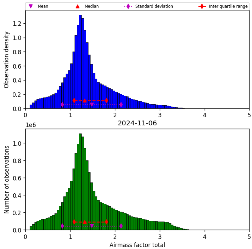
Figure 40: Histogram of “Airmass factor total” for 2024-11-05 to 2024-11-07
