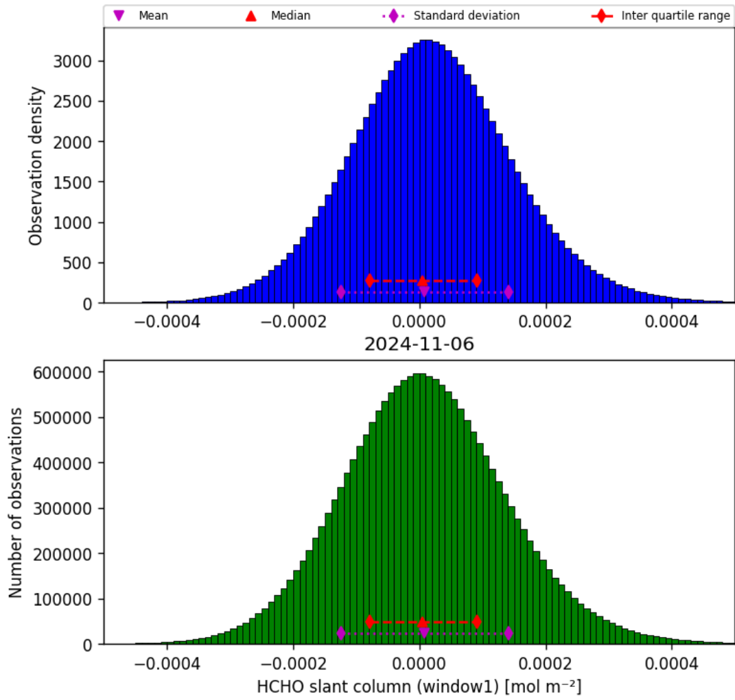
Figure 38: Histogram of “HCHO slant column (window1)” for 2024-11-05 to 2024-11-07
