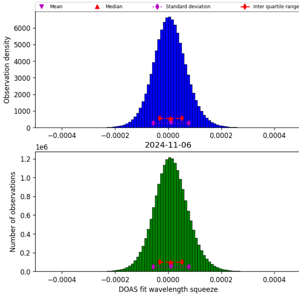
Figure 45: Histogram of “DOAS fit wavelength squeeze” for 2024-11-05 to 2024-11-07
