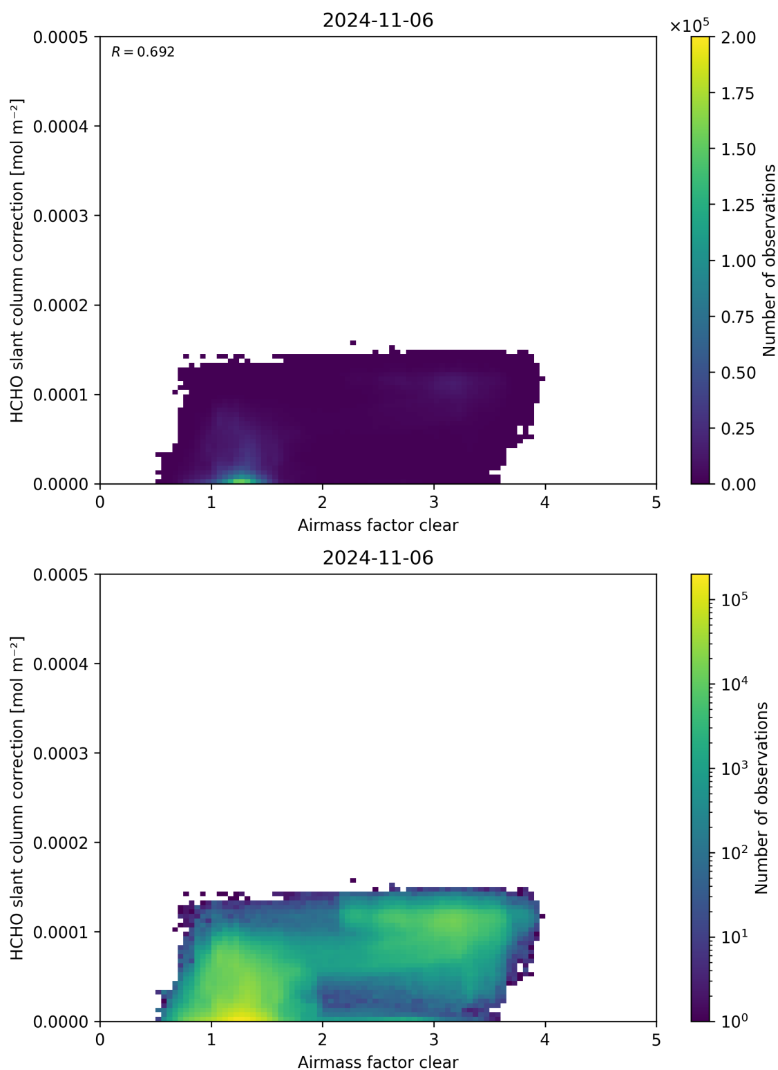
Figure 75: Scatter density plot of “Airmass factor clear” against “HCHO slant column correction” for 2024-11-05 to 2024-11-07.
