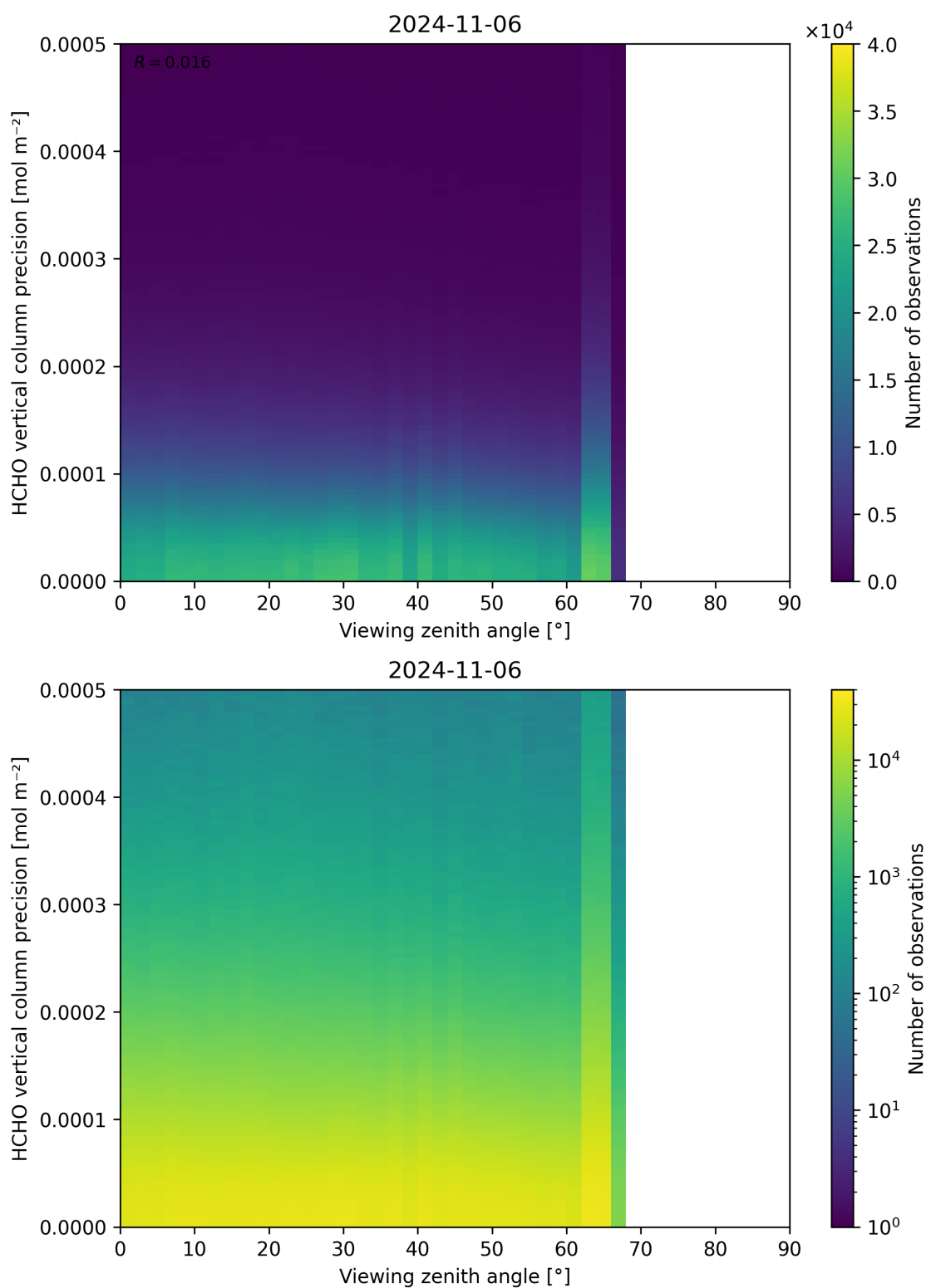
Figure 194: Scatter density plot of “Viewing zenith angle” against “HCHO vertical column precision” for 2024-11-05 to 2024-11-07.
