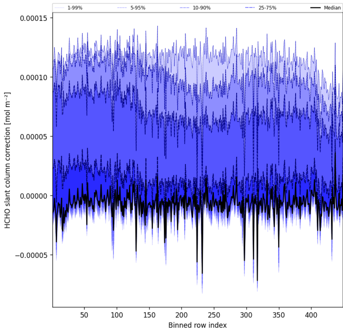
Figure 61: Along track statistics of “HCHO slant column correction” for 2024-11-05 to 2024-11-07
