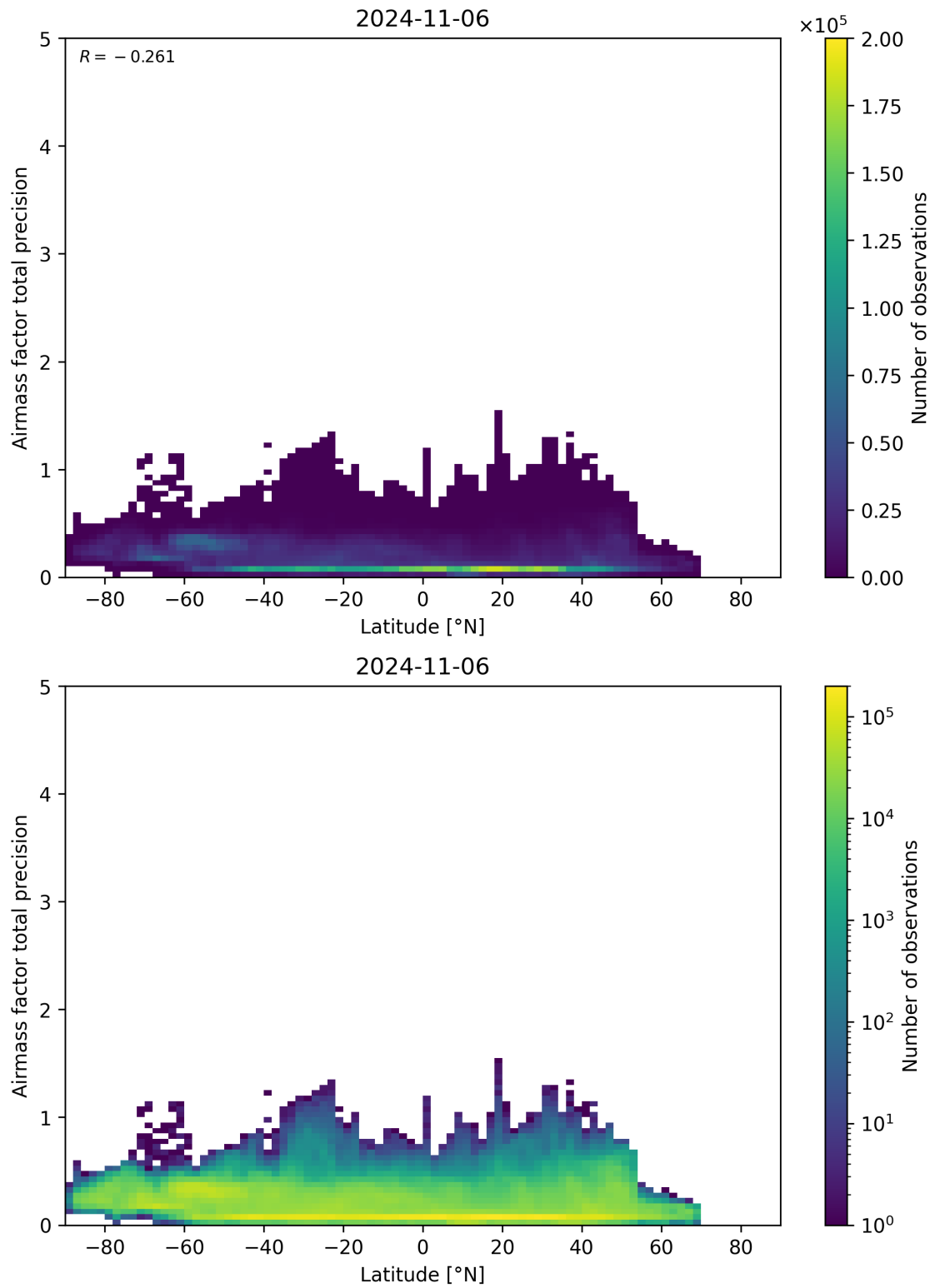
Figure 162: Scatter density plot of “Latitude” against “Airmass factor total precision” for 2024-11-05 to 2024-11-07.
