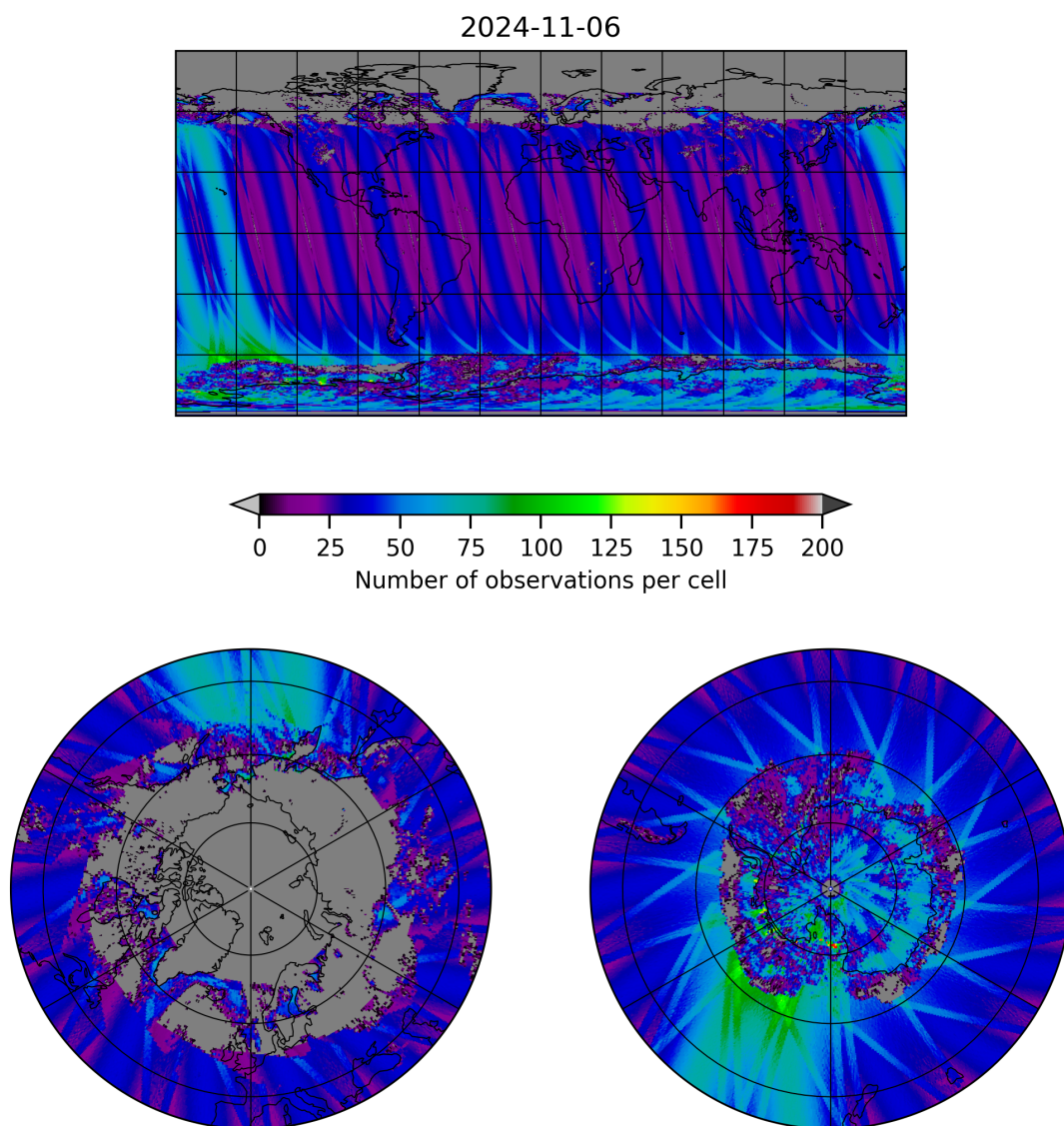
Figure 19: Map of the number of observations for 2024-11-05 to 2024-11-07
