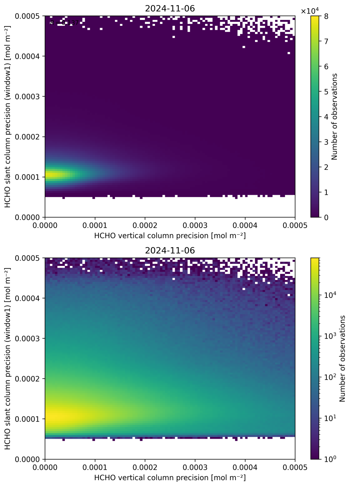
Figure 143: Scatter density plot of “HCHO vertical column precision” against “HCHO slant column precision (window1)” for 2024-11-05 to 2024-11-07.
