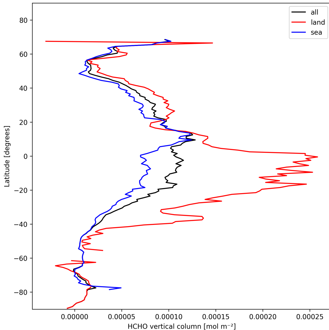
Figure 21: Zonal average of “HCHO vertical column” for 2024-11-05 to 2024-11-07.
