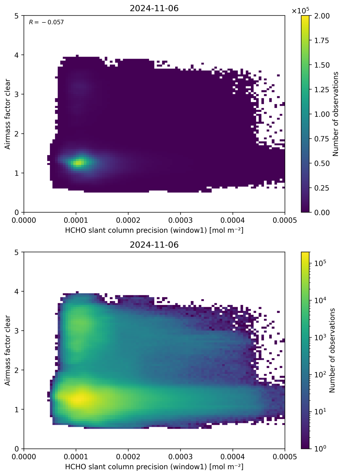
Figure 91: Scatter density plot of “HCHO slant column precision (window1)” against “Airmass factor clear” for 2024-11-05 to 2024-11-07.
