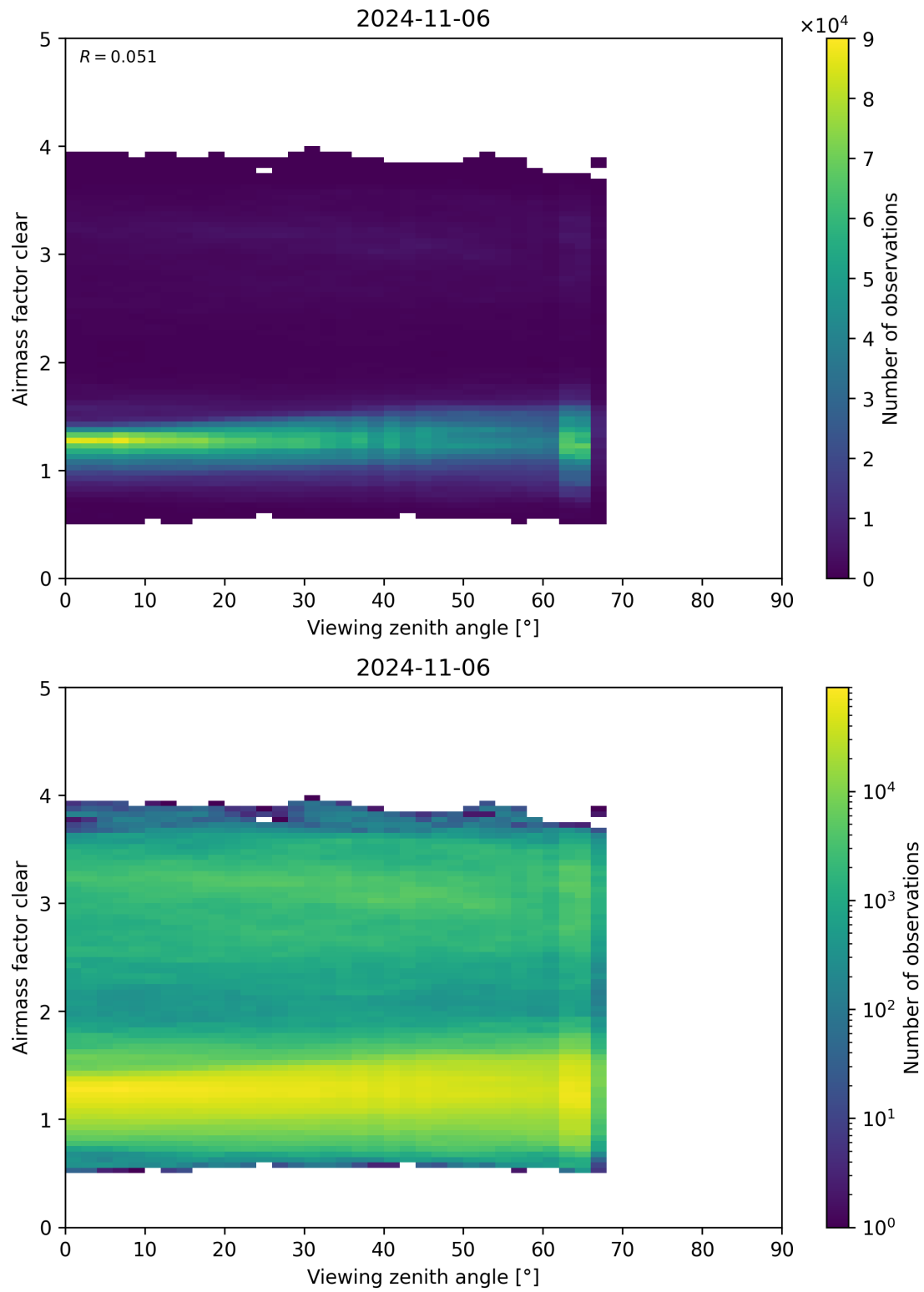
Figure 185: Scatter density plot of “Viewing zenith angle” against “Airmass factor clear” for 2024-11-05 to 2024-11-07.
