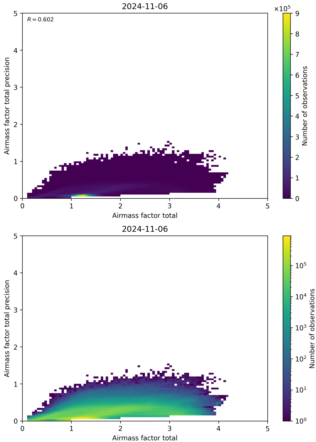
Figure 103: Scatter density plot of “Airmass factor total” against “Airmass factor total precision” for 2024-11-05 to 2024-11-07.
