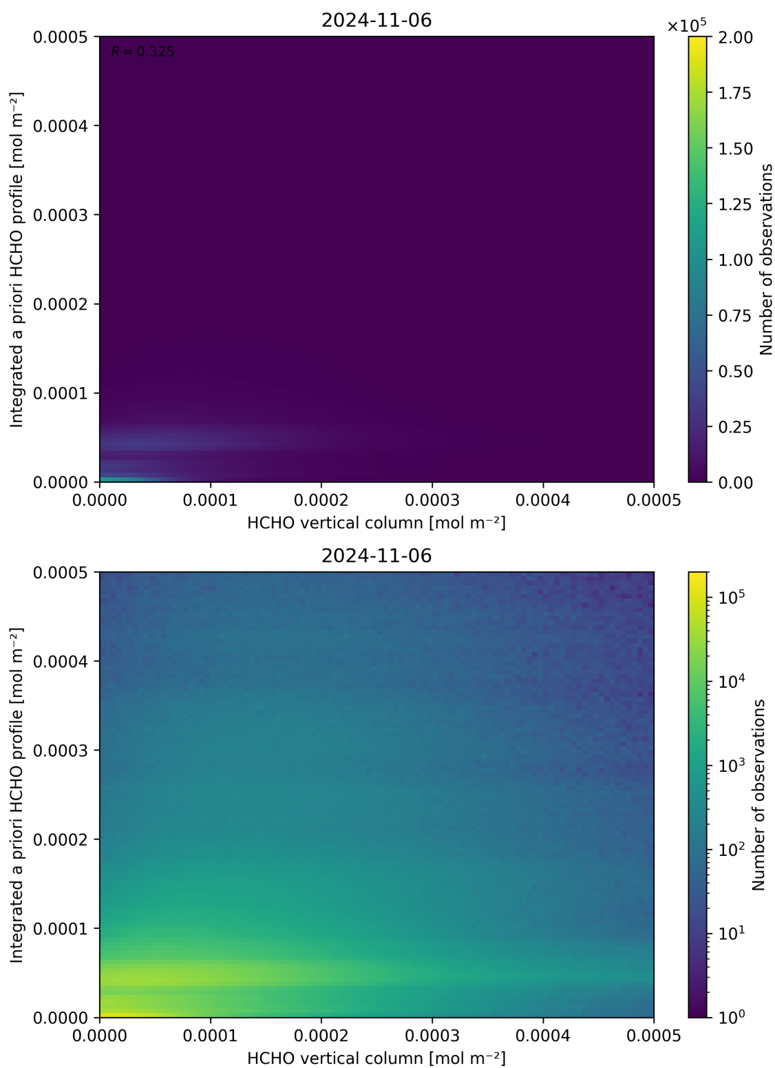
Figure 135: Scatter density plot of “HCHO vertical column” against “Integrated a priori HCHO profile” for 2024-11-05 to 2024-11-07.
