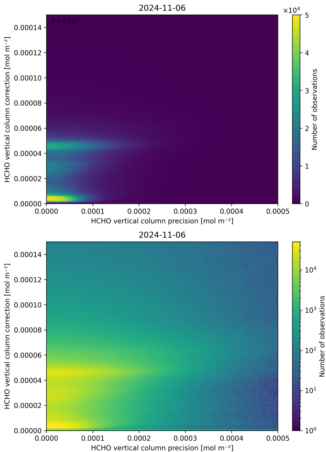
Figure 146: Scatter density plot of “HCHO vertical column precision” against “HCHO vertical column correction” for 2024-11-05 to 2024-11-07.
