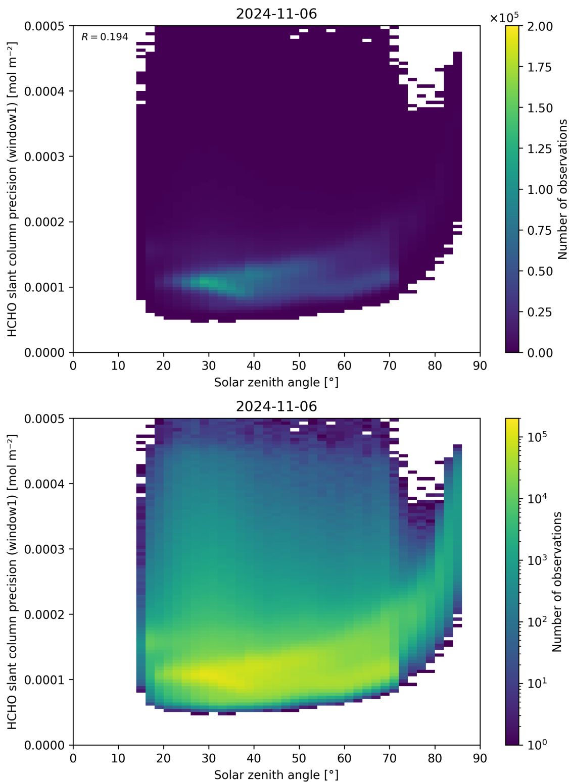
Figure 174: Scatter density plot of “Solar zenith angle” against “HCHO slant column precision (window1)” for 2024-11-05 to 2024-11-07.
