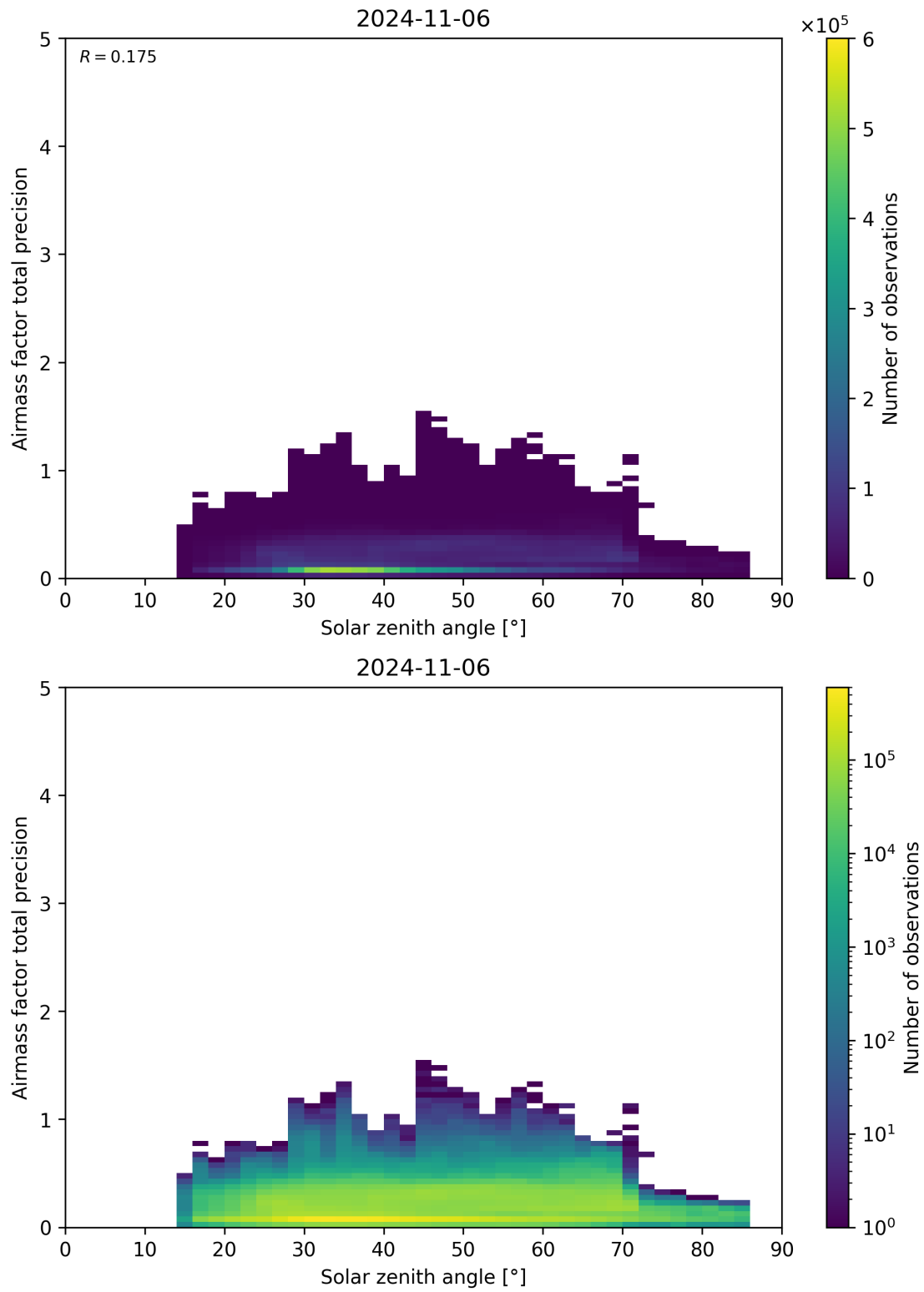
Figure 176: Scatter density plot of “Solar zenith angle” against “Airmass factor total precision” for 2024-11-05 to 2024-11-07.
