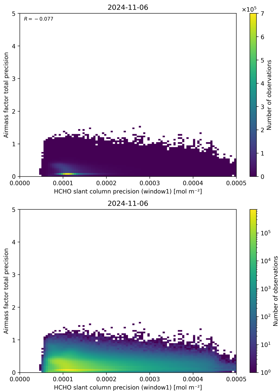
Figure 95: Scatter density plot of “HCHO slant column precision (window1)” against “Airmass factor total precision” for 2024-11-05 to 2024-11-07.
