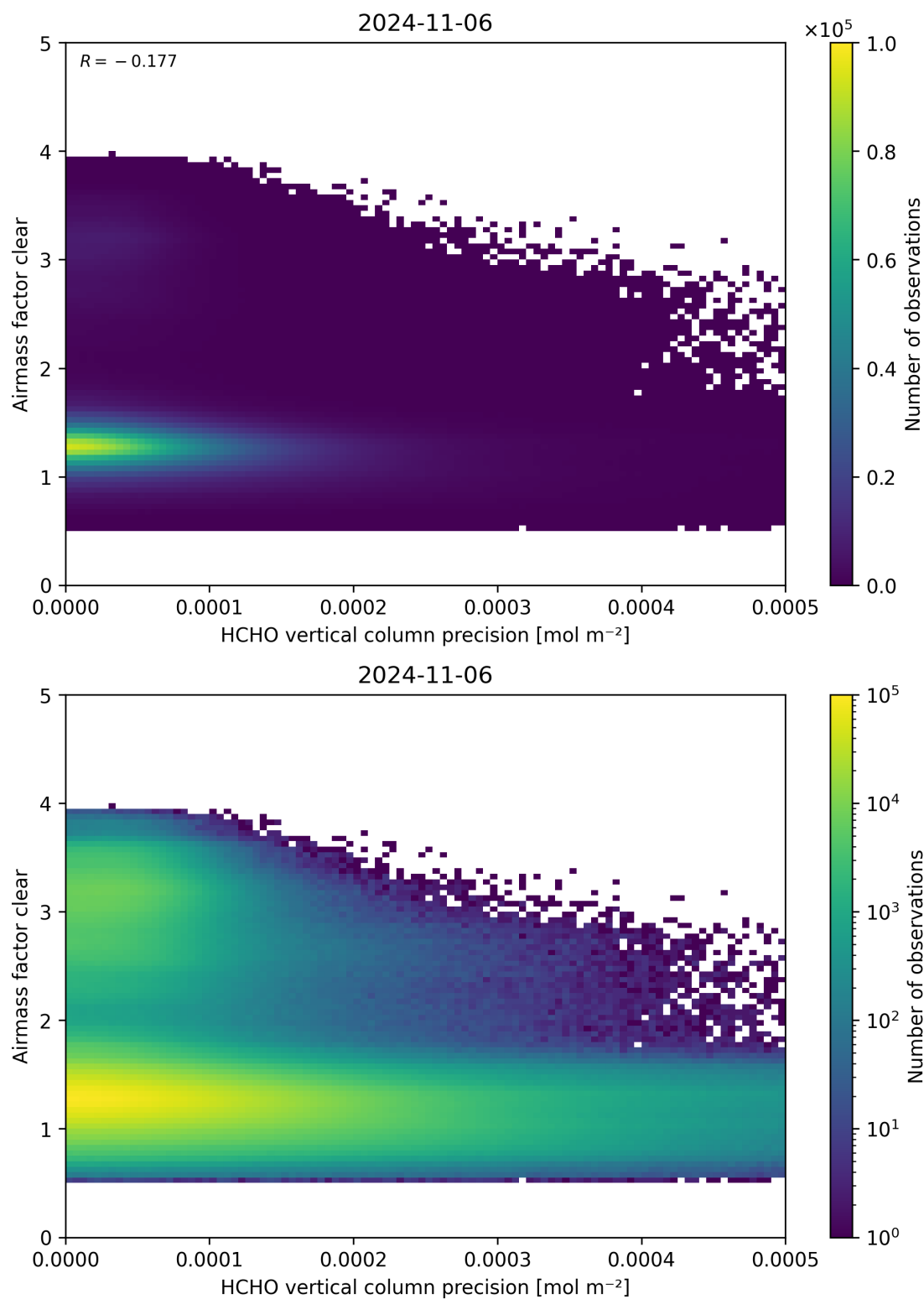
Figure 139: Scatter density plot of “HCHO vertical column precision” against “Airmass factor clear” for 2024-11-05 to 2024-11-07.
