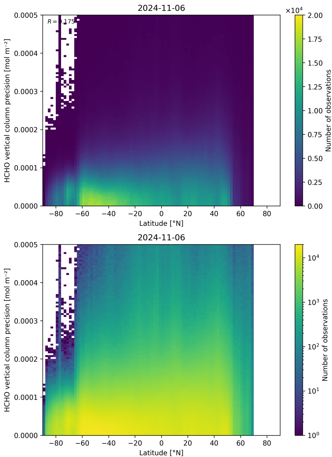
Figure 165: Scatter density plot of “Latitude” against “HCHO vertical column precision” for 2024-11-05 to 2024-11-07.
