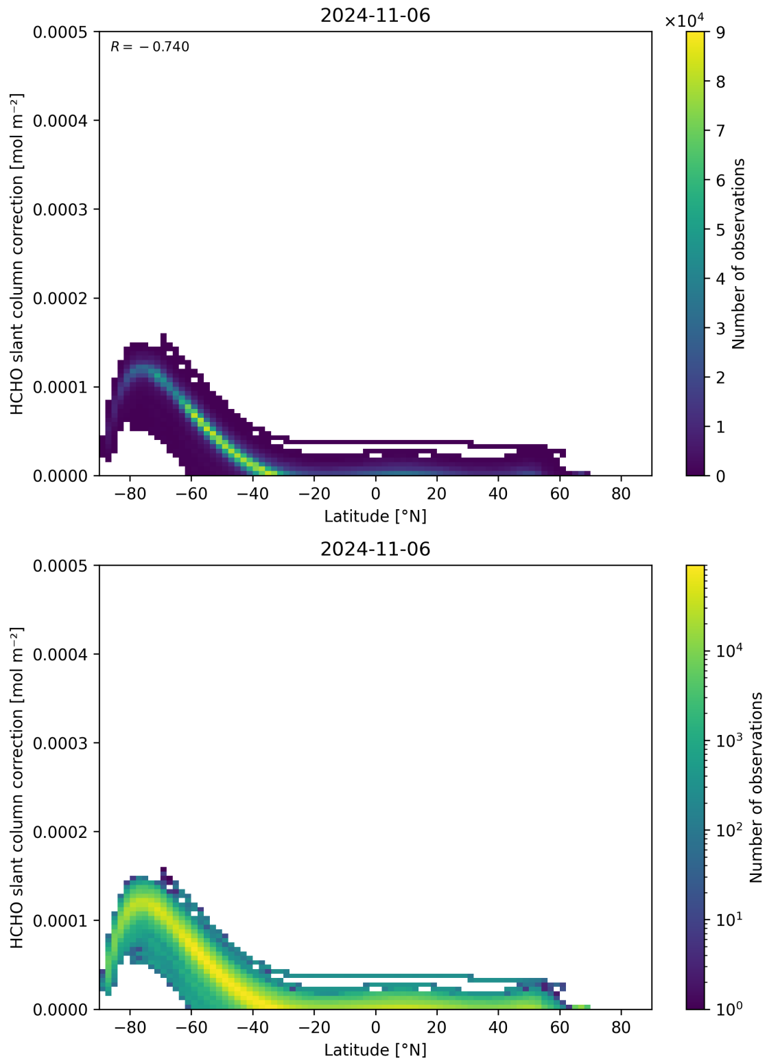
Figure 158: Scatter density plot of “Latitude” against “HCHO slant column correction” for 2024-11-05 to 2024-11-07.
