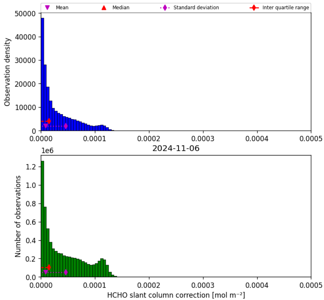
Figure 47: Histogram of "HCHO slant column correction" for 2024-11-05 to 2024-11-07
