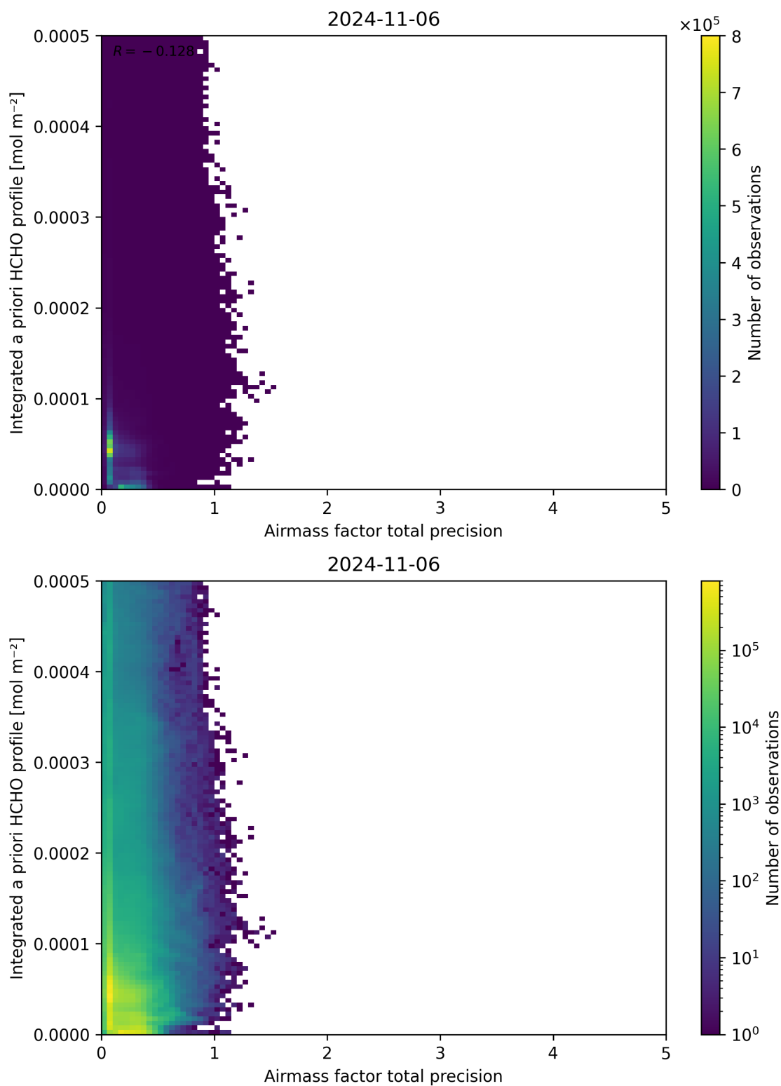
Figure 111: Scatter density plot of “Airmass factor total precision” against “Integrated a priori HCHO profile” for 2024-11-05 to 2024-11-07.
