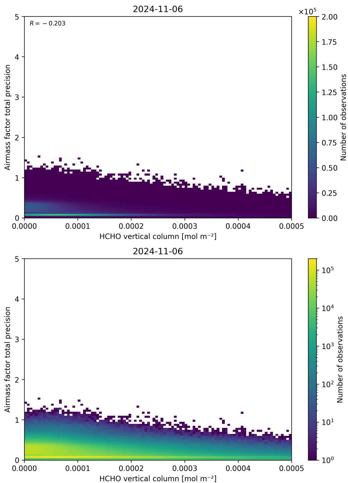
Figure 132: Scatter density plot of “HCHO vertical column” against “Airmass factor total precision” for 2024-11-05 to 2024-11-07.
