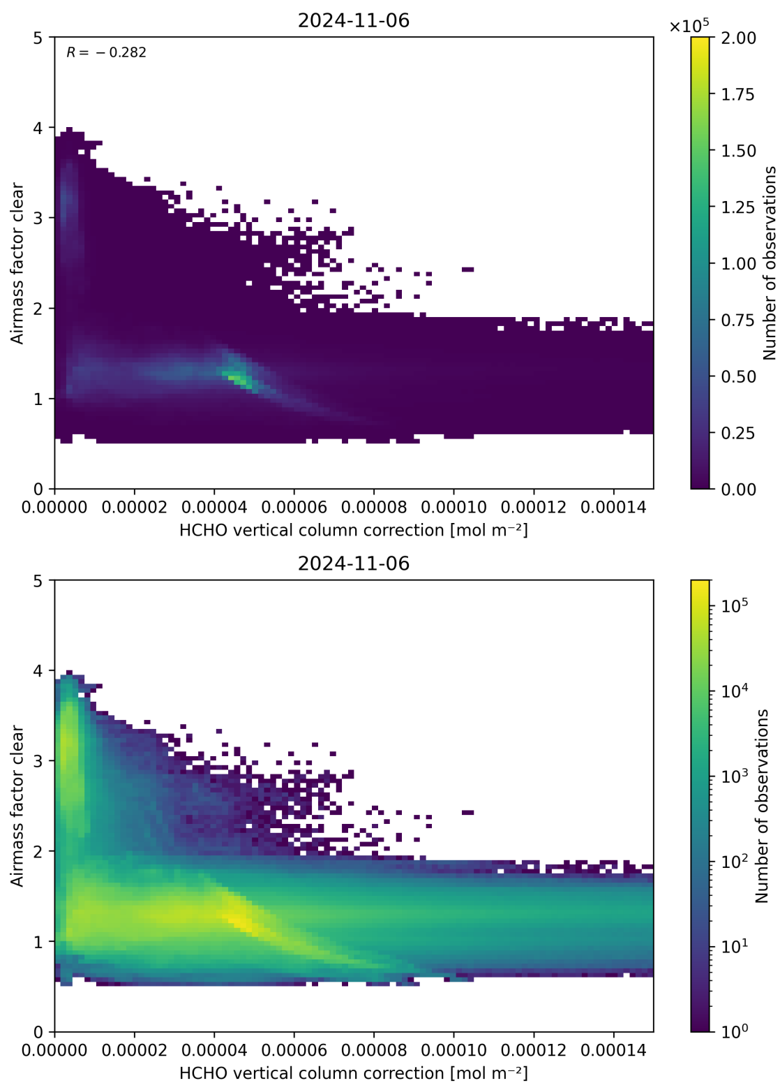
Figure 115: Scatter density plot of “HCHO vertical column correction” against “Airmass factor clear” for 2024-11-05 to 2024-11-07.
