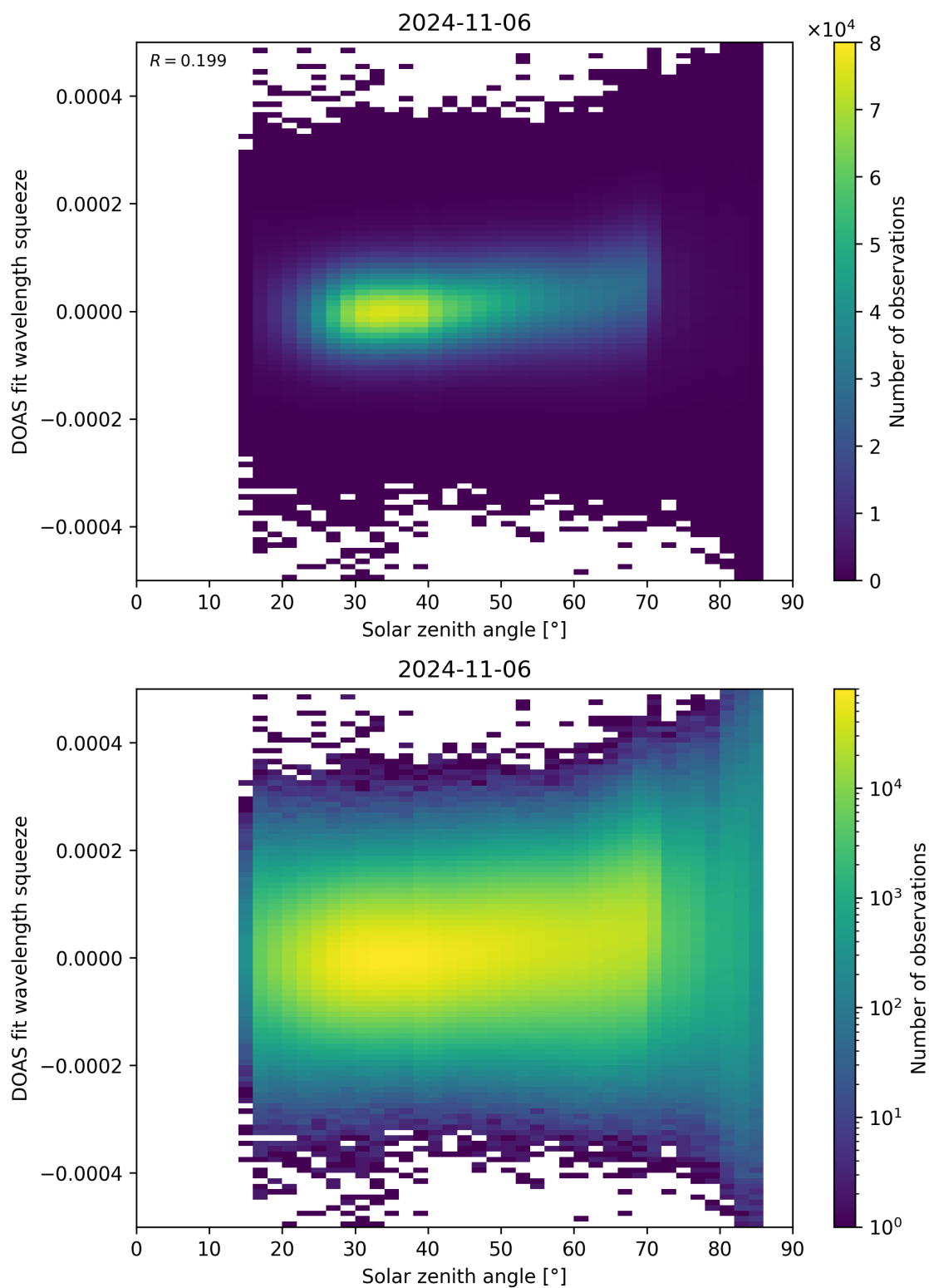
Figure 169: Scatter density plot of “Solar zenith angle” against “DOAS fit wavelength squeeze” for 2024-11-05 to 2024-11-07.
