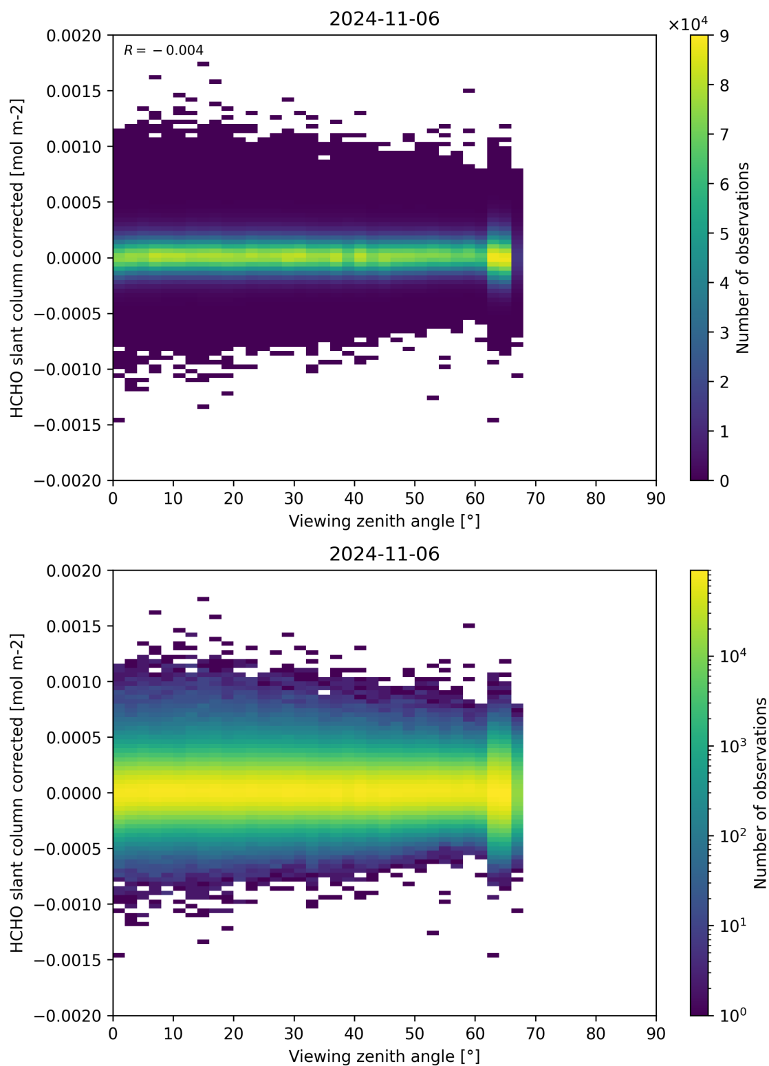
Figure 186: Scatter density plot of “Viewing zenith angle” against “HCHO slant column corrected” for 2024-11-05 to 2024-11-07.
