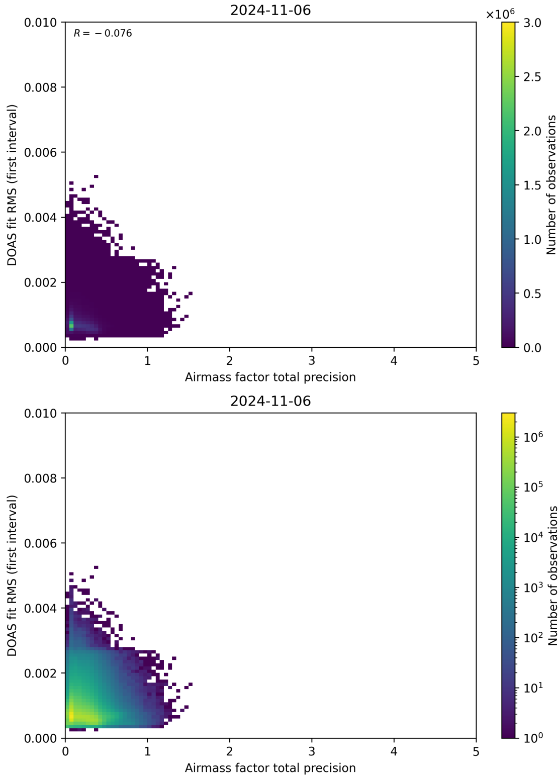
Figure 105: Scatter density plot of “Airmass factor total precision” against “DOAS fit RMS (first interval)” for 2024-11-05 to 2024-11-07.
