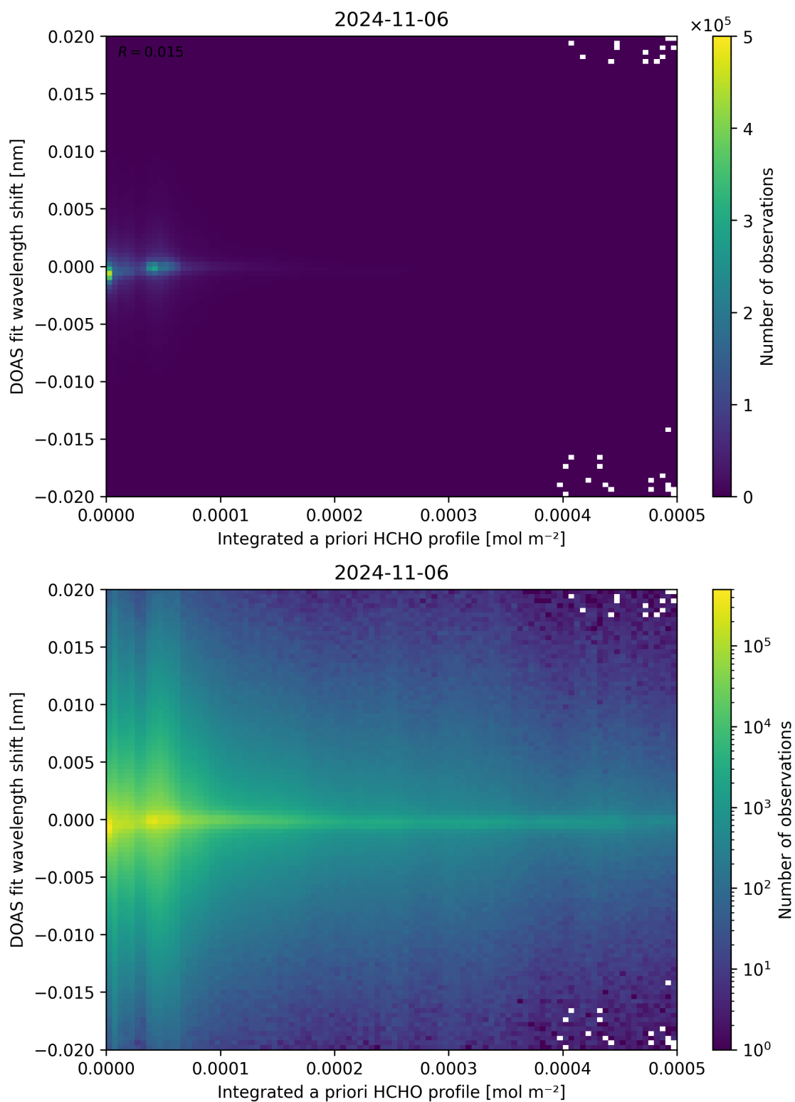
Figure 149: Scatter density plot of “Integrated a priori HCHO profile” against “DOAS fit wavelength shift” for 2024-11-05 to 2024-11-07.
