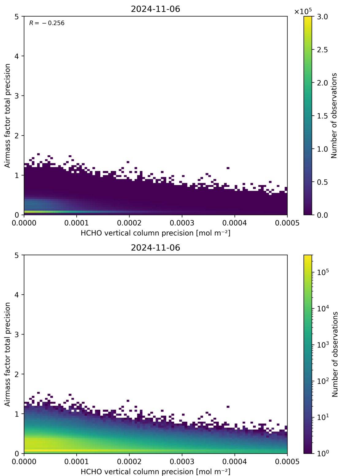
Figure 145: Scatter density plot of “HCHO vertical column precision” against “Airmass factor total precision” for 2024-11-05 to 2024-11-07.
