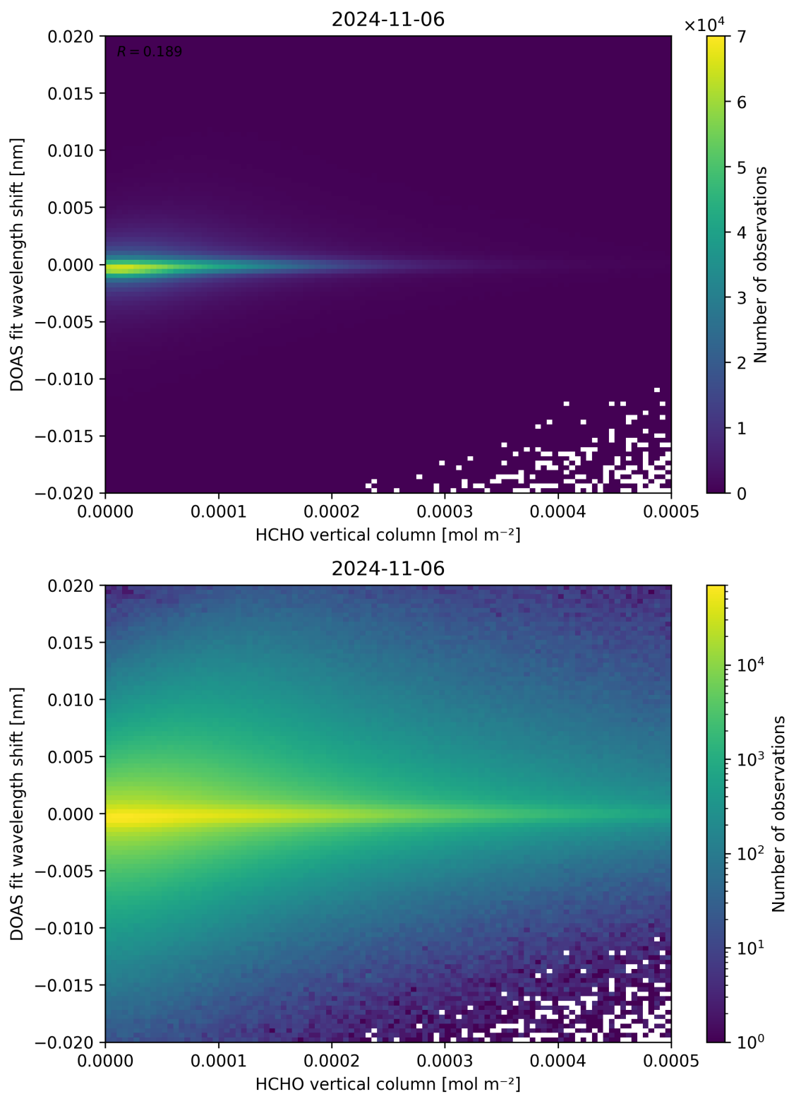
Figure 124: Scatter density plot of “HCHO vertical column” against “DOAS fit wavelength shift” for 2024-11-05 to 2024-11-07.
