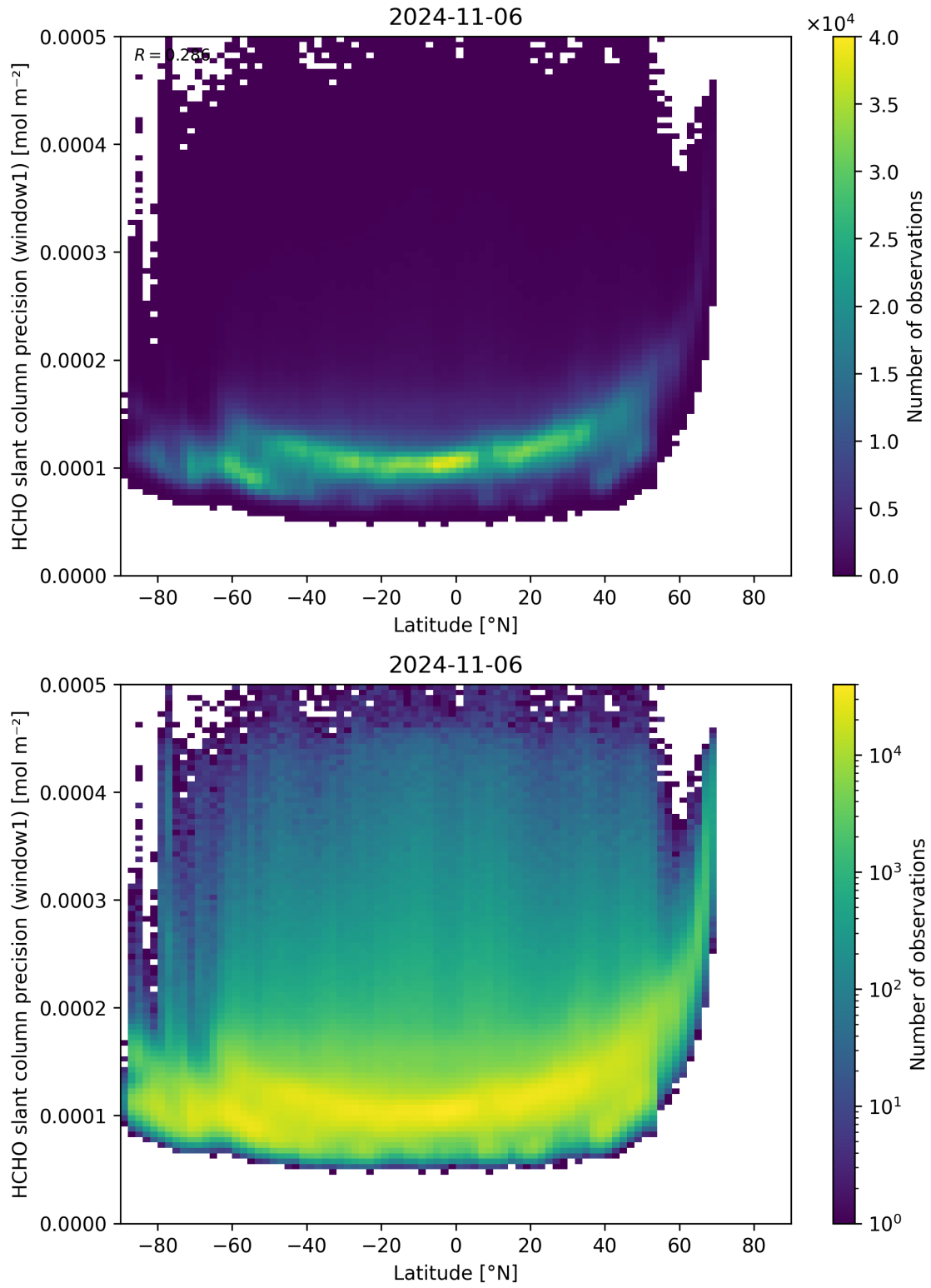
Figure 160: Scatter density plot of “Latitude” against “HCHO slant column precision (window1)” for 2024-11-05 to 2024-11-07.
