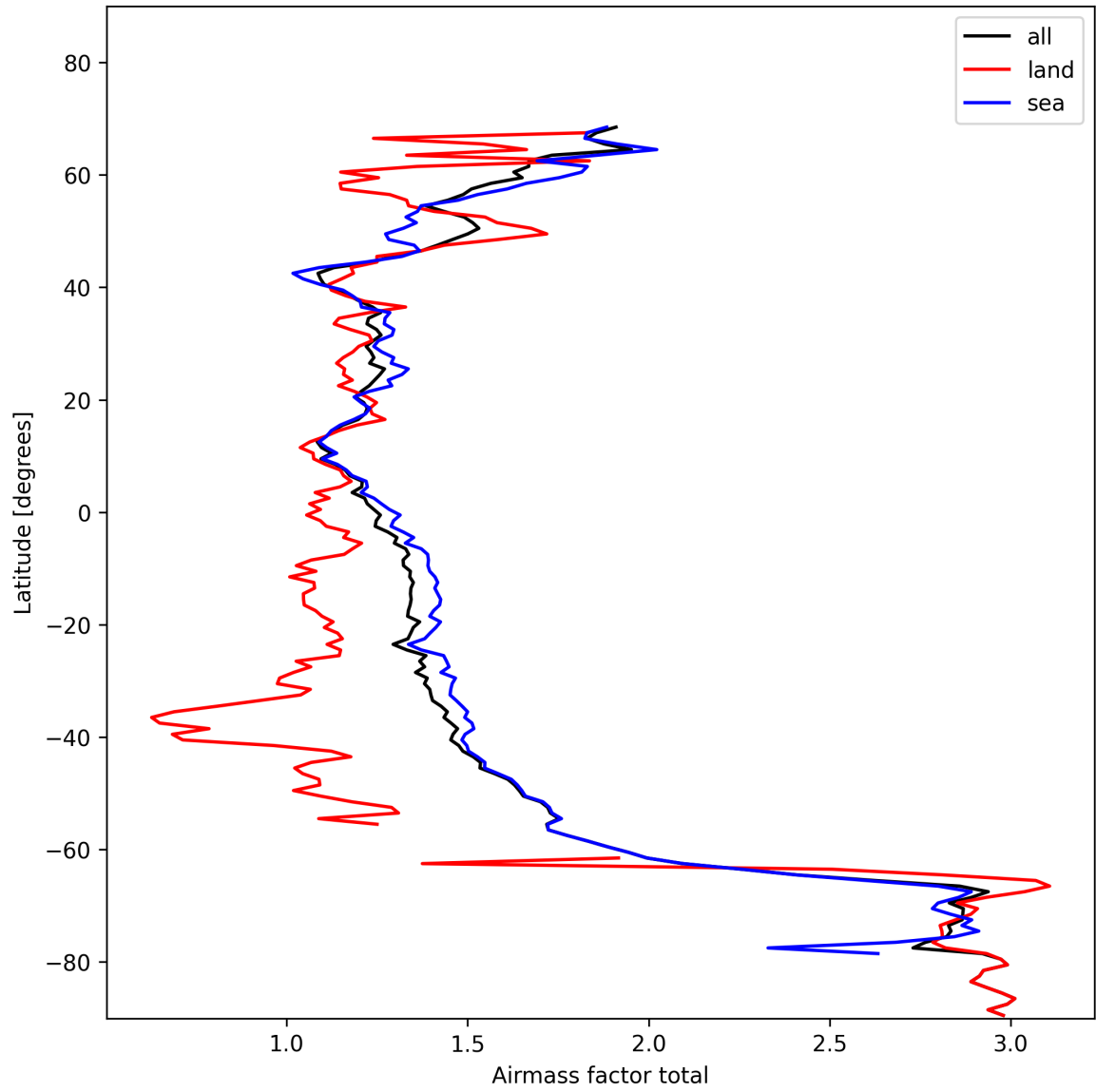
Figure 26: Zonal average of “Airmass factor total” for 2024-11-05 to 2024-11-07.
