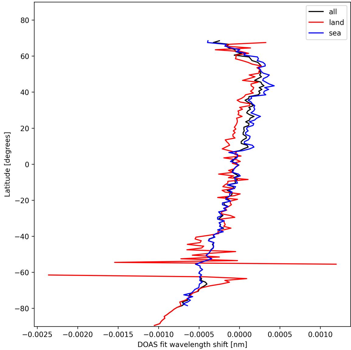
Figure 30: Zonal average of "DOAS fit wavelength shift" for 2024-11-05 to 2024-11-07.
