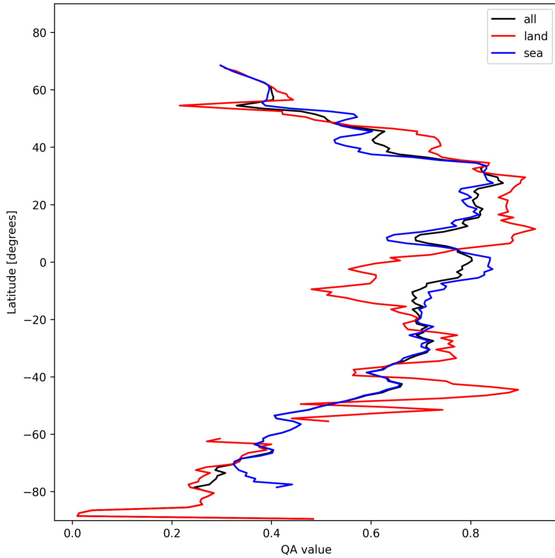
Figure 20: Zonal average of “QA value” for 2024-11-05 to 2024-11-07.
