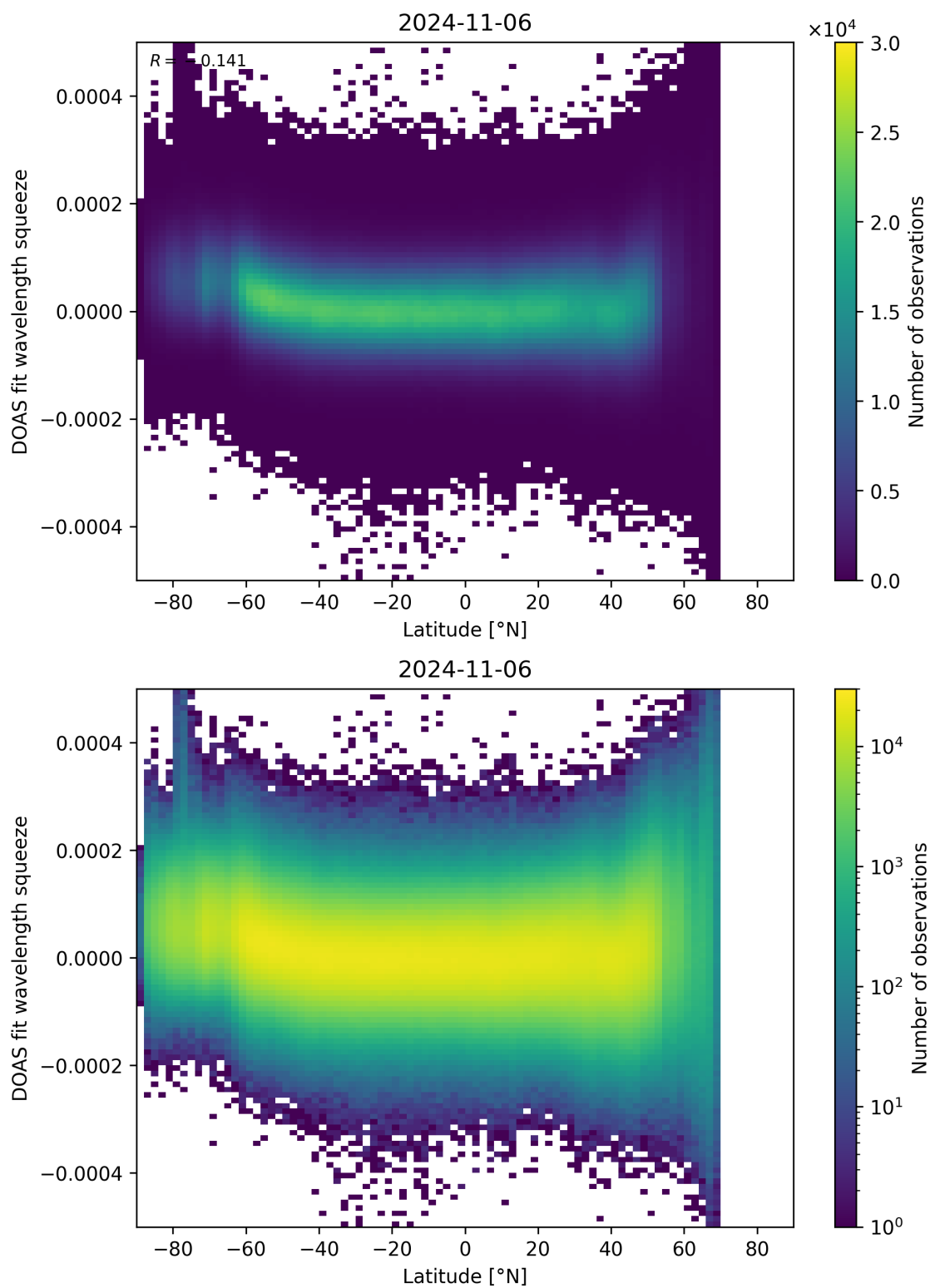
Figure 155: Scatter density plot of “Latitude” against “DOAS fit wavelength squeeze” for 2024-11-05 to 2024-11-07.
