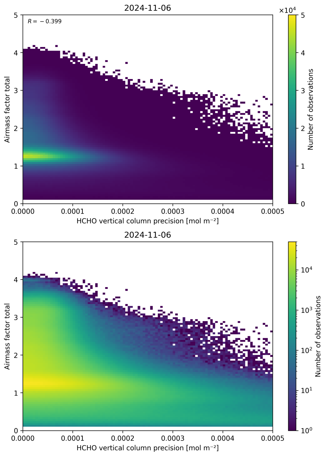
Figure 144: Scatter density plot of “HCHO vertical column precision” against “Airmass factor total” for 2024-11-05 to 2024-11-07.
