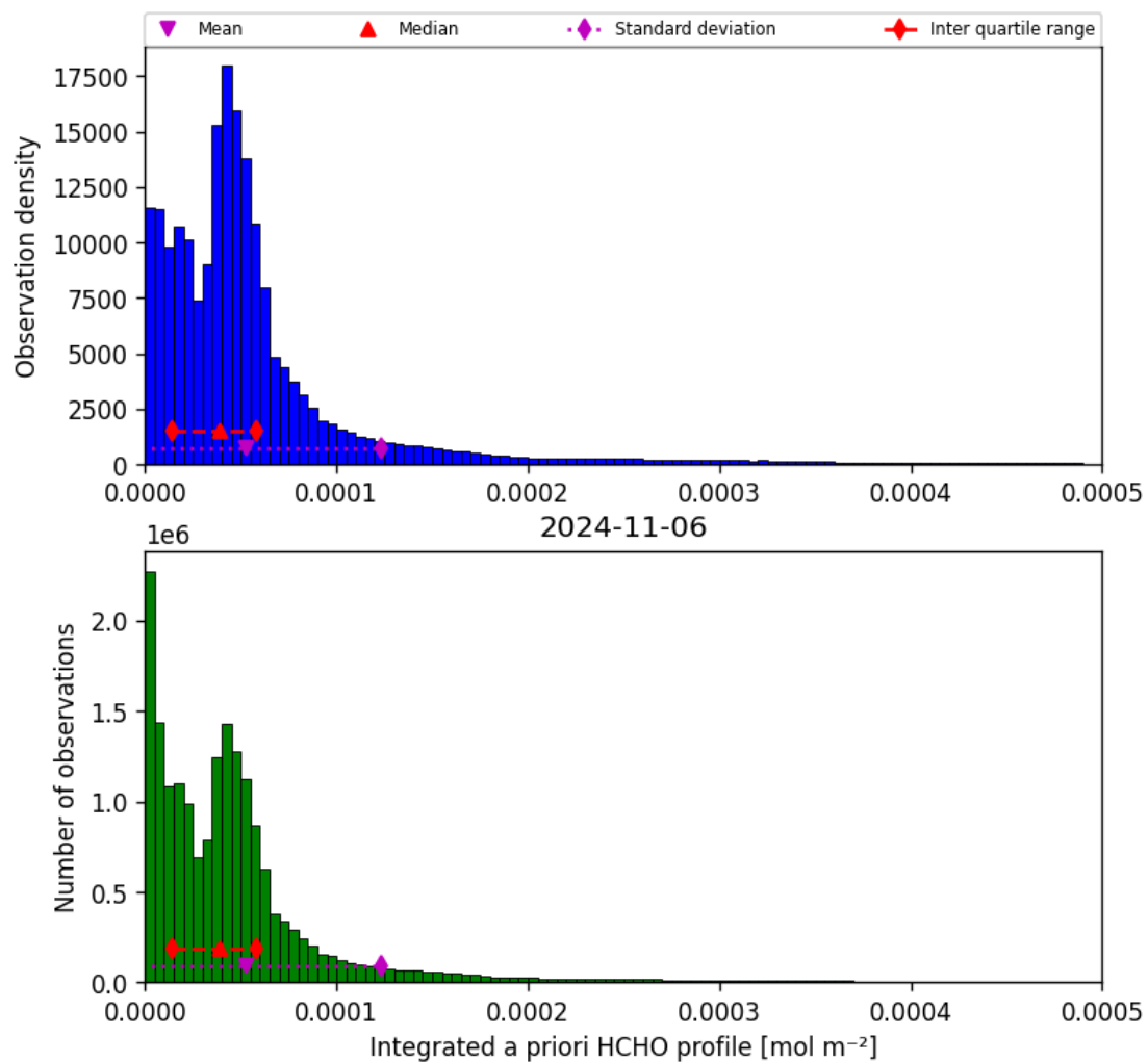
Figure 43: Histogram of “Integrated a priori HCHO profile” for 2024-11-05 to 2024-11-07
