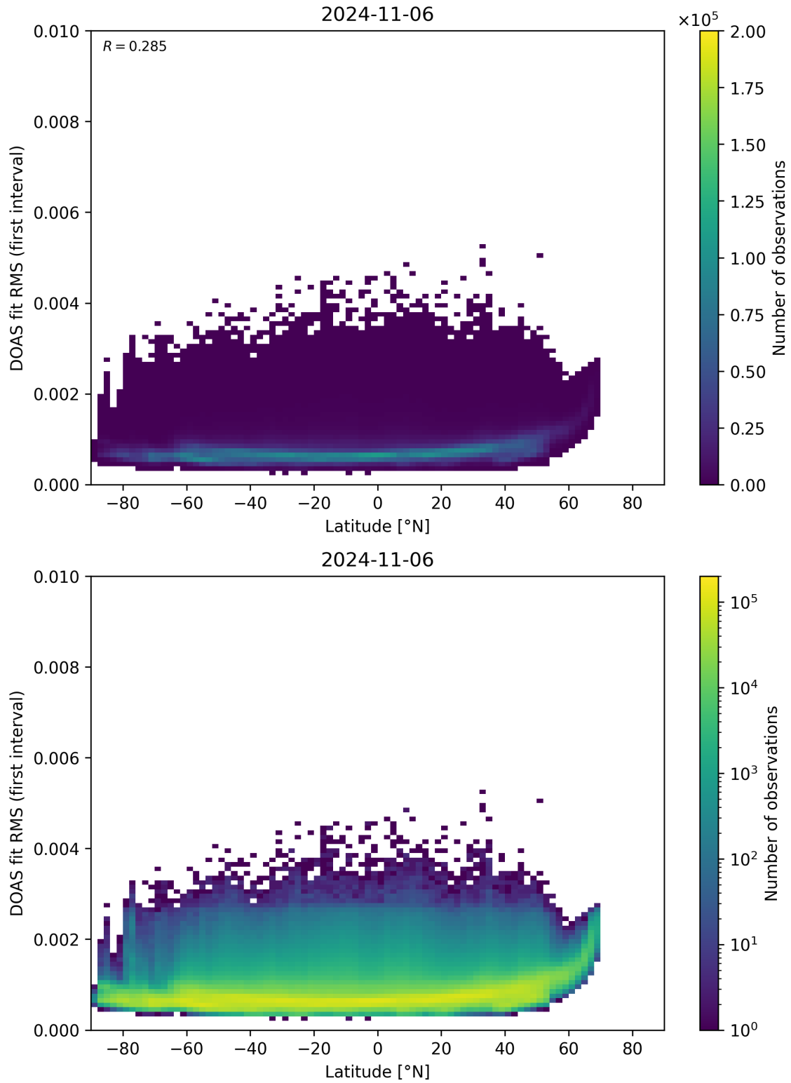
Figure 153: Scatter density plot of “Latitude” against “DOAS fit RMS (first interval)” for 2024-11-05 to 2024-11-07.
