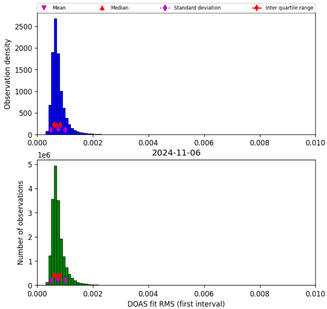
Figure 46: Histogram of “DOAS fit RMS (first interval)” for 2024-11-05 to 2024-11-07
