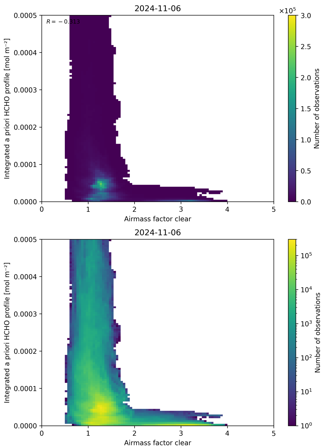
Figure 76: Scatter density plot of “Airmass factor clear” against “Integrated a priori HCHO profile” for 2024-11-05 to 2024-11-07.
