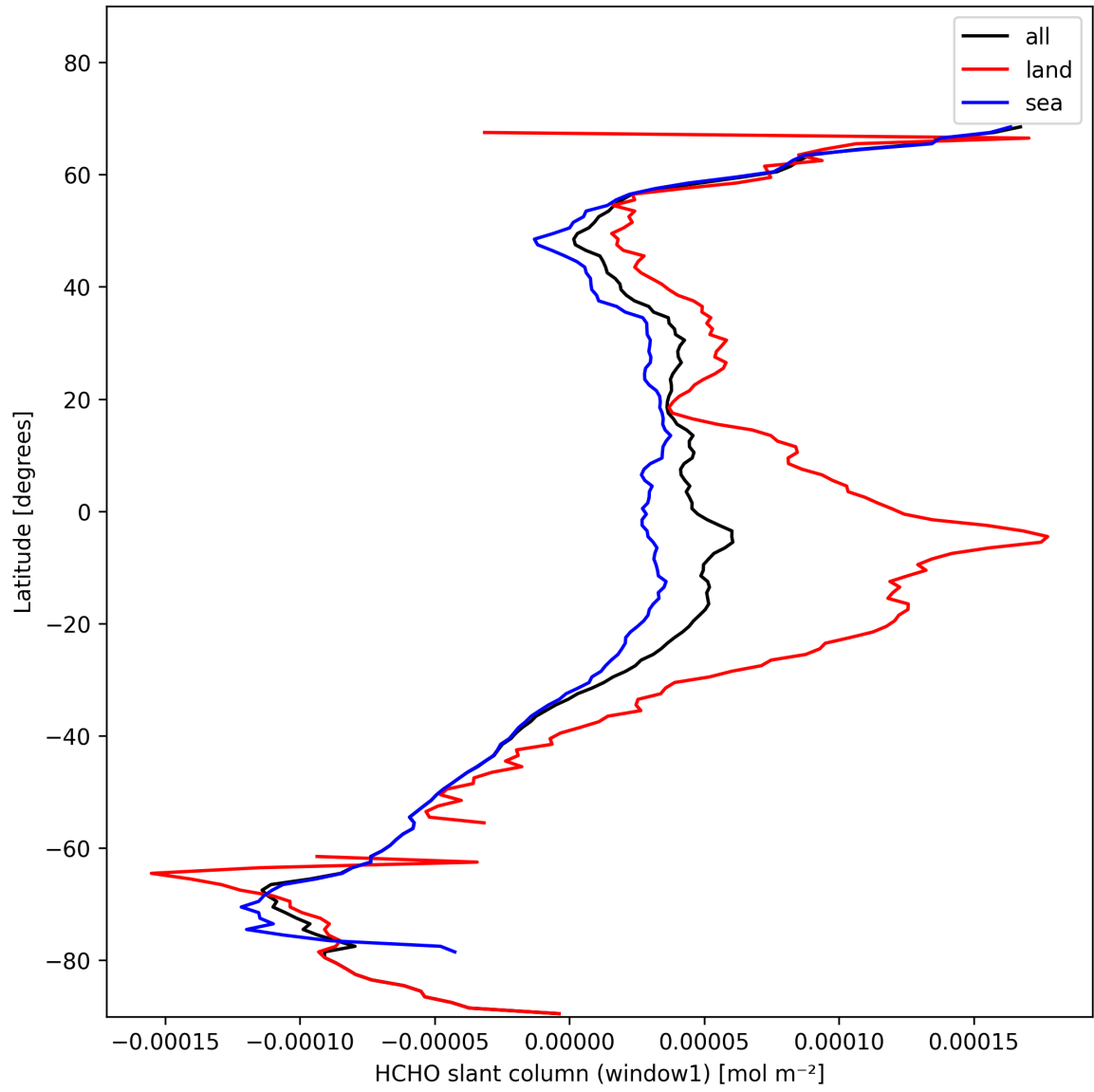
Figure 24: Zonal average of “HCHO slant column (window1)” for 2024-11-05 to 2024-11-07.
