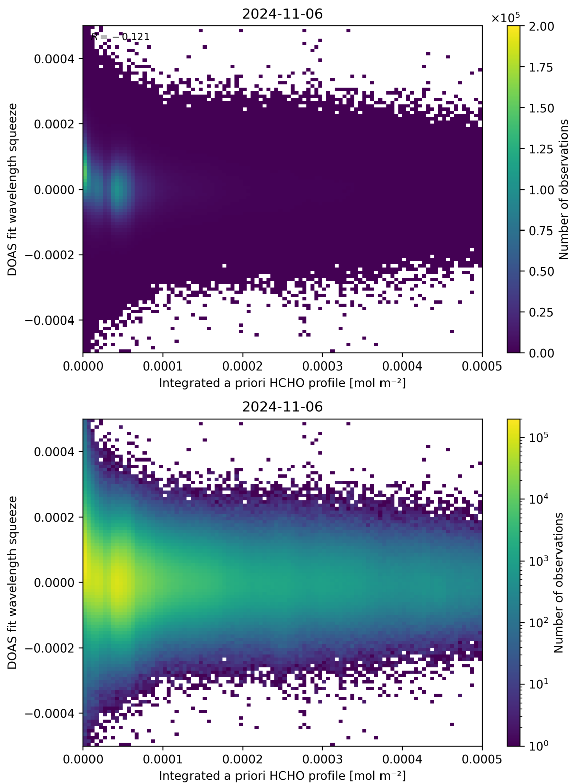
Figure 150: Scatter density plot of “Integrated a priori HCHO profile” against “DOAS fit wavelength squeeze” for 2024-11-05 to 2024-11-07.
