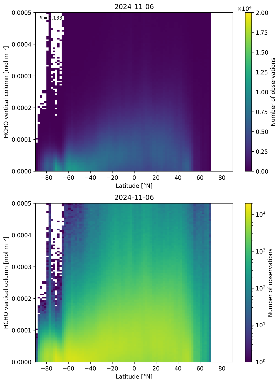
Figure 163: Scatter density plot of “Latitude” against “HCHO vertical column” for 2024-11-05 to 2024-11-07.
