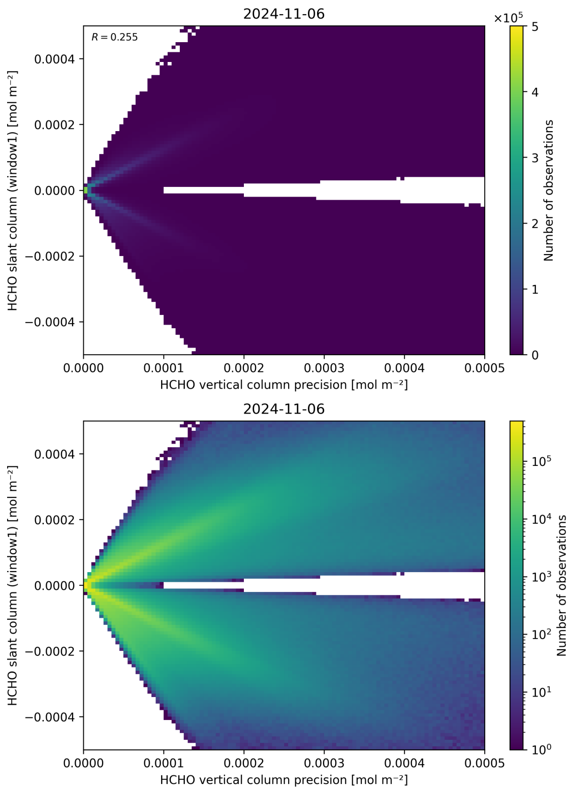
Figure 142: Scatter density plot of “HCHO vertical column precision” against “HCHO slant column (window1)” for 2024-11-05 to 2024-11-07.
