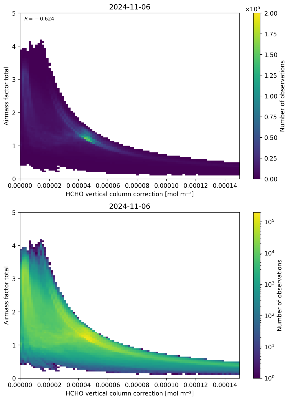
Figure 120: Scatter density plot of “HCHO vertical column correction” against “Airmass factor total” for 2024-11-05 to 2024-11-07.
