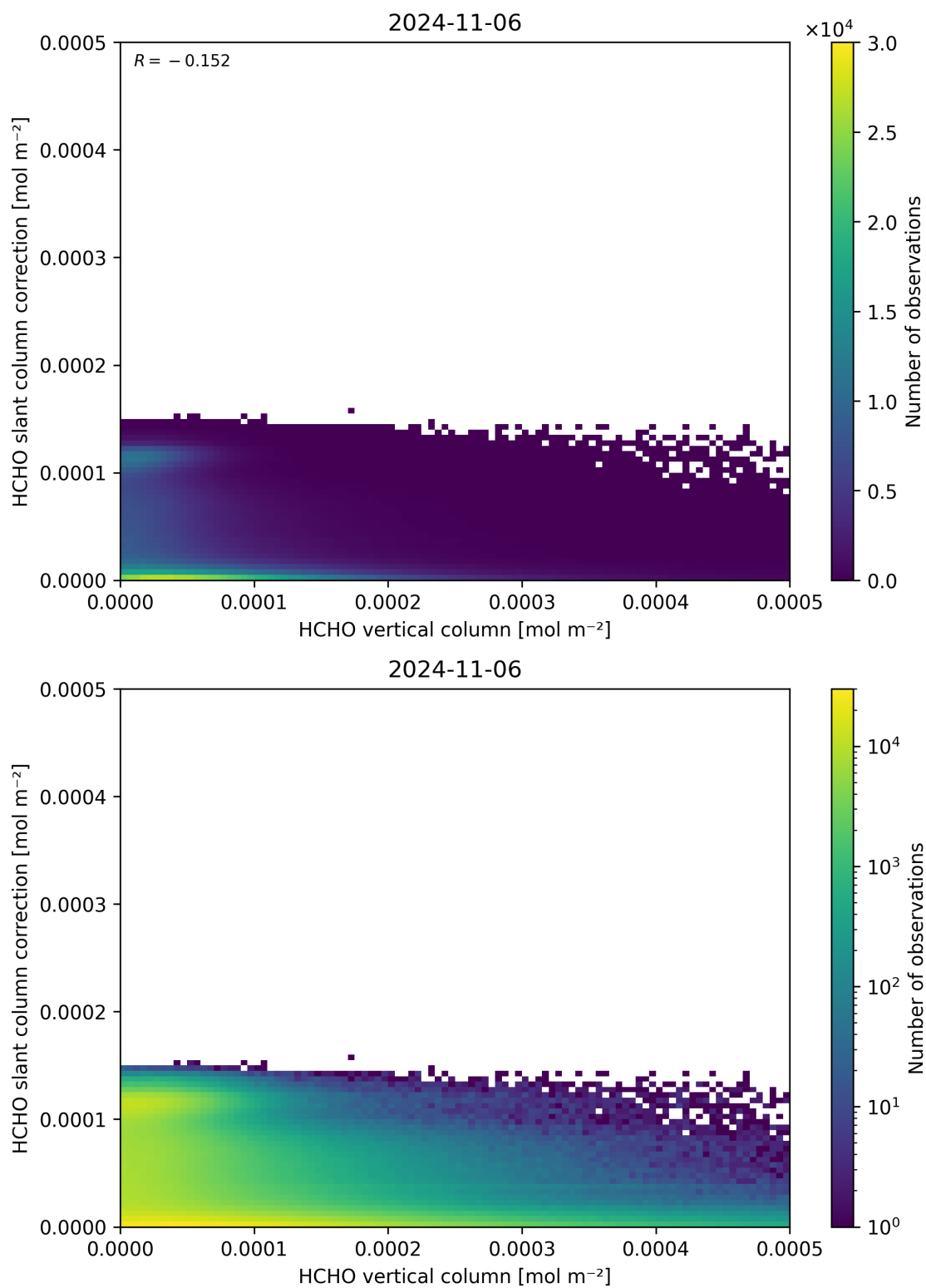
Figure 128: Scatter density plot of “HCHO vertical column” against “HCHO slant column correction” for 2024-11-05 to 2024-11-07.
