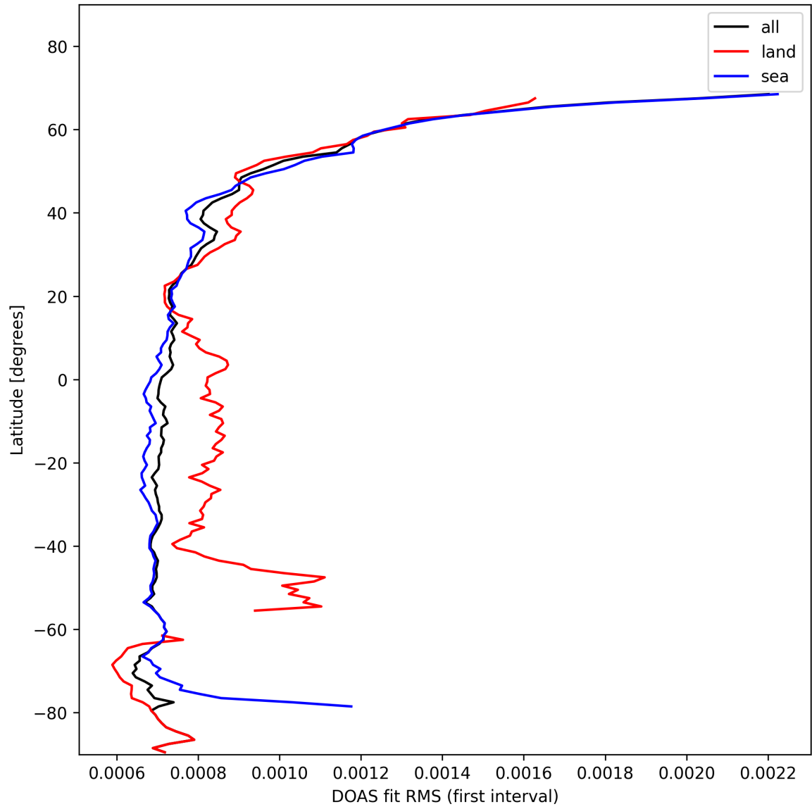
Figure 32: Zonal average of “DOAS fit RMS (first interval)” for 2024-11-05 to 2024-11-07.
