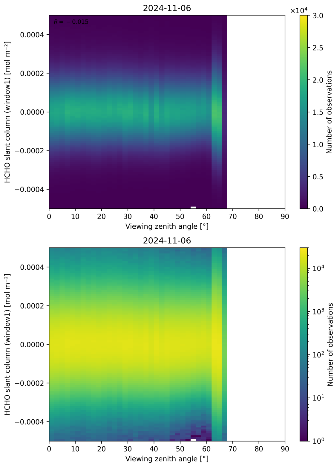
Figure 188: Scatter density plot of “Viewing zenith angle” against “HCHO slant column (window1)” for 2024-11-05 to 2024-11-07.
