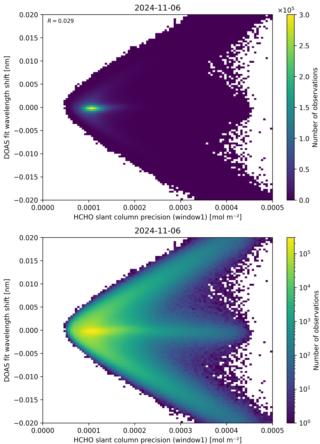
Figure 89: Scatter density plot of “HCHO slant column precision (window1)” against “DOAS fit wavelength shift” for 2024-11-05 to 2024-11-07.
