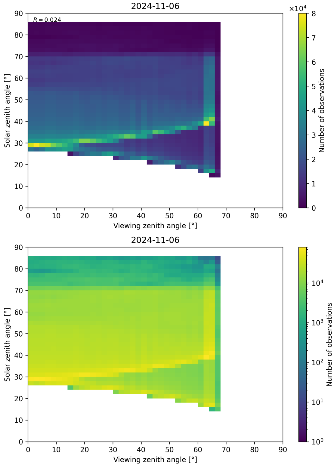
Figure 197: Scatter density plot of “Viewing zenith angle” against “Solar zenith angle” for 2024-11-05 to 2024-11-07.
