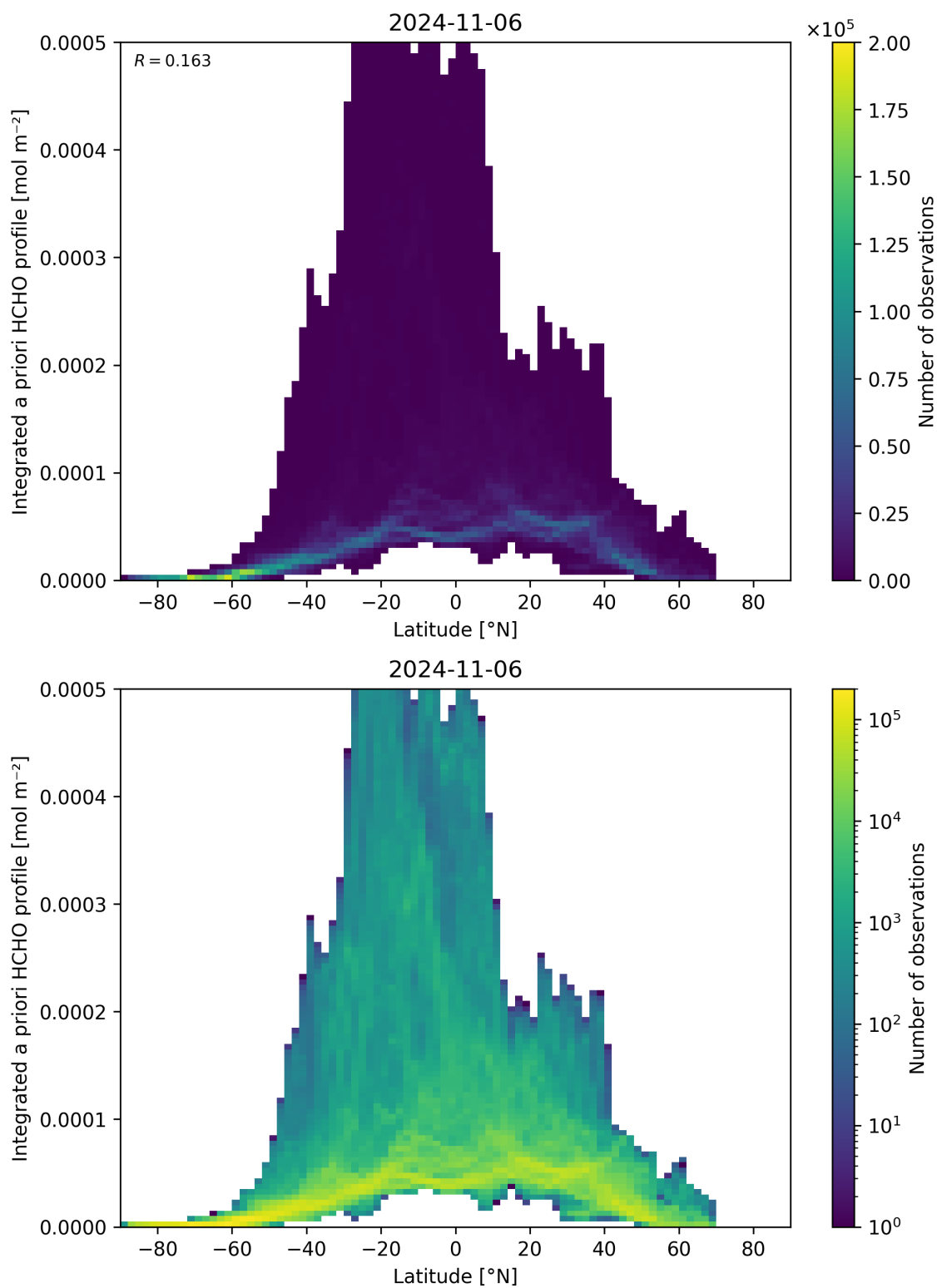
Figure 166: Scatter density plot of “Latitude” against “Integrated a priori HCHO profile” for 2024-11-05 to 2024-11-07.
