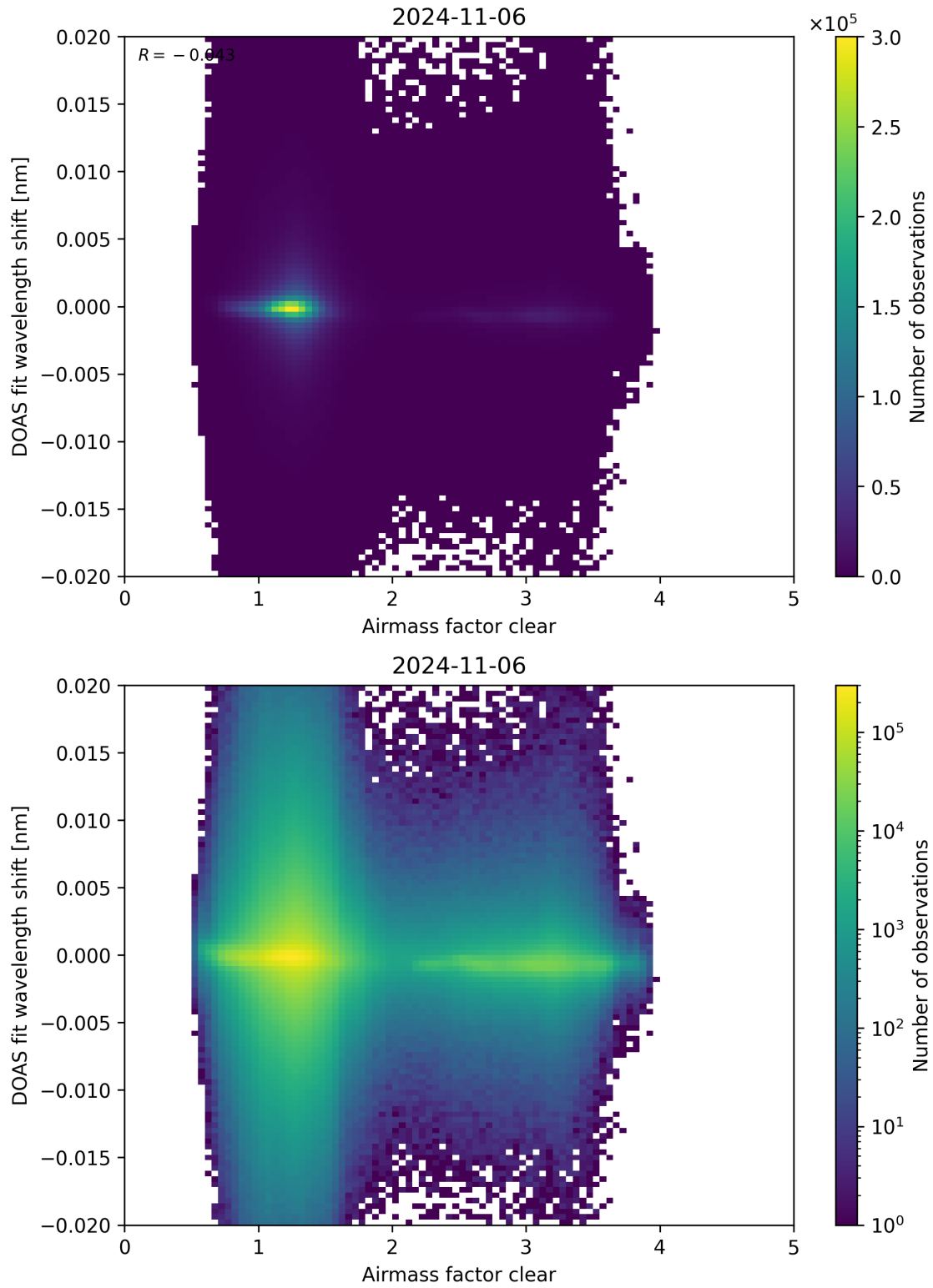
Figure 72: Scatter density plot of “Airmass factor clear” against “DOAS fit wavelength shift” for 2024-11-05 to 2024-11-07.
