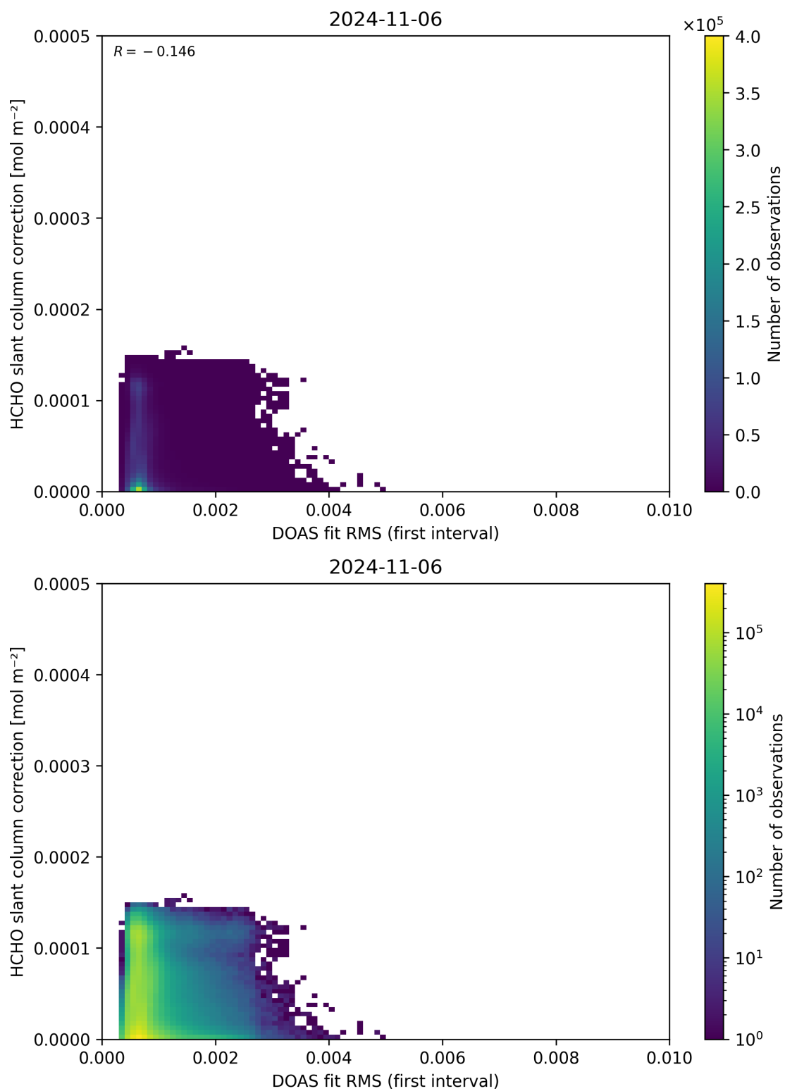
Figure 63: Scatter density plot of “DOAS fit RMS (first interval)” against “HCHO slant column correction” for 2024-11-05 to 2024-11-07.
