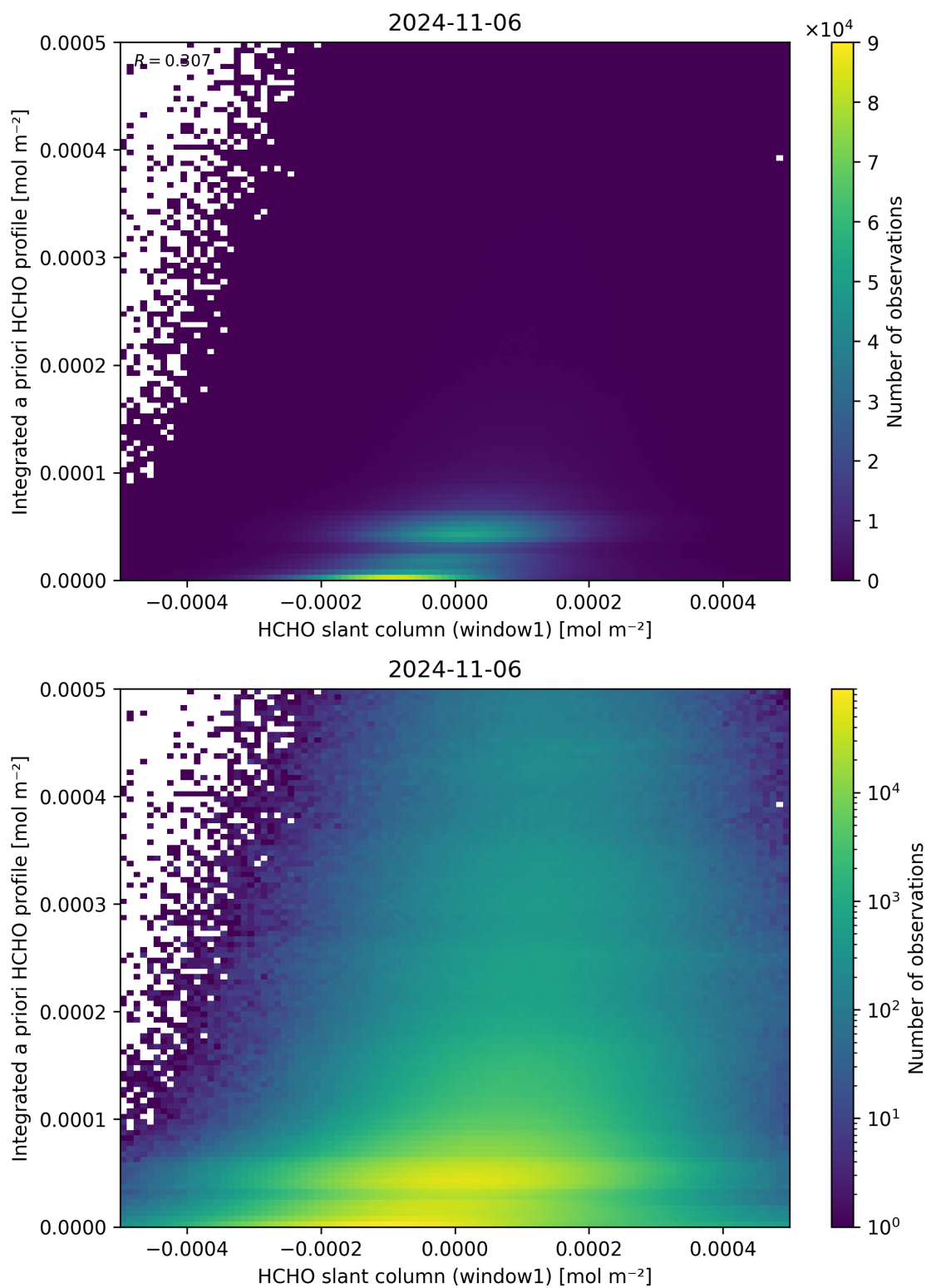
Figure 87: Scatter density plot of “HCHO slant column (window1)” against “Integrated a priori HCHO profile” for 2024-11-05 to 2024-11-07.
