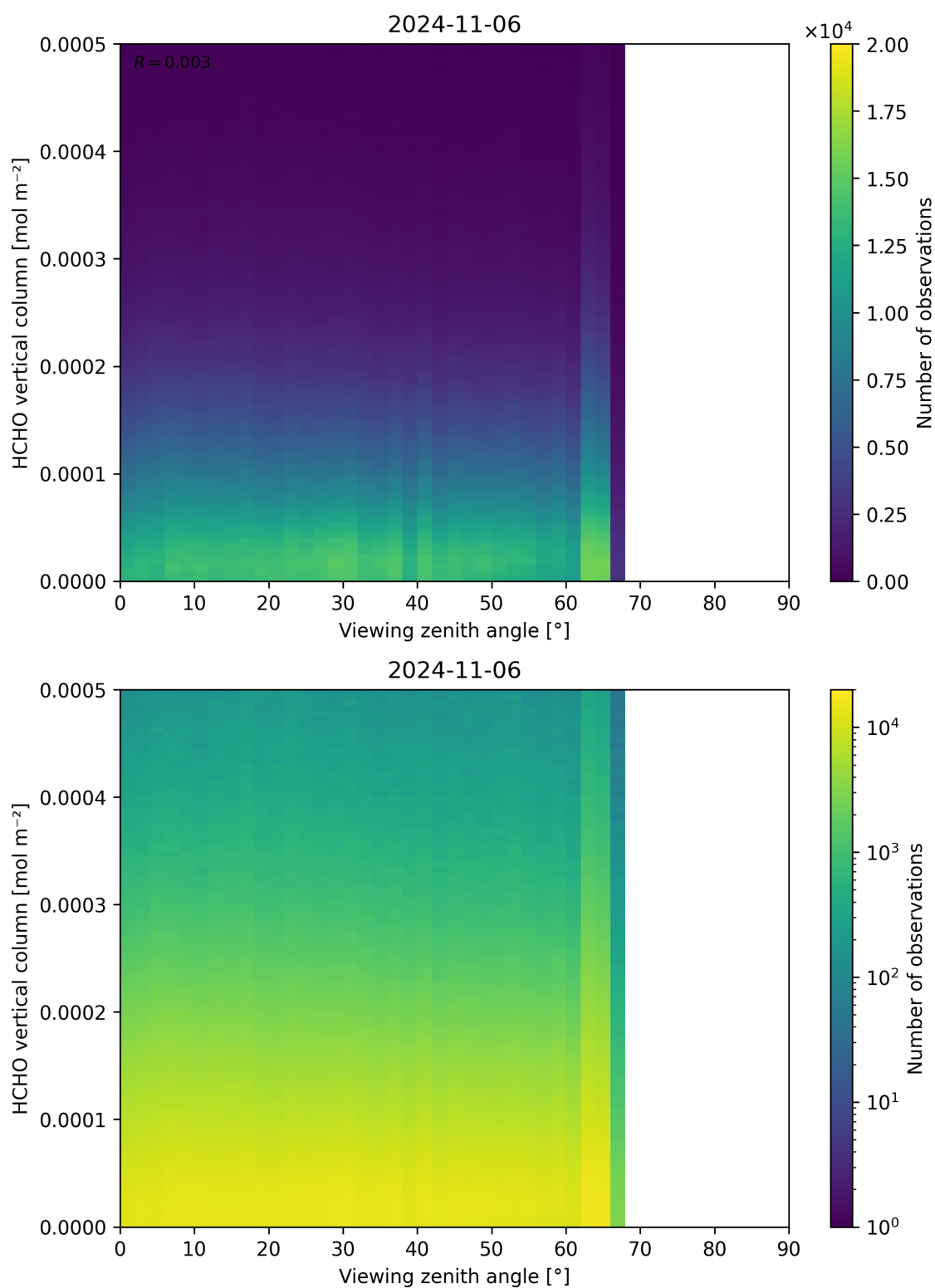
Figure 192: Scatter density plot of “Viewing zenith angle” against “HCHO vertical column” for 2024-11-05 to 2024-11-07.
