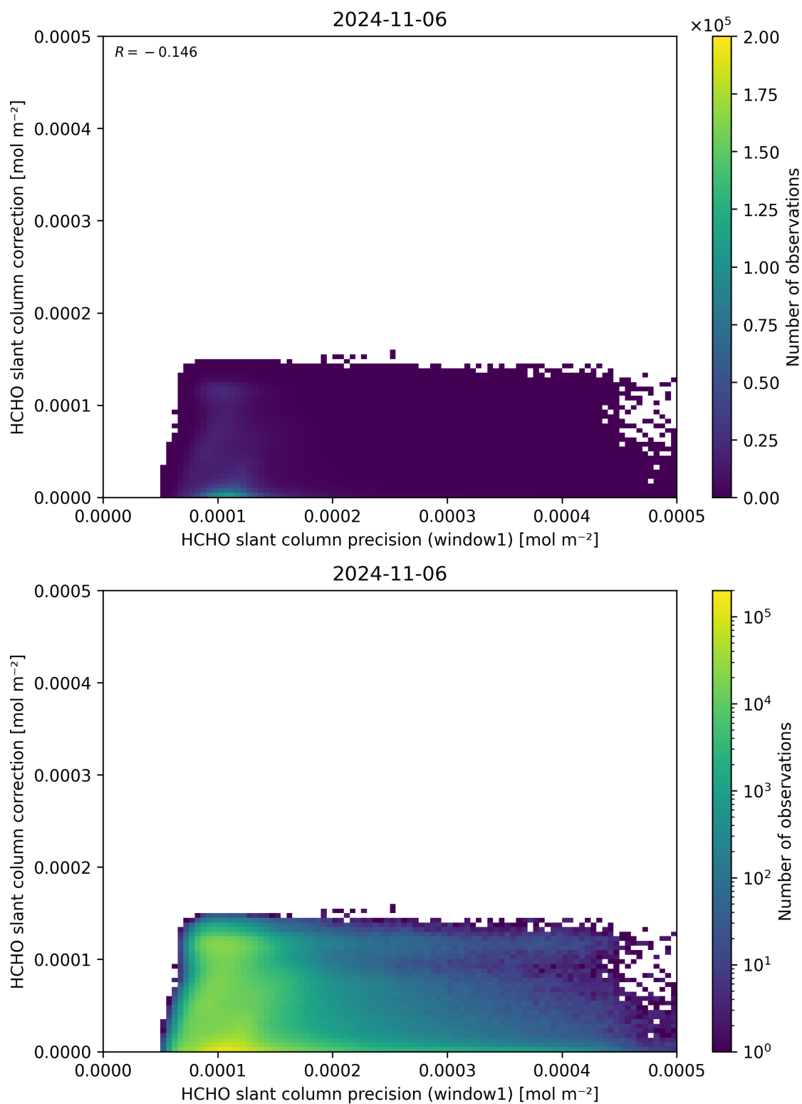
Figure 93: Scatter density plot of “HCHO slant column precision (window1)” against “HCHO slant column correction” for 2024-11-05 to 2024-11-07.
