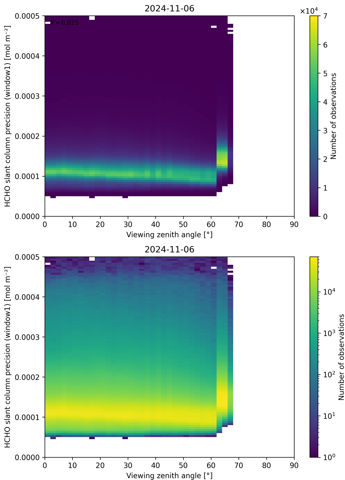
Figure 189: Scatter density plot of “Viewing zenith angle” against “HCHO slant column precision (window1)” for 2024-11-05 to 2024-11-07.
