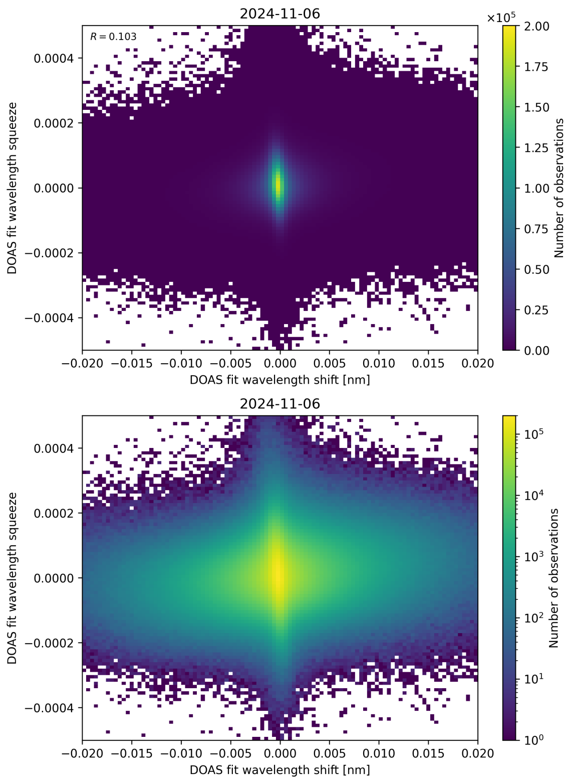
Figure 65: Scatter density plot of “DOAS fit wavelength shift” against “DOAS fit wavelength squeeze” for 2024-11-05 to 2024-11-07.
