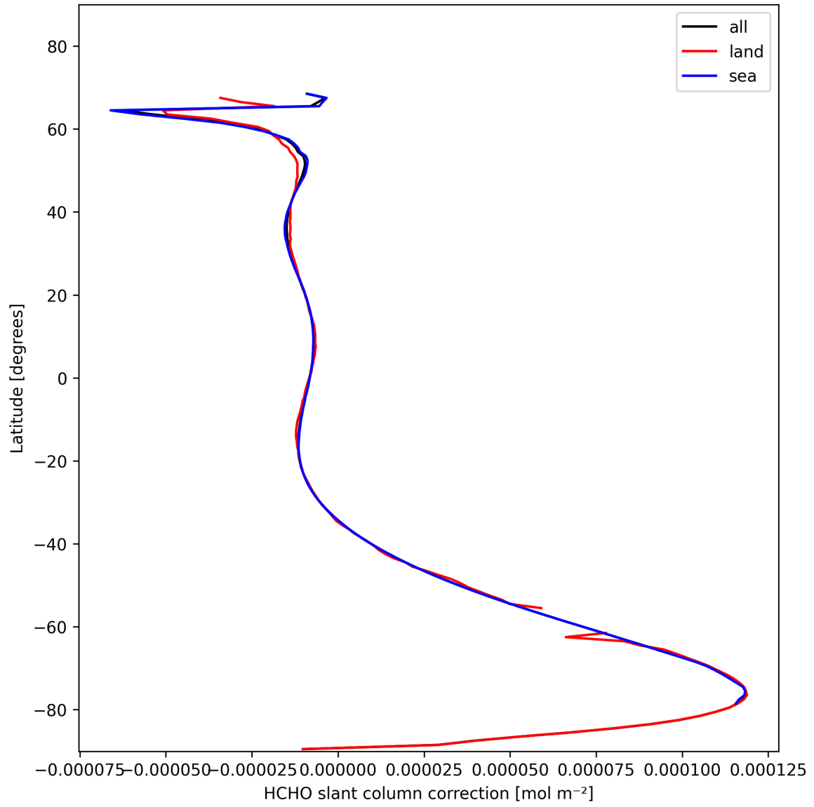
Figure 33: Zonal average of “HCHO slant column correction” for 2024-11-05 to 2024-11-07.
