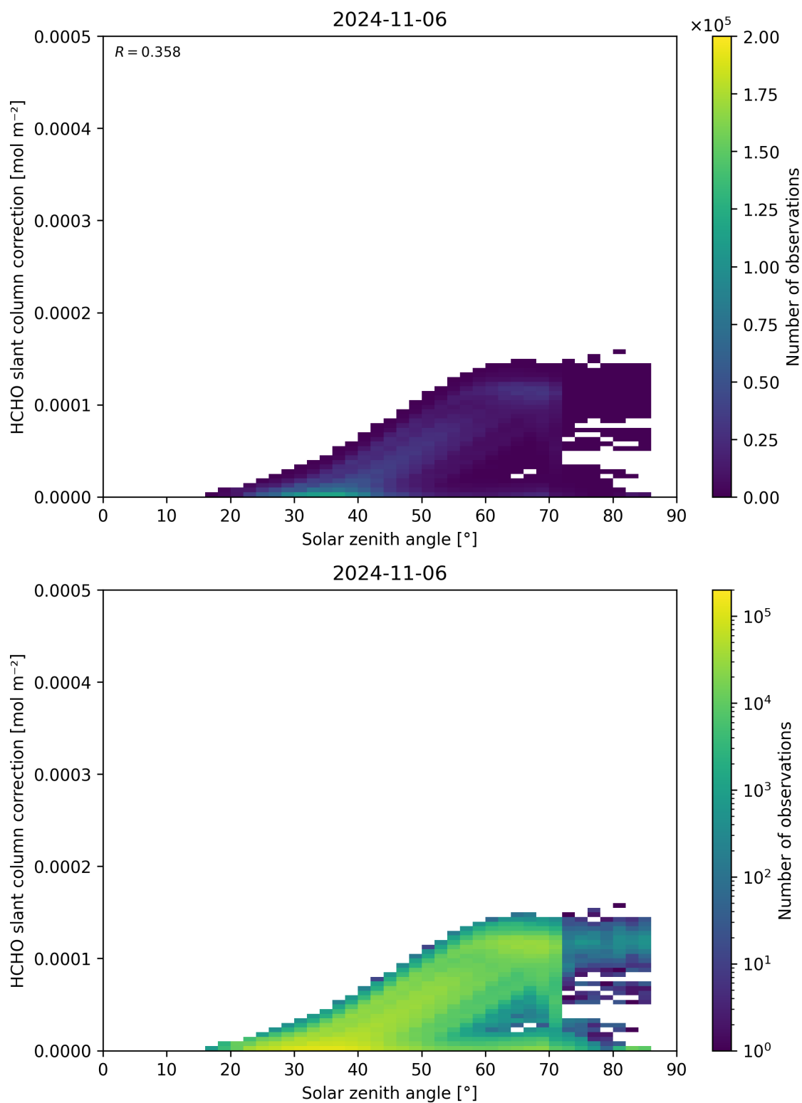
Figure 172: Scatter density plot of “Solar zenith angle” against “HCHO slant column correction” for 2024-11-05 to 2024-11-07.
