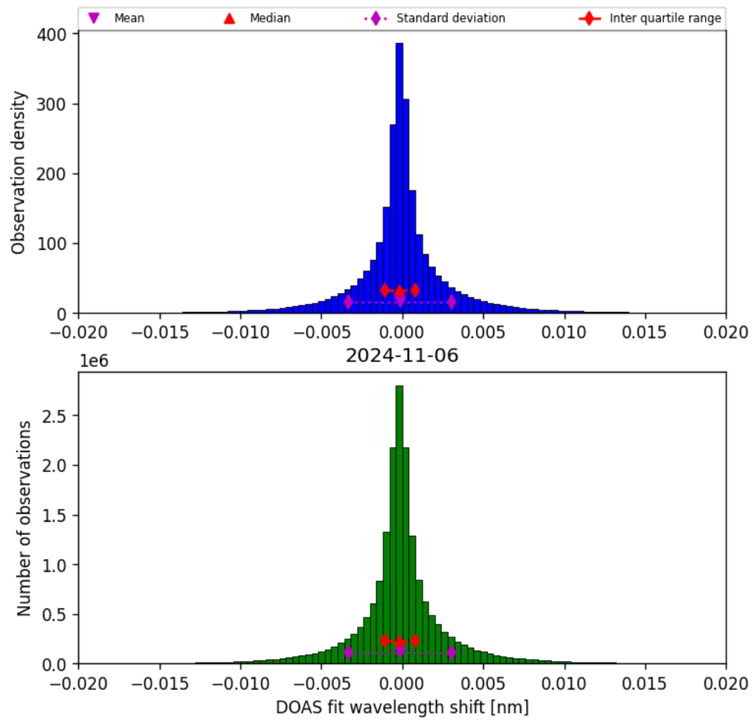
Figure 44: Histogram of “DOAS fit wavelength shift” for 2024-11-05 to 2024-11-07
