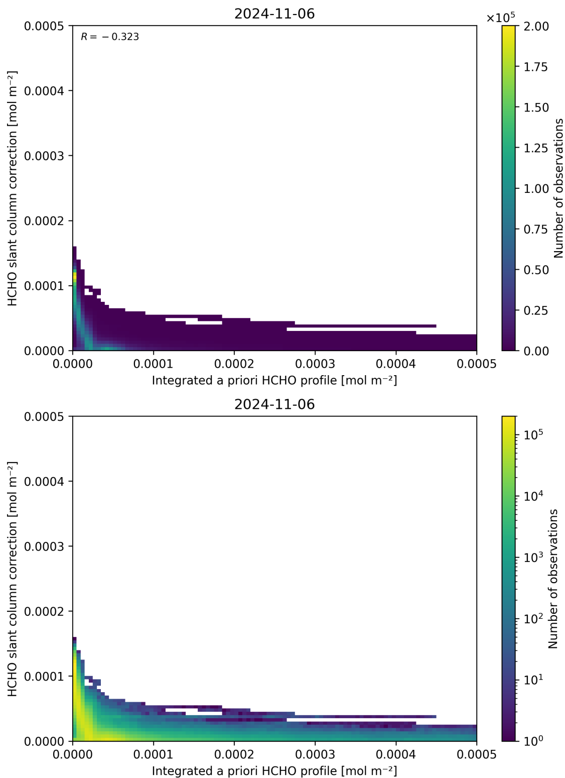
Figure 152: Scatter density plot of “Integrated a priori HCHO profile” against “HCHO slant column correction” for 2024-11-05 to 2024-11-07.
