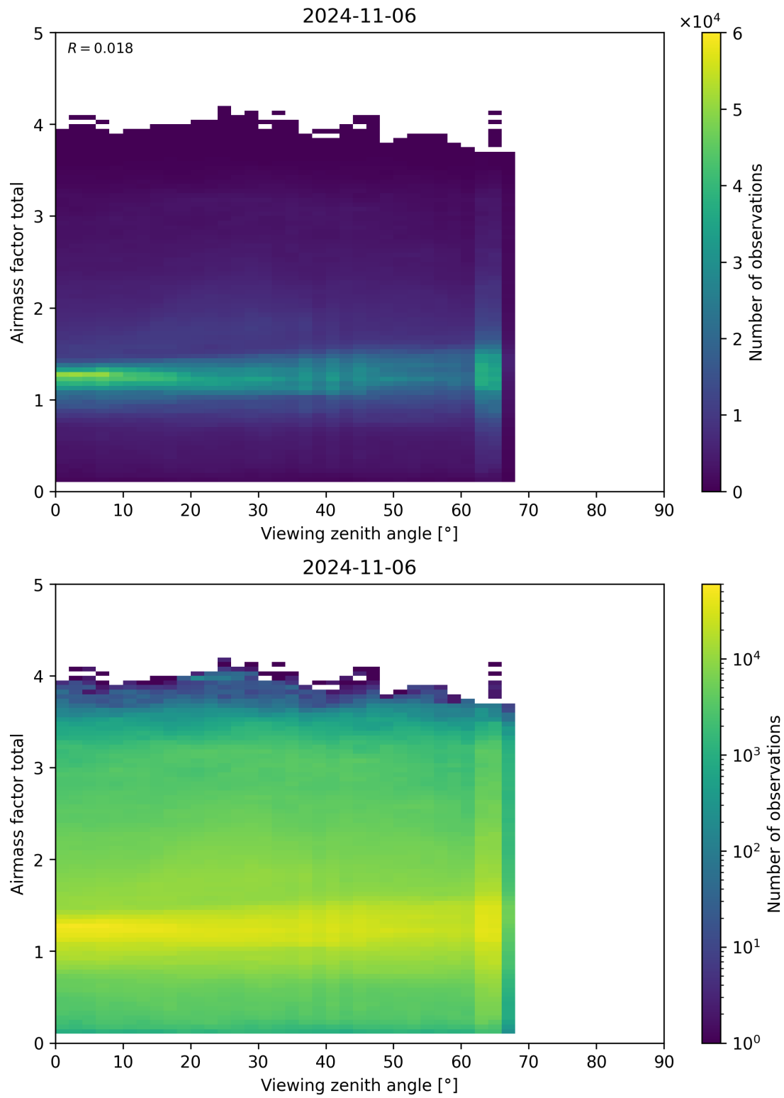
Figure 190: Scatter density plot of “Viewing zenith angle” against “Airmass factor total” for 2024-11-05 to 2024-11-07.
