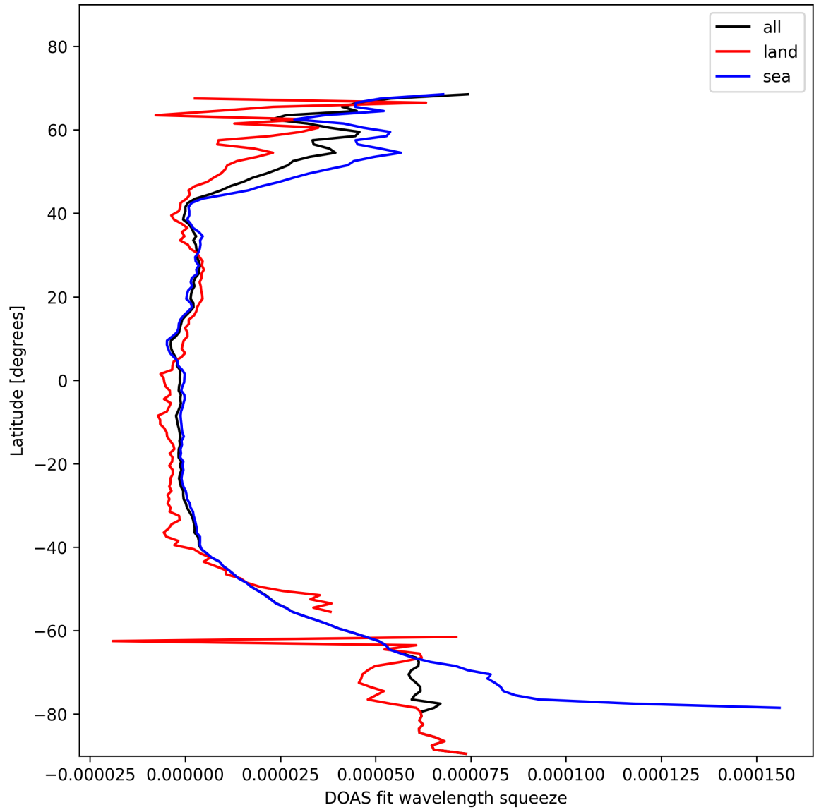
Figure 31: Zonal average of “DOAS fit wavelength squeeze” for 2024-11-05 to 2024-11-07.
