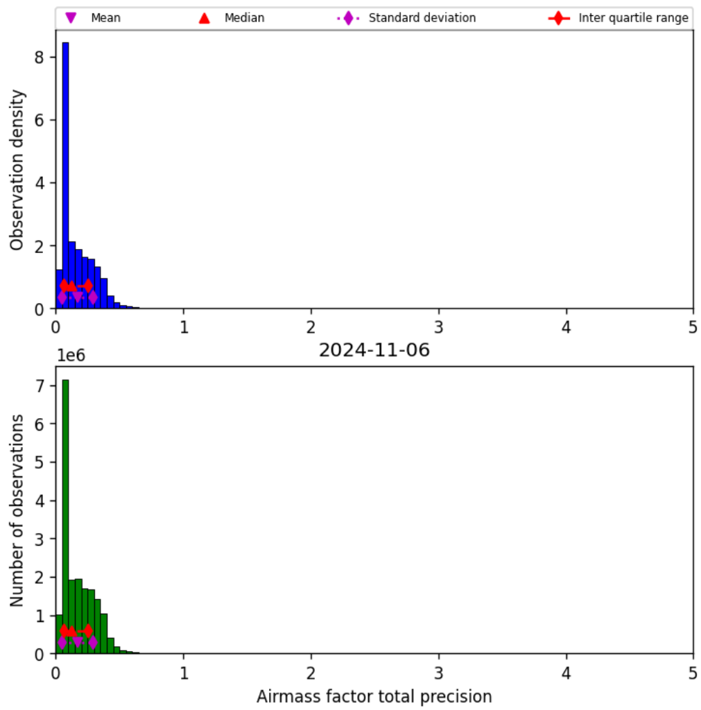
Figure 41: Histogram of “Airmass factor total precision” for 2024-11-05 to 2024-11-07
