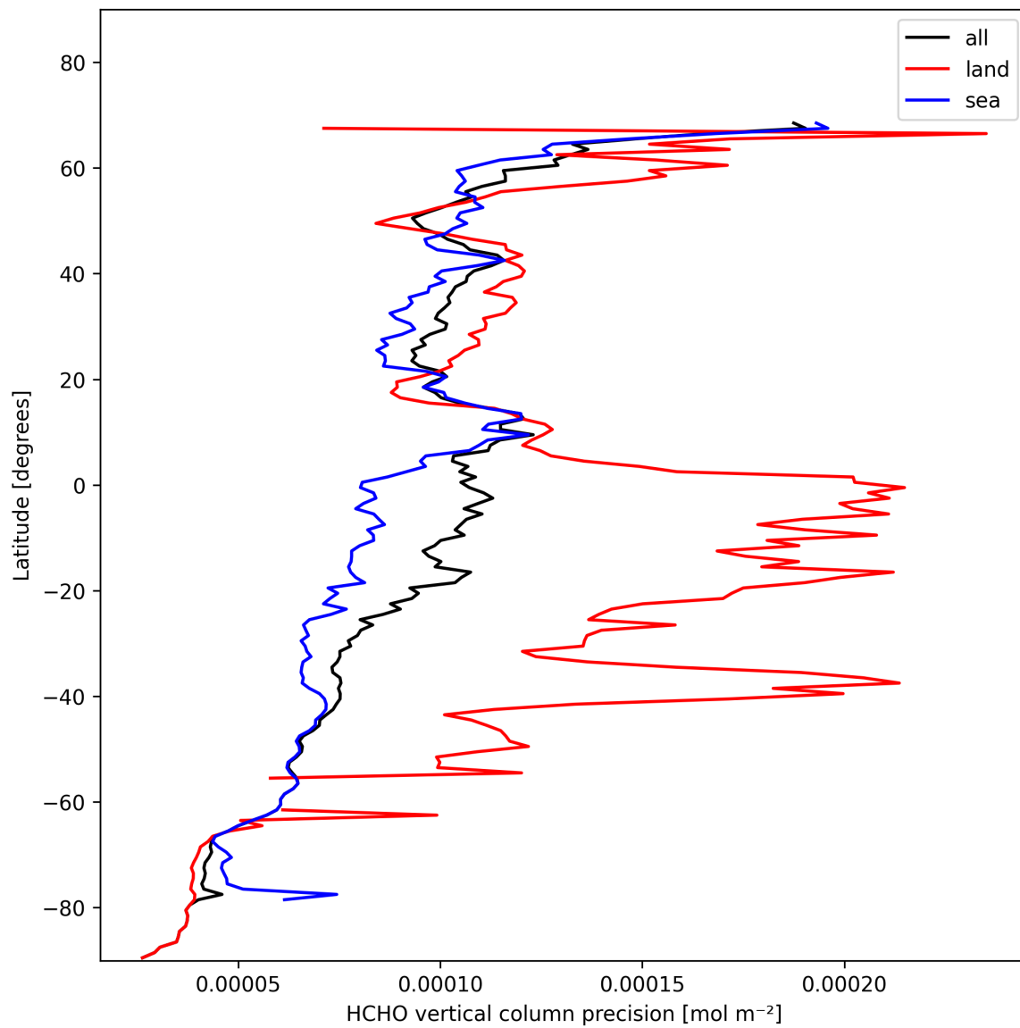
Figure 22: Zonal average of “HCHO vertical column precision” for 2024-11-05 to 2024-11-07.
