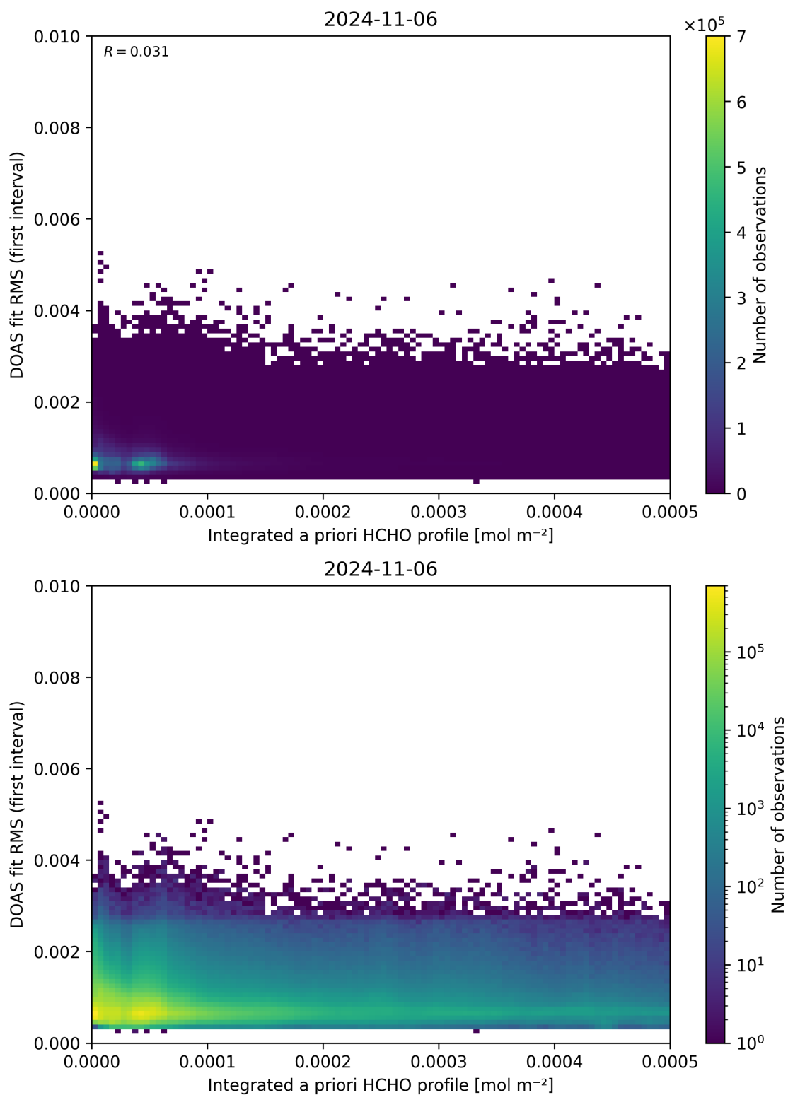
Figure 148: Scatter density plot of “Integrated a priori HCHO profile” against “DOAS fit RMS (first interval)” for 2024-11-05 to 2024-11-07.
