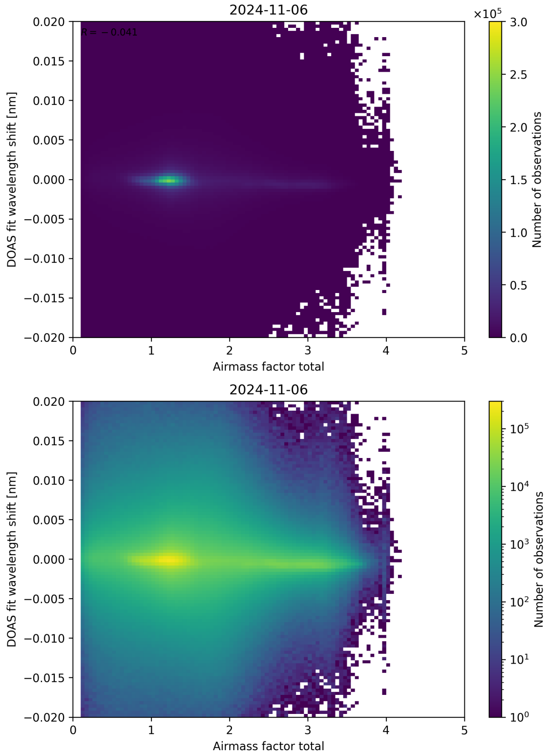
Figure 98: Scatter density plot of “Airmass factor total” against “DOAS fit wavelength shift” for 2024-11-05 to 2024-11-07.
