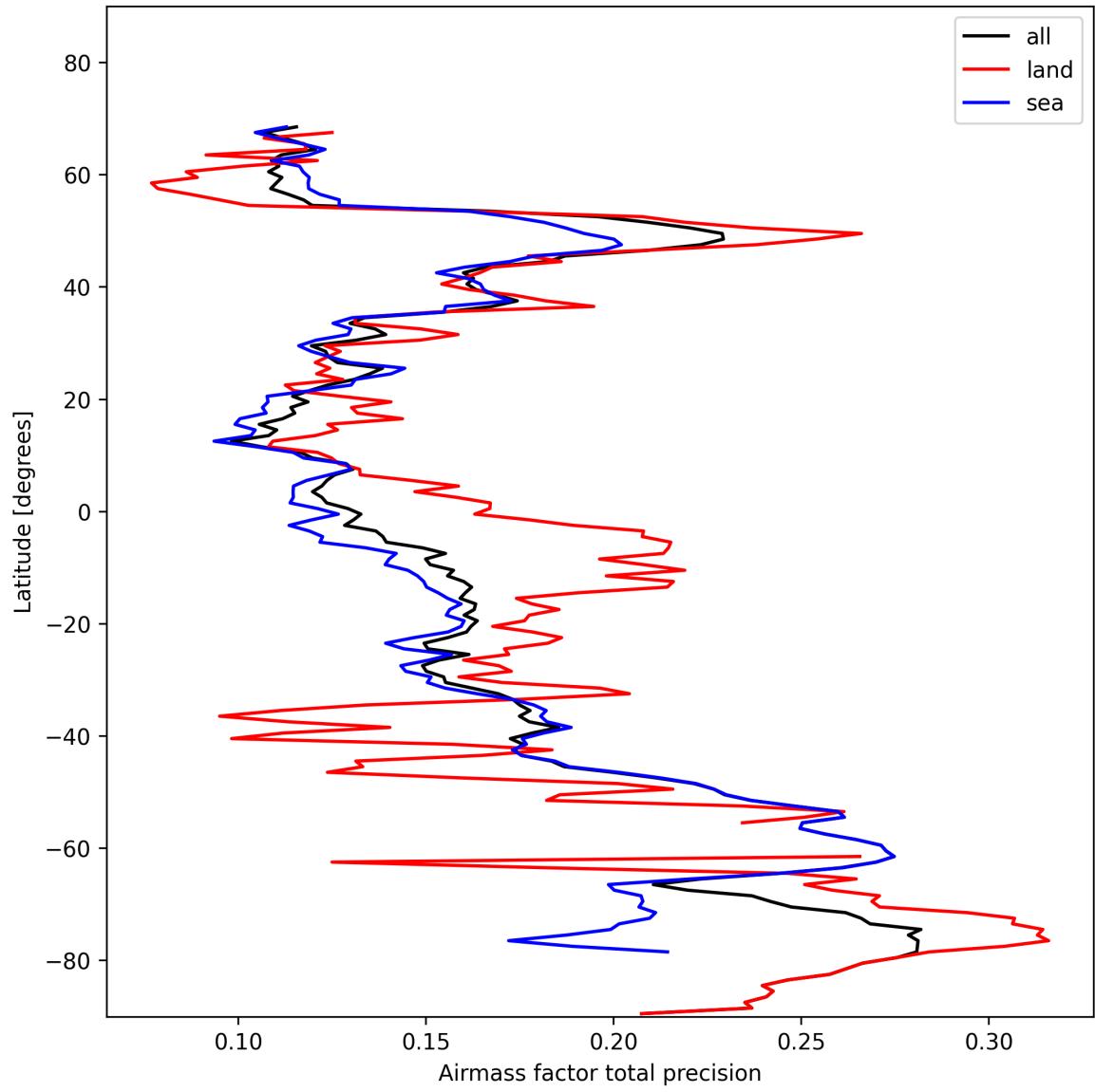
Figure 27: Zonal average of “Airmass factor total precision” for 2024-11-05 to 2024-11-07.
