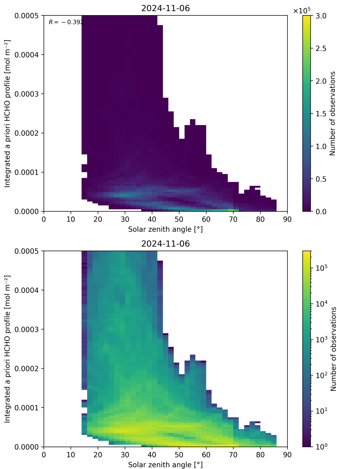
Figure 180: Scatter density plot of “Solar zenith angle” against “Integrated a priori HCHO profile” for 2024-11-05 to 2024-11-07.
