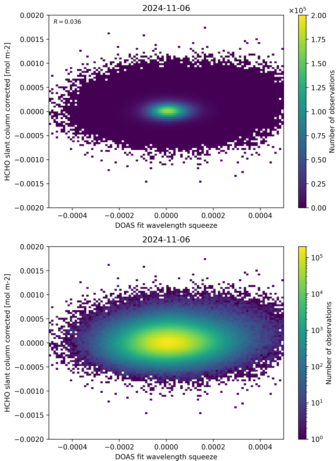
Figure 69: Scatter density plot of “DOAS fit wavelength squeeze” against “HCHO slant column corrected” for 2024-11-05 to 2024-11-07.
