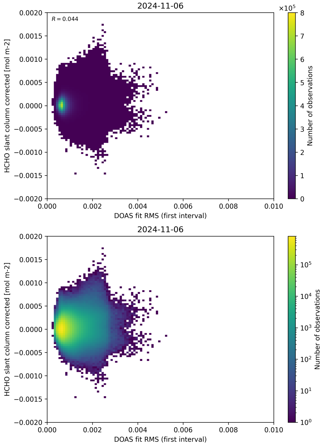
Figure 62: Scatter density plot of “DOAS fit RMS (first interval)” against “HCHO slant column corrected” for 2024-11-05 to 2024-11-07.
