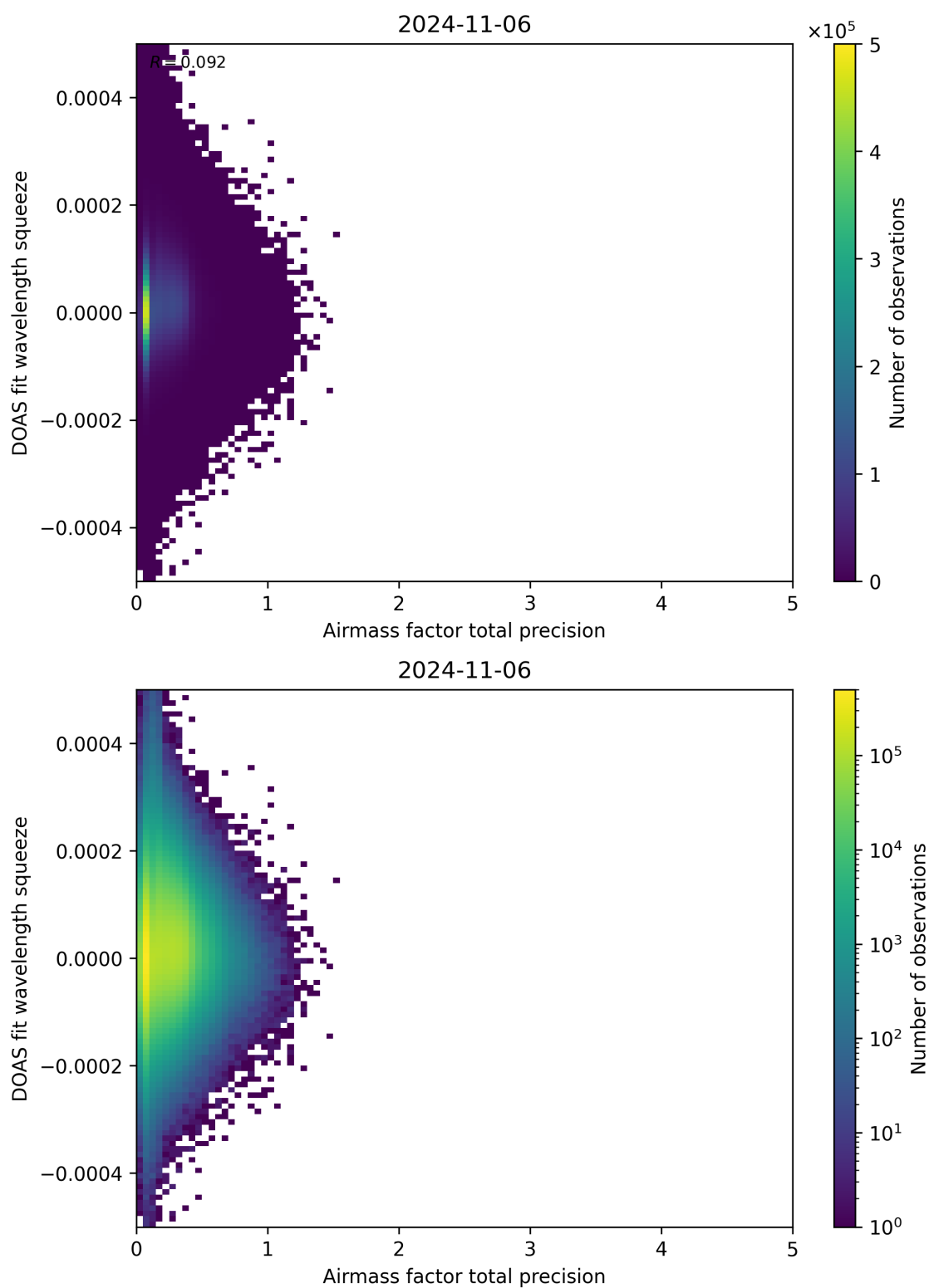
Figure 107: Scatter density plot of “Airmass factor total precision” against “DOAS fit wavelength squeeze” for 2024-11-05 to 2024-11-07.
