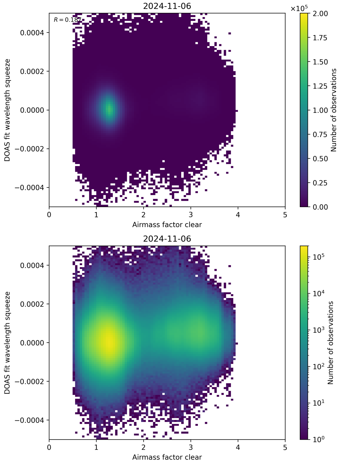
Figure 73: Scatter density plot of “Airmass factor clear” against “DOAS fit wavelength squeeze” for 2024-11-05 to 2024-11-07.
