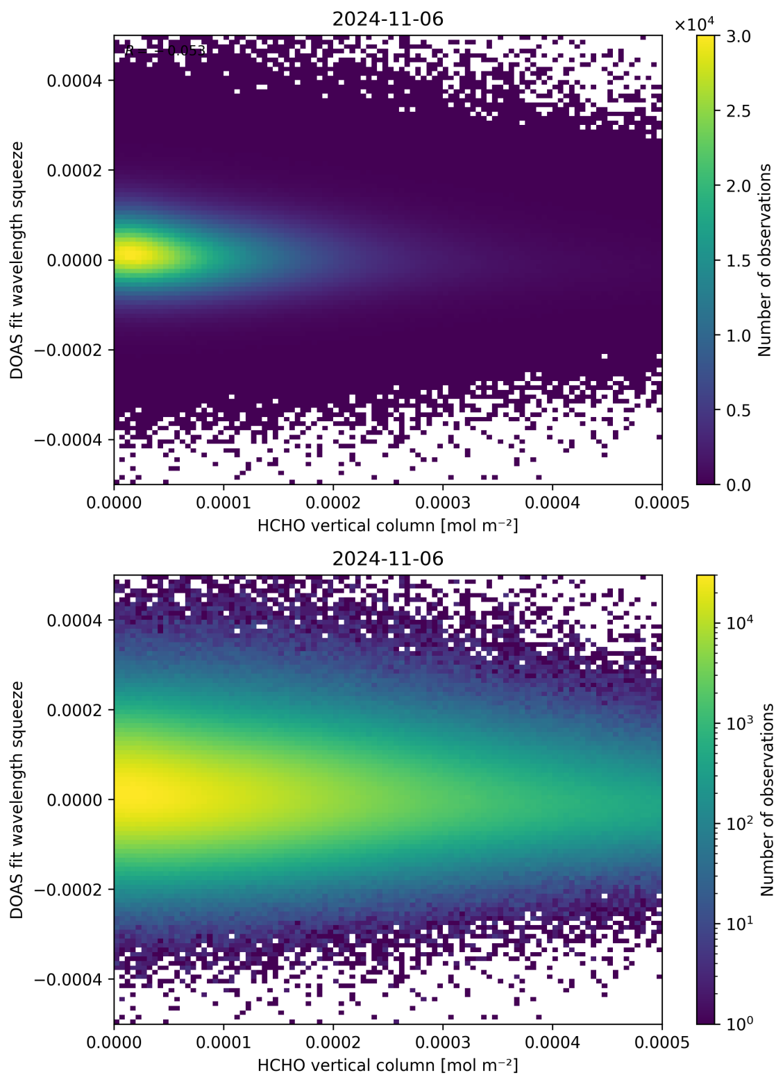
Figure 125: Scatter density plot of “HCHO vertical column” against “DOAS fit wavelength squeeze” for 2024-11-05 to 2024-11-07.
