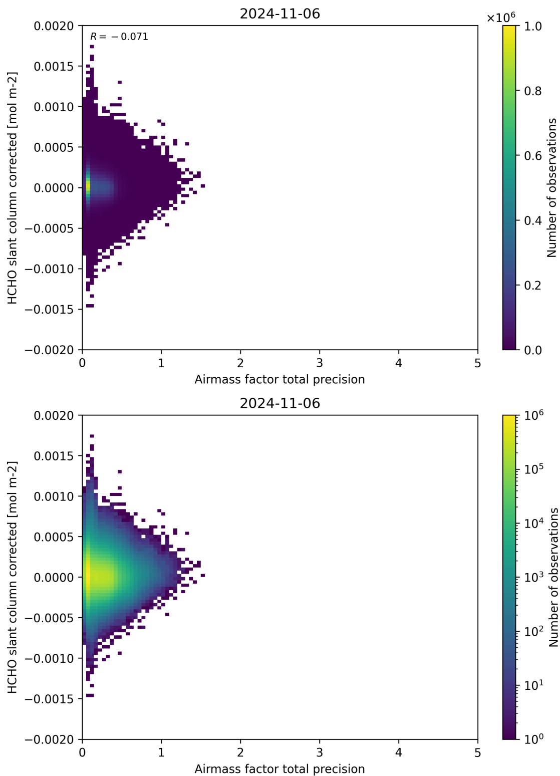
Figure 109: Scatter density plot of “Airmass factor total precision” against “HCHO slant column corrected” for 2024-11-05 to 2024-11-07.
