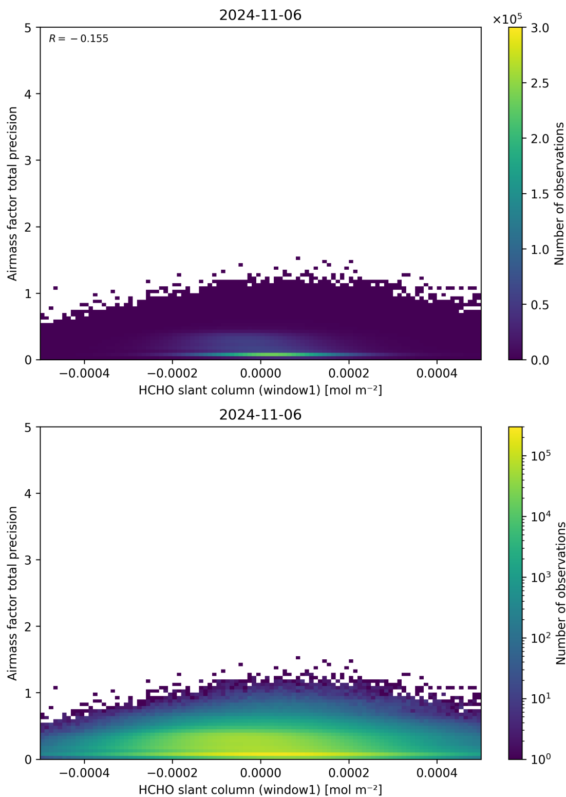
Figure 86: Scatter density plot of “HCHO slant column (window1)” against “Airmass factor total precision” for 2024-11-05 to 2024-11-07.
