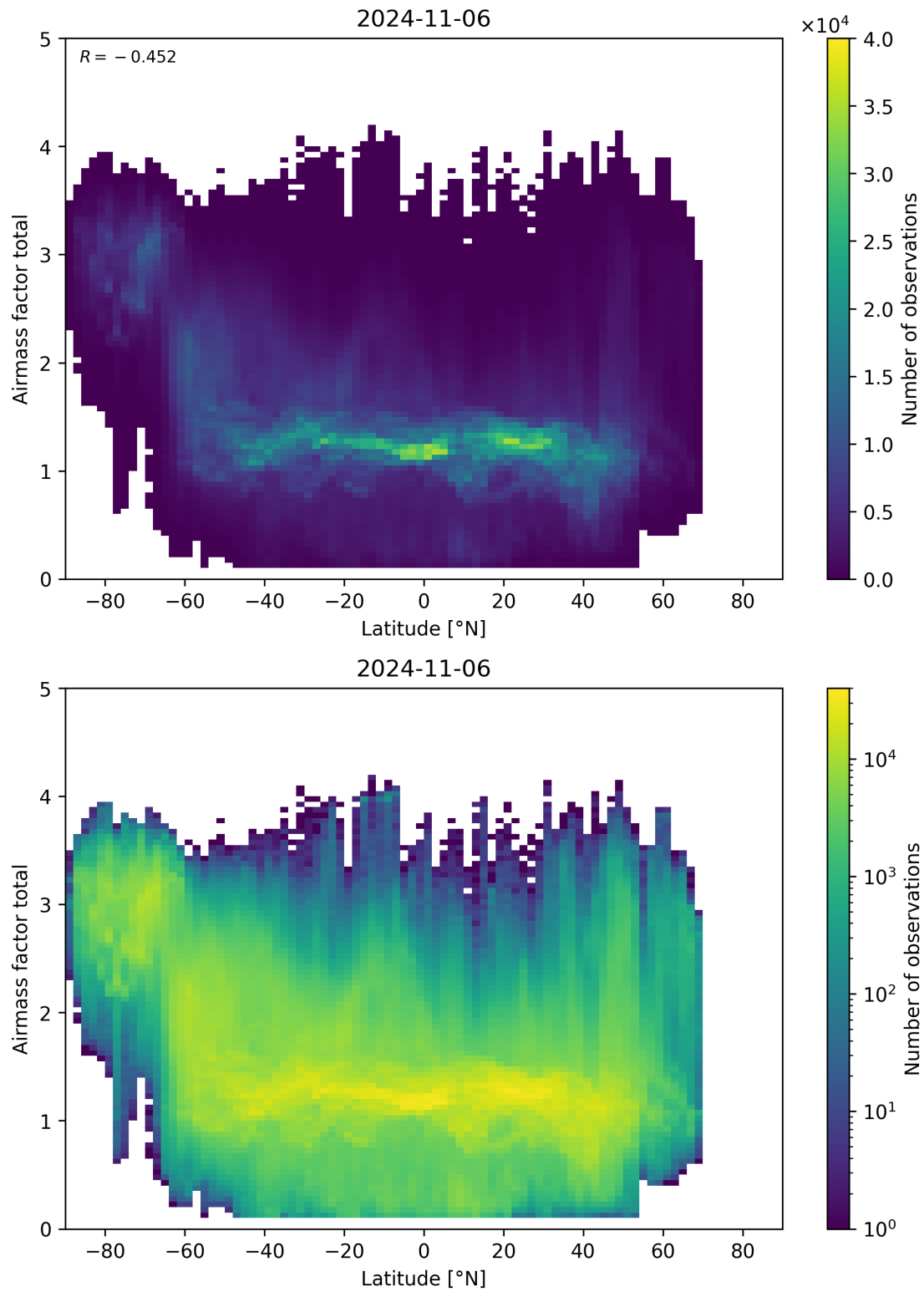
Figure 161: Scatter density plot of “Latitude” against “Airmass factor total” for 2024-11-05 to 2024-11-07.
