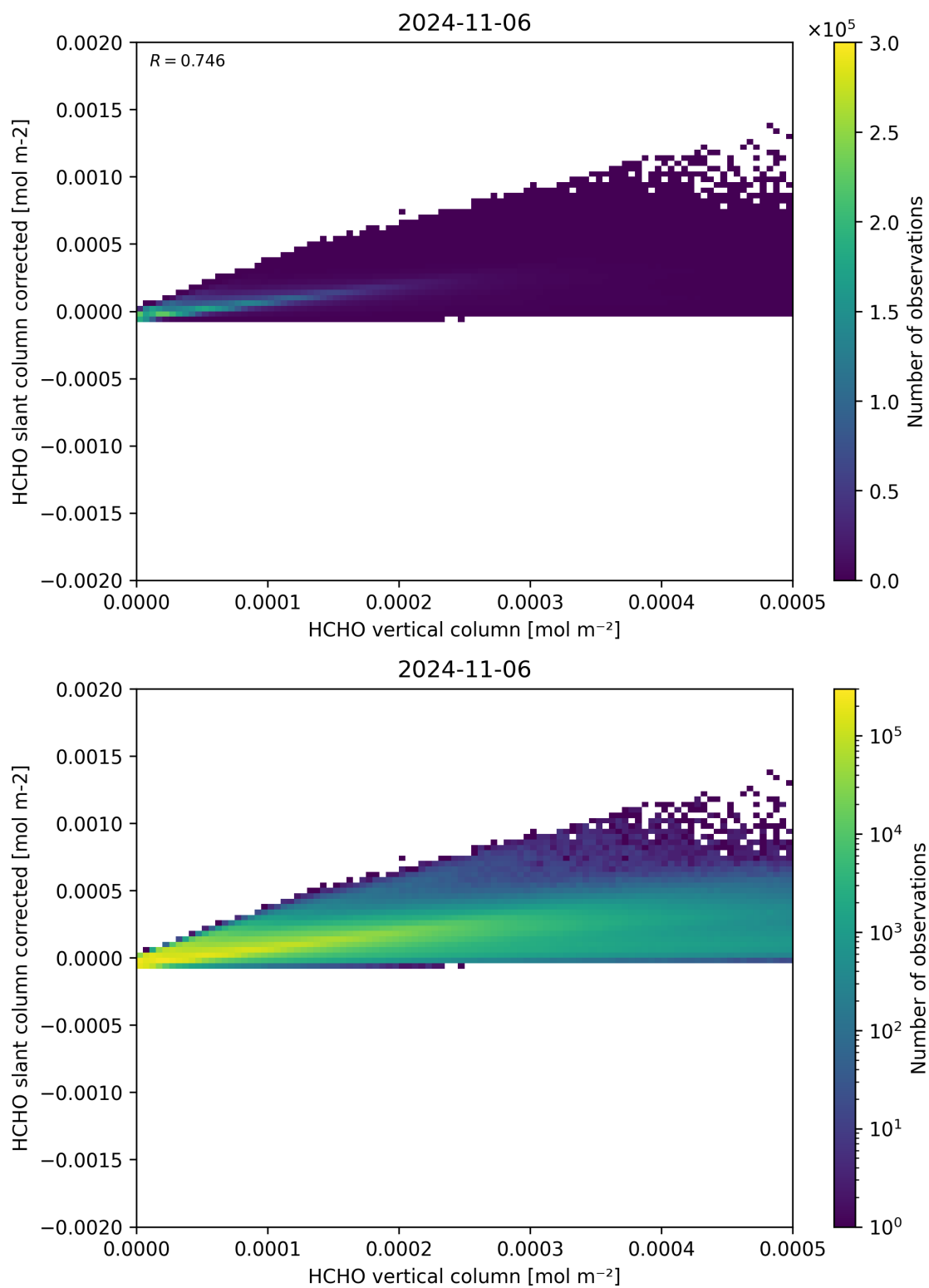
Figure 127: Scatter density plot of “HCHO vertical column” against “HCHO slant column corrected” for 2024-11-05 to 2024-11-07.
