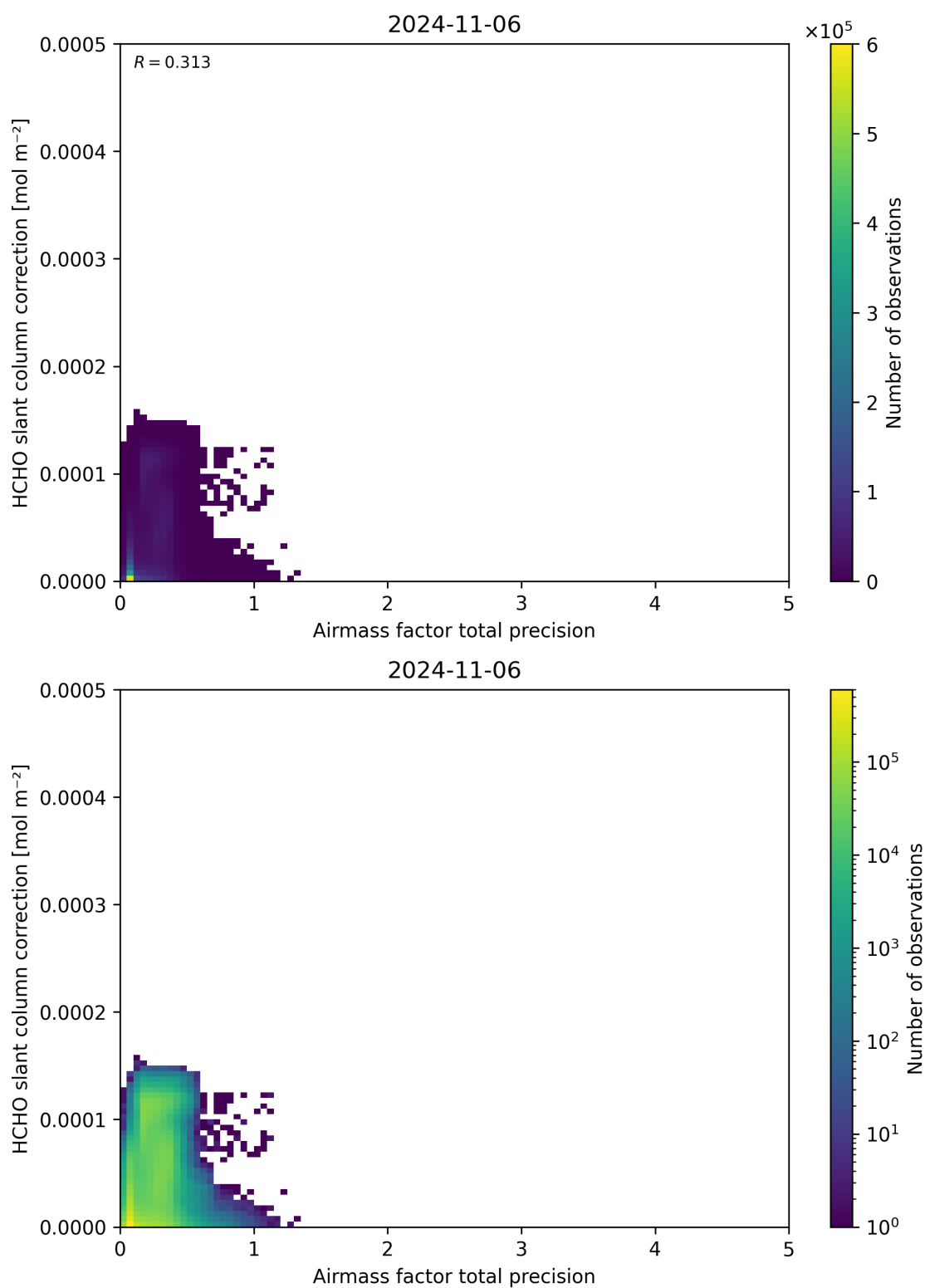
Figure 110: Scatter density plot of “Airmass factor total precision” against “HCHO slant column correction” for 2024-11-05 to 2024-11-07.
