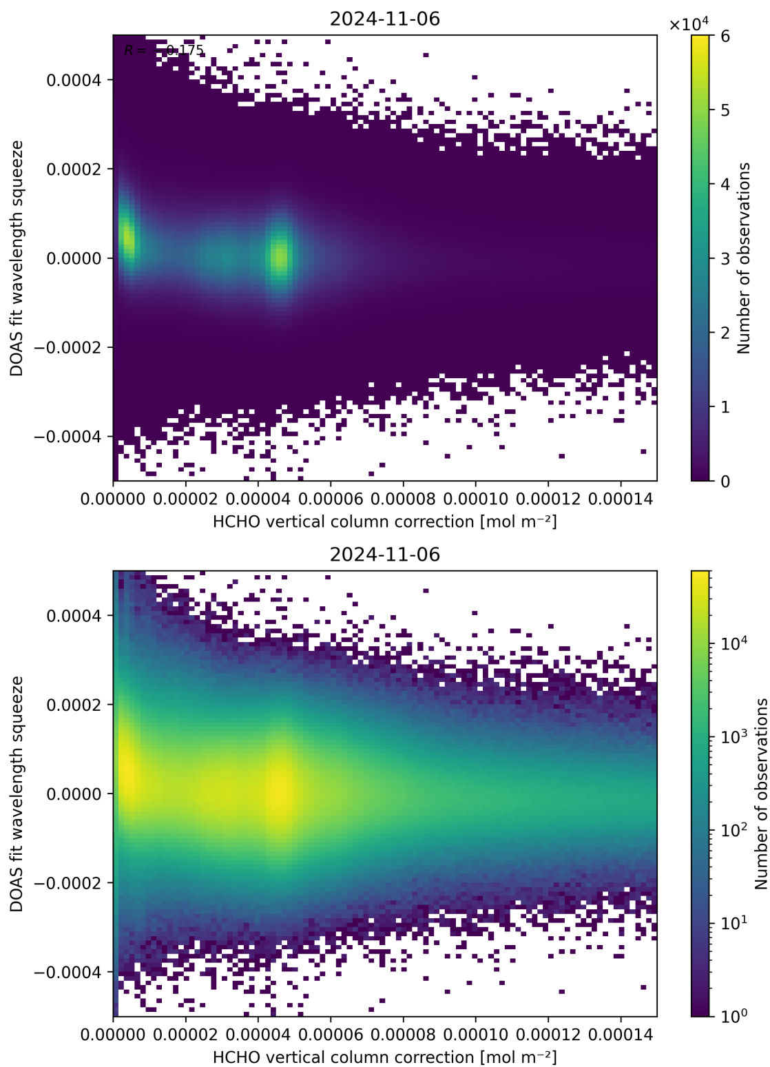
Figure 114: Scatter density plot of “HCHO vertical column correction” against “DOAS fit wavelength squeeze” for 2024-11-05 to 2024-11-07.
