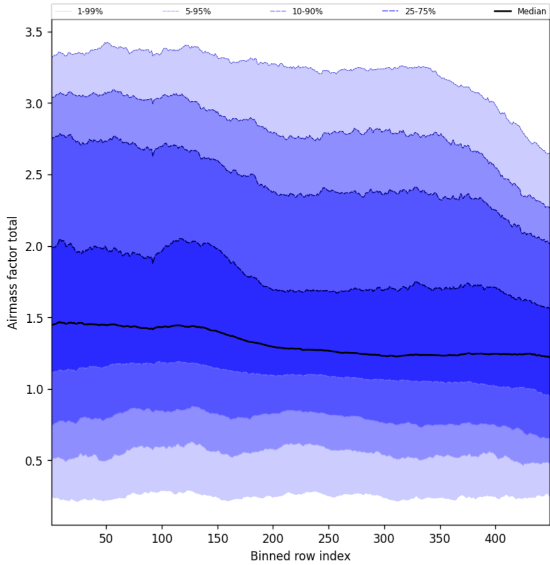
Figure 54: Along track statistics of “Airmass factor total” for 2024-11-05 to 2024-11-07
