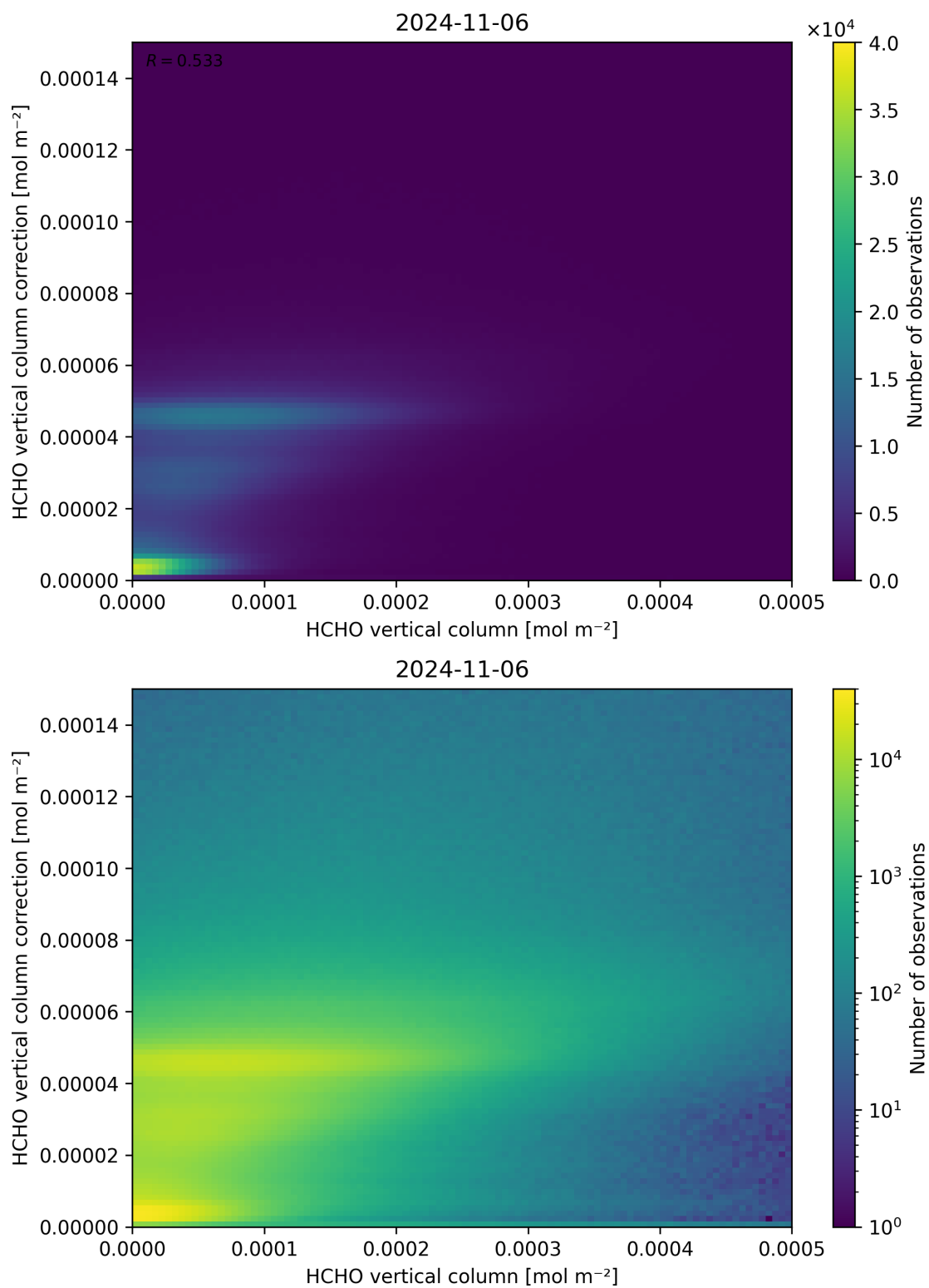
Figure 133: Scatter density plot of “HCHO vertical column” against “HCHO vertical column correction” for 2024-11-05 to 2024-11-07.
