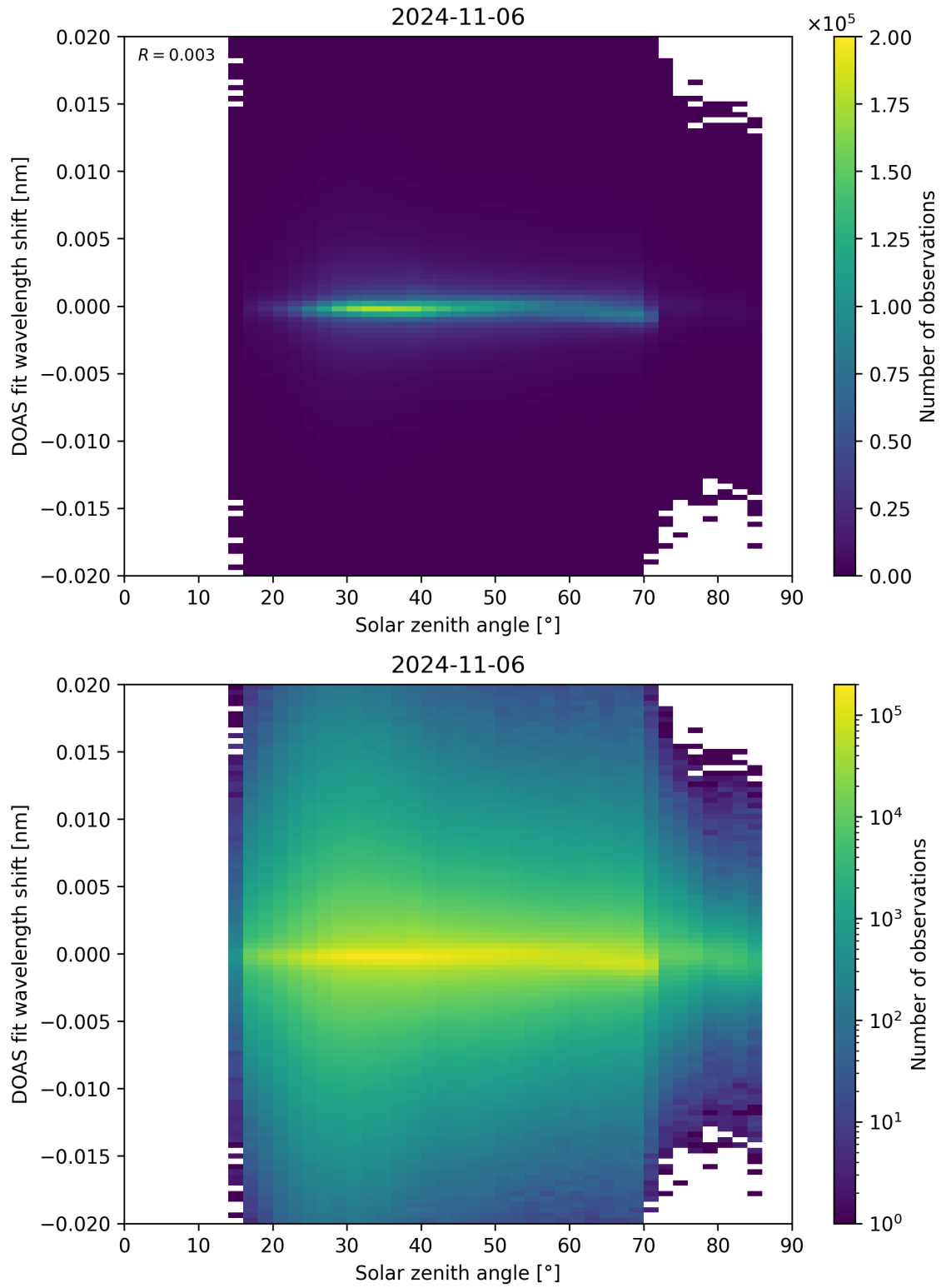
Figure 168: Scatter density plot of “Solar zenith angle” against “DOAS fit wavelength shift” for 2024-11-05 to 2024-11-07.
