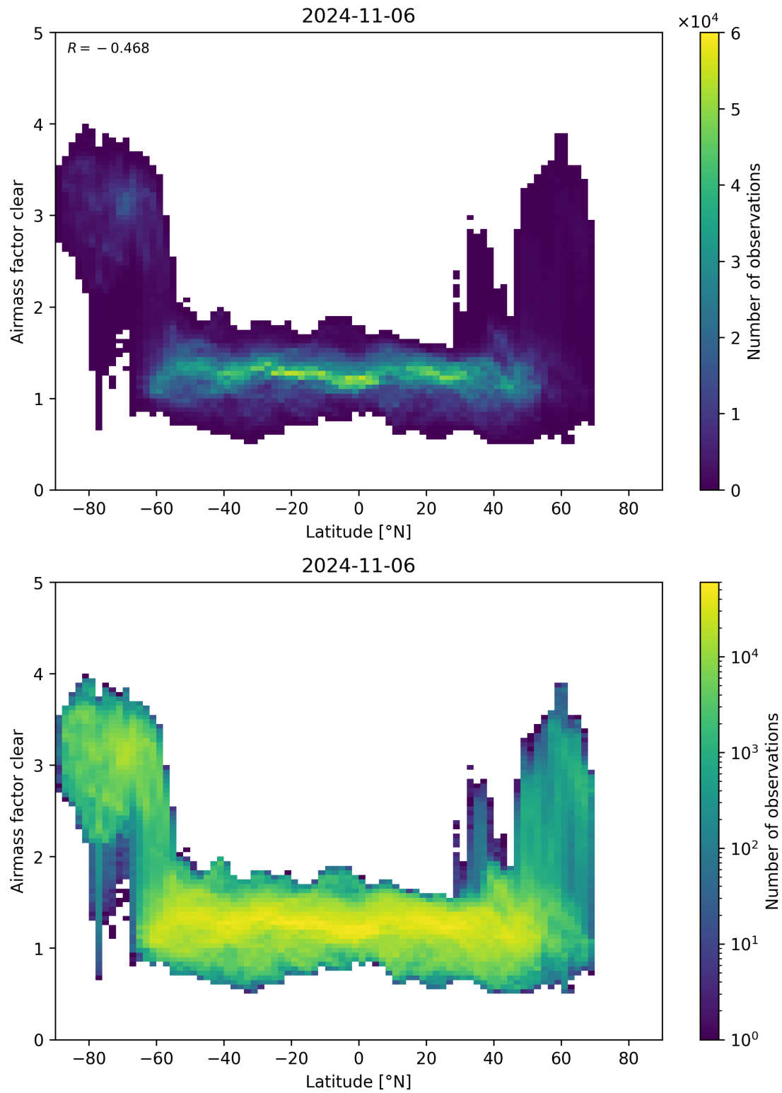
Figure 156: Scatter density plot of “Latitude” against “Airmass factor clear” for 2024-11-05 to 2024-11-07.
