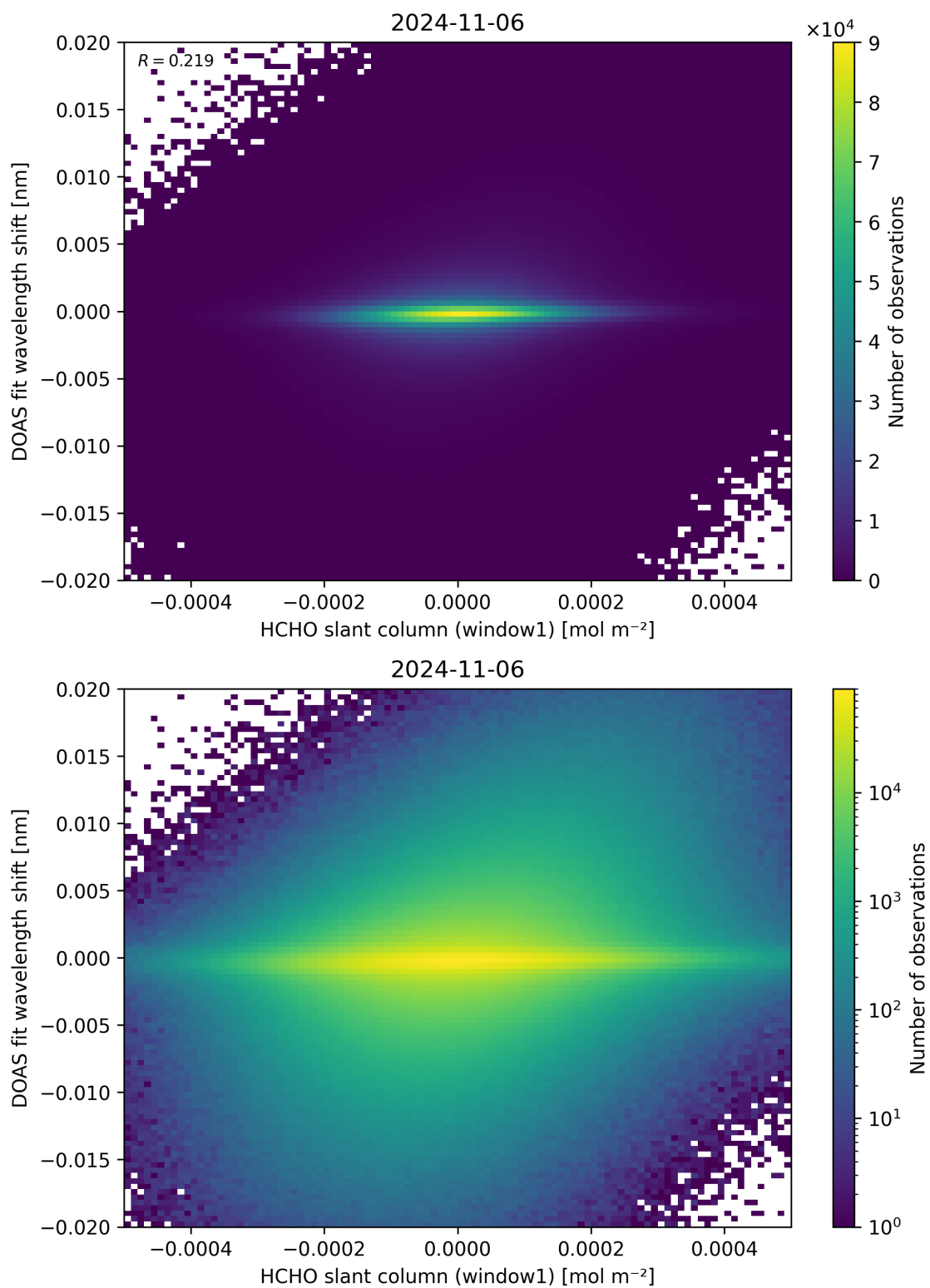
Figure 79: Scatter density plot of “HCHO slant column (window1)” against “DOAS fit wavelength shift” for 2024-11-05 to 2024-11-07.
