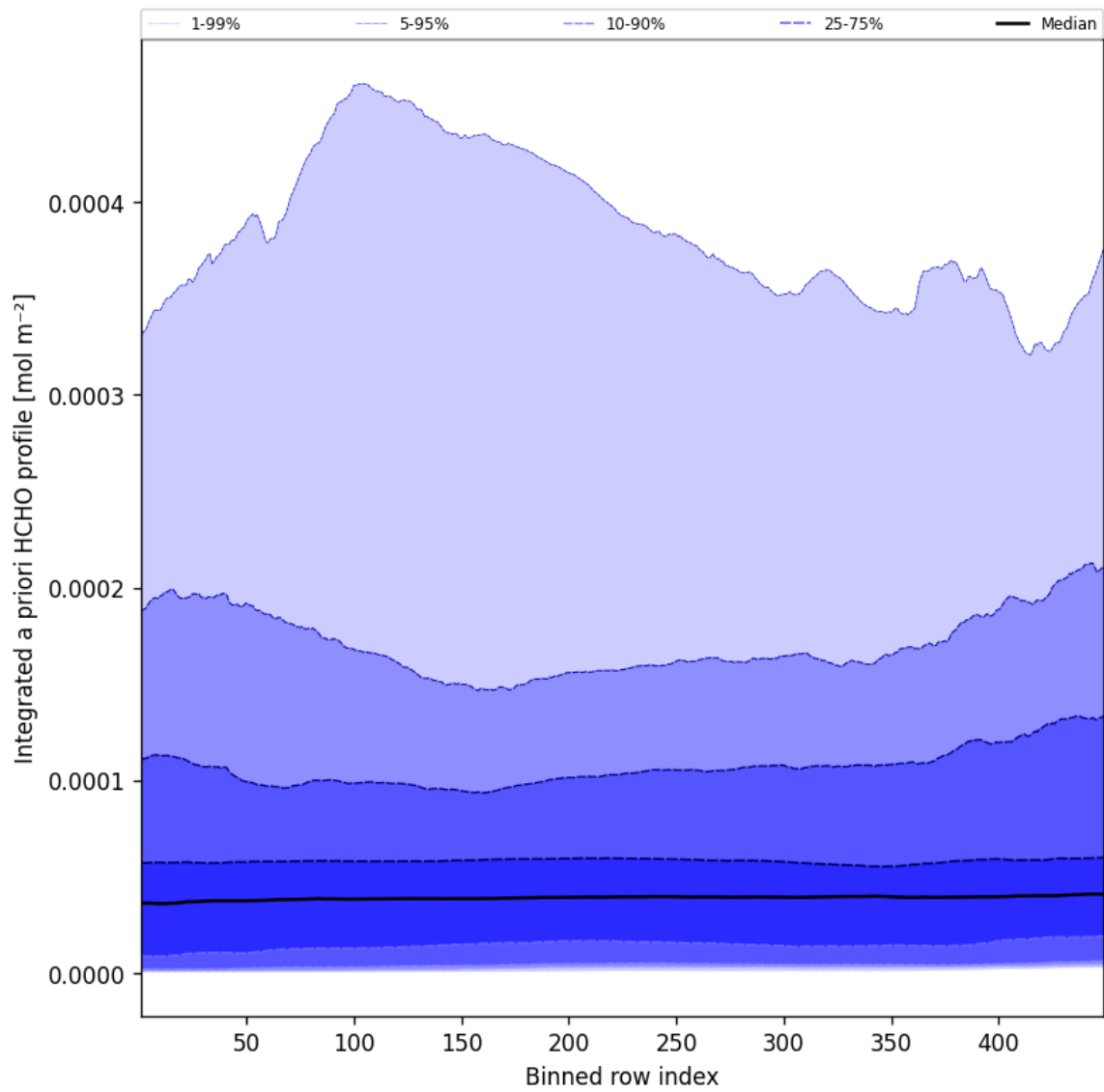
Figure 57: Along track statistics of "Integrated a priori HCHO profile" for 2024-11-05 to 2024-11-07
