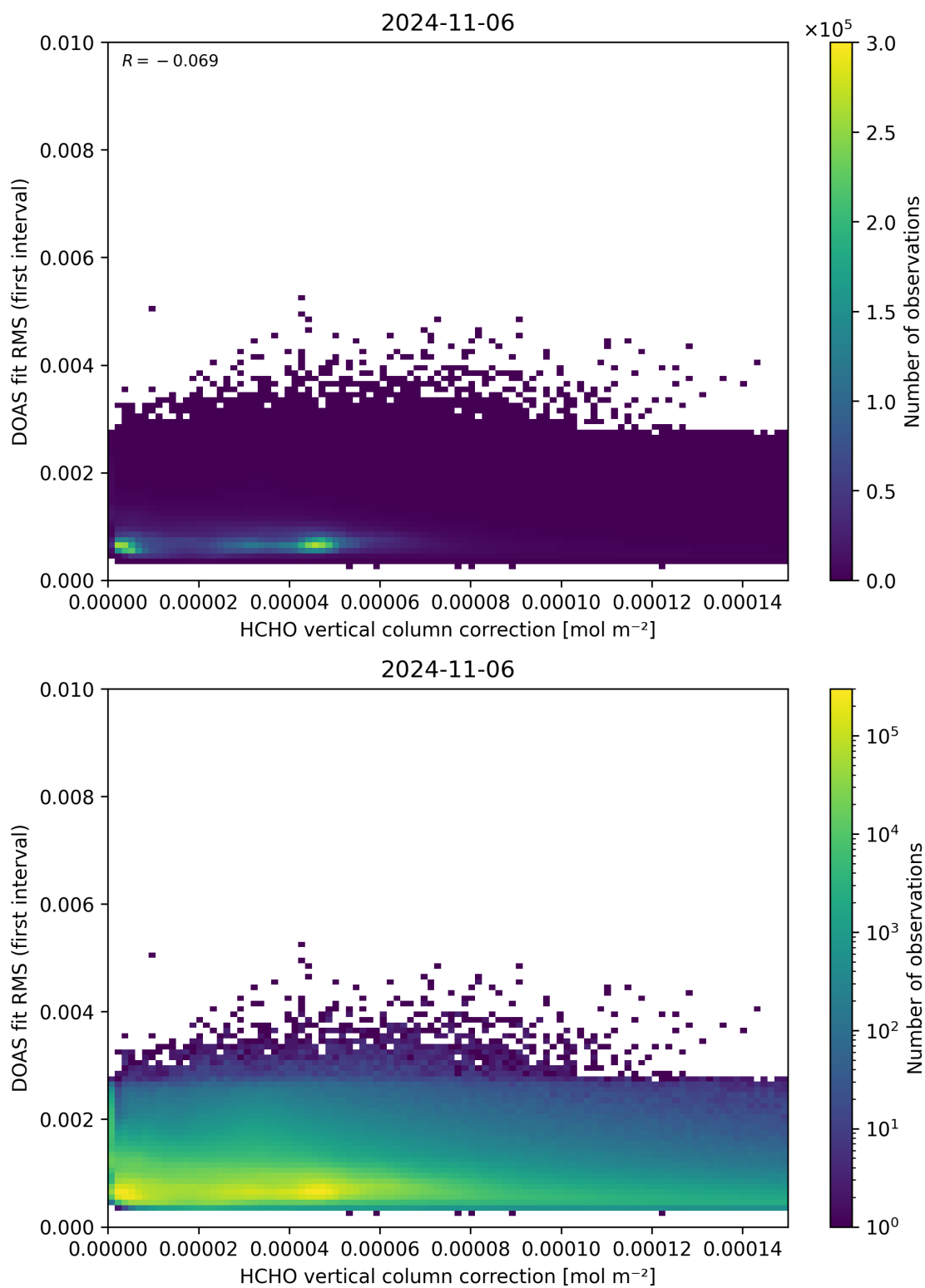
Figure 112: Scatter density plot of “HCHO vertical column correction” against “DOAS fit RMS (first interval)” for 2024-11-05 to 2024-11-07.
