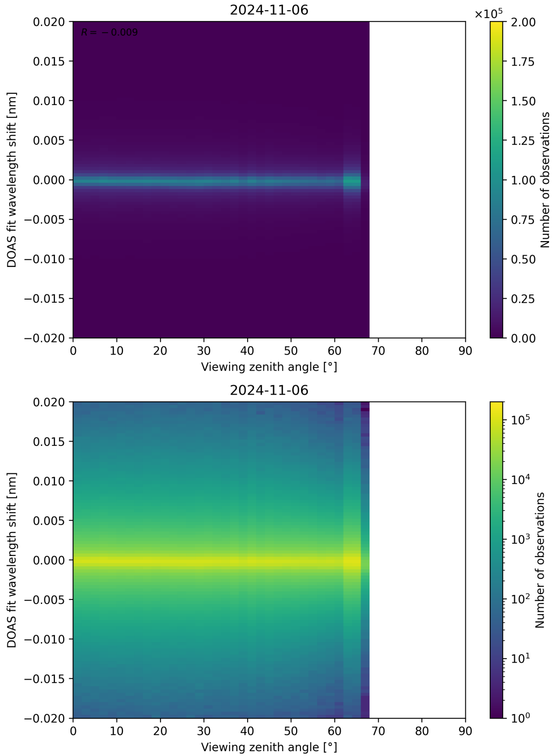
Figure 183: Scatter density plot of “Viewing zenith angle” against “DOAS fit wavelength shift” for 2024-11-05 to 2024-11-07.
