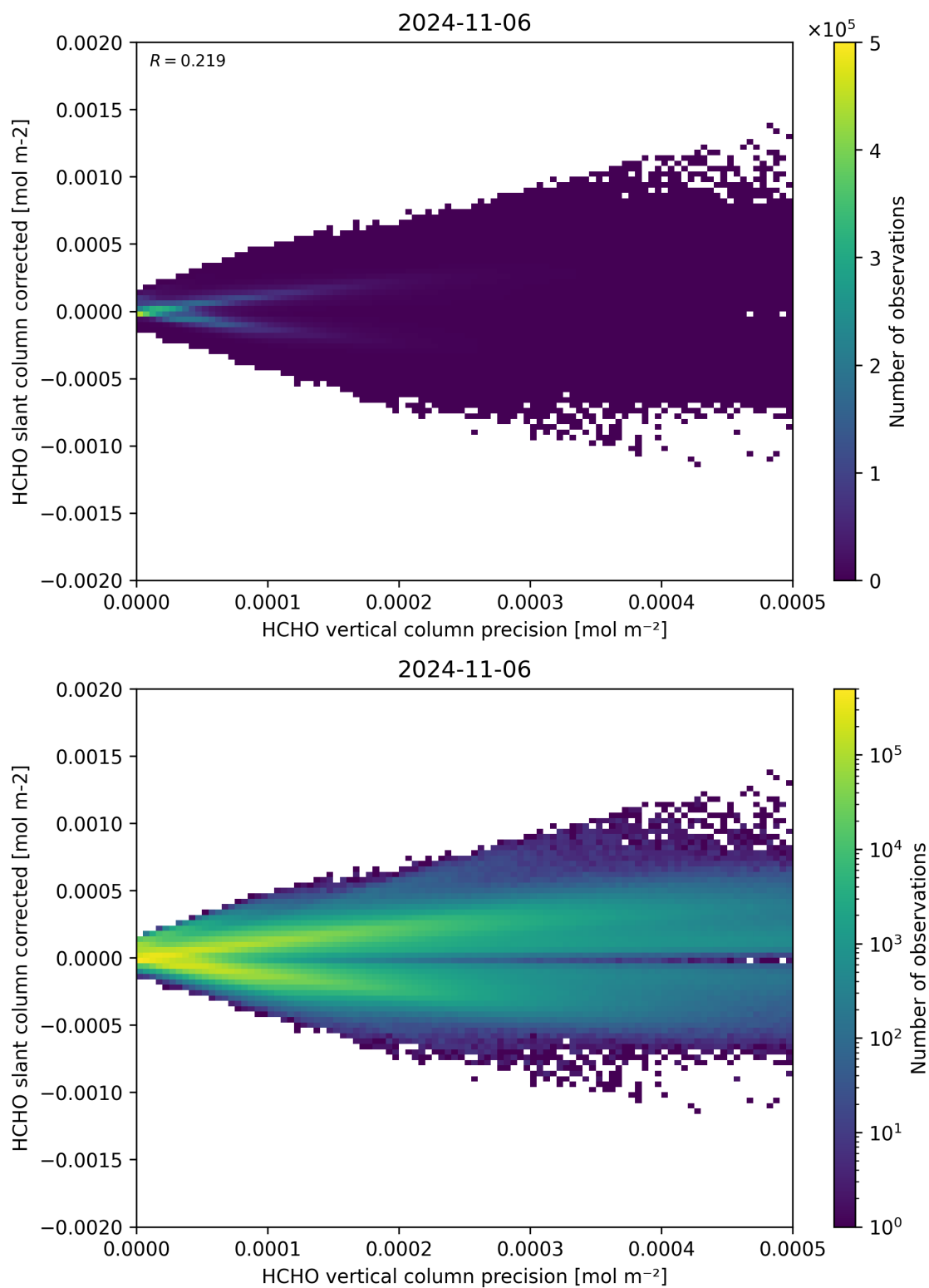
Figure 140: Scatter density plot of “HCHO vertical column precision” against “HCHO slant column corrected” for 2024-11-05 to 2024-11-07.
