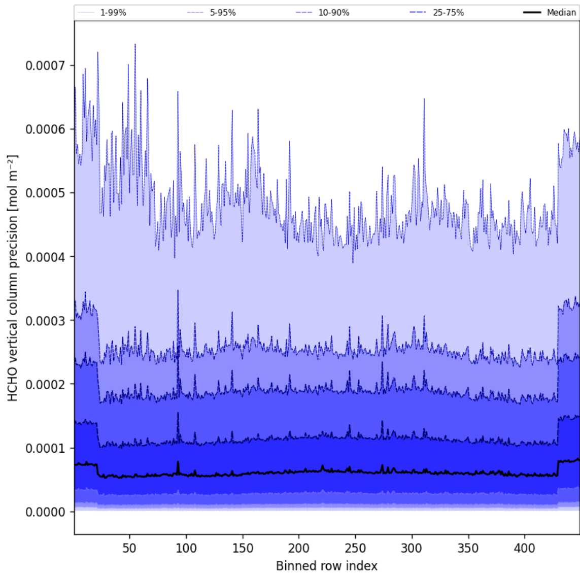
Figure 50: Along track statistics of “HCHO vertical column precision” for 2024-11-05 to 2024-11-07
