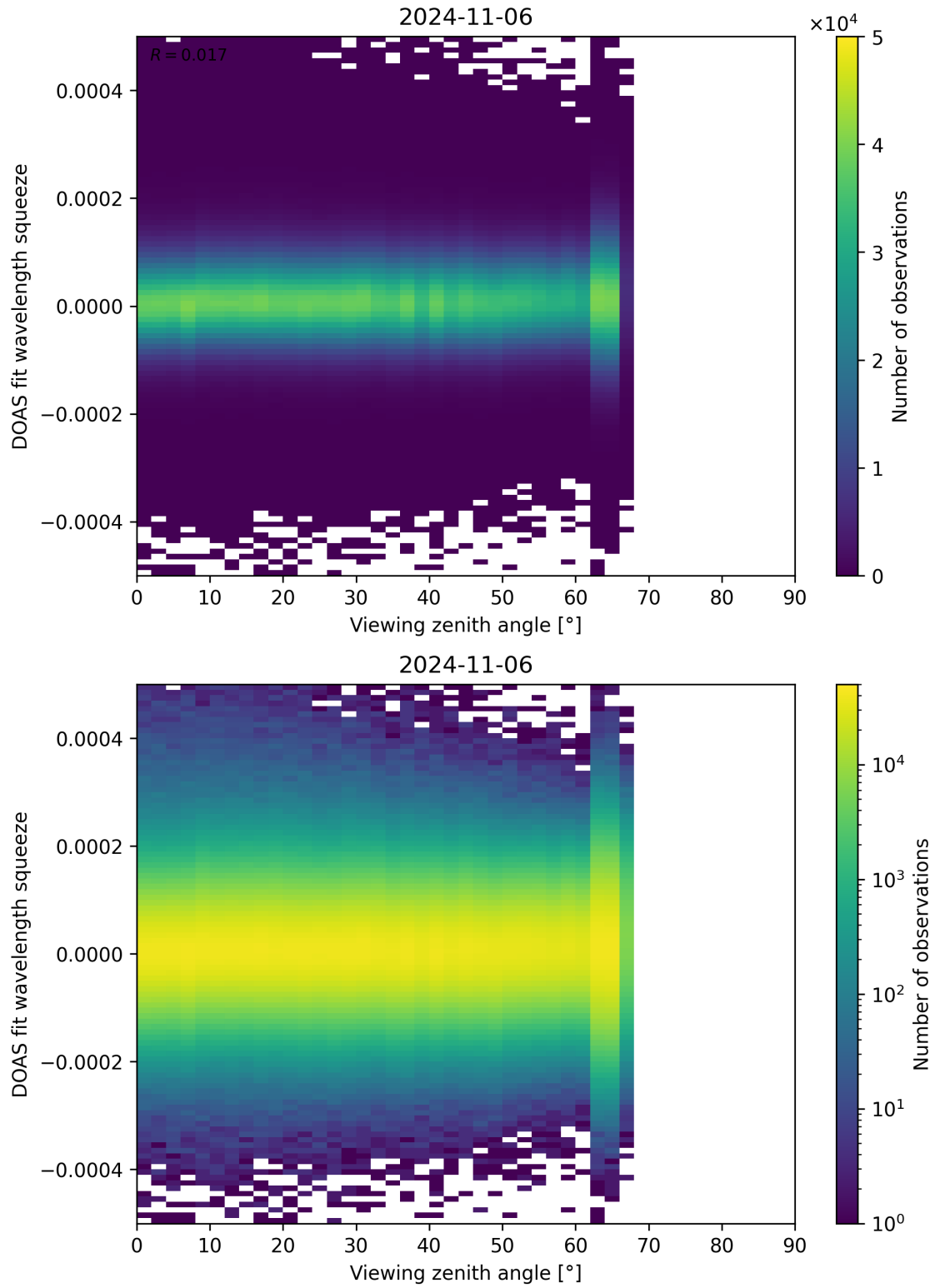
Figure 184: Scatter density plot of “Viewing zenith angle” against “DOAS fit wavelength squeeze” for 2024-11-05 to 2024-11-07.
