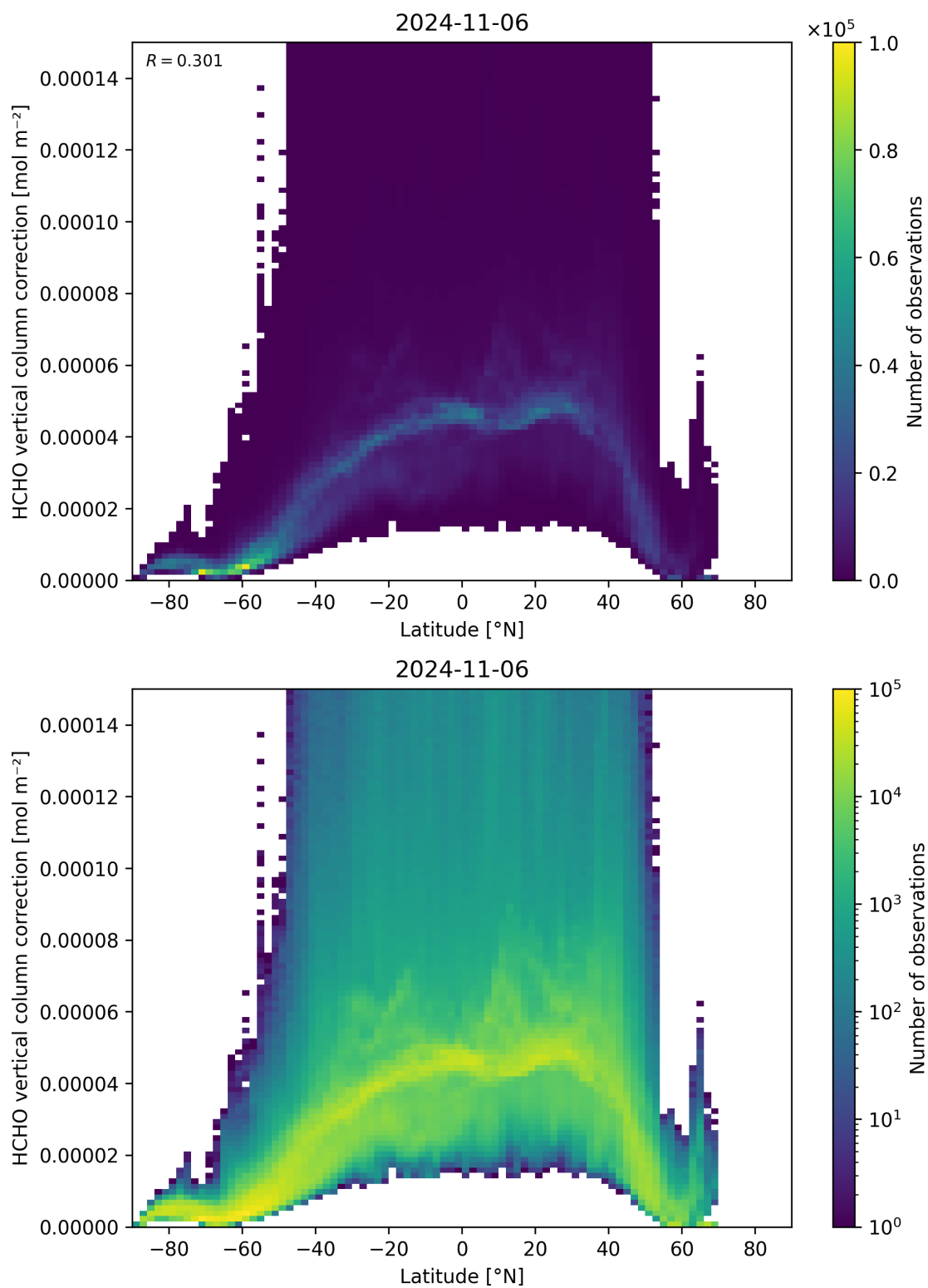
Figure 164: Scatter density plot of “Latitude” against “HCHO vertical column correction” for 2024-11-05 to 2024-11-07.
