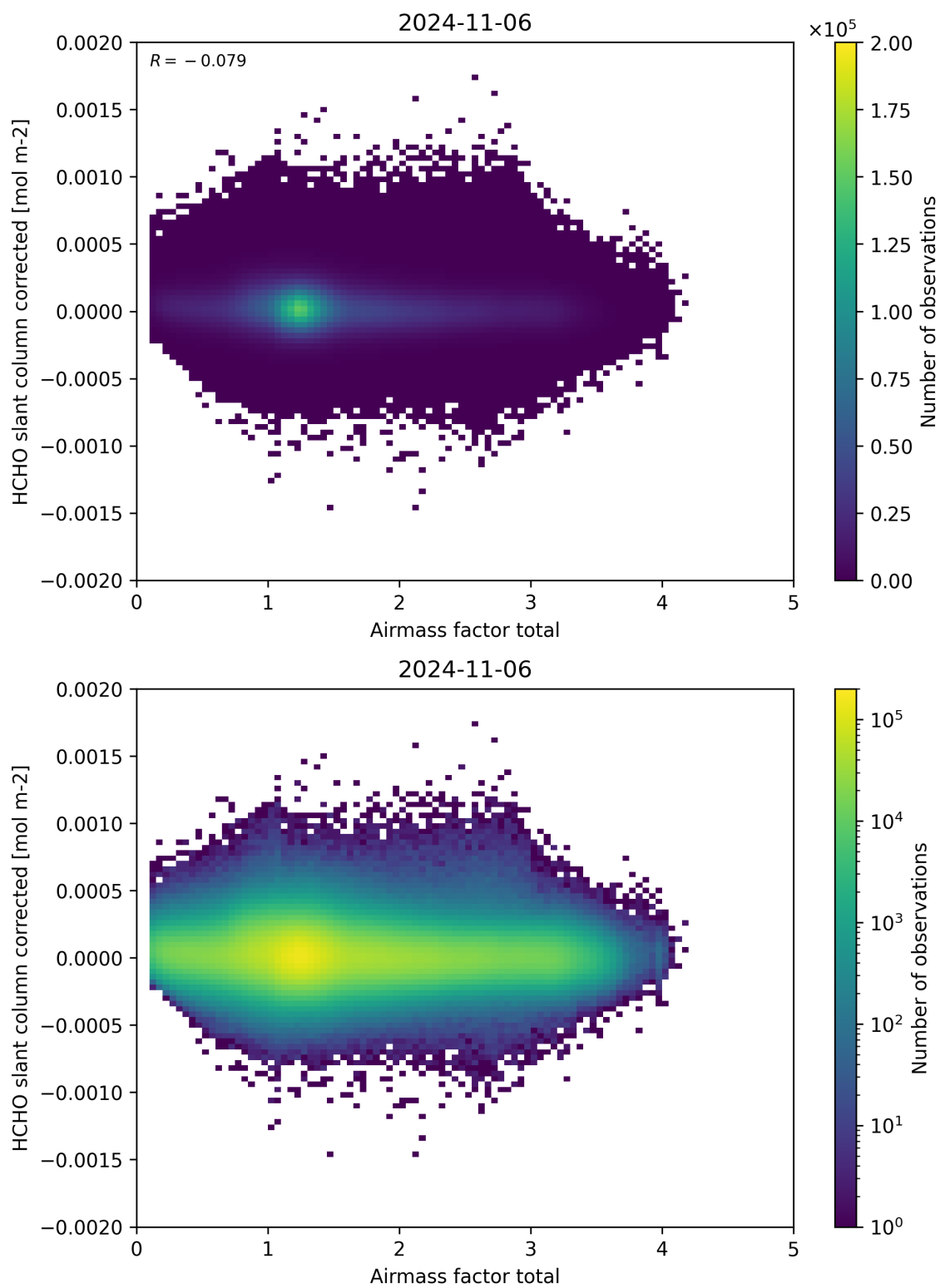
Figure 101: Scatter density plot of “Airmass factor total” against “HCHO slant column corrected” for 2024-11-05 to 2024-11-07.
