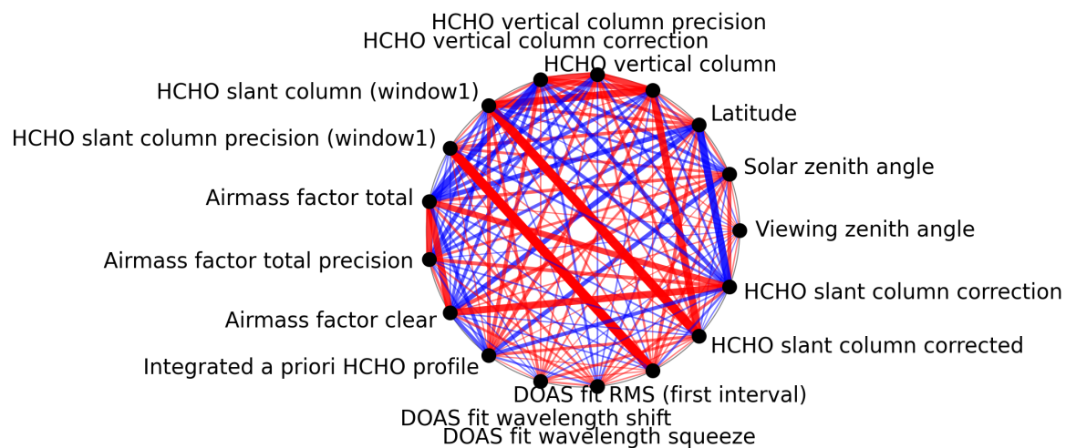
Figure 1: Map of correlation graph for 2024-11-05 to 2024-11-07.
