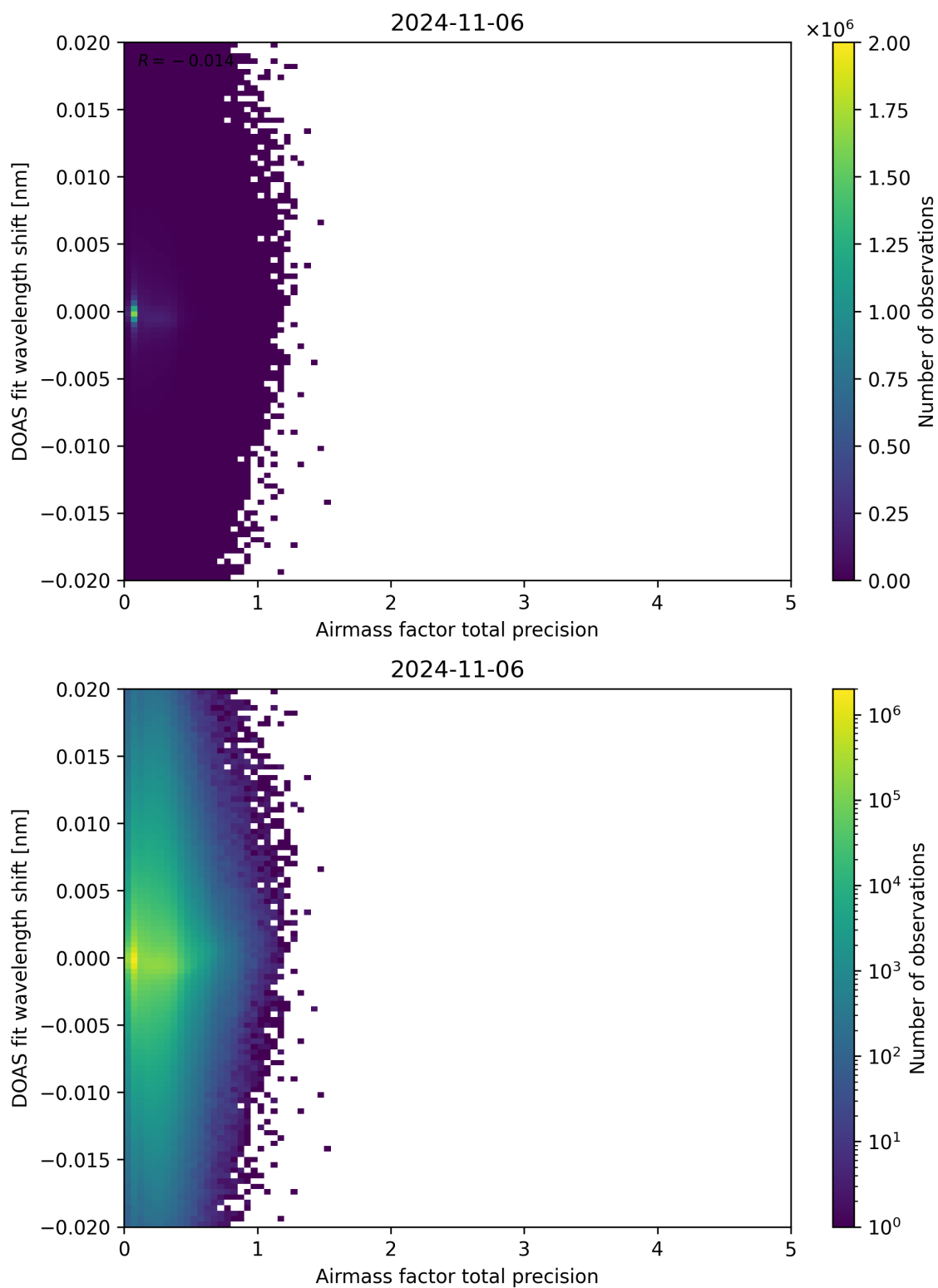
Figure 106: Scatter density plot of “Airmass factor total precision” against “DOAS fit wavelength shift” for 2024-11-05 to 2024-11-07.
