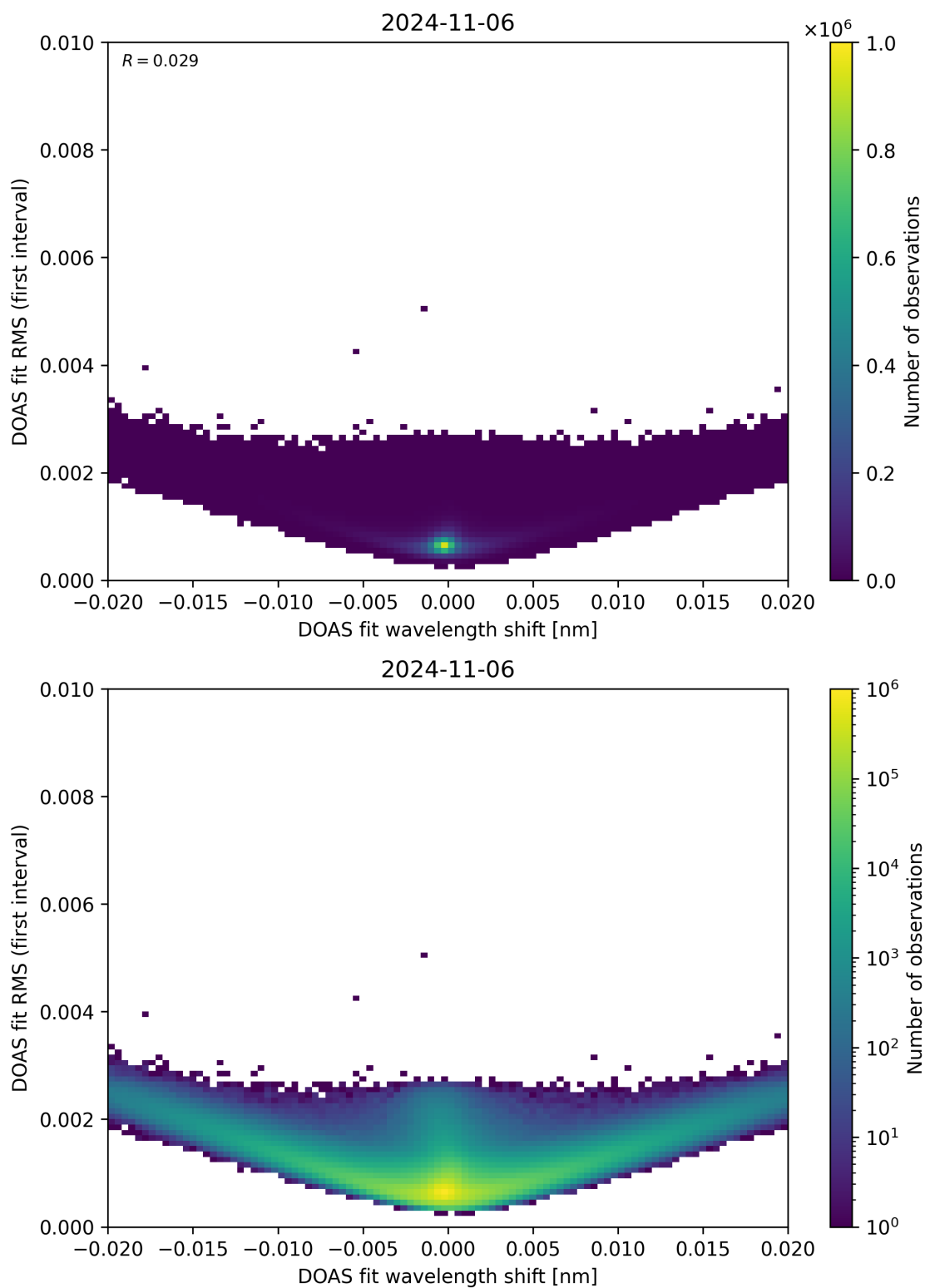
Figure 64: Scatter density plot of “DOAS fit wavelength shift” against “DOAS fit RMS (first interval)” for 2024-11-05 to 2024-11-07.
