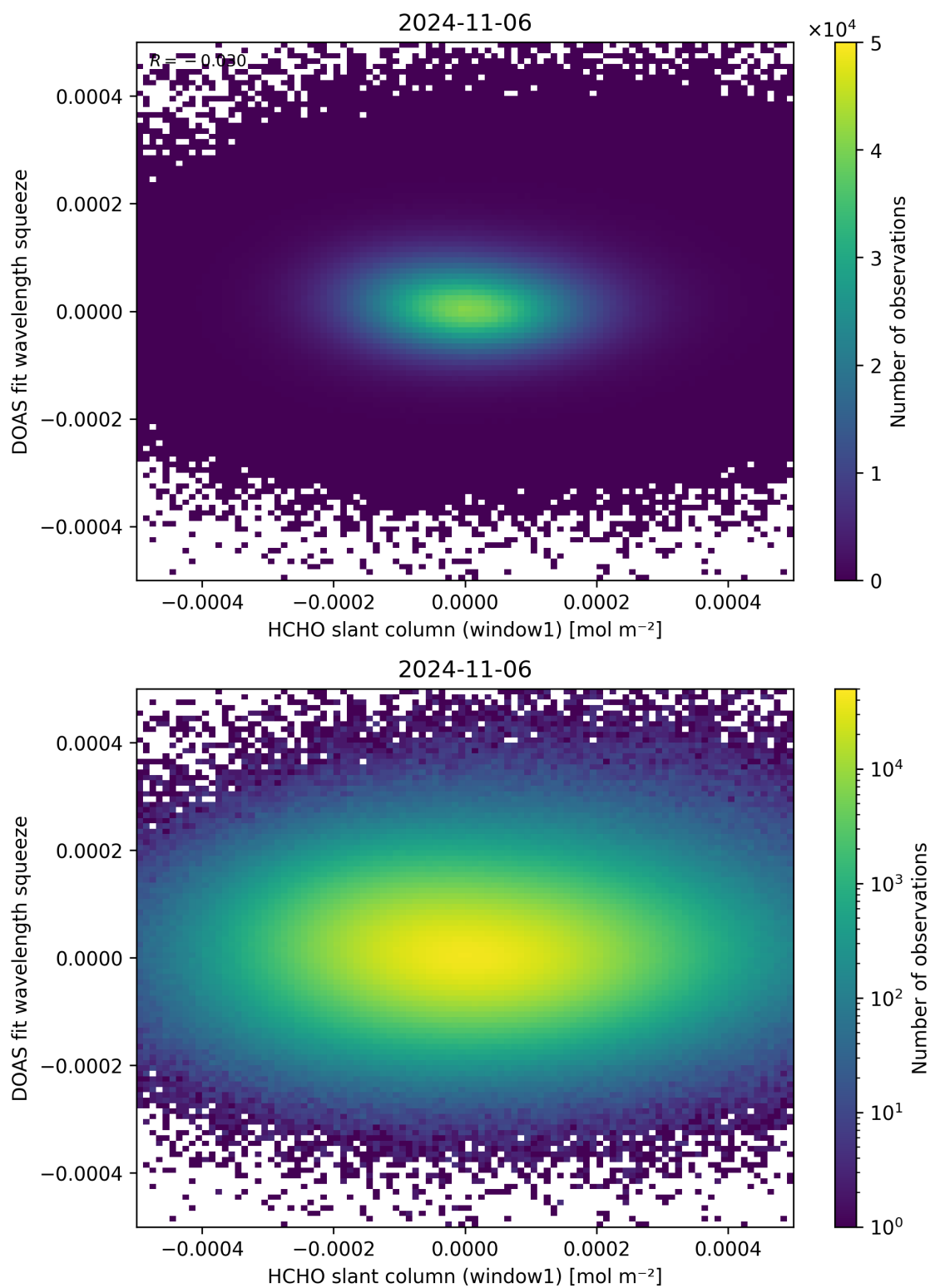
Figure 80: Scatter density plot of “HCHO slant column (window1)” against “DOAS fit wavelength squeeze” for 2024-11-05 to 2024-11-07.
