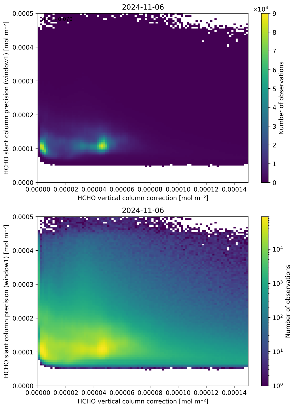
Figure 119: Scatter density plot of “HCHO vertical column correction” against “HCHO slant column precision (window1)” for 2024-11-05 to 2024-11-07.
