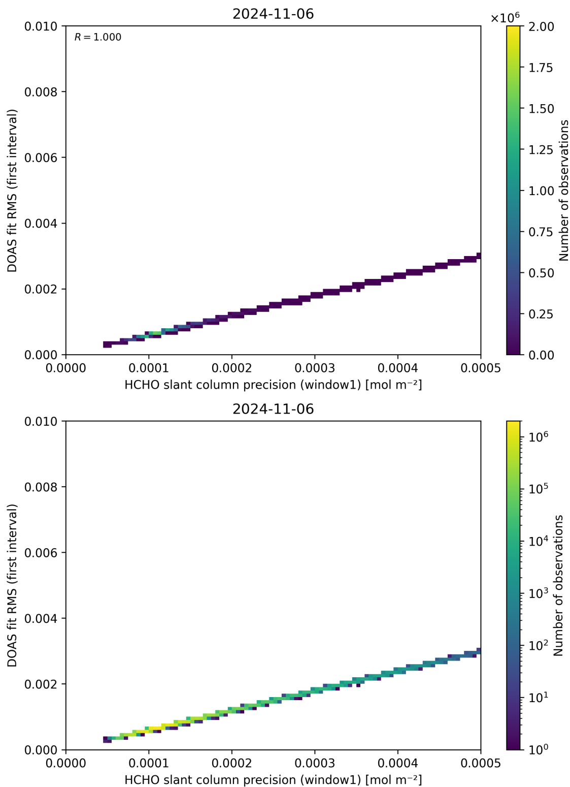
Figure 88: Scatter density plot of “HCHO slant column precision (window1)” against “DOAS fit RMS (first interval)” for 2024-11-05 to 2024-11-07.
