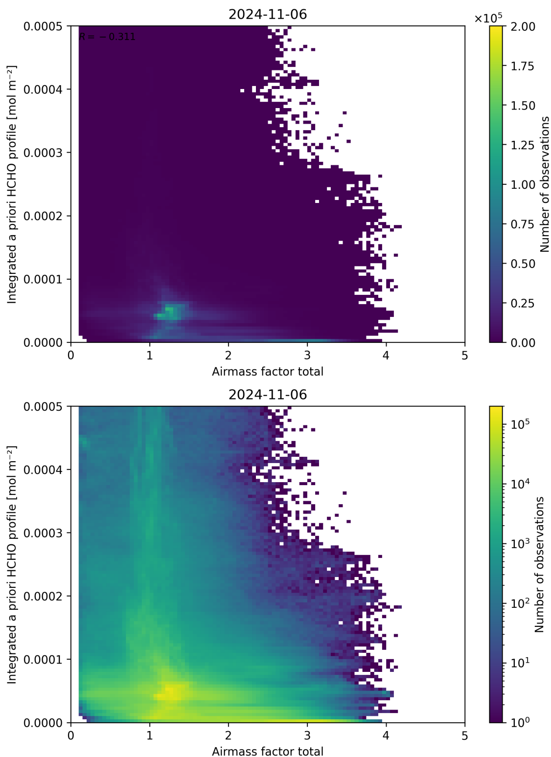
Figure 104: Scatter density plot of “Airmass factor total” against “Integrated a priori HCHO profile” for 2024-11-05 to 2024-11-07.
