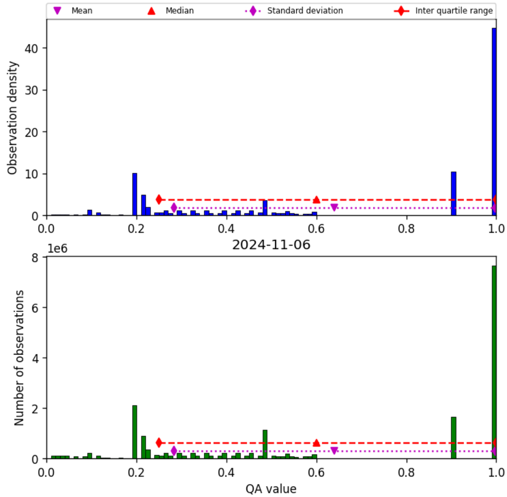
Figure 34: Histogram of “QA value” for 2024-11-05 to 2024-11-07
