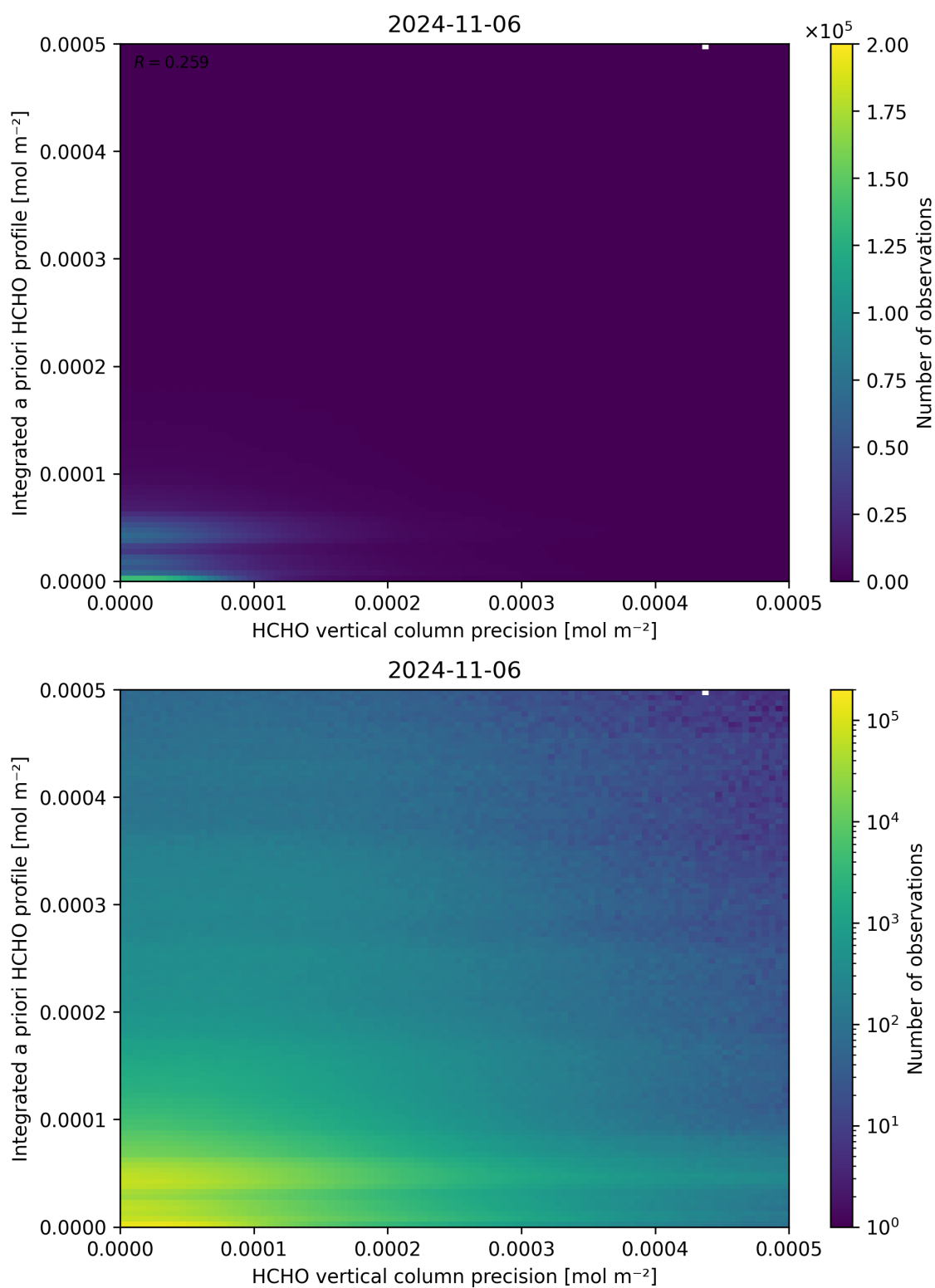
Figure 147: Scatter density plot of “HCHO vertical column precision” against “Integrated a priori HCHO profile” for 2024-11-05 to 2024-11-07.
