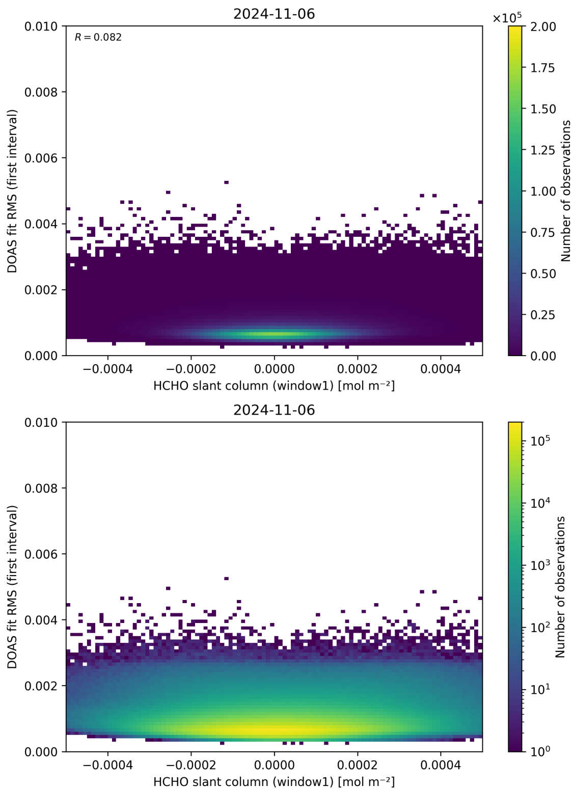
Figure 78: Scatter density plot of “HCHO slant column (window1)” against “DOAS fit RMS (first interval)” for 2024-11-05 to 2024-11-07.
