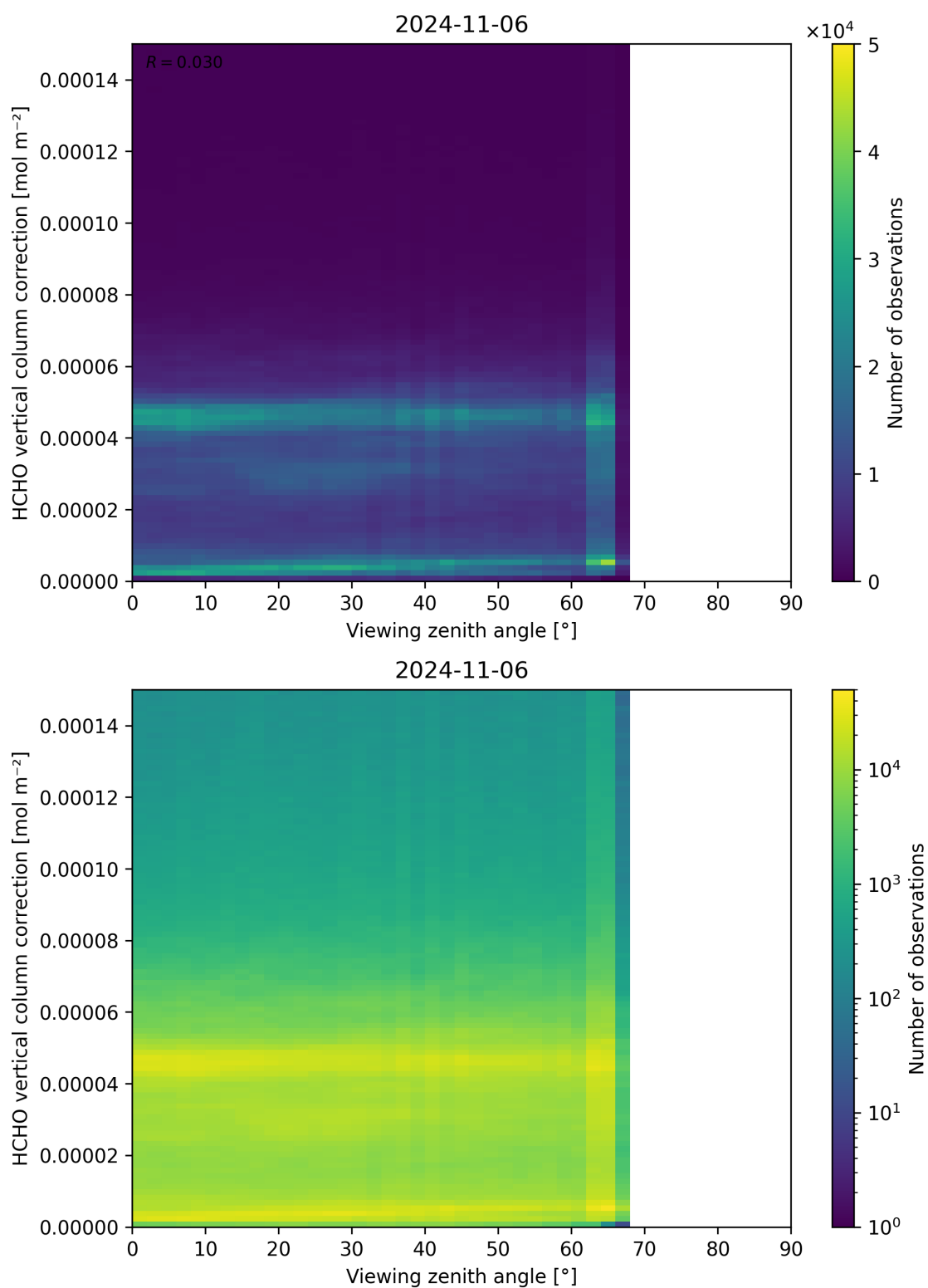
Figure 193: Scatter density plot of “Viewing zenith angle” against “HCHO vertical column correction” for 2024-11-05 to 2024-11-07.
