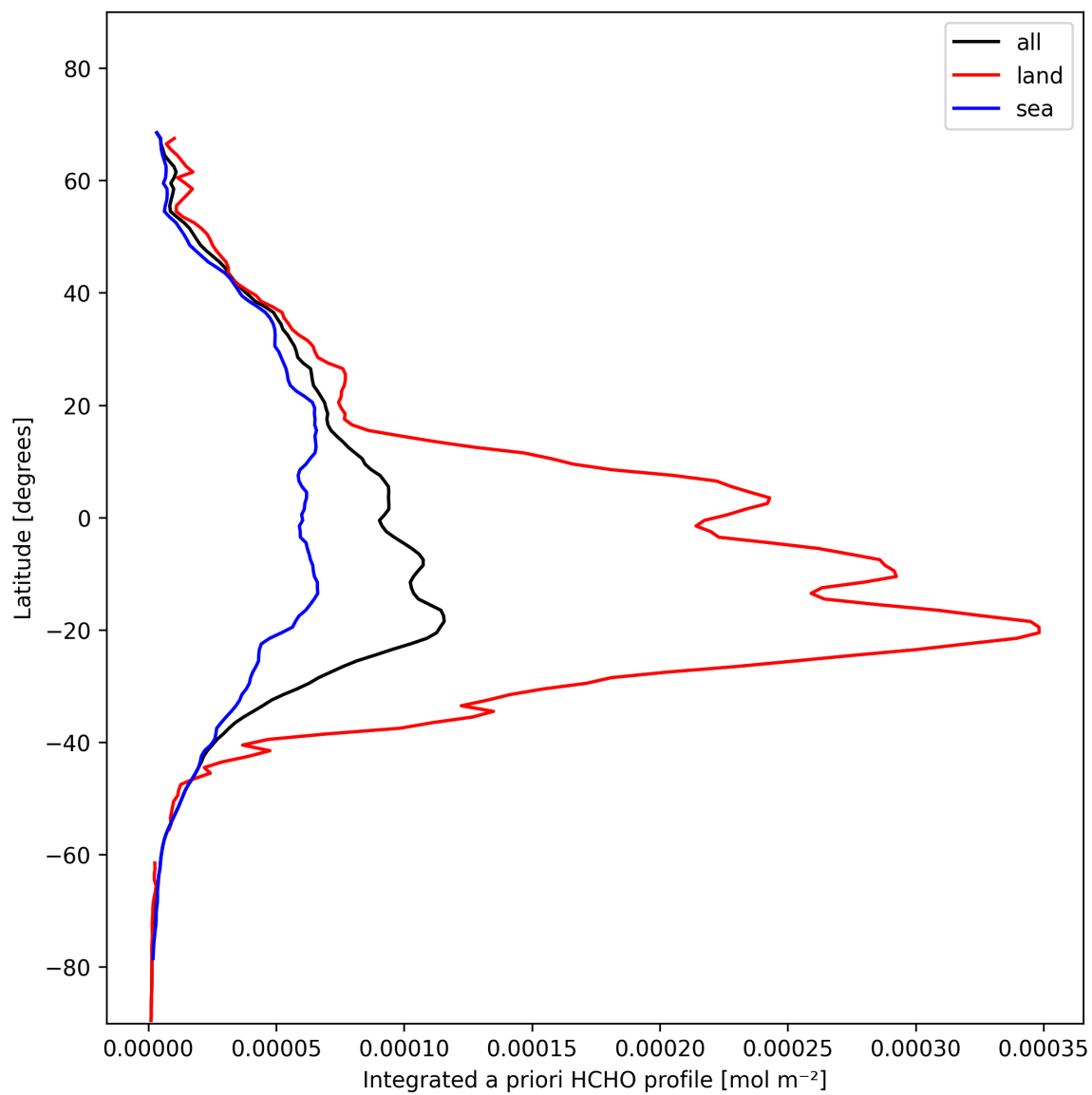
Figure 29: Zonal average of “Integrated a priori HCHO profile” for 2024-11-05 to 2024-11-07.
