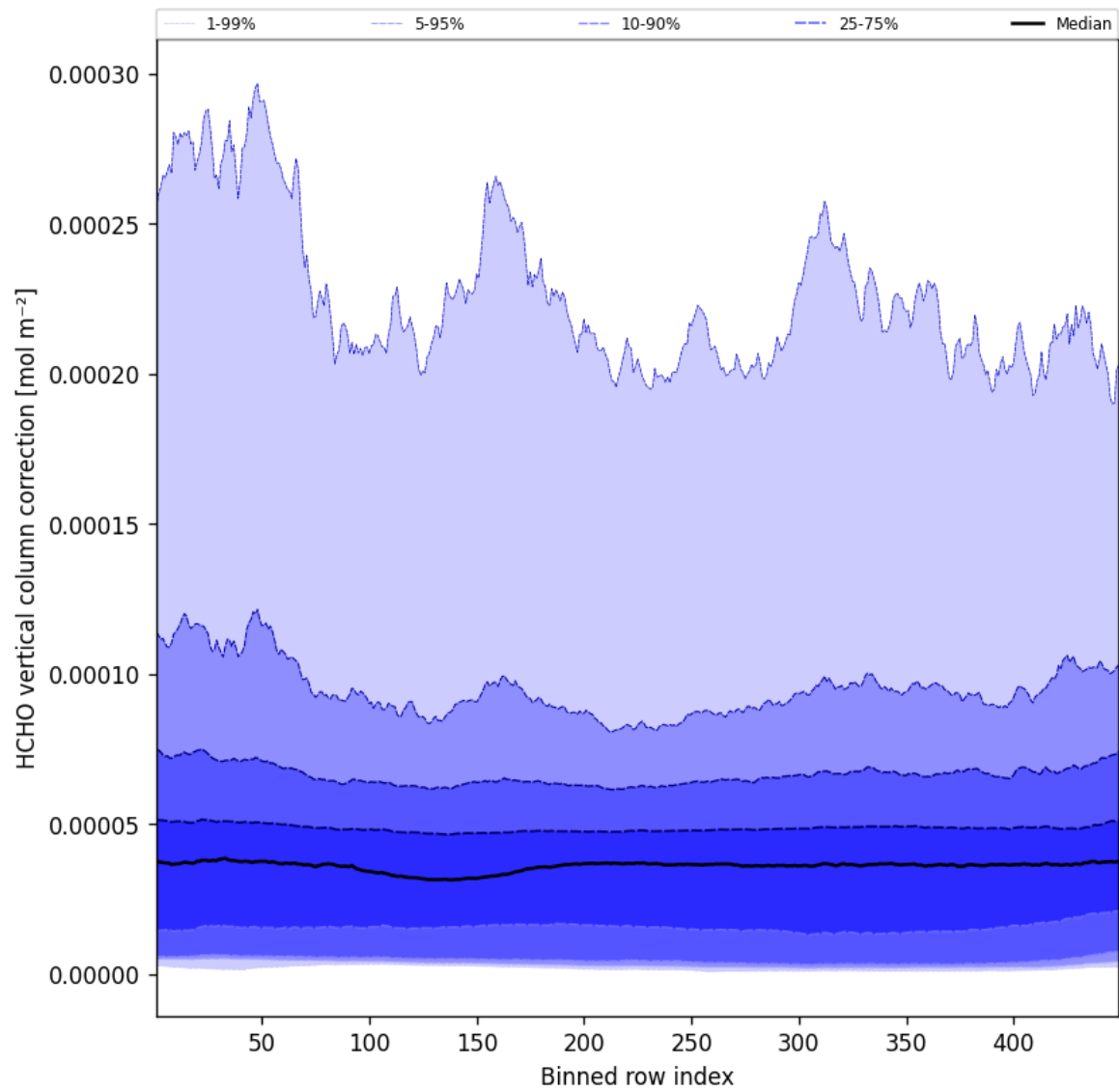
Figure 51: Along track statistics of “HCHO vertical column correction” for 2024-11-05 to 2024-11-07
