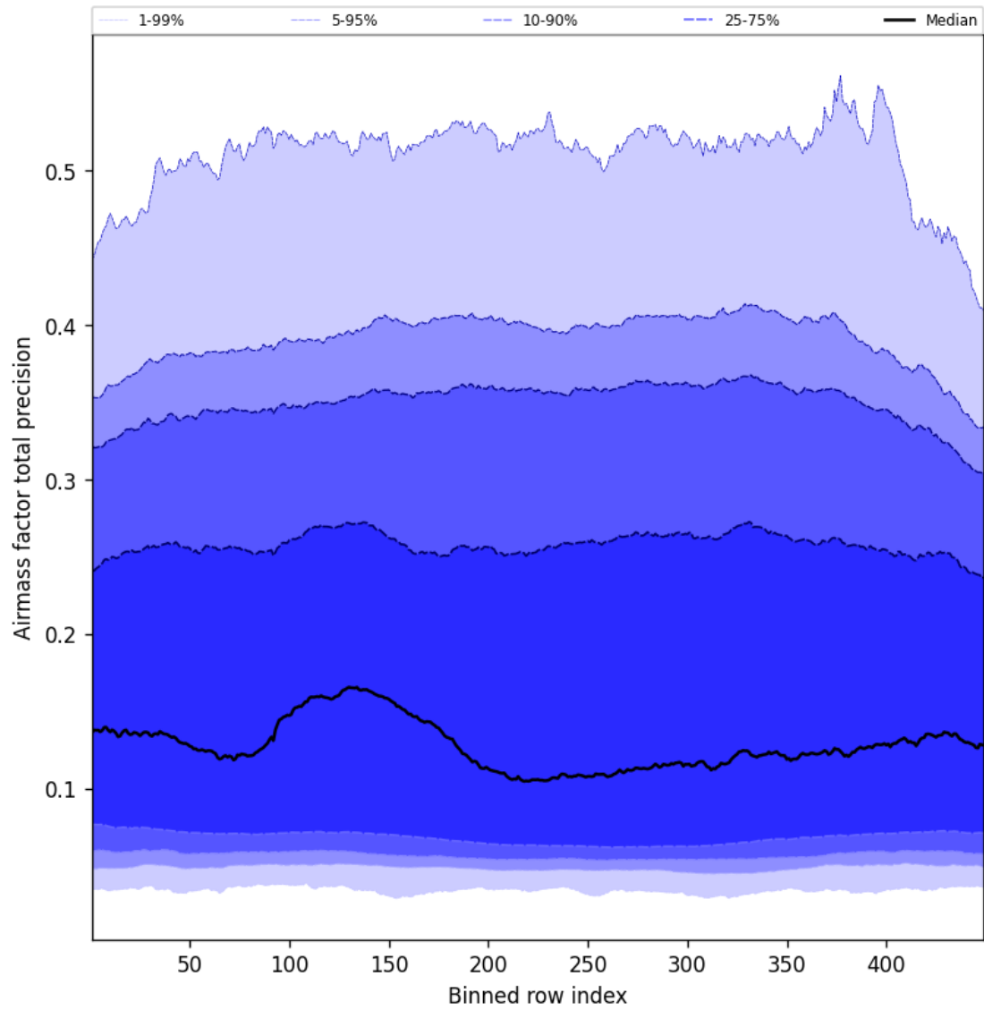
Figure 55: Along track statistics of “Airmass factor total precision” for 2024-11-05 to 2024-11-07
