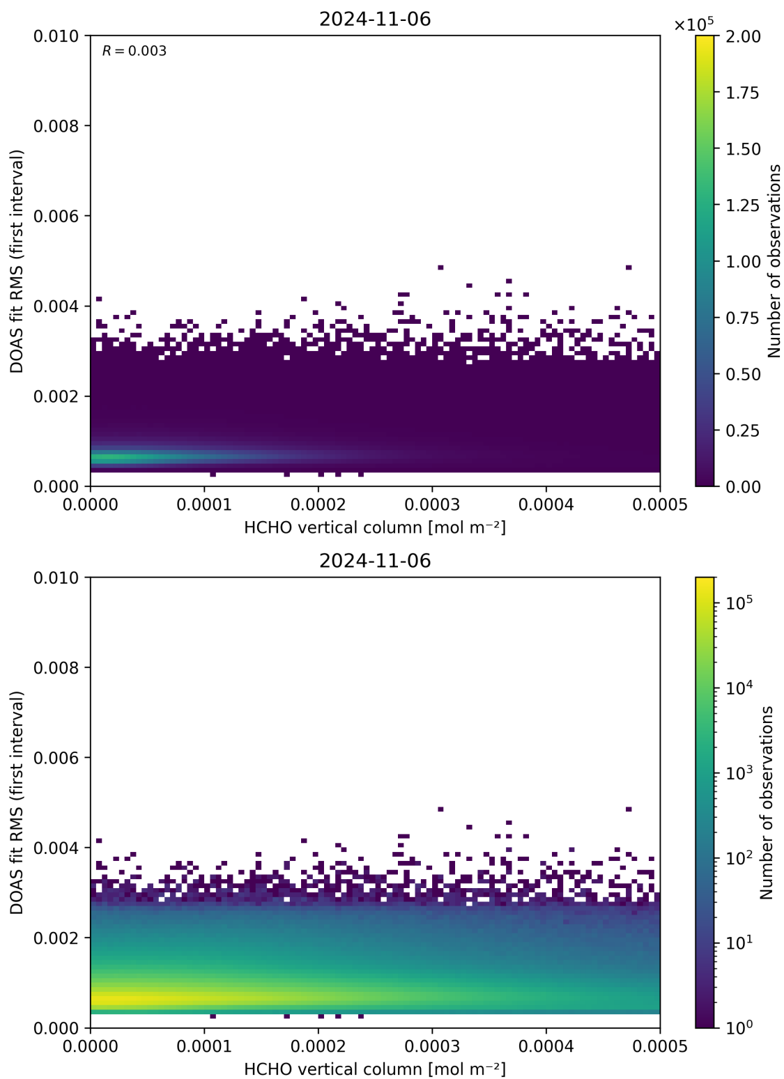
Figure 123: Scatter density plot of “HCHO vertical column” against “DOAS fit RMS (first interval)” for 2024-11-05 to 2024-11-07.
