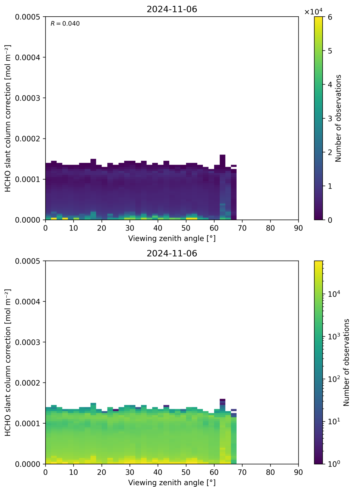
Figure 187: Scatter density plot of “Viewing zenith angle” against “HCHO slant column correction” for 2024-11-05 to 2024-11-07.
