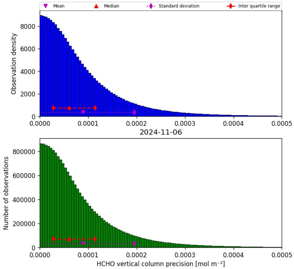
Figure 36: Histogram of “HCHO vertical column precision” for 2024-11-05 to 2024-11-07
