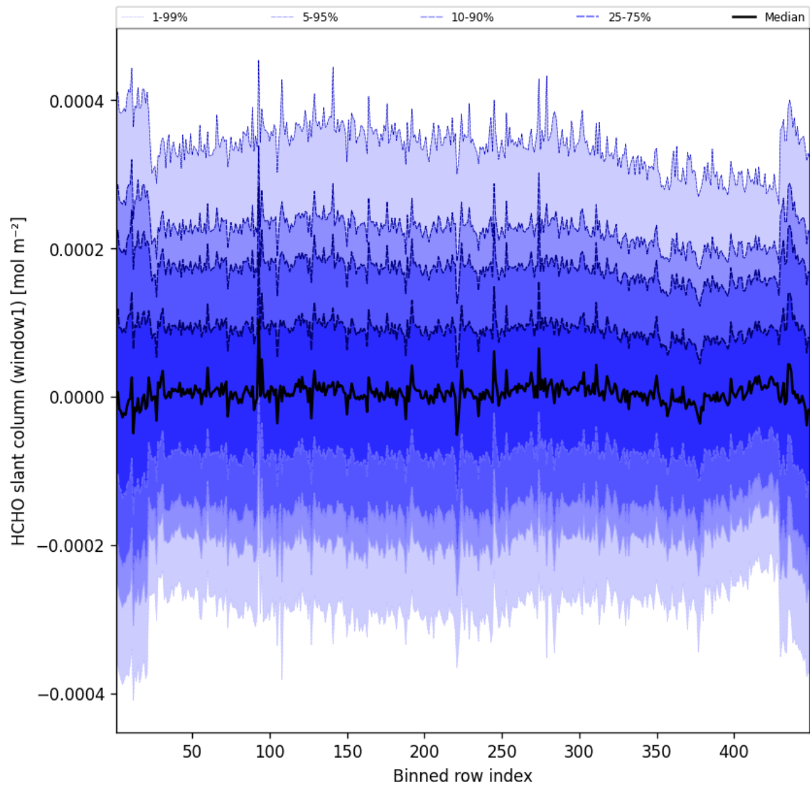
Figure 52: Along track statistics of “HCHO slant column (window1)” for 2024-11-05 to 2024-11-07
