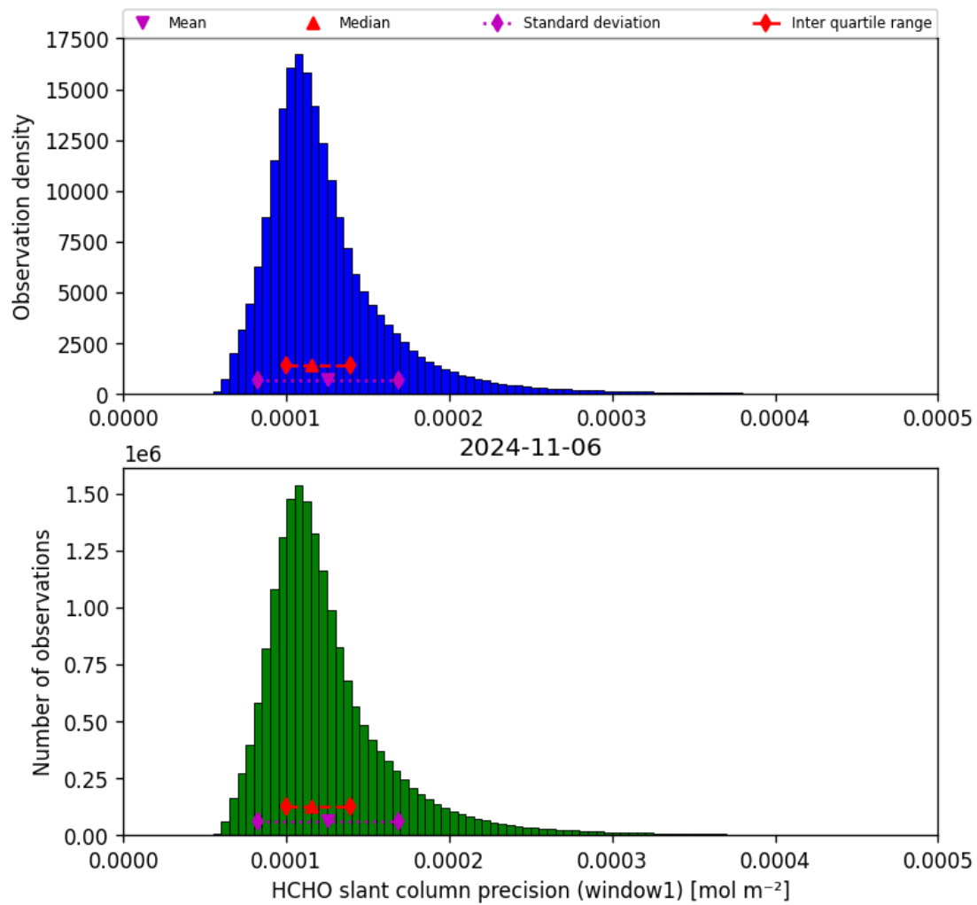
Figure 39: Histogram of “HCHO slant column precision (window1)” for 2024-11-05 to 2024-11-07
