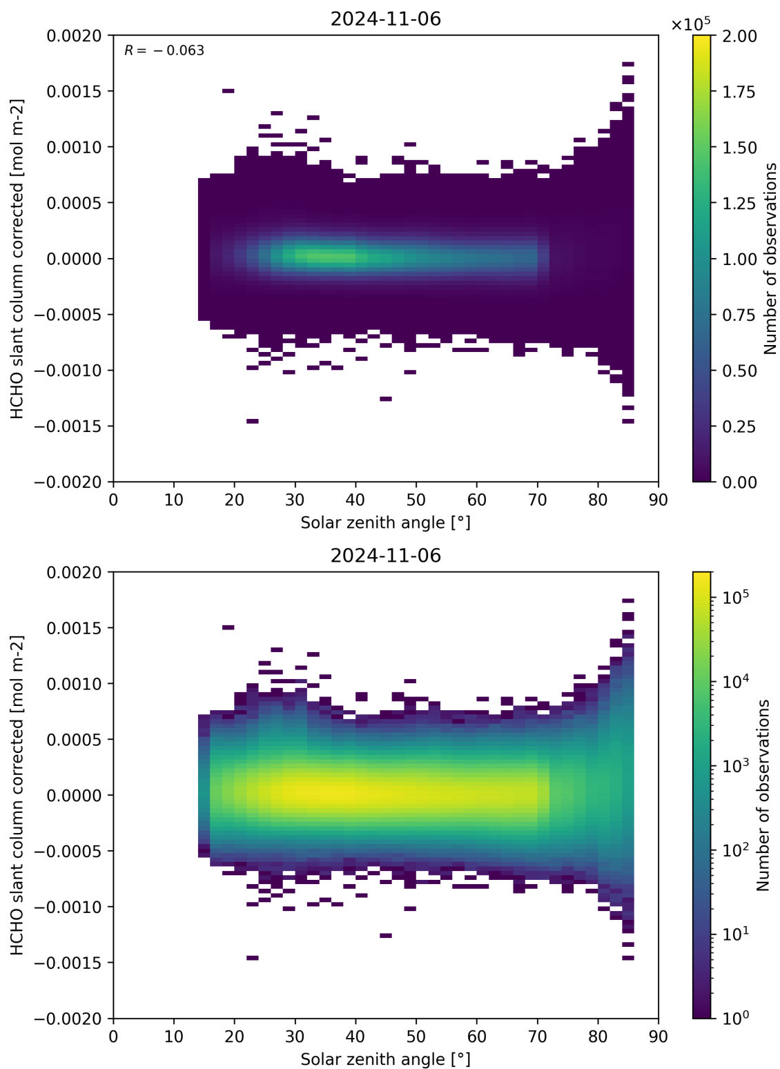
Figure 171: Scatter density plot of “Solar zenith angle” against “HCHO slant column corrected” for 2024-11-05 to 2024-11-07.
