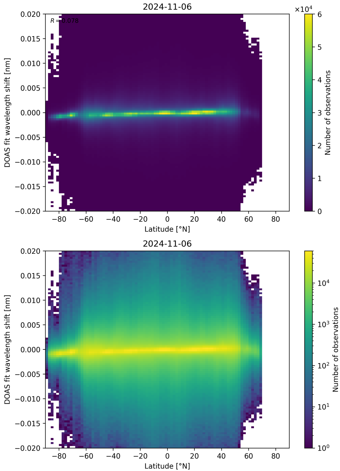
Figure 154: Scatter density plot of “Latitude” against “DOAS fit wavelength shift” for 2024-11-05 to 2024-11-07.
