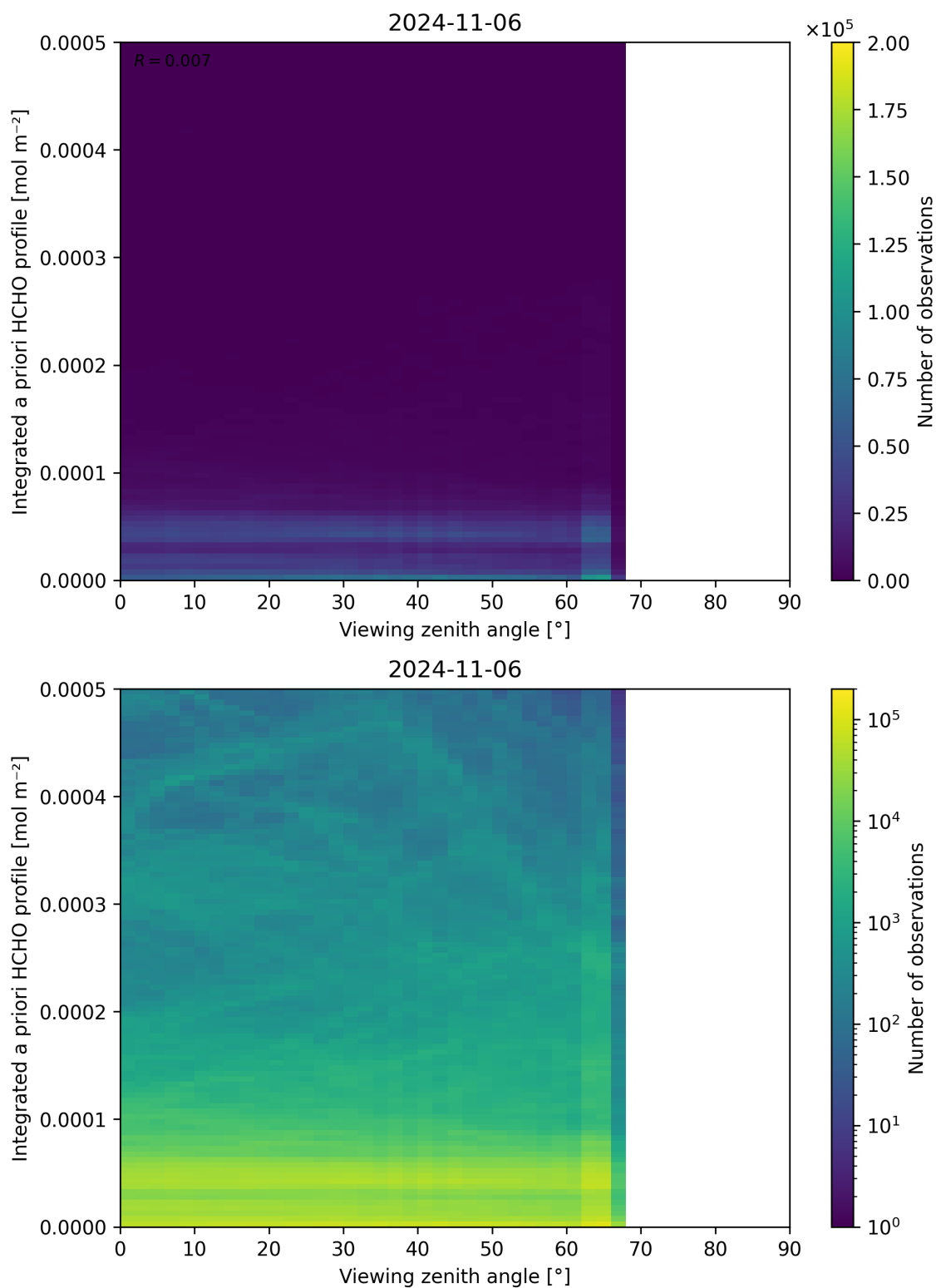
Figure 195: Scatter density plot of “Viewing zenith angle” against “Integrated a priori HCHO profile” for 2024-11-05 to 2024-11-07.
