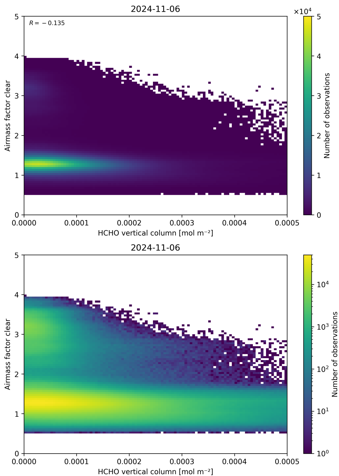
Figure 126: Scatter density plot of “HCHO vertical column” against “Airmass factor clear” for 2024-11-05 to 2024-11-07.
