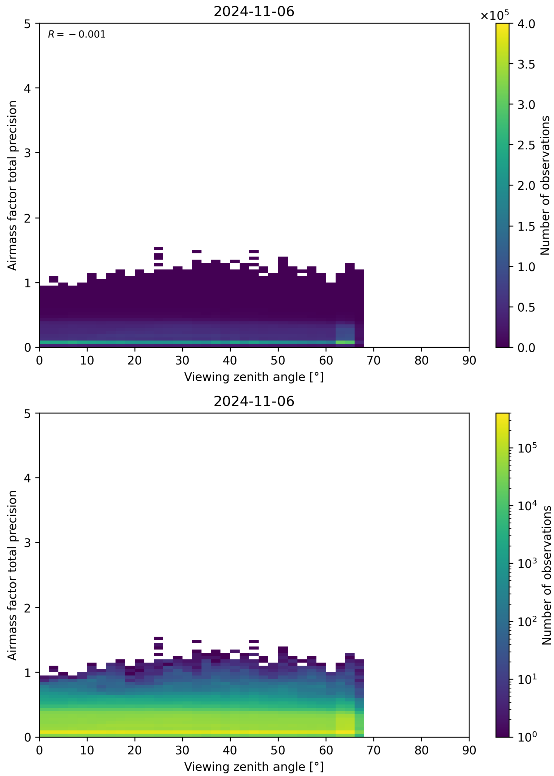
Figure 191: Scatter density plot of “Viewing zenith angle” against “Airmass factor total precision” for 2024-11-05 to 2024-11-07.
