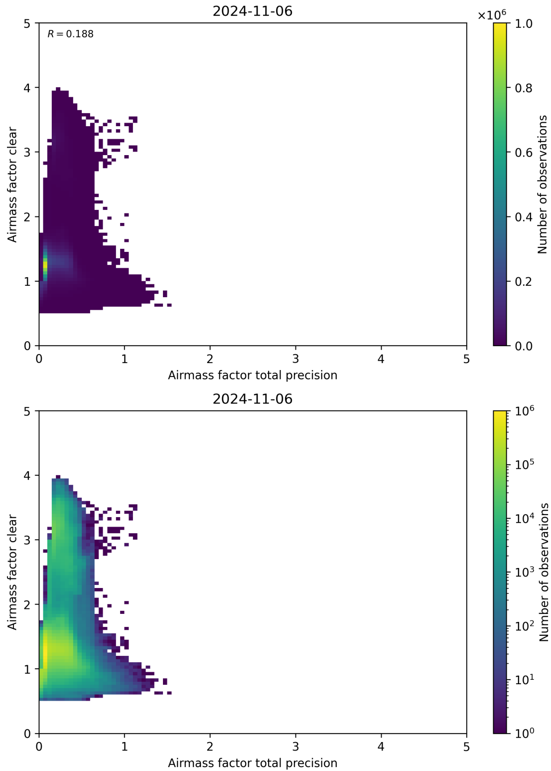
Figure 108: Scatter density plot of “Airmass factor total precision” against “Airmass factor clear” for 2024-11-05 to 2024-11-07.
