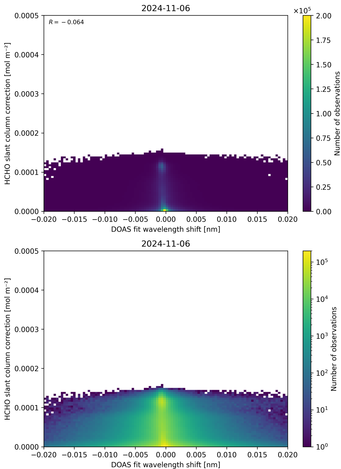
Figure 67: Scatter density plot of “DOAS fit wavelength shift” against “HCHO slant column correction” for 2024-11-05 to 2024-11-07.
