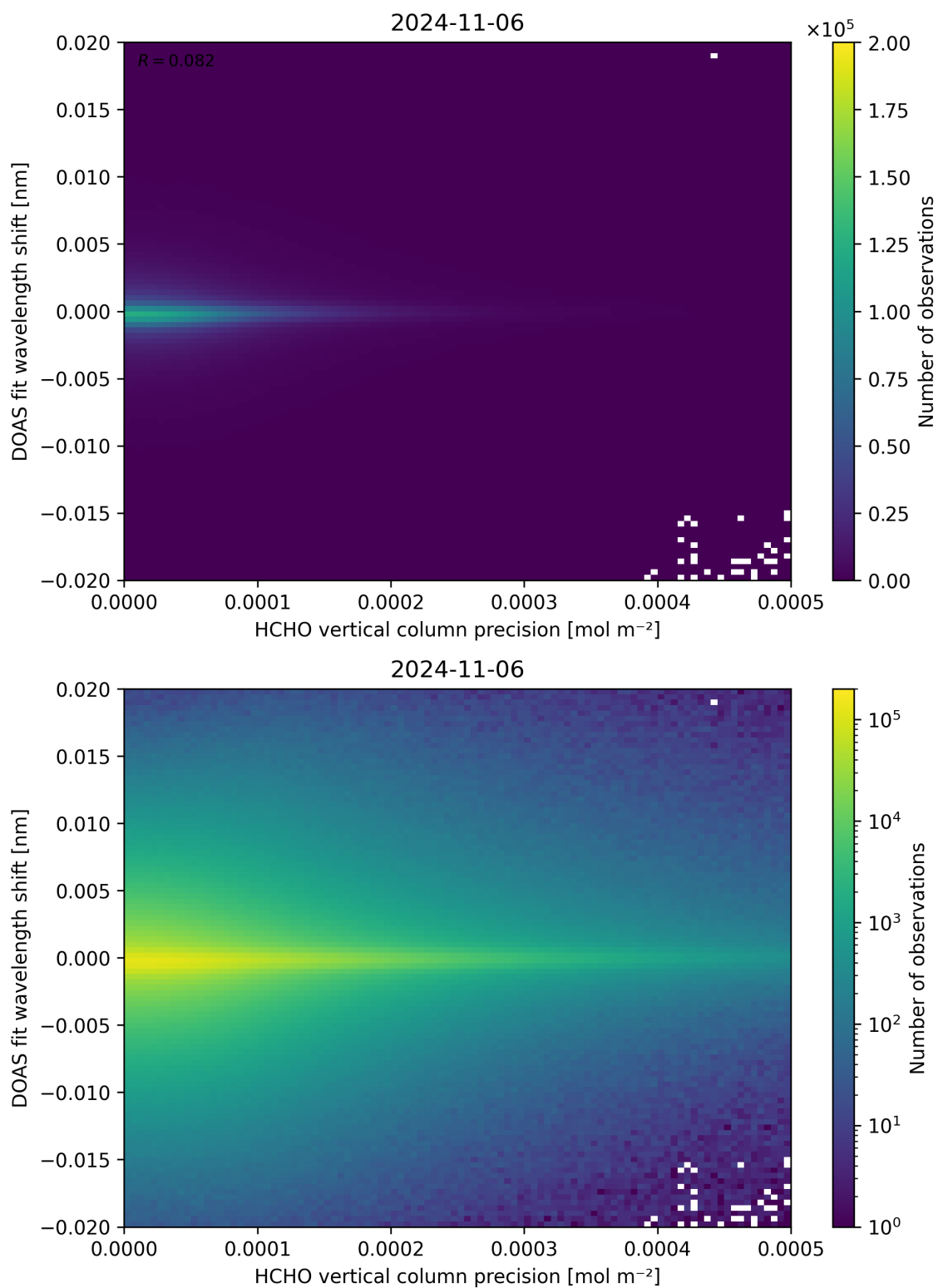
Figure 137: Scatter density plot of “HCHO vertical column precision” against “DOAS fit wavelength shift” for 2024-11-05 to 2024-11-07.
