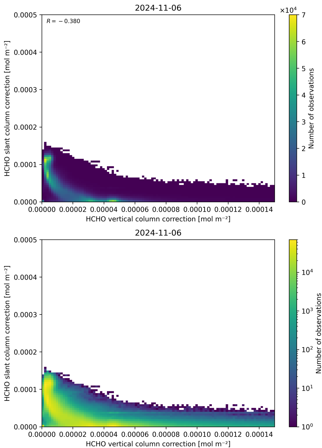
Figure 117: Scatter density plot of “HCHO vertical column correction” against “HCHO slant column correction” for 2024-11-05 to 2024-11-07.
