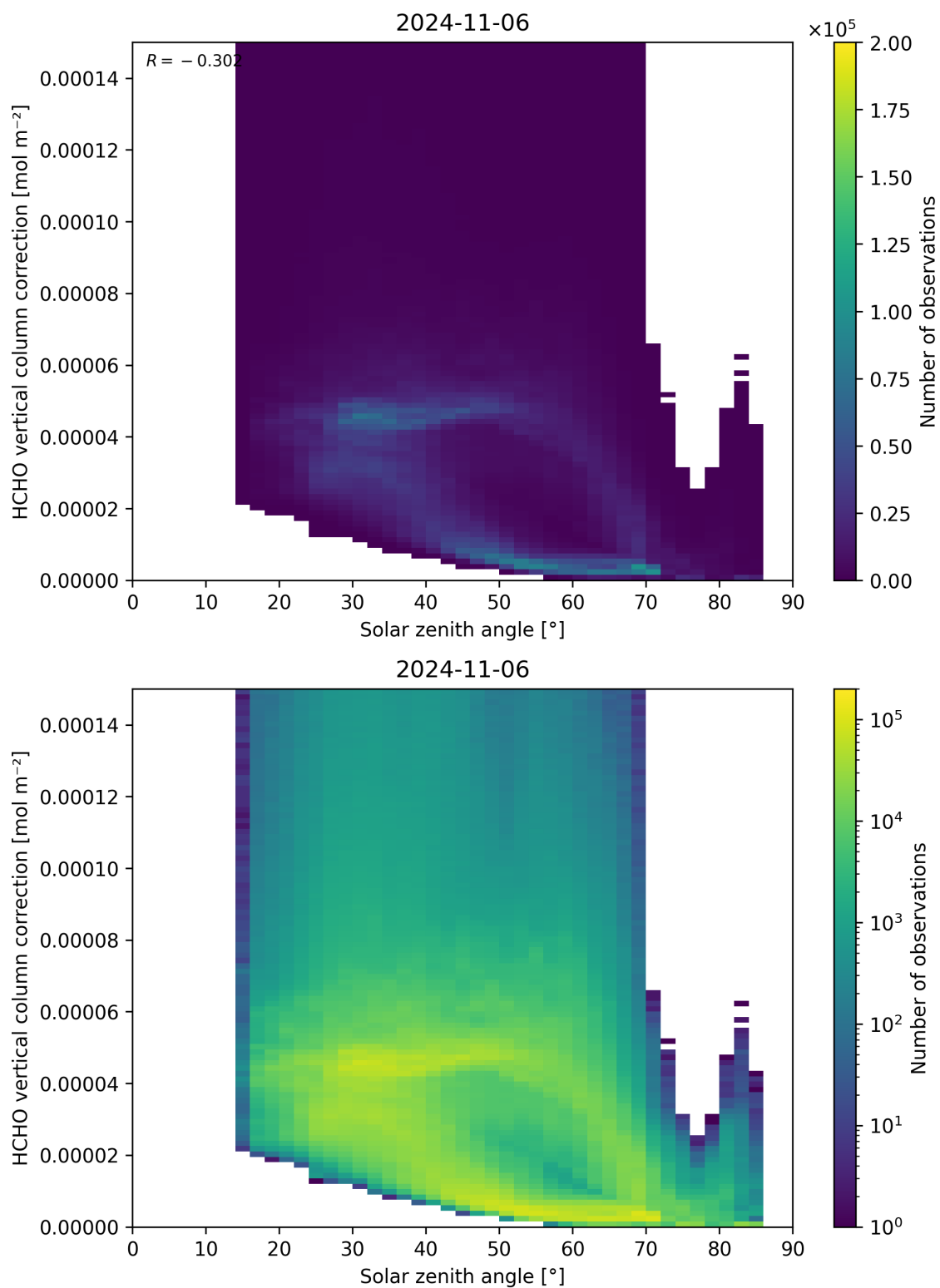
Figure 178: Scatter density plot of “Solar zenith angle” against “HCHO vertical column correction” for 2024-11-05 to 2024-11-07.
