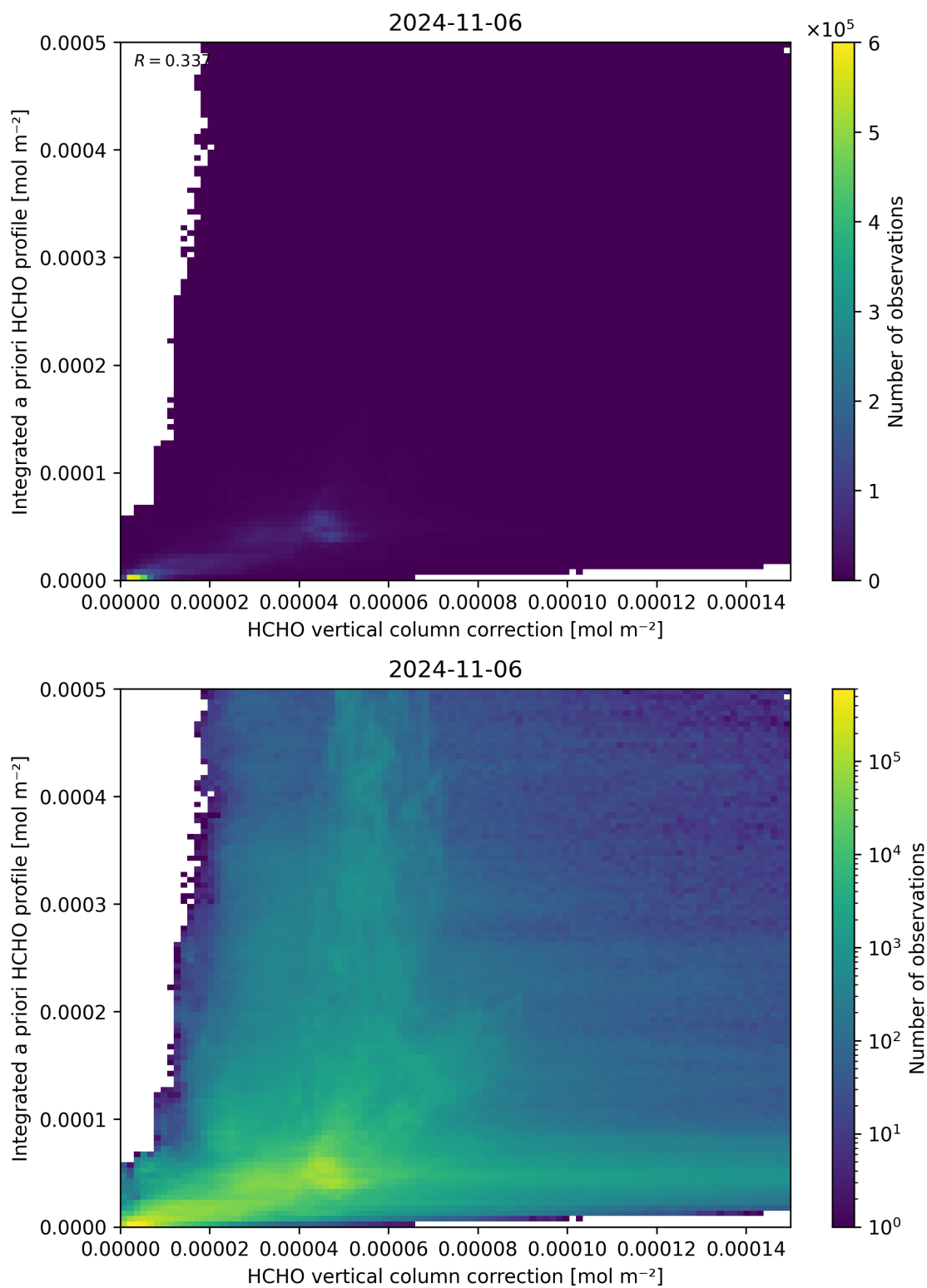
Figure 122: Scatter density plot of “HCHO vertical column correction” against “Integrated a priori HCHO profile” for 2024-11-05 to 2024-11-07.
