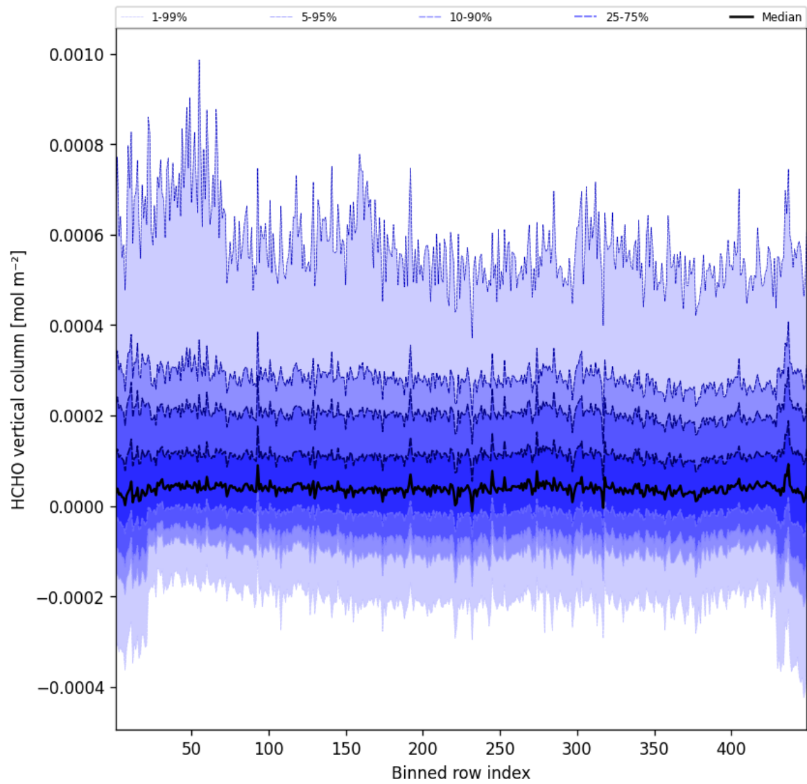
Figure 49: Along track statistics of “HCHO vertical column” for 2024-11-05 to 2024-11-07
