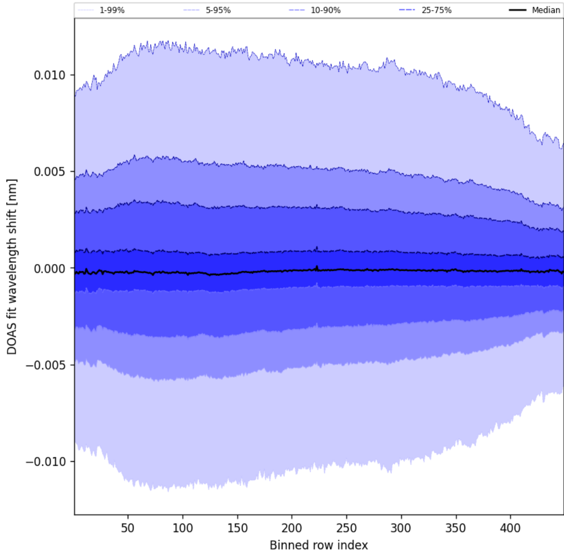
Figure 58: Along track statistics of “DOAS fit wavelength shift” for 2024-11-05 to 2024-11-07
