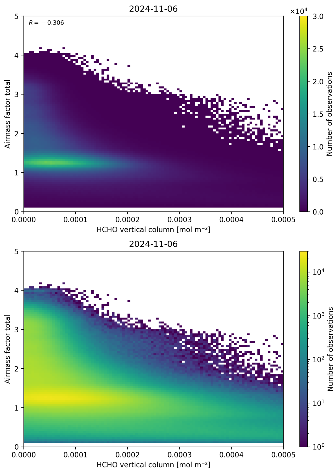
Figure 131: Scatter density plot of “HCHO vertical column” against “Airmass factor total” for 2024-11-05 to 2024-11-07.
