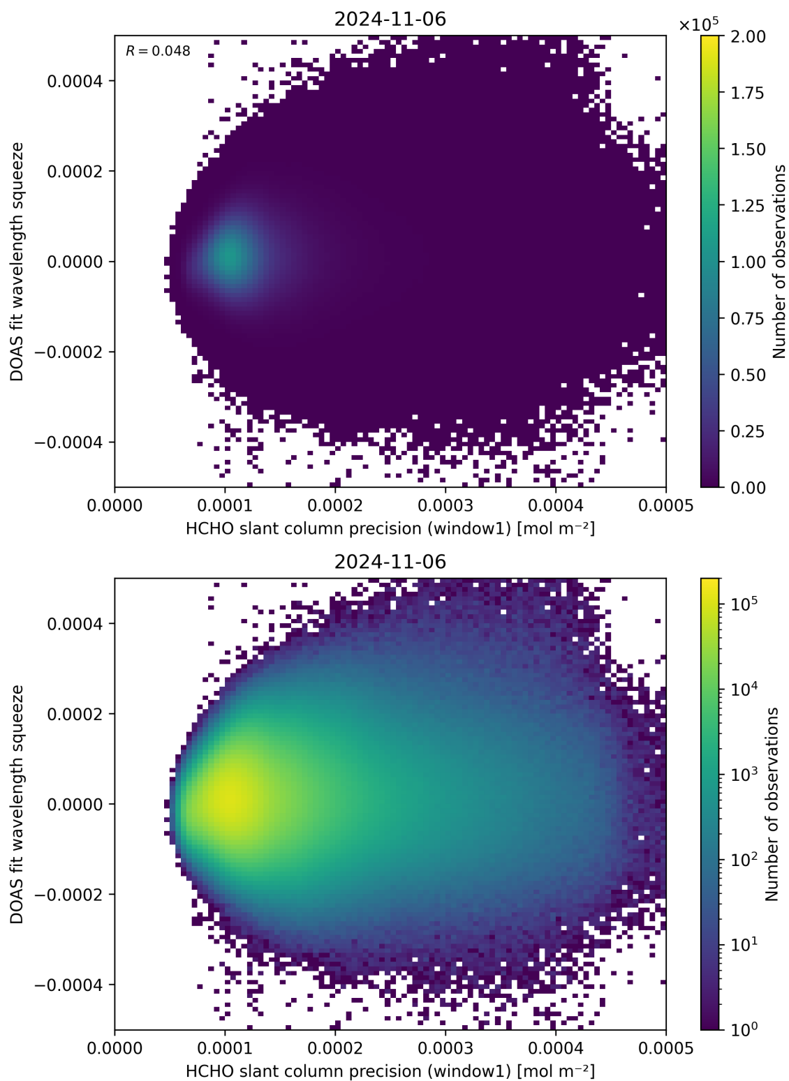
Figure 90: Scatter density plot of “HCHO slant column precision (window1)” against “DOAS fit wavelength squeeze” for 2024-11-05 to 2024-11-07.
