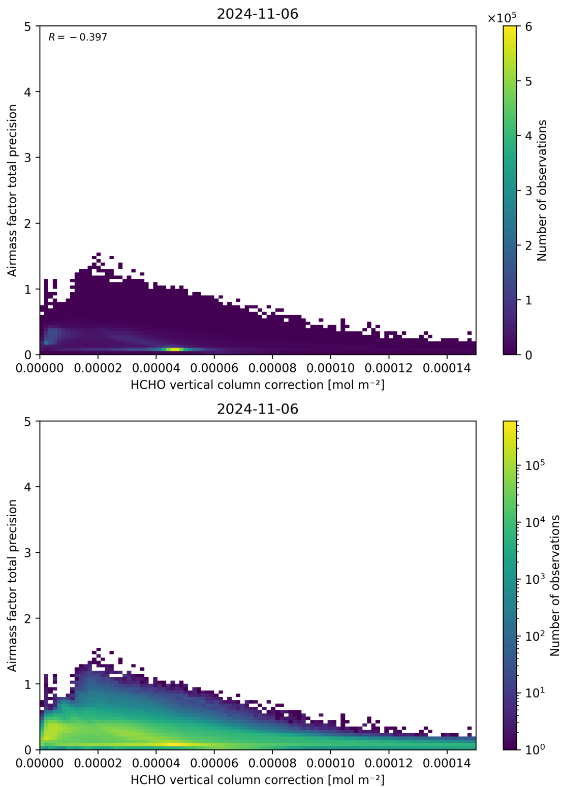
Figure 121: Scatter density plot of “HCHO vertical column correction” against “Airmass factor total precision” for 2024-11-05 to 2024-11-07.
