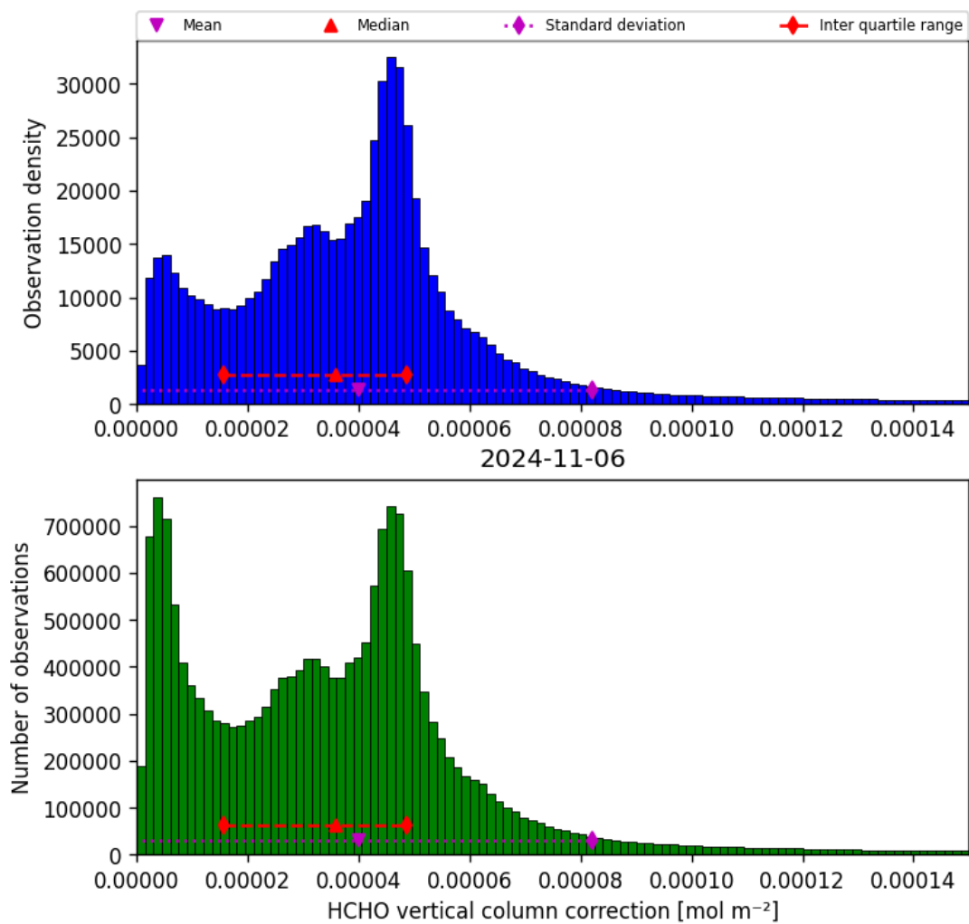
Figure 37: Histogram of “HCHO vertical column correction” for 2024-11-05 to 2024-11-07
