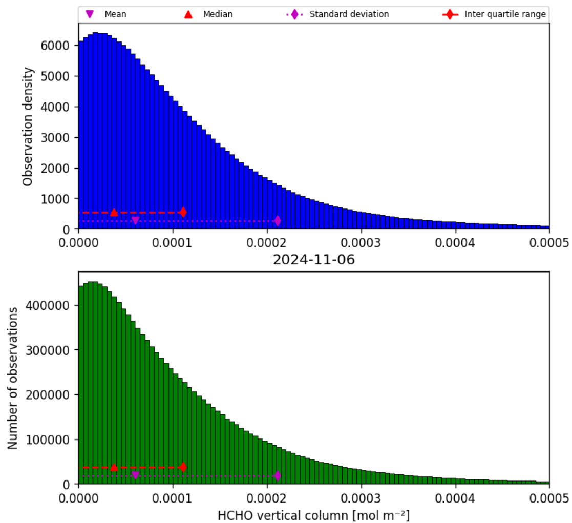
Figure 35: Histogram of “HCHO vertical column” for 2024-11-05 to 2024-11-07
