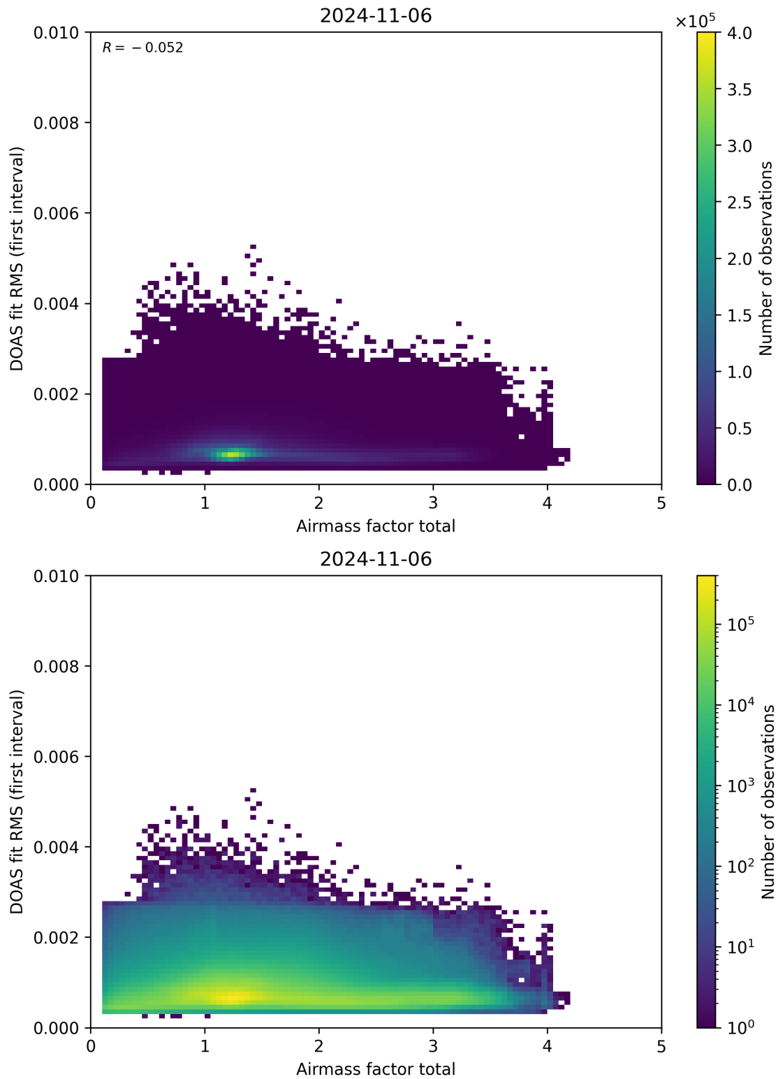
Figure 97: Scatter density plot of “Airmass factor total” against “DOAS fit RMS (first interval)” for 2024-11-05 to 2024-11-07.
