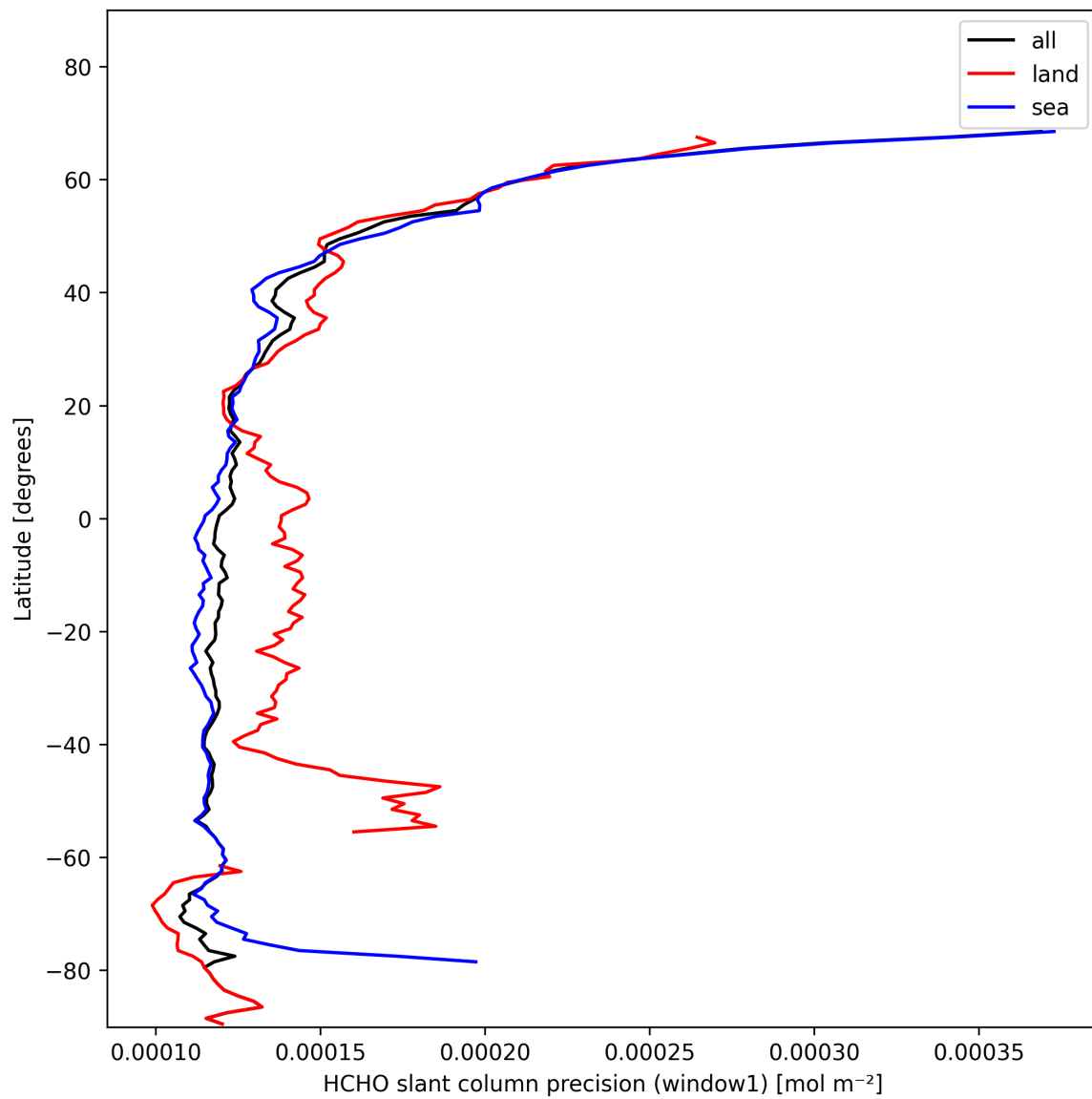
Figure 25: Zonal average of “HCHO slant column precision (window1)” for 2024-11-05 to 2024-11-07.
