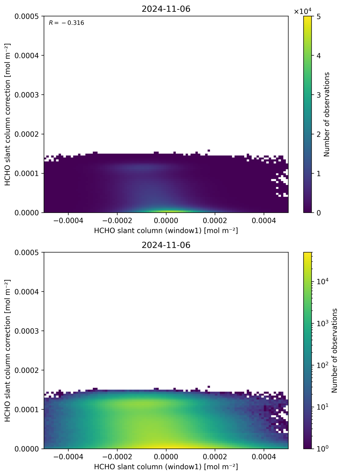
Figure 83: Scatter density plot of “HCHO slant column (window1)” against “HCHO slant column correction” for 2024-11-05 to 2024-11-07.
