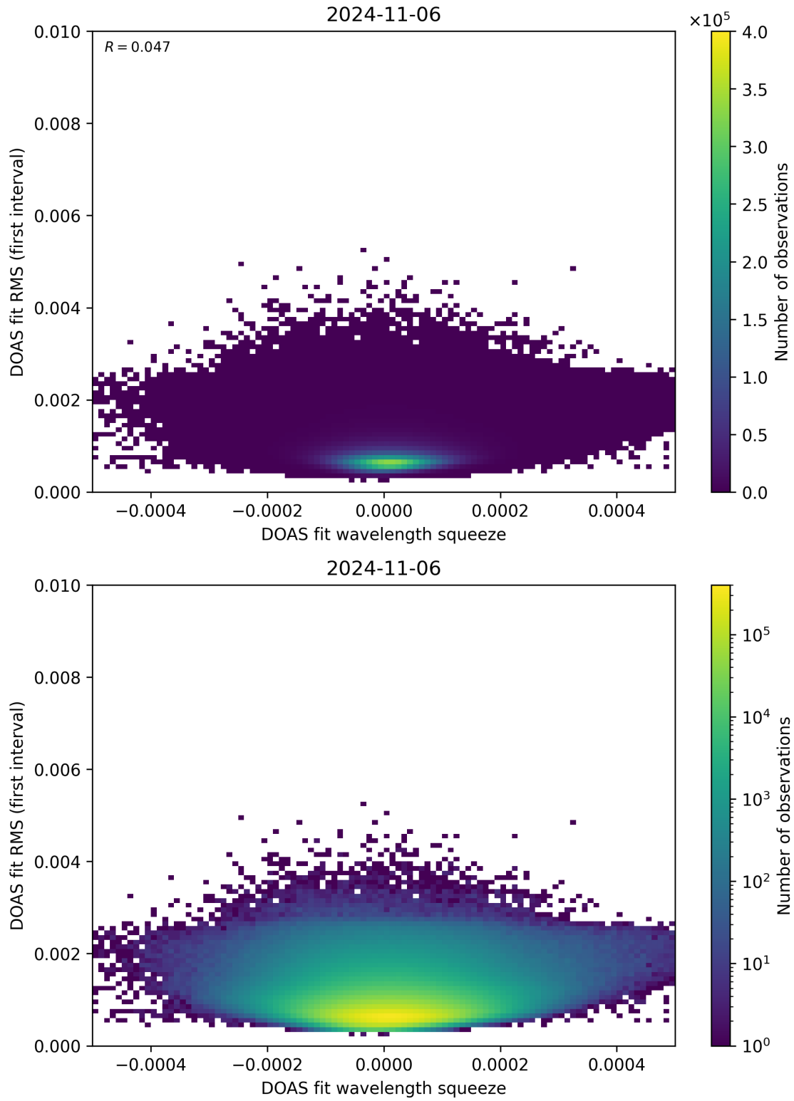
Figure 68: Scatter density plot of “DOAS fit wavelength squeeze” against “DOAS fit RMS (first interval)” for 2024-11-05 to 2024-11-07.
