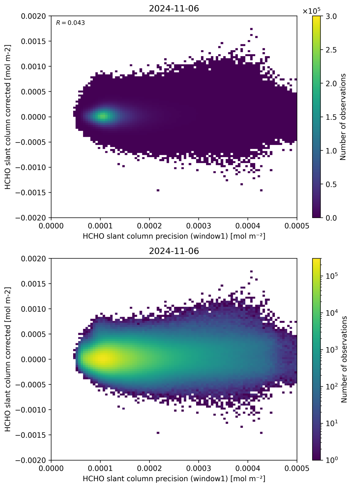
Figure 92: Scatter density plot of “HCHO slant column precision (window1)” against “HCHO slant column corrected” for 2024-11-05 to 2024-11-07.
