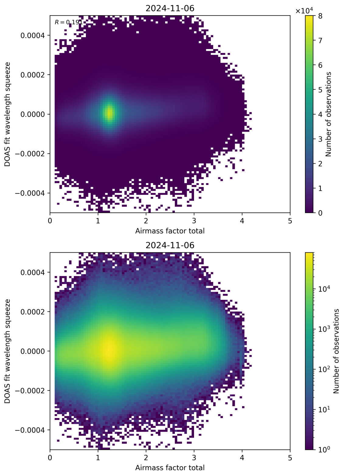
Figure 99: Scatter density plot of “Airmass factor total” against “DOAS fit wavelength squeeze” for 2024-11-05 to 2024-11-07.
