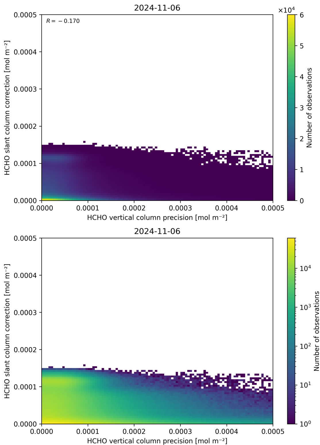
Figure 141: Scatter density plot of “HCHO vertical column precision” against “HCHO slant column correction” for 2024-11-05 to 2024-11-07.
