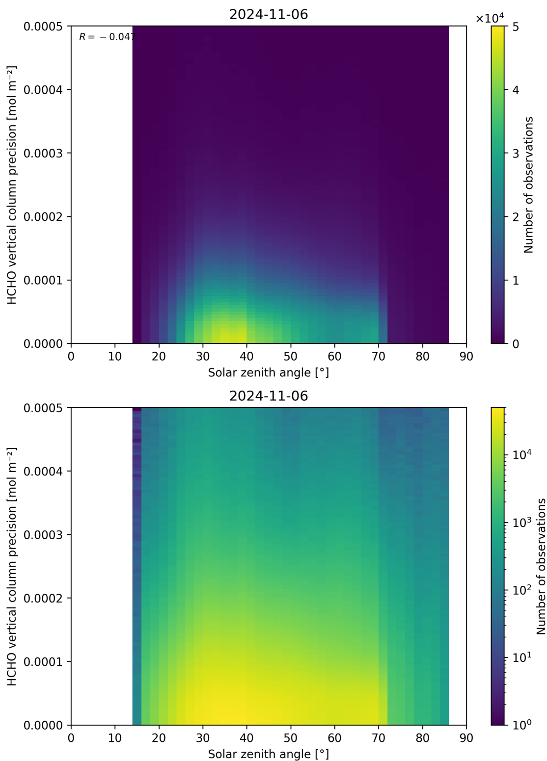
Figure 179: Scatter density plot of “Solar zenith angle” against “HCHO vertical column precision” for 2024-11-05 to 2024-11-07.
