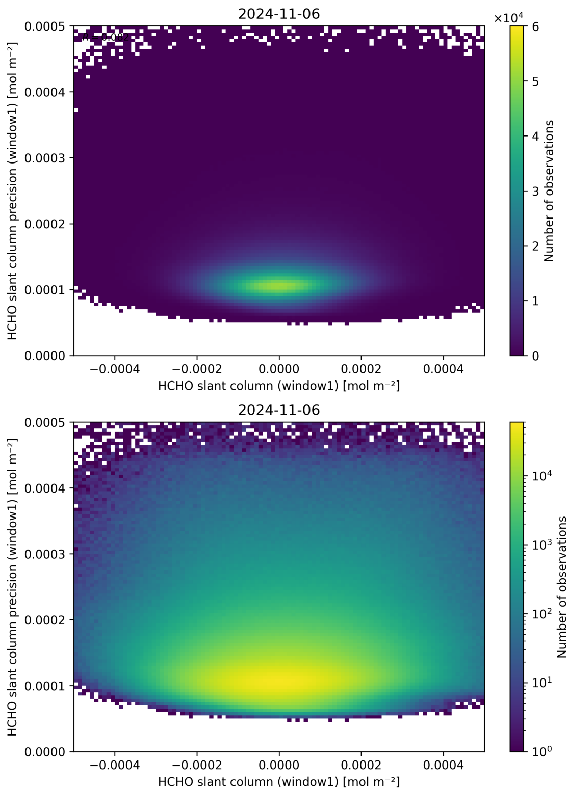
Figure 84: Scatter density plot of “HCHO slant column (window1)” against “HCHO slant column precision (window1)” for 2024-11-05 to 2024-11-07.
