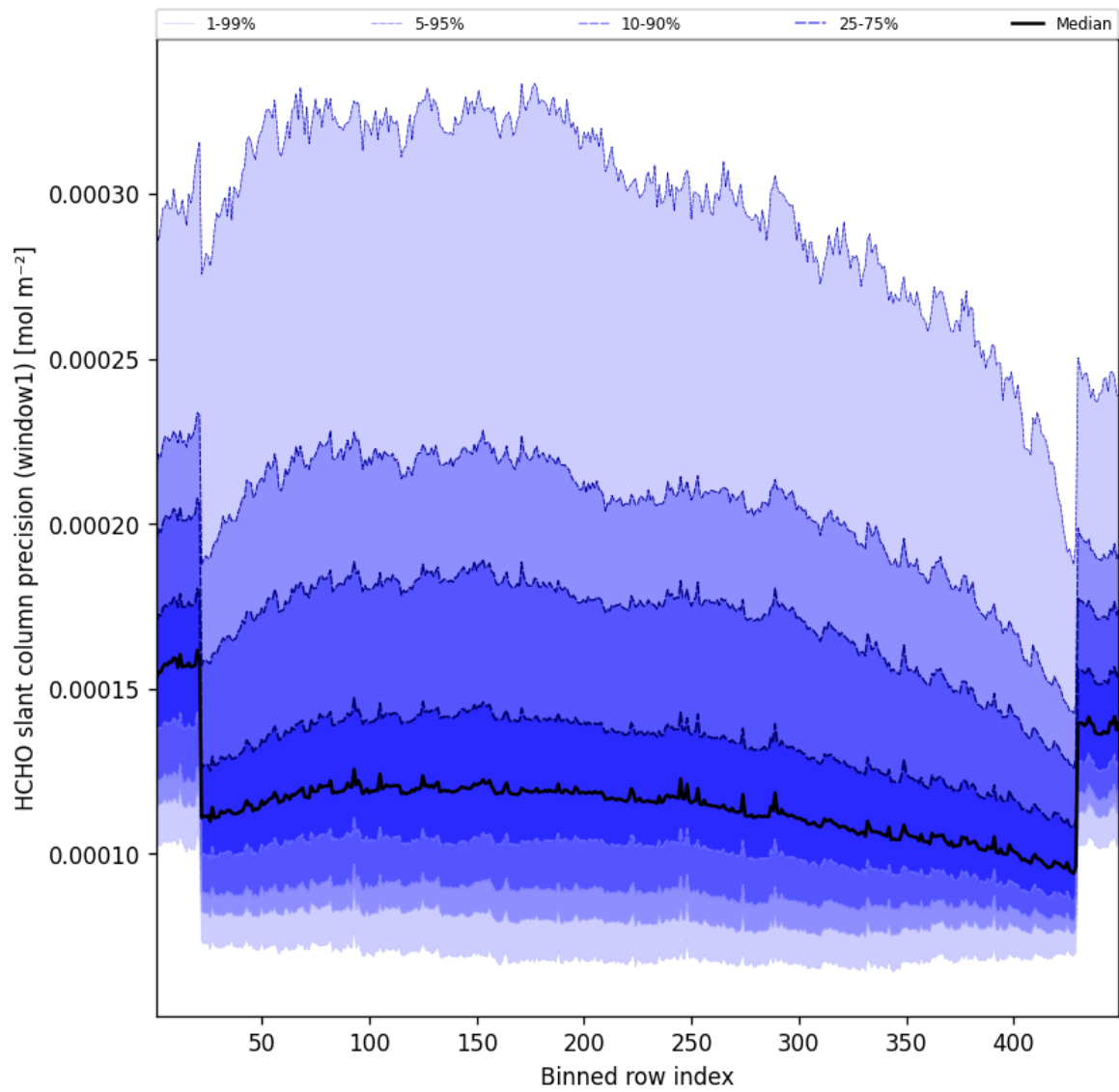
Figure 53: Along track statistics of "HCHO slant column precision (window1)" for 2024-11-05 to 2024-11-07
