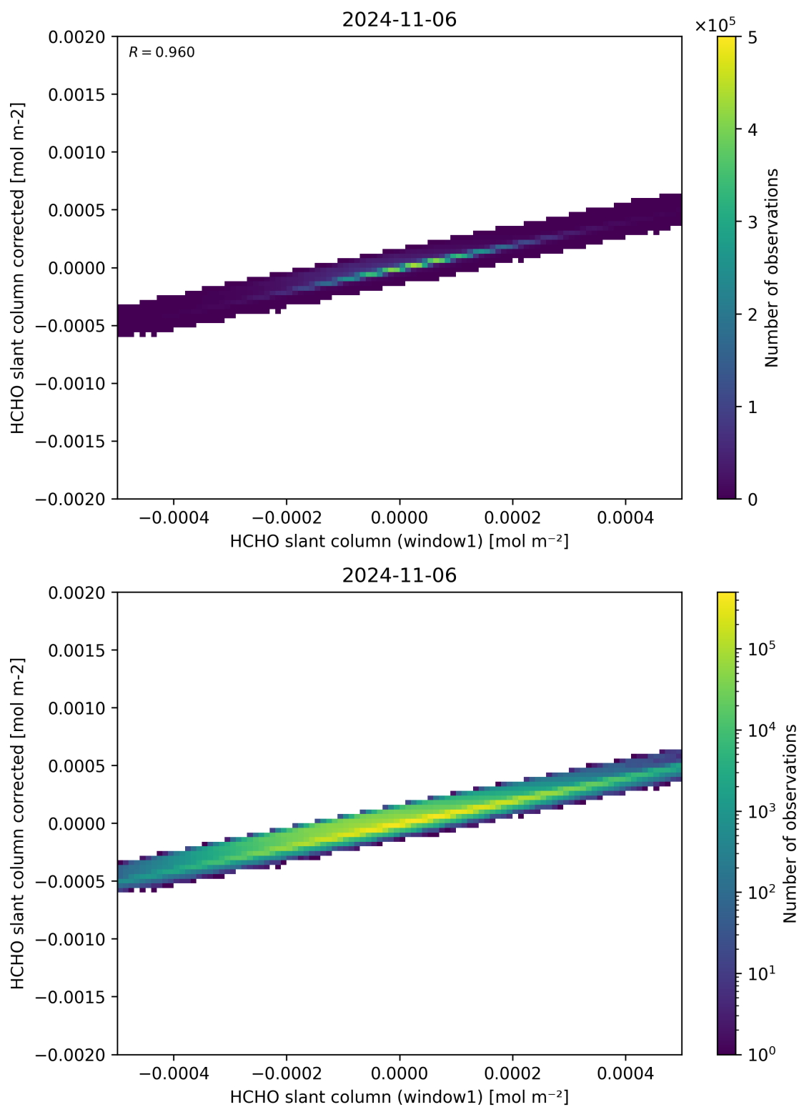
Figure 82: Scatter density plot of “HCHO slant column (window1)” against “HCHO slant column corrected” for 2024-11-05 to 2024-11-07.
