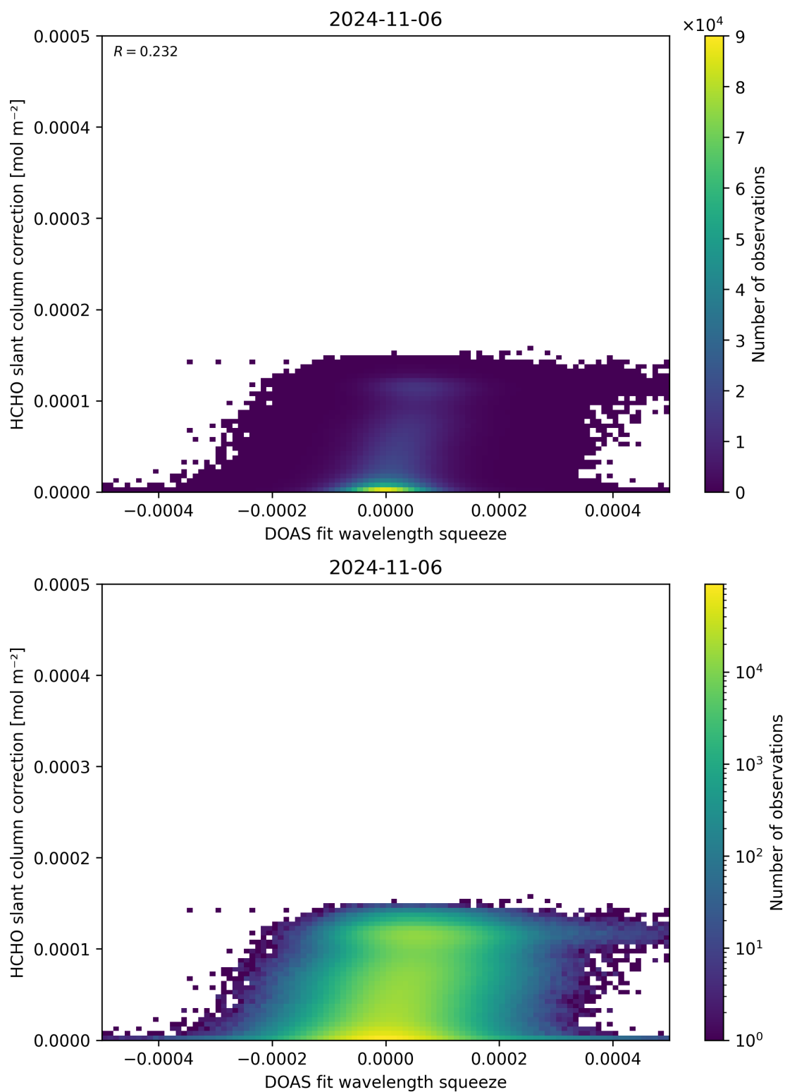
Figure 70: Scatter density plot of “DOAS fit wavelength squeeze” against “HCHO slant column correction” for 2024-11-05 to 2024-11-07.
