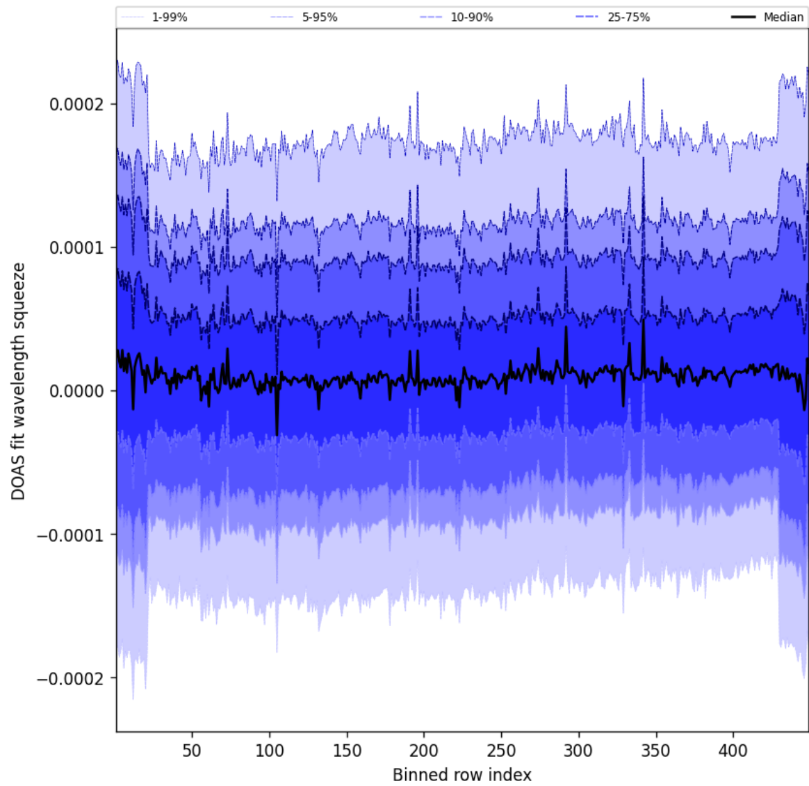
Figure 59: Along track statistics of “DOAS fit wavelength squeeze” for 2024-11-05 to 2024-11-07
