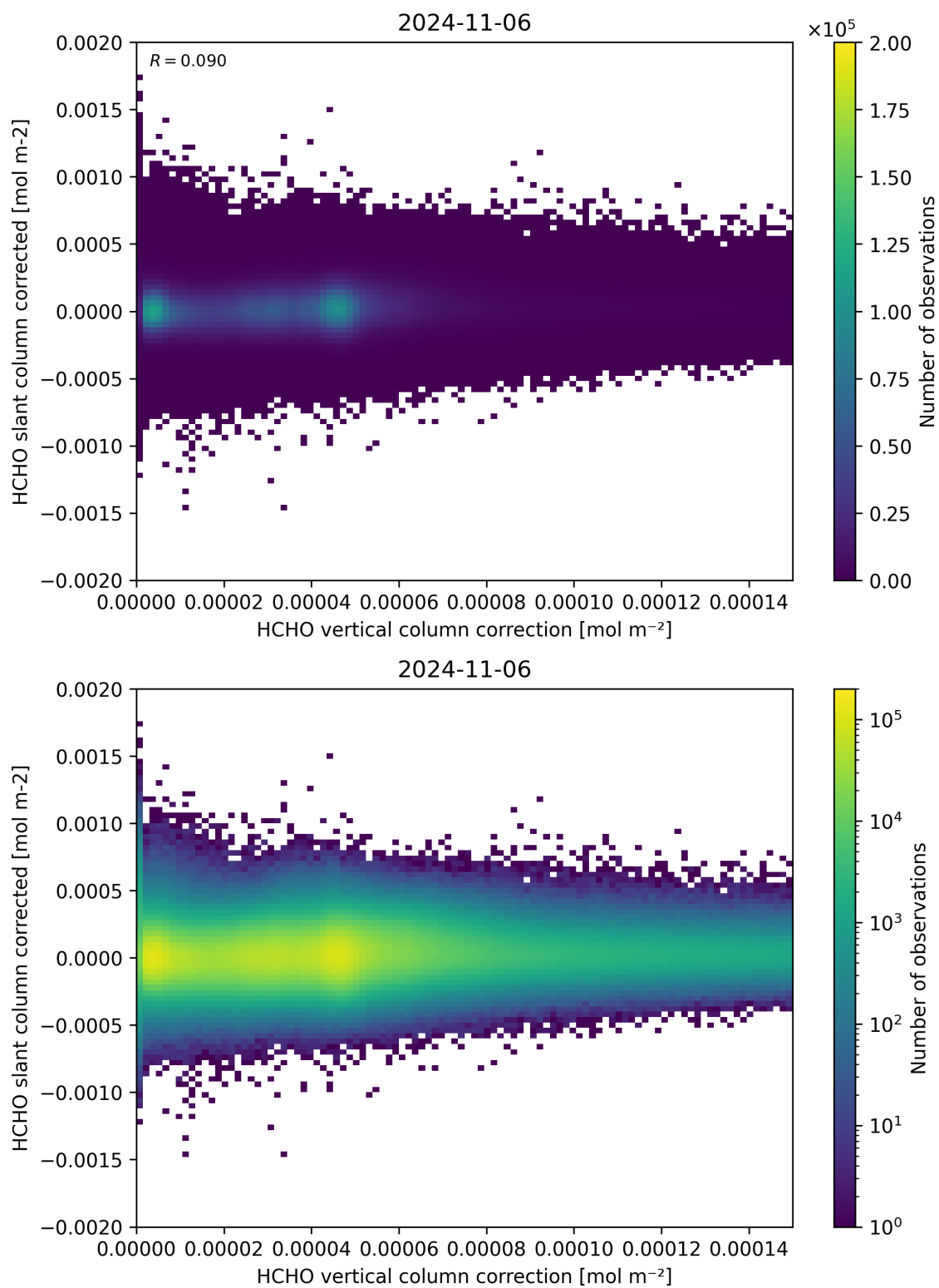
Figure 116: Scatter density plot of “HCHO vertical column correction” against “HCHO slant column corrected” for 2024-11-05 to 2024-11-07.
