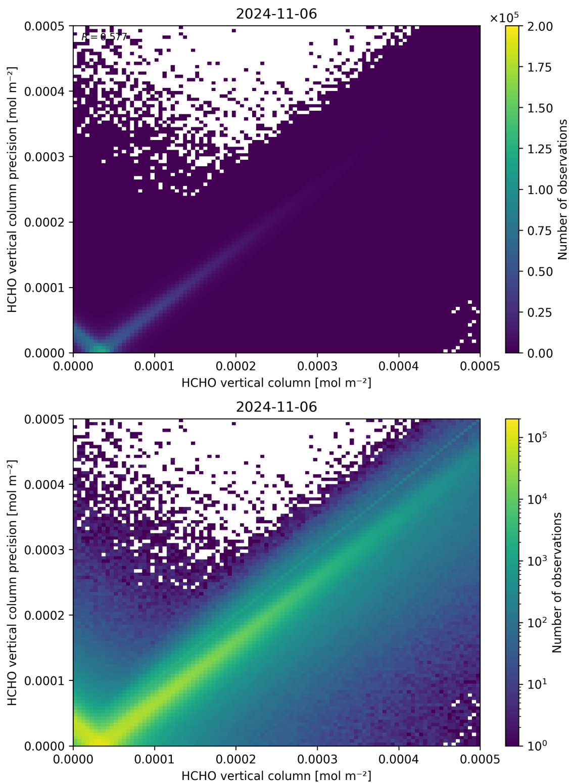
Figure 134: Scatter density plot of “HCHO vertical column” against “HCHO vertical column precision” for 2024-11-05 to 2024-11-07.
