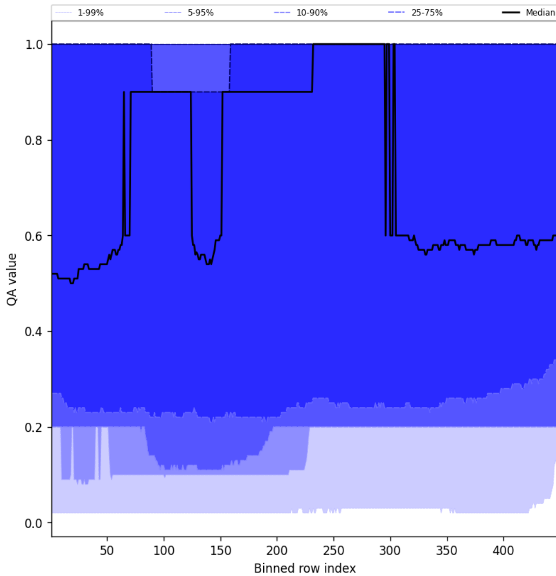
Figure 48: Along track statistics of “QA value” for 2024-11-05 to 2024-11-07
