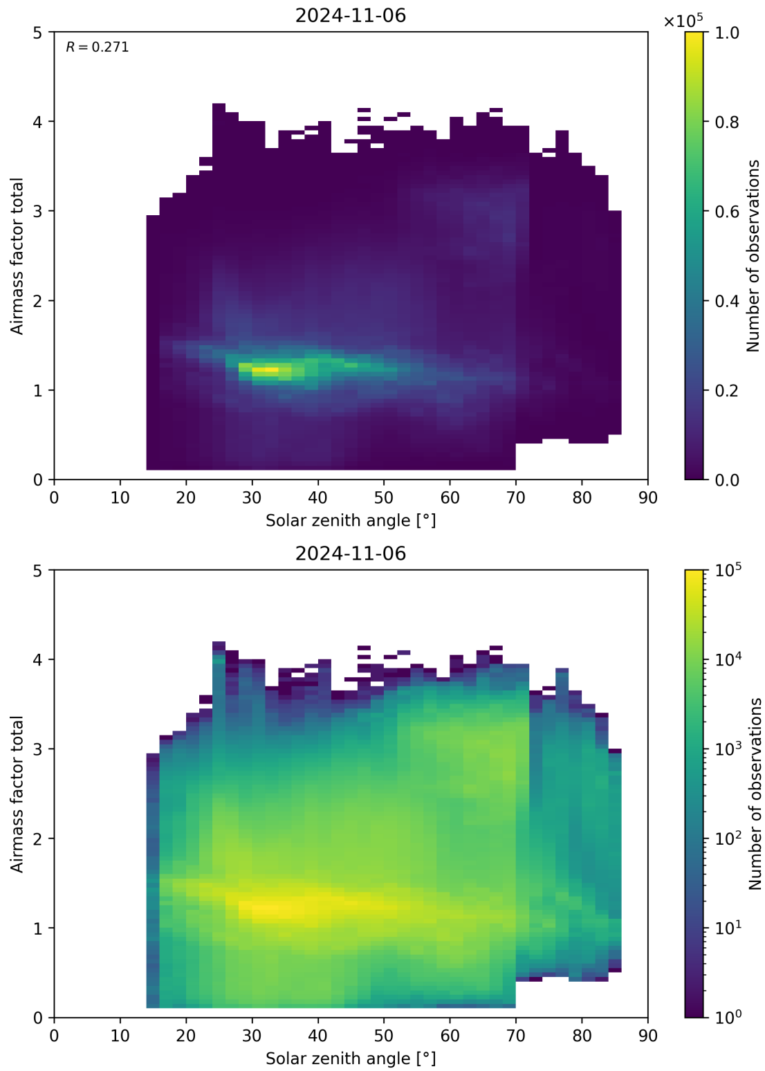
Figure 175: Scatter density plot of “Solar zenith angle” against “Airmass factor total” for 2024-11-05 to 2024-11-07.
