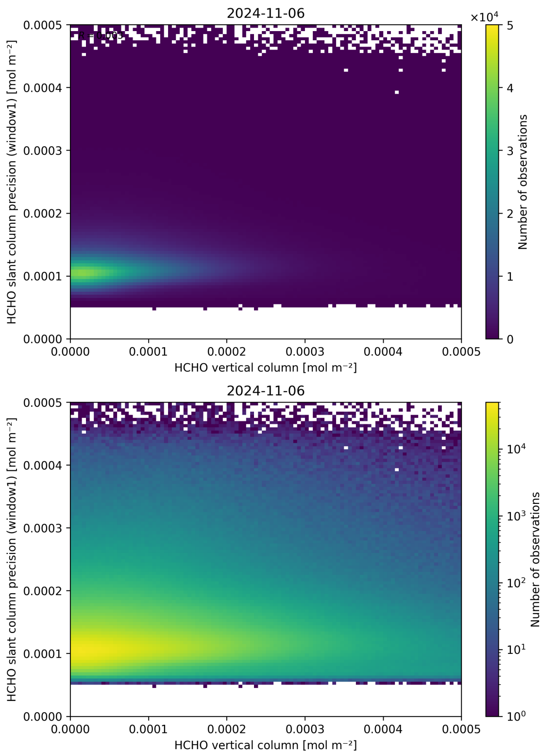
Figure 130: Scatter density plot of “HCHO vertical column” against “HCHO slant column precision (window1)” for 2024-11-05 to 2024-11-07.
