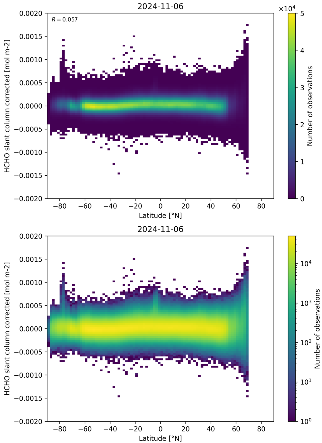
Figure 157: Scatter density plot of “Latitude” against “HCHO slant column corrected” for 2024-11-05 to 2024-11-07.
