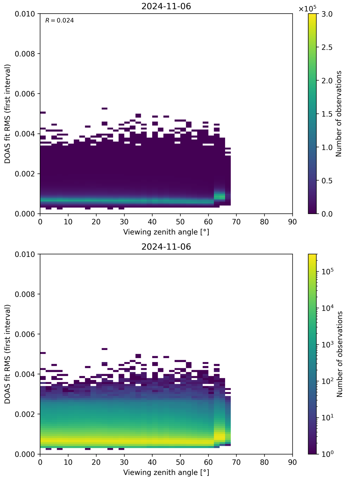
Figure 182: Scatter density plot of “Viewing zenith angle” against “DOAS fit RMS (first interval)” for 2024-11-05 to 2024-11-07.
