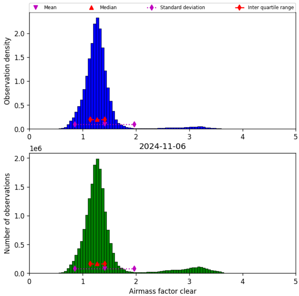
Figure 42: Histogram of “Airmass factor clear” for 2024-11-05 to 2024-11-07
