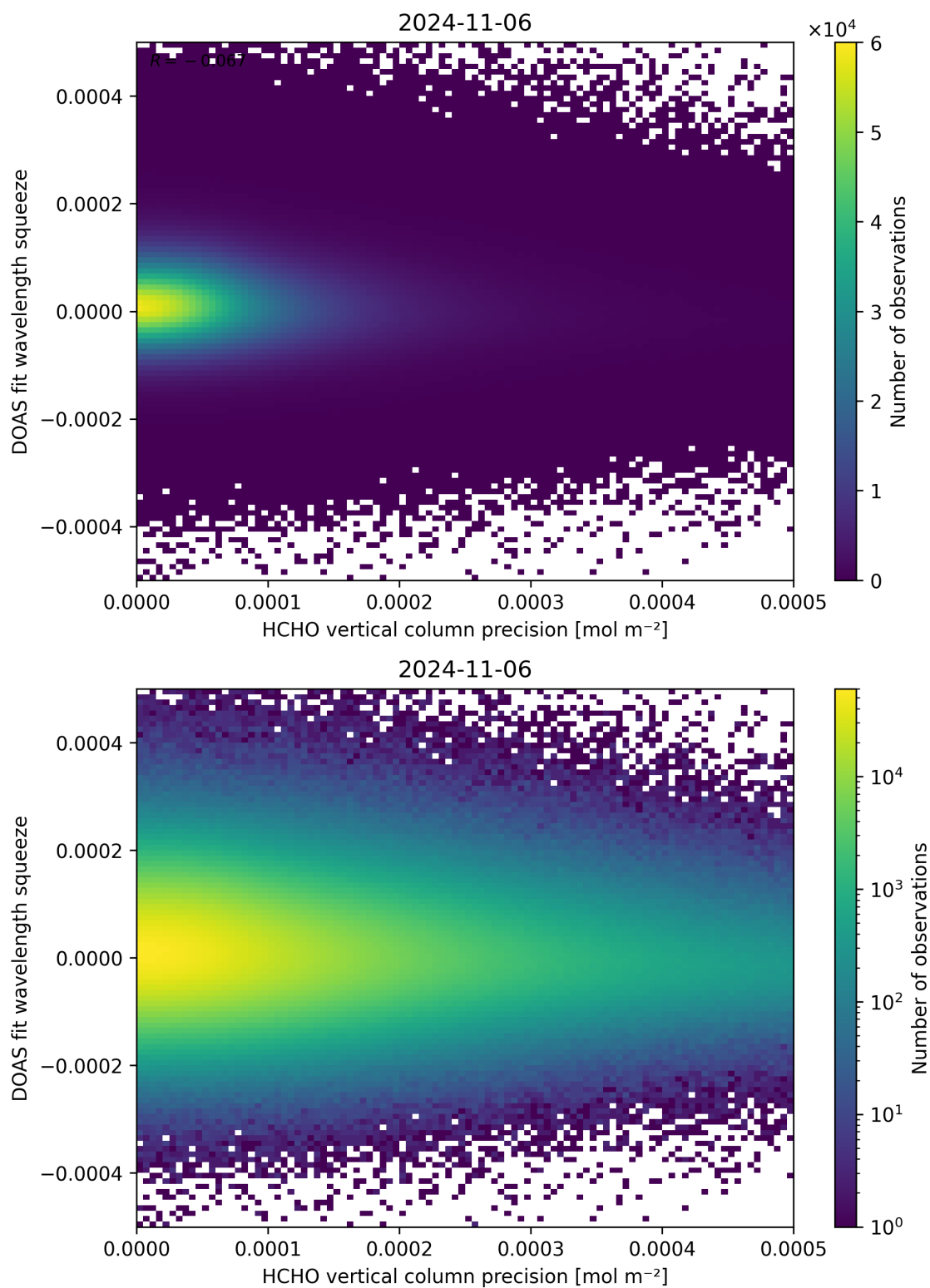
Figure 138: Scatter density plot of “HCHO vertical column precision” against “DOAS fit wavelength squeeze” for 2024-11-05 to 2024-11-07.
