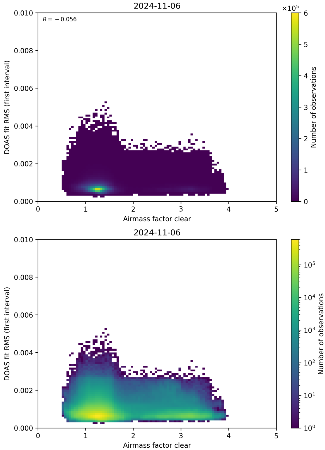
Figure 71: Scatter density plot of “Airmass factor clear” against “DOAS fit RMS (first interval)” for 2024-11-05 to 2024-11-07.
