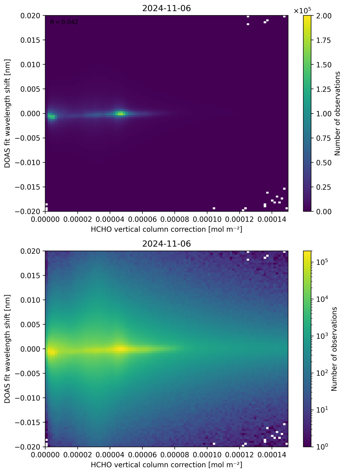
Figure 113: Scatter density plot of “HCHO vertical column correction” against “DOAS fit wavelength shift” for 2024-11-05 to 2024-11-07.
