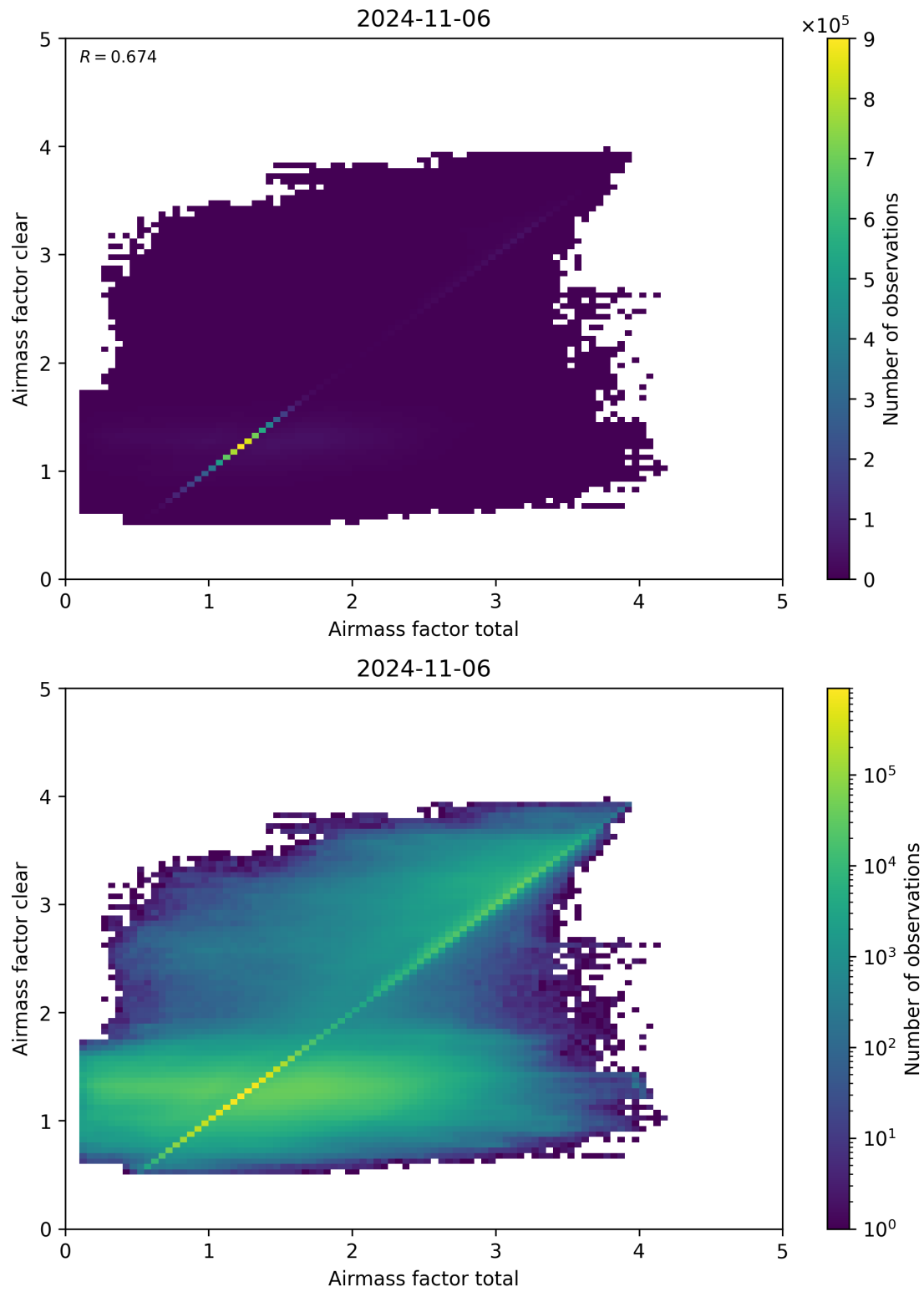
Figure 100: Scatter density plot of “Airmass factor total” against “Airmass factor clear” for 2024-11-05 to 2024-11-07.
