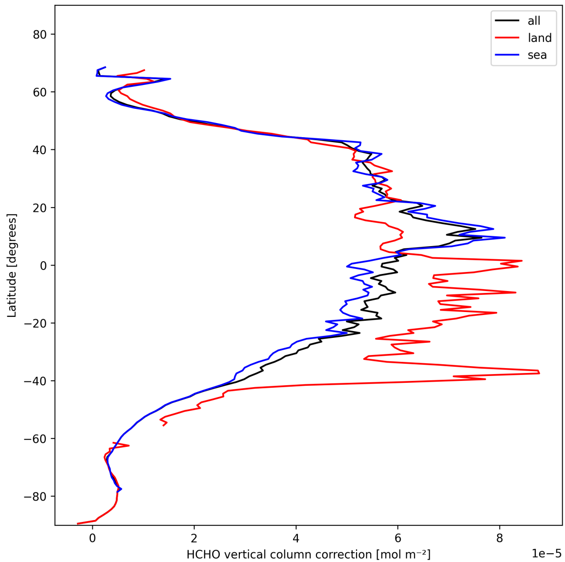
Figure 23: Zonal average of “HCHO vertical column correction” for 2024-11-05 to 2024-11-07.
