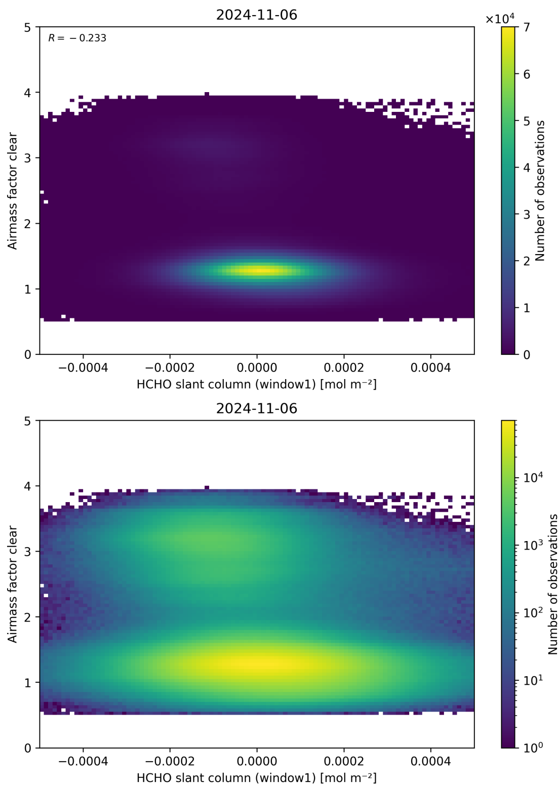
Figure 81: Scatter density plot of “HCHO slant column (window1)” against “Airmass factor clear” for 2024-11-05 to 2024-11-07.
