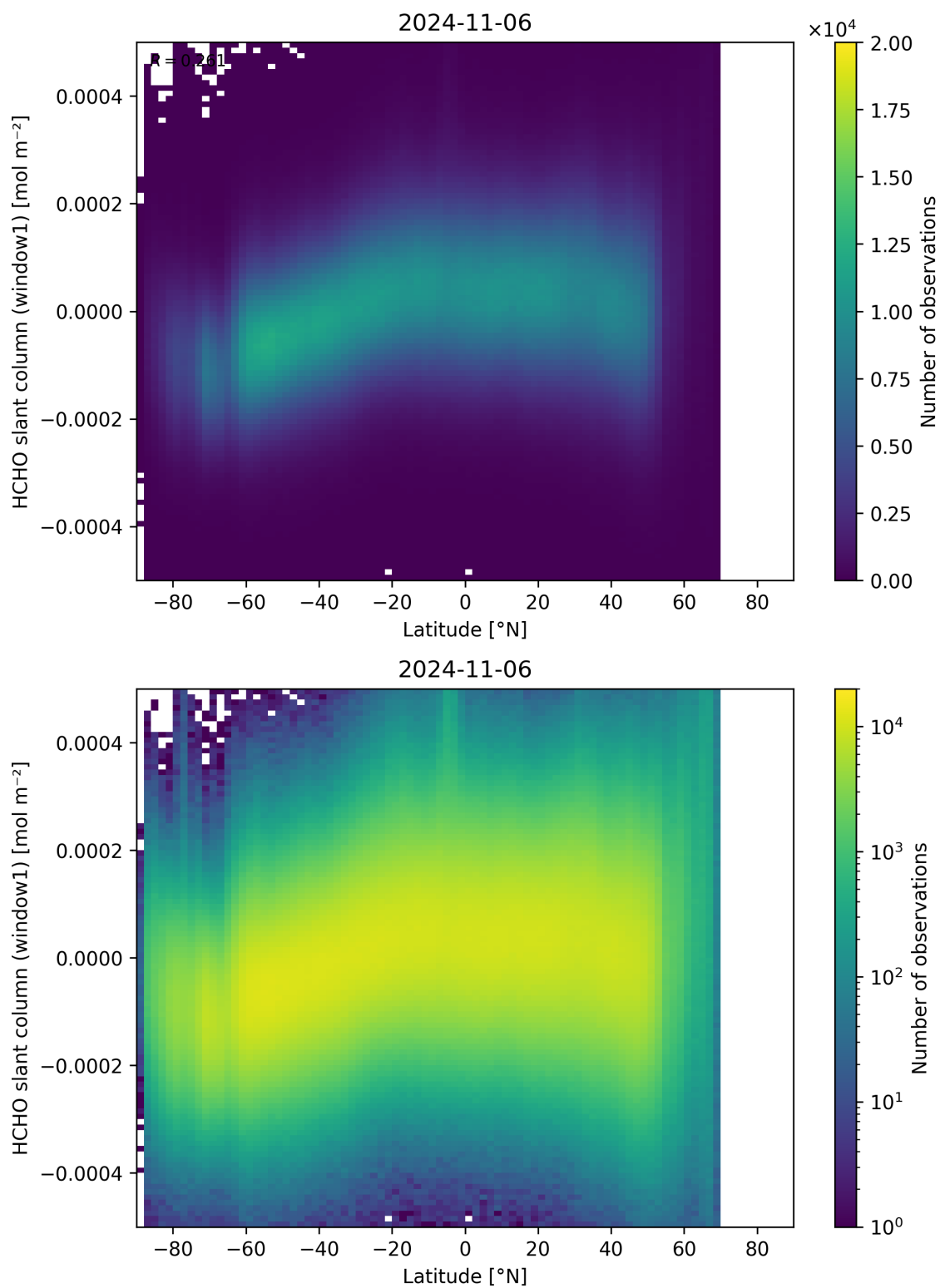
Figure 159: Scatter density plot of “Latitude” against “HCHO slant column (window1)” for 2024-11-05 to 2024-11-07.
