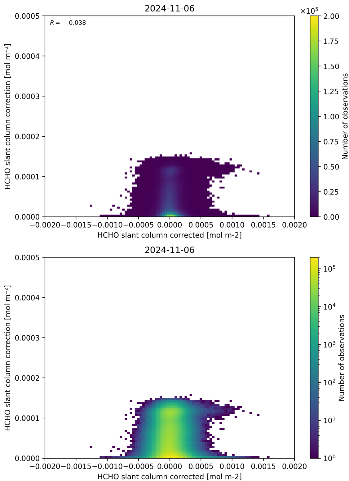
Figure 77: Scatter density plot of “HCHO slant column corrected” against “HCHO slant column correction” for 2024-11-05 to 2024-11-07.
