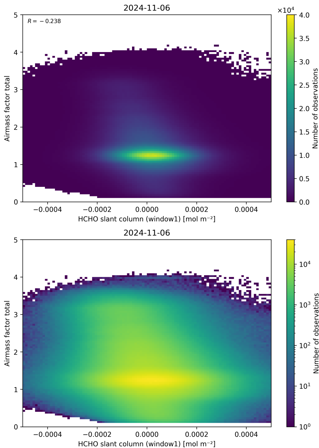
Figure 85: Scatter density plot of “HCHO slant column (window1)” against “Airmass factor total” for 2024-11-05 to 2024-11-07.
