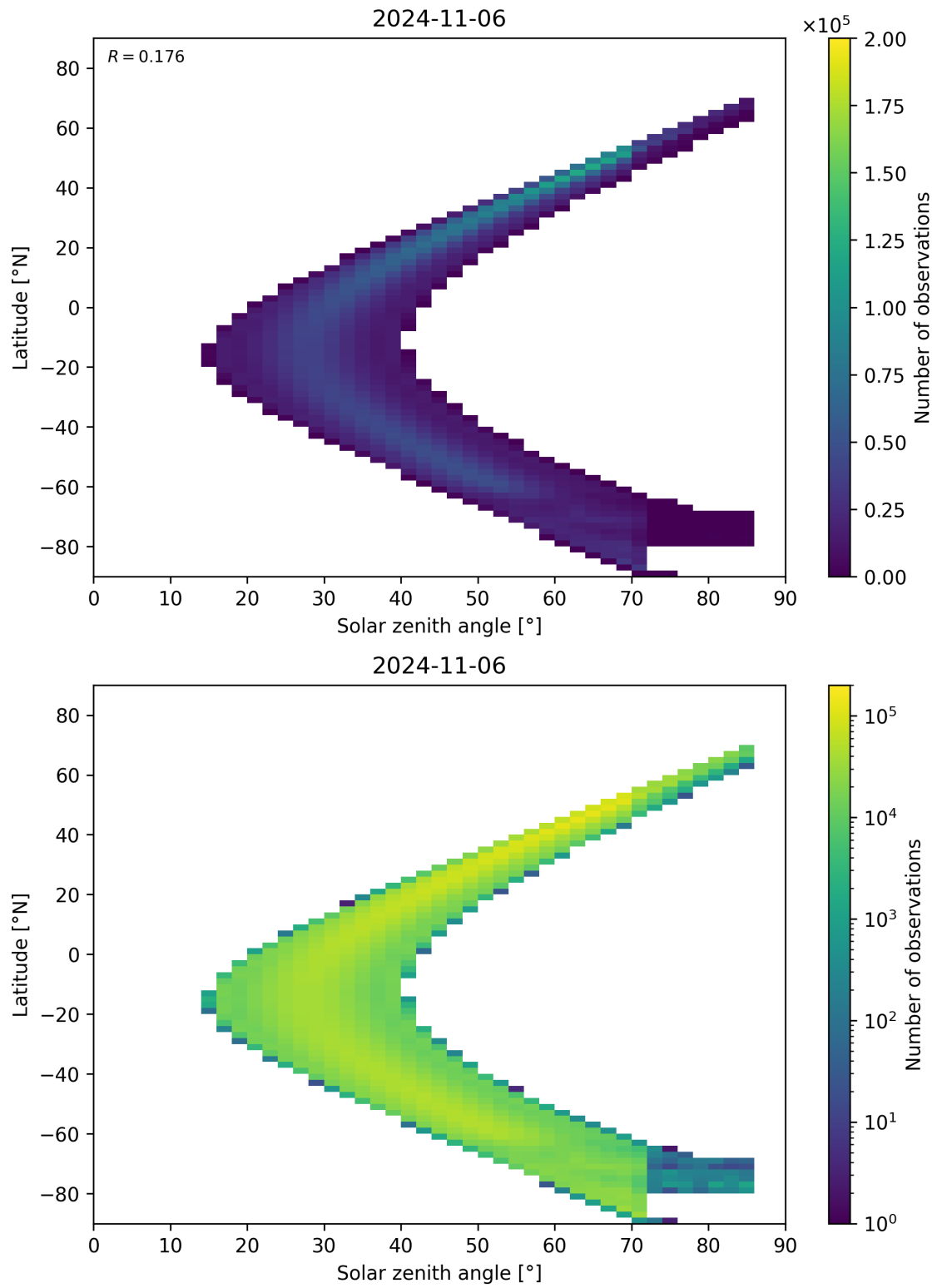
Figure 181: Scatter density plot of “Solar zenith angle” against “Latitude” for 2024-11-05 to 2024-11-07.
