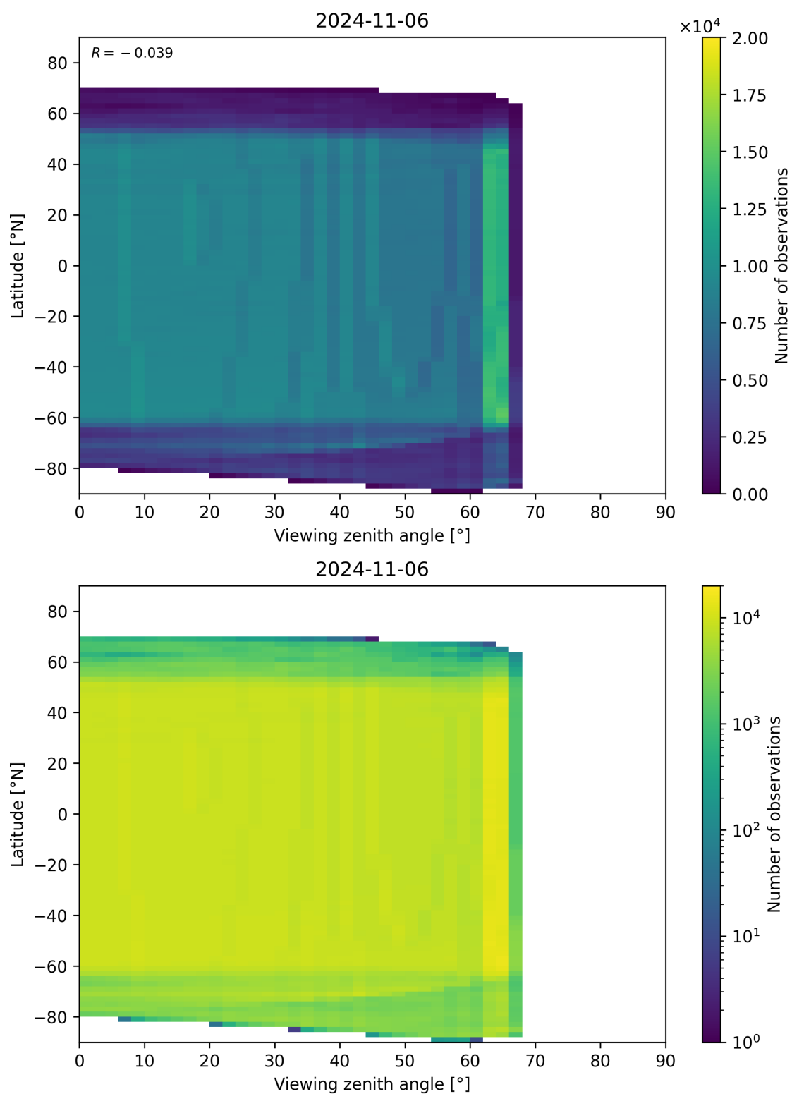
Figure 196: Scatter density plot of “Viewing zenith angle” against “Latitude” for 2024-11-05 to 2024-11-07.
