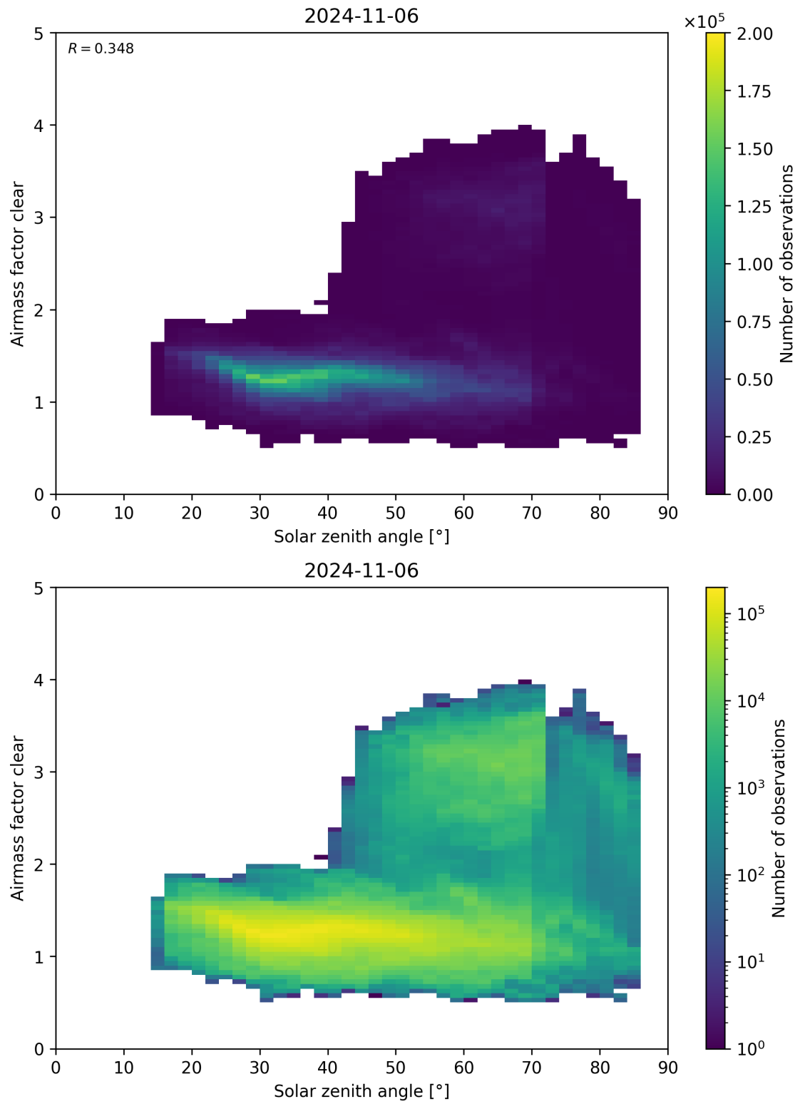
Figure 170: Scatter density plot of “Solar zenith angle” against “Airmass factor clear” for 2024-11-05 to 2024-11-07.
