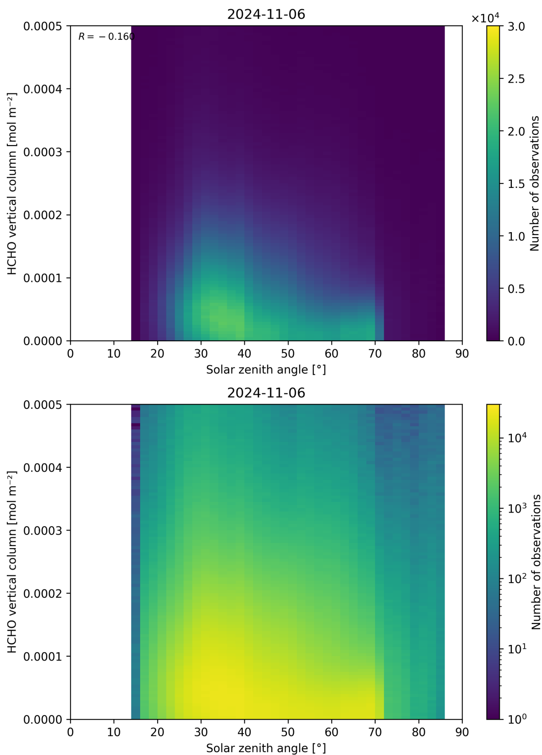
Figure 177: Scatter density plot of “Solar zenith angle” against “HCHO vertical column” for 2024-11-05 to 2024-11-07.
