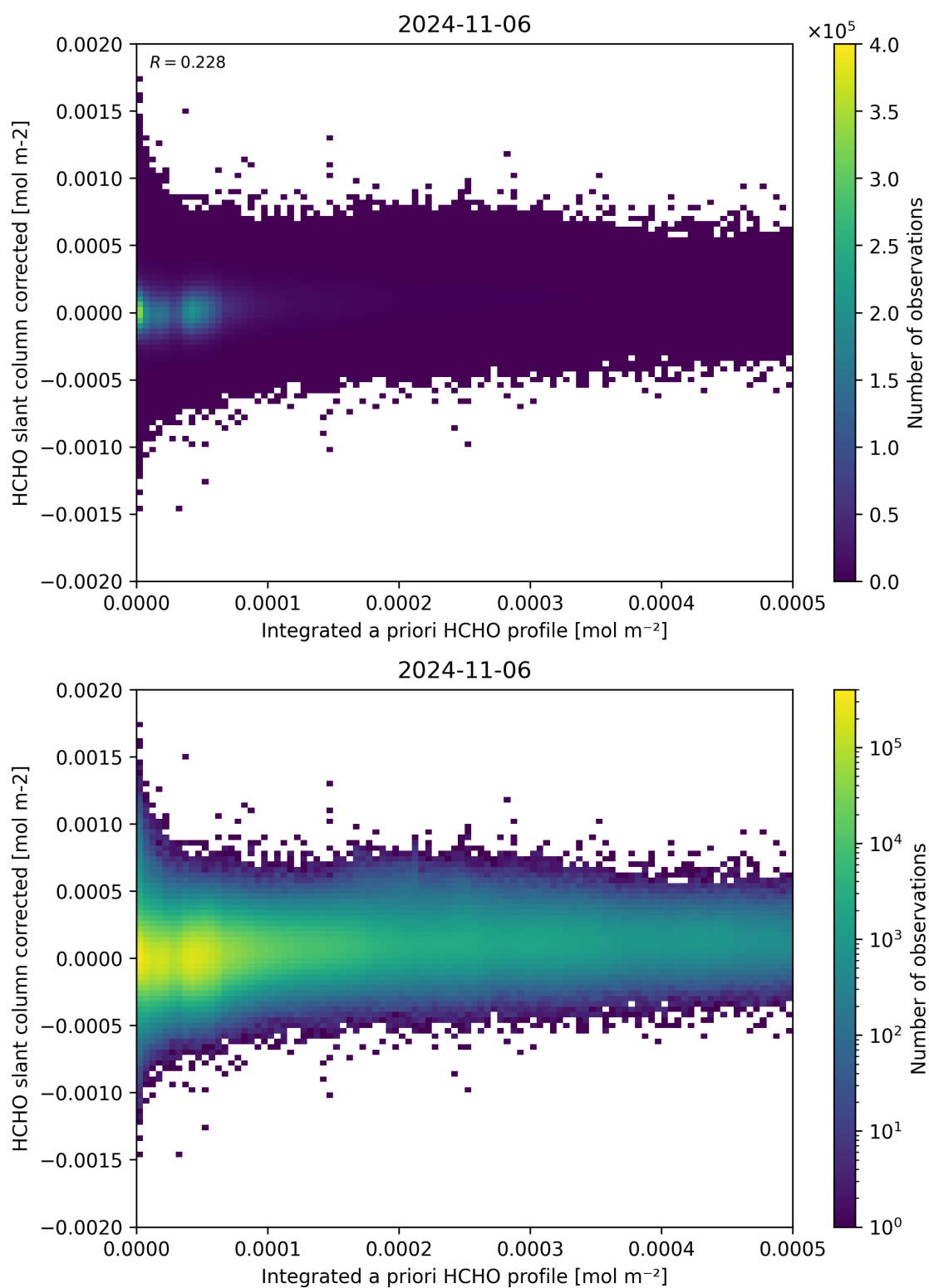
Figure 151: Scatter density plot of “Integrated a priori HCHO profile” against “HCHO slant column corrected” for 2024-11-05 to 2024-11-07.
