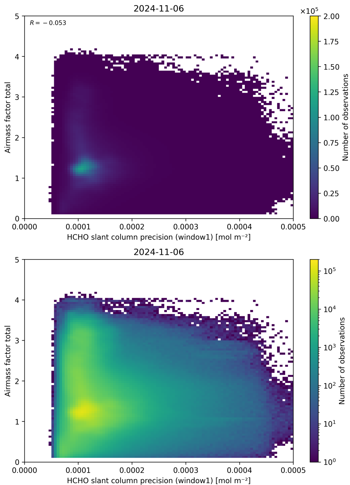
Figure 94: Scatter density plot of “HCHO slant column precision (window1)” against “Airmass factor total” for 2024-11-05 to 2024-11-07.
