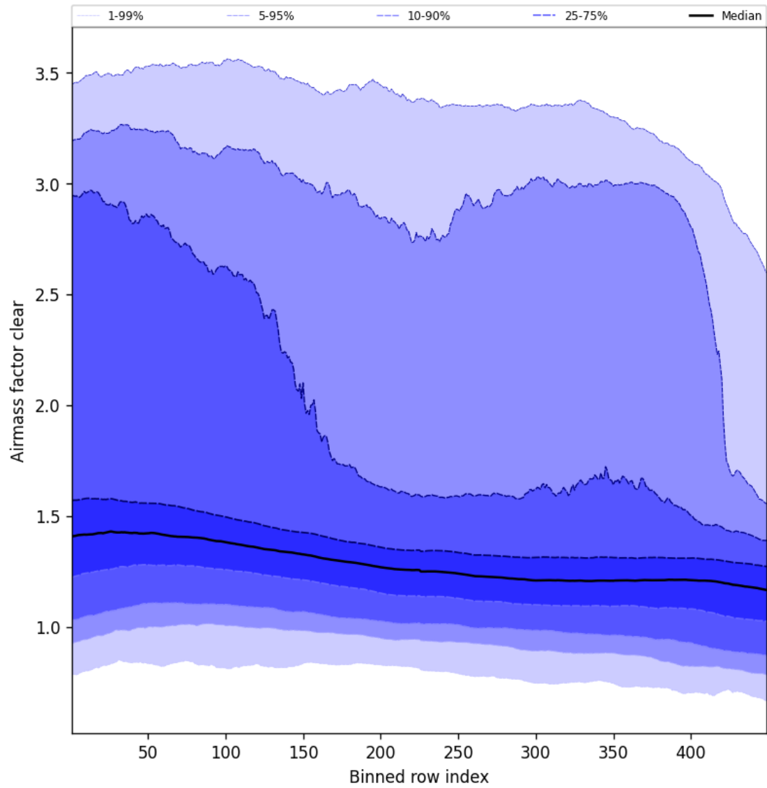
Figure 56: Along track statistics of “Airmass factor clear” for 2024-11-05 to 2024-11-07
