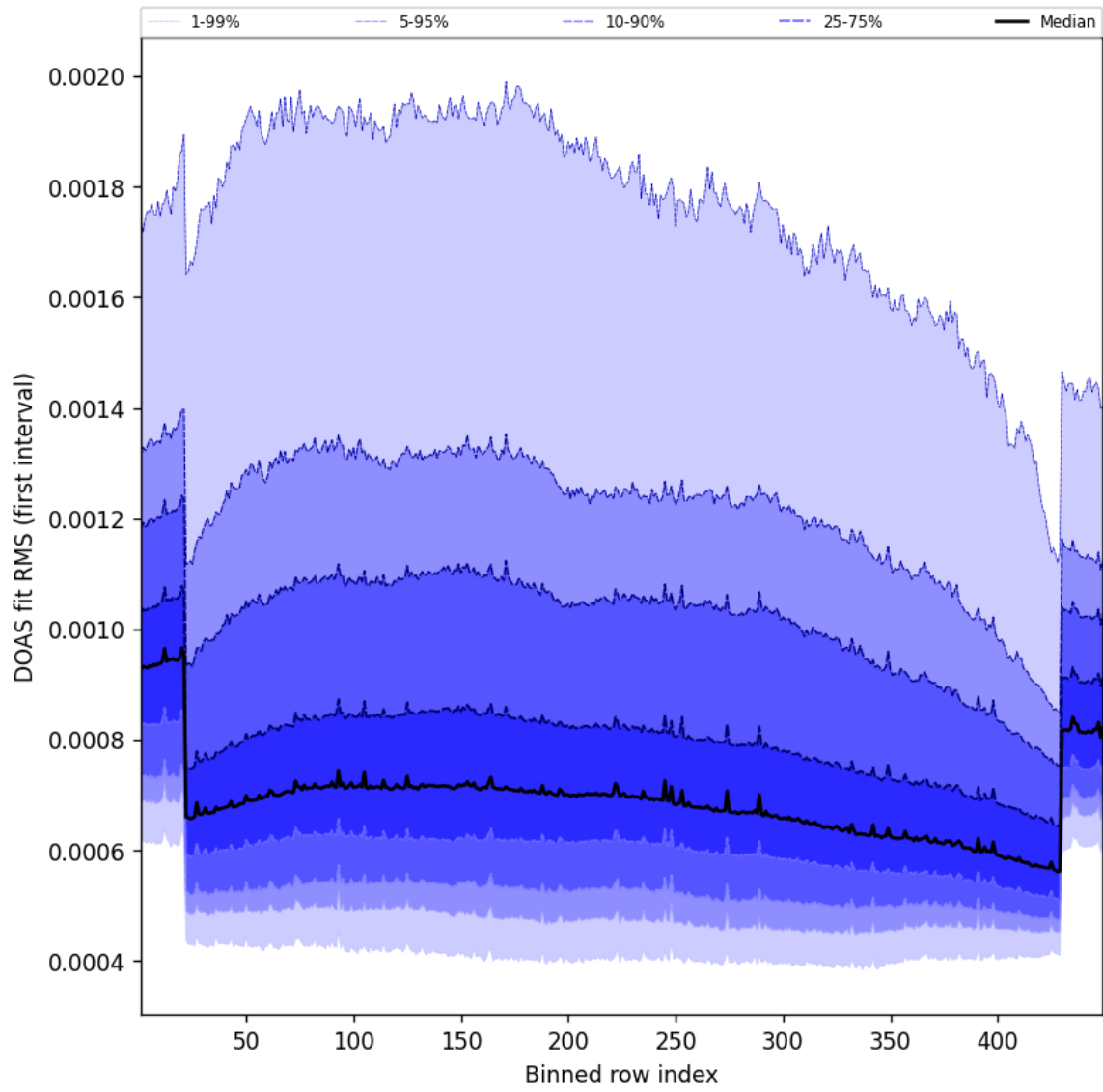
Figure 60: Along track statistics of “DOAS fit RMS (first interval)” for 2024-11-05 to 2024-11-07
