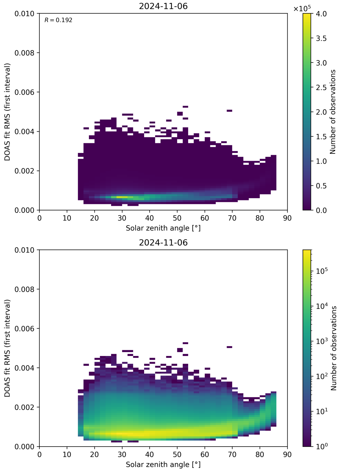
Figure 167: Scatter density plot of “Solar zenith angle” against “DOAS fit RMS (first interval)” for 2024-11-05 to 2024-11-07.
