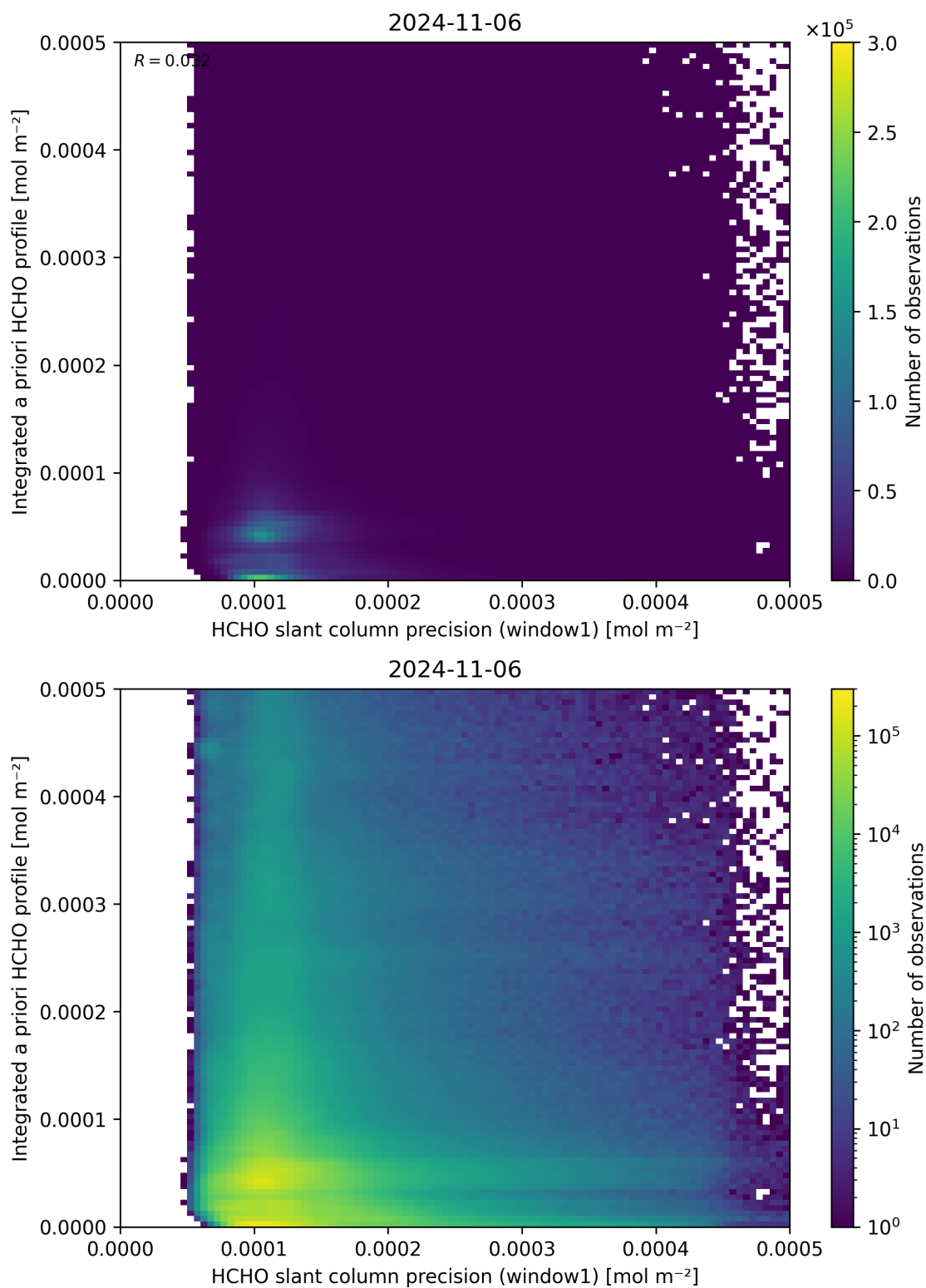
Figure 96: Scatter density plot of “HCHO slant column precision (window1)” against “Integrated a priori HCHO profile” for 2024-11-05 to 2024-11-07.
