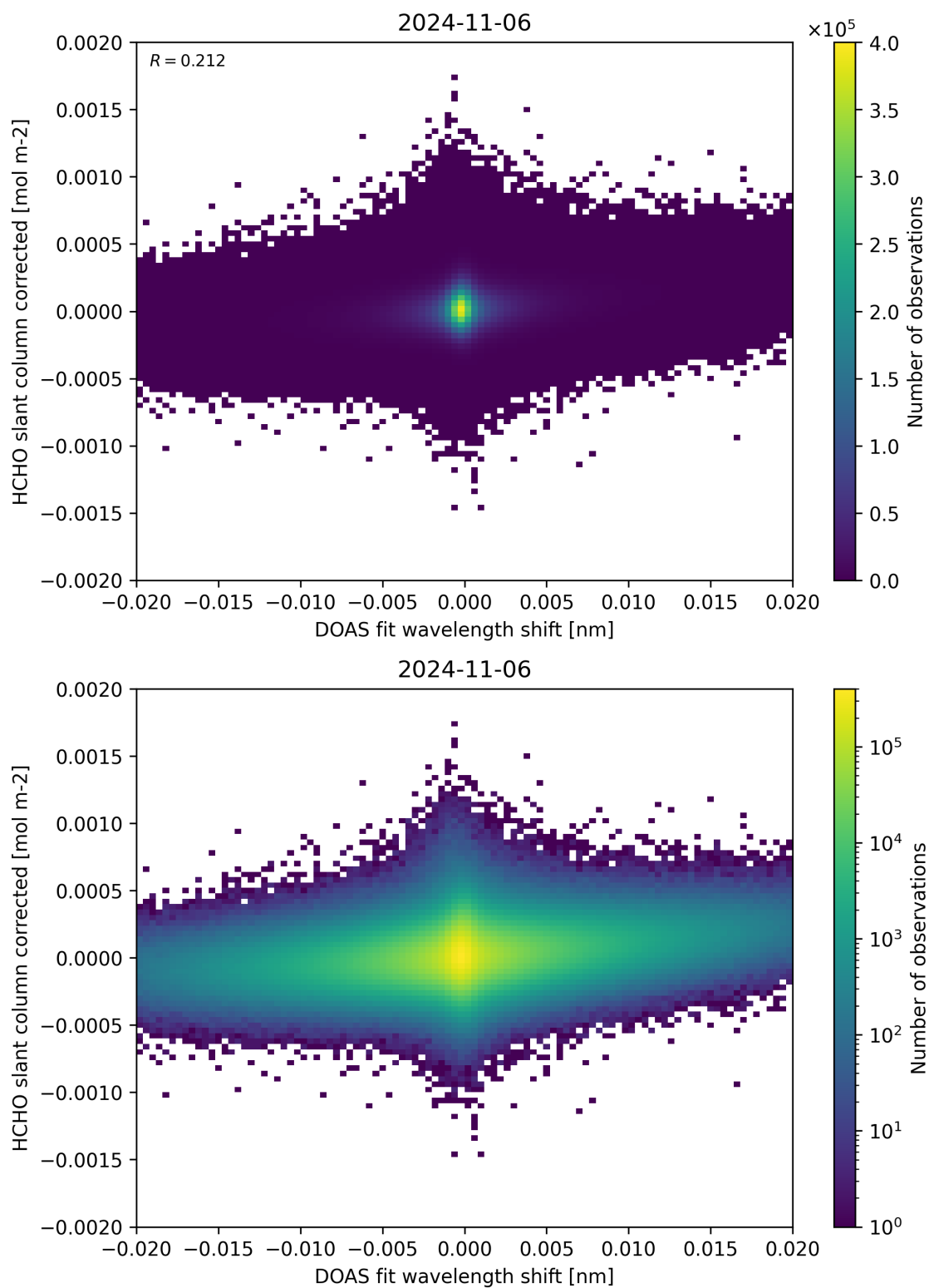
Figure 66: Scatter density plot of “DOAS fit wavelength shift” against “HCHO slant column corrected” for 2024-11-05 to 2024-11-07.
