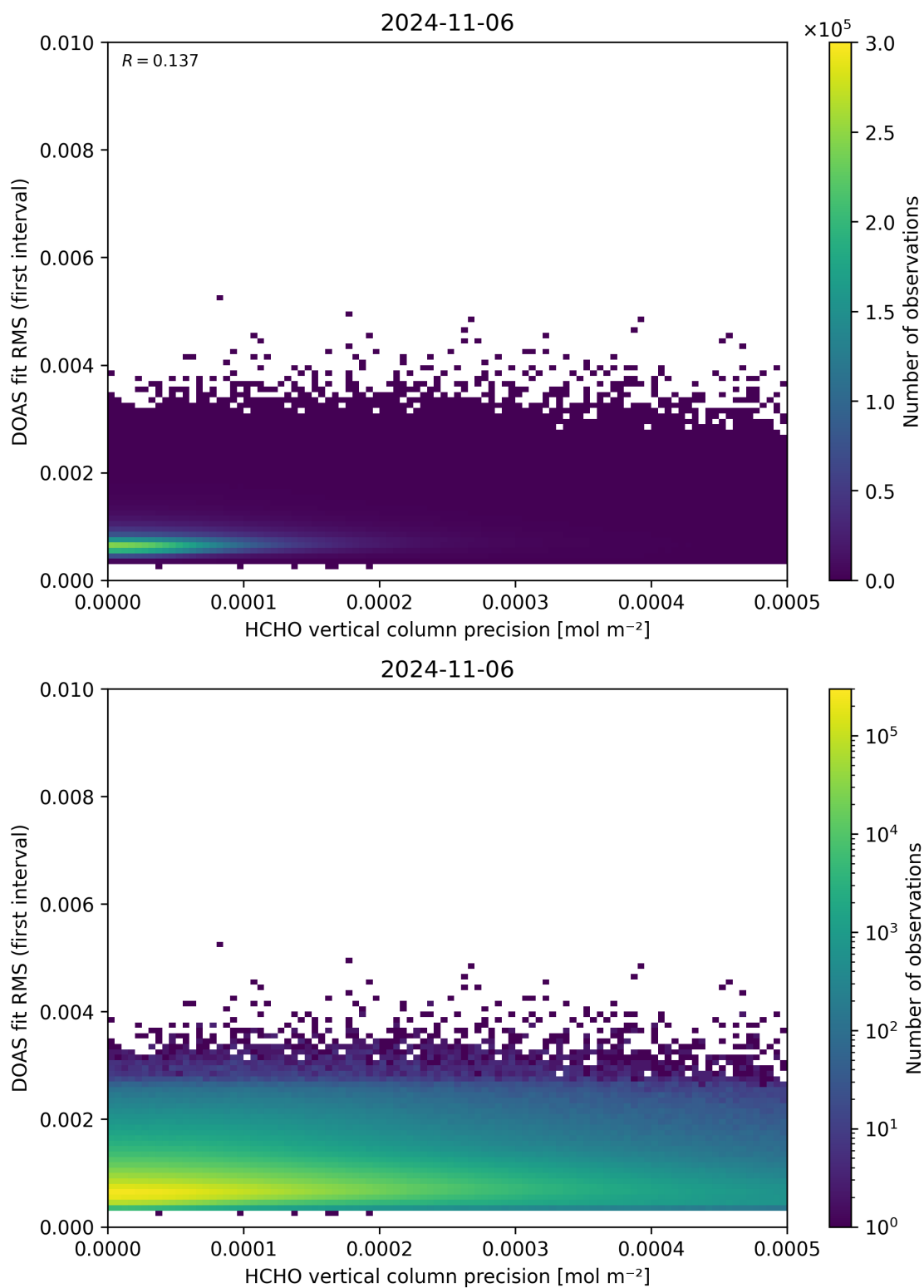
Figure 136: Scatter density plot of “HCHO vertical column precision” against “DOAS fit RMS (first interval)” for 2024-11-05 to 2024-11-07.
