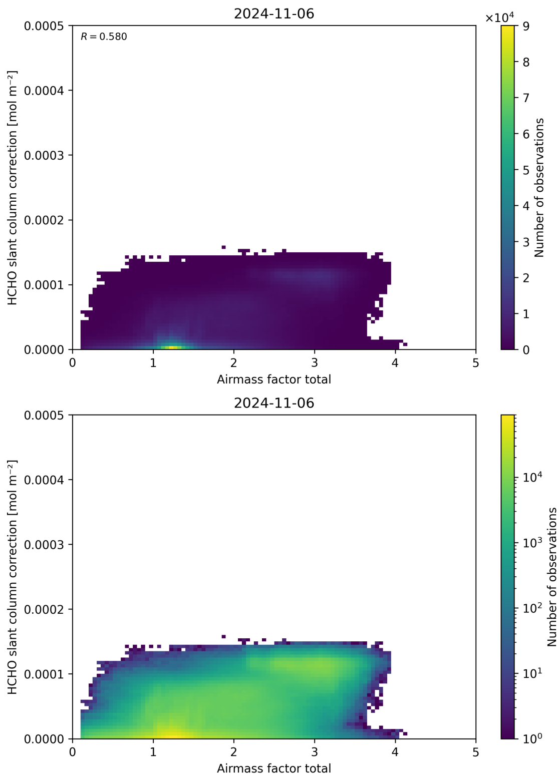
Figure 102: Scatter density plot of “Airmass factor total” against “HCHO slant column correction” for 2024-11-05 to 2024-11-07.
