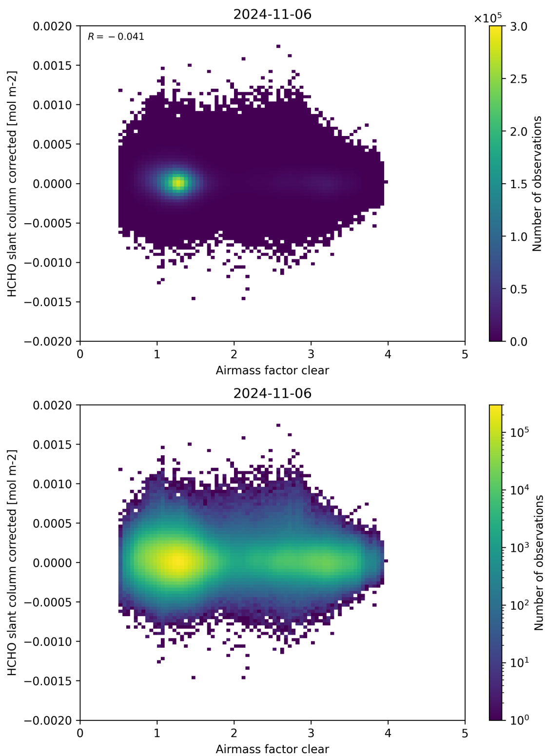
Figure 74: Scatter density plot of “Airmass factor clear” against “HCHO slant column corrected” for 2024-11-05 to 2024-11-07.
