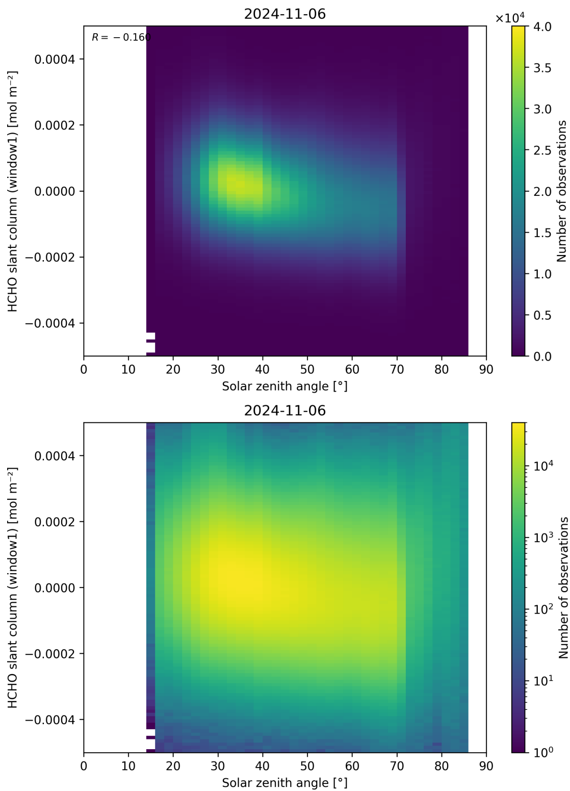
Figure 173: Scatter density plot of “Solar zenith angle” against “HCHO slant column (window1)” for 2024-11-05 to 2024-11-07.
