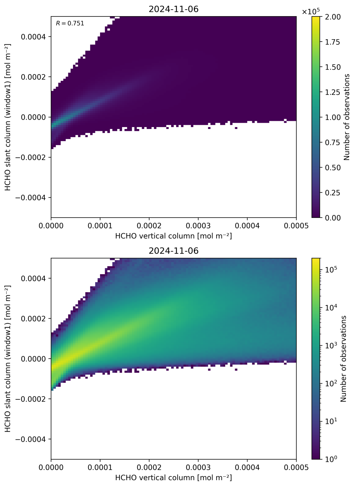
Figure 129: Scatter density plot of “HCHO vertical column” against “HCHO slant column (window1)” for 2024-11-05 to 2024-11-07.
