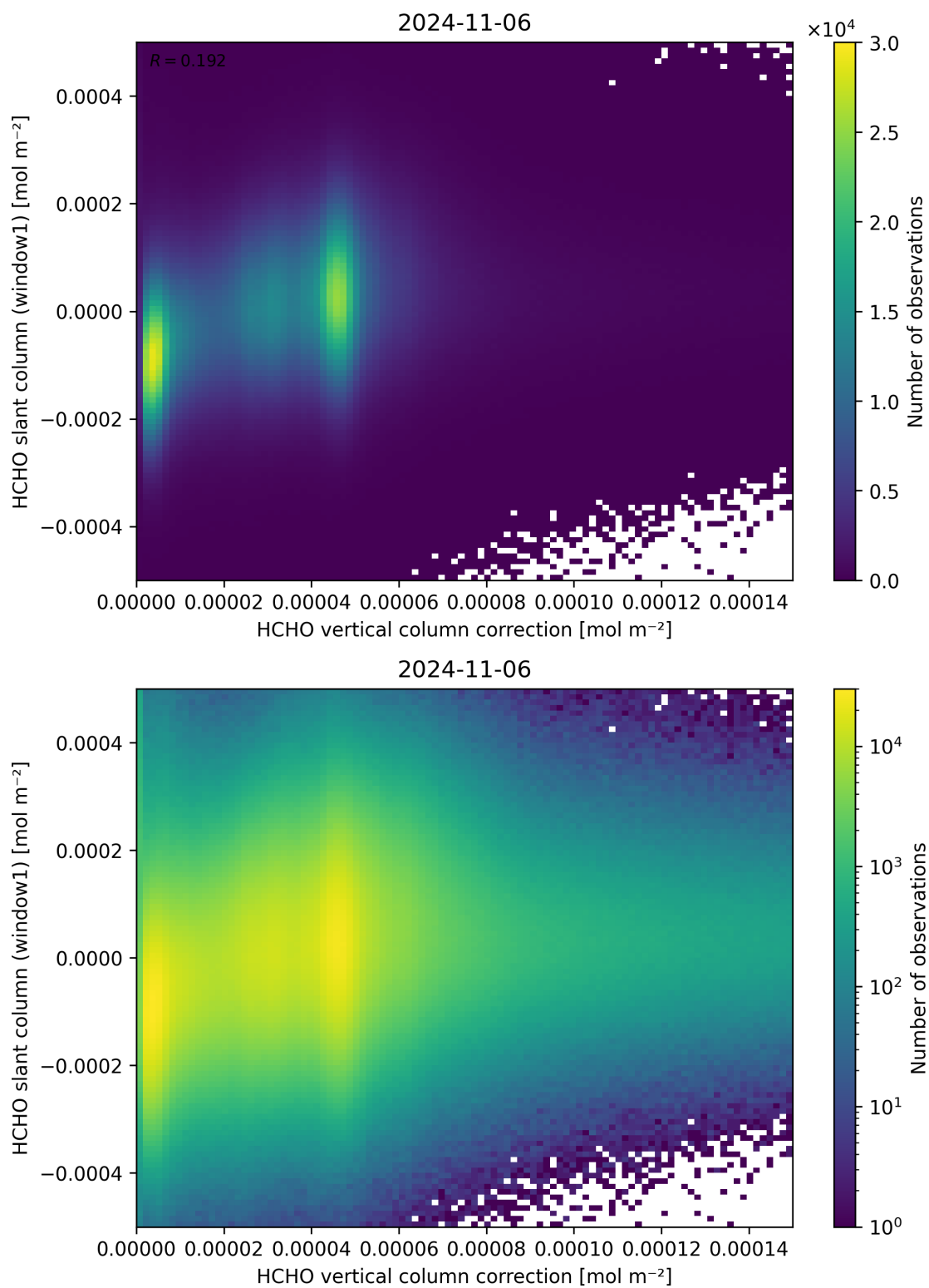
Figure 118: Scatter density plot of “HCHO vertical column correction” against “HCHO slant column (window1)” for 2024-11-05 to 2024-11-07.
