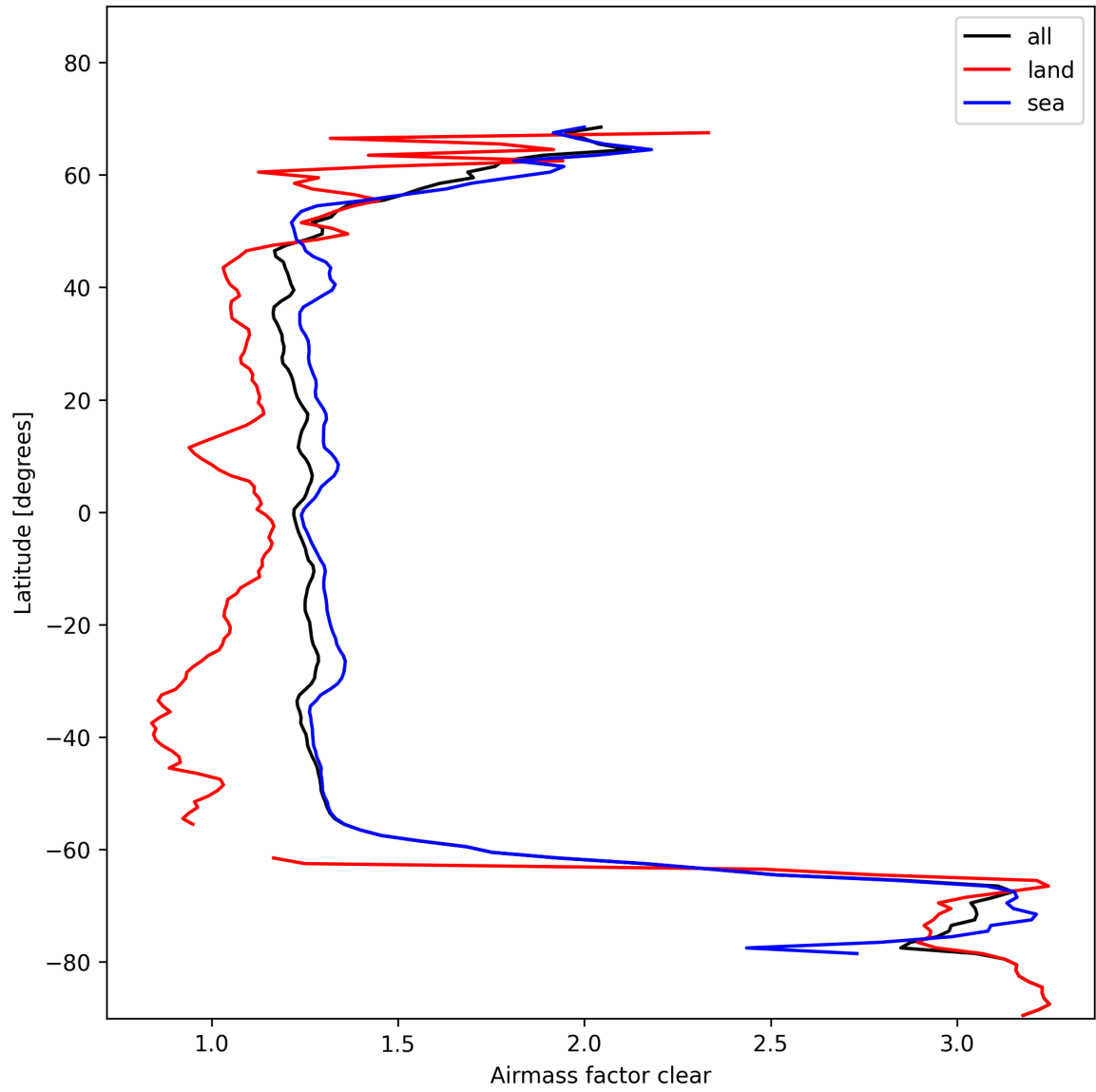
Figure 28: Zonal average of “Airmass factor clear” for 2024-11-05 to 2024-11-07.
