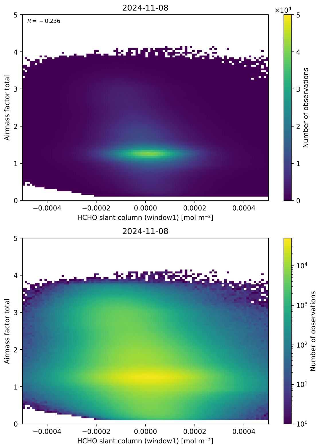
Figure 85: Scatter density plot of “HCHO slant column (window1)” against “Airmass factor total” for 2024-11-07 to 2024-11-09.
