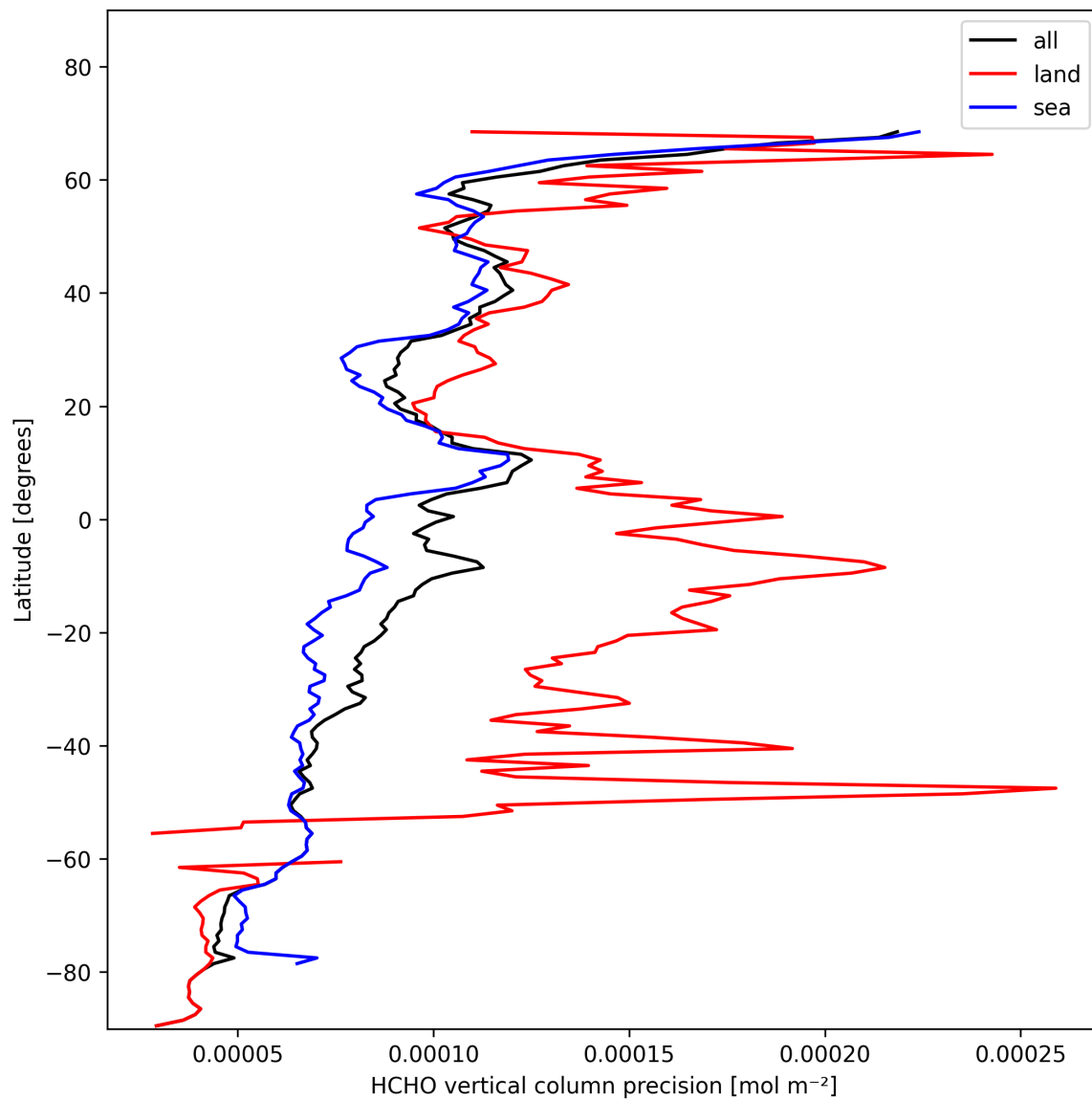
Figure 22: Zonal average of “HCHO vertical column precision” for 2024-11-07 to 2024-11-09.
