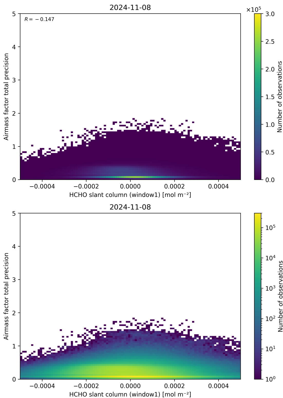
Figure 86: Scatter density plot of “HCHO slant column (window1)” against “Airmass factor total precision” for 2024-11-07 to 2024-11-09.
