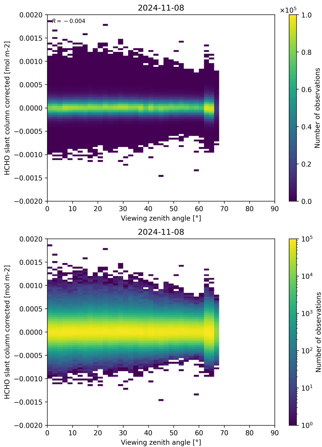
Figure 186: Scatter density plot of “Viewing zenith angle” against “HCHO slant column corrected” for 2024-11-07 to 2024-11-09.
