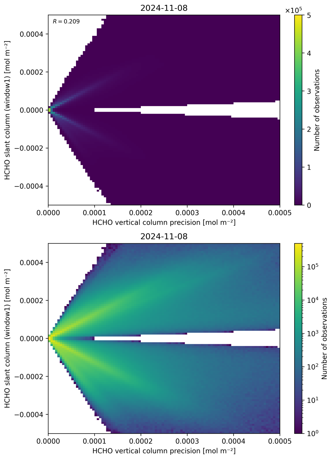
Figure 142: Scatter density plot of “HCHO vertical column precision” against “HCHO slant column (window1)” for 2024-11-07 to 2024-11-09.
