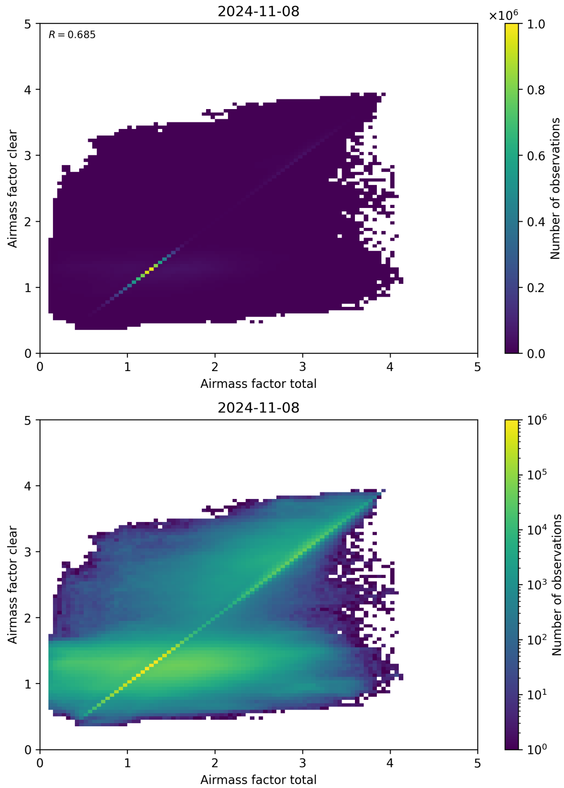
Figure 100: Scatter density plot of “Airmass factor total” against “Airmass factor clear” for 2024-11-07 to 2024-11-09.
