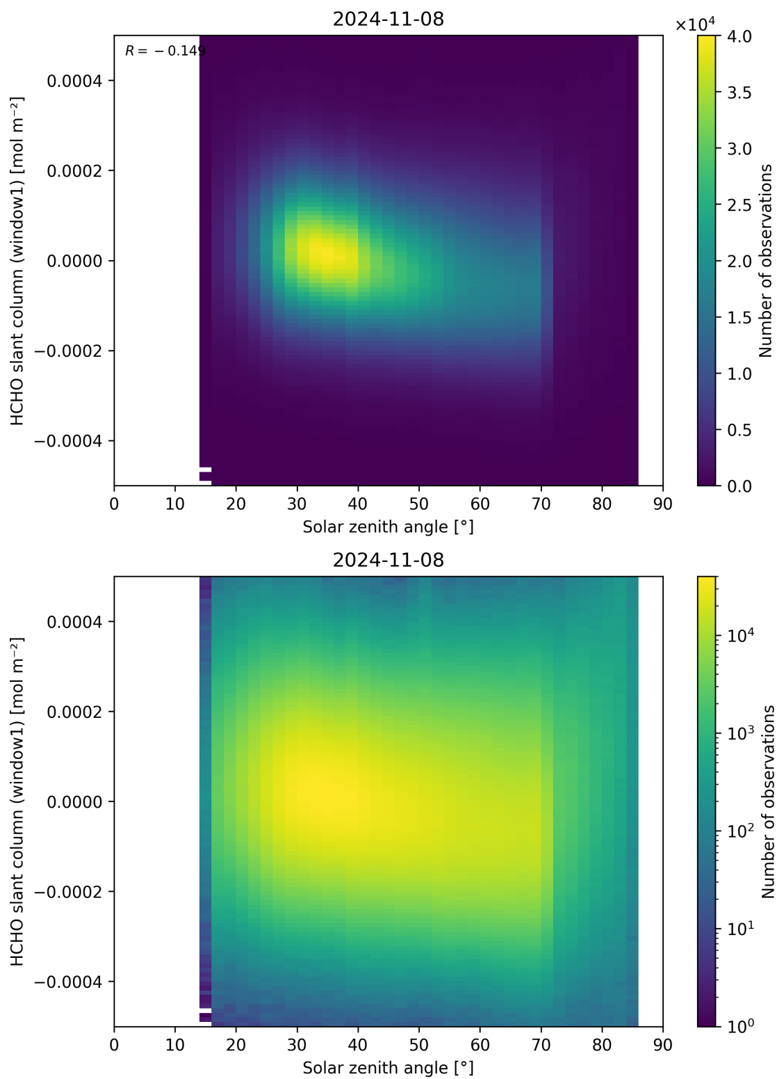
Figure 173: Scatter density plot of “Solar zenith angle” against “HCHO slant column (window1)” for 2024-11-07 to 2024-11-09.
