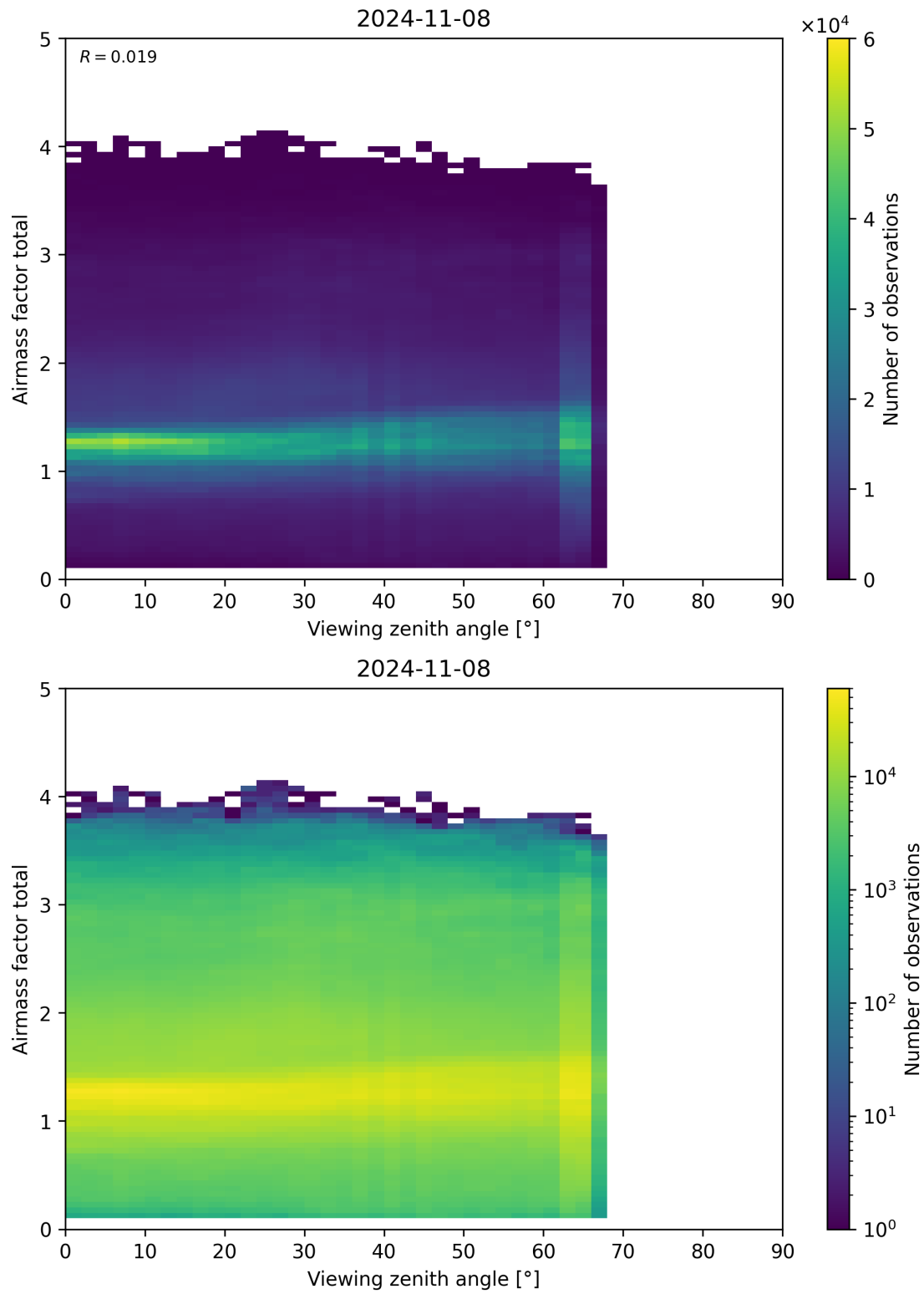
Figure 190: Scatter density plot of “Viewing zenith angle” against “Airmass factor total” for 2024-11-07 to 2024-11-09.
