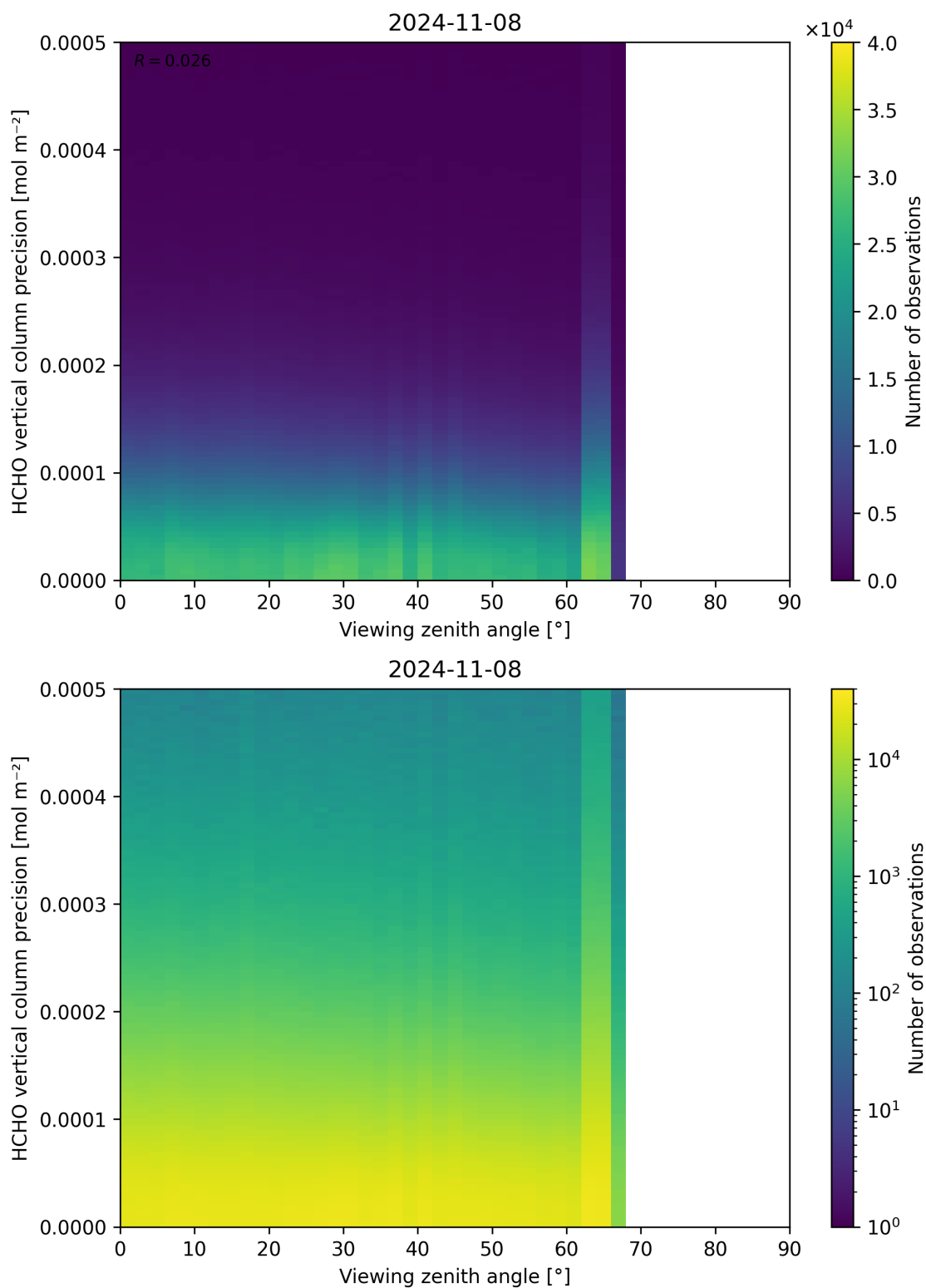
Figure 194: Scatter density plot of “Viewing zenith angle” against “HCHO vertical column precision” for 2024-11-07 to 2024-11-09.
