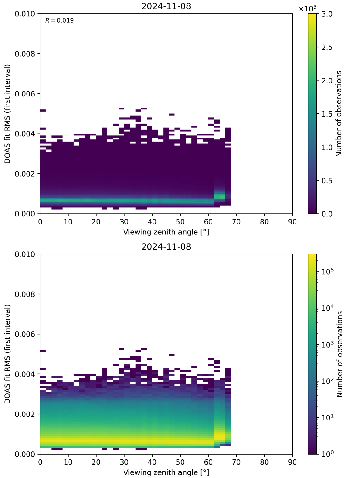
Figure 182: Scatter density plot of “Viewing zenith angle” against “DOAS fit RMS (first interval)” for 2024-11-07 to 2024-11-09.
