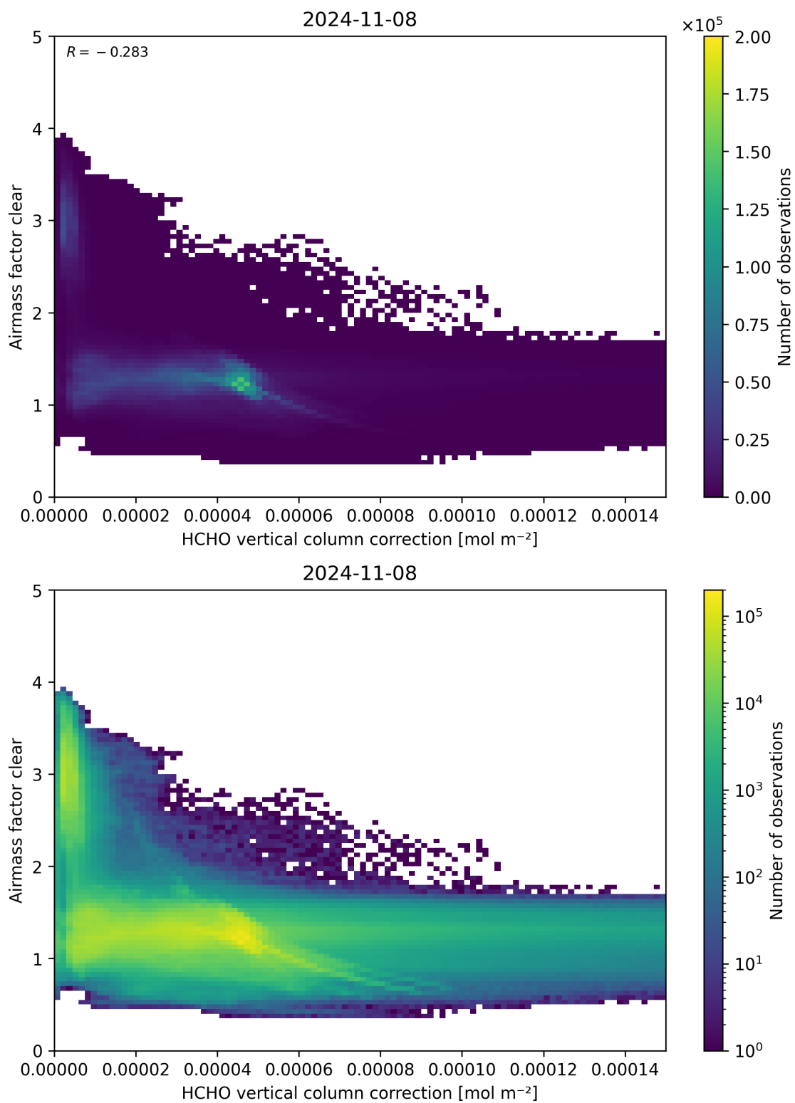
Figure 115: Scatter density plot of “HCHO vertical column correction” against “Airmass factor clear” for 2024-11-07 to 2024-11-09.
