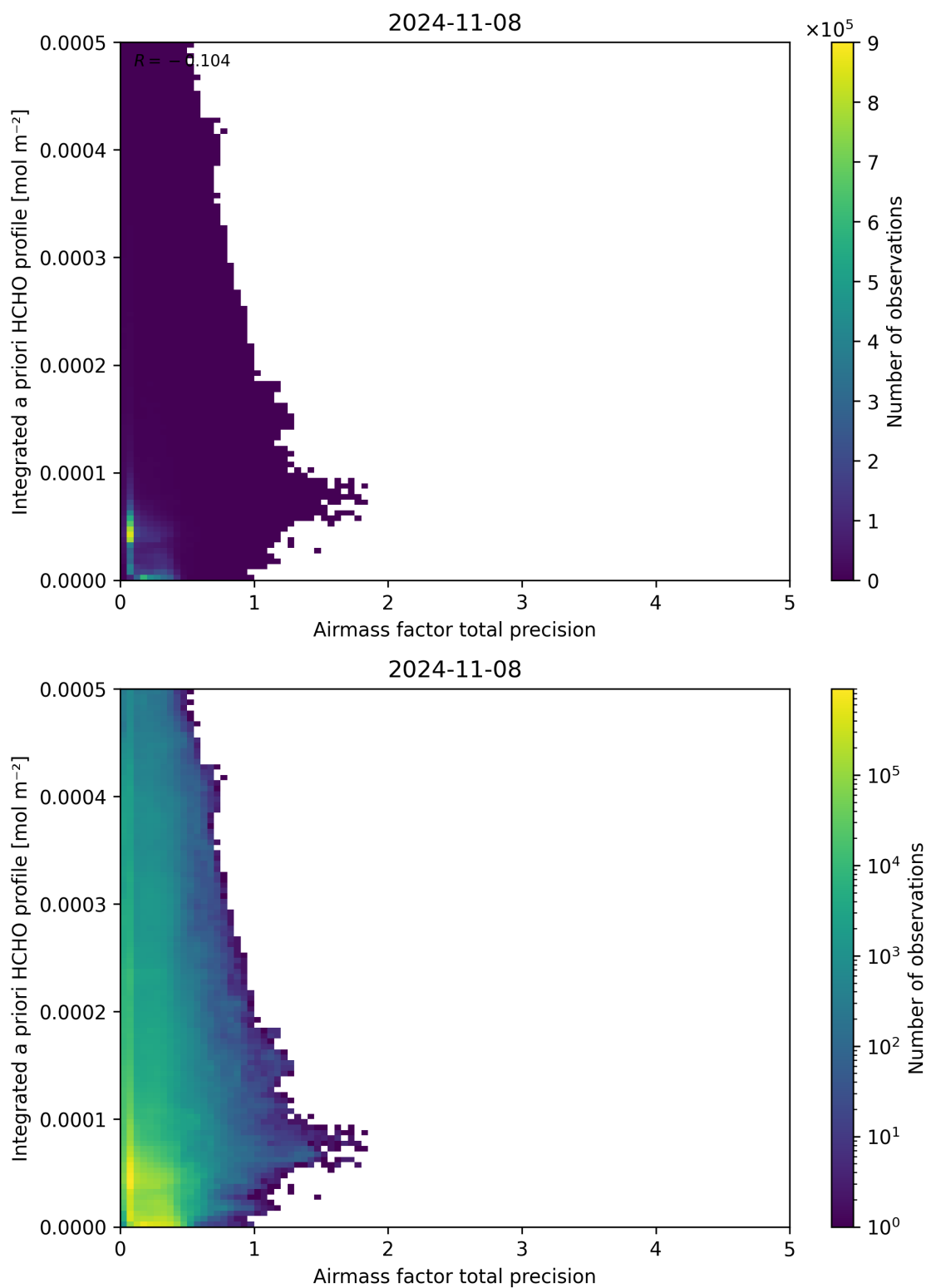
Figure 111: Scatter density plot of “Airmass factor total precision” against “Integrated a priori HCHO profile” for 2024-11-07 to 2024-11-09.
