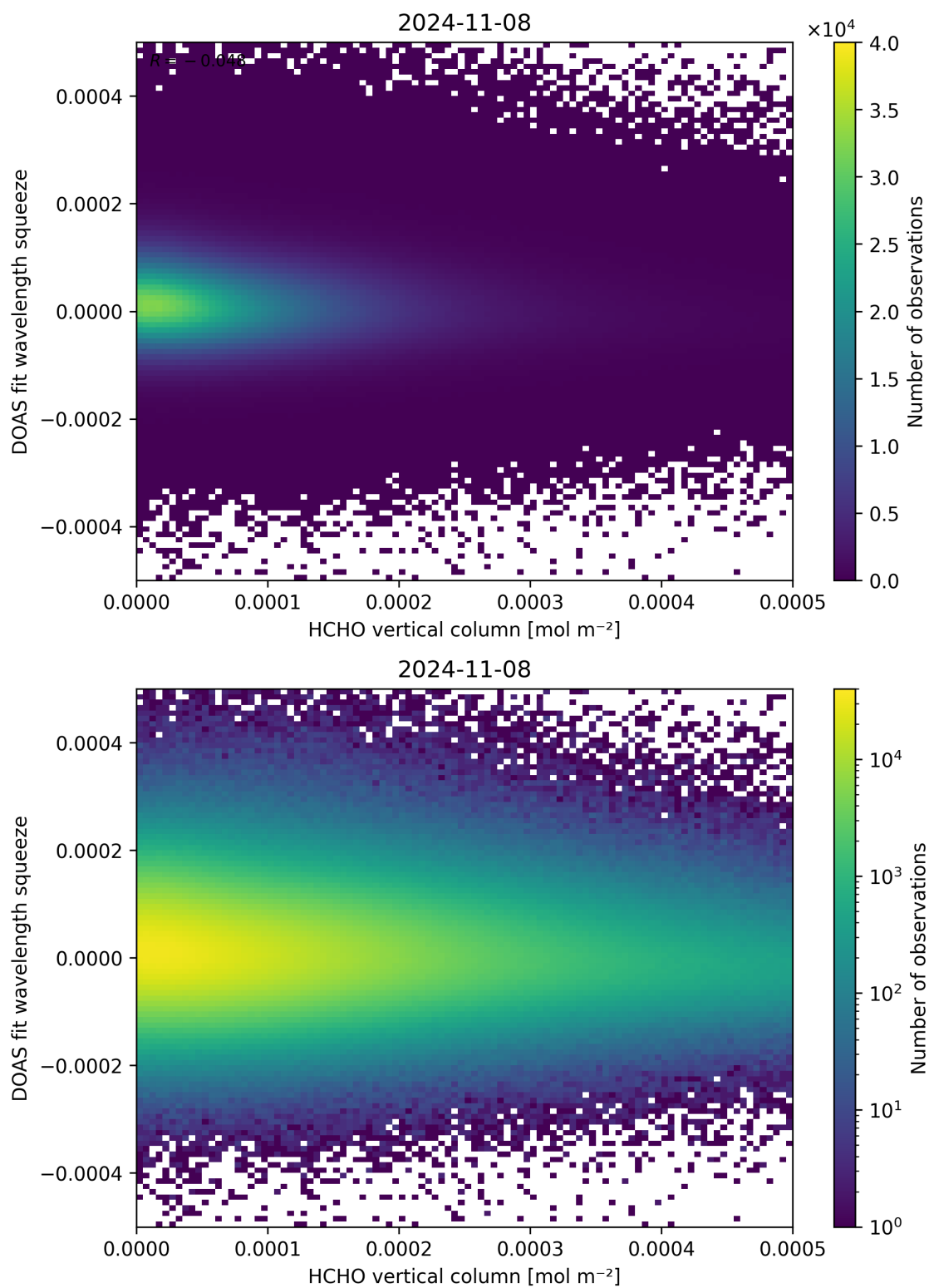
Figure 125: Scatter density plot of “HCHO vertical column” against “DOAS fit wavelength squeeze” for 2024-11-07 to 2024-11-09.
