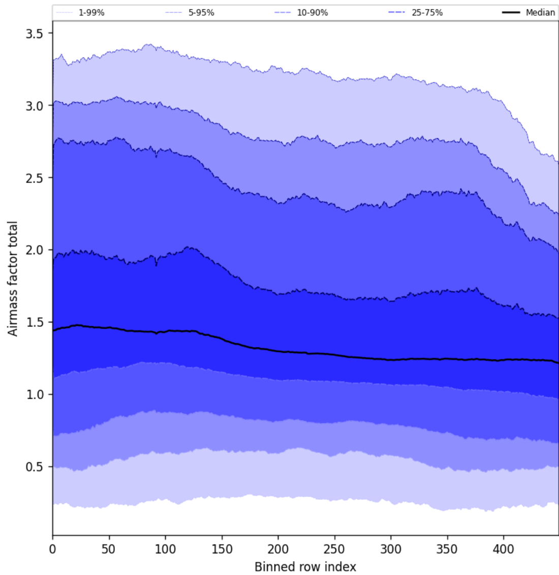
Figure 54: Along track statistics of “Airmass factor total” for 2024-11-07 to 2024-11-09
