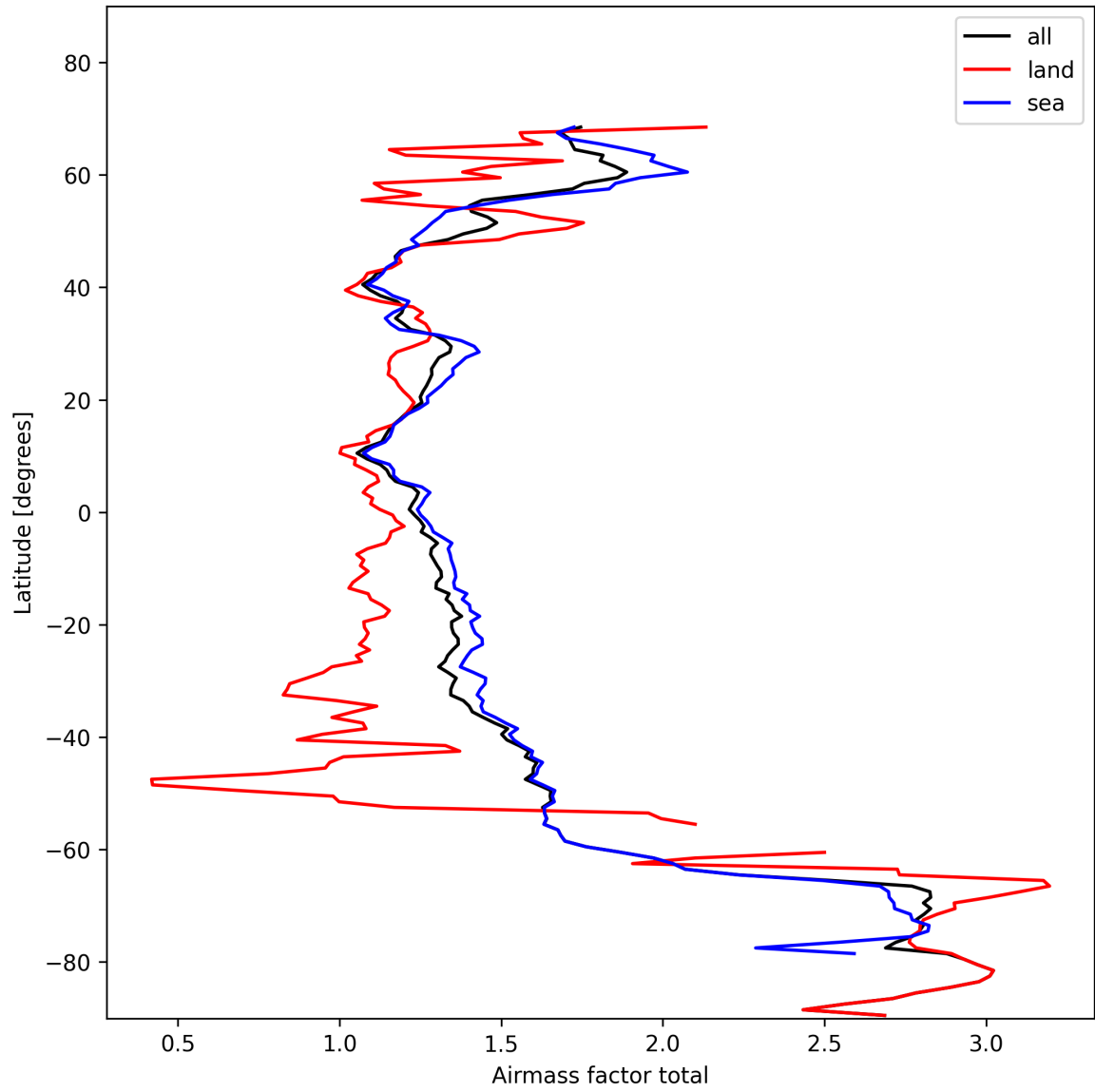
Figure 26: Zonal average of “Airmass factor total” for 2024-11-07 to 2024-11-09.
