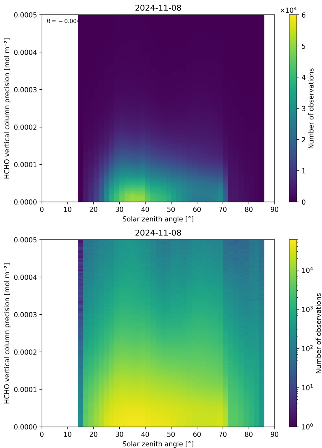
Figure 179: Scatter density plot of “Solar zenith angle” against “HCHO vertical column precision” for 2024-11-07 to 2024-11-09.
