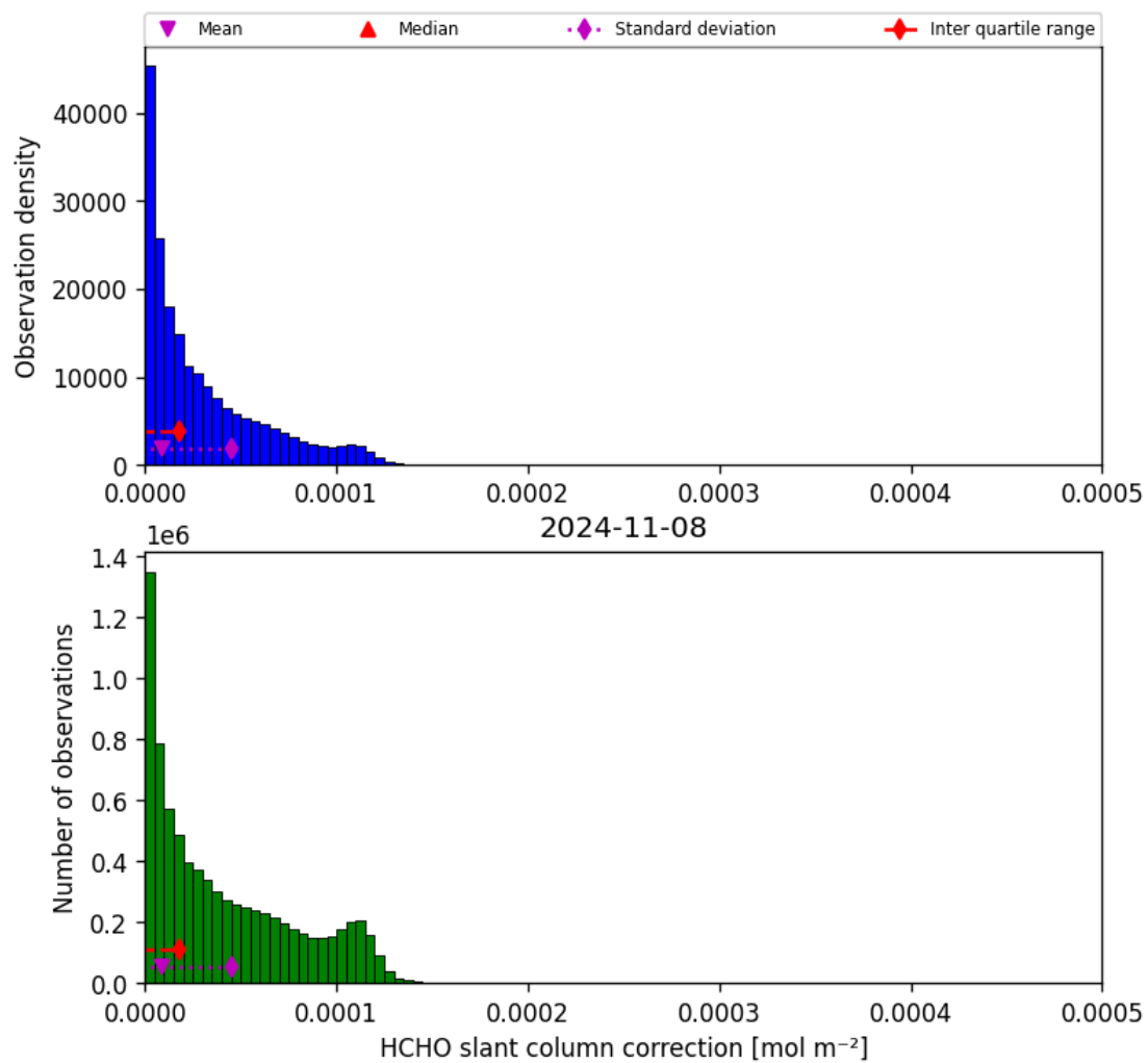
Figure 47: Histogram of “HCHO slant column correction” for 2024-11-07 to 2024-11-09
