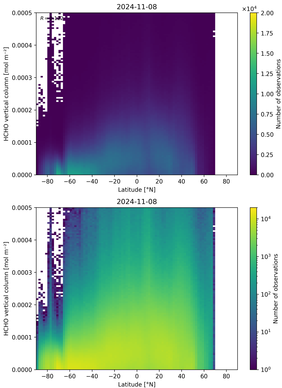
Figure 163: Scatter density plot of “Latitude” against “HCHO vertical column” for 2024-11-07 to 2024-11-09.
