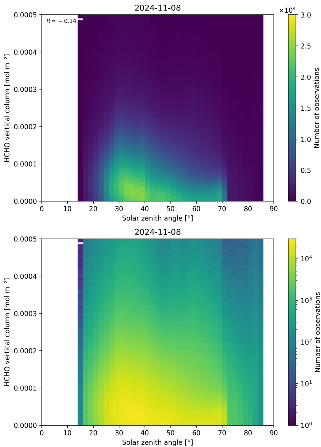
Figure 177: Scatter density plot of “Solar zenith angle” against “HCHO vertical column” for 2024-11-07 to 2024-11-09.
