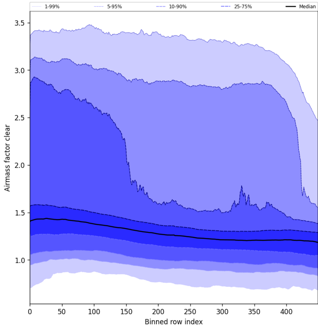
Figure 56: Along track statistics of “Airmass factor clear” for 2024-11-07 to 2024-11-09
