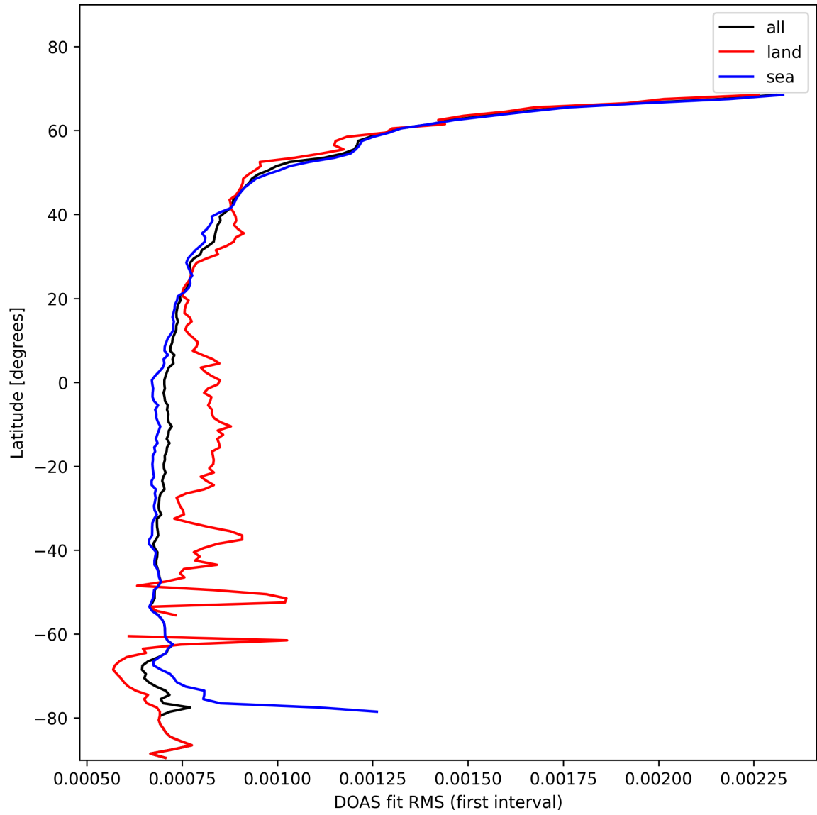
Figure 32: Zonal average of “DOAS fit RMS (first interval)” for 2024-11-07 to 2024-11-09.
