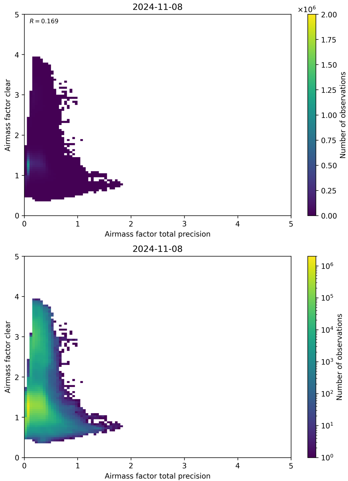
Figure 108: Scatter density plot of “Airmass factor total precision” against “Airmass factor clear” for 2024-11-07 to 2024-11-09.
