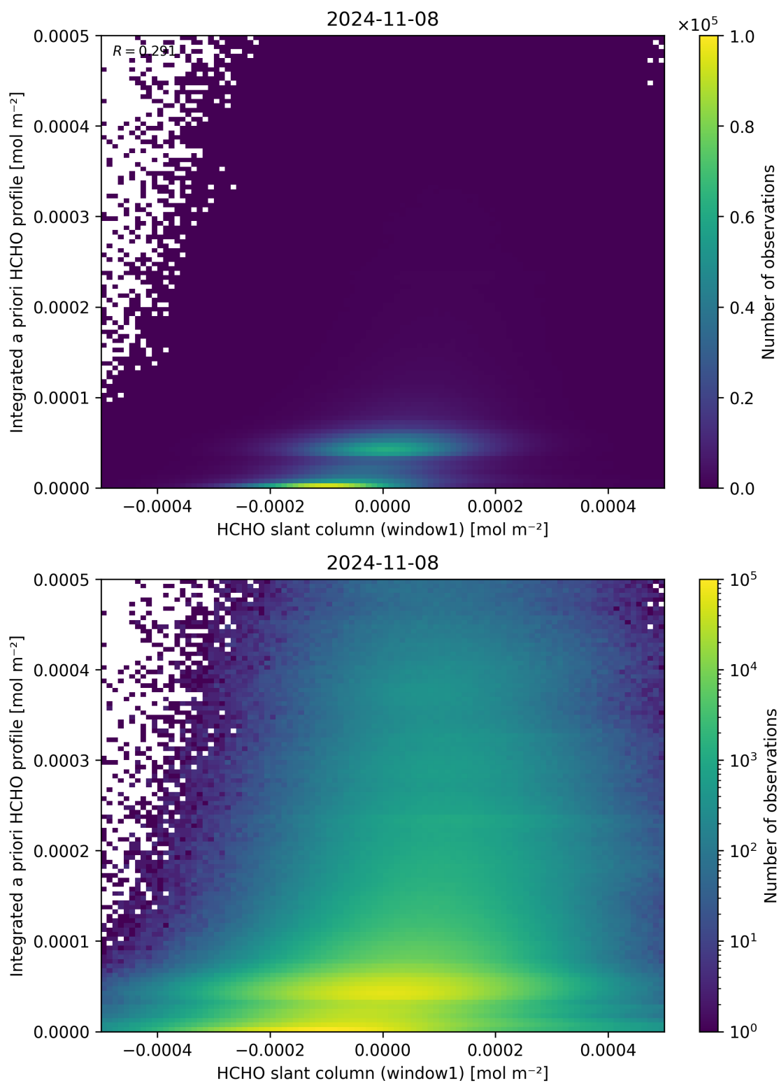
Figure 87: Scatter density plot of “HCHO slant column (window1)” against “Integrated a priori HCHO profile” for 2024-11-07 to 2024-11-09.
