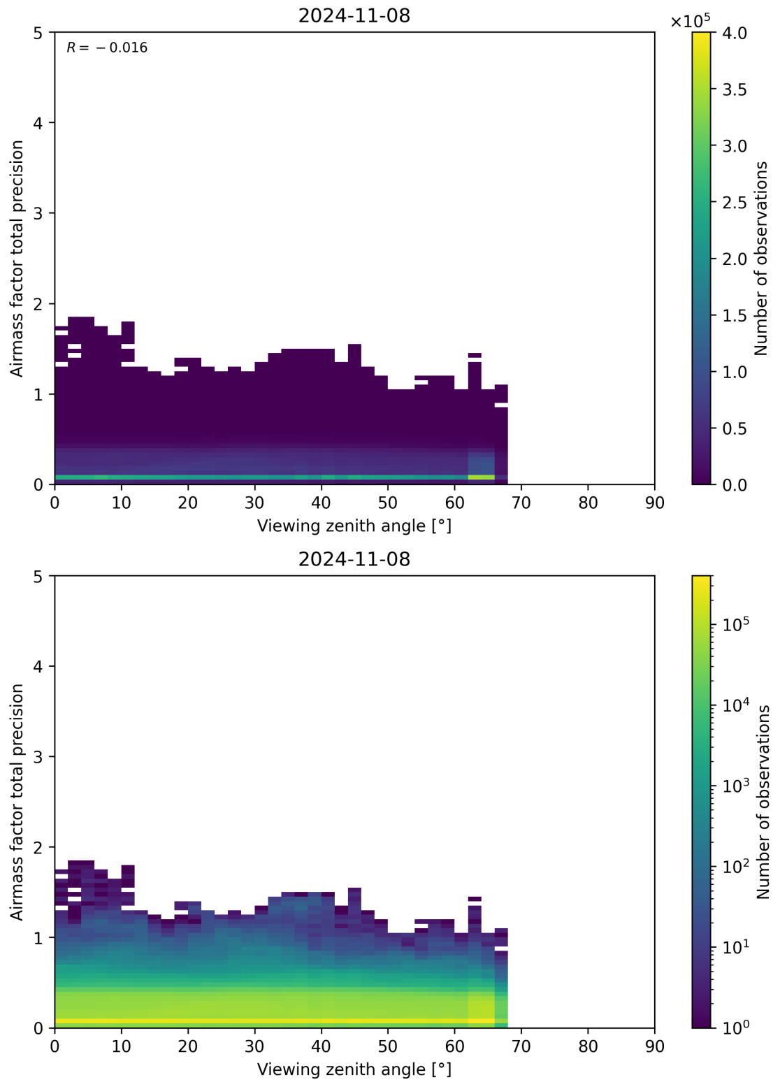
Figure 191: Scatter density plot of “Viewing zenith angle” against “Airmass factor total precision” for 2024-11-07 to 2024-11-09.
