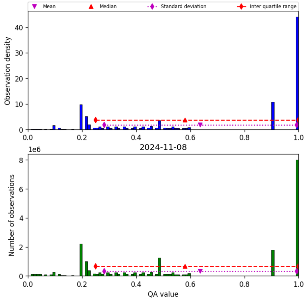
Figure 34: Histogram of “QA value” for 2024-11-07 to 2024-11-09
