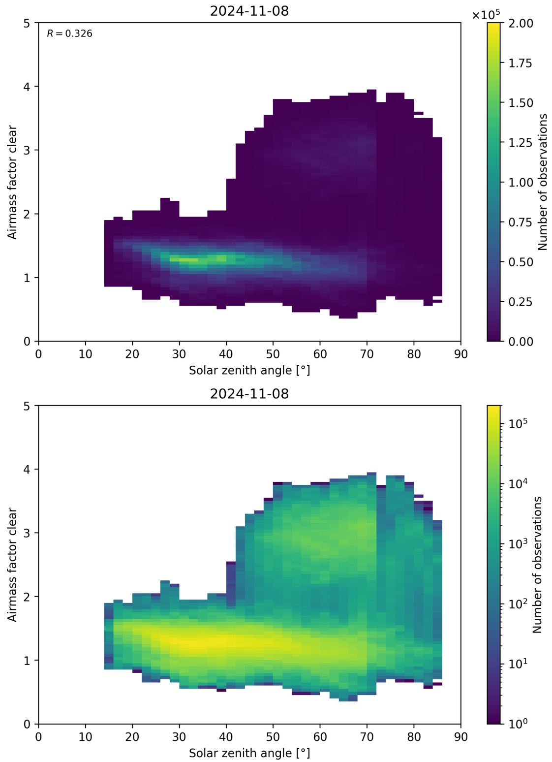
Figure 170: Scatter density plot of “Solar zenith angle” against “Airmass factor clear” for 2024-11-07 to 2024-11-09.
