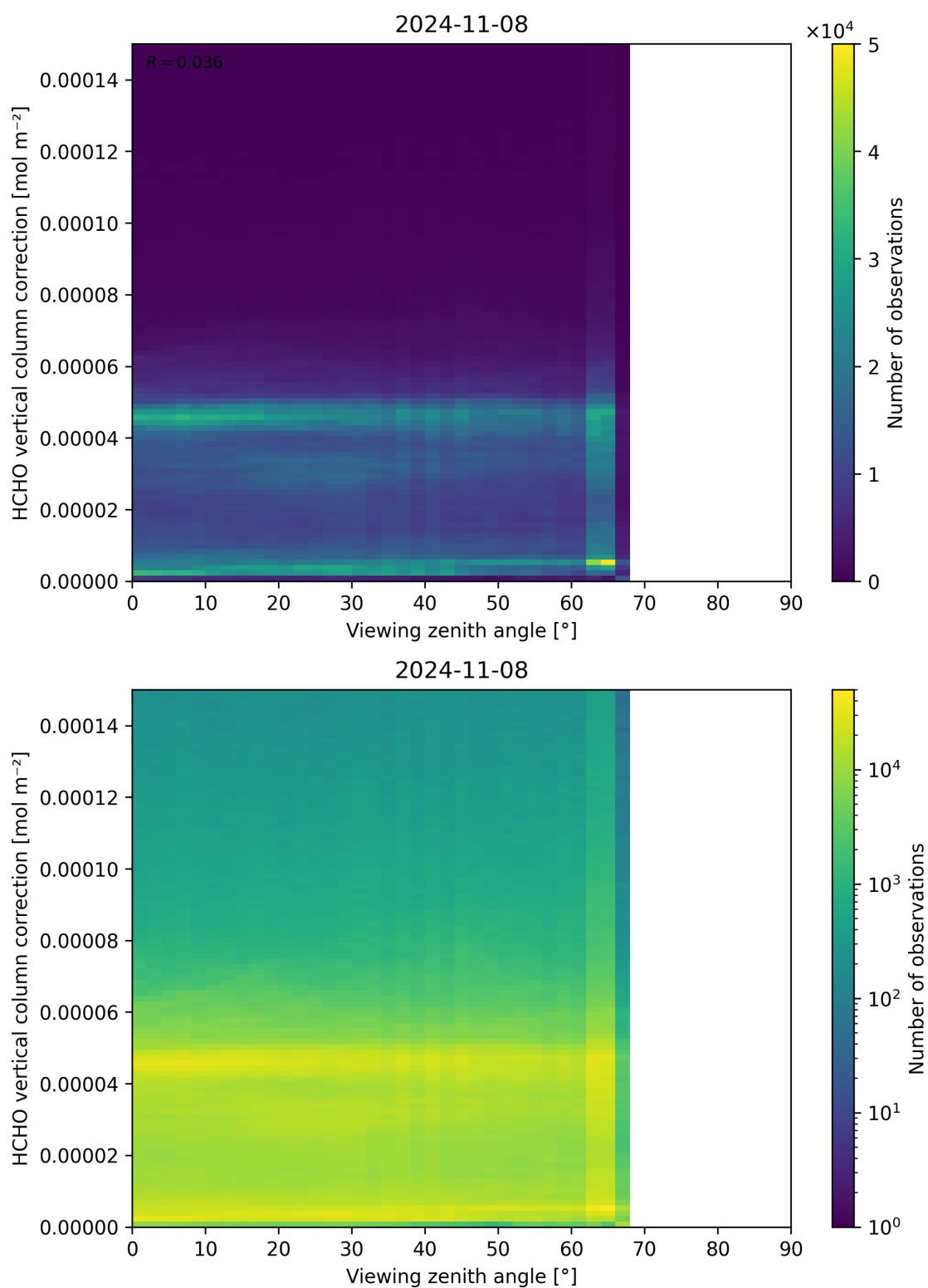
Figure 193: Scatter density plot of “Viewing zenith angle” against “HCHO vertical column correction” for 2024-11-07 to 2024-11-09.
