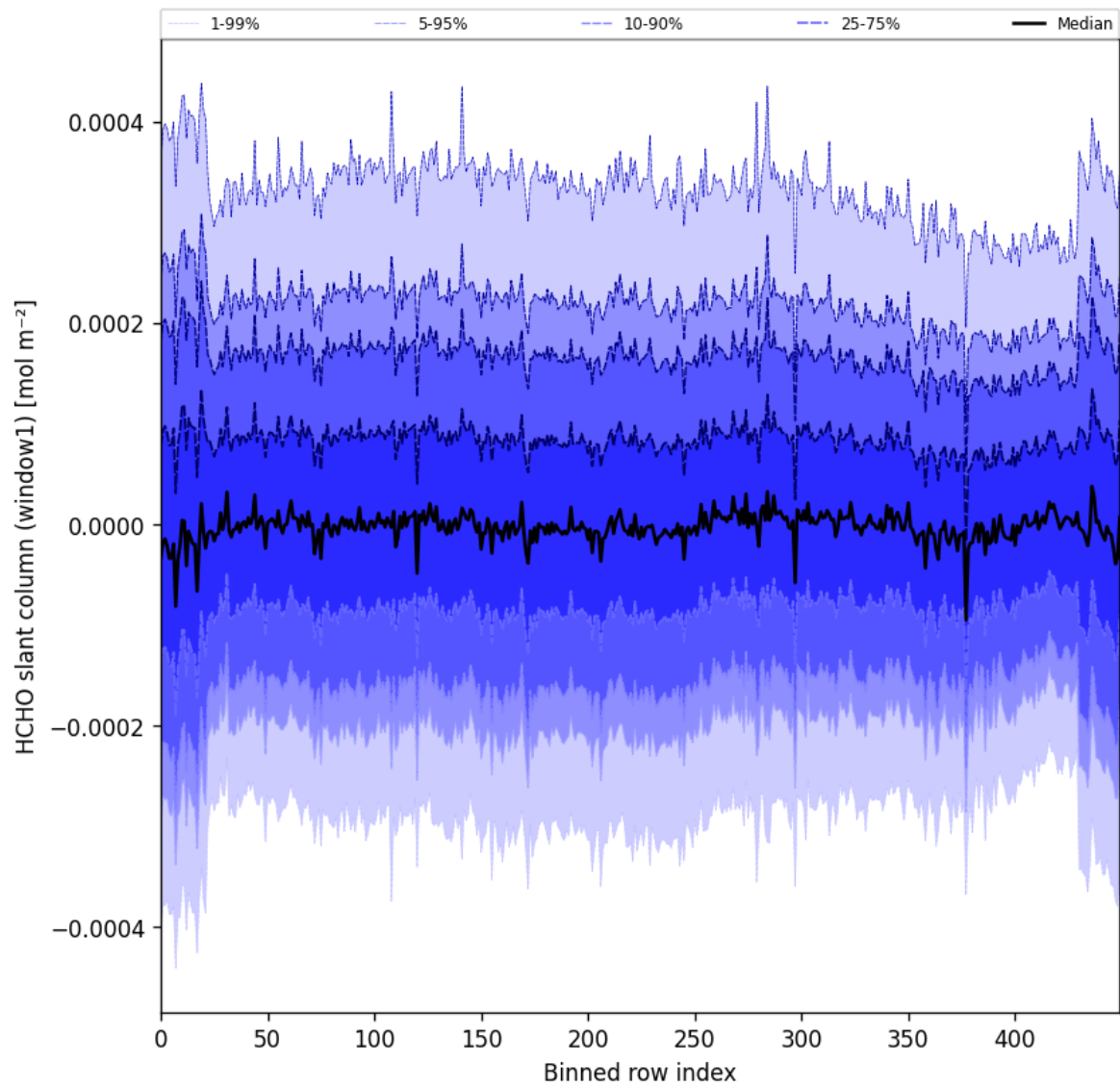
Figure 52: Along track statistics of "HCHO slant column (window1)" for 2024-11-07 to 2024-11-09
