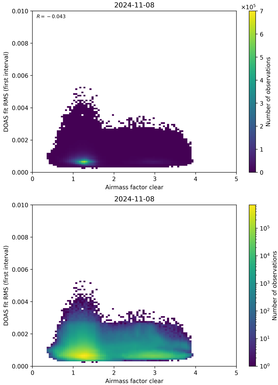
Figure 71: Scatter density plot of “Airmass factor clear” against “DOAS fit RMS (first interval)” for 2024-11-07 to 2024-11-09.
