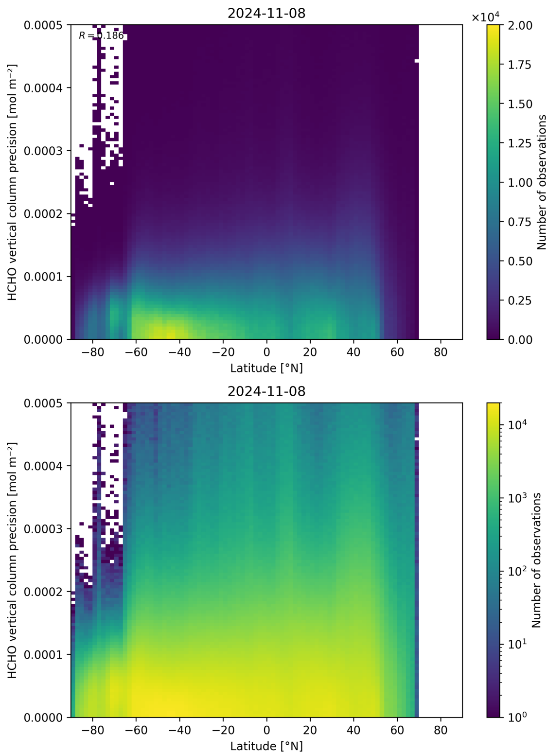
Figure 165: Scatter density plot of “Latitude” against “HCHO vertical column precision” for 2024-11-07 to 2024-11-09.
