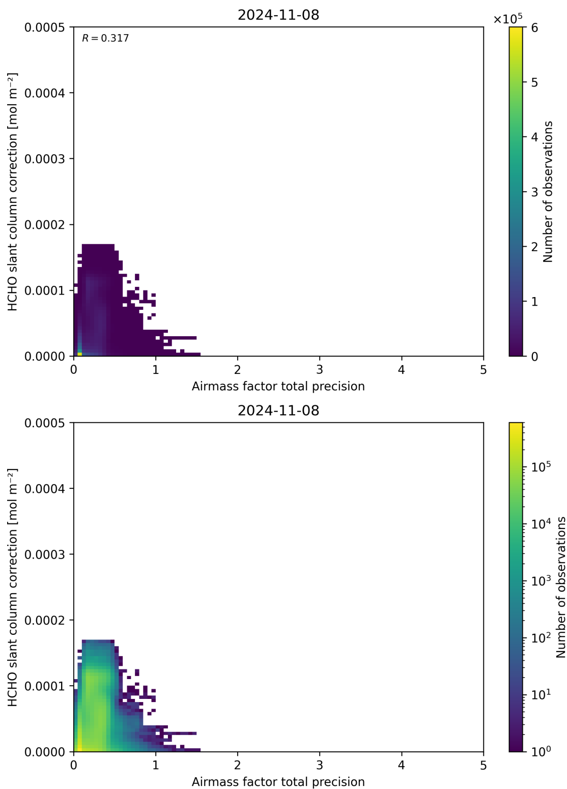
Figure 110: Scatter density plot of “Airmass factor total precision” against “HCHO slant column correction” for 2024-11-07 to 2024-11-09.
