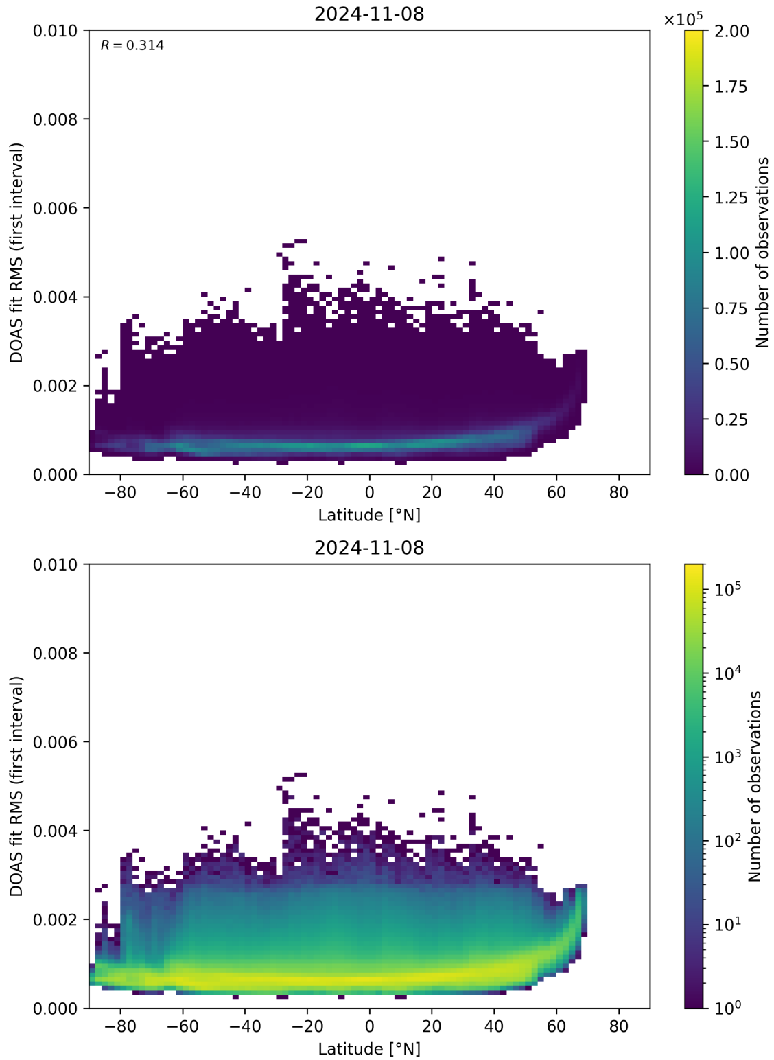
Figure 153: Scatter density plot of “Latitude” against “DOAS fit RMS (first interval)” for 2024-11-07 to 2024-11-09.
