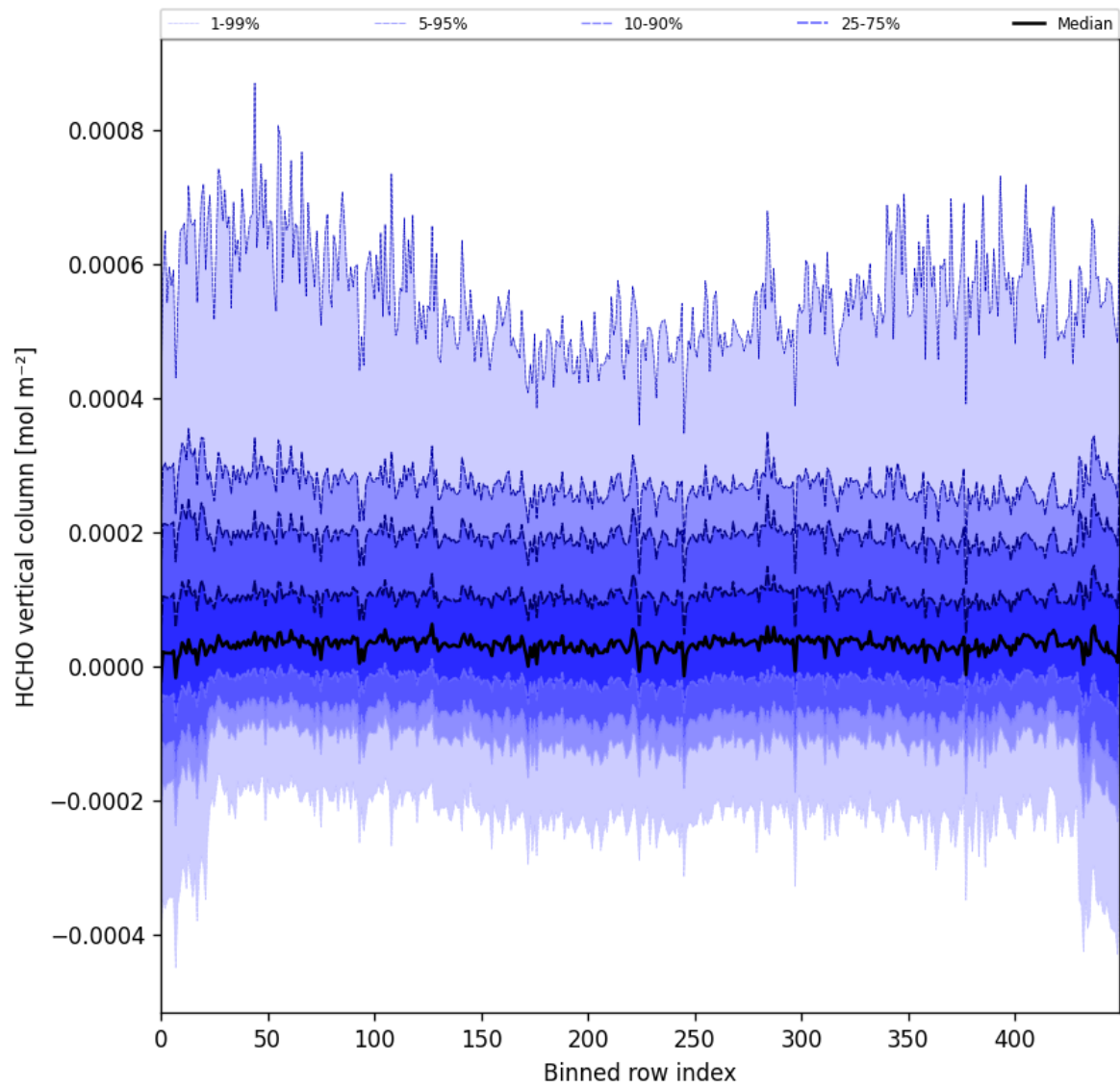
Figure 49: Along track statistics of “HCHO vertical column” for 2024-11-07 to 2024-11-09
