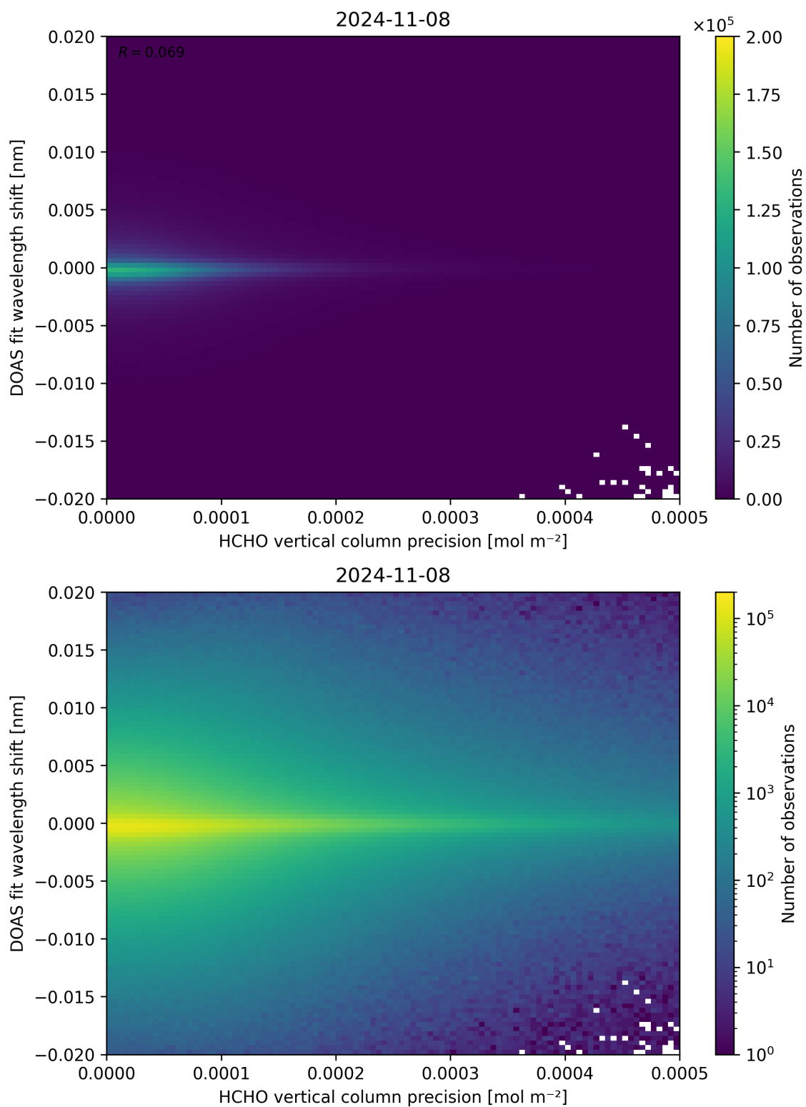
Figure 137: Scatter density plot of “HCHO vertical column precision” against “DOAS fit wavelength shift” for 2024-11-07 to 2024-11-09.
