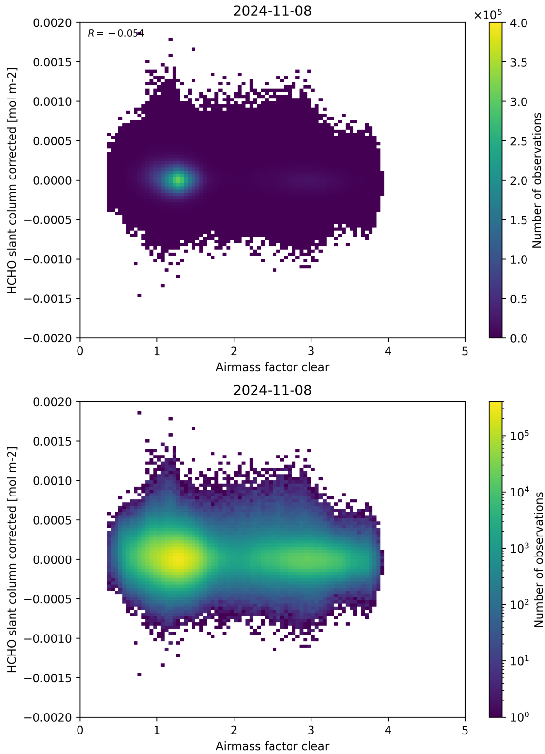
Figure 74: Scatter density plot of “Airmass factor clear” against “HCHO slant column corrected” for 2024-11-07 to 2024-11-09.
