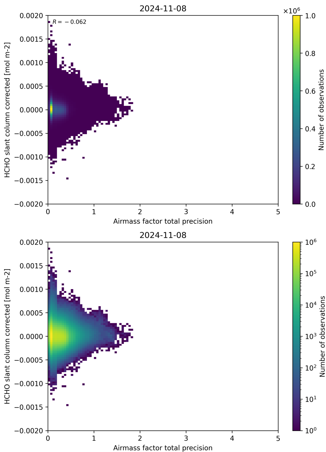
Figure 109: Scatter density plot of “Airmass factor total precision” against “HCHO slant column corrected” for 2024-11-07 to 2024-11-09.
