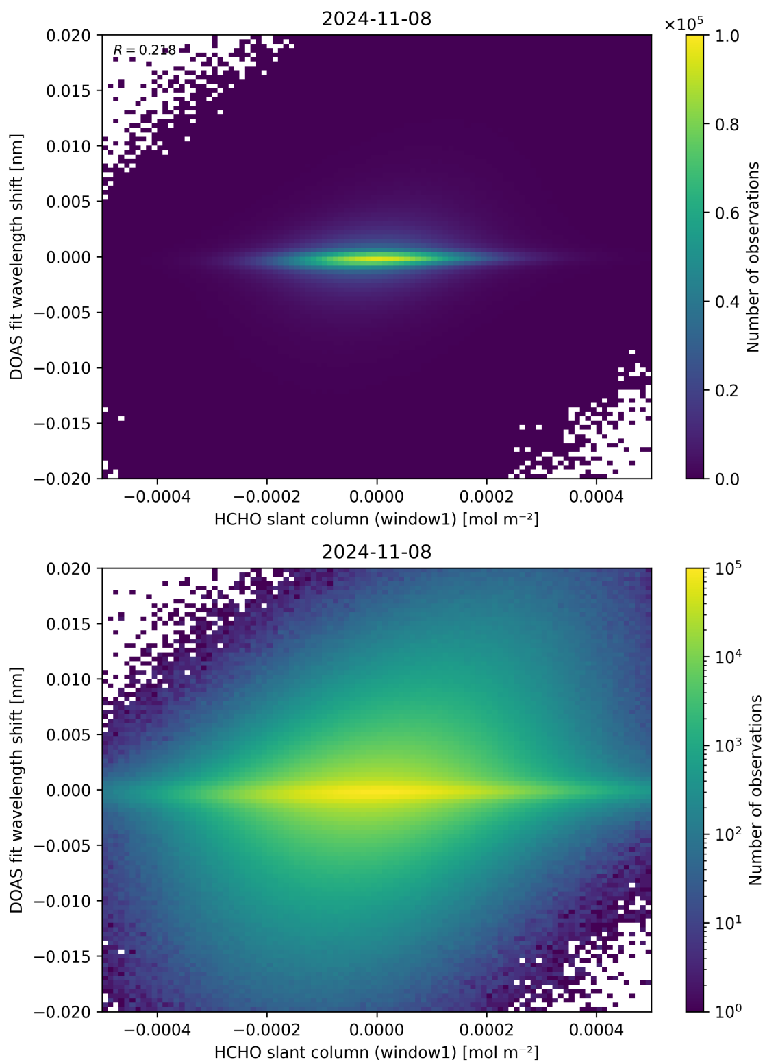
Figure 79: Scatter density plot of “HCHO slant column (window1)” against “DOAS fit wavelength shift” for 2024-11-07 to 2024-11-09.
