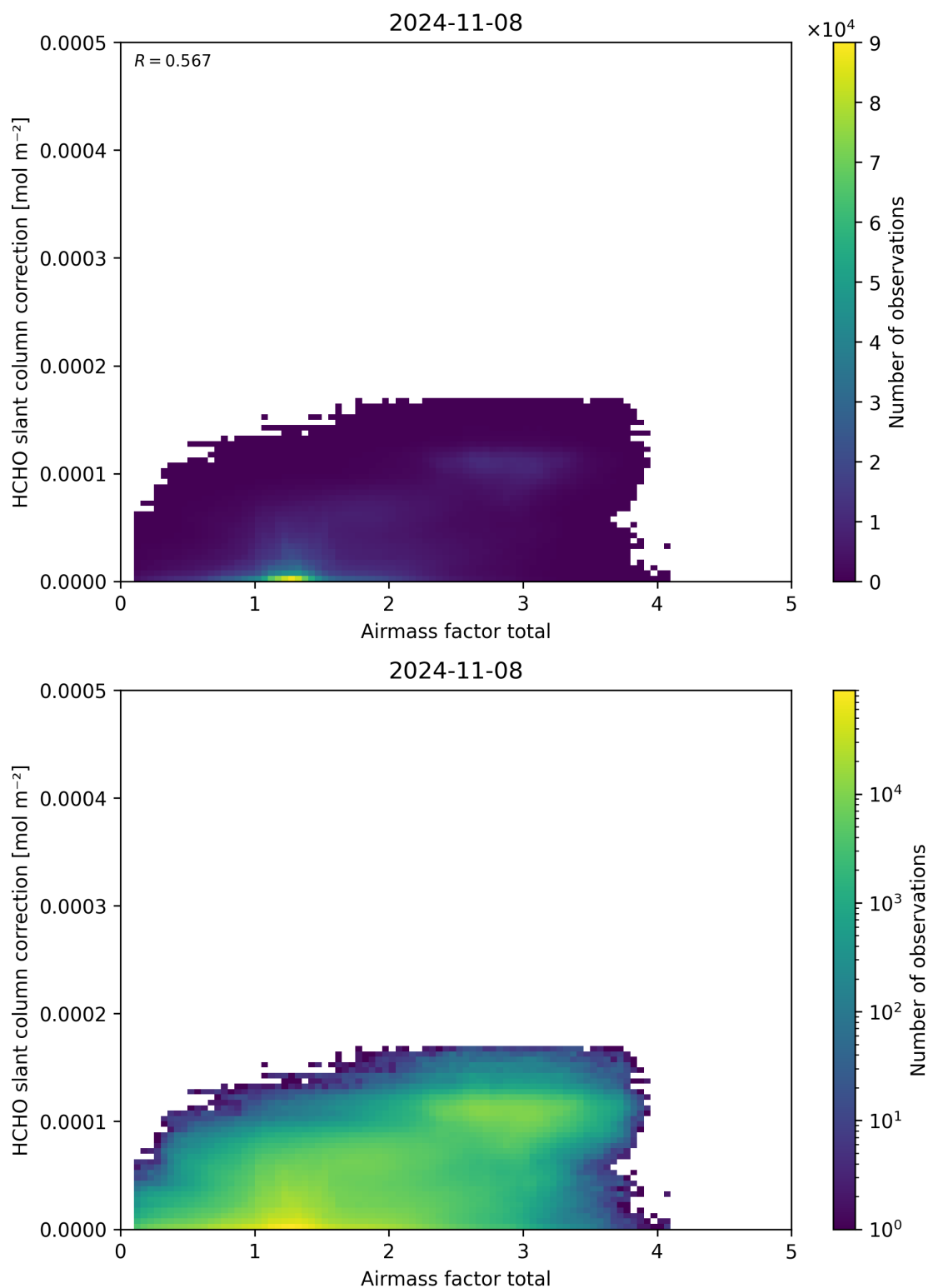
Figure 102: Scatter density plot of “Airmass factor total” against “HCHO slant column correction” for 2024-11-07 to 2024-11-09.
