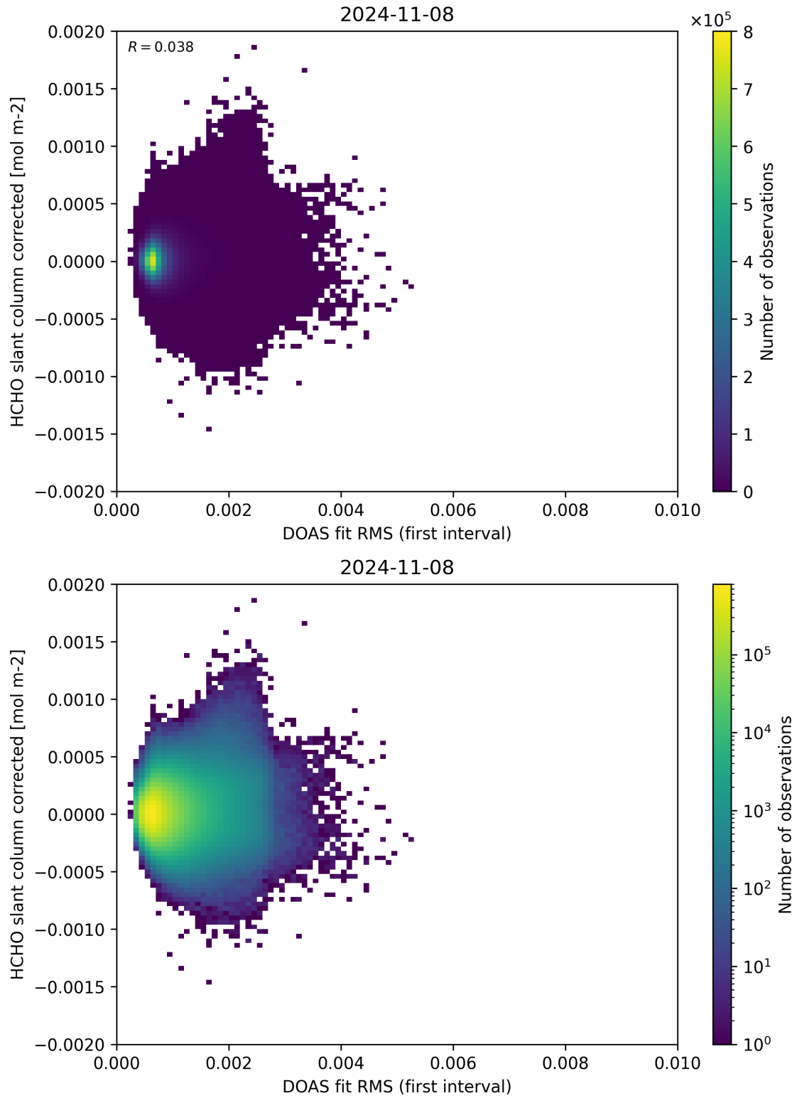
Figure 62: Scatter density plot of “DOAS fit RMS (first interval)” against “HCHO slant column corrected” for 2024-11-07 to 2024-11-09.
