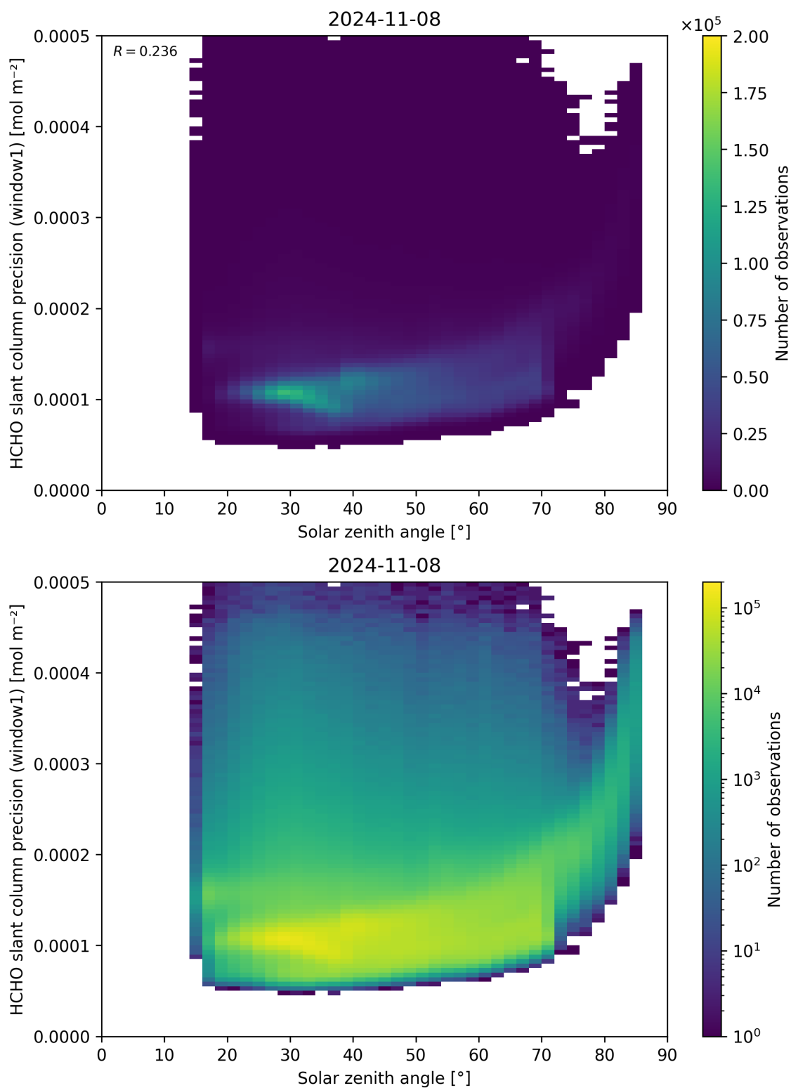
Figure 174: Scatter density plot of “Solar zenith angle” against “HCHO slant column precision (window1)” for 2024-11-07 to 2024-11-09.
