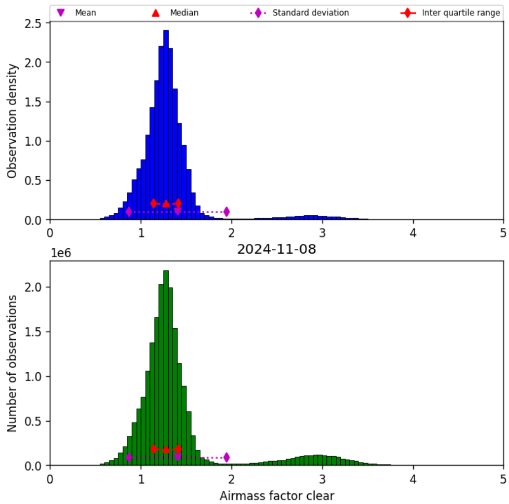
Figure 42: Histogram of “Airmass factor clear” for 2024-11-07 to 2024-11-09
