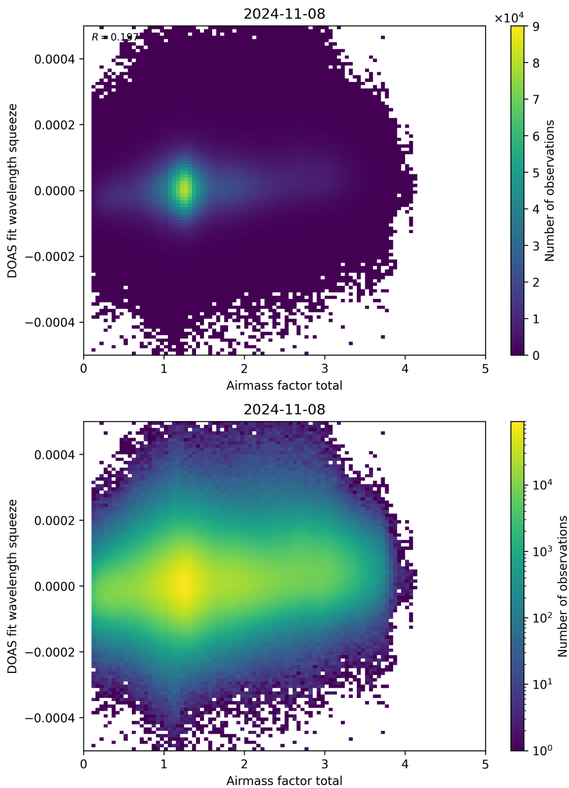
Figure 99: Scatter density plot of “Airmass factor total” against “DOAS fit wavelength squeeze” for 2024-11-07 to 2024-11-09.
