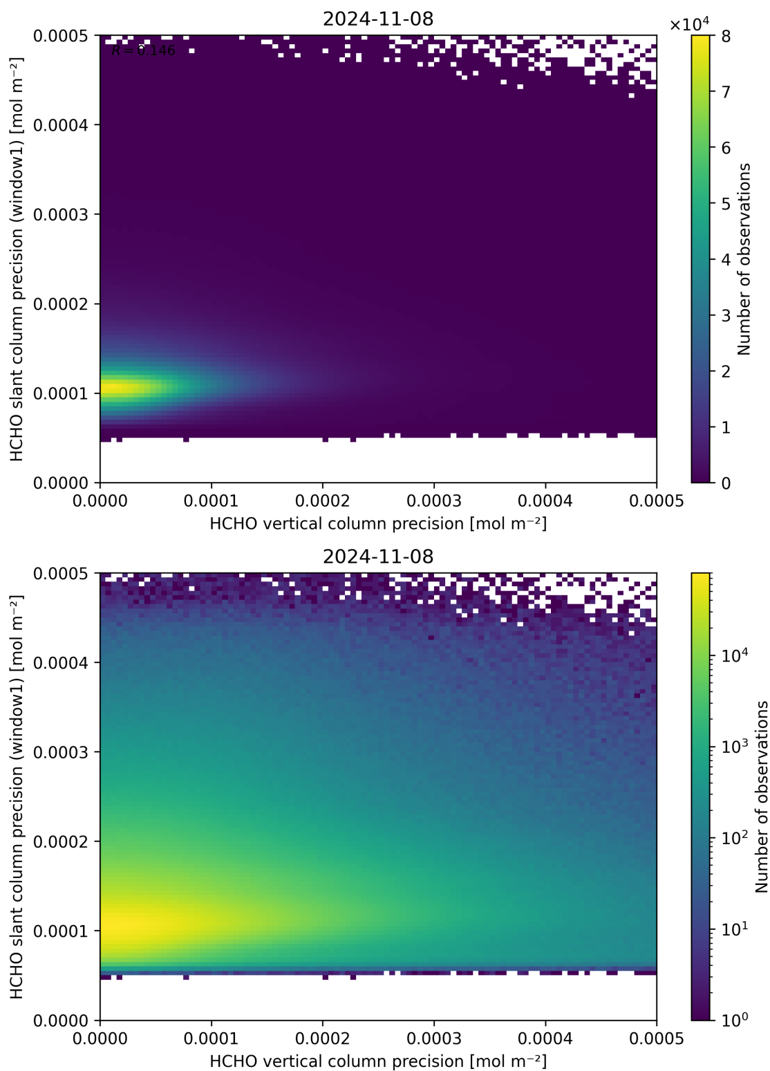
Figure 143: Scatter density plot of “HCHO vertical column precision” against “HCHO slant column precision (window1)” for 2024-11-07 to 2024-11-09.
