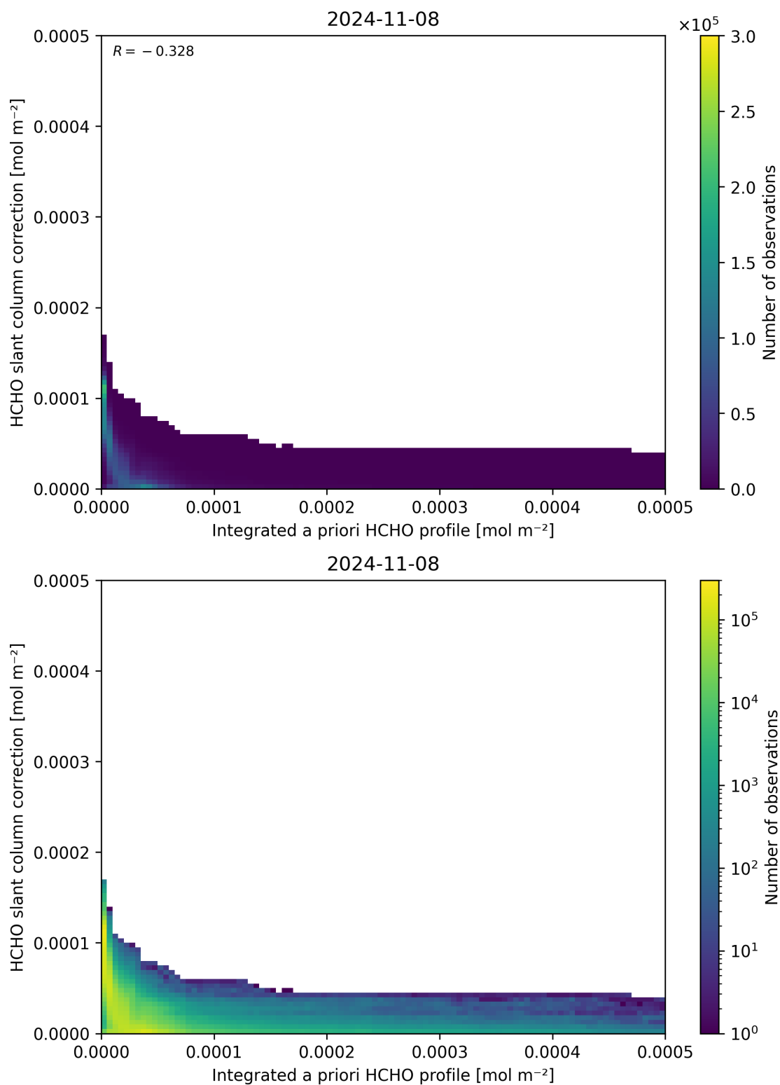
Figure 152: Scatter density plot of “Integrated a priori HCHO profile” against “HCHO slant column correction” for 2024-11-07 to 2024-11-09.
