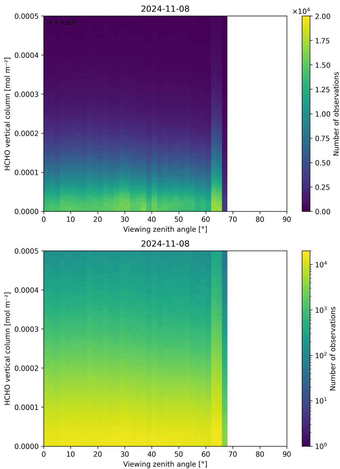
Figure 192: Scatter density plot of “Viewing zenith angle” against “HCHO vertical column” for 2024-11-07 to 2024-11-09.
