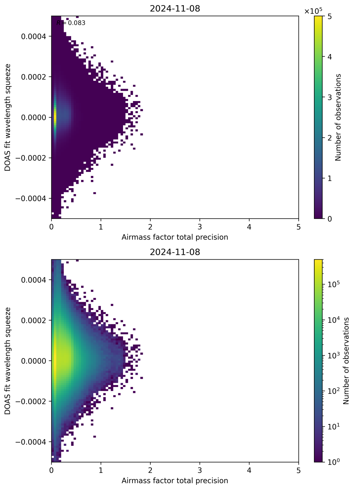
Figure 107: Scatter density plot of “Airmass factor total precision” against “DOAS fit wavelength squeeze” for 2024-11-07 to 2024-11-09.
