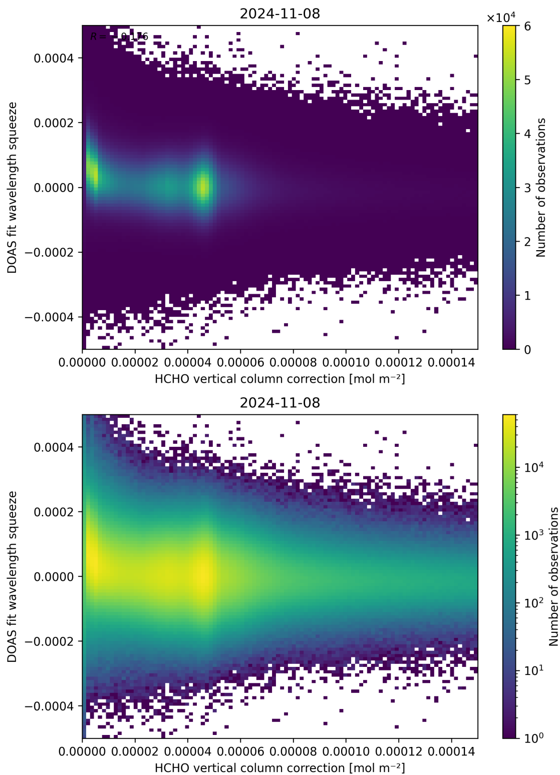
Figure 114: Scatter density plot of “HCHO vertical column correction” against “DOAS fit wavelength squeeze” for 2024-11-07 to 2024-11-09.
