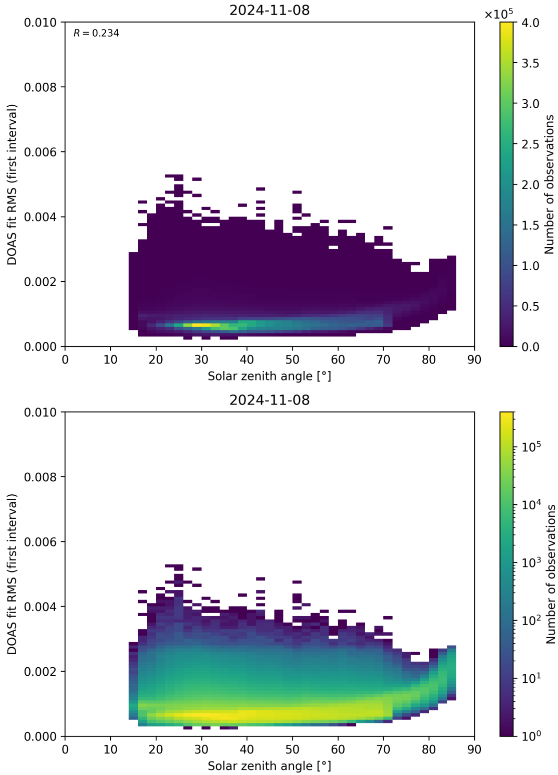
Figure 167: Scatter density plot of “Solar zenith angle” against “DOAS fit RMS (first interval)” for 2024-11-07 to 2024-11-09.
