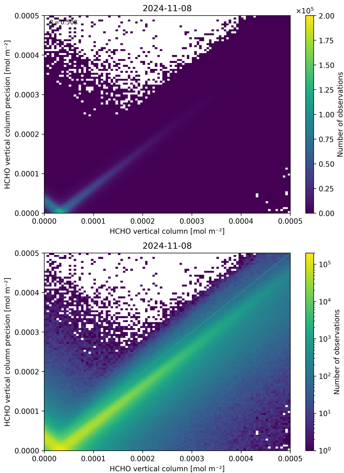
Figure 134: Scatter density plot of “HCHO vertical column” against “HCHO vertical column precision” for 2024-11-07 to 2024-11-09.
