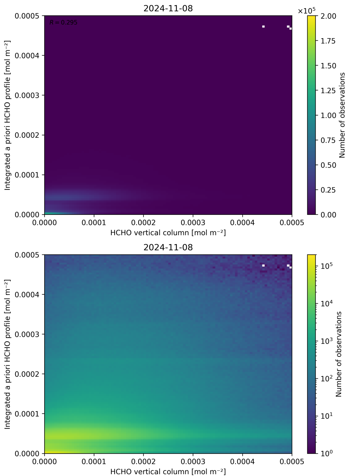
Figure 135: Scatter density plot of “HCHO vertical column” against “Integrated a priori HCHO profile” for 2024-11-07 to 2024-11-09.
