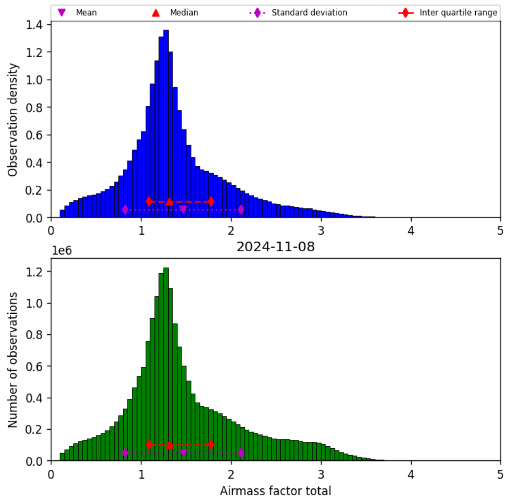
Figure 40: Histogram of “Airmass factor total” for 2024-11-07 to 2024-11-09
