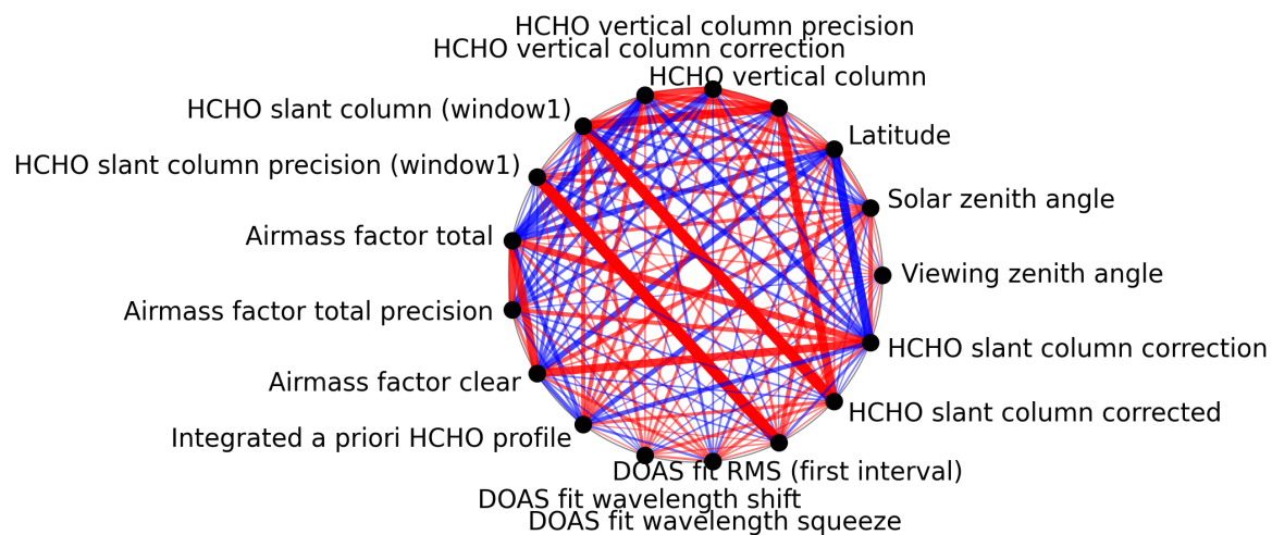
Figure 1: Map of correlation graph for 2024-11-07 to 2024-11-09.
