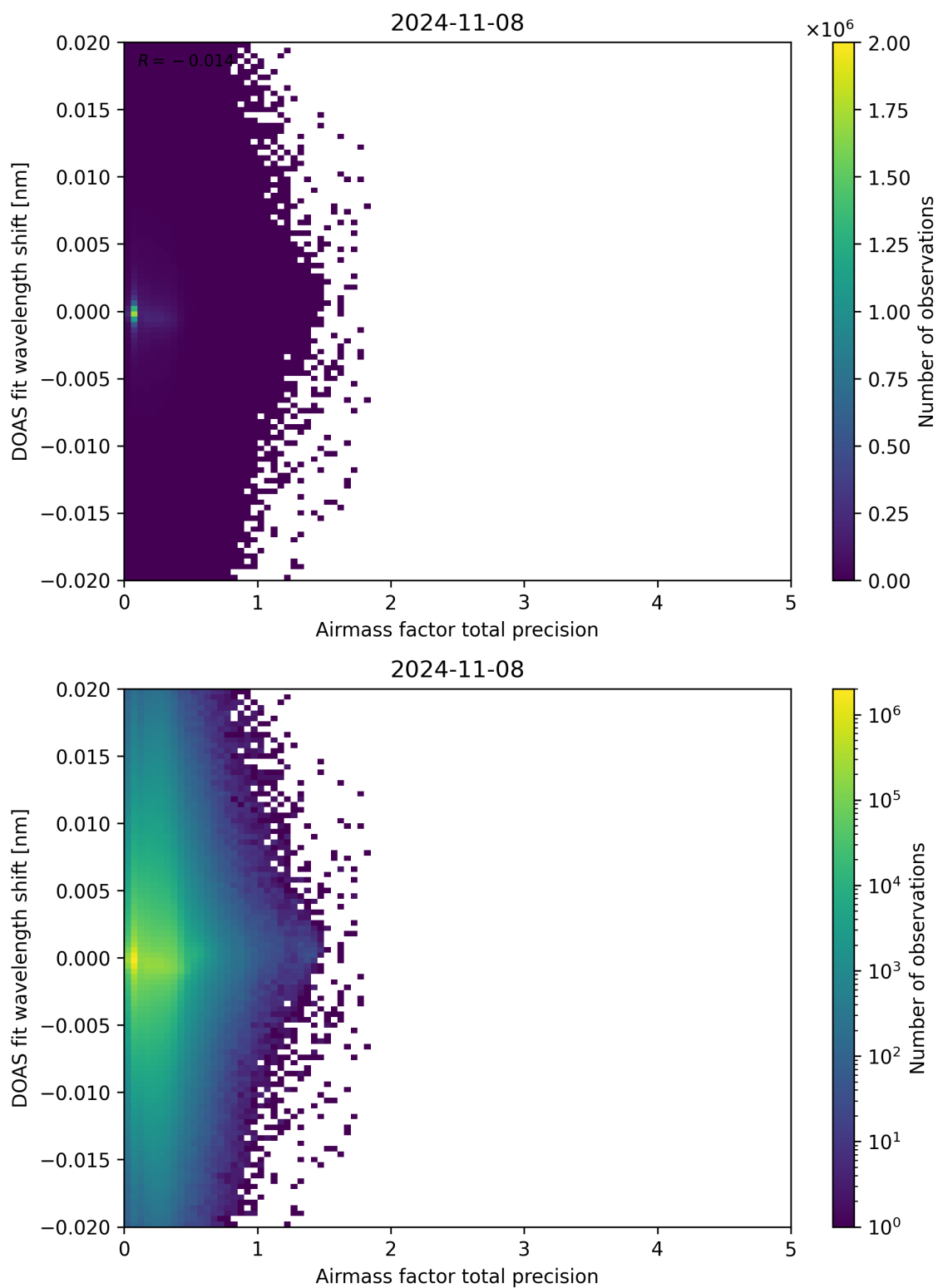
Figure 106: Scatter density plot of “Airmass factor total precision” against “DOAS fit wavelength shift” for 2024-11-07 to 2024-11-09.
