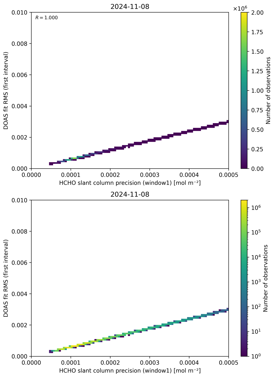
Figure 88: Scatter density plot of “HCHO slant column precision (window1)” against “DOAS fit RMS (first interval)” for 2024-11-07 to 2024-11-09.
