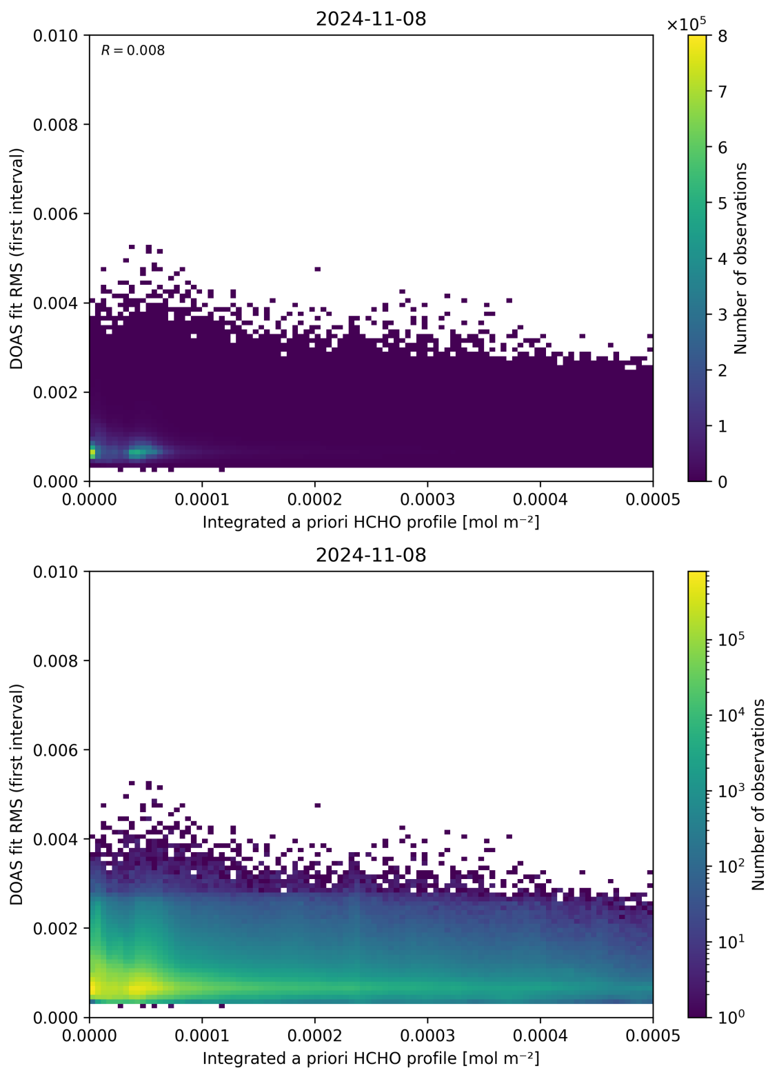
Figure 148: Scatter density plot of “Integrated a priori HCHO profile” against “DOAS fit RMS (first interval)” for 2024-11-07 to 2024-11-09.
