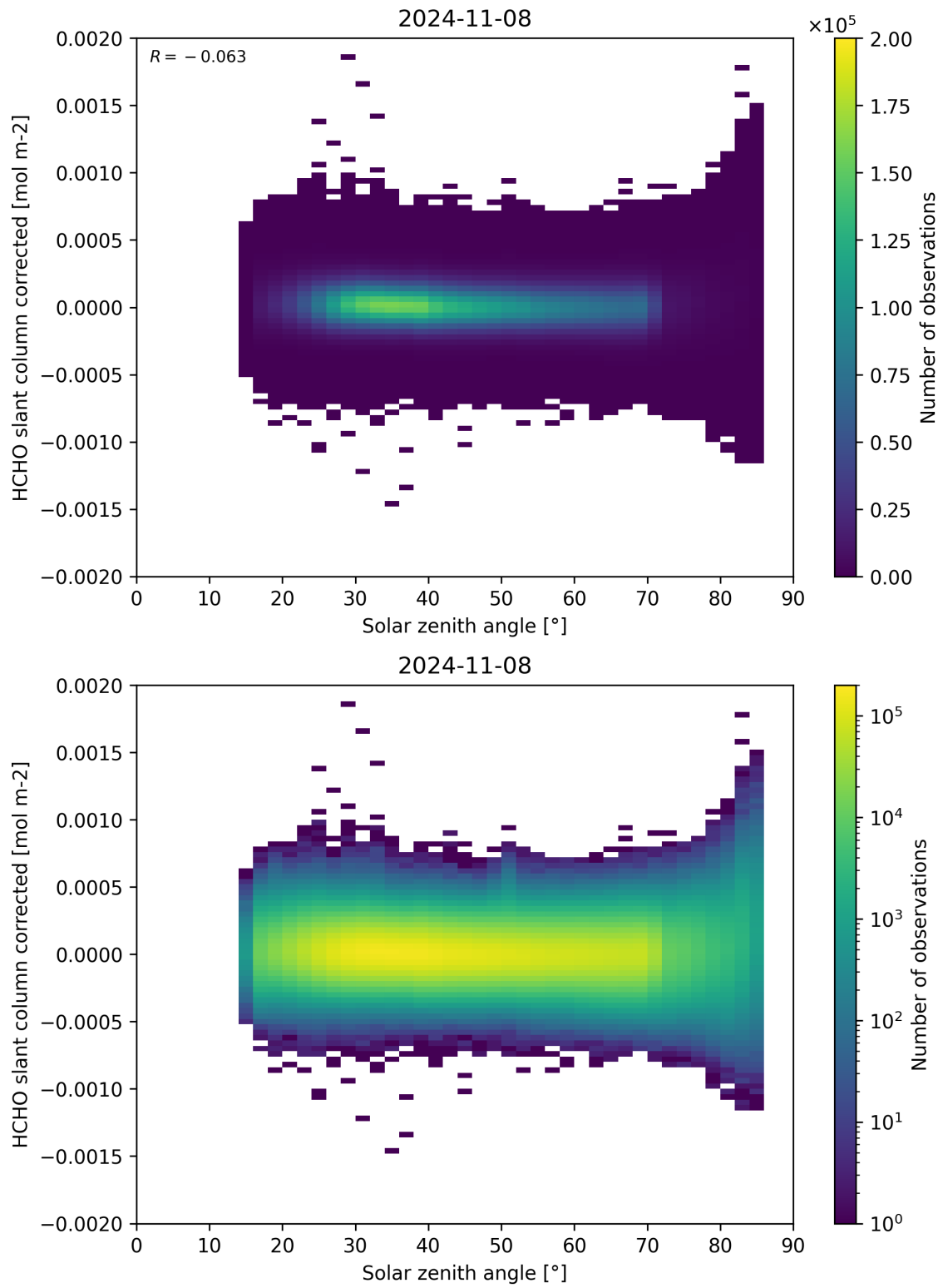
Figure 171: Scatter density plot of “Solar zenith angle” against “HCHO slant column corrected” for 2024-11-07 to 2024-11-09.
