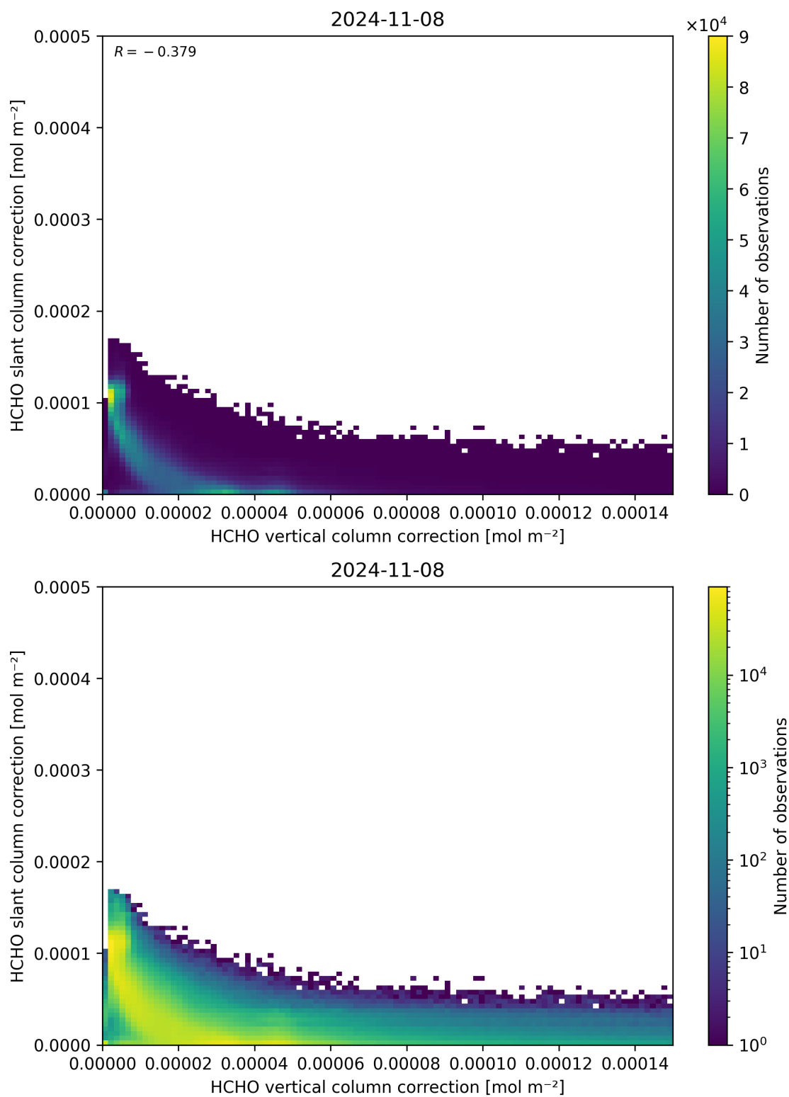
Figure 117: Scatter density plot of “HCHO vertical column correction” against “HCHO slant column correction” for 2024-11-07 to 2024-11-09.
