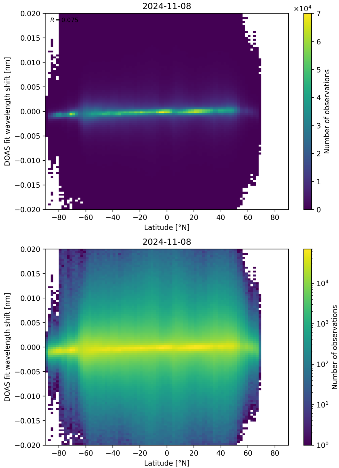
Figure 154: Scatter density plot of “Latitude” against “DOAS fit wavelength shift” for 2024-11-07 to 2024-11-09.
