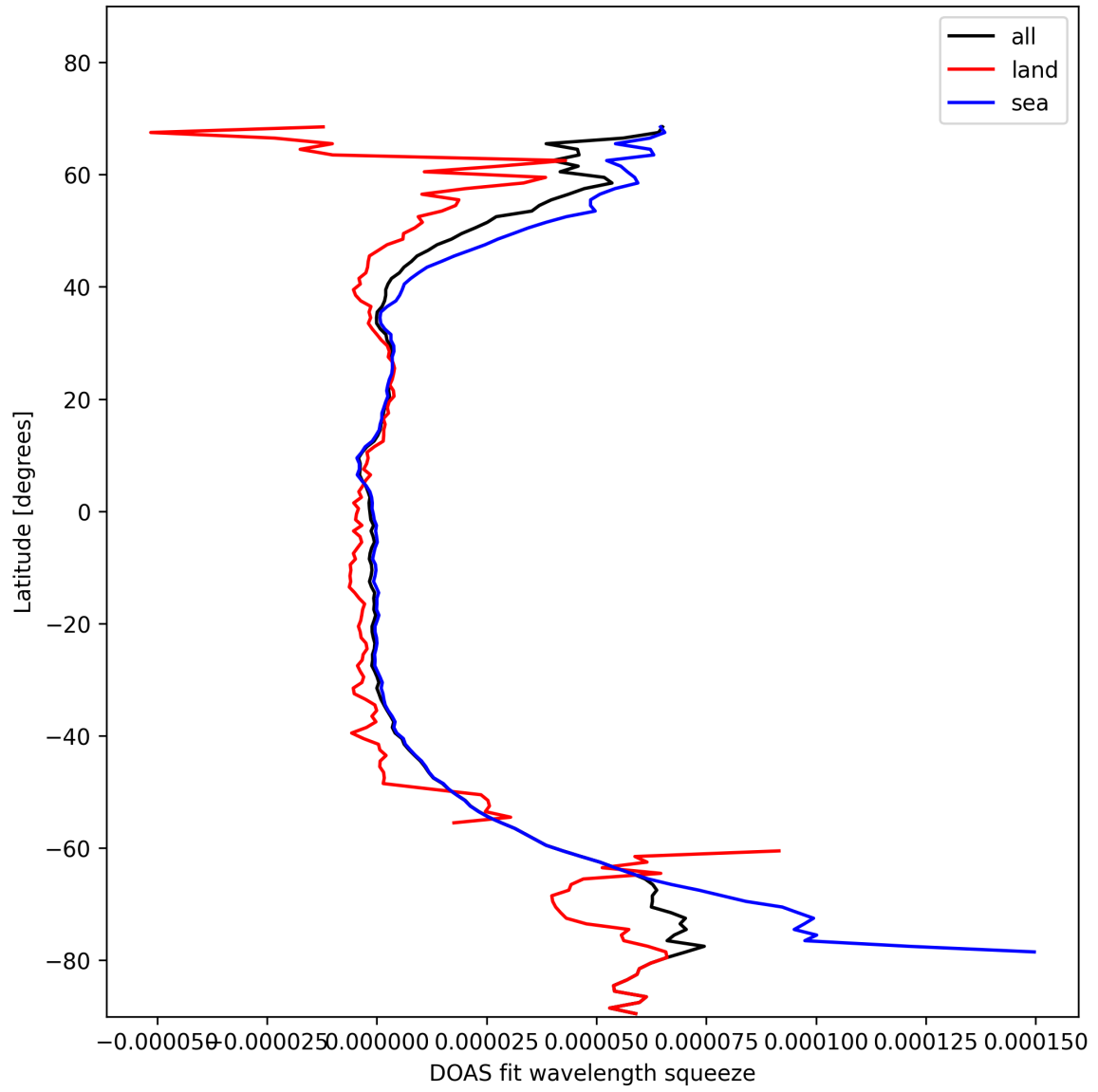
Figure 31: Zonal average of “DOAS fit wavelength squeeze” for 2024-11-07 to 2024-11-09.
