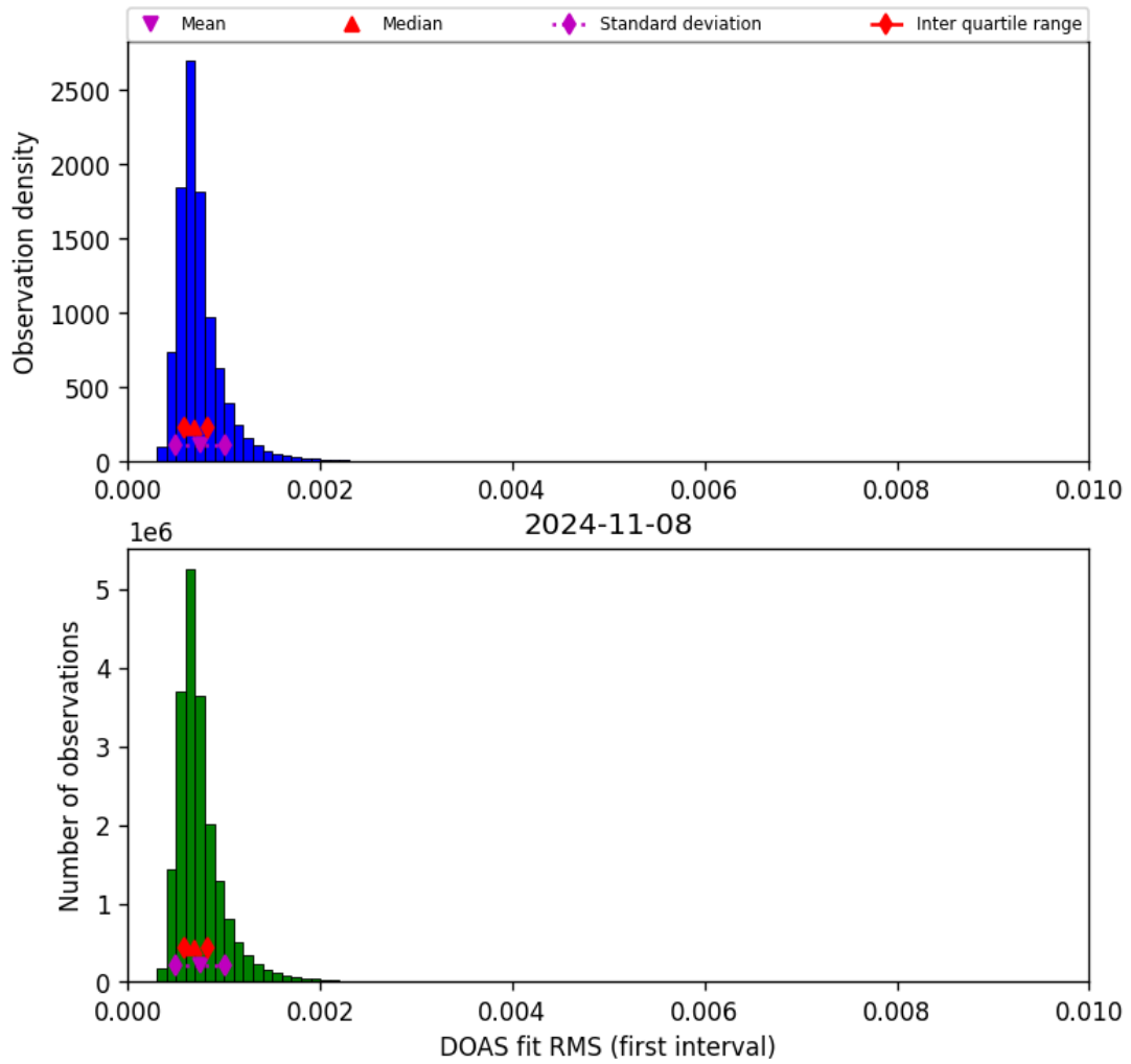
Figure 46: Histogram of “DOAS fit RMS (first interval)” for 2024-11-07 to 2024-11-09
