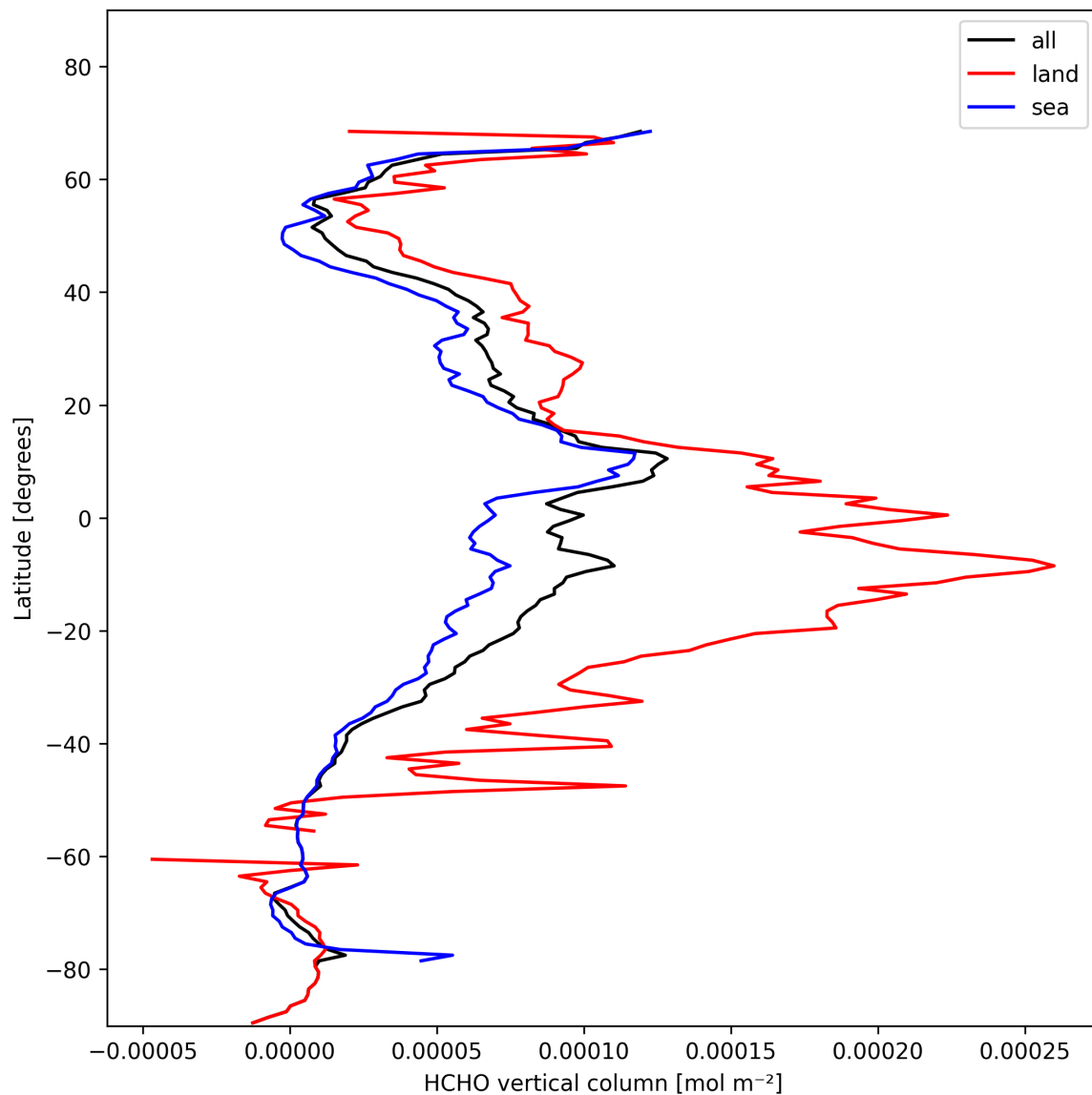
Figure 21: Zonal average of “HCHO vertical column” for 2024-11-07 to 2024-11-09.
