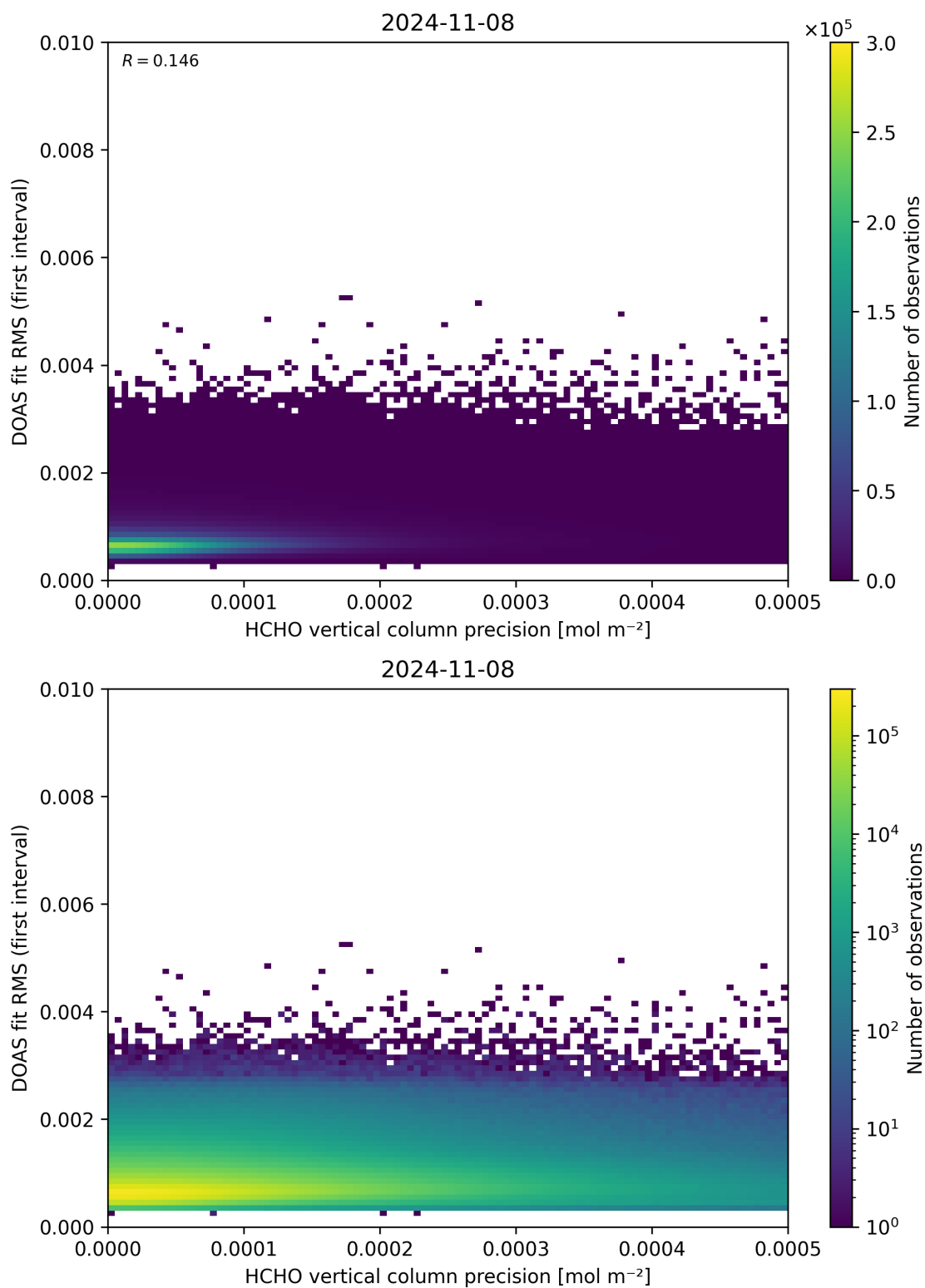
Figure 136: Scatter density plot of “HCHO vertical column precision” against “DOAS fit RMS (first interval)” for 2024-11-07 to 2024-11-09.
