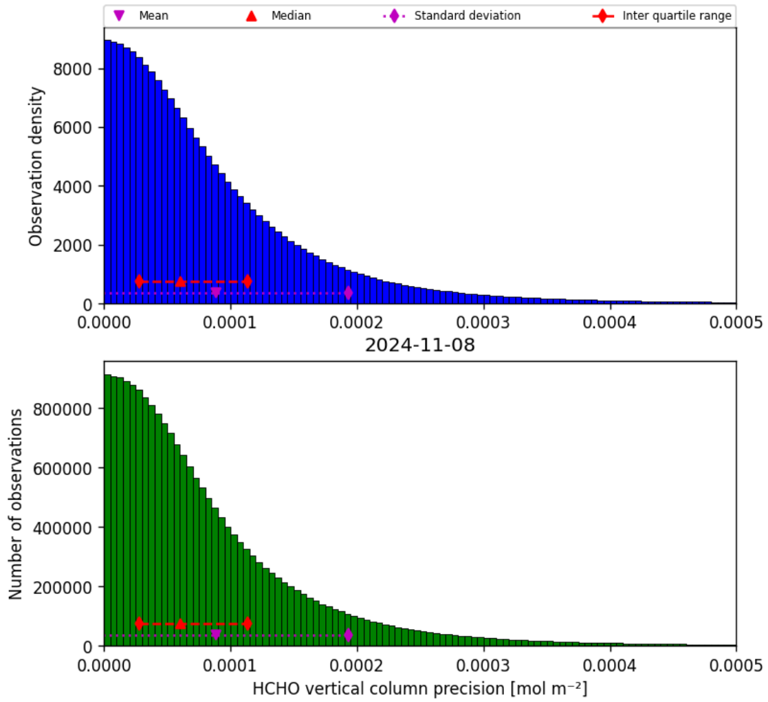
Figure 36: Histogram of “HCHO vertical column precision” for 2024-11-07 to 2024-11-09
