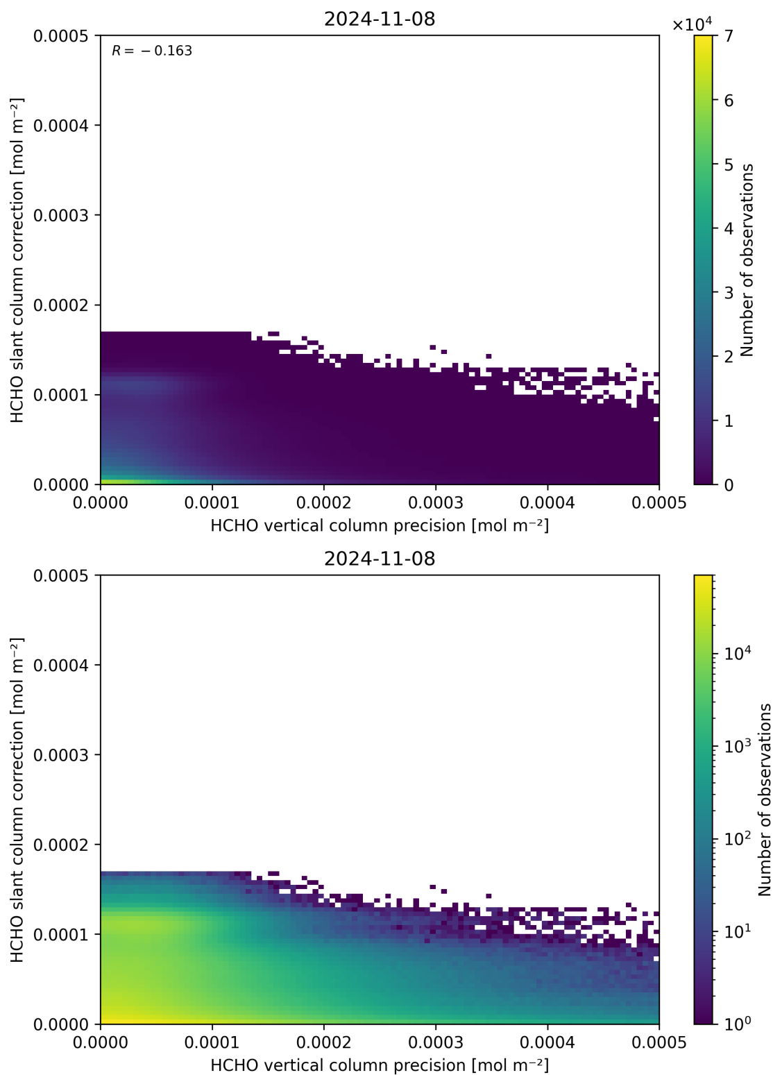
Figure 141: Scatter density plot of “HCHO vertical column precision” against “HCHO slant column correction” for 2024-11-07 to 2024-11-09.
