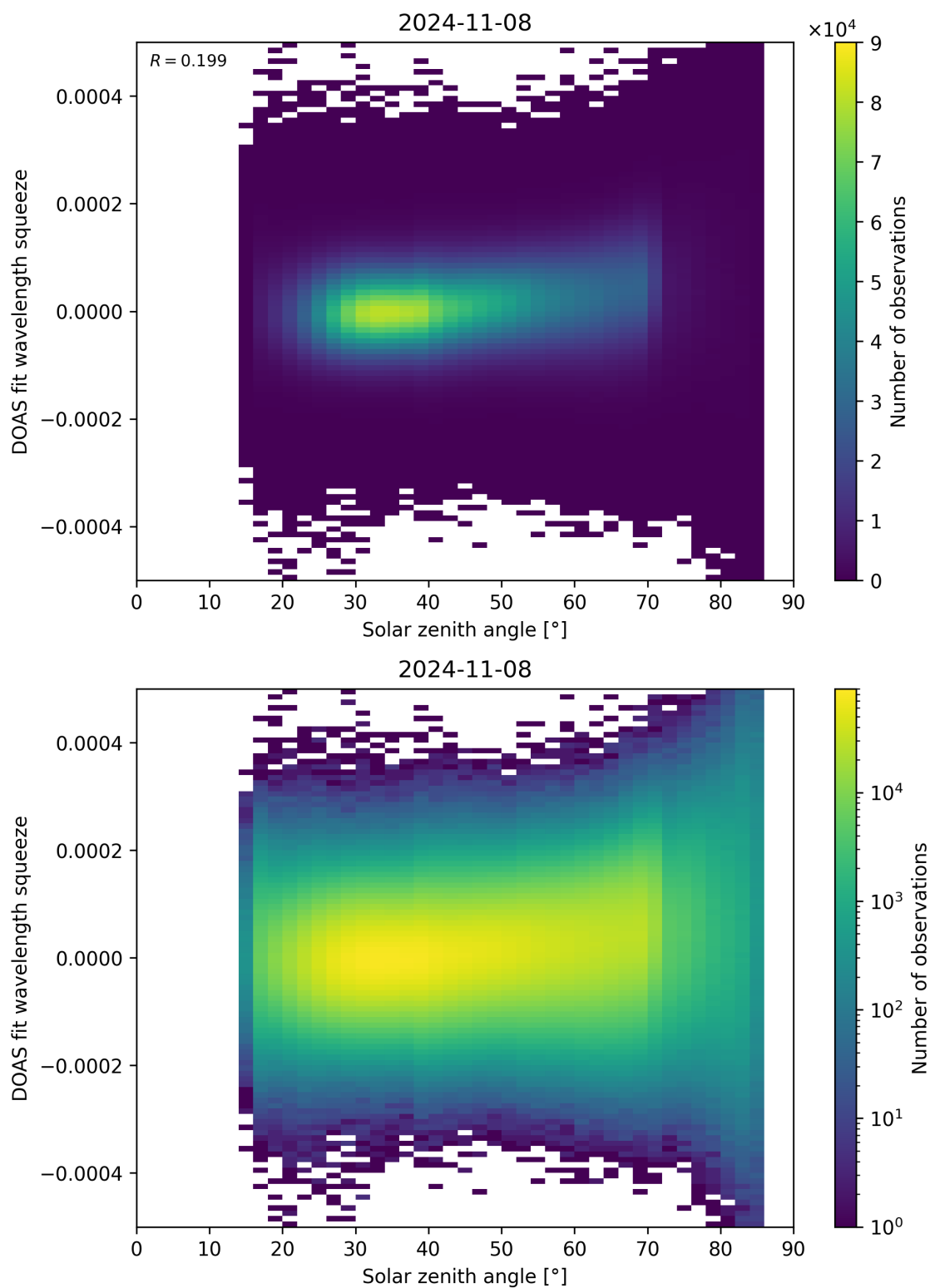
Figure 169: Scatter density plot of “Solar zenith angle” against “DOAS fit wavelength squeeze” for 2024-11-07 to 2024-11-09.
