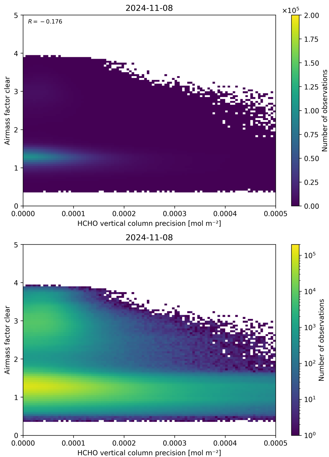
Figure 139: Scatter density plot of “HCHO vertical column precision” against “Airmass factor clear” for 2024-11-07 to 2024-11-09.
