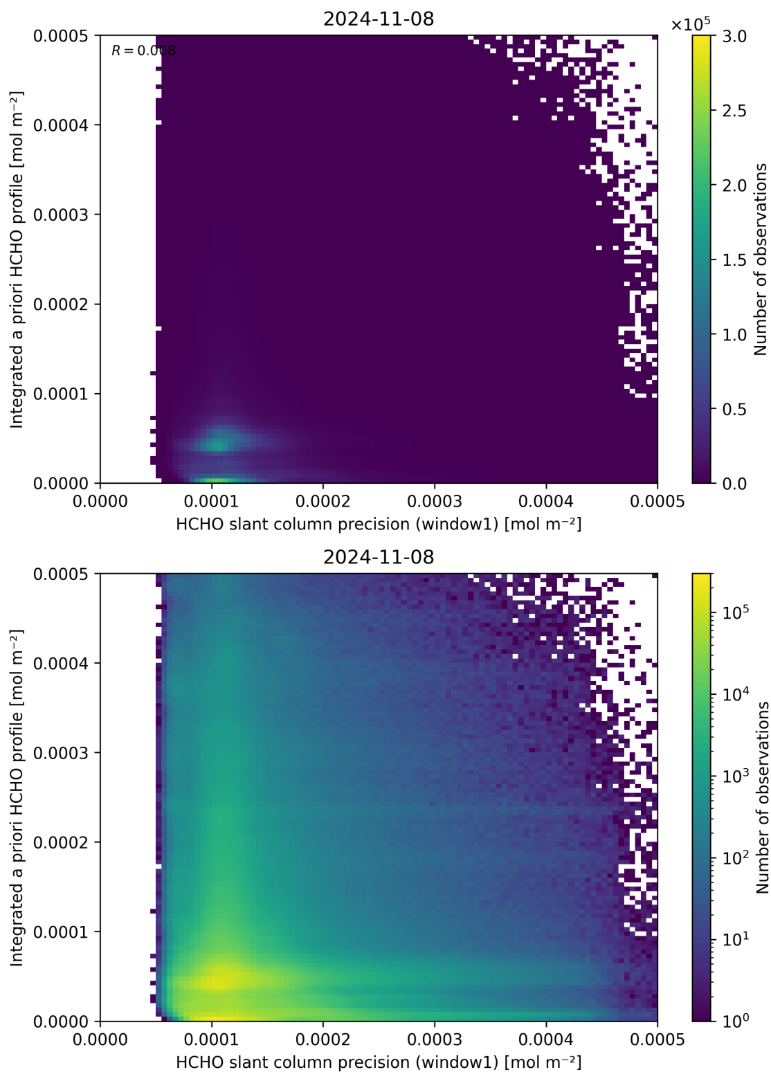
Figure 96: Scatter density plot of “HCHO slant column precision (window1)” against “Integrated a priori HCHO profile” for 2024-11-07 to 2024-11-09.
