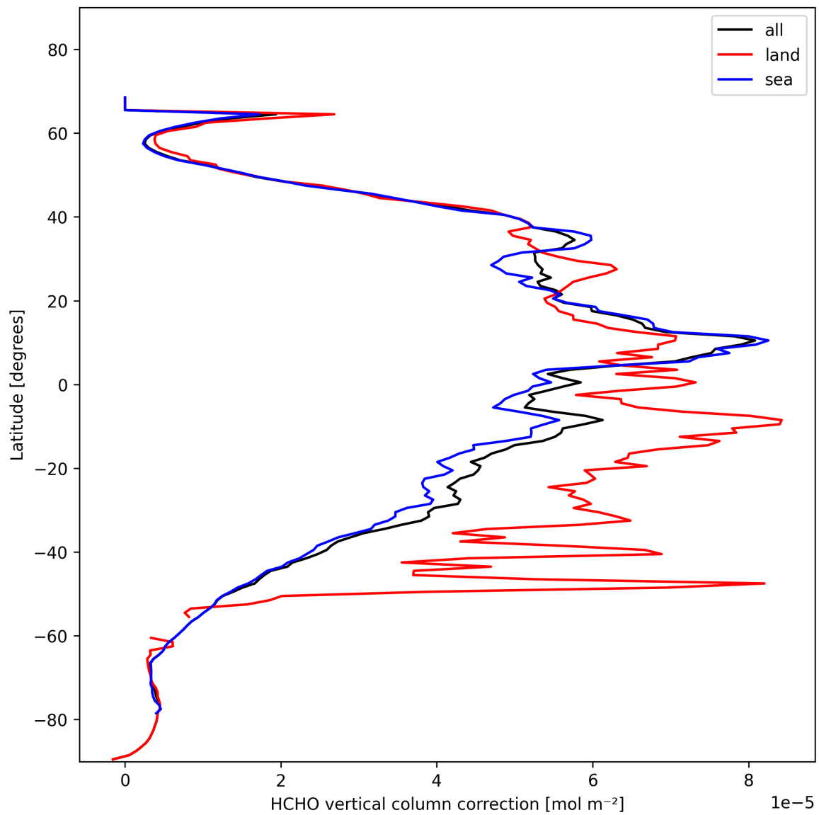
Figure 23: Zonal average of “HCHO vertical column correction” for 2024-11-07 to 2024-11-09.
