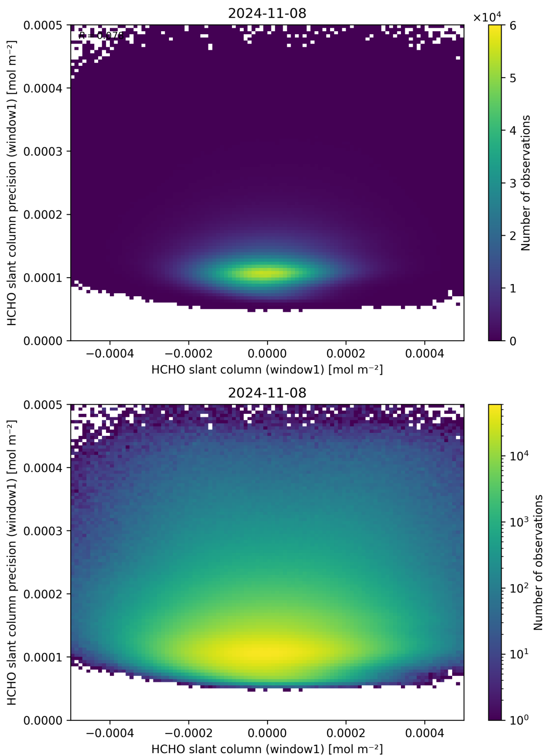
Figure 84: Scatter density plot of “HCHO slant column (window1)” against “HCHO slant column precision (window1)” for 2024-11-07 to 2024-11-09.
