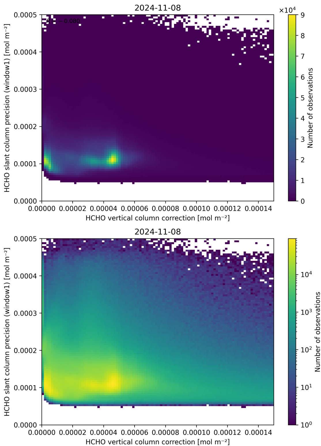
Figure 119: Scatter density plot of “HCHO vertical column correction” against “HCHO slant column precision (window1)” for 2024-11-07 to 2024-11-09.
