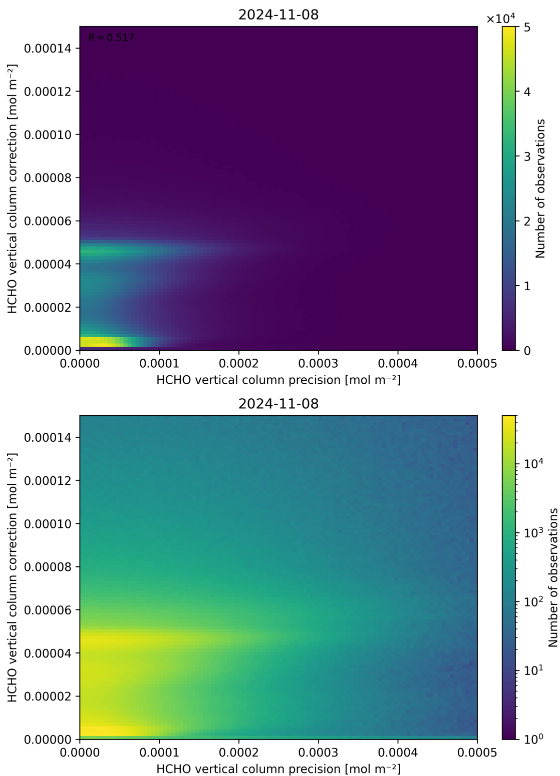
Figure 146: Scatter density plot of “HCHO vertical column precision” against “HCHO vertical column correction” for 2024-11-07 to 2024-11-09.
