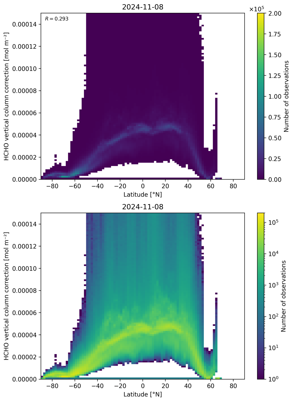
Figure 164: Scatter density plot of “Latitude” against “HCHO vertical column correction” for 2024-11-07 to 2024-11-09.
