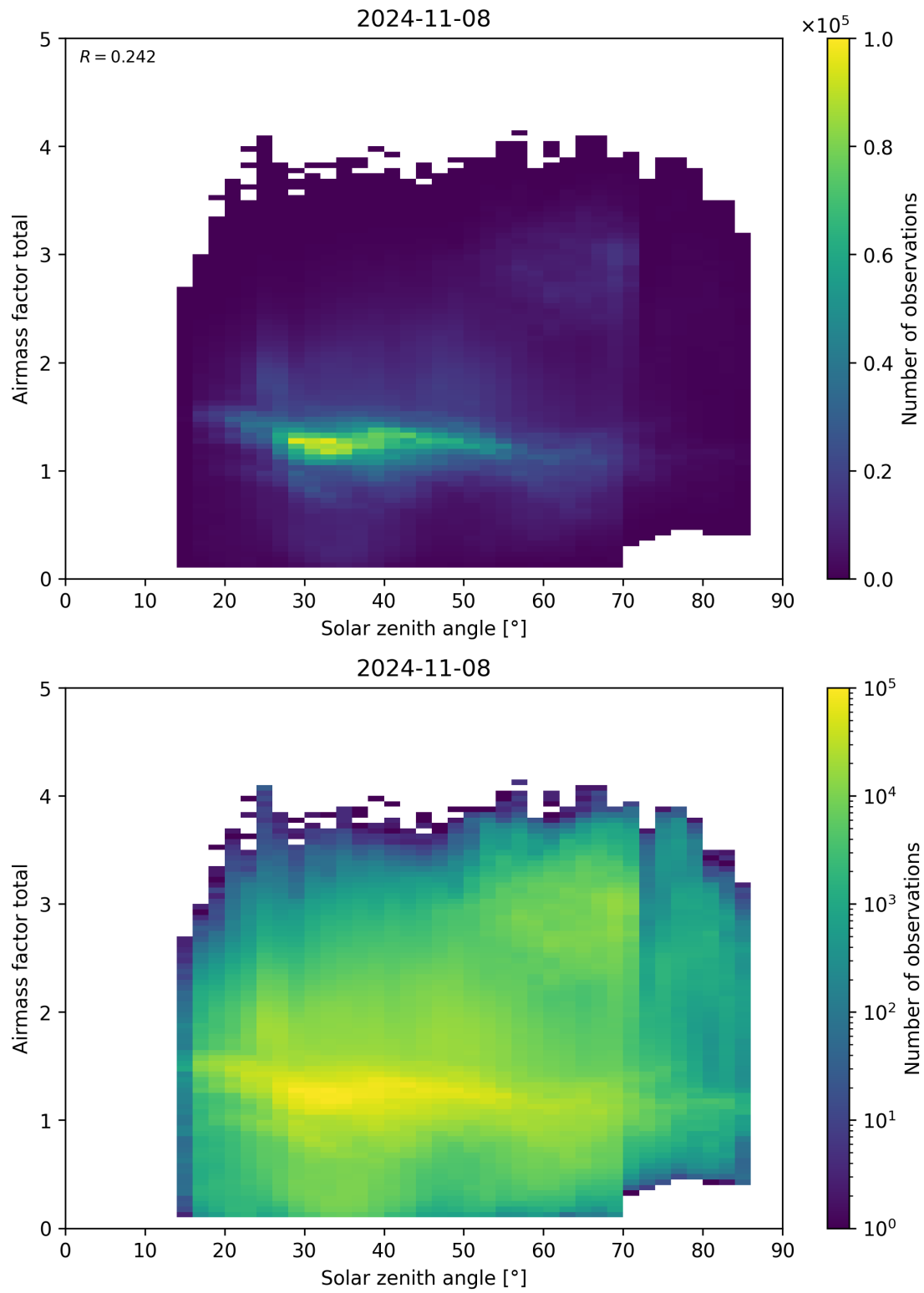
Figure 175: Scatter density plot of “Solar zenith angle” against “Airmass factor total” for 2024-11-07 to 2024-11-09.
