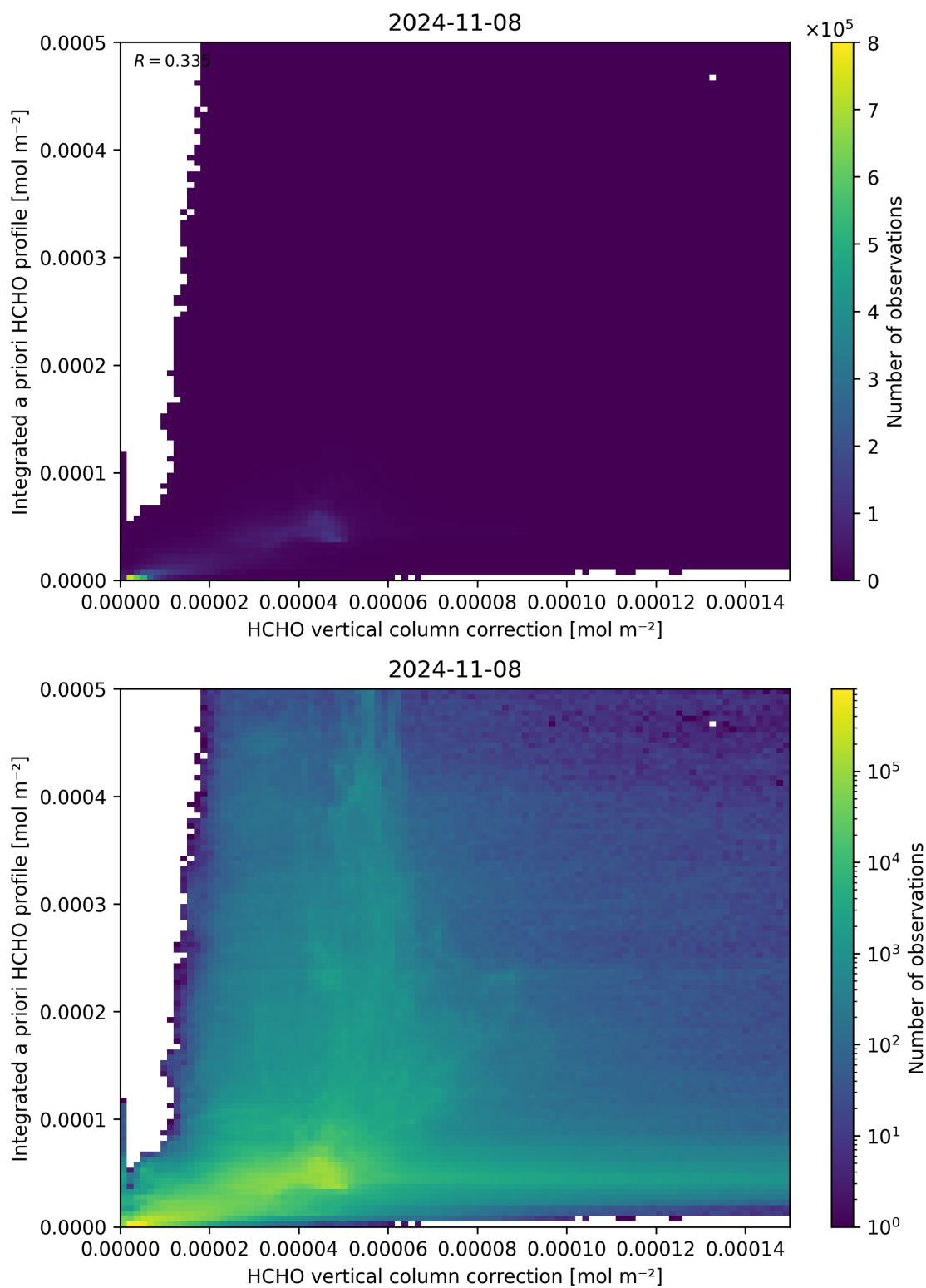
Figure 122: Scatter density plot of “HCHO vertical column correction” against “Integrated a priori HCHO profile” for 2024-11-07 to 2024-11-09.
