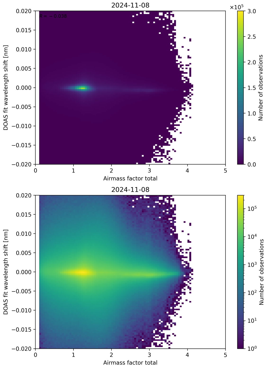
Figure 98: Scatter density plot of “Airmass factor total” against “DOAS fit wavelength shift” for 2024-11-07 to 2024-11-09.
