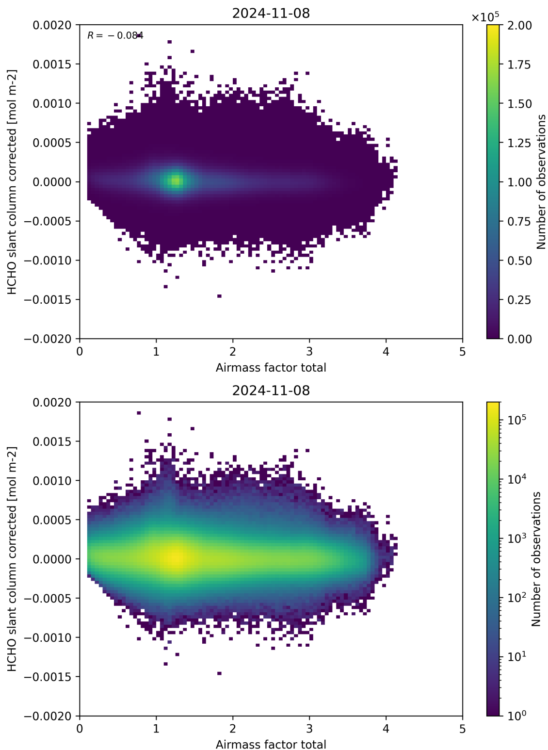
Figure 101: Scatter density plot of “Airmass factor total” against “HCHO slant column corrected” for 2024-11-07 to 2024-11-09.
