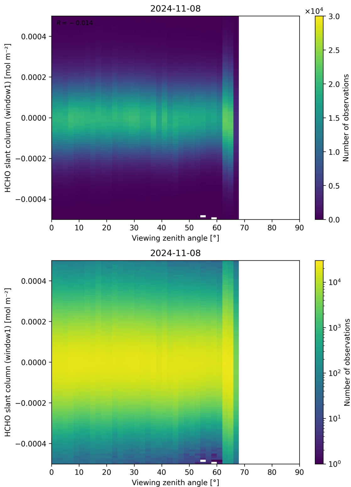
Figure 188: Scatter density plot of “Viewing zenith angle” against “HCHO slant column (window1)” for 2024-11-07 to 2024-11-09.
