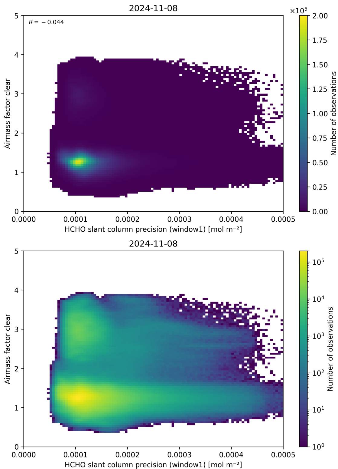
Figure 91: Scatter density plot of “HCHO slant column precision (window1)” against “Airmass factor clear” for 2024-11-07 to 2024-11-09.
