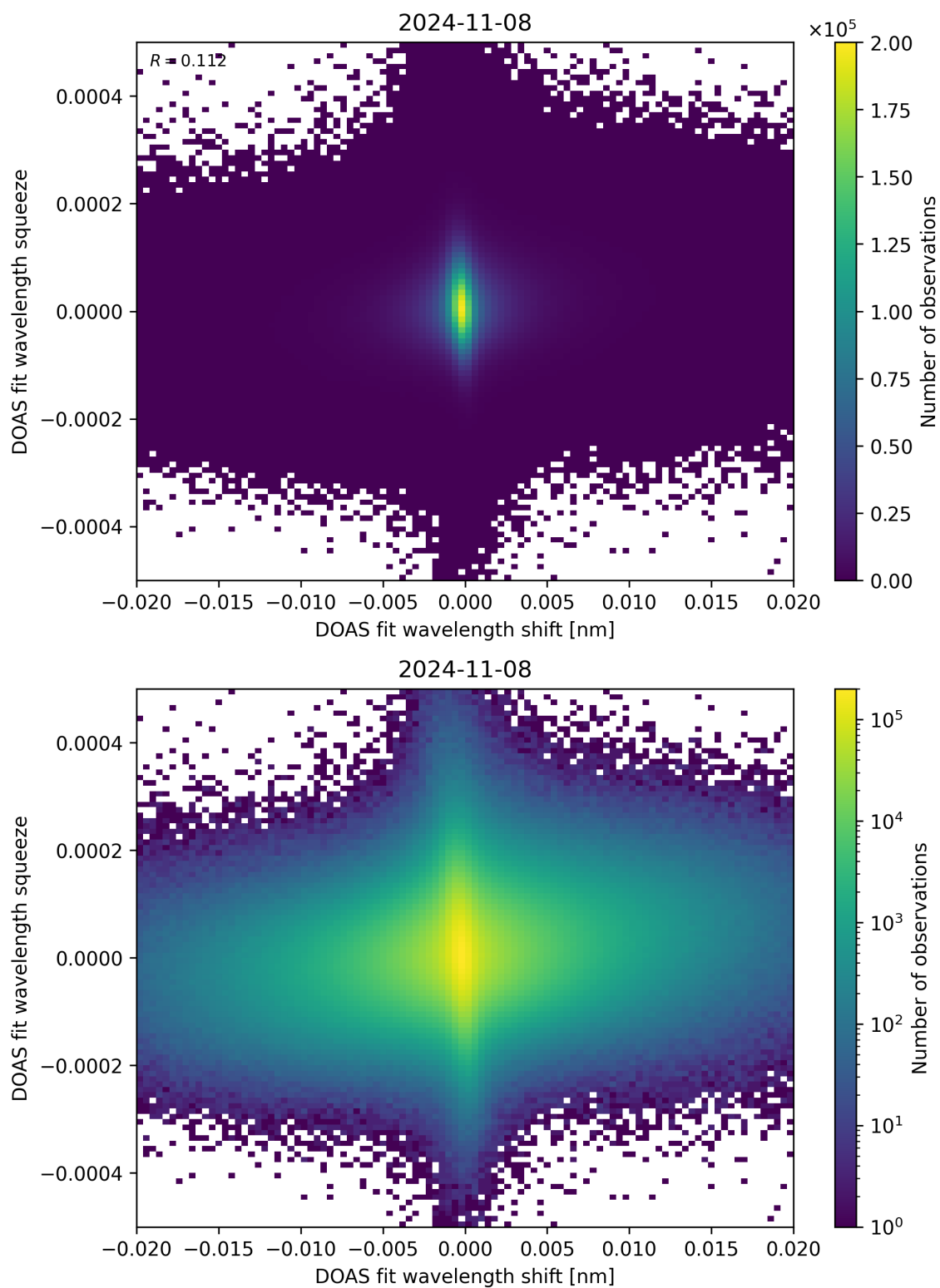
Figure 65: Scatter density plot of “DOAS fit wavelength shift” against “DOAS fit wavelength squeeze” for 2024-11-07 to 2024-11-09.
