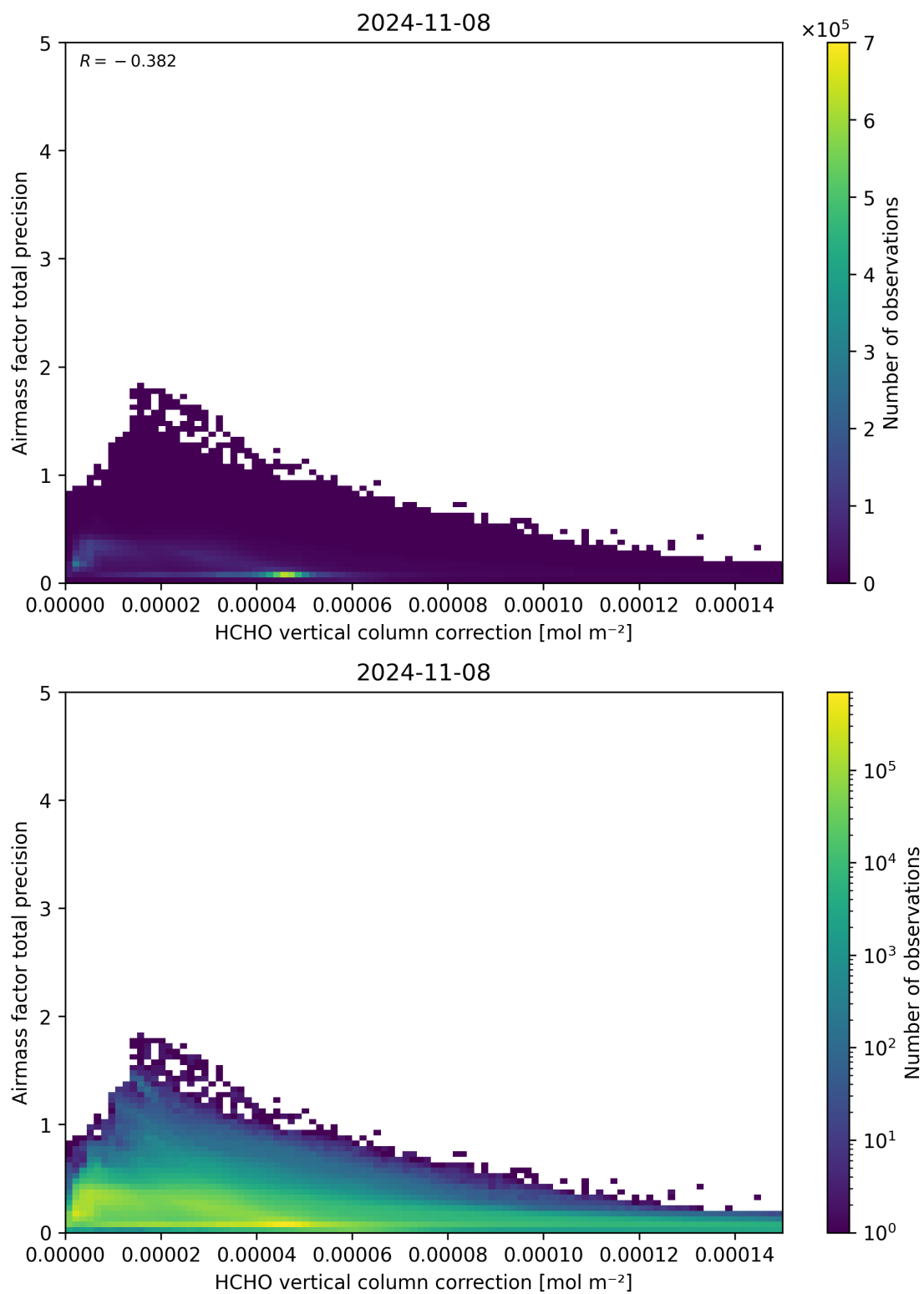
Figure 121: Scatter density plot of “HCHO vertical column correction” against “Airmass factor total precision” for 2024-11-07 to 2024-11-09.
