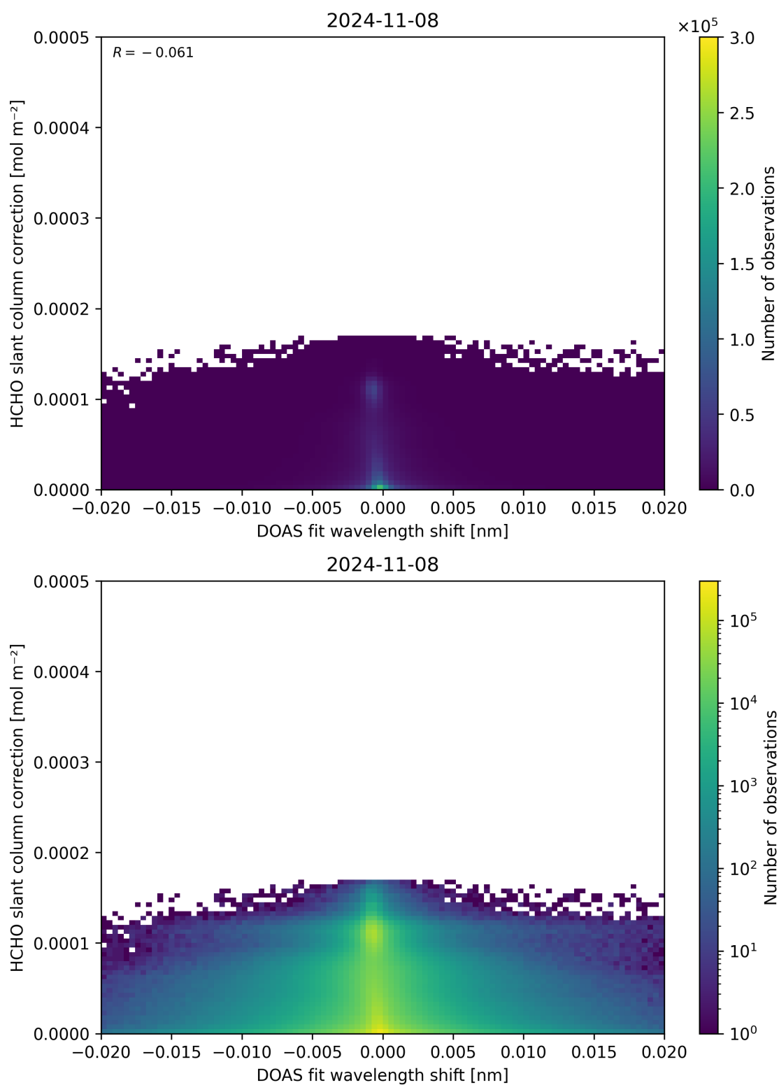
Figure 67: Scatter density plot of “DOAS fit wavelength shift” against “HCHO slant column correction” for 2024-11-07 to 2024-11-09.
