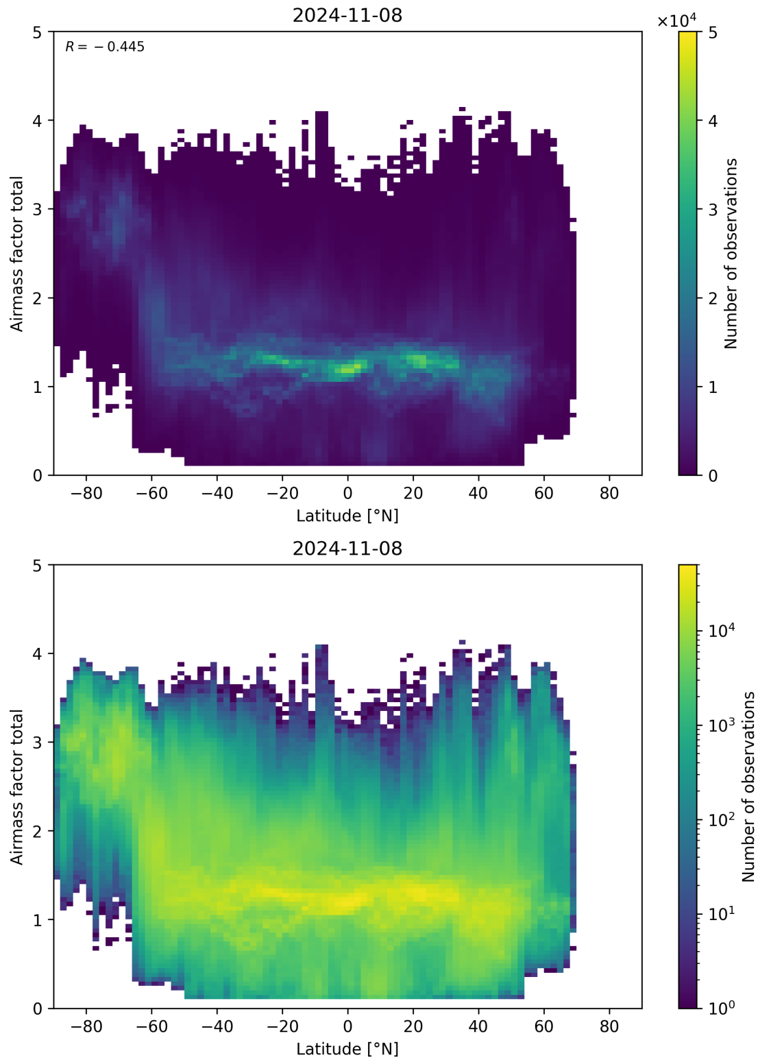
Figure 161: Scatter density plot of “Latitude” against “Airmass factor total” for 2024-11-07 to 2024-11-09.
