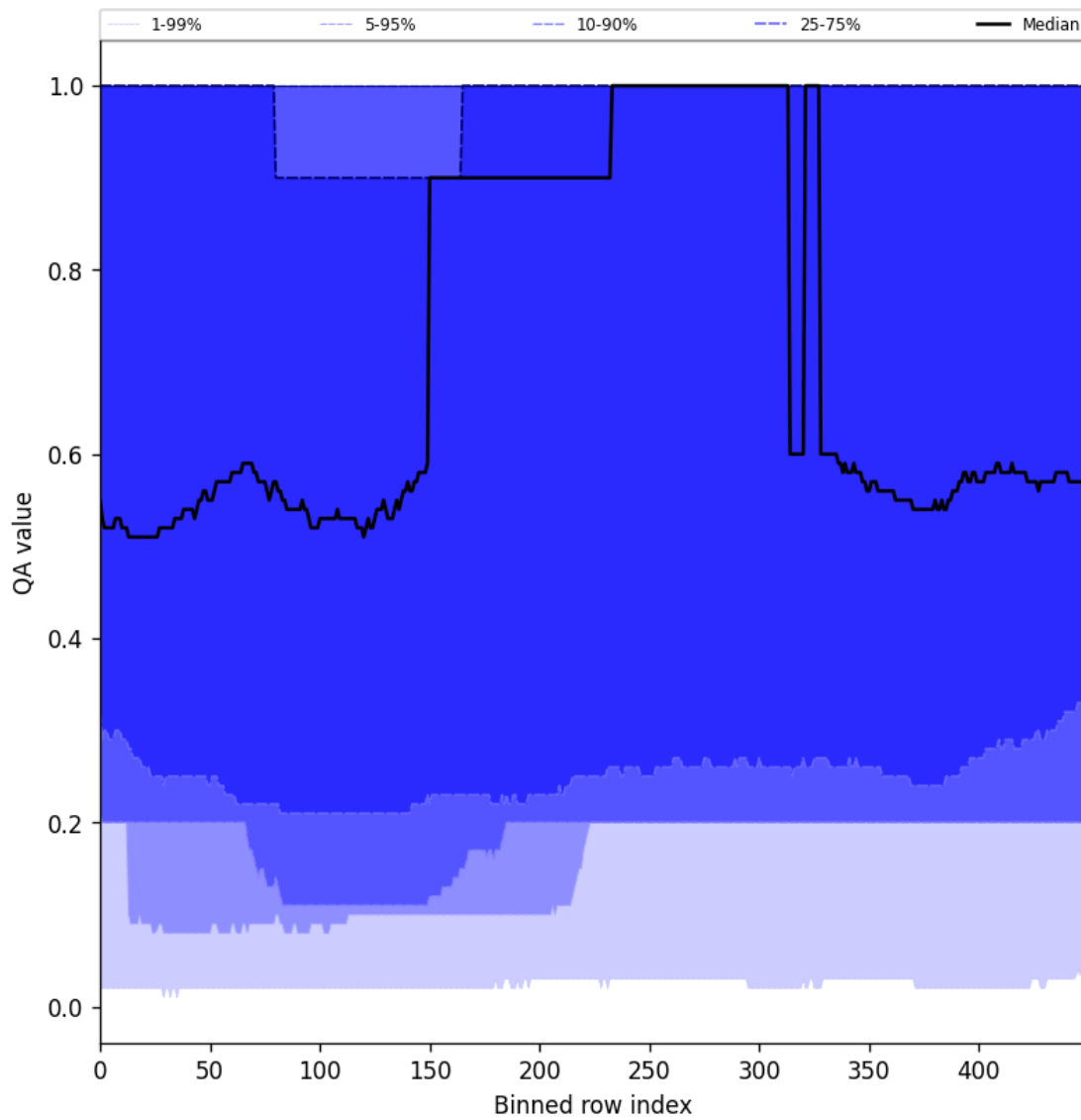
Figure 48: Along track statistics of “QA value” for 2024-11-07 to 2024-11-09
