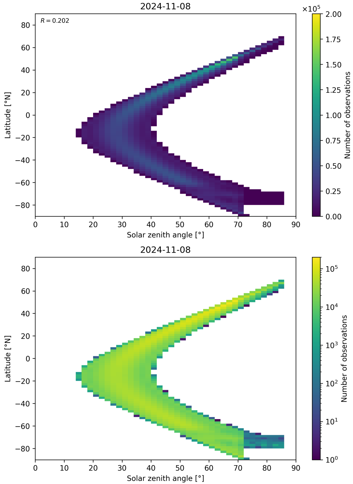
Figure 181: Scatter density plot of “Solar zenith angle” against “Latitude” for 2024-11-07 to 2024-11-09.
