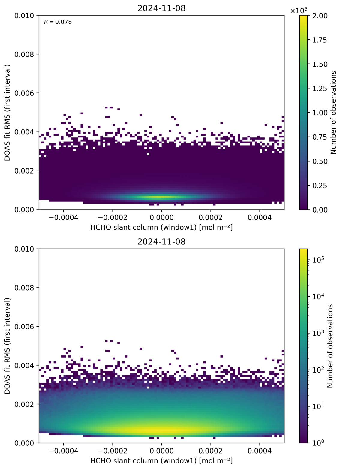
Figure 78: Scatter density plot of “HCHO slant column (window1)” against “DOAS fit RMS (first interval)” for 2024-11-07 to 2024-11-09.
