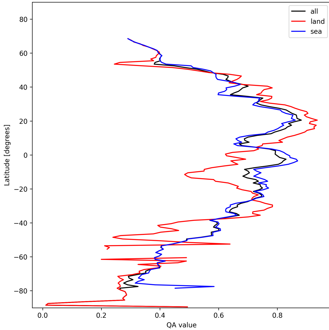
Figure 20: Zonal average of “QA value” for 2024-11-07 to 2024-11-09.
