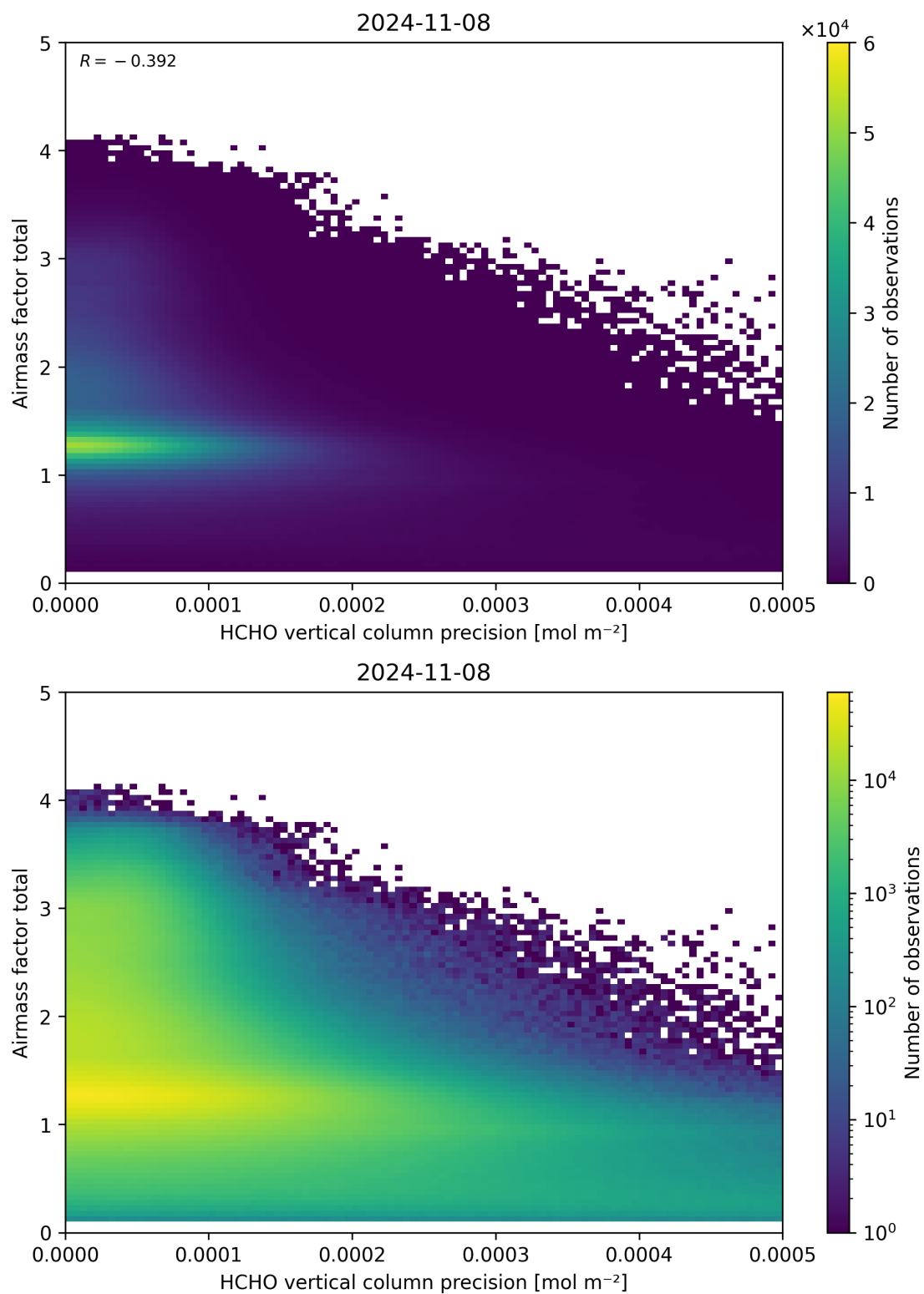
Figure 144: Scatter density plot of “HCHO vertical column precision” against “Airmass factor total” for 2024-11-07 to 2024-11-09.
