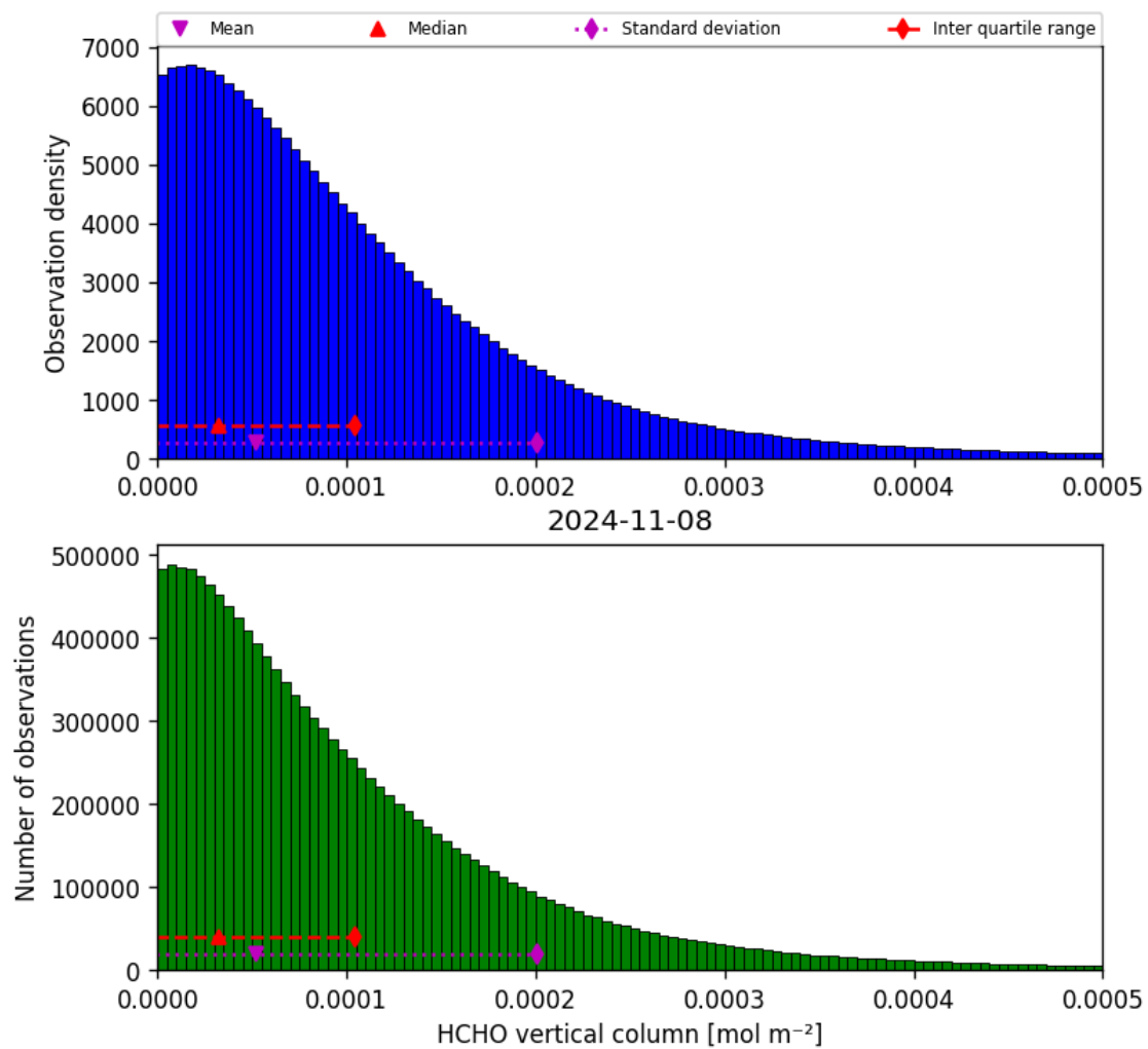
Figure 35: Histogram of “HCHO vertical column” for 2024-11-07 to 2024-11-09
