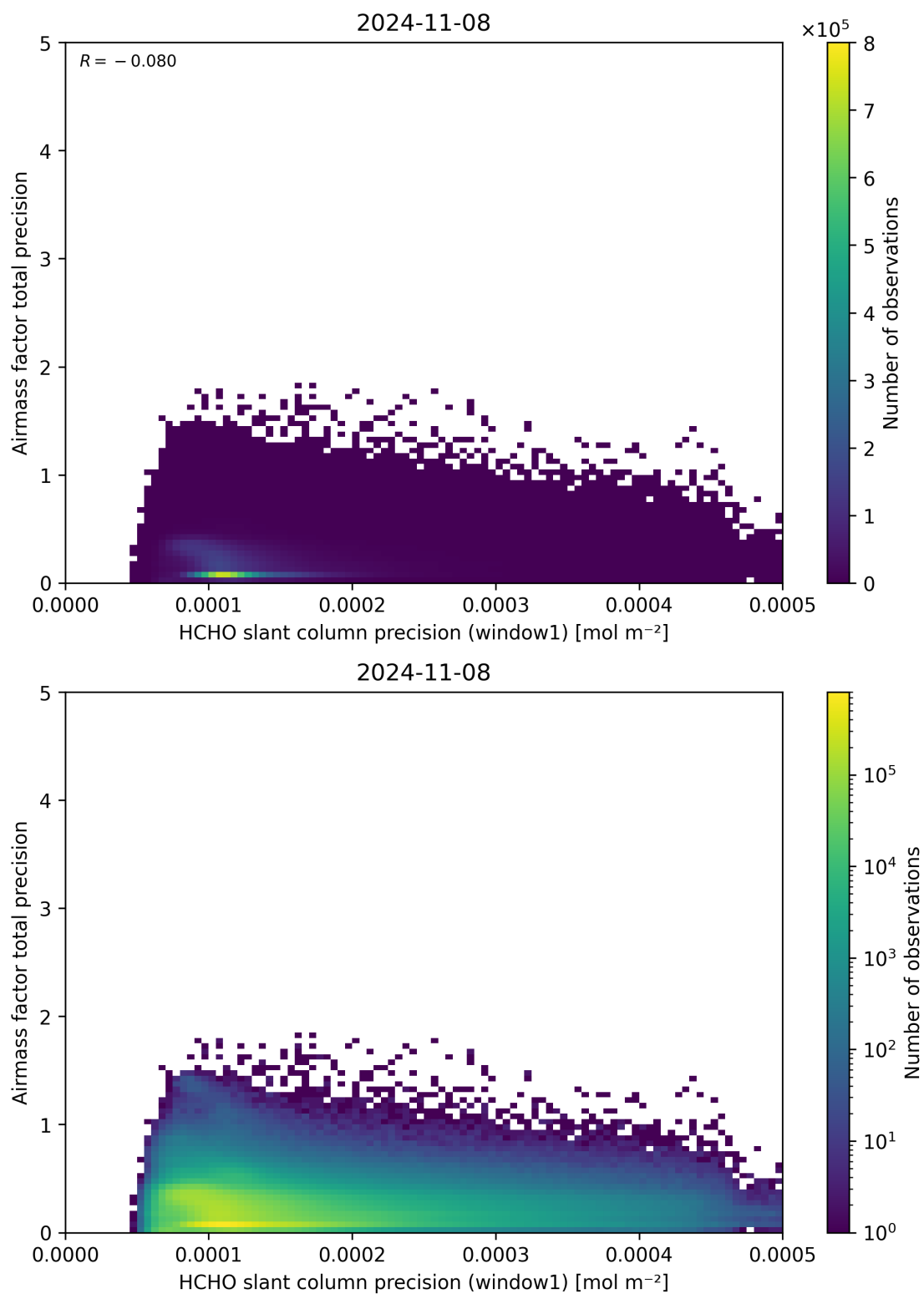
Figure 95: Scatter density plot of “HCHO slant column precision (window1)” against “Airmass factor total precision” for 2024-11-07 to 2024-11-09.
