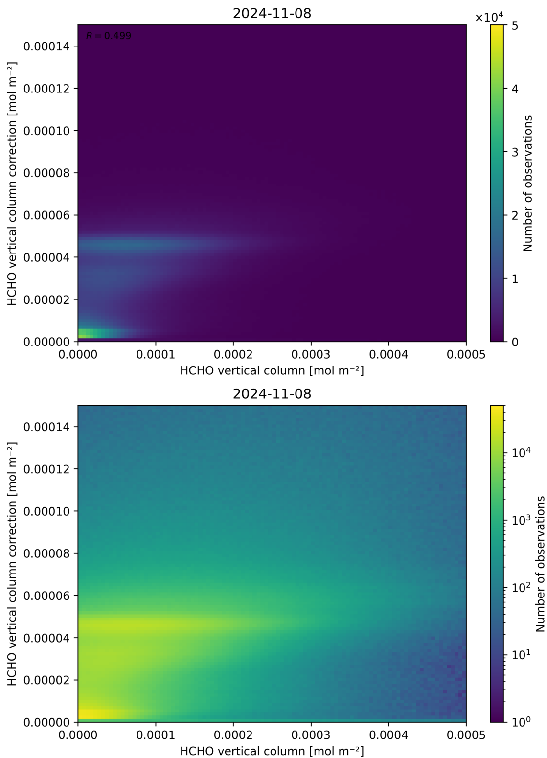
Figure 133: Scatter density plot of “HCHO vertical column” against “HCHO vertical column correction” for 2024-11-07 to 2024-11-09.
