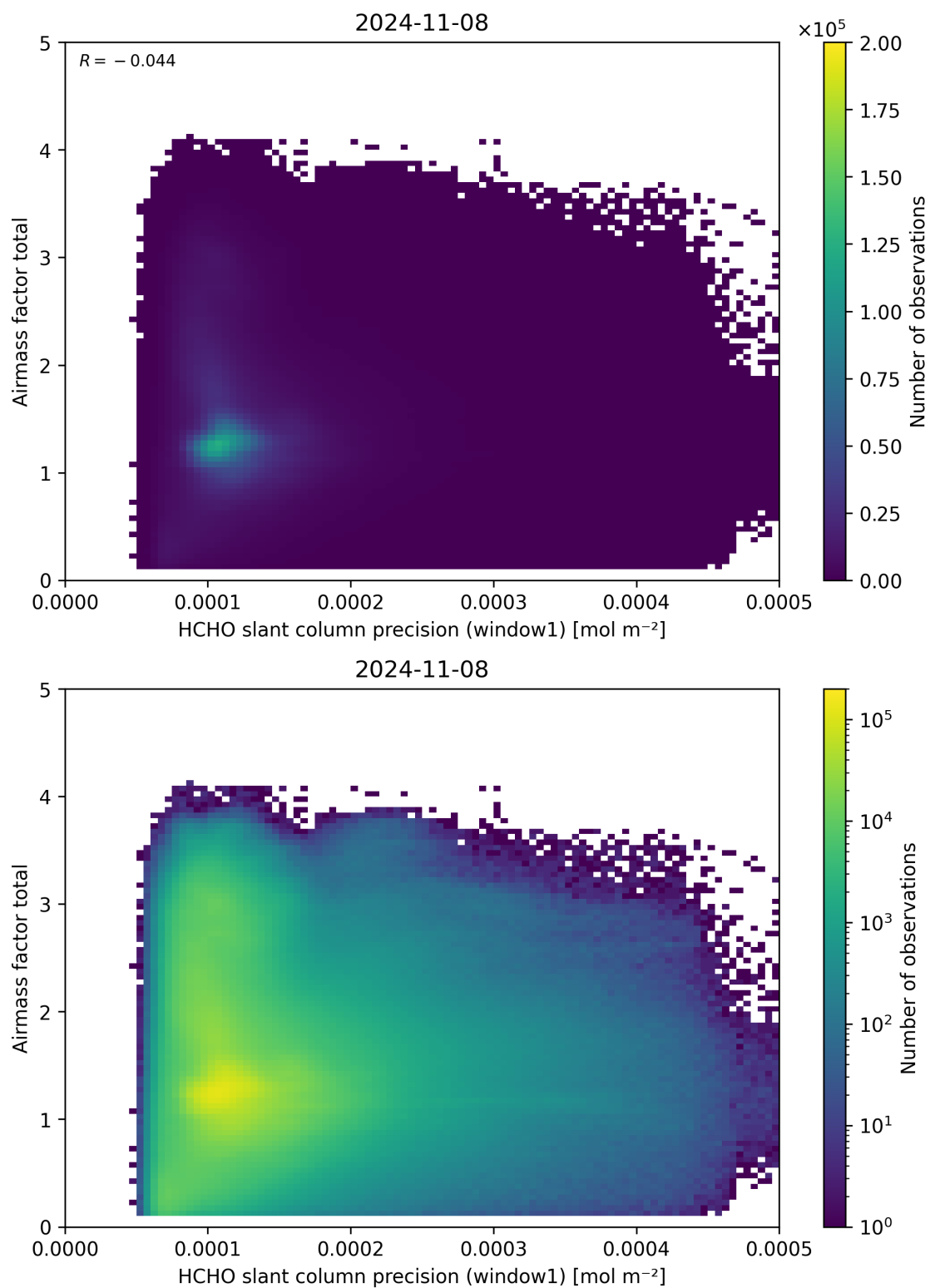
Figure 94: Scatter density plot of “HCHO slant column precision (window1)” against “Airmass factor total” for 2024-11-07 to 2024-11-09.
