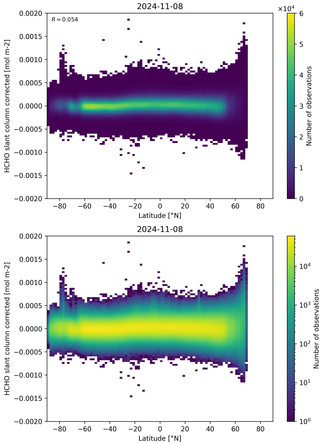
Figure 157: Scatter density plot of “Latitude” against “HCHO slant column corrected” for 2024-11-07 to 2024-11-09.
