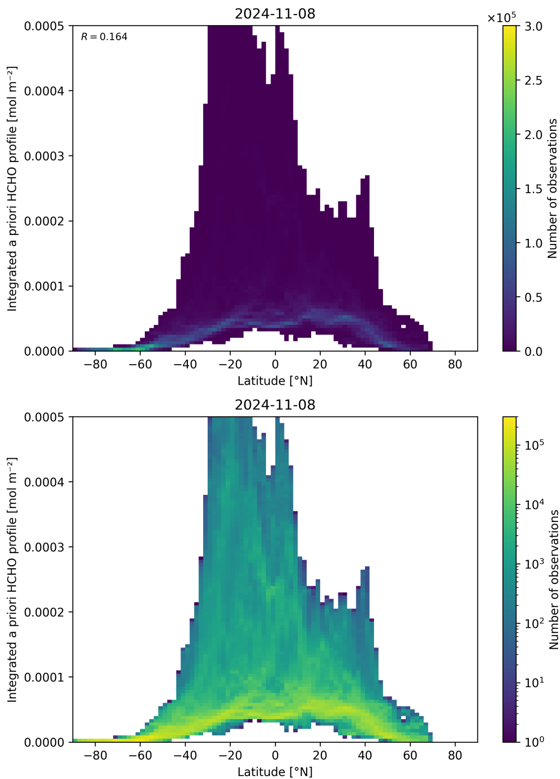
Figure 166: Scatter density plot of “Latitude” against “Integrated a priori HCHO profile” for 2024-11-07 to 2024-11-09.
