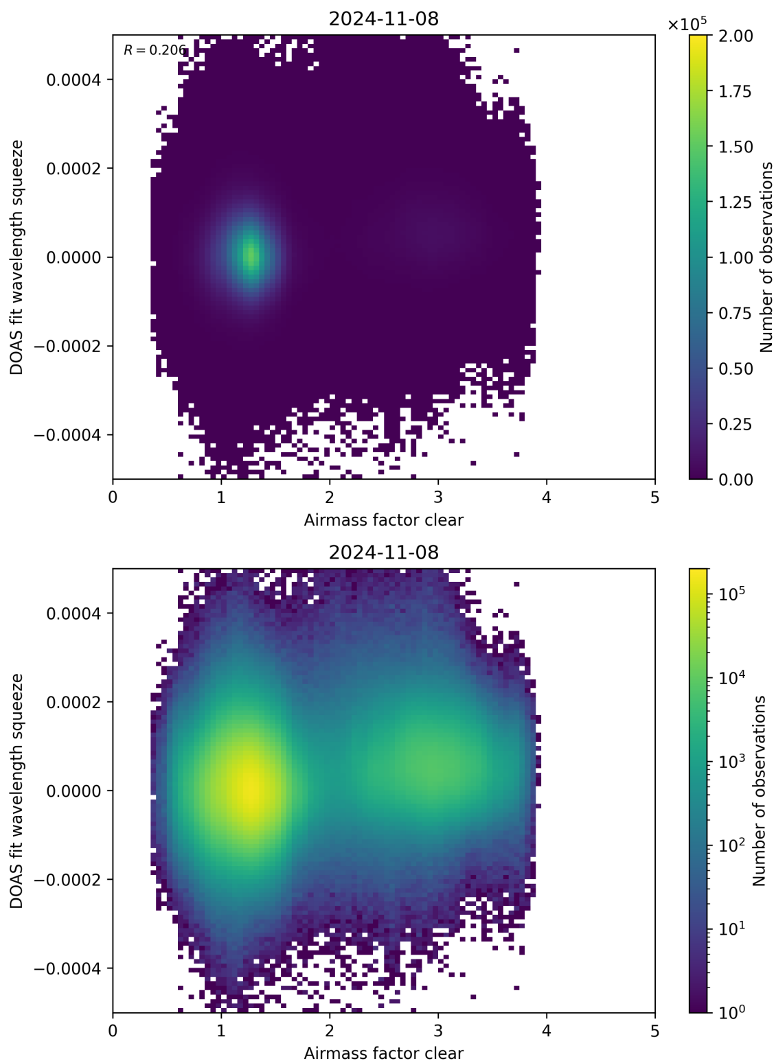
Figure 73: Scatter density plot of “Airmass factor clear” against “DOAS fit wavelength squeeze” for 2024-11-07 to 2024-11-09.
