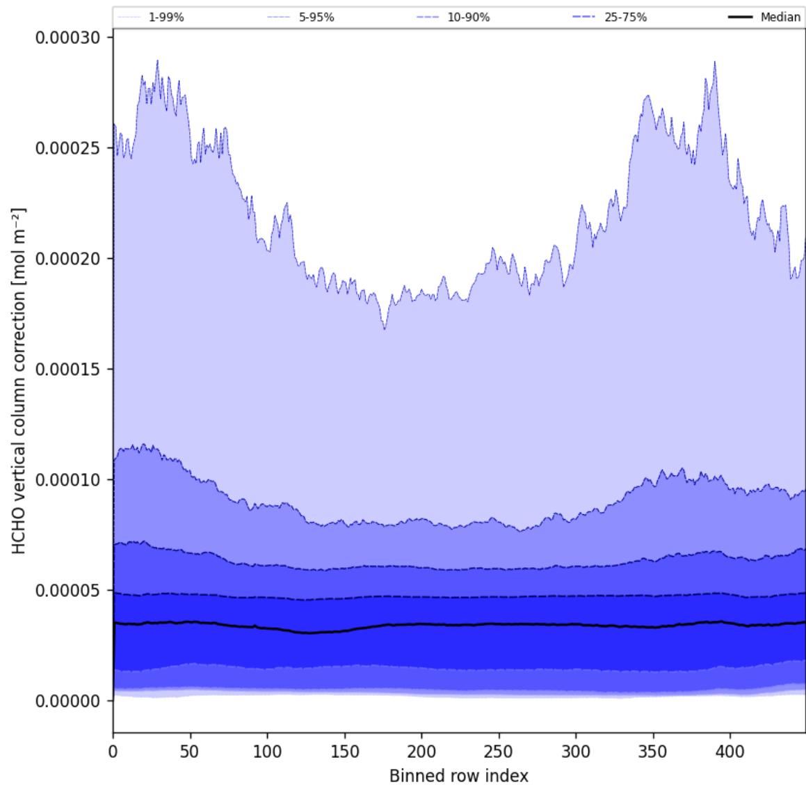
Figure 51: Along track statistics of "HCHO vertical column correction" for 2024-11-07 to 2024-11-09
