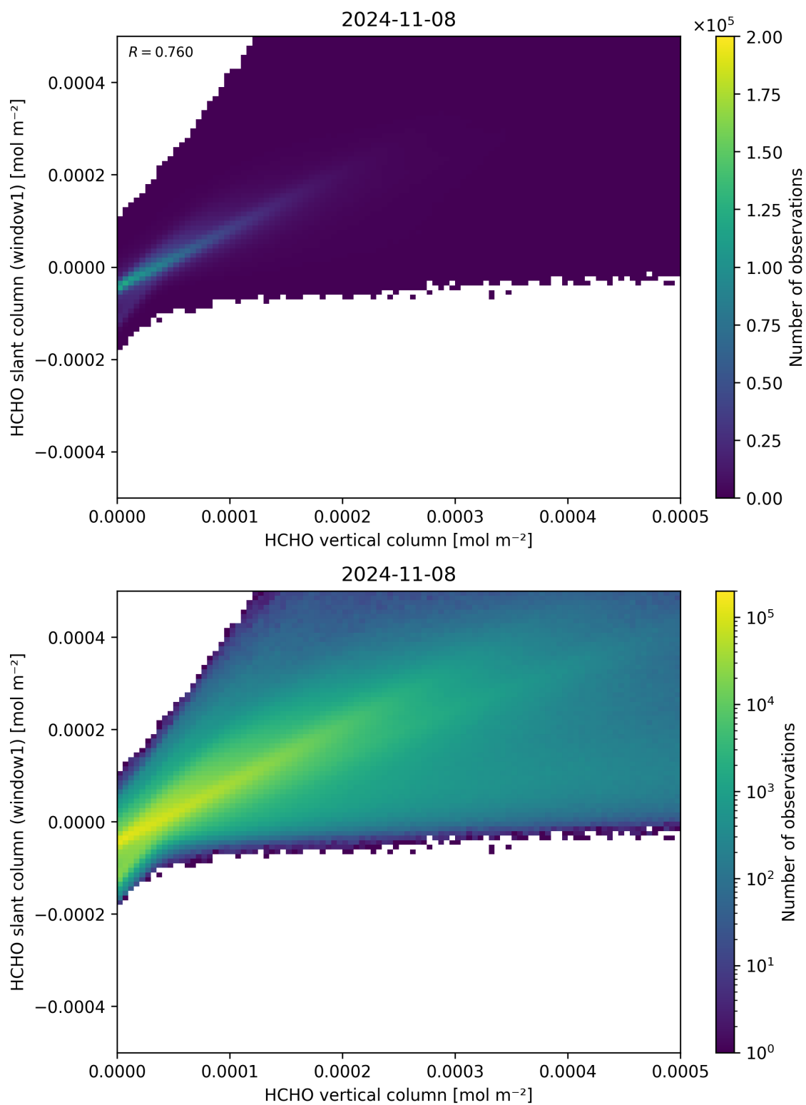
Figure 129: Scatter density plot of “HCHO vertical column” against “HCHO slant column (window1)” for 2024-11-07 to 2024-11-09.
