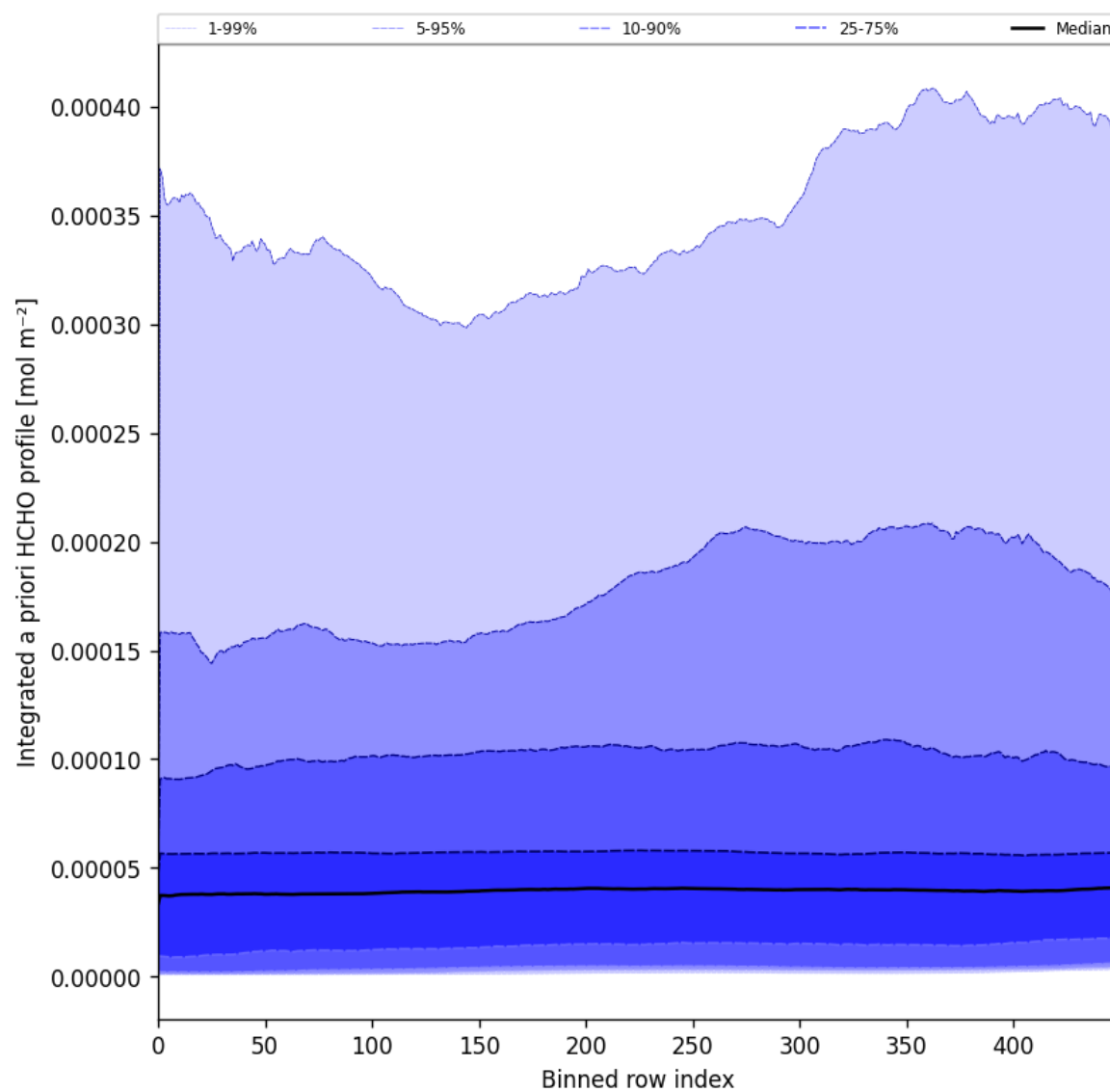
Figure 57: Along track statistics of "Integrated a priori HCHO profile" for 2024-11-07 to 2024-11-09
