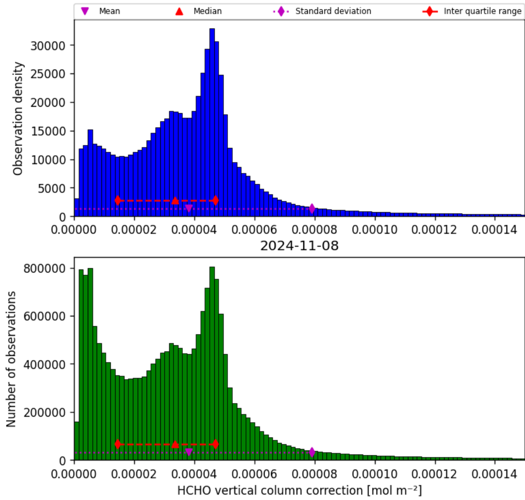
Figure 37: Histogram of “HCHO vertical column correction” for 2024-11-07 to 2024-11-09
