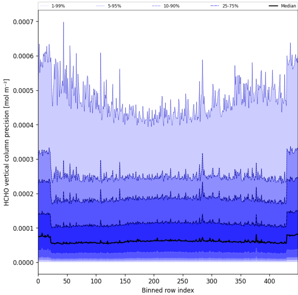
Figure 50: Along track statistics of “HCHO vertical column precision” for 2024-11-07 to 2024-11-09
