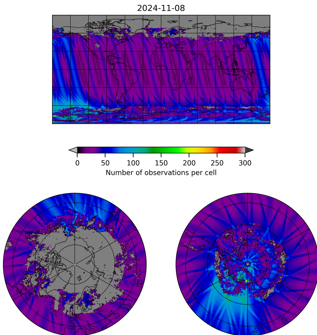
Figure 19: Map of the number of observations for 2024-11-07 to 2024-11-09
