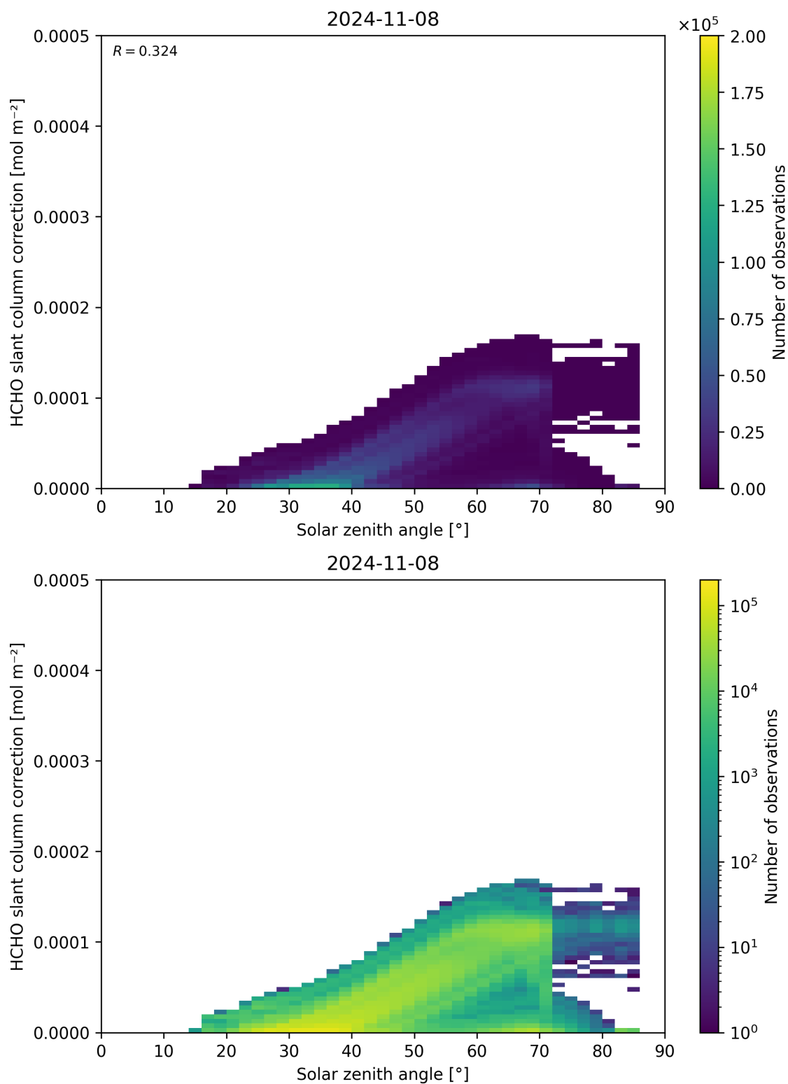
Figure 172: Scatter density plot of “Solar zenith angle” against “HCHO slant column correction” for 2024-11-07 to 2024-11-09.
