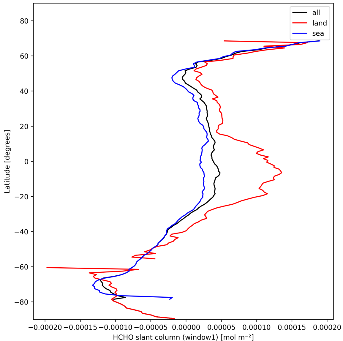
Figure 24: Zonal average of “HCHO slant column (window1)” for 2024-11-07 to 2024-11-09.
