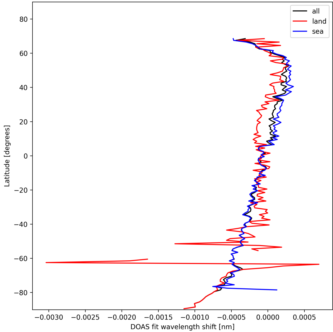
Figure 30: Zonal average of “DOAS fit wavelength shift” for 2024-11-07 to 2024-11-09.
