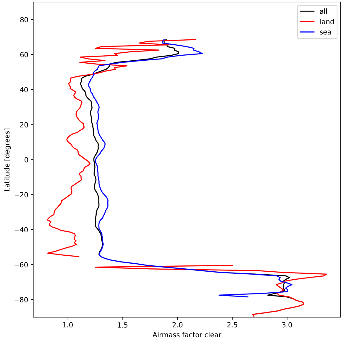
Figure 28: Zonal average of “Airmass factor clear” for 2024-11-07 to 2024-11-09.
