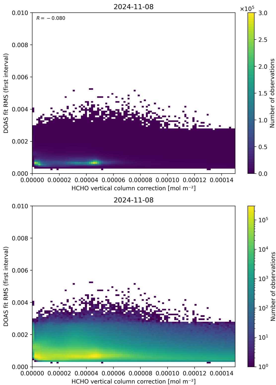
Figure 112: Scatter density plot of “HCHO vertical column correction” against “DOAS fit RMS (first interval)” for 2024-11-07 to 2024-11-09.
