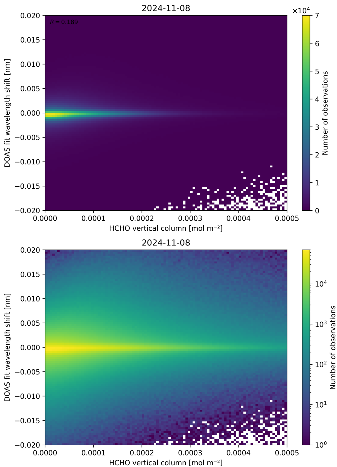
Figure 124: Scatter density plot of “HCHO vertical column” against “DOAS fit wavelength shift” for 2024-11-07 to 2024-11-09.
