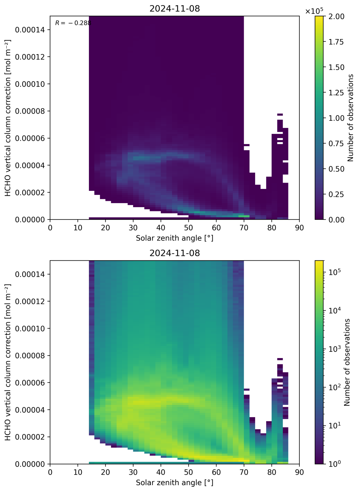
Figure 178: Scatter density plot of “Solar zenith angle” against “HCHO vertical column correction” for 2024-11-07 to 2024-11-09.
