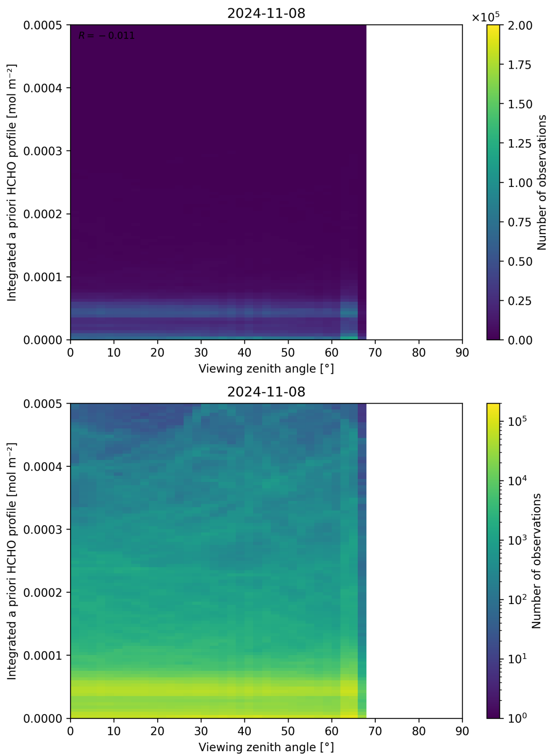
Figure 195: Scatter density plot of “Viewing zenith angle” against “Integrated a priori HCHO profile” for 2024-11-07 to 2024-11-09.
