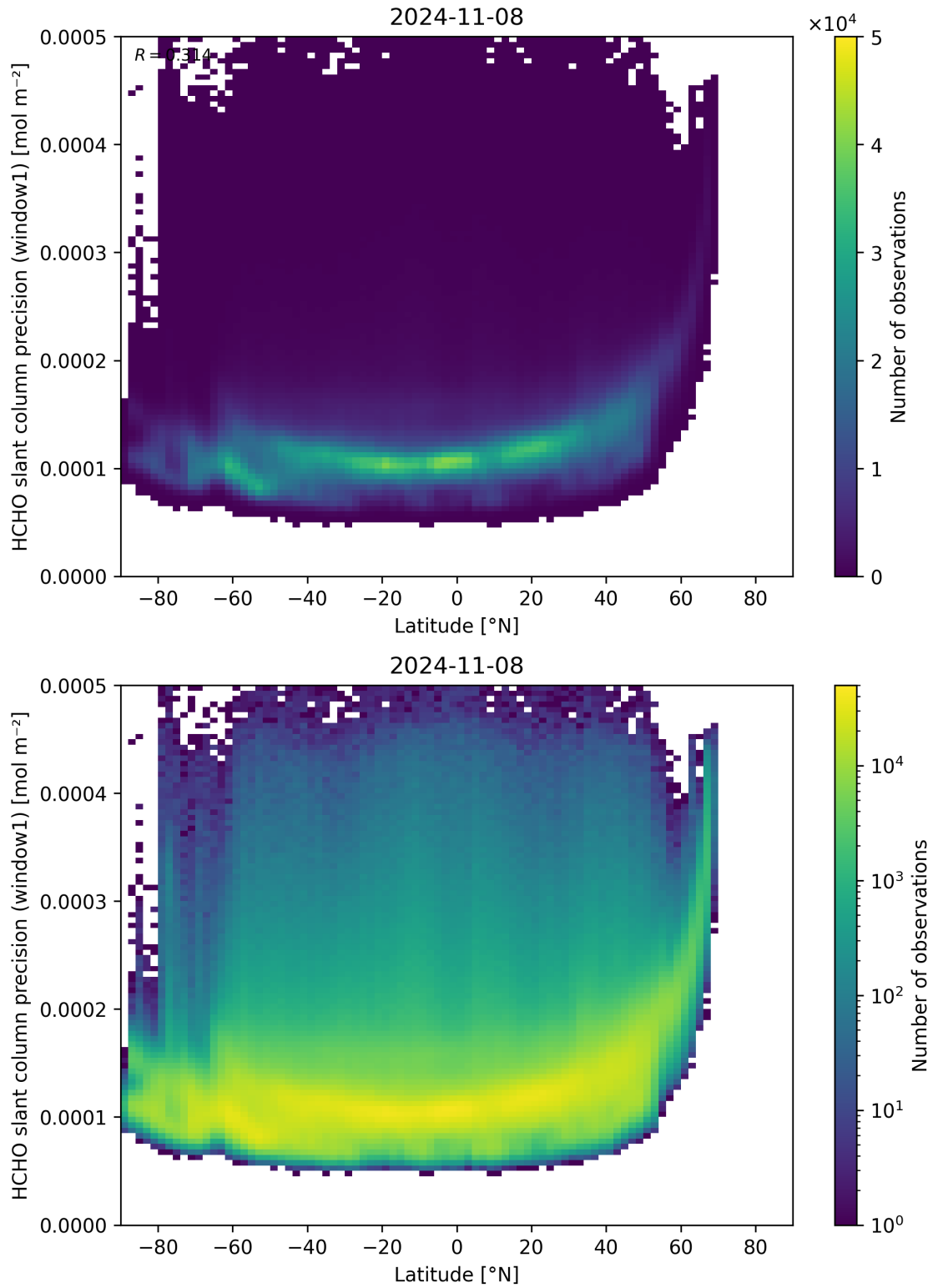
Figure 160: Scatter density plot of “Latitude” against “HCHO slant column precision (window1)” for 2024-11-07 to 2024-11-09.
