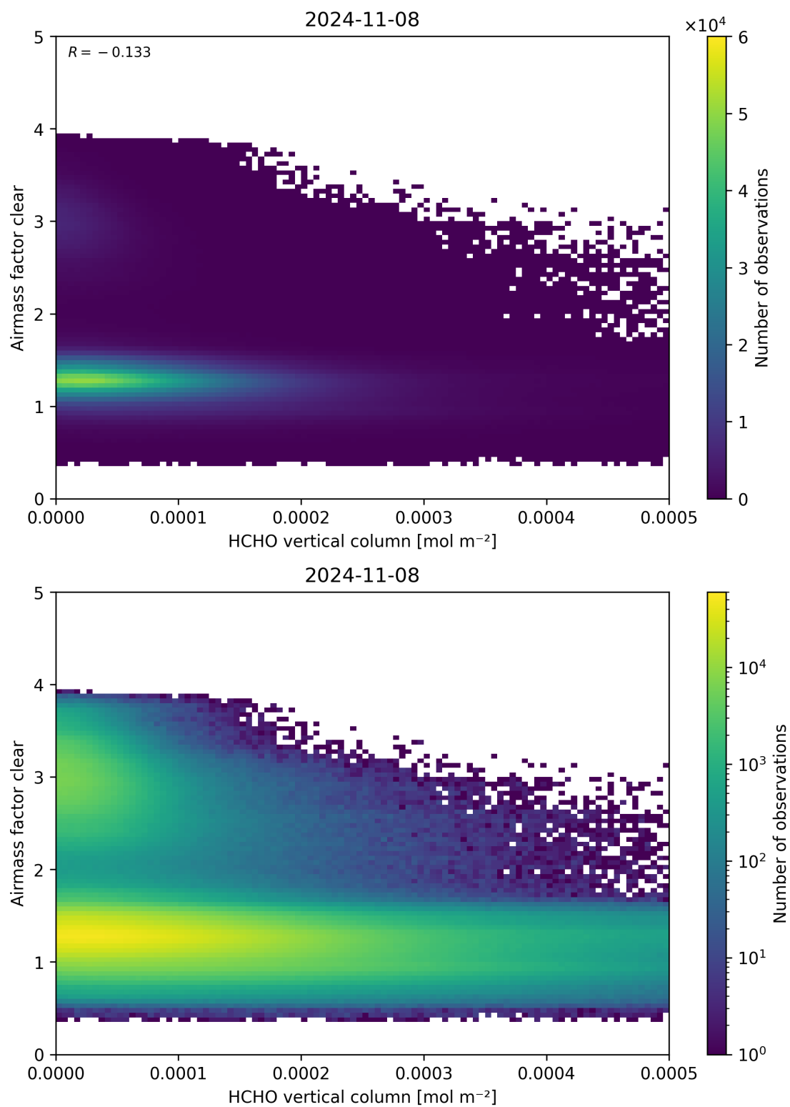
Figure 126: Scatter density plot of “HCHO vertical column” against “Airmass factor clear” for 2024-11-07 to 2024-11-09.
