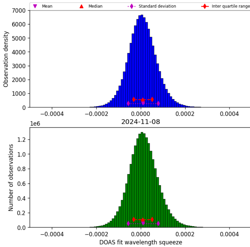
Figure 45: Histogram of “DOAS fit wavelength squeeze” for 2024-11-07 to 2024-11-09
