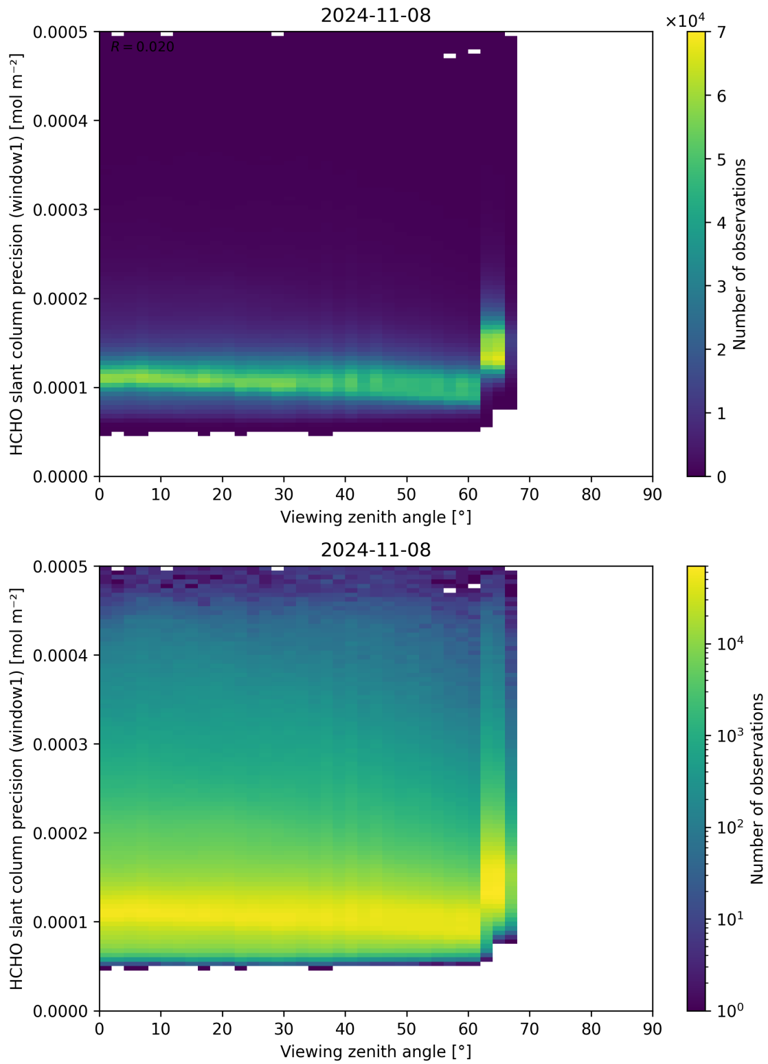
Figure 189: Scatter density plot of “Viewing zenith angle” against “HCHO slant column precision (window1)” for 2024-11-07 to 2024-11-09.
