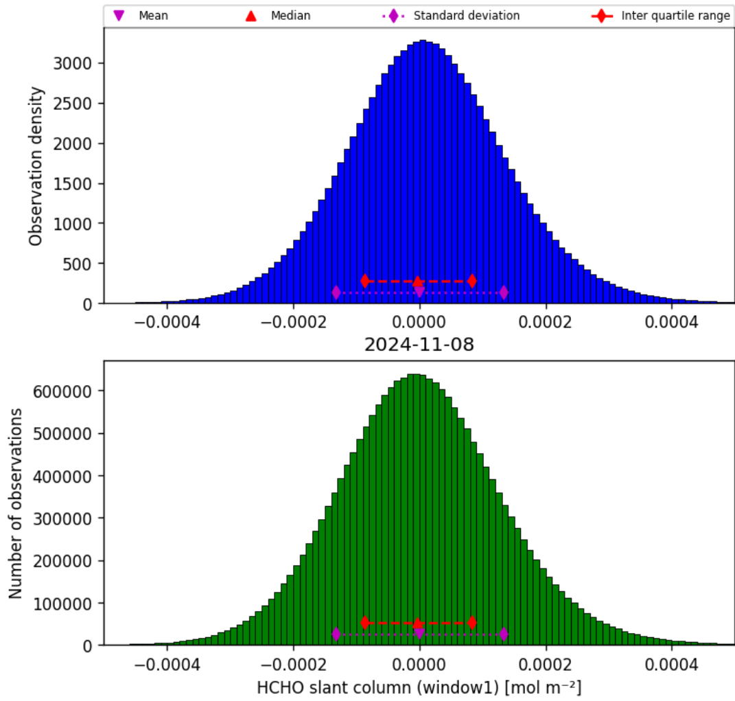
Figure 38: Histogram of “HCHO slant column (window1)” for 2024-11-07 to 2024-11-09
