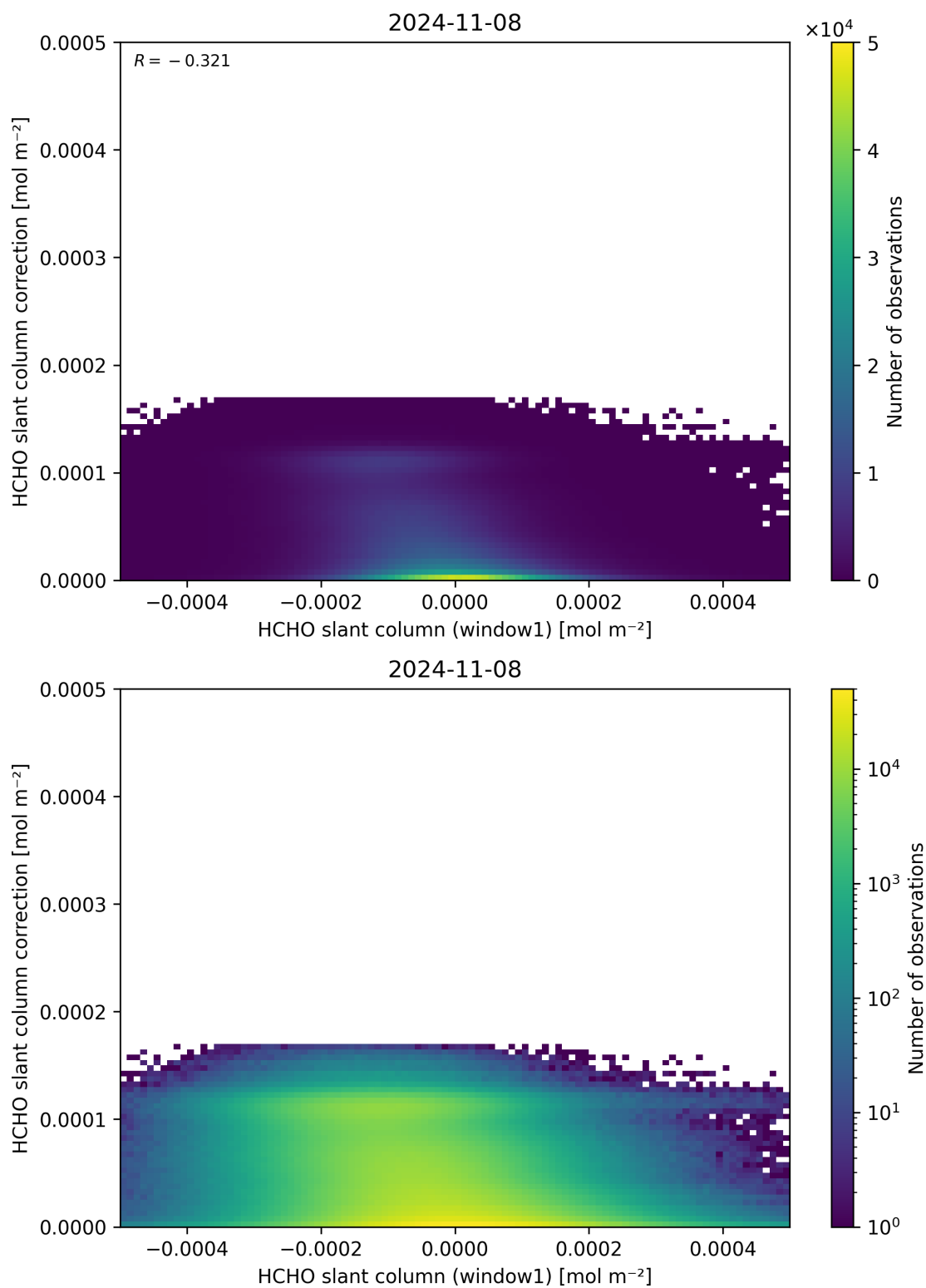
Figure 83: Scatter density plot of “HCHO slant column (window1)” against “HCHO slant column correction” for 2024-11-07 to 2024-11-09.
