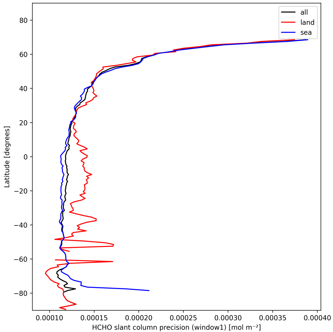
Figure 25: Zonal average of “HCHO slant column precision (window1)” for 2024-11-07 to 2024-11-09.
