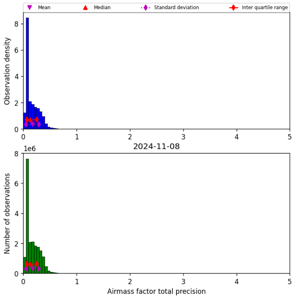
Figure 41: Histogram of “Airmass factor total precision” for 2024-11-07 to 2024-11-09
