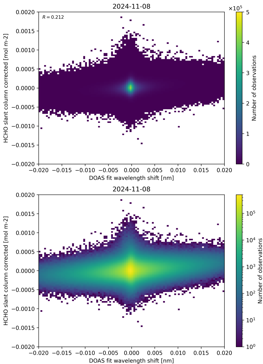
Figure 66: Scatter density plot of “DOAS fit wavelength shift” against “HCHO slant column corrected” for 2024-11-07 to 2024-11-09.
