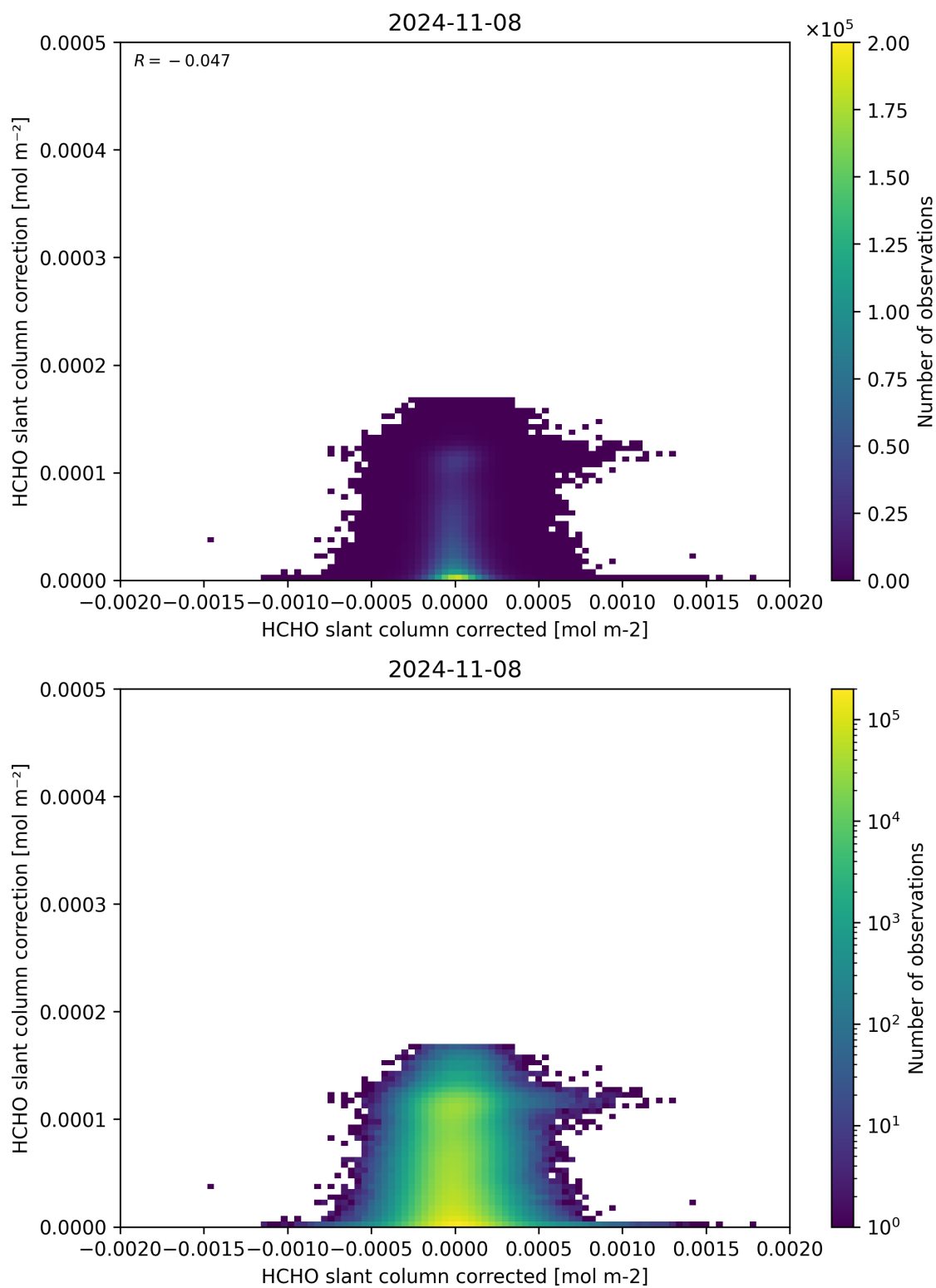
Figure 77: Scatter density plot of “HCHO slant column corrected” against “HCHO slant column correction” for 2024-11-07 to 2024-11-09.
