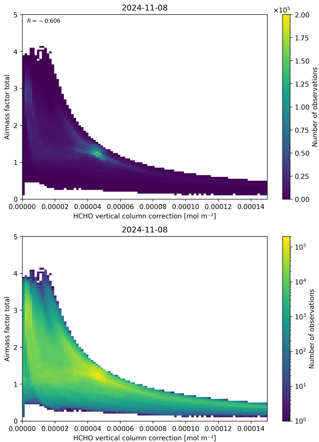
Figure 120: Scatter density plot of “HCHO vertical column correction” against “Airmass factor total” for 2024-11-07 to 2024-11-09.
