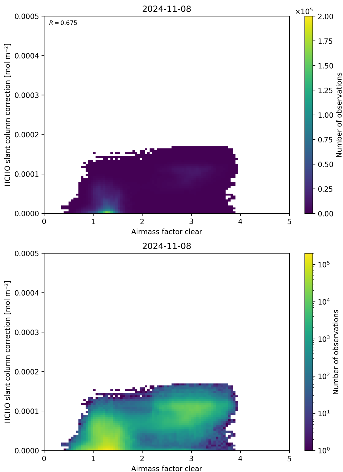
Figure 75: Scatter density plot of “Airmass factor clear” against “HCHO slant column correction” for 2024-11-07 to 2024-11-09.
