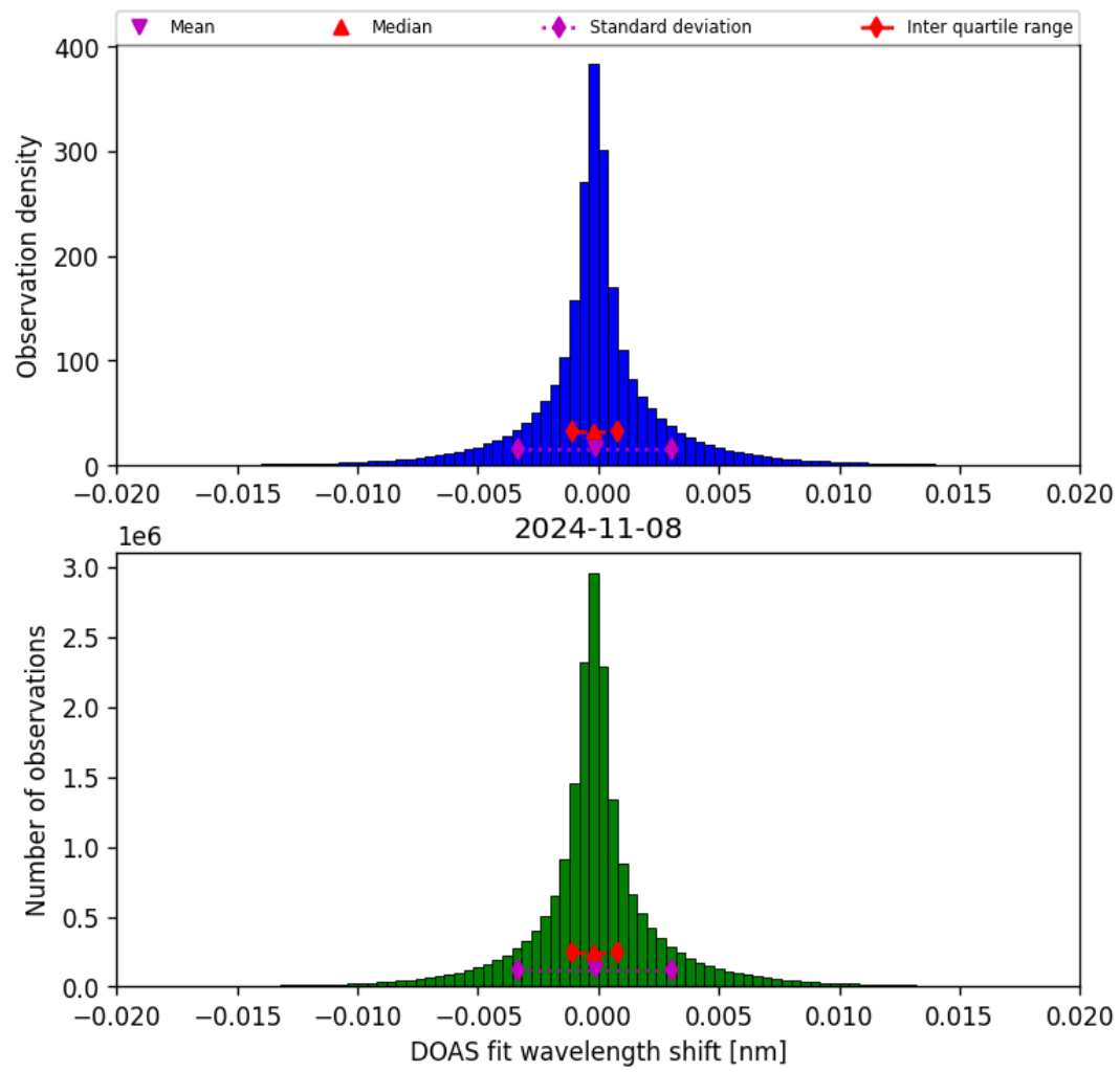
Figure 44: Histogram of “DOAS fit wavelength shift” for 2024-11-07 to 2024-11-09
