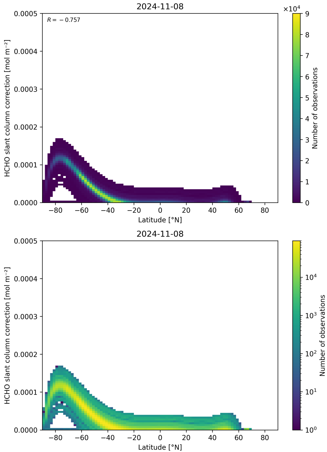
Figure 158: Scatter density plot of “Latitude” against “HCHO slant column correction” for 2024-11-07 to 2024-11-09.
