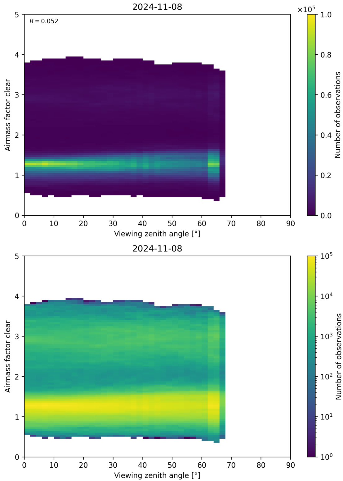
Figure 185: Scatter density plot of “Viewing zenith angle” against “Airmass factor clear” for 2024-11-07 to 2024-11-09.
