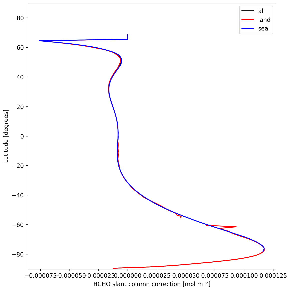
Figure 33: Zonal average of “HCHO slant column correction” for 2024-11-07 to 2024-11-09.
