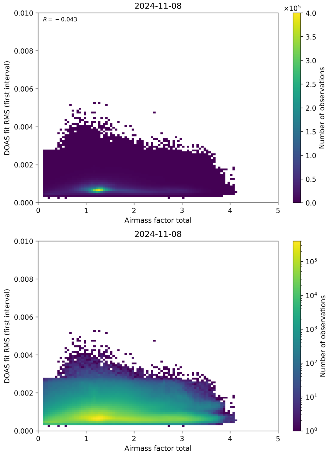
Figure 97: Scatter density plot of “Airmass factor total” against “DOAS fit RMS (first interval)” for 2024-11-07 to 2024-11-09.
