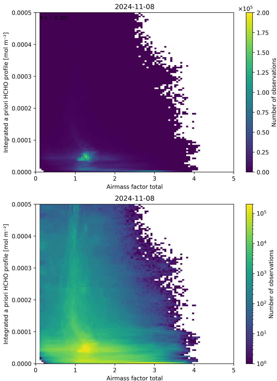
Figure 104: Scatter density plot of “Airmass factor total” against “Integrated a priori HCHO profile” for 2024-11-07 to 2024-11-09.
