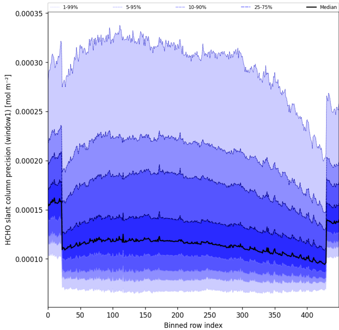
Figure 53: Along track statistics of “HCHO slant column precision (window1)” for 2024-11-07 to 2024-11-09
