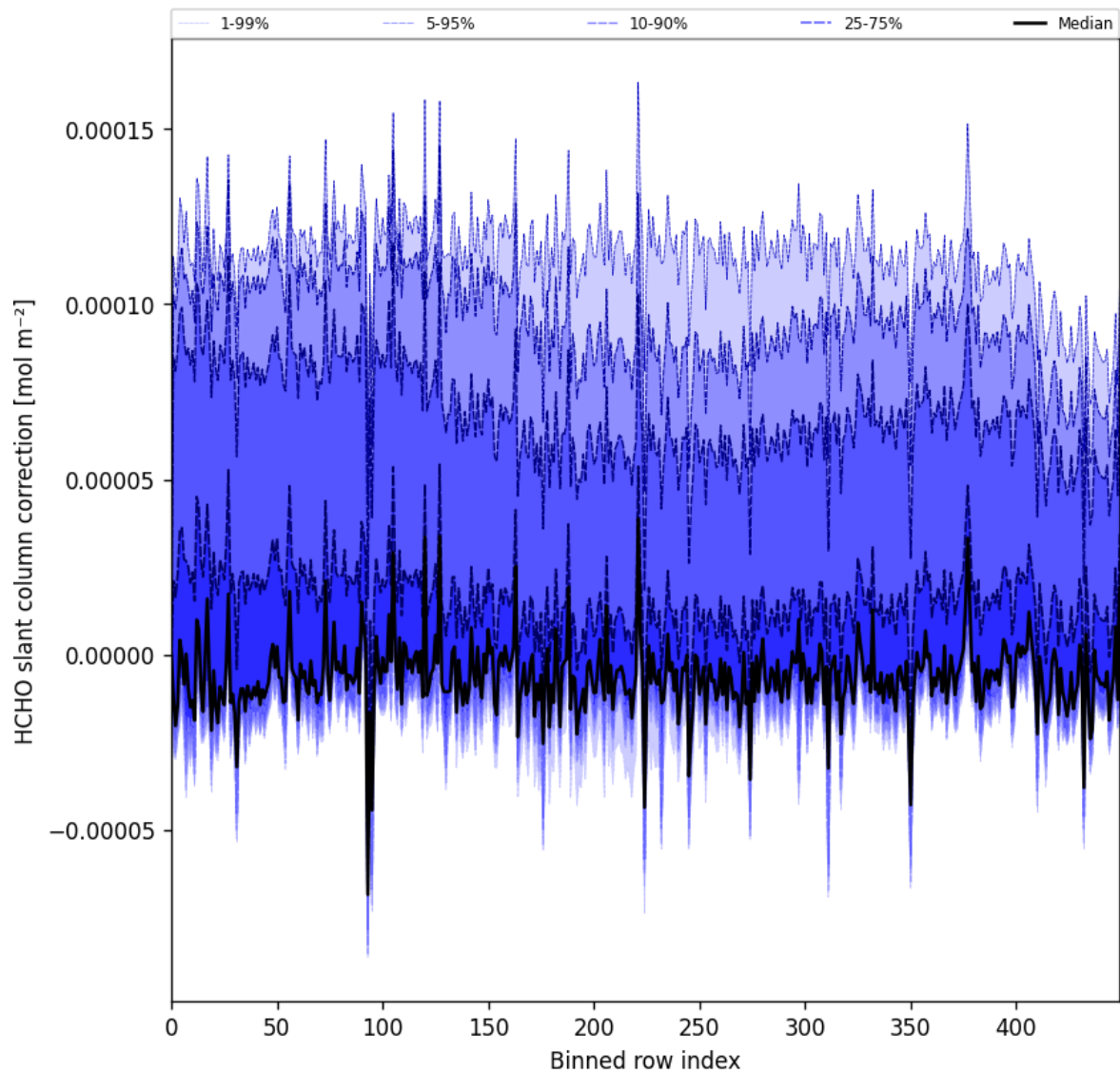
Figure 61: Along track statistics of “HCHO slant column correction” for 2024-11-07 to 2024-11-09
