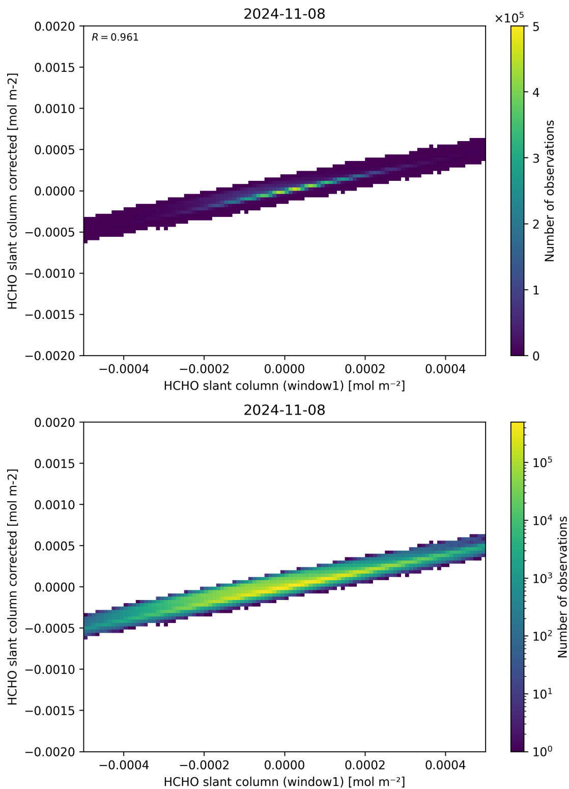
Figure 82: Scatter density plot of “HCHO slant column (window1)” against “HCHO slant column corrected” for 2024-11-07 to 2024-11-09.
