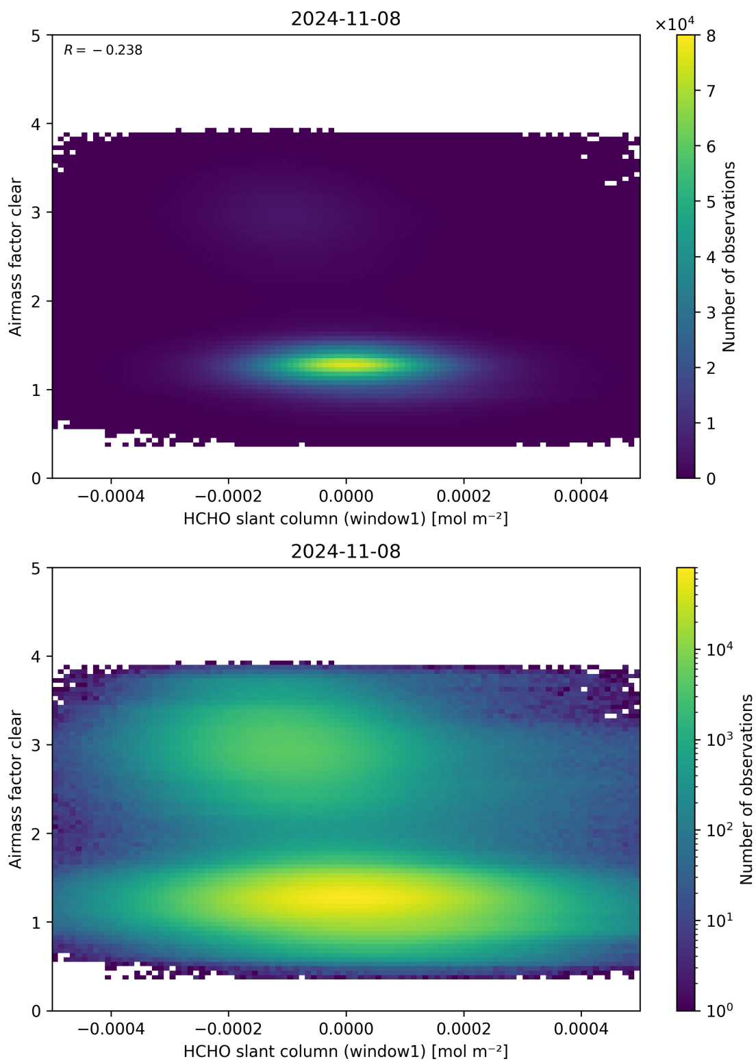
Figure 81: Scatter density plot of “HCHO slant column (window1)” against “Airmass factor clear” for 2024-11-07 to 2024-11-09.
