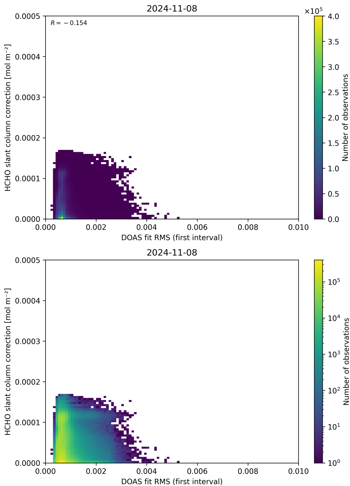
Figure 63: Scatter density plot of “DOAS fit RMS (first interval)” against “HCHO slant column correction” for 2024-11-07 to 2024-11-09.
