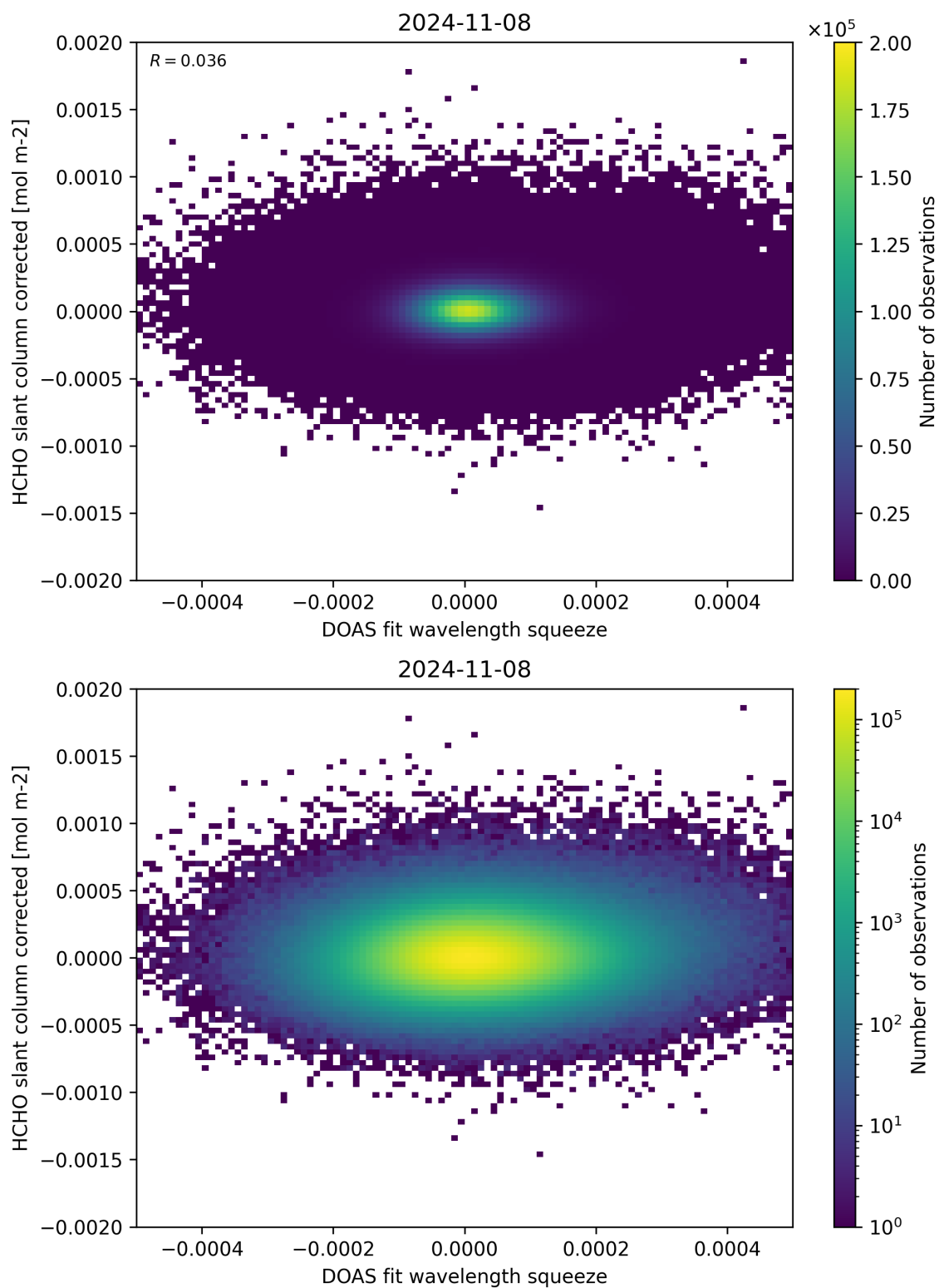
Figure 69: Scatter density plot of “DOAS fit wavelength squeeze” against “HCHO slant column corrected” for 2024-11-07 to 2024-11-09.
