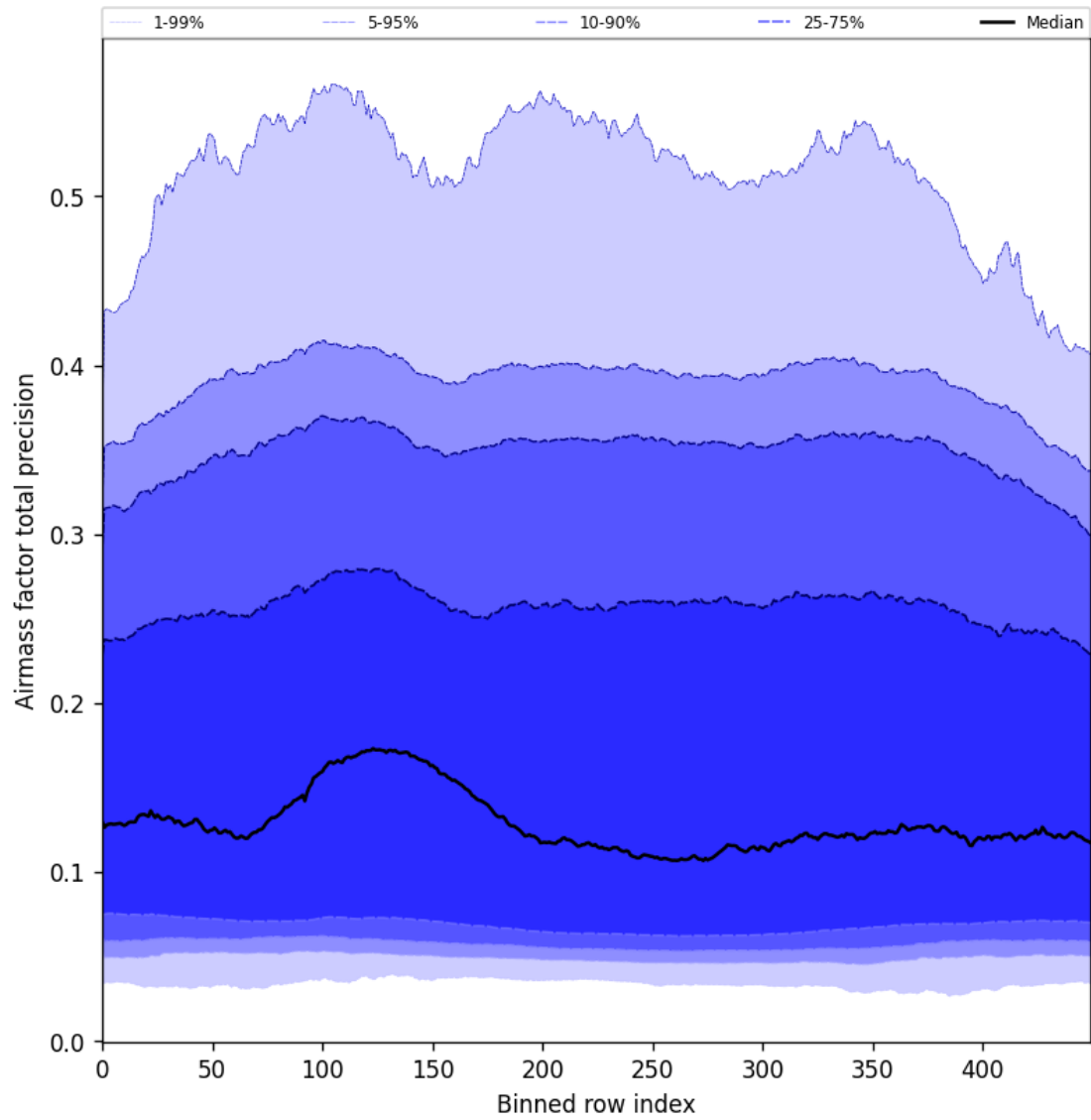
Figure 55: Along track statistics of “Airmass factor total precision” for 2024-11-07 to 2024-11-09
