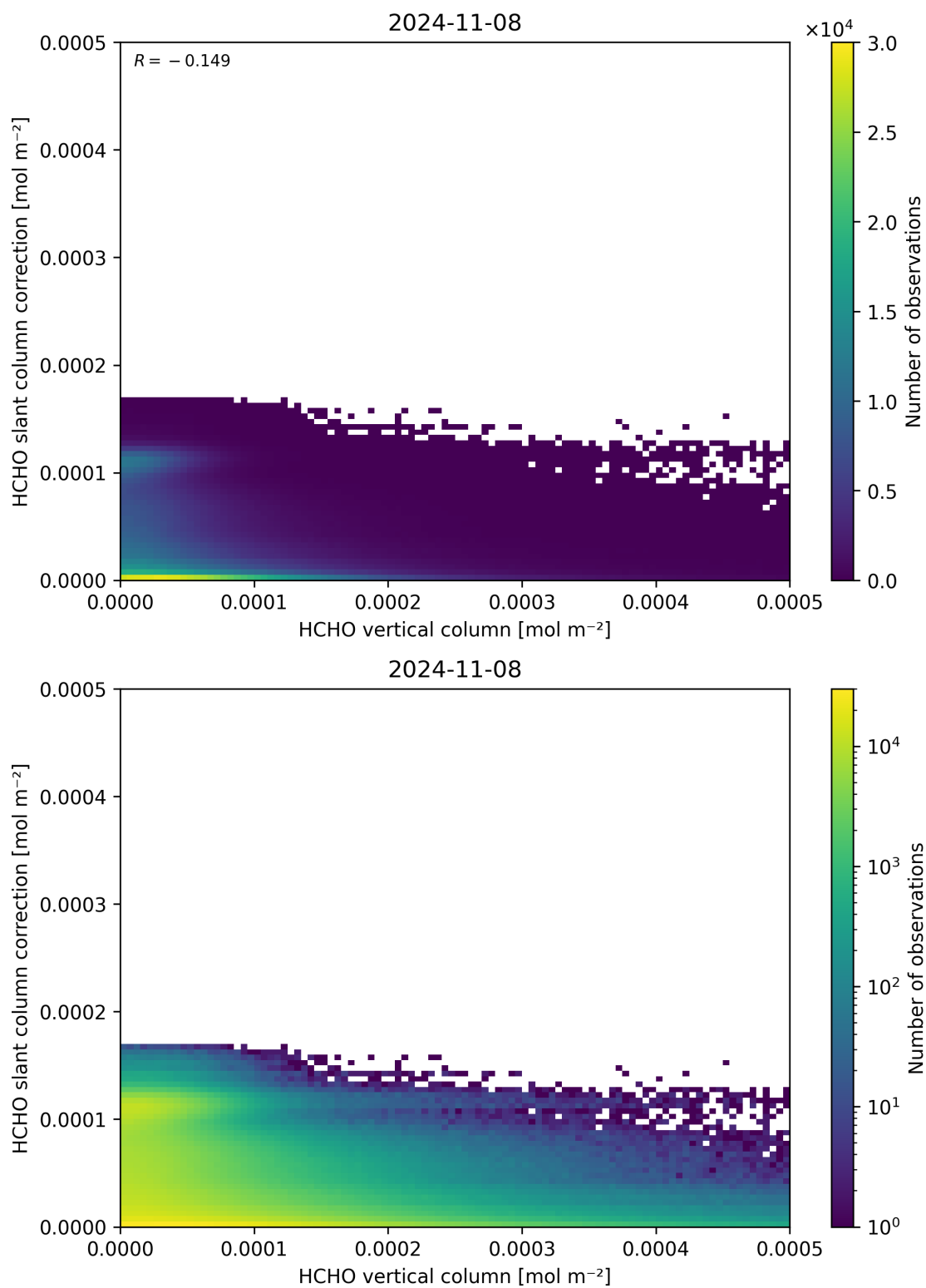
Figure 128: Scatter density plot of “HCHO vertical column” against “HCHO slant column correction” for 2024-11-07 to 2024-11-09.
