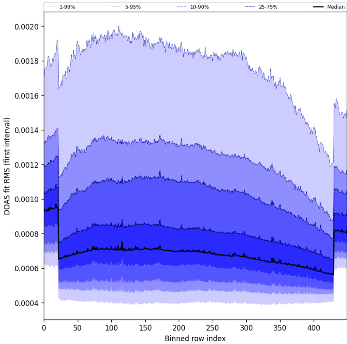
Figure 60: Along track statistics of “DOAS fit RMS (first interval)” for 2024-11-07 to 2024-11-09
