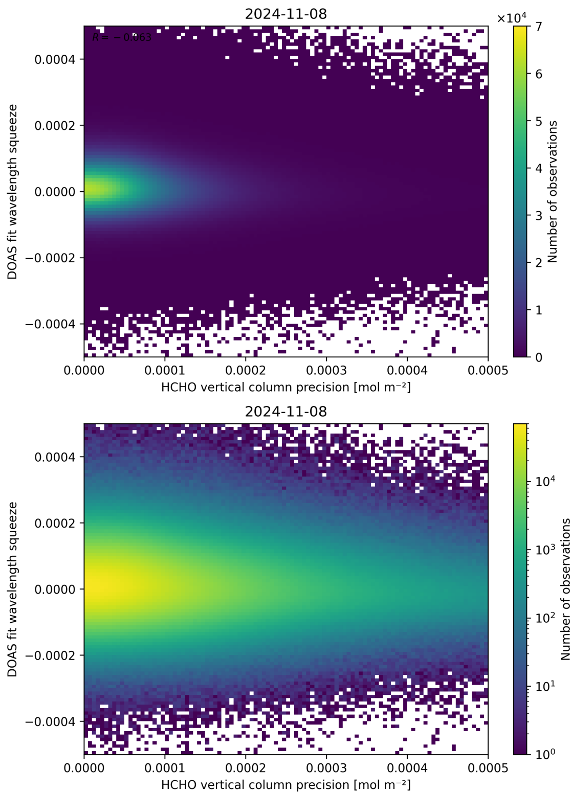
Figure 138: Scatter density plot of “HCHO vertical column precision” against “DOAS fit wavelength squeeze” for 2024-11-07 to 2024-11-09.
