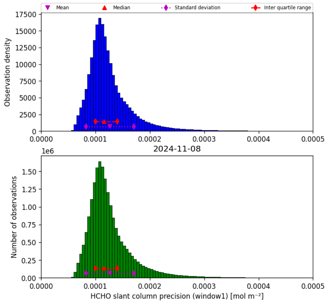
Figure 39: Histogram of “HCHO slant column precision (window1)” for 2024-11-07 to 2024-11-09
