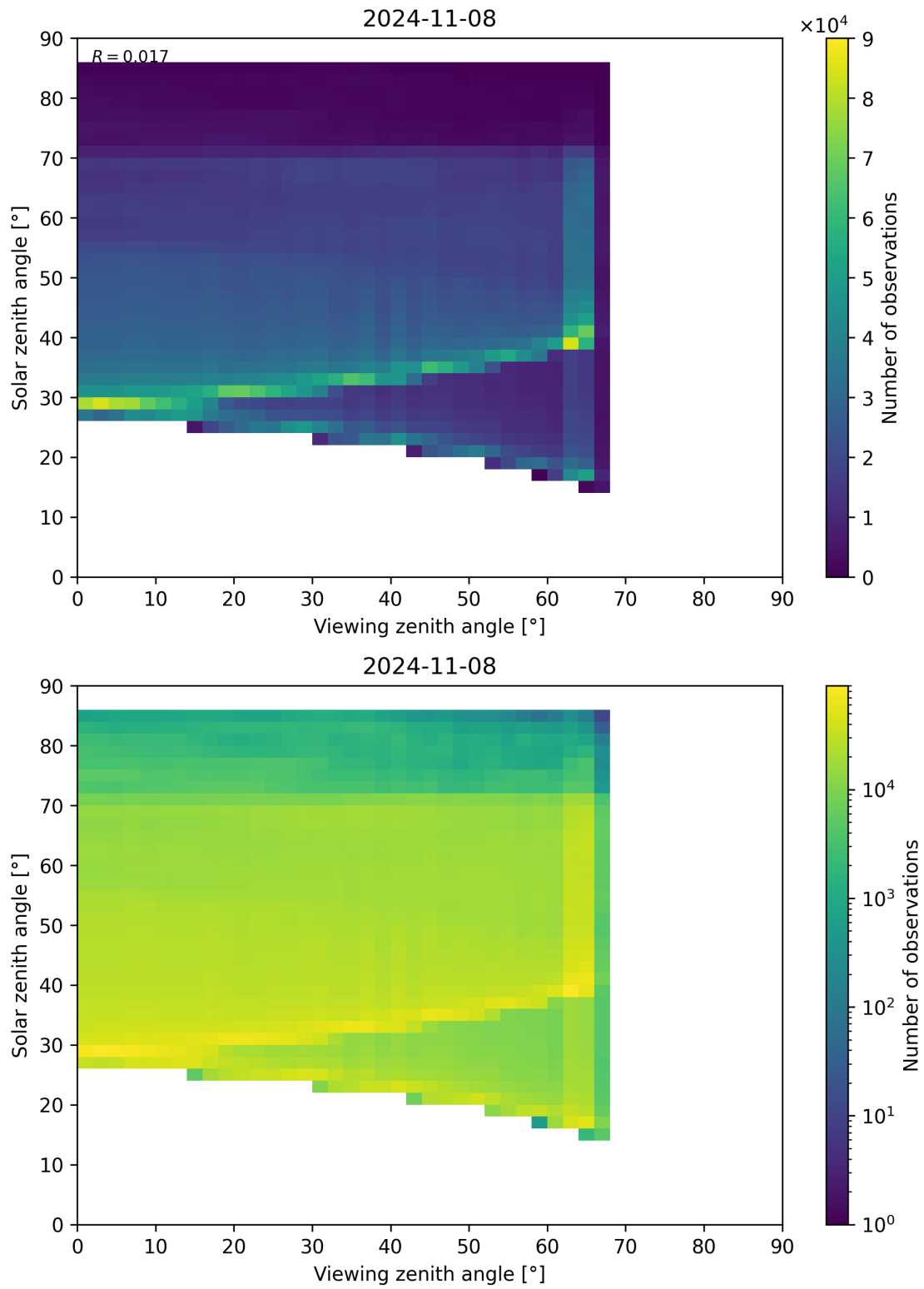
Figure 197: Scatter density plot of “Viewing zenith angle” against “Solar zenith angle” for 2024-11-07 to 2024-11-09.
