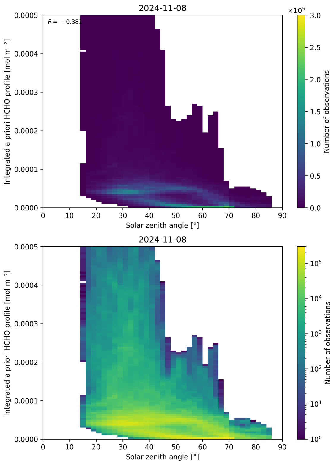
Figure 180: Scatter density plot of “Solar zenith angle” against “Integrated a priori HCHO profile” for 2024-11-07 to 2024-11-09.
