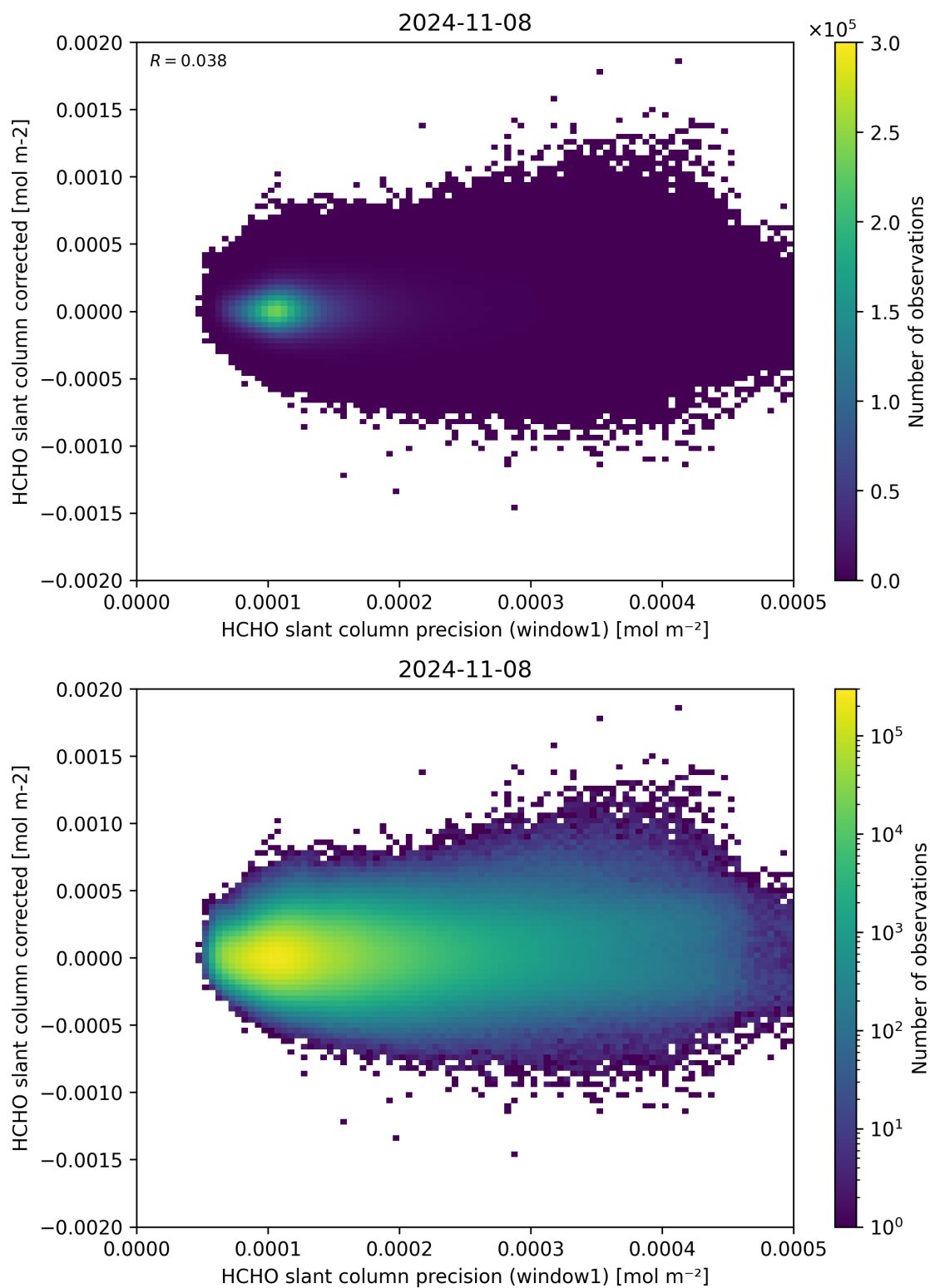
Figure 92: Scatter density plot of “HCHO slant column precision (window1)” against “HCHO slant column corrected” for 2024-11-07 to 2024-11-09.
