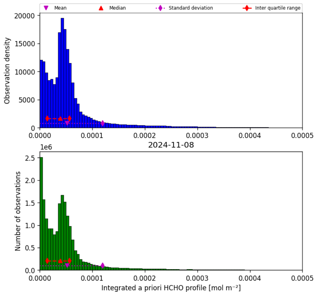
Figure 43: Histogram of “Integrated a priori HCHO profile” for 2024-11-07 to 2024-11-09
