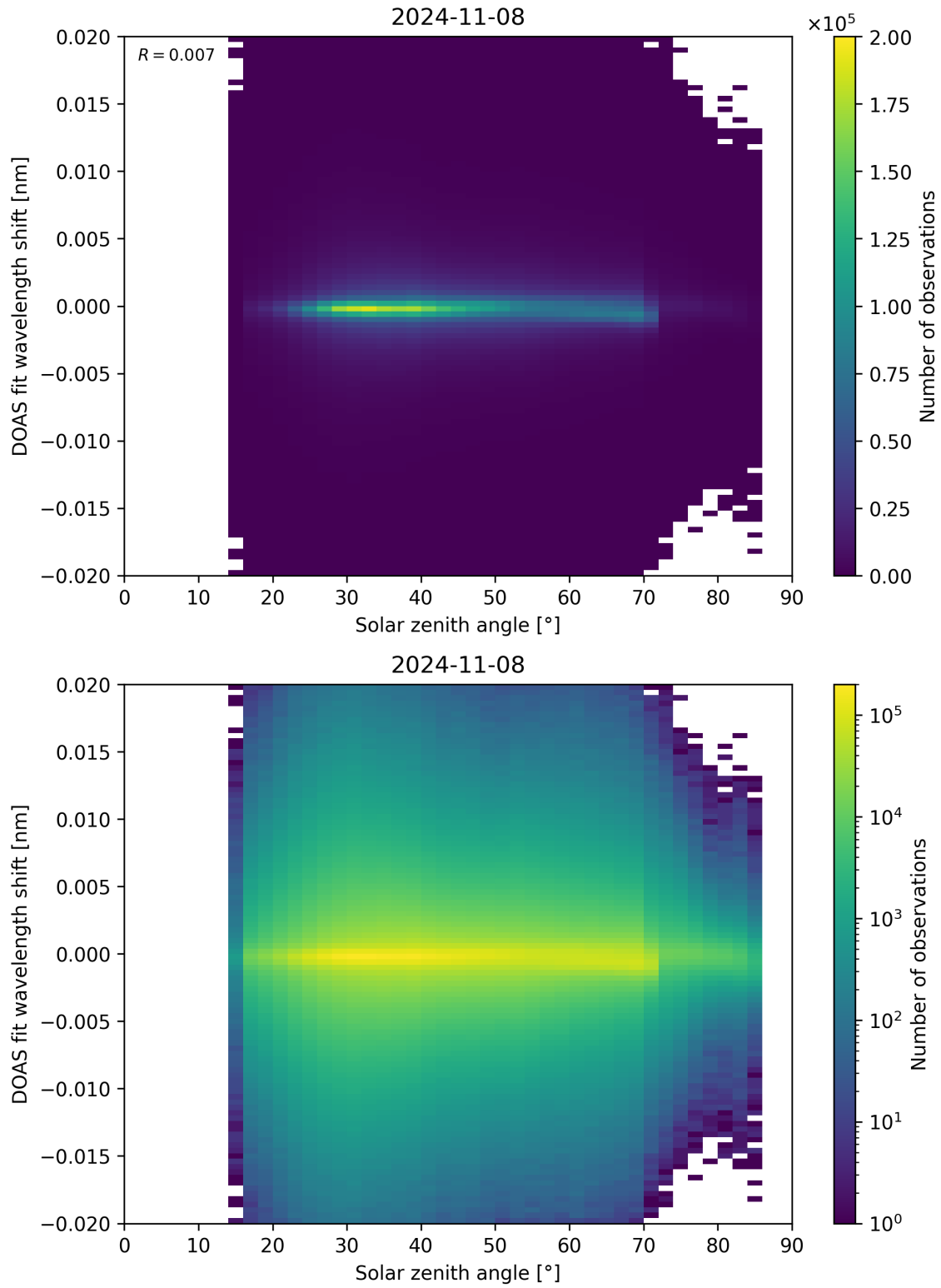
Figure 168: Scatter density plot of “Solar zenith angle” against “DOAS fit wavelength shift” for 2024-11-07 to 2024-11-09.
