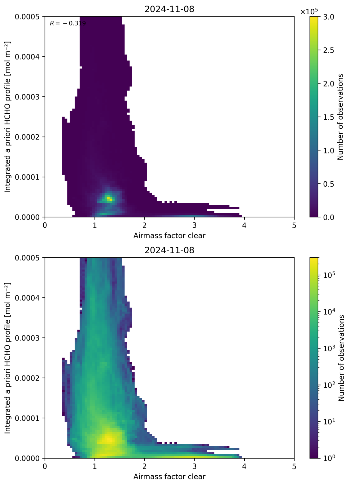
Figure 76: Scatter density plot of “Airmass factor clear” against “Integrated a priori HCHO profile” for 2024-11-07 to 2024-11-09.
