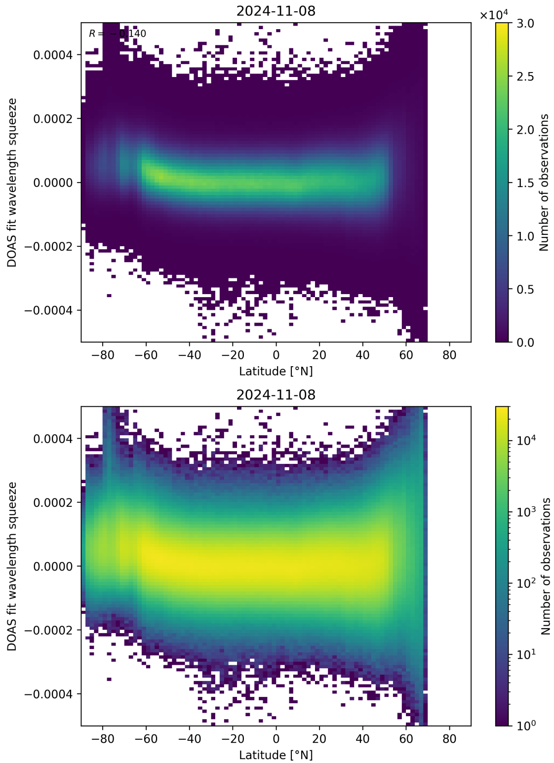
Figure 155: Scatter density plot of “Latitude” against “DOAS fit wavelength squeeze” for 2024-11-07 to 2024-11-09.
