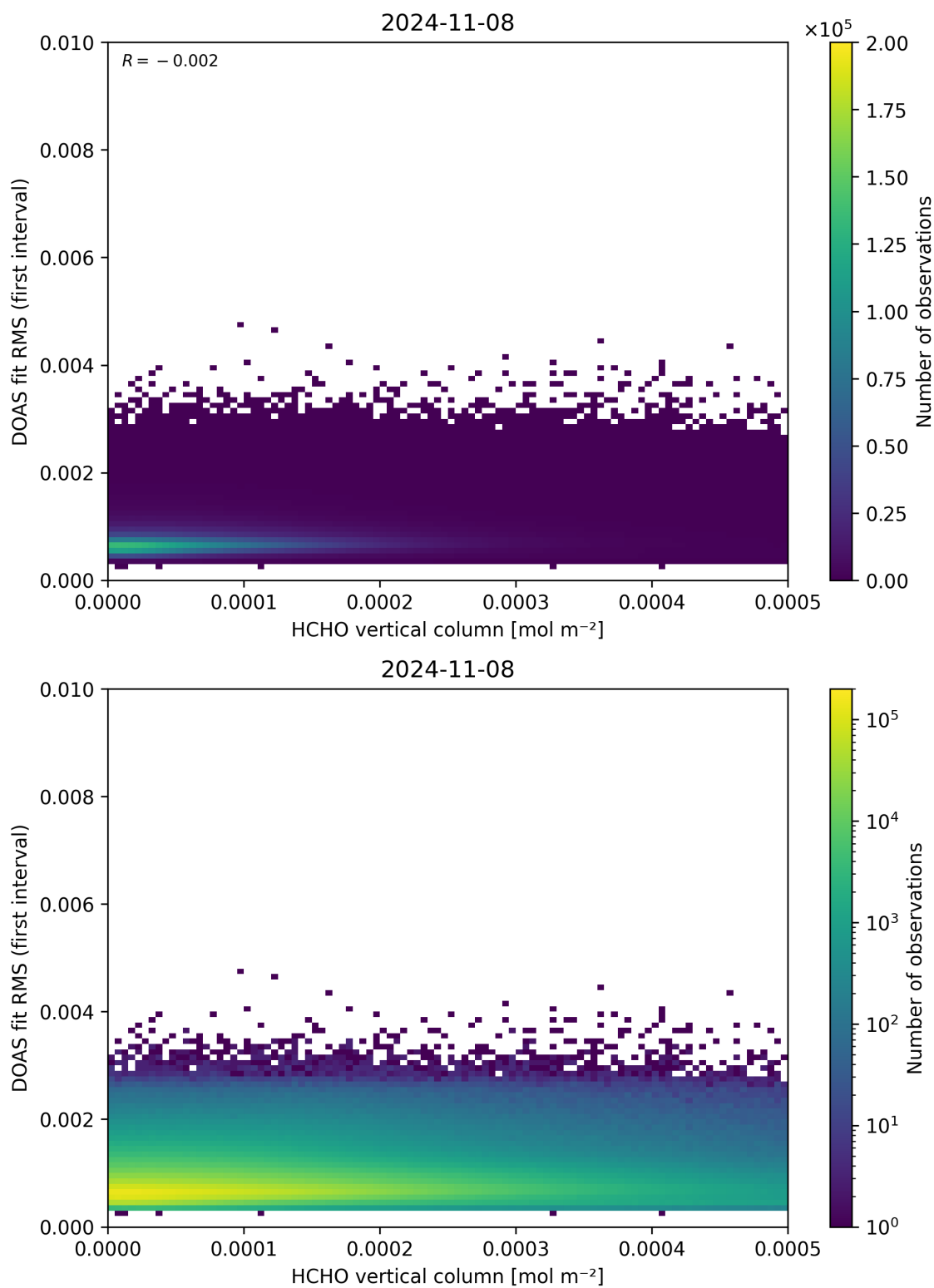
Figure 123: Scatter density plot of “HCHO vertical column” against “DOAS fit RMS (first interval)” for 2024-11-07 to 2024-11-09.
