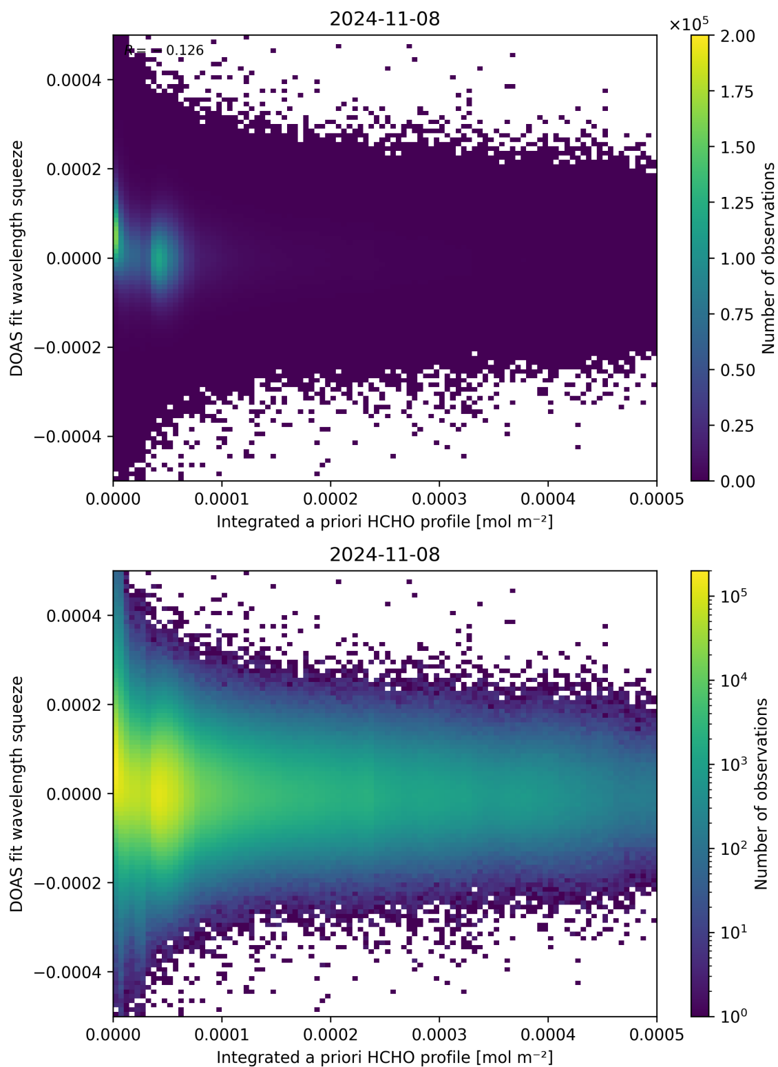
Figure 150: Scatter density plot of “Integrated a priori HCHO profile” against “DOAS fit wavelength squeeze” for 2024-11-07 to 2024-11-09.
