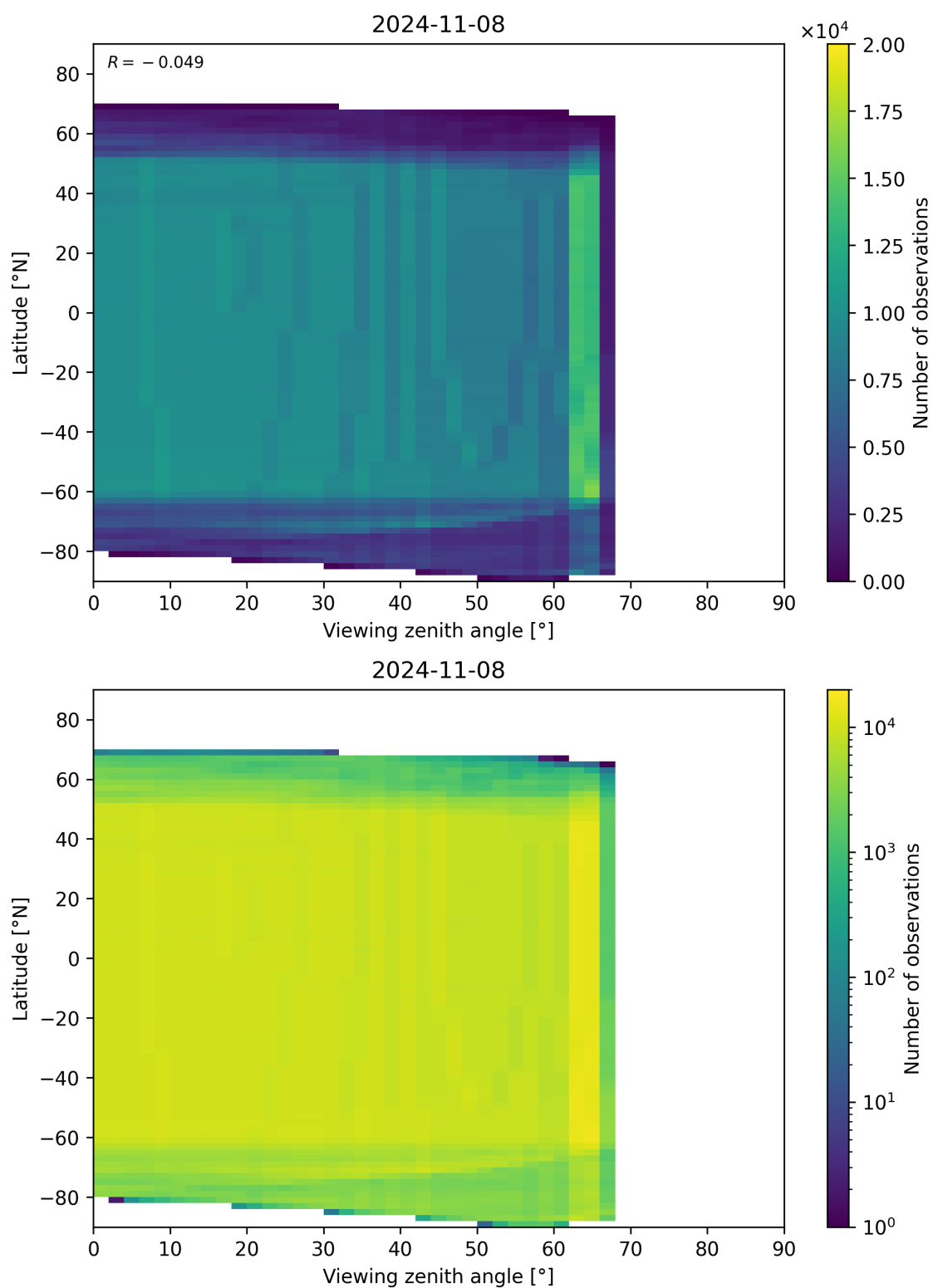
Figure 196: Scatter density plot of “Viewing zenith angle” against “Latitude” for 2024-11-07 to 2024-11-09.
