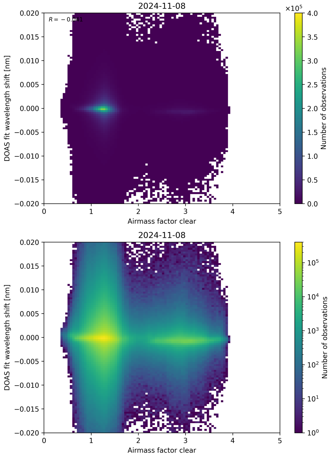
Figure 72: Scatter density plot of “Airmass factor clear” against “DOAS fit wavelength shift” for 2024-11-07 to 2024-11-09.
