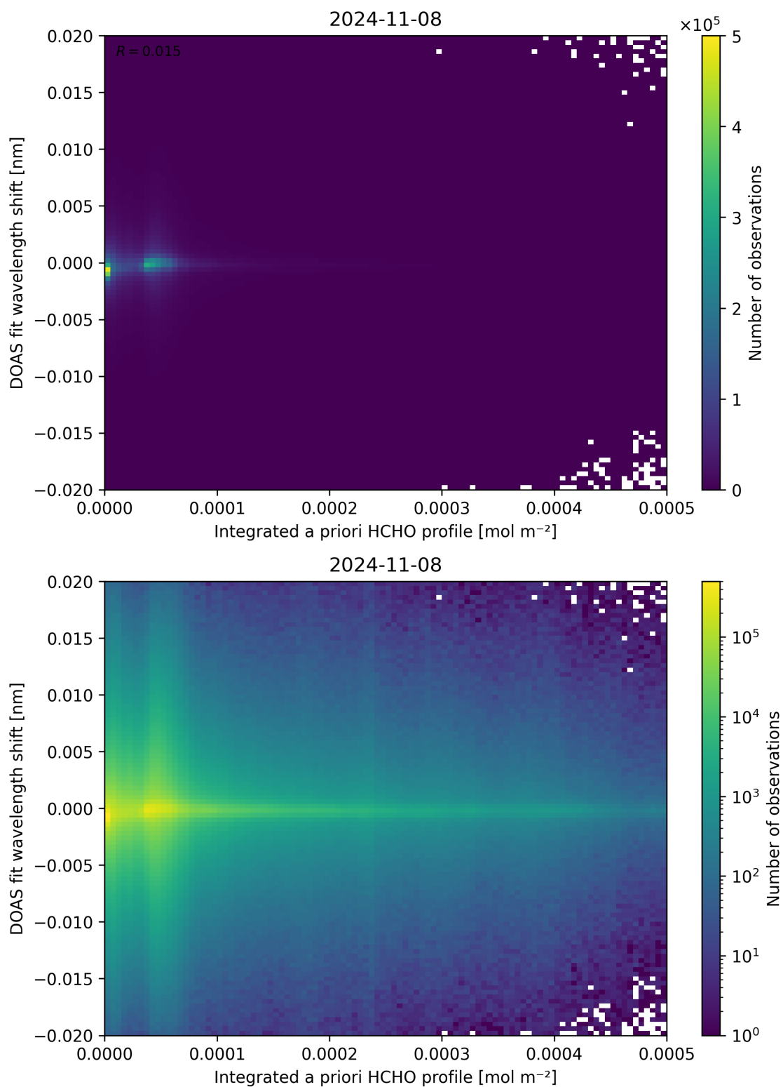
Figure 149: Scatter density plot of “Integrated a priori HCHO profile” against “DOAS fit wavelength shift” for 2024-11-07 to 2024-11-09.
