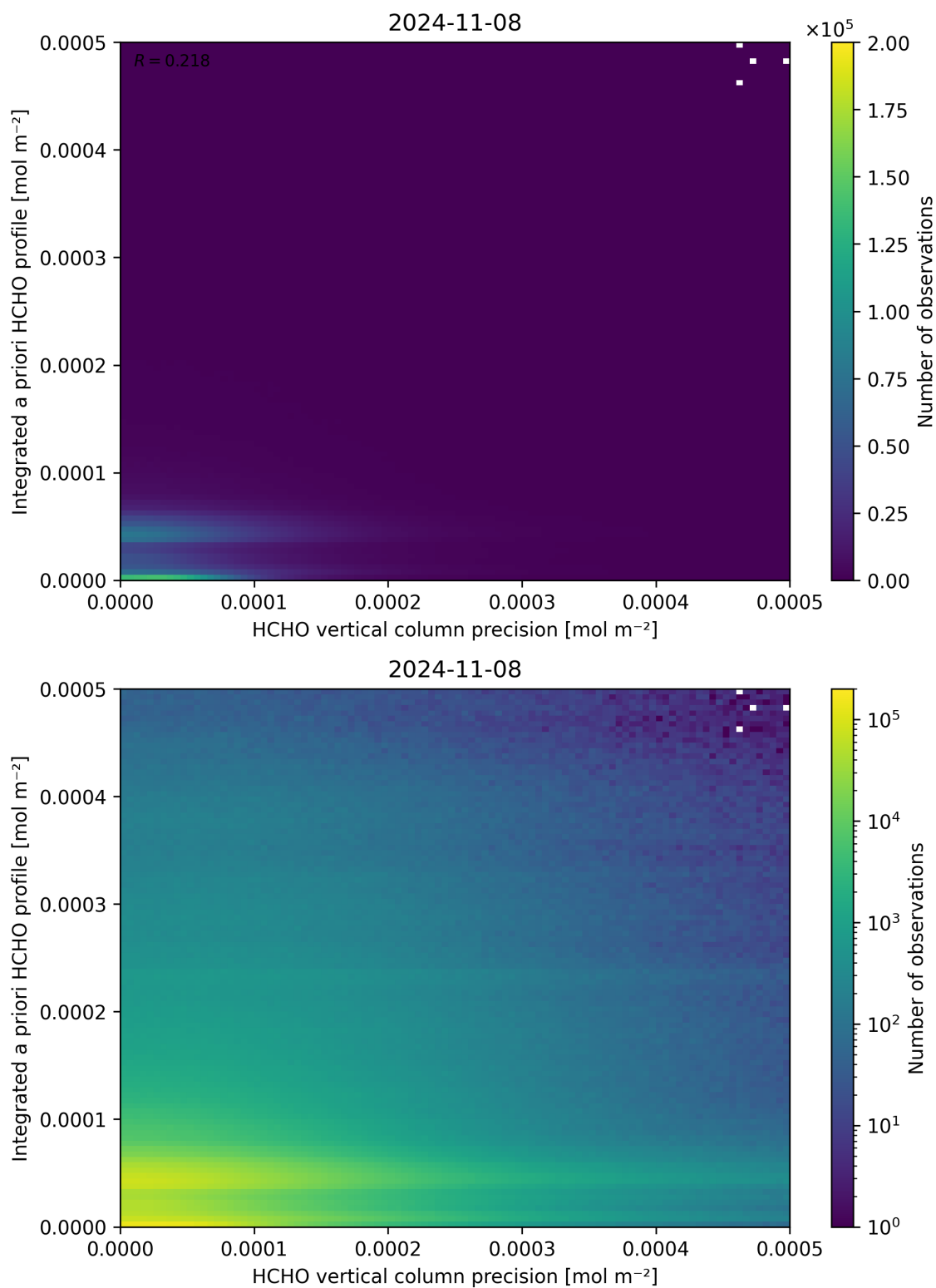
Figure 147: Scatter density plot of “HCHO vertical column precision” against “Integrated a priori HCHO profile” for 2024-11-07 to 2024-11-09.
