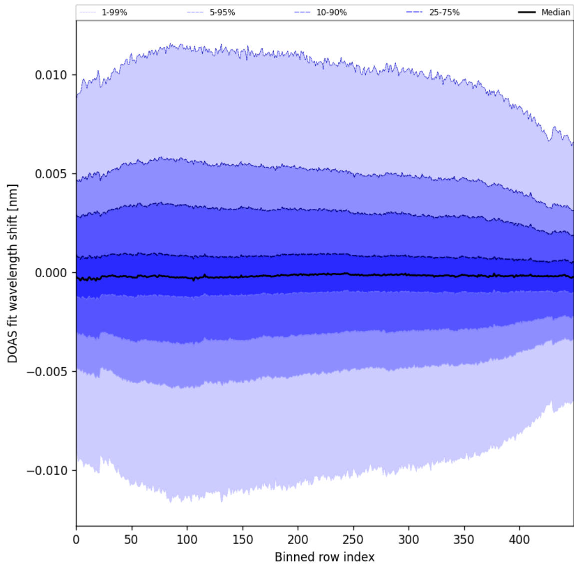
Figure 58: Along track statistics of “DOAS fit wavelength shift” for 2024-11-07 to 2024-11-09
