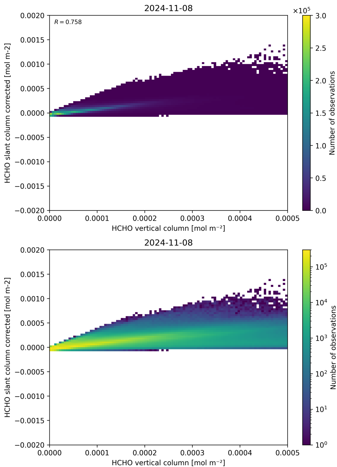
Figure 127: Scatter density plot of “HCHO vertical column” against “HCHO slant column corrected” for 2024-11-07 to 2024-11-09.
