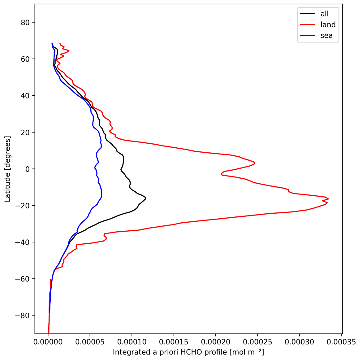
Figure 29: Zonal average of “Integrated a priori HCHO profile” for 2024-11-07 to 2024-11-09.
