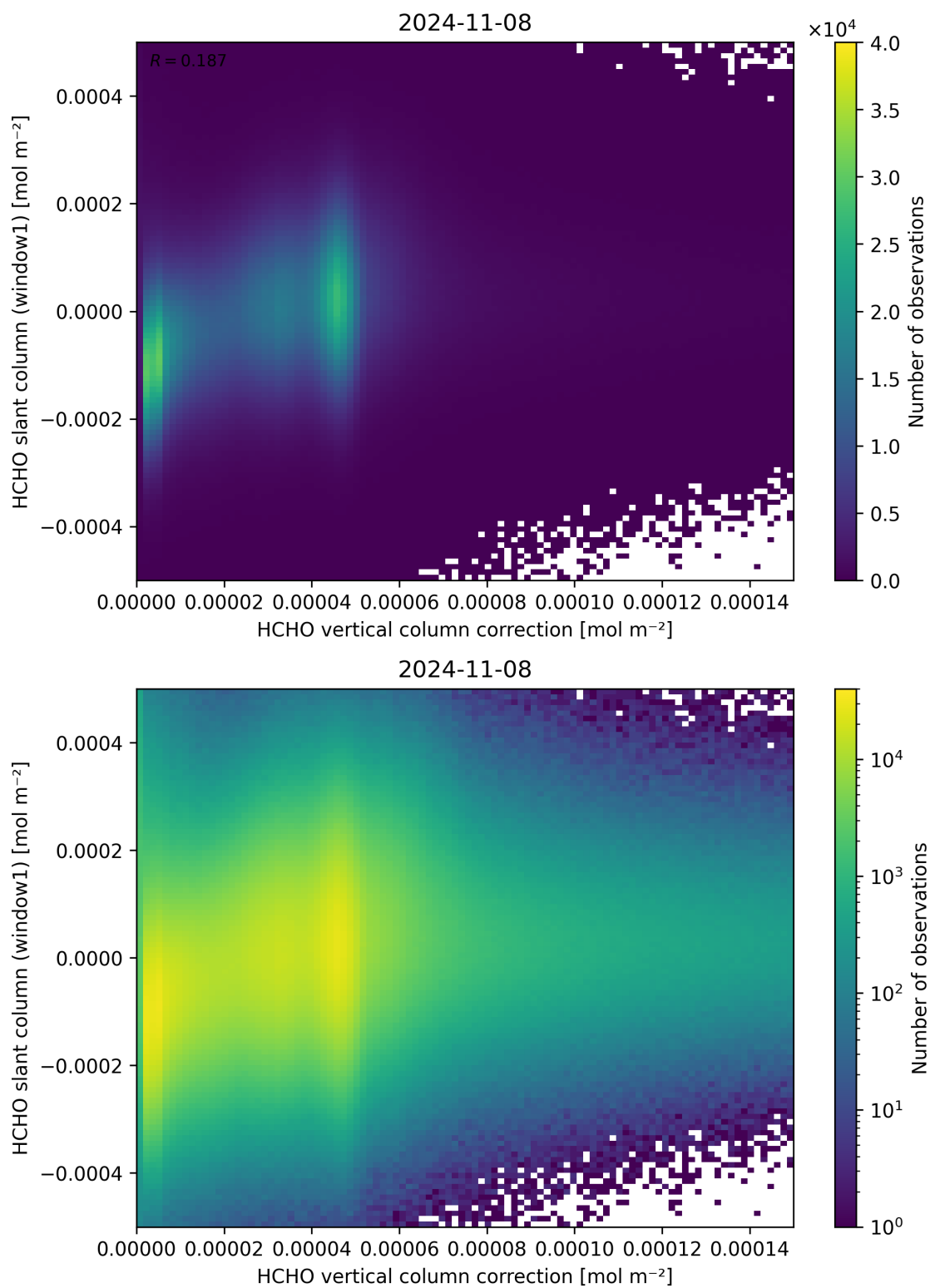
Figure 118: Scatter density plot of “HCHO vertical column correction” against “HCHO slant column (window1)” for 2024-11-07 to 2024-11-09.
