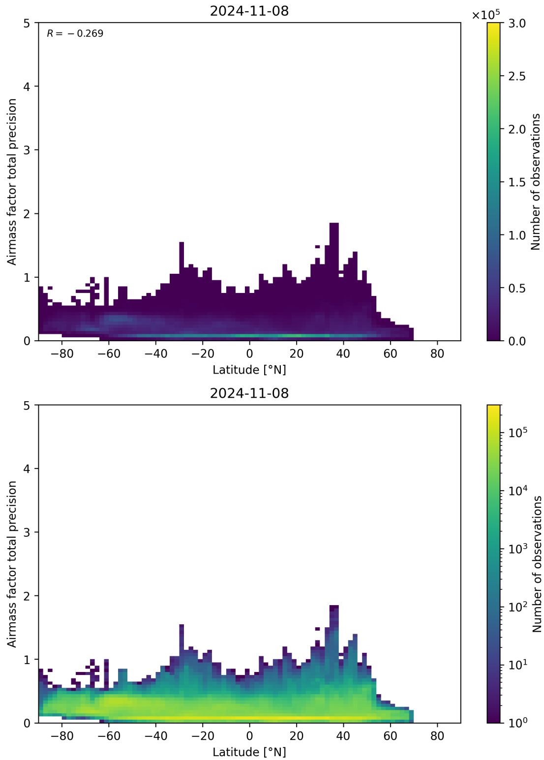
Figure 162: Scatter density plot of “Latitude” against “Airmass factor total precision” for 2024-11-07 to 2024-11-09.
