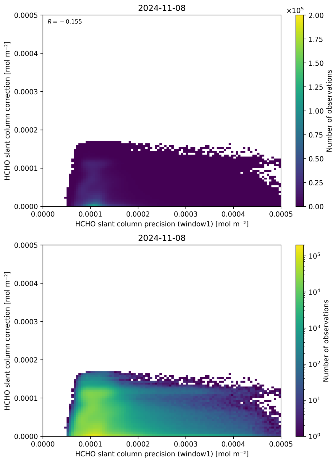
Figure 93: Scatter density plot of “HCHO slant column precision (window1)” against “HCHO slant column correction” for 2024-11-07 to 2024-11-09.
