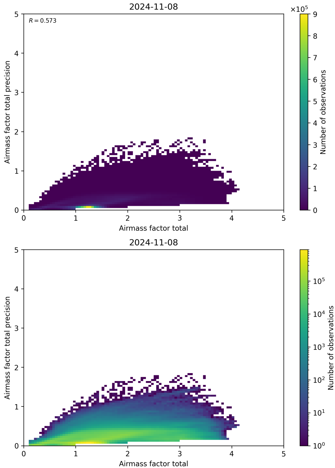
Figure 103: Scatter density plot of “Airmass factor total” against “Airmass factor total precision” for 2024-11-07 to 2024-11-09.
