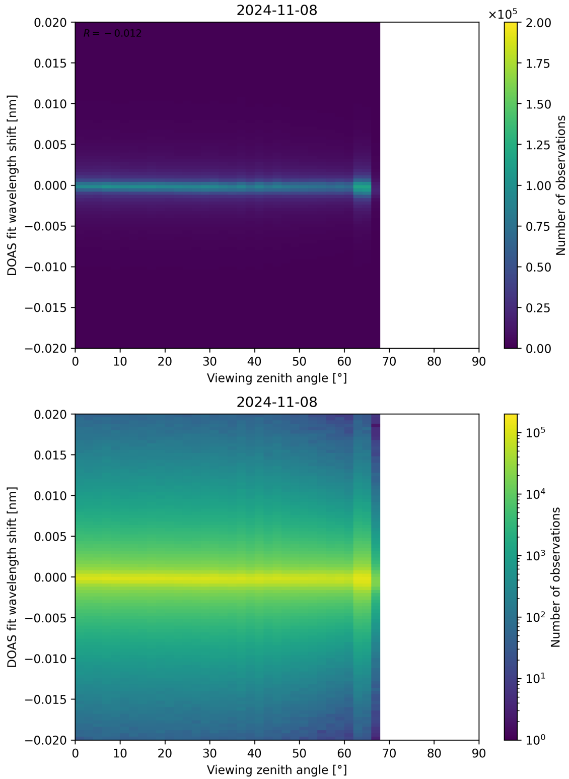
Figure 183: Scatter density plot of “Viewing zenith angle” against “DOAS fit wavelength shift” for 2024-11-07 to 2024-11-09.
