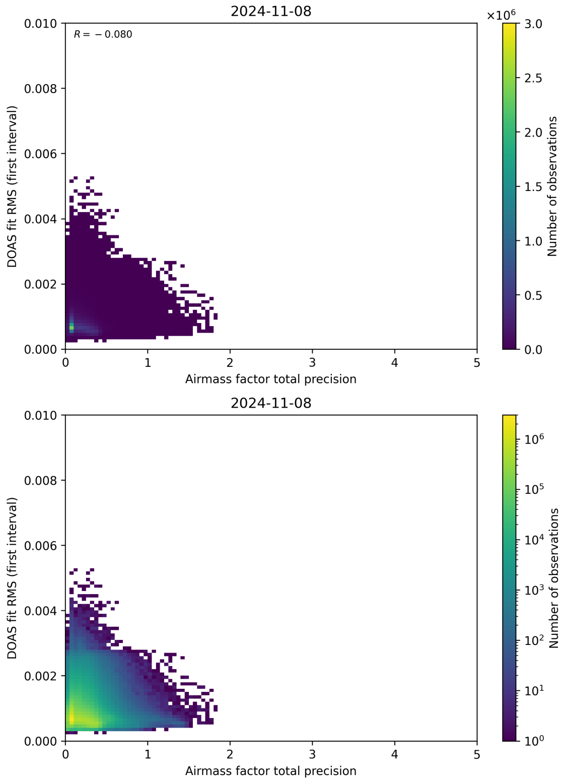
Figure 105: Scatter density plot of “Airmass factor total precision” against “DOAS fit RMS (first interval)” for 2024-11-07 to 2024-11-09.
