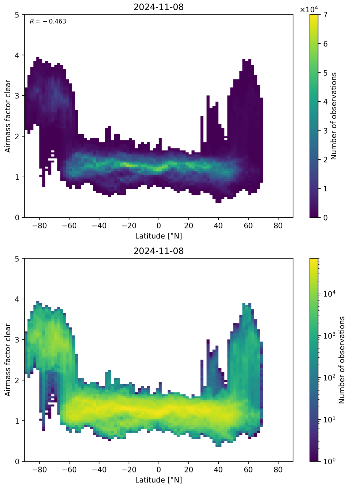
Figure 156: Scatter density plot of “Latitude” against “Airmass factor clear” for 2024-11-07 to 2024-11-09.
