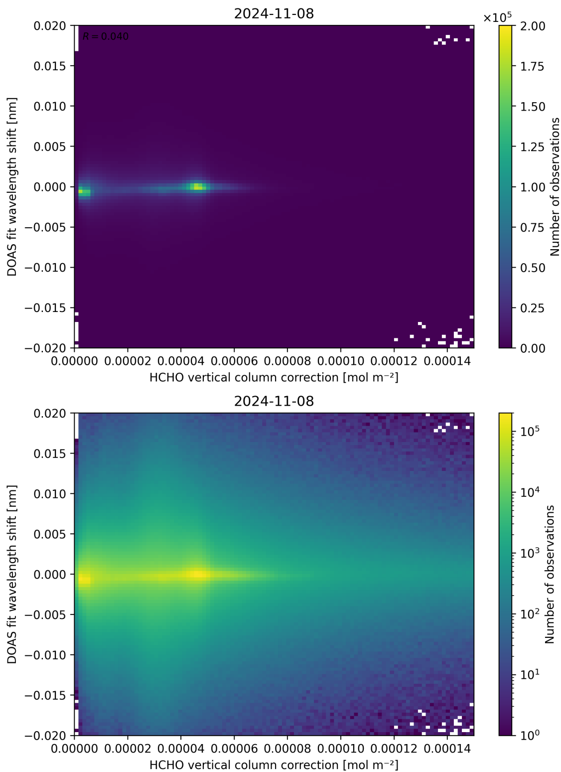
Figure 113: Scatter density plot of “HCHO vertical column correction” against “DOAS fit wavelength shift” for 2024-11-07 to 2024-11-09.
