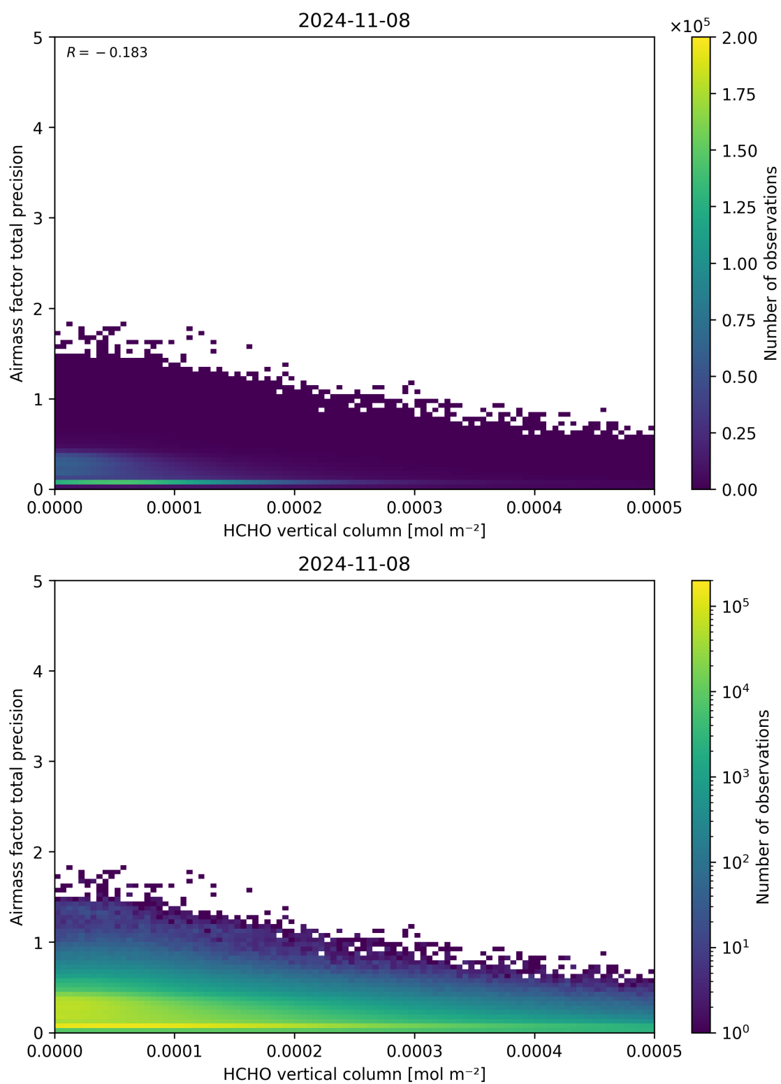
Figure 132: Scatter density plot of “HCHO vertical column” against “Airmass factor total precision” for 2024-11-07 to 2024-11-09.
