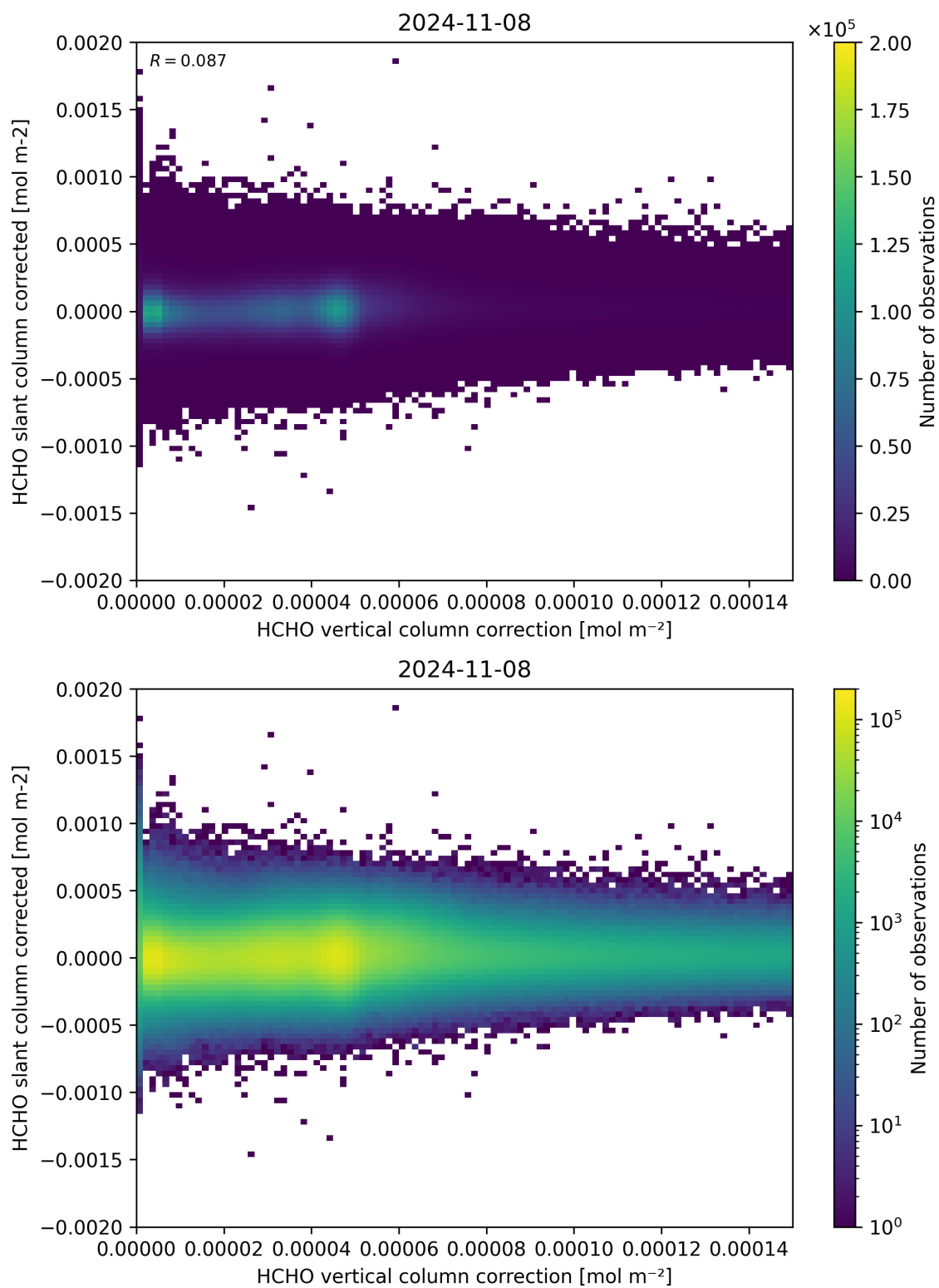
Figure 116: Scatter density plot of “HCHO vertical column correction” against “HCHO slant column corrected” for 2024-11-07 to 2024-11-09.
