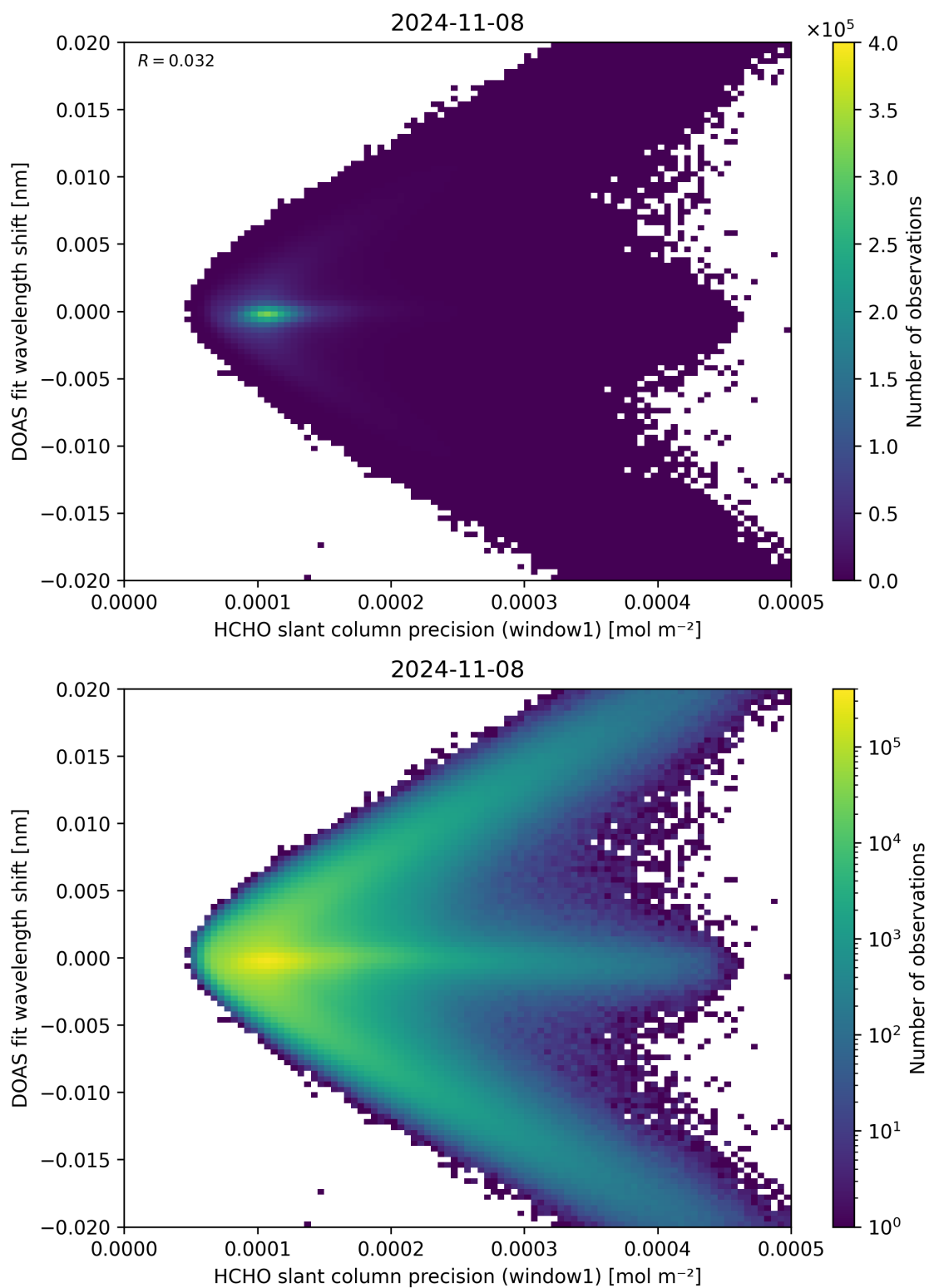
Figure 89: Scatter density plot of “HCHO slant column precision (window1)” against “DOAS fit wavelength shift” for 2024-11-07 to 2024-11-09.
