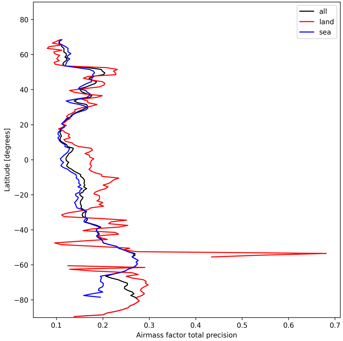
Figure 27: Zonal average of “Airmass factor total precision” for 2024-11-07 to 2024-11-09.
