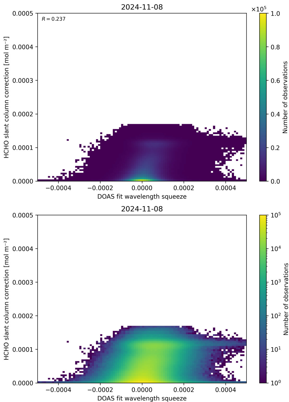
Figure 70: Scatter density plot of “DOAS fit wavelength squeeze” against “HCHO slant column correction” for 2024-11-07 to 2024-11-09.
