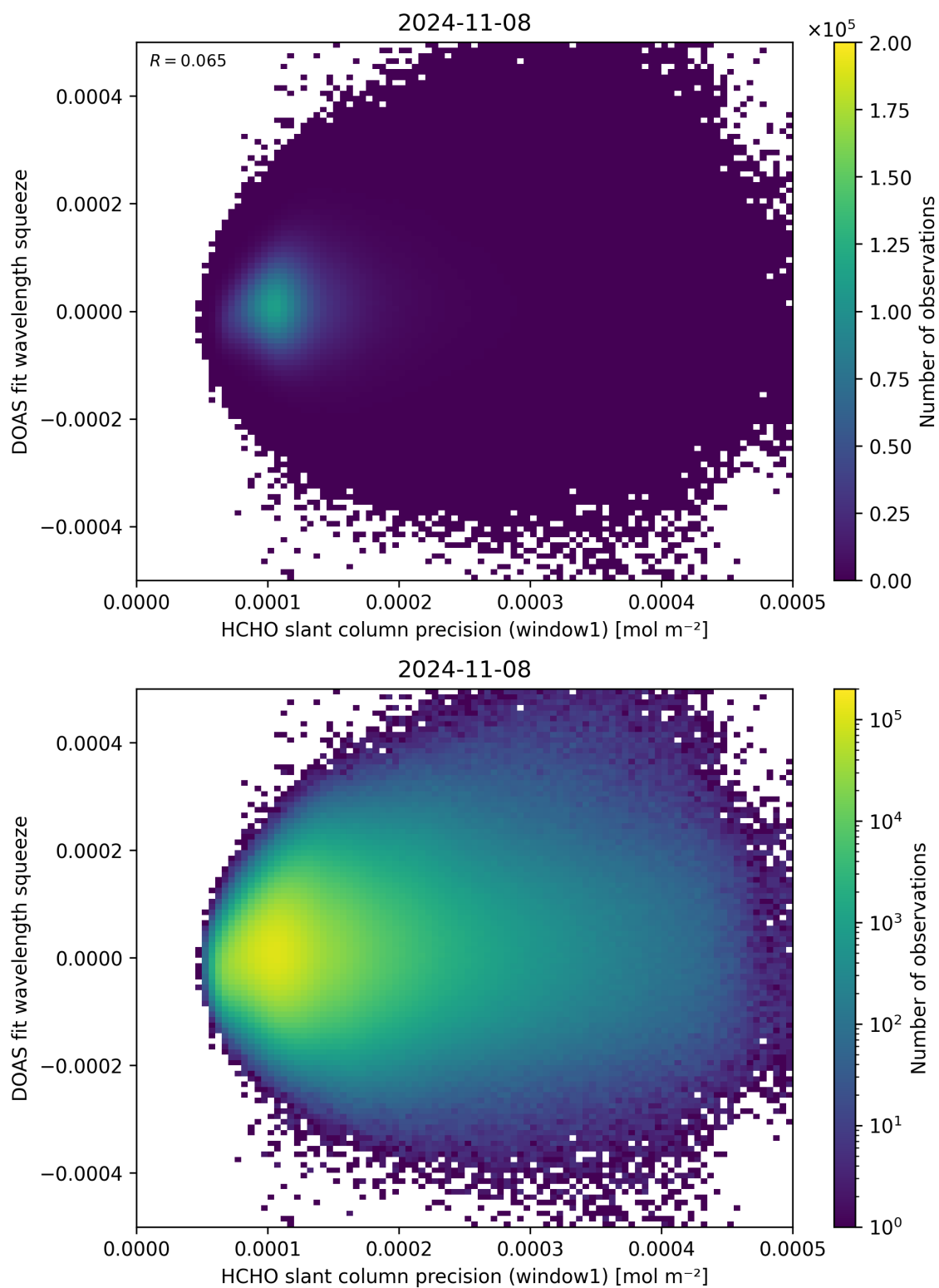
Figure 90: Scatter density plot of “HCHO slant column precision (window1)” against “DOAS fit wavelength squeeze” for 2024-11-07 to 2024-11-09.
