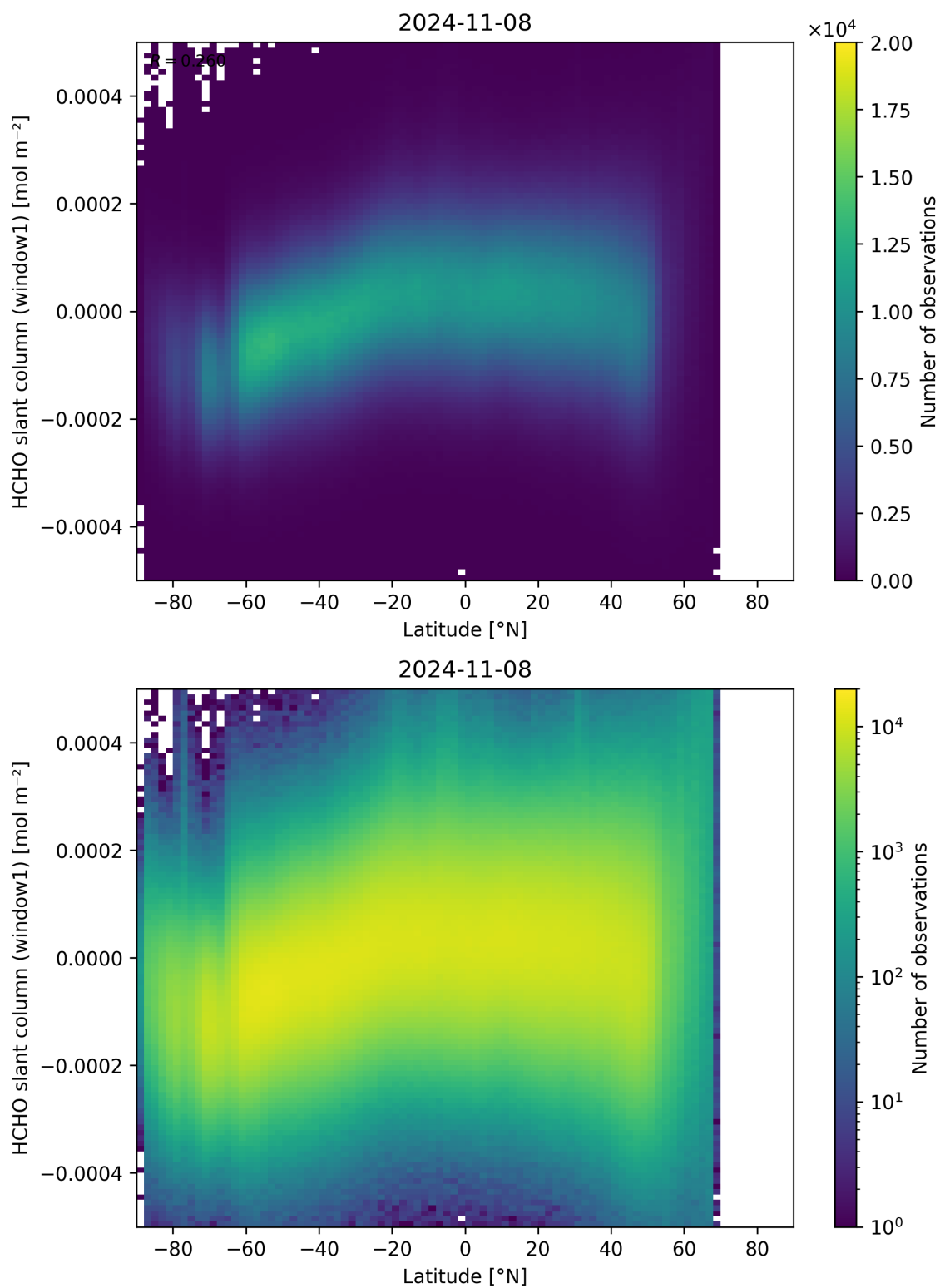
Figure 159: Scatter density plot of “Latitude” against “HCHO slant column (window1)” for 2024-11-07 to 2024-11-09.
