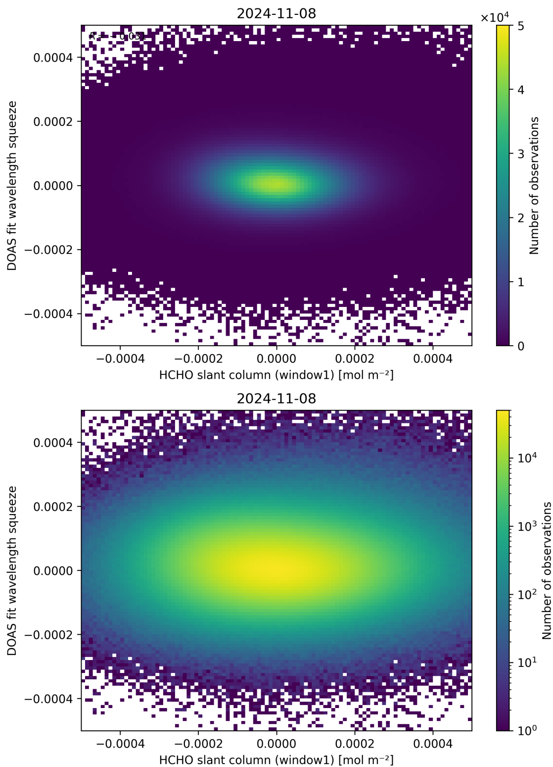
Figure 80: Scatter density plot of “HCHO slant column (window1)” against “DOAS fit wavelength squeeze” for 2024-11-07 to 2024-11-09.
