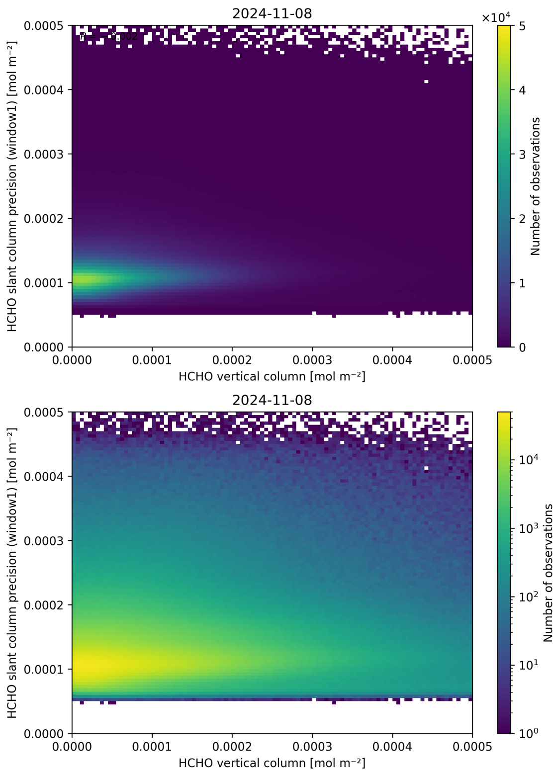
Figure 130: Scatter density plot of “HCHO vertical column” against “HCHO slant column precision (window1)” for 2024-11-07 to 2024-11-09.
