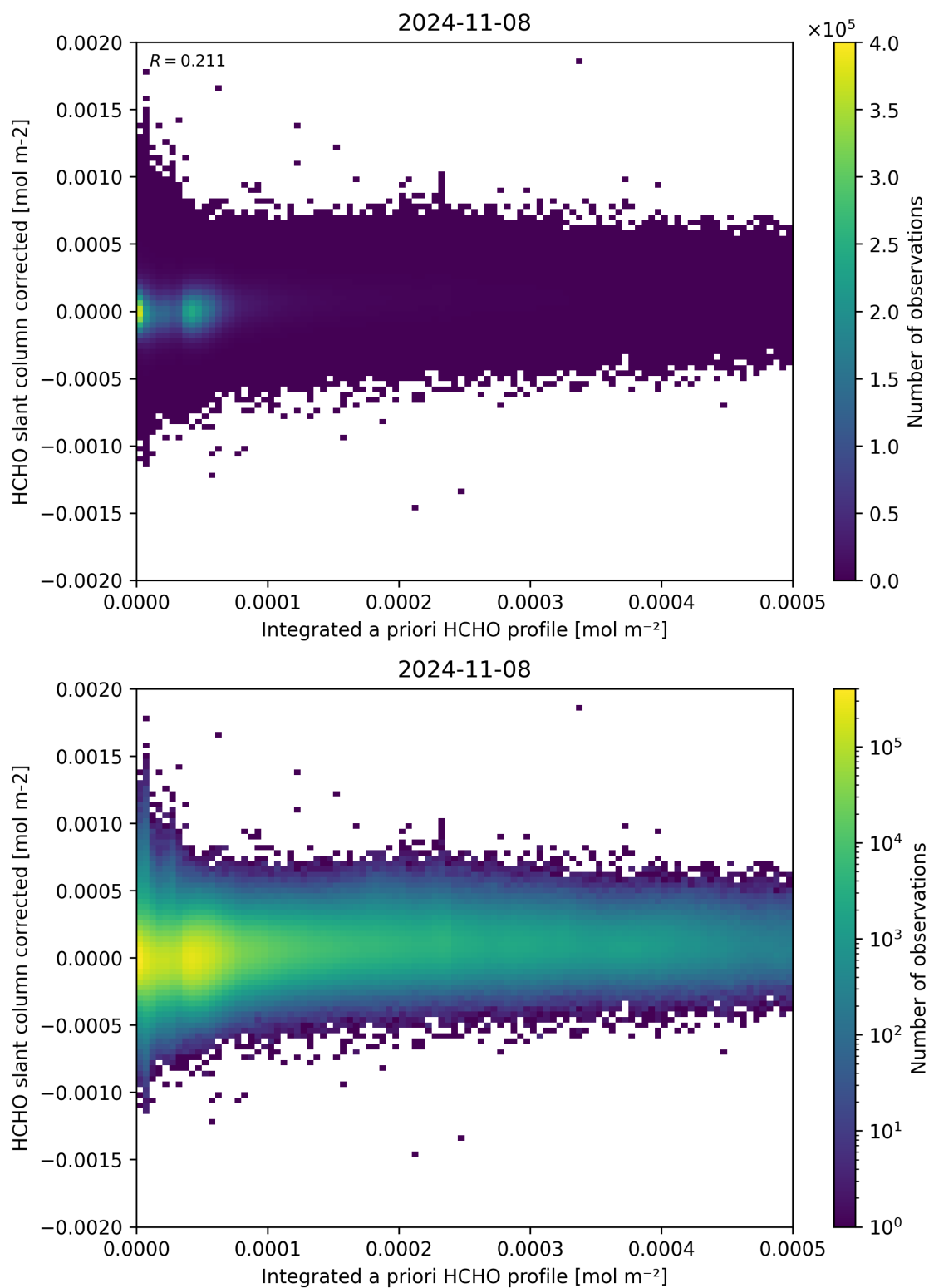
Figure 151: Scatter density plot of “Integrated a priori HCHO profile” against “HCHO slant column corrected” for 2024-11-07 to 2024-11-09.
