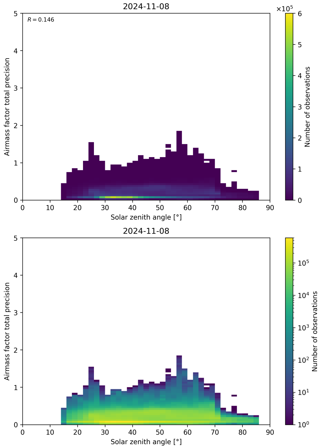
Figure 176: Scatter density plot of “Solar zenith angle” against “Airmass factor total precision” for 2024-11-07 to 2024-11-09.
