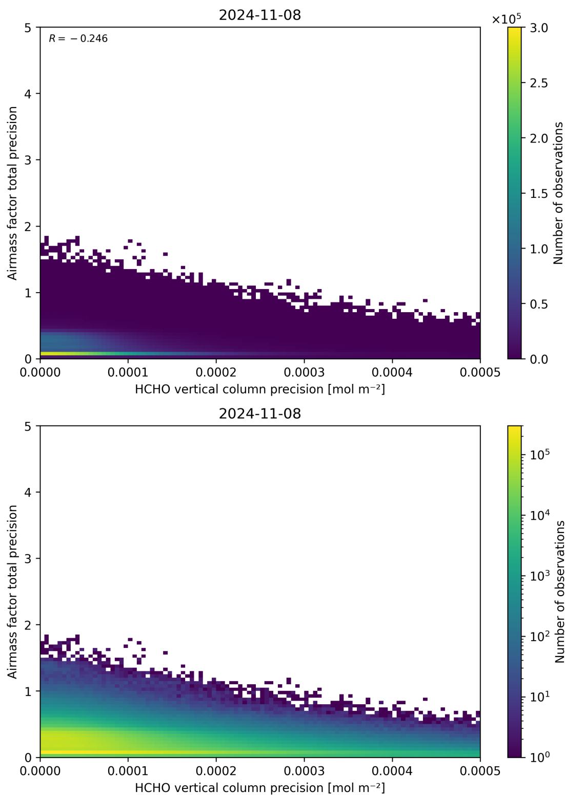
Figure 145: Scatter density plot of “HCHO vertical column precision” against “Airmass factor total precision” for 2024-11-07 to 2024-11-09.
