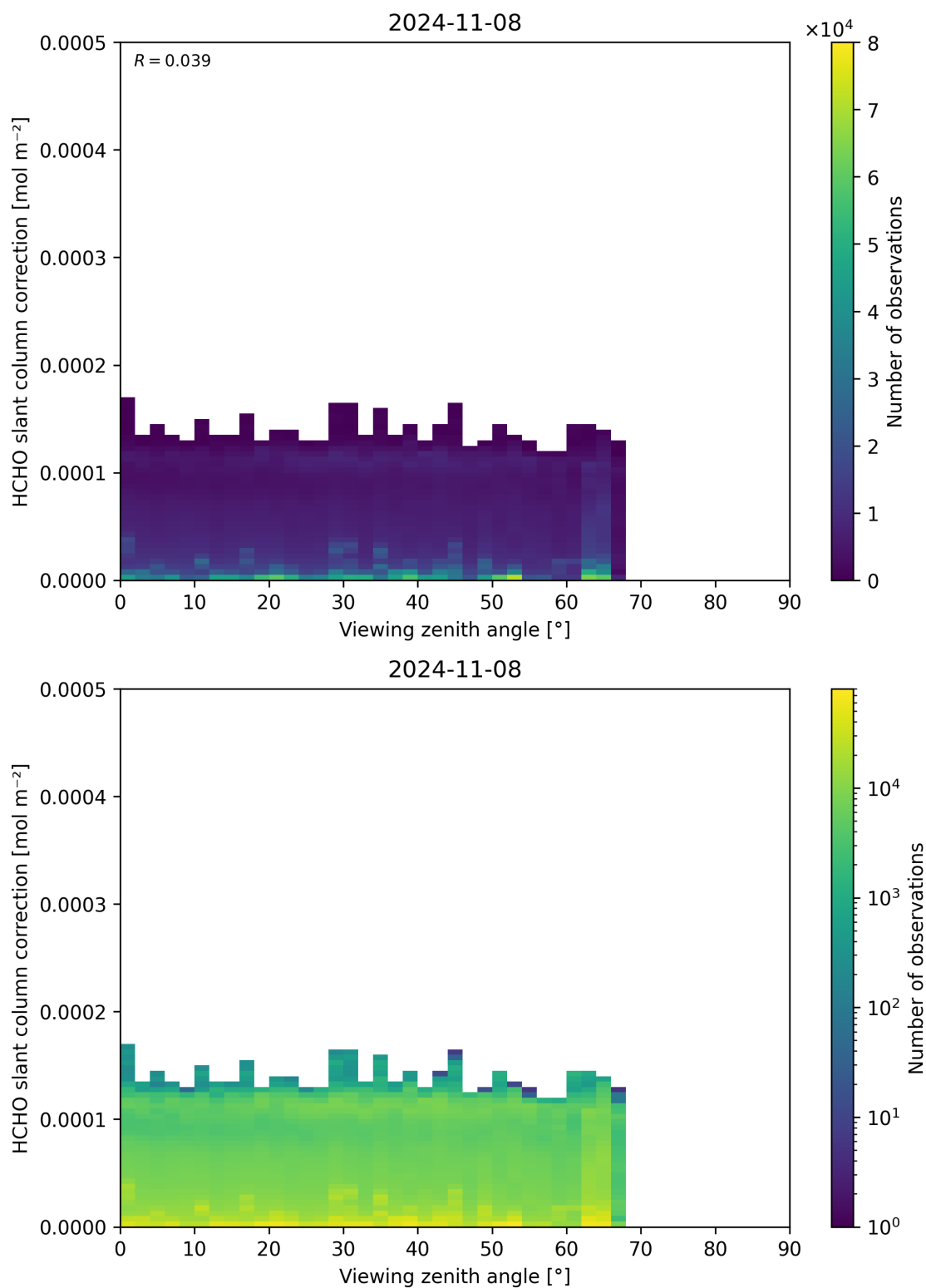
Figure 187: Scatter density plot of “Viewing zenith angle” against “HCHO slant column correction” for 2024-11-07 to 2024-11-09.
