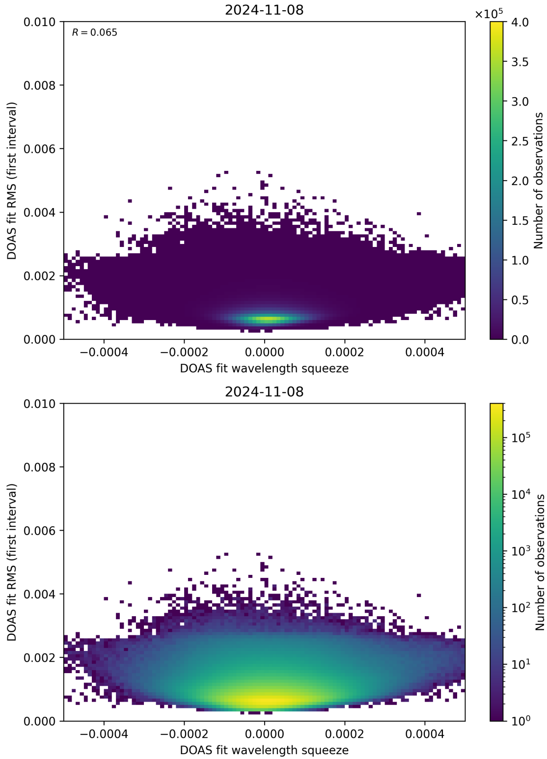
Figure 68: Scatter density plot of “DOAS fit wavelength squeeze” against “DOAS fit RMS (first interval)” for 2024-11-07 to 2024-11-09.
