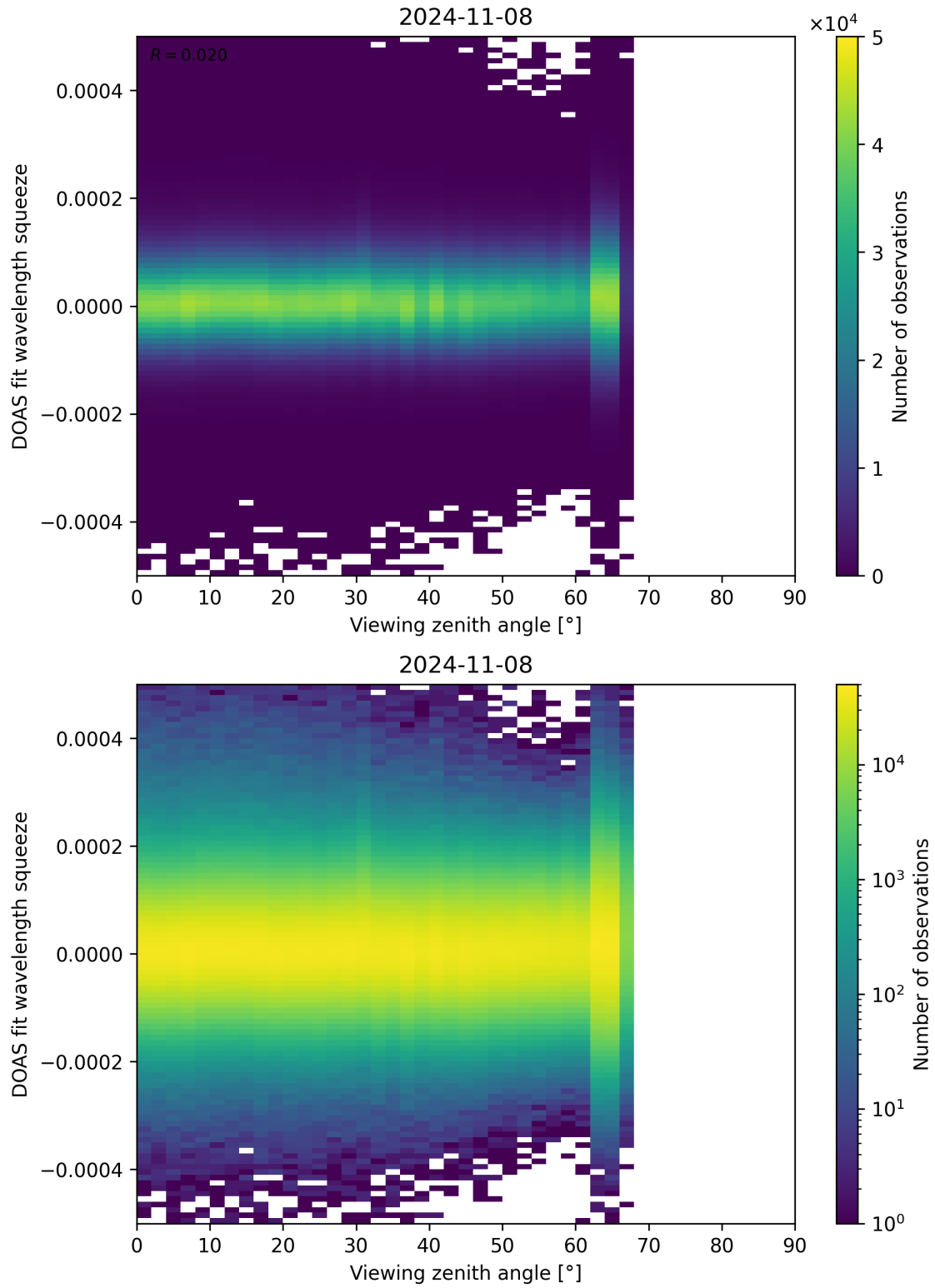
Figure 184: Scatter density plot of “Viewing zenith angle” against “DOAS fit wavelength squeeze” for 2024-11-07 to 2024-11-09.
