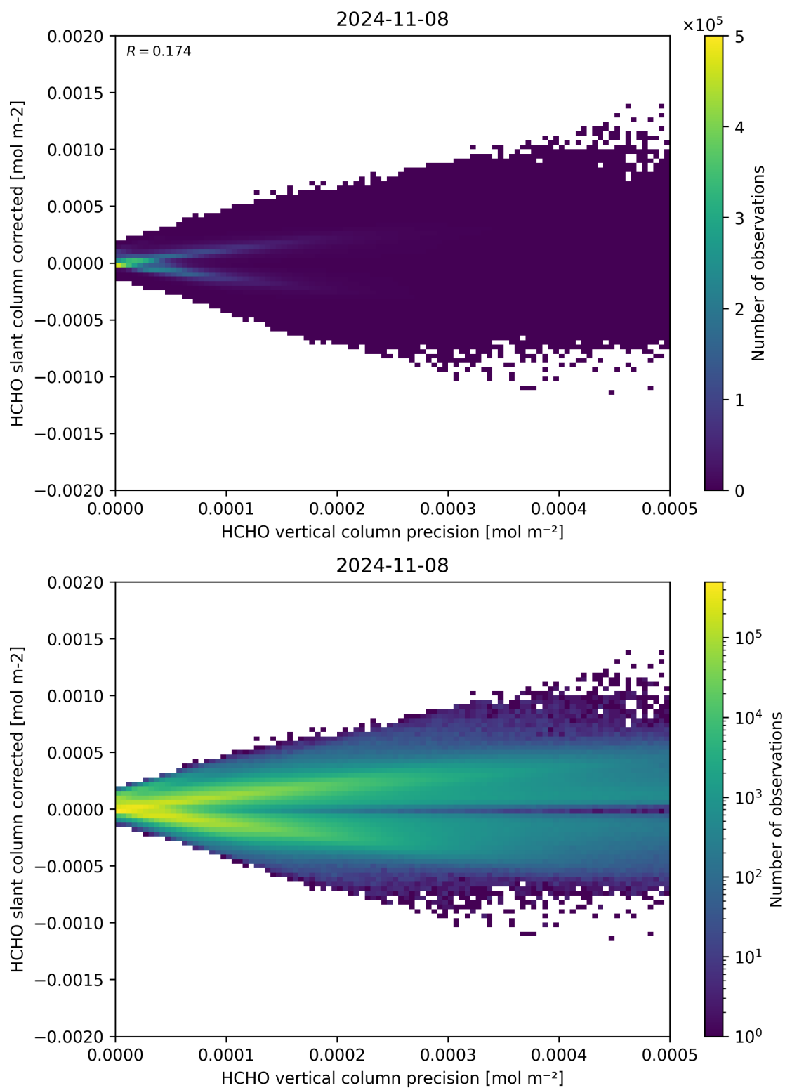
Figure 140: Scatter density plot of “HCHO vertical column precision” against “HCHO slant column corrected” for 2024-11-07 to 2024-11-09.
