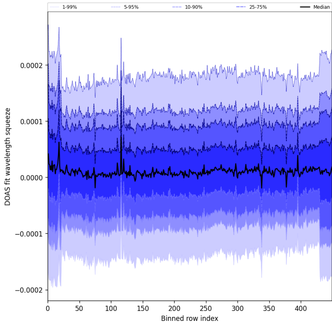
Figure 59: Along track statistics of “DOAS fit wavelength squeeze” for 2024-11-07 to 2024-11-09
