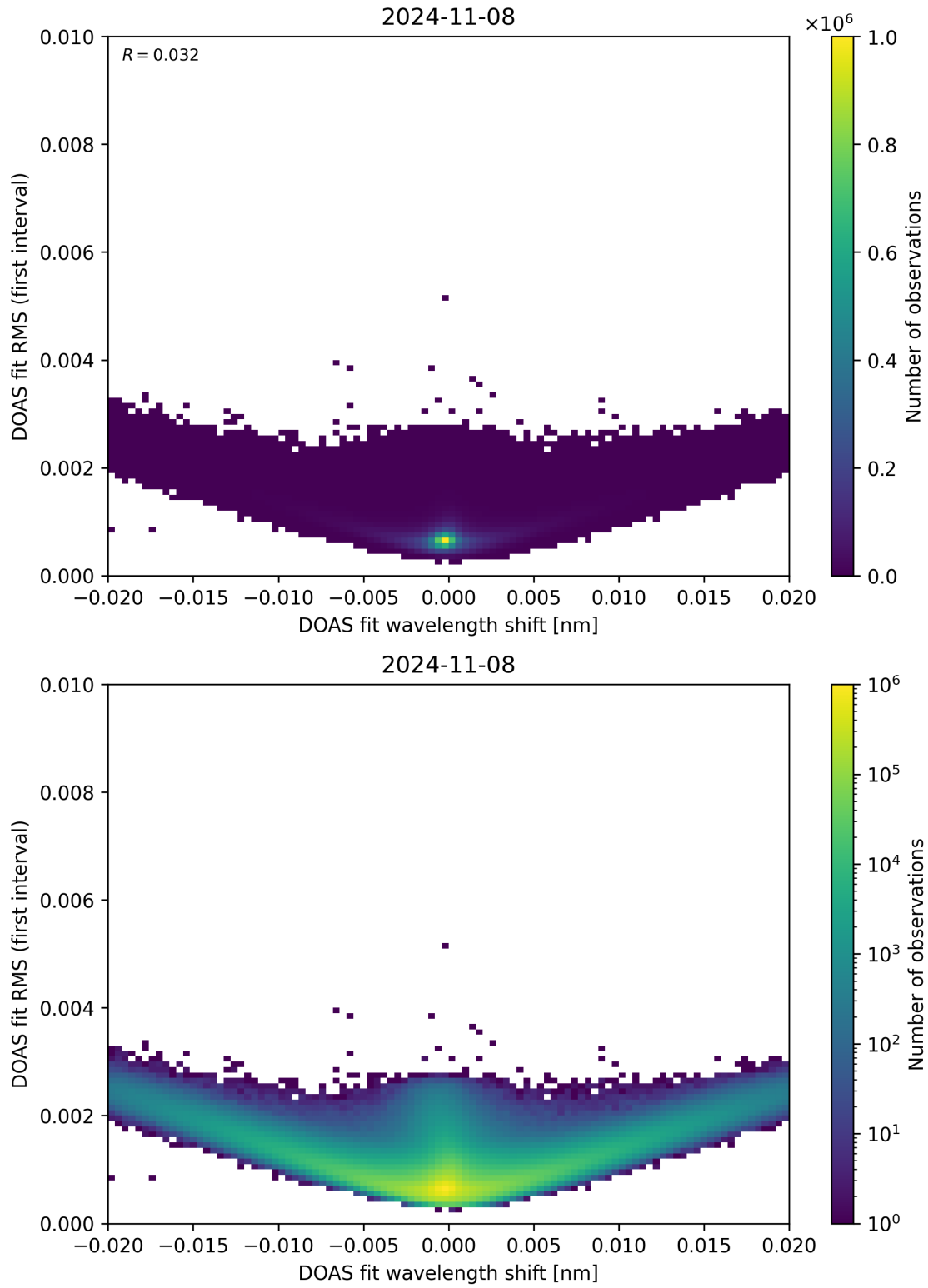
Figure 64: Scatter density plot of “DOAS fit wavelength shift” against “DOAS fit RMS (first interval)” for 2024-11-07 to 2024-11-09.
