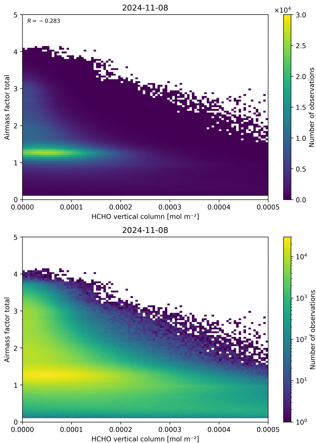
Figure 131: Scatter density plot of “HCHO vertical column” against “Airmass factor total” for 2024-11-07 to 2024-11-09.
