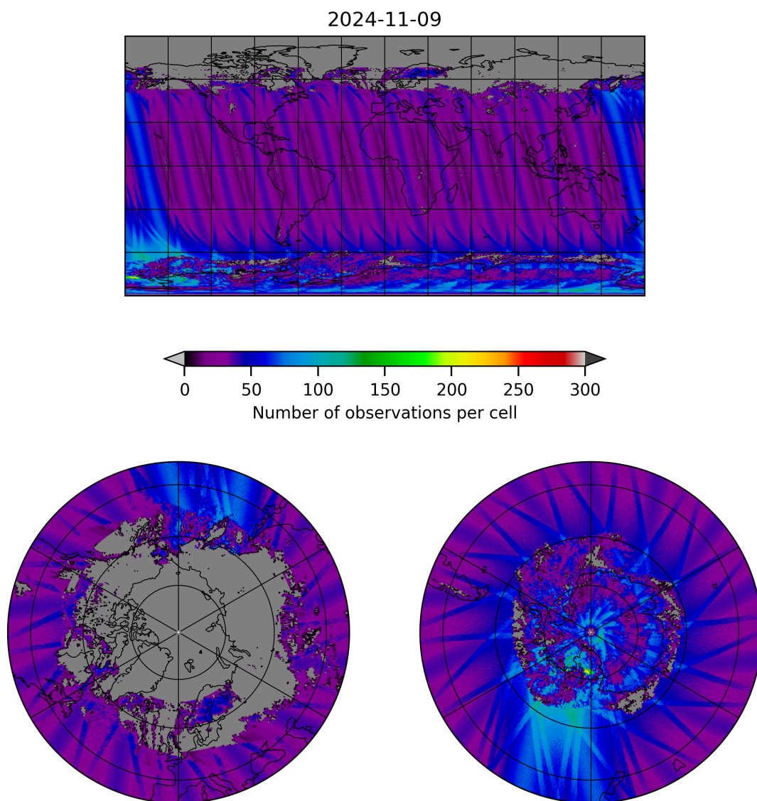
Figure 19: Map of the number of observations for 2024-11-09 to 2024-11-10
