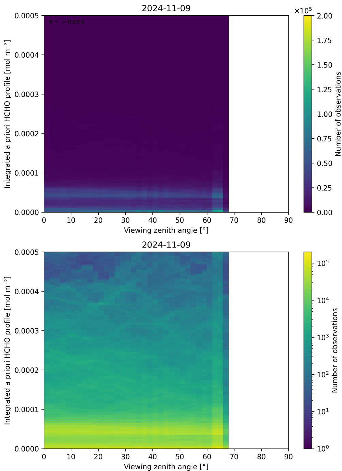
Figure 195: Scatter density plot of “Viewing zenith angle” against “Integrated a priori HCHO profile” for 2024-11-09 to 2024-11-10.
