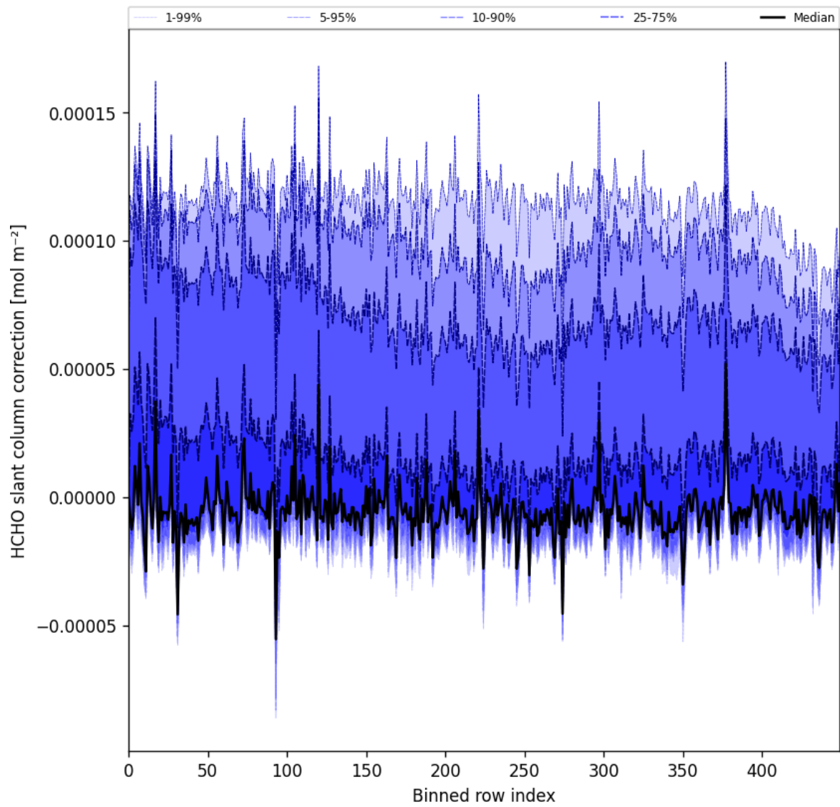
Figure 61: Along track statistics of “HCHO slant column correction” for 2024-11-09 to 2024-11-10
