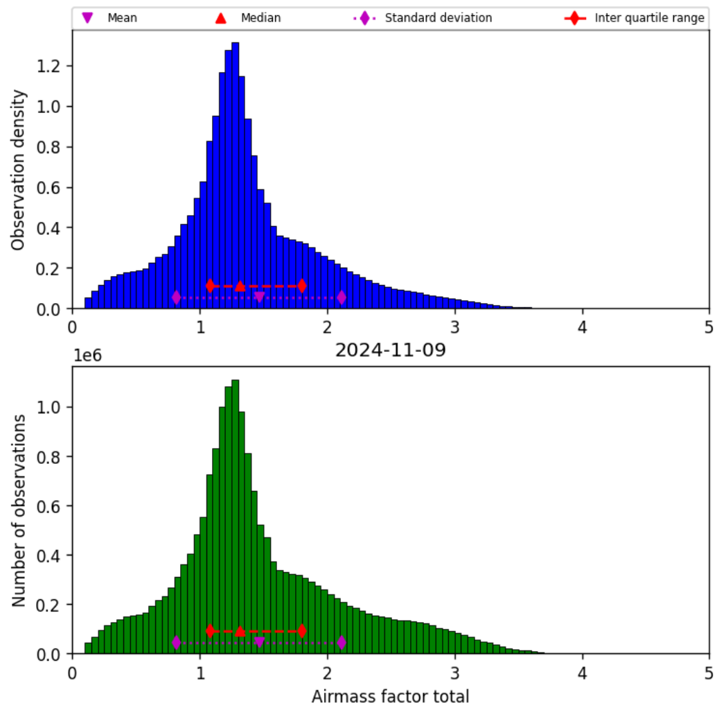
Figure 40: Histogram of “Airmass factor total” for 2024-11-09 to 2024-11-10
