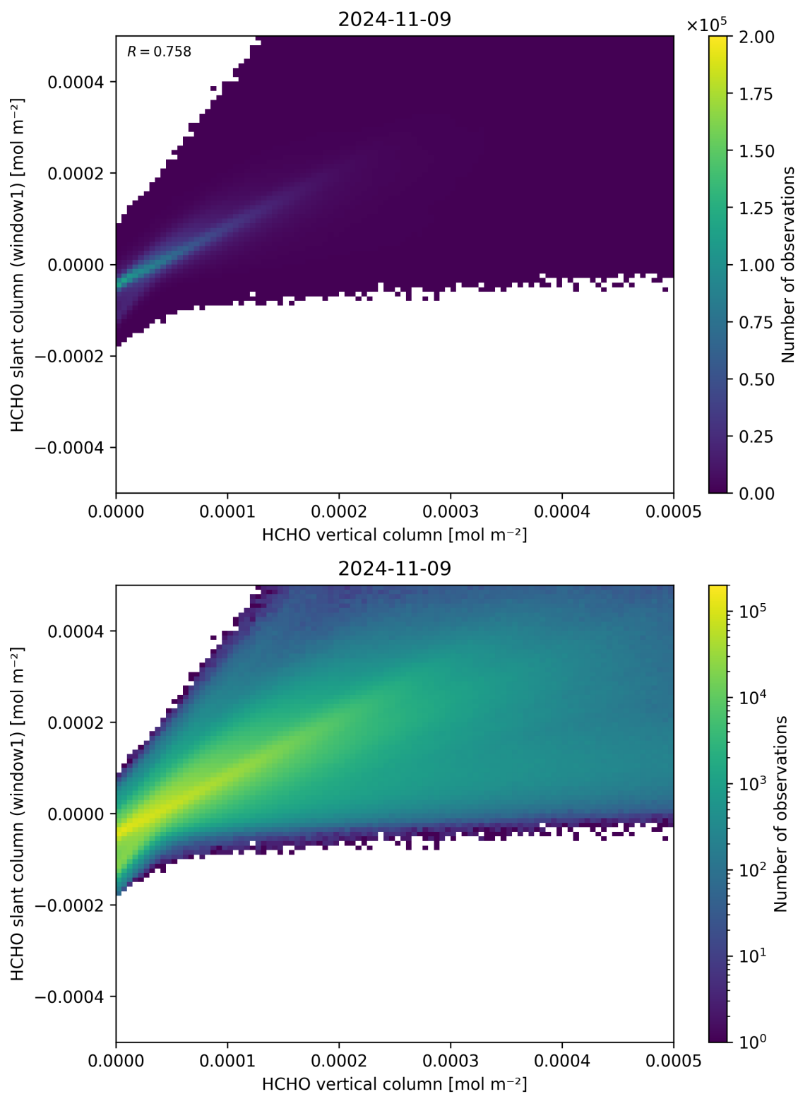
Figure 129: Scatter density plot of “HCHO vertical column” against “HCHO slant column (window1)” for 2024-11-09 to 2024-11-10.
