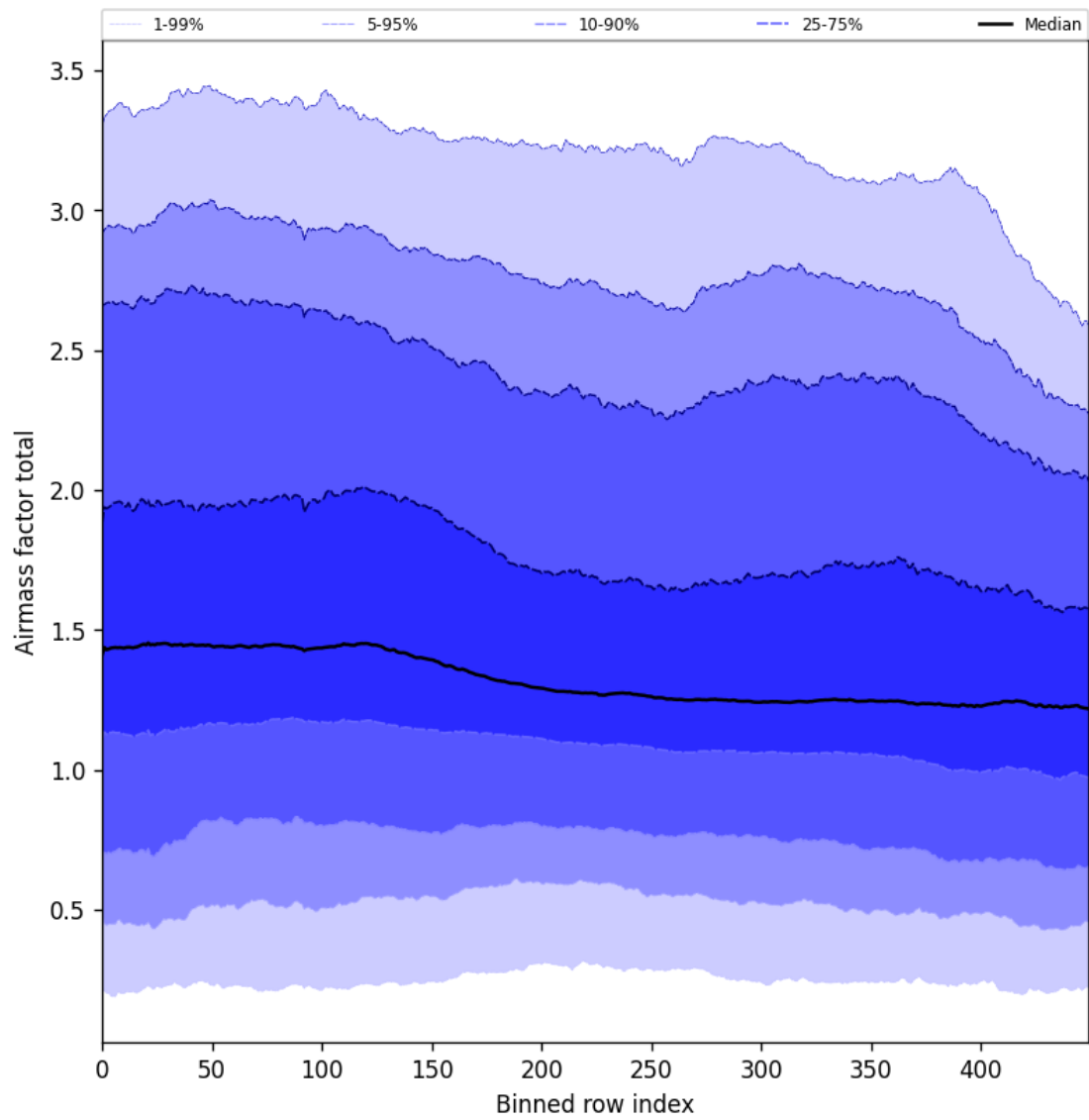
Figure 54: Along track statistics of “Airmass factor total” for 2024-11-09 to 2024-11-10
