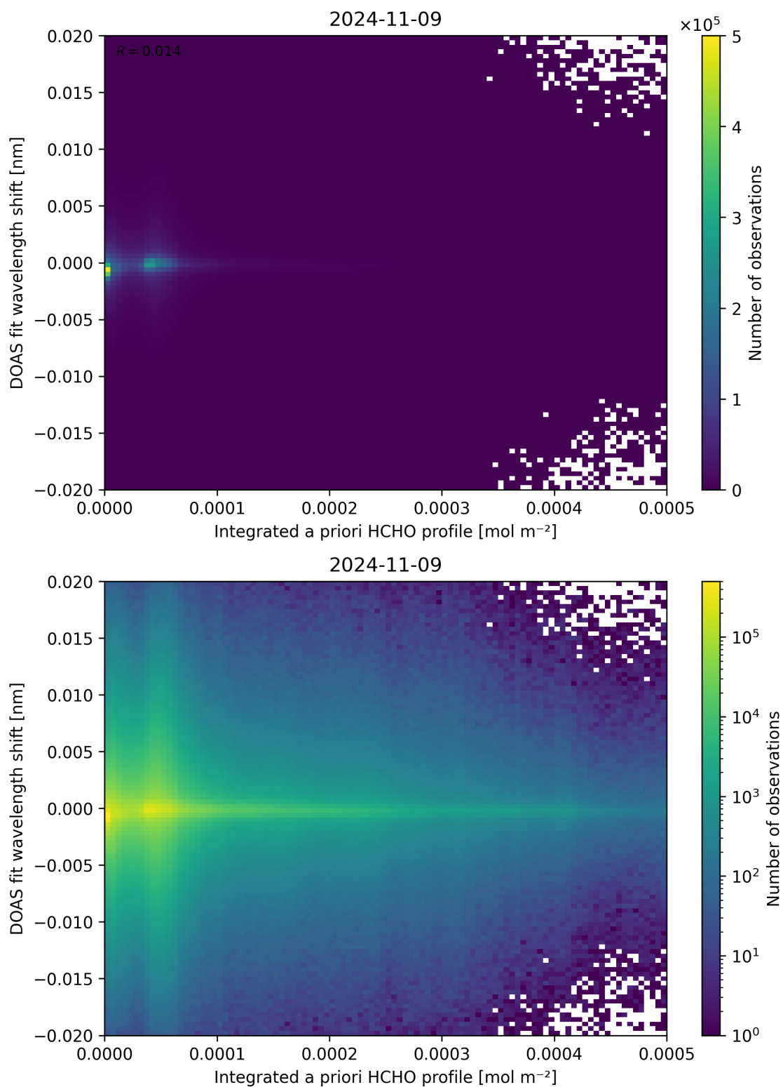
Figure 149: Scatter density plot of “Integrated a priori HCHO profile” against “DOAS fit wavelength shift” for 2024-11-09 to 2024-11-10.
