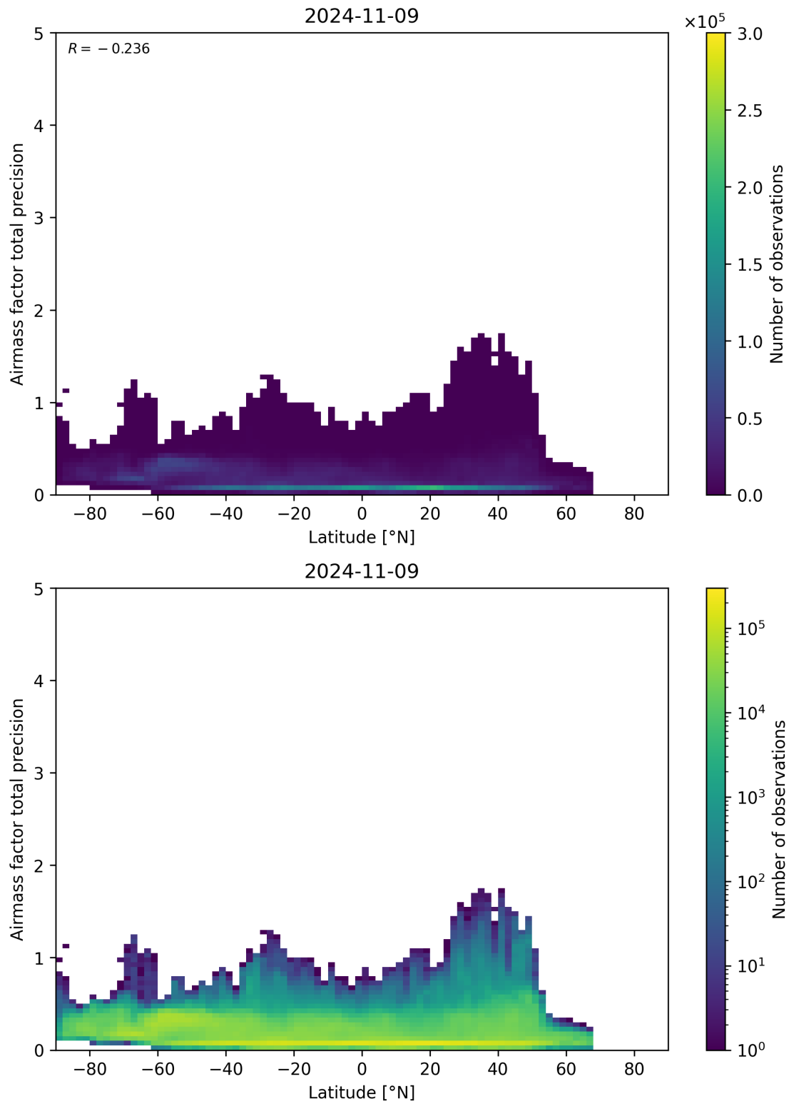
Figure 162: Scatter density plot of “Latitude” against “Airmass factor total precision” for 2024-11-09 to 2024-11-10.
