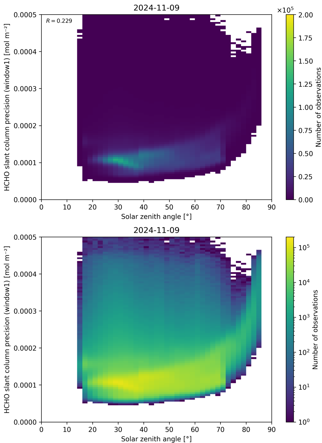
Figure 174: Scatter density plot of “Solar zenith angle” against “HCHO slant column precision (window1)” for 2024-11-09 to 2024-11-10.
