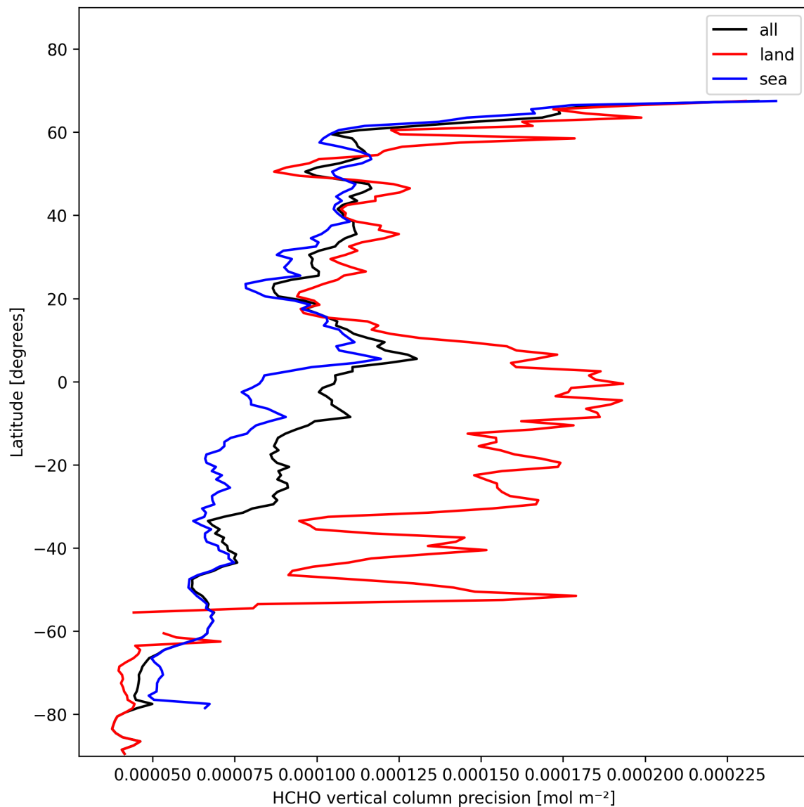
Figure 22: Zonal average of “HCHO vertical column precision” for 2024-11-09 to 2024-11-10.
