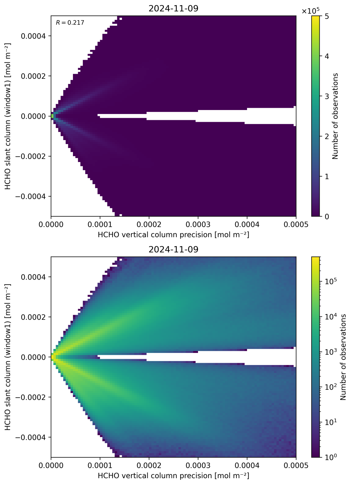
Figure 142: Scatter density plot of “HCHO vertical column precision” against “HCHO slant column (window1)” for 2024-11-09 to 2024-11-10.
