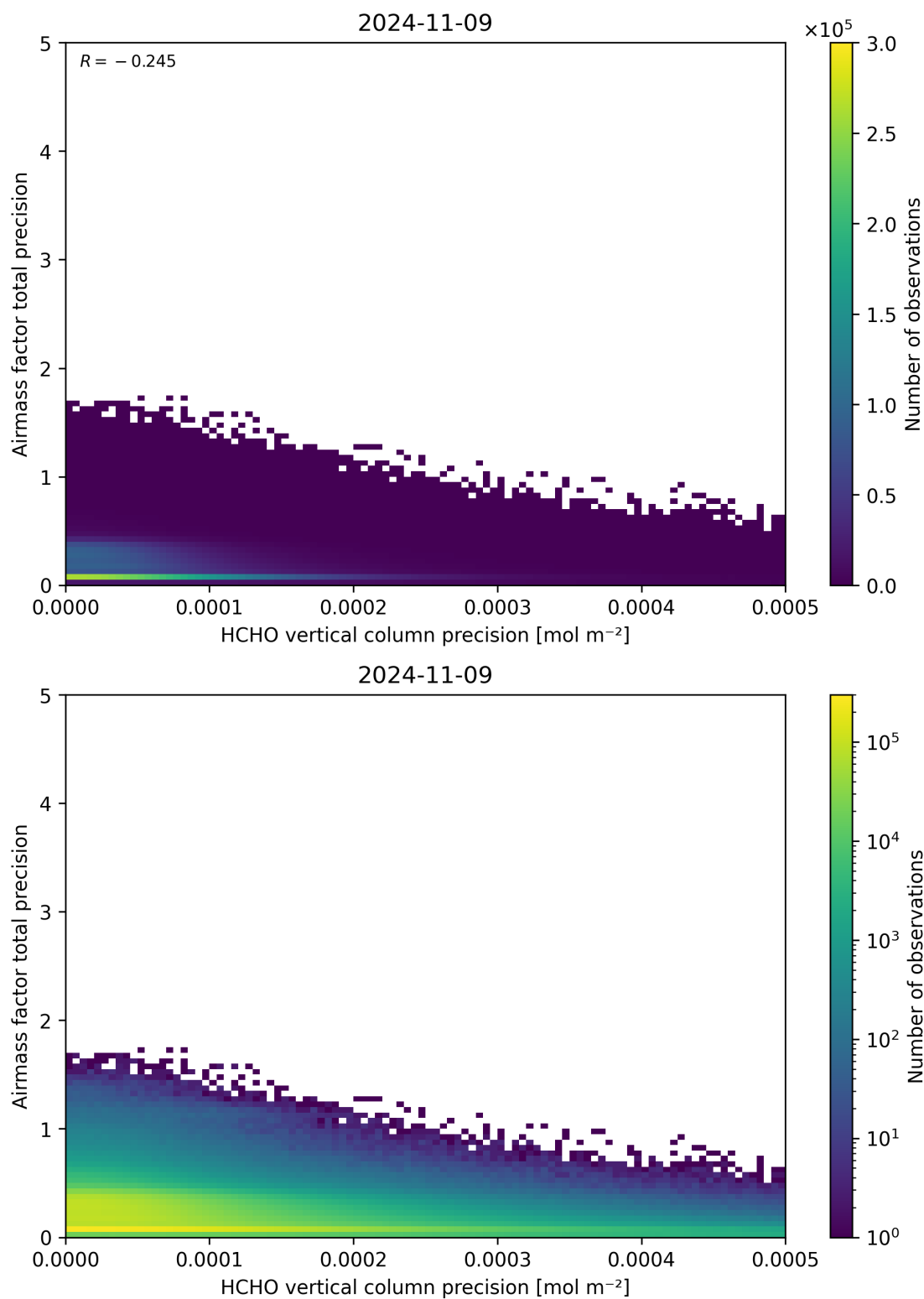
Figure 145: Scatter density plot of “HCHO vertical column precision” against “Airmass factor total precision” for 2024-11-09 to 2024-11-10.
