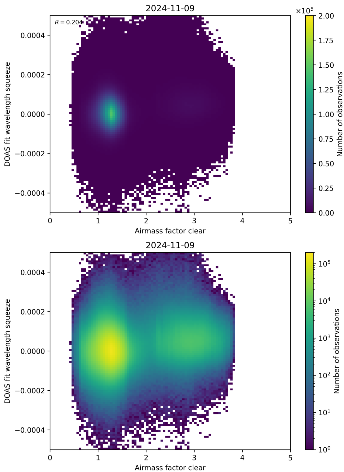
Figure 73: Scatter density plot of “Airmass factor clear” against “DOAS fit wavelength squeeze” for 2024-11-09 to 2024-11-10.
