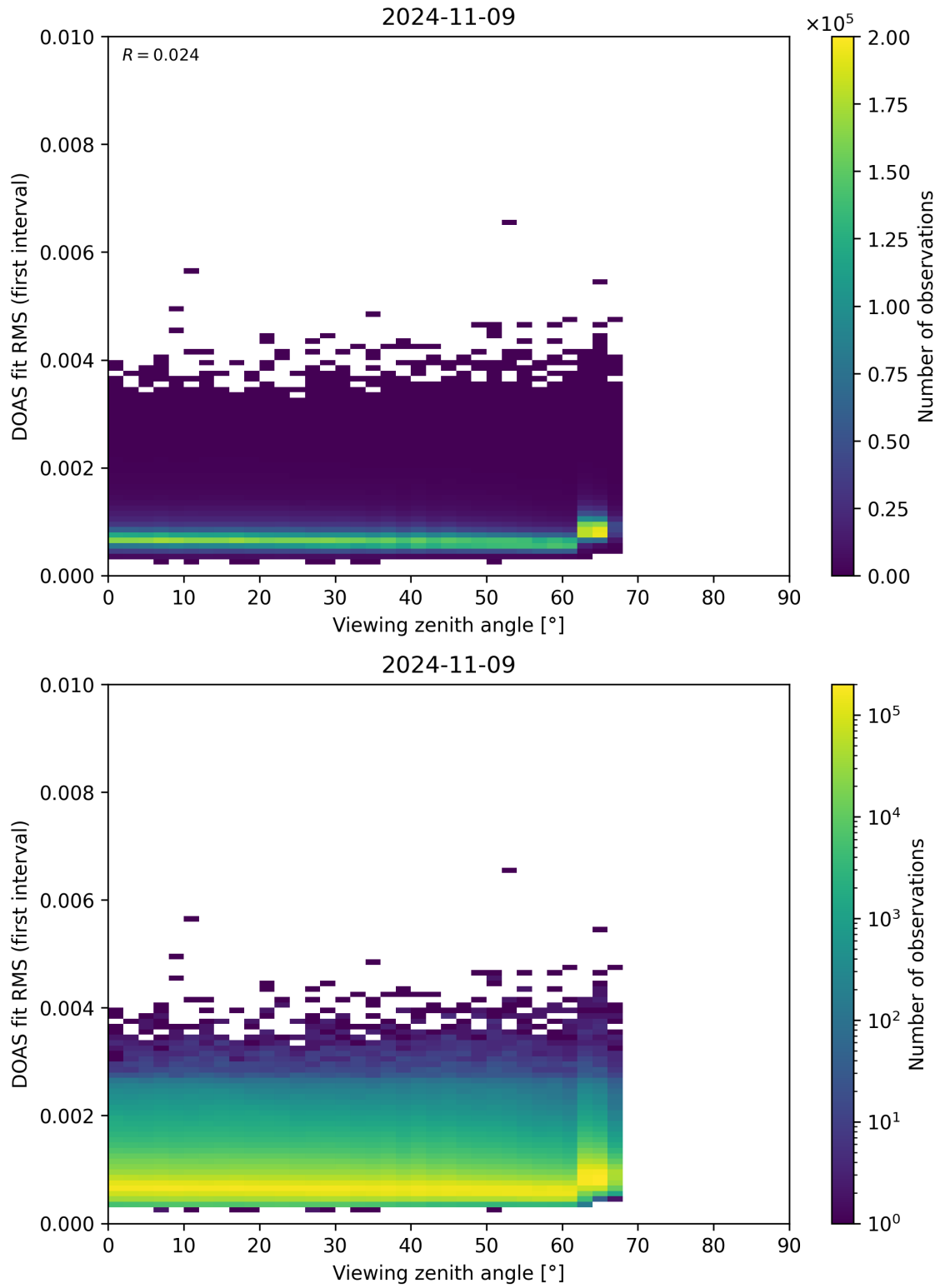
Figure 182: Scatter density plot of “Viewing zenith angle” against “DOAS fit RMS (first interval)” for 2024-11-09 to 2024-11-10.
