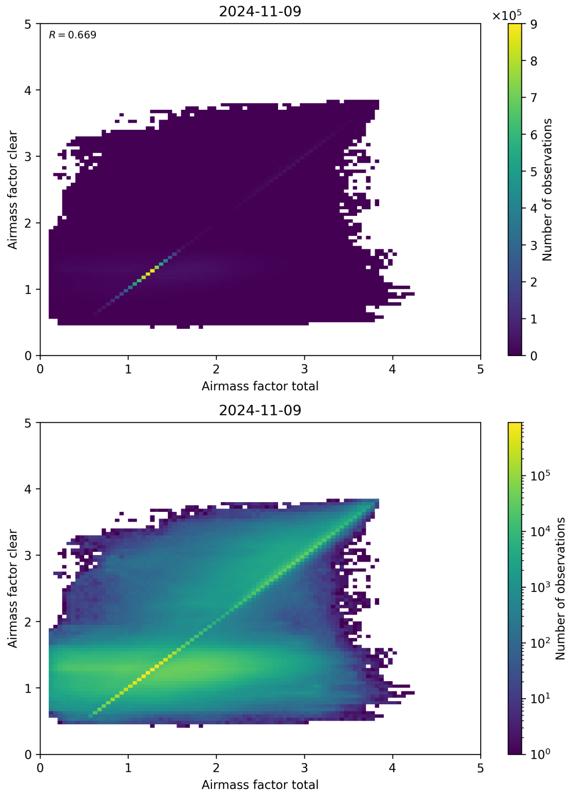
Figure 100: Scatter density plot of “Airmass factor total” against “Airmass factor clear” for 2024-11-09 to 2024-11-10.
