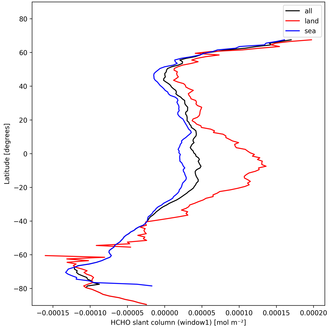
Figure 24: Zonal average of “HCHO slant column (window1)” for 2024-11-09 to 2024-11-10.
