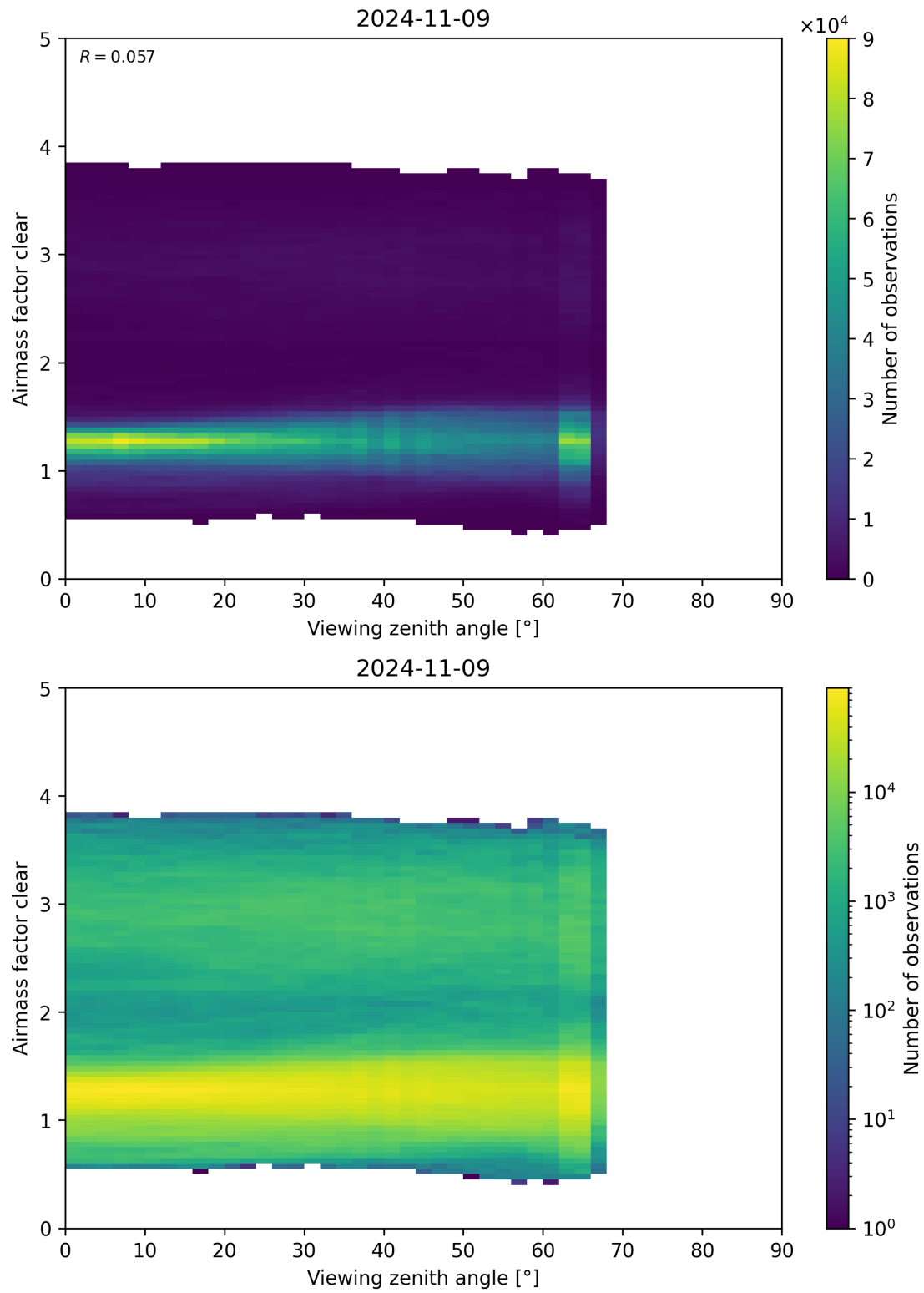
Figure 185: Scatter density plot of “Viewing zenith angle” against “Airmass factor clear” for 2024-11-09 to 2024-11-10.
