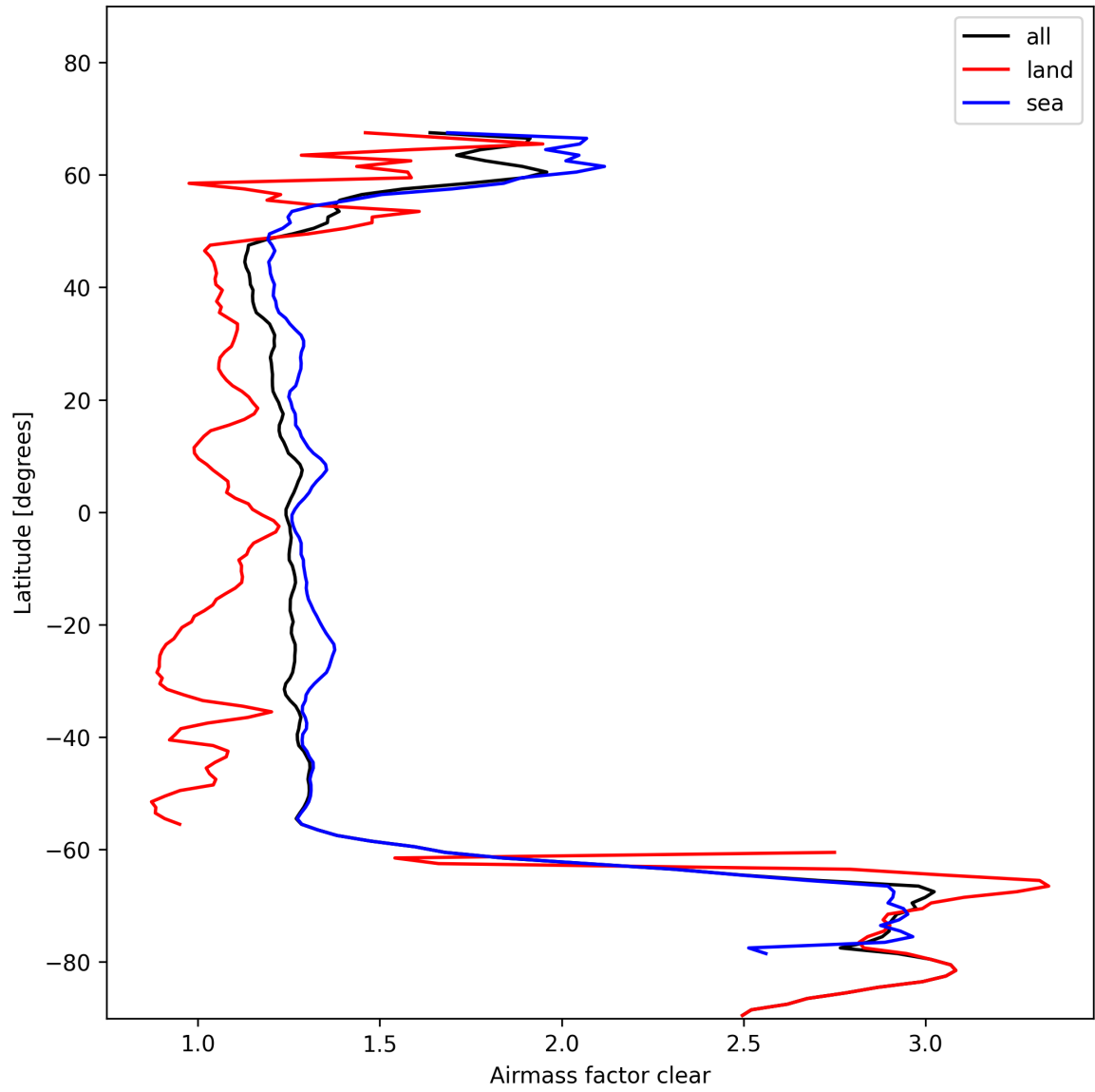
Figure 28: Zonal average of “Airmass factor clear” for 2024-11-09 to 2024-11-10.
