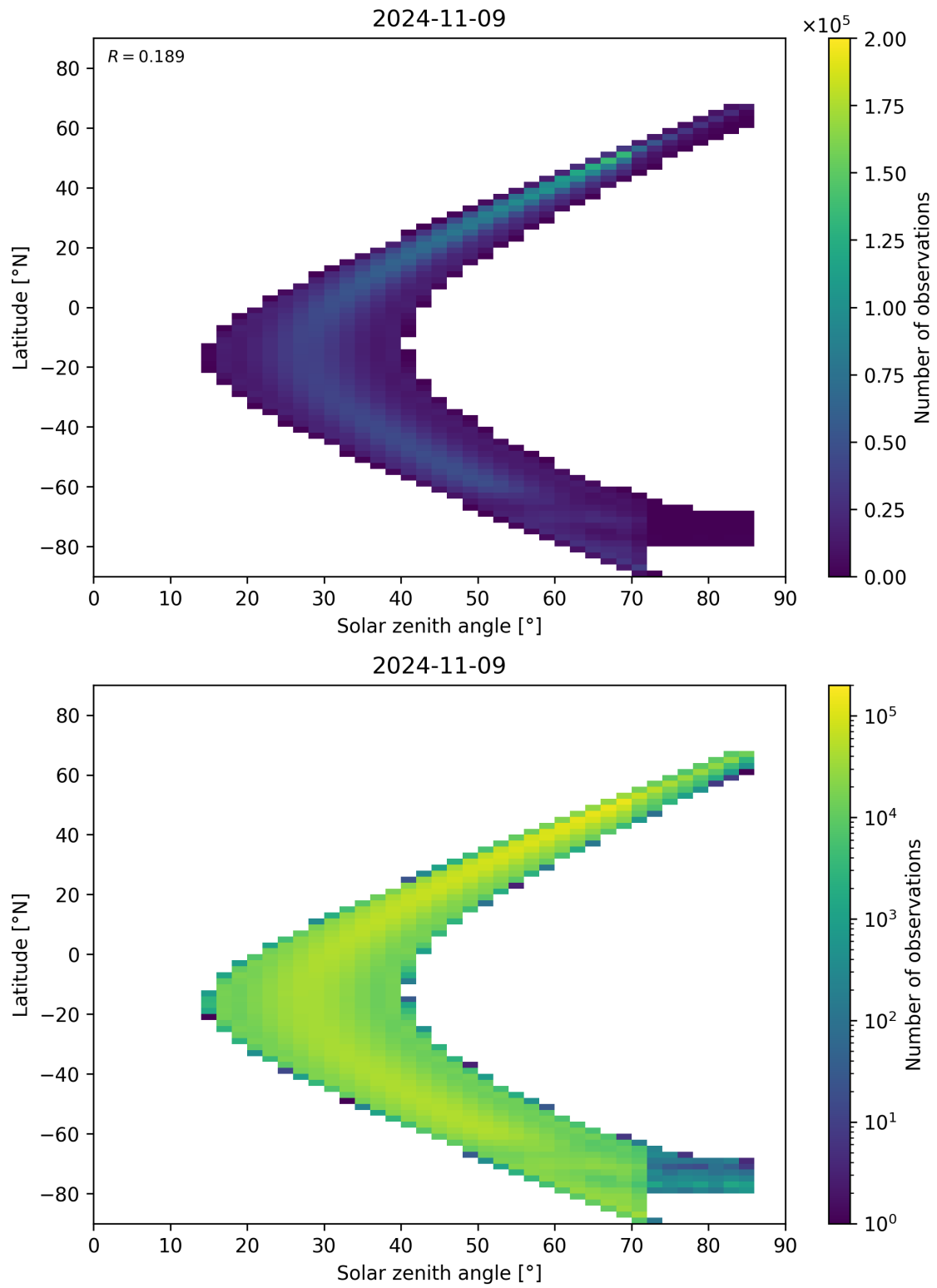
Figure 181: Scatter density plot of “Solar zenith angle” against “Latitude” for 2024-11-09 to 2024-11-10.
