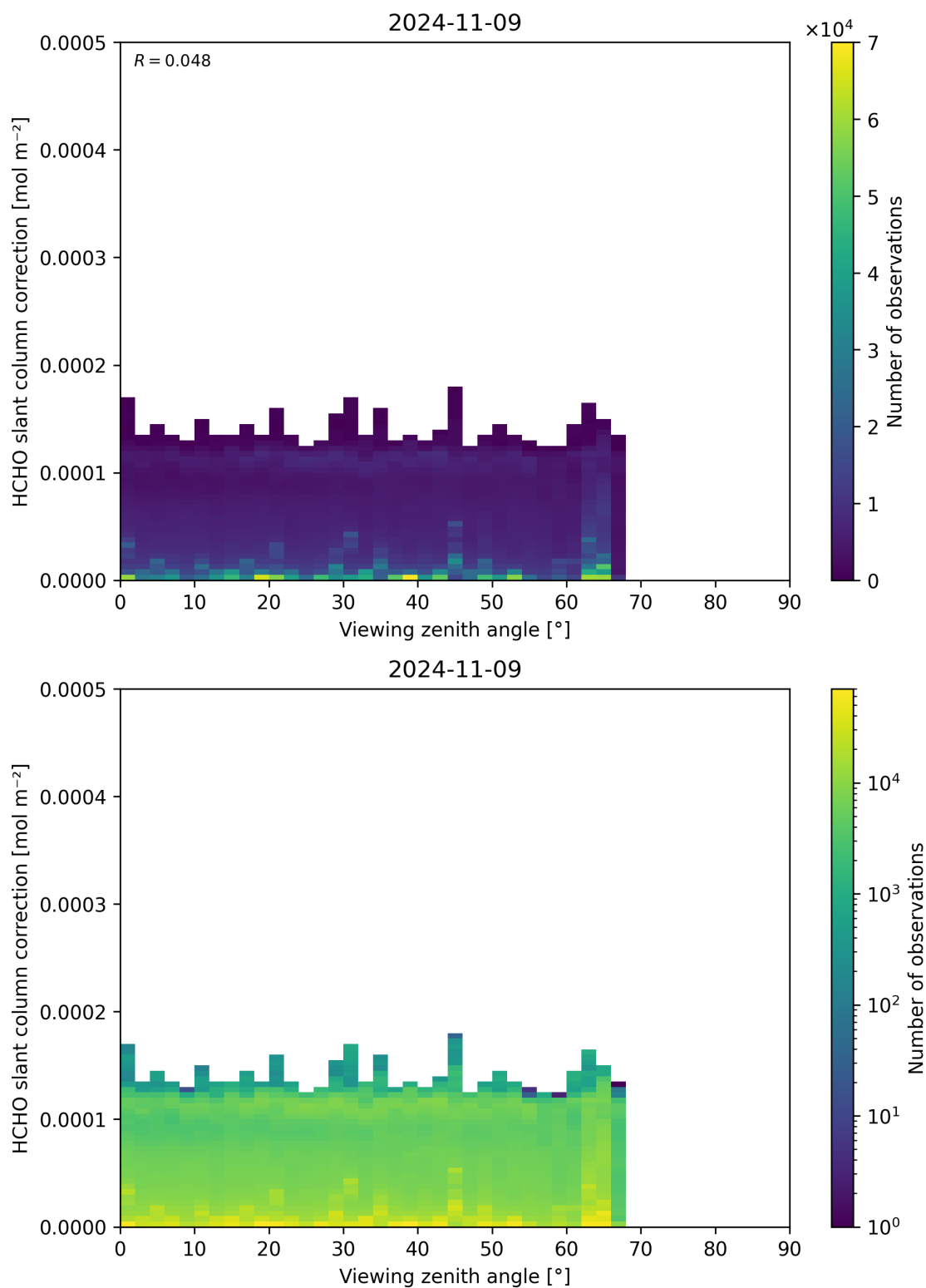
Figure 187: Scatter density plot of “Viewing zenith angle” against “HCHO slant column correction” for 2024-11-09 to 2024-11-10.
