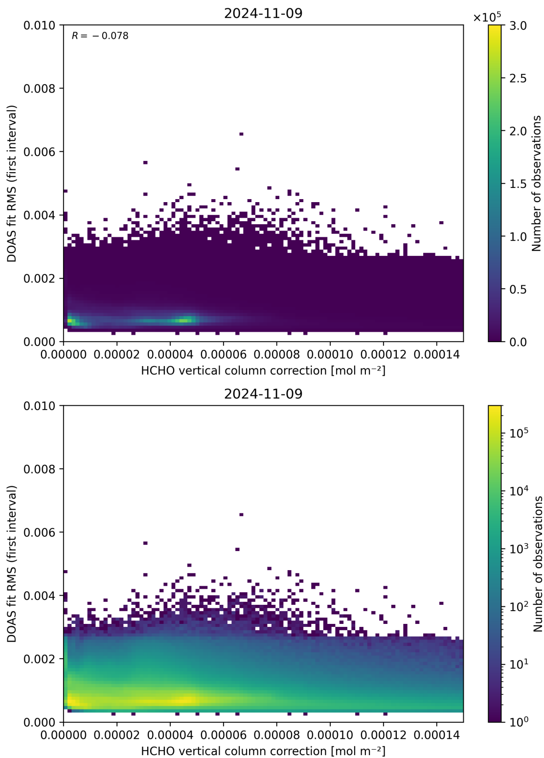
Figure 112: Scatter density plot of “HCHO vertical column correction” against “DOAS fit RMS (first interval)” for 2024-11-09 to 2024-11-10.
