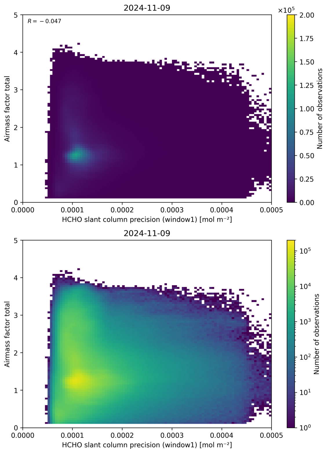
Figure 94: Scatter density plot of “HCHO slant column precision (window1)” against “Airmass factor total” for 2024-11-09 to 2024-11-10.
