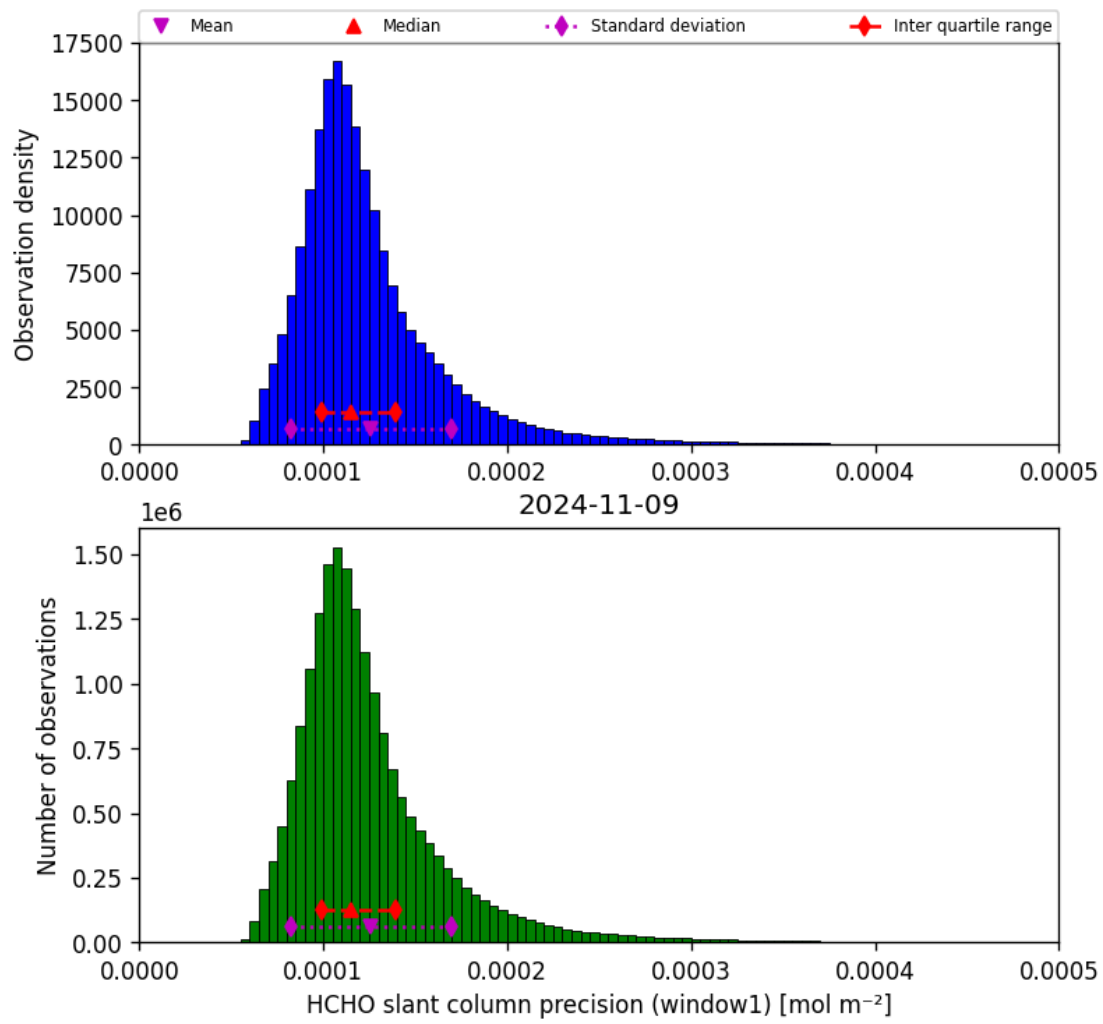
Figure 39: Histogram of “HCHO slant column precision (window1)” for 2024-11-09 to 2024-11-10
