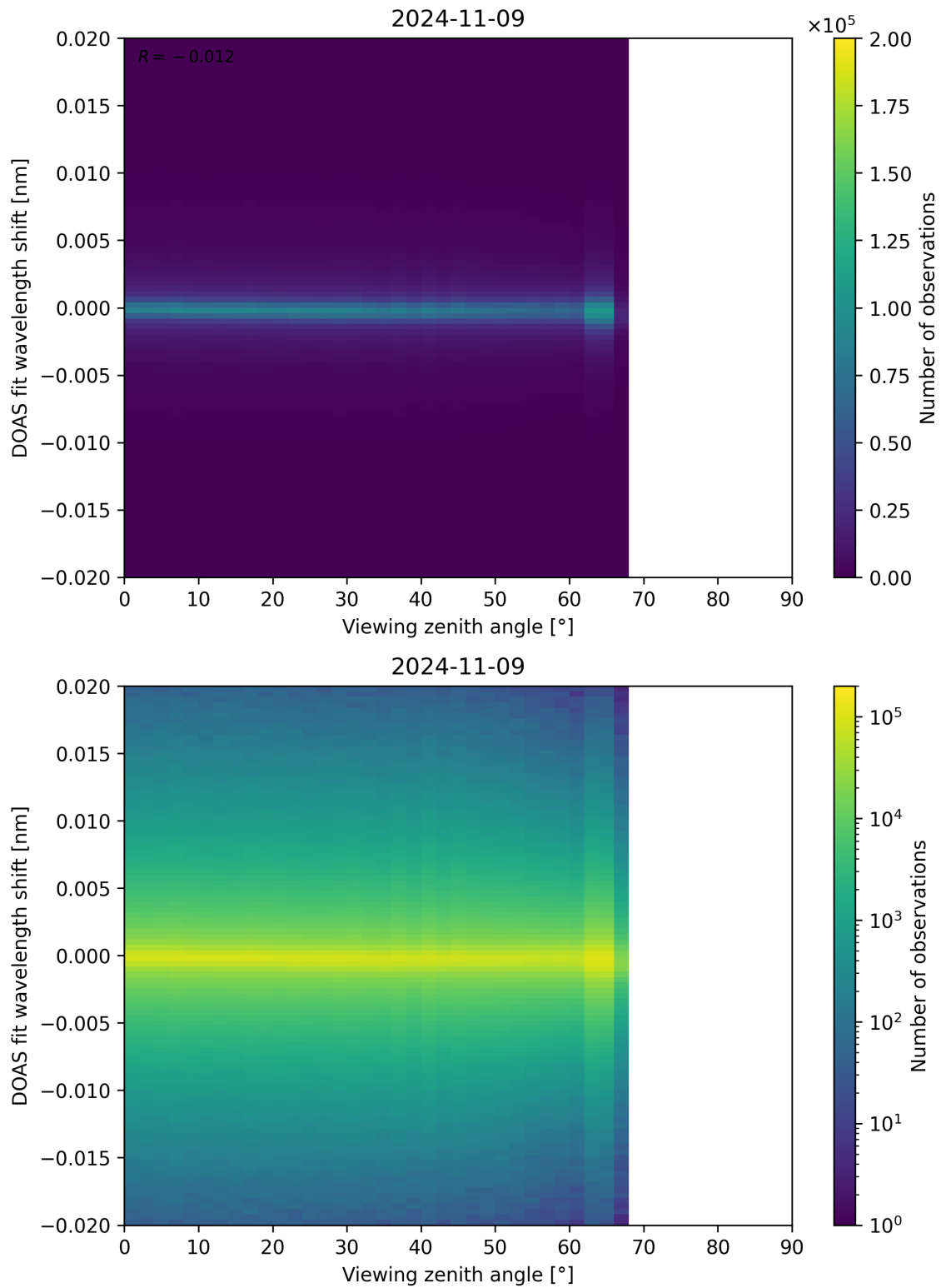
Figure 183: Scatter density plot of “Viewing zenith angle” against “DOAS fit wavelength shift” for 2024-11-09 to 2024-11-10.
