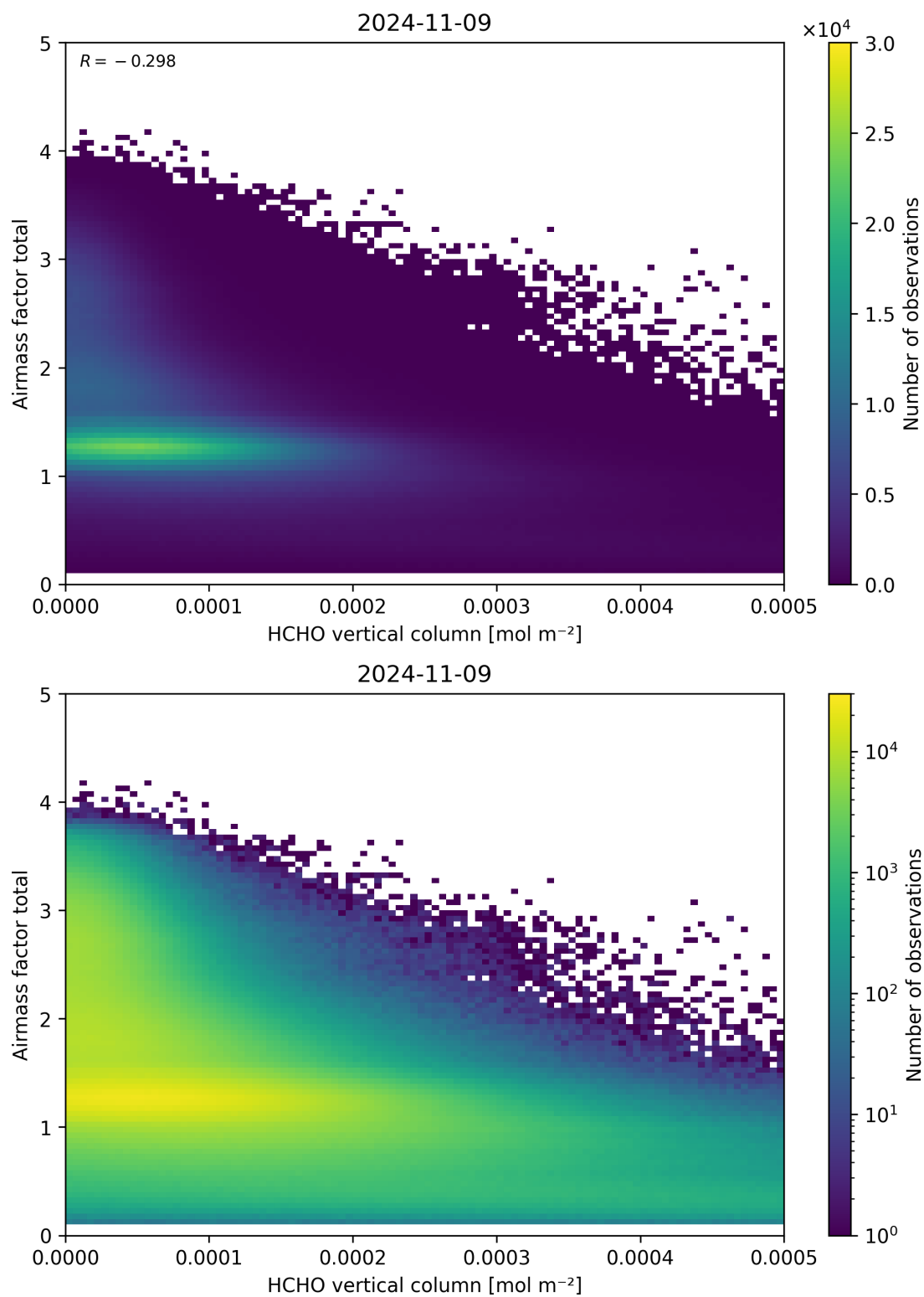
Figure 131: Scatter density plot of “HCHO vertical column” against “Airmass factor total” for 2024-11-09 to 2024-11-10.
