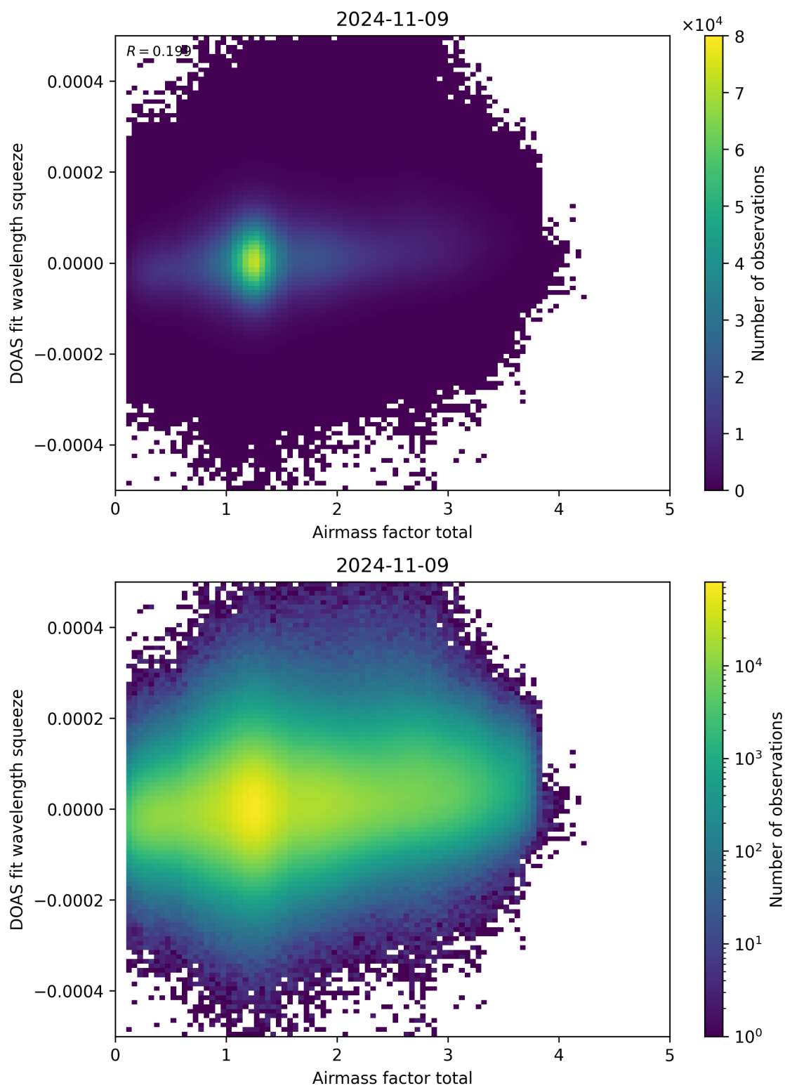
Figure 99: Scatter density plot of “Airmass factor total” against “DOAS fit wavelength squeeze” for 2024-11-09 to 2024-11-10.
