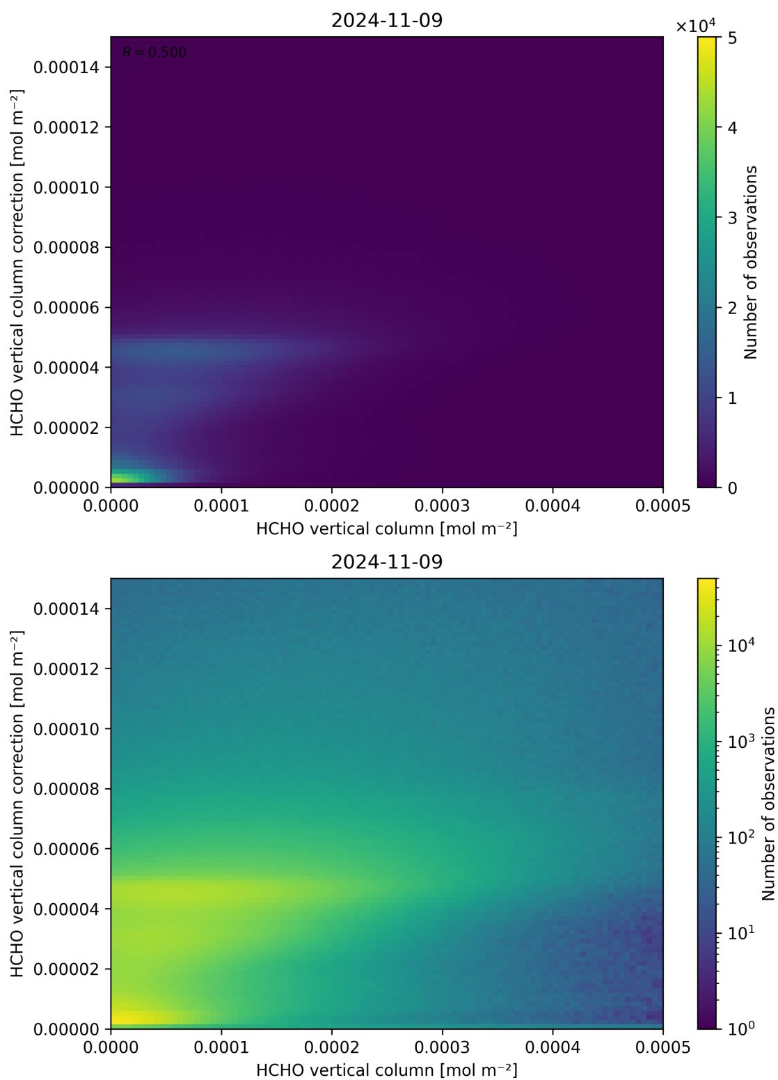
Figure 133: Scatter density plot of “HCHO vertical column” against “HCHO vertical column correction” for 2024-11-09 to 2024-11-10.
