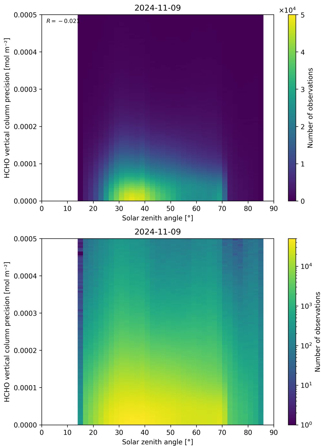
Figure 179: Scatter density plot of “Solar zenith angle” against “HCHO vertical column precision” for 2024-11-09 to 2024-11-10.
