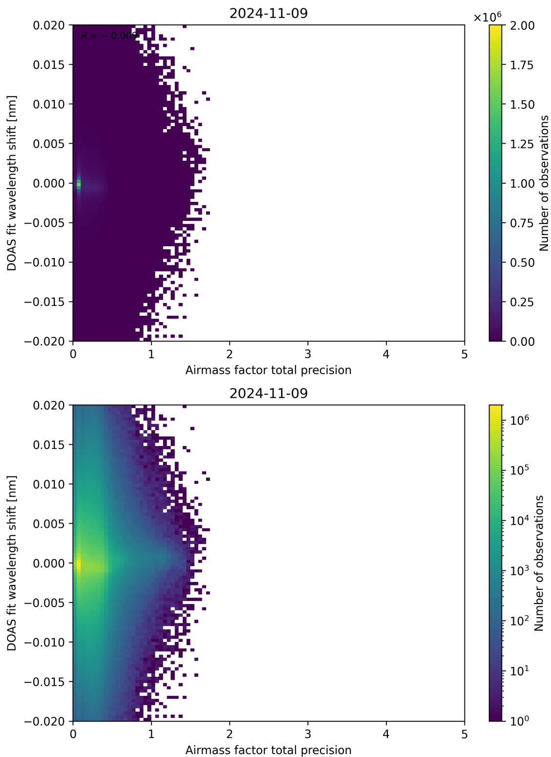
Figure 106: Scatter density plot of “Airmass factor total precision” against “DOAS fit wavelength shift” for 2024-11-09 to 2024-11-10.
