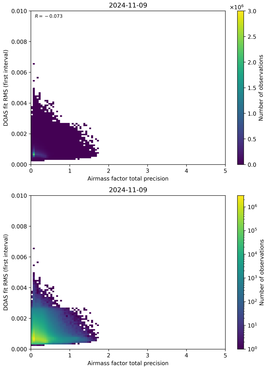
Figure 105: Scatter density plot of “Airmass factor total precision” against “DOAS fit RMS (first interval)” for 2024-11-09 to 2024-11-10.
