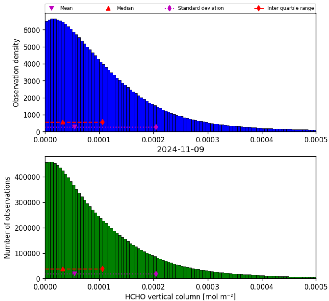
Figure 35: Histogram of “HCHO vertical column” for 2024-11-09 to 2024-11-10
