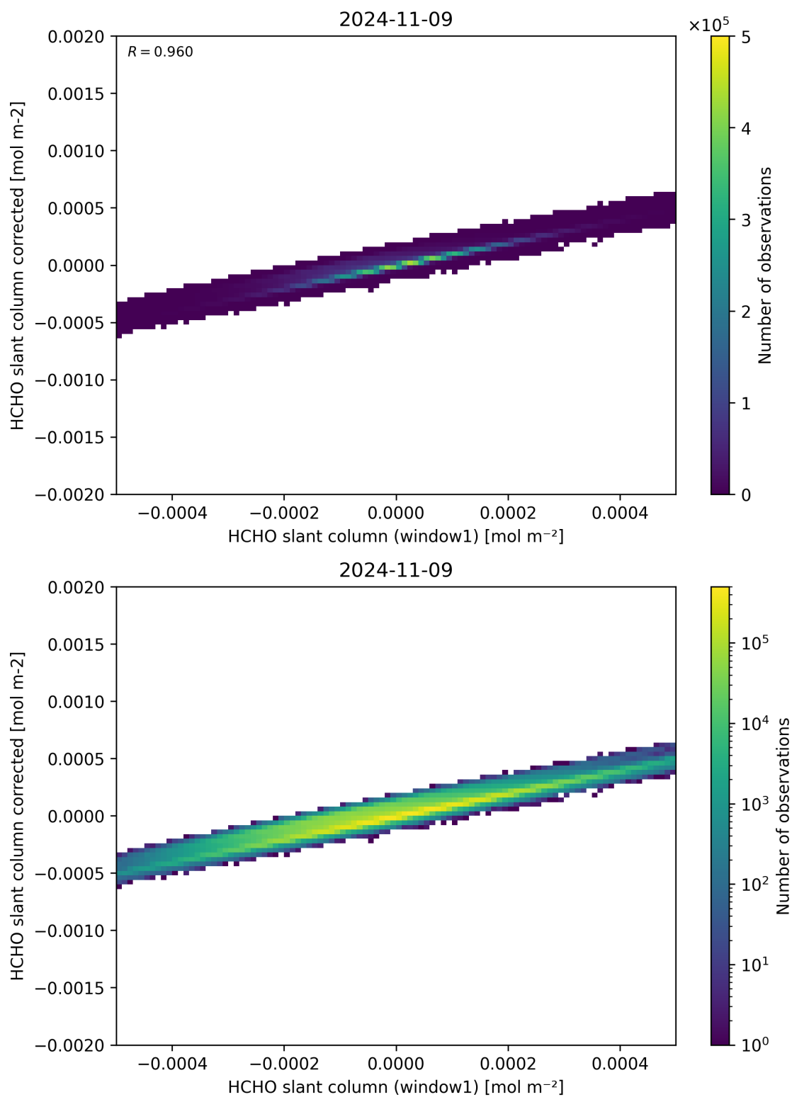
Figure 82: Scatter density plot of “HCHO slant column (window1)” against “HCHO slant column corrected” for 2024-11-09 to 2024-11-10.
