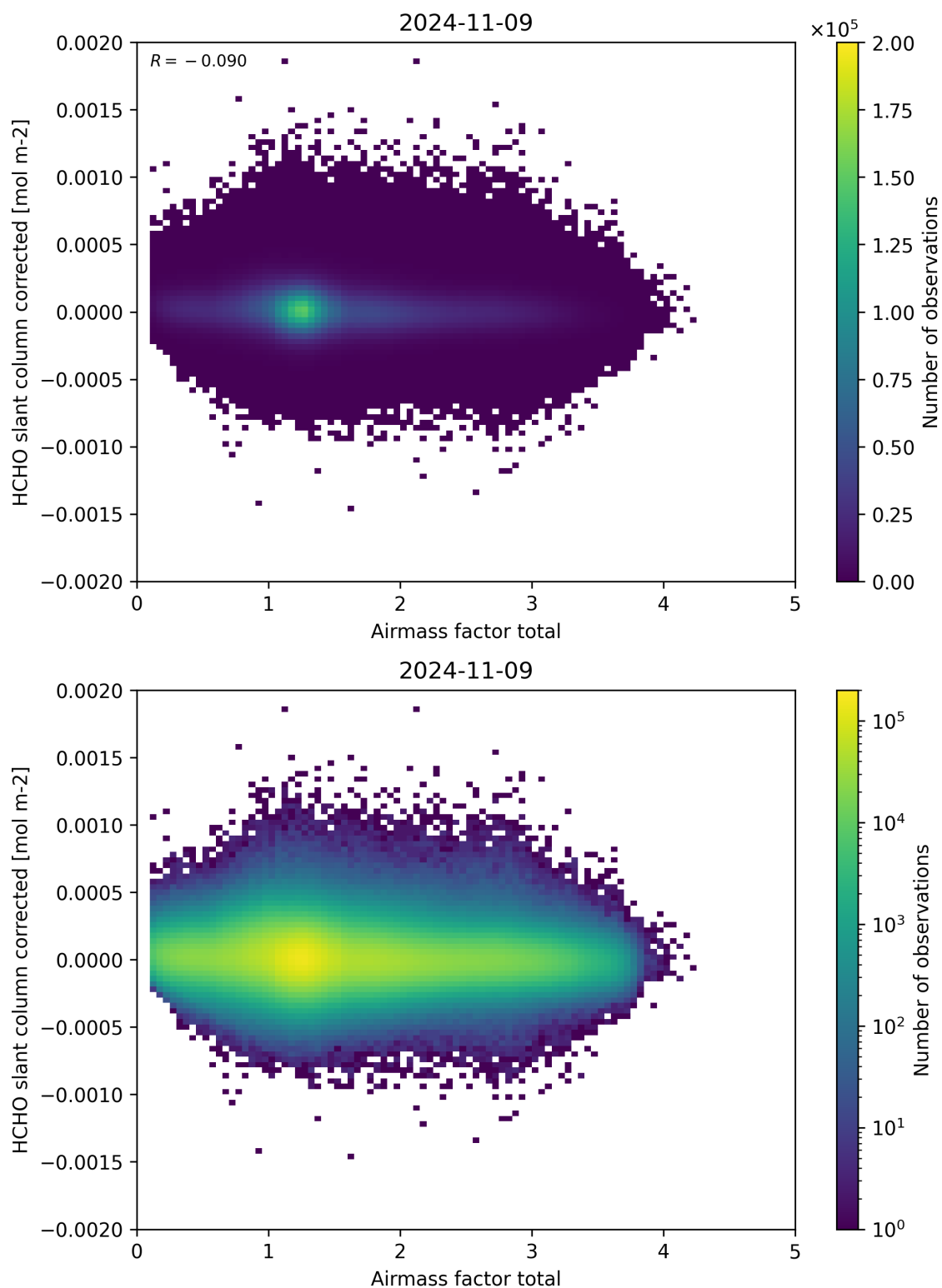
Figure 101: Scatter density plot of “Airmass factor total” against “HCHO slant column corrected” for 2024-11-09 to 2024-11-10.
