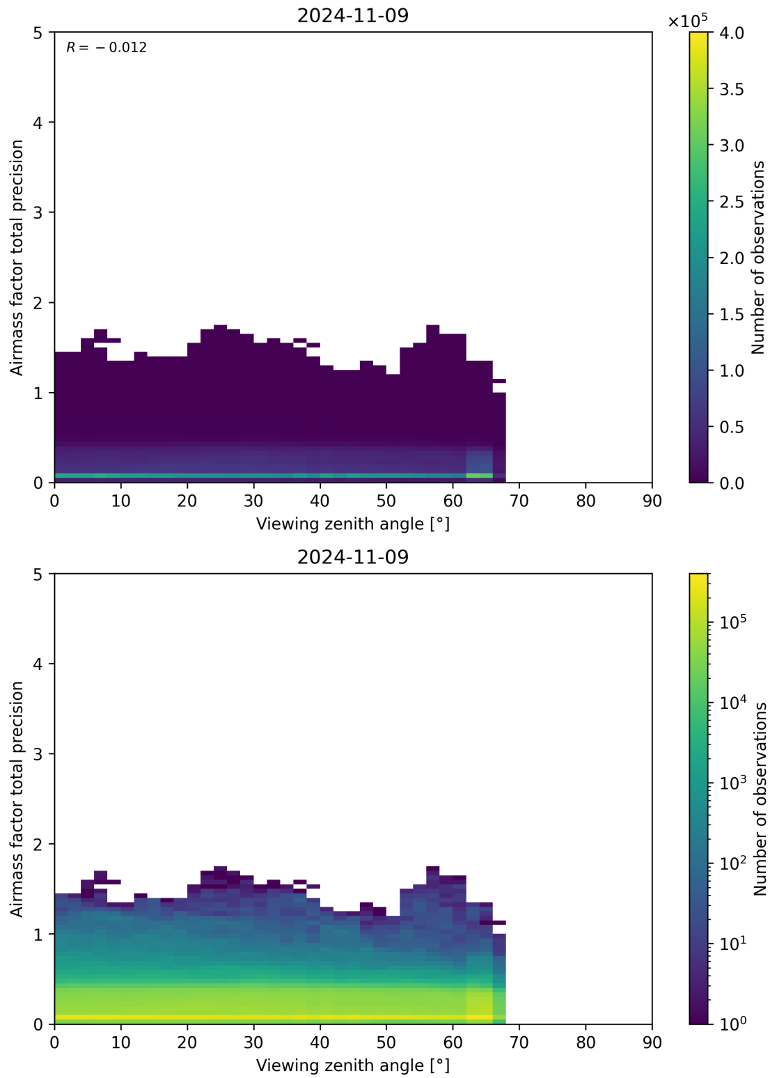
Figure 191: Scatter density plot of “Viewing zenith angle” against “Airmass factor total precision” for 2024-11-09 to 2024-11-10.
