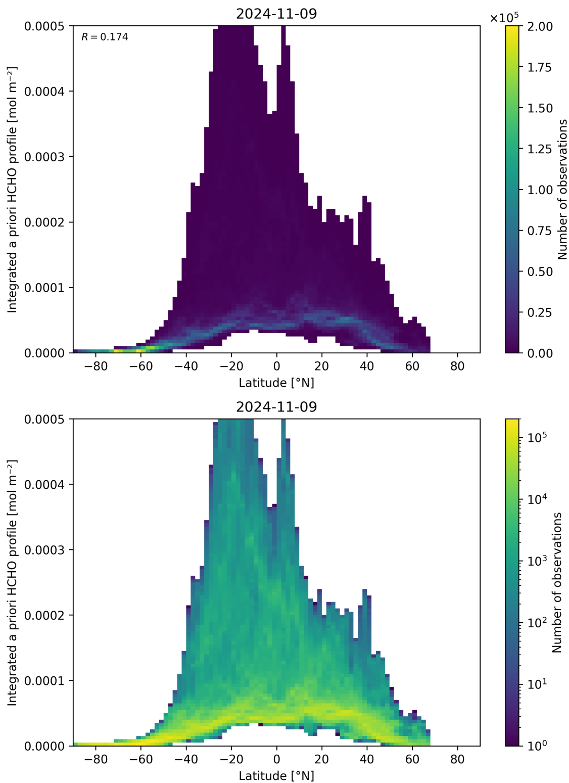
Figure 166: Scatter density plot of “Latitude” against “Integrated a priori HCHO profile” for 2024-11-09 to 2024-11-10.
