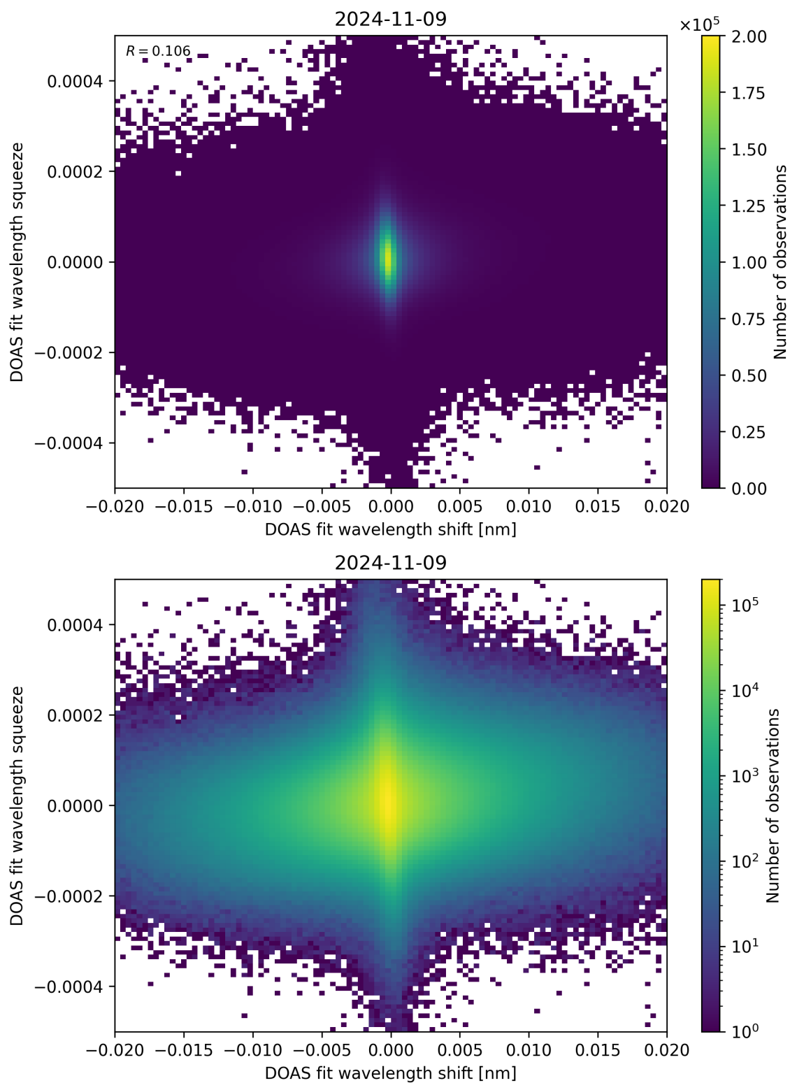
Figure 65: Scatter density plot of “DOAS fit wavelength shift” against “DOAS fit wavelength squeeze” for 2024-11-09 to 2024-11-10.
