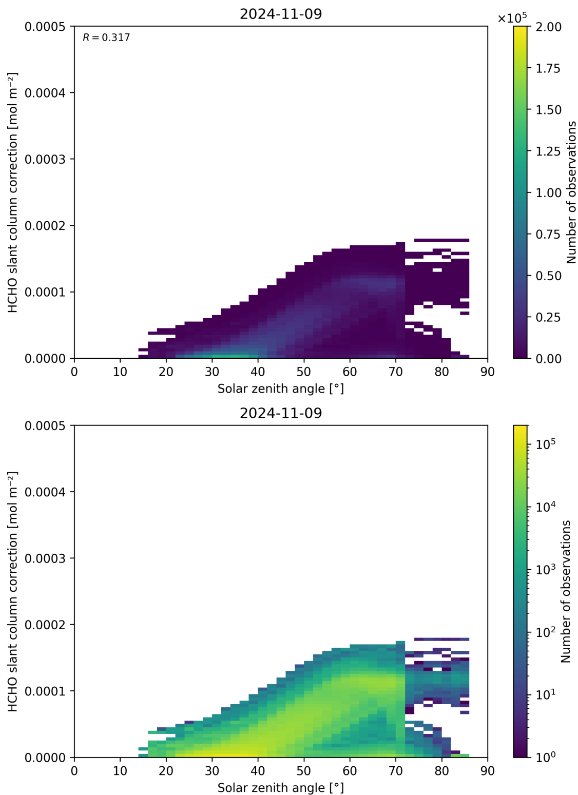
Figure 172: Scatter density plot of “Solar zenith angle” against “HCHO slant column correction” for 2024-11-09 to 2024-11-10.
