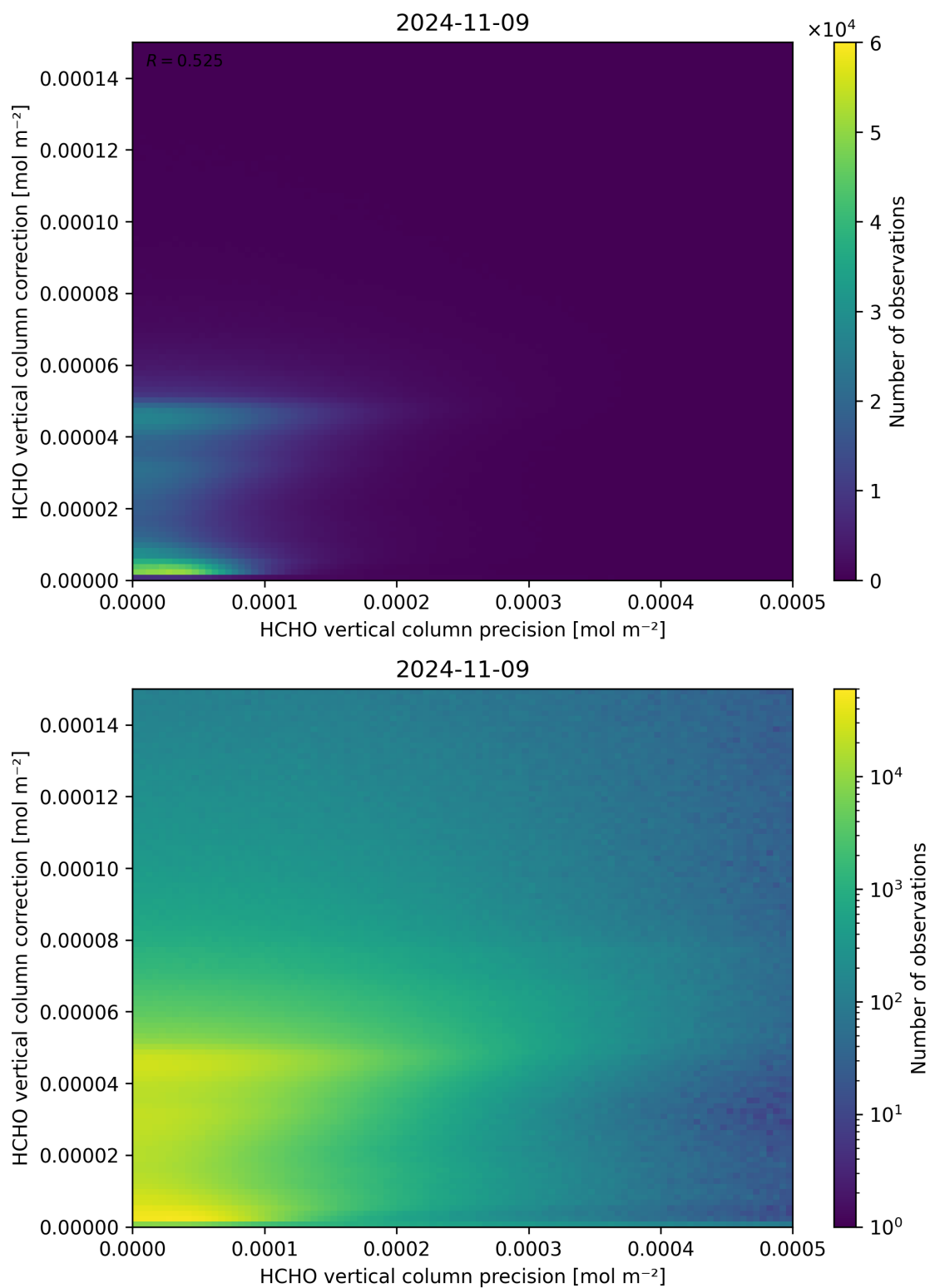
Figure 146: Scatter density plot of “HCHO vertical column precision” against “HCHO vertical column correction” for 2024-11-09 to 2024-11-10.
