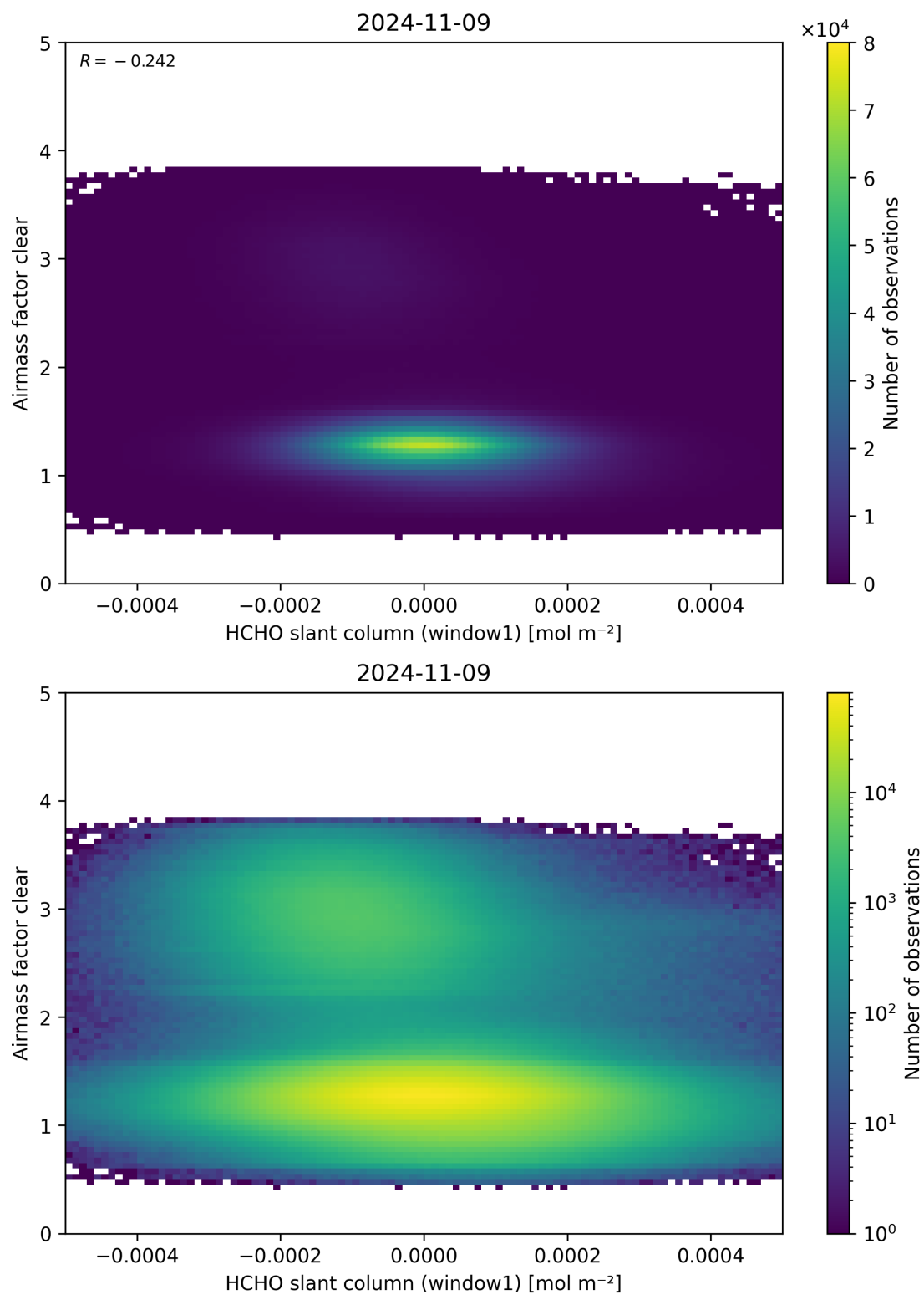
Figure 81: Scatter density plot of “HCHO slant column (window1)” against “Airmass factor clear” for 2024-11-09 to 2024-11-10.
