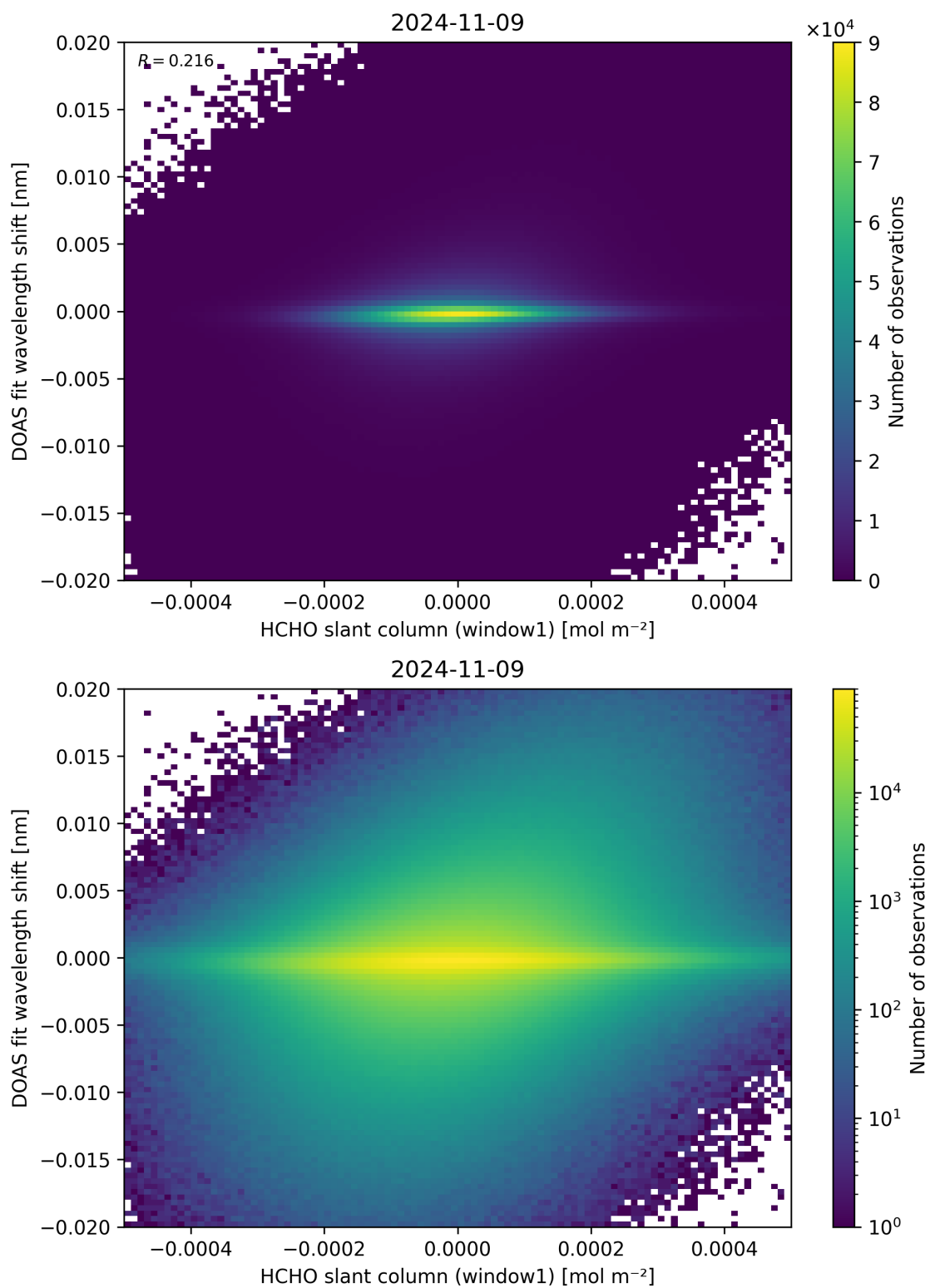
Figure 79: Scatter density plot of “HCHO slant column (window1)” against “DOAS fit wavelength shift” for 2024-11-09 to 2024-11-10.
