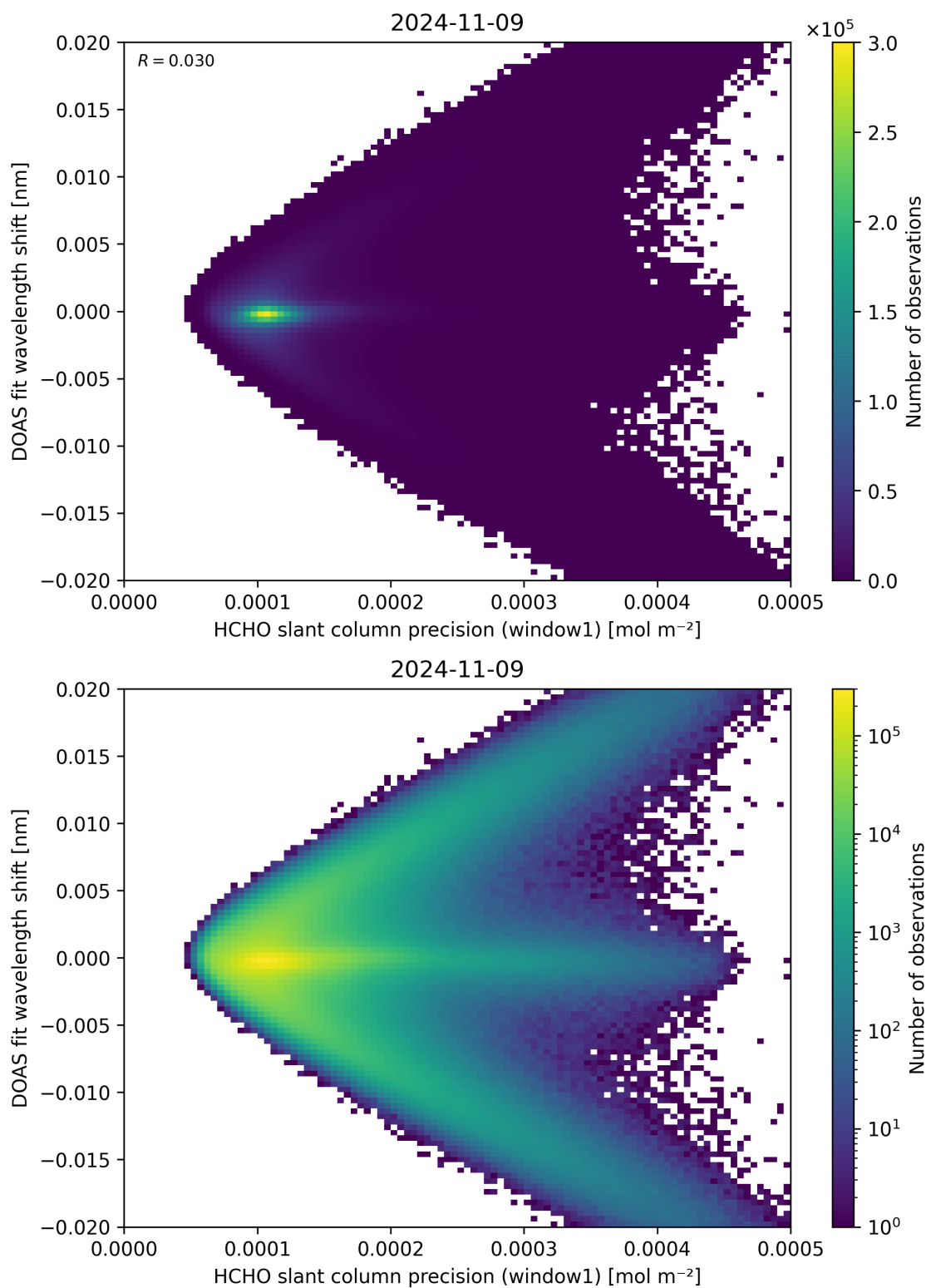
Figure 89: Scatter density plot of “HCHO slant column precision (window1)” against “DOAS fit wavelength shift” for 2024-11-09 to 2024-11-10.
