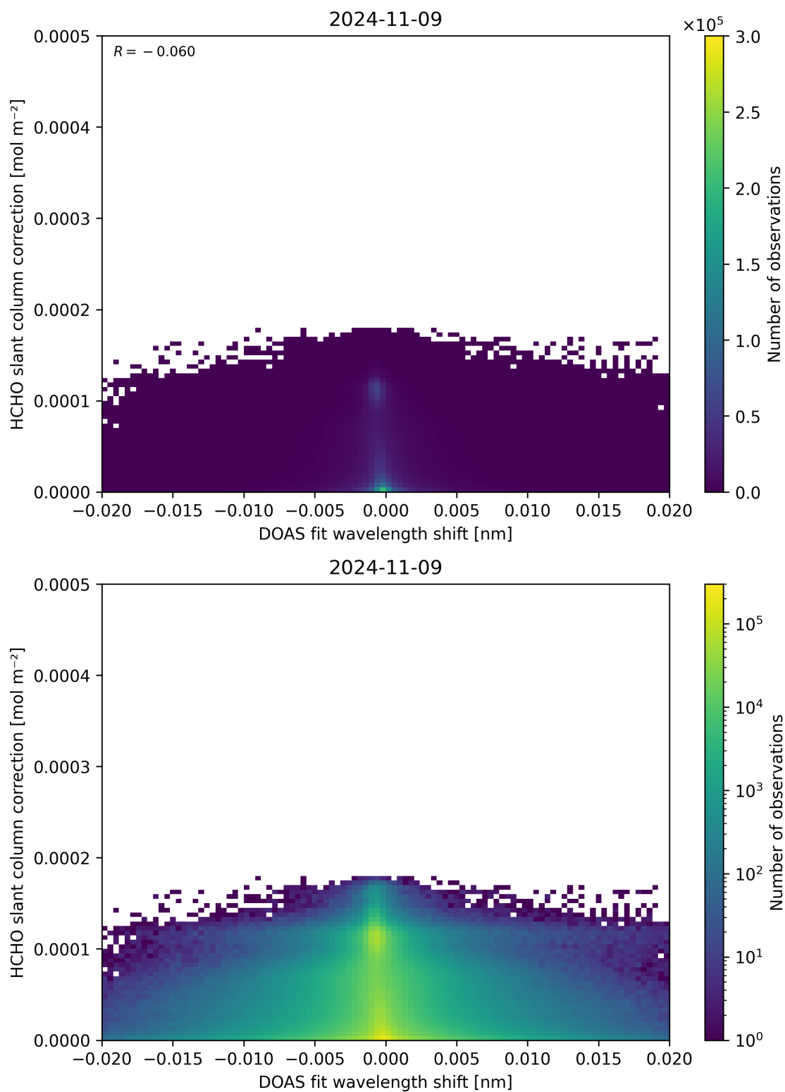
Figure 67: Scatter density plot of “DOAS fit wavelength shift” against “HCHO slant column correction” for 2024-11-09 to 2024-11-10.
