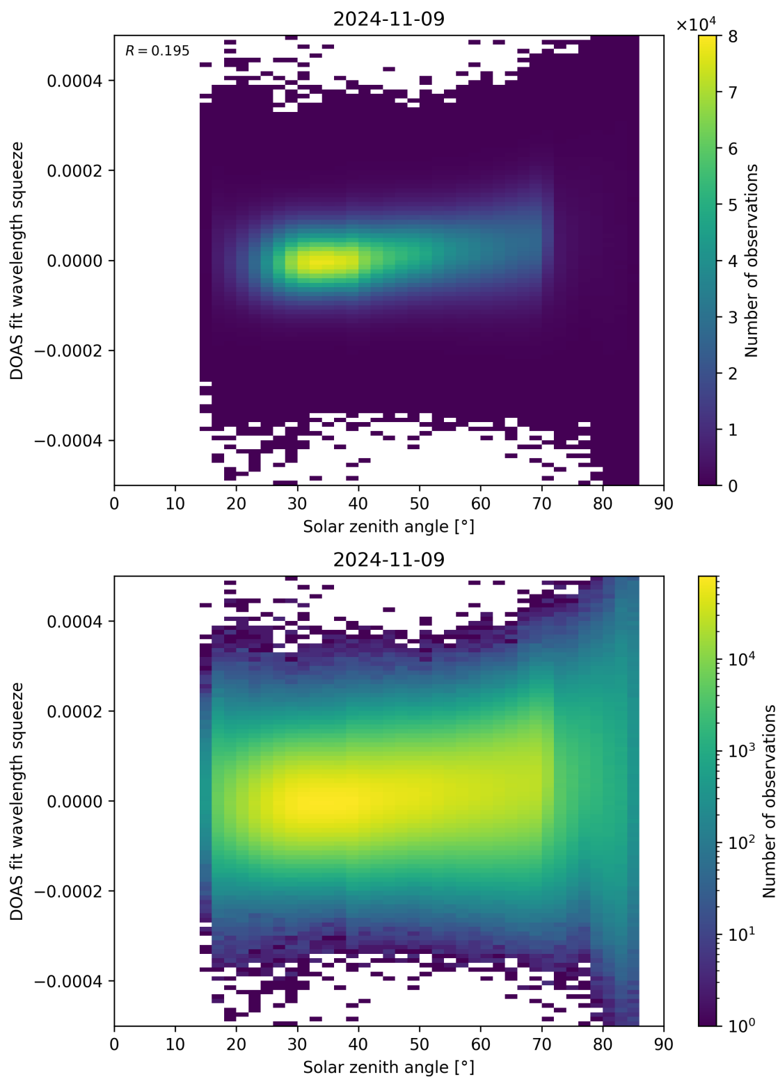
Figure 169: Scatter density plot of “Solar zenith angle” against “DOAS fit wavelength squeeze” for 2024-11-09 to 2024-11-10.
