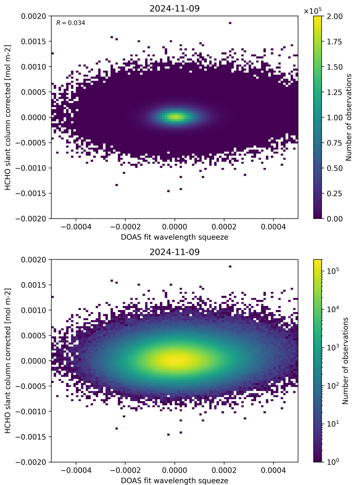
Figure 69: Scatter density plot of “DOAS fit wavelength squeeze” against “HCHO slant column corrected” for 2024-11-09 to 2024-11-10.
