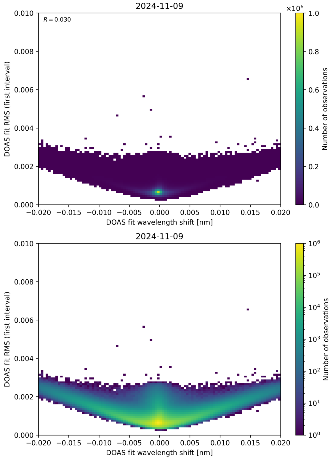
Figure 64: Scatter density plot of “DOAS fit wavelength shift” against “DOAS fit RMS (first interval)” for 2024-11-09 to 2024-11-10.
