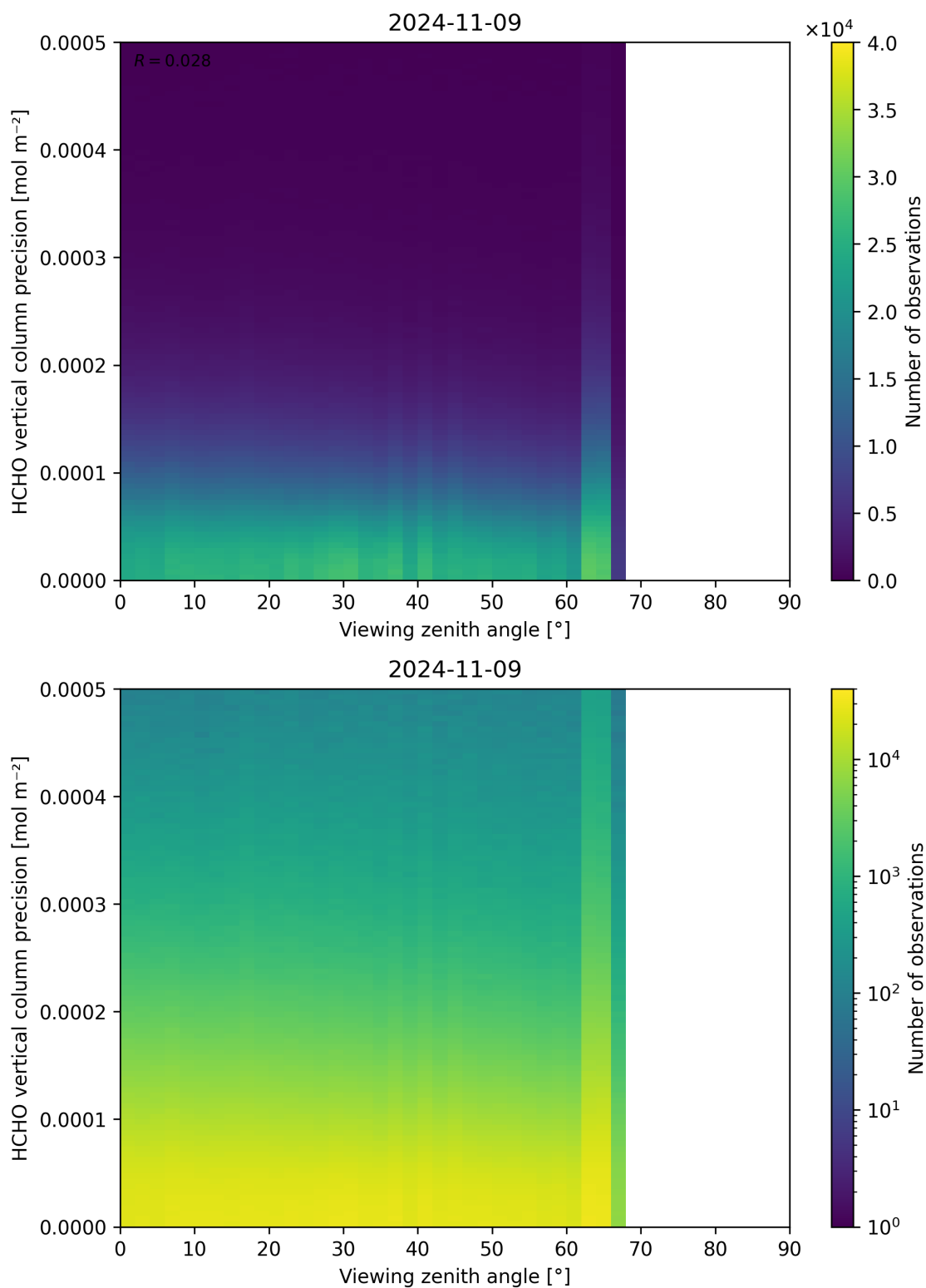
Figure 194: Scatter density plot of “Viewing zenith angle” against “HCHO vertical column precision” for 2024-11-09 to 2024-11-10.
