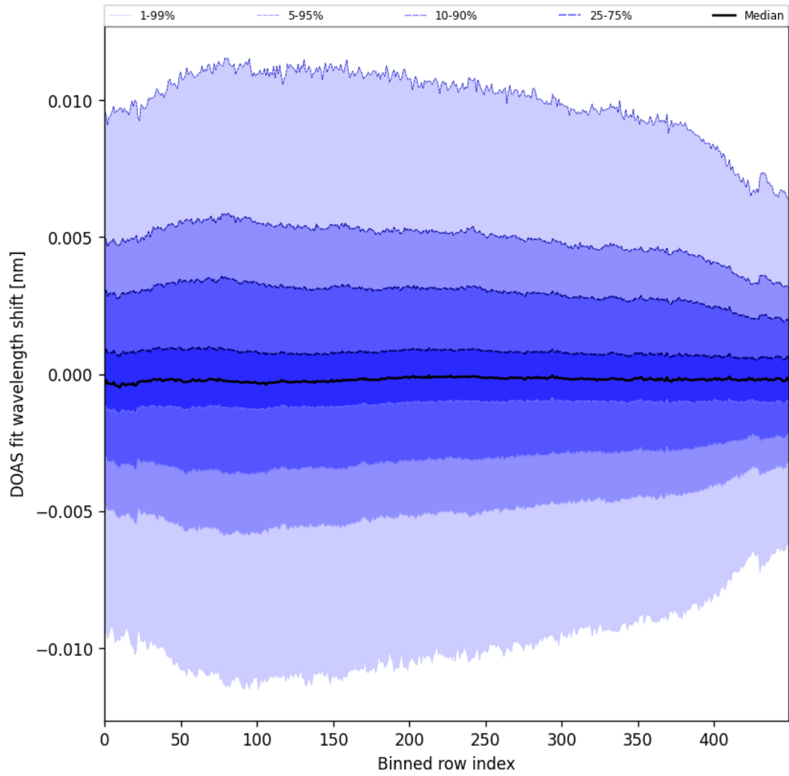
Figure 58: Along track statistics of “DOAS fit wavelength shift” for 2024-11-09 to 2024-11-10
