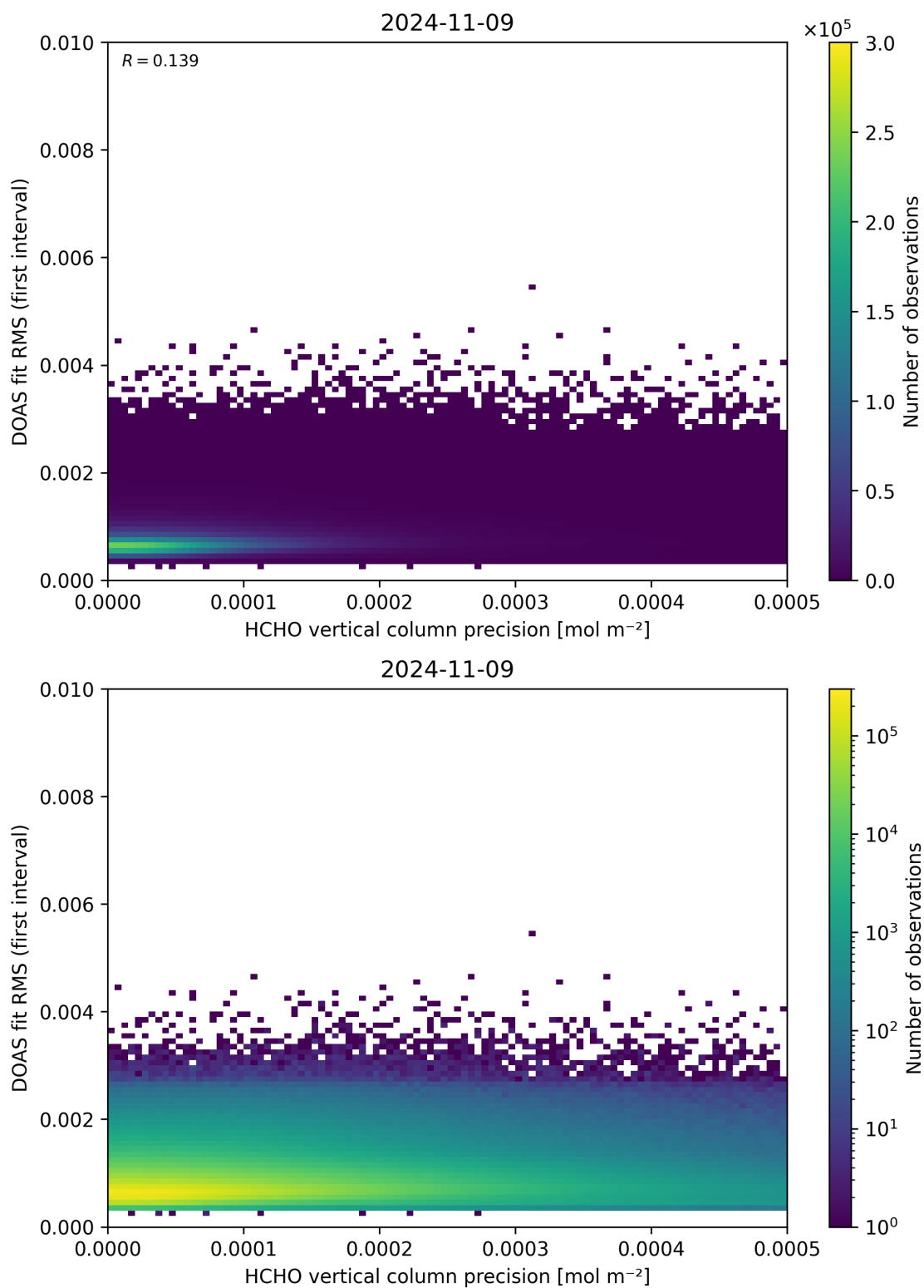
Figure 136: Scatter density plot of “HCHO vertical column precision” against “DOAS fit RMS (first interval)” for 2024-11-09 to 2024-11-10.
