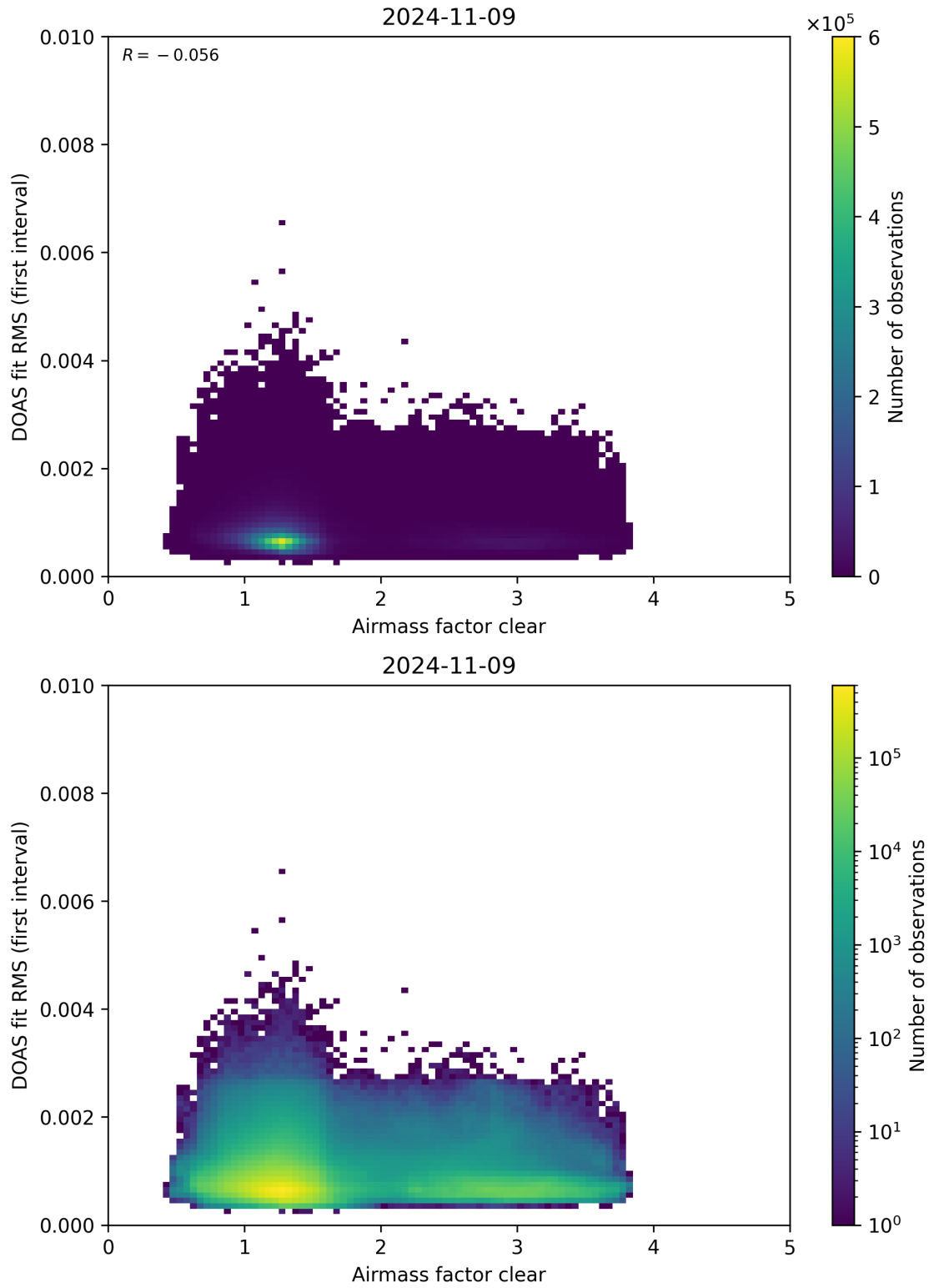
Figure 71: Scatter density plot of “Airmass factor clear” against “DOAS fit RMS (first interval)” for 2024-11-09 to 2024-11-10.
