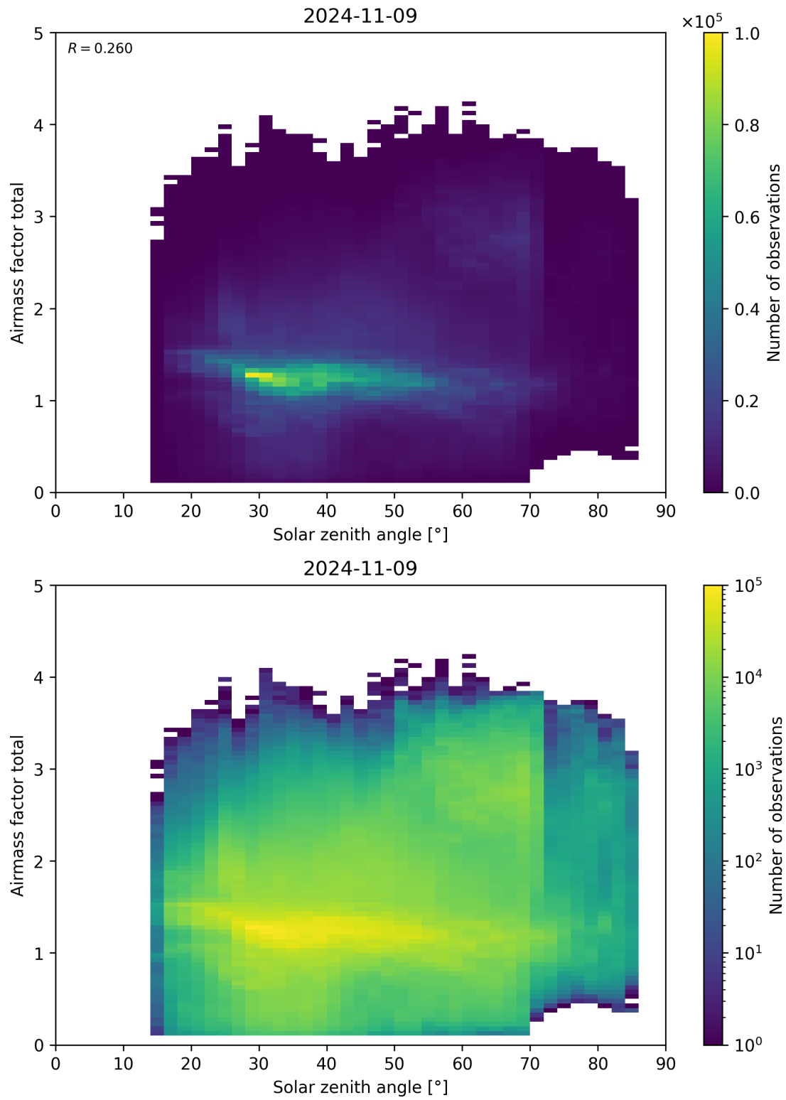
Figure 175: Scatter density plot of “Solar zenith angle” against “Airmass factor total” for 2024-11-09 to 2024-11-10.
