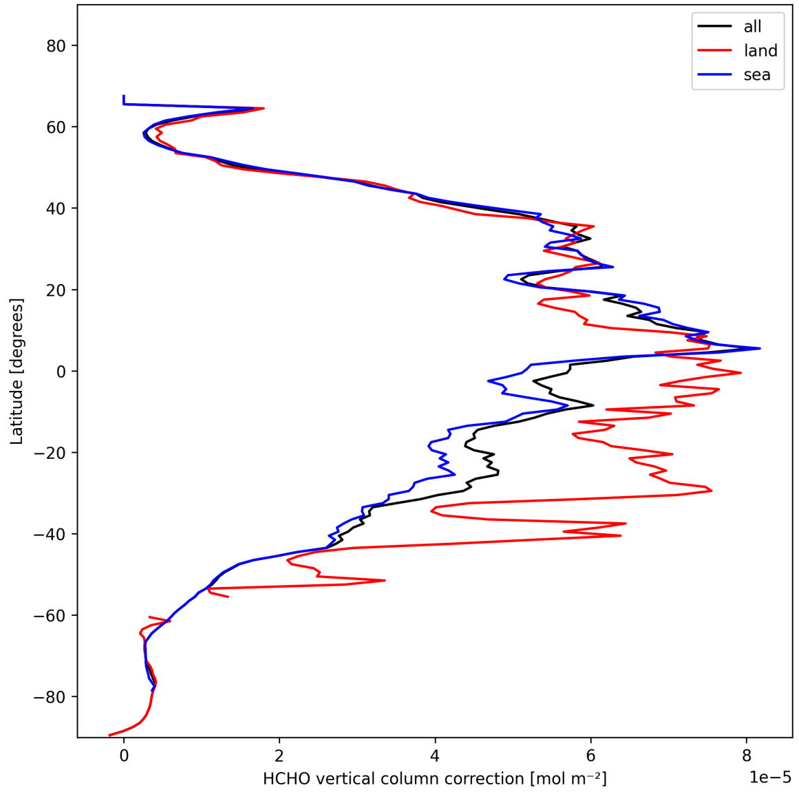
Figure 23: Zonal average of "HCHO vertical column correction" for 2024-11-09 to 2024-11-10.
