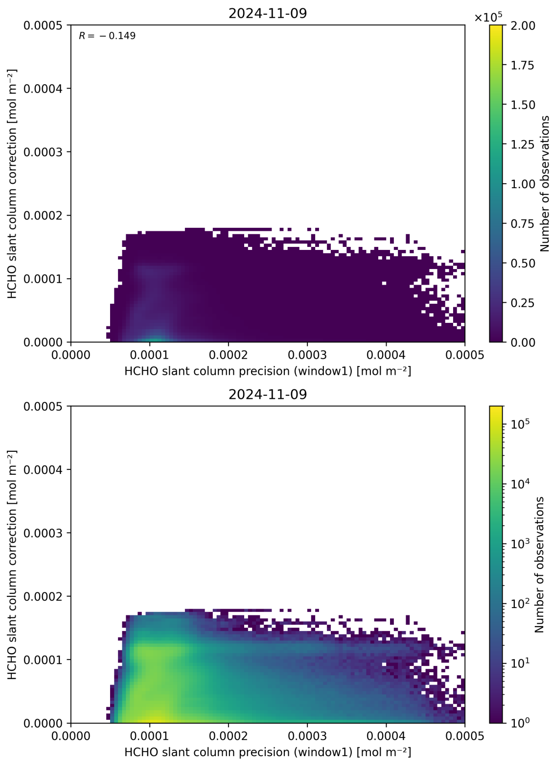
Figure 93: Scatter density plot of “HCHO slant column precision (window1)” against “HCHO slant column correction” for 2024-11-09 to 2024-11-10.
