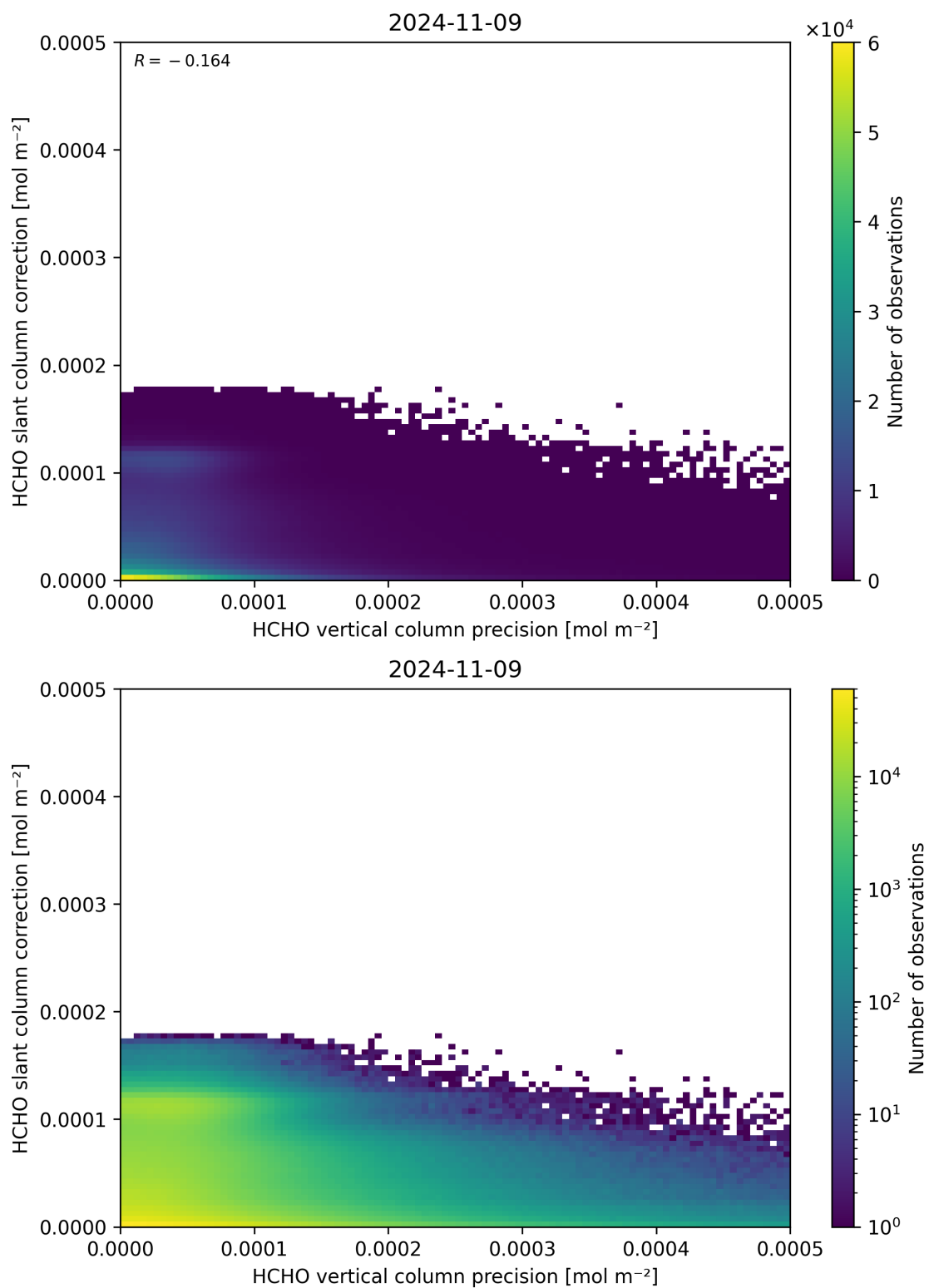
Figure 141: Scatter density plot of “HCHO vertical column precision” against “HCHO slant column correction” for 2024-11-09 to 2024-11-10.
