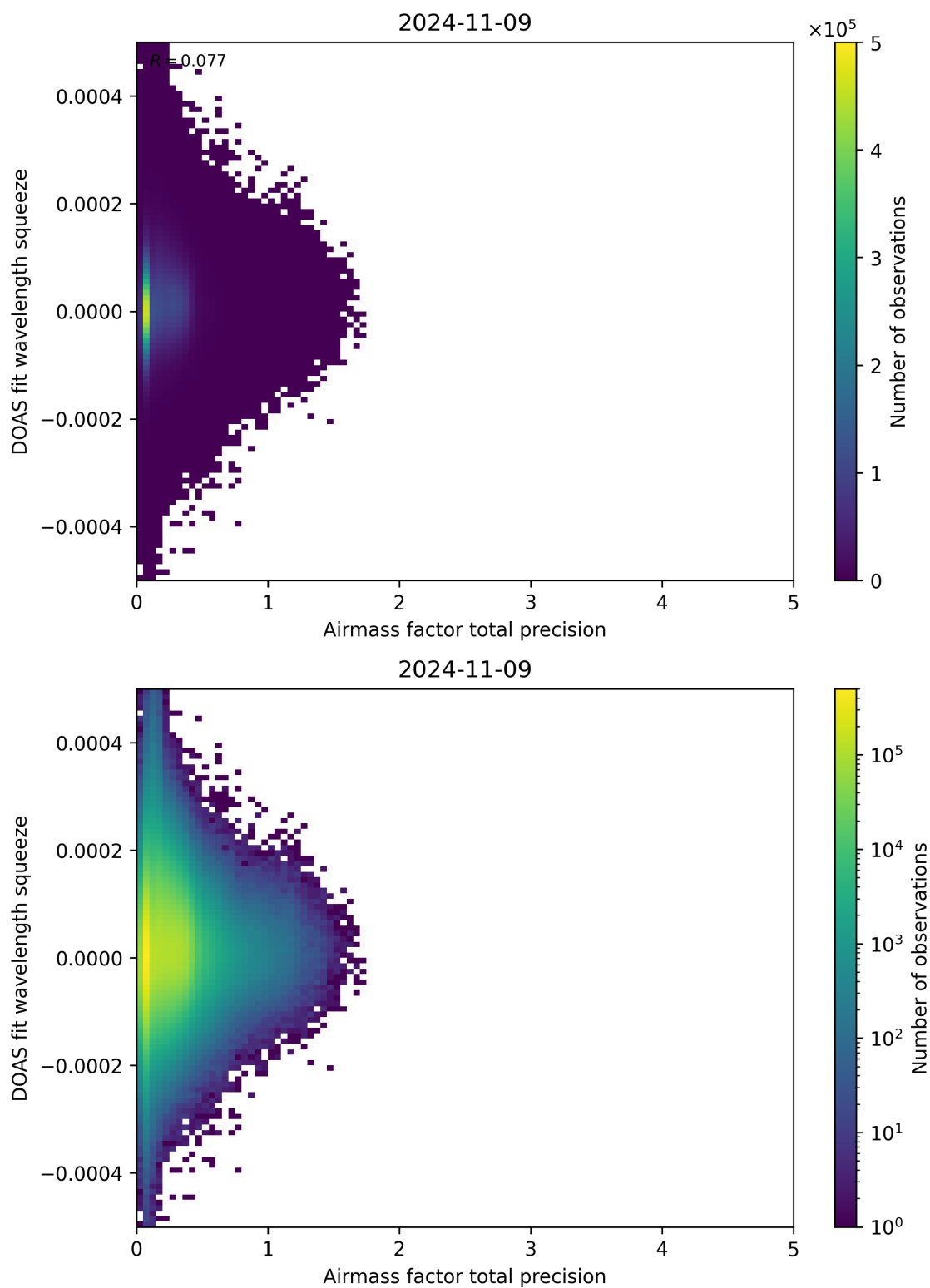
Figure 107: Scatter density plot of “Airmass factor total precision” against “DOAS fit wavelength squeeze” for 2024-11-09 to 2024-11-10.
