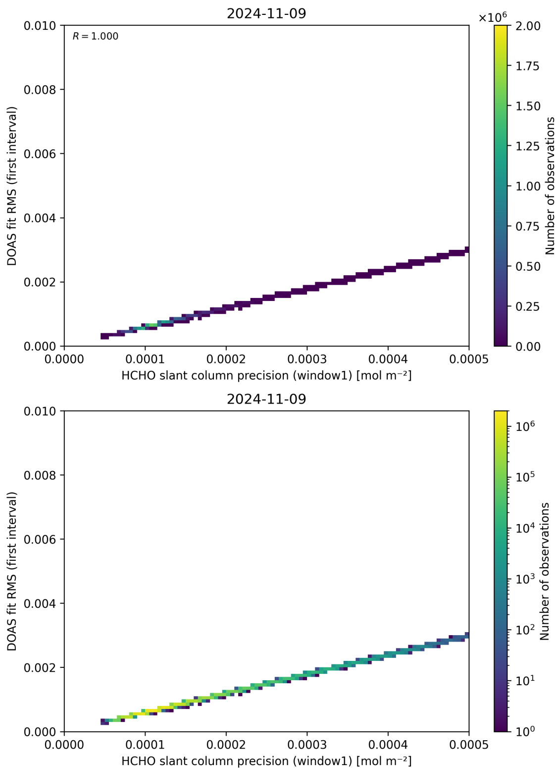
Figure 88: Scatter density plot of “HCHO slant column precision (window1)” against “DOAS fit RMS (first interval)” for 2024-11-09 to 2024-11-10.
