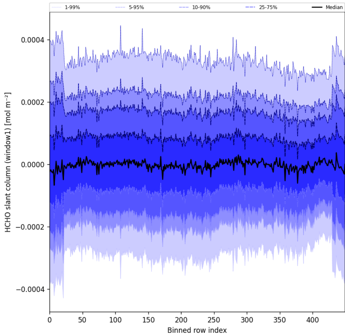
Figure 52: Along track statistics of “HCHO slant column (window1)” for 2024-11-09 to 2024-11-10
