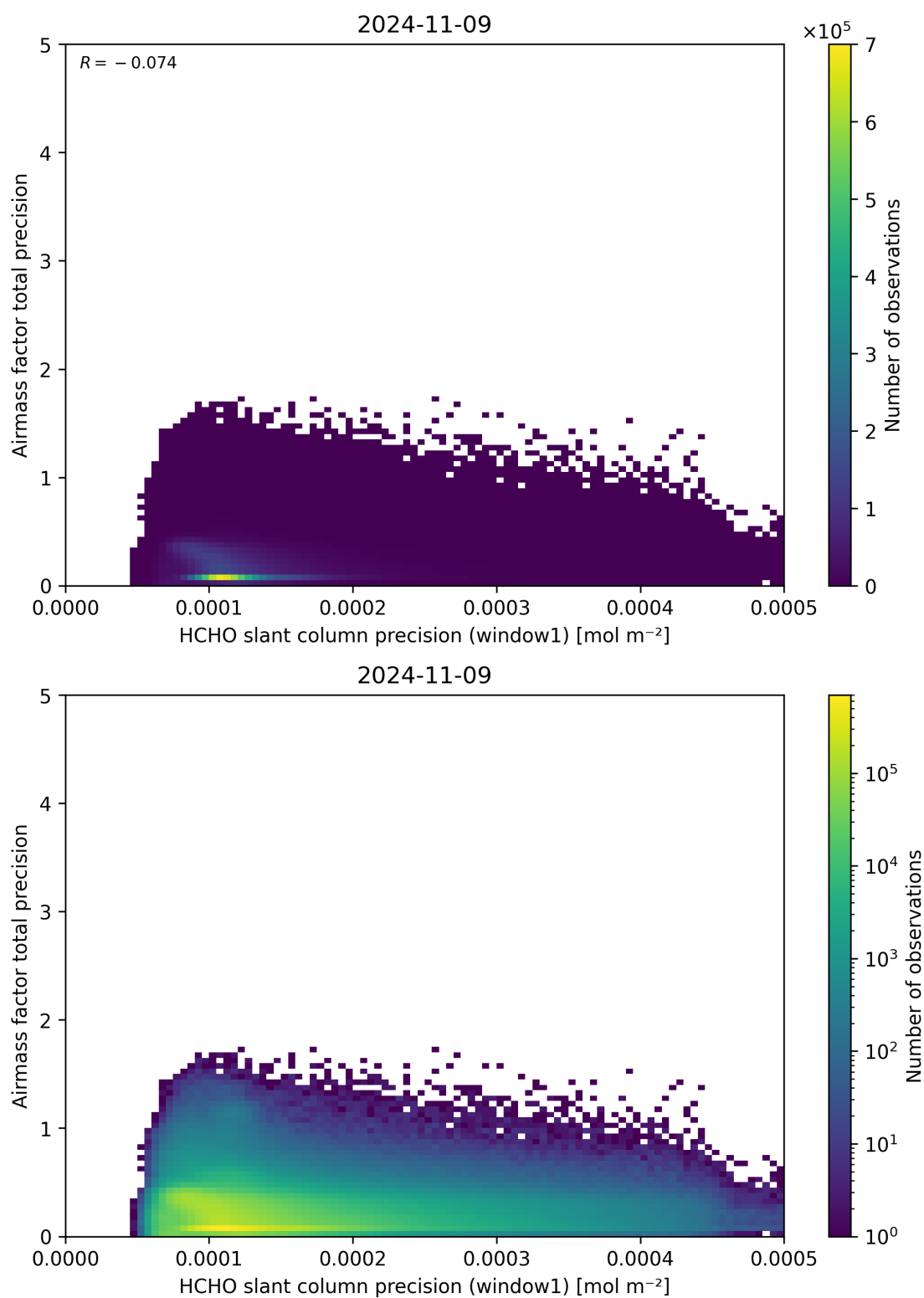
Figure 95: Scatter density plot of “HCHO slant column precision (window1)” against “Airmass factor total precision” for 2024-11-09 to 2024-11-10.
