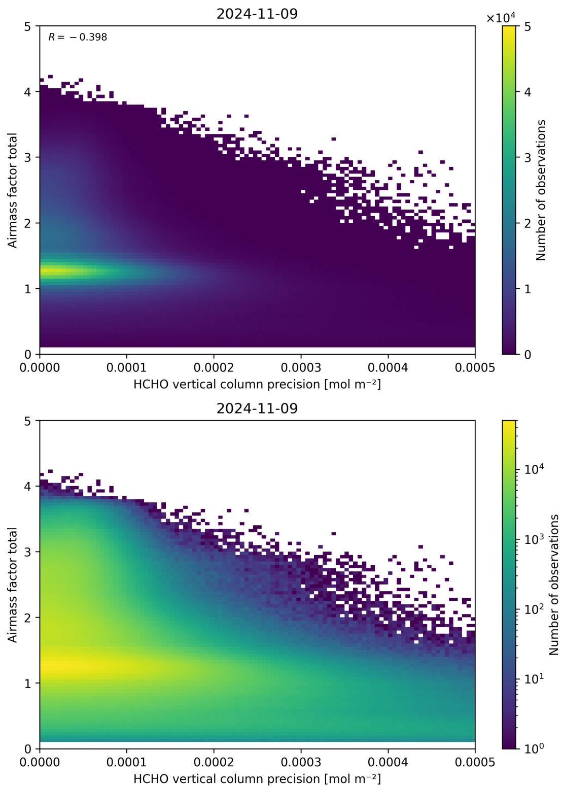
Figure 144: Scatter density plot of “HCHO vertical column precision” against “Airmass factor total” for 2024-11-09 to 2024-11-10.
