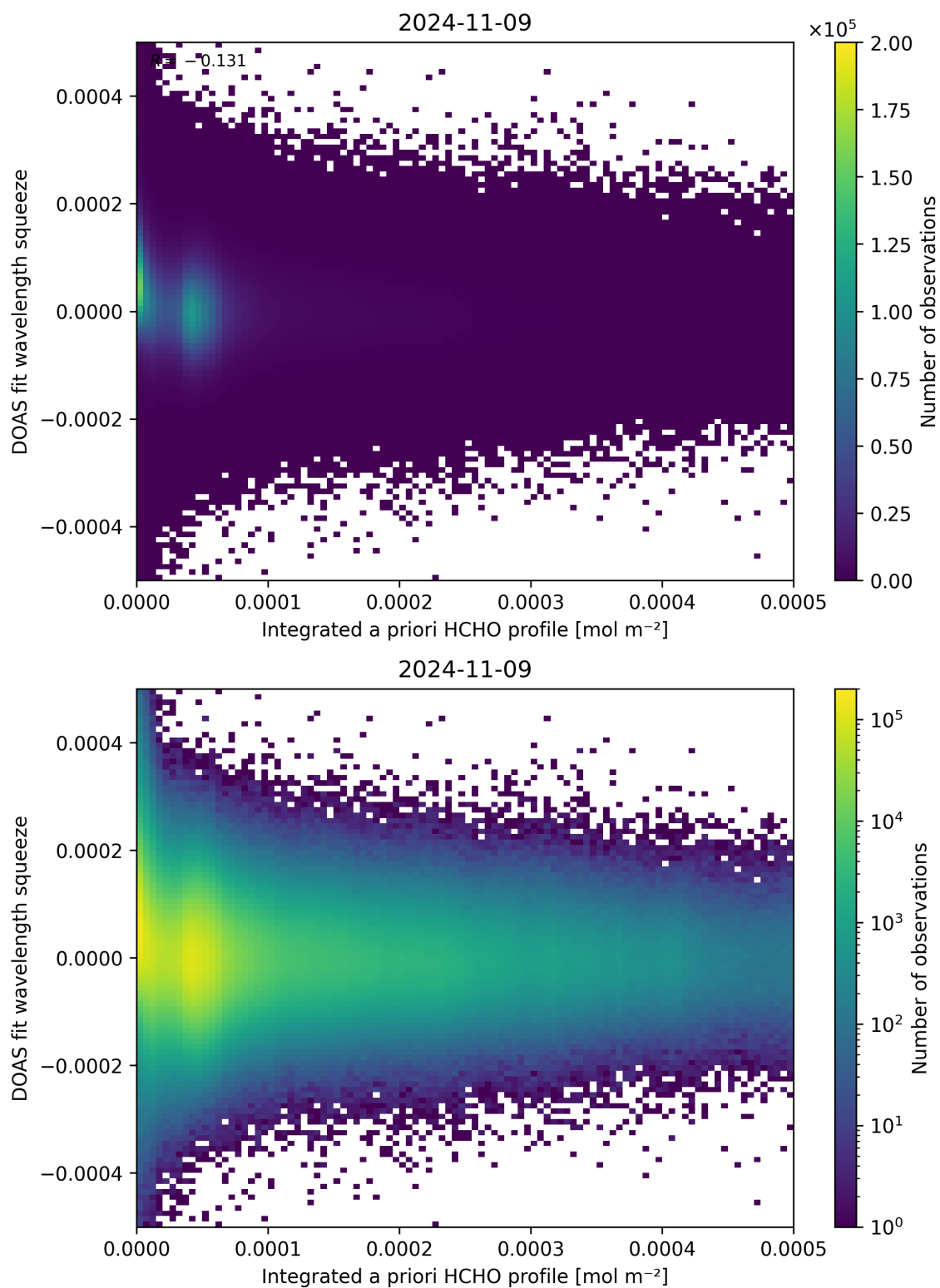
Figure 150: Scatter density plot of “Integrated a priori HCHO profile” against “DOAS fit wavelength squeeze” for 2024-11-09 to 2024-11-10.
