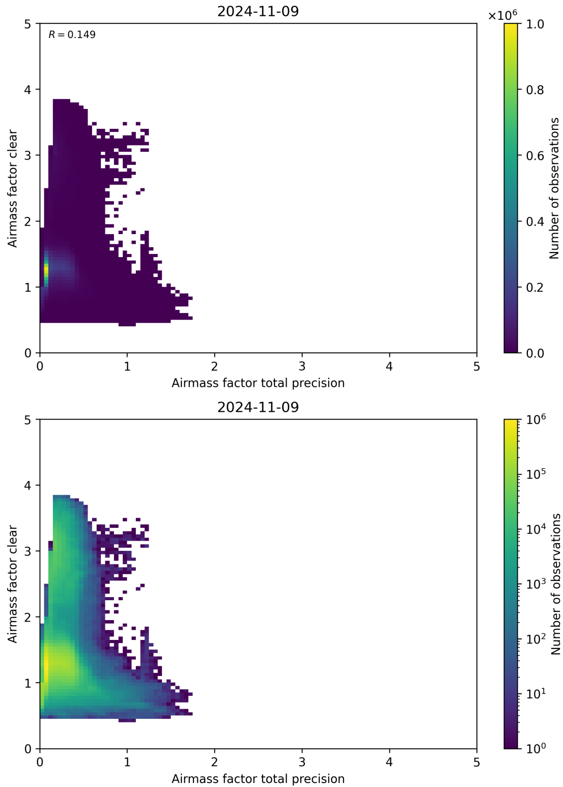
Figure 108: Scatter density plot of “Airmass factor total precision” against “Airmass factor clear” for 2024-11-09 to 2024-11-10.
