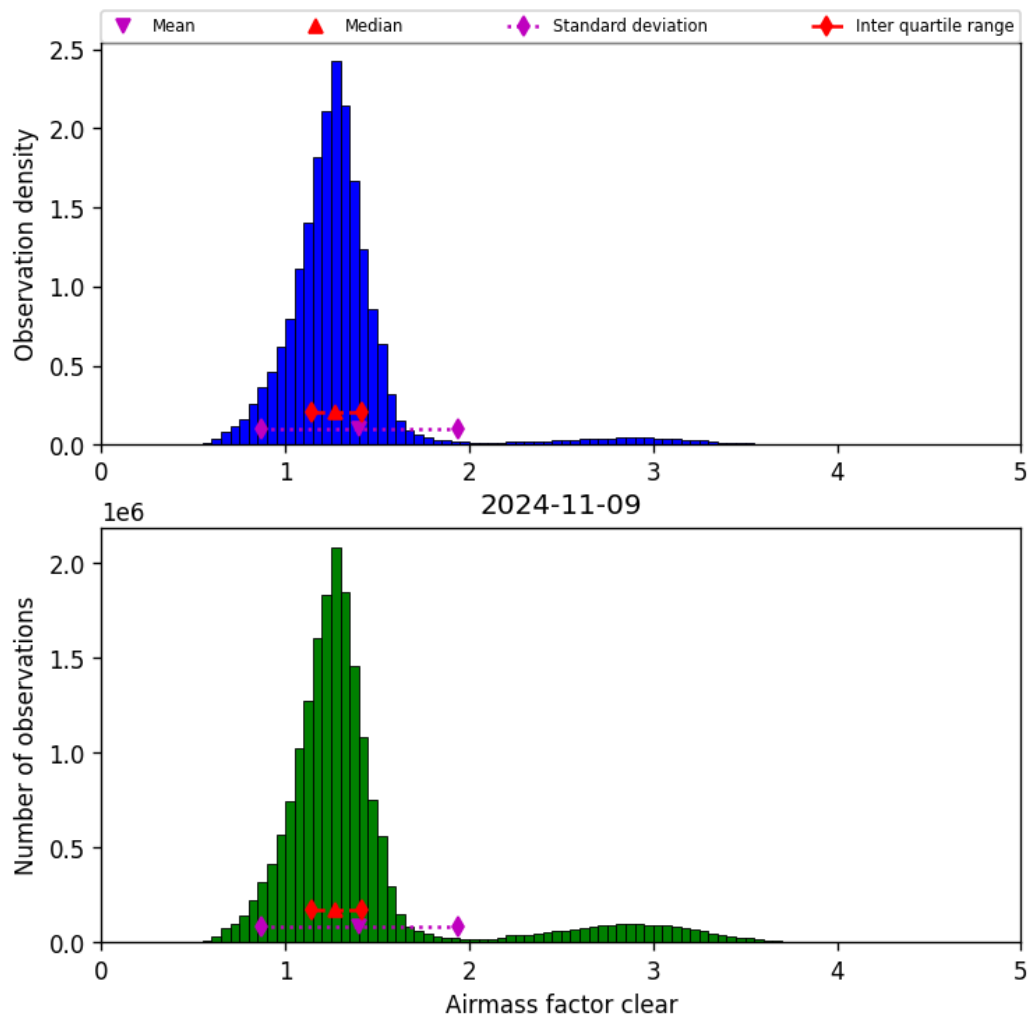
Figure 42: Histogram of “Airmass factor clear” for 2024-11-09 to 2024-11-10
