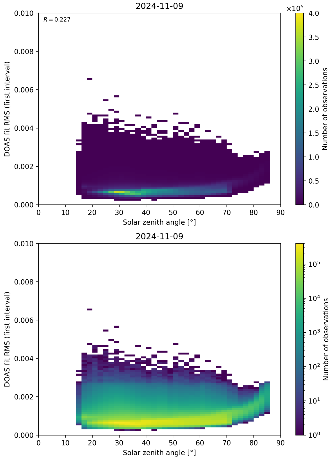
Figure 167: Scatter density plot of “Solar zenith angle” against “DOAS fit RMS (first interval)” for 2024-11-09 to 2024-11-10.
