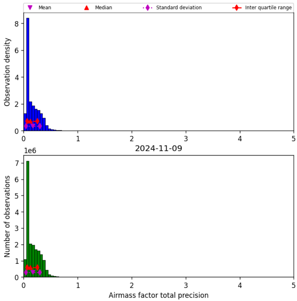
Figure 41: Histogram of “Airmass factor total precision” for 2024-11-09 to 2024-11-10
