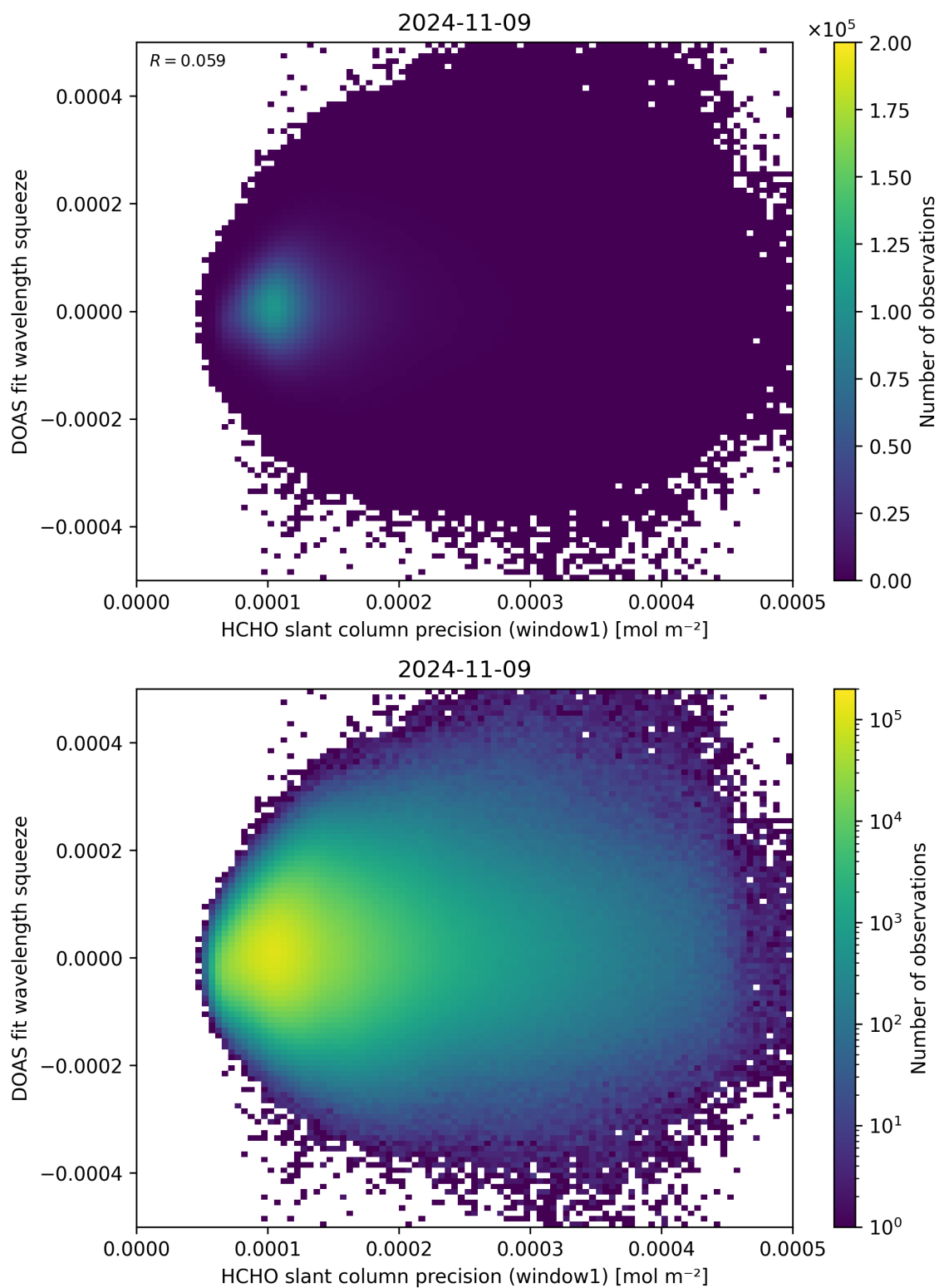
Figure 90: Scatter density plot of “HCHO slant column precision (window1)” against “DOAS fit wavelength squeeze” for 2024-11-09 to 2024-11-10.
