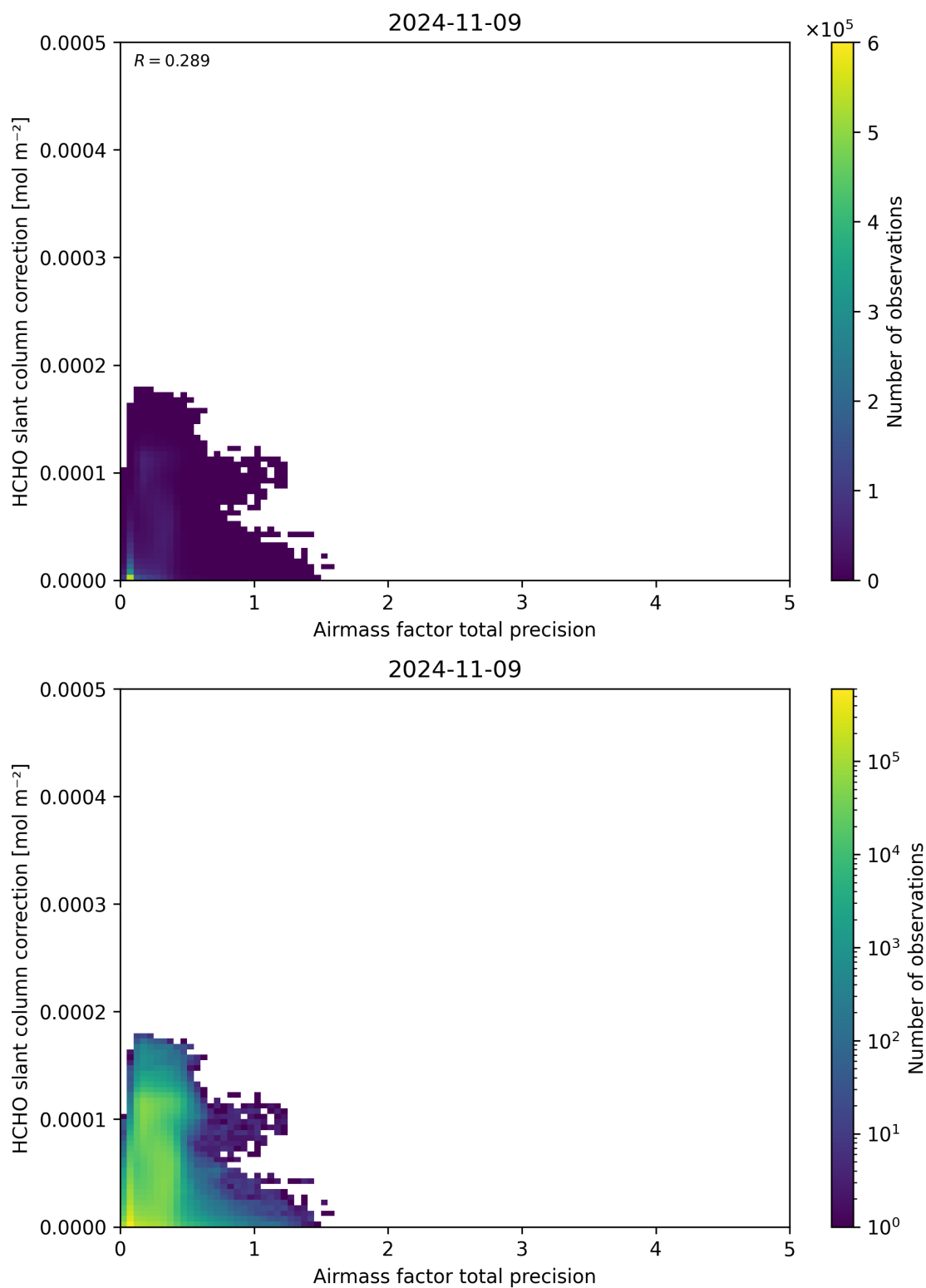
Figure 110: Scatter density plot of “Airmass factor total precision” against “HCHO slant column correction” for 2024-11-09 to 2024-11-10.
