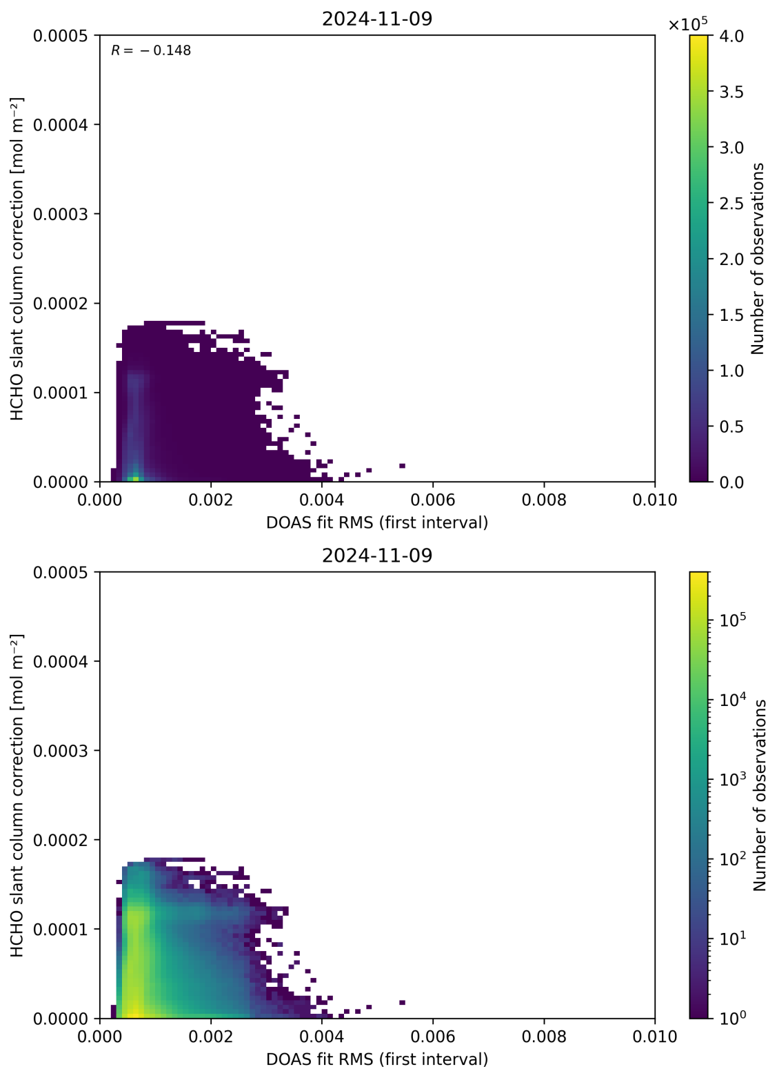
Figure 63: Scatter density plot of “DOAS fit RMS (first interval)” against “HCHO slant column correction” for 2024-11-09 to 2024-11-10.
