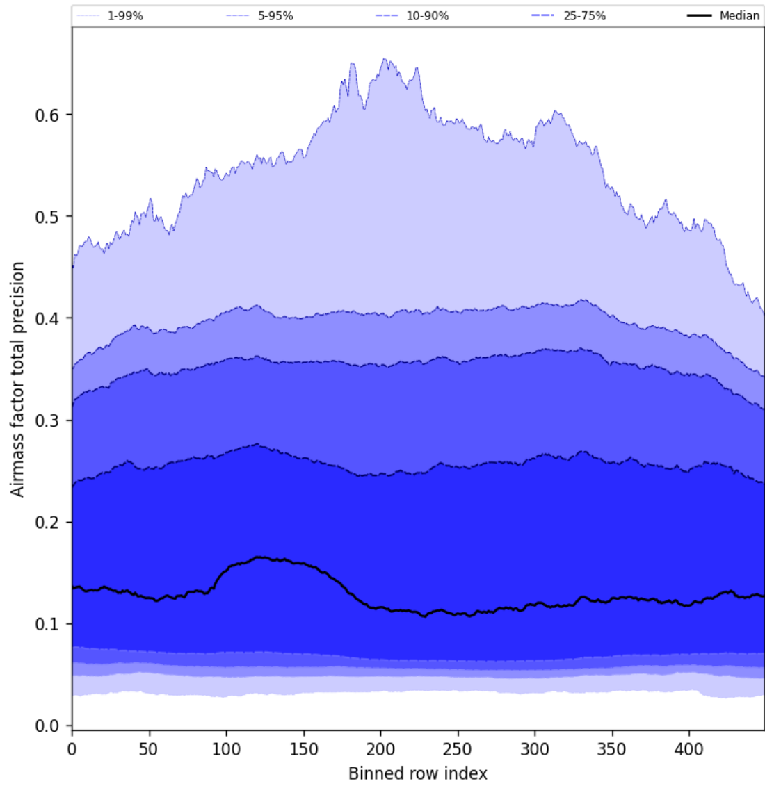
Figure 55: Along track statistics of “Airmass factor total precision” for 2024-11-09 to 2024-11-10
