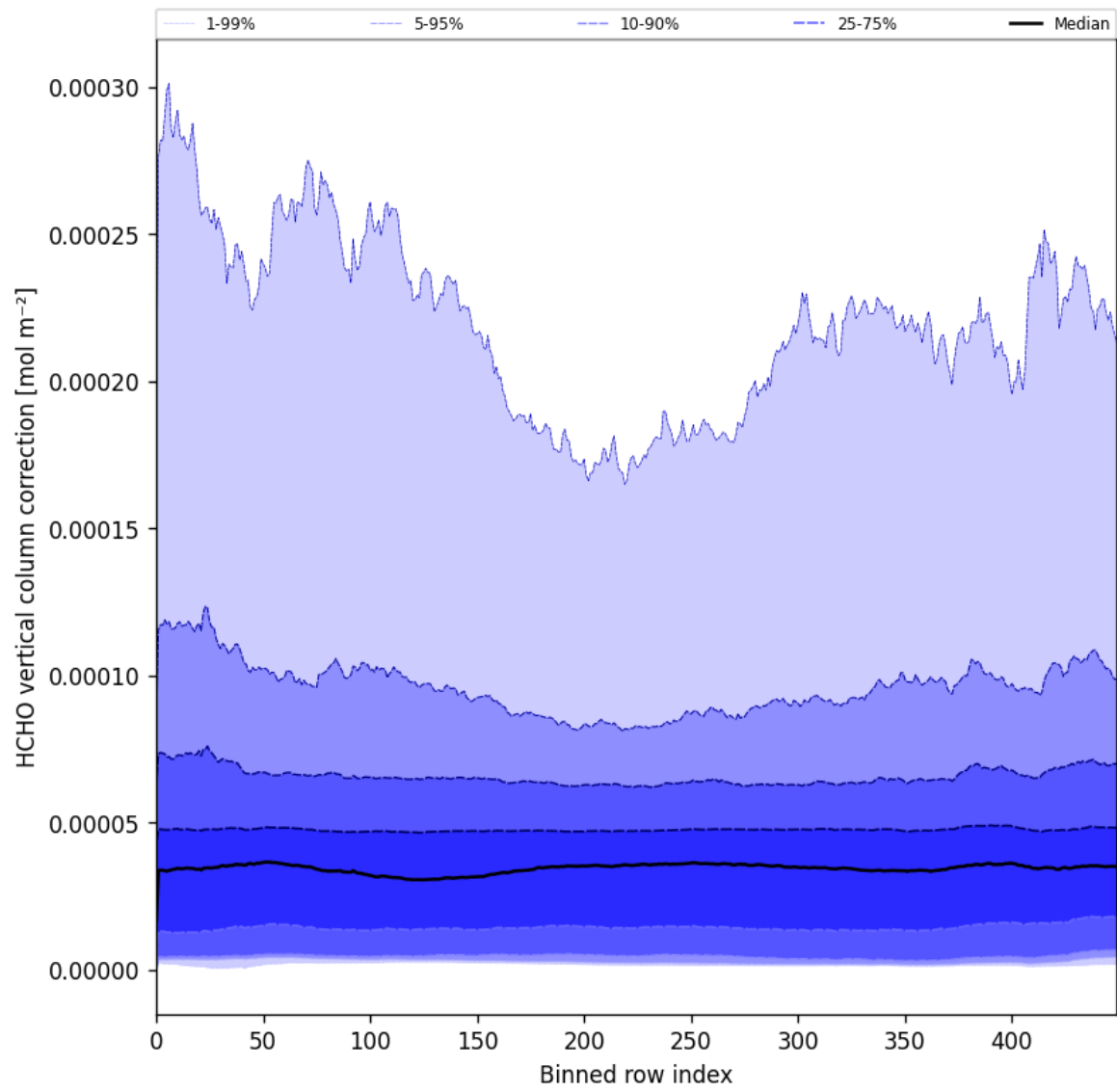
Figure 51: Along track statistics of “HCHO vertical column correction” for 2024-11-09 to 2024-11-10
