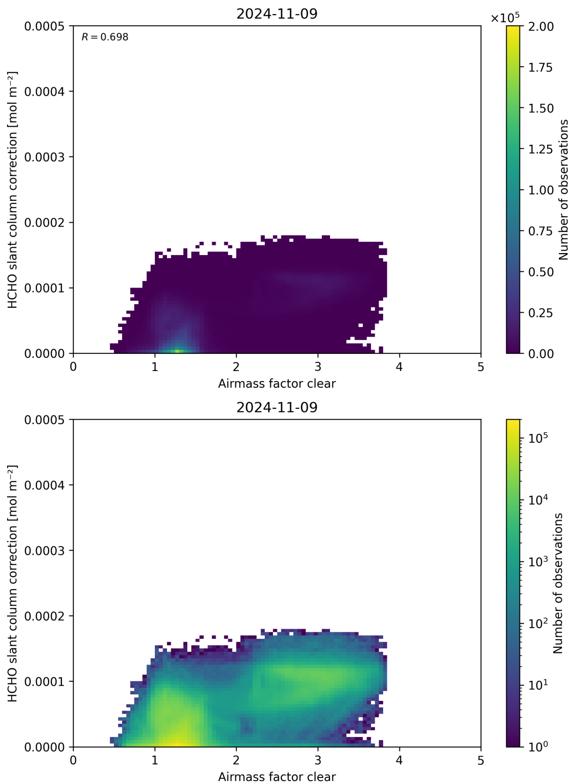
Figure 75: Scatter density plot of “Airmass factor clear” against “HCHO slant column correction” for 2024-11-09 to 2024-11-10.
