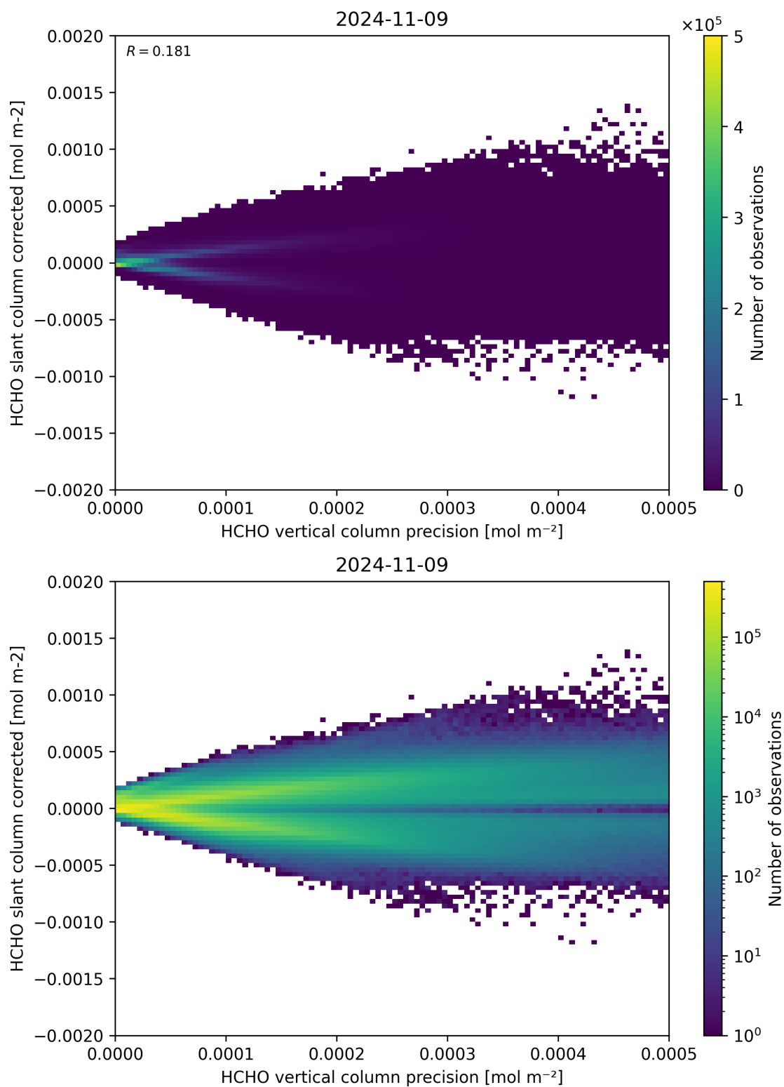
Figure 140: Scatter density plot of “HCHO vertical column precision” against “HCHO slant column corrected” for 2024-11-09 to 2024-11-10.
