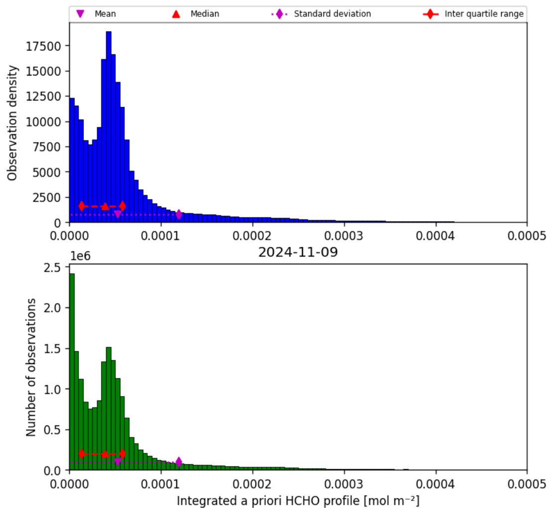
Figure 43: Histogram of “Integrated a priori HCHO profile” for 2024-11-09 to 2024-11-10
