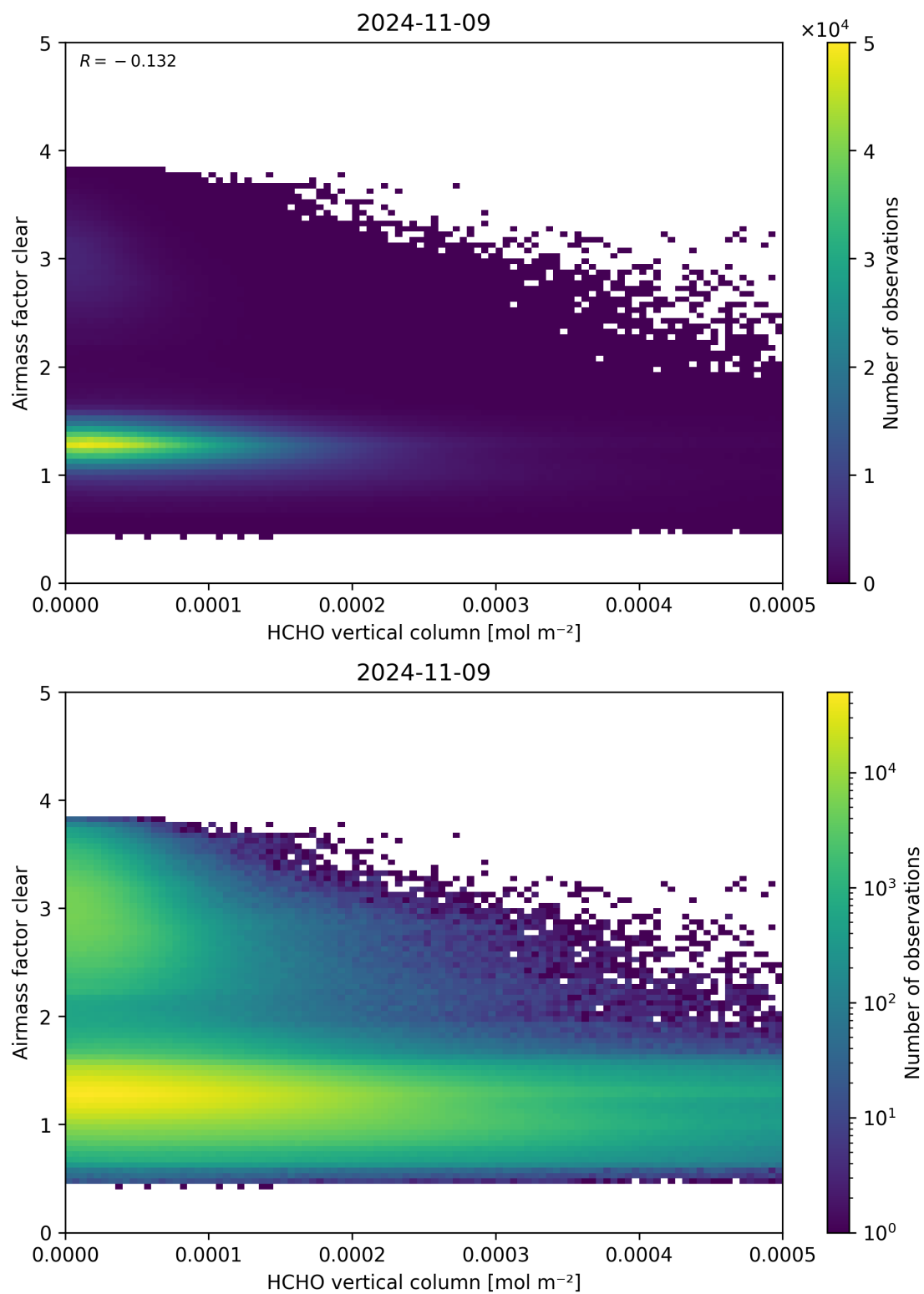
Figure 126: Scatter density plot of “HCHO vertical column” against “Airmass factor clear” for 2024-11-09 to 2024-11-10.
