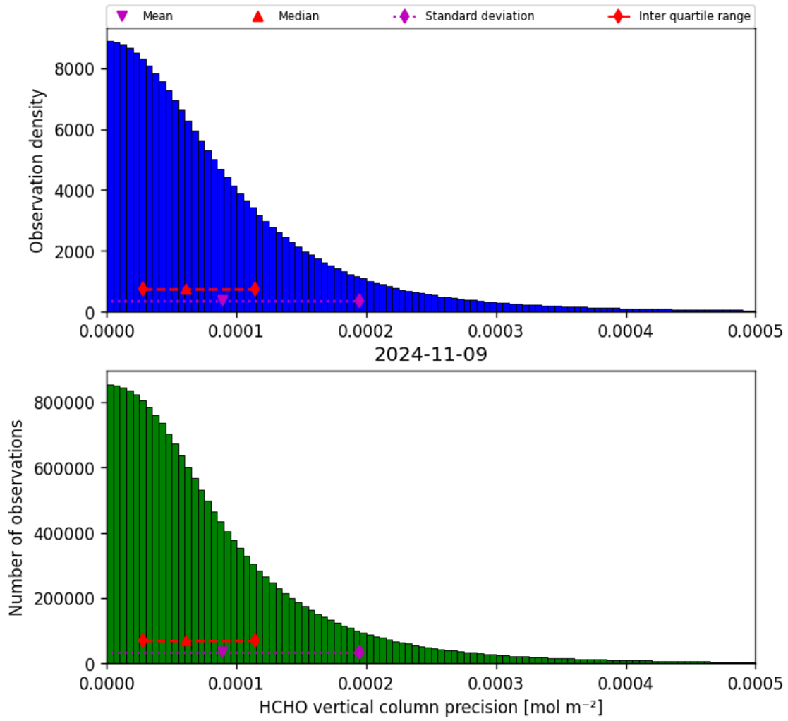
Figure 36: Histogram of “HCHO vertical column precision” for 2024-11-09 to 2024-11-10
