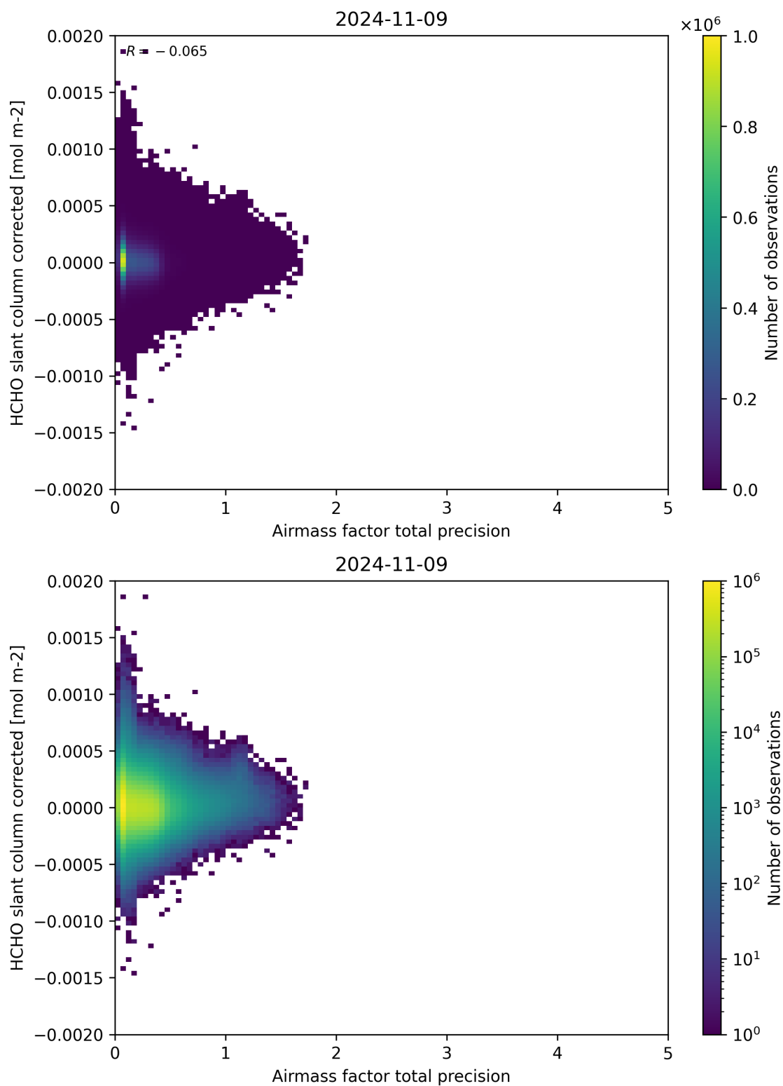
Figure 109: Scatter density plot of “Airmass factor total precision” against “HCHO slant column corrected” for 2024-11-09 to 2024-11-10.
