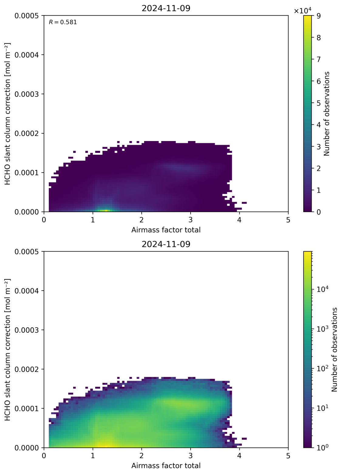
Figure 102: Scatter density plot of “Airmass factor total” against “HCHO slant column correction” for 2024-11-09 to 2024-11-10.
