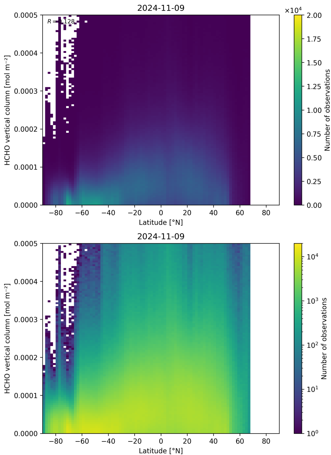
Figure 163: Scatter density plot of “Latitude” against “HCHO vertical column” for 2024-11-09 to 2024-11-10.
