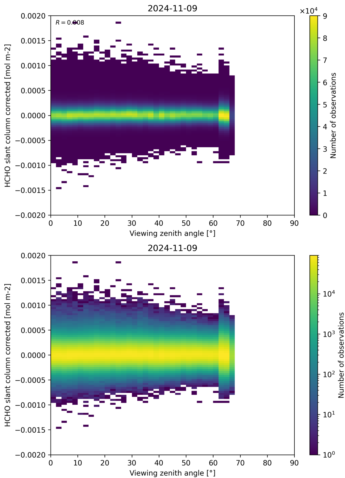
Figure 186: Scatter density plot of “Viewing zenith angle” against “HCHO slant column corrected” for 2024-11-09 to 2024-11-10.
