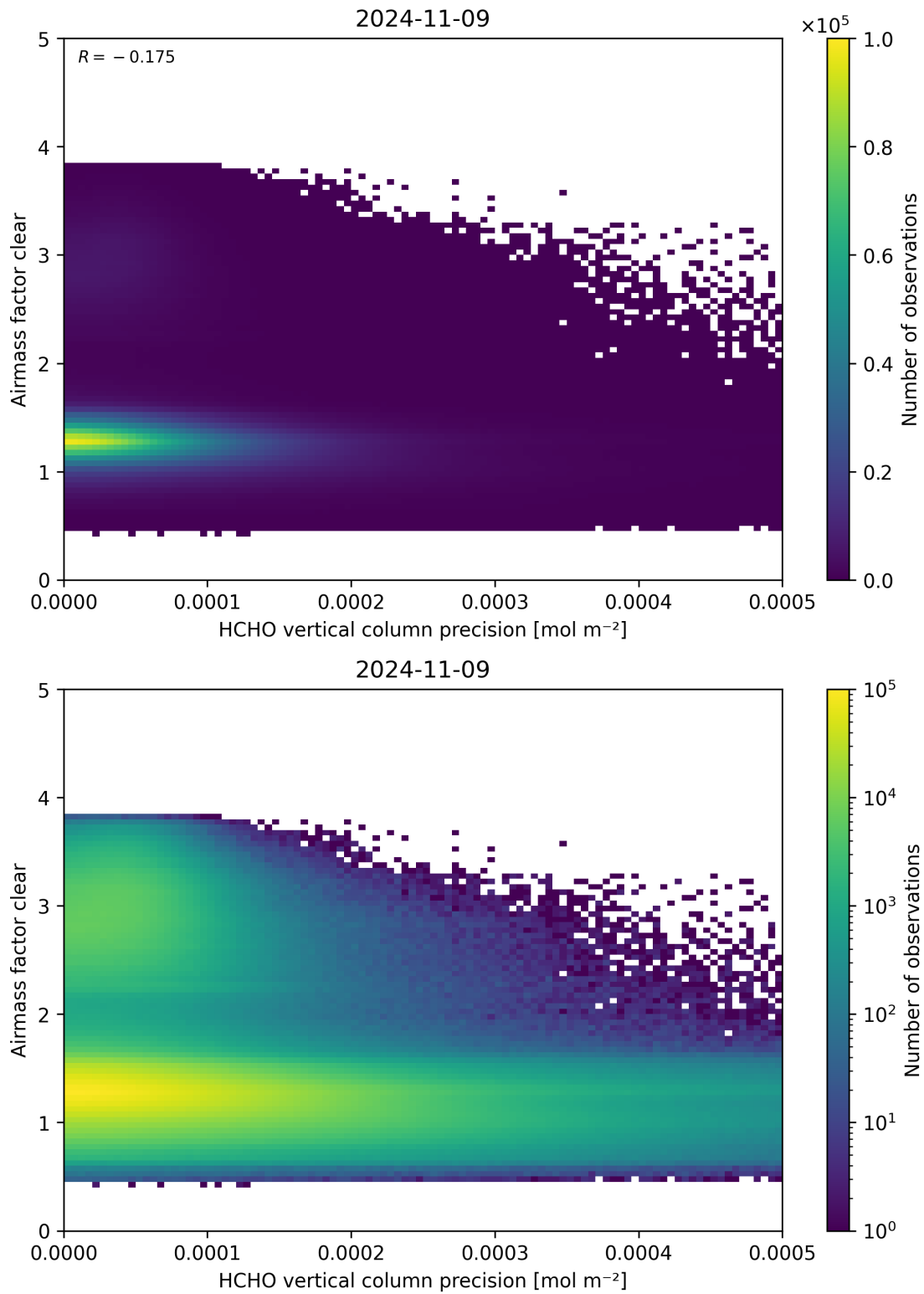
Figure 139: Scatter density plot of “HCHO vertical column precision” against “Airmass factor clear” for 2024-11-09 to 2024-11-10.
