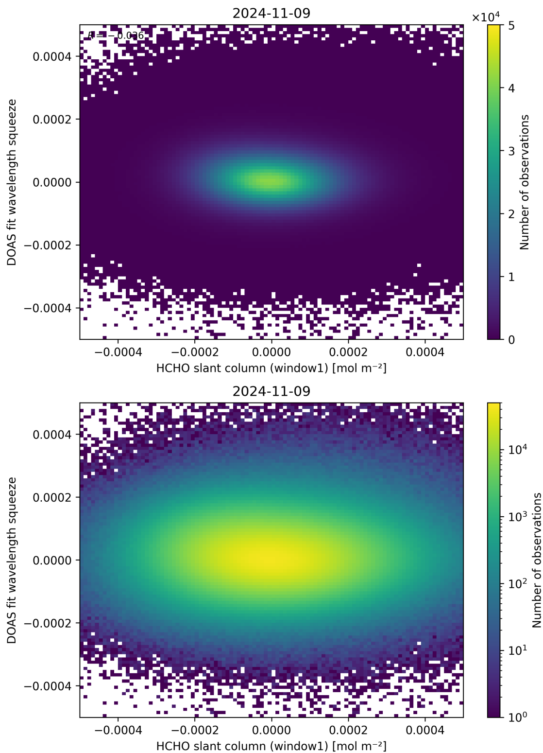
Figure 80: Scatter density plot of “HCHO slant column (window1)” against “DOAS fit wavelength squeeze” for 2024-11-09 to 2024-11-10.
