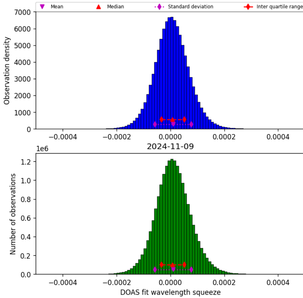
Figure 45: Histogram of “DOAS fit wavelength squeeze” for 2024-11-09 to 2024-11-10
