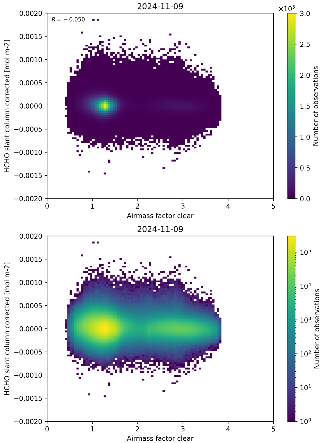
Figure 74: Scatter density plot of “Airmass factor clear” against “HCHO slant column corrected” for 2024-11-09 to 2024-11-10.
