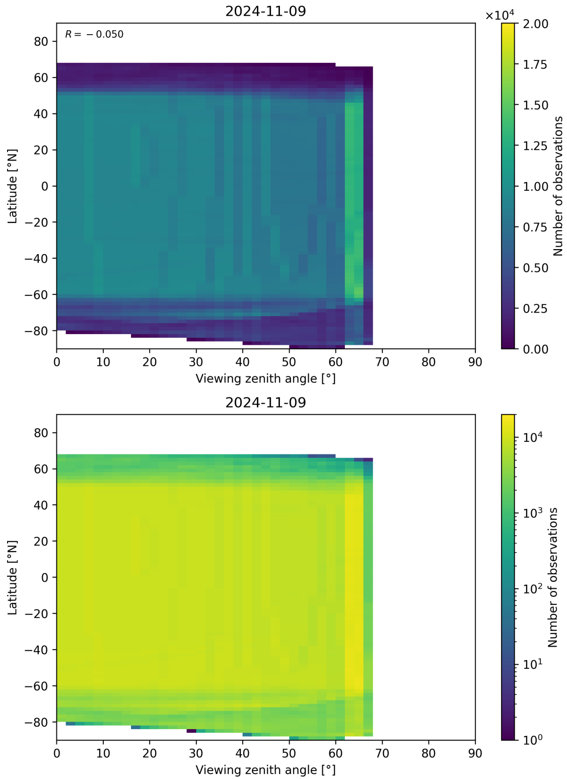
Figure 196: Scatter density plot of “Viewing zenith angle” against “Latitude” for 2024-11-09 to 2024-11-10.
