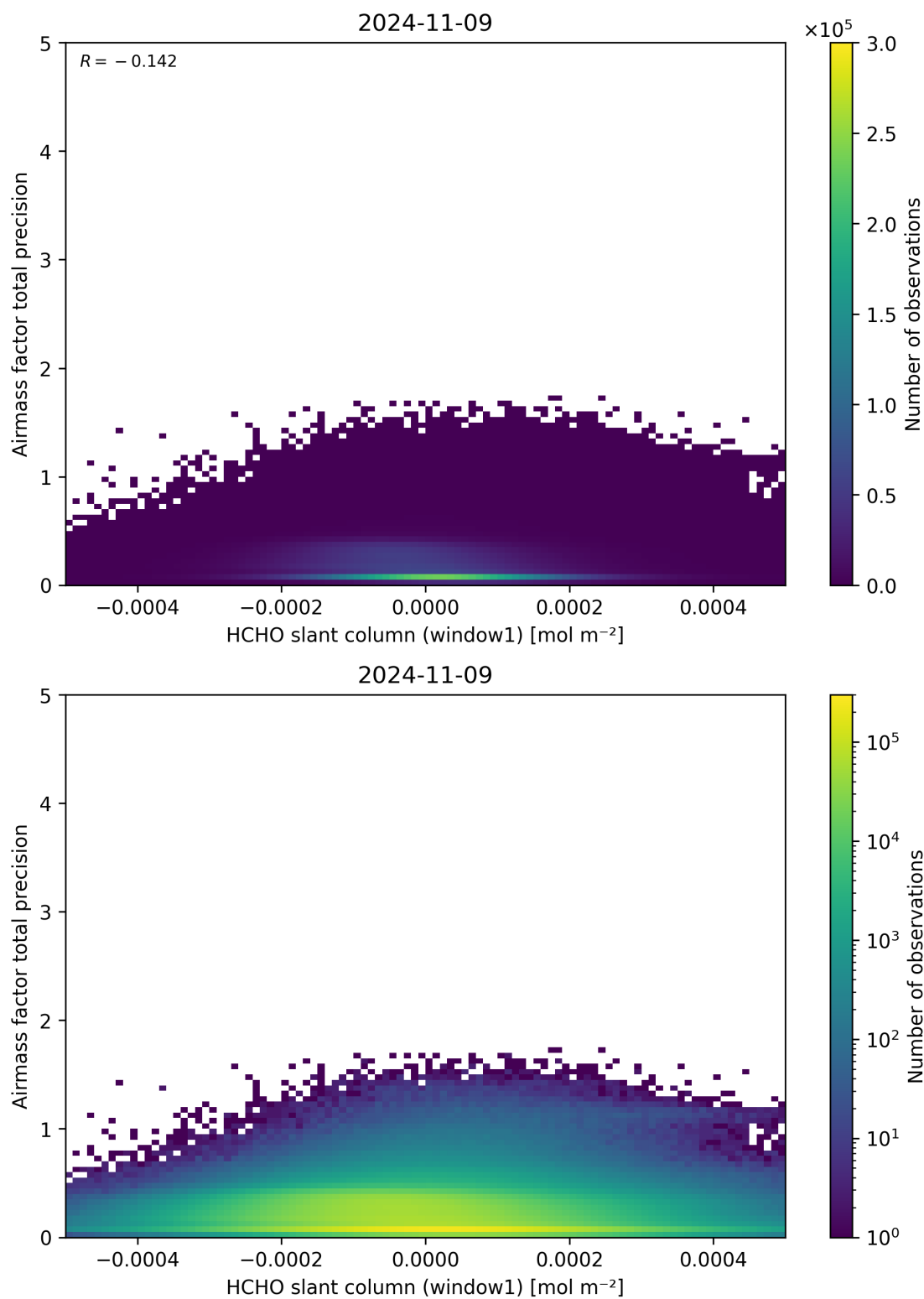
Figure 86: Scatter density plot of “HCHO slant column (window1)” against “Airmass factor total precision” for 2024-11-09 to 2024-11-10.
