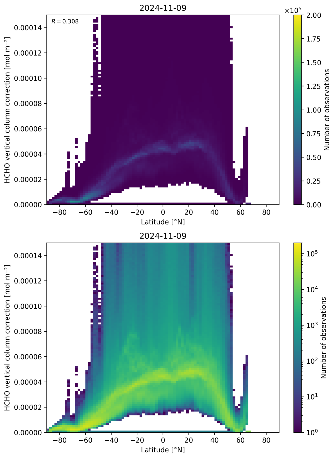
Figure 164: Scatter density plot of “Latitude” against “HCHO vertical column correction” for 2024-11-09 to 2024-11-10.
