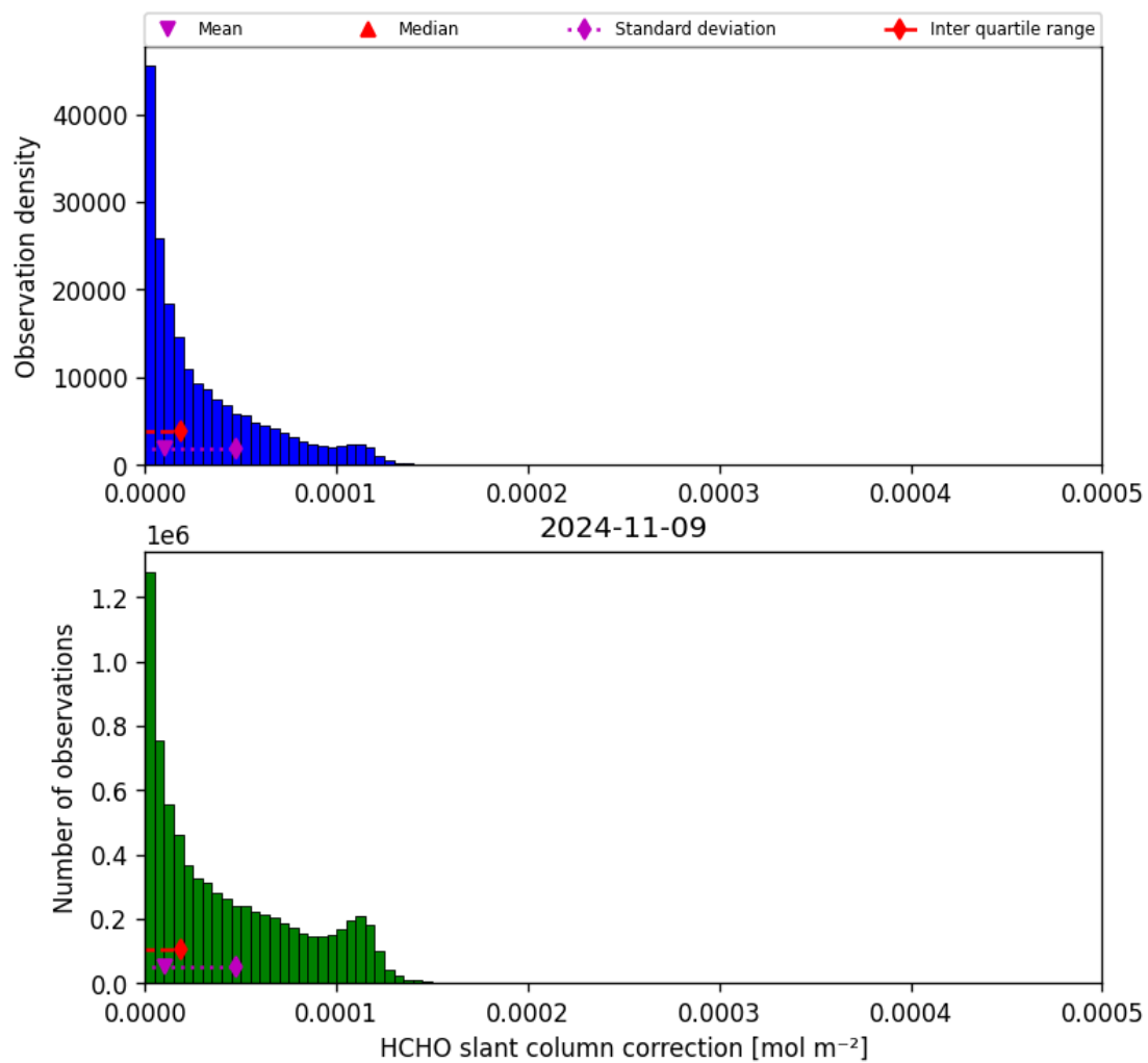
Figure 47: Histogram of “HCHO slant column correction” for 2024-11-09 to 2024-11-10
