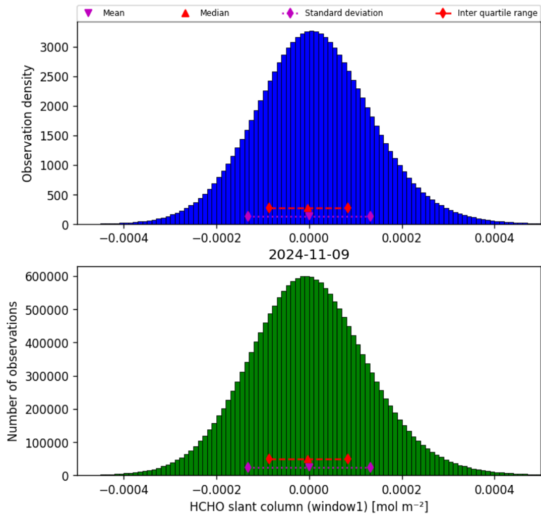
Figure 38: Histogram of “HCHO slant column (window1)” for 2024-11-09 to 2024-11-10
