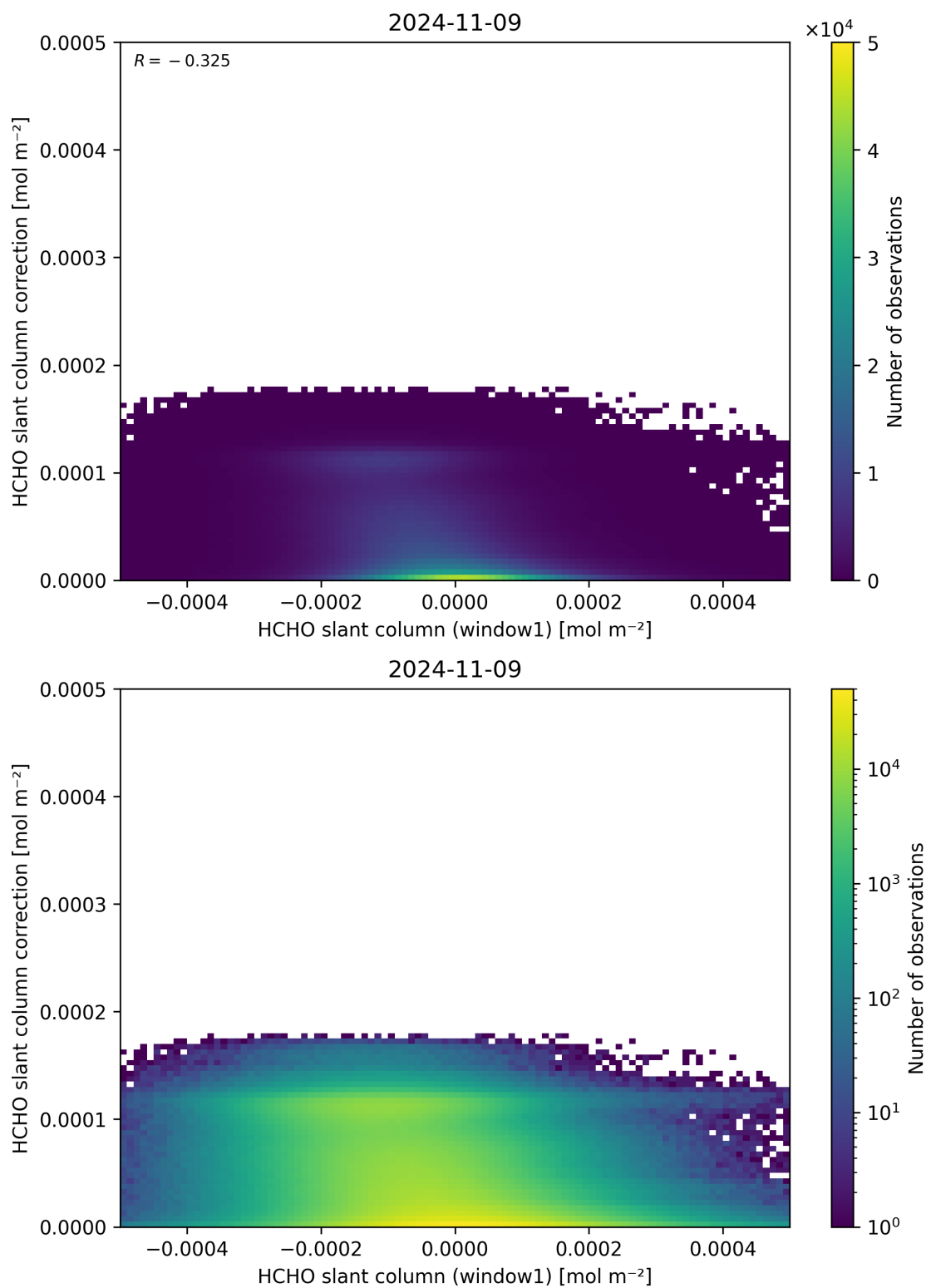
Figure 83: Scatter density plot of “HCHO slant column (window1)” against “HCHO slant column correction” for 2024-11-09 to 2024-11-10.
