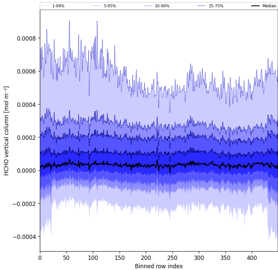
Figure 49: Along track statistics of “HCHO vertical column” for 2024-11-09 to 2024-11-10
