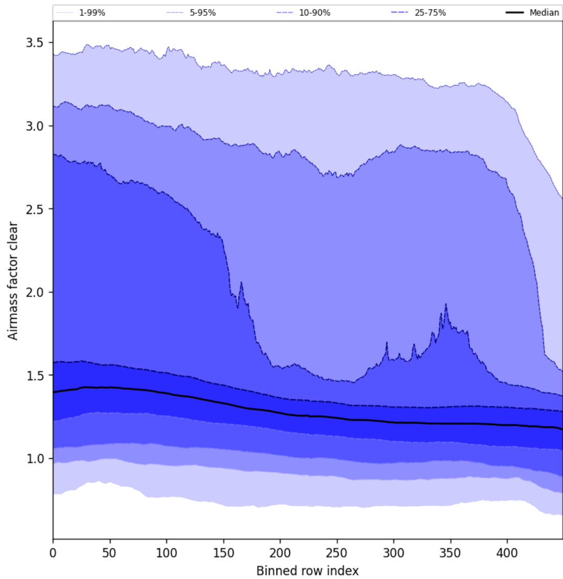
Figure 56: Along track statistics of “Air mass factor clear” for 2024-11-09 to 2024-11-10
