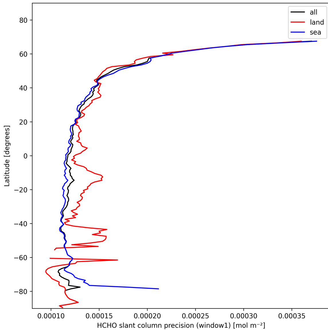
Figure 25: Zonal average of “HCHO slant column precision (window1)” for 2024-11-09 to 2024-11-10.
