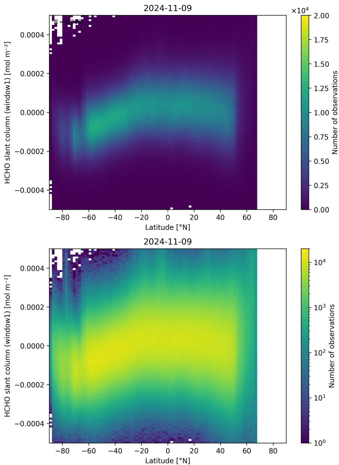
Figure 159: Scatter density plot of “Latitude” against “HCHO slant column (window1)” for 2024-11-09 to 2024-11-10.
