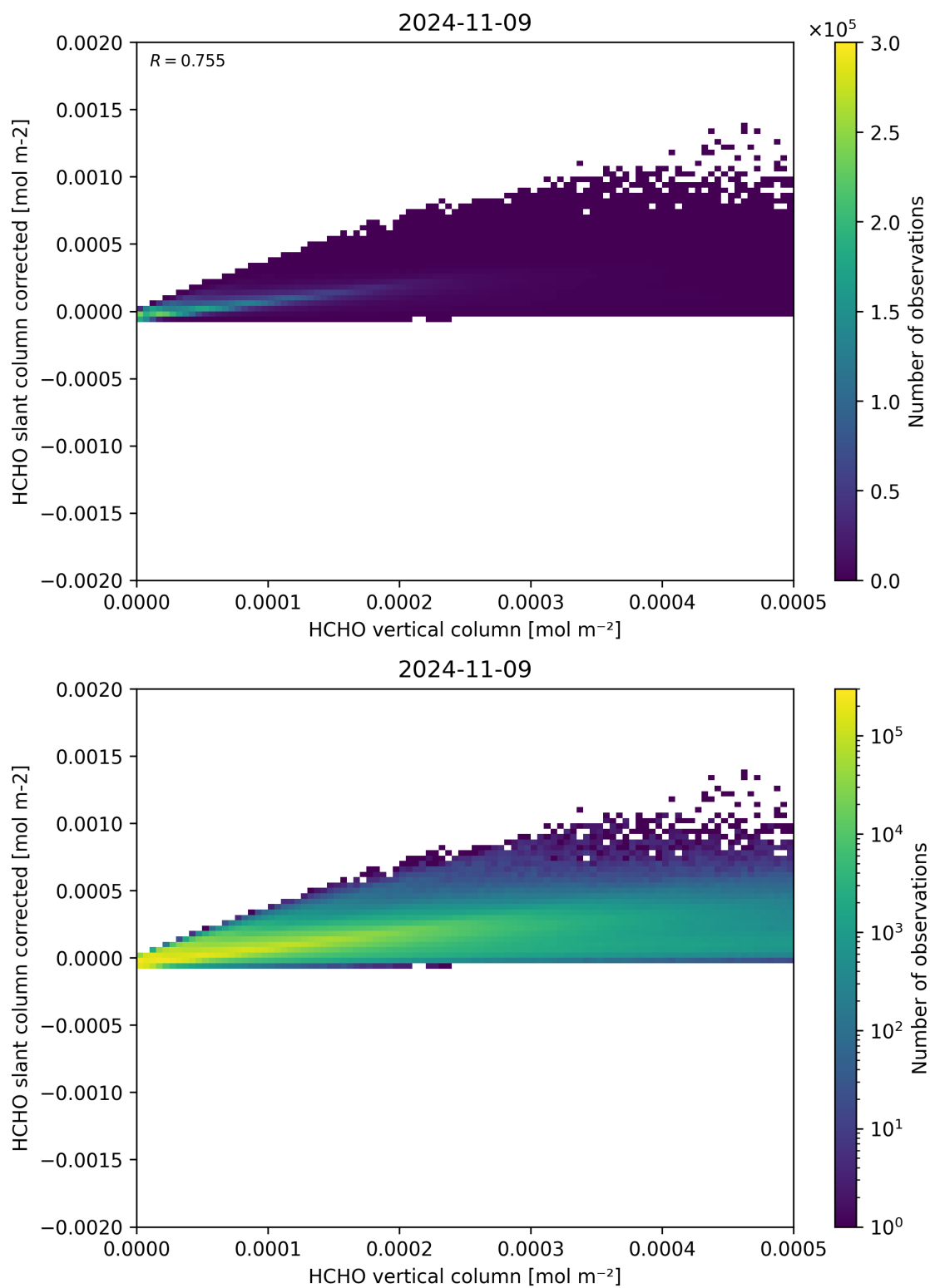
Figure 127: Scatter density plot of “HCHO vertical column” against “HCHO slant column corrected” for 2024-11-09 to 2024-11-10.
