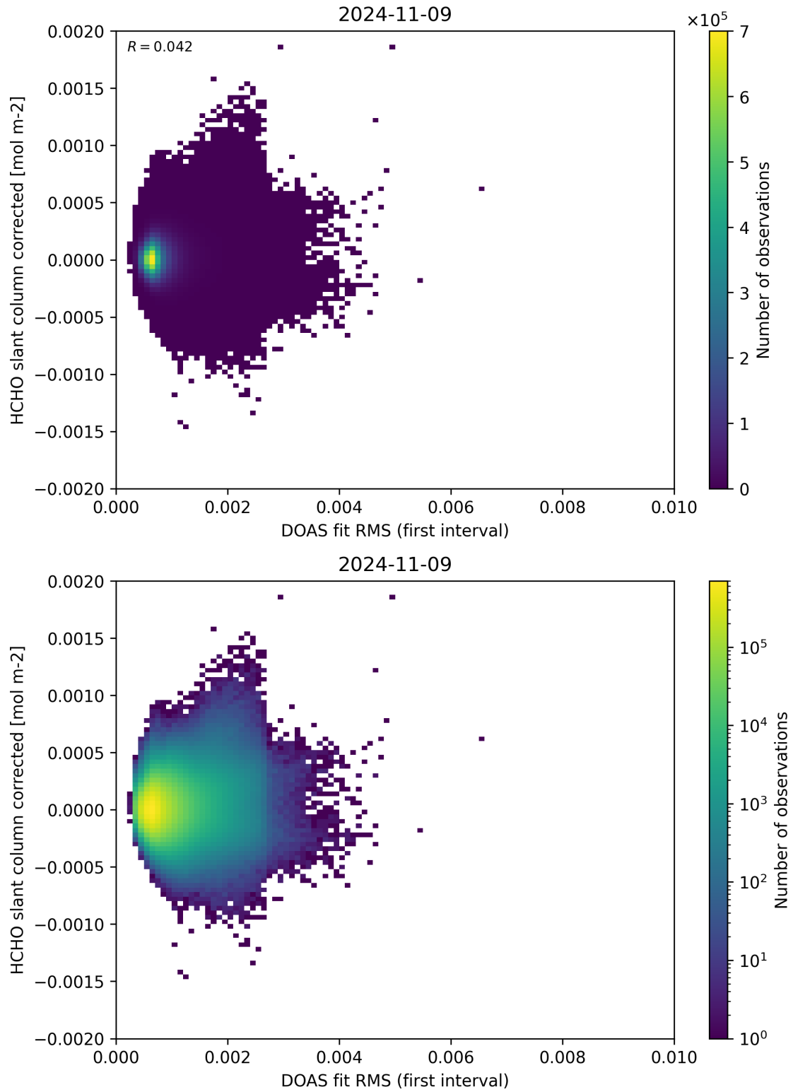
Figure 62: Scatter density plot of “DOAS fit RMS (first interval)” against “HCHO slant column corrected” for 2024-11-09 to 2024-11-10.
