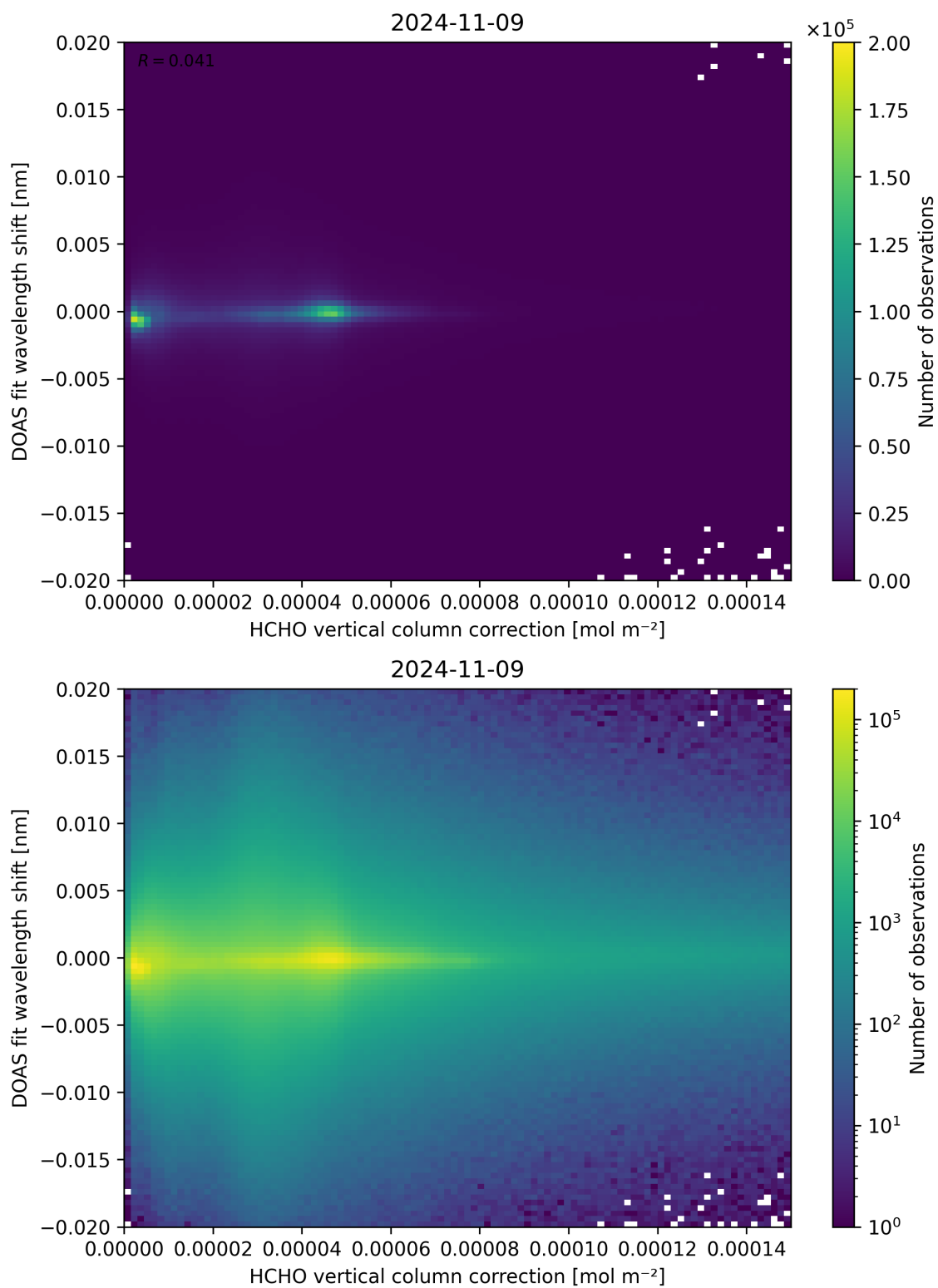
Figure 113: Scatter density plot of “HCHO vertical column correction” against “DOAS fit wavelength shift” for 2024-11-09 to 2024-11-10.
