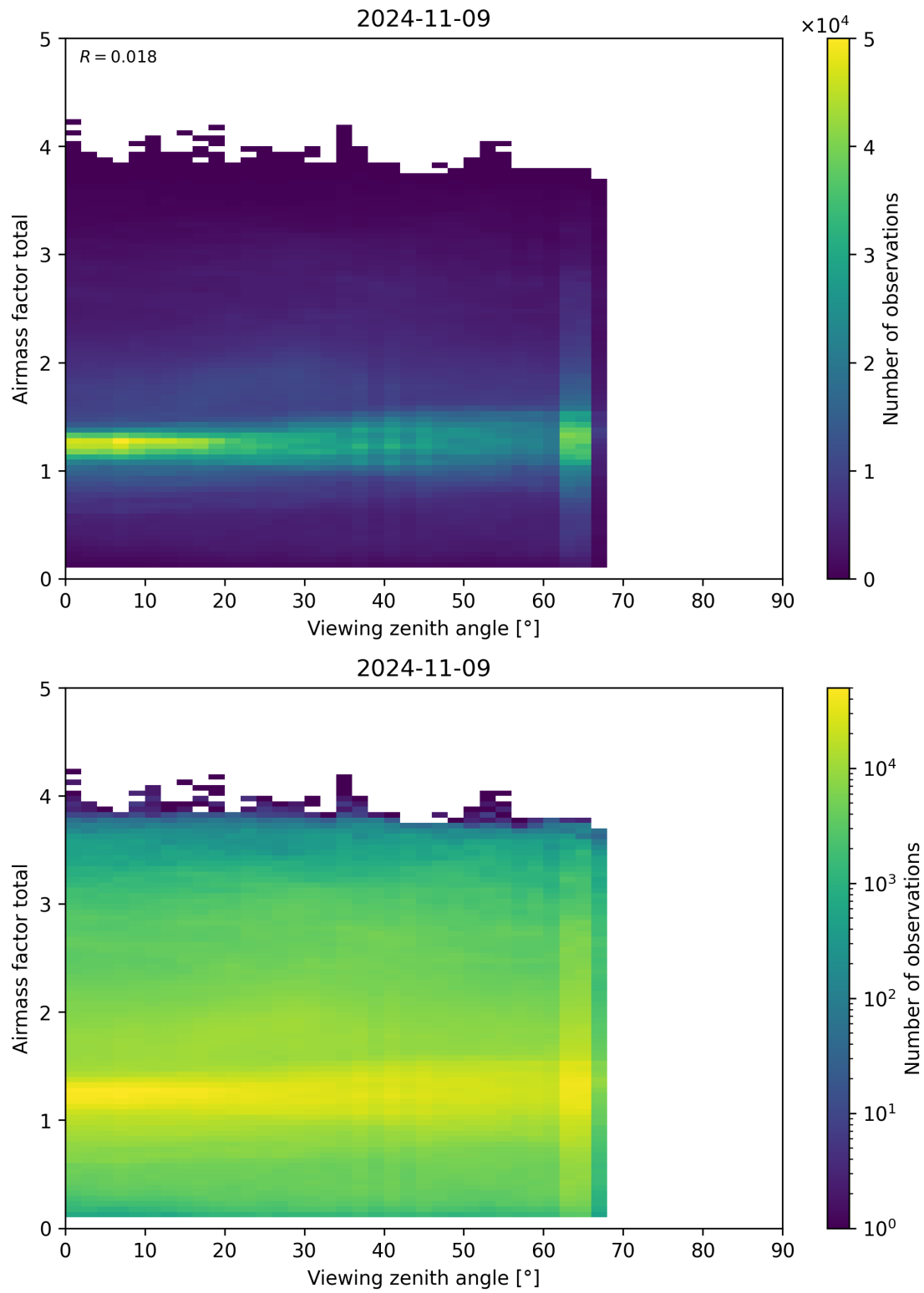
Figure 190: Scatter density plot of “Viewing zenith angle” against “Airmass factor total” for 2024-11-09 to 2024-11-10.
