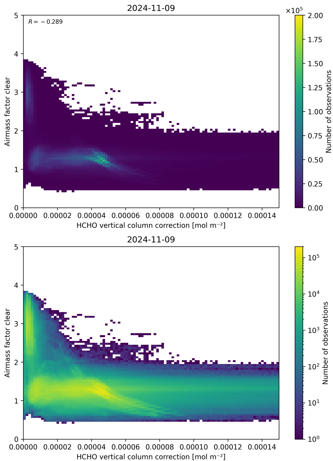
Figure 115: Scatter density plot of “HCHO vertical column correction” against “Airmass factor clear” for 2024-11-09 to 2024-11-10.
