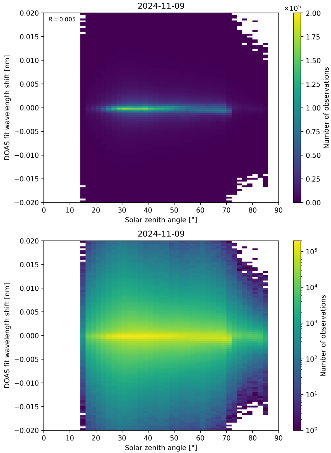
Figure 168: Scatter density plot of “Solar zenith angle” against “DOAS fit wavelength shift” for 2024-11-09 to 2024-11-10.
