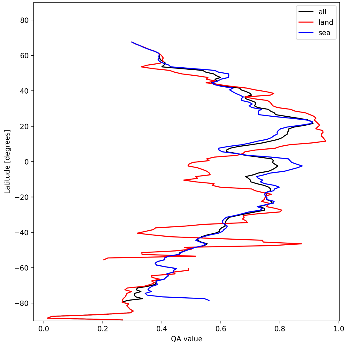
Figure 20: Zonal average of “QA value” for 2024-11-09 to 2024-11-10.
