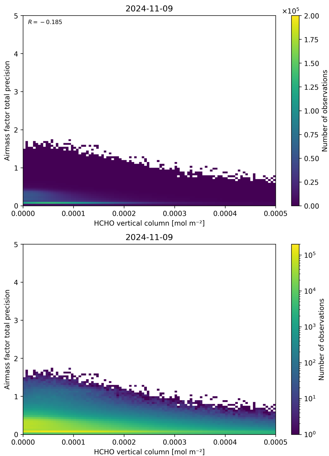
Figure 132: Scatter density plot of “HCHO vertical column” against “Airmass factor total precision” for 2024-11-09 to 2024-11-10.
