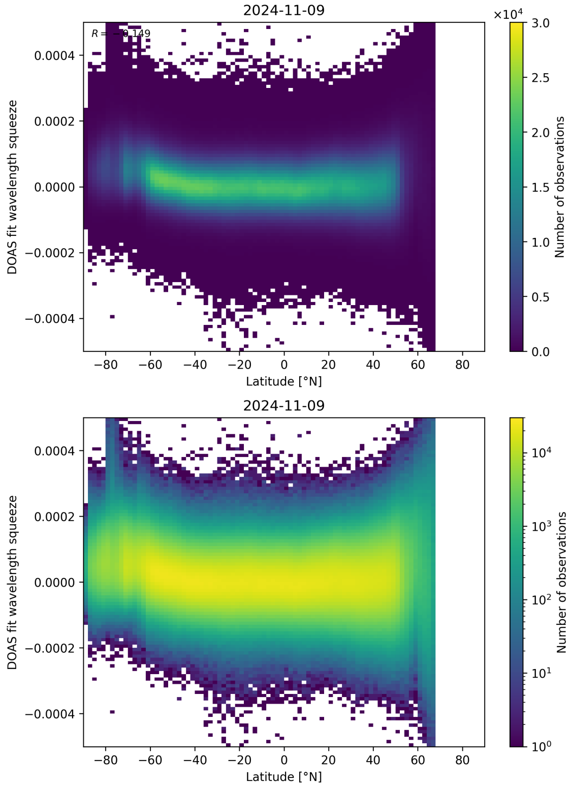
Figure 155: Scatter density plot of “Latitude” against “DOAS fit wavelength squeeze” for 2024-11-09 to 2024-11-10.
