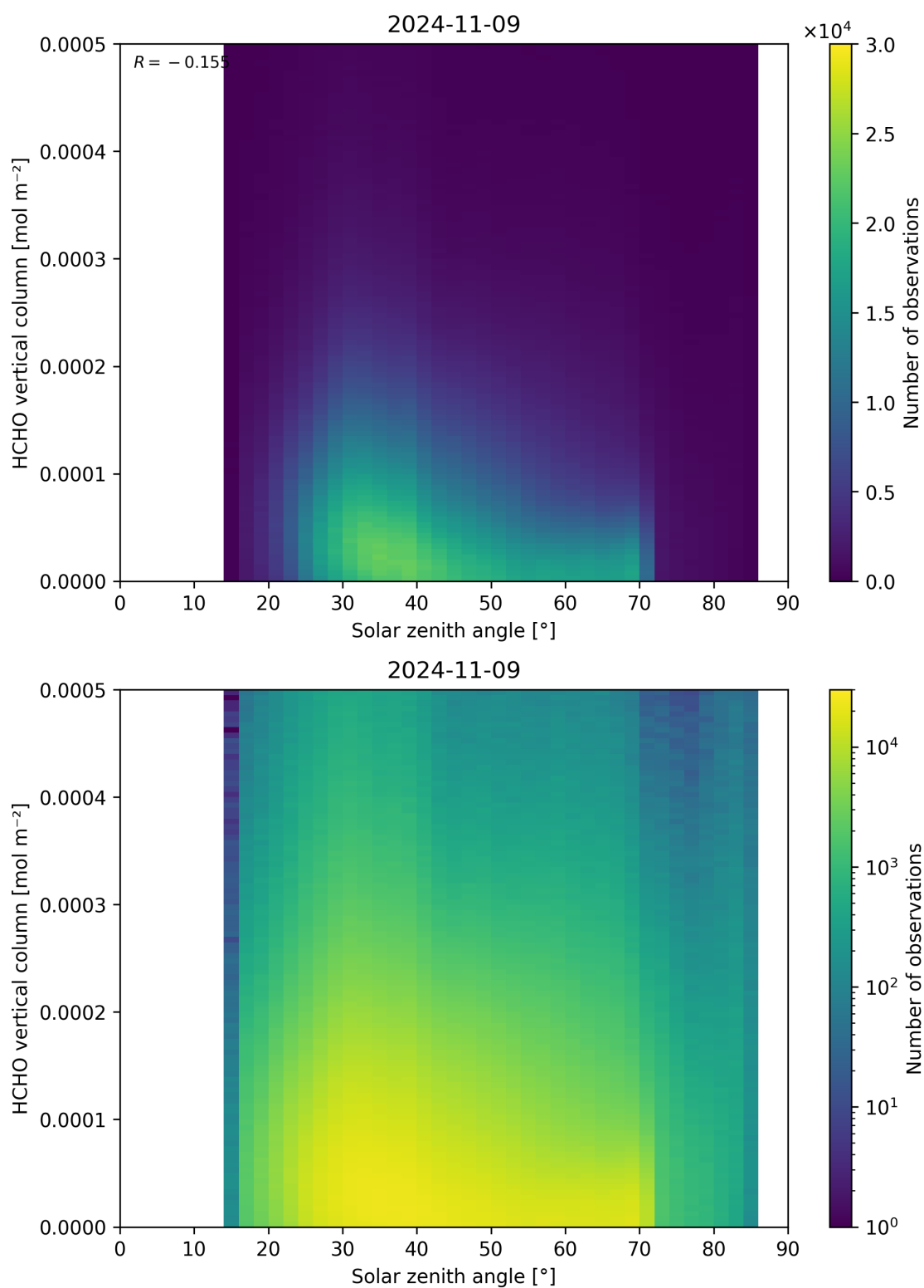
Figure 177: Scatter density plot of “Solar zenith angle” against “HCHO vertical column” for 2024-11-09 to 2024-11-10.
