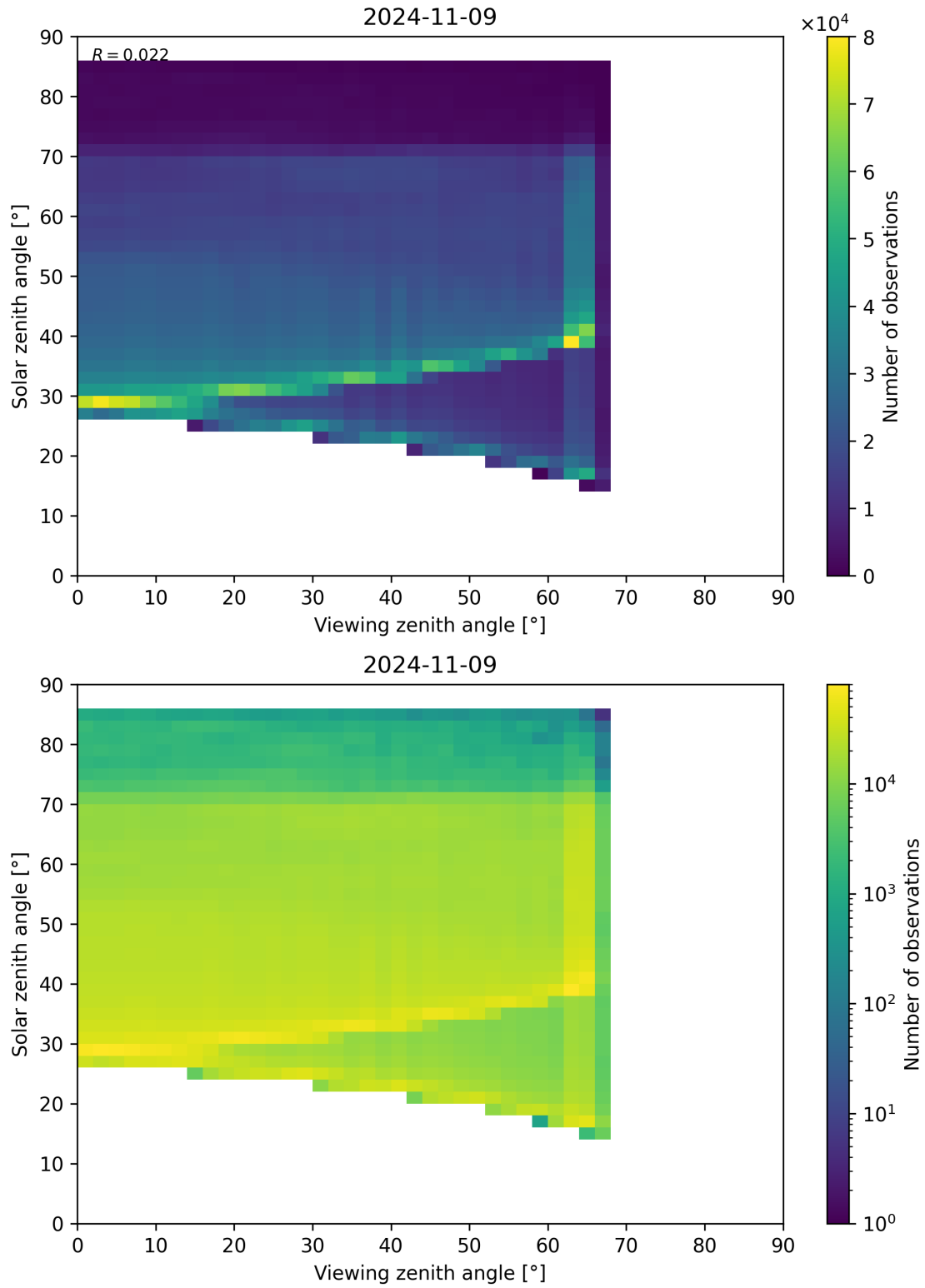
Figure 197: Scatter density plot of “Viewing zenith angle” against “Solar zenith angle” for 2024-11-09 to 2024-11-10.
