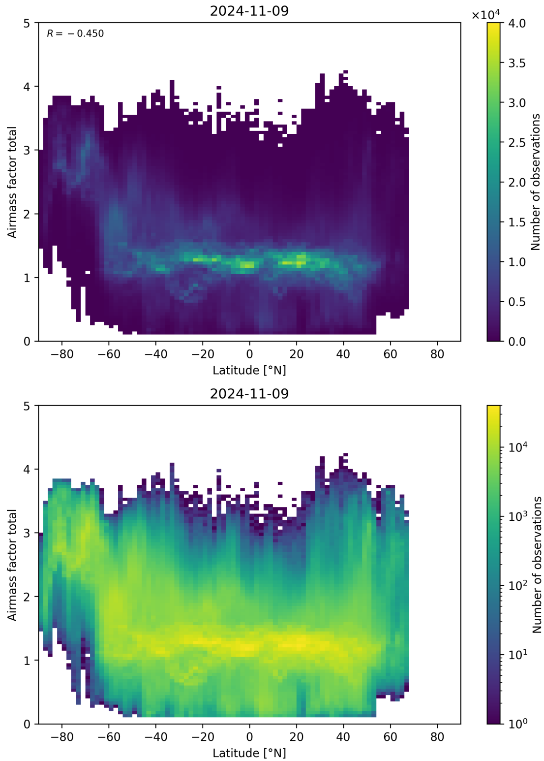
Figure 161: Scatter density plot of “Latitude” against “Airmass factor total” for 2024-11-09 to 2024-11-10.
