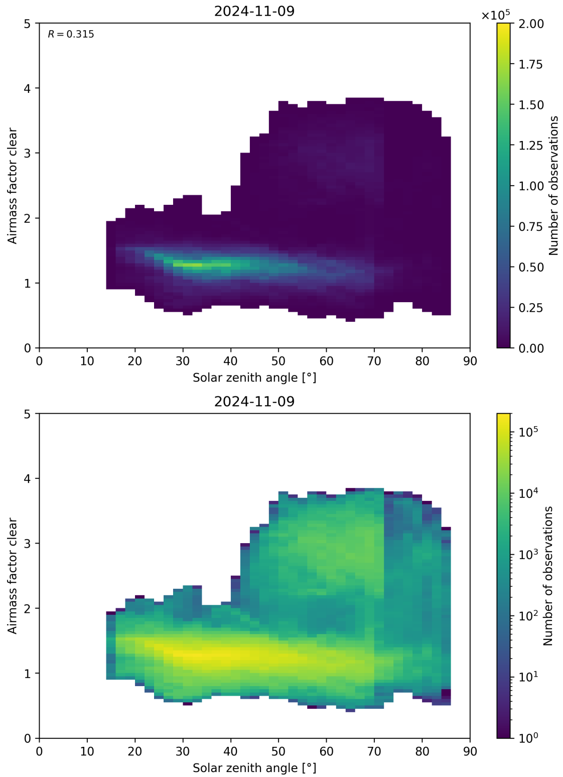
Figure 170: Scatter density plot of “Solar zenith angle” against “Airmass factor clear” for 2024-11-09 to 2024-11-10.
