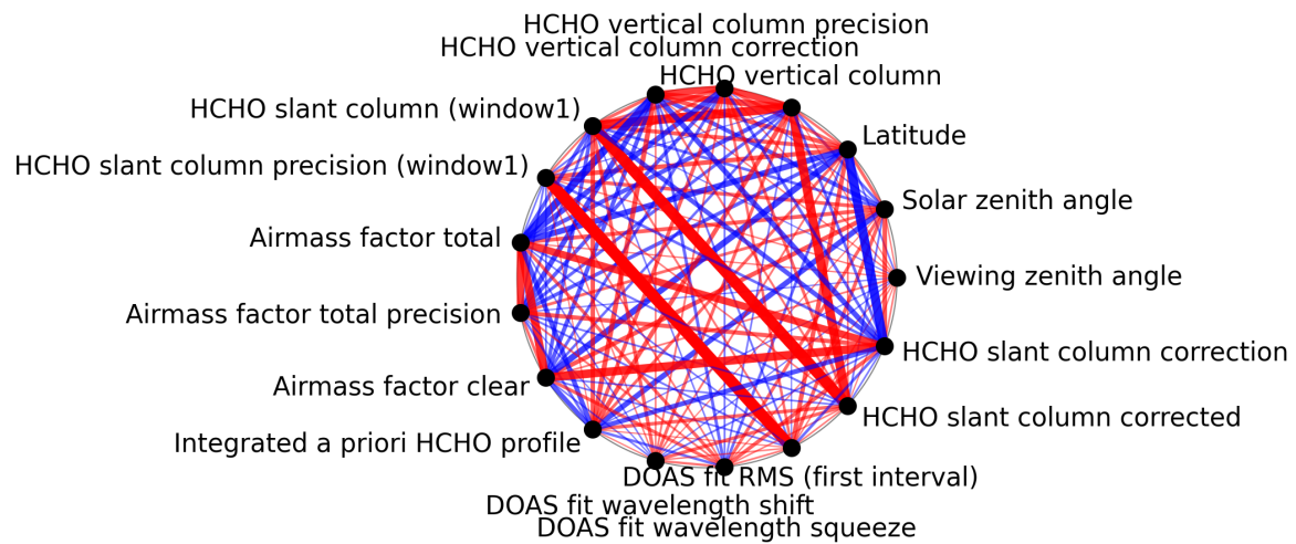
Figure 1: Map of correlation graph for 2024-11-09 to 2024-11-10.
