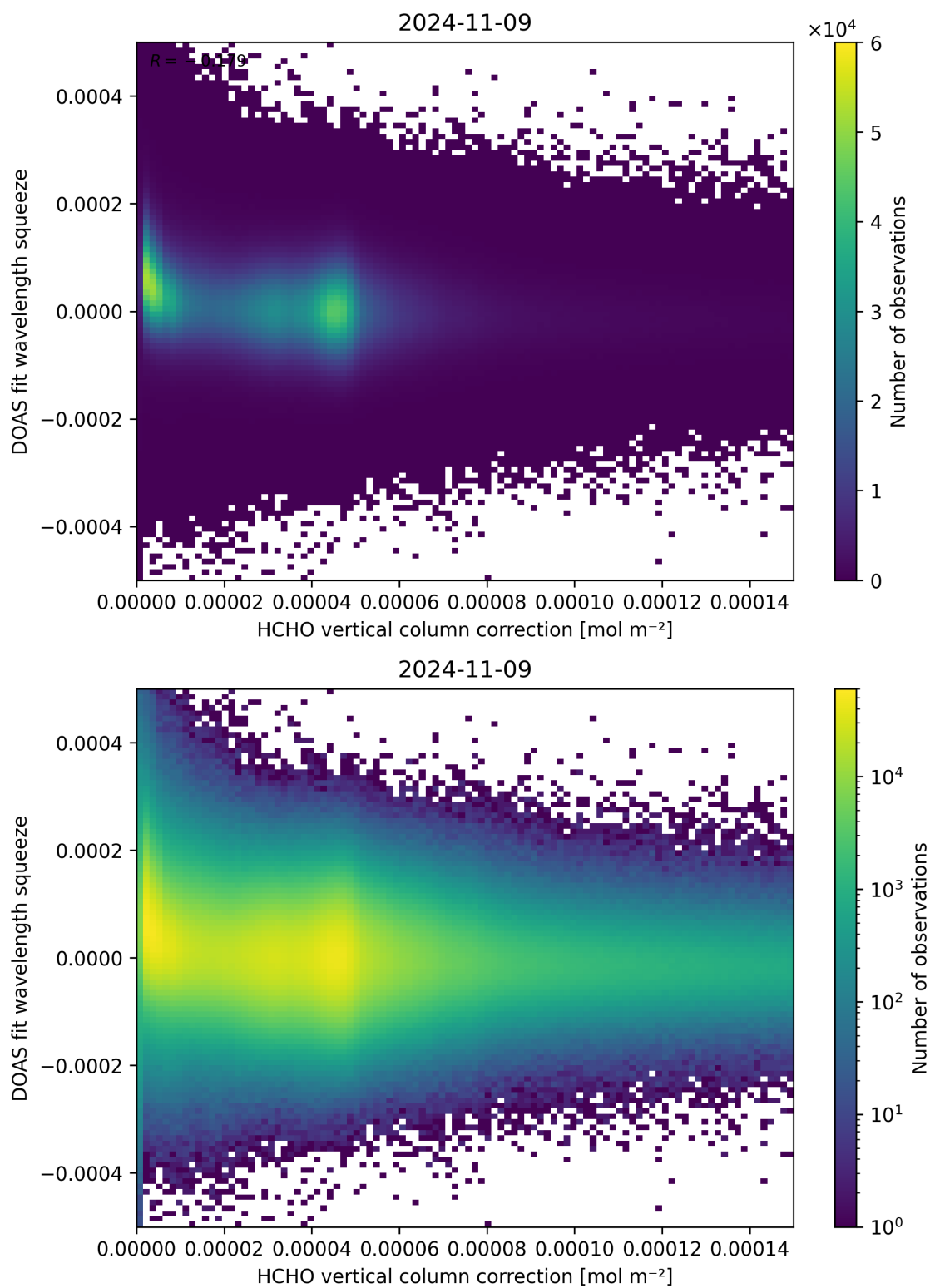
Figure 114: Scatter density plot of “HCHO vertical column correction” against “DOAS fit wavelength squeeze” for 2024-11-09 to 2024-11-10.
