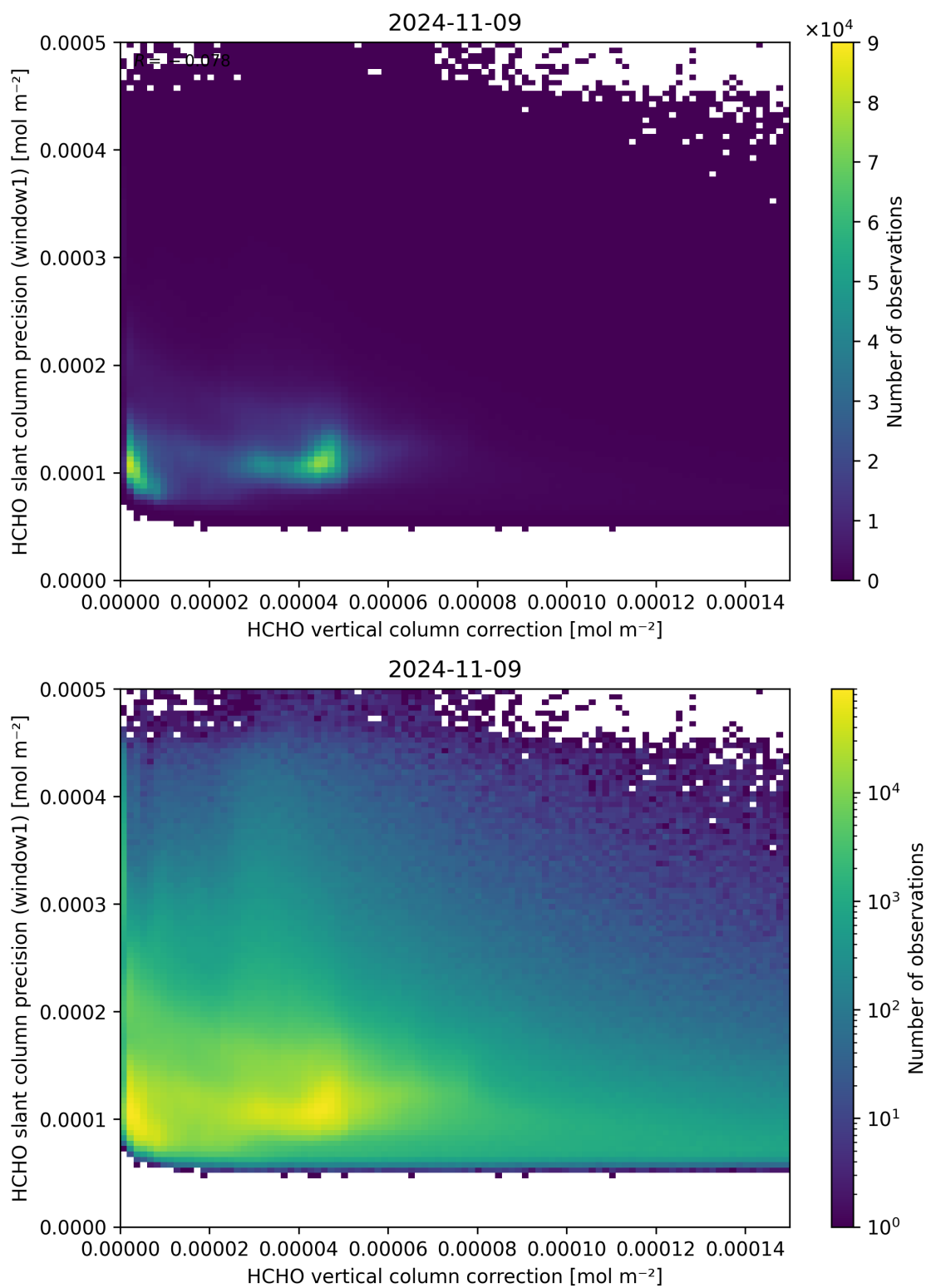
Figure 119: Scatter density plot of “HCHO vertical column correction” against “HCHO slant column precision (window1)” for 2024-11-09 to 2024-11-10.
