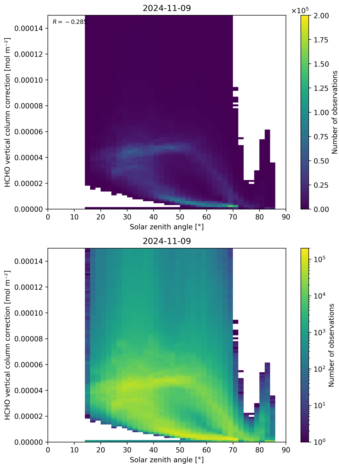
Figure 178: Scatter density plot of “Solar zenith angle” against “HCHO vertical column correction” for 2024-11-09 to 2024-11-10.
