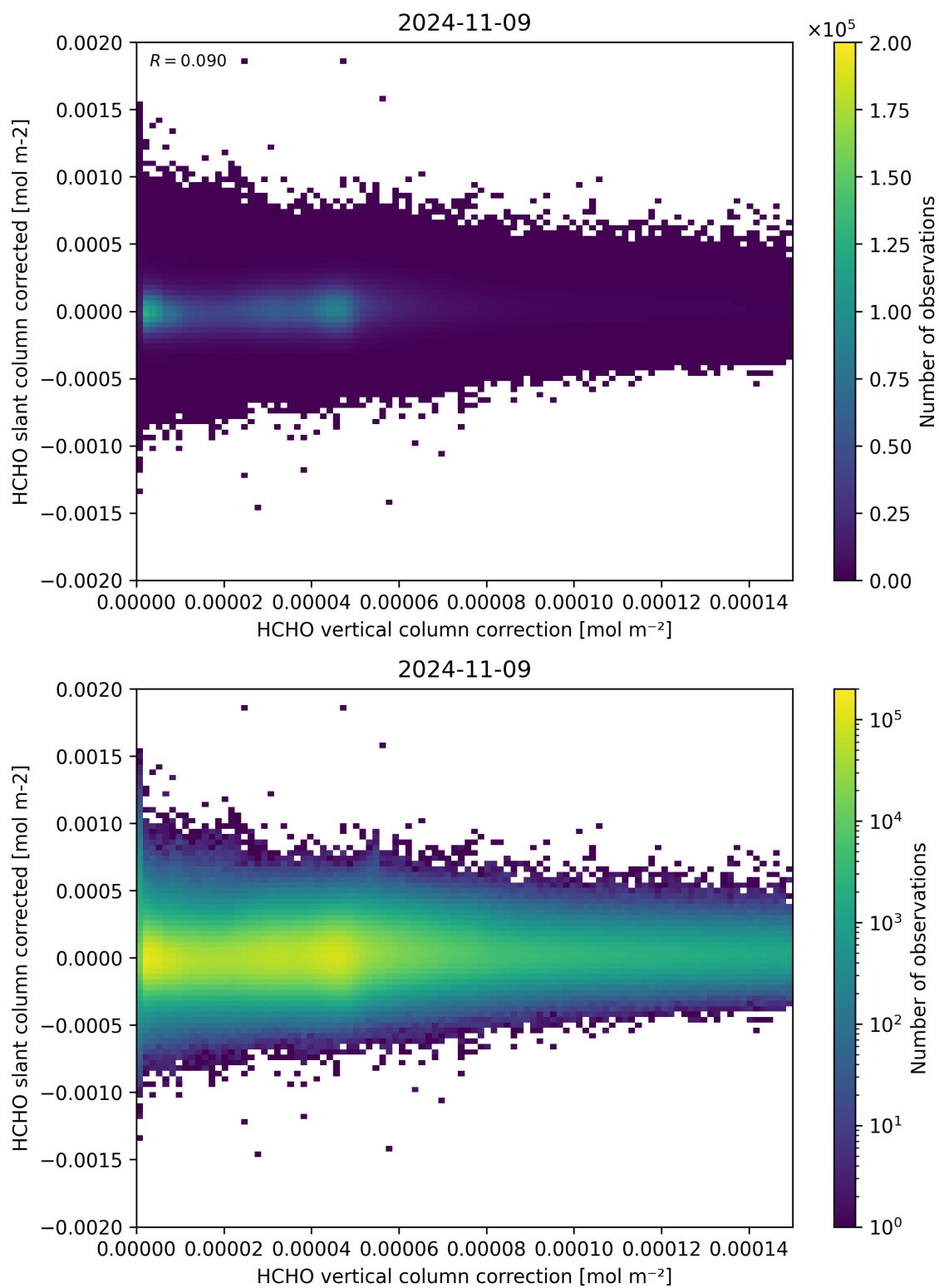
Figure 116: Scatter density plot of “HCHO vertical column correction” against “HCHO slant column corrected” for 2024-11-09 to 2024-11-10.
