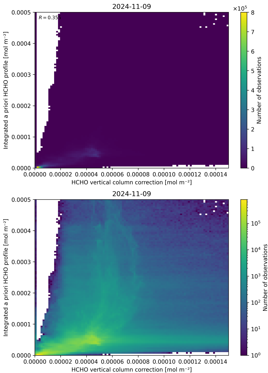
Figure 122: Scatter density plot of “HCHO vertical column correction” against “Integrated a priori HCHO profile” for 2024-11-09 to 2024-11-10.
