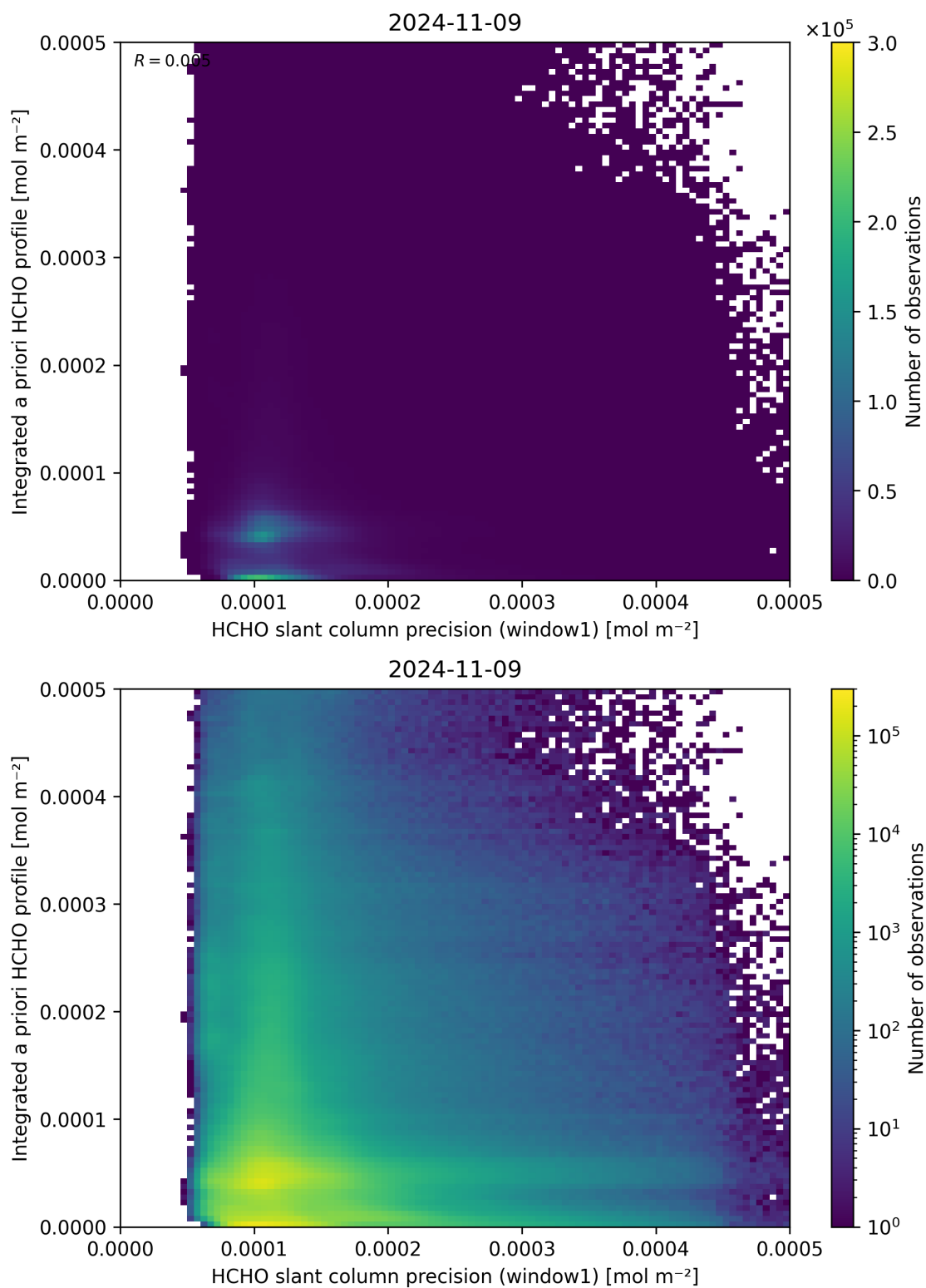
Figure 96: Scatter density plot of “HCHO slant column precision (window1)” against “Integrated a priori HCHO profile” for 2024-11-09 to 2024-11-10.
