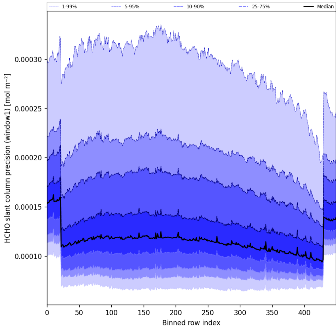
Figure 53: Along track statistics of “HCHO slant column precision (window1)” for 2024-11-09 to 2024-11-10
