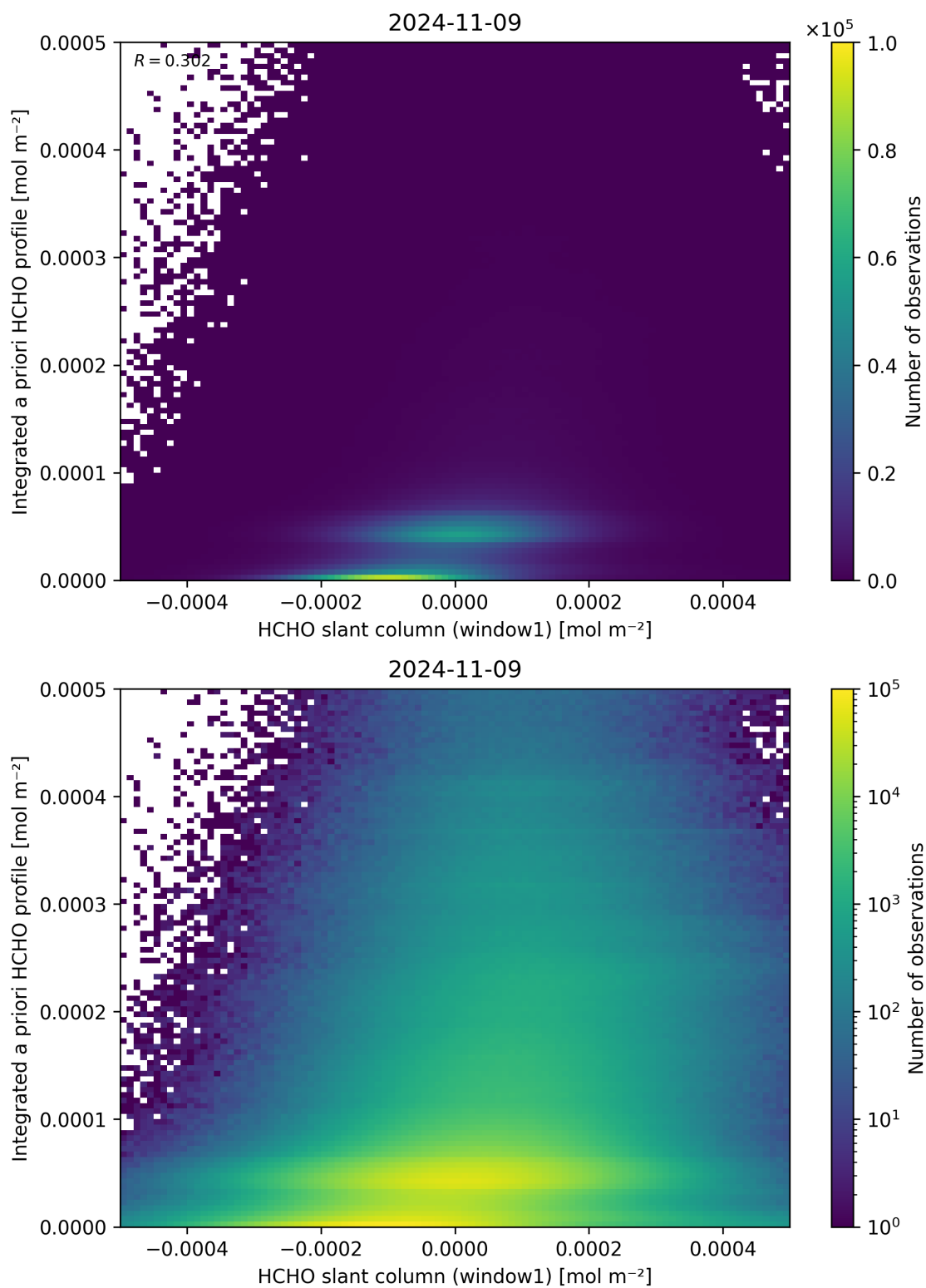
Figure 87: Scatter density plot of “HCHO slant column (window1)” against “Integrated a priori HCHO profile” for 2024-11-09 to 2024-11-10.
