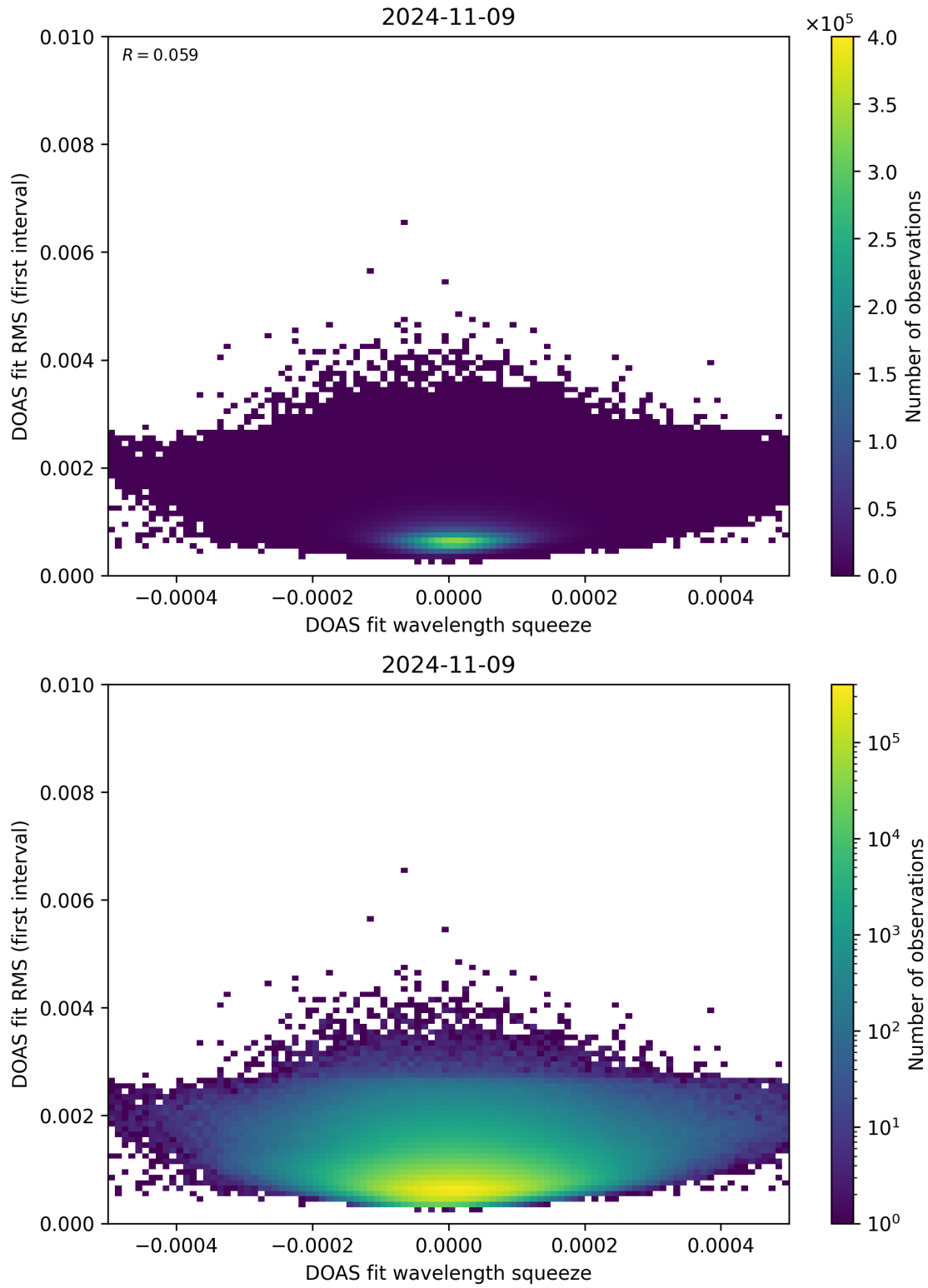
Figure 68: Scatter density plot of “DOAS fit wavelength squeeze” against “DOAS fit RMS (first interval)” for 2024-11-09 to 2024-11-10.
