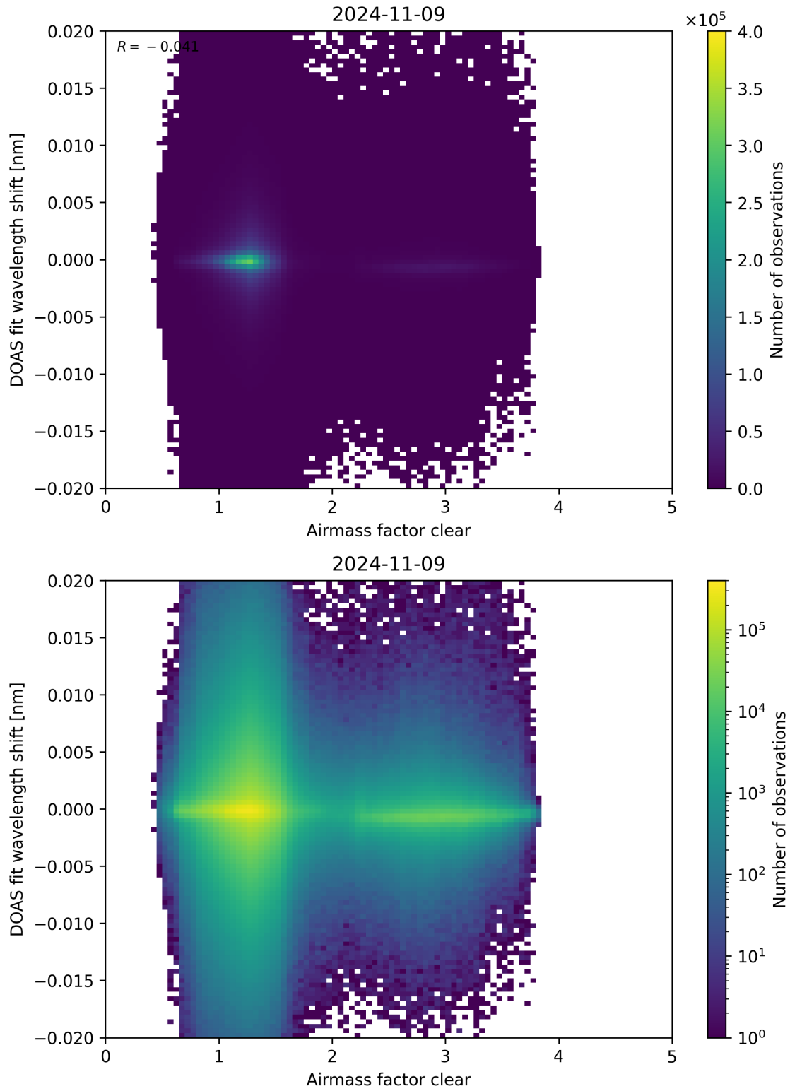
Figure 72: Scatter density plot of “Airmass factor clear” against “DOAS fit wavelength shift” for 2024-11-09 to 2024-11-10.
