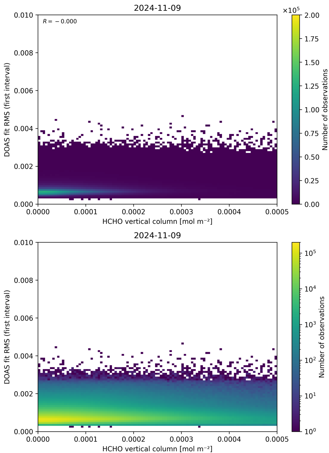
Figure 123: Scatter density plot of “HCHO vertical column” against “DOAS fit RMS (first interval)” for 2024-11-09 to 2024-11-10.
