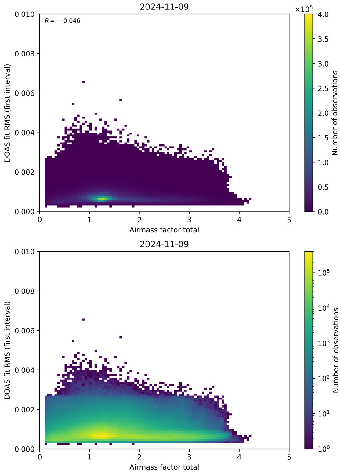
Figure 97: Scatter density plot of “Airmass factor total” against “DOAS fit RMS (first interval)” for 2024-11-09 to 2024-11-10.
