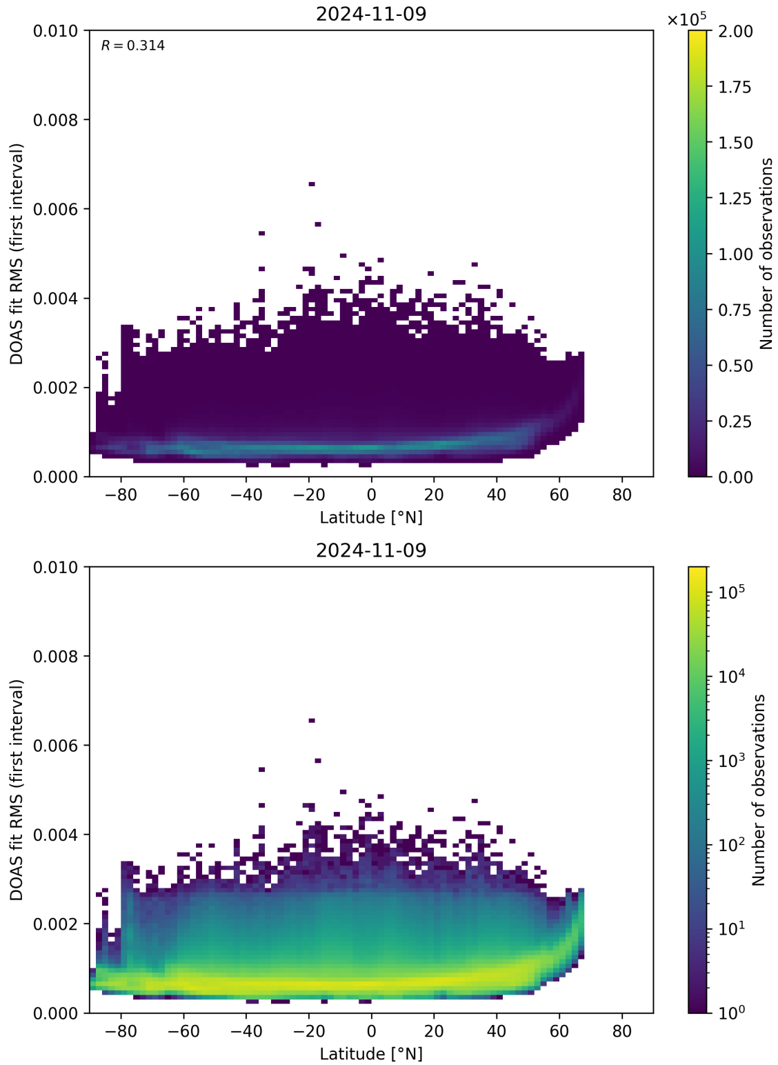
Figure 153: Scatter density plot of “Latitude” against “DOAS fit RMS (first interval)” for 2024-11-09 to 2024-11-10.
