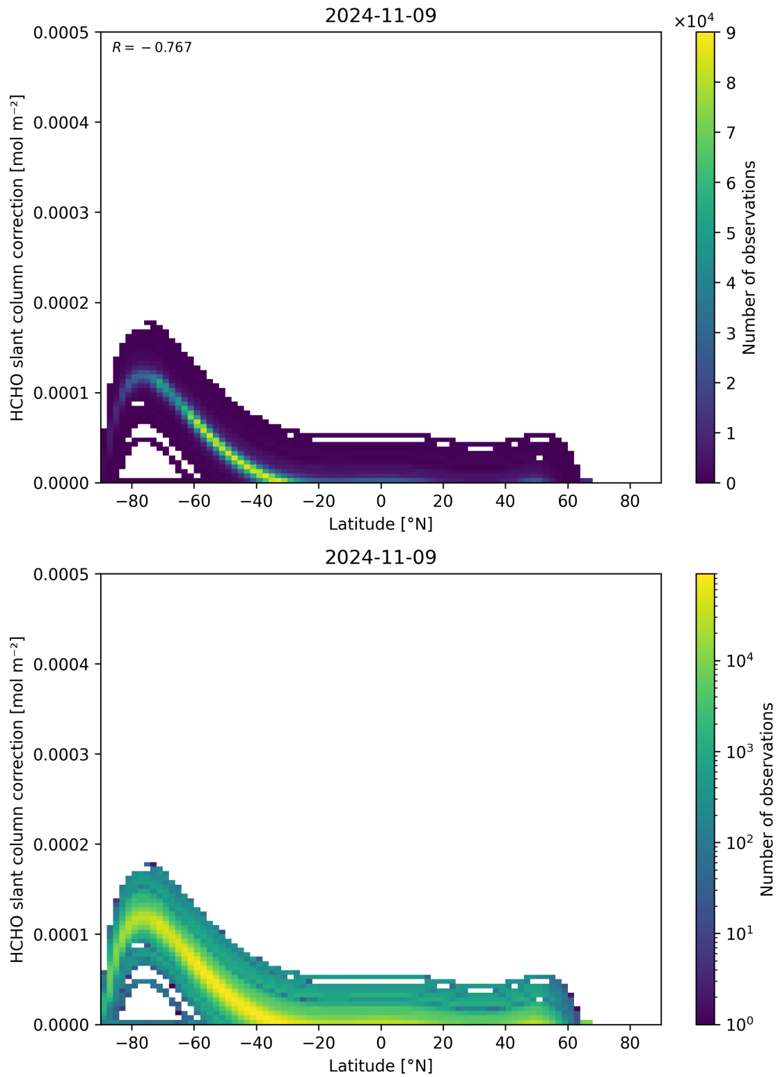
Figure 158: Scatter density plot of “Latitude” against “HCHO slant column correction” for 2024-11-09 to 2024-11-10.
