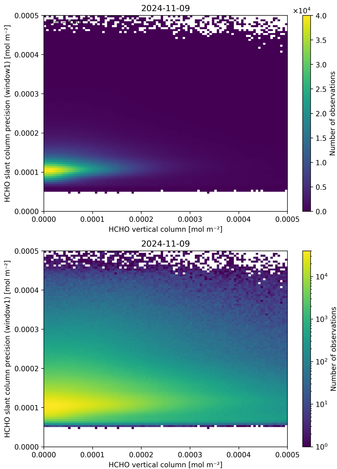
Figure 130: Scatter density plot of “HCHO vertical column” against “HCHO slant column precision (window1)” for 2024-11-09 to 2024-11-10.
