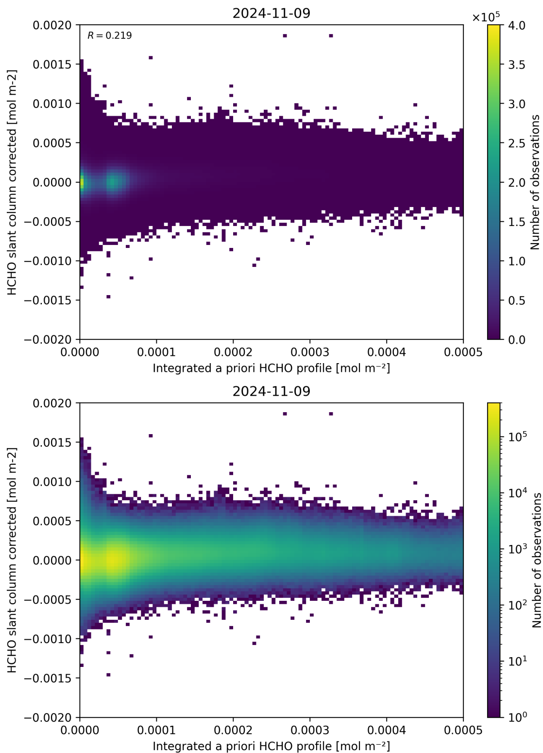
Figure 151: Scatter density plot of “Integrated a priori HCHO profile” against “HCHO slant column corrected” for 2024-11-09 to 2024-11-10.
