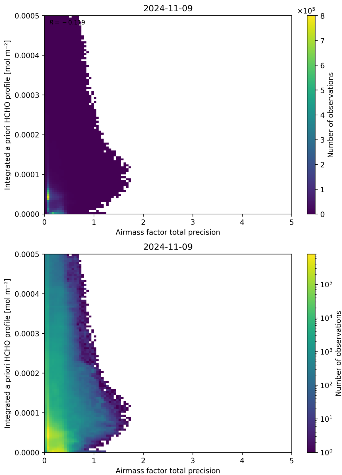
Figure 111: Scatter density plot of “Airmass factor total precision” against “Integrated a priori HCHO profile” for 2024-11-09 to 2024-11-10.
