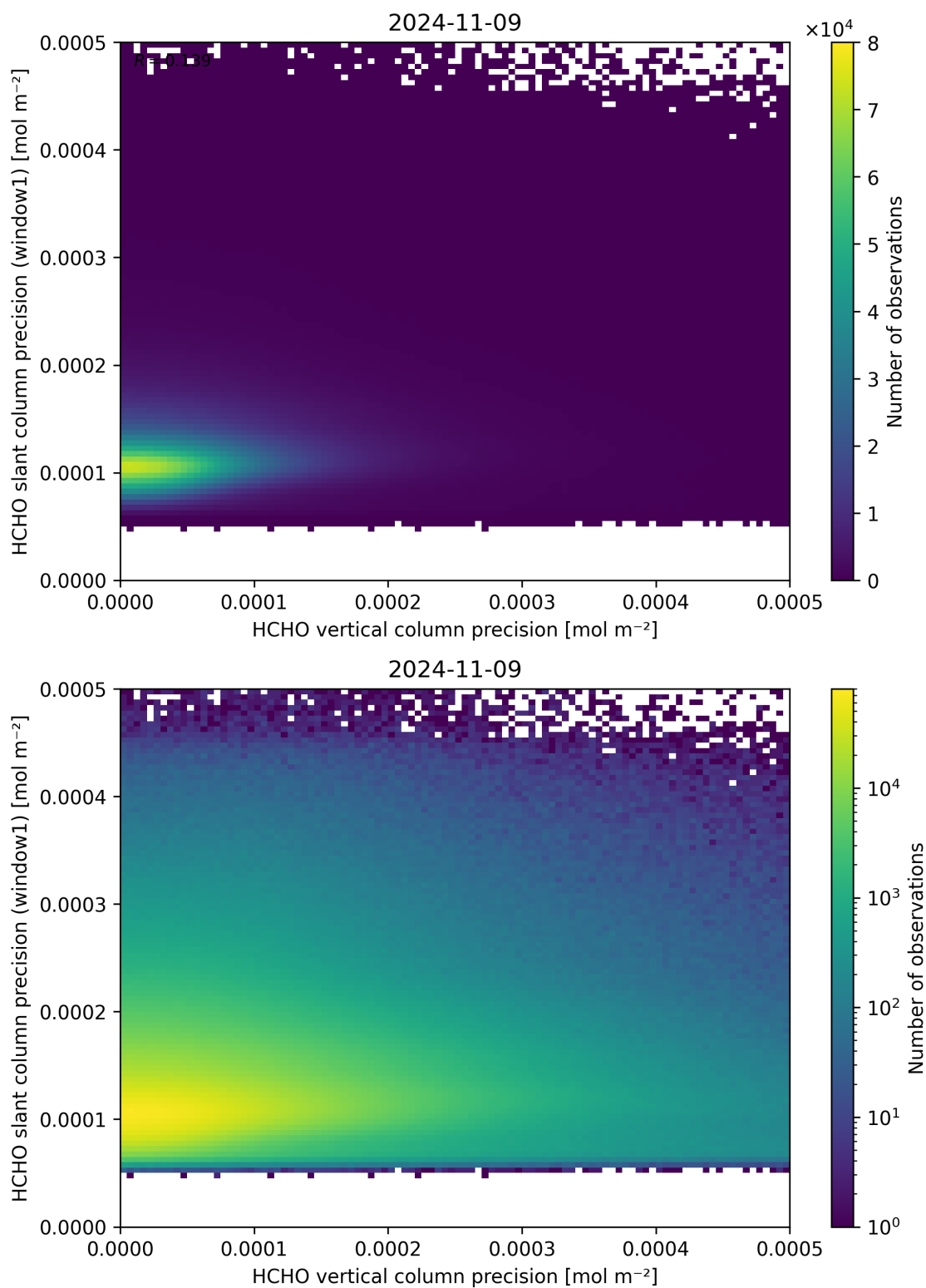
Figure 143: Scatter density plot of “HCHO vertical column precision” against “HCHO slant column precision (window1)” for 2024-11-09 to 2024-11-10.
