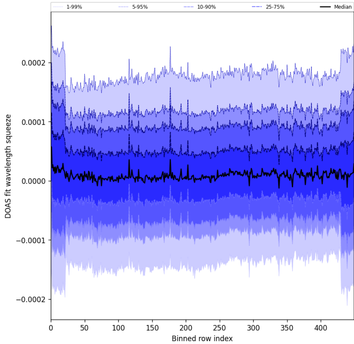
Figure 59: Along track statistics of “DOAS fit wavelength squeeze” for 2024-11-09 to 2024-11-10
