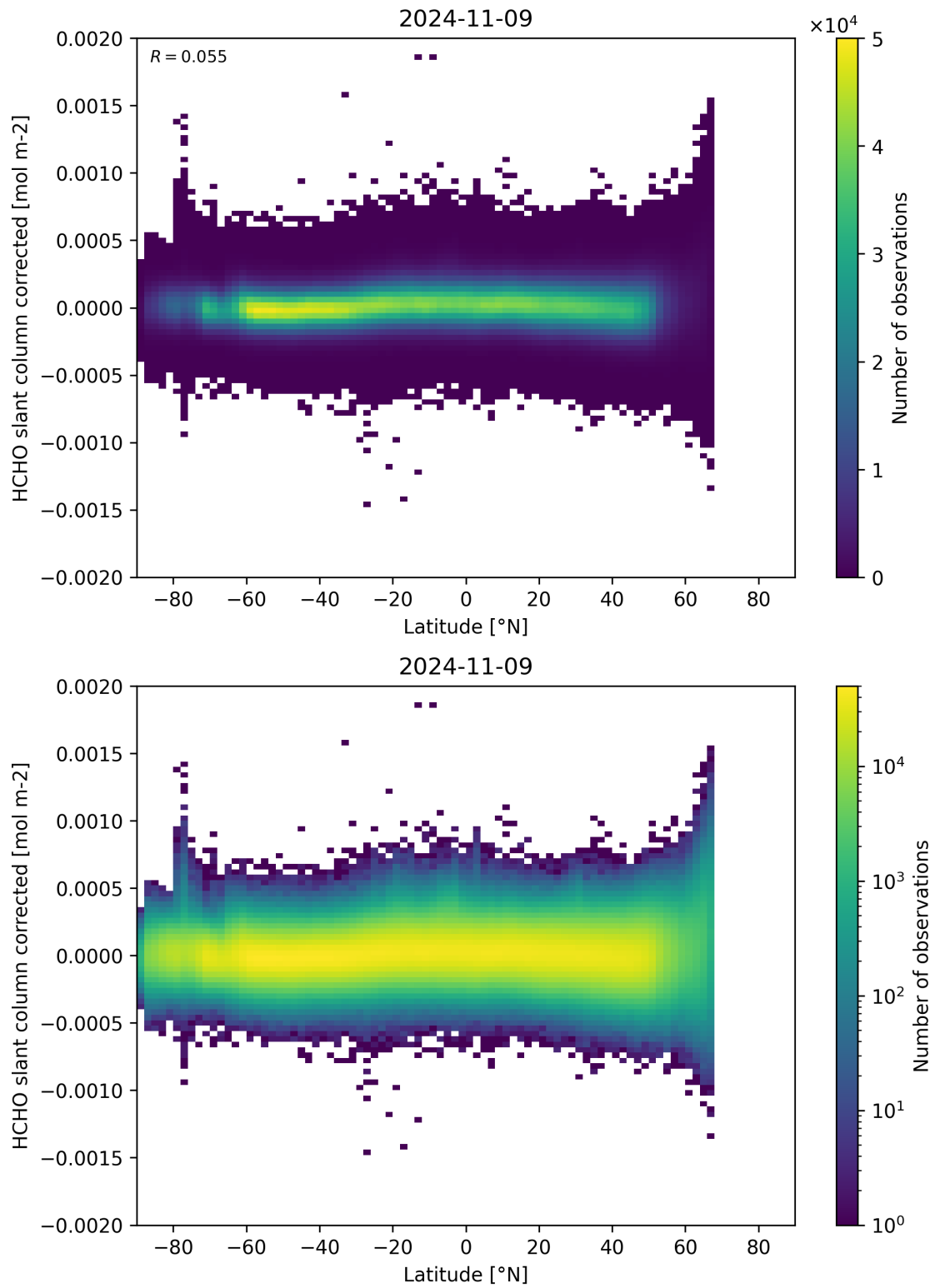
Figure 157: Scatter density plot of “Latitude” against “HCHO slant column corrected” for 2024-11-09 to 2024-11-10.
