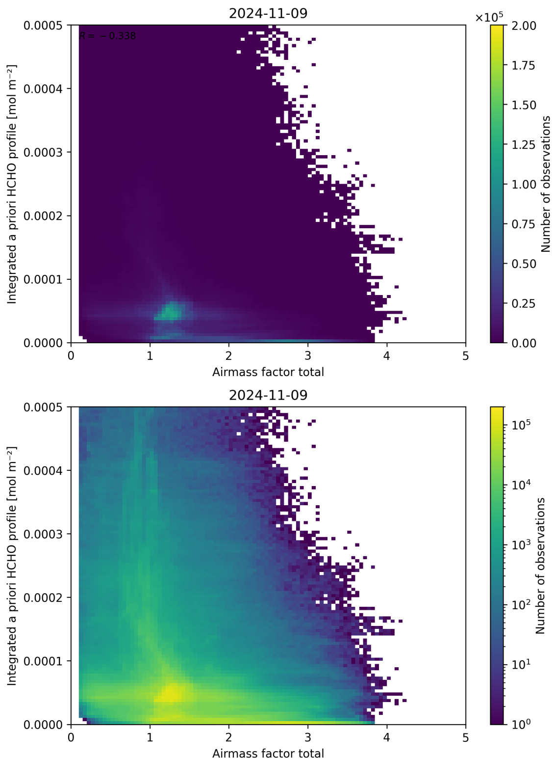
Figure 104: Scatter density plot of “Airmass factor total” against “Integrated a priori HCHO profile” for 2024-11-09 to 2024-11-10.
