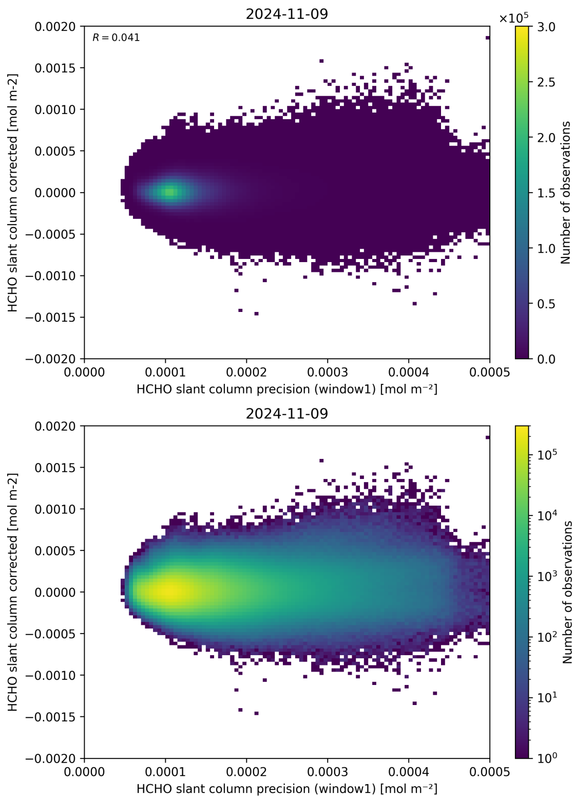
Figure 92: Scatter density plot of “HCHO slant column precision (window1)” against “HCHO slant column corrected” for 2024-11-09 to 2024-11-10.
