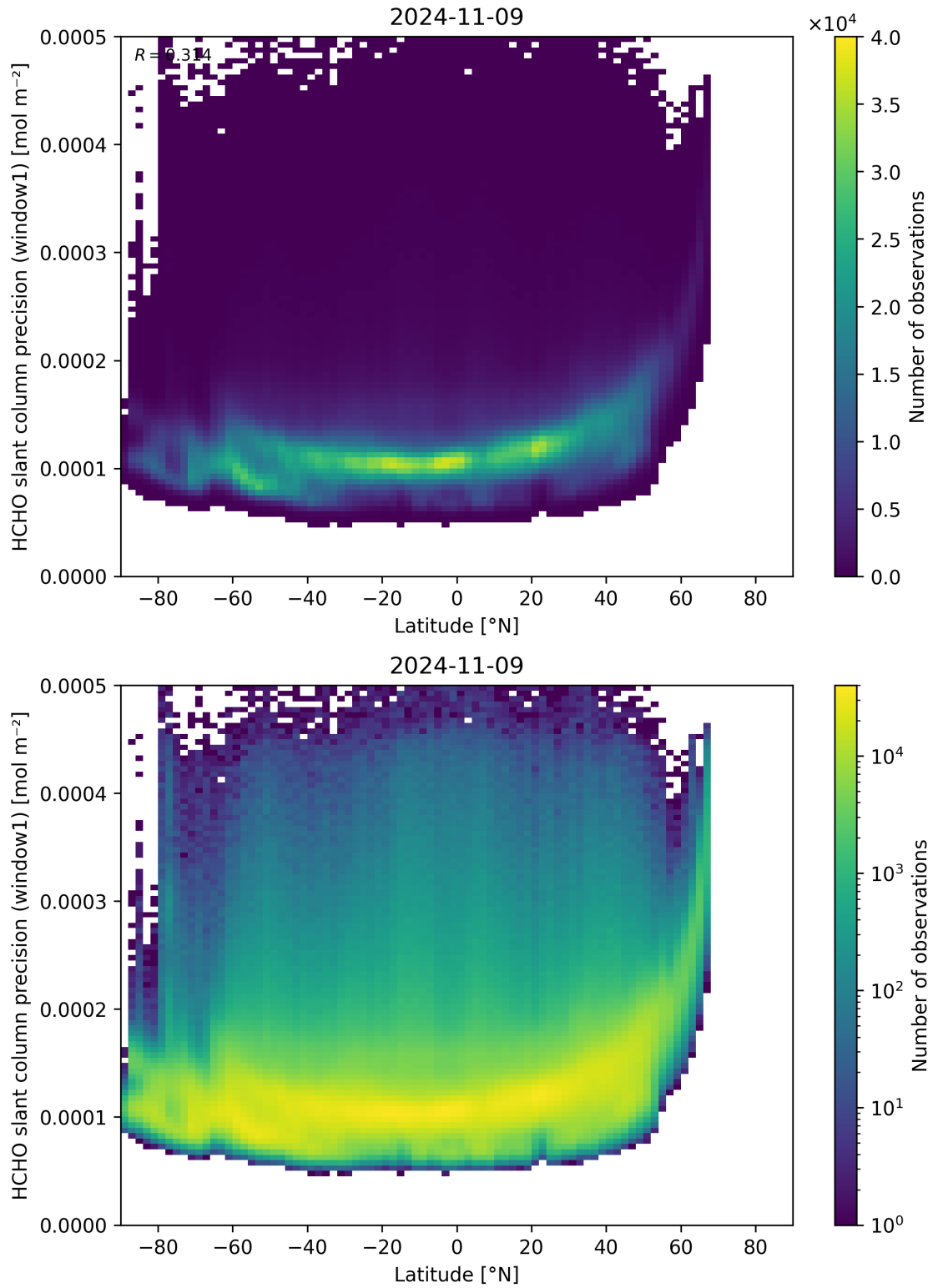
Figure 160: Scatter density plot of “Latitude” against “HCHO slant column precision (window1)” for 2024-11-09 to 2024-11-10.
