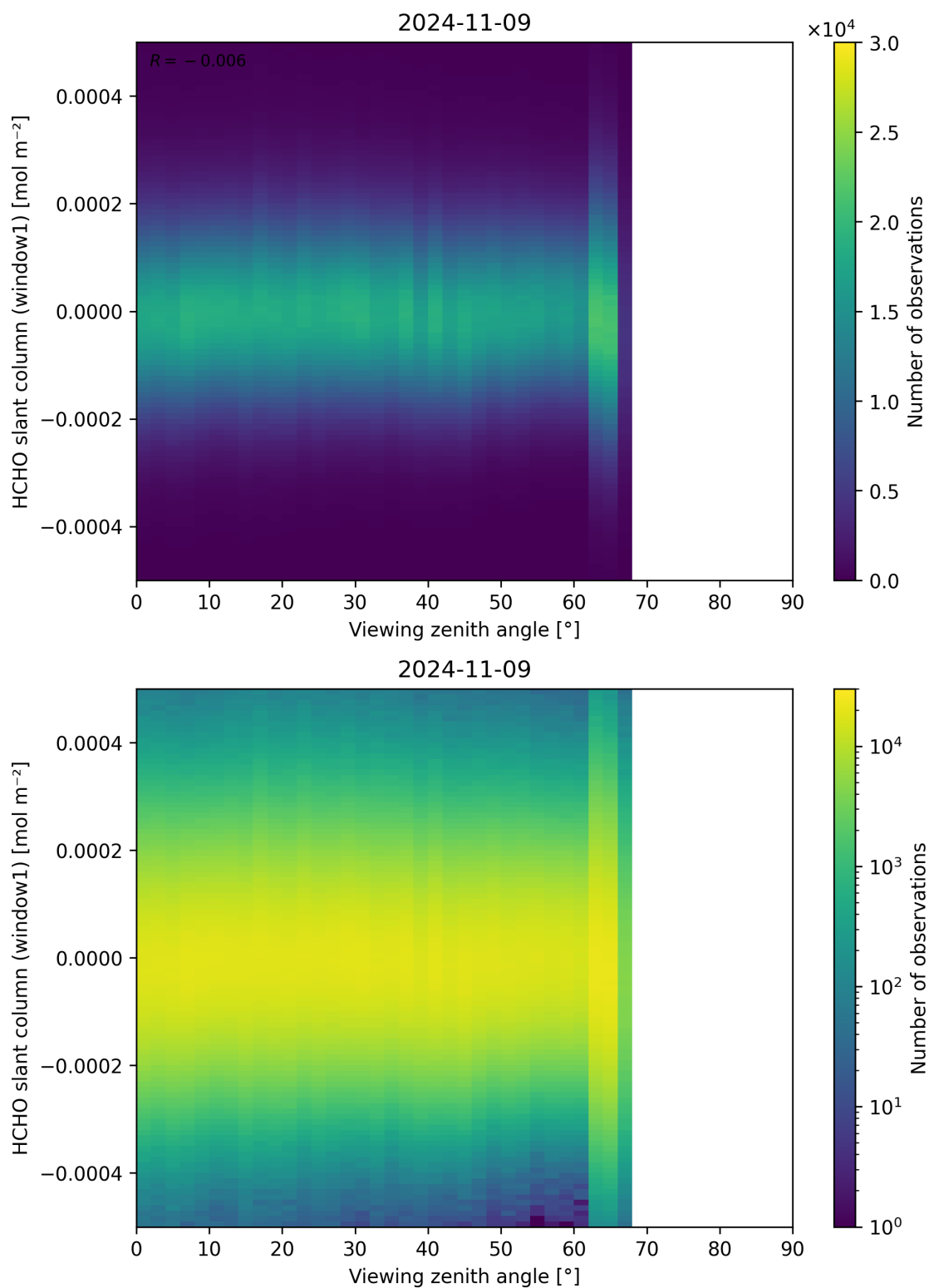
Figure 188: Scatter density plot of “Viewing zenith angle” against “HCHO slant column (window1)” for 2024-11-09 to 2024-11-10.
