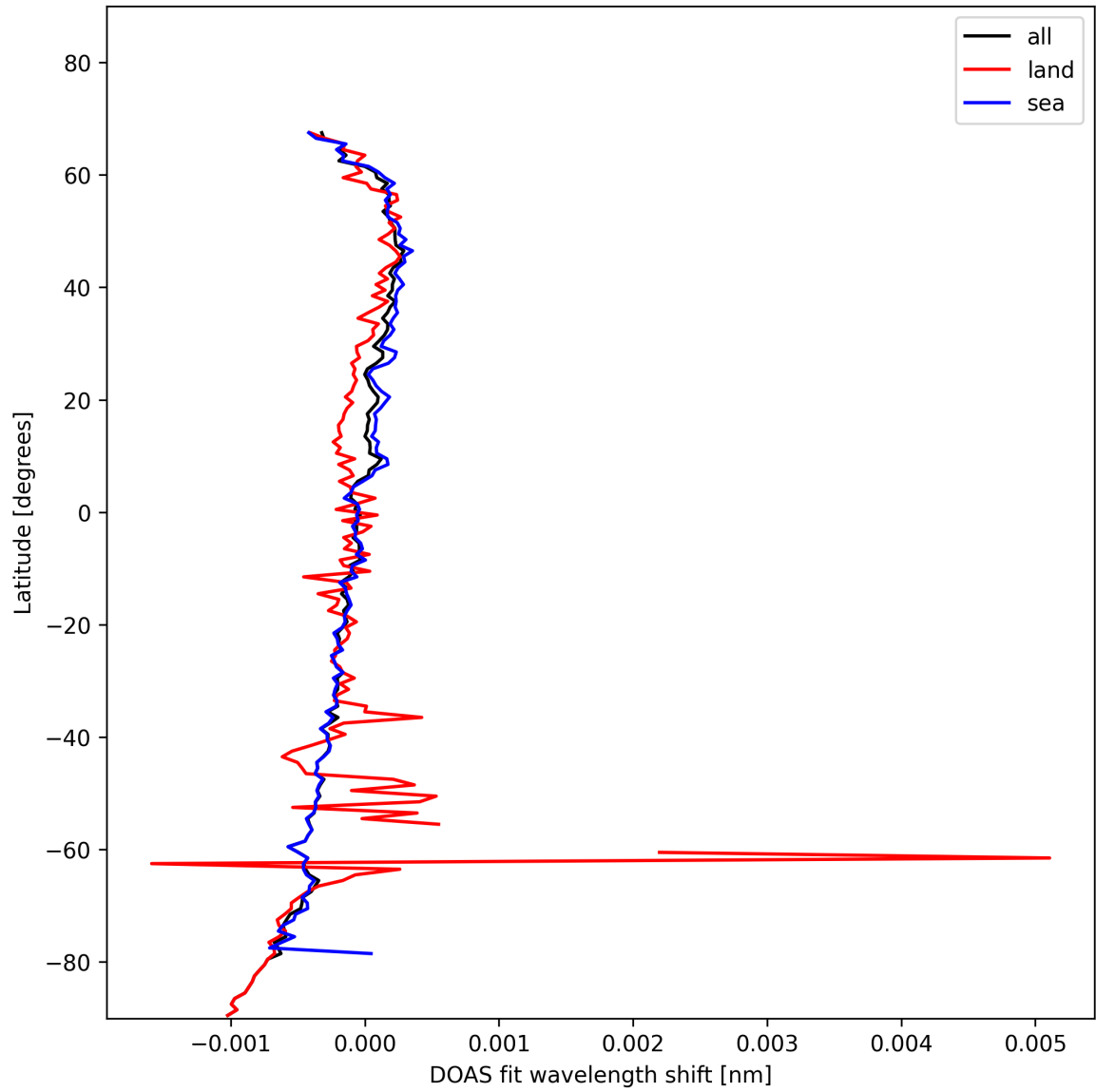
Figure 30: Zonal average of "DOAS fit wavelength shift" for 2024-11-09 to 2024-11-10.
