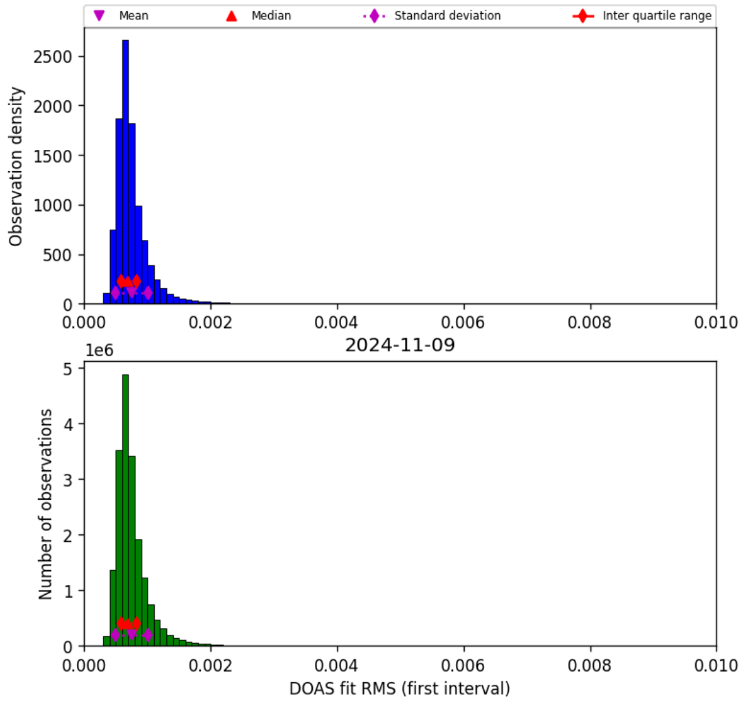
Figure 46: Histogram of “DOAS fit RMS (first interval)” for 2024-11-09 to 2024-11-10
