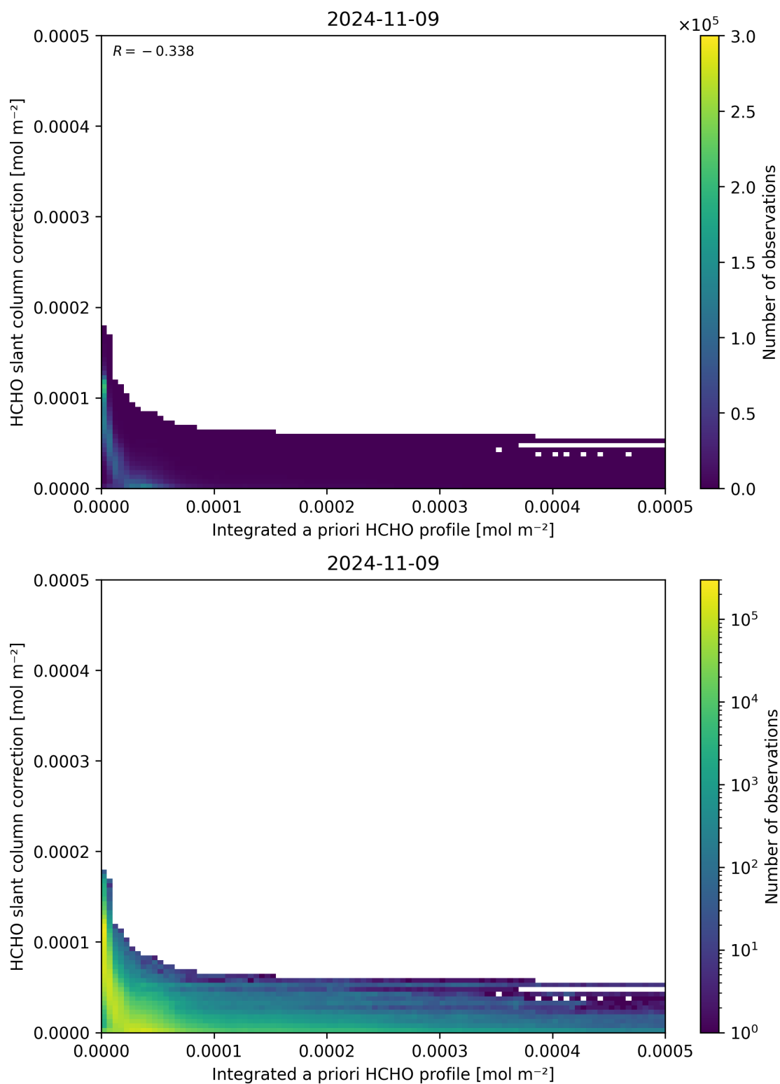
Figure 152: Scatter density plot of “Integrated a priori HCHO profile” against “HCHO slant column correction” for 2024-11-09 to 2024-11-10.
