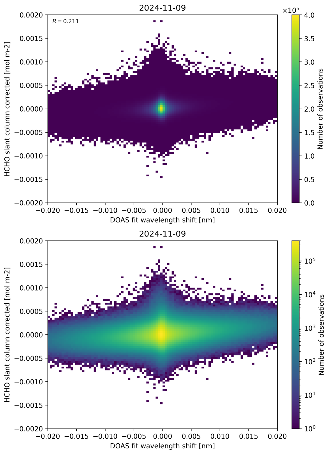
Figure 66: Scatter density plot of “DOAS fit wavelength shift” against “HCHO slant column corrected” for 2024-11-09 to 2024-11-10.
