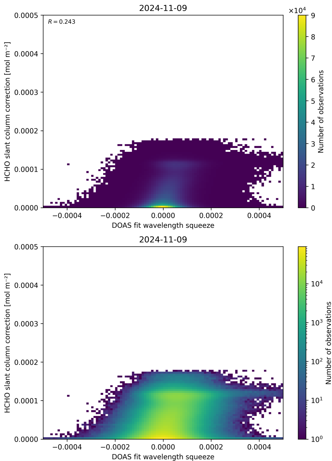
Figure 70: Scatter density plot of “DOAS fit wavelength squeeze” against “HCHO slant column correction” for 2024-11-09 to 2024-11-10.
