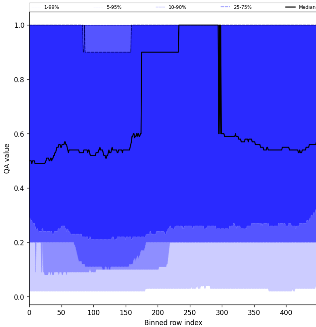
Figure 48: Along track statistics of “QA value” for 2024-11-09 to 2024-11-10
