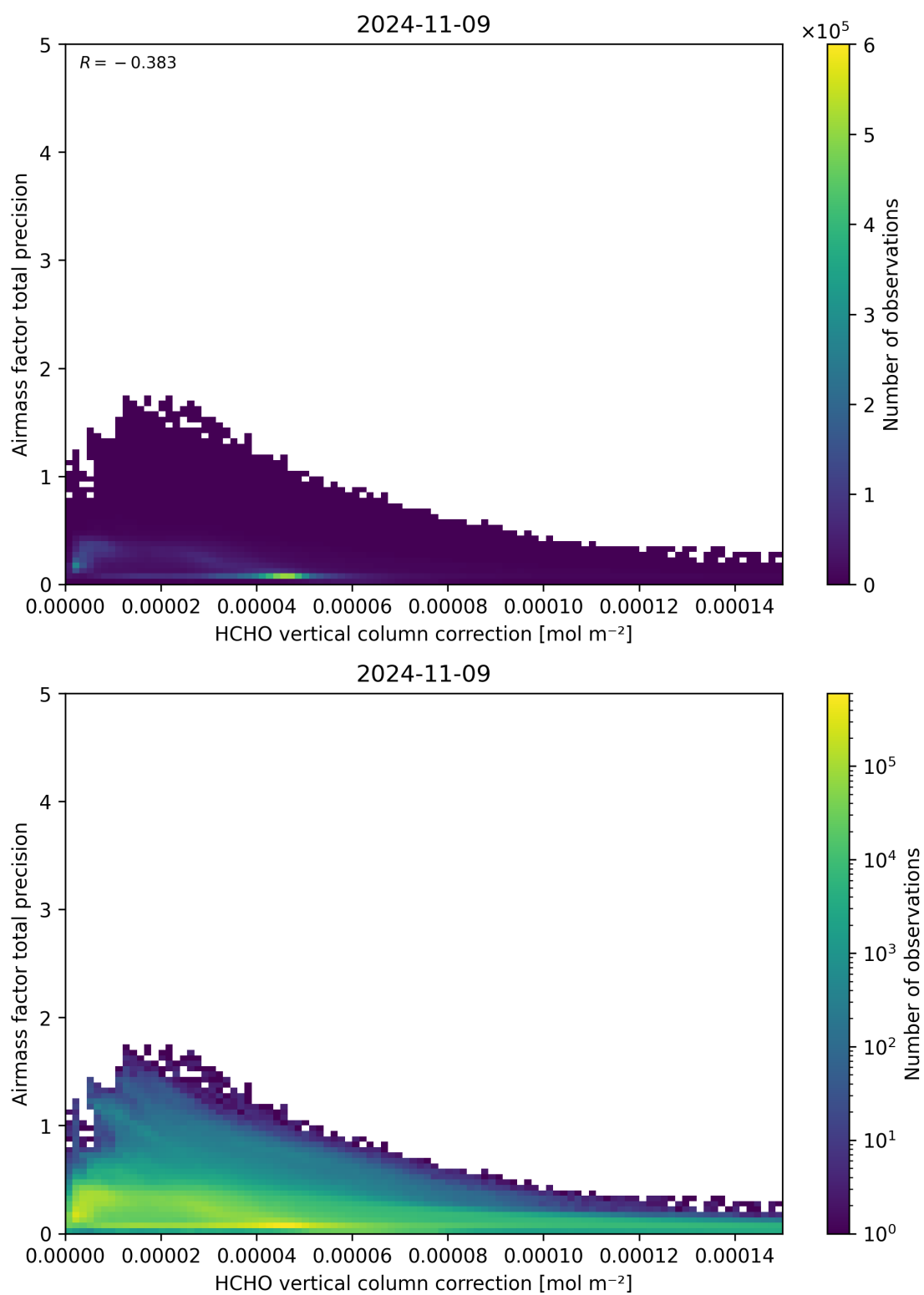
Figure 121: Scatter density plot of “HCHO vertical column correction” against “Airmass factor total precision” for 2024-11-09 to 2024-11-10.
