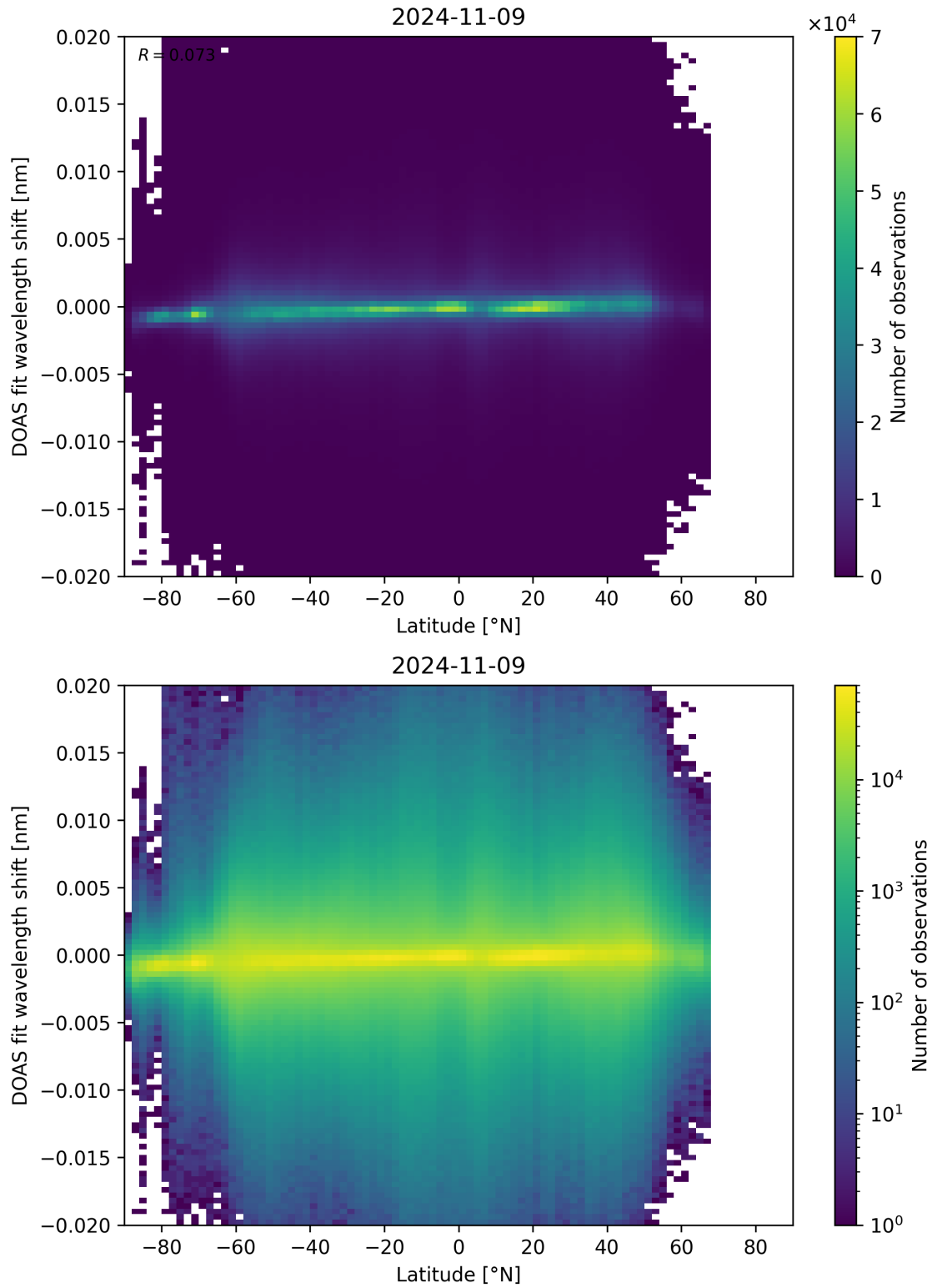
Figure 154: Scatter density plot of “Latitude” against “DOAS fit wavelength shift” for 2024-11-09 to 2024-11-10.
