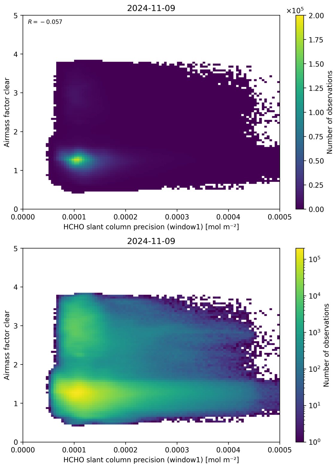
Figure 91: Scatter density plot of “HCHO slant column precision (window1)” against “Airmass factor clear” for 2024-11-09 to 2024-11-10.
