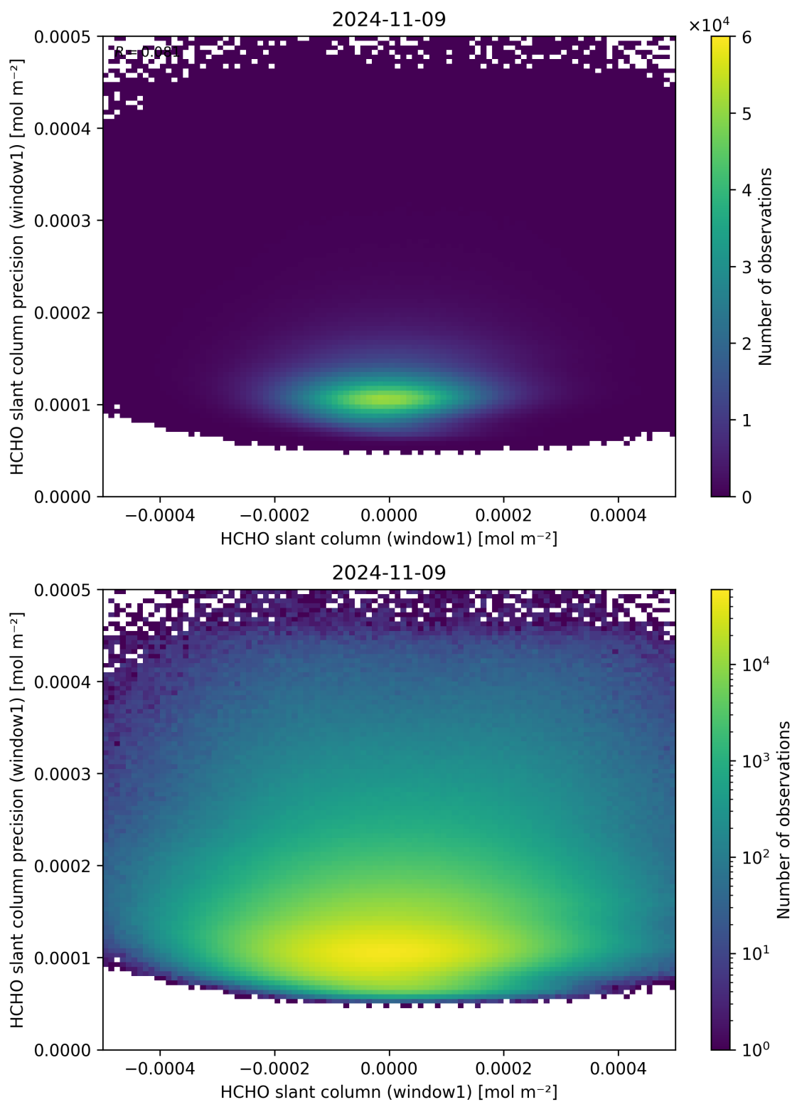
Figure 84: Scatter density plot of “HCHO slant column (window1)” against “HCHO slant column precision (window1)” for 2024-11-09 to 2024-11-10.
