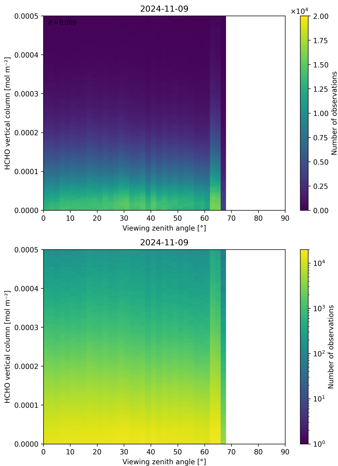
Figure 192: Scatter density plot of “Viewing zenith angle” against “HCHO vertical column” for 2024-11-09 to 2024-11-10.
