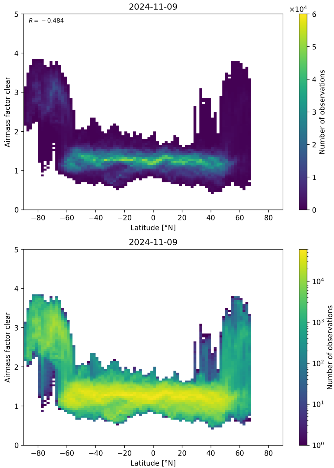
Figure 156: Scatter density plot of “Latitude” against “Airmass factor clear” for 2024-11-09 to 2024-11-10.
