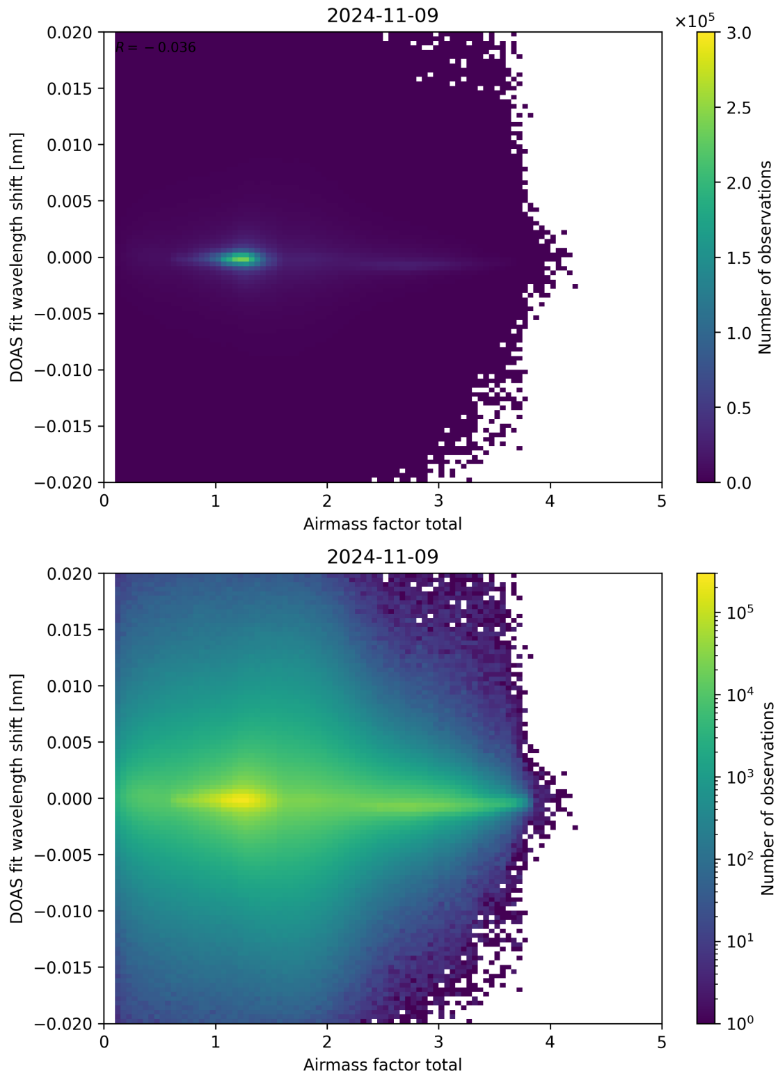
Figure 98: Scatter density plot of “Airmass factor total” against “DOAS fit wavelength shift” for 2024-11-09 to 2024-11-10.
