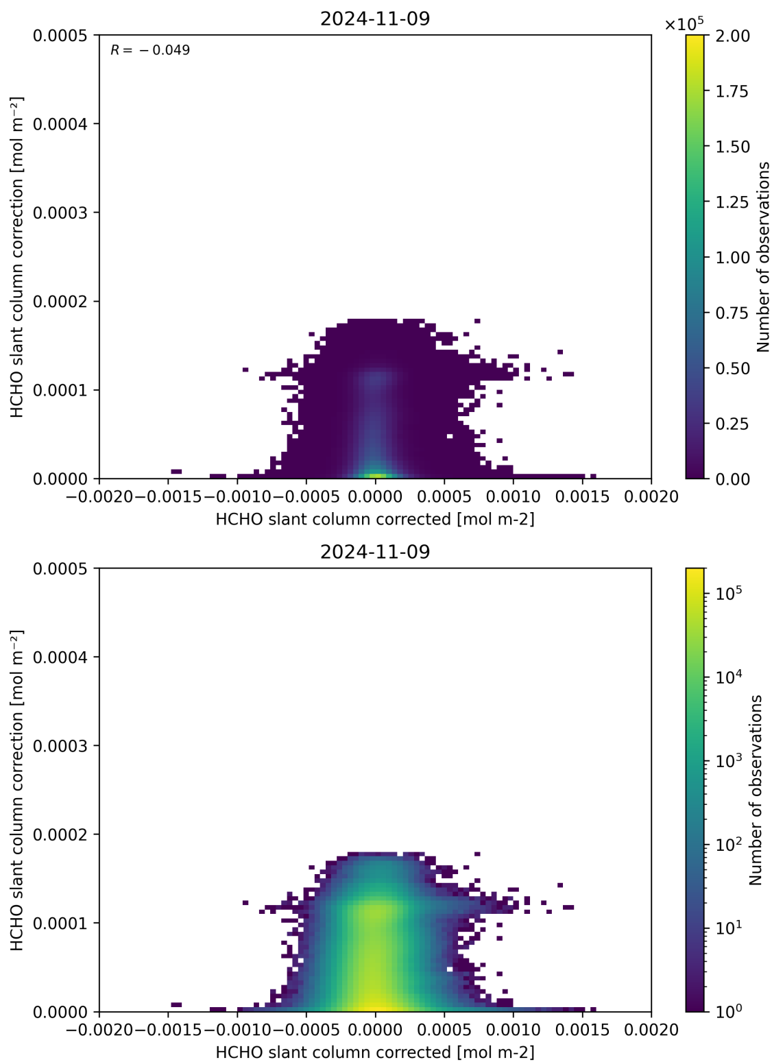
Figure 77: Scatter density plot of “HCHO slant column corrected” against “HCHO slant column correction” for 2024-11-09 to 2024-11-10.
