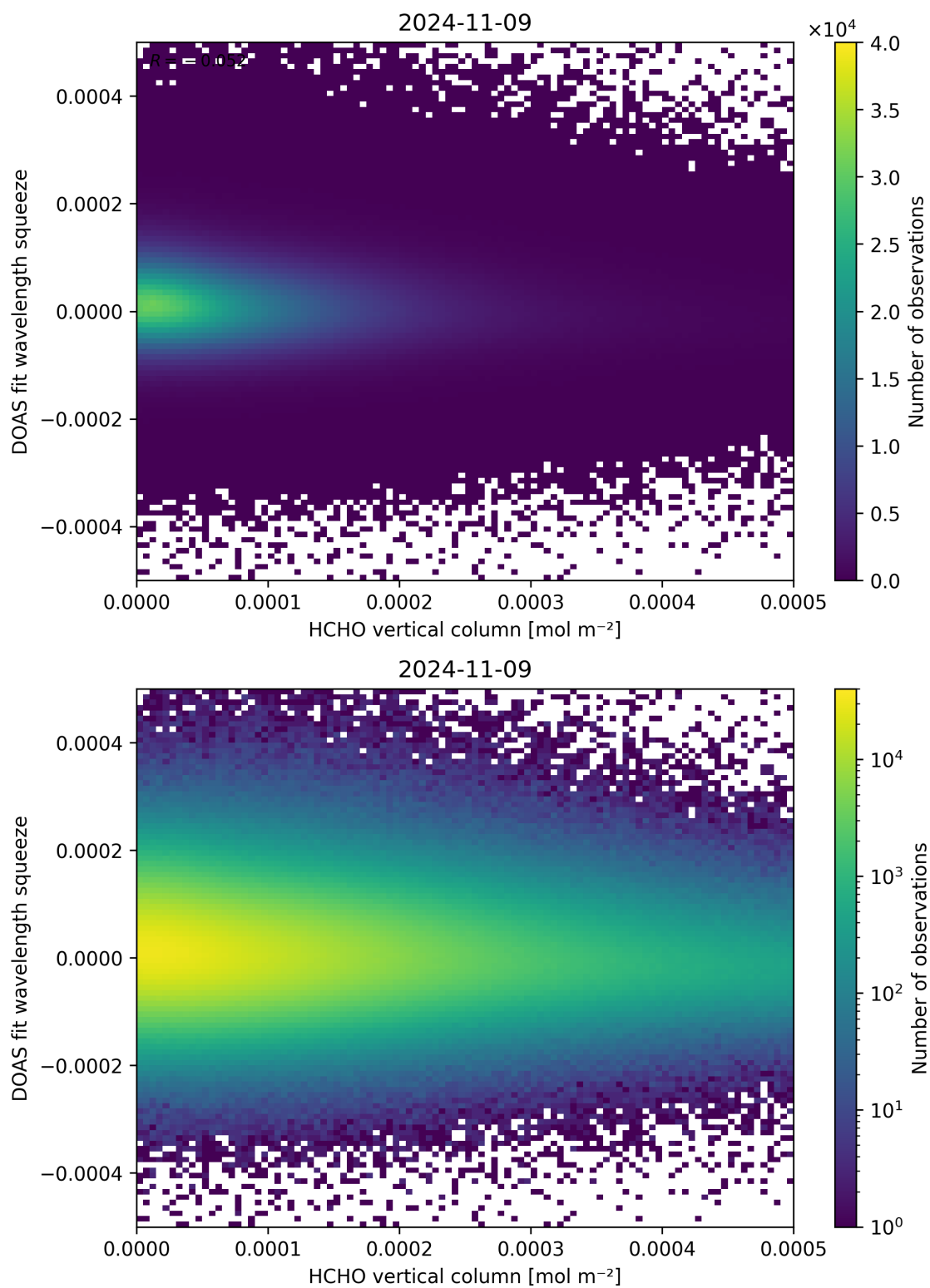
Figure 125: Scatter density plot of “HCHO vertical column” against “DOAS fit wavelength squeeze” for 2024-11-09 to 2024-11-10.
