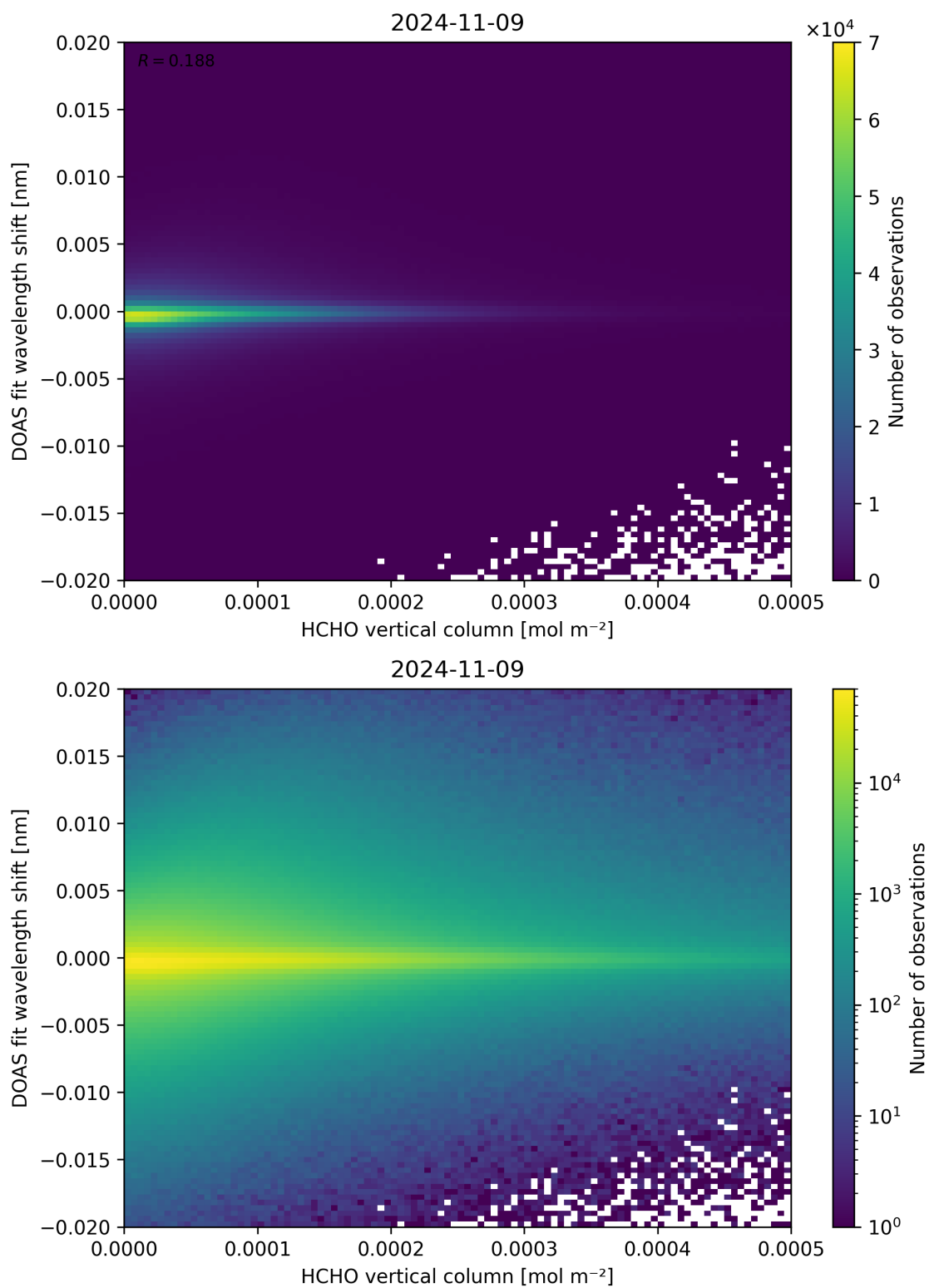
Figure 124: Scatter density plot of “HCHO vertical column” against “DOAS fit wavelength shift” for 2024-11-09 to 2024-11-10.
