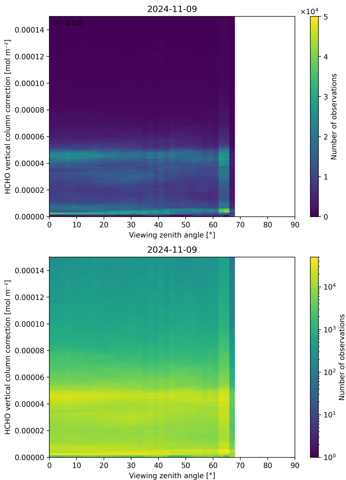
Figure 193: Scatter density plot of “Viewing zenith angle” against “HCHO vertical column correction” for 2024-11-09 to 2024-11-10.
