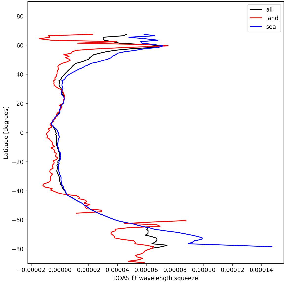
Figure 31: Zonal average of “DOAS fit wavelength squeeze” for 2024-11-09 to 2024-11-10.
