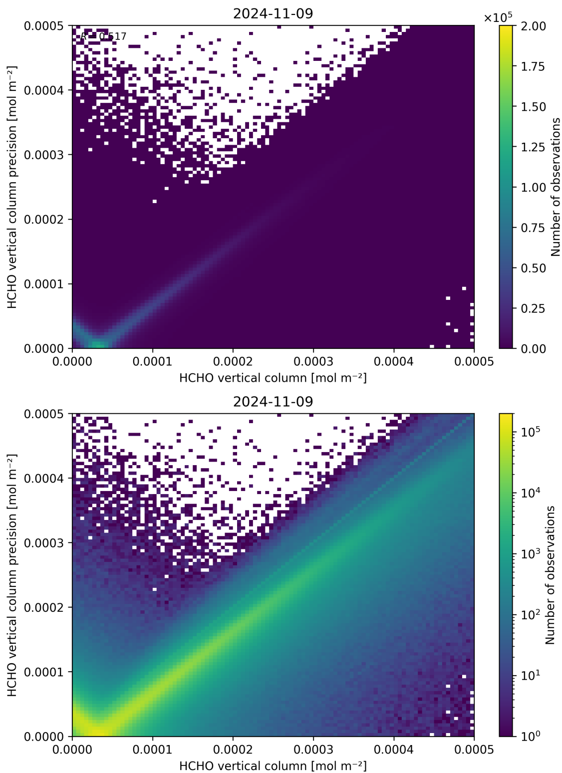
Figure 134: Scatter density plot of “HCHO vertical column” against “HCHO vertical column precision” for 2024-11-09 to 2024-11-10.
