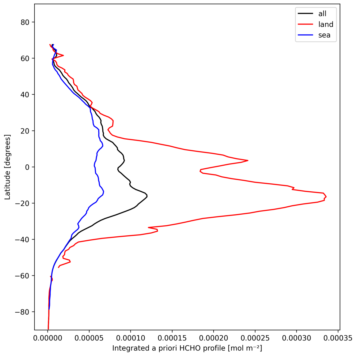
Figure 29: Zonal average of “Integrated a priori HCHO profile” for 2024-11-09 to 2024-11-10.
