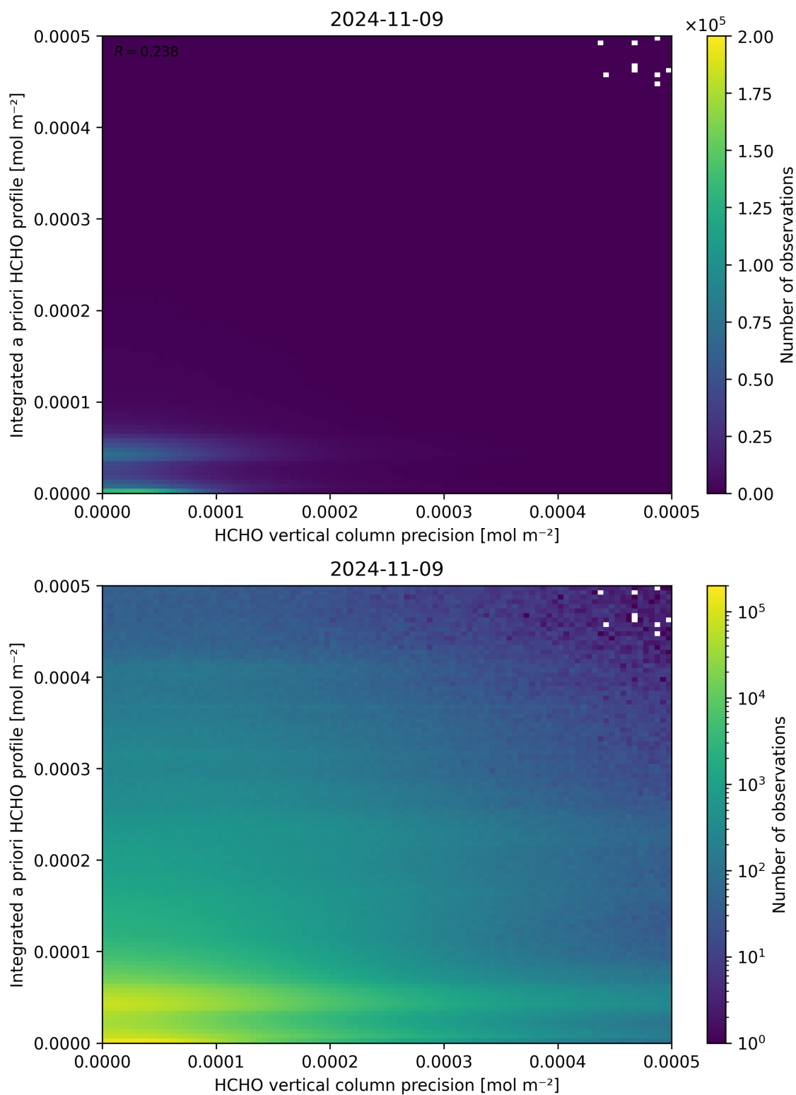
Figure 147: Scatter density plot of “HCHO vertical column precision” against “Integrated a priori HCHO profile” for 2024-11-09 to 2024-11-10.
