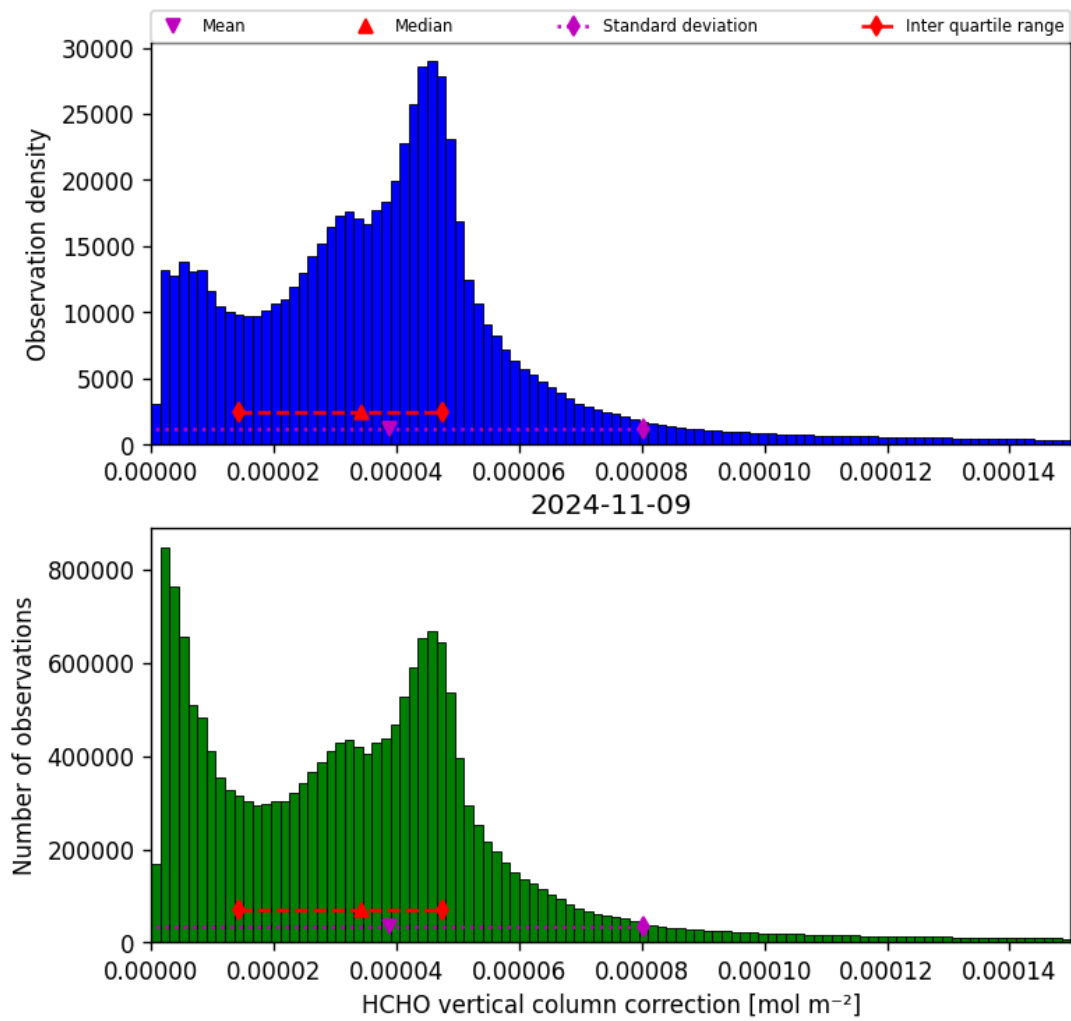
Figure 37: Histogram of “HCHO vertical column correction” for 2024-11-09 to 2024-11-10
