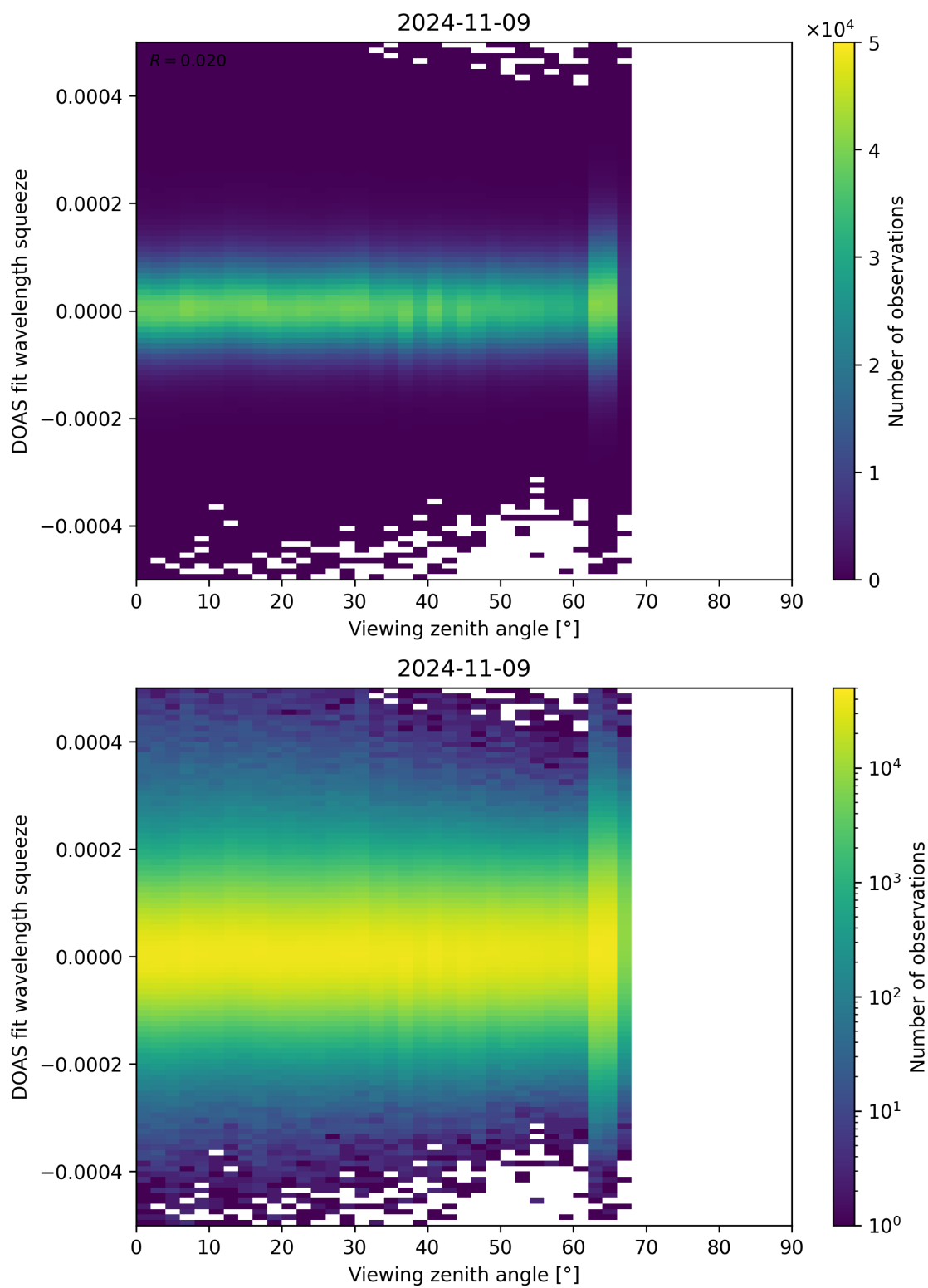
Figure 184: Scatter density plot of “Viewing zenith angle” against “DOAS fit wavelength squeeze” for 2024-11-09 to 2024-11-10.
