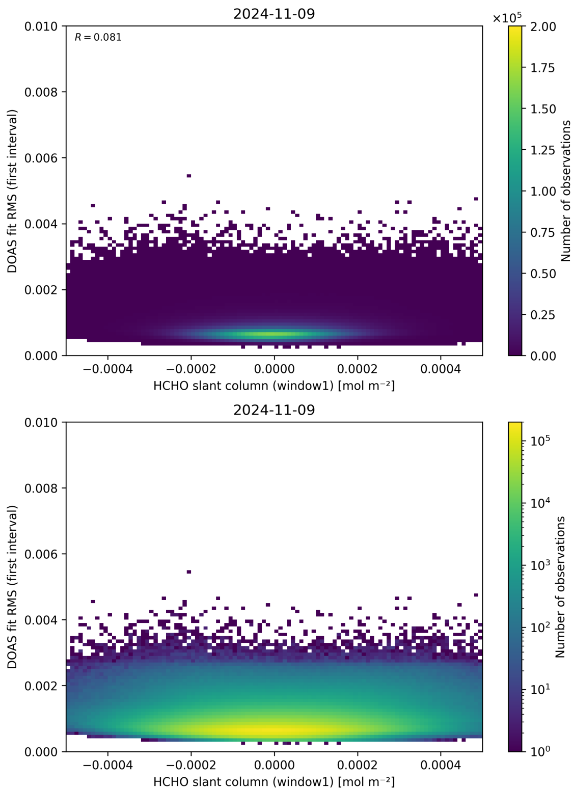
Figure 78: Scatter density plot of “HCHO slant column (window1)” against “DOAS fit RMS (first interval)” for 2024-11-09 to 2024-11-10.
