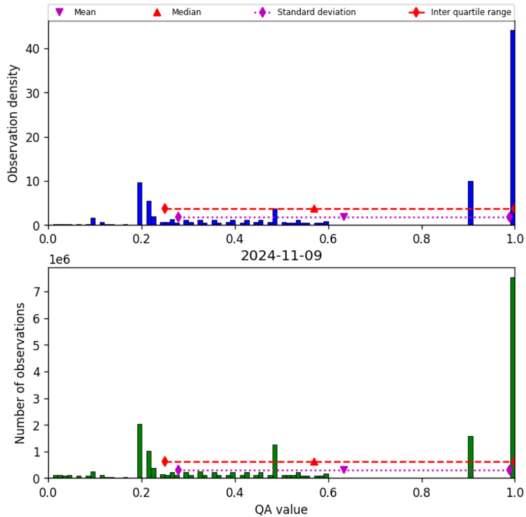
Figure 34: Histogram of “QA value” for 2024-11-09 to 2024-11-10
