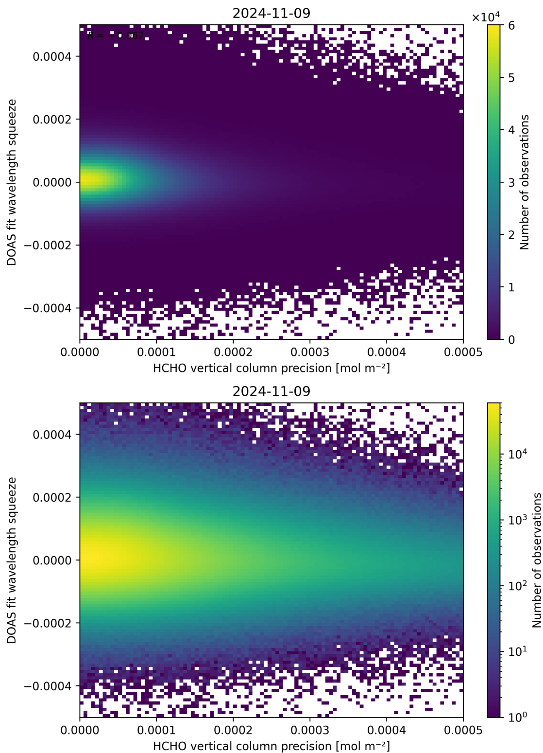
Figure 138: Scatter density plot of “HCHO vertical column precision” against “DOAS fit wavelength squeeze” for 2024-11-09 to 2024-11-10.
