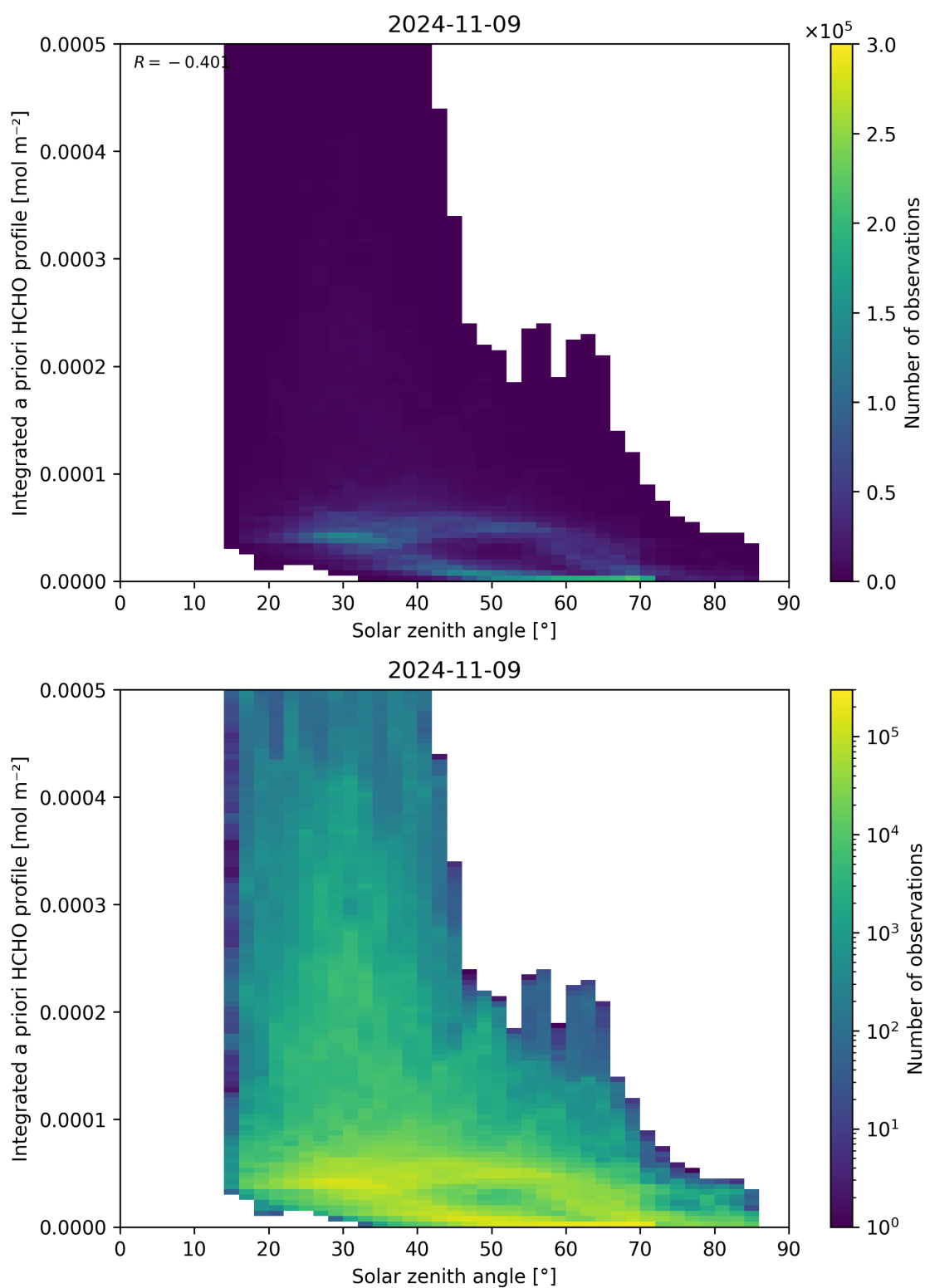
Figure 180: Scatter density plot of “Solar zenith angle” against “Integrated a priori HCHO profile” for 2024-11-09 to 2024-11-10.
