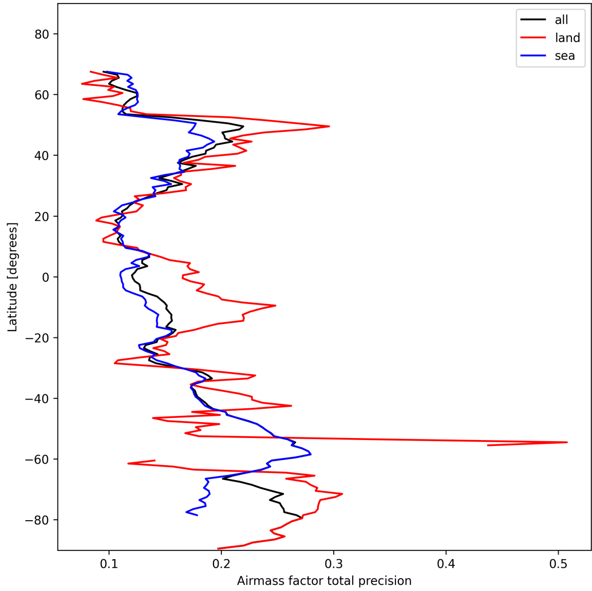
Figure 27: Zonal average of “Airmass factor total precision” for 2024-11-09 to 2024-11-10.
