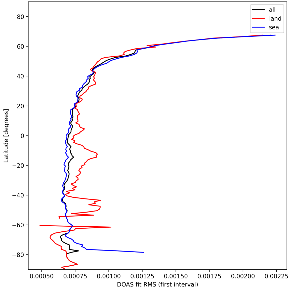
Figure 32: Zonal average of “DOAS fit RMS (first interval)” for 2024-11-09 to 2024-11-10.
