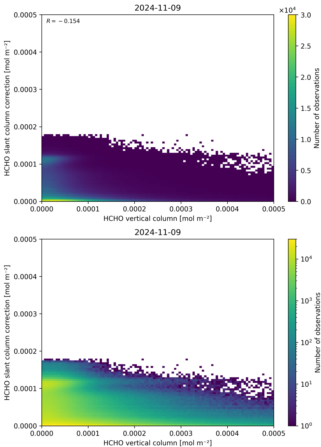
Figure 128: Scatter density plot of “HCHO vertical column” against “HCHO slant column correction” for 2024-11-09 to 2024-11-10.
