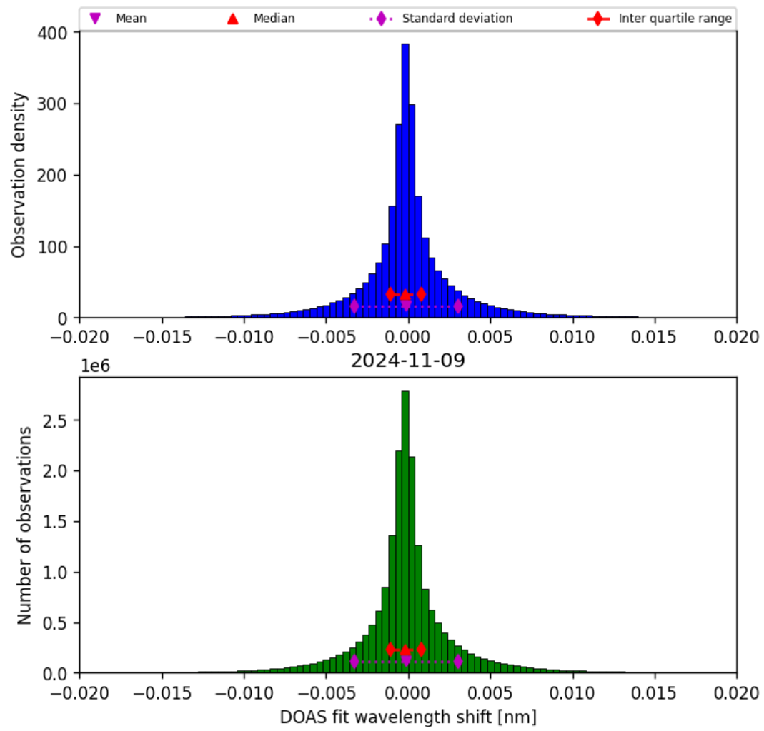
Figure 44: Histogram of “DOAS fit wavelength shift” for 2024-11-09 to 2024-11-10
