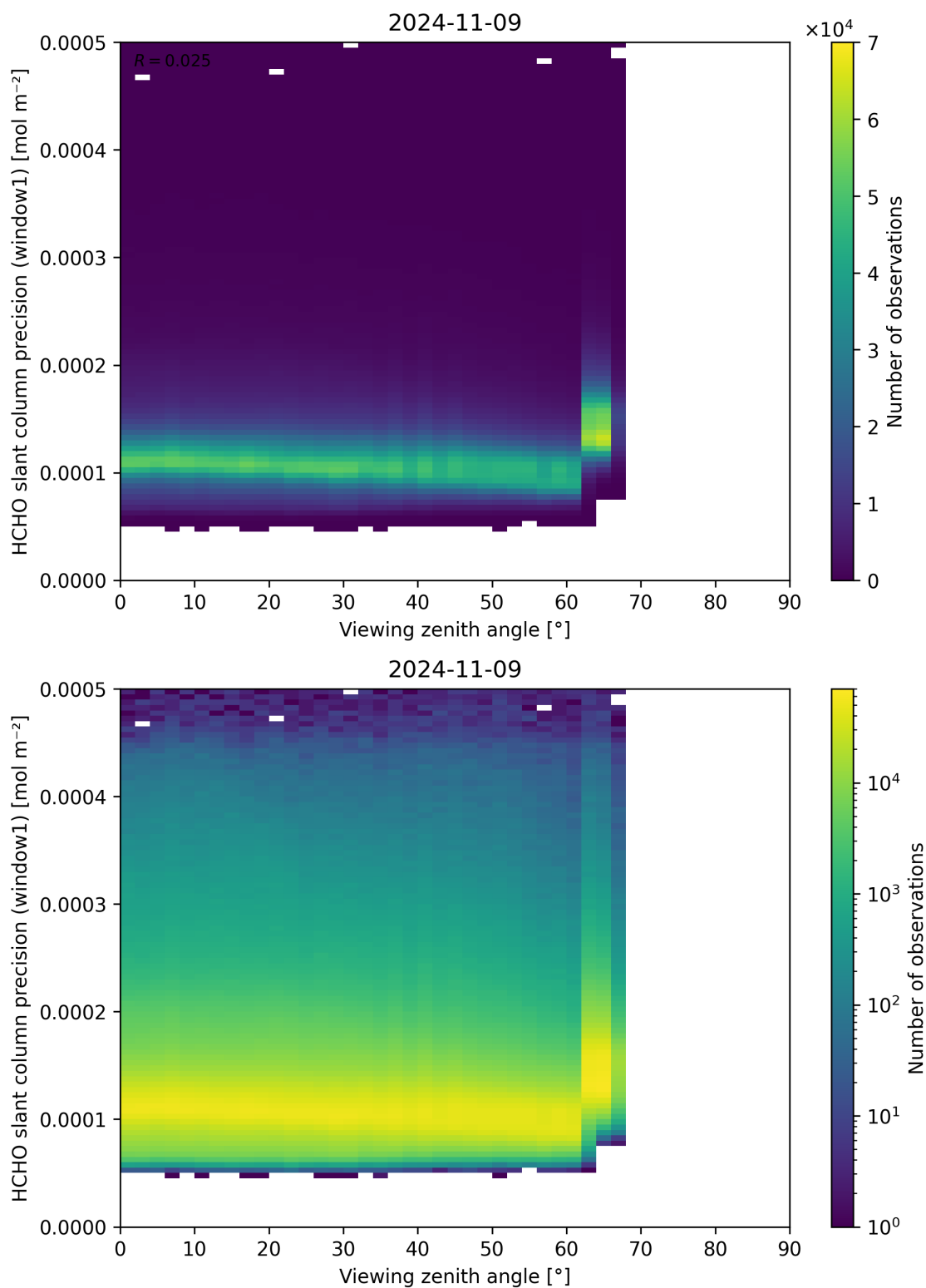
Figure 189: Scatter density plot of “Viewing zenith angle” against “HCHO slant column precision (window1)” for 2024-11-09 to 2024-11-10.
