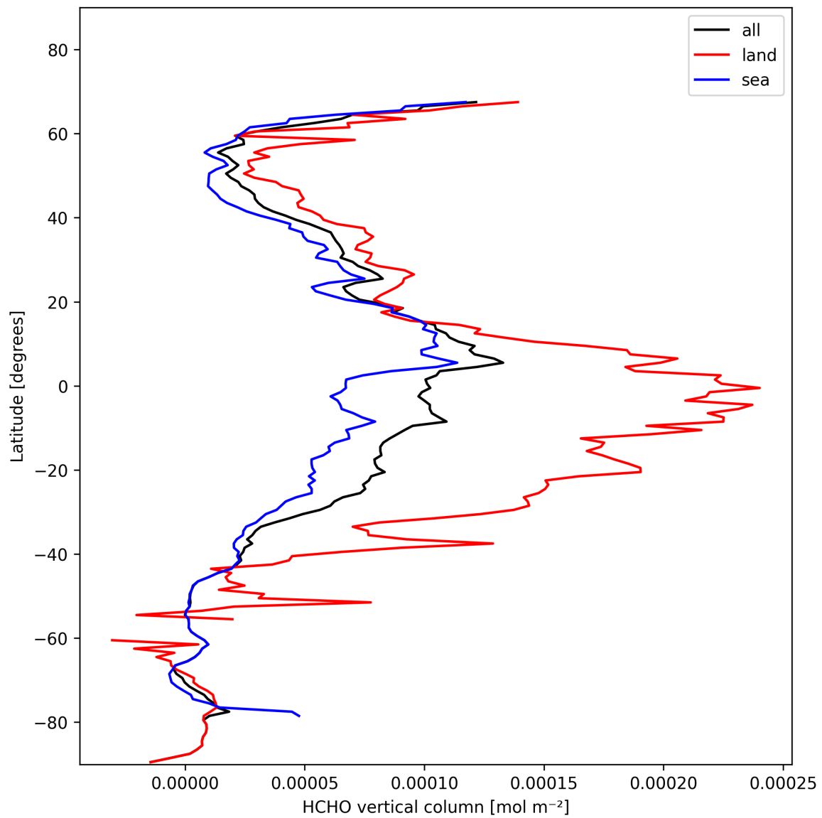
Figure 21: Zonal average of “HCHO vertical column” for 2024-11-09 to 2024-11-10.
