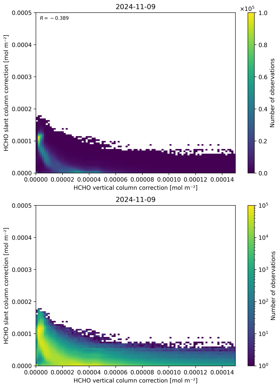
Figure 117: Scatter density plot of “HCHO vertical column correction” against “HCHO slant column correction” for 2024-11-09 to 2024-11-10.
