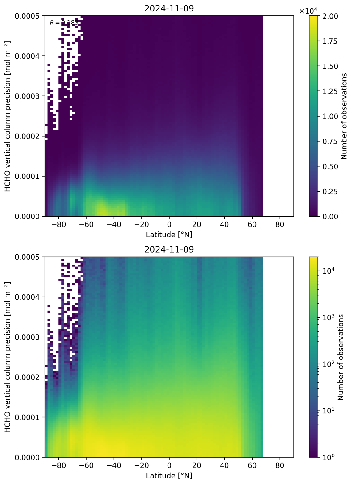
Figure 165: Scatter density plot of “Latitude” against “HCHO vertical column precision” for 2024-11-09 to 2024-11-10.
