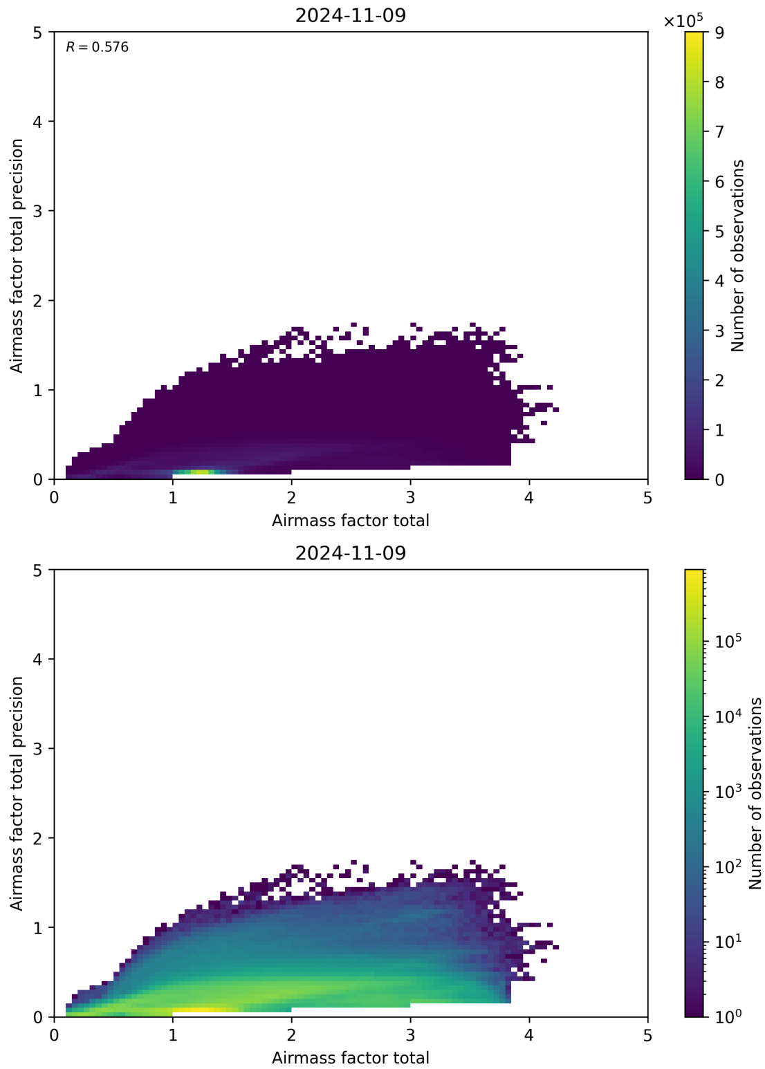
Figure 103: Scatter density plot of “Airmass factor total” against “Airmass factor total precision” for 2024-11-09 to 2024-11-10.
