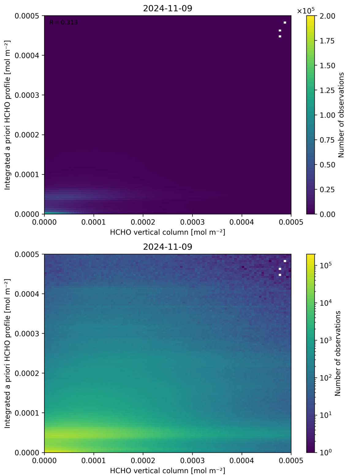
Figure 135: Scatter density plot of “HCHO vertical column” against “Integrated a priori HCHO profile” for 2024-11-09 to 2024-11-10.
