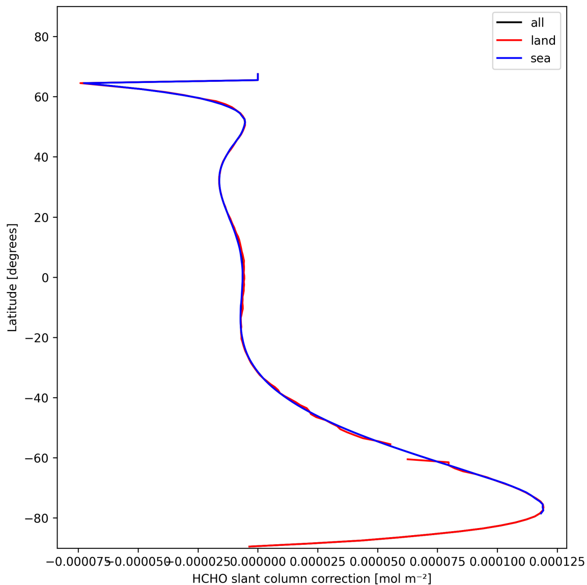
Figure 33: Zonal average of “HCHO slant column correction” for 2024-11-09 to 2024-11-10.
