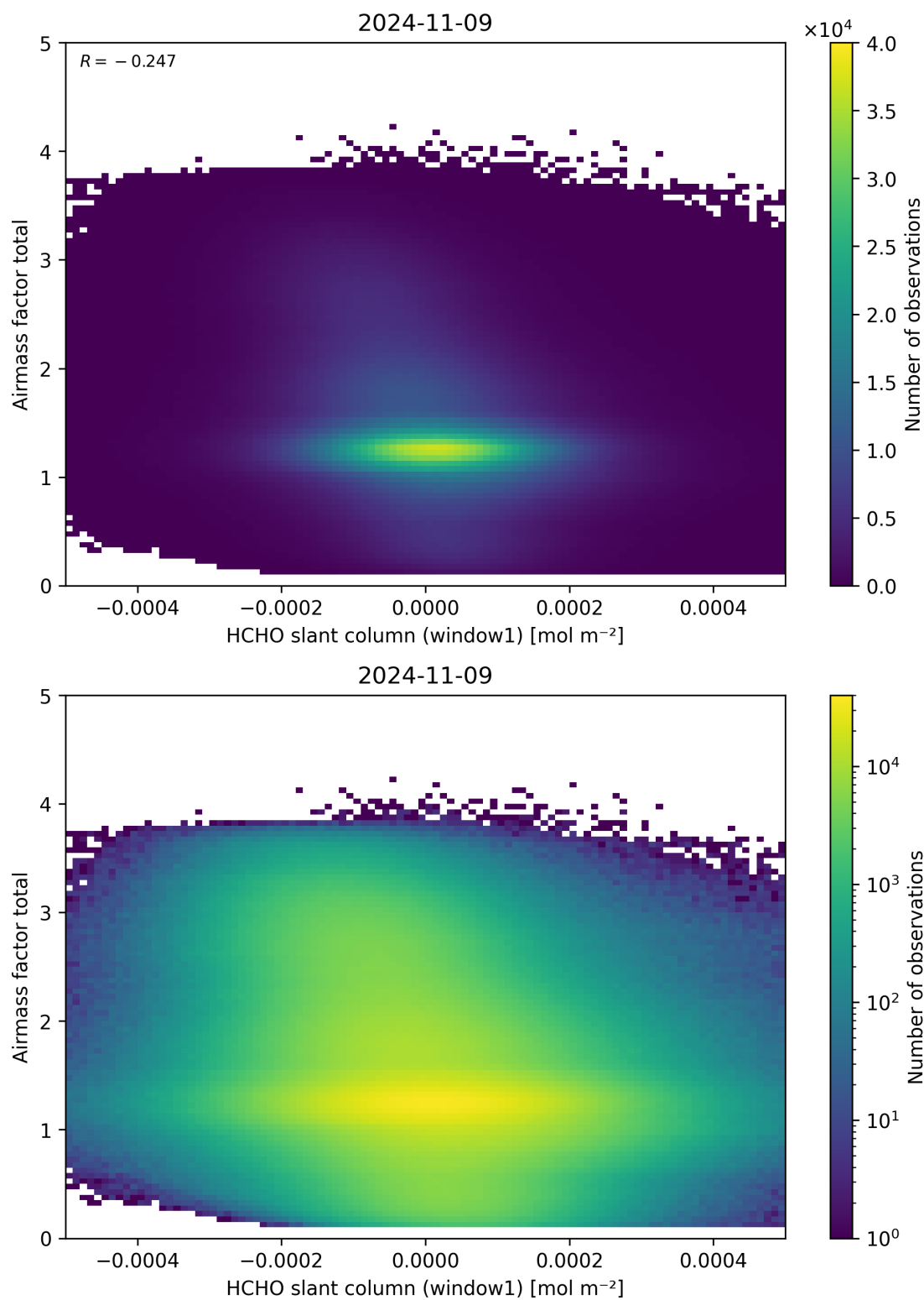
Figure 85: Scatter density plot of “HCHO slant column (window1)” against “Airmass factor total” for 2024-11-09 to 2024-11-10.
