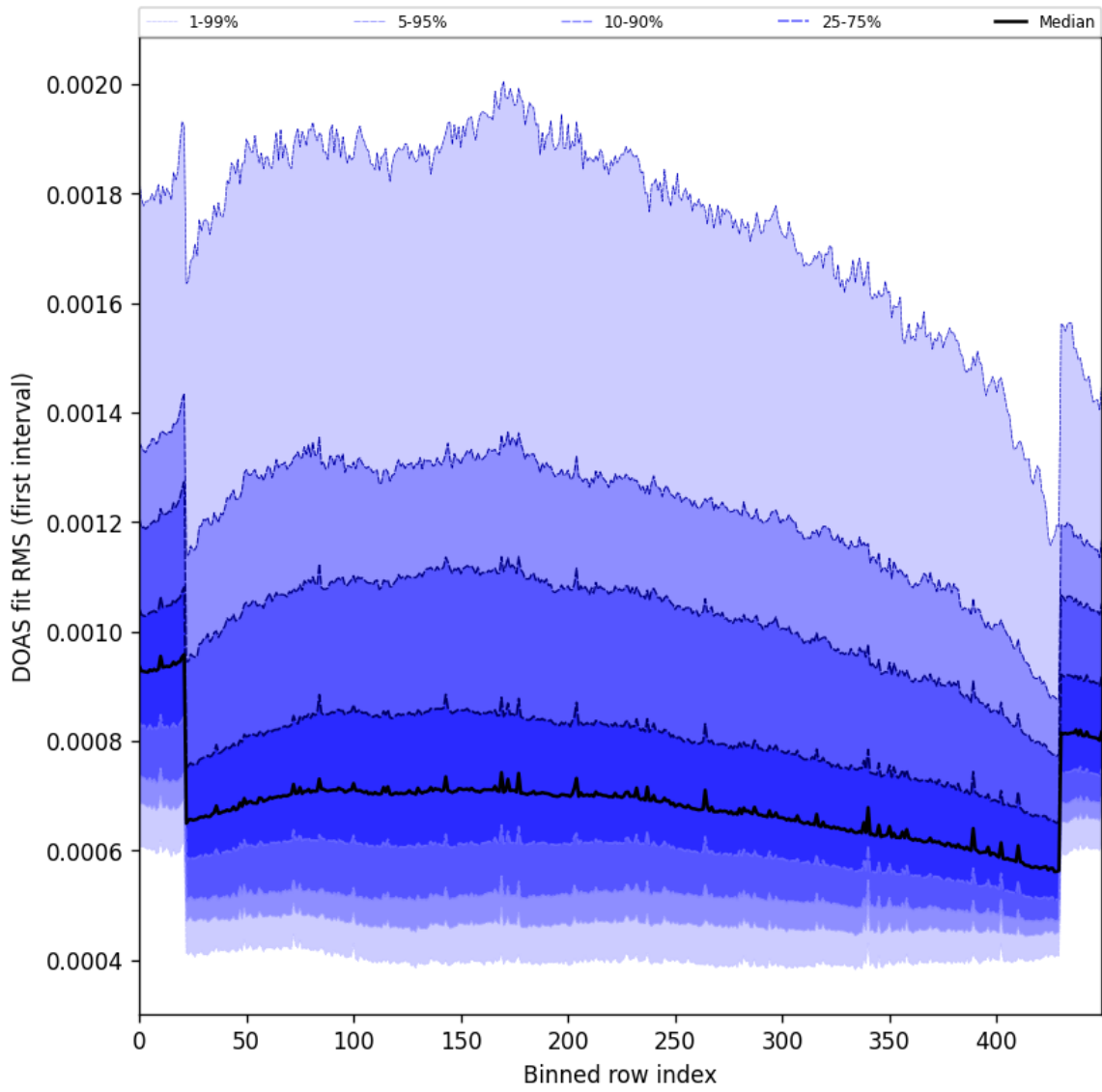
Figure 60: Along track statistics of “DOAS fit RMS (first interval)” for 2024-11-09 to 2024-11-10
