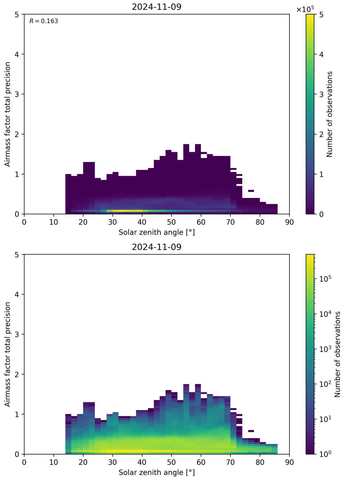
Figure 176: Scatter density plot of “Solar zenith angle” against “Airmass factor total precision” for 2024-11-09 to 2024-11-10.
