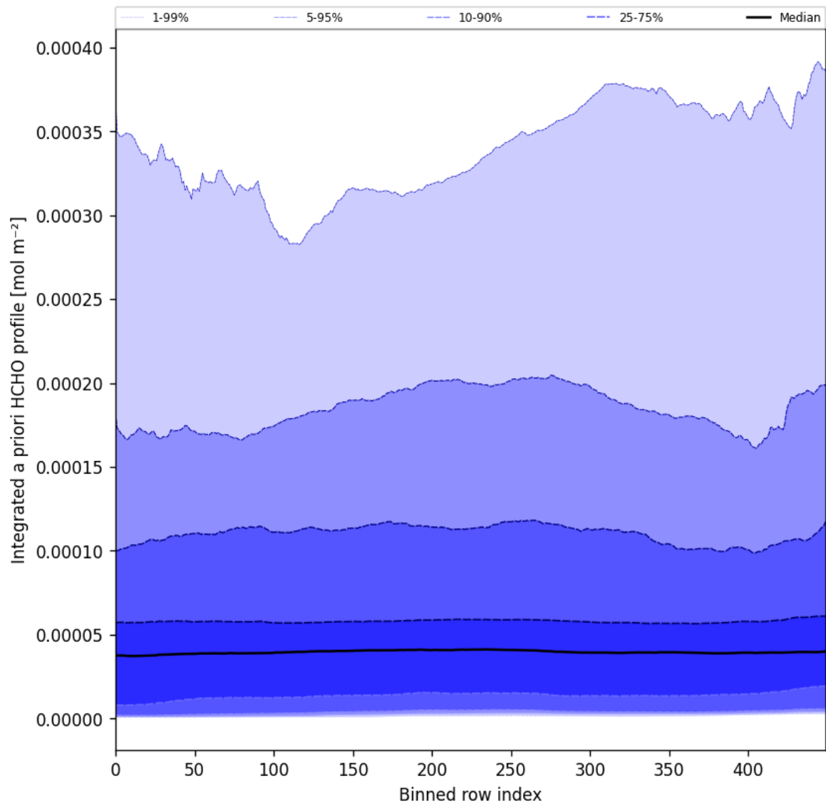
Figure 57: Along track statistics of “Integrated a priori HCHO profile” for 2024-11-09 to 2024-11-10
