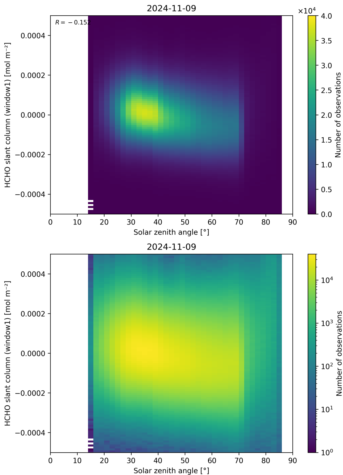
Figure 173: Scatter density plot of “Solar zenith angle” against “HCHO slant column (window1)” for 2024-11-09 to 2024-11-10.
