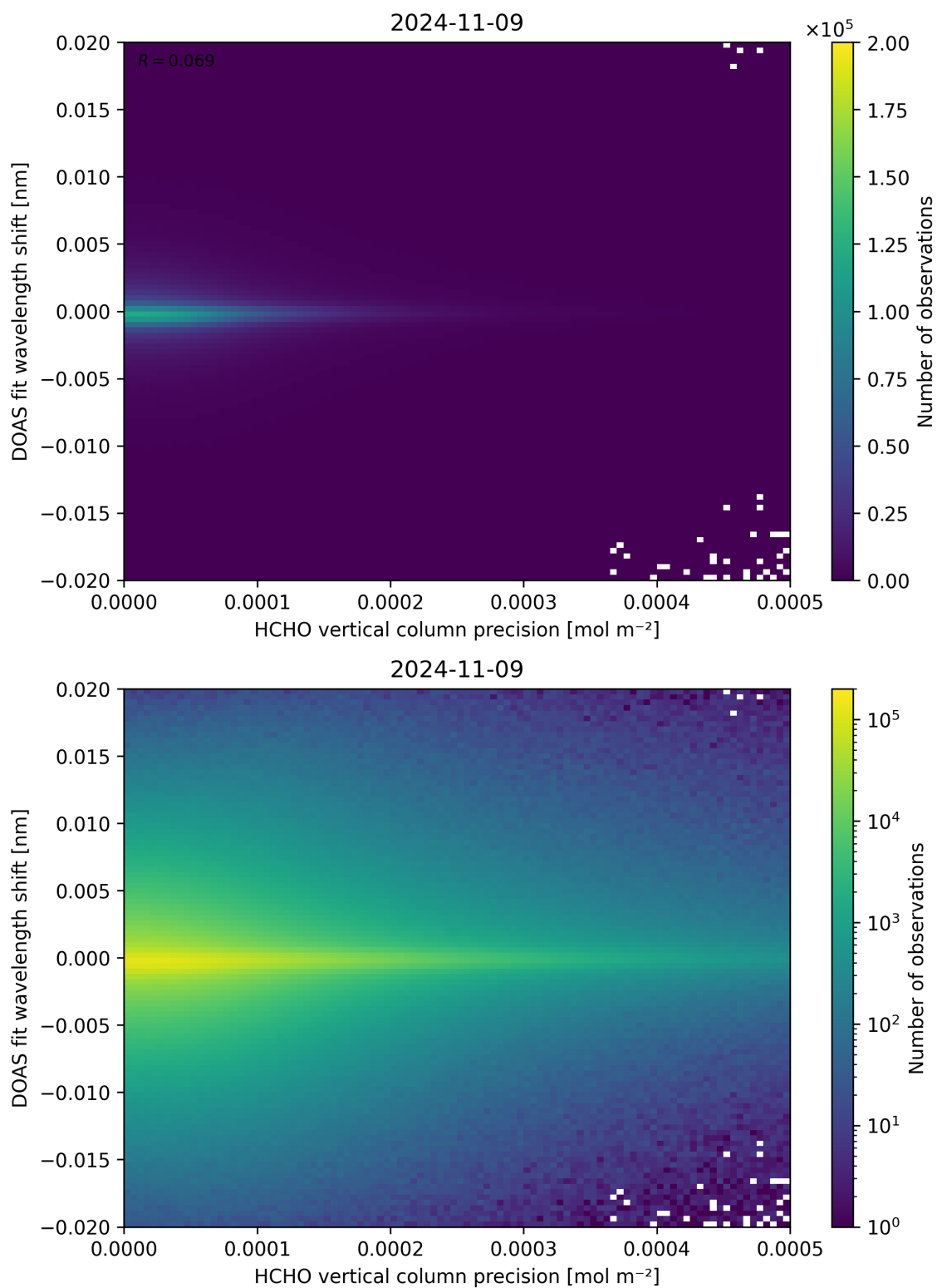
Figure 137: Scatter density plot of “HCHO vertical column precision” against “DOAS fit wavelength shift” for 2024-11-09 to 2024-11-10.
