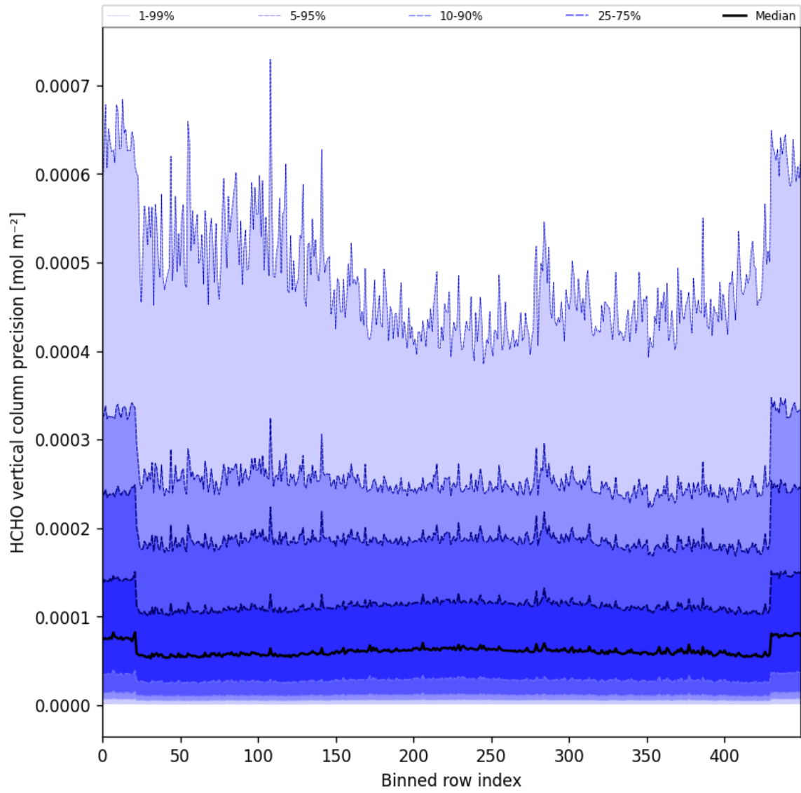
Figure 50: Along track statistics of "HCHO vertical column precision" for 2024-11-09 to 2024-11-10
