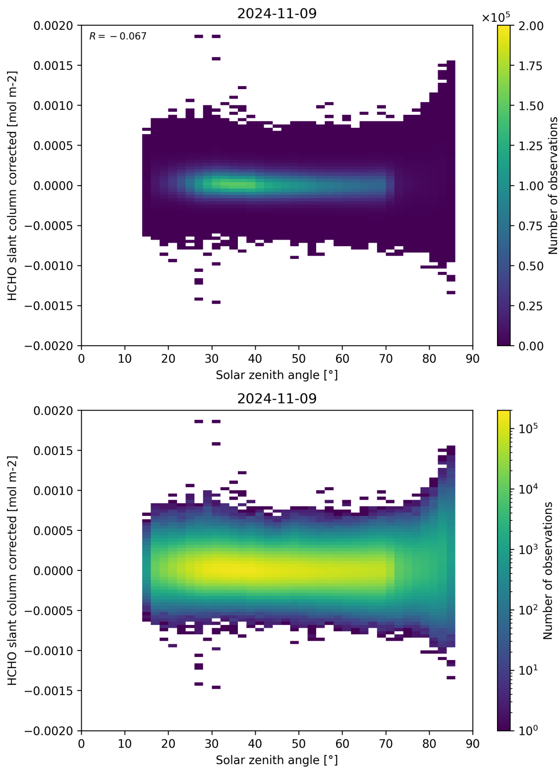
Figure 171: Scatter density plot of “Solar zenith angle” against “HCHO slant column corrected” for 2024-11-09 to 2024-11-10.
