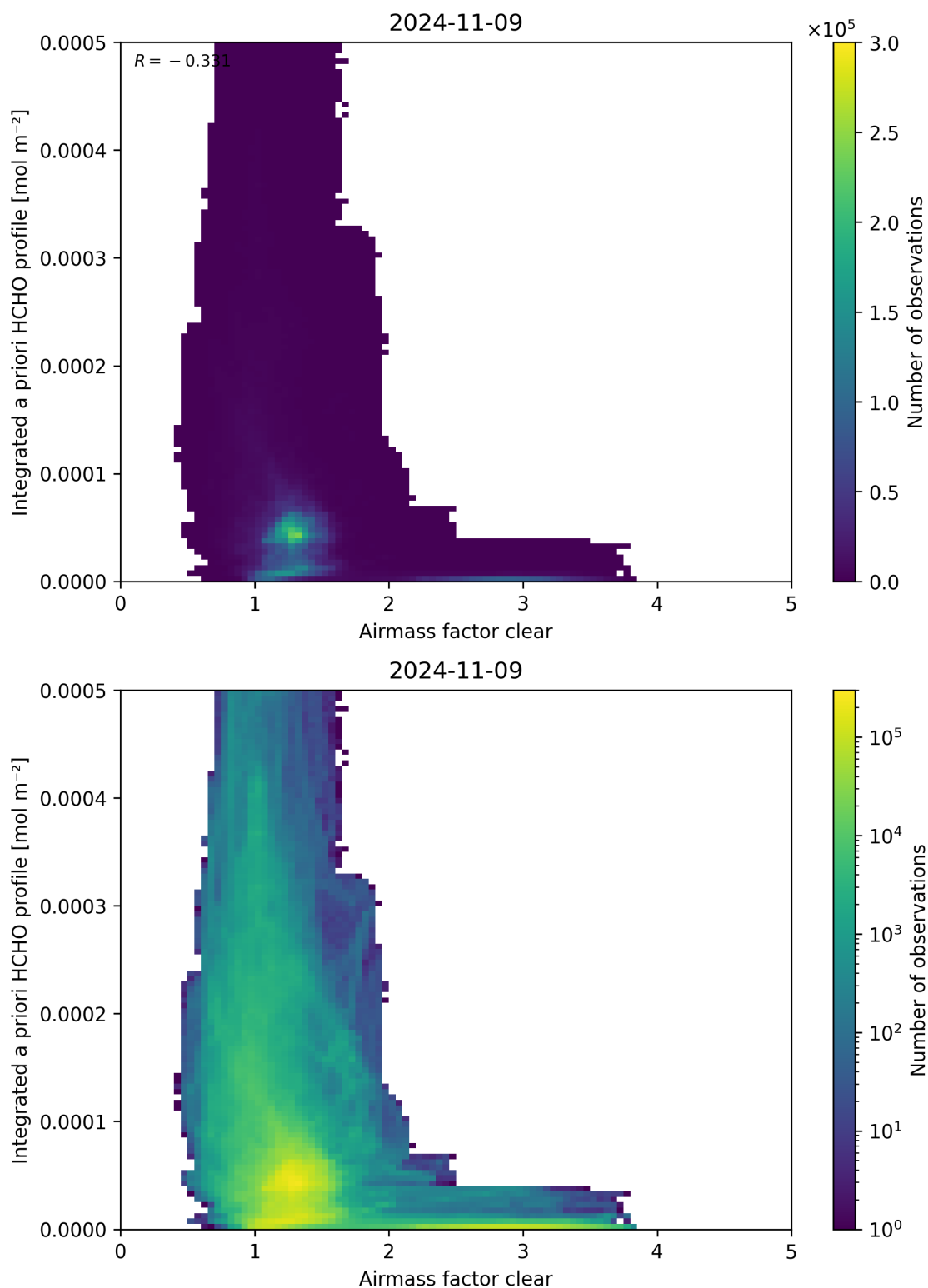
Figure 76: Scatter density plot of “Airmass factor clear” against “Integrated a priori HCHO profile” for 2024-11-09 to 2024-11-10.
