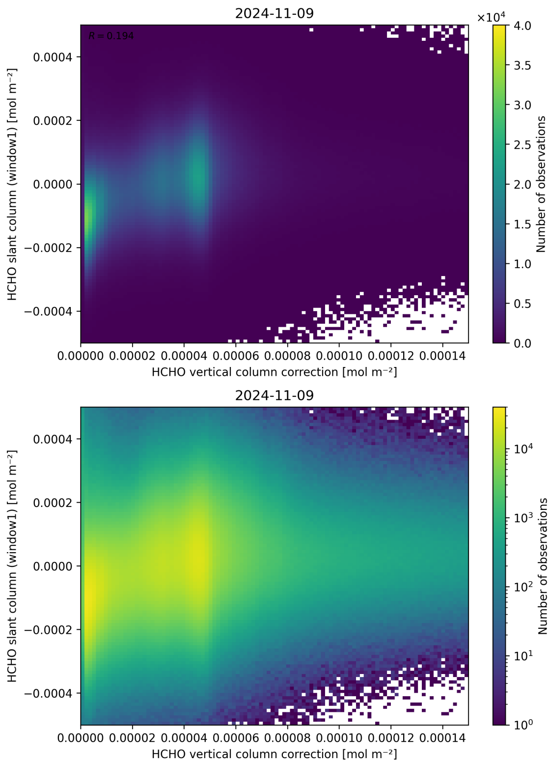
Figure 118: Scatter density plot of “HCHO vertical column correction” against “HCHO slant column (window1)” for 2024-11-09 to 2024-11-10.
