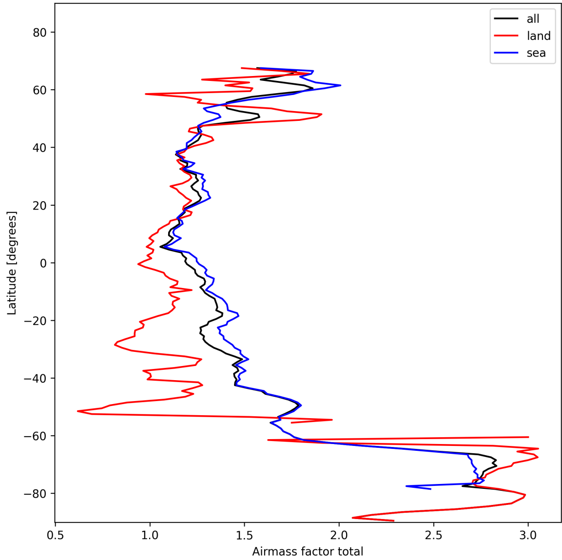
Figure 26: Zonal average of “Airmass factor total” for 2024-11-09 to 2024-11-10.
