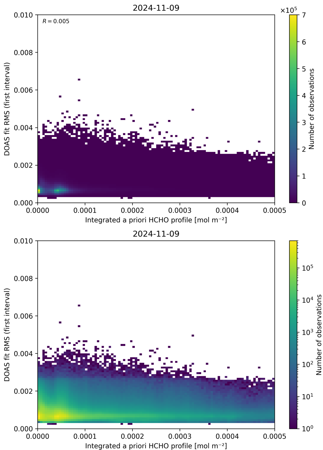
Figure 148: Scatter density plot of “Integrated a priori HCHO profile” against “DOAS fit RMS (first interval)” for 2024-11-09 to 2024-11-10.
