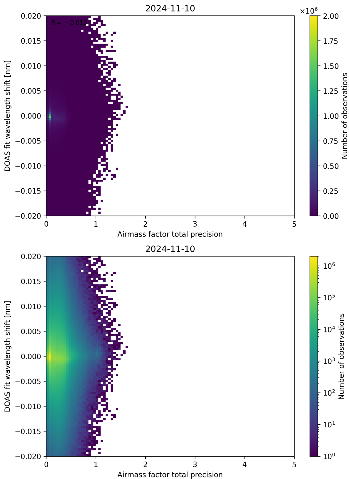
Figure 106: Scatter density plot of “Airmass factor total precision” against “DOAS fit wavelength shift” for 2024-11-09 to 2024-11-11.
