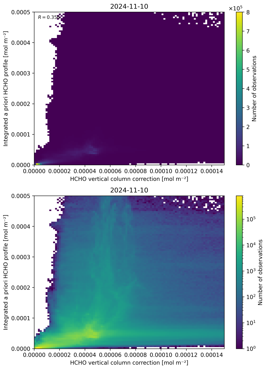
Figure 122: Scatter density plot of “HCHO vertical column correction” against “Integrated a priori HCHO profile” for 2024-11-09 to 2024-11-11.
