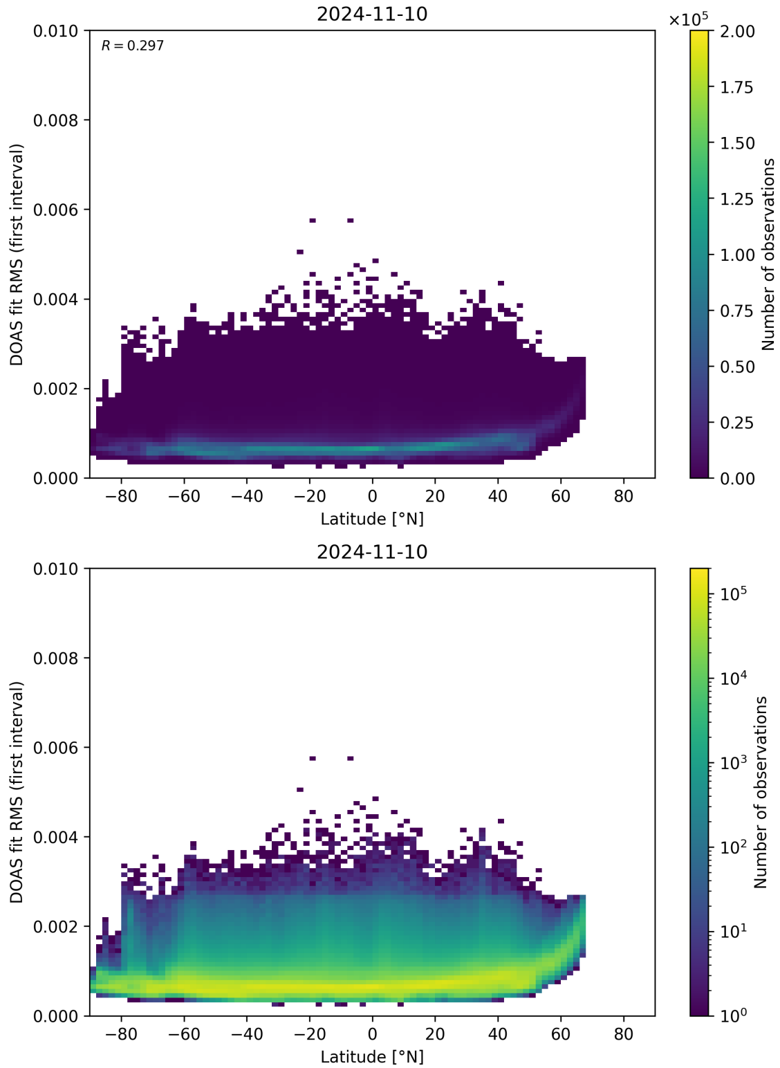
Figure 153: Scatter density plot of “Latitude” against “DOAS fit RMS (first interval)” for 2024-11-09 to 2024-11-11.
