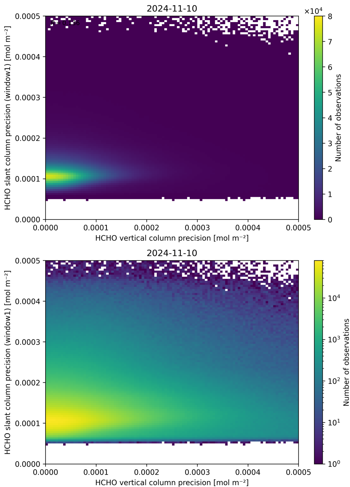
Figure 143: Scatter density plot of “HCHO vertical column precision” against “HCHO slant column precision (window1)” for 2024-11-09 to 2024-11-11.
