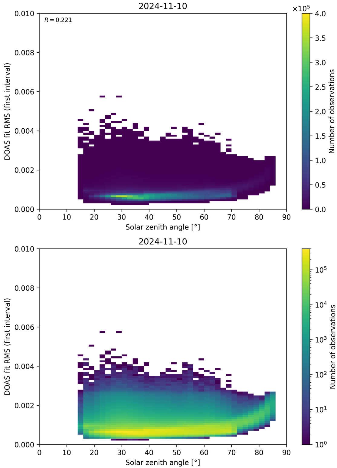
Figure 167: Scatter density plot of “Solar zenith angle” against “DOAS fit RMS (first interval)” for 2024-11-09 to 2024-11-11.
