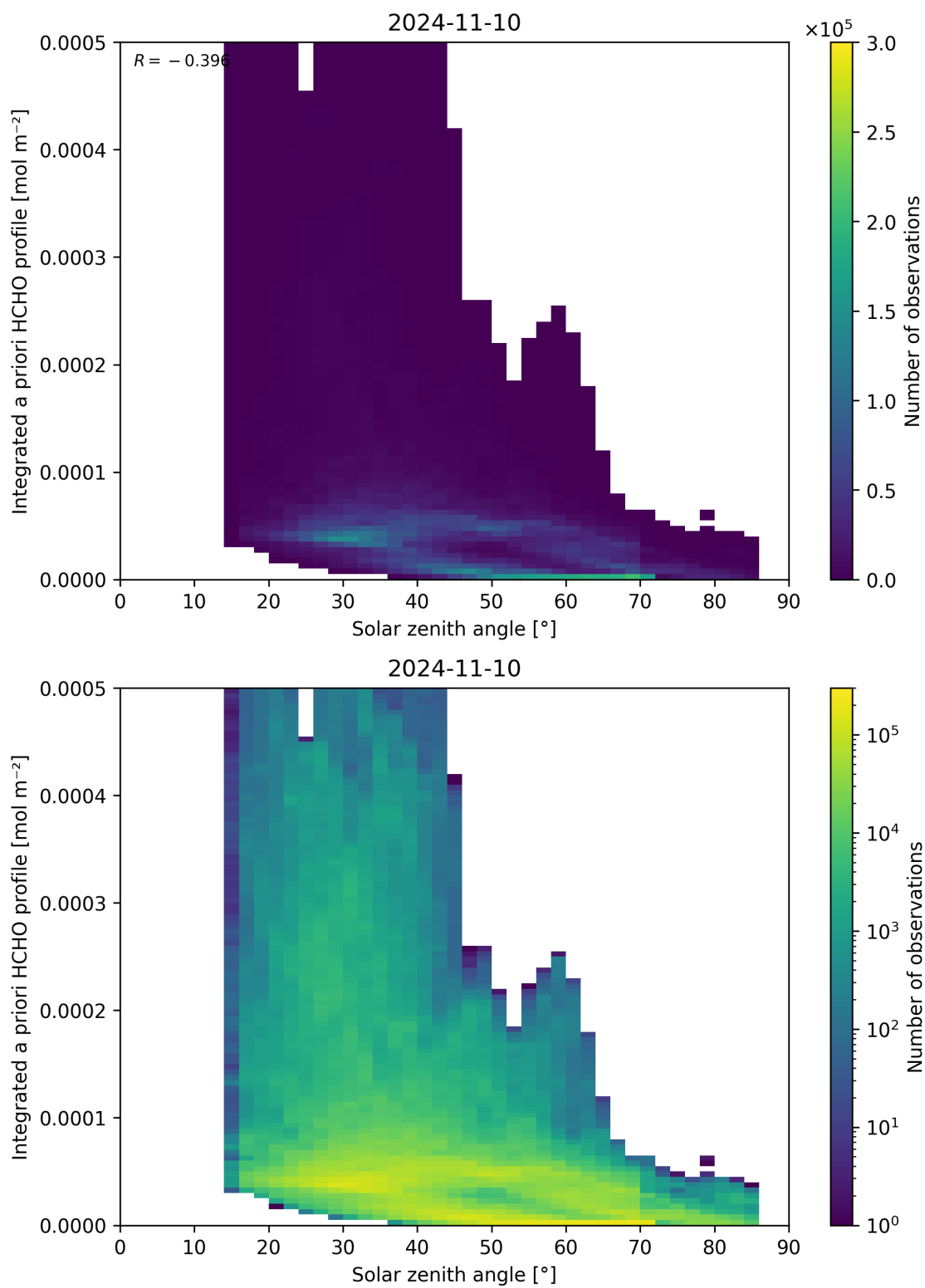
Figure 180: Scatter density plot of “Solar zenith angle” against “Integrated a priori HCHO profile” for 2024-11-09 to 2024-11-11.
