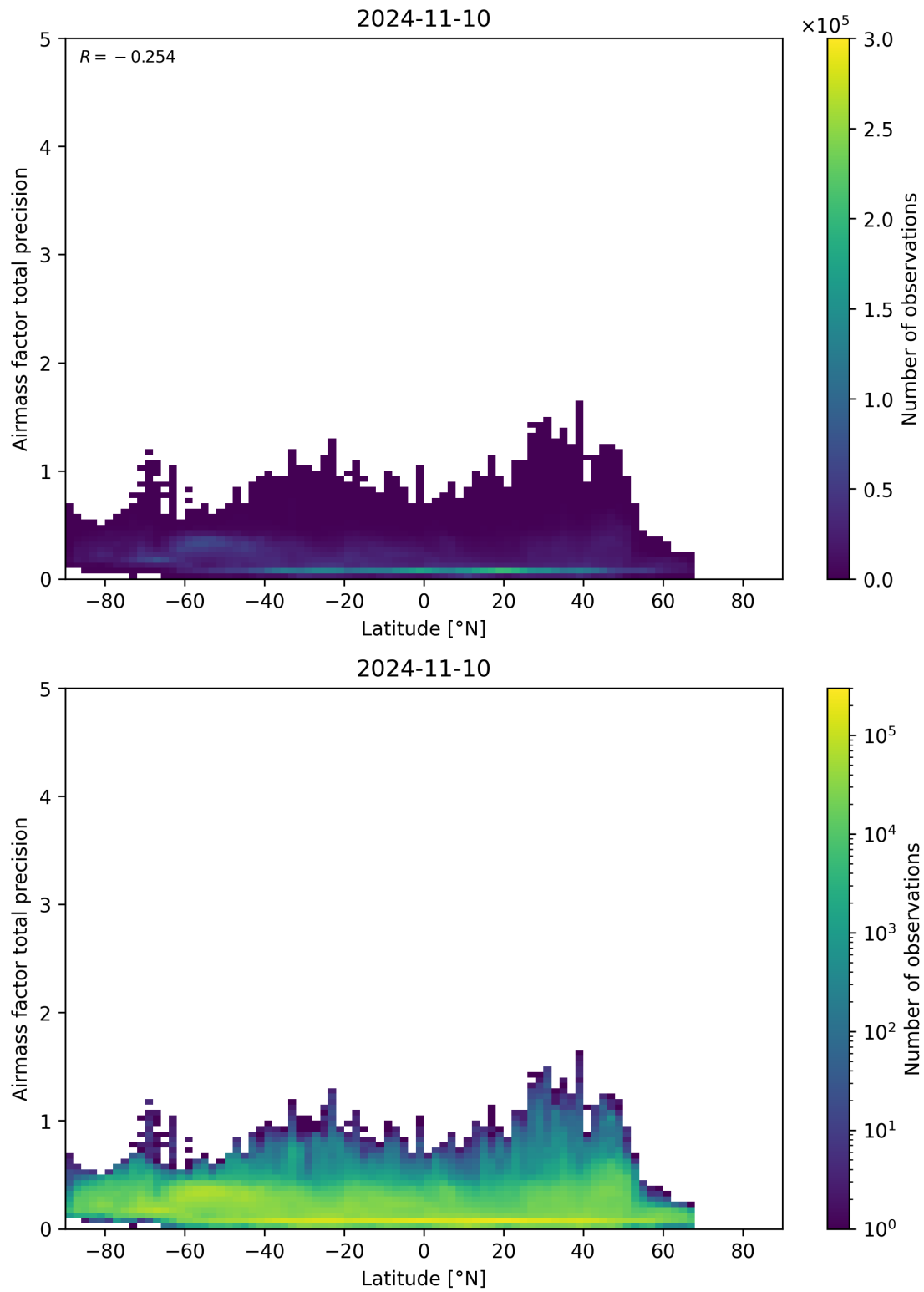
Figure 162: Scatter density plot of “Latitude” against “Airmass factor total precision” for 2024-11-09 to 2024-11-11.
