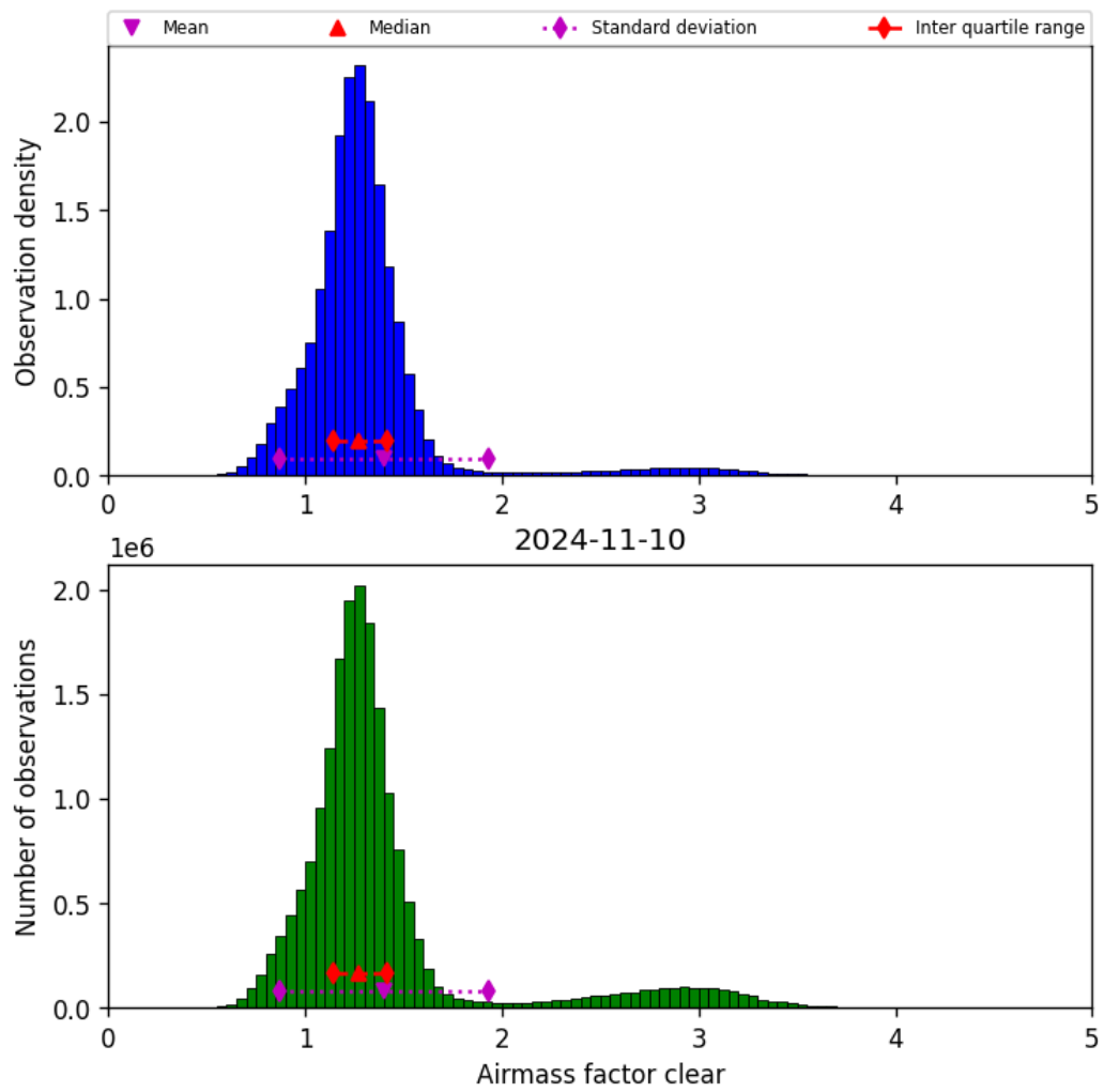
Figure 42: Histogram of “Airmass factor clear” for 2024-11-09 to 2024-11-11
