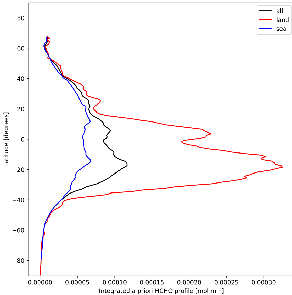
Figure 29: Zonal average of “Integrated a priori HCHO profile” for 2024-11-09 to 2024-11-11.
