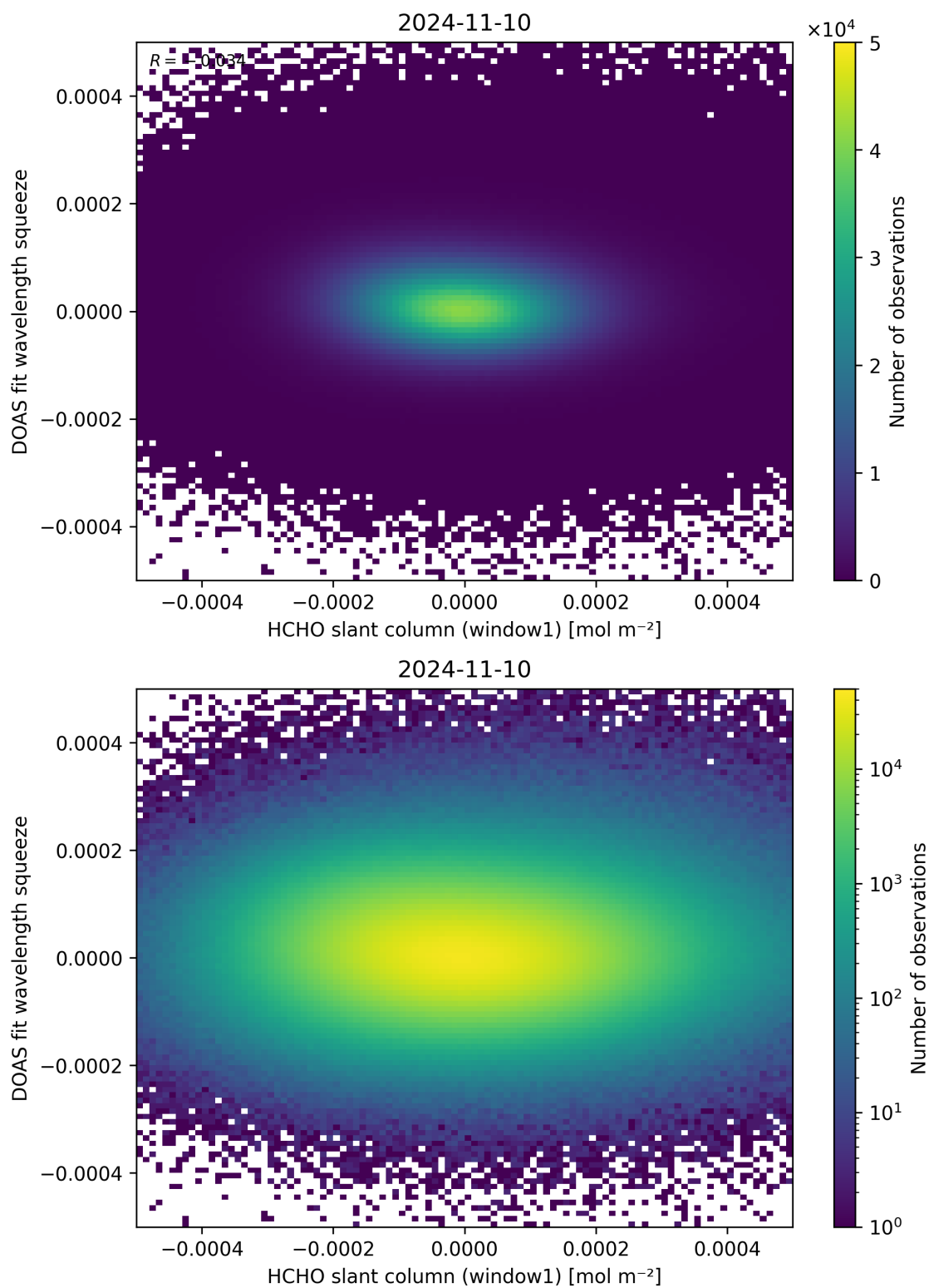
Figure 80: Scatter density plot of “HCHO slant column (window1)” against “DOAS fit wavelength squeeze” for 2024-11-09 to 2024-11-11.
