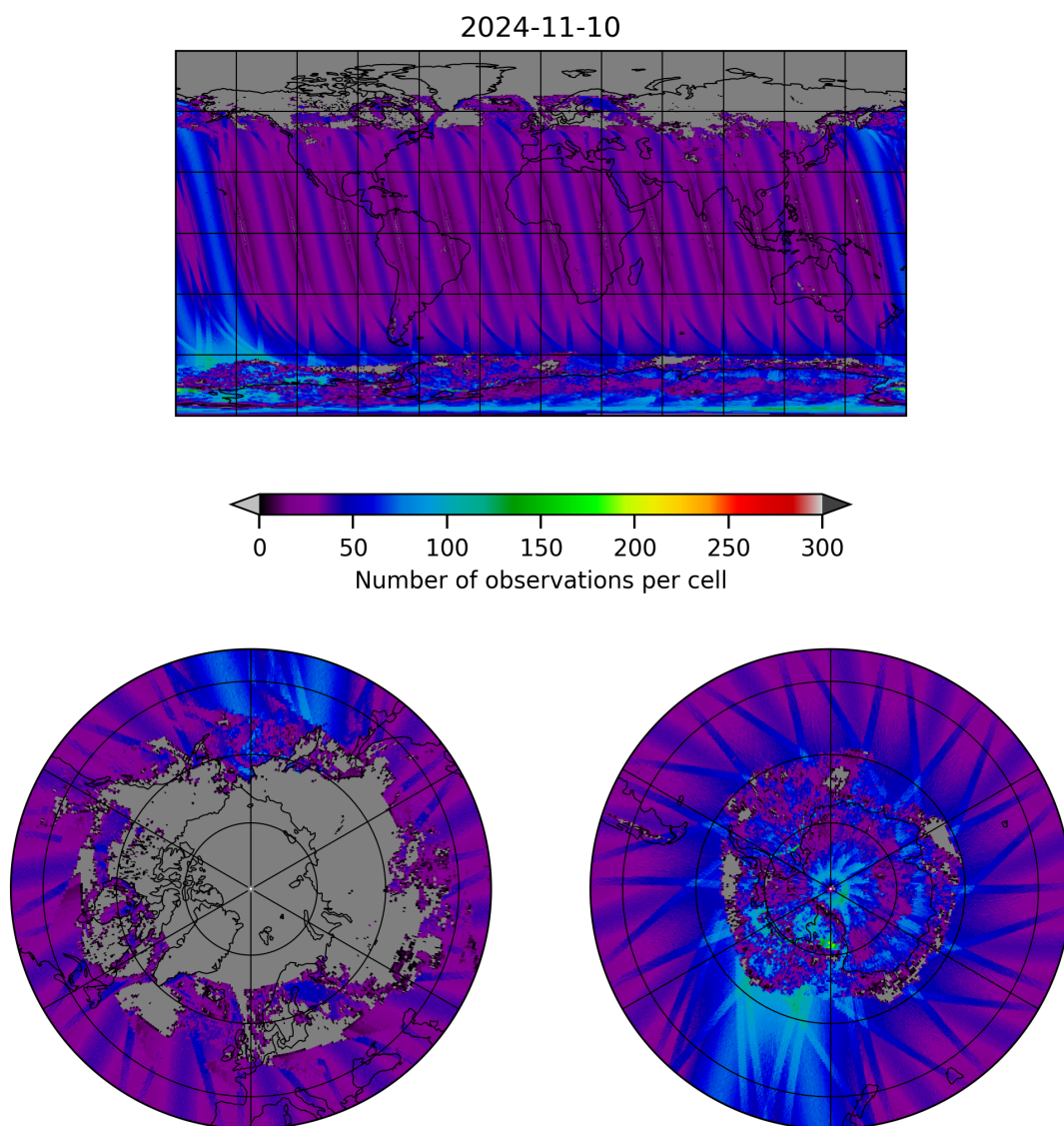
Figure 19: Map of the number of observations for 2024-11-09 to 2024-11-11
