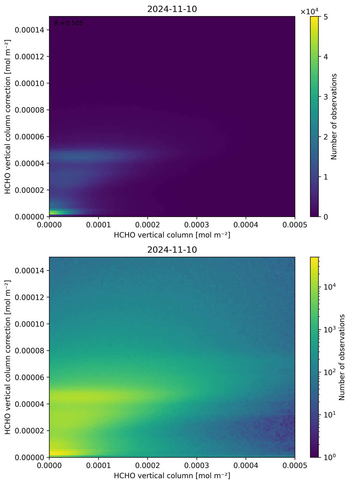
Figure 133: Scatter density plot of “HCHO vertical column” against “HCHO vertical column correction” for 2024-11-09 to 2024-11-11.
