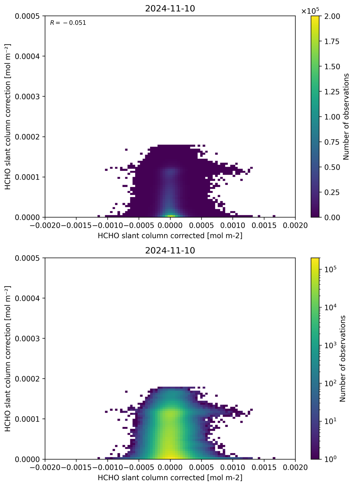
Figure 77: Scatter density plot of “HCHO slant column corrected” against “HCHO slant column correction” for 2024-11-09 to 2024-11-11.
