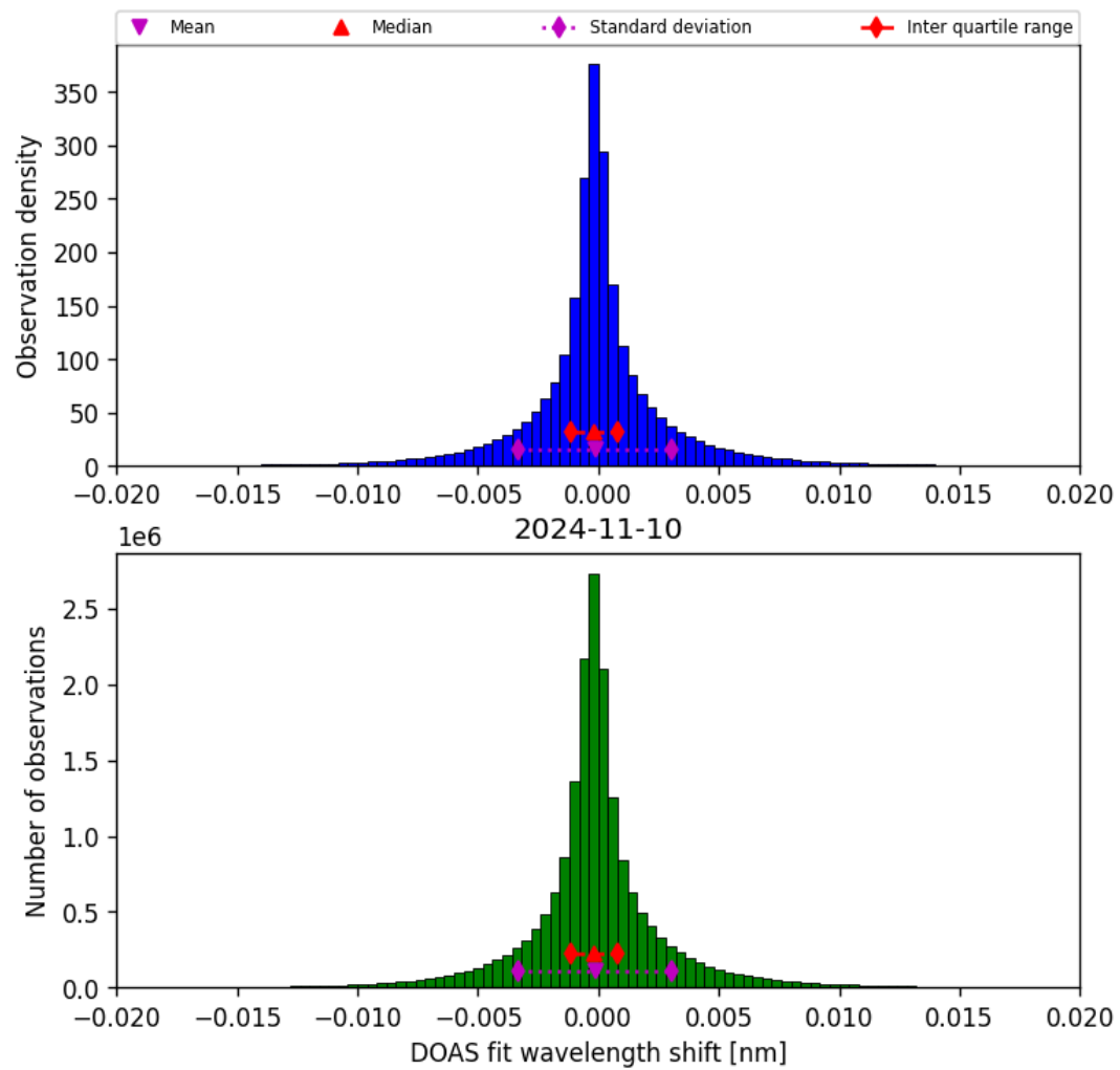
Figure 44: Histogram of “DOAS fit wavelength shift” for 2024-11-09 to 2024-11-11
