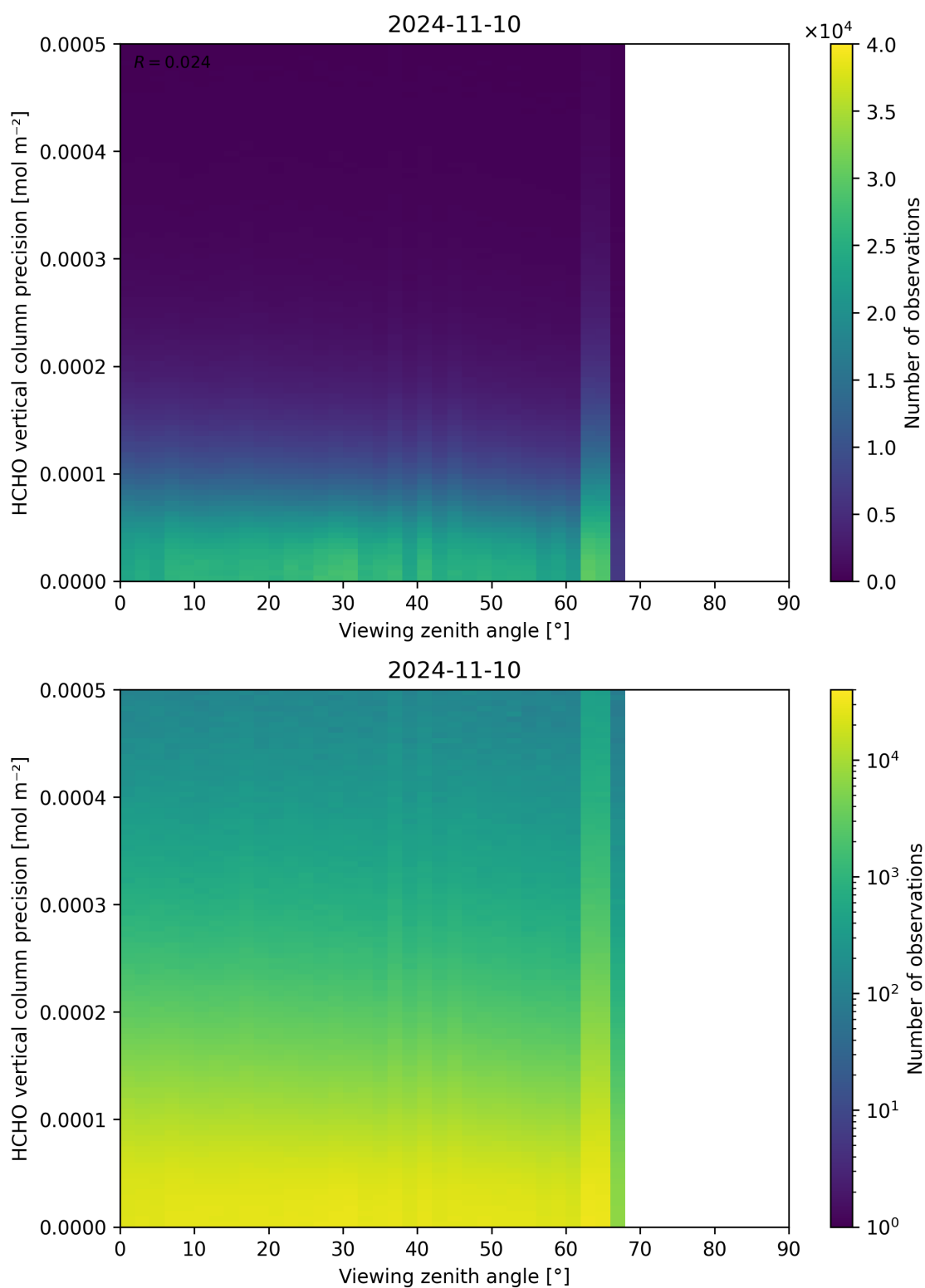
Figure 194: Scatter density plot of “Viewing zenith angle” against “HCHO vertical column precision” for 2024-11-09 to 2024-11-11.
