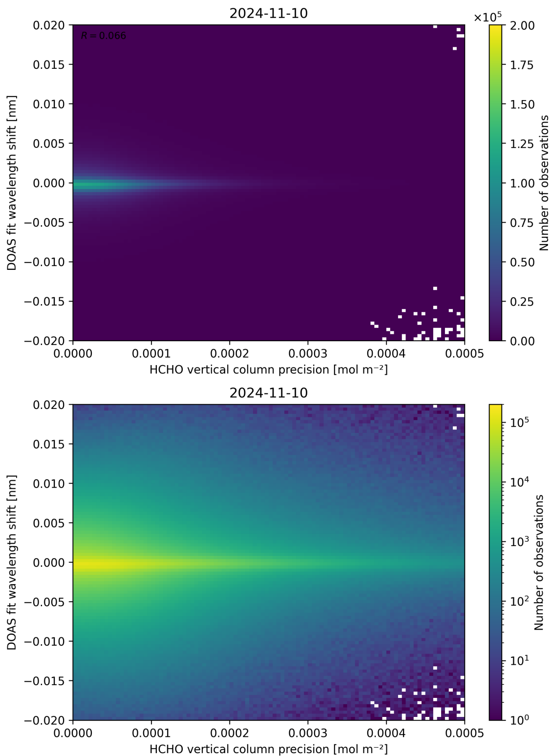
Figure 137: Scatter density plot of “HCHO vertical column precision” against “DOAS fit wavelength shift” for 2024-11-09 to 2024-11-11.
