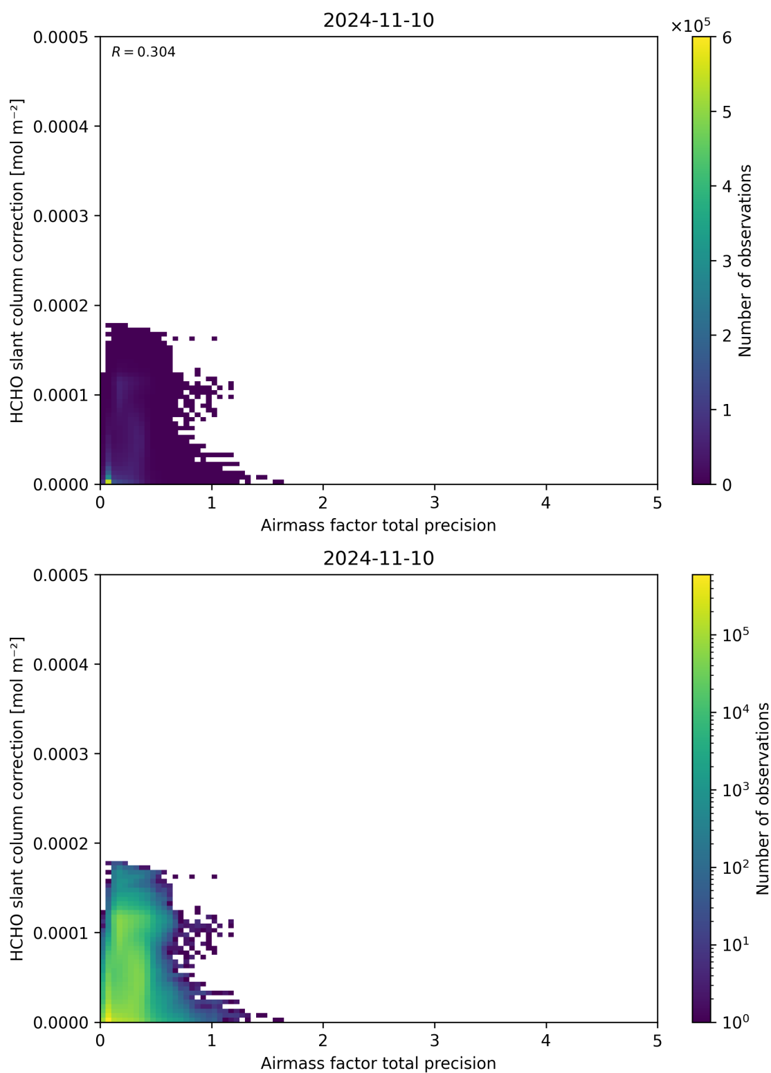
Figure 110: Scatter density plot of “Airmass factor total precision” against “HCHO slant column correction” for 2024-11-09 to 2024-11-11.
