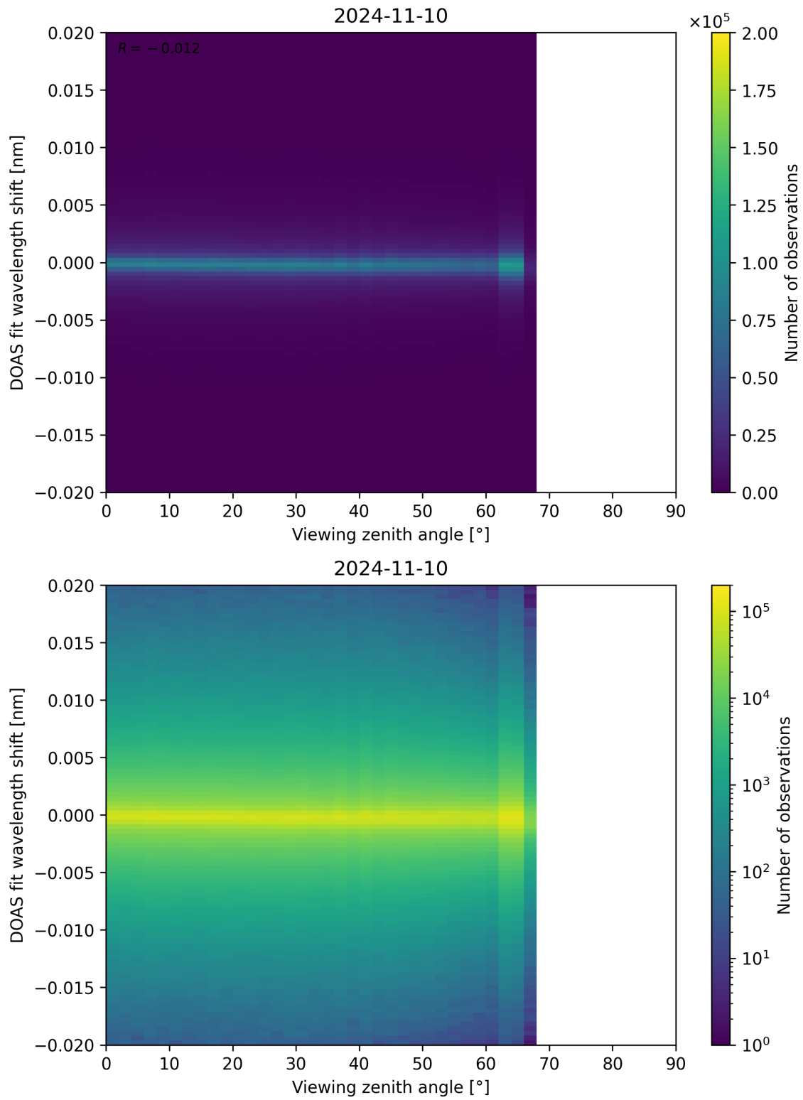
Figure 183: Scatter density plot of “Viewing zenith angle” against “DOAS fit wavelength shift” for 2024-11-09 to 2024-11-11.
