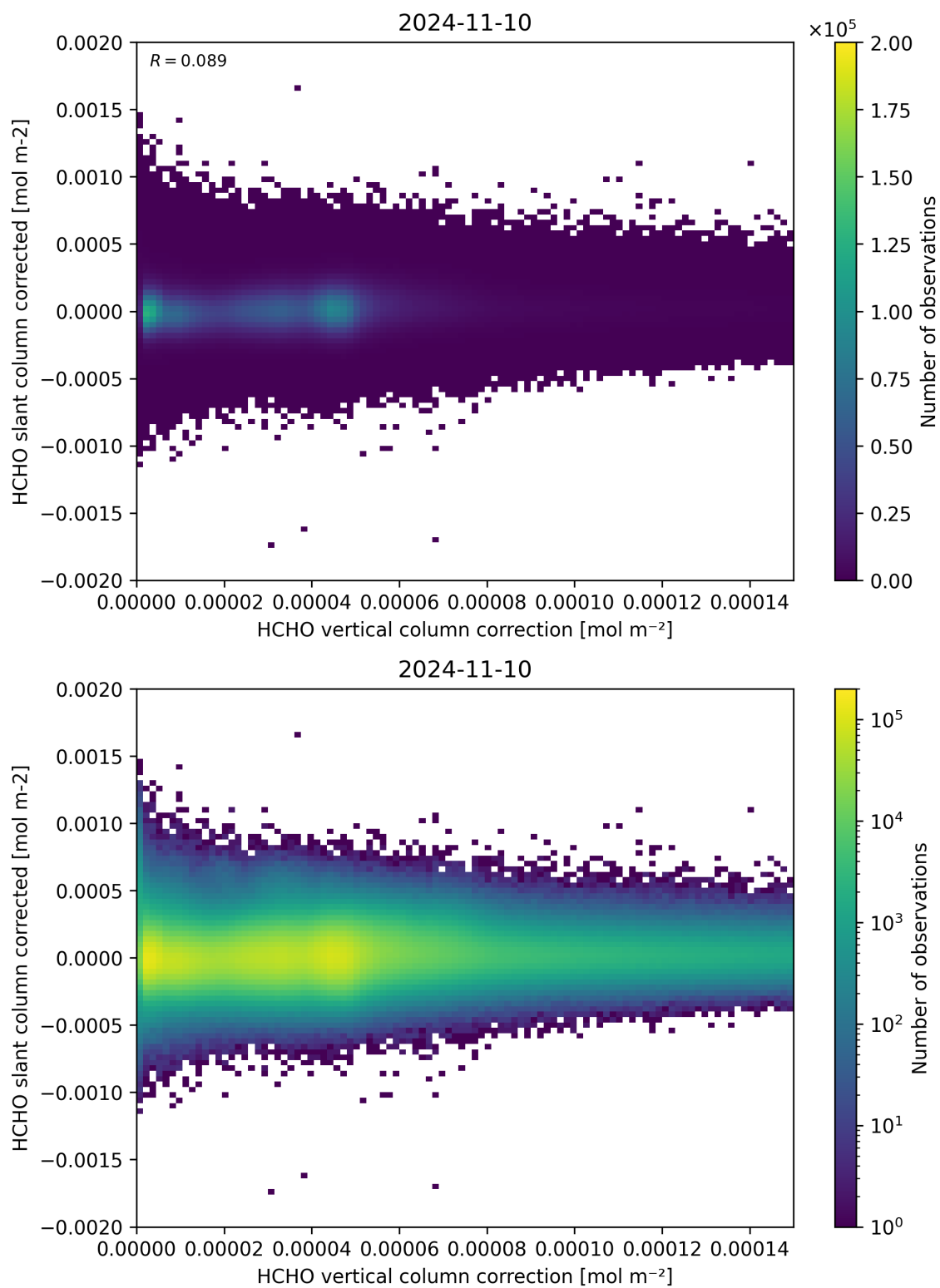
Figure 116: Scatter density plot of “HCHO vertical column correction” against “HCHO slant column corrected” for 2024-11-09 to 2024-11-11.
