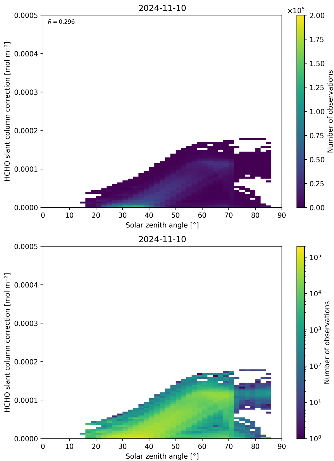
Figure 172: Scatter density plot of “Solar zenith angle” against “HCHO slant column correction” for 2024-11-09 to 2024-11-11.
