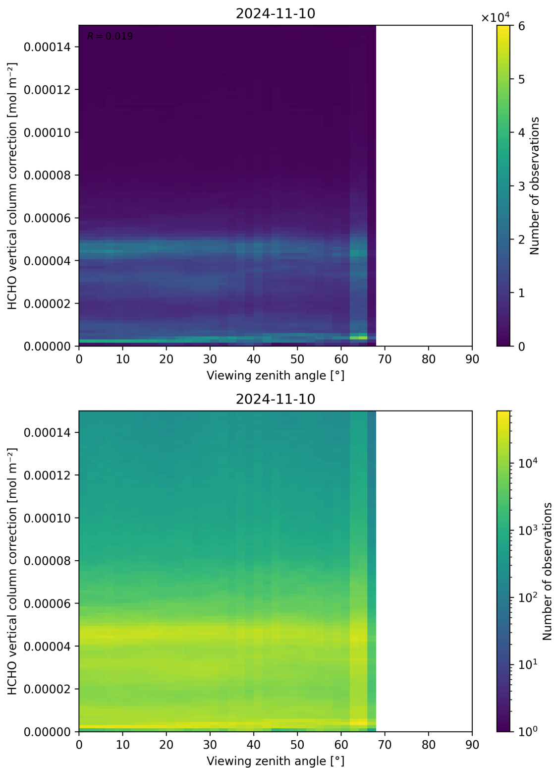
Figure 193: Scatter density plot of “Viewing zenith angle” against “HCHO vertical column correction” for 2024-11-09 to 2024-11-11.
