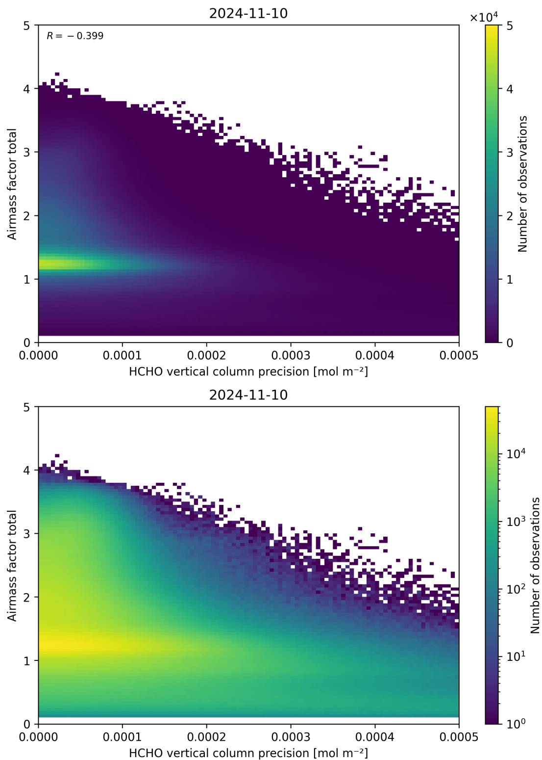
Figure 144: Scatter density plot of “HCHO vertical column precision” against “Airmass factor total” for 2024-11-09 to 2024-11-11.
