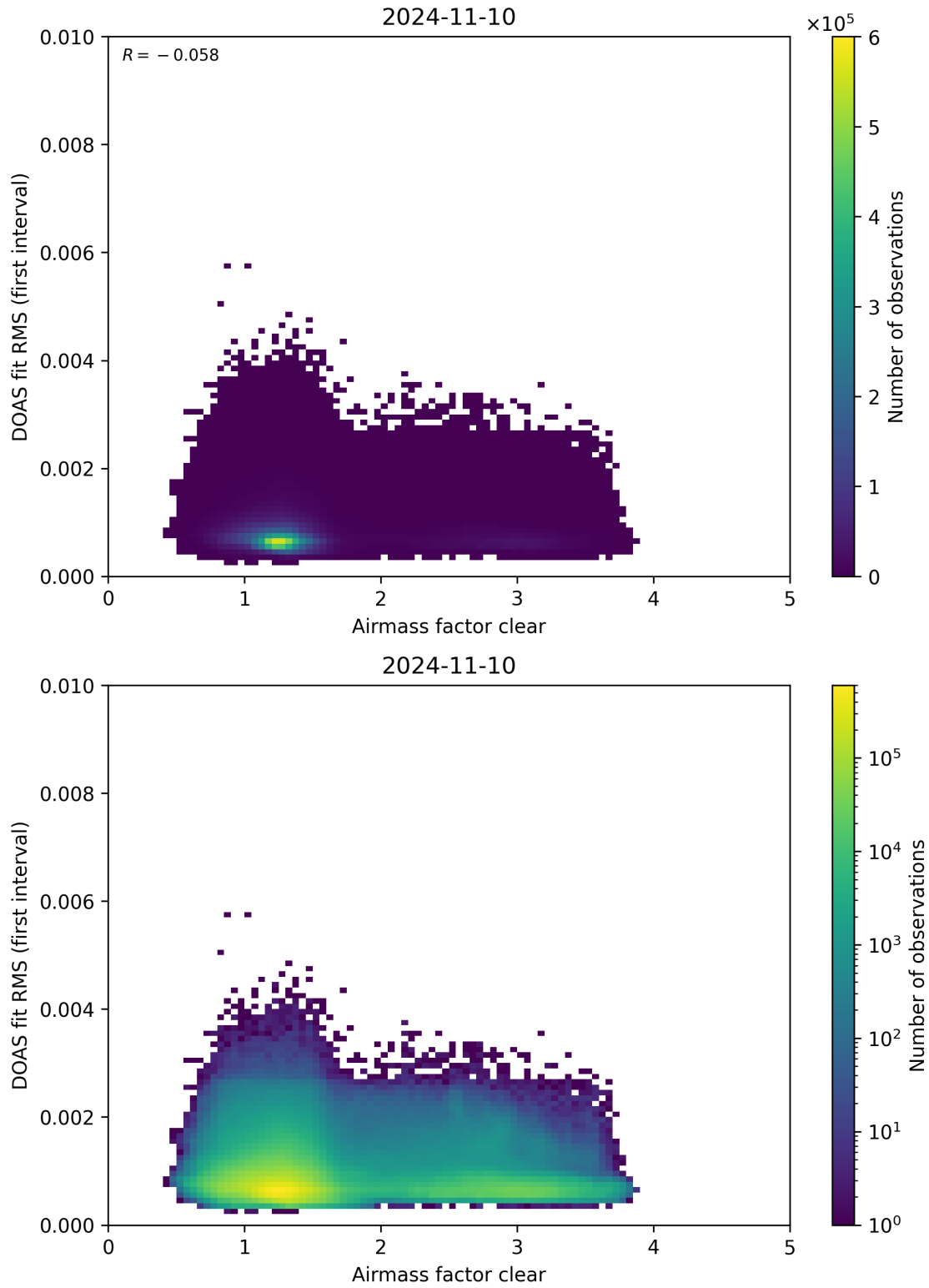
Figure 71: Scatter density plot of “Airmass factor clear” against “DOAS fit RMS (first interval)” for 2024-11-09 to 2024-11-11.
