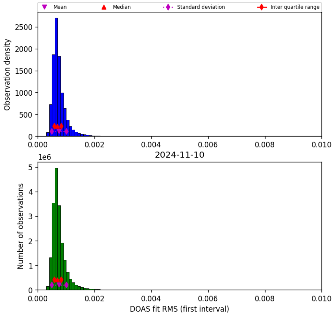
Figure 46: Histogram of “DOAS fit RMS (first interval)” for 2024-11-09 to 2024-11-11
