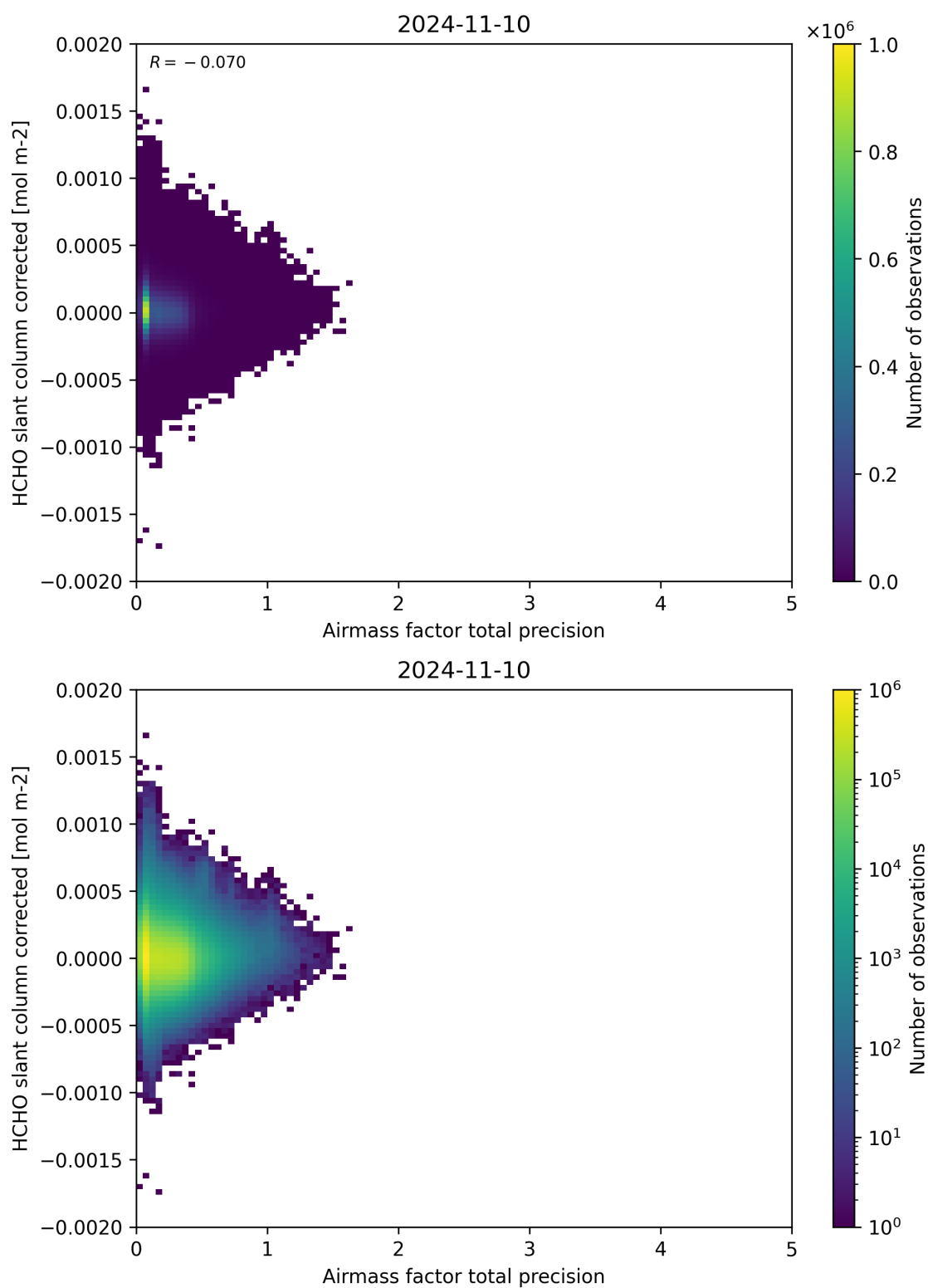
Figure 109: Scatter density plot of “Airmass factor total precision” against “HCHO slant column corrected” for 2024-11-09 to 2024-11-11.
