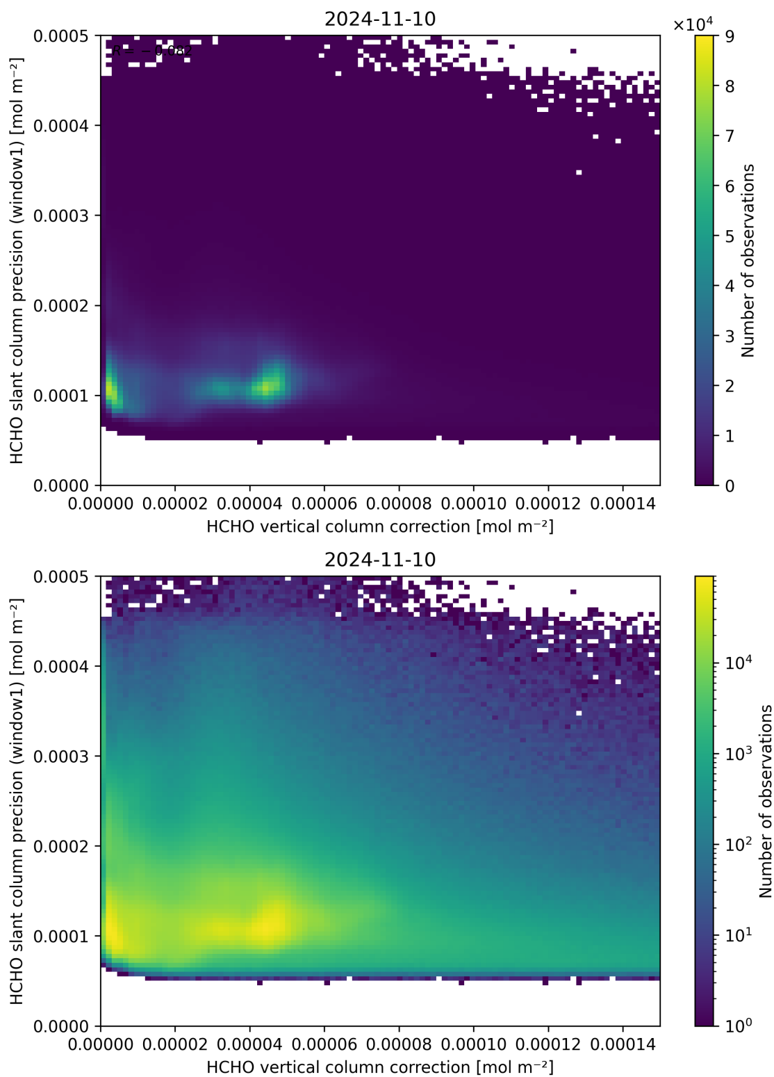
Figure 119: Scatter density plot of “HCHO vertical column correction” against “HCHO slant column precision (window1)” for 2024-11-09 to 2024-11-11.
