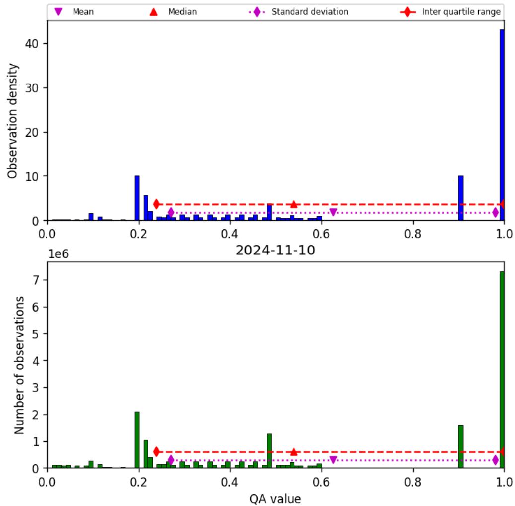
Figure 34: Histogram of “QA value” for 2024-11-09 to 2024-11-11
