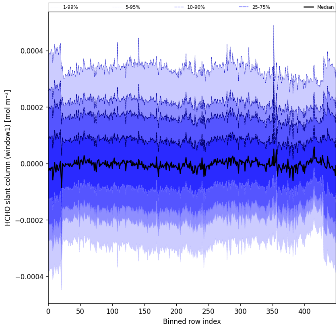
Figure 52: Along track statistics of “HCHO slant column (window1)” for 2024-11-09 to 2024-11-11
