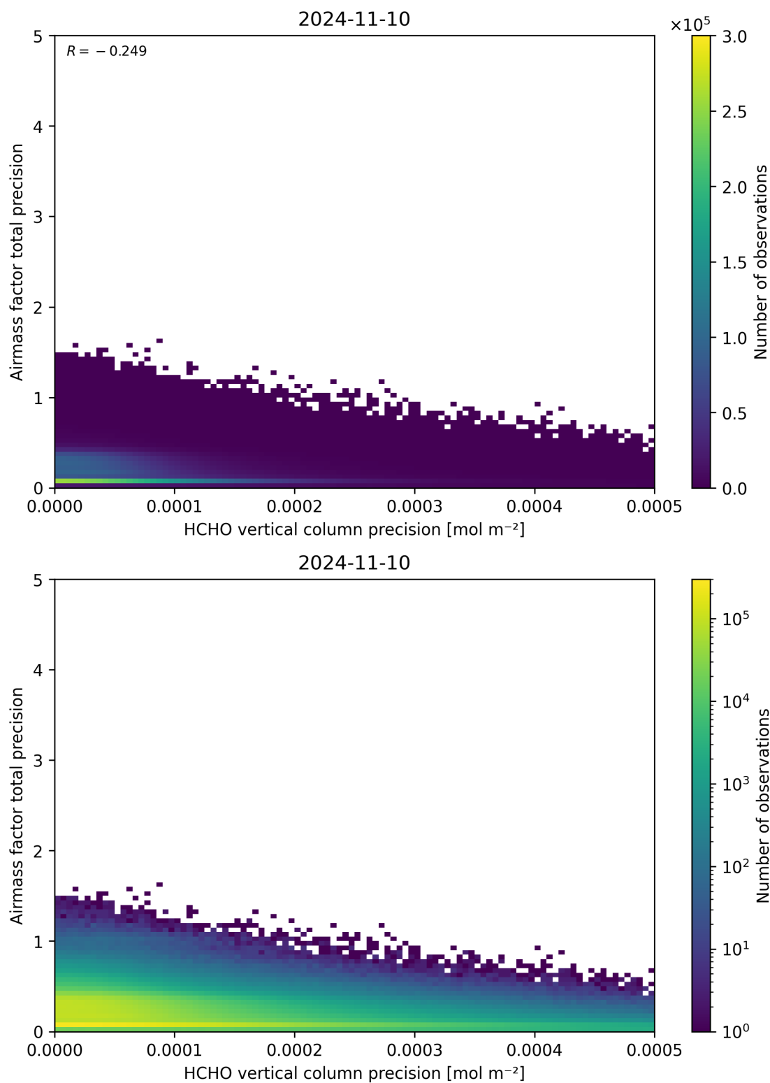
Figure 145: Scatter density plot of “HCHO vertical column precision” against “Airmass factor total precision” for 2024-11-09 to 2024-11-11.
