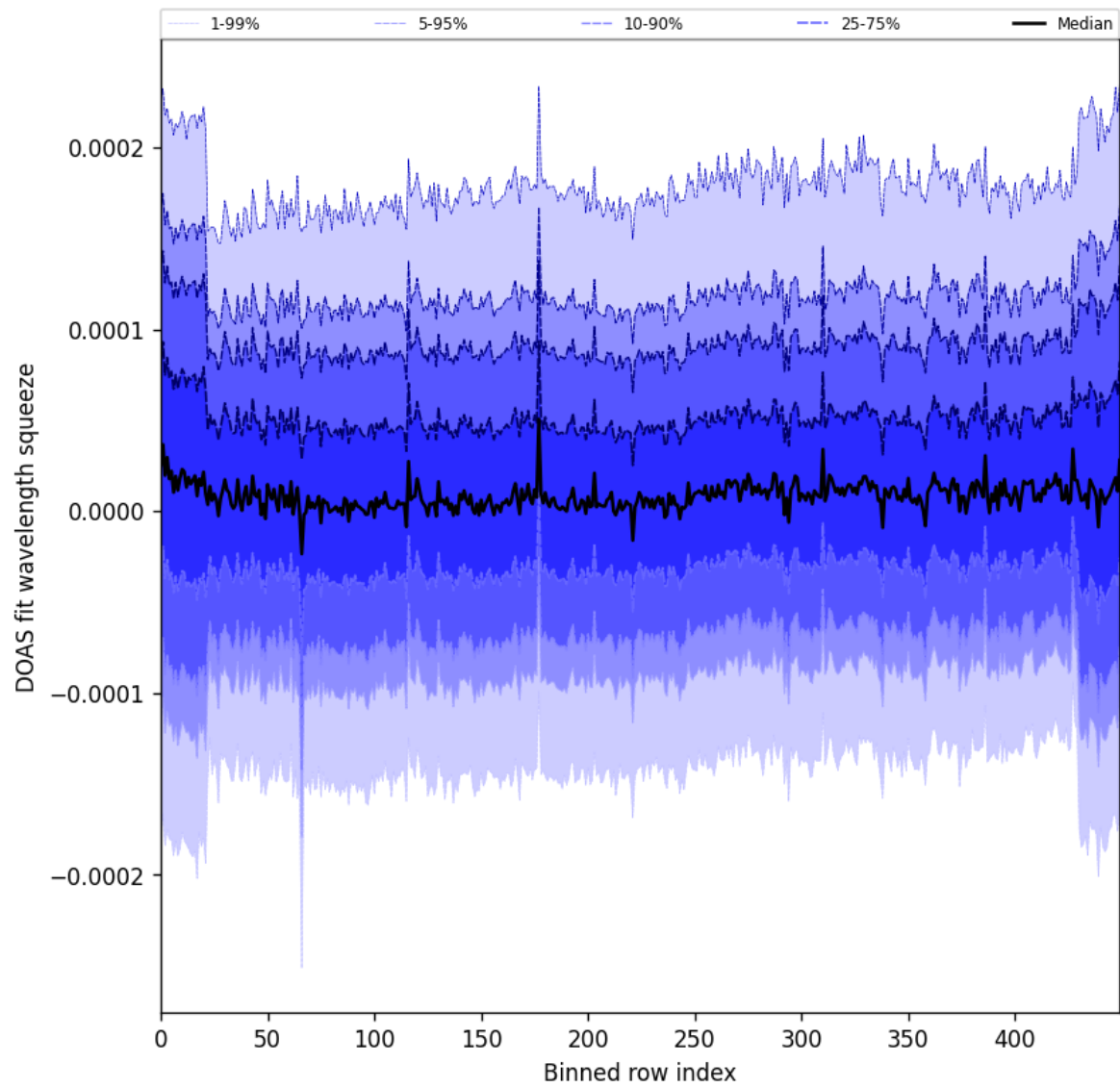
Figure 59: Along track statistics of “DOAS fit wavelength squeeze” for 2024-11-09 to 2024-11-11
