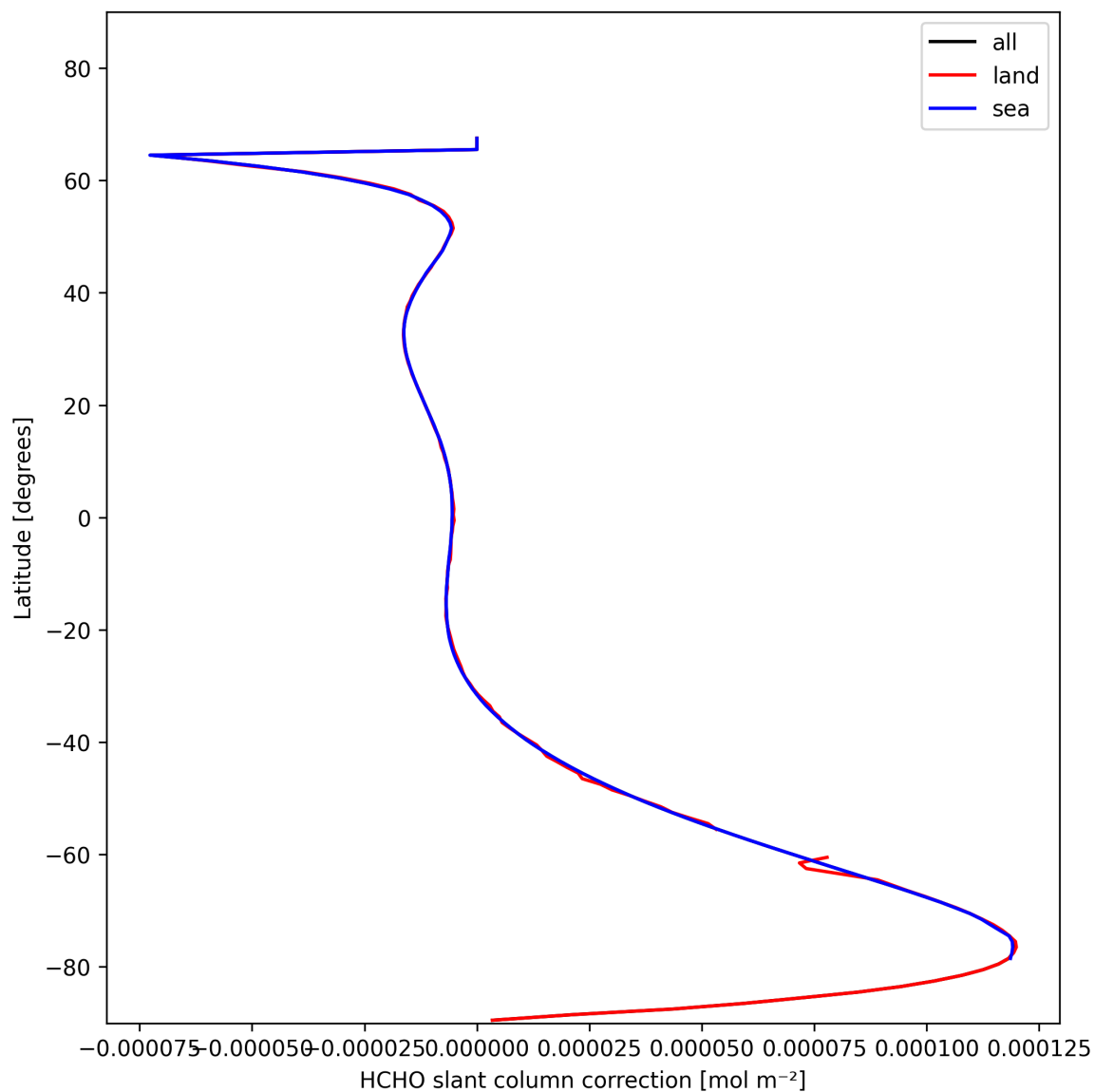
Figure 33: Zonal average of “HCHO slant column correction” for 2024-11-09 to 2024-11-11.
