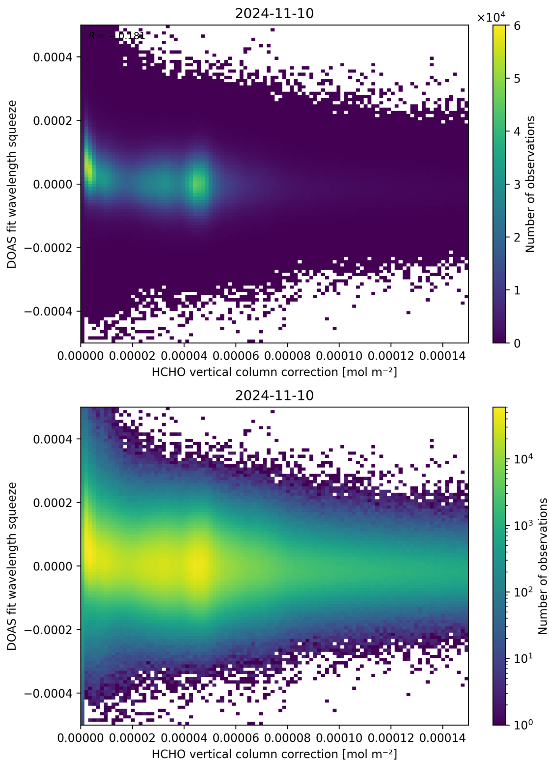
Figure 114: Scatter density plot of “HCHO vertical column correction” against “DOAS fit wavelength squeeze” for 2024-11-09 to 2024-11-11.
