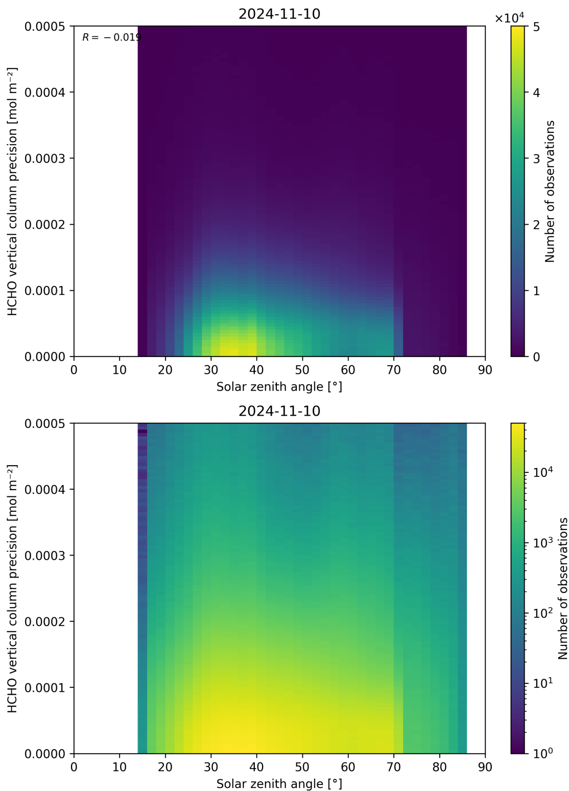
Figure 179: Scatter density plot of “Solar zenith angle” against “HCHO vertical column precision” for 2024-11-09 to 2024-11-11.
