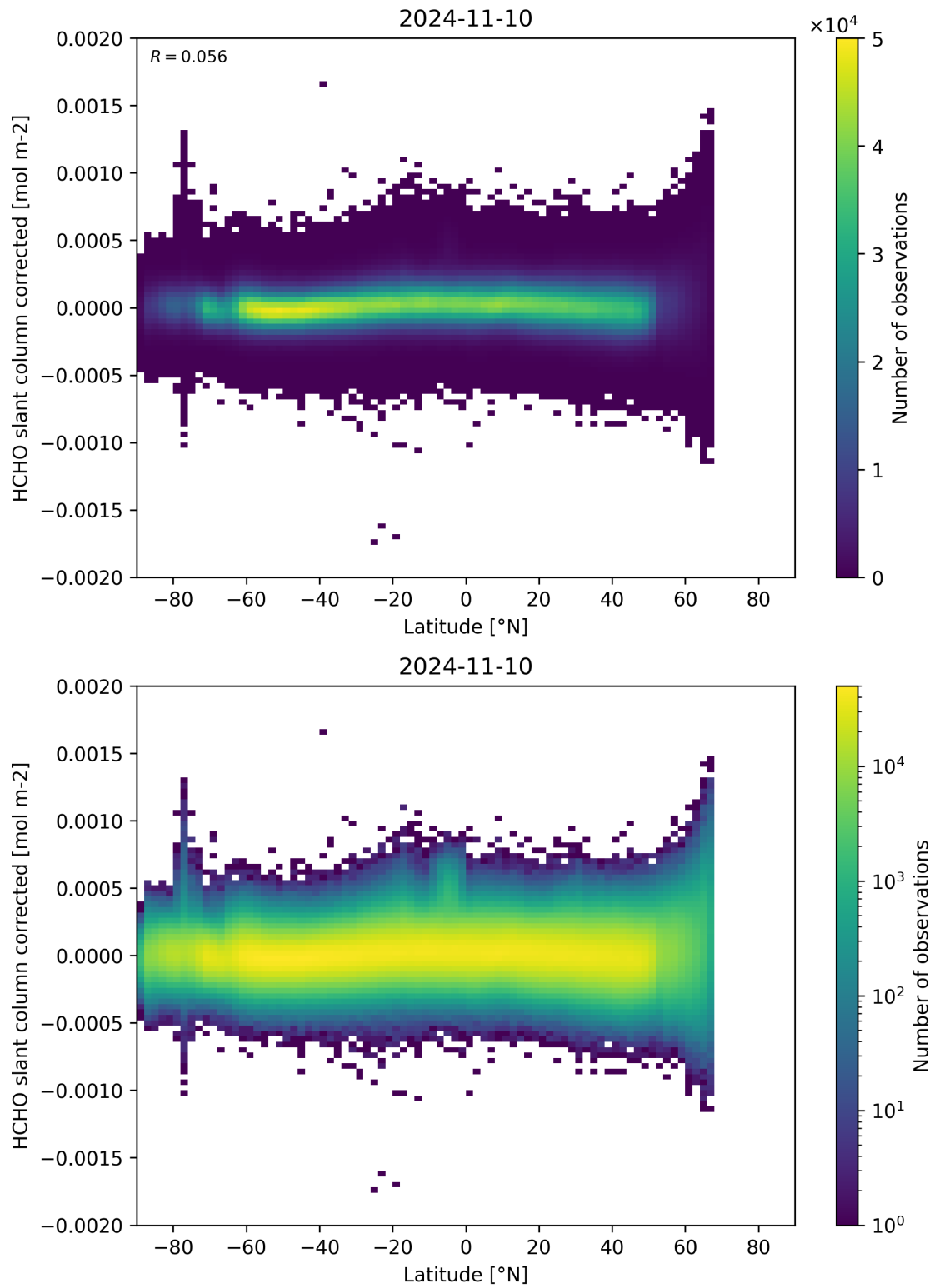
Figure 157: Scatter density plot of “Latitude” against “HCHO slant column corrected” for 2024-11-09 to 2024-11-11.
