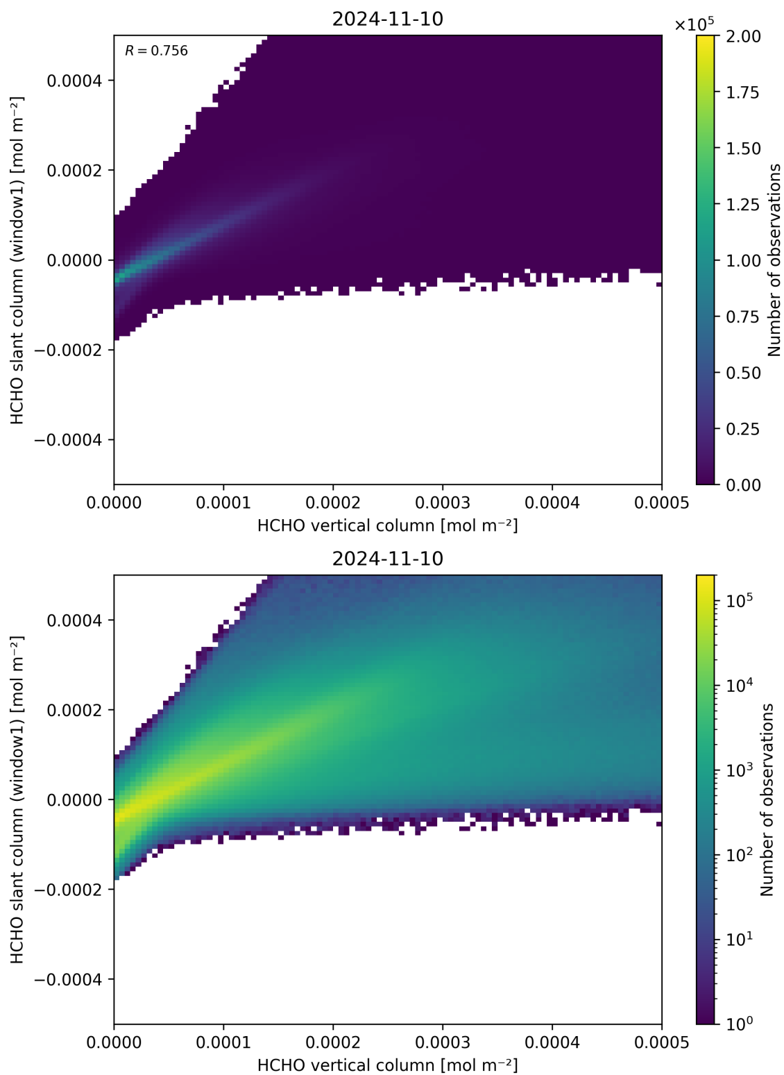
Figure 129: Scatter density plot of “HCHO vertical column” against “HCHO slant column (window1)” for 2024-11-09 to 2024-11-11.
