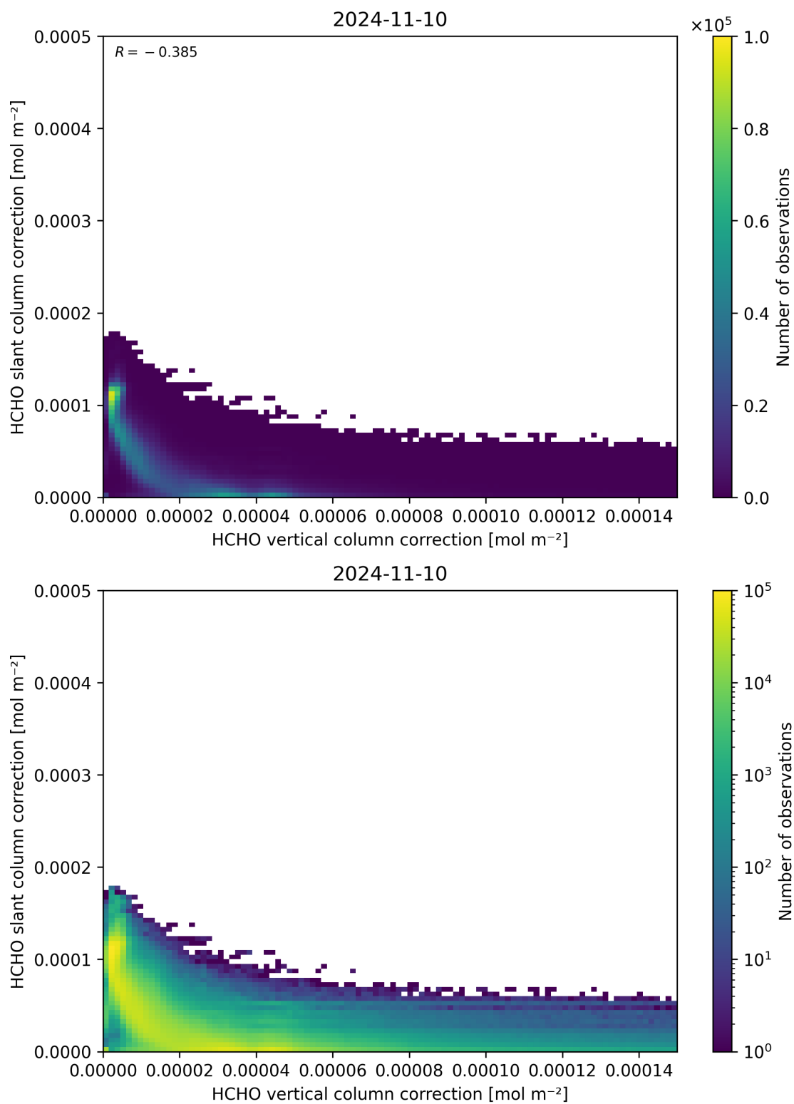
Figure 117: Scatter density plot of “HCHO vertical column correction” against “HCHO slant column correction” for 2024-11-09 to 2024-11-11.
