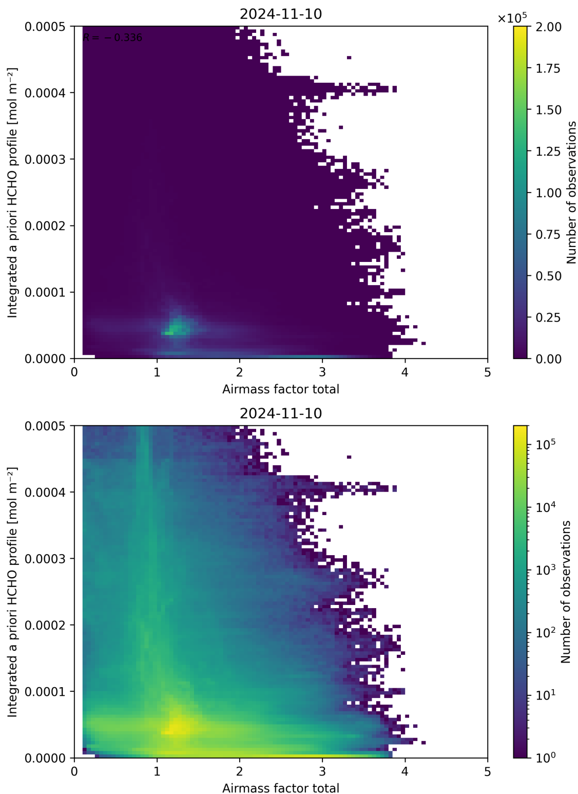
Figure 104: Scatter density plot of “Airmass factor total” against “Integrated a priori HCHO profile” for 2024-11-09 to 2024-11-11.
