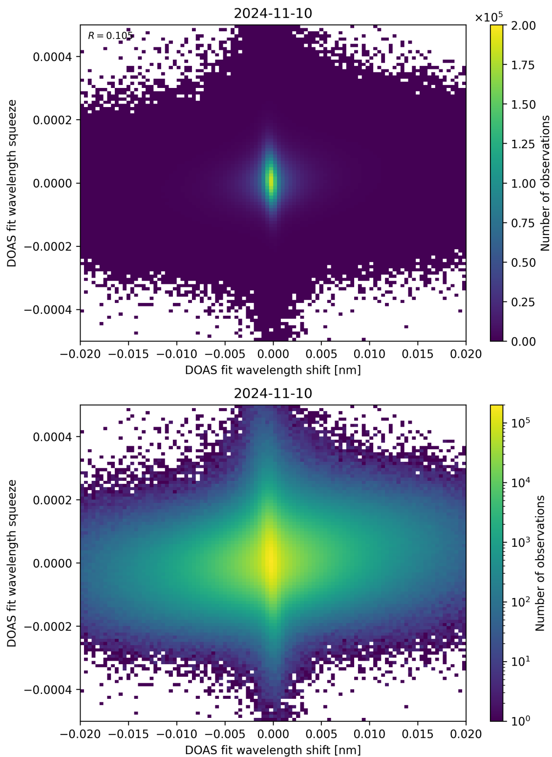
Figure 65: Scatter density plot of “DOAS fit wavelength shift” against “DOAS fit wavelength squeeze” for 2024-11-09 to 2024-11-11.
