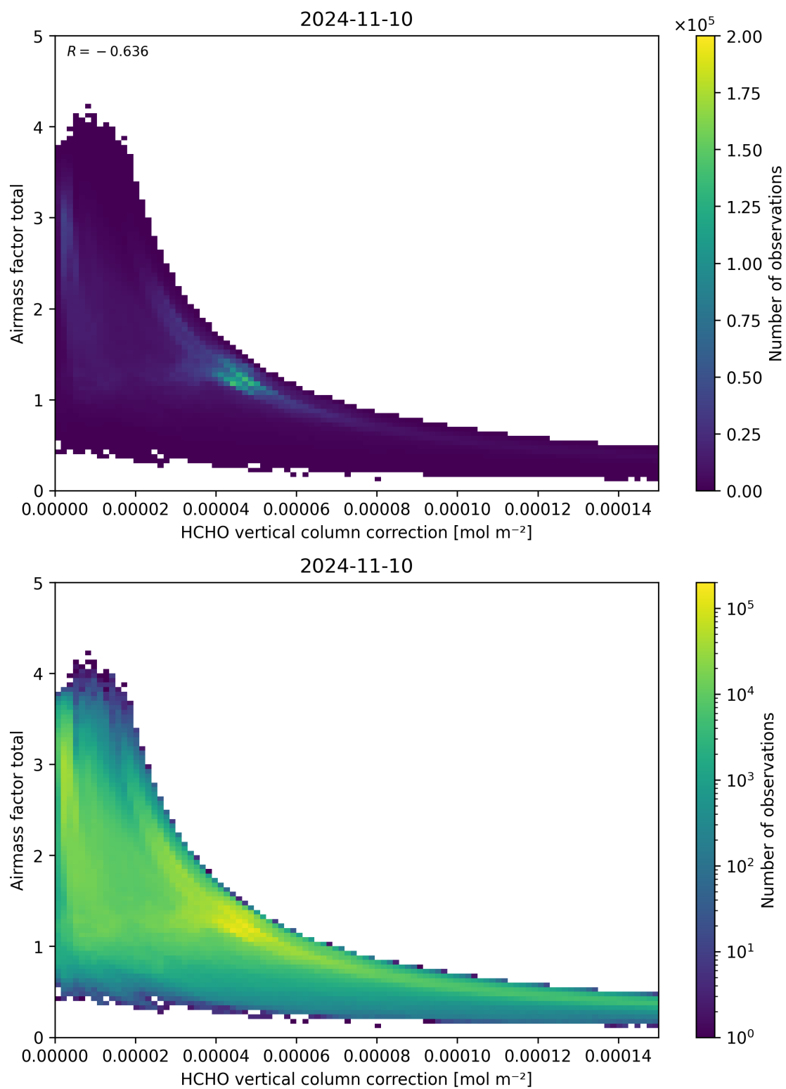
Figure 120: Scatter density plot of “HCHO vertical column correction” against “Airmass factor total” for 2024-11-09 to 2024-11-11.
