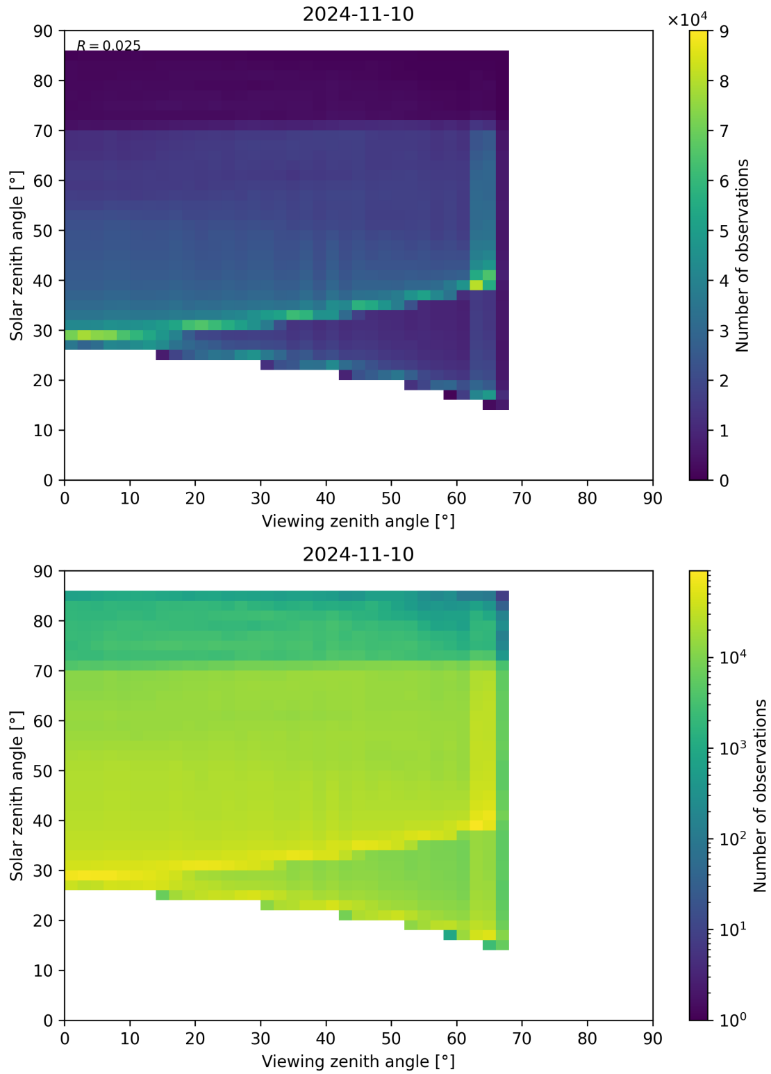
Figure 197: Scatter density plot of “Viewing zenith angle” against “Solar zenith angle” for 2024-11-09 to 2024-11-11.
