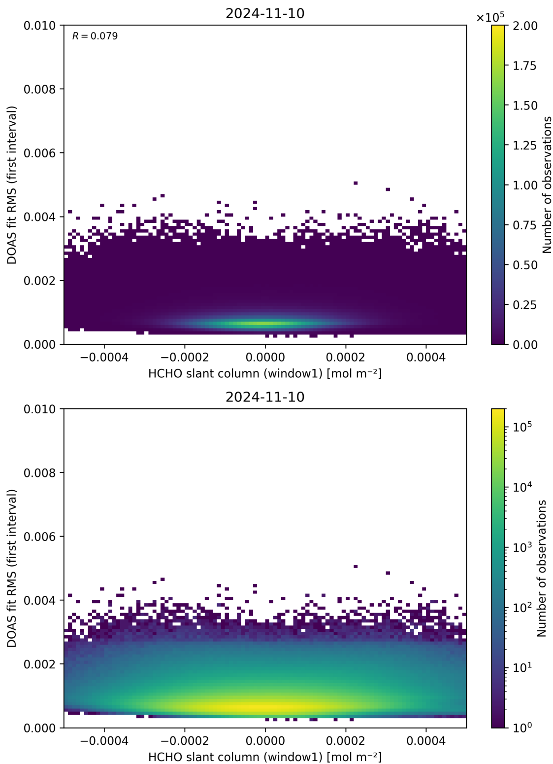
Figure 78: Scatter density plot of “HCHO slant column (window1)” against “DOAS fit RMS (first interval)” for 2024-11-09 to 2024-11-11.
