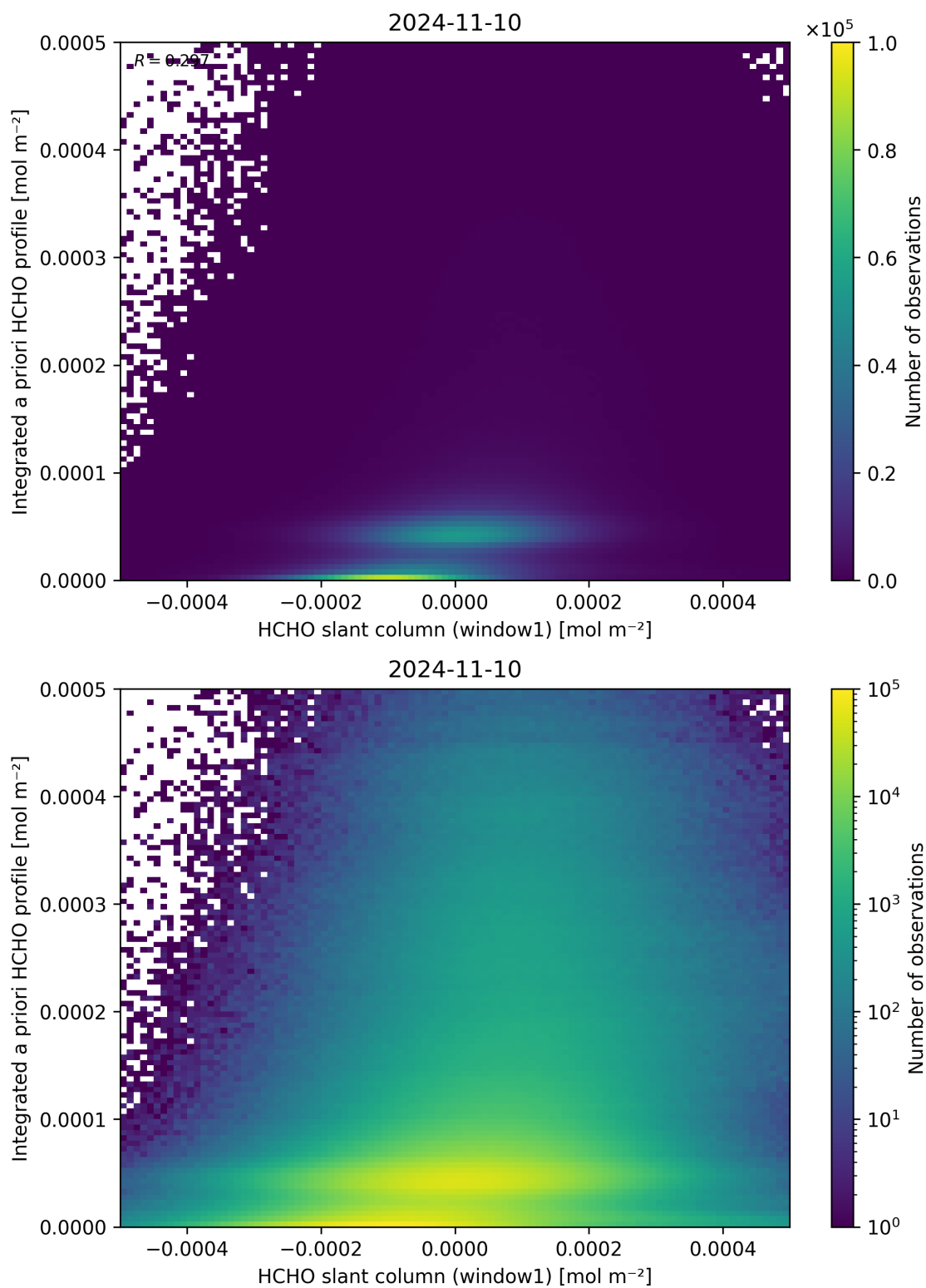
Figure 87: Scatter density plot of “HCHO slant column (window1)” against “Integrated a priori HCHO profile” for 2024-11-09 to 2024-11-11.
