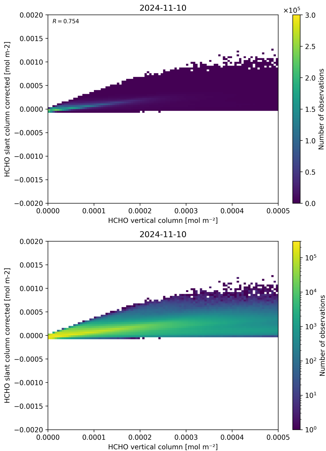
Figure 127: Scatter density plot of “HCHO vertical column” against “HCHO slant column corrected” for 2024-11-09 to 2024-11-11.
