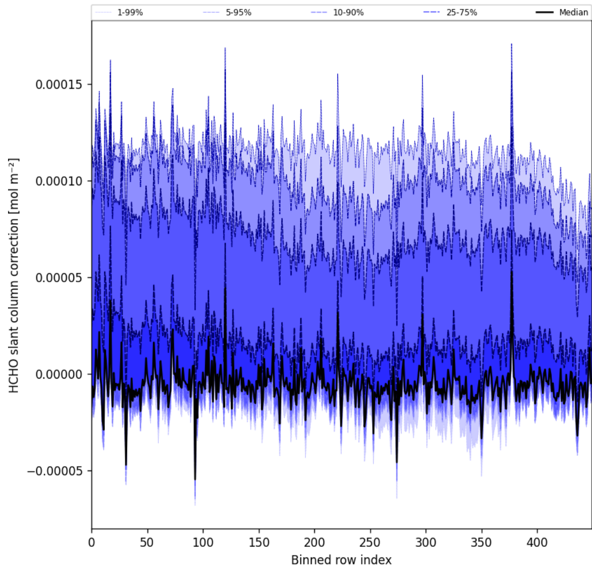
Figure 61: Along track statistics of “HCHO slant column correction” for 2024-11-09 to 2024-11-11
