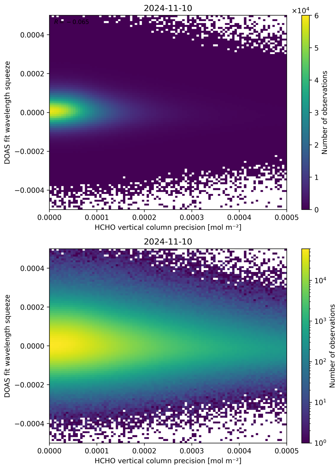
Figure 138: Scatter density plot of “HCHO vertical column precision” against “DOAS fit wavelength squeeze” for 2024-11-09 to 2024-11-11.
