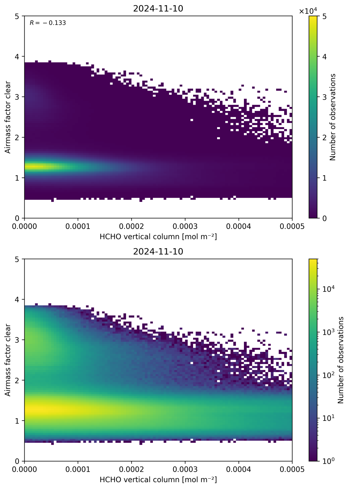
Figure 126: Scatter density plot of “HCHO vertical column” against “Airmass factor clear” for 2024-11-09 to 2024-11-11.
