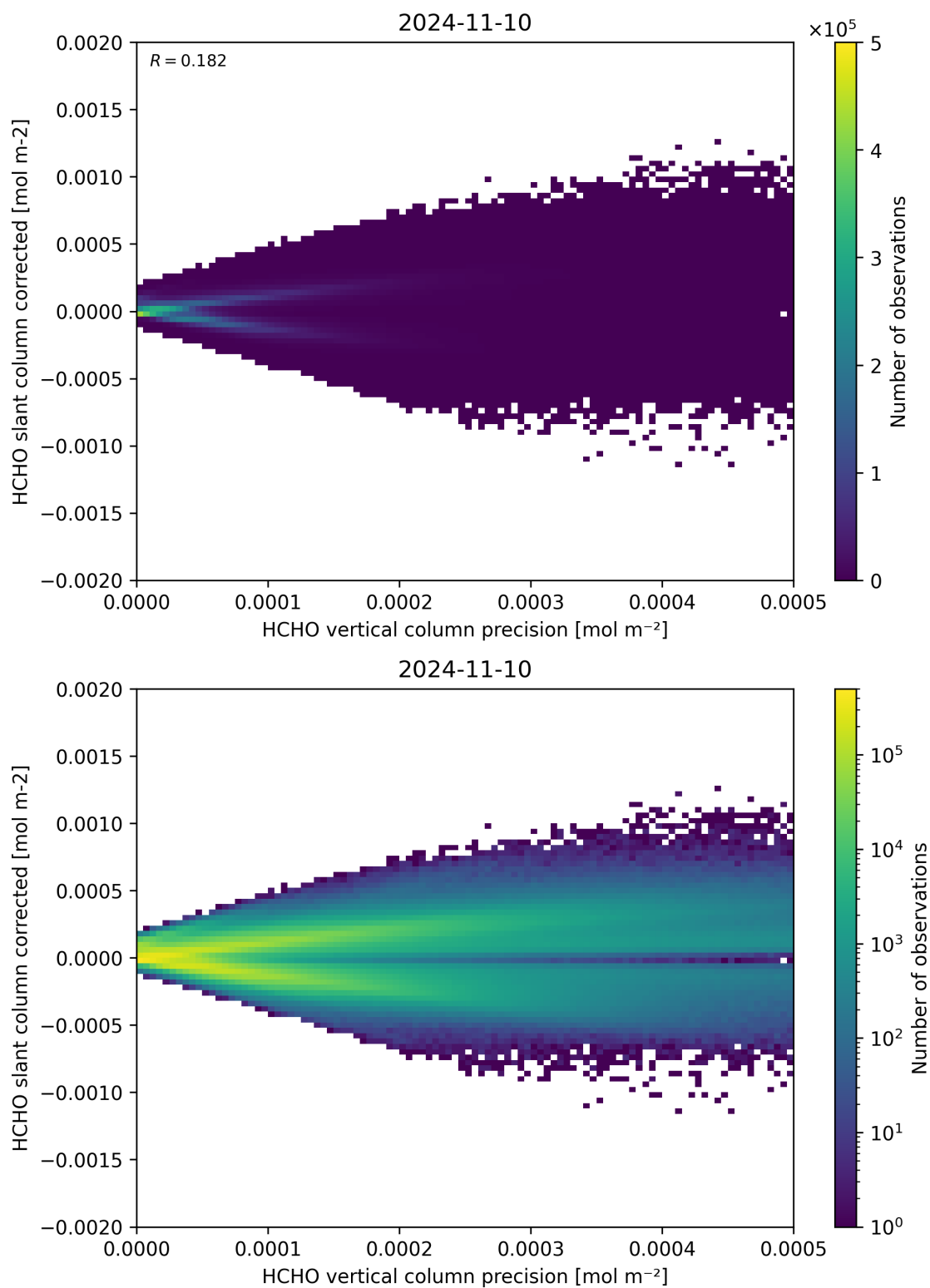
Figure 140: Scatter density plot of “HCHO vertical column precision” against “HCHO slant column corrected” for 2024-11-09 to 2024-11-11.
