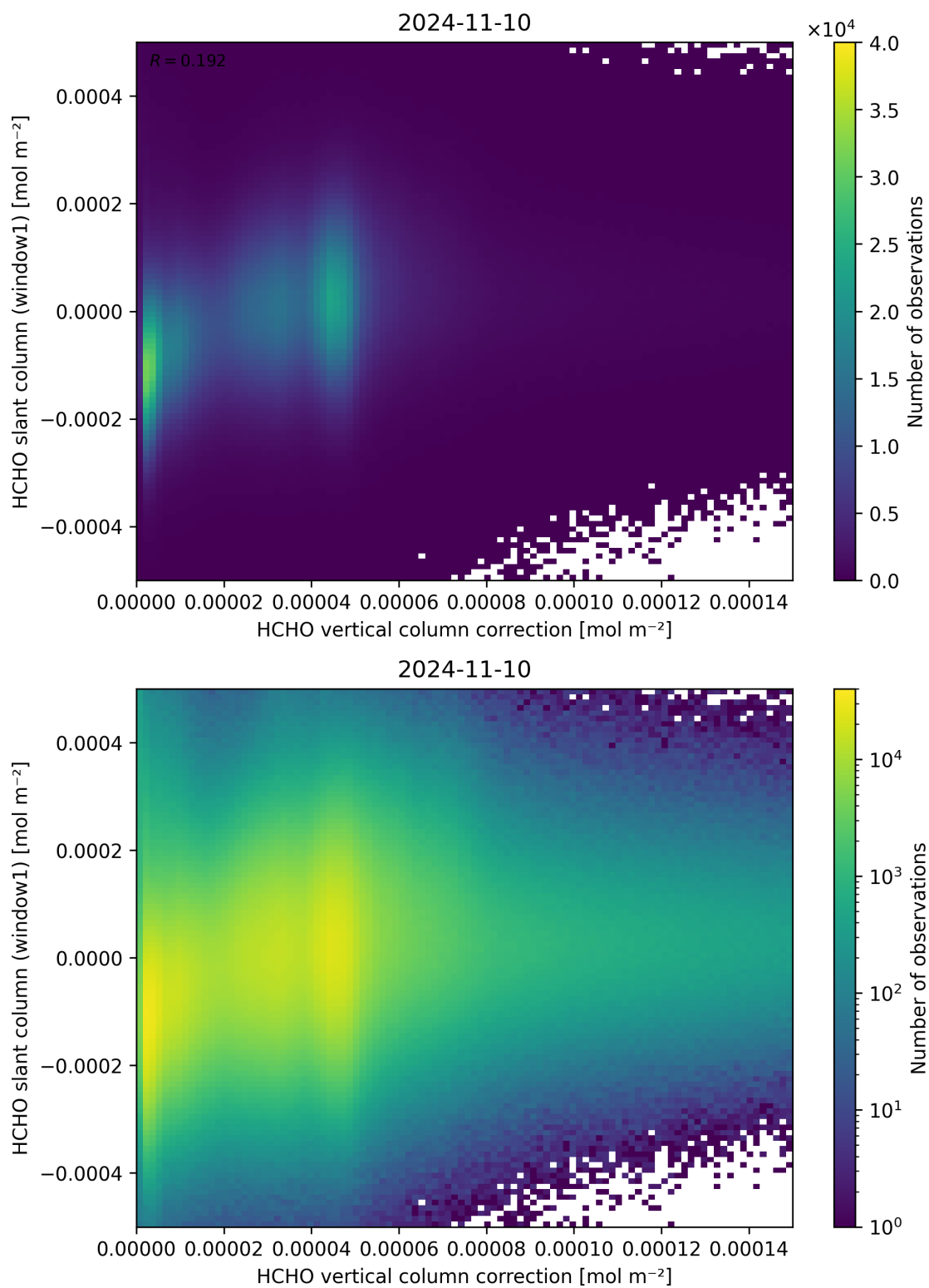
Figure 118: Scatter density plot of “HCHO vertical column correction” against “HCHO slant column (window1)” for 2024-11-09 to 2024-11-11.
