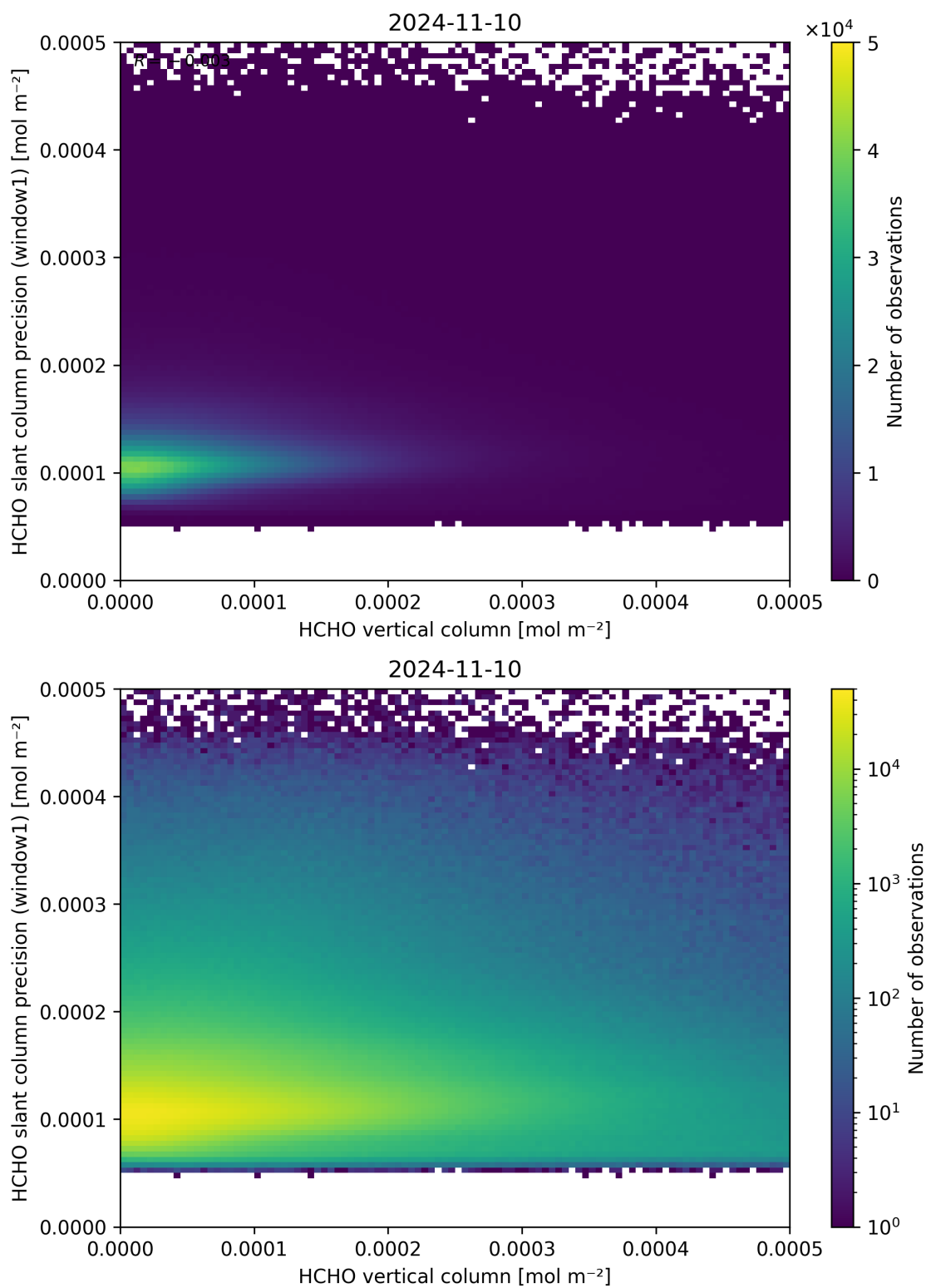
Figure 130: Scatter density plot of “HCHO vertical column” against “HCHO slant column precision (window1)” for 2024-11-09 to 2024-11-11.
