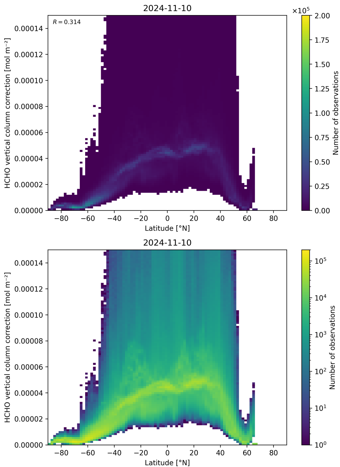
Figure 164: Scatter density plot of “Latitude” against “HCHO vertical column correction” for 2024-11-09 to 2024-11-11.
