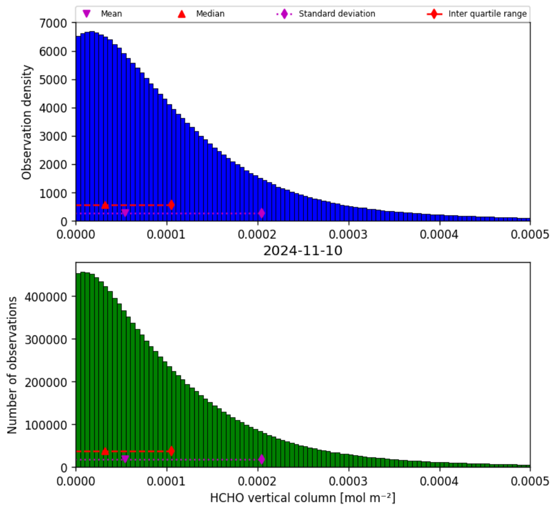
Figure 35: Histogram of “HCHO vertical column” for 2024-11-09 to 2024-11-11
