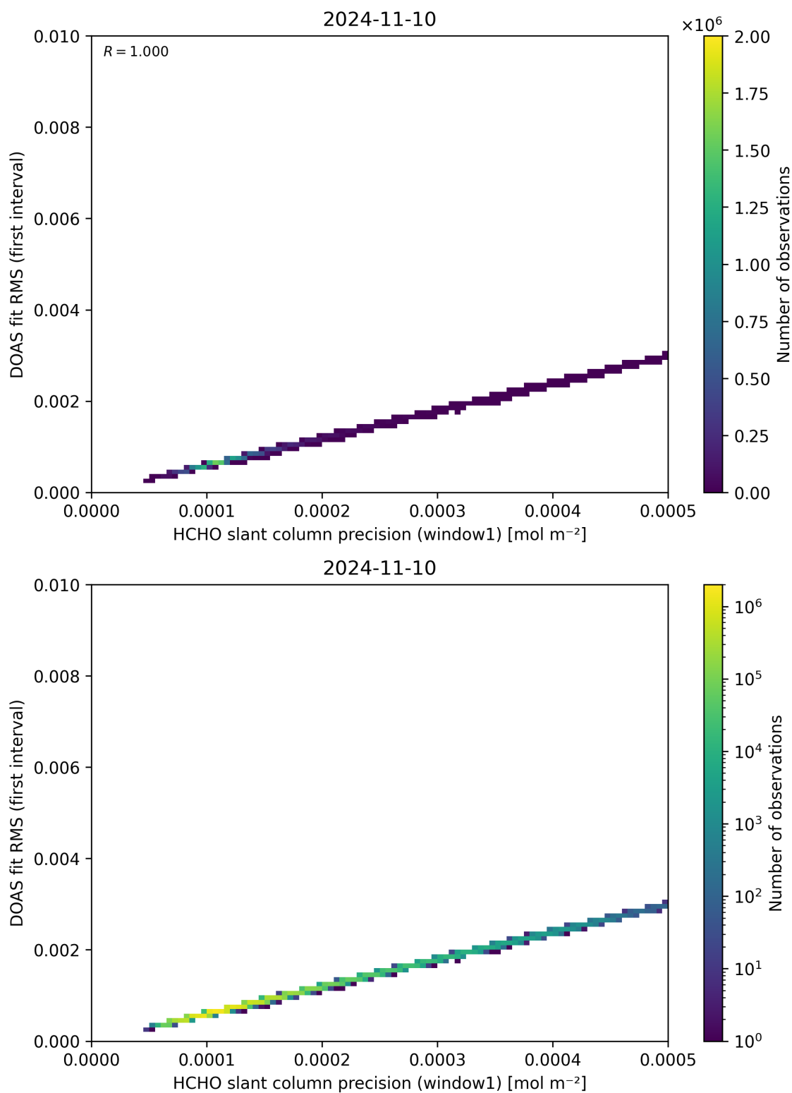
Figure 88: Scatter density plot of “HCHO slant column precision (window1)” against “DOAS fit RMS (first interval)” for 2024-11-09 to 2024-11-11.
