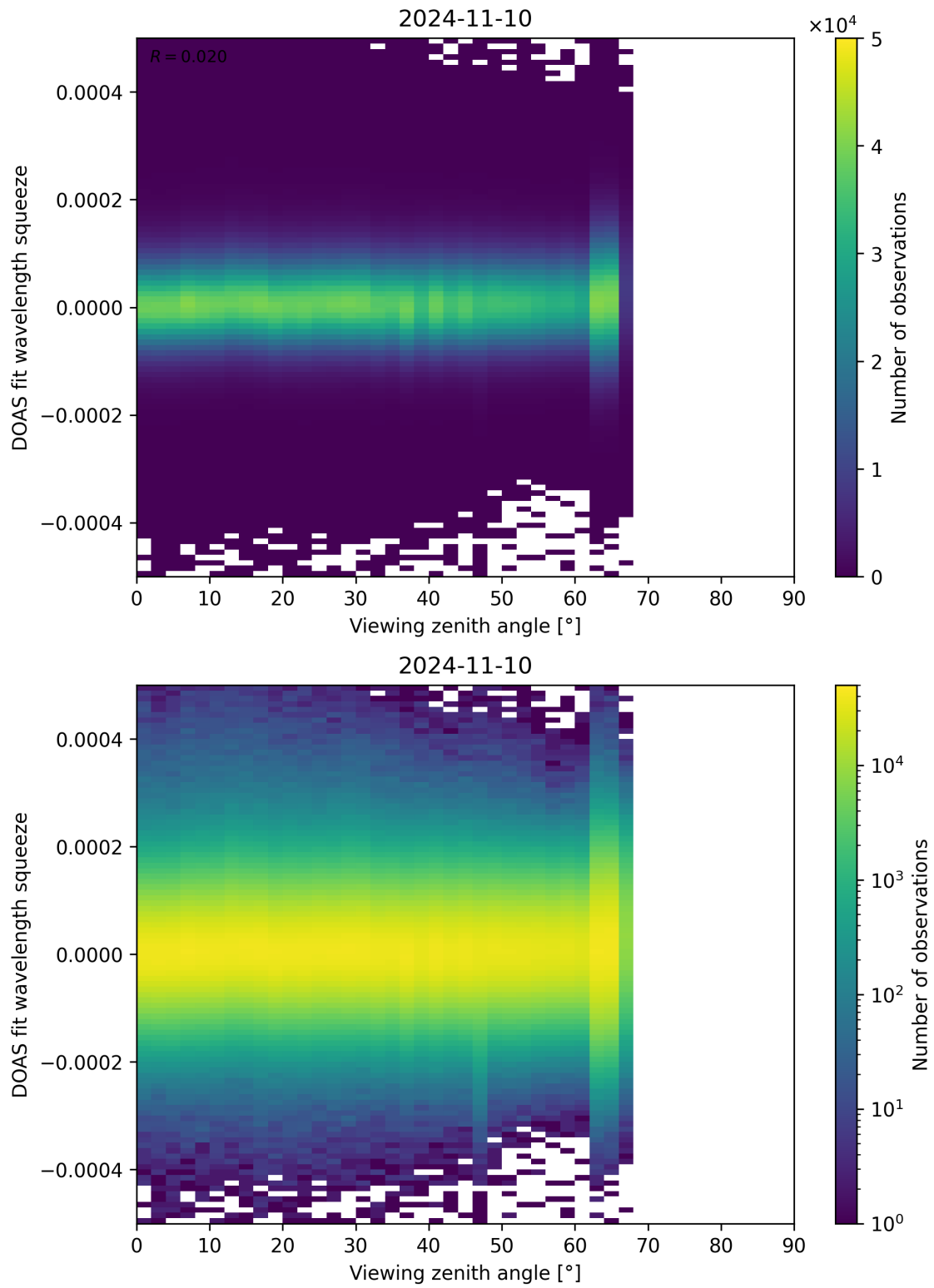
Figure 184: Scatter density plot of “Viewing zenith angle” against “DOAS fit wavelength squeeze” for 2024-11-09 to 2024-11-11.
