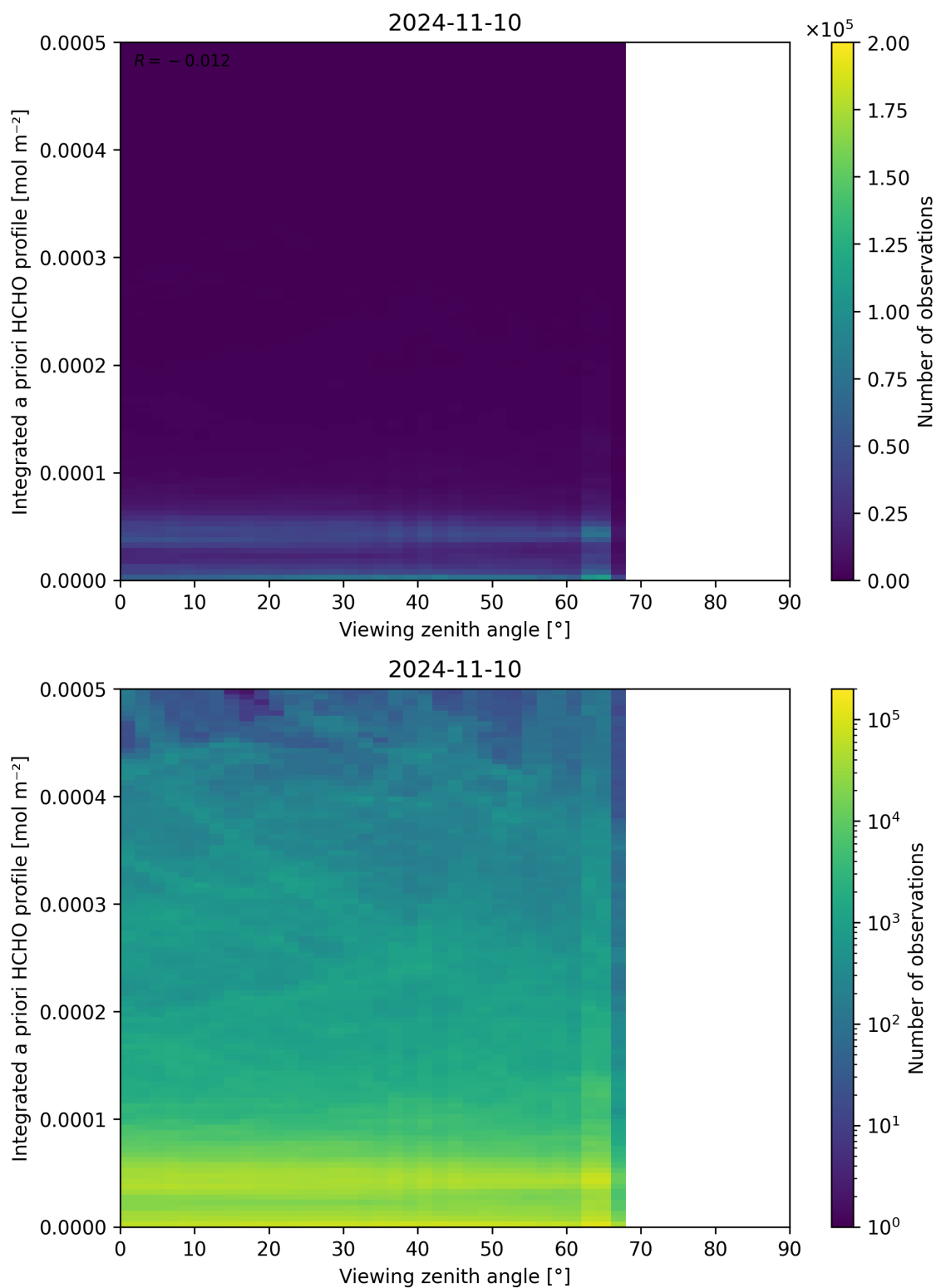
Figure 195: Scatter density plot of “Viewing zenith angle” against “Integrated a priori HCHO profile” for 2024-11-09 to 2024-11-11.
