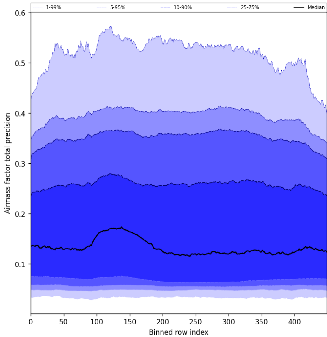
Figure 55: Along track statistics of “Airmass factor total precision” for 2024-11-09 to 2024-11-11
