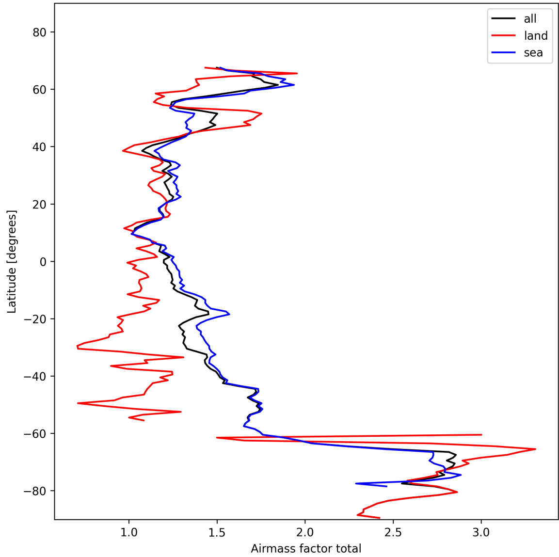
Figure 26: Zonal average of “Airmass factor total” for 2024-11-09 to 2024-11-11.
