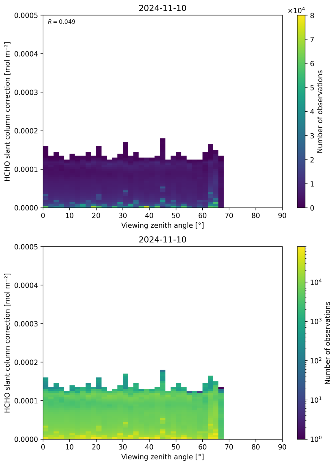
Figure 187: Scatter density plot of “Viewing zenith angle” against “HCHO slant column correction” for 2024-11-09 to 2024-11-11.
