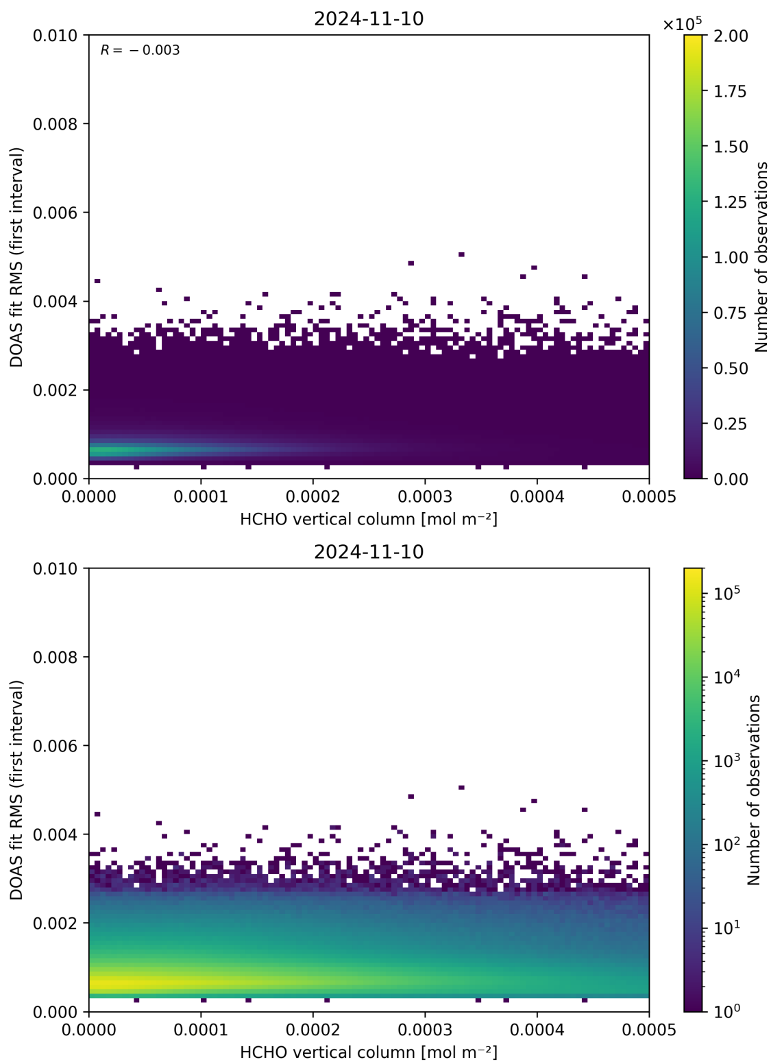
Figure 123: Scatter density plot of “HCHO vertical column” against “DOAS fit RMS (first interval)” for 2024-11-09 to 2024-11-11.
