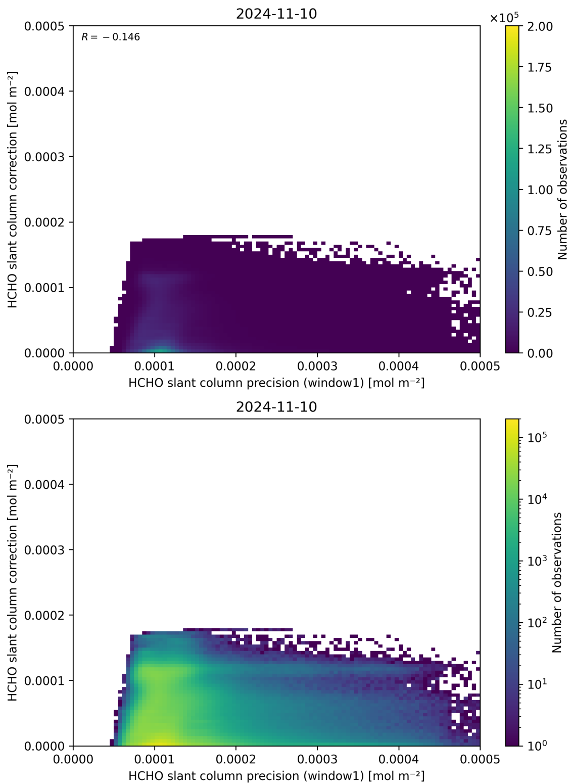
Figure 93: Scatter density plot of “HCHO slant column precision (window1)” against “HCHO slant column correction” for 2024-11-09 to 2024-11-11.
