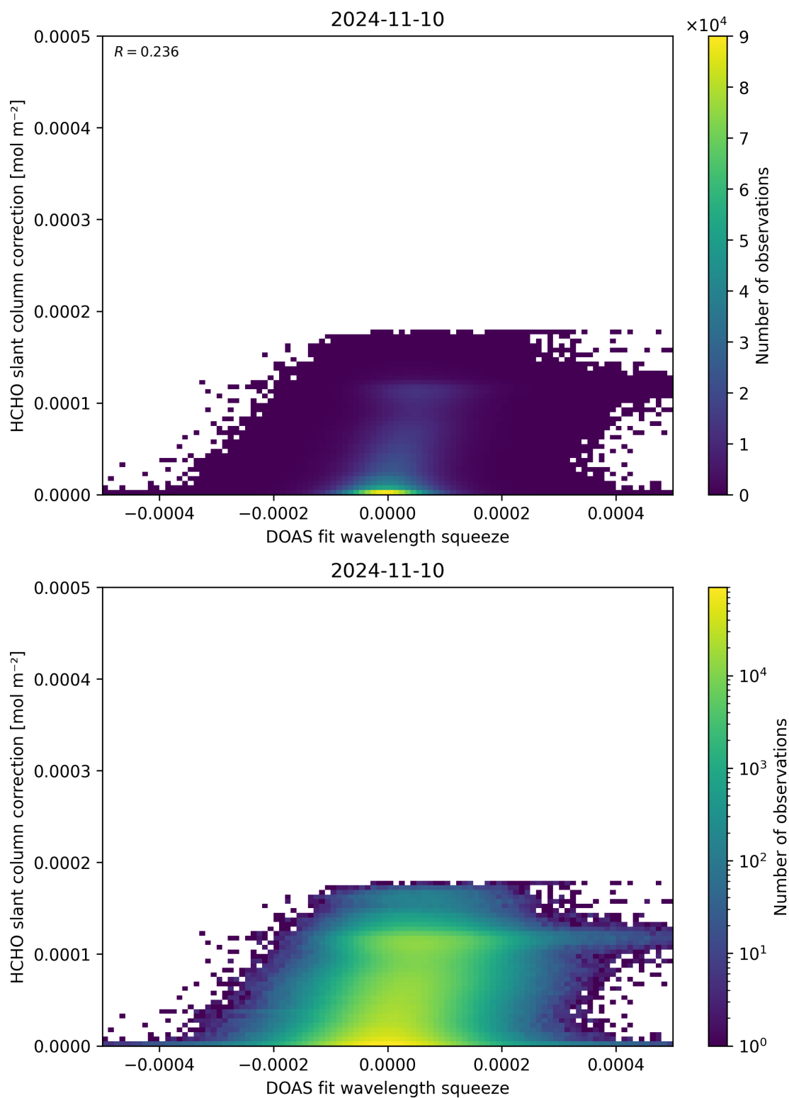
Figure 70: Scatter density plot of “DOAS fit wavelength squeeze” against “HCHO slant column correction” for 2024-11-09 to 2024-11-11.
