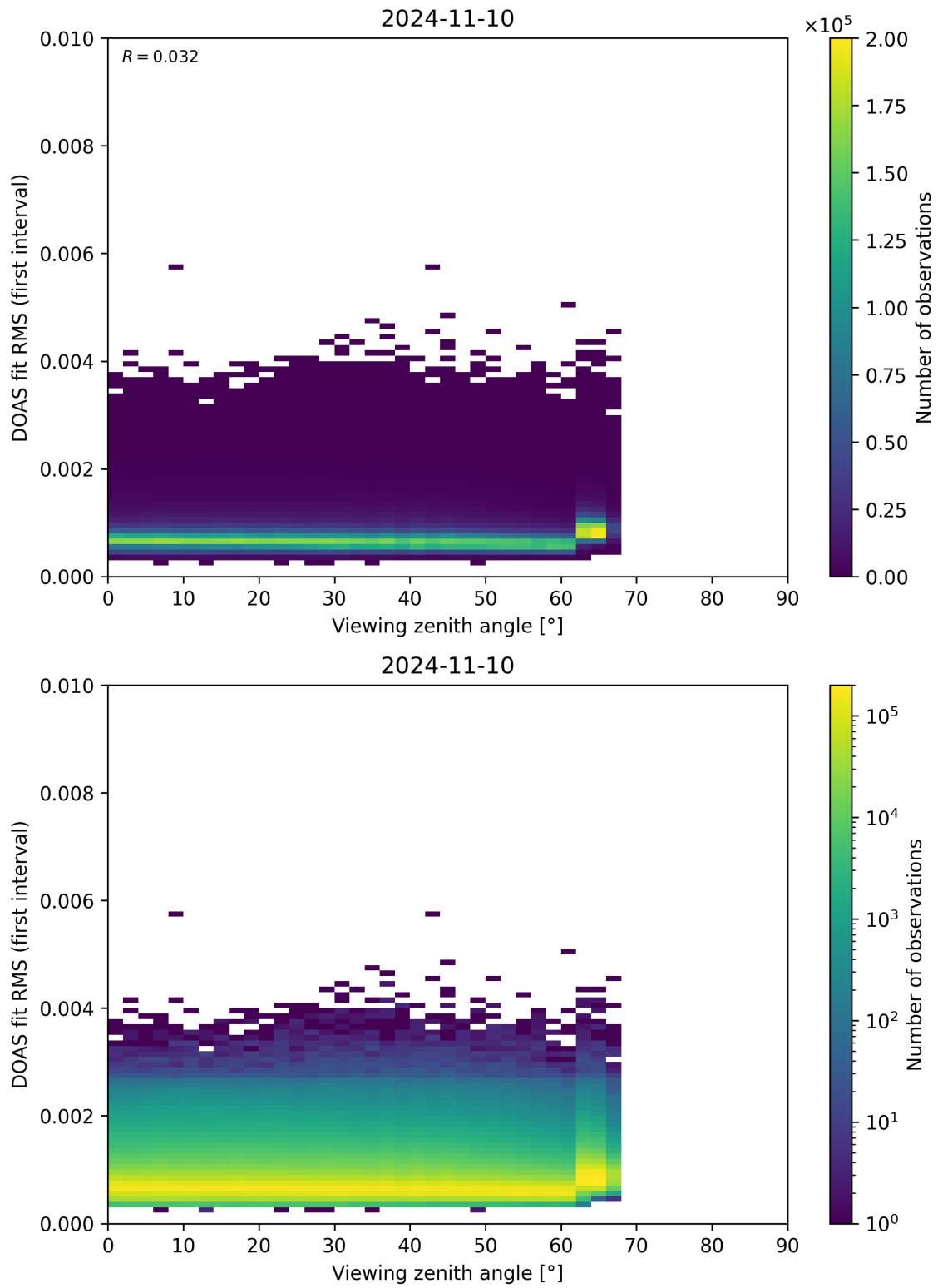
Figure 182: Scatter density plot of “Viewing zenith angle” against “DOAS fit RMS (first interval)” for 2024-11-09 to 2024-11-11.
