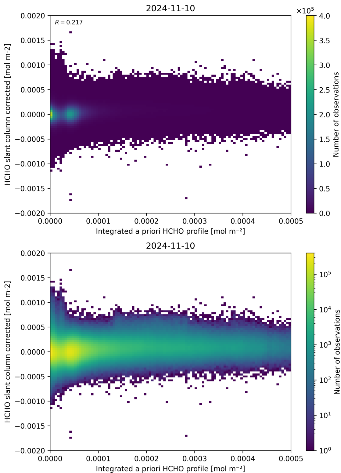
Figure 151: Scatter density plot of “Integrated a priori HCHO profile” against “HCHO slant column corrected” for 2024-11-09 to 2024-11-11.
