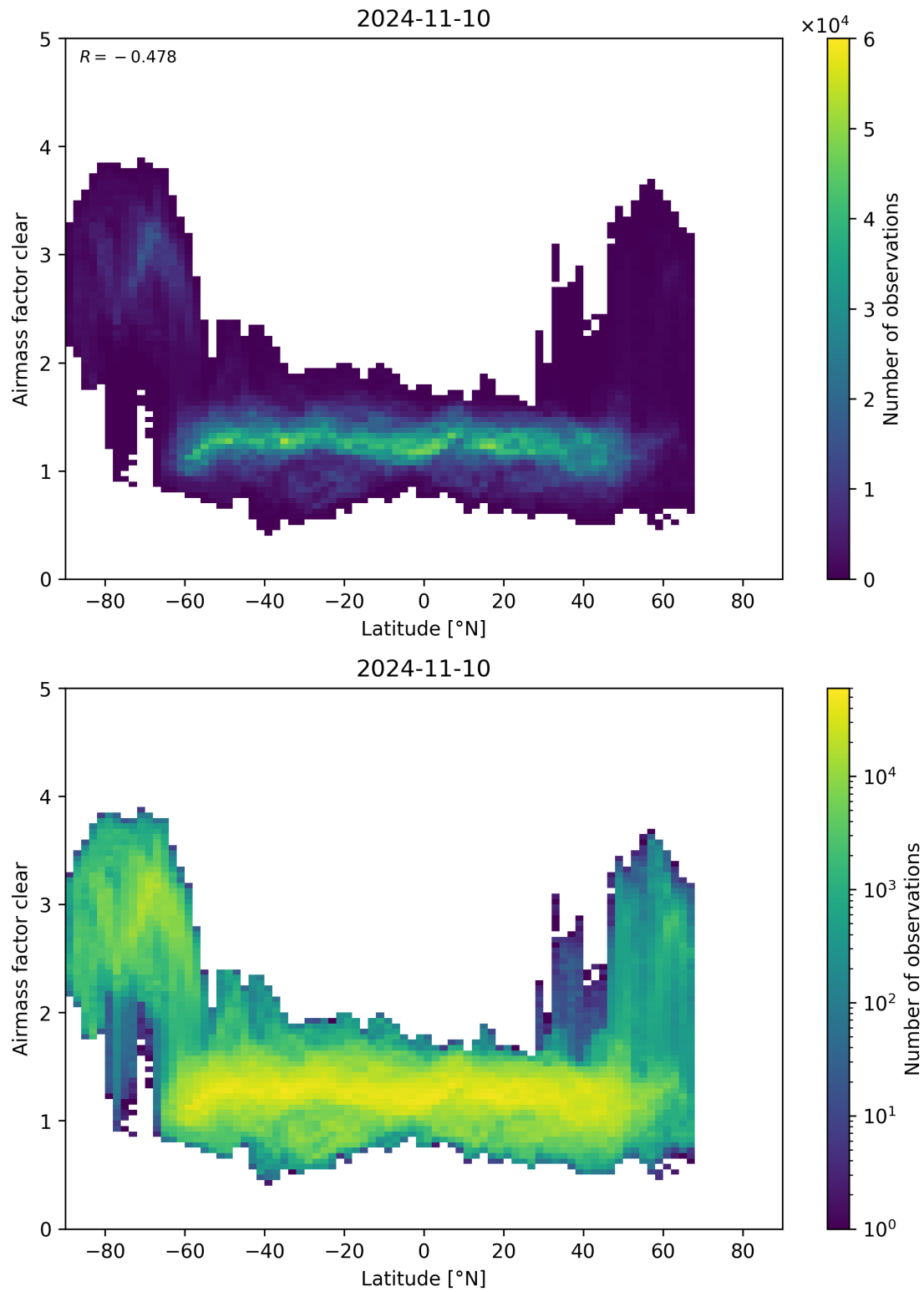
Figure 156: Scatter density plot of “Latitude” against “Airmass factor clear” for 2024-11-09 to 2024-11-11.
