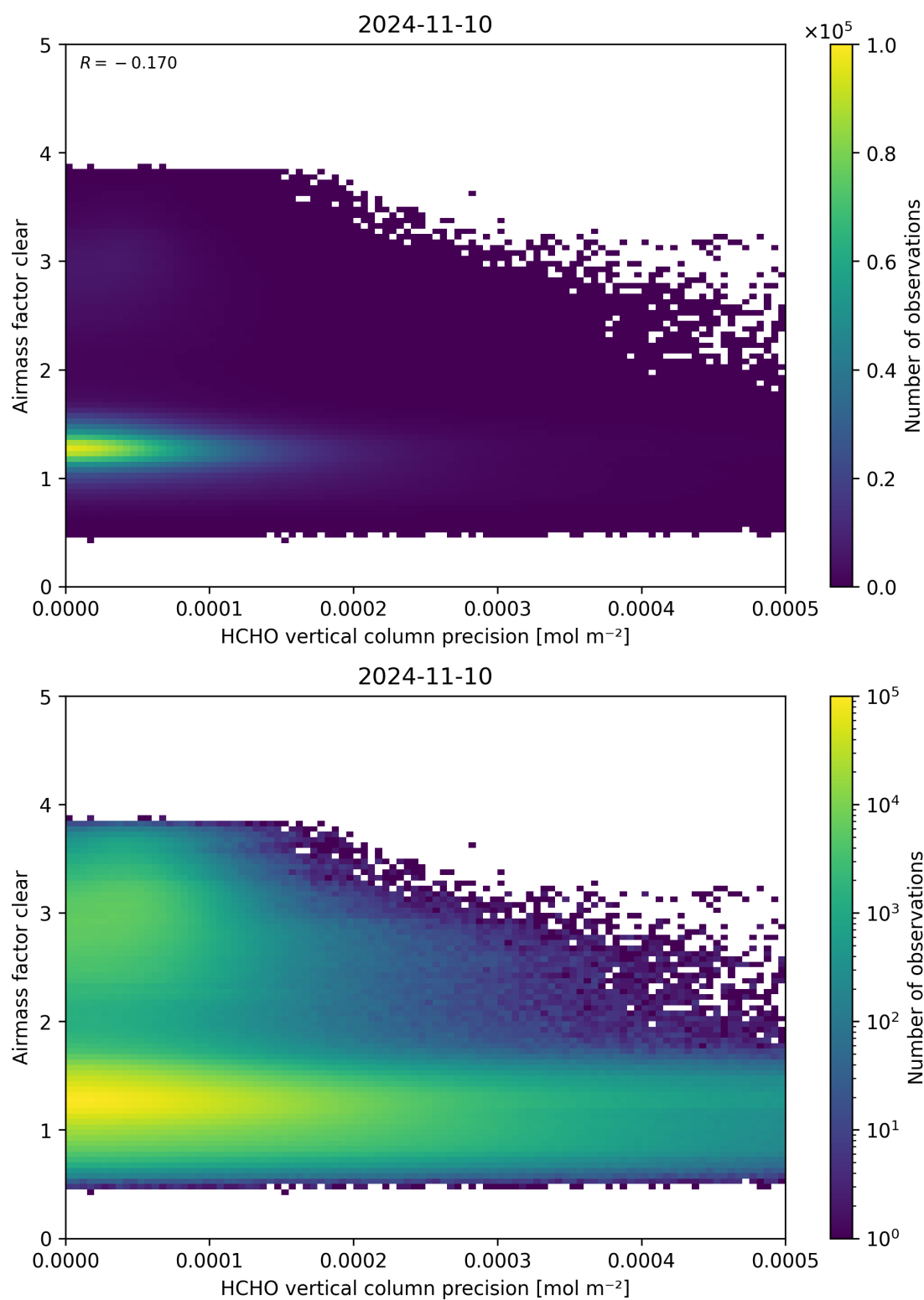
Figure 139: Scatter density plot of “HCHO vertical column precision” against “Airmass factor clear” for 2024-11-09 to 2024-11-11.
