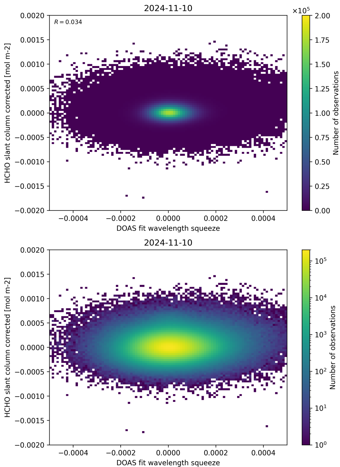
Figure 69: Scatter density plot of “DOAS fit wavelength squeeze” against “HCHO slant column corrected” for 2024-11-09 to 2024-11-11.
