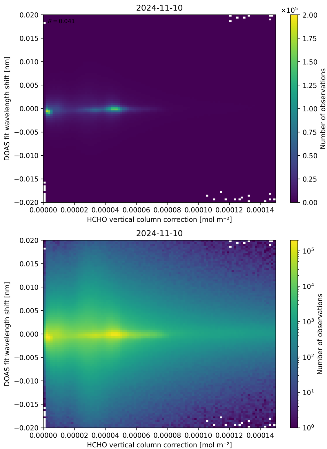
Figure 113: Scatter density plot of “HCHO vertical column correction” against “DOAS fit wavelength shift” for 2024-11-09 to 2024-11-11.
