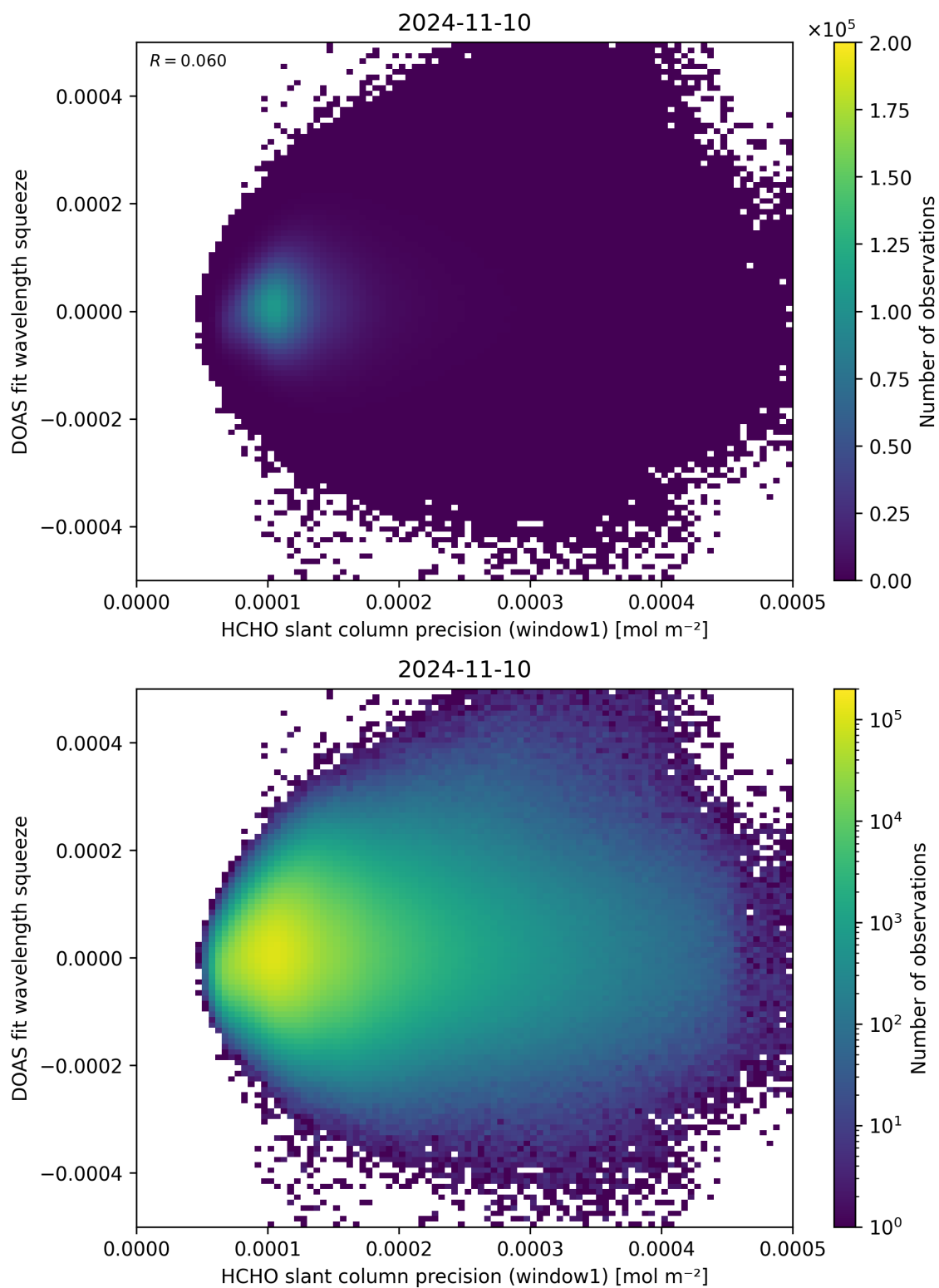
Figure 90: Scatter density plot of “HCHO slant column precision (window1)” against “DOAS fit wavelength squeeze” for 2024-11-09 to 2024-11-11.
