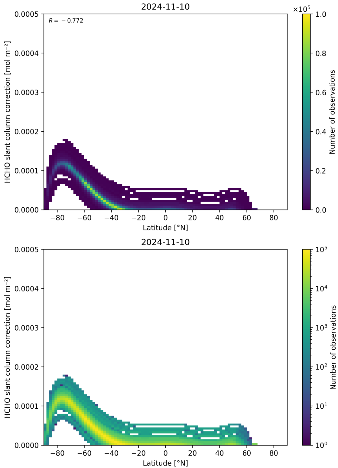
Figure 158: Scatter density plot of “Latitude” against “HCHO slant column correction” for 2024-11-09 to 2024-11-11.
