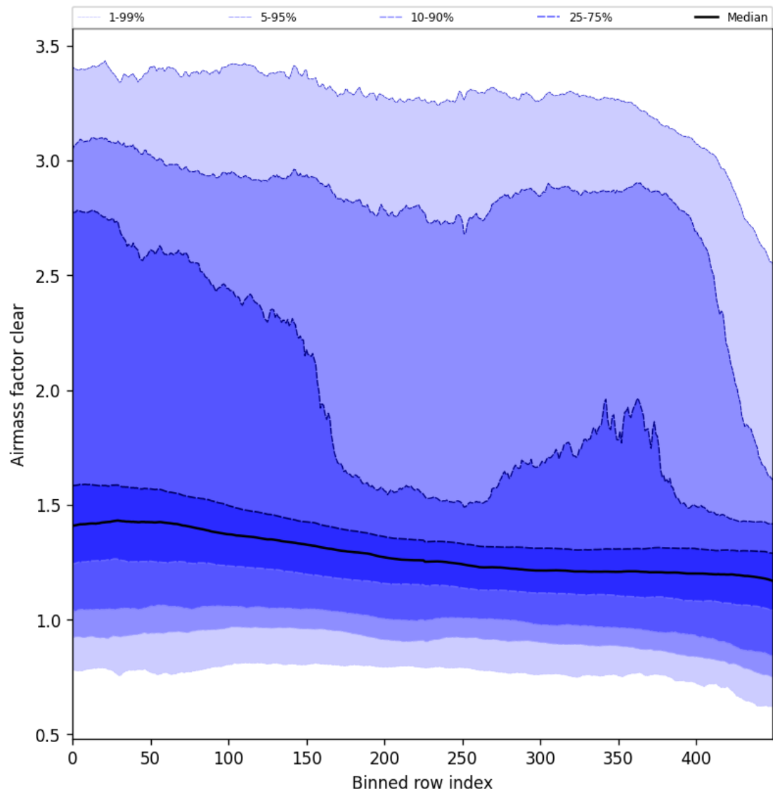
Figure 56: Along track statistics of “Air mass factor clear” for 2024-11-09 to 2024-11-11
