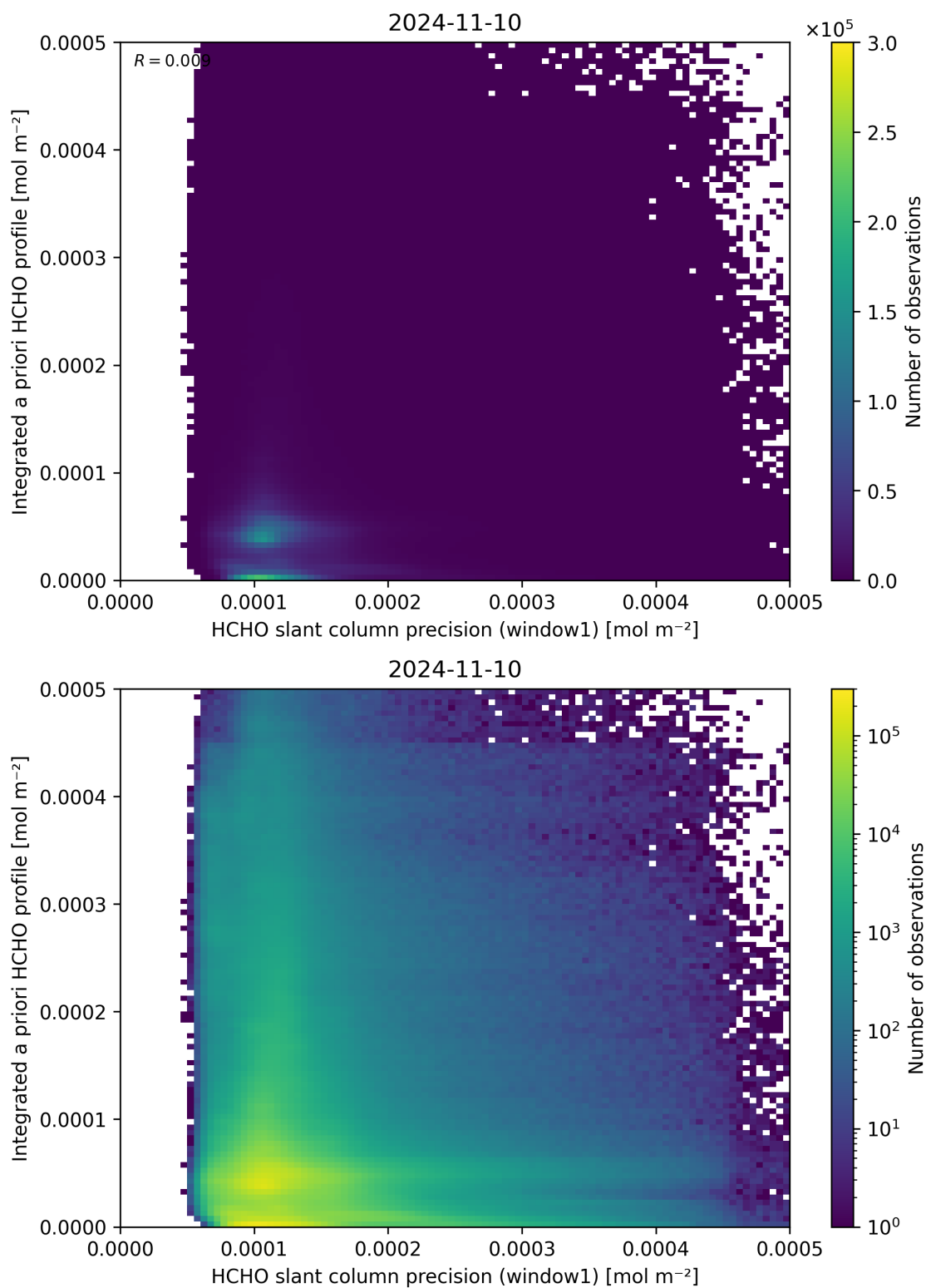
Figure 96: Scatter density plot of “HCHO slant column precision (window1)” against “Integrated a priori HCHO profile” for 2024-11-09 to 2024-11-11.
