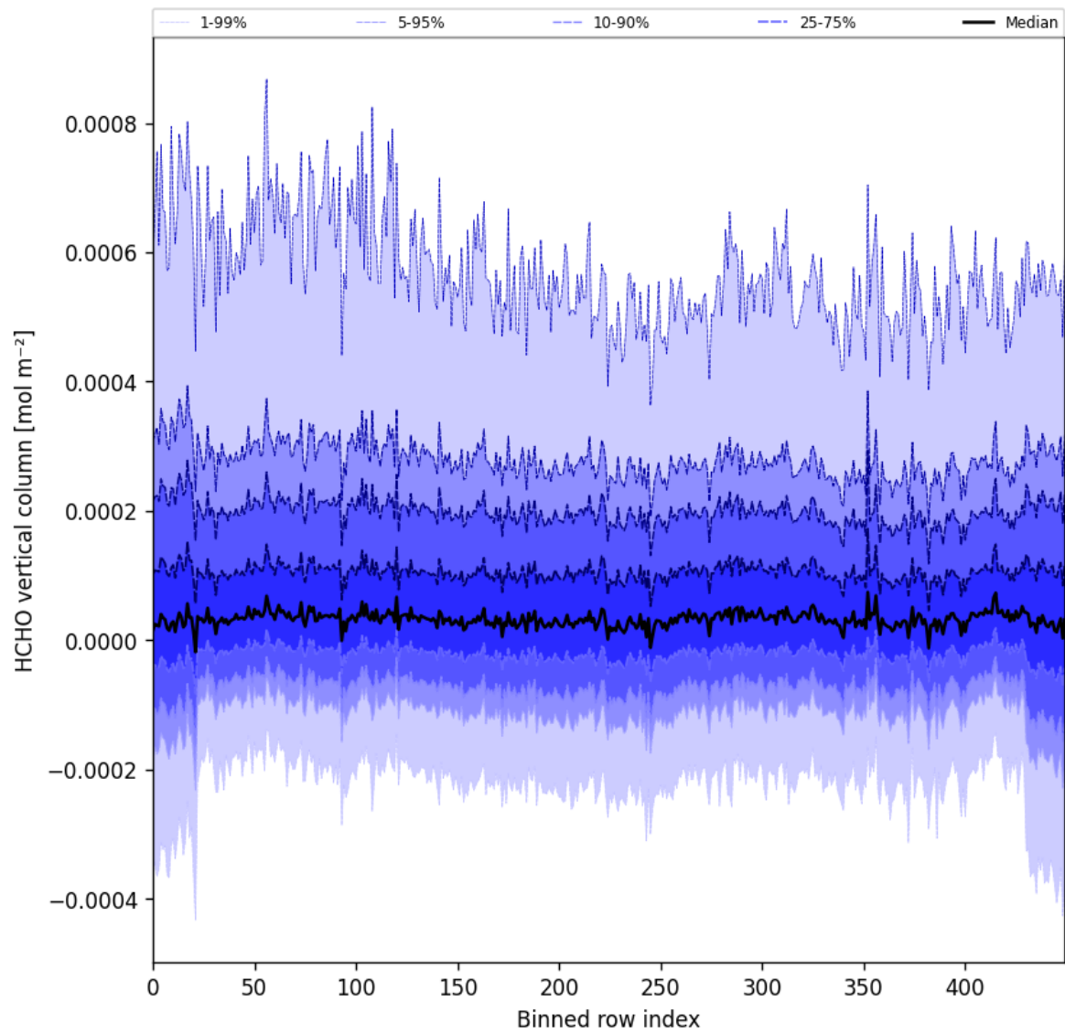
Figure 49: Along track statistics of “HCHO vertical column” for 2024-11-09 to 2024-11-11
