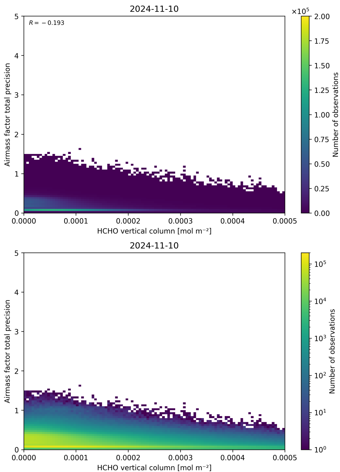
Figure 132: Scatter density plot of “HCHO vertical column” against “Airmass factor total precision” for 2024-11-09 to 2024-11-11.
