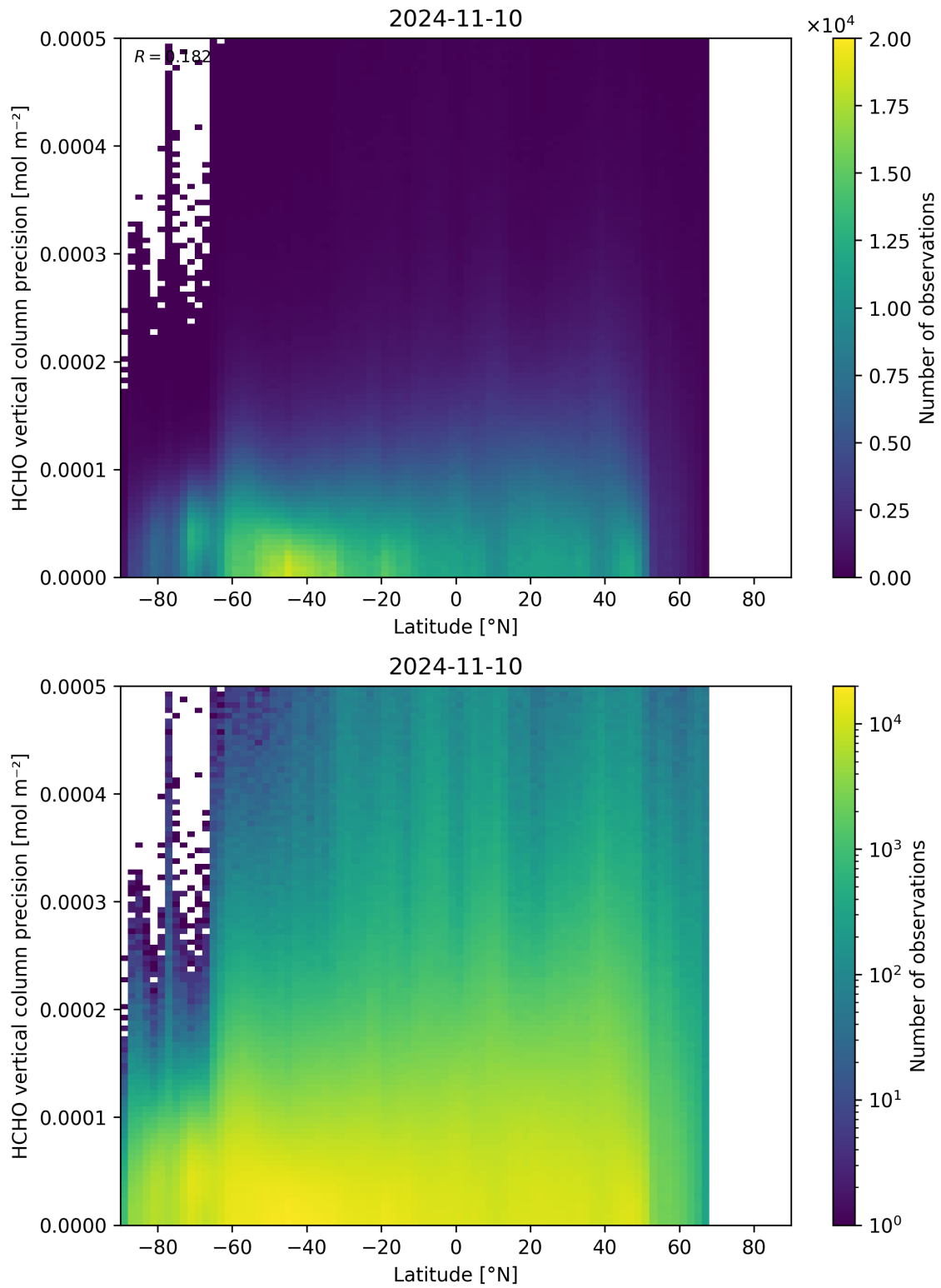
Figure 165: Scatter density plot of “Latitude” against “HCHO vertical column precision” for 2024-11-09 to 2024-11-11.
