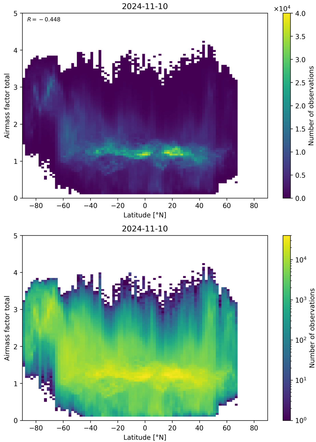
Figure 161: Scatter density plot of “Latitude” against “Airmass factor total” for 2024-11-09 to 2024-11-11.
