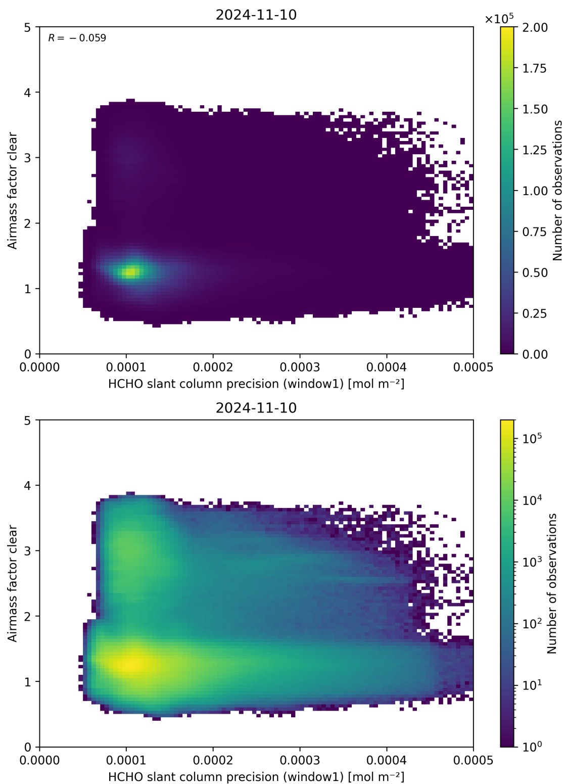
Figure 91: Scatter density plot of “HCHO slant column precision (window1)” against “Airmass factor clear” for 2024-11-09 to 2024-11-11.
