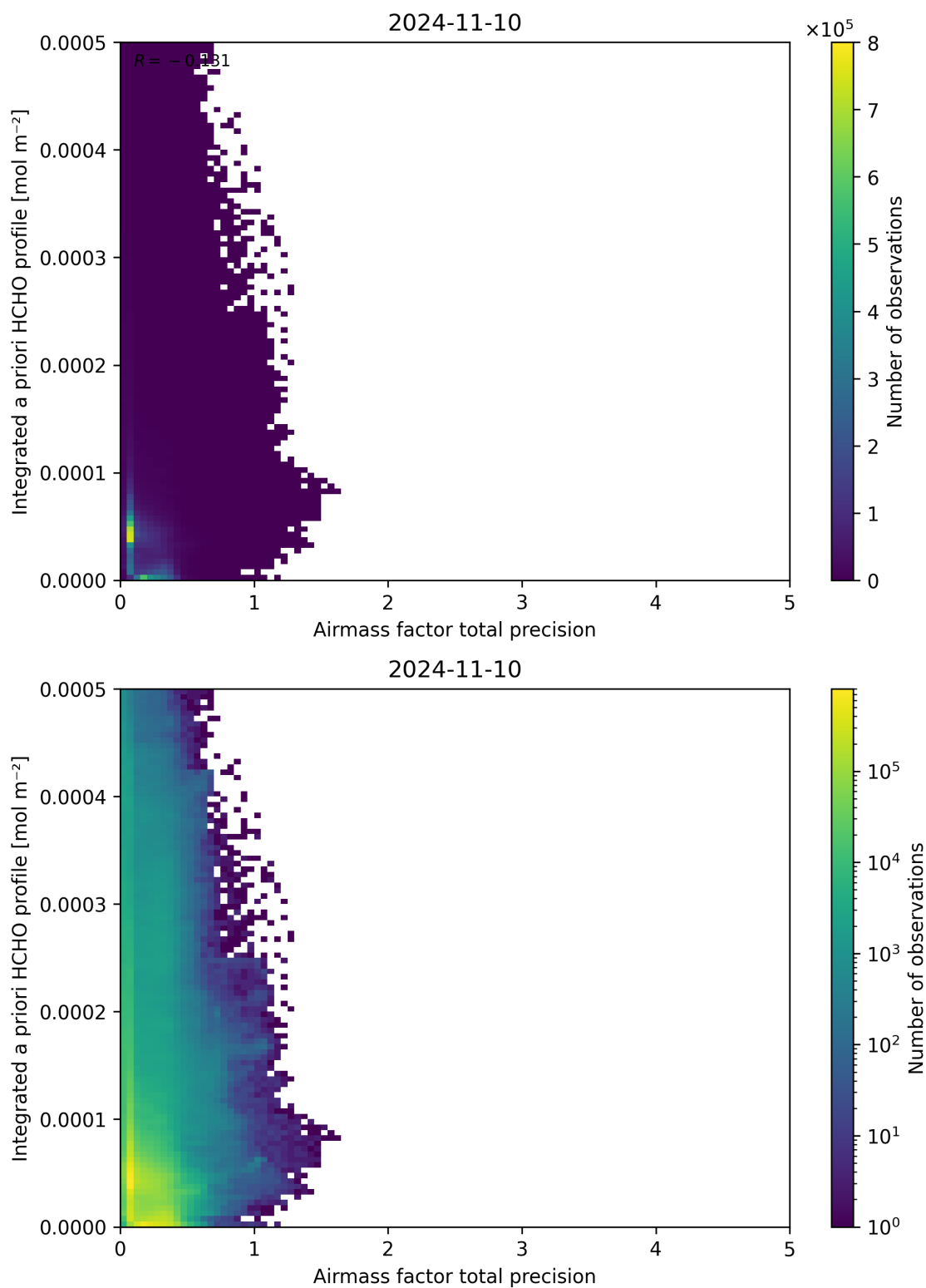
Figure 111: Scatter density plot of “Airmass factor total precision” against “Integrated a priori HCHO profile” for 2024-11-09 to 2024-11-11.
