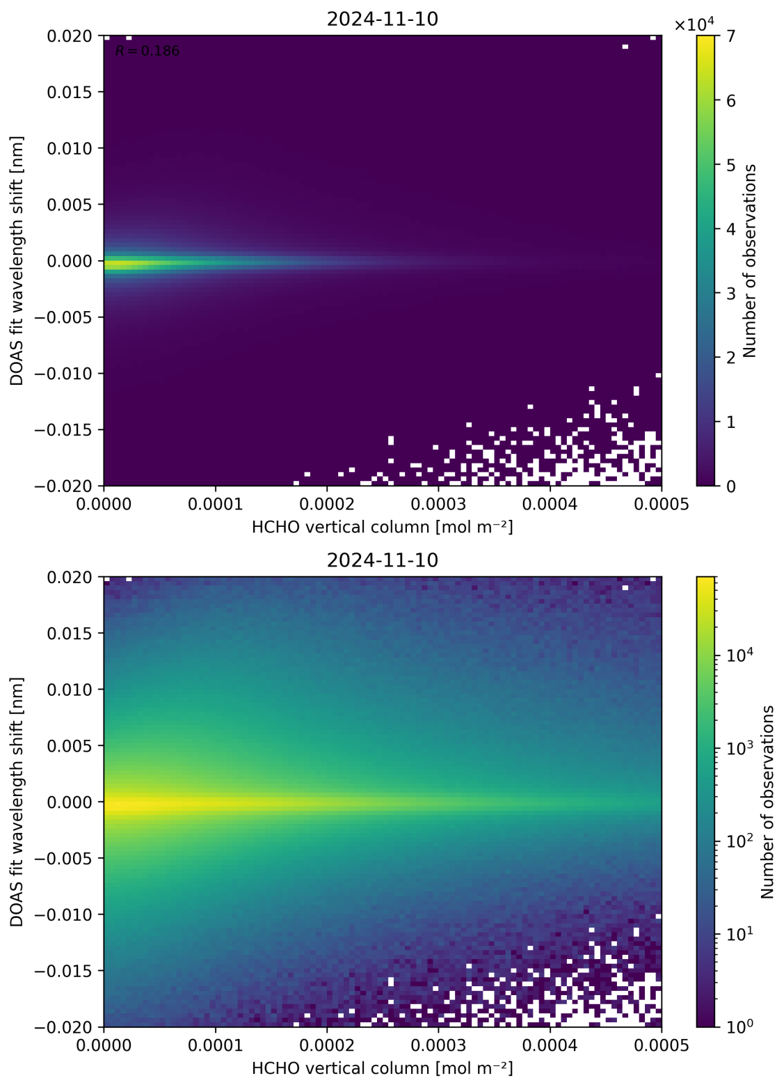
Figure 124: Scatter density plot of “HCHO vertical column” against “DOAS fit wavelength shift” for 2024-11-09 to 2024-11-11.
