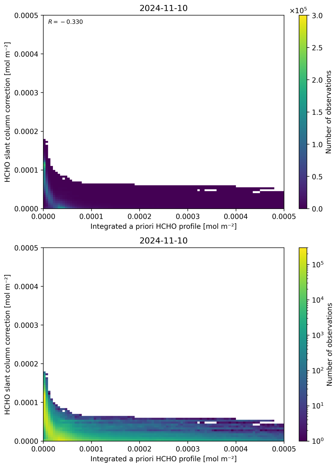
Figure 152: Scatter density plot of “Integrated a priori HCHO profile” against “HCHO slant column correction” for 2024-11-09 to 2024-11-11.
