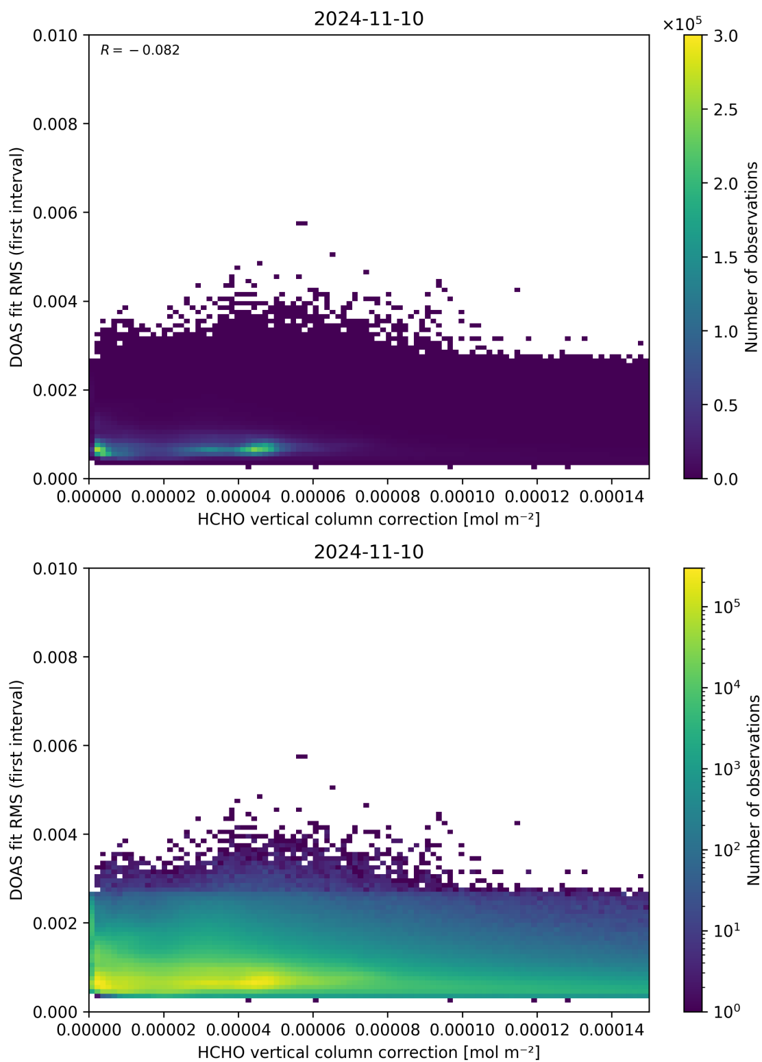
Figure 112: Scatter density plot of “HCHO vertical column correction” against “DOAS fit RMS (first interval)” for 2024-11-09 to 2024-11-11.
