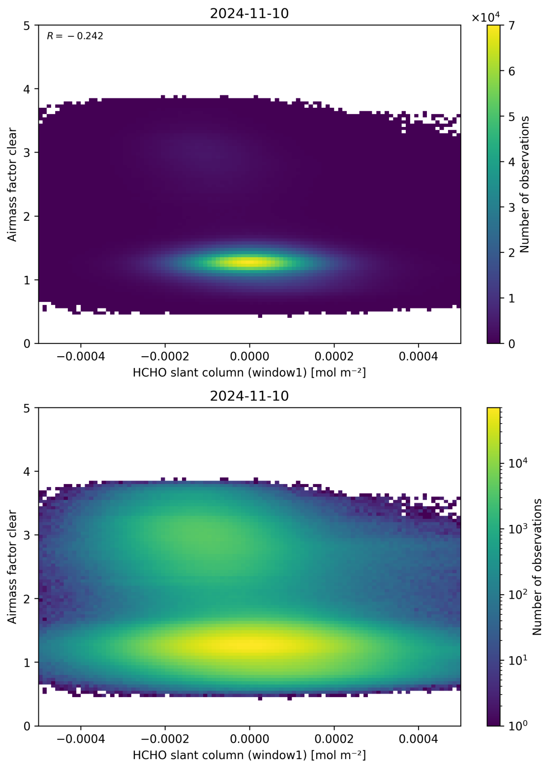
Figure 81: Scatter density plot of “HCHO slant column (window1)” against “Airmass factor clear” for 2024-11-09 to 2024-11-11.
