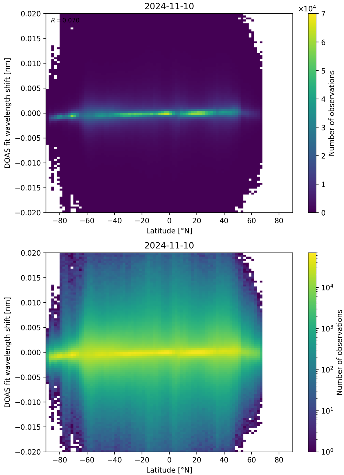
Figure 154: Scatter density plot of “Latitude” against “DOAS fit wavelength shift” for 2024-11-09 to 2024-11-11.
