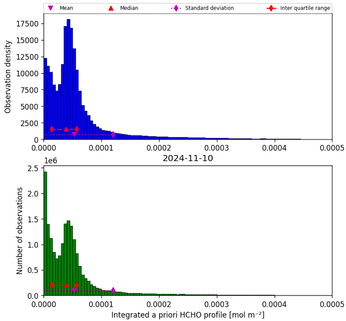
Figure 43: Histogram of “Integrated a priori HCHO profile” for 2024-11-09 to 2024-11-11
