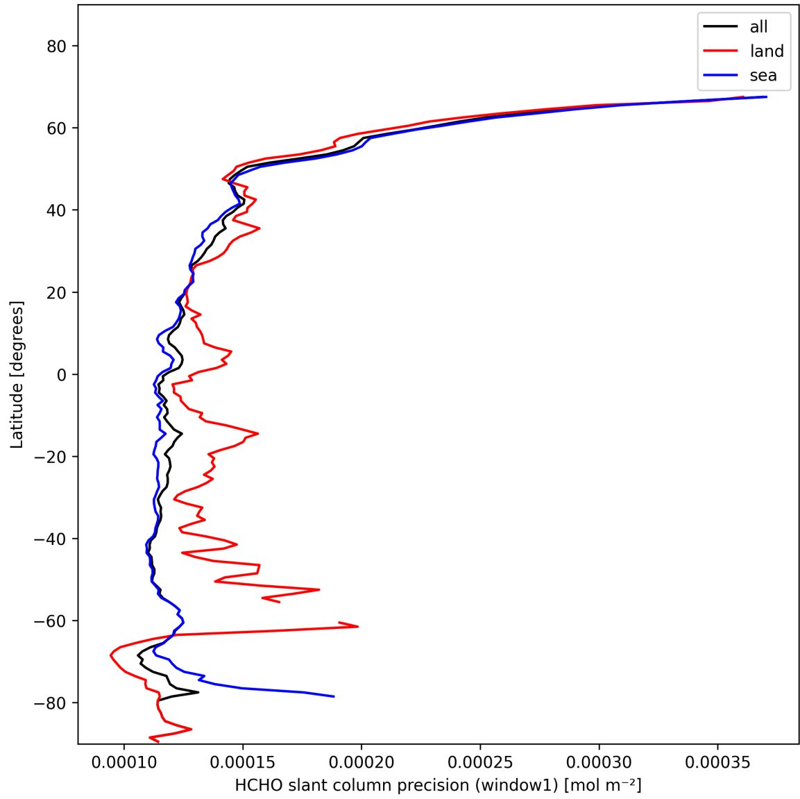
Figure 25: Zonal average of “HCHO slant column precision (window1)” for 2024-11-09 to 2024-11-11.
