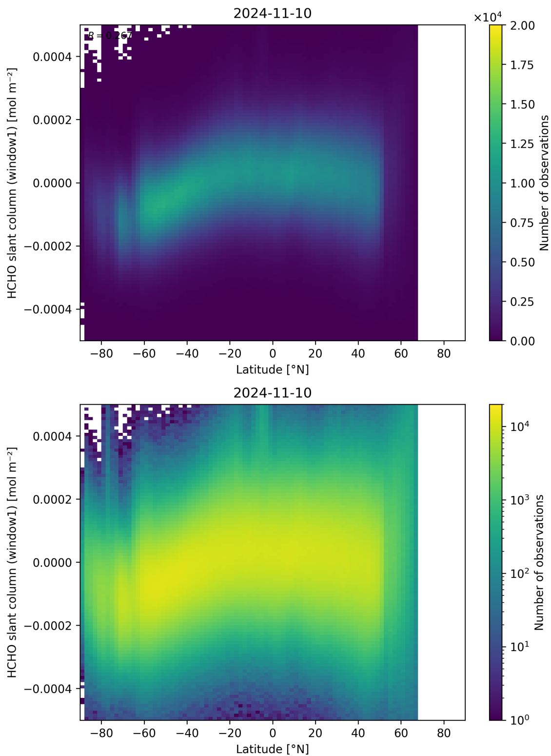
Figure 159: Scatter density plot of “Latitude” against “HCHO slant column (window1)” for 2024-11-09 to 2024-11-11.
