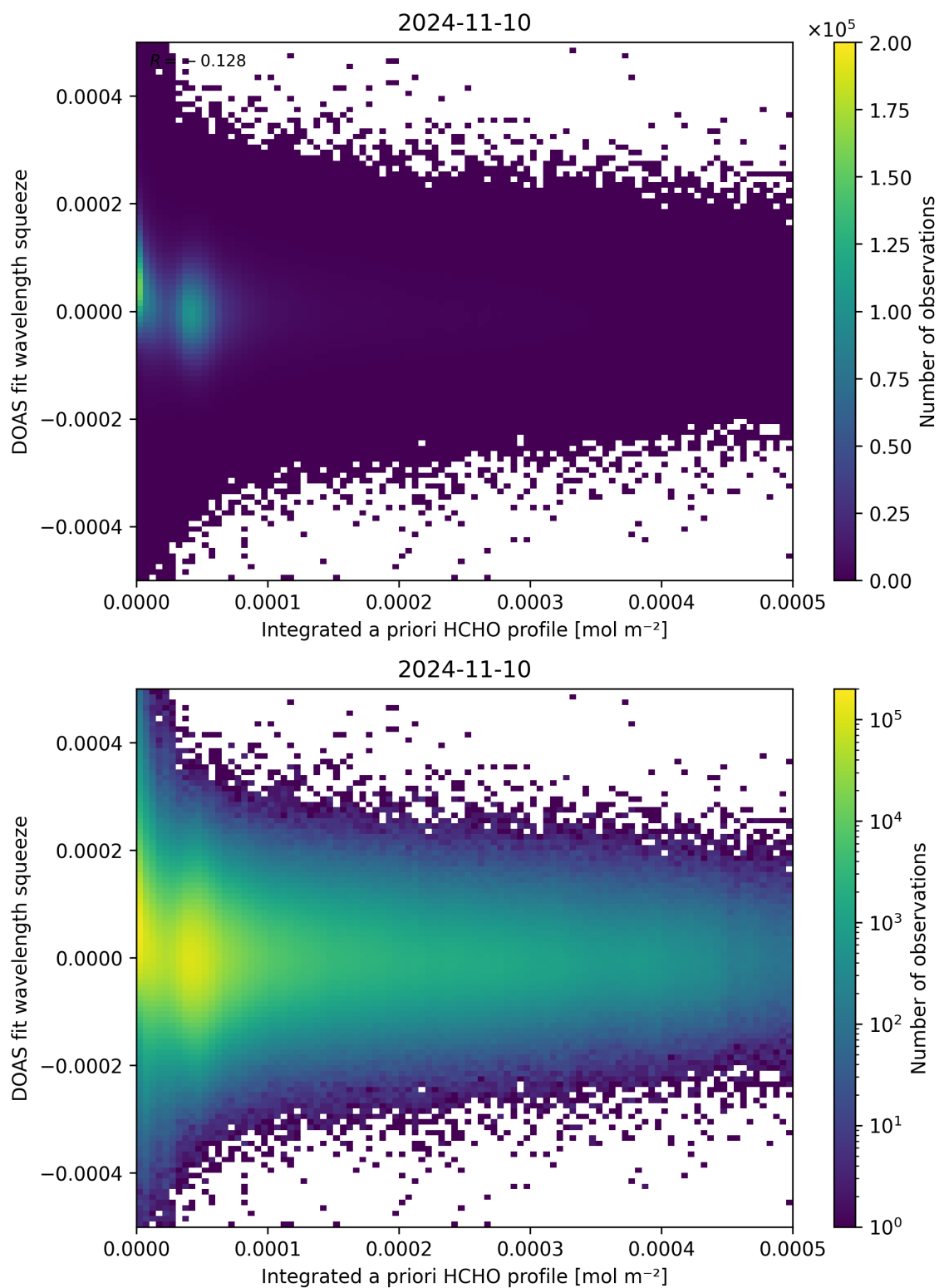
Figure 150: Scatter density plot of “Integrated a priori HCHO profile” against “DOAS fit wavelength squeeze” for 2024-11-09 to 2024-11-11.
