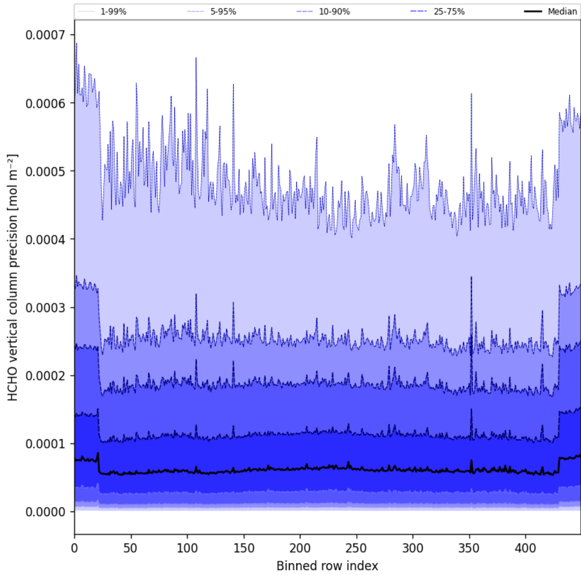
Figure 50: Along track statistics of “HCHO vertical column precision” for 2024-11-09 to 2024-11-11
