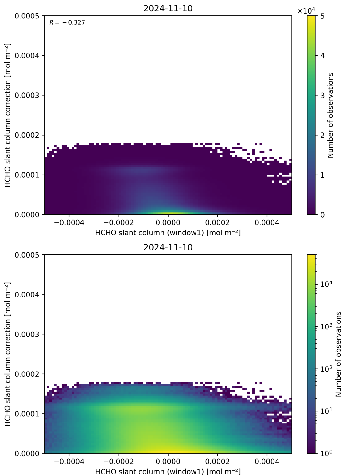
Figure 83: Scatter density plot of “HCHO slant column (window1)” against “HCHO slant column correction” for 2024-11-09 to 2024-11-11.
