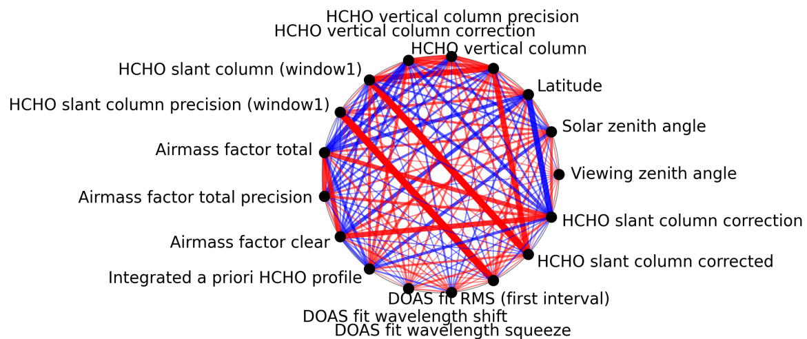
Figure 1: Map of correlation graph for 2024-11-09 to 2024-11-11.
