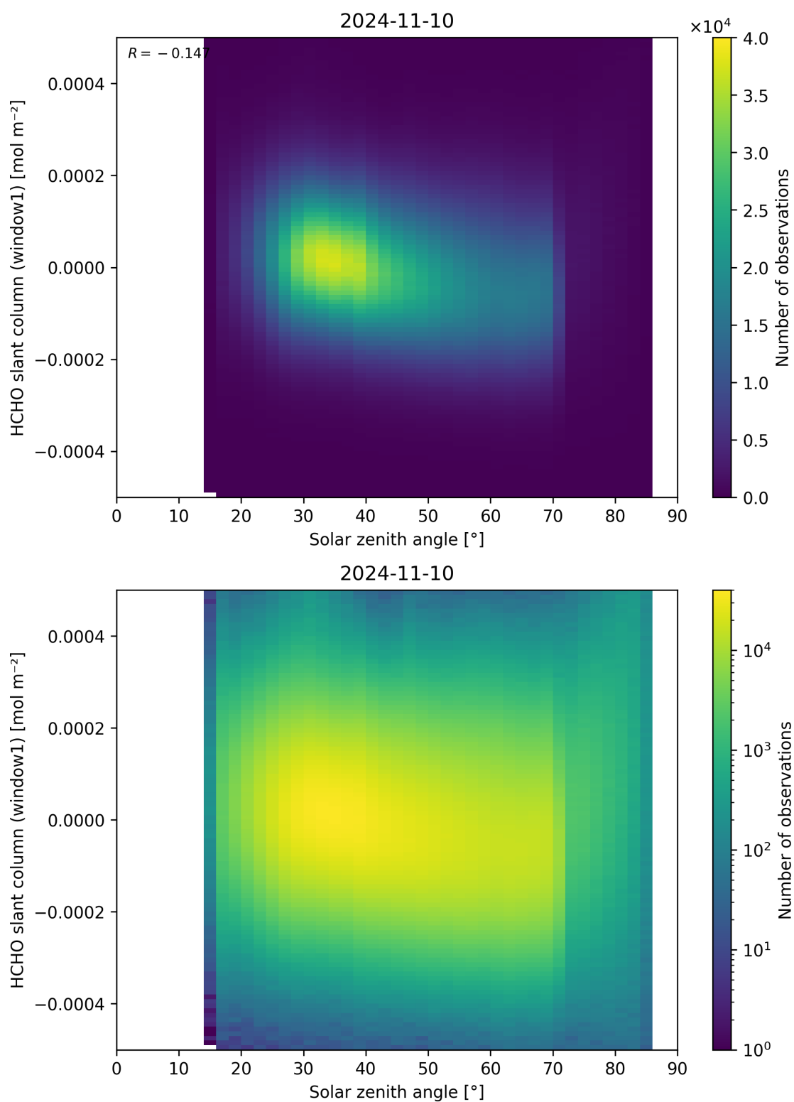
Figure 173: Scatter density plot of “Solar zenith angle” against “HCHO slant column (window1)” for 2024-11-09 to 2024-11-11.
