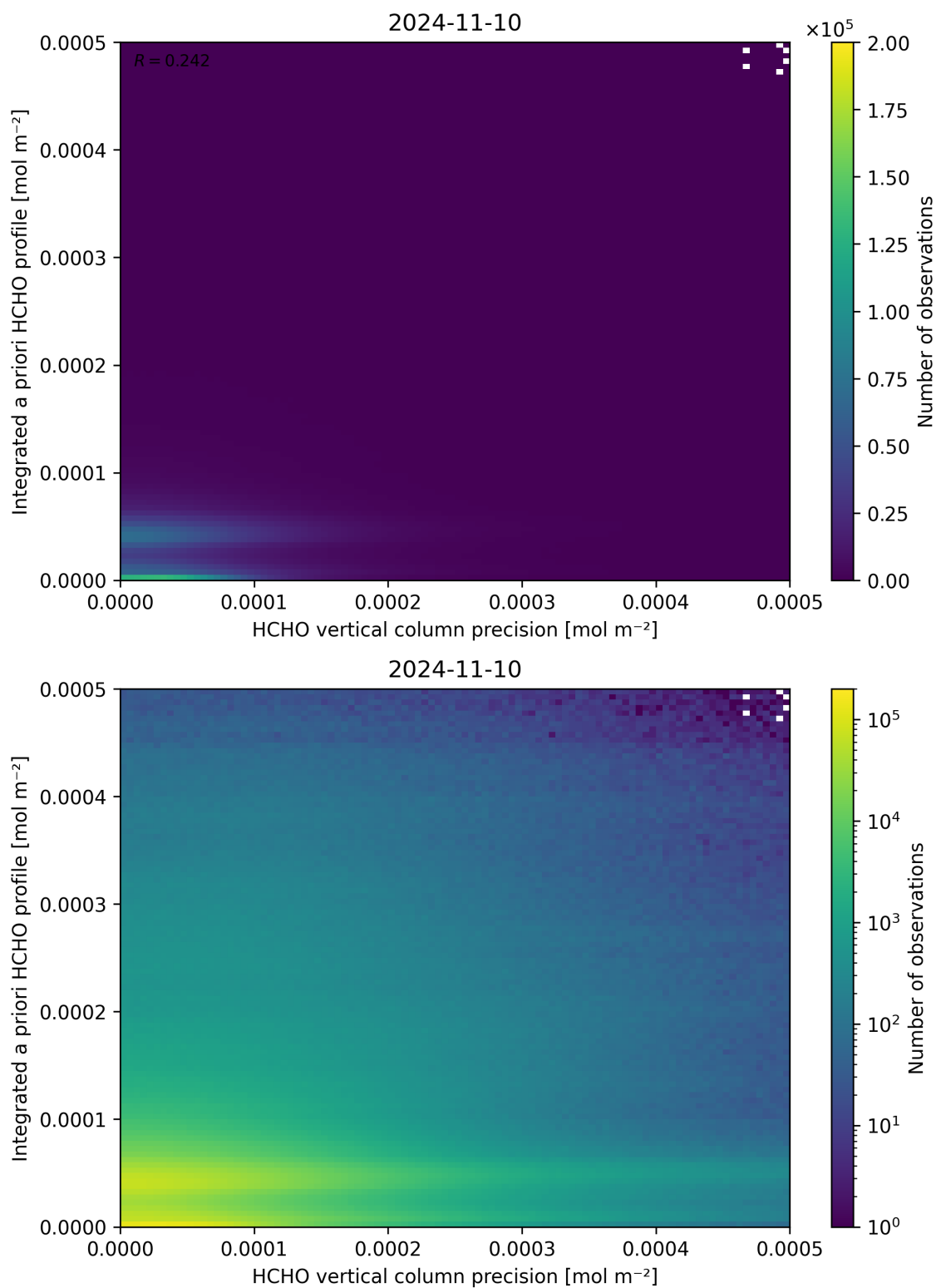
Figure 147: Scatter density plot of “HCHO vertical column precision” against “Integrated a priori HCHO profile” for 2024-11-09 to 2024-11-11.
