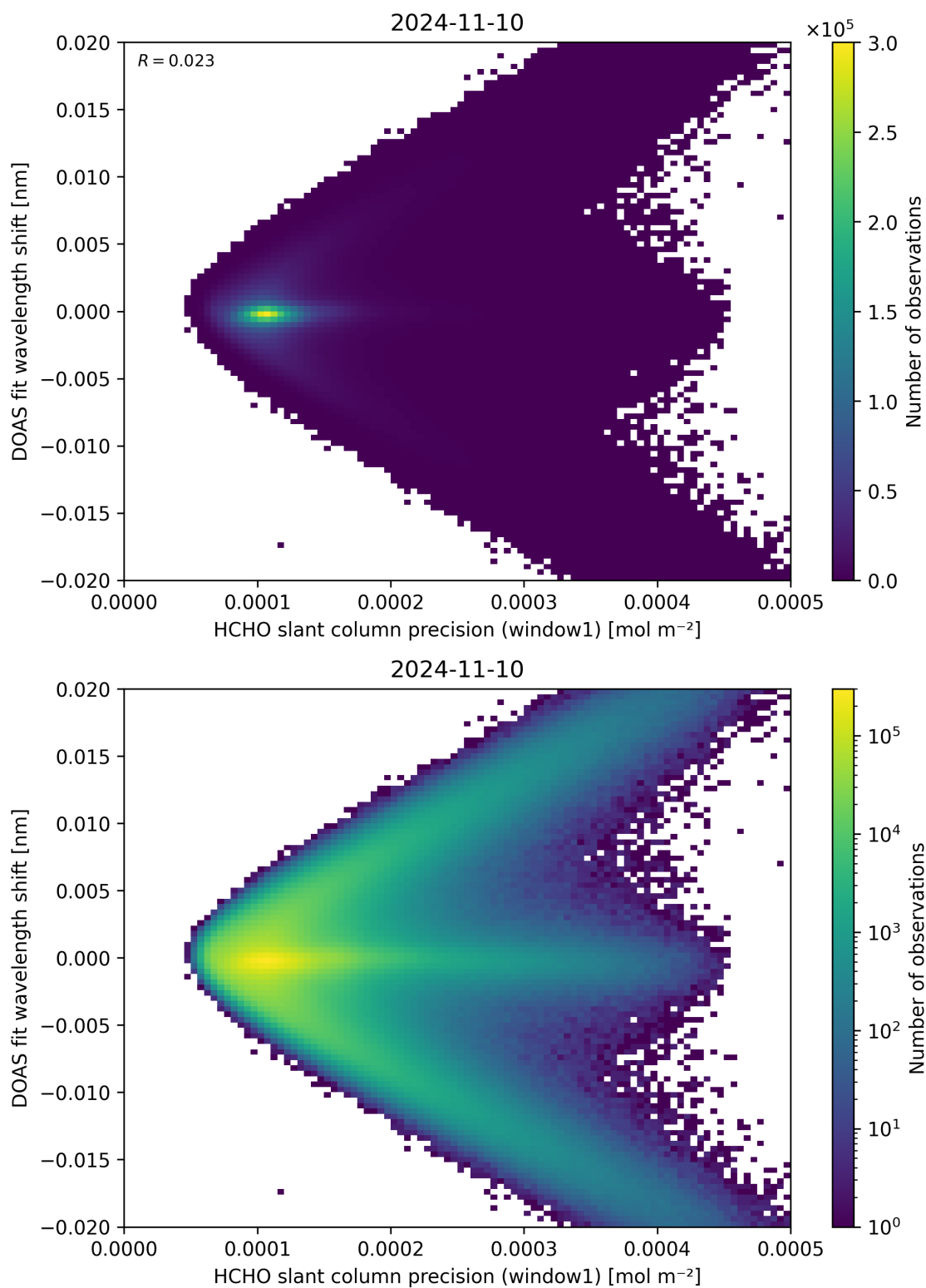
Figure 89: Scatter density plot of “HCHO slant column precision (window1)” against “DOAS fit wavelength shift” for 2024-11-09 to 2024-11-11.
