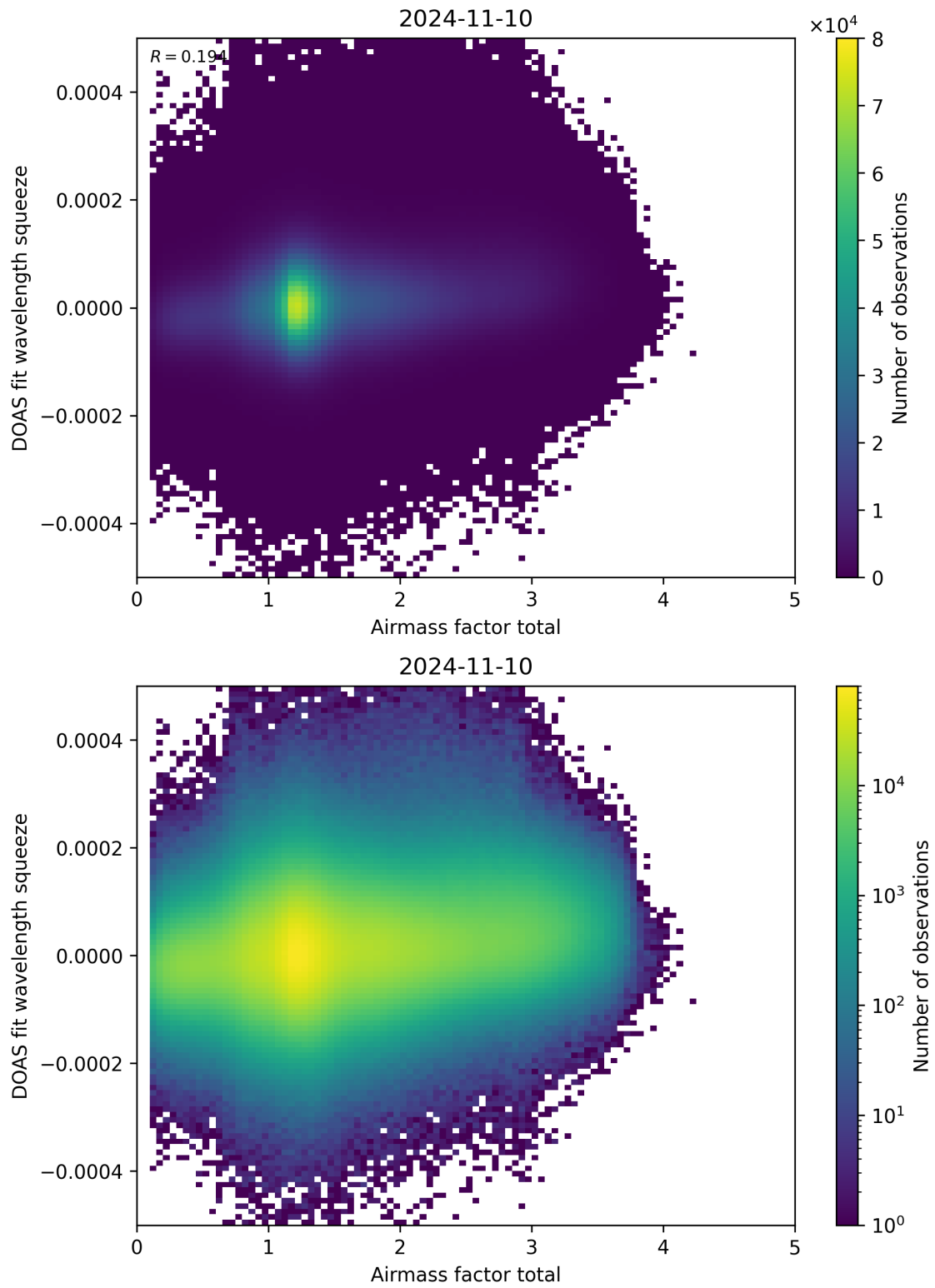
Figure 99: Scatter density plot of “Airmass factor total” against “DOAS fit wavelength squeeze” for 2024-11-09 to 2024-11-11.
