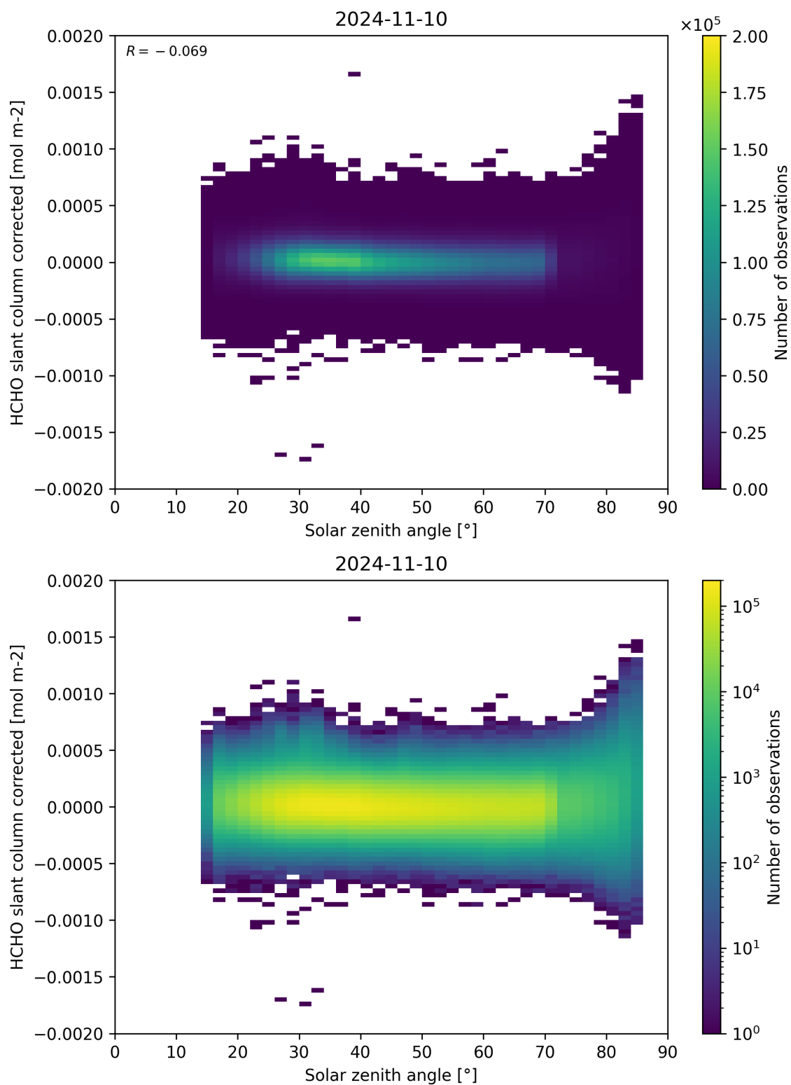
Figure 171: Scatter density plot of “Solar zenith angle” against “HCHO slant column corrected” for 2024-11-09 to 2024-11-11.
