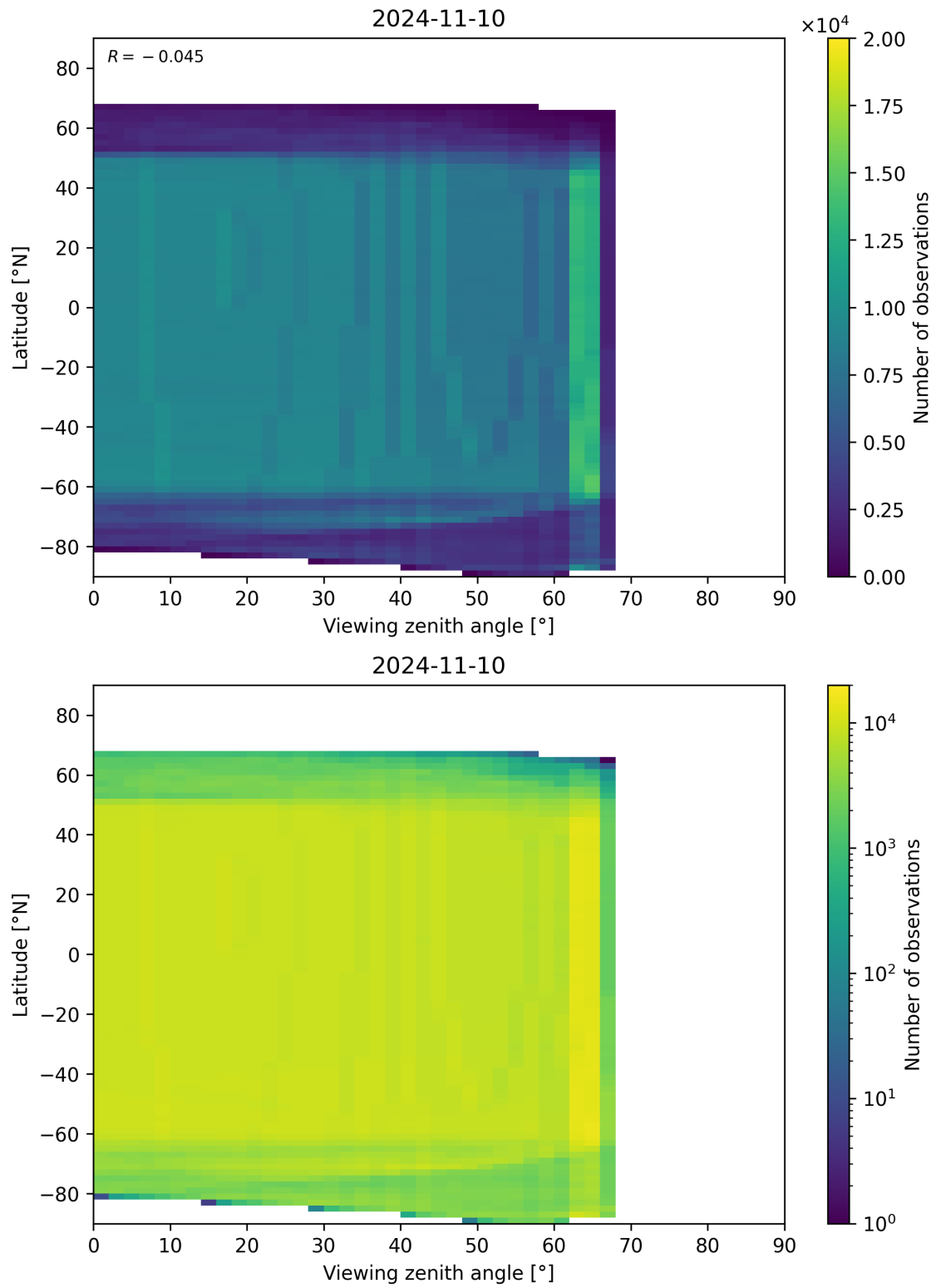
Figure 196: Scatter density plot of “Viewing zenith angle” against “Latitude” for 2024-11-09 to 2024-11-11.
