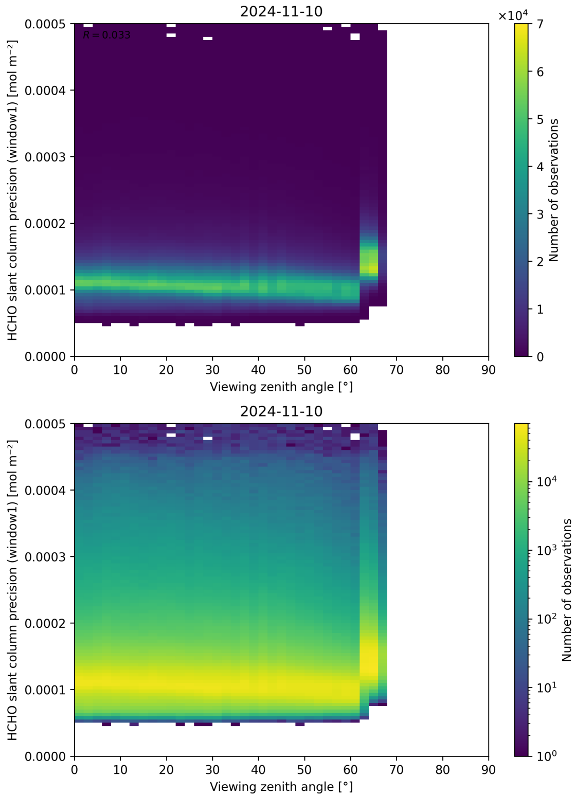
Figure 189: Scatter density plot of “Viewing zenith angle” against “HCHO slant column precision (window1)” for 2024-11-09 to 2024-11-11.
