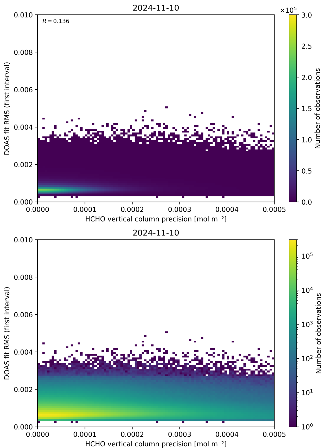
Figure 136: Scatter density plot of “HCHO vertical column precision” against “DOAS fit RMS (first interval)” for 2024-11-09 to 2024-11-11.
