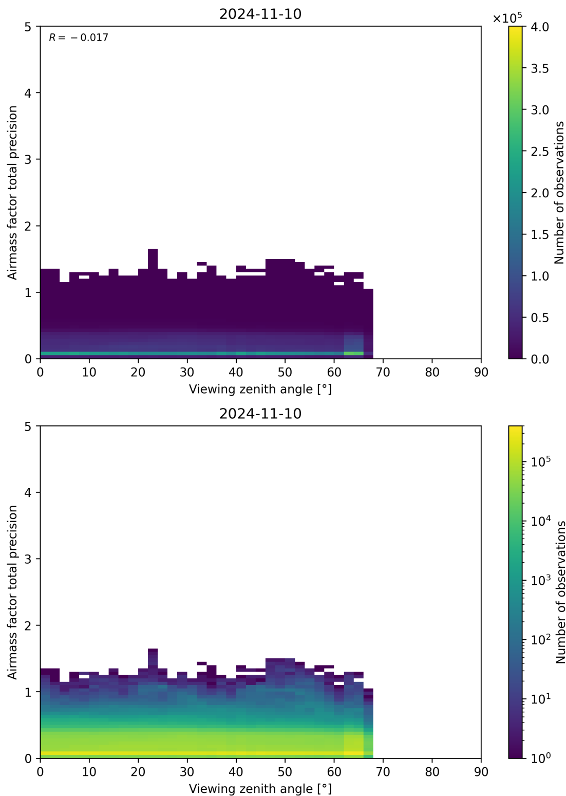
Figure 191: Scatter density plot of “Viewing zenith angle” against “Airmass factor total precision” for 2024-11-09 to 2024-11-11.
