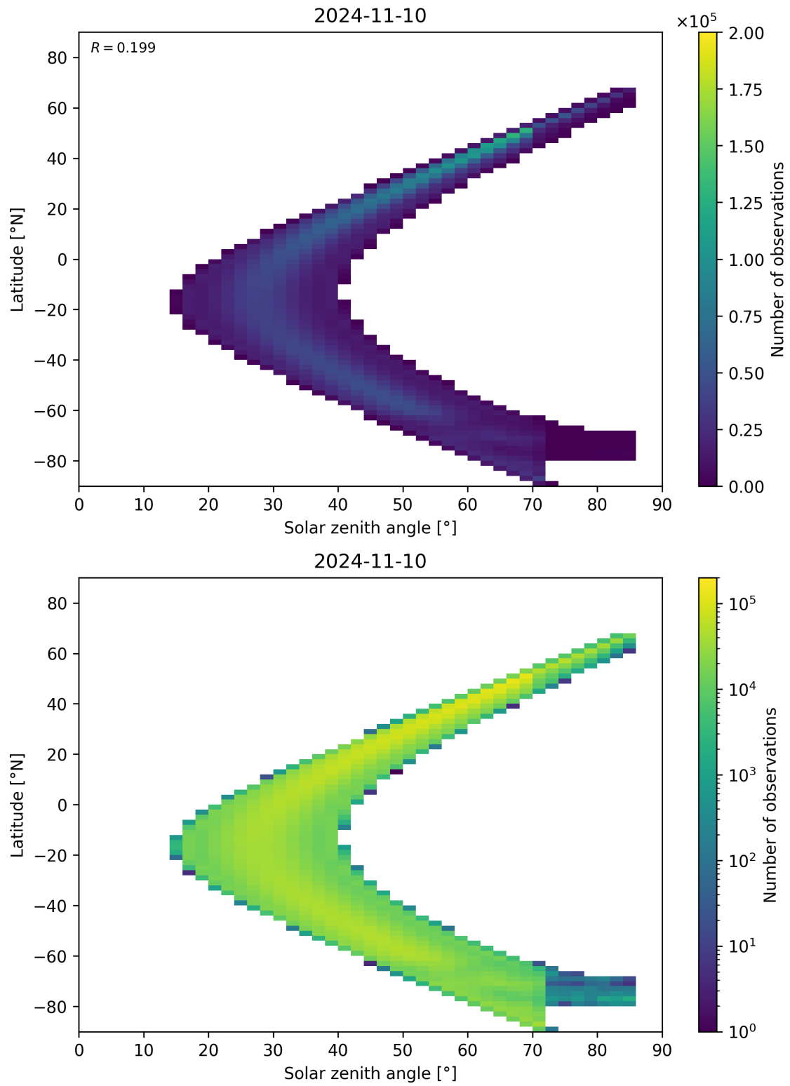
Figure 181: Scatter density plot of “Solar zenith angle” against “Latitude” for 2024-11-09 to 2024-11-11.
