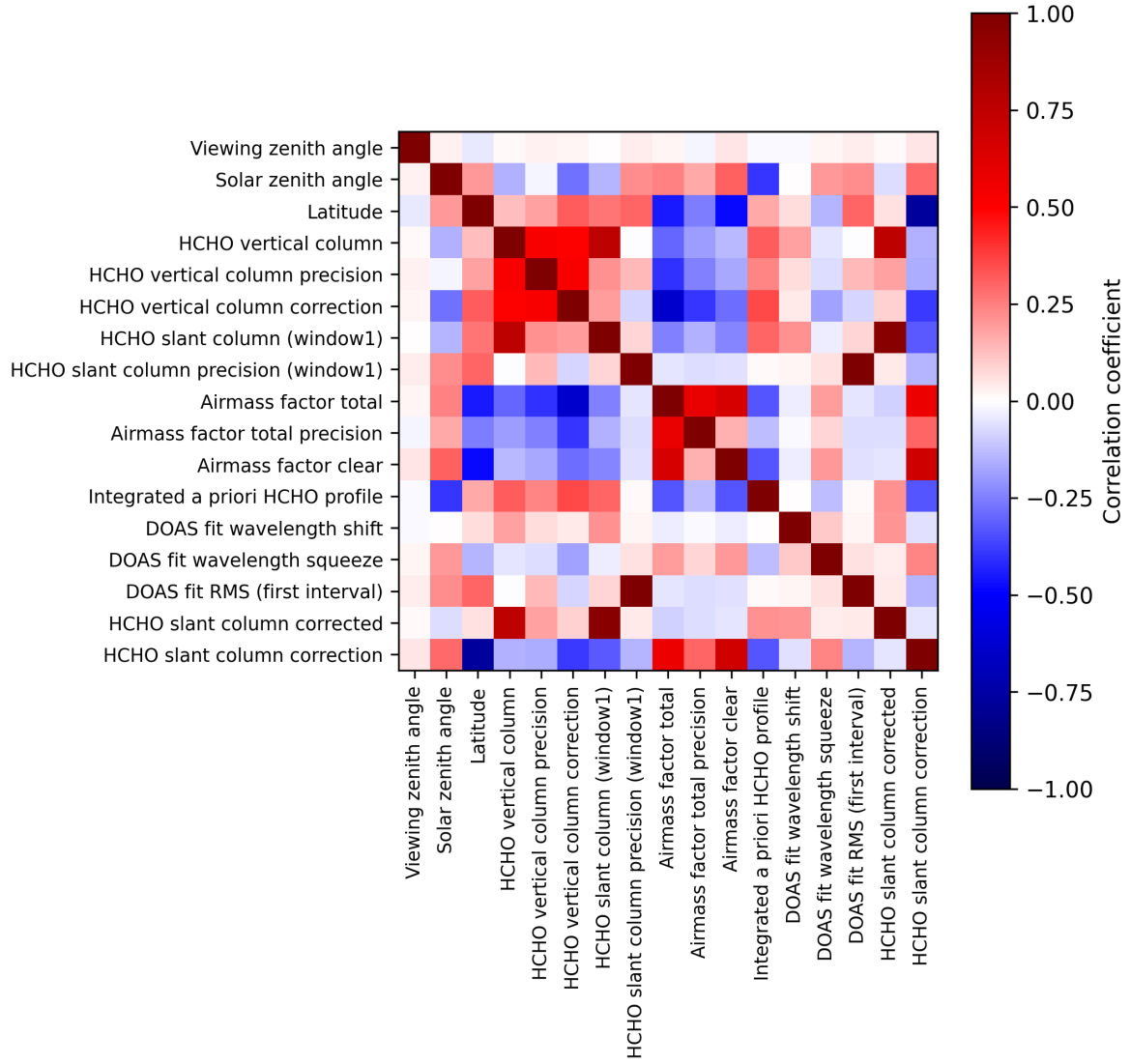
Figure 2: Map of correlation matrix for 2024-11-09 to 2024-11-11.
