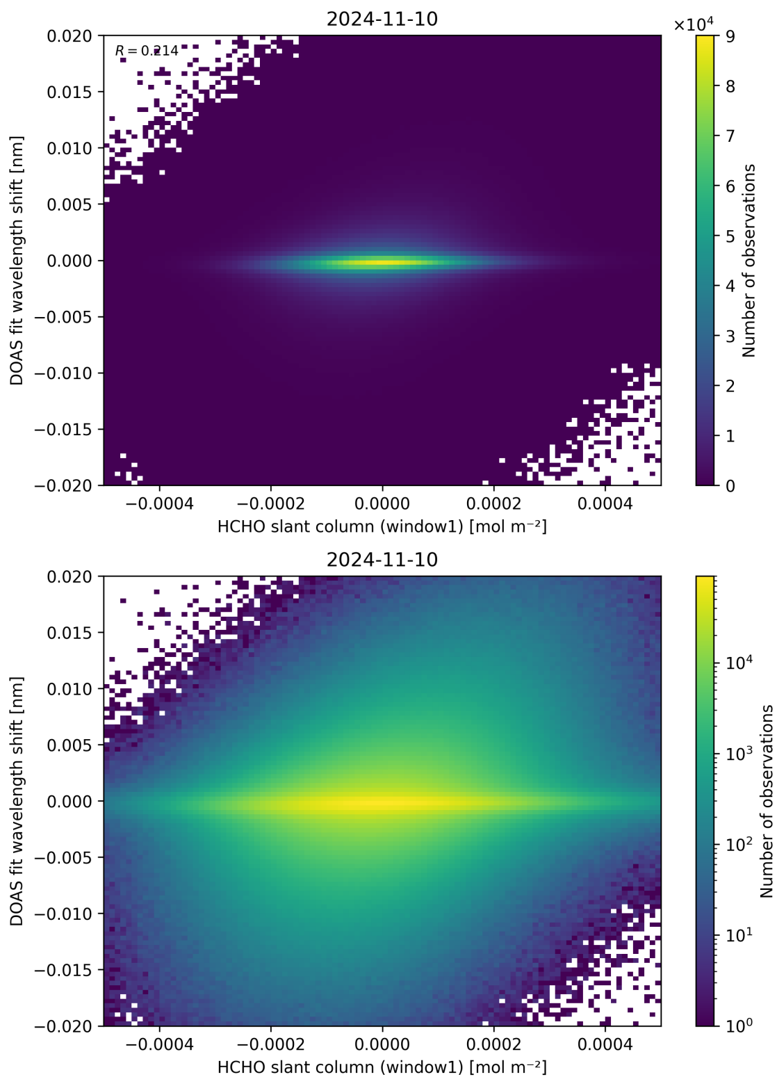
Figure 79: Scatter density plot of “HCHO slant column (window1)” against “DOAS fit wavelength shift” for 2024-11-09 to 2024-11-11.
