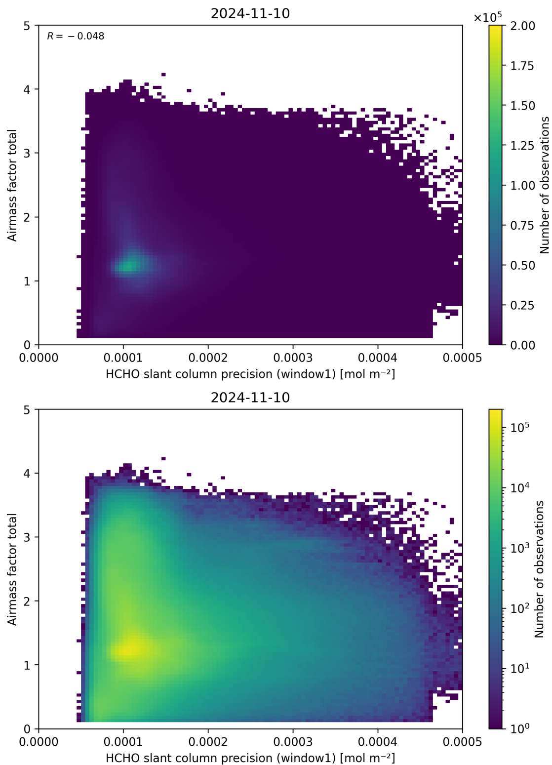
Figure 94: Scatter density plot of “HCHO slant column precision (window1)” against “Airmass factor total” for 2024-11-09 to 2024-11-11.
