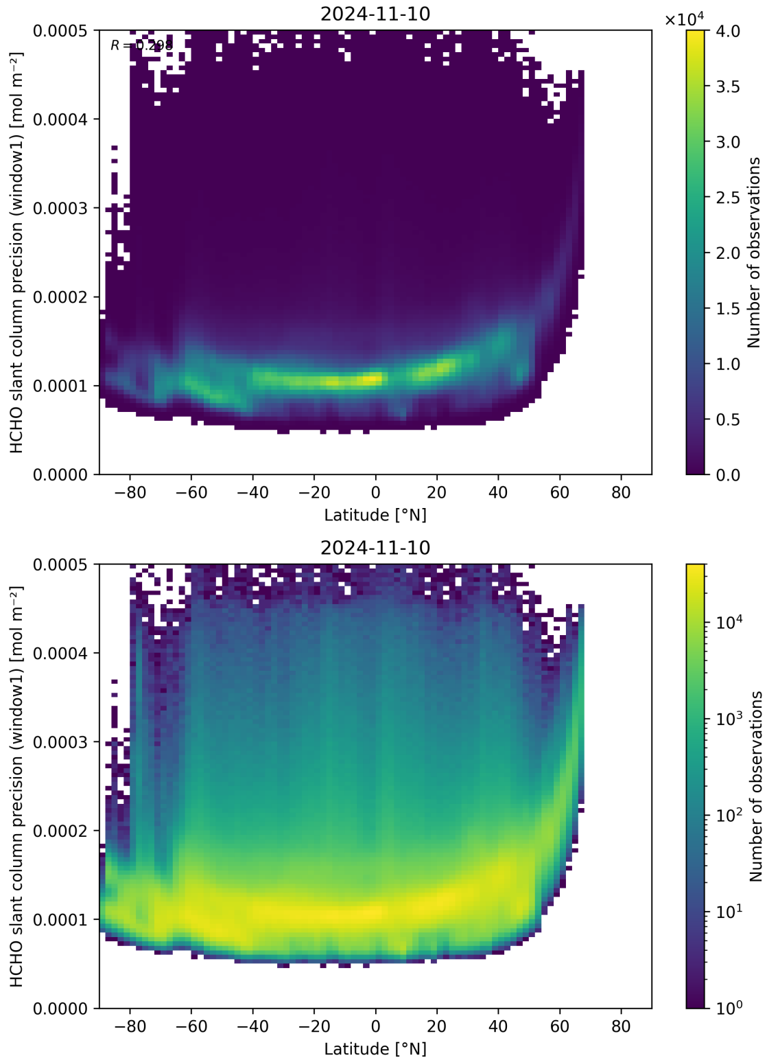
Figure 160: Scatter density plot of “Latitude” against “HCHO slant column precision (window1)” for 2024-11-09 to 2024-11-11.
