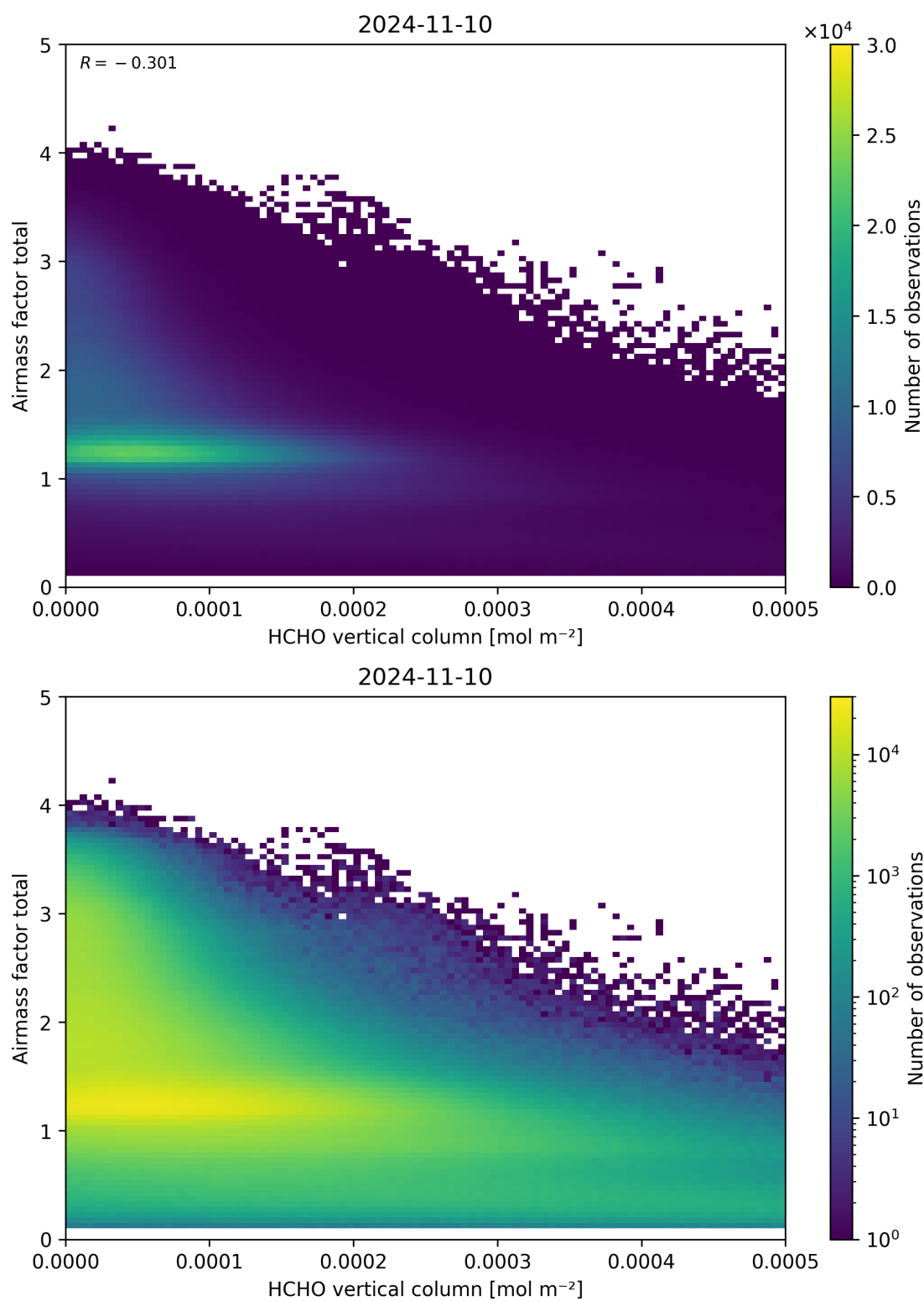
Figure 131: Scatter density plot of “HCHO vertical column” against “Airmass factor total” for 2024-11-09 to 2024-11-11.
