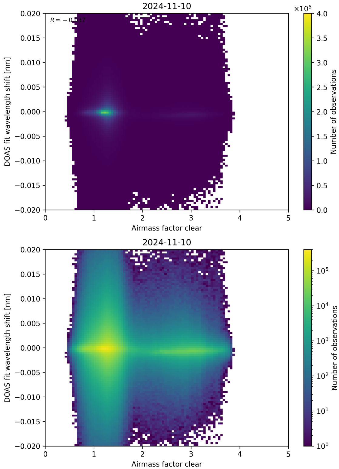
Figure 72: Scatter density plot of “Airmass factor clear” against “DOAS fit wavelength shift” for 2024-11-09 to 2024-11-11.
