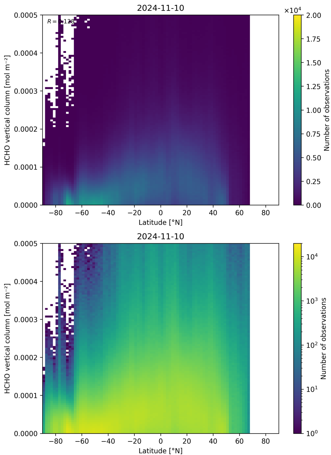
Figure 163: Scatter density plot of “Latitude” against “HCHO vertical column” for 2024-11-09 to 2024-11-11.
