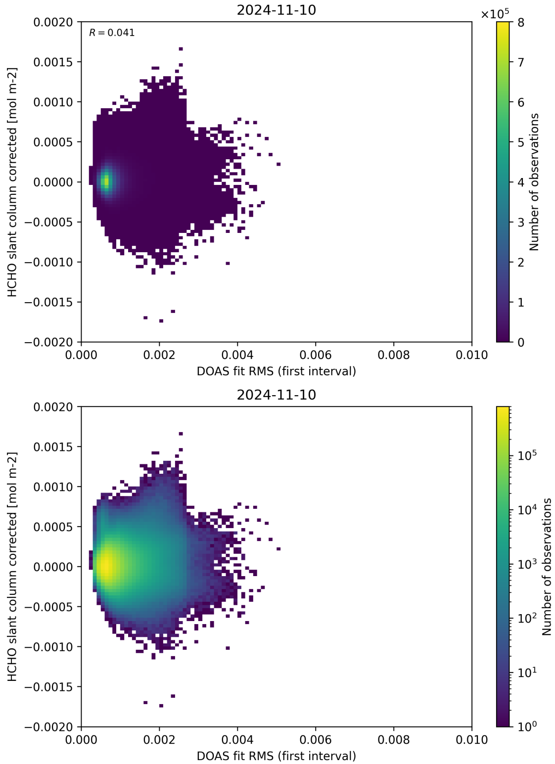
Figure 62: Scatter density plot of “DOAS fit RMS (first interval)” against “HCHO slant column corrected” for 2024-11-09 to 2024-11-11.
