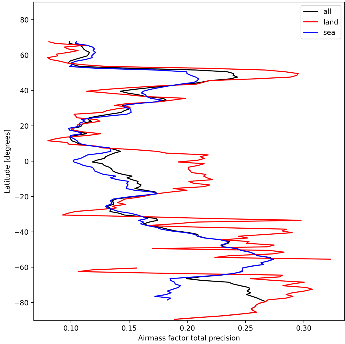
Figure 27: Zonal average of “Airmass factor total precision” for 2024-11-09 to 2024-11-11.
