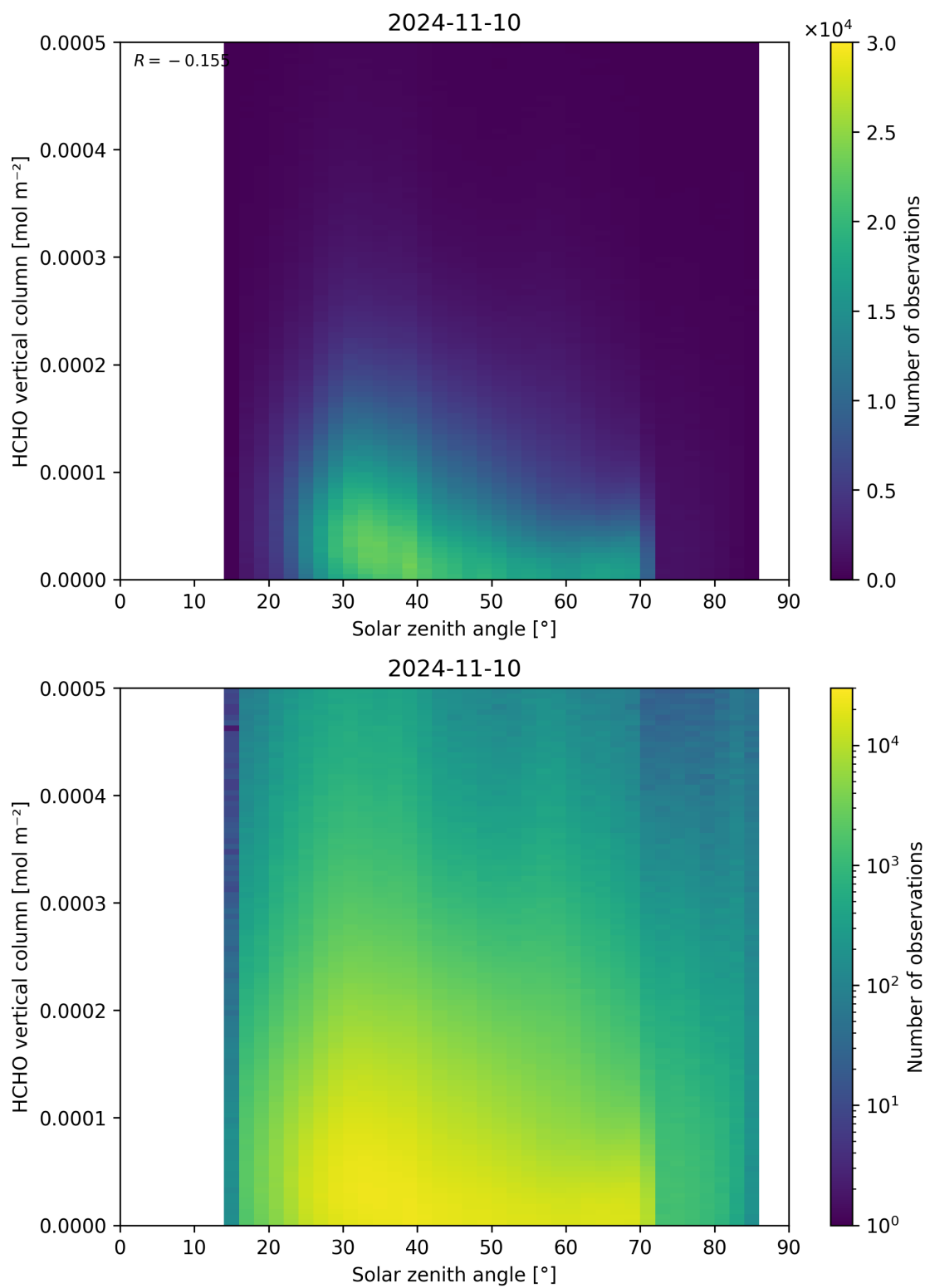
Figure 177: Scatter density plot of “Solar zenith angle” against “HCHO vertical column” for 2024-11-09 to 2024-11-11.
