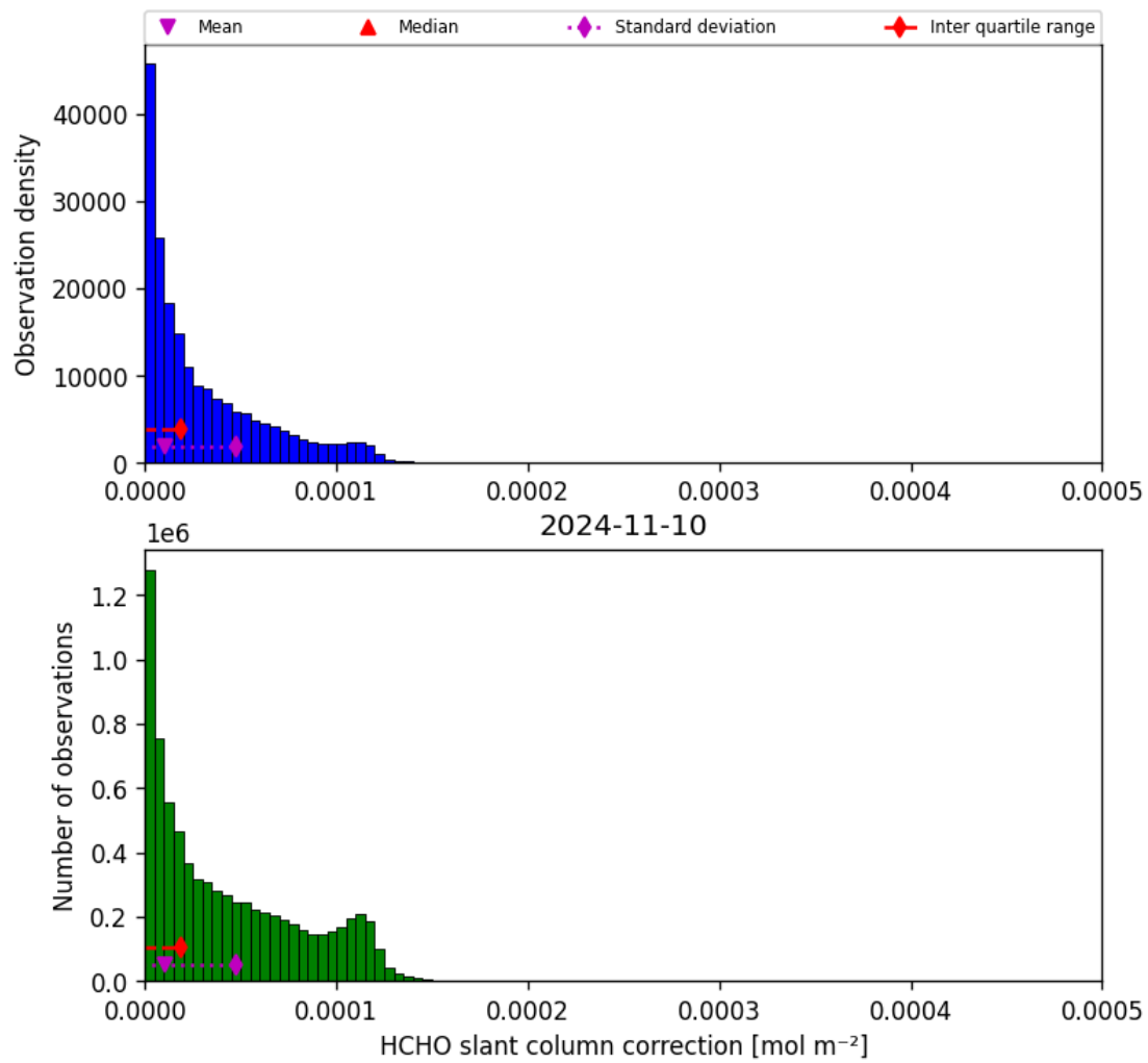
Figure 47: Histogram of “HCHO slant column correction” for 2024-11-09 to 2024-11-11
