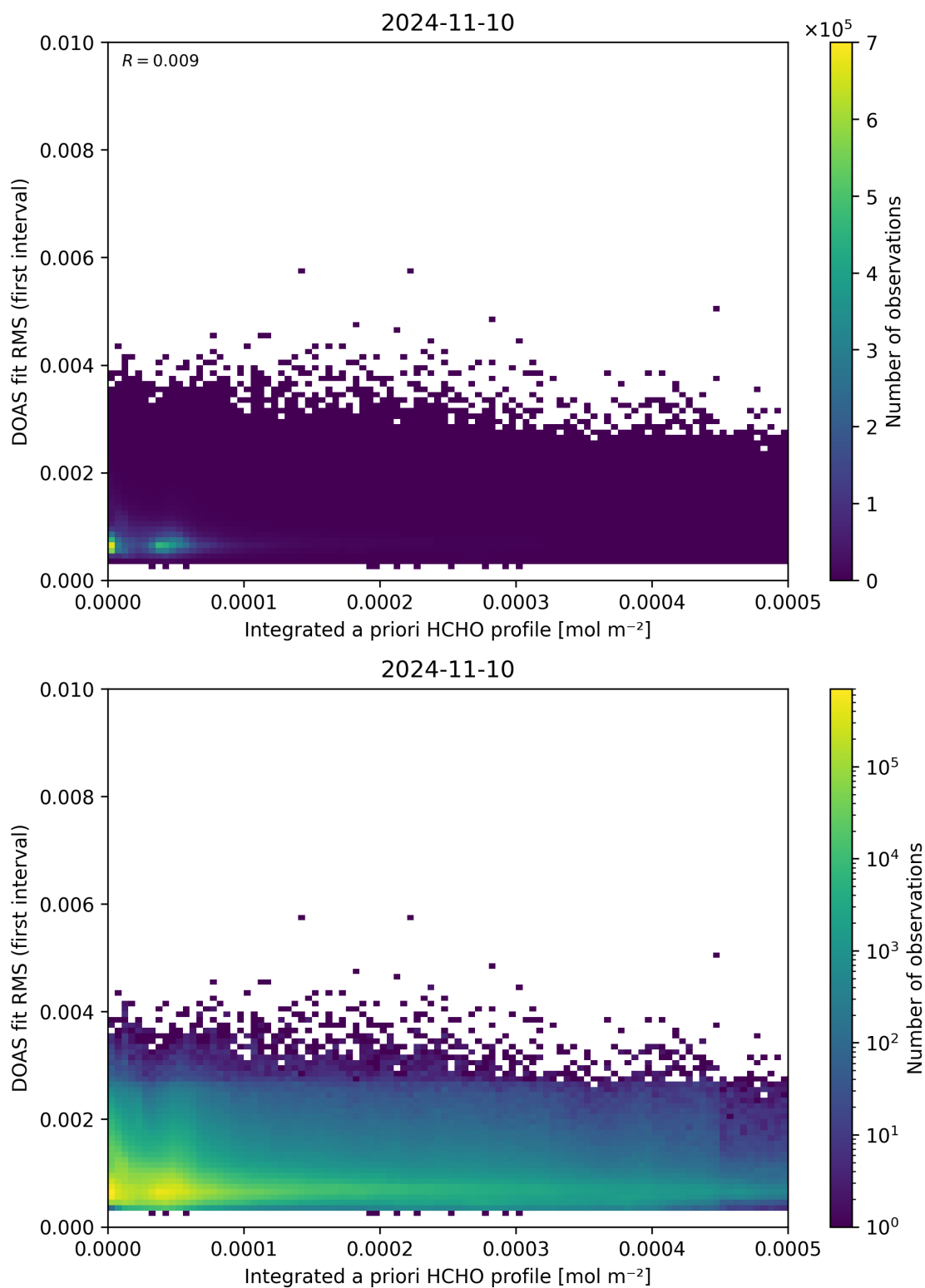
Figure 148: Scatter density plot of “Integrated a priori HCHO profile” against “DOAS fit RMS (first interval)” for 2024-11-09 to 2024-11-11.
