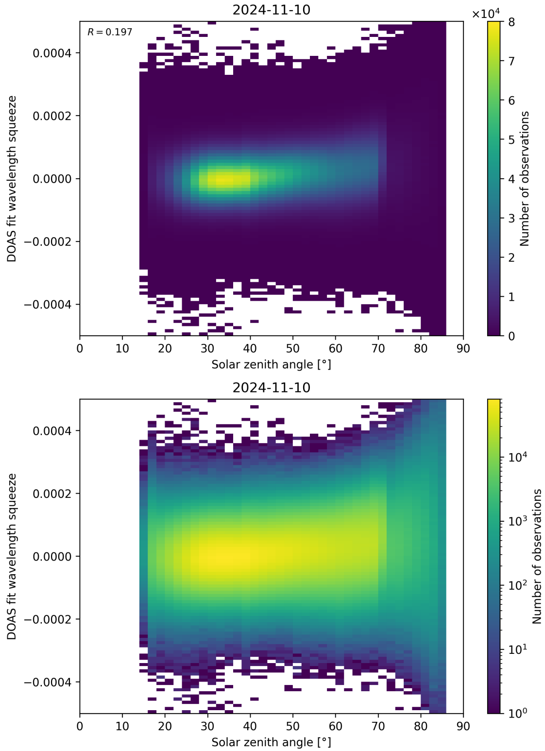
Figure 169: Scatter density plot of “Solar zenith angle” against “DOAS fit wavelength squeeze” for 2024-11-09 to 2024-11-11.
