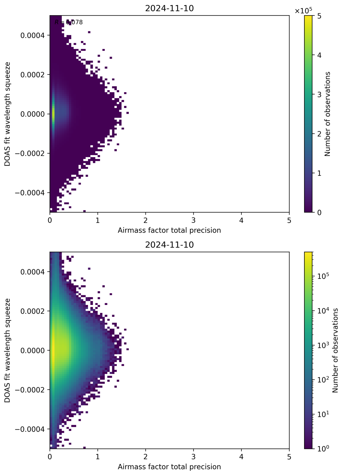
Figure 107: Scatter density plot of “Airmass factor total precision” against “DOAS fit wavelength squeeze” for 2024-11-09 to 2024-11-11.
