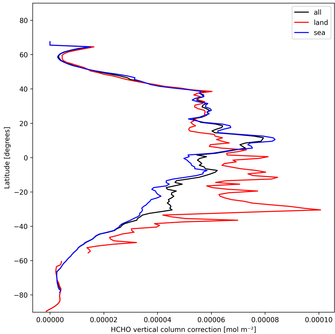
Figure 23: Zonal average of “HCHO vertical column correction” for 2024-11-09 to 2024-11-11.
