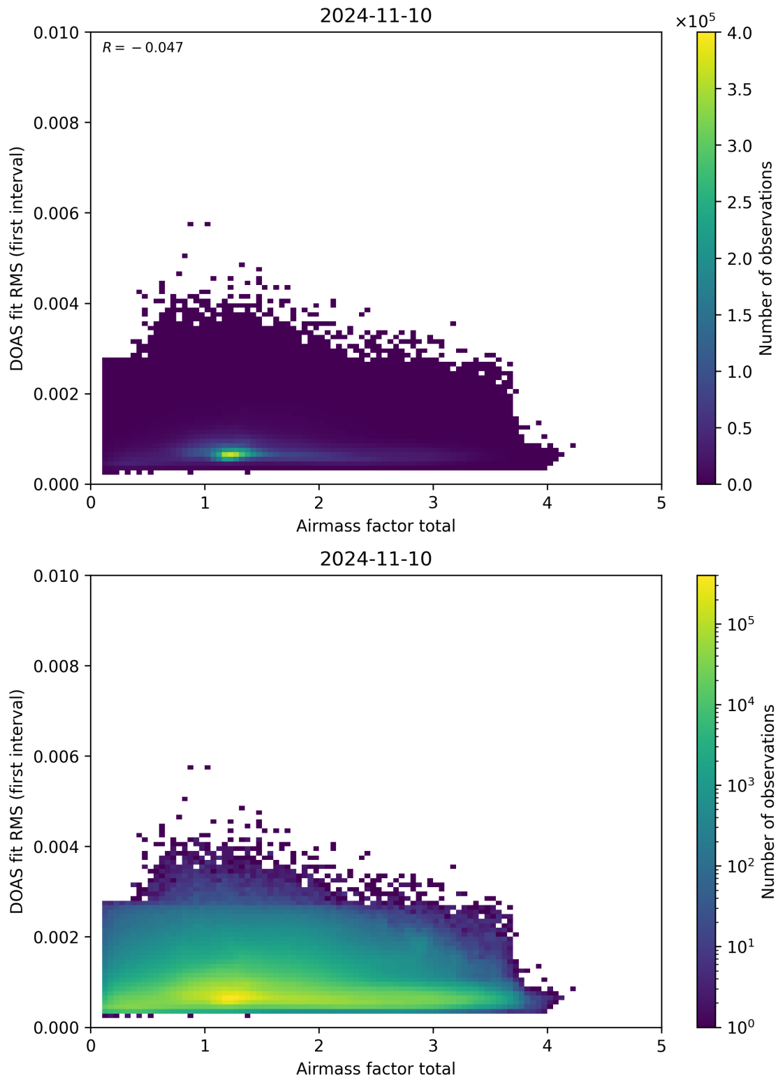
Figure 97: Scatter density plot of “Airmass factor total” against “DOAS fit RMS (first interval)” for 2024-11-09 to 2024-11-11.
