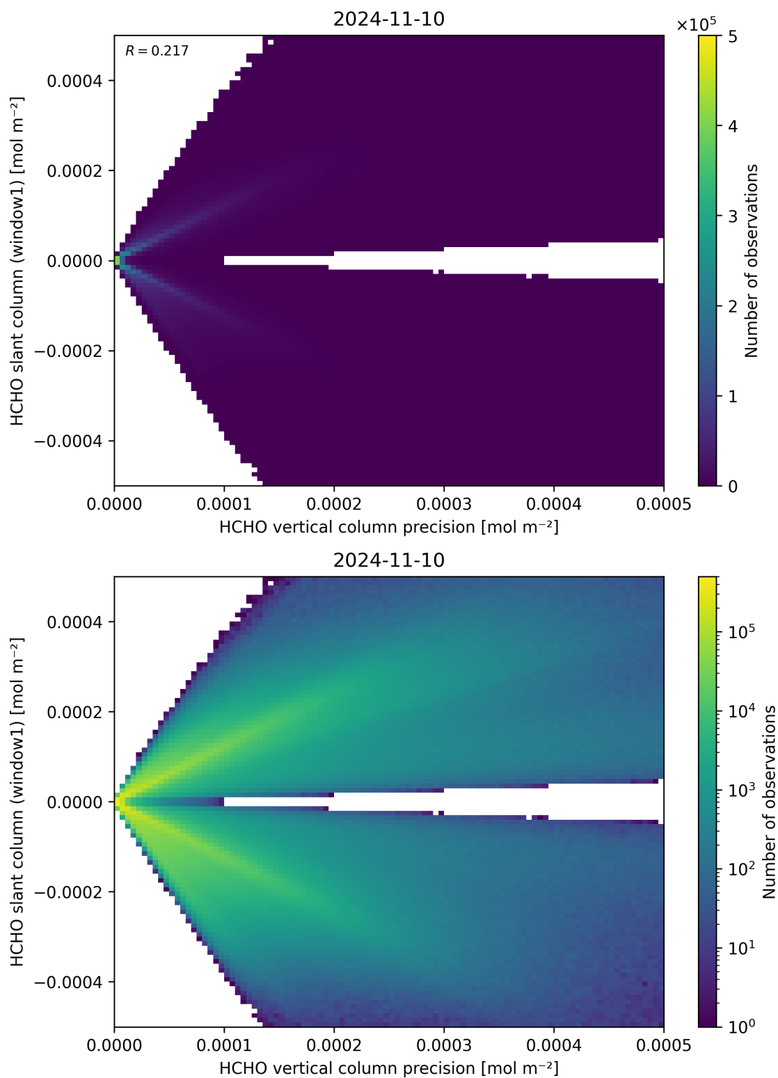
Figure 142: Scatter density plot of “HCHO vertical column precision” against “HCHO slant column (window1)” for 2024-11-09 to 2024-11-11.
