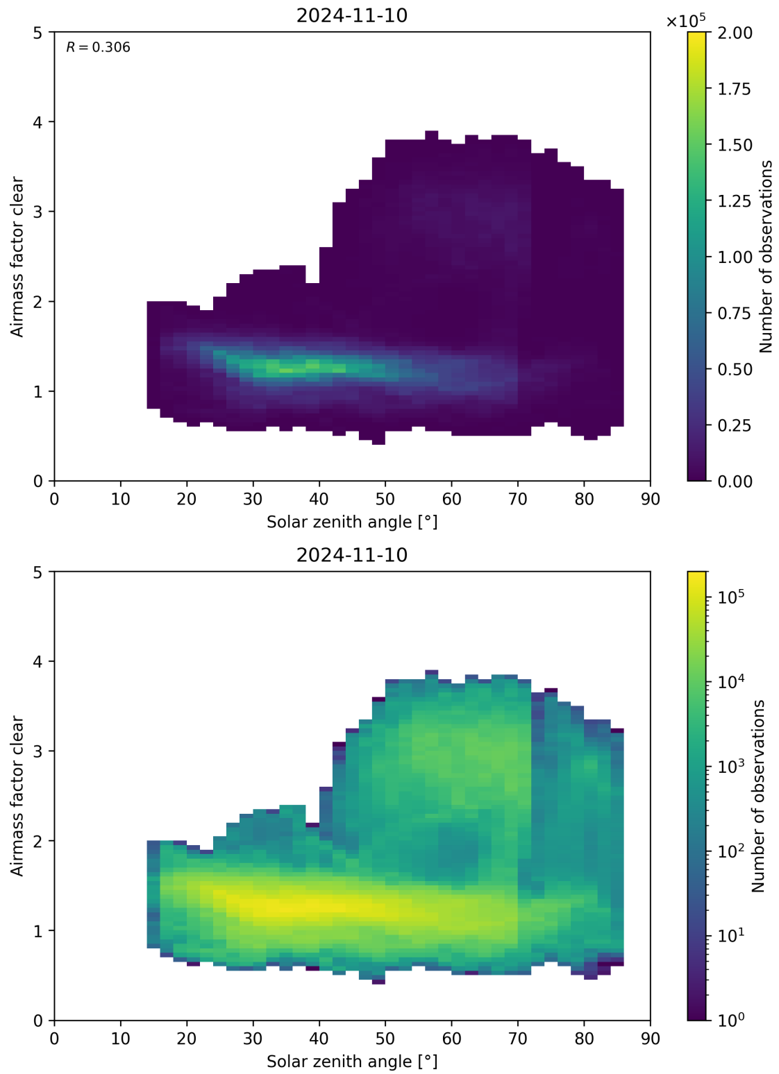
Figure 170: Scatter density plot of “Solar zenith angle” against “Airmass factor clear” for 2024-11-09 to 2024-11-11.
