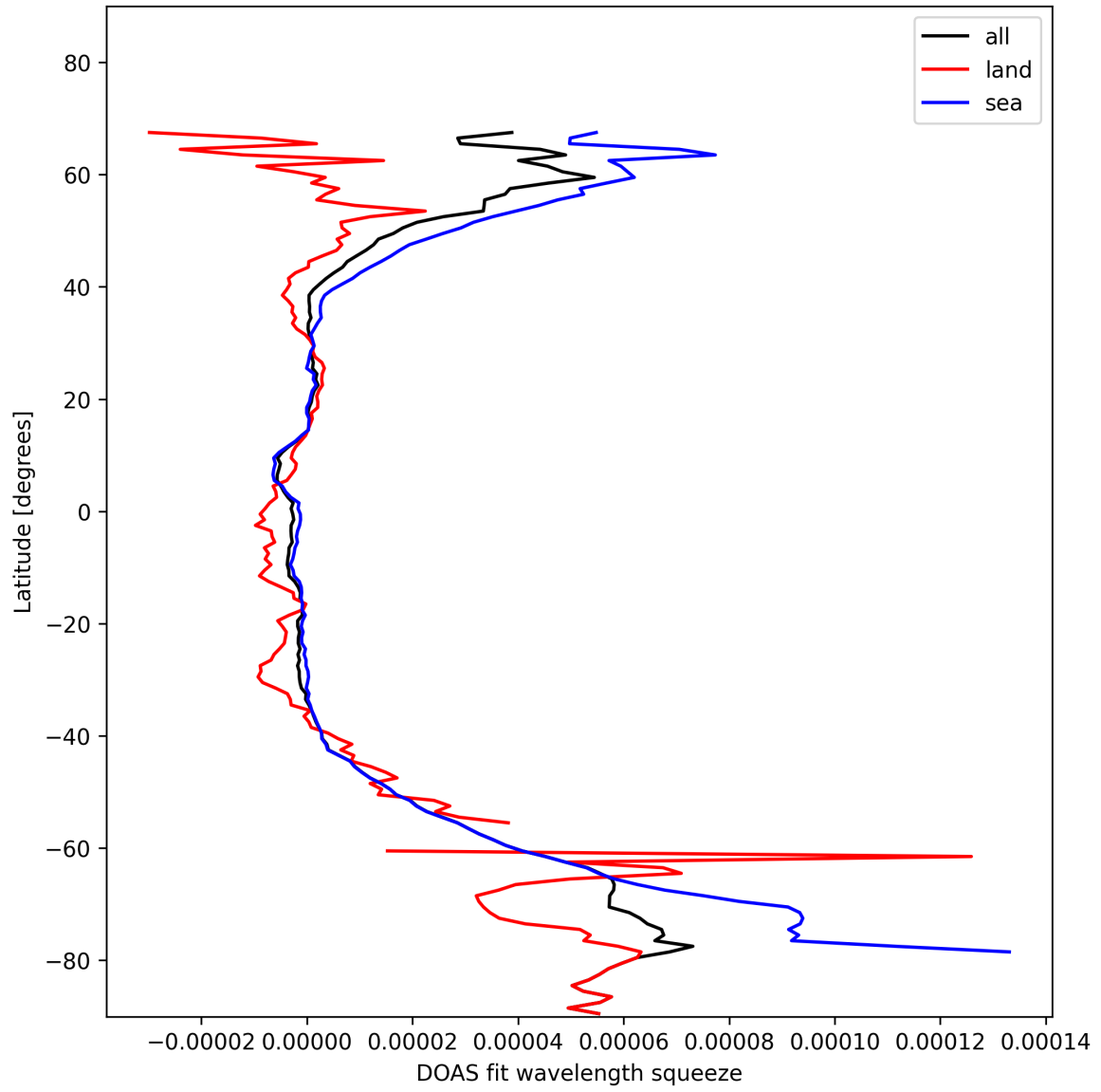
Figure 31: Zonal average of “DOAS fit wavelength squeeze” for 2024-11-09 to 2024-11-11.
