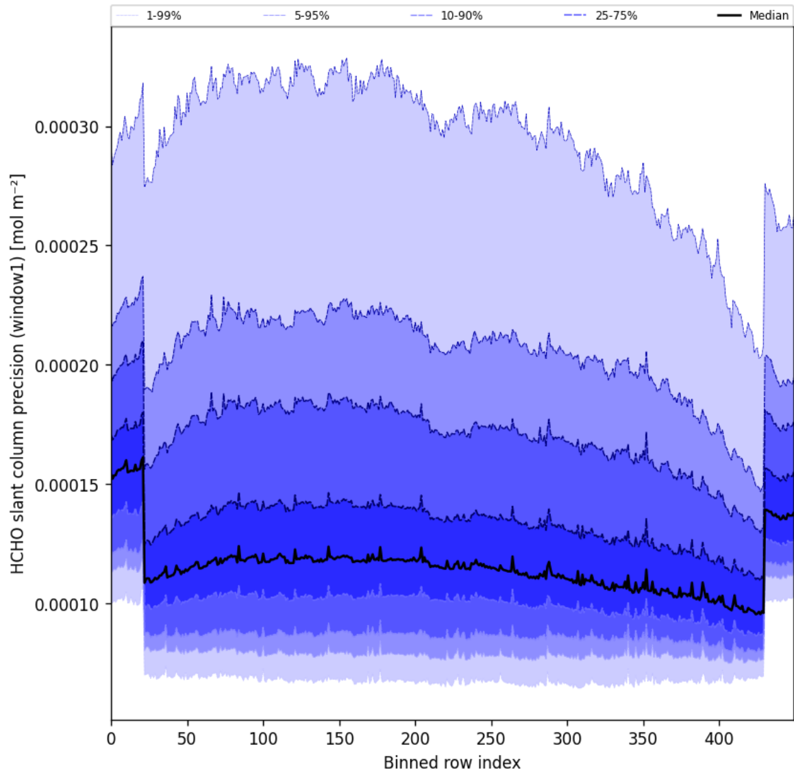
Figure 53: Along track statistics of "HCHO slant column precision (window1)" for 2024-11-09 to 2024-11-11
