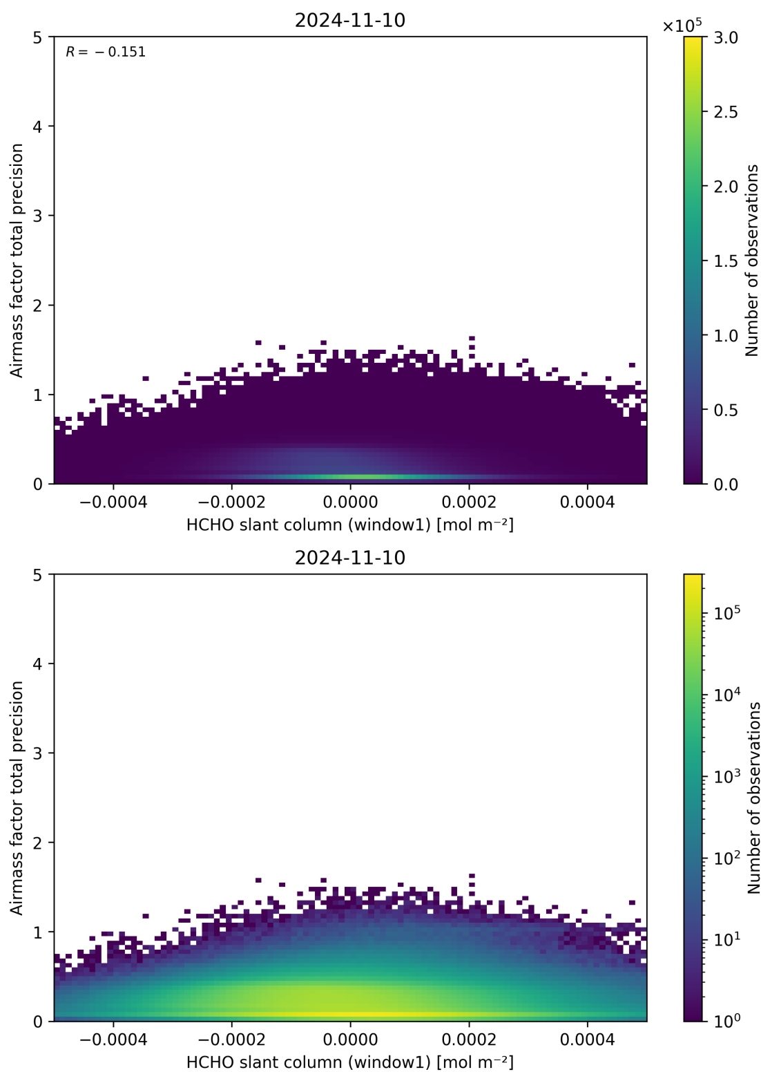
Figure 86: Scatter density plot of “HCHO slant column (window1)” against “Airmass factor total precision” for 2024-11-09 to 2024-11-11.
