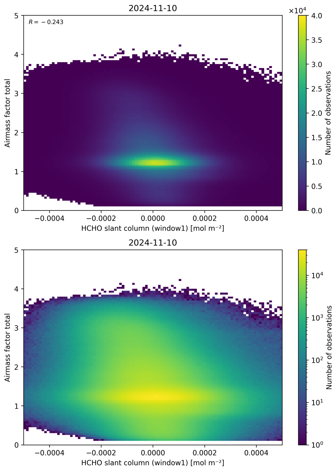
Figure 85: Scatter density plot of “HCHO slant column (window1)” against “Airmass factor total” for 2024-11-09 to 2024-11-11.
