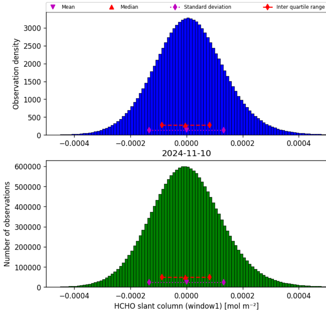
Figure 38: Histogram of “HCHO slant column (window1)” for 2024-11-09 to 2024-11-11
