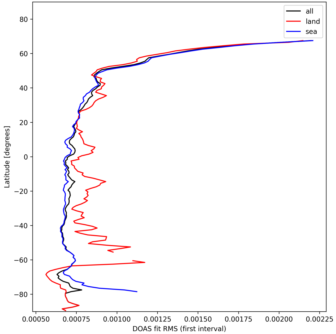
Figure 32: Zonal average of “DOAS fit RMS (first interval)” for 2024-11-09 to 2024-11-11.
