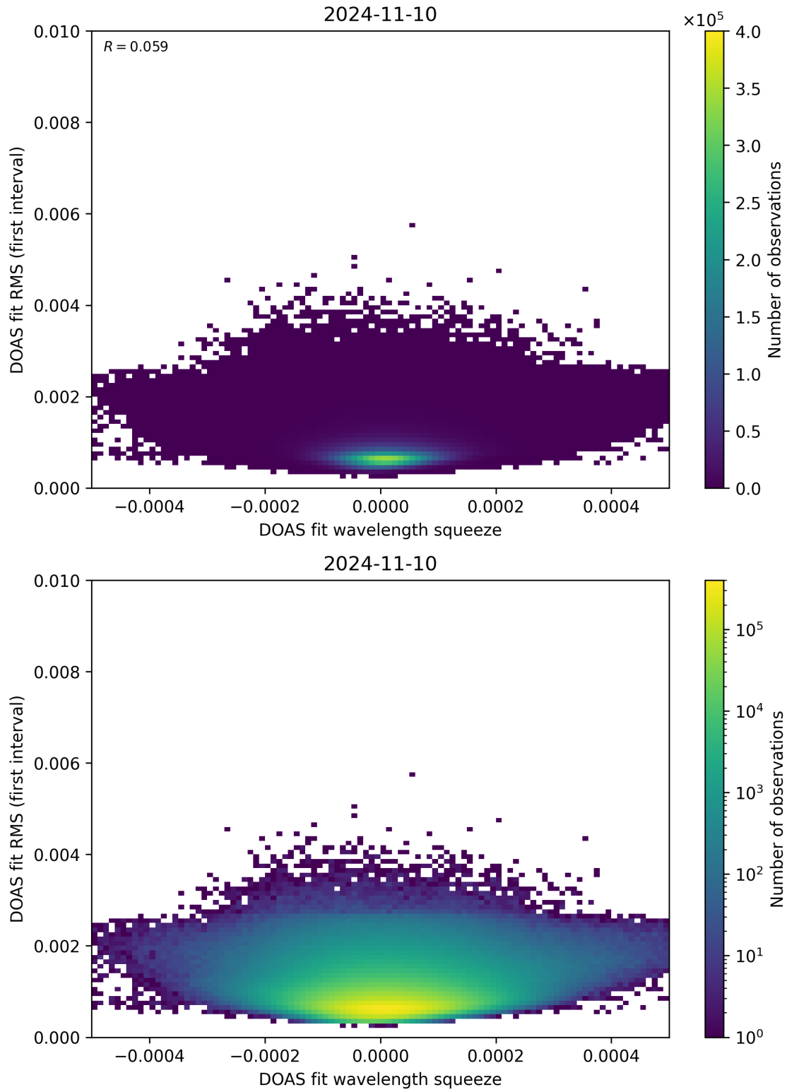
Figure 68: Scatter density plot of “DOAS fit wavelength squeeze” against “DOAS fit RMS (first interval)” for 2024-11-09 to 2024-11-11.
