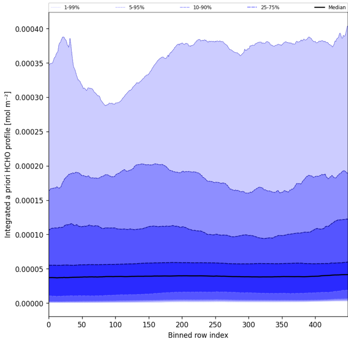
Figure 57: Along track statistics of "Integrated a priori HCHO profile" for 2024-11-09 to 2024-11-11
