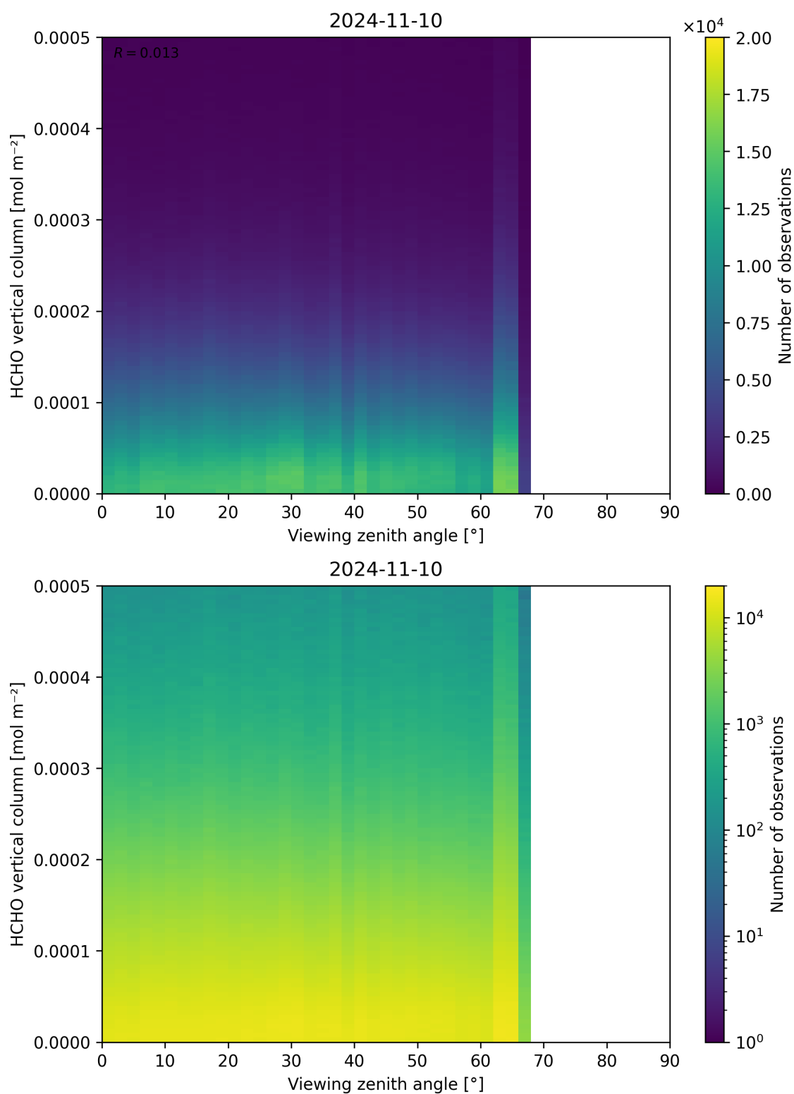
Figure 192: Scatter density plot of “Viewing zenith angle” against “HCHO vertical column” for 2024-11-09 to 2024-11-11.
