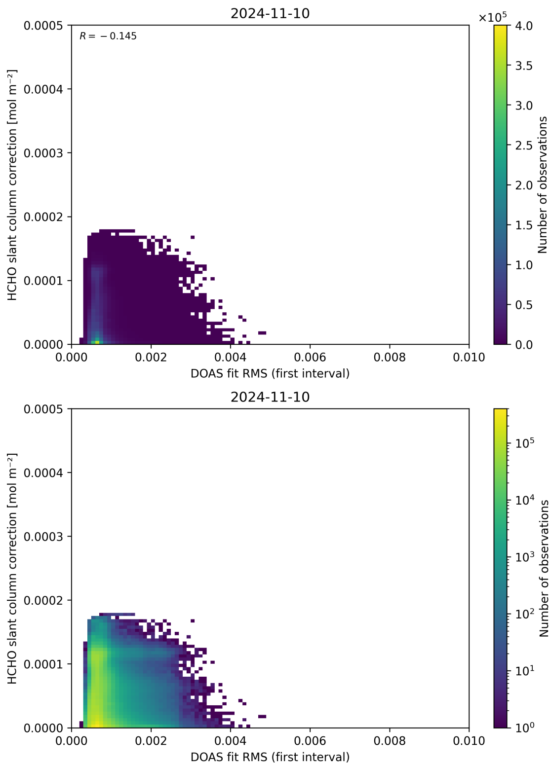
Figure 63: Scatter density plot of “DOAS fit RMS (first interval)” against “HCHO slant column correction” for 2024-11-09 to 2024-11-11.
