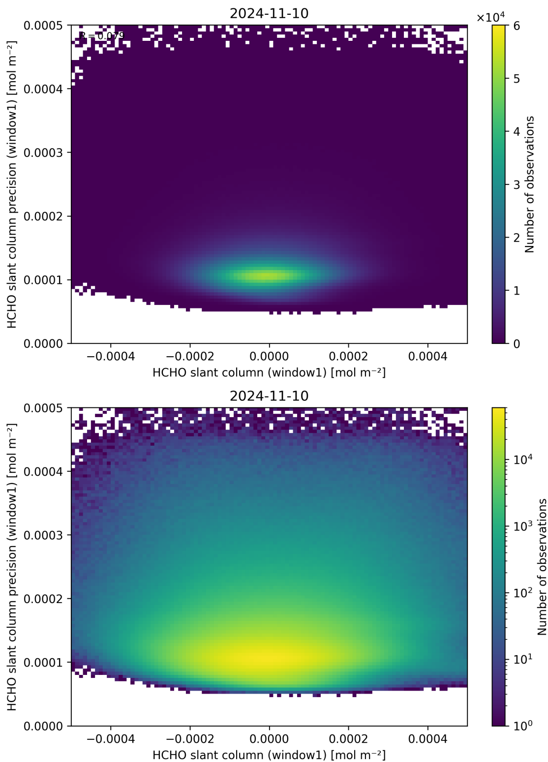
Figure 84: Scatter density plot of “HCHO slant column (window1)” against “HCHO slant column precision (window1)” for 2024-11-09 to 2024-11-11.
