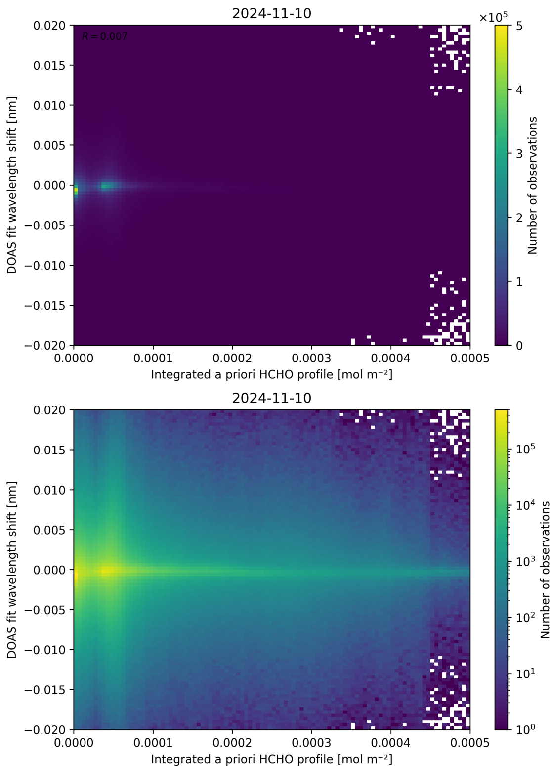
Figure 149: Scatter density plot of “Integrated a priori HCHO profile” against “DOAS fit wavelength shift” for 2024-11-09 to 2024-11-11.
