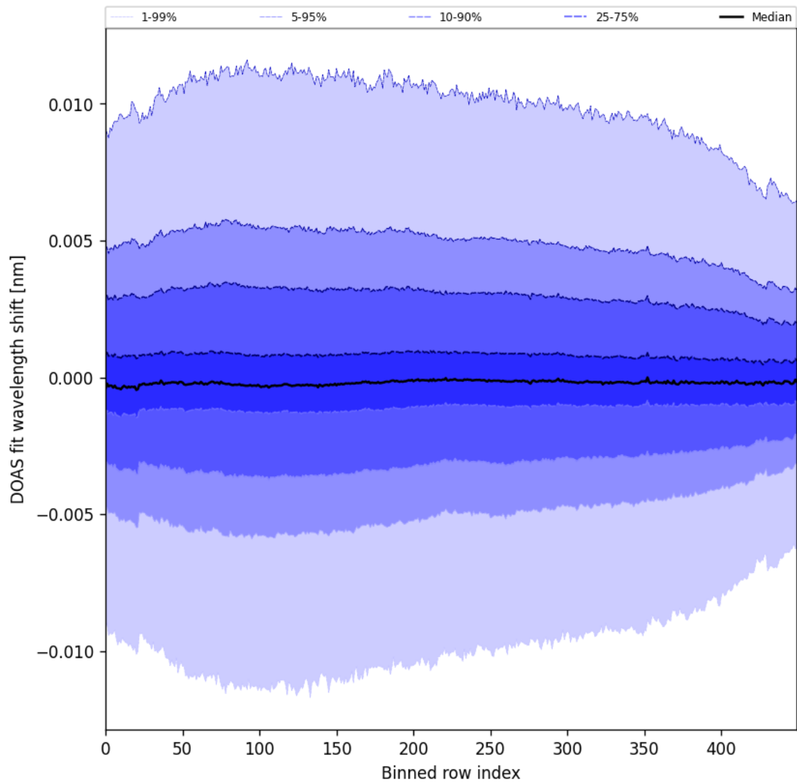
Figure 58: Along track statistics of “DOAS fit wavelength shift” for 2024-11-09 to 2024-11-11
