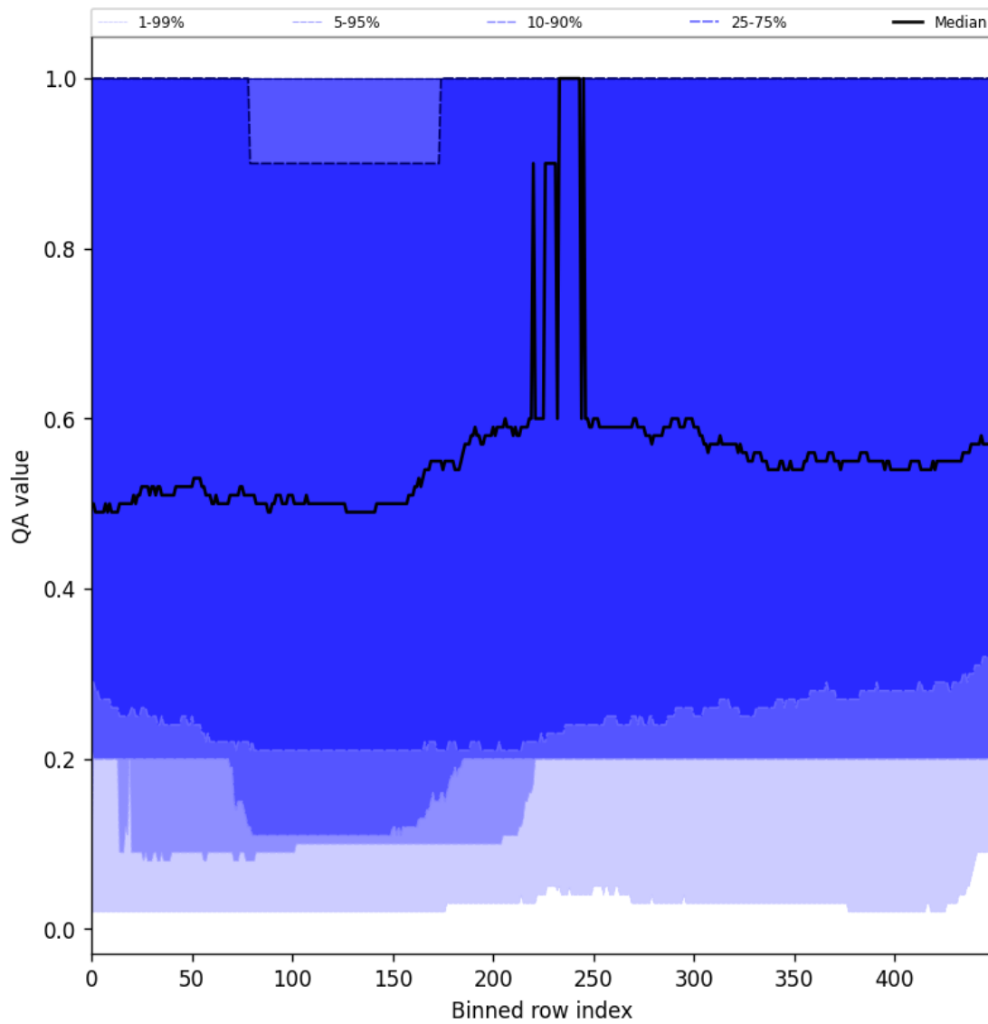
Figure 48: Along track statistics of “QA value” for 2024-11-09 to 2024-11-11
