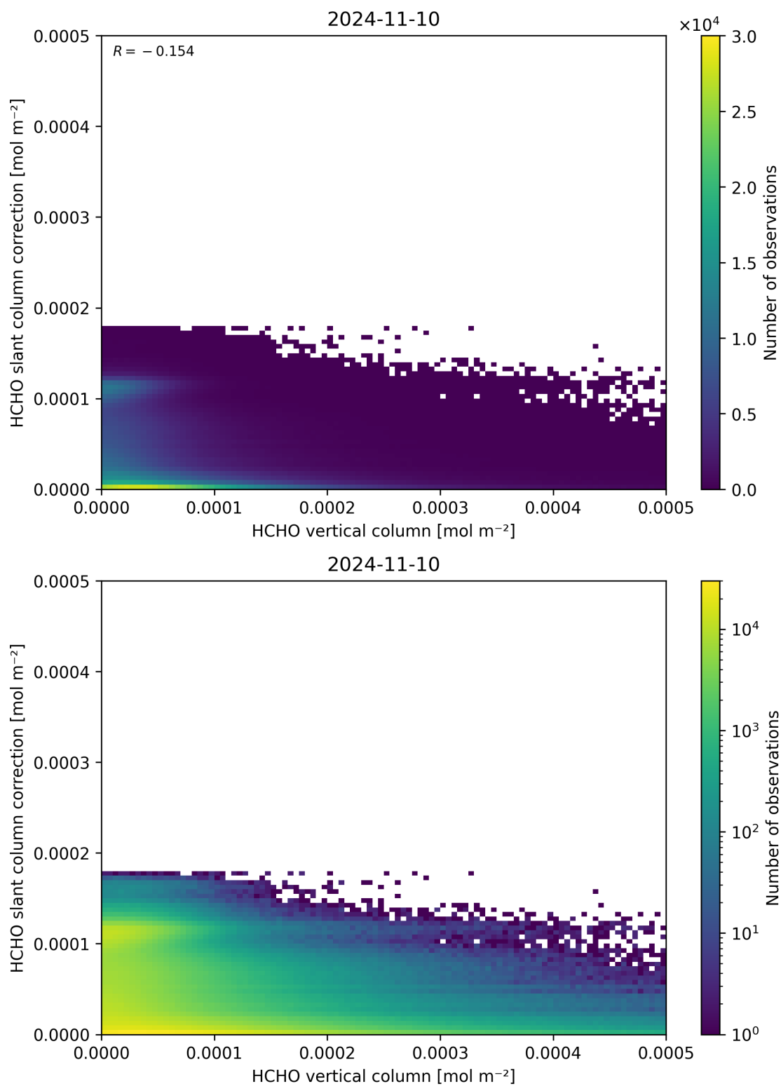
Figure 128: Scatter density plot of “HCHO vertical column” against “HCHO slant column correction” for 2024-11-09 to 2024-11-11.
