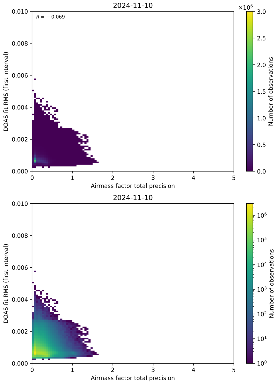
Figure 105: Scatter density plot of “Airmass factor total precision” against “DOAS fit RMS (first interval)” for 2024-11-09 to 2024-11-11.
