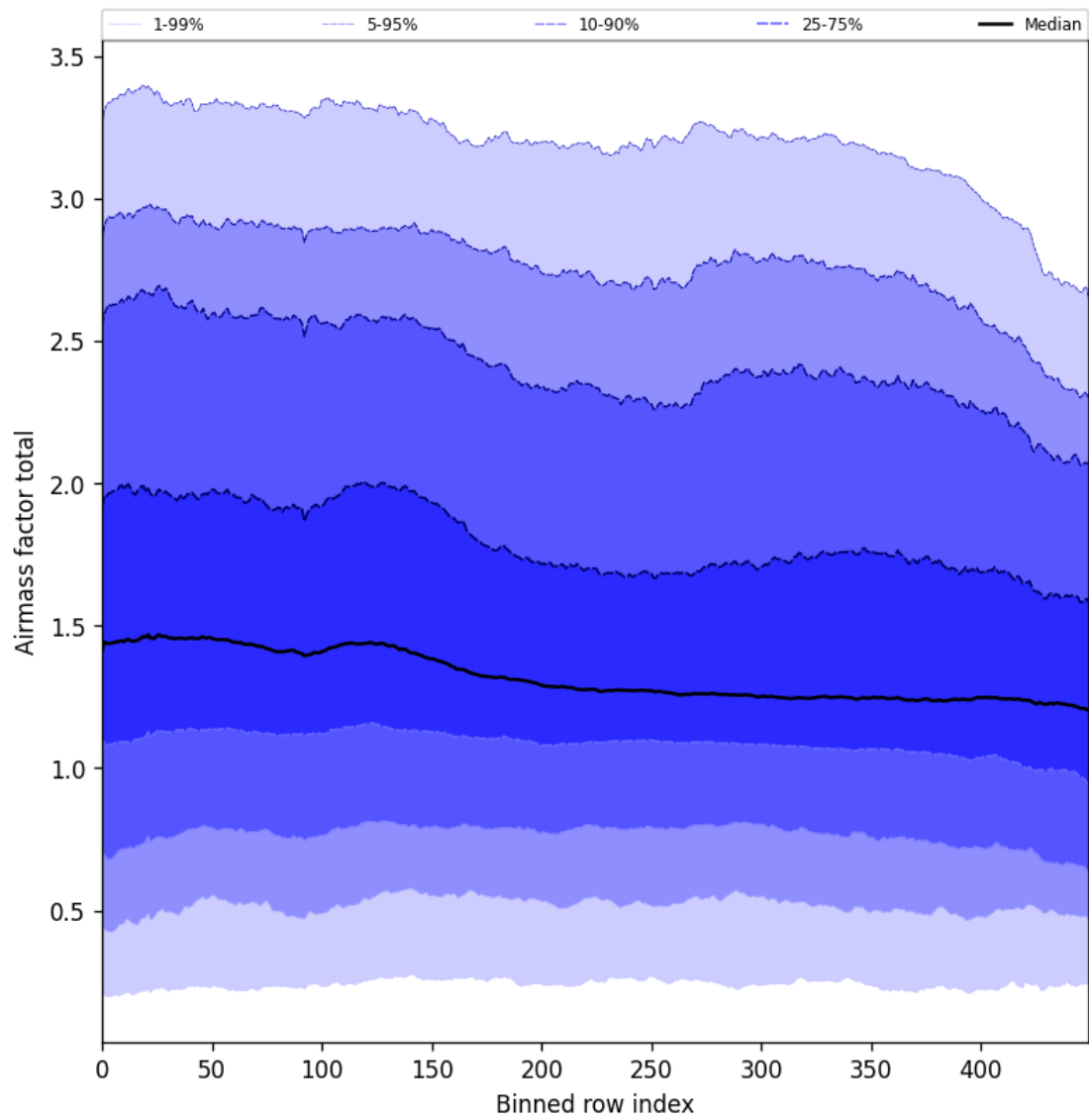
Figure 54: Along track statistics of “Airmass factor total” for 2024-11-09 to 2024-11-11
