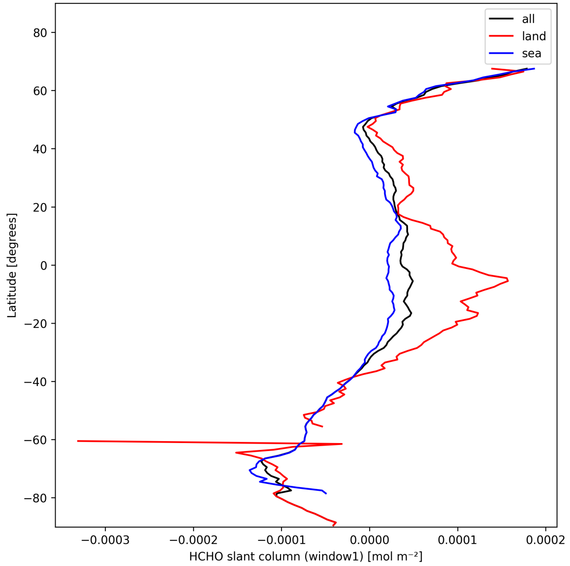
Figure 24: Zonal average of “HCHO slant column (window1)” for 2024-11-09 to 2024-11-11.
