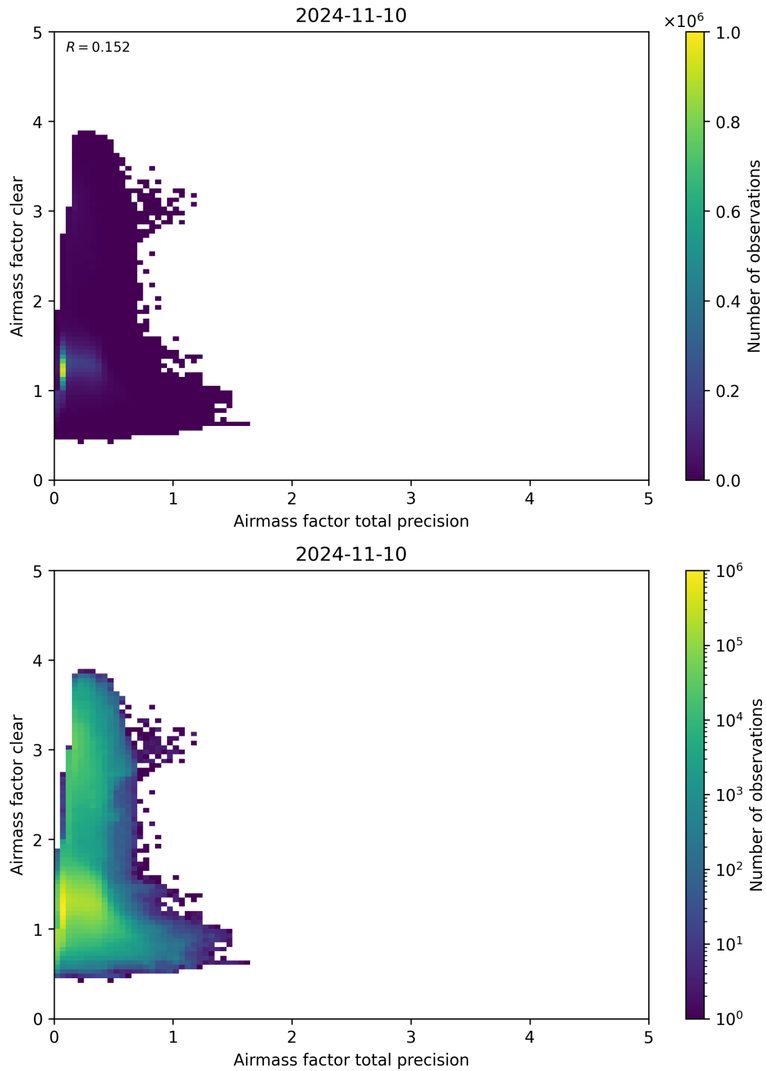
Figure 108: Scatter density plot of “Airmass factor total precision” against “Airmass factor clear” for 2024-11-09 to 2024-11-11.
