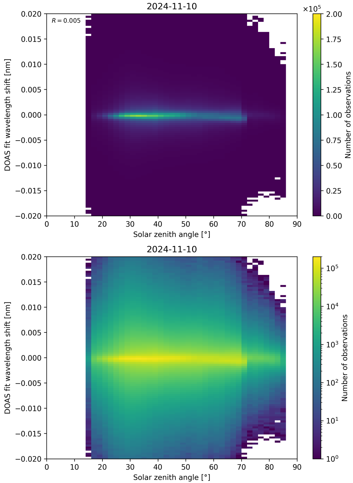
Figure 168: Scatter density plot of “Solar zenith angle” against “DOAS fit wavelength shift” for 2024-11-09 to 2024-11-11.
