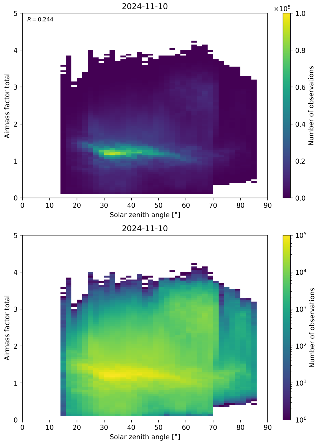
Figure 175: Scatter density plot of “Solar zenith angle” against “Airmass factor total” for 2024-11-09 to 2024-11-11.
