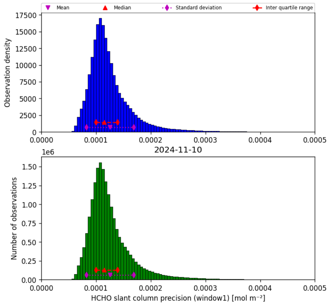
Figure 39: Histogram of “HCHO slant column precision (window1)” for 2024-11-09 to 2024-11-11
