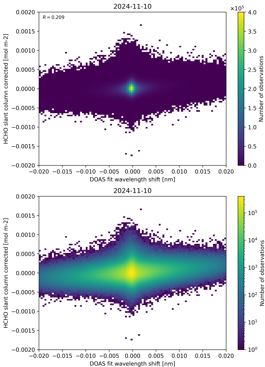
Figure 66: Scatter density plot of “DOAS fit wavelength shift” against “HCHO slant column corrected” for 2024-11-09 to 2024-11-11.
