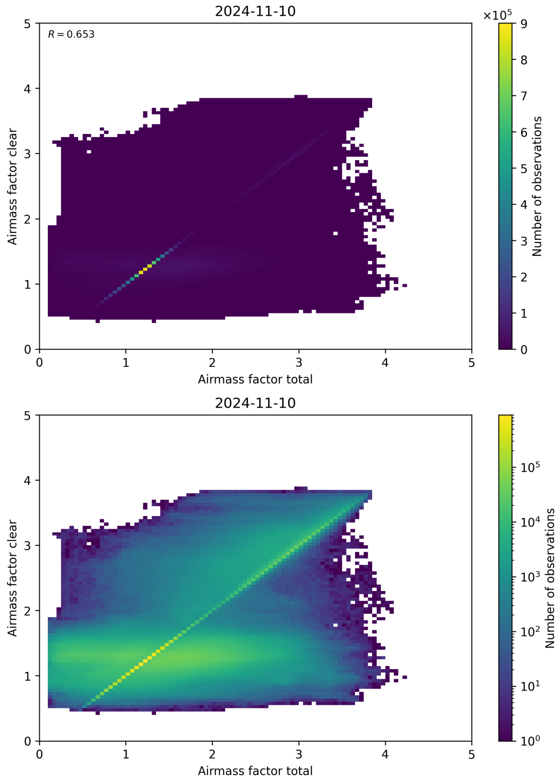
Figure 100: Scatter density plot of “Airmass factor total” against “Airmass factor clear” for 2024-11-09 to 2024-11-11.
