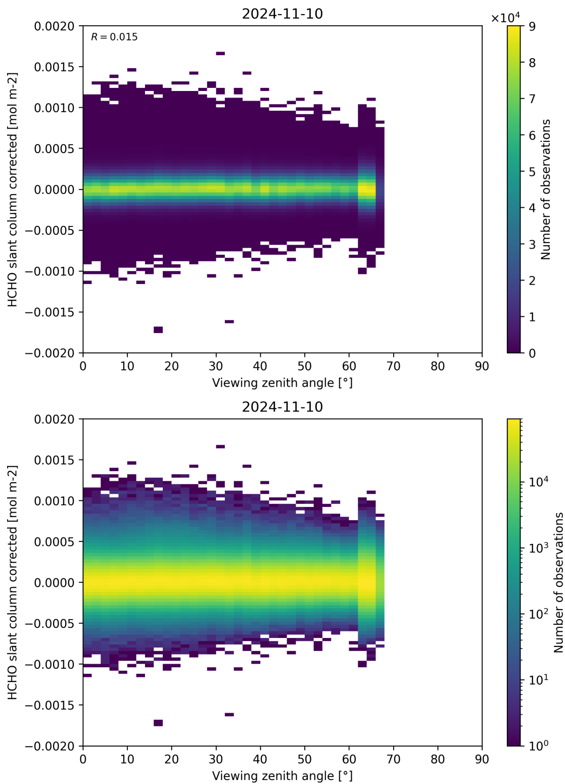
Figure 186: Scatter density plot of “Viewing zenith angle” against “HCHO slant column corrected” for 2024-11-09 to 2024-11-11.
