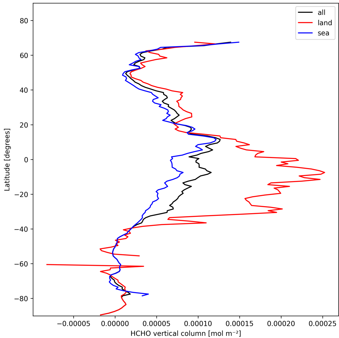
Figure 21: Zonal average of “HCHO vertical column” for 2024-11-09 to 2024-11-11.
