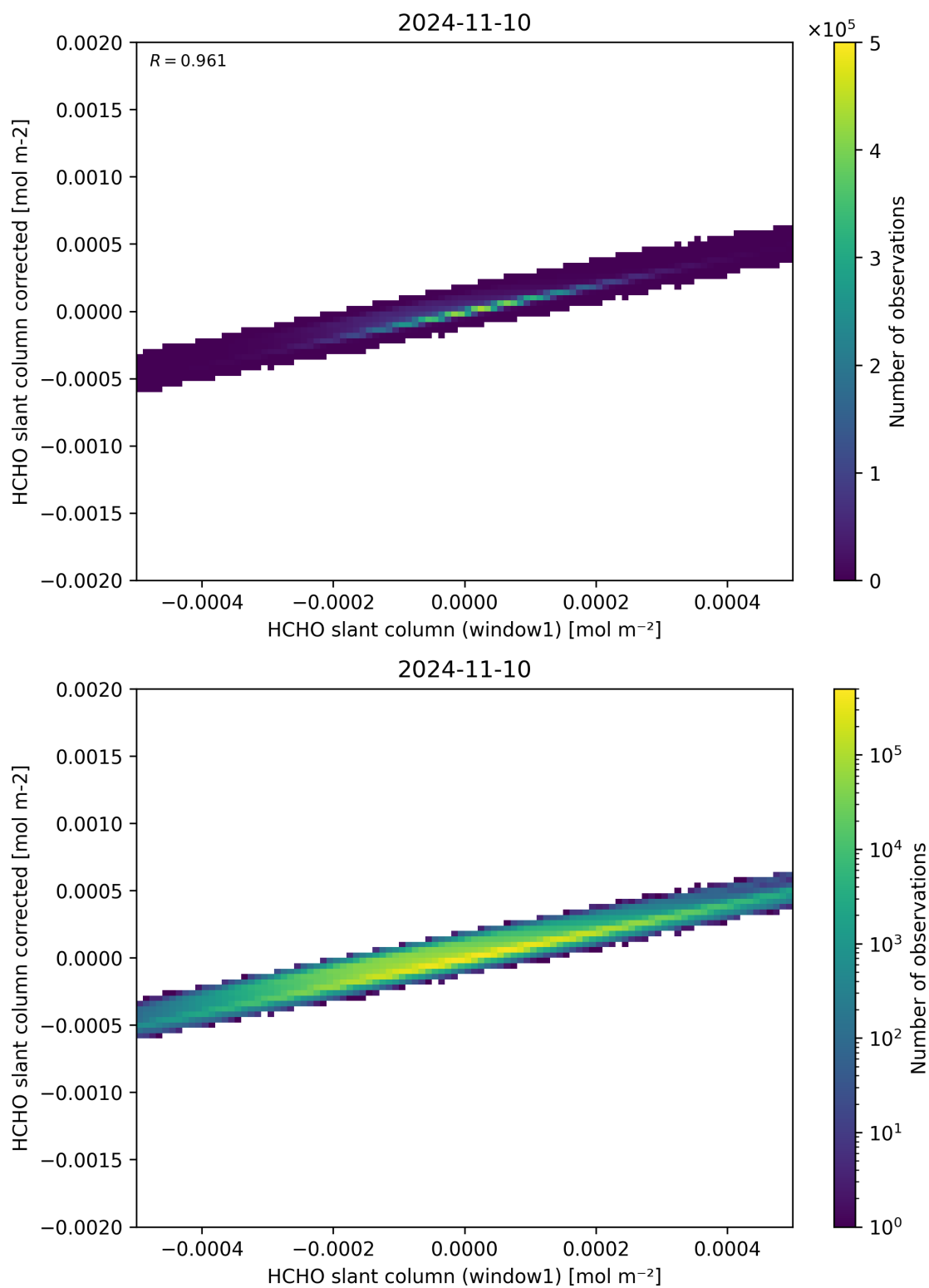
Figure 82: Scatter density plot of “HCHO slant column (window1)” against “HCHO slant column corrected” for 2024-11-09 to 2024-11-11.
