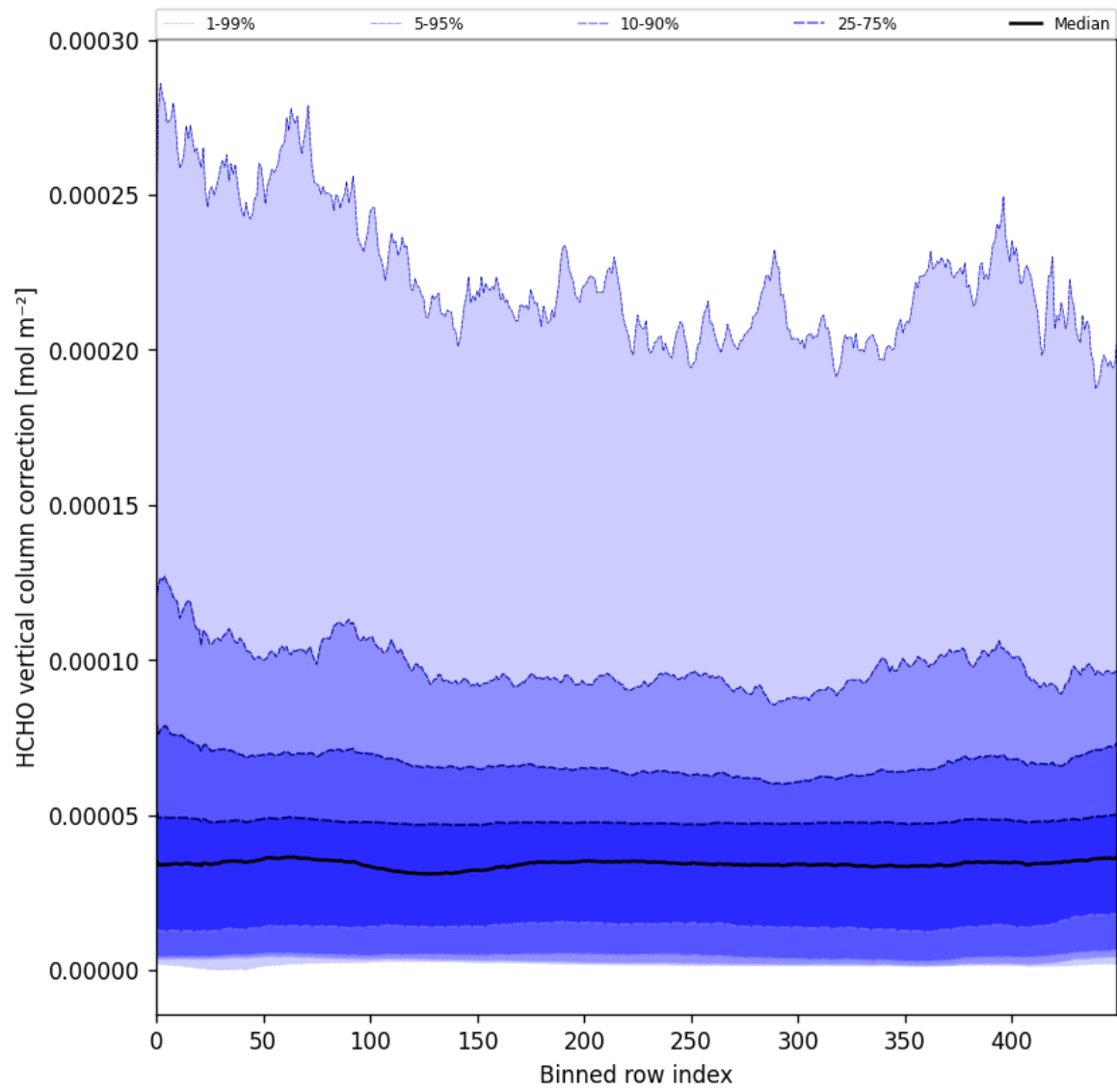
Figure 51: Along track statistics of “HCHO vertical column correction” for 2024-11-09 to 2024-11-11
