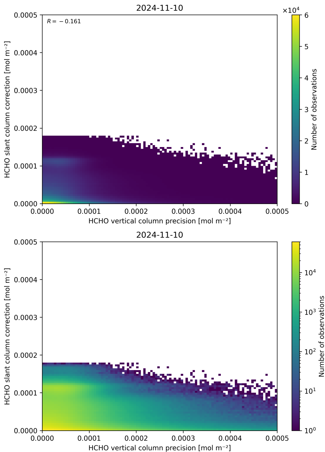
Figure 141: Scatter density plot of “HCHO vertical column precision” against “HCHO slant column correction” for 2024-11-09 to 2024-11-11.
