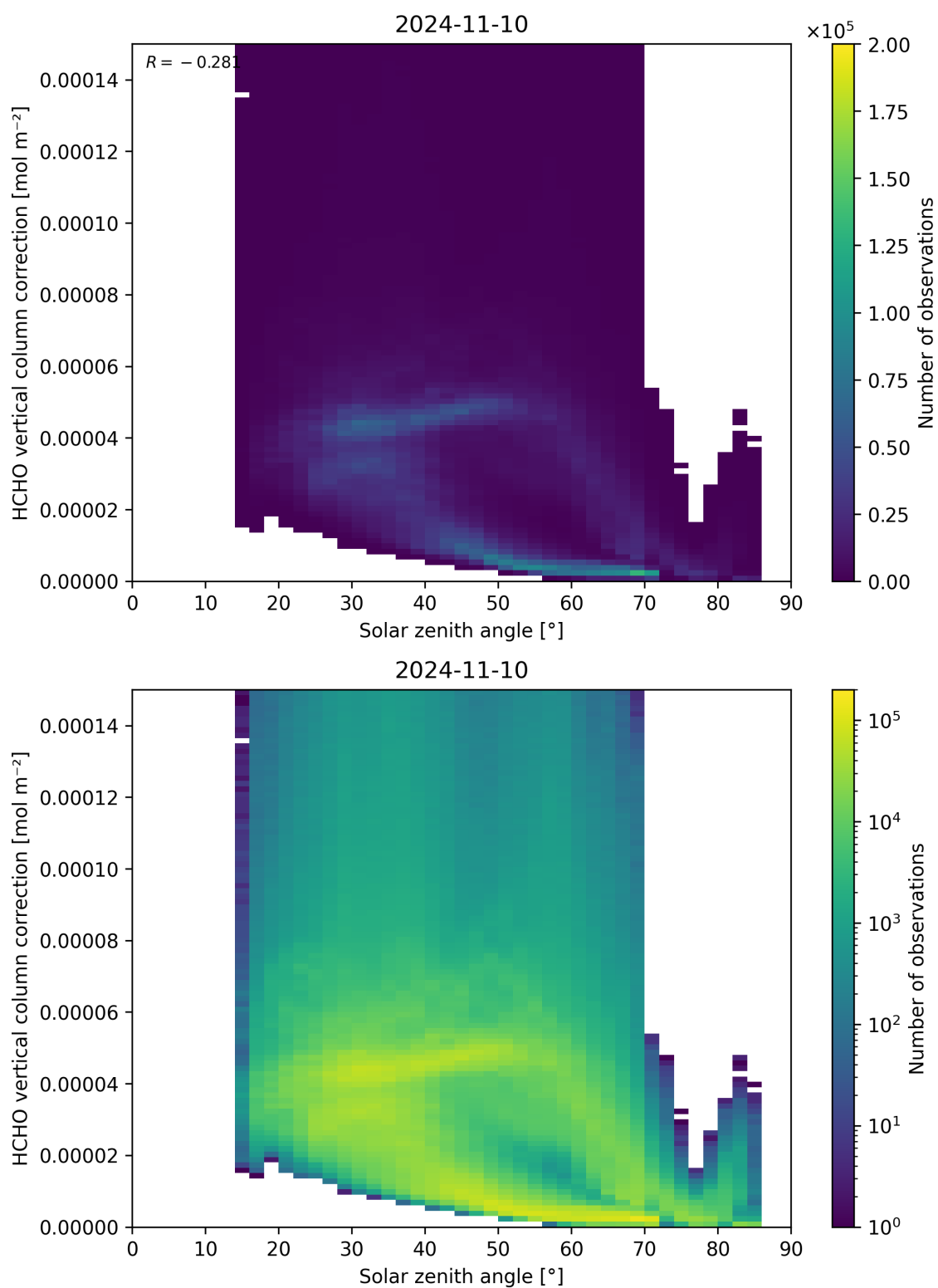
Figure 178: Scatter density plot of “Solar zenith angle” against “HCHO vertical column correction” for 2024-11-09 to 2024-11-11.
