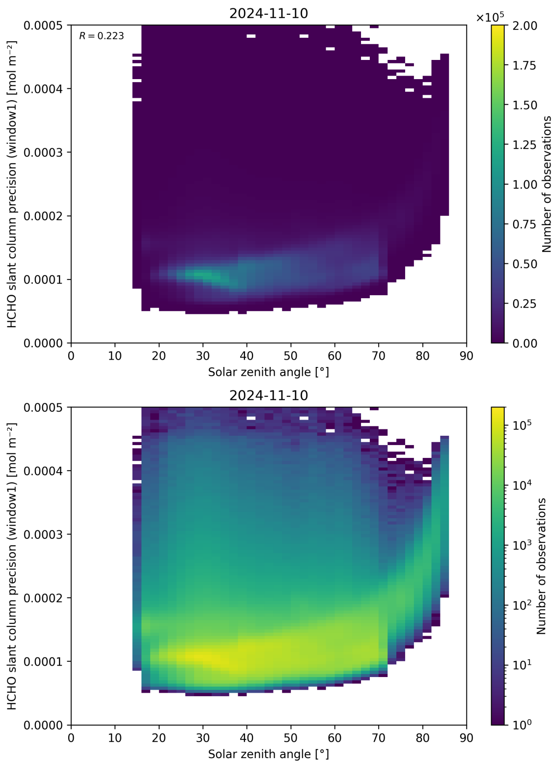
Figure 174: Scatter density plot of “Solar zenith angle” against “HCHO slant column precision (window1)” for 2024-11-09 to 2024-11-11.
