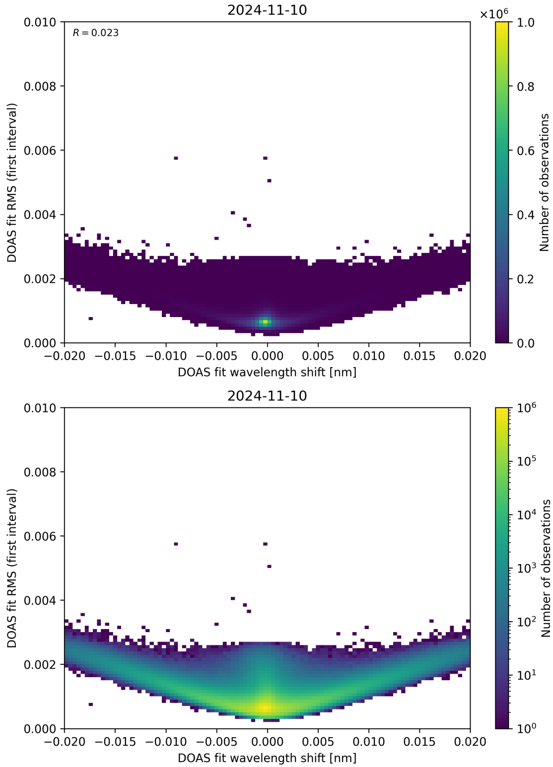
Figure 64: Scatter density plot of “DOAS fit wavelength shift” against “DOAS fit RMS (first interval)” for 2024-11-09 to 2024-11-11.
