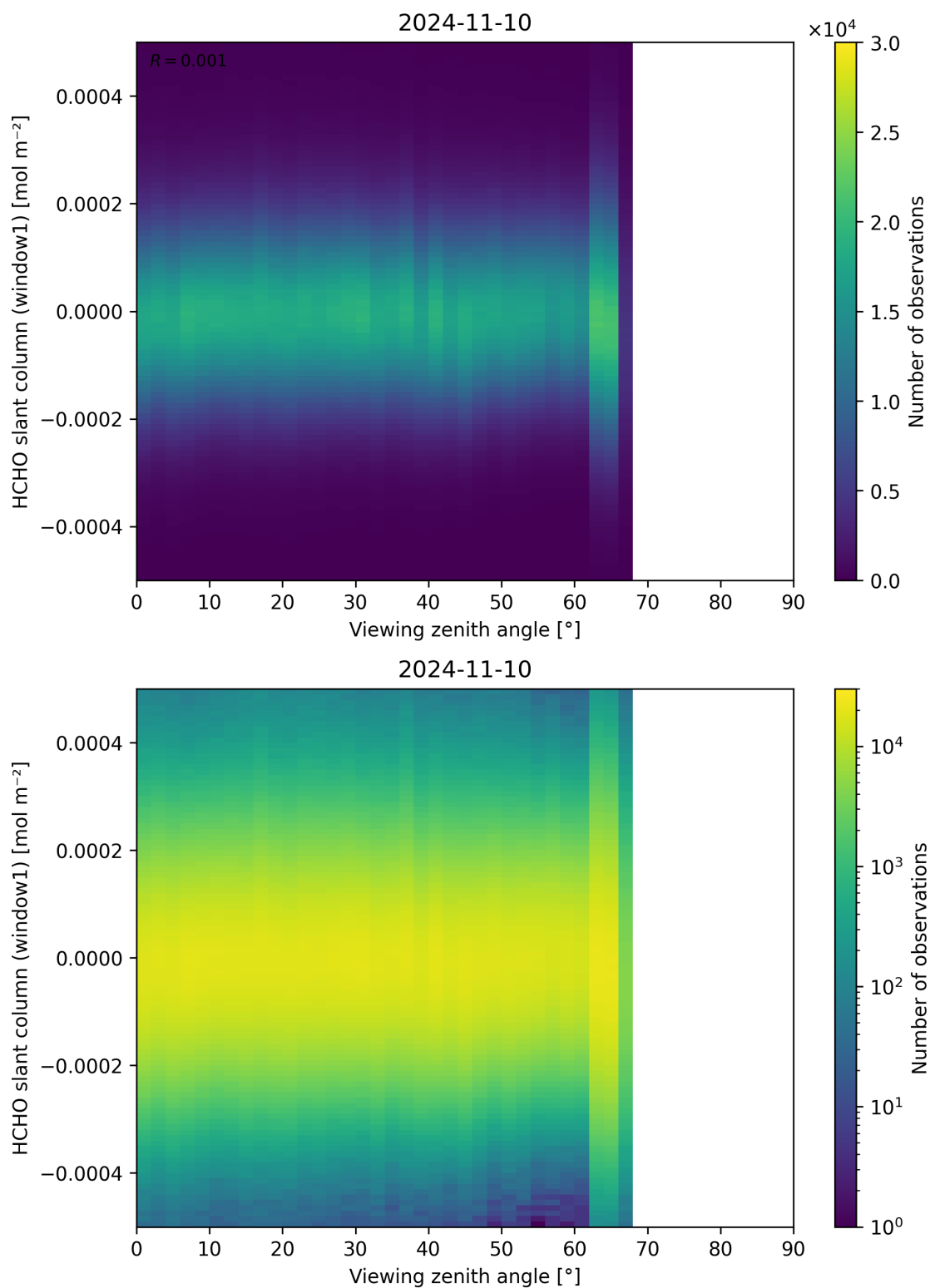
Figure 188: Scatter density plot of “Viewing zenith angle” against “HCHO slant column (window1)” for 2024-11-09 to 2024-11-11.
