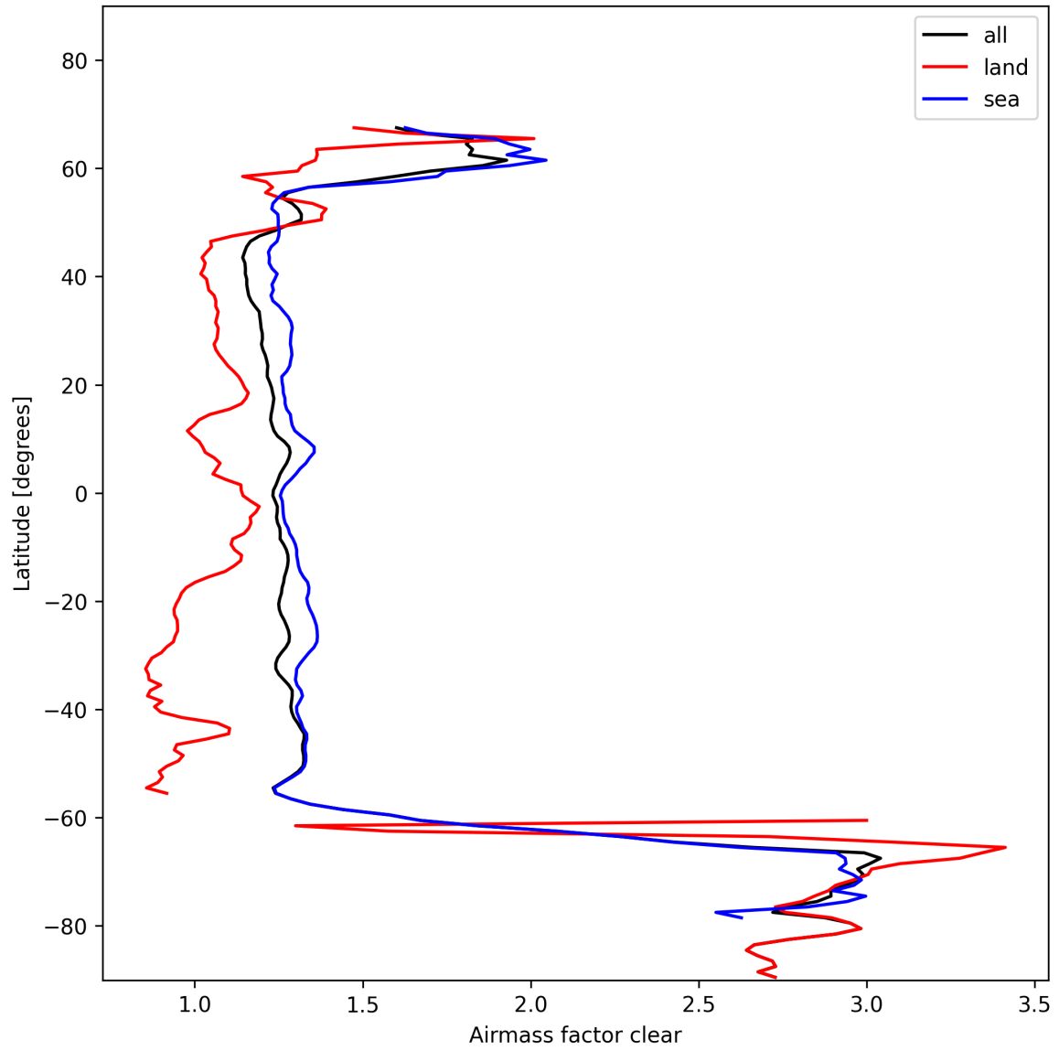
Figure 28: Zonal average of “Airmass factor clear” for 2024-11-09 to 2024-11-11.
