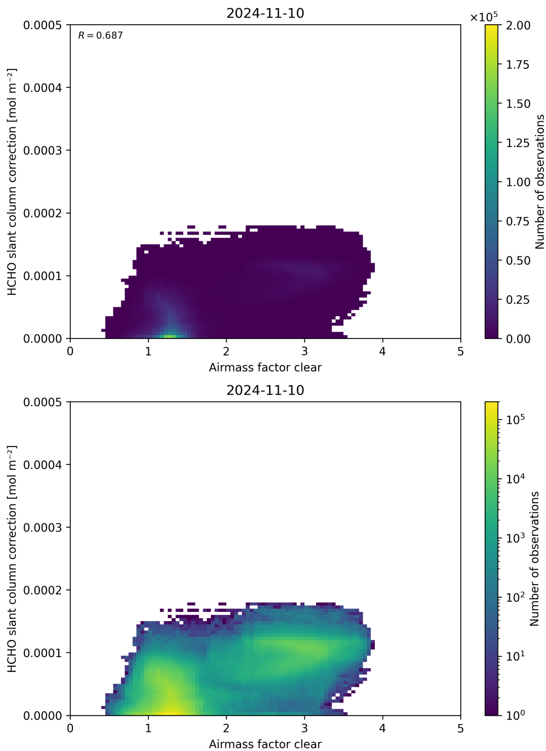
Figure 75: Scatter density plot of “Airmass factor clear” against “HCHO slant column correction” for 2024-11-09 to 2024-11-11.
