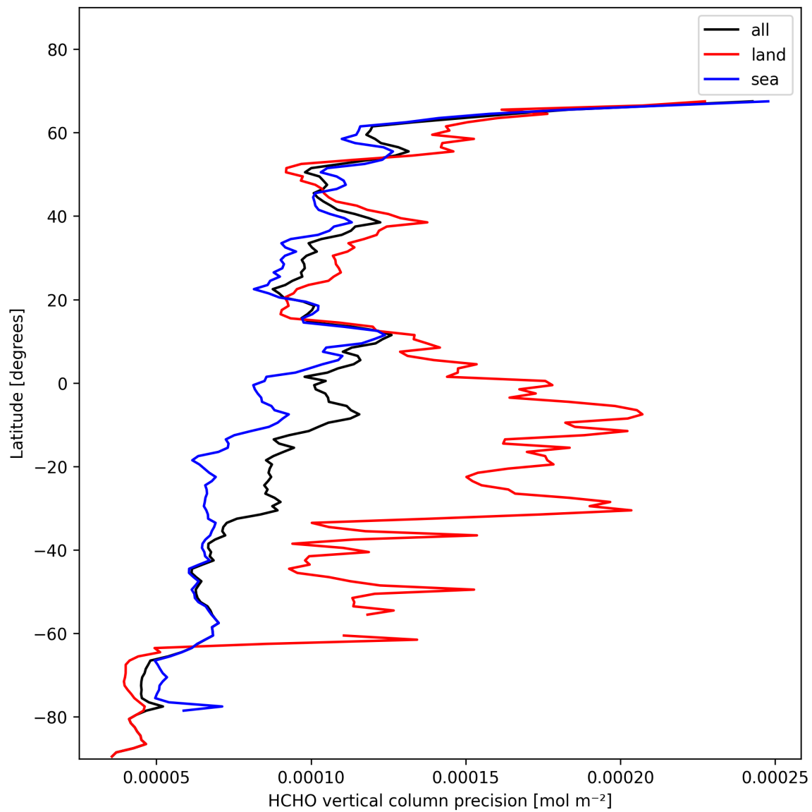
Figure 22: Zonal average of “HCHO vertical column precision” for 2024-11-09 to 2024-11-11.
