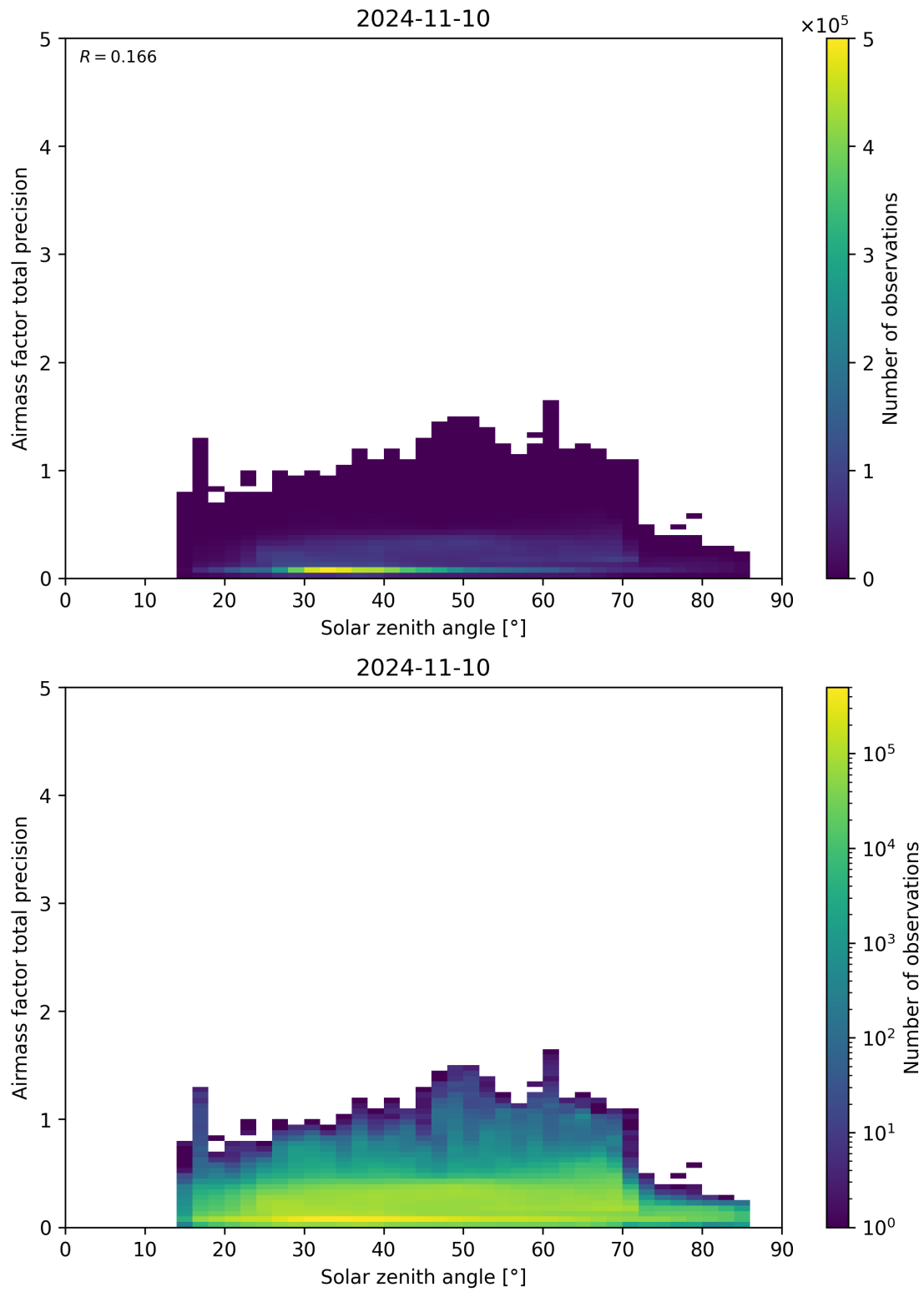
Figure 176: Scatter density plot of “Solar zenith angle” against “Airmass factor total precision” for 2024-11-09 to 2024-11-11.
