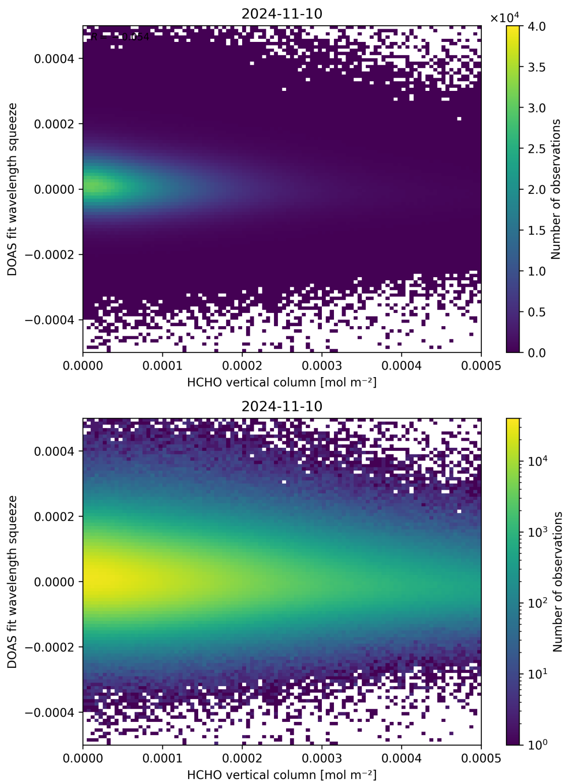
Figure 125: Scatter density plot of “HCHO vertical column” against “DOAS fit wavelength squeeze” for 2024-11-09 to 2024-11-11.
