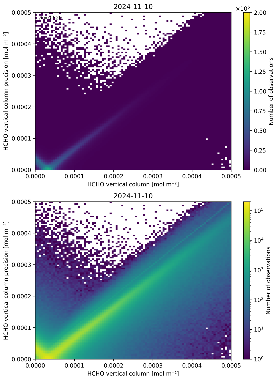
Figure 134: Scatter density plot of “HCHO vertical column” against “HCHO vertical column precision” for 2024-11-09 to 2024-11-11.
