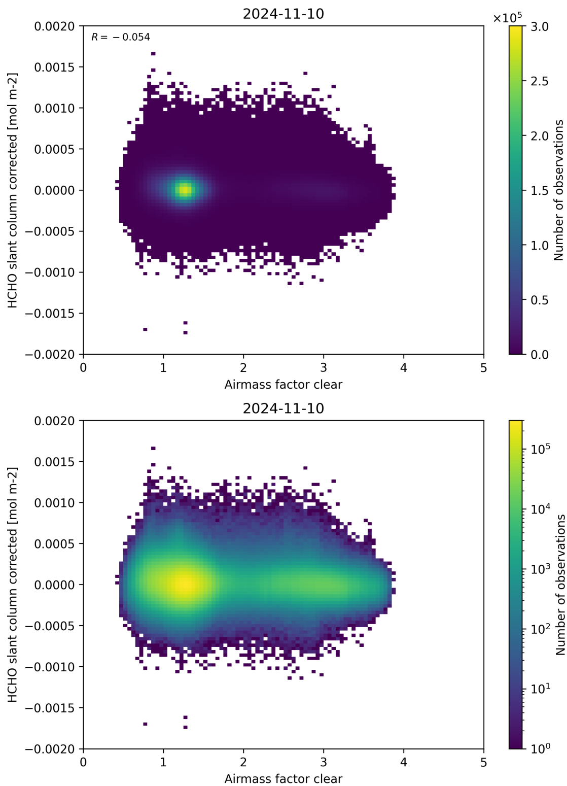
Figure 74: Scatter density plot of “Airmass factor clear” against “HCHO slant column corrected” for 2024-11-09 to 2024-11-11.
