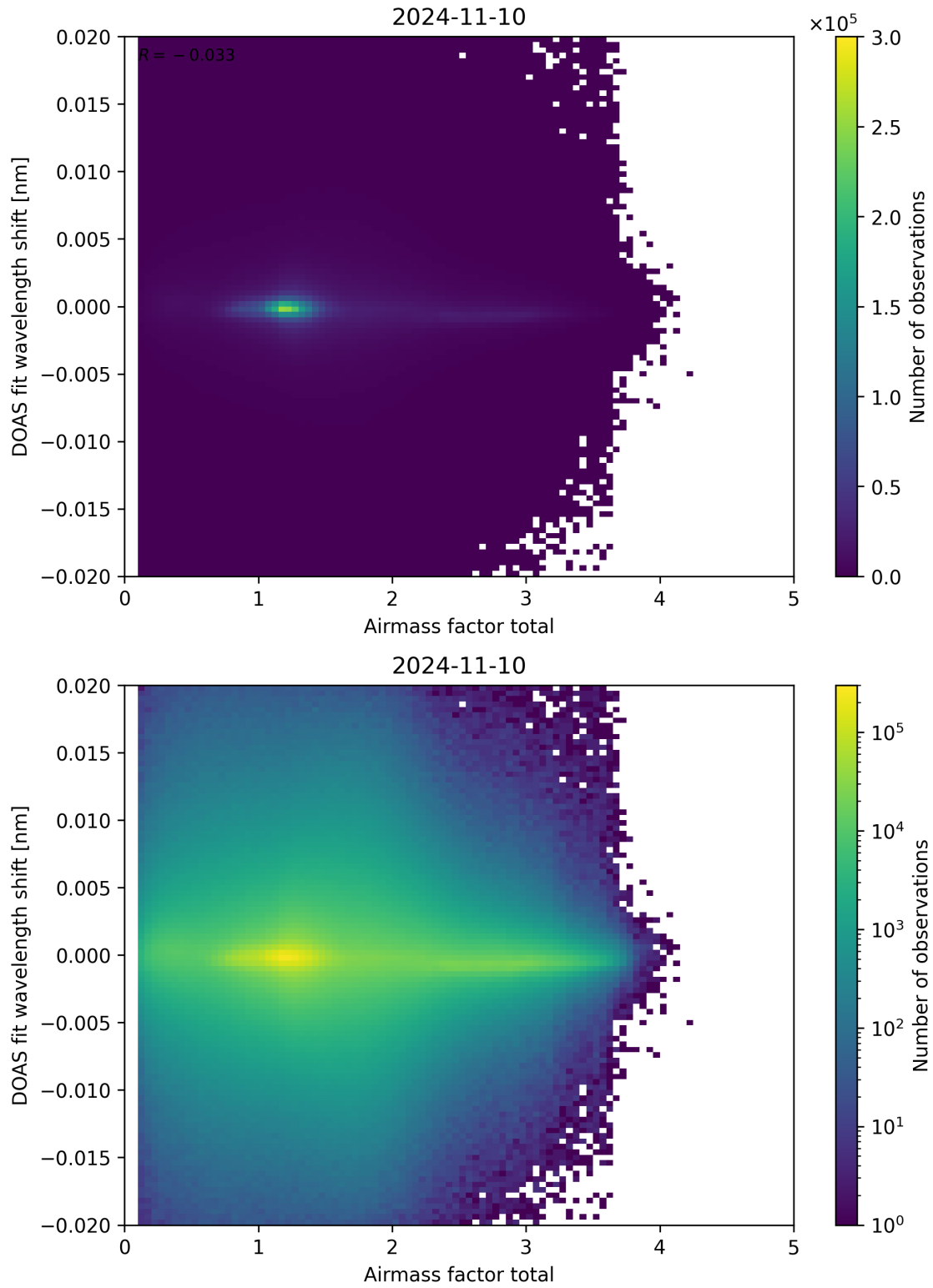
Figure 98: Scatter density plot of “Airmass factor total” against “DOAS fit wavelength shift” for 2024-11-09 to 2024-11-11.
