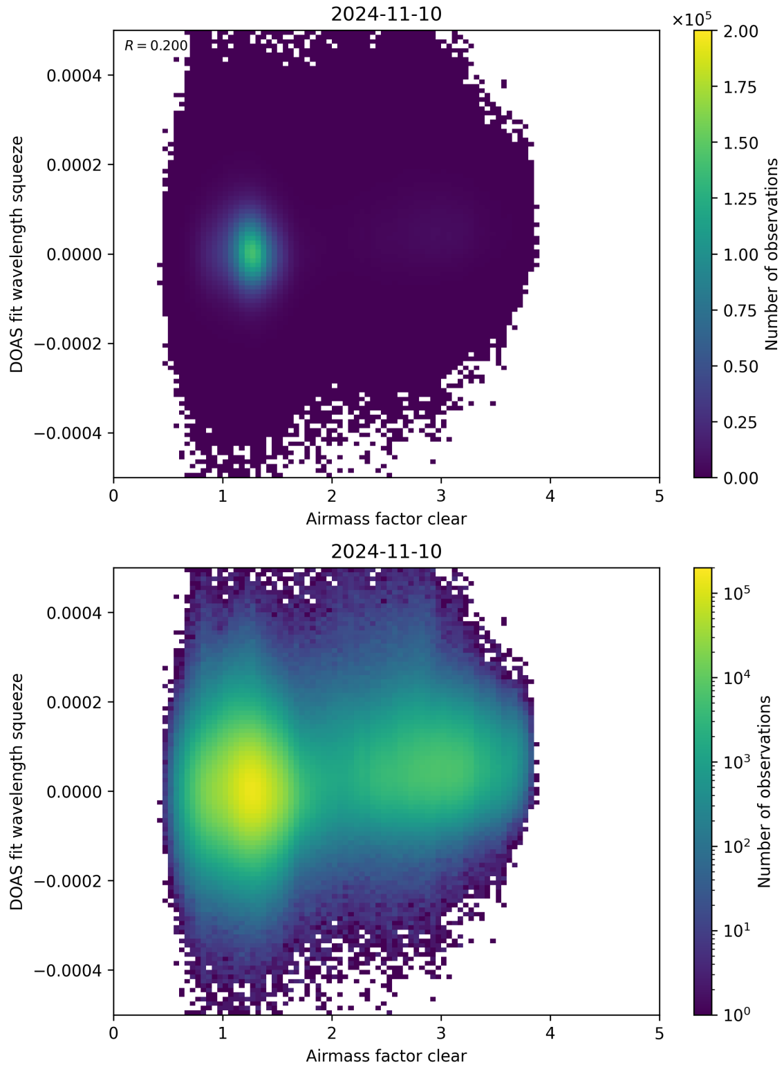
Figure 73: Scatter density plot of “Airmass factor clear” against “DOAS fit wavelength squeeze” for 2024-11-09 to 2024-11-11.
