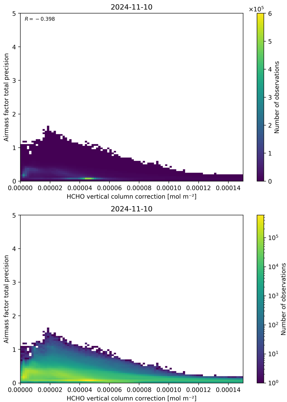
Figure 121: Scatter density plot of “HCHO vertical column correction” against “Airmass factor total precision” for 2024-11-09 to 2024-11-11.
