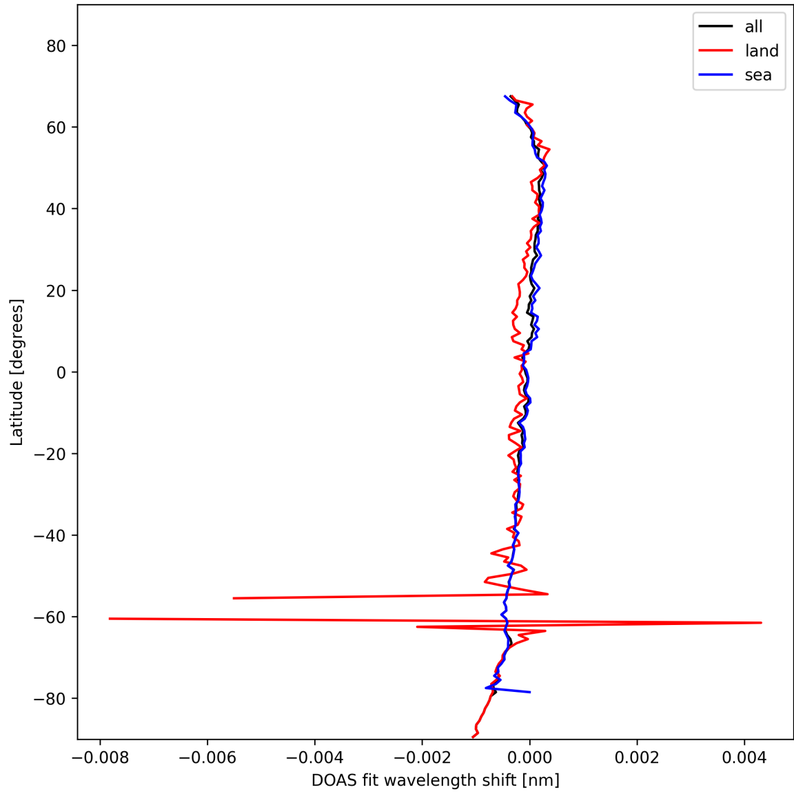
Figure 30: Zonal average of “DOAS fit wavelength shift” for 2024-11-09 to 2024-11-11.
