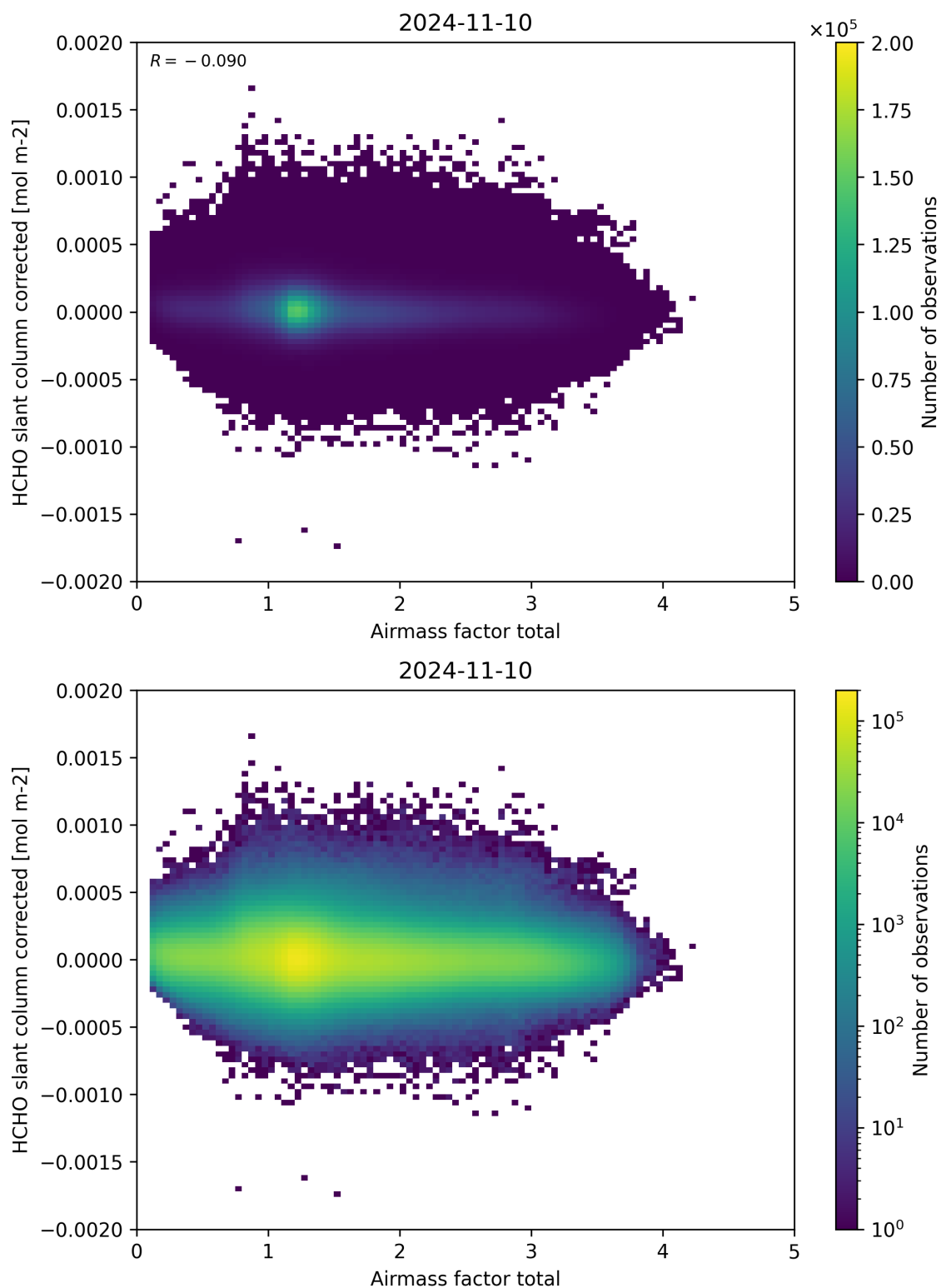
Figure 101: Scatter density plot of “Airmass factor total” against “HCHO slant column corrected” for 2024-11-09 to 2024-11-11.
