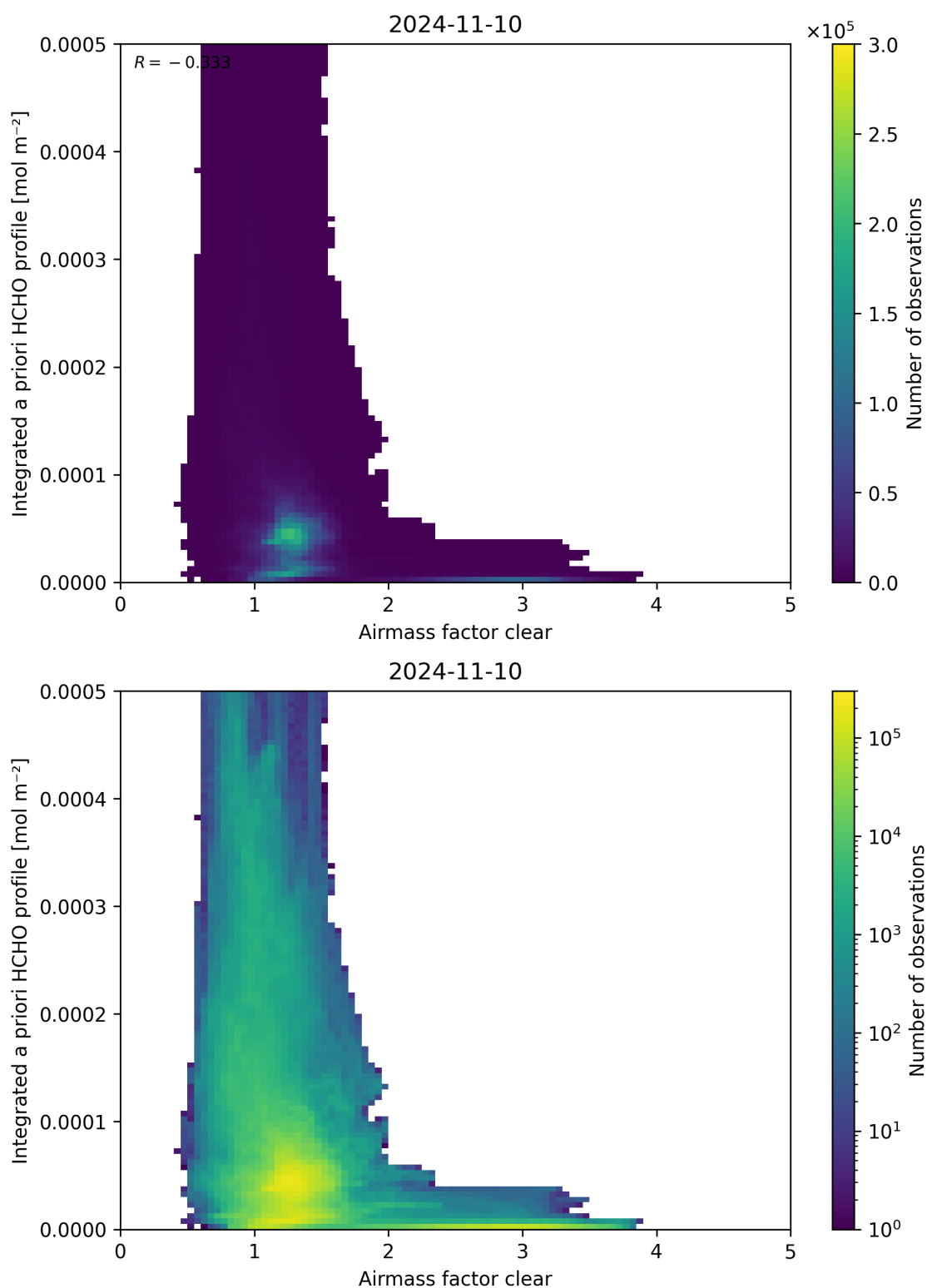
Figure 76: Scatter density plot of “Airmass factor clear” against “Integrated a priori HCHO profile” for 2024-11-09 to 2024-11-11.
