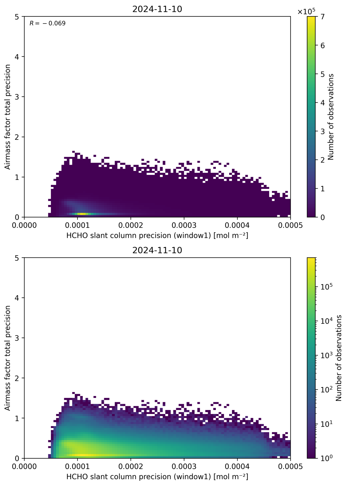
Figure 95: Scatter density plot of “HCHO slant column precision (window1)” against “Airmass factor total precision” for 2024-11-09 to 2024-11-11.
