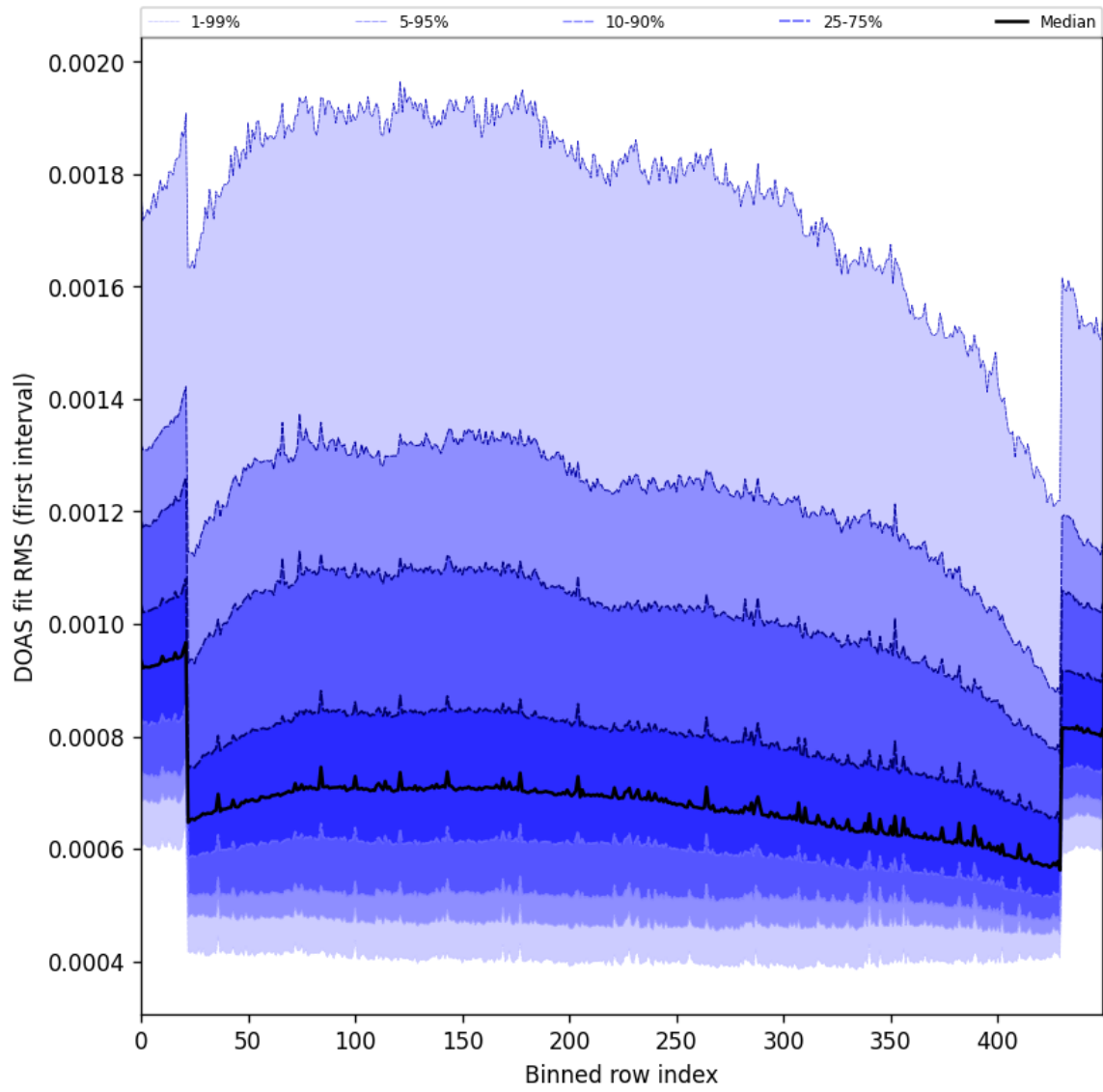
Figure 60: Along track statistics of “DOAS fit RMS (first interval)” for 2024-11-09 to 2024-11-11
