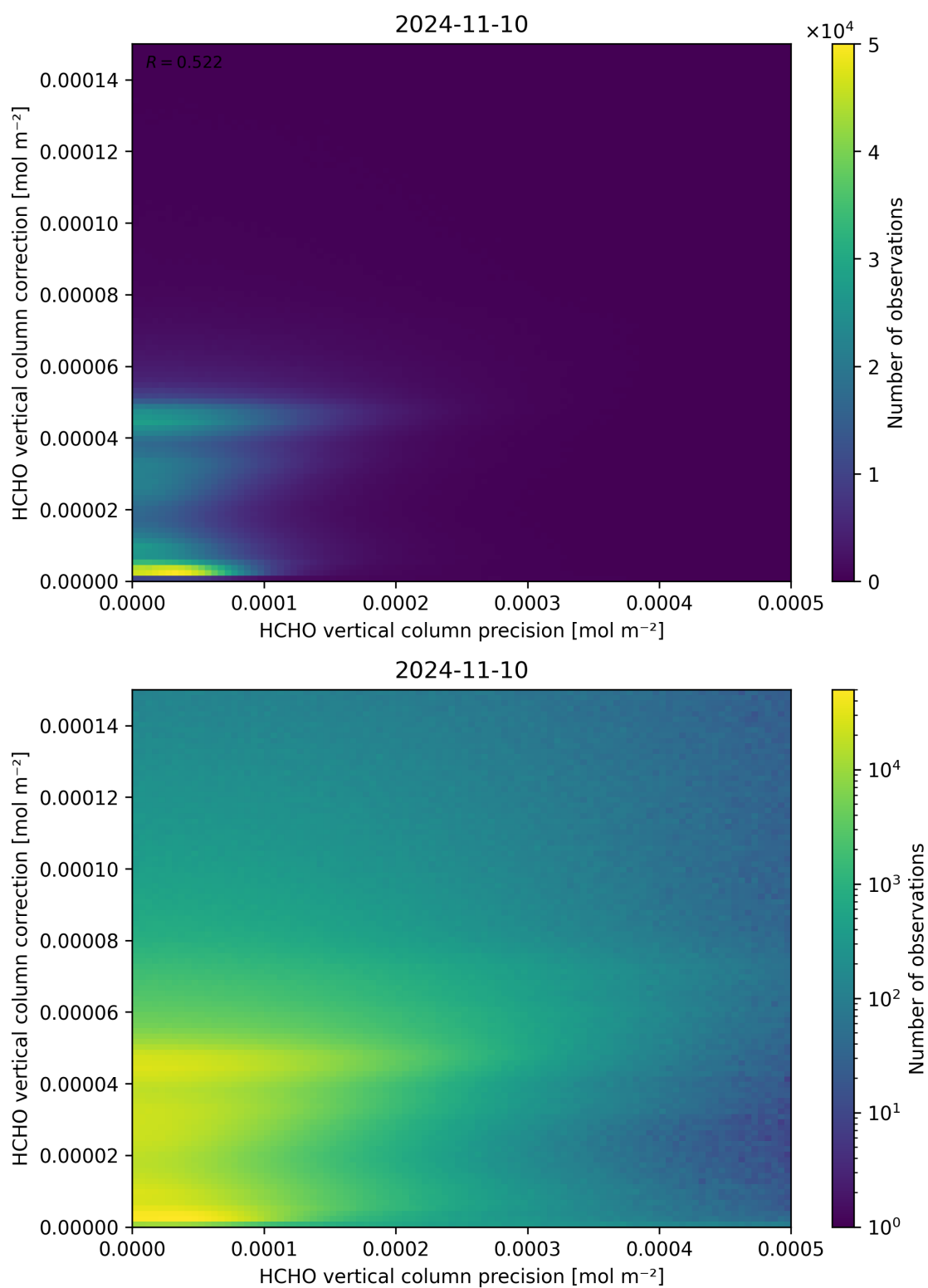
Figure 146: Scatter density plot of “HCHO vertical column precision” against “HCHO vertical column correction” for 2024-11-09 to 2024-11-11.
