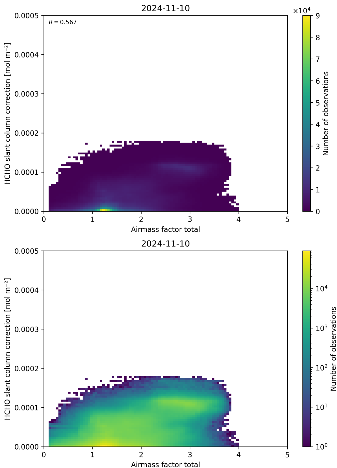
Figure 102: Scatter density plot of “Airmass factor total” against “HCHO slant column correction” for 2024-11-09 to 2024-11-11.
