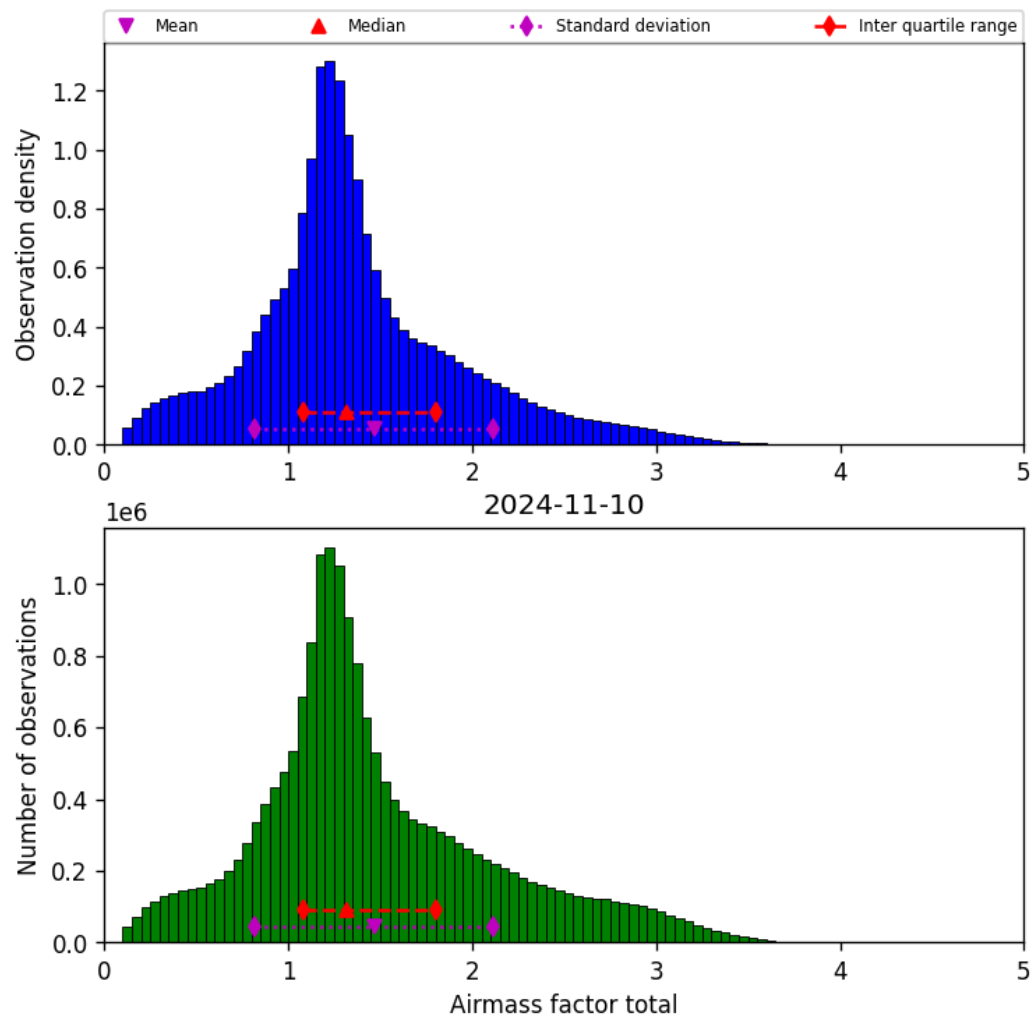
Figure 40: Histogram of “Airmass factor total” for 2024-11-09 to 2024-11-11
