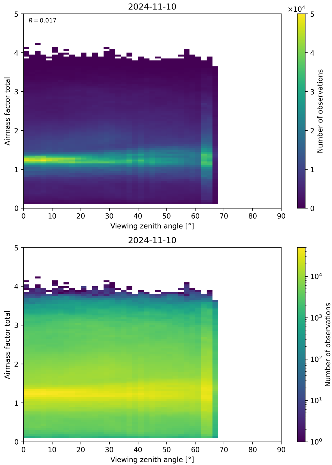
Figure 190: Scatter density plot of “Viewing zenith angle” against “Airmass factor total” for 2024-11-09 to 2024-11-11.
