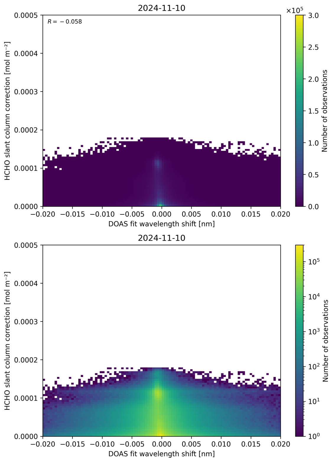
Figure 67: Scatter density plot of “DOAS fit wavelength shift” against “HCHO slant column correction” for 2024-11-09 to 2024-11-11.
