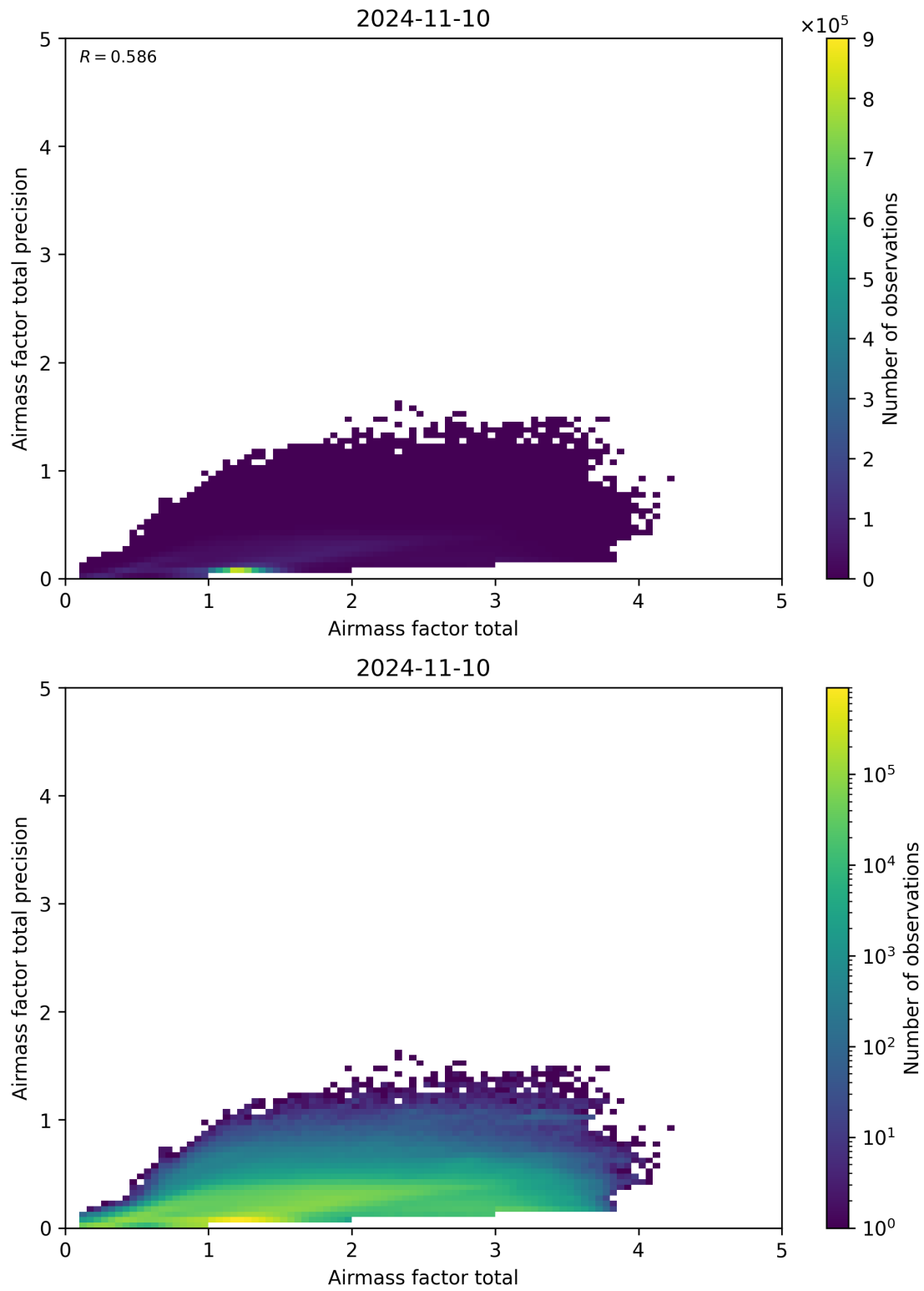
Figure 103: Scatter density plot of “Airmass factor total” against “Airmass factor total precision” for 2024-11-09 to 2024-11-11.
