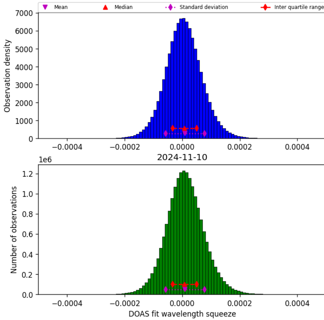
Figure 45: Histogram of “DOAS fit wavelength squeeze” for 2024-11-09 to 2024-11-11
