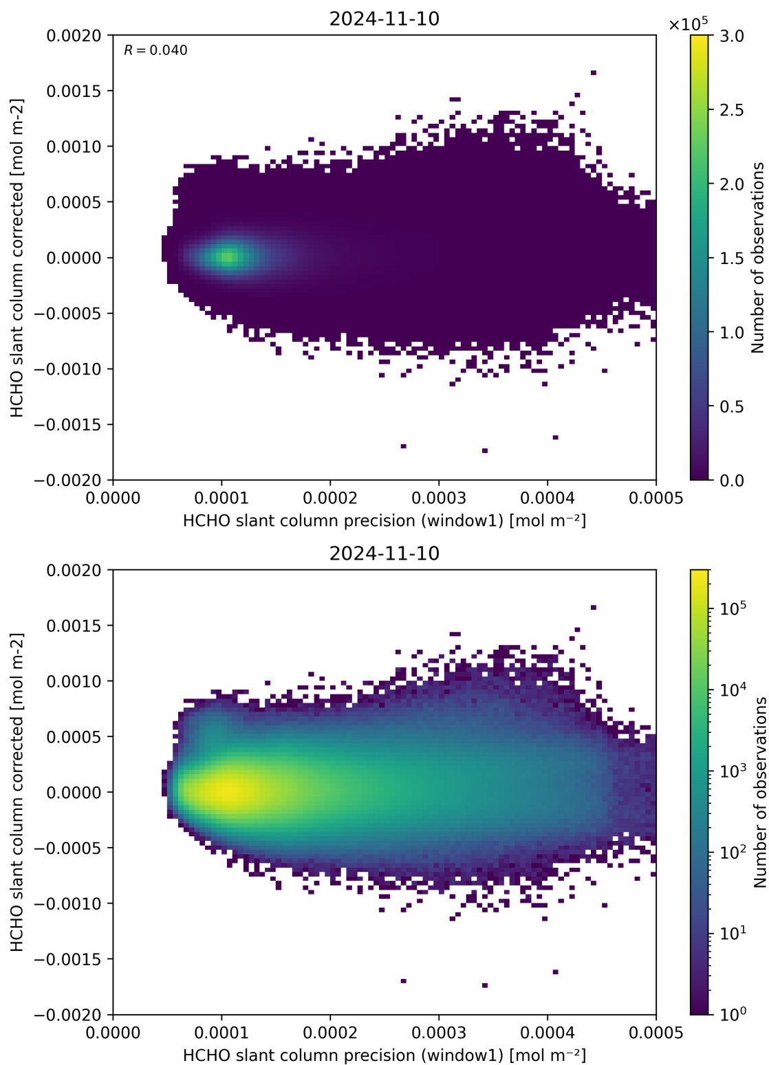
Figure 92: Scatter density plot of “HCHO slant column precision (window1)” against “HCHO slant column corrected” for 2024-11-09 to 2024-11-11.
