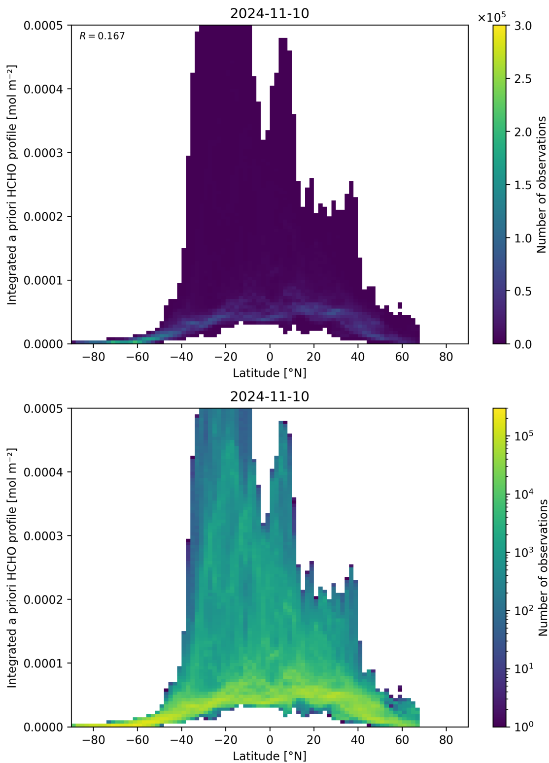
Figure 166: Scatter density plot of “Latitude” against “Integrated a priori HCHO profile” for 2024-11-09 to 2024-11-11.
