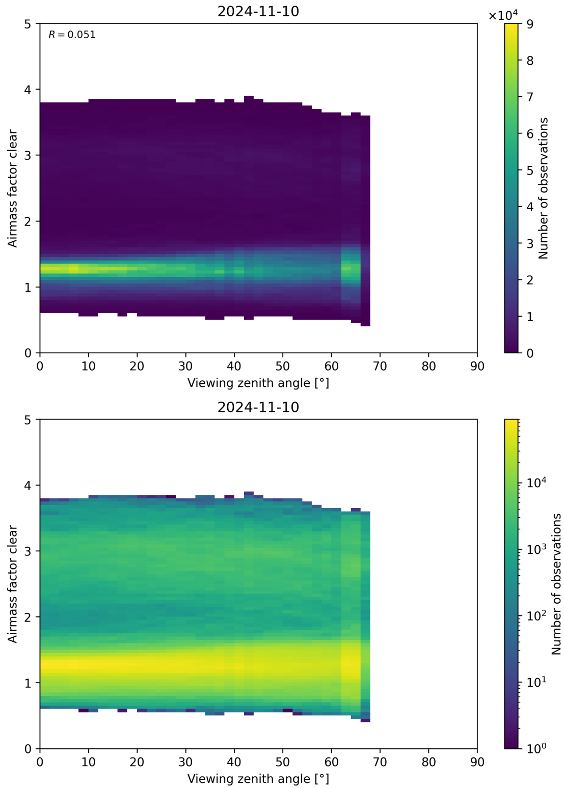
Figure 185: Scatter density plot of “Viewing zenith angle” against “Airmass factor clear” for 2024-11-09 to 2024-11-11.
