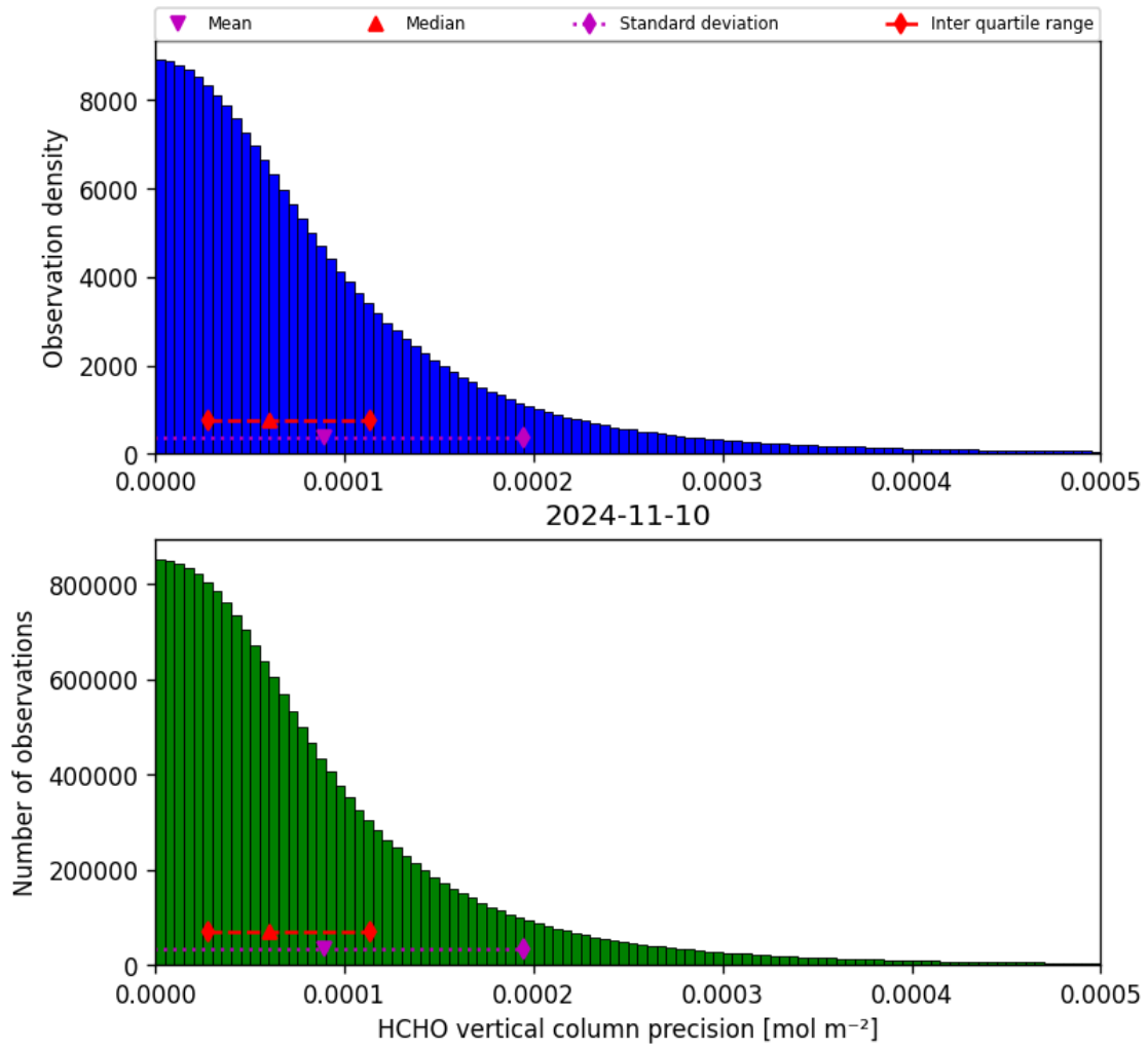
Figure 36: Histogram of “HCHO vertical column precision” for 2024-11-09 to 2024-11-11
