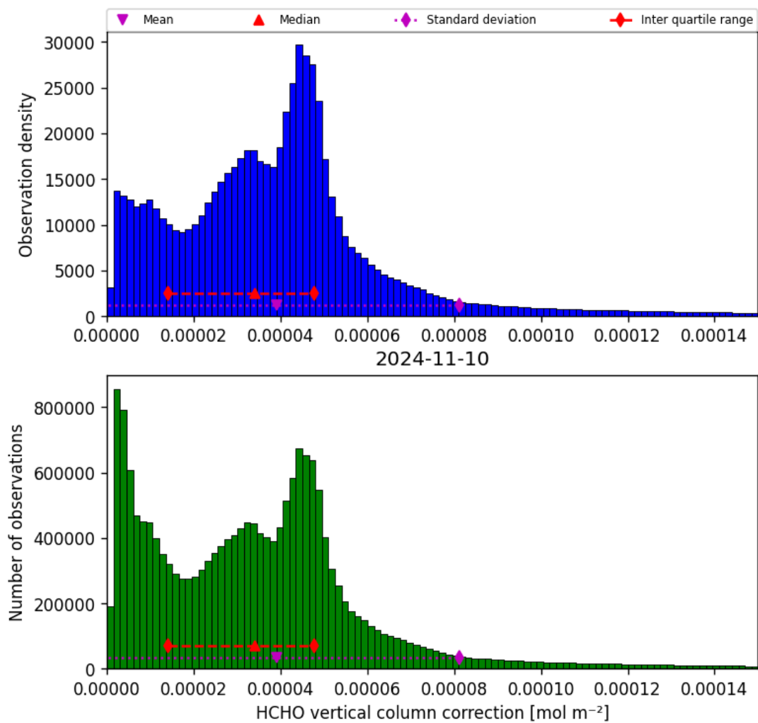
Figure 37: Histogram of “HCHO vertical column correction” for 2024-11-09 to 2024-11-11
