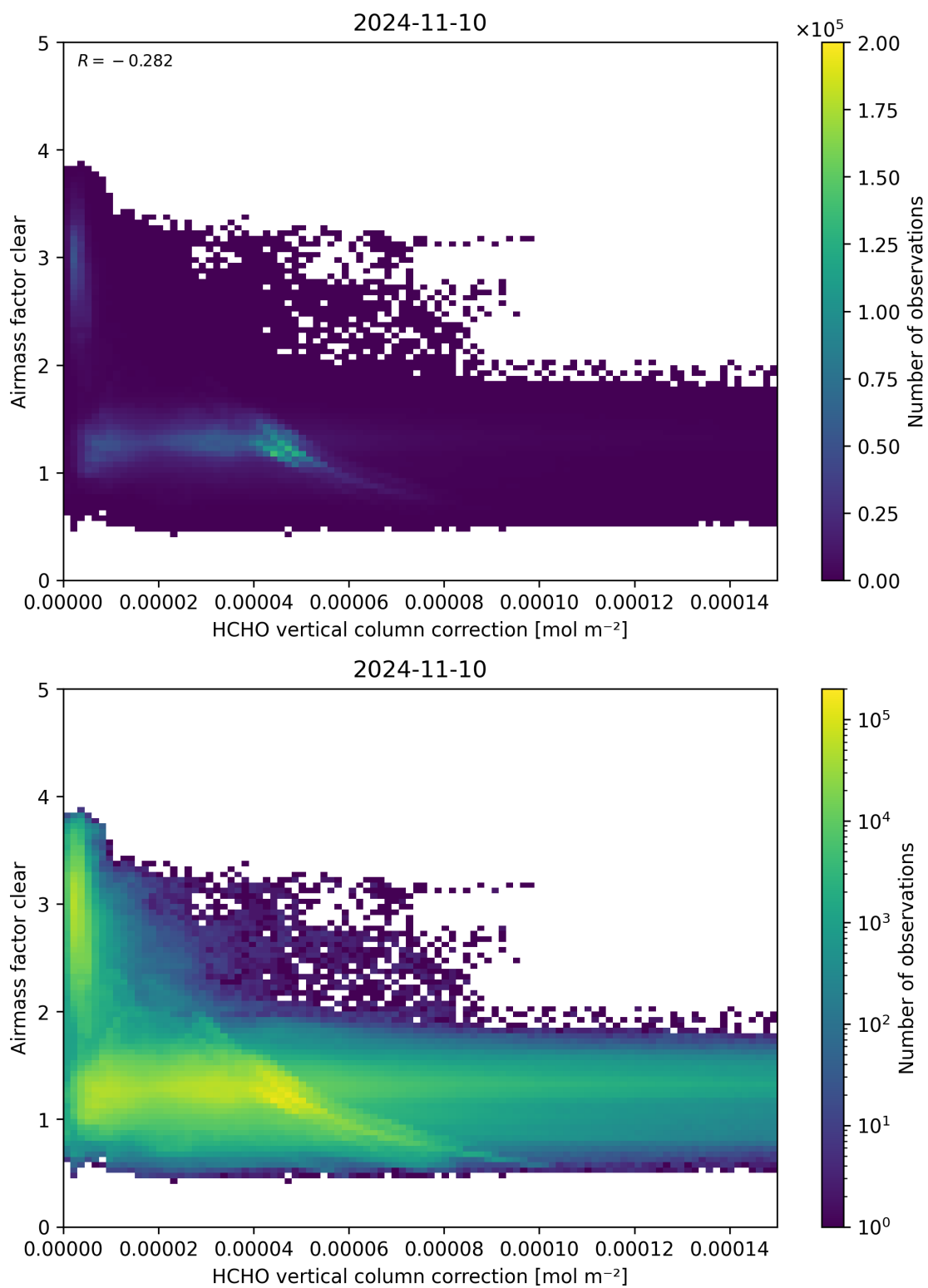
Figure 115: Scatter density plot of “HCHO vertical column correction” against “Airmass factor clear” for 2024-11-09 to 2024-11-11.
