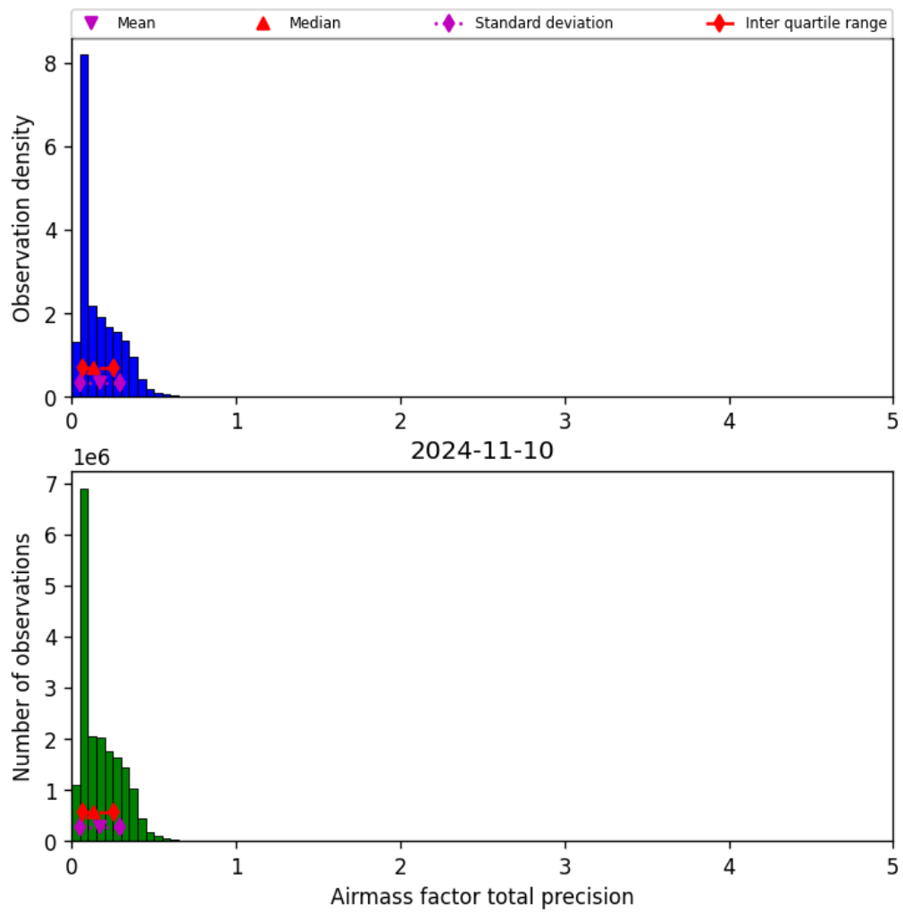
Figure 41: Histogram of “Airmass factor total precision” for 2024-11-09 to 2024-11-11
