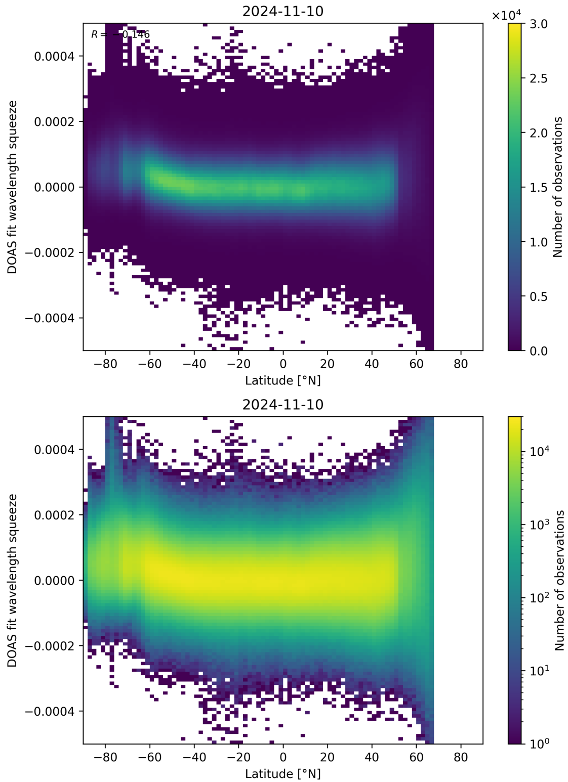
Figure 155: Scatter density plot of “Latitude” against “DOAS fit wavelength squeeze” for 2024-11-09 to 2024-11-11.
