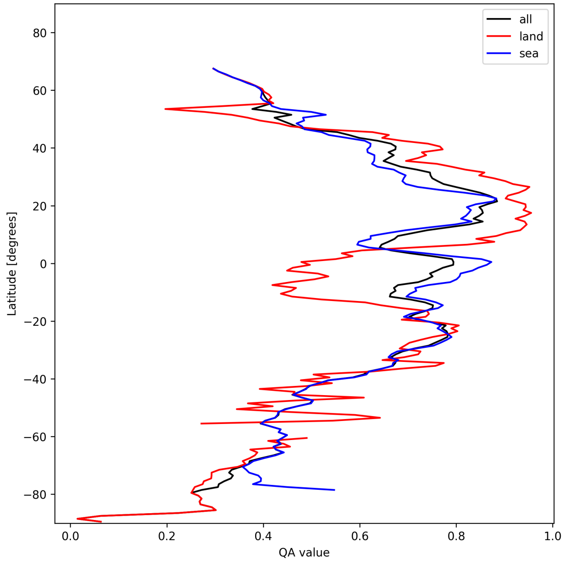
Figure 20: Zonal average of “QA value” for 2024-11-09 to 2024-11-11.
