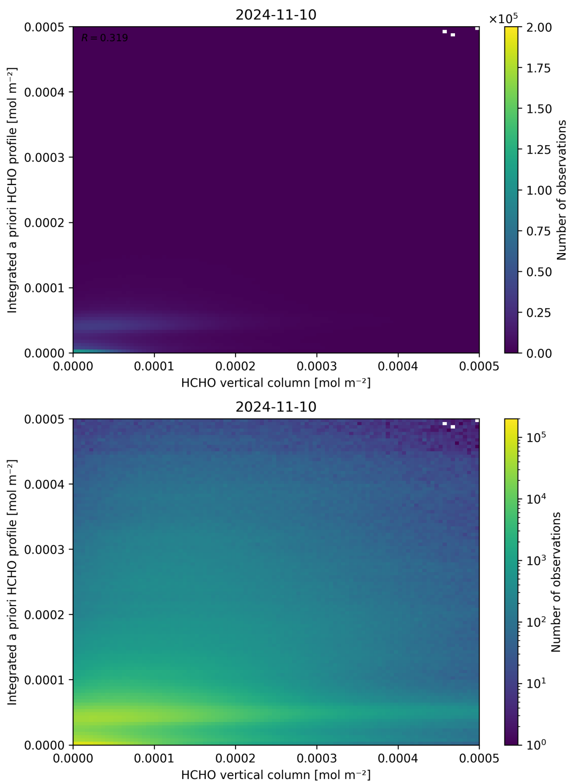
Figure 135: Scatter density plot of “HCHO vertical column” against “Integrated a priori HCHO profile” for 2024-11-09 to 2024-11-11.
