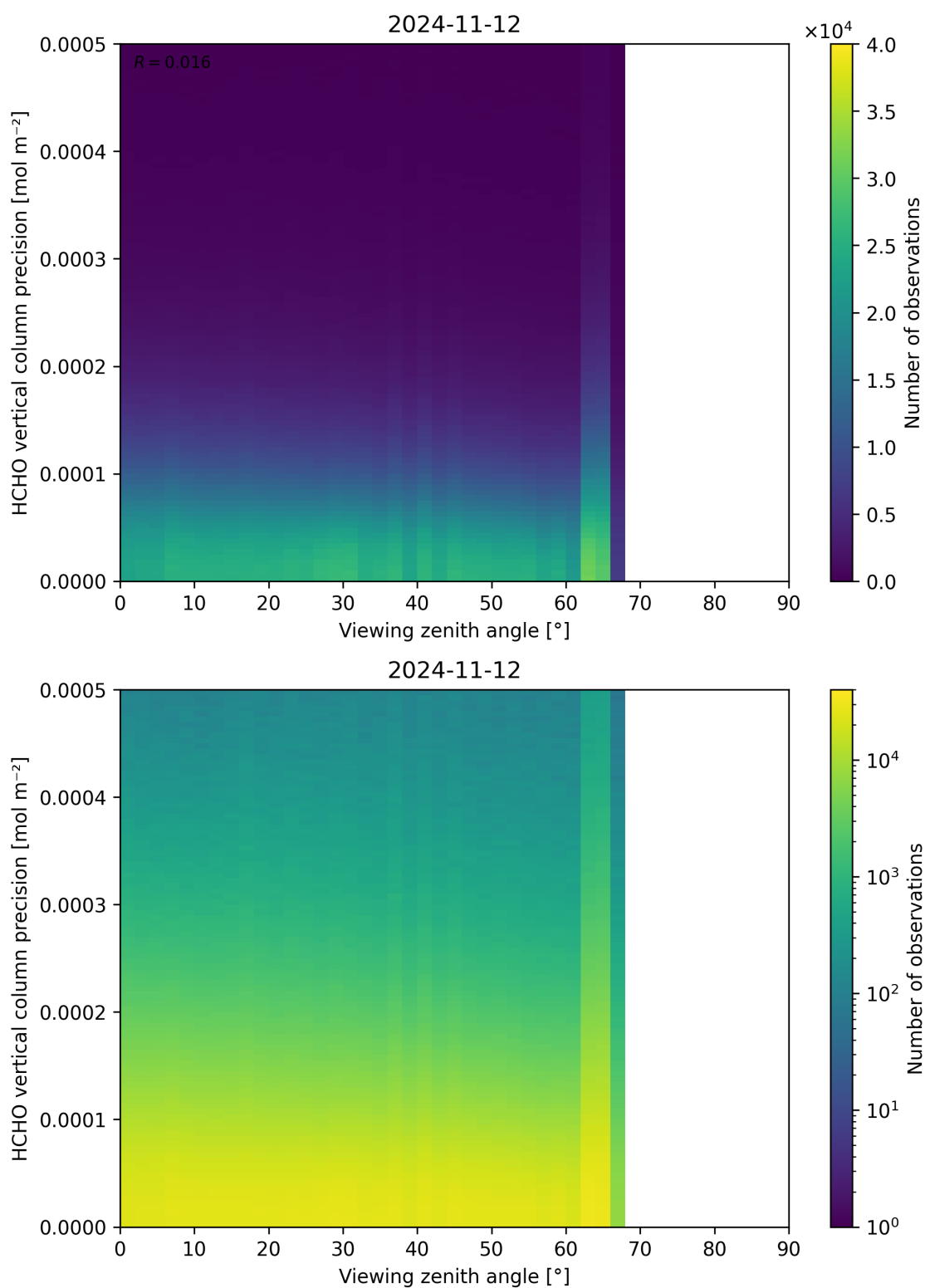
Figure 194: Scatter density plot of “Viewing zenith angle” against “HCHO vertical column precision” for 2024-11-11 to 2024-11-13.
