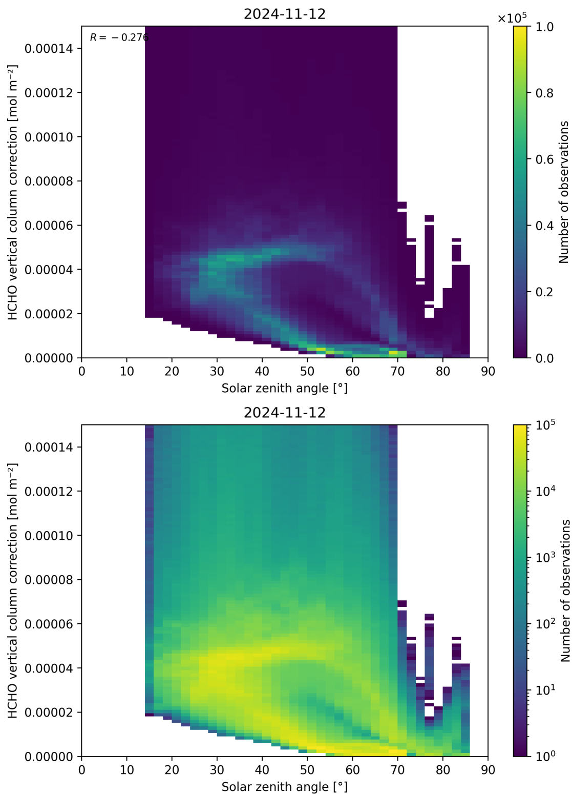
Figure 178: Scatter density plot of “Solar zenith angle” against “HCHO vertical column correction” for 2024-11-11 to 2024-11-13.
