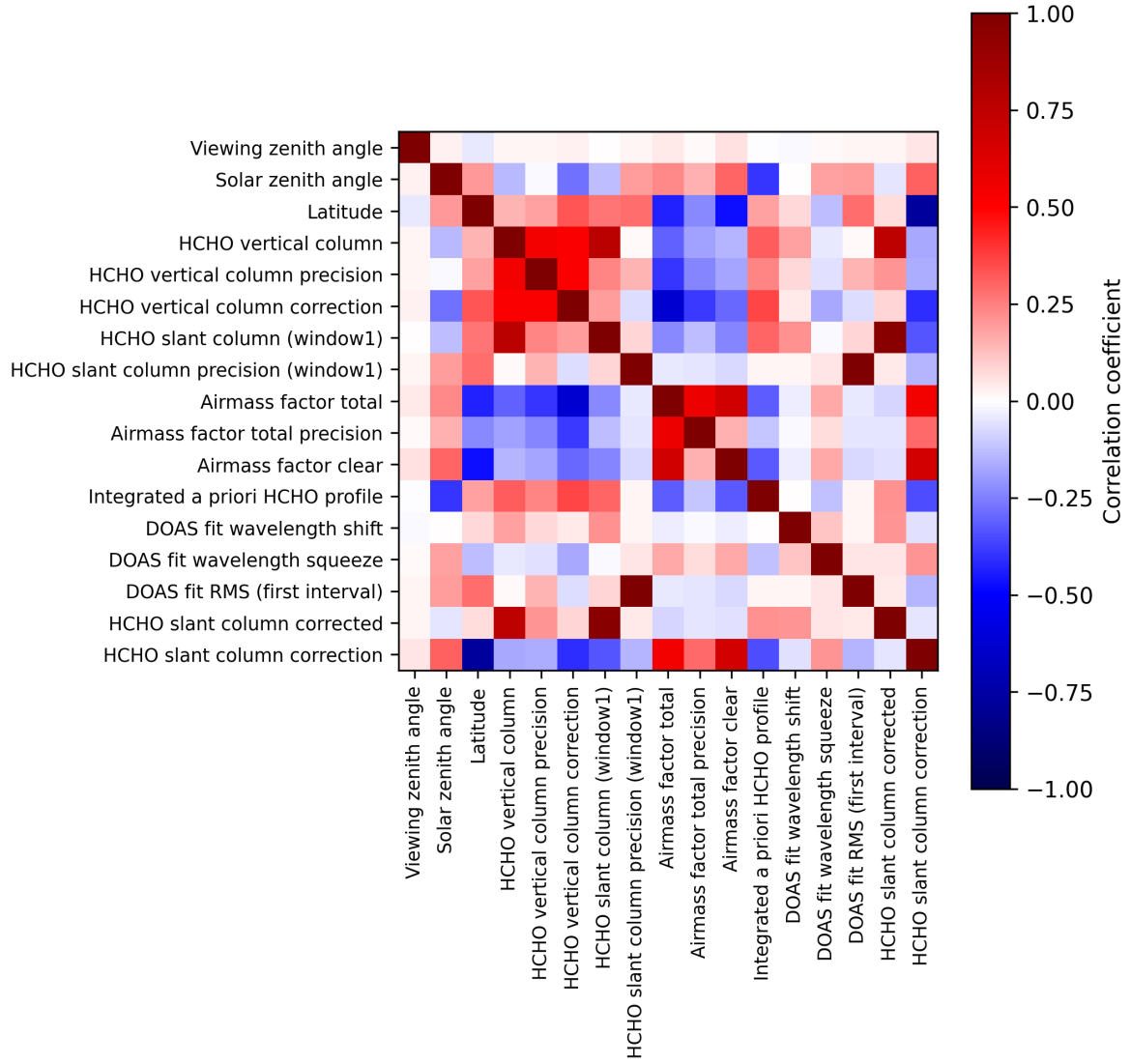
Figure 2: Map of correlation matrix for 2024-11-11 to 2024-11-13.
