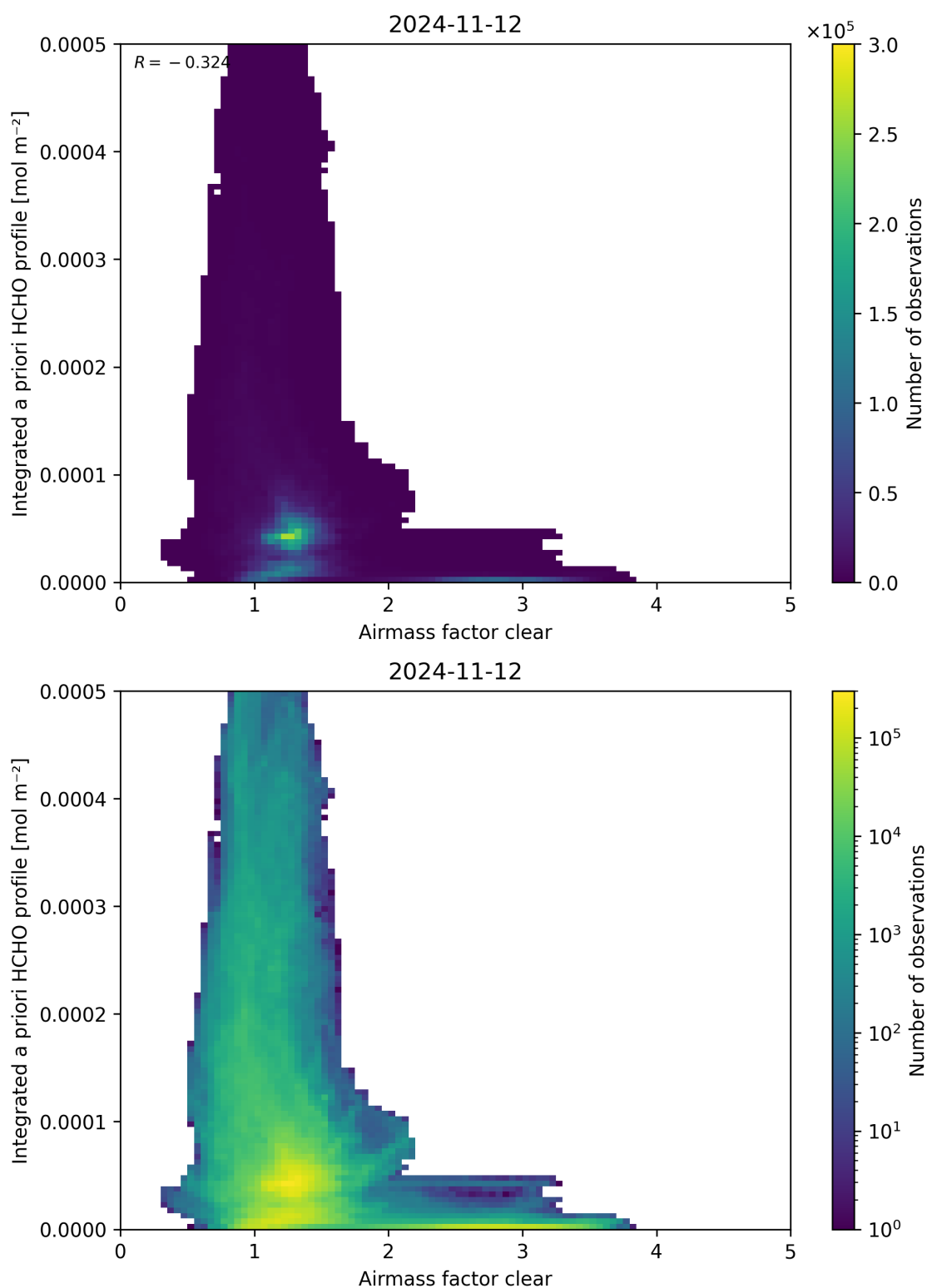
Figure 76: Scatter density plot of “Airmass factor clear” against “Integrated a priori HCHO profile” for 2024-11-11 to 2024-11-13.
