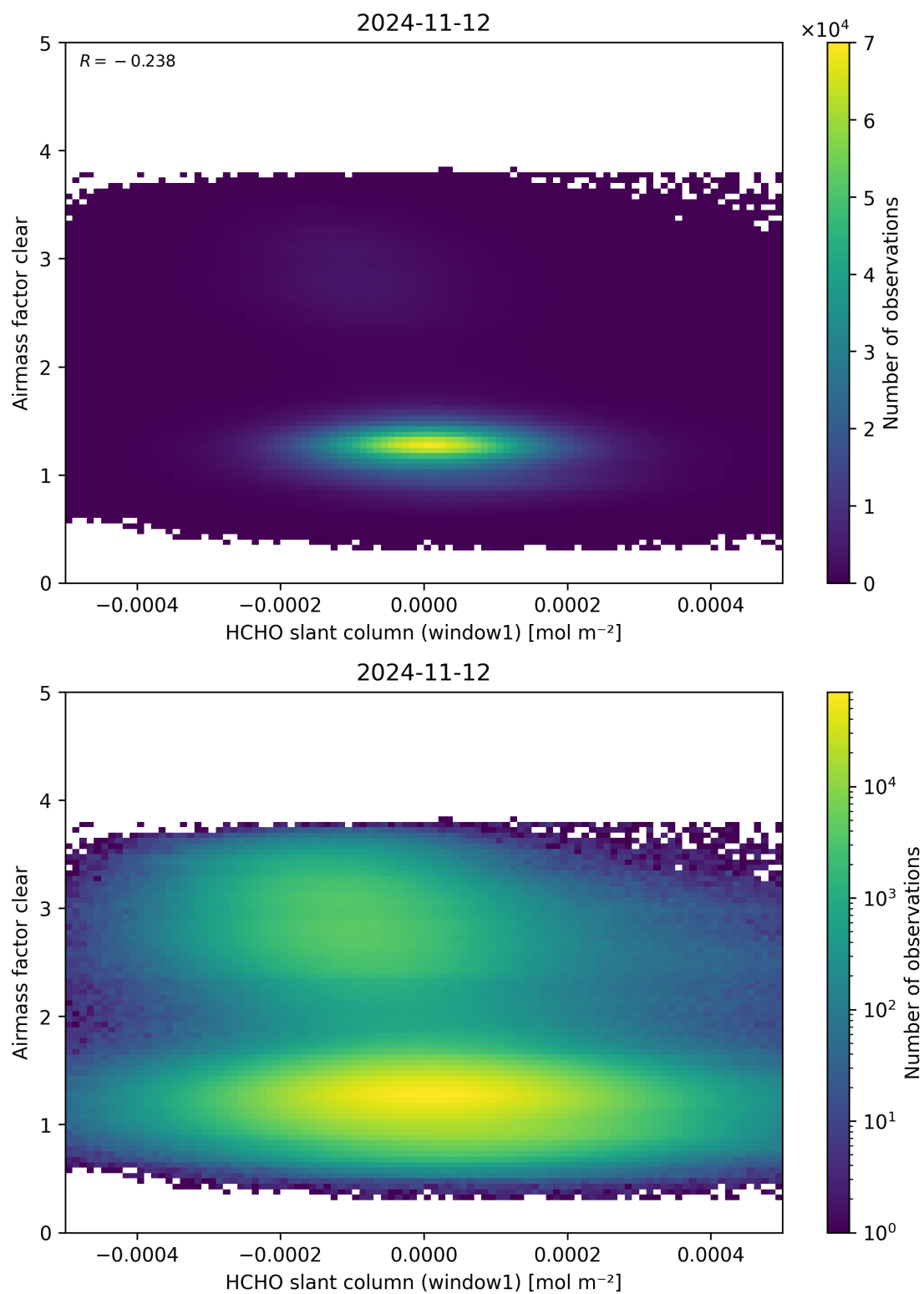
Figure 81: Scatter density plot of “HCHO slant column (window1)” against “Airmass factor clear” for 2024-11-11 to 2024-11-13.
