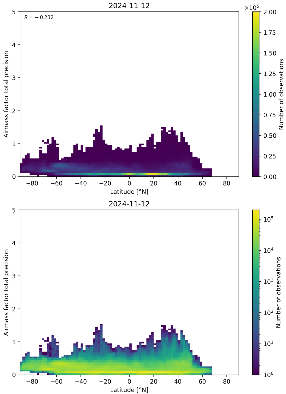
Figure 162: Scatter density plot of “Latitude” against “Airmass factor total precision” for 2024-11-11 to 2024-11-13.
