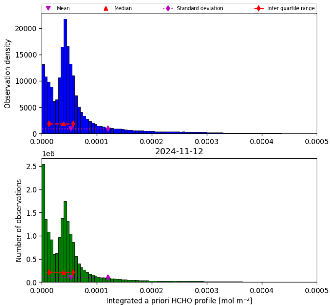
Figure 43: Histogram of “Integrated a priori HCHO profile” for 2024-11-11 to 2024-11-13
