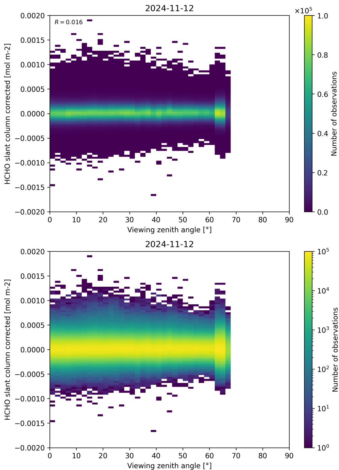
Figure 186: Scatter density plot of “Viewing zenith angle” against “HCHO slant column corrected” for 2024-11-11 to 2024-11-13.
