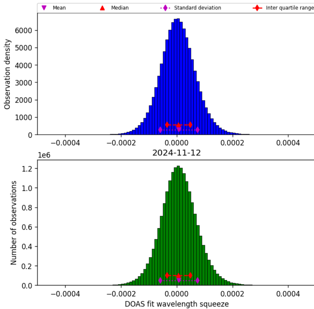
Figure 45: Histogram of “DOAS fit wavelength squeeze” for 2024-11-11 to 2024-11-13
