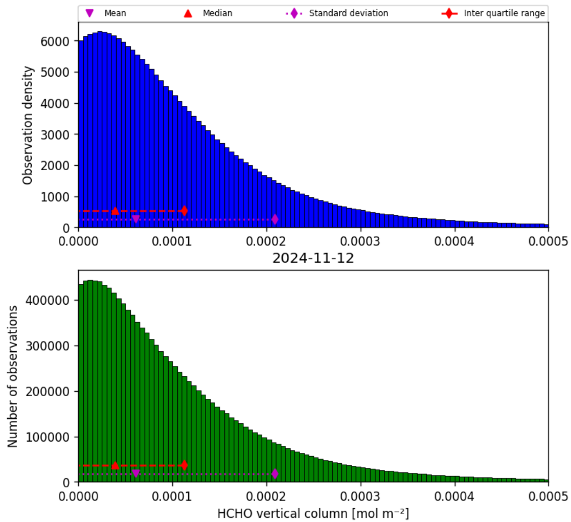
Figure 35: Histogram of “HCHO vertical column” for 2024-11-11 to 2024-11-13
