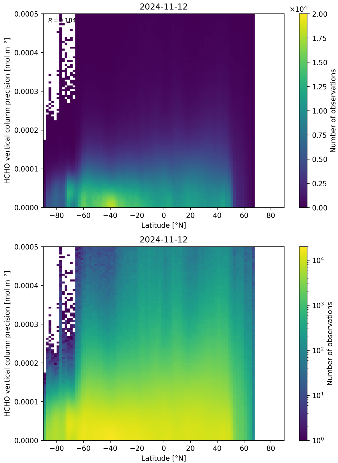
Figure 165: Scatter density plot of “Latitude” against “HCHO vertical column precision” for 2024-11-11 to 2024-11-13.
