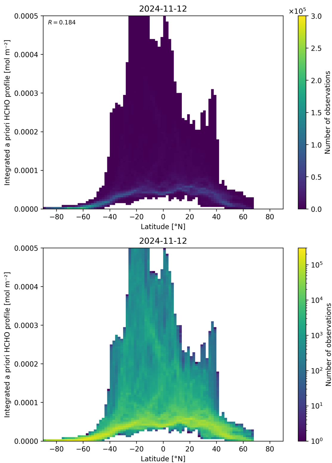
Figure 166: Scatter density plot of “Latitude” against “Integrated a priori HCHO profile” for 2024-11-11 to 2024-11-13.
