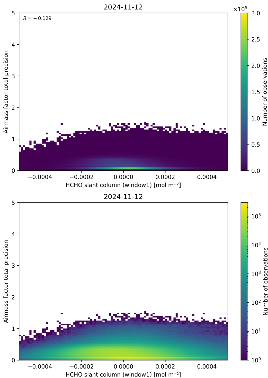
Figure 86: Scatter density plot of “HCHO slant column (window1)” against “Airmass factor total precision” for 2024-11-11 to 2024-11-13.
