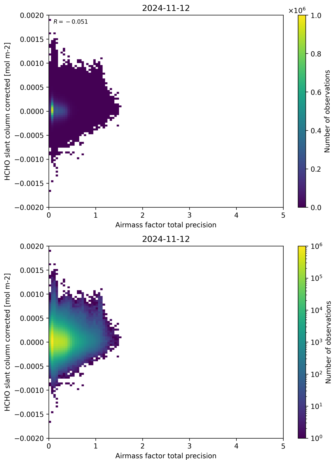
Figure 109: Scatter density plot of “Airmass factor total precision” against “HCHO slant column corrected” for 2024-11-11 to 2024-11-13.
