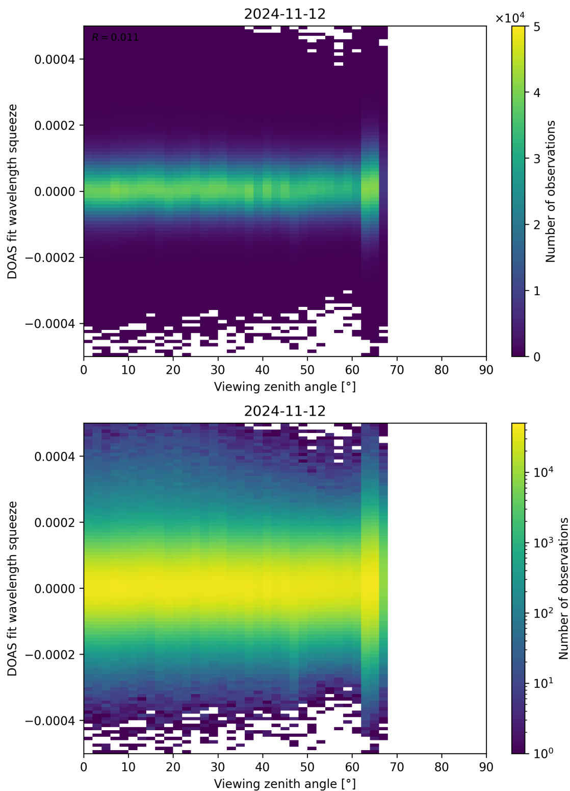
Figure 184: Scatter density plot of “Viewing zenith angle” against “DOAS fit wavelength squeeze” for 2024-11-11 to 2024-11-13.
