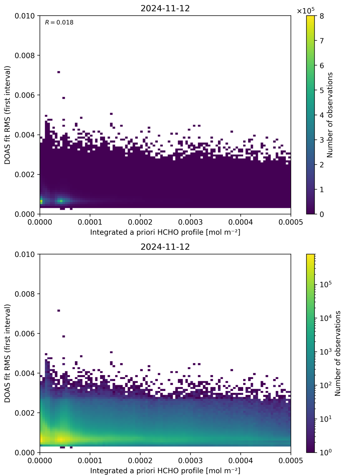
Figure 148: Scatter density plot of “Integrated a priori HCHO profile” against “DOAS fit RMS (first interval)” for 2024-11-11 to 2024-11-13.
