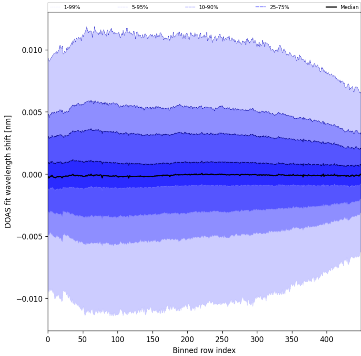
Figure 58: Along track statistics of “DOAS fit wavelength shift” for 2024-11-11 to 2024-11-13
