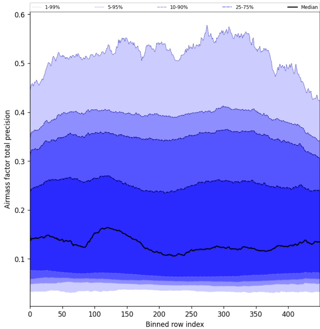
Figure 55: Along track statistics of “Airmass factor total precision” for 2024-11-11 to 2024-11-13
