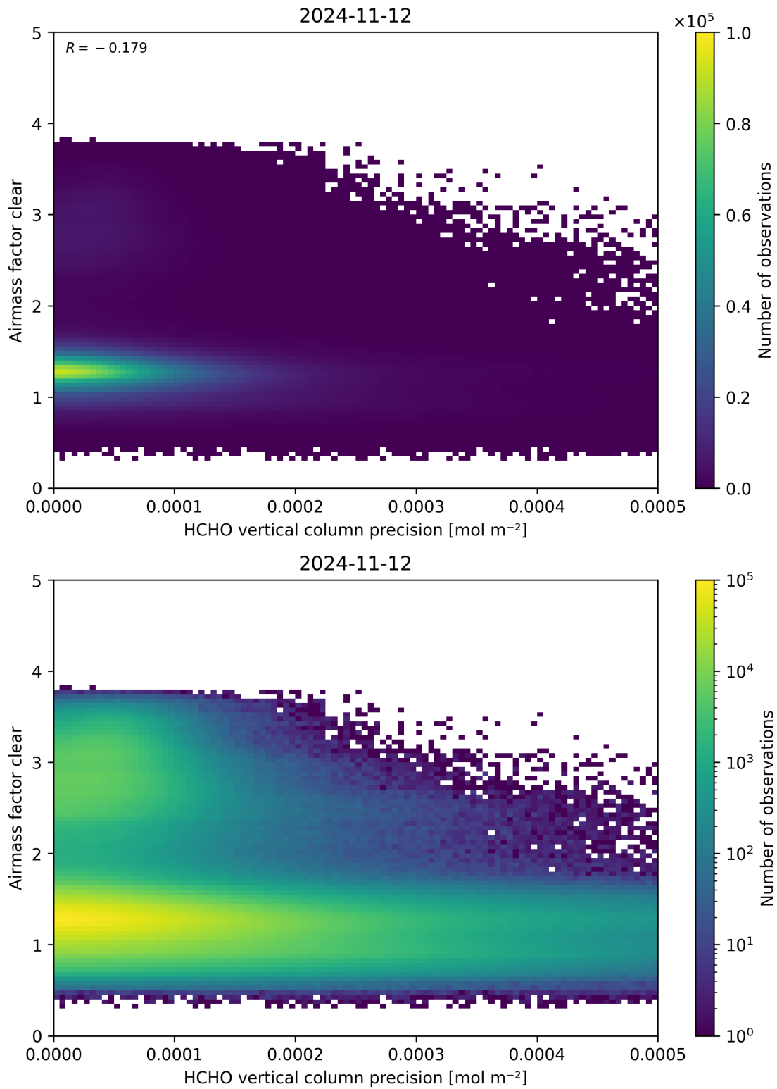
Figure 139: Scatter density plot of “HCHO vertical column precision” against “Airmass factor clear” for 2024-11-11 to 2024-11-13.
