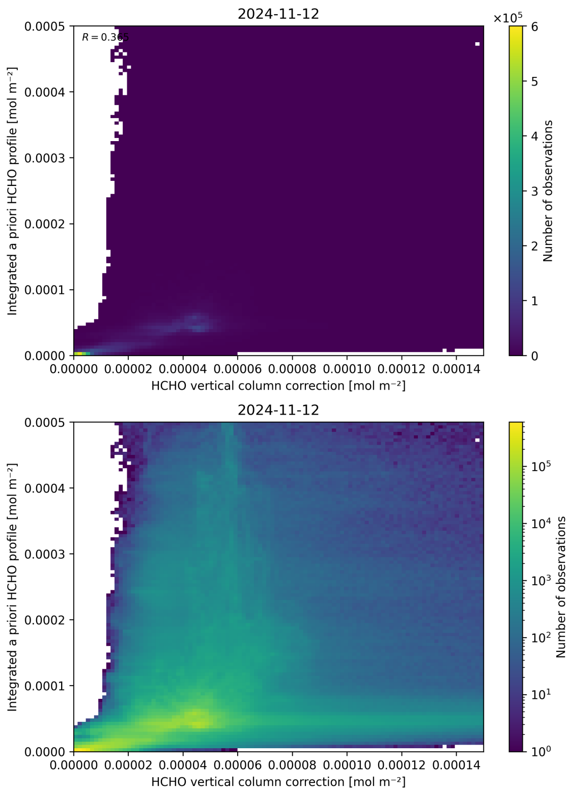
Figure 122: Scatter density plot of “HCHO vertical column correction” against “Integrated a priori HCHO profile” for 2024-11-11 to 2024-11-13.
