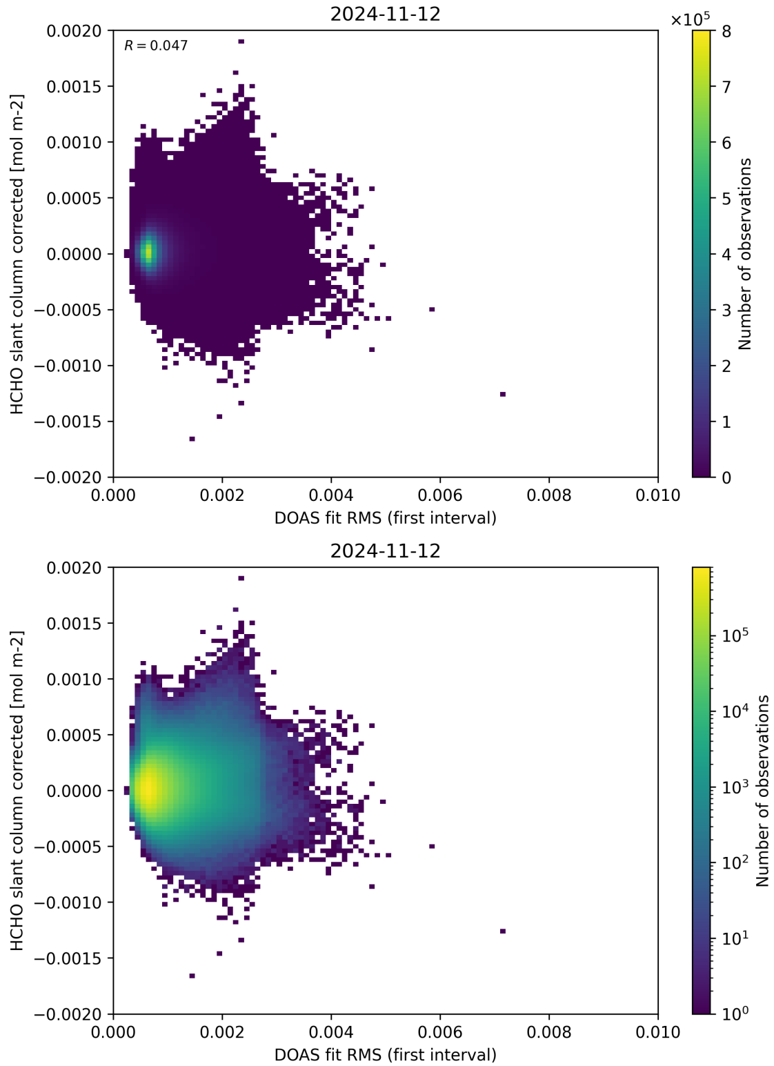
Figure 62: Scatter density plot of “DOAS fit RMS (first interval)” against “HCHO slant column corrected” for 2024-11-11 to 2024-11-13.
