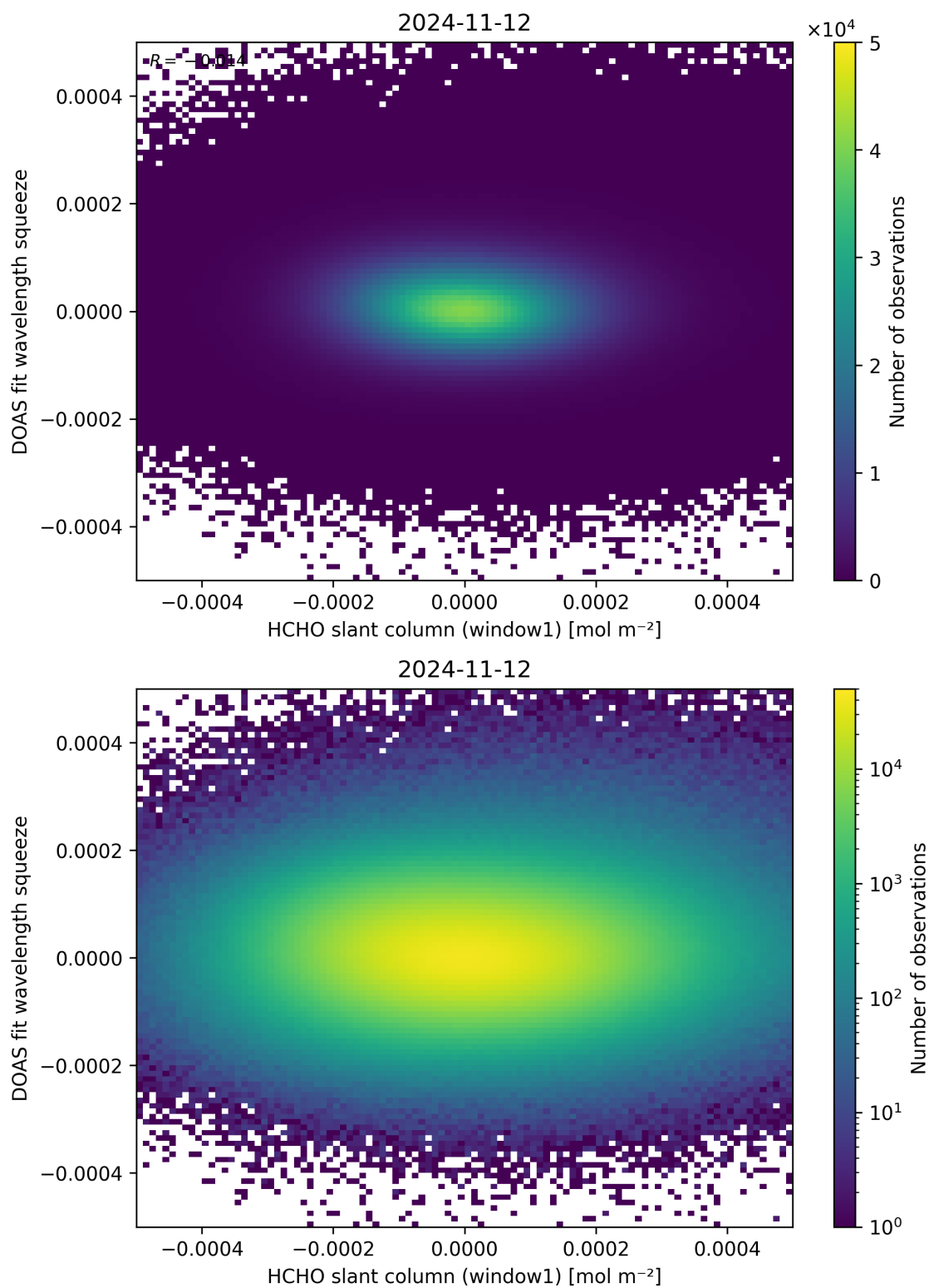
Figure 80: Scatter density plot of “HCHO slant column (window1)” against “DOAS fit wavelength squeeze” for 2024-11-11 to 2024-11-13.
