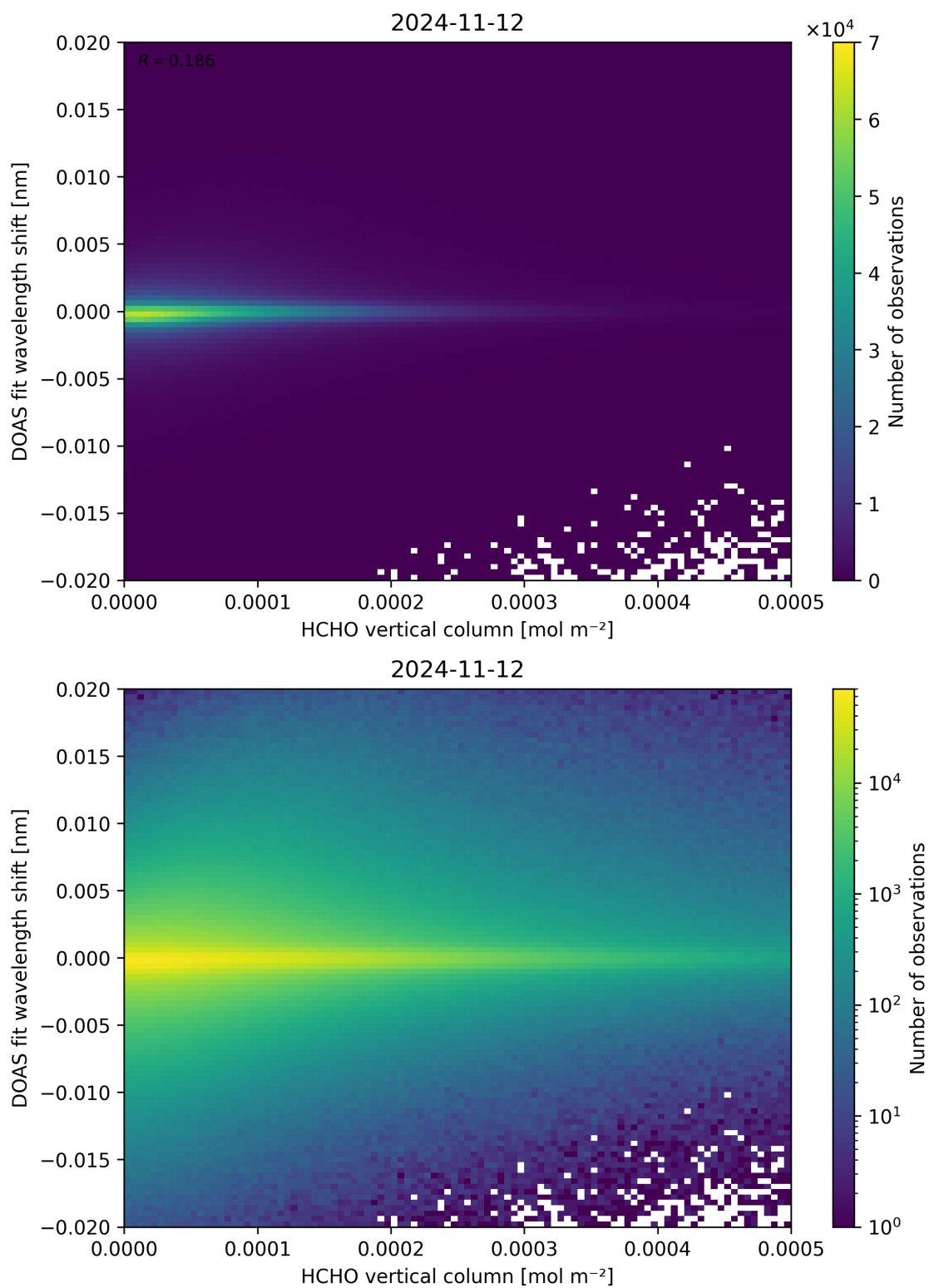
Figure 124: Scatter density plot of “HCHO vertical column” against “DOAS fit wavelength shift” for 2024-11-11 to 2024-11-13.
