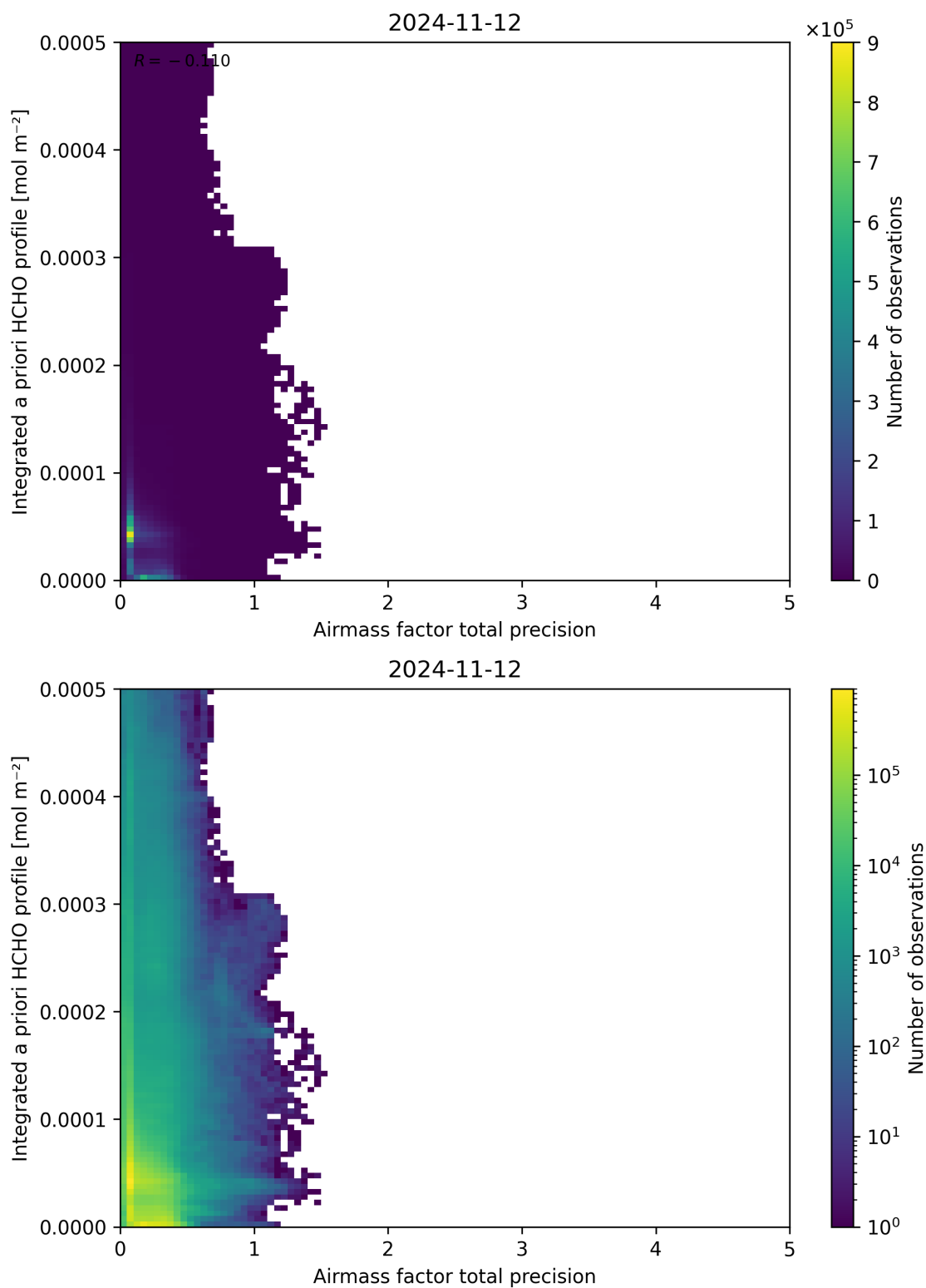
Figure 111: Scatter density plot of “Airmass factor total precision” against “Integrated a priori HCHO profile” for 2024-11-11 to 2024-11-13.
