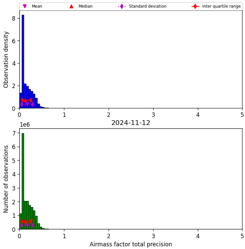
Figure 41: Histogram of “Airmass factor total precision” for 2024-11-11 to 2024-11-13
