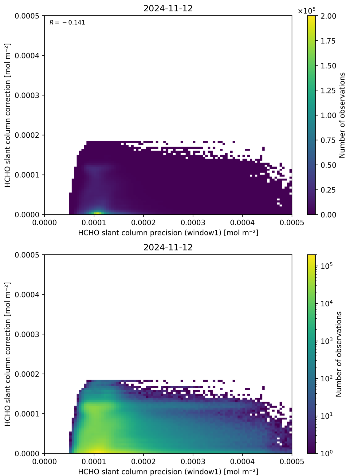
Figure 93: Scatter density plot of “HCHO slant column precision (window1)” against “HCHO slant column correction” for 2024-11-11 to 2024-11-13.
