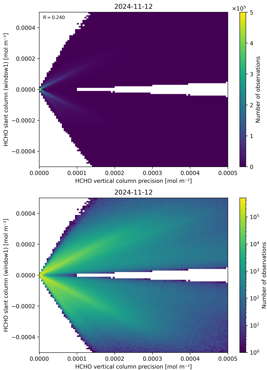
Figure 142: Scatter density plot of “HCHO vertical column precision” against “HCHO slant column (window1)” for 2024-11-11 to 2024-11-13.
