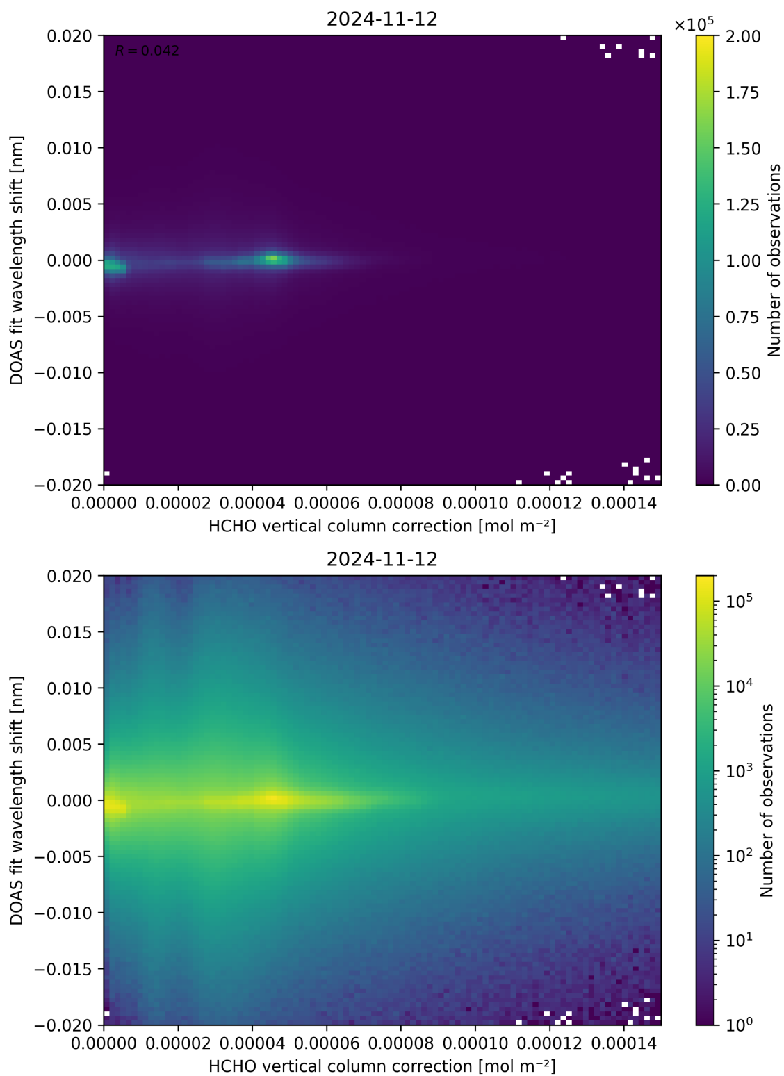
Figure 113: Scatter density plot of “HCHO vertical column correction” against “DOAS fit wavelength shift” for 2024-11-11 to 2024-11-13.
