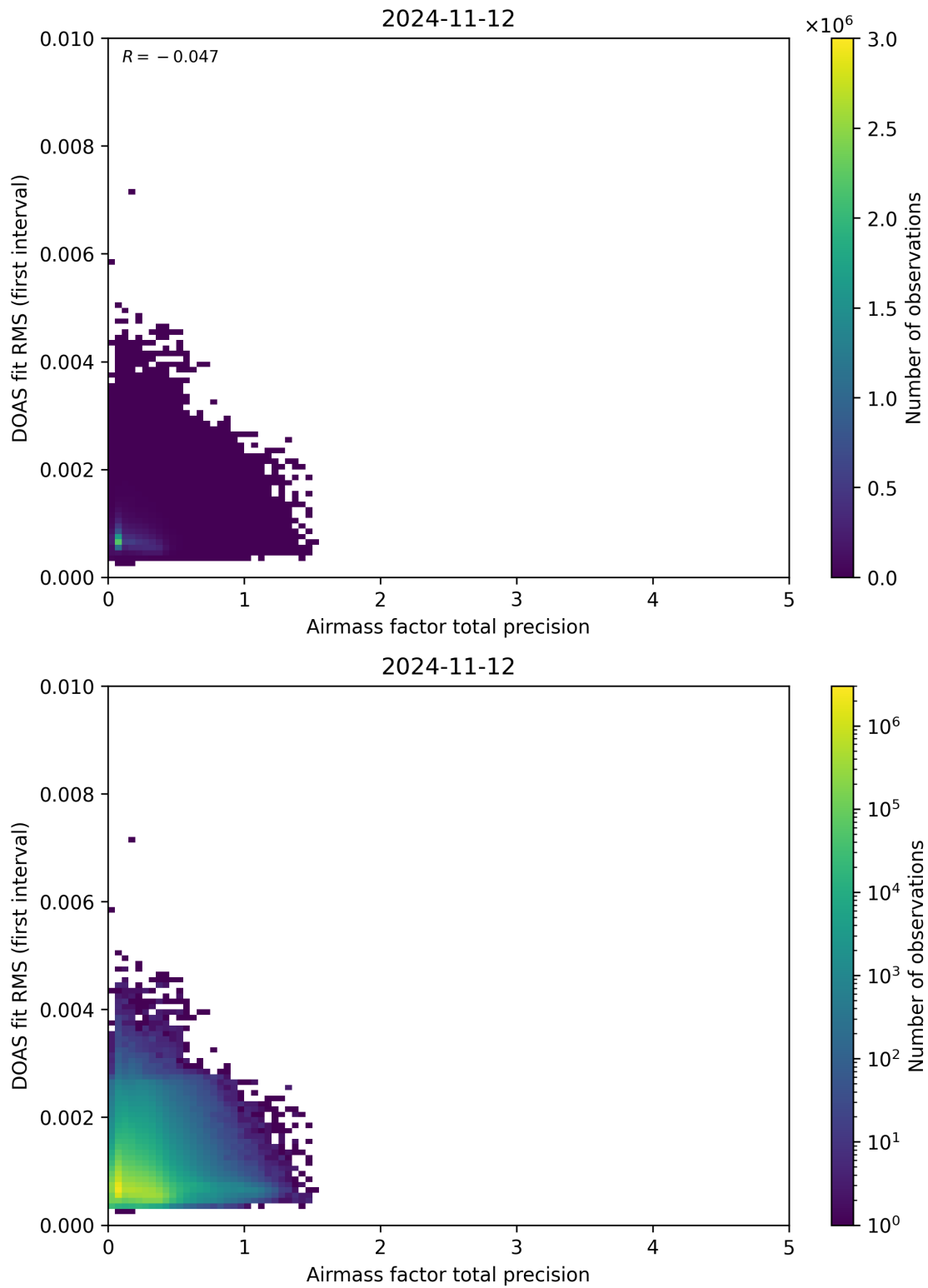
Figure 105: Scatter density plot of “Airmass factor total precision” against “DOAS fit RMS (first interval)” for 2024-11-11 to 2024-11-13.
