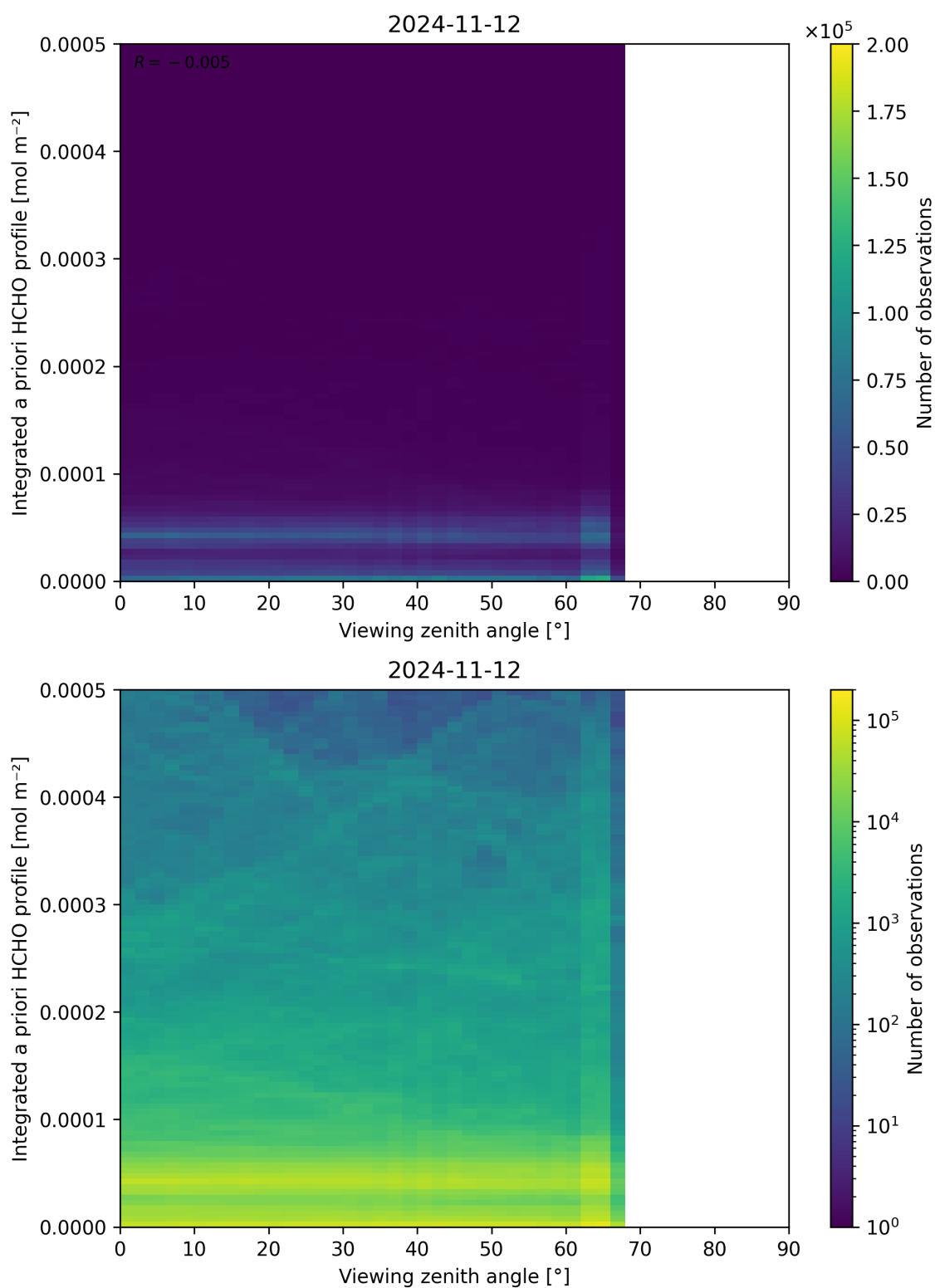
Figure 195: Scatter density plot of “Viewing zenith angle” against “Integrated a priori HCHO profile” for 2024-11-11 to 2024-11-13.
