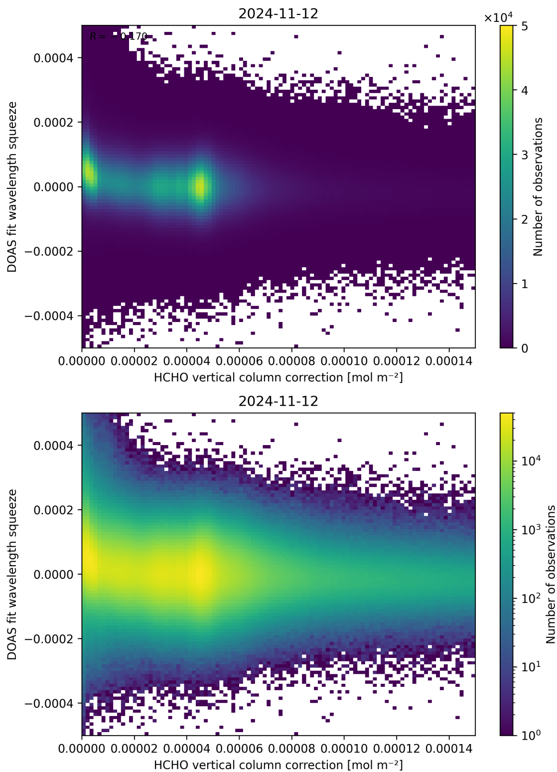
Figure 114: Scatter density plot of “HCHO vertical column correction” against “DOAS fit wavelength squeeze” for 2024-11-11 to 2024-11-13.
