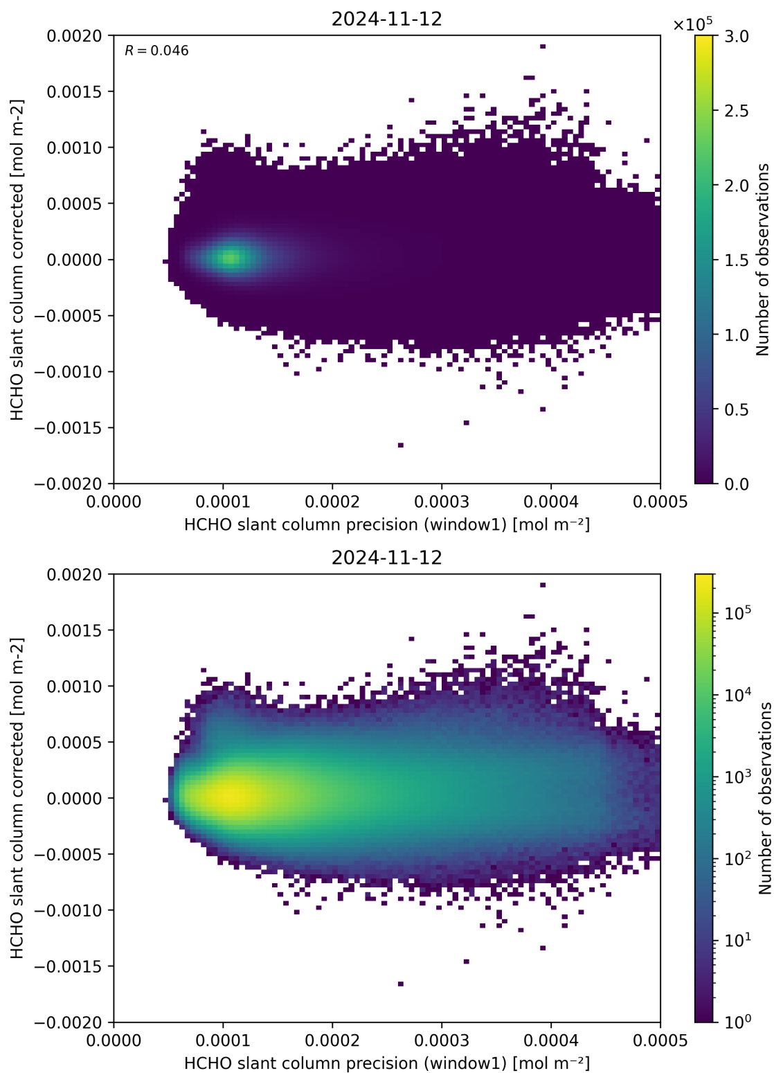
Figure 92: Scatter density plot of “HCHO slant column precision (window1)” against “HCHO slant column corrected” for 2024-11-11 to 2024-11-13.
