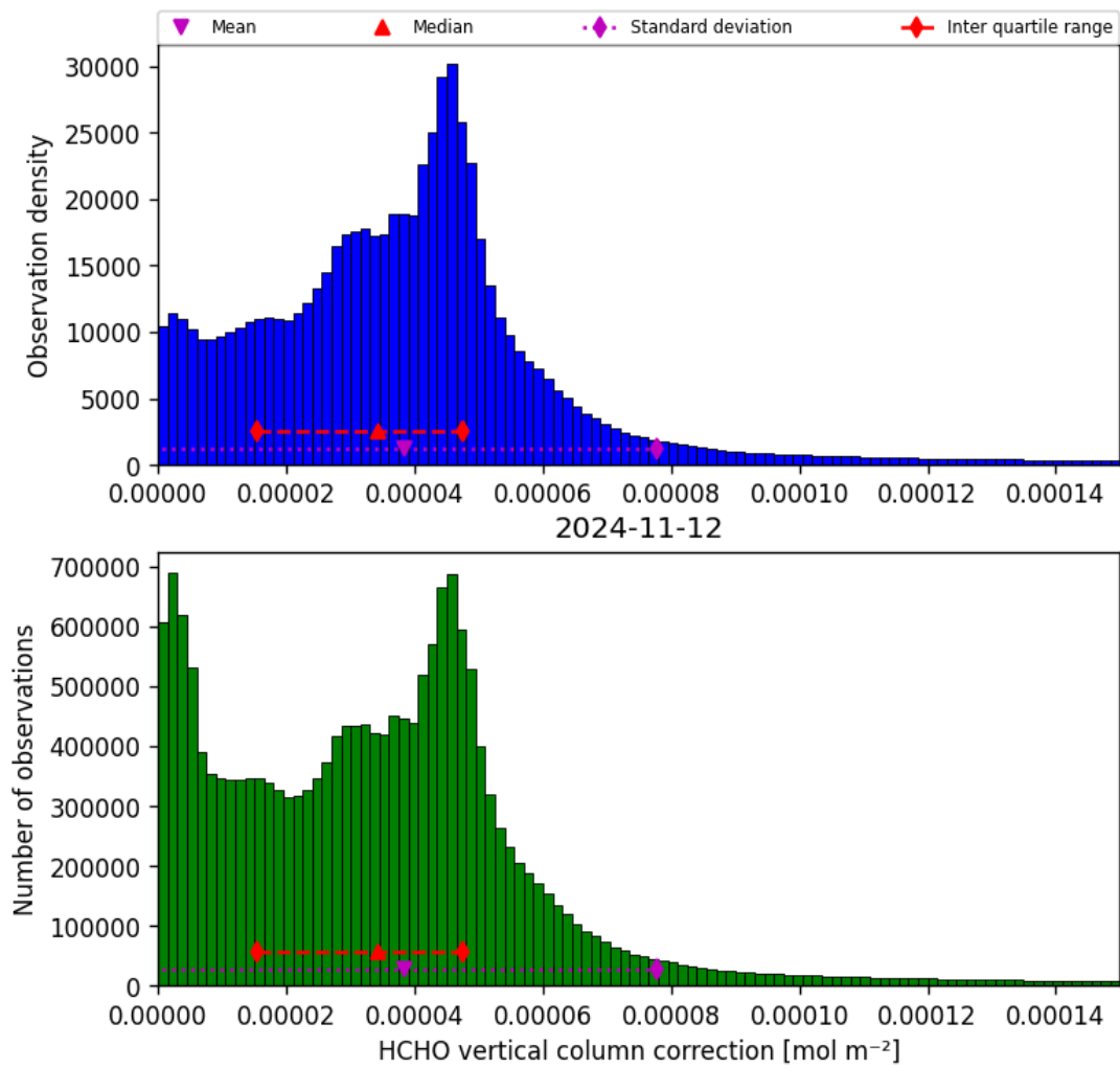
Figure 37: Histogram of “HCHO vertical column correction” for 2024-11-11 to 2024-11-13
