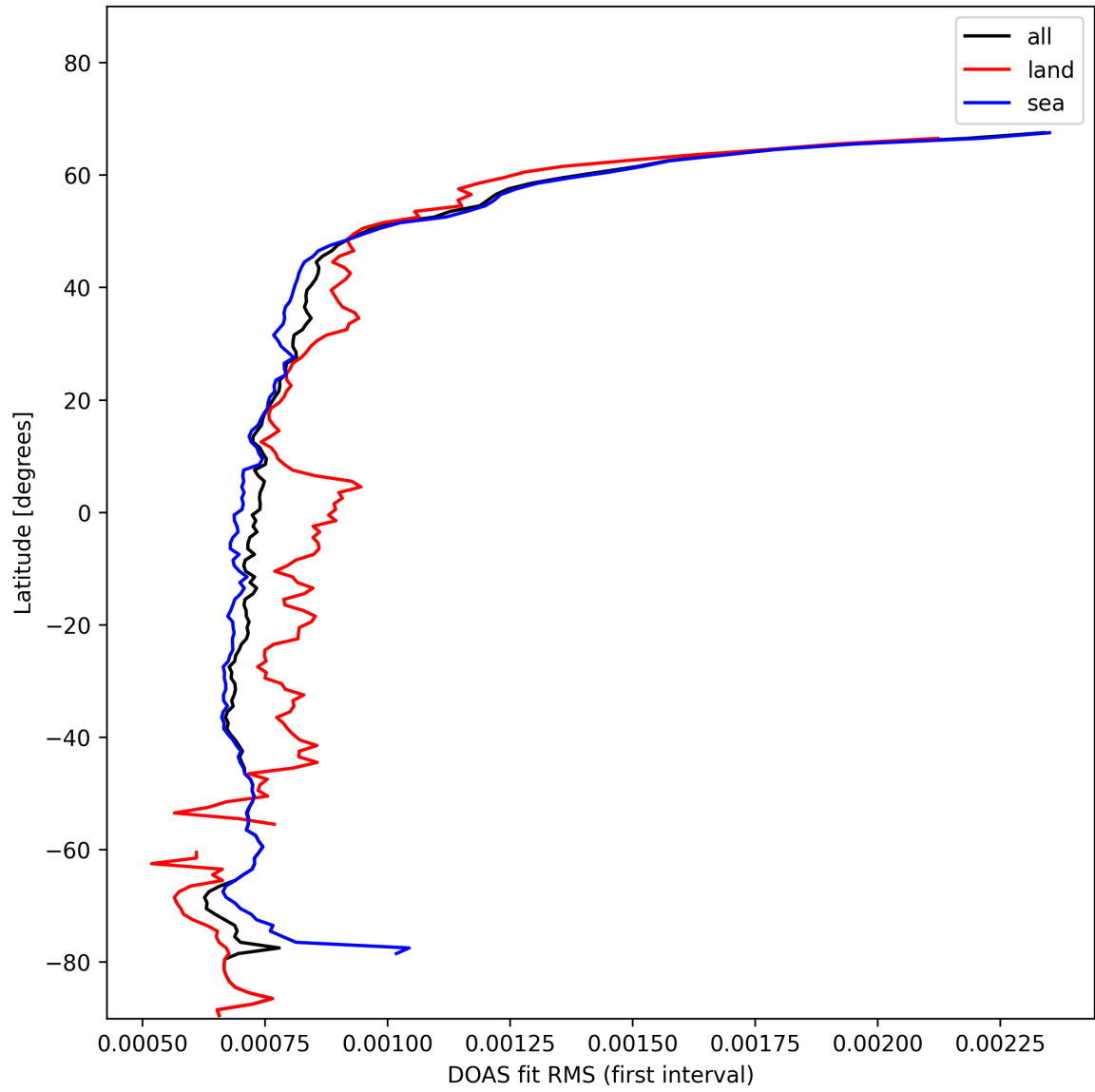
Figure 32: Zonal average of “DOAS fit RMS (first interval)” for 2024-11-11 to 2024-11-13.
