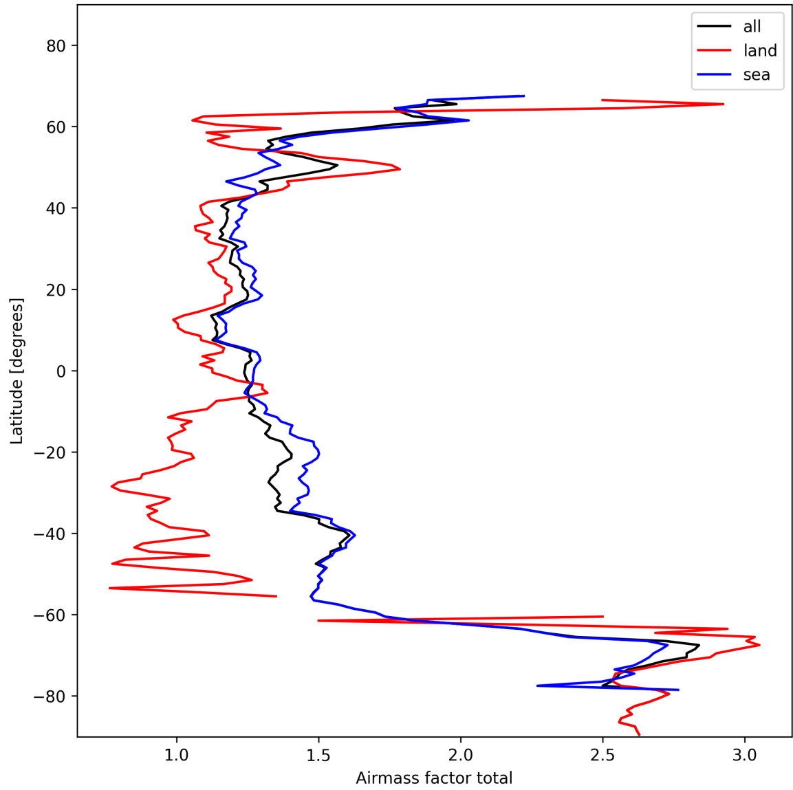
Figure 26: Zonal average of “Airmass factor total” for 2024-11-11 to 2024-11-13.
