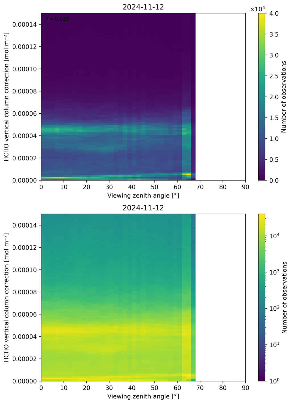
Figure 193: Scatter density plot of “Viewing zenith angle” against “HCHO vertical column correction” for 2024-11-11 to 2024-11-13.
