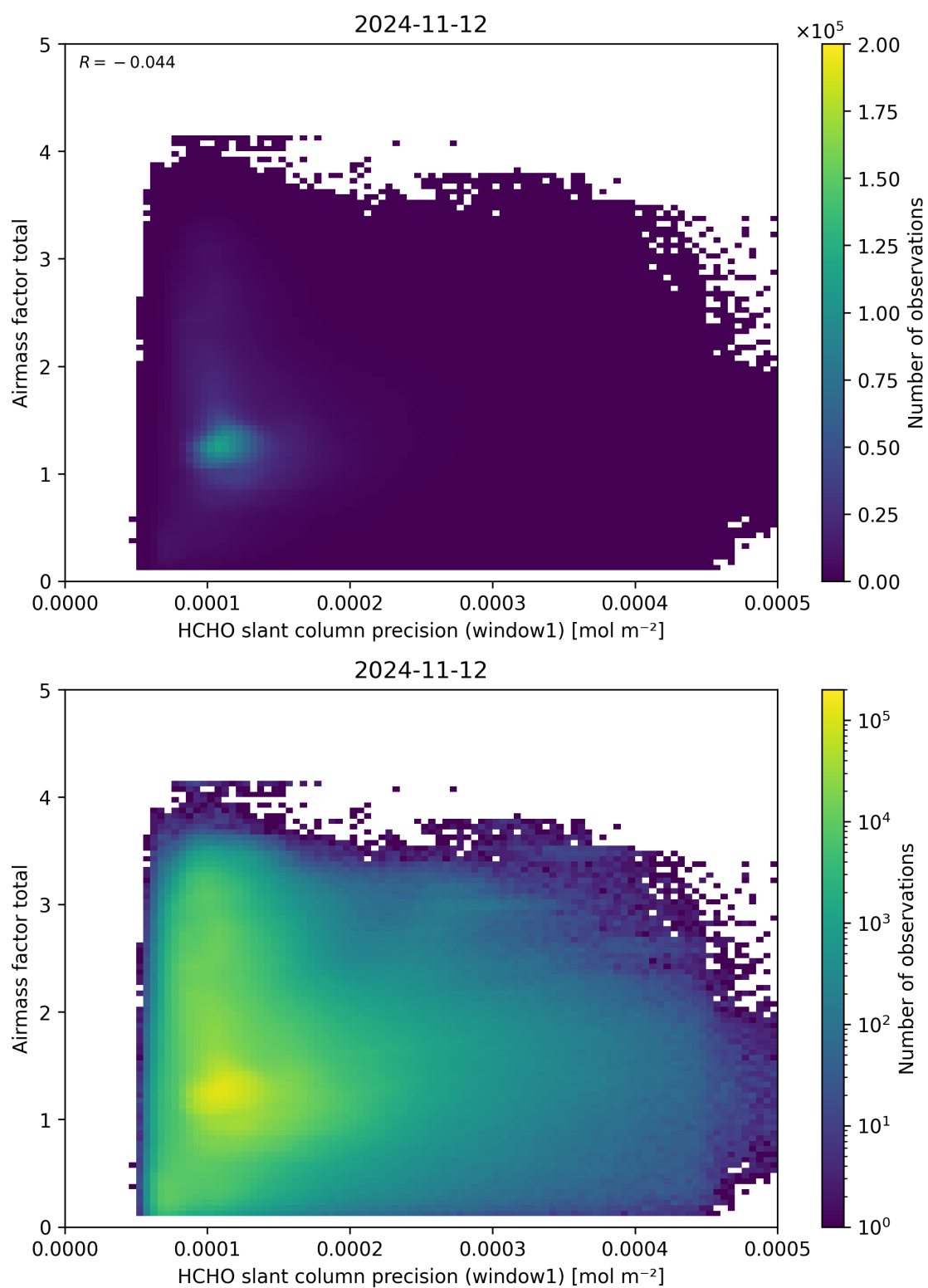
Figure 94: Scatter density plot of “HCHO slant column precision (window1)” against “Airmass factor total” for 2024-11-11 to 2024-11-13.
