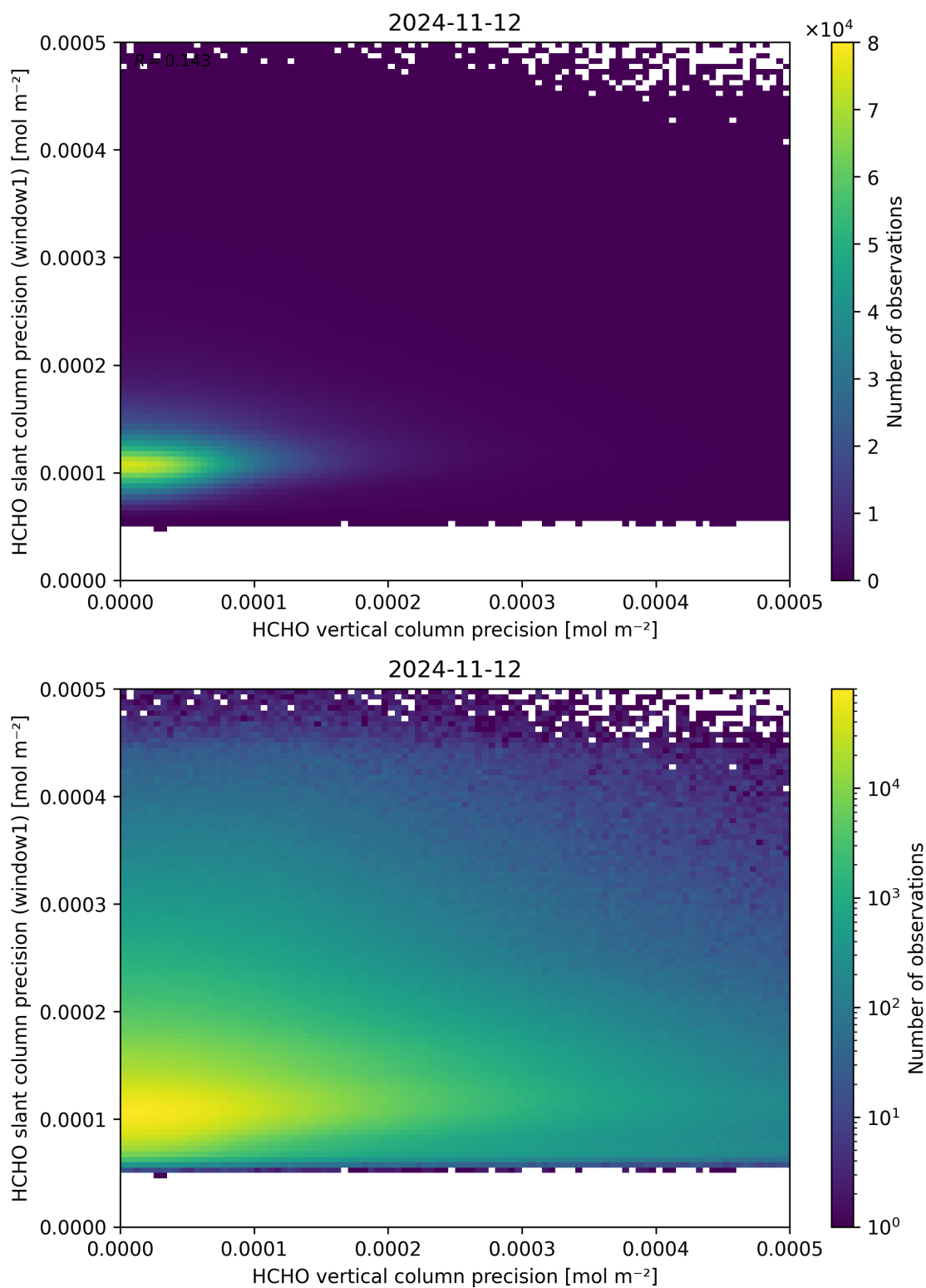
Figure 143: Scatter density plot of “HCHO vertical column precision” against “HCHO slant column precision (window1)” for 2024-11-11 to 2024-11-13.
