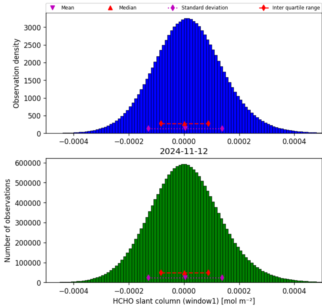
Figure 38: Histogram of “HCHO slant column (window1)” for 2024-11-11 to 2024-11-13
