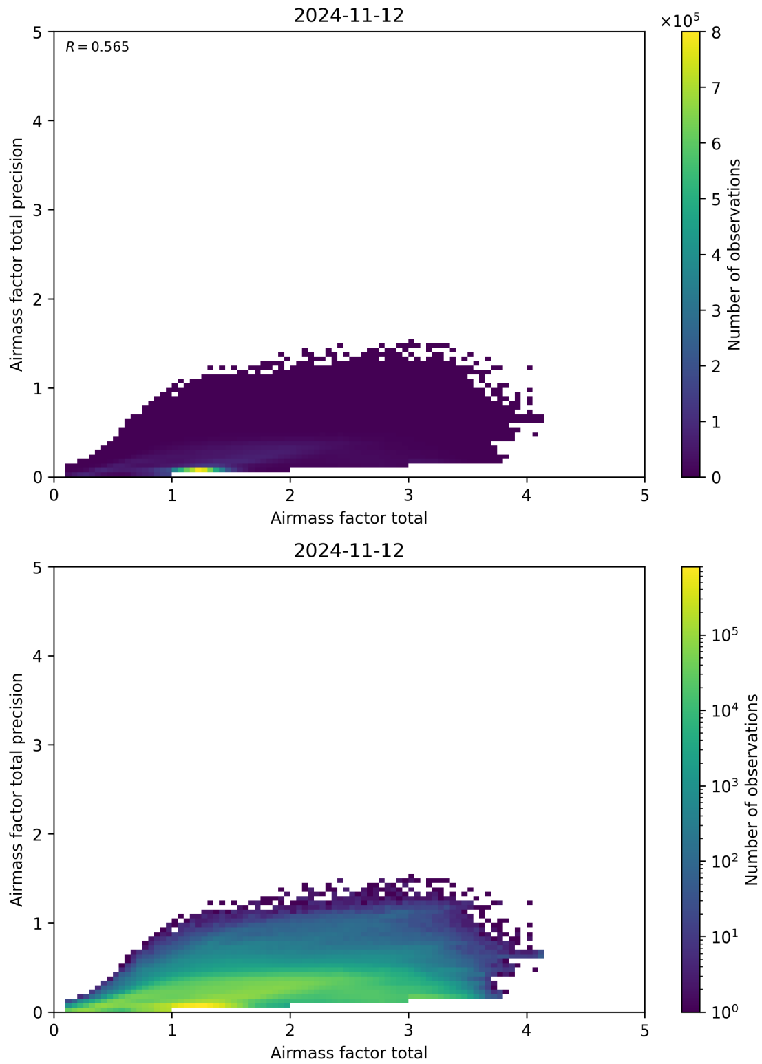
Figure 103: Scatter density plot of “Airmass factor total” against “Airmass factor total precision” for 2024-11-11 to 2024-11-13.
