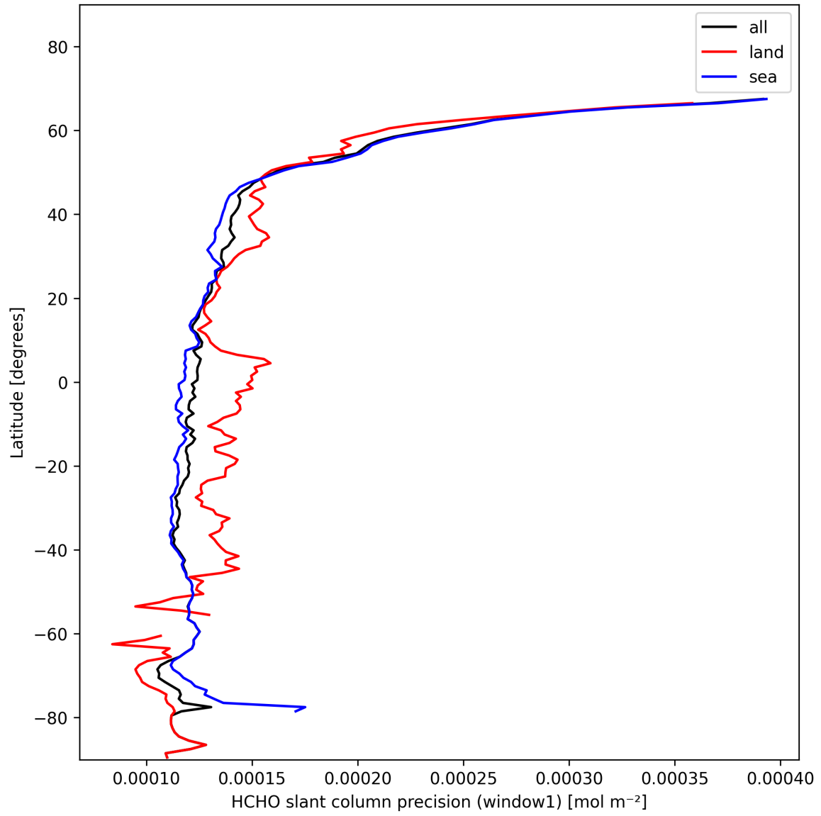
Figure 25: Zonal average of “HCHO slant column precision (window1)” for 2024-11-11 to 2024-11-13.
