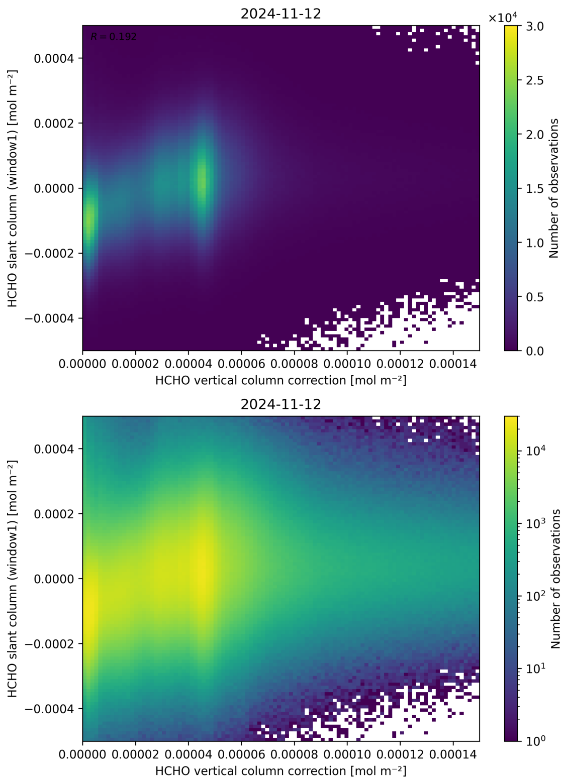
Figure 118: Scatter density plot of “HCHO vertical column correction” against “HCHO slant column (window1)” for 2024-11-11 to 2024-11-13.
