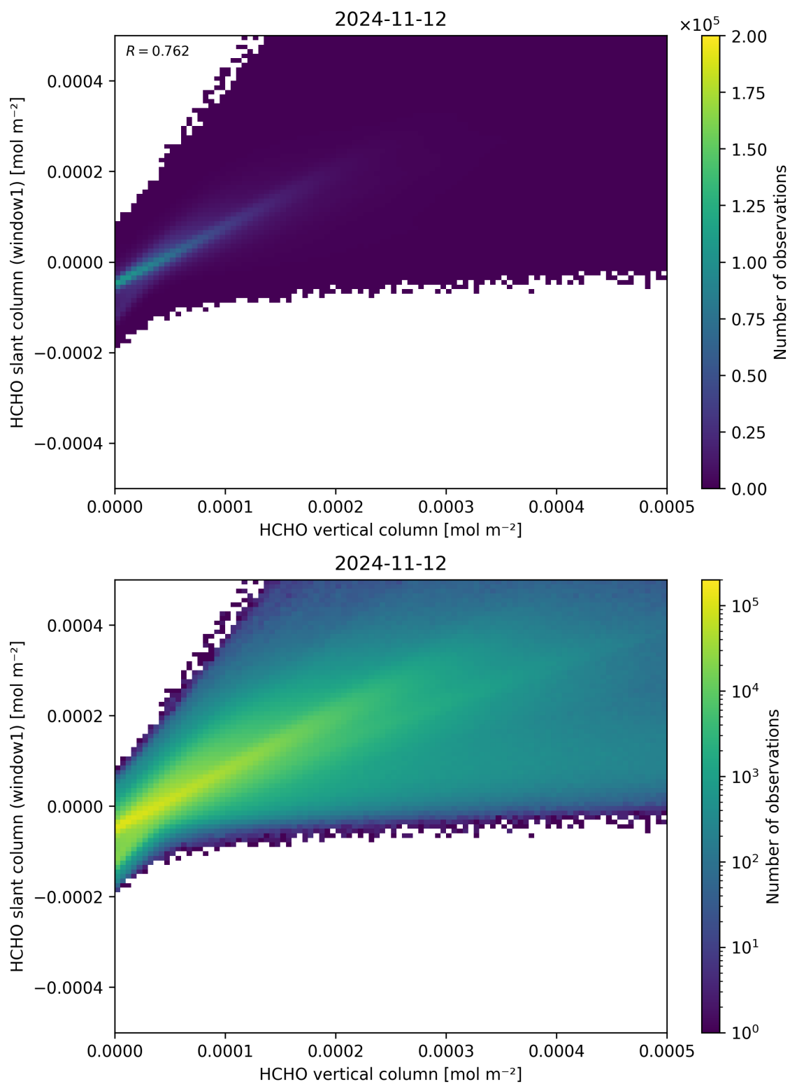
Figure 129: Scatter density plot of “HCHO vertical column” against “HCHO slant column (window1)” for 2024-11-11 to 2024-11-13.
