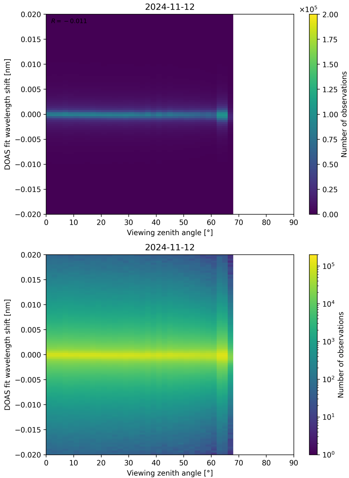
Figure 183: Scatter density plot of “Viewing zenith angle” against “DOAS fit wavelength shift” for 2024-11-11 to 2024-11-13.
