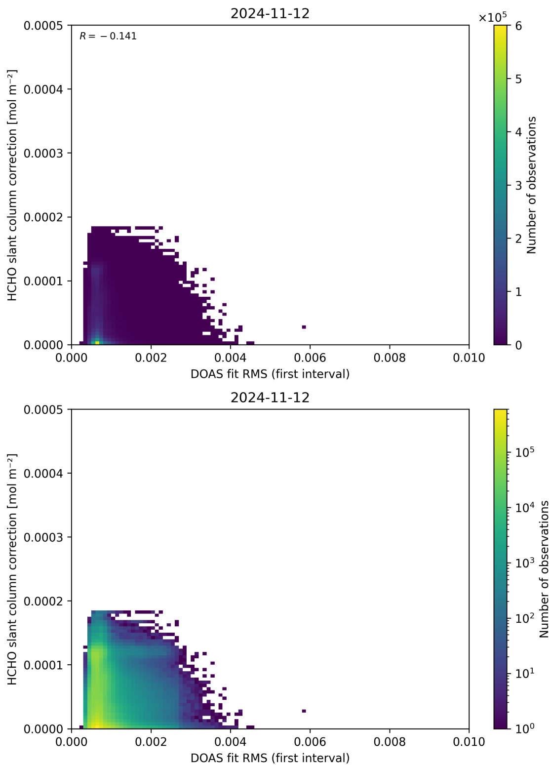
Figure 63: Scatter density plot of “DOAS fit RMS (first interval)” against “HCHO slant column correction” for 2024-11-11 to 2024-11-13.
