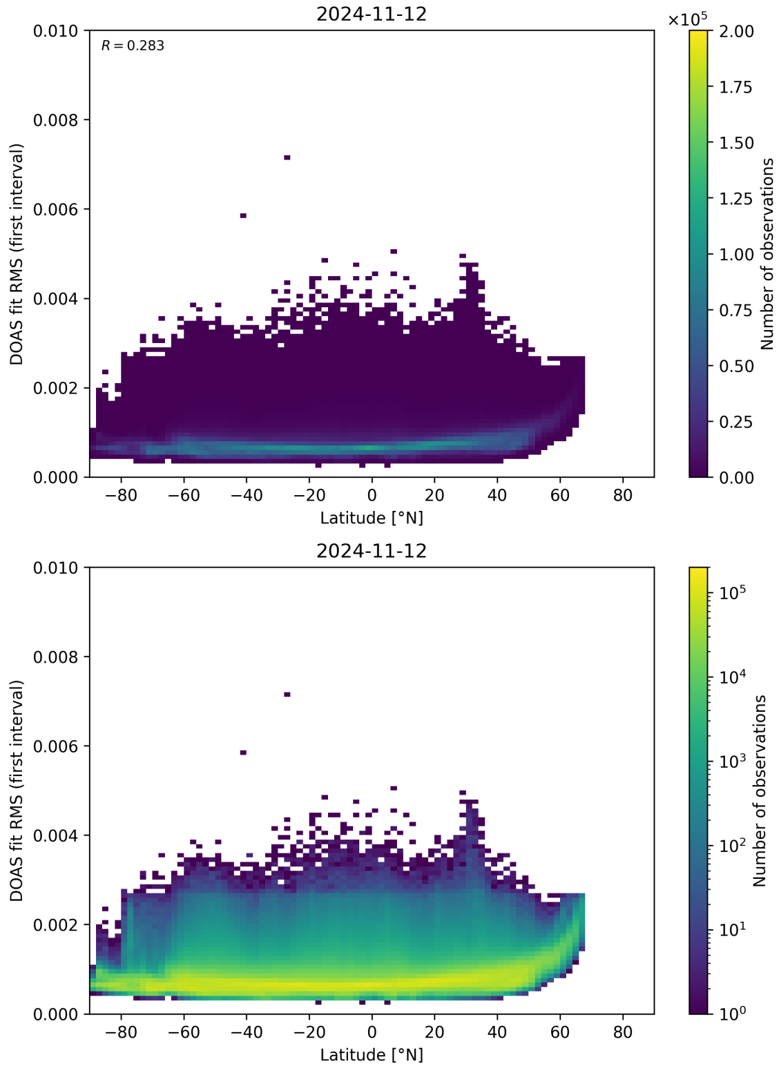
Figure 153: Scatter density plot of “Latitude” against “DOAS fit RMS (first interval)” for 2024-11-11 to 2024-11-13.
