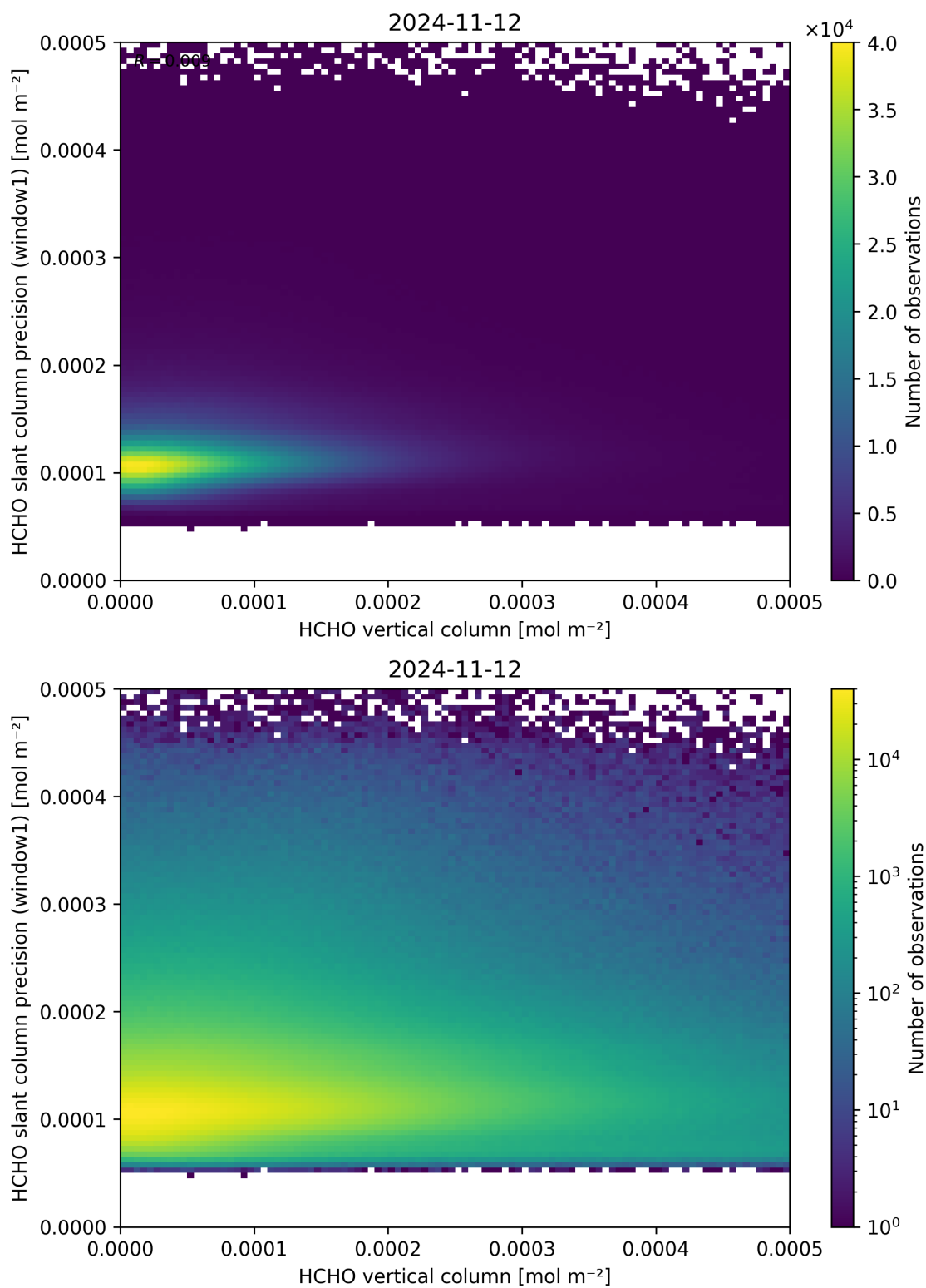
Figure 130: Scatter density plot of “HCHO vertical column” against “HCHO slant column precision (window1)” for 2024-11-11 to 2024-11-13.
