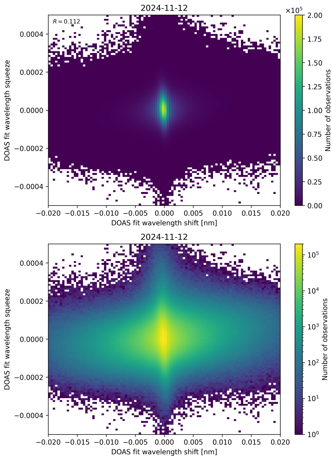
Figure 65: Scatter density plot of “DOAS fit wavelength shift” against “DOAS fit wavelength squeeze” for 2024-11-11 to 2024-11-13.
