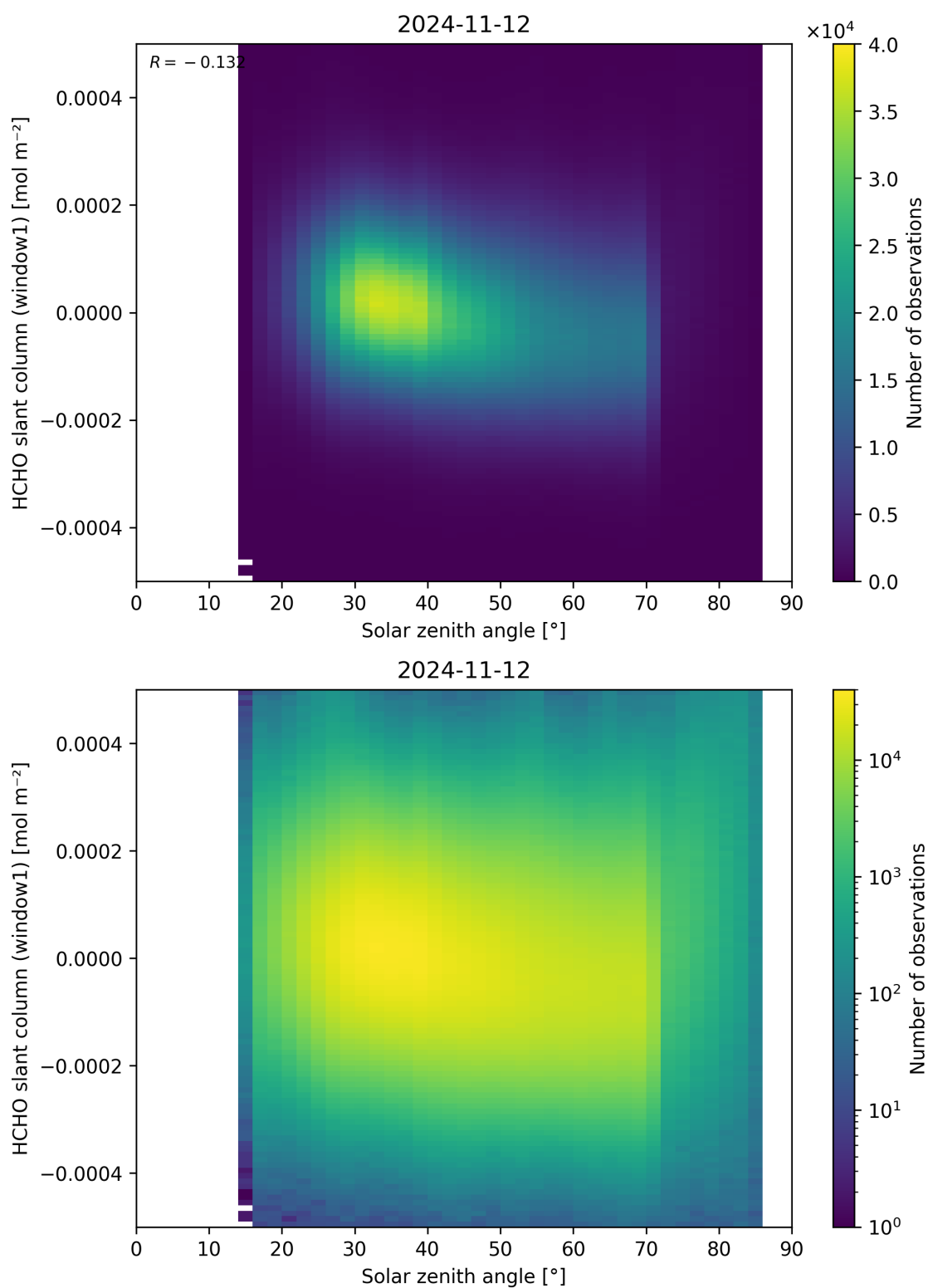
Figure 173: Scatter density plot of “Solar zenith angle” against “HCHO slant column (window1)” for 2024-11-11 to 2024-11-13.
