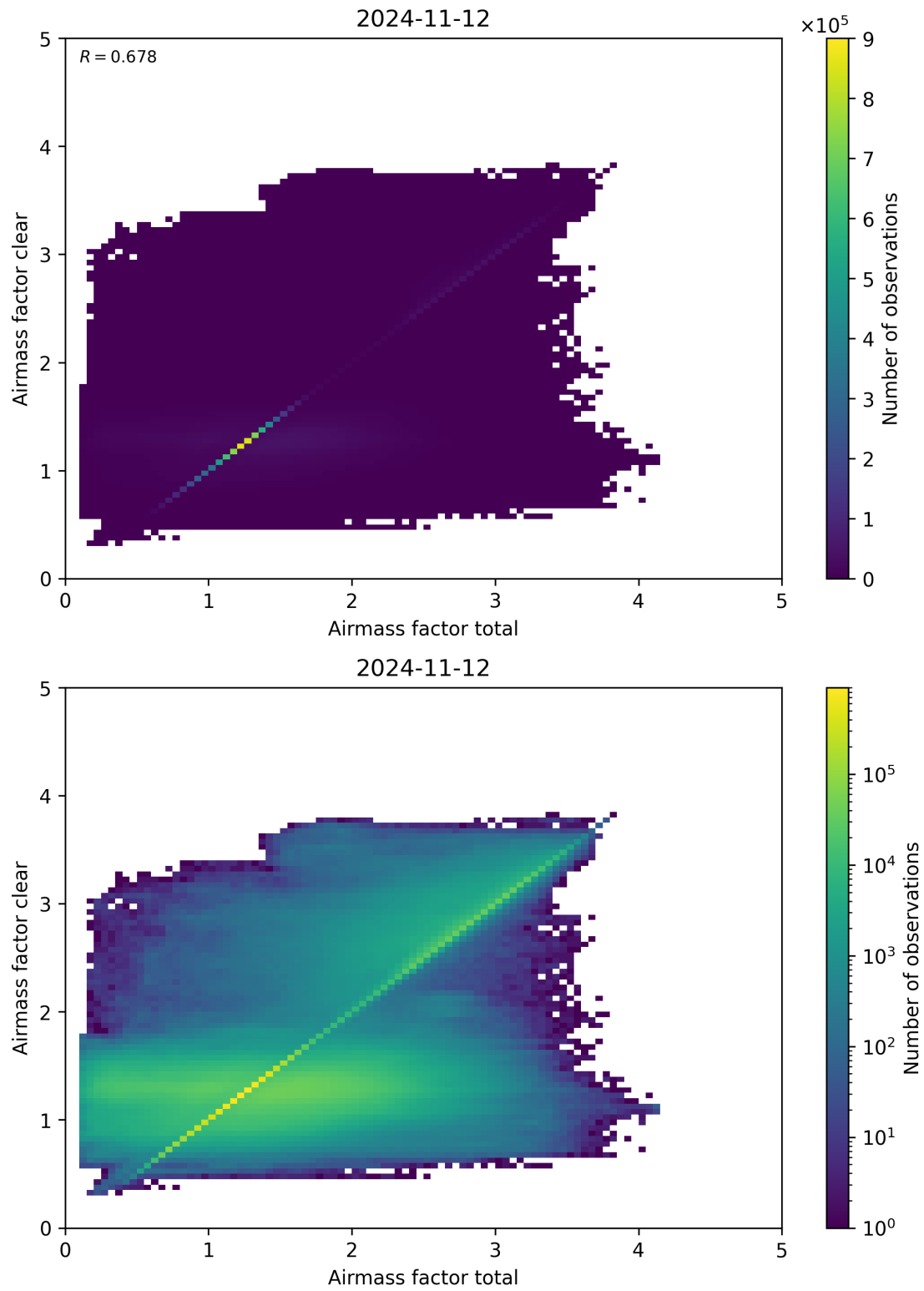
Figure 100: Scatter density plot of “Airmass factor total” against “Airmass factor clear” for 2024-11-11 to 2024-11-13.
