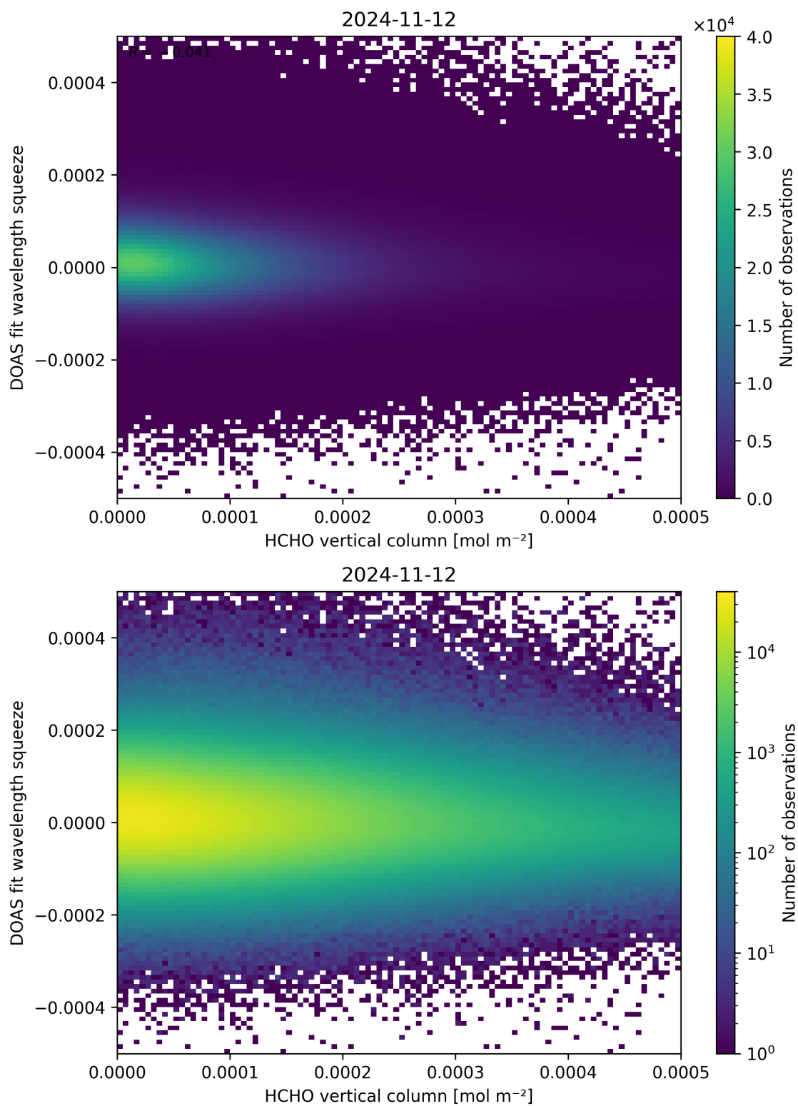
Figure 125: Scatter density plot of “HCHO vertical column” against “DOAS fit wavelength squeeze” for 2024-11-11 to 2024-11-13.
