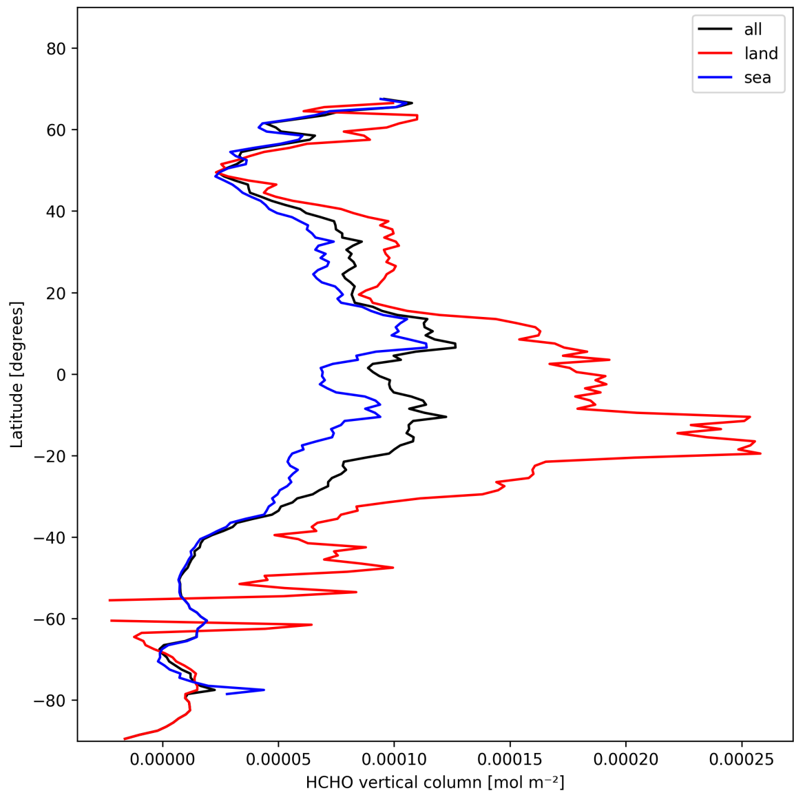
Figure 21: Zonal average of “HCHO vertical column” for 2024-11-11 to 2024-11-13.
