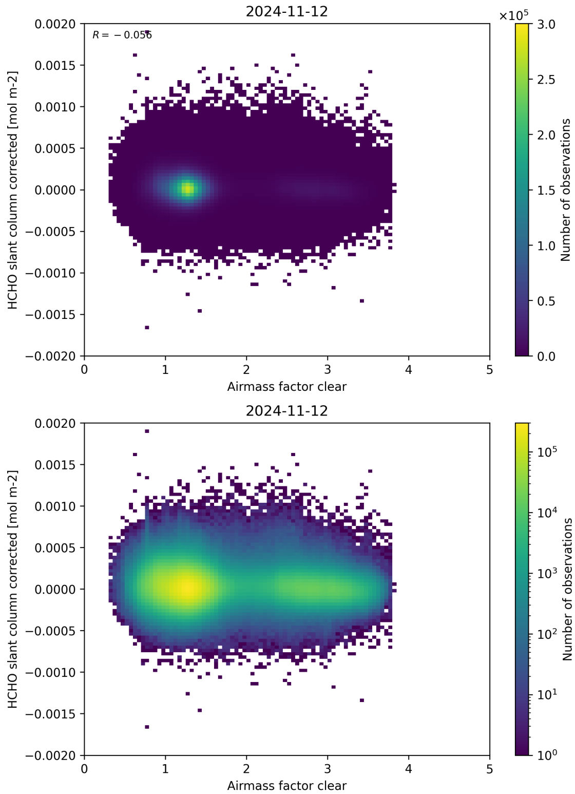
Figure 74: Scatter density plot of “Airmass factor clear” against “HCHO slant column corrected” for 2024-11-11 to 2024-11-13.
