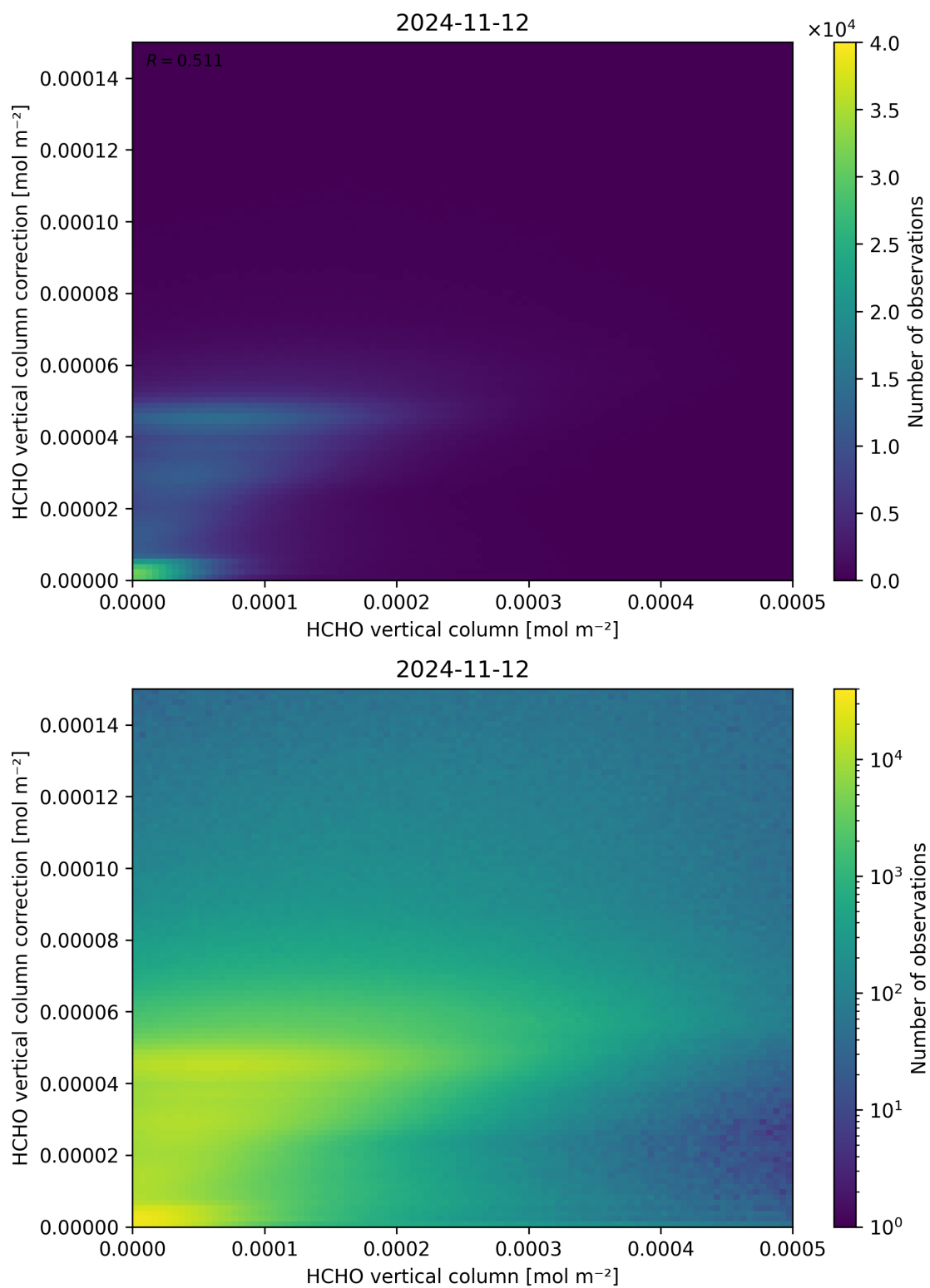
Figure 133: Scatter density plot of “HCHO vertical column” against “HCHO vertical column correction” for 2024-11-11 to 2024-11-13.
