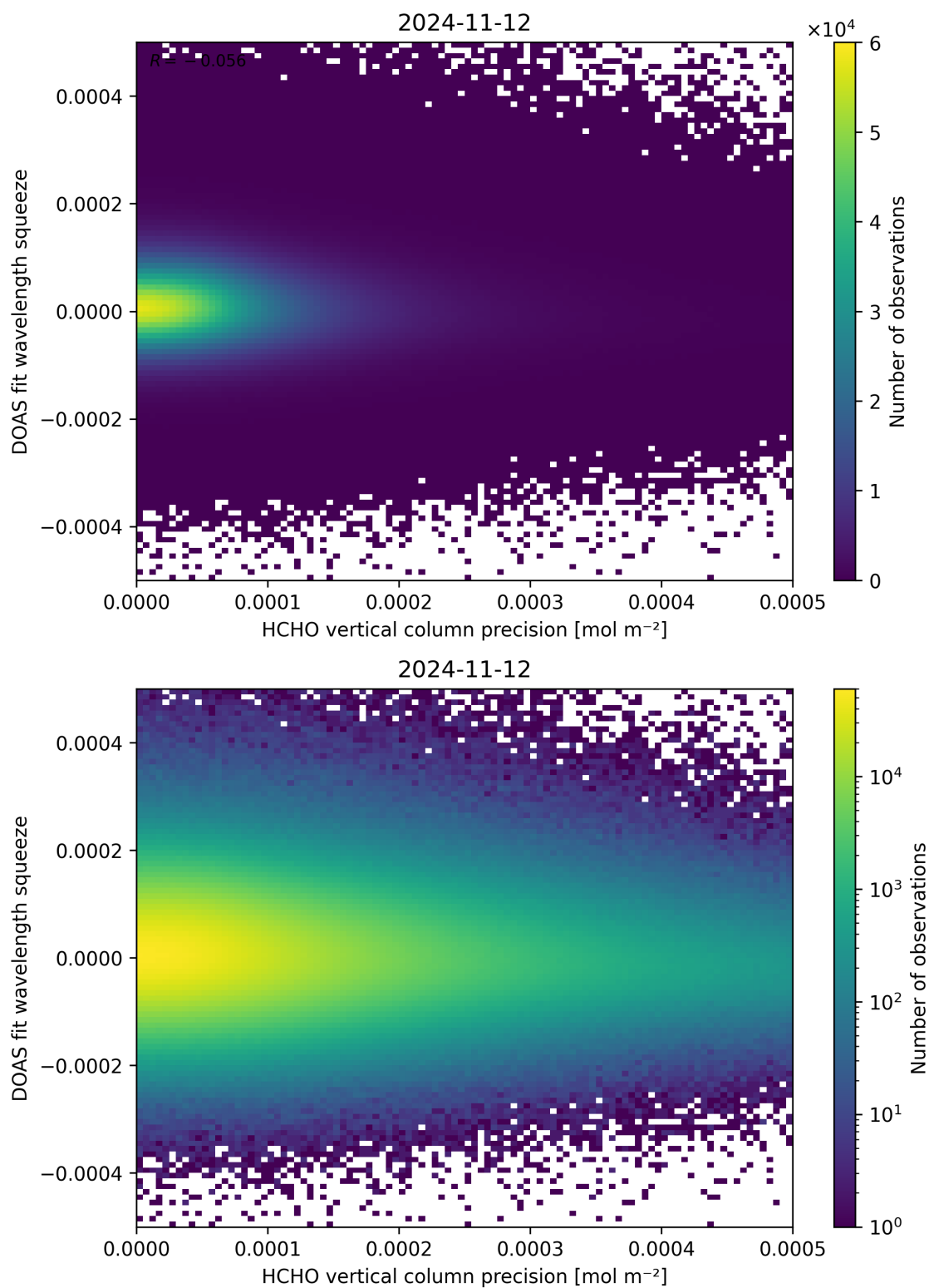
Figure 138: Scatter density plot of “HCHO vertical column precision” against “DOAS fit wavelength squeeze” for 2024-11-11 to 2024-11-13.
