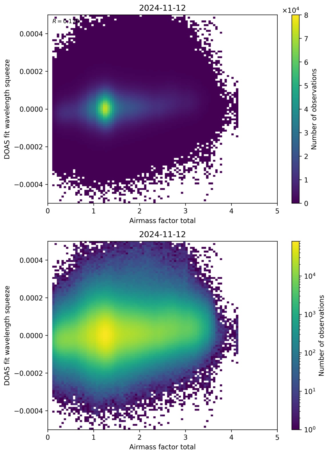
Figure 99: Scatter density plot of “Airmass factor total” against “DOAS fit wavelength squeeze” for 2024-11-11 to 2024-11-13.
