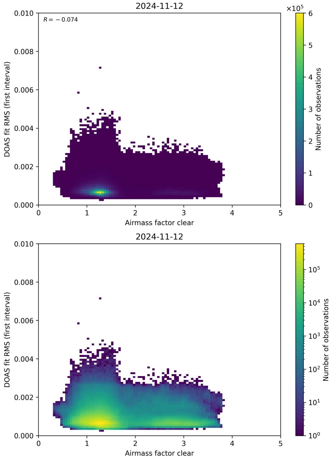
Figure 71: Scatter density plot of “Airmass factor clear” against “DOAS fit RMS (first interval)” for 2024-11-11 to 2024-11-13.
