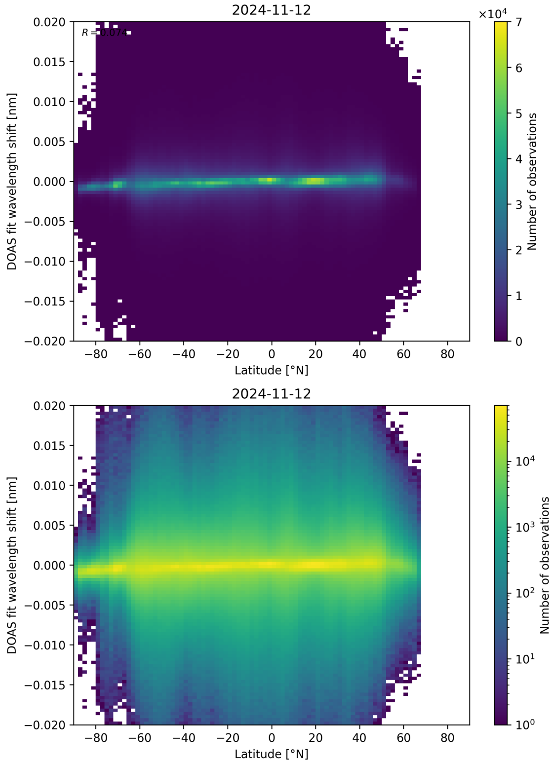
Figure 154: Scatter density plot of “Latitude” against “DOAS fit wavelength shift” for 2024-11-11 to 2024-11-13.
