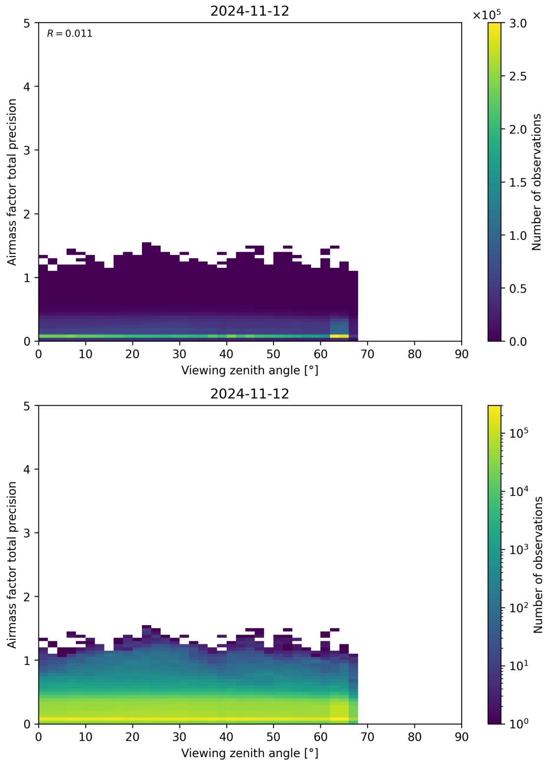
Figure 191: Scatter density plot of “Viewing zenith angle” against “Airmass factor total precision” for 2024-11-11 to 2024-11-13.
