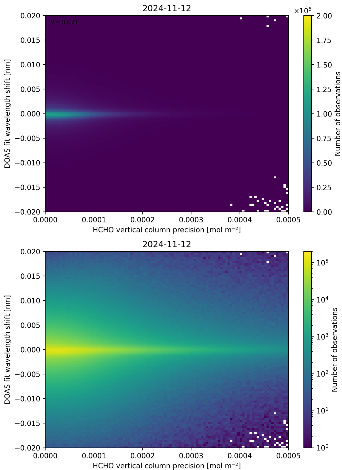
Figure 137: Scatter density plot of “HCHO vertical column precision” against “DOAS fit wavelength shift” for 2024-11-11 to 2024-11-13.
