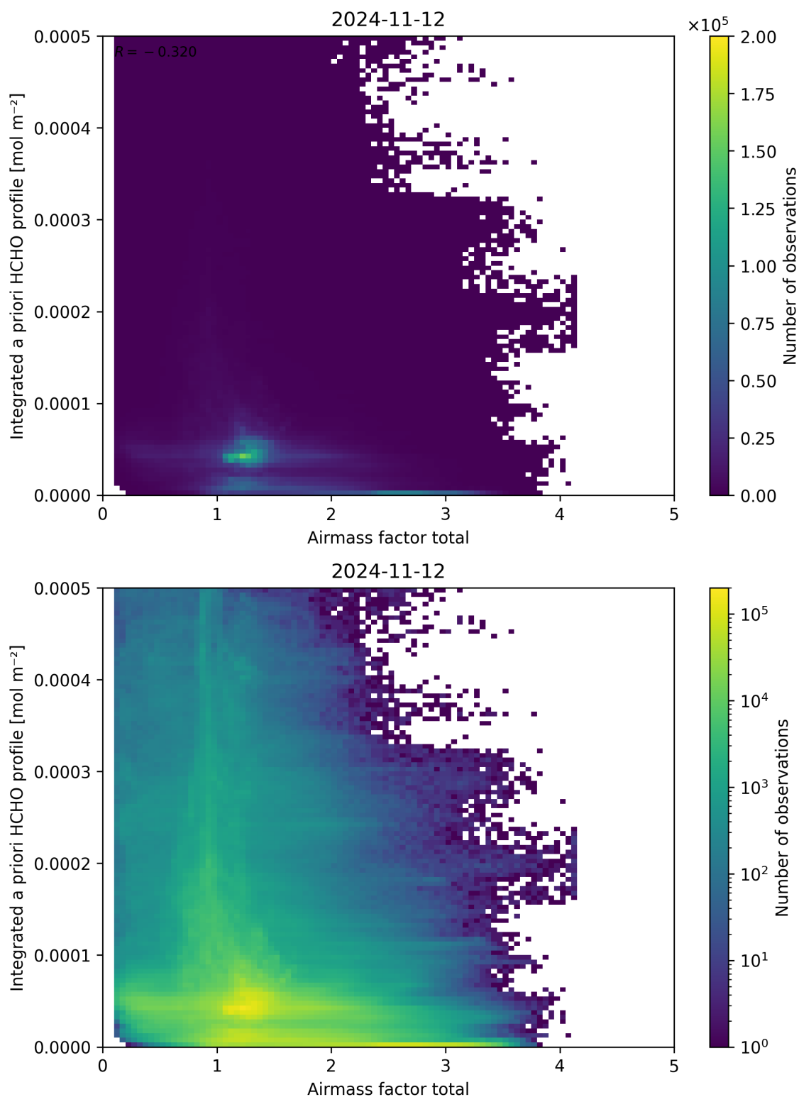
Figure 104: Scatter density plot of “Airmass factor total” against “Integrated a priori HCHO profile” for 2024-11-11 to 2024-11-13.
