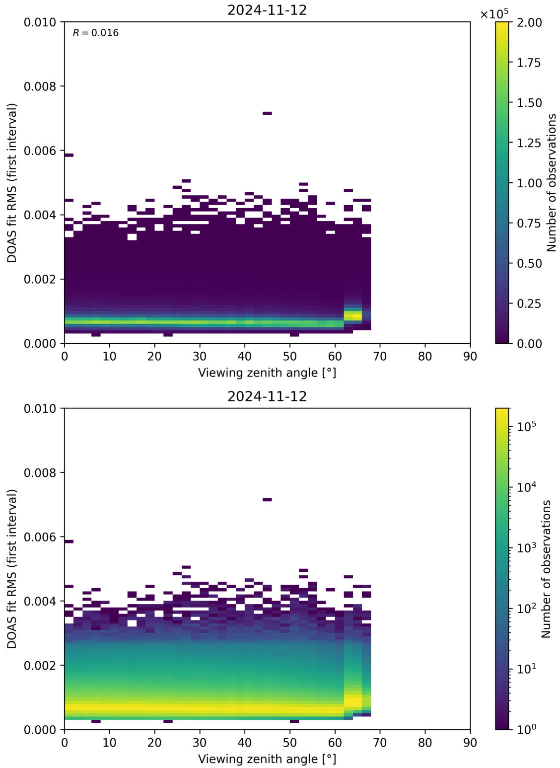
Figure 182: Scatter density plot of “Viewing zenith angle” against “DOAS fit RMS (first interval)” for 2024-11-11 to 2024-11-13.
