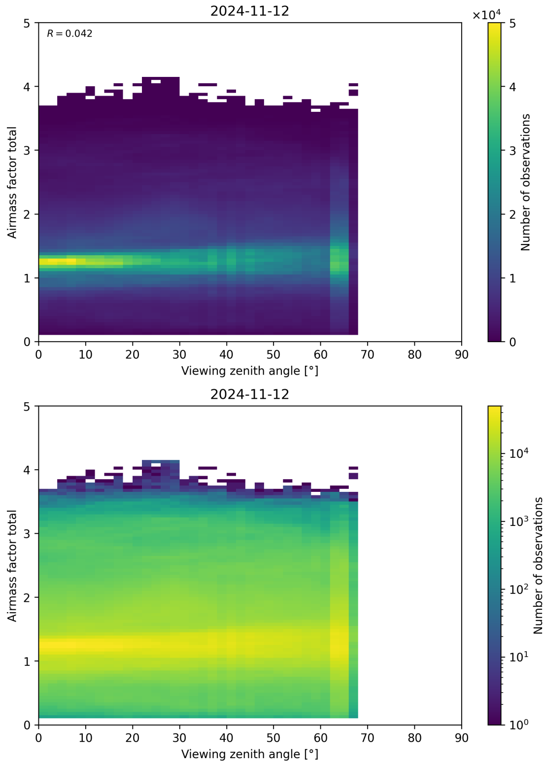
Figure 190: Scatter density plot of “Viewing zenith angle” against “Airmass factor total” for 2024-11-11 to 2024-11-13.
