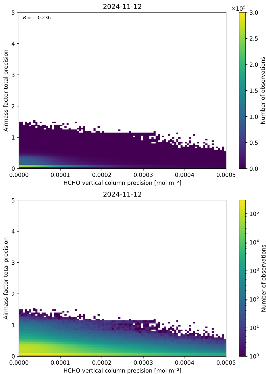
Figure 145: Scatter density plot of “HCHO vertical column precision” against “Airmass factor total precision” for 2024-11-11 to 2024-11-13.
