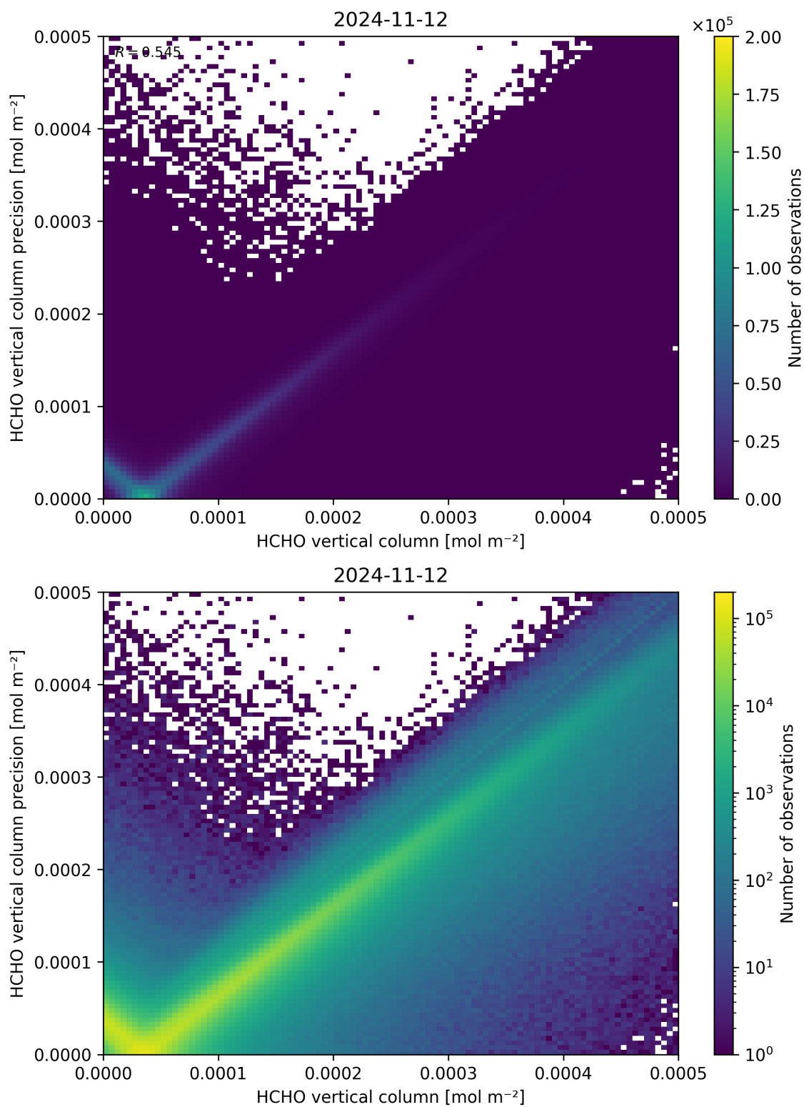
Figure 134: Scatter density plot of “HCHO vertical column” against “HCHO vertical column precision” for 2024-11-11 to 2024-11-13.
