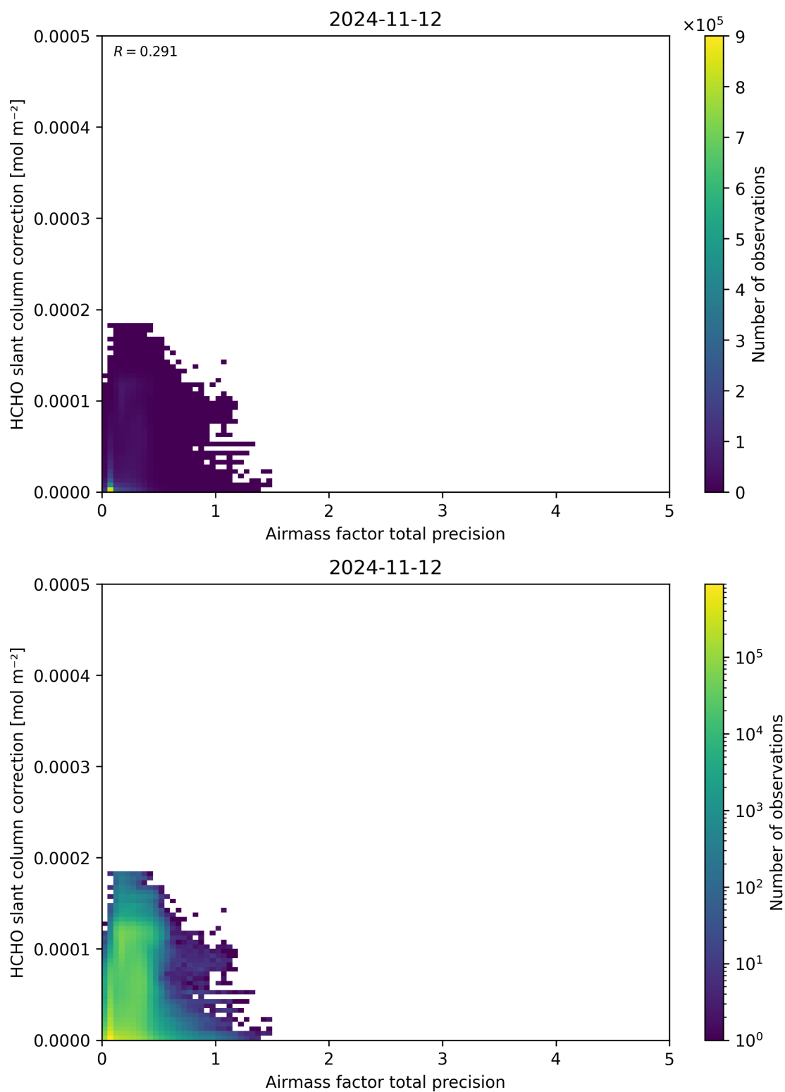
Figure 110: Scatter density plot of “Airmass factor total precision” against “HCHO slant column correction” for 2024-11-11 to 2024-11-13.
