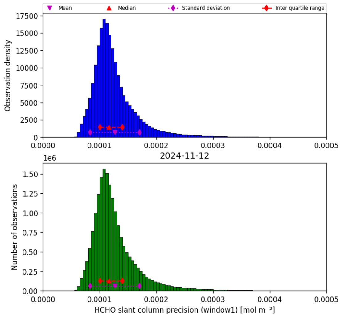
Figure 39: Histogram of “HCHO slant column precision (window1)” for 2024-11-11 to 2024-11-13
