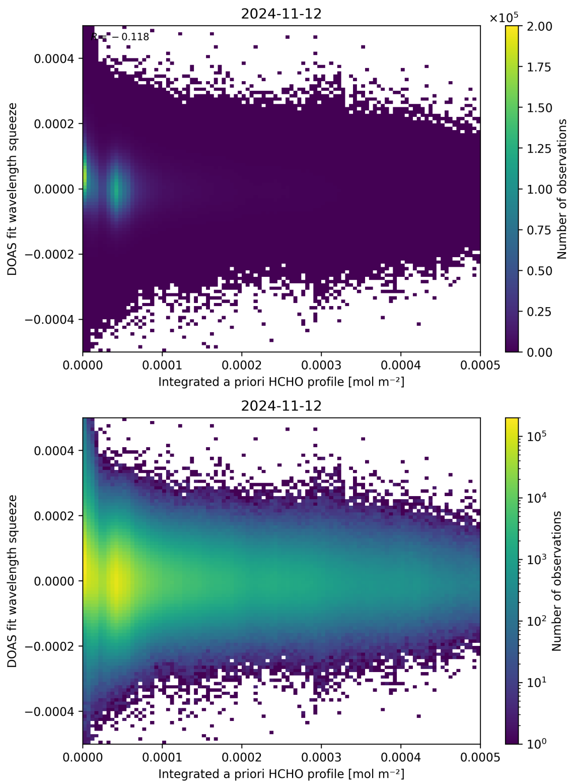
Figure 150: Scatter density plot of “Integrated a priori HCHO profile” against “DOAS fit wavelength squeeze” for 2024-11-11 to 2024-11-13.
