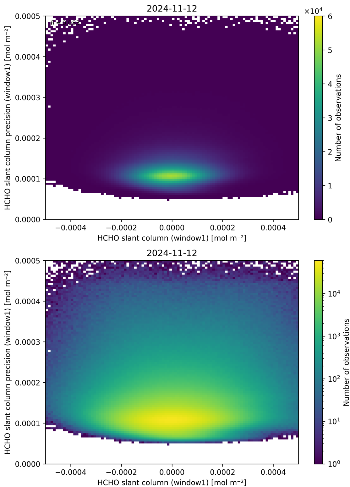
Figure 84: Scatter density plot of “HCHO slant column (window1)” against “HCHO slant column precision (window1)” for 2024-11-11 to 2024-11-13.
