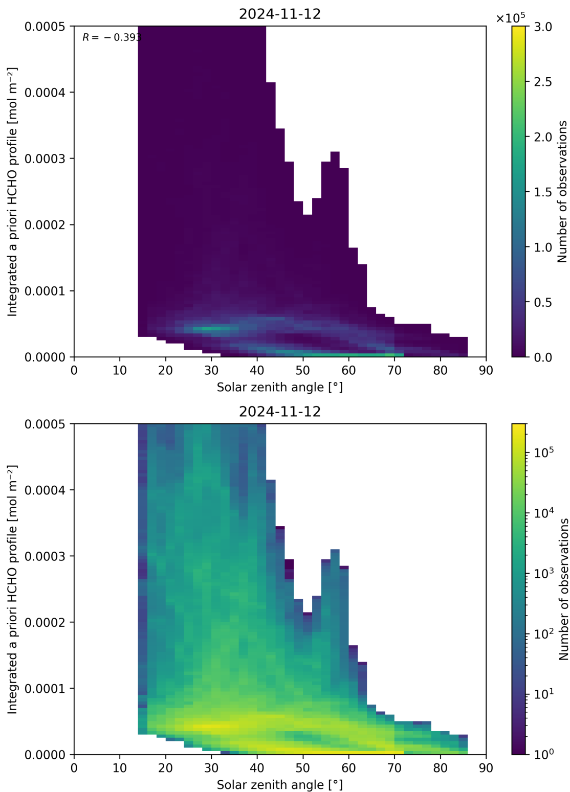
Figure 180: Scatter density plot of “Solar zenith angle” against “Integrated a priori HCHO profile” for 2024-11-11 to 2024-11-13.
