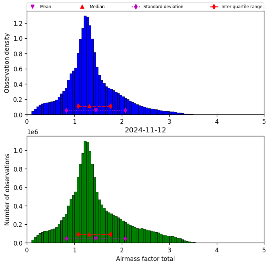
Figure 40: Histogram of “Airmass factor total” for 2024-11-11 to 2024-11-13
