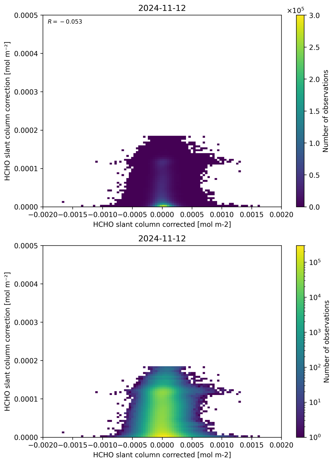
Figure 77: Scatter density plot of “HCHO slant column corrected” against “HCHO slant column correction” for 2024-11-11 to 2024-11-13.
