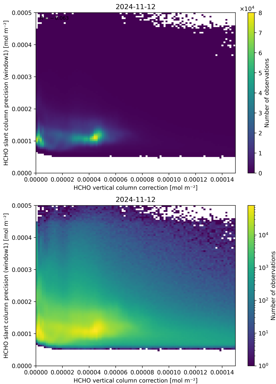
Figure 119: Scatter density plot of “HCHO vertical column correction” against “HCHO slant column precision (window1)” for 2024-11-11 to 2024-11-13.
