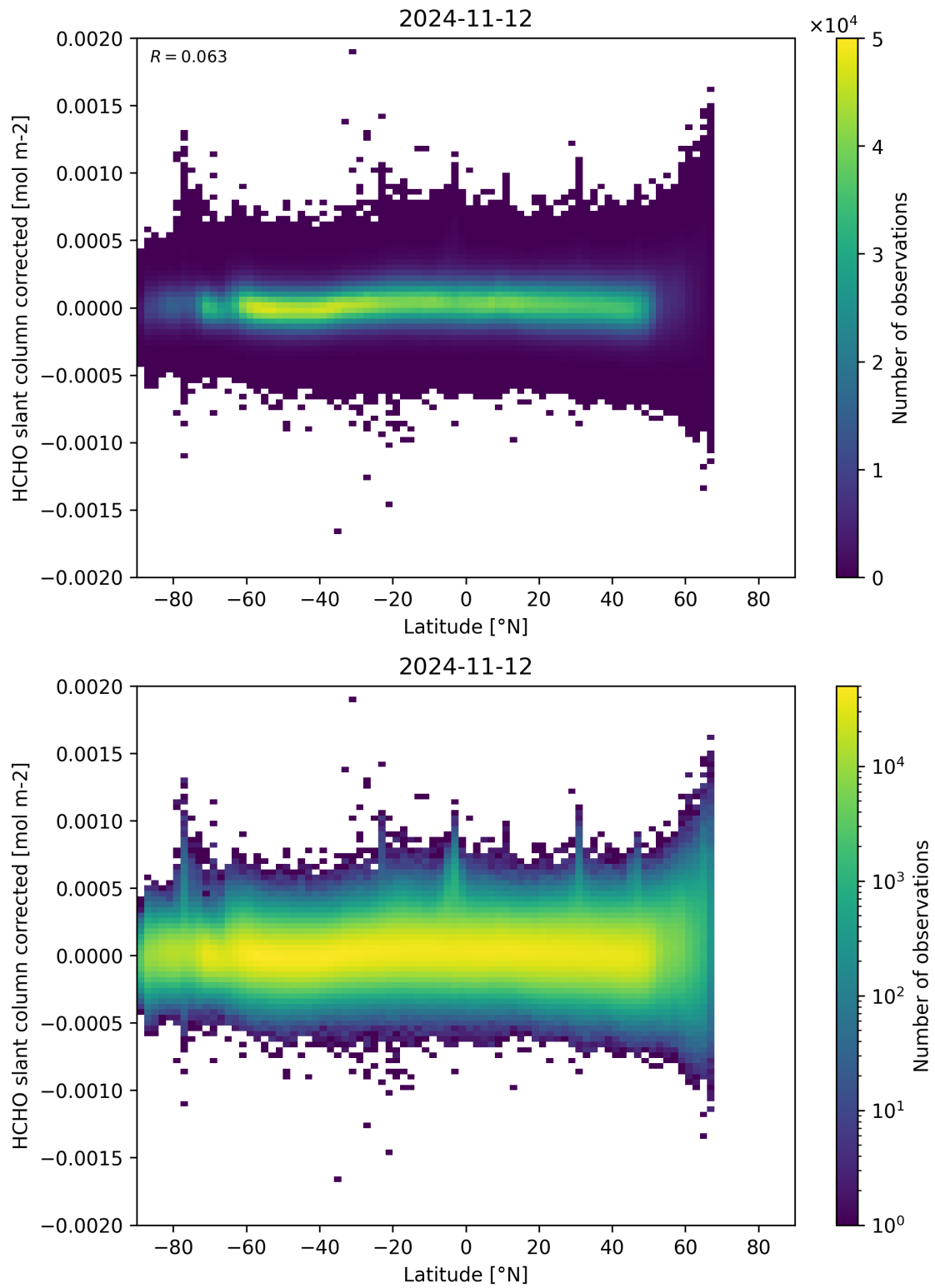
Figure 157: Scatter density plot of “Latitude” against “HCHO slant column corrected” for 2024-11-11 to 2024-11-13.
