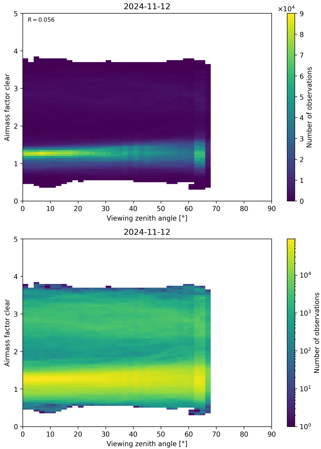
Figure 185: Scatter density plot of “Viewing zenith angle” against “Airmass factor clear” for 2024-11-11 to 2024-11-13.
