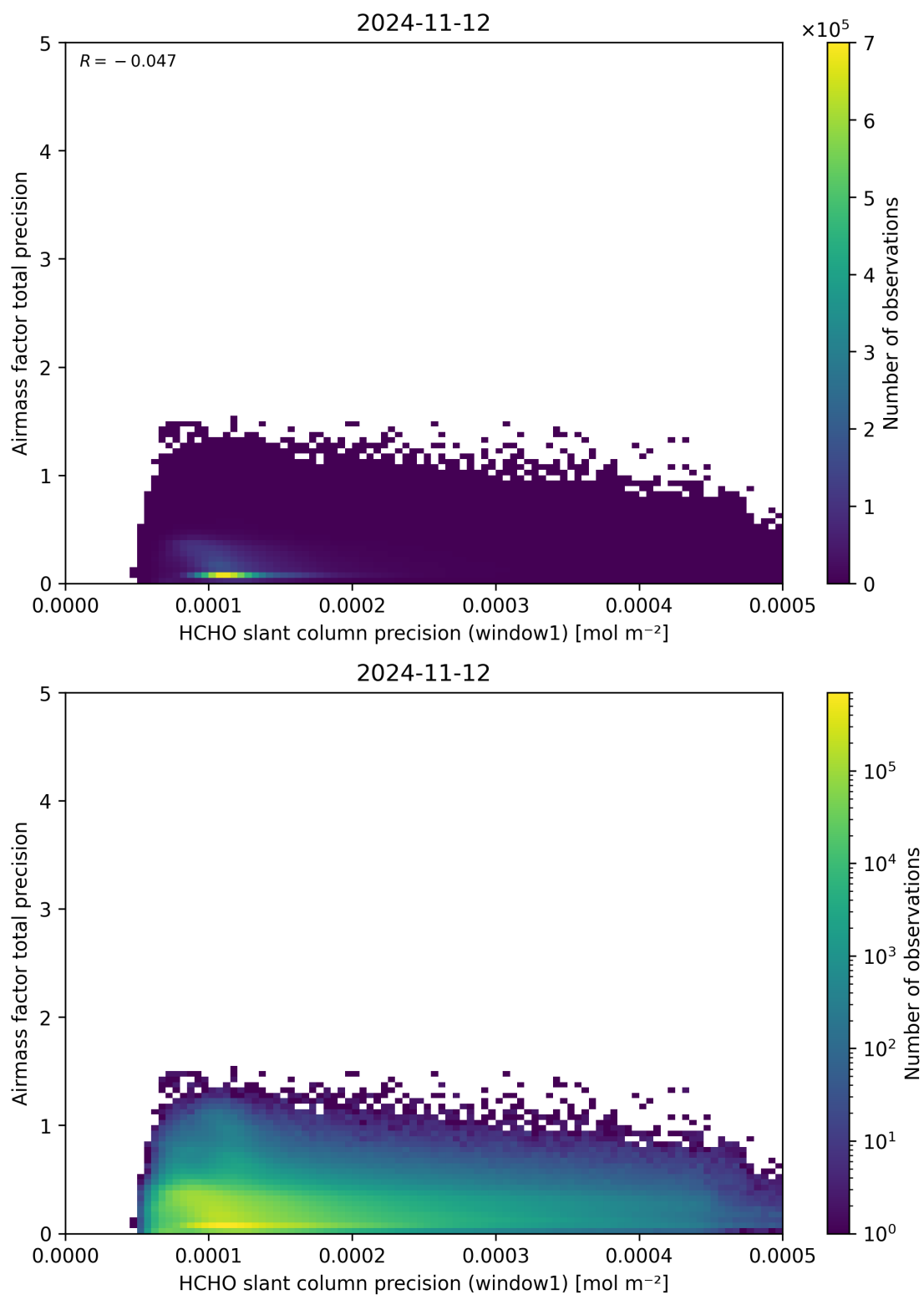
Figure 95: Scatter density plot of “HCHO slant column precision (window1)” against “Airmass factor total precision” for 2024-11-11 to 2024-11-13.
