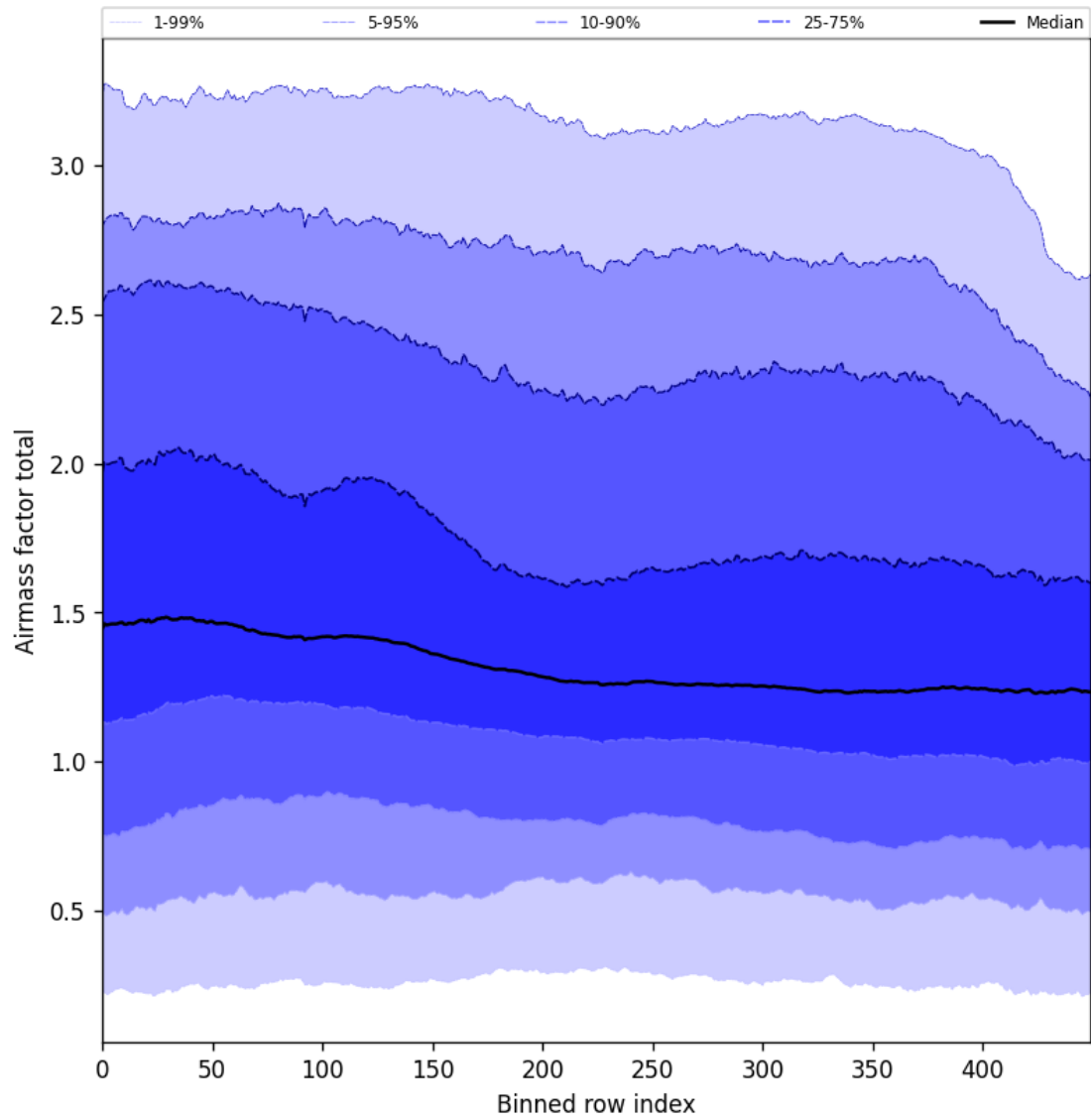
Figure 54: Along track statistics of “Airmass factor total” for 2024-11-11 to 2024-11-13
