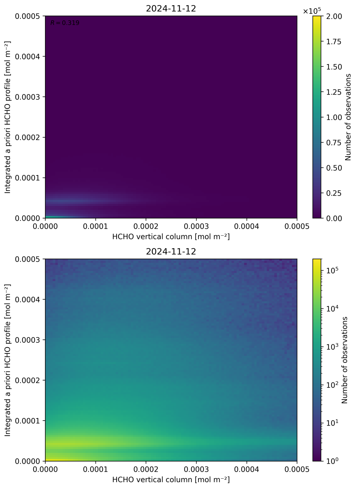
Figure 135: Scatter density plot of “HCHO vertical column” against “Integrated a priori HCHO profile” for 2024-11-11 to 2024-11-13.
