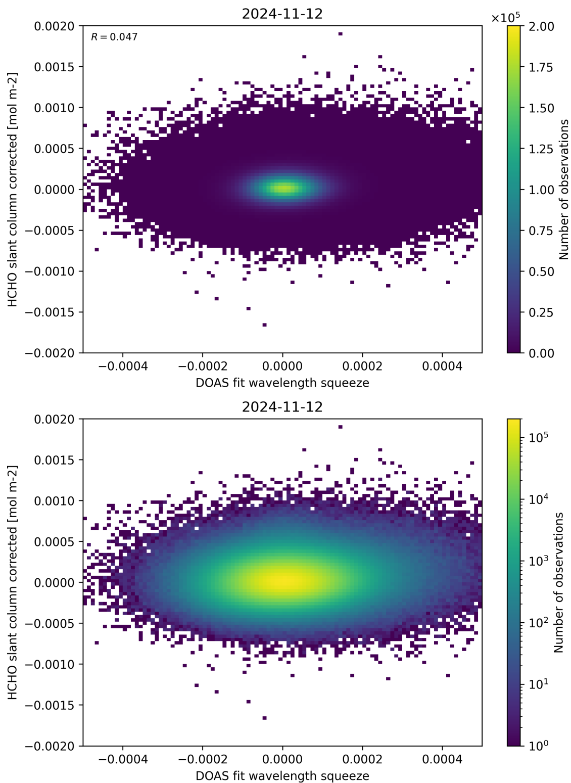
Figure 69: Scatter density plot of “DOAS fit wavelength squeeze” against “HCHO slant column corrected” for 2024-11-11 to 2024-11-13.
