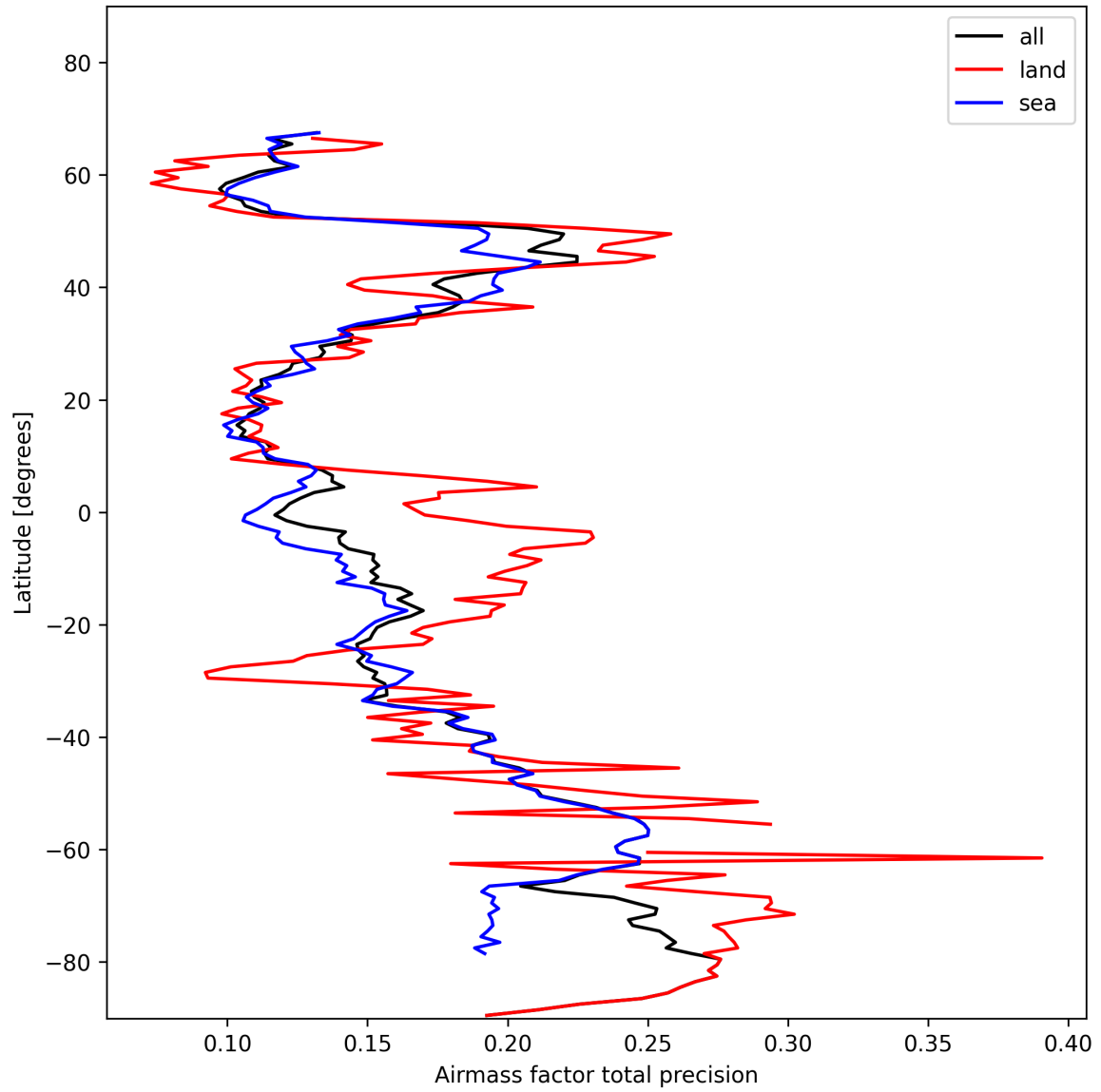
Figure 27: Zonal average of “Airmass factor total precision” for 2024-11-11 to 2024-11-13.
