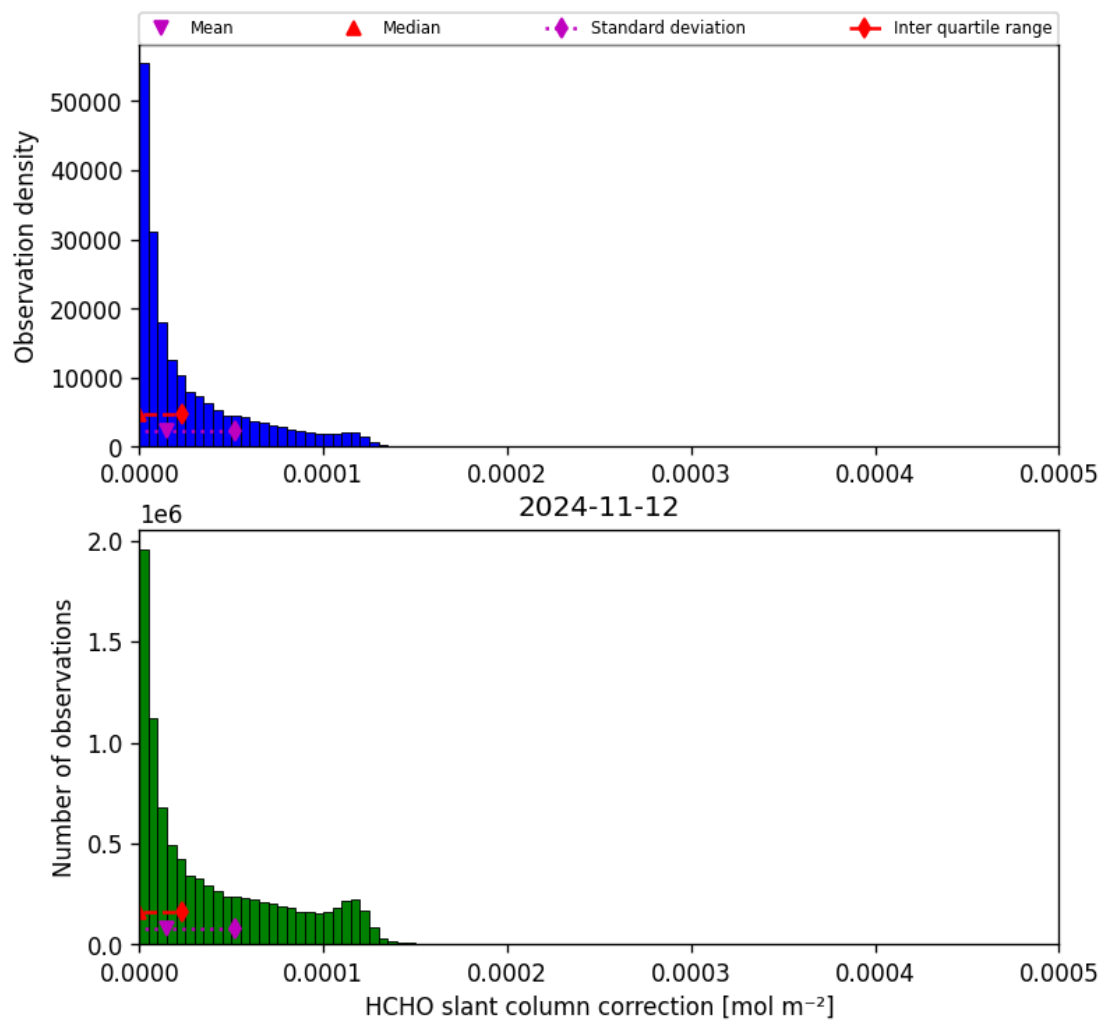
Figure 47: Histogram of “HCHO slant column correction” for 2024-11-11 to 2024-11-13
