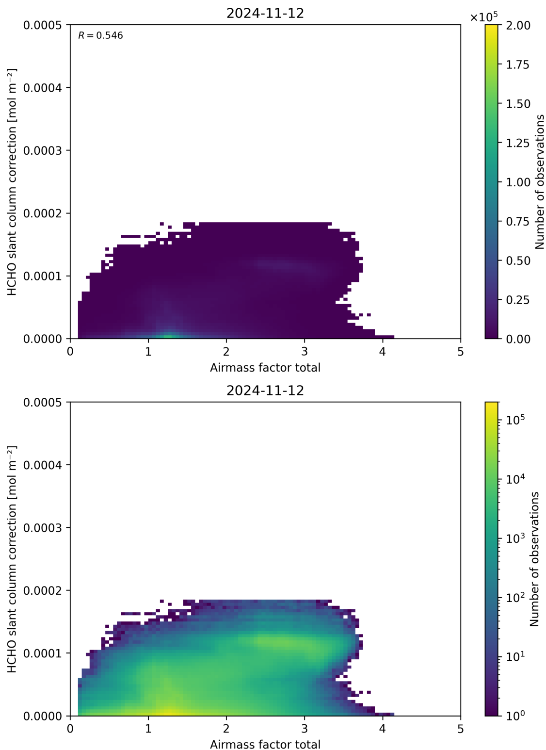
Figure 102: Scatter density plot of “Airmass factor total” against “HCHO slant column correction” for 2024-11-11 to 2024-11-13.
