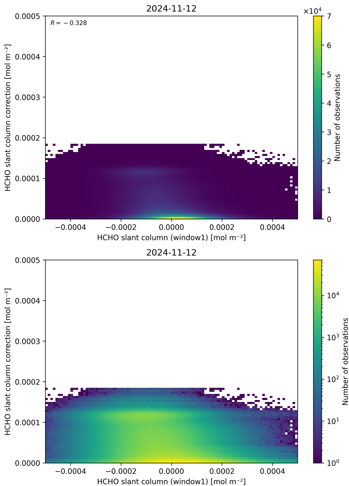
Figure 83: Scatter density plot of “HCHO slant column (window1)” against “HCHO slant column correction” for 2024-11-11 to 2024-11-13.
