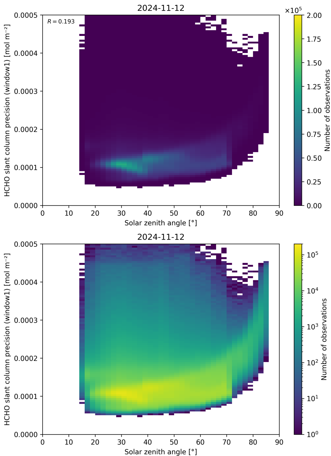
Figure 174: Scatter density plot of “Solar zenith angle” against “HCHO slant column precision (window1)” for 2024-11-11 to 2024-11-13.
