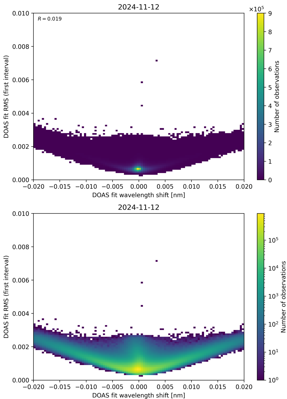
Figure 64: Scatter density plot of “DOAS fit wavelength shift” against “DOAS fit RMS (first interval)” for 2024-11-11 to 2024-11-13.
