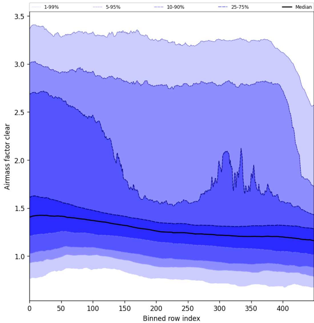
Figure 56: Along track statistics of “Airmass factor clear” for 2024-11-11 to 2024-11-13
