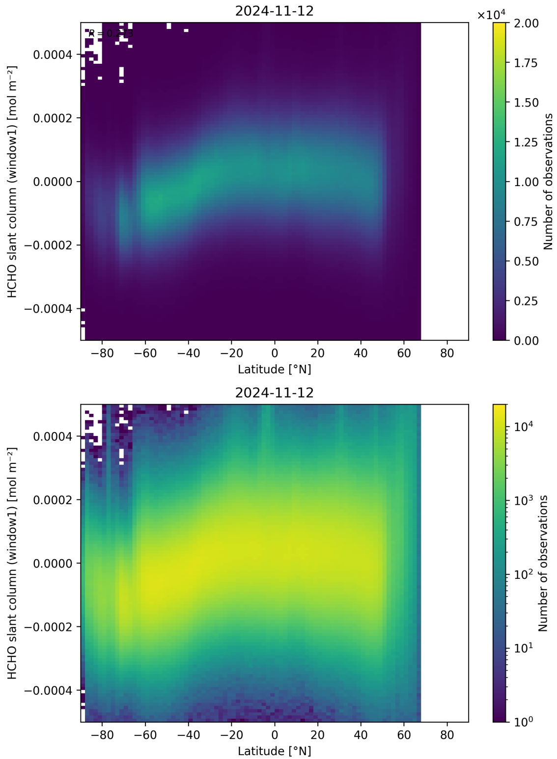
Figure 159: Scatter density plot of “Latitude” against “HCHO slant column (window1)” for 2024-11-11 to 2024-11-13.
