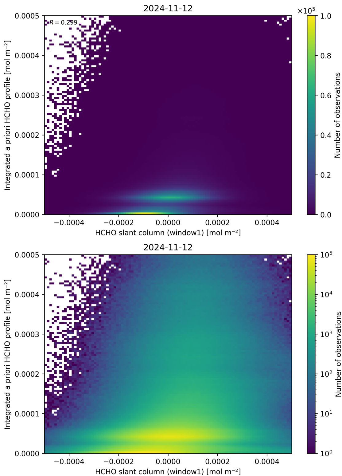
Figure 87: Scatter density plot of “HCHO slant column (window1)” against “Integrated a priori HCHO profile” for 2024-11-11 to 2024-11-13.
