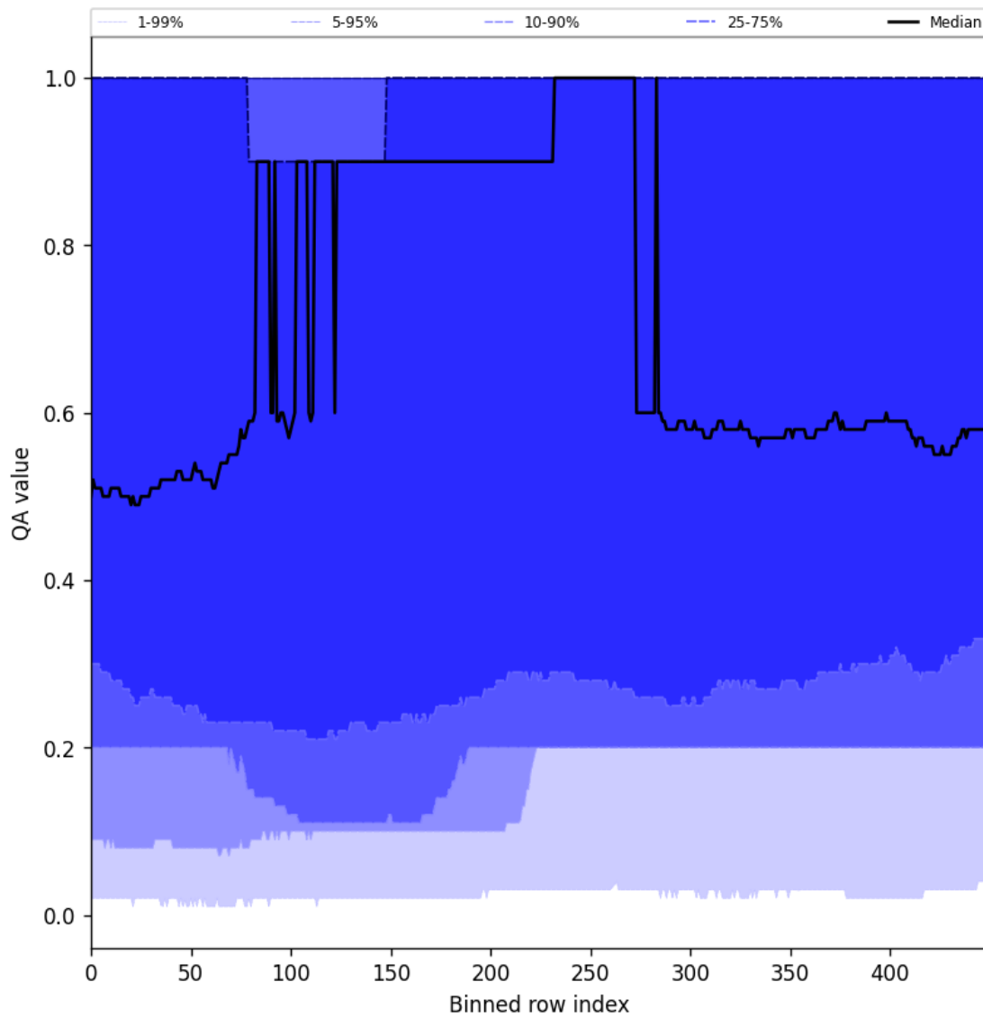
Figure 48: Along track statistics of “QA value” for 2024-11-11 to 2024-11-13
