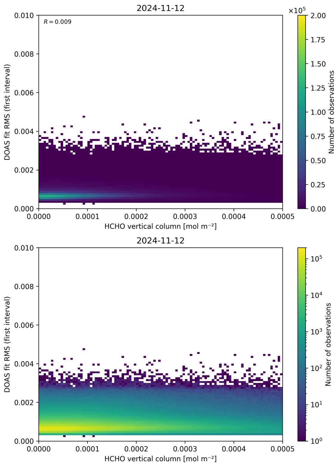
Figure 123: Scatter density plot of “HCHO vertical column” against “DOAS fit RMS (first interval)” for 2024-11-11 to 2024-11-13.
