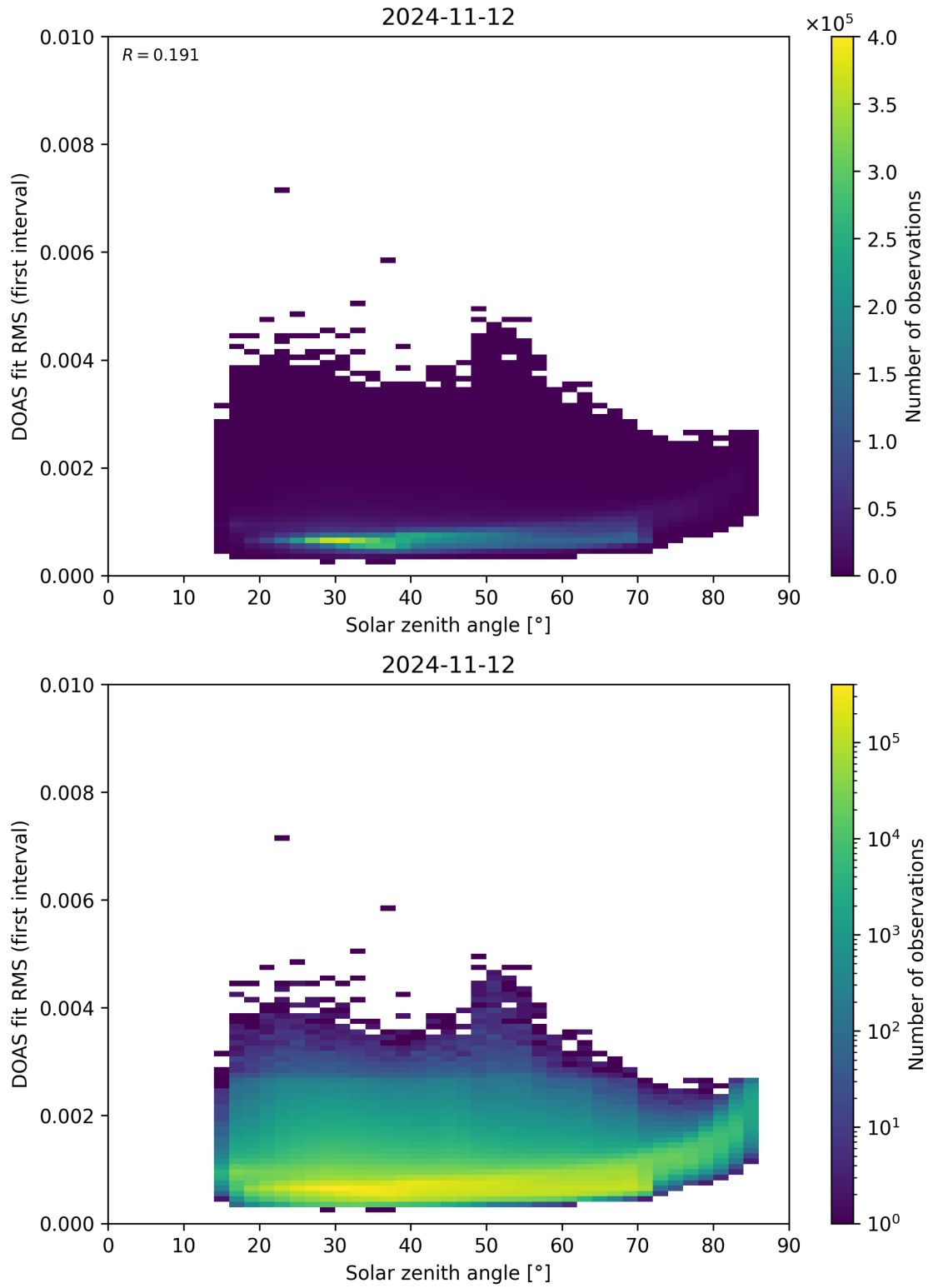
Figure 167: Scatter density plot of “Solar zenith angle” against “DOAS fit RMS (first interval)” for 2024-11-11 to 2024-11-13.
