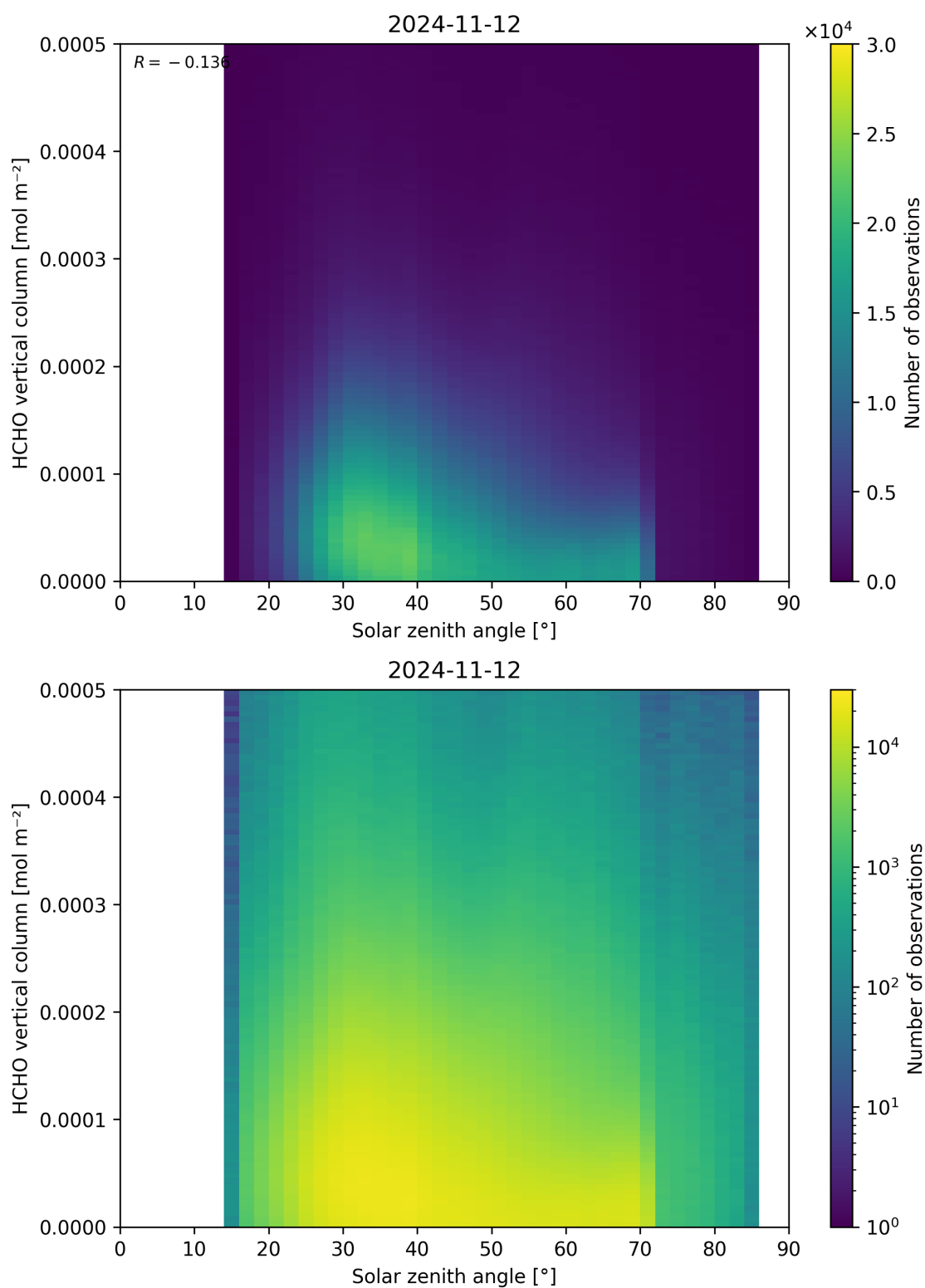
Figure 177: Scatter density plot of “Solar zenith angle” against “HCHO vertical column” for 2024-11-11 to 2024-11-13.
