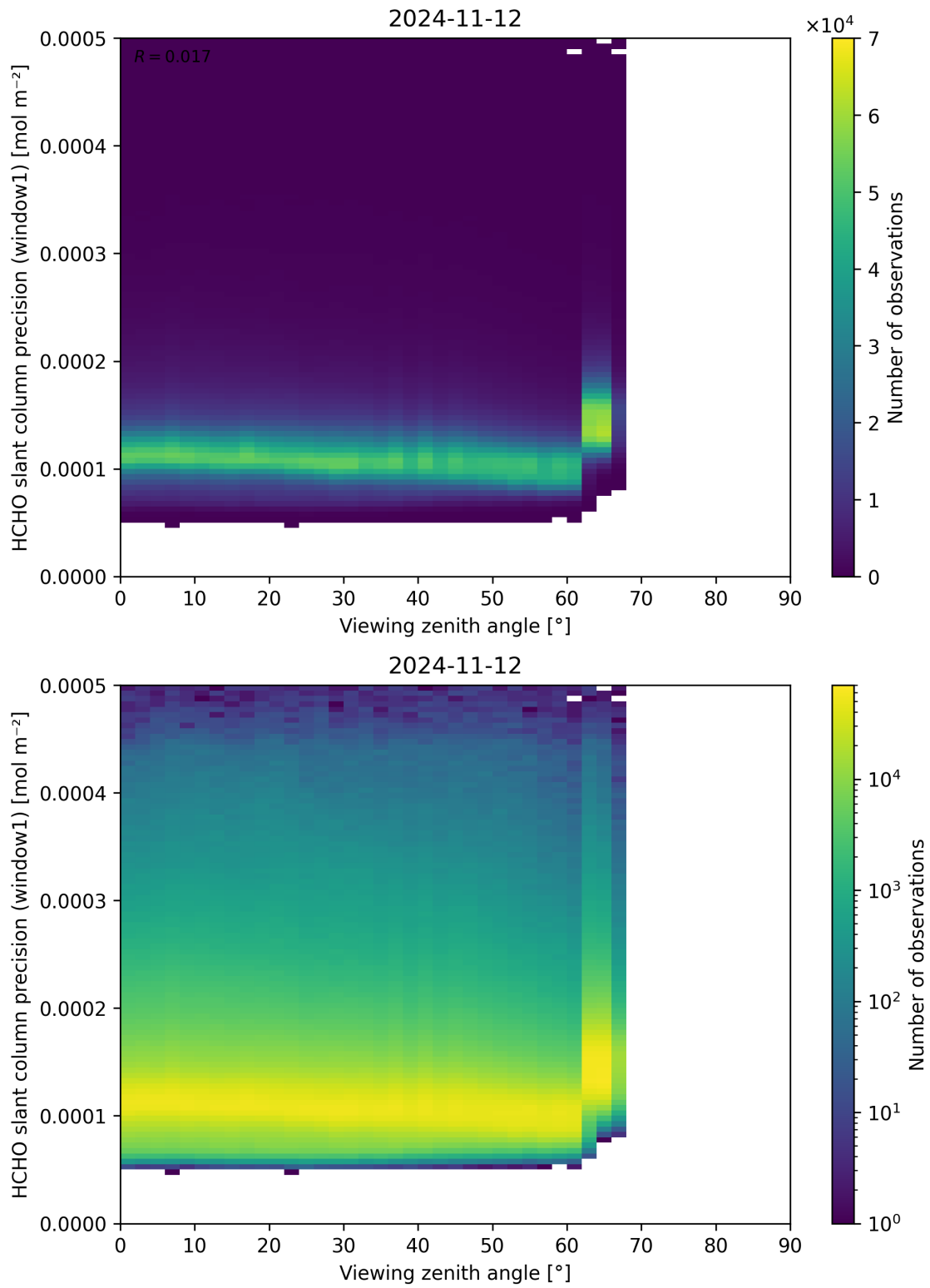
Figure 189: Scatter density plot of “Viewing zenith angle” against “HCHO slant column precision (window1)” for 2024-11-11 to 2024-11-13.
