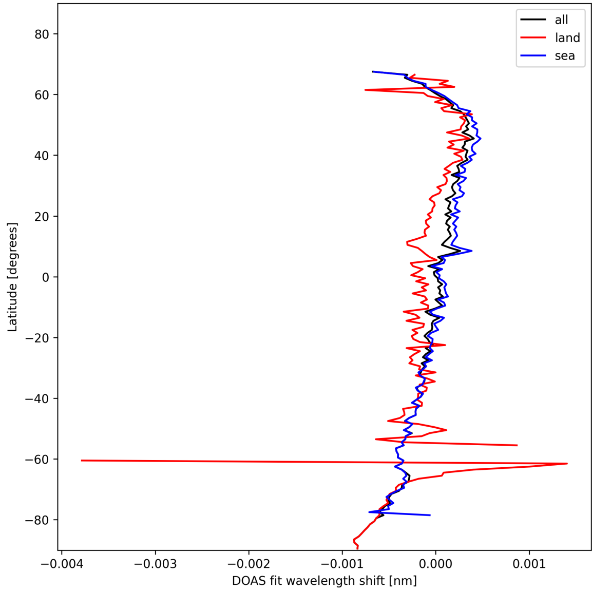
Figure 30: Zonal average of “DOAS fit wavelength shift” for 2024-11-11 to 2024-11-13.
