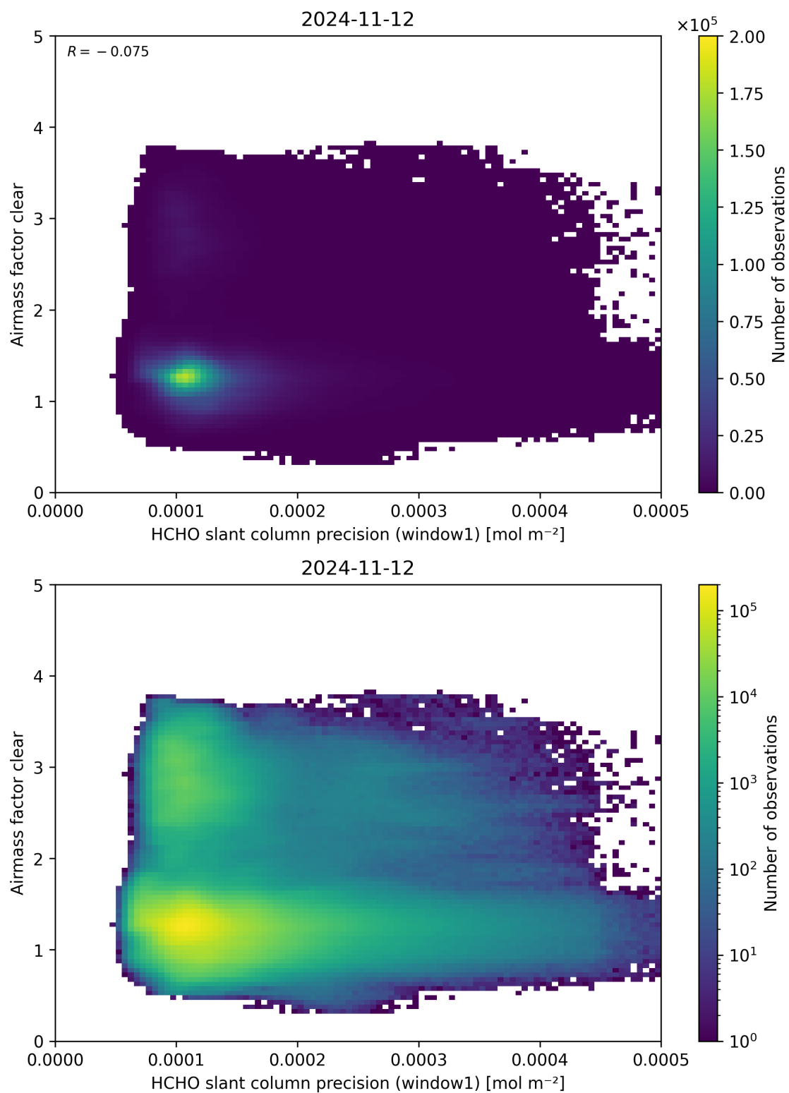
Figure 91: Scatter density plot of “HCHO slant column precision (window1)” against “Airmass factor clear” for 2024-11-11 to 2024-11-13.
