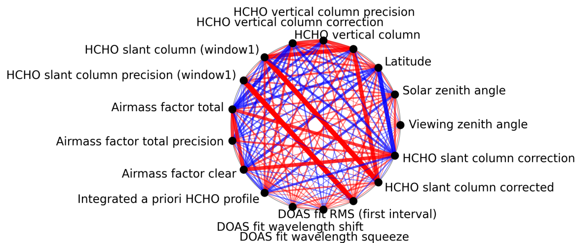
Figure 1: Map of correlation graph for 2024-11-11 to 2024-11-13.
