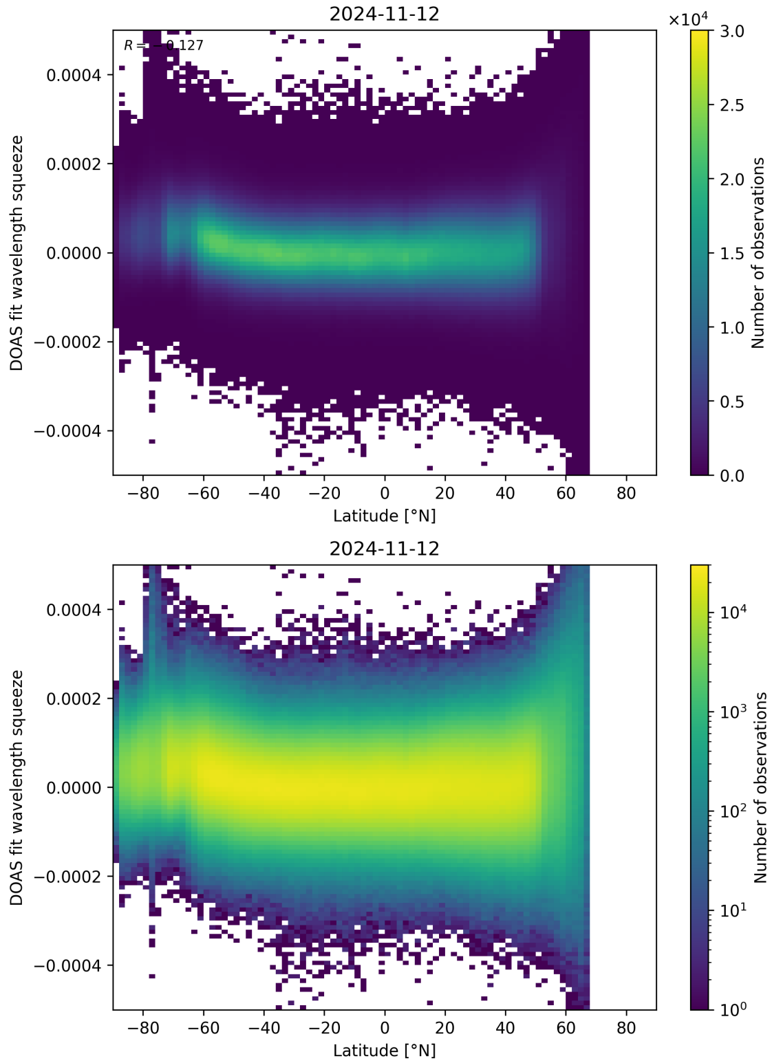
Figure 155: Scatter density plot of “Latitude” against “DOAS fit wavelength squeeze” for 2024-11-11 to 2024-11-13.
