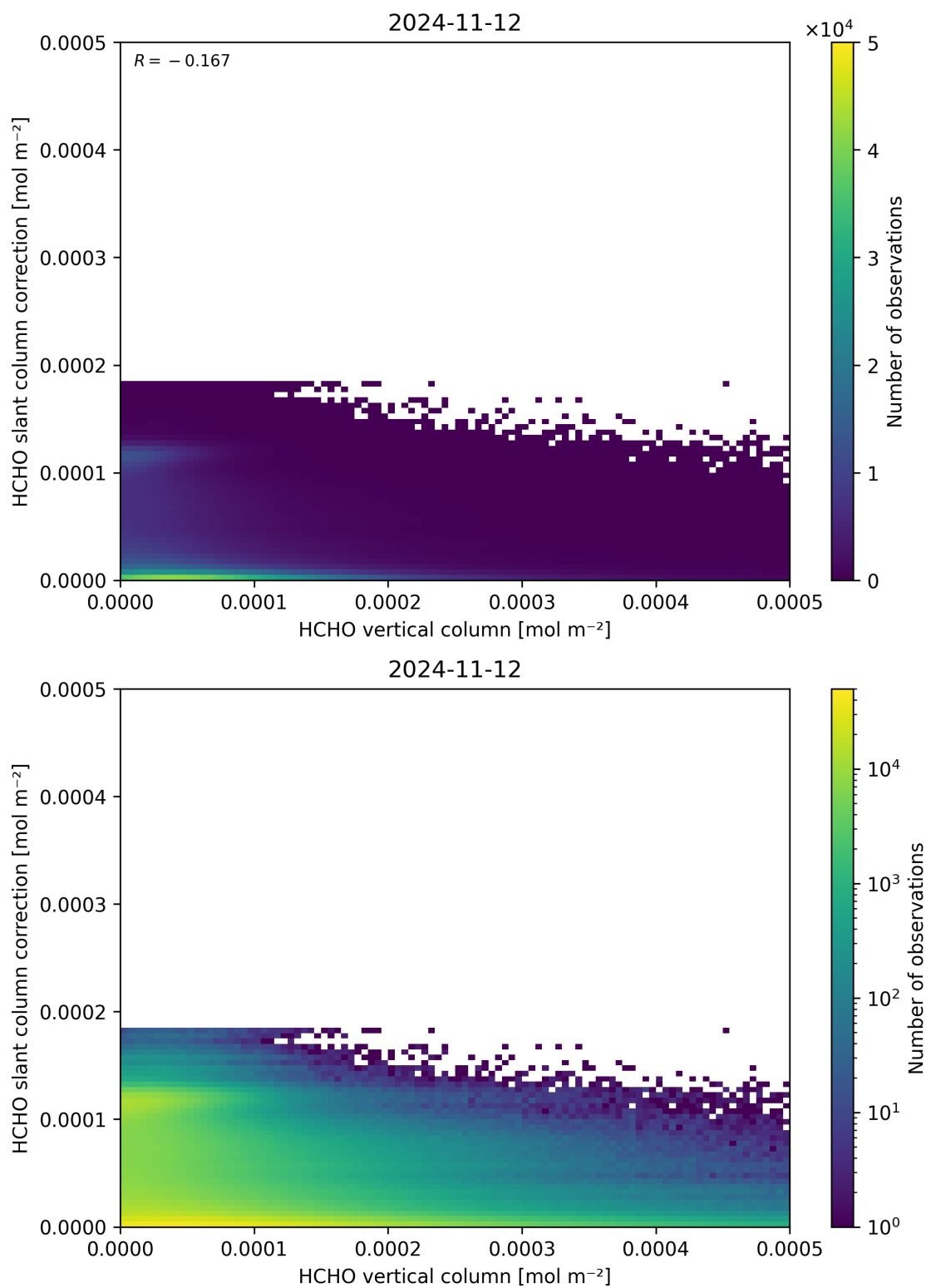
Figure 128: Scatter density plot of “HCHO vertical column” against “HCHO slant column correction” for 2024-11-11 to 2024-11-13.
