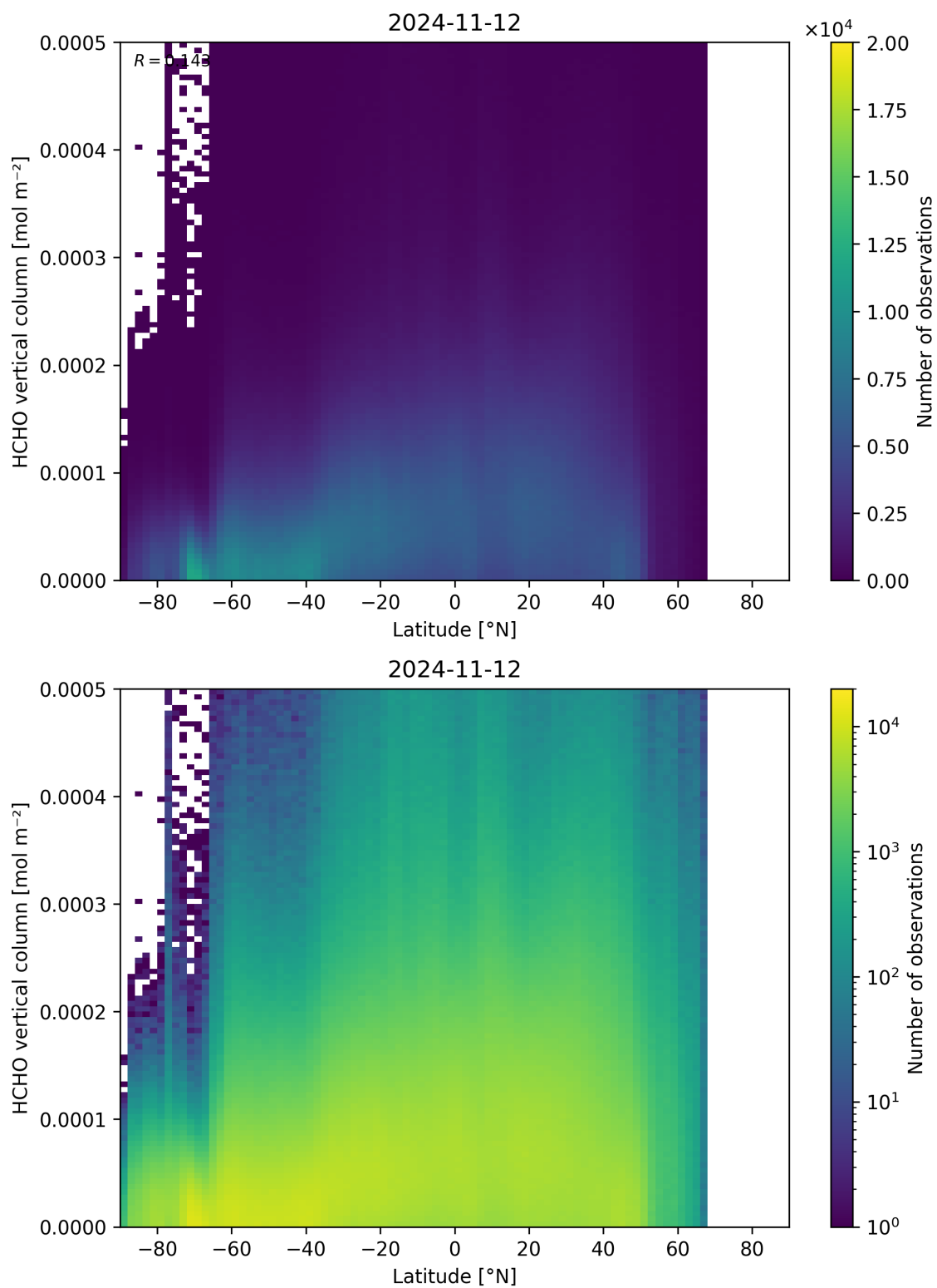
Figure 163: Scatter density plot of “Latitude” against “HCHO vertical column” for 2024-11-11 to 2024-11-13.
