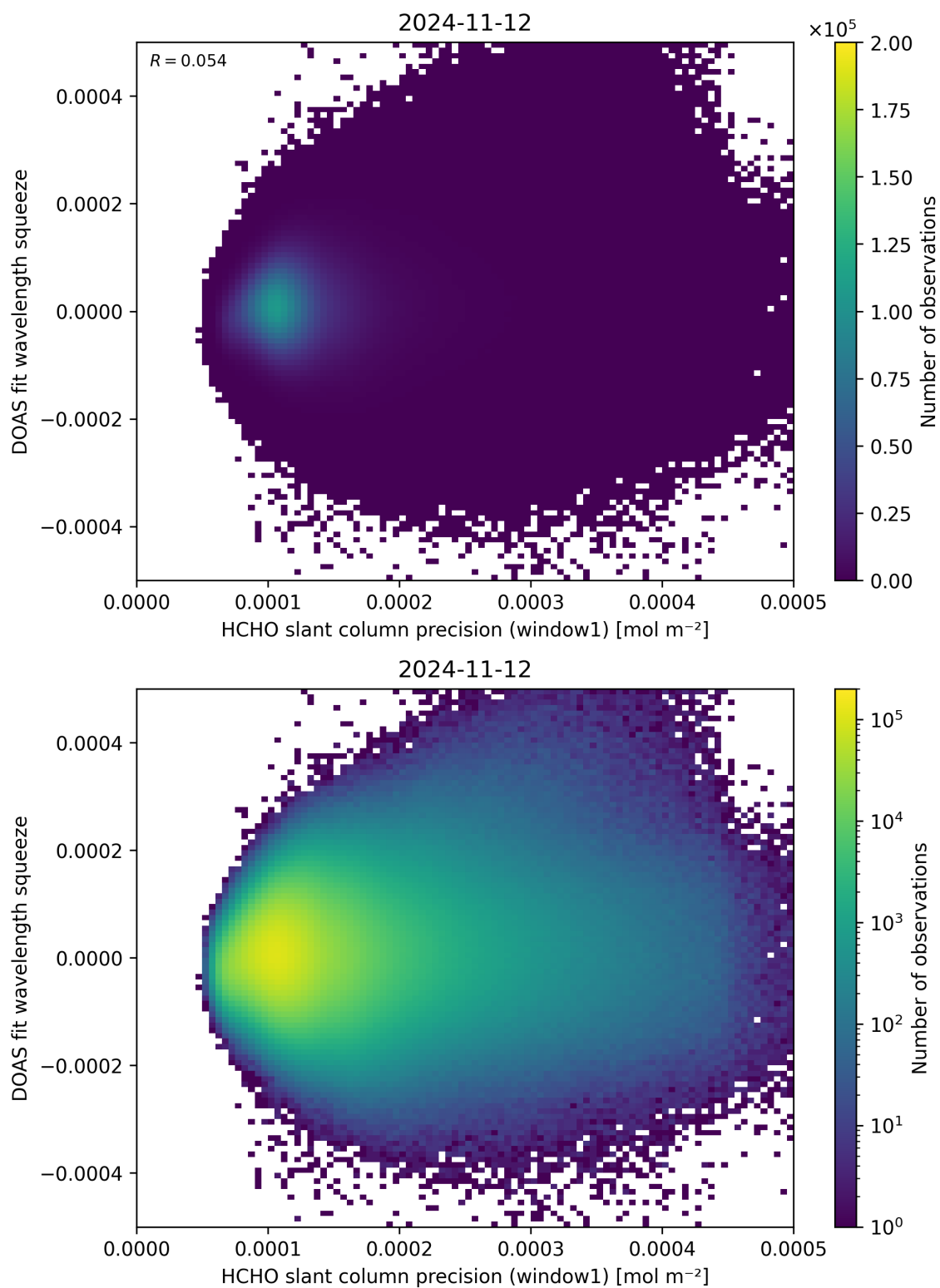
Figure 90: Scatter density plot of “HCHO slant column precision (window1)” against “DOAS fit wavelength squeeze” for 2024-11-11 to 2024-11-13.
