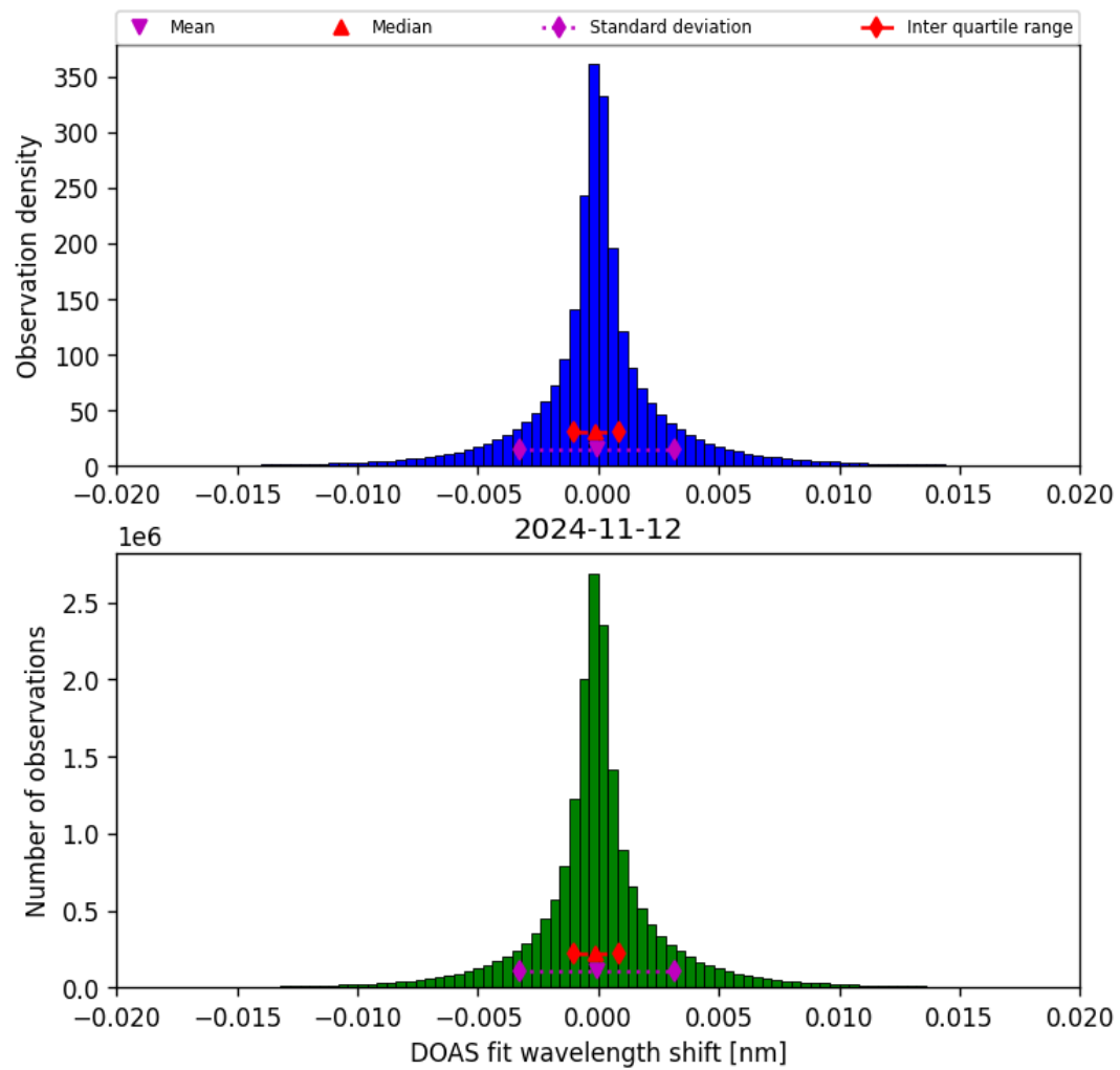
Figure 44: Histogram of “DOAS fit wavelength shift” for 2024-11-11 to 2024-11-13
