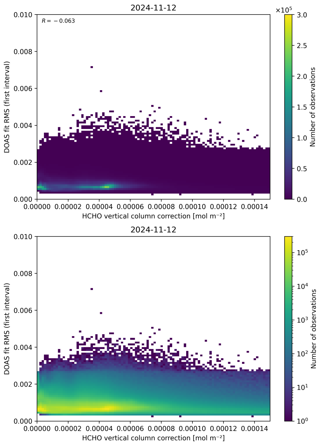
Figure 112: Scatter density plot of “HCHO vertical column correction” against “DOAS fit RMS (first interval)” for 2024-11-11 to 2024-11-13.
