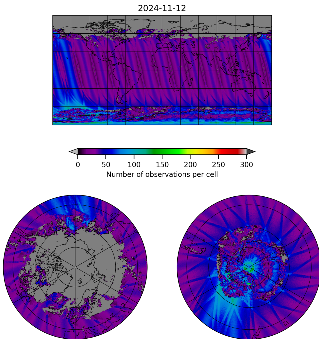
Figure 19: Map of the number of observations for 2024-11-11 to 2024-11-13
