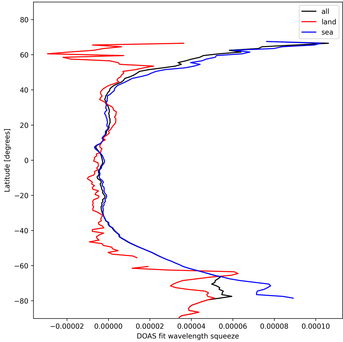
Figure 31: Zonal average of “DOAS fit wavelength squeeze” for 2024-11-11 to 2024-11-13.
