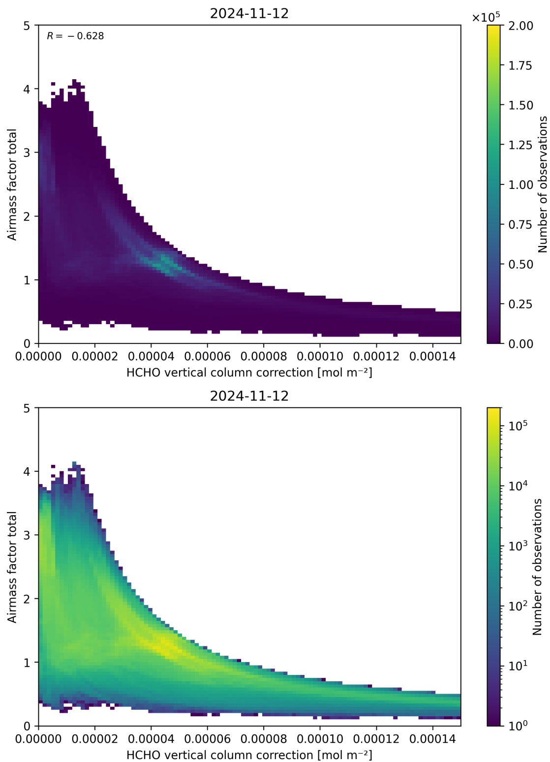
Figure 120: Scatter density plot of “HCHO vertical column correction” against “Airmass factor total” for 2024-11-11 to 2024-11-13.
