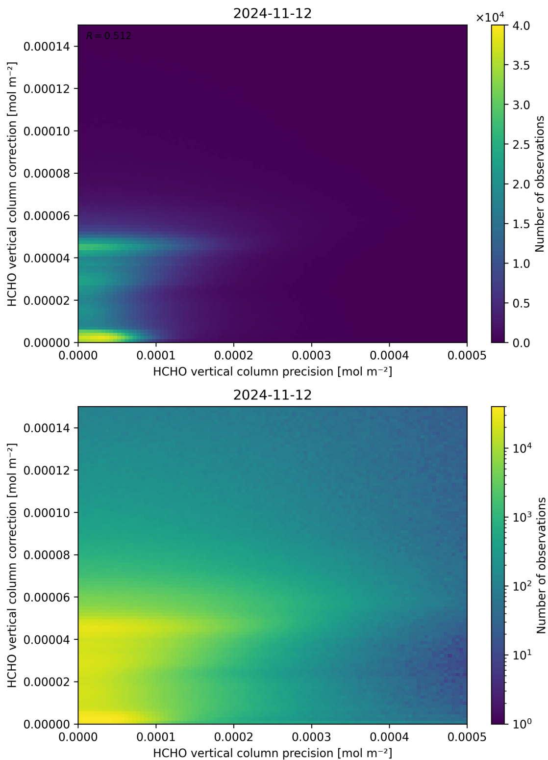
Figure 146: Scatter density plot of “HCHO vertical column precision” against “HCHO vertical column correction” for 2024-11-11 to 2024-11-13.
