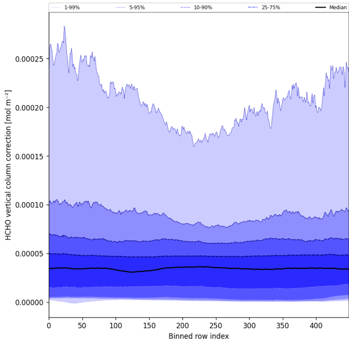
Figure 51: Along track statistics of “HCHO vertical column correction” for 2024-11-11 to 2024-11-13
