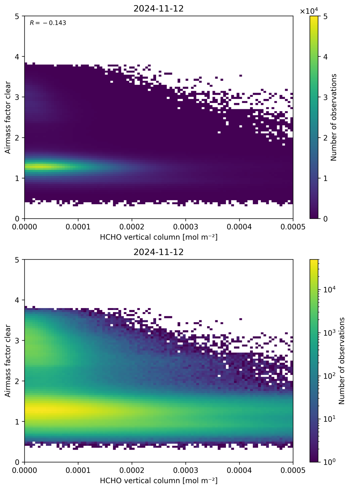
Figure 126: Scatter density plot of “HCHO vertical column” against “Airmass factor clear” for 2024-11-11 to 2024-11-13.
