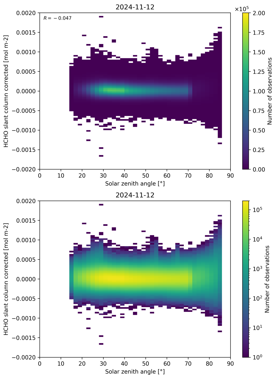
Figure 171: Scatter density plot of “Solar zenith angle” against “HCHO slant column corrected” for 2024-11-11 to 2024-11-13.
