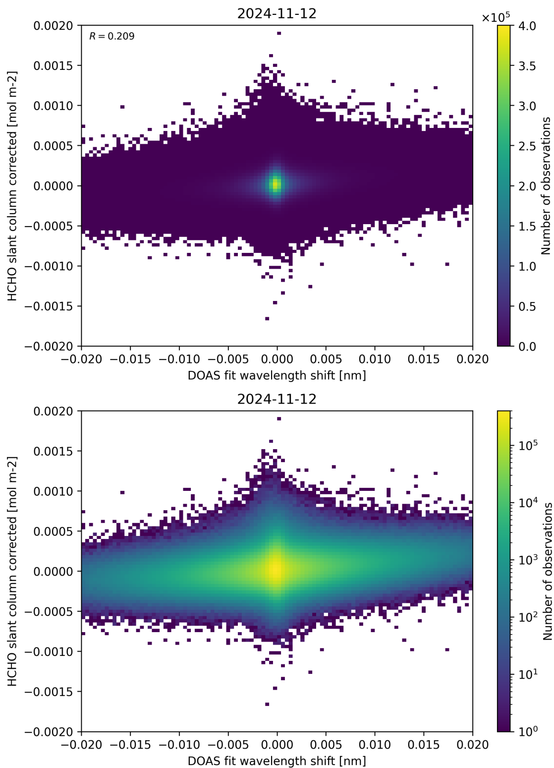
Figure 66: Scatter density plot of “DOAS fit wavelength shift” against “HCHO slant column corrected” for 2024-11-11 to 2024-11-13.
