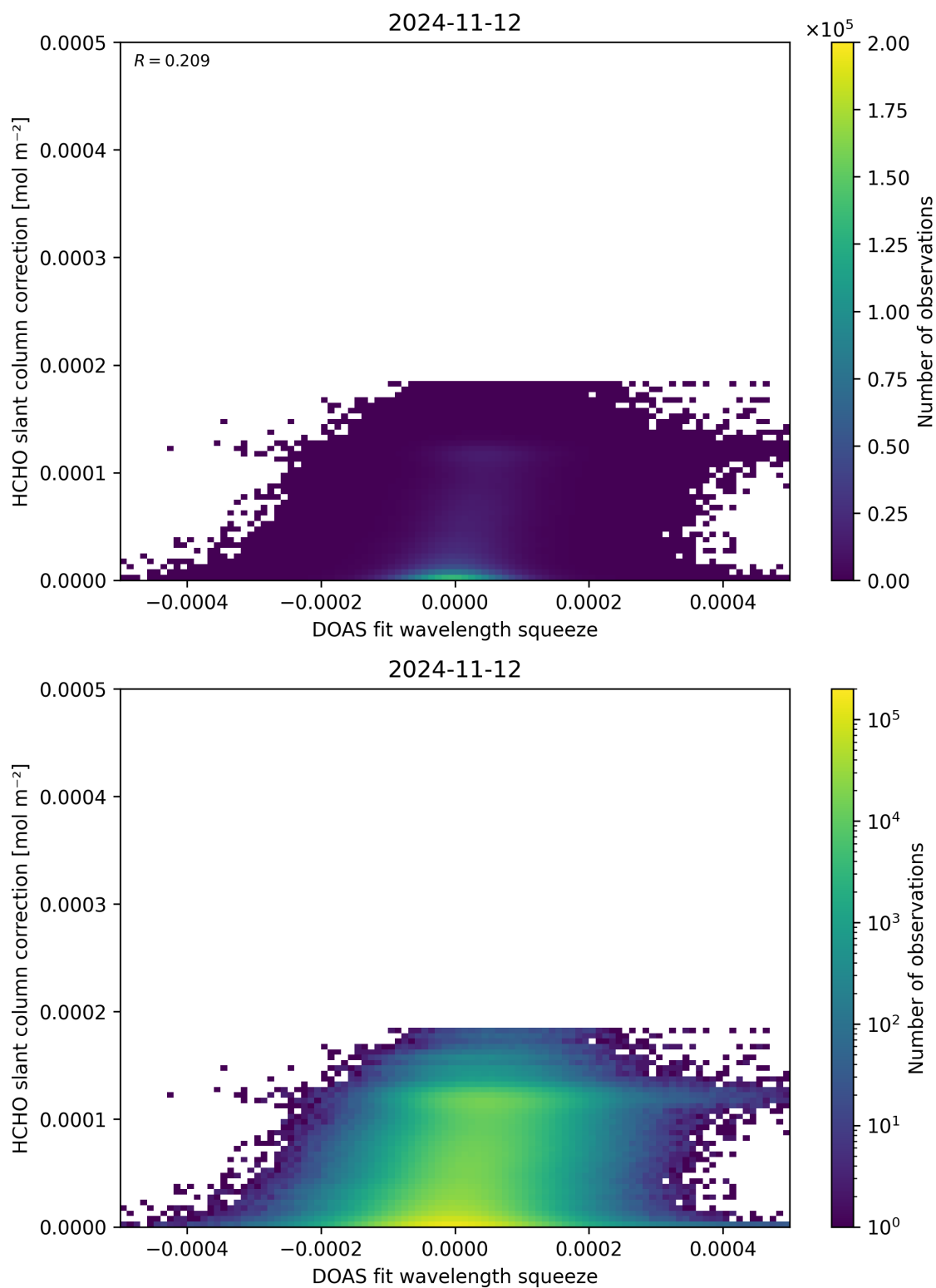
Figure 70: Scatter density plot of “DOAS fit wavelength squeeze” against “HCHO slant column correction” for 2024-11-11 to 2024-11-13.
