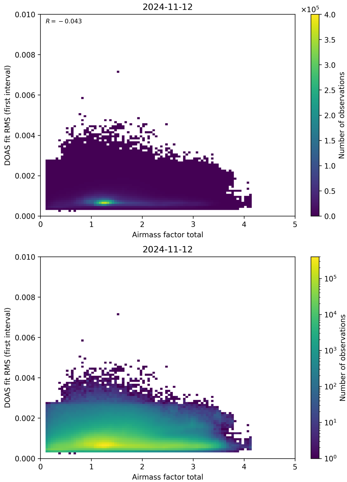
Figure 97: Scatter density plot of “Airmass factor total” against “DOAS fit RMS (first interval)” for 2024-11-11 to 2024-11-13.
