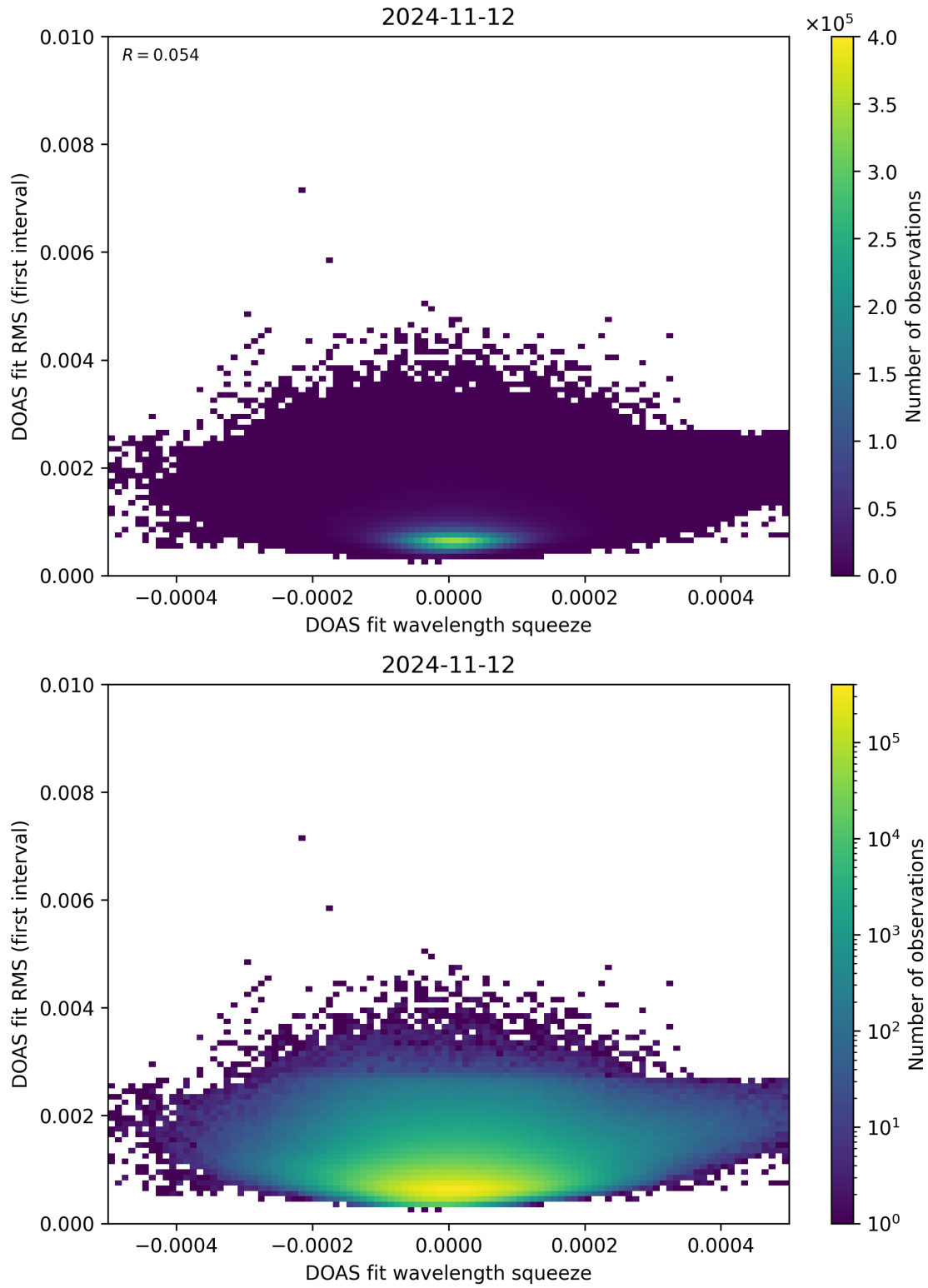
Figure 68: Scatter density plot of “DOAS fit wavelength squeeze” against “DOAS fit RMS (first interval)” for 2024-11-11 to 2024-11-13.
