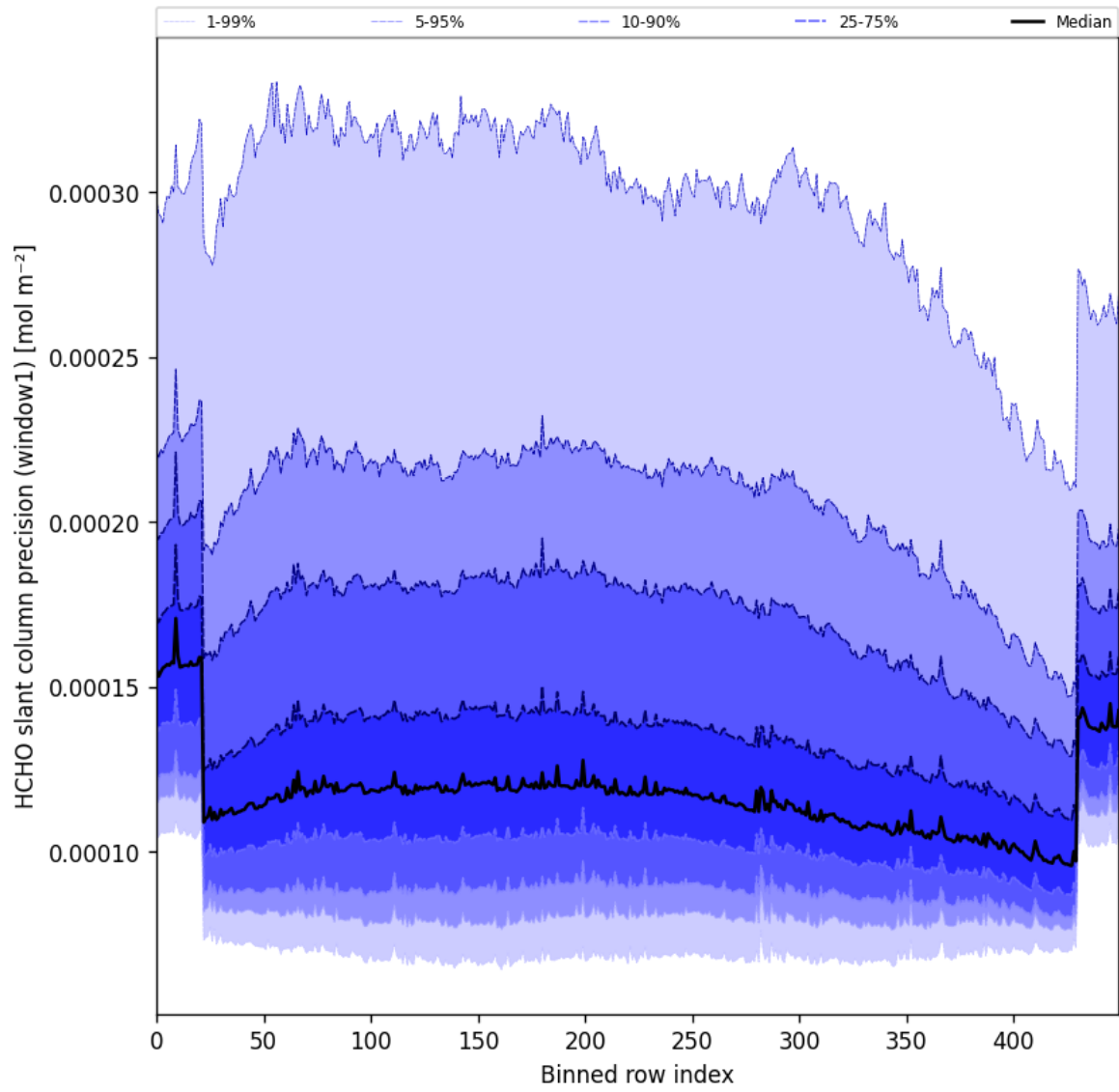
Figure 53: Along track statistics of “HCHO slant column precision (window1)” for 2024-11-11 to 2024-11-13
