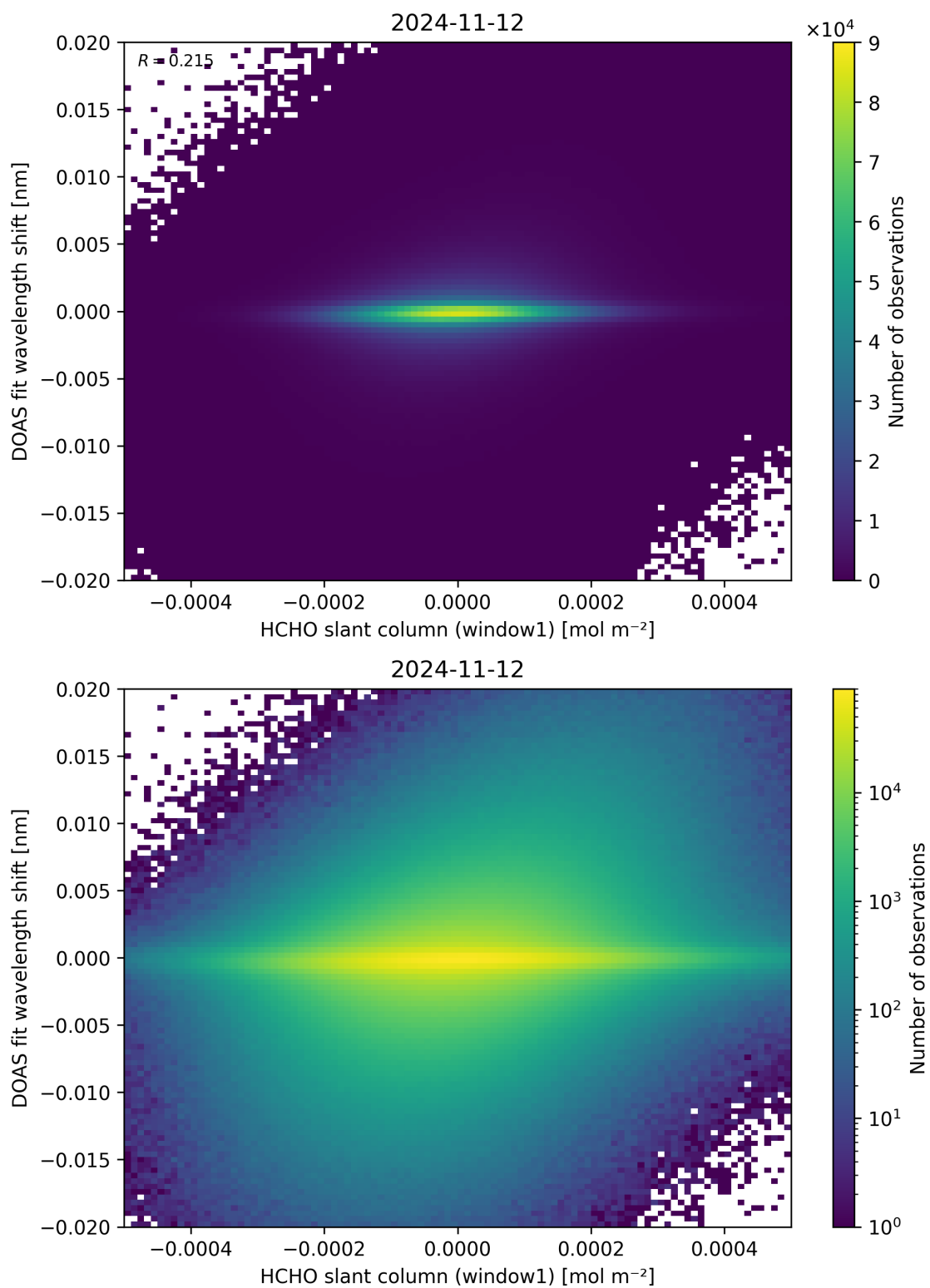
Figure 79: Scatter density plot of “HCHO slant column (window1)” against “DOAS fit wavelength shift” for 2024-11-11 to 2024-11-13.
