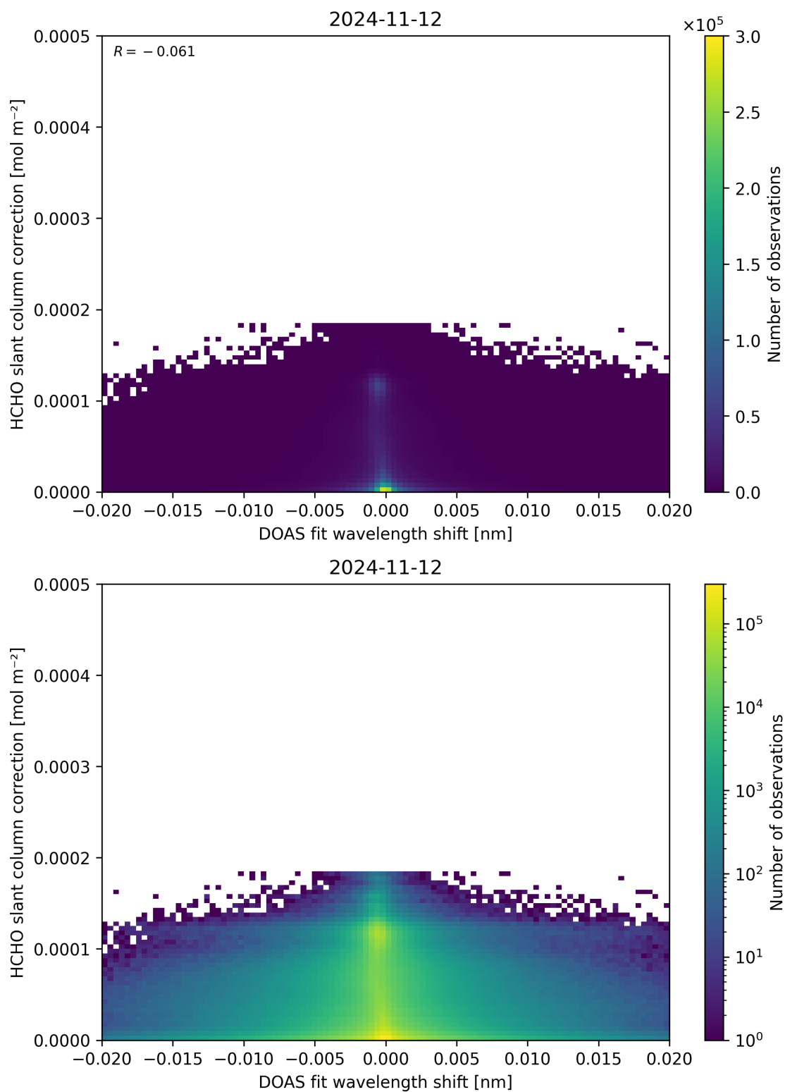
Figure 67: Scatter density plot of “DOAS fit wavelength shift” against “HCHO slant column correction” for 2024-11-11 to 2024-11-13.
