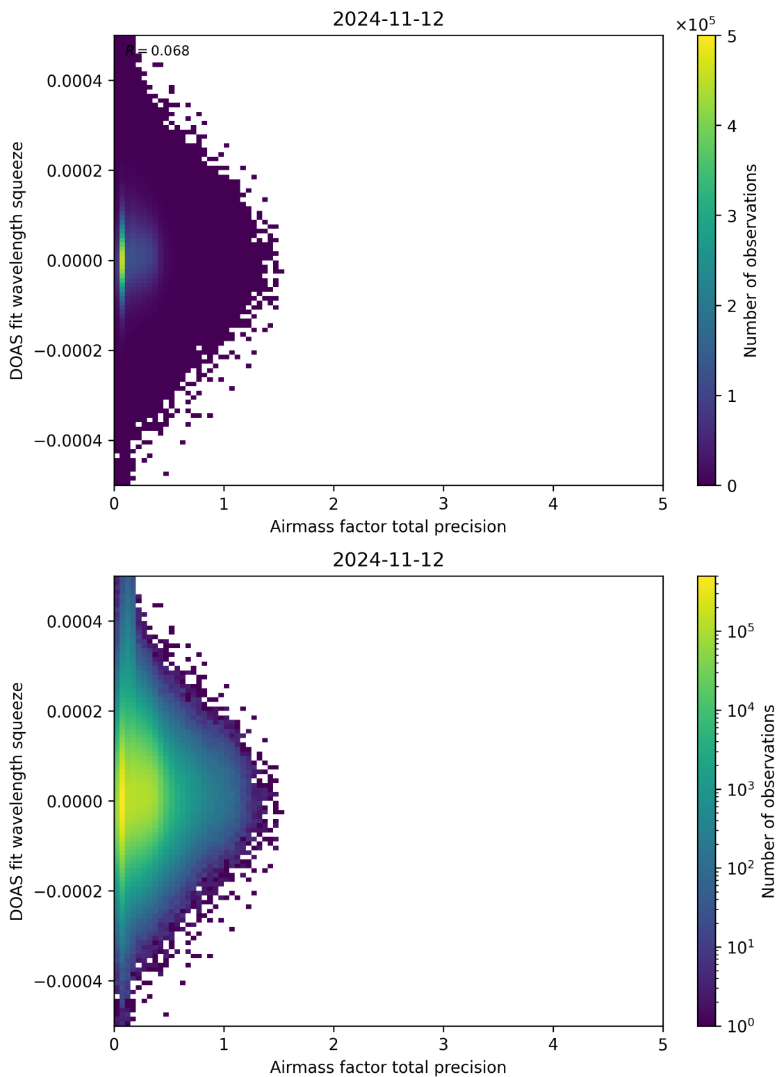
Figure 107: Scatter density plot of “Airmass factor total precision” against “DOAS fit wavelength squeeze” for 2024-11-11 to 2024-11-13.
