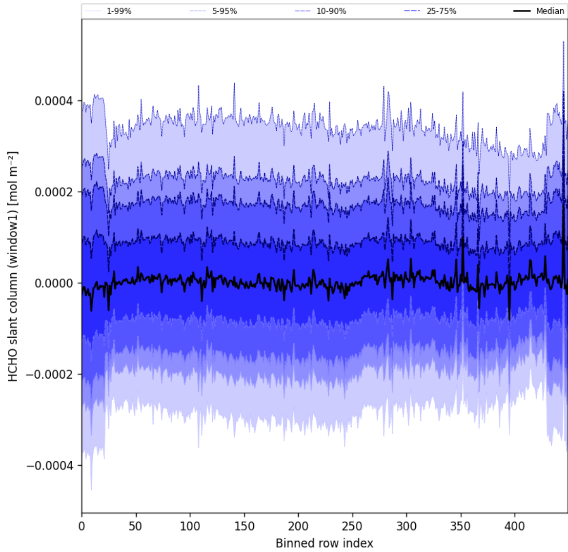
Figure 52: Along track statistics of “HCHO slant column (window1)” for 2024-11-11 to 2024-11-13
