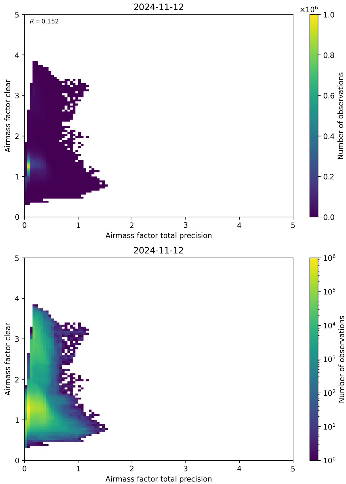
Figure 108: Scatter density plot of “Airmass factor total precision” against “Airmass factor clear” for 2024-11-11 to 2024-11-13.
