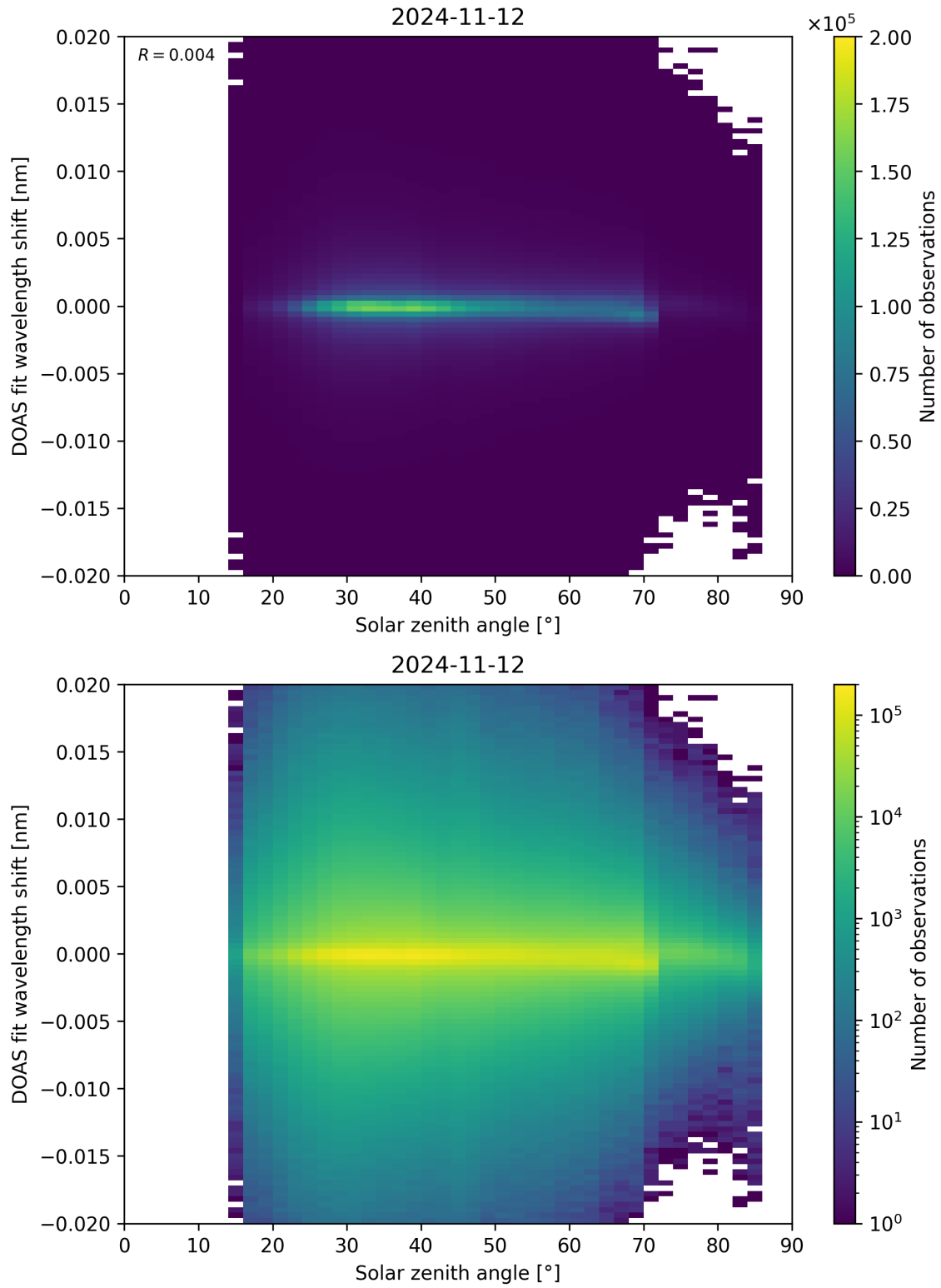
Figure 168: Scatter density plot of “Solar zenith angle” against “DOAS fit wavelength shift” for 2024-11-11 to 2024-11-13.
