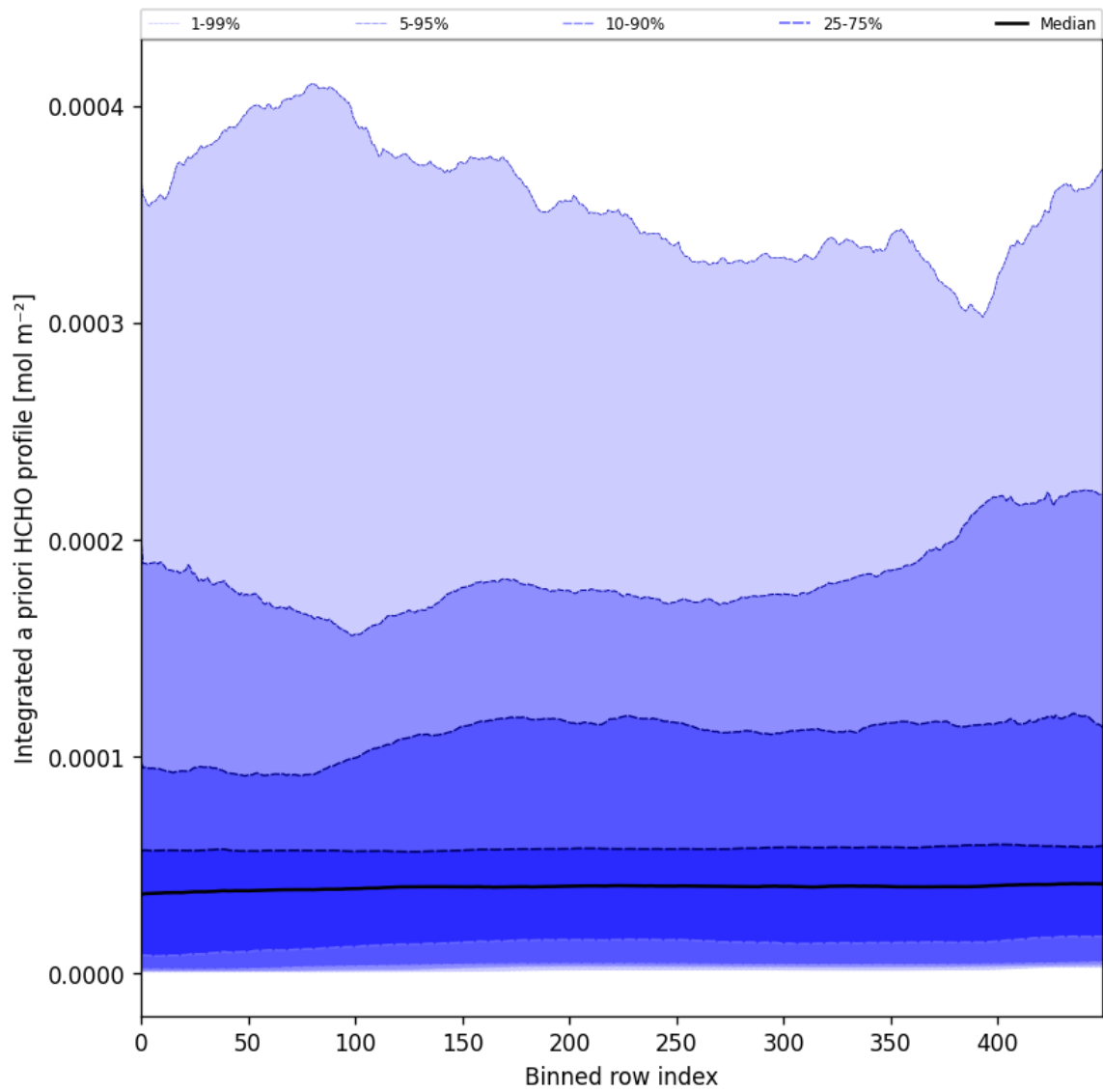
Figure 57: Along track statistics of "Integrated a priori HCHO profile" for 2024-11-11 to 2024-11-13
