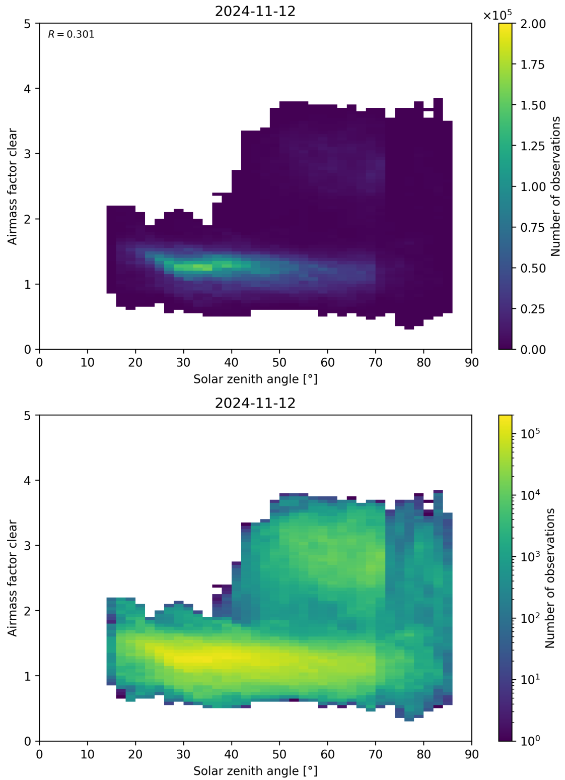
Figure 170: Scatter density plot of “Solar zenith angle” against “Airmass factor clear” for 2024-11-11 to 2024-11-13.
