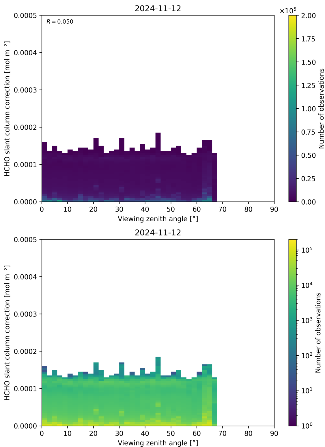
Figure 187: Scatter density plot of “Viewing zenith angle” against “HCHO slant column correction” for 2024-11-11 to 2024-11-13.
