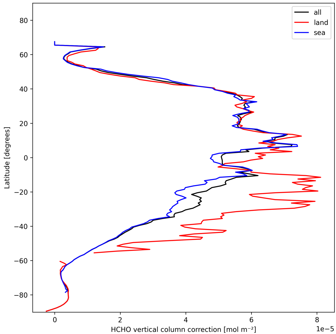
Figure 23: Zonal average of “HCHO vertical column correction” for 2024-11-11 to 2024-11-13.
