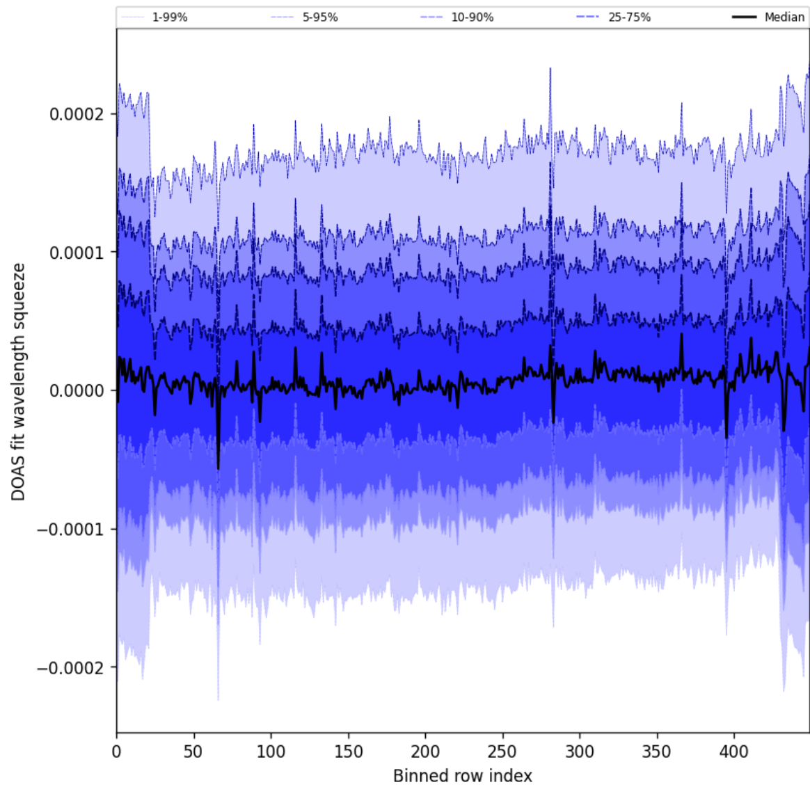
Figure 59: Along track statistics of “DOAS fit wavelength squeeze” for 2024-11-12 to 2024-11-14
