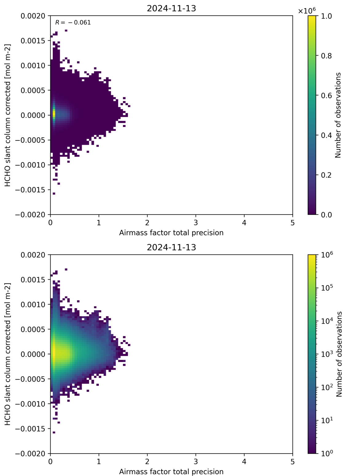
Figure 109: Scatter density plot of “Airmass factor total precision” against “HCHO slant column corrected” for 2024-11-12 to 2024-11-14.
