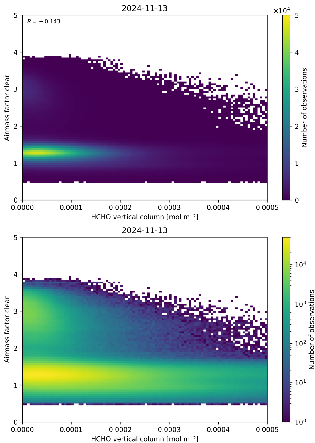
Figure 126: Scatter density plot of “HCHO vertical column” against “Airmass factor clear” for 2024-11-12 to 2024-11-14.
