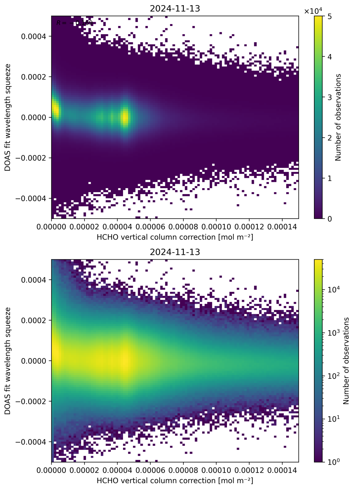
Figure 114: Scatter density plot of “HCHO vertical column correction” against “DOAS fit wavelength squeeze” for 2024-11-12 to 2024-11-14.
