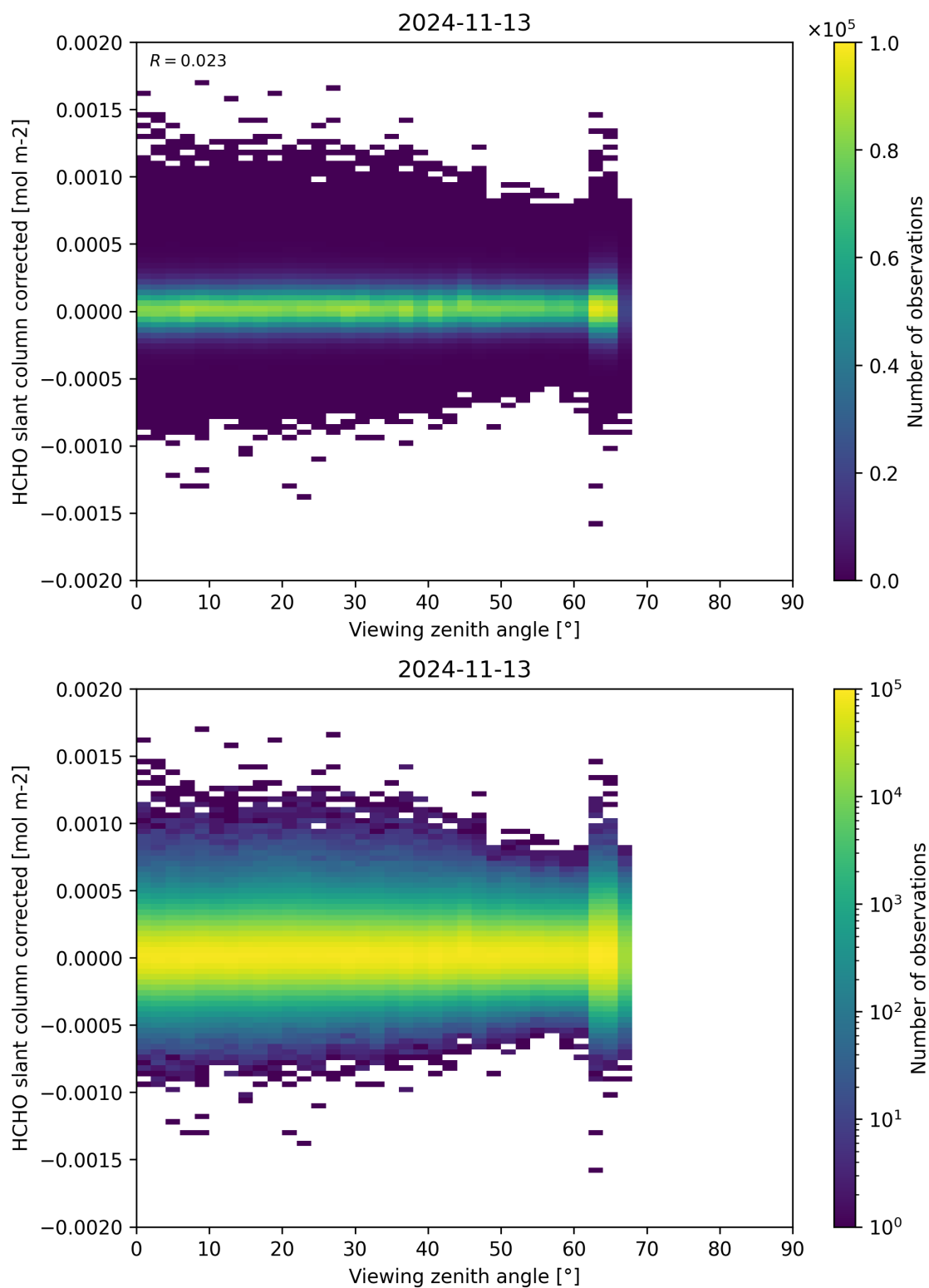
Figure 186: Scatter density plot of “Viewing zenith angle” against “HCHO slant column corrected” for 2024-11-12 to 2024-11-14.
