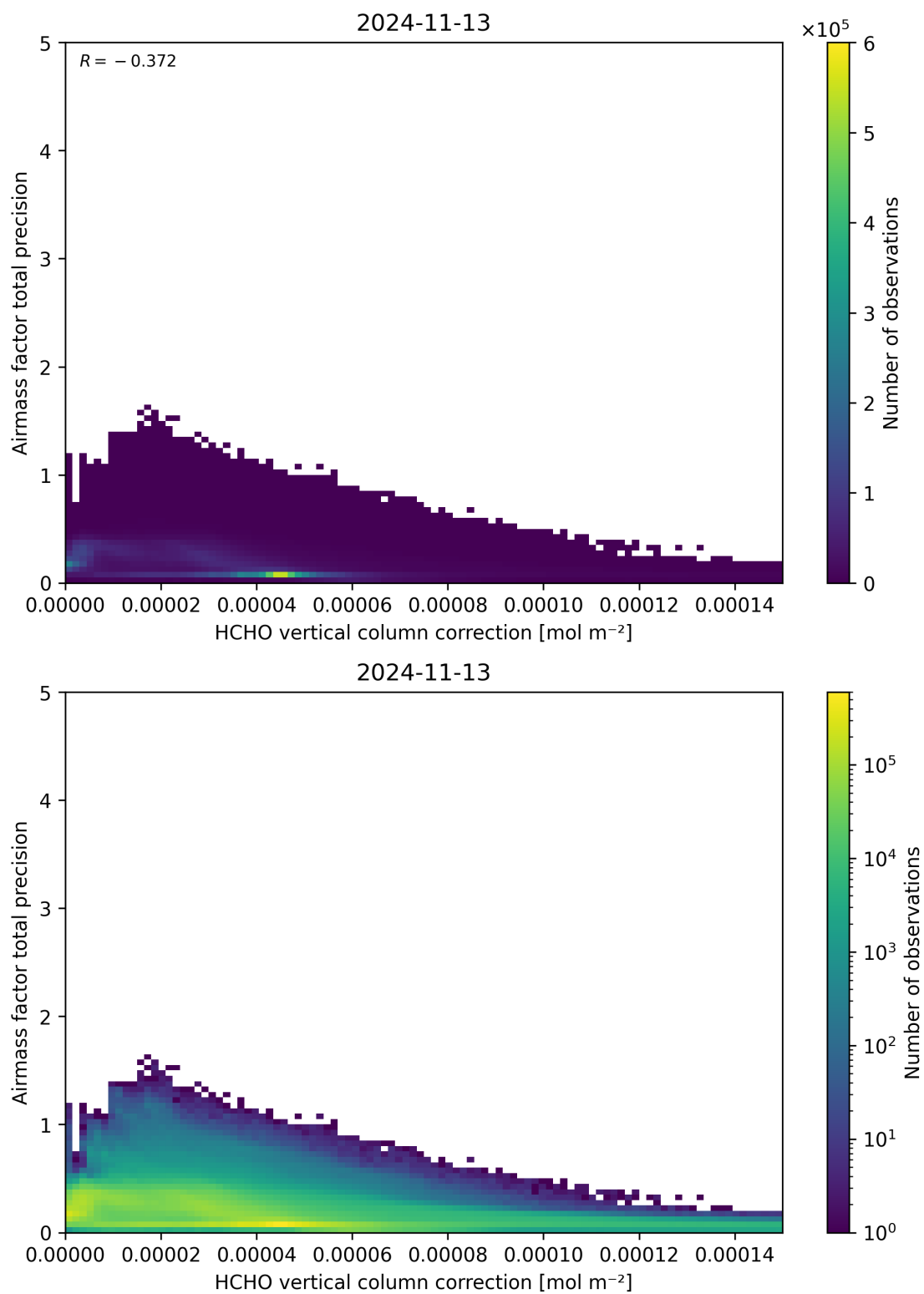
Figure 121: Scatter density plot of “HCHO vertical column correction” against “Airmass factor total precision” for 2024-11-12 to 2024-11-14.
