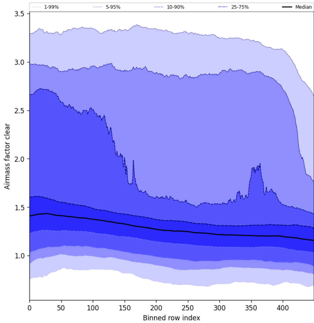
Figure 56: Along track statistics of “Airmass factor clear” for 2024-11-12 to 2024-11-14
