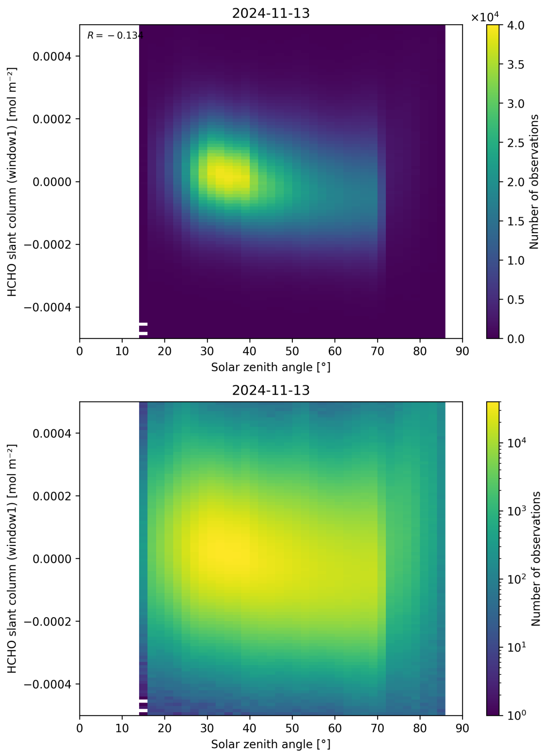
Figure 173: Scatter density plot of “Solar zenith angle” against “HCHO slant column (window1)” for 2024-11-12 to 2024-11-14.
