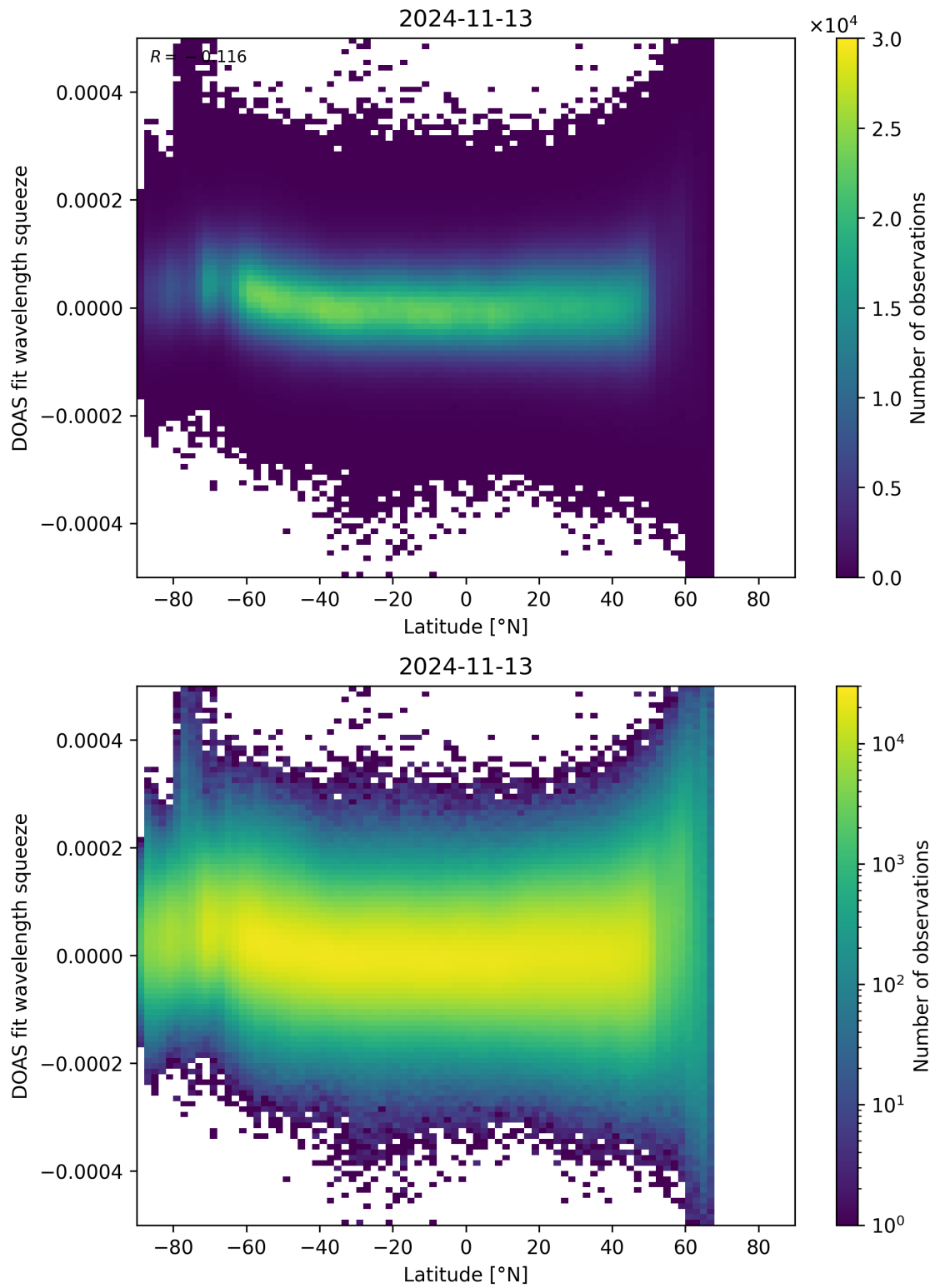
Figure 155: Scatter density plot of “Latitude” against “DOAS fit wavelength squeeze” for 2024-11-12 to 2024-11-14.
