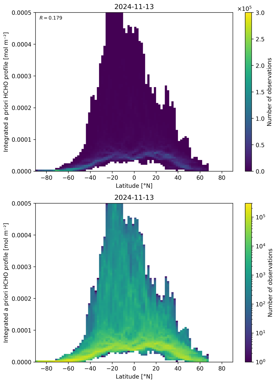
Figure 166: Scatter density plot of “Latitude” against “Integrated a priori HCHO profile” for 2024-11-12 to 2024-11-14.
