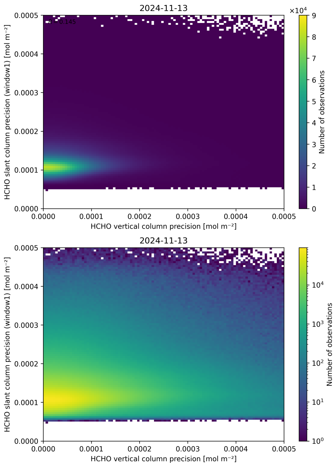
Figure 143: Scatter density plot of “HCHO vertical column precision” against “HCHO slant column precision (window1)” for 2024-11-12 to 2024-11-14.
