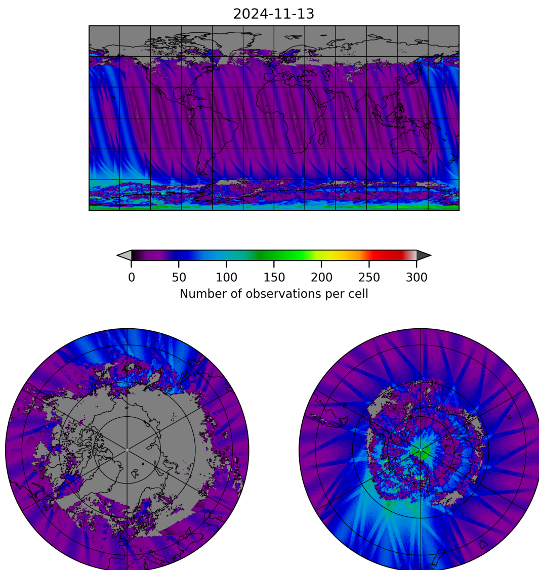
Figure 19: Map of the number of observations for 2024-11-12 to 2024-11-14
