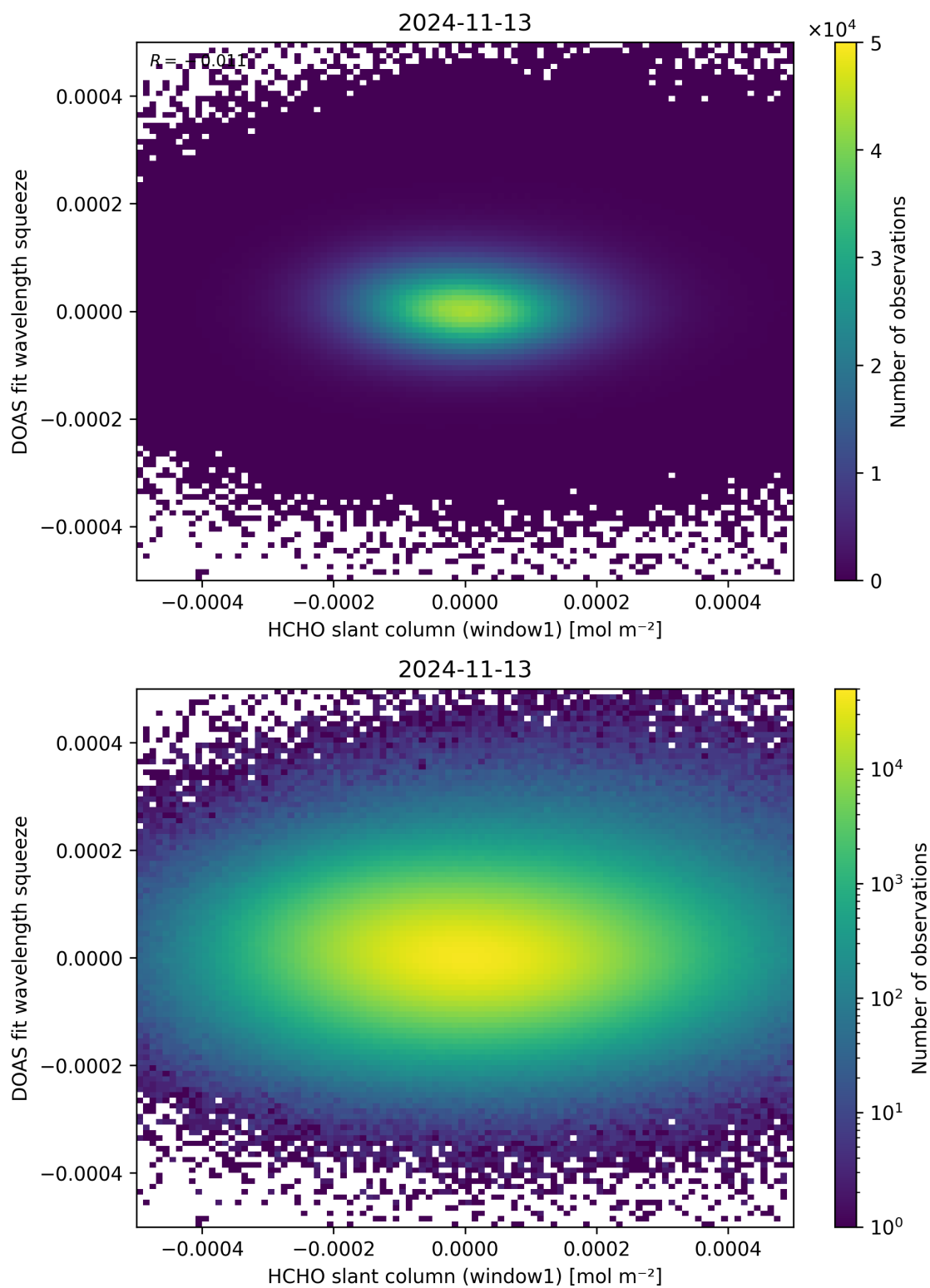
Figure 80: Scatter density plot of “HCHO slant column (window1)” against “DOAS fit wavelength squeeze” for 2024-11-12 to 2024-11-14.
