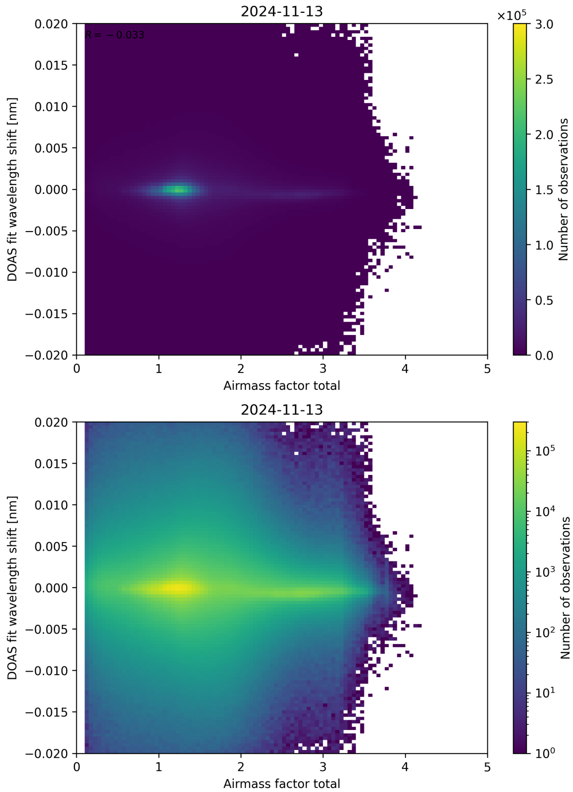
Figure 98: Scatter density plot of “Airmass factor total” against “DOAS fit wavelength shift” for 2024-11-12 to 2024-11-14.
