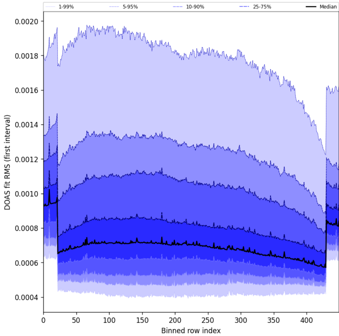
Figure 60: Along track statistics of “DOAS fit RMS (first interval)” for 2024-11-12 to 2024-11-14
