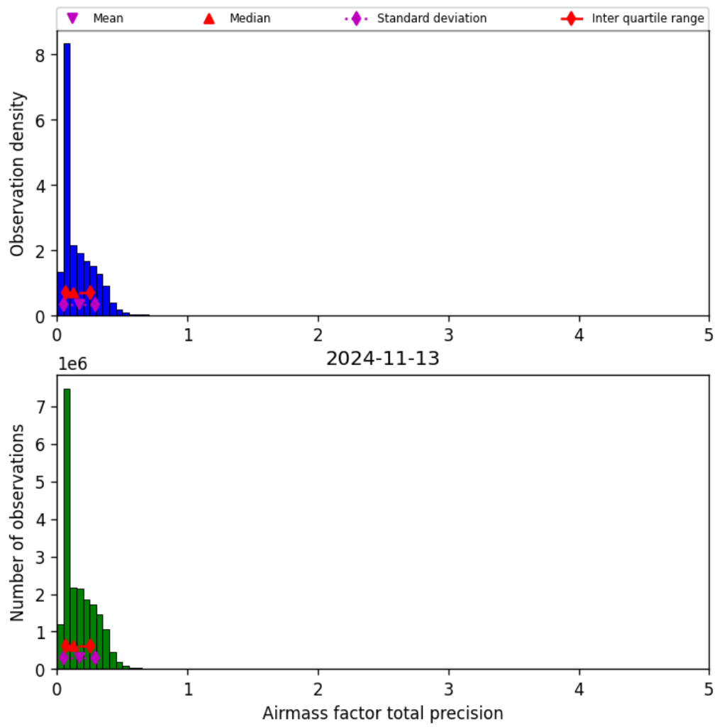
Figure 41: Histogram of “Airmass factor total precision” for 2024-11-12 to 2024-11-14
