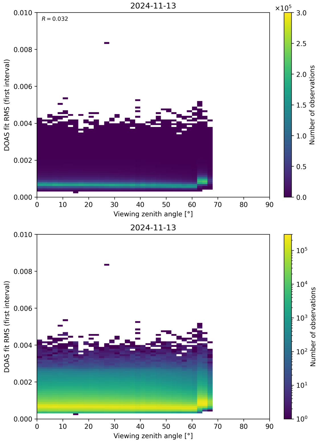
Figure 182: Scatter density plot of “Viewing zenith angle” against “DOAS fit RMS (first interval)” for 2024-11-12 to 2024-11-14.
