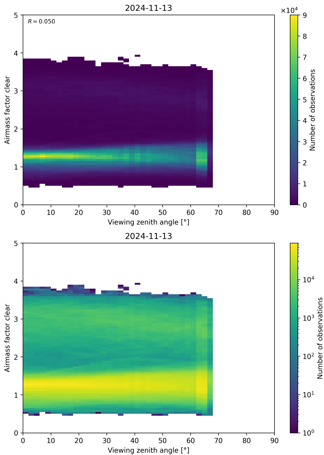
Figure 185: Scatter density plot of “Viewing zenith angle” against “Airmass factor clear” for 2024-11-12 to 2024-11-14.
