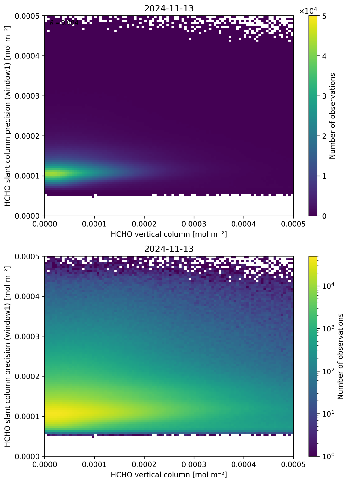
Figure 130: Scatter density plot of “HCHO vertical column” against “HCHO slant column precision (window1)” for 2024-11-12 to 2024-11-14.
