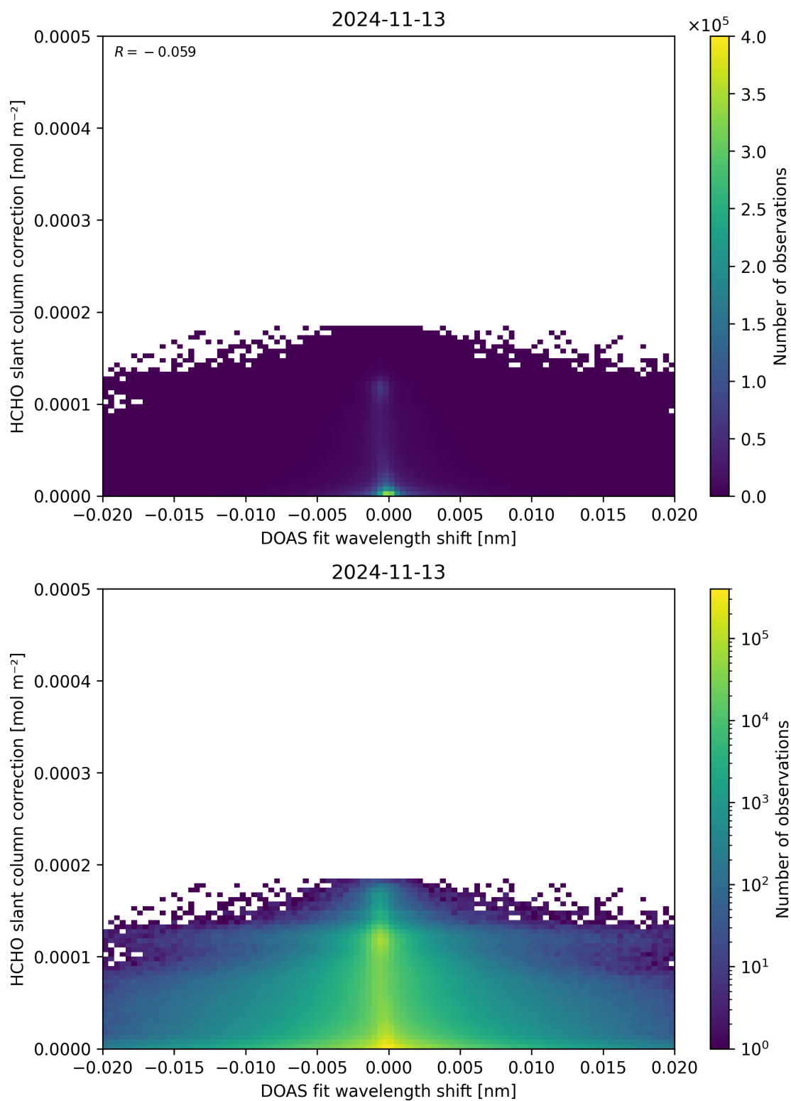
Figure 67: Scatter density plot of “DOAS fit wavelength shift” against “HCHO slant column correction” for 2024-11-12 to 2024-11-14.
