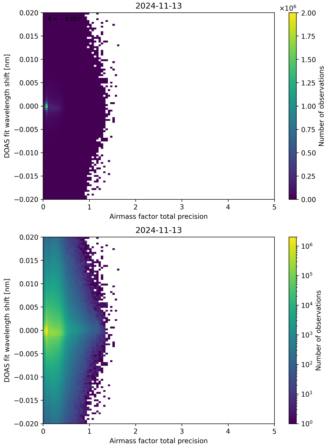
Figure 106: Scatter density plot of “Airmass factor total precision” against “DOAS fit wavelength shift” for 2024-11-12 to 2024-11-14.
