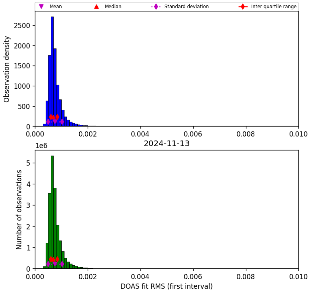
Figure 46: Histogram of “DOAS fit RMS (first interval)” for 2024-11-12 to 2024-11-14
