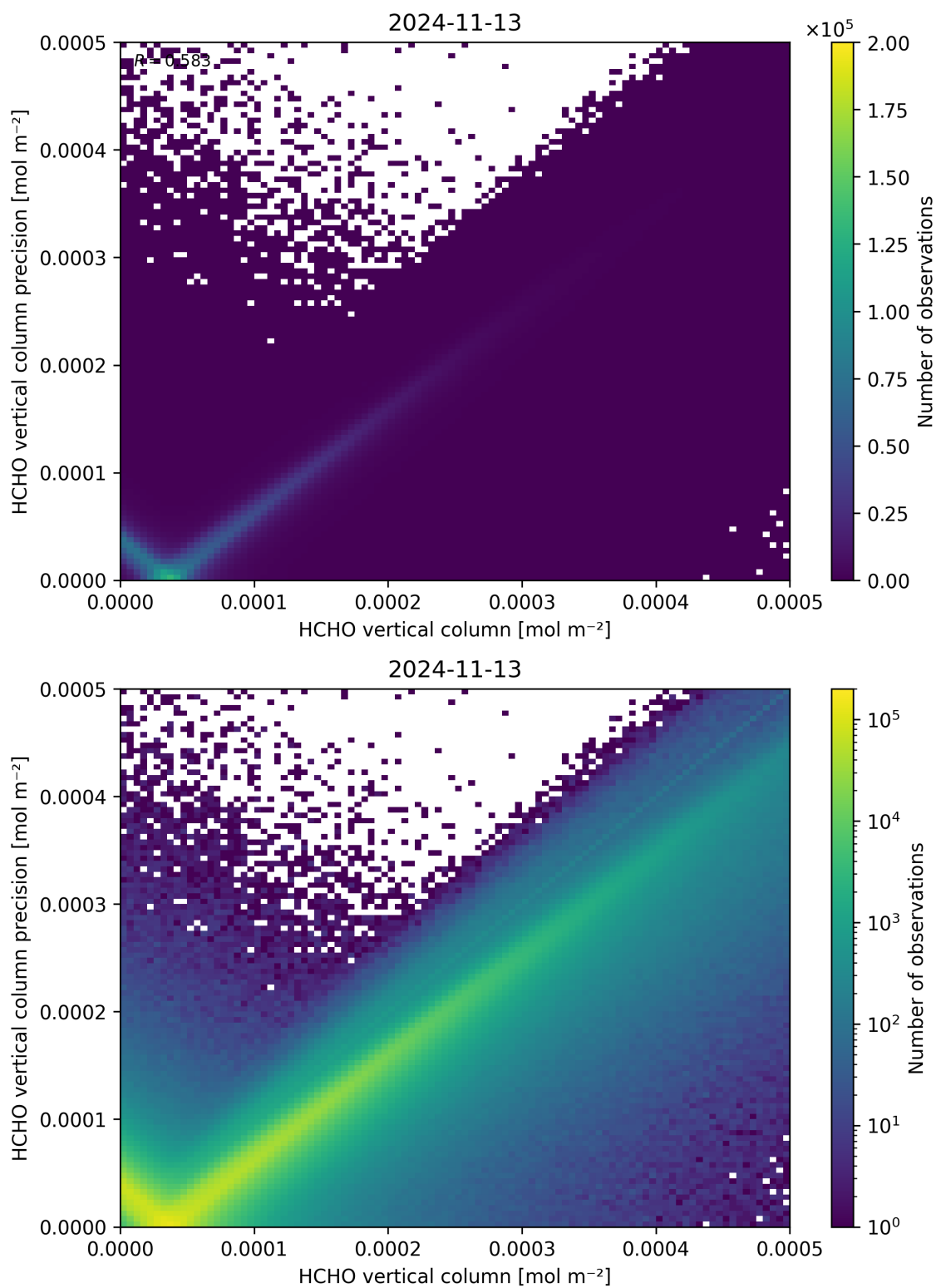
Figure 134: Scatter density plot of “HCHO vertical column” against “HCHO vertical column precision” for 2024-11-12 to 2024-11-14.
