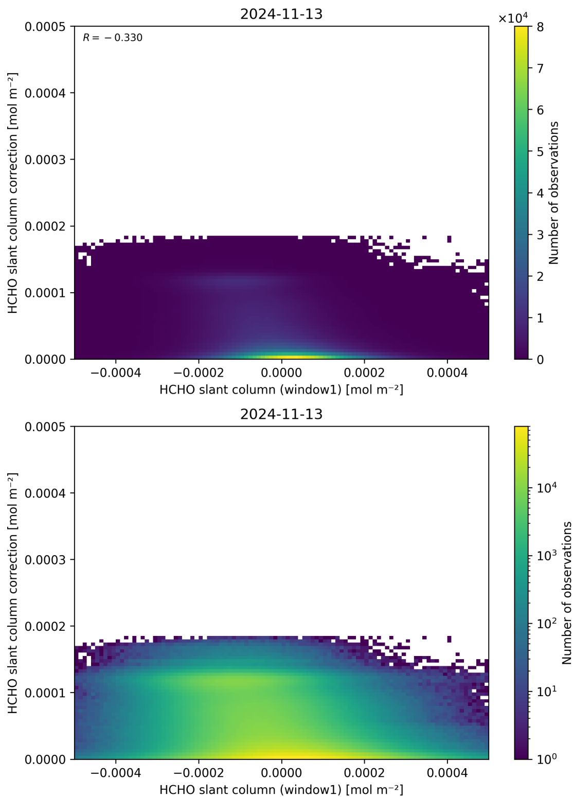
Figure 83: Scatter density plot of “HCHO slant column (window1)” against “HCHO slant column correction” for 2024-11-12 to 2024-11-14.
