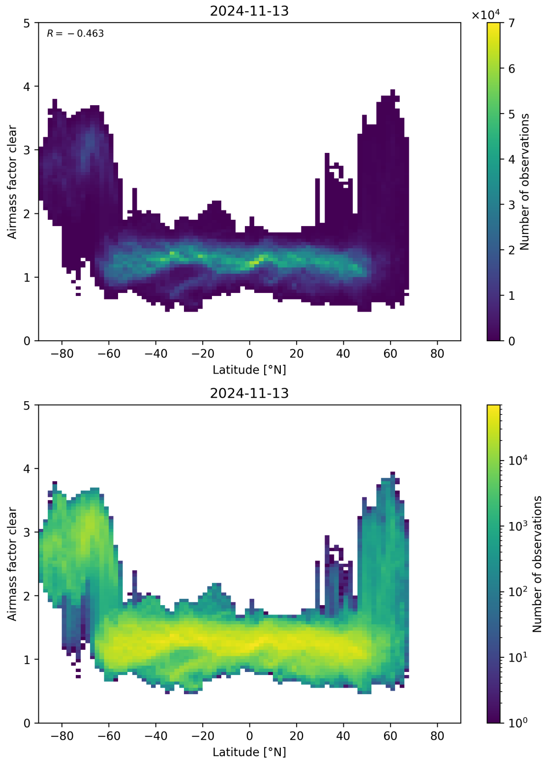
Figure 156: Scatter density plot of “Latitude” against “Airmass factor clear” for 2024-11-12 to 2024-11-14.
