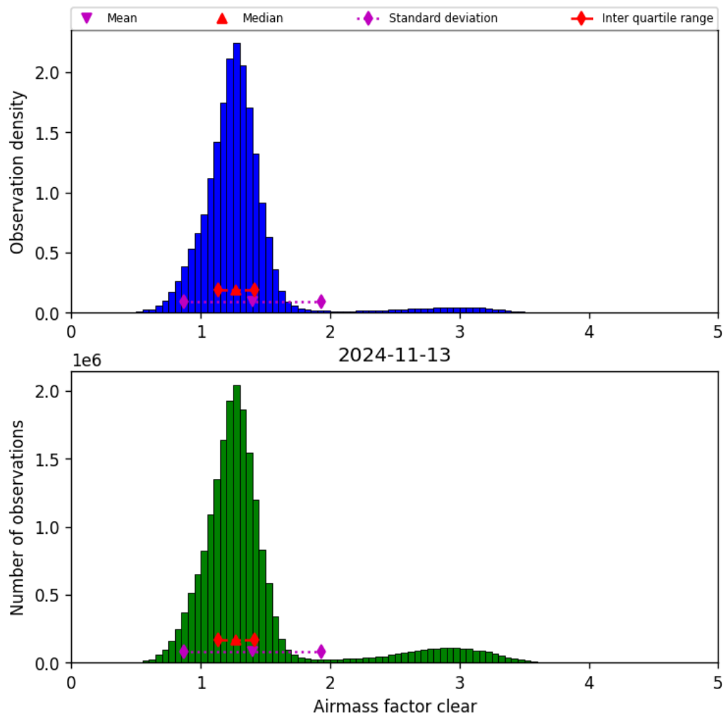
Figure 42: Histogram of “Airmass factor clear” for 2024-11-12 to 2024-11-14
