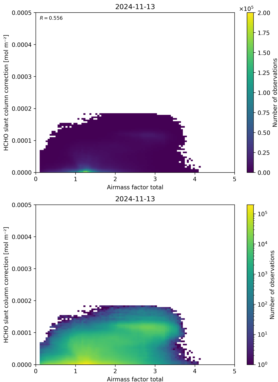
Figure 102: Scatter density plot of “Airmass factor total” against “HCHO slant column correction” for 2024-11-12 to 2024-11-14.
