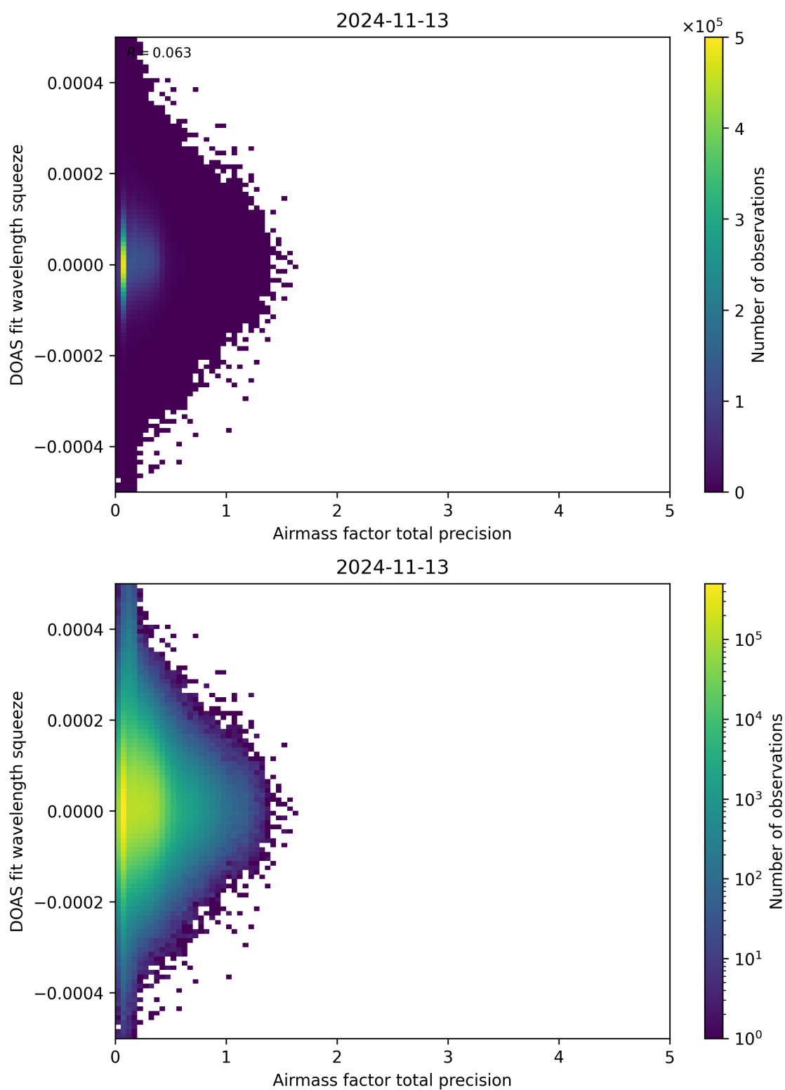
Figure 107: Scatter density plot of “Airmass factor total precision” against “DOAS fit wavelength squeeze” for 2024-11-12 to 2024-11-14.
