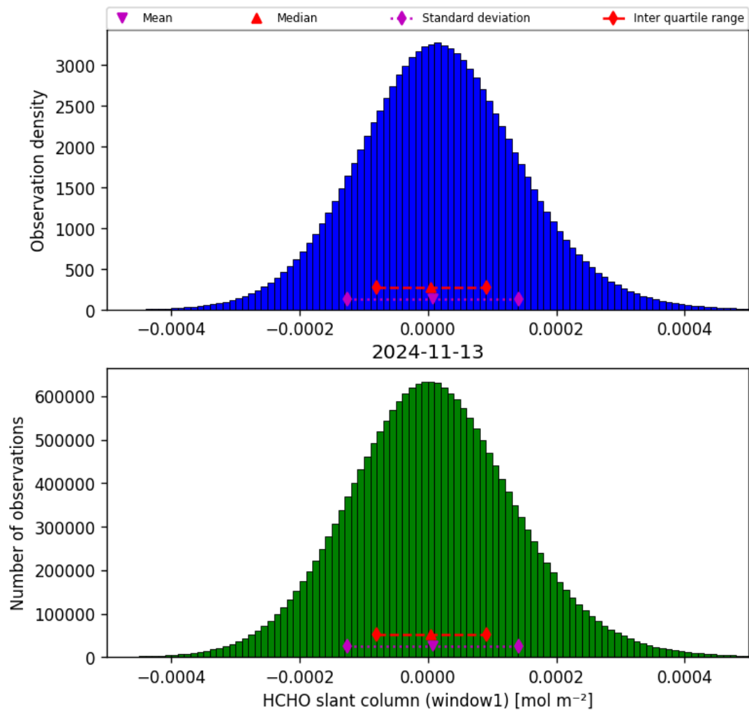
Figure 38: Histogram of “HCHO slant column (window1)” for 2024-11-12 to 2024-11-14
