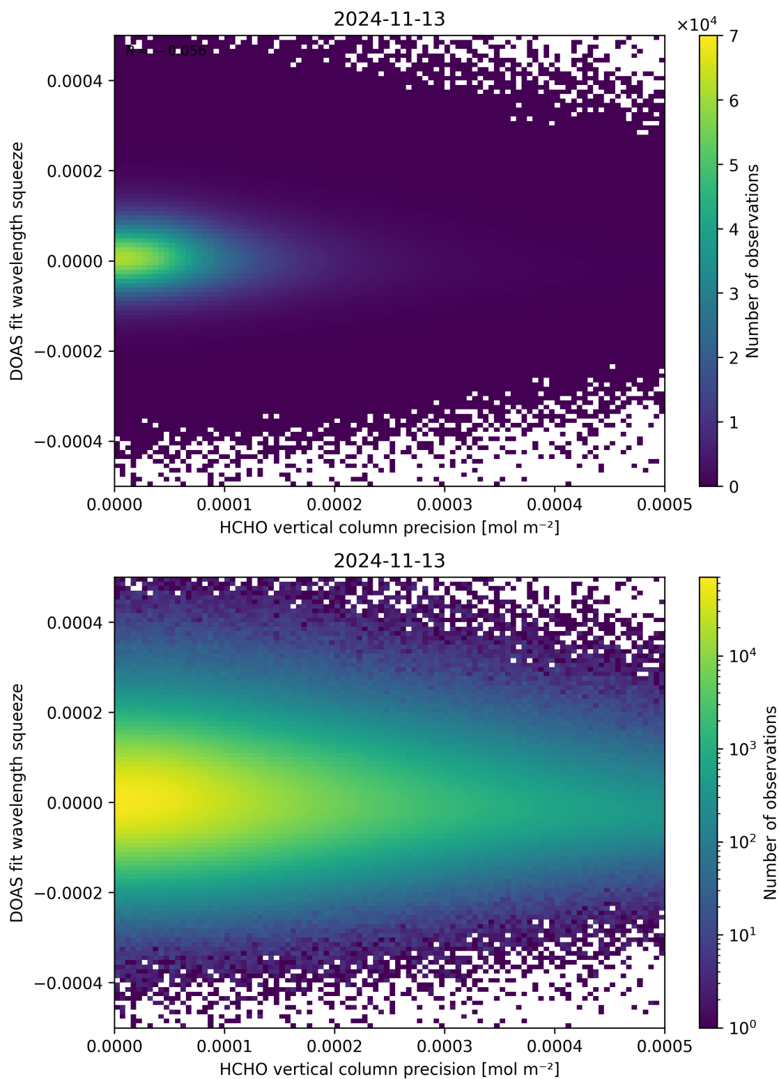
Figure 138: Scatter density plot of “HCHO vertical column precision” against “DOAS fit wavelength squeeze” for 2024-11-12 to 2024-11-14.
