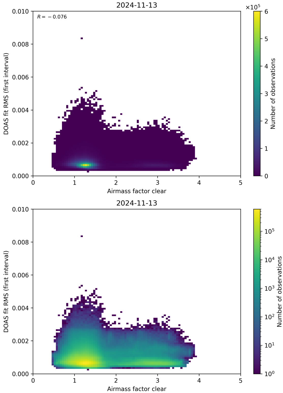
Figure 71: Scatter density plot of “Airmass factor clear” against “DOAS fit RMS (first interval)” for 2024-11-12 to 2024-11-14.
