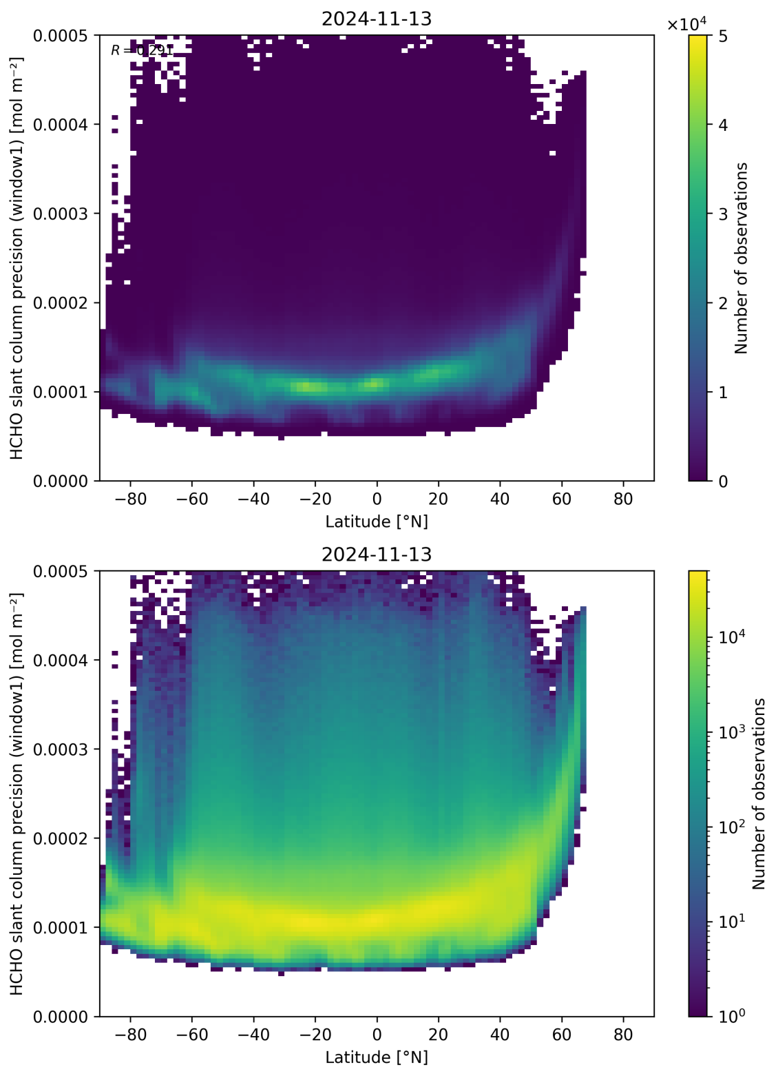
Figure 160: Scatter density plot of “Latitude” against “HCHO slant column precision (window1)” for 2024-11-12 to 2024-11-14.
