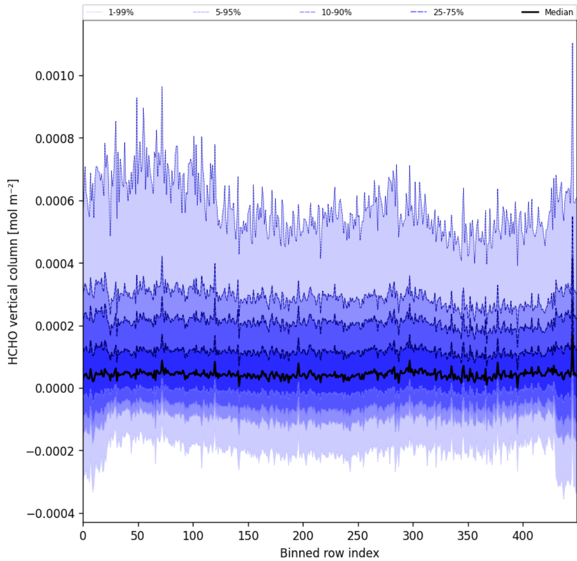
Figure 49: Along track statistics of “HCHO vertical column” for 2024-11-12 to 2024-11-14
