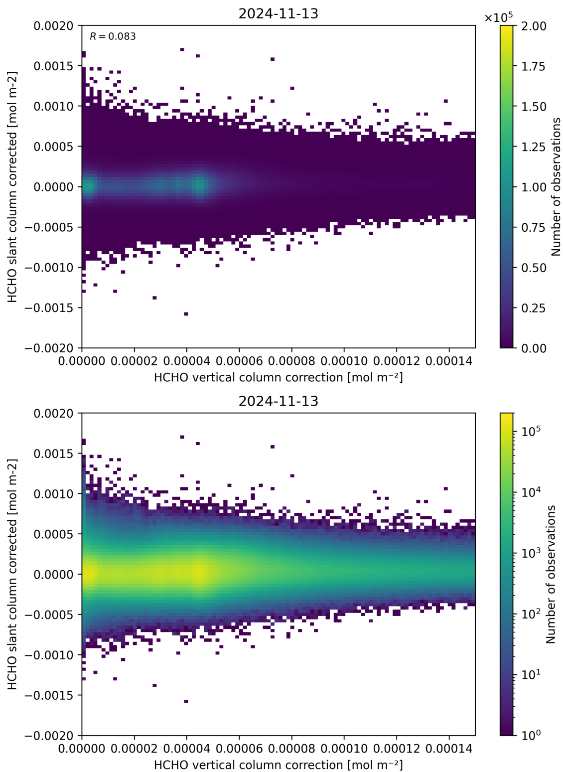
Figure 116: Scatter density plot of “HCHO vertical column correction” against “HCHO slant column corrected” for 2024-11-12 to 2024-11-14.
