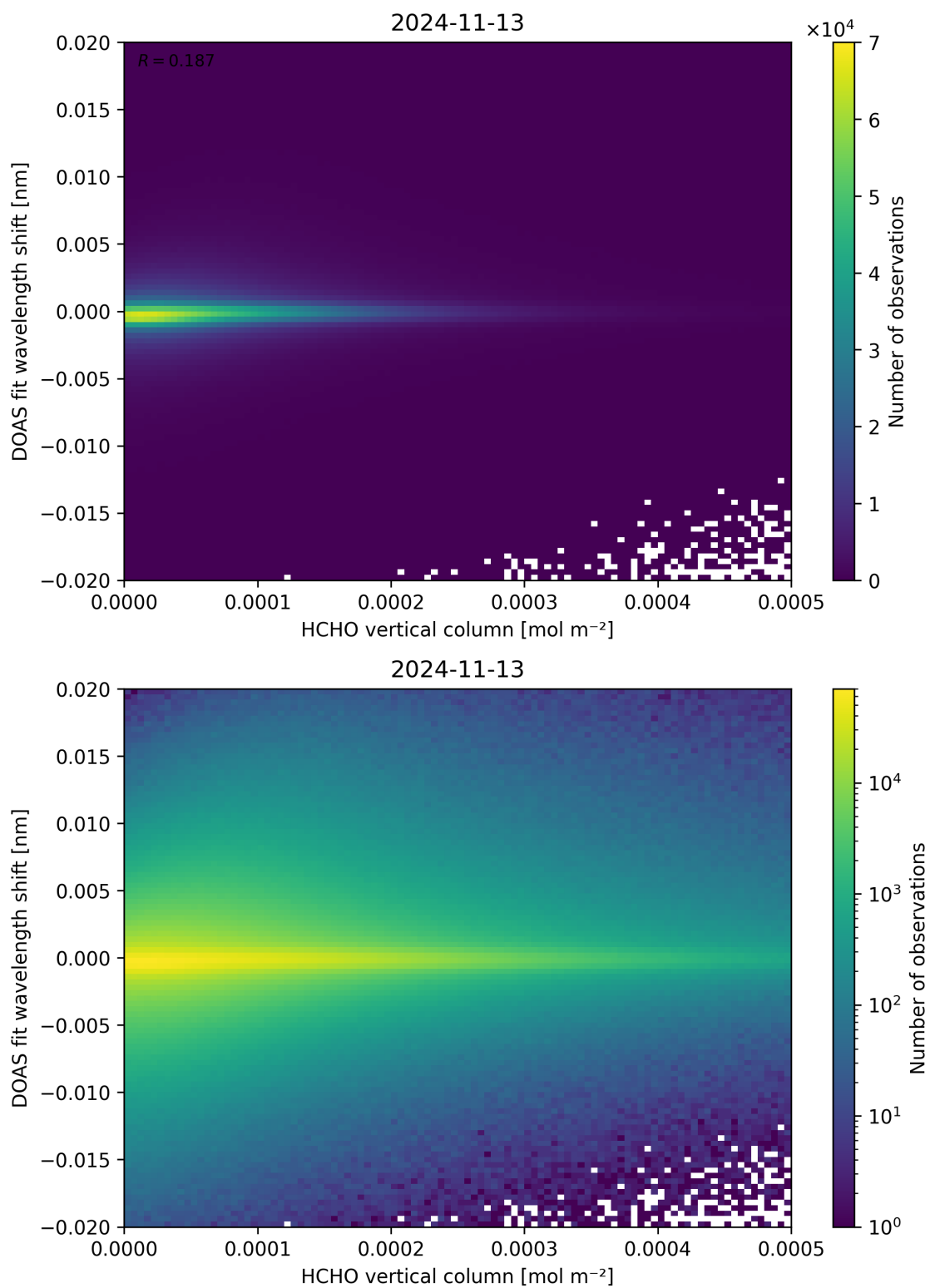
Figure 124: Scatter density plot of “HCHO vertical column” against “DOAS fit wavelength shift” for 2024-11-12 to 2024-11-14.
