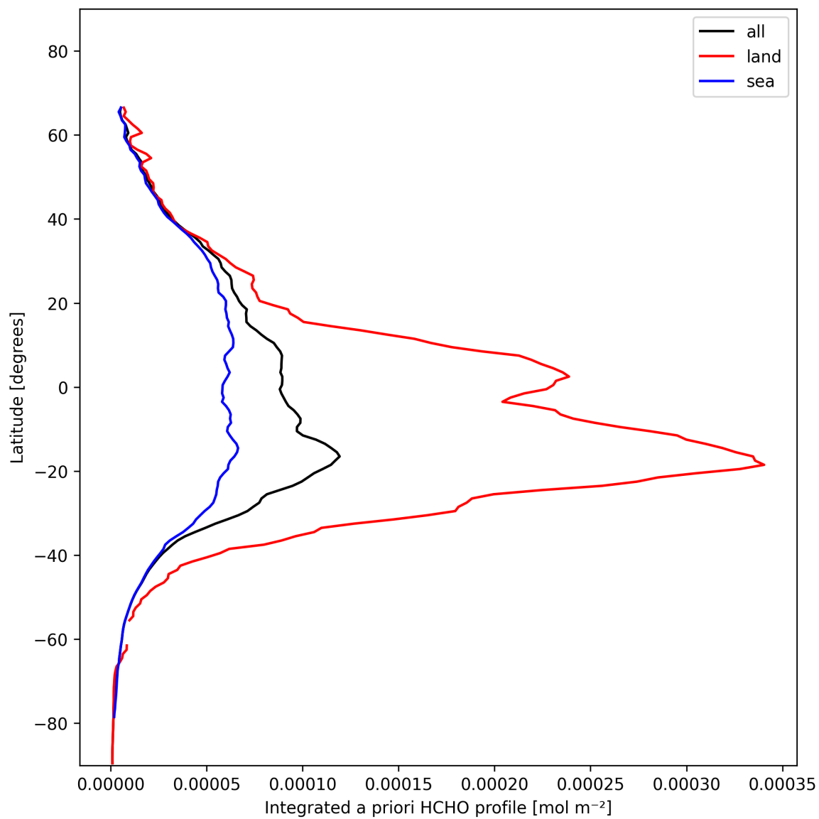
Figure 29: Zonal average of “Integrated a priori HCHO profile” for 2024-11-12 to 2024-11-14.
