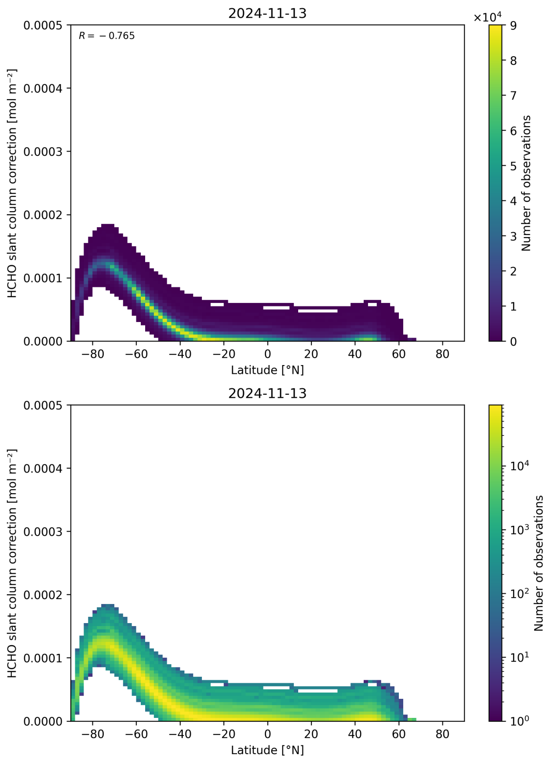
Figure 158: Scatter density plot of “Latitude” against “HCHO slant column correction” for 2024-11-12 to 2024-11-14.
