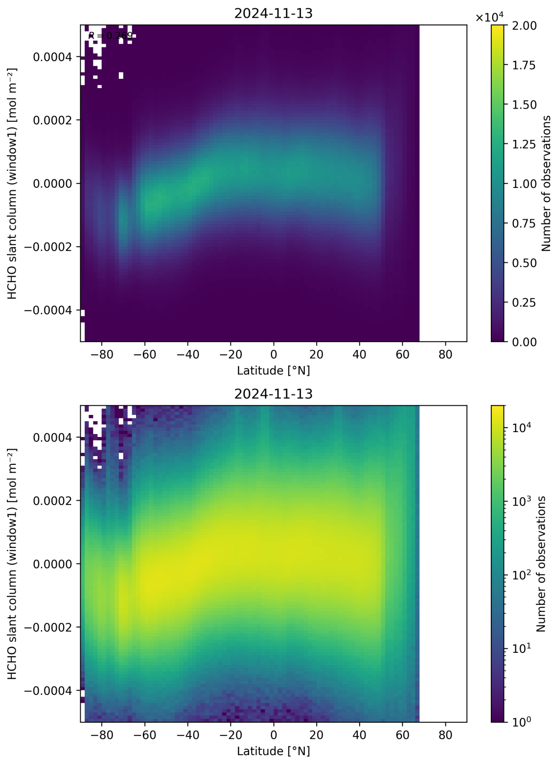
Figure 159: Scatter density plot of “Latitude” against “HCHO slant column (window1)” for 2024-11-12 to 2024-11-14.
