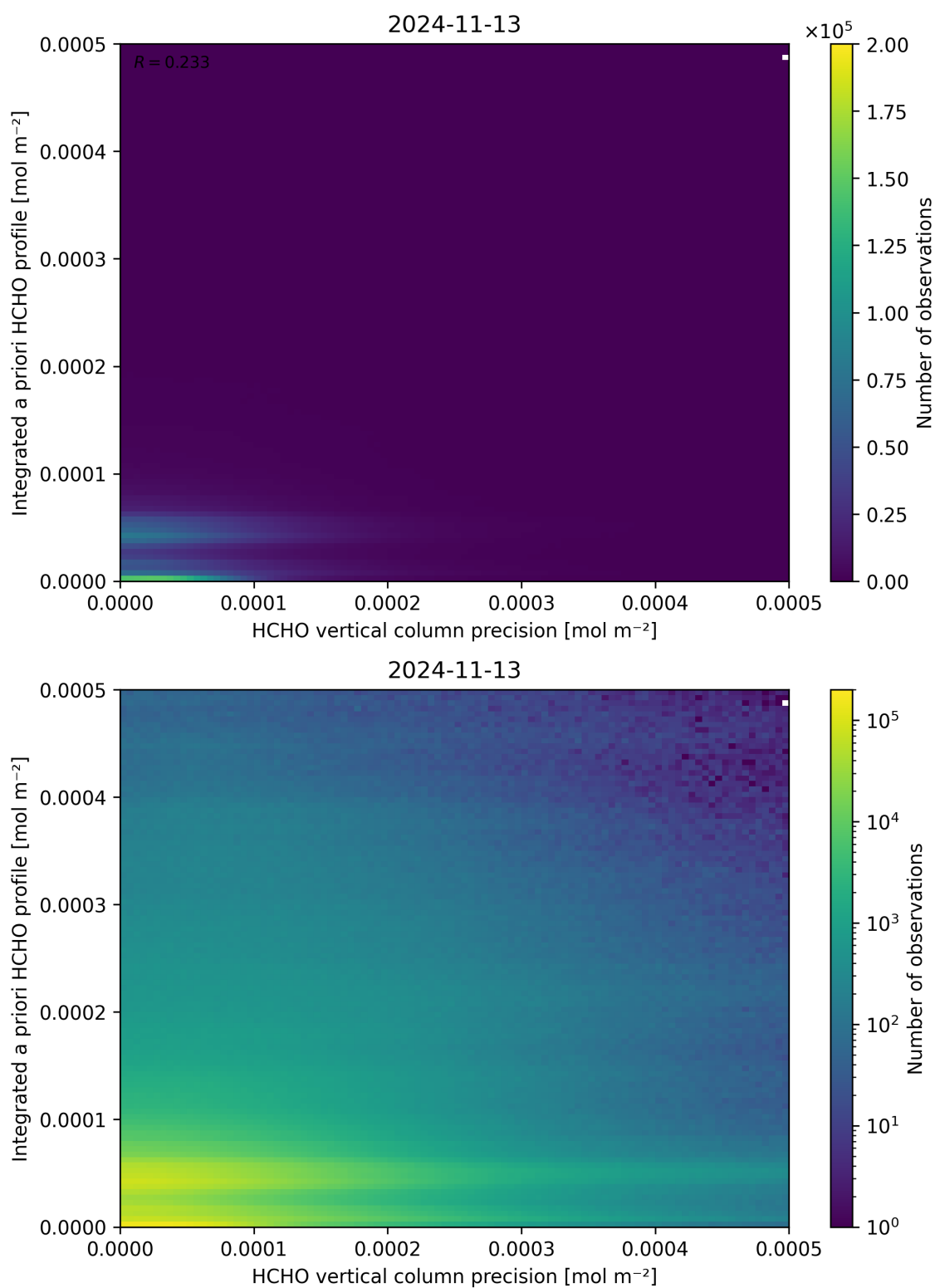
Figure 147: Scatter density plot of “HCHO vertical column precision” against “Integrated a priori HCHO profile” for 2024-11-12 to 2024-11-14.
