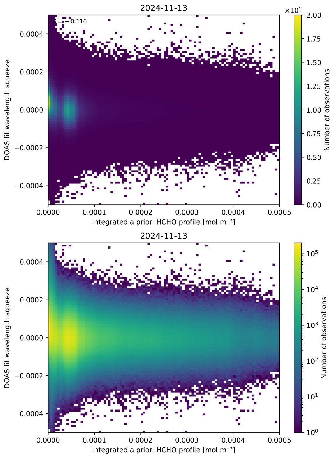
Figure 150: Scatter density plot of “Integrated a priori HCHO profile” against “DOAS fit wavelength squeeze” for 2024-11-12 to 2024-11-14.
