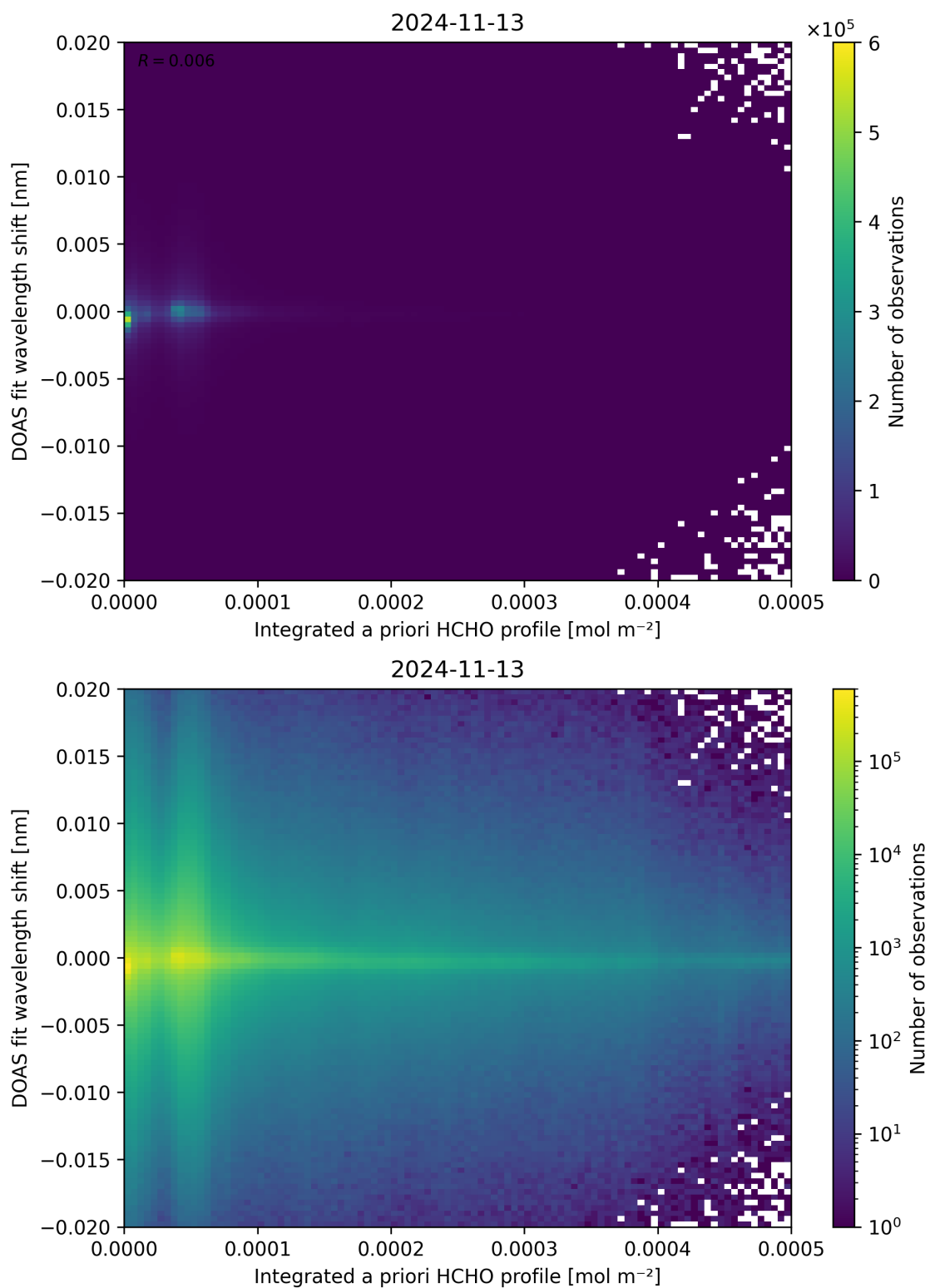
Figure 149: Scatter density plot of “Integrated a priori HCHO profile” against “DOAS fit wavelength shift” for 2024-11-12 to 2024-11-14.
