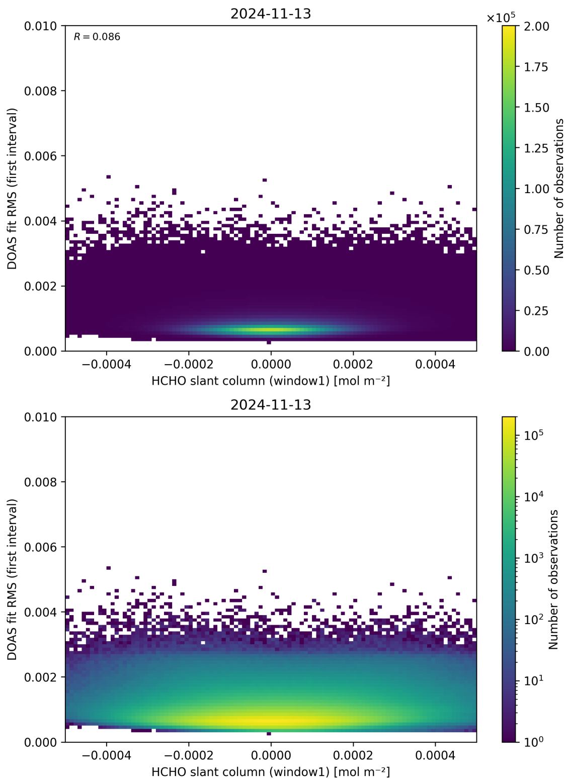
Figure 78: Scatter density plot of “HCHO slant column (window1)” against “DOAS fit RMS (first interval)” for 2024-11-12 to 2024-11-14.
