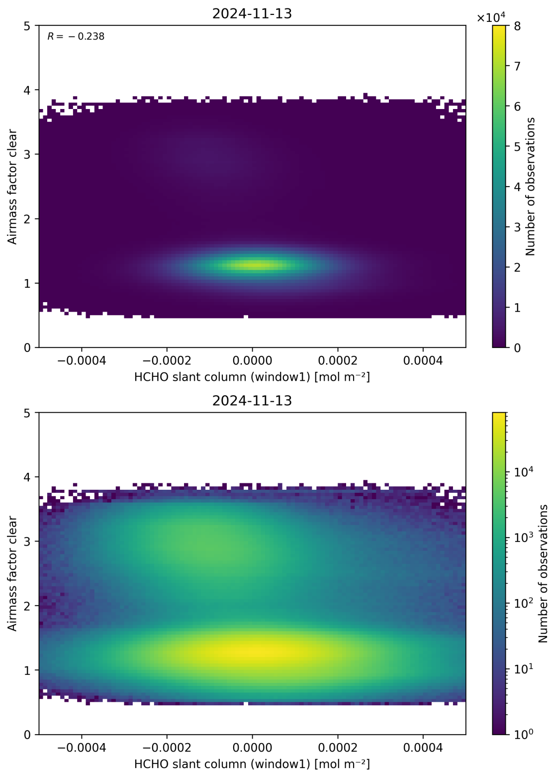
Figure 81: Scatter density plot of “HCHO slant column (window1)” against “Airmass factor clear” for 2024-11-12 to 2024-11-14.
