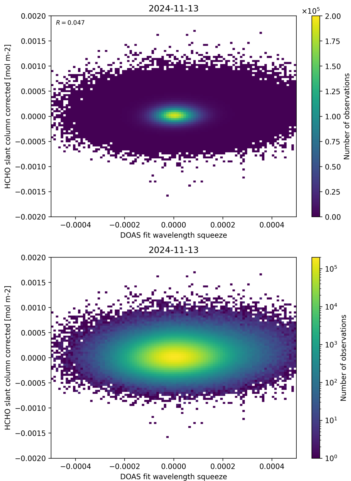
Figure 69: Scatter density plot of “DOAS fit wavelength squeeze” against “HCHO slant column corrected” for 2024-11-12 to 2024-11-14.
