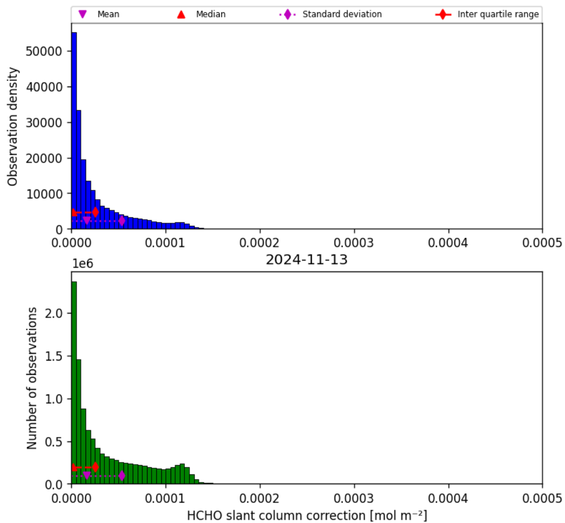
Figure 47: Histogram of “HCHO slant column correction” for 2024-11-12 to 2024-11-14
