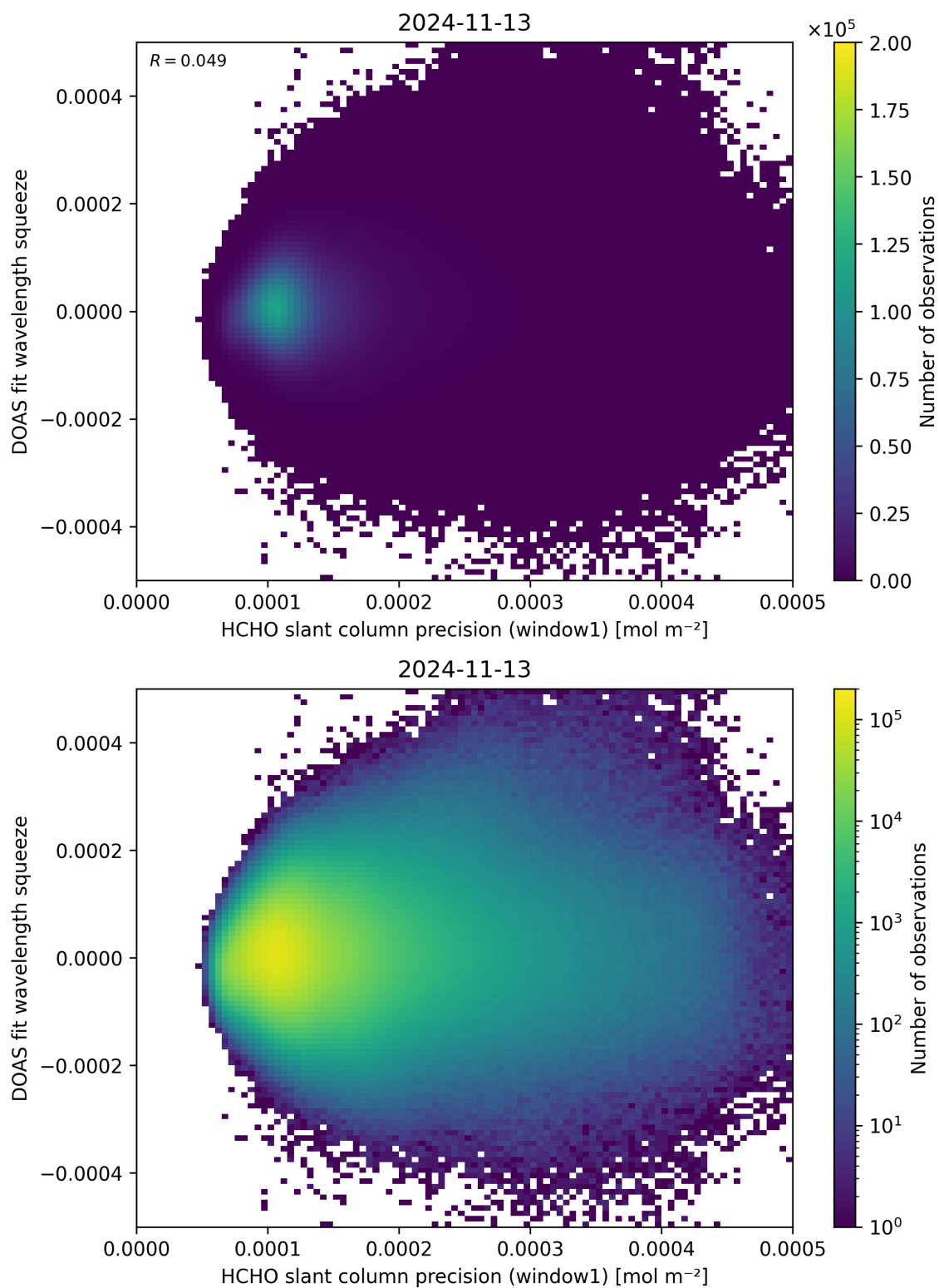
Figure 90: Scatter density plot of “HCHO slant column precision (window1)” against “DOAS fit wavelength squeeze” for 2024-11-12 to 2024-11-14.
