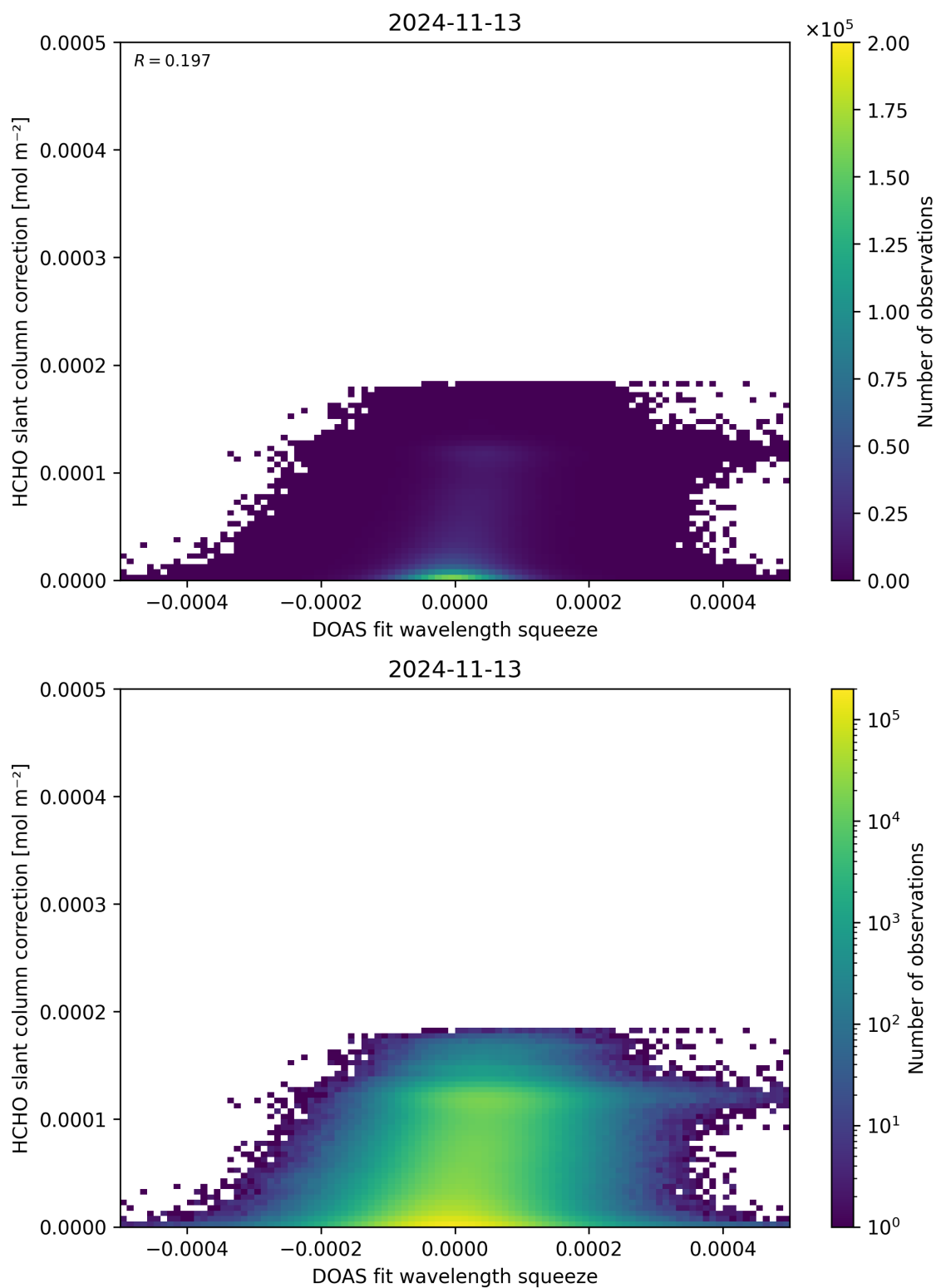
Figure 70: Scatter density plot of “DOAS fit wavelength squeeze” against “HCHO slant column correction” for 2024-11-12 to 2024-11-14.
