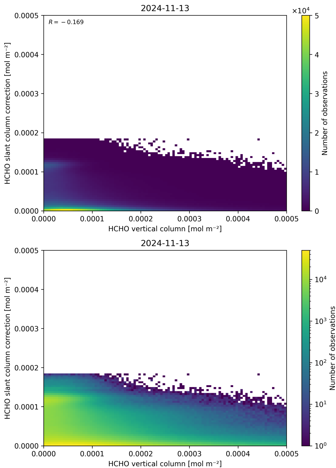
Figure 128: Scatter density plot of “HCHO vertical column” against “HCHO slant column correction” for 2024-11-12 to 2024-11-14.
