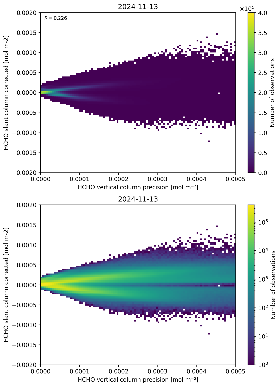
Figure 140: Scatter density plot of “HCHO vertical column precision” against “HCHO slant column corrected” for 2024-11-12 to 2024-11-14.
