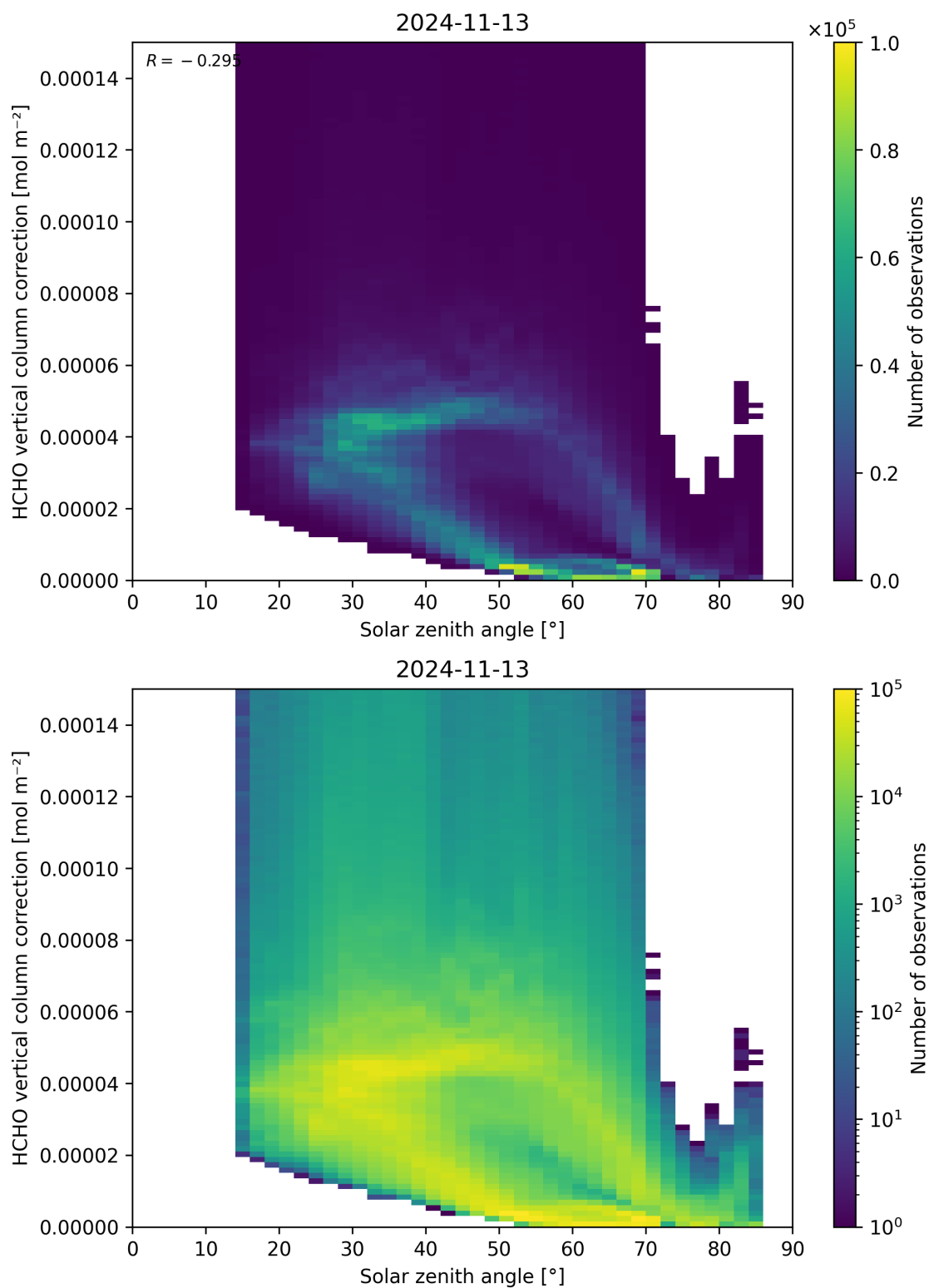
Figure 178: Scatter density plot of “Solar zenith angle” against “HCHO vertical column correction” for 2024-11-12 to 2024-11-14.
