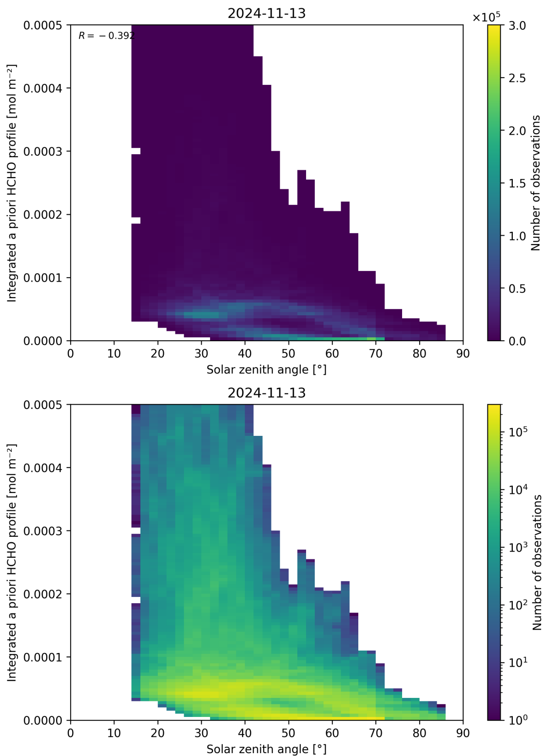
Figure 180: Scatter density plot of “Solar zenith angle” against “Integrated a priori HCHO profile” for 2024-11-12 to 2024-11-14.
