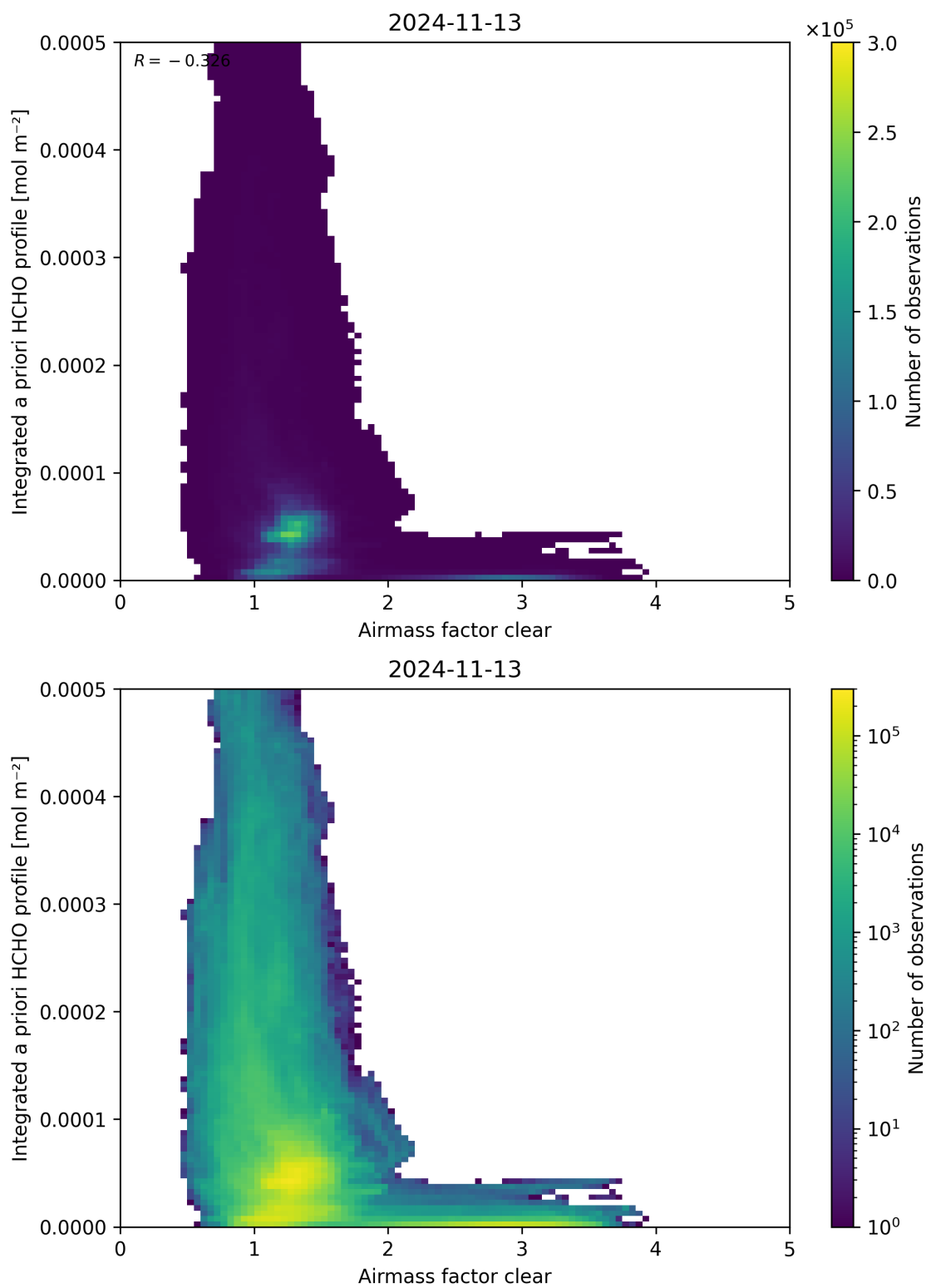
Figure 76: Scatter density plot of “Airmass factor clear” against “Integrated a priori HCHO profile” for 2024-11-12 to 2024-11-14.
