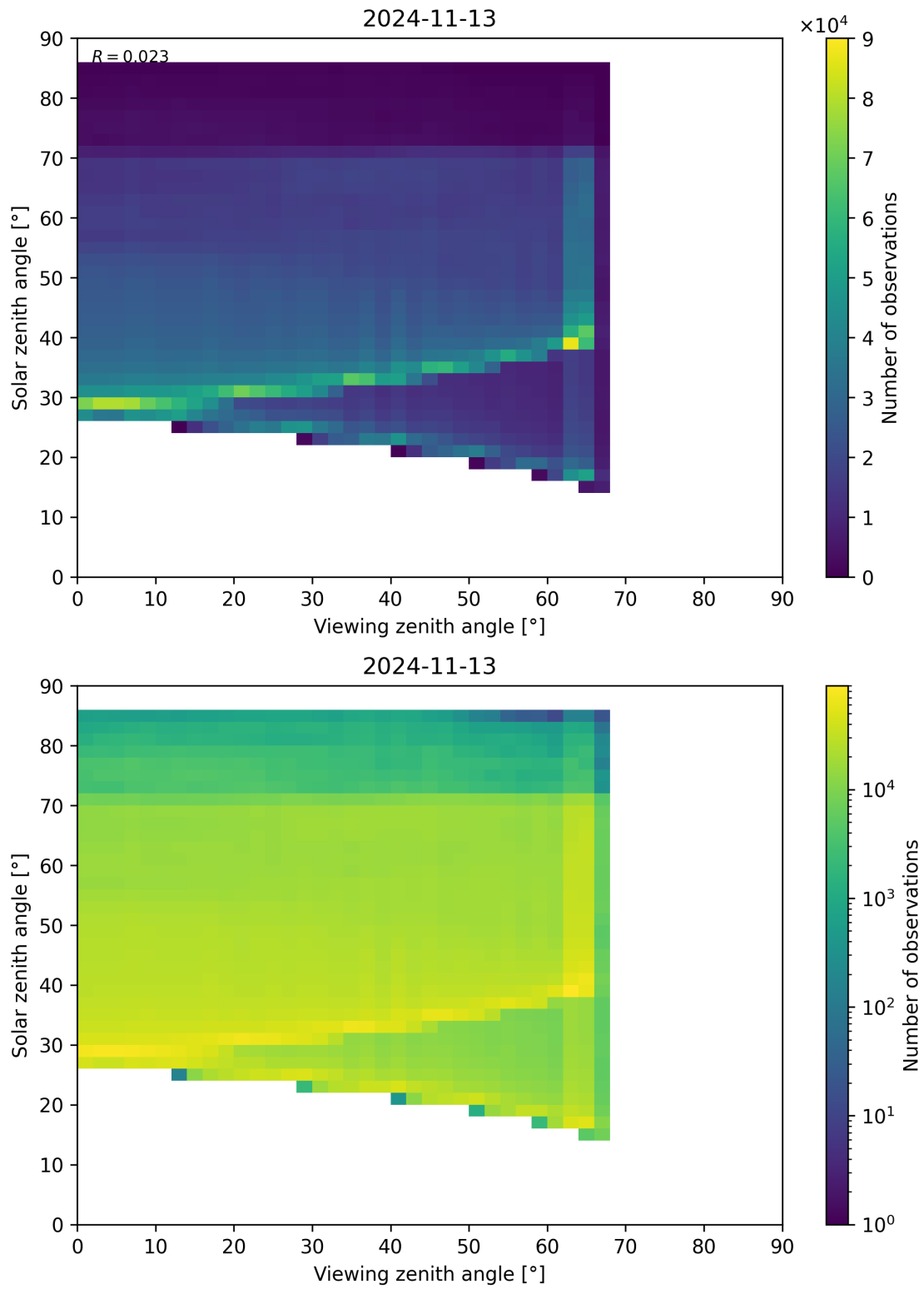
Figure 197: Scatter density plot of “Viewing zenith angle” against “Solar zenith angle” for 2024-11-12 to 2024-11-14.
