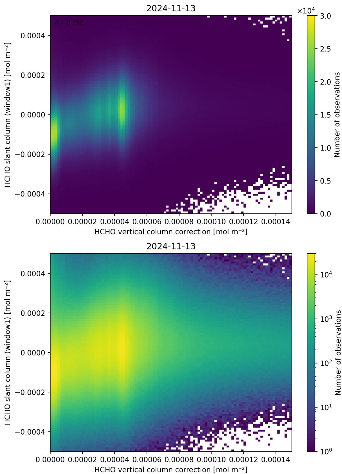
Figure 118: Scatter density plot of “HCHO vertical column correction” against “HCHO slant column (window1)” for 2024-11-12 to 2024-11-14.
