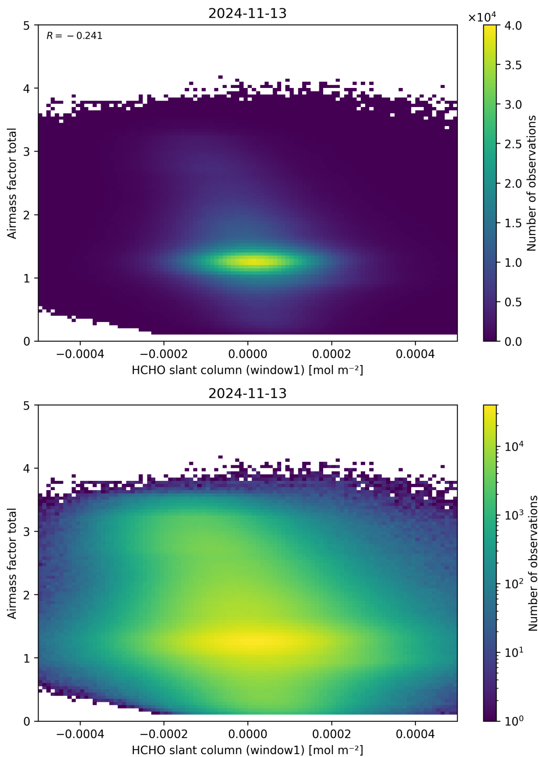
Figure 85: Scatter density plot of “HCHO slant column (window1)” against “Airmass factor total” for 2024-11-12 to 2024-11-14.
