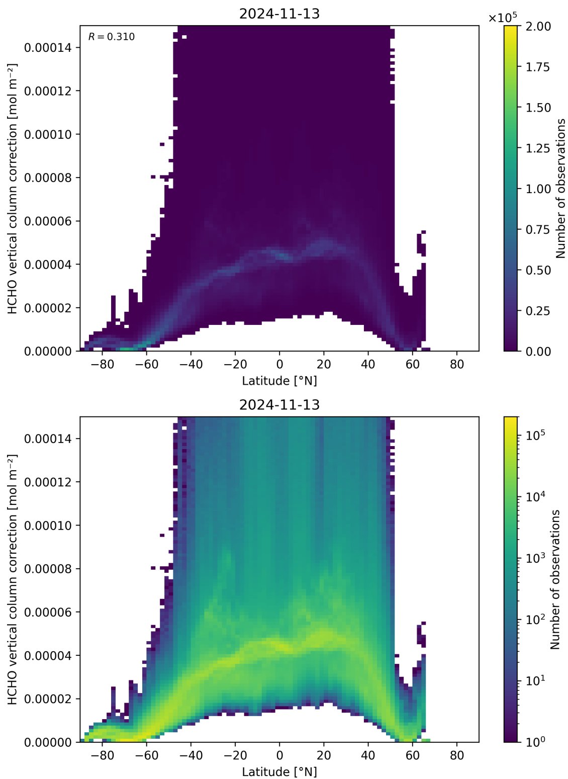
Figure 164: Scatter density plot of “Latitude” against “HCHO vertical column correction” for 2024-11-12 to 2024-11-14.
