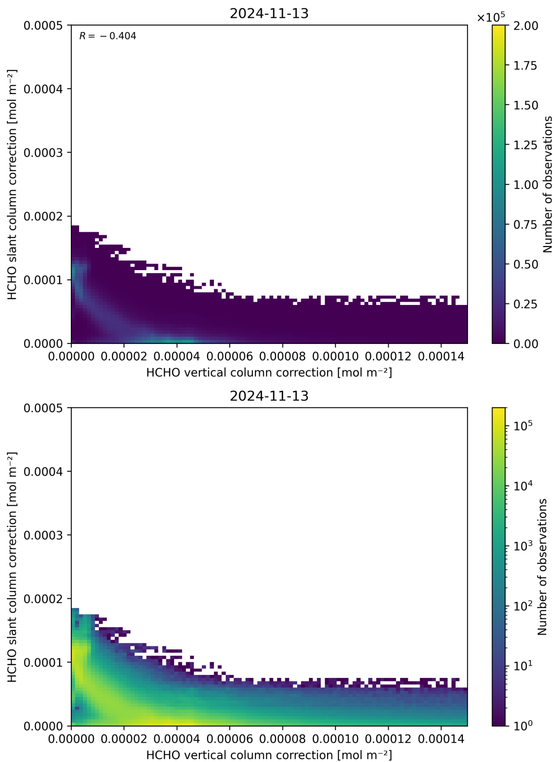
Figure 117: Scatter density plot of “HCHO vertical column correction” against “HCHO slant column correction” for 2024-11-12 to 2024-11-14.
