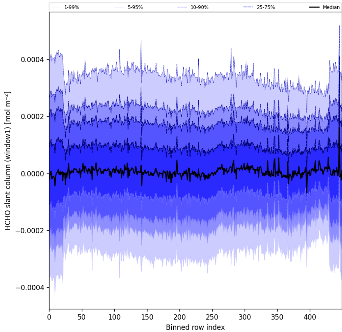
Figure 52: Along track statistics of “HCHO slant column (window1)” for 2024-11-12 to 2024-11-14
