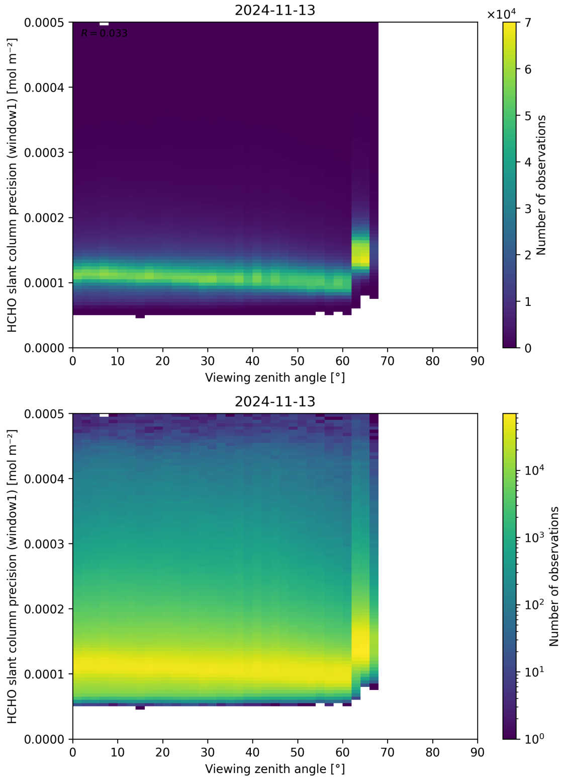
Figure 189: Scatter density plot of “Viewing zenith angle” against “HCHO slant column precision (window1)” for 2024-11-12 to 2024-11-14.
