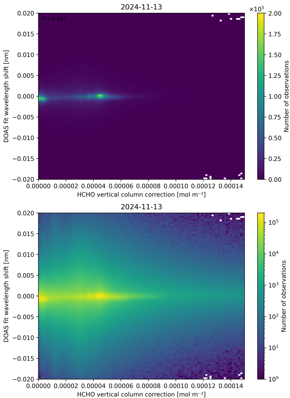
Figure 113: Scatter density plot of “HCHO vertical column correction” against “DOAS fit wavelength shift” for 2024-11-12 to 2024-11-14.
