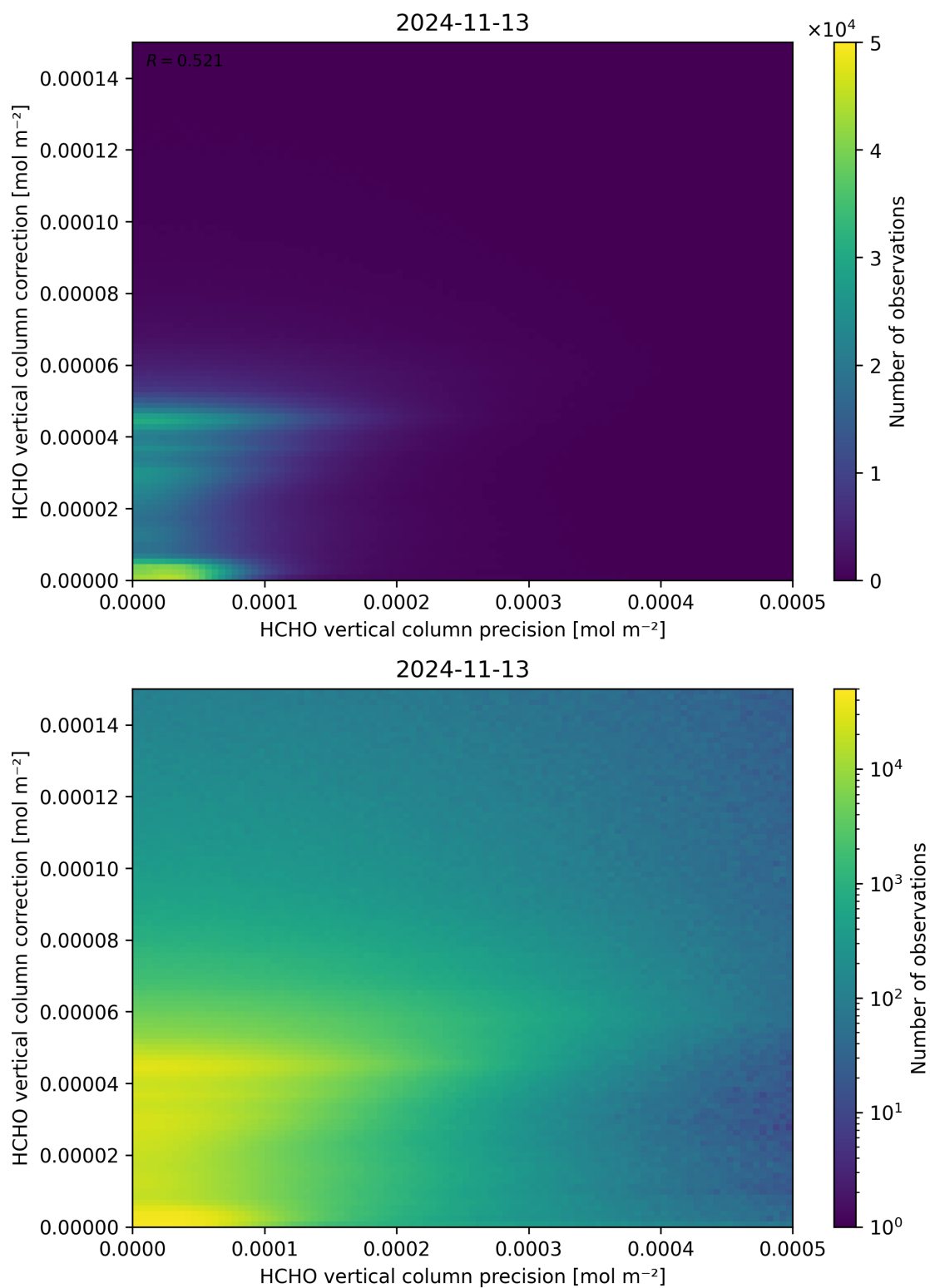
Figure 146: Scatter density plot of “HCHO vertical column precision” against “HCHO vertical column correction” for 2024-11-12 to 2024-11-14.
