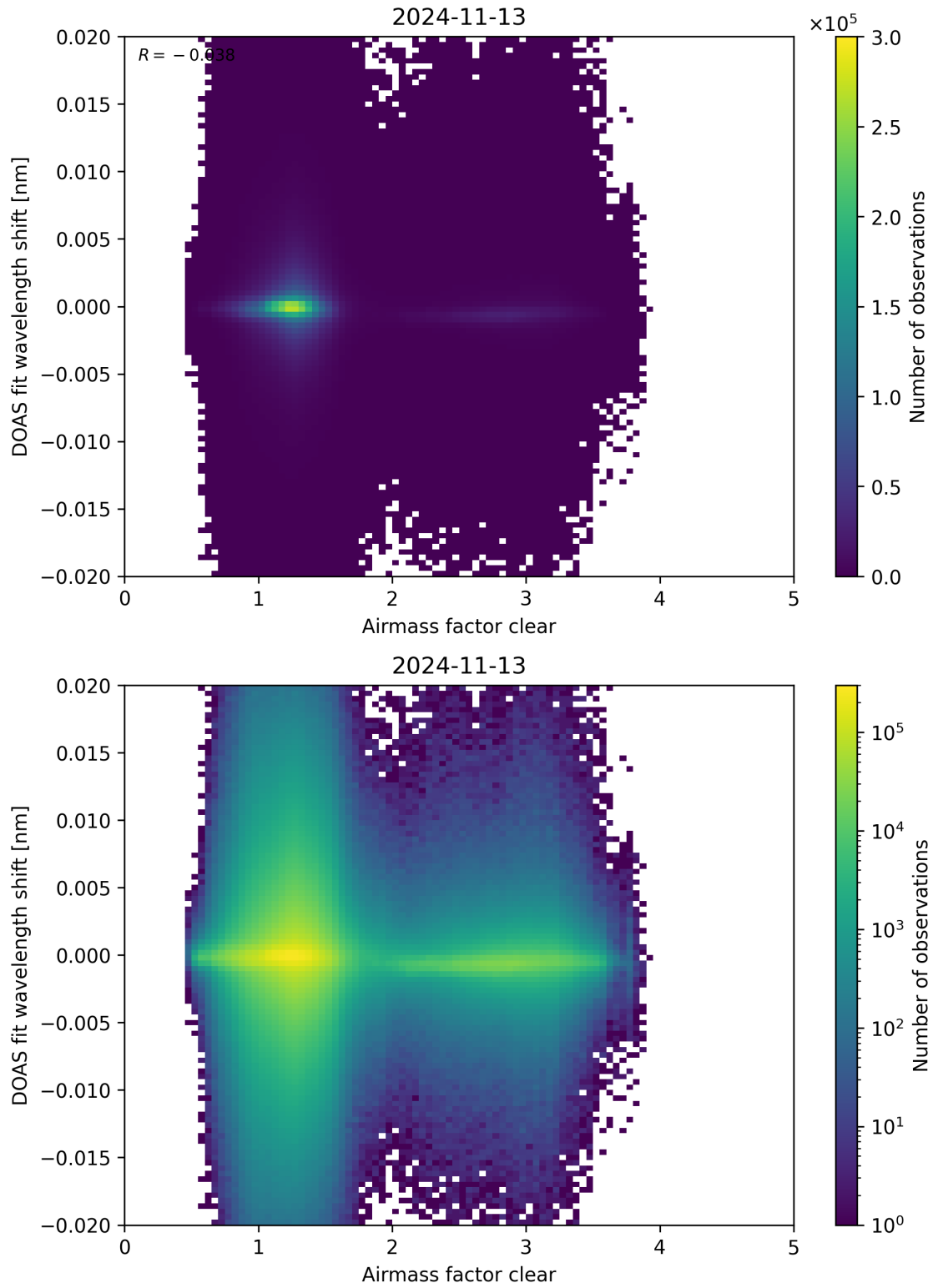
Figure 72: Scatter density plot of “Airmass factor clear” against “DOAS fit wavelength shift” for 2024-11-12 to 2024-11-14.
