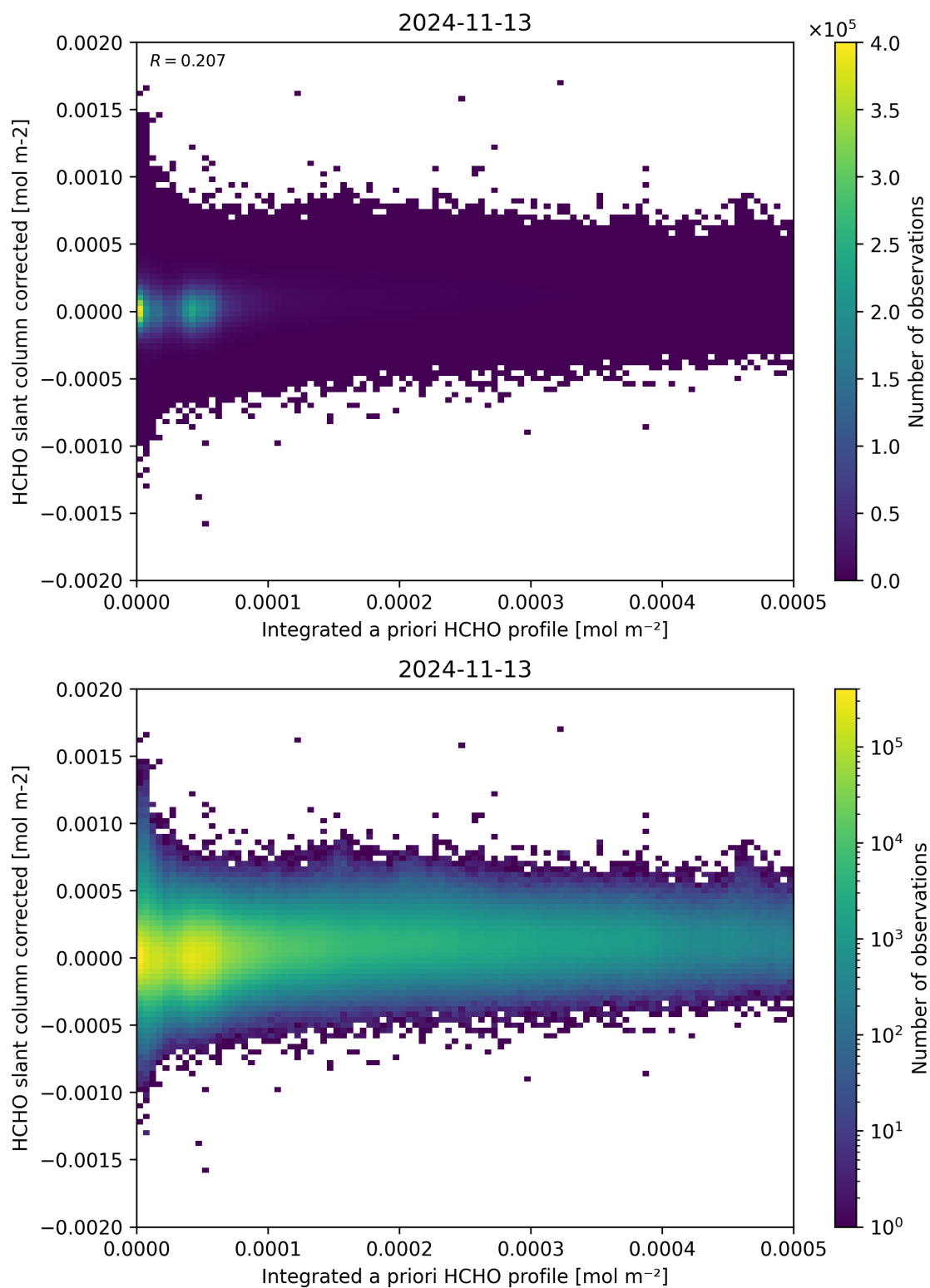
Figure 151: Scatter density plot of “Integrated a priori HCHO profile” against “HCHO slant column corrected” for 2024-11-12 to 2024-11-14.
