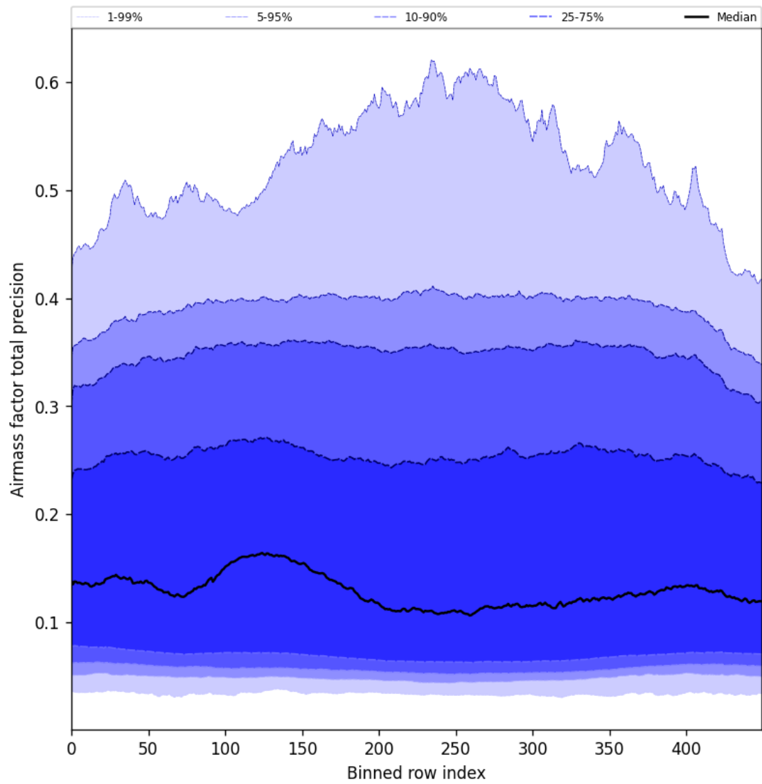
Figure 55: Along track statistics of “Airmass factor total precision” for 2024-11-12 to 2024-11-14
