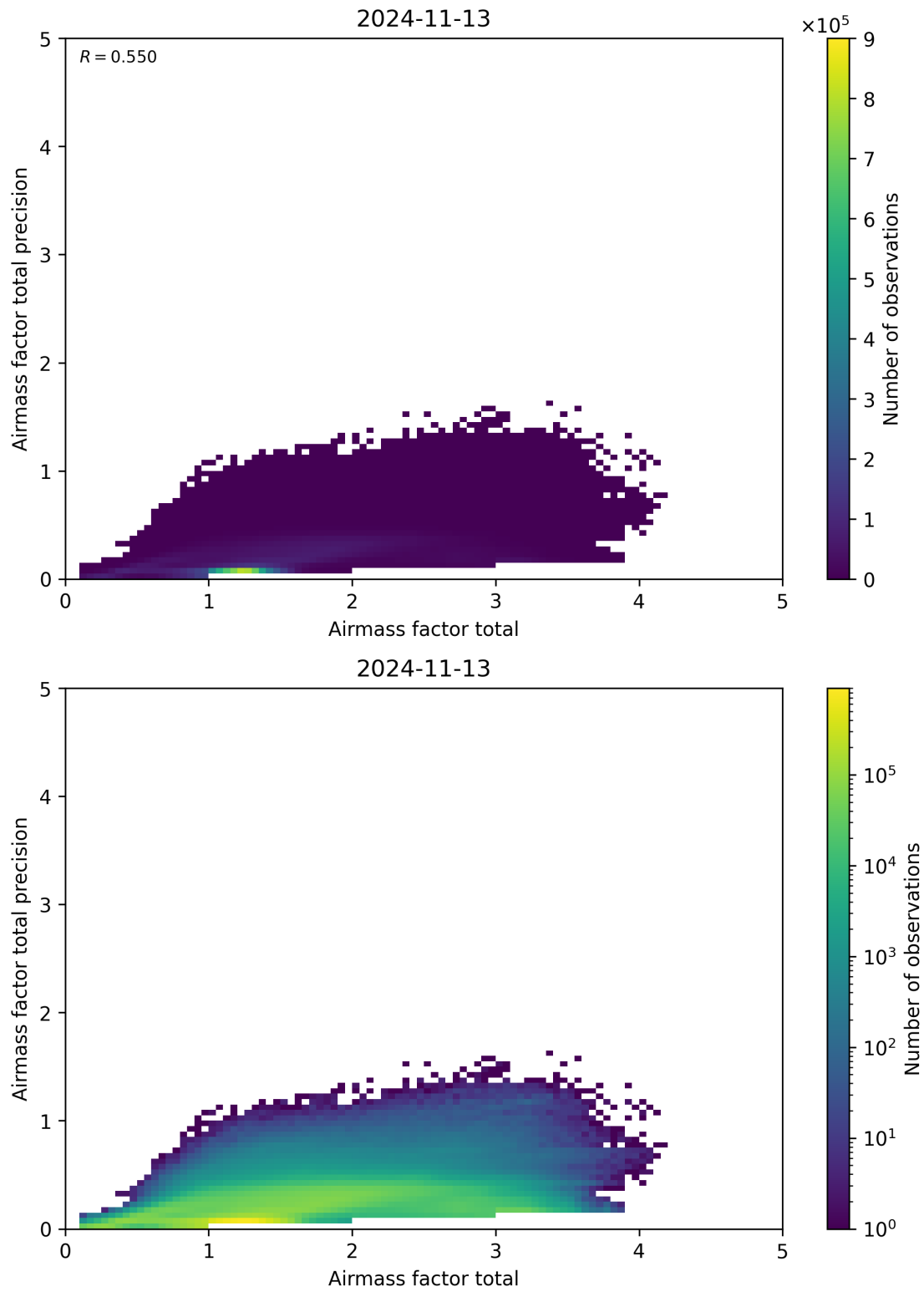
Figure 103: Scatter density plot of “Airmass factor total” against “Airmass factor total precision” for 2024-11-12 to 2024-11-14.
