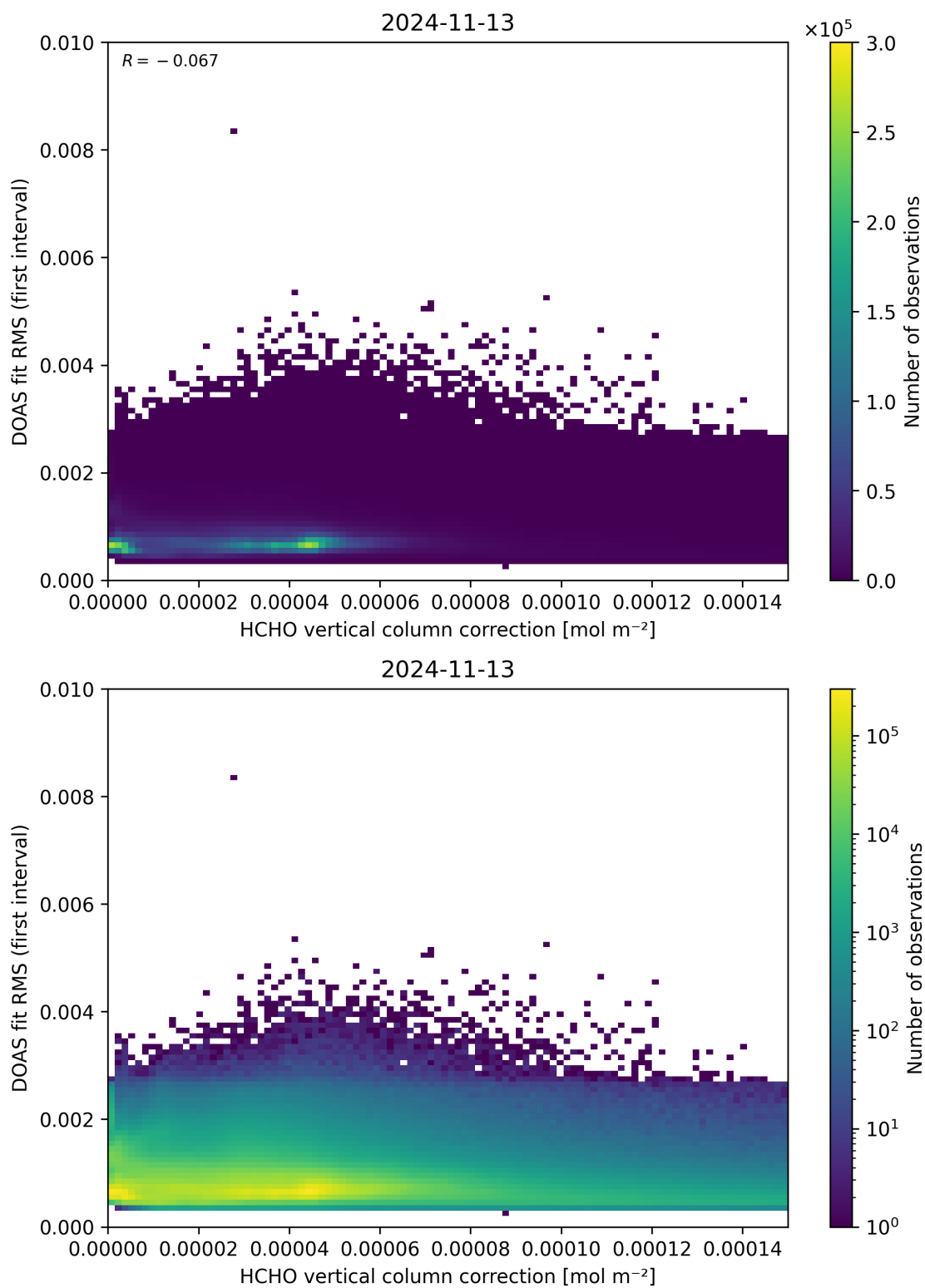
Figure 112: Scatter density plot of “HCHO vertical column correction” against “DOAS fit RMS (first interval)” for 2024-11-12 to 2024-11-14.
