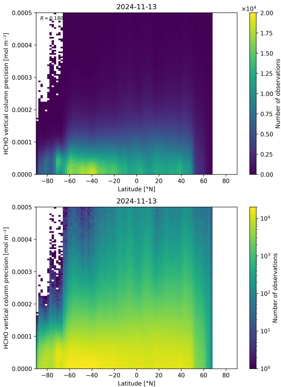
Figure 165: Scatter density plot of “Latitude” against “HCHO vertical column precision” for 2024-11-12 to 2024-11-14.
