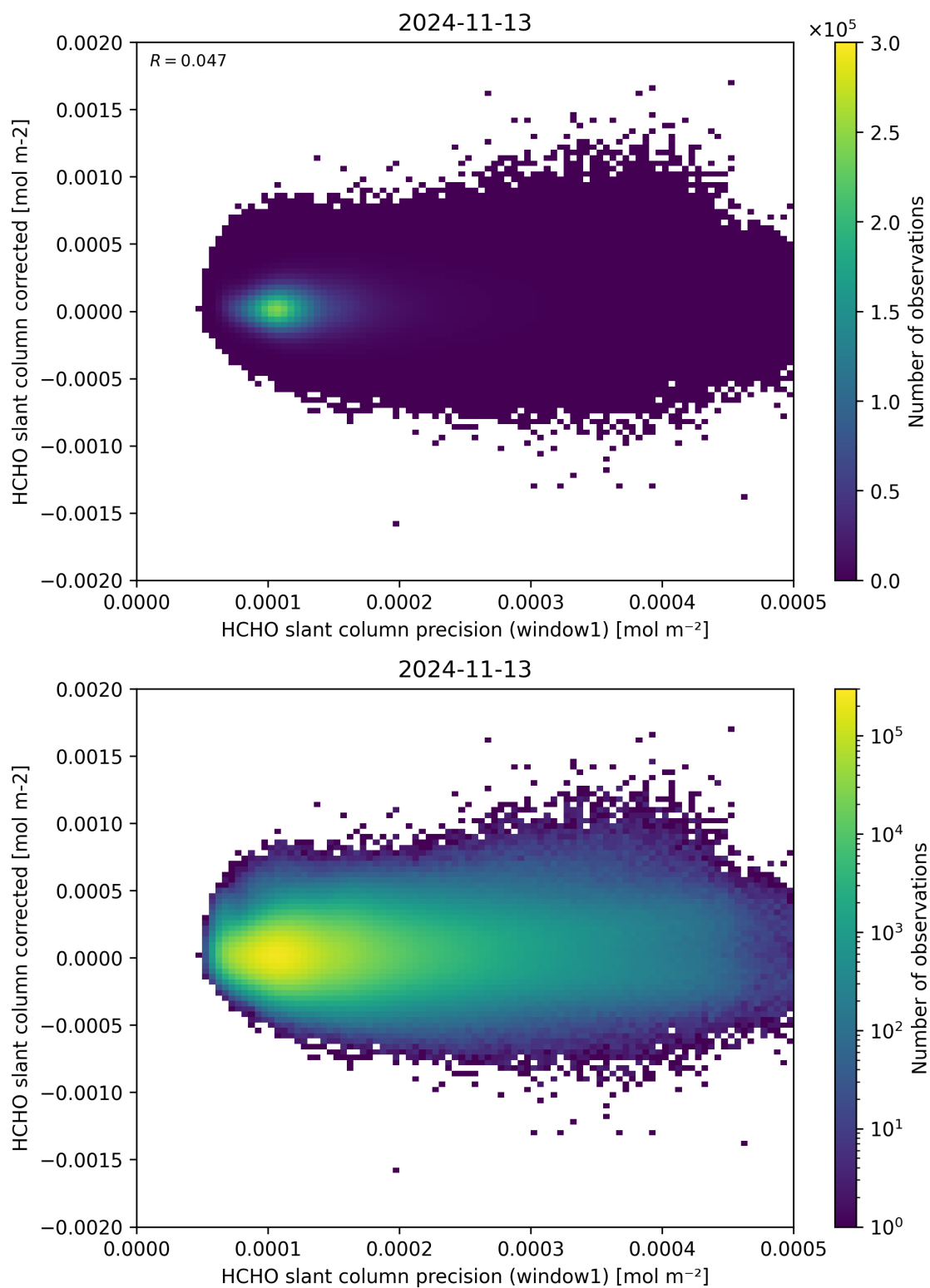
Figure 92: Scatter density plot of “HCHO slant column precision (window1)” against “HCHO slant column corrected” for 2024-11-12 to 2024-11-14.
