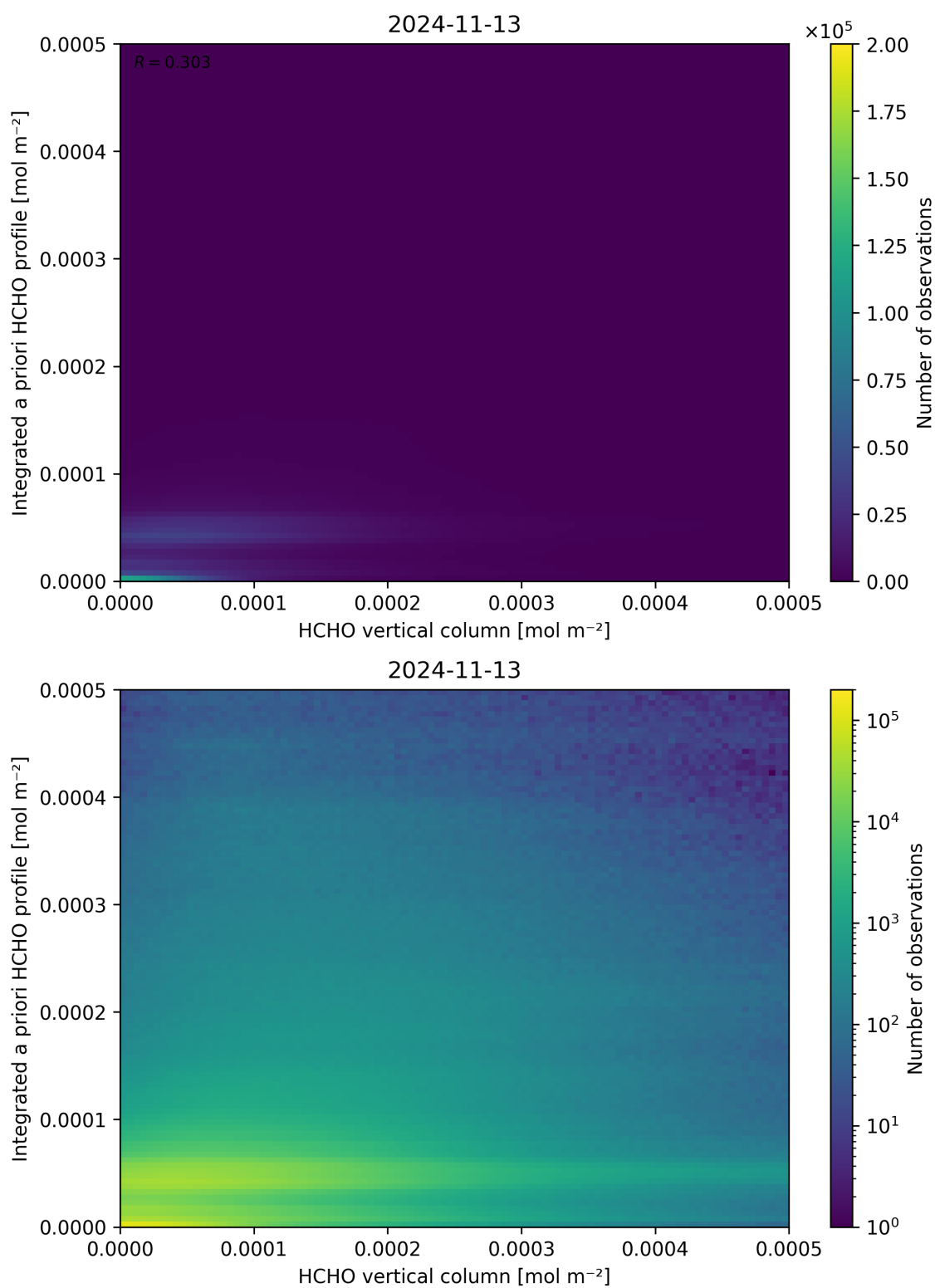
Figure 135: Scatter density plot of “HCHO vertical column” against “Integrated a priori HCHO profile” for 2024-11-12 to 2024-11-14.
