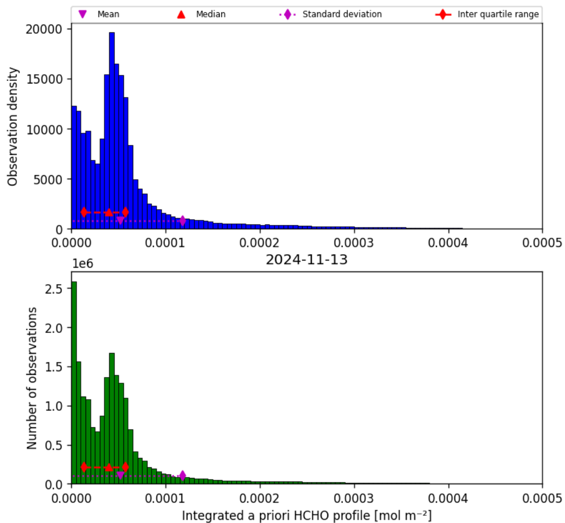
Figure 43: Histogram of “Integrated a priori HCHO profile” for 2024-11-12 to 2024-11-14
