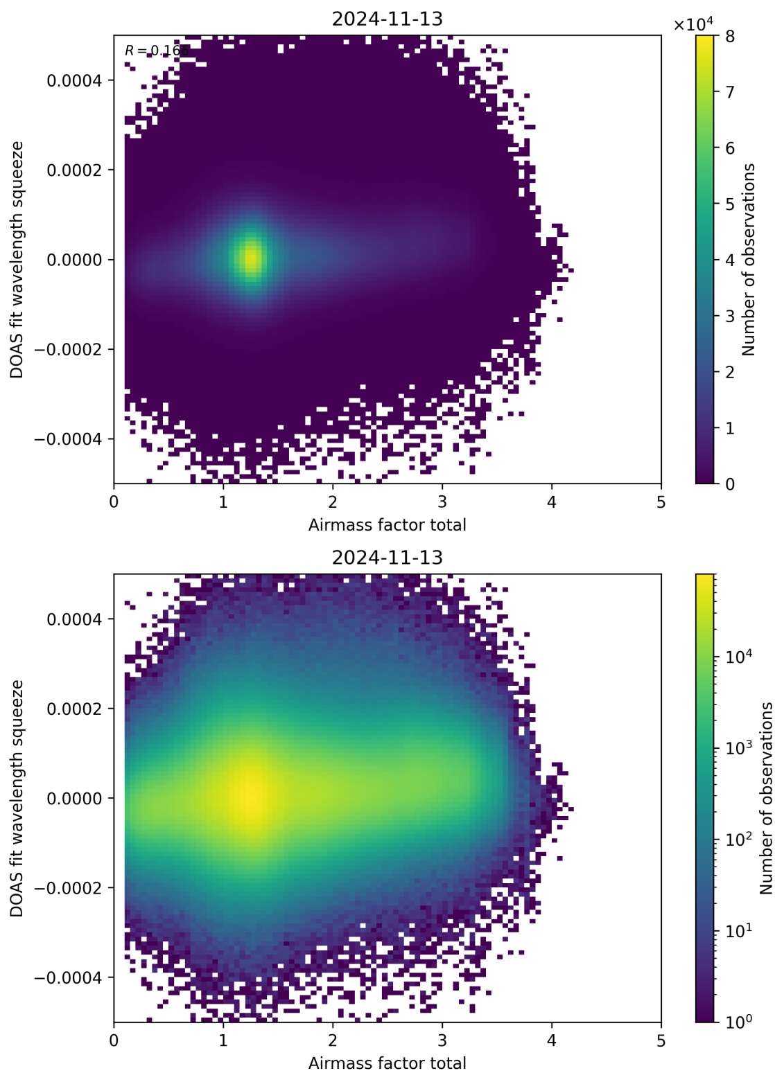
Figure 99: Scatter density plot of “Airmass factor total” against “DOAS fit wavelength squeeze” for 2024-11-12 to 2024-11-14.
