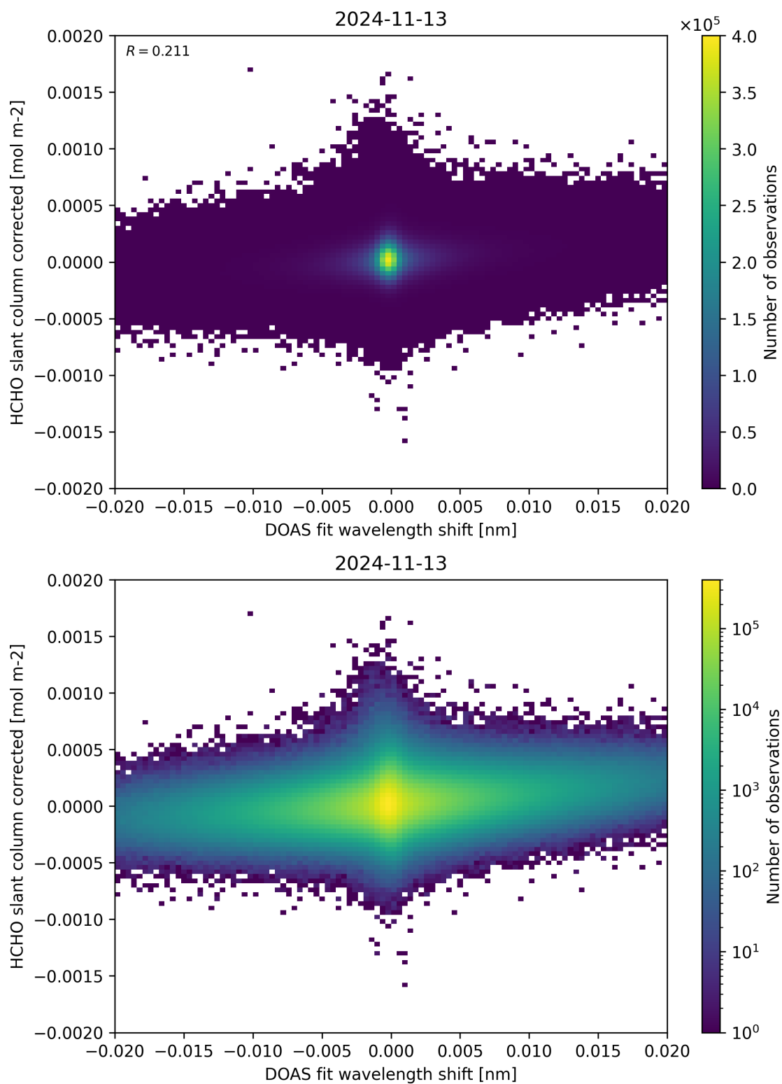
Figure 66: Scatter density plot of “DOAS fit wavelength shift” against “HCHO slant column corrected” for 2024-11-12 to 2024-11-14.
