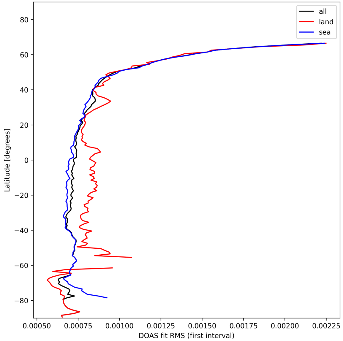
Figure 32: Zonal average of “DOAS fit RMS (first interval)” for 2024-11-12 to 2024-11-14.
