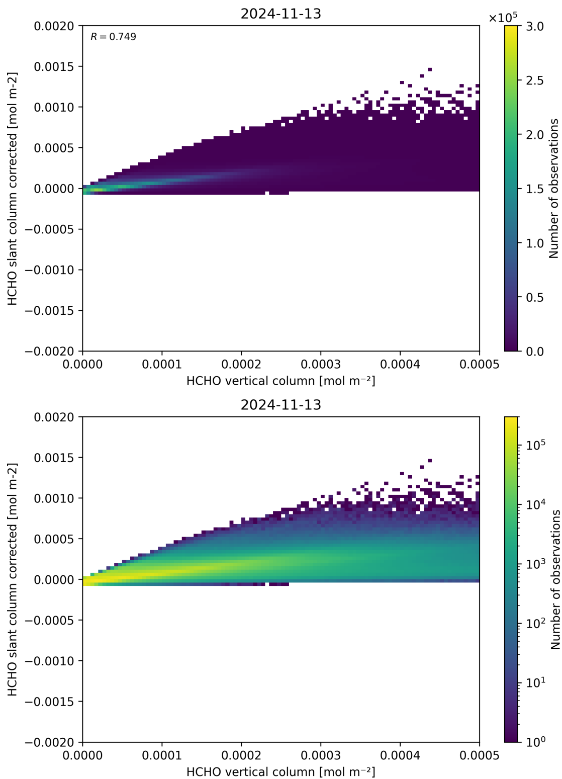
Figure 127: Scatter density plot of “HCHO vertical column” against “HCHO slant column corrected” for 2024-11-12 to 2024-11-14.
