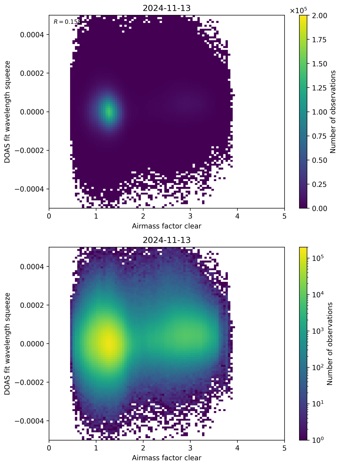
Figure 73: Scatter density plot of “Airmass factor clear” against “DOAS fit wavelength squeeze” for 2024-11-12 to 2024-11-14.
