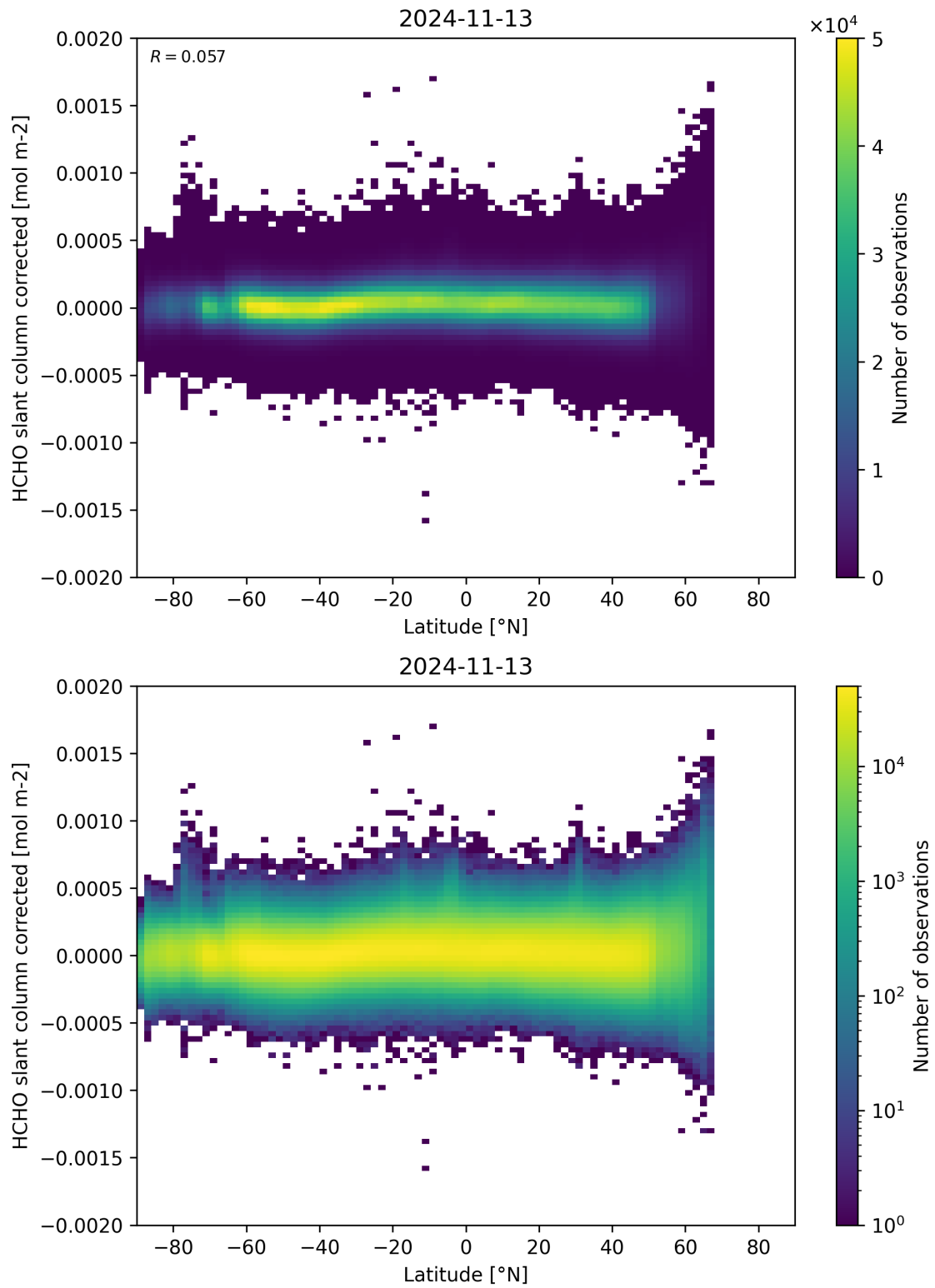
Figure 157: Scatter density plot of “Latitude” against “HCHO slant column corrected” for 2024-11-12 to 2024-11-14.
