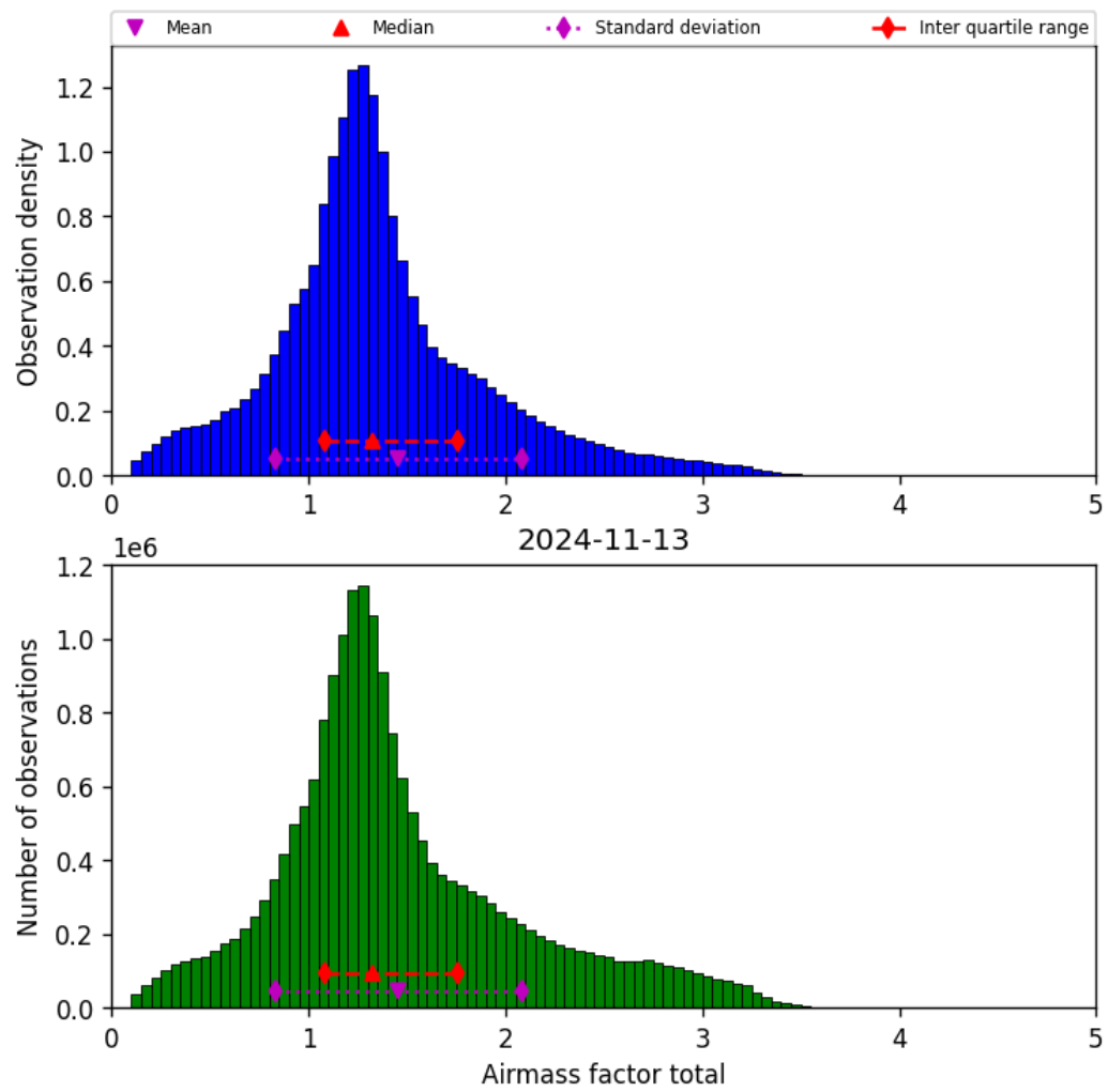
Figure 40: Histogram of “Airmass factor total” for 2024-11-12 to 2024-11-14
