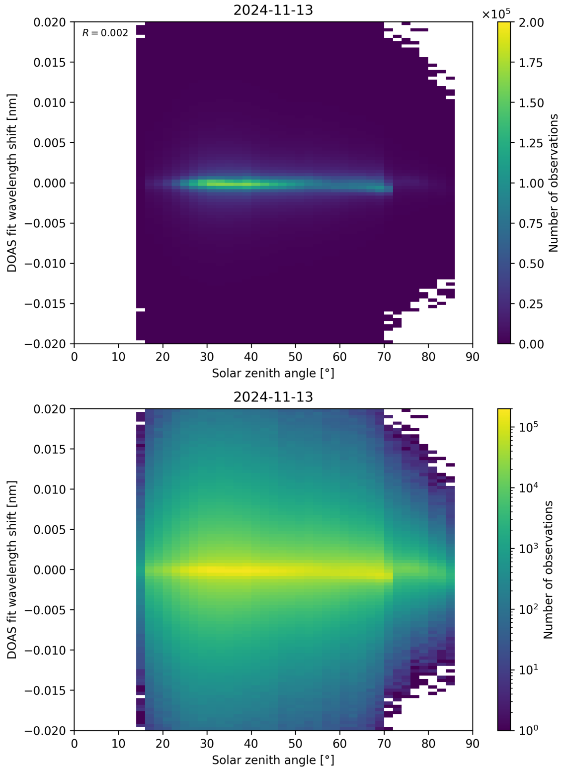
Figure 168: Scatter density plot of “Solar zenith angle” against “DOAS fit wavelength shift” for 2024-11-12 to 2024-11-14.
