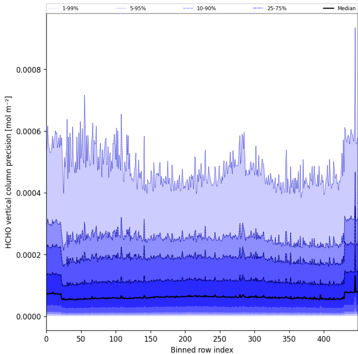
Figure 50: Along track statistics of “HCHO vertical column precision” for 2024-11-12 to 2024-11-14
