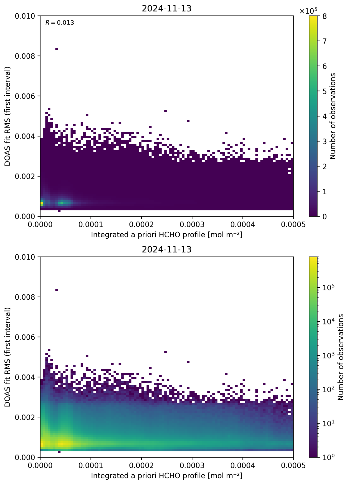
Figure 148: Scatter density plot of “Integrated a priori HCHO profile” against “DOAS fit RMS (first interval)” for 2024-11-12 to 2024-11-14.
