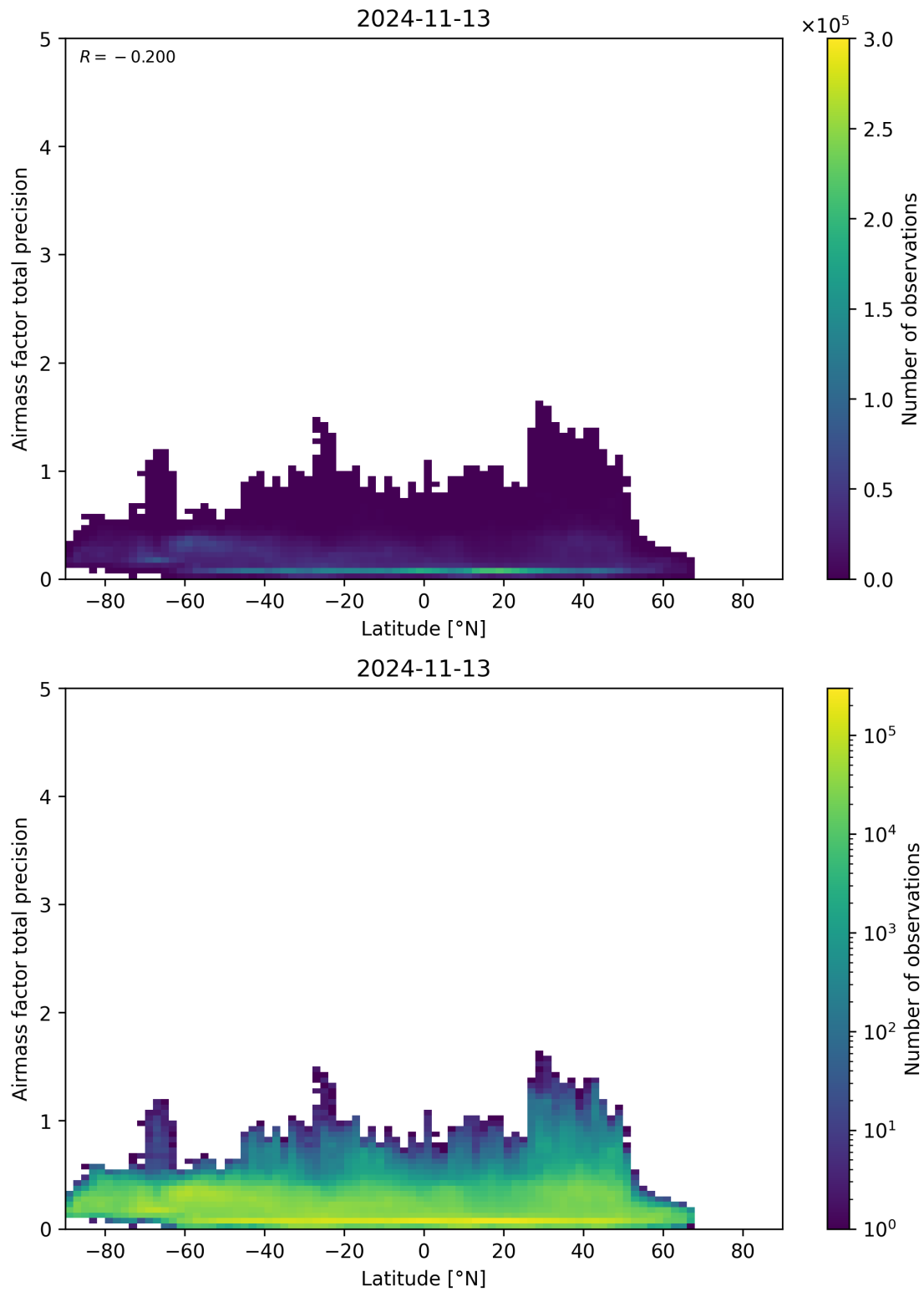
Figure 162: Scatter density plot of “Latitude” against “Airmass factor total precision” for 2024-11-12 to 2024-11-14.
