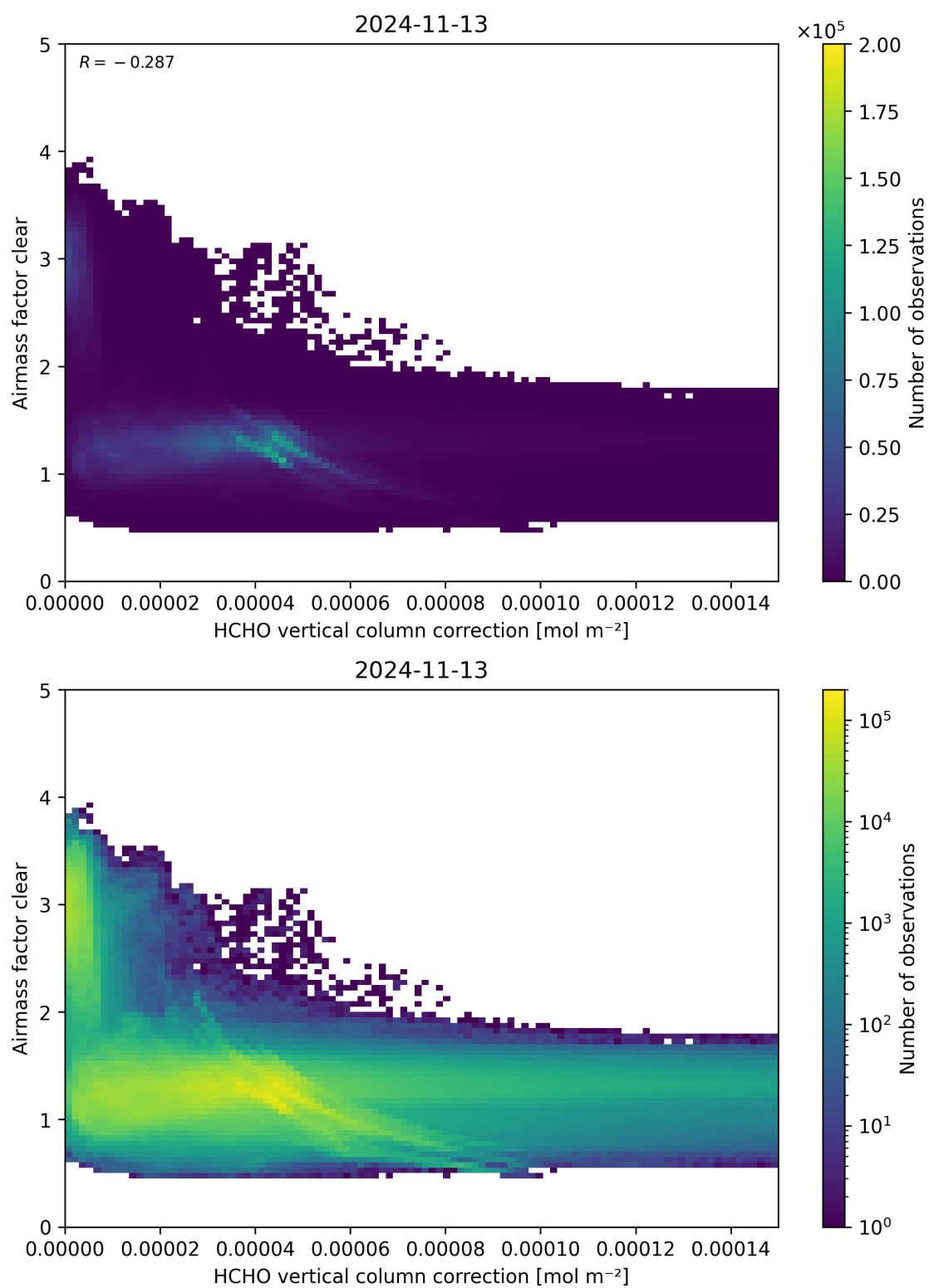
Figure 115: Scatter density plot of “HCHO vertical column correction” against “Airmass factor clear” for 2024-11-12 to 2024-11-14.
