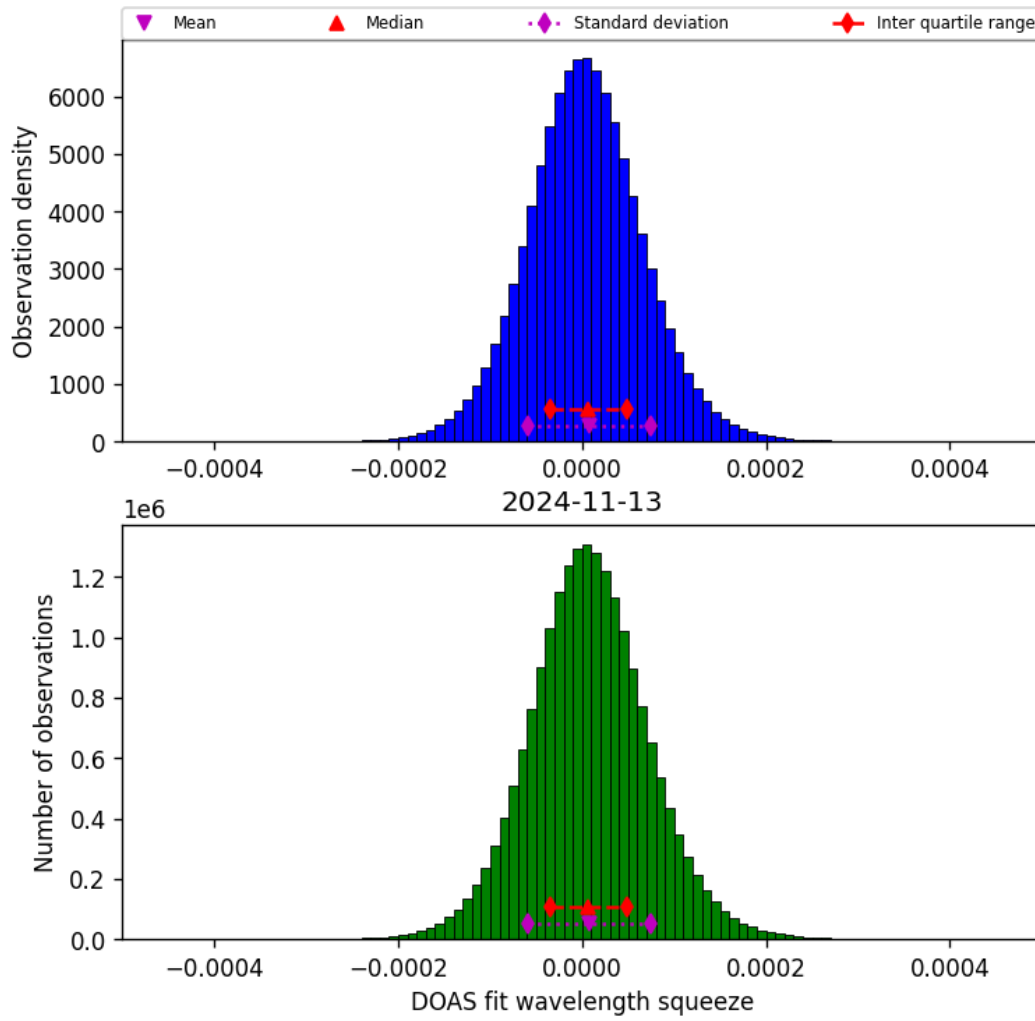
Figure 45: Histogram of “DOAS fit wavelength squeeze” for 2024-11-12 to 2024-11-14
