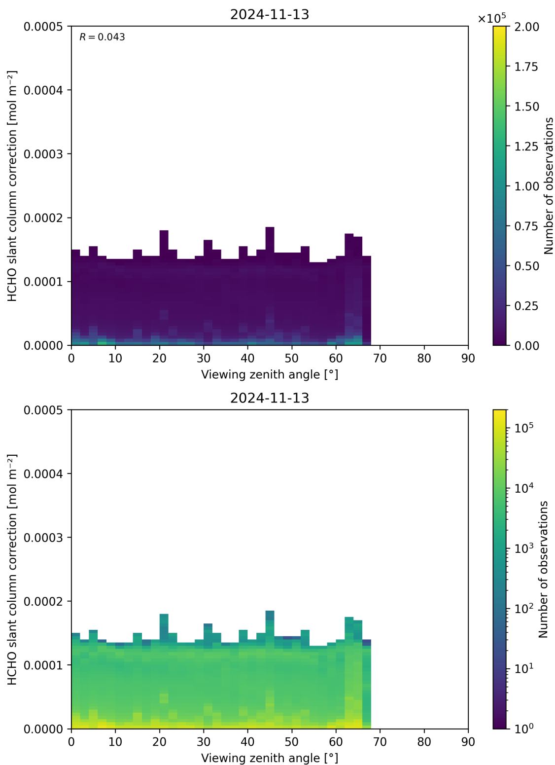
Figure 187: Scatter density plot of “Viewing zenith angle” against “HCHO slant column correction” for 2024-11-12 to 2024-11-14.
