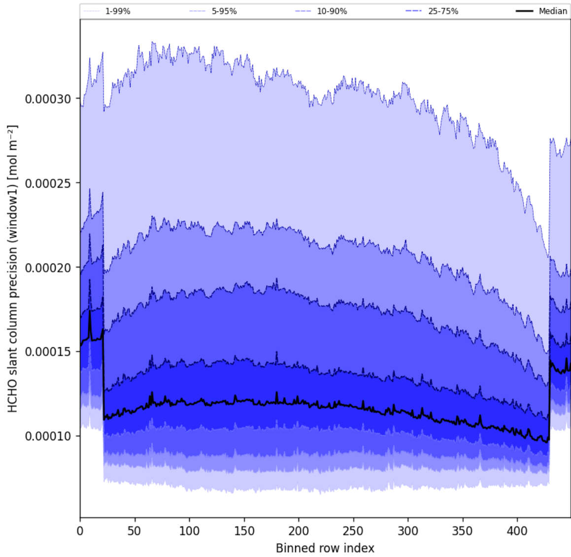
Figure 53: Along track statistics of “HCHO slant column precision (window1)” for 2024-11-12 to 2024-11-14
