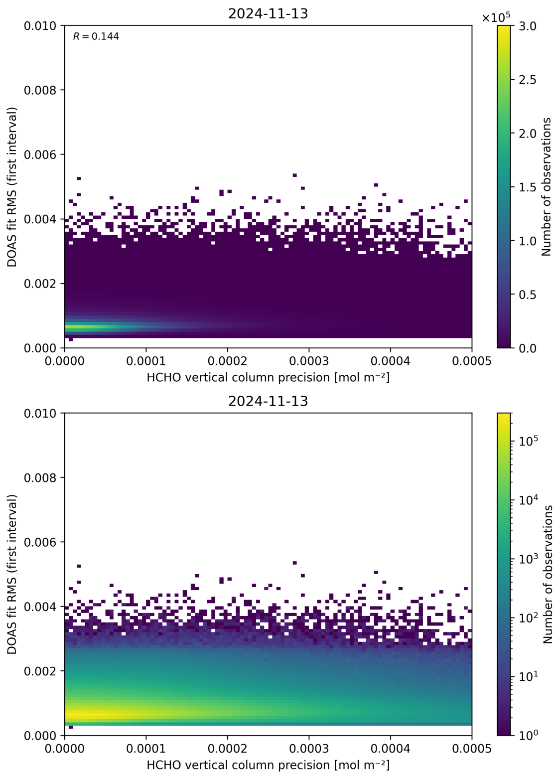
Figure 136: Scatter density plot of “HCHO vertical column precision” against “DOAS fit RMS (first interval)” for 2024-11-12 to 2024-11-14.
