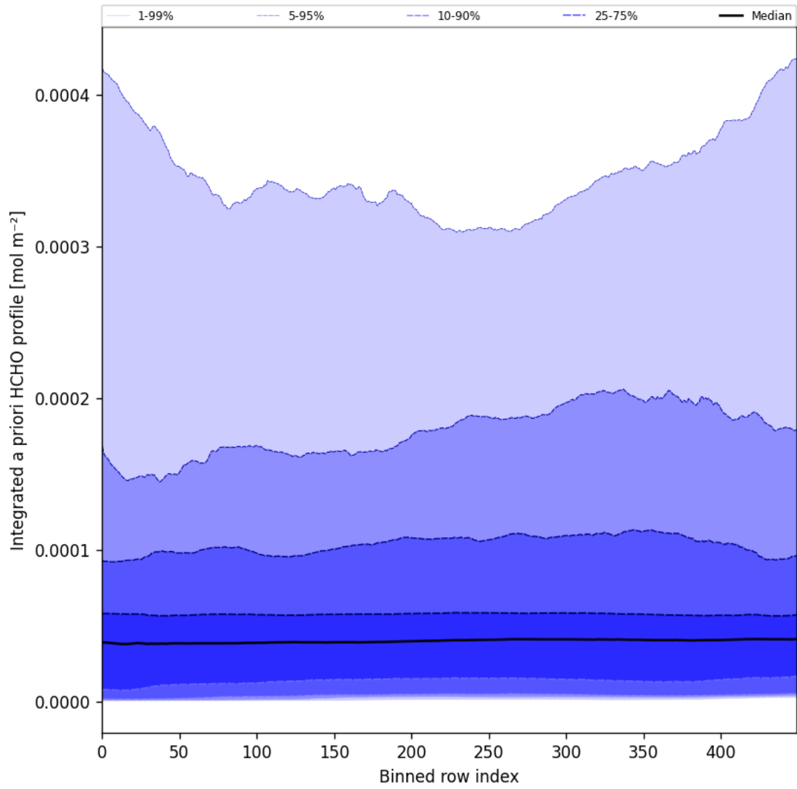
Figure 57: Along track statistics of "Integrated a priori HCHO profile" for 2024-11-12 to 2024-11-14
