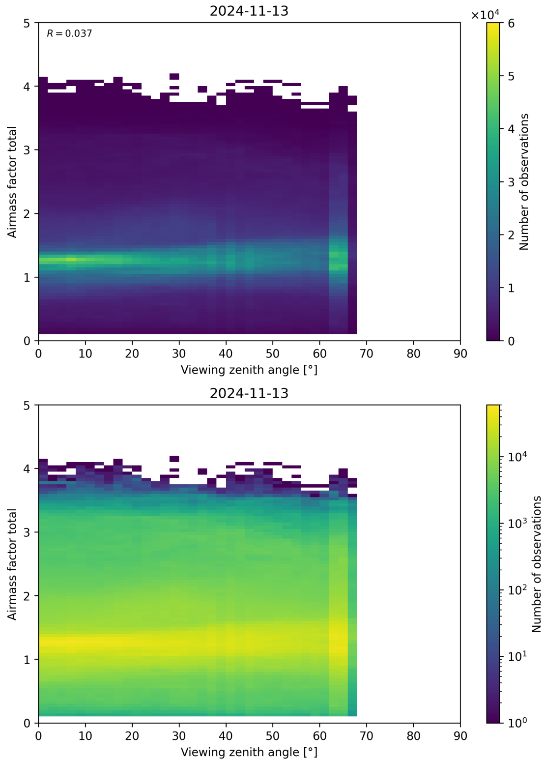
Figure 190: Scatter density plot of “Viewing zenith angle” against “Airmass factor total” for 2024-11-12 to 2024-11-14.
