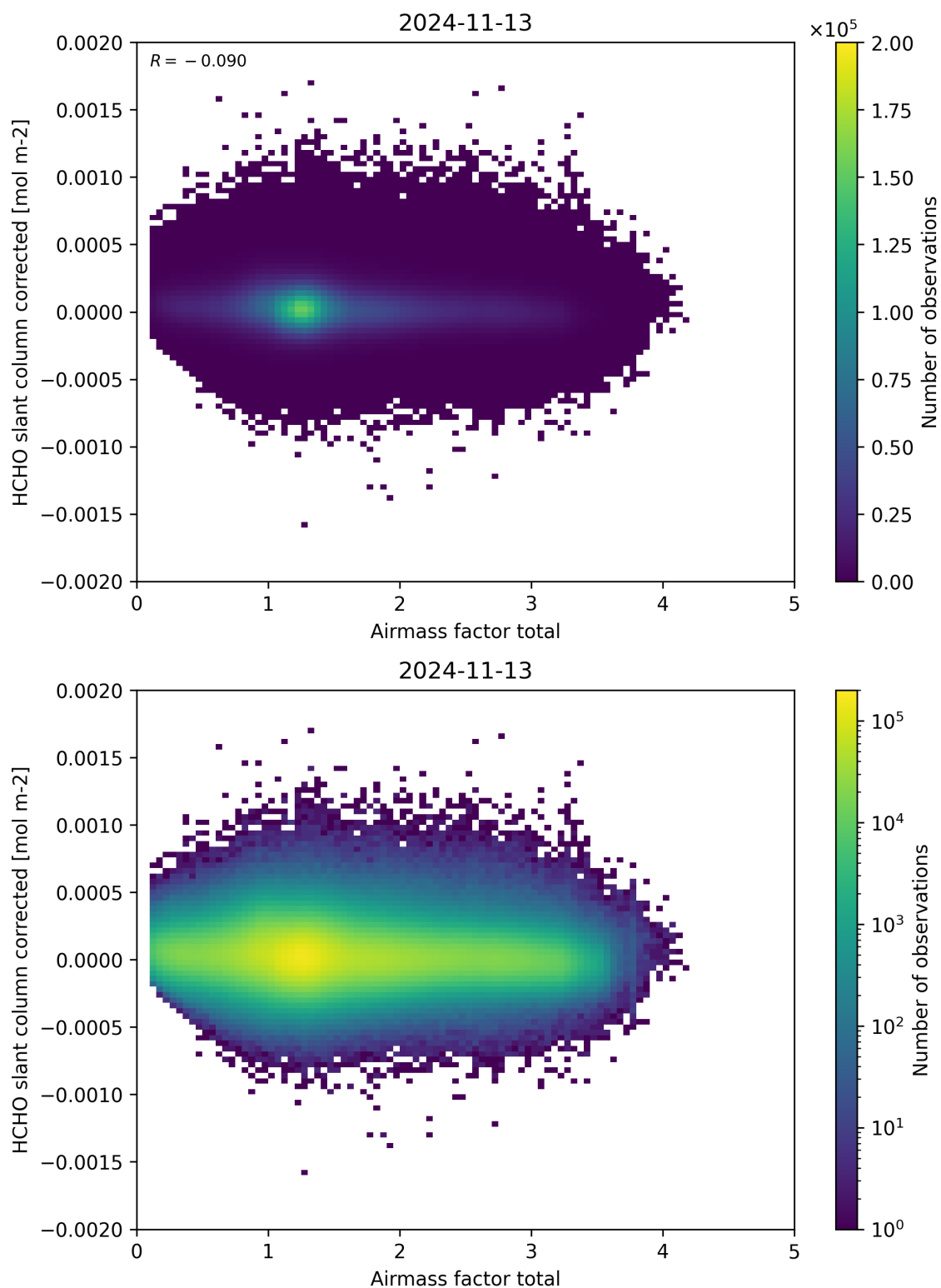
Figure 101: Scatter density plot of “Airmass factor total” against “HCHO slant column corrected” for 2024-11-12 to 2024-11-14.
