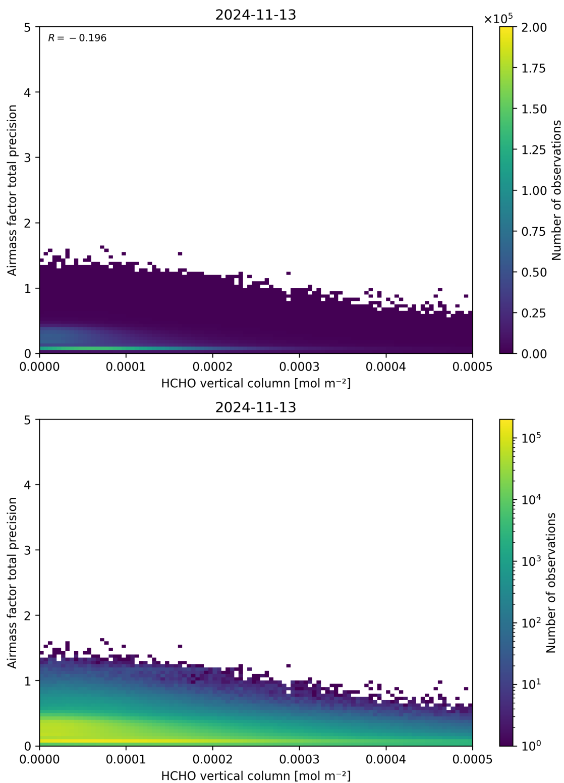
Figure 132: Scatter density plot of “HCHO vertical column” against “Airmass factor total precision” for 2024-11-12 to 2024-11-14.
