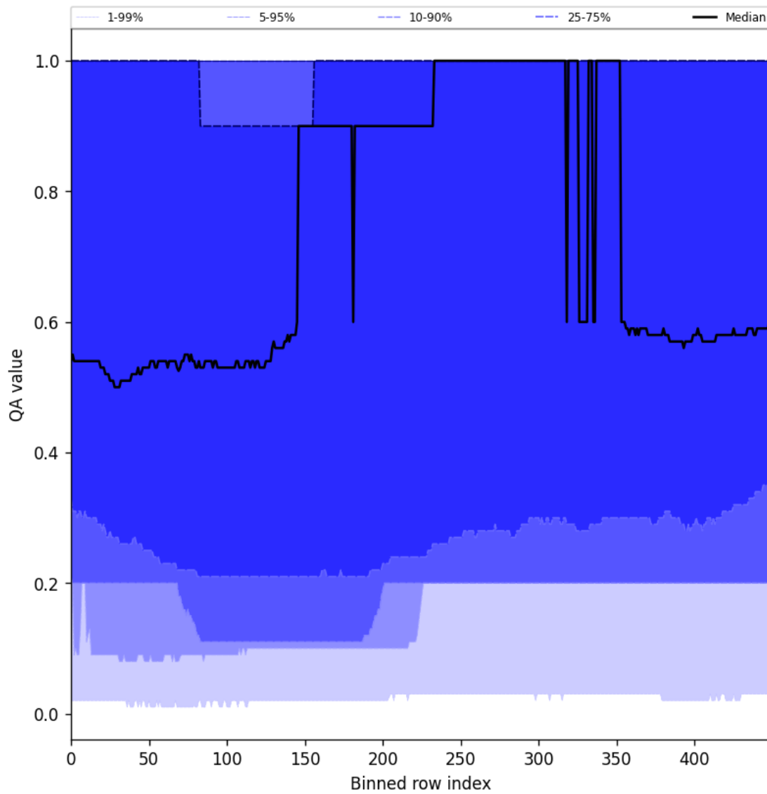
Figure 48: Along track statistics of “QA value” for 2024-11-12 to 2024-11-14
