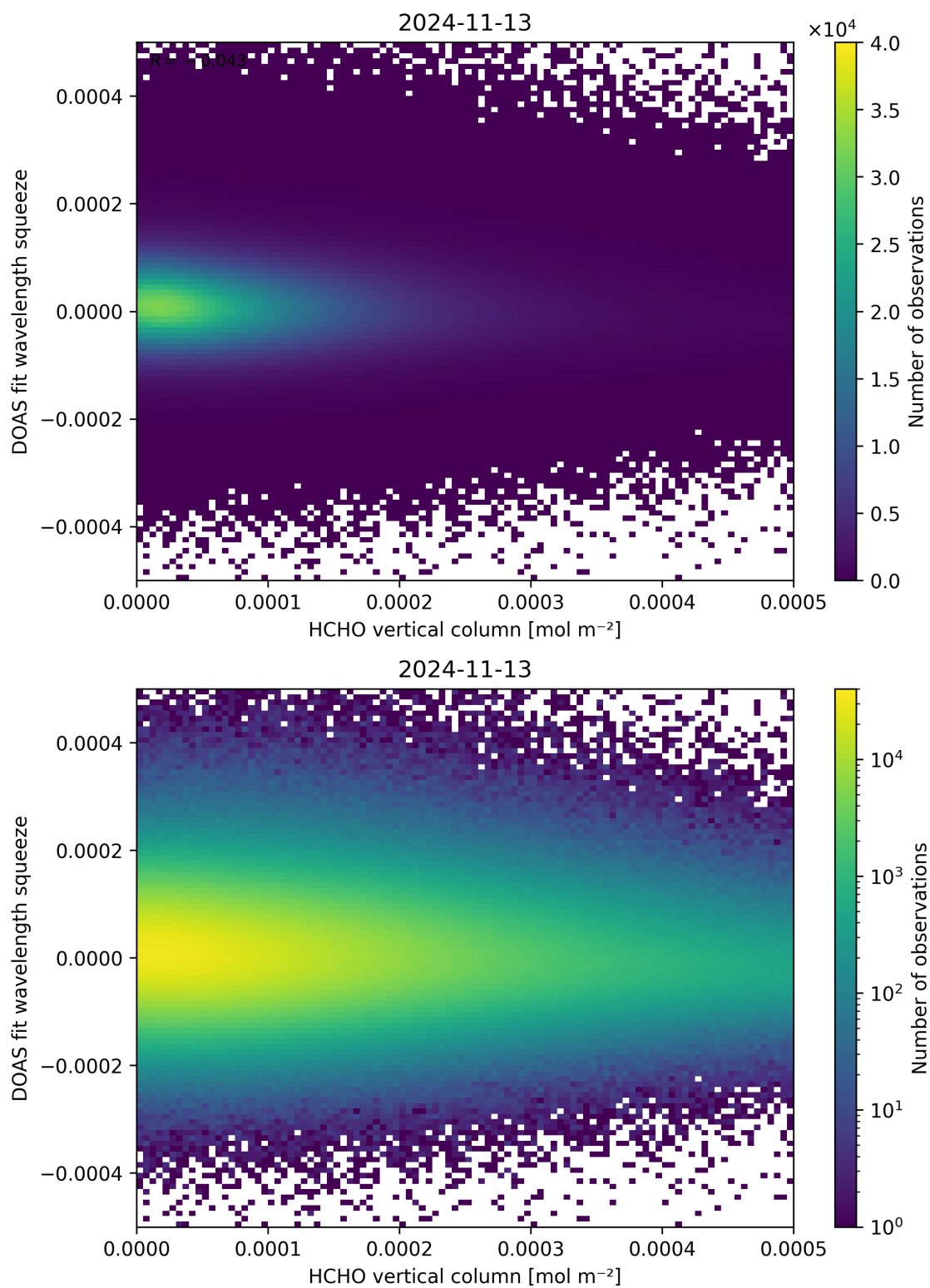
Figure 125: Scatter density plot of “HCHO vertical column” against “DOAS fit wavelength squeeze” for 2024-11-12 to 2024-11-14.
