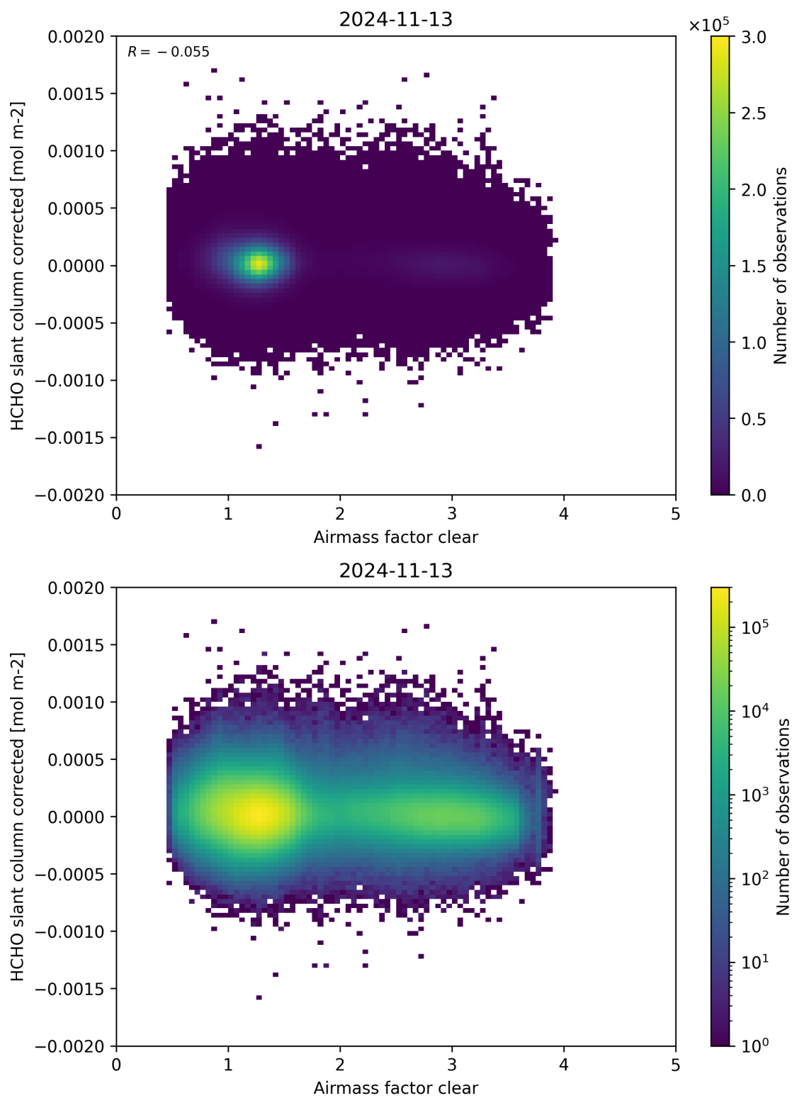
Figure 74: Scatter density plot of “Airmass factor clear” against “HCHO slant column corrected” for 2024-11-12 to 2024-11-14.
