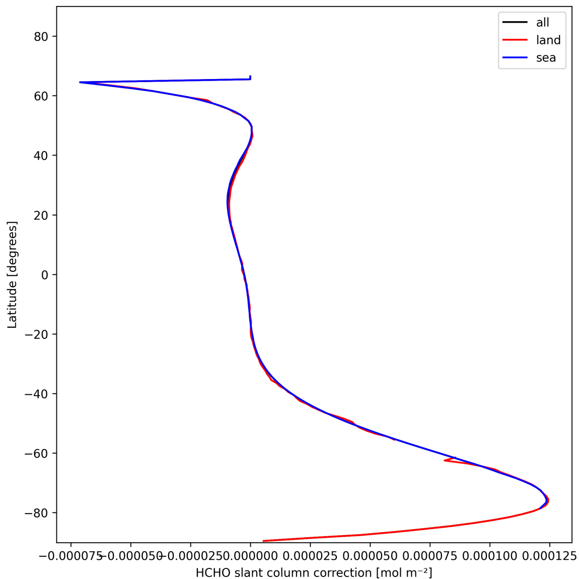
Figure 33: Zonal average of “HCHO slant column correction” for 2024-11-12 to 2024-11-14.
