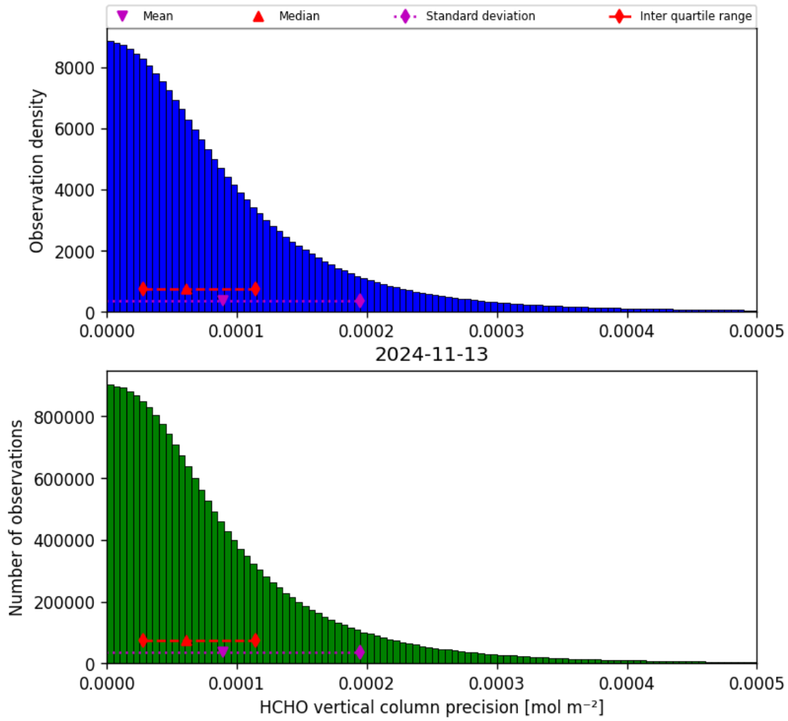
Figure 36: Histogram of “HCHO vertical column precision” for 2024-11-12 to 2024-11-14
