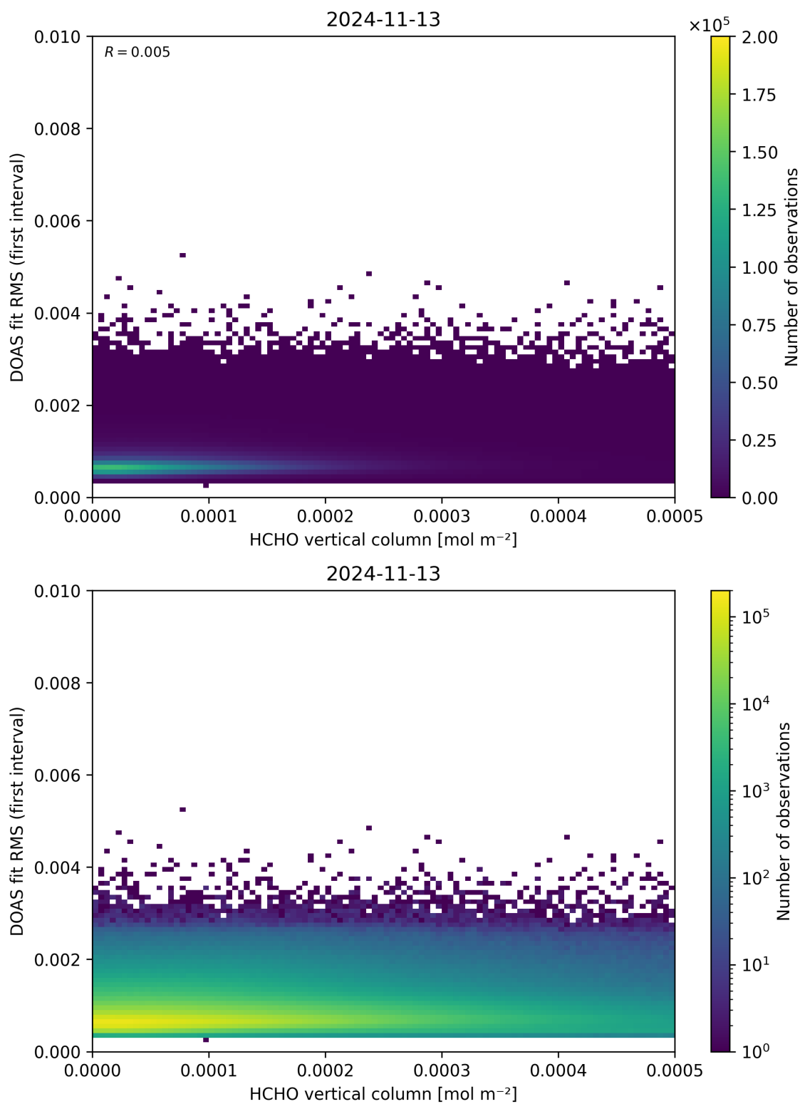
Figure 123: Scatter density plot of “HCHO vertical column” against “DOAS fit RMS (first interval)” for 2024-11-12 to 2024-11-14.
