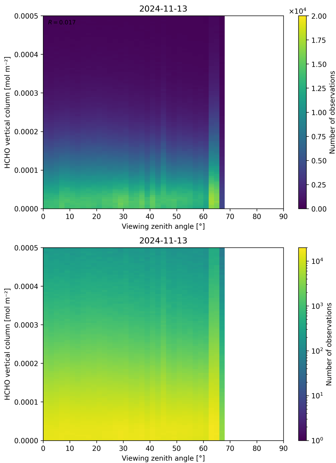
Figure 192: Scatter density plot of “Viewing zenith angle” against “HCHO vertical column” for 2024-11-12 to 2024-11-14.
