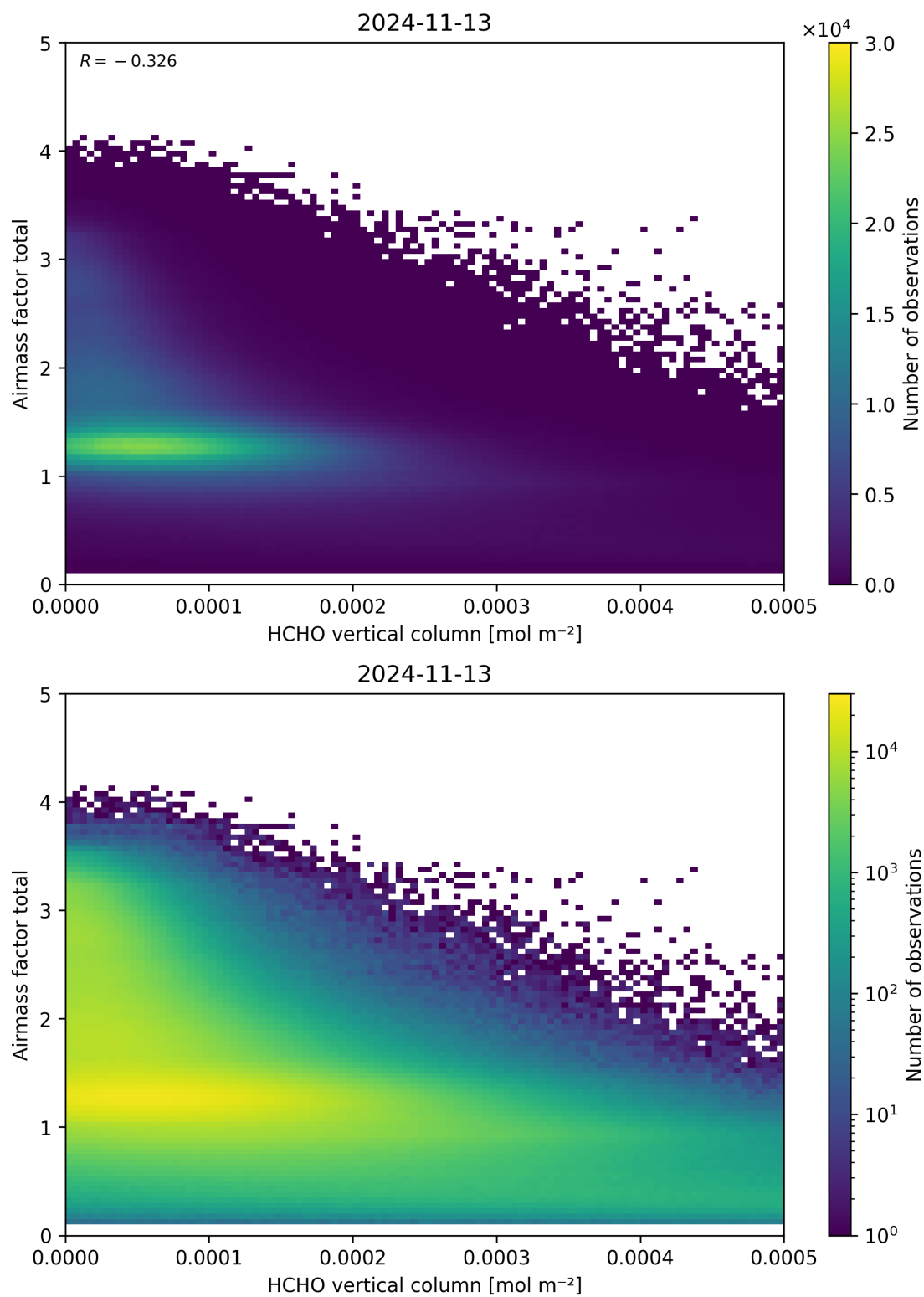
Figure 131: Scatter density plot of “HCHO vertical column” against “Airmass factor total” for 2024-11-12 to 2024-11-14.
