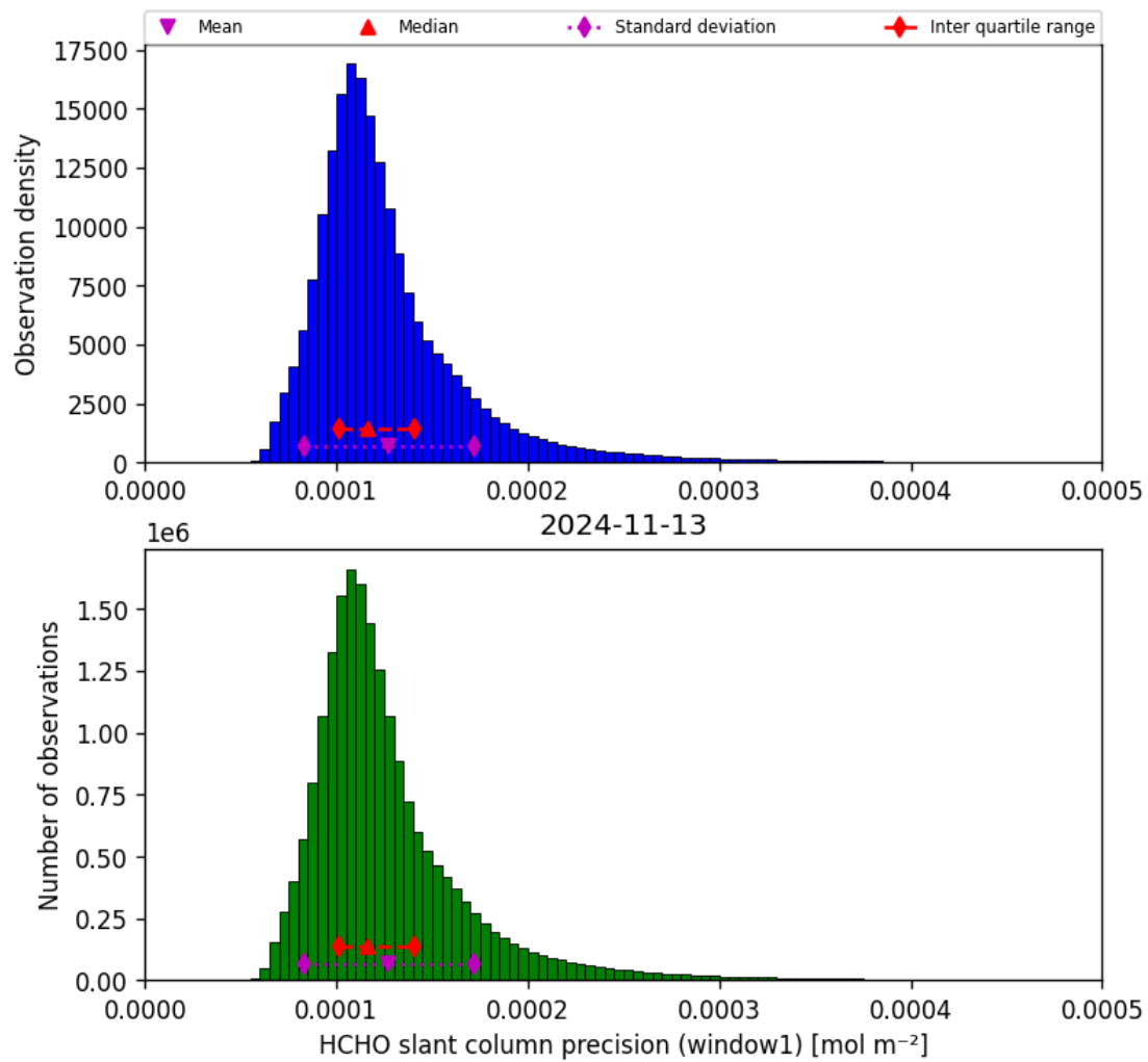
Figure 39: Histogram of “HCHO slant column precision (window1)” for 2024-11-12 to 2024-11-14
