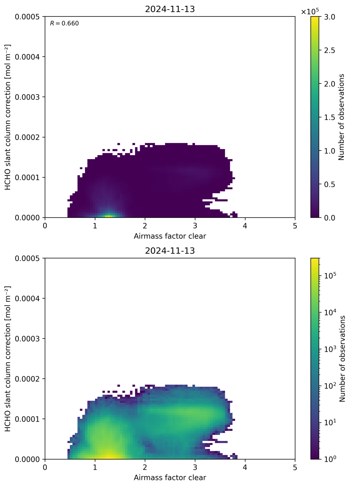
Figure 75: Scatter density plot of “Airmass factor clear” against “HCHO slant column correction” for 2024-11-12 to 2024-11-14.
