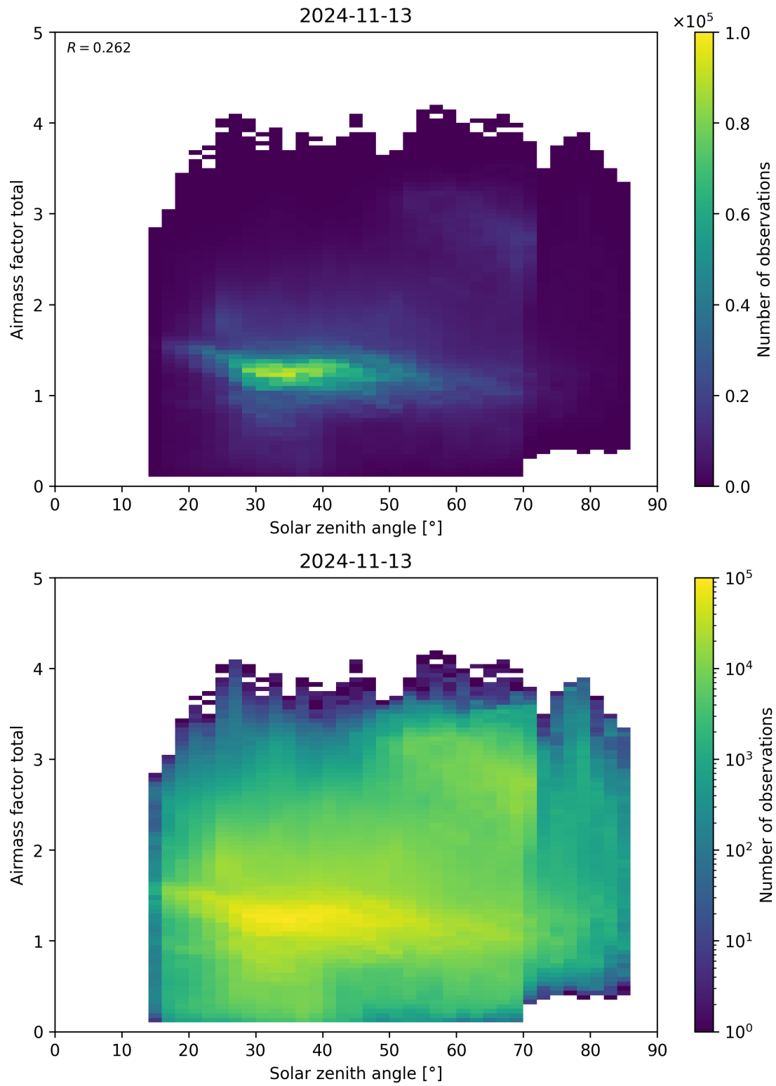
Figure 175: Scatter density plot of “Solar zenith angle” against “Airmass factor total” for 2024-11-12 to 2024-11-14.
