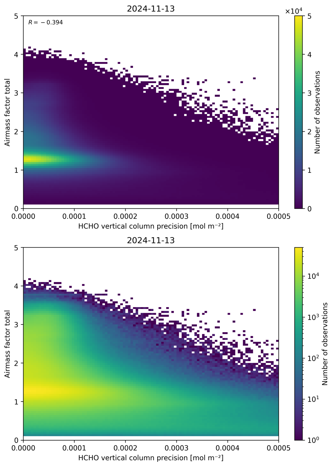
Figure 144: Scatter density plot of “HCHO vertical column precision” against “Airmass factor total” for 2024-11-12 to 2024-11-14.
