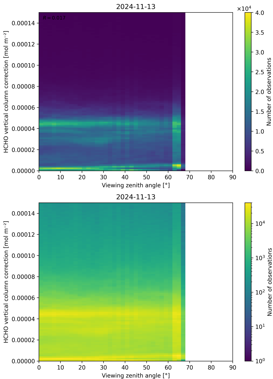
Figure 193: Scatter density plot of “Viewing zenith angle” against “HCHO vertical column correction” for 2024-11-12 to 2024-11-14.
