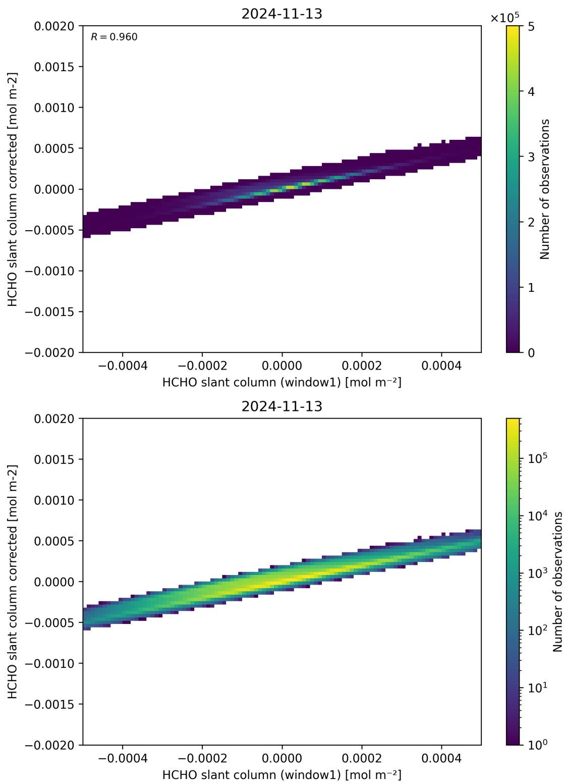
Figure 82: Scatter density plot of “HCHO slant column (window1)” against “HCHO slant column corrected” for 2024-11-12 to 2024-11-14.
