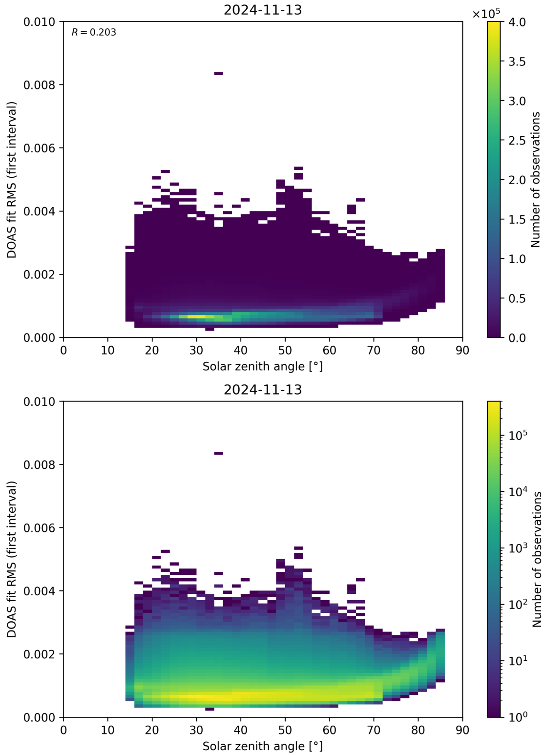
Figure 167: Scatter density plot of “Solar zenith angle” against “DOAS fit RMS (first interval)” for 2024-11-12 to 2024-11-14.
