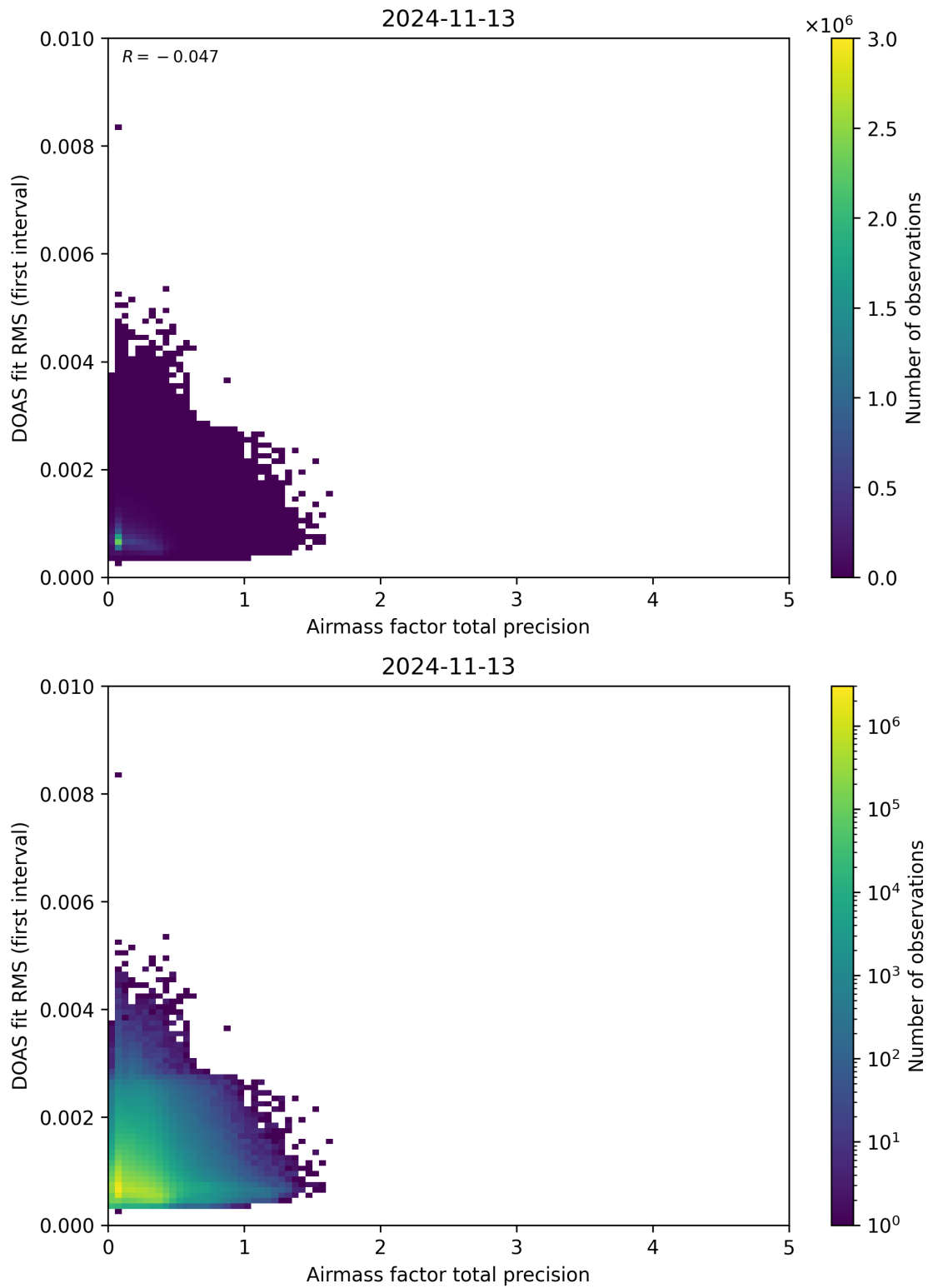
Figure 105: Scatter density plot of “Airmass factor total precision” against “DOAS fit RMS (first interval)” for 2024-11-12 to 2024-11-14.
