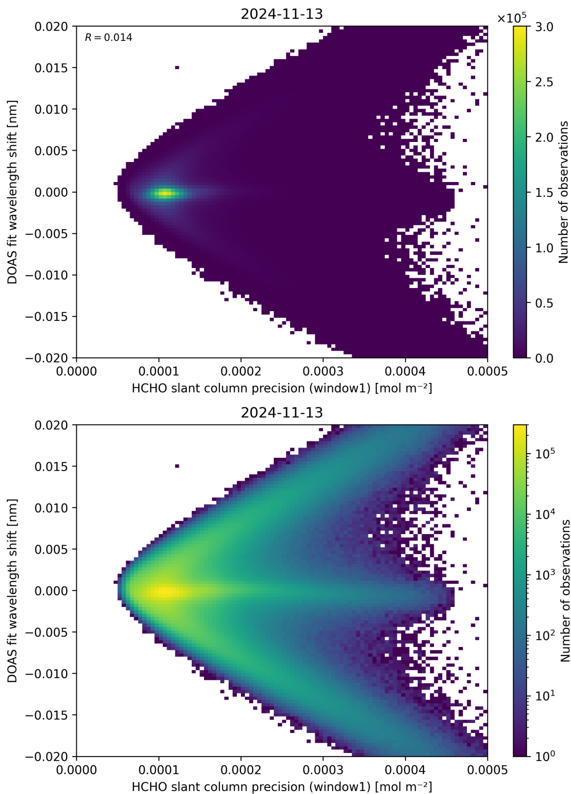
Figure 89: Scatter density plot of “HCHO slant column precision (window1)” against “DOAS fit wavelength shift” for 2024-11-12 to 2024-11-14.
