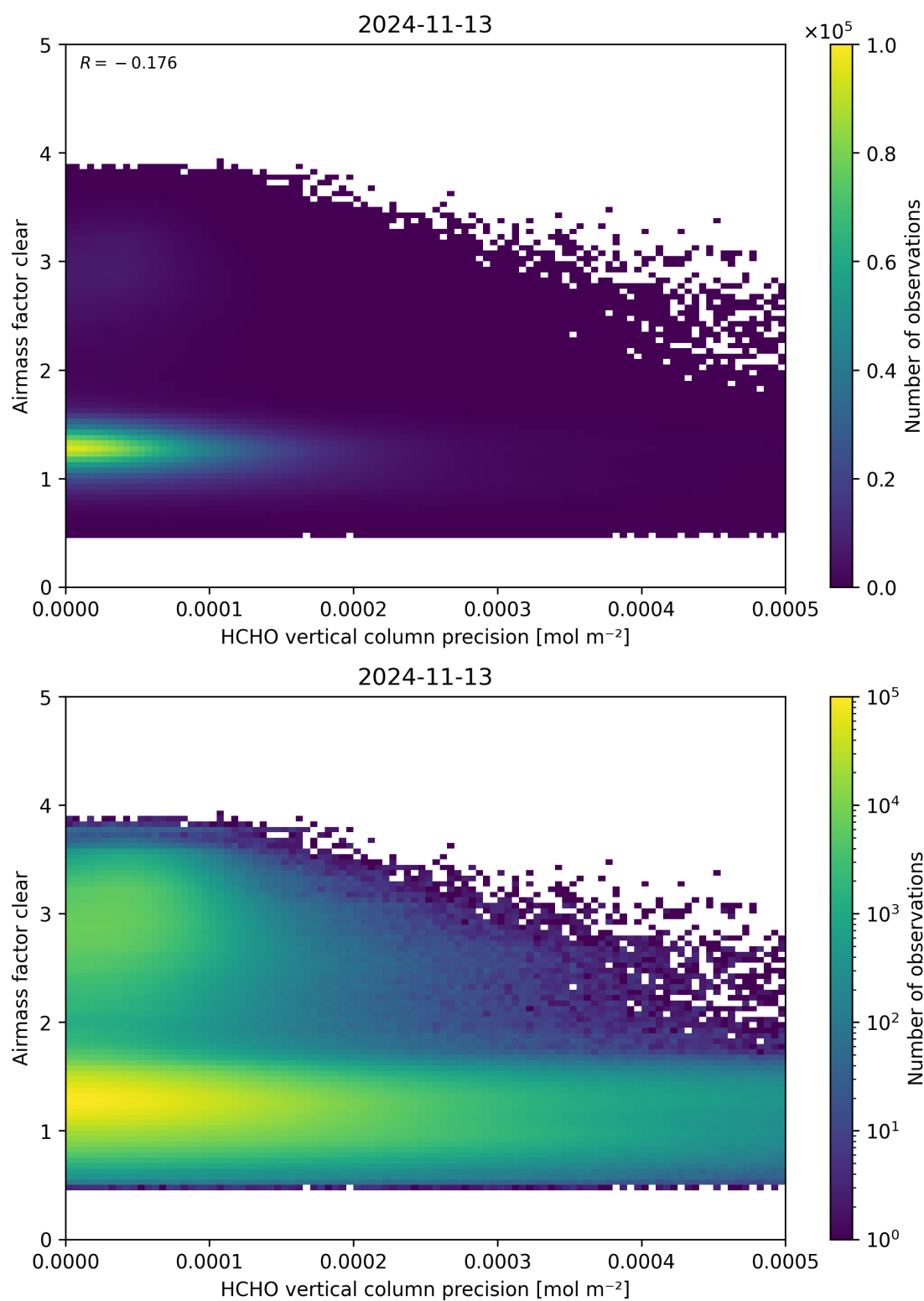
Figure 139: Scatter density plot of “HCHO vertical column precision” against “Airmass factor clear” for 2024-11-12 to 2024-11-14.
