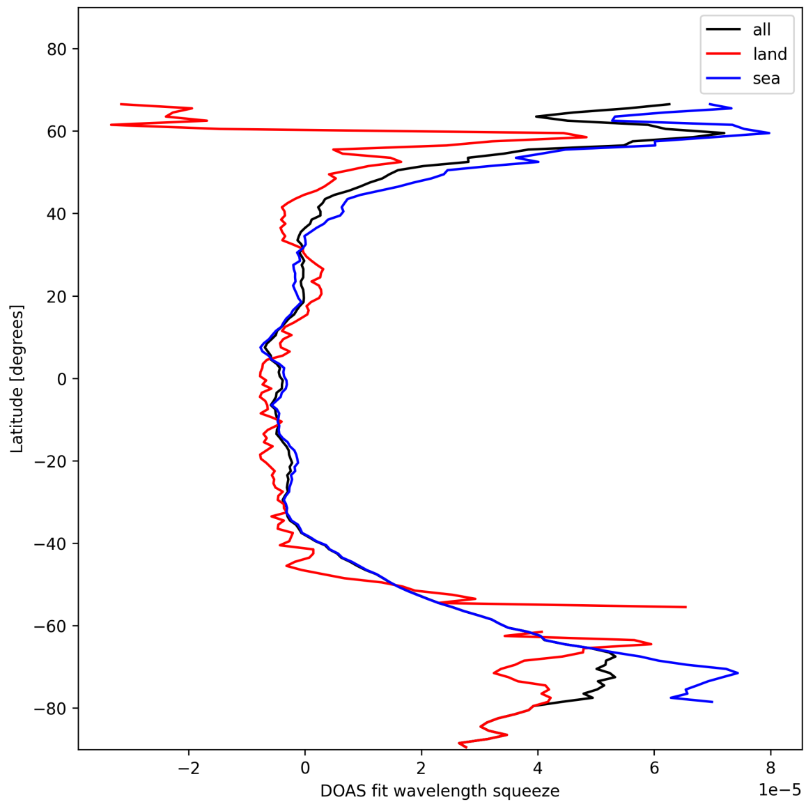
Figure 31: Zonal average of “DOAS fit wavelength squeeze” for 2024-11-12 to 2024-11-14.
