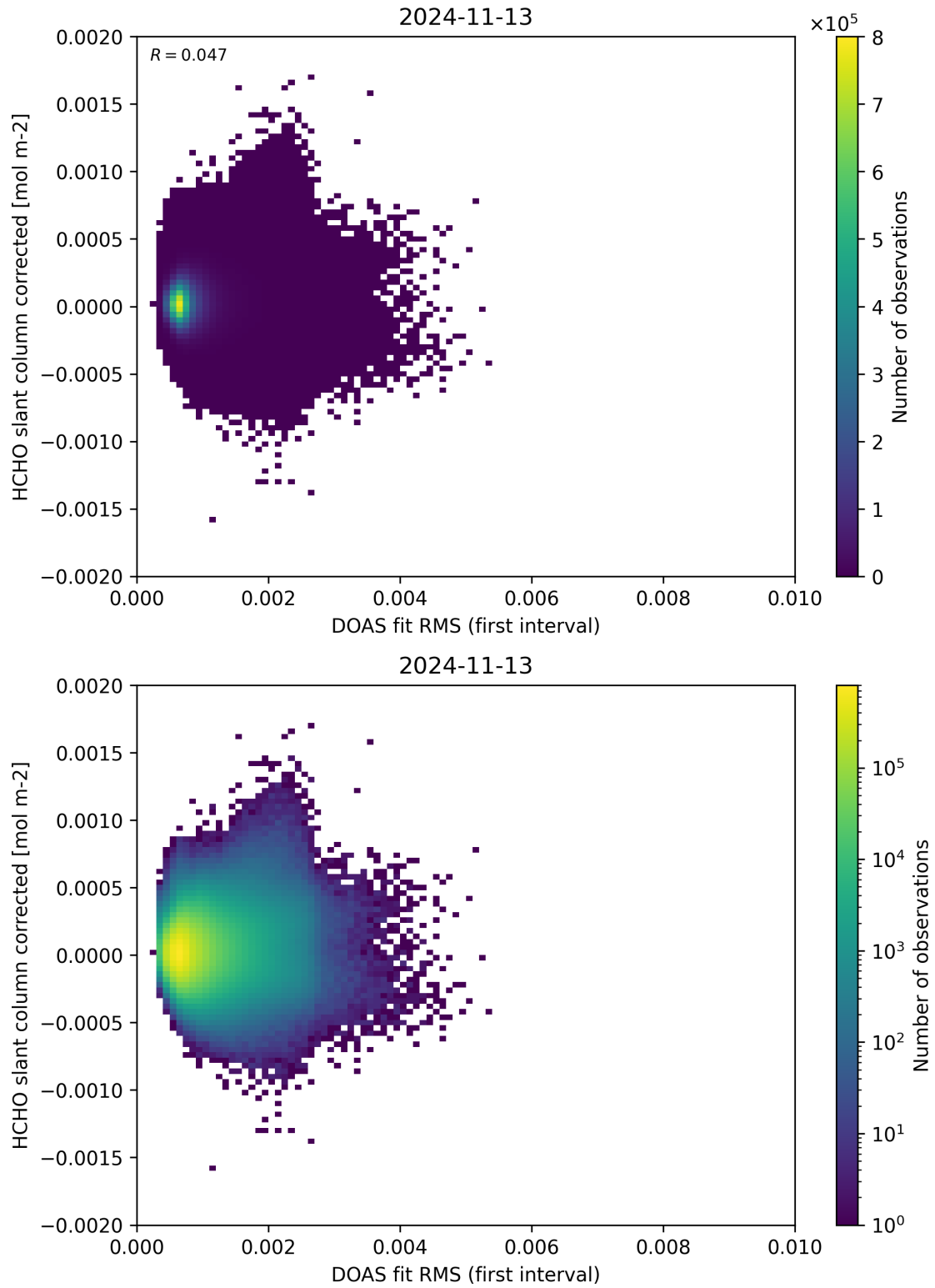
Figure 62: Scatter density plot of “DOAS fit RMS (first interval)” against “HCHO slant column corrected” for 2024-11-12 to 2024-11-14.
