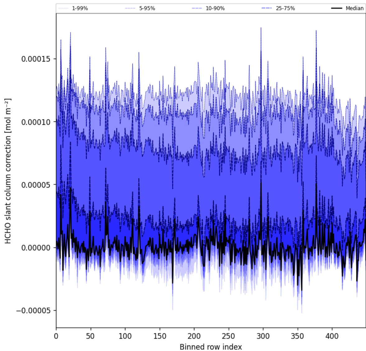
Figure 61: Along track statistics of “HCHO slant column correction” for 2024-11-12 to 2024-11-14
