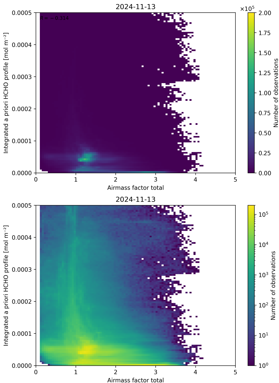
Figure 104: Scatter density plot of “Airmass factor total” against “Integrated a priori HCHO profile” for 2024-11-12 to 2024-11-14.
