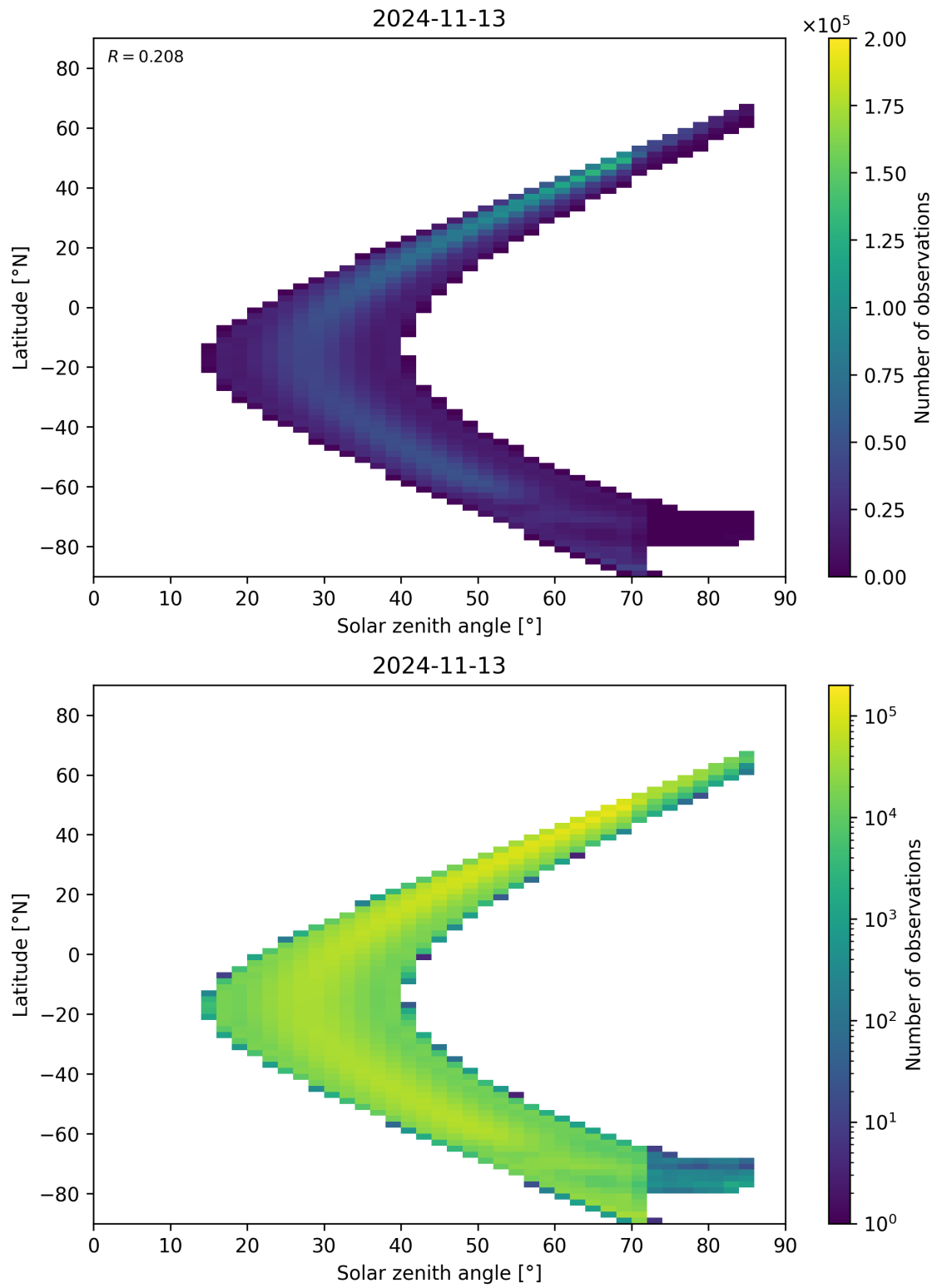
Figure 181: Scatter density plot of “Solar zenith angle” against “Latitude” for 2024-11-12 to 2024-11-14.
