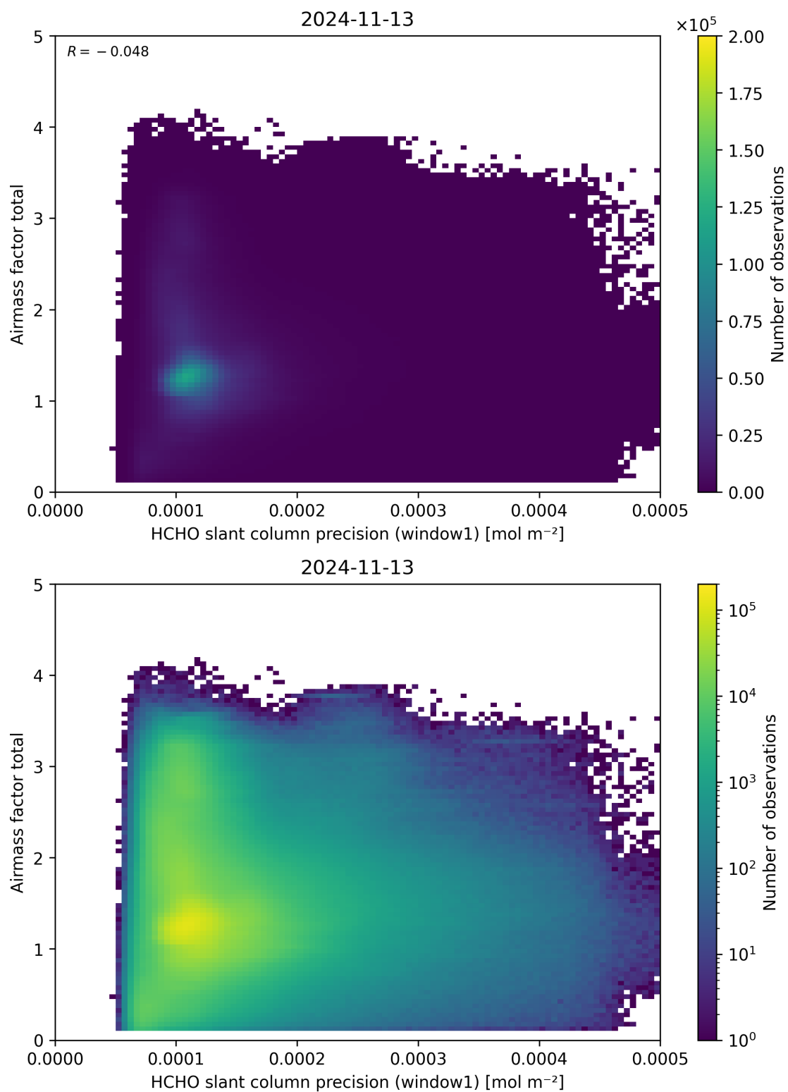
Figure 94: Scatter density plot of “HCHO slant column precision (window1)” against “Airmass factor total” for 2024-11-12 to 2024-11-14.
