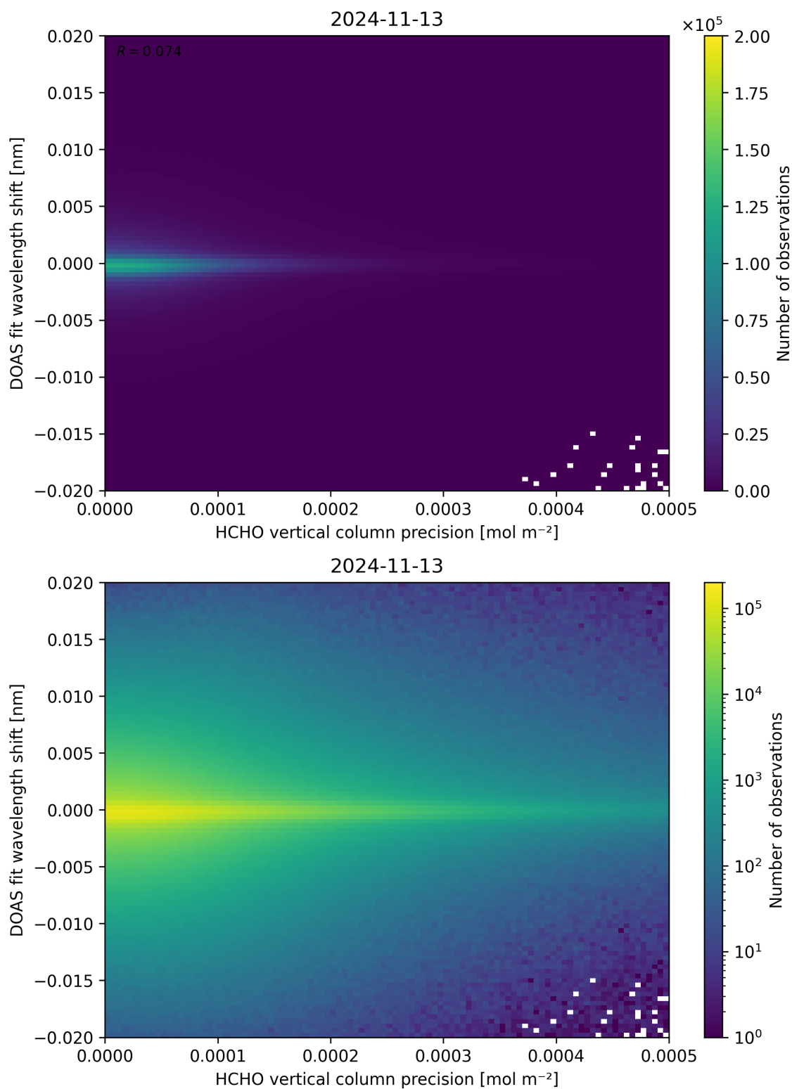
Figure 137: Scatter density plot of “HCHO vertical column precision” against “DOAS fit wavelength shift” for 2024-11-12 to 2024-11-14.
