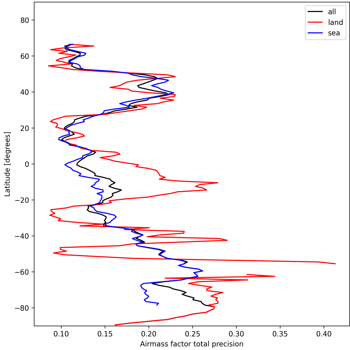
Figure 27: Zonal average of “Airmass factor total precision” for 2024-11-12 to 2024-11-14.
