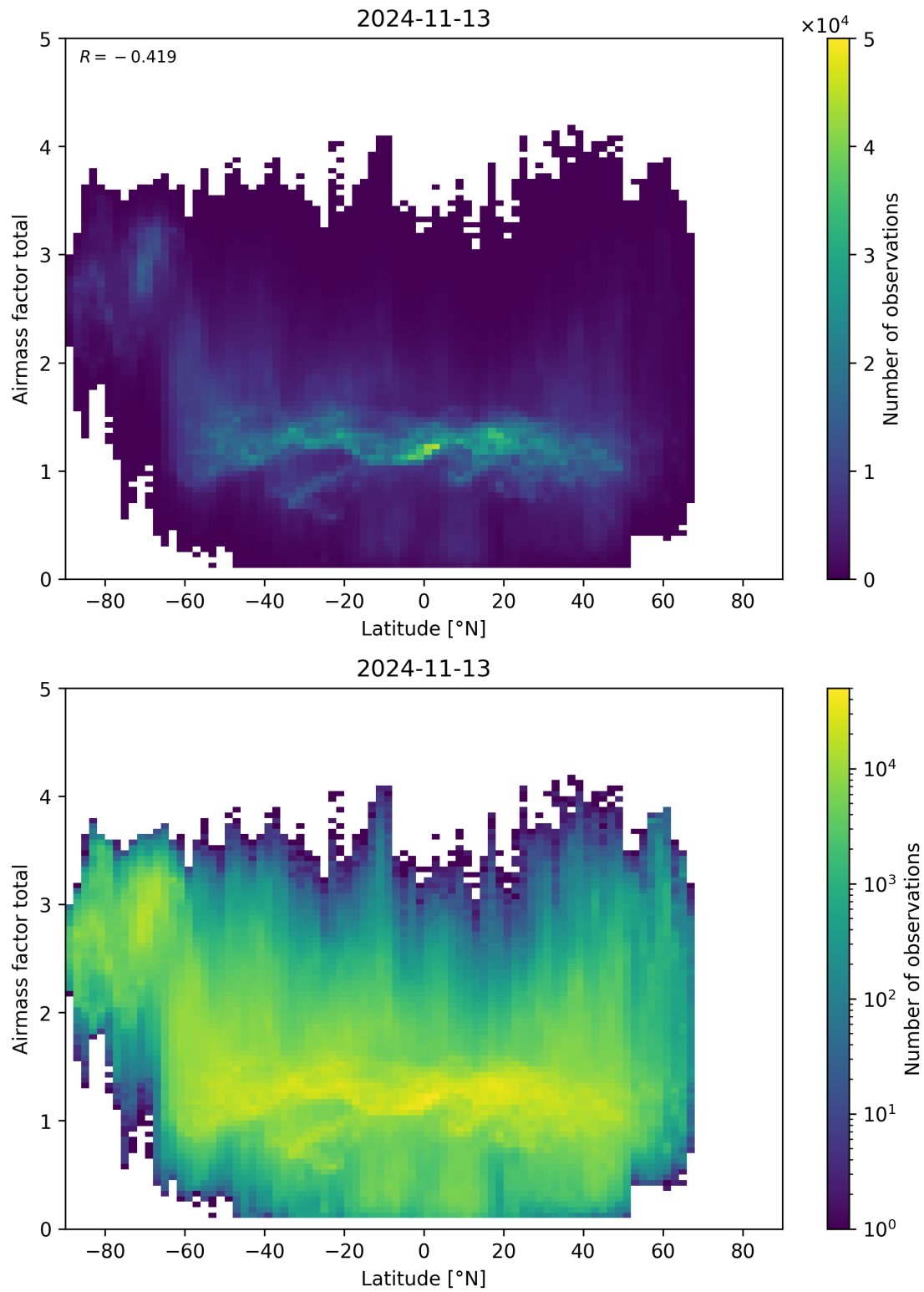
Figure 161: Scatter density plot of “Latitude” against “Airmass factor total” for 2024-11-12 to 2024-11-14.
