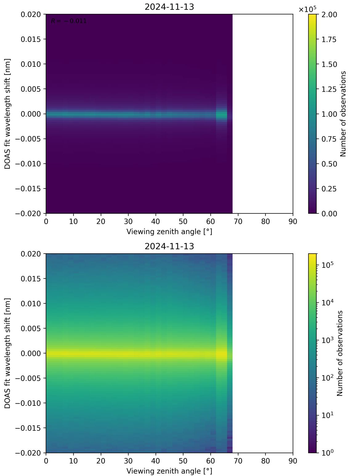
Figure 183: Scatter density plot of “Viewing zenith angle” against “DOAS fit wavelength shift” for 2024-11-12 to 2024-11-14.
