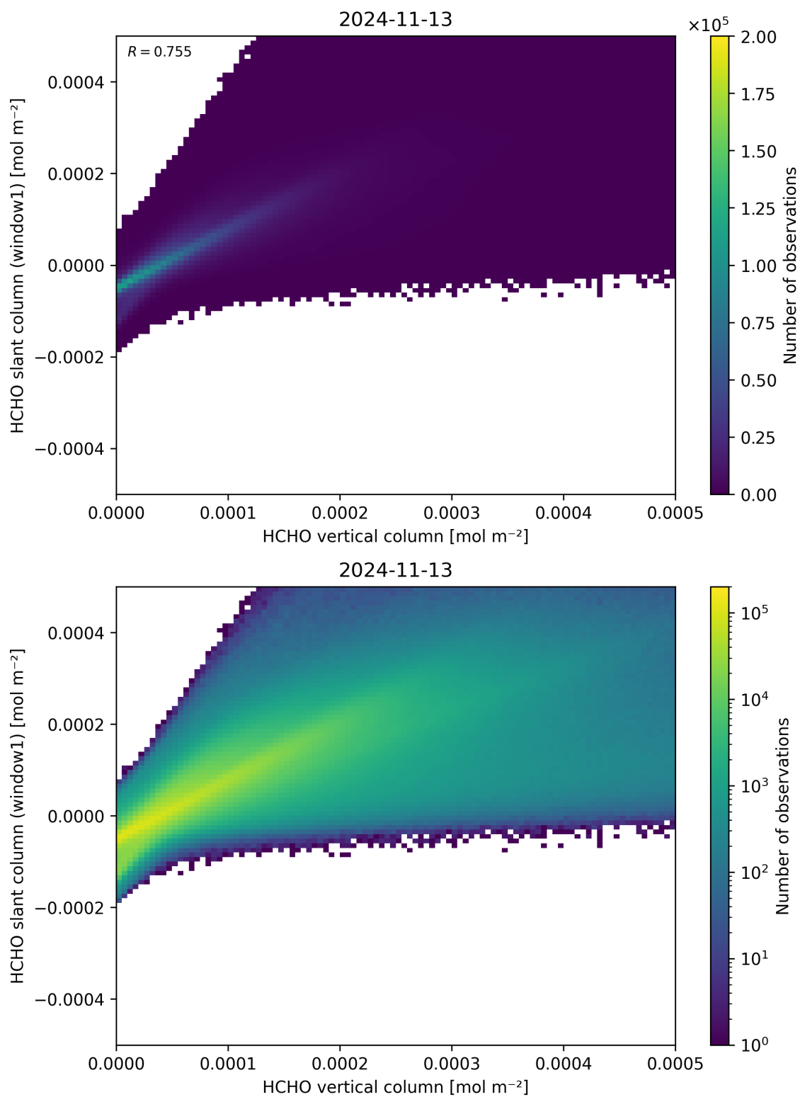
Figure 129: Scatter density plot of “HCHO vertical column” against “HCHO slant column (window1)” for 2024-11-12 to 2024-11-14.
