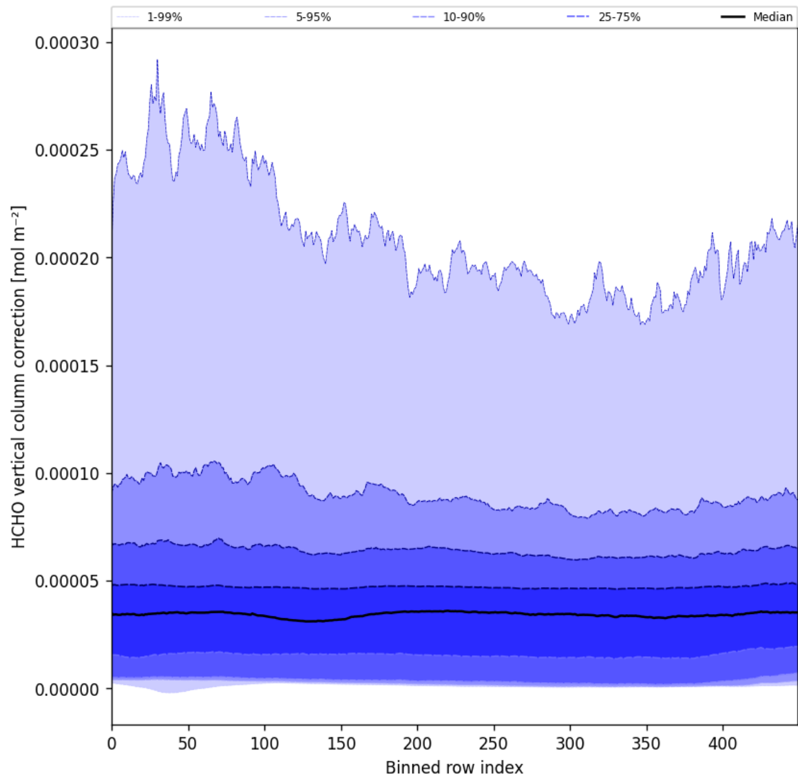
Figure 51: Along track statistics of “HCHO vertical column correction” for 2024-11-12 to 2024-11-14
