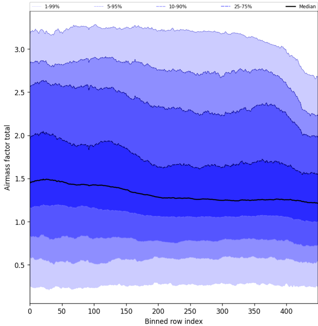
Figure 54: Along track statistics of “Airmass factor total” for 2024-11-12 to 2024-11-14
