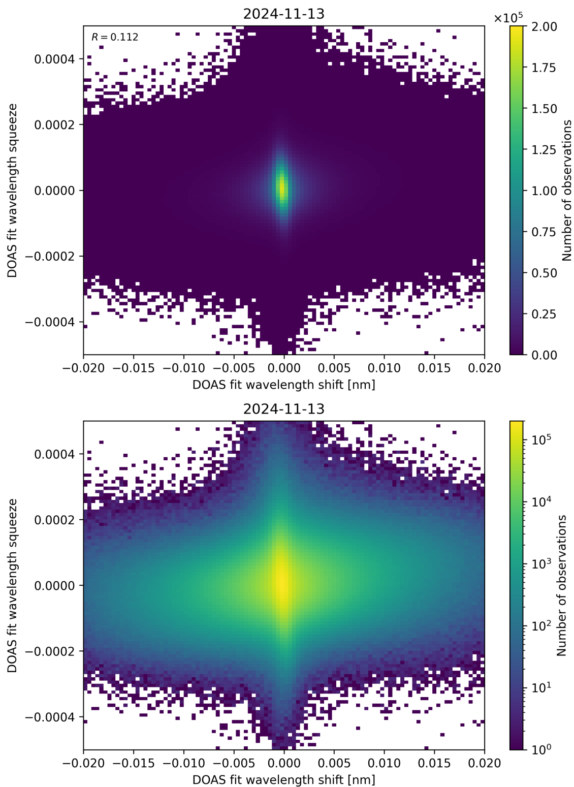
Figure 65: Scatter density plot of “DOAS fit wavelength shift” against “DOAS fit wavelength squeeze” for 2024-11-12 to 2024-11-14.
