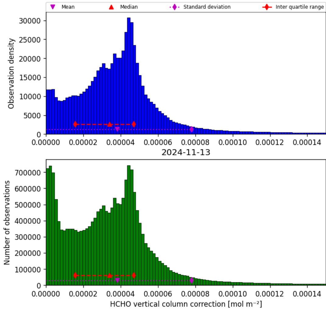
Figure 37: Histogram of “HCHO vertical column correction” for 2024-11-12 to 2024-11-14
