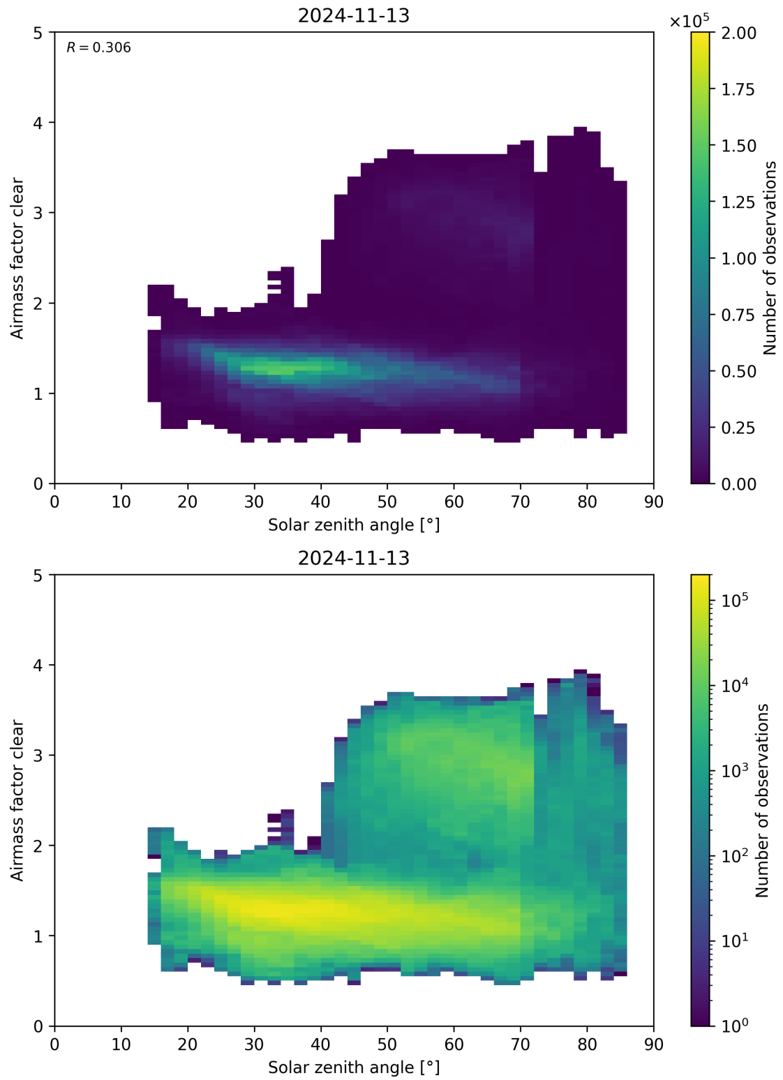
Figure 170: Scatter density plot of “Solar zenith angle” against “Airmass factor clear” for 2024-11-12 to 2024-11-14.
