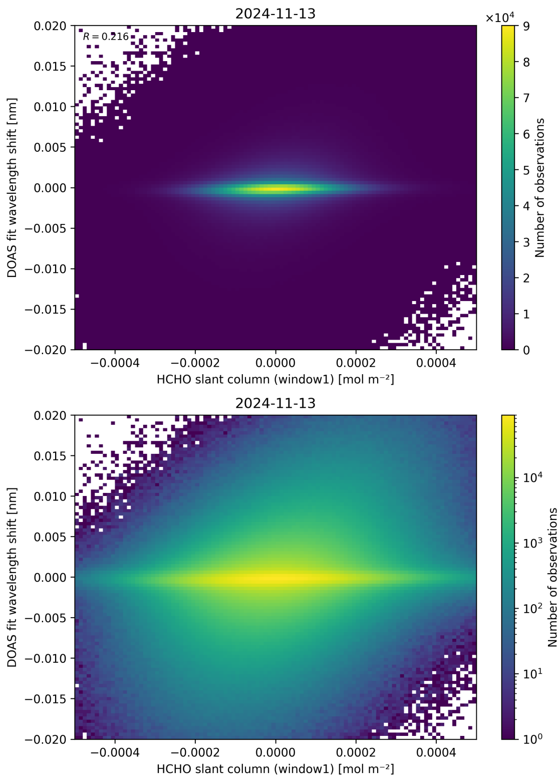
Figure 79: Scatter density plot of “HCHO slant column (window1)” against “DOAS fit wavelength shift” for 2024-11-12 to 2024-11-14.
