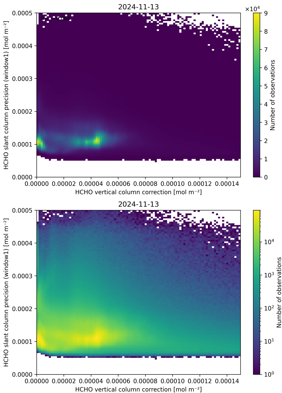
Figure 119: Scatter density plot of “HCHO vertical column correction” against “HCHO slant column precision (window1)” for 2024-11-12 to 2024-11-14.
