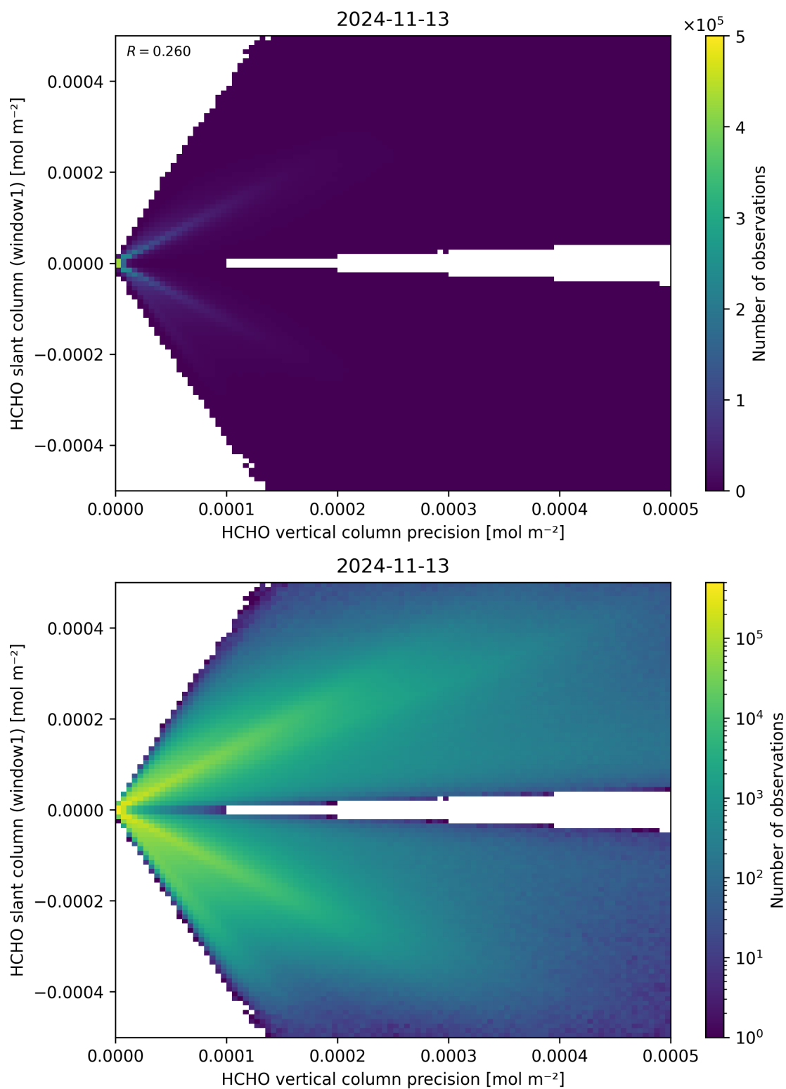
Figure 142: Scatter density plot of “HCHO vertical column precision” against “HCHO slant column (window1)” for 2024-11-12 to 2024-11-14.
