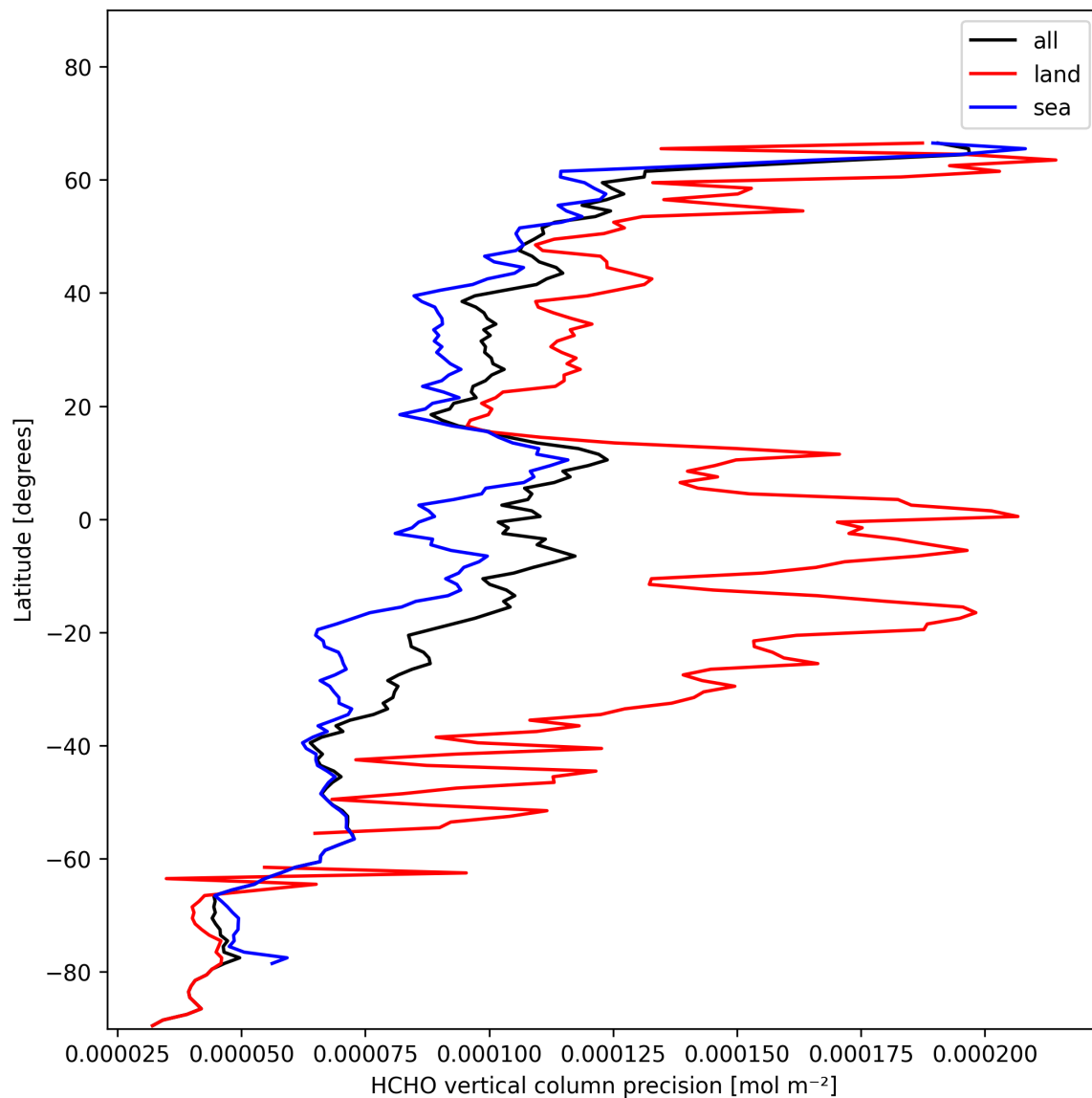
Figure 22: Zonal average of “HCHO vertical column precision” for 2024-11-12 to 2024-11-14.
