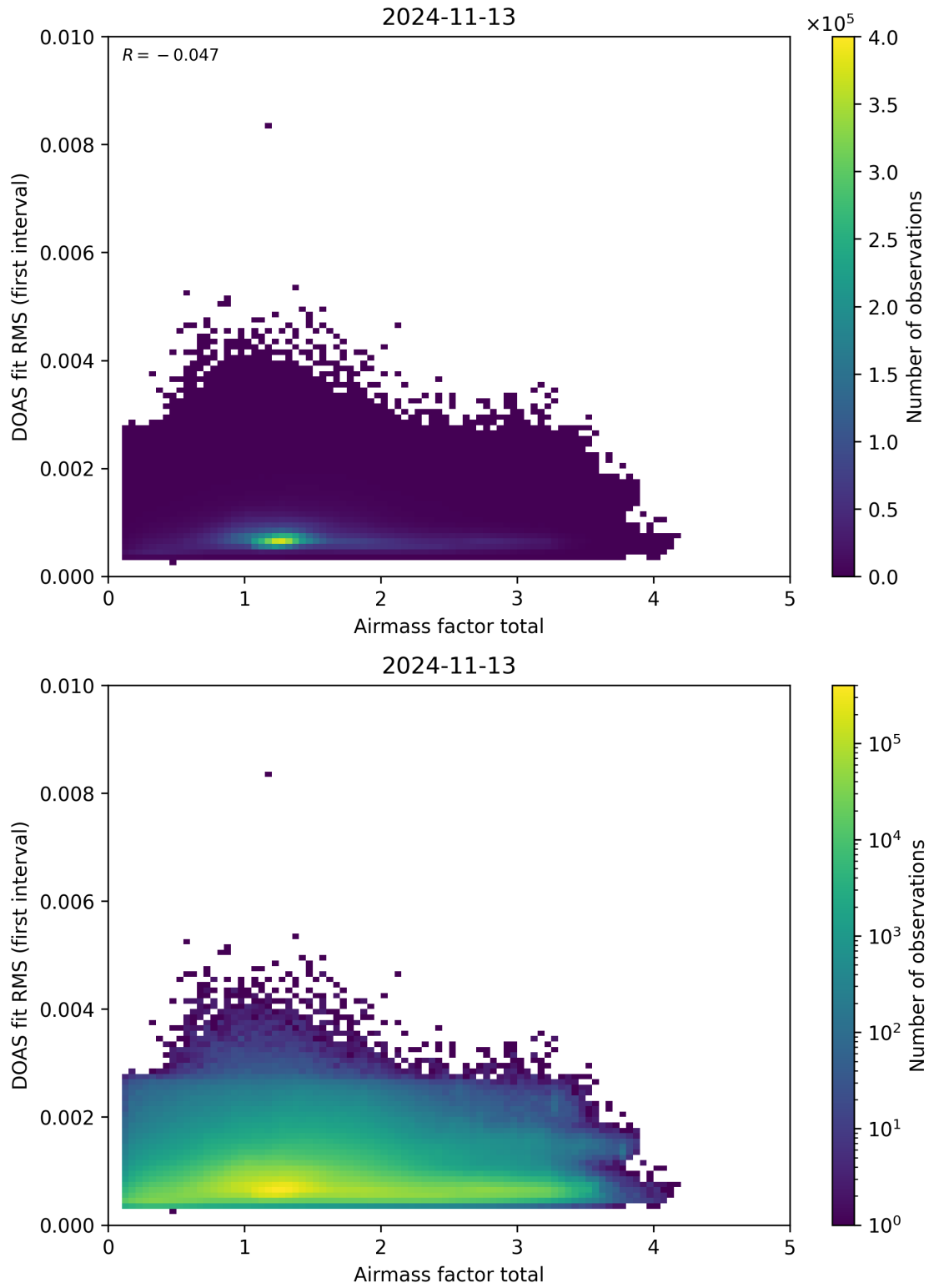
Figure 97: Scatter density plot of “Airmass factor total” against “DOAS fit RMS (first interval)” for 2024-11-12 to 2024-11-14.
