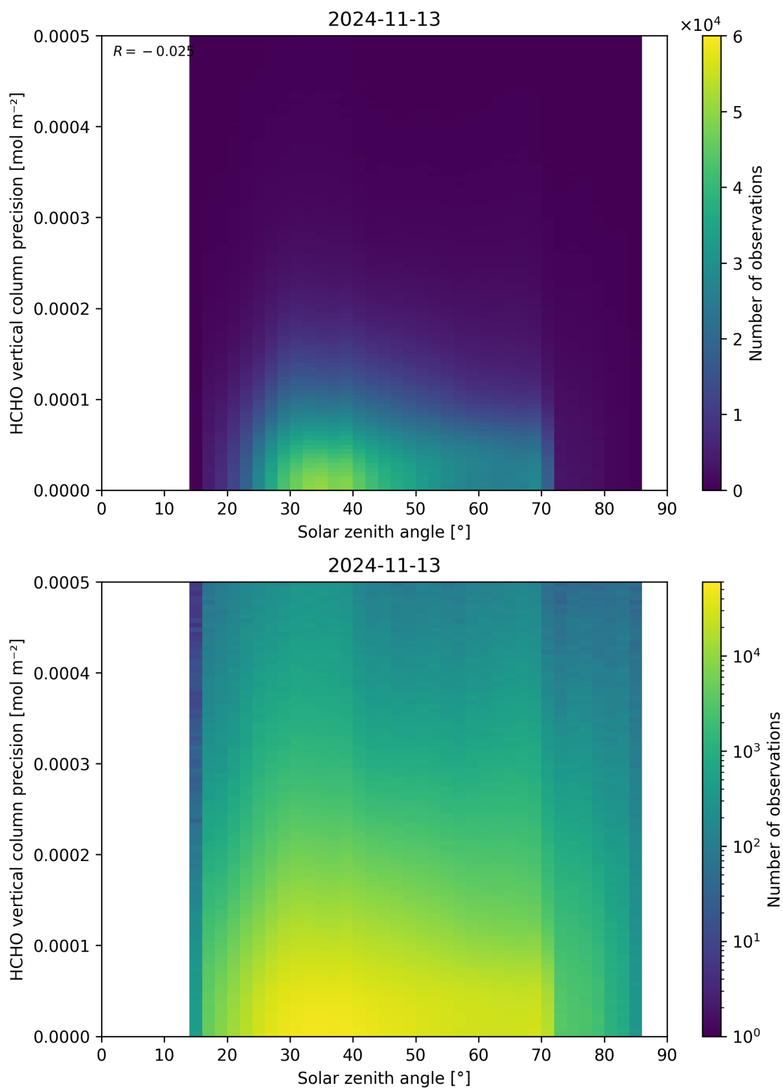
Figure 179: Scatter density plot of “Solar zenith angle” against “HCHO vertical column precision” for 2024-11-12 to 2024-11-14.
