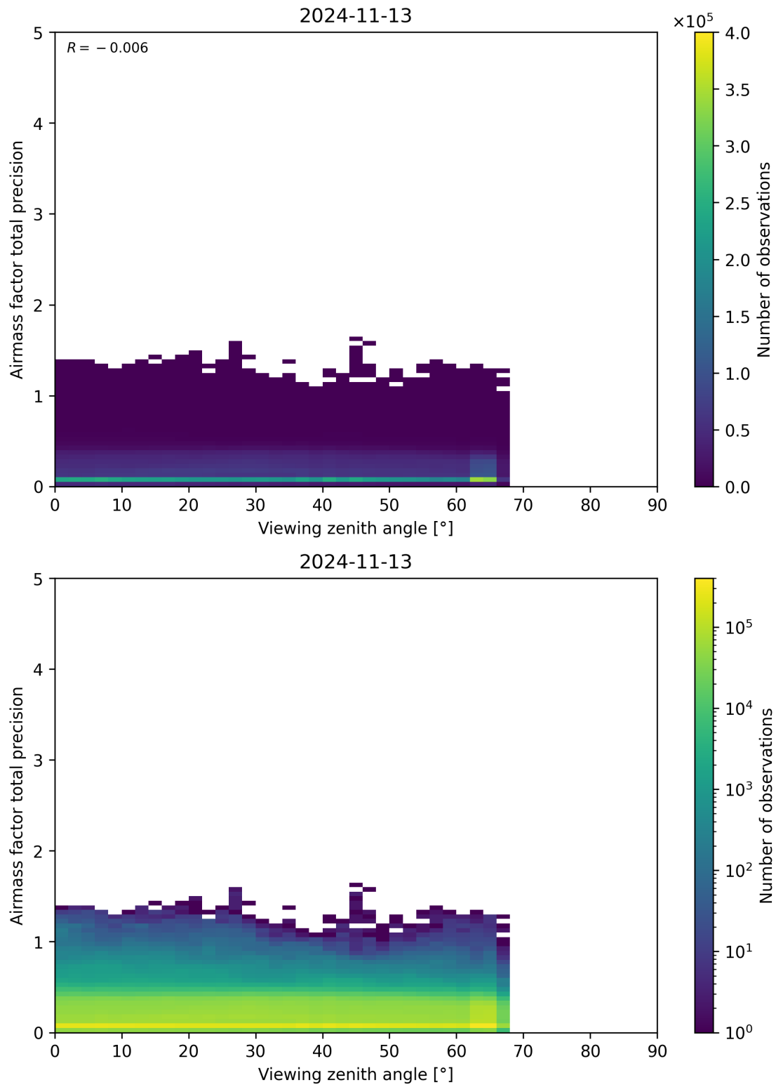
Figure 191: Scatter density plot of “Viewing zenith angle” against “Airmass factor total precision” for 2024-11-12 to 2024-11-14.
