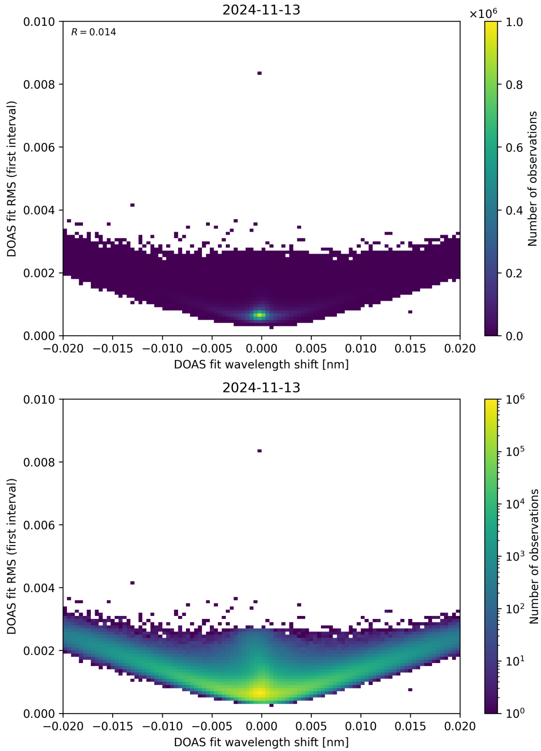
Figure 64: Scatter density plot of “DOAS fit wavelength shift” against “DOAS fit RMS (first interval)” for 2024-11-12 to 2024-11-14.
