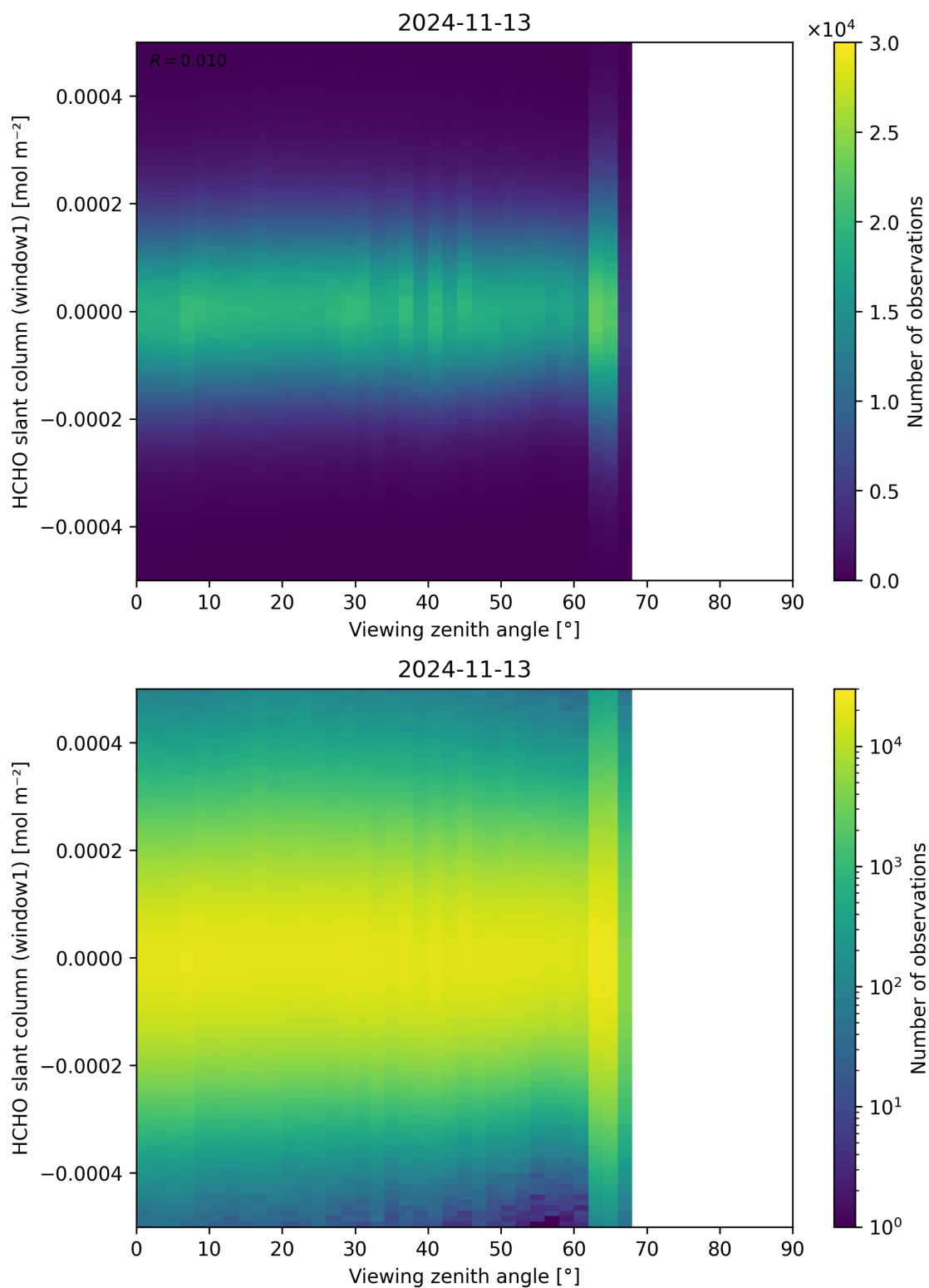
Figure 188: Scatter density plot of “Viewing zenith angle” against “HCHO slant column (window1)” for 2024-11-12 to 2024-11-14.
