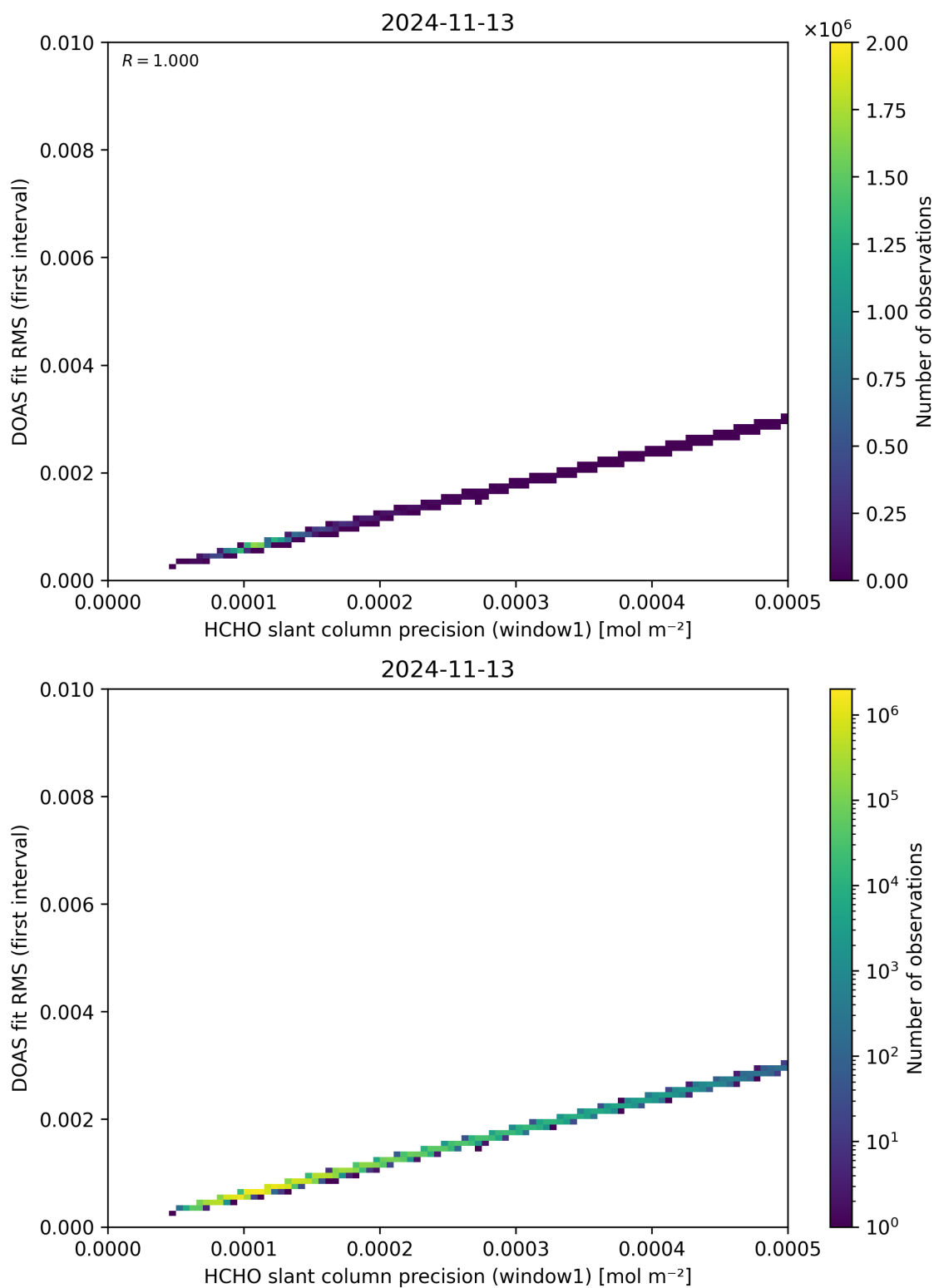
Figure 88: Scatter density plot of “HCHO slant column precision (window1)” against “DOAS fit RMS (first interval)” for 2024-11-12 to 2024-11-14.
