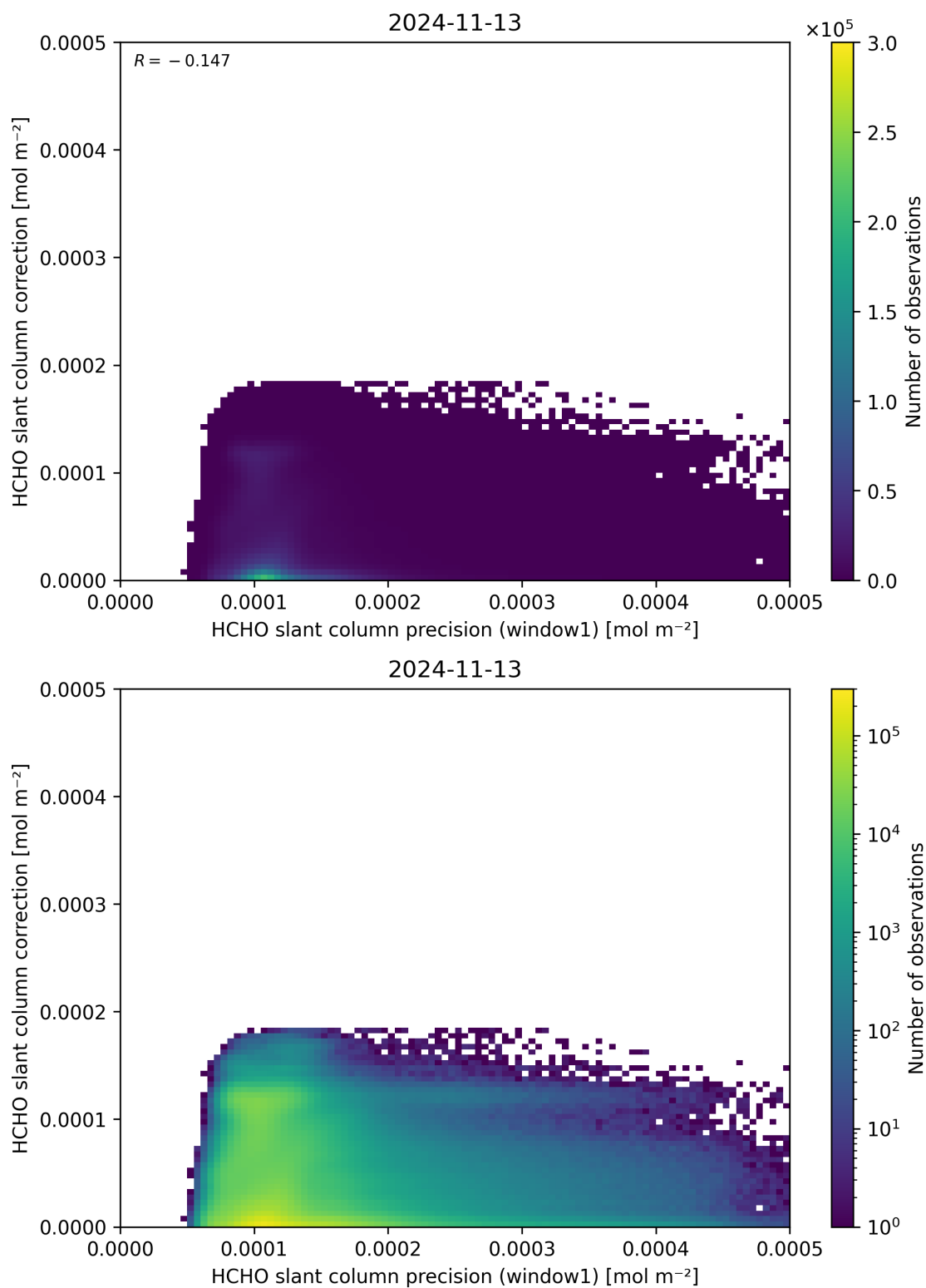
Figure 93: Scatter density plot of “HCHO slant column precision (window1)” against “HCHO slant column correction” for 2024-11-12 to 2024-11-14.
