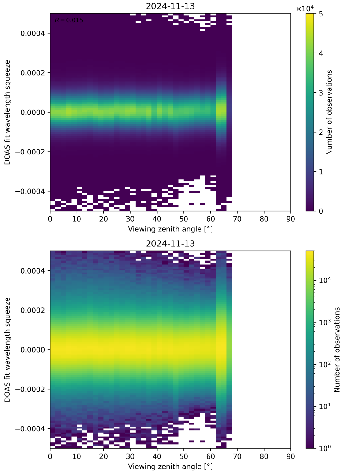
Figure 184: Scatter density plot of “Viewing zenith angle” against “DOAS fit wavelength squeeze” for 2024-11-12 to 2024-11-14.
