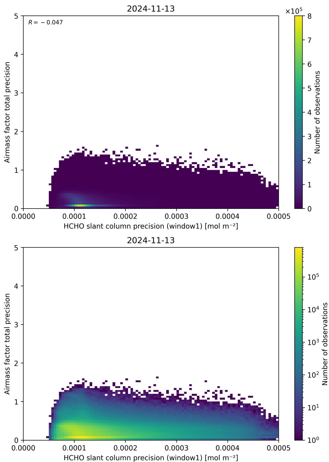
Figure 95: Scatter density plot of “HCHO slant column precision (window1)” against “Airmass factor total precision” for 2024-11-12 to 2024-11-14.
