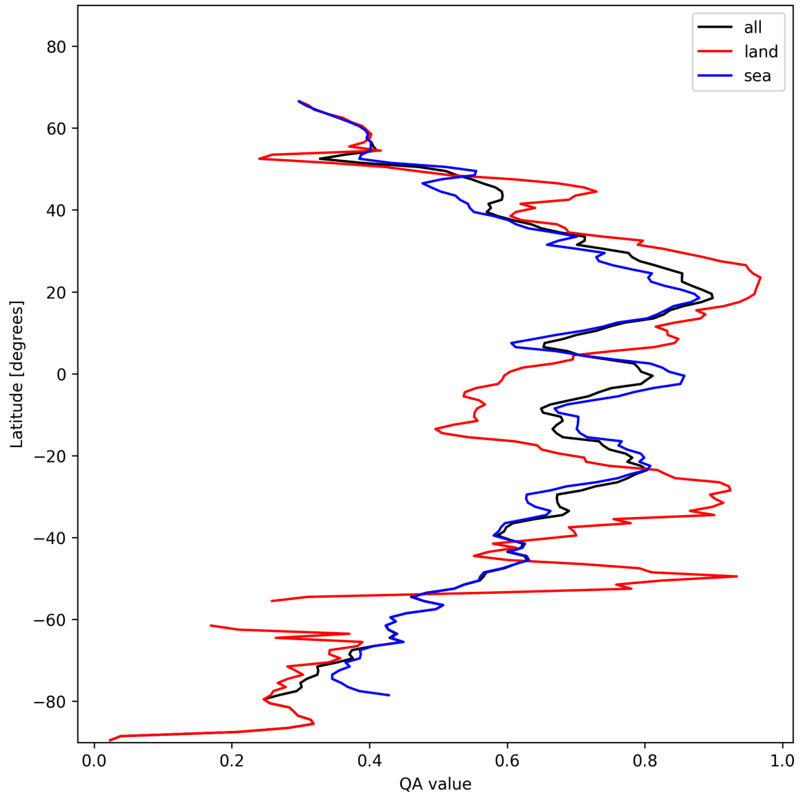
Figure 20: Zonal average of “QA value” for 2024-11-12 to 2024-11-14.
