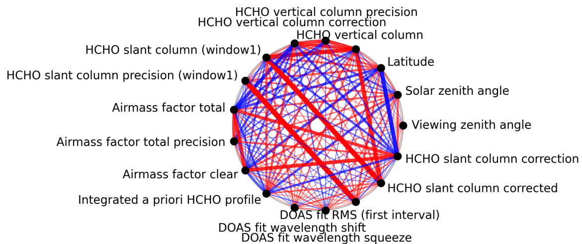
Figure 1: Map of correlation graph for 2024-11-12 to 2024-11-14.
