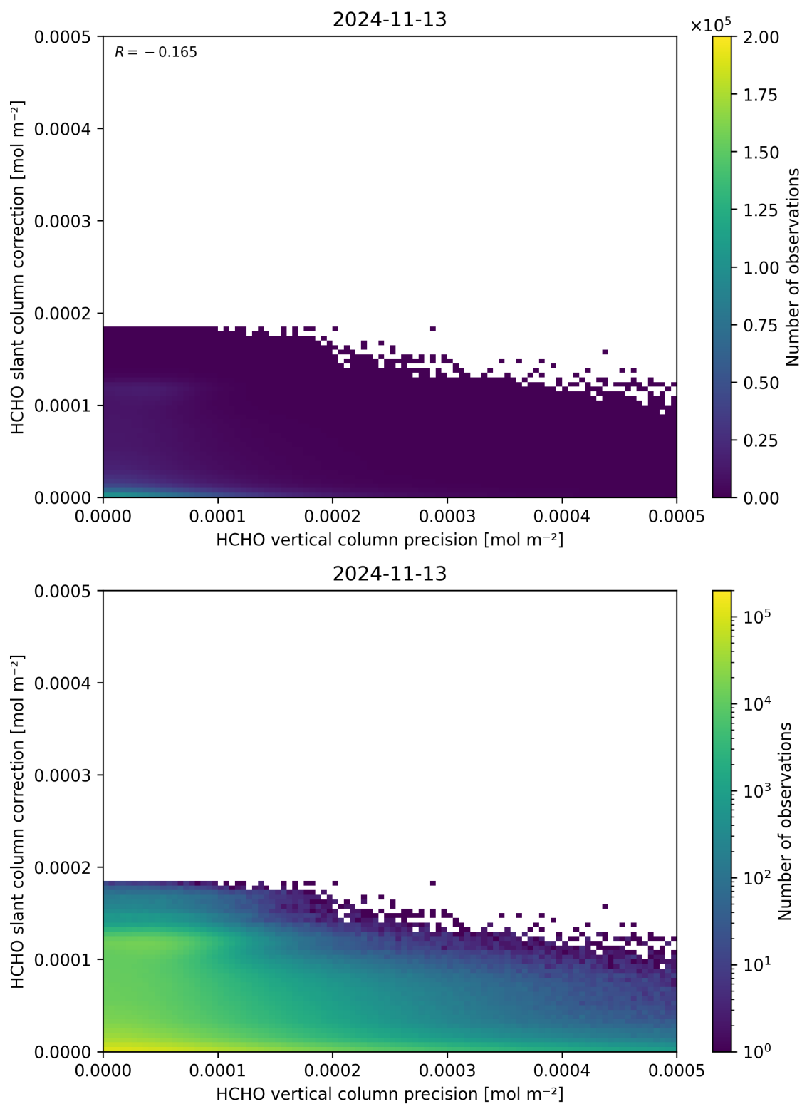
Figure 141: Scatter density plot of “HCHO vertical column precision” against “HCHO slant column correction” for 2024-11-12 to 2024-11-14.
