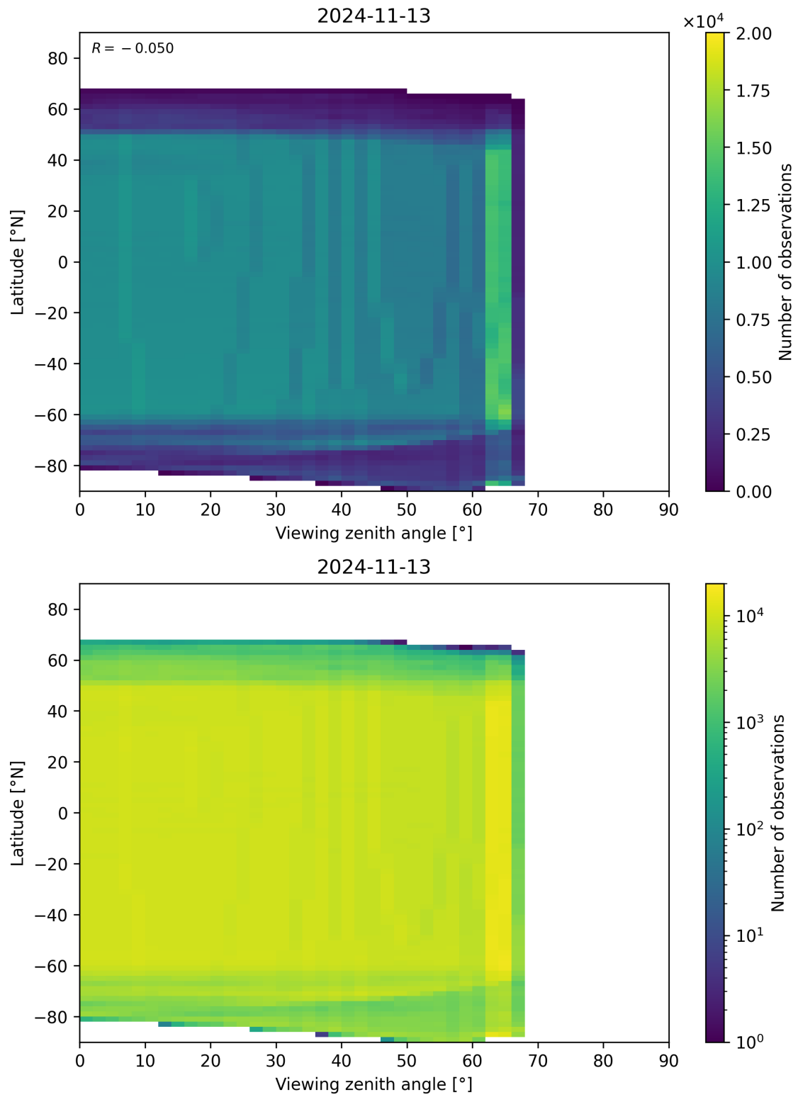
Figure 196: Scatter density plot of “Viewing zenith angle” against “Latitude” for 2024-11-12 to 2024-11-14.
