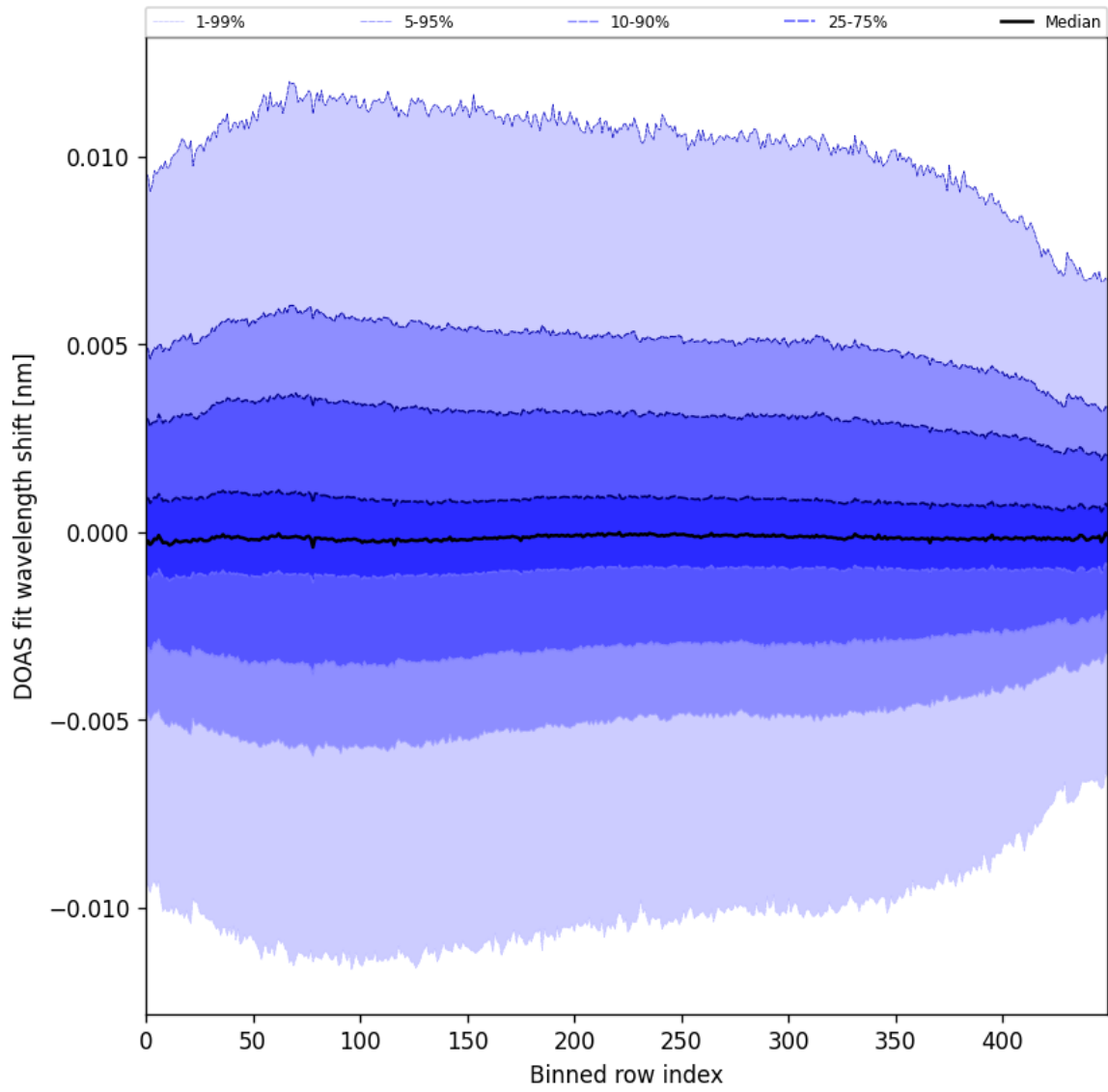
Figure 58: Along track statistics of “DOAS fit wavelength shift” for 2024-11-12 to 2024-11-14
