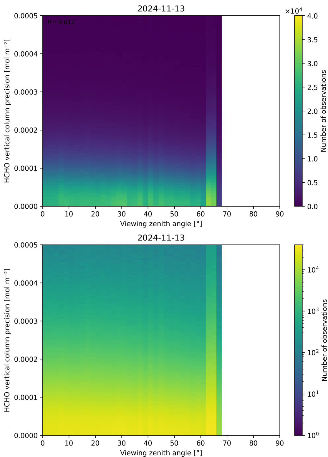
Figure 194: Scatter density plot of “Viewing zenith angle” against “HCHO vertical column precision” for 2024-11-12 to 2024-11-14.
