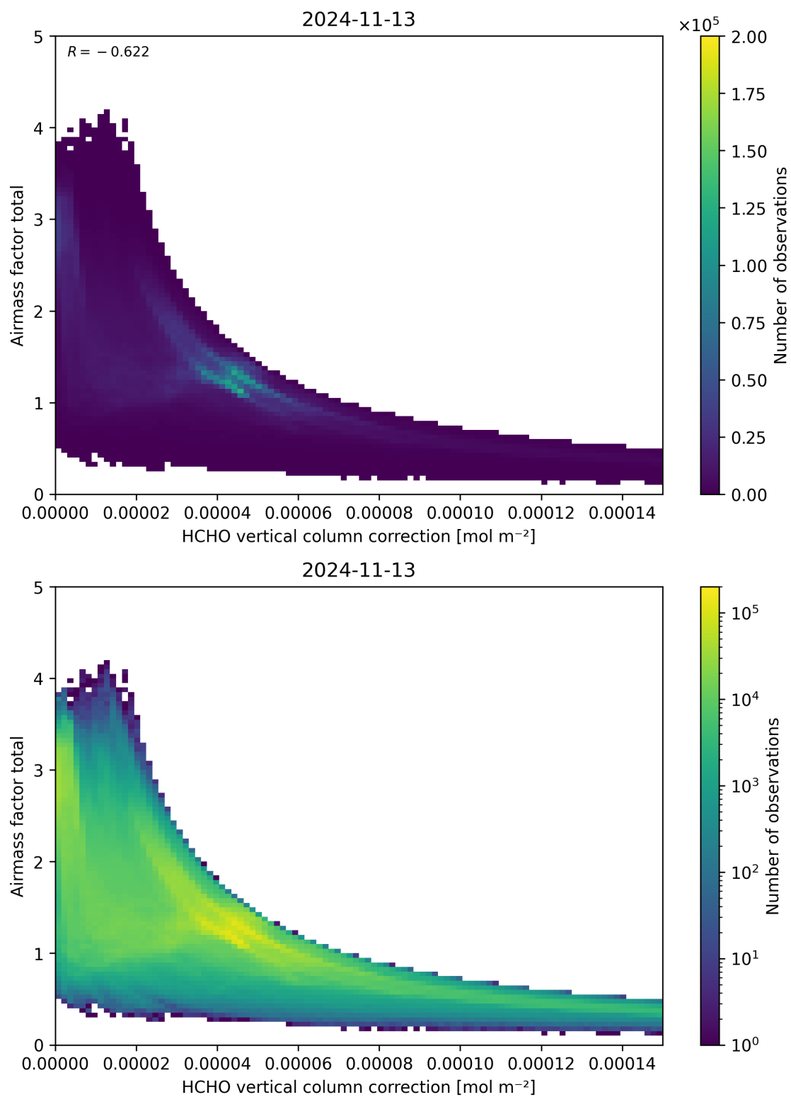
Figure 120: Scatter density plot of “HCHO vertical column correction” against “Airmass factor total” for 2024-11-12 to 2024-11-14.
