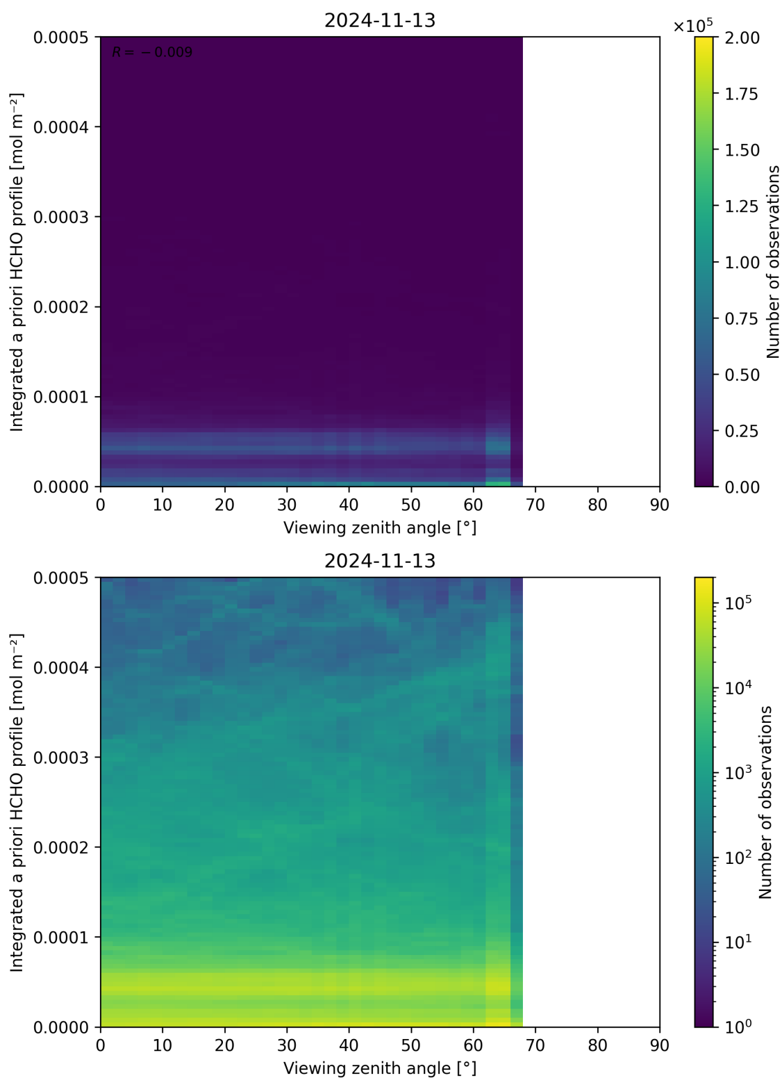
Figure 195: Scatter density plot of “Viewing zenith angle” against “Integrated a priori HCHO profile” for 2024-11-12 to 2024-11-14.
