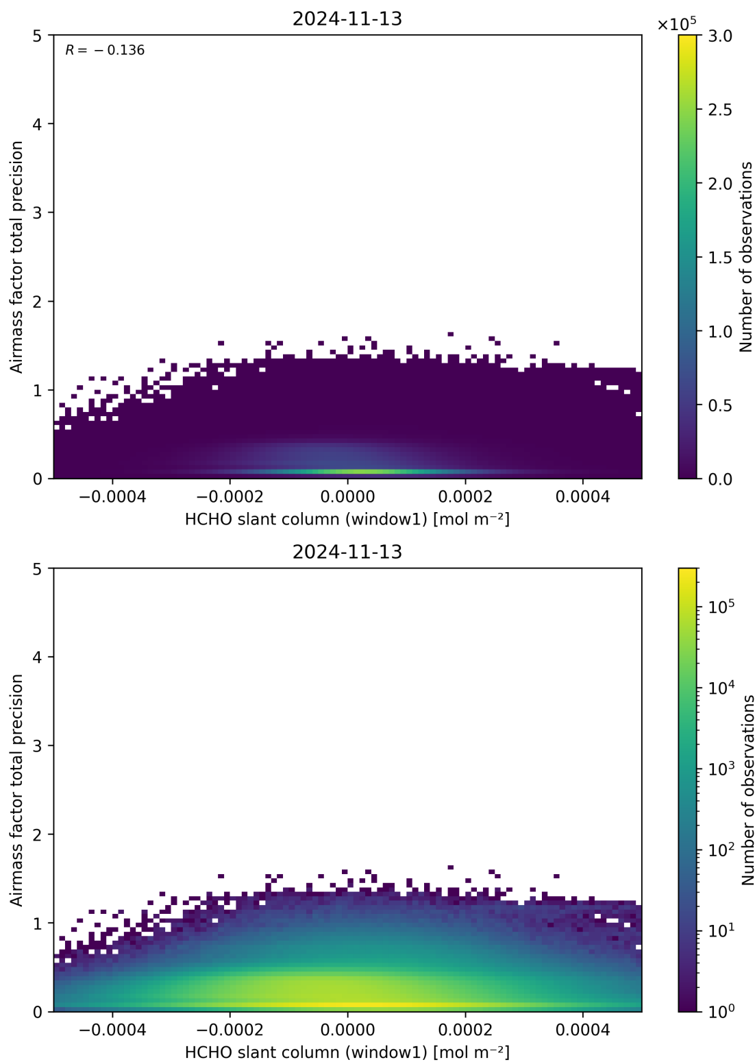
Figure 86: Scatter density plot of “HCHO slant column (window1)” against “Airmass factor total precision” for 2024-11-12 to 2024-11-14.
