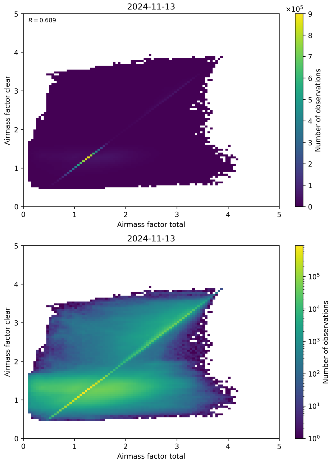
Figure 100: Scatter density plot of “Airmass factor total” against “Airmass factor clear” for 2024-11-12 to 2024-11-14.
