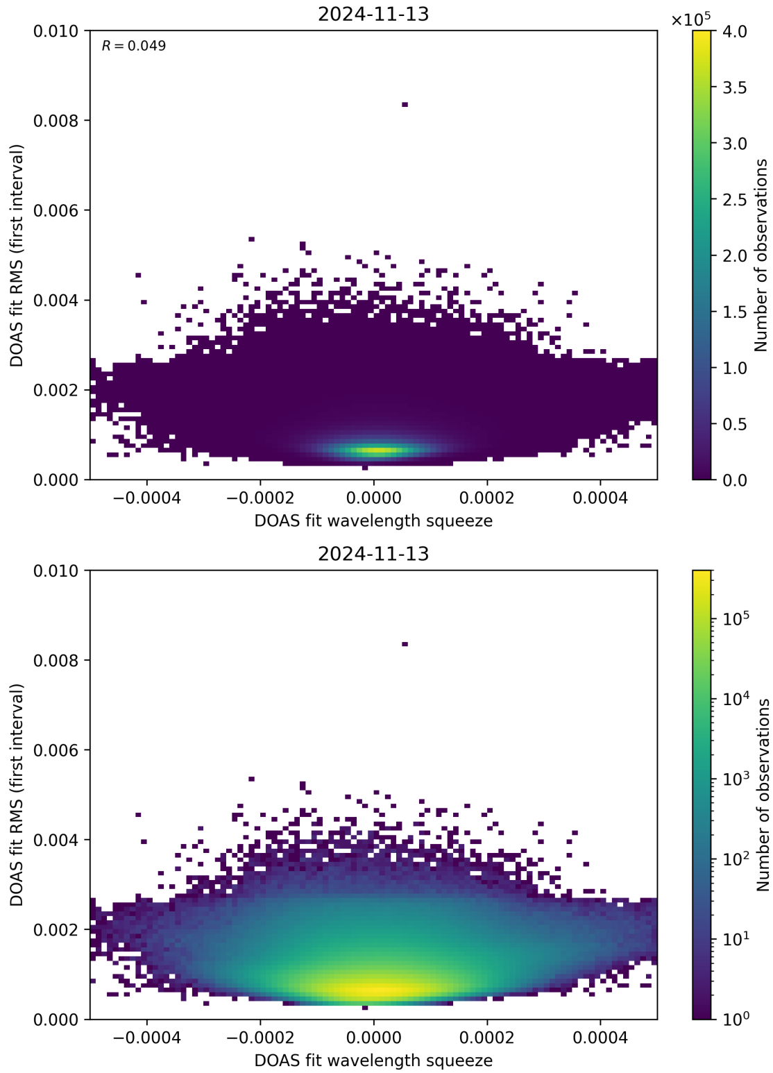
Figure 68: Scatter density plot of “DOAS fit wavelength squeeze” against “DOAS fit RMS (first interval)” for 2024-11-12 to 2024-11-14.
