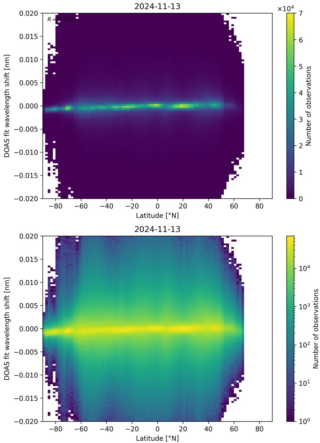
Figure 154: Scatter density plot of “Latitude” against “DOAS fit wavelength shift” for 2024-11-12 to 2024-11-14.
