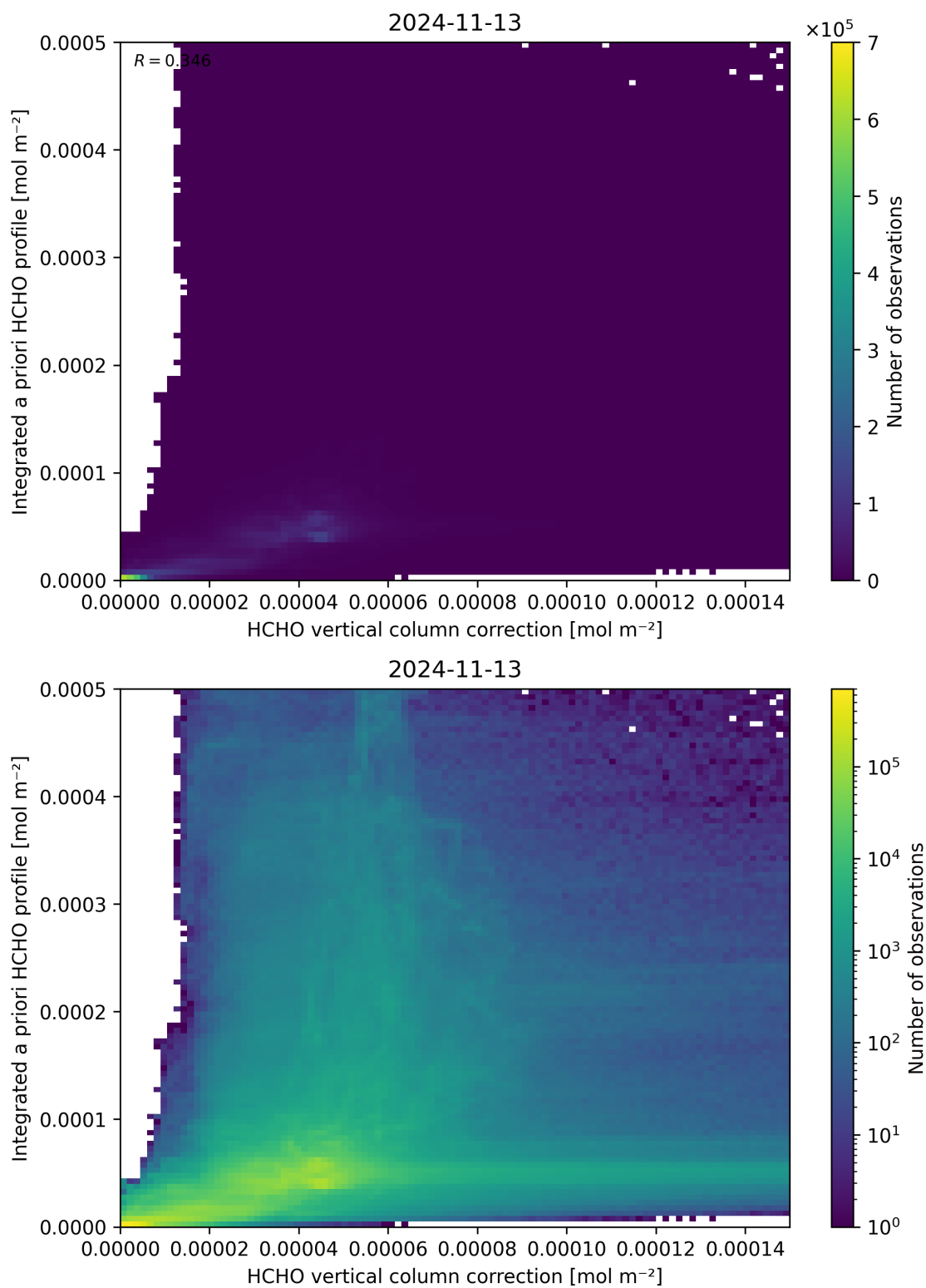
Figure 122: Scatter density plot of “HCHO vertical column correction” against “Integrated a priori HCHO profile” for 2024-11-12 to 2024-11-14.
