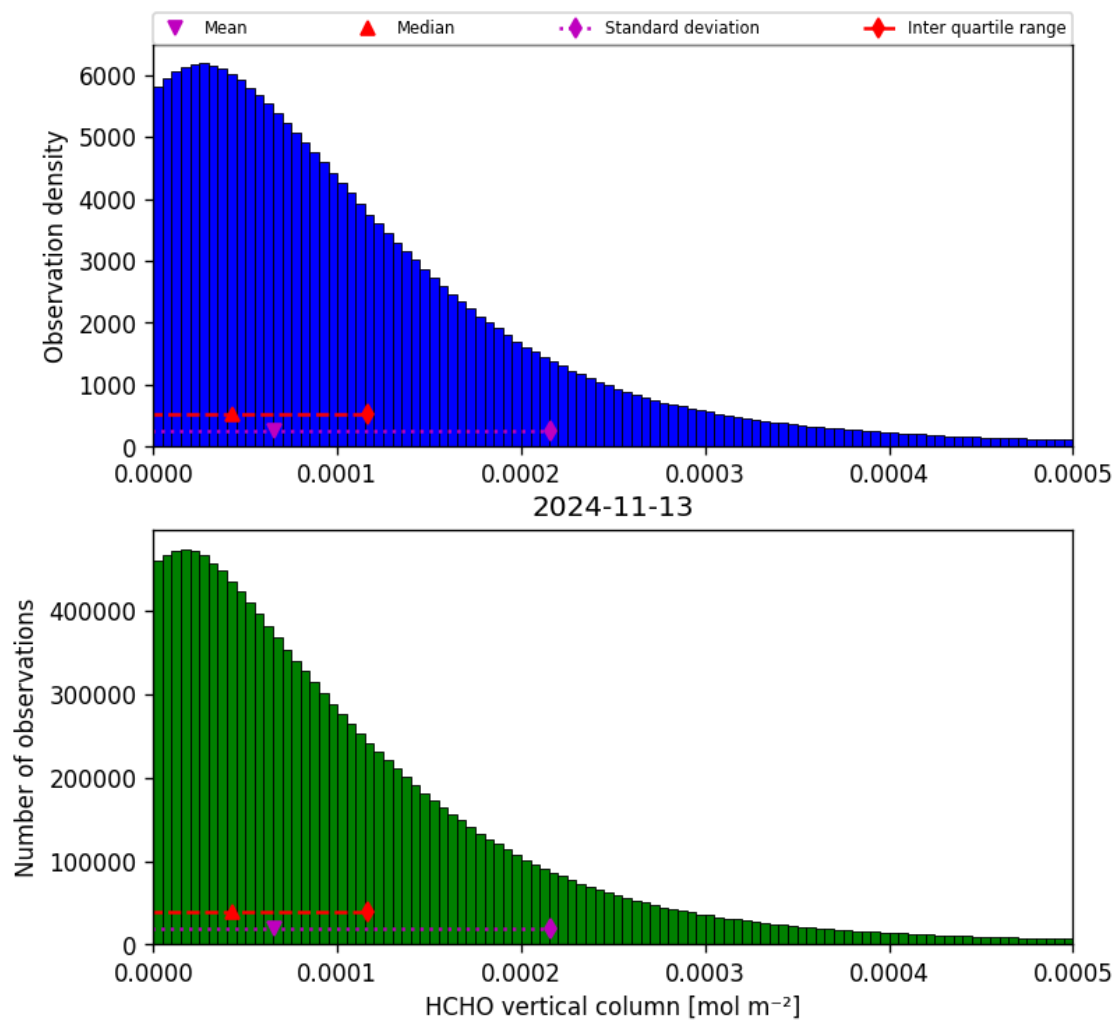
Figure 35: Histogram of “HCHO vertical column” for 2024-11-12 to 2024-11-14
