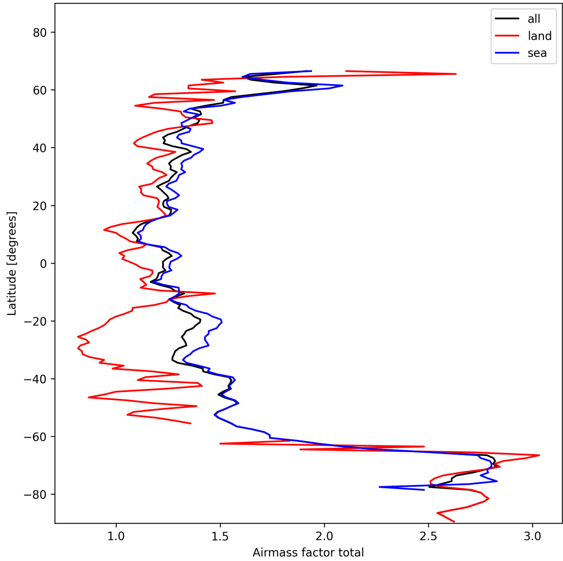
Figure 26: Zonal average of “Airmass factor total” for 2024-11-12 to 2024-11-14.
