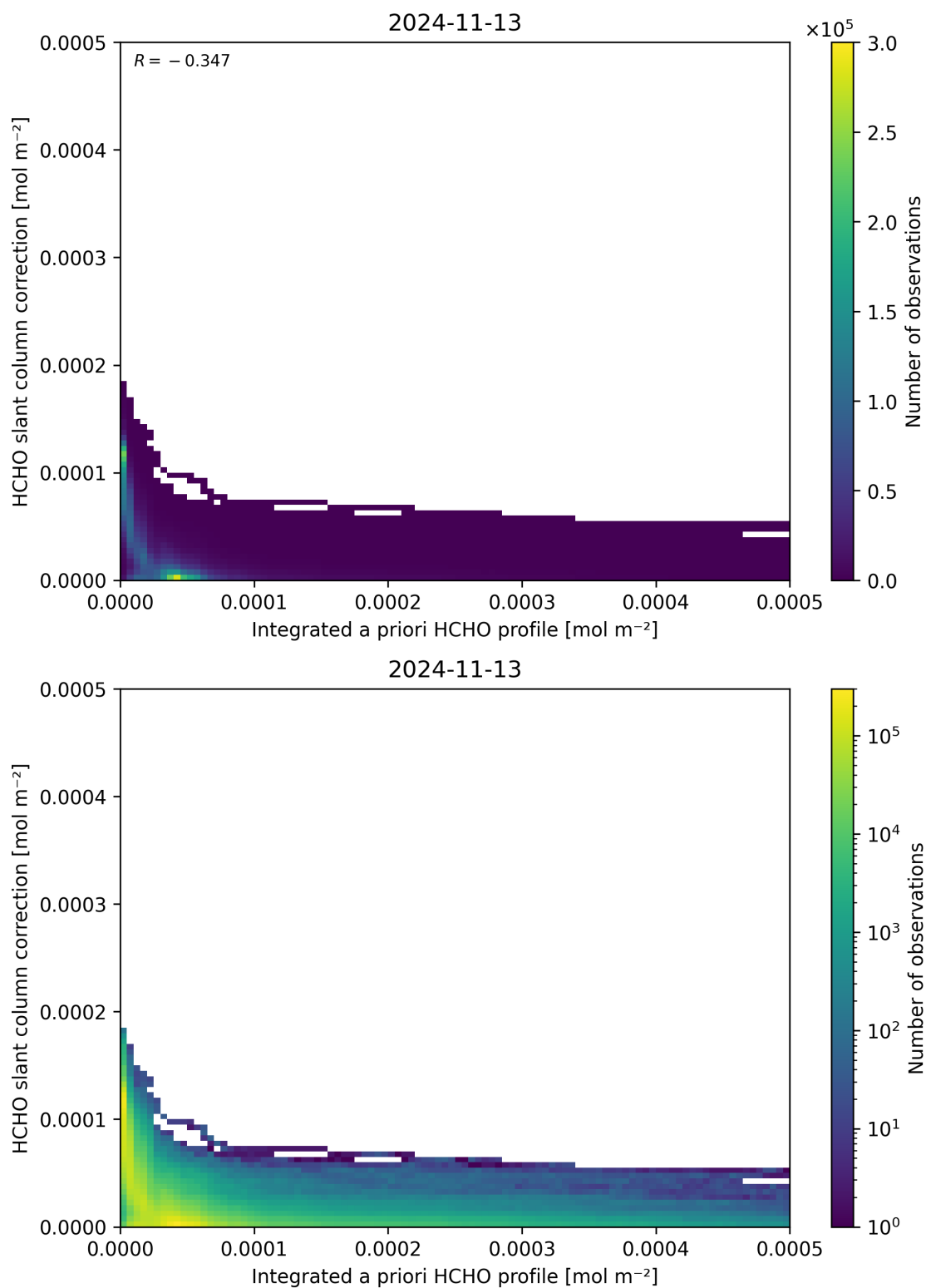
Figure 152: Scatter density plot of “Integrated a priori HCHO profile” against “HCHO slant column correction” for 2024-11-12 to 2024-11-14.
