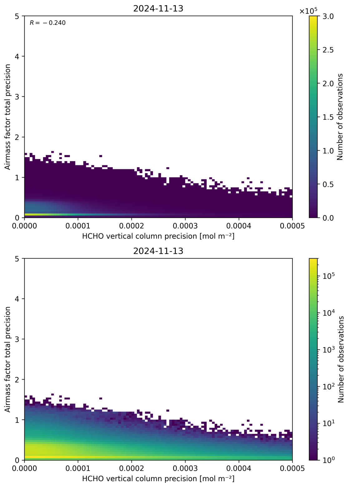
Figure 145: Scatter density plot of “HCHO vertical column precision” against “Airmass factor total precision” for 2024-11-12 to 2024-11-14.
