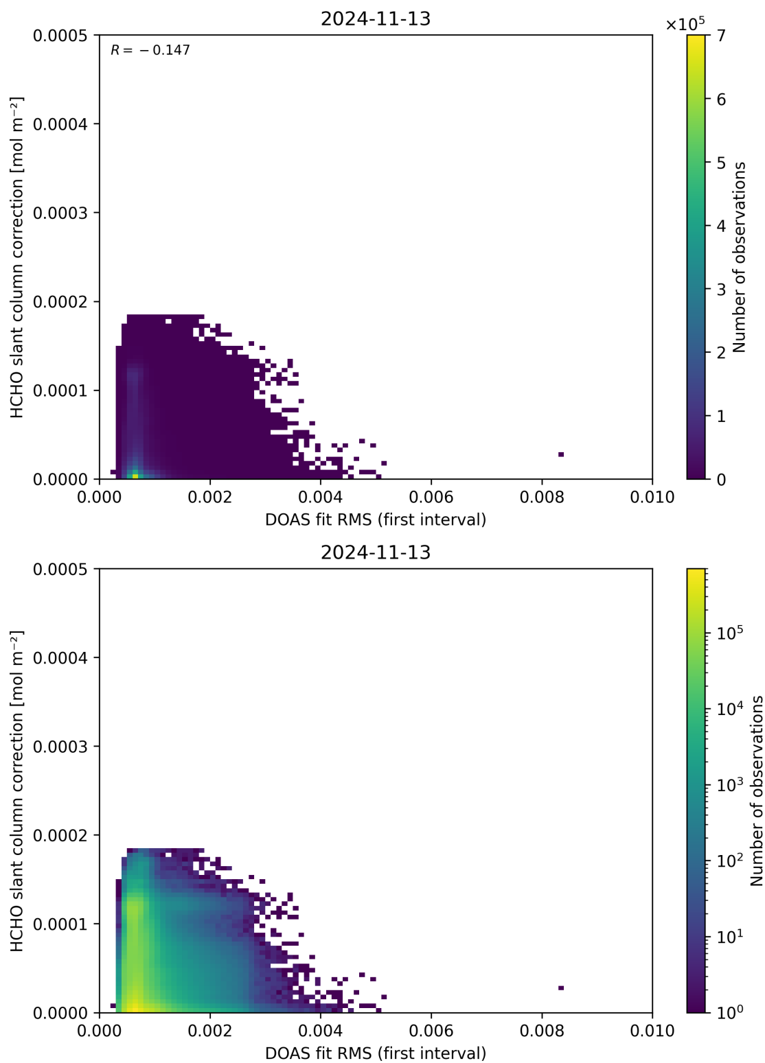
Figure 63: Scatter density plot of “DOAS fit RMS (first interval)” against “HCHO slant column correction” for 2024-11-12 to 2024-11-14.
