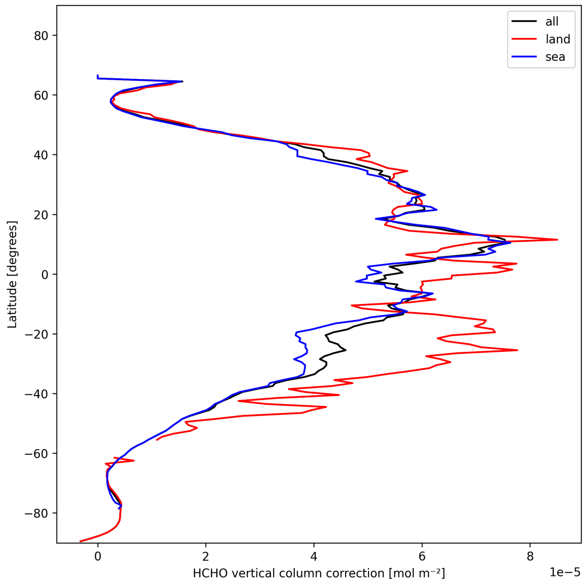
Figure 23: Zonal average of “HCHO vertical column correction” for 2024-11-12 to 2024-11-14.
