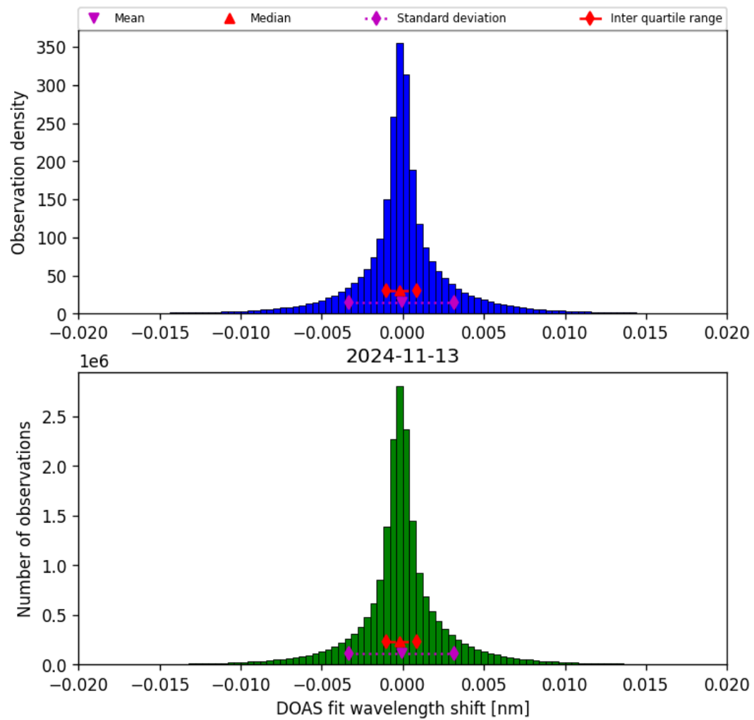
Figure 44: Histogram of “DOAS fit wavelength shift” for 2024-11-12 to 2024-11-14
