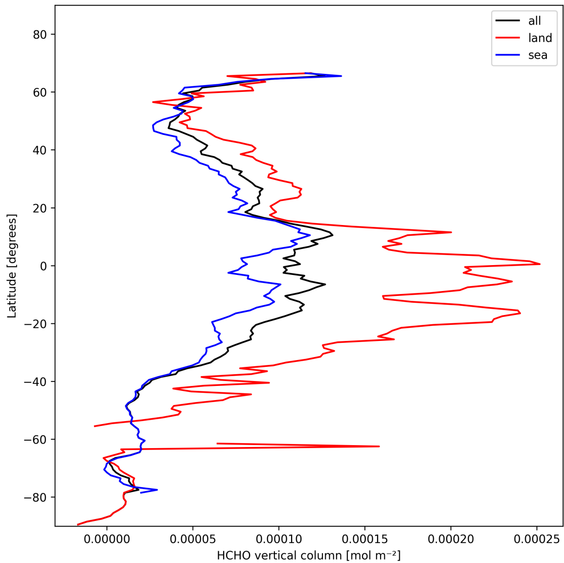
Figure 21: Zonal average of “HCHO vertical column” for 2024-11-12 to 2024-11-14.
