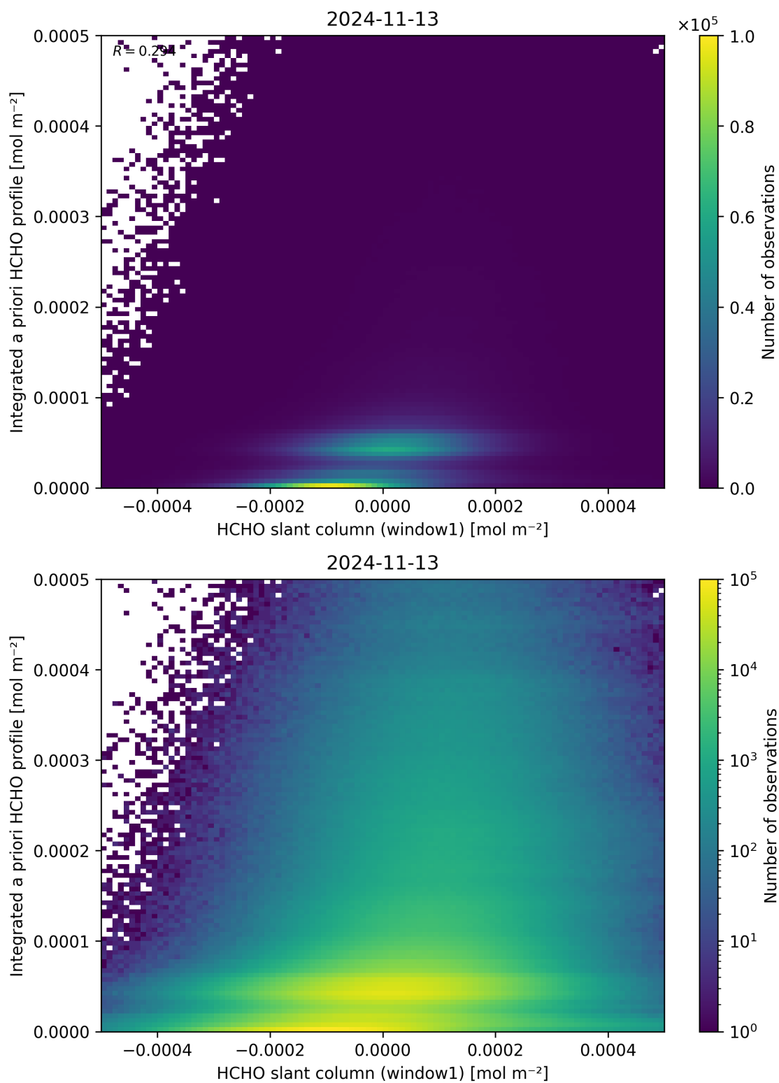
Figure 87: Scatter density plot of “HCHO slant column (window1)” against “Integrated a priori HCHO profile” for 2024-11-12 to 2024-11-14.
