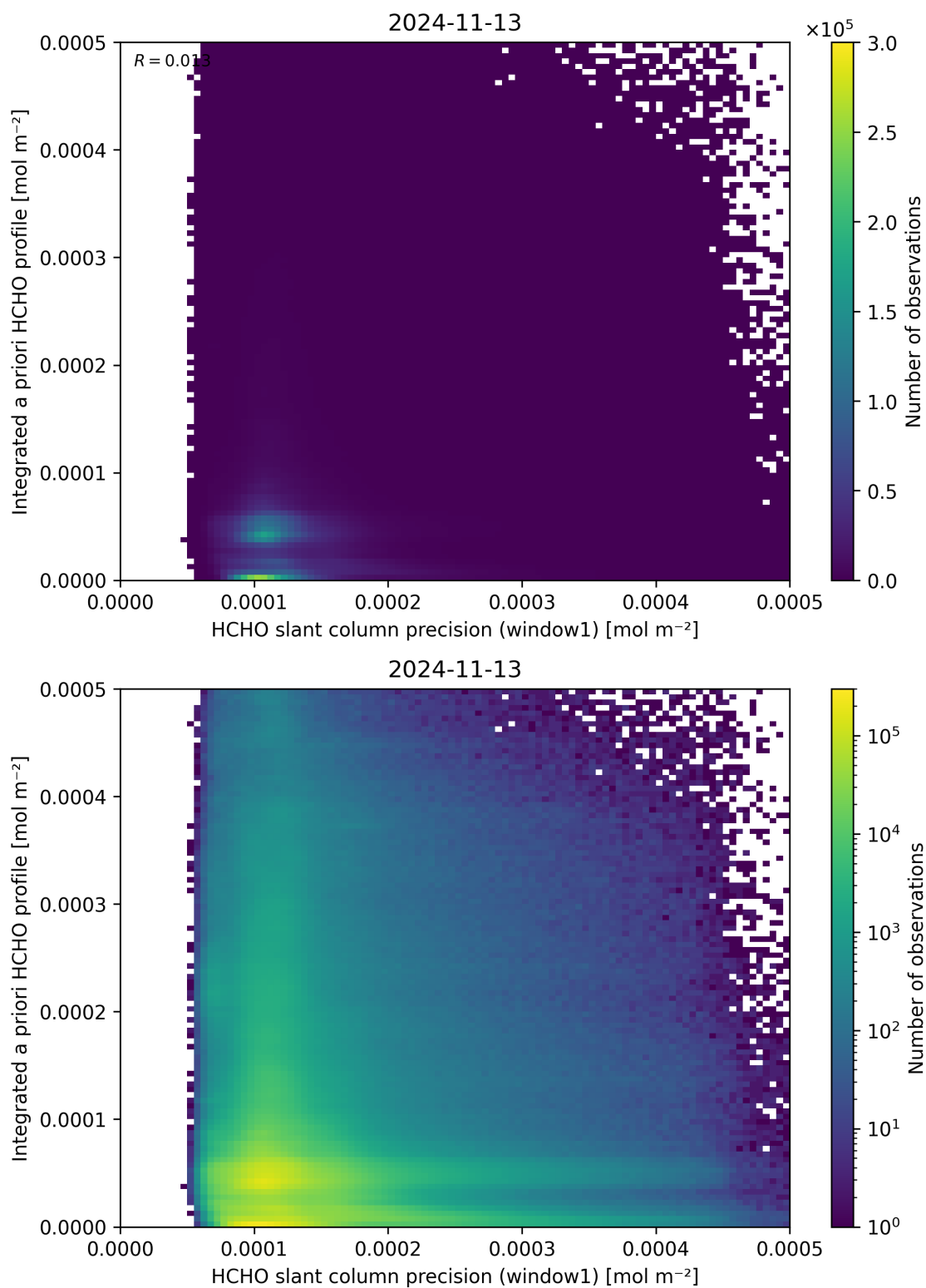
Figure 96: Scatter density plot of “HCHO slant column precision (window1)” against “Integrated a priori HCHO profile” for 2024-11-12 to 2024-11-14.
