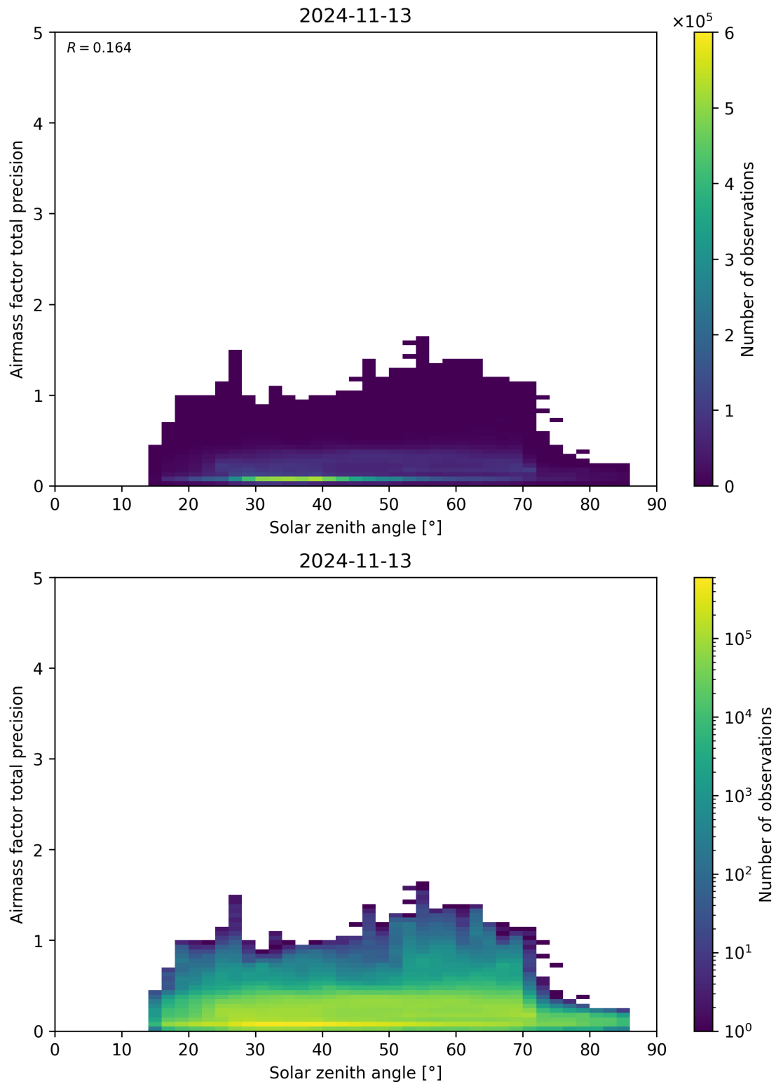
Figure 176: Scatter density plot of “Solar zenith angle” against “Airmass factor total precision” for 2024-11-12 to 2024-11-14.
