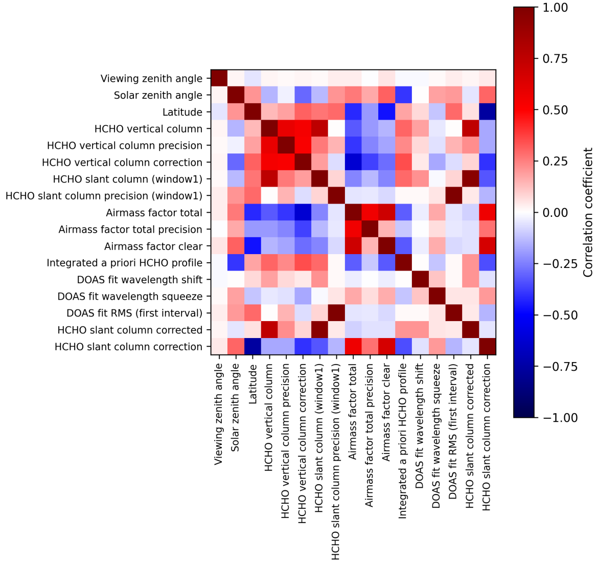
Figure 2: Map of correlation matrix for 2024-11-12 to 2024-11-14.
