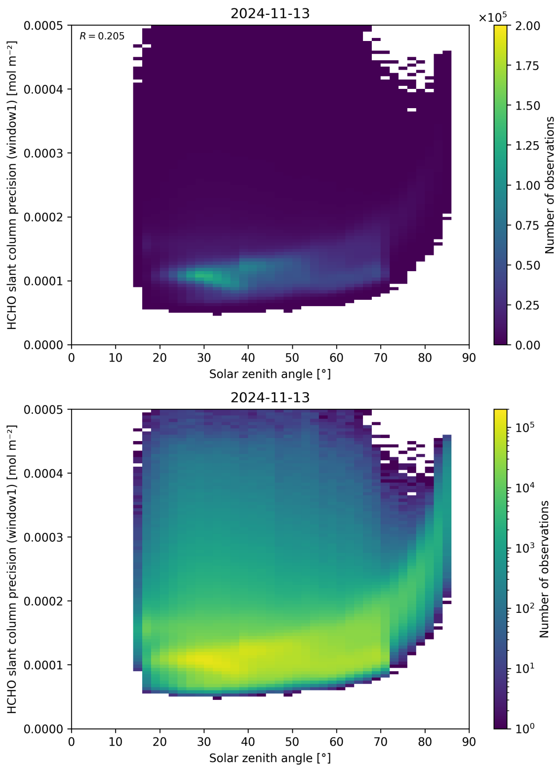
Figure 174: Scatter density plot of “Solar zenith angle” against “HCHO slant column precision (window1)” for 2024-11-12 to 2024-11-14.
