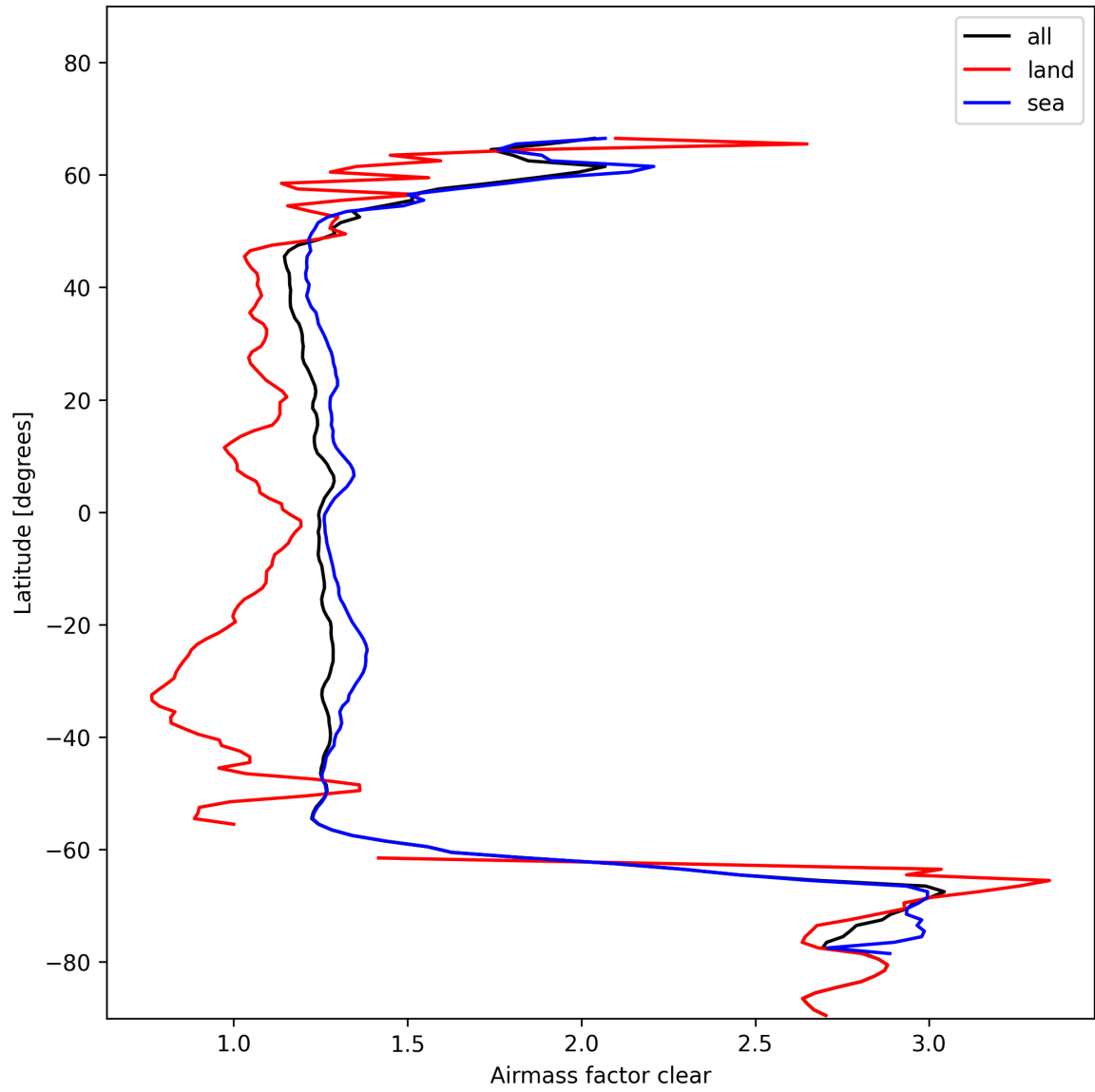
Figure 28: Zonal average of “Airmass factor clear” for 2024-11-12 to 2024-11-14.
