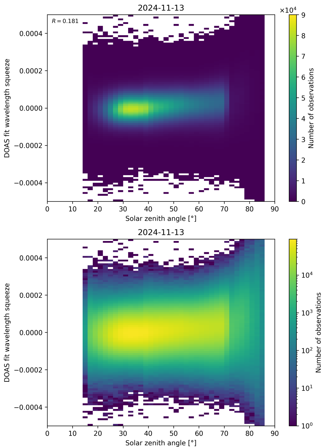
Figure 169: Scatter density plot of “Solar zenith angle” against “DOAS fit wavelength squeeze” for 2024-11-12 to 2024-11-14.
