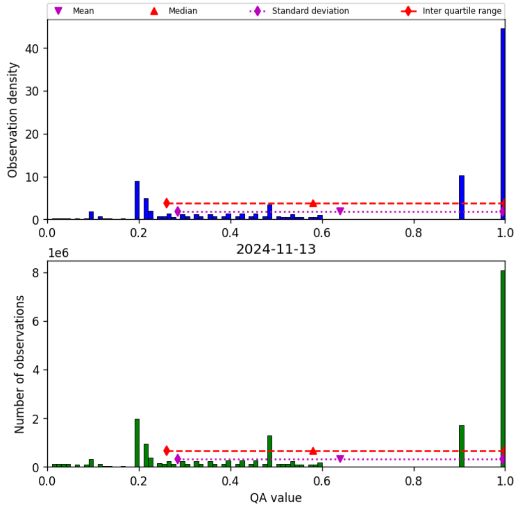
Figure 34: Histogram of “QA value” for 2024-11-12 to 2024-11-14
