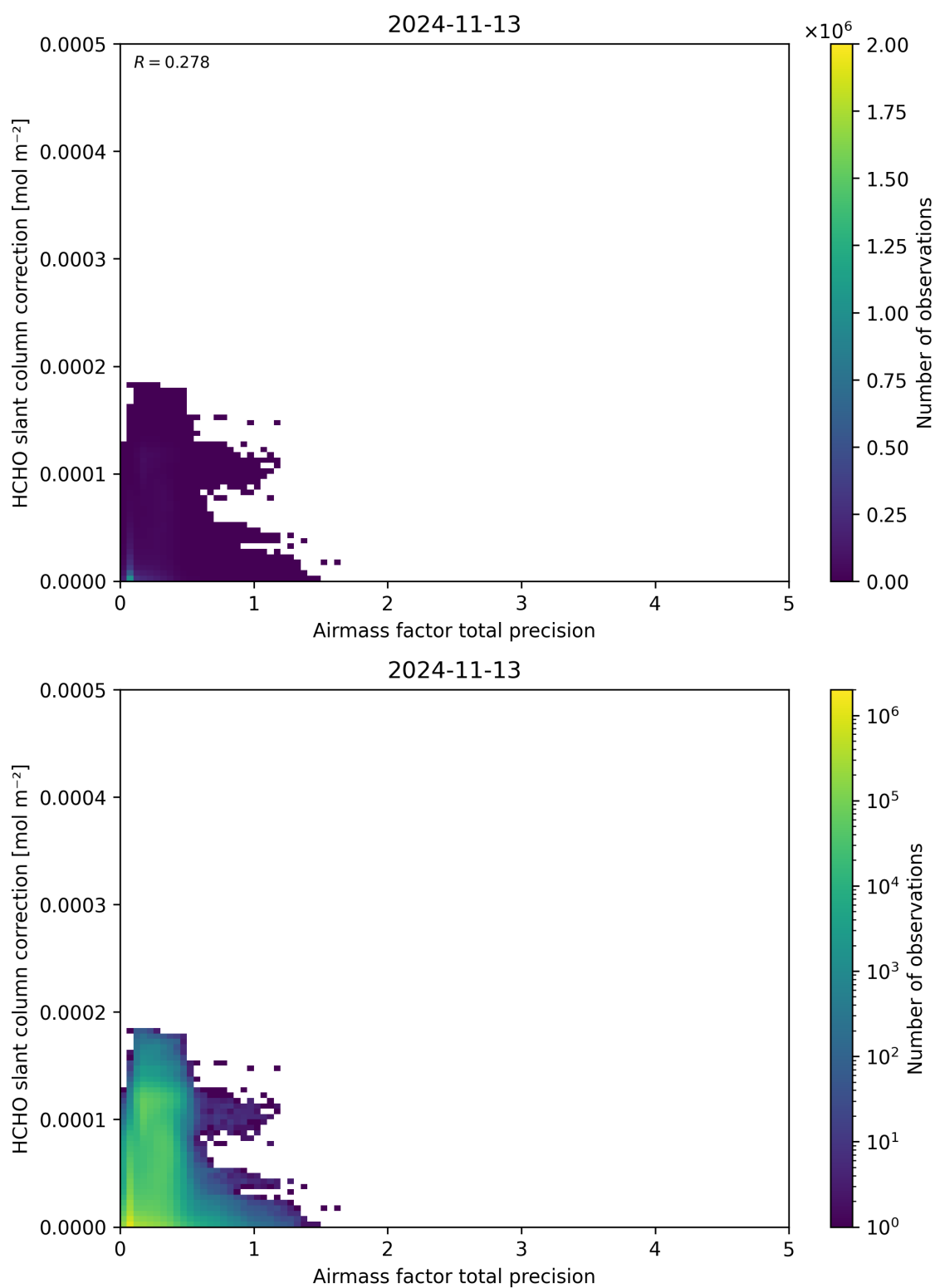
Figure 110: Scatter density plot of “Airmass factor total precision” against “HCHO slant column correction” for 2024-11-12 to 2024-11-14.
