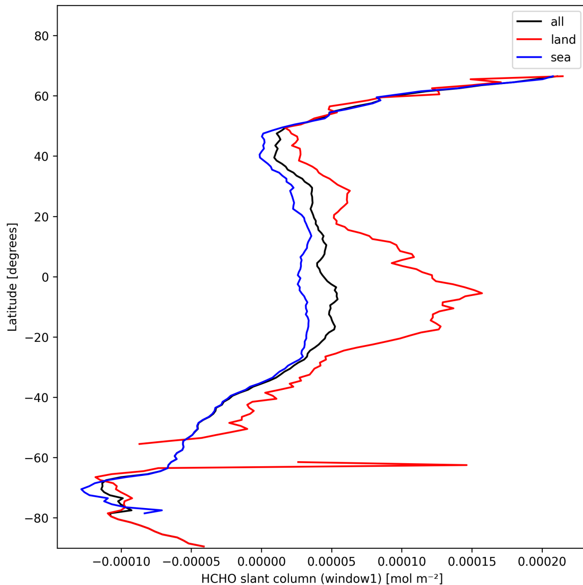
Figure 24: Zonal average of “HCHO slant column (window1)” for 2024-11-12 to 2024-11-14.
