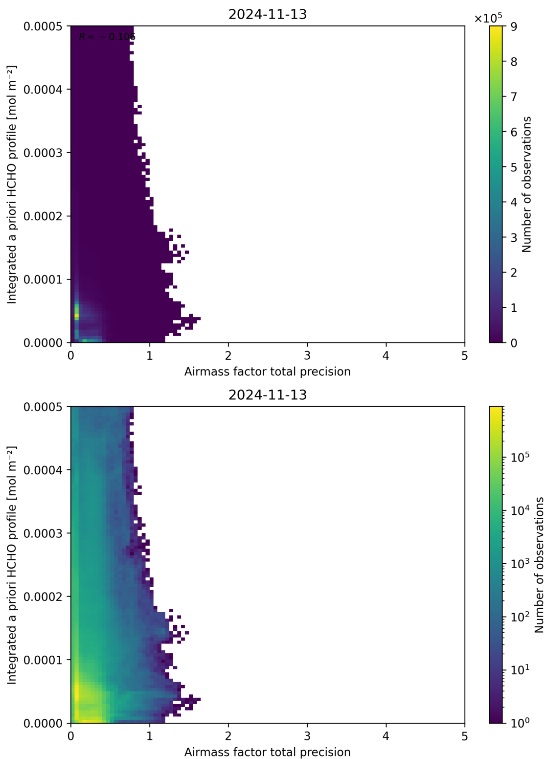
Figure 111: Scatter density plot of “Airmass factor total precision” against “Integrated a priori HCHO profile” for 2024-11-12 to 2024-11-14.
