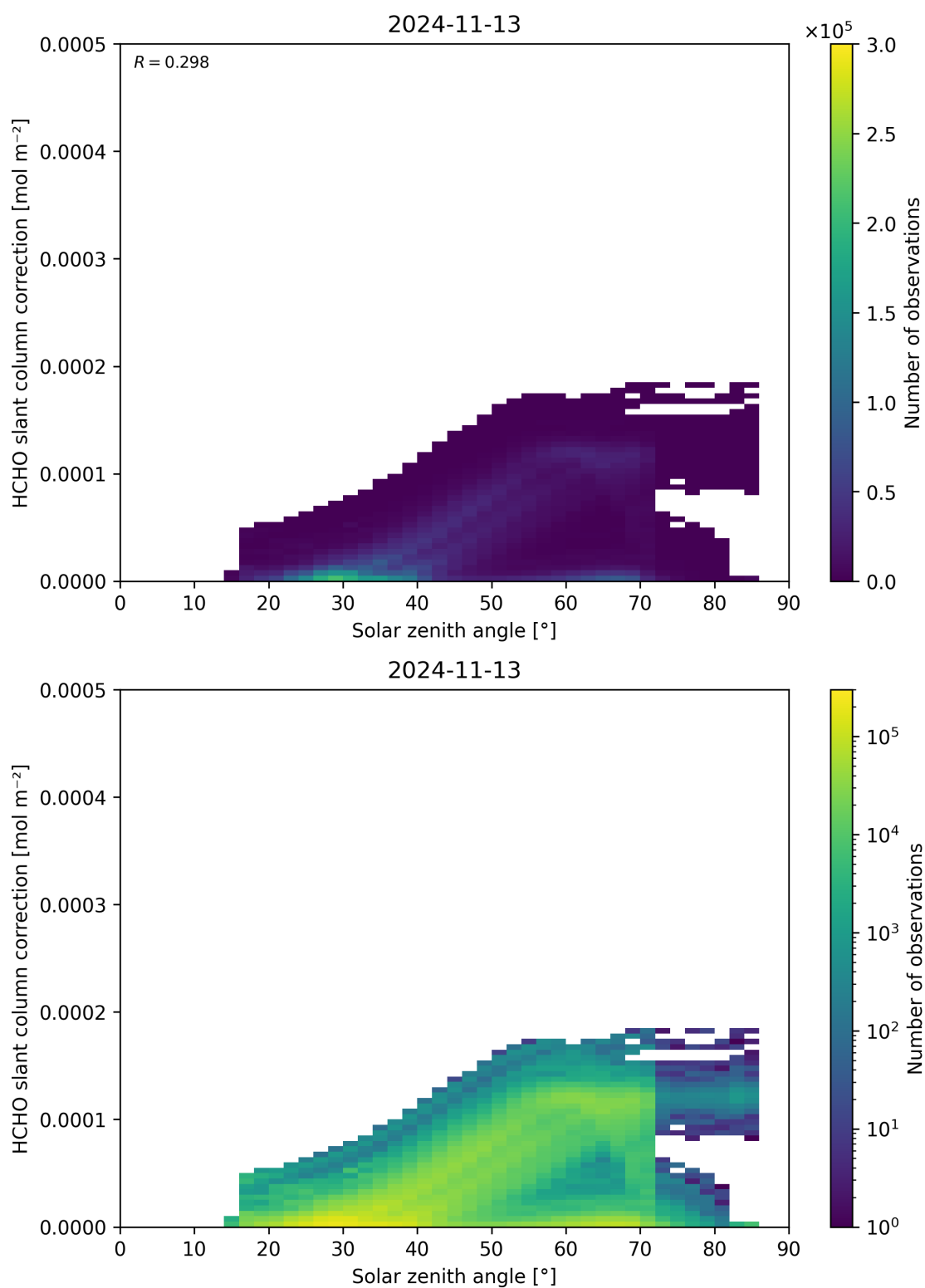
Figure 172: Scatter density plot of “Solar zenith angle” against “HCHO slant column correction” for 2024-11-12 to 2024-11-14.
