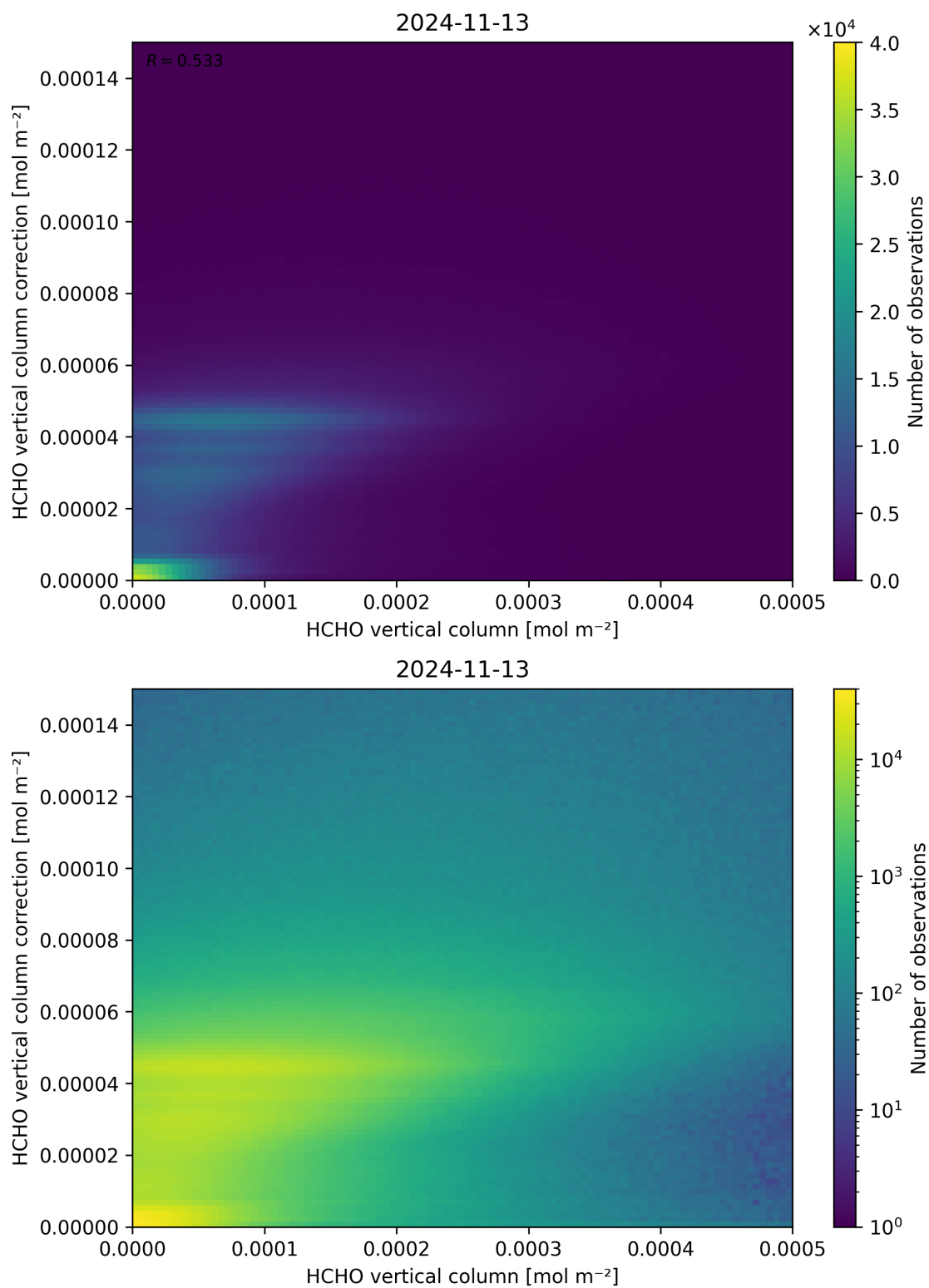
Figure 133: Scatter density plot of “HCHO vertical column” against “HCHO vertical column correction” for 2024-11-12 to 2024-11-14.
