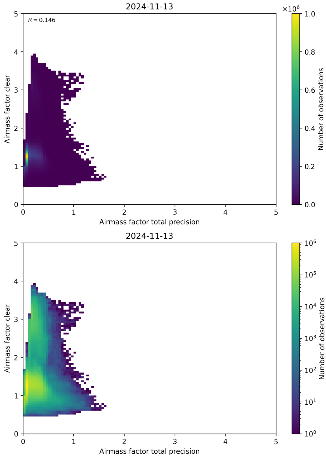
Figure 108: Scatter density plot of “Airmass factor total precision” against “Airmass factor clear” for 2024-11-12 to 2024-11-14.
