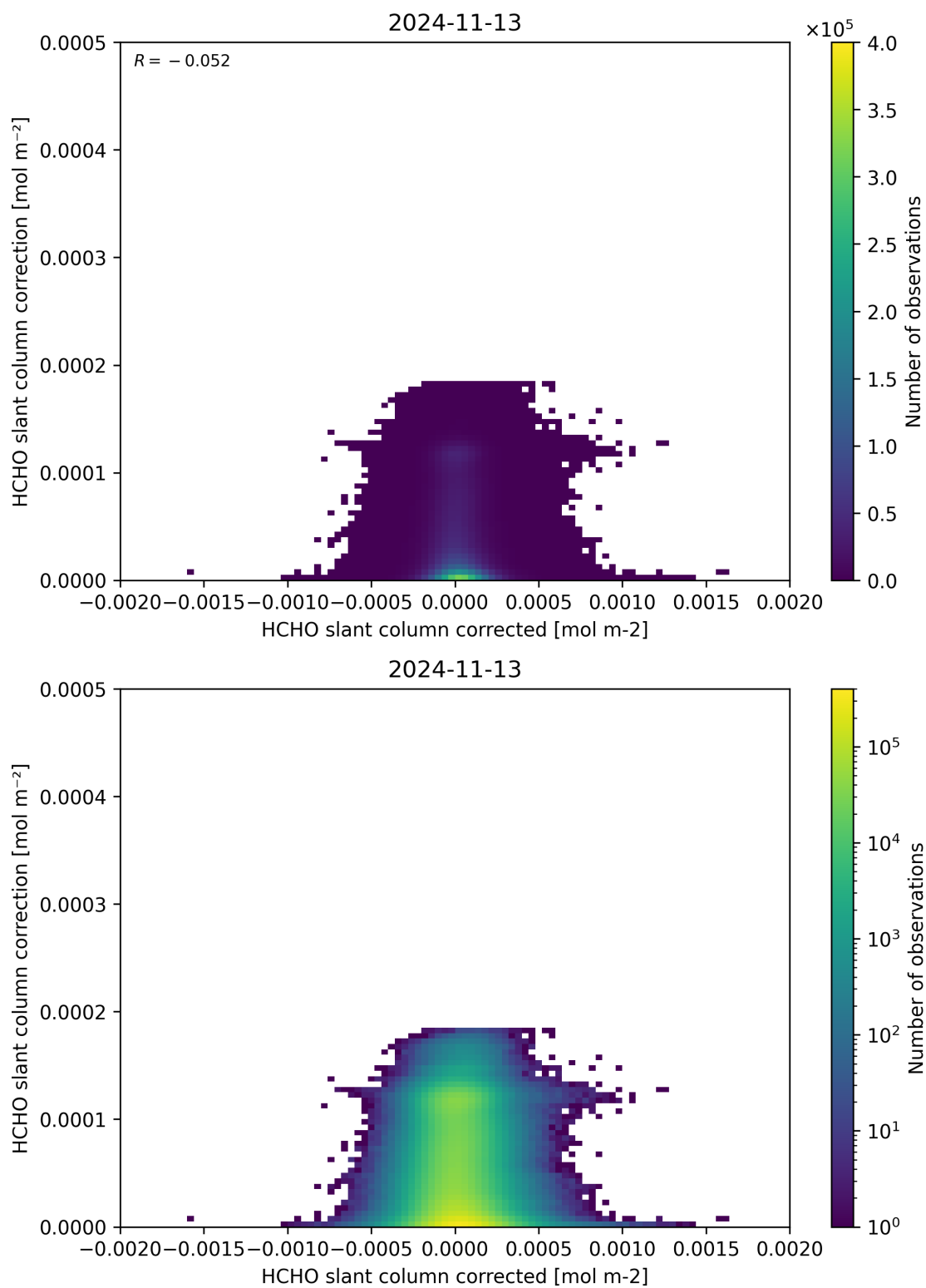
Figure 77: Scatter density plot of “HCHO slant column corrected” against “HCHO slant column correction” for 2024-11-12 to 2024-11-14.
