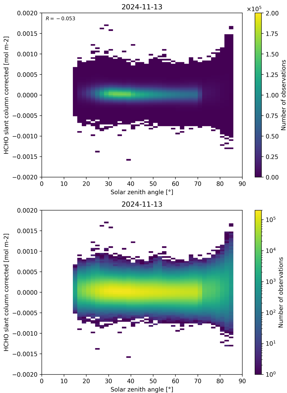
Figure 171: Scatter density plot of “Solar zenith angle” against “HCHO slant column corrected” for 2024-11-12 to 2024-11-14.
