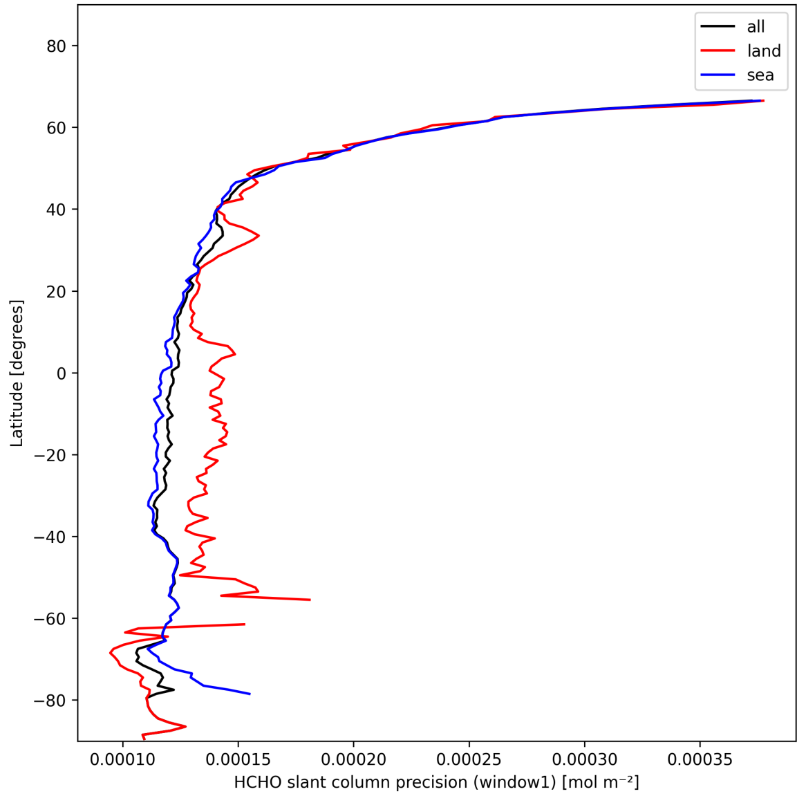
Figure 25: Zonal average of “HCHO slant column precision (window1)” for 2024-11-12 to 2024-11-14.
