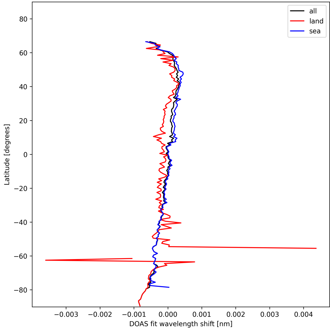
Figure 30: Zonal average of "DOAS fit wavelength shift" for 2024-11-12 to 2024-11-14.
