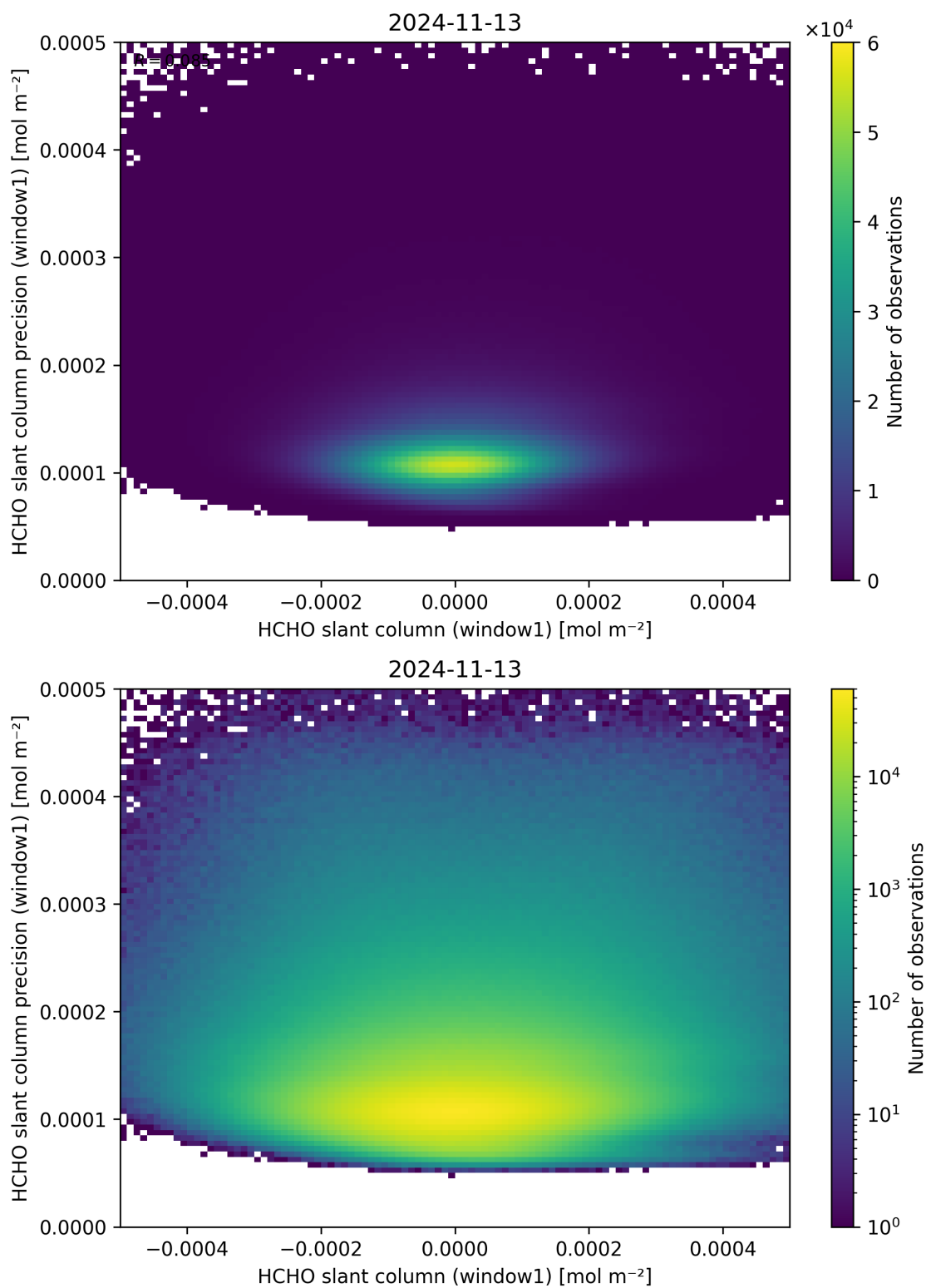
Figure 84: Scatter density plot of “HCHO slant column (window1)” against “HCHO slant column precision (window1)” for 2024-11-12 to 2024-11-14.
