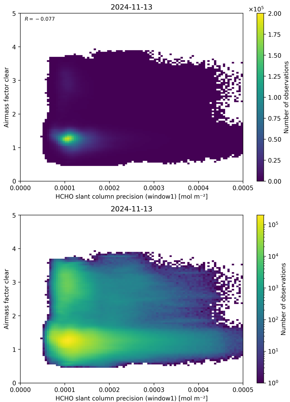
Figure 91: Scatter density plot of “HCHO slant column precision (window1)” against “Airmass factor clear” for 2024-11-12 to 2024-11-14.
