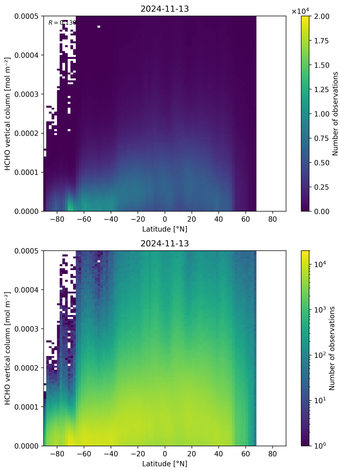
Figure 163: Scatter density plot of “Latitude” against “HCHO vertical column” for 2024-11-12 to 2024-11-14.
