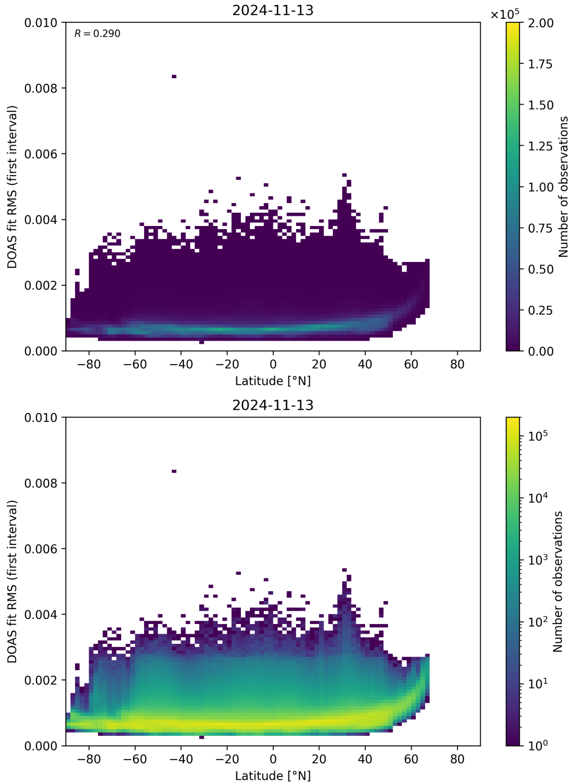
Figure 153: Scatter density plot of “Latitude” against “DOAS fit RMS (first interval)” for 2024-11-12 to 2024-11-14.
