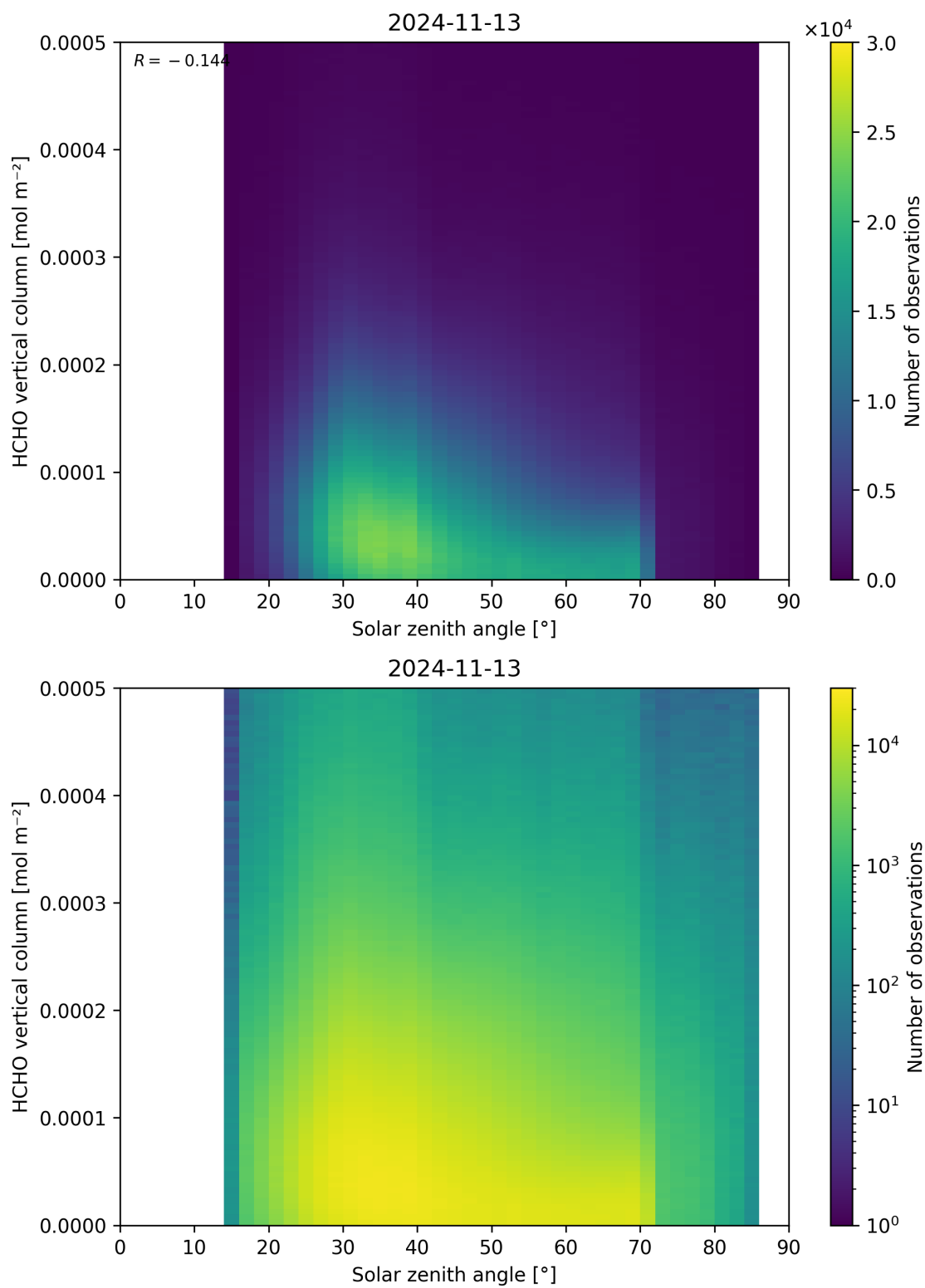
Figure 177: Scatter density plot of “Solar zenith angle” against “HCHO vertical column” for 2024-11-12 to 2024-11-14.
