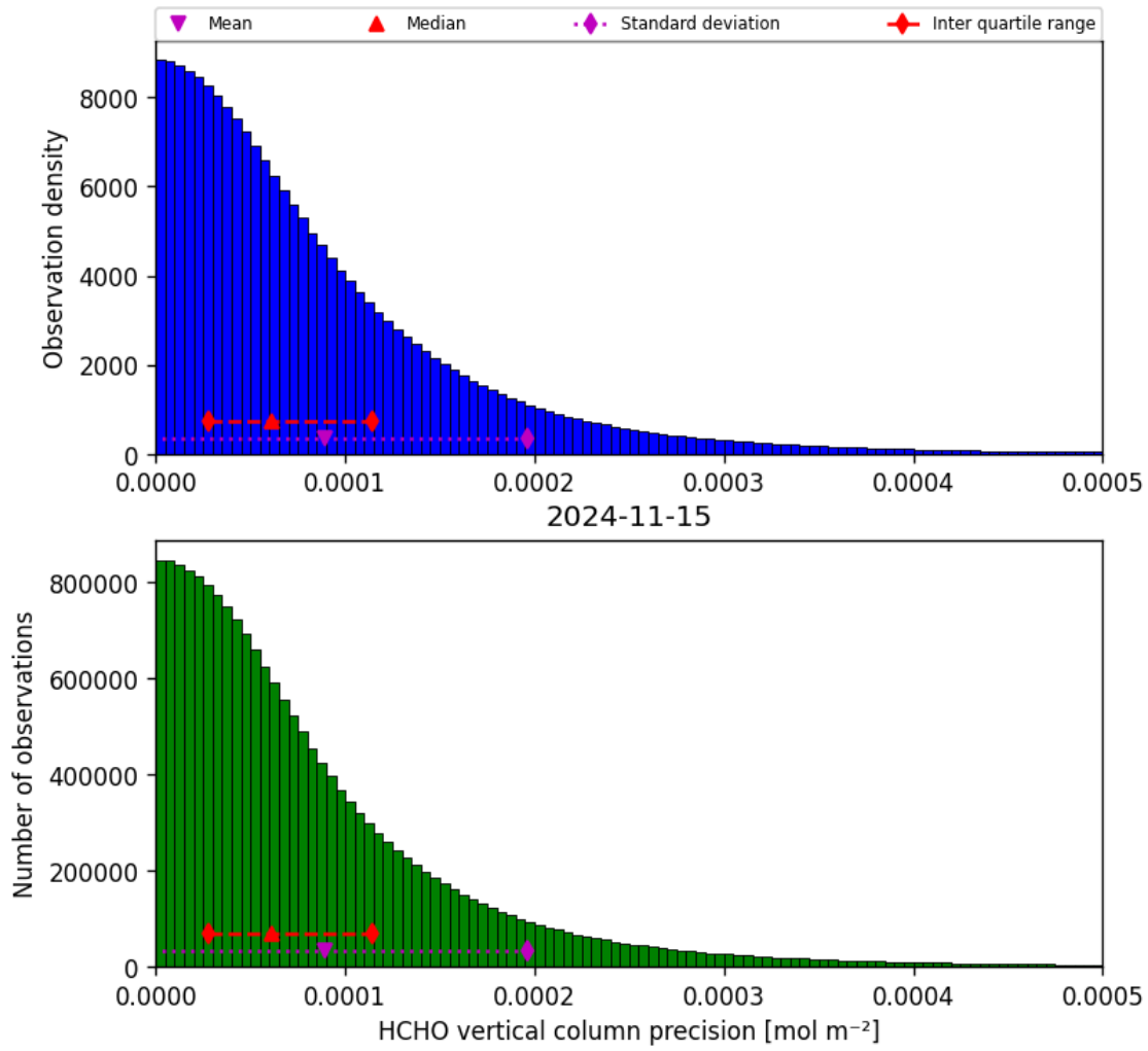
Figure 36: Histogram of “HCHO vertical column precision” for 2024-11-14 to 2024-11-16
