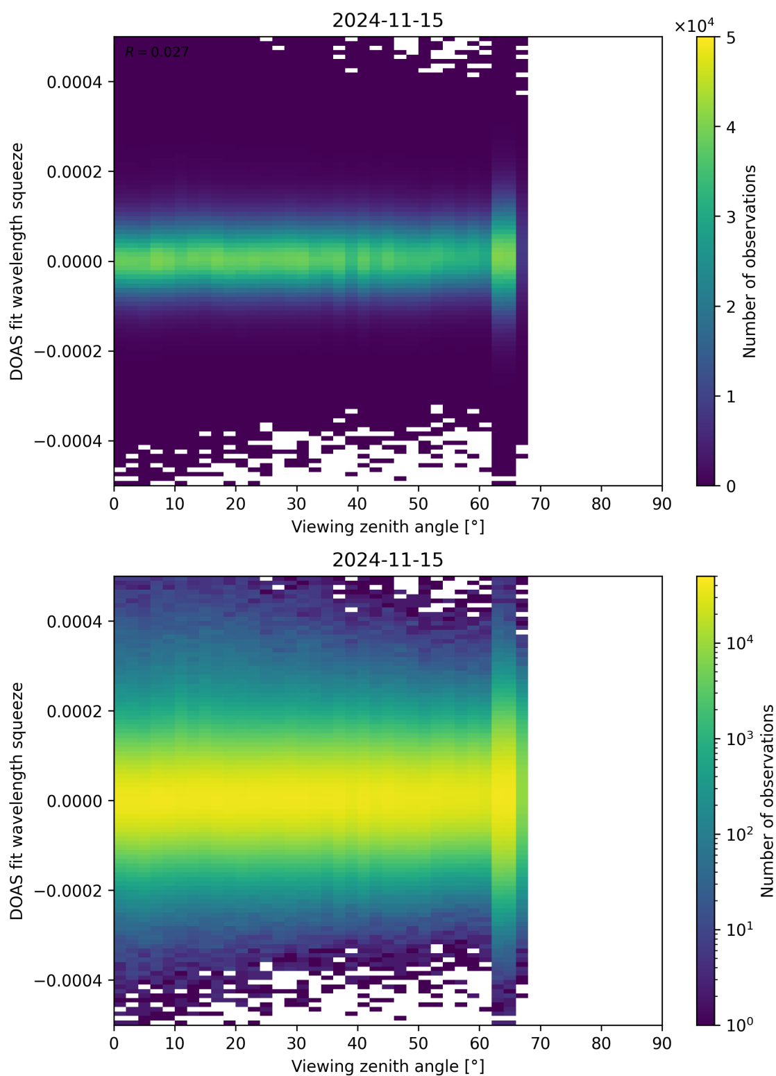
Figure 184: Scatter density plot of “Viewing zenith angle” against “DOAS fit wavelength squeeze” for 2024-11-14 to 2024-11-16.
