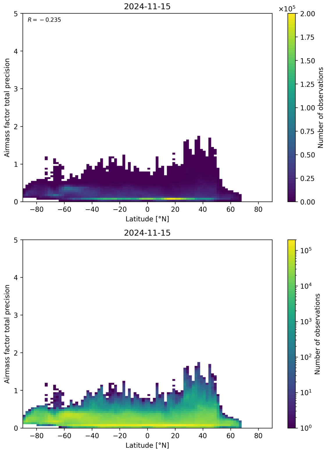
Figure 162: Scatter density plot of “Latitude” against “Airmass factor total precision” for 2024-11-14 to 2024-11-16.
