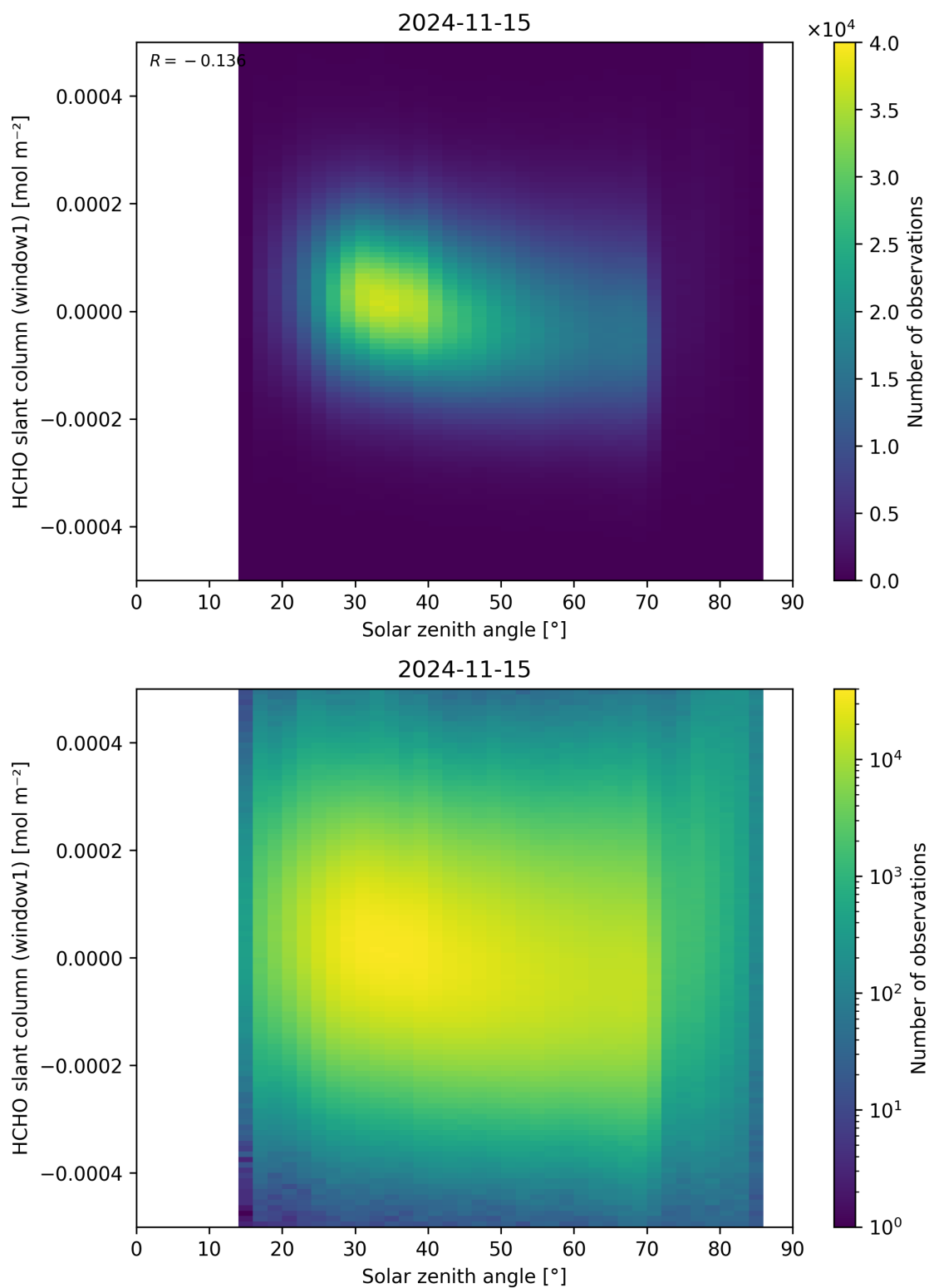
Figure 173: Scatter density plot of “Solar zenith angle” against “HCHO slant column (window1)” for 2024-11-14 to 2024-11-16.
