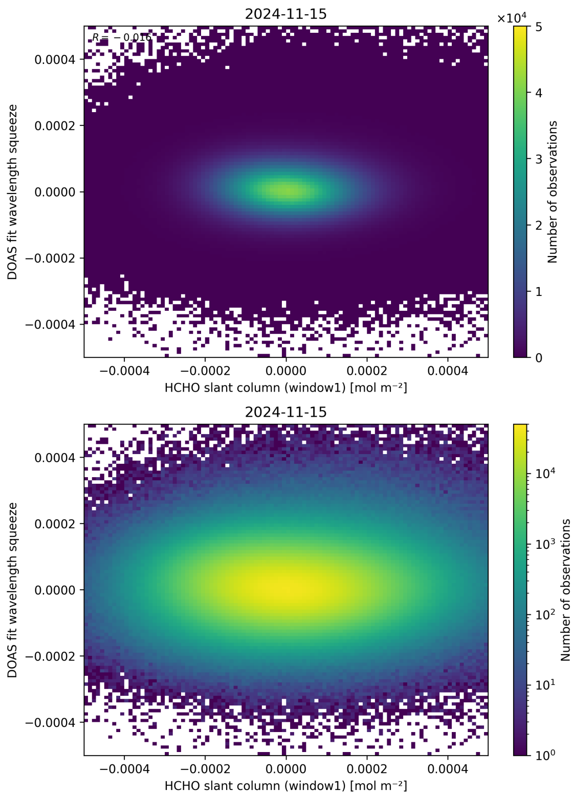
Figure 80: Scatter density plot of “HCHO slant column (window1)” against “DOAS fit wavelength squeeze” for 2024-11-14 to 2024-11-16.
