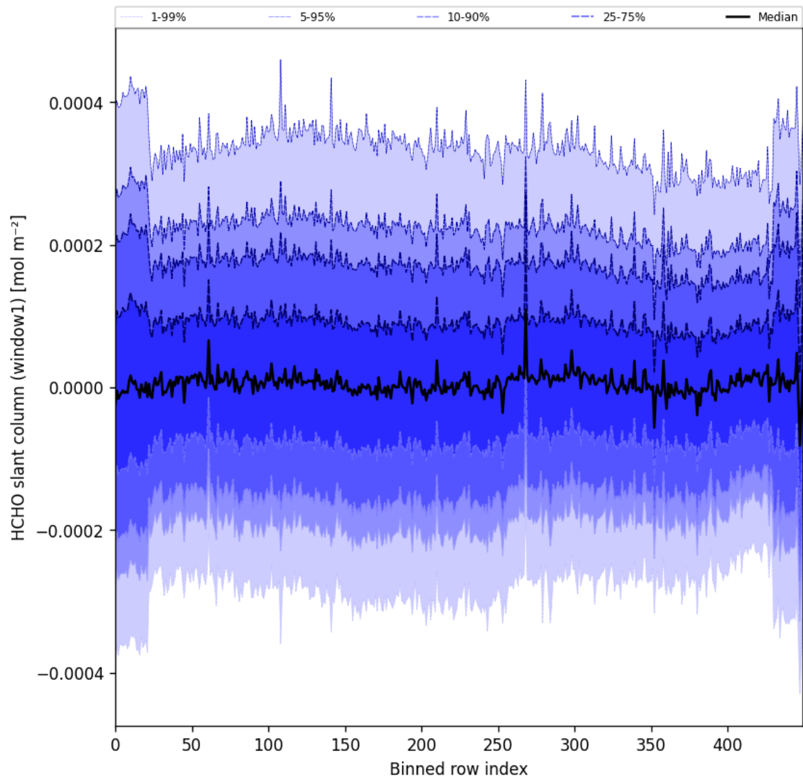
Figure 52: Along track statistics of “HCHO slant column (window1)” for 2024-11-14 to 2024-11-16
