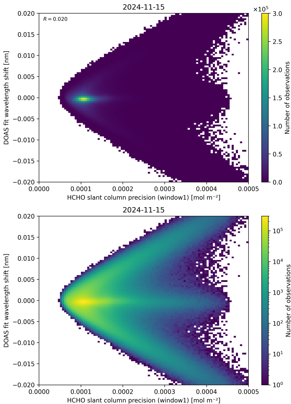
Figure 89: Scatter density plot of “HCHO slant column precision (window1)” against “DOAS fit wavelength shift” for 2024-11-14 to 2024-11-16.
