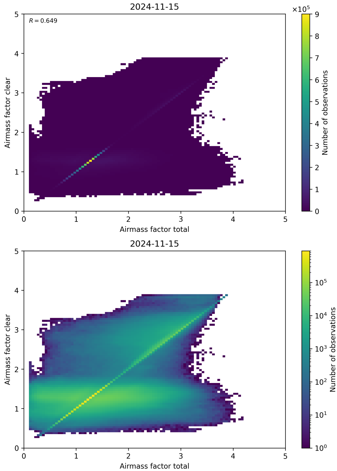
Figure 100: Scatter density plot of “Airmass factor total” against “Airmass factor clear” for 2024-11-14 to 2024-11-16.
