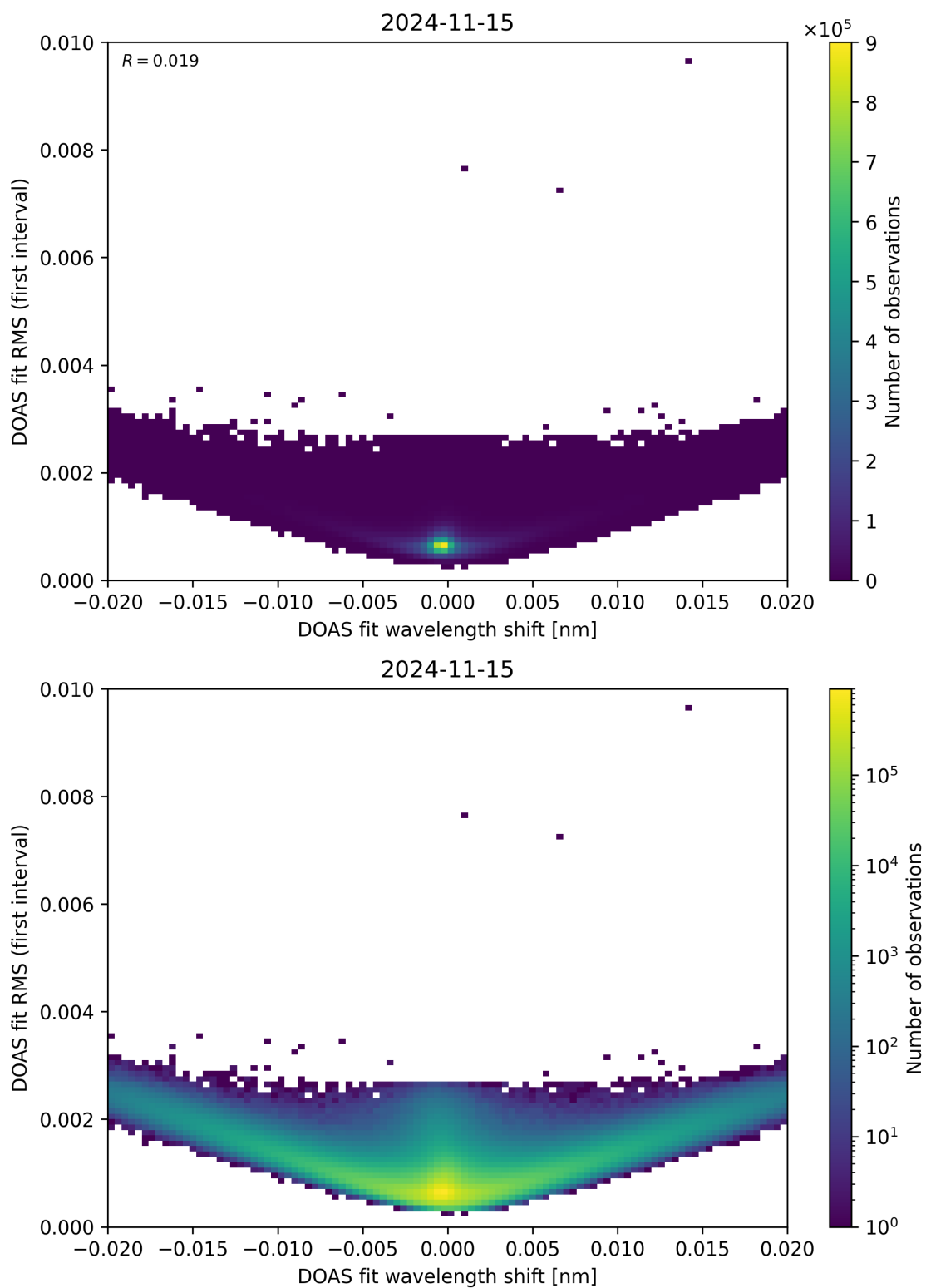
Figure 64: Scatter density plot of “DOAS fit wavelength shift” against “DOAS fit RMS (first interval)” for 2024-11-14 to 2024-11-16.
