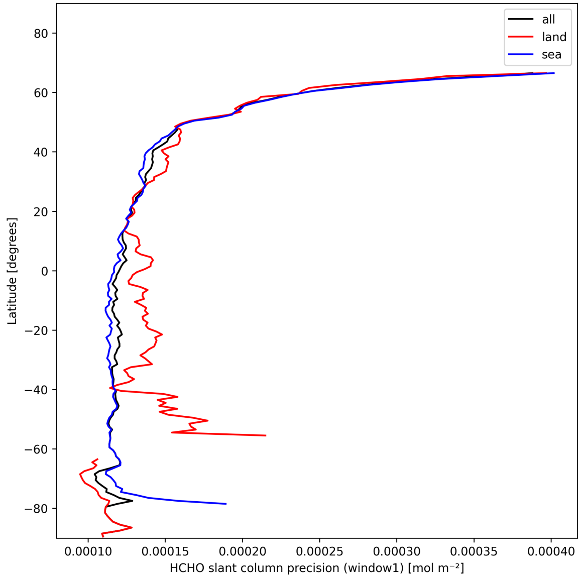
Figure 25: Zonal average of “HCHO slant column precision (window1)” for 2024-11-14 to 2024-11-16.
