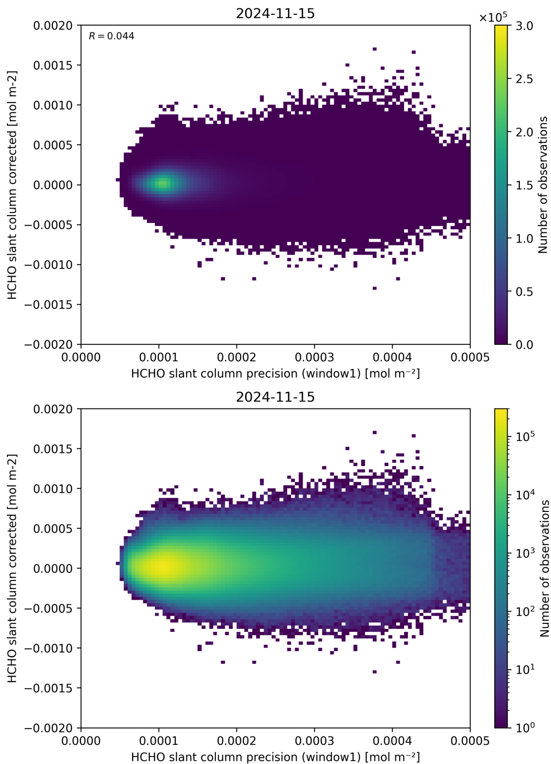
Figure 92: Scatter density plot of “HCHO slant column precision (window1)” against “HCHO slant column corrected” for 2024-11-14 to 2024-11-16.
