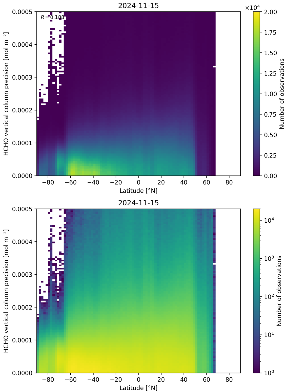
Figure 165: Scatter density plot of “Latitude” against “HCHO vertical column precision” for 2024-11-14 to 2024-11-16.
