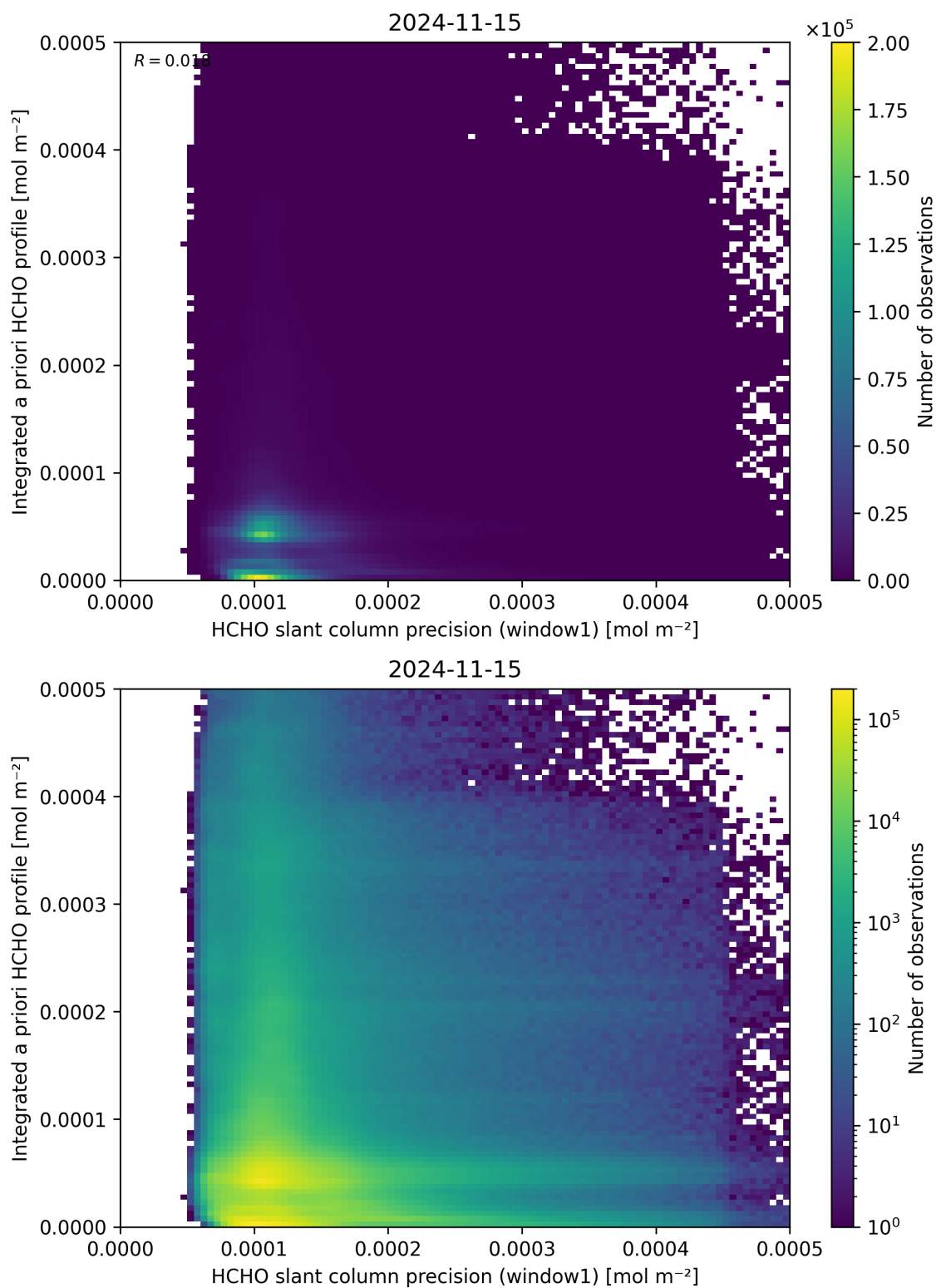
Figure 96: Scatter density plot of “HCHO slant column precision (window1)” against “Integrated a priori HCHO profile” for 2024-11-14 to 2024-11-16.
