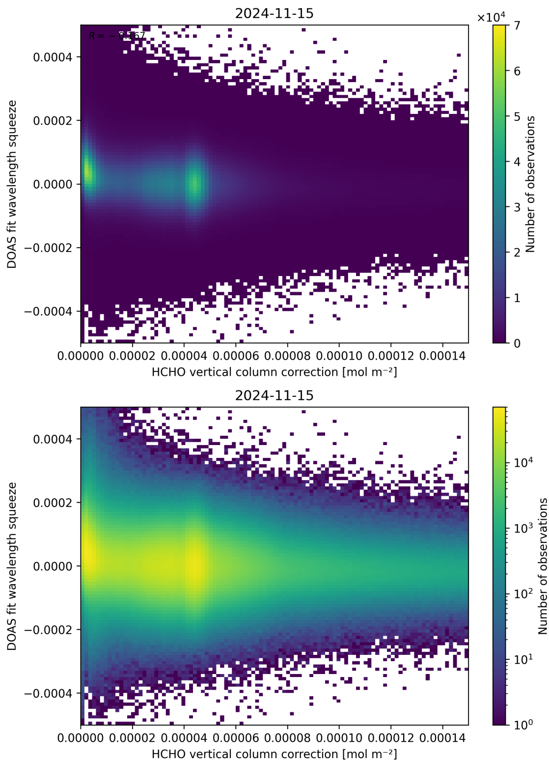
Figure 114: Scatter density plot of “HCHO vertical column correction” against “DOAS fit wavelength squeeze” for 2024-11-14 to 2024-11-16.
