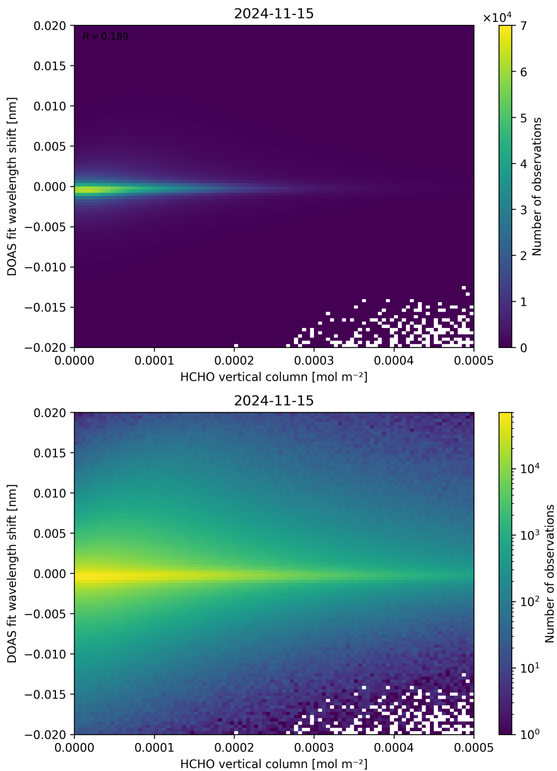
Figure 124: Scatter density plot of “HCHO vertical column” against “DOAS fit wavelength shift” for 2024-11-14 to 2024-11-16.
