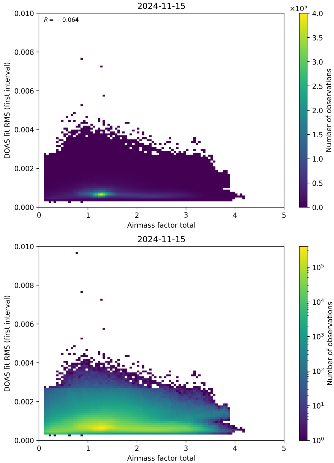
Figure 97: Scatter density plot of “Airmass factor total” against “DOAS fit RMS (first interval)” for 2024-11-14 to 2024-11-16.
