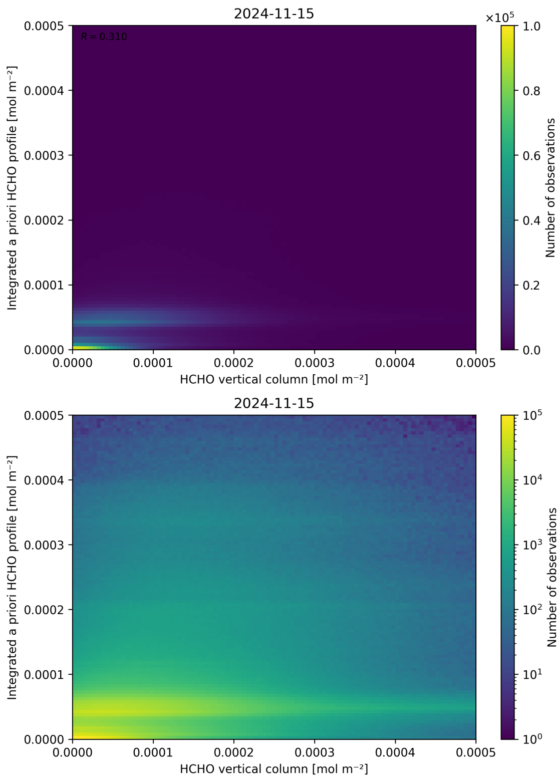
Figure 135: Scatter density plot of “HCHO vertical column” against “Integrated a priori HCHO profile” for 2024-11-14 to 2024-11-16.
