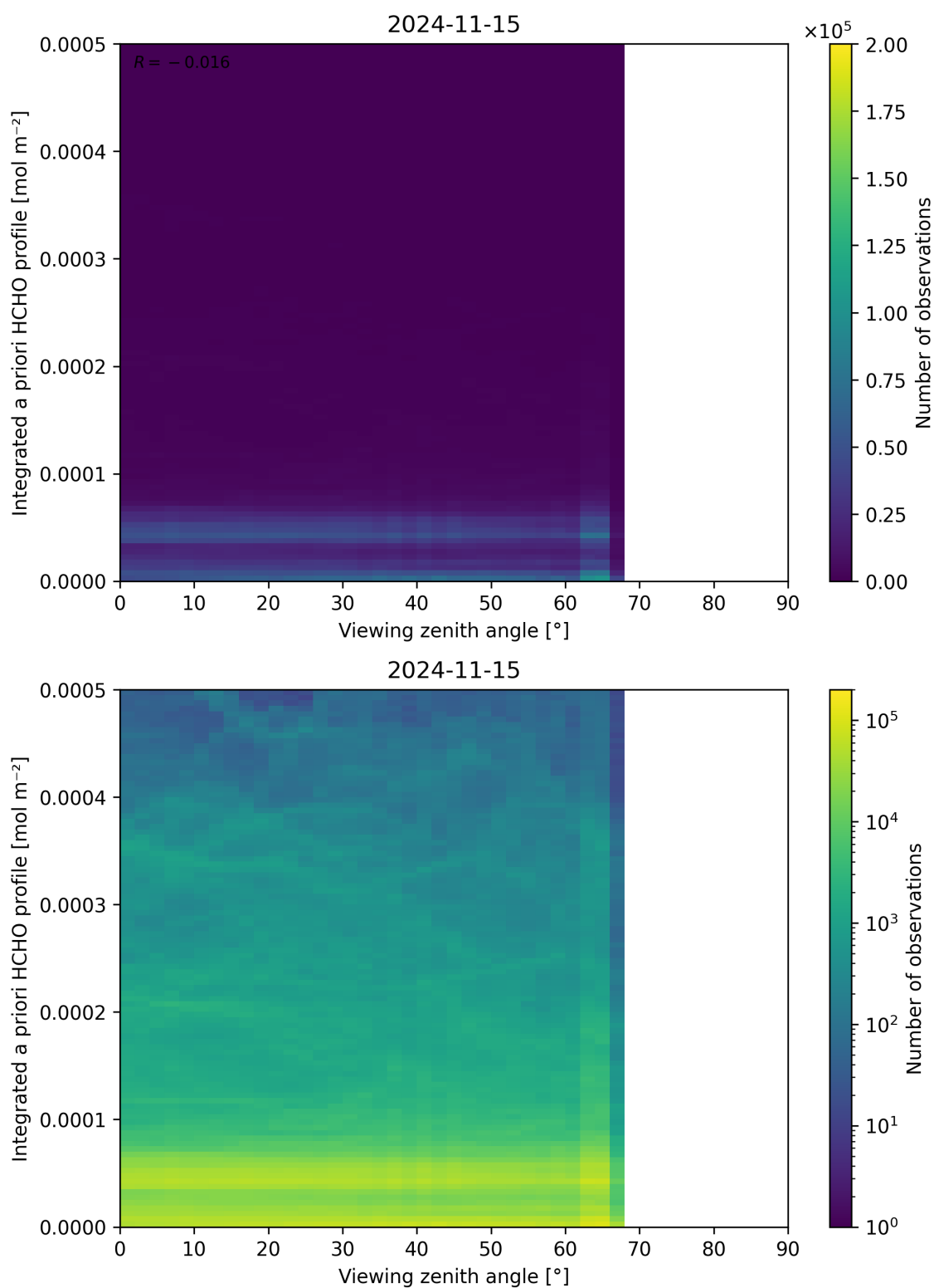
Figure 195: Scatter density plot of “Viewing zenith angle” against “Integrated a priori HCHO profile” for 2024-11-14 to 2024-11-16.
