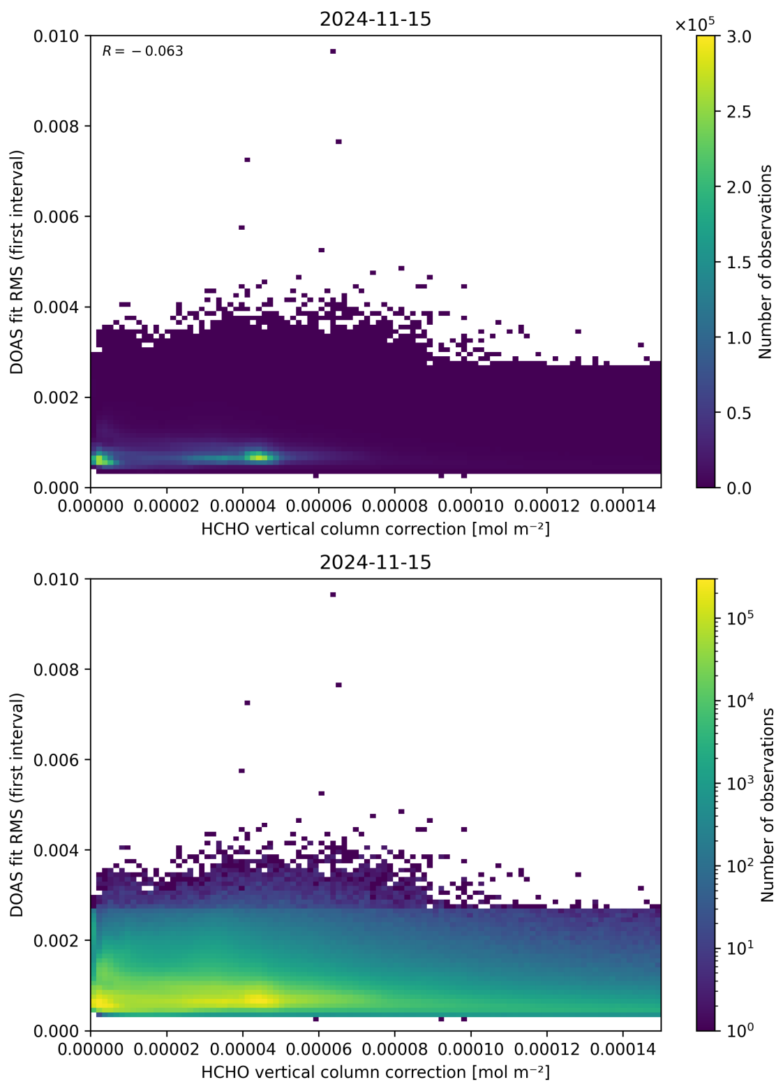
Figure 112: Scatter density plot of “HCHO vertical column correction” against “DOAS fit RMS (first interval)” for 2024-11-14 to 2024-11-16.
