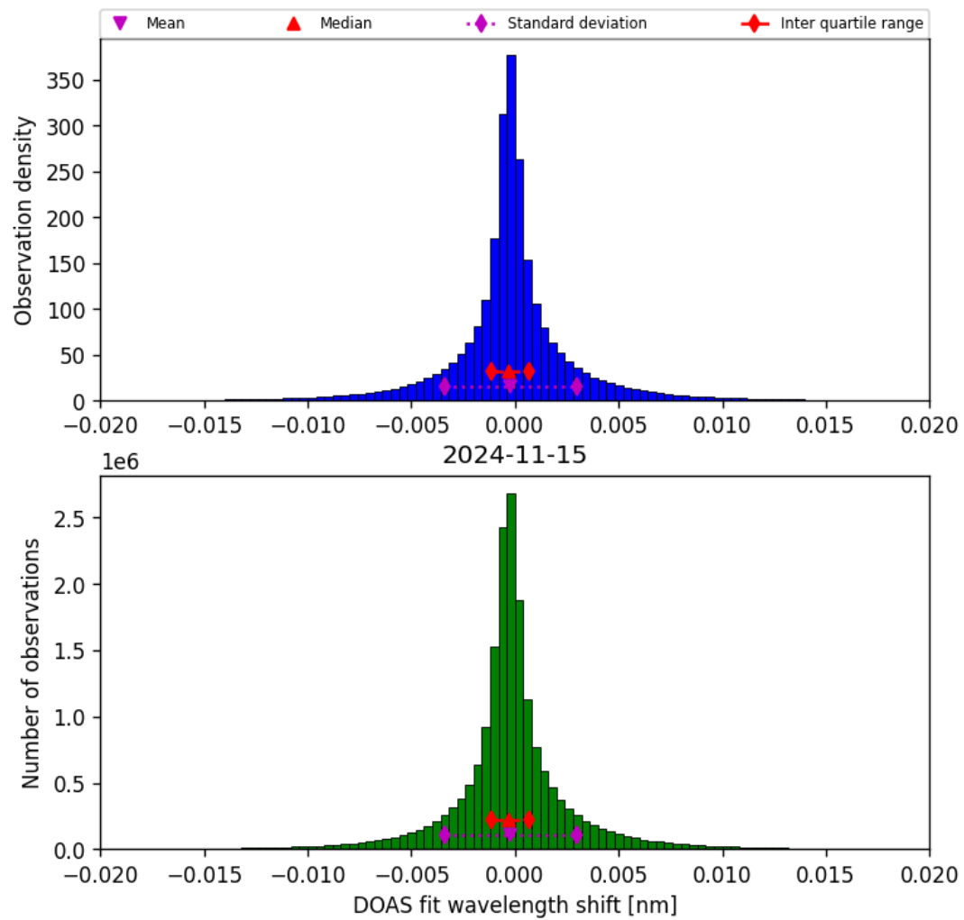
Figure 44: Histogram of “DOAS fit wavelength shift” for 2024-11-14 to 2024-11-16
