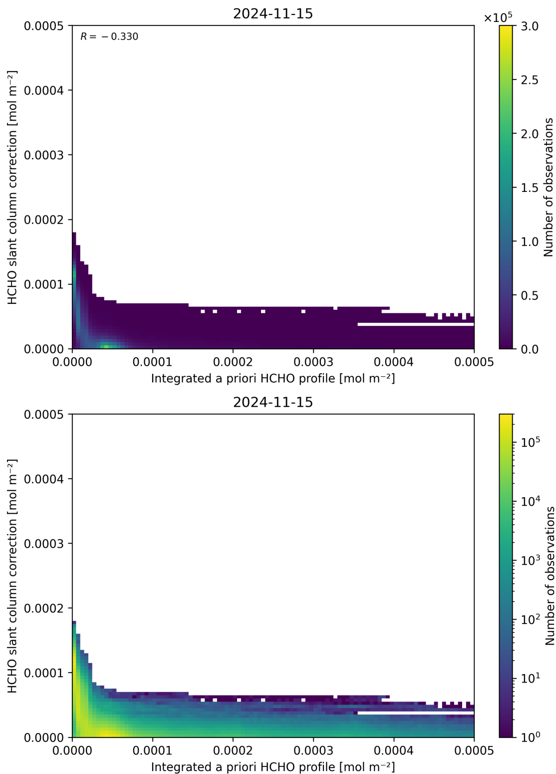
Figure 152: Scatter density plot of “Integrated a priori HCHO profile” against “HCHO slant column correction” for 2024-11-14 to 2024-11-16.
