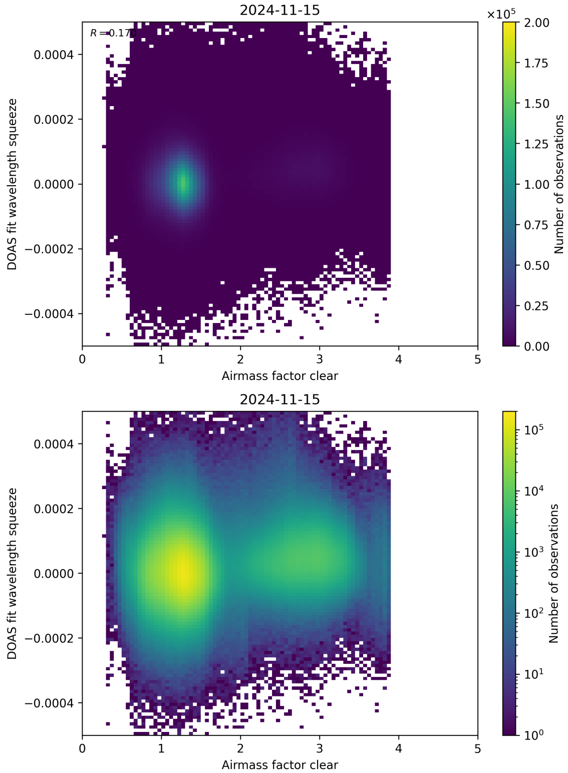
Figure 73: Scatter density plot of “Airmass factor clear” against “DOAS fit wavelength squeeze” for 2024-11-14 to 2024-11-16.
