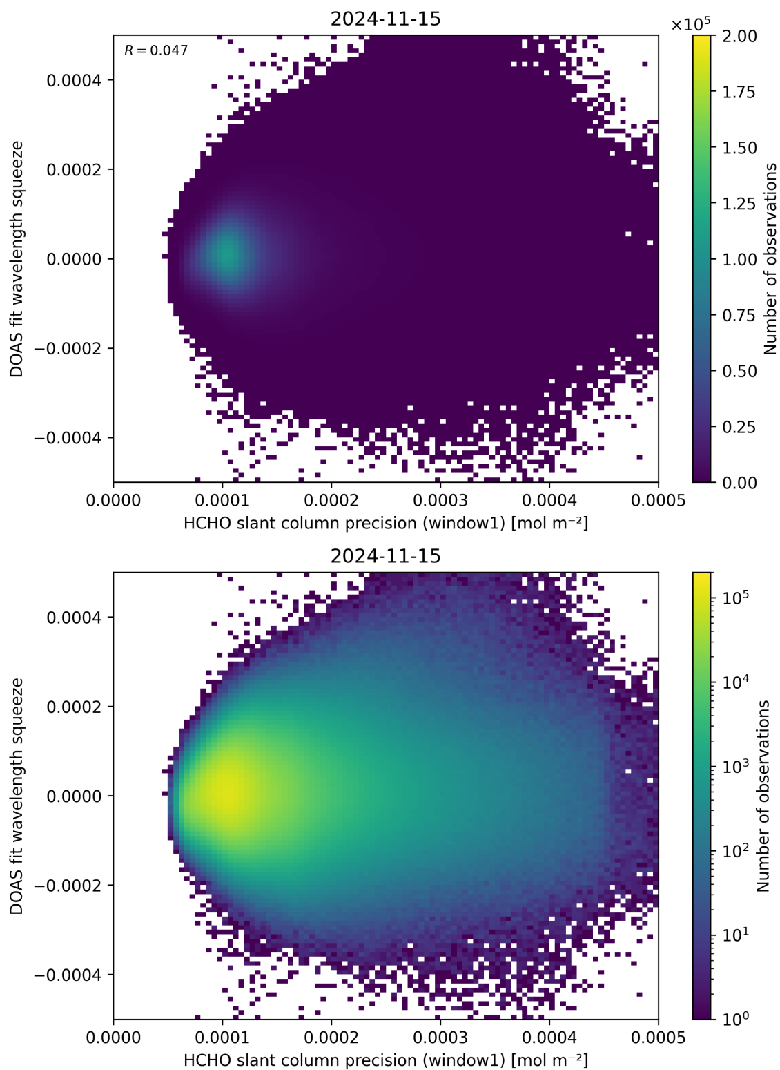
Figure 90: Scatter density plot of “HCHO slant column precision (window1)” against “DOAS fit wavelength squeeze” for 2024-11-14 to 2024-11-16.
