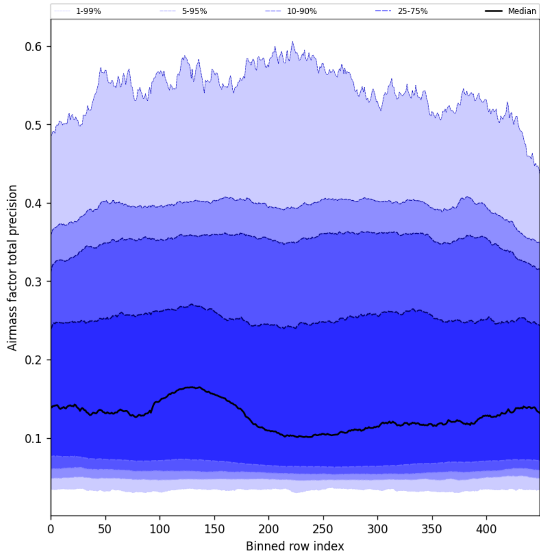
Figure 55: Along track statistics of “Airmass factor total precision” for 2024-11-14 to 2024-11-16
