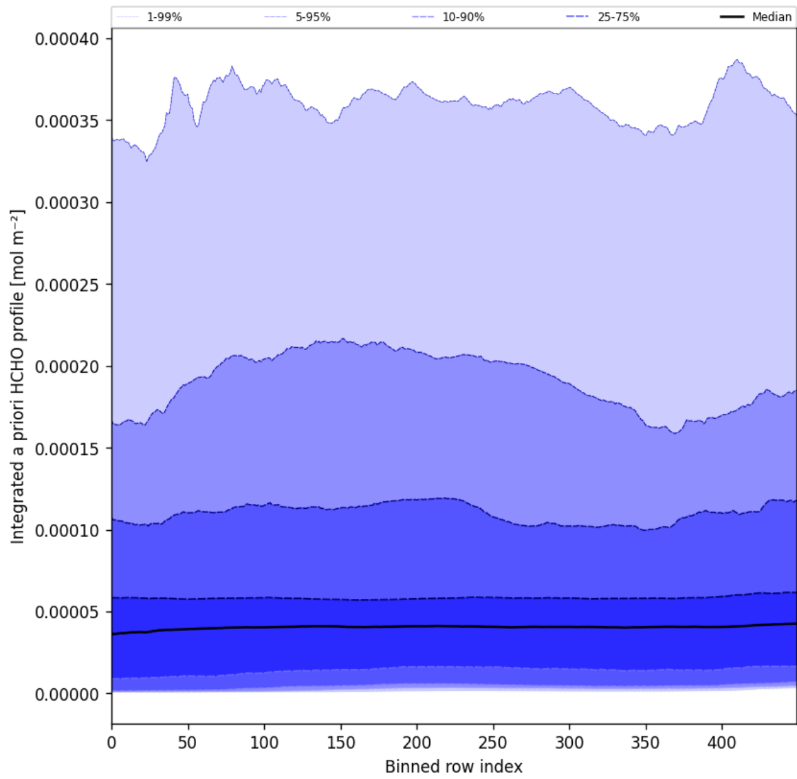
Figure 57: Along track statistics of “Integrated a priori HCHO profile” for 2024-11-14 to 2024-11-16
