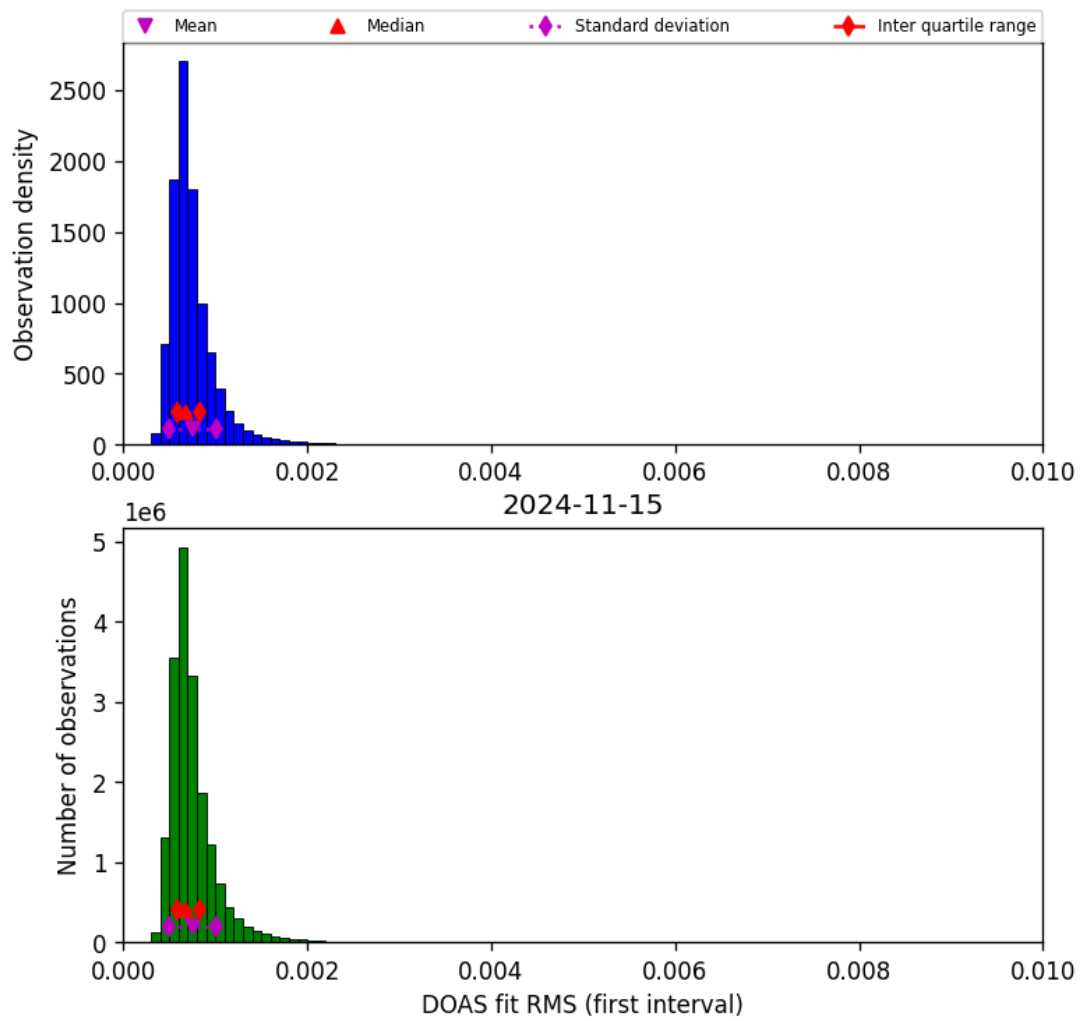
Figure 46: Histogram of “DOAS fit RMS (first interval)” for 2024-11-14 to 2024-11-16
