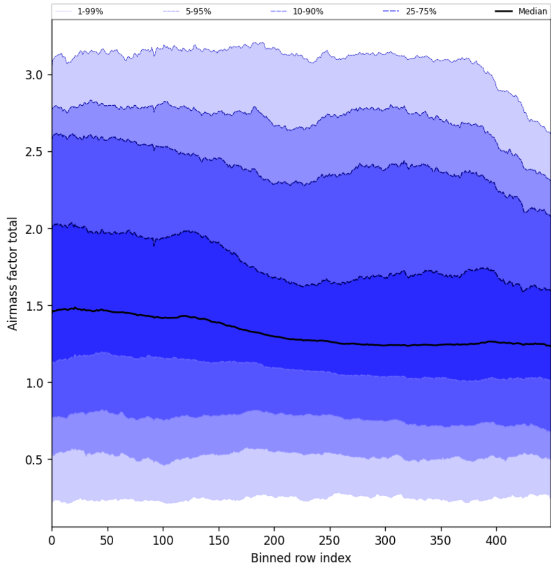
Figure 54: Along track statistics of “Airmass factor total” for 2024-11-14 to 2024-11-16
