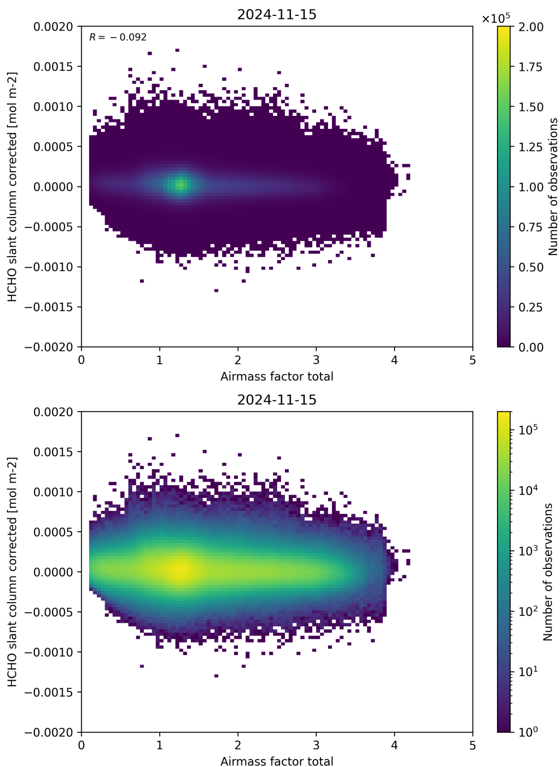
Figure 101: Scatter density plot of “Airmass factor total” against “HCHO slant column corrected” for 2024-11-14 to 2024-11-16.
