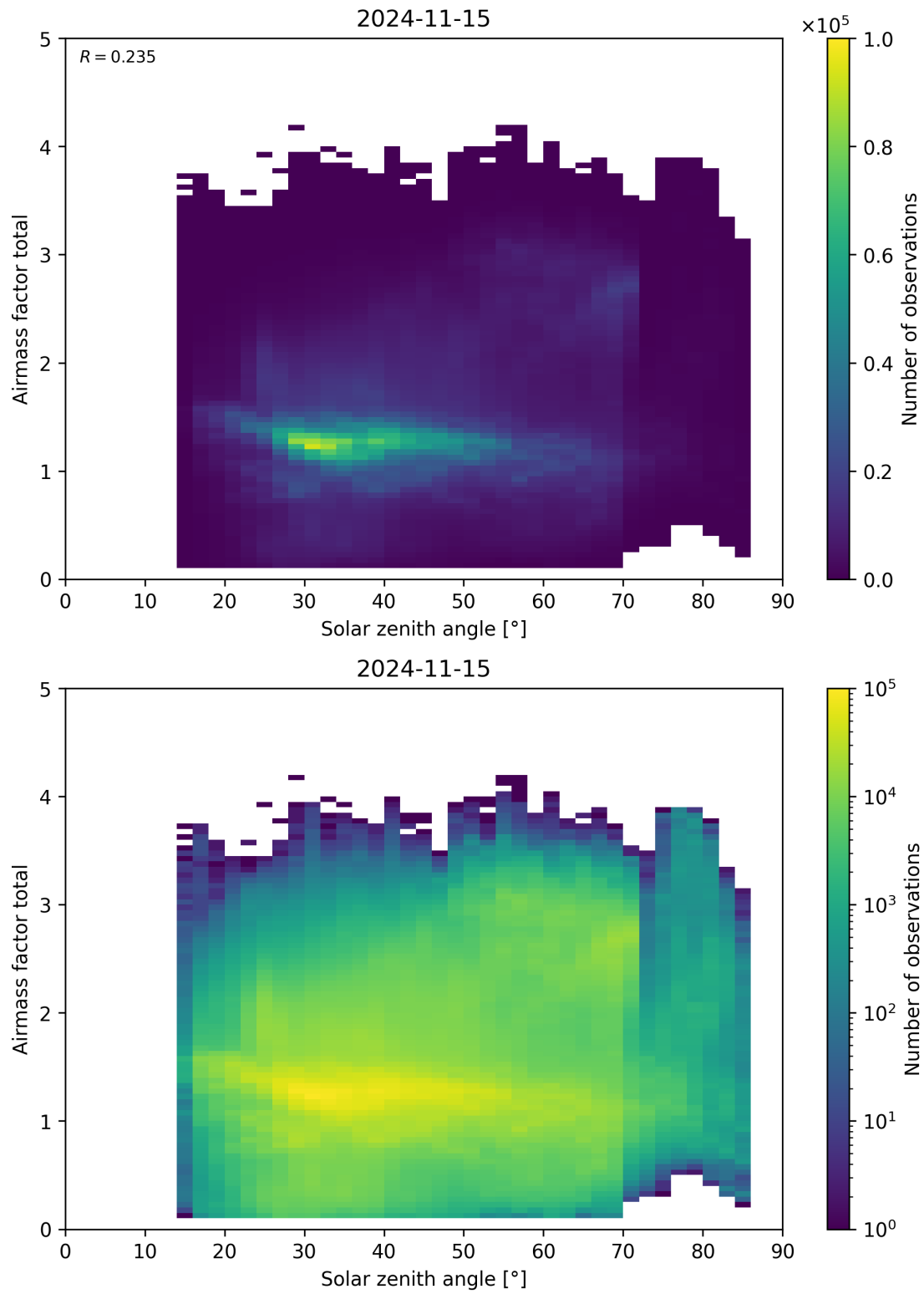
Figure 175: Scatter density plot of “Solar zenith angle” against “Airmass factor total” for 2024-11-14 to 2024-11-16.
