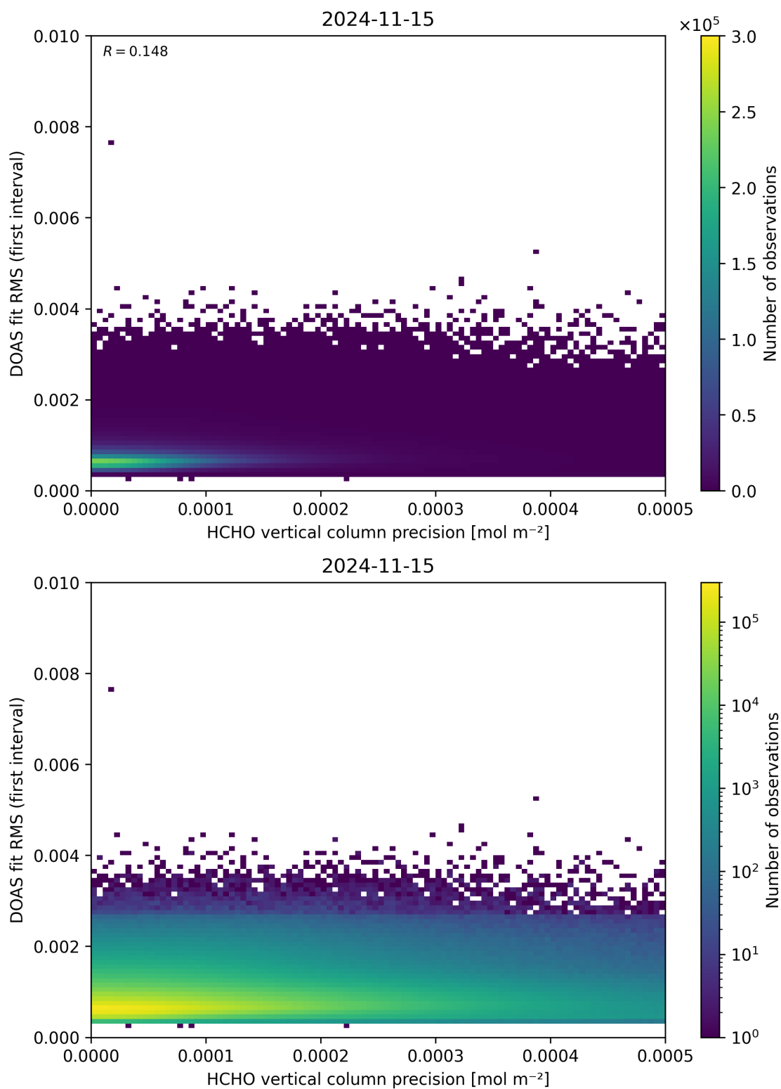
Figure 136: Scatter density plot of “HCHO vertical column precision” against “DOAS fit RMS (first interval)” for 2024-11-14 to 2024-11-16.
