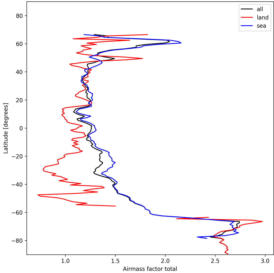
Figure 26: Zonal average of “Airmass factor total” for 2024-11-14 to 2024-11-16.
