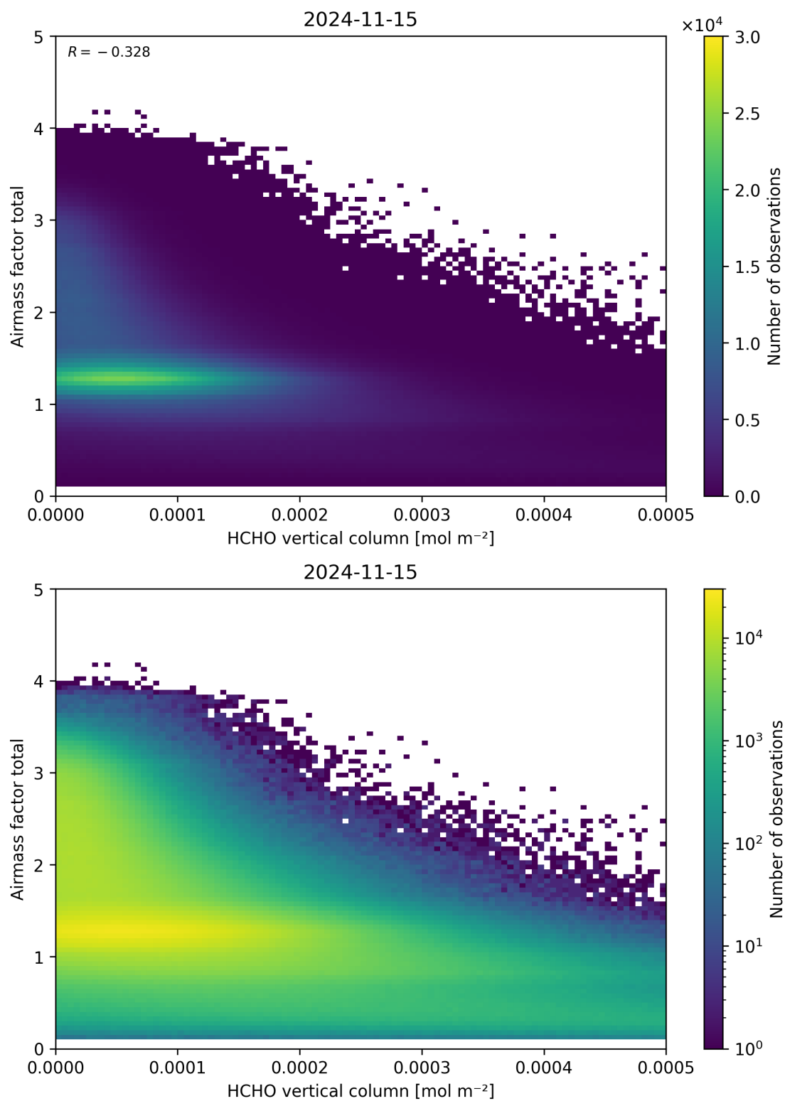
Figure 131: Scatter density plot of “HCHO vertical column” against “Airmass factor total” for 2024-11-14 to 2024-11-16.
