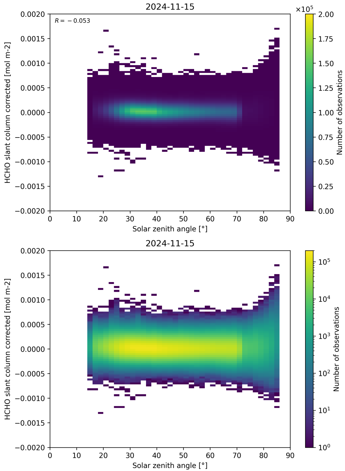
Figure 171: Scatter density plot of “Solar zenith angle” against “HCHO slant column corrected” for 2024-11-14 to 2024-11-16.
