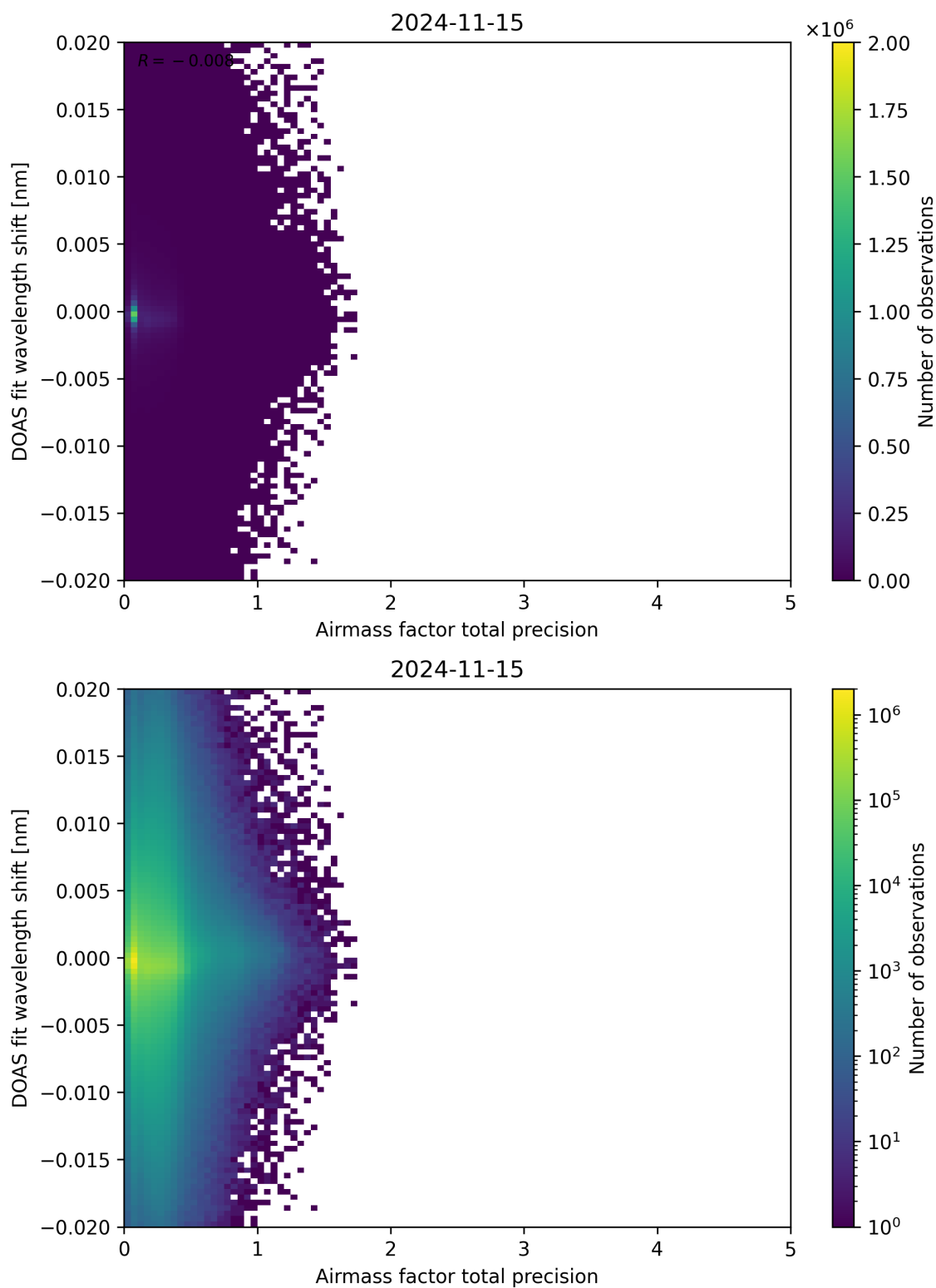
Figure 106: Scatter density plot of “Airmass factor total precision” against “DOAS fit wavelength shift” for 2024-11-14 to 2024-11-16.
