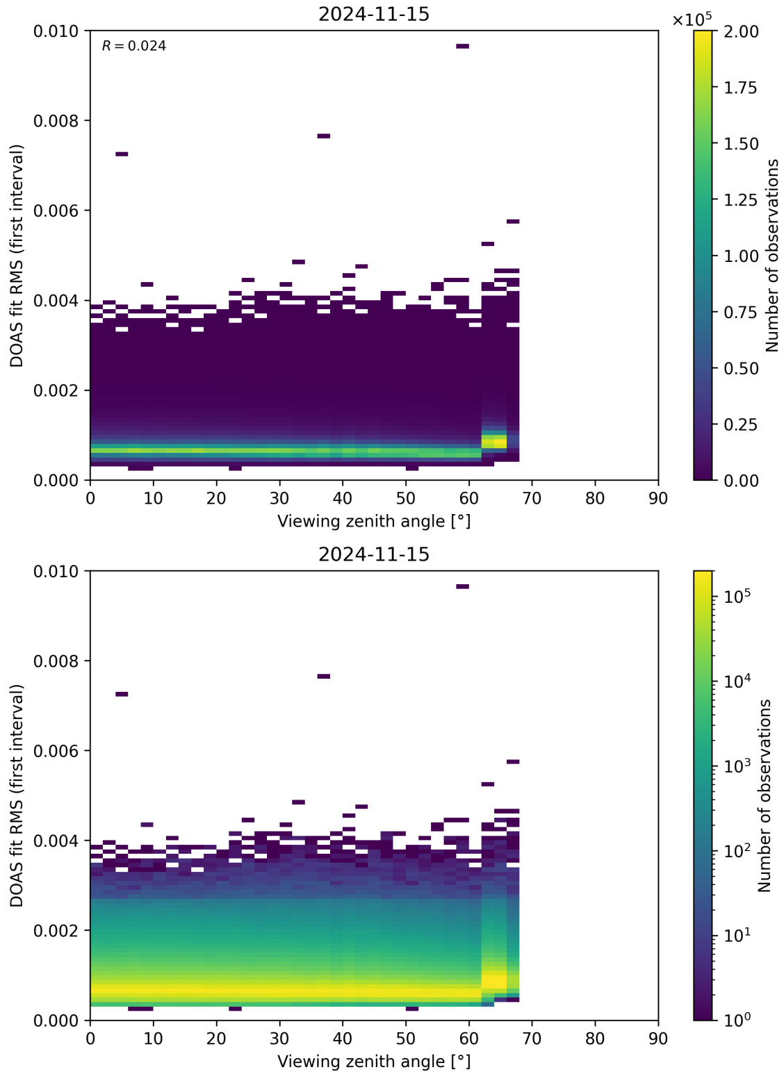
Figure 182: Scatter density plot of “Viewing zenith angle” against “DOAS fit RMS (first interval)” for 2024-11-14 to 2024-11-16.
