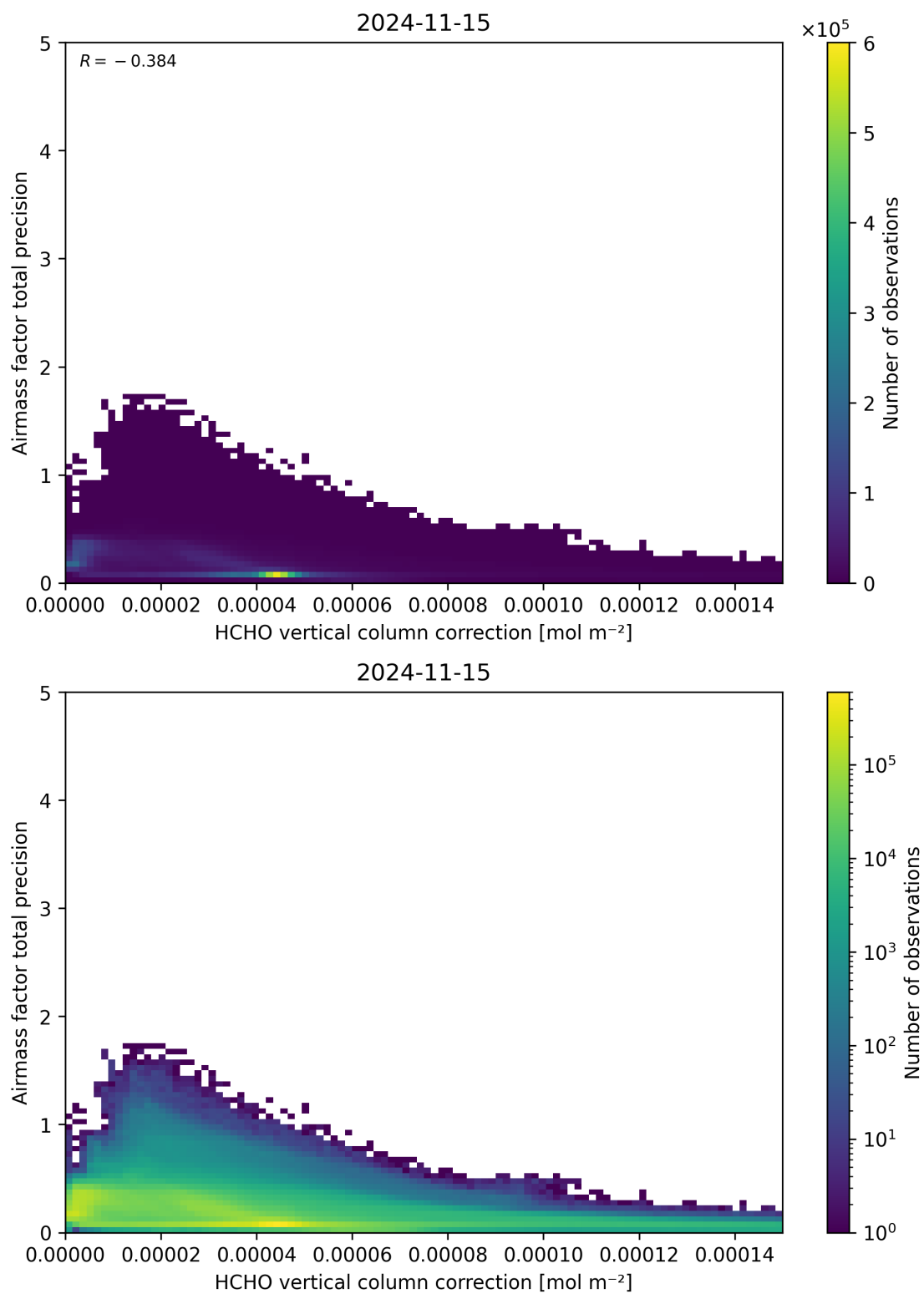
Figure 121: Scatter density plot of “HCHO vertical column correction” against “Airmass factor total precision” for 2024-11-14 to 2024-11-16.
