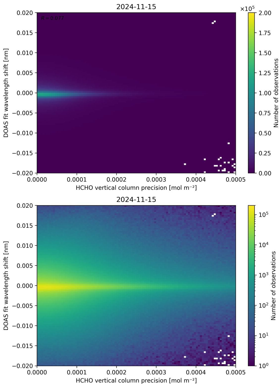
Figure 137: Scatter density plot of “HCHO vertical column precision” against “DOAS fit wavelength shift” for 2024-11-14 to 2024-11-16.
