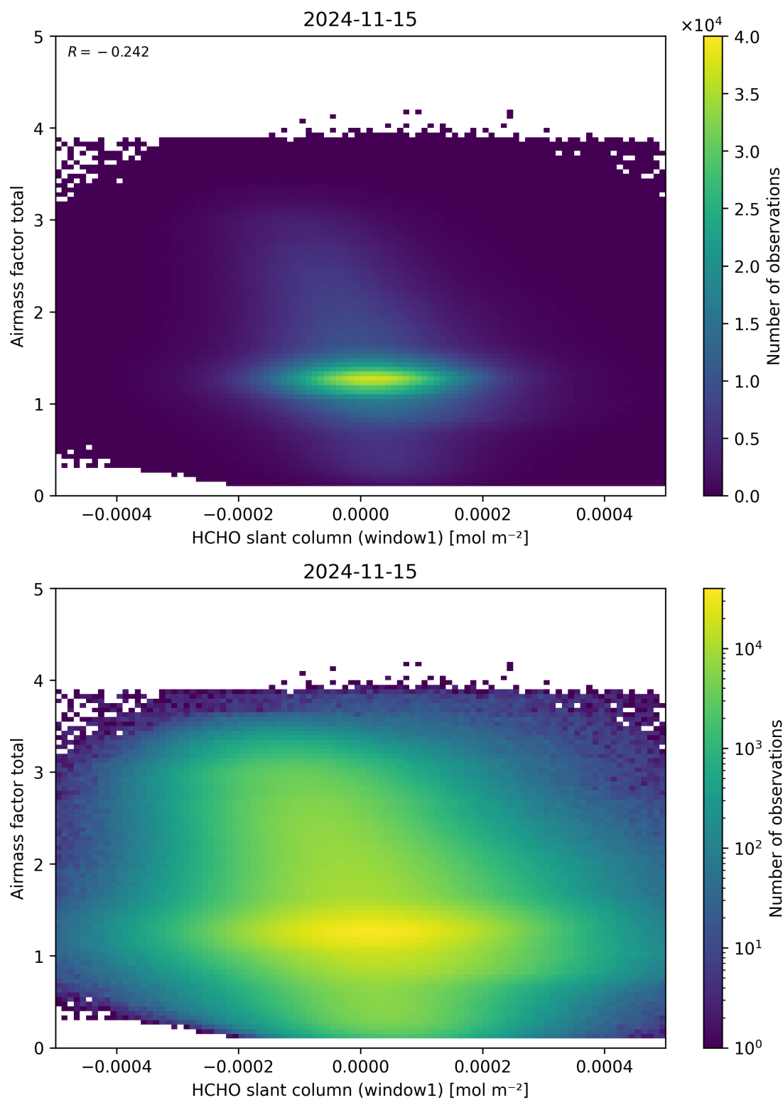
Figure 85: Scatter density plot of “HCHO slant column (window1)” against “Airmass factor total” for 2024-11-14 to 2024-11-16.
