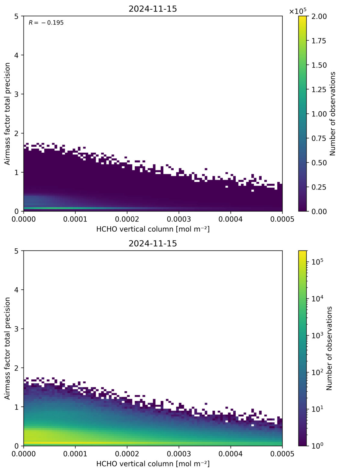
Figure 132: Scatter density plot of “HCHO vertical column” against “Airmass factor total precision” for 2024-11-14 to 2024-11-16.
