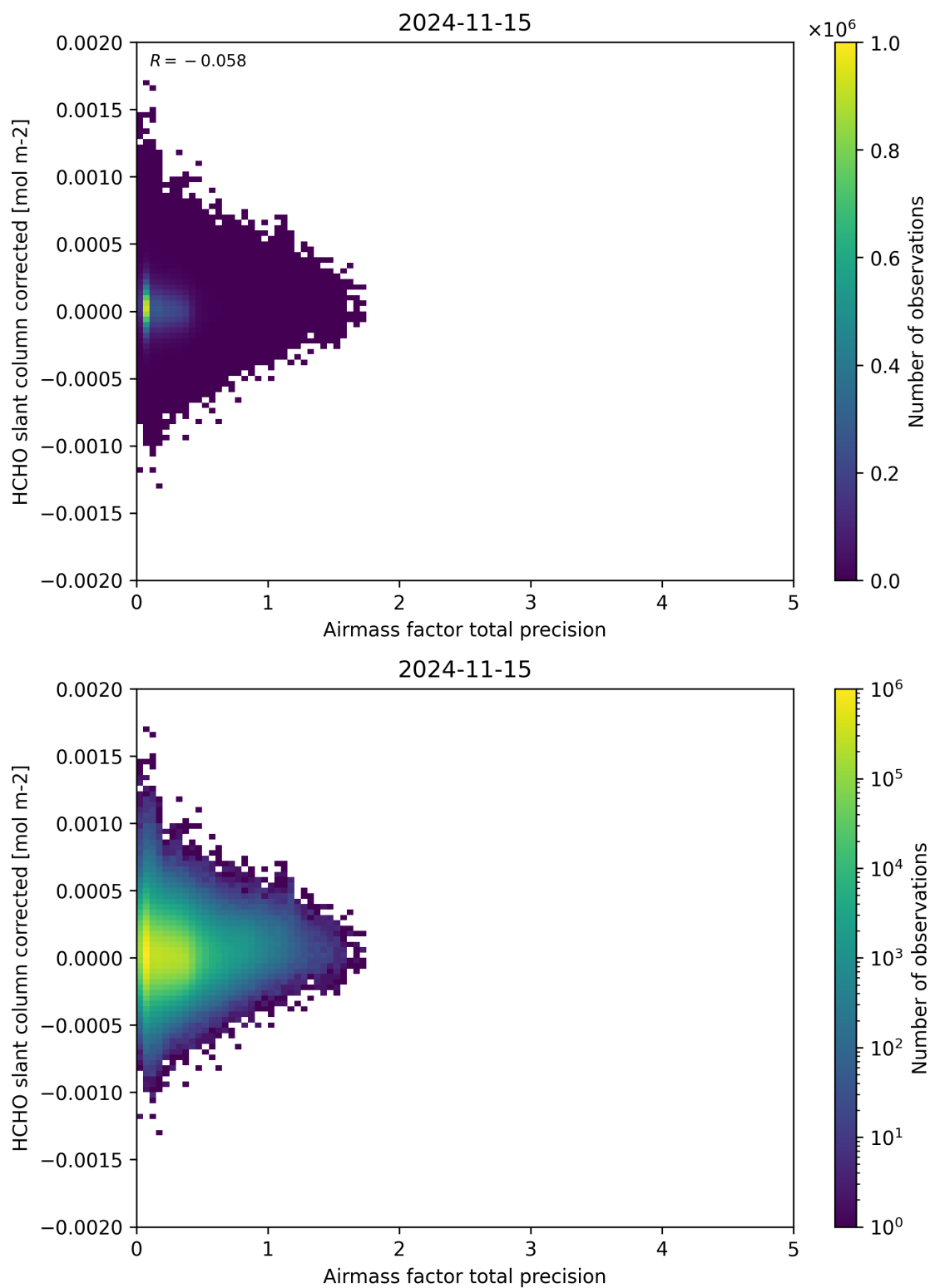
Figure 109: Scatter density plot of “Airmass factor total precision” against “HCHO slant column corrected” for 2024-11-14 to 2024-11-16.
