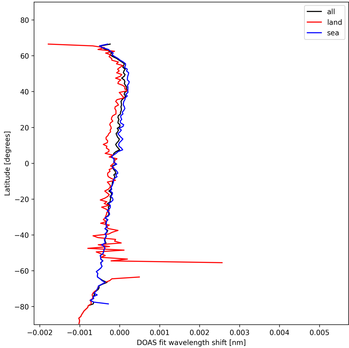
Figure 30: Zonal average of “DOAS fit wavelength shift” for 2024-11-14 to 2024-11-16.
