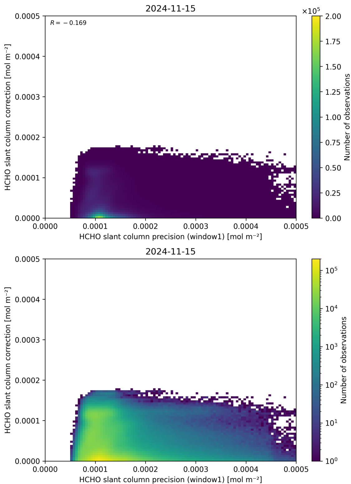
Figure 93: Scatter density plot of “HCHO slant column precision (window1)” against “HCHO slant column correction” for 2024-11-14 to 2024-11-16.
