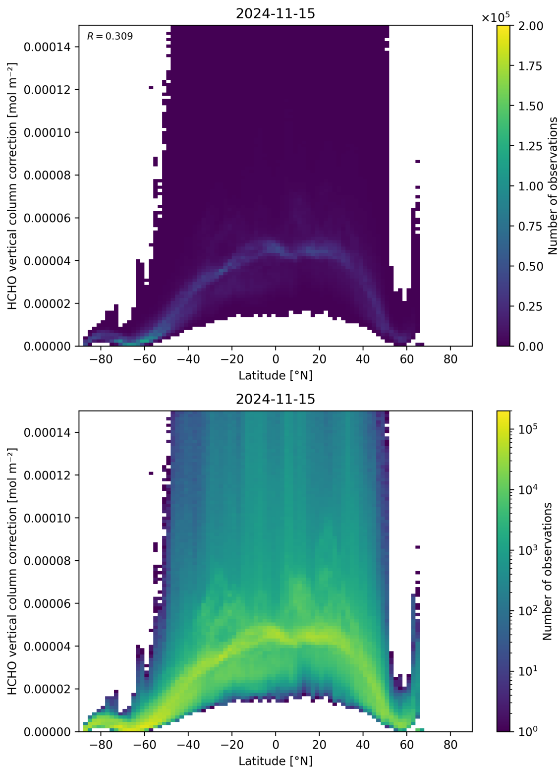
Figure 164: Scatter density plot of “Latitude” against “HCHO vertical column correction” for 2024-11-14 to 2024-11-16.
