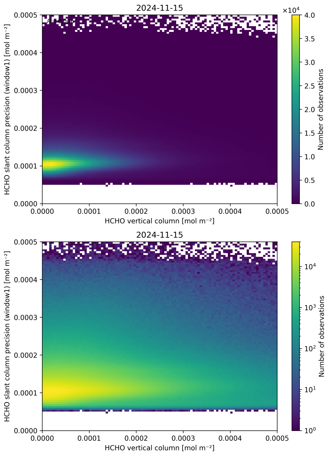
Figure 130: Scatter density plot of “HCHO vertical column” against “HCHO slant column precision (window1)” for 2024-11-14 to 2024-11-16.
