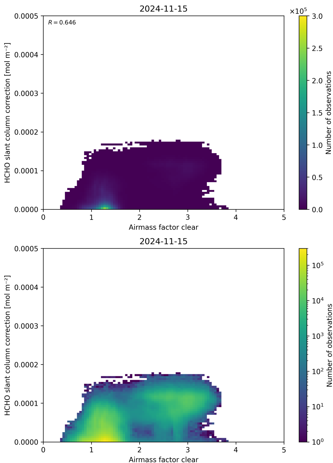
Figure 75: Scatter density plot of “Airmass factor clear” against “HCHO slant column correction” for 2024-11-14 to 2024-11-16.
