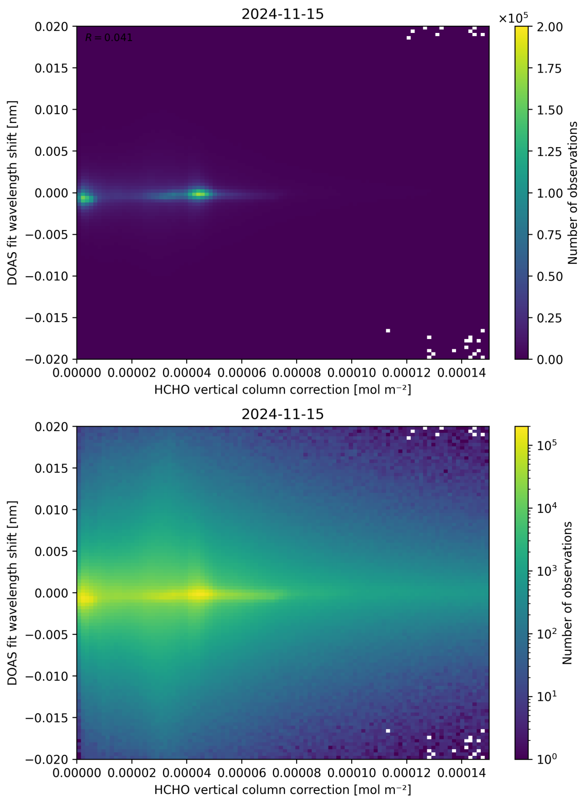
Figure 113: Scatter density plot of “HCHO vertical column correction” against “DOAS fit wavelength shift” for 2024-11-14 to 2024-11-16.
