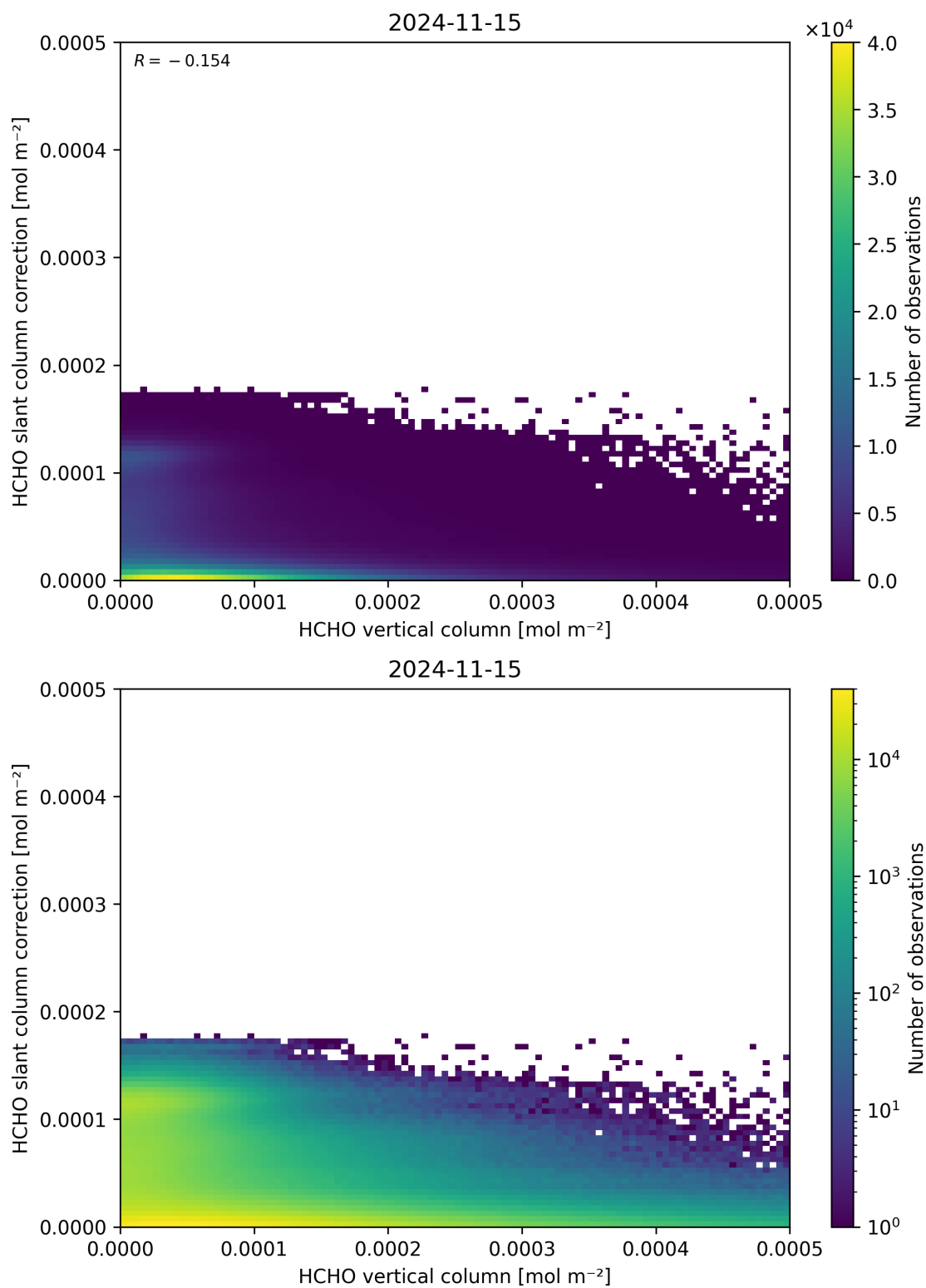
Figure 128: Scatter density plot of “HCHO vertical column” against “HCHO slant column correction” for 2024-11-14 to 2024-11-16.
