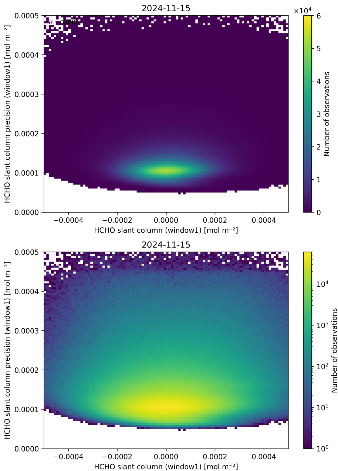
Figure 84: Scatter density plot of “HCHO slant column (window1)” against “HCHO slant column precision (window1)” for 2024-11-14 to 2024-11-16.
