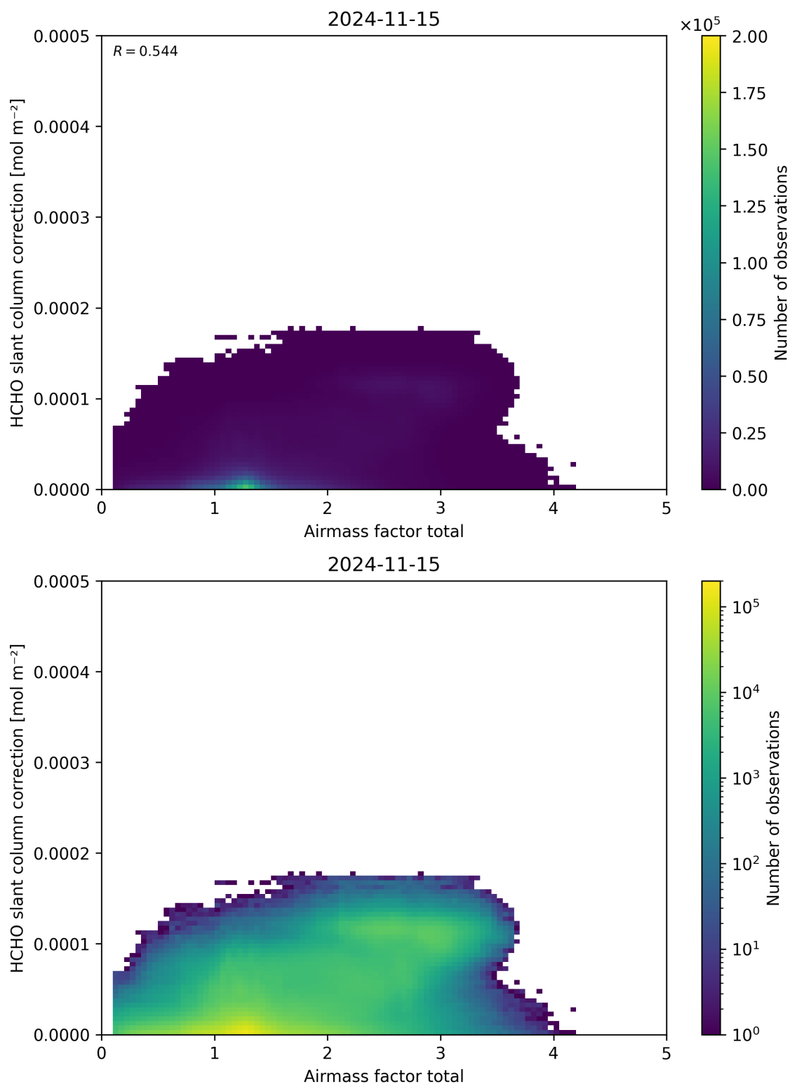
Figure 102: Scatter density plot of “Airmass factor total” against “HCHO slant column correction” for 2024-11-14 to 2024-11-16.
