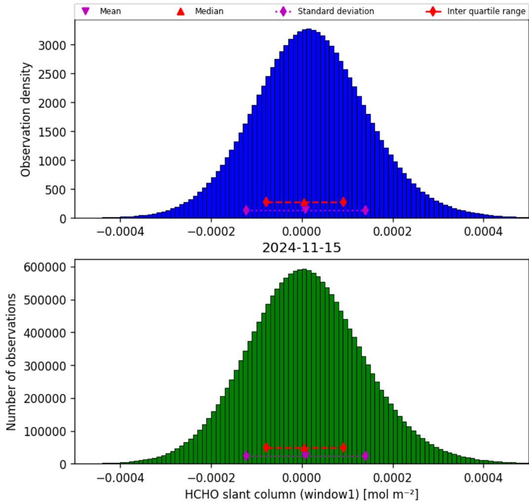
Figure 38: Histogram of “HCHO slant column (window1)” for 2024-11-14 to 2024-11-16
