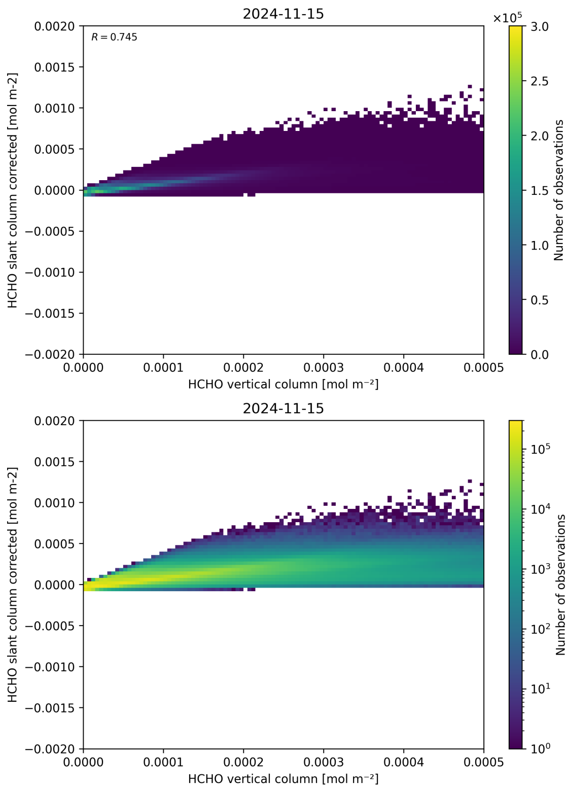
Figure 127: Scatter density plot of “HCHO vertical column” against “HCHO slant column corrected” for 2024-11-14 to 2024-11-16.
