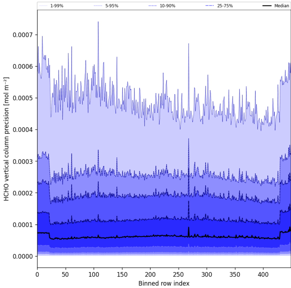
Figure 50: Along track statistics of “HCHO vertical column precision” for 2024-11-14 to 2024-11-16
