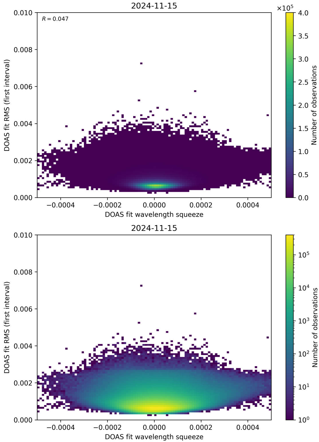
Figure 68: Scatter density plot of “DOAS fit wavelength squeeze” against “DOAS fit RMS (first interval)” for 2024-11-14 to 2024-11-16.
