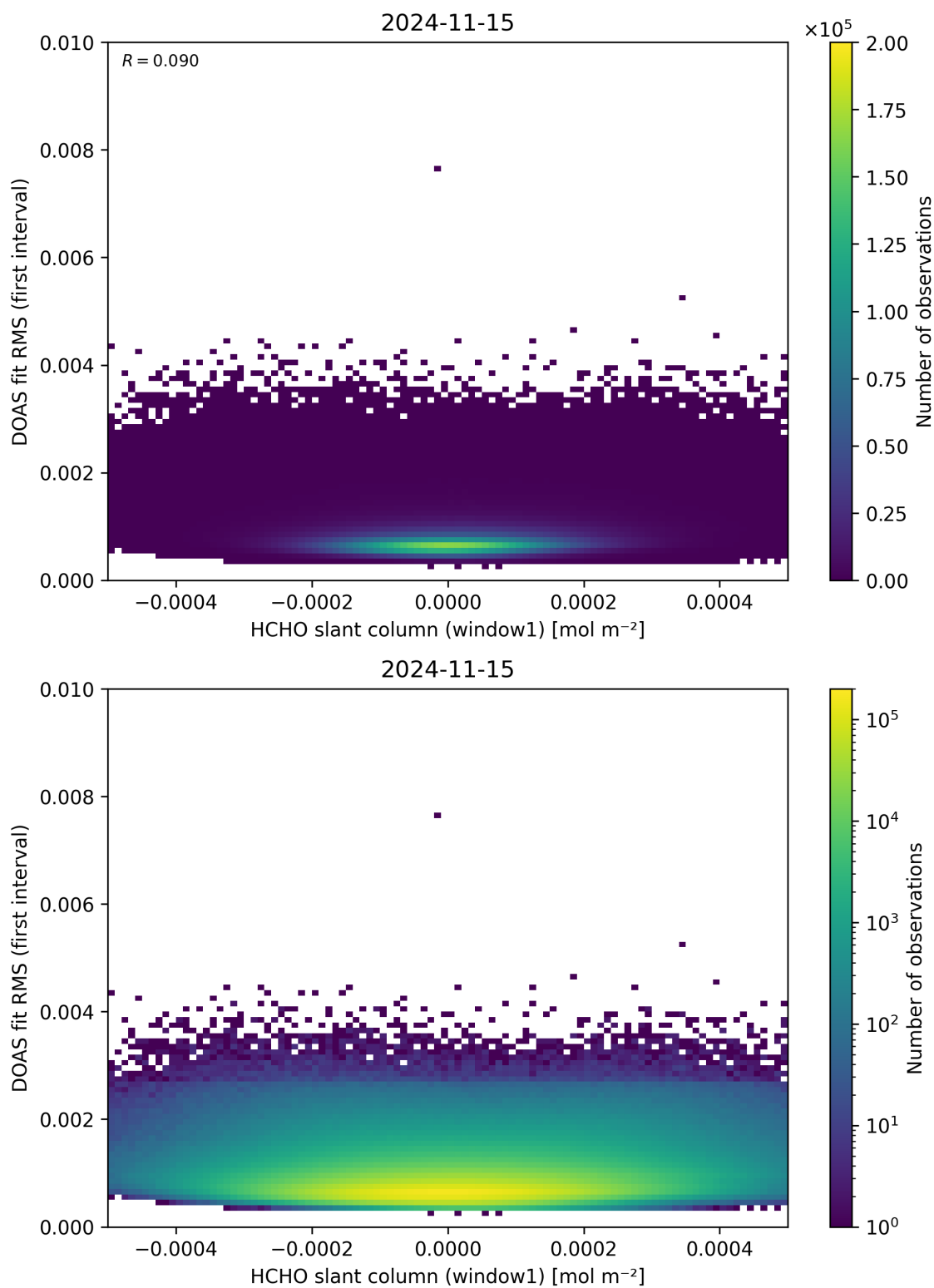
Figure 78: Scatter density plot of “HCHO slant column (window1)” against “DOAS fit RMS (first interval)” for 2024-11-14 to 2024-11-16.
