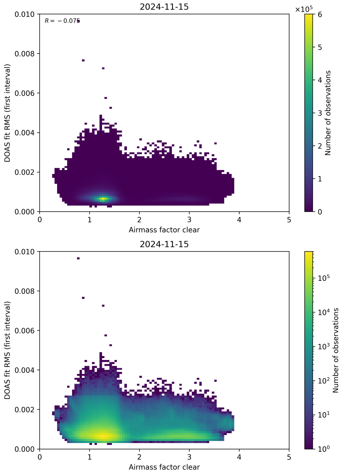
Figure 71: Scatter density plot of “Airmass factor clear” against “DOAS fit RMS (first interval)” for 2024-11-14 to 2024-11-16.
