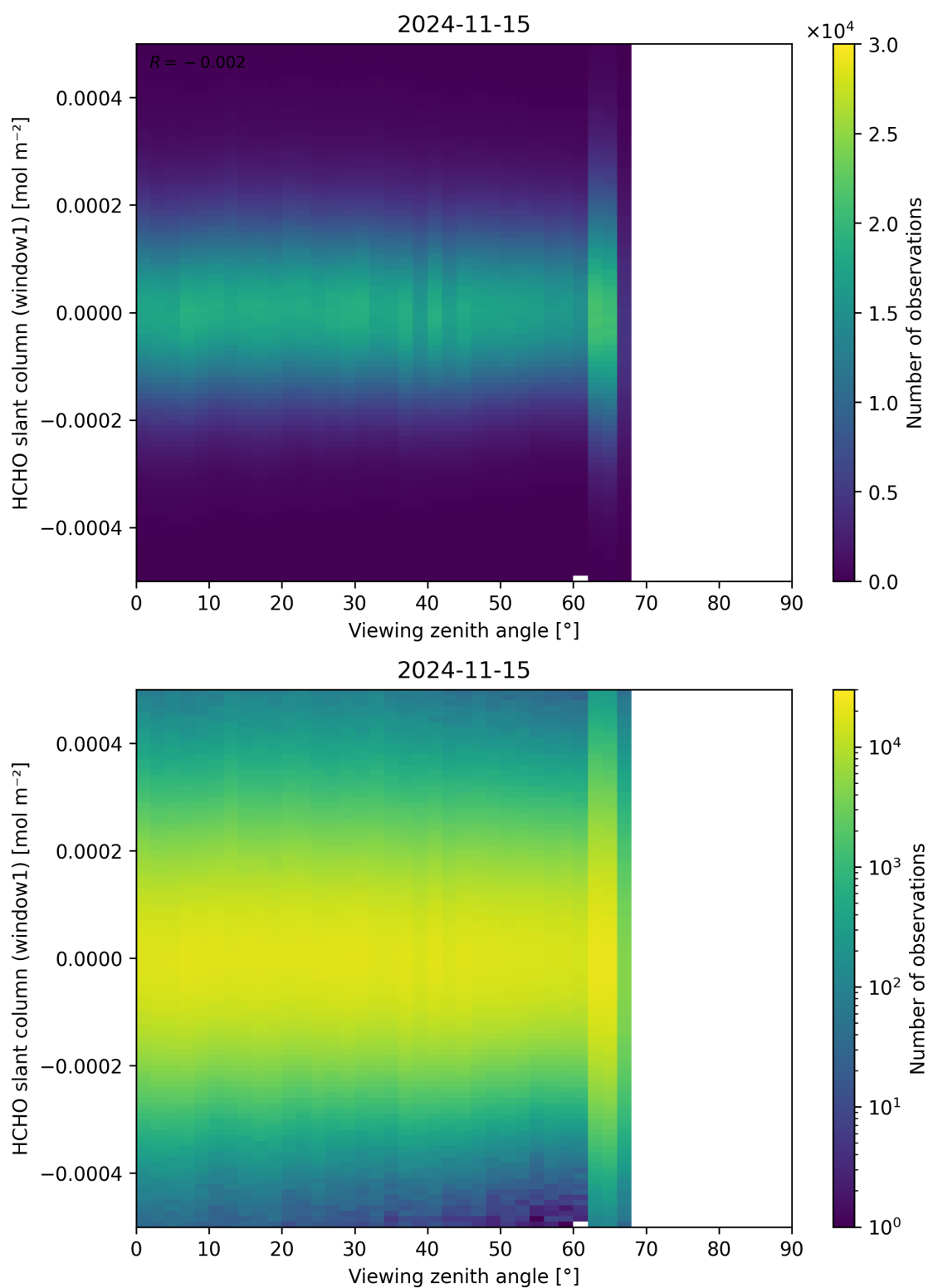
Figure 188: Scatter density plot of “Viewing zenith angle” against “HCHO slant column (window1)” for 2024-11-14 to 2024-11-16.
