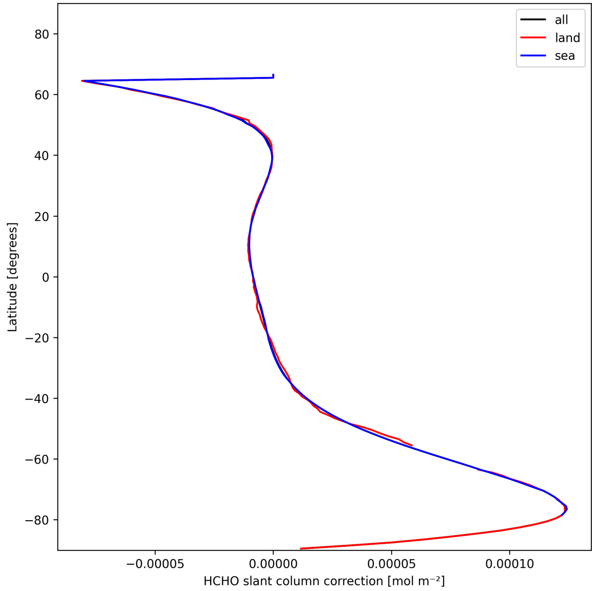
Figure 33: Zonal average of “HCHO slant column correction” for 2024-11-14 to 2024-11-16.
