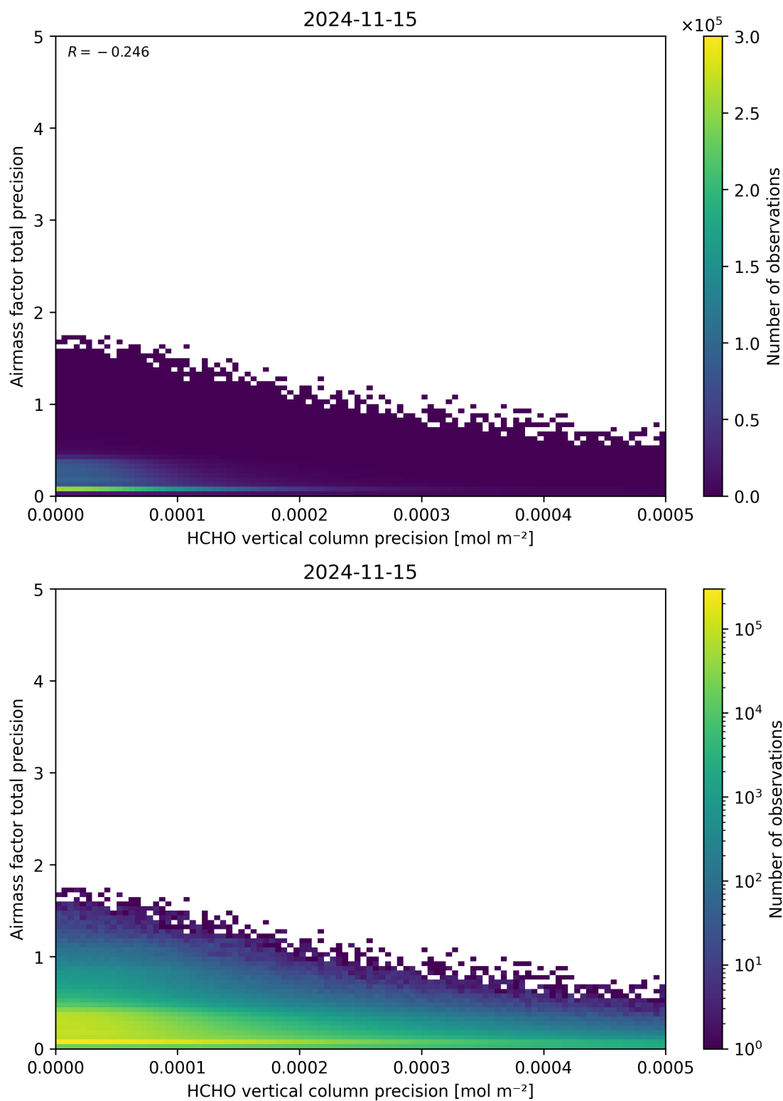
Figure 145: Scatter density plot of “HCHO vertical column precision” against “Airmass factor total precision” for 2024-11-14 to 2024-11-16.
