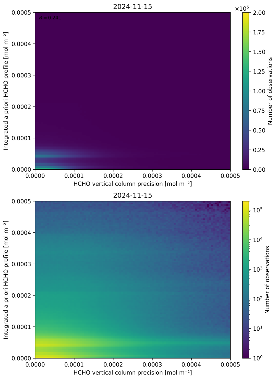
Figure 147: Scatter density plot of “HCHO vertical column precision” against “Integrated a priori HCHO profile” for 2024-11-14 to 2024-11-16.
