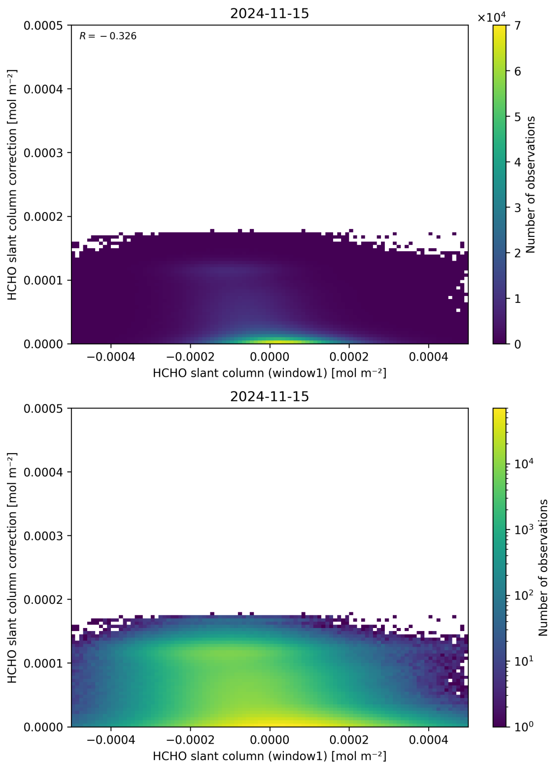
Figure 83: Scatter density plot of “HCHO slant column (window1)” against “HCHO slant column correction” for 2024-11-14 to 2024-11-16.
