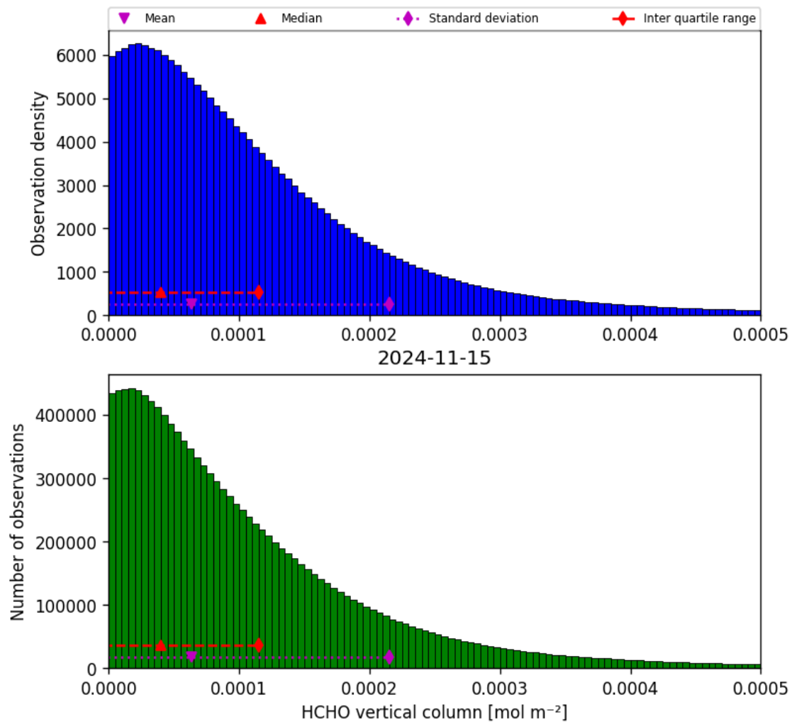
Figure 35: Histogram of “HCHO vertical column” for 2024-11-14 to 2024-11-16
