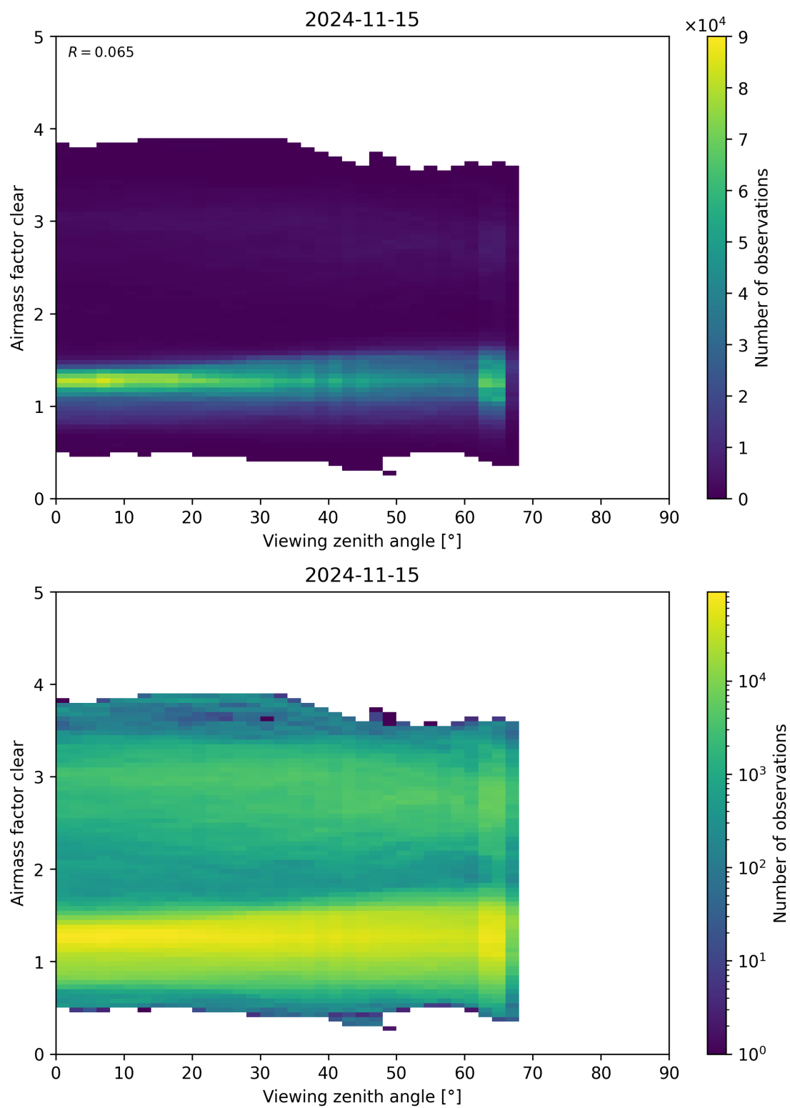
Figure 185: Scatter density plot of “Viewing zenith angle” against “Airmass factor clear” for 2024-11-14 to 2024-11-16.
