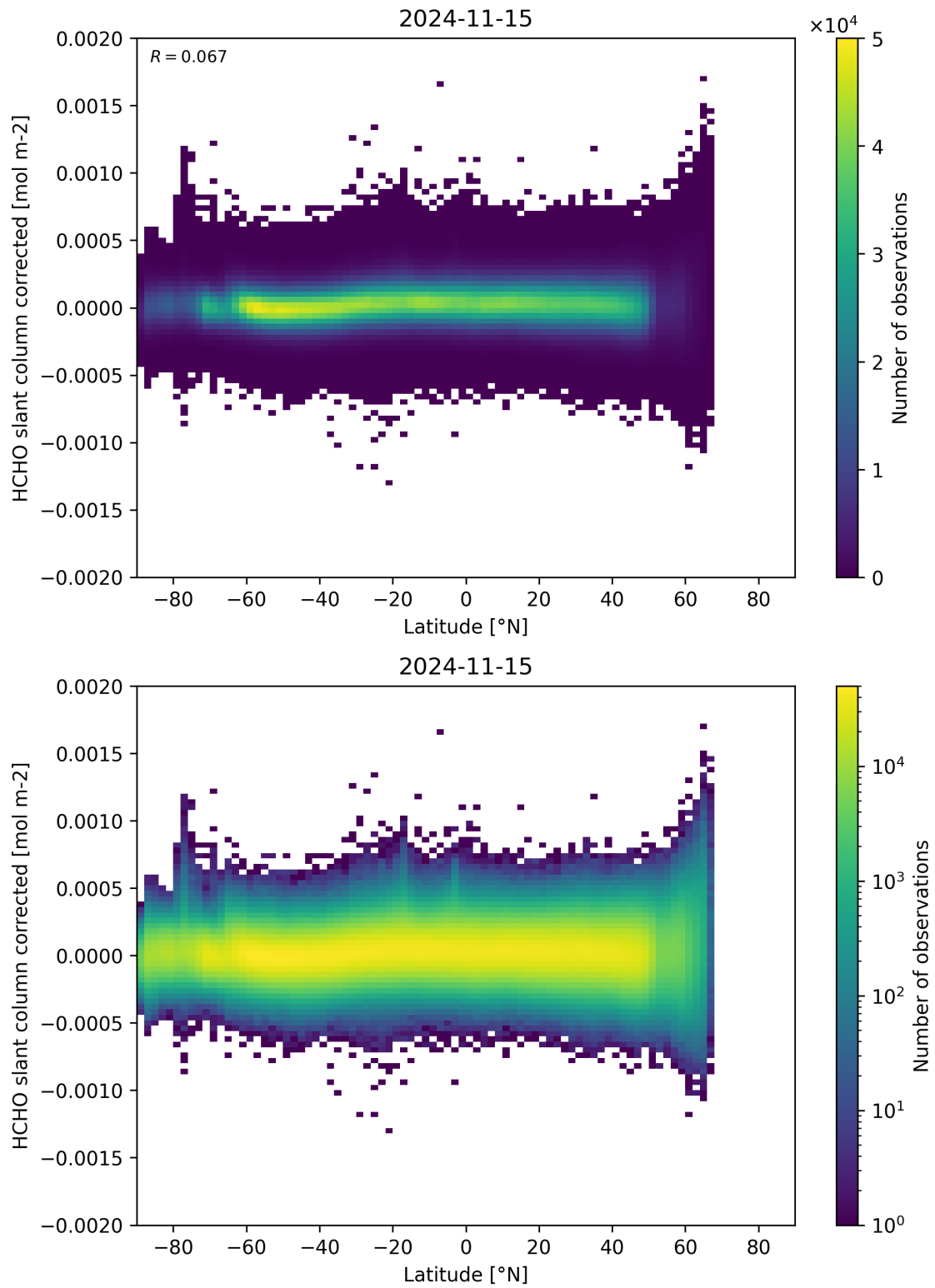
Figure 157: Scatter density plot of “Latitude” against “HCHO slant column corrected” for 2024-11-14 to 2024-11-16.
