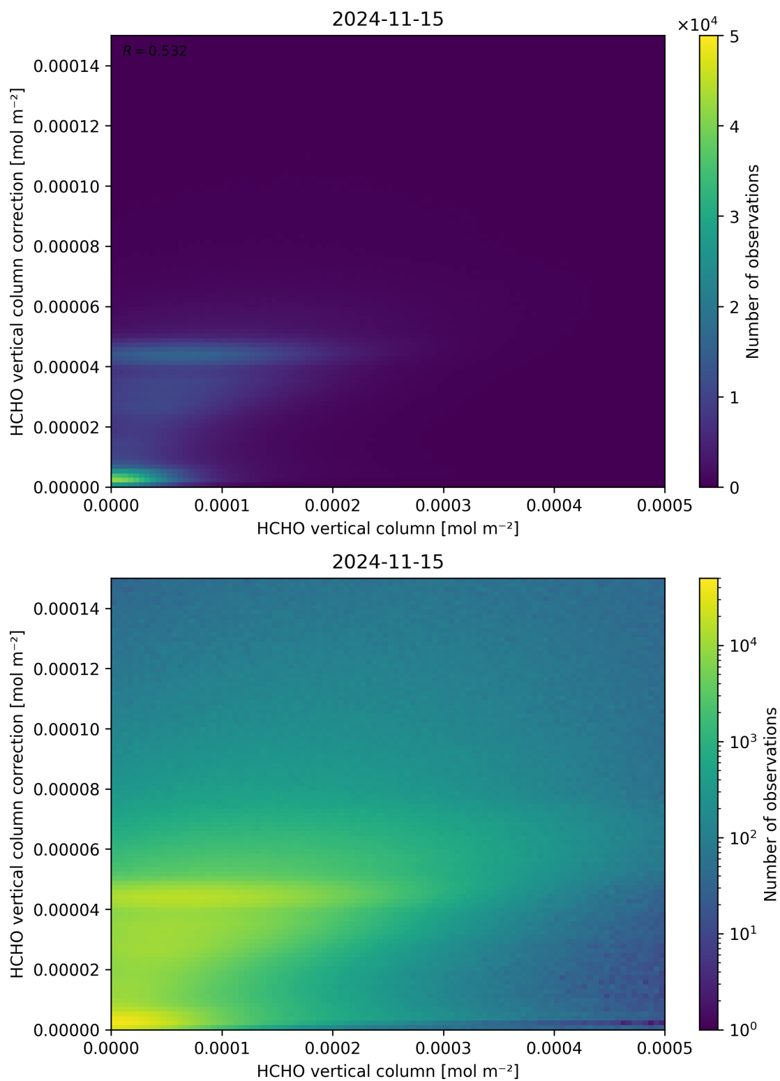
Figure 133: Scatter density plot of “HCHO vertical column” against “HCHO vertical column correction” for 2024-11-14 to 2024-11-16.
