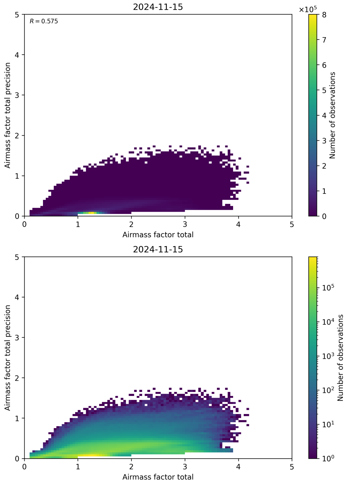
Figure 103: Scatter density plot of “Airmass factor total” against “Airmass factor total precision” for 2024-11-14 to 2024-11-16.
