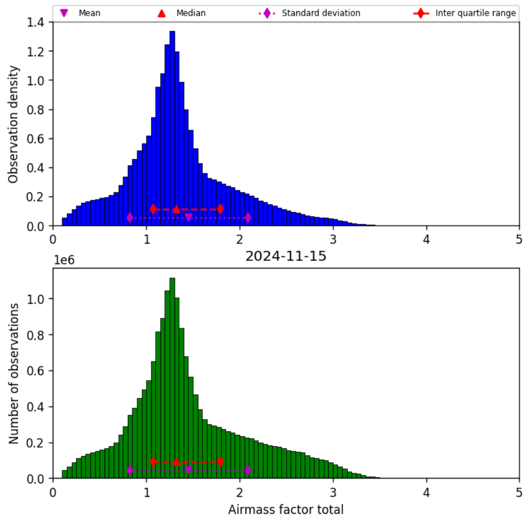
Figure 40: Histogram of “Airmass factor total” for 2024-11-14 to 2024-11-16
