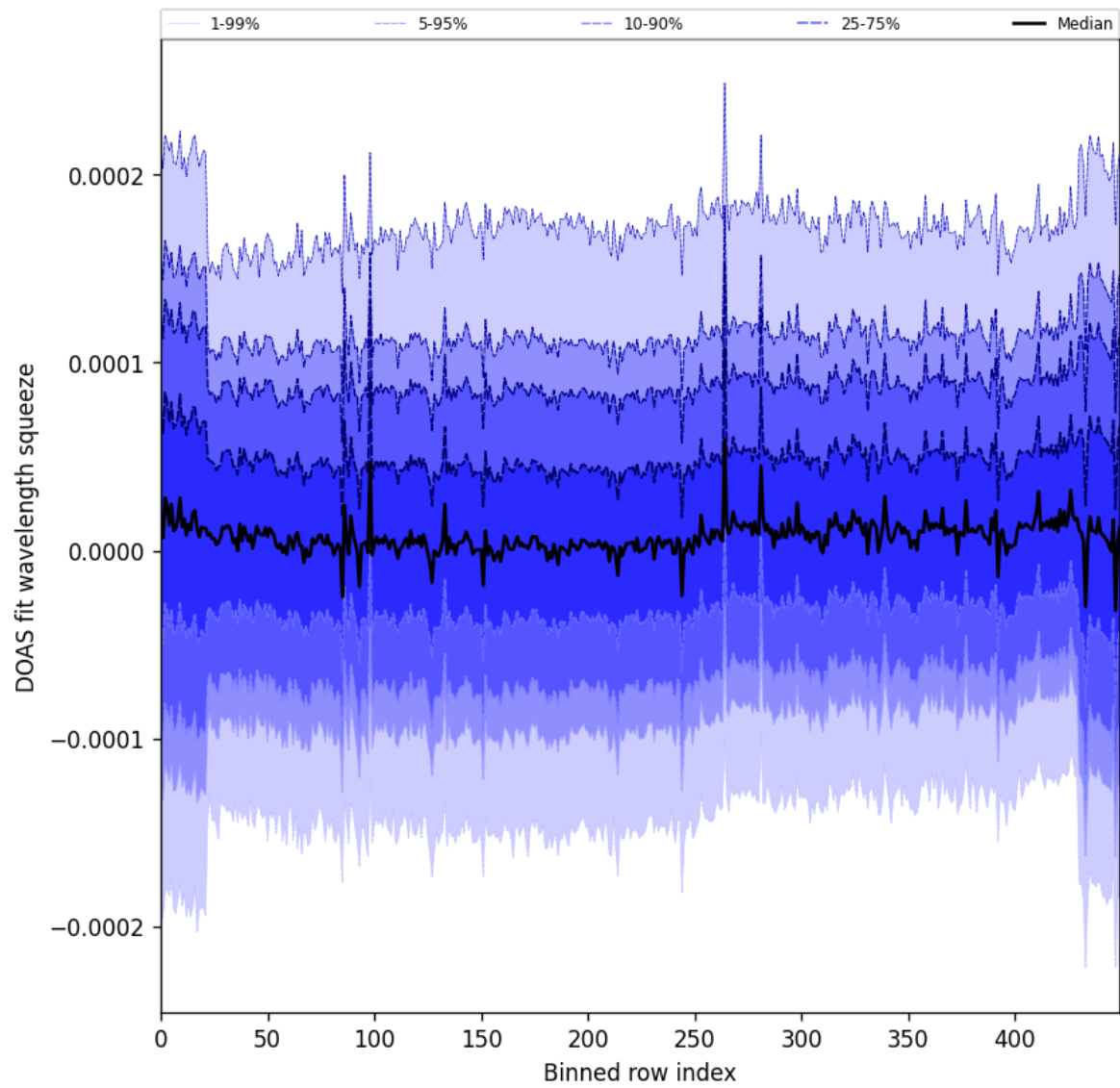
Figure 59: Along track statistics of “DOAS fit wavelength squeeze” for 2024-11-14 to 2024-11-16
