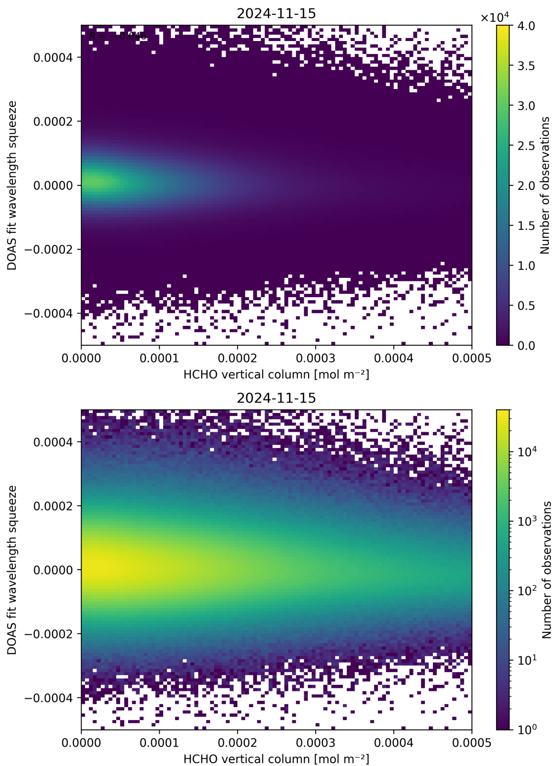
Figure 125: Scatter density plot of “HCHO vertical column” against “DOAS fit wavelength squeeze” for 2024-11-14 to 2024-11-16.
