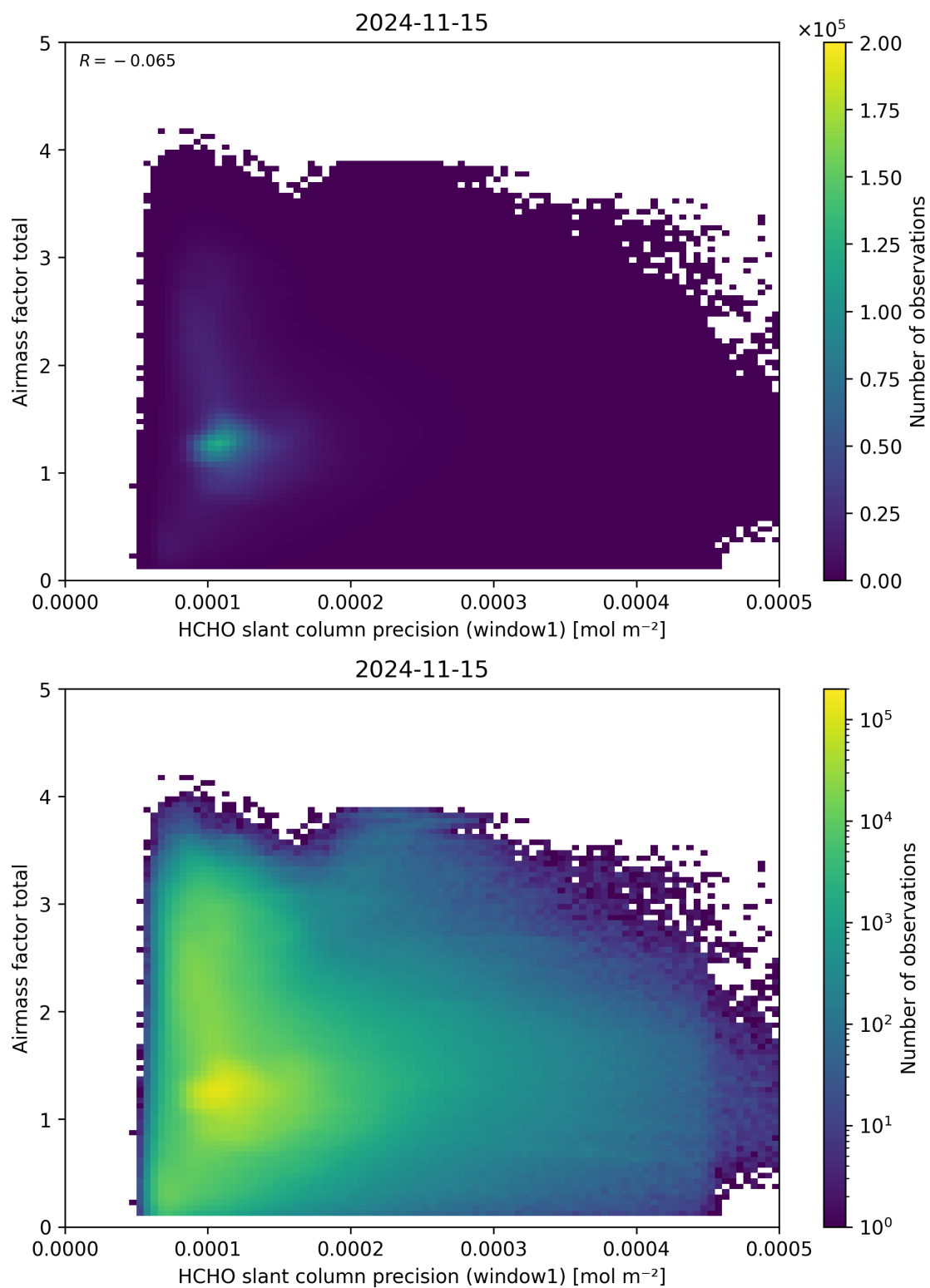
Figure 94: Scatter density plot of “HCHO slant column precision (window1)” against “Airmass factor total” for 2024-11-14 to 2024-11-16.
