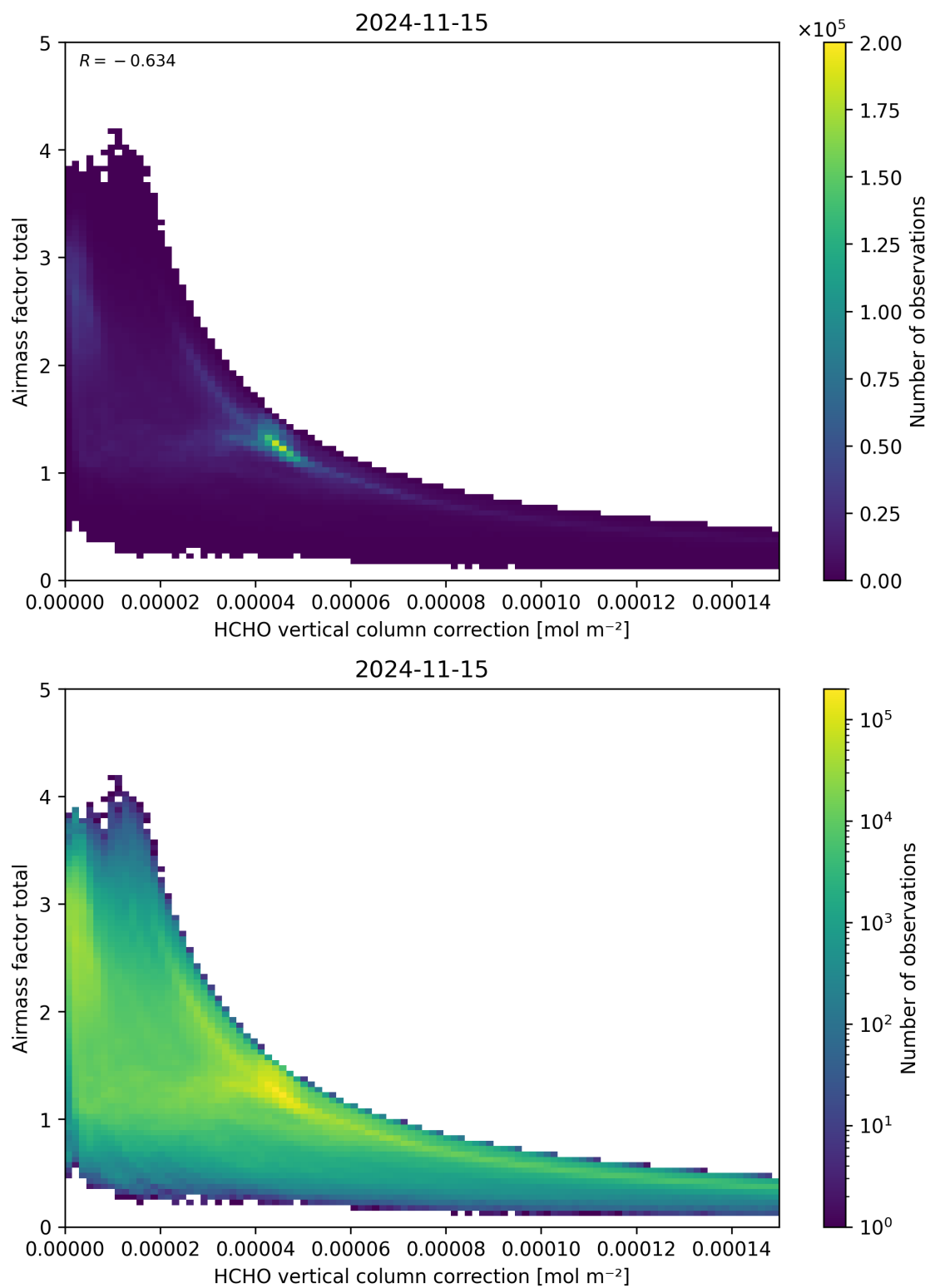
Figure 120: Scatter density plot of “HCHO vertical column correction” against “Airmass factor total” for 2024-11-14 to 2024-11-16.
