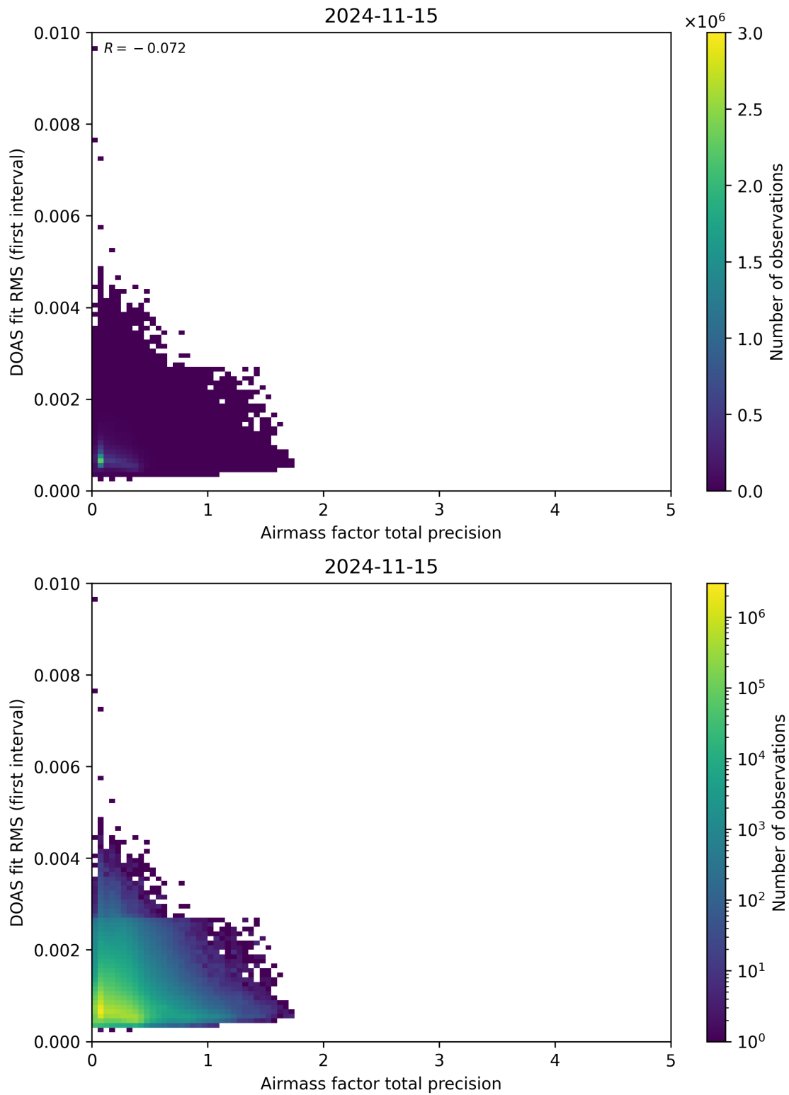
Figure 105: Scatter density plot of “Airmass factor total precision” against “DOAS fit RMS (first interval)” for 2024-11-14 to 2024-11-16.
