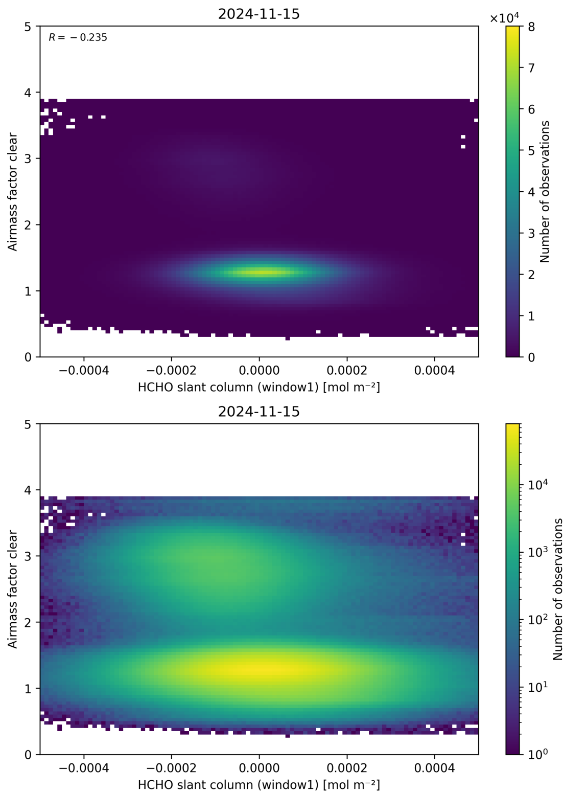
Figure 81: Scatter density plot of “HCHO slant column (window1)” against “Airmass factor clear” for 2024-11-14 to 2024-11-16.
