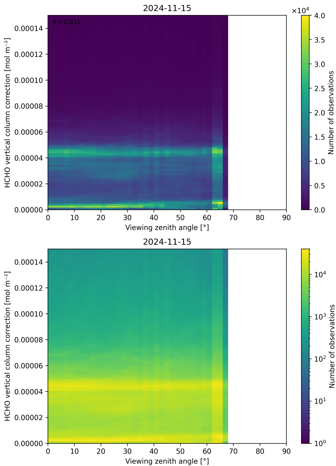
Figure 193: Scatter density plot of “Viewing zenith angle” against “HCHO vertical column correction” for 2024-11-14 to 2024-11-16.
