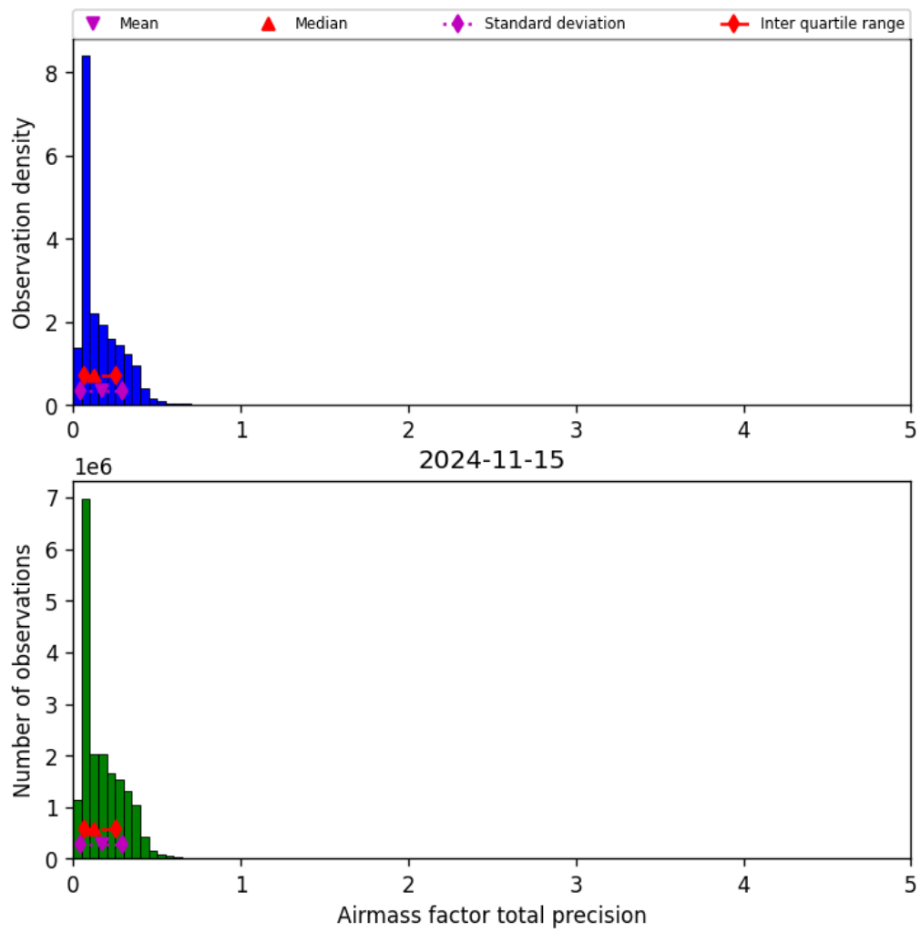
Figure 41: Histogram of “Airmass factor total precision” for 2024-11-14 to 2024-11-16
