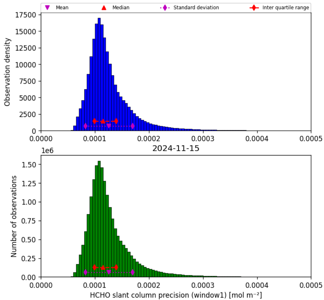
Figure 39: Histogram of “HCHO slant column precision (window1)” for 2024-11-14 to 2024-11-16
