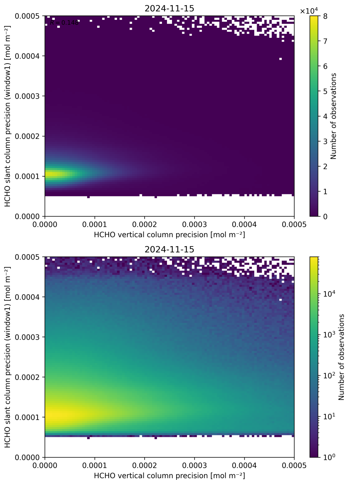
Figure 143: Scatter density plot of “HCHO vertical column precision” against “HCHO slant column precision (window1)” for 2024-11-14 to 2024-11-16.
