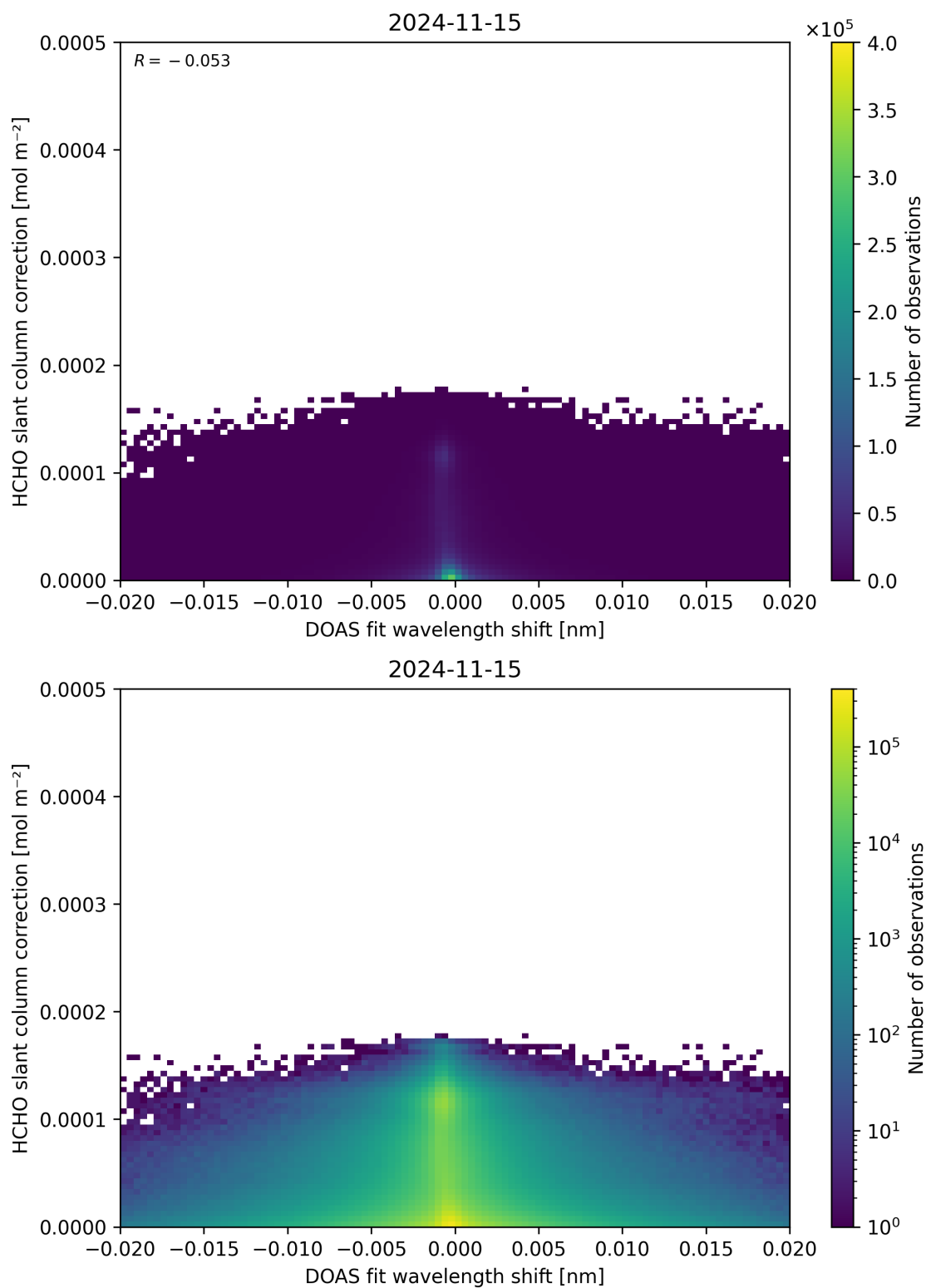
Figure 67: Scatter density plot of “DOAS fit wavelength shift” against “HCHO slant column correction” for 2024-11-14 to 2024-11-16.
