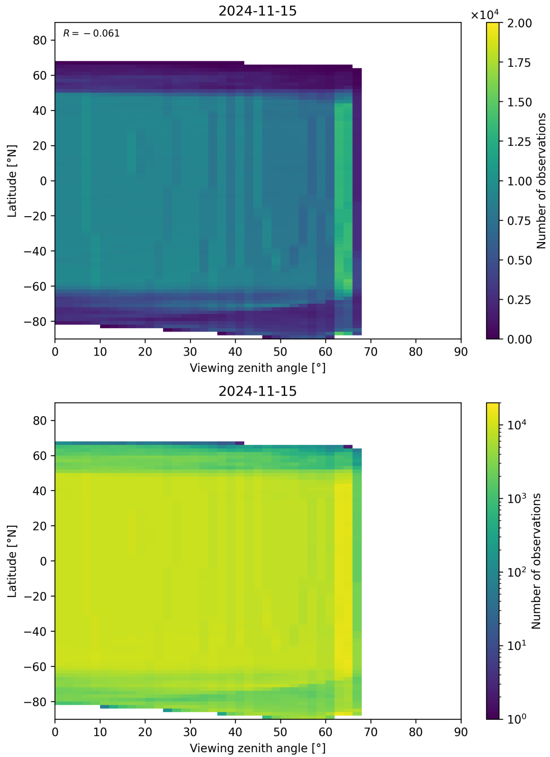
Figure 196: Scatter density plot of “Viewing zenith angle” against “Latitude” for 2024-11-14 to 2024-11-16.
