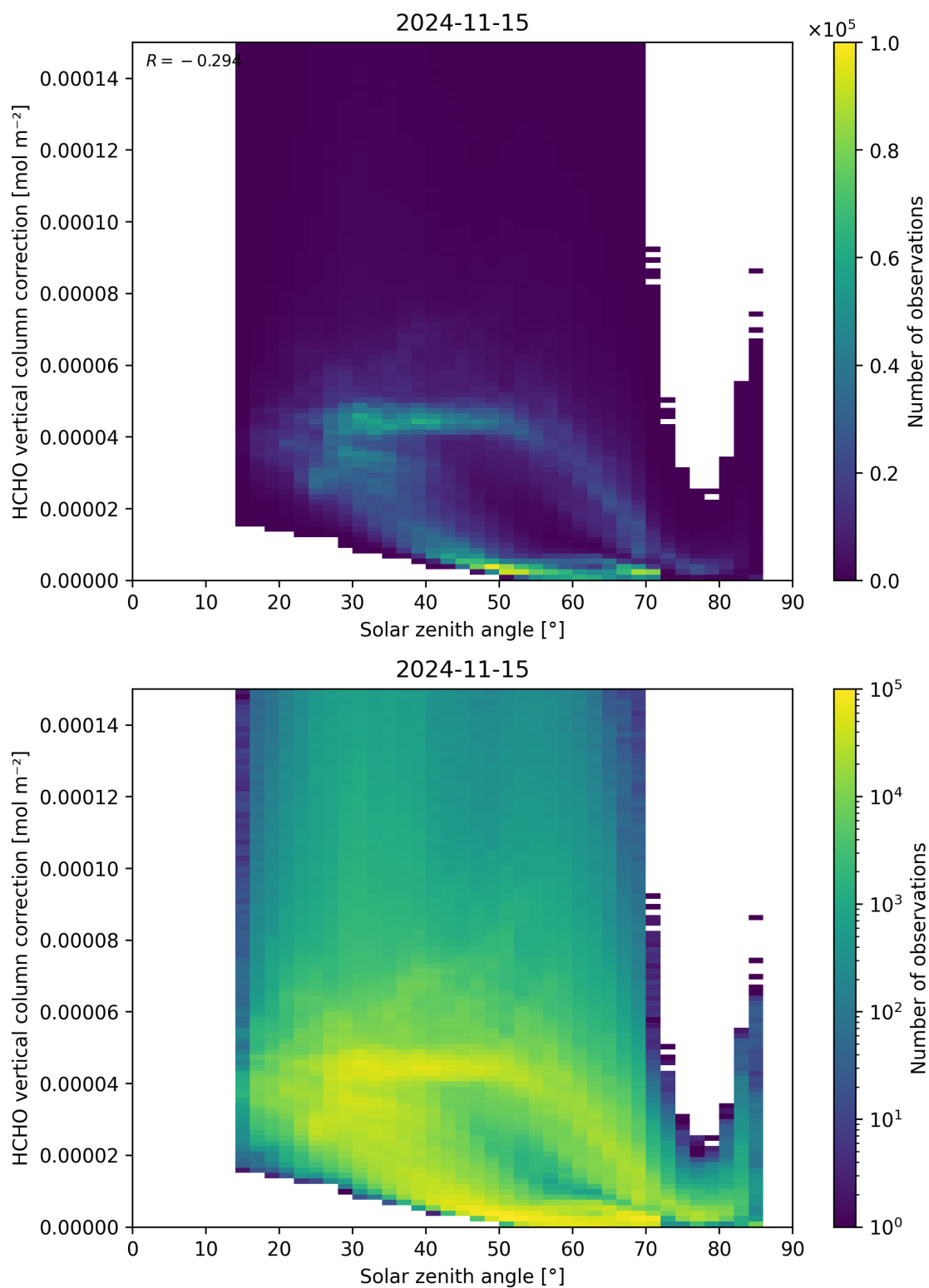
Figure 178: Scatter density plot of “Solar zenith angle” against “HCHO vertical column correction” for 2024-11-14 to 2024-11-16.
