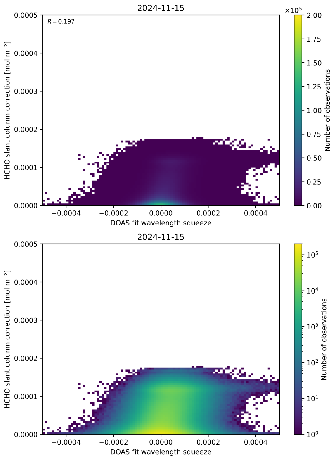
Figure 70: Scatter density plot of “DOAS fit wavelength squeeze” against “HCHO slant column correction” for 2024-11-14 to 2024-11-16.
