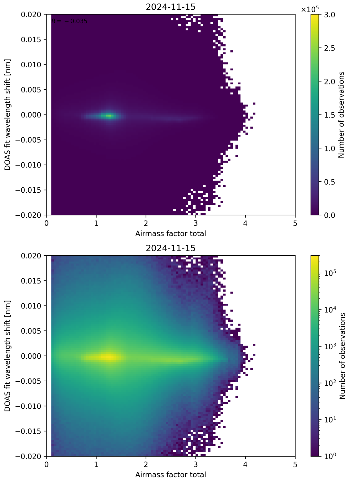
Figure 98: Scatter density plot of “Airmass factor total” against “DOAS fit wavelength shift” for 2024-11-14 to 2024-11-16.
