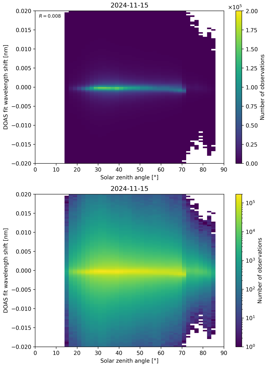
Figure 168: Scatter density plot of “Solar zenith angle” against “DOAS fit wavelength shift” for 2024-11-14 to 2024-11-16.
