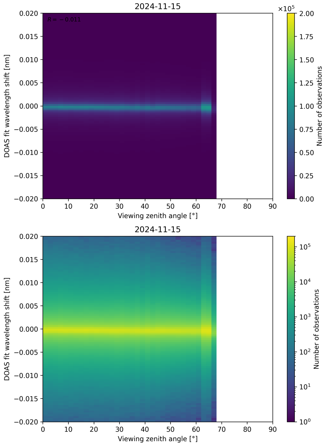
Figure 183: Scatter density plot of “Viewing zenith angle” against “DOAS fit wavelength shift” for 2024-11-14 to 2024-11-16.
