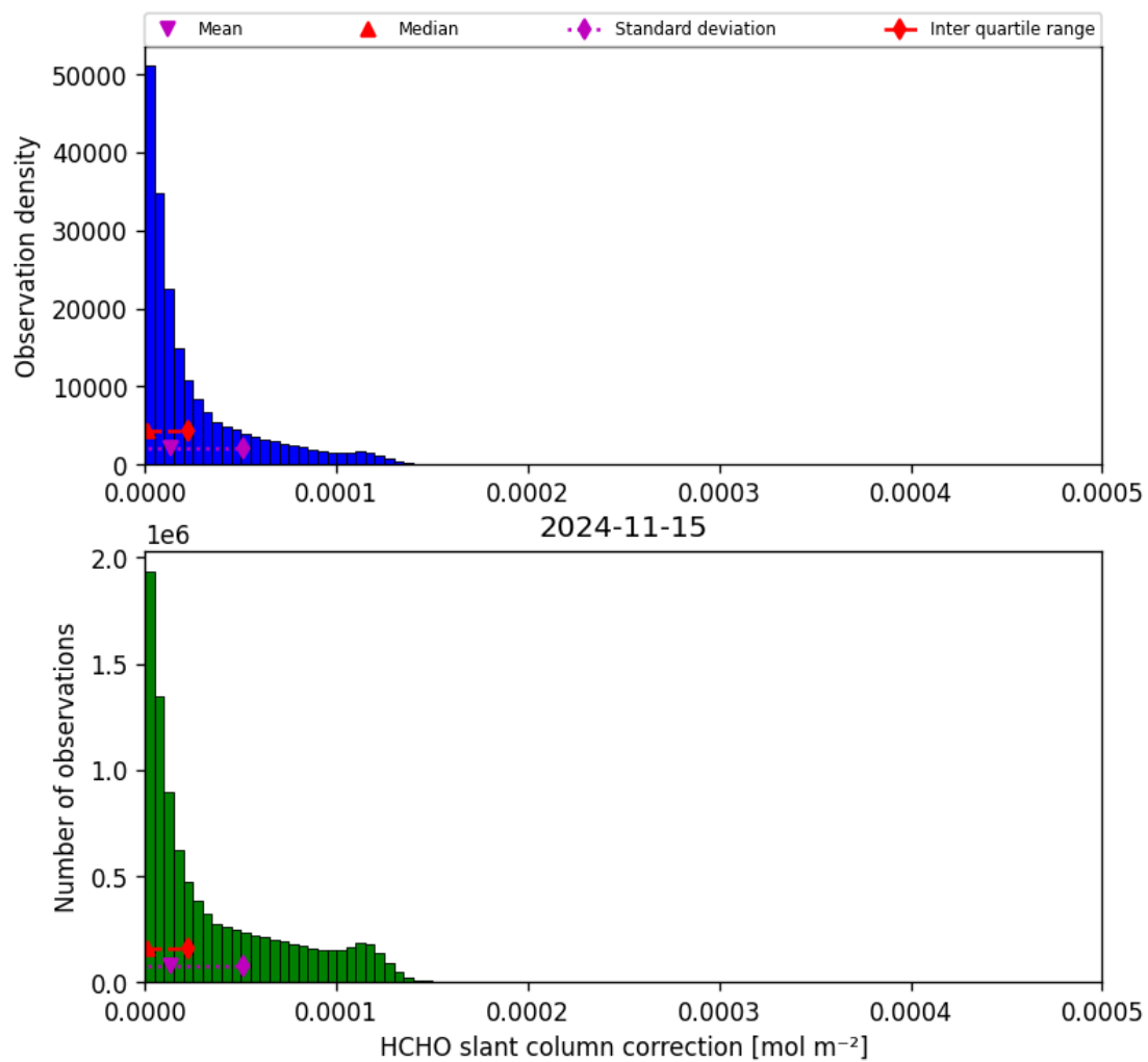
Figure 47: Histogram of “HCHO slant column correction” for 2024-11-14 to 2024-11-16
