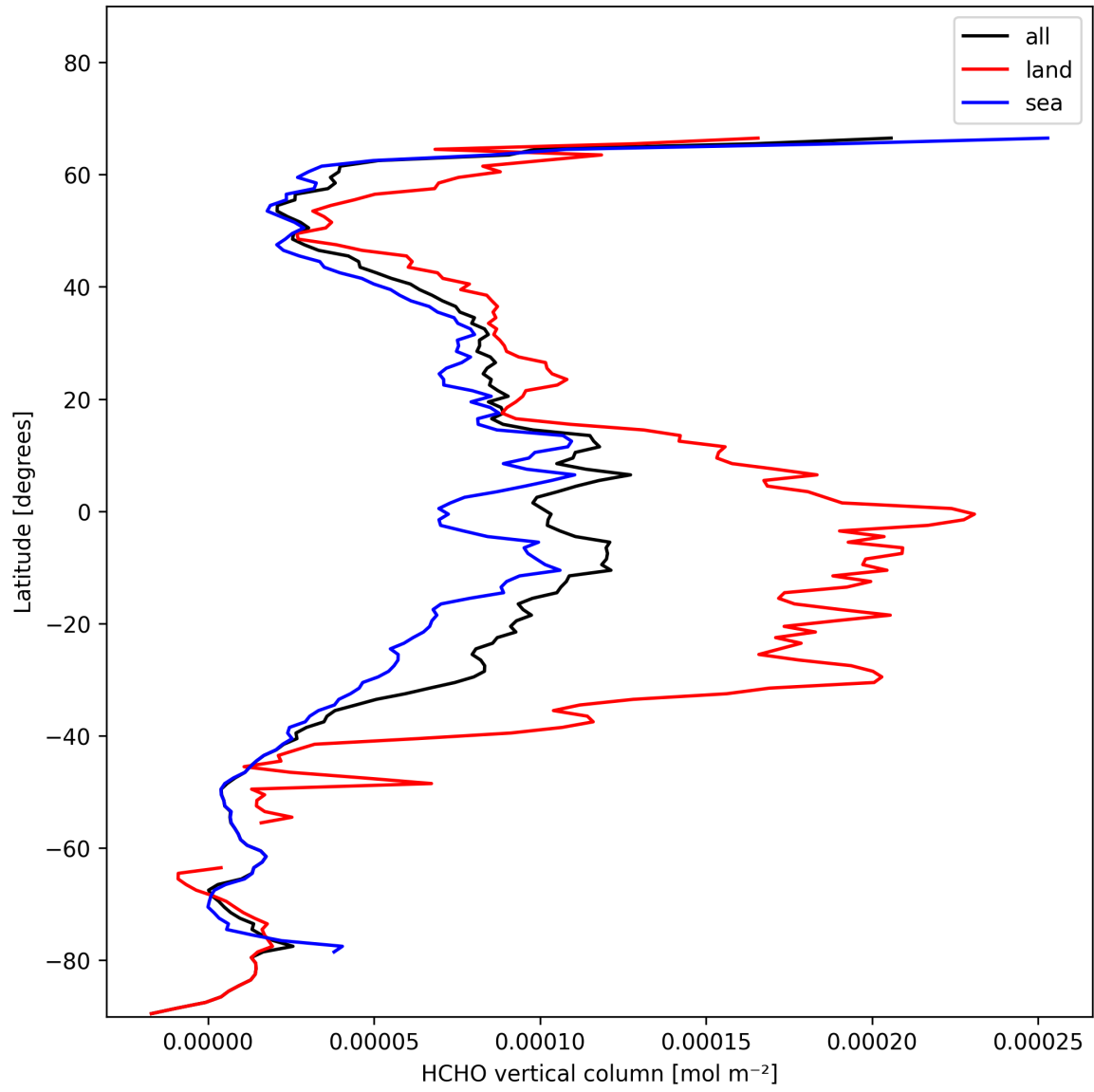
Figure 21: Zonal average of “HCHO vertical column” for 2024-11-14 to 2024-11-16.
