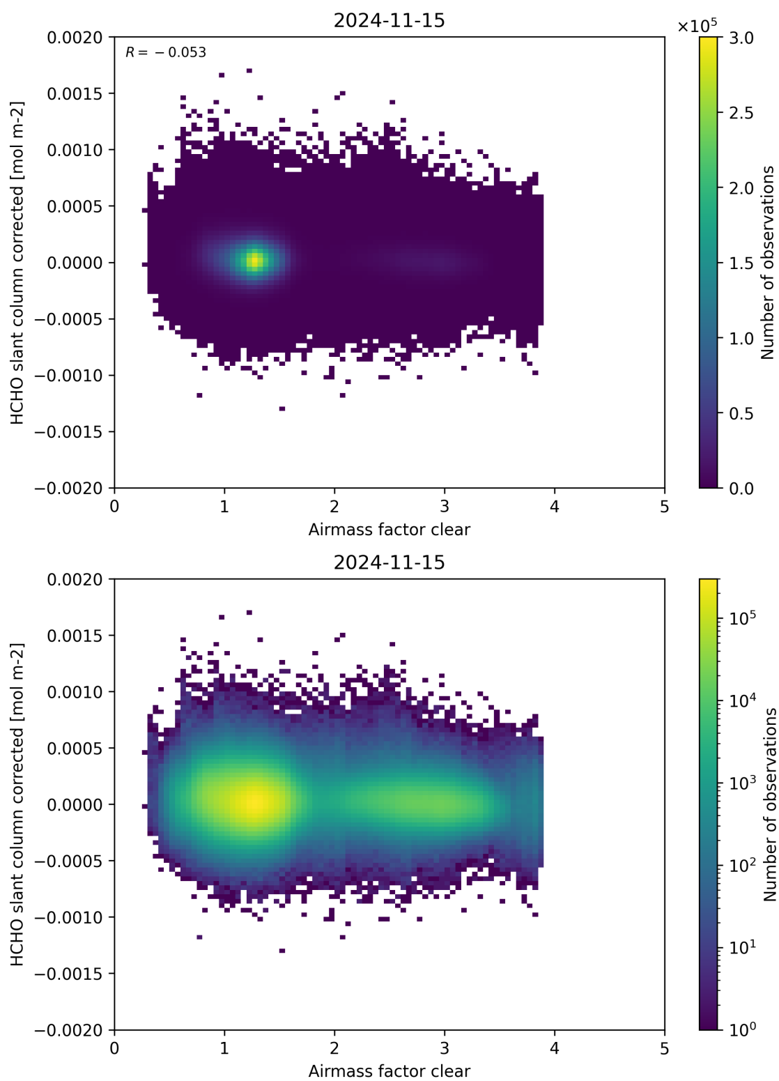
Figure 74: Scatter density plot of “Airmass factor clear” against “HCHO slant column corrected” for 2024-11-14 to 2024-11-16.
