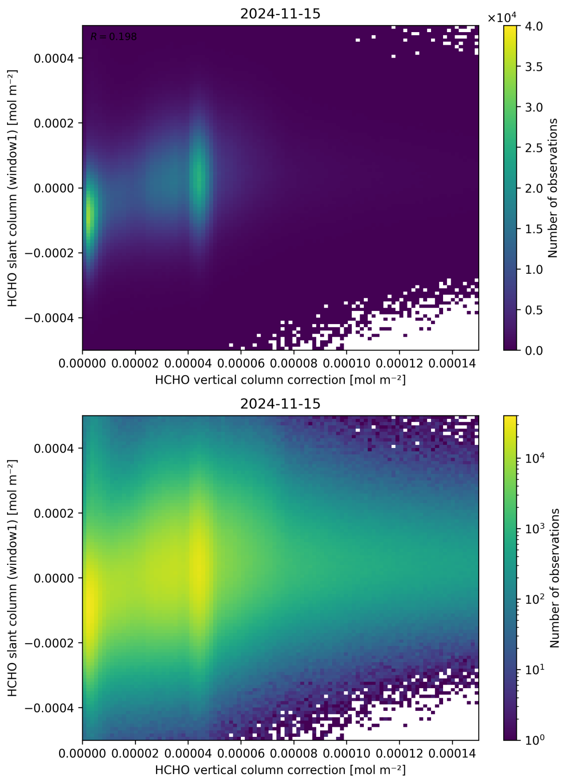
Figure 118: Scatter density plot of “HCHO vertical column correction” against “HCHO slant column (window1)” for 2024-11-14 to 2024-11-16.
