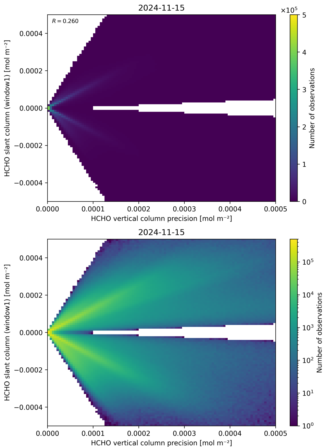
Figure 142: Scatter density plot of “HCHO vertical column precision” against “HCHO slant column (window1)” for 2024-11-14 to 2024-11-16.
