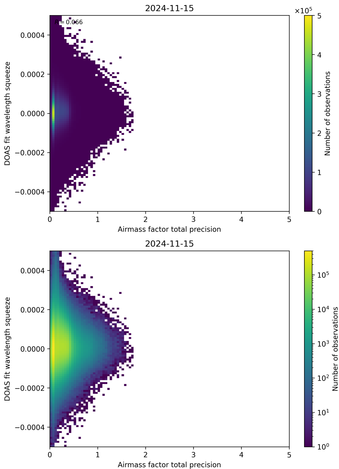
Figure 107: Scatter density plot of “Airmass factor total precision” against “DOAS fit wavelength squeeze” for 2024-11-14 to 2024-11-16.
