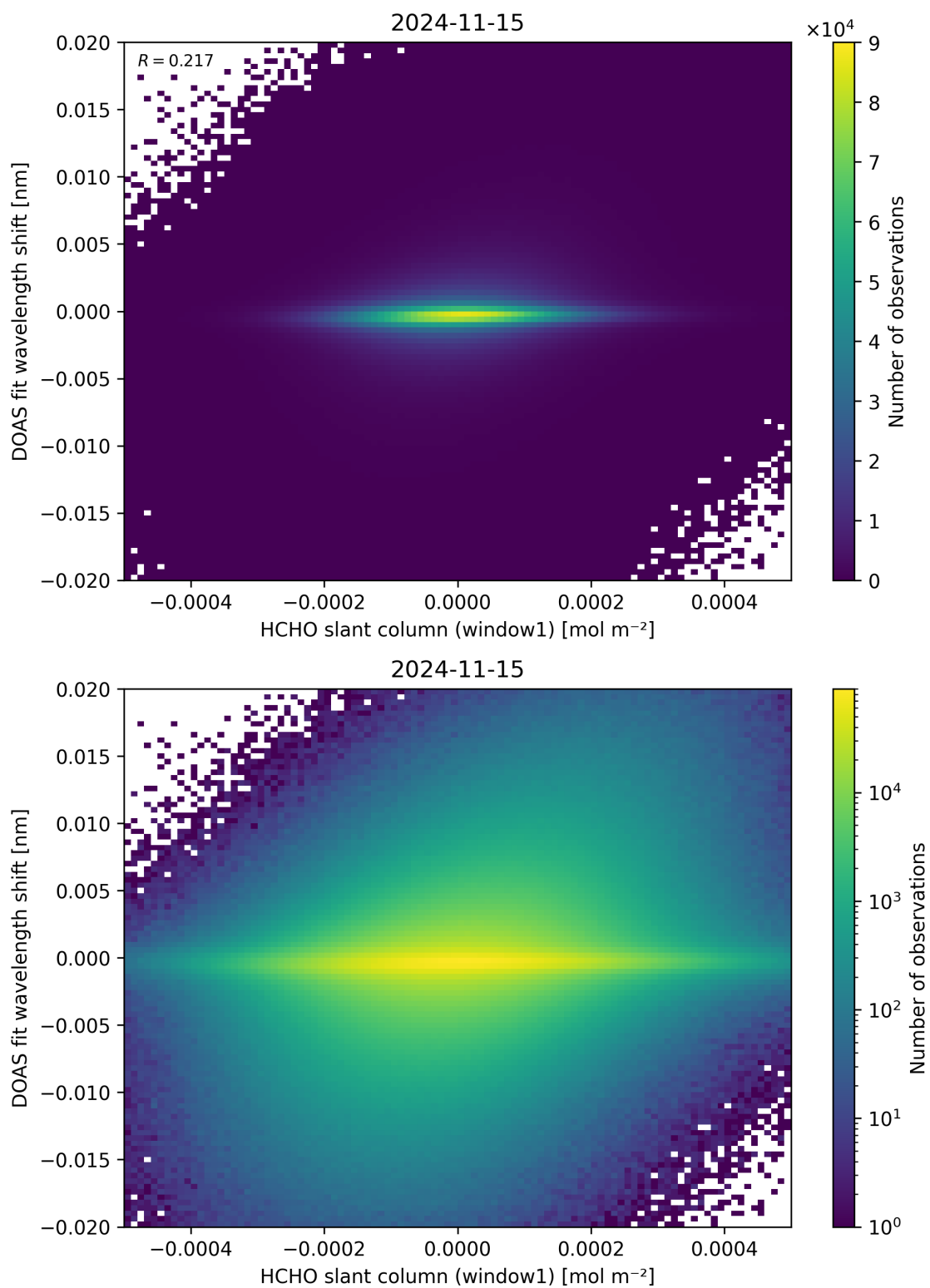
Figure 79: Scatter density plot of “HCHO slant column (window1)” against “DOAS fit wavelength shift” for 2024-11-14 to 2024-11-16.
