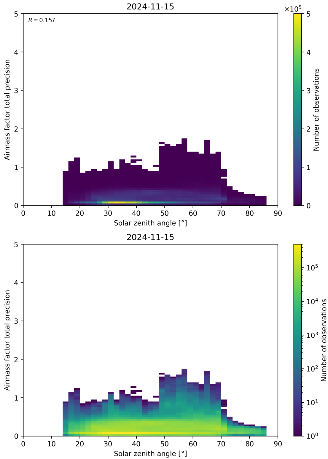
Figure 176: Scatter density plot of “Solar zenith angle” against “Airmass factor total precision” for 2024-11-14 to 2024-11-16.
