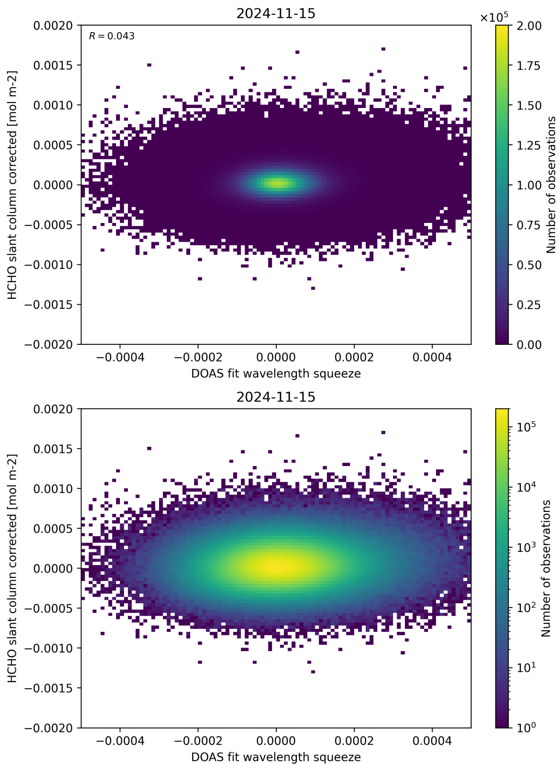
Figure 69: Scatter density plot of “DOAS fit wavelength squeeze” against “HCHO slant column corrected” for 2024-11-14 to 2024-11-16.
