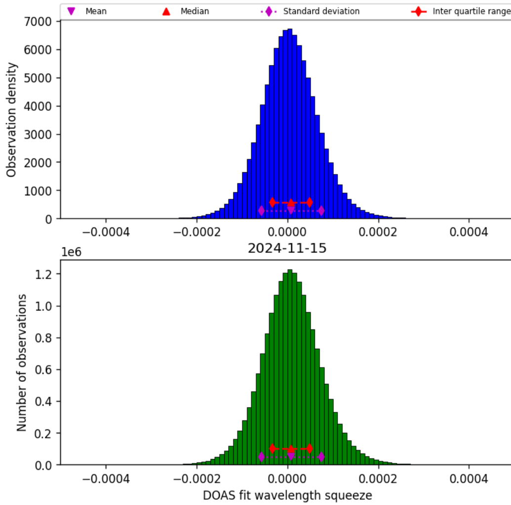
Figure 45: Histogram of “DOAS fit wavelength squeeze” for 2024-11-14 to 2024-11-16
