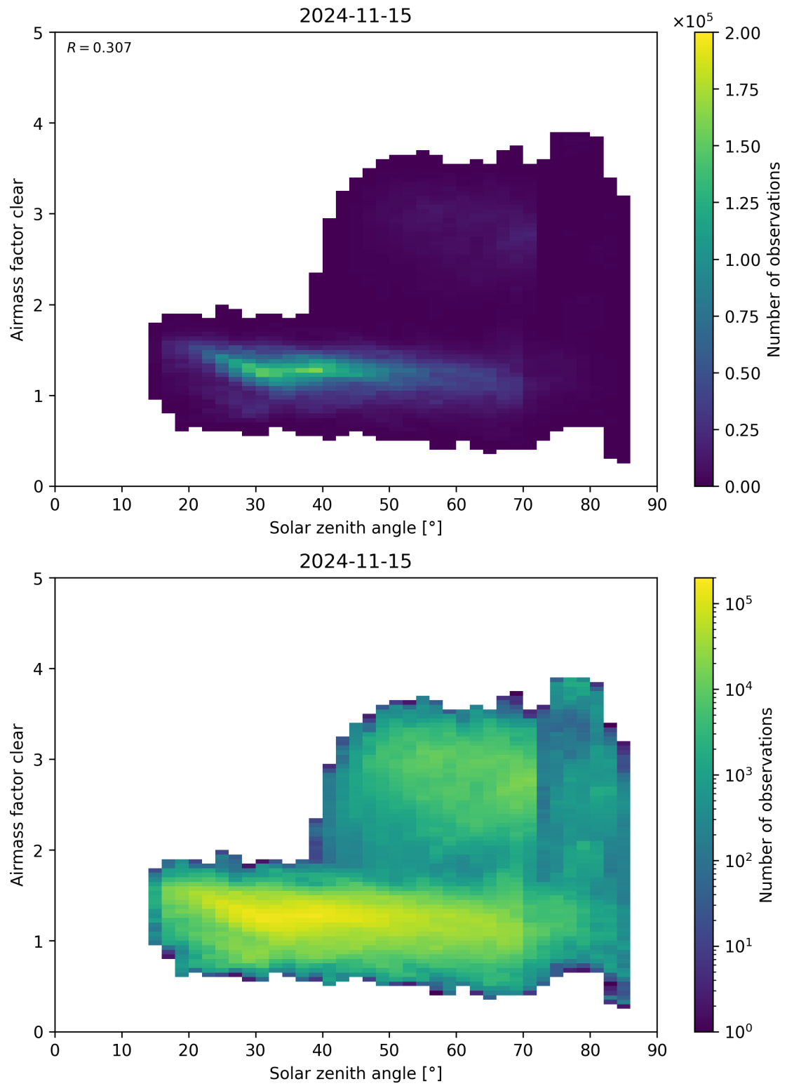
Figure 170: Scatter density plot of “Solar zenith angle” against “Airmass factor clear” for 2024-11-14 to 2024-11-16.
