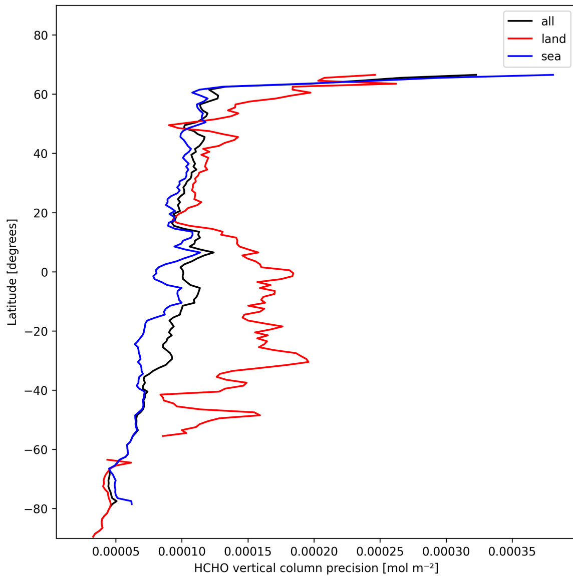
Figure 22: Zonal average of “HCHO vertical column precision” for 2024-11-14 to 2024-11-16.
