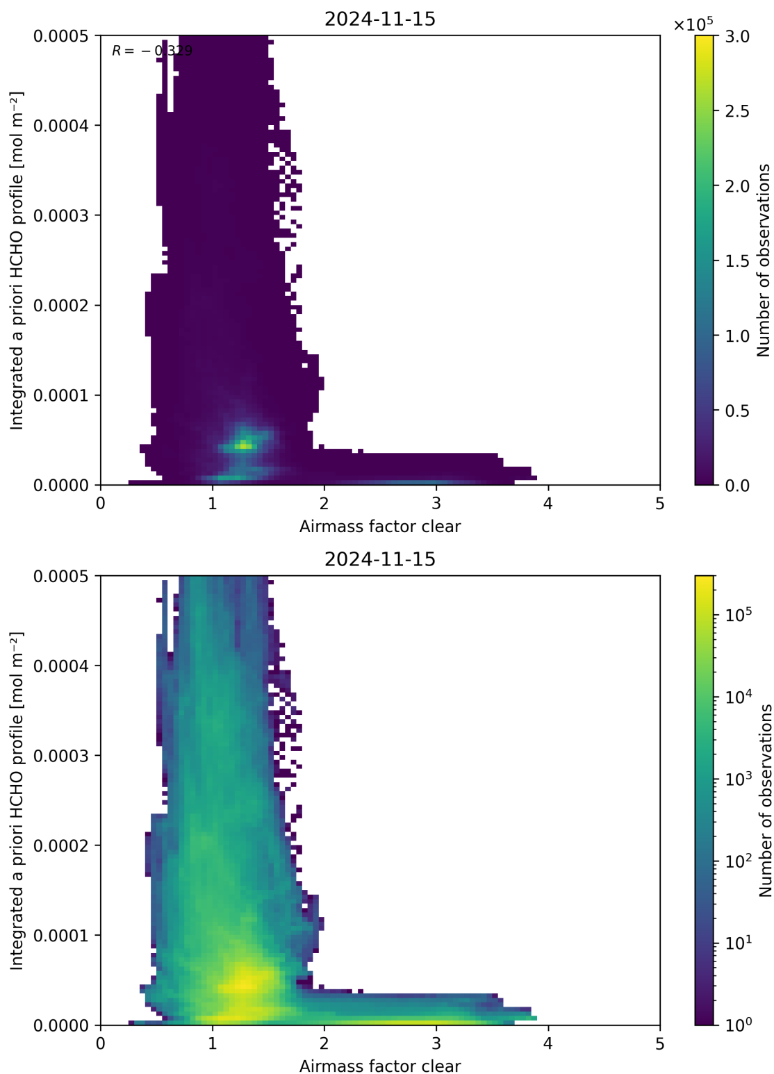
Figure 76: Scatter density plot of “Airmass factor clear” against “Integrated a priori HCHO profile” for 2024-11-14 to 2024-11-16.
