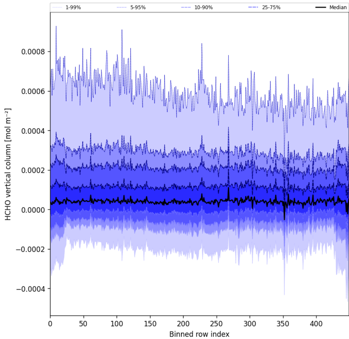
Figure 49: Along track statistics of “HCHO vertical column” for 2024-11-14 to 2024-11-16
