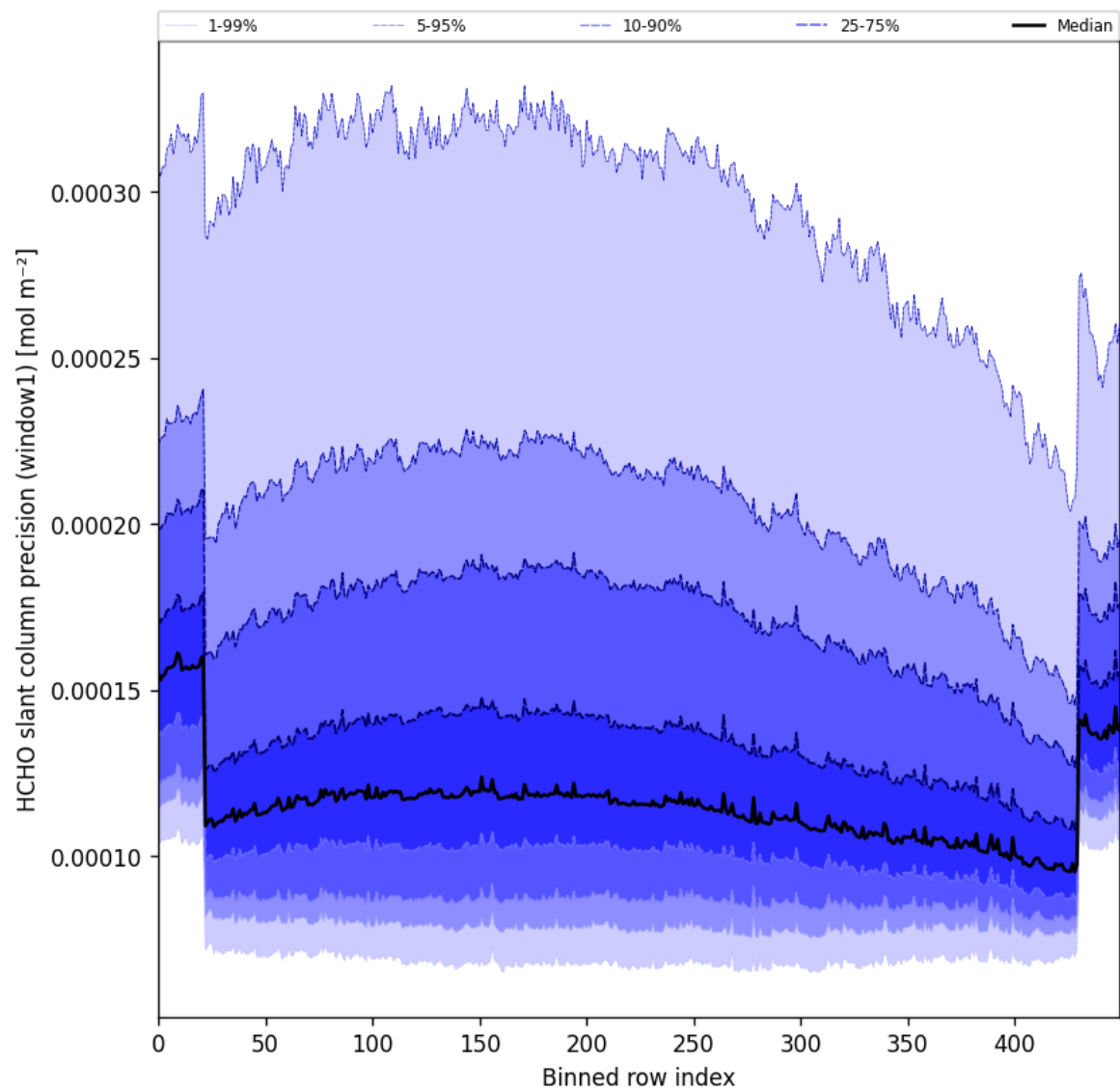
Figure 53: Along track statistics of “HCHO slant column precision (window1)” for 2024-11-14 to 2024-11-16
