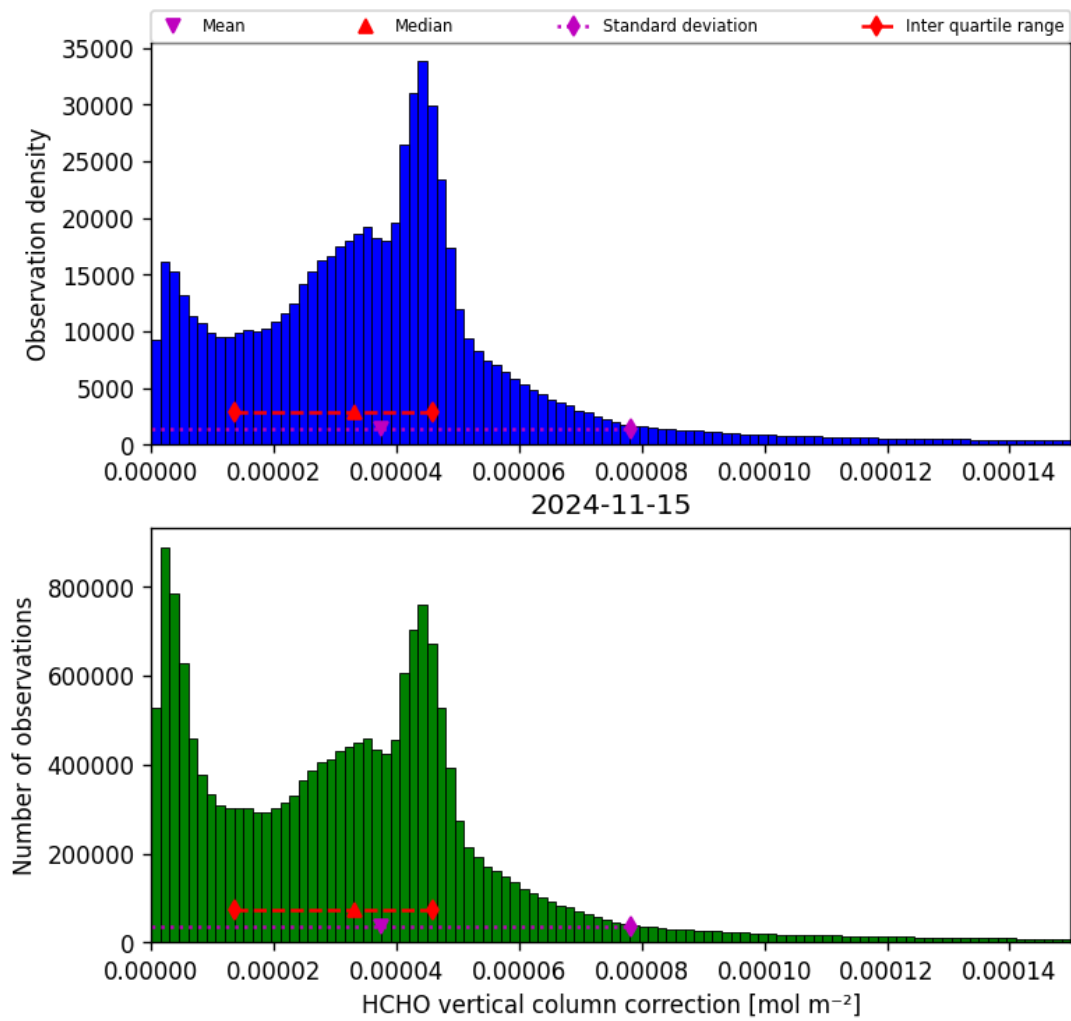
Figure 37: Histogram of “HCHO vertical column correction” for 2024-11-14 to 2024-11-16
