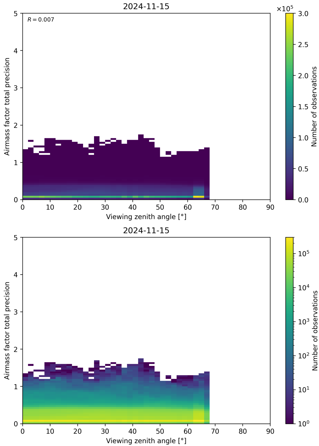
Figure 191: Scatter density plot of “Viewing zenith angle” against “Airmass factor total precision” for 2024-11-14 to 2024-11-16.
