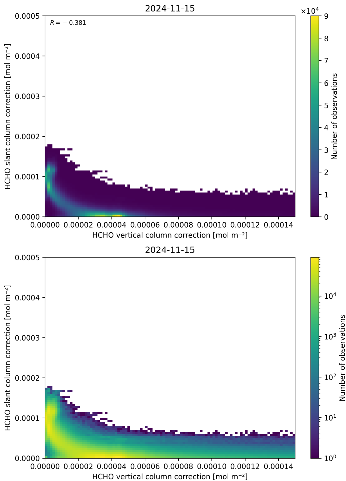
Figure 117: Scatter density plot of “HCHO vertical column correction” against “HCHO slant column correction” for 2024-11-14 to 2024-11-16.
