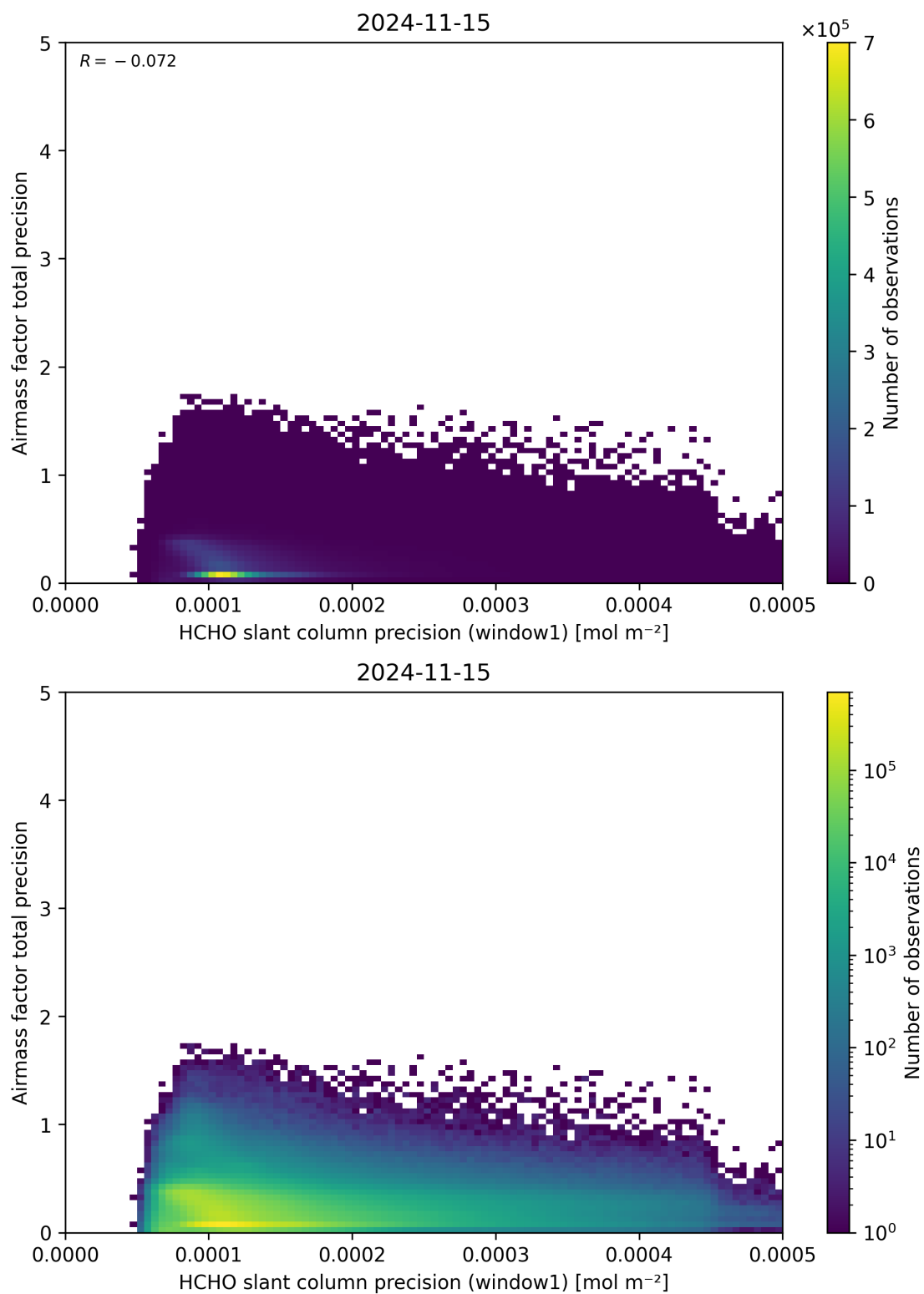
Figure 95: Scatter density plot of “HCHO slant column precision (window1)” against “Airmass factor total precision” for 2024-11-14 to 2024-11-16.
