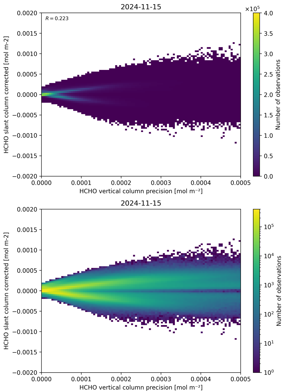
Figure 140: Scatter density plot of “HCHO vertical column precision” against “HCHO slant column corrected” for 2024-11-14 to 2024-11-16.
