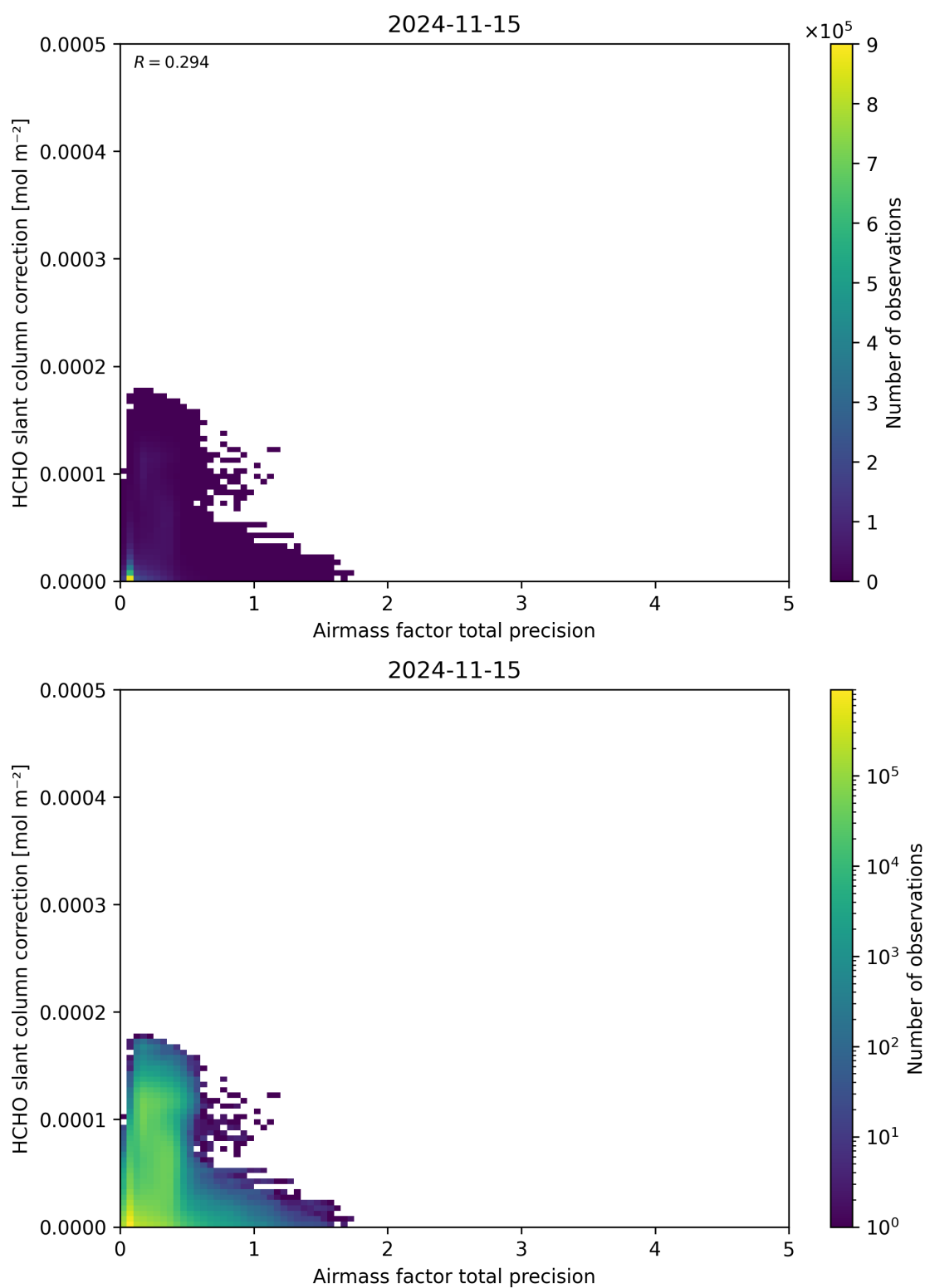
Figure 110: Scatter density plot of “Airmass factor total precision” against “HCHO slant column correction” for 2024-11-14 to 2024-11-16.
