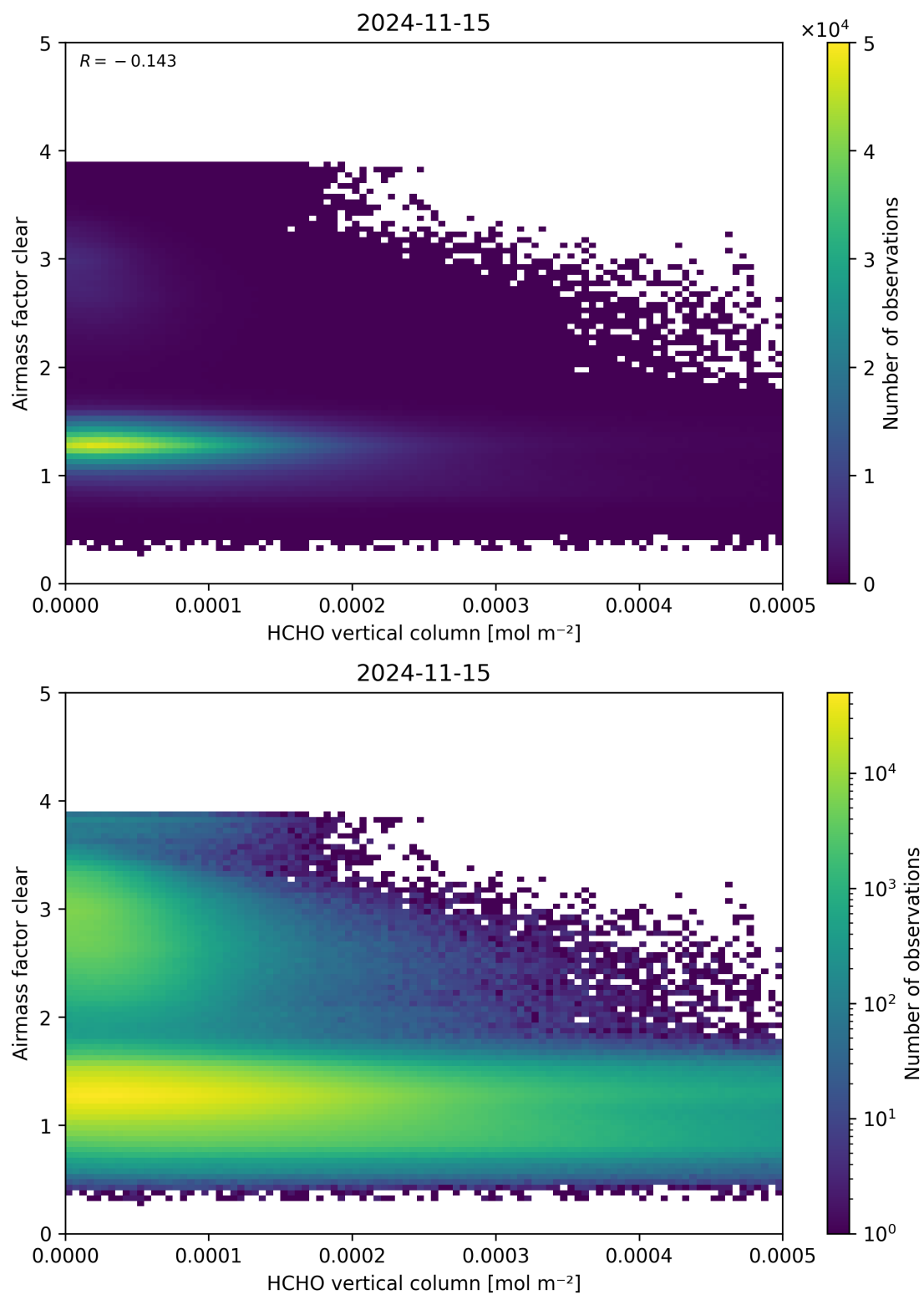
Figure 126: Scatter density plot of “HCHO vertical column” against “Airmass factor clear” for 2024-11-14 to 2024-11-16.
