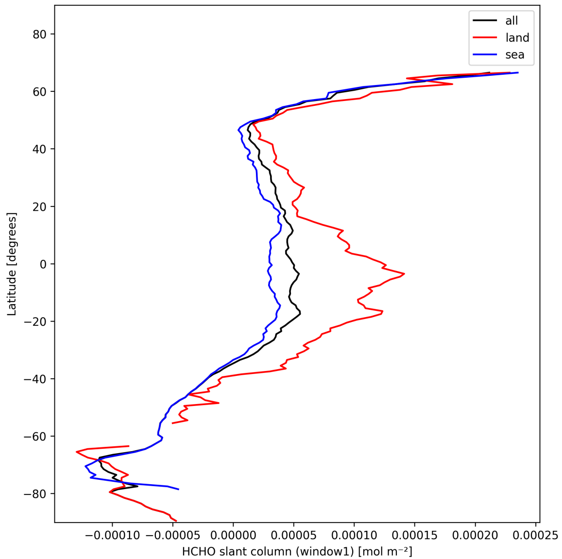
Figure 24: Zonal average of “HCHO slant column (window1)” for 2024-11-14 to 2024-11-16.
