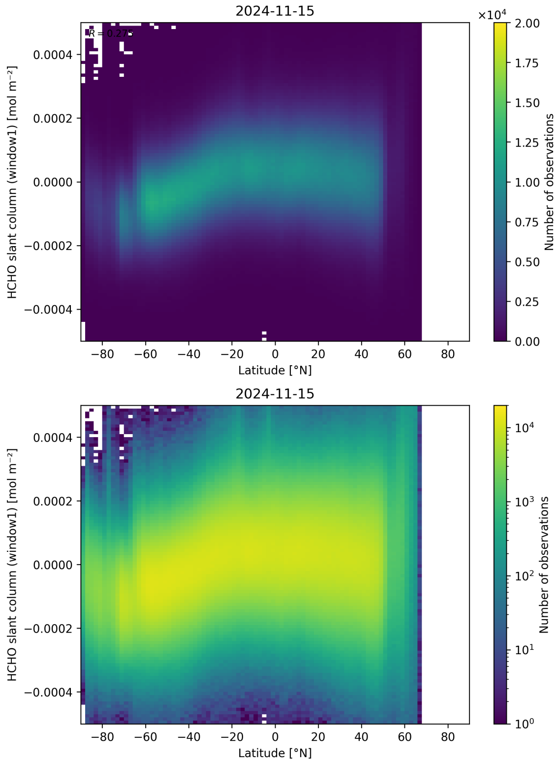
Figure 159: Scatter density plot of “Latitude” against “HCHO slant column (window1)” for 2024-11-14 to 2024-11-16.
