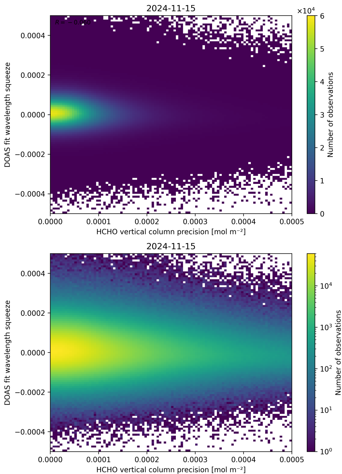
Figure 138: Scatter density plot of “HCHO vertical column precision” against “DOAS fit wavelength squeeze” for 2024-11-14 to 2024-11-16.
