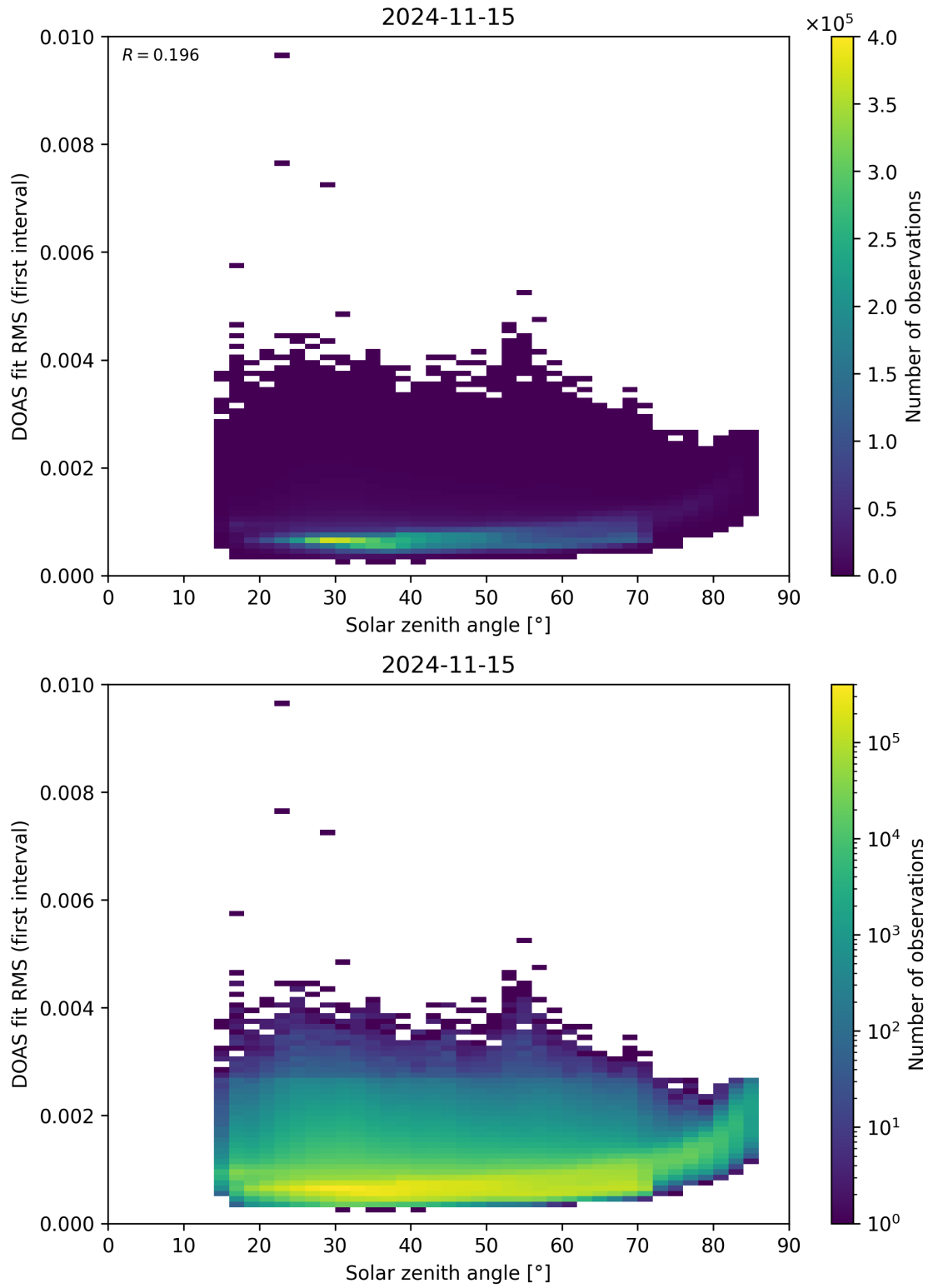
Figure 167: Scatter density plot of “Solar zenith angle” against “DOAS fit RMS (first interval)” for 2024-11-14 to 2024-11-16.
