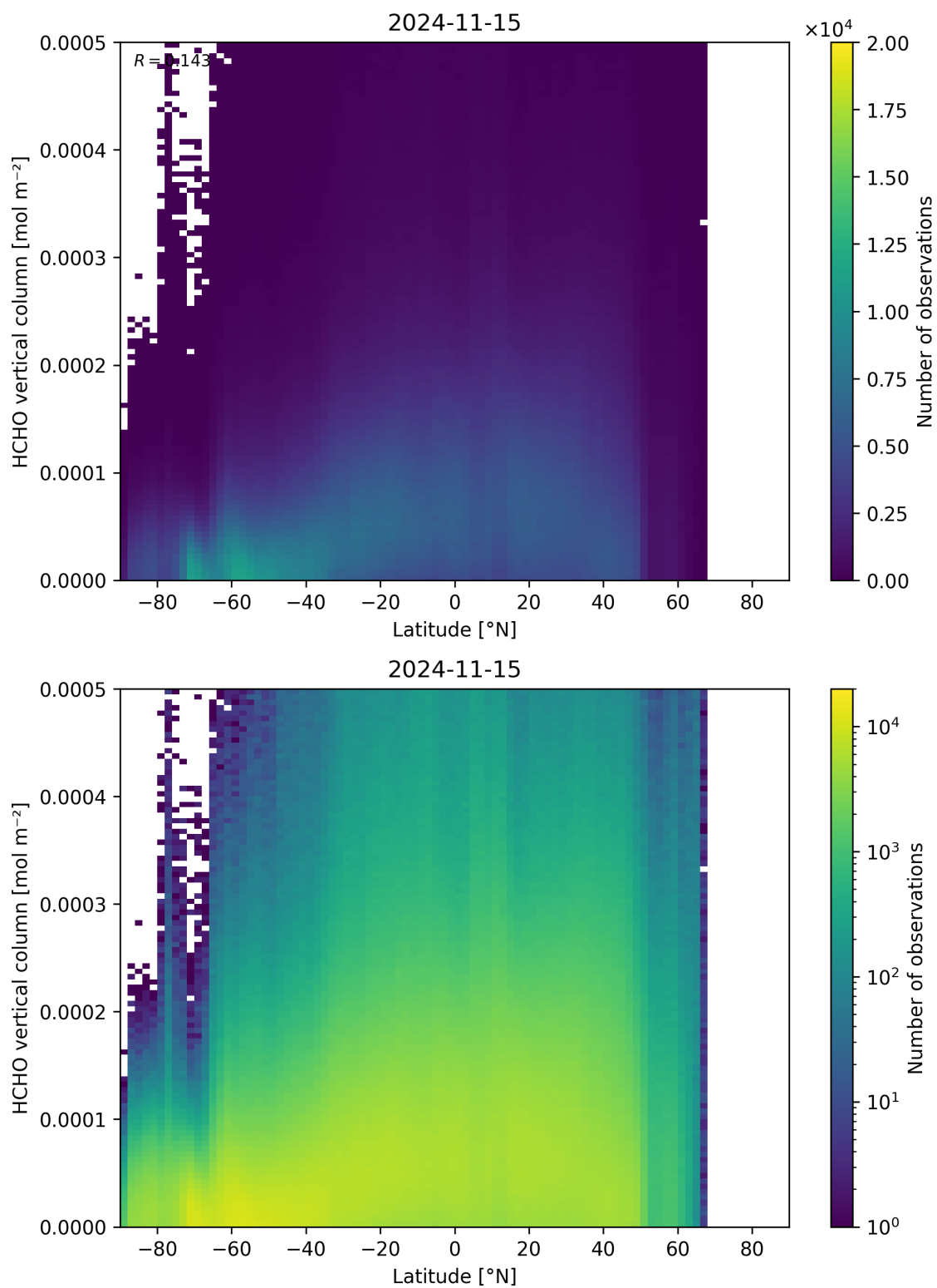
Figure 163: Scatter density plot of “Latitude” against “HCHO vertical column” for 2024-11-14 to 2024-11-16.
