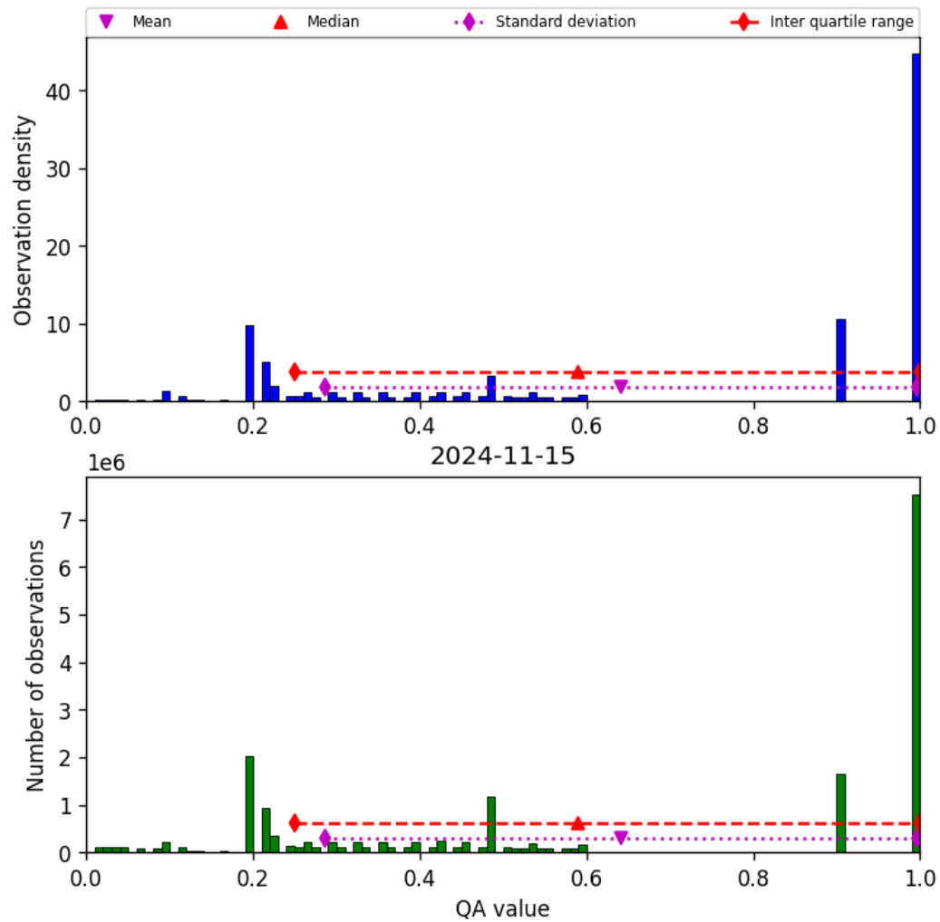
Figure 34: Histogram of “QA value” for 2024-11-14 to 2024-11-16
