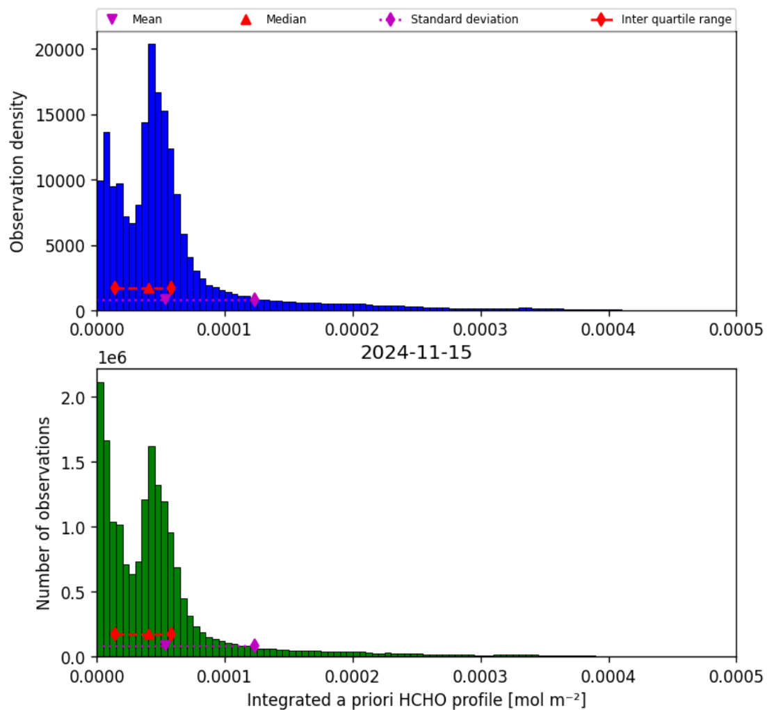
Figure 43: Histogram of “Integrated a priori HCHO profile” for 2024-11-14 to 2024-11-16
