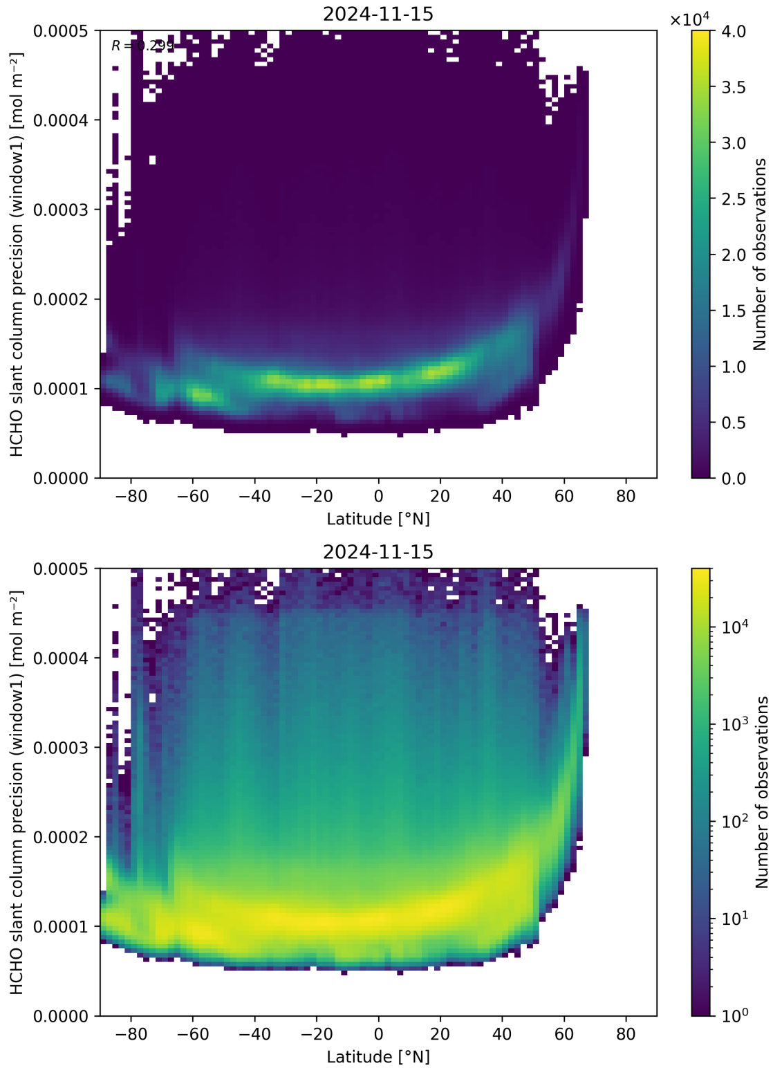
Figure 160: Scatter density plot of “Latitude” against “HCHO slant column precision (window1)” for 2024-11-14 to 2024-11-16.
