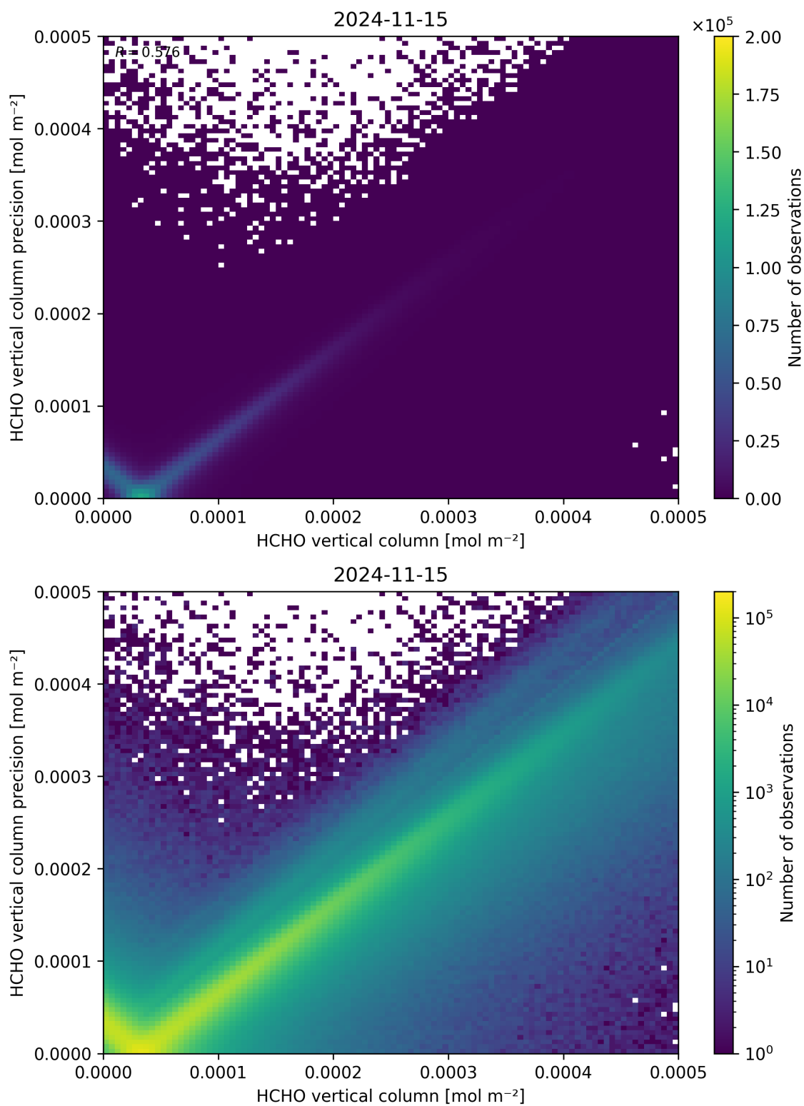
Figure 134: Scatter density plot of “HCHO vertical column” against “HCHO vertical column precision” for 2024-11-14 to 2024-11-16.
