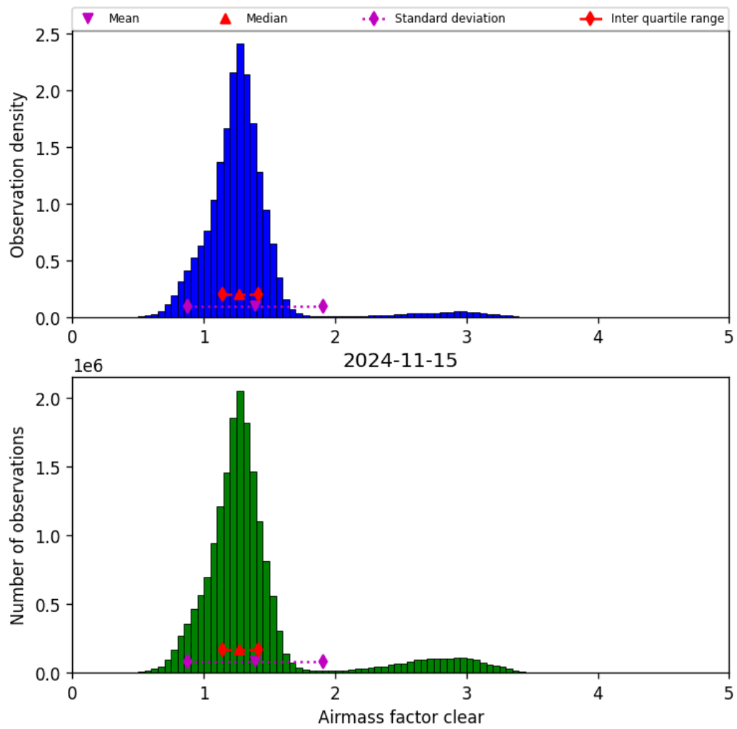
Figure 42: Histogram of “Airmass factor clear” for 2024-11-14 to 2024-11-16
