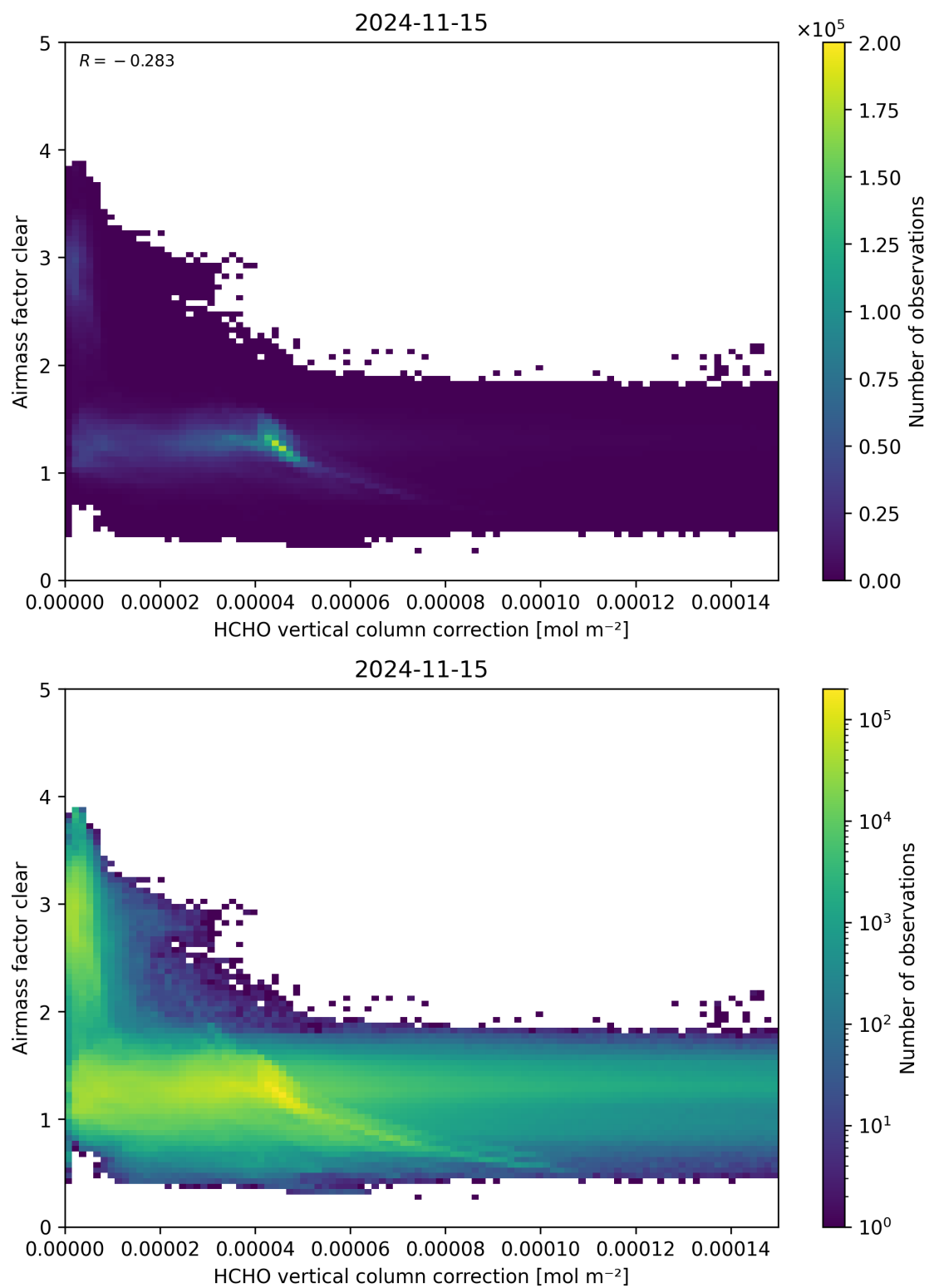
Figure 115: Scatter density plot of “HCHO vertical column correction” against “Airmass factor clear” for 2024-11-14 to 2024-11-16.
