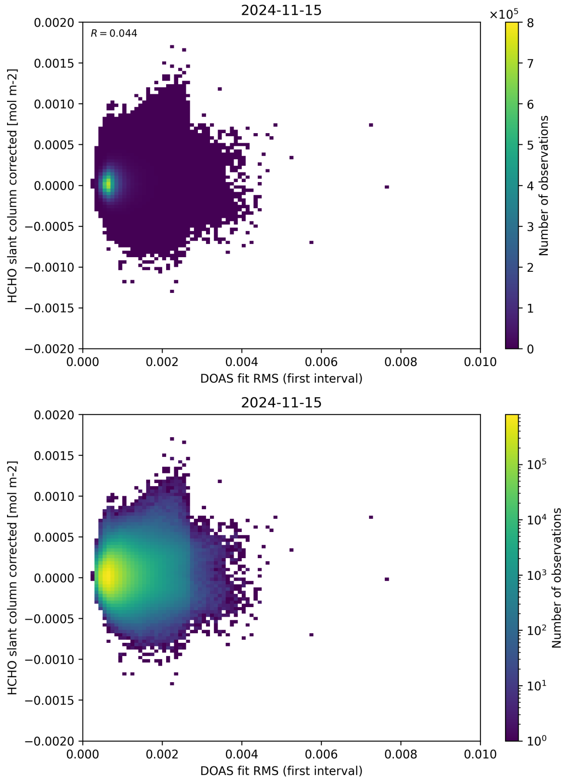
Figure 62: Scatter density plot of “DOAS fit RMS (first interval)” against “HCHO slant column corrected” for 2024-11-14 to 2024-11-16.
