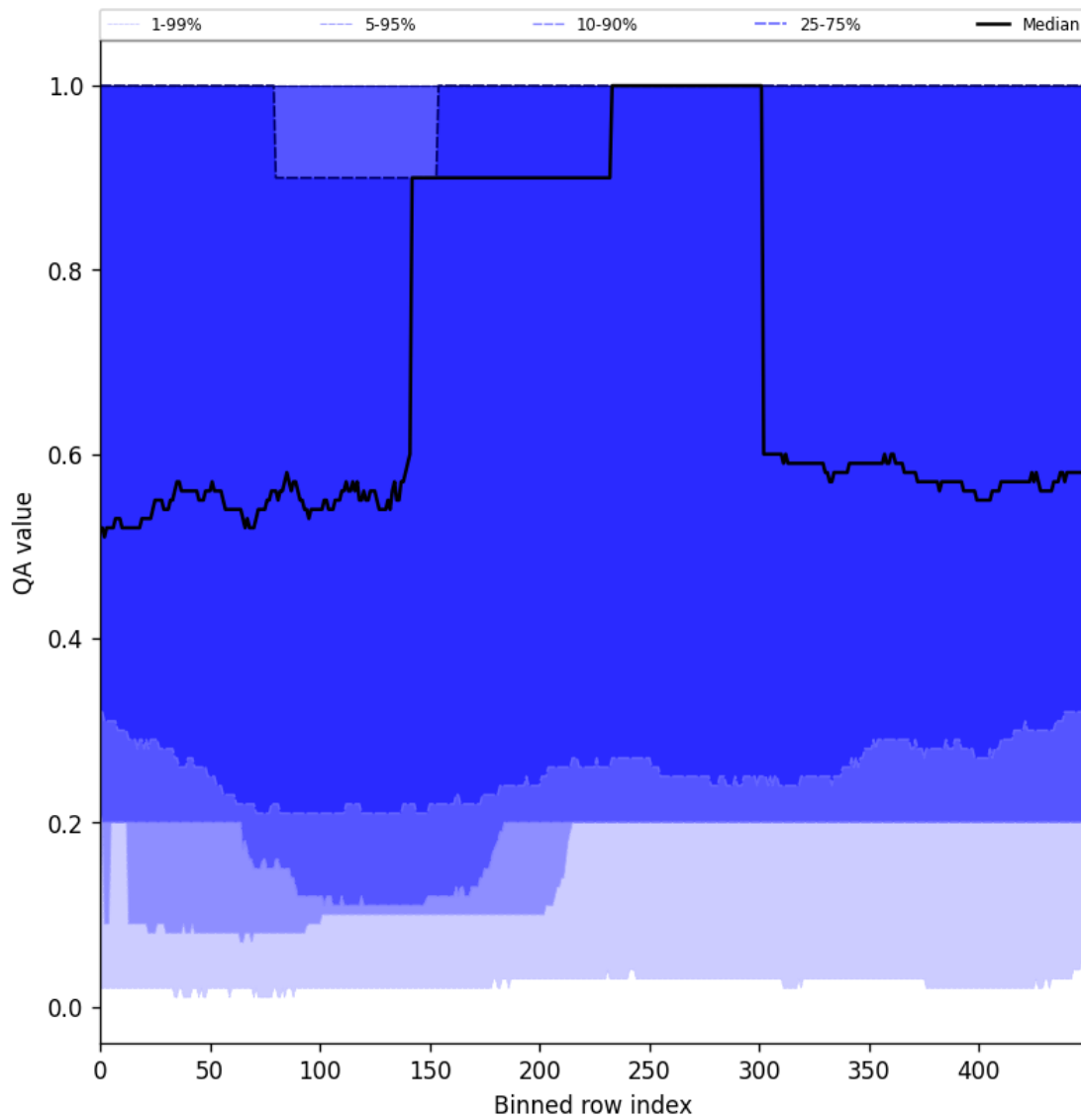
Figure 48: Along track statistics of “QA value” for 2024-11-14 to 2024-11-16
