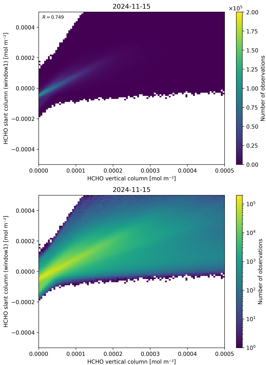
Figure 129: Scatter density plot of “HCHO vertical column” against “HCHO slant column (window1)” for 2024-11-14 to 2024-11-16.
