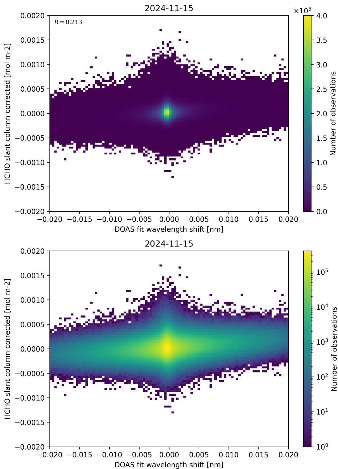
Figure 66: Scatter density plot of “DOAS fit wavelength shift” against “HCHO slant column corrected” for 2024-11-14 to 2024-11-16.
