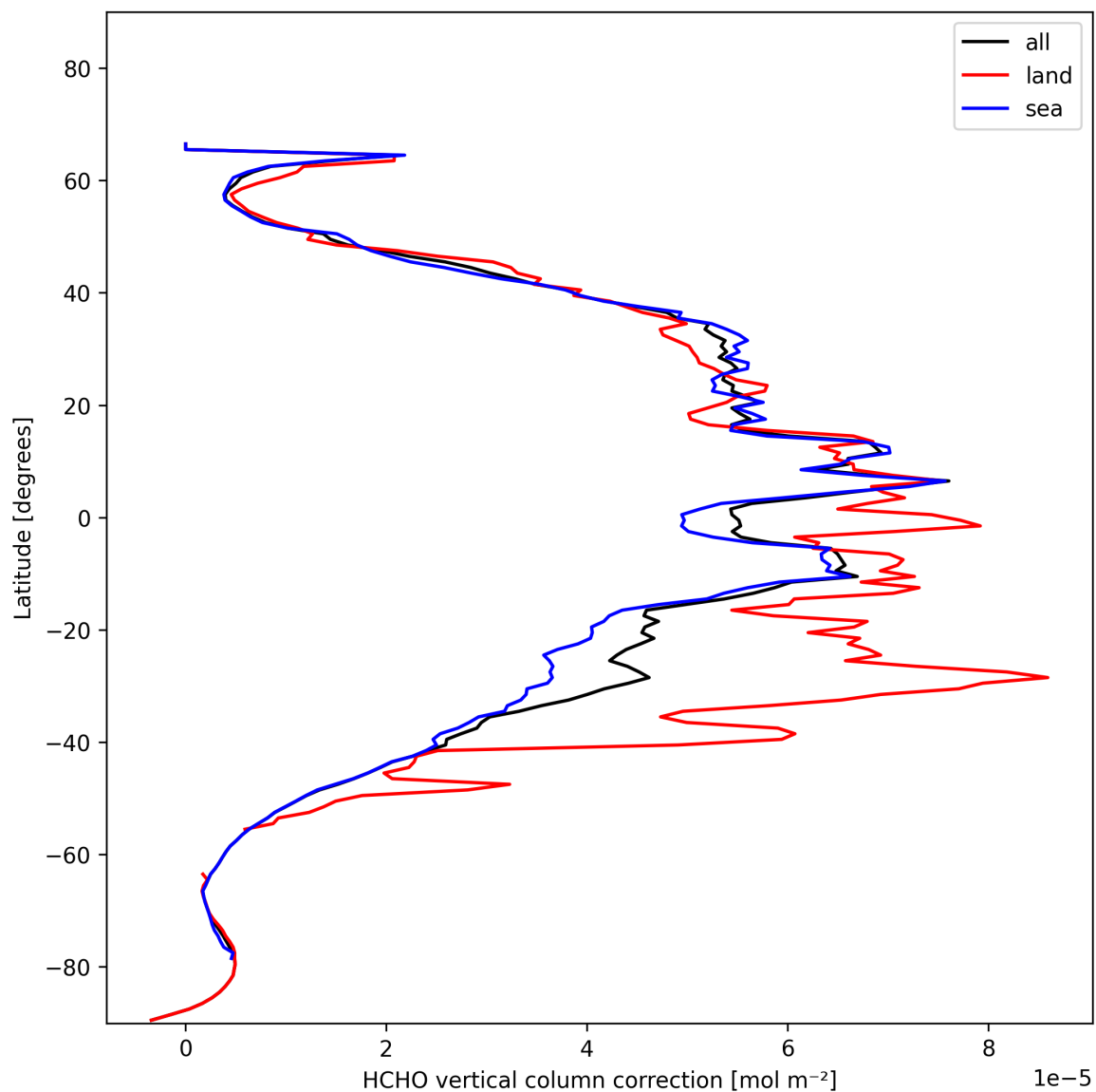
Figure 23: Zonal average of “HCHO vertical column correction” for 2024-11-14 to 2024-11-16.
