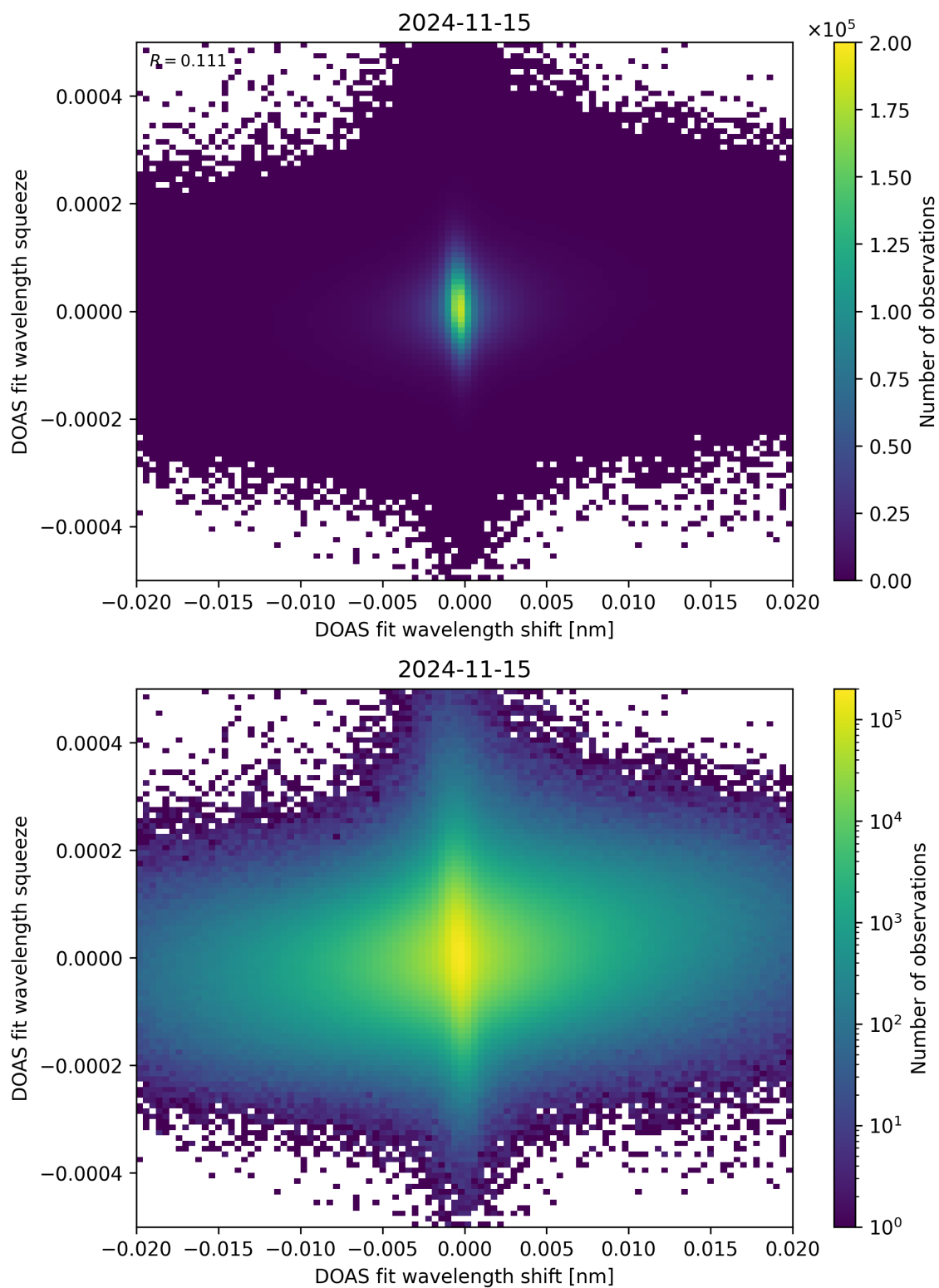
Figure 65: Scatter density plot of “DOAS fit wavelength shift” against “DOAS fit wavelength squeeze” for 2024-11-14 to 2024-11-16.
