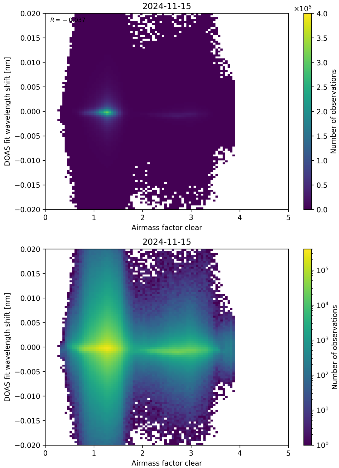
Figure 72: Scatter density plot of “Airmass factor clear” against “DOAS fit wavelength shift” for 2024-11-14 to 2024-11-16.
