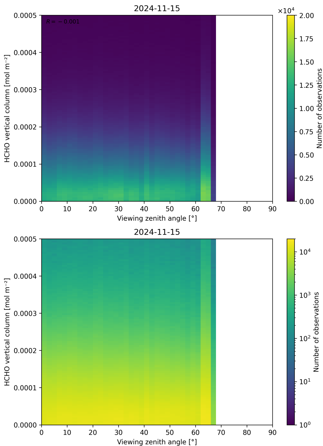
Figure 192: Scatter density plot of “Viewing zenith angle” against “HCHO vertical column” for 2024-11-14 to 2024-11-16.
