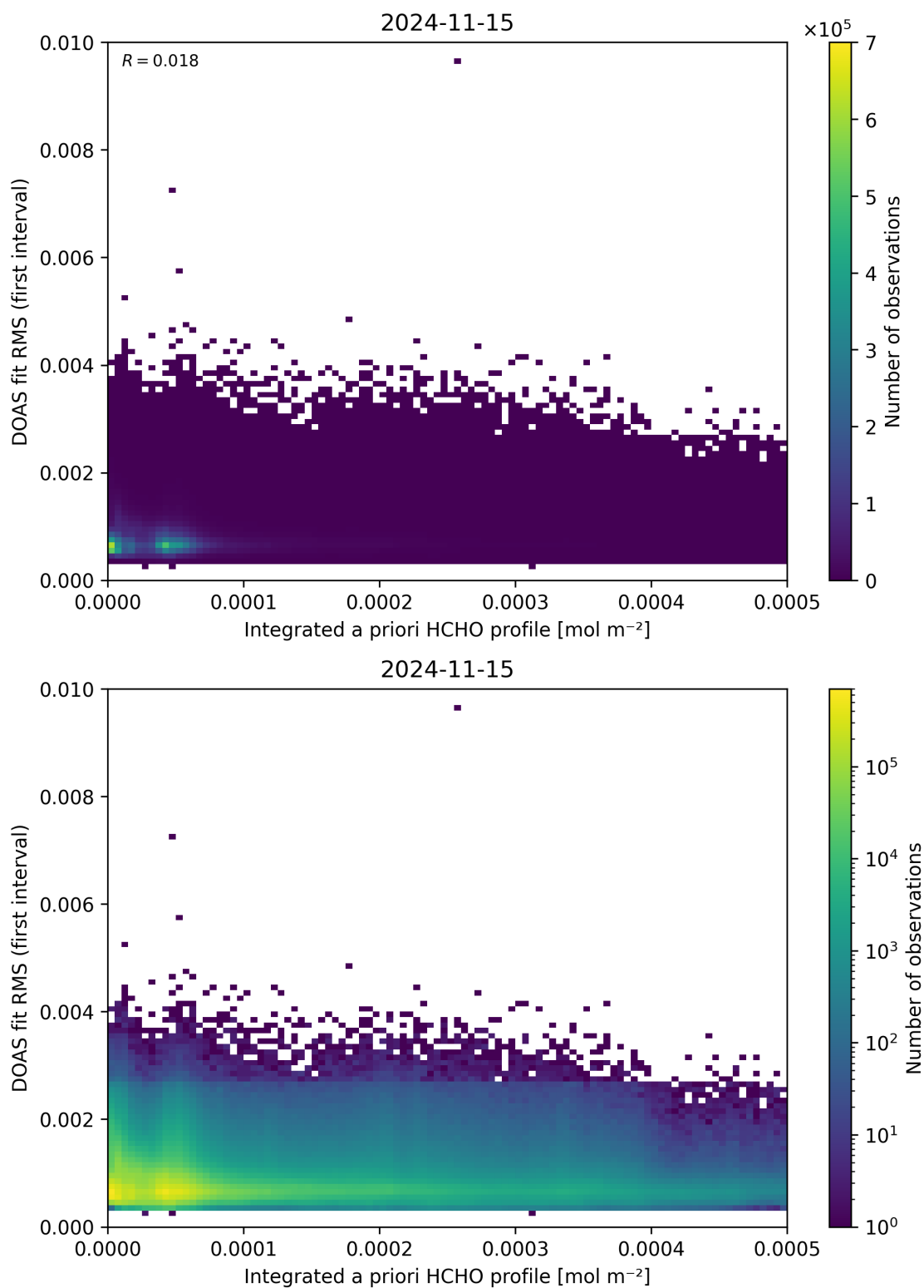
Figure 148: Scatter density plot of “Integrated a priori HCHO profile” against “DOAS fit RMS (first interval)” for 2024-11-14 to 2024-11-16.
