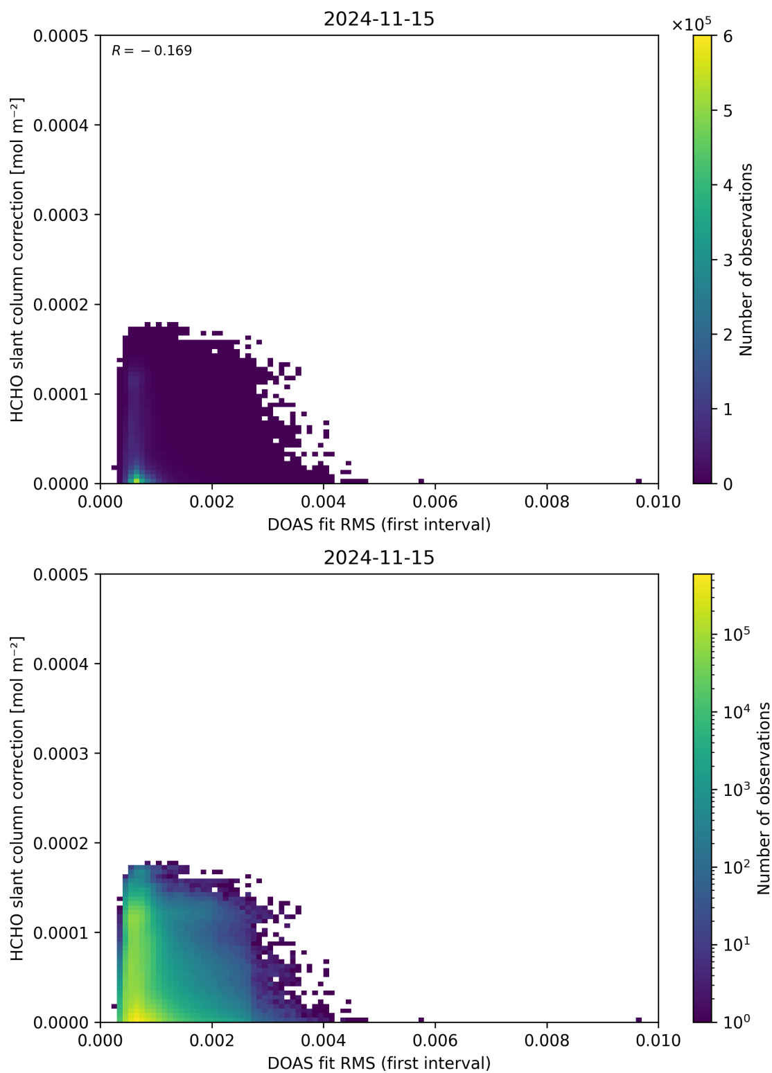
Figure 63: Scatter density plot of “DOAS fit RMS (first interval)” against “HCHO slant column correction” for 2024-11-14 to 2024-11-16.
