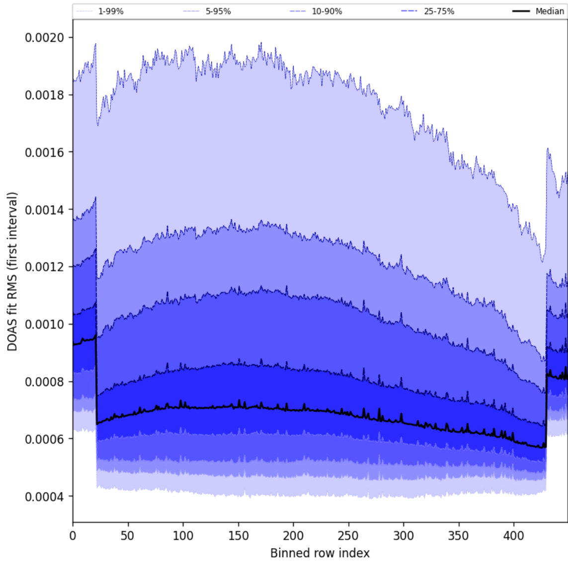
Figure 60: Along track statistics of “DOAS fit RMS (first interval)” for 2024-11-14 to 2024-11-16
