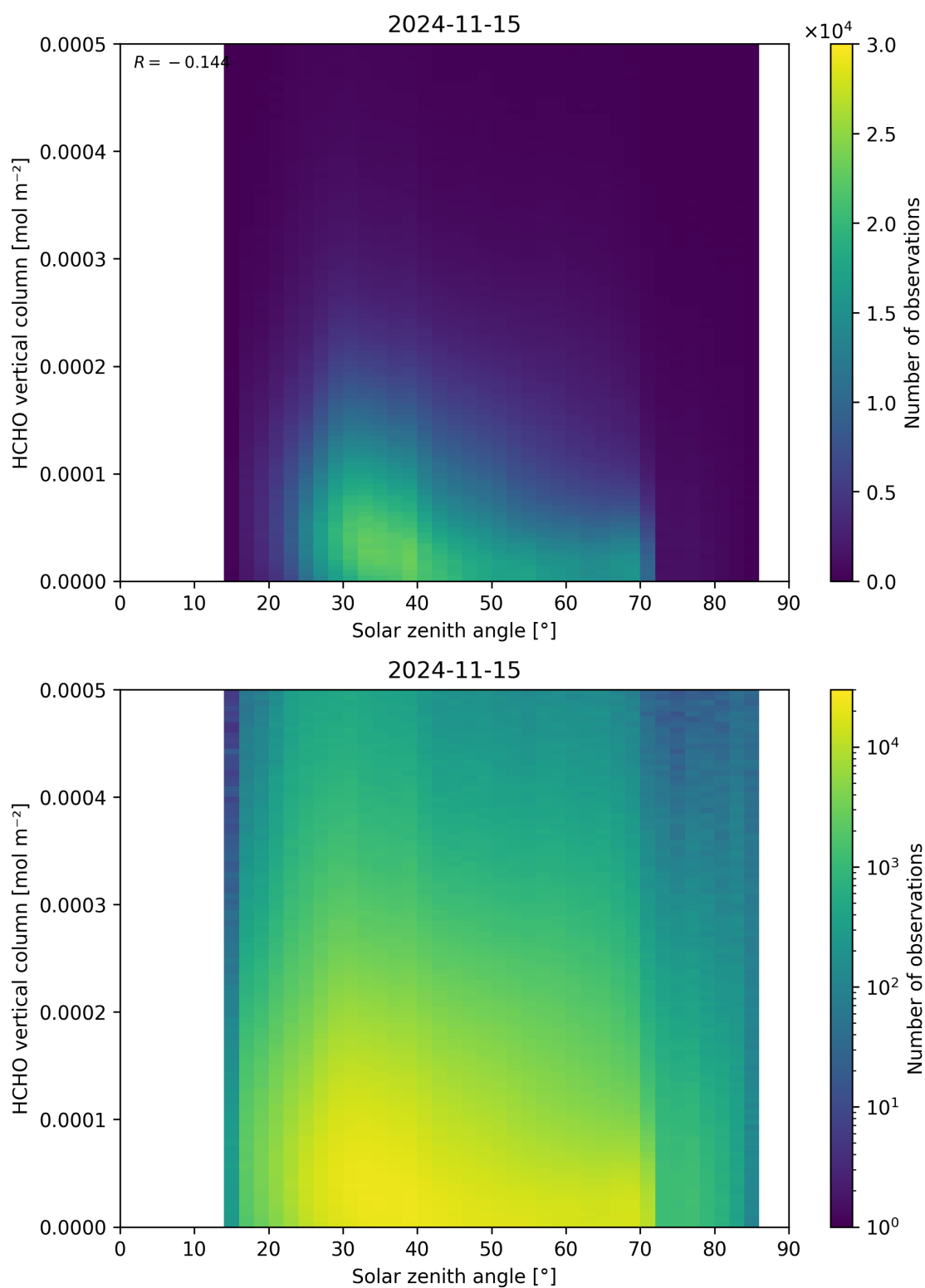
Figure 177: Scatter density plot of “Solar zenith angle” against “HCHO vertical column” for 2024-11-14 to 2024-11-16.
