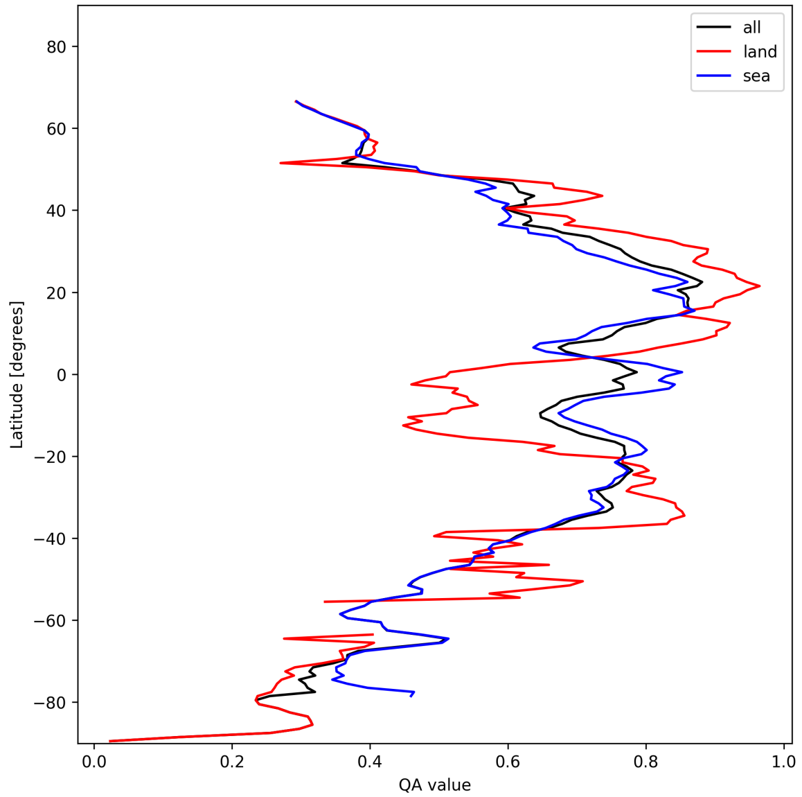
Figure 20: Zonal average of “QA value” for 2024-11-14 to 2024-11-16.
