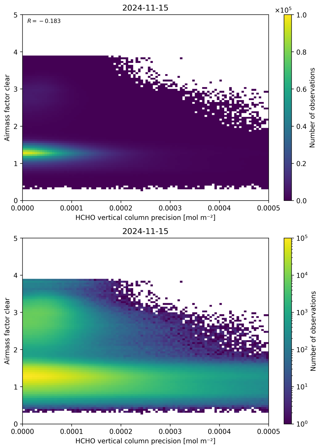
Figure 139: Scatter density plot of “HCHO vertical column precision” against “Airmass factor clear” for 2024-11-14 to 2024-11-16.
