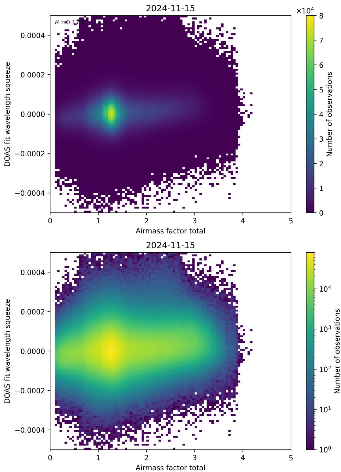
Figure 99: Scatter density plot of “Airmass factor total” against “DOAS fit wavelength squeeze” for 2024-11-14 to 2024-11-16.
