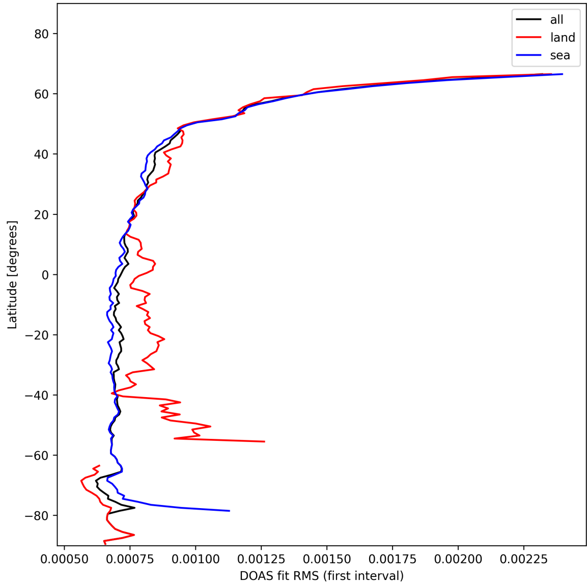
Figure 32: Zonal average of “DOAS fit RMS (first interval)” for 2024-11-14 to 2024-11-16.
