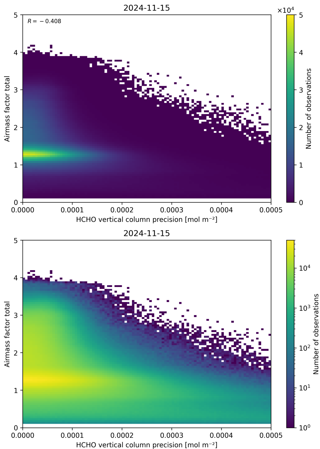
Figure 144: Scatter density plot of “HCHO vertical column precision” against “Airmass factor total” for 2024-11-14 to 2024-11-16.
