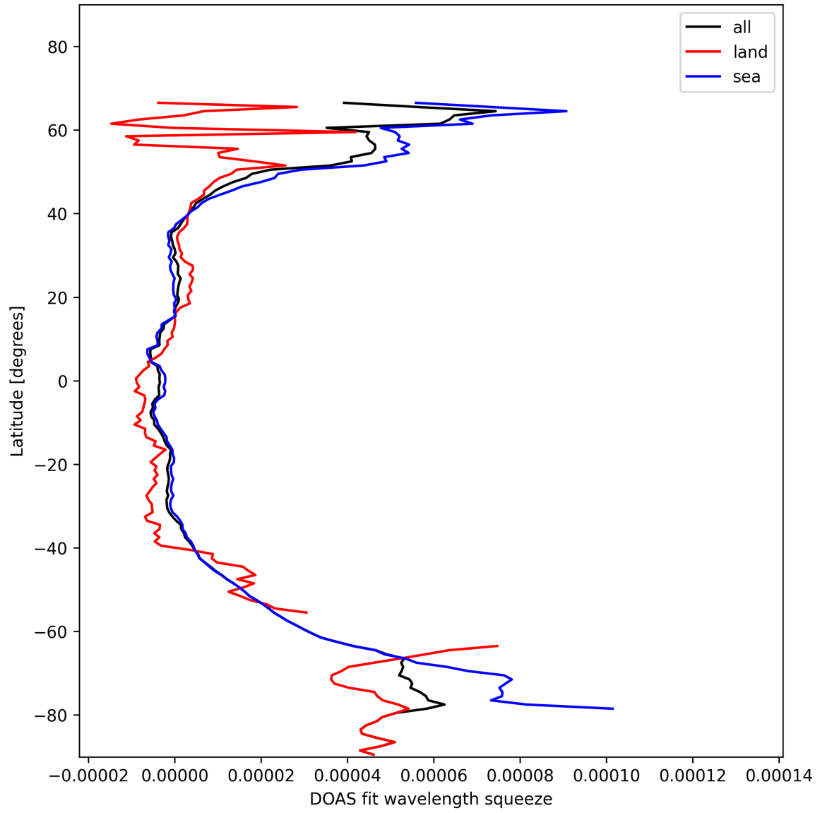
Figure 31: Zonal average of “DOAS fit wavelength squeeze” for 2024-11-14 to 2024-11-16.
