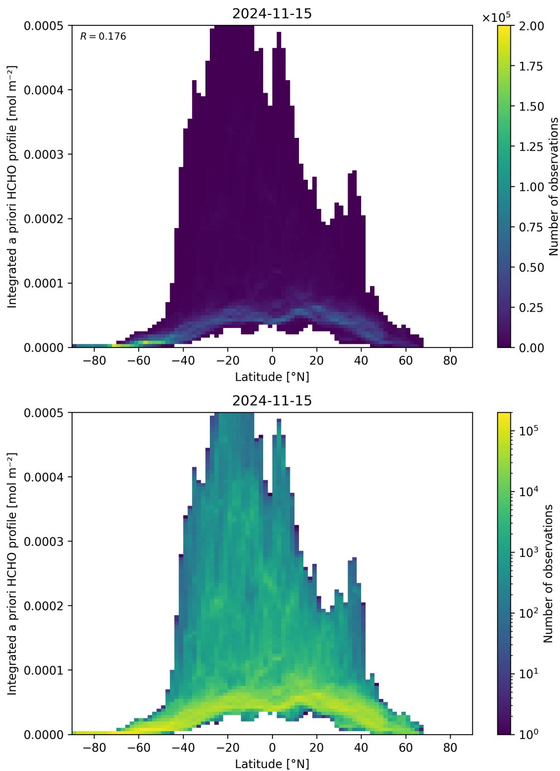
Figure 166: Scatter density plot of “Latitude” against “Integrated a priori HCHO profile” for 2024-11-14 to 2024-11-16.
