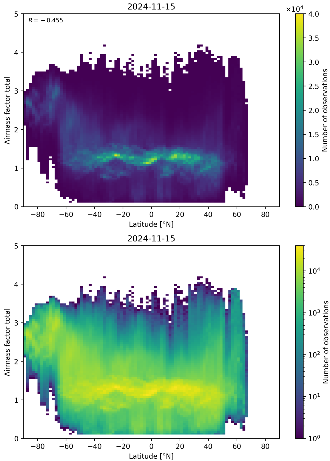
Figure 161: Scatter density plot of “Latitude” against “Airmass factor total” for 2024-11-14 to 2024-11-16.
