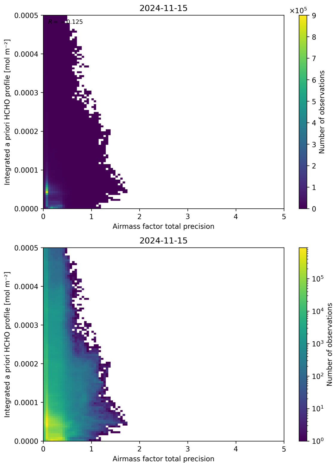
Figure 111: Scatter density plot of “Airmass factor total precision” against “Integrated a priori HCHO profile” for 2024-11-14 to 2024-11-16.
