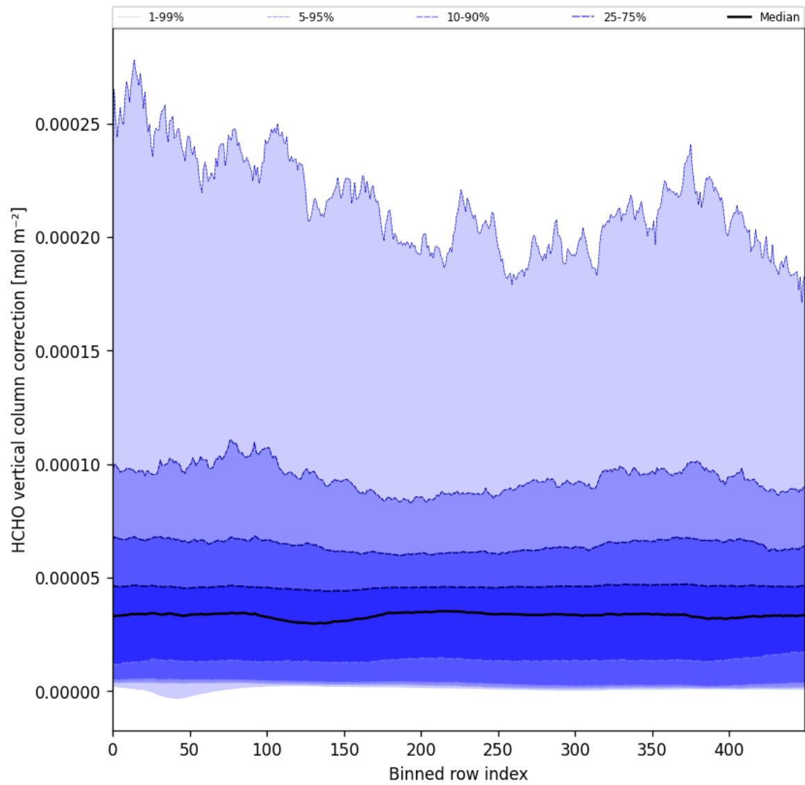
Figure 51: Along track statistics of “HCHO vertical column correction” for 2024-11-14 to 2024-11-16
