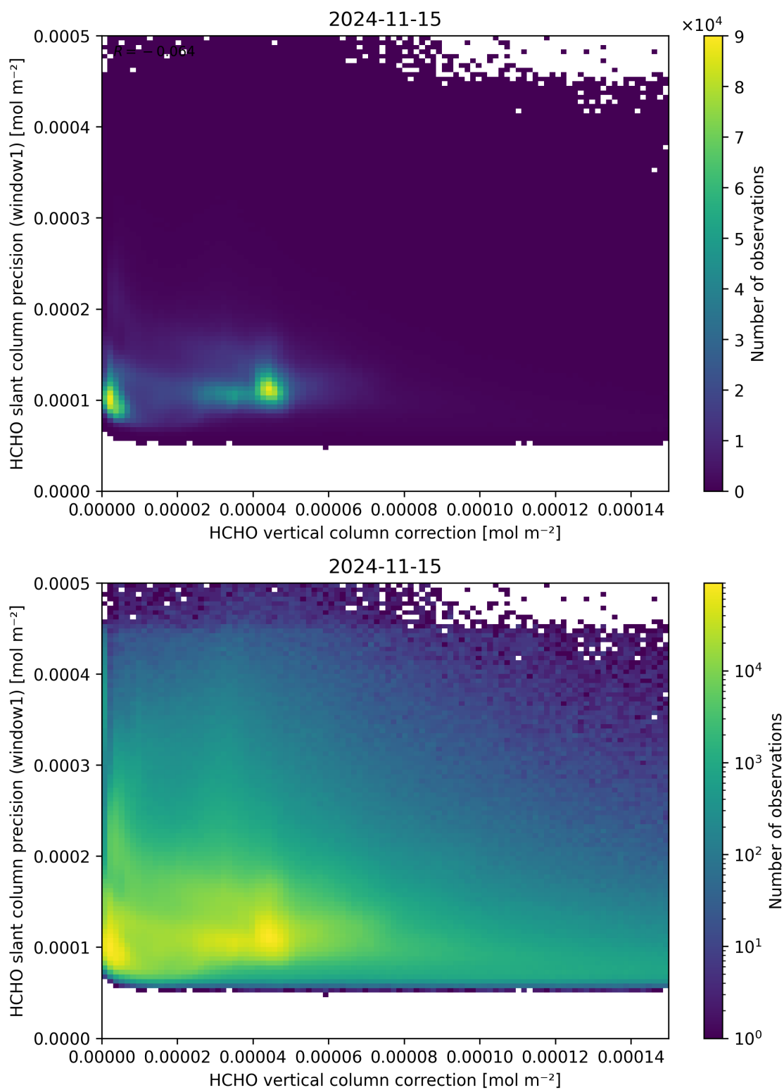
Figure 119: Scatter density plot of “HCHO vertical column correction” against “HCHO slant column precision (window1)” for 2024-11-14 to 2024-11-16.
