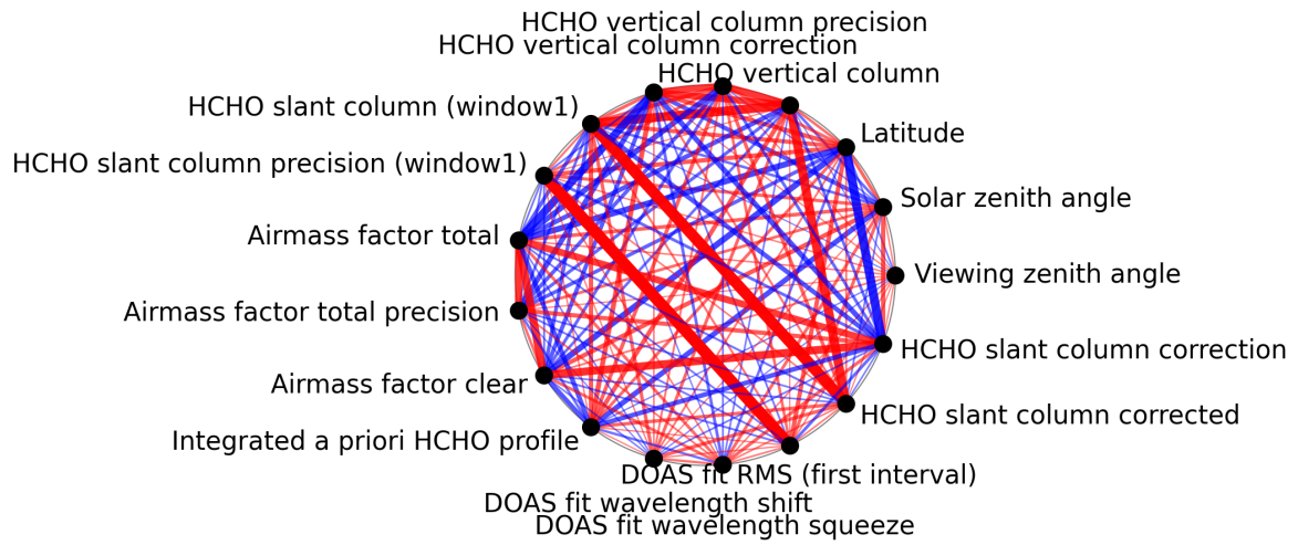
Figure 1: Map of correlation graph for 2024-11-14 to 2024-11-16.
