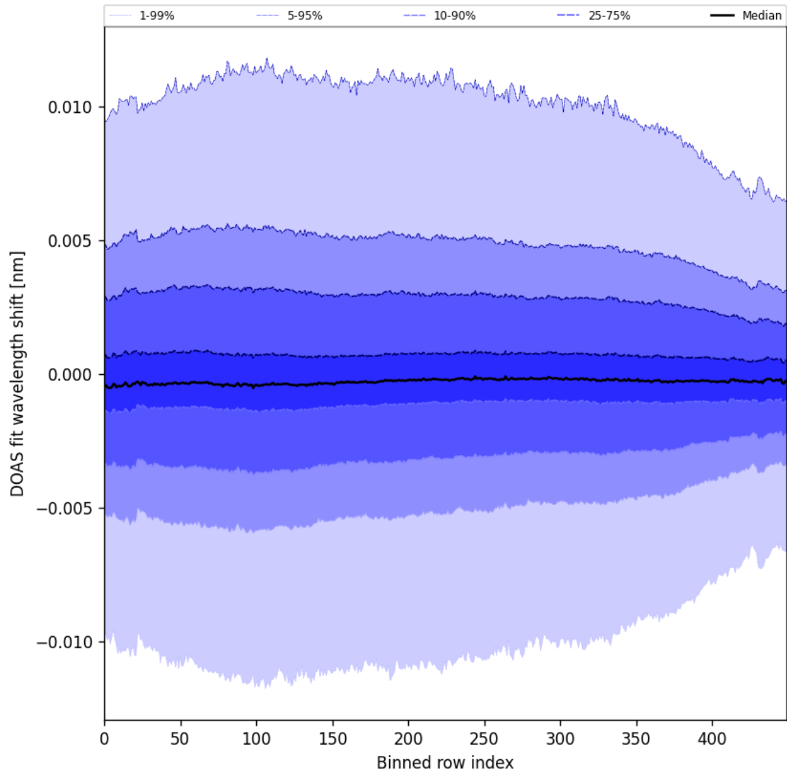
Figure 58: Along track statistics of “DOAS fit wavelength shift” for 2024-11-14 to 2024-11-16
