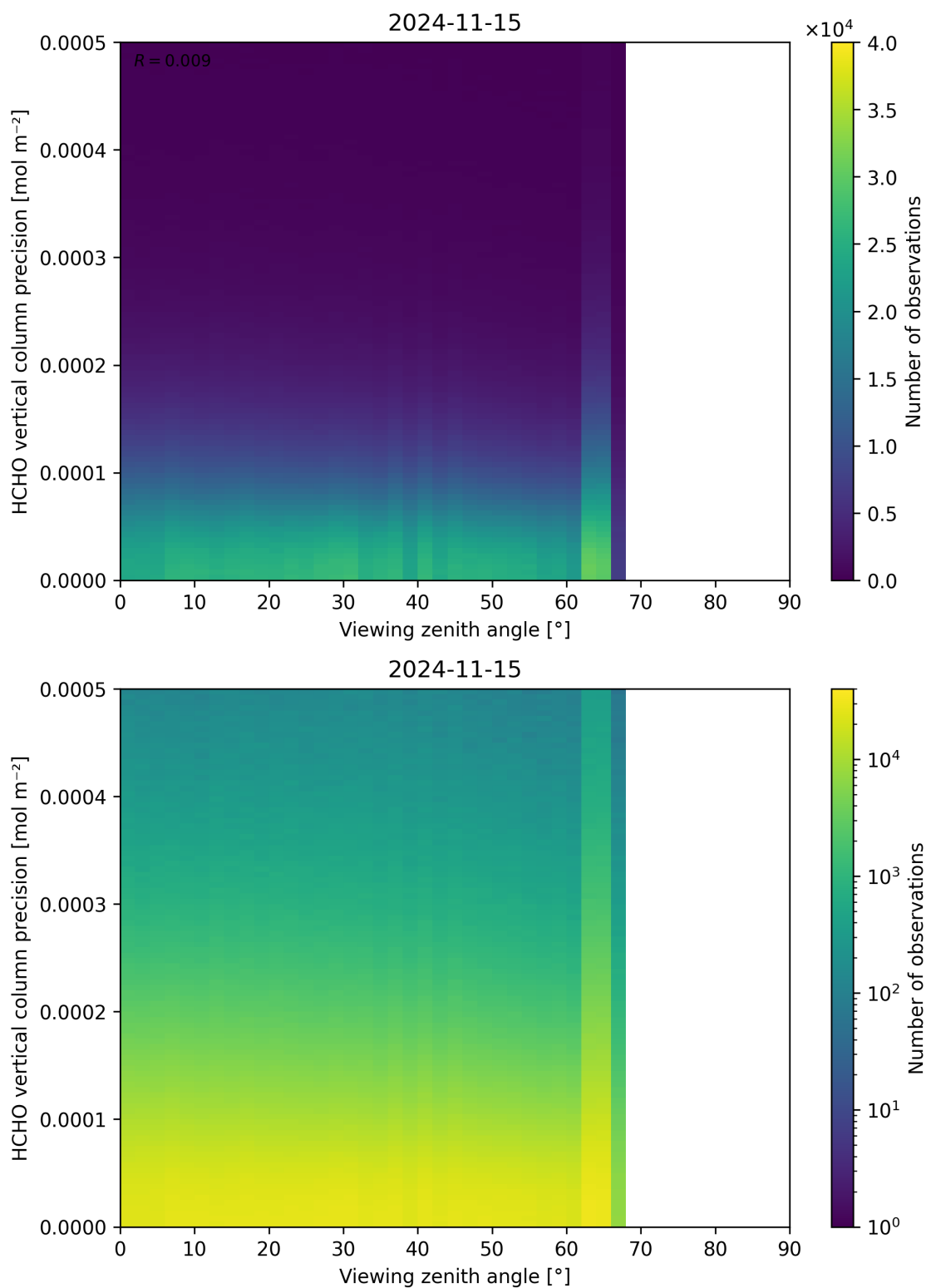
Figure 194: Scatter density plot of “Viewing zenith angle” against “HCHO vertical column precision” for 2024-11-14 to 2024-11-16.
