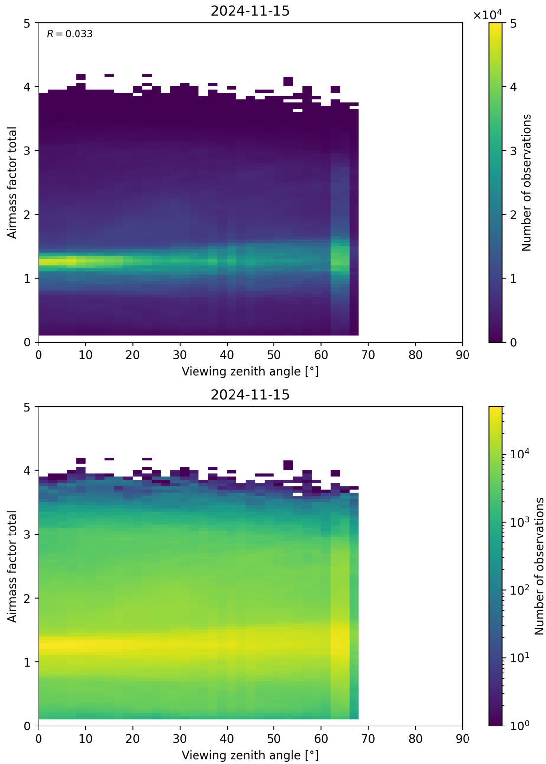
Figure 190: Scatter density plot of “Viewing zenith angle” against “Airmass factor total” for 2024-11-14 to 2024-11-16.
