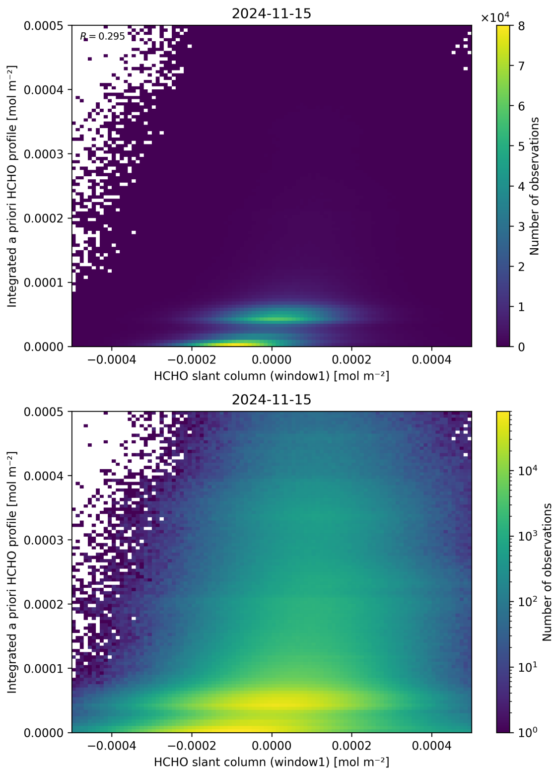
Figure 87: Scatter density plot of “HCHO slant column (window1)” against “Integrated a priori HCHO profile” for 2024-11-14 to 2024-11-16.
