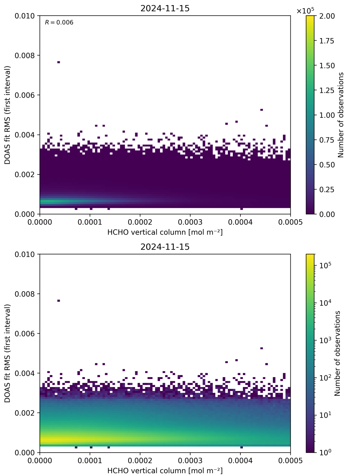
Figure 123: Scatter density plot of “HCHO vertical column” against “DOAS fit RMS (first interval)” for 2024-11-14 to 2024-11-16.
