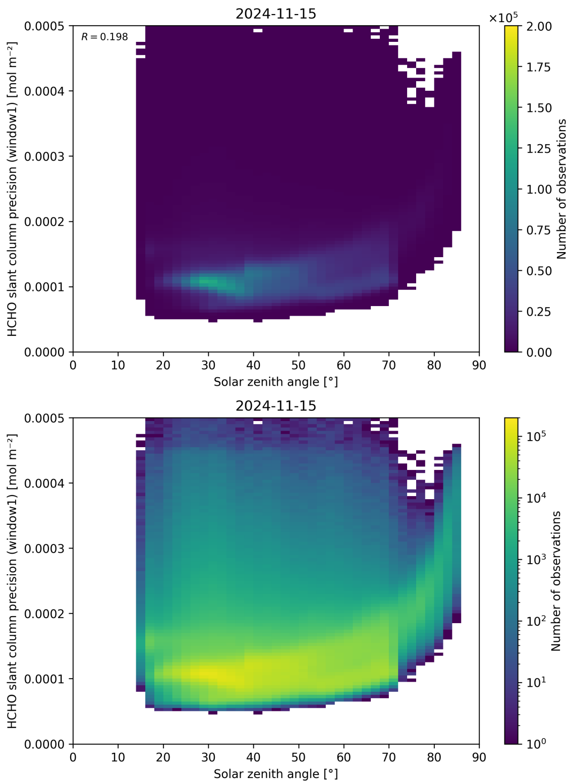
Figure 174: Scatter density plot of “Solar zenith angle” against “HCHO slant column precision (window1)” for 2024-11-14 to 2024-11-16.
