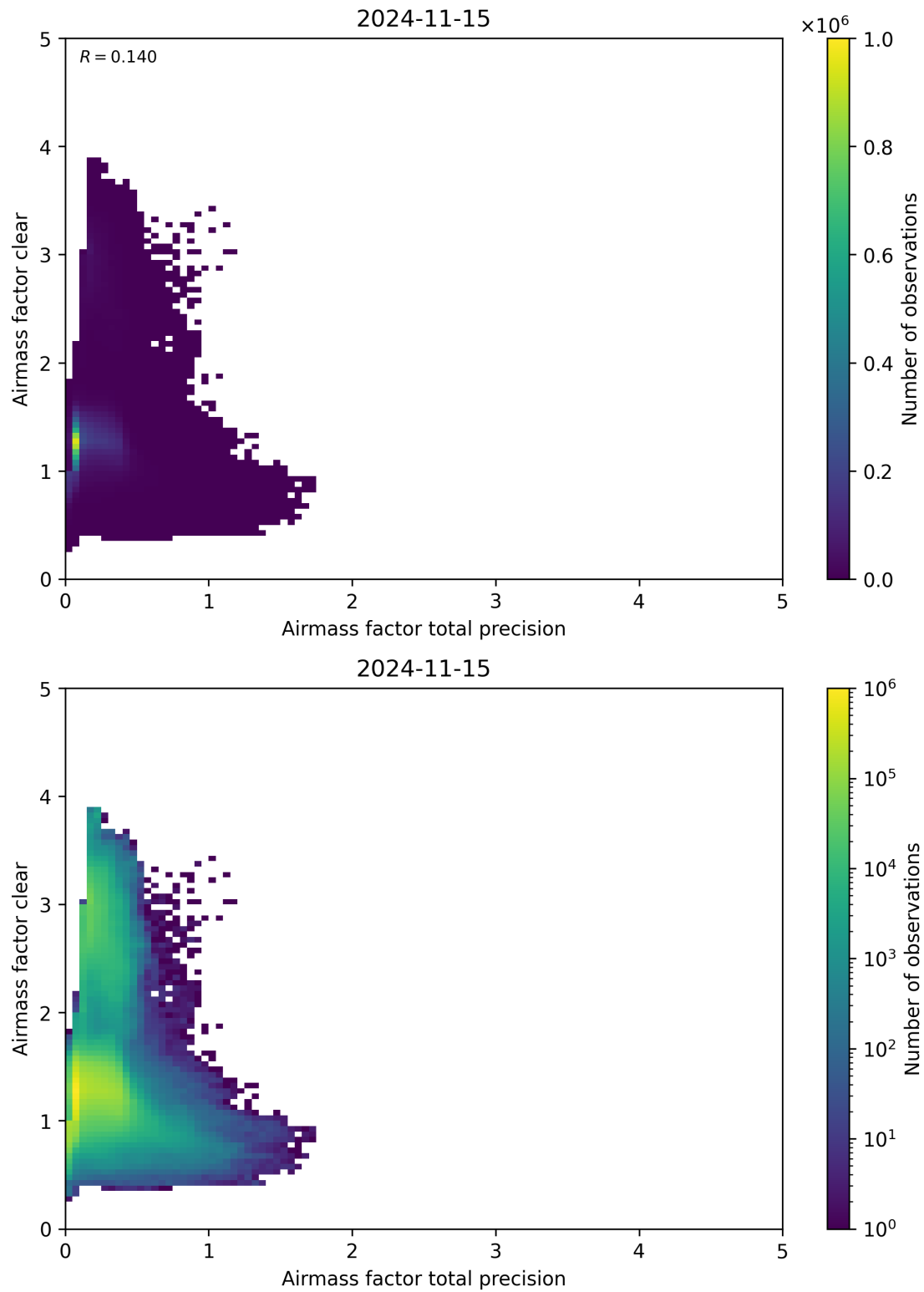
Figure 108: Scatter density plot of “Airmass factor total precision” against “Airmass factor clear” for 2024-11-14 to 2024-11-16.
