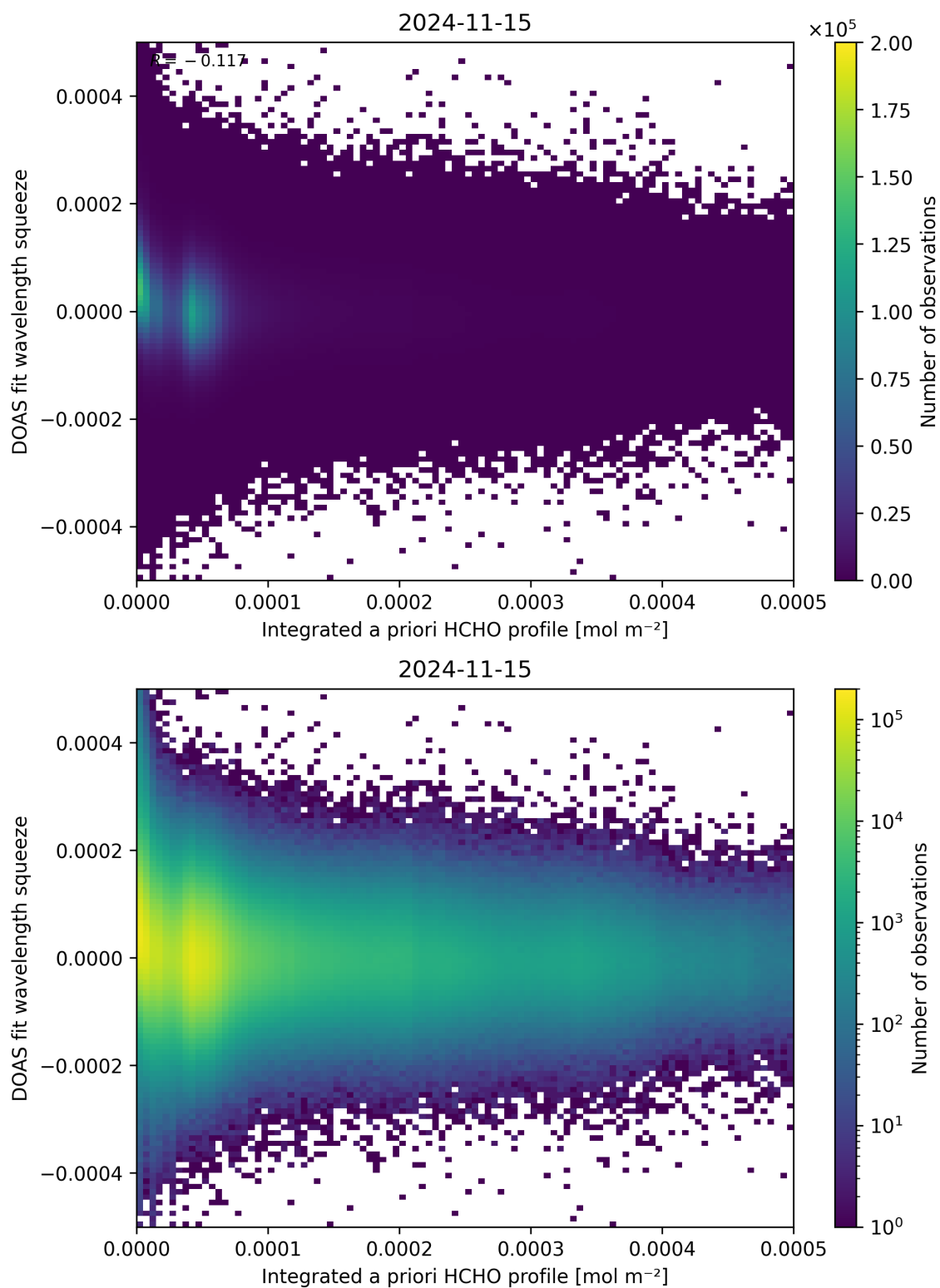
Figure 150: Scatter density plot of “Integrated a priori HCHO profile” against “DOAS fit wavelength squeeze” for 2024-11-14 to 2024-11-16.
