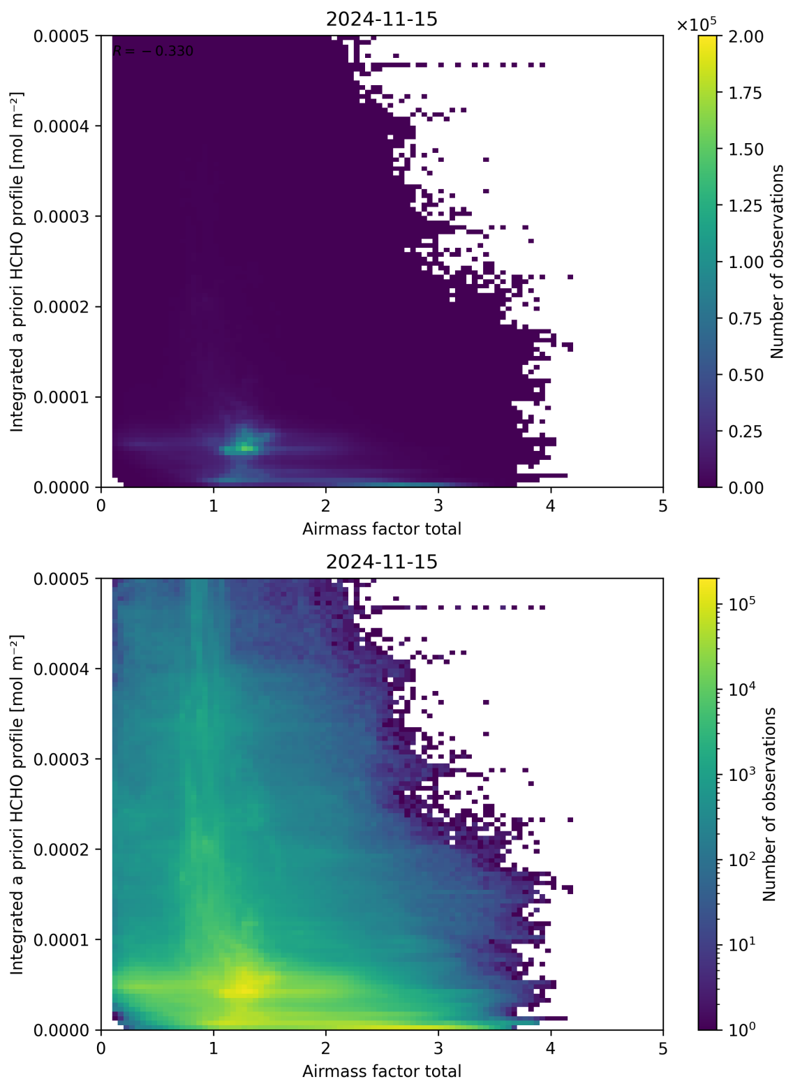
Figure 104: Scatter density plot of “Airmass factor total” against “Integrated a priori HCHO profile” for 2024-11-14 to 2024-11-16.
