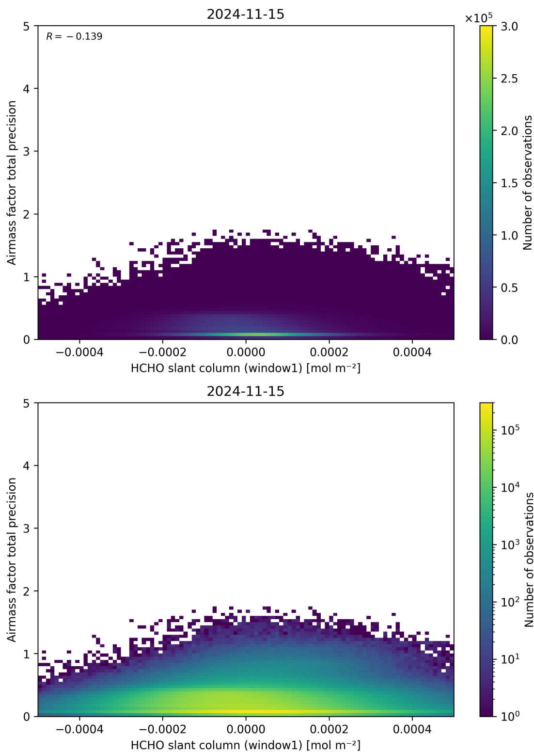
Figure 86: Scatter density plot of “HCHO slant column (window1)” against “Airmass factor total precision” for 2024-11-14 to 2024-11-16.
