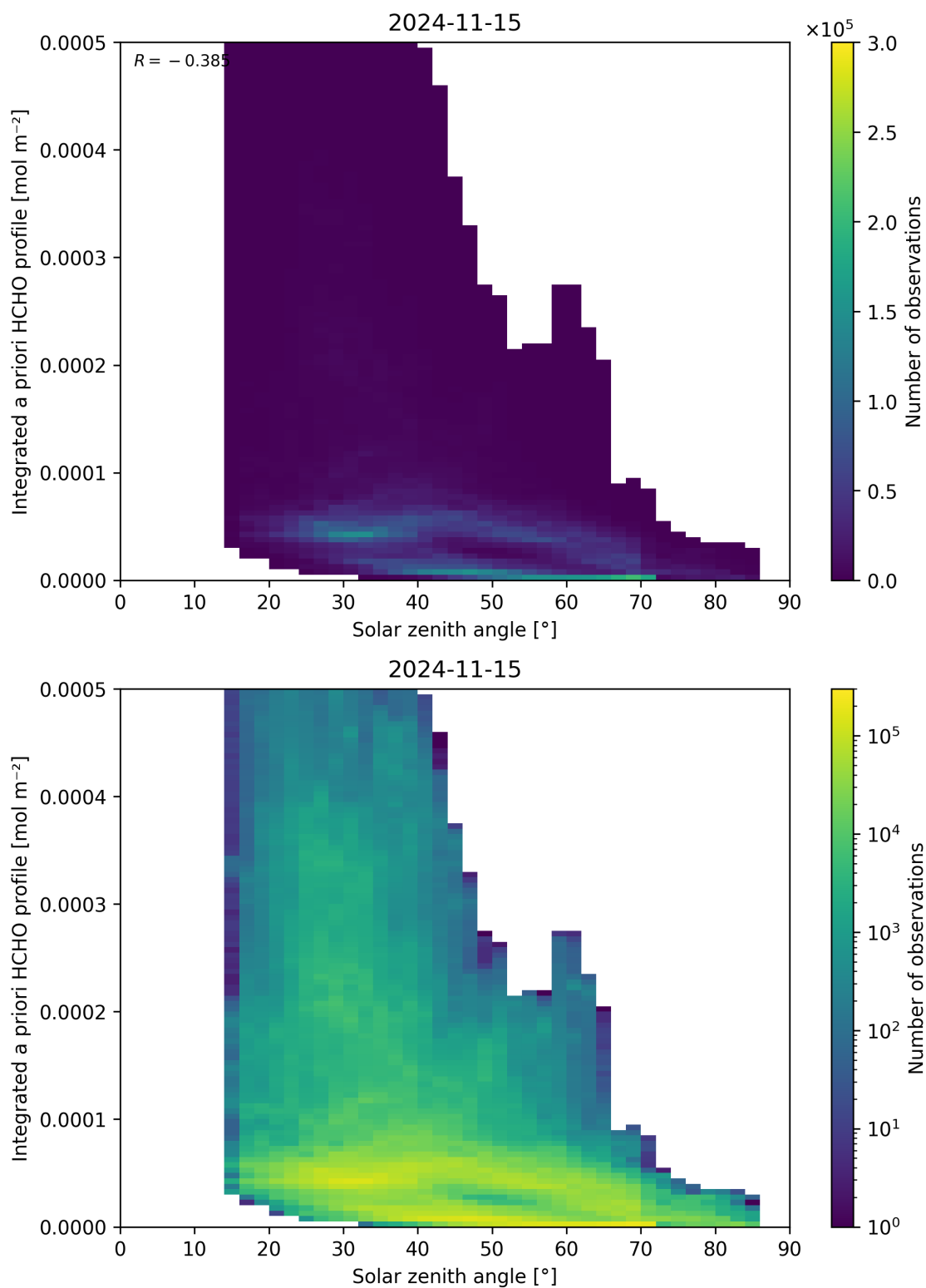
Figure 180: Scatter density plot of “Solar zenith angle” against “Integrated a priori HCHO profile” for 2024-11-14 to 2024-11-16.
