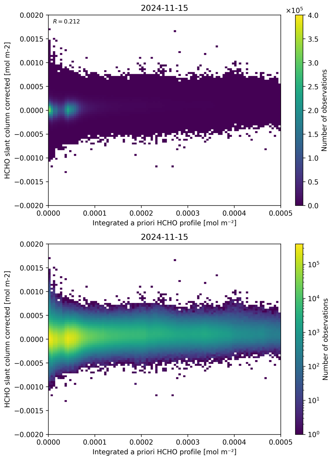
Figure 151: Scatter density plot of “Integrated a priori HCHO profile” against “HCHO slant column corrected” for 2024-11-14 to 2024-11-16.
