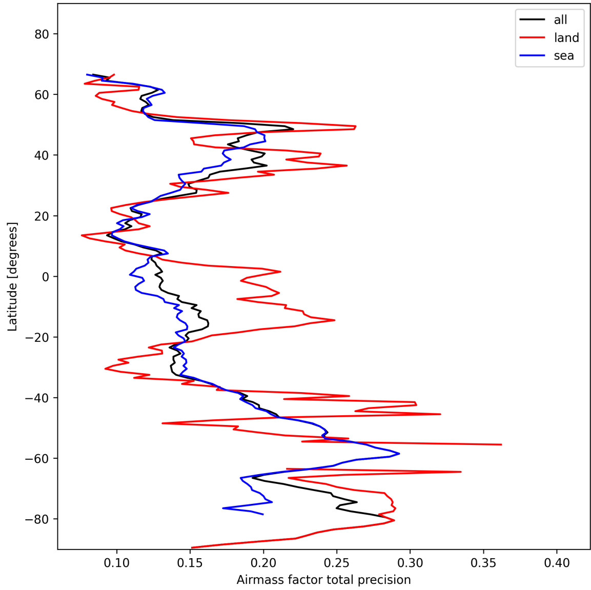
Figure 27: Zonal average of “Airmass factor total precision” for 2024-11-14 to 2024-11-16.
