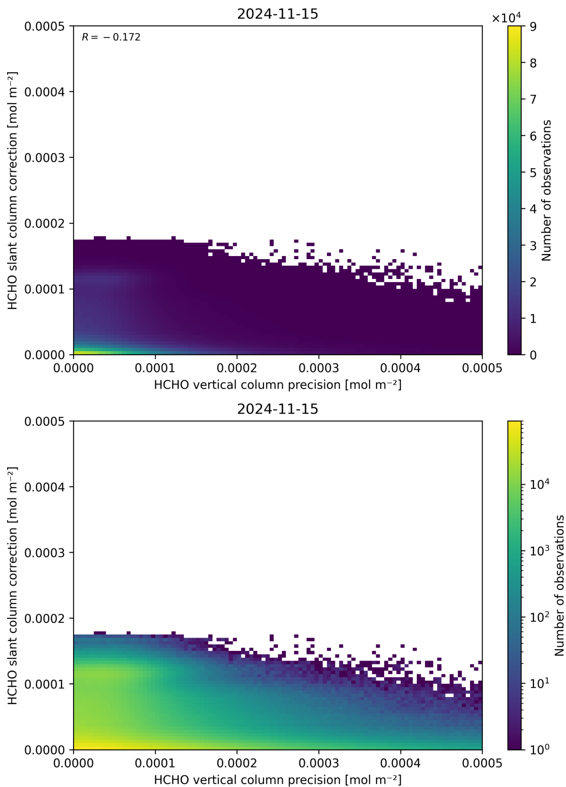
Figure 141: Scatter density plot of “HCHO vertical column precision” against “HCHO slant column correction” for 2024-11-14 to 2024-11-16.
