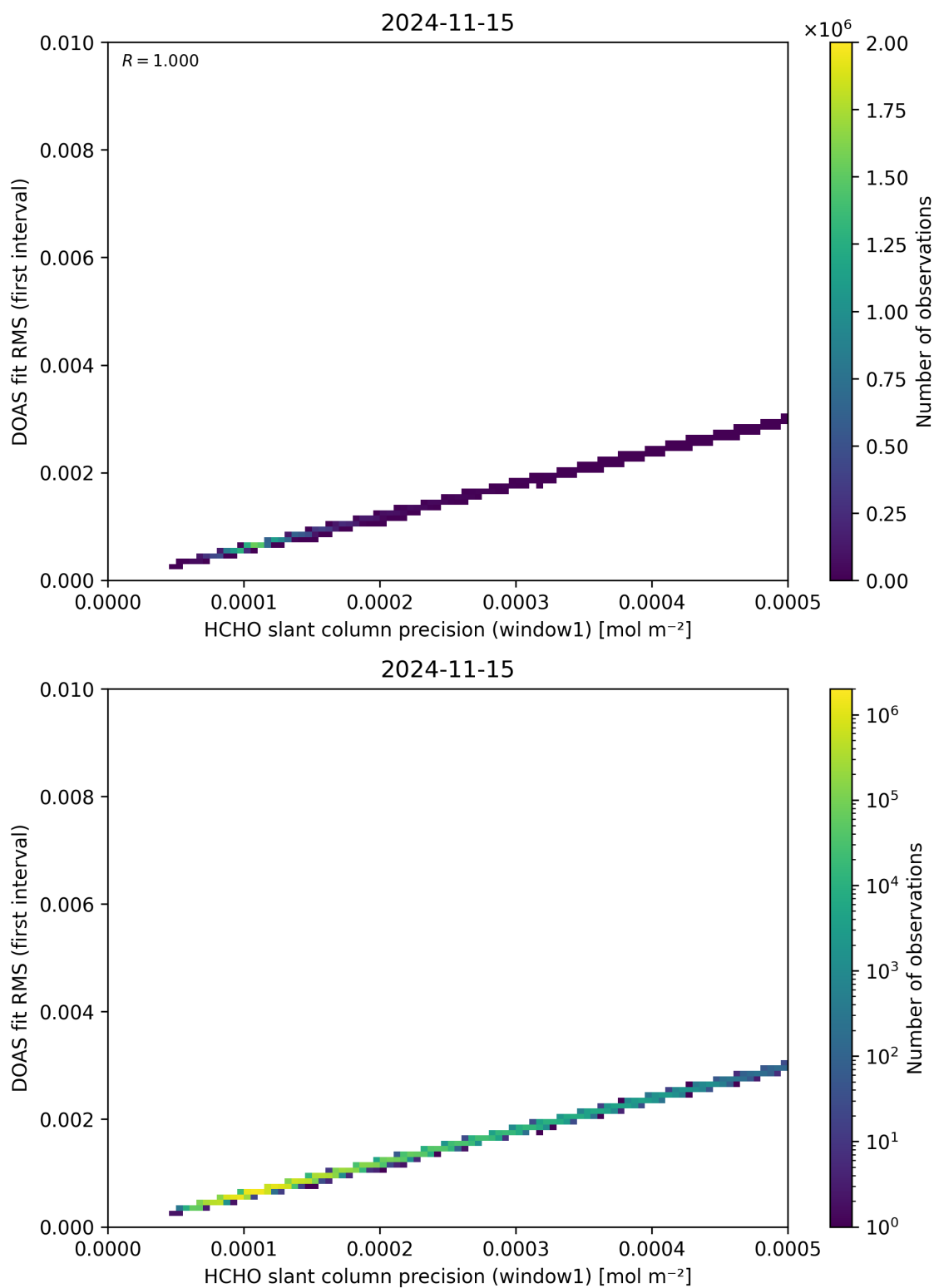
Figure 88: Scatter density plot of “HCHO slant column precision (window1)” against “DOAS fit RMS (first interval)” for 2024-11-14 to 2024-11-16.
