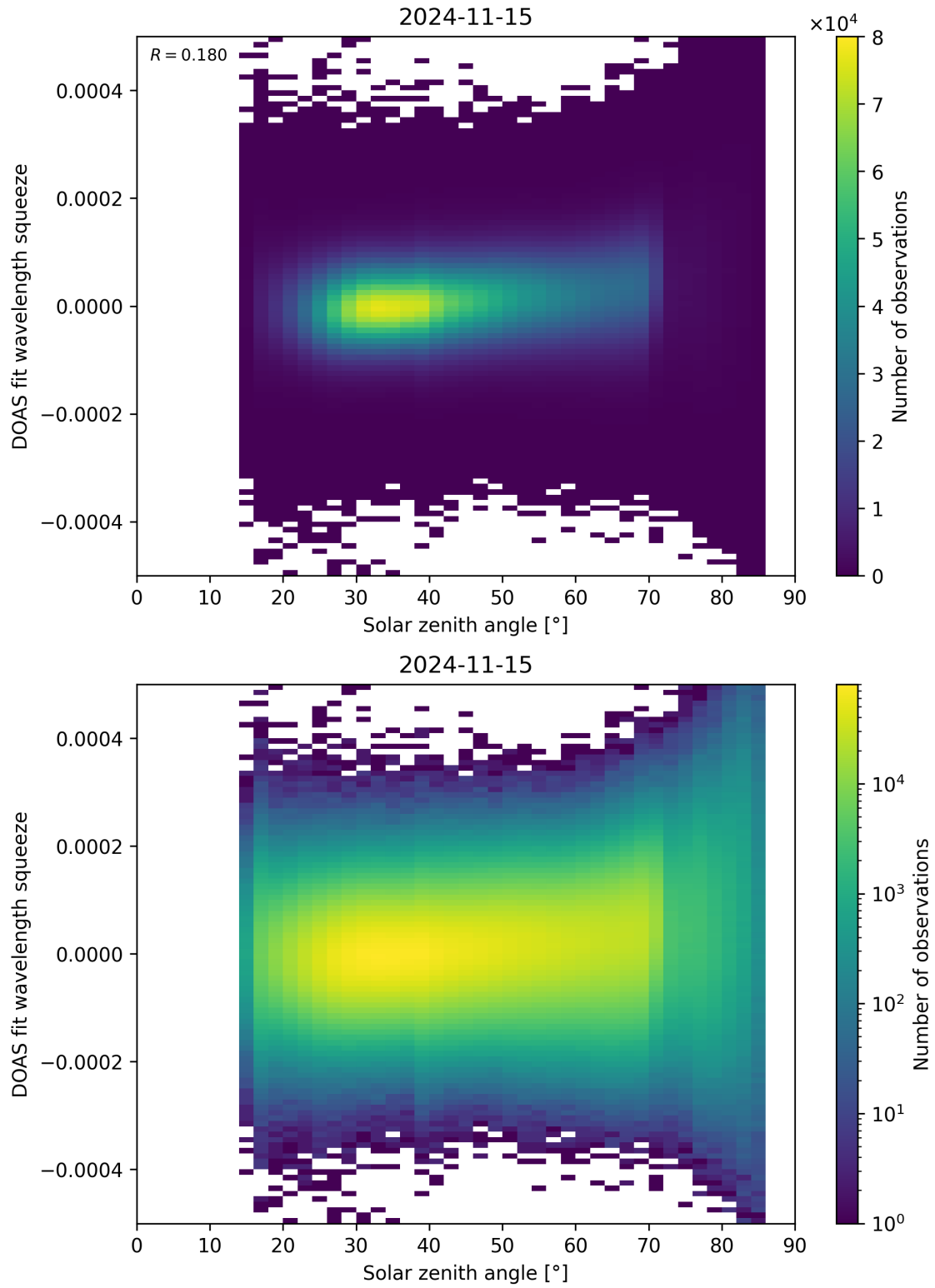
Figure 169: Scatter density plot of “Solar zenith angle” against “DOAS fit wavelength squeeze” for 2024-11-14 to 2024-11-16.
