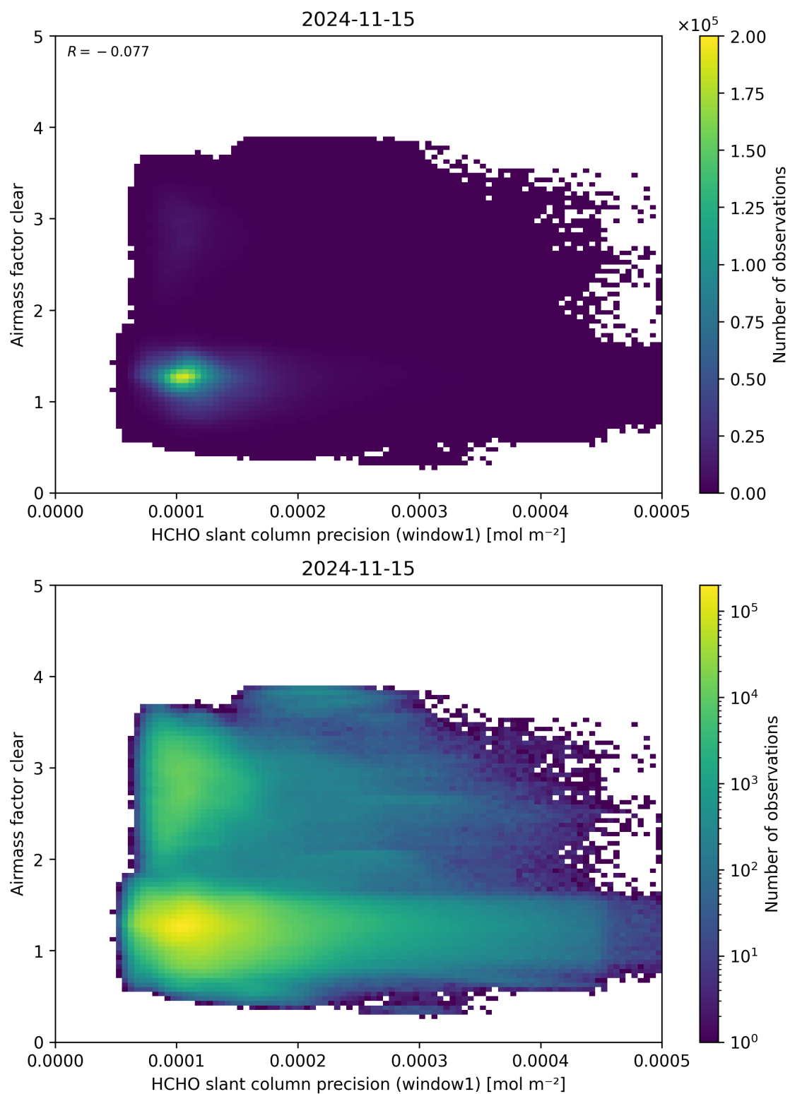
Figure 91: Scatter density plot of “HCHO slant column precision (window1)” against “Airmass factor clear” for 2024-11-14 to 2024-11-16.
