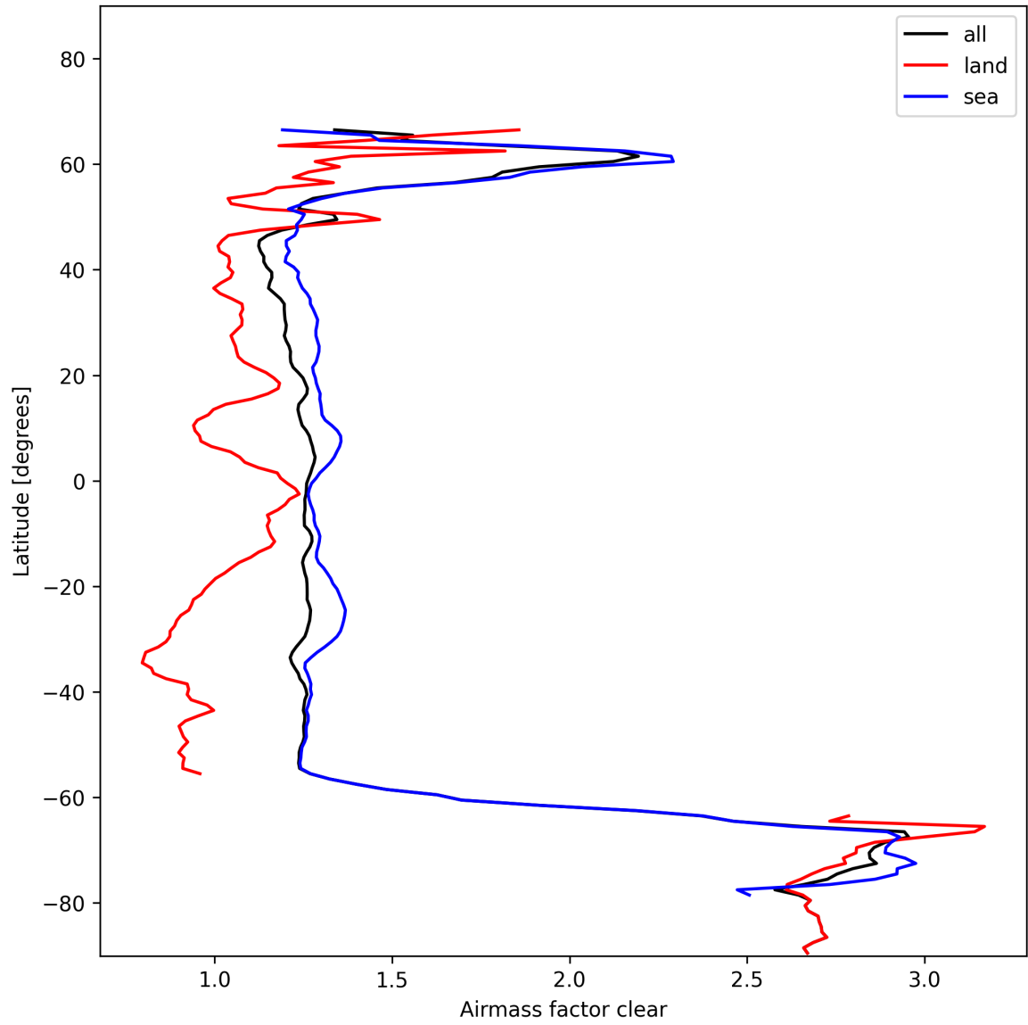
Figure 28: Zonal average of “Airmass factor clear” for 2024-11-14 to 2024-11-16.
