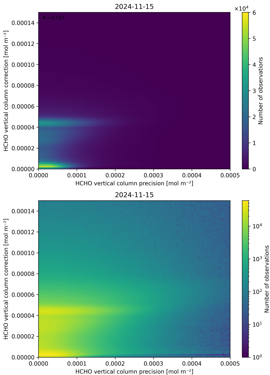
Figure 146: Scatter density plot of “HCHO vertical column precision” against “HCHO vertical column correction” for 2024-11-14 to 2024-11-16.
