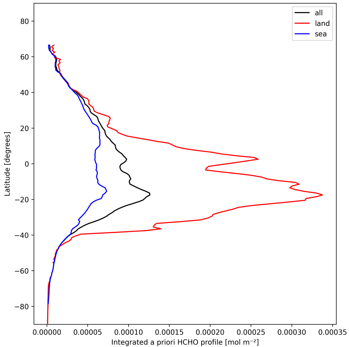
Figure 29: Zonal average of “Integrated a priori HCHO profile” for 2024-11-14 to 2024-11-16.
