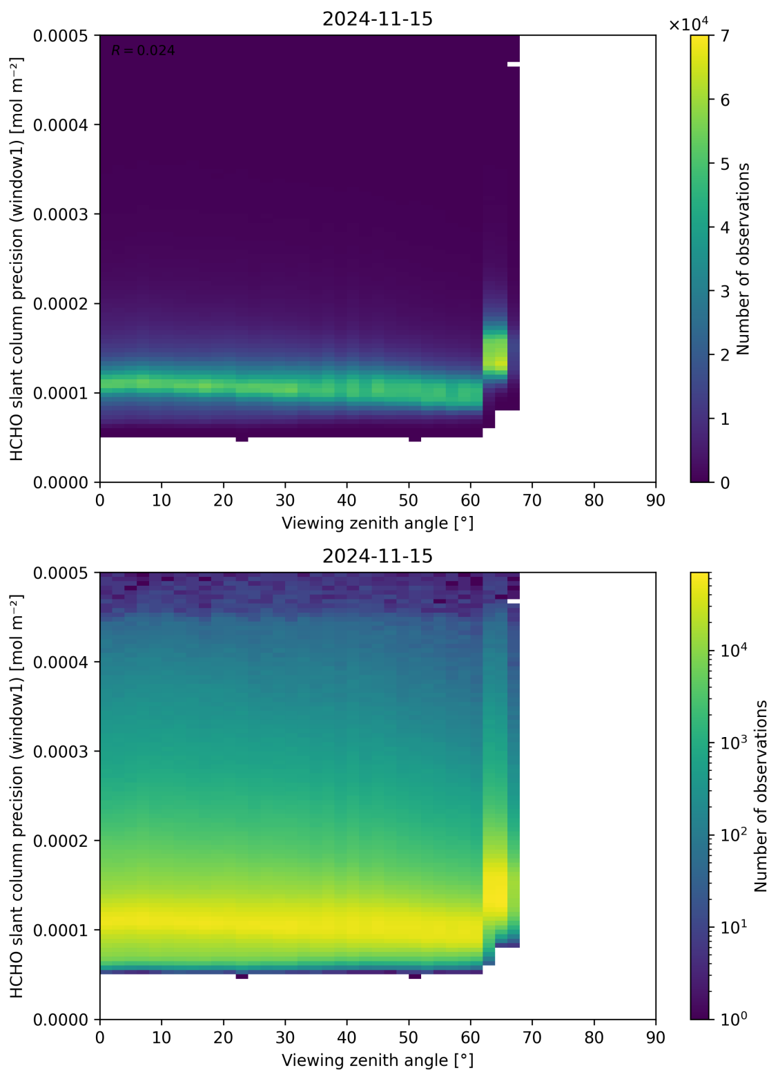
Figure 189: Scatter density plot of “Viewing zenith angle” against “HCHO slant column precision (window1)” for 2024-11-14 to 2024-11-16.
