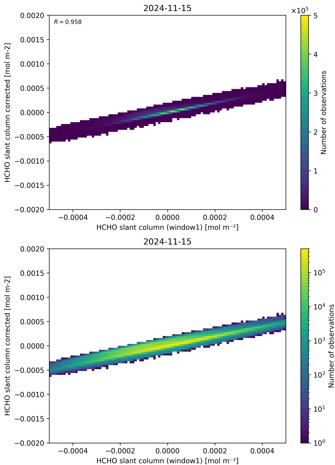
Figure 82: Scatter density plot of “HCHO slant column (window1)” against “HCHO slant column corrected” for 2024-11-14 to 2024-11-16.
