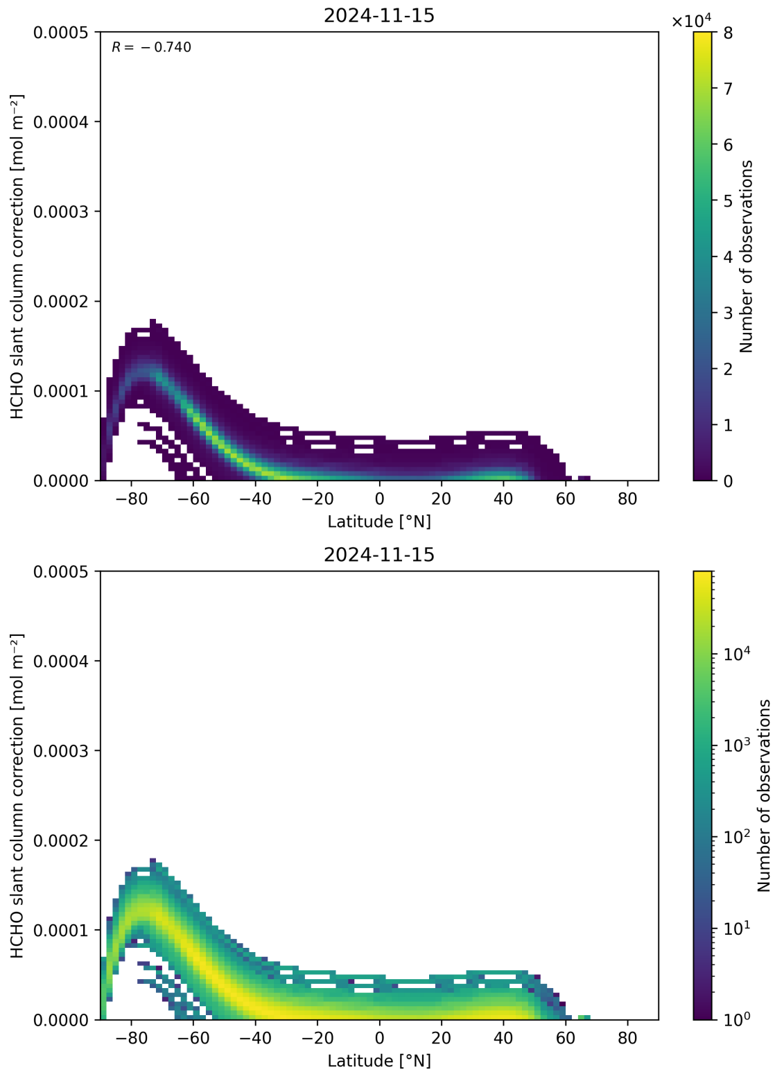
Figure 158: Scatter density plot of “Latitude” against “HCHO slant column correction” for 2024-11-14 to 2024-11-16.
