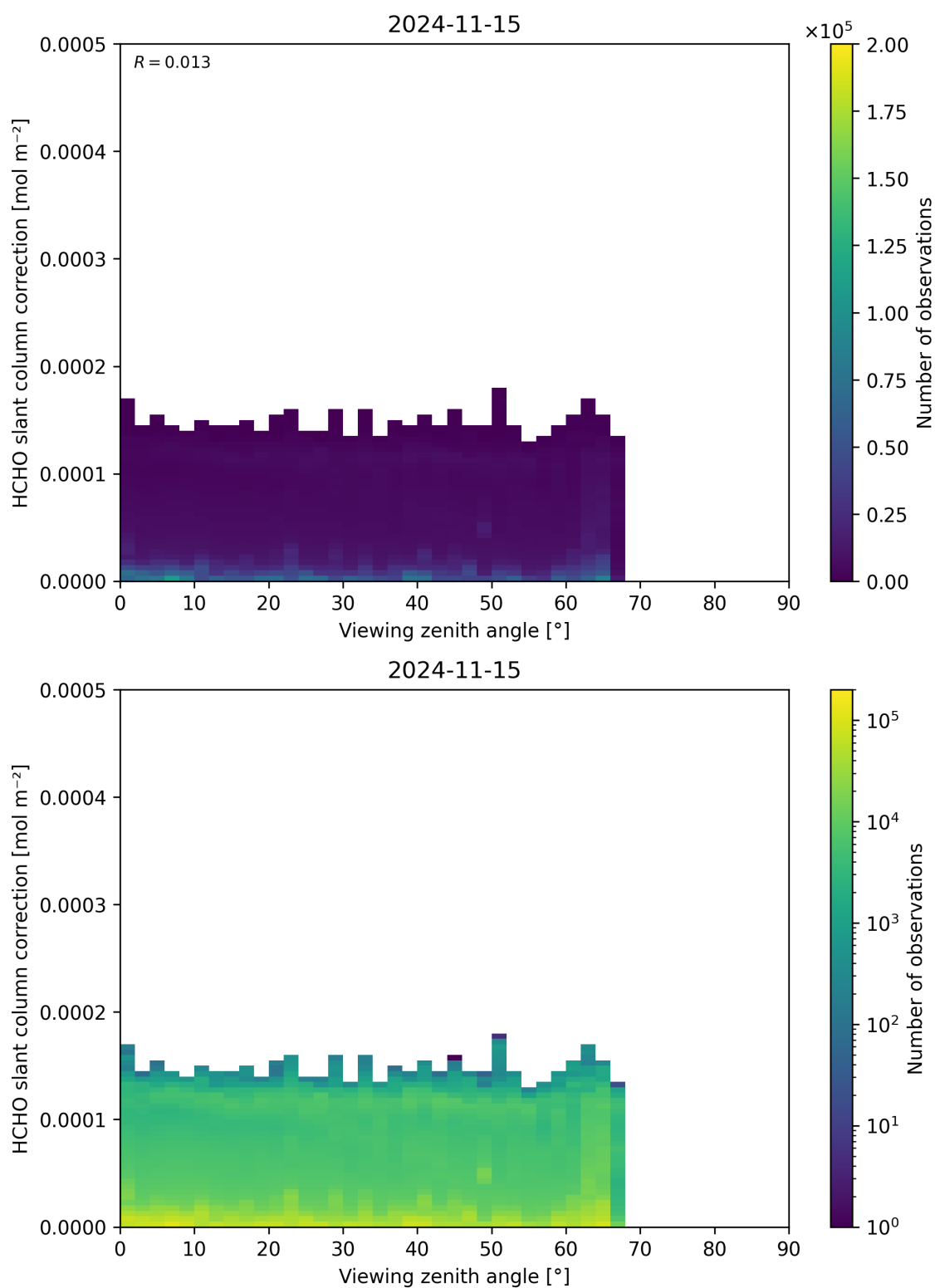
Figure 187: Scatter density plot of “Viewing zenith angle” against “HCHO slant column correction” for 2024-11-14 to 2024-11-16.
