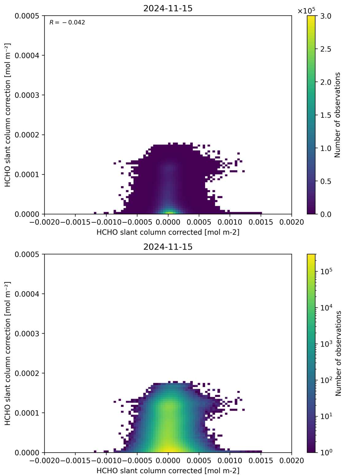
Figure 77: Scatter density plot of “HCHO slant column corrected” against “HCHO slant column correction” for 2024-11-14 to 2024-11-16.
