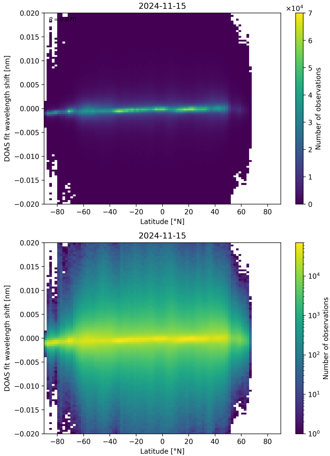
Figure 154: Scatter density plot of “Latitude” against “DOAS fit wavelength shift” for 2024-11-14 to 2024-11-16.
