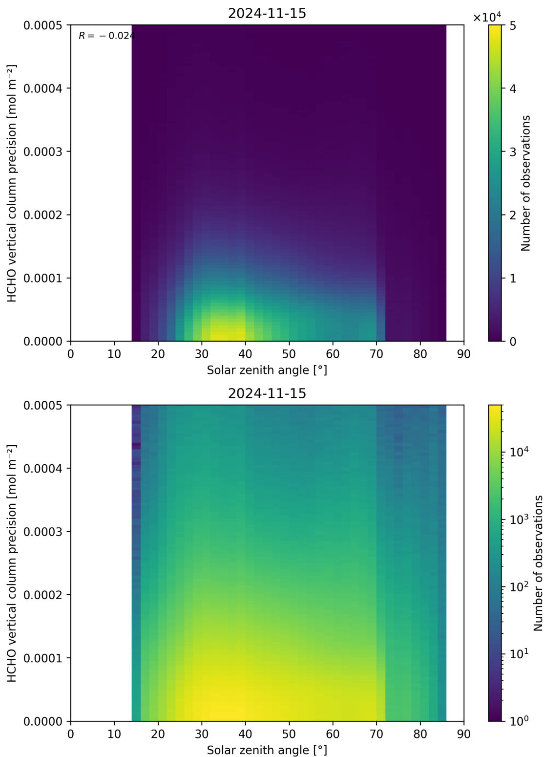
Figure 179: Scatter density plot of “Solar zenith angle” against “HCHO vertical column precision” for 2024-11-14 to 2024-11-16.
