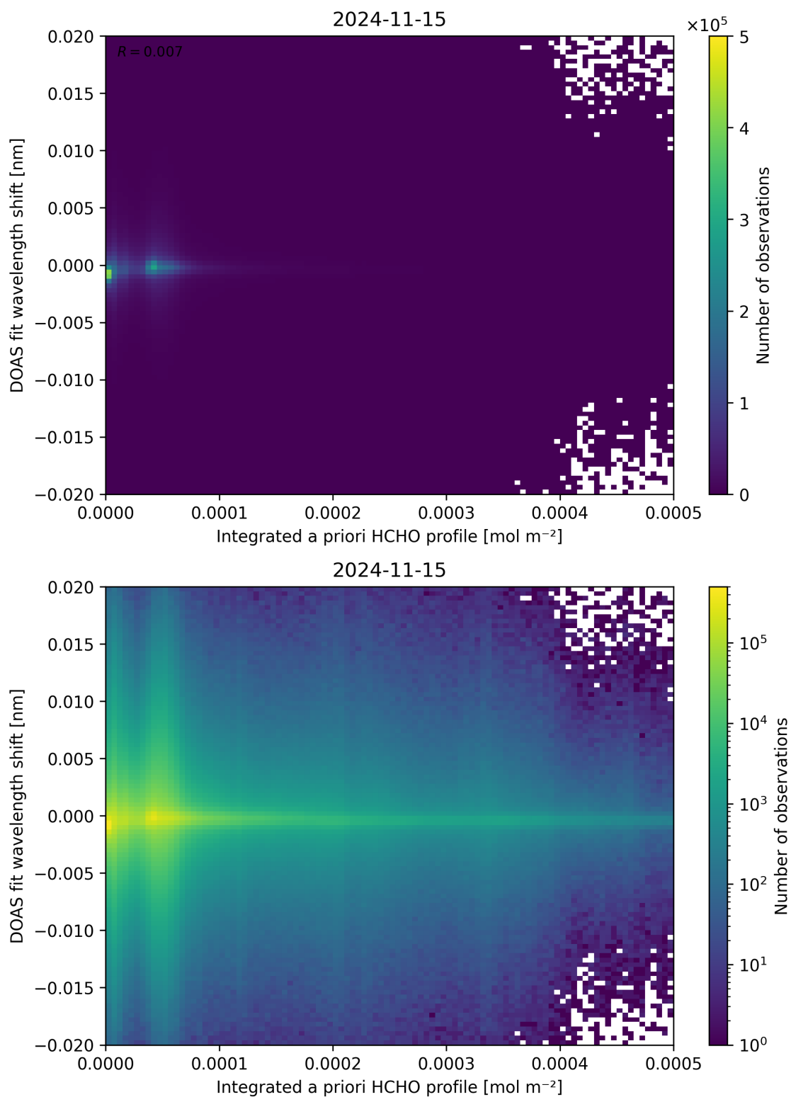
Figure 149: Scatter density plot of “Integrated a priori HCHO profile” against “DOAS fit wavelength shift” for 2024-11-14 to 2024-11-16.
