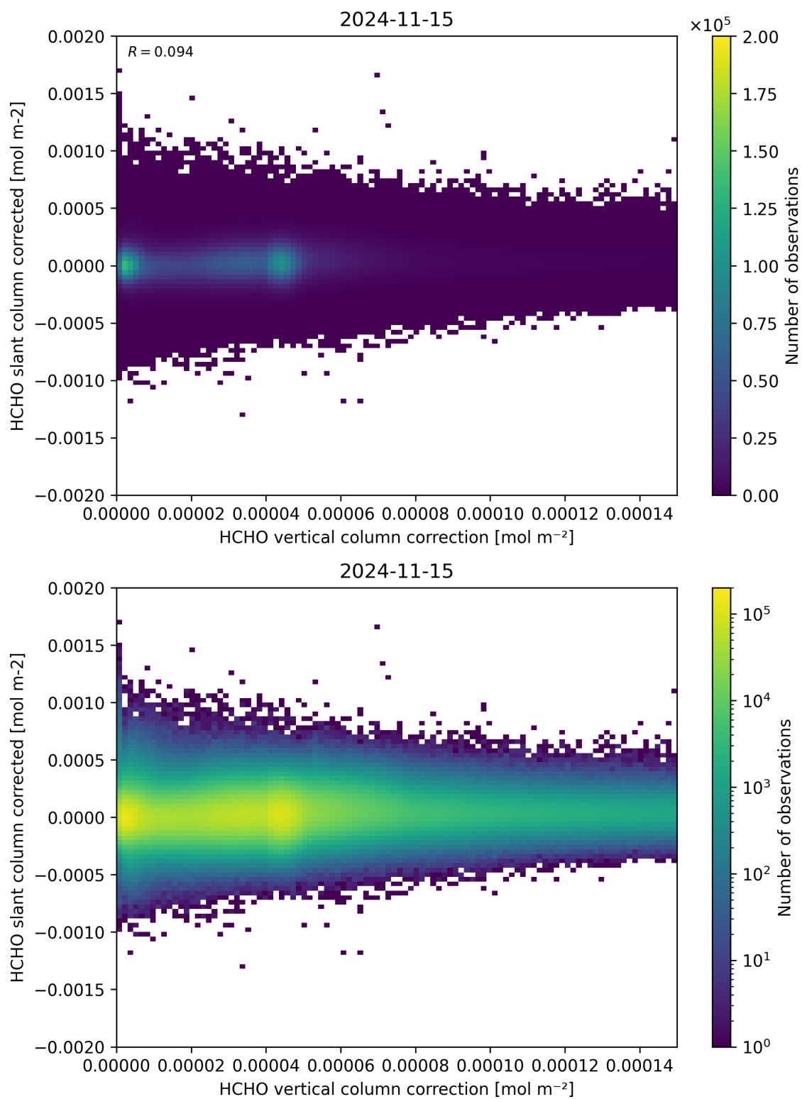
Figure 116: Scatter density plot of “HCHO vertical column correction” against “HCHO slant column corrected” for 2024-11-14 to 2024-11-16.
