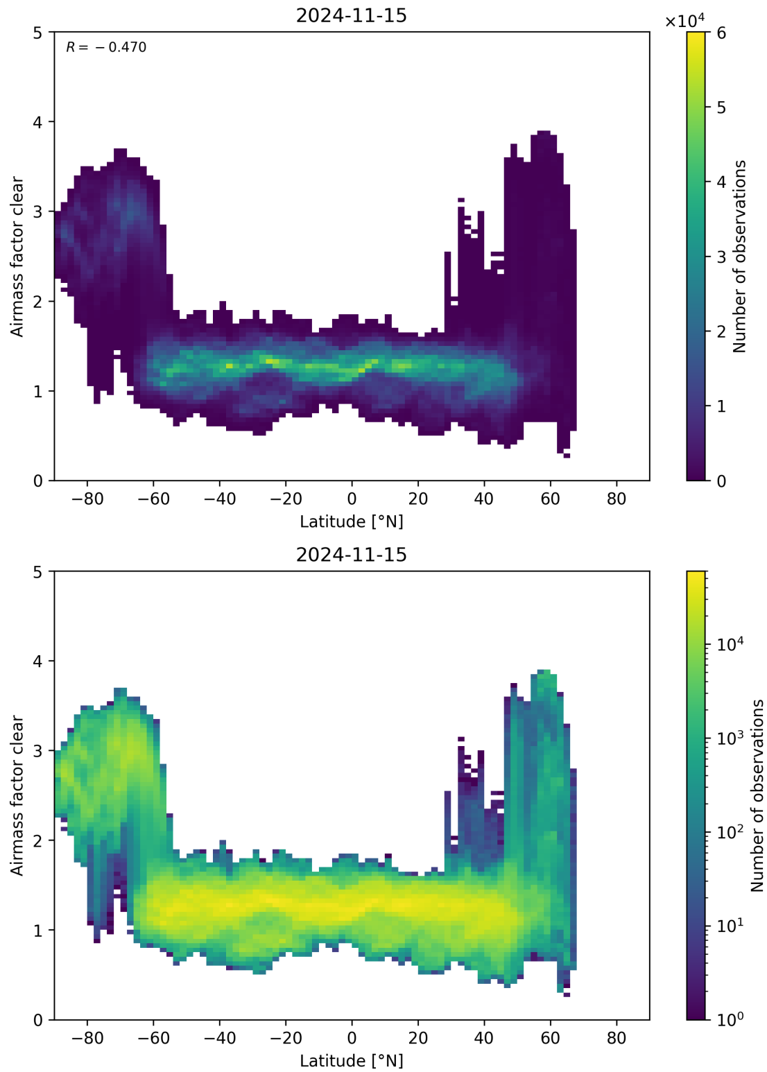
Figure 156: Scatter density plot of “Latitude” against “Airmass factor clear” for 2024-11-14 to 2024-11-16.
