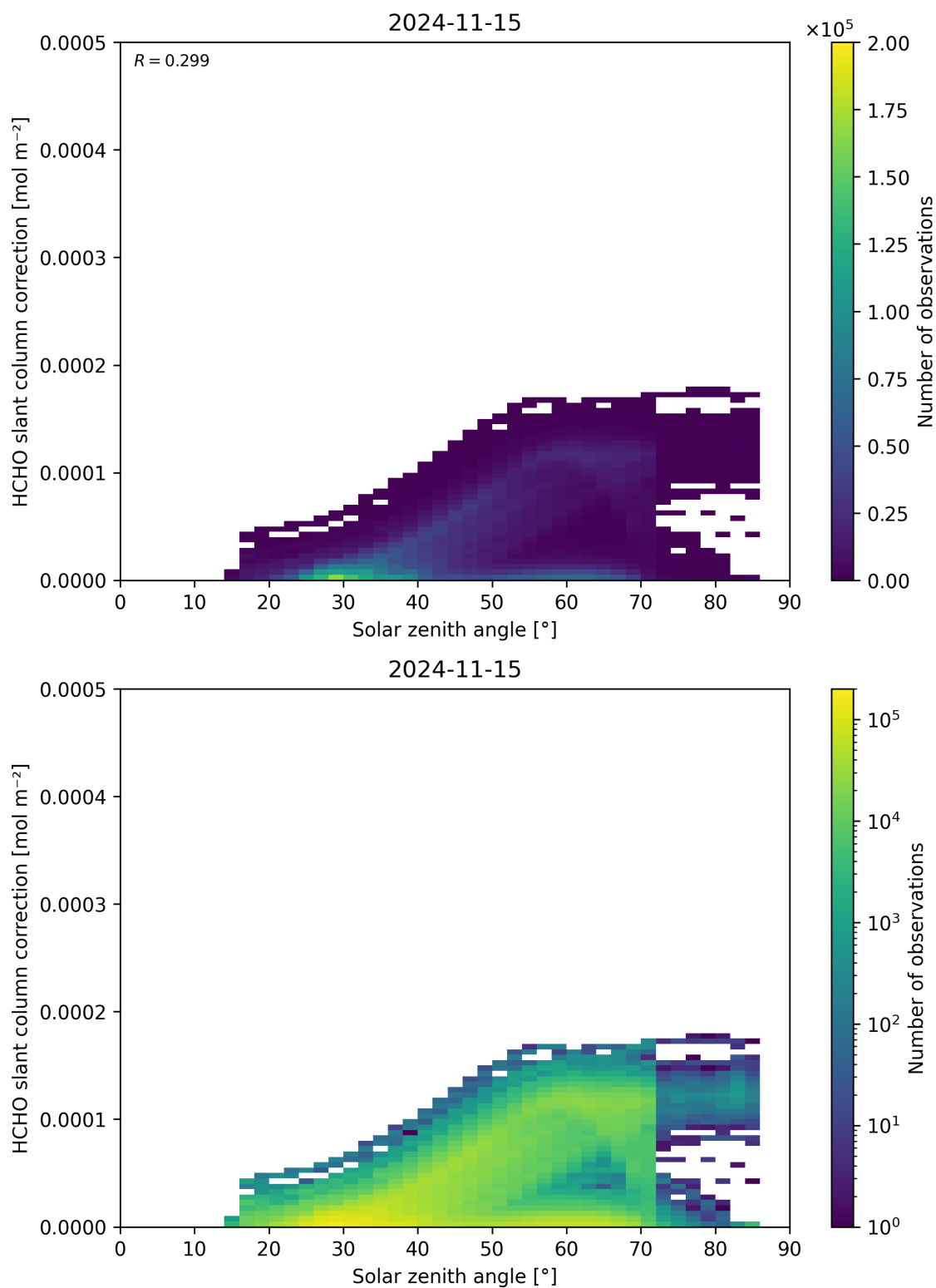
Figure 172: Scatter density plot of “Solar zenith angle” against “HCHO slant column correction” for 2024-11-14 to 2024-11-16.
