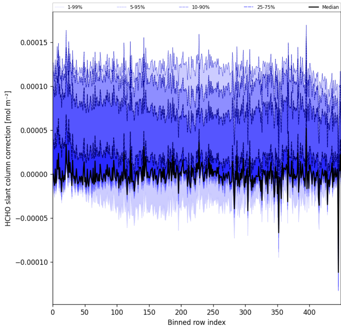
Figure 61: Along track statistics of “HCHO slant column correction” for 2024-11-14 to 2024-11-16
