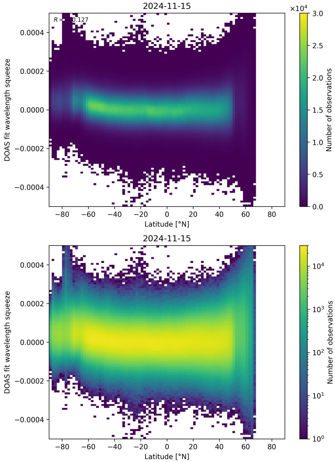
Figure 155: Scatter density plot of “Latitude” against “DOAS fit wavelength squeeze” for 2024-11-14 to 2024-11-16.
