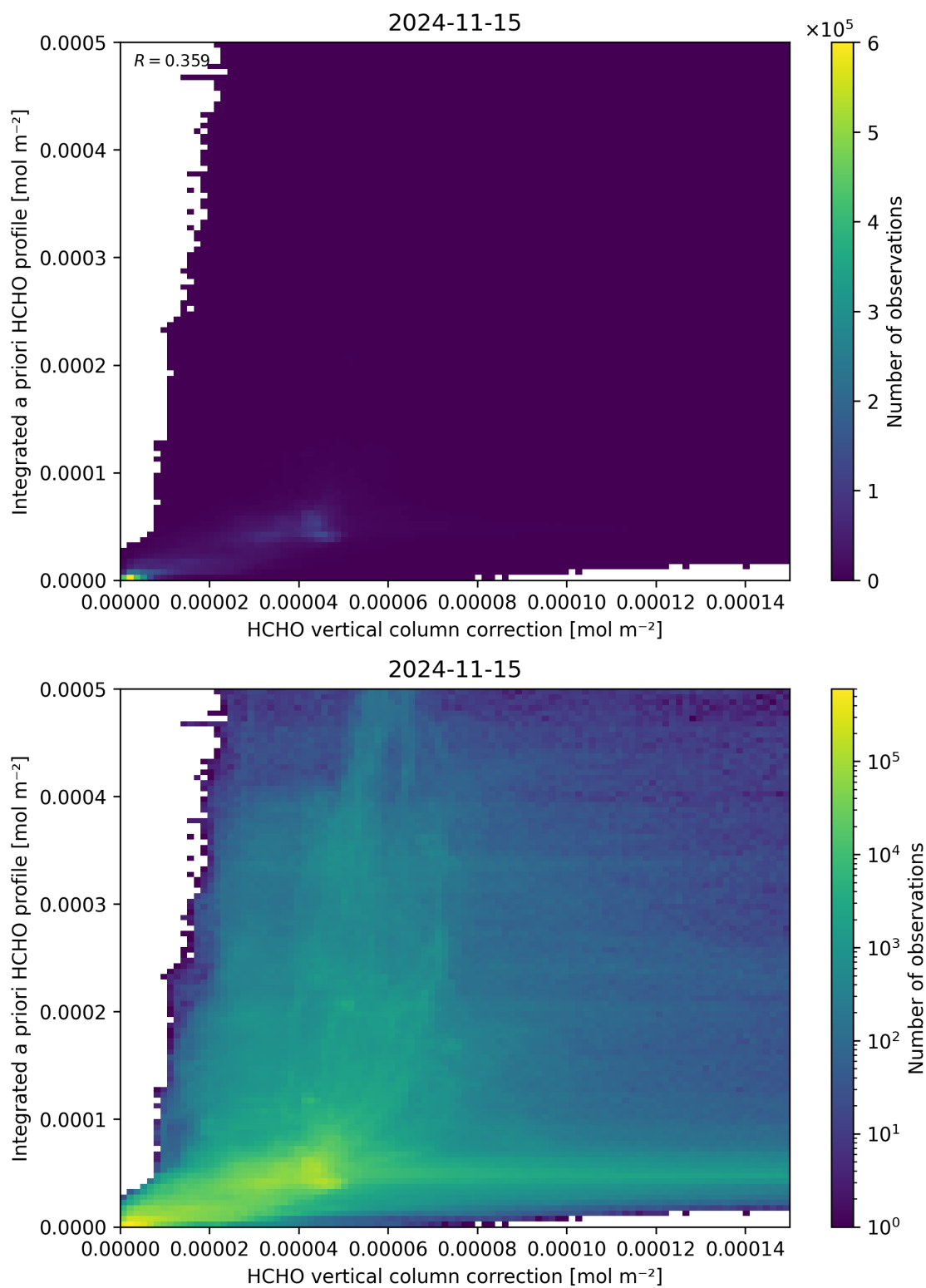
Figure 122: Scatter density plot of “HCHO vertical column correction” against “Integrated a priori HCHO profile” for 2024-11-14 to 2024-11-16.
