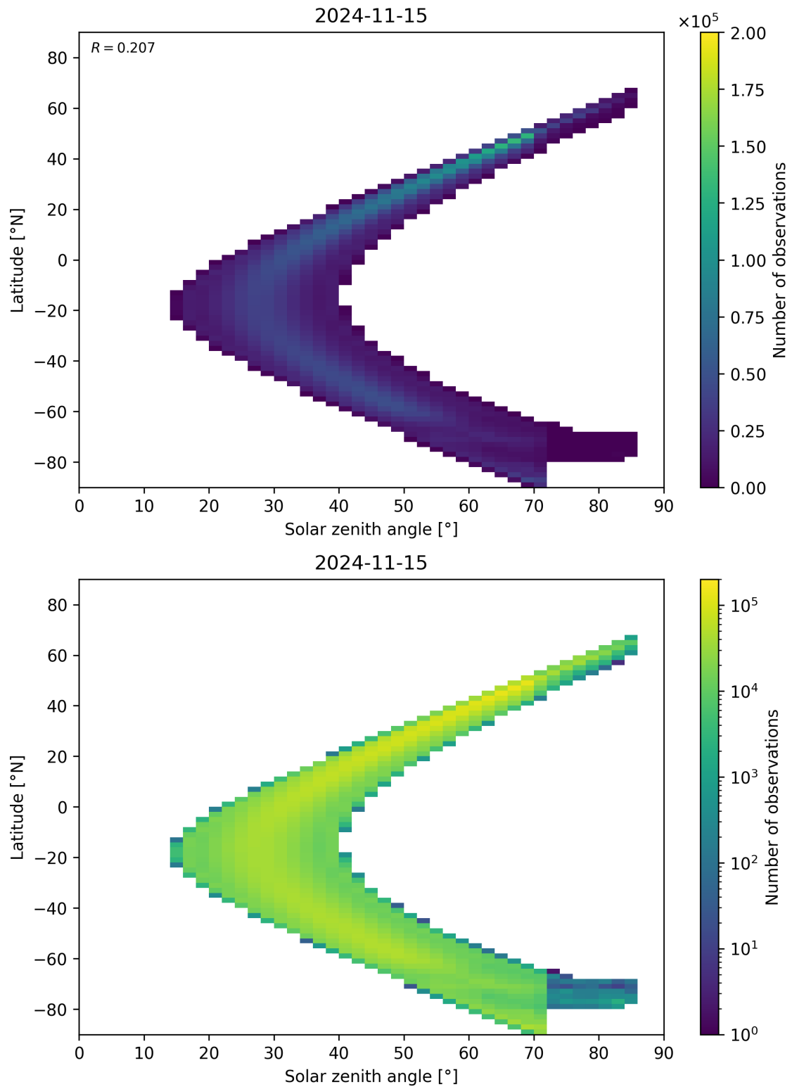
Figure 181: Scatter density plot of “Solar zenith angle” against “Latitude” for 2024-11-14 to 2024-11-16.
