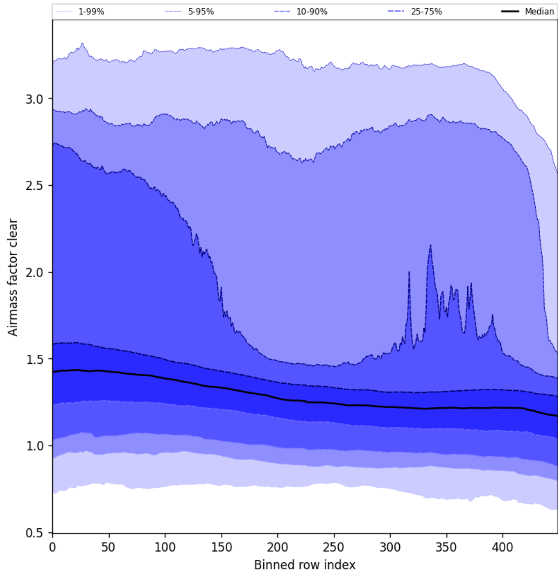
Figure 56: Along track statistics of “Airmass factor clear” for 2024-11-14 to 2024-11-16
