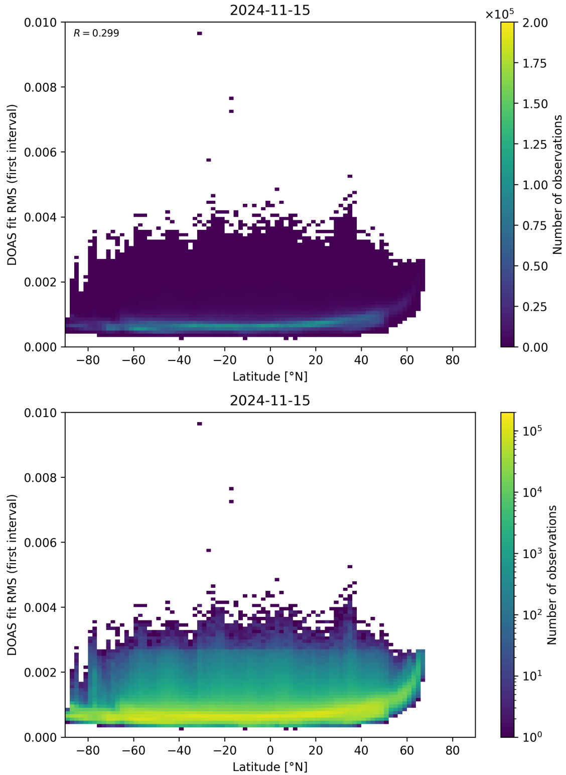
Figure 153: Scatter density plot of “Latitude” against “DOAS fit RMS (first interval)” for 2024-11-14 to 2024-11-16.
