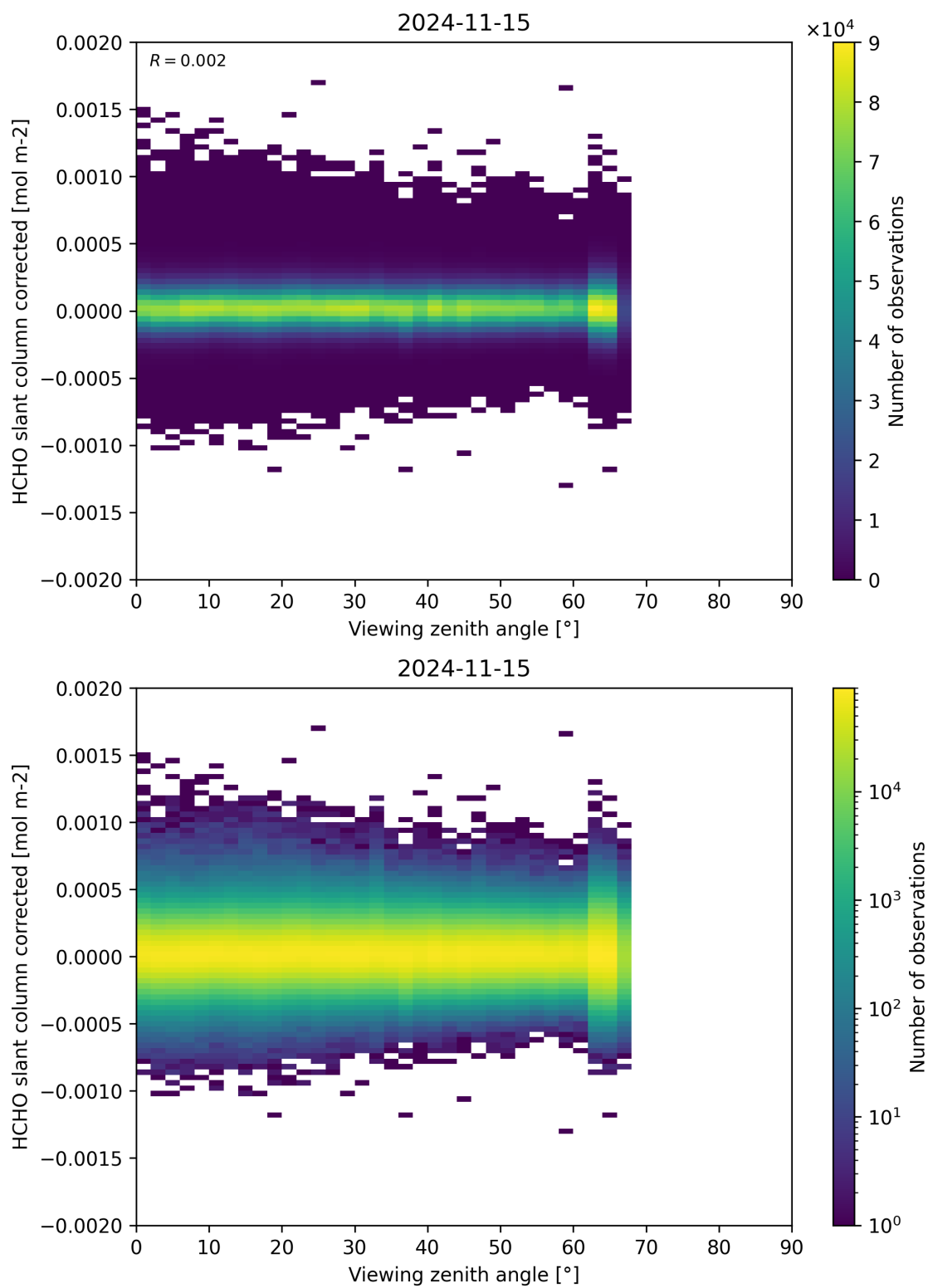
Figure 186: Scatter density plot of “Viewing zenith angle” against “HCHO slant column corrected” for 2024-11-14 to 2024-11-16.
