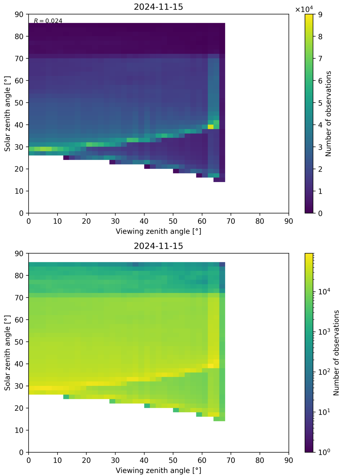
Figure 197: Scatter density plot of “Viewing zenith angle” against “Solar zenith angle” for 2024-11-14 to 2024-11-16.
