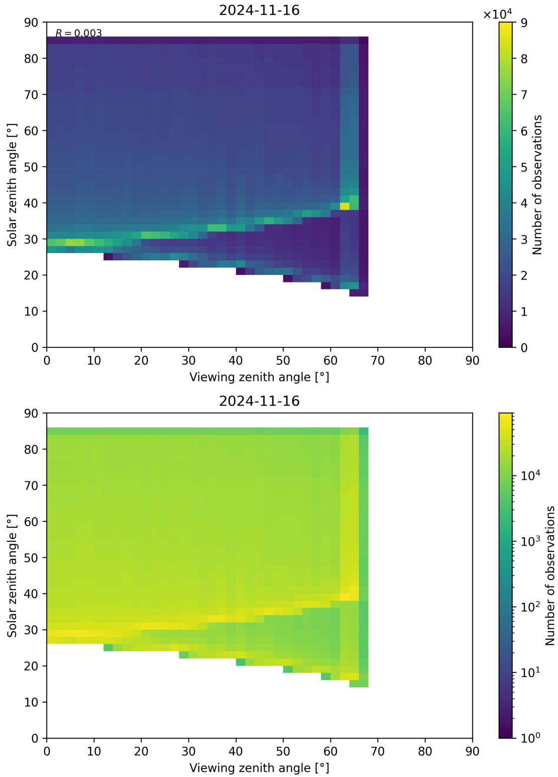
Figure 197: Scatter density plot of “Viewing zenith angle” against “Solar zenith angle” for 2024-11-15 to 2024-11-17.
