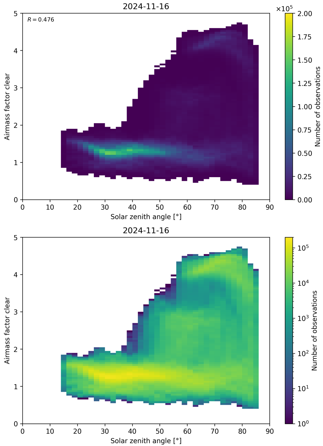
Figure 170: Scatter density plot of “Solar zenith angle” against “Airmass factor clear” for 2024-11-15 to 2024-11-17.
