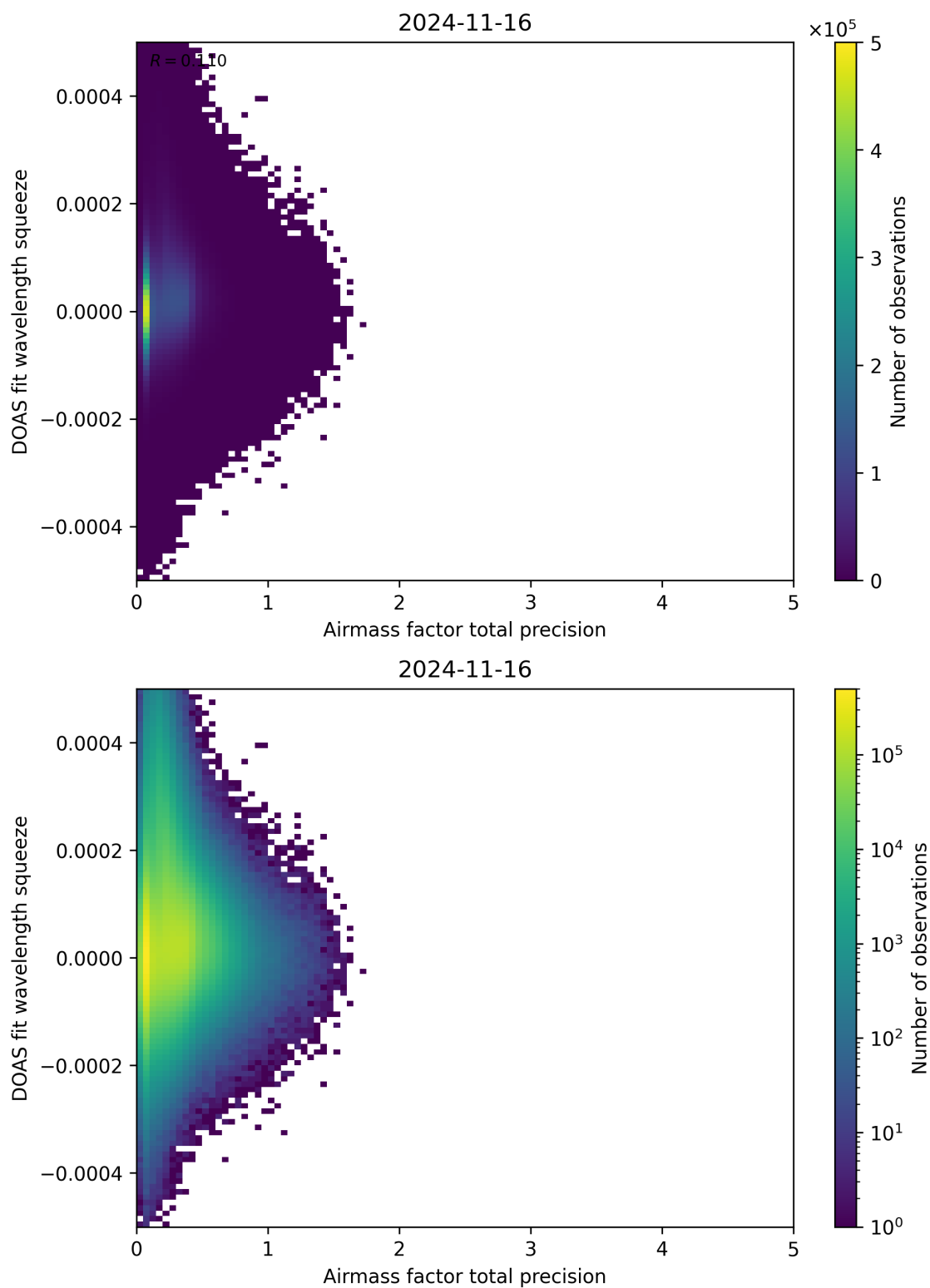
Figure 107: Scatter density plot of “Airmass factor total precision” against “DOAS fit wavelength squeeze” for 2024-11-15 to 2024-11-17.
