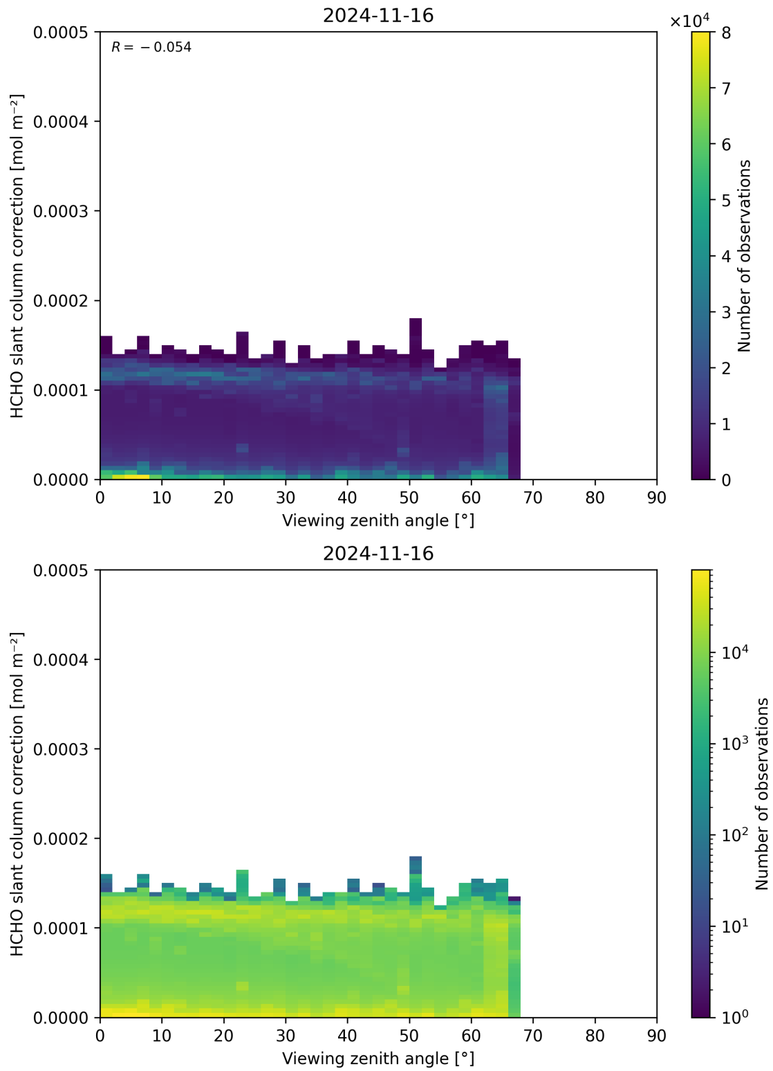
Figure 187: Scatter density plot of “Viewing zenith angle” against “HCHO slant column correction” for 2024-11-15 to 2024-11-17.
