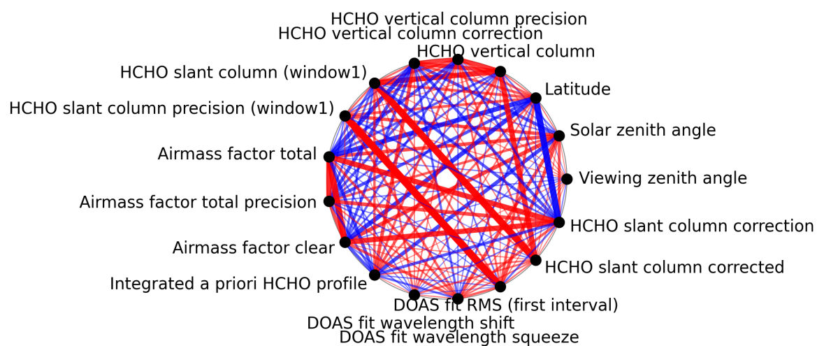
Figure 1: Map of correlation graph for 2024-11-15 to 2024-11-17.
