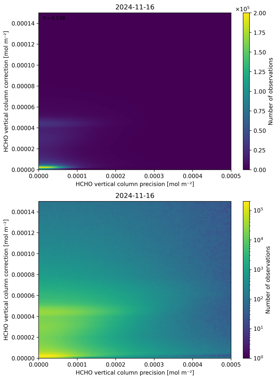
Figure 146: Scatter density plot of “HCHO vertical column precision” against “HCHO vertical column correction” for 2024-11-15 to 2024-11-17.
