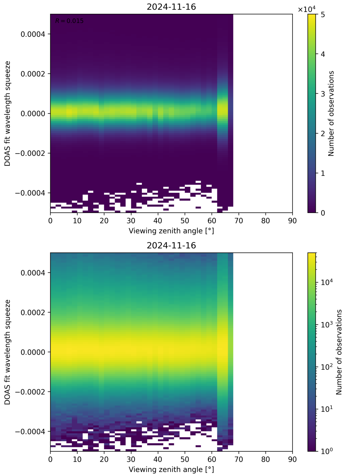
Figure 184: Scatter density plot of “Viewing zenith angle” against “DOAS fit wavelength squeeze” for 2024-11-15 to 2024-11-17.
