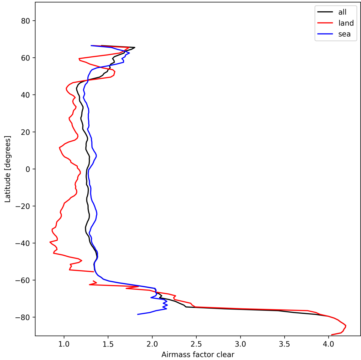
Figure 28: Zonal average of “Airmass factor clear” for 2024-11-15 to 2024-11-17.
