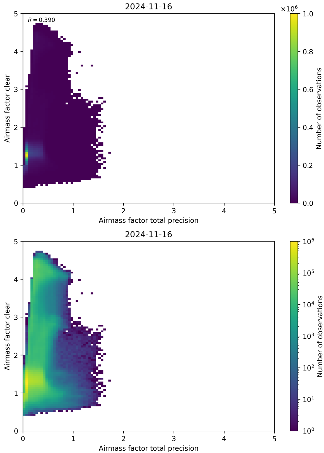
Figure 108: Scatter density plot of “Airmass factor total precision” against “Airmass factor clear” for 2024-11-15 to 2024-11-17.
