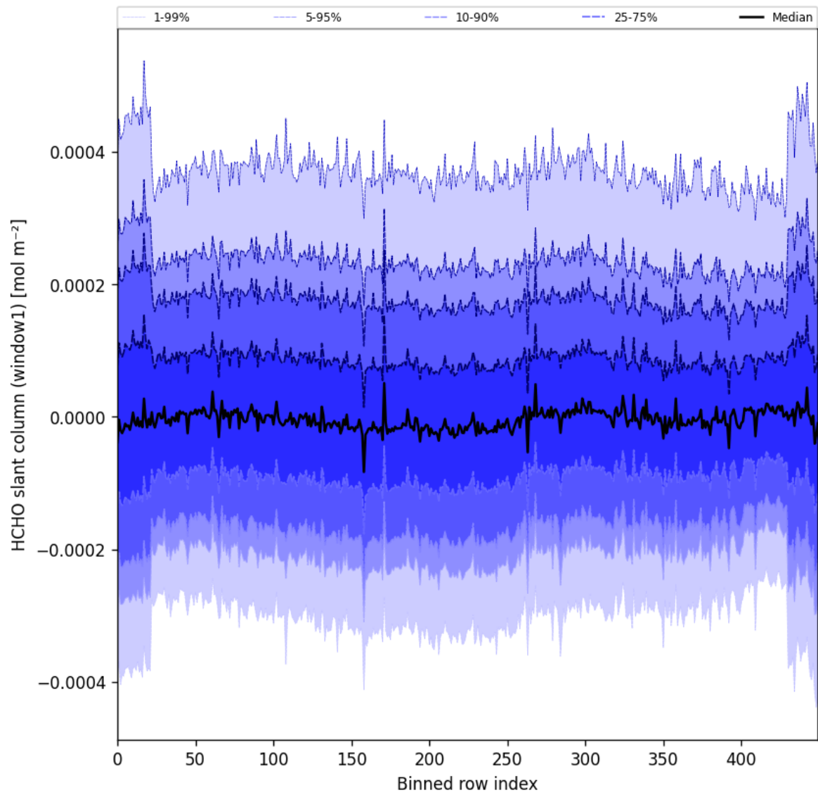
Figure 52: Along track statistics of “HCHO slant column (window1)” for 2024-11-15 to 2024-11-17
