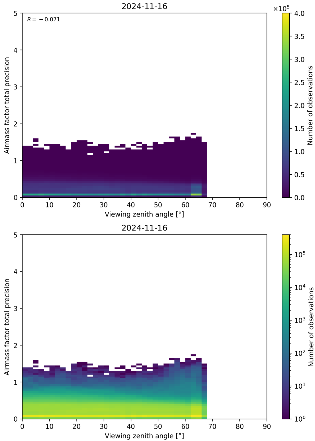
Figure 191: Scatter density plot of “Viewing zenith angle” against “Airmass factor total precision” for 2024-11-15 to 2024-11-17.
