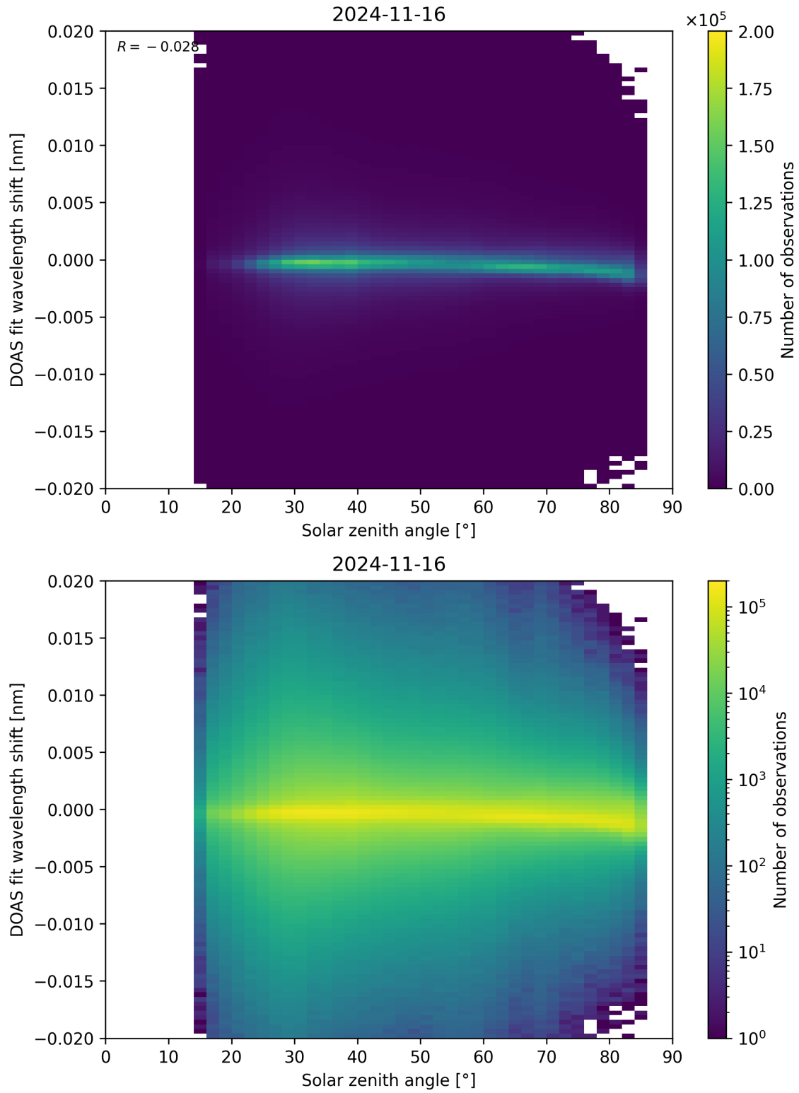
Figure 168: Scatter density plot of “Solar zenith angle” against “DOAS fit wavelength shift” for 2024-11-15 to 2024-11-17.
