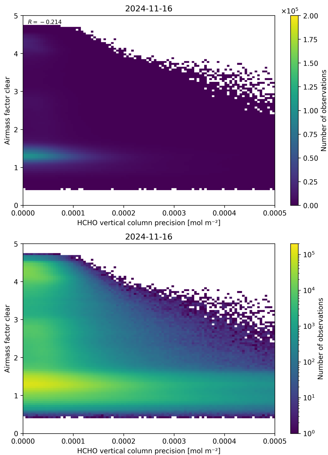
Figure 139: Scatter density plot of “HCHO vertical column precision” against “Airmass factor clear” for 2024-11-15 to 2024-11-17.
