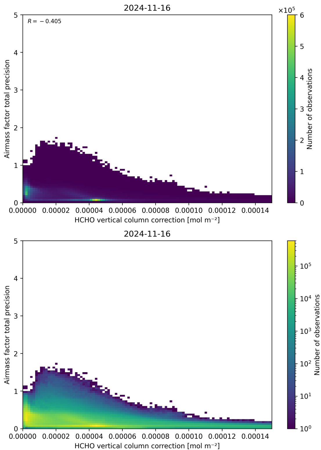
Figure 121: Scatter density plot of “HCHO vertical column correction” against “Airmass factor total precision” for 2024-11-15 to 2024-11-17.
