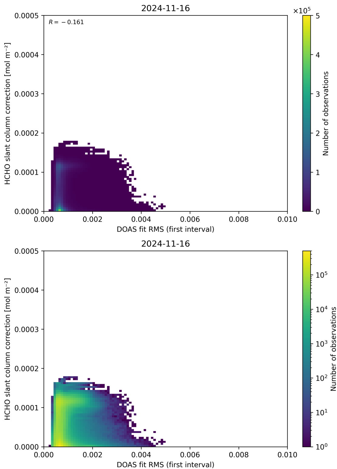
Figure 63: Scatter density plot of “DOAS fit RMS (first interval)” against “HCHO slant column correction” for 2024-11-15 to 2024-11-17.
