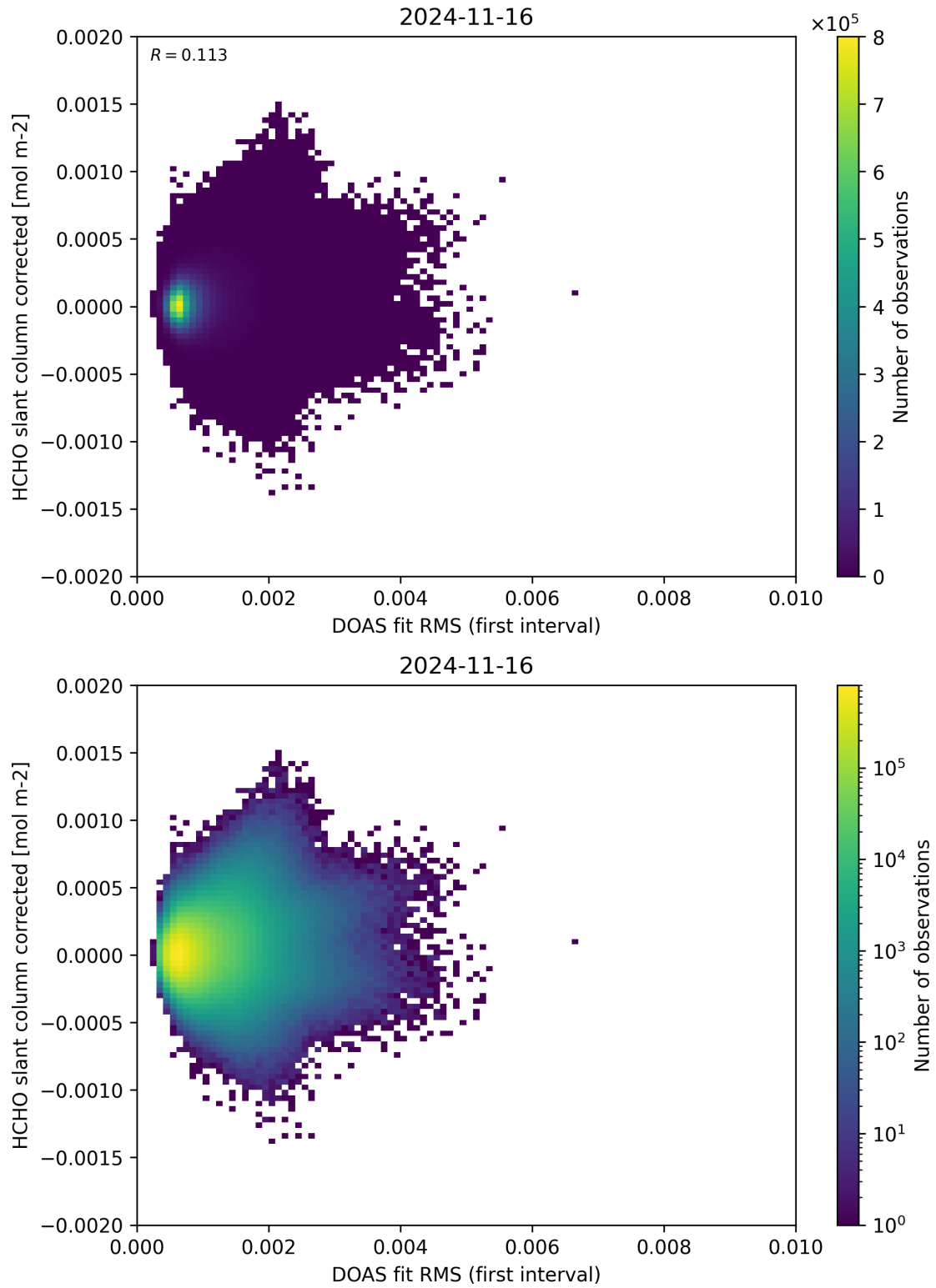
Figure 62: Scatter density plot of “DOAS fit RMS (first interval)” against “HCHO slant column corrected” for 2024-11-15 to 2024-11-17.
