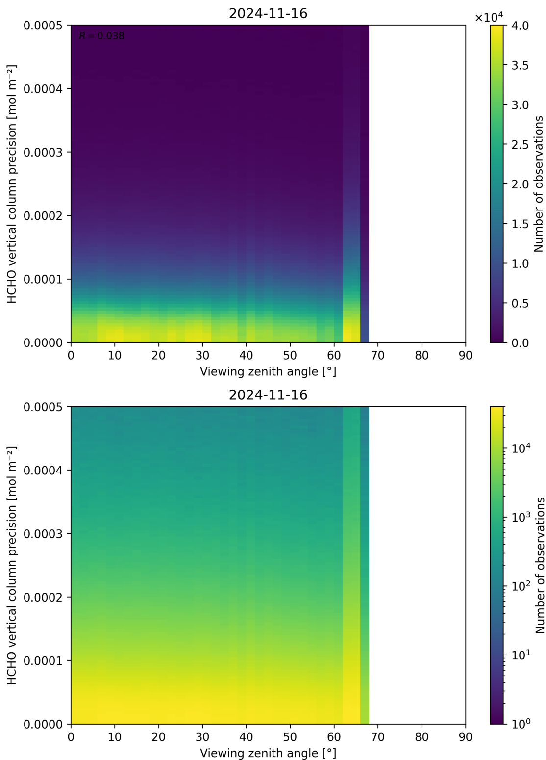
Figure 194: Scatter density plot of “Viewing zenith angle” against “HCHO vertical column precision” for 2024-11-15 to 2024-11-17.
