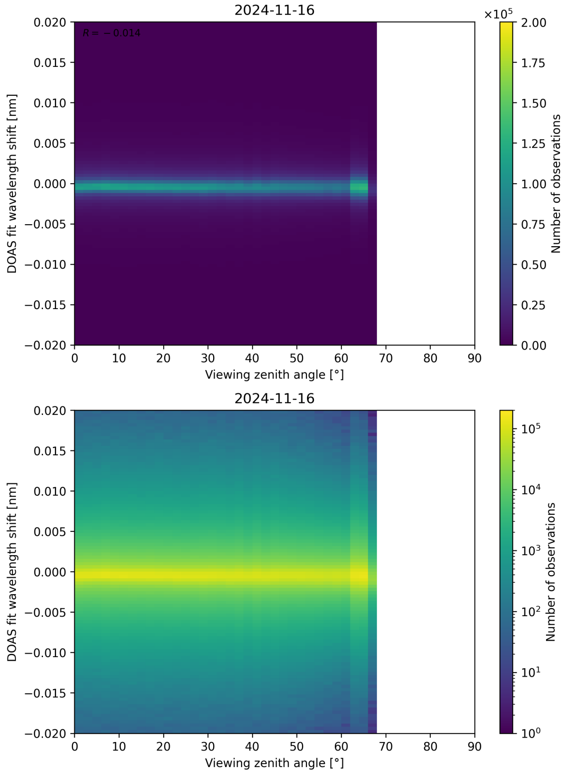
Figure 183: Scatter density plot of “Viewing zenith angle” against “DOAS fit wavelength shift” for 2024-11-15 to 2024-11-17.
