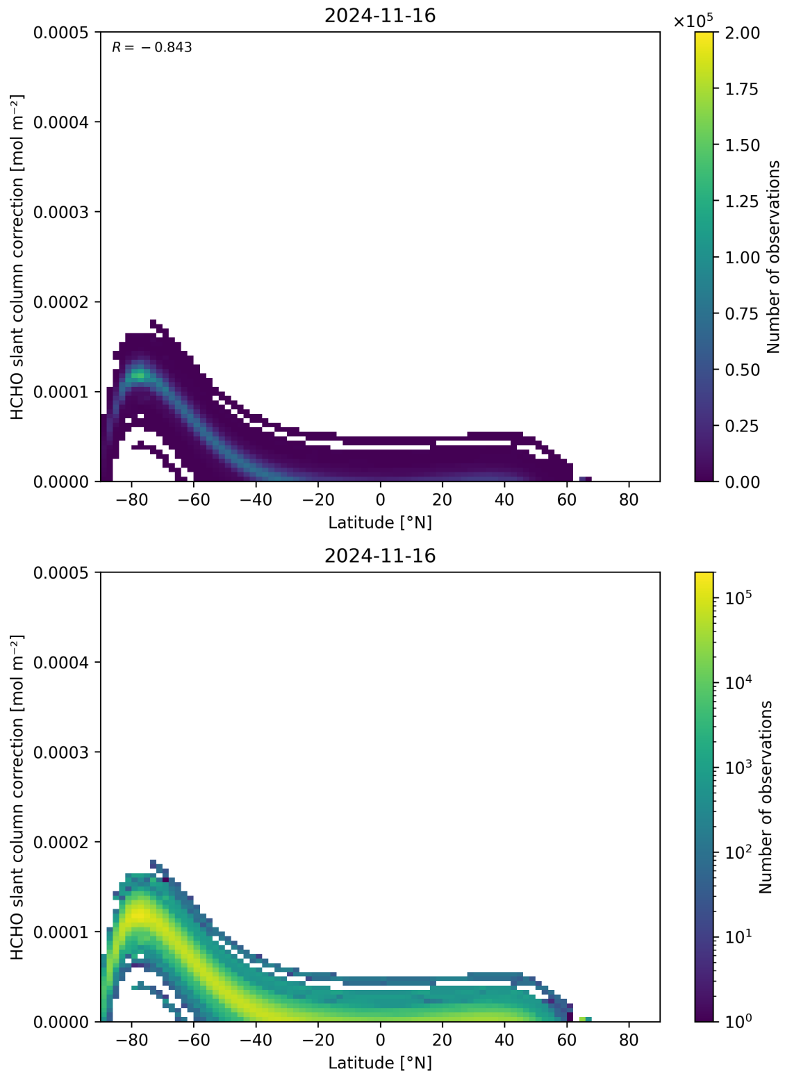
Figure 158: Scatter density plot of “Latitude” against “HCHO slant column correction” for 2024-11-15 to 2024-11-17.
