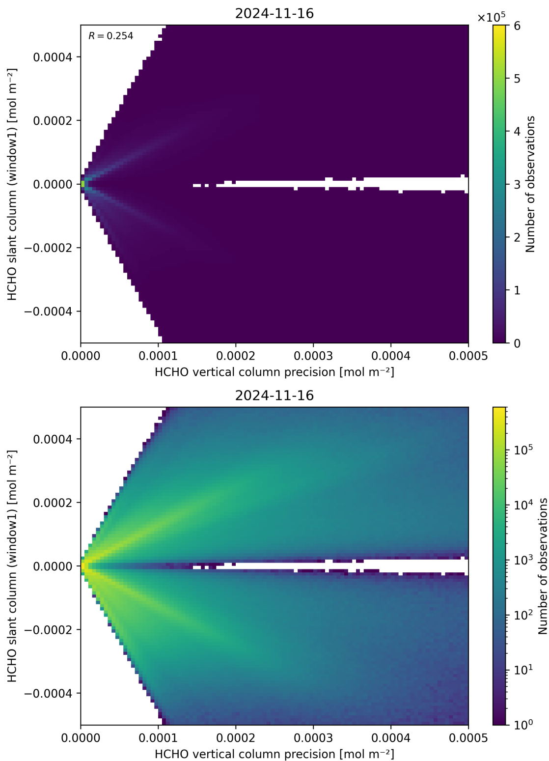
Figure 142: Scatter density plot of “HCHO vertical column precision” against “HCHO slant column (window1)” for 2024-11-15 to 2024-11-17.
