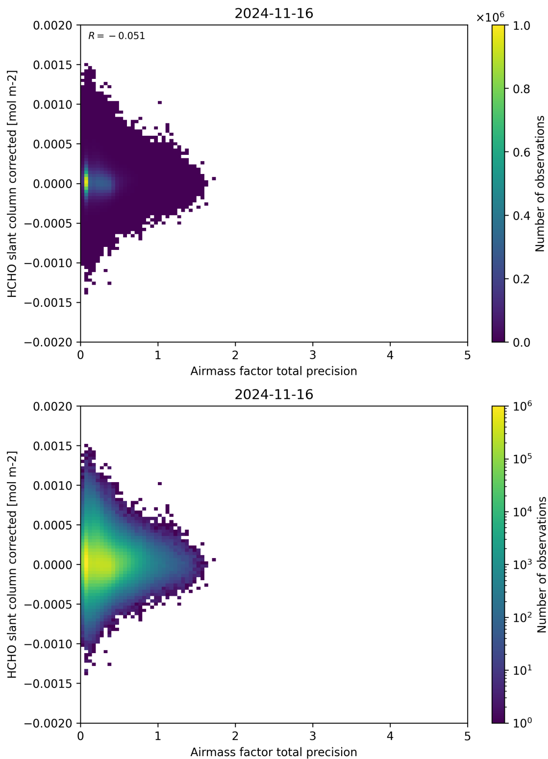
Figure 109: Scatter density plot of “Airmass factor total precision” against “HCHO slant column corrected” for 2024-11-15 to 2024-11-17.
