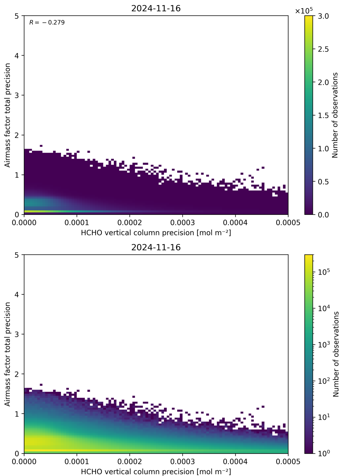
Figure 145: Scatter density plot of “HCHO vertical column precision” against “Airmass factor total precision” for 2024-11-15 to 2024-11-17.
