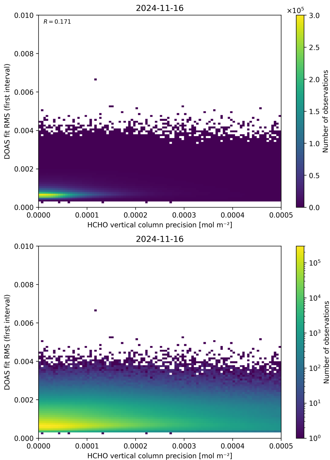
Figure 136: Scatter density plot of “HCHO vertical column precision” against “DOAS fit RMS (first interval)” for 2024-11-15 to 2024-11-17.
