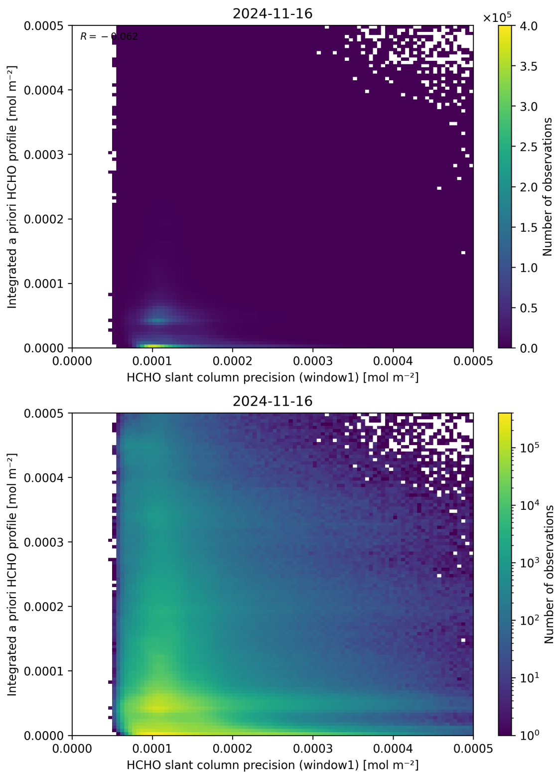
Figure 96: Scatter density plot of “HCHO slant column precision (window1)” against “Integrated a priori HCHO profile” for 2024-11-15 to 2024-11-17.
