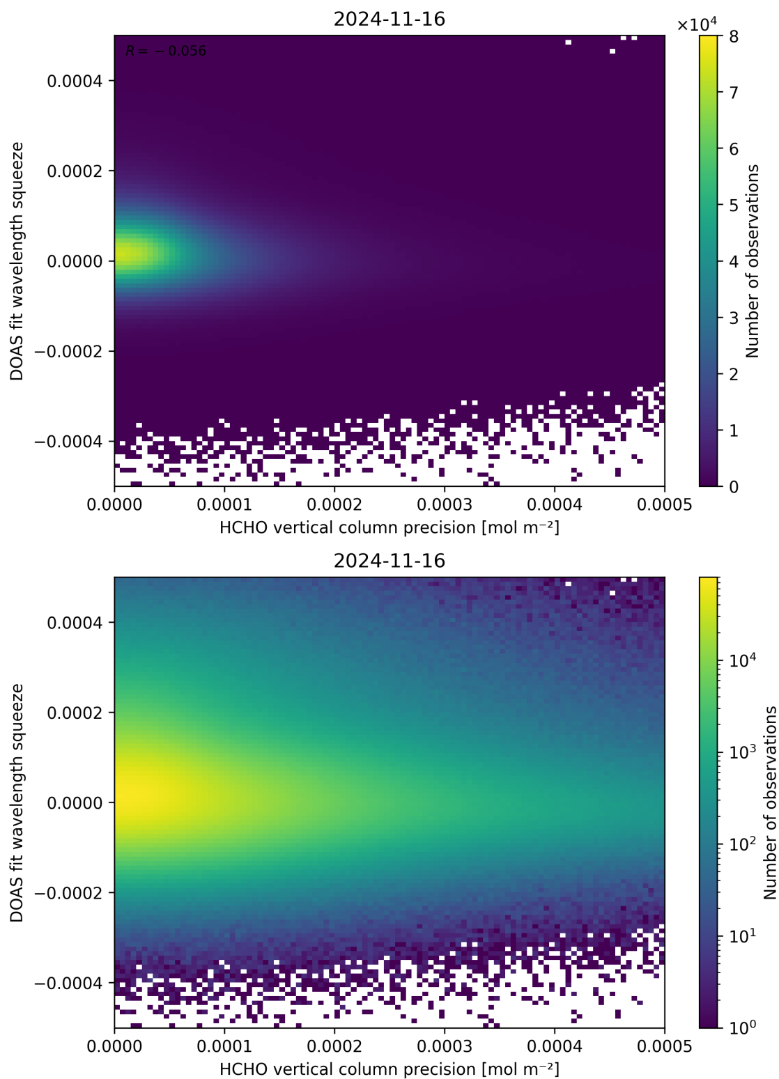
Figure 138: Scatter density plot of “HCHO vertical column precision” against “DOAS fit wavelength squeeze” for 2024-11-15 to 2024-11-17.
