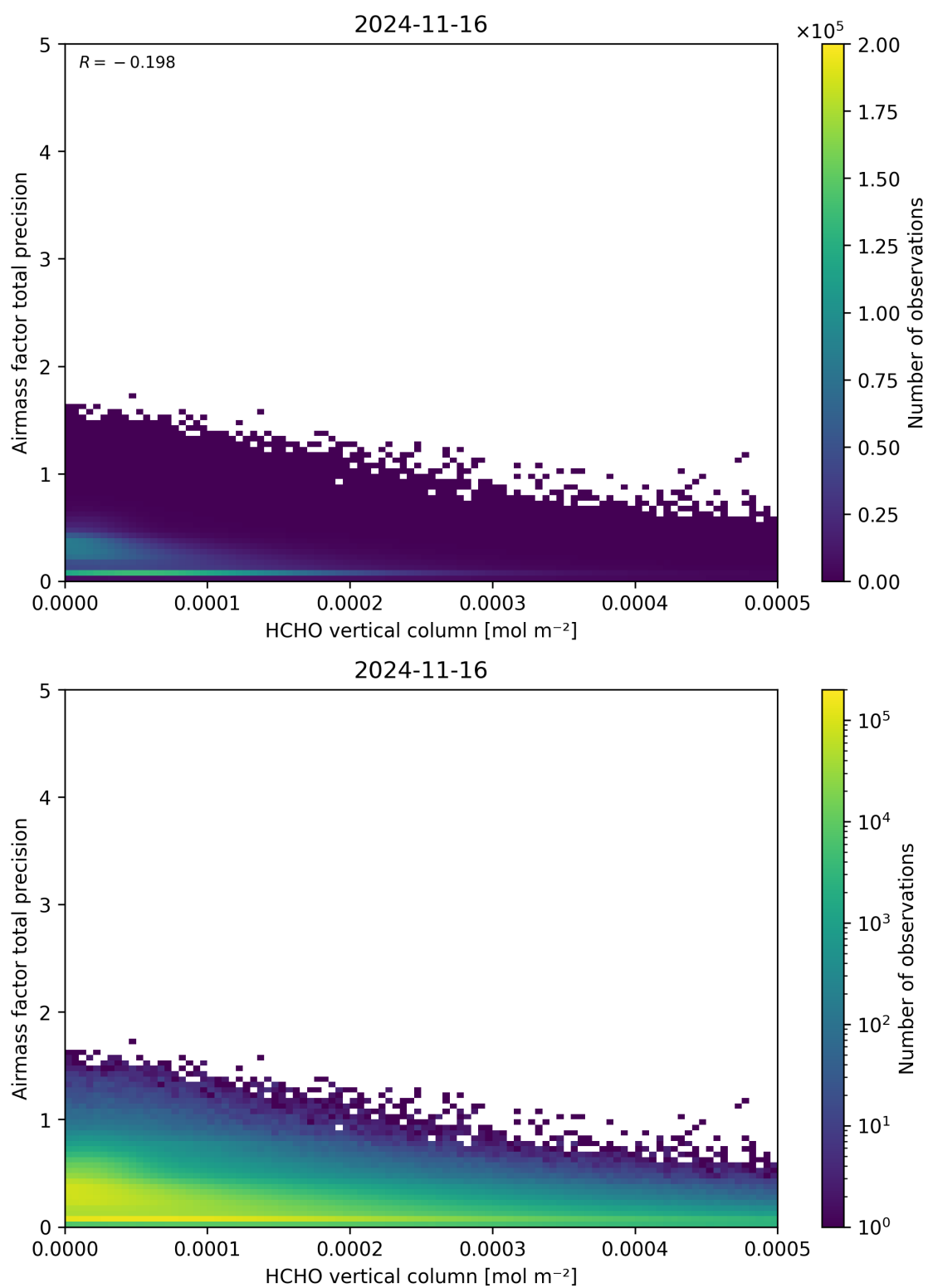
Figure 132: Scatter density plot of “HCHO vertical column” against “Airmass factor total precision” for 2024-11-15 to 2024-11-17.
