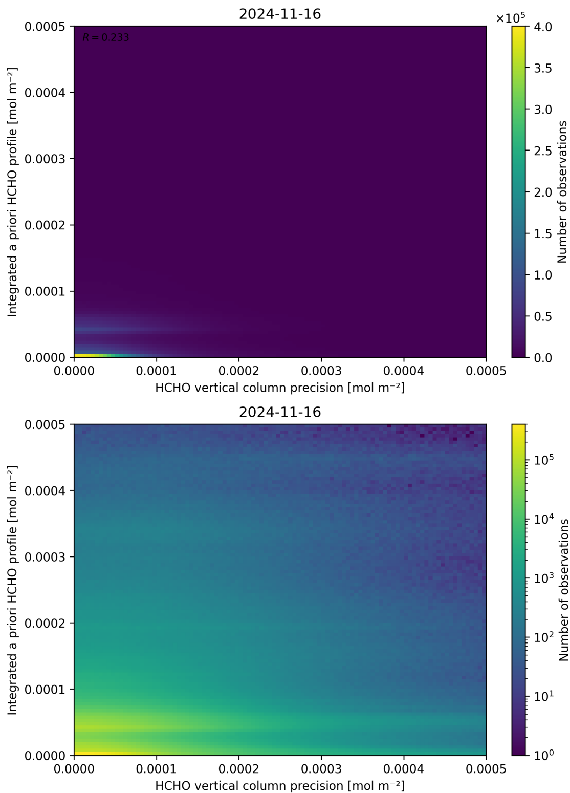
Figure 147: Scatter density plot of “HCHO vertical column precision” against “Integrated a priori HCHO profile” for 2024-11-15 to 2024-11-17.
