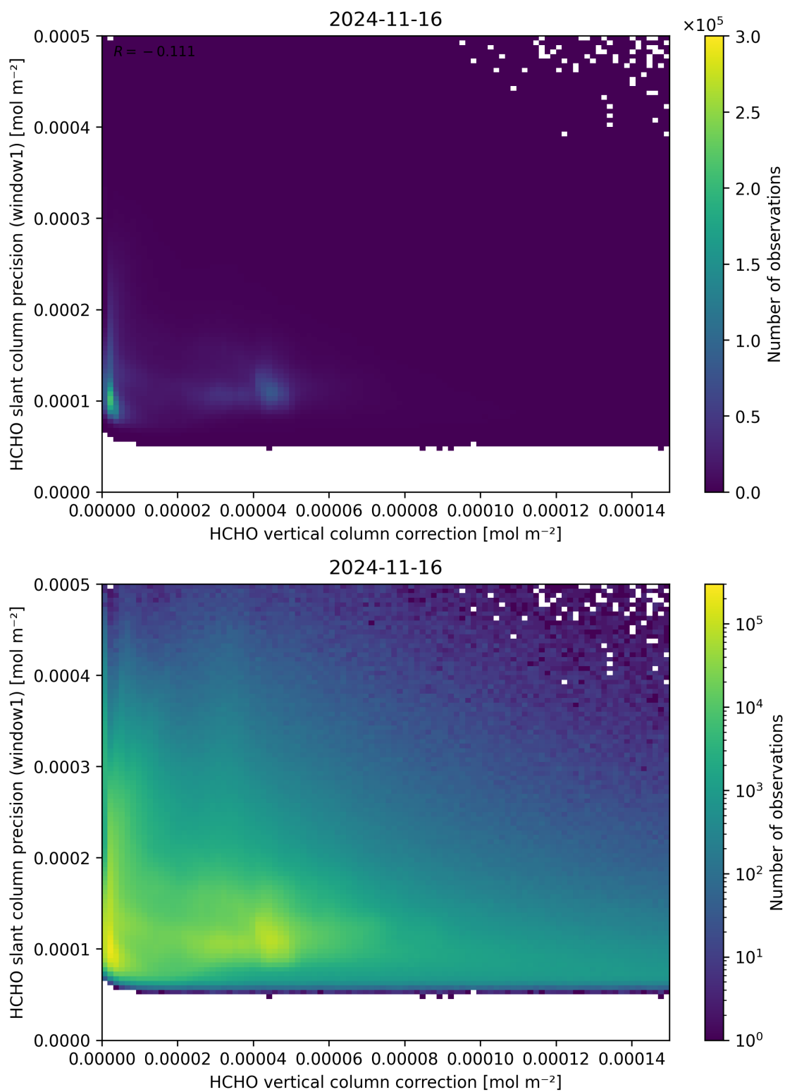
Figure 119: Scatter density plot of “HCHO vertical column correction” against “HCHO slant column precision (window1)” for 2024-11-15 to 2024-11-17.
