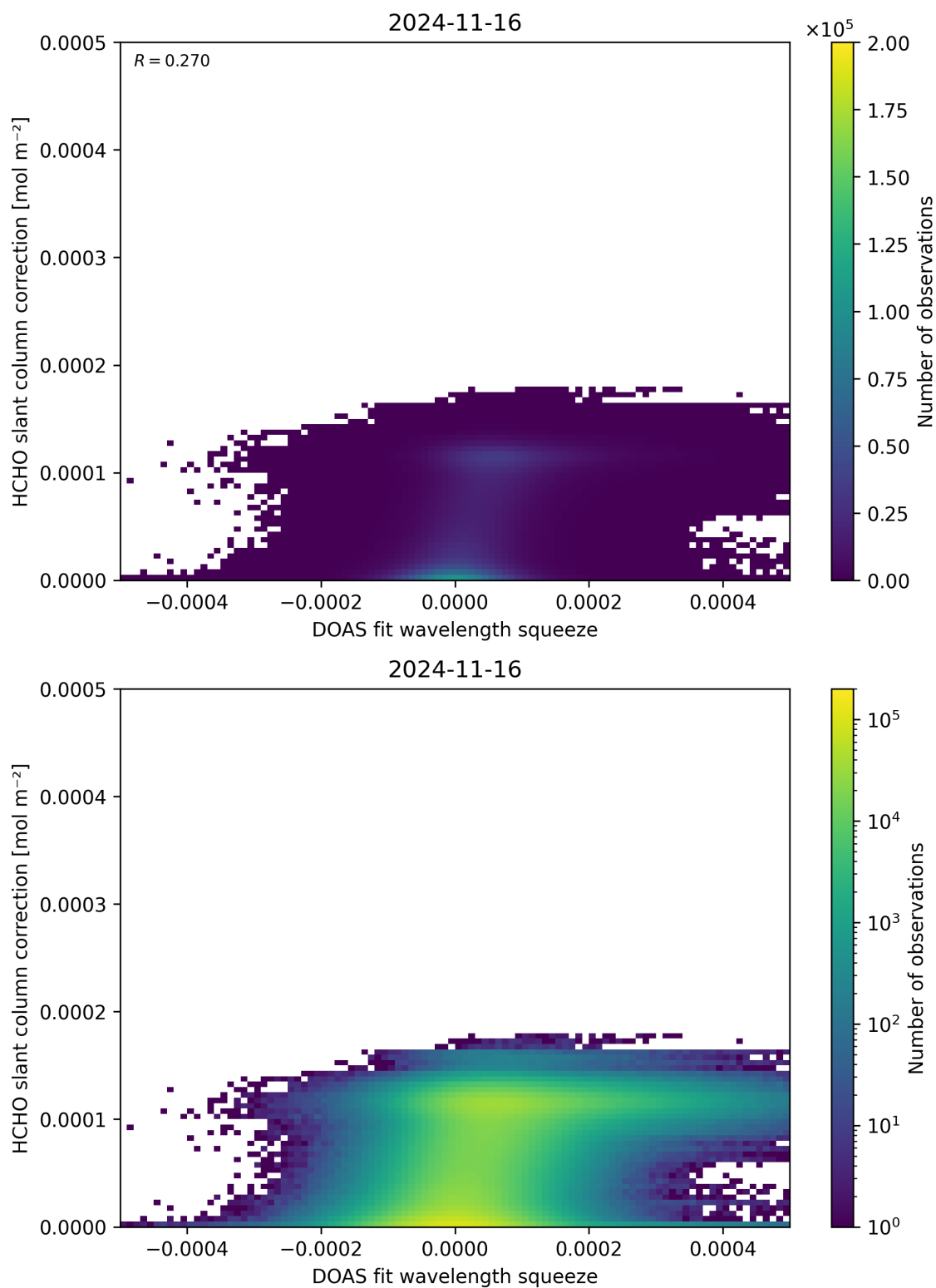
Figure 70: Scatter density plot of “DOAS fit wavelength squeeze” against “HCHO slant column correction” for 2024-11-15 to 2024-11-17.
