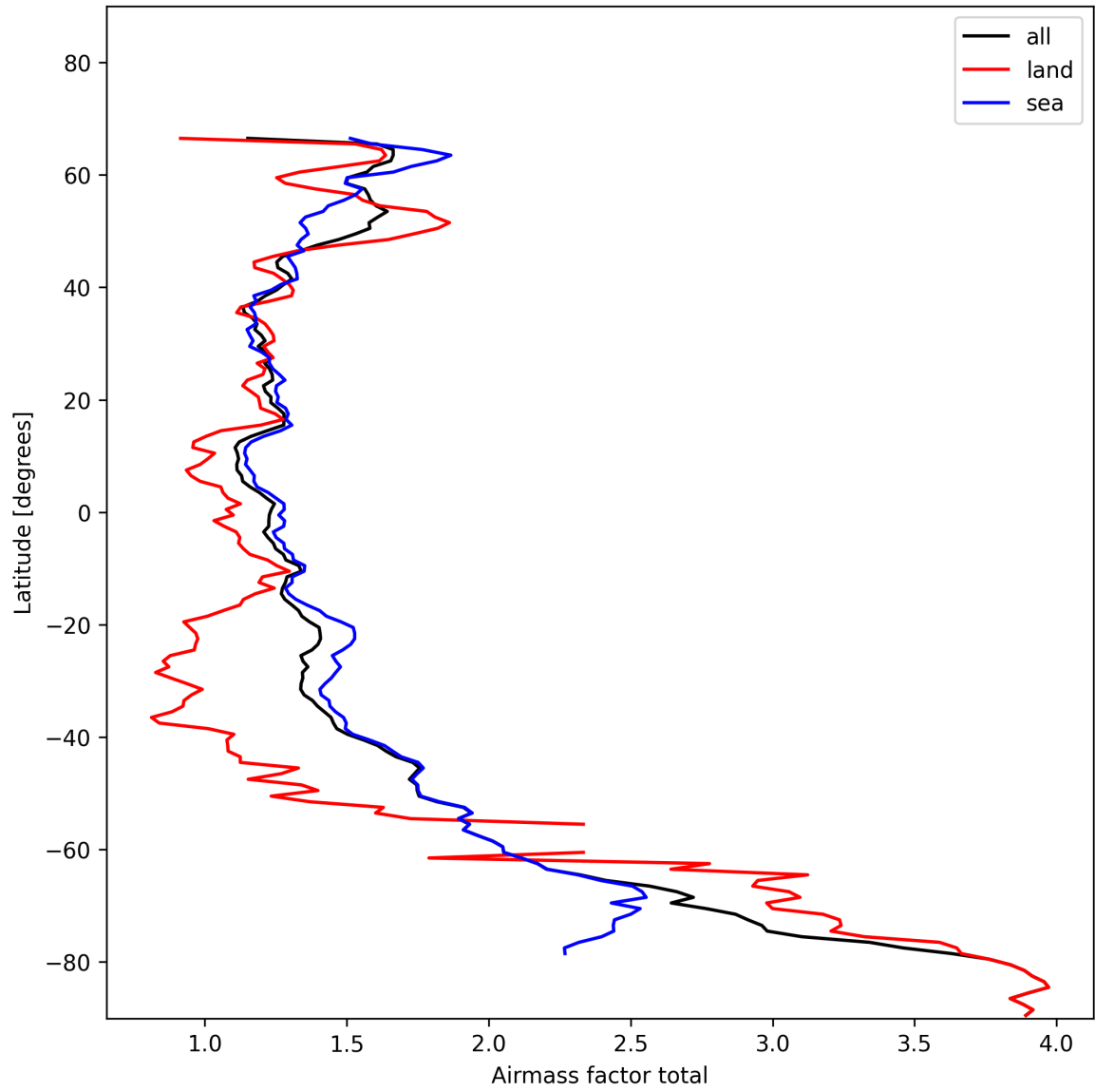
Figure 26: Zonal average of “Airmass factor total” for 2024-11-15 to 2024-11-17.
