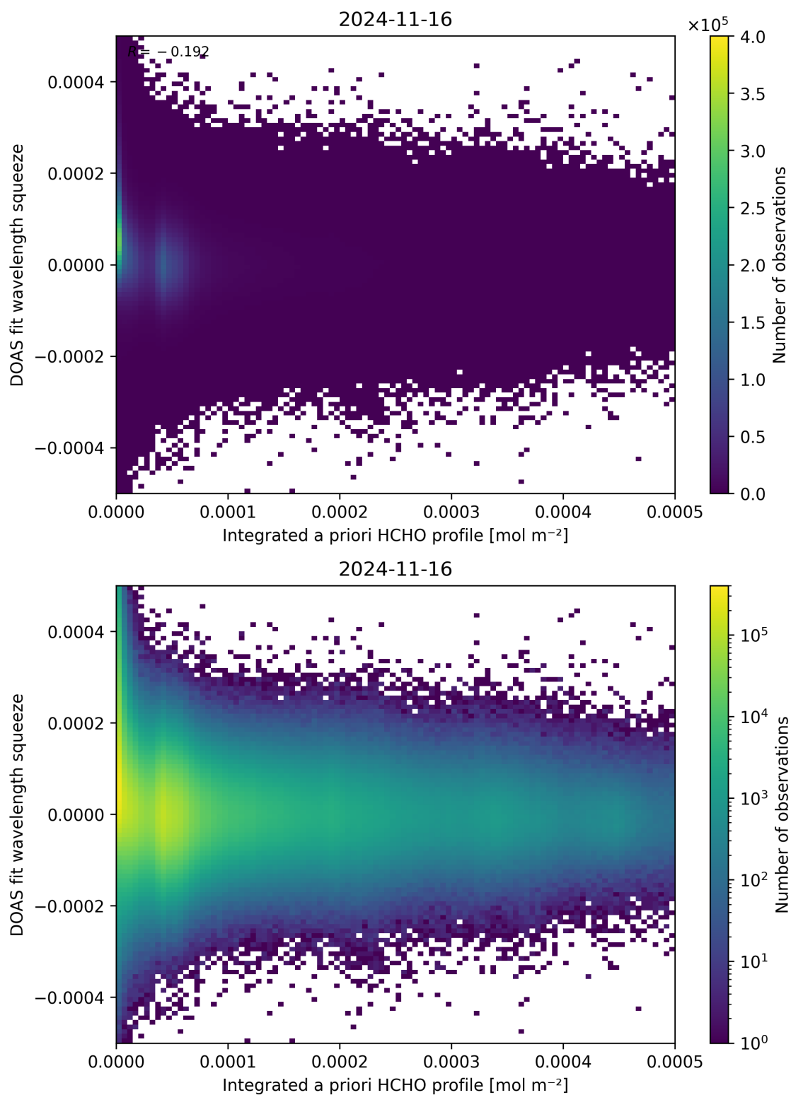
Figure 150: Scatter density plot of “Integrated a priori HCHO profile” against “DOAS fit wavelength squeeze” for 2024-11-15 to 2024-11-17.
