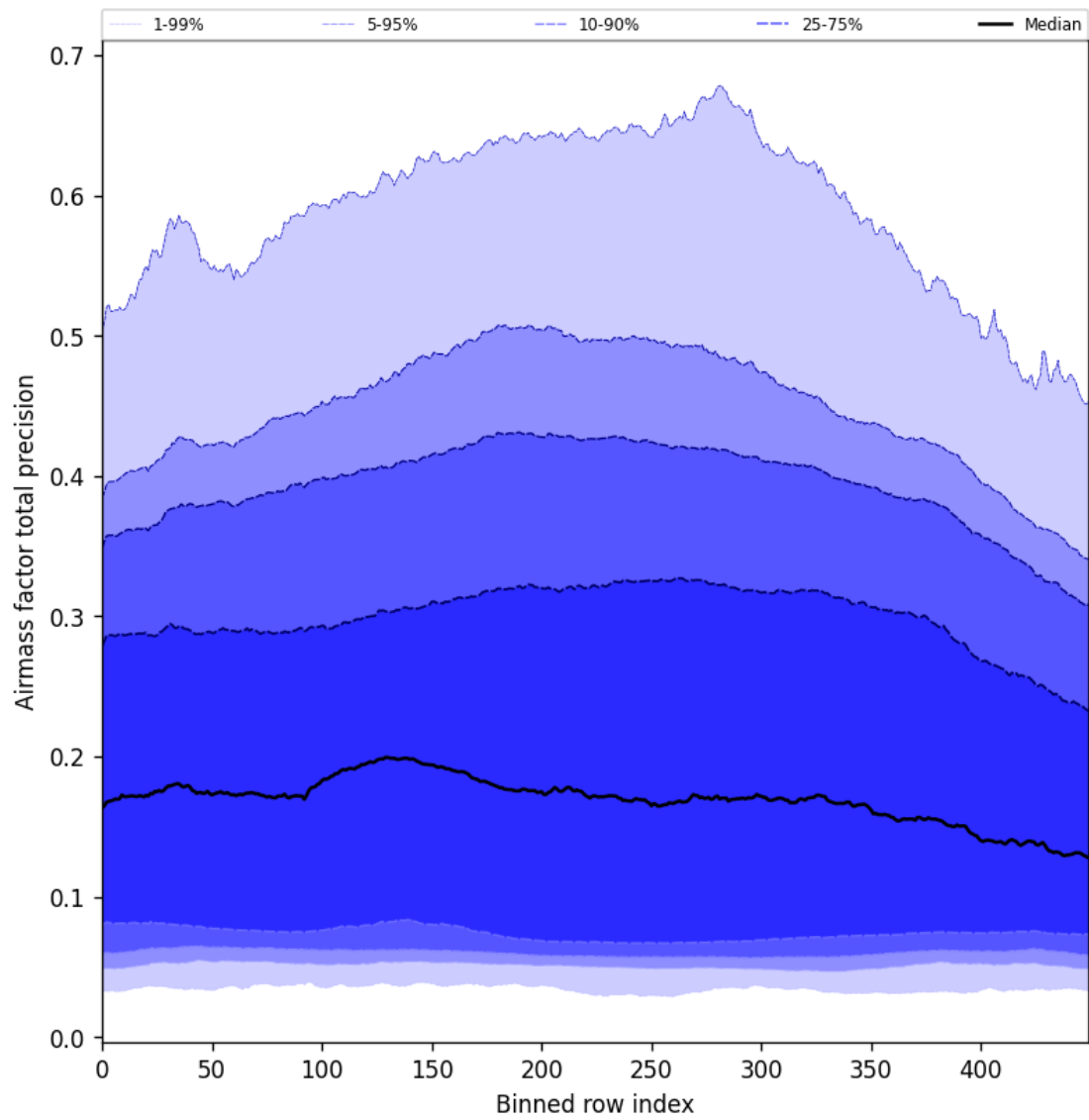
Figure 55: Along track statistics of “Airmass factor total precision” for 2024-11-15 to 2024-11-17
