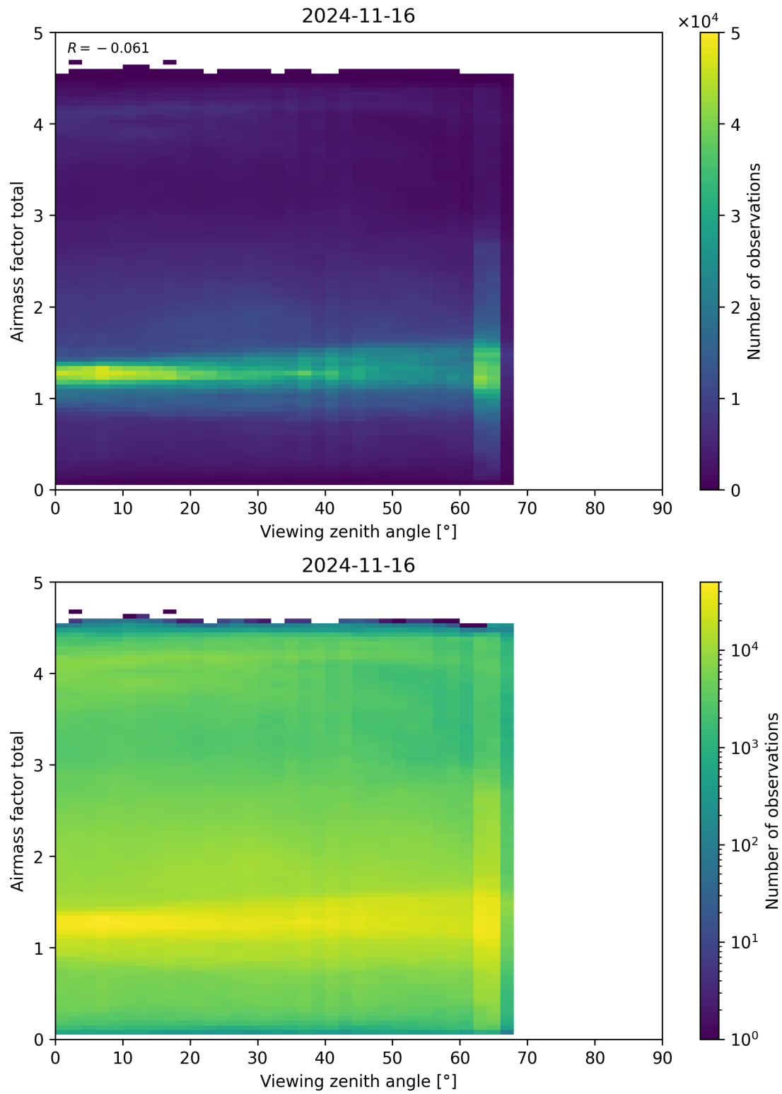
Figure 190: Scatter density plot of “Viewing zenith angle” against “Airmass factor total” for 2024-11-15 to 2024-11-17.
