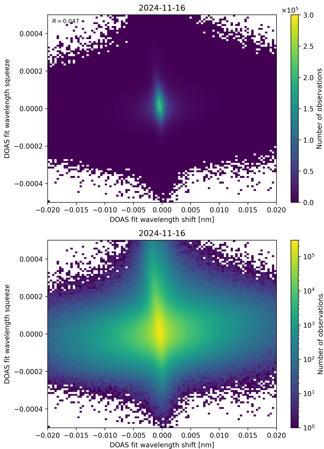
Figure 65: Scatter density plot of “DOAS fit wavelength shift” against “DOAS fit wavelength squeeze” for 2024-11-15 to 2024-11-17.
