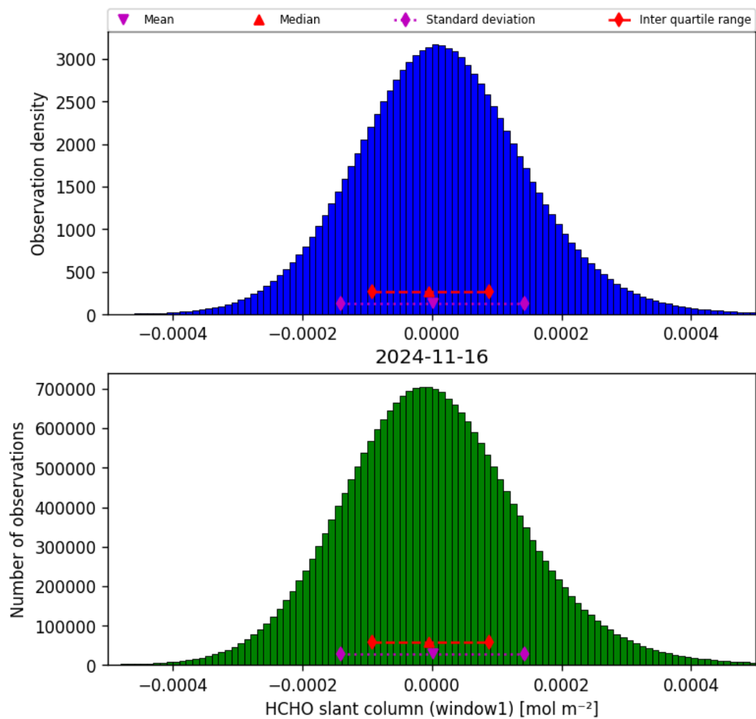
Figure 38: Histogram of “HCHO slant column (window1)” for 2024-11-15 to 2024-11-17
