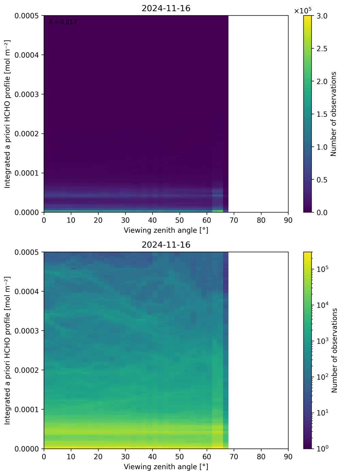
Figure 195: Scatter density plot of “Viewing zenith angle” against “Integrated a priori HCHO profile” for 2024-11-15 to 2024-11-17.
