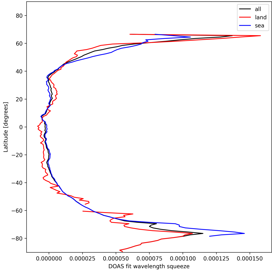
Figure 31: Zonal average of “DOAS fit wavelength squeeze” for 2024-11-15 to 2024-11-17.
