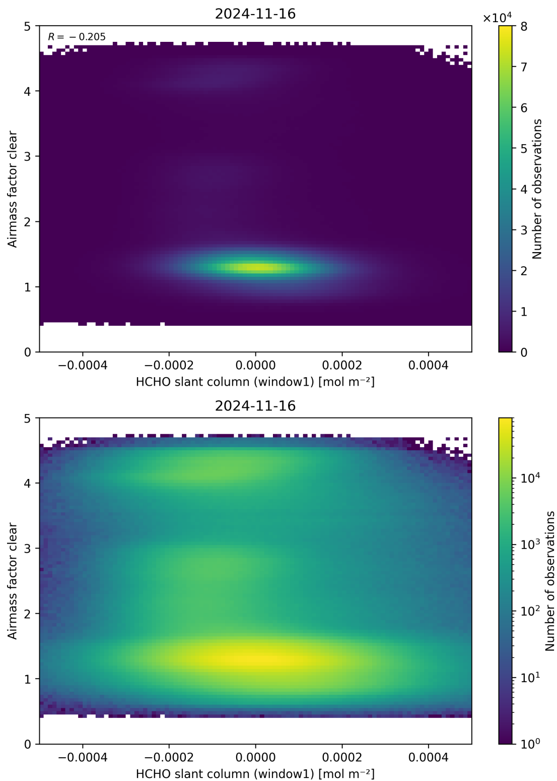
Figure 81: Scatter density plot of “HCHO slant column (window1)” against “Airmass factor clear” for 2024-11-15 to 2024-11-17.
