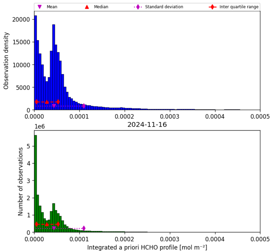
Figure 43: Histogram of “Integrated a priori HCHO profile” for 2024-11-15 to 2024-11-17
