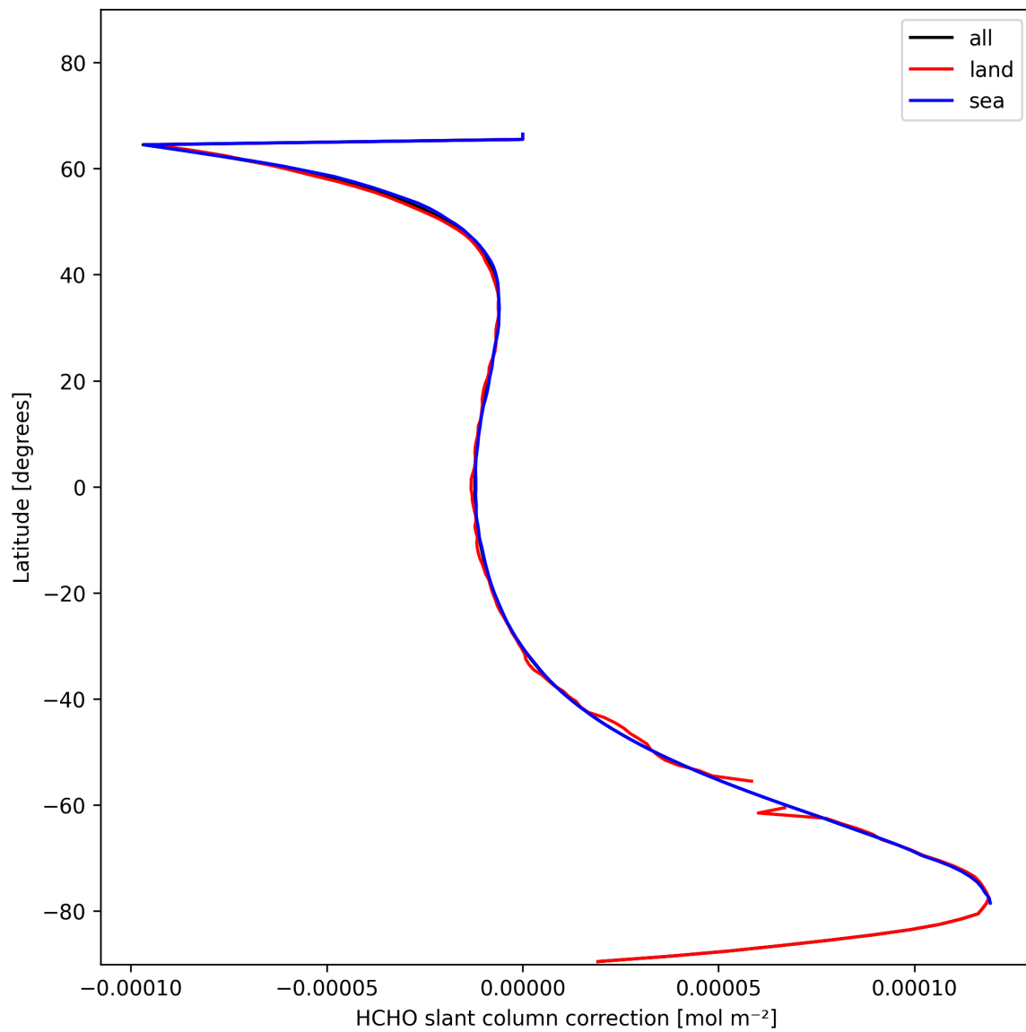
Figure 33: Zonal average of “HCHO slant column correction” for 2024-11-15 to 2024-11-17.
