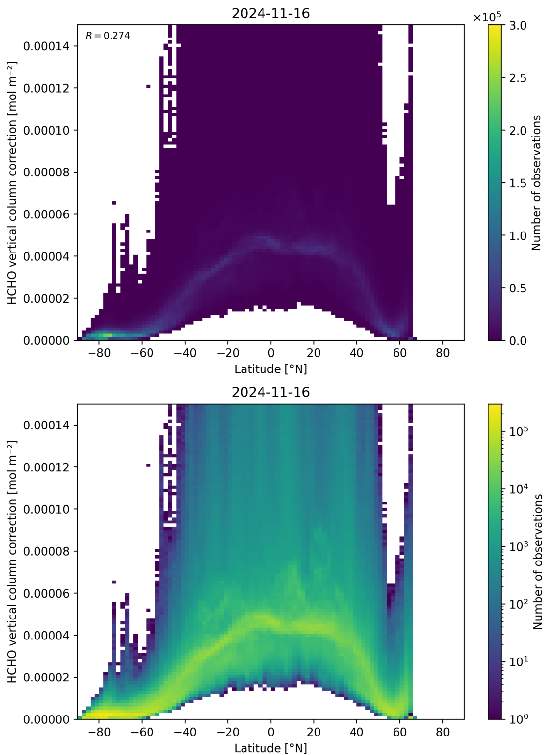
Figure 164: Scatter density plot of “Latitude” against “HCHO vertical column correction” for 2024-11-15 to 2024-11-17.
