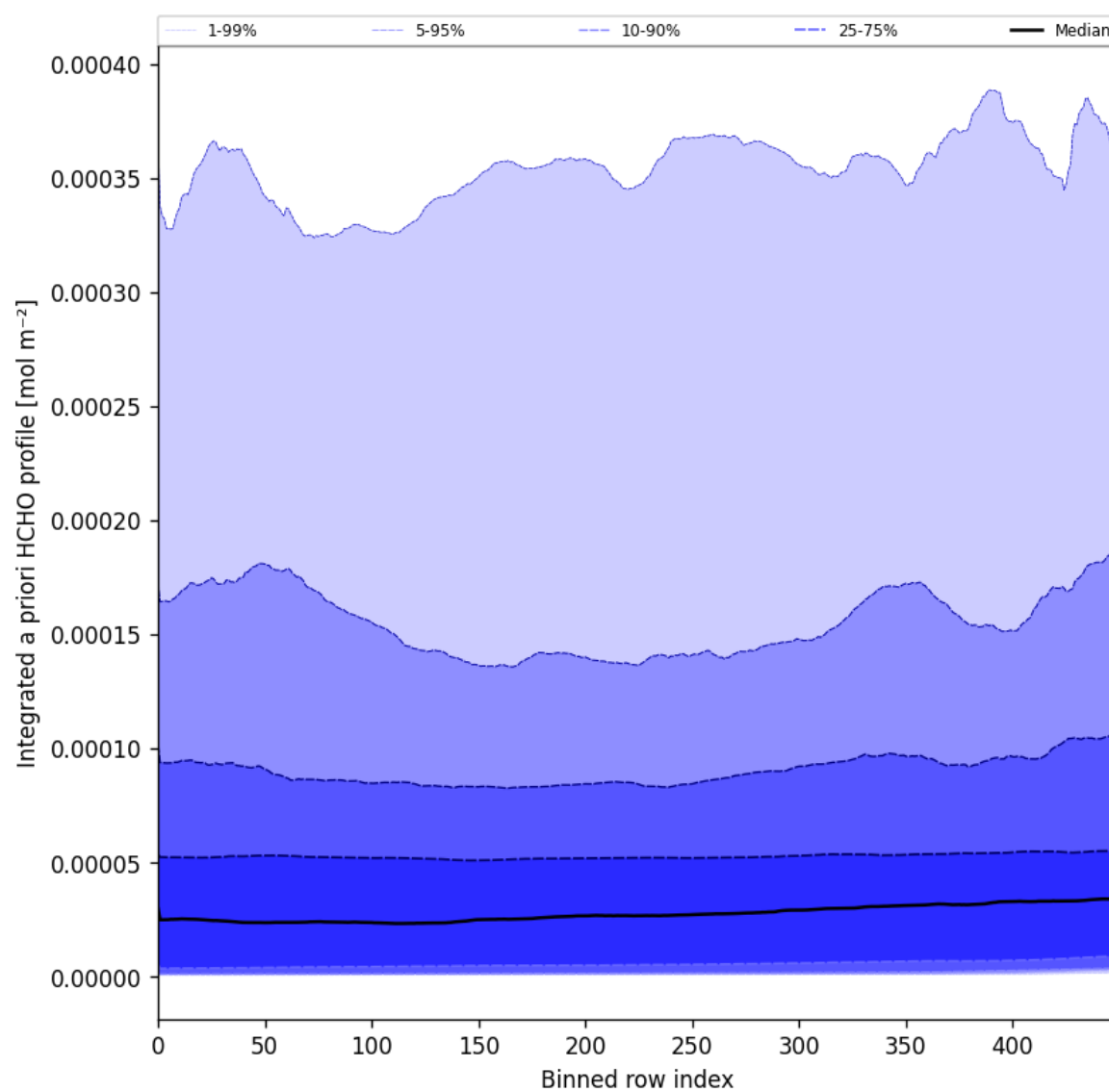
Figure 57: Along track statistics of “Integrated a priori HCHO profile” for 2024-11-15 to 2024-11-17
