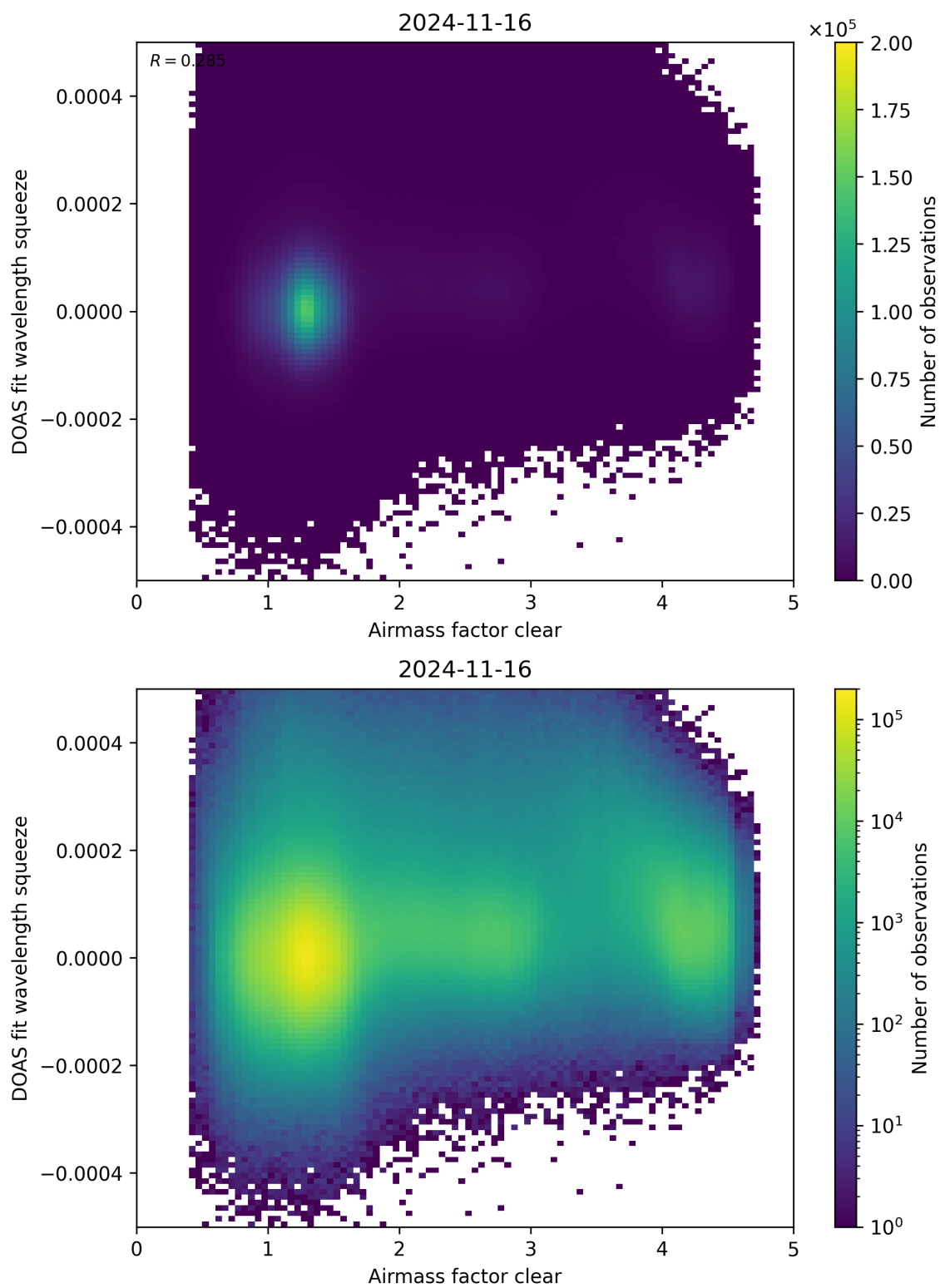
Figure 73: Scatter density plot of “Airmass factor clear” against “DOAS fit wavelength squeeze” for 2024-11-15 to 2024-11-17.
