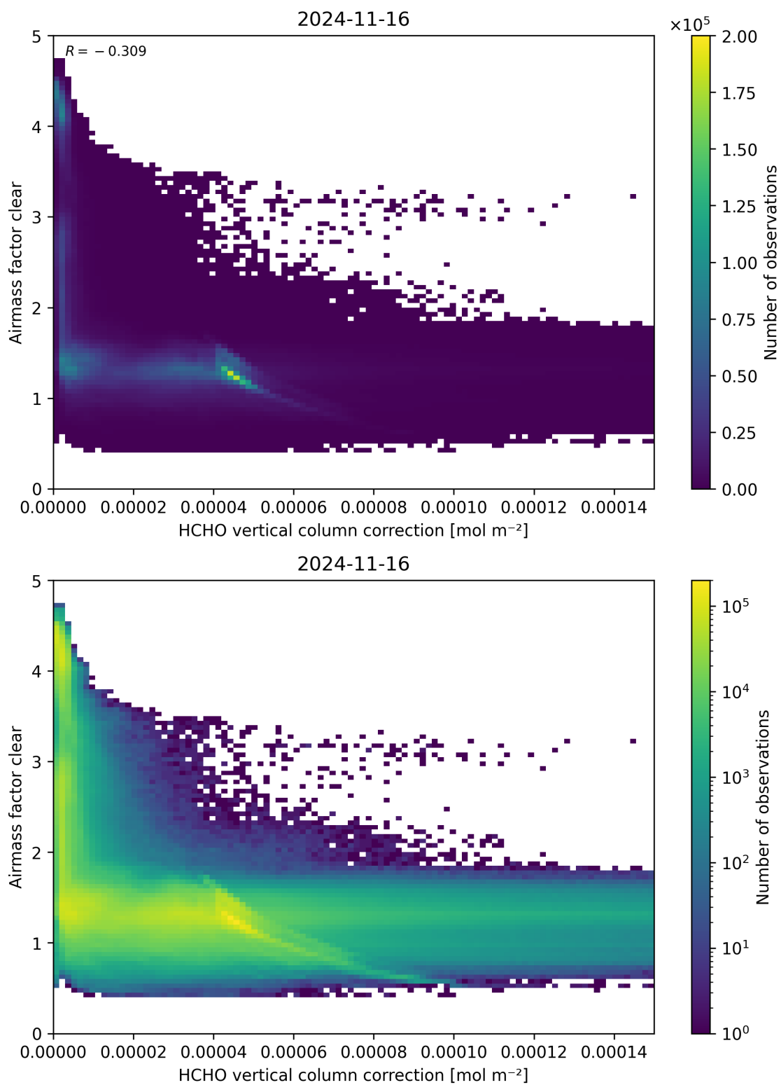
Figure 115: Scatter density plot of “HCHO vertical column correction” against “Airmass factor clear” for 2024-11-15 to 2024-11-17.
