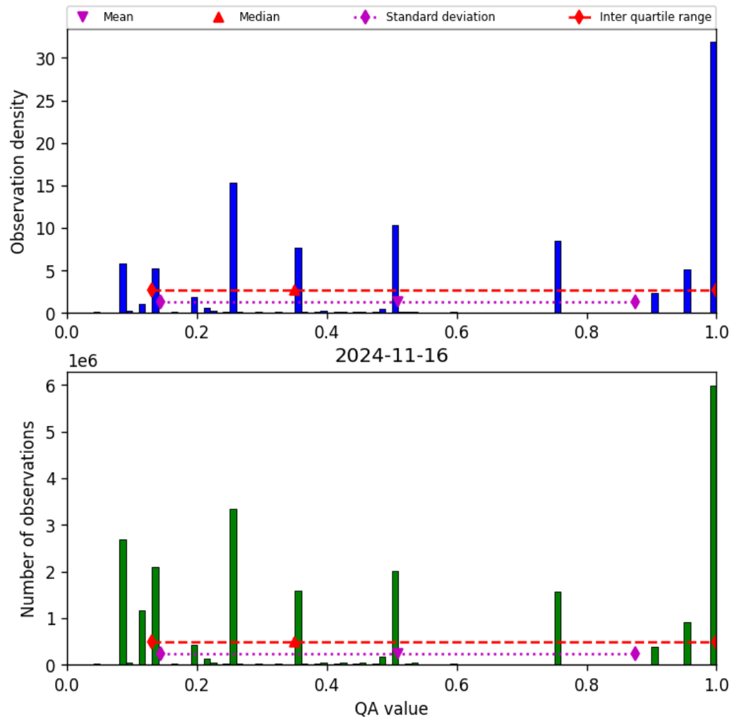
Figure 34: Histogram of “QA value” for 2024-11-15 to 2024-11-17
