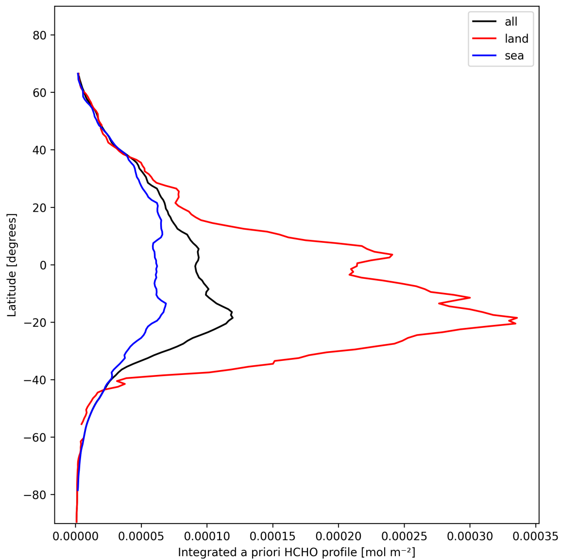
Figure 29: Zonal average of “Integrated a priori HCHO profile” for 2024-11-15 to 2024-11-17.
