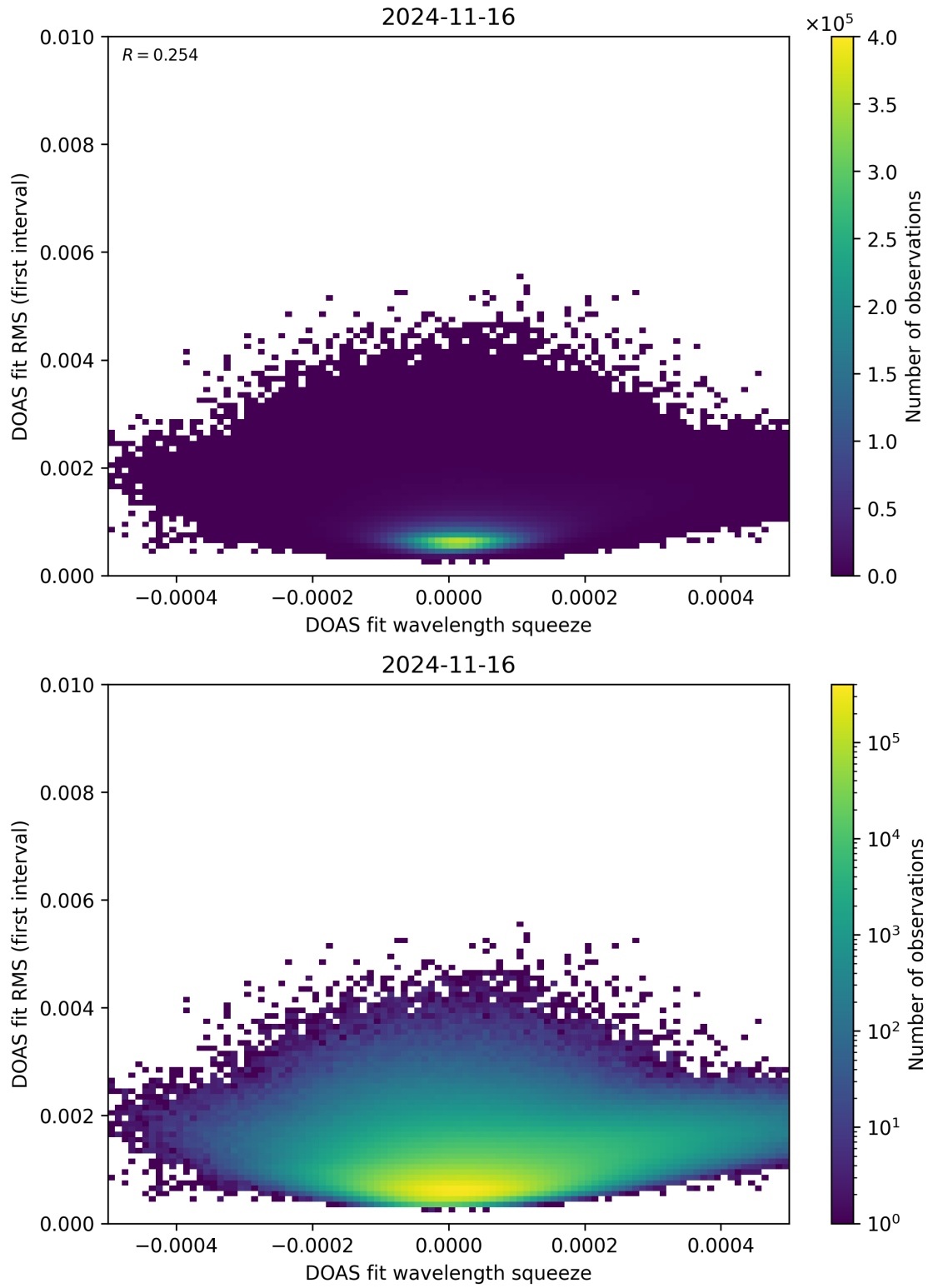
Figure 68: Scatter density plot of “DOAS fit wavelength squeeze” against “DOAS fit RMS (first interval)” for 2024-11-15 to 2024-11-17.
