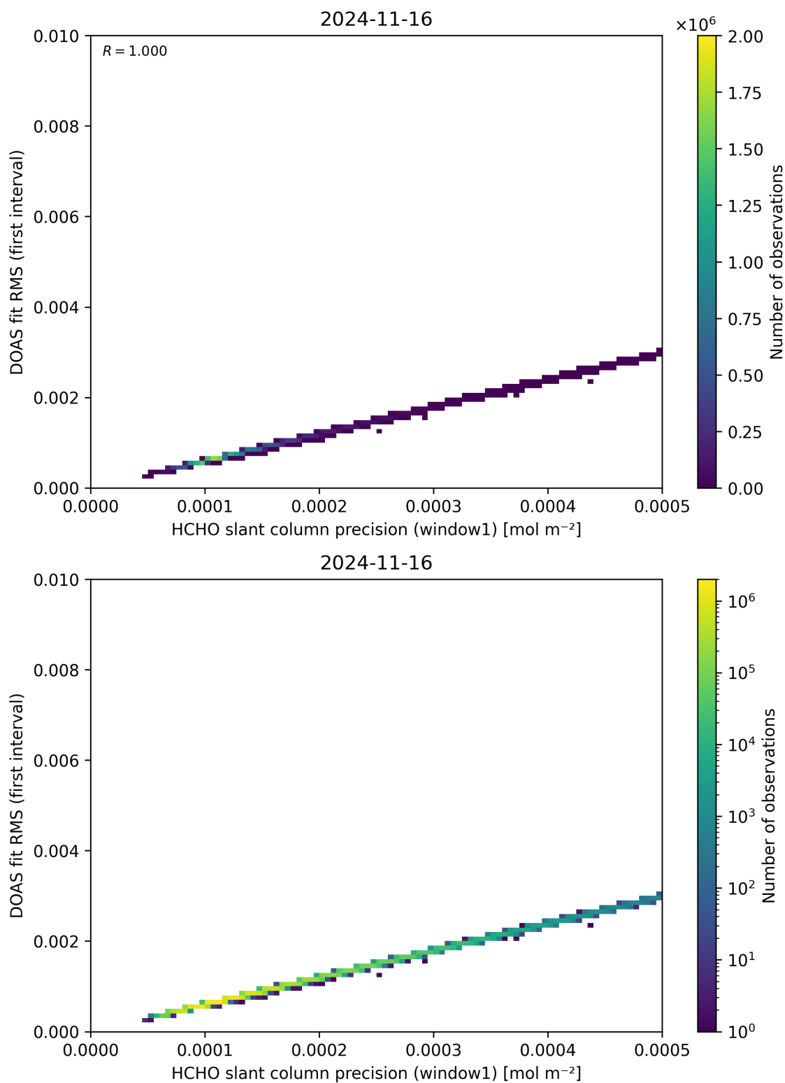
Figure 88: Scatter density plot of “HCHO slant column precision (window1)” against “DOAS fit RMS (first interval)” for 2024-11-15 to 2024-11-17.
