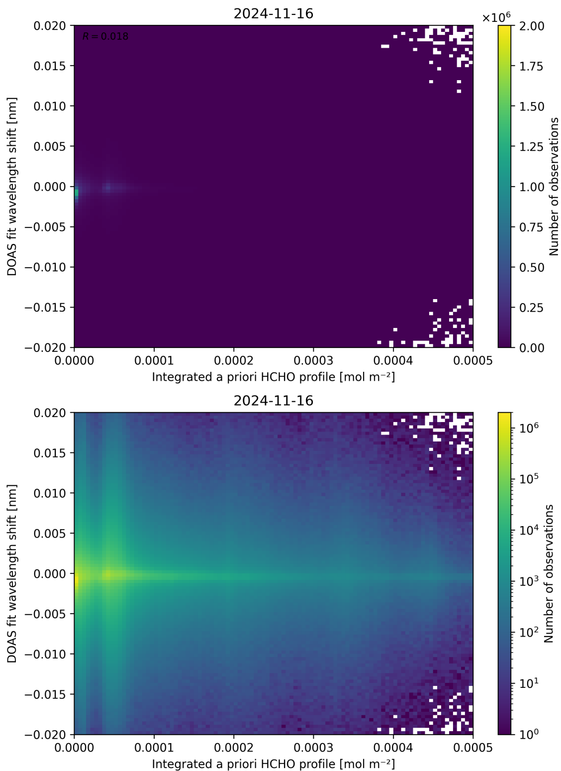
Figure 149: Scatter density plot of “Integrated a priori HCHO profile” against “DOAS fit wavelength shift” for 2024-11-15 to 2024-11-17.
