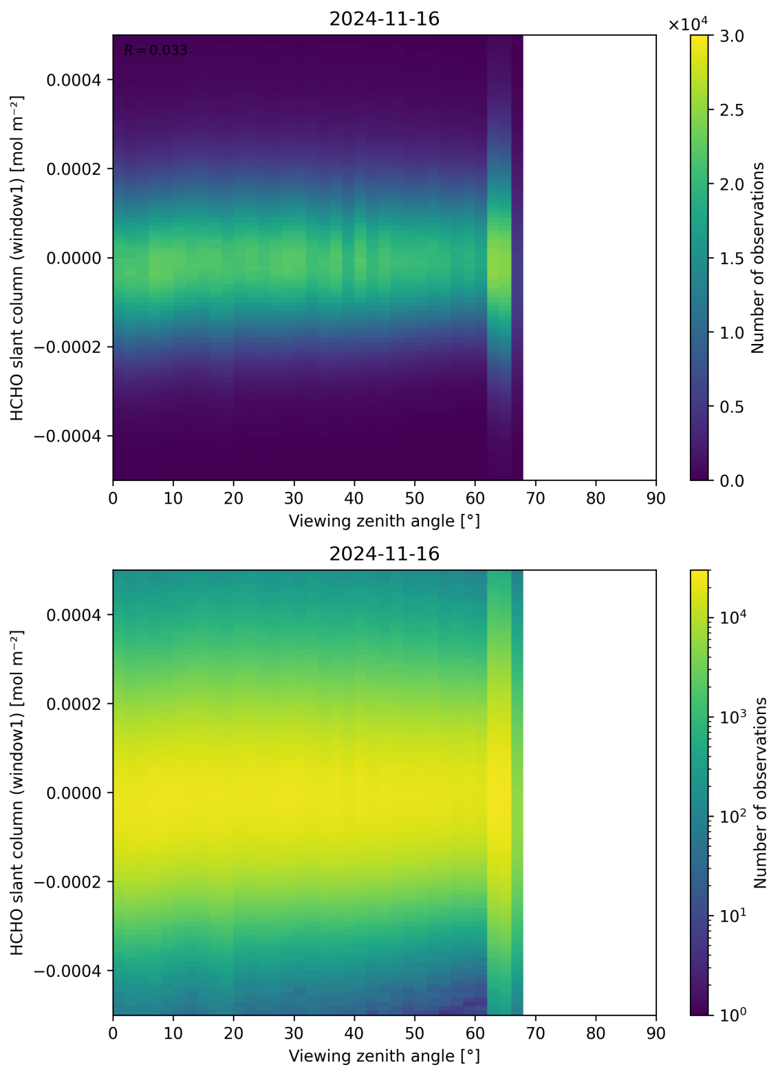
Figure 188: Scatter density plot of “Viewing zenith angle” against “HCHO slant column (window1)” for 2024-11-15 to 2024-11-17.
