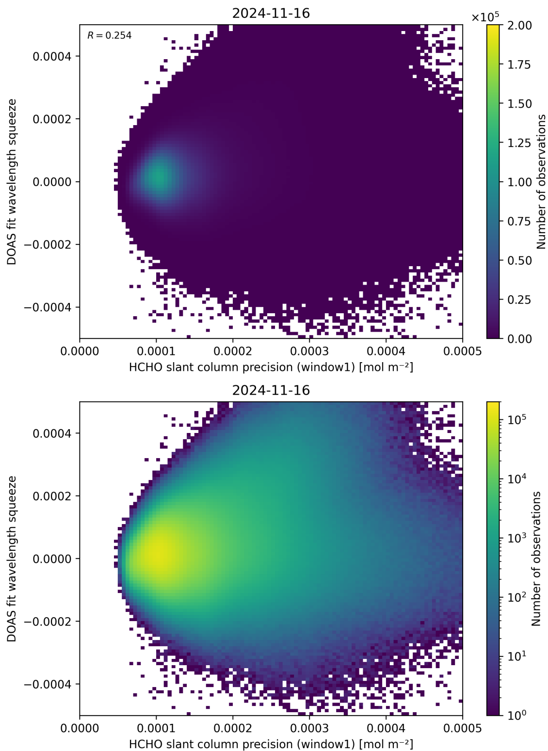
Figure 90: Scatter density plot of “HCHO slant column precision (window1)” against “DOAS fit wavelength squeeze” for 2024-11-15 to 2024-11-17.
