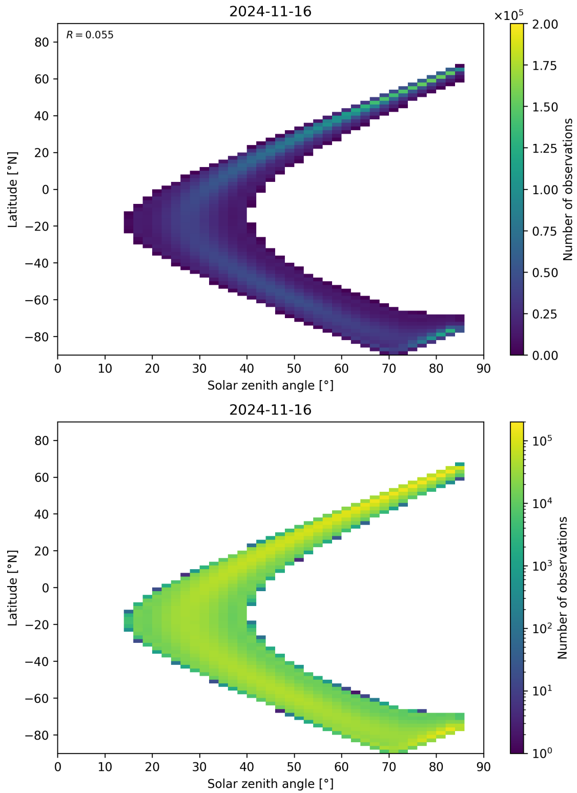
Figure 181: Scatter density plot of “Solar zenith angle” against “Latitude” for 2024-11-15 to 2024-11-17.
