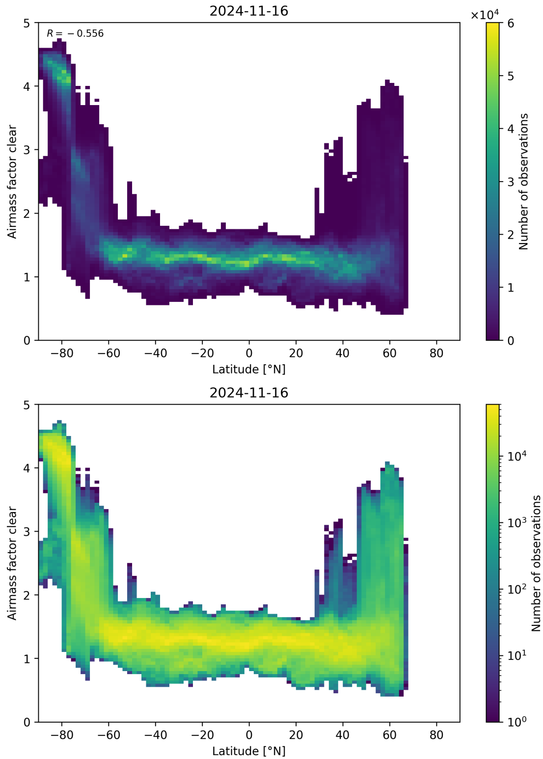
Figure 156: Scatter density plot of “Latitude” against “Airmass factor clear” for 2024-11-15 to 2024-11-17.
