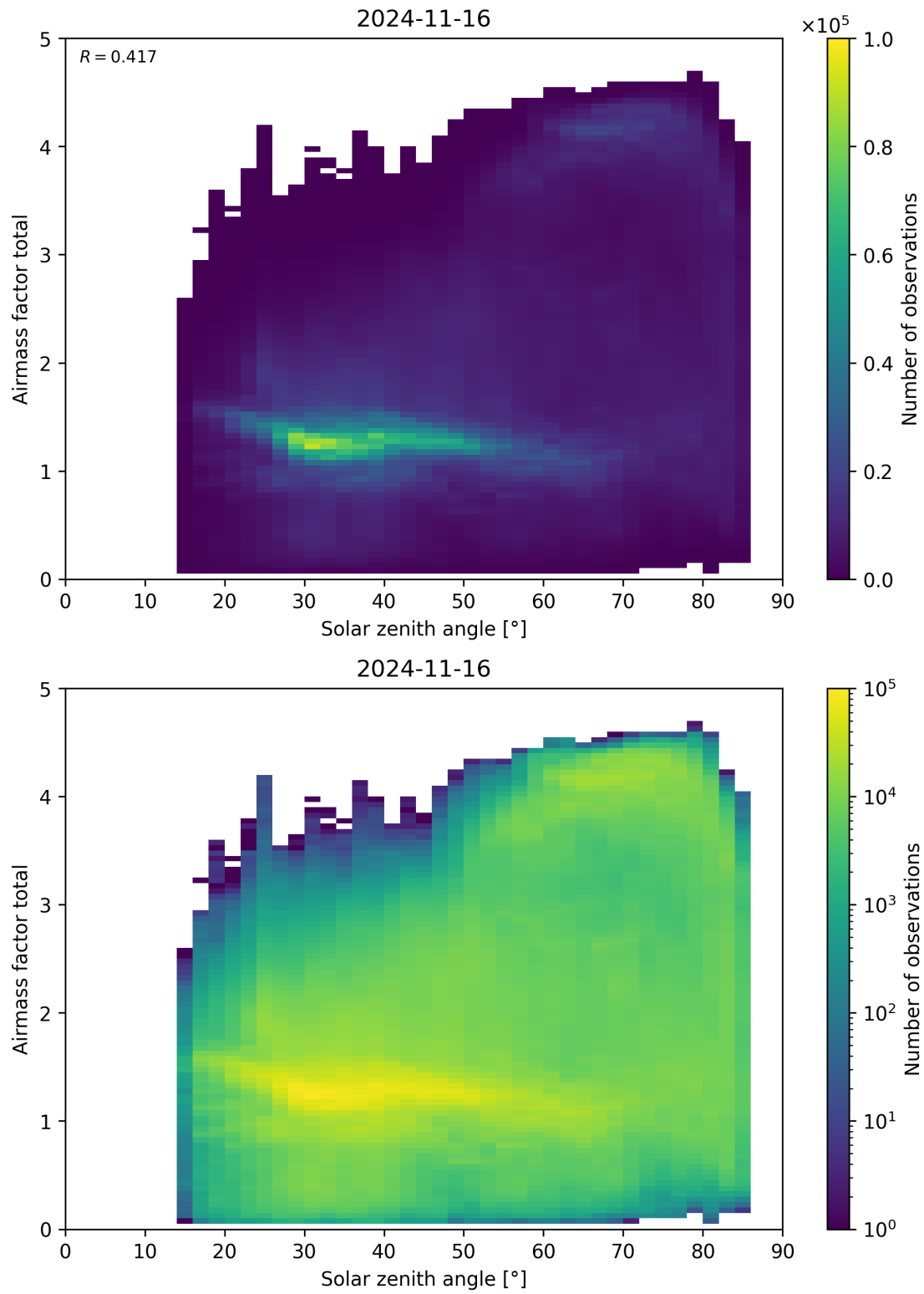
Figure 175: Scatter density plot of “Solar zenith angle” against “Airmass factor total” for 2024-11-15 to 2024-11-17.
