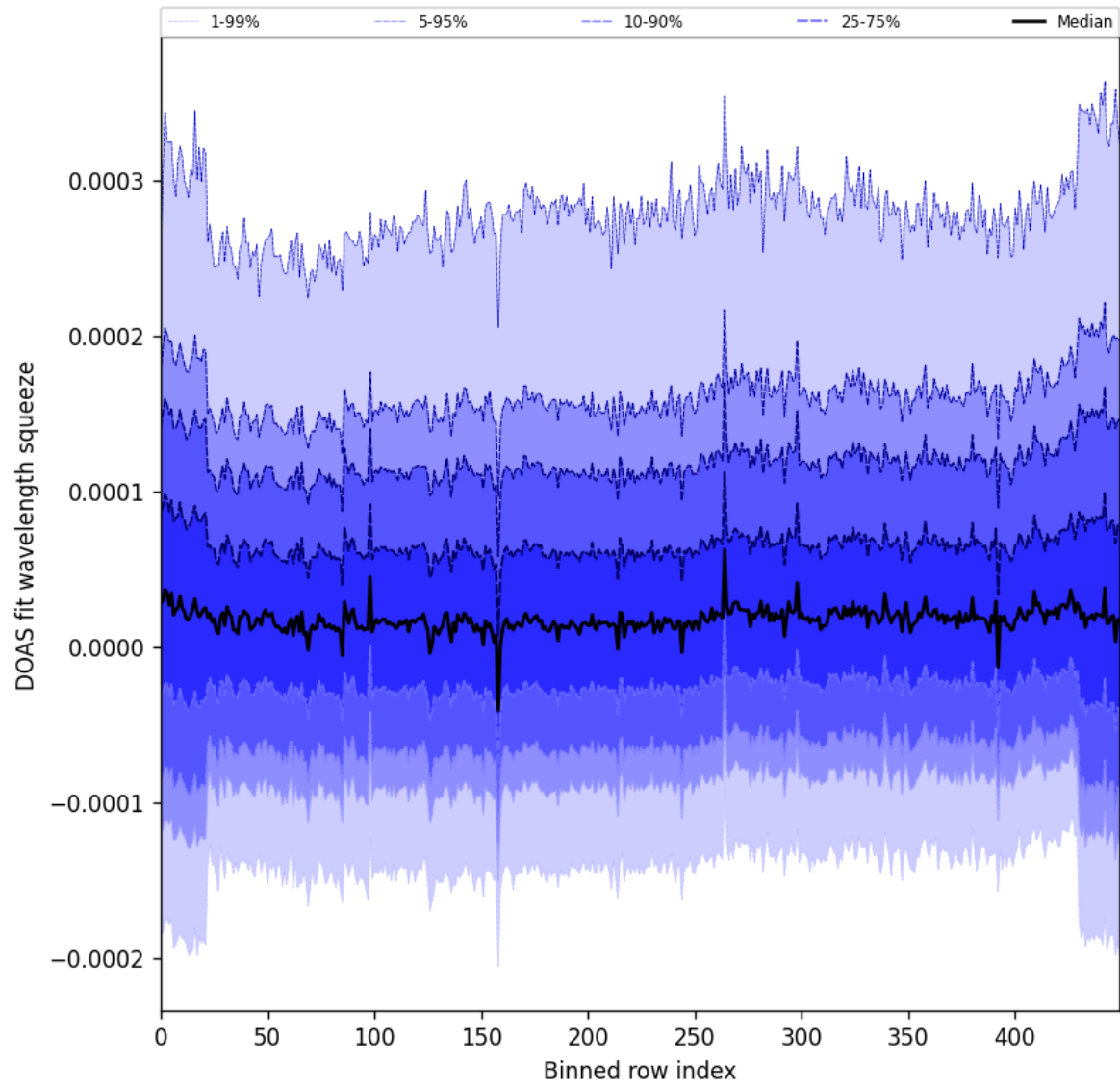
Figure 59: Along track statistics of “DOAS fit wavelength squeeze” for 2024-11-15 to 2024-11-17
