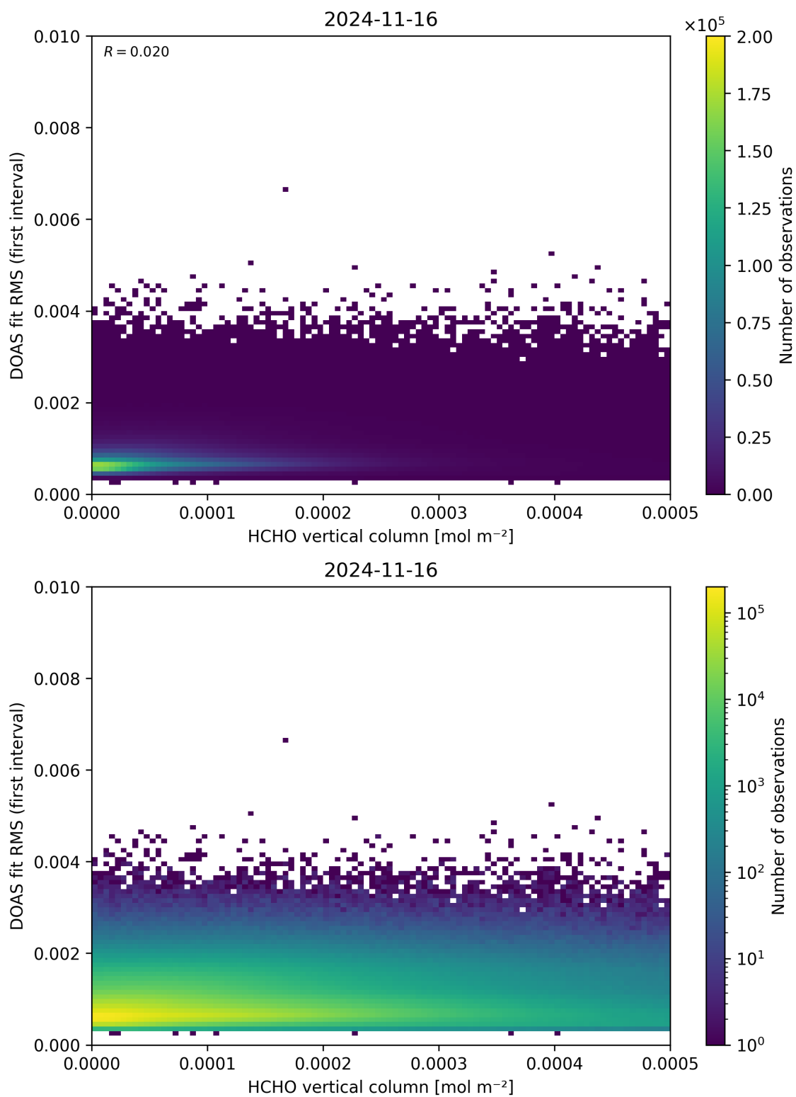
Figure 123: Scatter density plot of “HCHO vertical column” against “DOAS fit RMS (first interval)” for 2024-11-15 to 2024-11-17.
