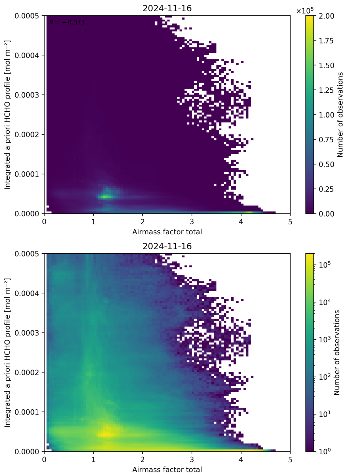
Figure 104: Scatter density plot of “Airmass factor total” against “Integrated a priori HCHO profile” for 2024-11-15 to 2024-11-17.
