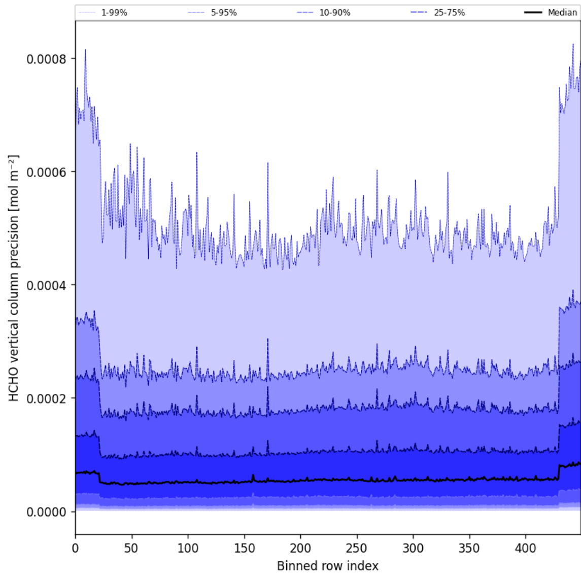
Figure 50: Along track statistics of "HCHO vertical column precision" for 2024-11-15 to 2024-11-17
