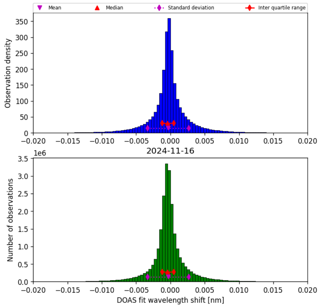
Figure 44: Histogram of “DOAS fit wavelength shift” for 2024-11-15 to 2024-11-17
