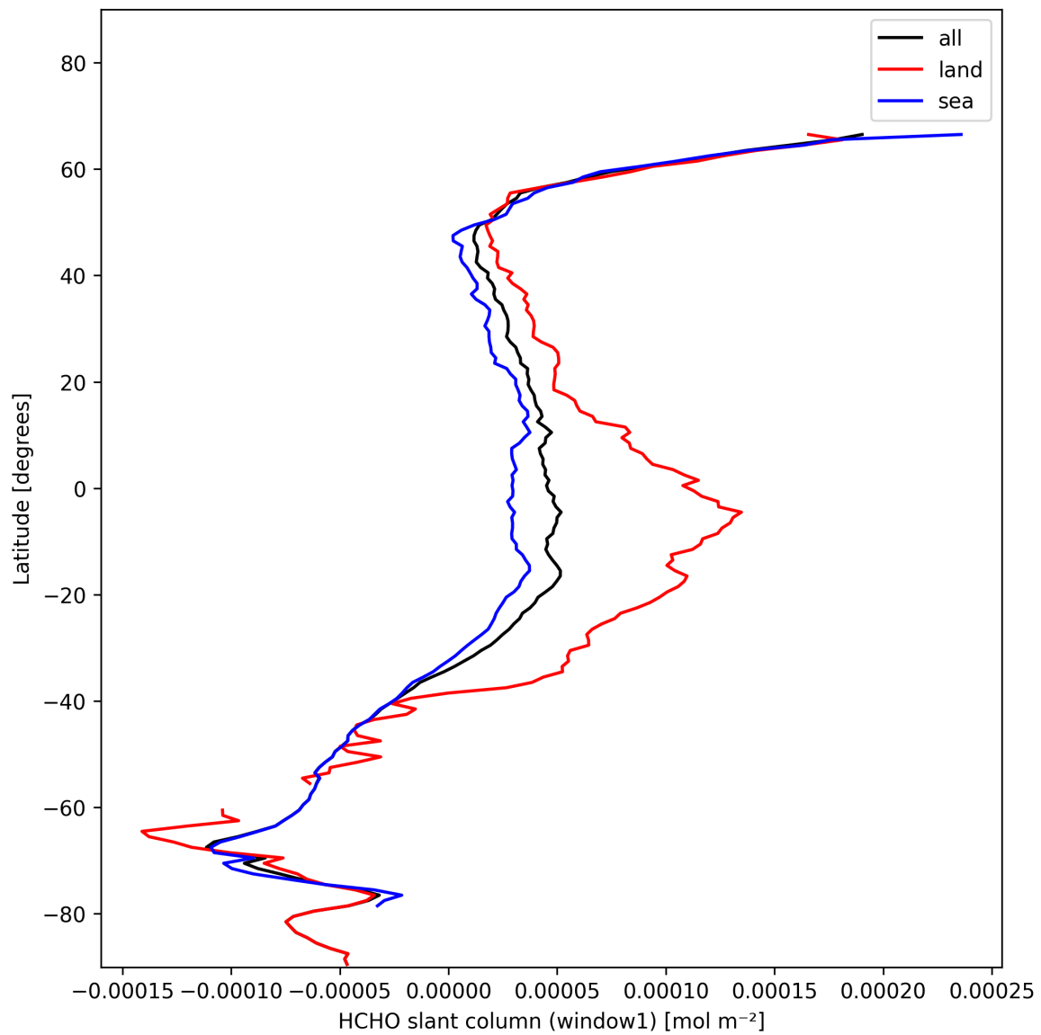
Figure 24: Zonal average of “HCHO slant column (window1)” for 2024-11-15 to 2024-11-17.
