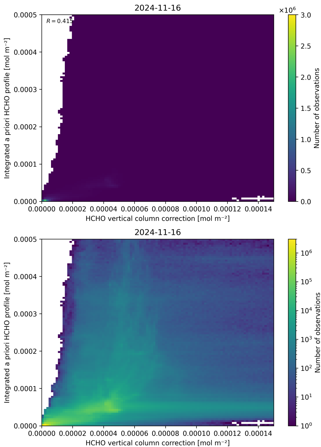
Figure 122: Scatter density plot of “HCHO vertical column correction” against “Integrated a priori HCHO profile” for 2024-11-15 to 2024-11-17.
