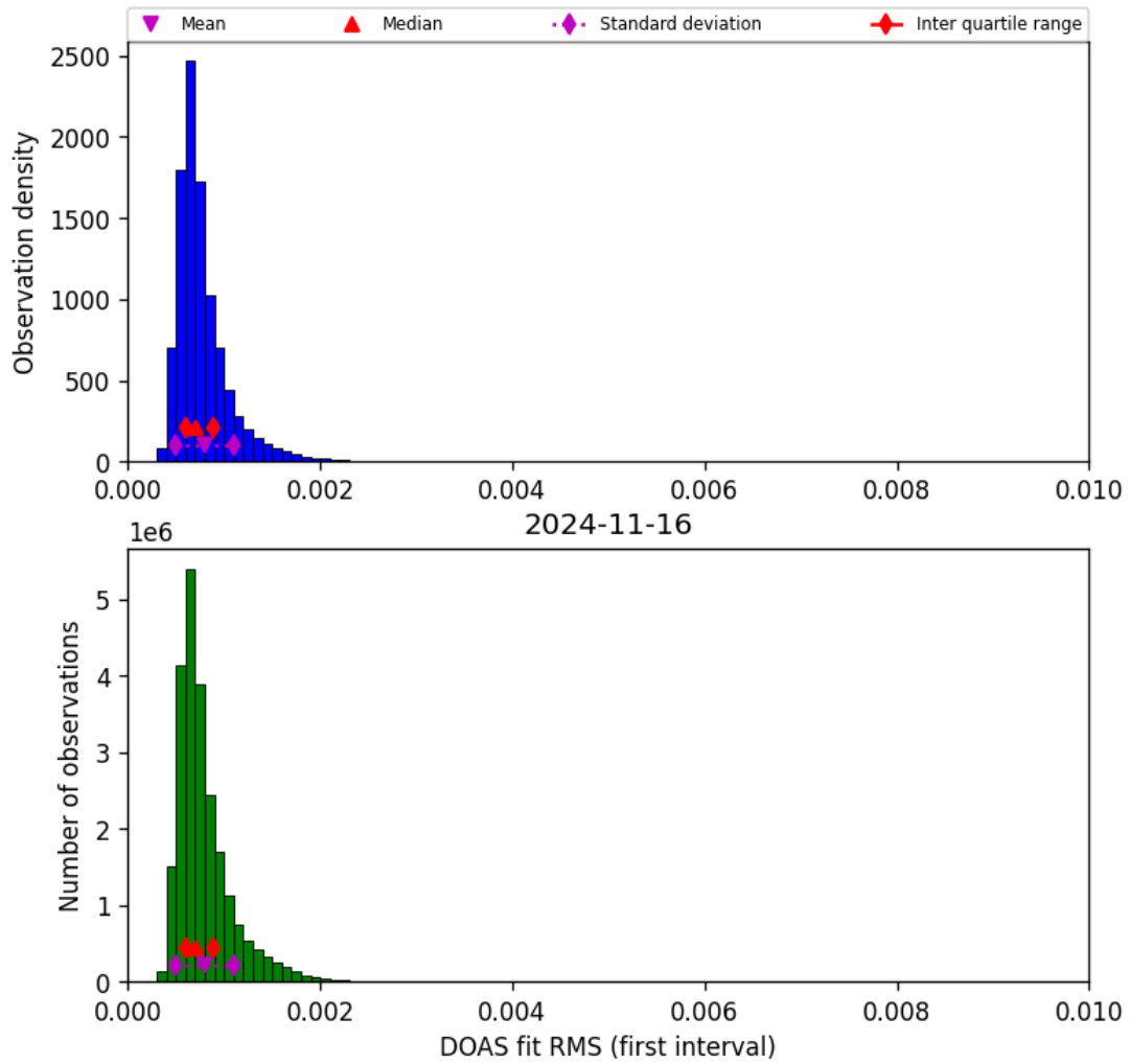
Figure 46: Histogram of “DOAS fit RMS (first interval)” for 2024-11-15 to 2024-11-17
