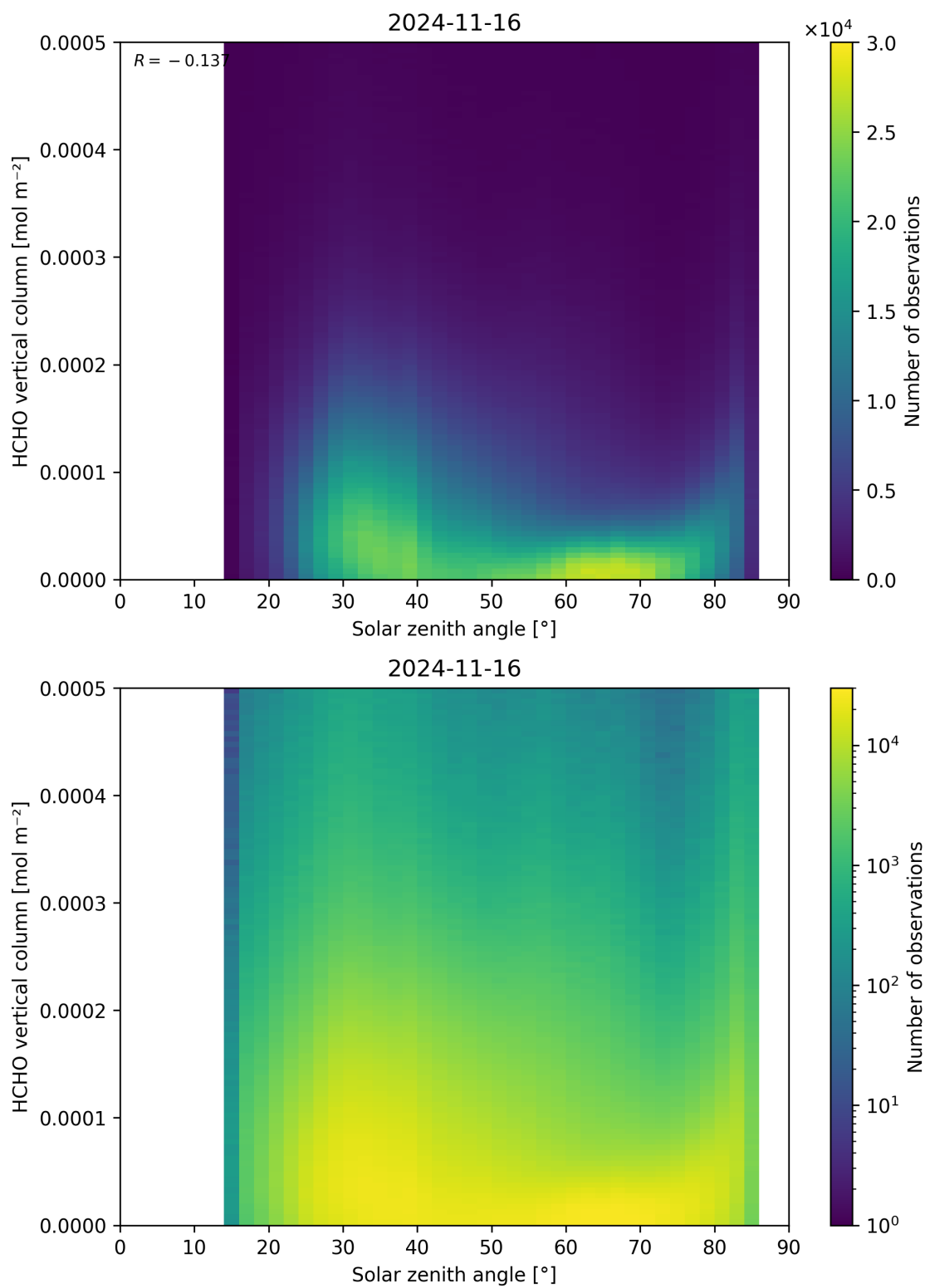
Figure 177: Scatter density plot of “Solar zenith angle” against “HCHO vertical column” for 2024-11-15 to 2024-11-17.
