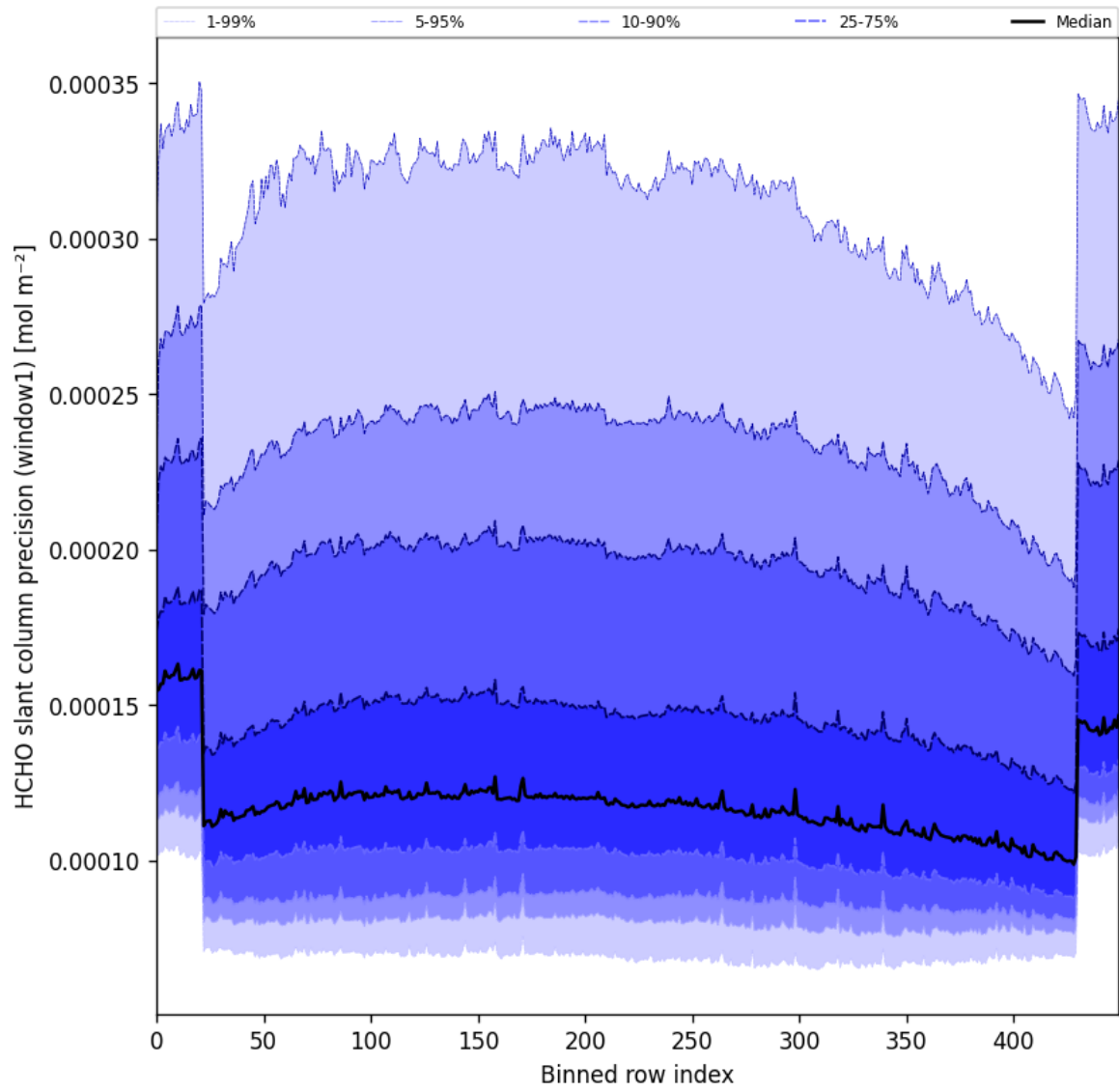
Figure 53: Along track statistics of “HCHO slant column precision (window1)” for 2024-11-15 to 2024-11-17
