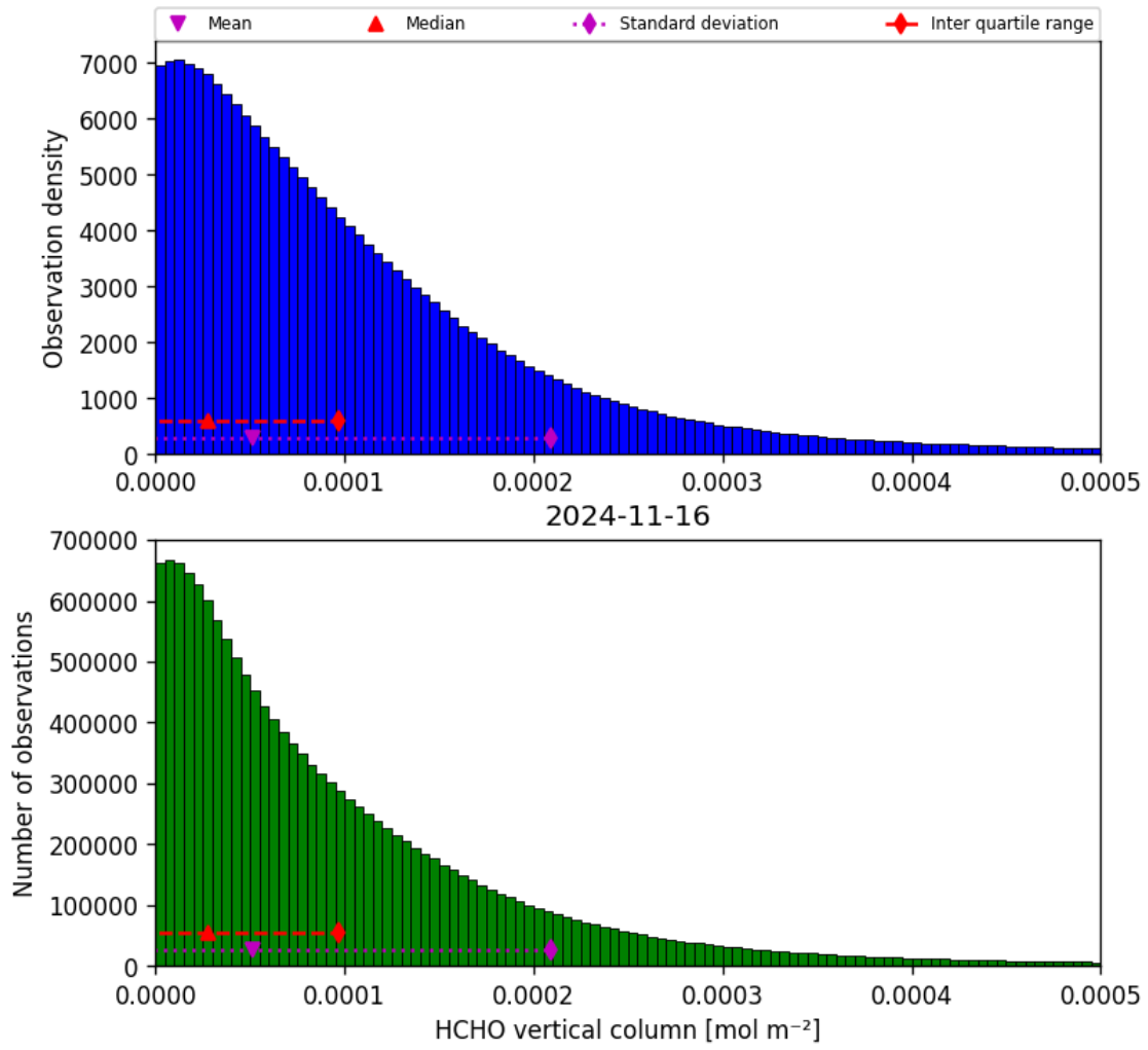
Figure 35: Histogram of “HCHO vertical column” for 2024-11-15 to 2024-11-17
