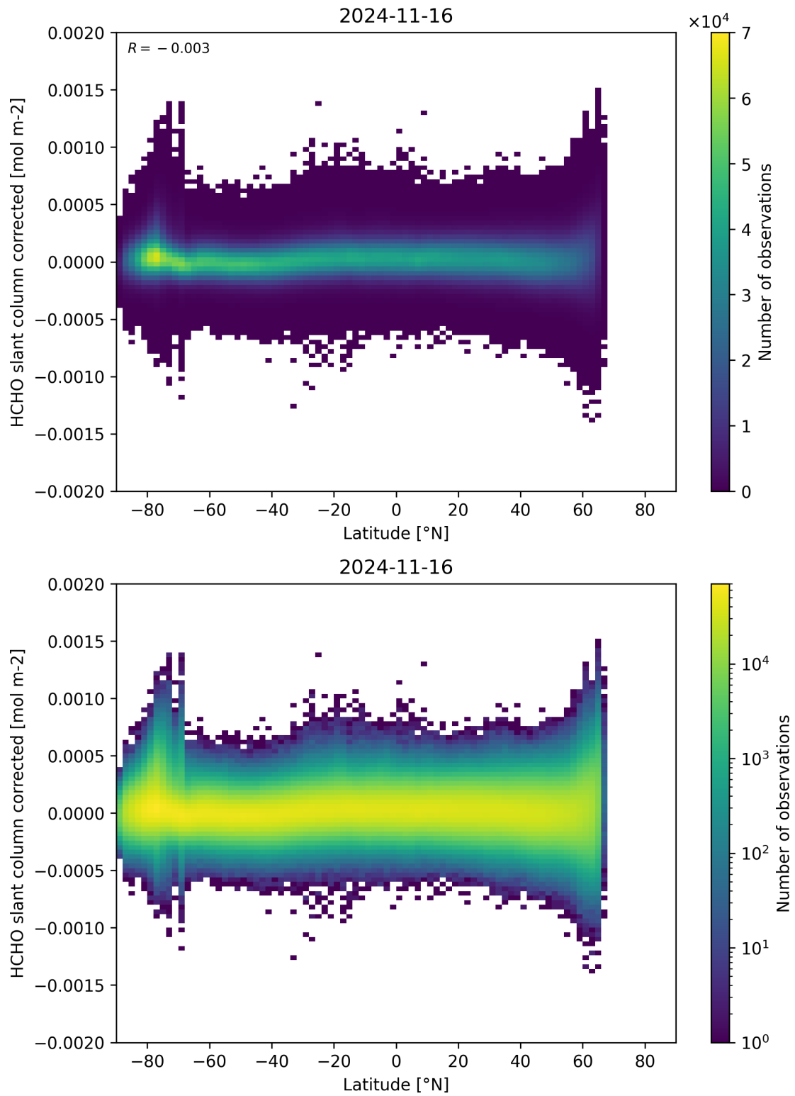
Figure 157: Scatter density plot of “Latitude” against “HCHO slant column corrected” for 2024-11-15 to 2024-11-17.
