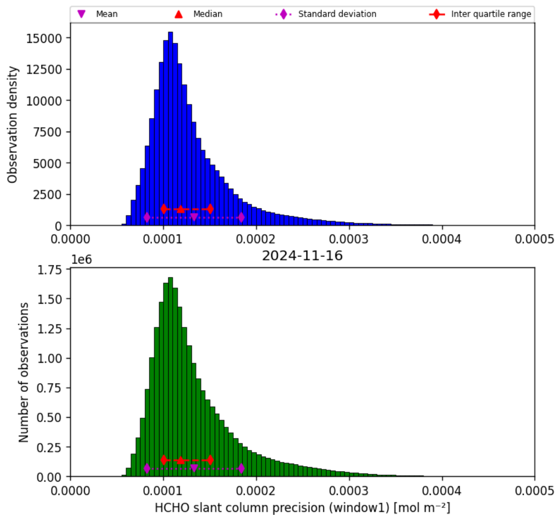
Figure 39: Histogram of “HCHO slant column precision (window1)” for 2024-11-15 to 2024-11-17
