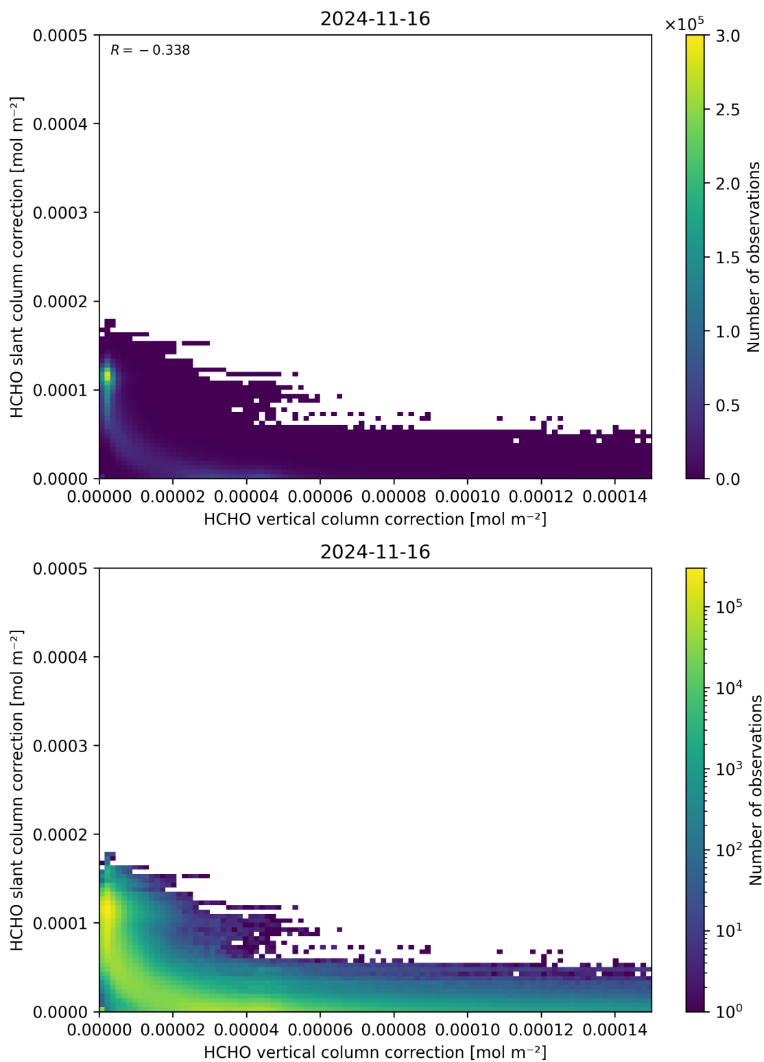
Figure 117: Scatter density plot of “HCHO vertical column correction” against “HCHO slant column correction” for 2024-11-15 to 2024-11-17.
