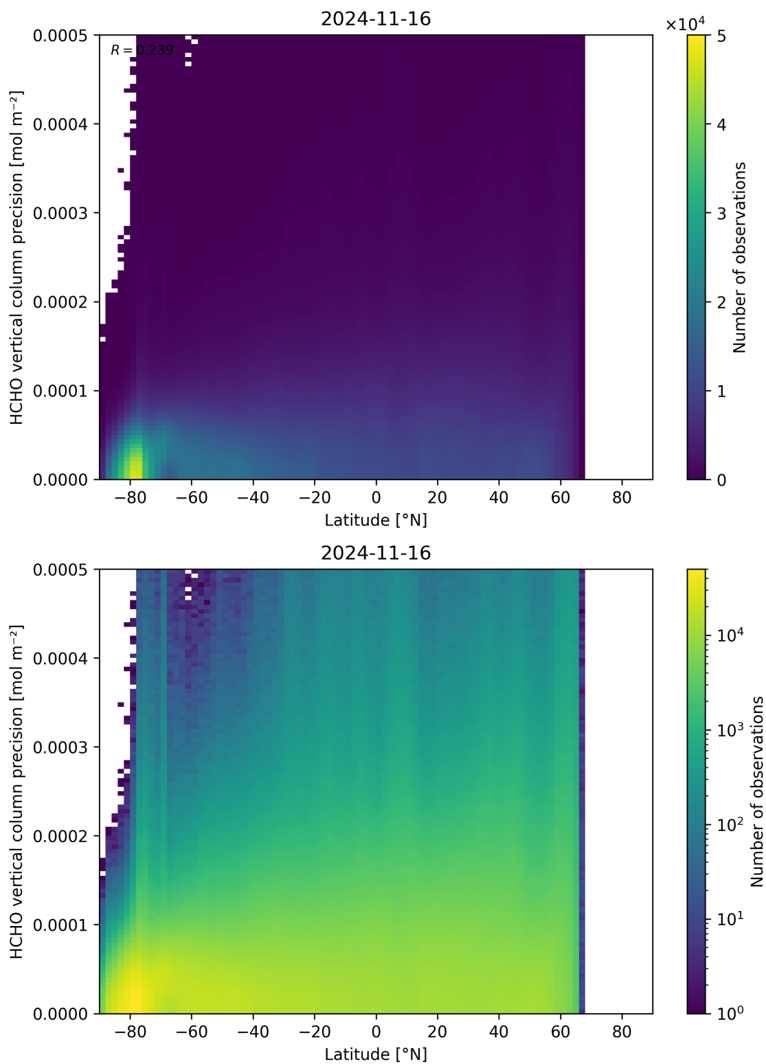
Figure 165: Scatter density plot of “Latitude” against “HCHO vertical column precision” for 2024-11-15 to 2024-11-17.
