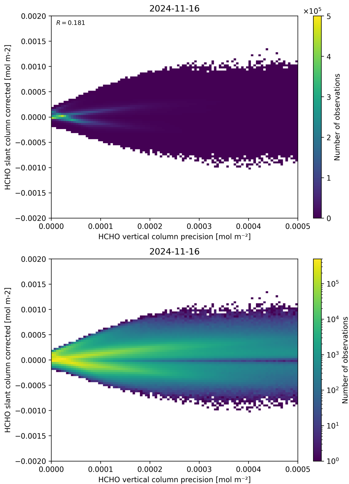
Figure 140: Scatter density plot of “HCHO vertical column precision” against “HCHO slant column corrected” for 2024-11-15 to 2024-11-17.
