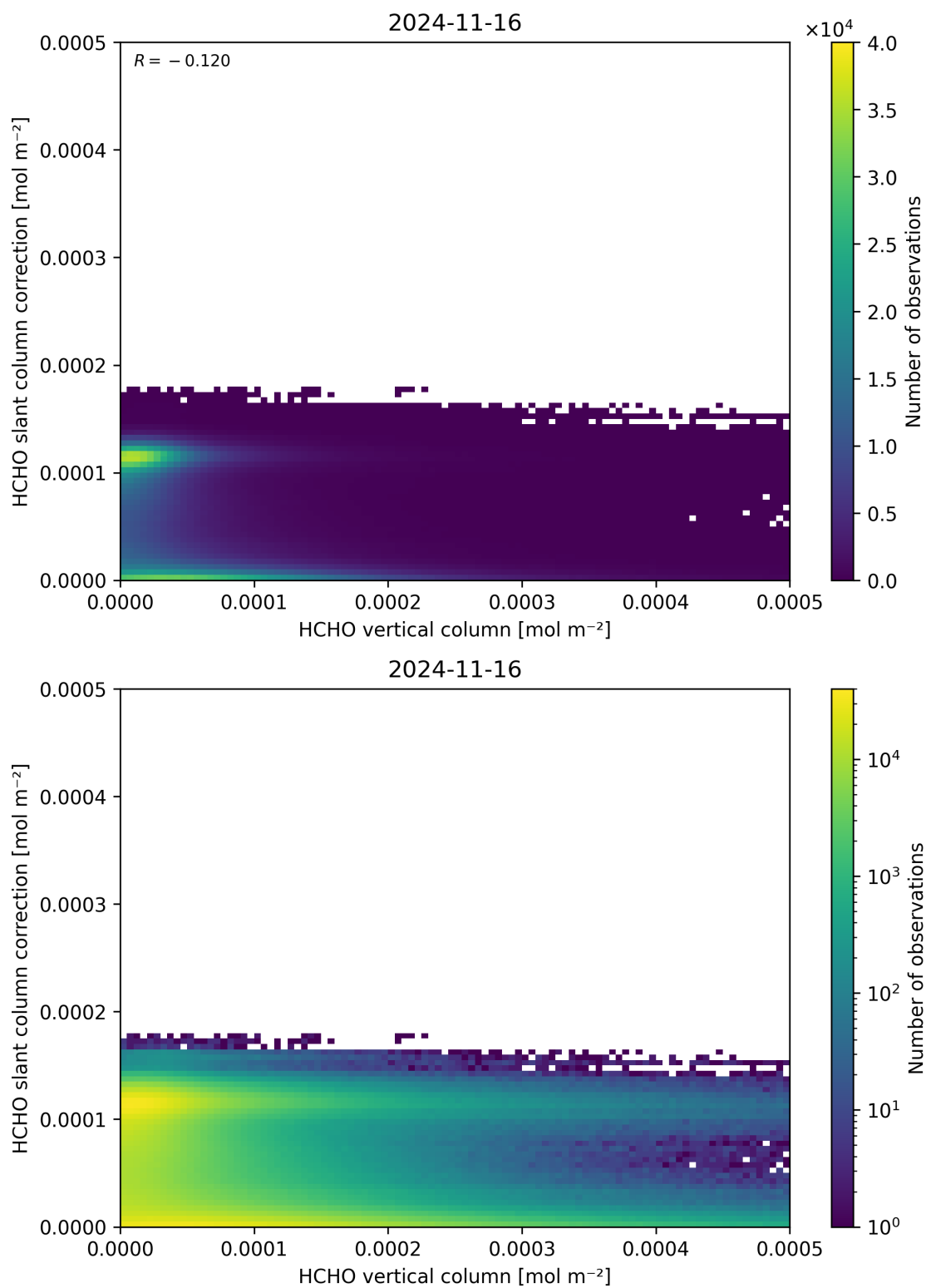
Figure 128: Scatter density plot of “HCHO vertical column” against “HCHO slant column correction” for 2024-11-15 to 2024-11-17.
