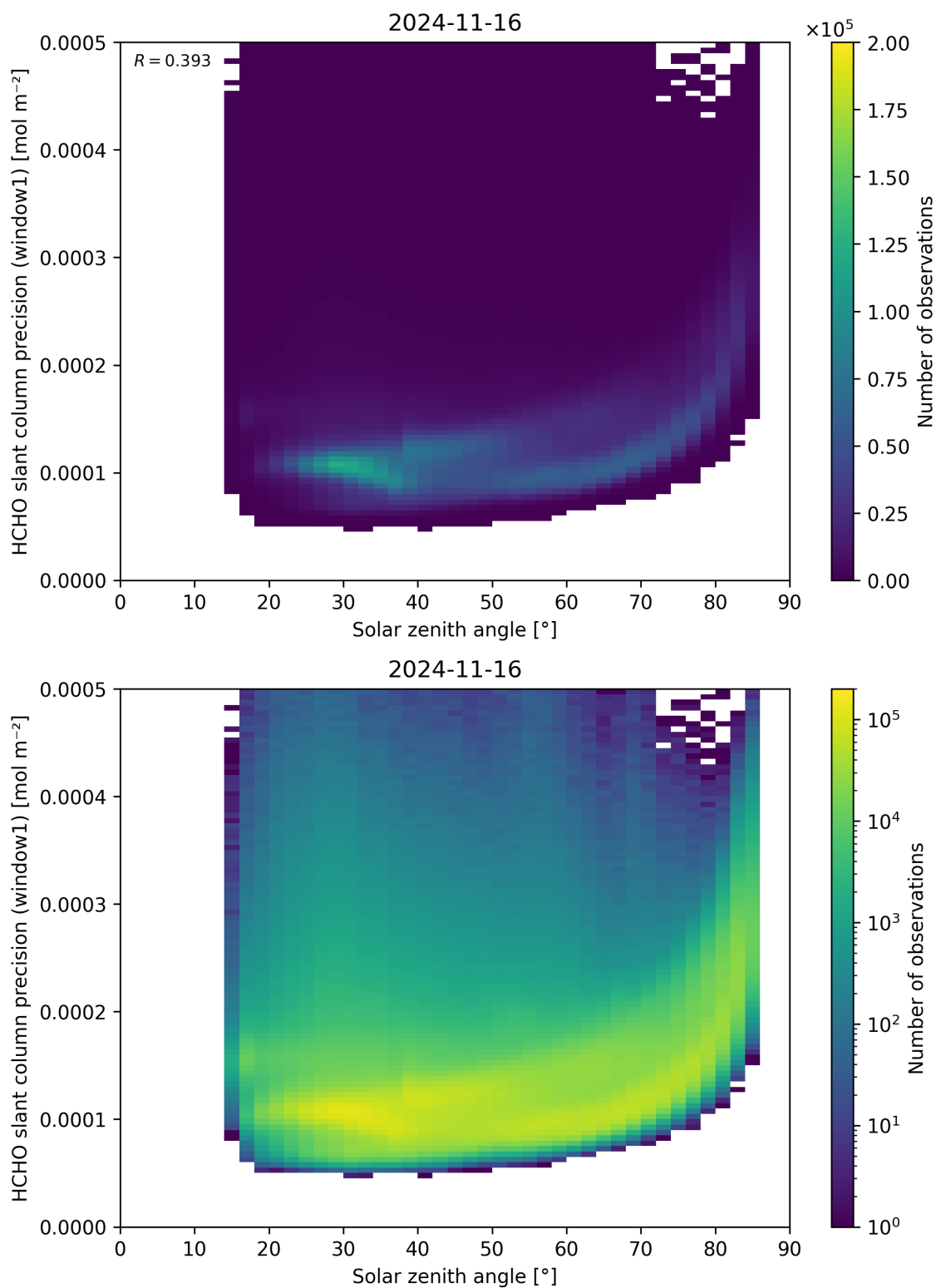
Figure 174: Scatter density plot of “Solar zenith angle” against “HCHO slant column precision (window1)” for 2024-11-15 to 2024-11-17.
