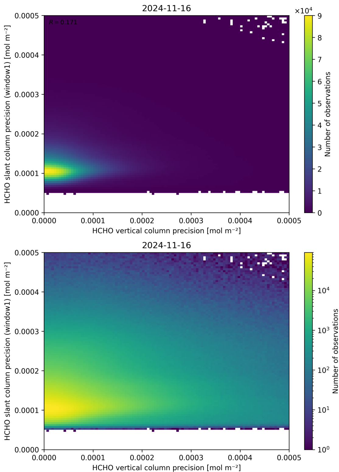
Figure 143: Scatter density plot of “HCHO vertical column precision” against “HCHO slant column precision (window1)” for 2024-11-15 to 2024-11-17.
