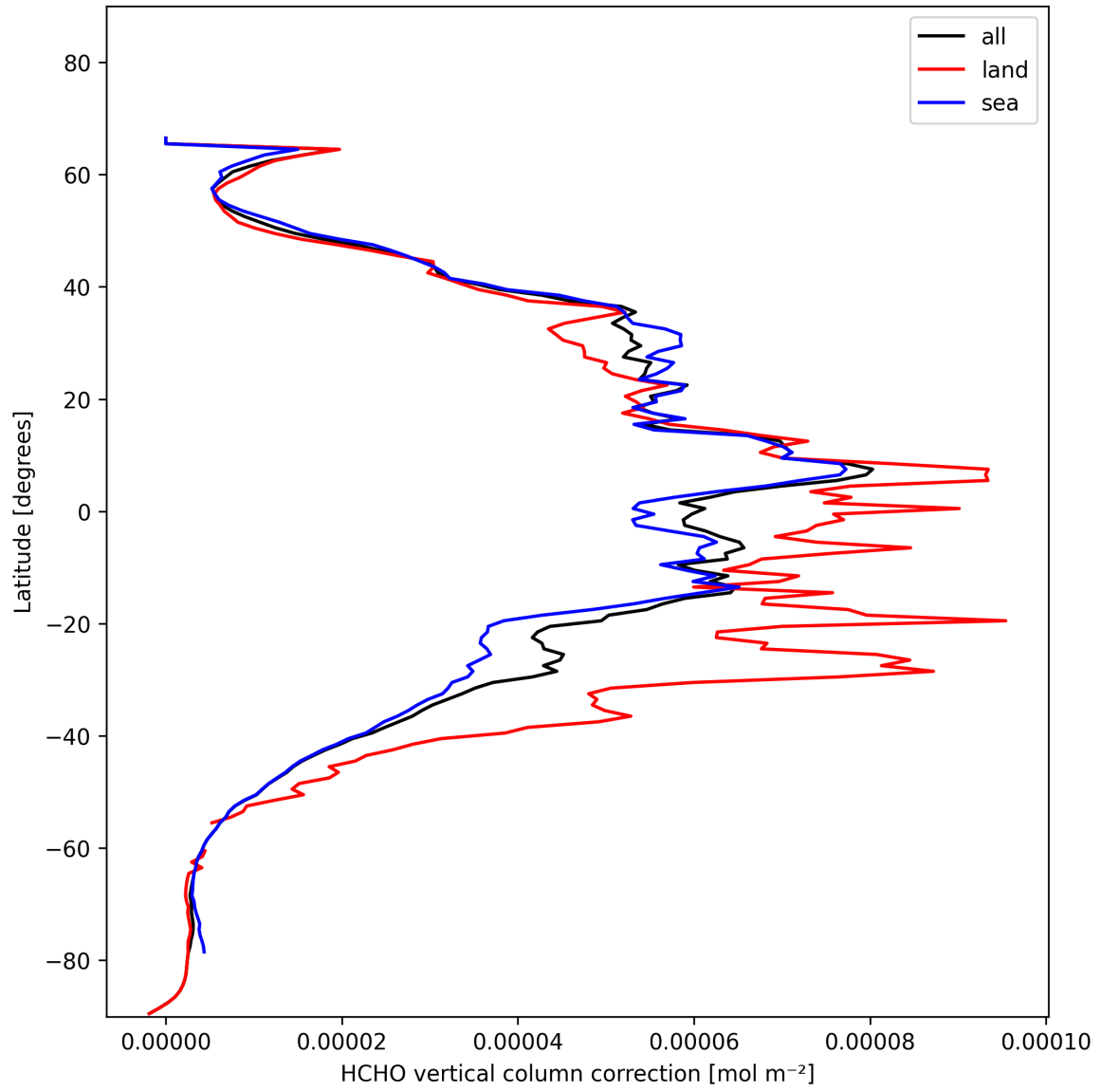
Figure 23: Zonal average of “HCHO vertical column correction” for 2024-11-15 to 2024-11-17.
