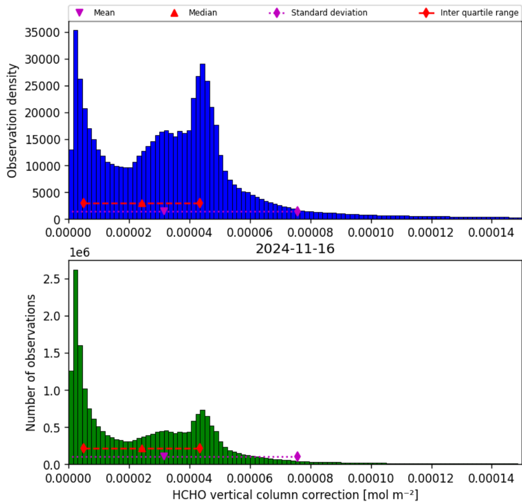
Figure 37: Histogram of “HCHO vertical column correction” for 2024-11-15 to 2024-11-17
