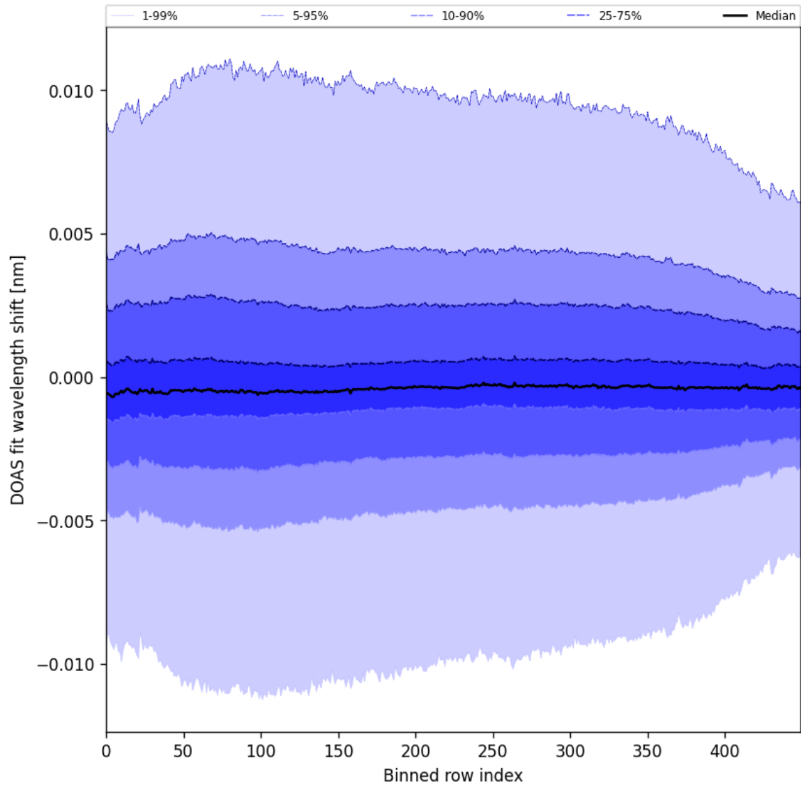
Figure 58: Along track statistics of “DOAS fit wavelength shift” for 2024-11-15 to 2024-11-17
