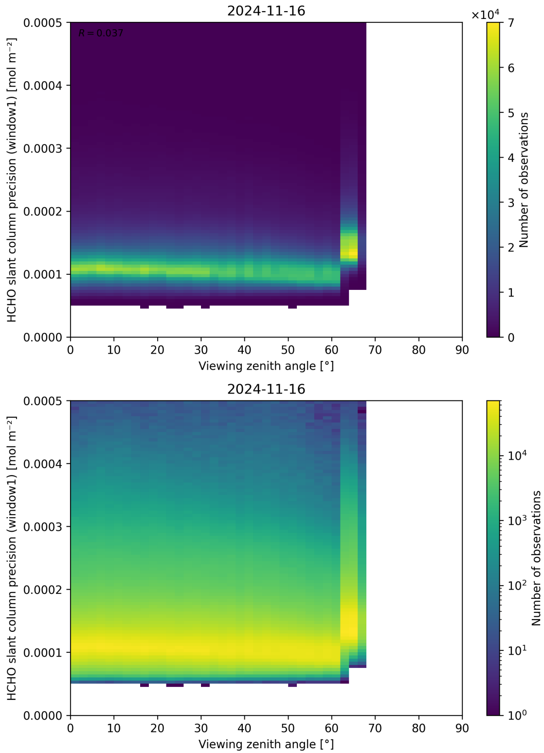
Figure 189: Scatter density plot of “Viewing zenith angle” against “HCHO slant column precision (window1)” for 2024-11-15 to 2024-11-17.
