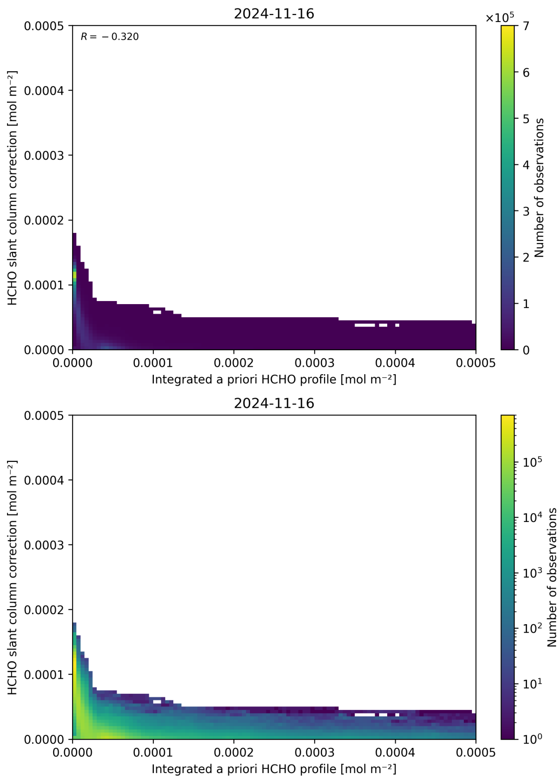
Figure 152: Scatter density plot of “Integrated a priori HCHO profile” against “HCHO slant column correction” for 2024-11-15 to 2024-11-17.
