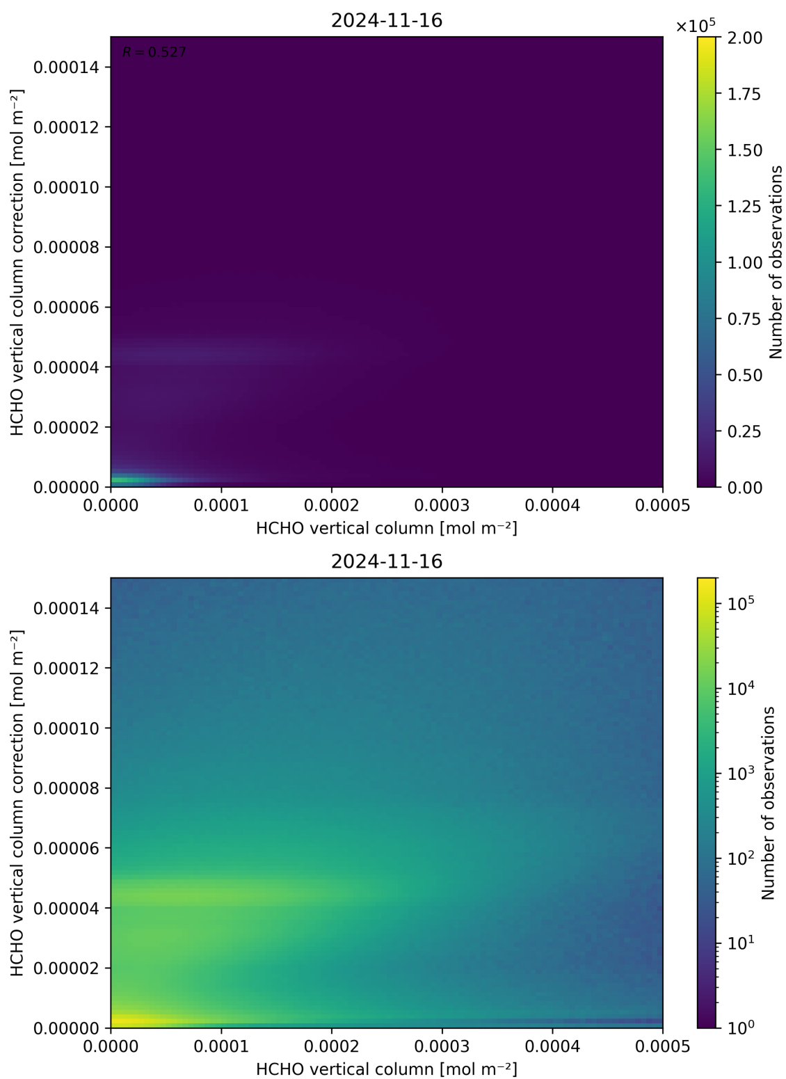
Figure 133: Scatter density plot of “HCHO vertical column” against “HCHO vertical column correction” for 2024-11-15 to 2024-11-17.
