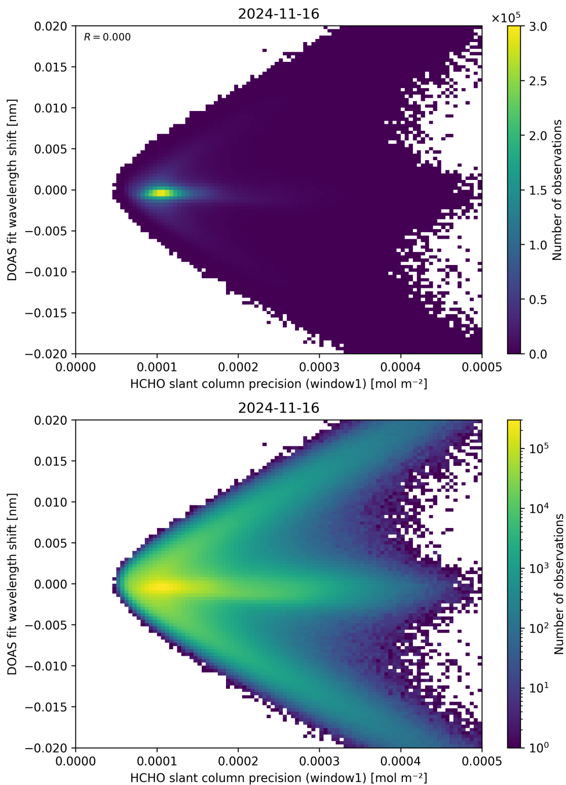
Figure 89: Scatter density plot of “HCHO slant column precision (window1)” against “DOAS fit wavelength shift” for 2024-11-15 to 2024-11-17.
