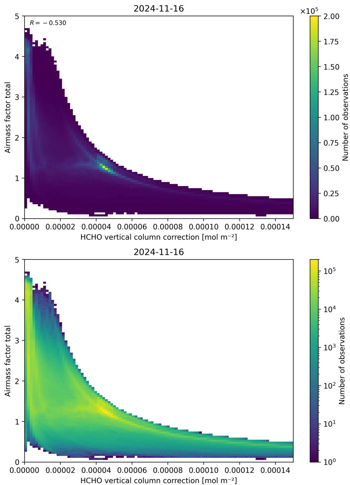
Figure 120: Scatter density plot of “HCHO vertical column correction” against “Airmass factor total” for 2024-11-15 to 2024-11-17.
