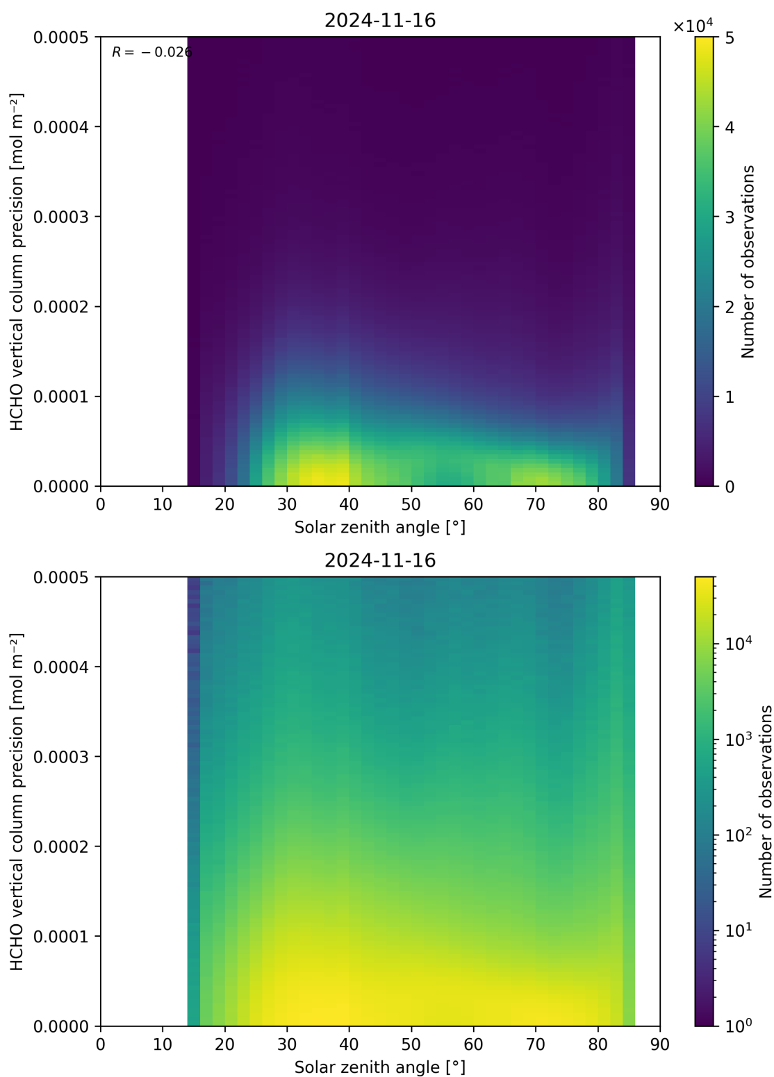
Figure 179: Scatter density plot of “Solar zenith angle” against “HCHO vertical column precision” for 2024-11-15 to 2024-11-17.
