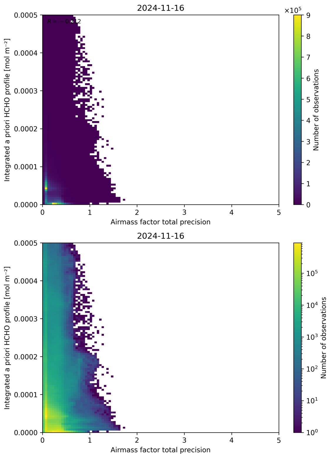
Figure 111: Scatter density plot of “Airmass factor total precision” against “Integrated a priori HCHO profile” for 2024-11-15 to 2024-11-17.
