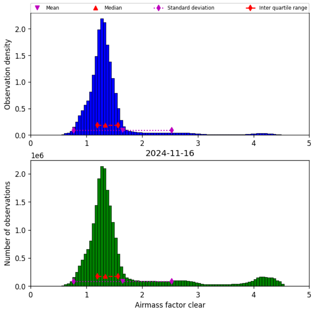
Figure 42: Histogram of “Airmass factor clear” for 2024-11-15 to 2024-11-17
