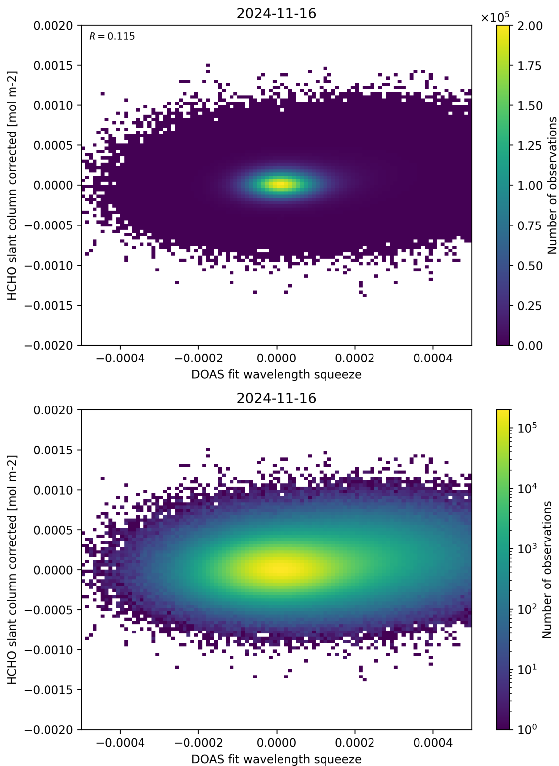
Figure 69: Scatter density plot of “DOAS fit wavelength squeeze” against “HCHO slant column corrected” for 2024-11-15 to 2024-11-17.
