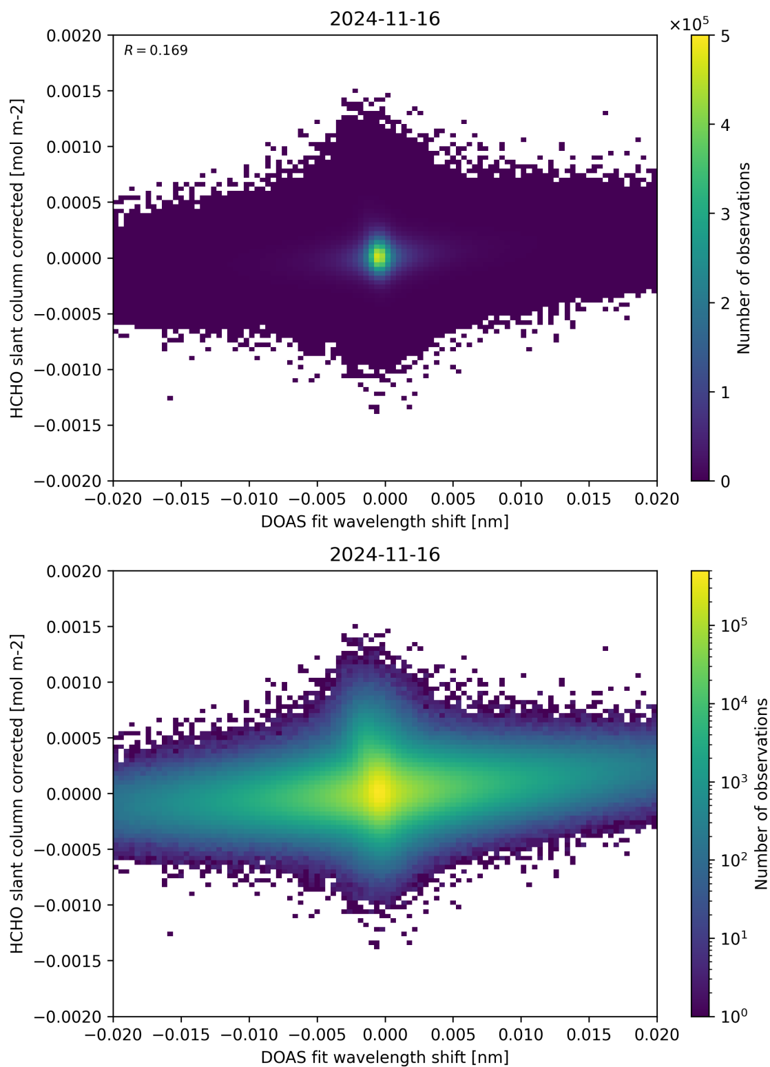
Figure 66: Scatter density plot of “DOAS fit wavelength shift” against “HCHO slant column corrected” for 2024-11-15 to 2024-11-17.
