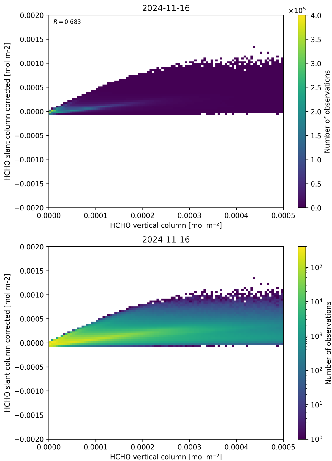
Figure 127: Scatter density plot of “HCHO vertical column” against “HCHO slant column corrected” for 2024-11-15 to 2024-11-17.
