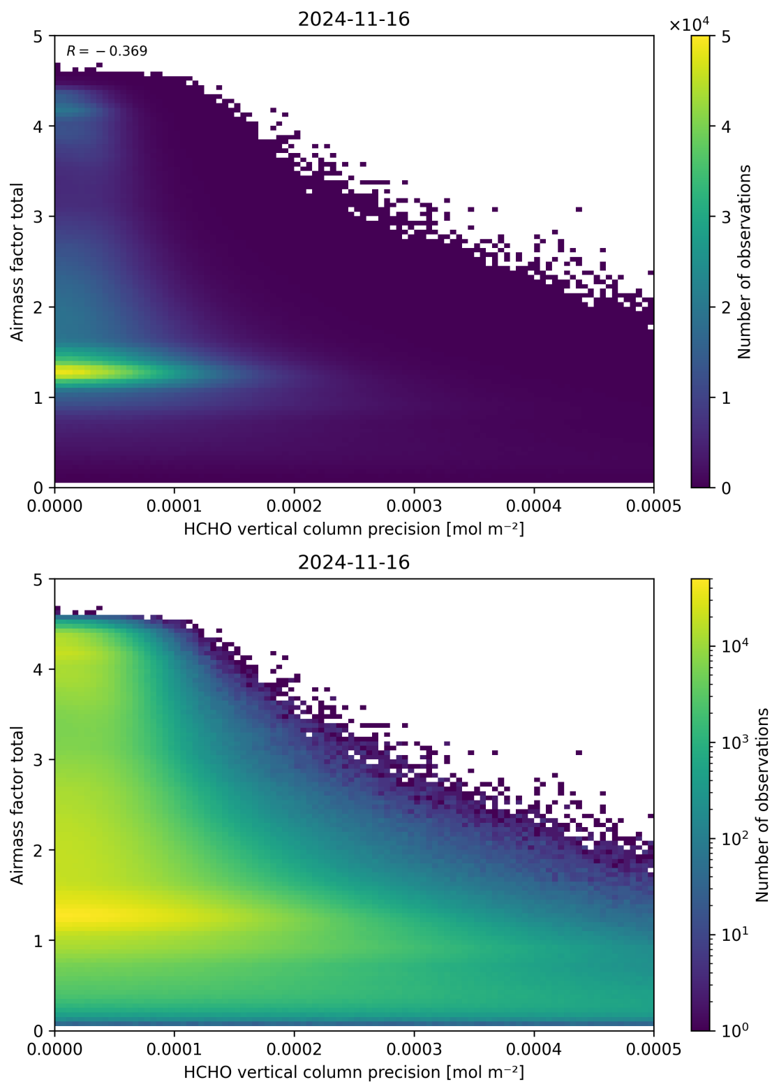
Figure 144: Scatter density plot of “HCHO vertical column precision” against “Airmass factor total” for 2024-11-15 to 2024-11-17.
