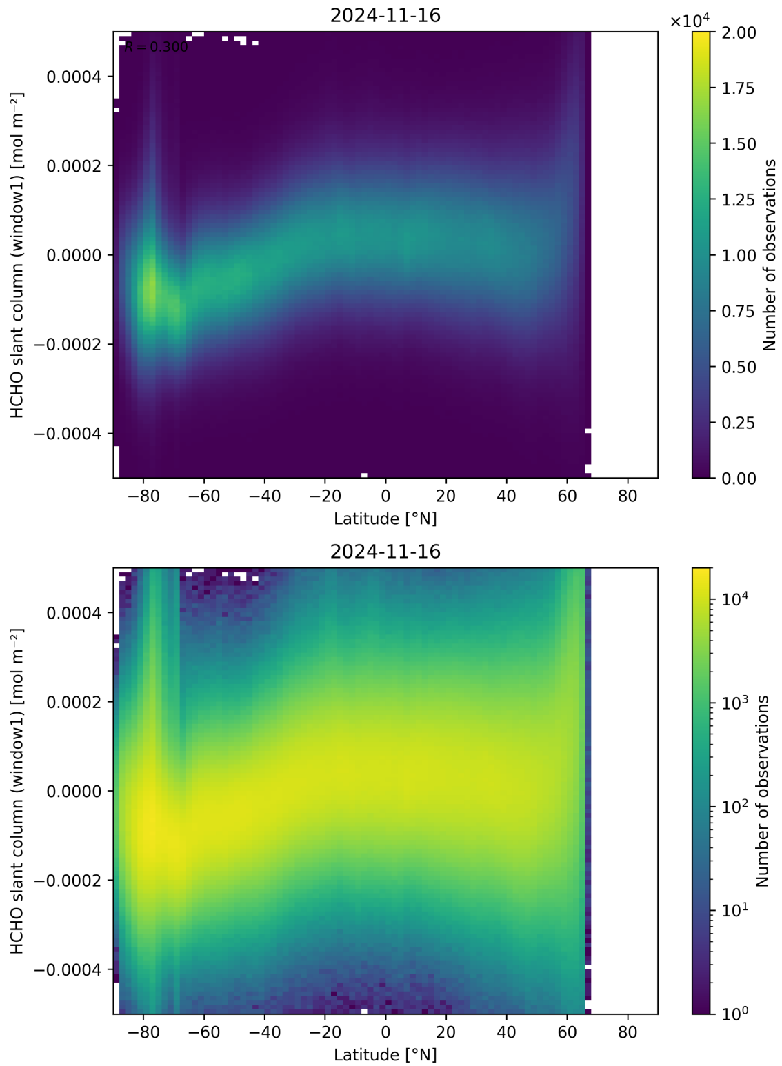
Figure 159: Scatter density plot of “Latitude” against “HCHO slant column (window1)” for 2024-11-15 to 2024-11-17.
