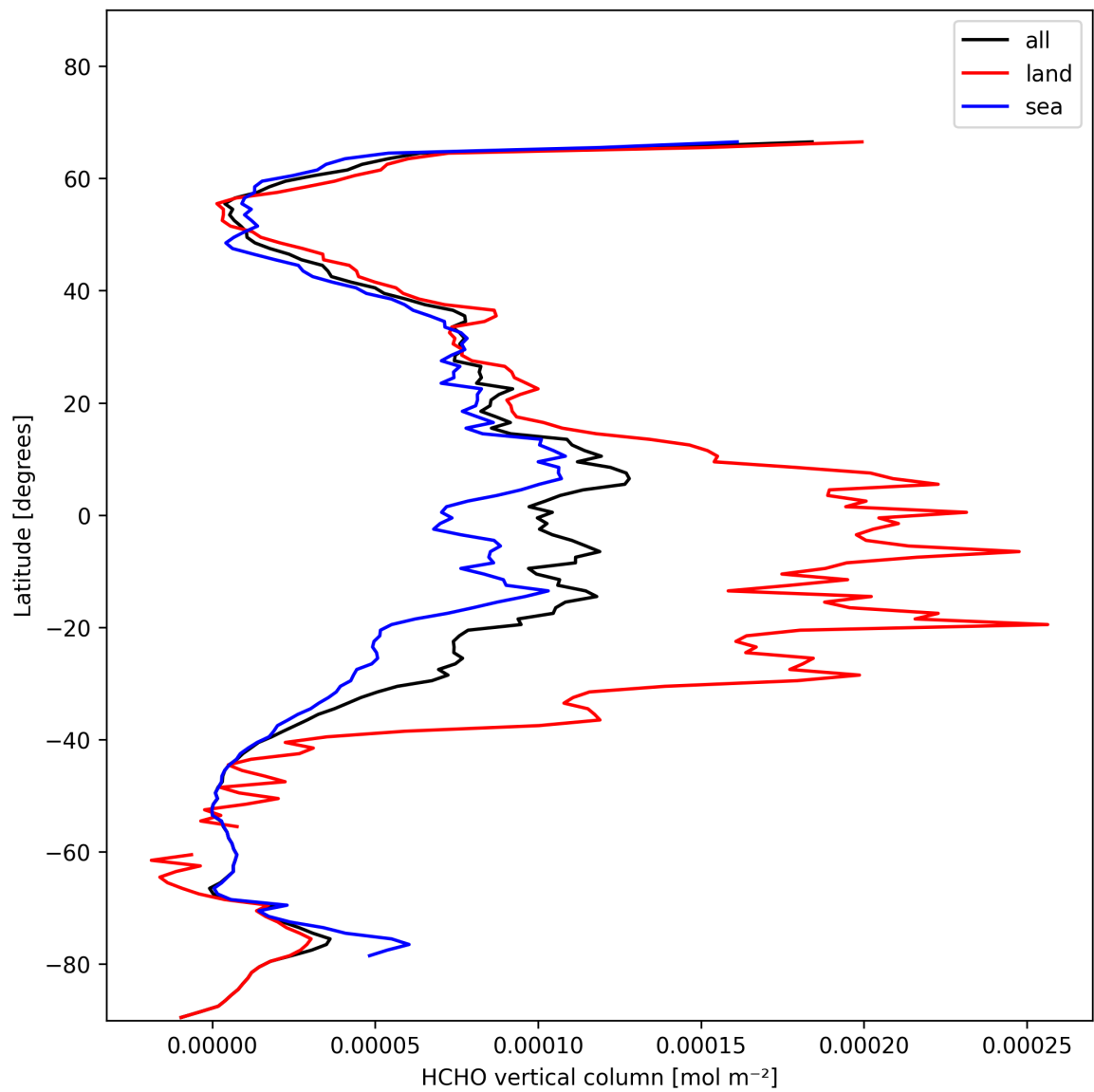
Figure 21: Zonal average of “HCHO vertical column” for 2024-11-15 to 2024-11-17.
