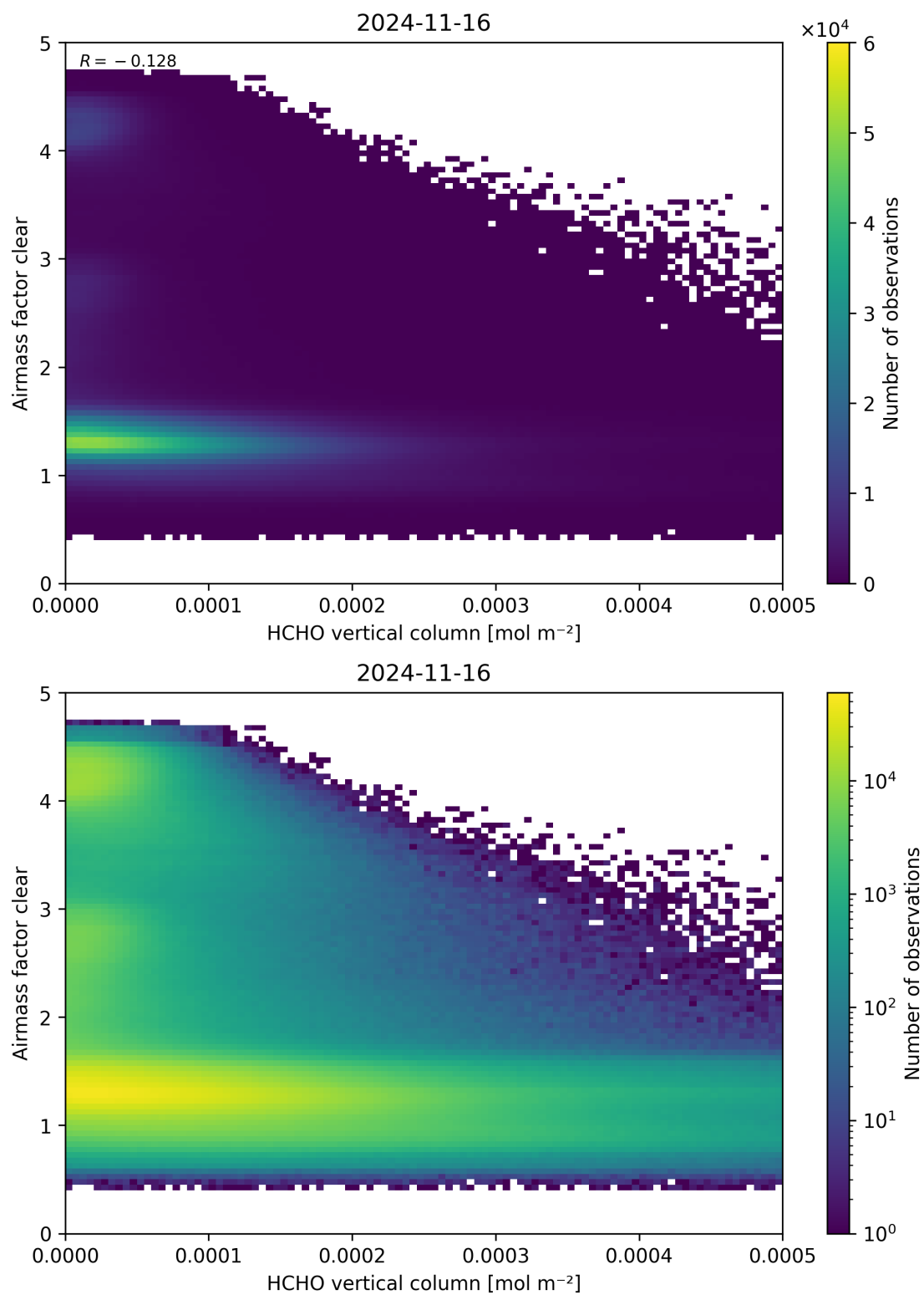
Figure 126: Scatter density plot of “HCHO vertical column” against “Airmass factor clear” for 2024-11-15 to 2024-11-17.
