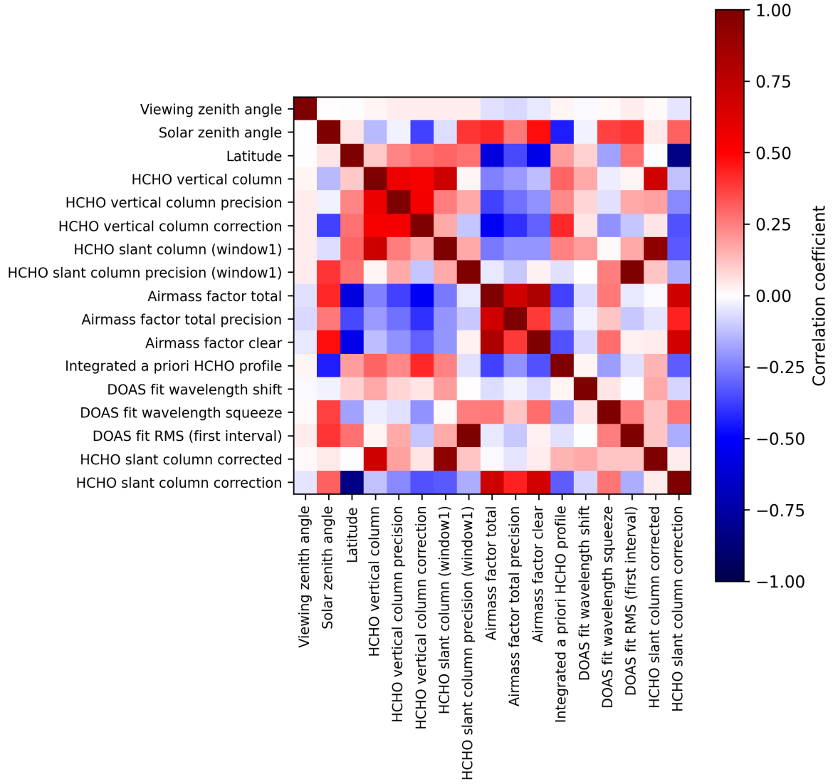
Figure 2: Map of correlation matrix for 2024-11-15 to 2024-11-17.
