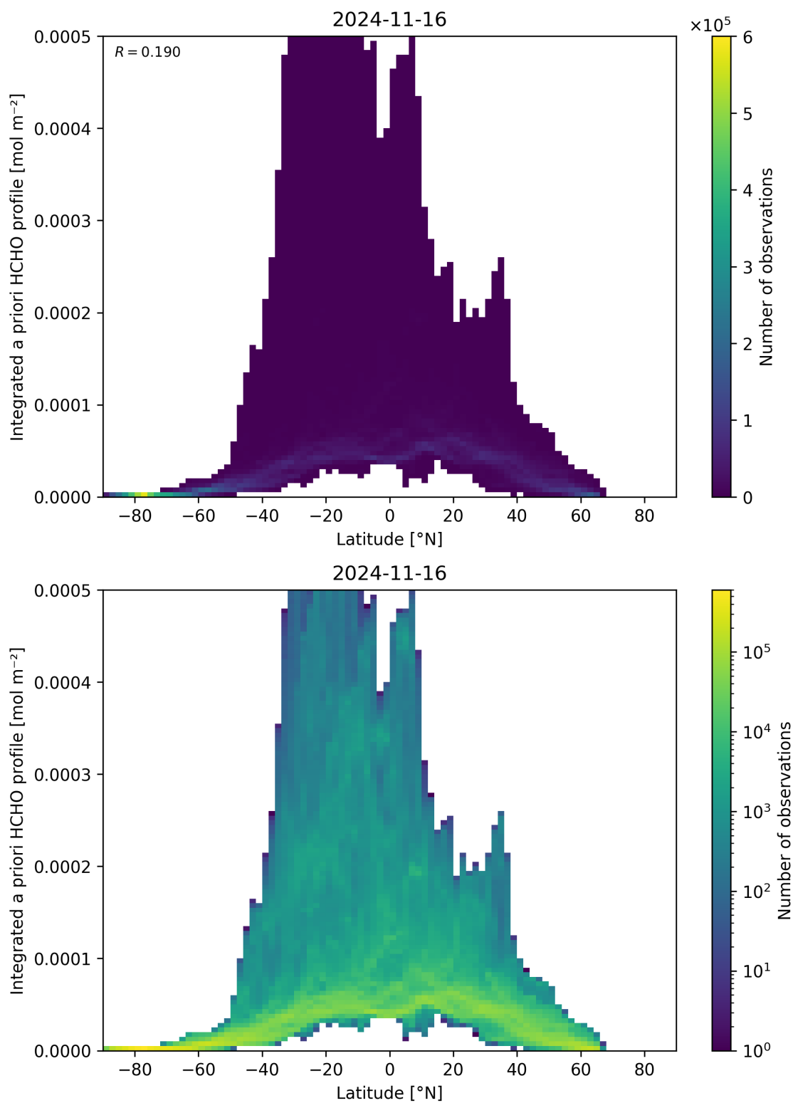
Figure 166: Scatter density plot of “Latitude” against “Integrated a priori HCHO profile” for 2024-11-15 to 2024-11-17.
