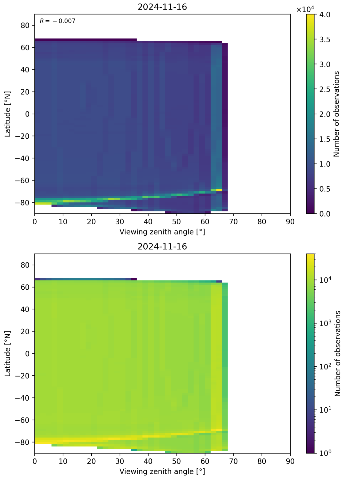
Figure 196: Scatter density plot of “Viewing zenith angle” against “Latitude” for 2024-11-15 to 2024-11-17.
