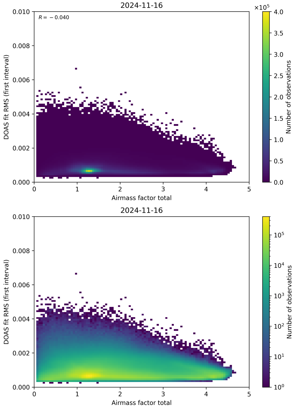
Figure 97: Scatter density plot of “Airmass factor total” against “DOAS fit RMS (first interval)” for 2024-11-15 to 2024-11-17.
