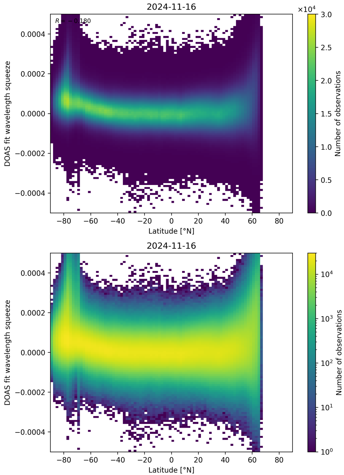
Figure 155: Scatter density plot of “Latitude” against “DOAS fit wavelength squeeze” for 2024-11-15 to 2024-11-17.
