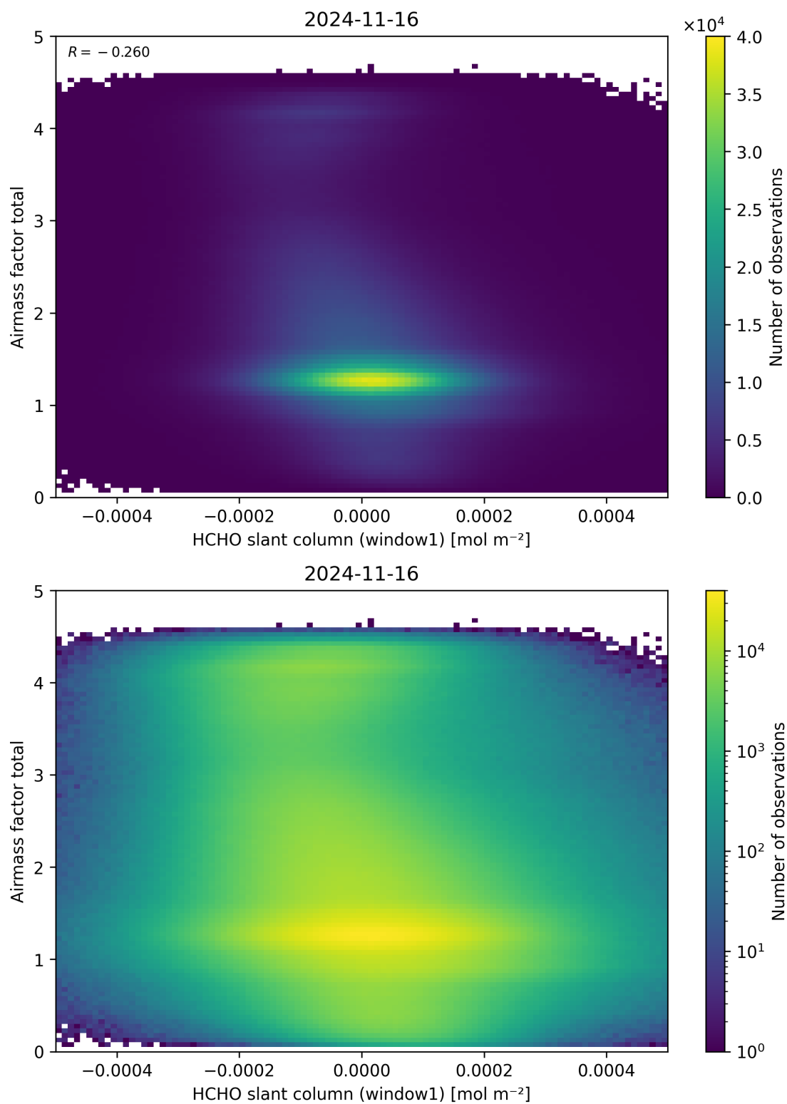
Figure 85: Scatter density plot of “HCHO slant column (window1)” against “Airmass factor total” for 2024-11-15 to 2024-11-17.
