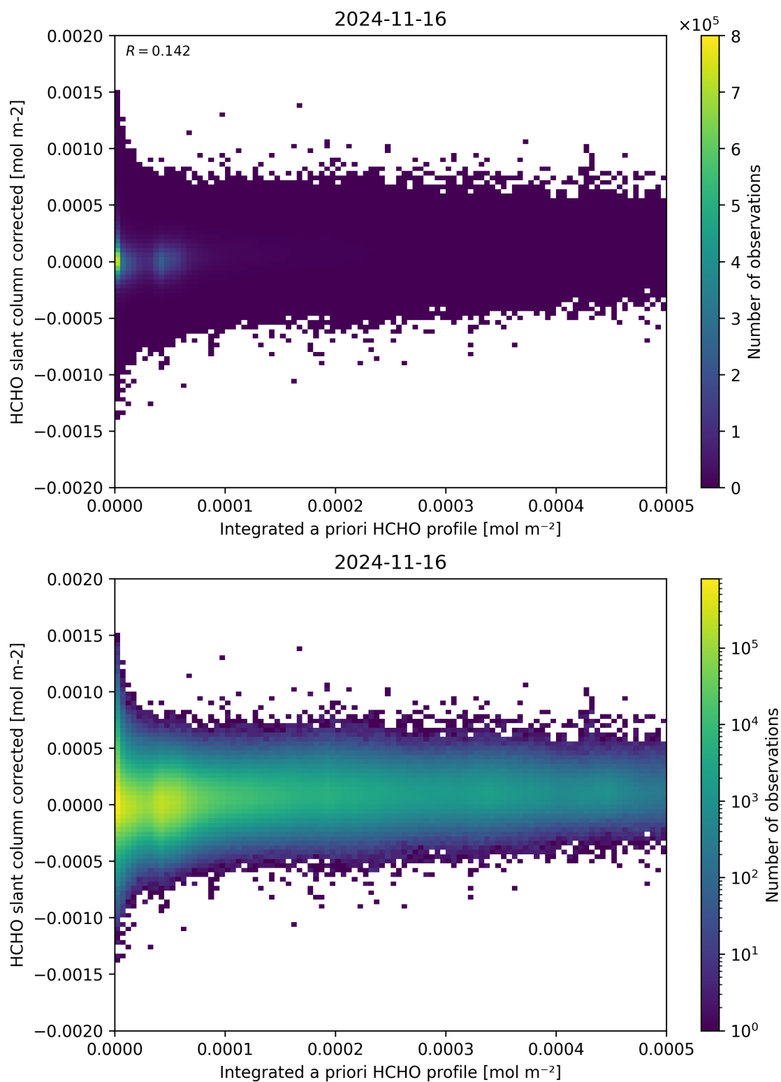
Figure 151: Scatter density plot of “Integrated a priori HCHO profile” against “HCHO slant column corrected” for 2024-11-15 to 2024-11-17.
