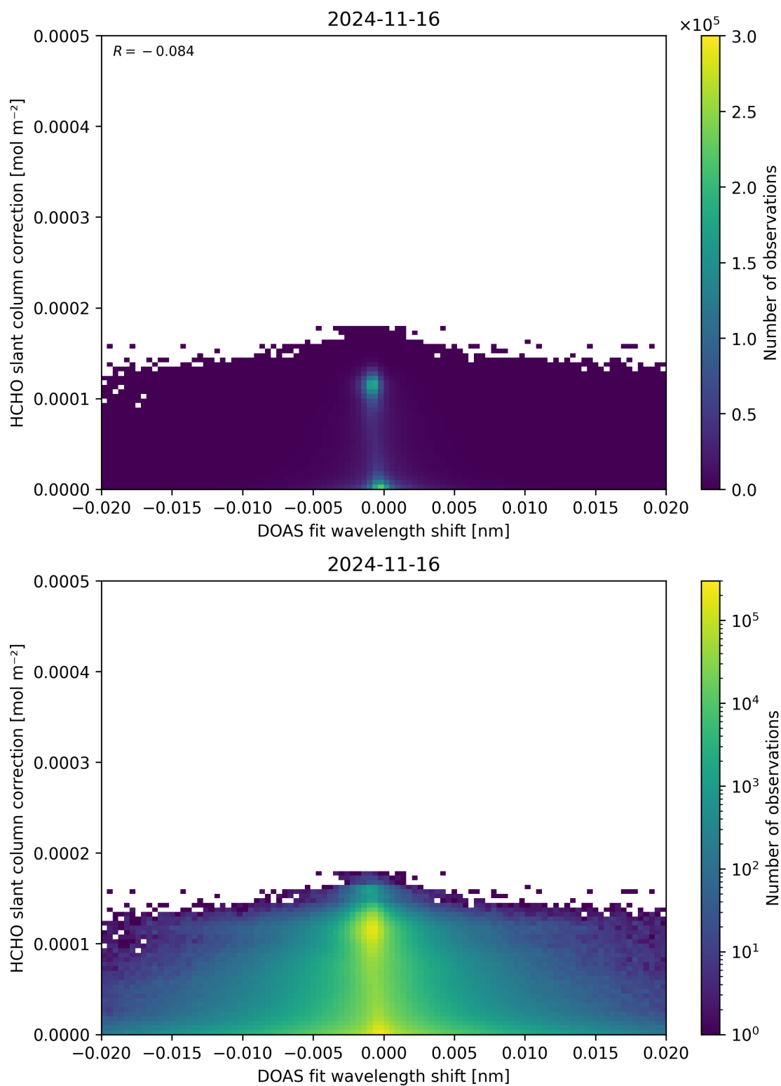
Figure 67: Scatter density plot of “DOAS fit wavelength shift” against “HCHO slant column correction” for 2024-11-15 to 2024-11-17.
