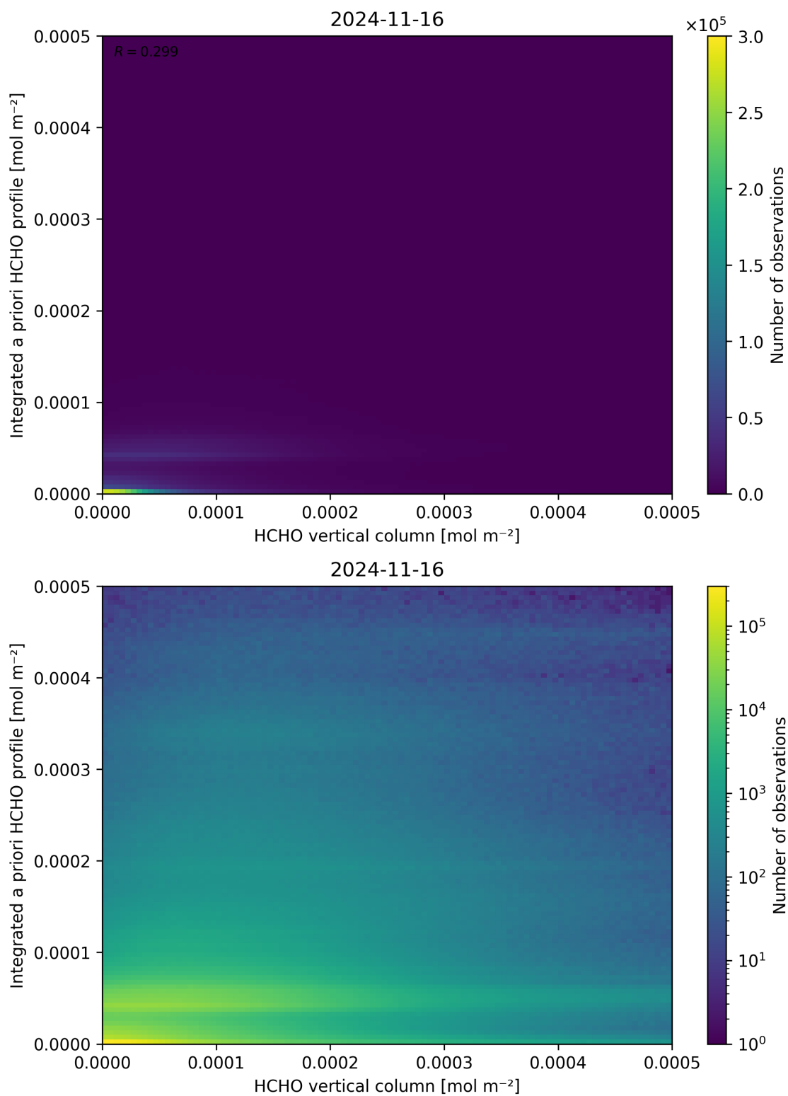
Figure 135: Scatter density plot of “HCHO vertical column” against “Integrated a priori HCHO profile” for 2024-11-15 to 2024-11-17.
