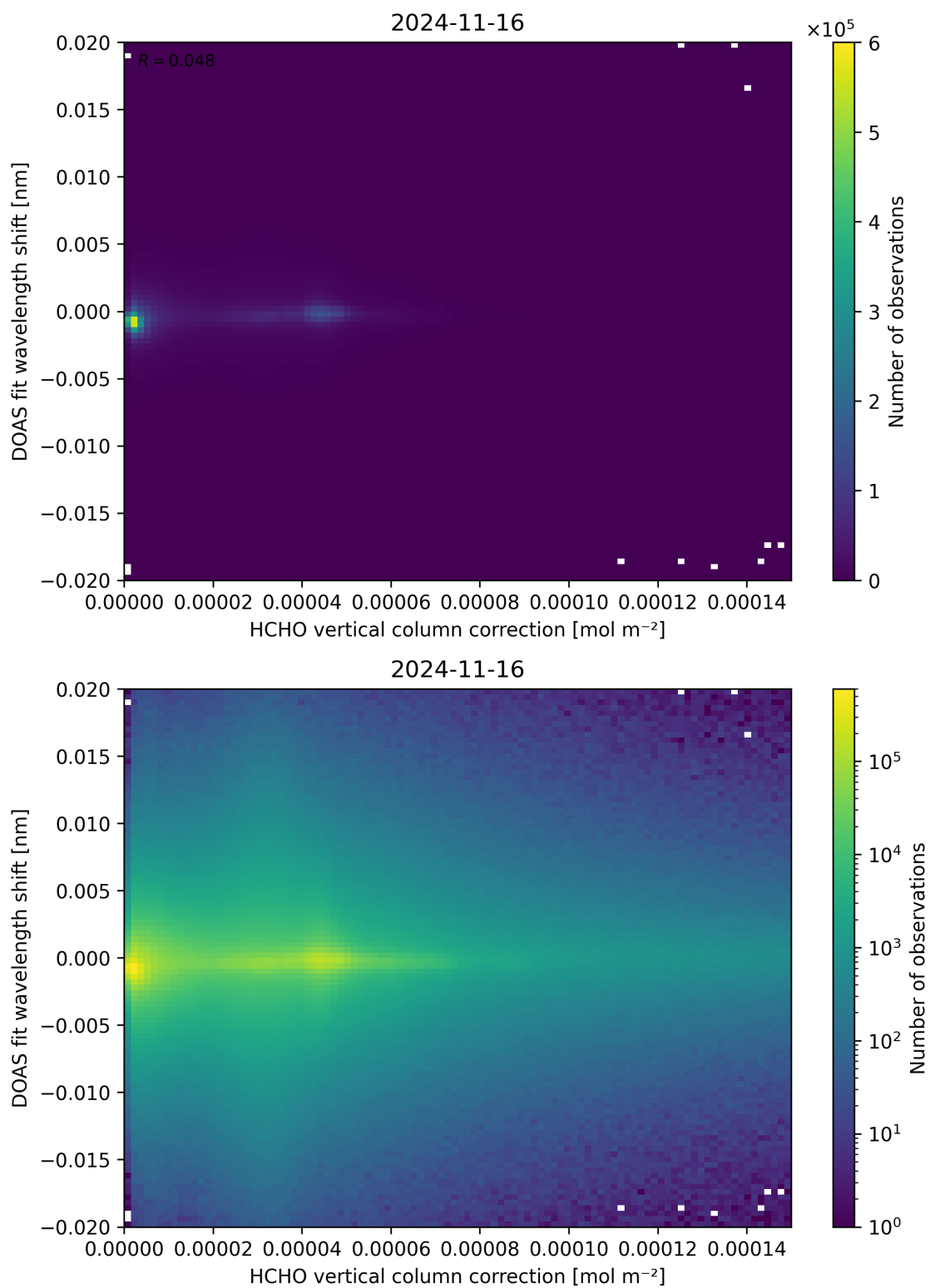
Figure 113: Scatter density plot of “HCHO vertical column correction” against “DOAS fit wavelength shift” for 2024-11-15 to 2024-11-17.
