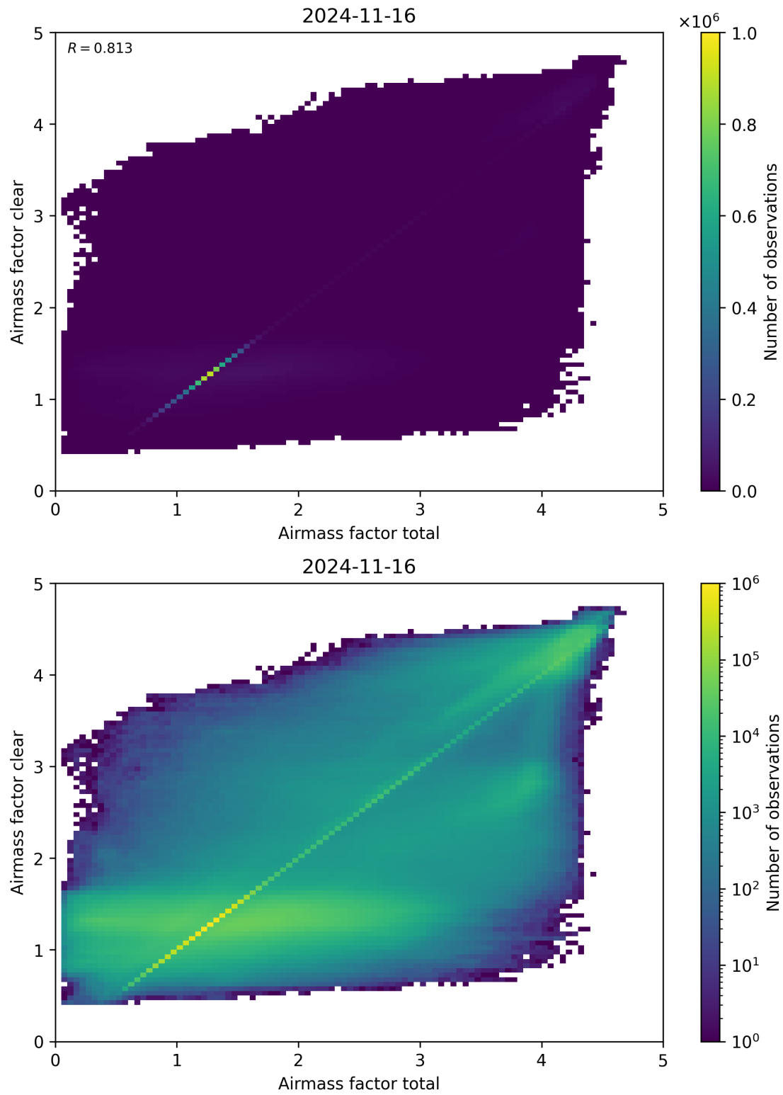
Figure 100: Scatter density plot of “Airmass factor total” against “Airmass factor clear” for 2024-11-15 to 2024-11-17.
