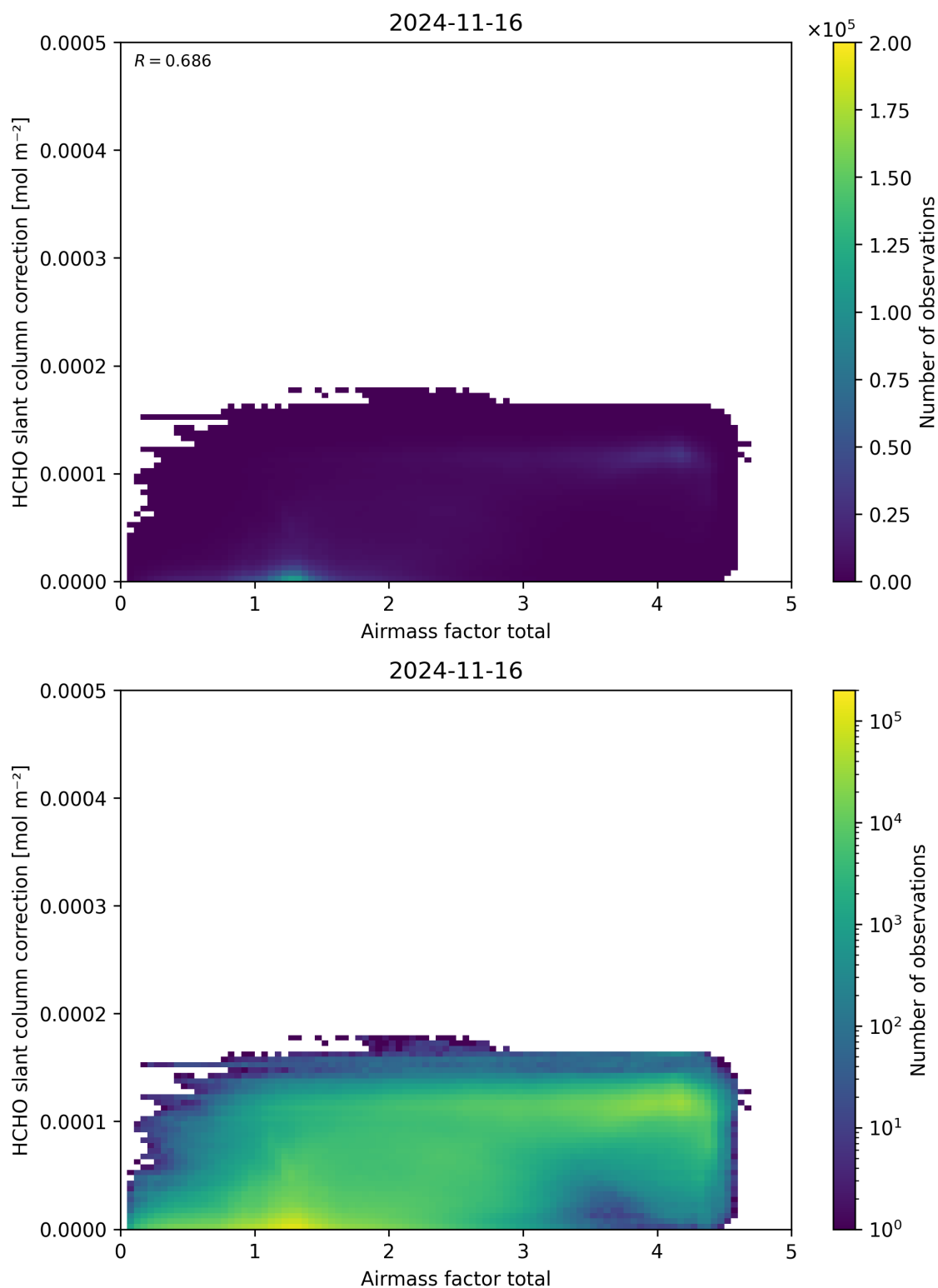
Figure 102: Scatter density plot of “Airmass factor total” against “HCHO slant column correction” for 2024-11-15 to 2024-11-17.
