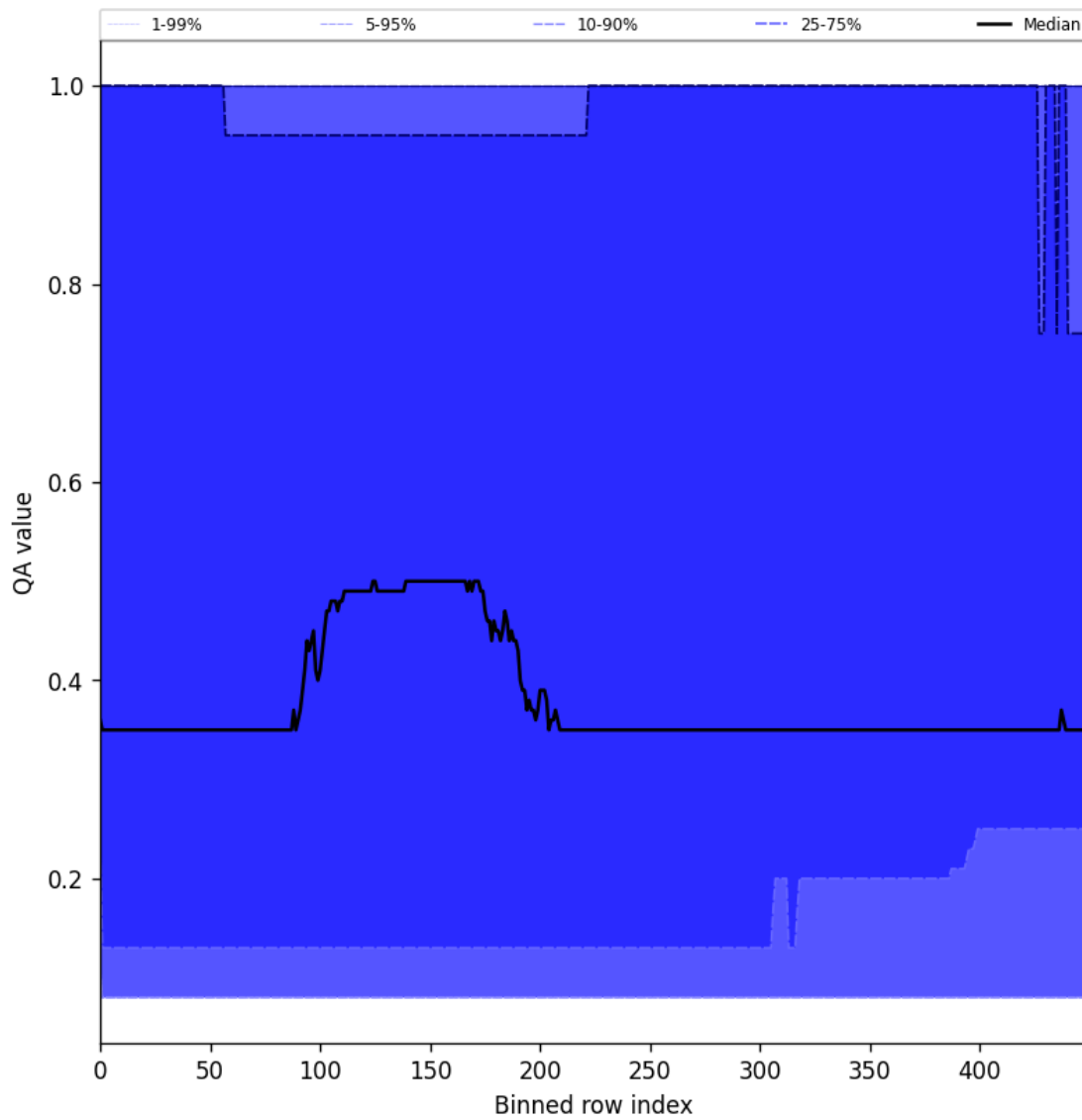
Figure 48: Along track statistics of “QA value” for 2024-11-15 to 2024-11-17
