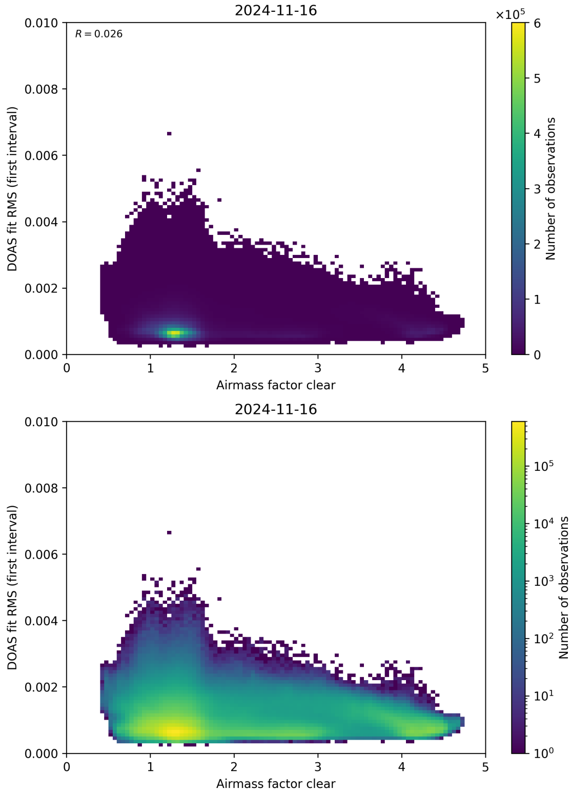
Figure 71: Scatter density plot of “Airmass factor clear” against “DOAS fit RMS (first interval)” for 2024-11-15 to 2024-11-17.
