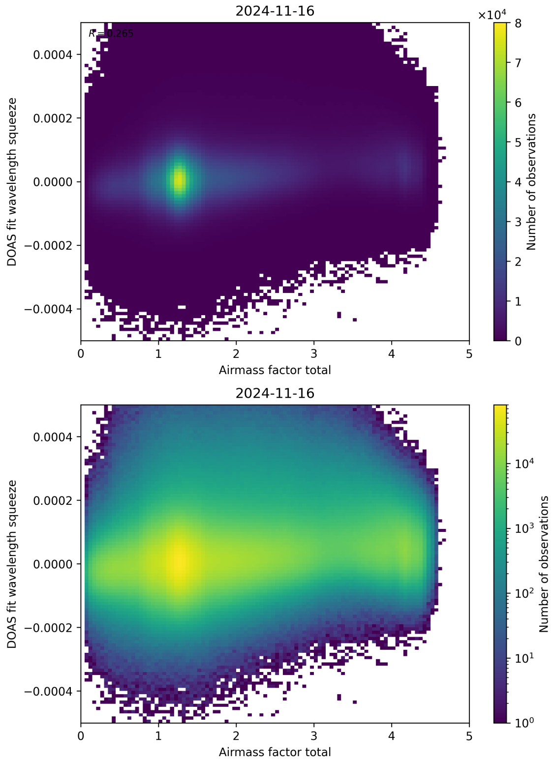
Figure 99: Scatter density plot of “Airmass factor total” against “DOAS fit wavelength squeeze” for 2024-11-15 to 2024-11-17.
