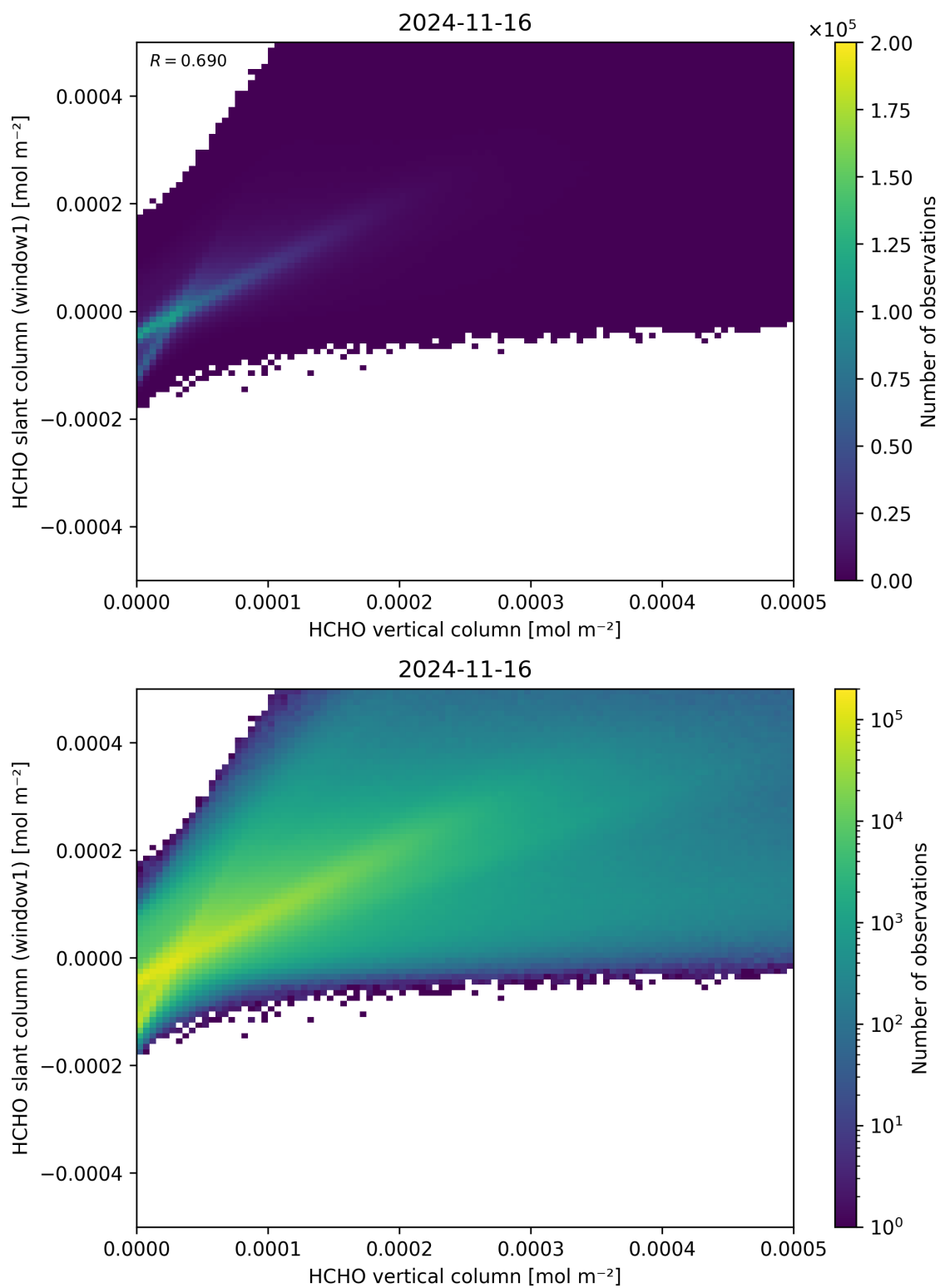
Figure 129: Scatter density plot of “HCHO vertical column” against “HCHO slant column (window1)” for 2024-11-15 to 2024-11-17.
