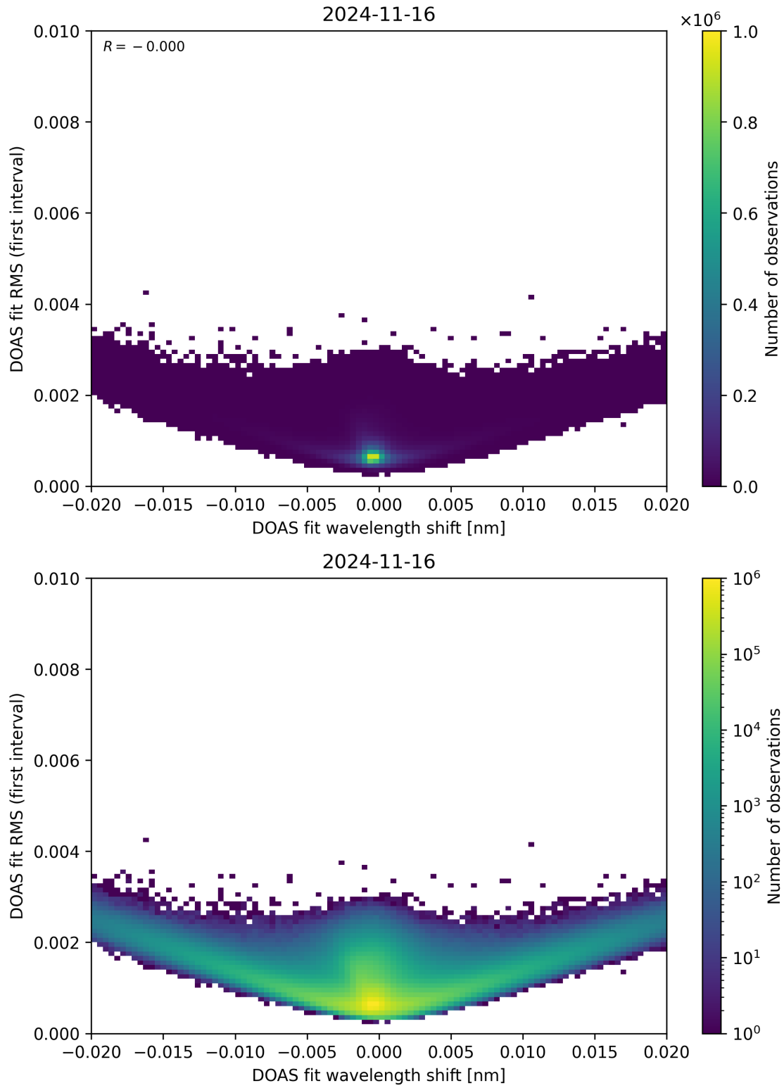
Figure 64: Scatter density plot of “DOAS fit wavelength shift” against “DOAS fit RMS (first interval)” for 2024-11-15 to 2024-11-17.
