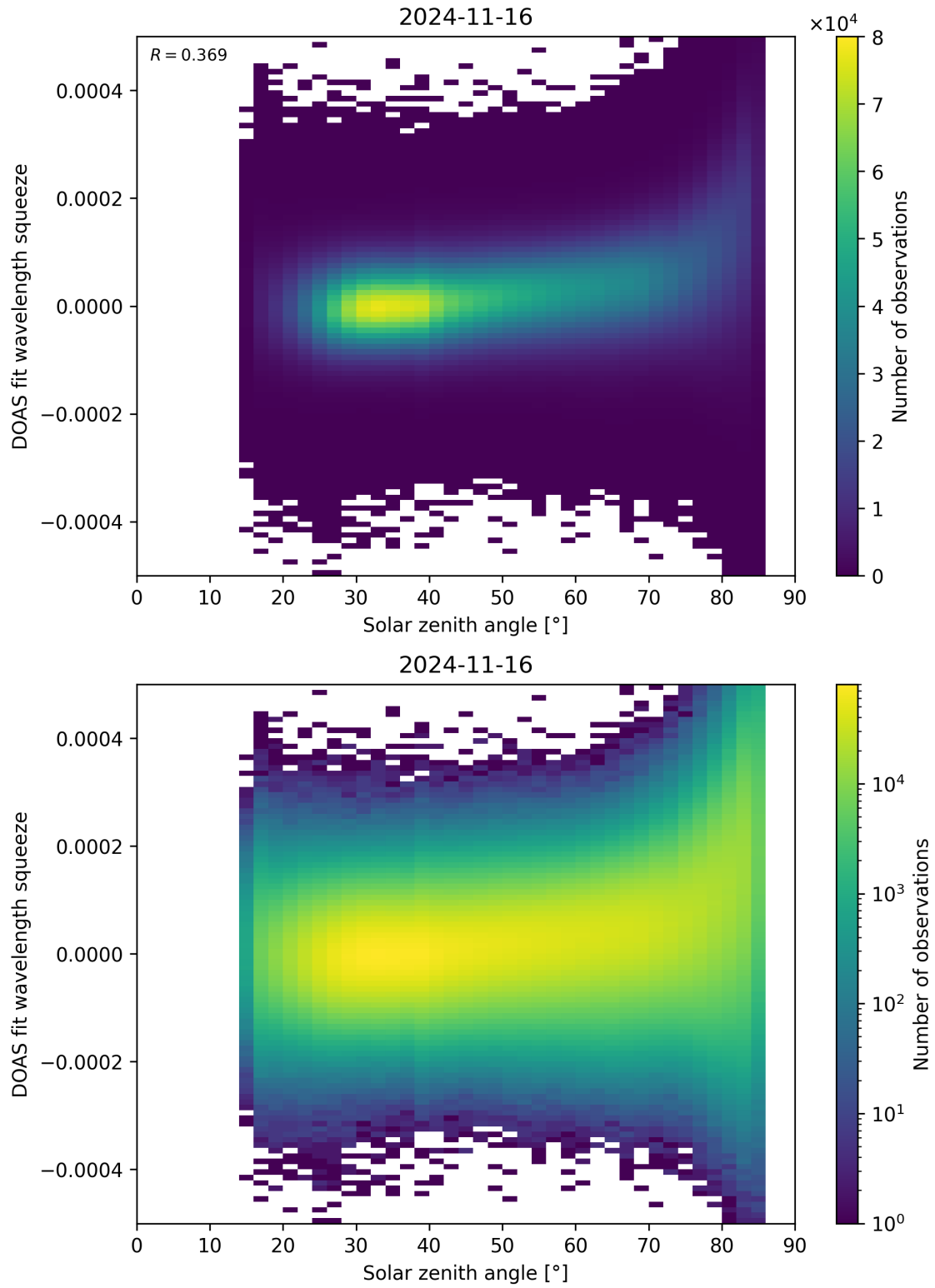
Figure 169: Scatter density plot of “Solar zenith angle” against “DOAS fit wavelength squeeze” for 2024-11-15 to 2024-11-17.
