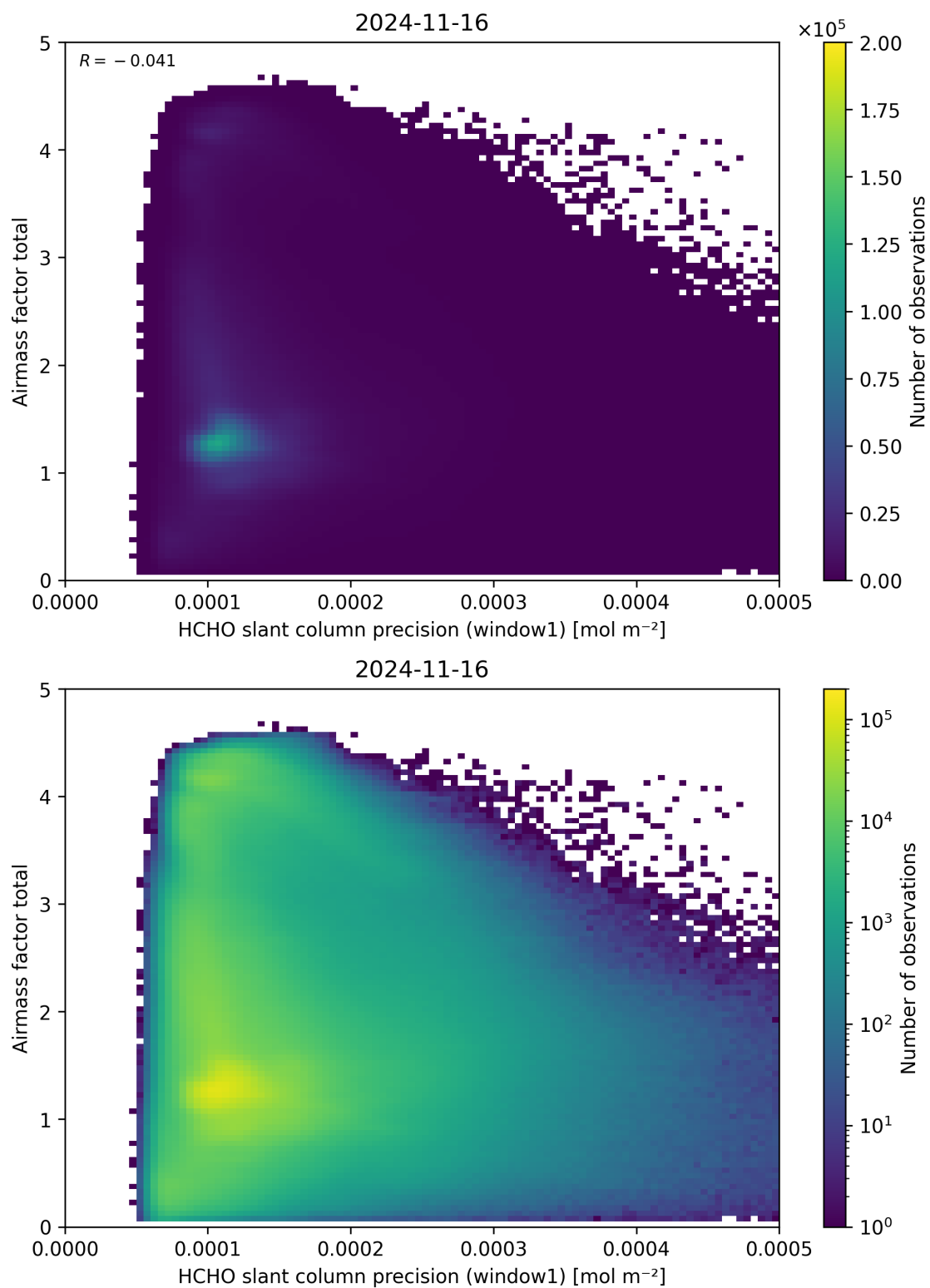
Figure 94: Scatter density plot of “HCHO slant column precision (window1)” against “Airmass factor total” for 2024-11-15 to 2024-11-17.
