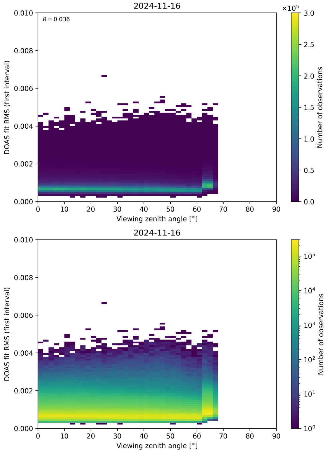
Figure 182: Scatter density plot of “Viewing zenith angle” against “DOAS fit RMS (first interval)” for 2024-11-15 to 2024-11-17.
