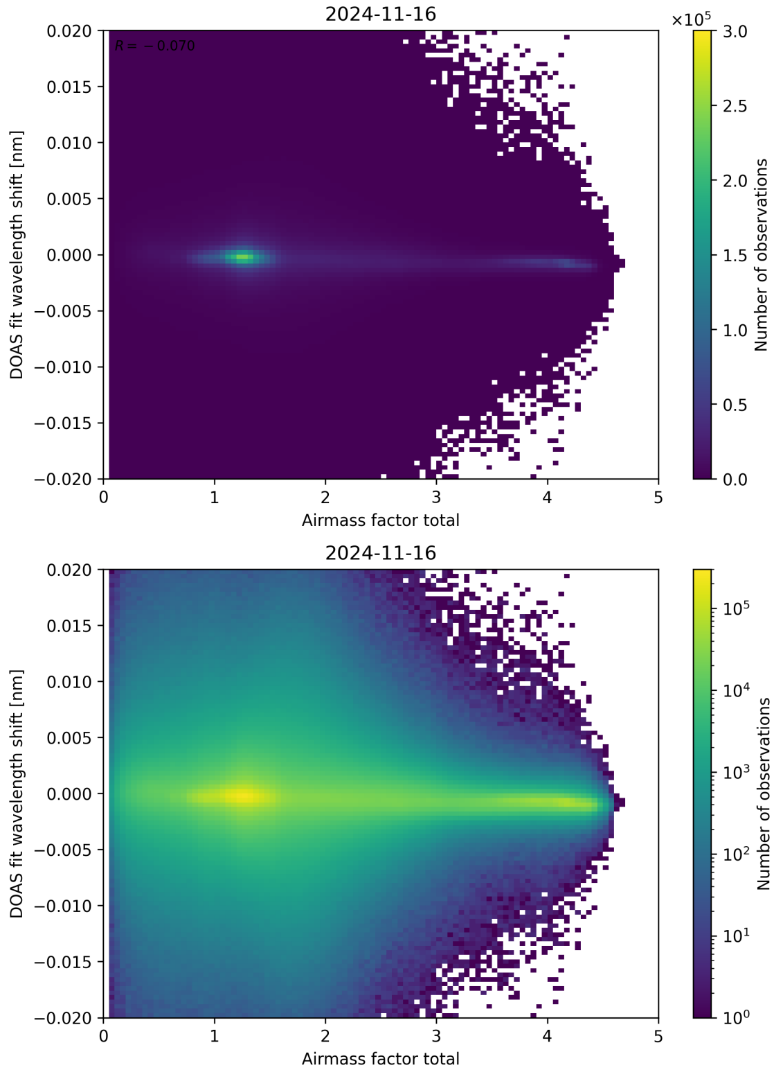
Figure 98: Scatter density plot of “Airmass factor total” against “DOAS fit wavelength shift” for 2024-11-15 to 2024-11-17.
