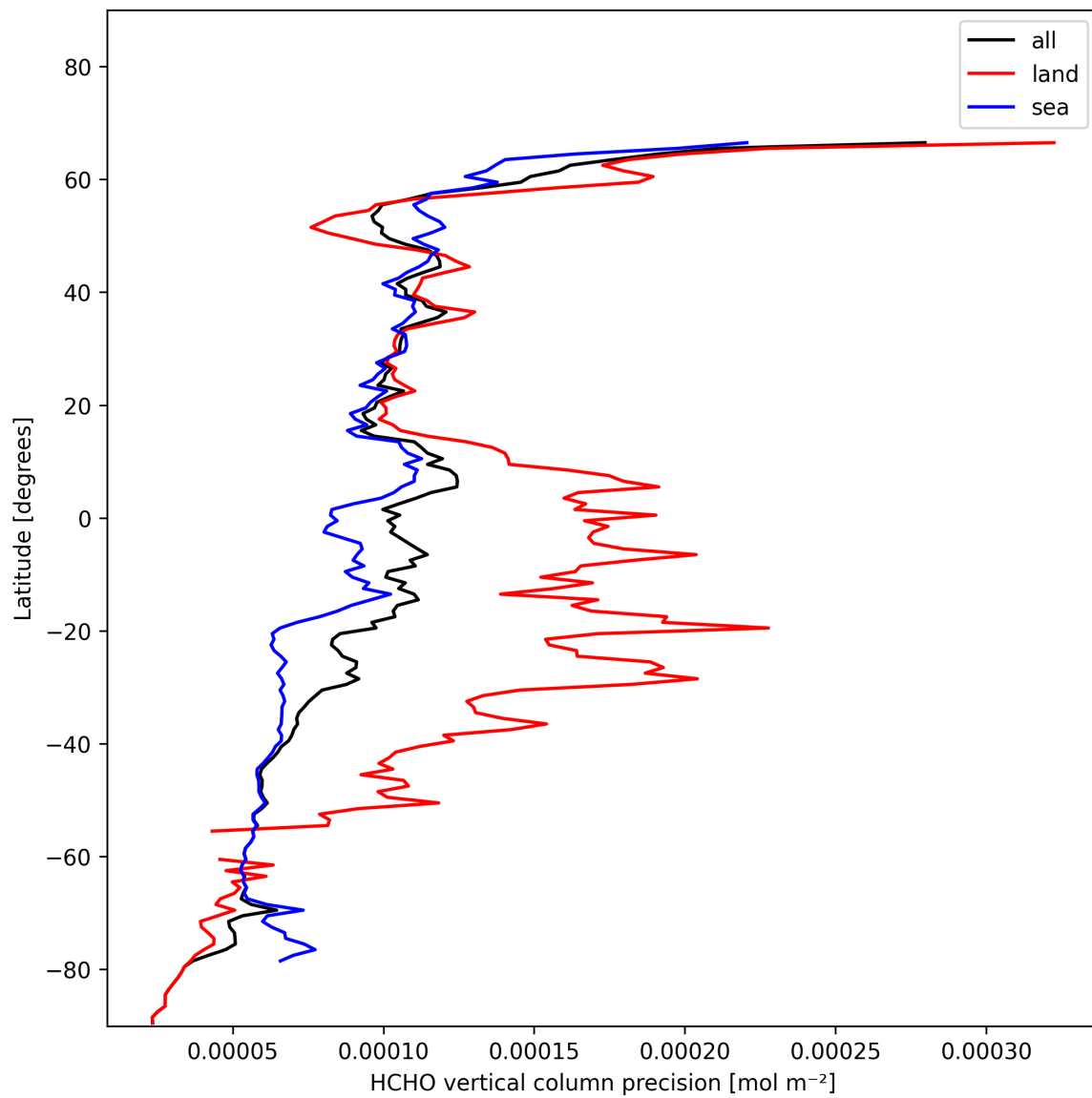
Figure 22: Zonal average of “HCHO vertical column precision” for 2024-11-15 to 2024-11-17.
