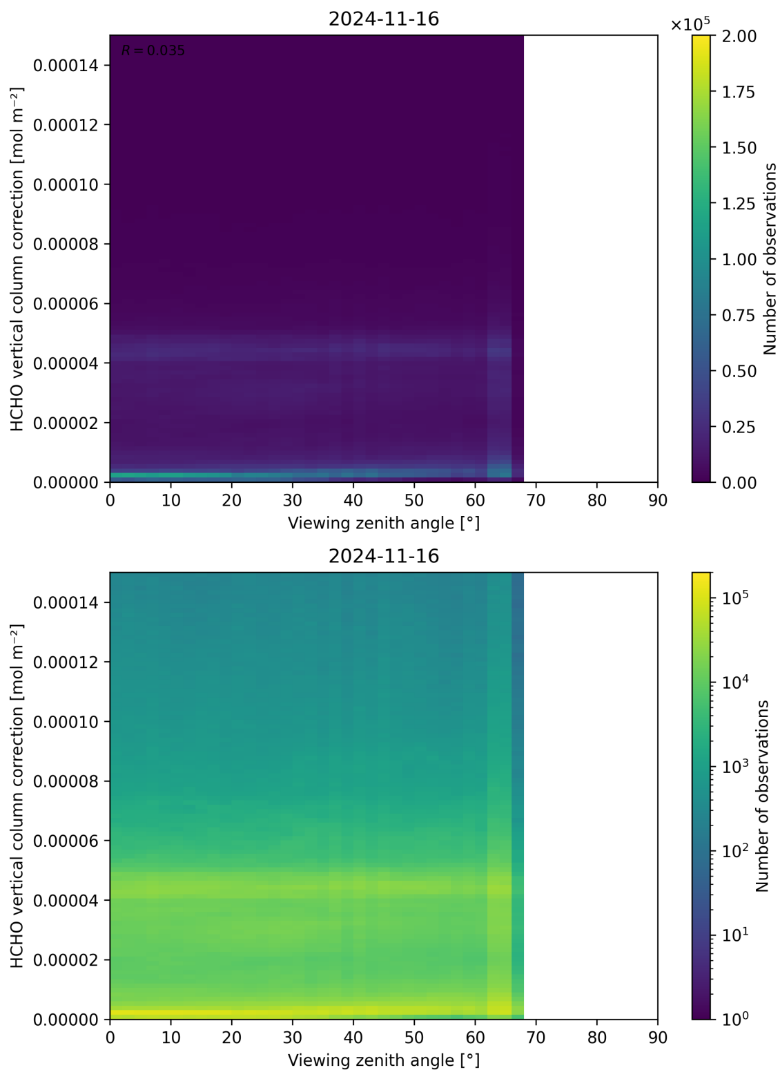
Figure 193: Scatter density plot of “Viewing zenith angle” against “HCHO vertical column correction” for 2024-11-15 to 2024-11-17.
