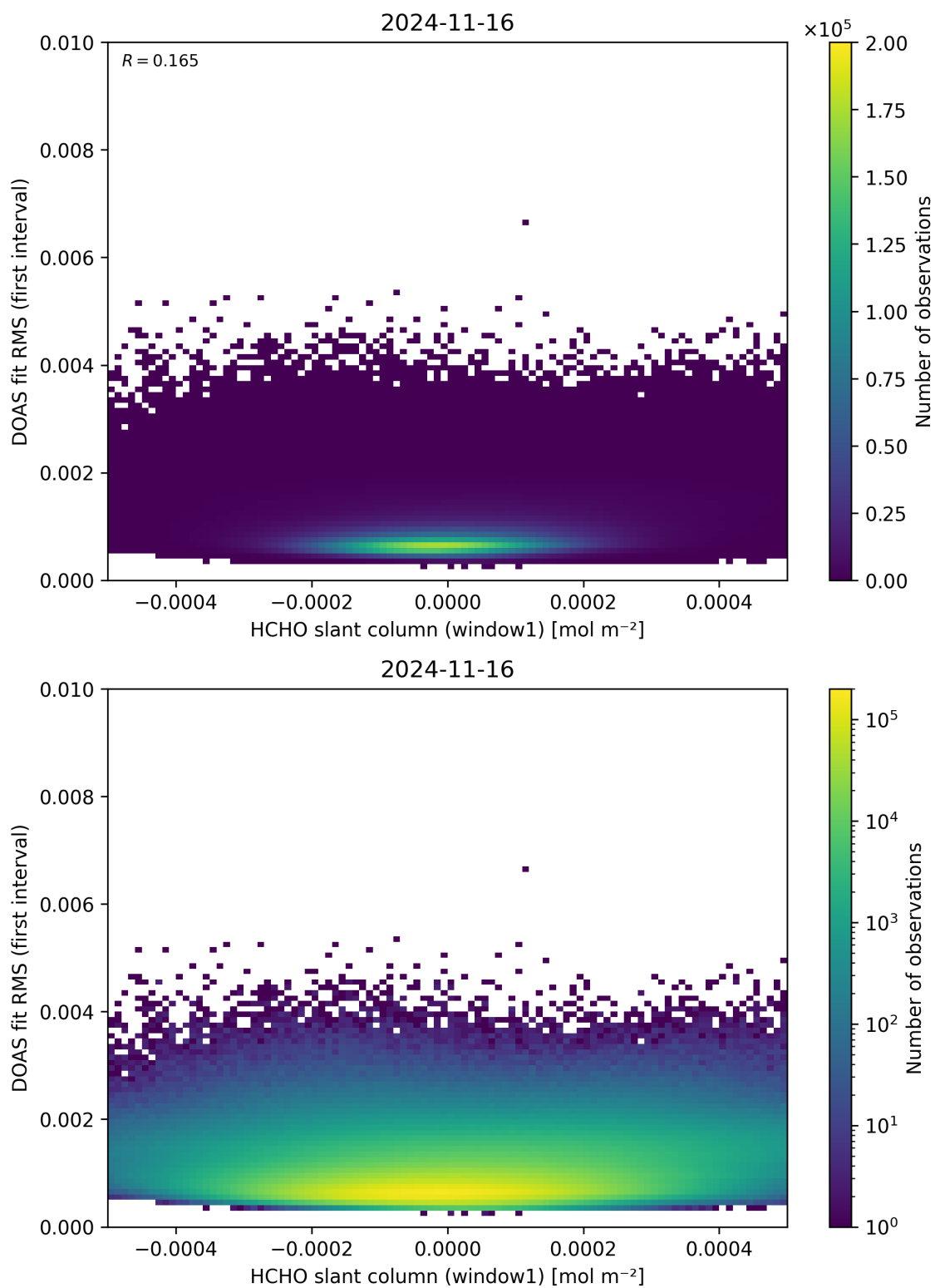
Figure 78: Scatter density plot of “HCHO slant column (window1)” against “DOAS fit RMS (first interval)” for 2024-11-15 to 2024-11-17.
