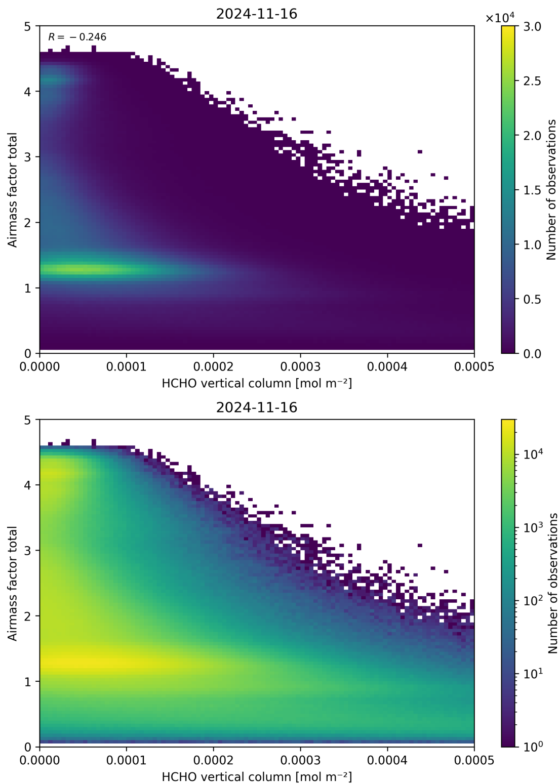
Figure 131: Scatter density plot of “HCHO vertical column” against “Airmass factor total” for 2024-11-15 to 2024-11-17.
