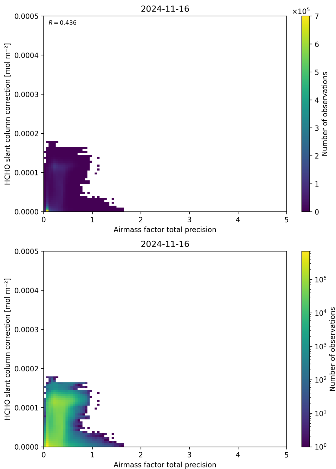
Figure 110: Scatter density plot of “Airmass factor total precision” against “HCHO slant column correction” for 2024-11-15 to 2024-11-17.
