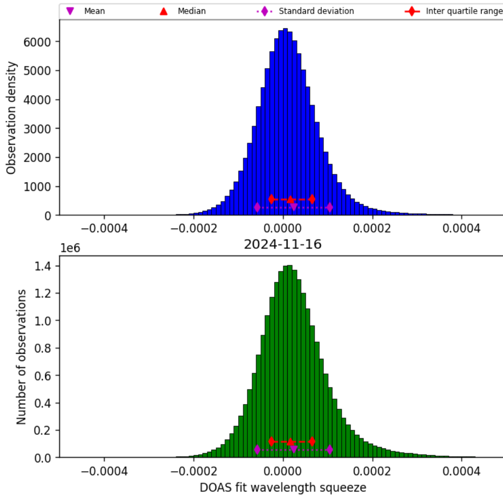
Figure 45: Histogram of “DOAS fit wavelength squeeze” for 2024-11-15 to 2024-11-17
