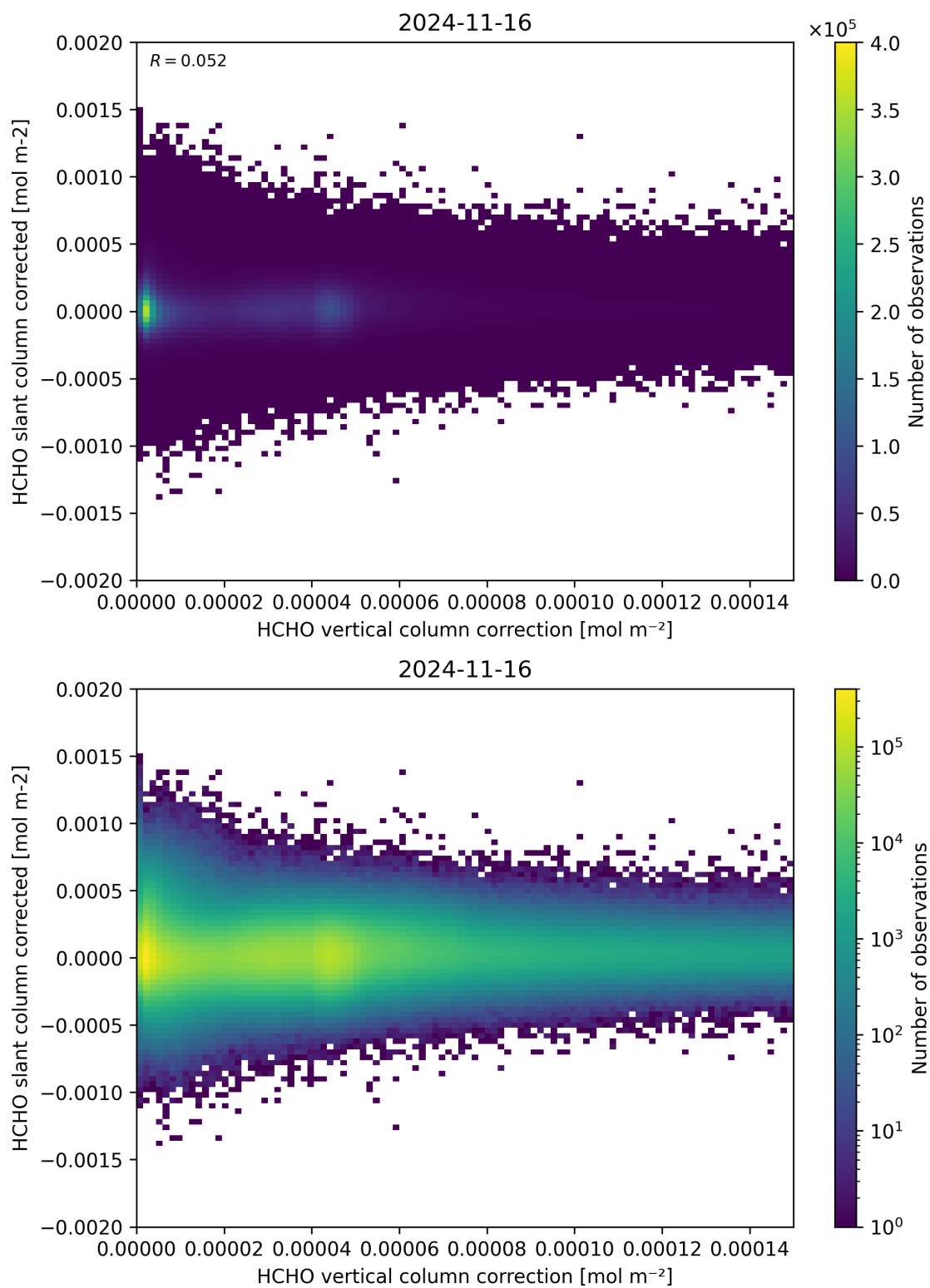
Figure 116: Scatter density plot of “HCHO vertical column correction” against “HCHO slant column corrected” for 2024-11-15 to 2024-11-17.
