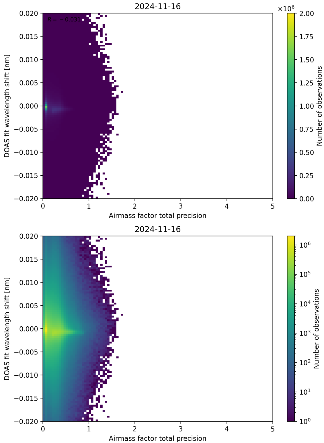
Figure 106: Scatter density plot of “Airmass factor total precision” against “DOAS fit wavelength shift” for 2024-11-15 to 2024-11-17.
