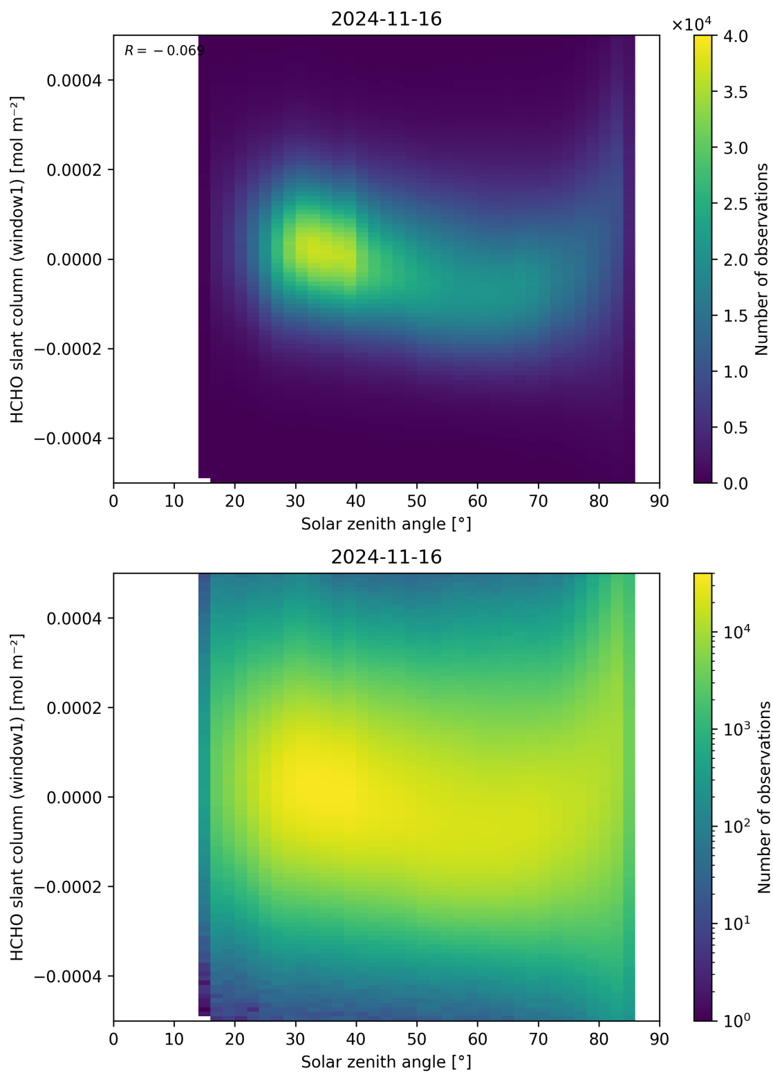
Figure 173: Scatter density plot of “Solar zenith angle” against “HCHO slant column (window1)” for 2024-11-15 to 2024-11-17.
