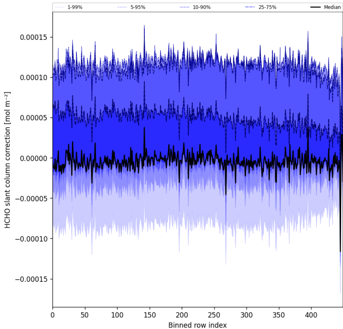
Figure 61: Along track statistics of “HCHO slant column correction” for 2024-11-15 to 2024-11-17
