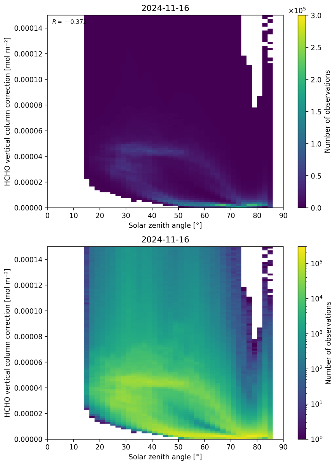
Figure 178: Scatter density plot of “Solar zenith angle” against “HCHO vertical column correction” for 2024-11-15 to 2024-11-17.
