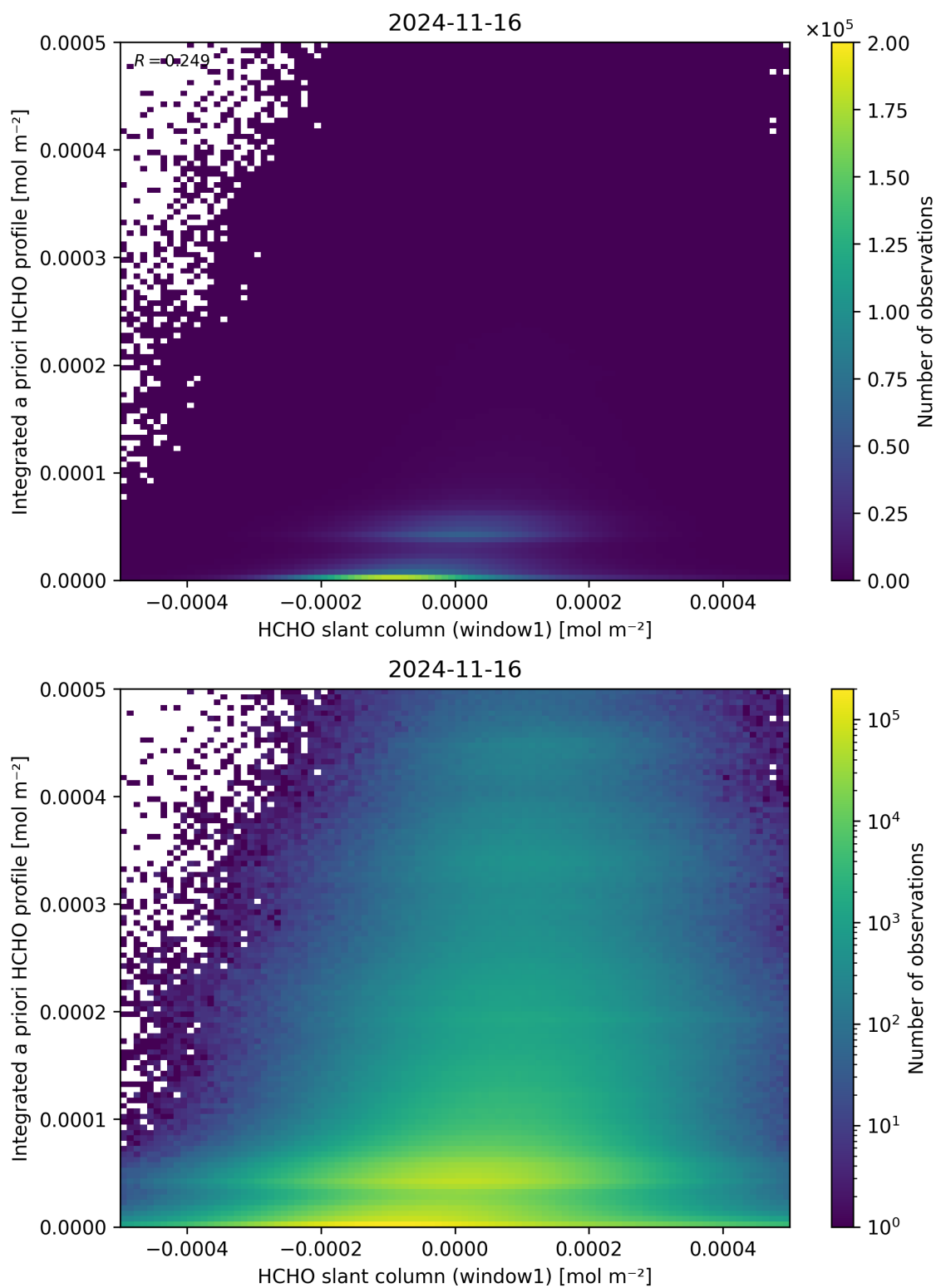
Figure 87: Scatter density plot of “HCHO slant column (window1)” against “Integrated a priori HCHO profile” for 2024-11-15 to 2024-11-17.
