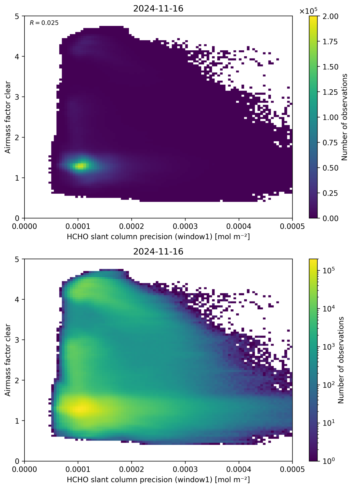
Figure 91: Scatter density plot of “HCHO slant column precision (window1)” against “Airmass factor clear” for 2024-11-15 to 2024-11-17.
