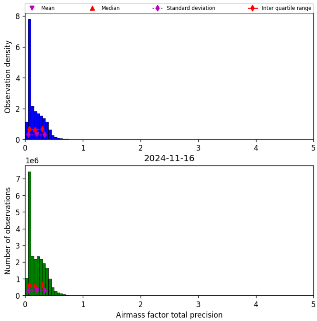
Figure 41: Histogram of “Airmass factor total precision” for 2024-11-15 to 2024-11-17
