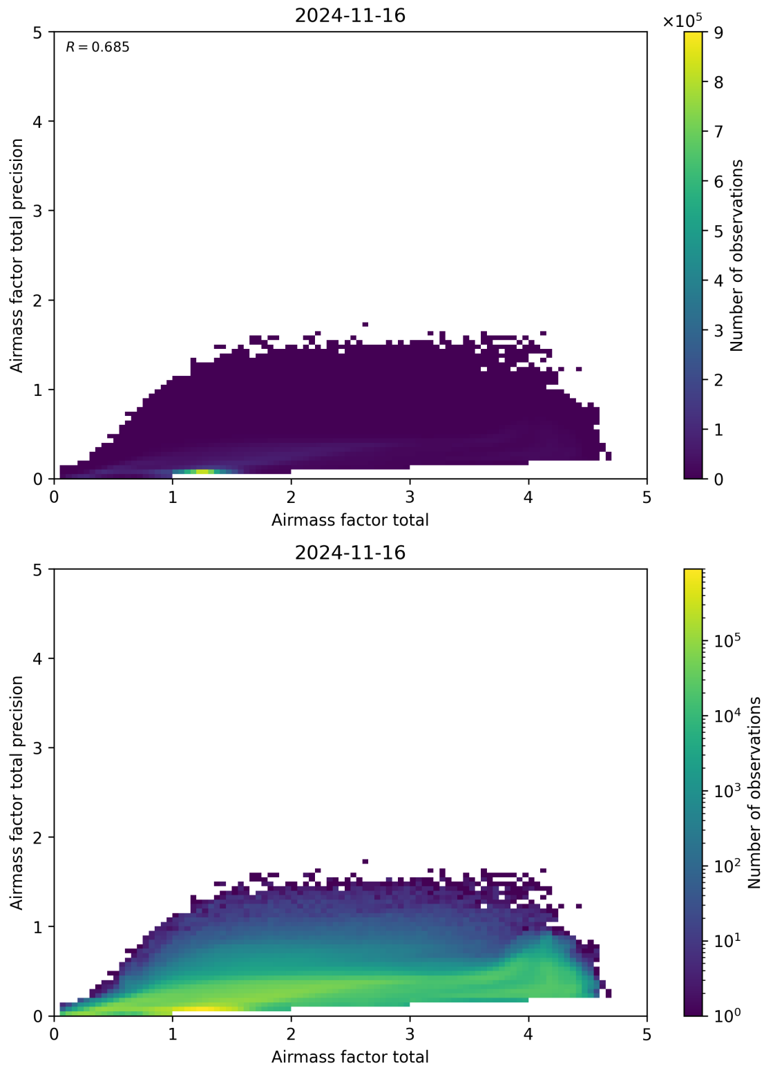
Figure 103: Scatter density plot of “Airmass factor total” against “Airmass factor total precision” for 2024-11-15 to 2024-11-17.
