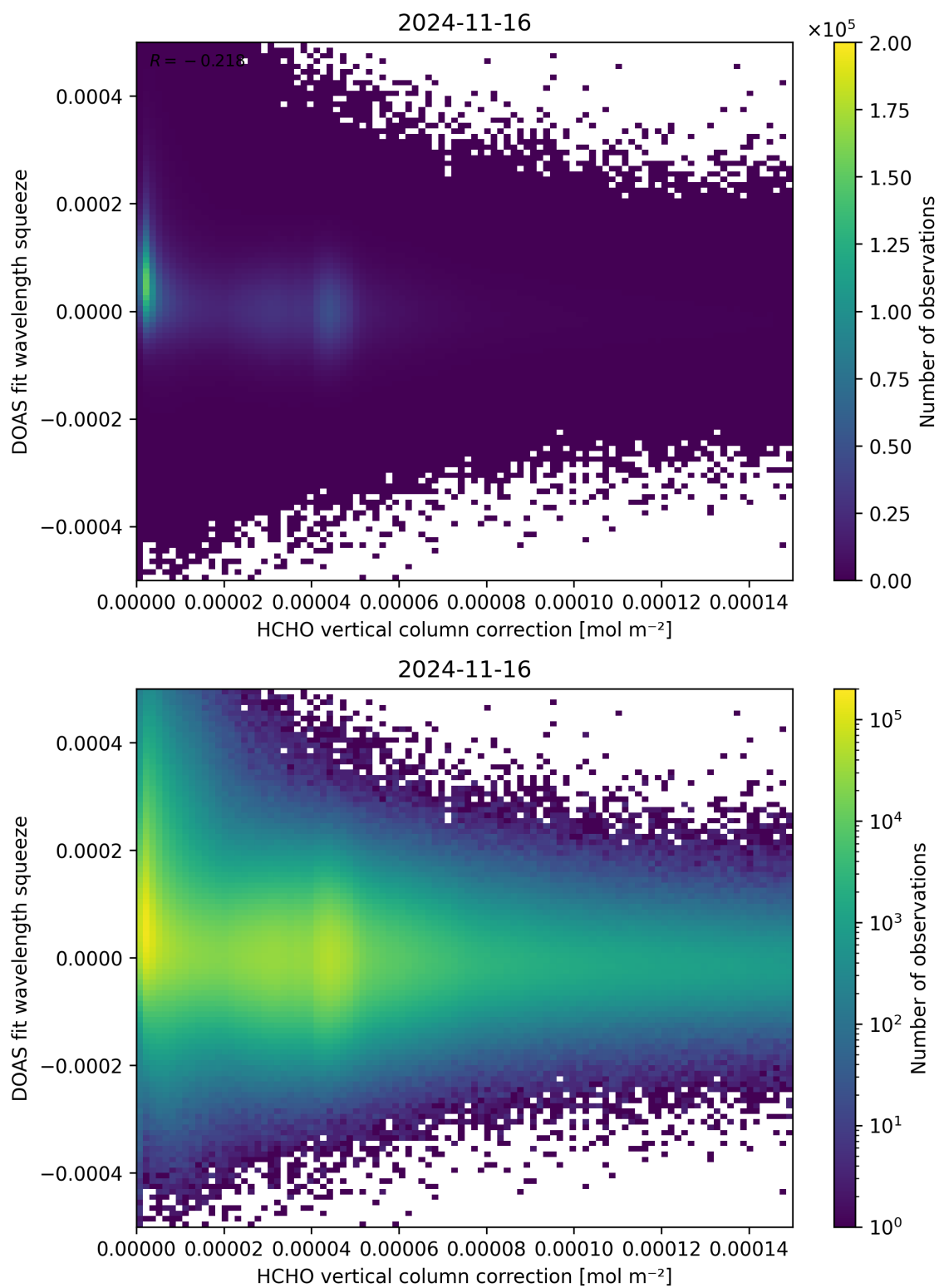
Figure 114: Scatter density plot of “HCHO vertical column correction” against “DOAS fit wavelength squeeze” for 2024-11-15 to 2024-11-17.
