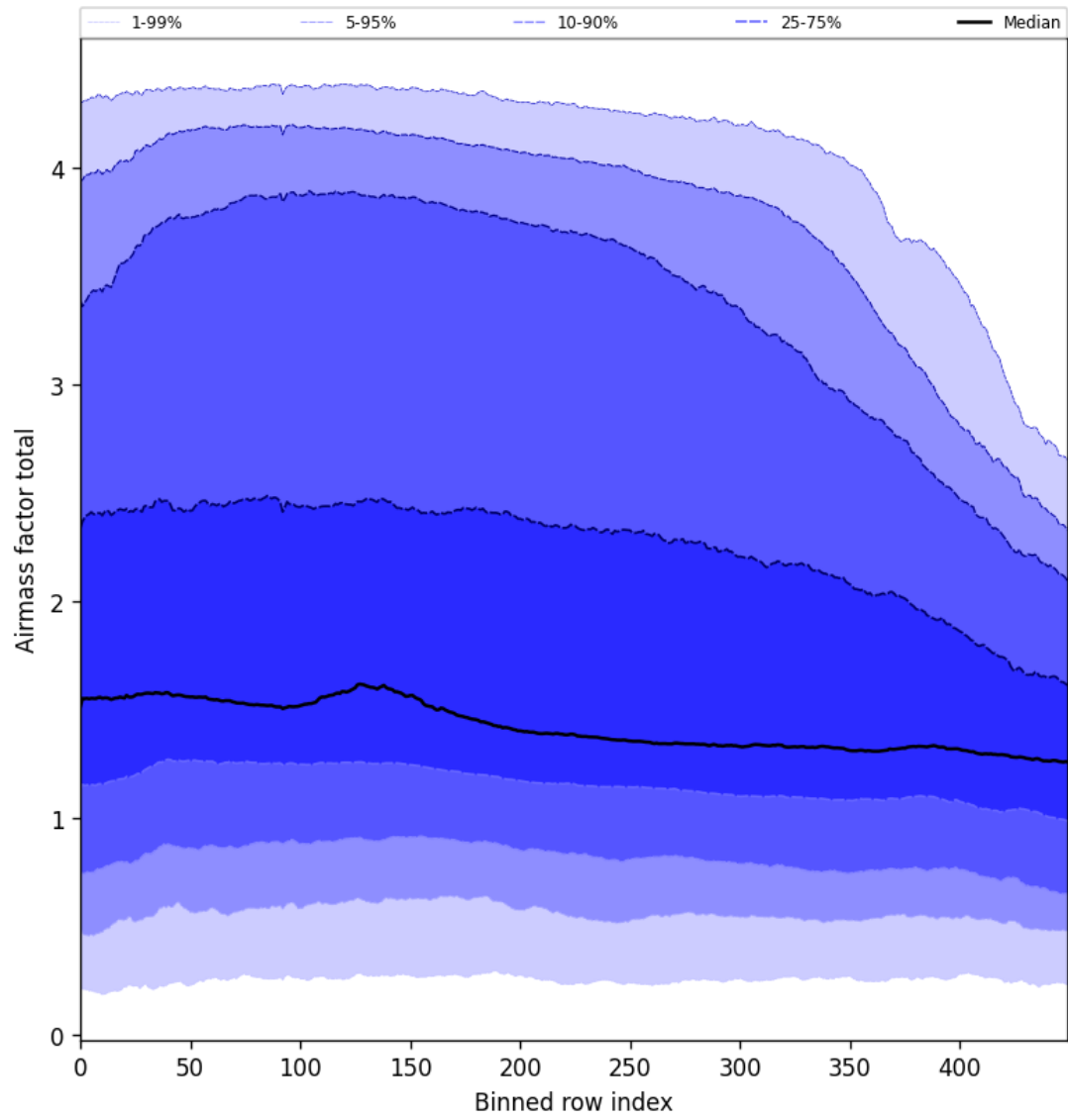
Figure 54: Along track statistics of “Airmass factor total” for 2024-11-15 to 2024-11-17
