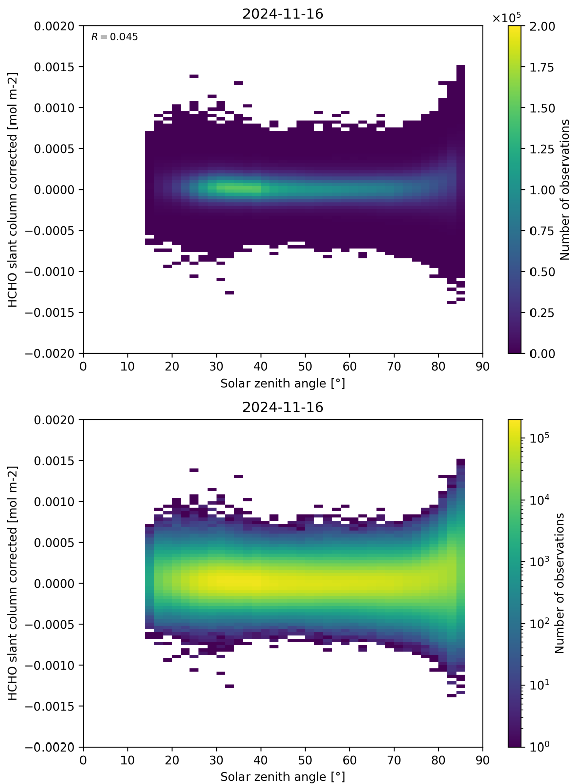
Figure 171: Scatter density plot of “Solar zenith angle” against “HCHO slant column corrected” for 2024-11-15 to 2024-11-17.
