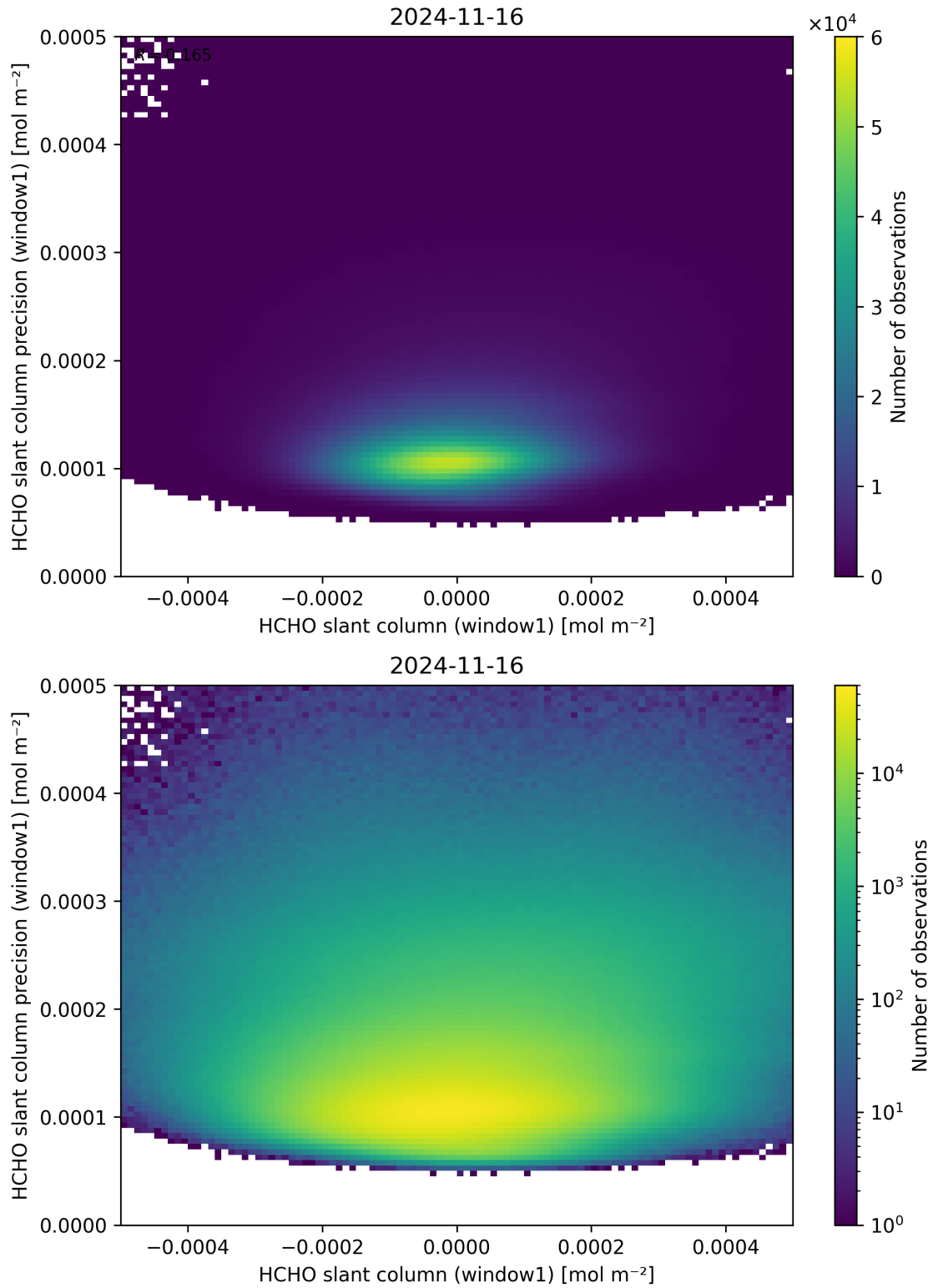
Figure 84: Scatter density plot of “HCHO slant column (window1)” against “HCHO slant column precision (window1)” for 2024-11-15 to 2024-11-17.
