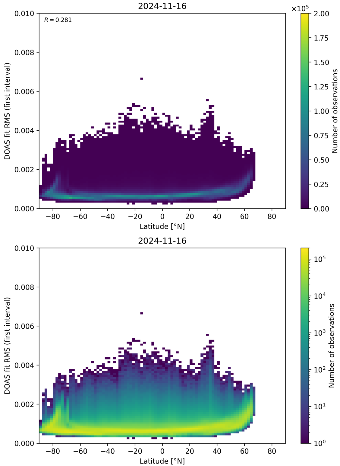
Figure 153: Scatter density plot of “Latitude” against “DOAS fit RMS (first interval)” for 2024-11-15 to 2024-11-17.
