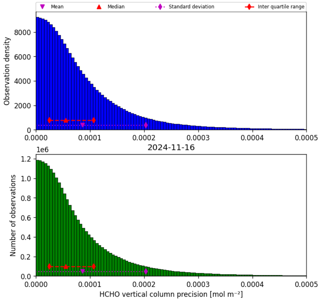
Figure 36: Histogram of “HCHO vertical column precision” for 2024-11-15 to 2024-11-17
