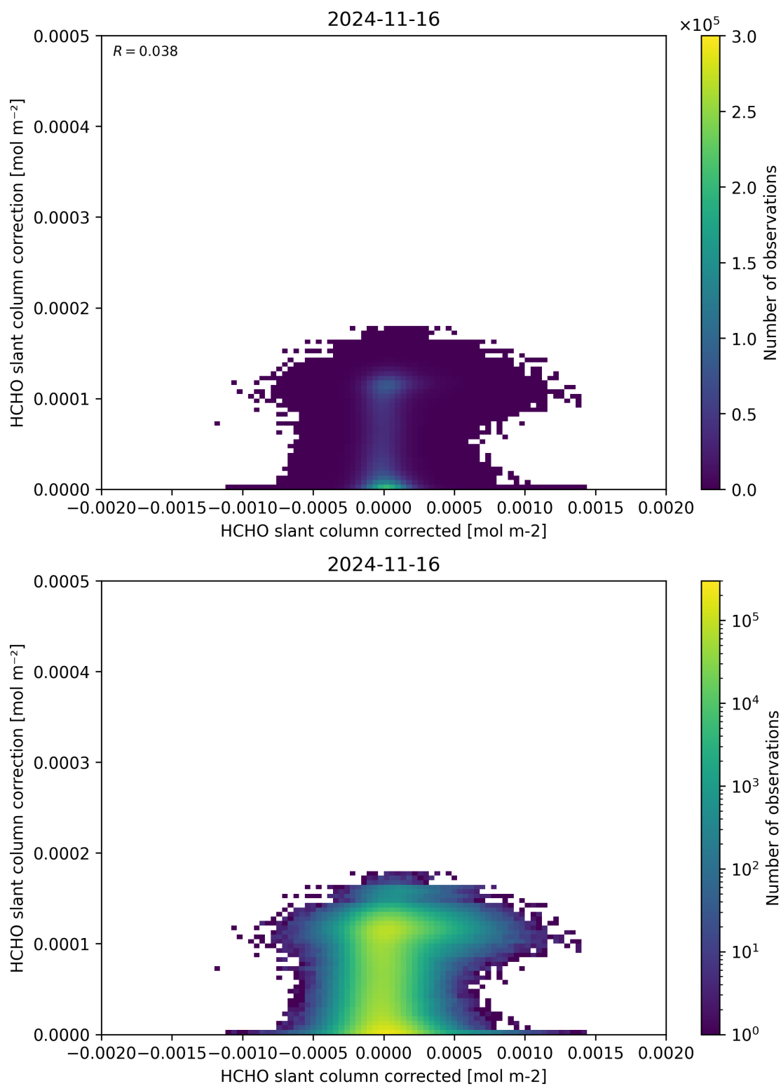
Figure 77: Scatter density plot of “HCHO slant column corrected” against “HCHO slant column correction” for 2024-11-15 to 2024-11-17.
