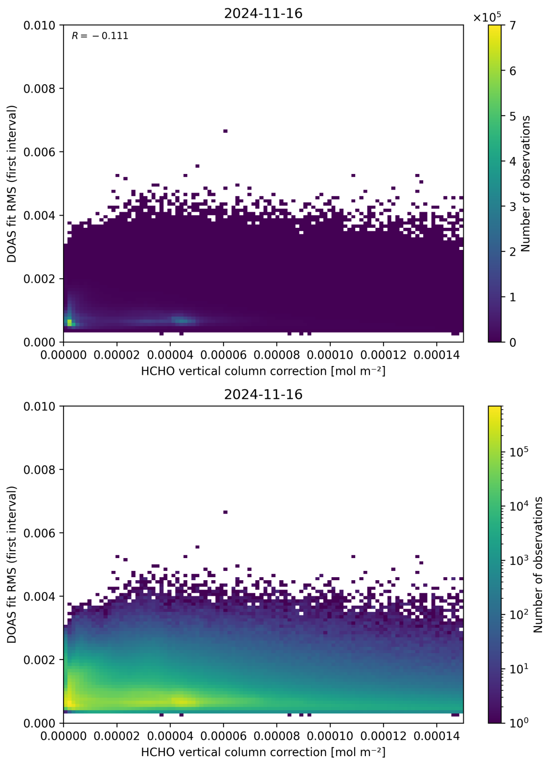
Figure 112: Scatter density plot of “HCHO vertical column correction” against “DOAS fit RMS (first interval)” for 2024-11-15 to 2024-11-17.
