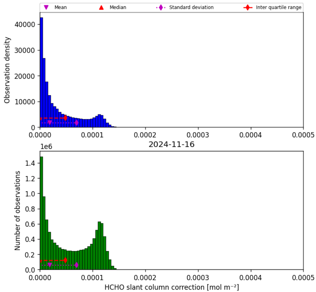
Figure 47: Histogram of “HCHO slant column correction” for 2024-11-15 to 2024-11-17
