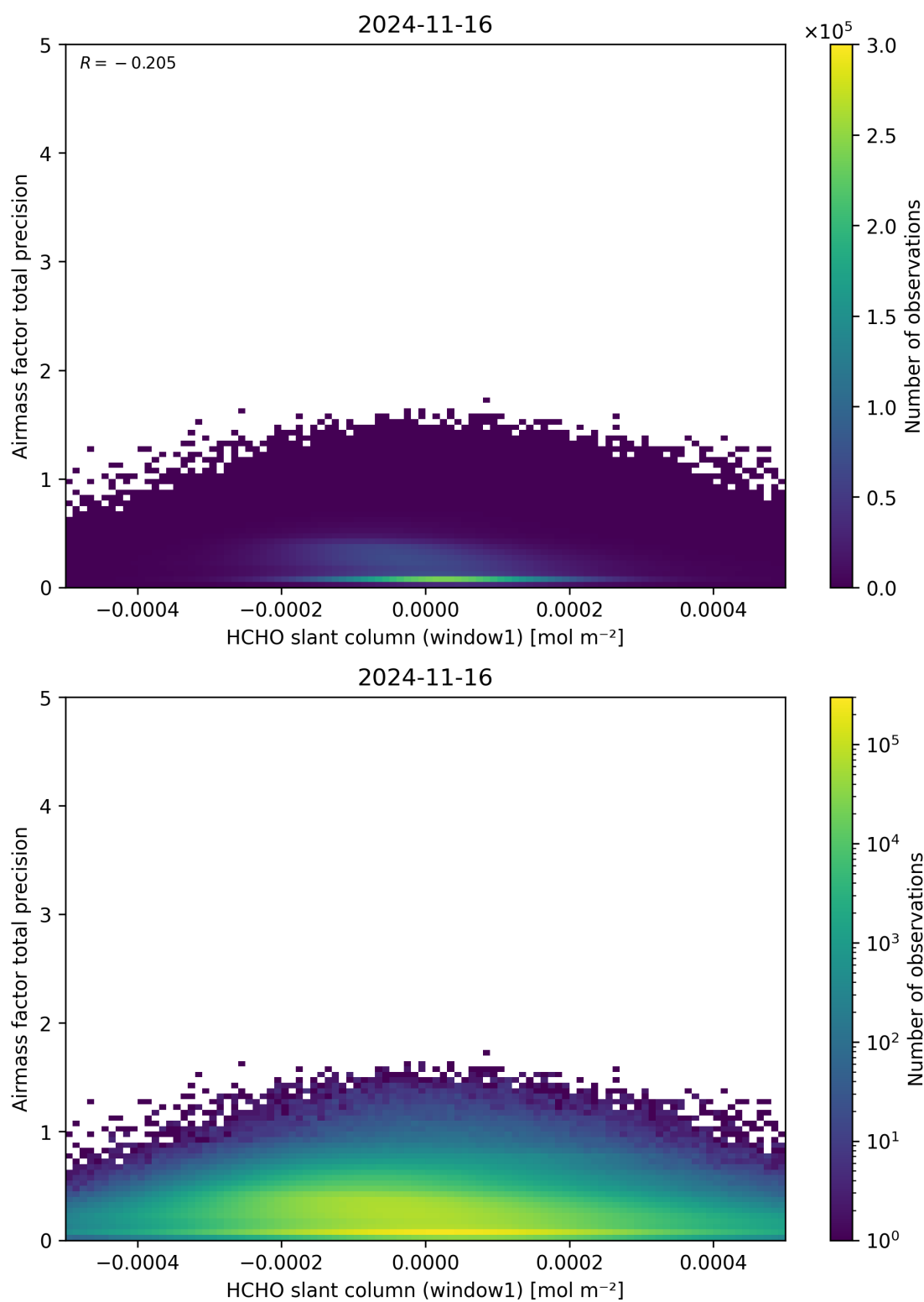
Figure 86: Scatter density plot of “HCHO slant column (window1)” against “Airmass factor total precision” for 2024-11-15 to 2024-11-17.
