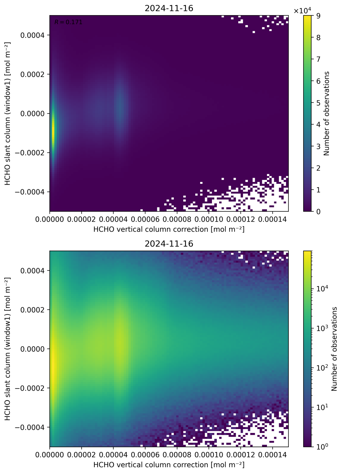
Figure 118: Scatter density plot of “HCHO vertical column correction” against “HCHO slant column (window1)” for 2024-11-15 to 2024-11-17.
