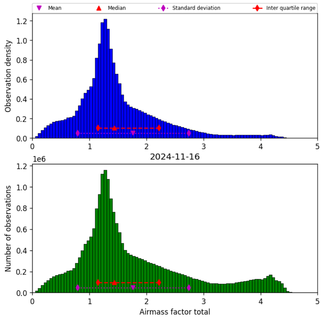
Figure 40: Histogram of “Airmass factor total” for 2024-11-15 to 2024-11-17
