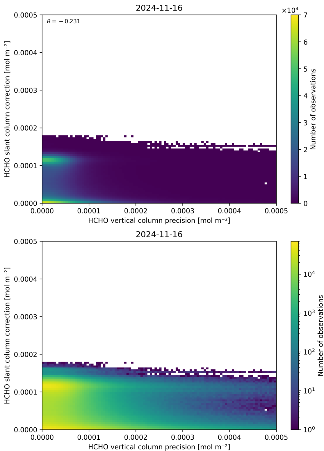
Figure 141: Scatter density plot of “HCHO vertical column precision” against “HCHO slant column correction” for 2024-11-15 to 2024-11-17.
