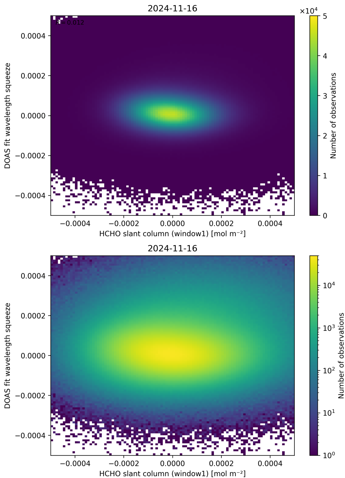
Figure 80: Scatter density plot of “HCHO slant column (window1)” against “DOAS fit wavelength squeeze” for 2024-11-15 to 2024-11-17.
