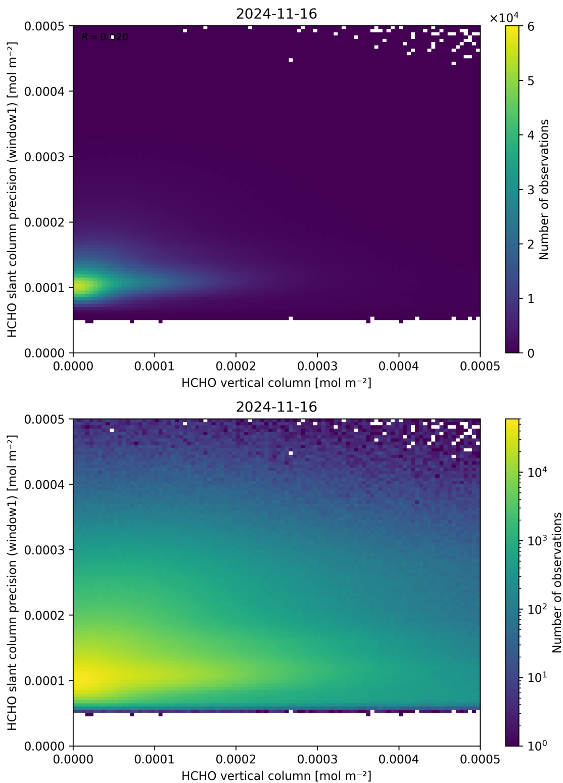
Figure 130: Scatter density plot of “HCHO vertical column” against “HCHO slant column precision (window1)” for 2024-11-15 to 2024-11-17.
