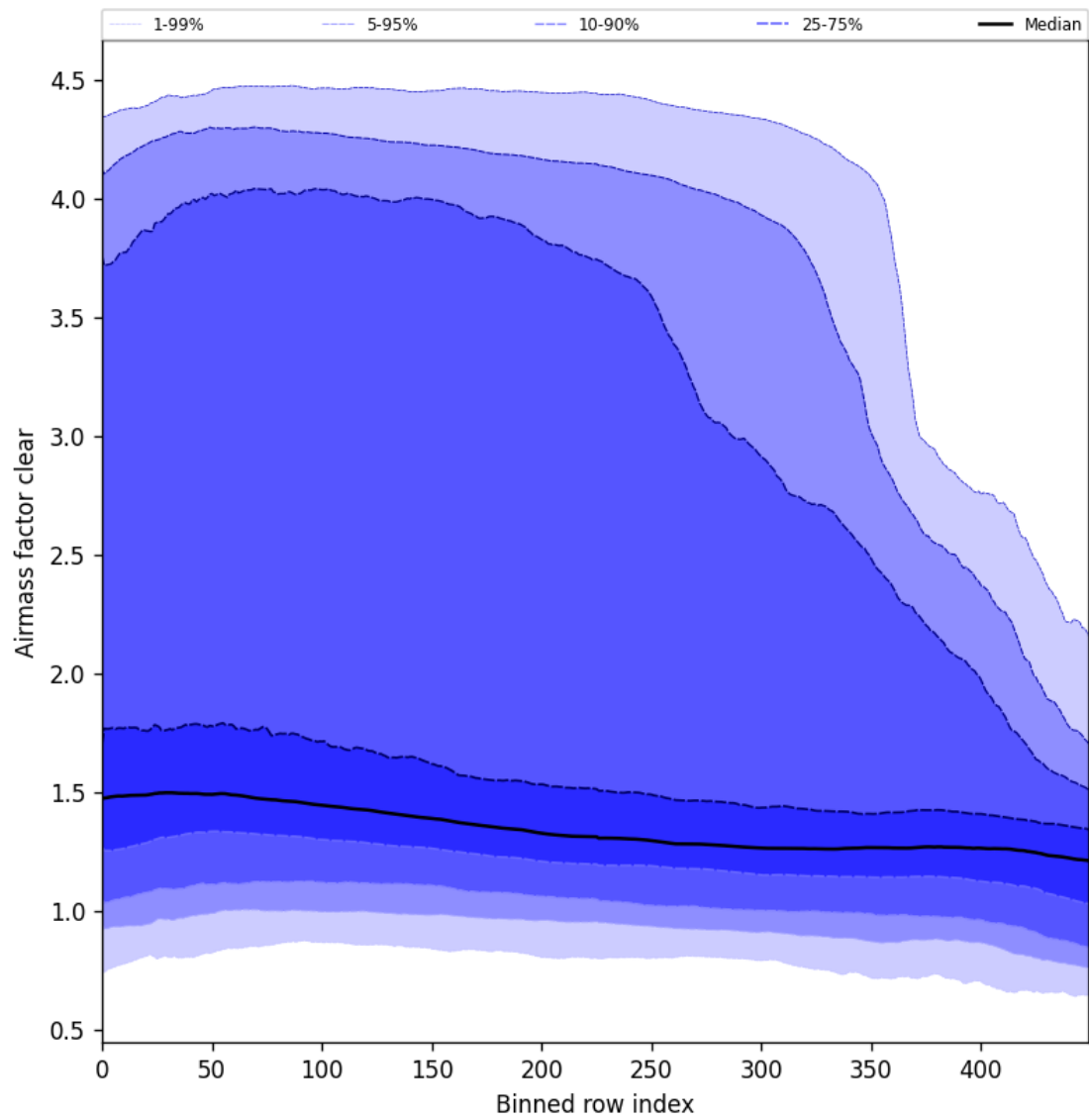
Figure 56: Along track statistics of “Air mass factor clear” for 2024-11-15 to 2024-11-17
