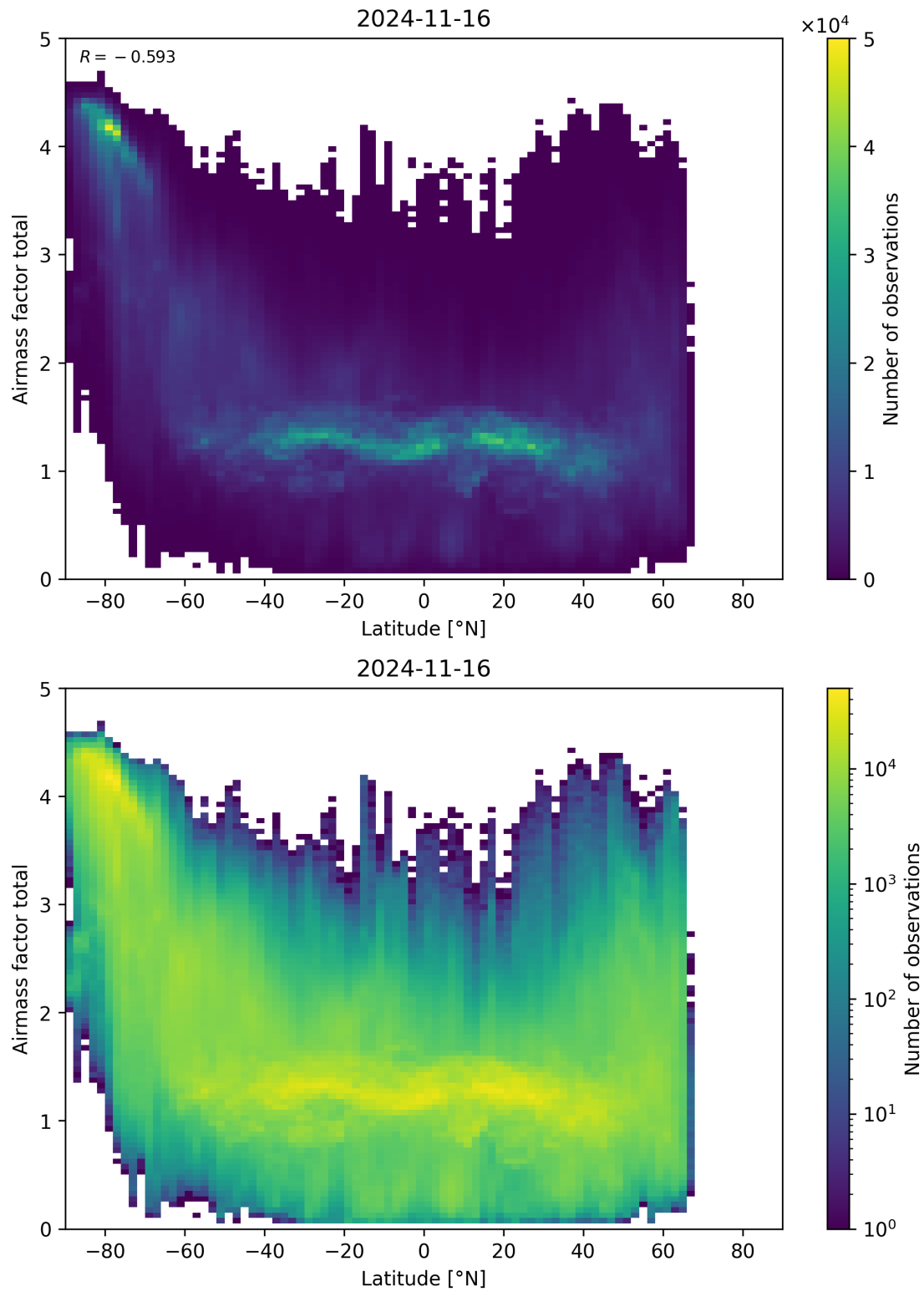
Figure 161: Scatter density plot of “Latitude” against “Airmass factor total” for 2024-11-15 to 2024-11-17.
