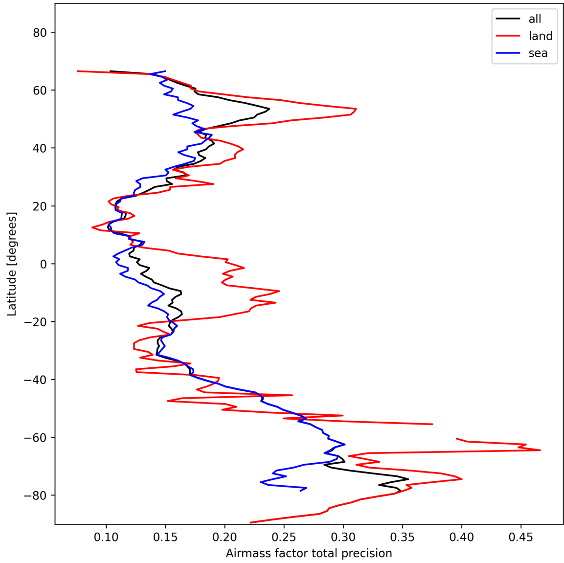
Figure 27: Zonal average of “Airmass factor total precision” for 2024-11-15 to 2024-11-17.
