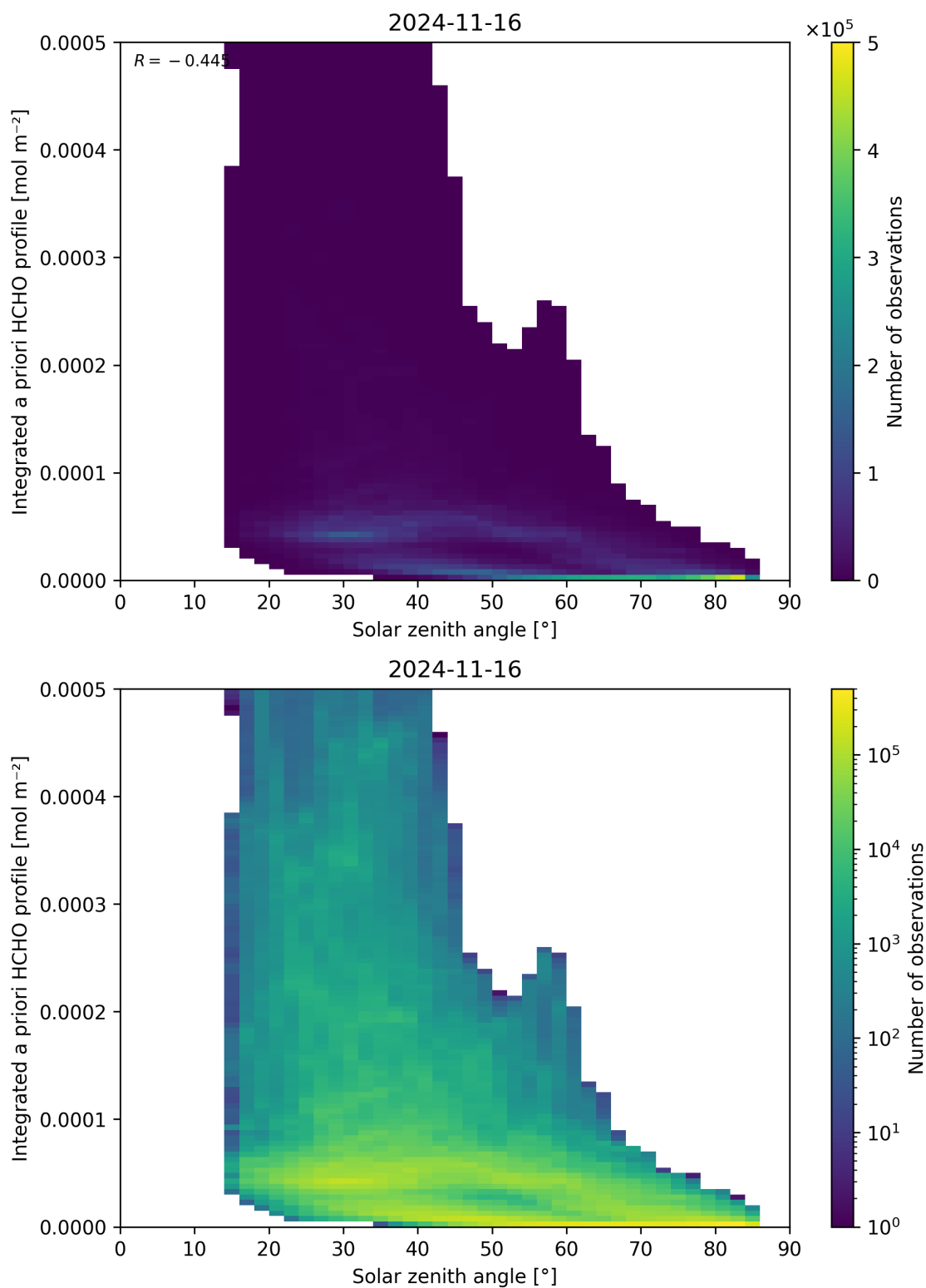
Figure 180: Scatter density plot of “Solar zenith angle” against “Integrated a priori HCHO profile” for 2024-11-15 to 2024-11-17.
