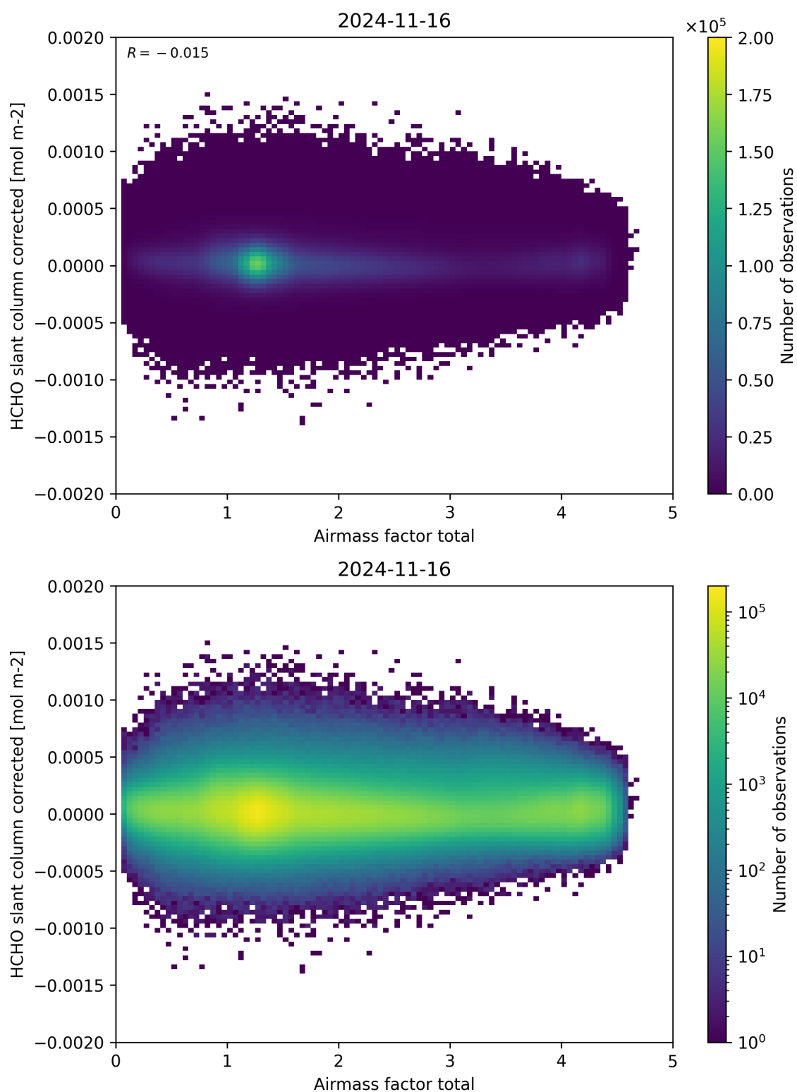
Figure 101: Scatter density plot of “Airmass factor total” against “HCHO slant column corrected” for 2024-11-15 to 2024-11-17.
