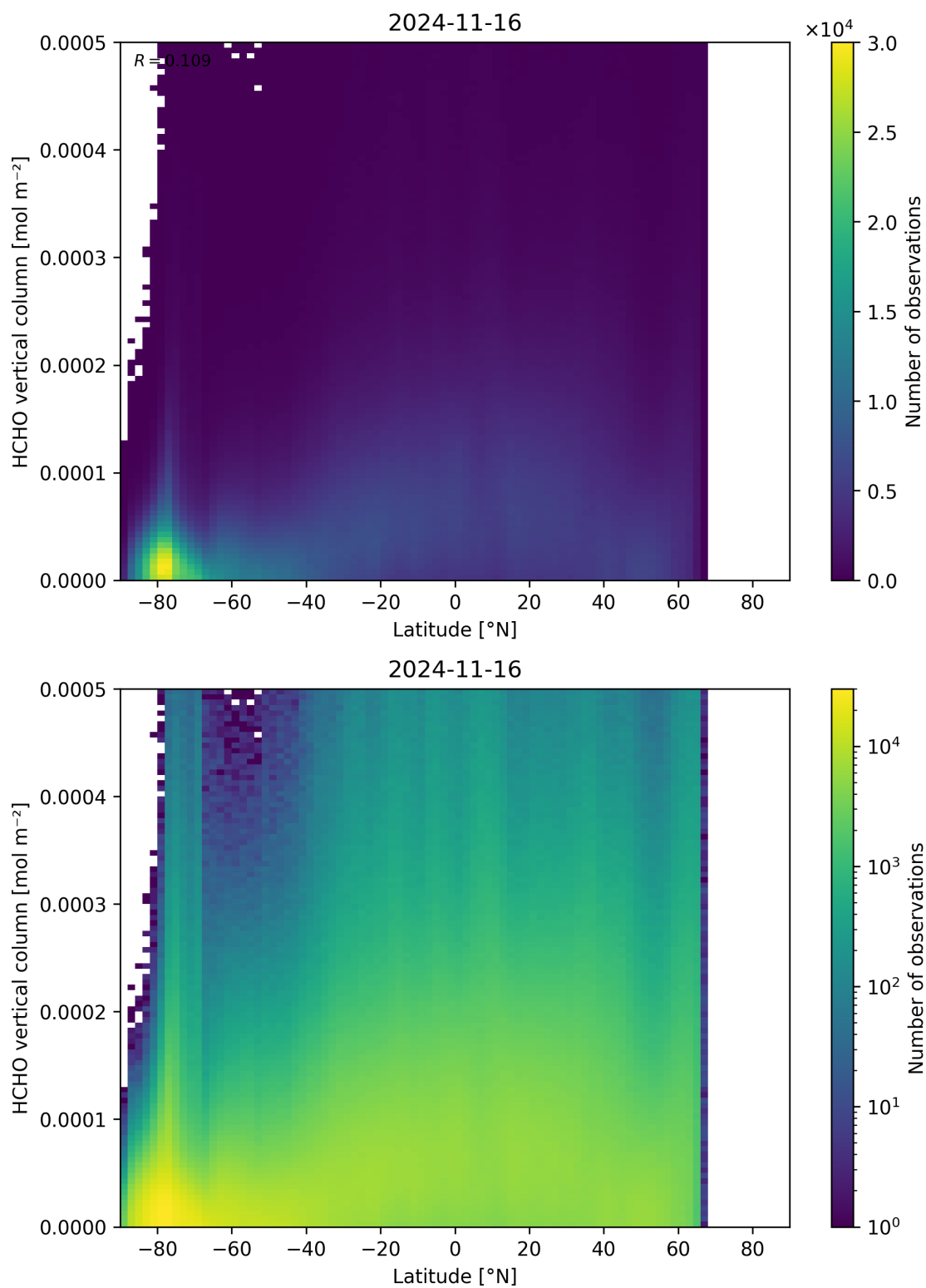
Figure 163: Scatter density plot of “Latitude” against “HCHO vertical column” for 2024-11-15 to 2024-11-17.
