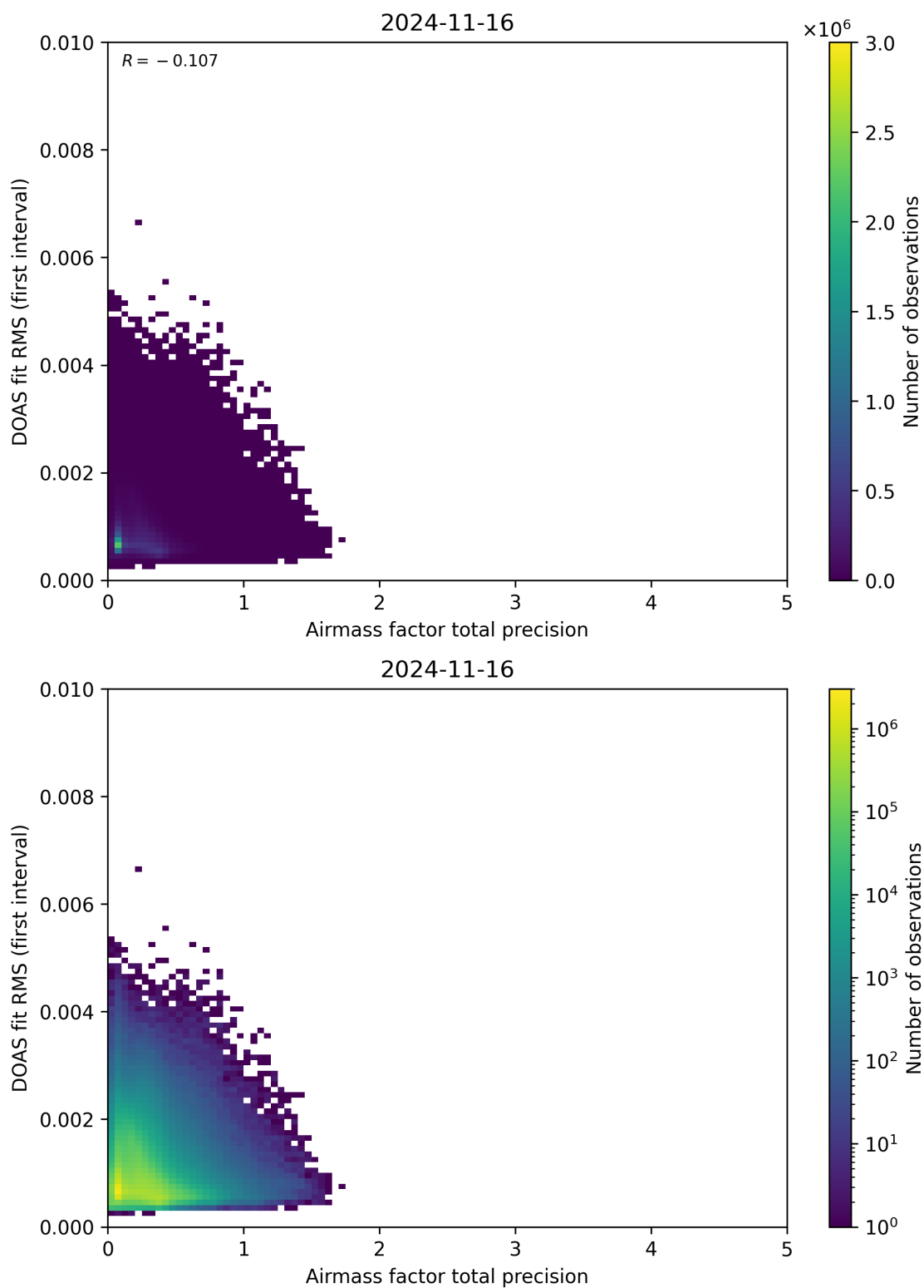
Figure 105: Scatter density plot of “Airmass factor total precision” against “DOAS fit RMS (first interval)” for 2024-11-15 to 2024-11-17.
