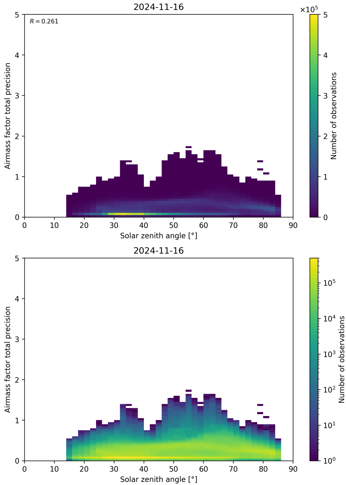
Figure 176: Scatter density plot of “Solar zenith angle” against “Airmass factor total precision” for 2024-11-15 to 2024-11-17.
