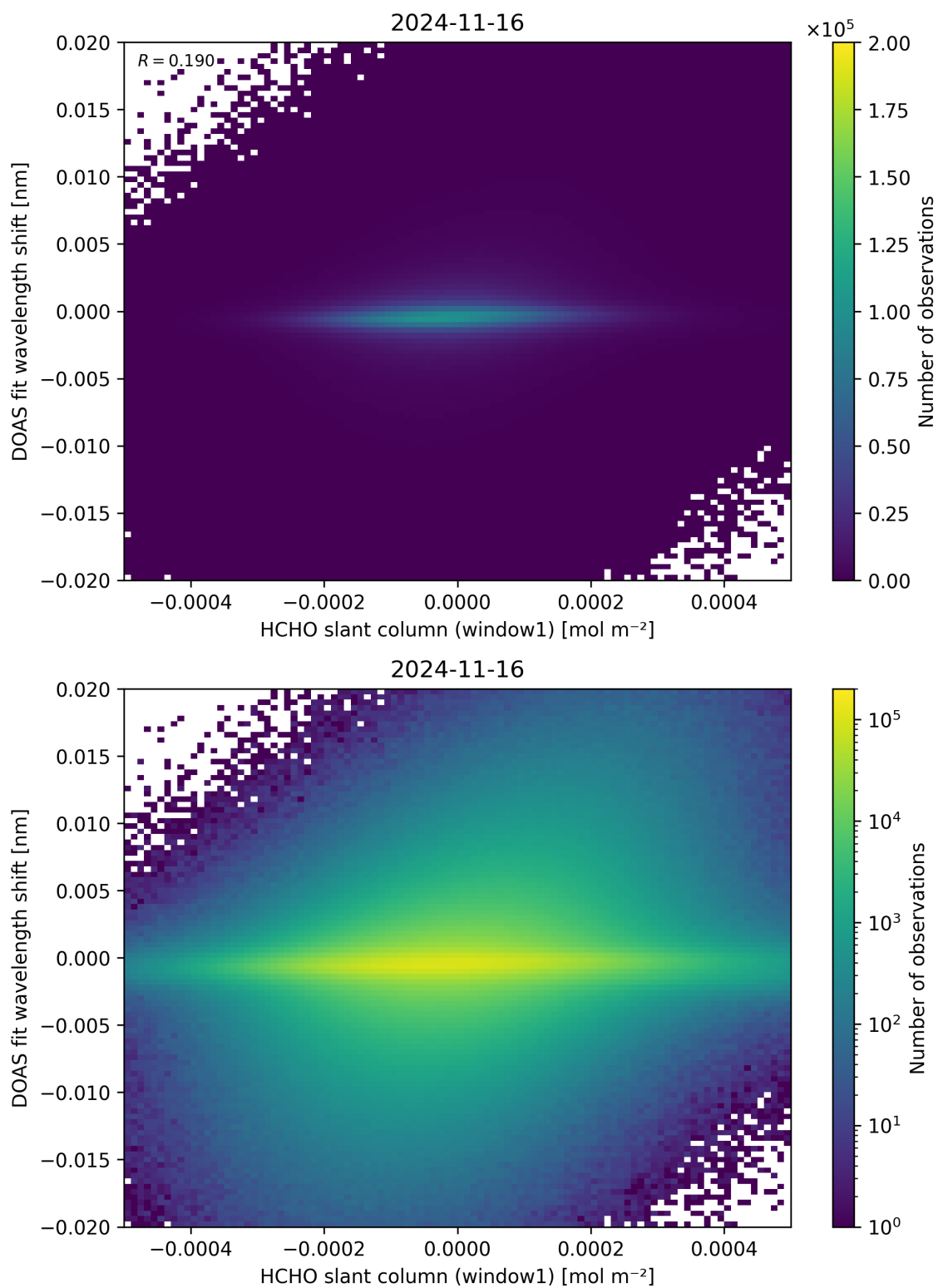
Figure 79: Scatter density plot of “HCHO slant column (window1)” against “DOAS fit wavelength shift” for 2024-11-15 to 2024-11-17.
