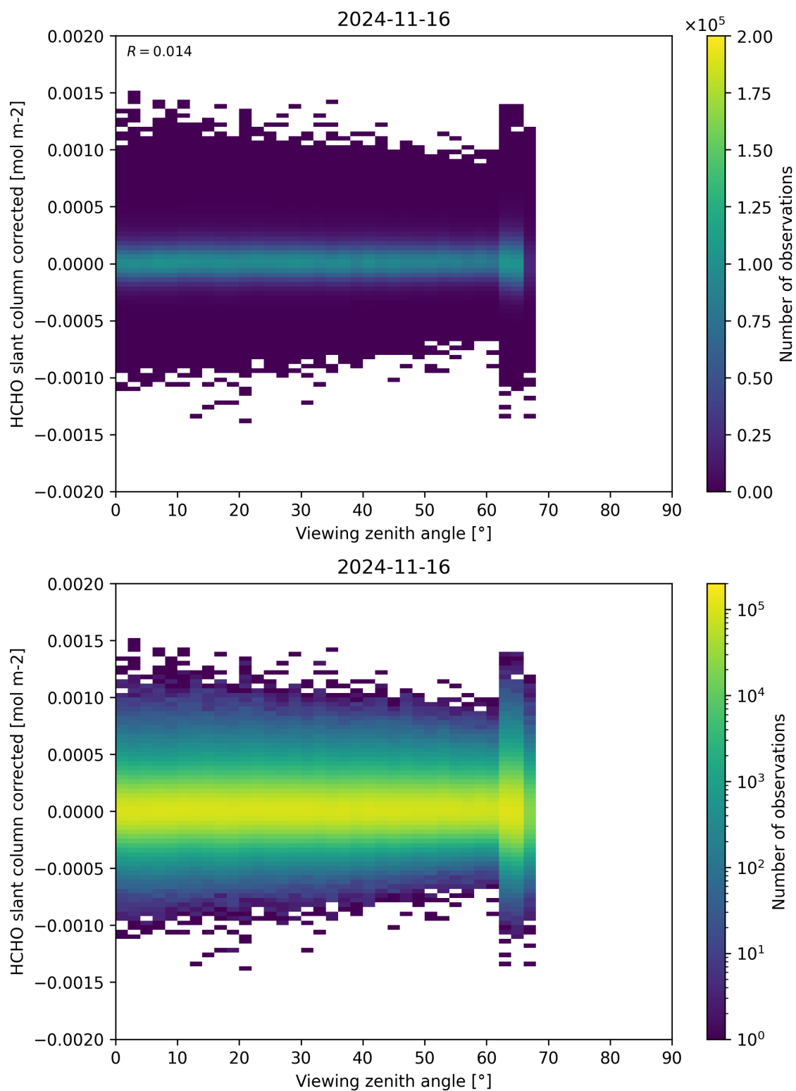
Figure 186: Scatter density plot of “Viewing zenith angle” against “HCHO slant column corrected” for 2024-11-15 to 2024-11-17.
