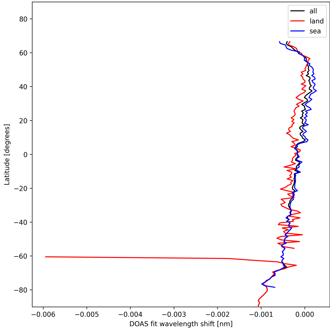
Figure 30: Zonal average of "DOAS fit wavelength shift" for 2024-11-15 to 2024-11-17.
