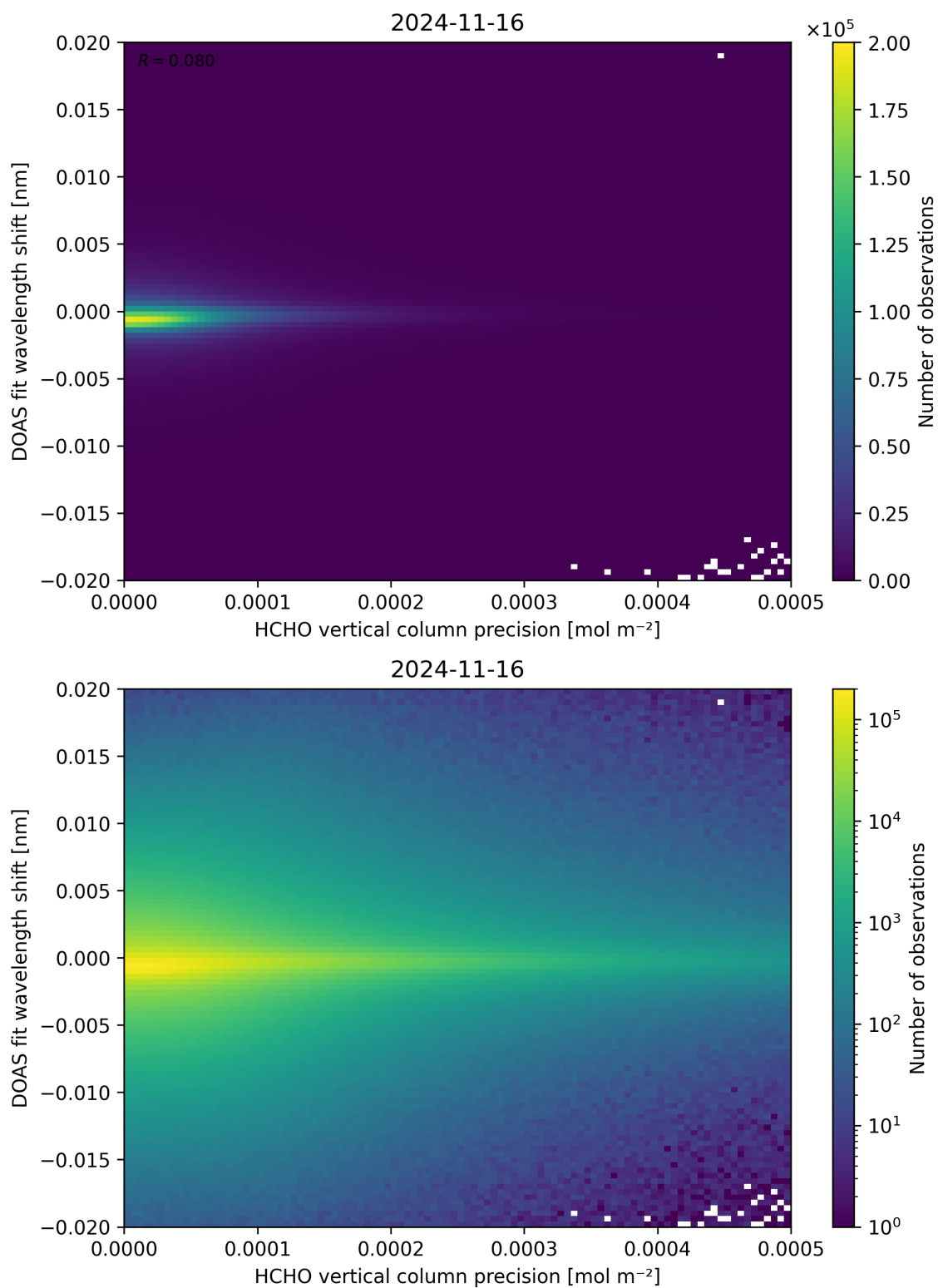
Figure 137: Scatter density plot of “HCHO vertical column precision” against “DOAS fit wavelength shift” for 2024-11-15 to 2024-11-17.
