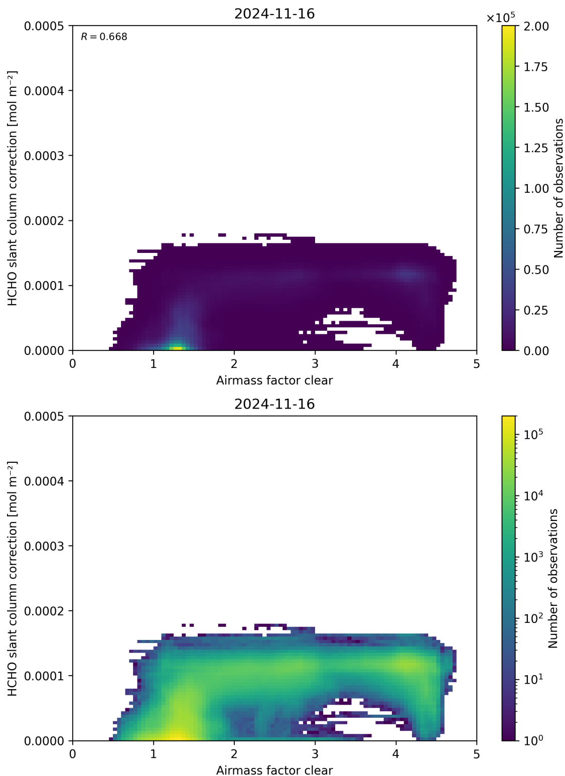
Figure 75: Scatter density plot of “Airmass factor clear” against “HCHO slant column correction” for 2024-11-15 to 2024-11-17.
