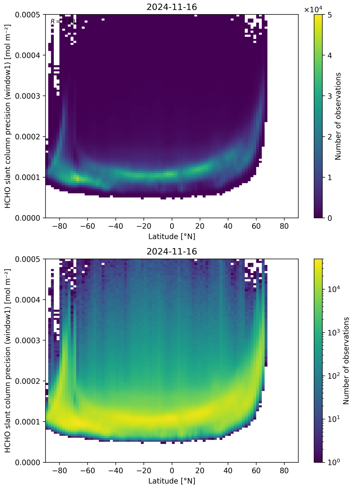
Figure 160: Scatter density plot of “Latitude” against “HCHO slant column precision (window1)” for 2024-11-15 to 2024-11-17.
