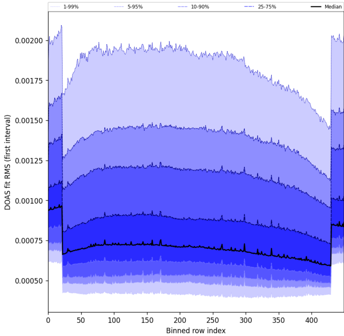
Figure 60: Along track statistics of “DOAS fit RMS (first interval)” for 2024-11-15 to 2024-11-17
