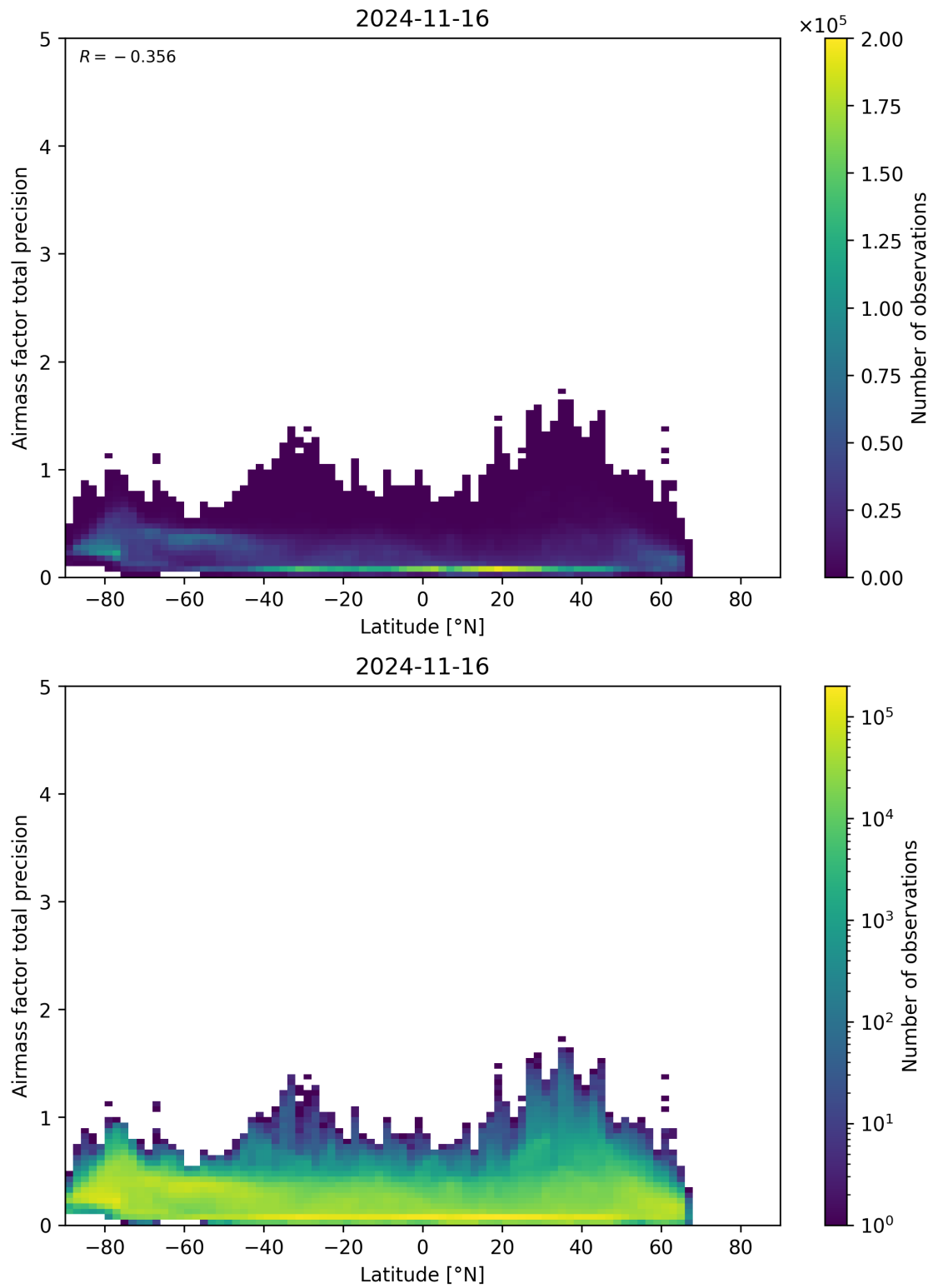
Figure 162: Scatter density plot of “Latitude” against “Airmass factor total precision” for 2024-11-15 to 2024-11-17.
