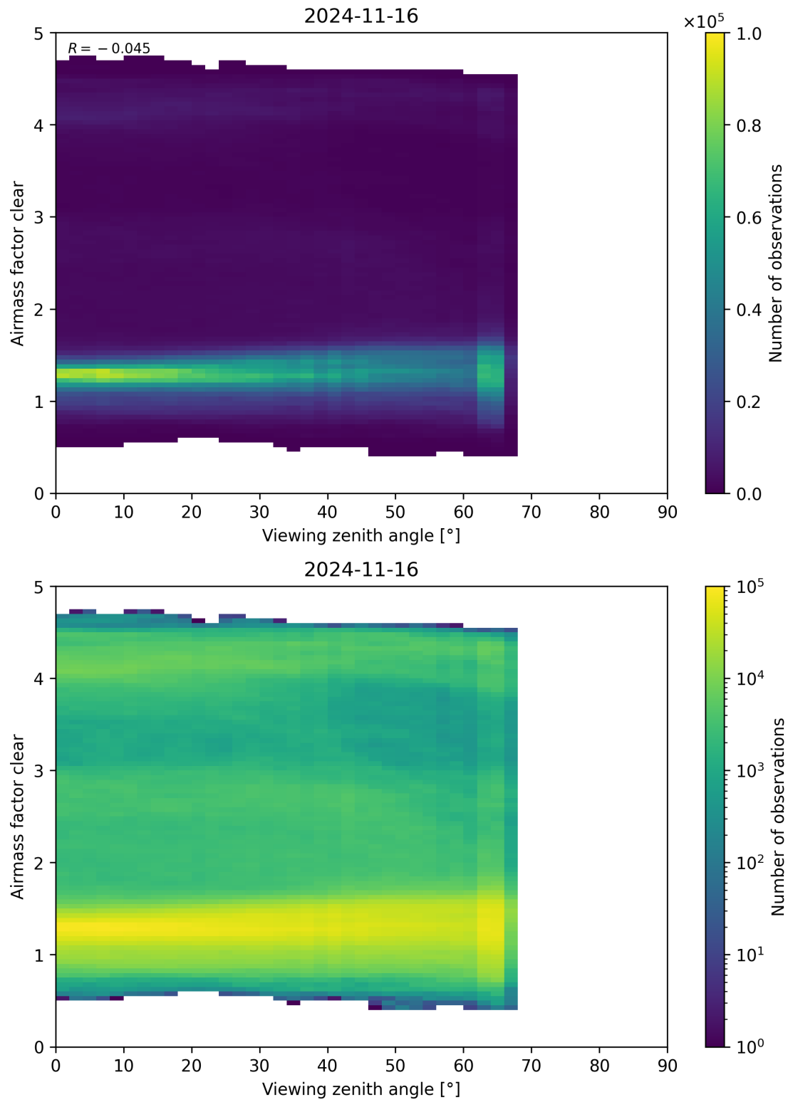
Figure 185: Scatter density plot of “Viewing zenith angle” against “Airmass factor clear” for 2024-11-15 to 2024-11-17.
