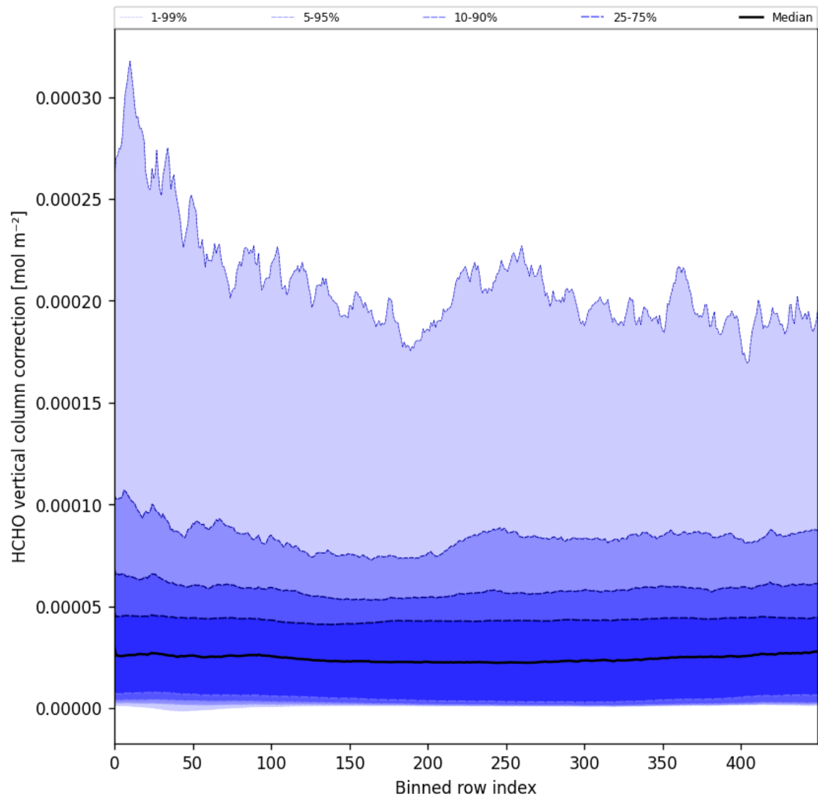
Figure 51: Along track statistics of “HCHO vertical column correction” for 2024-11-15 to 2024-11-17
