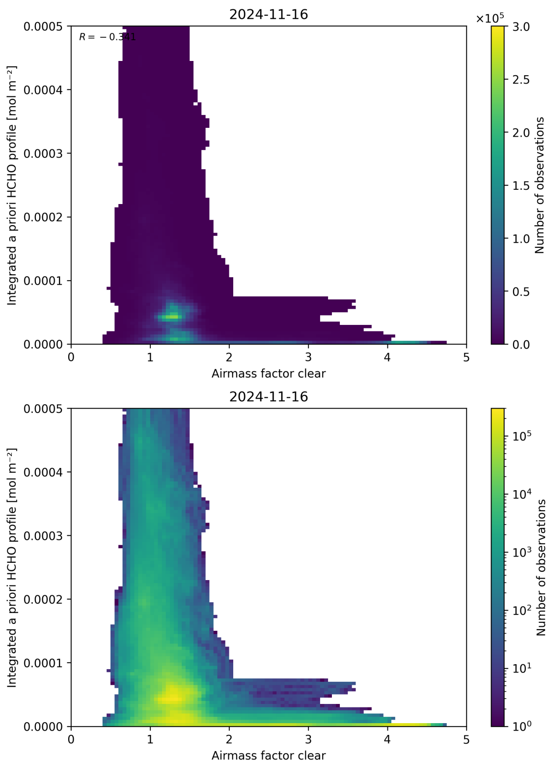
Figure 76: Scatter density plot of “Airmass factor clear” against “Integrated a priori HCHO profile” for 2024-11-15 to 2024-11-17.
