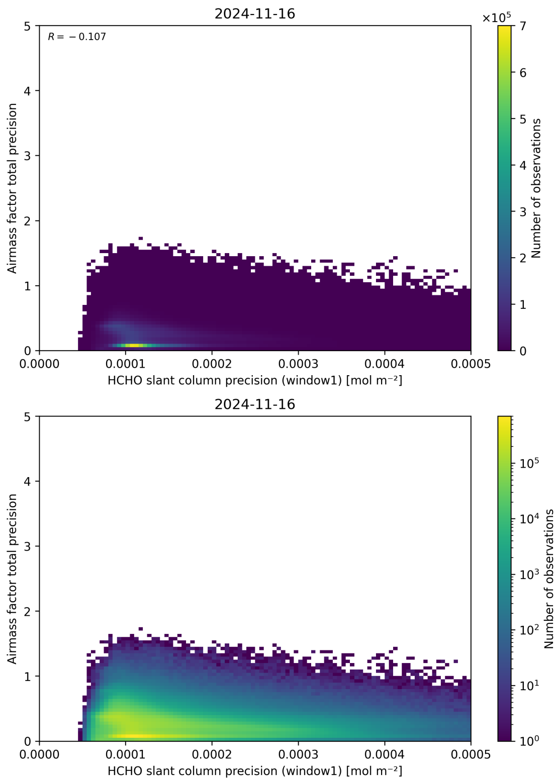
Figure 95: Scatter density plot of “HCHO slant column precision (window1)” against “Airmass factor total precision” for 2024-11-15 to 2024-11-17.
