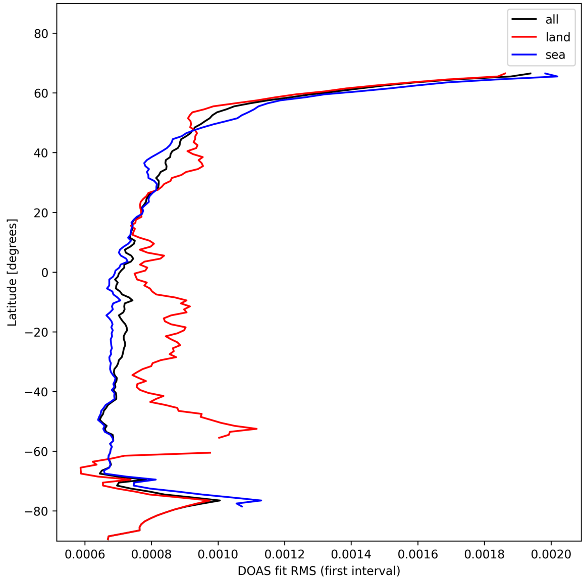
Figure 32: Zonal average of “DOAS fit RMS (first interval)” for 2024-11-15 to 2024-11-17.
