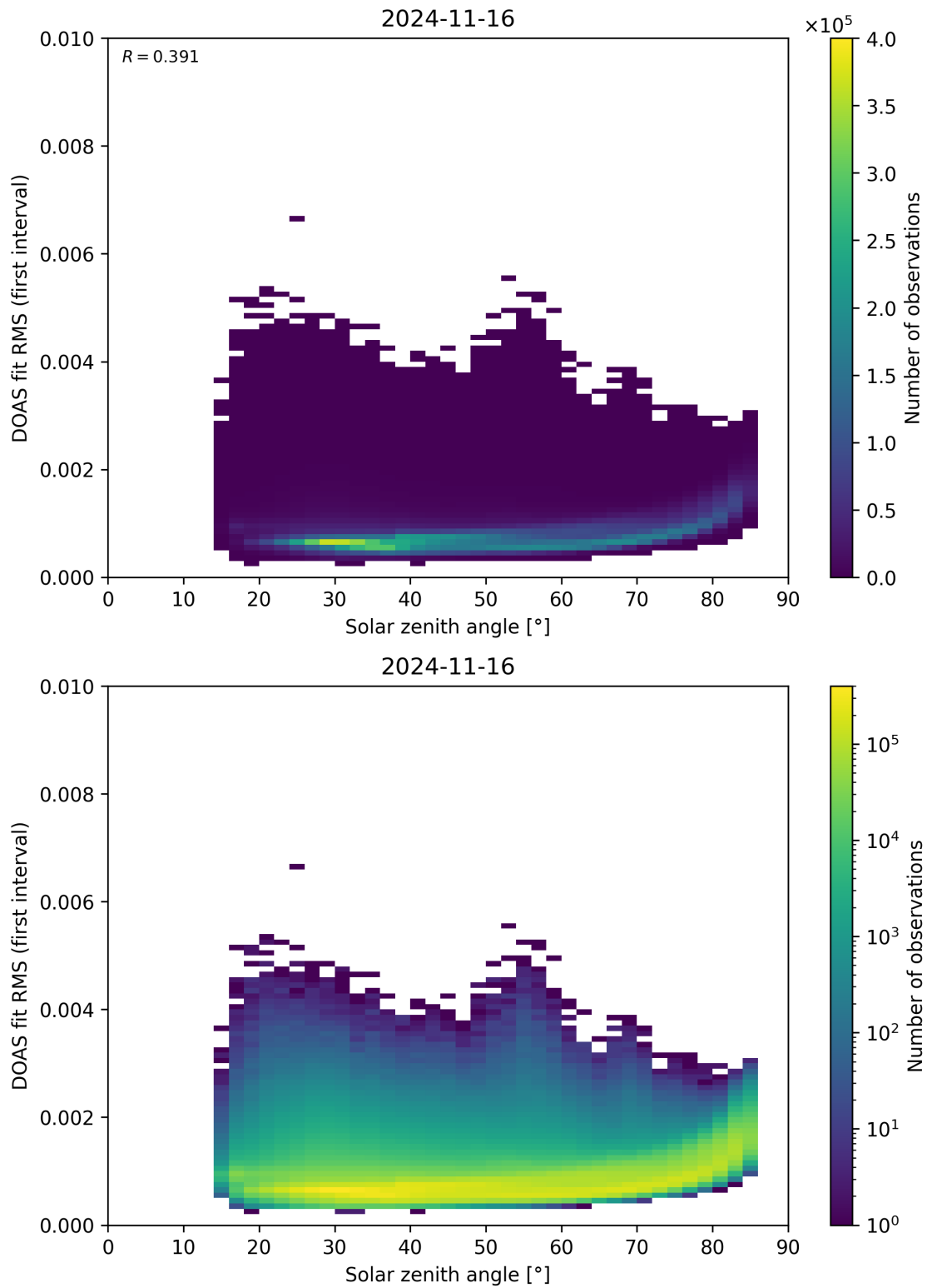
Figure 167: Scatter density plot of “Solar zenith angle” against “DOAS fit RMS (first interval)” for 2024-11-15 to 2024-11-17.
