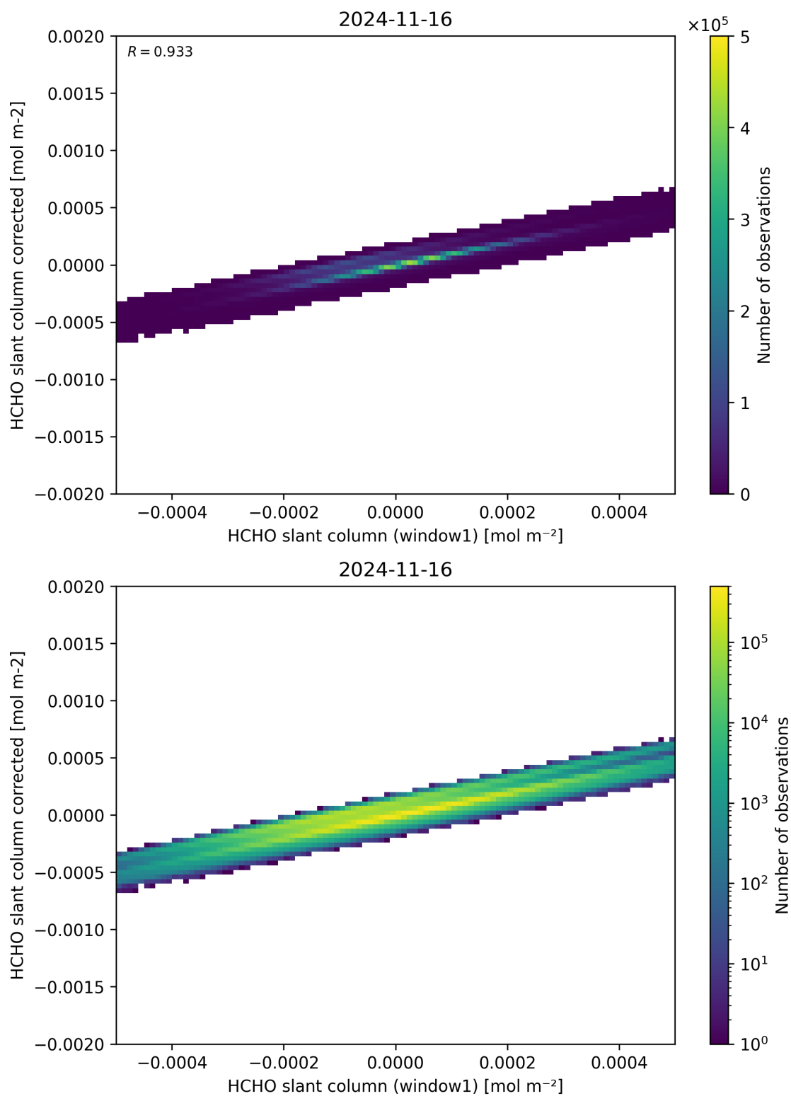
Figure 82: Scatter density plot of “HCHO slant column (window1)” against “HCHO slant column corrected” for 2024-11-15 to 2024-11-17.
