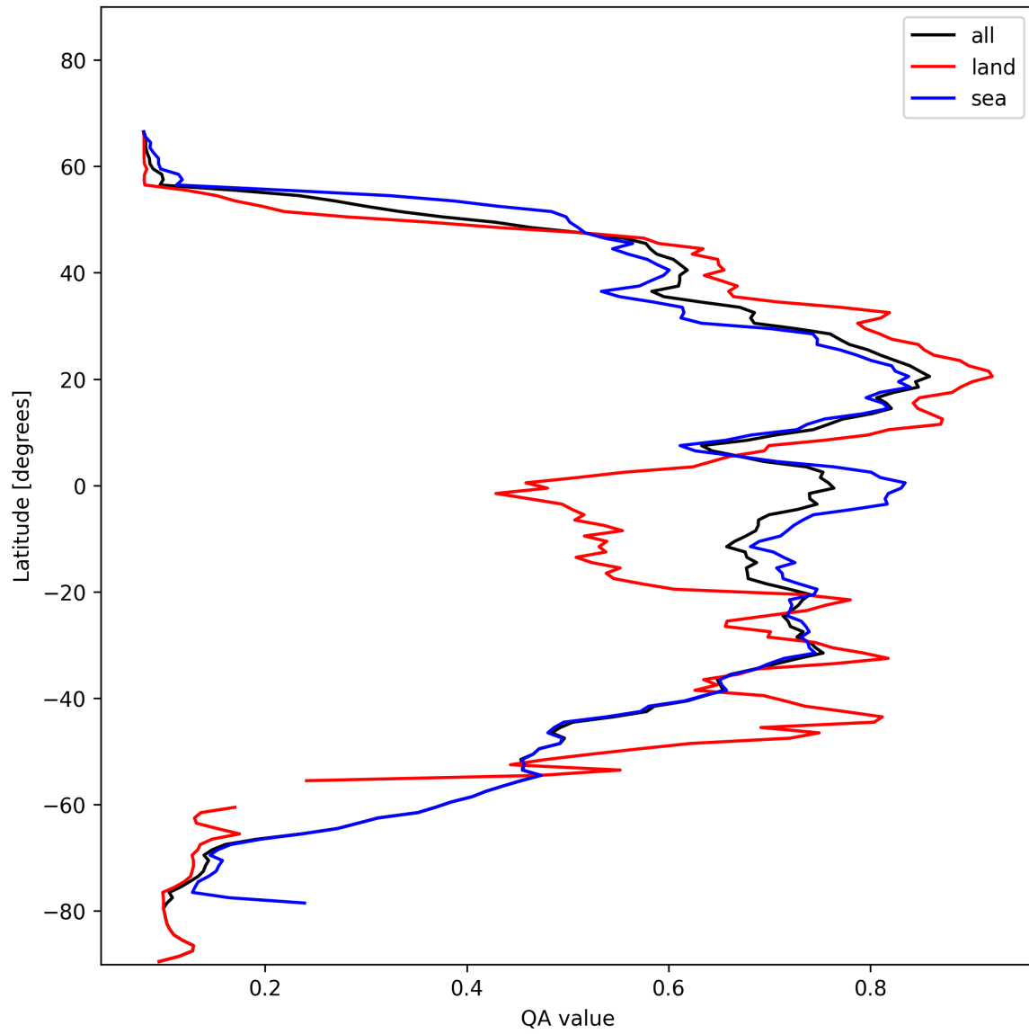
Figure 20: Zonal average of “QA value” for 2024-11-15 to 2024-11-17.
