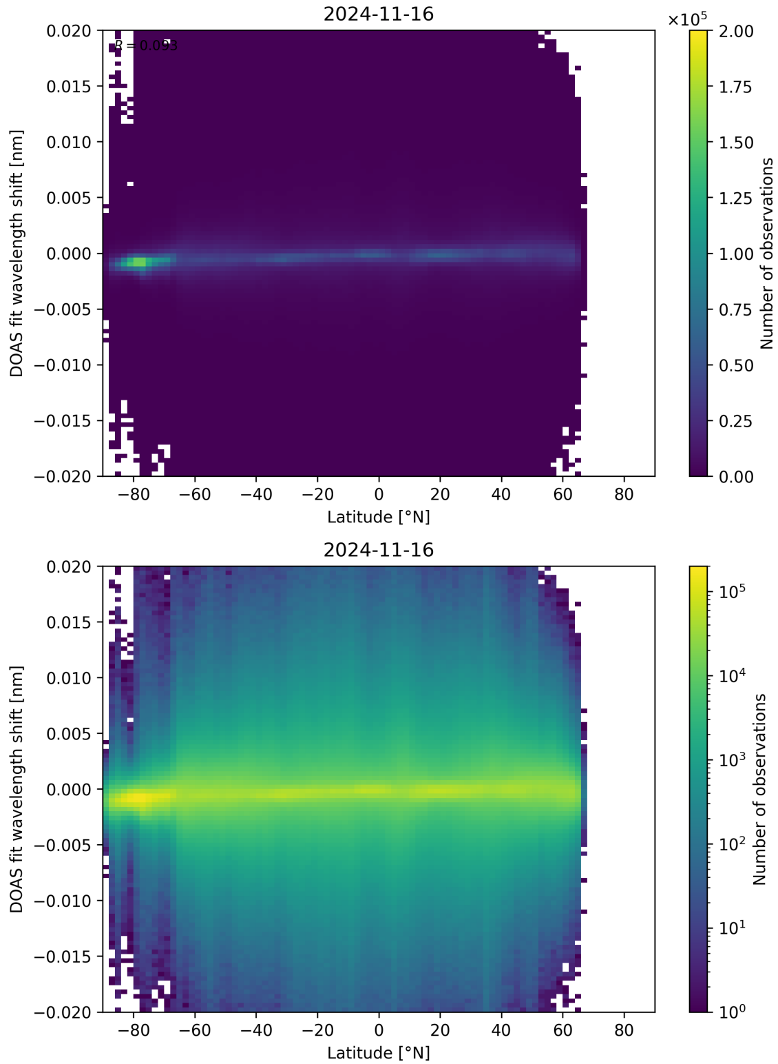
Figure 154: Scatter density plot of “Latitude” against “DOAS fit wavelength shift” for 2024-11-15 to 2024-11-17.
