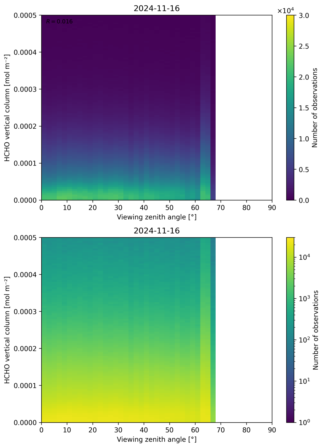
Figure 192: Scatter density plot of “Viewing zenith angle” against “HCHO vertical column” for 2024-11-15 to 2024-11-17.
