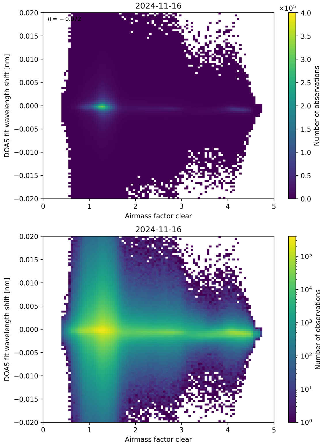
Figure 72: Scatter density plot of “Airmass factor clear” against “DOAS fit wavelength shift” for 2024-11-15 to 2024-11-17.
