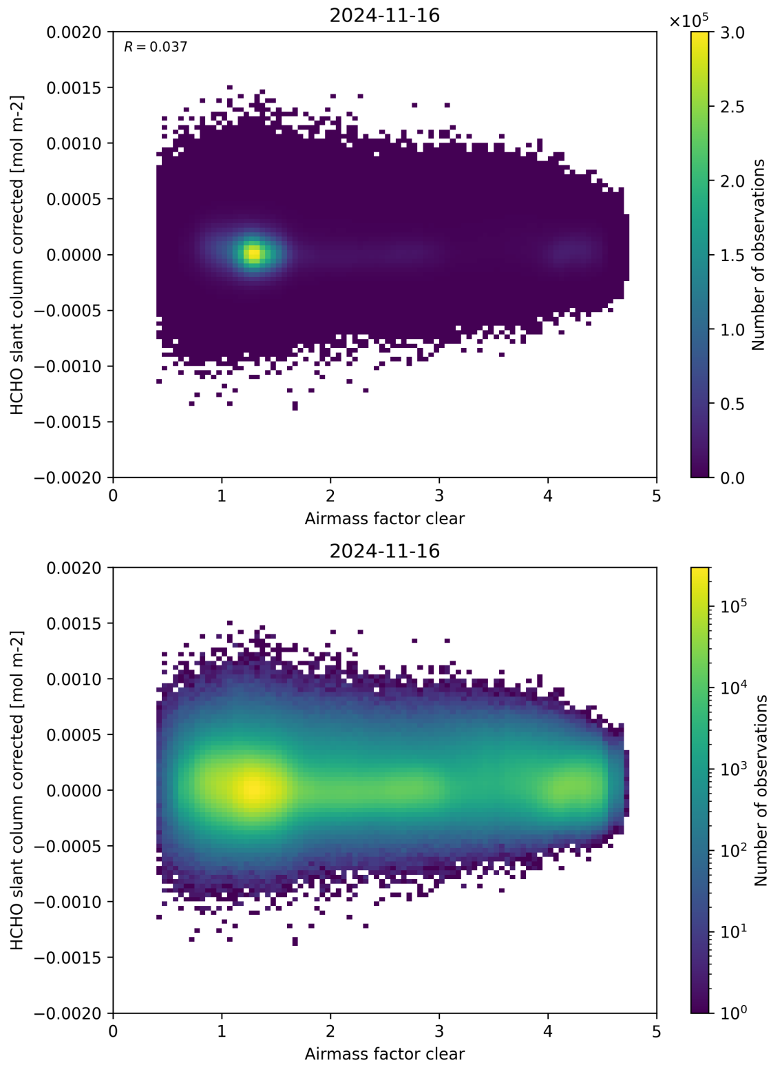
Figure 74: Scatter density plot of “Airmass factor clear” against “HCHO slant column corrected” for 2024-11-15 to 2024-11-17.
