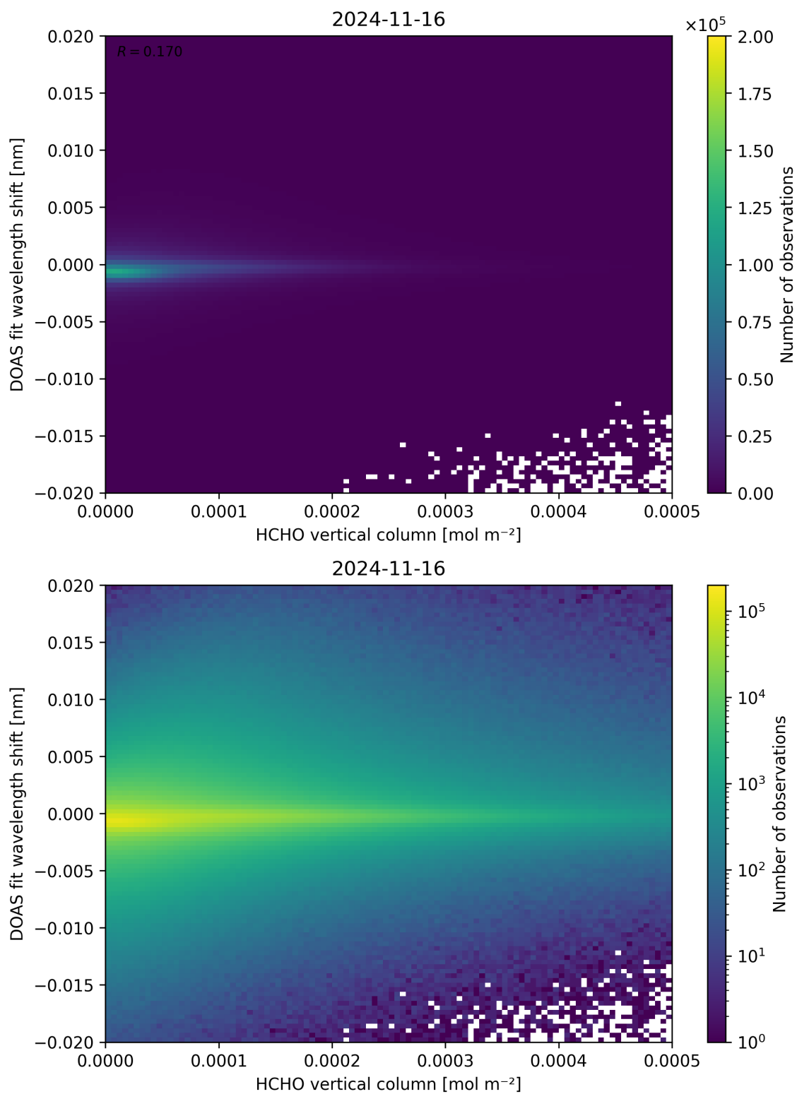
Figure 124: Scatter density plot of “HCHO vertical column” against “DOAS fit wavelength shift” for 2024-11-15 to 2024-11-17.
