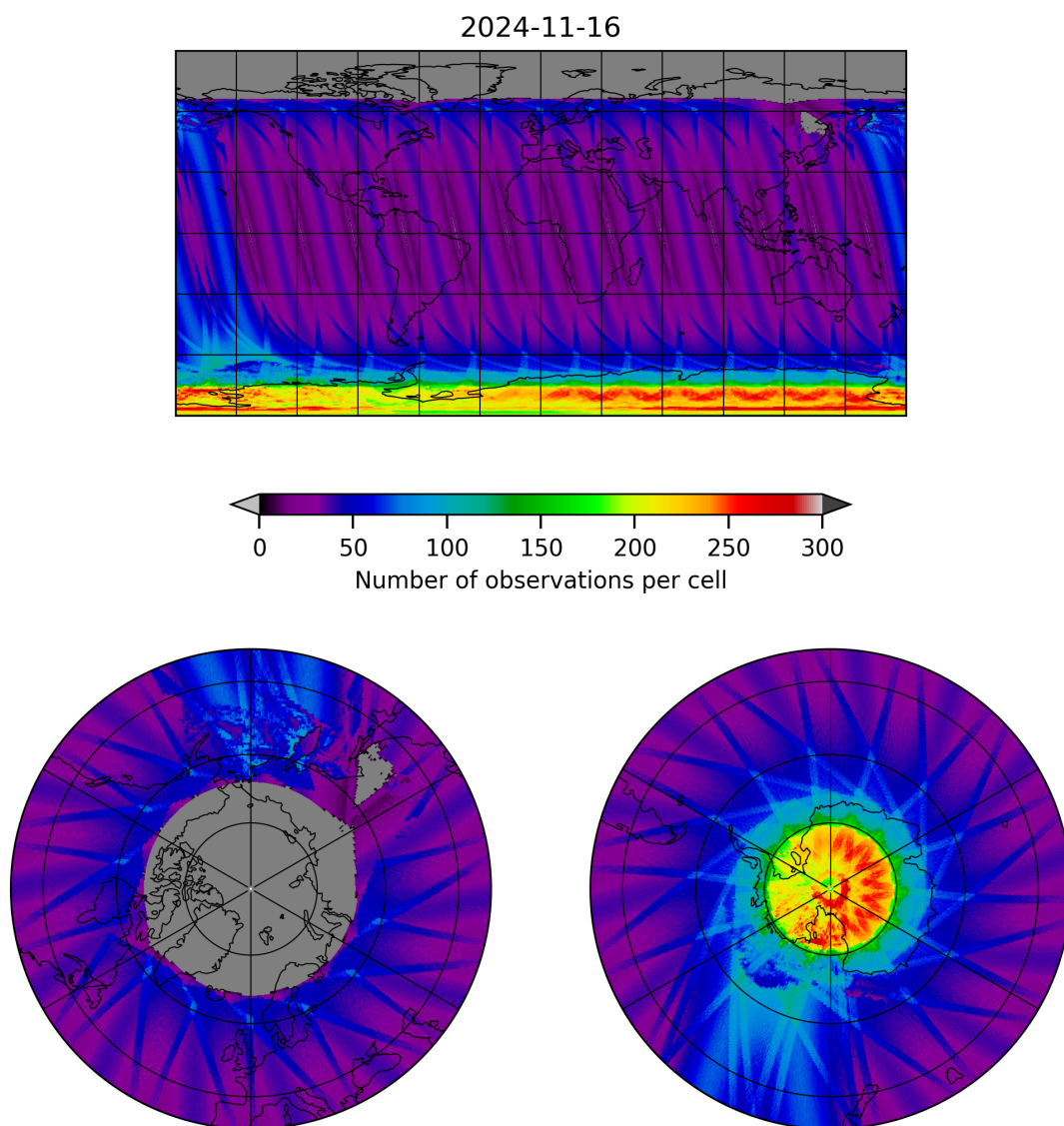
Figure 19: Map of the number of observations for 2024-11-15 to 2024-11-17
