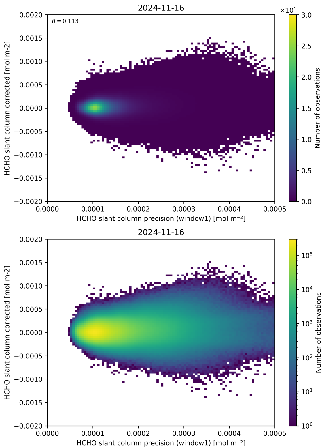
Figure 92: Scatter density plot of “HCHO slant column precision (window1)” against “HCHO slant column corrected” for 2024-11-15 to 2024-11-17.
