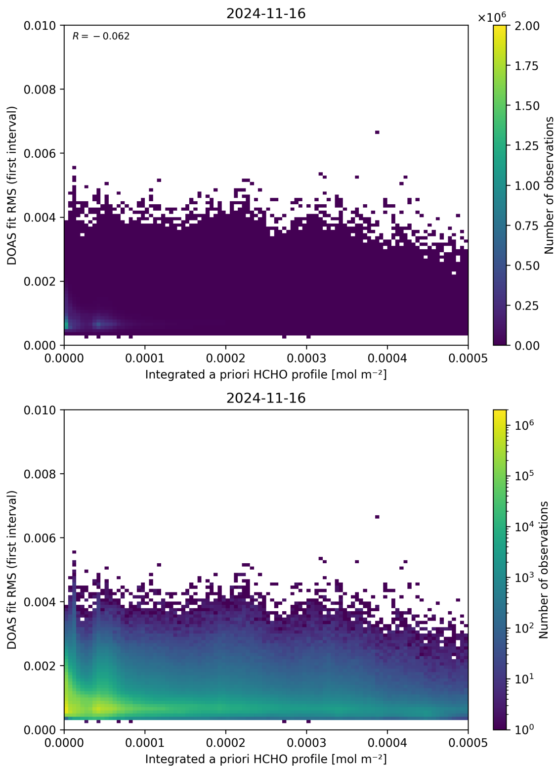
Figure 148: Scatter density plot of “Integrated a priori HCHO profile” against “DOAS fit RMS (first interval)” for 2024-11-15 to 2024-11-17.
