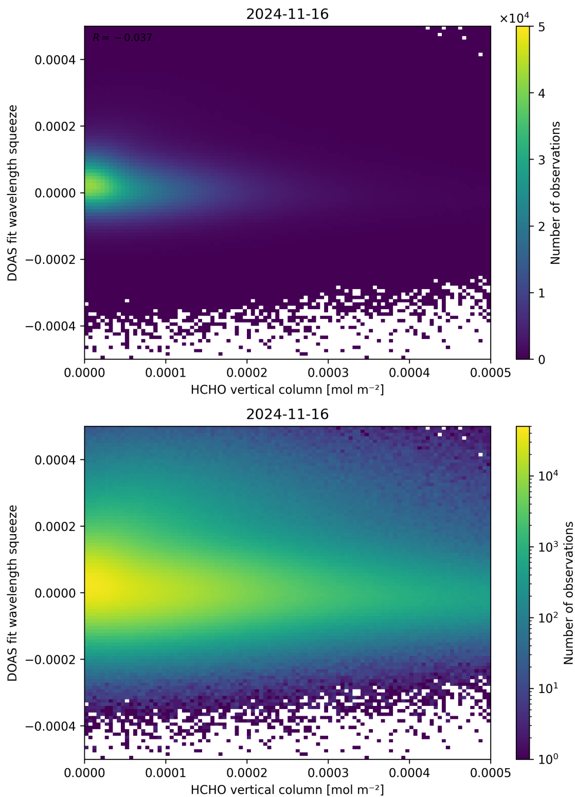
Figure 125: Scatter density plot of “HCHO vertical column” against “DOAS fit wavelength squeeze” for 2024-11-15 to 2024-11-17.
