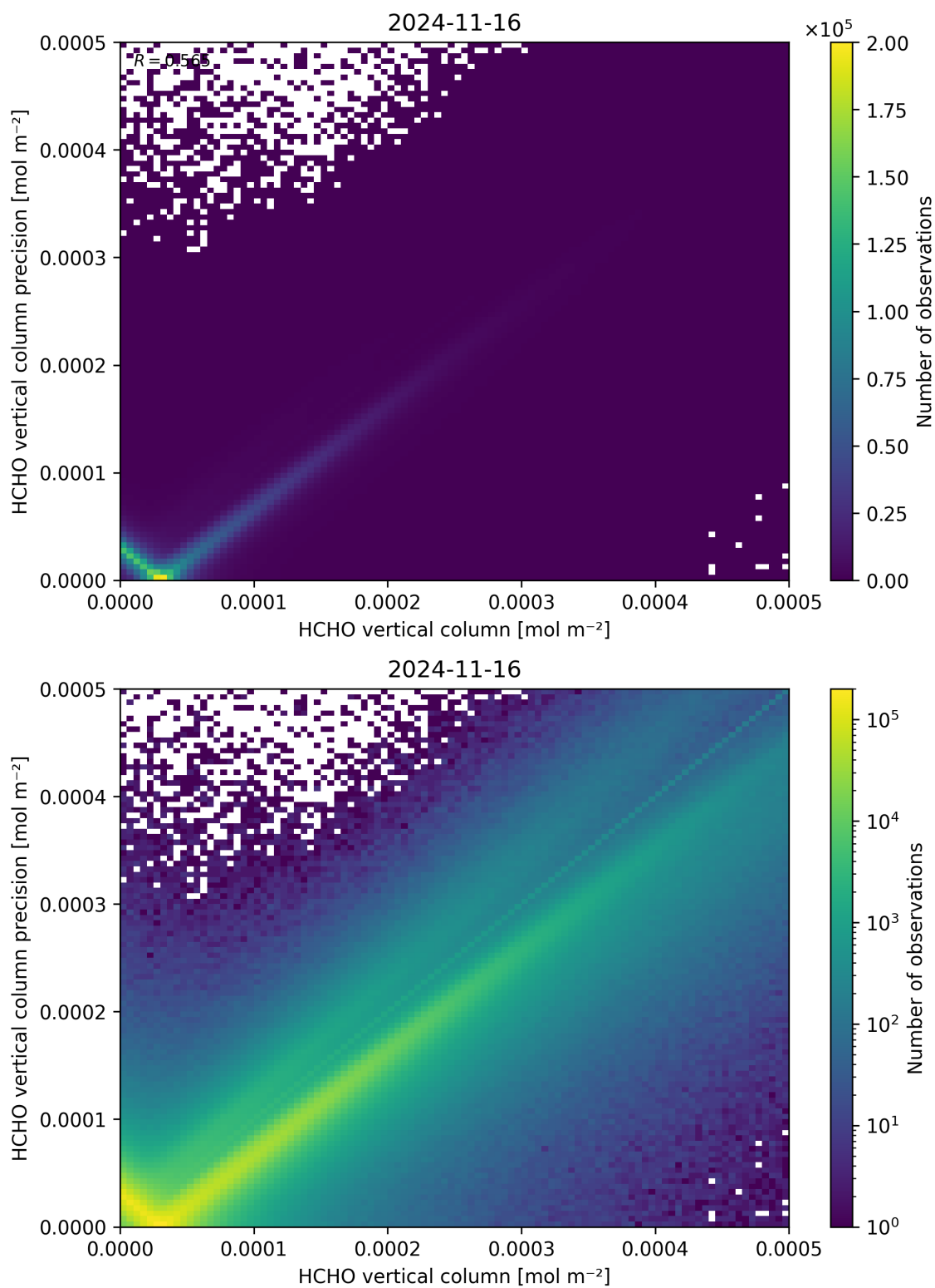
Figure 134: Scatter density plot of “HCHO vertical column” against “HCHO vertical column precision” for 2024-11-15 to 2024-11-17.
