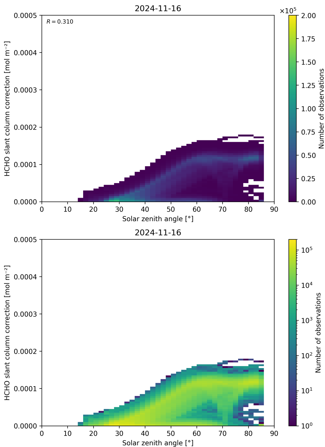
Figure 172: Scatter density plot of “Solar zenith angle” against “HCHO slant column correction” for 2024-11-15 to 2024-11-17.
