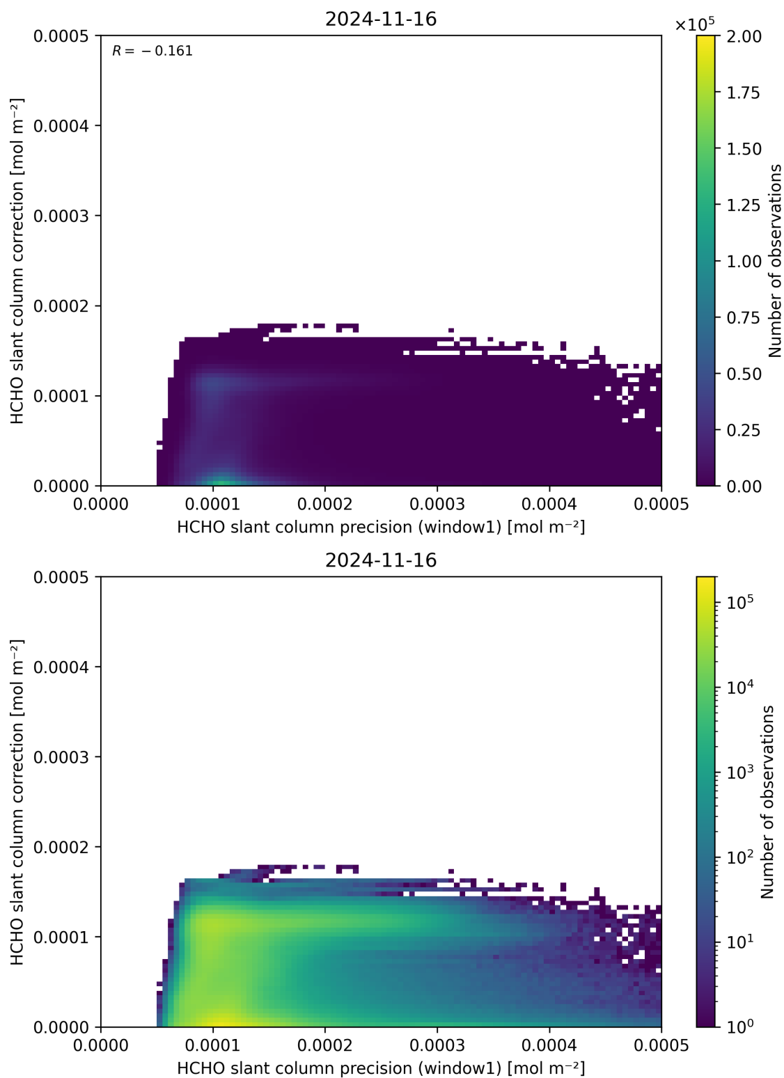
Figure 93: Scatter density plot of “HCHO slant column precision (window1)” against “HCHO slant column correction” for 2024-11-15 to 2024-11-17.
