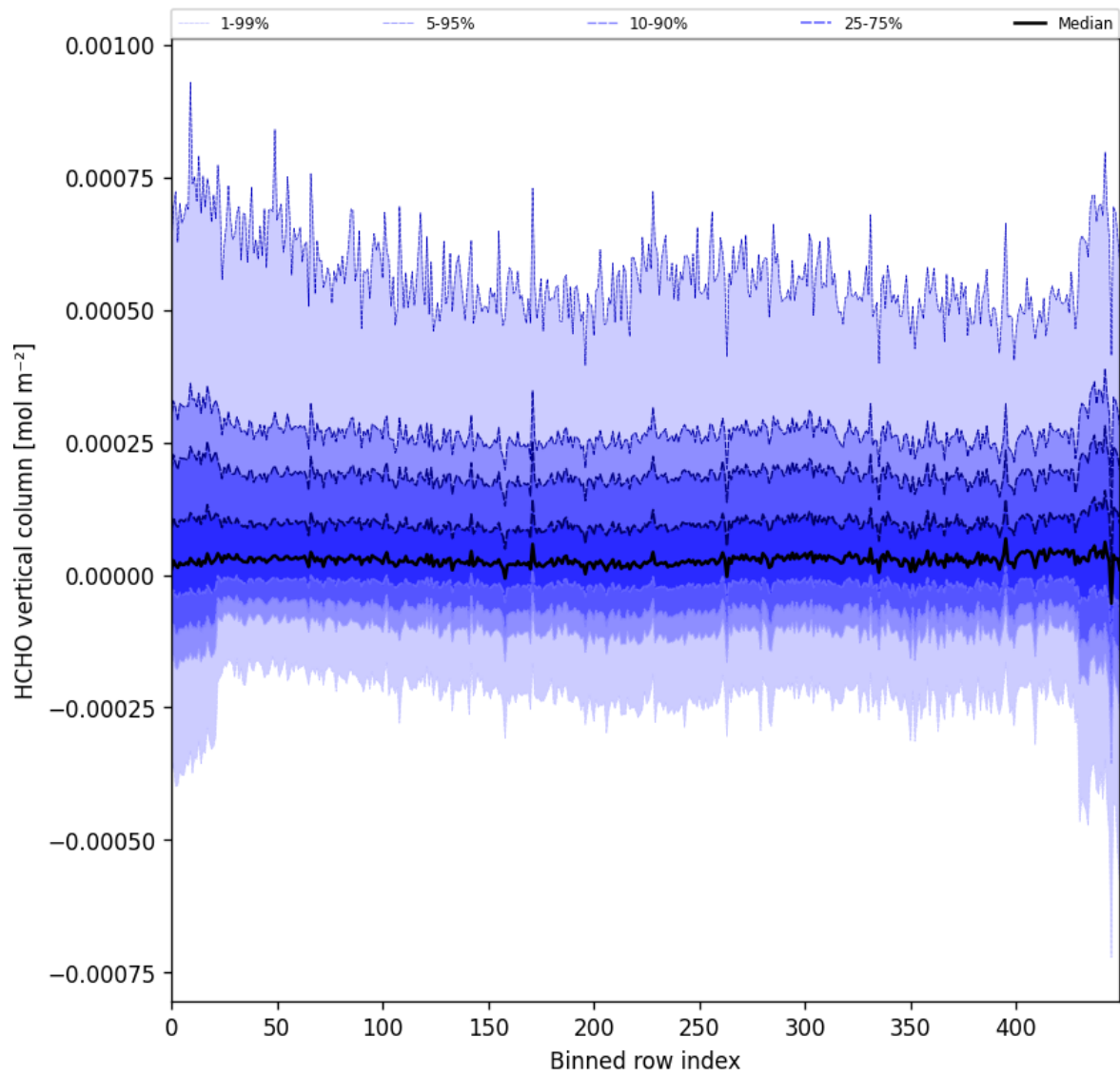
Figure 49: Along track statistics of “HCHO vertical column” for 2024-11-15 to 2024-11-17
