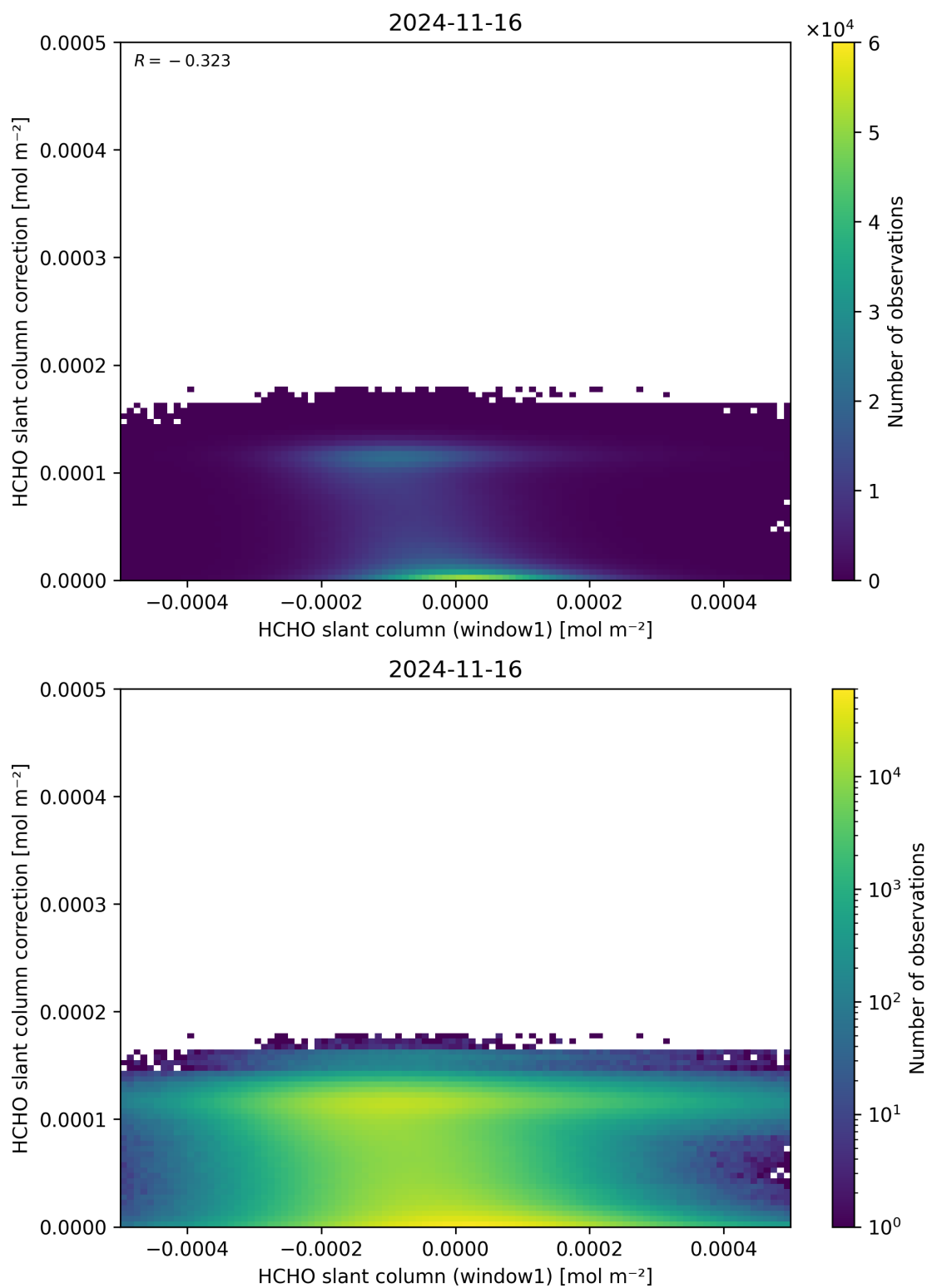
Figure 83: Scatter density plot of “HCHO slant column (window1)” against “HCHO slant column correction” for 2024-11-15 to 2024-11-17.
