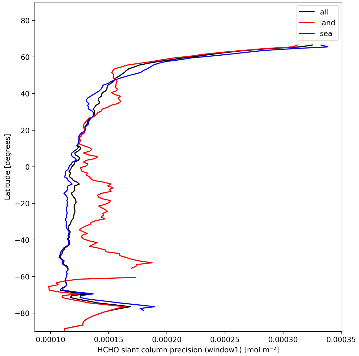
Figure 25: Zonal average of “HCHO slant column precision (window1)” for 2024-11-15 to 2024-11-17.
