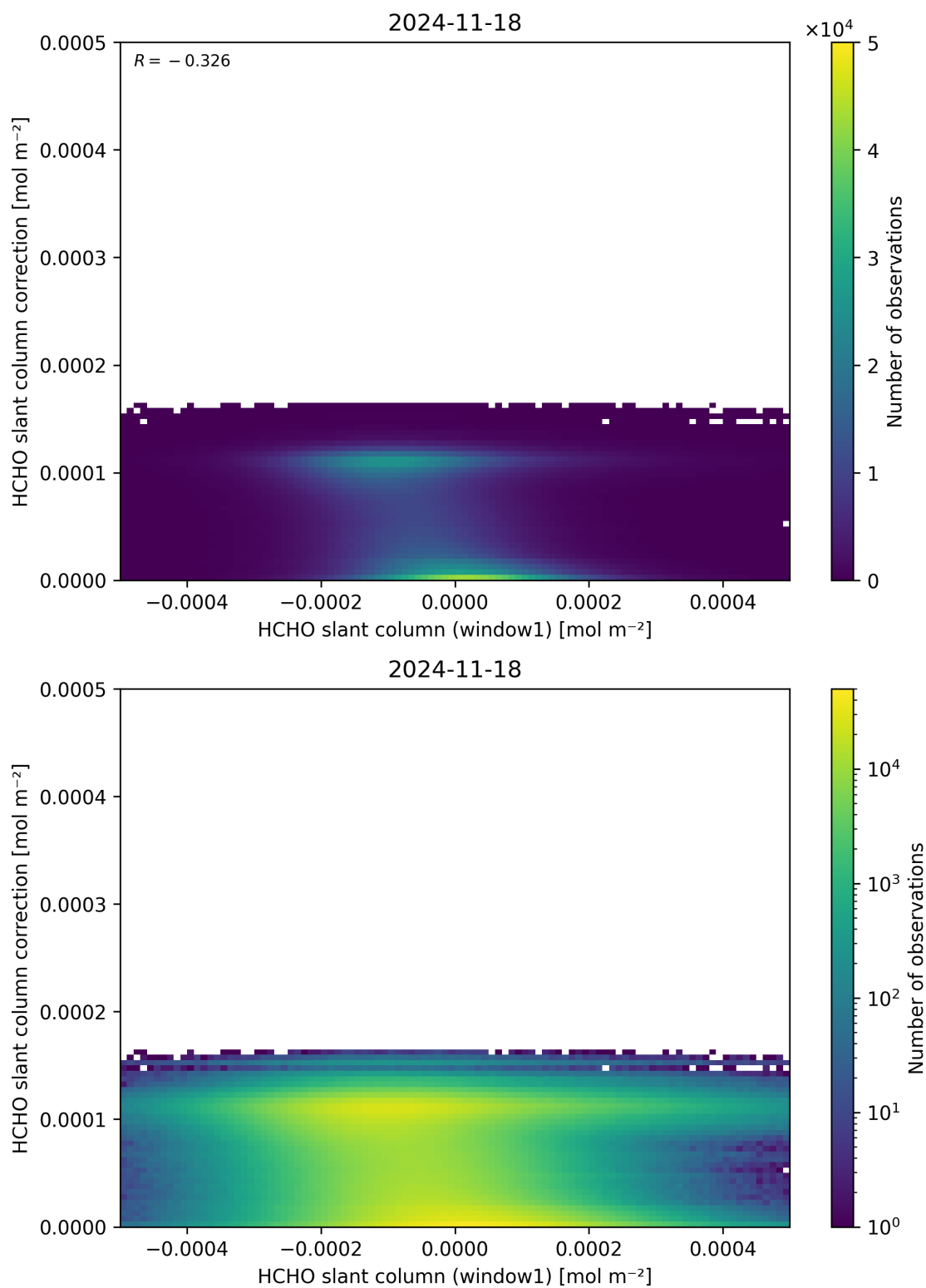
Figure 83: Scatter density plot of “HCHO slant column (window1)” against “HCHO slant column correction” for 2024-11-17 to 2024-11-19.
