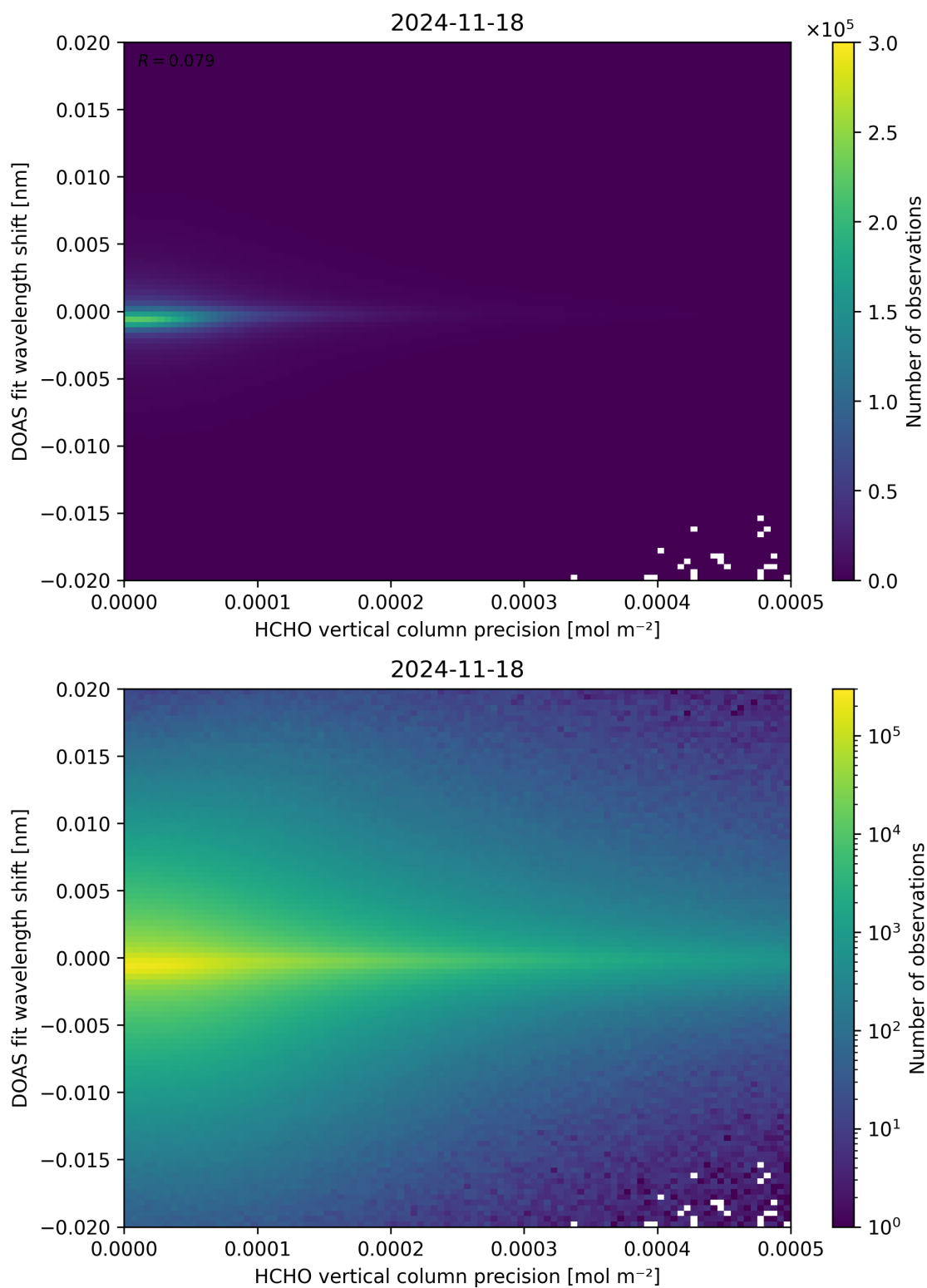
Figure 137: Scatter density plot of “HCHO vertical column precision” against “DOAS fit wavelength shift” for 2024-11-17 to 2024-11-19.
