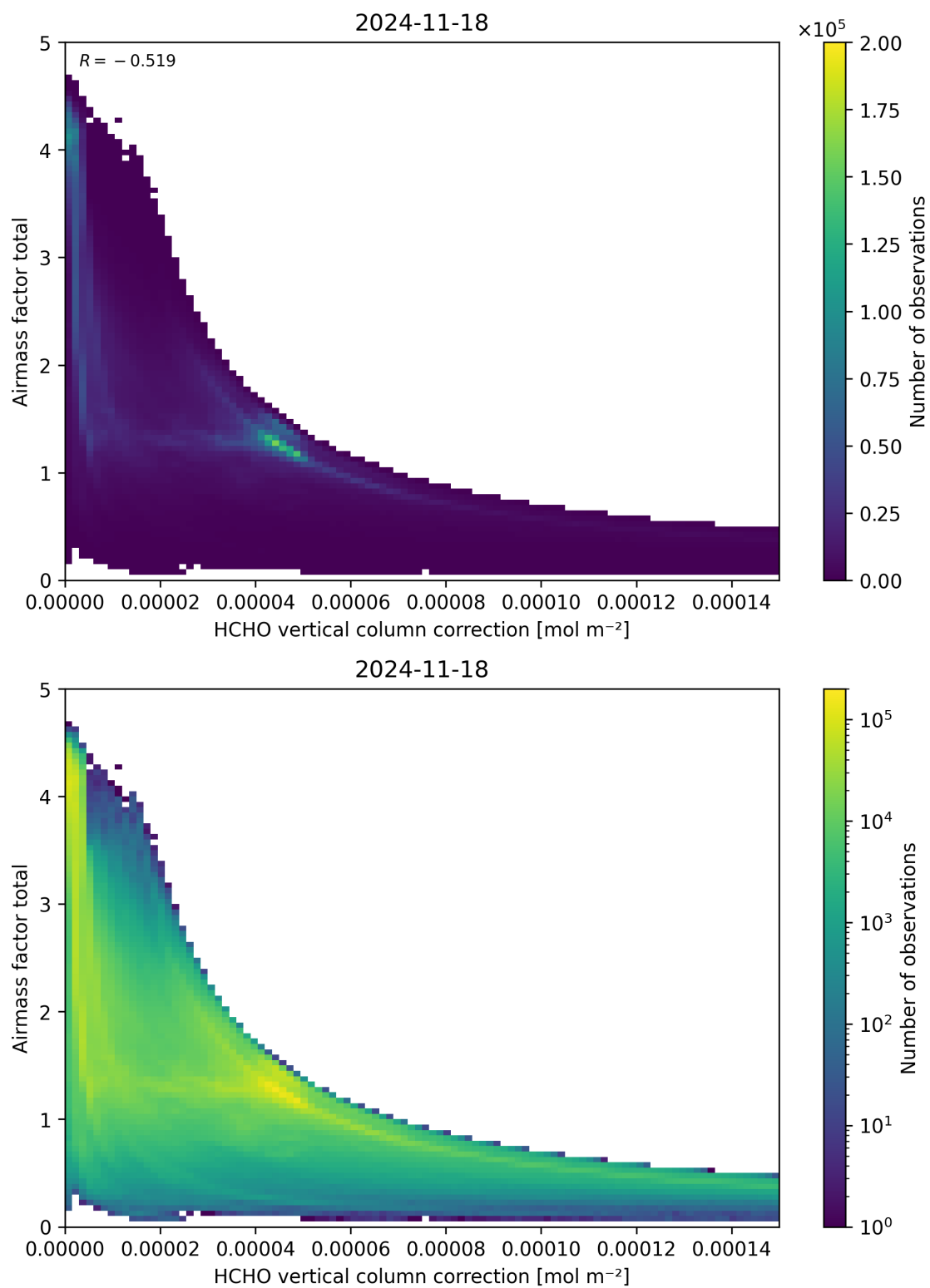
Figure 120: Scatter density plot of “HCHO vertical column correction” against “Airmass factor total” for 2024-11-17 to 2024-11-19.
