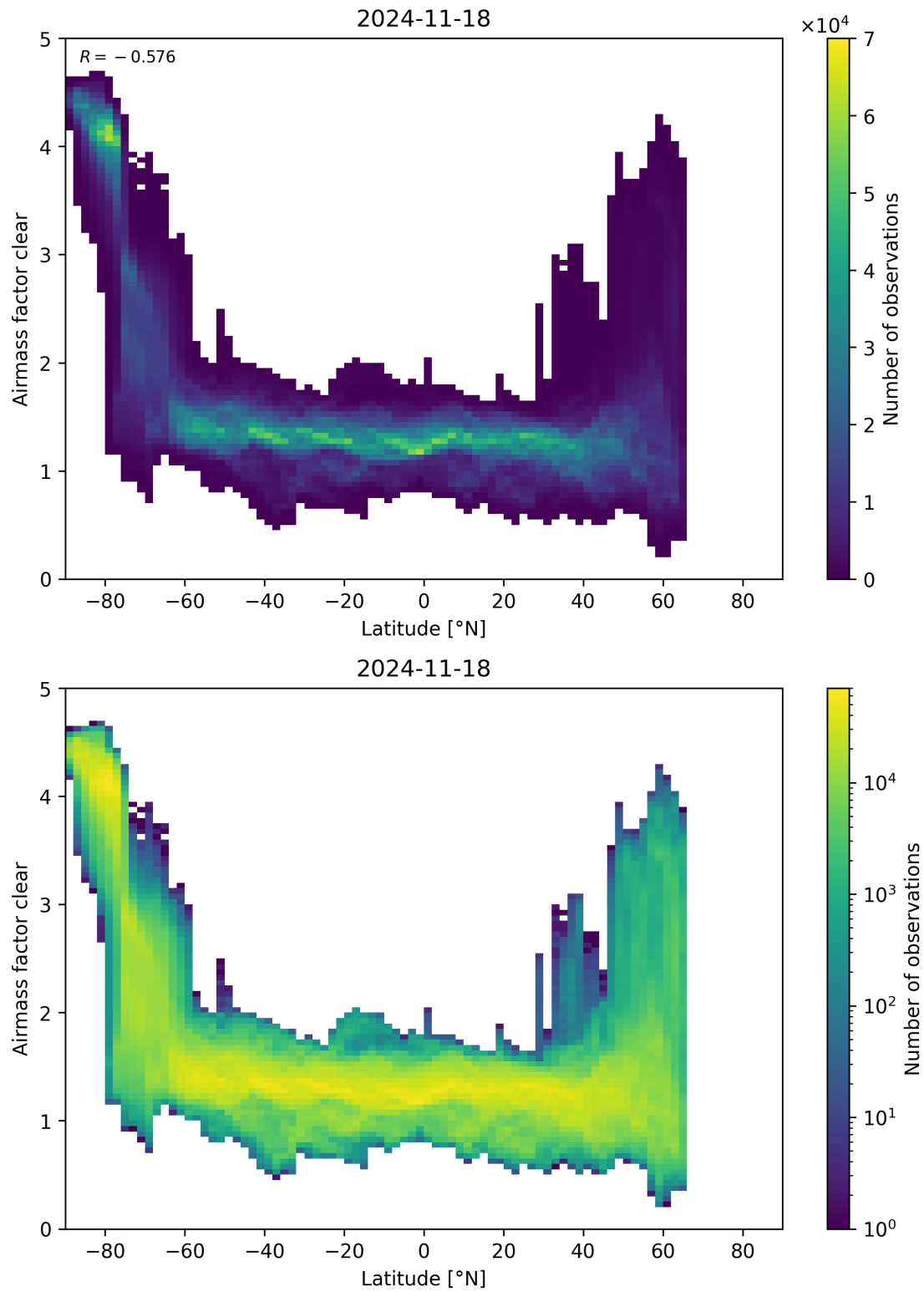
Figure 156: Scatter density plot of “Latitude” against “Airmass factor clear” for 2024-11-17 to 2024-11-19.
