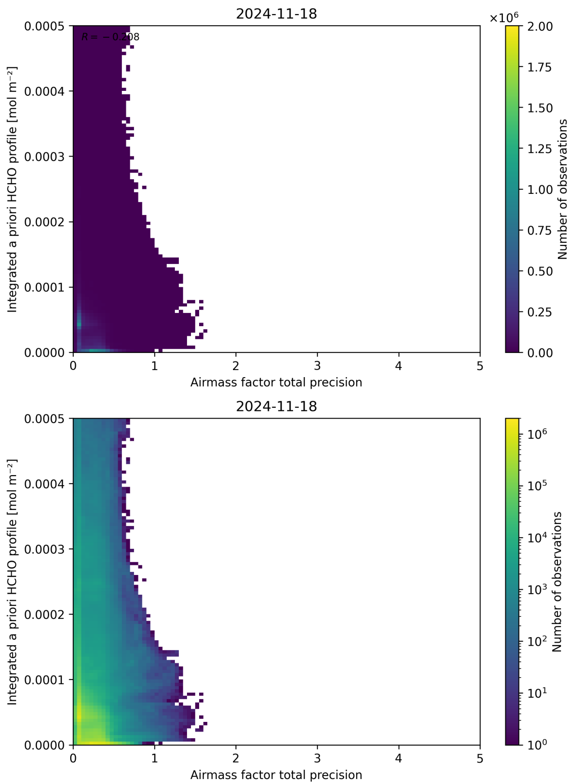
Figure 111: Scatter density plot of “Airmass factor total precision” against “Integrated a priori HCHO profile” for 2024-11-17 to 2024-11-19.
