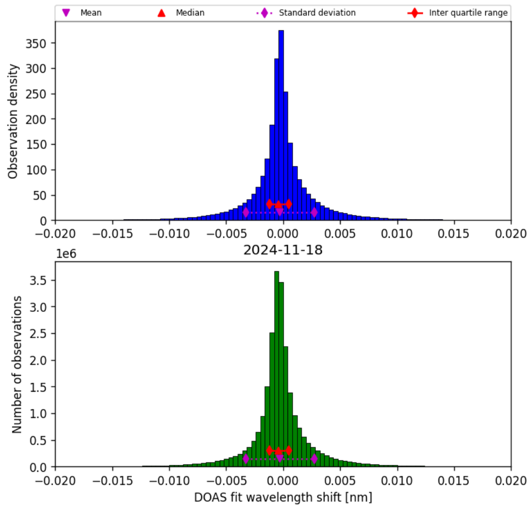
Figure 44: Histogram of “DOAS fit wavelength shift” for 2024-11-17 to 2024-11-19
