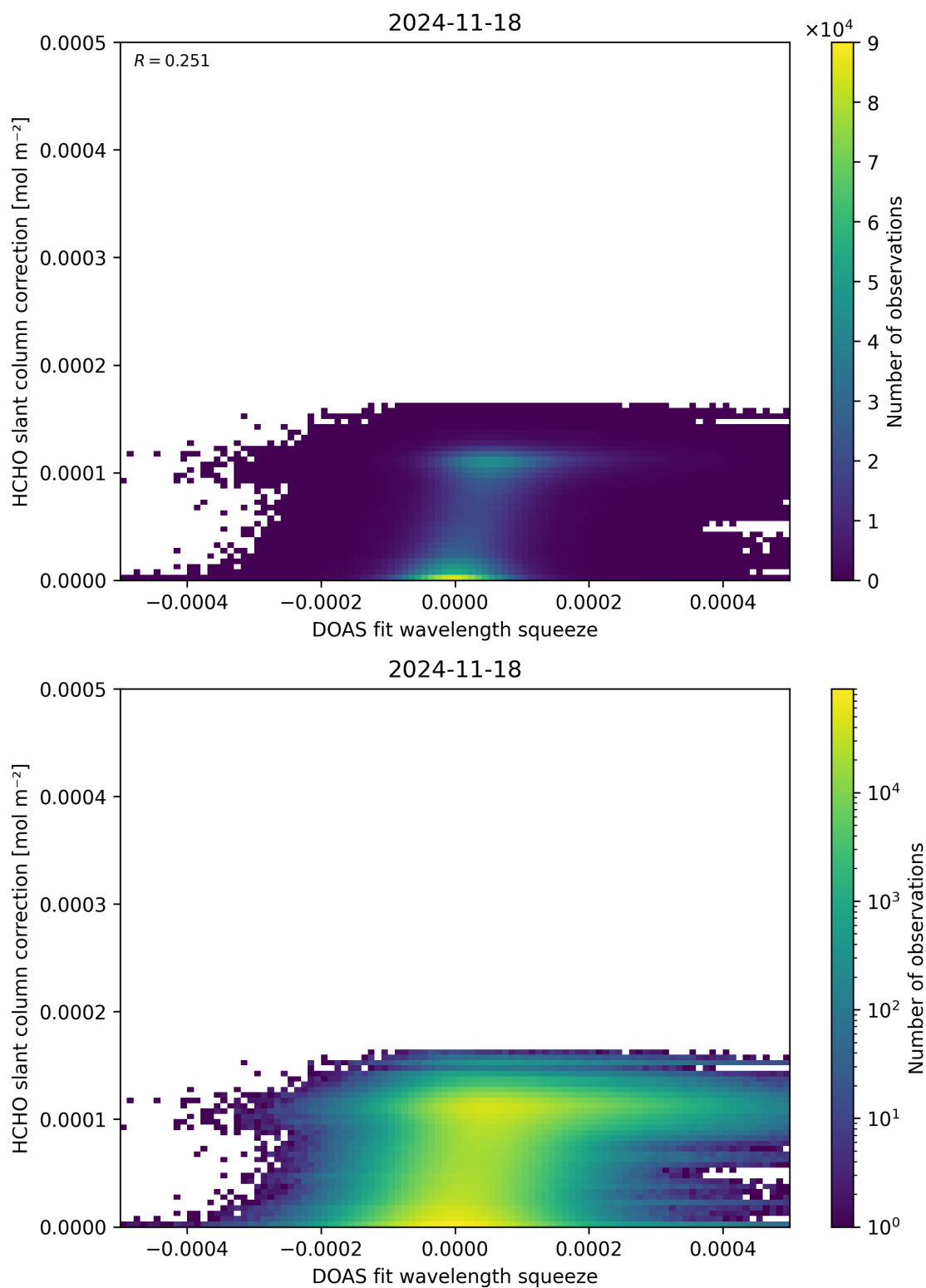
Figure 70: Scatter density plot of “DOAS fit wavelength squeeze” against “HCHO slant column correction” for 2024-11-17 to 2024-11-19.
