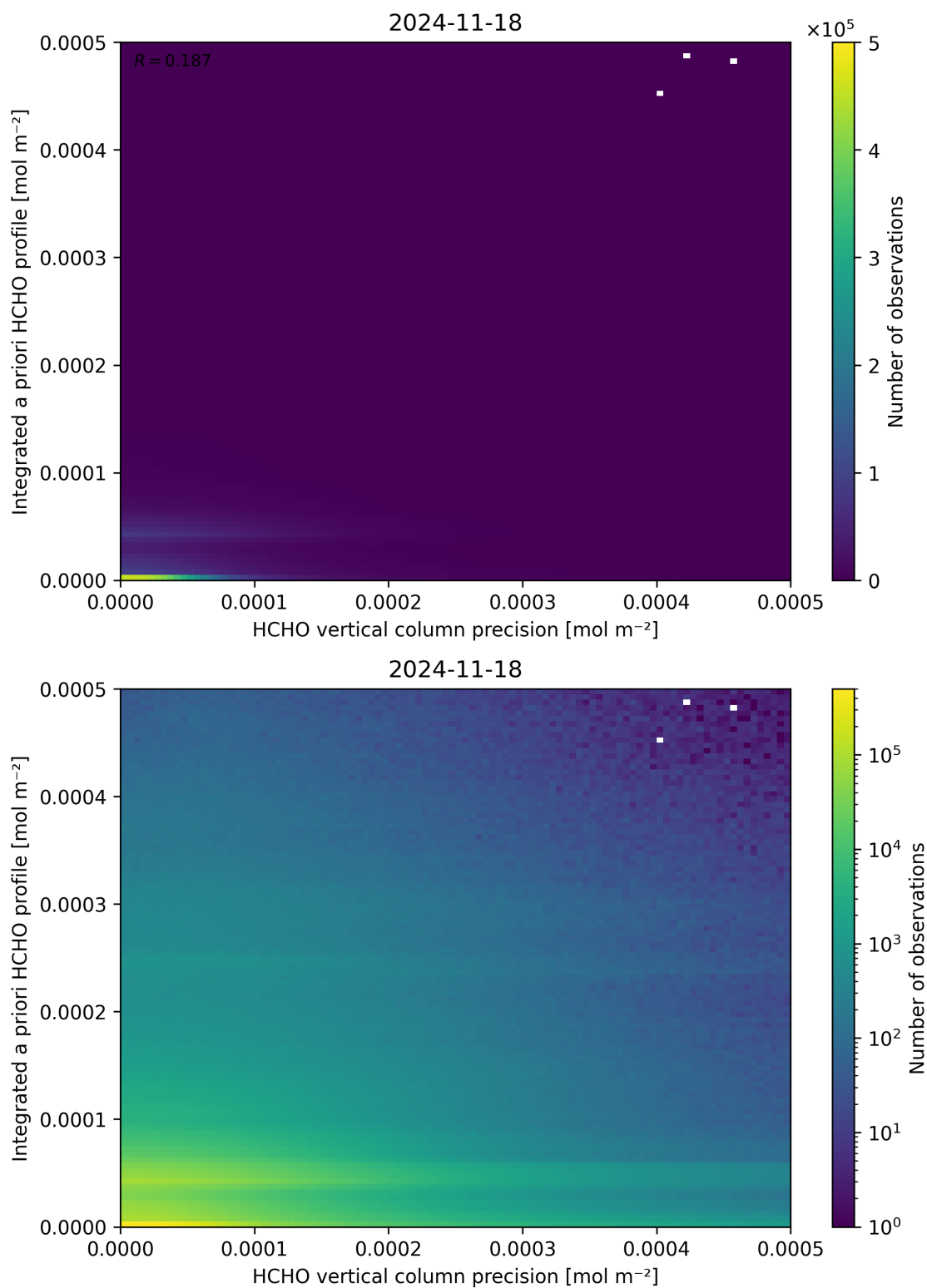
Figure 147: Scatter density plot of “HCHO vertical column precision” against “Integrated a priori HCHO profile” for 2024-11-17 to 2024-11-19.
