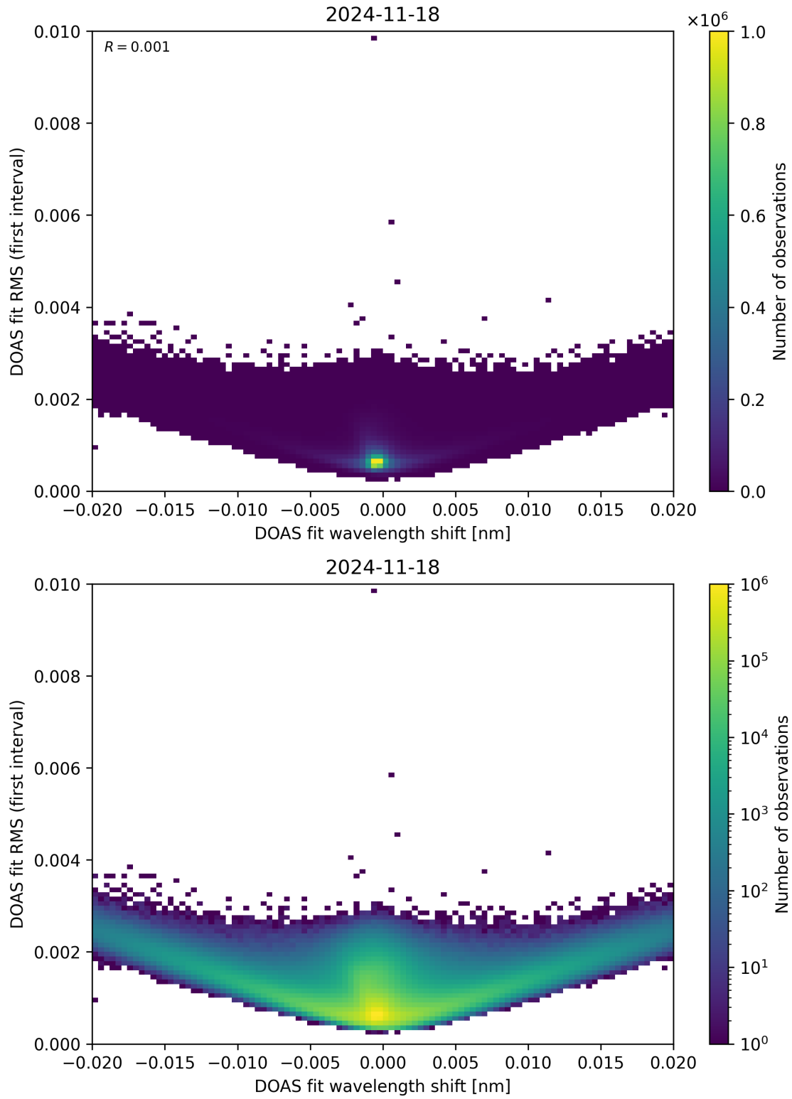
Figure 64: Scatter density plot of “DOAS fit wavelength shift” against “DOAS fit RMS (first interval)” for 2024-11-17 to 2024-11-19.
