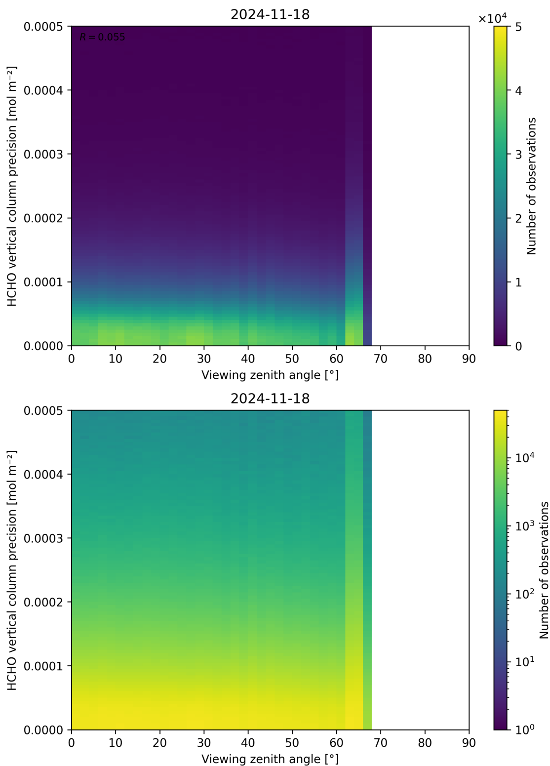
Figure 194: Scatter density plot of “Viewing zenith angle” against “HCHO vertical column precision” for 2024-11-17 to 2024-11-19.
