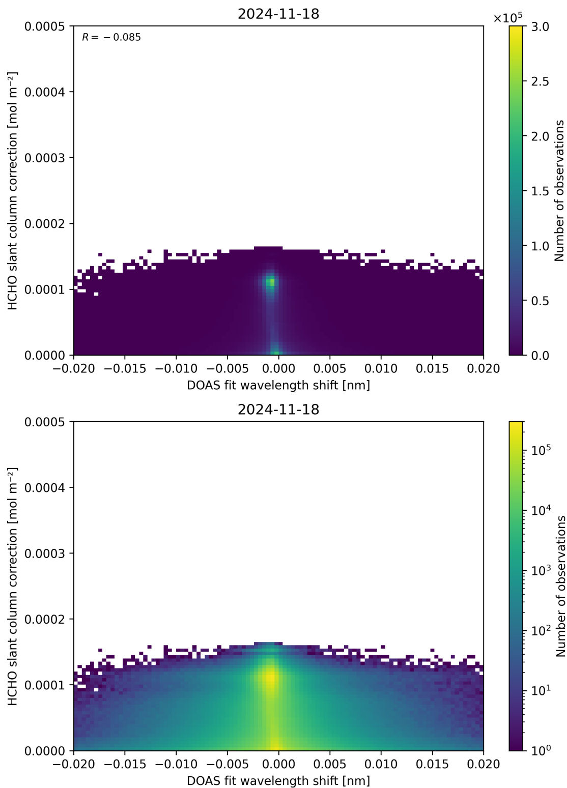
Figure 67: Scatter density plot of “DOAS fit wavelength shift” against “HCHO slant column correction” for 2024-11-17 to 2024-11-19.
