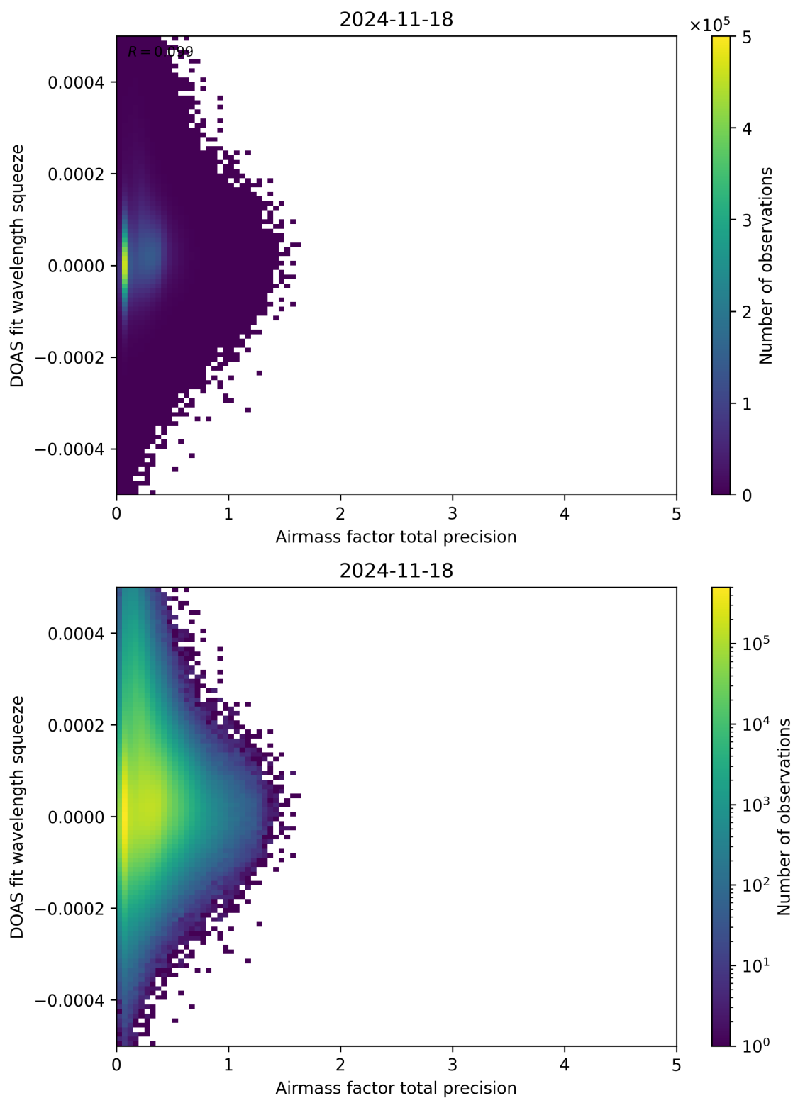
Figure 107: Scatter density plot of “Airmass factor total precision” against “DOAS fit wavelength squeeze” for 2024-11-17 to 2024-11-19.
