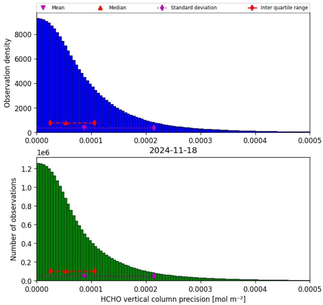
Figure 36: Histogram of “HCHO vertical column precision” for 2024-11-17 to 2024-11-19
