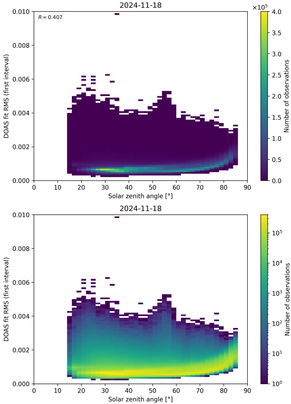
Figure 167: Scatter density plot of “Solar zenith angle” against “DOAS fit RMS (first interval)” for 2024-11-17 to 2024-11-19.
