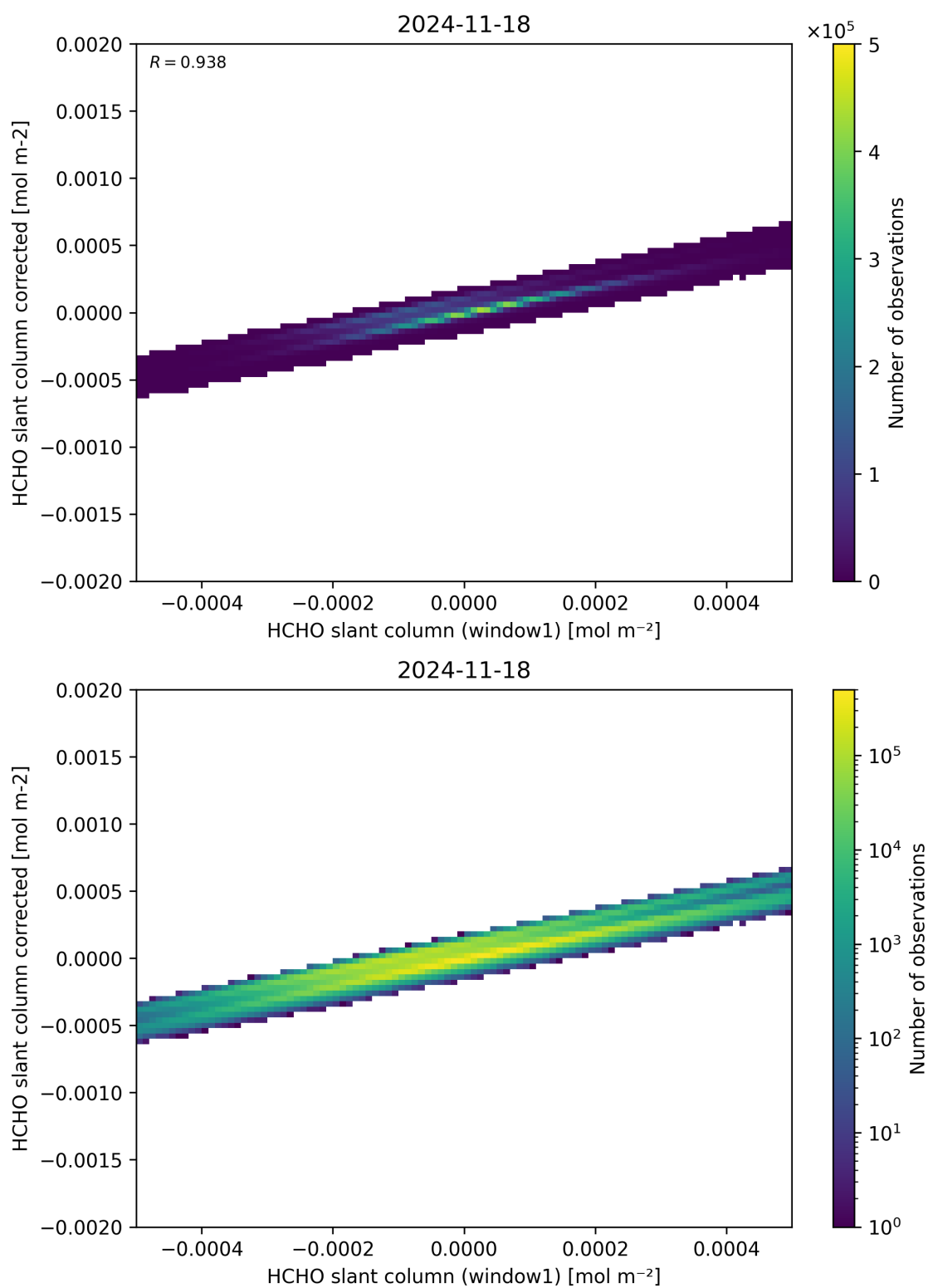
Figure 82: Scatter density plot of “HCHO slant column (window1)” against “HCHO slant column corrected” for 2024-11-17 to 2024-11-19.
