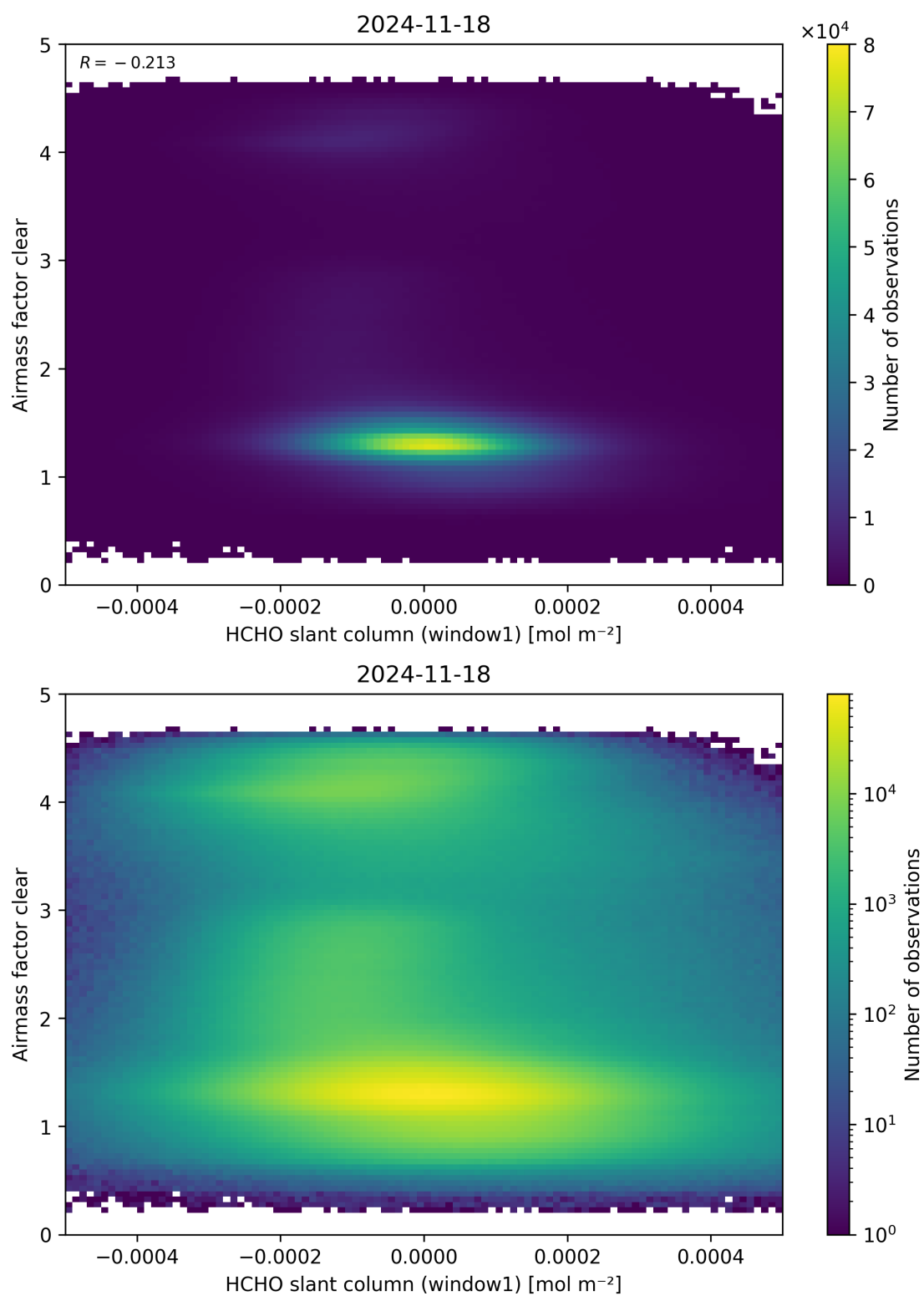
Figure 81: Scatter density plot of “HCHO slant column (window1)” against “Airmass factor clear” for 2024-11-17 to 2024-11-19.
