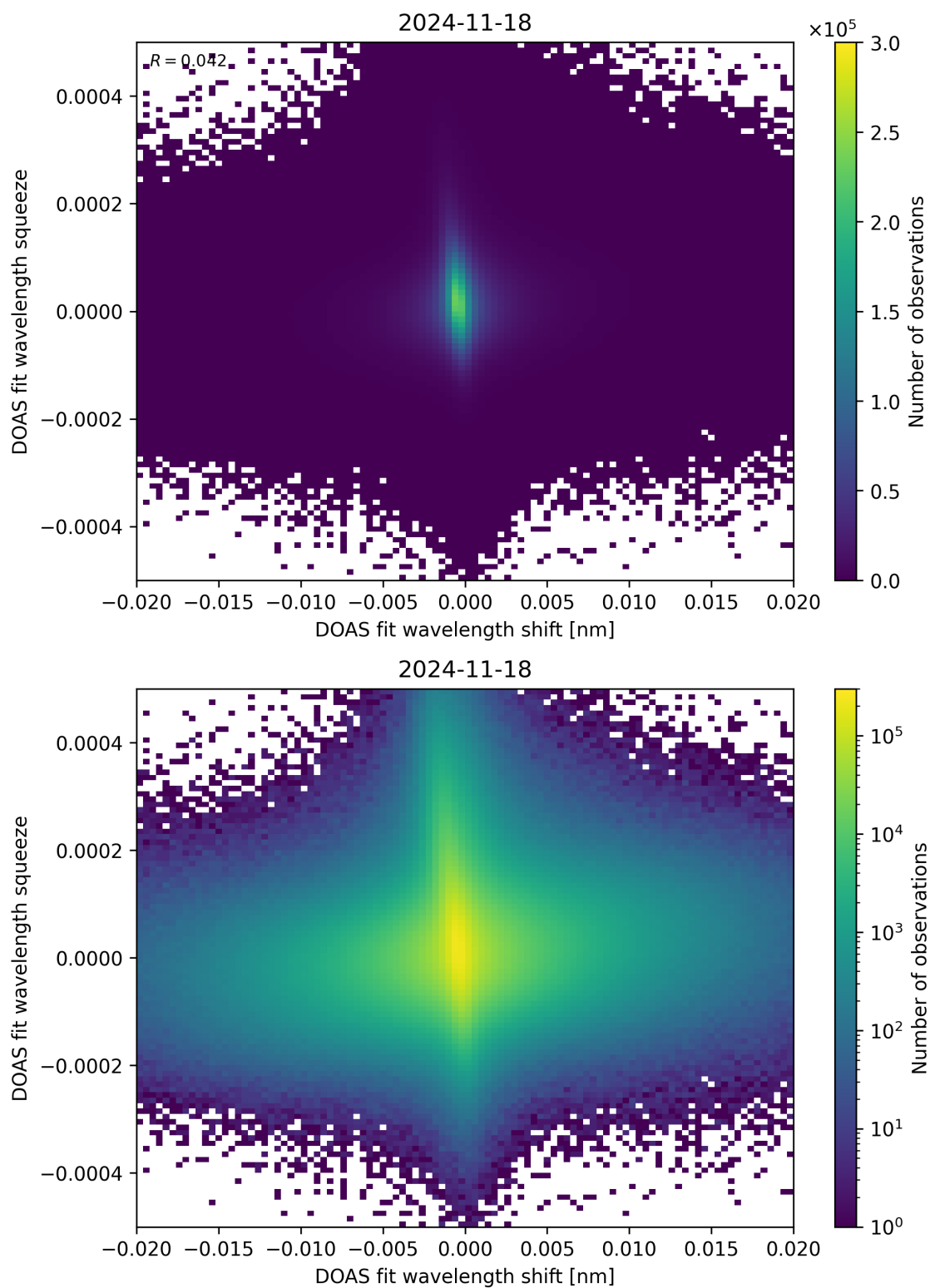
Figure 65: Scatter density plot of “DOAS fit wavelength shift” against “DOAS fit wavelength squeeze” for 2024-11-17 to 2024-11-19.
