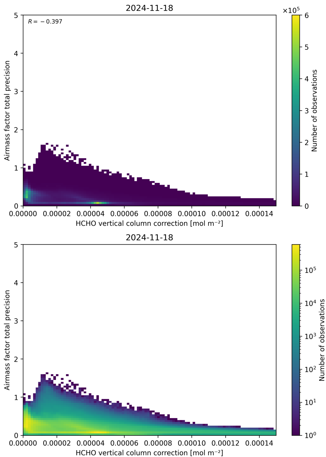
Figure 121: Scatter density plot of “HCHO vertical column correction” against “Airmass factor total precision” for 2024-11-17 to 2024-11-19.
