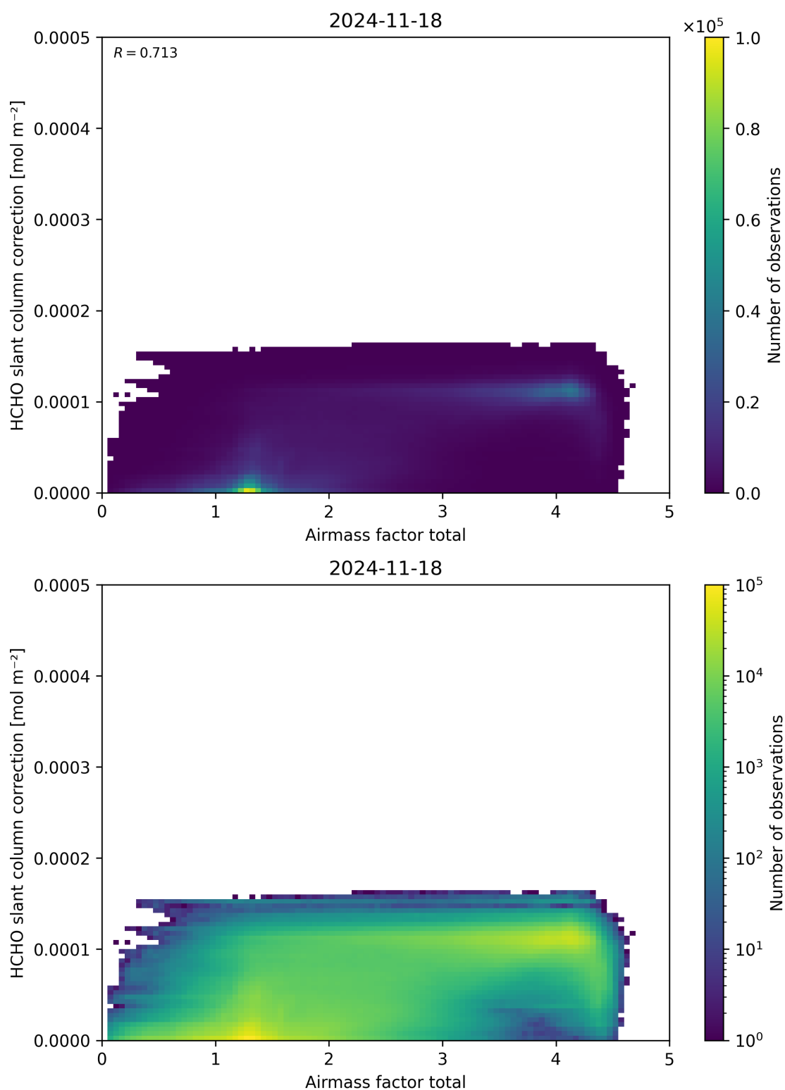
Figure 102: Scatter density plot of “Airmass factor total” against “HCHO slant column correction” for 2024-11-17 to 2024-11-19.
