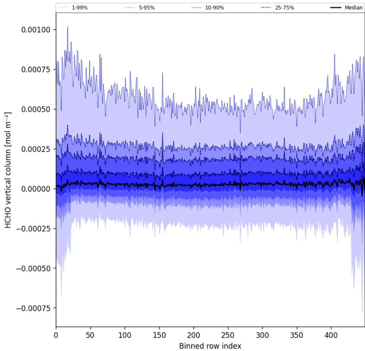
Figure 49: Along track statistics of “HCHO vertical column” for 2024-11-17 to 2024-11-19
