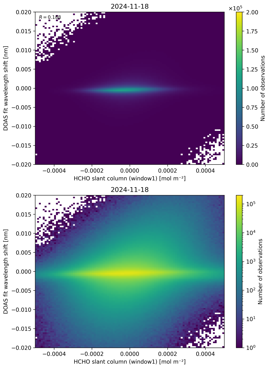
Figure 79: Scatter density plot of “HCHO slant column (window1)” against “DOAS fit wavelength shift” for 2024-11-17 to 2024-11-19.
