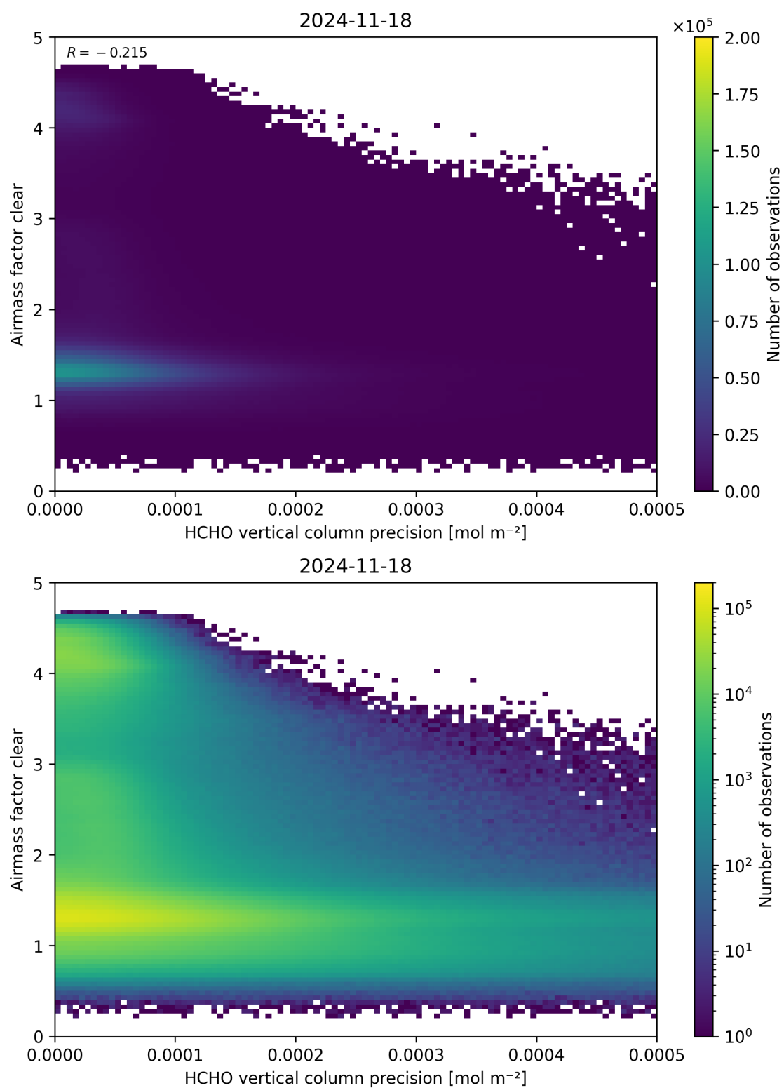
Figure 139: Scatter density plot of “HCHO vertical column precision” against “Airmass factor clear” for 2024-11-17 to 2024-11-19.
