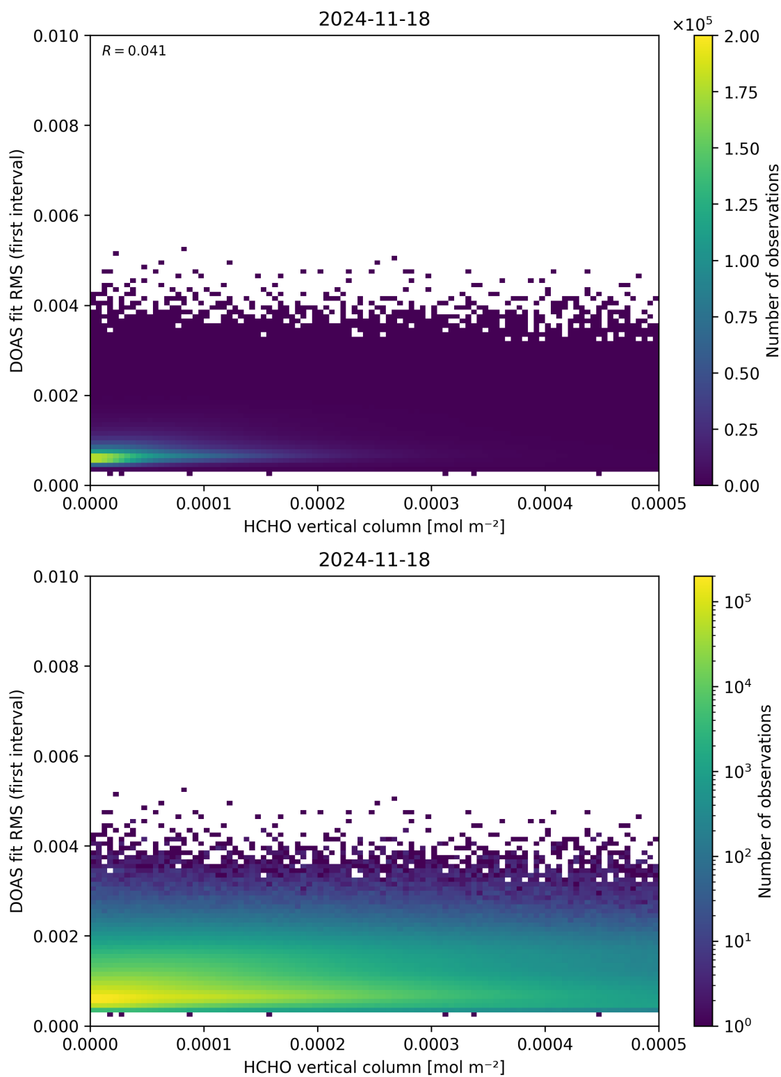
Figure 123: Scatter density plot of “HCHO vertical column” against “DOAS fit RMS (first interval)” for 2024-11-17 to 2024-11-19.
