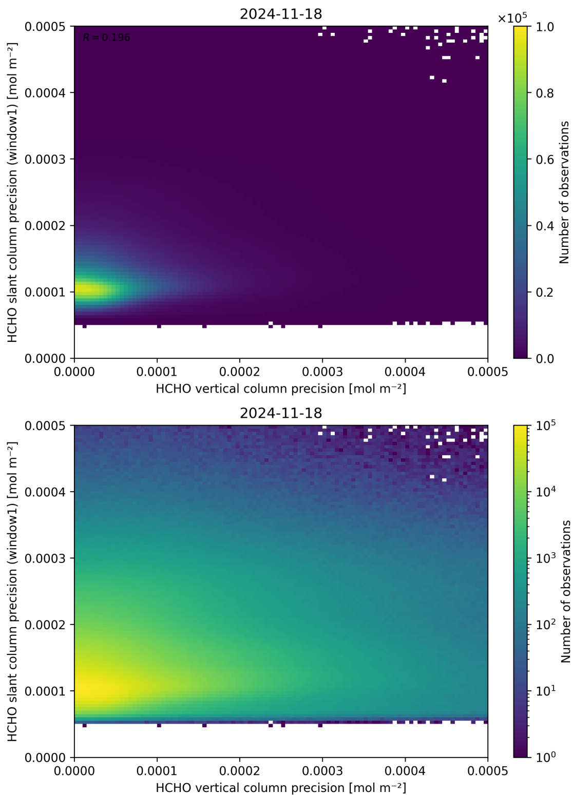
Figure 143: Scatter density plot of “HCHO vertical column precision” against “HCHO slant column precision (window1)” for 2024-11-17 to 2024-11-19.
