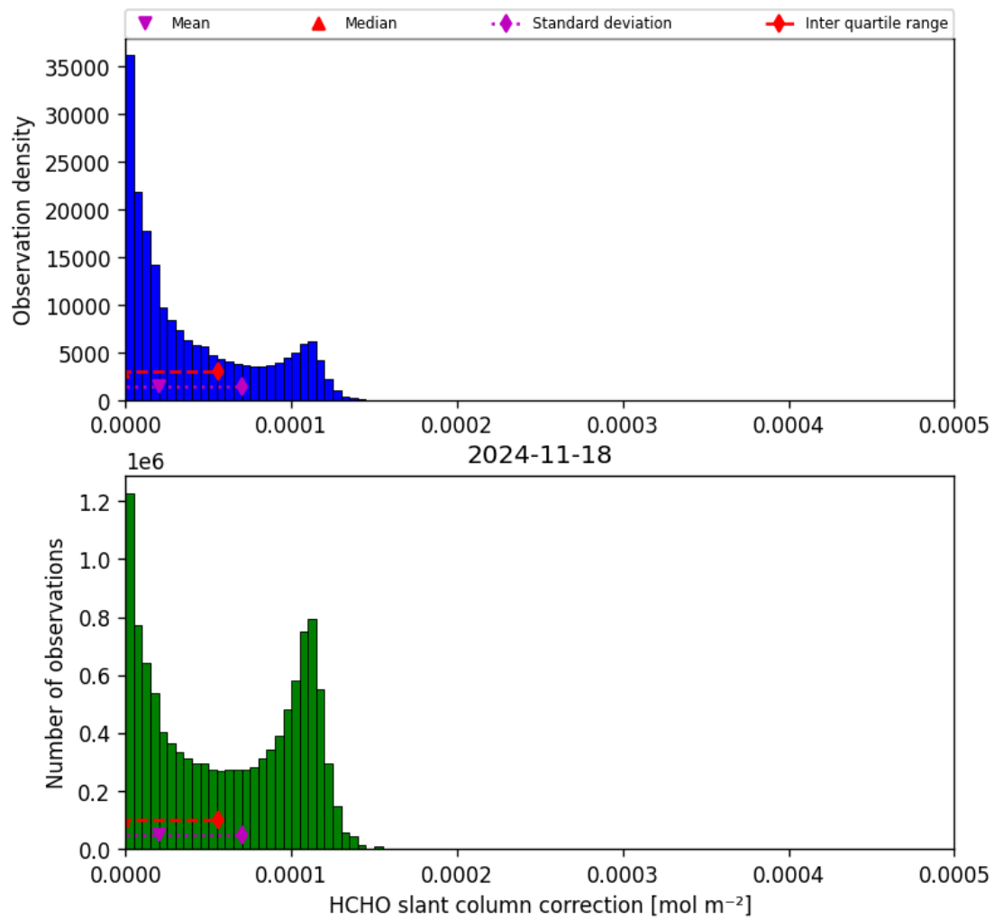
Figure 47: Histogram of “HCHO slant column correction” for 2024-11-17 to 2024-11-19
