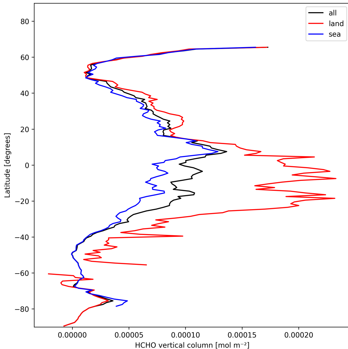
Figure 21: Zonal average of “HCHO vertical column” for 2024-11-17 to 2024-11-19.
