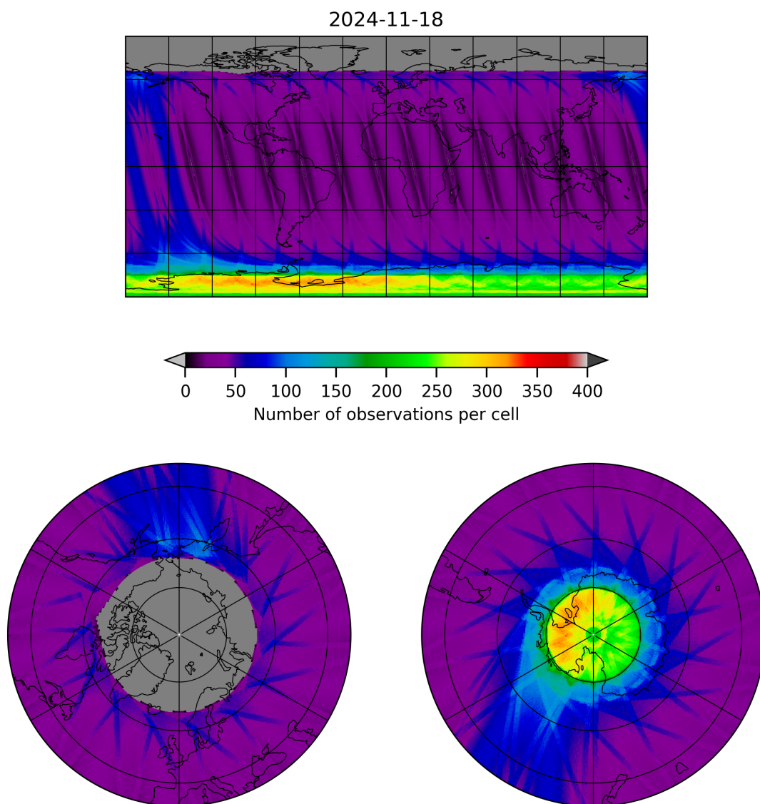
Figure 19: Map of the number of observations for 2024-11-17 to 2024-11-19
