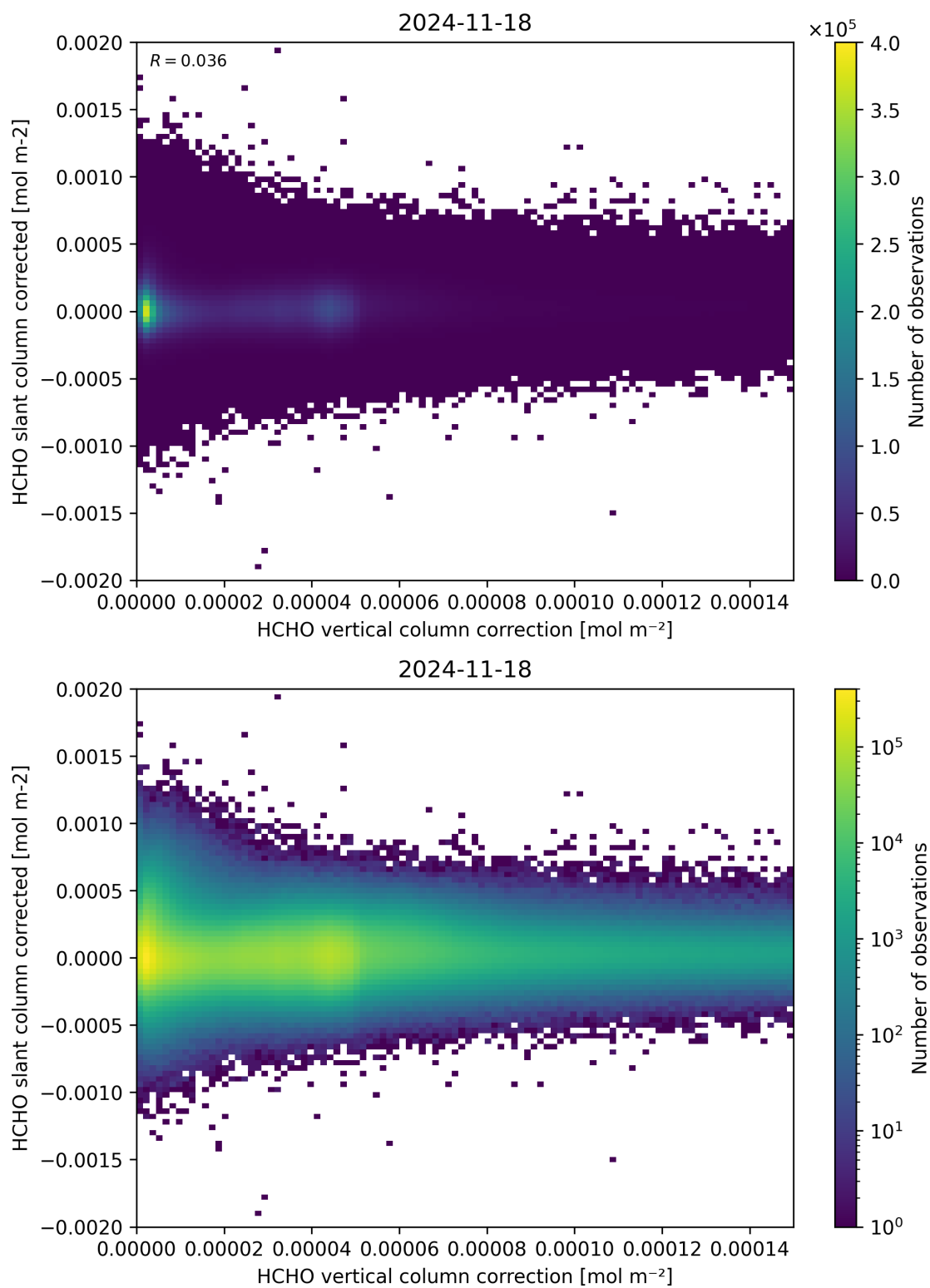
Figure 116: Scatter density plot of “HCHO vertical column correction” against “HCHO slant column corrected” for 2024-11-17 to 2024-11-19.
