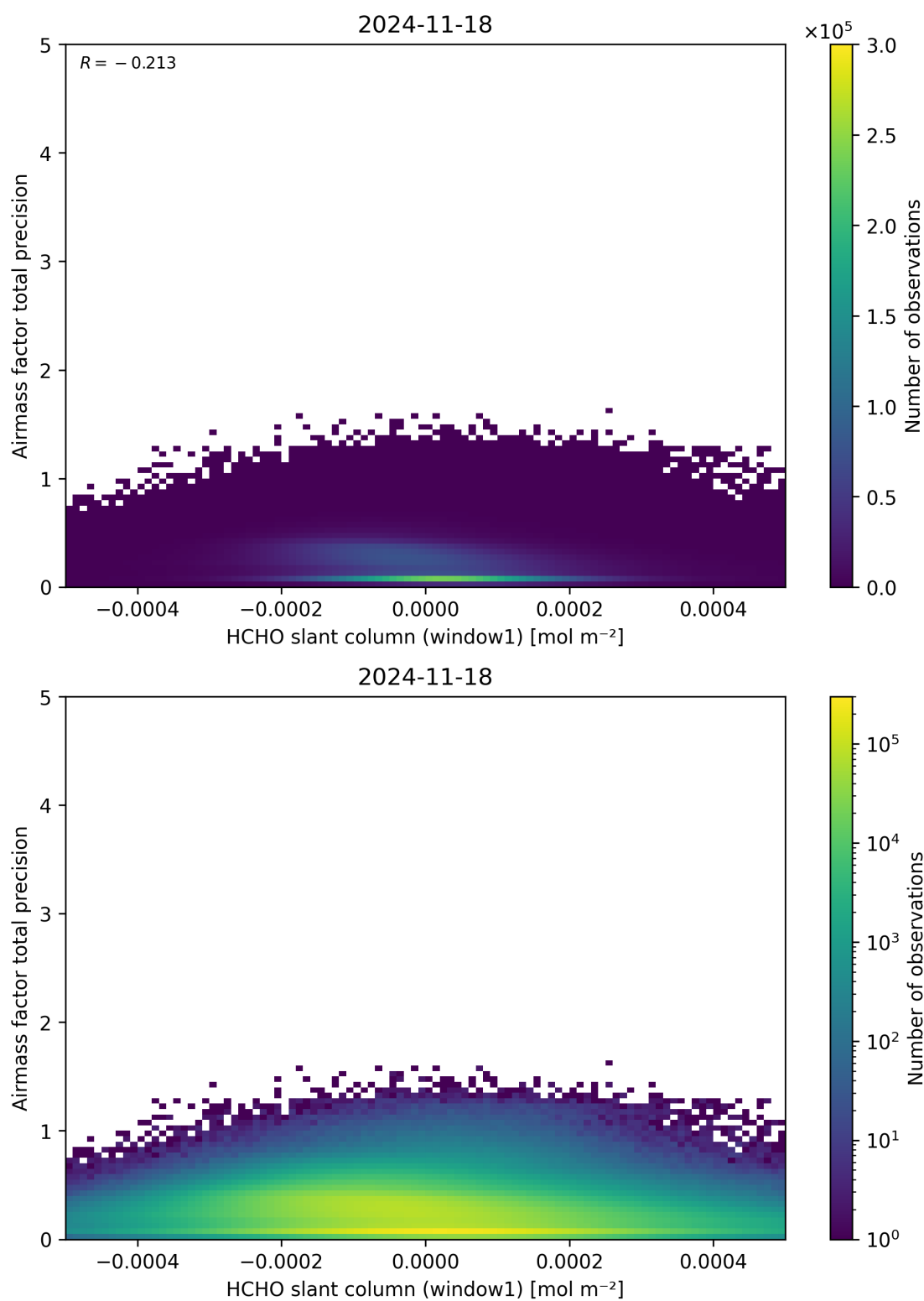
Figure 86: Scatter density plot of “HCHO slant column (window1)” against “Airmass factor total precision” for 2024-11-17 to 2024-11-19.
