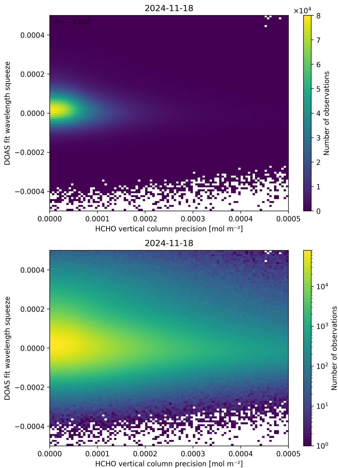
Figure 138: Scatter density plot of “HCHO vertical column precision” against “DOAS fit wavelength squeeze” for 2024-11-17 to 2024-11-19.
