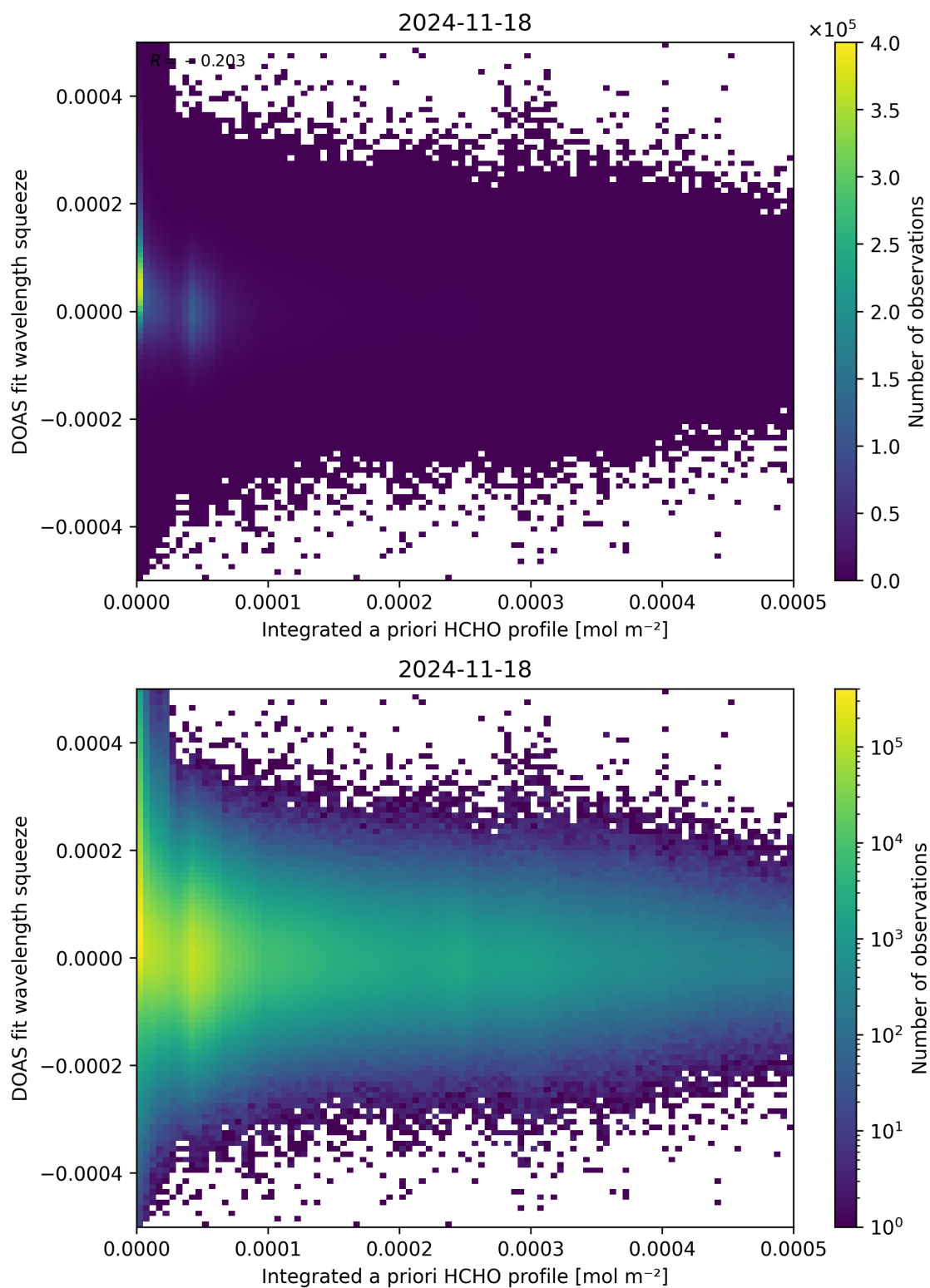
Figure 150: Scatter density plot of “Integrated a priori HCHO profile” against “DOAS fit wavelength squeeze” for 2024-11-17 to 2024-11-19.
