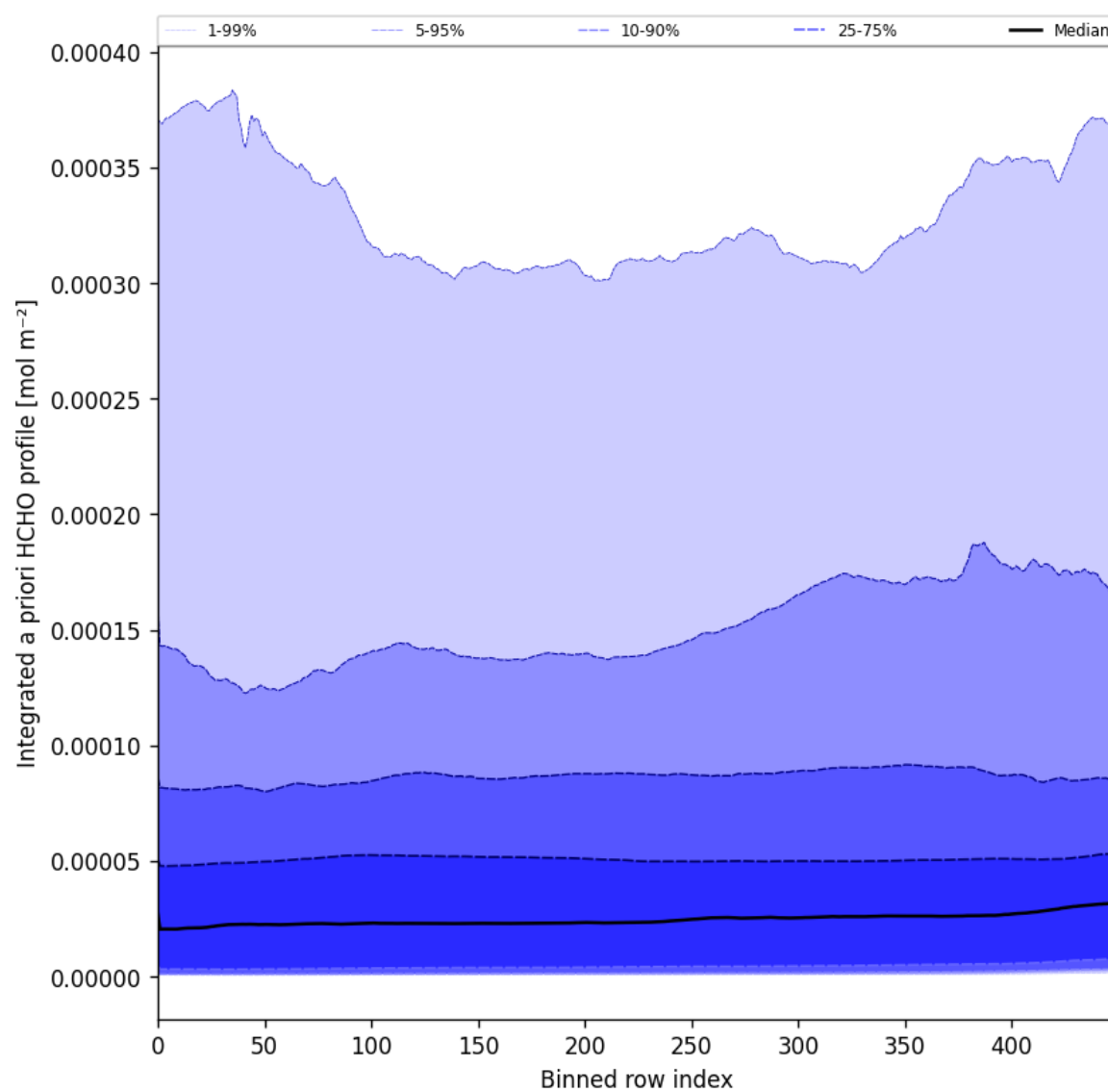
Figure 57: Along track statistics of “Integrated a priori HCHO profile” for 2024-11-17 to 2024-11-19
