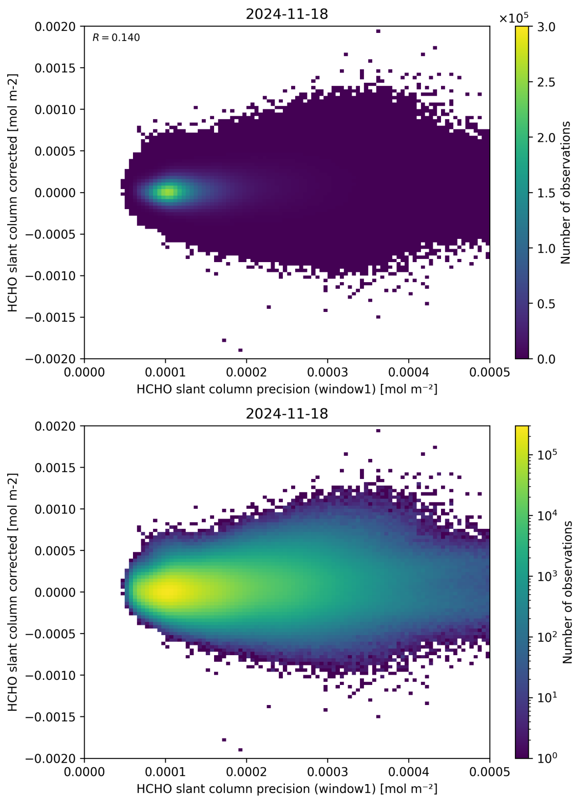
Figure 92: Scatter density plot of “HCHO slant column precision (window1)” against “HCHO slant column corrected” for 2024-11-17 to 2024-11-19.
