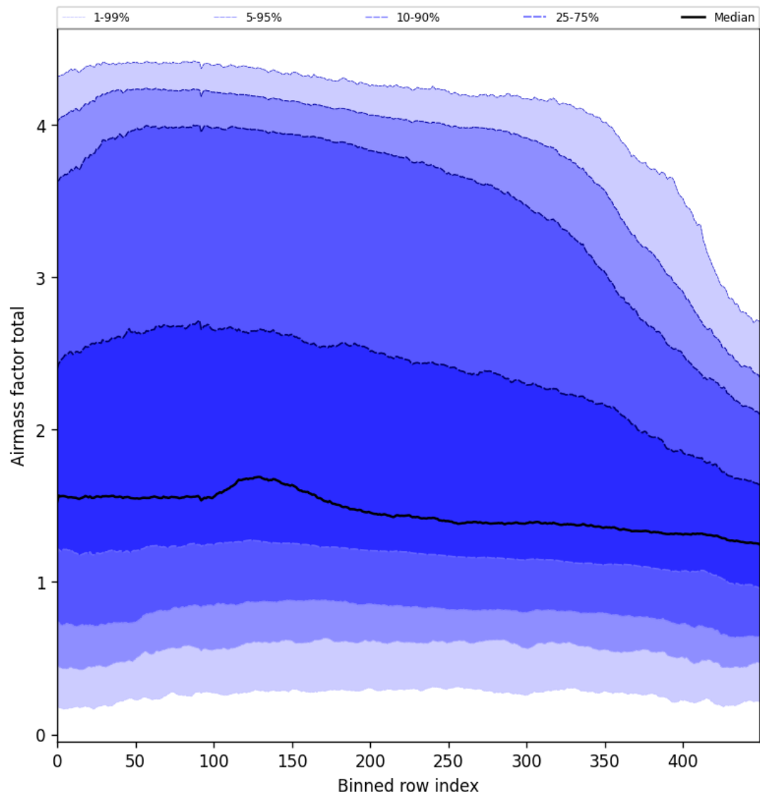
Figure 54: Along track statistics of “Airmass factor total” for 2024-11-17 to 2024-11-19
