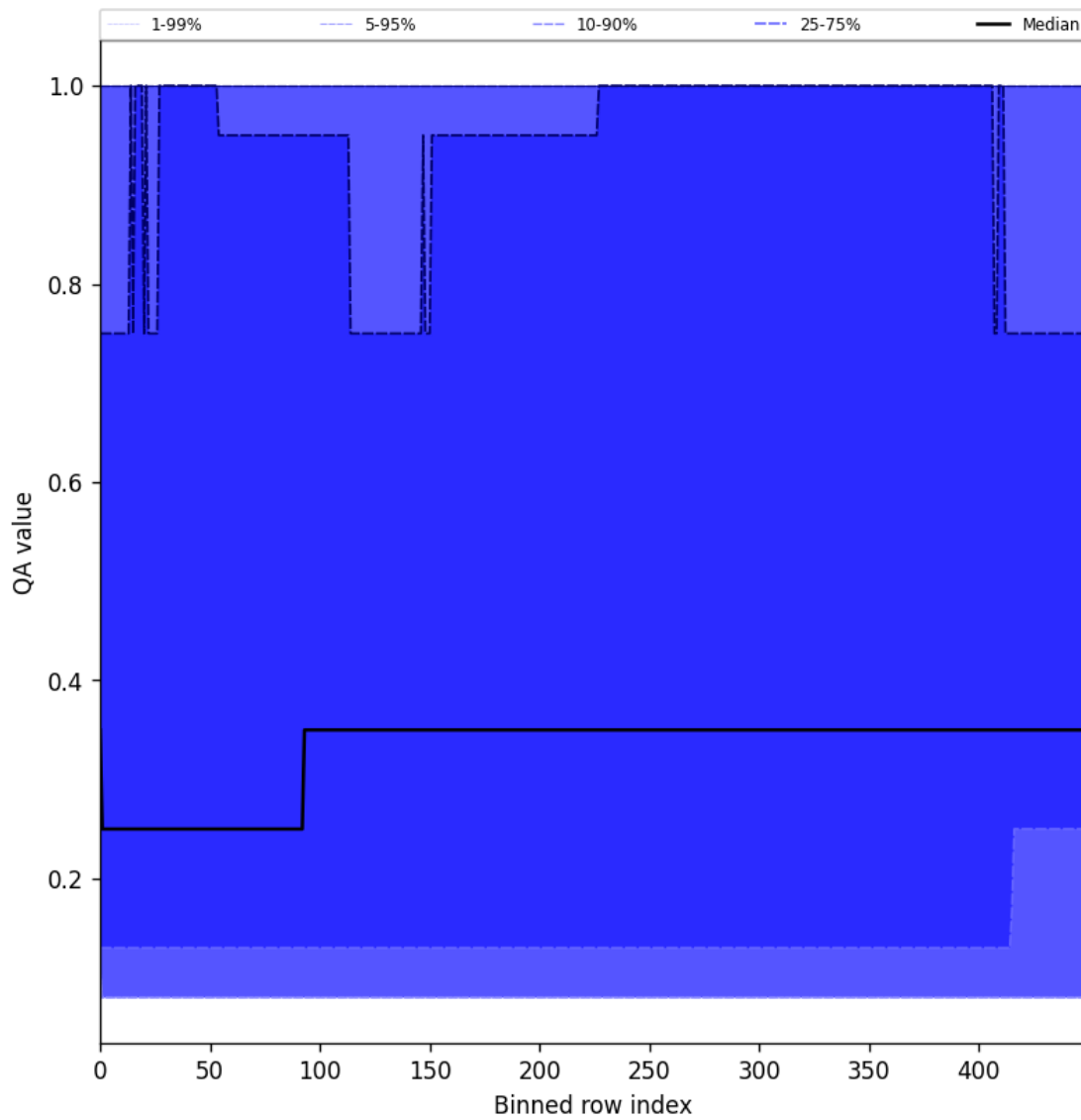
Figure 48: Along track statistics of “QA value” for 2024-11-17 to 2024-11-19
