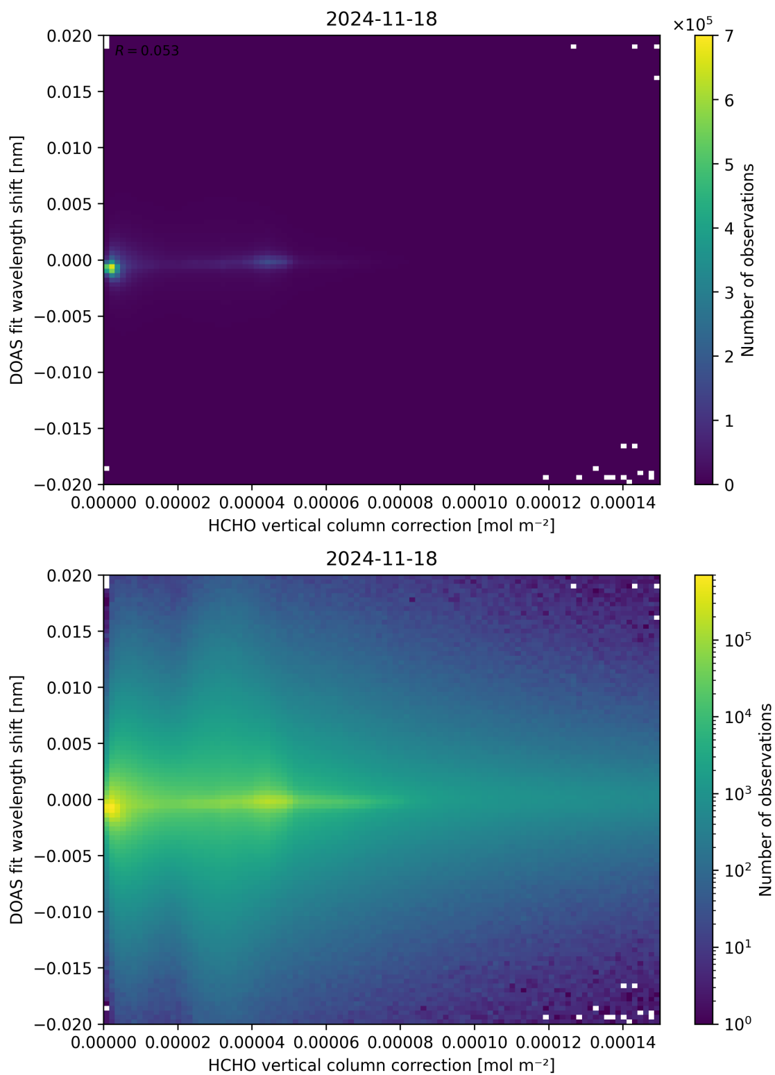
Figure 113: Scatter density plot of “HCHO vertical column correction” against “DOAS fit wavelength shift” for 2024-11-17 to 2024-11-19.
