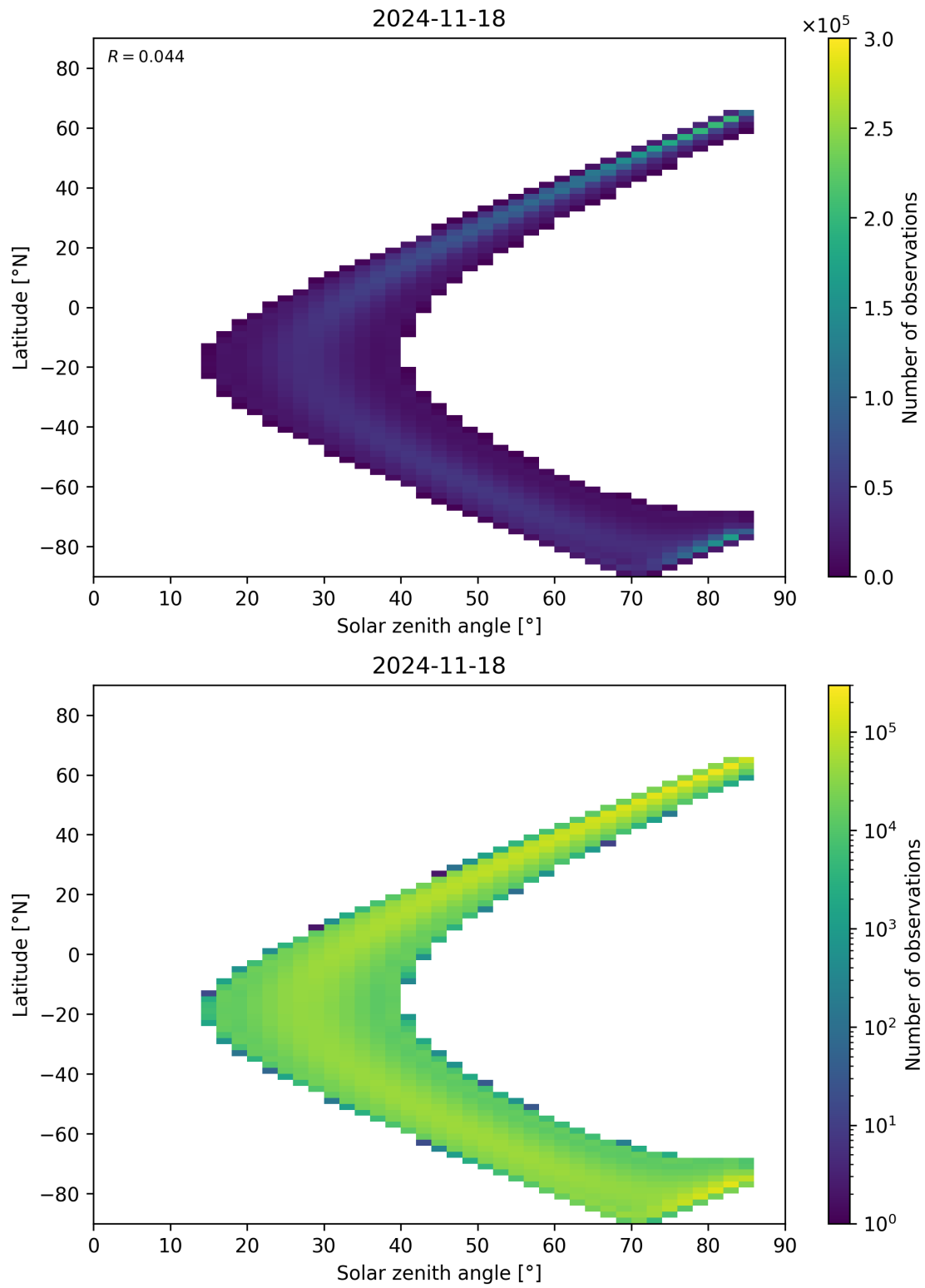
Figure 181: Scatter density plot of “Solar zenith angle” against “Latitude” for 2024-11-17 to 2024-11-19.
