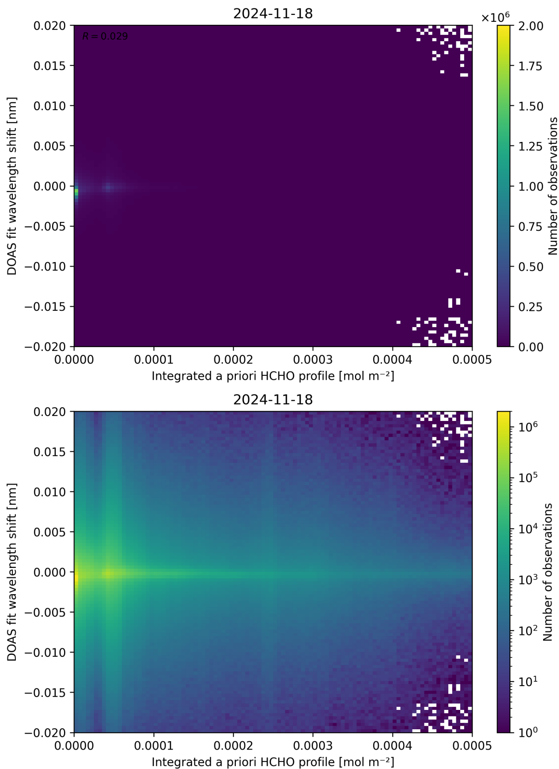
Figure 149: Scatter density plot of “Integrated a priori HCHO profile” against “DOAS fit wavelength shift” for 2024-11-17 to 2024-11-19.
