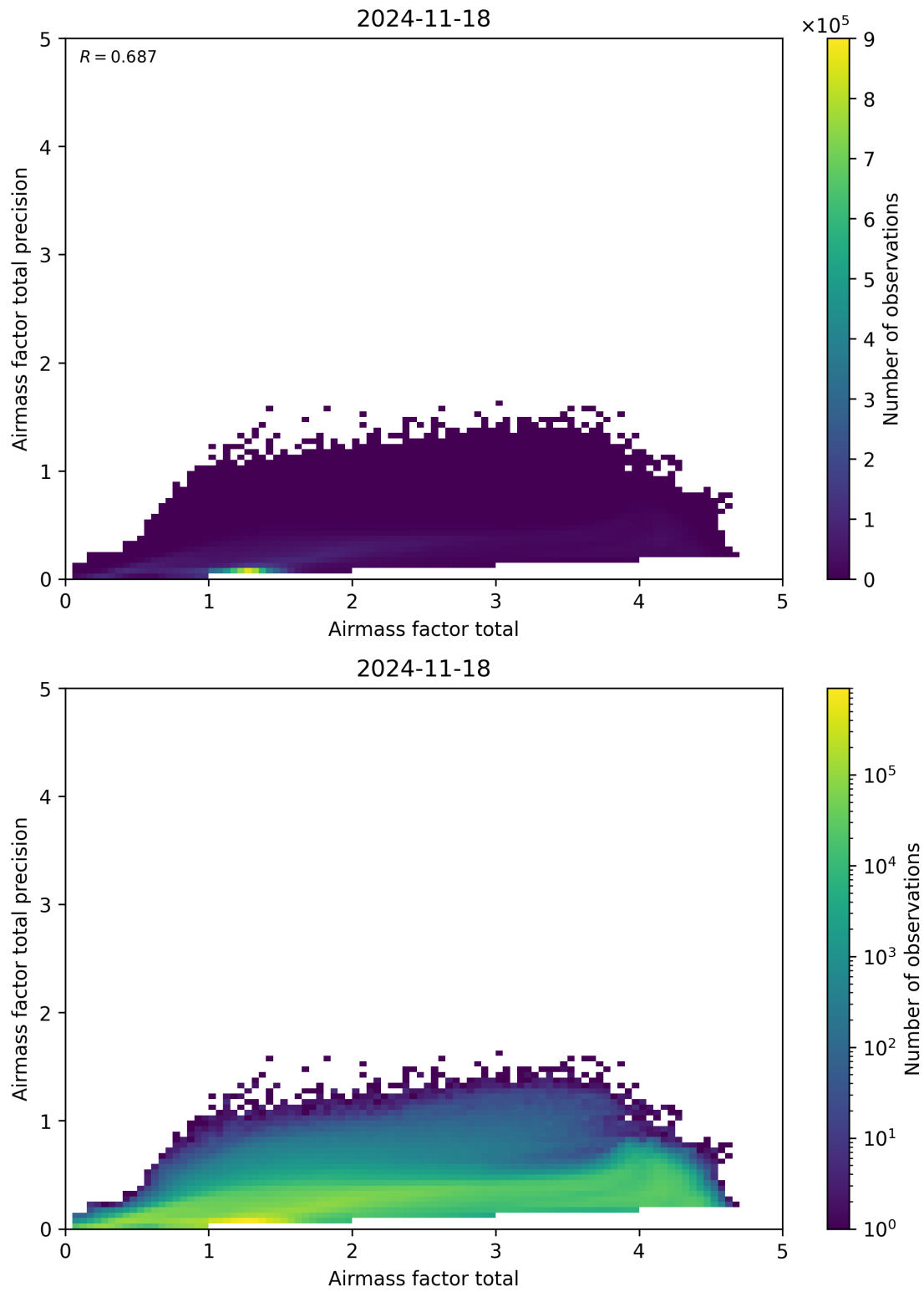
Figure 103: Scatter density plot of “Airmass factor total” against “Airmass factor total precision” for 2024-11-17 to 2024-11-19.
