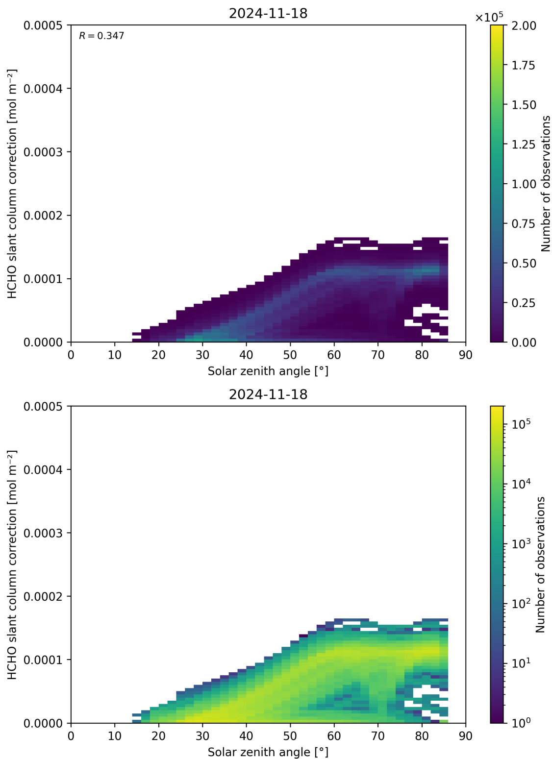
Figure 172: Scatter density plot of “Solar zenith angle” against “HCHO slant column correction” for 2024-11-17 to 2024-11-19.
