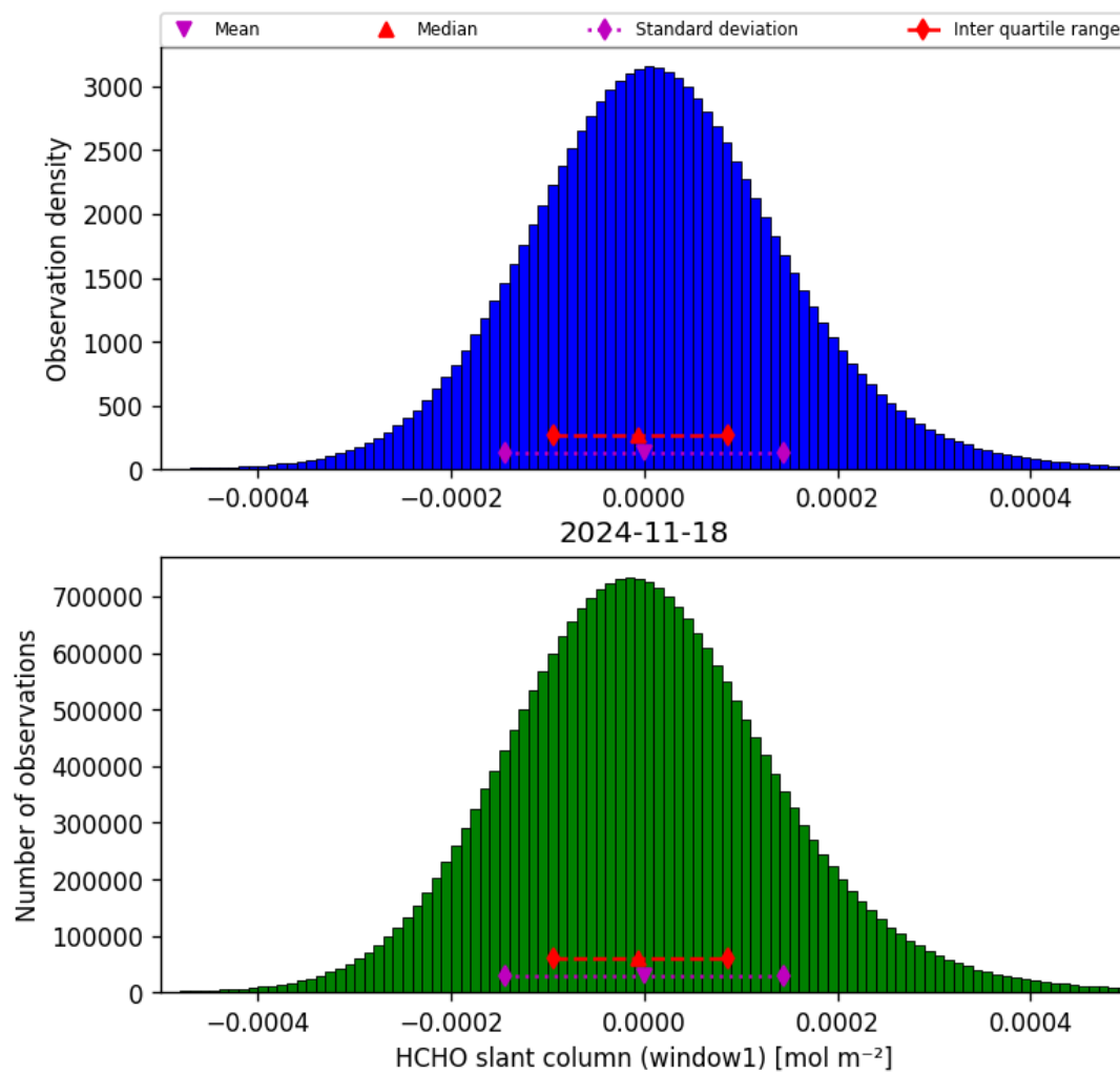
Figure 38: Histogram of “HCHO slant column (window1)” for 2024-11-17 to 2024-11-19
