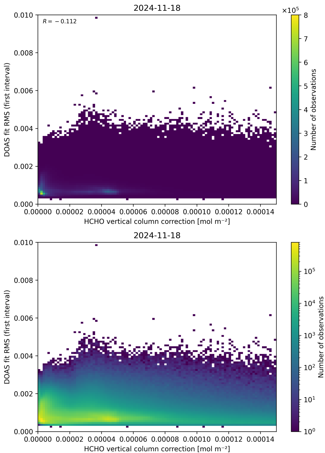
Figure 112: Scatter density plot of “HCHO vertical column correction” against “DOAS fit RMS (first interval)” for 2024-11-17 to 2024-11-19.
