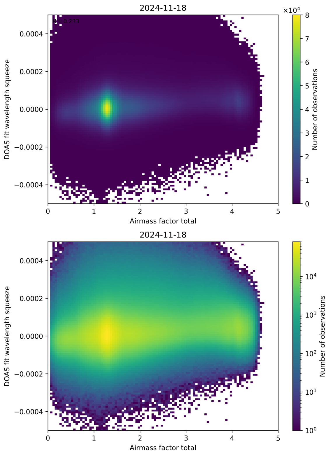
Figure 99: Scatter density plot of “Airmass factor total” against “DOAS fit wavelength squeeze” for 2024-11-17 to 2024-11-19.
