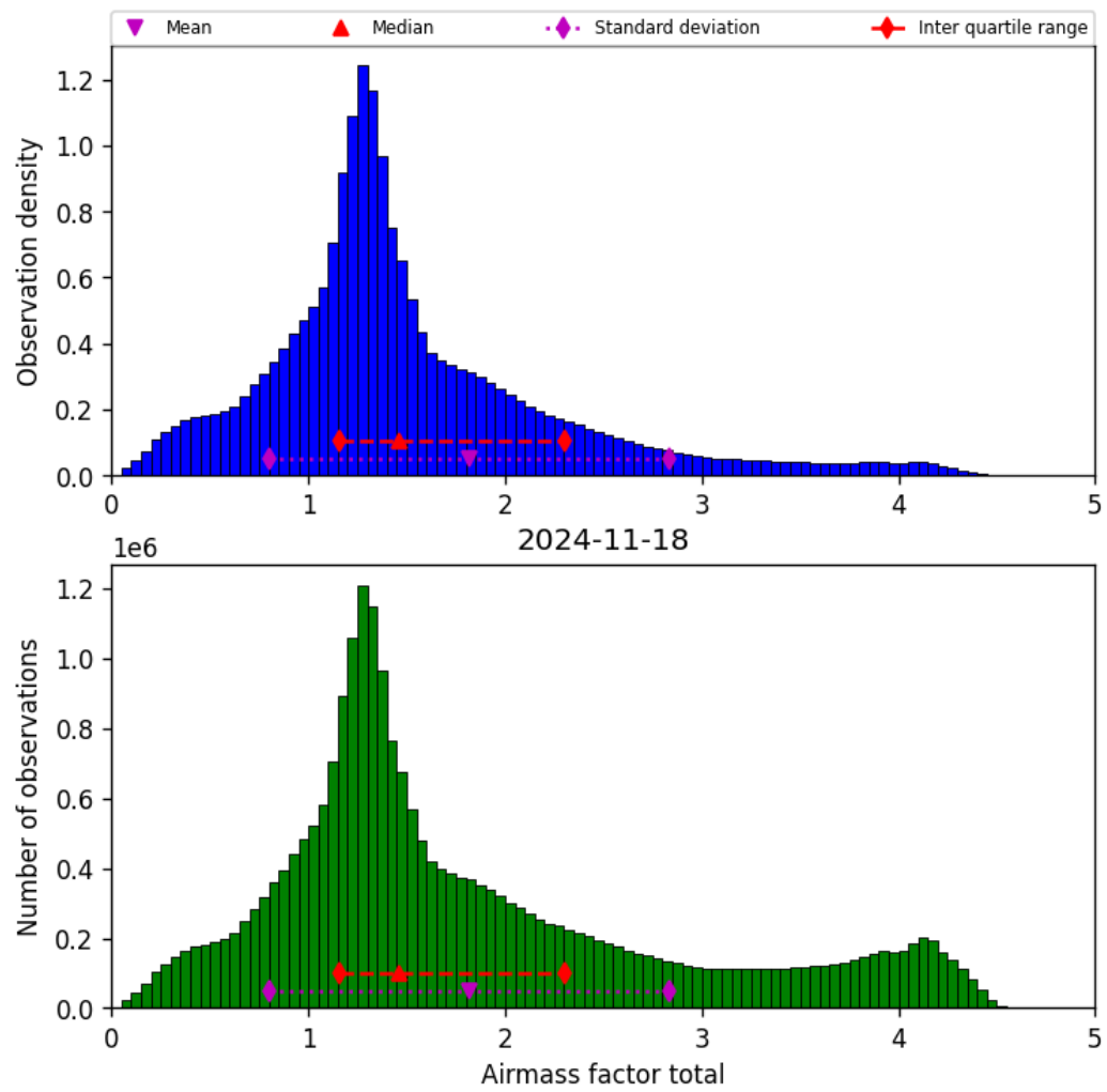
Figure 40: Histogram of “Airmass factor total” for 2024-11-17 to 2024-11-19
