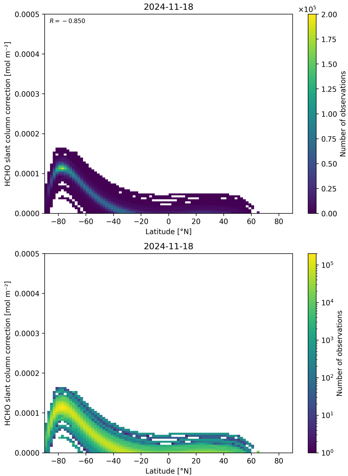
Figure 158: Scatter density plot of “Latitude” against “HCHO slant column correction” for 2024-11-17 to 2024-11-19.
