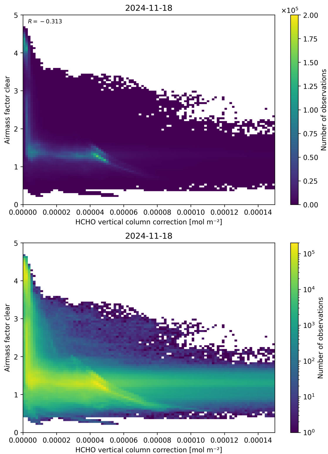
Figure 115: Scatter density plot of “HCHO vertical column correction” against “Airmass factor clear” for 2024-11-17 to 2024-11-19.
