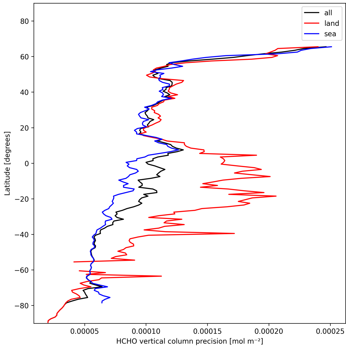
Figure 22: Zonal average of “HCHO vertical column precision” for 2024-11-17 to 2024-11-19.
