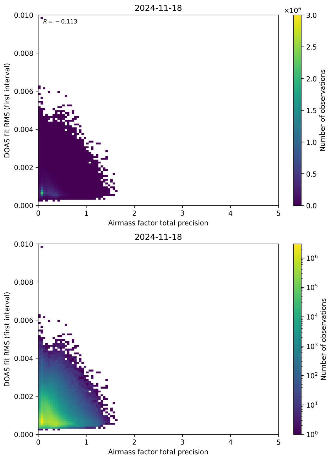
Figure 105: Scatter density plot of “Airmass factor total precision” against “DOAS fit RMS (first interval)” for 2024-11-17 to 2024-11-19.
