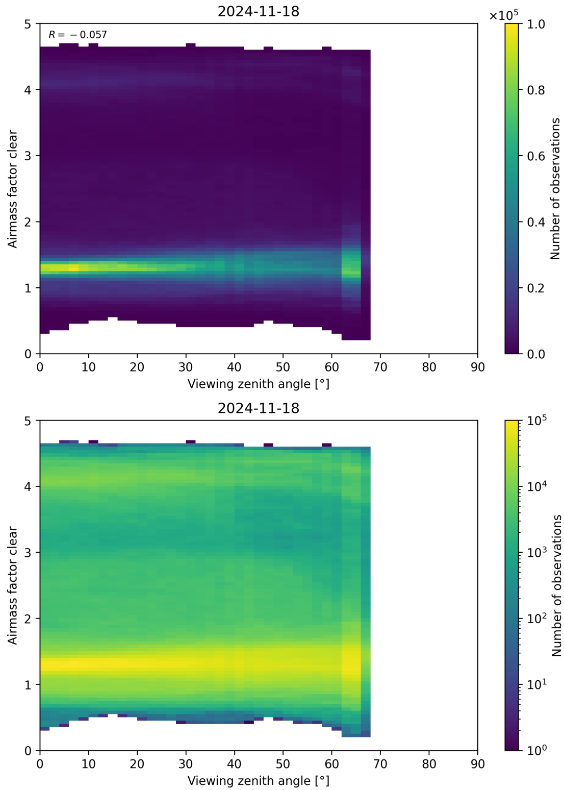
Figure 185: Scatter density plot of “Viewing zenith angle” against “Airmass factor clear” for 2024-11-17 to 2024-11-19.
