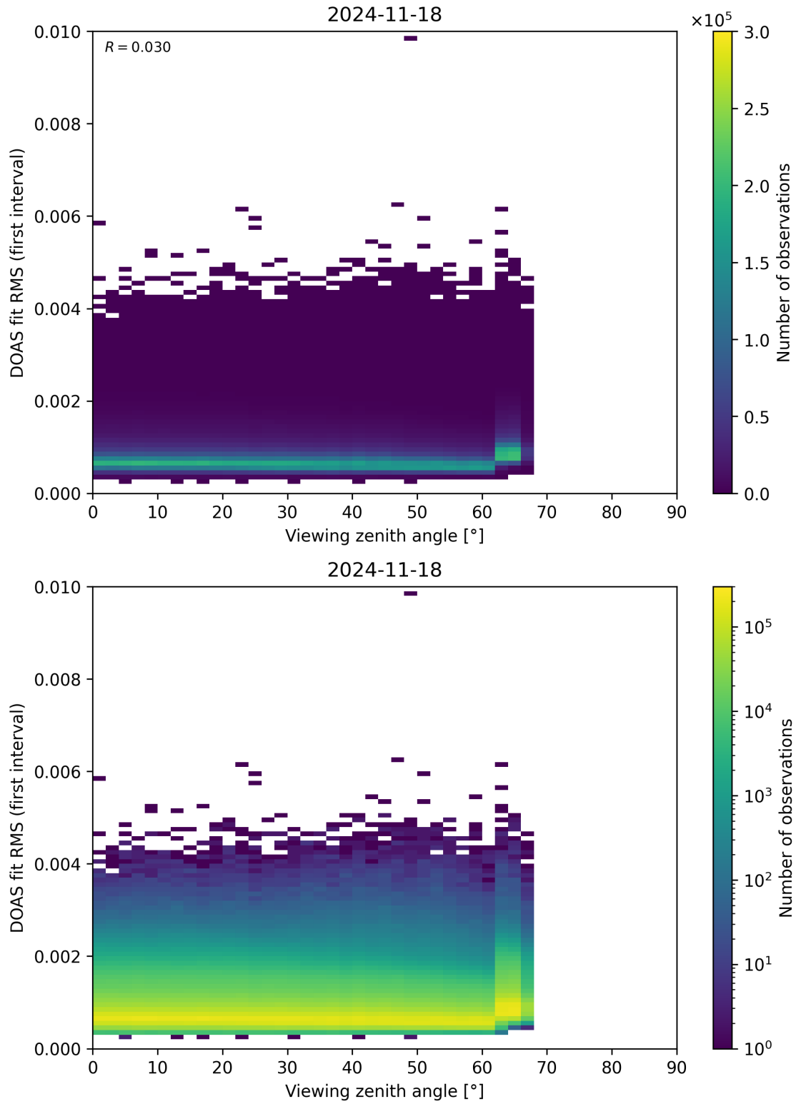
Figure 182: Scatter density plot of “Viewing zenith angle” against “DOAS fit RMS (first interval)” for 2024-11-17 to 2024-11-19.
