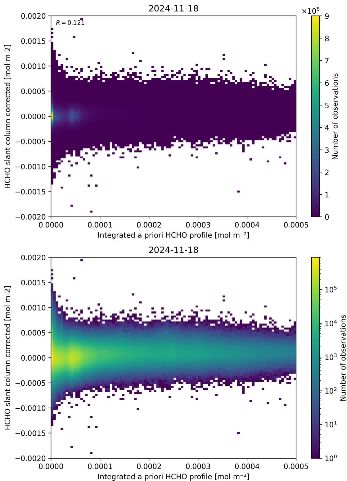
Figure 151: Scatter density plot of “Integrated a priori HCHO profile” against “HCHO slant column corrected” for 2024-11-17 to 2024-11-19.
