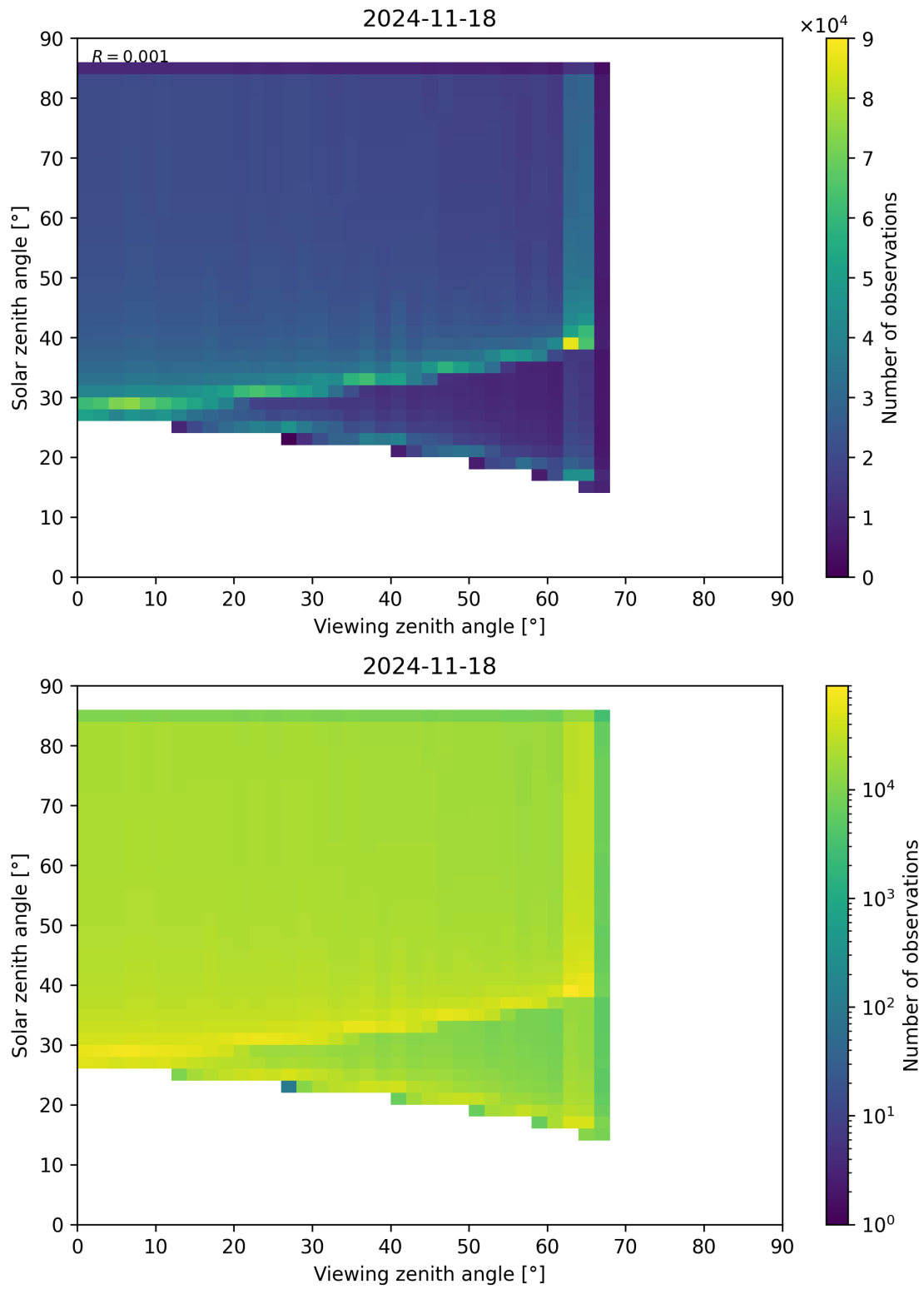
Figure 197: Scatter density plot of “Viewing zenith angle” against “Solar zenith angle” for 2024-11-17 to 2024-11-19.
