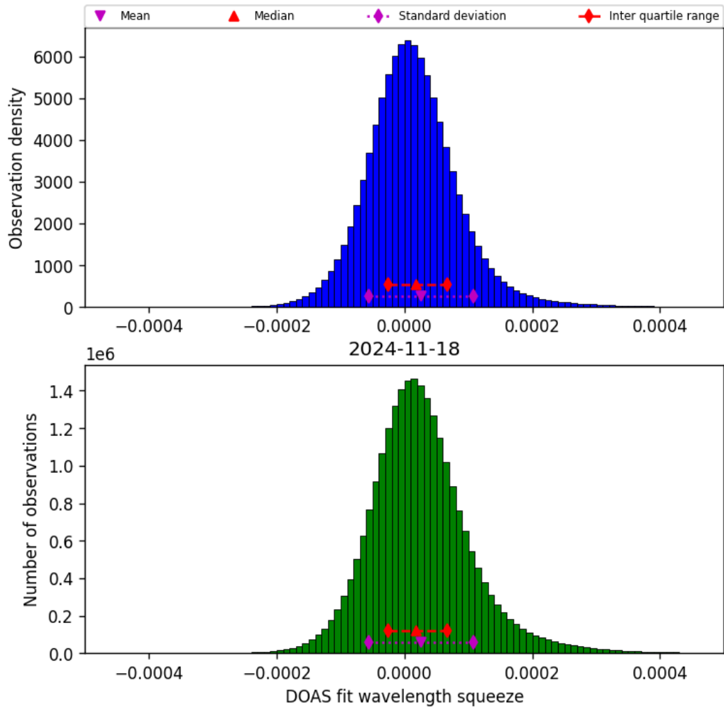
Figure 45: Histogram of “DOAS fit wavelength squeeze” for 2024-11-17 to 2024-11-19
