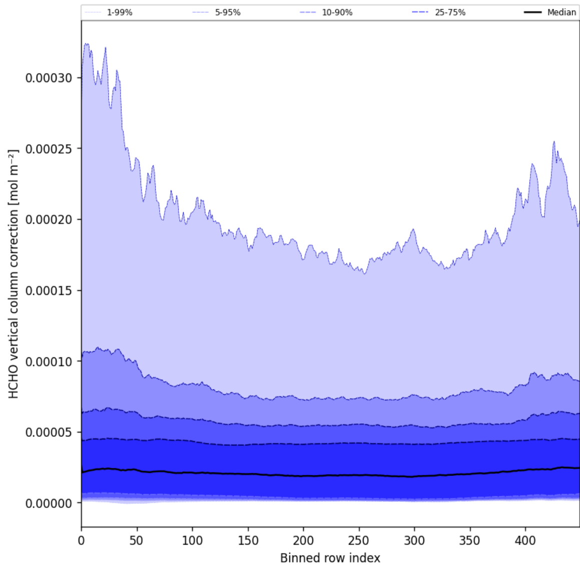
Figure 51: Along track statistics of “HCHO vertical column correction” for 2024-11-17 to 2024-11-19
