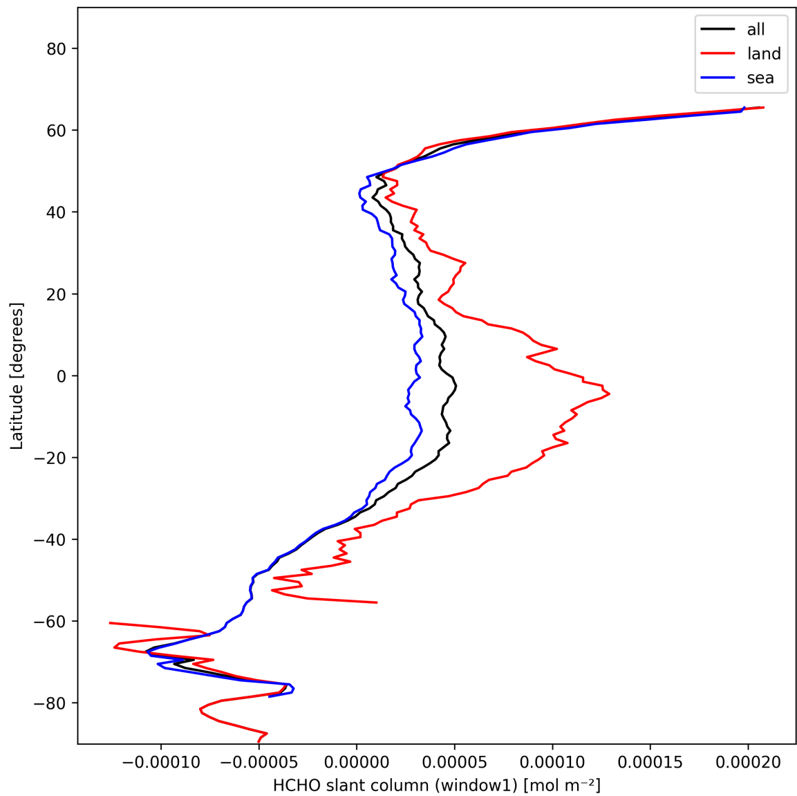
Figure 24: Zonal average of “HCHO slant column (window1)” for 2024-11-17 to 2024-11-19.
