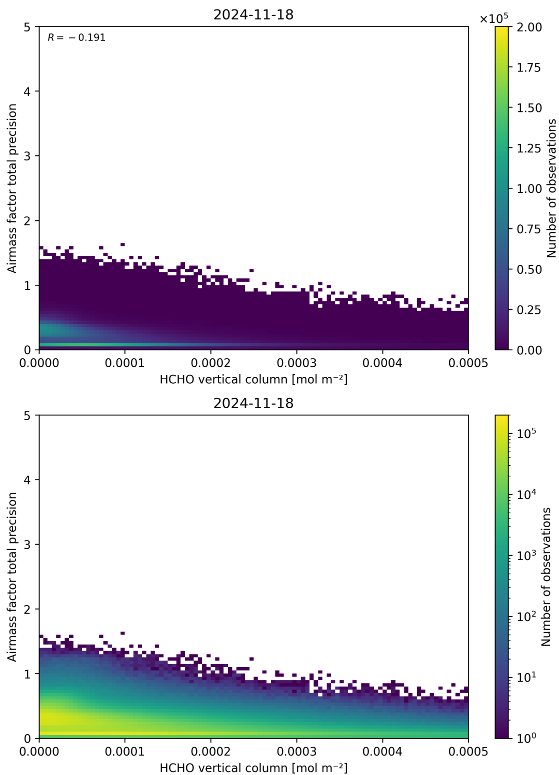
Figure 132: Scatter density plot of “HCHO vertical column” against “Airmass factor total precision” for 2024-11-17 to 2024-11-19.
