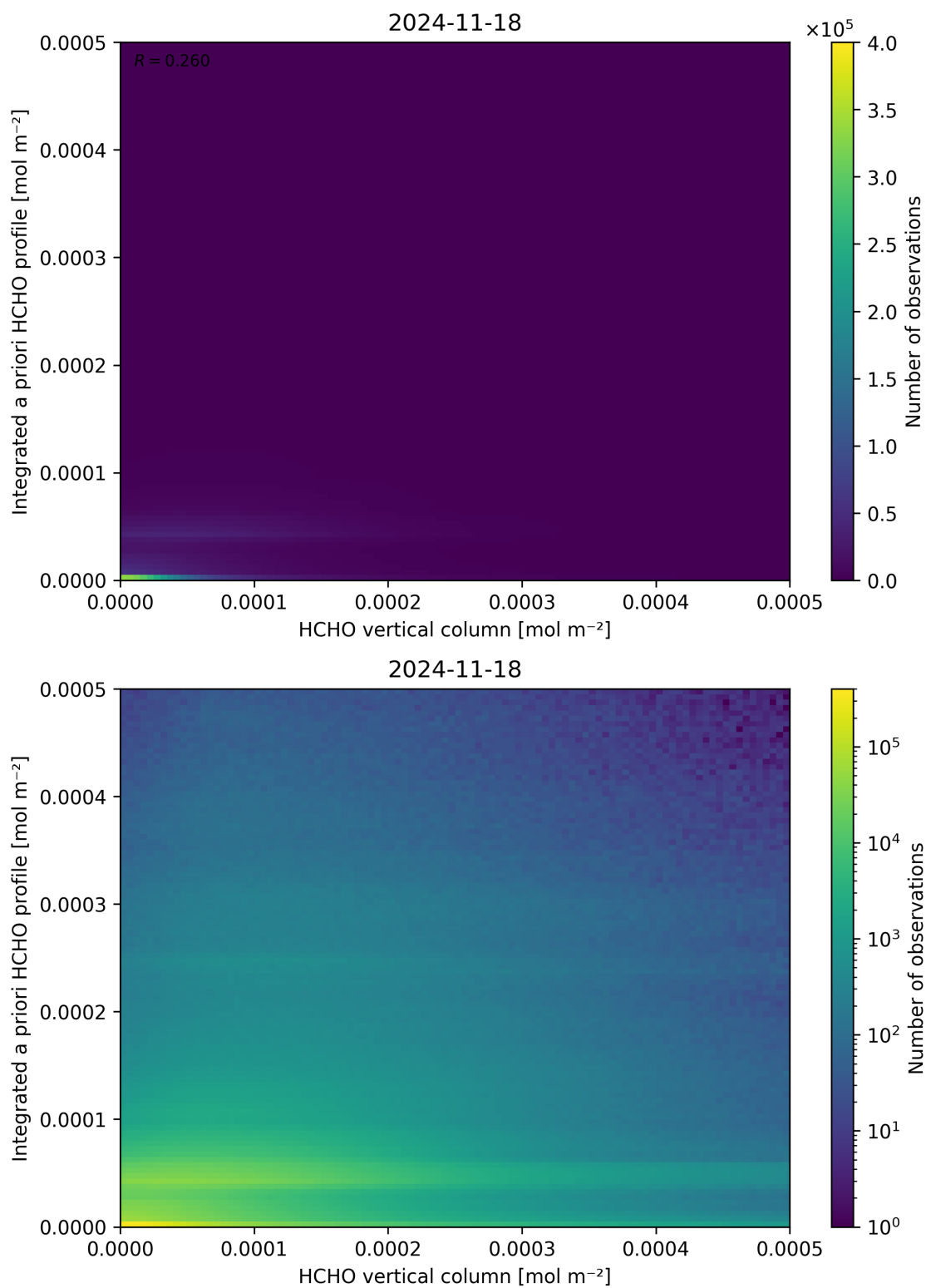
Figure 135: Scatter density plot of “HCHO vertical column” against “Integrated a priori HCHO profile” for 2024-11-17 to 2024-11-19.
