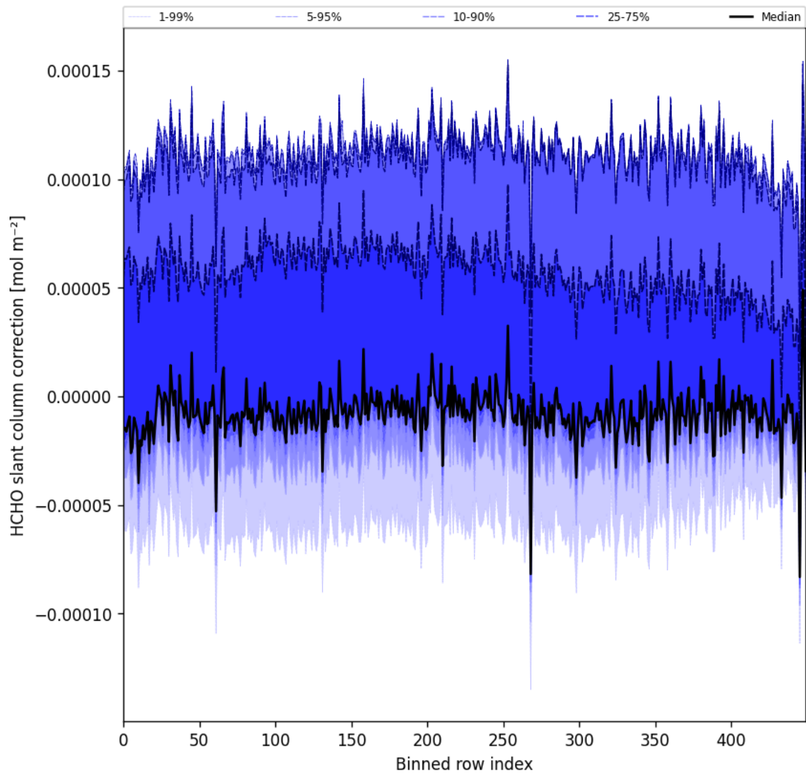
Figure 61: Along track statistics of “HCHO slant column correction” for 2024-11-17 to 2024-11-19
