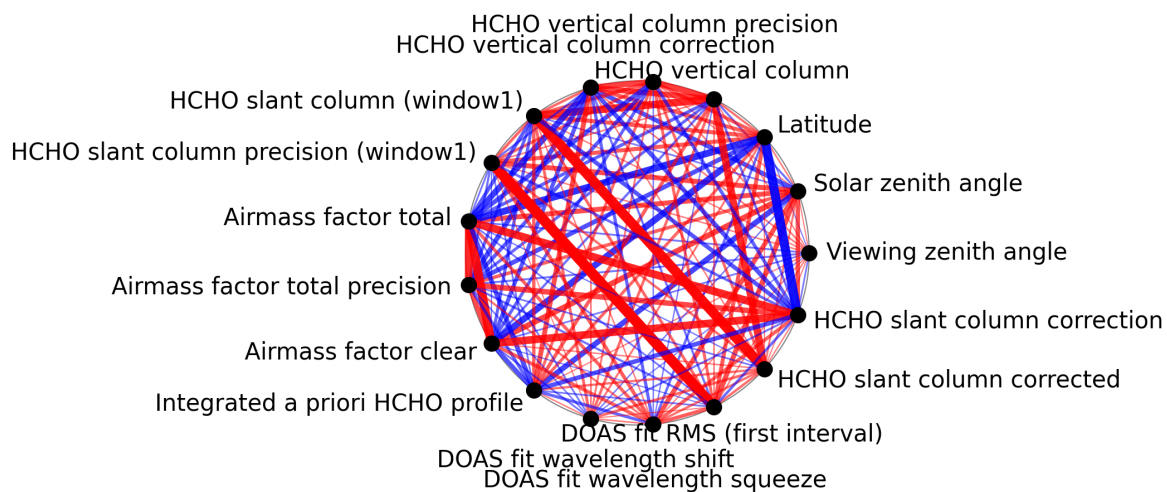
Figure 1: Map of correlation graph for 2024-11-17 to 2024-11-19.
