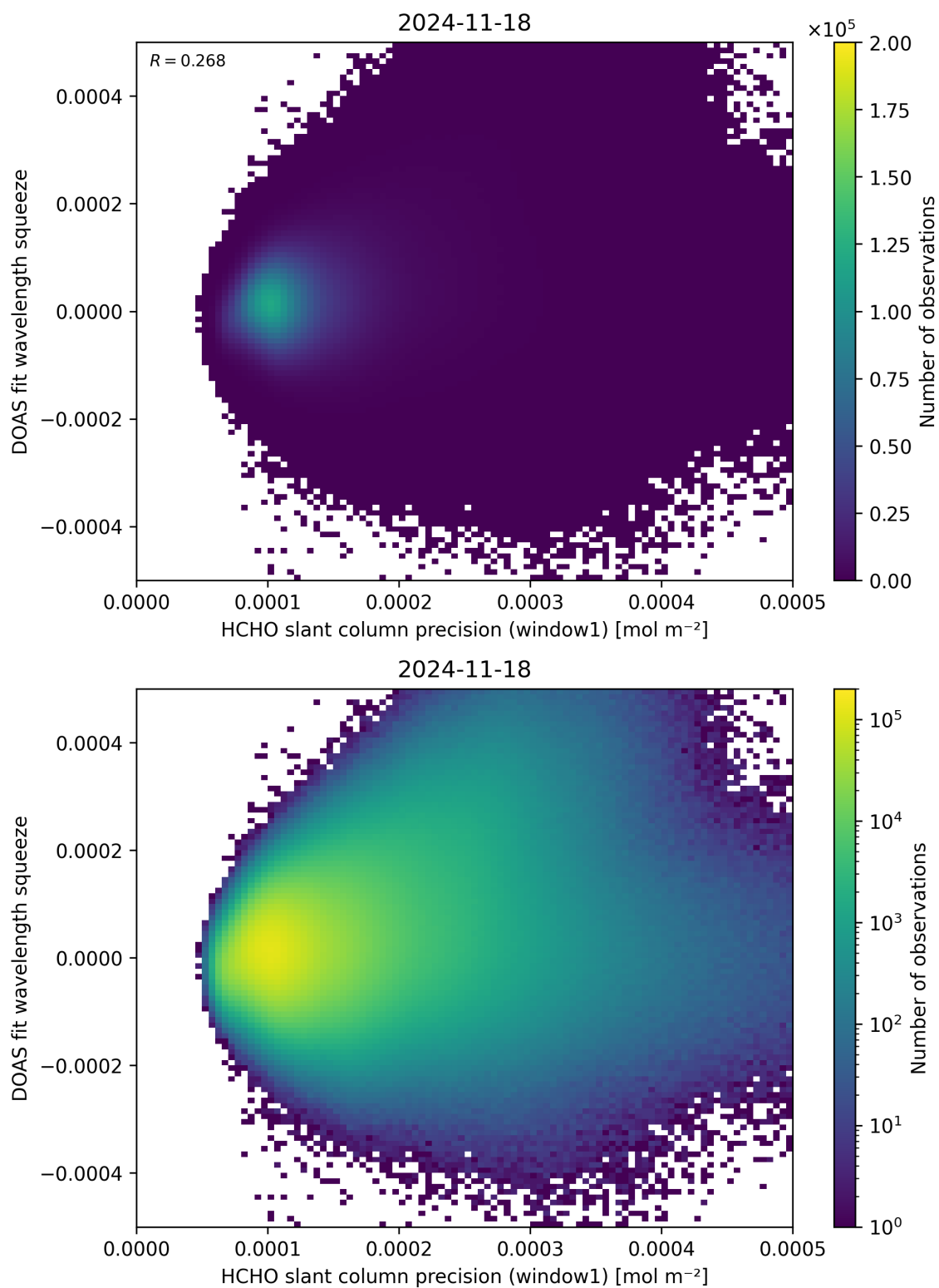
Figure 90: Scatter density plot of “HCHO slant column precision (window1)” against “DOAS fit wavelength squeeze” for 2024-11-17 to 2024-11-19.
