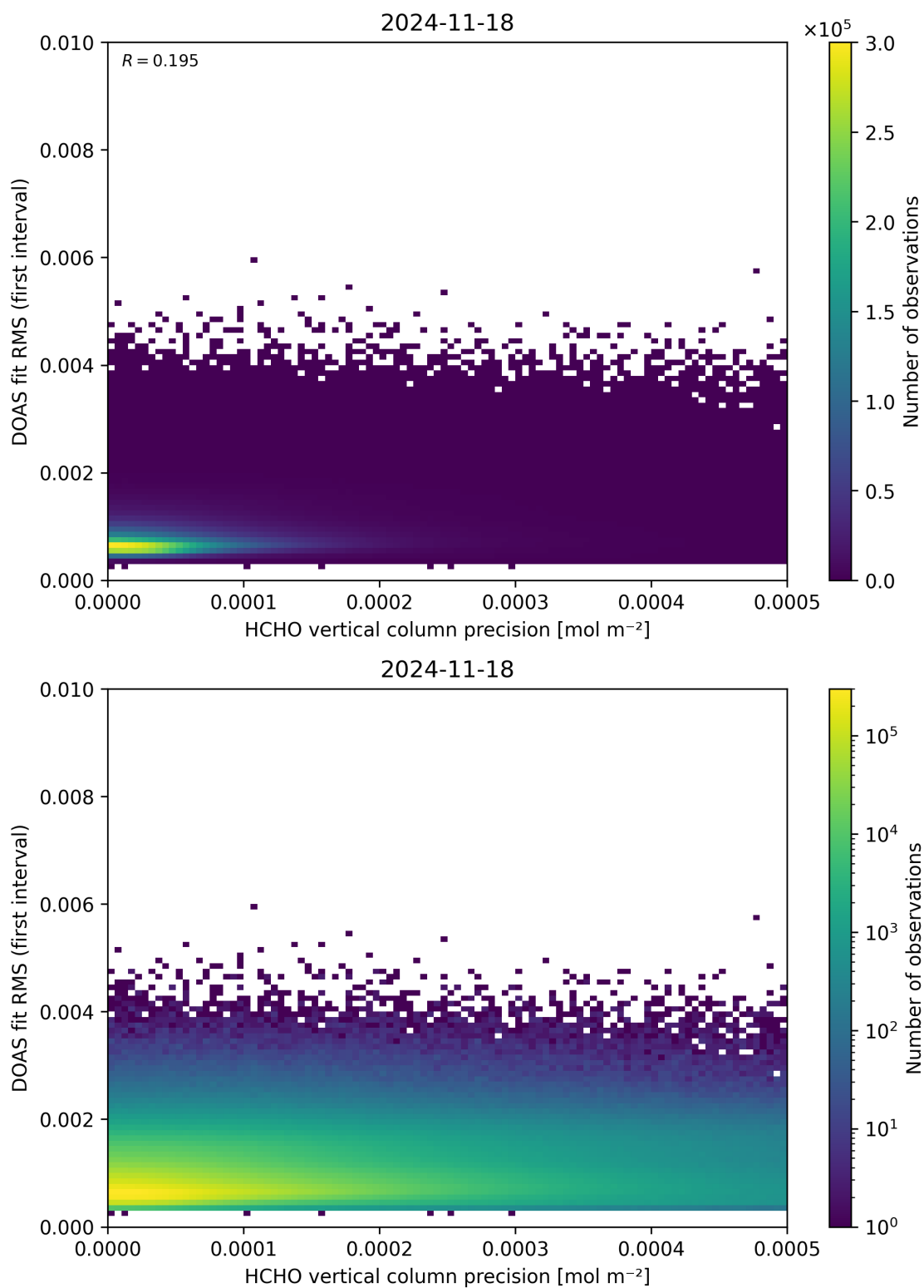
Figure 136: Scatter density plot of “HCHO vertical column precision” against “DOAS fit RMS (first interval)” for 2024-11-17 to 2024-11-19.
