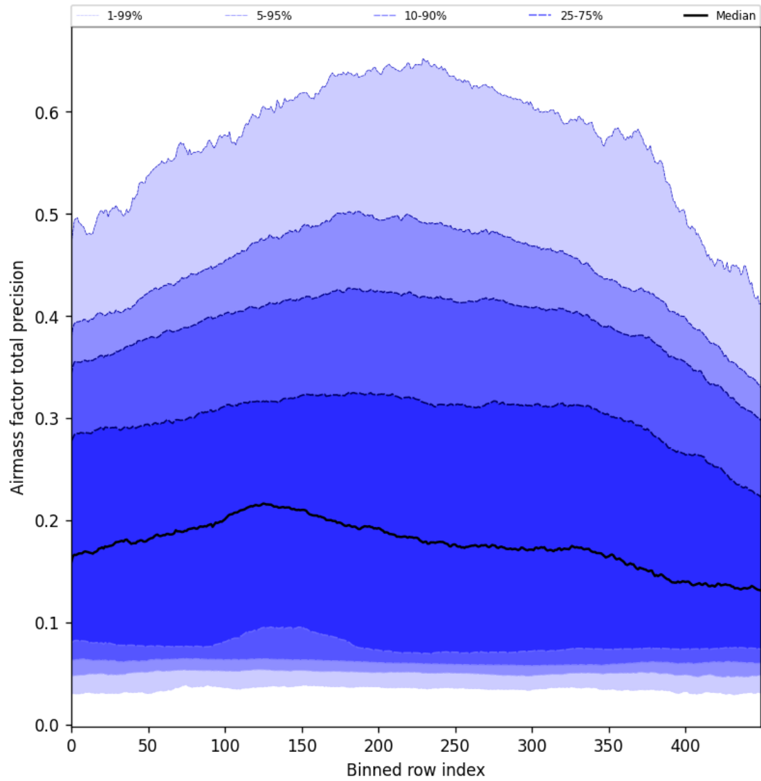
Figure 55: Along track statistics of “Airmass factor total precision” for 2024-11-17 to 2024-11-19
