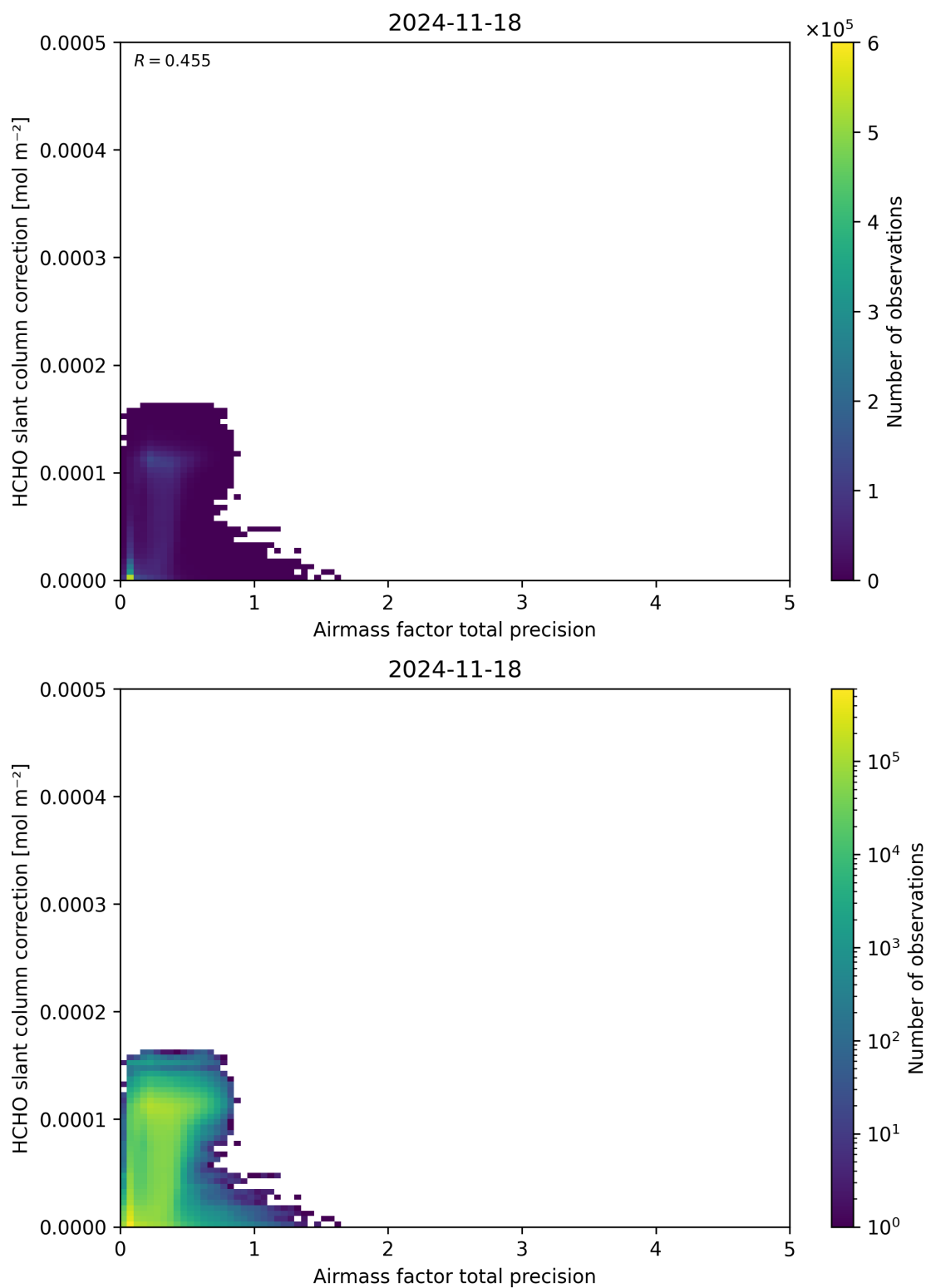
Figure 110: Scatter density plot of “Airmass factor total precision” against “HCHO slant column correction” for 2024-11-17 to 2024-11-19.
