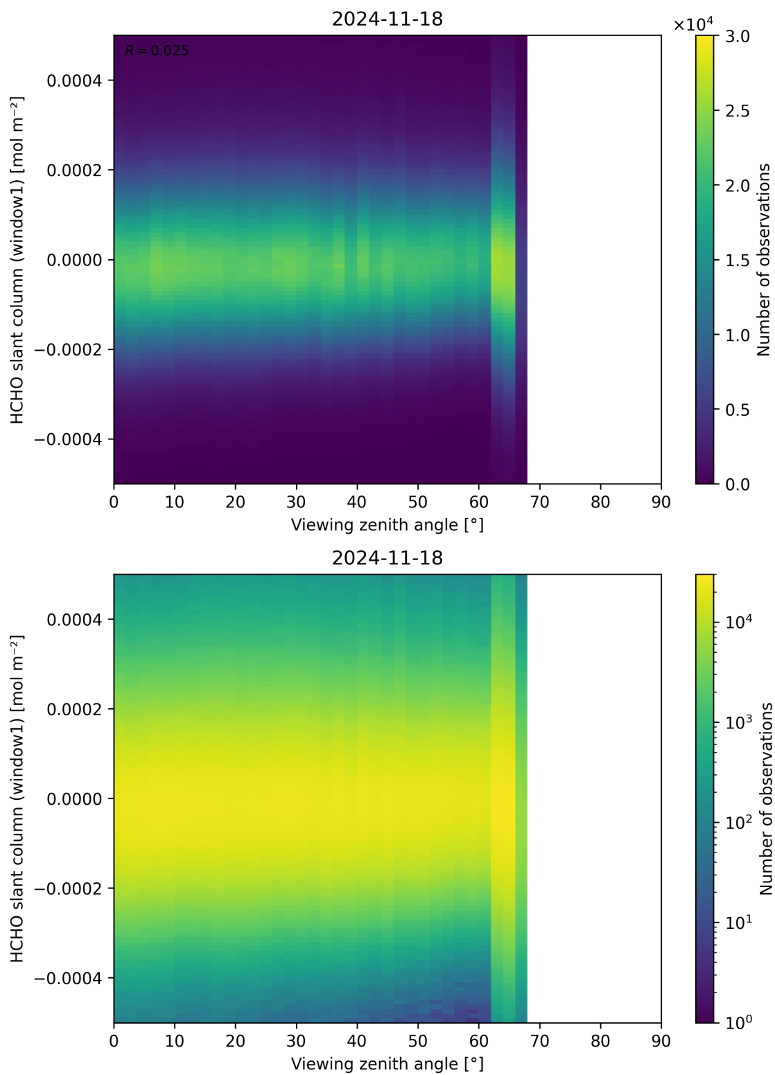
Figure 188: Scatter density plot of “Viewing zenith angle” against “HCHO slant column (window1)” for 2024-11-17 to 2024-11-19.
