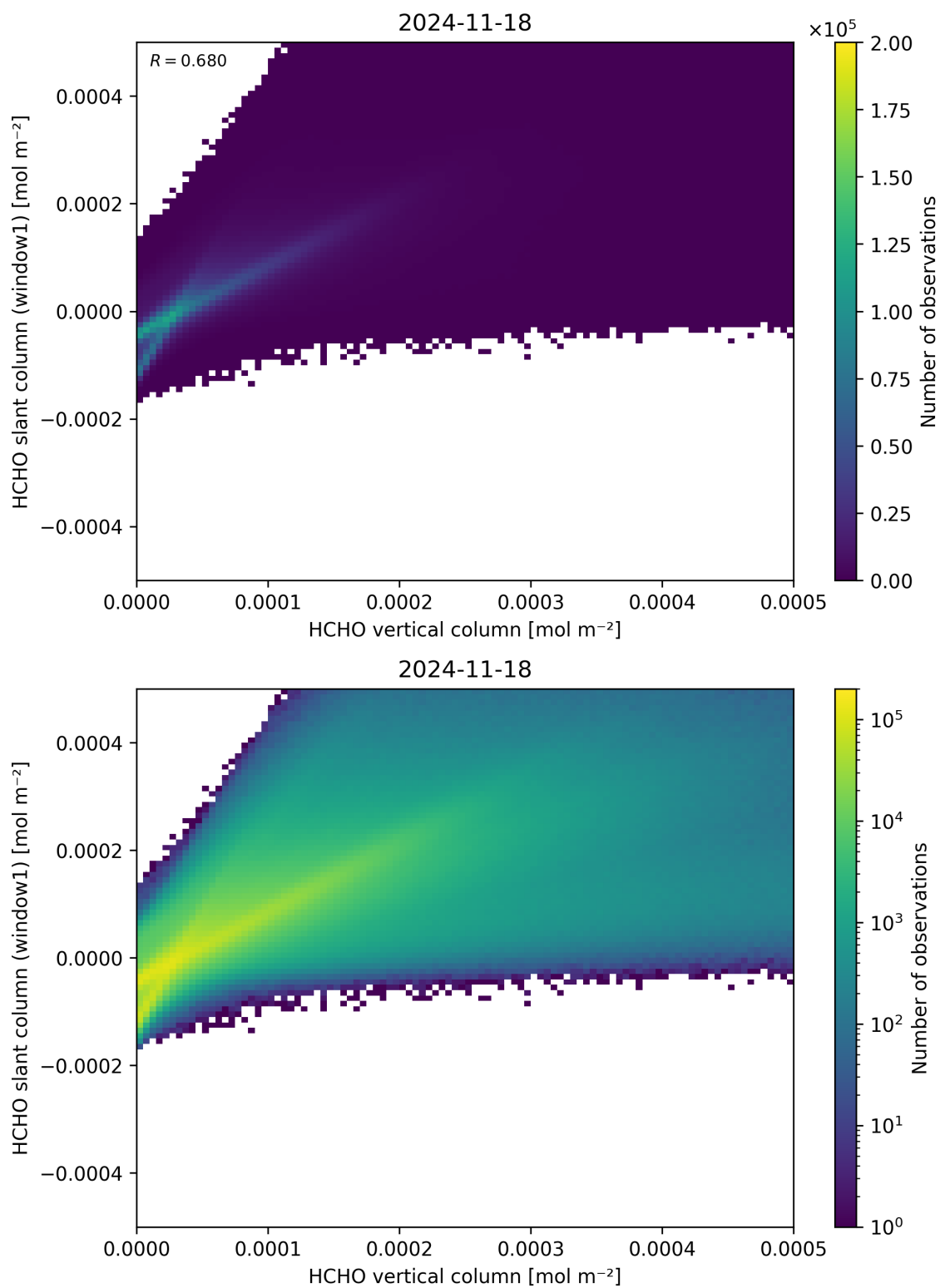
Figure 129: Scatter density plot of “HCHO vertical column” against “HCHO slant column (window1)” for 2024-11-17 to 2024-11-19.
