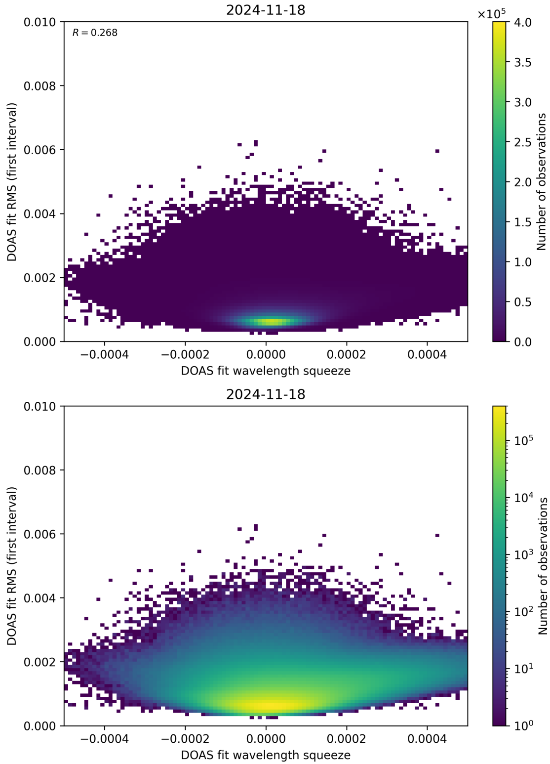
Figure 68: Scatter density plot of “DOAS fit wavelength squeeze” against “DOAS fit RMS (first interval)” for 2024-11-17 to 2024-11-19.
