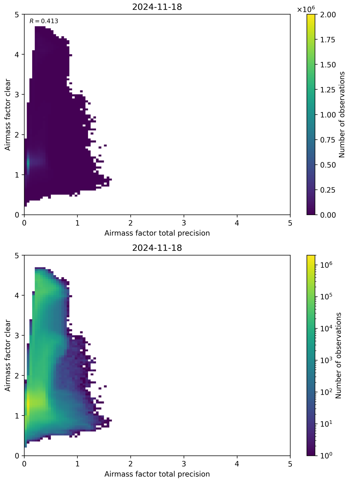
Figure 108: Scatter density plot of “Airmass factor total precision” against “Airmass factor clear” for 2024-11-17 to 2024-11-19.
