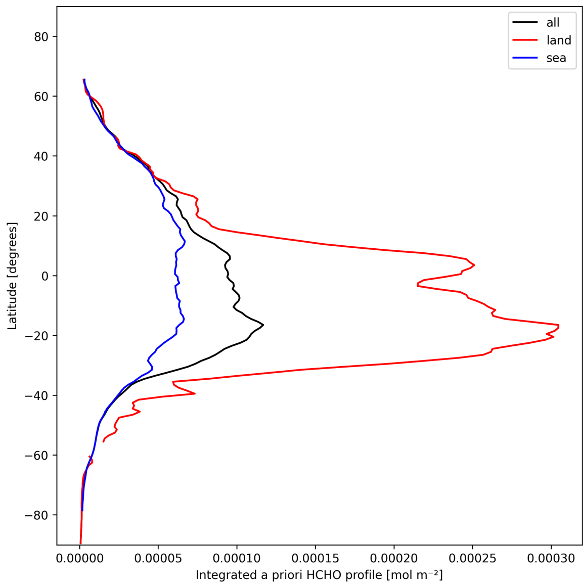
Figure 29: Zonal average of “Integrated a priori HCHO profile” for 2024-11-17 to 2024-11-19.
