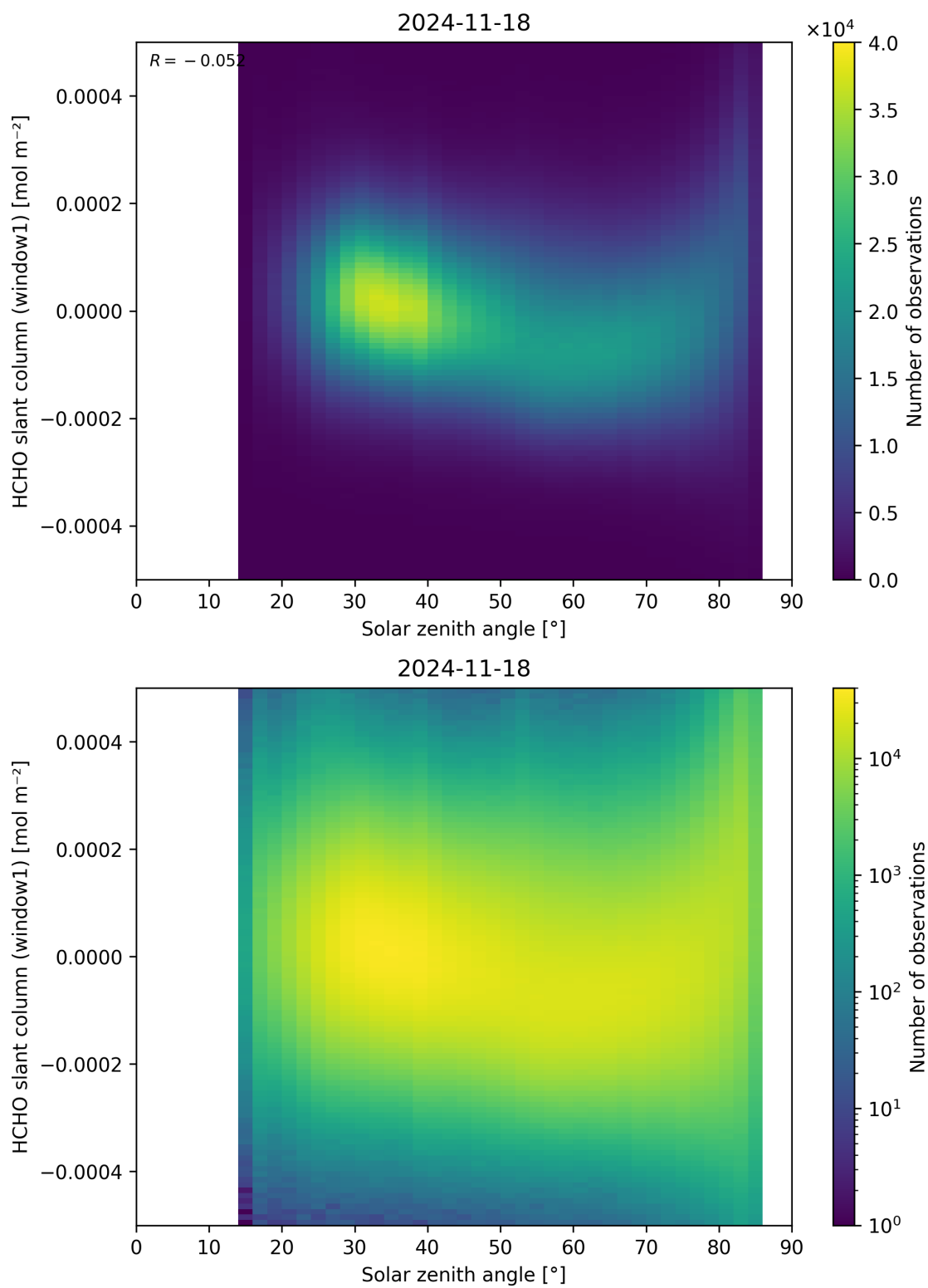
Figure 173: Scatter density plot of “Solar zenith angle” against “HCHO slant column (window1)” for 2024-11-17 to 2024-11-19.
