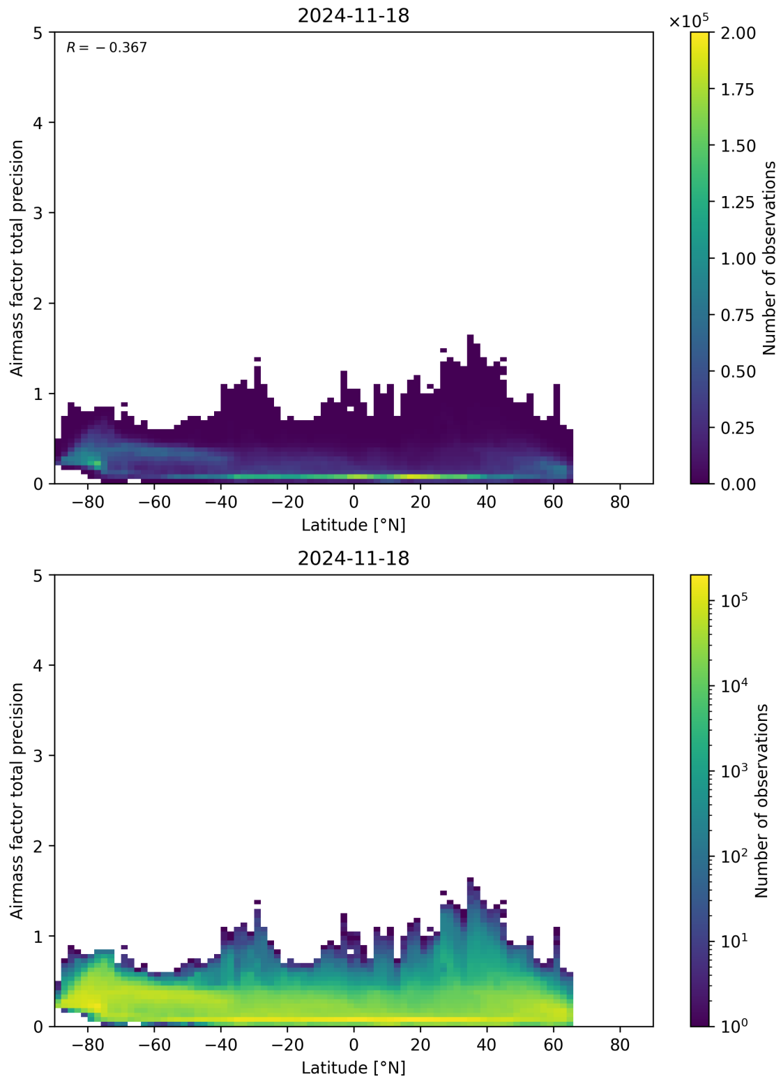
Figure 162: Scatter density plot of “Latitude” against “Airmass factor total precision” for 2024-11-17 to 2024-11-19.
