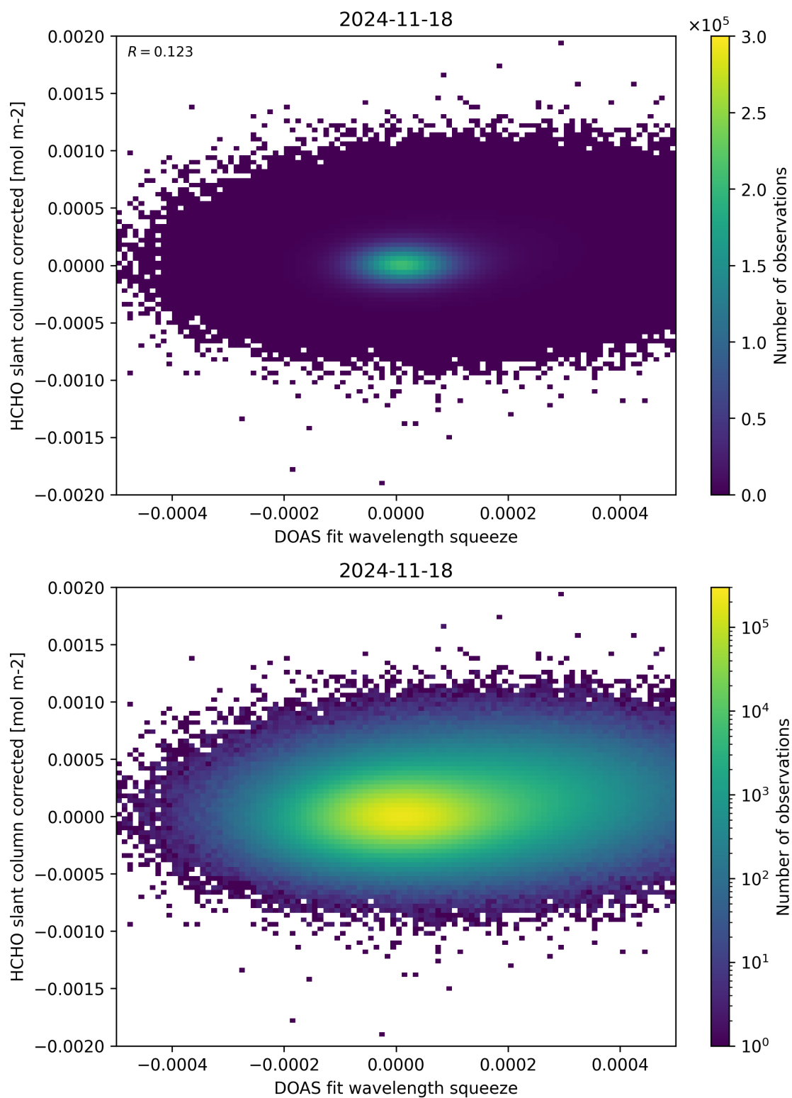
Figure 69: Scatter density plot of “DOAS fit wavelength squeeze” against “HCHO slant column corrected” for 2024-11-17 to 2024-11-19.
