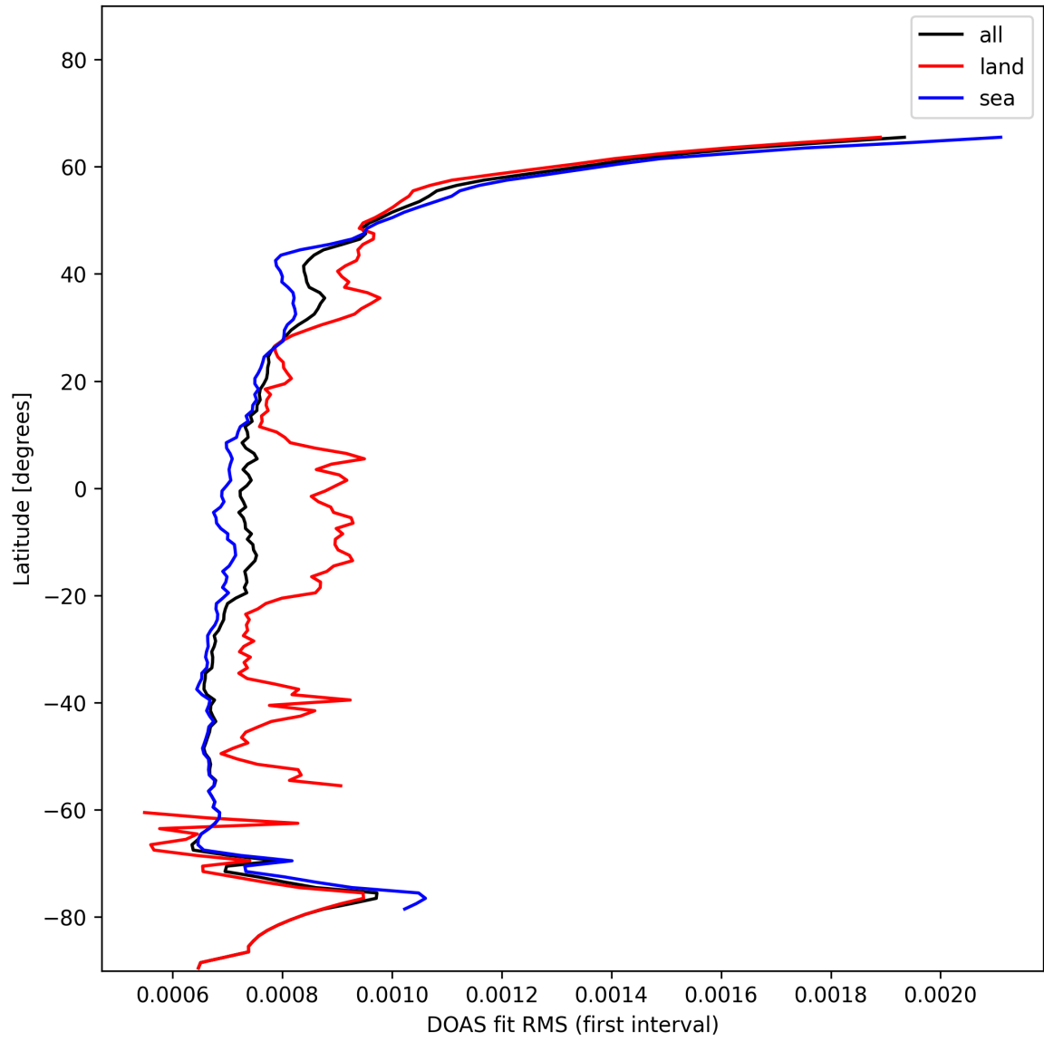
Figure 32: Zonal average of "DOAS fit RMS (first interval)" for 2024-11-17 to 2024-11-19.
