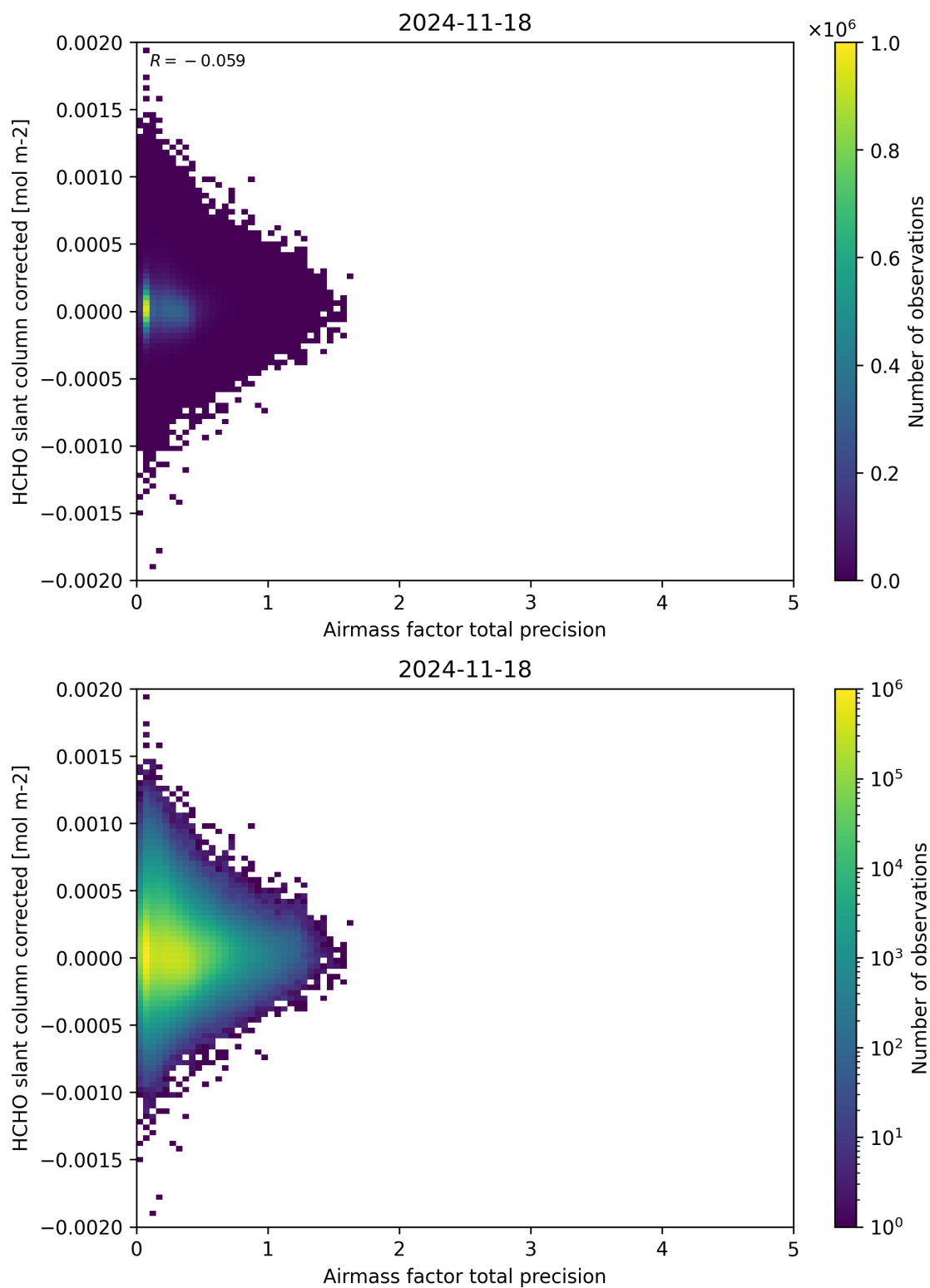
Figure 109: Scatter density plot of “Airmass factor total precision” against “HCHO slant column corrected” for 2024-11-17 to 2024-11-19.
