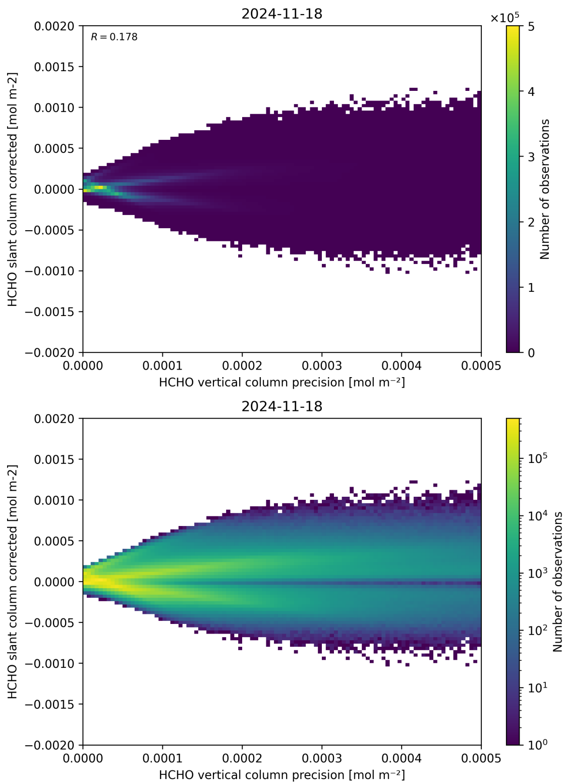
Figure 140: Scatter density plot of “HCHO vertical column precision” against “HCHO slant column corrected” for 2024-11-17 to 2024-11-19.
