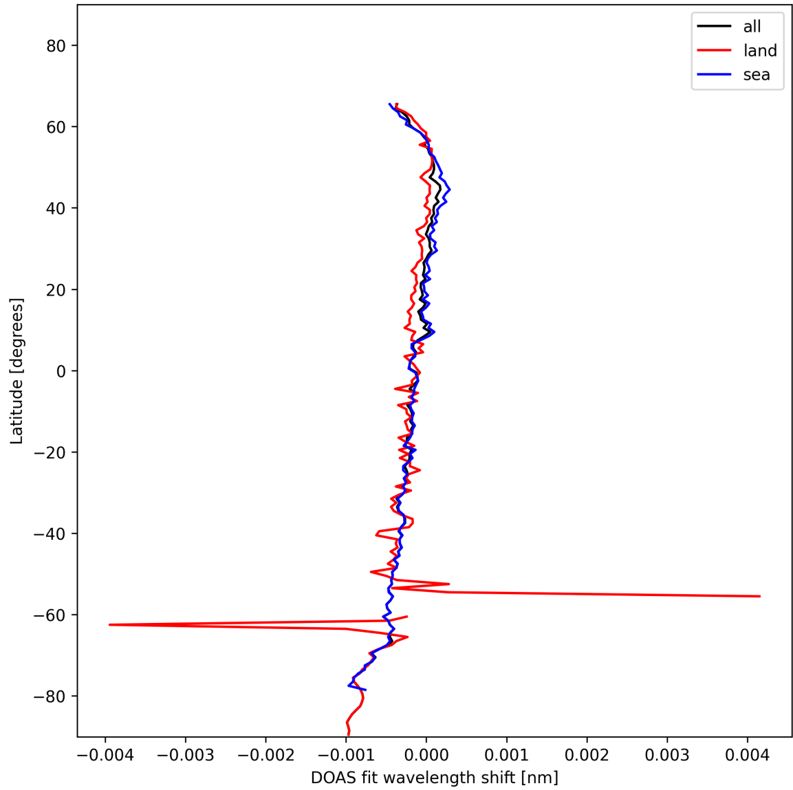
Figure 30: Zonal average of “DOAS fit wavelength shift” for 2024-11-17 to 2024-11-19.
