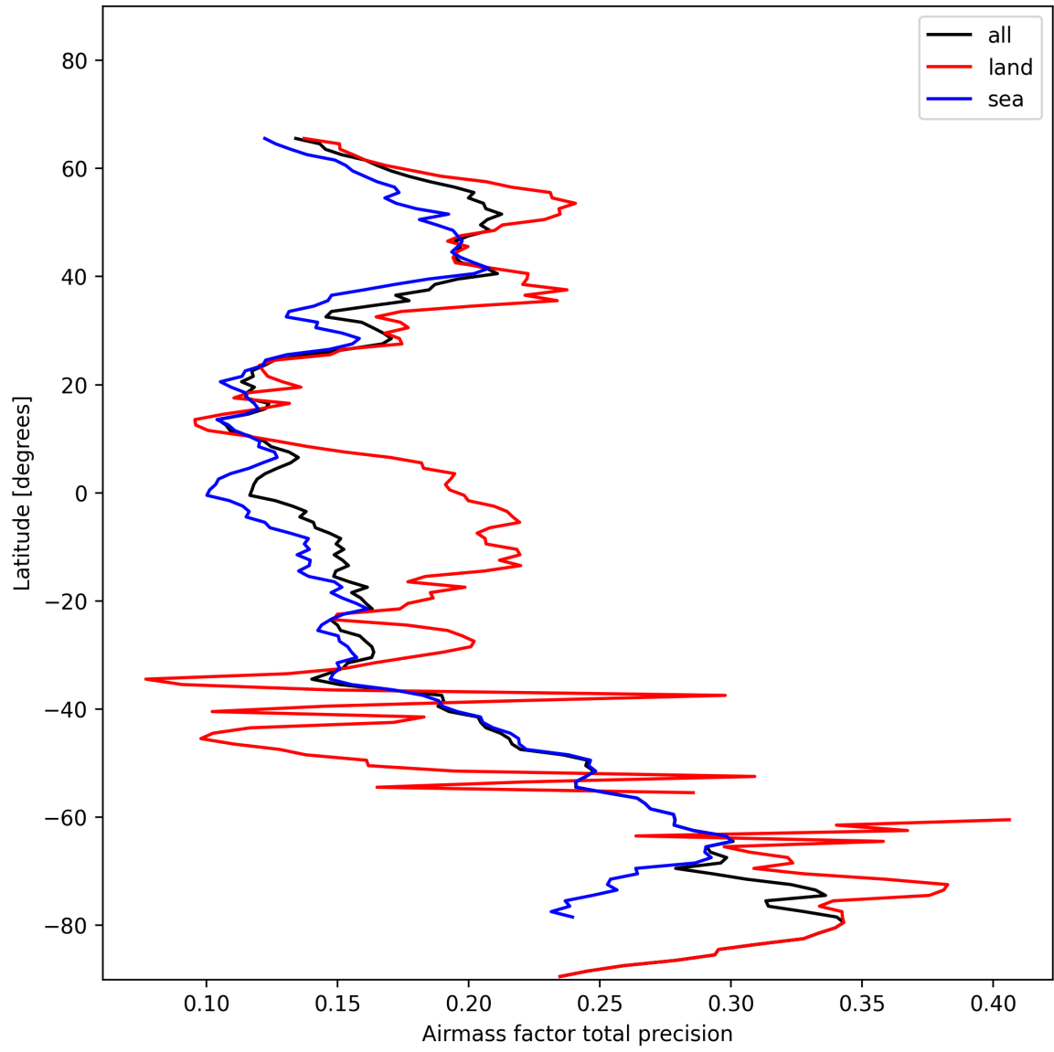
Figure 27: Zonal average of “Airmass factor total precision” for 2024-11-17 to 2024-11-19.
