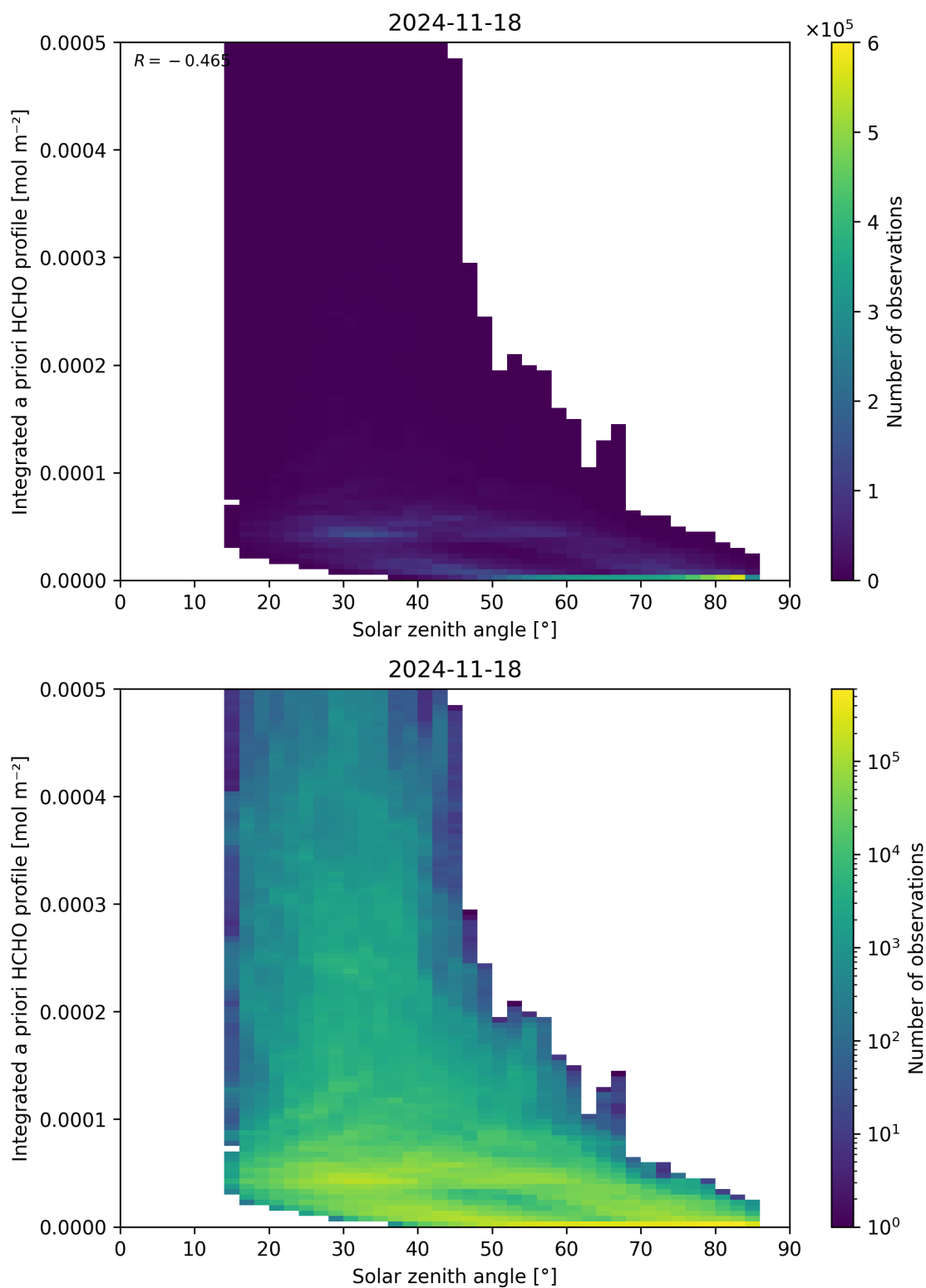
Figure 180: Scatter density plot of “Solar zenith angle” against “Integrated a priori HCHO profile” for 2024-11-17 to 2024-11-19.
