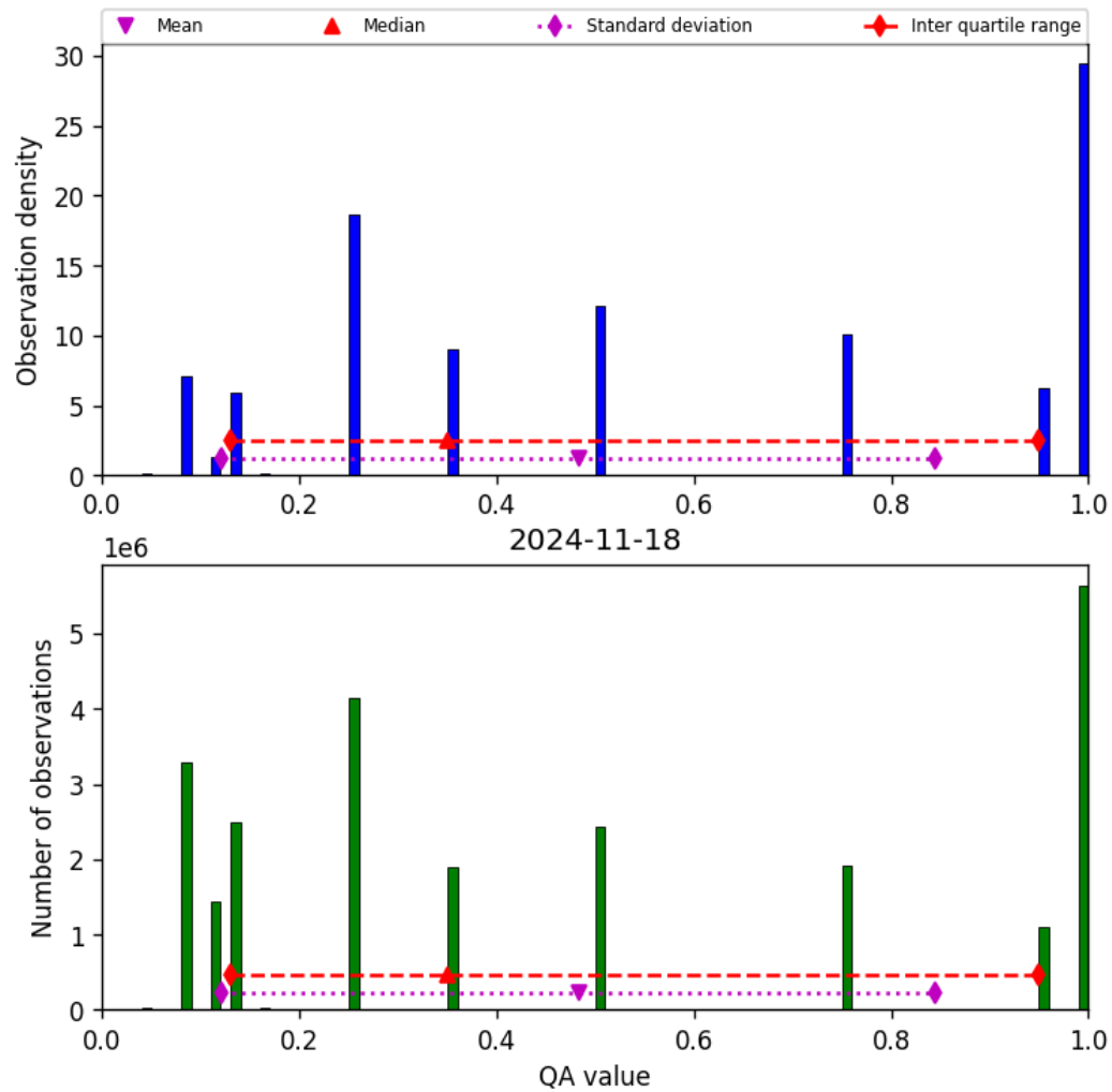
Figure 34: Histogram of “QA value” for 2024-11-17 to 2024-11-19
