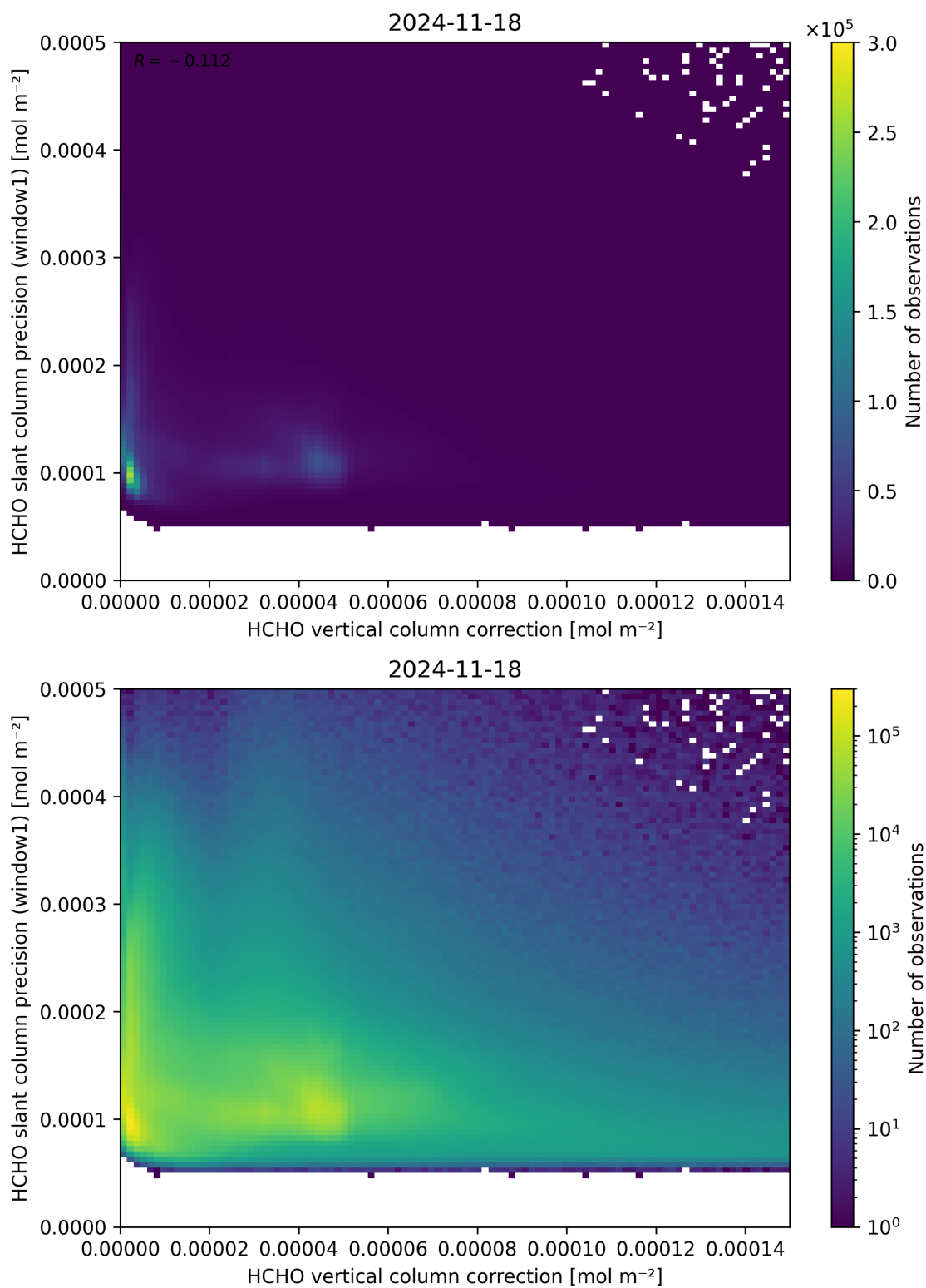
Figure 119: Scatter density plot of “HCHO vertical column correction” against “HCHO slant column precision (window1)” for 2024-11-17 to 2024-11-19.
