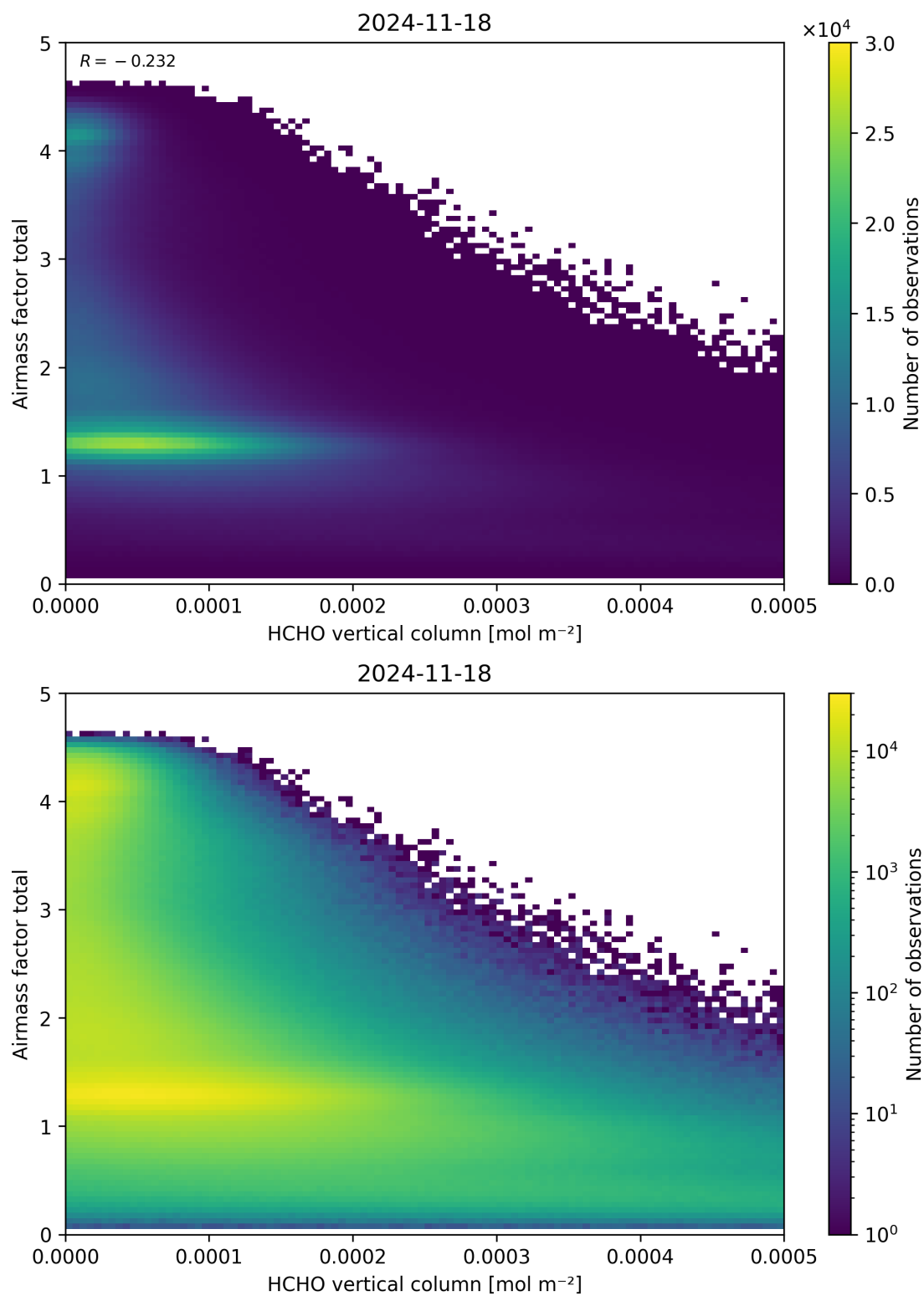
Figure 131: Scatter density plot of “HCHO vertical column” against “Airmass factor total” for 2024-11-17 to 2024-11-19.
