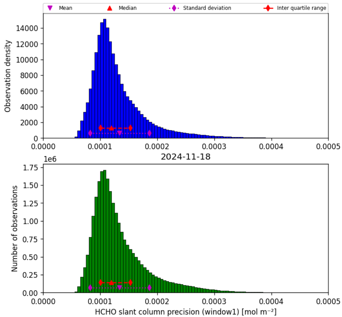
Figure 39: Histogram of “HCHO slant column precision (window1)” for 2024-11-17 to 2024-11-19
