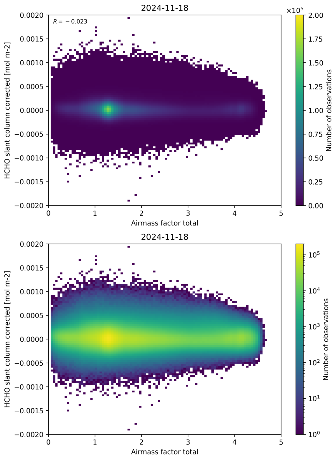
Figure 101: Scatter density plot of “Airmass factor total” against “HCHO slant column corrected” for 2024-11-17 to 2024-11-19.
