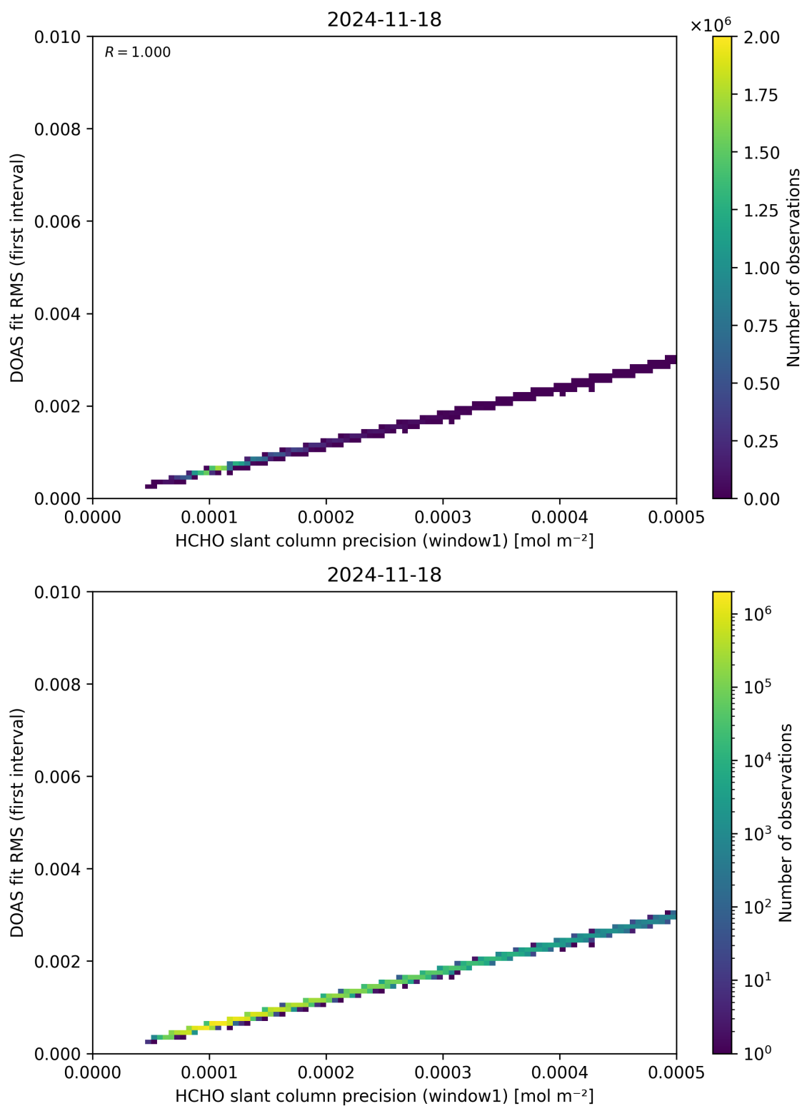
Figure 88: Scatter density plot of “HCHO slant column precision (window1)” against “DOAS fit RMS (first interval)” for 2024-11-17 to 2024-11-19.
