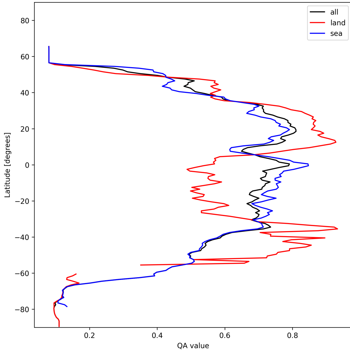
Figure 20: Zonal average of “QA value” for 2024-11-17 to 2024-11-19.
