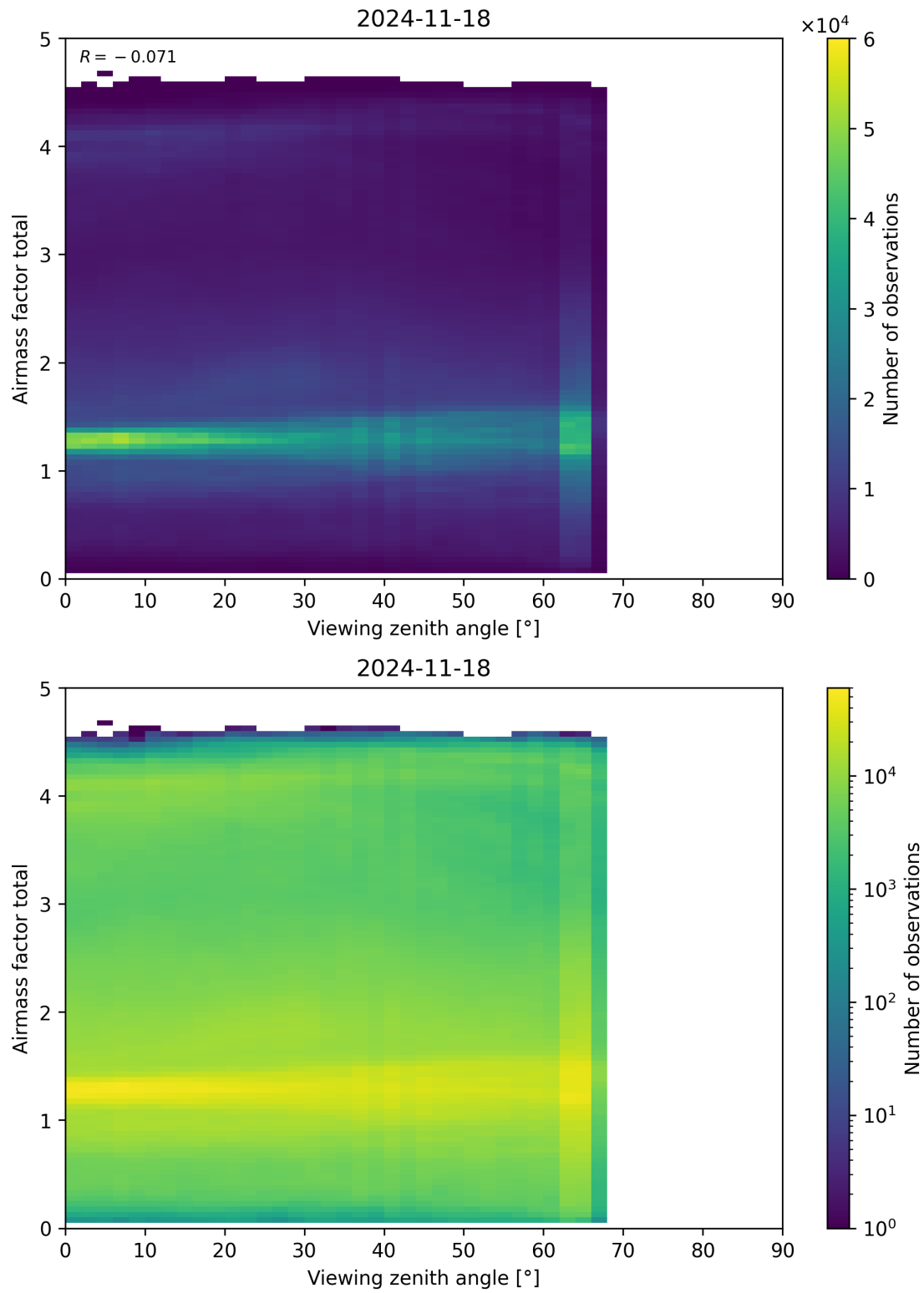
Figure 190: Scatter density plot of “Viewing zenith angle” against “Airmass factor total” for 2024-11-17 to 2024-11-19.
