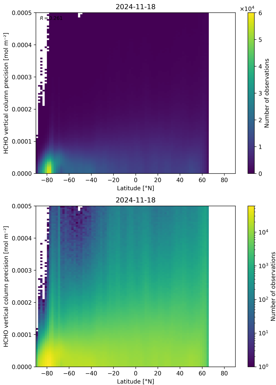
Figure 165: Scatter density plot of “Latitude” against “HCHO vertical column precision” for 2024-11-17 to 2024-11-19.
