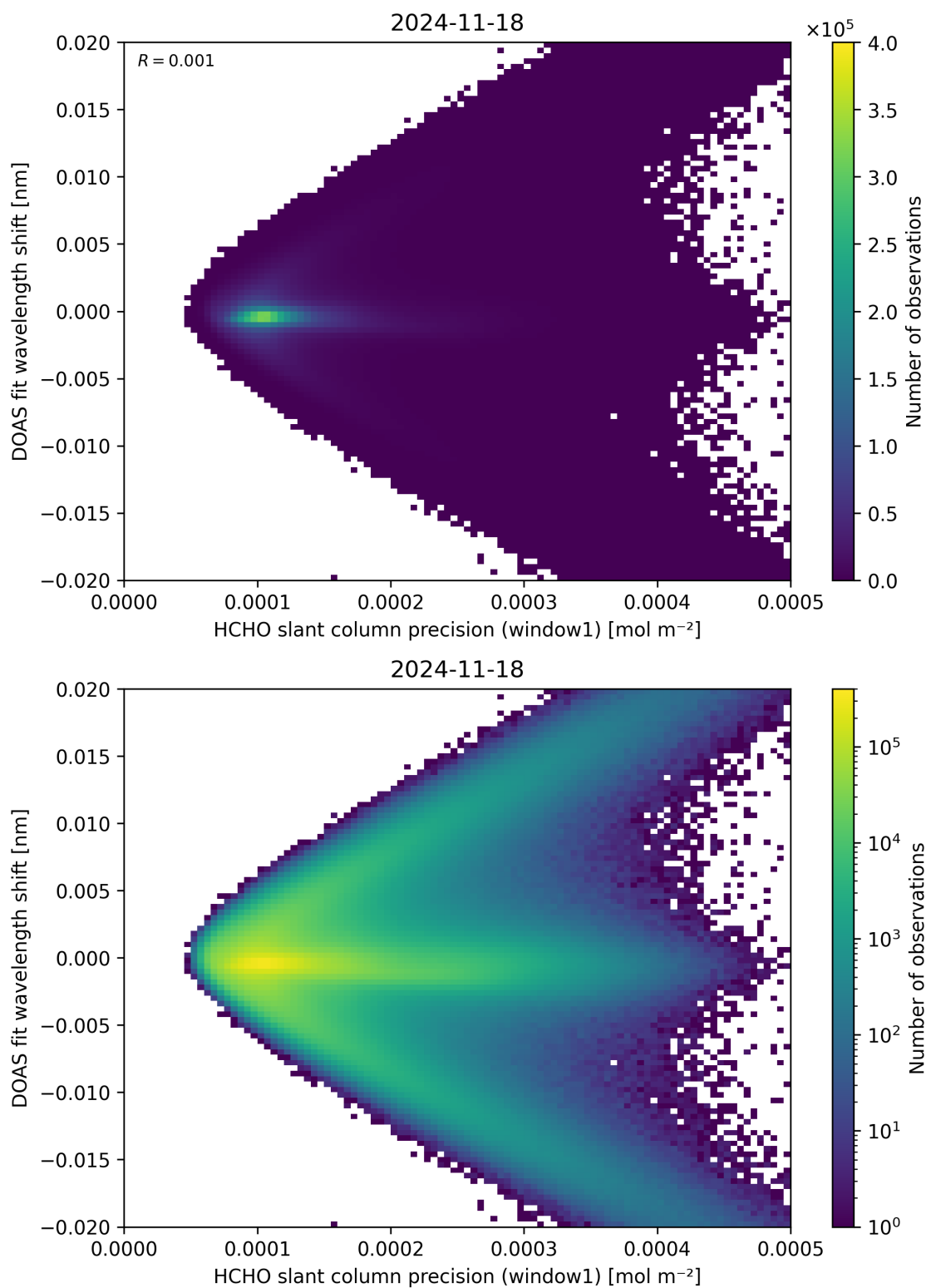
Figure 89: Scatter density plot of “HCHO slant column precision (window1)” against “DOAS fit wavelength shift” for 2024-11-17 to 2024-11-19.
