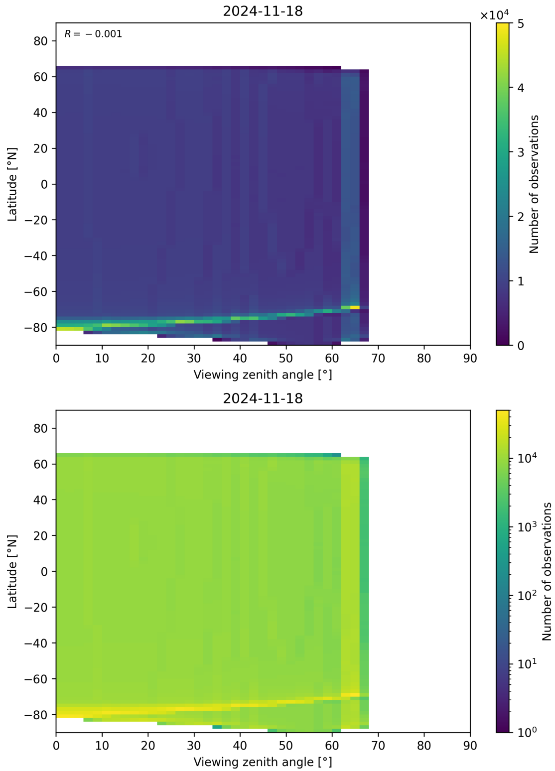
Figure 196: Scatter density plot of “Viewing zenith angle” against “Latitude” for 2024-11-17 to 2024-11-19.
