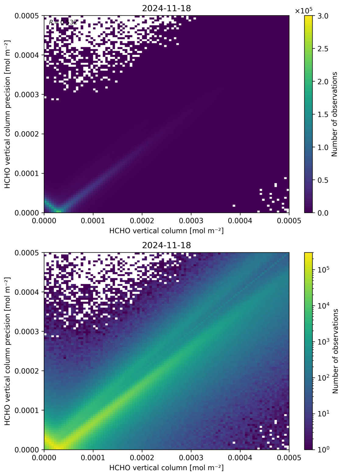
Figure 134: Scatter density plot of “HCHO vertical column” against “HCHO vertical column precision” for 2024-11-17 to 2024-11-19.
