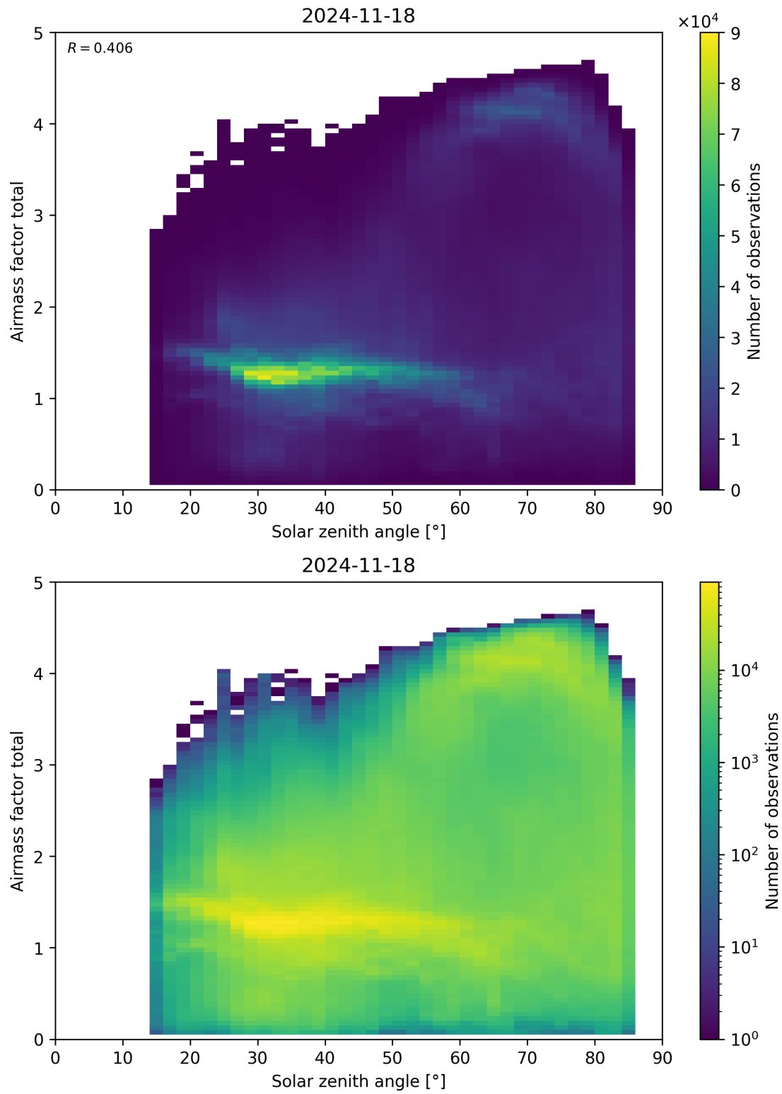
Figure 175: Scatter density plot of “Solar zenith angle” against “Airmass factor total” for 2024-11-17 to 2024-11-19.
