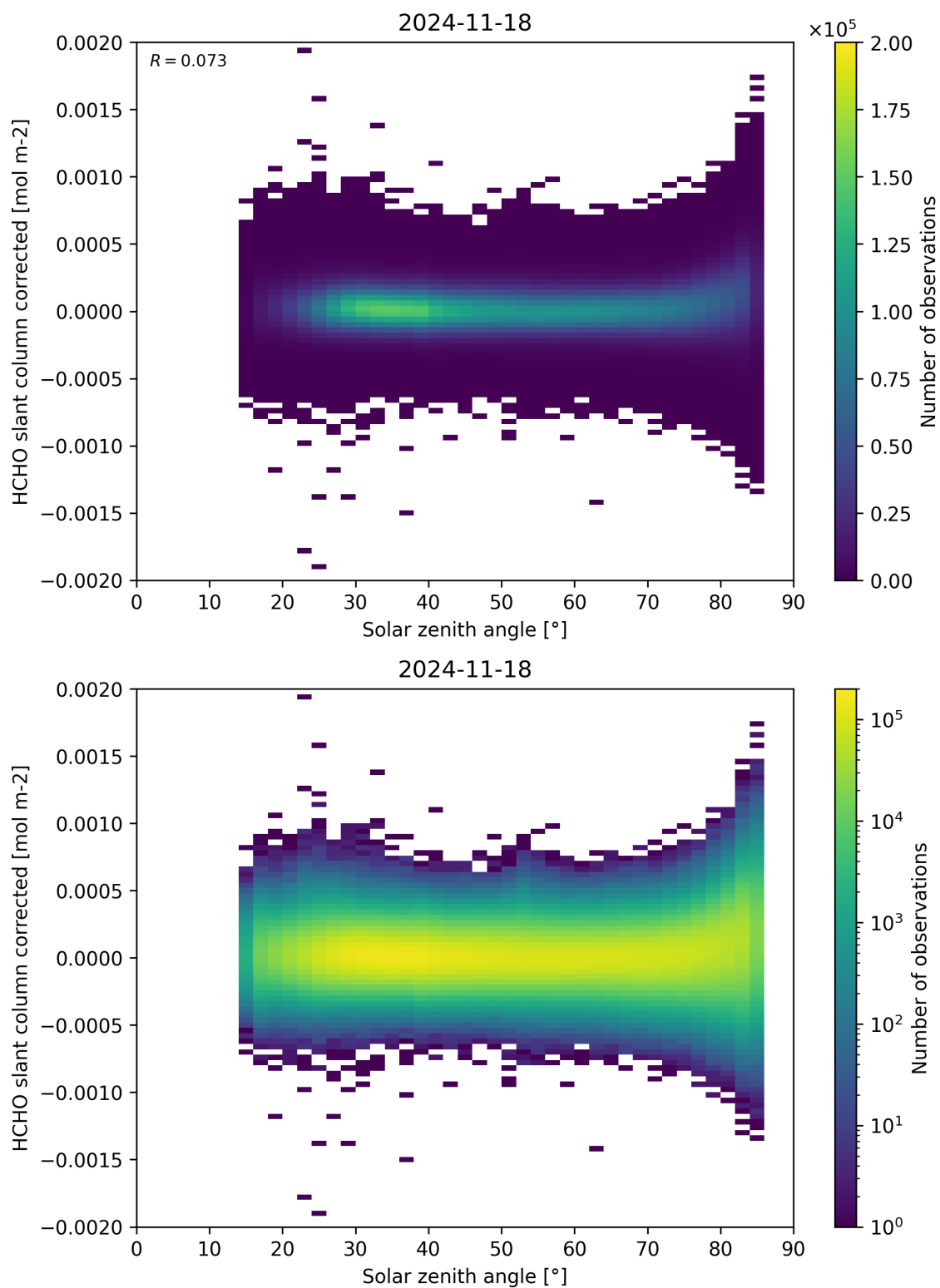
Figure 171: Scatter density plot of “Solar zenith angle” against “HCHO slant column corrected” for 2024-11-17 to 2024-11-19.
