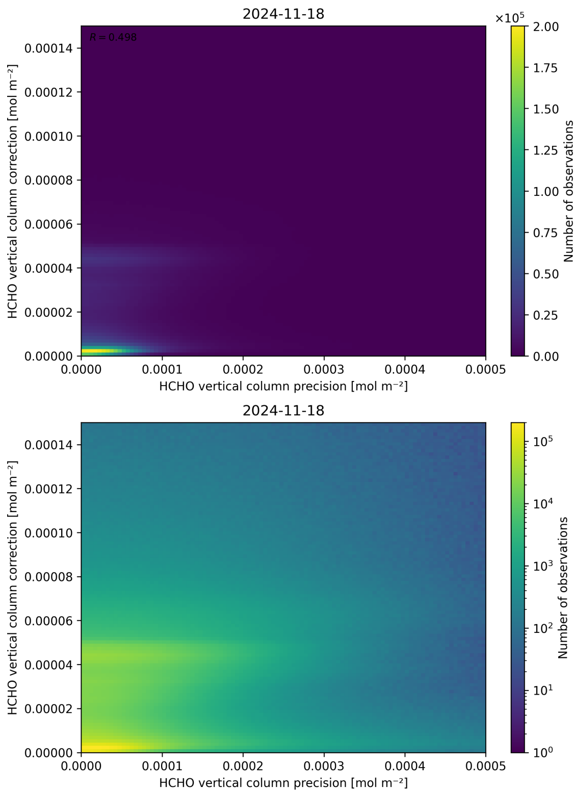
Figure 146: Scatter density plot of “HCHO vertical column precision” against “HCHO vertical column correction” for 2024-11-17 to 2024-11-19.
