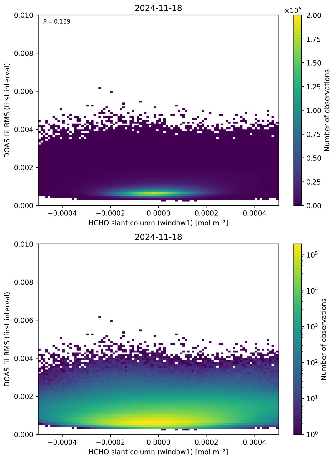
Figure 78: Scatter density plot of “HCHO slant column (window1)” against “DOAS fit RMS (first interval)” for 2024-11-17 to 2024-11-19.
