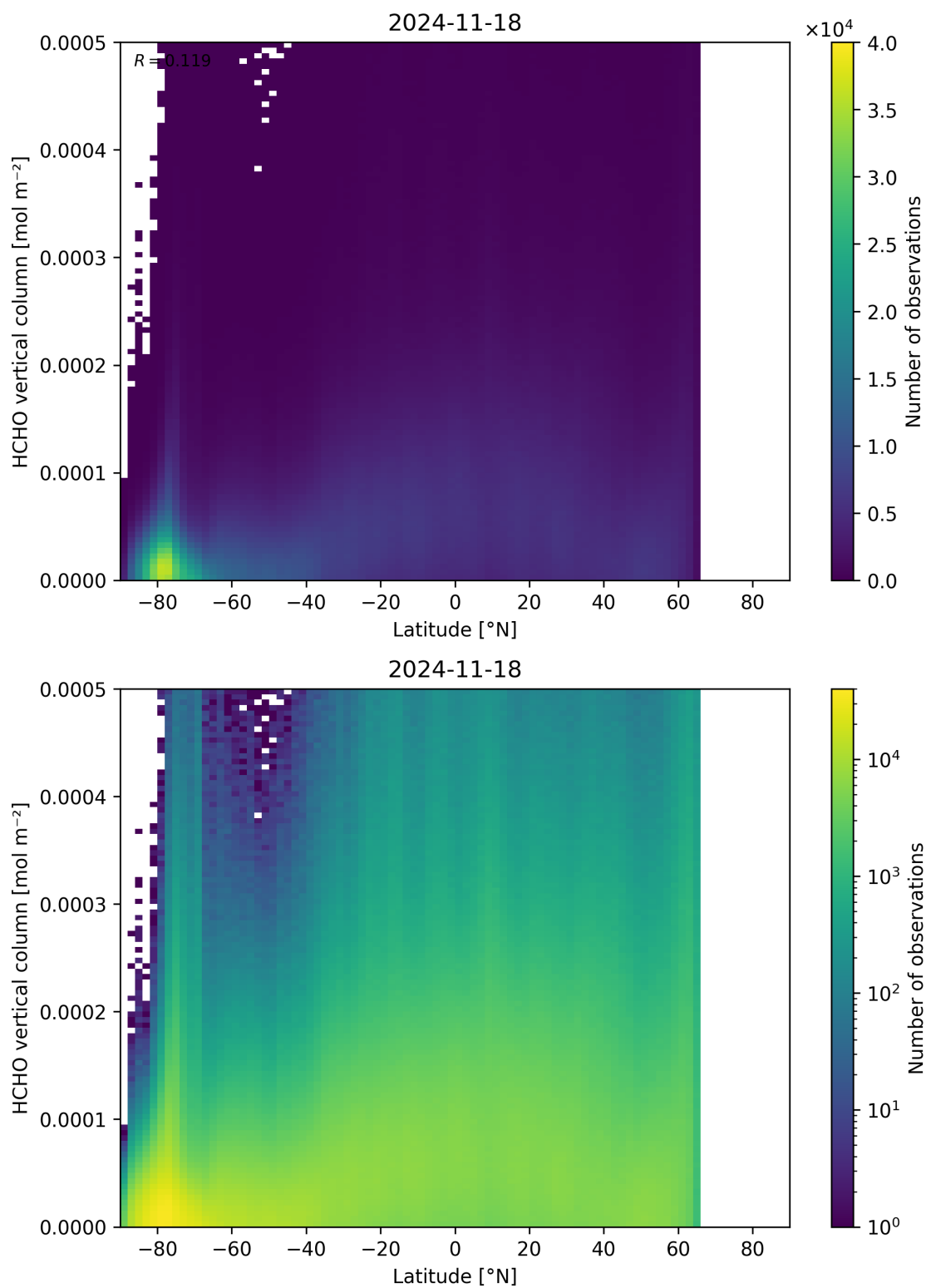
Figure 163: Scatter density plot of “Latitude” against “HCHO vertical column” for 2024-11-17 to 2024-11-19.
