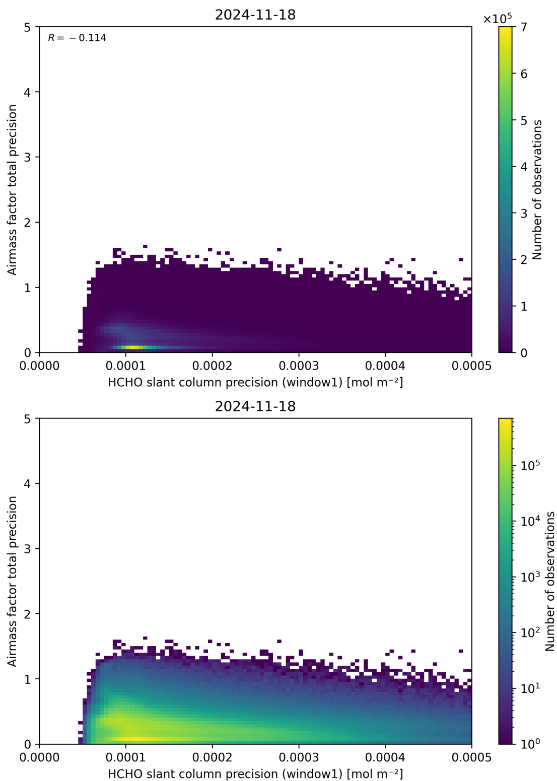
Figure 95: Scatter density plot of “HCHO slant column precision (window1)” against “Airmass factor total precision” for 2024-11-17 to 2024-11-19.
