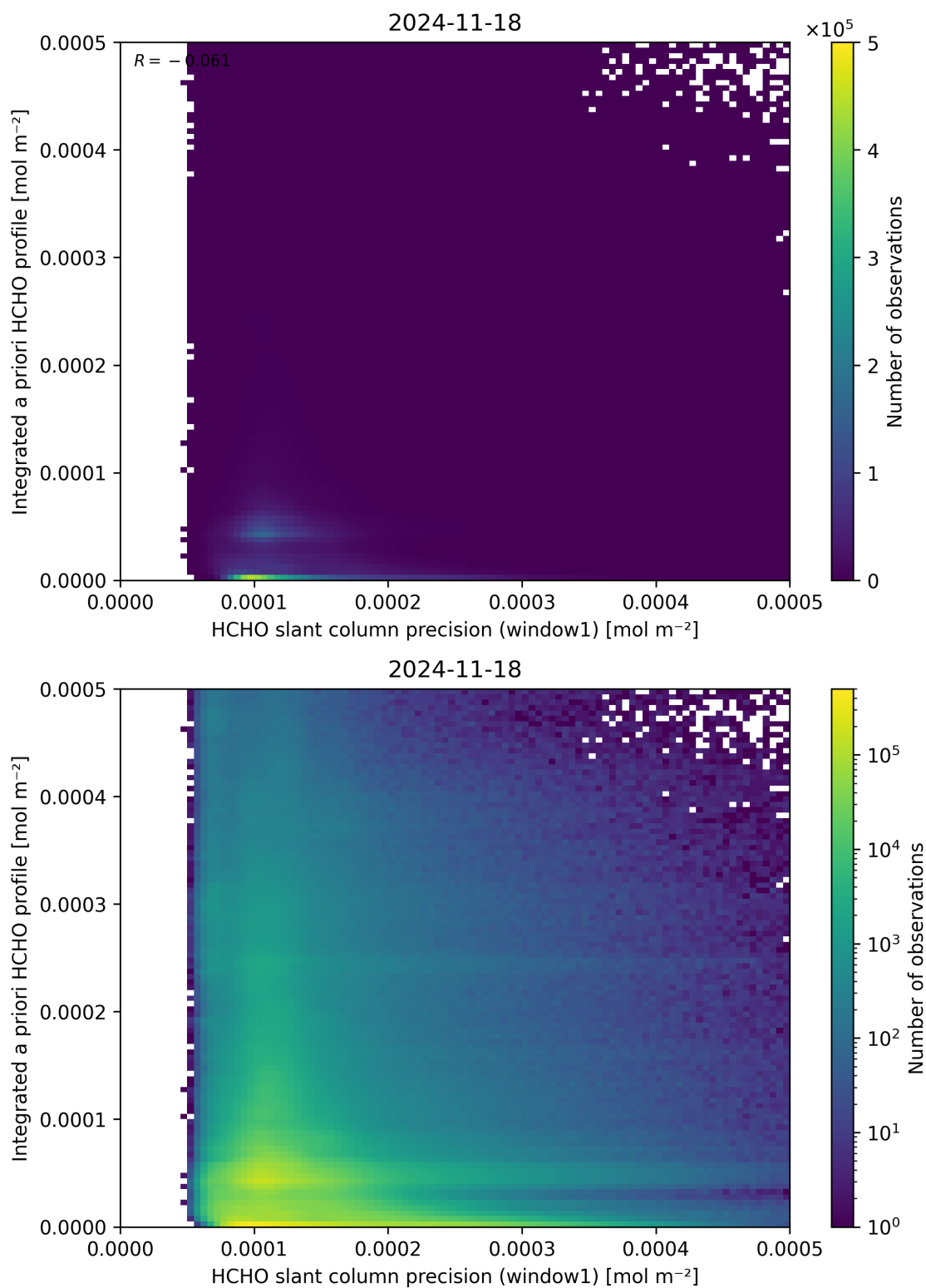
Figure 96: Scatter density plot of “HCHO slant column precision (window1)” against “Integrated a priori HCHO profile” for 2024-11-17 to 2024-11-19.
