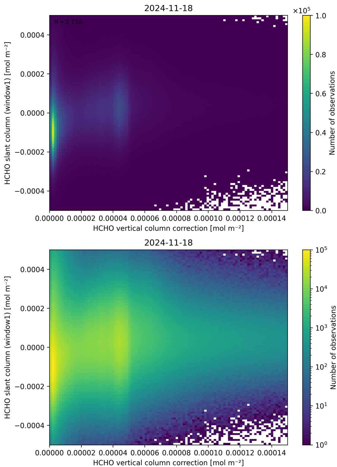
Figure 118: Scatter density plot of “HCHO vertical column correction” against “HCHO slant column (window1)” for 2024-11-17 to 2024-11-19.
