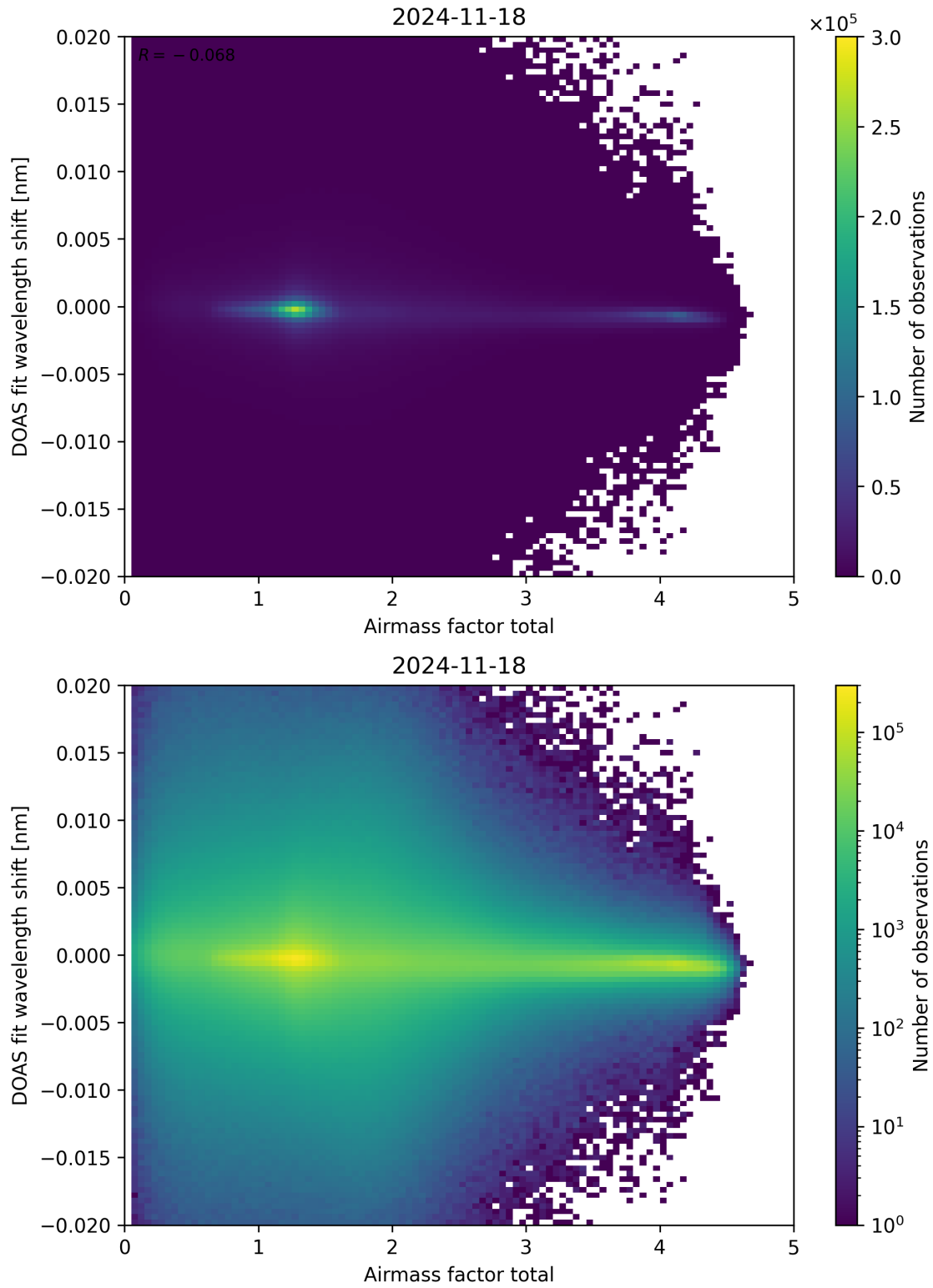
Figure 98: Scatter density plot of “Airmass factor total” against “DOAS fit wavelength shift” for 2024-11-17 to 2024-11-19.
