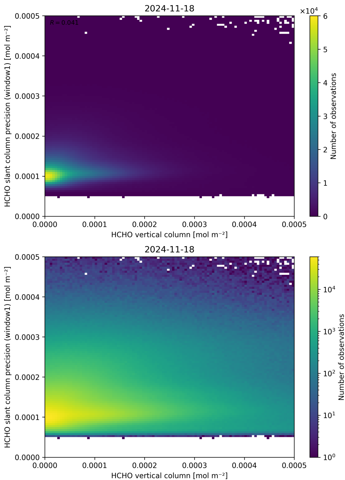
Figure 130: Scatter density plot of “HCHO vertical column” against “HCHO slant column precision (window1)” for 2024-11-17 to 2024-11-19.
