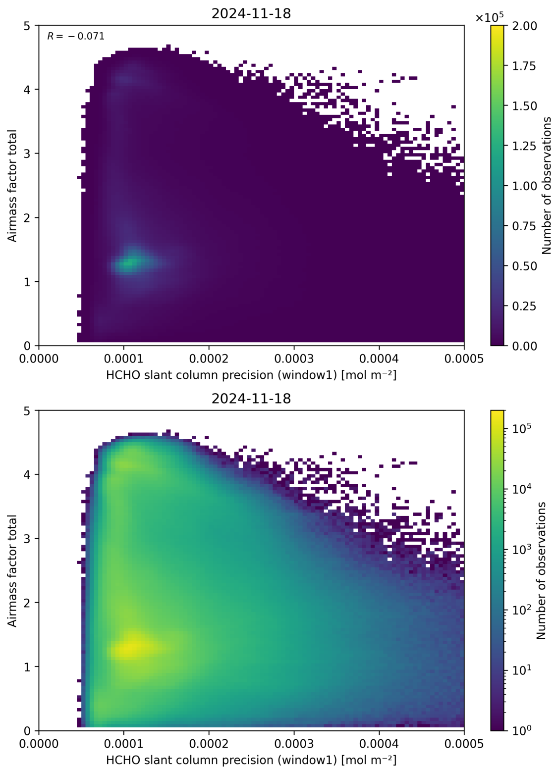
Figure 94: Scatter density plot of “HCHO slant column precision (window1)” against “Airmass factor total” for 2024-11-17 to 2024-11-19.
