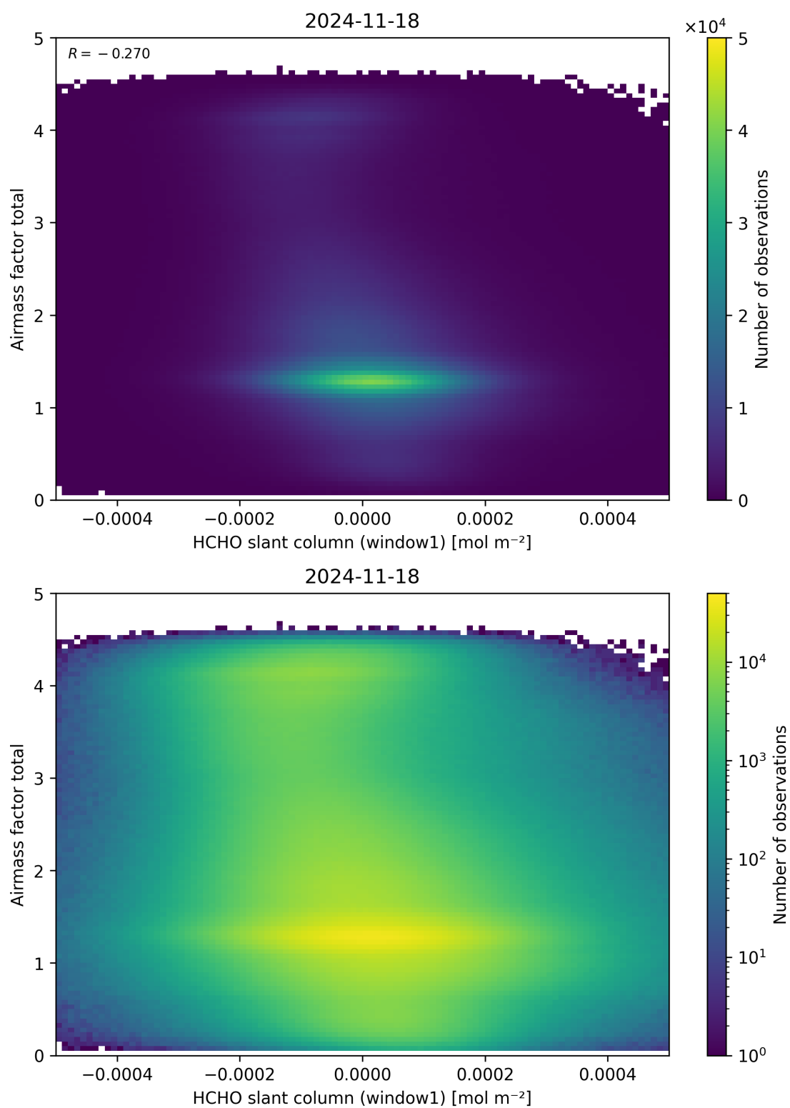
Figure 85: Scatter density plot of “HCHO slant column (window1)” against “Airmass factor total” for 2024-11-17 to 2024-11-19.
