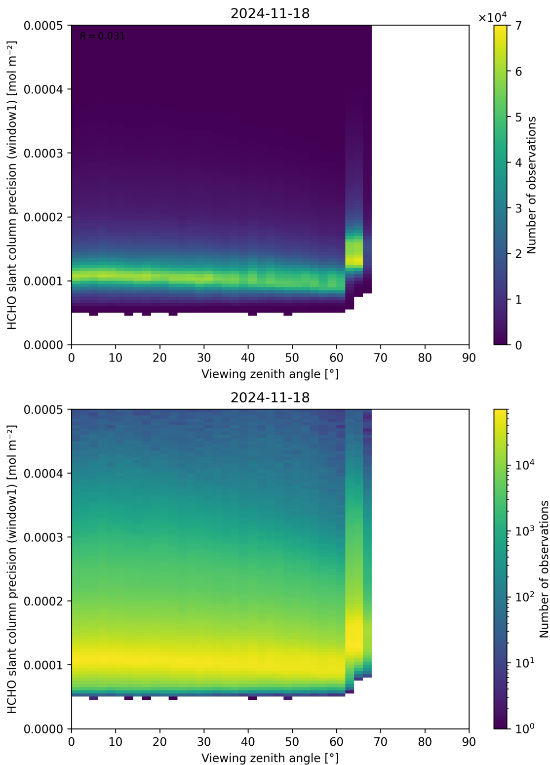
Figure 189: Scatter density plot of “Viewing zenith angle” against “HCHO slant column precision (window1)” for 2024-11-17 to 2024-11-19.
