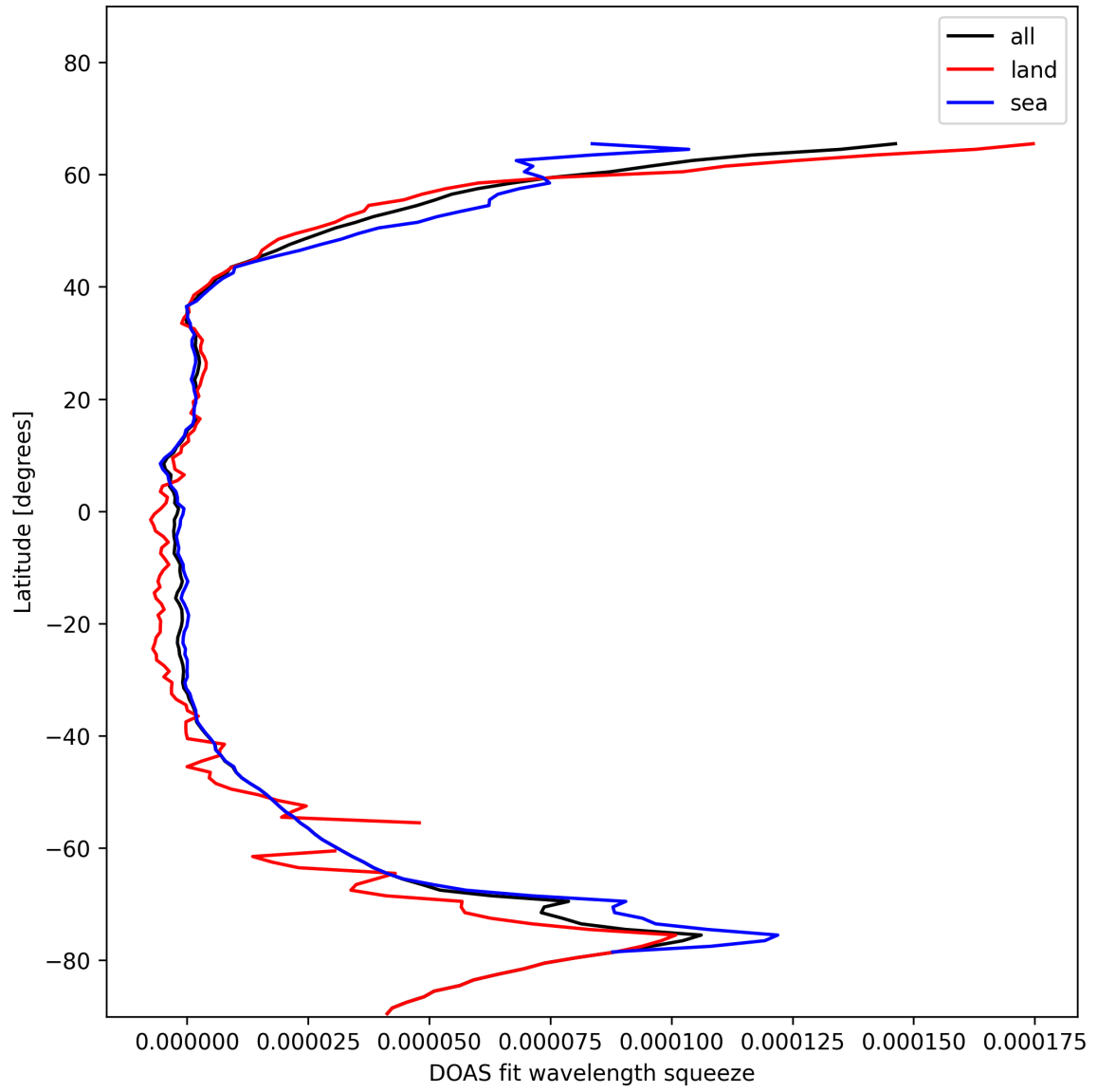
Figure 31: Zonal average of “DOAS fit wavelength squeeze” for 2024-11-17 to 2024-11-19.
