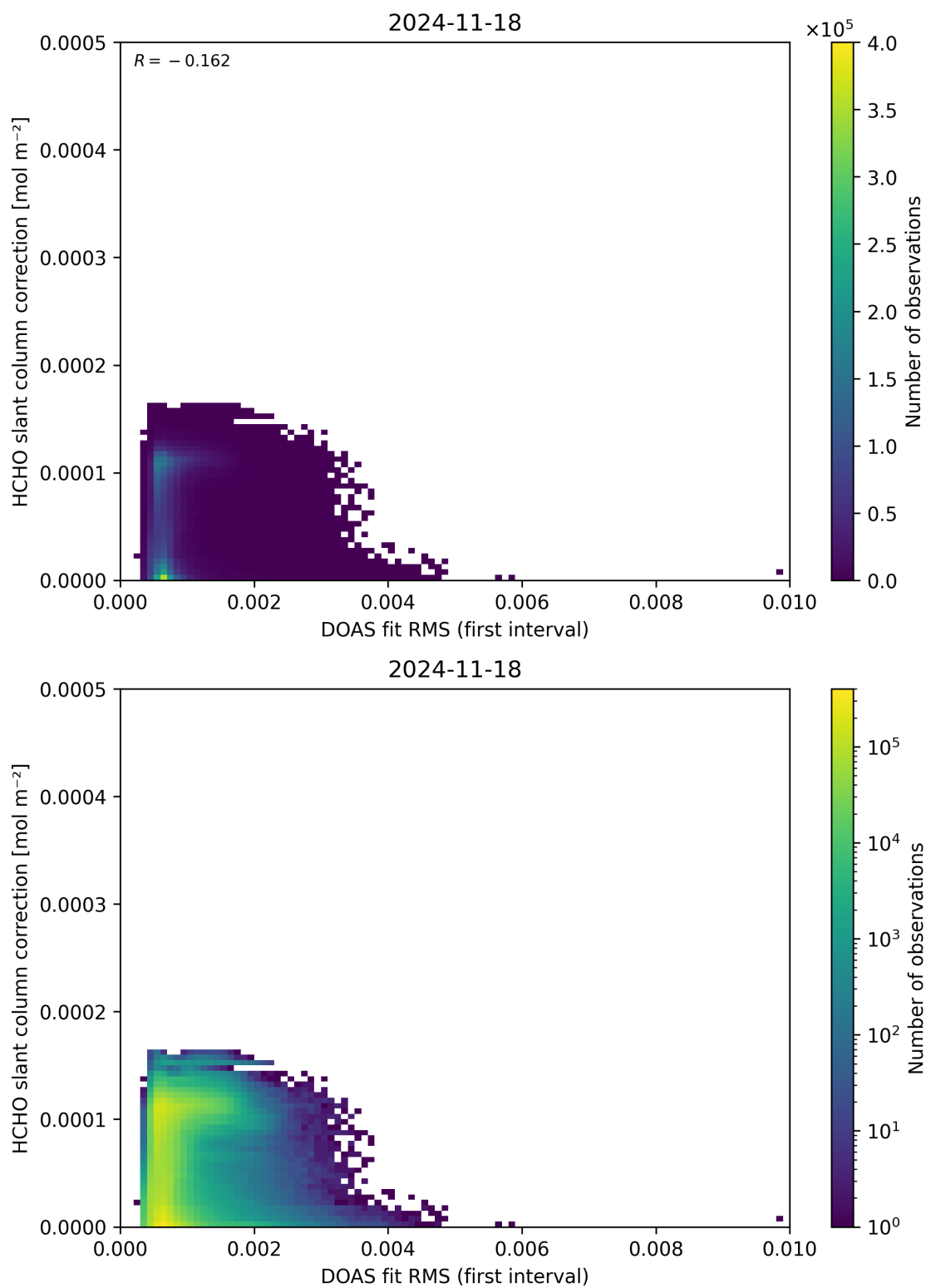
Figure 63: Scatter density plot of “DOAS fit RMS (first interval)” against “HCHO slant column correction” for 2024-11-17 to 2024-11-19.
