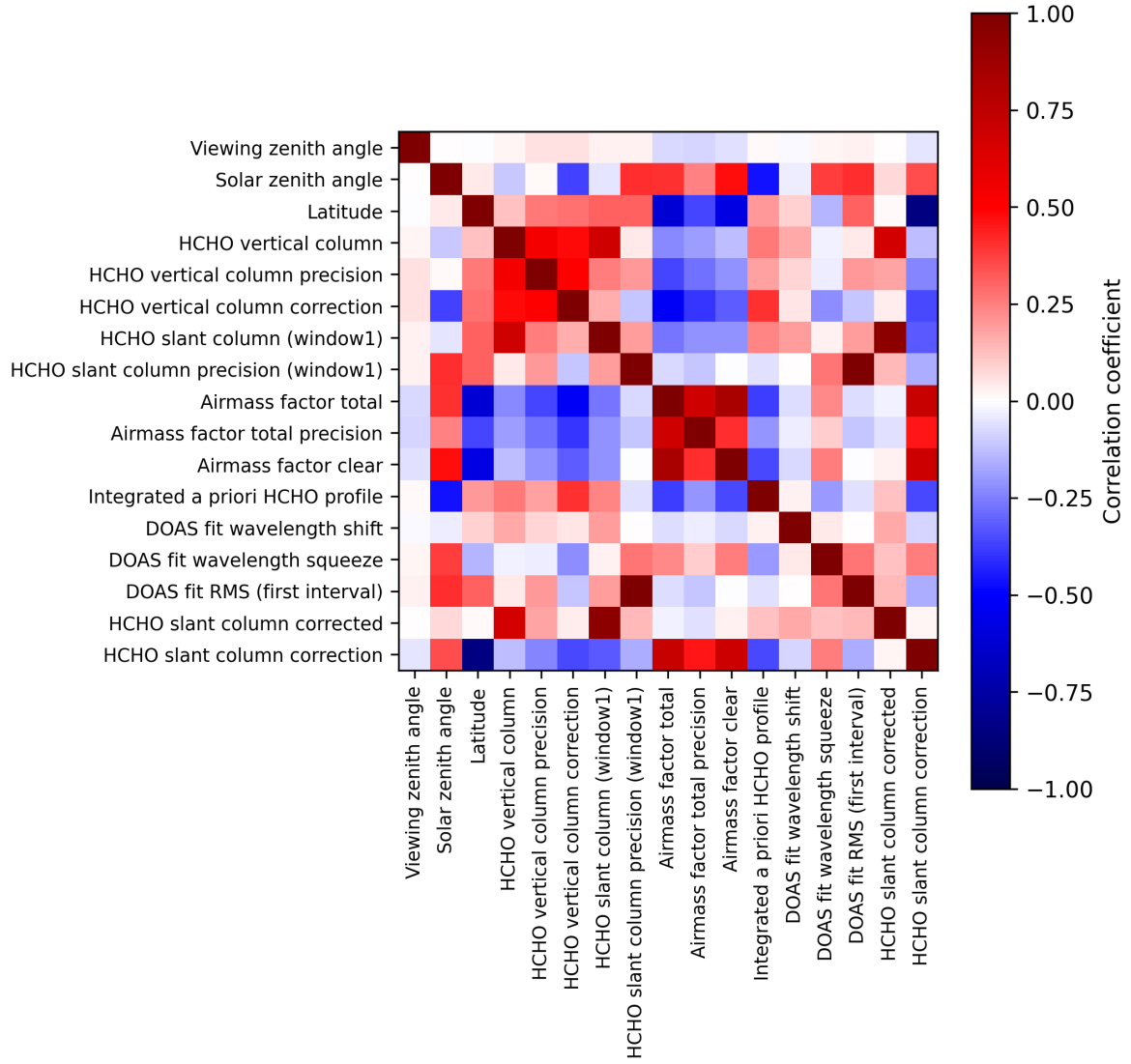
Figure 2: Map of correlation matrix for 2024-11-17 to 2024-11-19.
