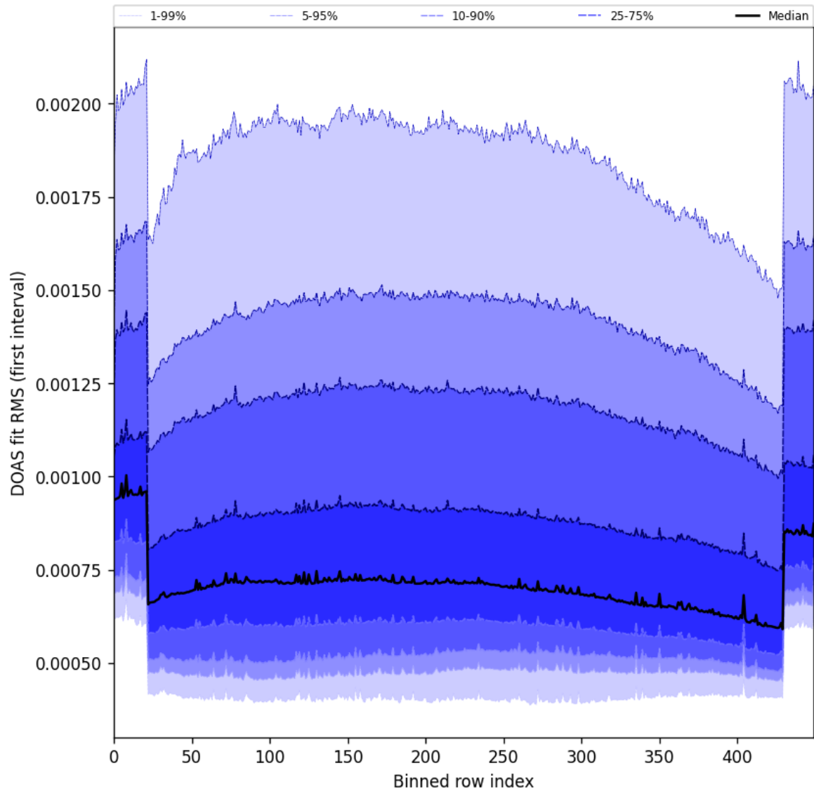
Figure 60: Along track statistics of “DOAS fit RMS (first interval)” for 2024-11-17 to 2024-11-19
