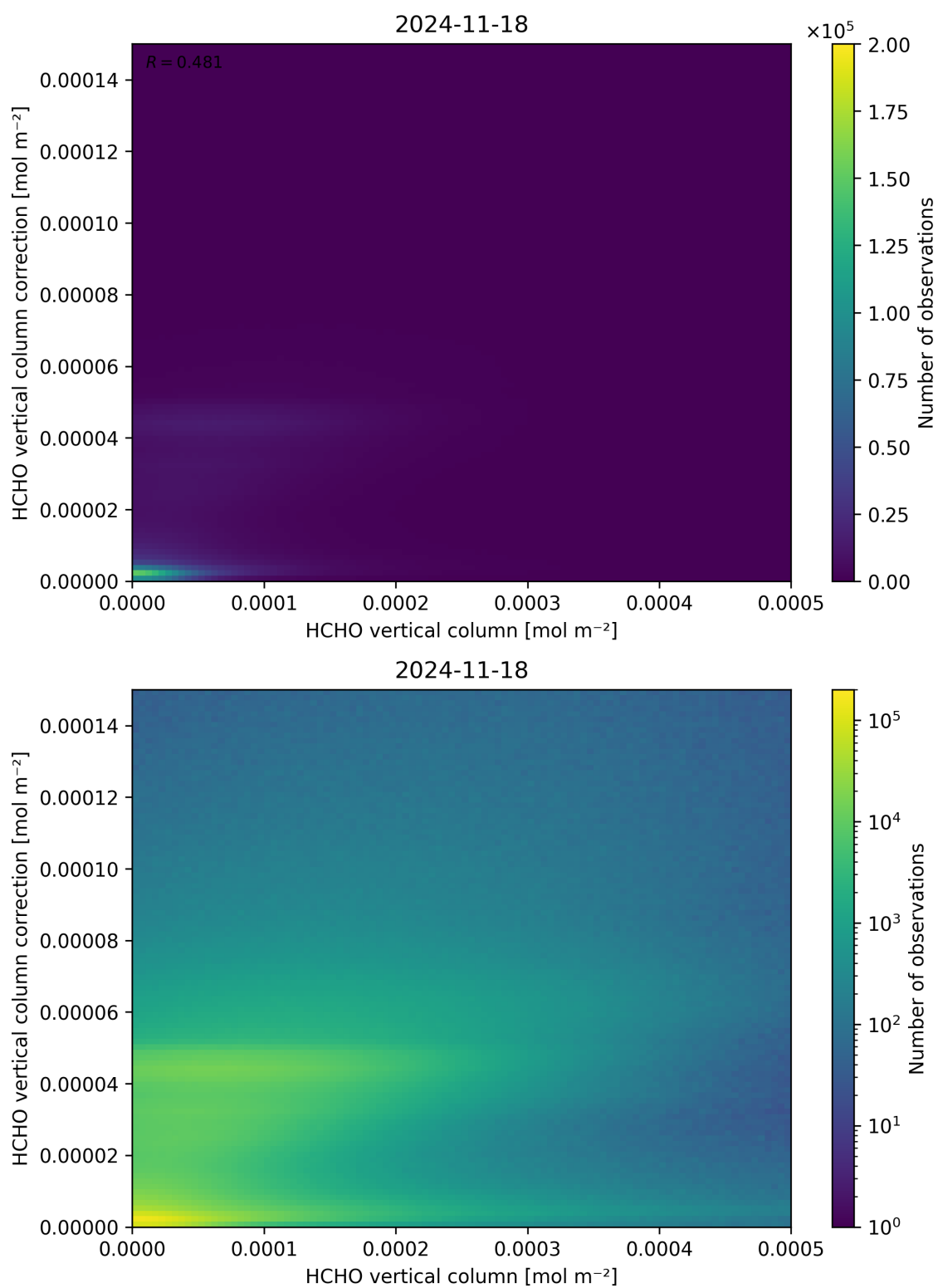
Figure 133: Scatter density plot of “HCHO vertical column” against “HCHO vertical column correction” for 2024-11-17 to 2024-11-19.
