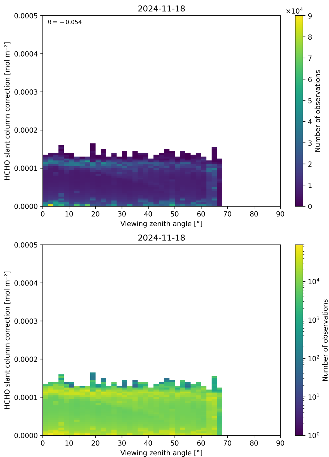
Figure 187: Scatter density plot of “Viewing zenith angle” against “HCHO slant column correction” for 2024-11-17 to 2024-11-19.
