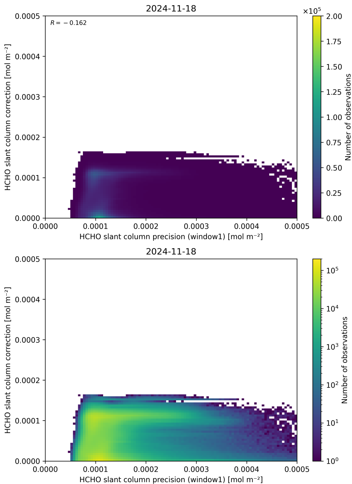
Figure 93: Scatter density plot of “HCHO slant column precision (window1)” against “HCHO slant column correction” for 2024-11-17 to 2024-11-19.
