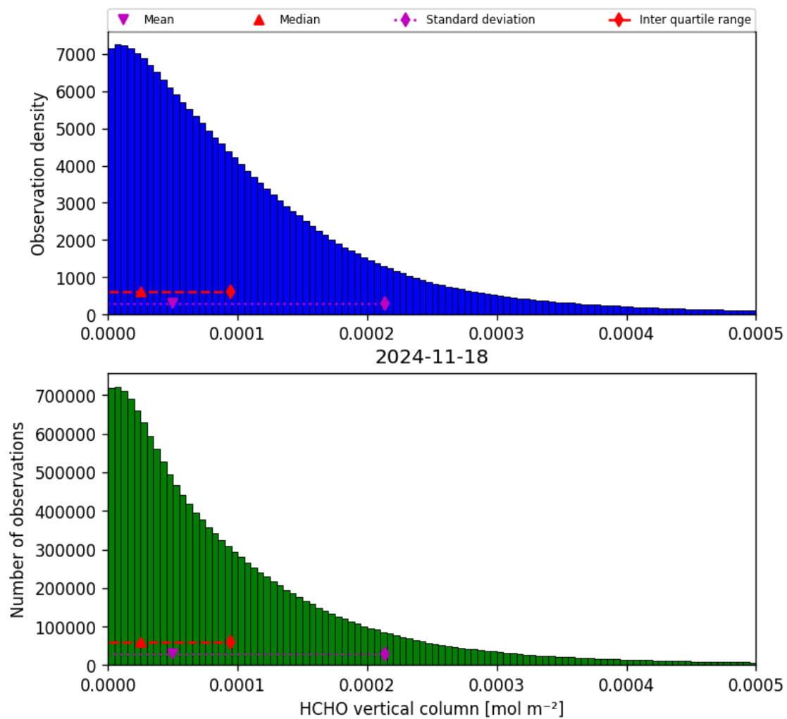
Figure 35: Histogram of “HCHO vertical column” for 2024-11-17 to 2024-11-19
