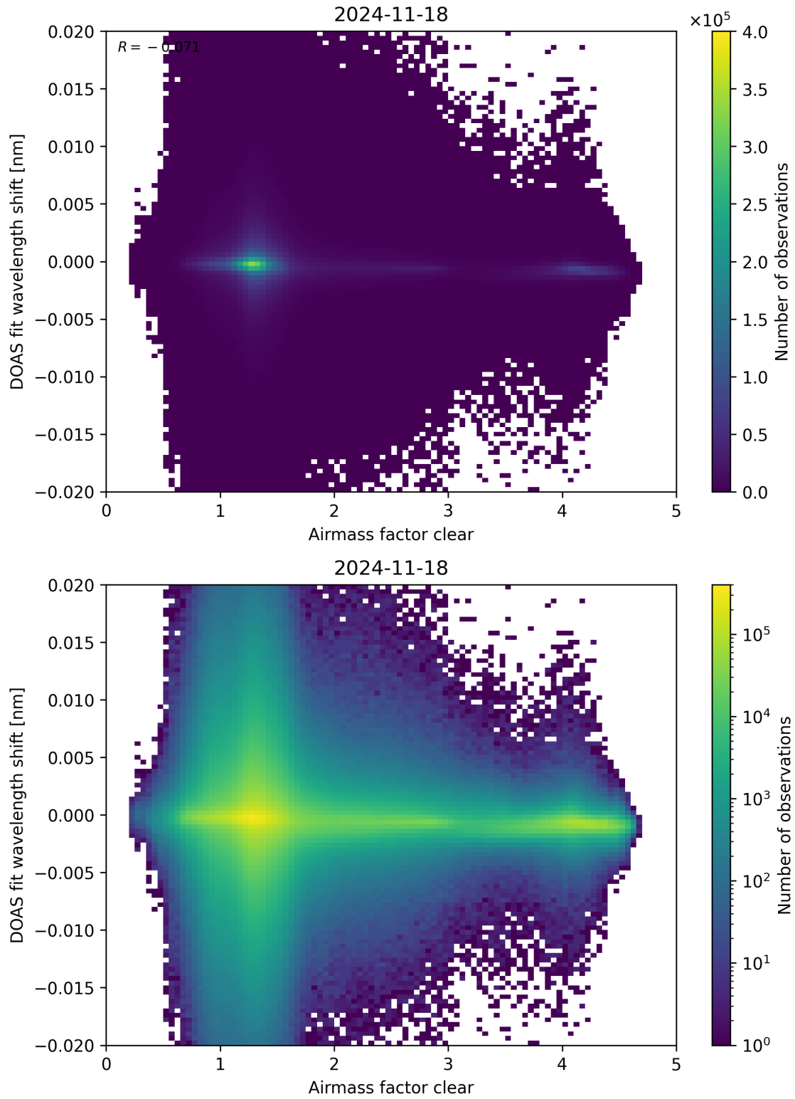
Figure 72: Scatter density plot of “Airmass factor clear” against “DOAS fit wavelength shift” for 2024-11-17 to 2024-11-19.
