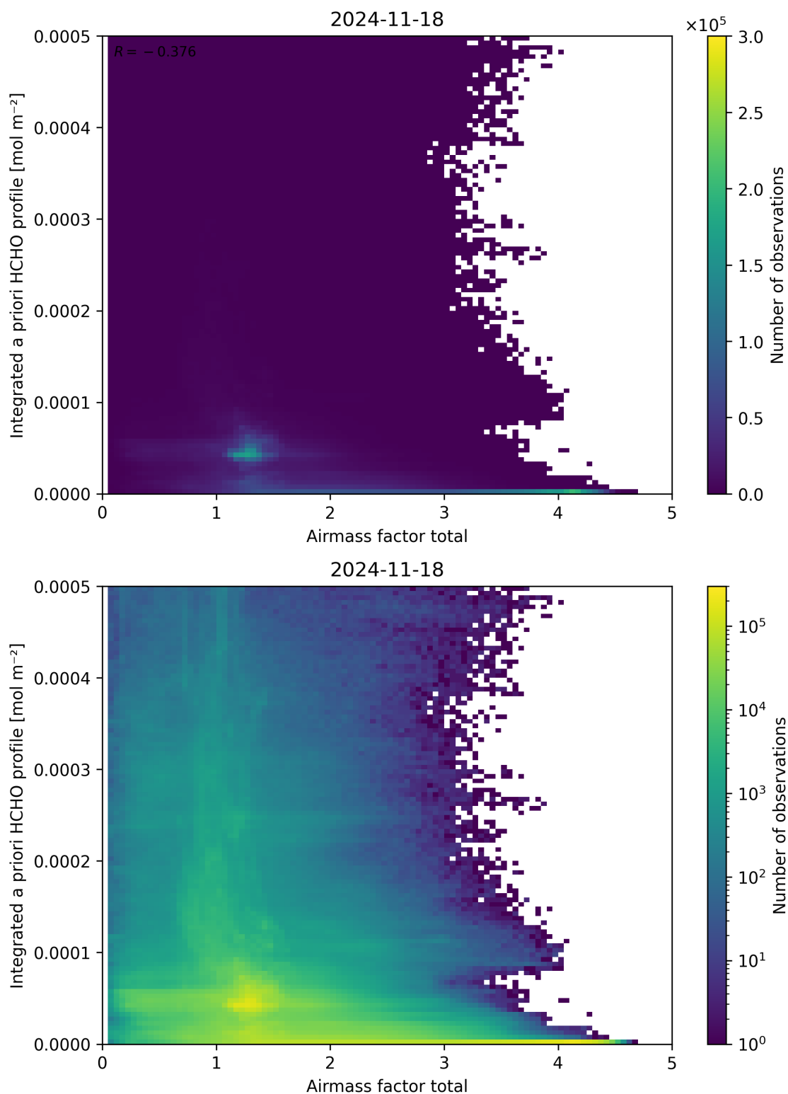
Figure 104: Scatter density plot of “Airmass factor total” against “Integrated a priori HCHO profile” for 2024-11-17 to 2024-11-19.
