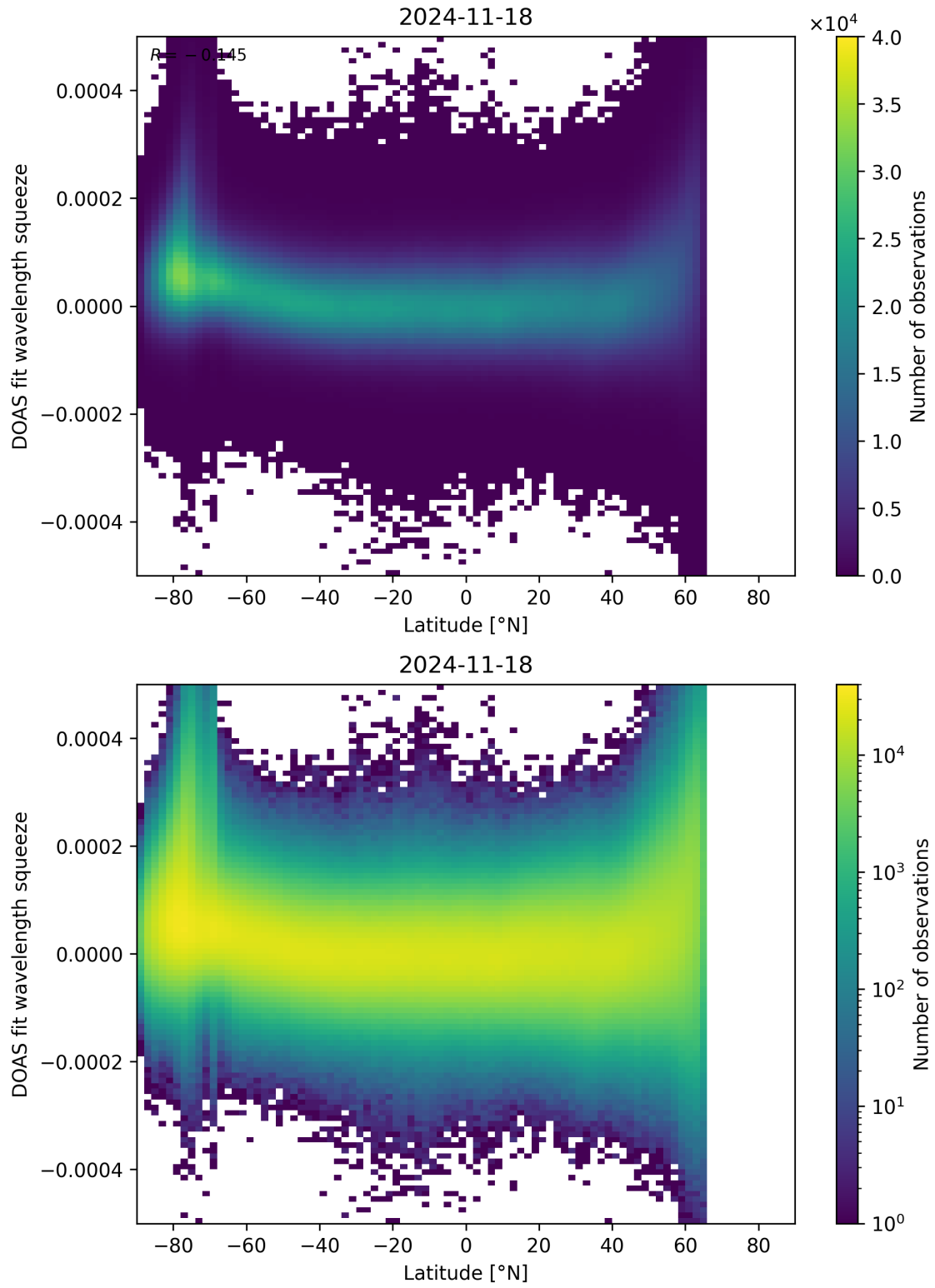
Figure 155: Scatter density plot of “Latitude” against “DOAS fit wavelength squeeze” for 2024-11-17 to 2024-11-19.
