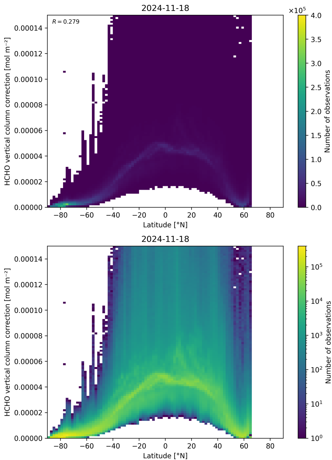
Figure 164: Scatter density plot of “Latitude” against “HCHO vertical column correction” for 2024-11-17 to 2024-11-19.
