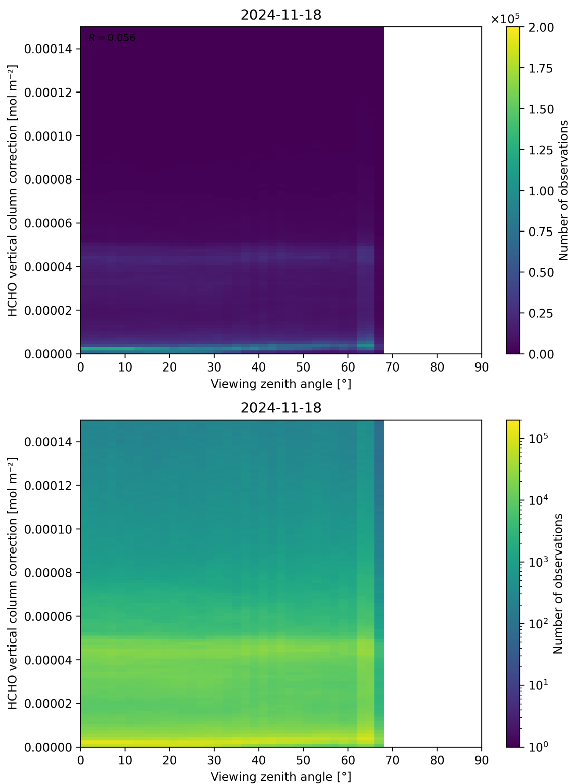
Figure 193: Scatter density plot of “Viewing zenith angle” against “HCHO vertical column correction” for 2024-11-17 to 2024-11-19.
