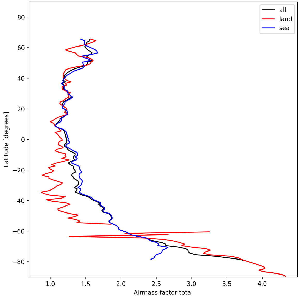
Figure 26: Zonal average of “Airmass factor total” for 2024-11-17 to 2024-11-19.
