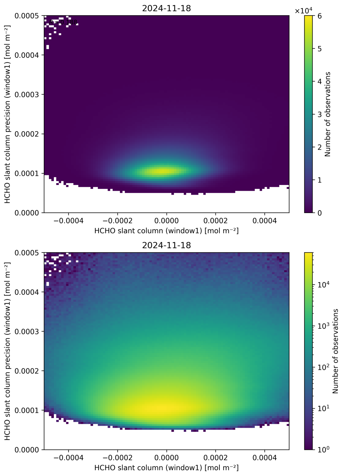
Figure 84: Scatter density plot of “HCHO slant column (window1)” against “HCHO slant column precision (window1)” for 2024-11-17 to 2024-11-19.
