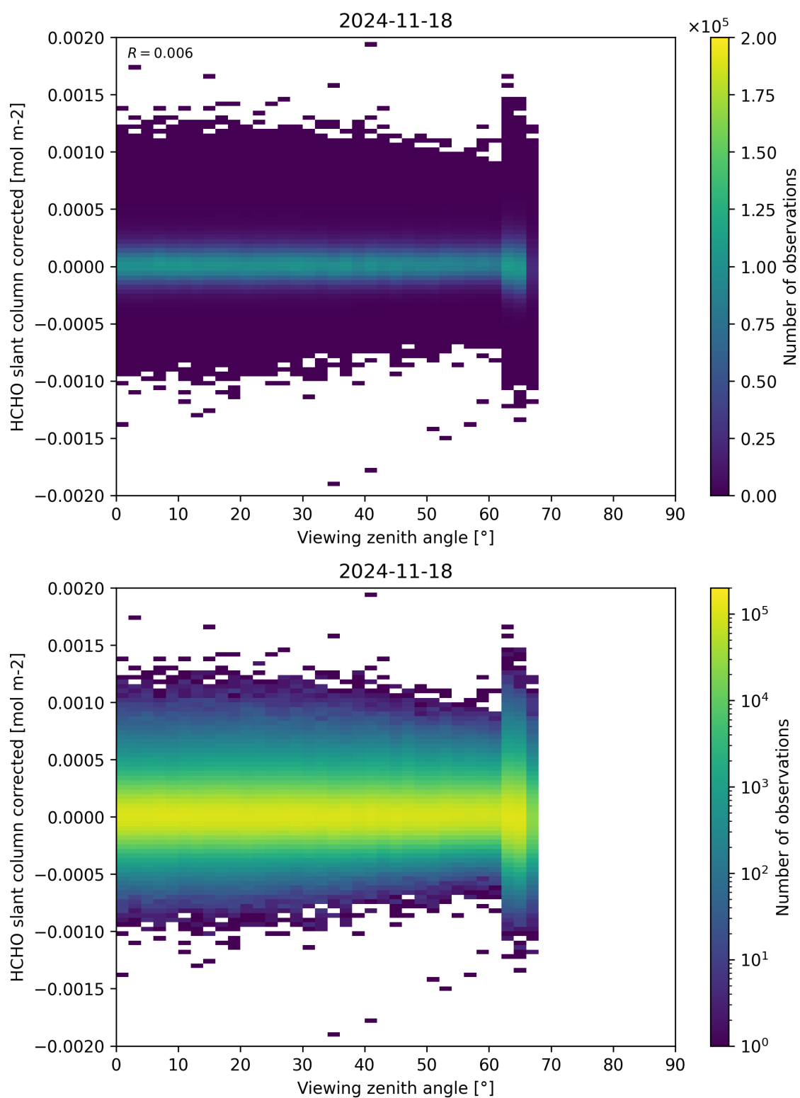
Figure 186: Scatter density plot of “Viewing zenith angle” against “HCHO slant column corrected” for 2024-11-17 to 2024-11-19.
