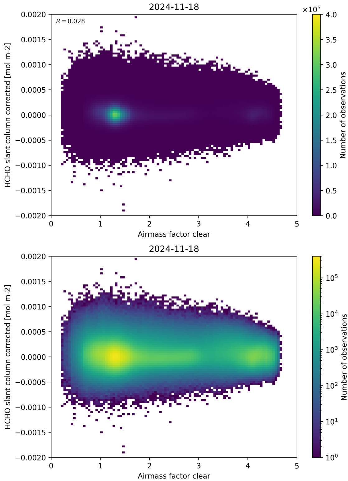
Figure 74: Scatter density plot of “Airmass factor clear” against “HCHO slant column corrected” for 2024-11-17 to 2024-11-19.
