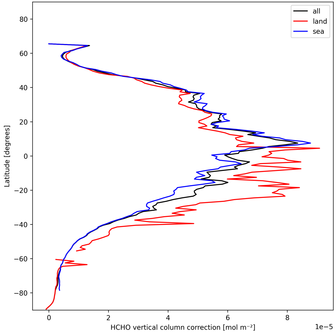
Figure 23: Zonal average of “HCHO vertical column correction” for 2024-11-17 to 2024-11-19.
