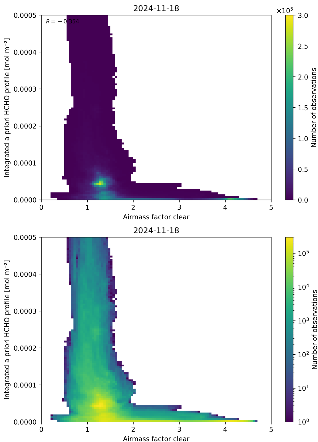
Figure 76: Scatter density plot of “Airmass factor clear” against “Integrated a priori HCHO profile” for 2024-11-17 to 2024-11-19.
