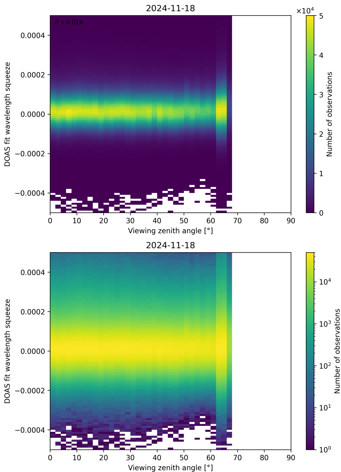
Figure 184: Scatter density plot of “Viewing zenith angle” against “DOAS fit wavelength squeeze” for 2024-11-17 to 2024-11-19.
