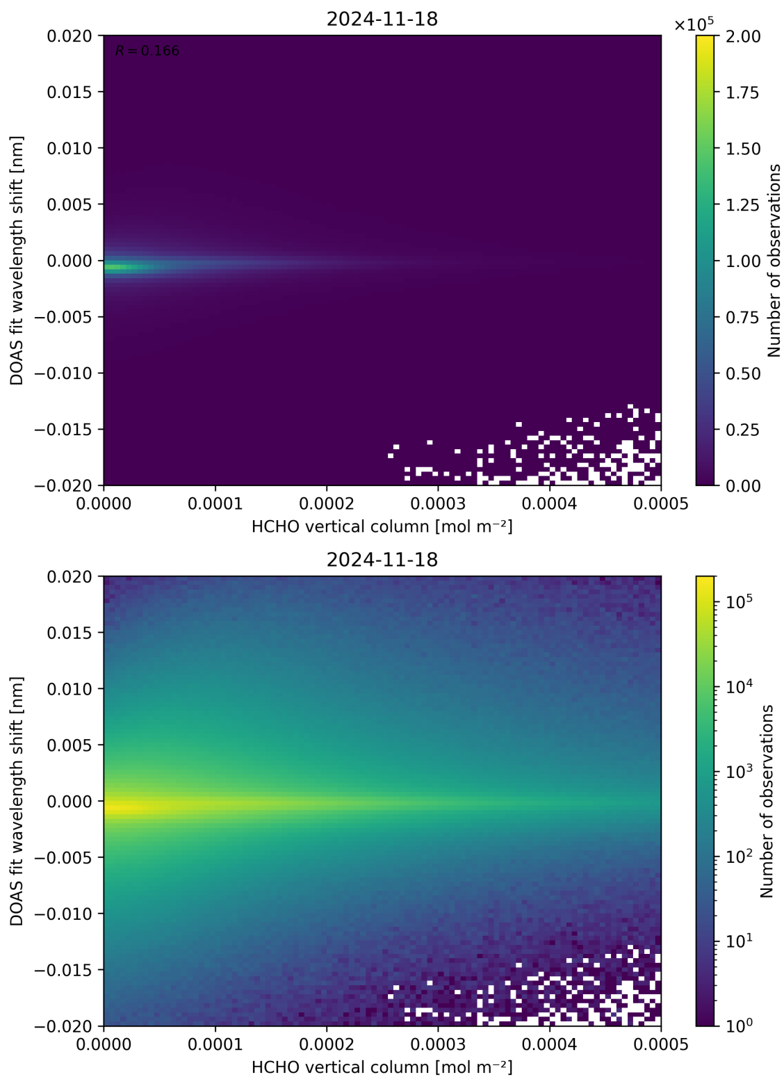
Figure 124: Scatter density plot of “HCHO vertical column” against “DOAS fit wavelength shift” for 2024-11-17 to 2024-11-19.
