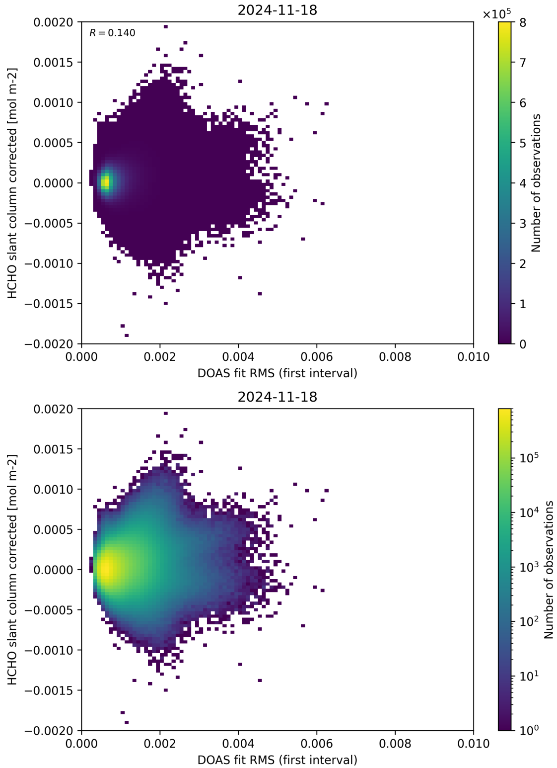
Figure 62: Scatter density plot of “DOAS fit RMS (first interval)” against “HCHO slant column corrected” for 2024-11-17 to 2024-11-19.
