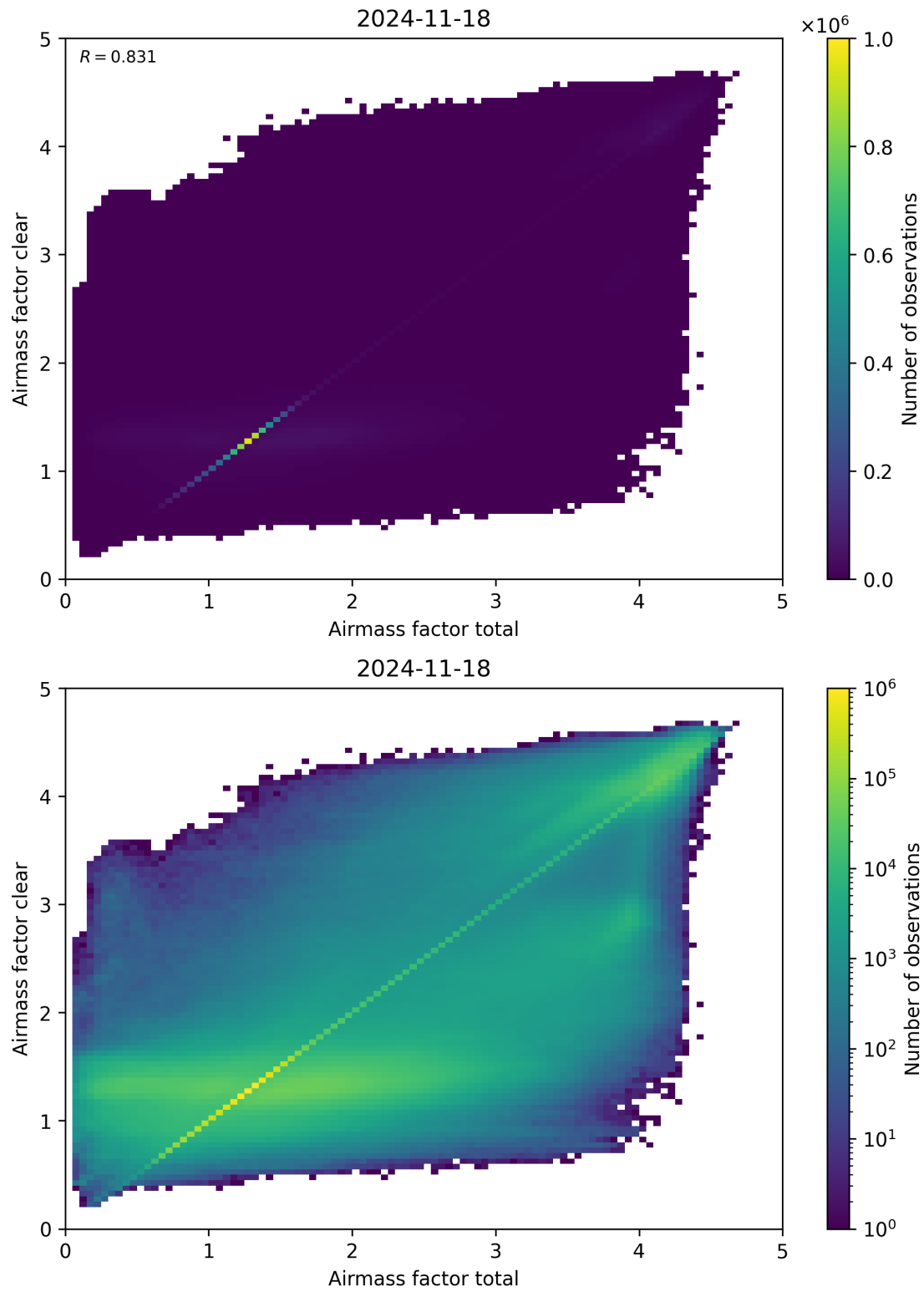
Figure 100: Scatter density plot of “Airmass factor total” against “Airmass factor clear” for 2024-11-17 to 2024-11-19.
