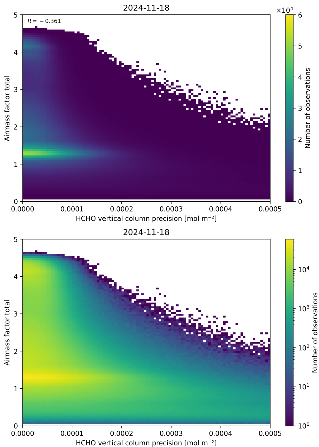
Figure 144: Scatter density plot of “HCHO vertical column precision” against “Airmass factor total” for 2024-11-17 to 2024-11-19.
