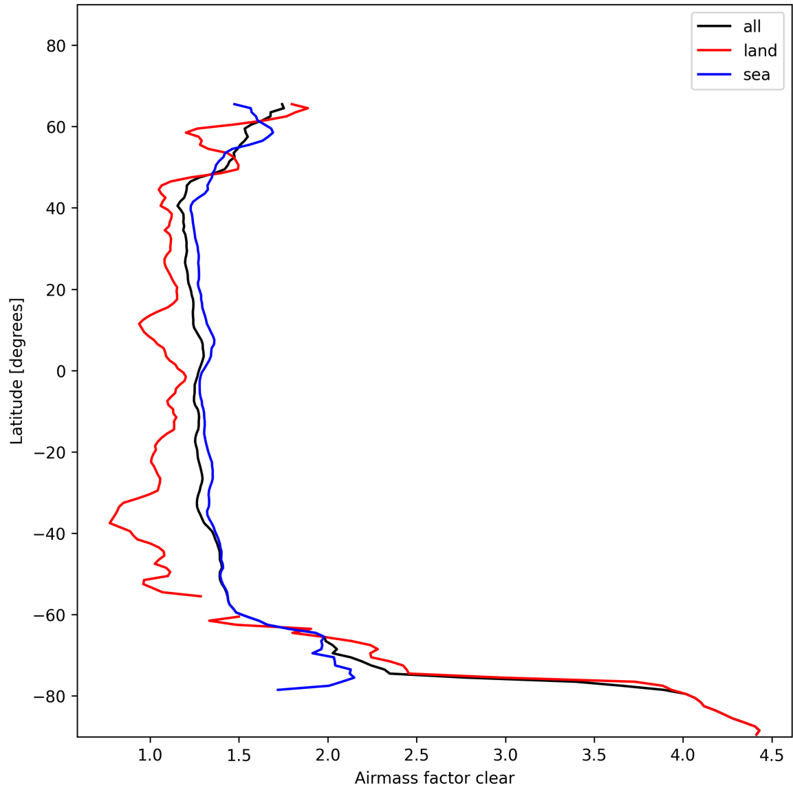
Figure 28: Zonal average of “Airmass factor clear” for 2024-11-17 to 2024-11-19.
