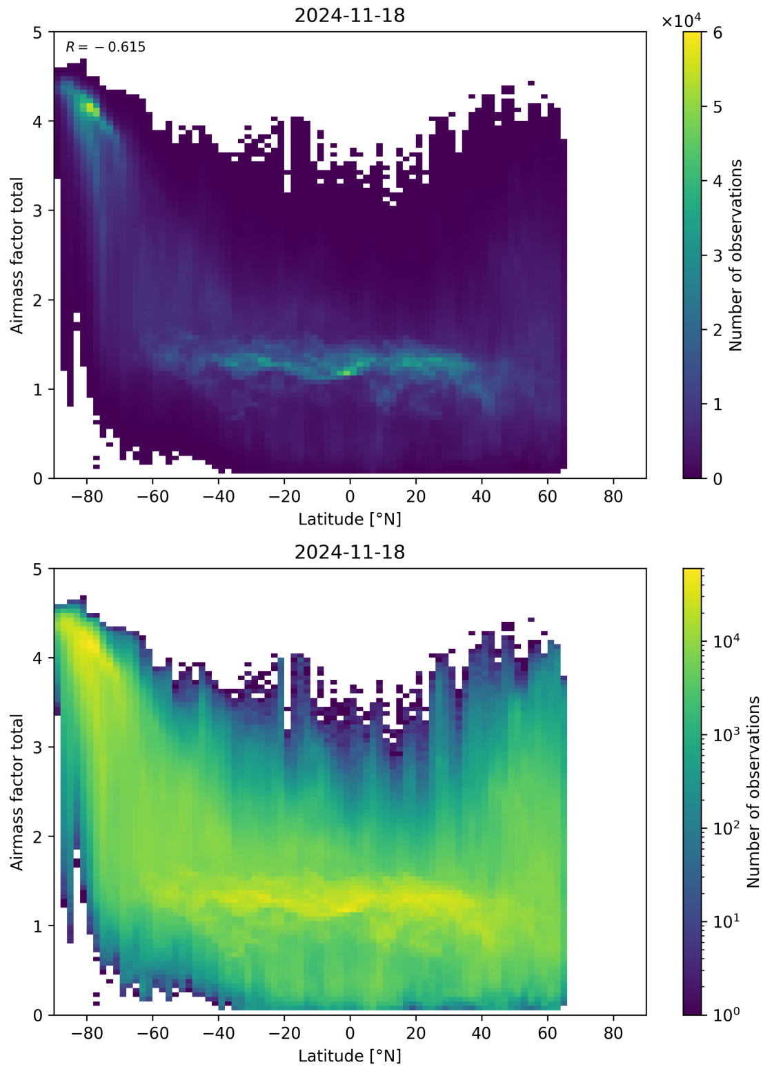
Figure 161: Scatter density plot of “Latitude” against “Airmass factor total” for 2024-11-17 to 2024-11-19.
