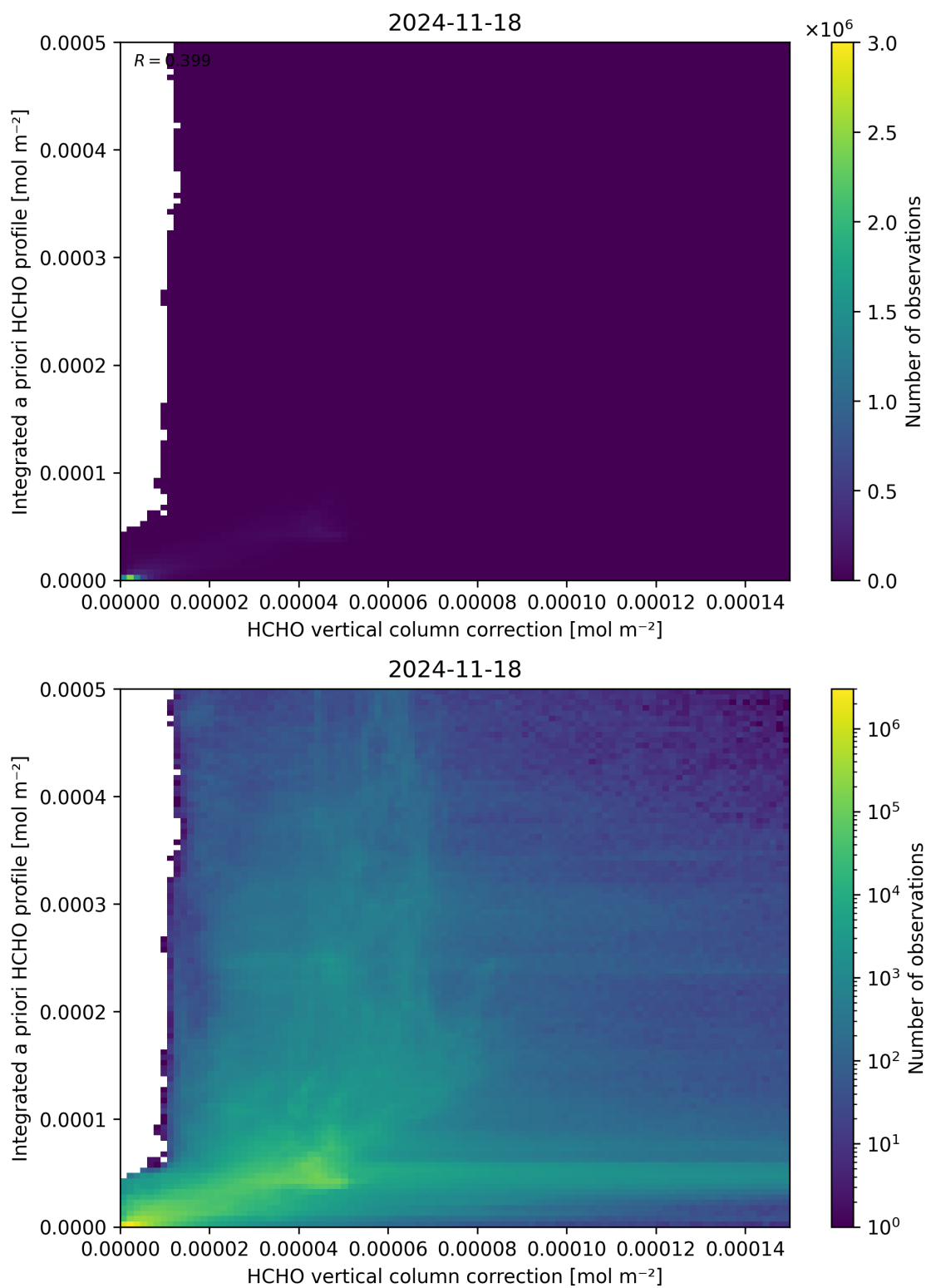
Figure 122: Scatter density plot of “HCHO vertical column correction” against “Integrated a priori HCHO profile” for 2024-11-17 to 2024-11-19.
