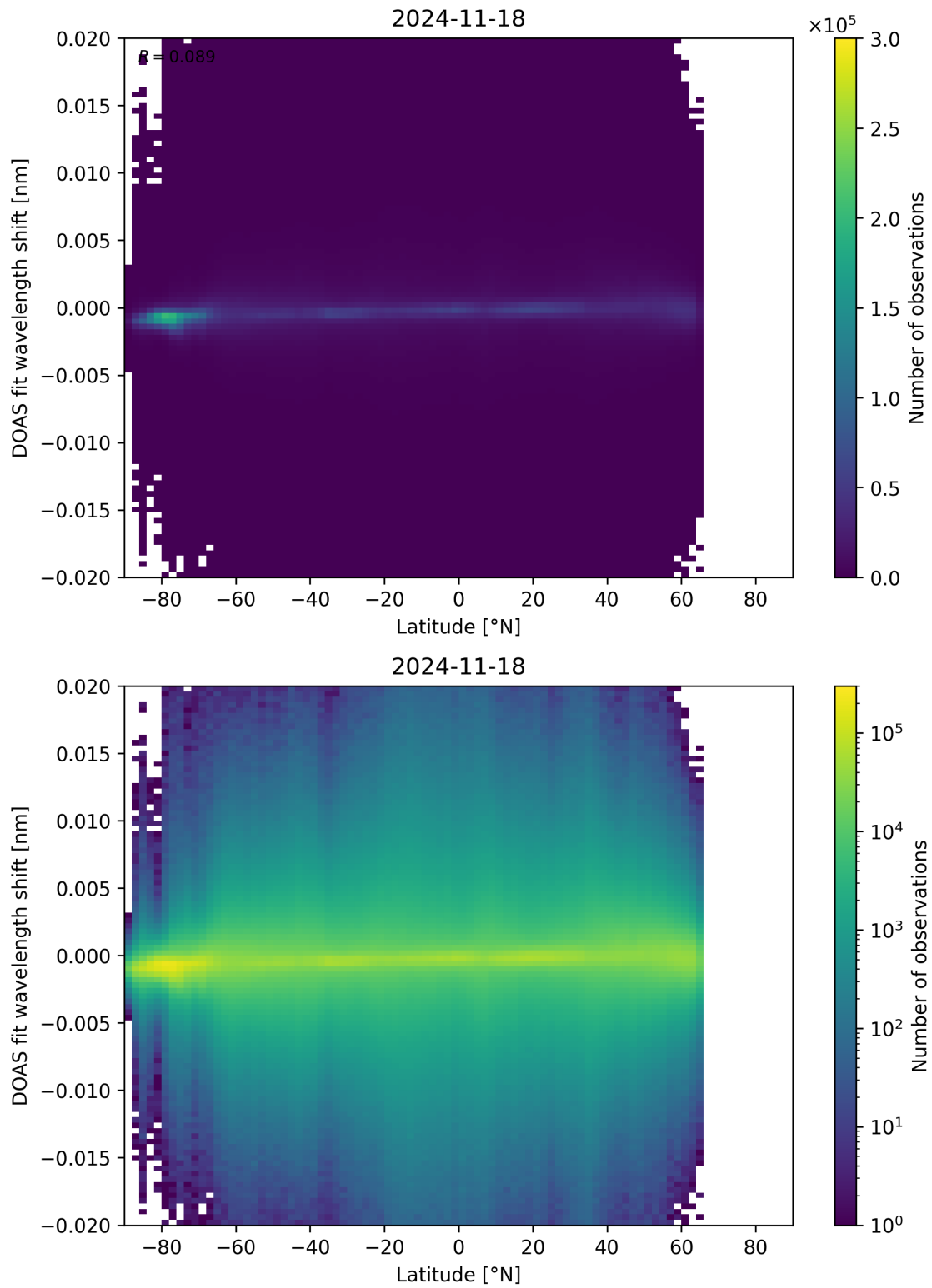
Figure 154: Scatter density plot of “Latitude” against “DOAS fit wavelength shift” for 2024-11-17 to 2024-11-19.
