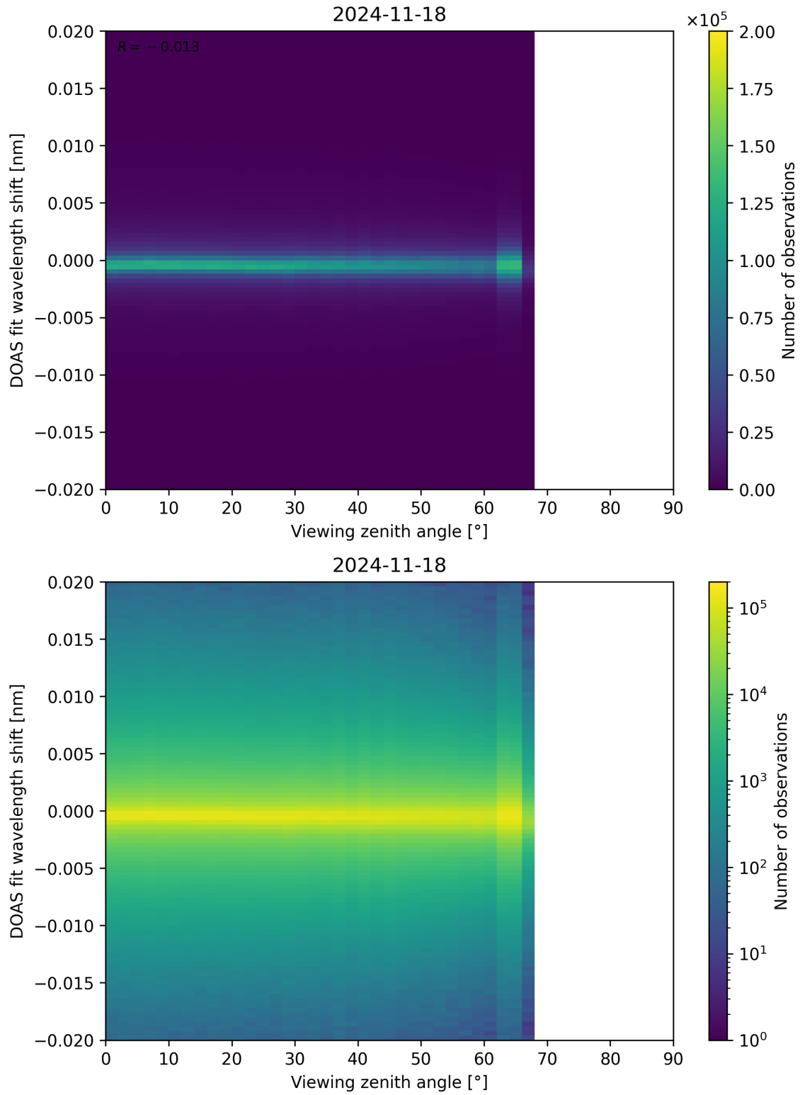
Figure 183: Scatter density plot of “Viewing zenith angle” against “DOAS fit wavelength shift” for 2024-11-17 to 2024-11-19.
