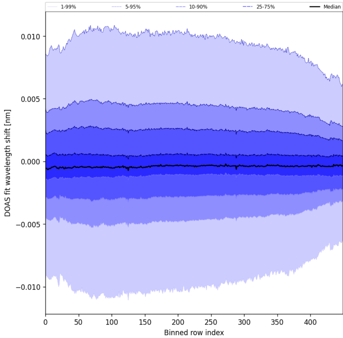
Figure 58: Along track statistics of "DOAS fit wavelength shift" for 2024-11-17 to 2024-11-19
