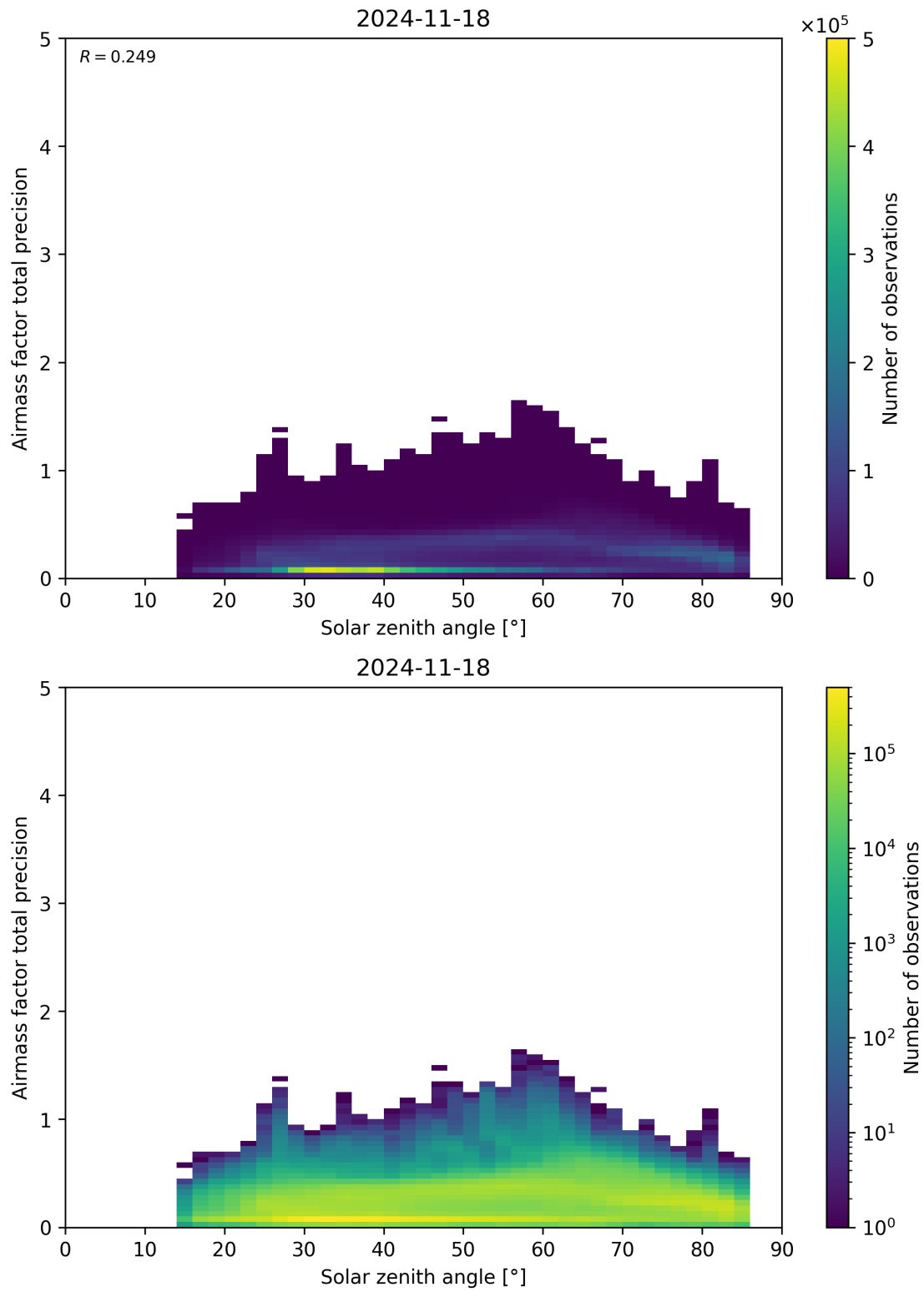
Figure 176: Scatter density plot of “Solar zenith angle” against “Airmass factor total precision” for 2024-11-17 to 2024-11-19.
