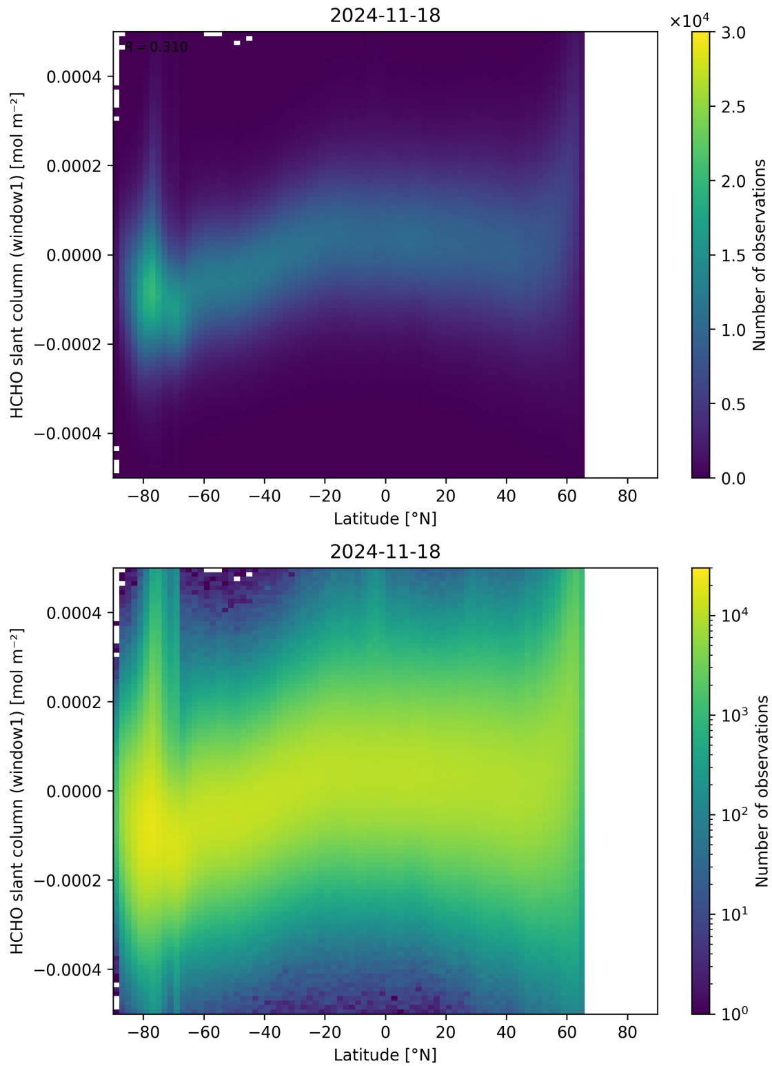
Figure 159: Scatter density plot of “Latitude” against “HCHO slant column (window1)” for 2024-11-17 to 2024-11-19.
