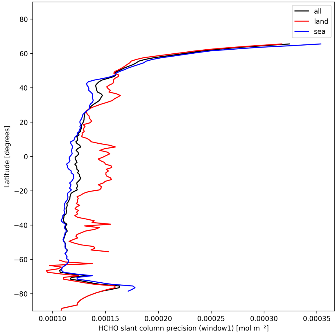
Figure 25: Zonal average of “HCHO slant column precision (window1)” for 2024-11-17 to 2024-11-19.
