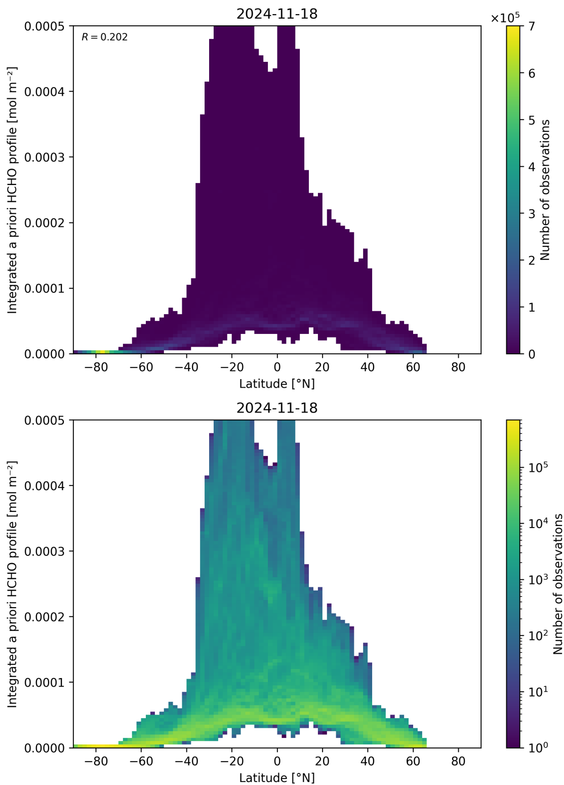
Figure 166: Scatter density plot of “Latitude” against “Integrated a priori HCHO profile” for 2024-11-17 to 2024-11-19.
