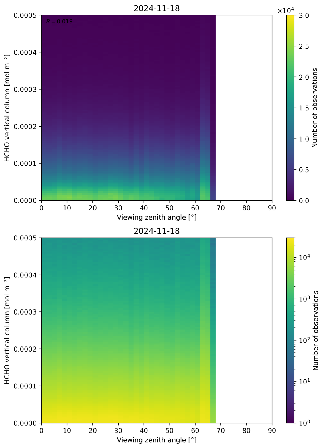
Figure 192: Scatter density plot of “Viewing zenith angle” against “HCHO vertical column” for 2024-11-17 to 2024-11-19.
