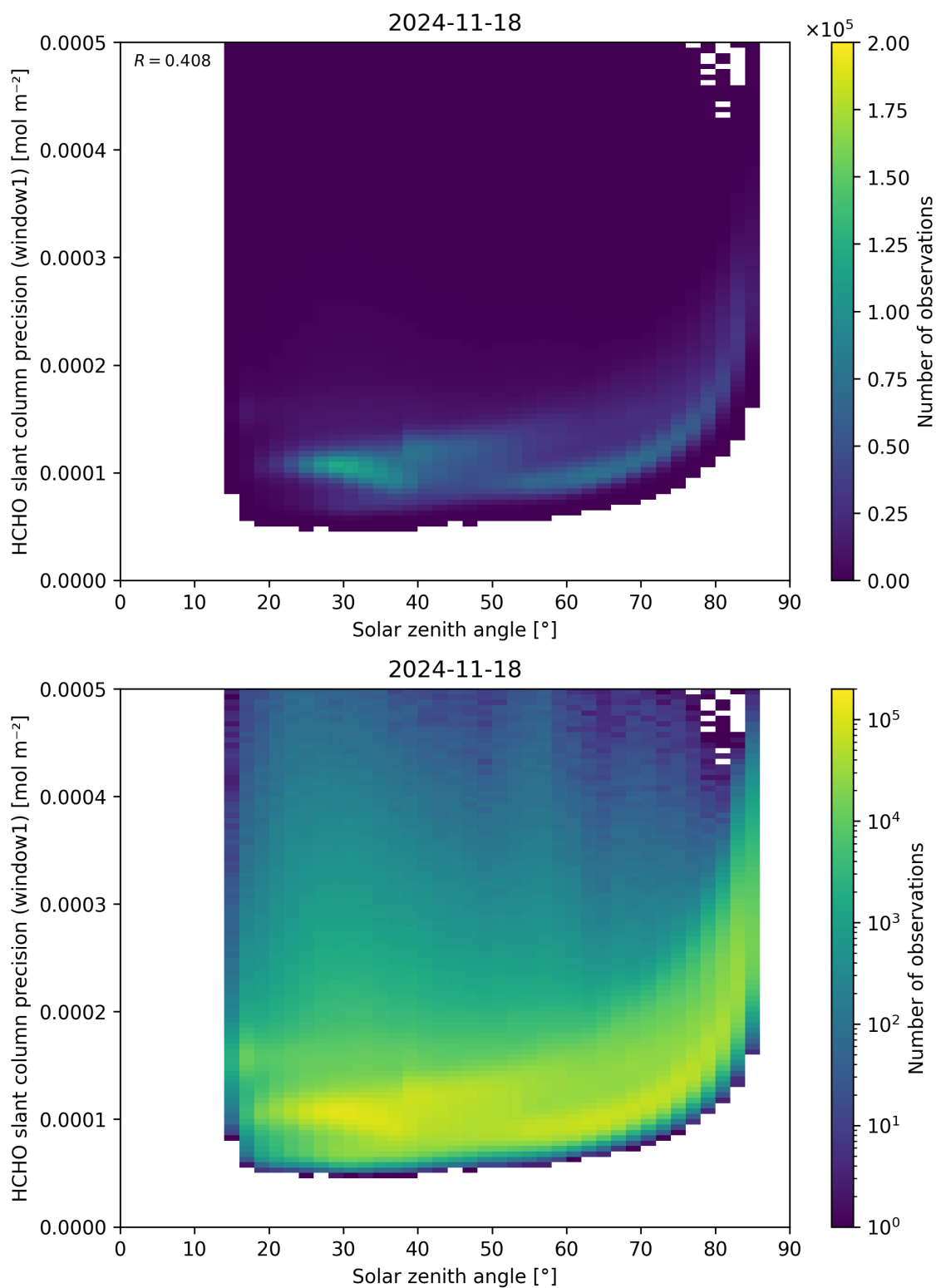
Figure 174: Scatter density plot of “Solar zenith angle” against “HCHO slant column precision (window1)” for 2024-11-17 to 2024-11-19.
