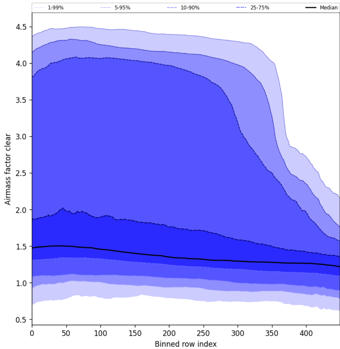
Figure 56: Along track statistics of “Air mass factor clear” for 2024-11-17 to 2024-11-19
