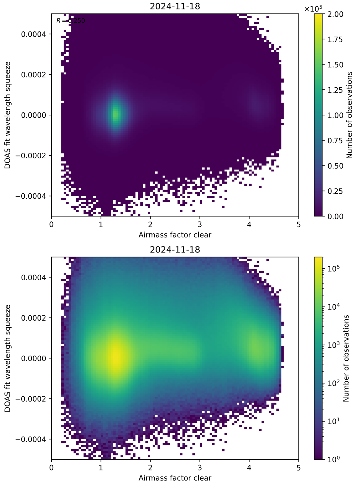
Figure 73: Scatter density plot of “Airmass factor clear” against “DOAS fit wavelength squeeze” for 2024-11-17 to 2024-11-19.
