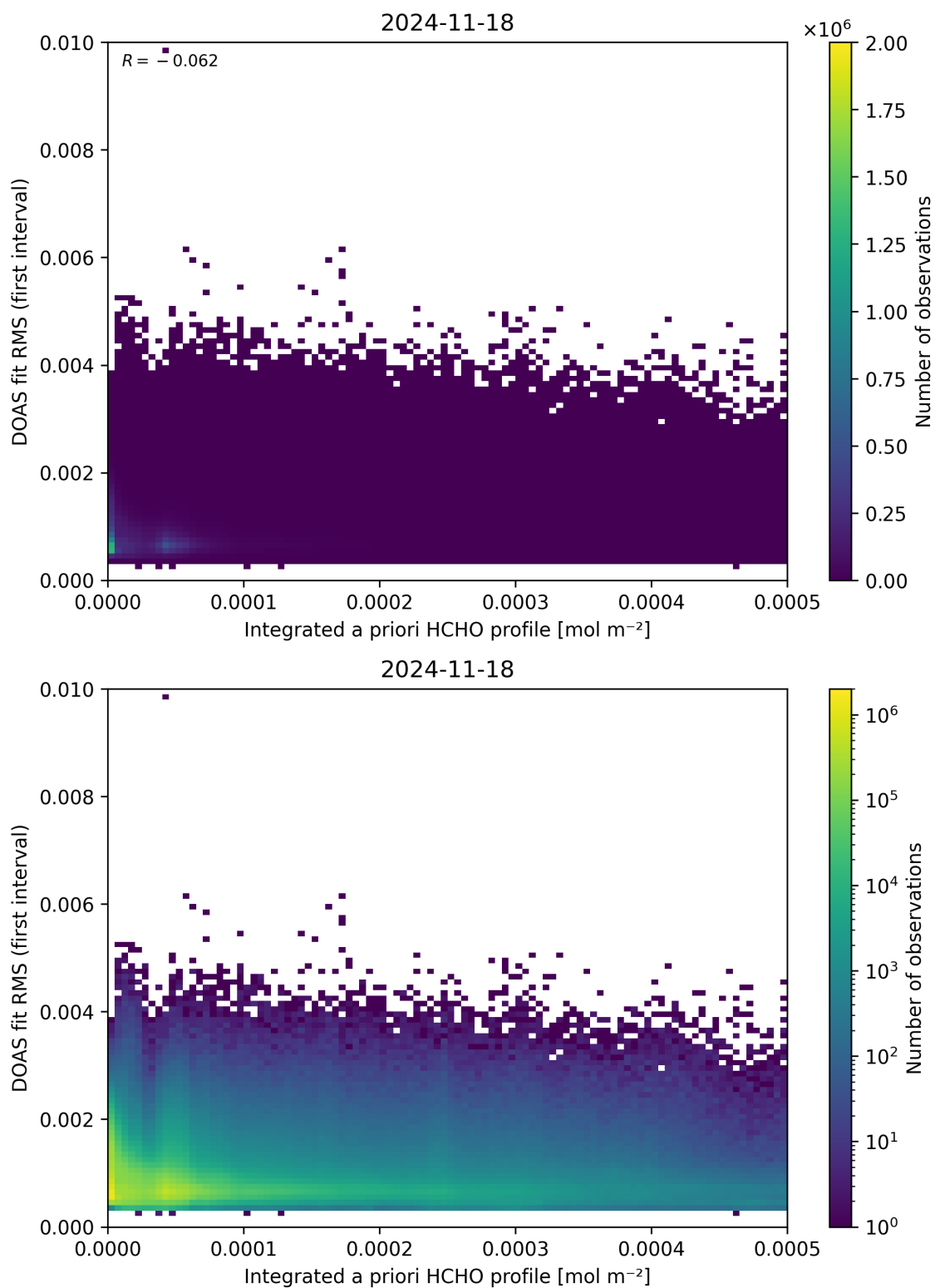
Figure 148: Scatter density plot of “Integrated a priori HCHO profile” against “DOAS fit RMS (first interval)” for 2024-11-17 to 2024-11-19.
