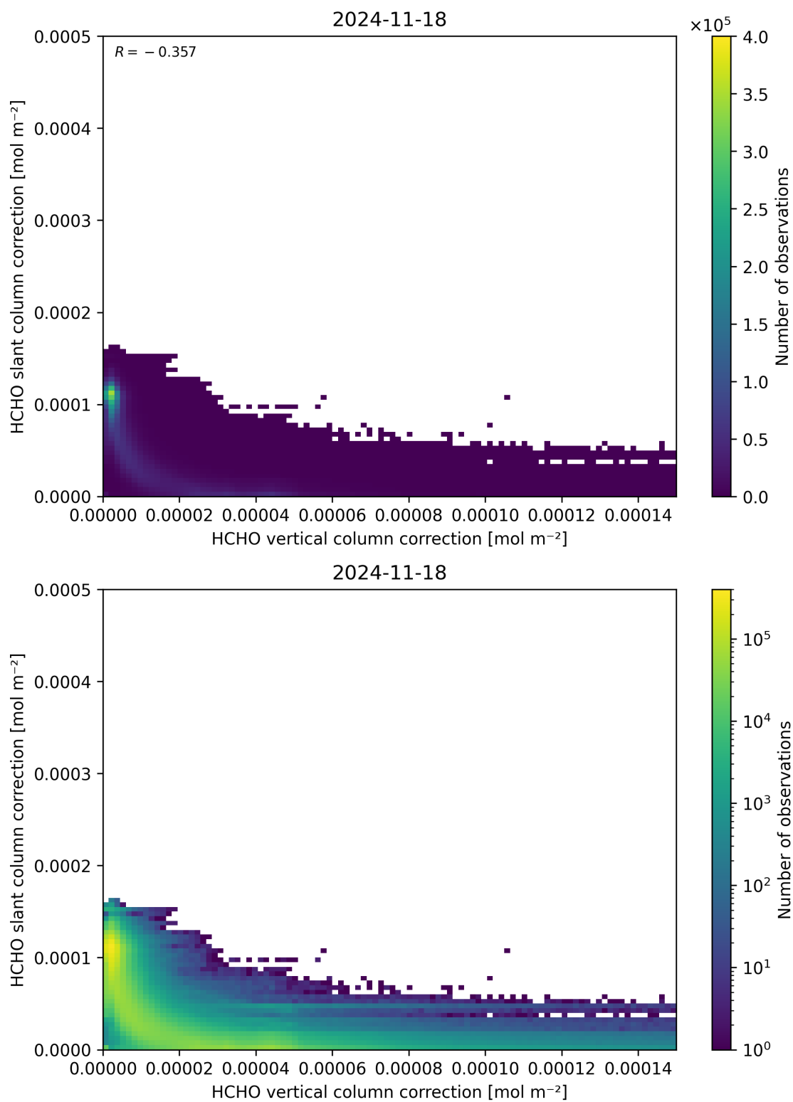
Figure 117: Scatter density plot of “HCHO vertical column correction” against “HCHO slant column correction” for 2024-11-17 to 2024-11-19.
