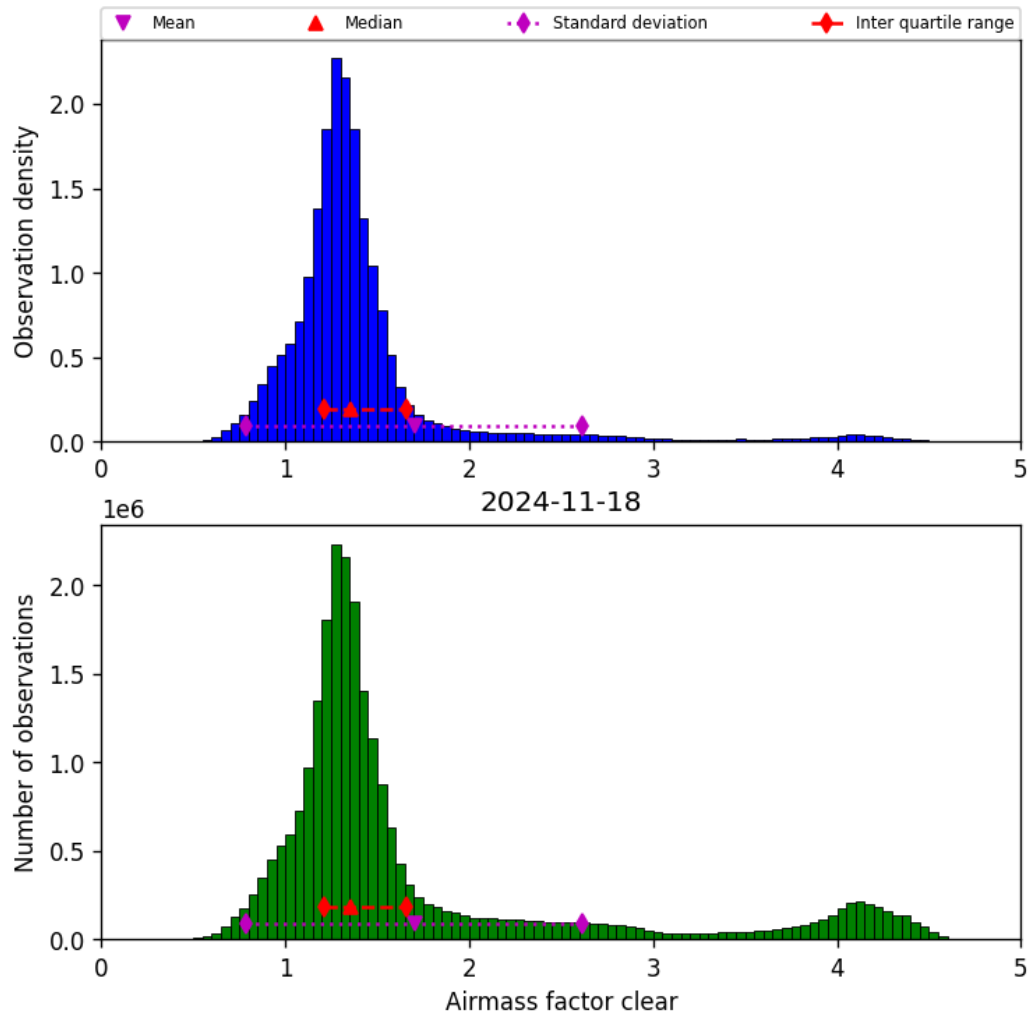
Figure 42: Histogram of “Airmass factor clear” for 2024-11-17 to 2024-11-19
