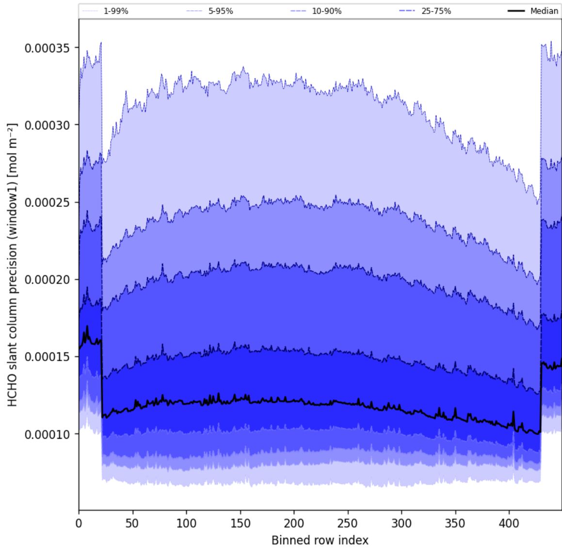
Figure 53: Along track statistics of “HCHO slant column precision (window1)” for 2024-11-17 to 2024-11-19
