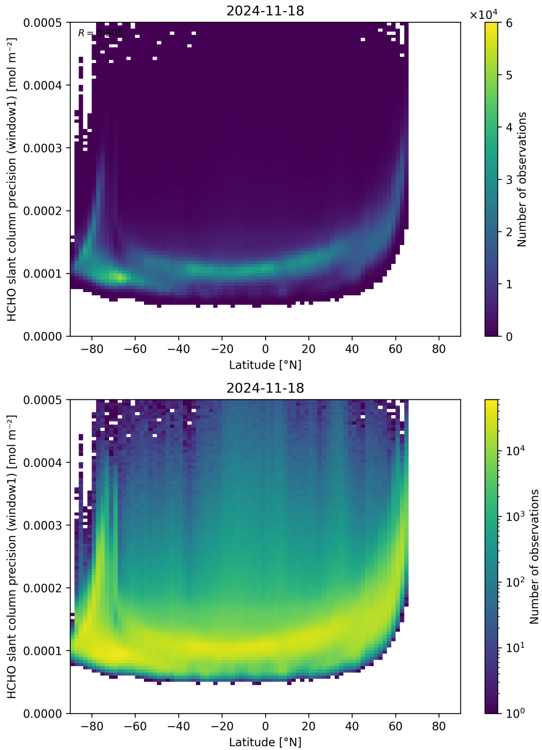
Figure 160: Scatter density plot of “Latitude” against “HCHO slant column precision (window1)” for 2024-11-17 to 2024-11-19.
