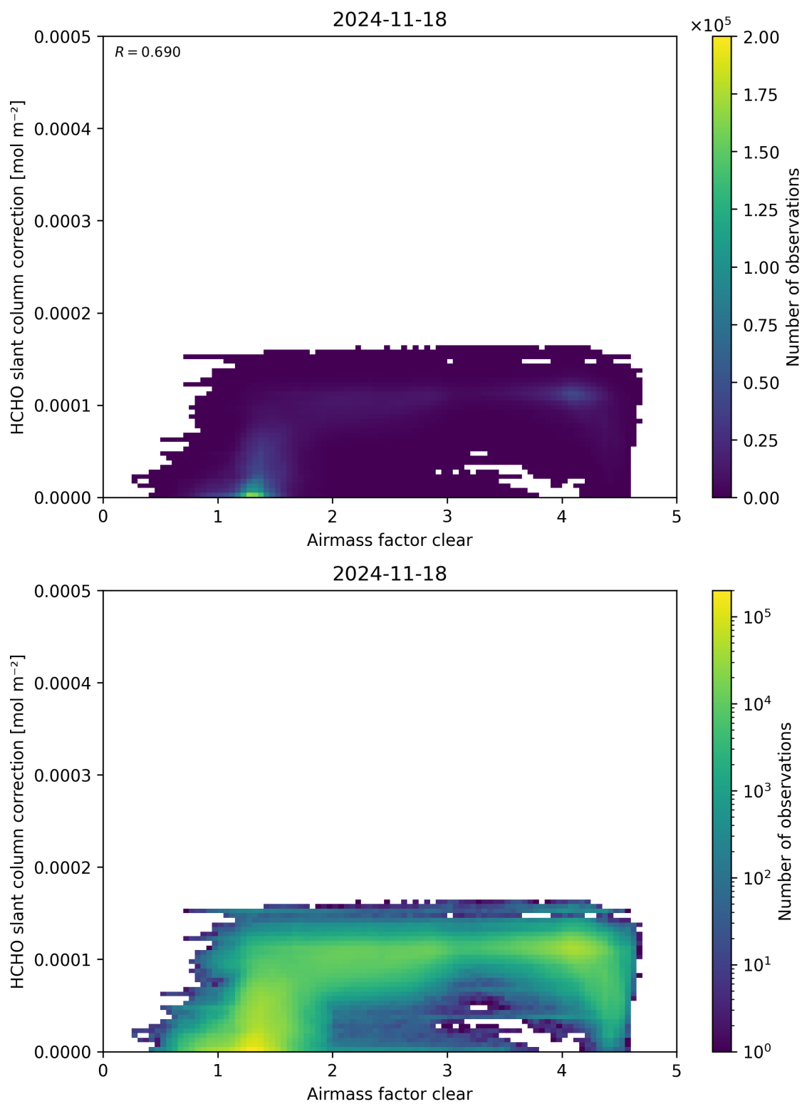
Figure 75: Scatter density plot of “Airmass factor clear” against “HCHO slant column correction” for 2024-11-17 to 2024-11-19.
