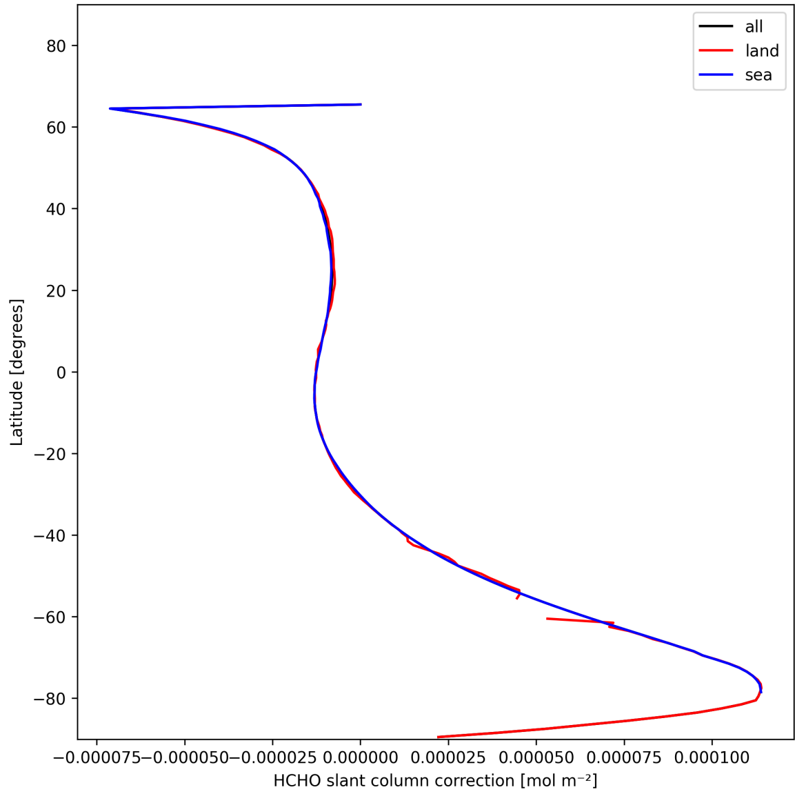
Figure 33: Zonal average of “HCHO slant column correction” for 2024-11-17 to 2024-11-19.
