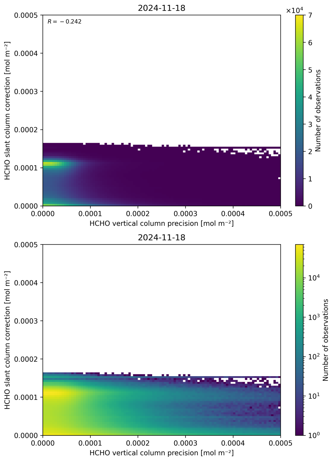
Figure 141: Scatter density plot of “HCHO vertical column precision” against “HCHO slant column correction” for 2024-11-17 to 2024-11-19.
