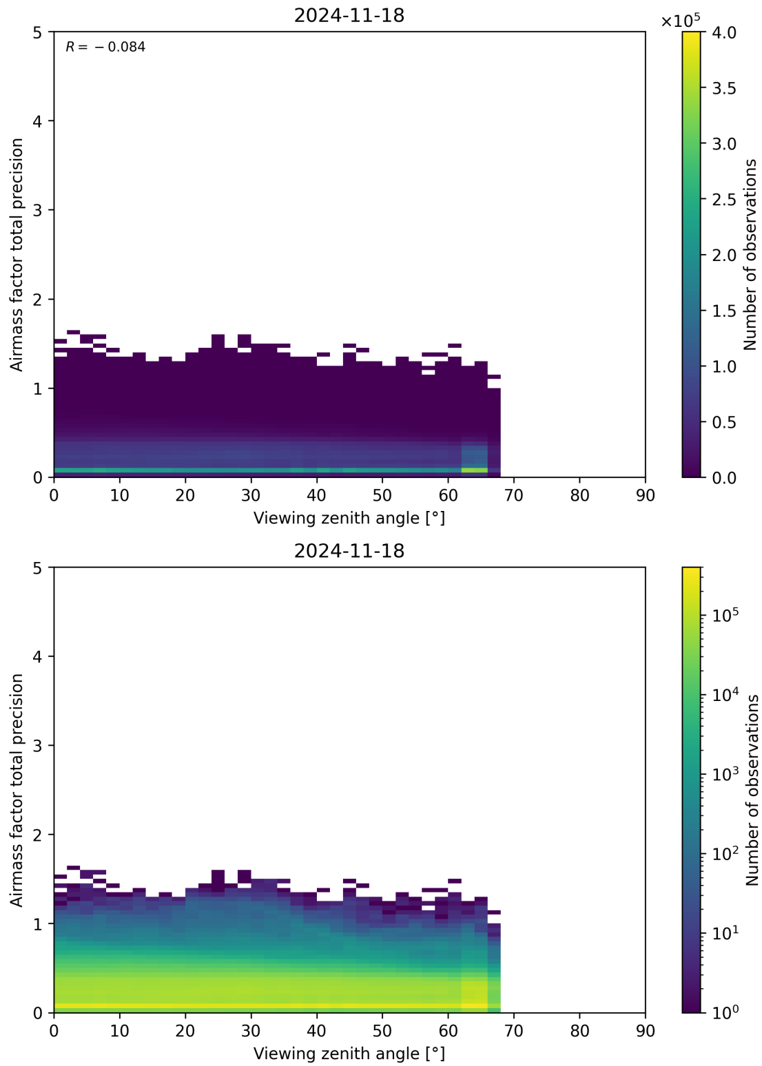
Figure 191: Scatter density plot of “Viewing zenith angle” against “Airmass factor total precision” for 2024-11-17 to 2024-11-19.
