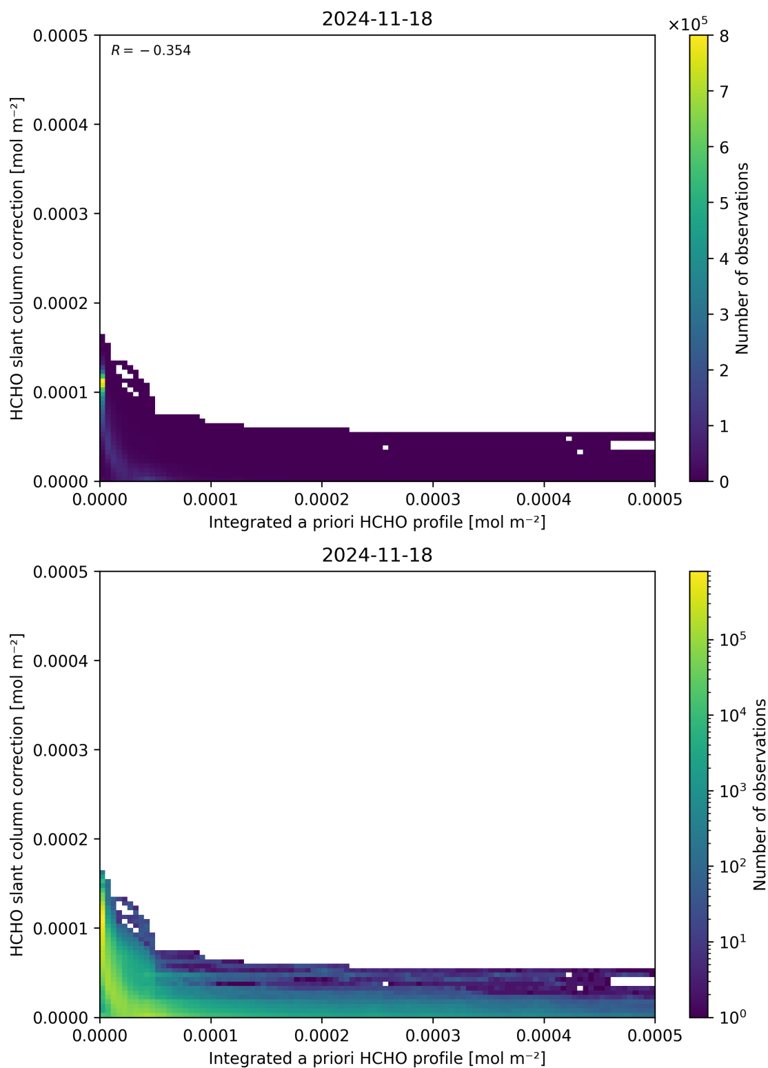
Figure 152: Scatter density plot of “Integrated a priori HCHO profile” against “HCHO slant column correction” for 2024-11-17 to 2024-11-19.
