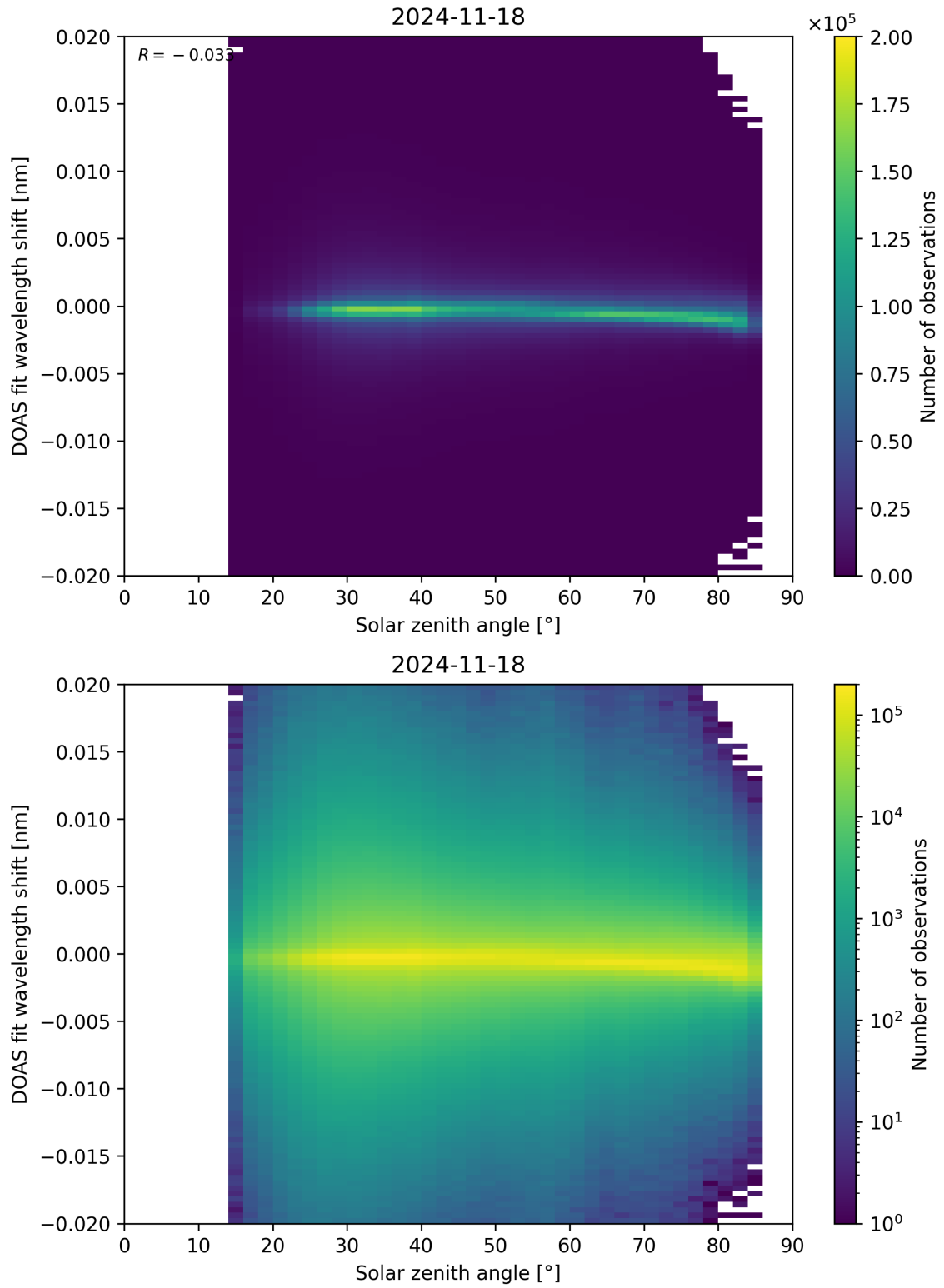
Figure 168: Scatter density plot of “Solar zenith angle” against “DOAS fit wavelength shift” for 2024-11-17 to 2024-11-19.
