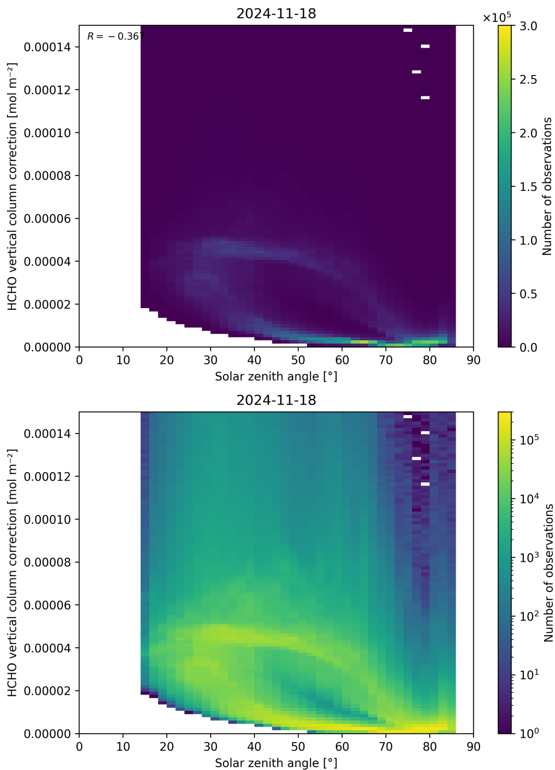
Figure 178: Scatter density plot of “Solar zenith angle” against “HCHO vertical column correction” for 2024-11-17 to 2024-11-19.
