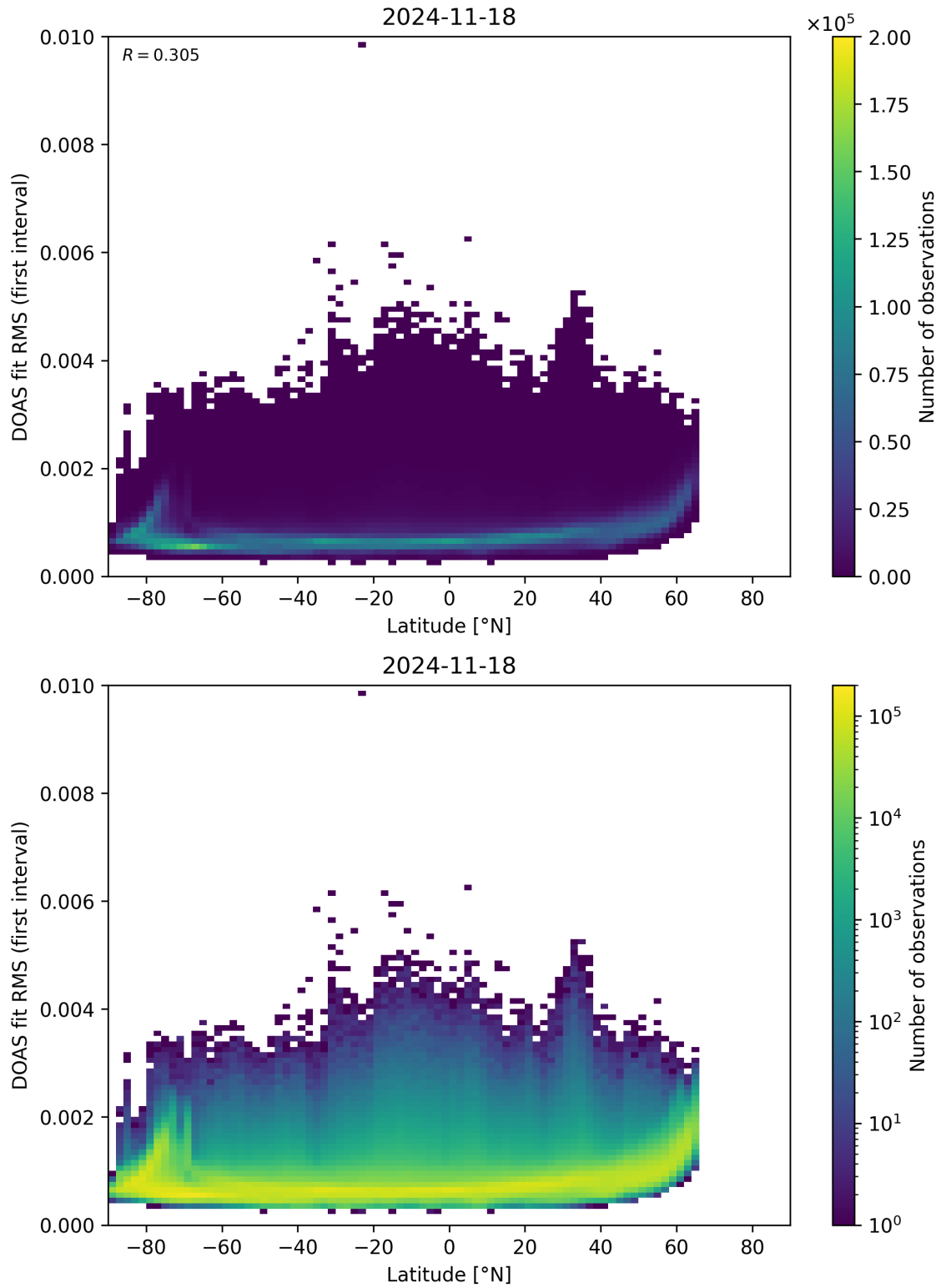
Figure 153: Scatter density plot of “Latitude” against “DOAS fit RMS (first interval)” for 2024-11-17 to 2024-11-19.
