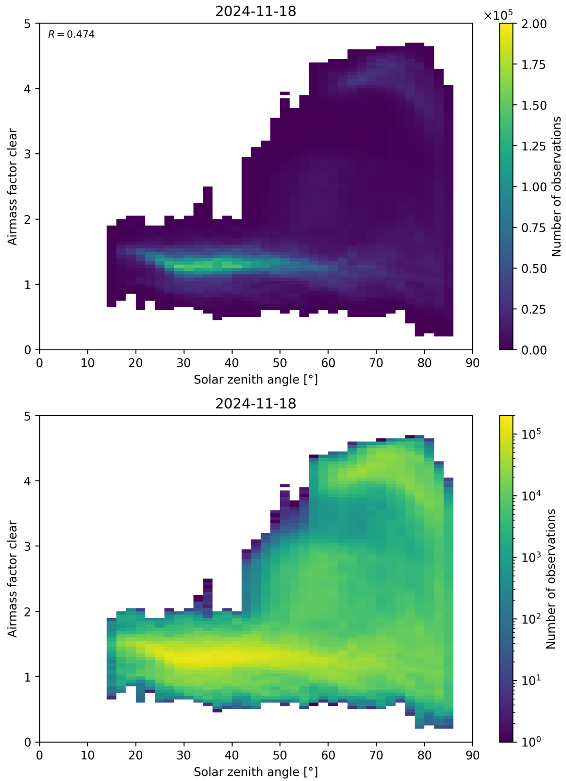
Figure 170: Scatter density plot of “Solar zenith angle” against “Airmass factor clear” for 2024-11-17 to 2024-11-19.
