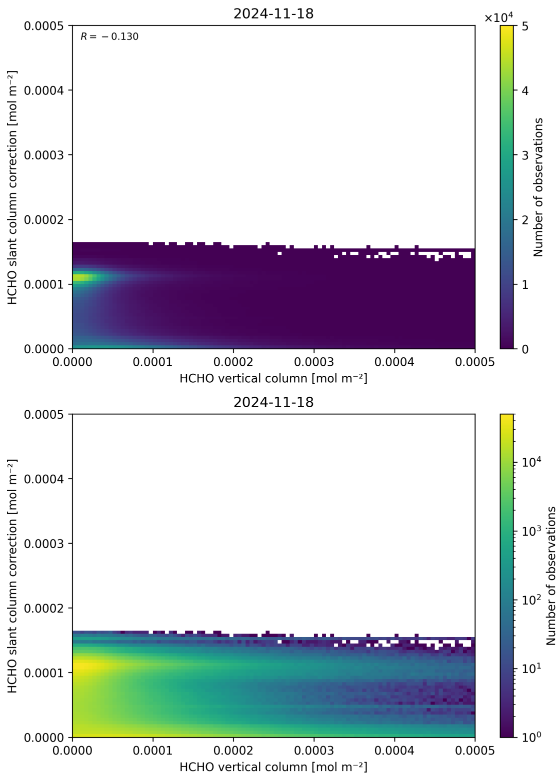
Figure 128: Scatter density plot of “HCHO vertical column” against “HCHO slant column correction” for 2024-11-17 to 2024-11-19.
