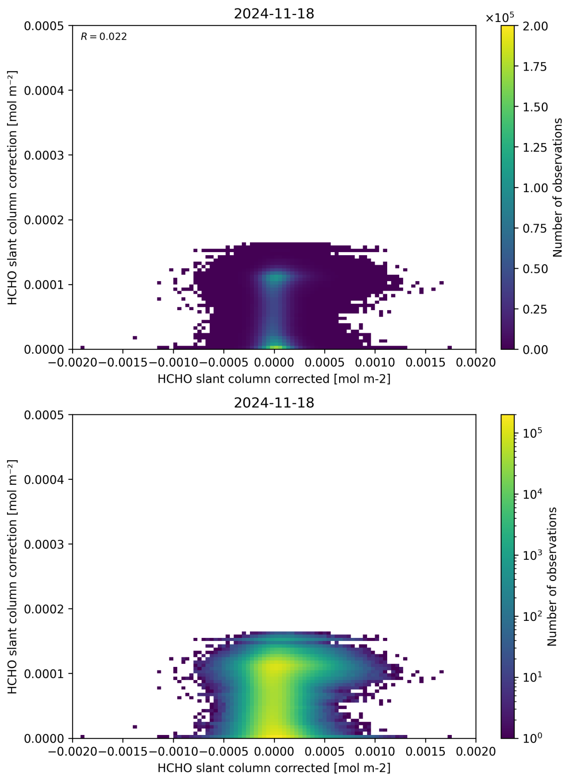
Figure 77: Scatter density plot of “HCHO slant column corrected” against “HCHO slant column correction” for 2024-11-17 to 2024-11-19.
