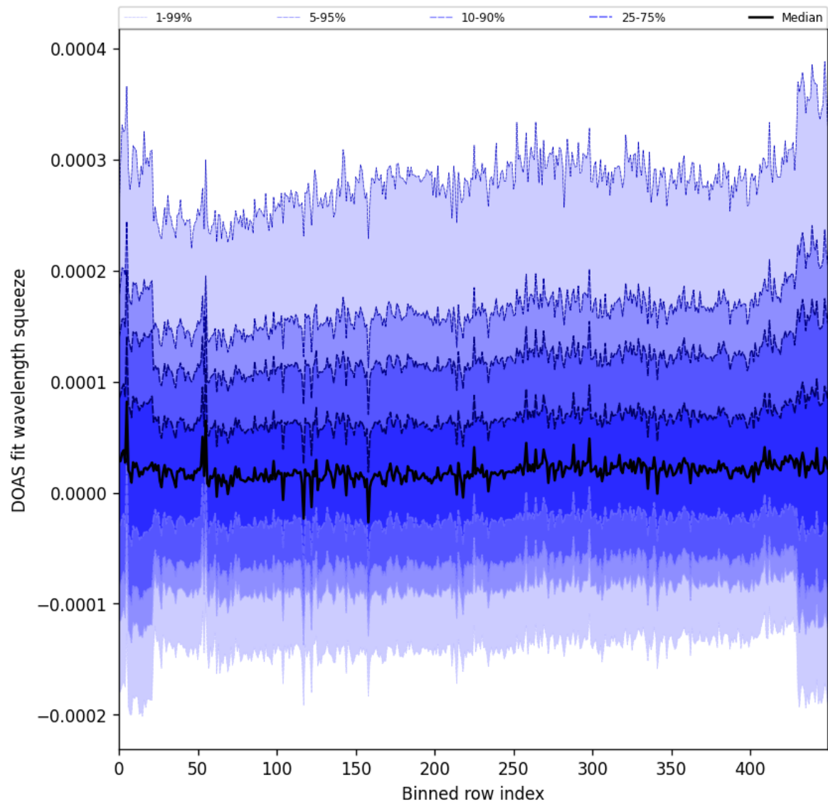
Figure 59: Along track statistics of “DOAS fit wavelength squeeze” for 2024-11-17 to 2024-11-19
