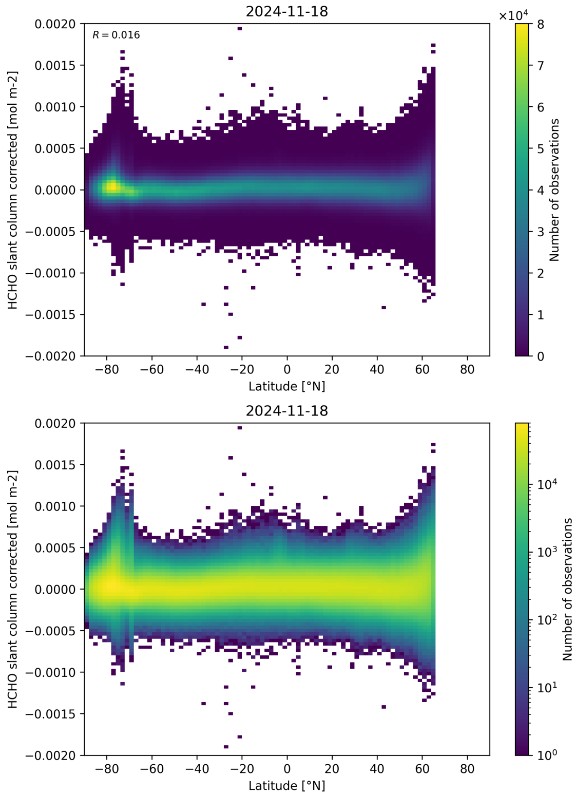
Figure 157: Scatter density plot of “Latitude” against “HCHO slant column corrected” for 2024-11-17 to 2024-11-19.
