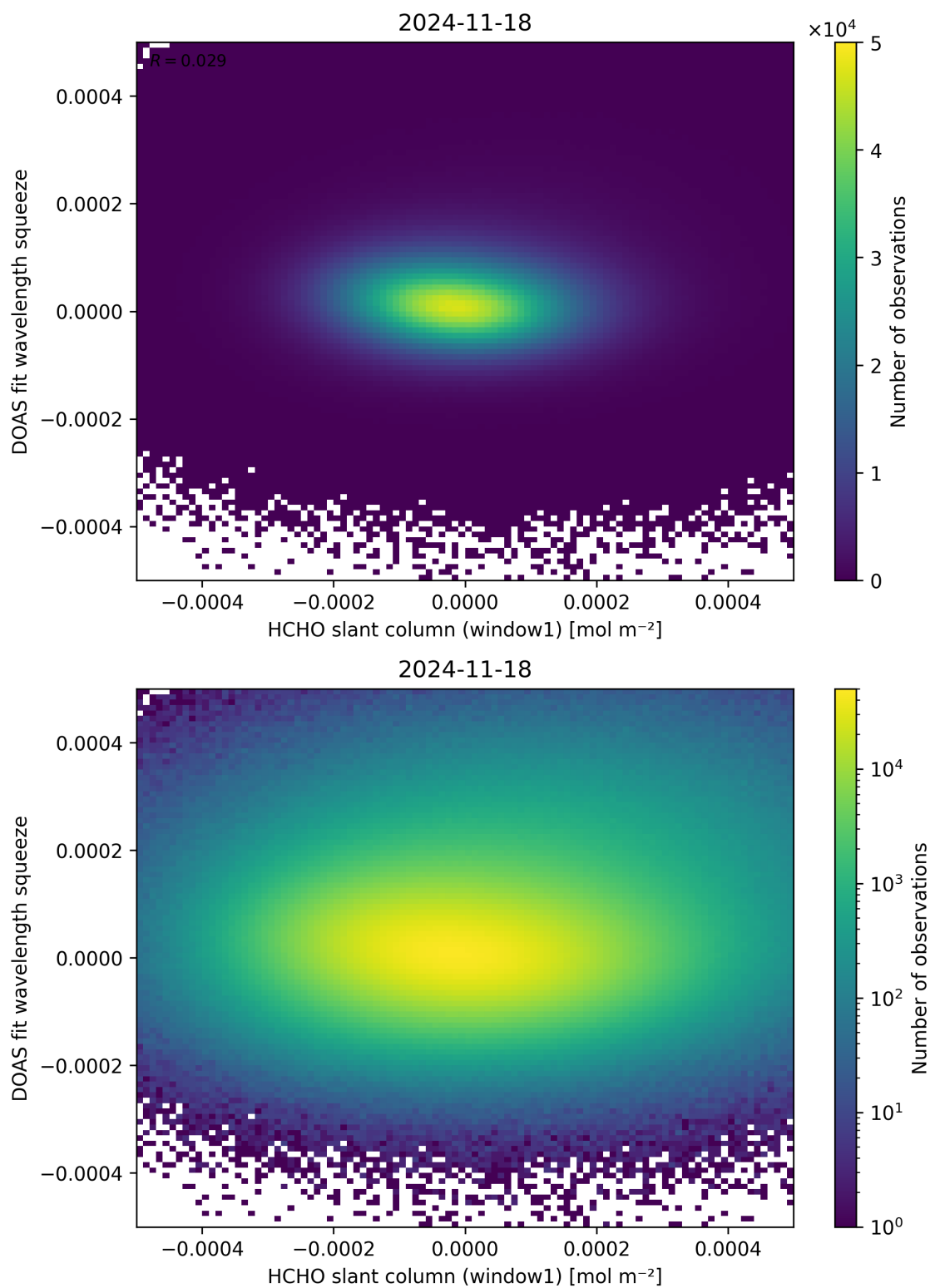
Figure 80: Scatter density plot of “HCHO slant column (window1)” against “DOAS fit wavelength squeeze” for 2024-11-17 to 2024-11-19.
