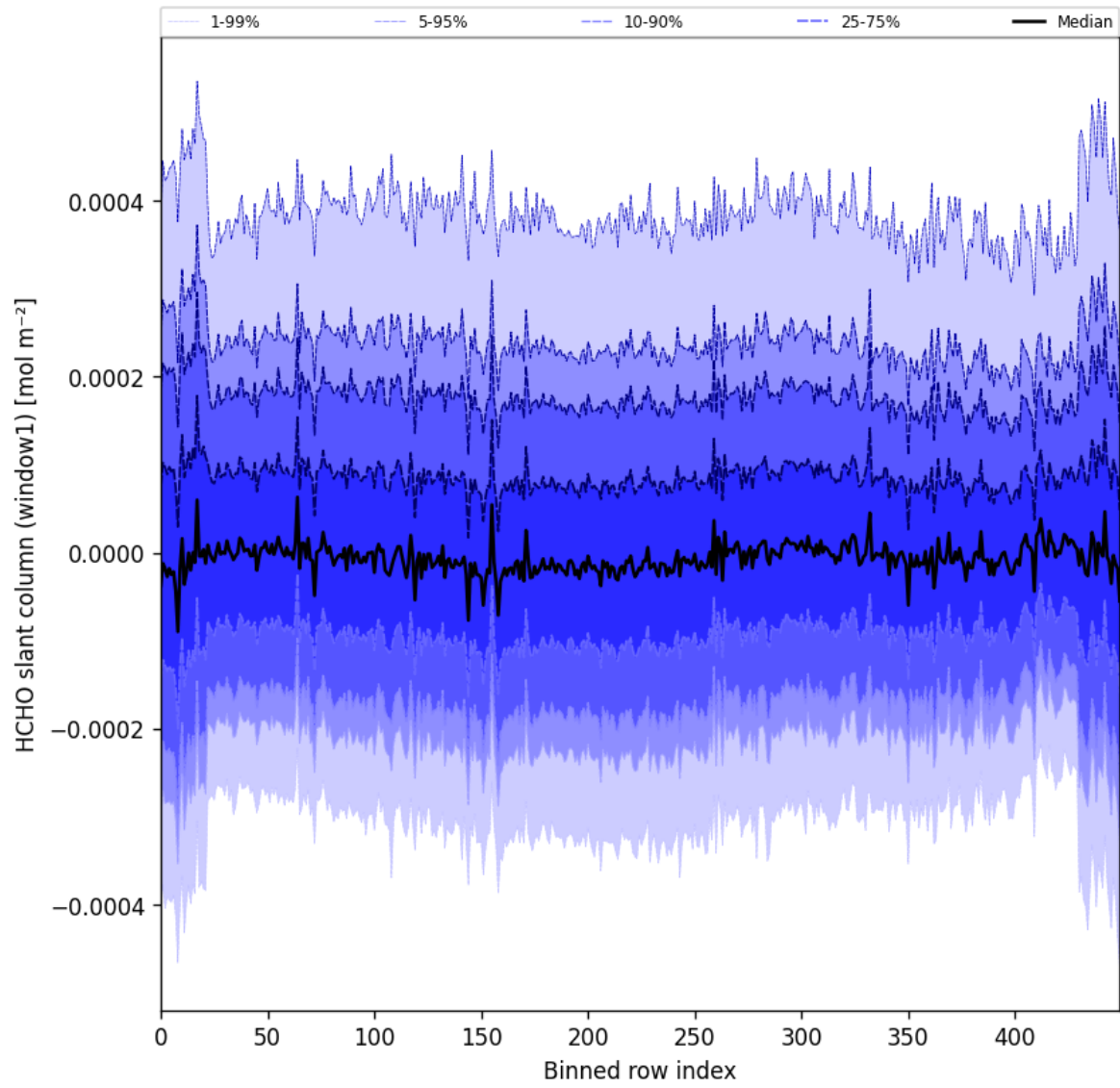
Figure 52: Along track statistics of “HCHO slant column (window1)” for 2024-11-17 to 2024-11-19
