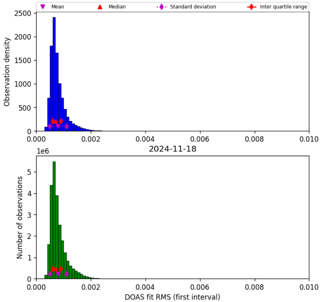
Figure 46: Histogram of “DOAS fit RMS (first interval)” for 2024-11-17 to 2024-11-19
