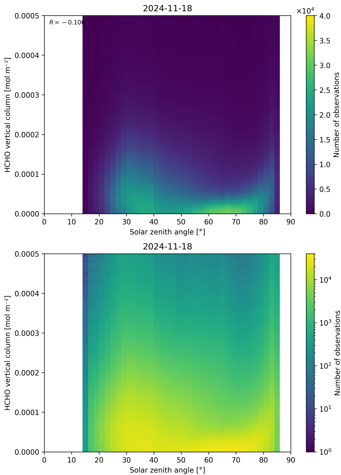
Figure 177: Scatter density plot of “Solar zenith angle” against “HCHO vertical column” for 2024-11-17 to 2024-11-19.
