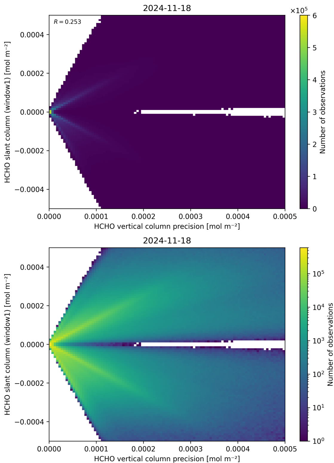
Figure 142: Scatter density plot of “HCHO vertical column precision” against “HCHO slant column (window1)” for 2024-11-17 to 2024-11-19.
