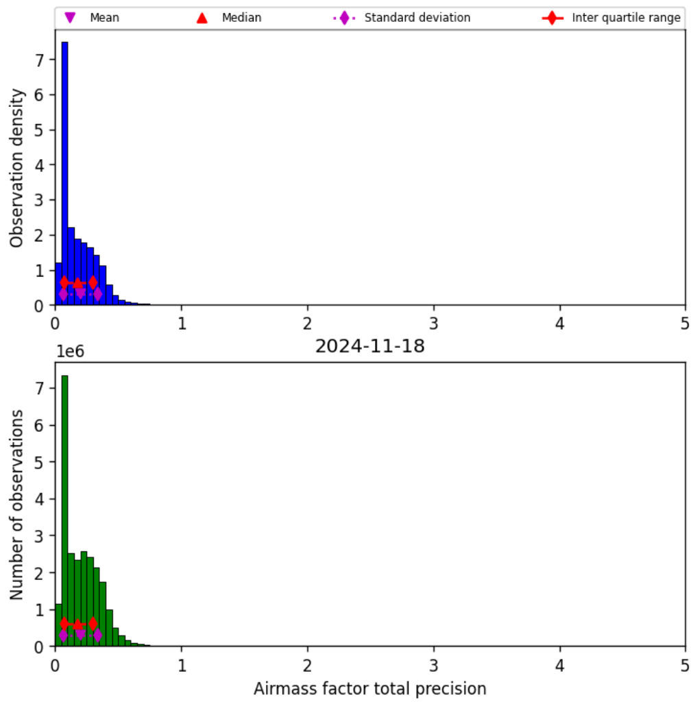
Figure 41: Histogram of “Airmass factor total precision” for 2024-11-17 to 2024-11-19
