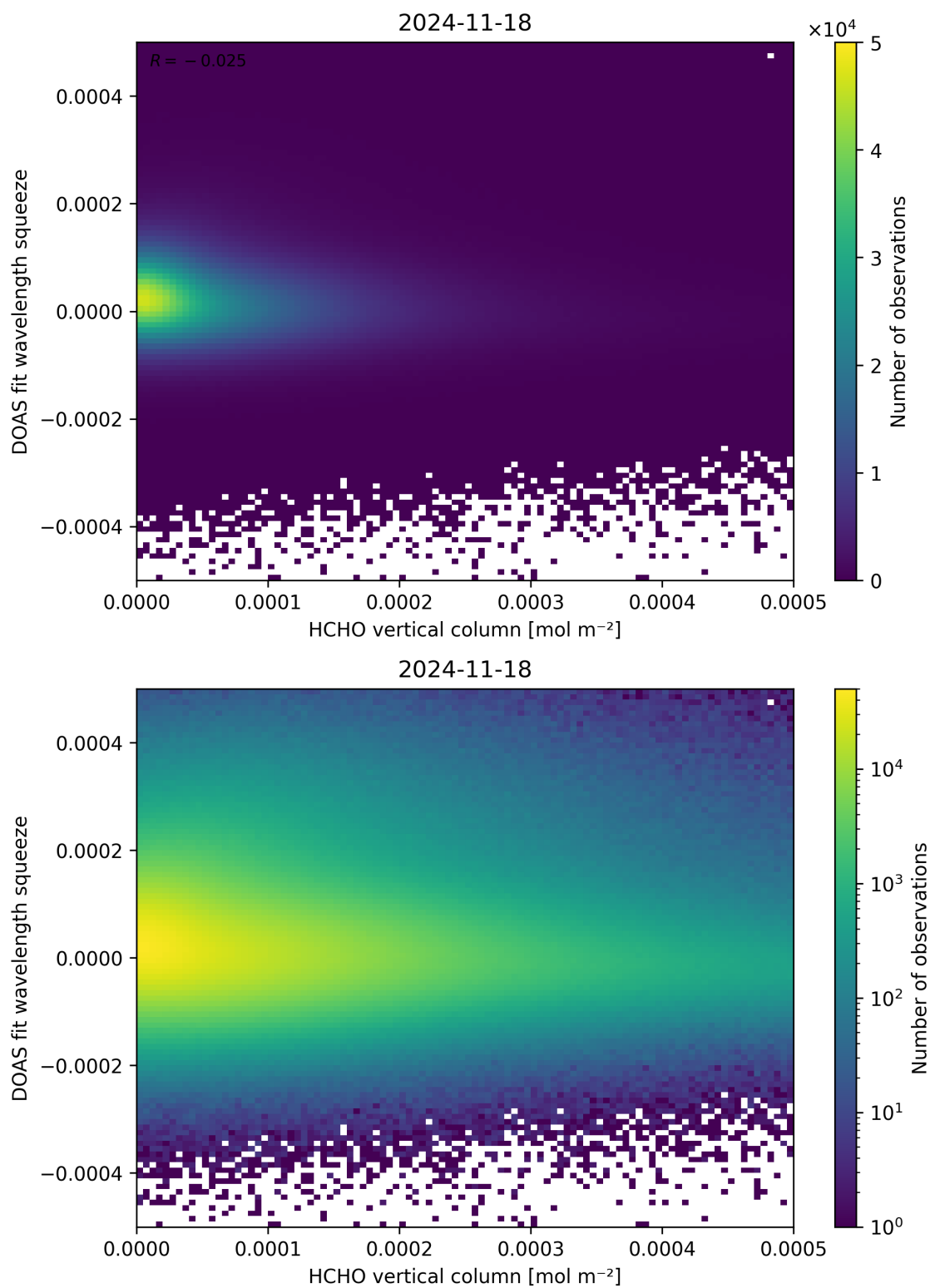
Figure 125: Scatter density plot of “HCHO vertical column” against “DOAS fit wavelength squeeze” for 2024-11-17 to 2024-11-19.
