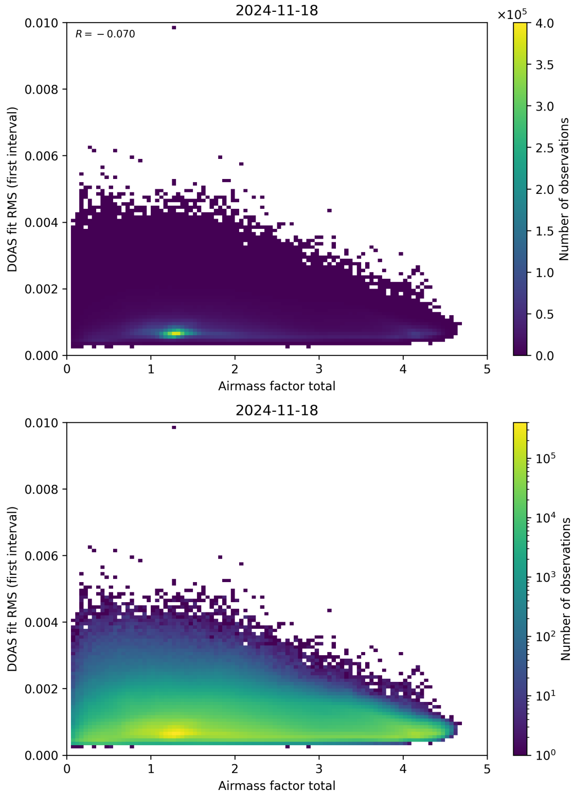
Figure 97: Scatter density plot of “Airmass factor total” against “DOAS fit RMS (first interval)” for 2024-11-17 to 2024-11-19.
