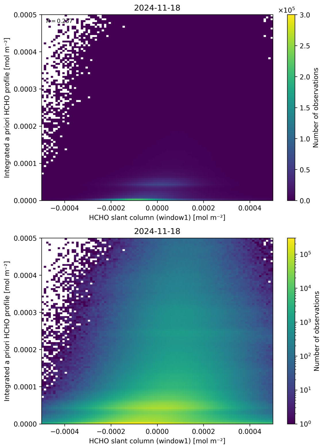
Figure 87: Scatter density plot of “HCHO slant column (window1)” against “Integrated a priori HCHO profile” for 2024-11-17 to 2024-11-19.
