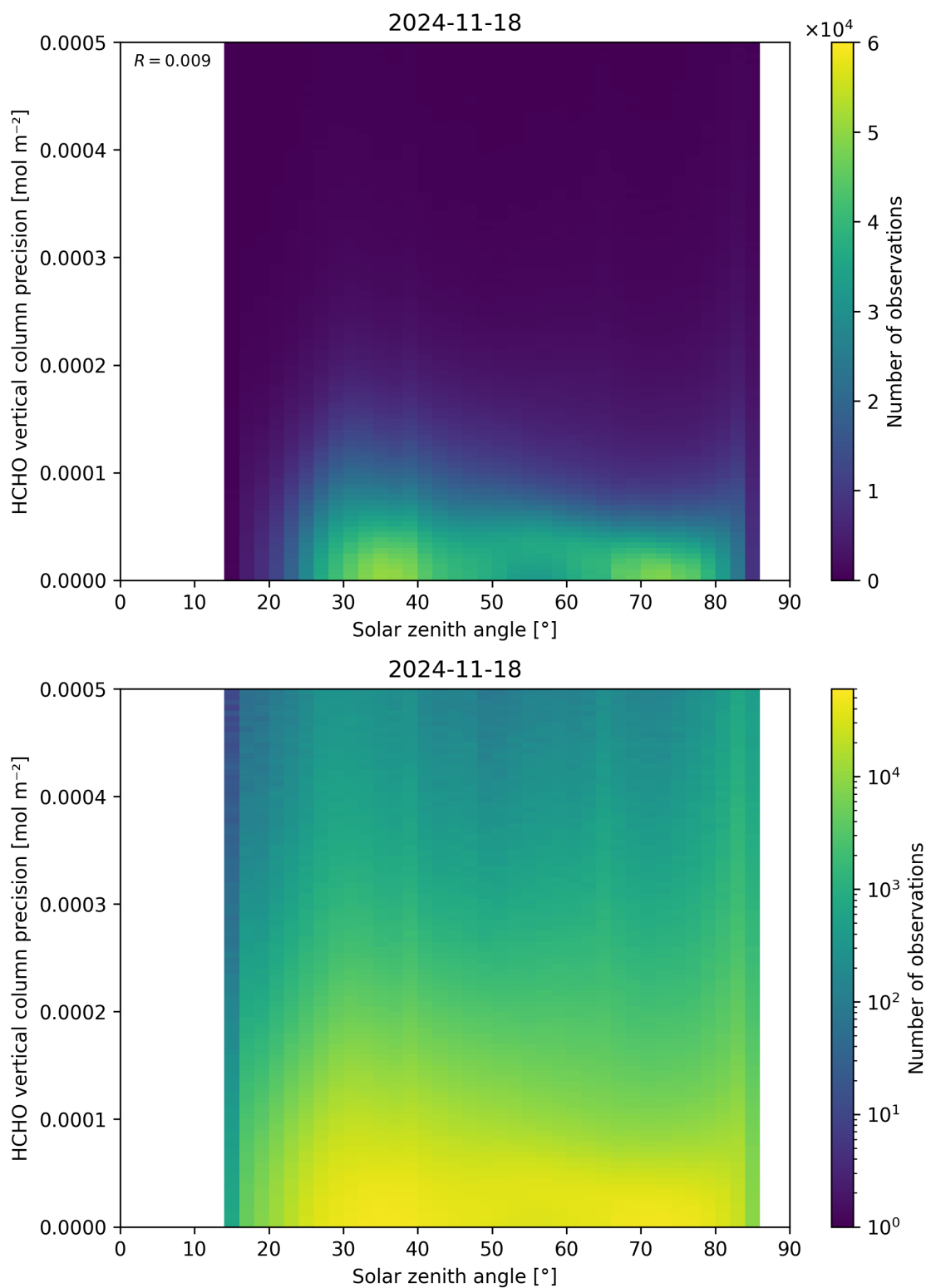
Figure 179: Scatter density plot of “Solar zenith angle” against “HCHO vertical column precision” for 2024-11-17 to 2024-11-19.
