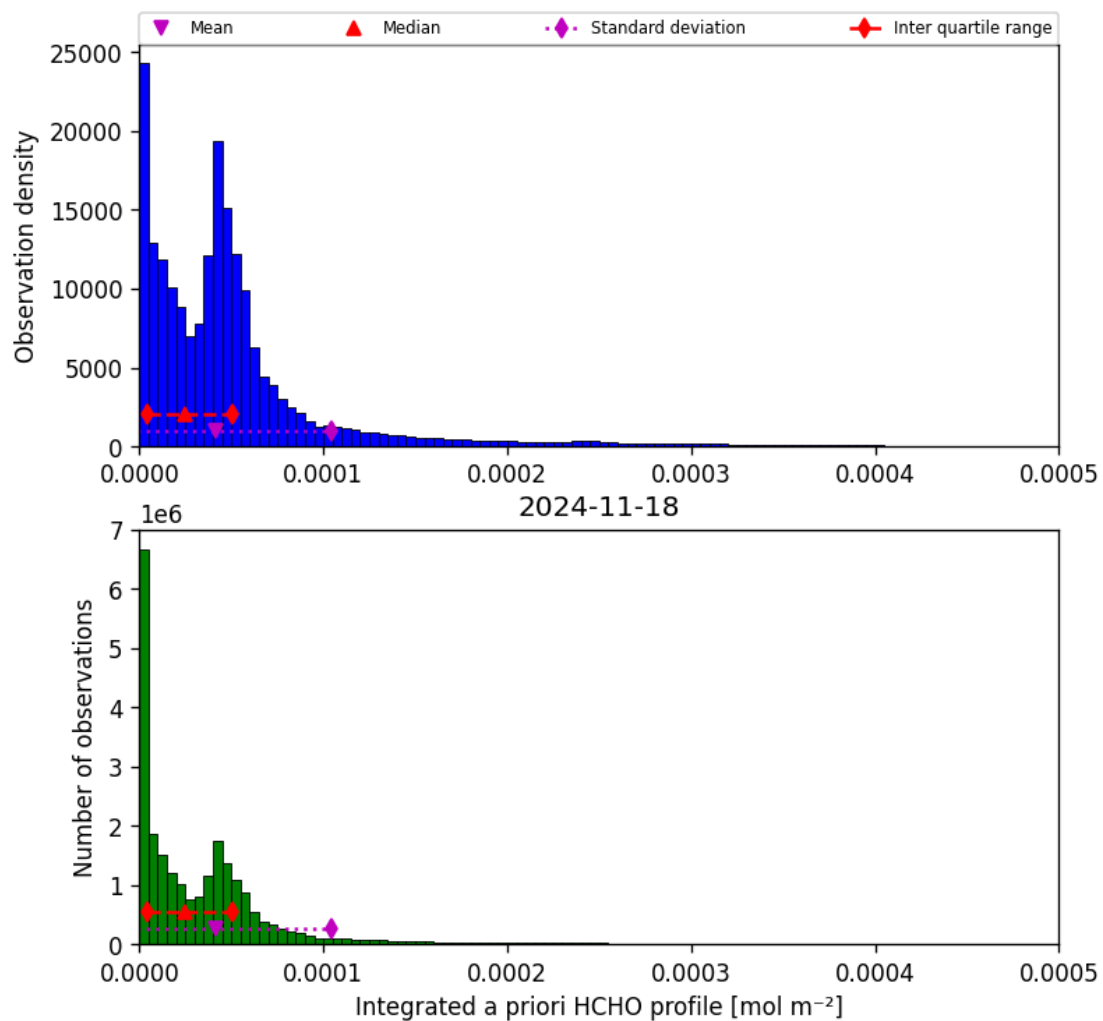
Figure 43: Histogram of “Integrated a priori HCHO profile” for 2024-11-17 to 2024-11-19
