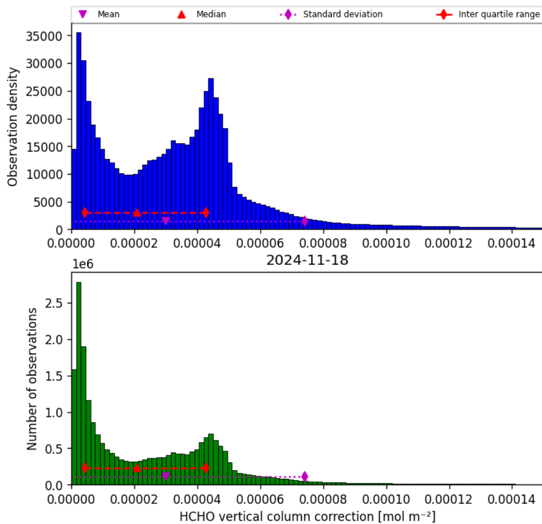
Figure 37: Histogram of “HCHO vertical column correction” for 2024-11-17 to 2024-11-19
