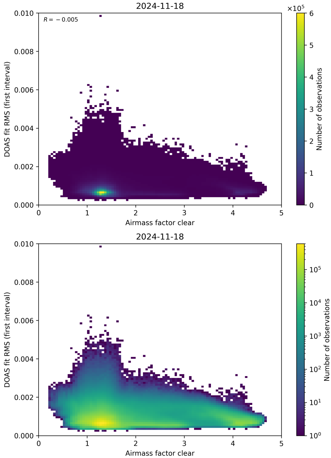
Figure 71: Scatter density plot of “Airmass factor clear” against “DOAS fit RMS (first interval)” for 2024-11-17 to 2024-11-19.
