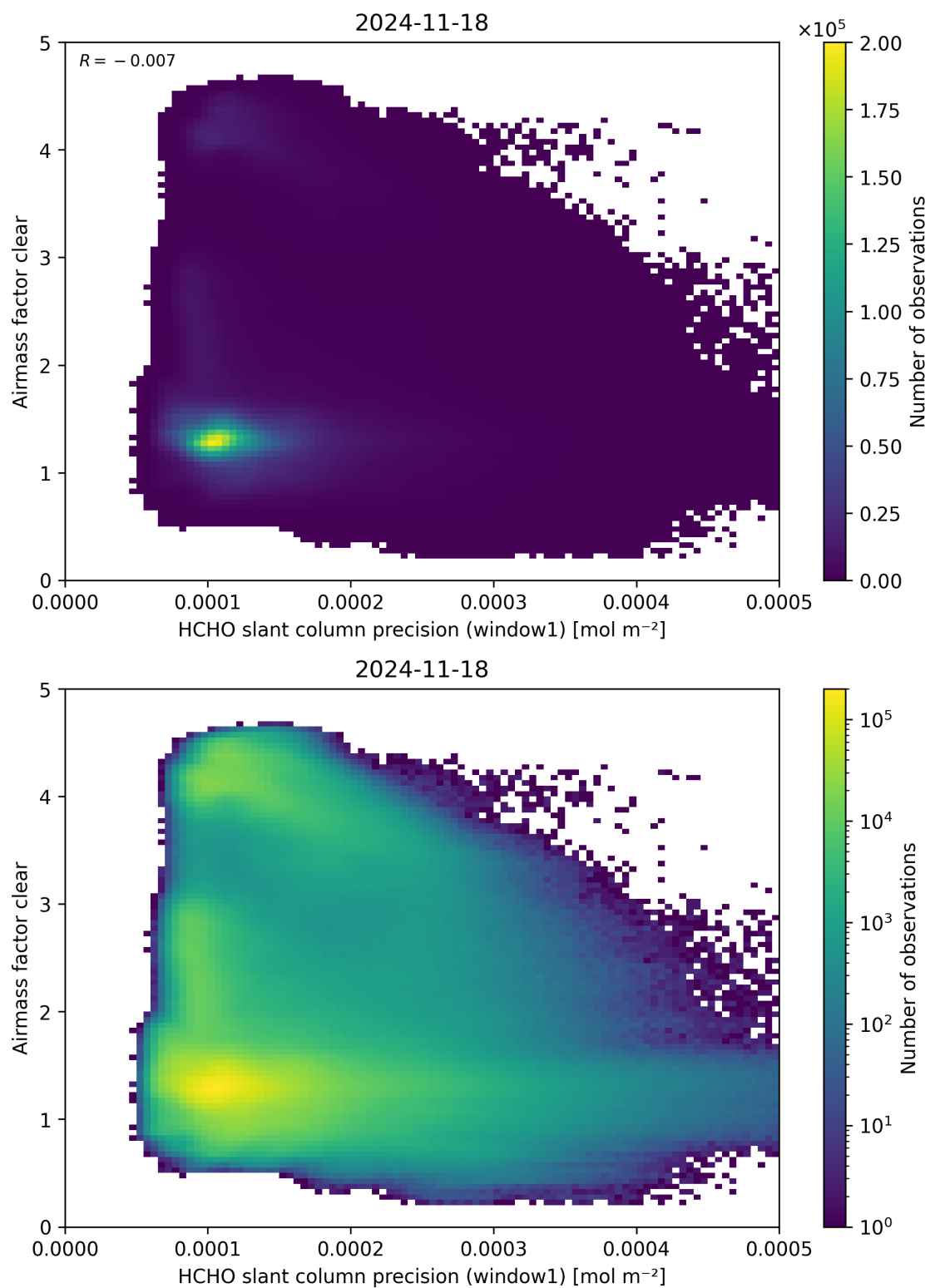
Figure 91: Scatter density plot of “HCHO slant column precision (window1)” against “Airmass factor clear” for 2024-11-17 to 2024-11-19.
