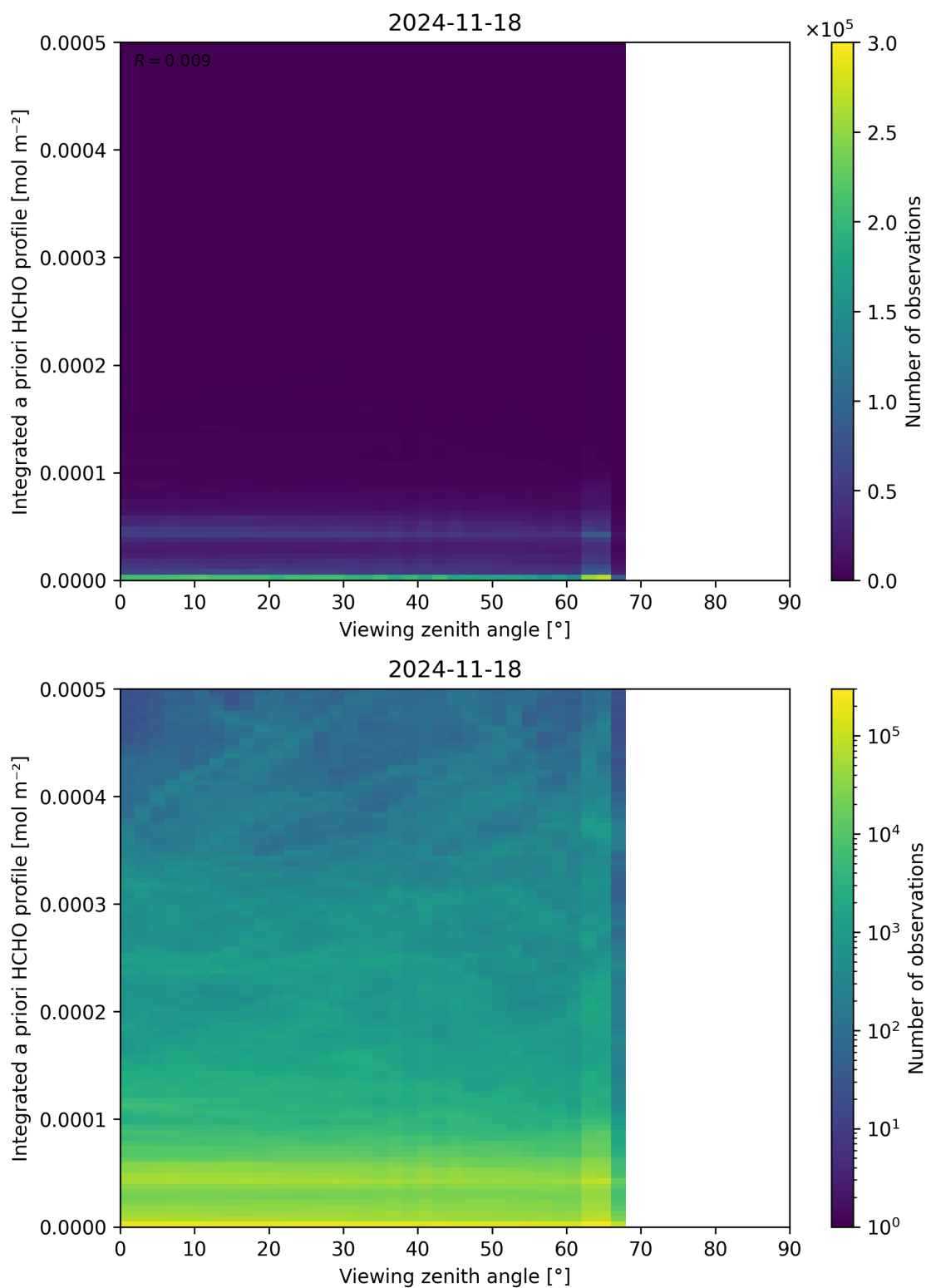
Figure 195: Scatter density plot of “Viewing zenith angle” against “Integrated a priori HCHO profile” for 2024-11-17 to 2024-11-19.
