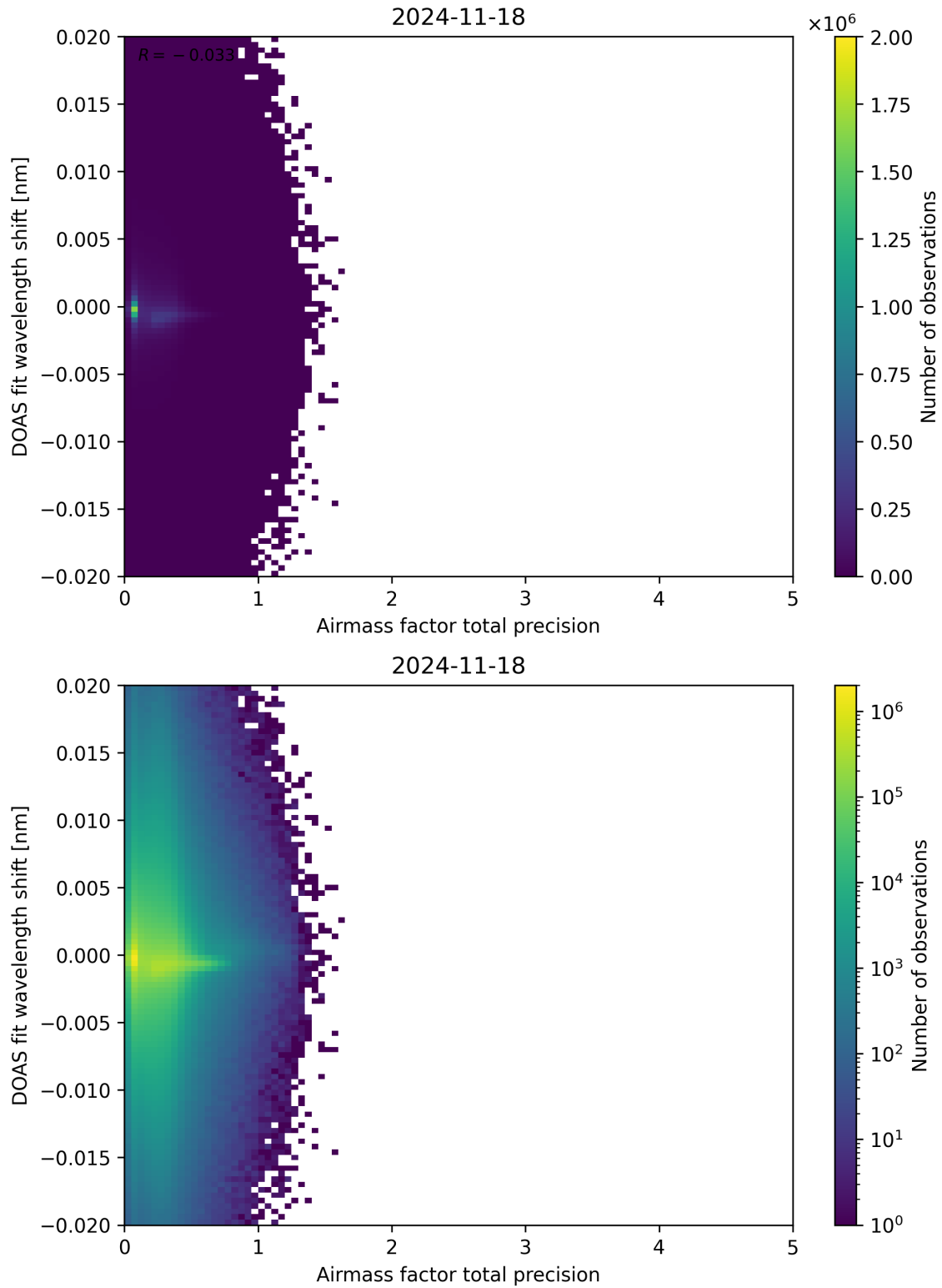
Figure 106: Scatter density plot of “Airmass factor total precision” against “DOAS fit wavelength shift” for 2024-11-17 to 2024-11-19.
