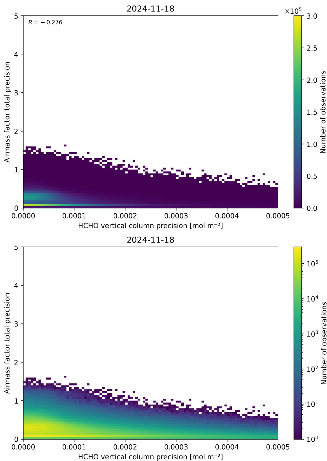
Figure 145: Scatter density plot of “HCHO vertical column precision” against “Airmass factor total precision” for 2024-11-17 to 2024-11-19.
