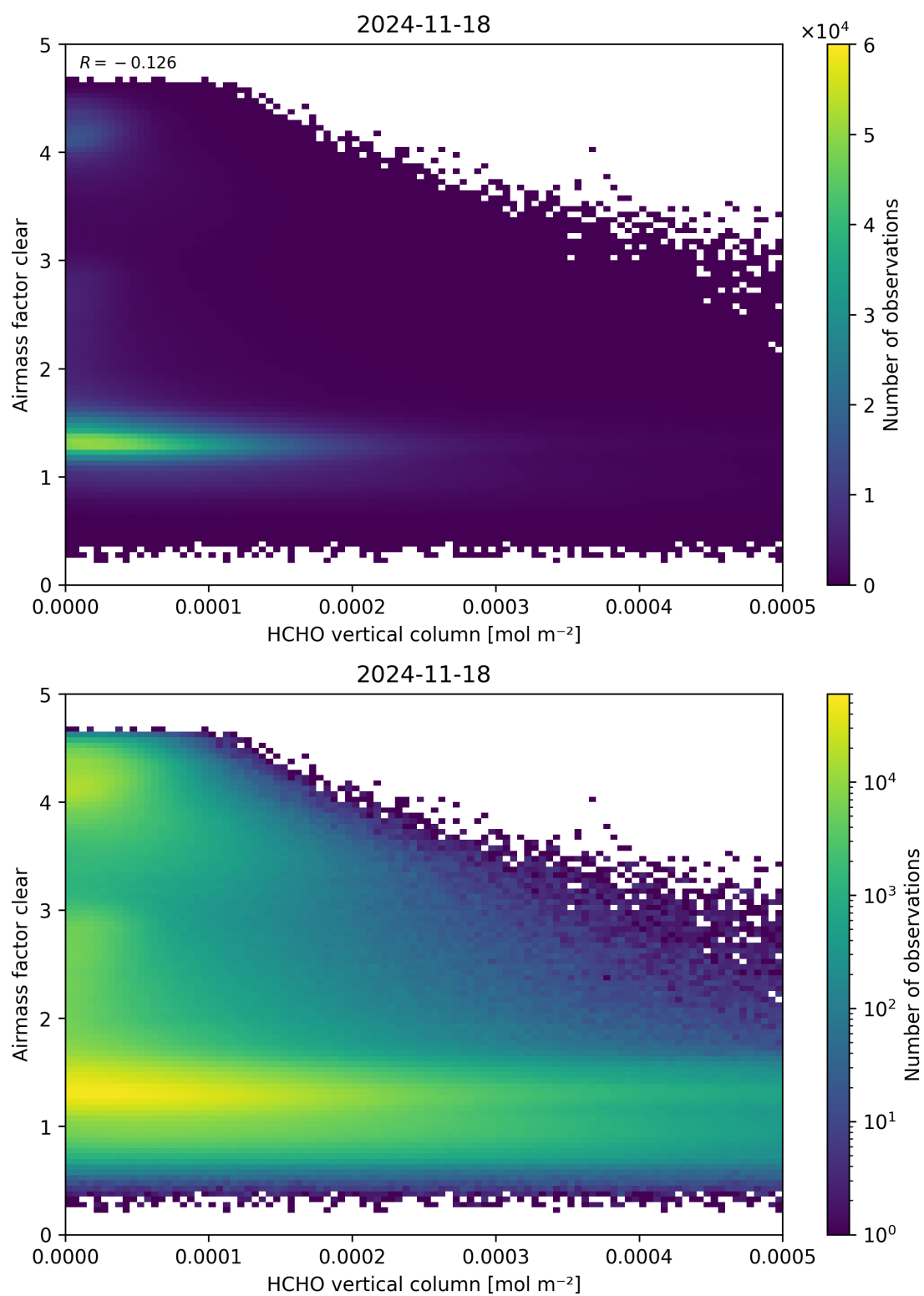
Figure 126: Scatter density plot of “HCHO vertical column” against “Airmass factor clear” for 2024-11-17 to 2024-11-19.
