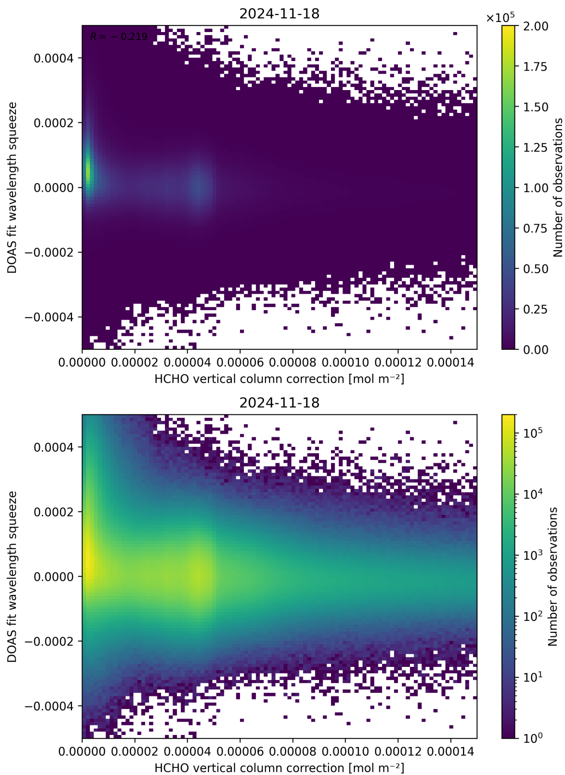
Figure 114: Scatter density plot of “HCHO vertical column correction” against “DOAS fit wavelength squeeze” for 2024-11-17 to 2024-11-19.
