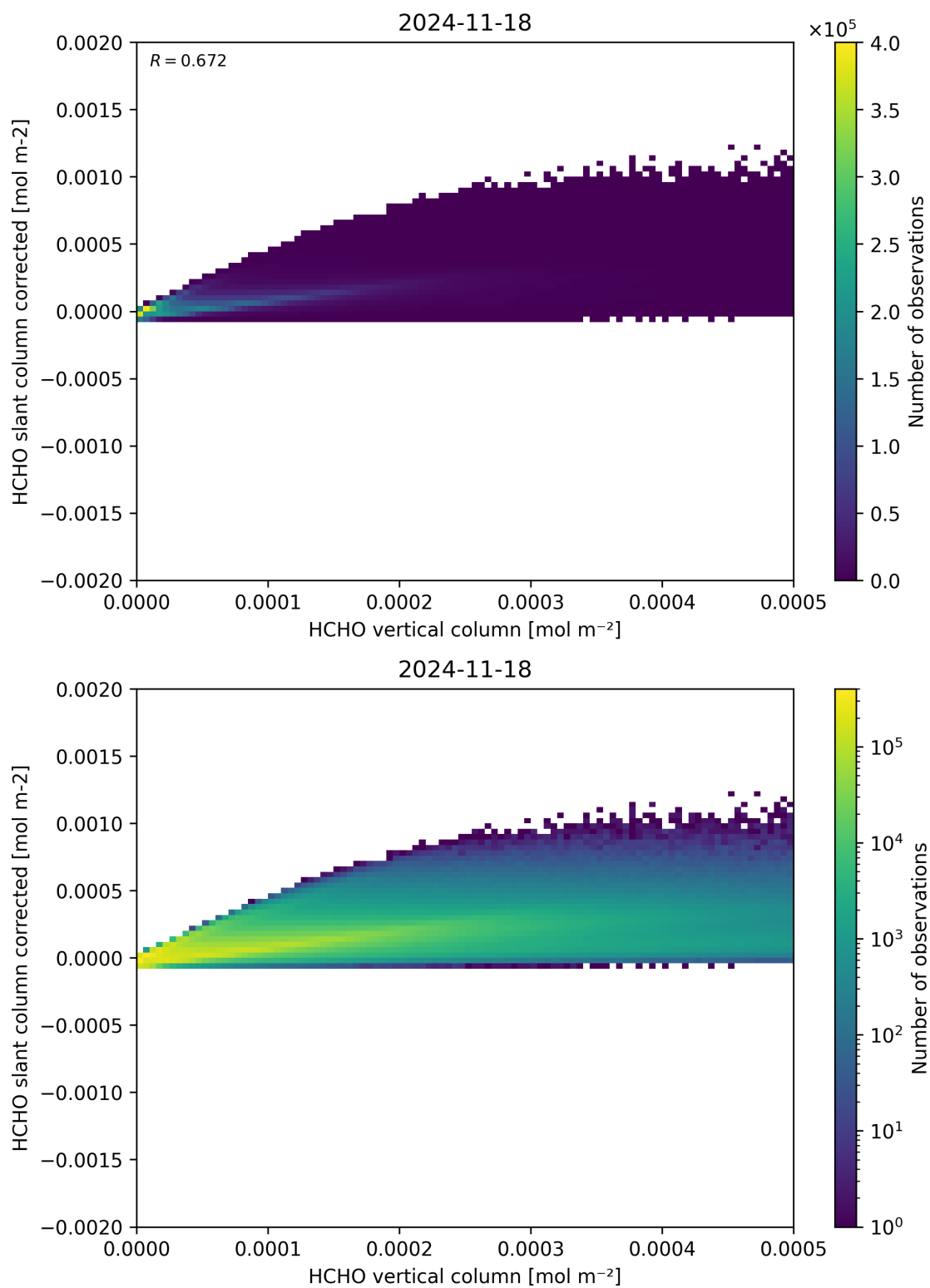
Figure 127: Scatter density plot of “HCHO vertical column” against “HCHO slant column corrected” for 2024-11-17 to 2024-11-19.
