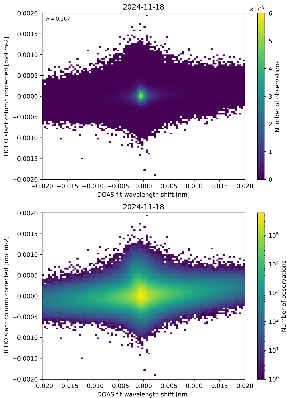
Figure 66: Scatter density plot of “DOAS fit wavelength shift” against “HCHO slant column corrected” for 2024-11-17 to 2024-11-19.
