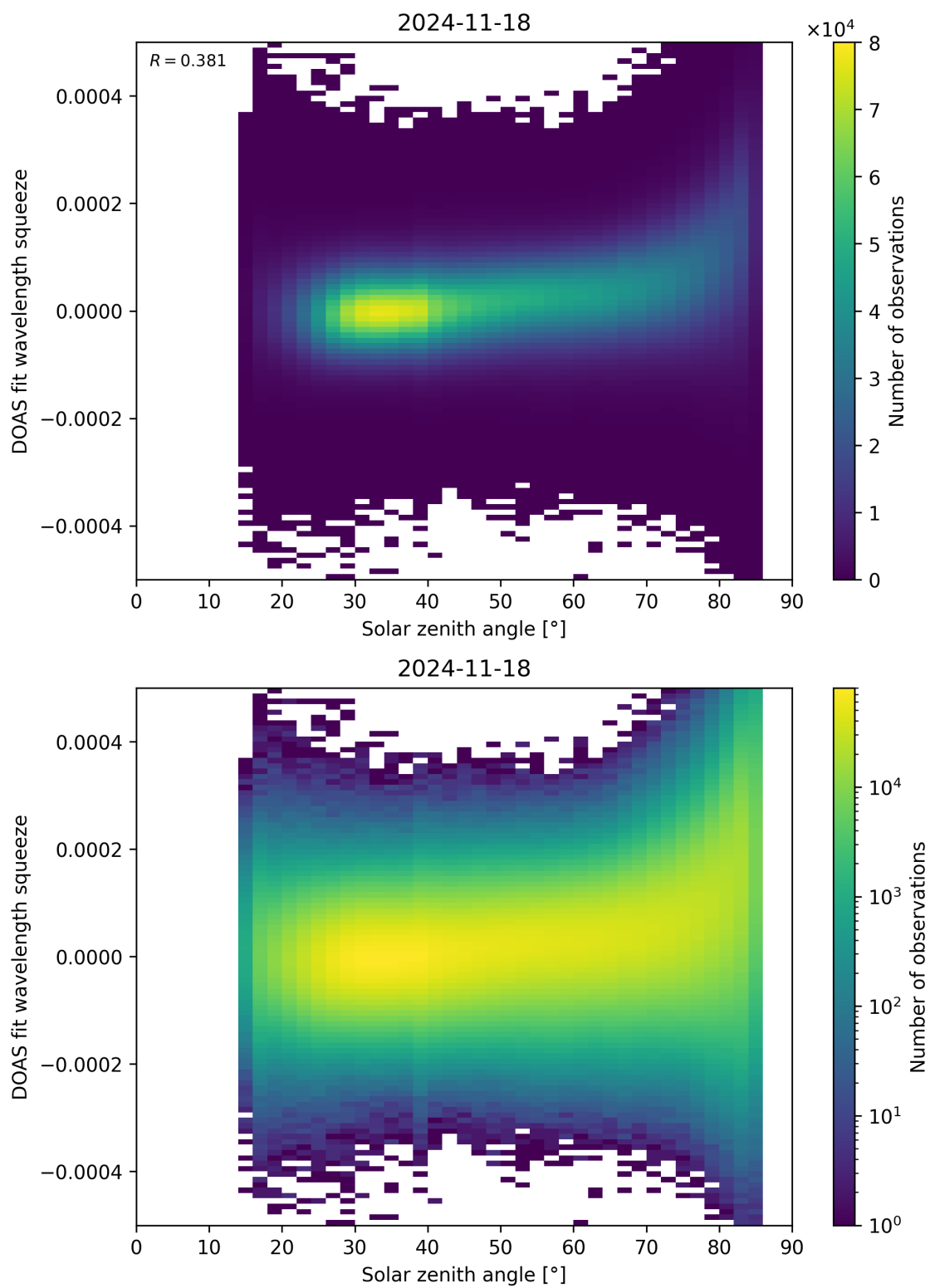
Figure 169: Scatter density plot of “Solar zenith angle” against “DOAS fit wavelength squeeze” for 2024-11-17 to 2024-11-19.
