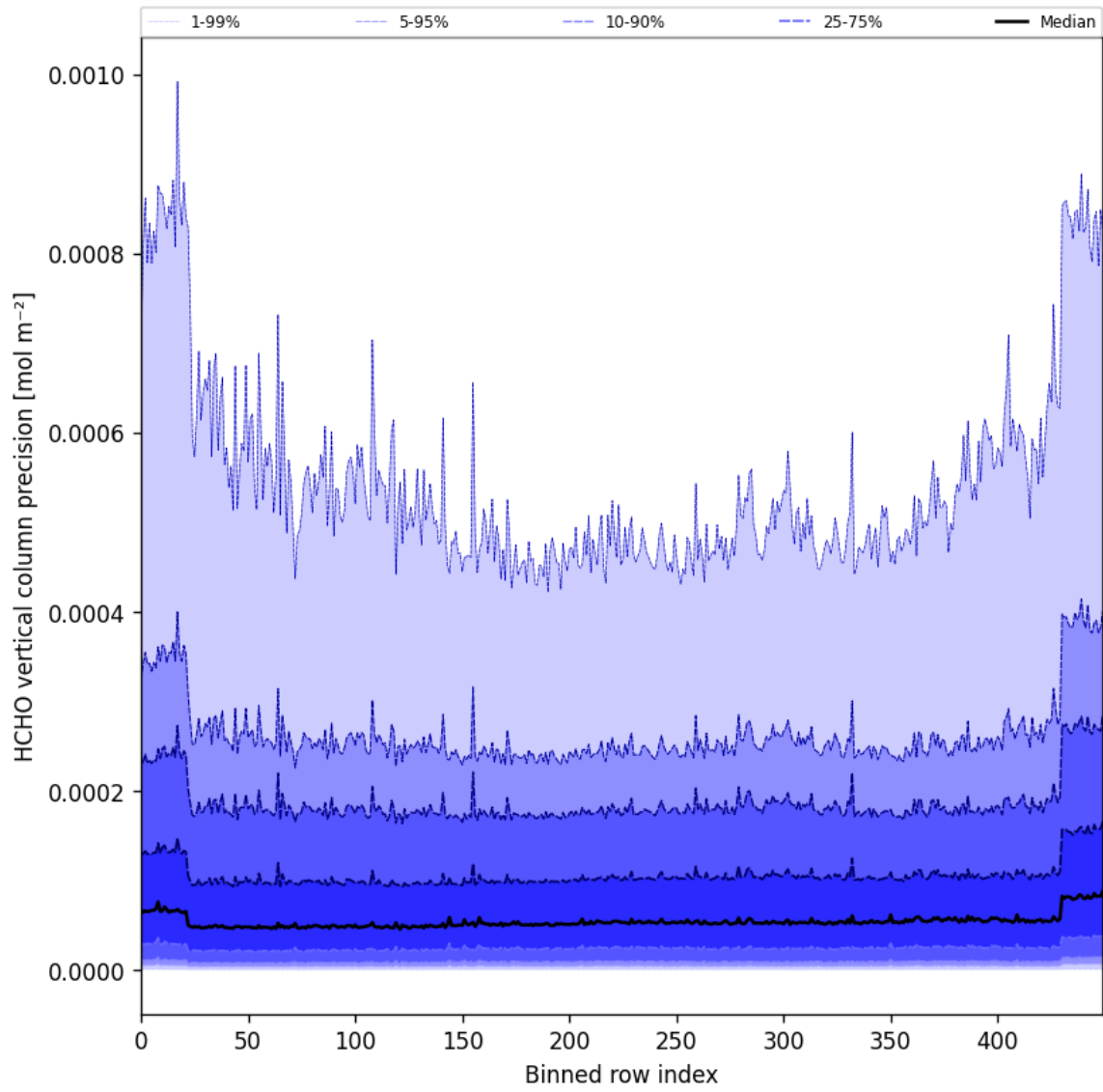
Figure 50: Along track statistics of “HCHO vertical column precision” for 2024-11-17 to 2024-11-19
