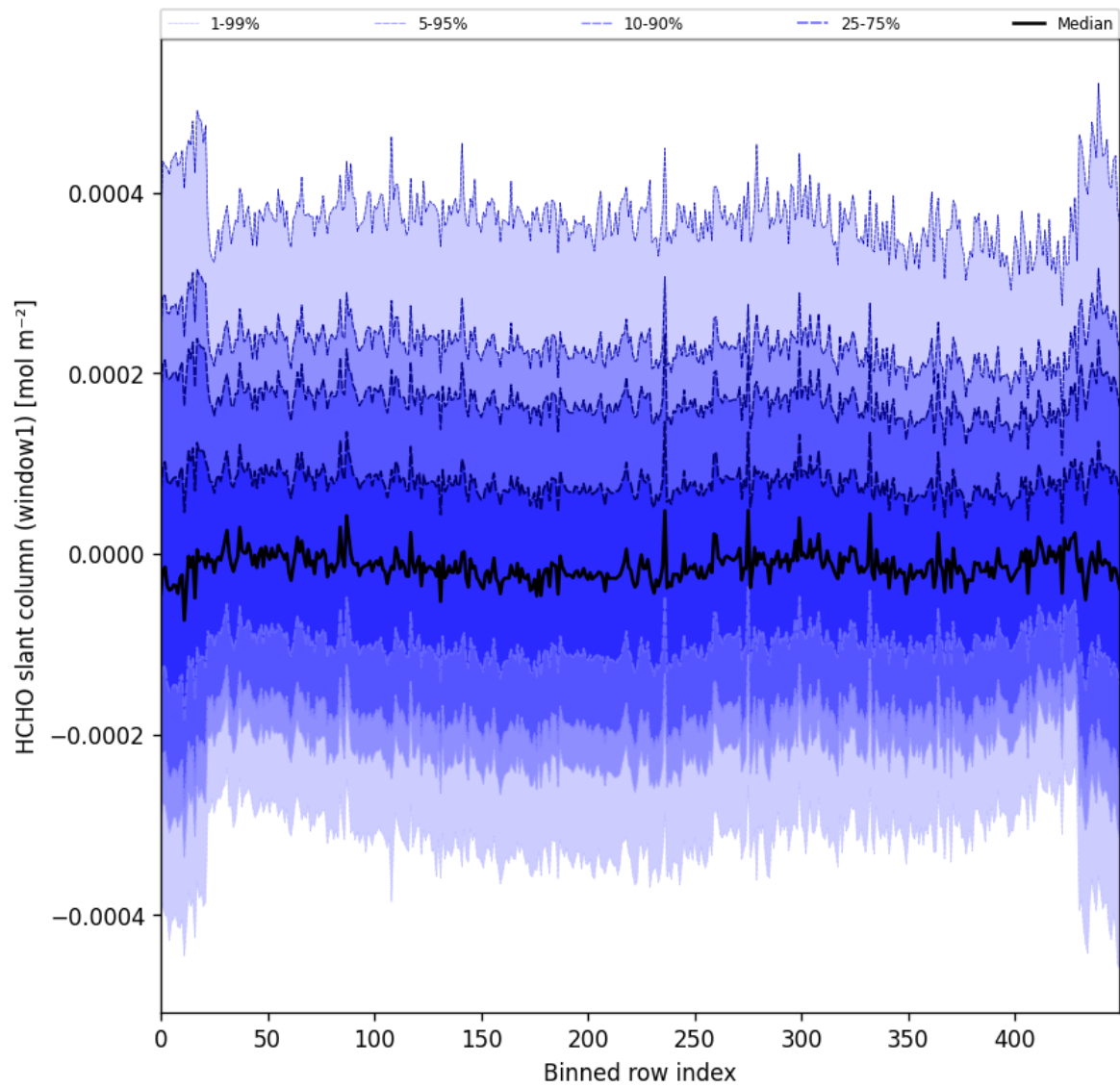
Figure 52: Along track statistics of “HCHO slant column (window1)” for 2024-11-20 to 2024-11-21
