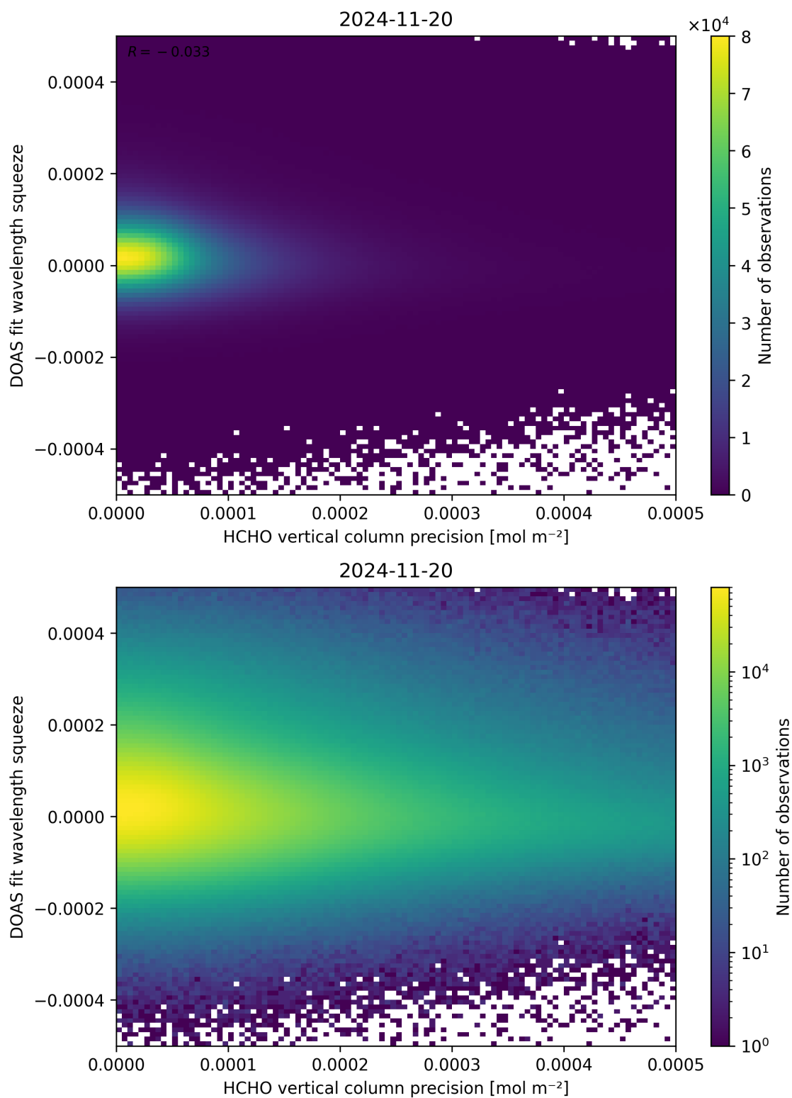
Figure 138: Scatter density plot of “HCHO vertical column precision” against “DOAS fit wavelength squeeze” for 2024-11-20 to 2024-11-21.
