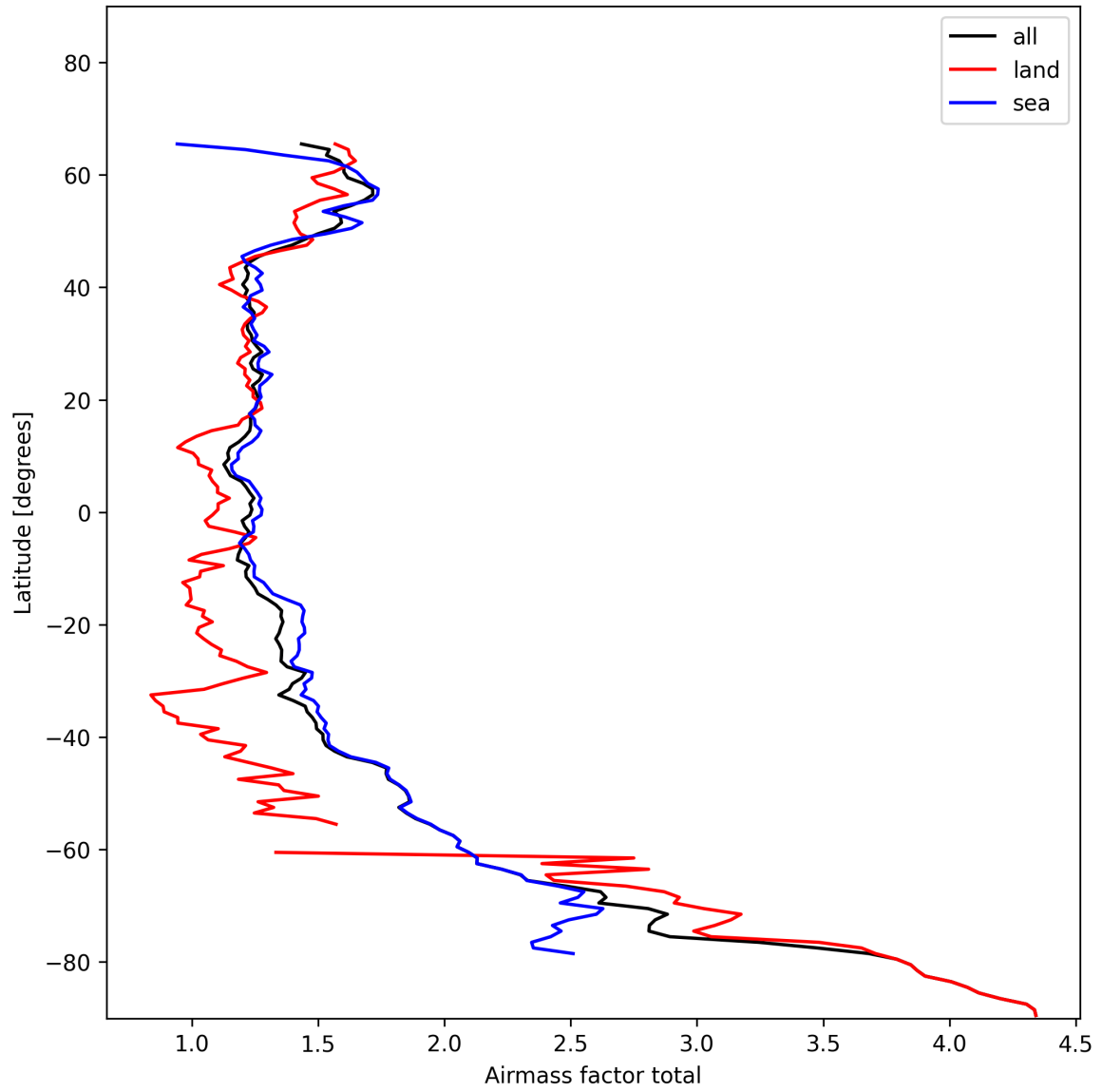
Figure 26: Zonal average of “Airmass factor total” for 2024-11-20 to 2024-11-21.
