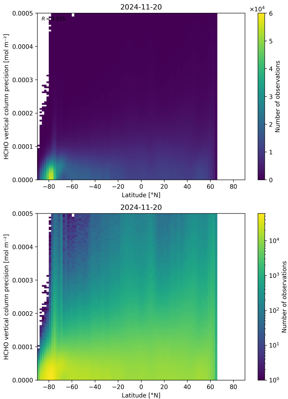
Figure 165: Scatter density plot of “Latitude” against “HCHO vertical column precision” for 2024-11-20 to 2024-11-21.
