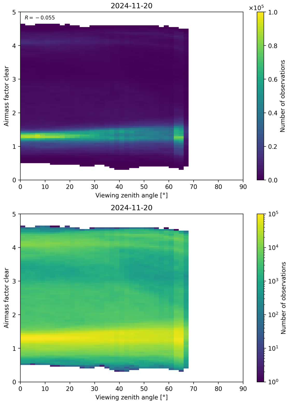
Figure 185: Scatter density plot of “Viewing zenith angle” against “Airmass factor clear” for 2024-11-20 to 2024-11-21.
