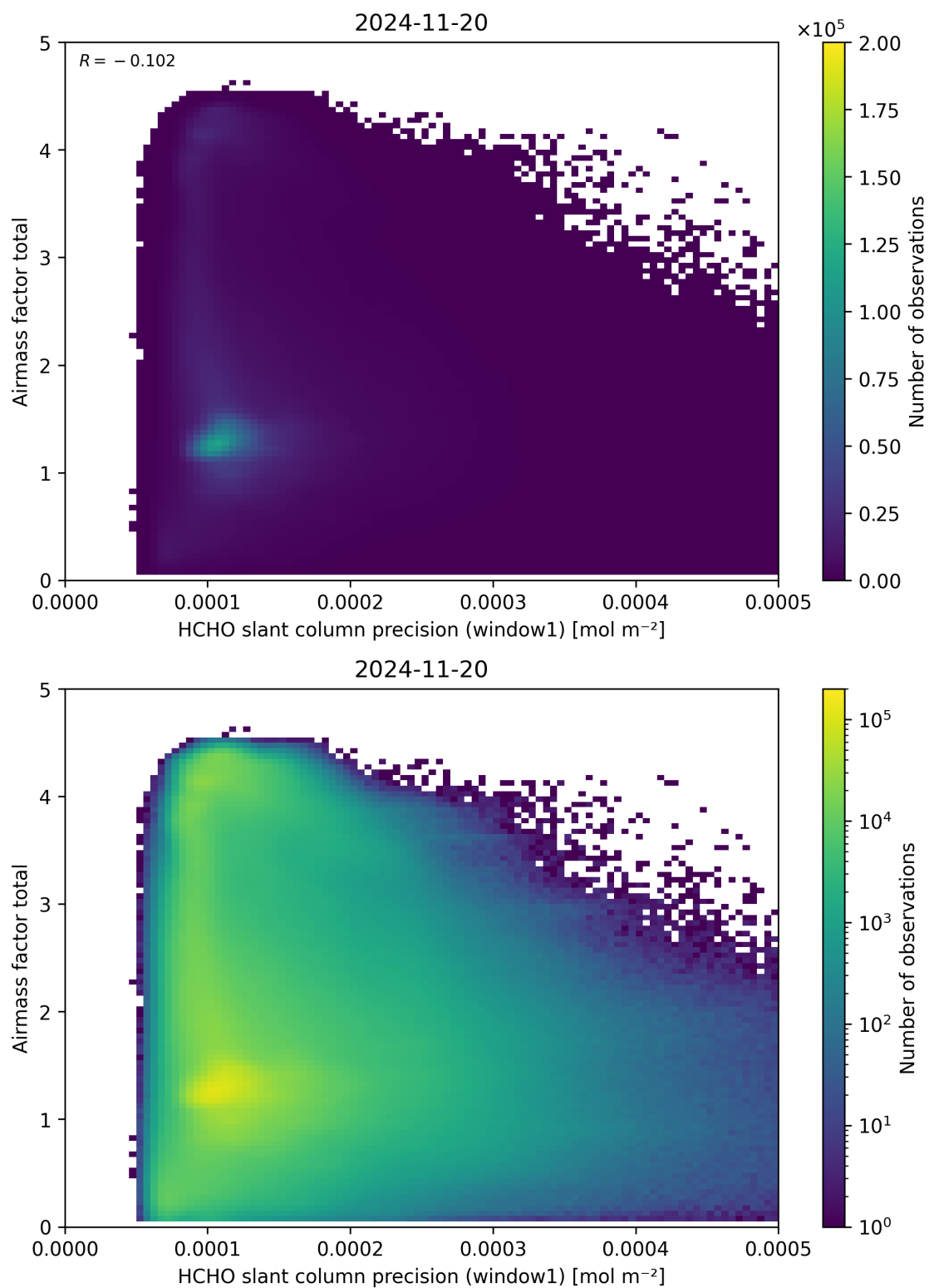
Figure 94: Scatter density plot of “HCHO slant column precision (window1)” against “Airmass factor total” for 2024-11-20 to 2024-11-21.
