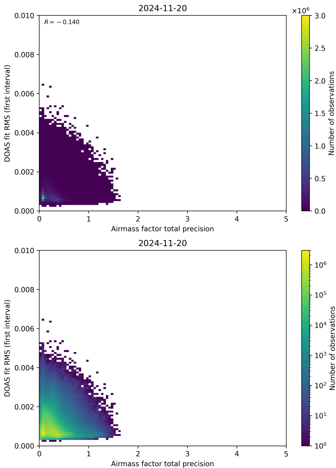
Figure 105: Scatter density plot of “Airmass factor total precision” against “DOAS fit RMS (first interval)” for 2024-11-20 to 2024-11-21.
