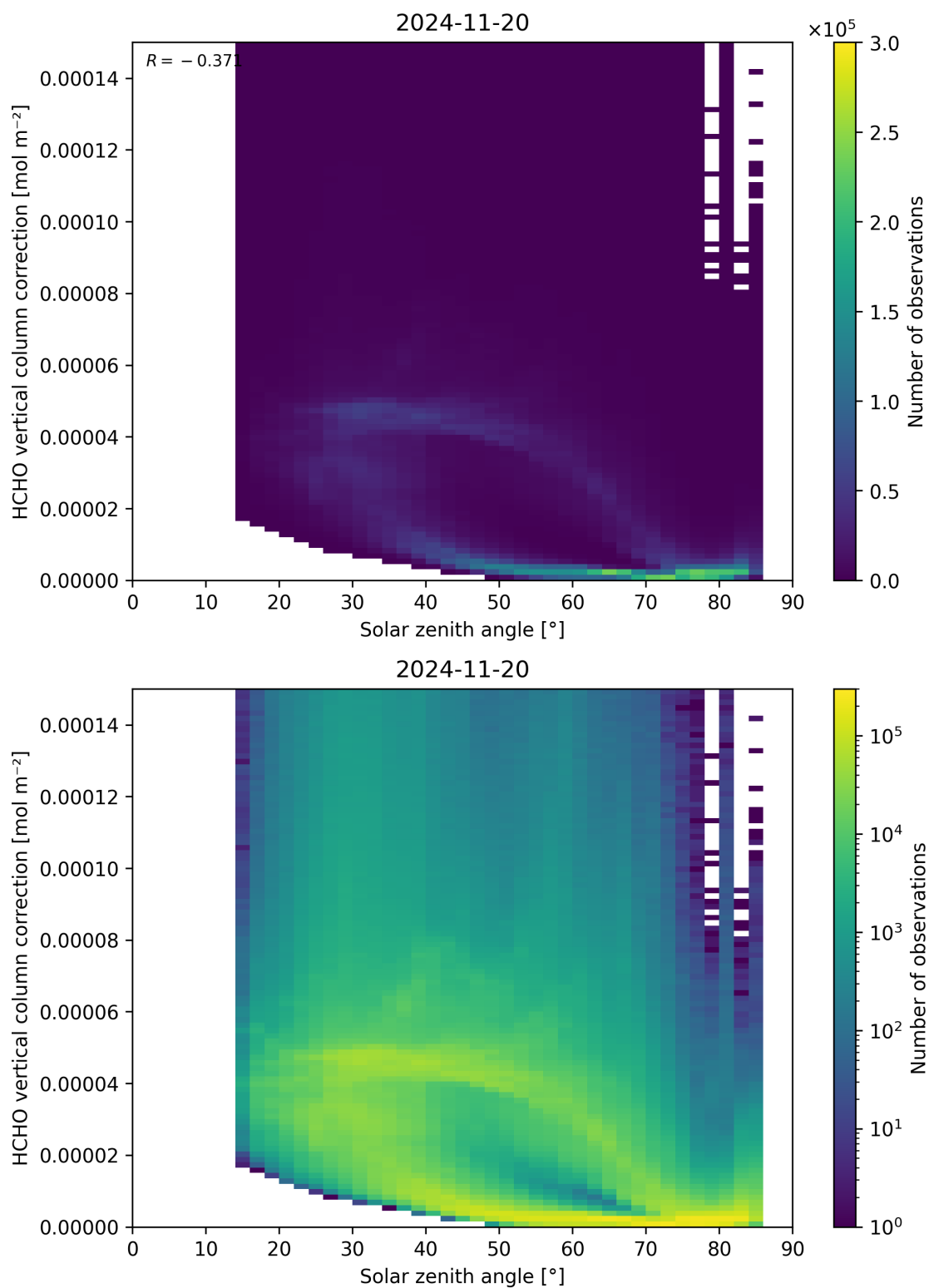
Figure 178: Scatter density plot of “Solar zenith angle” against “HCHO vertical column correction” for 2024-11-20 to 2024-11-21.
