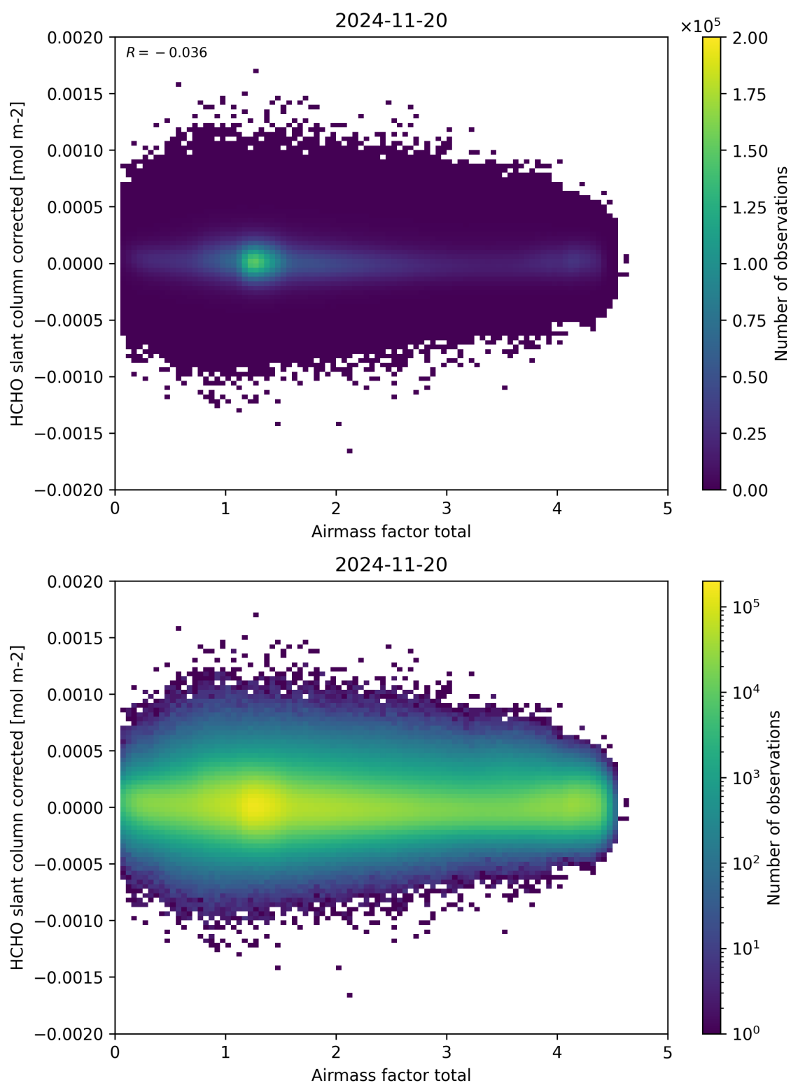
Figure 101: Scatter density plot of “Airmass factor total” against “HCHO slant column corrected” for 2024-11-20 to 2024-11-21.
