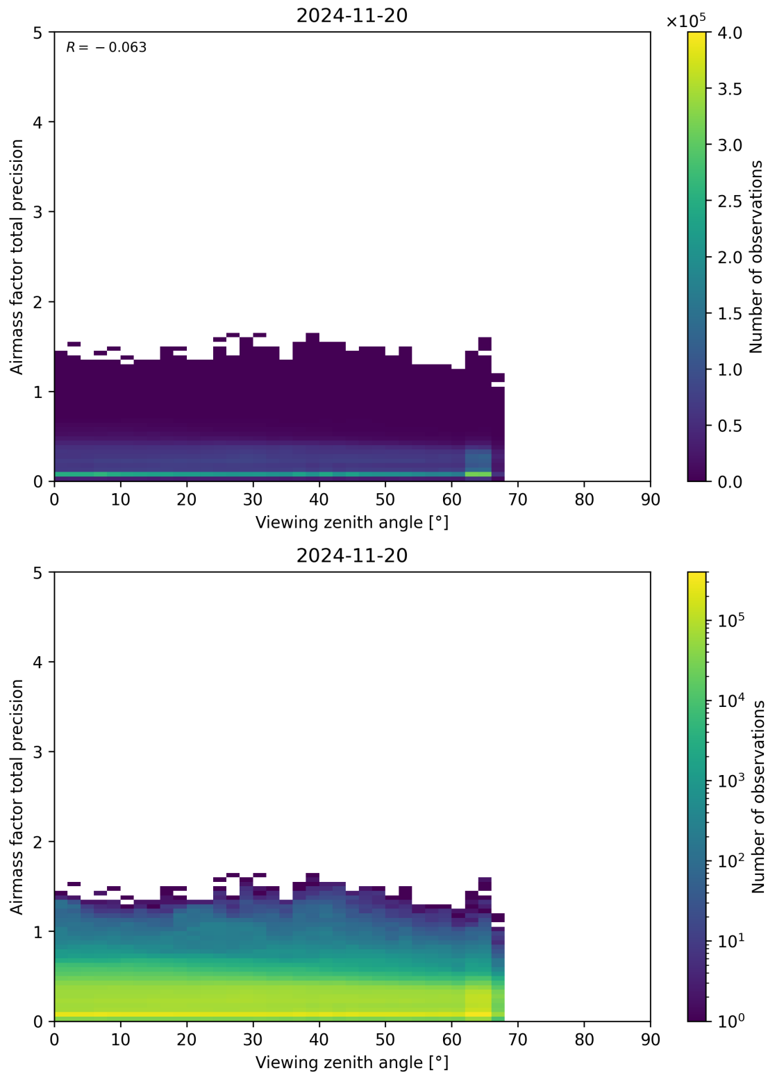
Figure 191: Scatter density plot of “Viewing zenith angle” against “Airmass factor total precision” for 2024-11-20 to 2024-11-21.
