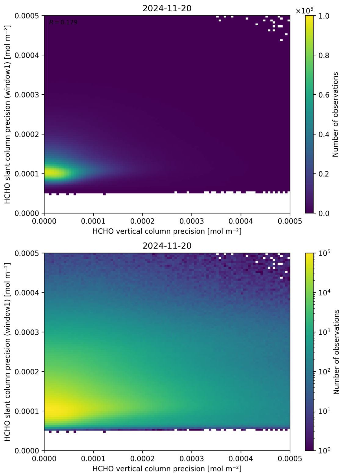
Figure 143: Scatter density plot of “HCHO vertical column precision” against “HCHO slant column precision (window1)” for 2024-11-20 to 2024-11-21.
