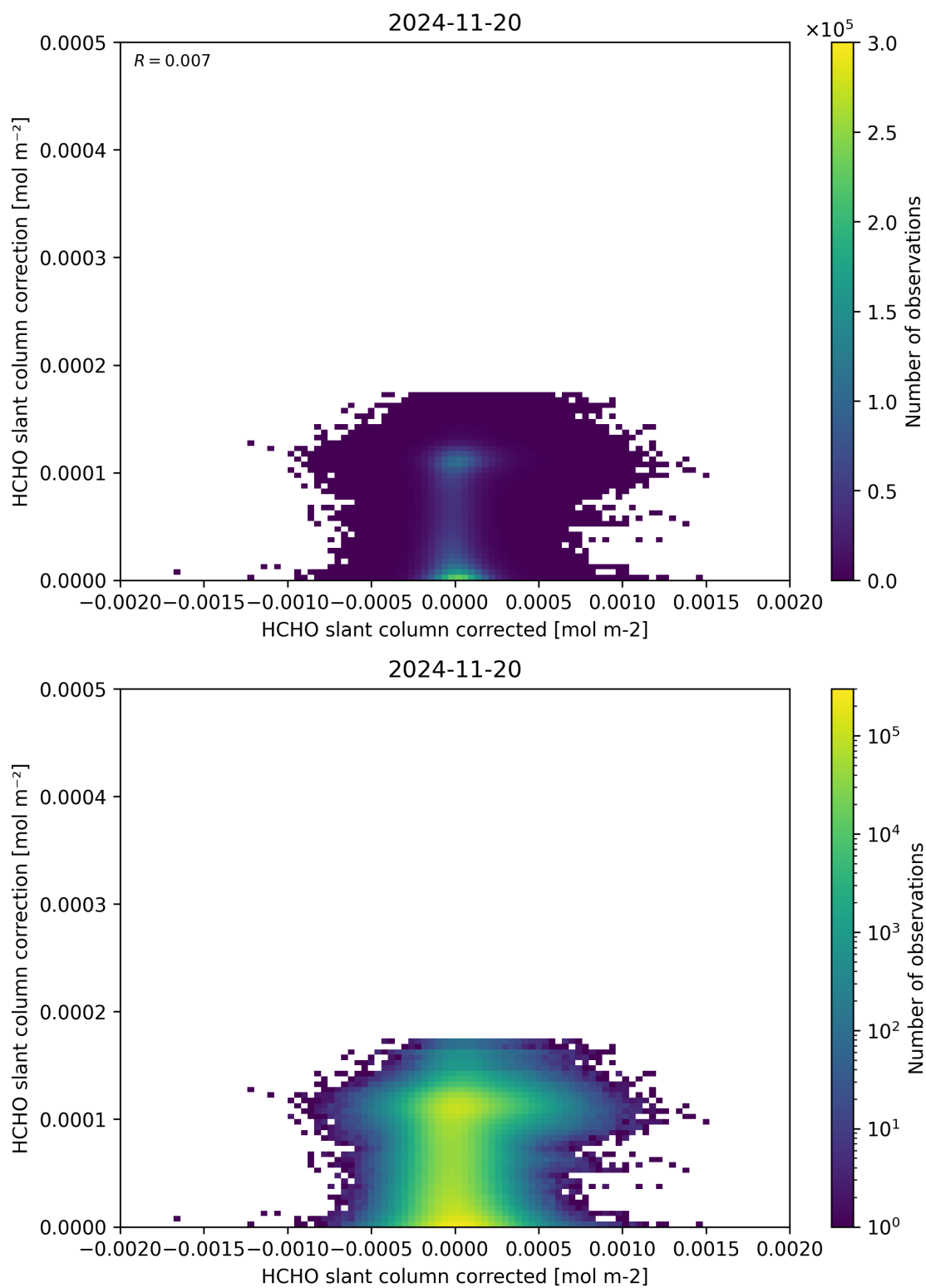
Figure 77: Scatter density plot of “HCHO slant column corrected” against “HCHO slant column correction” for 2024-11-20 to 2024-11-21.
