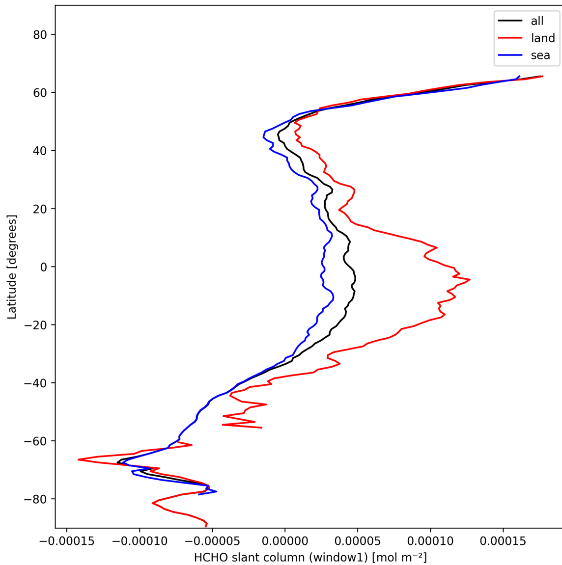
Figure 24: Zonal average of “HCHO slant column (window1)” for 2024-11-20 to 2024-11-21.
