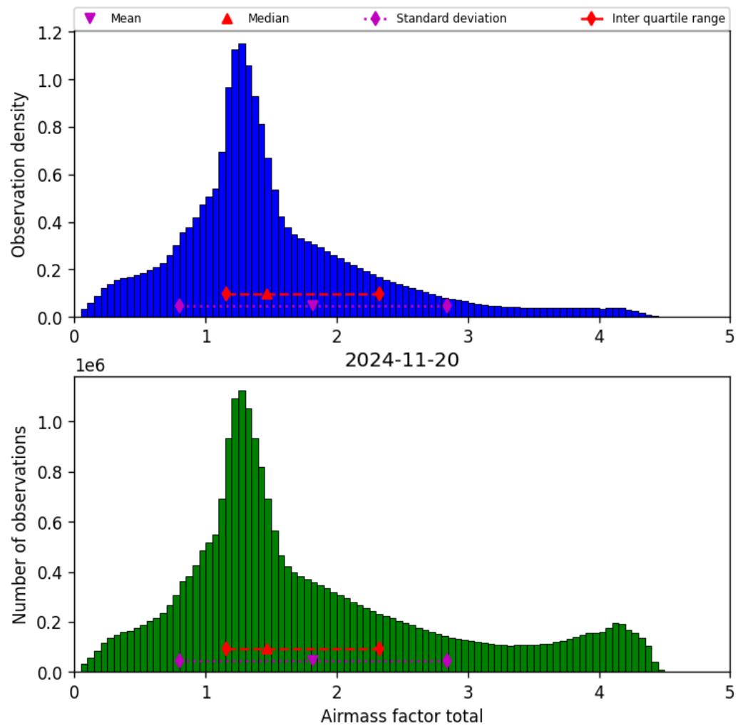
Figure 40: Histogram of “Airmass factor total” for 2024-11-20 to 2024-11-21
