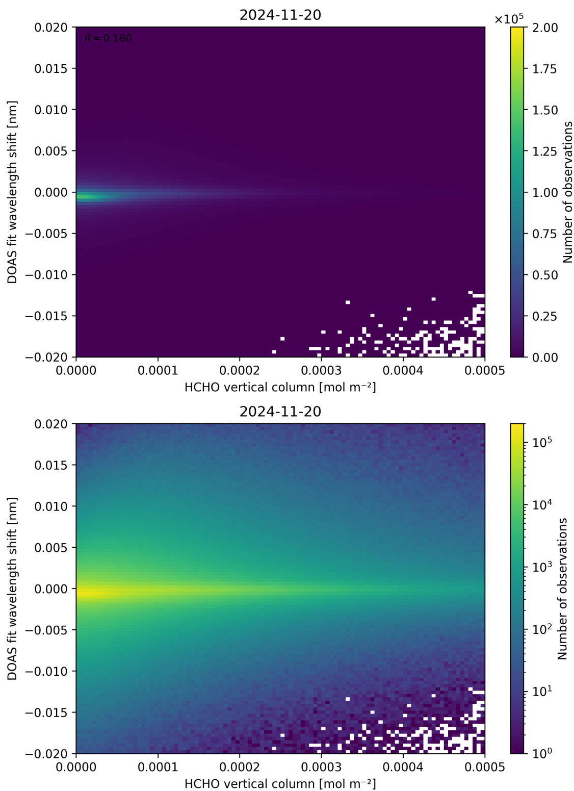
Figure 124: Scatter density plot of “HCHO vertical column” against “DOAS fit wavelength shift” for 2024-11-20 to 2024-11-21.
