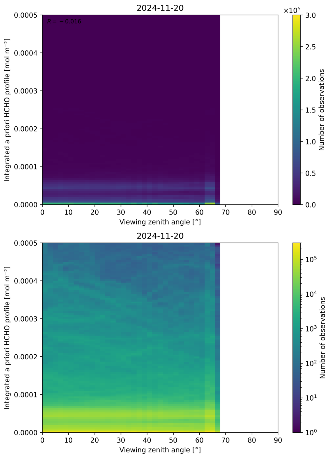
Figure 195: Scatter density plot of “Viewing zenith angle” against “Integrated a priori HCHO profile” for 2024-11-20 to 2024-11-21.
