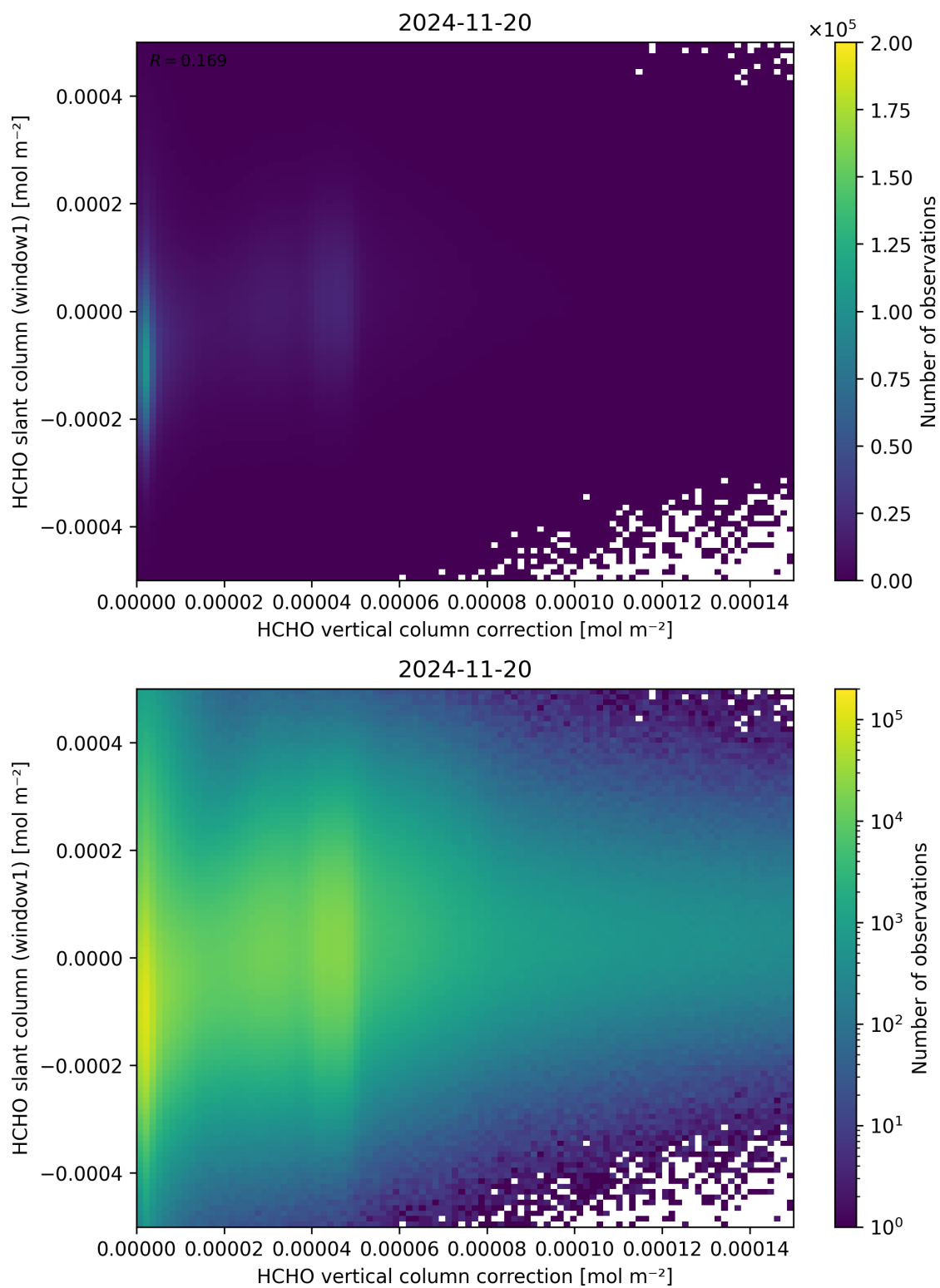
Figure 118: Scatter density plot of “HCHO vertical column correction” against “HCHO slant column (window1)” for 2024-11-20 to 2024-11-21.
