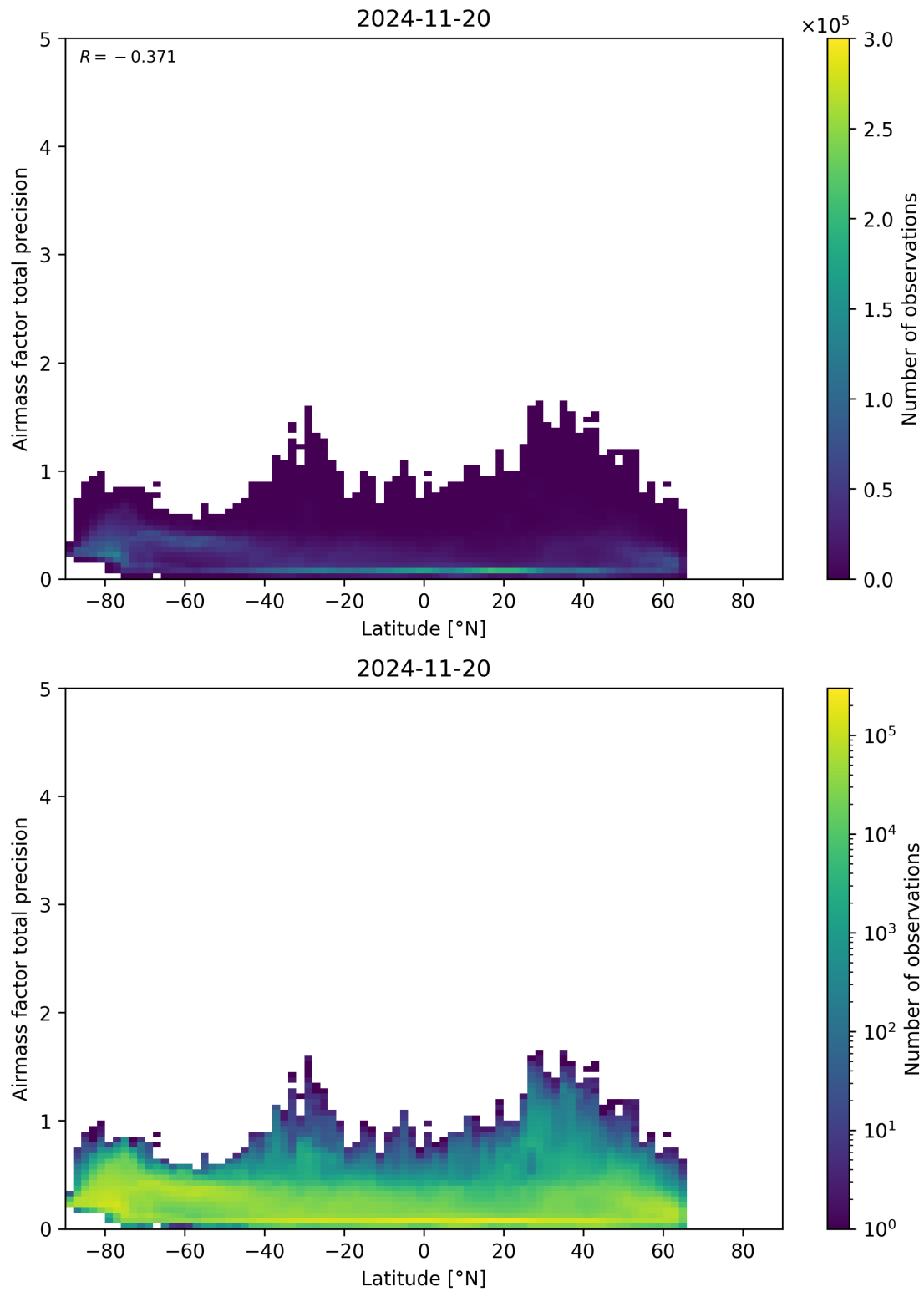
Figure 162: Scatter density plot of “Latitude” against “Airmass factor total precision” for 2024-11-20 to 2024-11-21.
