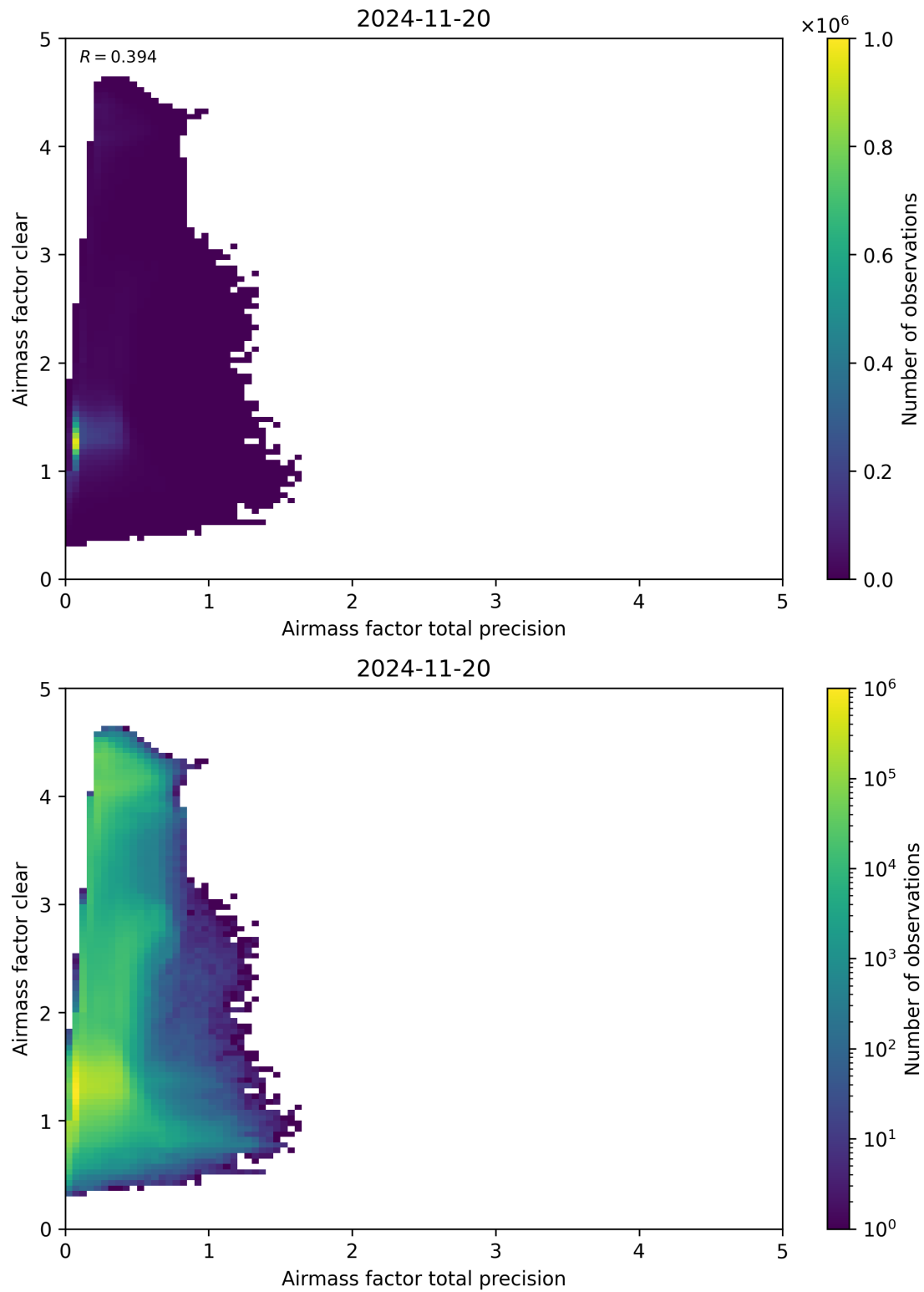
Figure 108: Scatter density plot of “Airmass factor total precision” against “Airmass factor clear” for 2024-11-20 to 2024-11-21.
