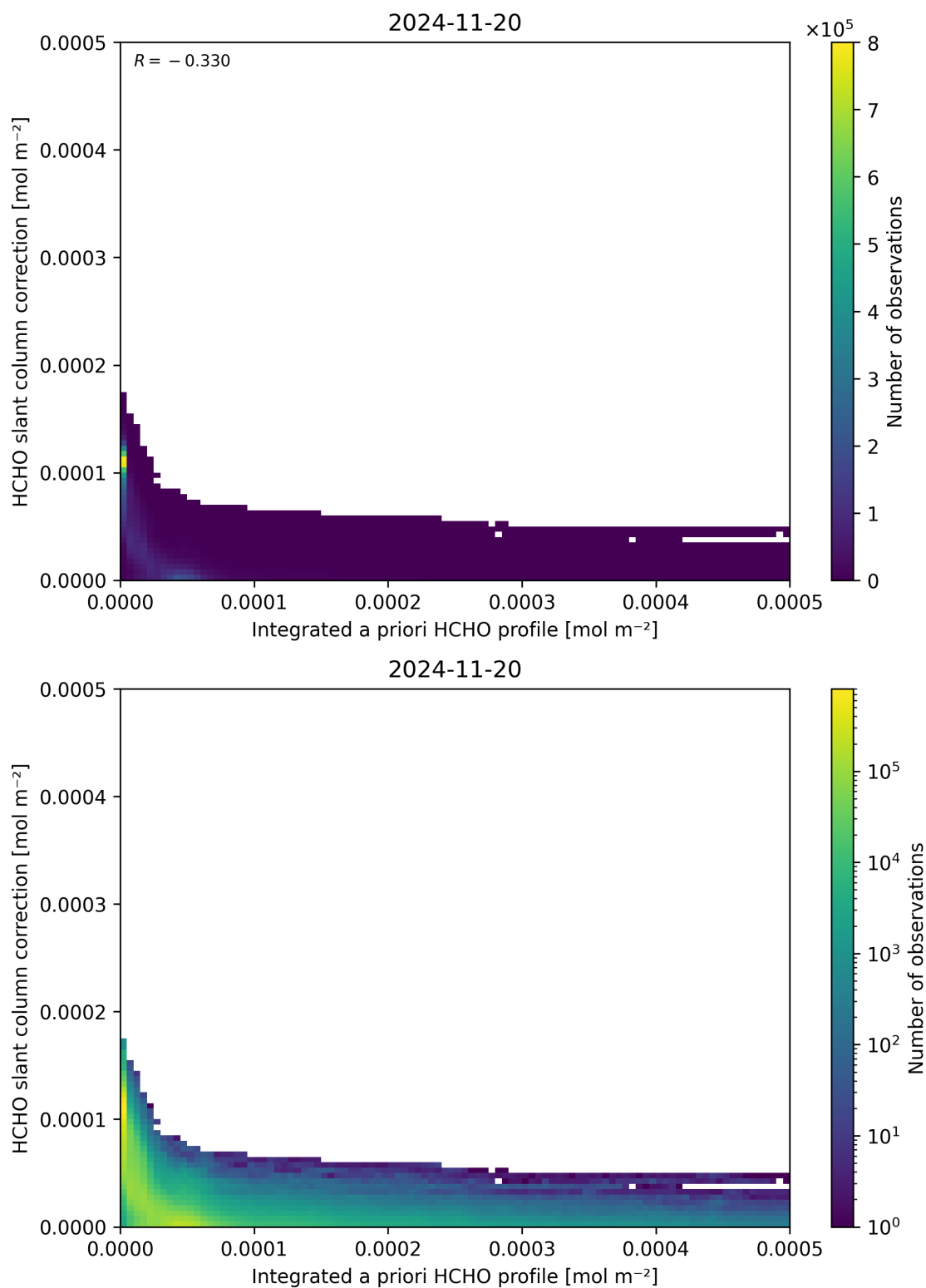
Figure 152: Scatter density plot of “Integrated a priori HCHO profile” against “HCHO slant column correction” for 2024-11-20 to 2024-11-21.
