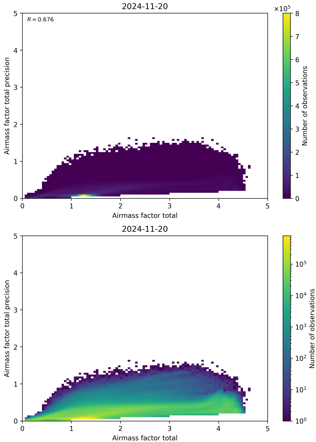
Figure 103: Scatter density plot of “Airmass factor total” against “Airmass factor total precision” for 2024-11-20 to 2024-11-21.
