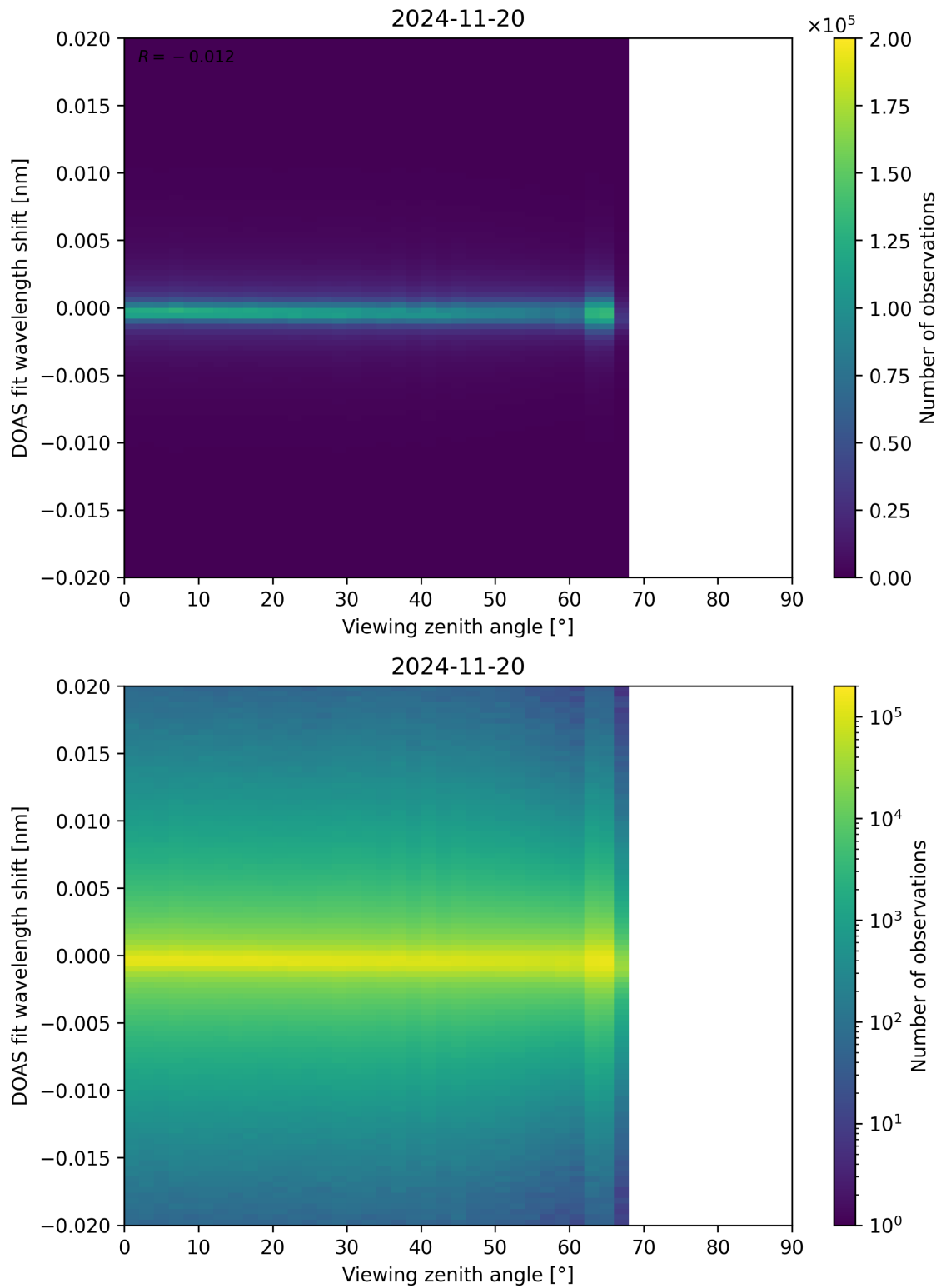
Figure 183: Scatter density plot of “Viewing zenith angle” against “DOAS fit wavelength shift” for 2024-11-20 to 2024-11-21.
