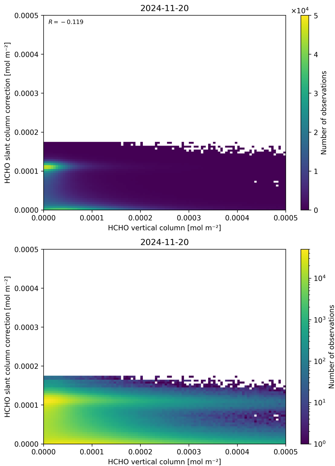
Figure 128: Scatter density plot of “HCHO vertical column” against “HCHO slant column correction” for 2024-11-20 to 2024-11-21.
