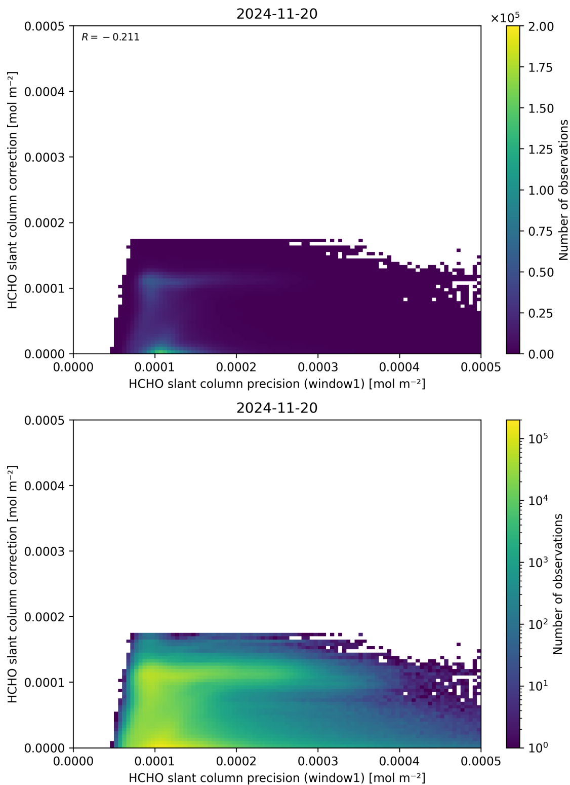
Figure 93: Scatter density plot of “HCHO slant column precision (window1)” against “HCHO slant column correction” for 2024-11-20 to 2024-11-21.
