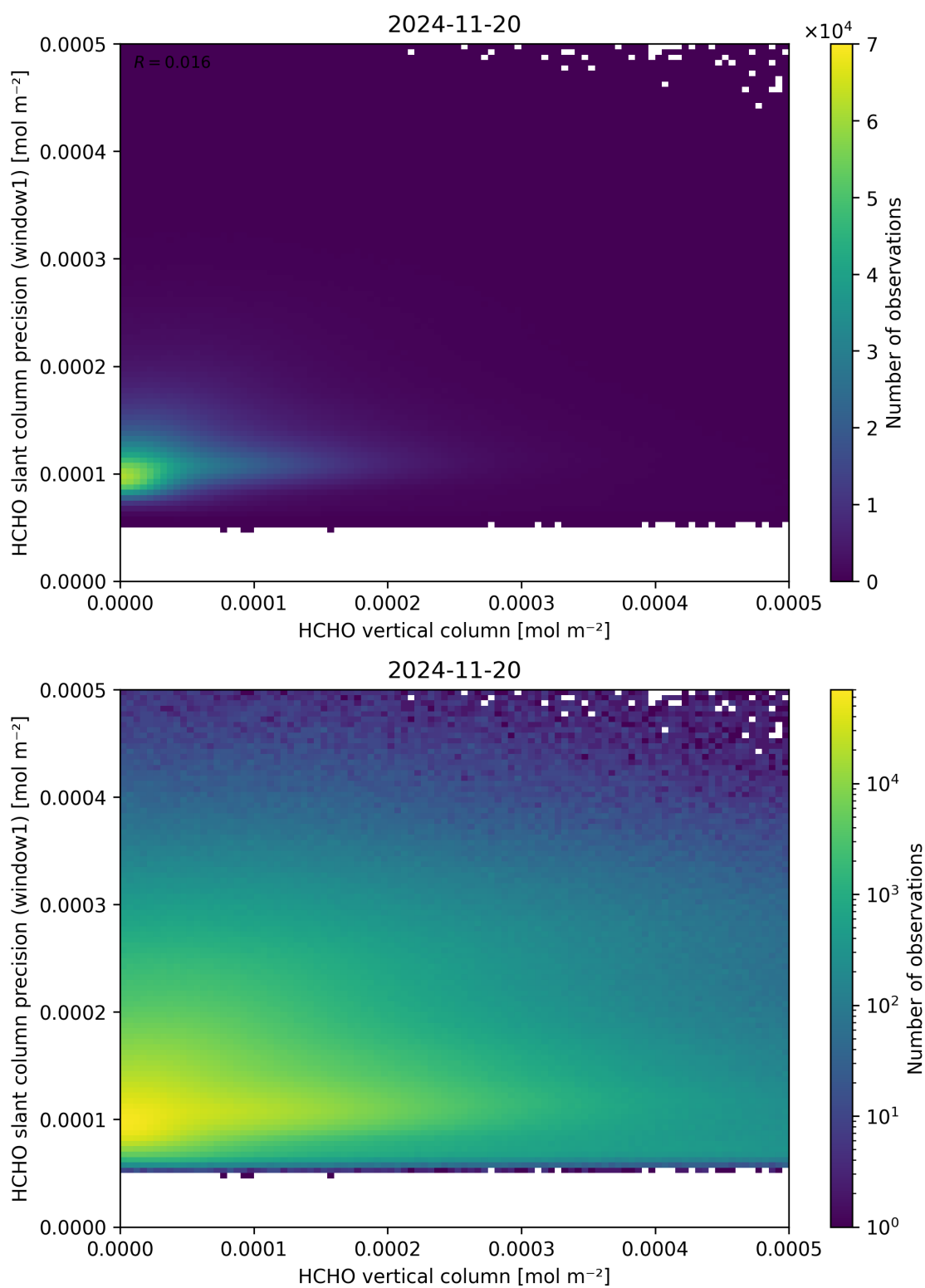
Figure 130: Scatter density plot of “HCHO vertical column” against “HCHO slant column precision (window1)” for 2024-11-20 to 2024-11-21.
