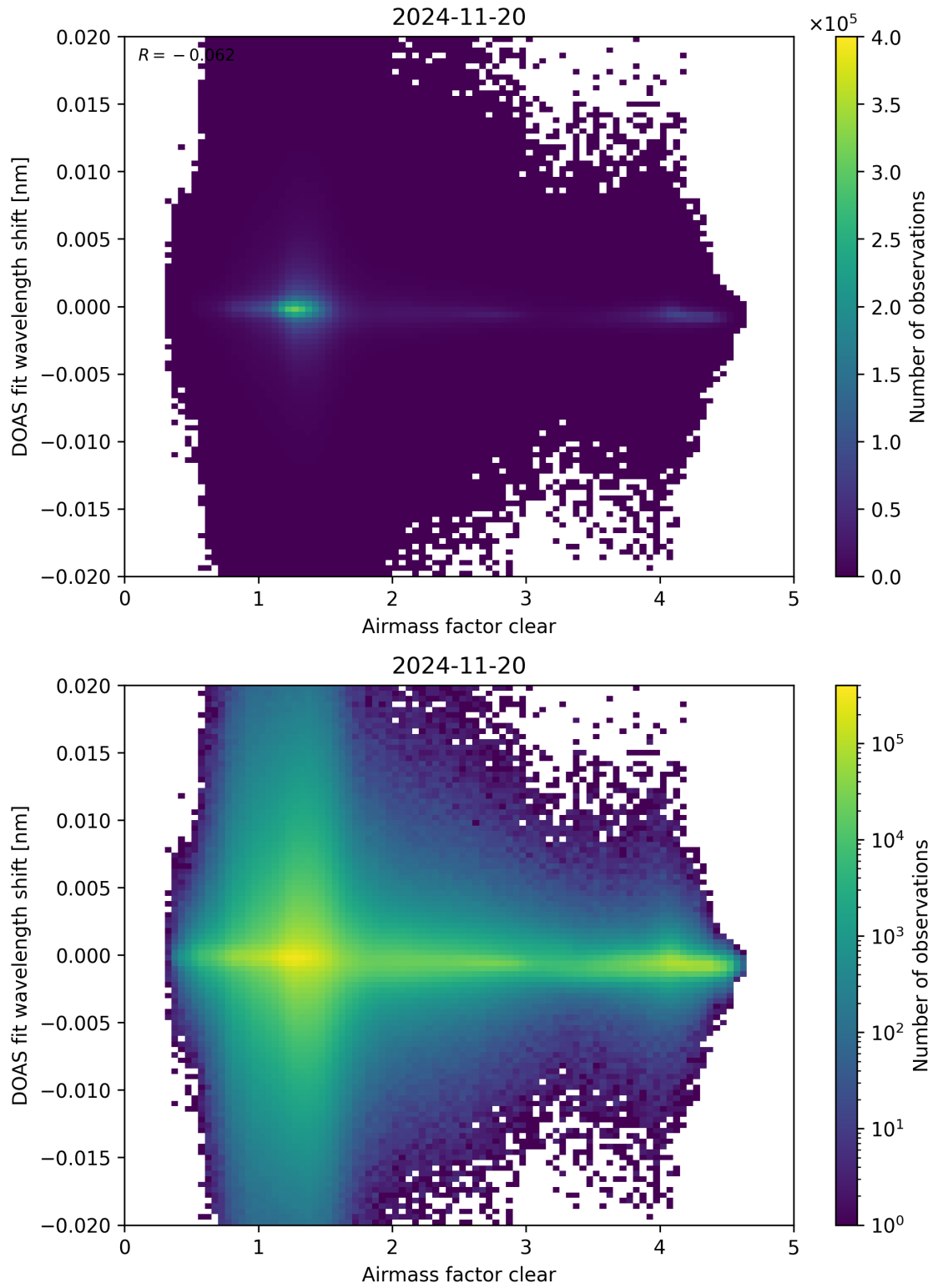
Figure 72: Scatter density plot of “Airmass factor clear” against “DOAS fit wavelength shift” for 2024-11-20 to 2024-11-21.
