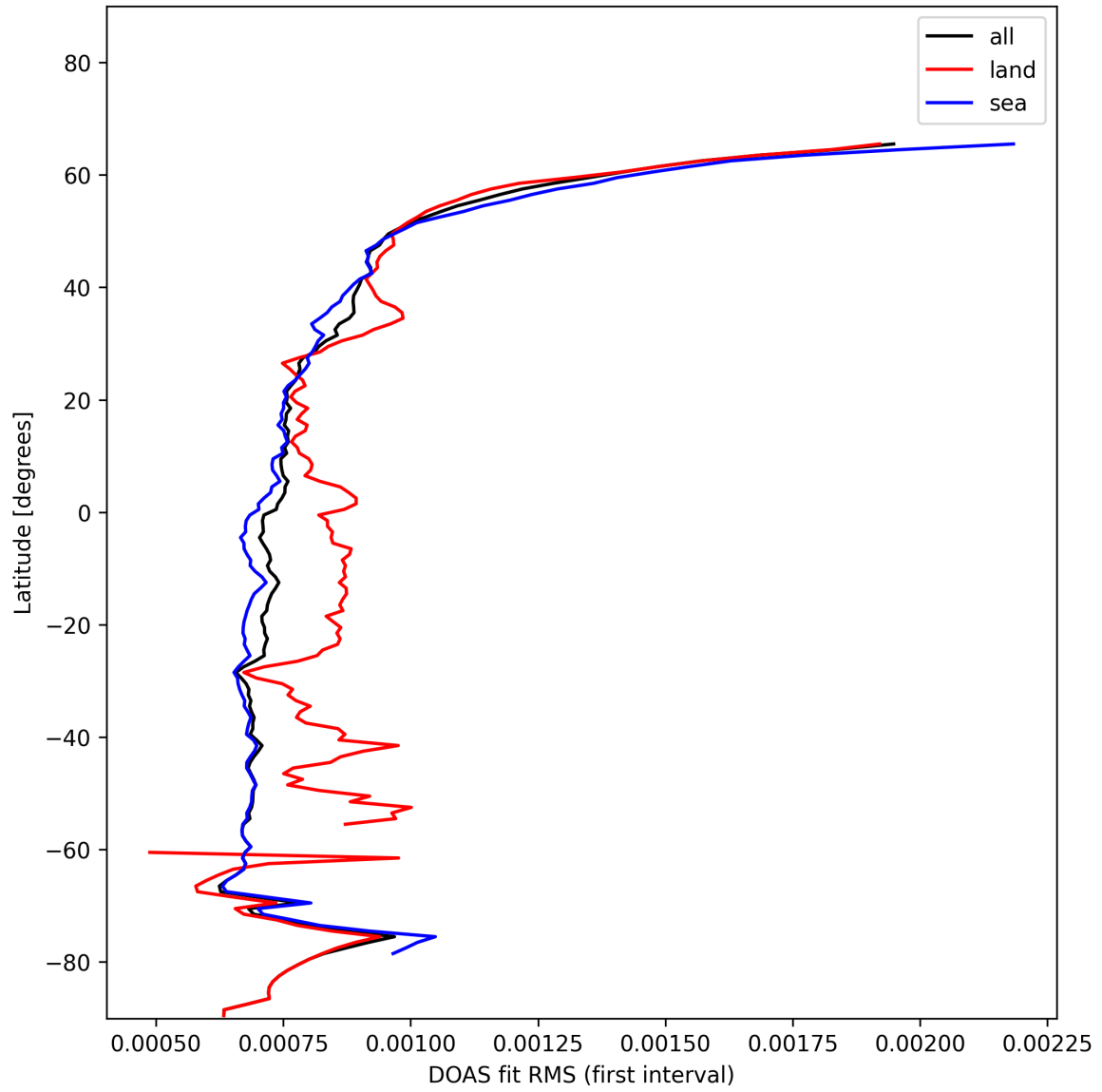
Figure 32: Zonal average of “DOAS fit RMS (first interval)” for 2024-11-20 to 2024-11-21.
