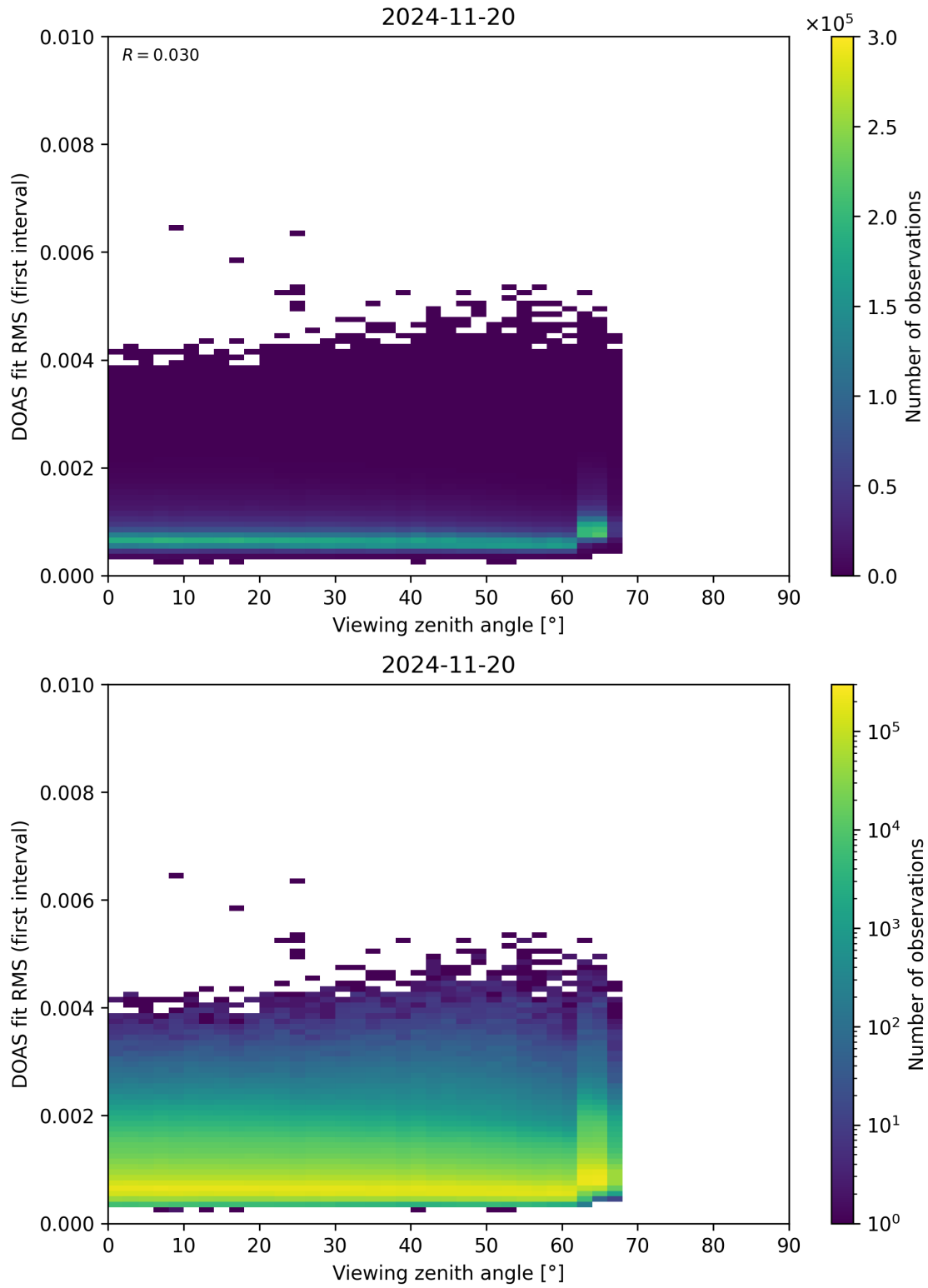
Figure 182: Scatter density plot of “Viewing zenith angle” against “DOAS fit RMS (first interval)” for 2024-11-20 to 2024-11-21.
