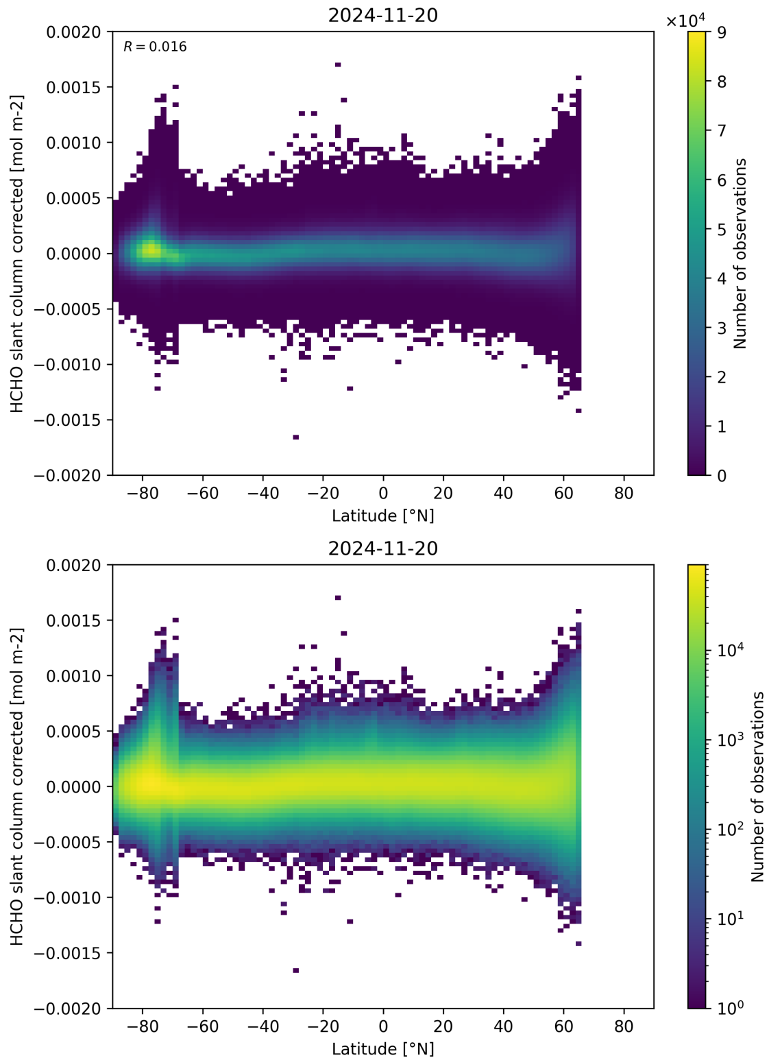
Figure 157: Scatter density plot of “Latitude” against “HCHO slant column corrected” for 2024-11-20 to 2024-11-21.
