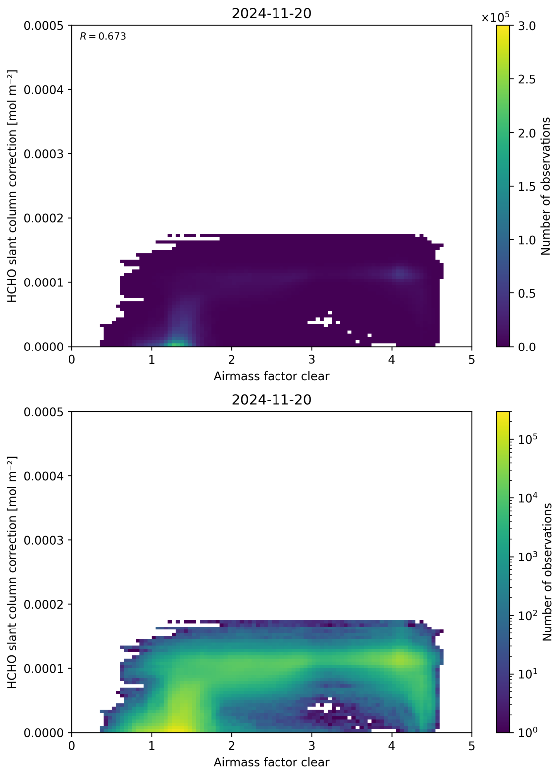
Figure 75: Scatter density plot of “Airmass factor clear” against “HCHO slant column correction” for 2024-11-20 to 2024-11-21.
