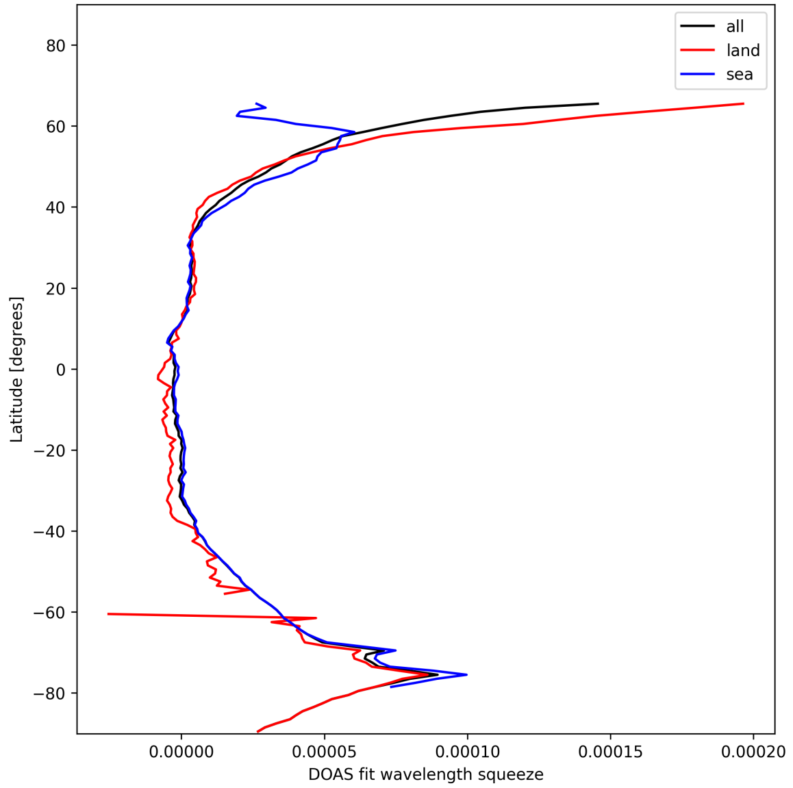
Figure 31: Zonal average of “DOAS fit wavelength squeeze” for 2024-11-20 to 2024-11-21.
