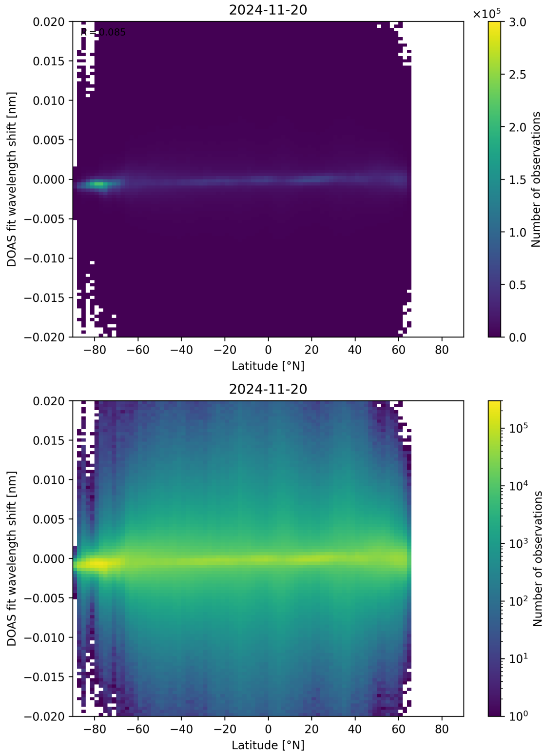
Figure 154: Scatter density plot of “Latitude” against “DOAS fit wavelength shift” for 2024-11-20 to 2024-11-21.
