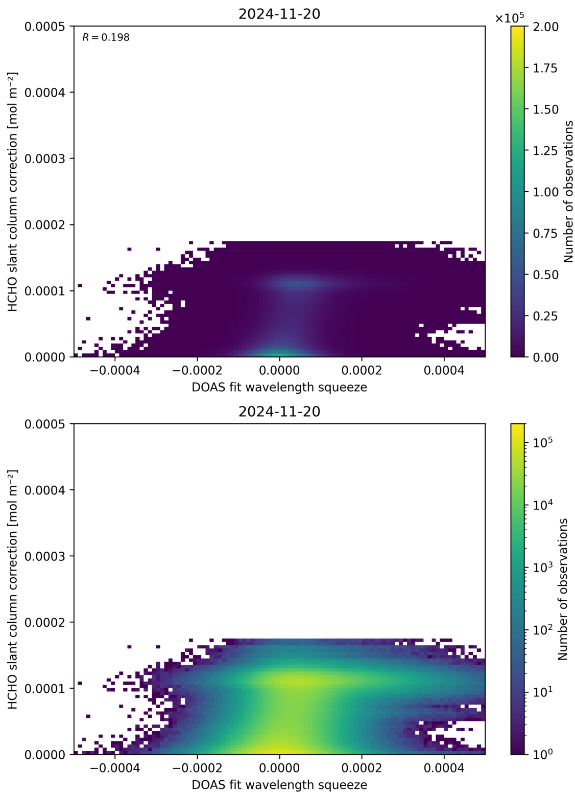
Figure 70: Scatter density plot of “DOAS fit wavelength squeeze” against “HCHO slant column correction” for 2024-11-20 to 2024-11-21.
