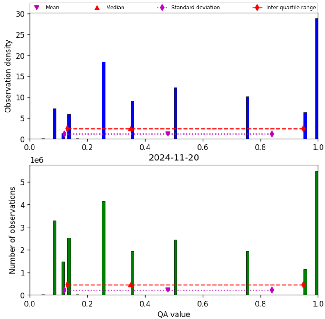
Figure 34: Histogram of “QA value” for 2024-11-20 to 2024-11-21
