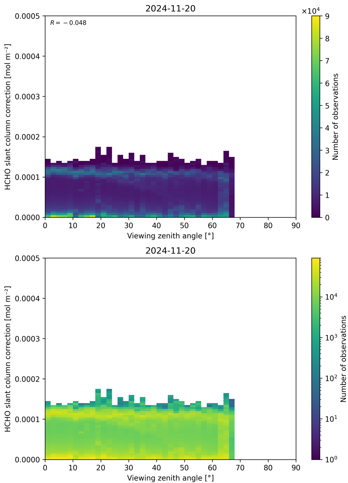
Figure 187: Scatter density plot of “Viewing zenith angle” against “HCHO slant column correction” for 2024-11-20 to 2024-11-21.
