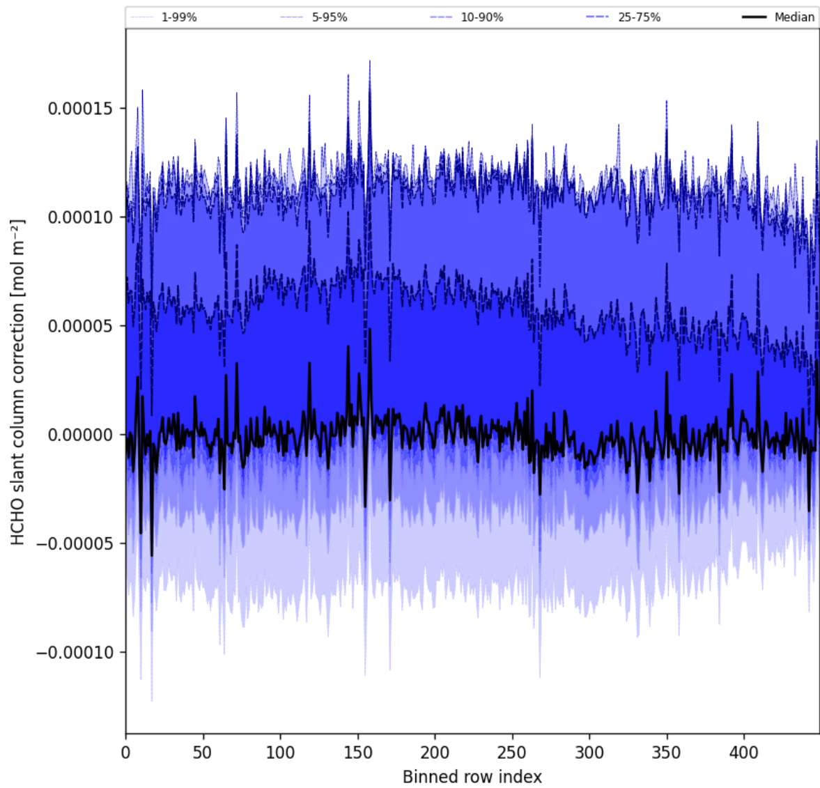
Figure 61: Along track statistics of “HCHO slant column correction” for 2024-11-20 to 2024-11-21
