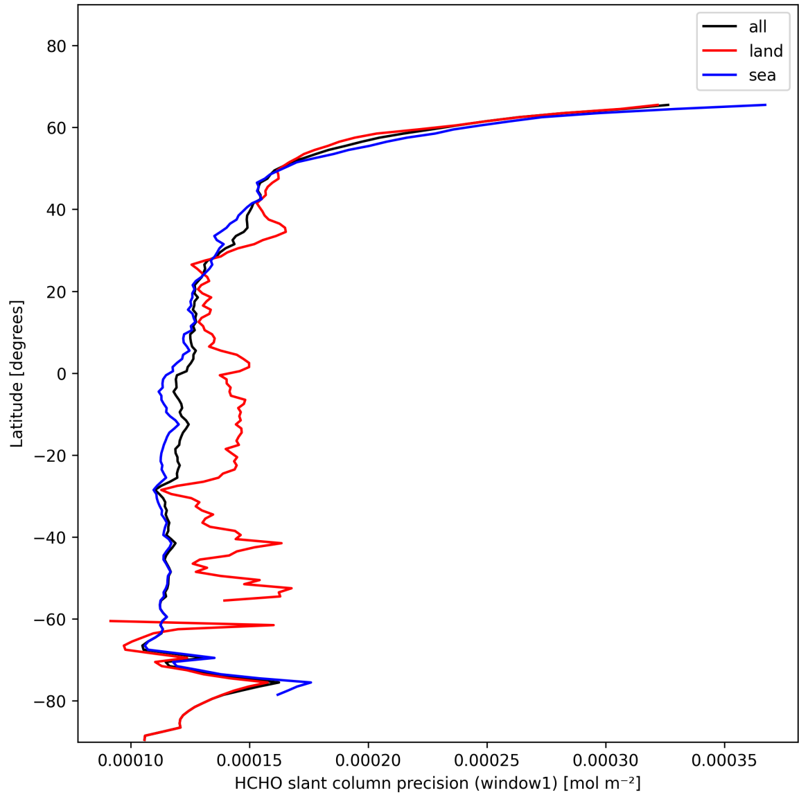
Figure 25: Zonal average of “HCHO slant column precision (window1)” for 2024-11-20 to 2024-11-21.
