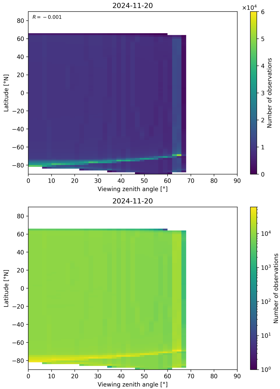
Figure 196: Scatter density plot of “Viewing zenith angle” against “Latitude” for 2024-11-20 to 2024-11-21.
