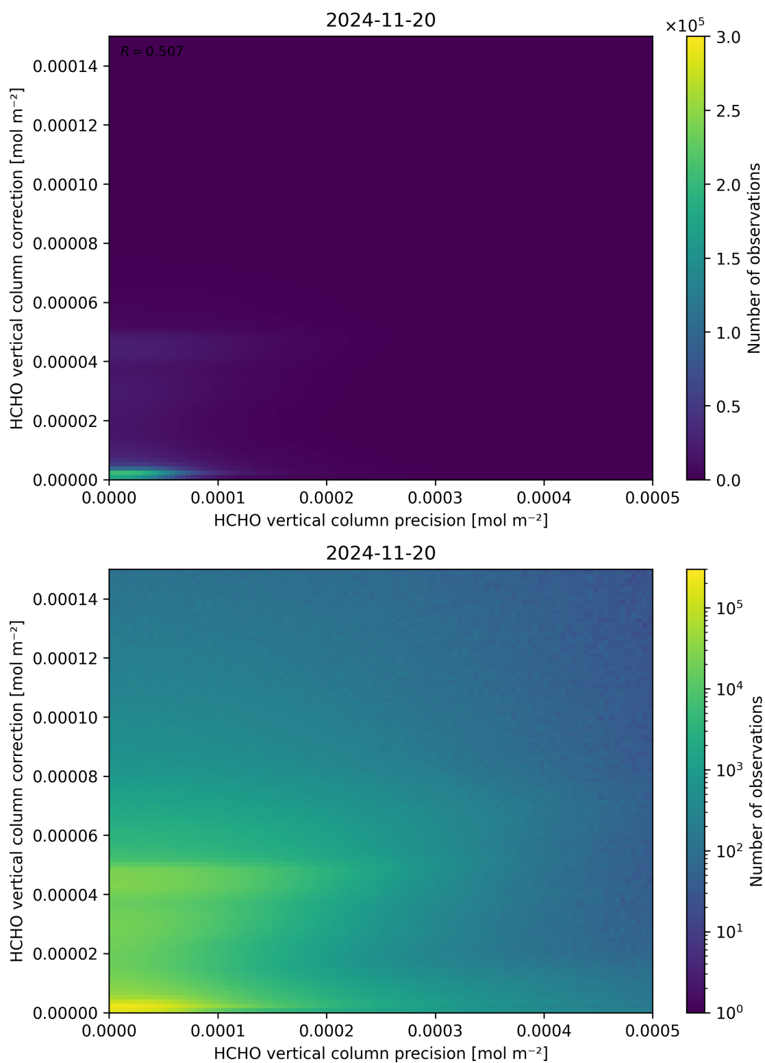
Figure 146: Scatter density plot of “HCHO vertical column precision” against “HCHO vertical column correction” for 2024-11-20 to 2024-11-21.
