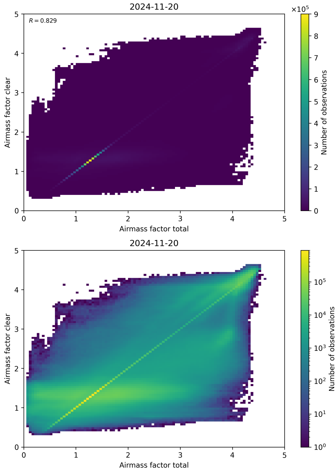
Figure 100: Scatter density plot of “Airmass factor total” against “Airmass factor clear” for 2024-11-20 to 2024-11-21.
