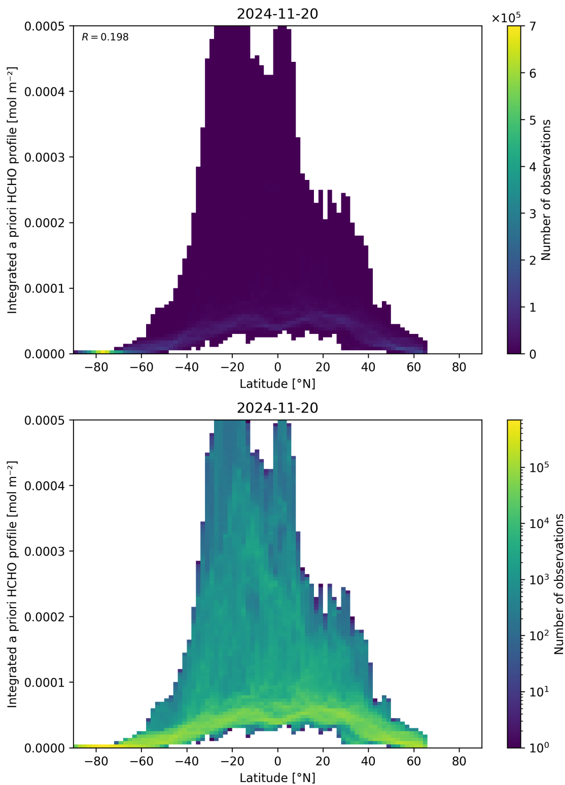
Figure 166: Scatter density plot of “Latitude” against “Integrated a priori HCHO profile” for 2024-11-20 to 2024-11-21.
