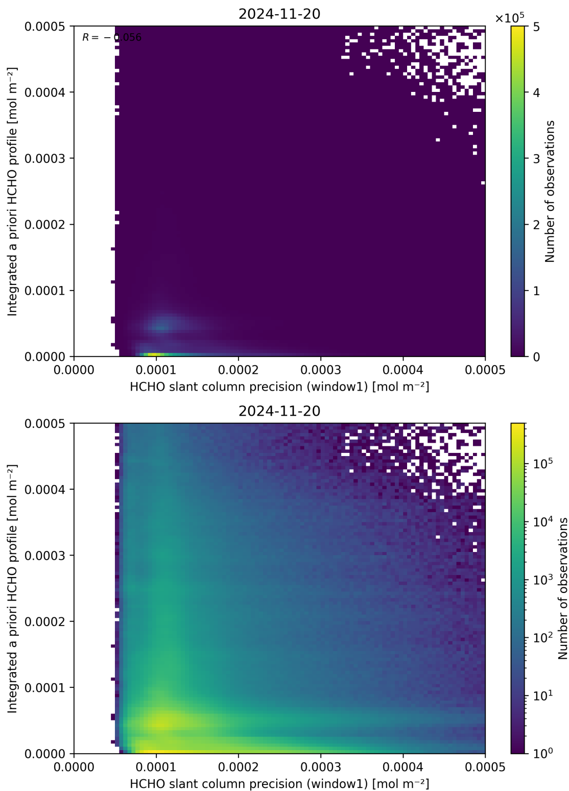
Figure 96: Scatter density plot of “HCHO slant column precision (window1)” against “Integrated a priori HCHO profile” for 2024-11-20 to 2024-11-21.
