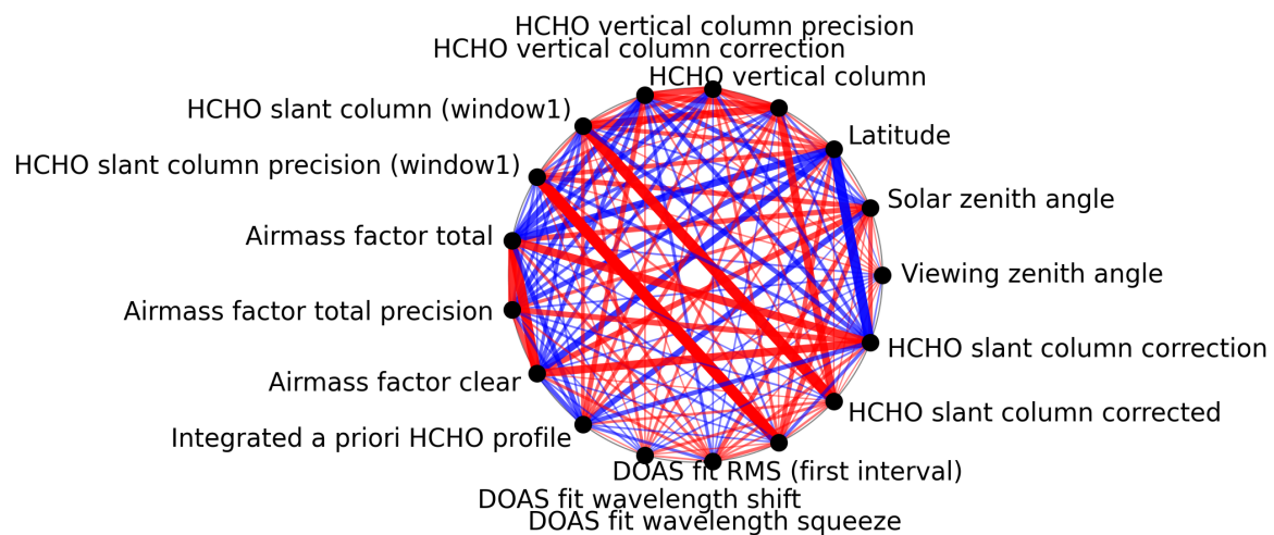
Figure 1: Map of correlation graph for 2024-11-20 to 2024-11-21.
