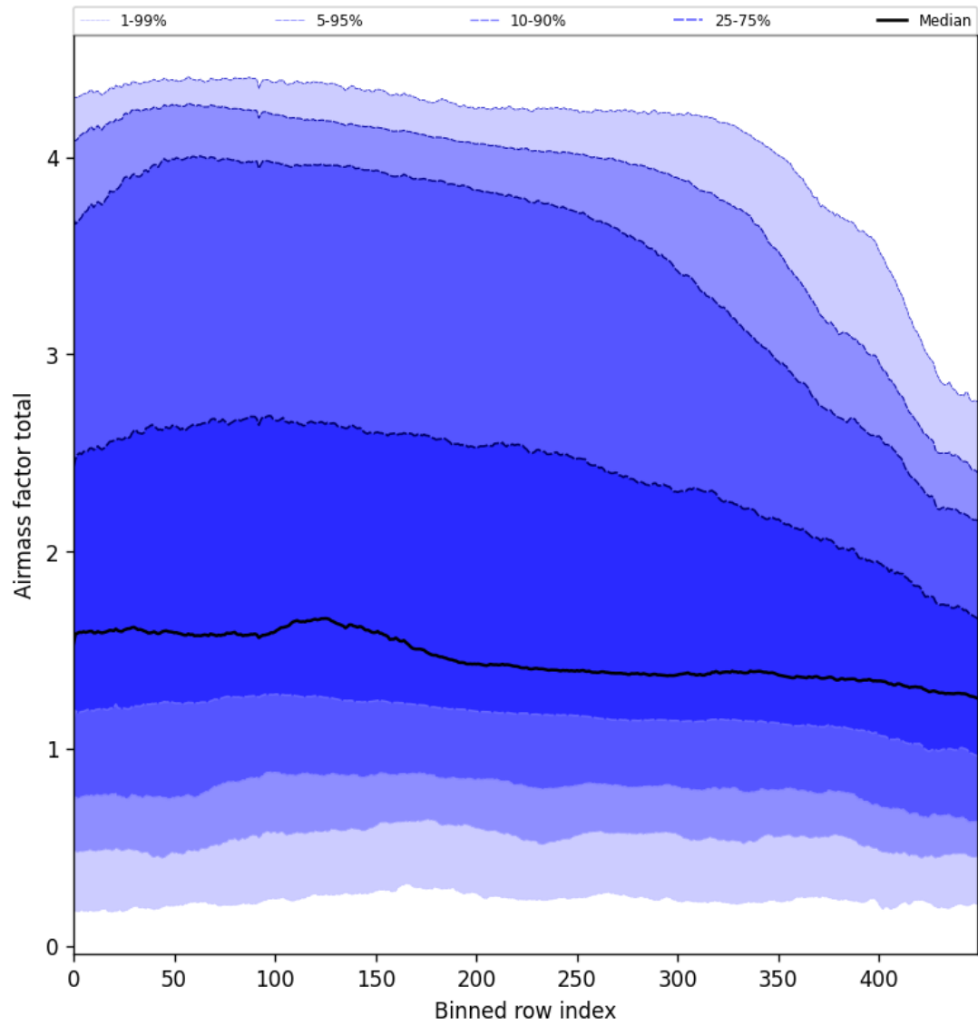
Figure 54: Along track statistics of “Airmass factor total” for 2024-11-20 to 2024-11-21
