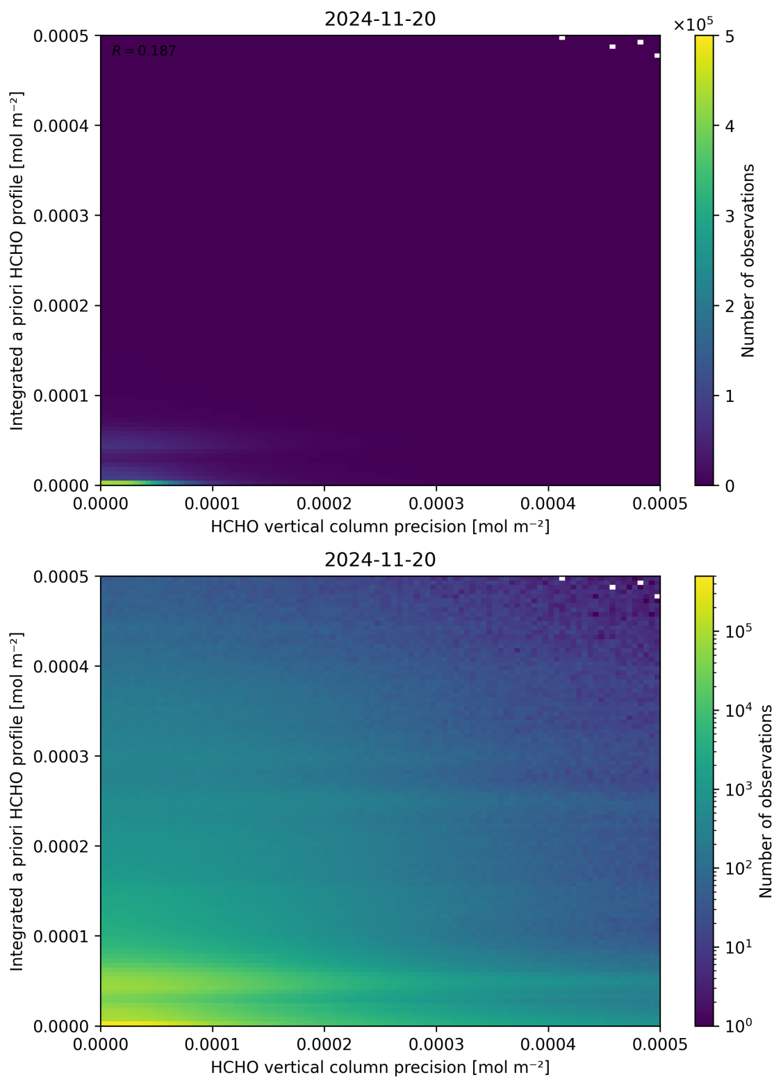
Figure 147: Scatter density plot of “HCHO vertical column precision” against “Integrated a priori HCHO profile” for 2024-11-20 to 2024-11-21.
