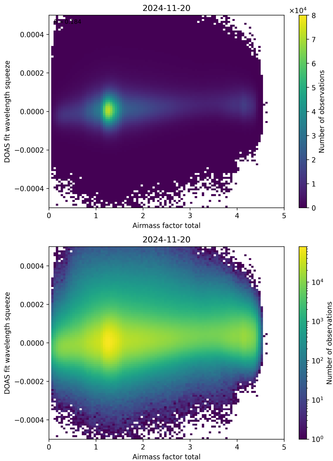
Figure 99: Scatter density plot of “Airmass factor total” against “DOAS fit wavelength squeeze” for 2024-11-20 to 2024-11-21.
