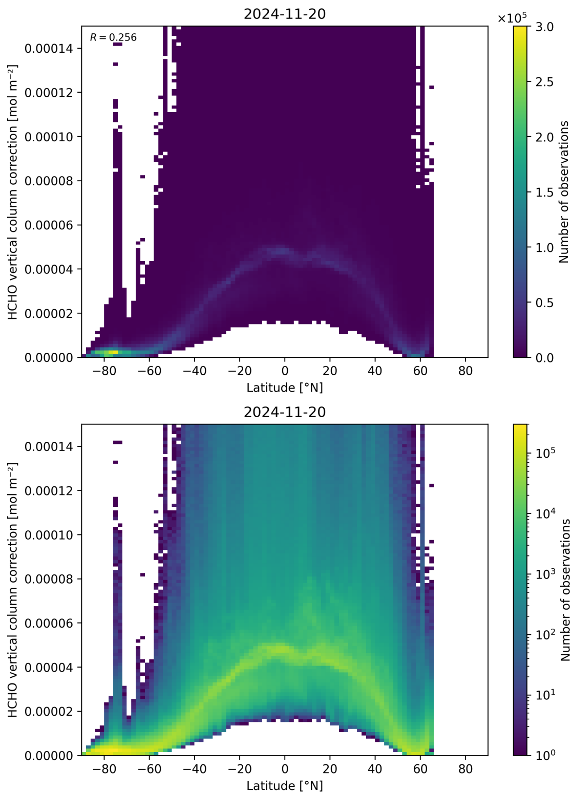
Figure 164: Scatter density plot of “Latitude” against “HCHO vertical column correction” for 2024-11-20 to 2024-11-21.
