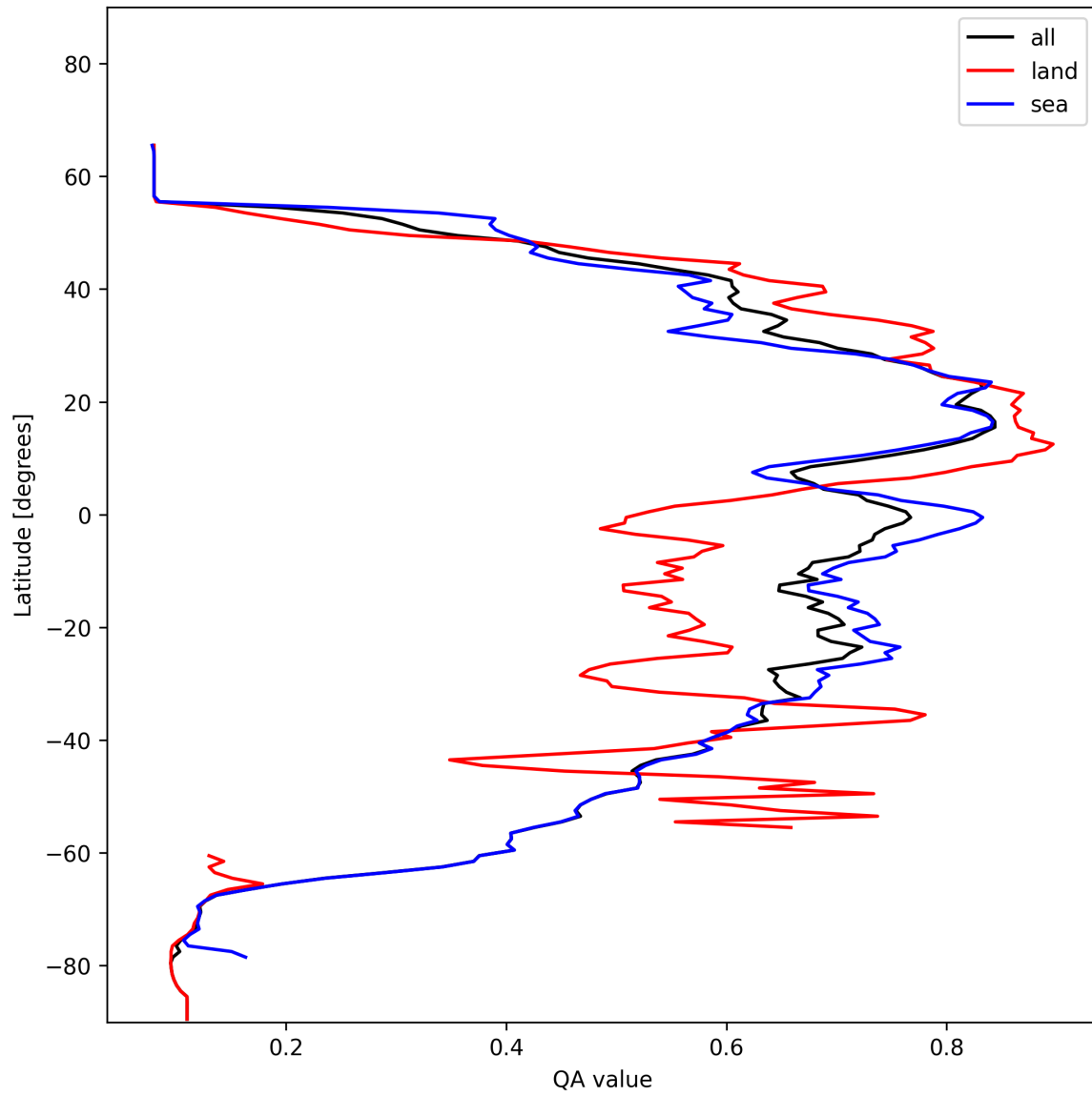
Figure 20: Zonal average of “QA value” for 2024-11-20 to 2024-11-21.
