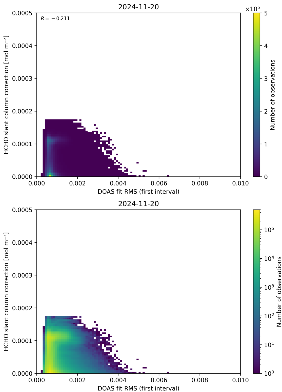
Figure 63: Scatter density plot of “DOAS fit RMS (first interval)” against “HCHO slant column correction” for 2024-11-20 to 2024-11-21.
