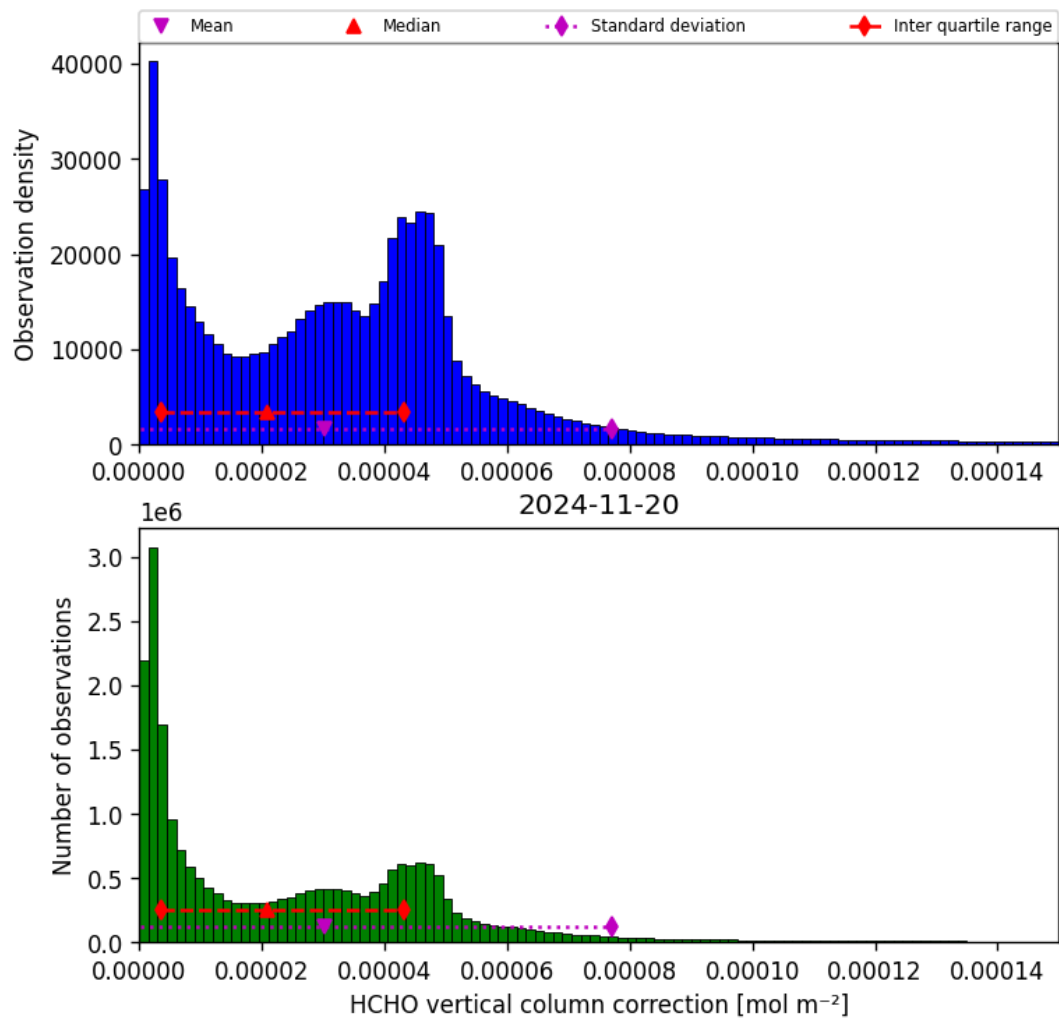
Figure 37: Histogram of “HCHO vertical column correction” for 2024-11-20 to 2024-11-21
