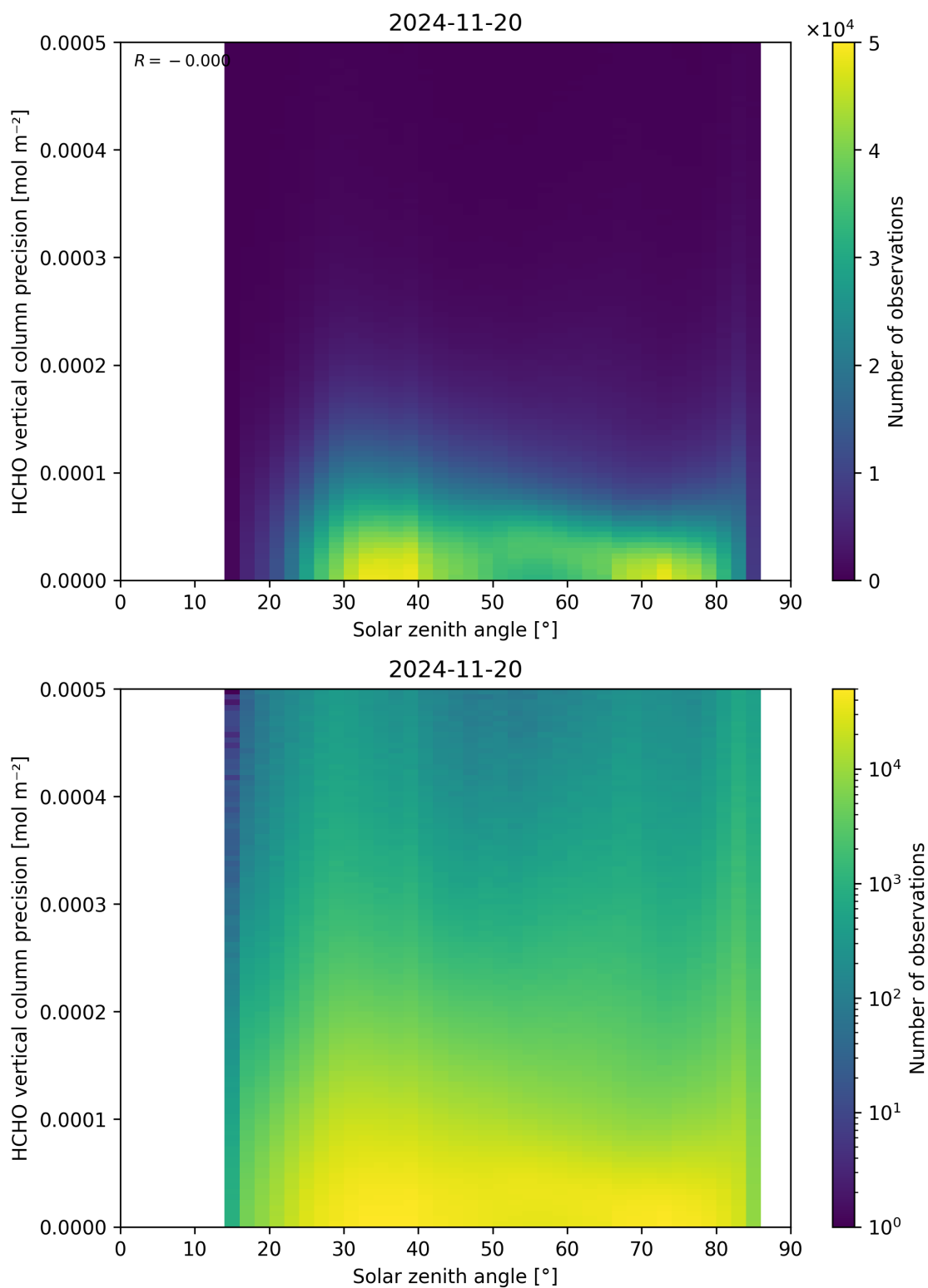
Figure 179: Scatter density plot of “Solar zenith angle” against “HCHO vertical column precision” for 2024-11-20 to 2024-11-21.
