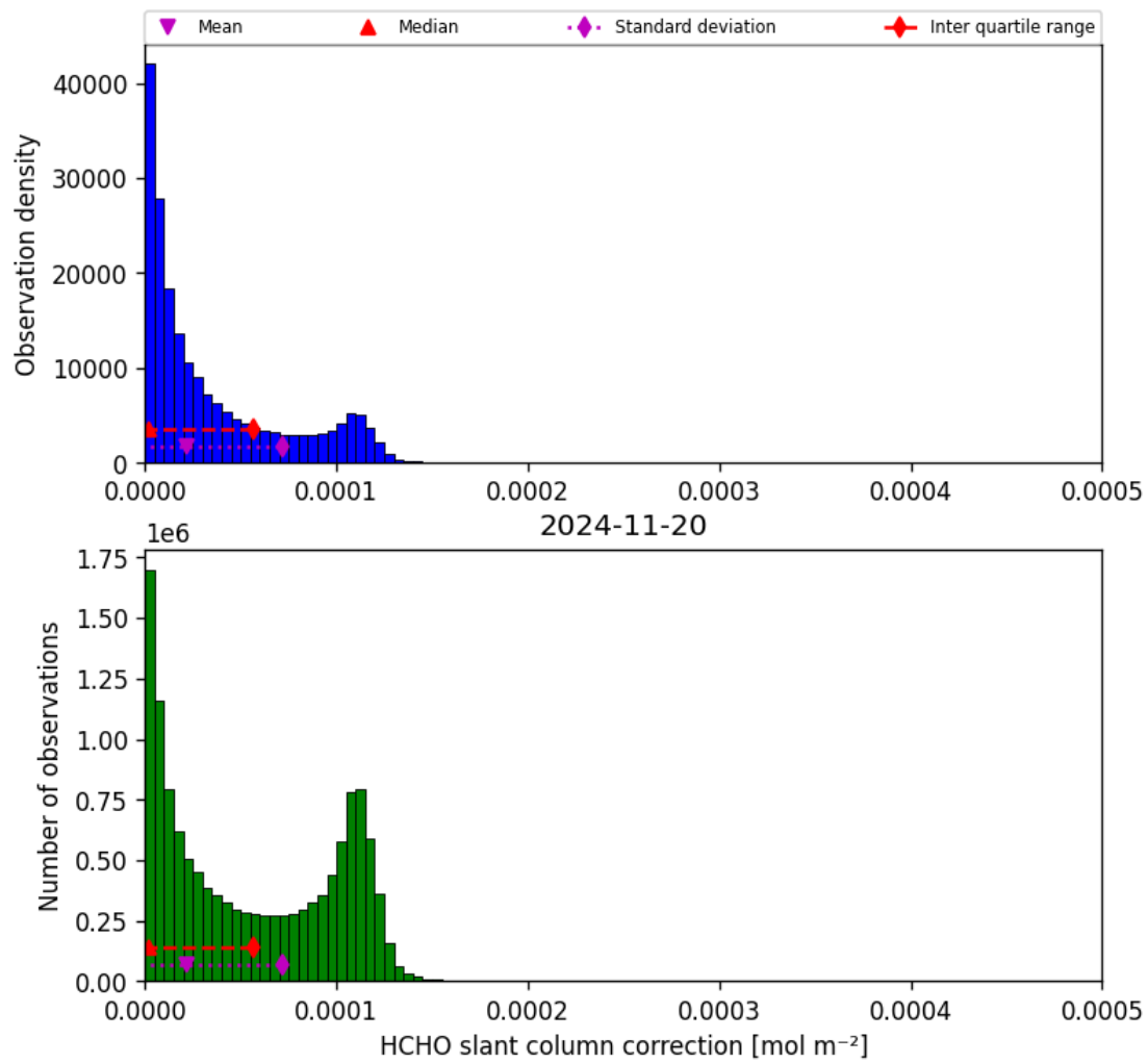
Figure 47: Histogram of “HCHO slant column correction” for 2024-11-20 to 2024-11-21
