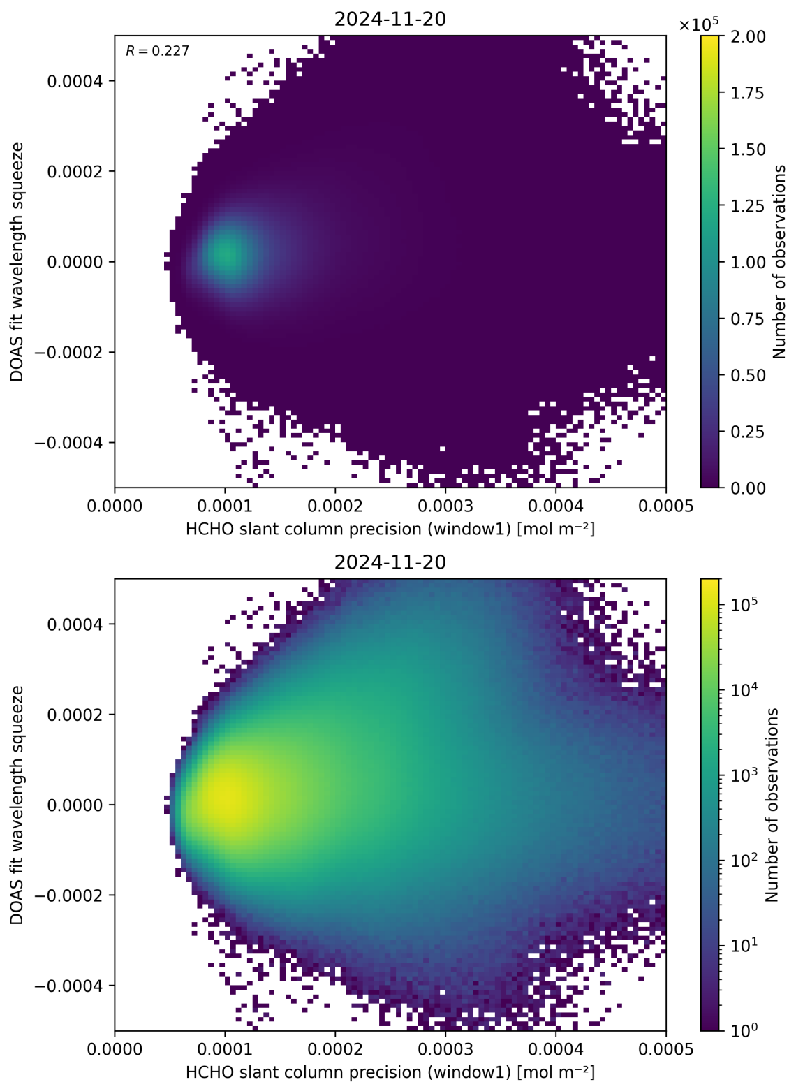
Figure 90: Scatter density plot of “HCHO slant column precision (window1)” against “DOAS fit wavelength squeeze” for 2024-11-20 to 2024-11-21.
