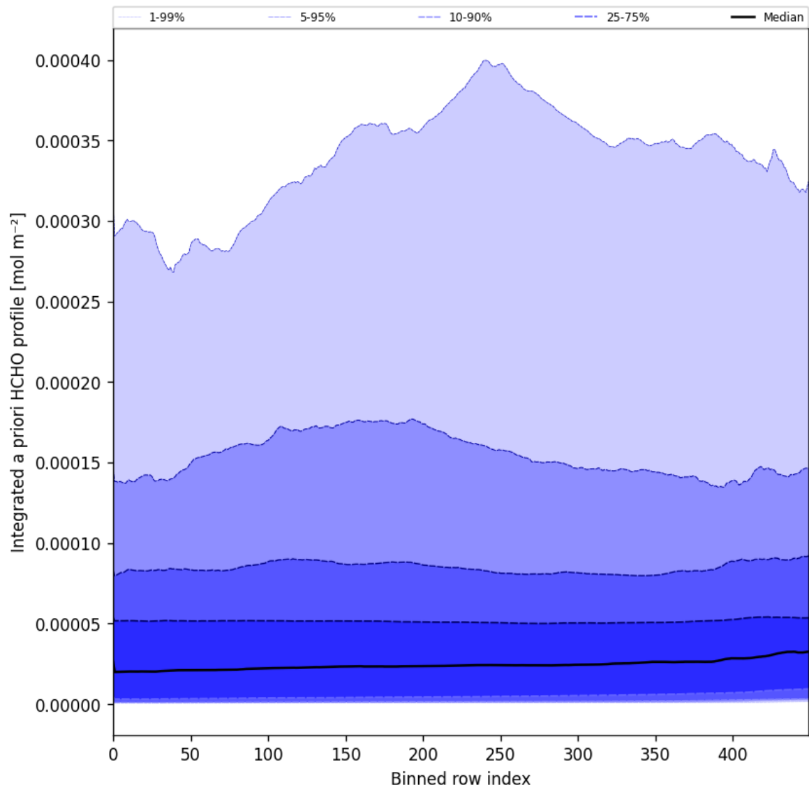
Figure 57: Along track statistics of "Integrated a priori HCHO profile" for 2024-11-20 to 2024-11-21
