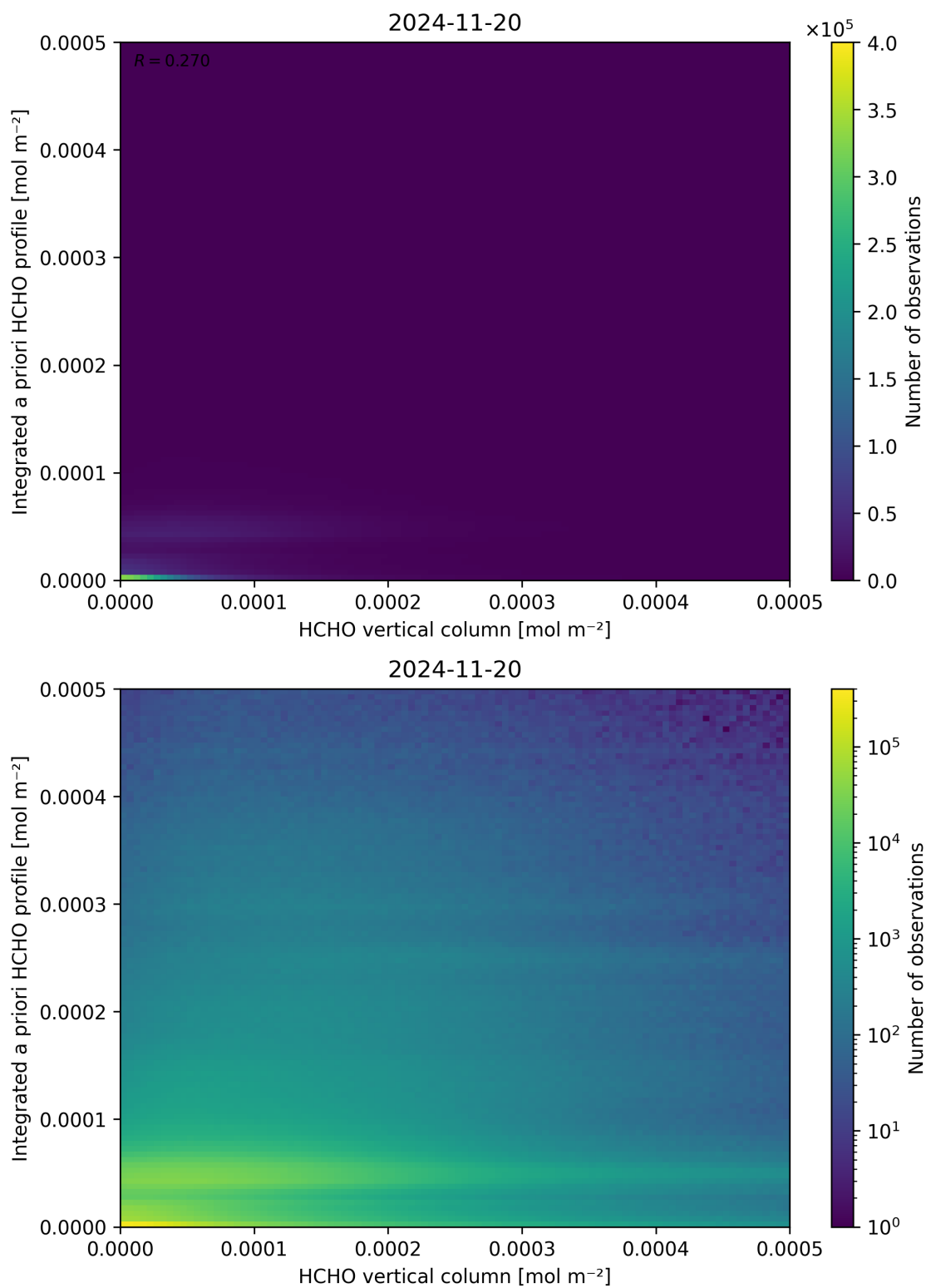
Figure 135: Scatter density plot of “HCHO vertical column” against “Integrated a priori HCHO profile” for 2024-11-20 to 2024-11-21.
