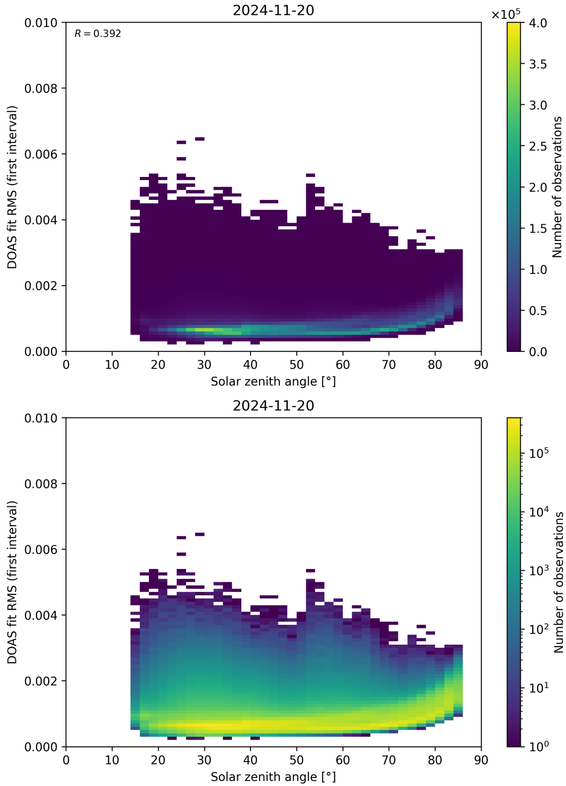
Figure 167: Scatter density plot of “Solar zenith angle” against “DOAS fit RMS (first interval)” for 2024-11-20 to 2024-11-21.
