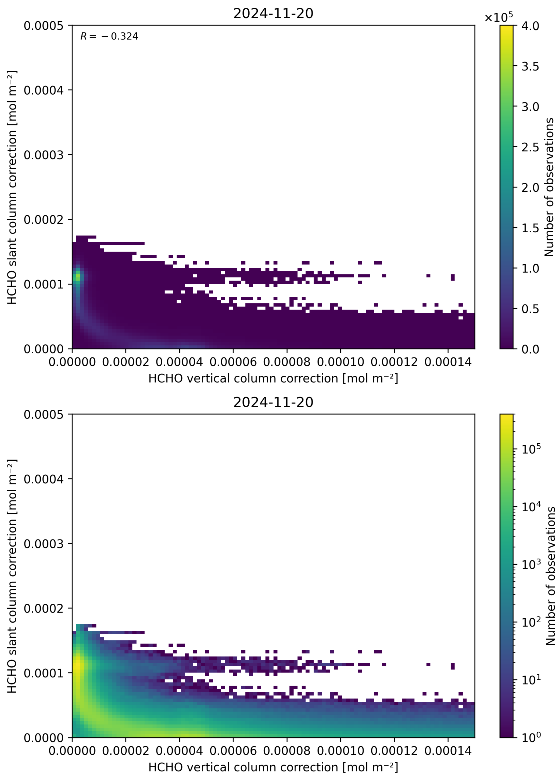
Figure 117: Scatter density plot of “HCHO vertical column correction” against “HCHO slant column correction” for 2024-11-20 to 2024-11-21.
