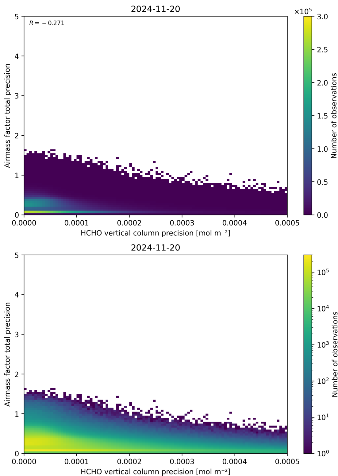
Figure 145: Scatter density plot of “HCHO vertical column precision” against “Airmass factor total precision” for 2024-11-20 to 2024-11-21.
