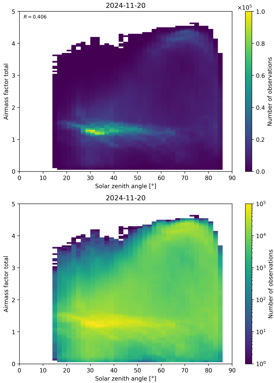
Figure 175: Scatter density plot of “Solar zenith angle” against “Airmass factor total” for 2024-11-20 to 2024-11-21.
