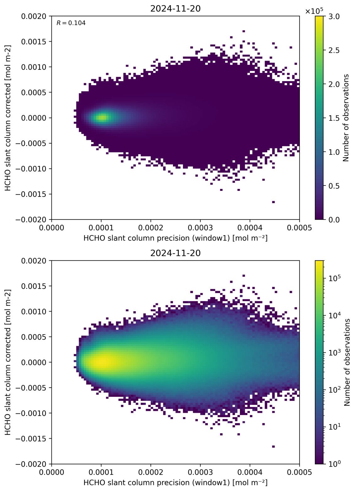
Figure 92: Scatter density plot of “HCHO slant column precision (window1)” against “HCHO slant column corrected” for 2024-11-20 to 2024-11-21.
