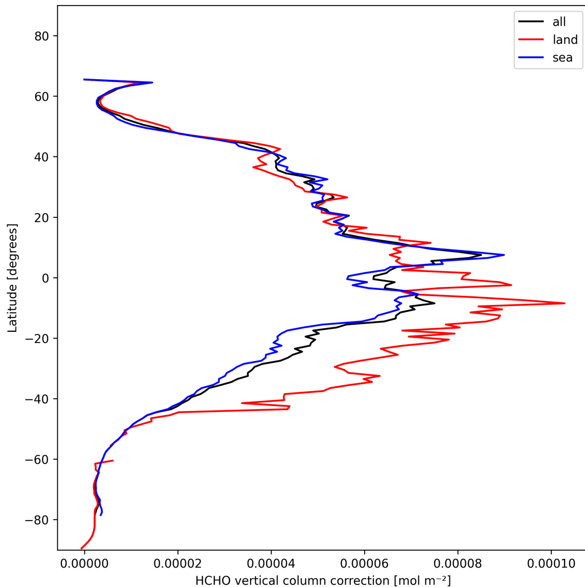
Figure 23: Zonal average of “HCHO vertical column correction” for 2024-11-20 to 2024-11-21.
