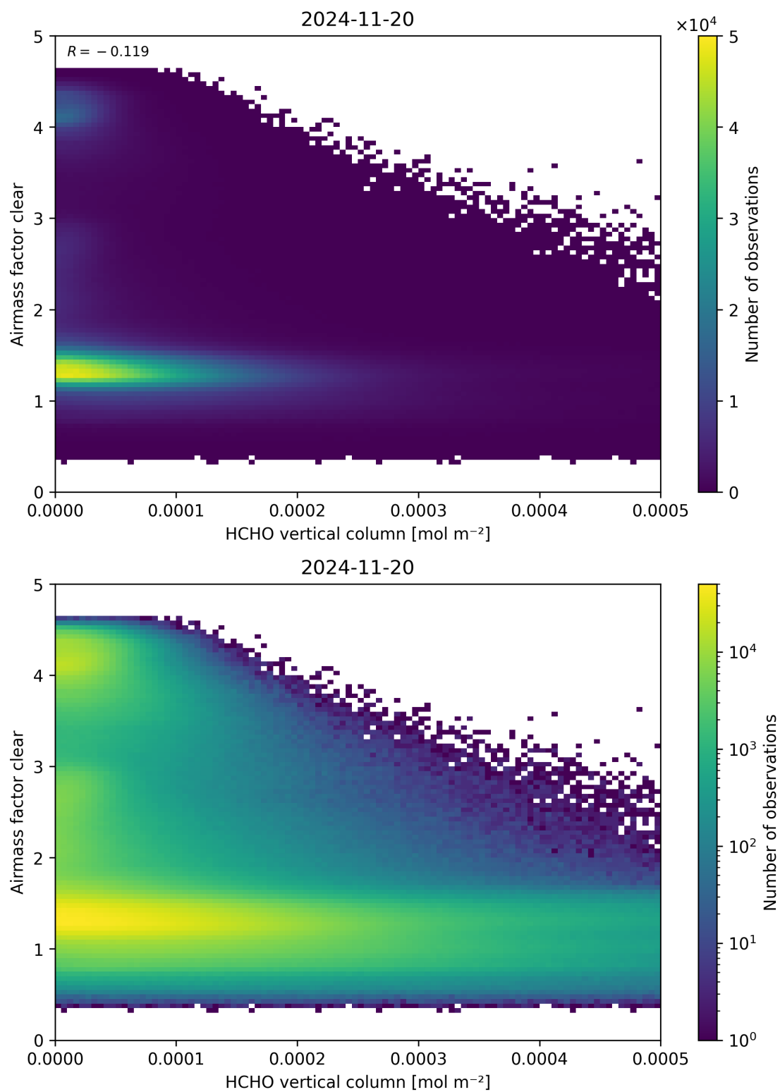
Figure 126: Scatter density plot of “HCHO vertical column” against “Airmass factor clear” for 2024-11-20 to 2024-11-21.
