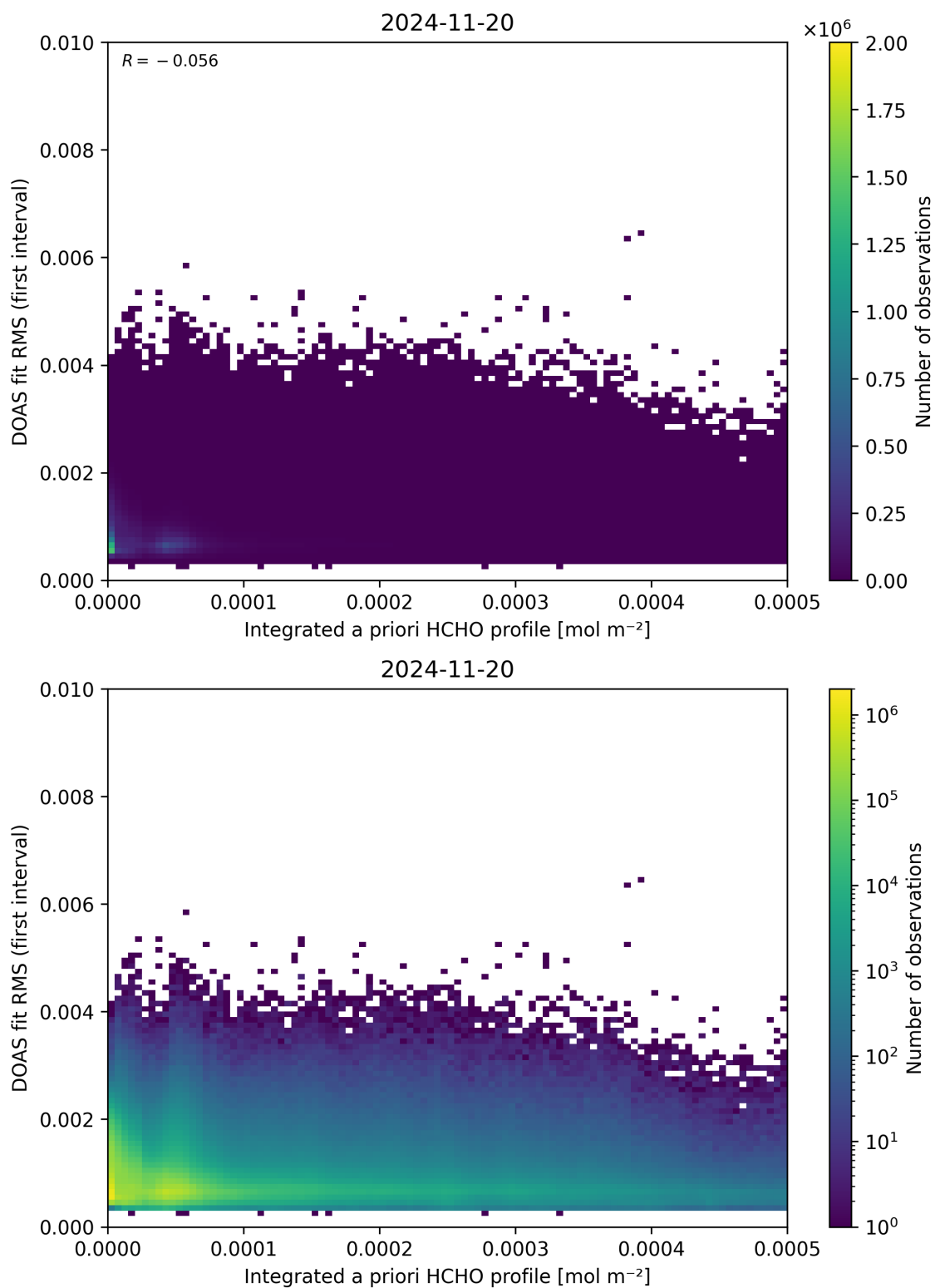
Figure 148: Scatter density plot of “Integrated a priori HCHO profile” against “DOAS fit RMS (first interval)” for 2024-11-20 to 2024-11-21.
