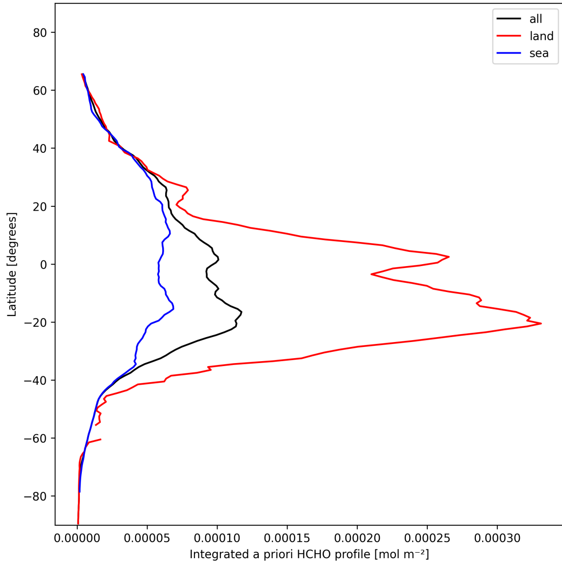
Figure 29: Zonal average of “Integrated a priori HCHO profile” for 2024-11-20 to 2024-11-21.
