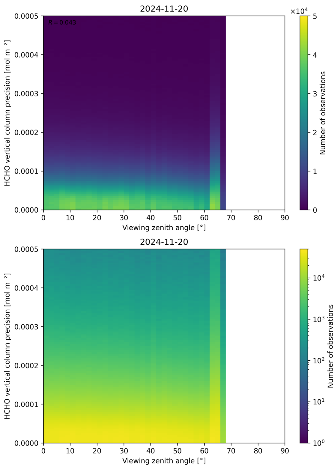
Figure 194: Scatter density plot of “Viewing zenith angle” against “HCHO vertical column precision” for 2024-11-20 to 2024-11-21.
