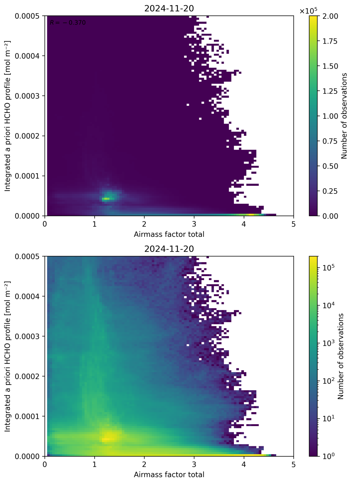
Figure 104: Scatter density plot of “Airmass factor total” against “Integrated a priori HCHO profile” for 2024-11-20 to 2024-11-21.
