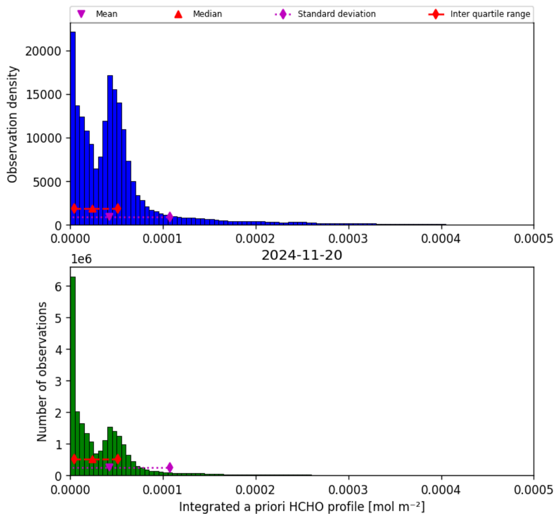
Figure 43: Histogram of “Integrated a priori HCHO profile” for 2024-11-20 to 2024-11-21
