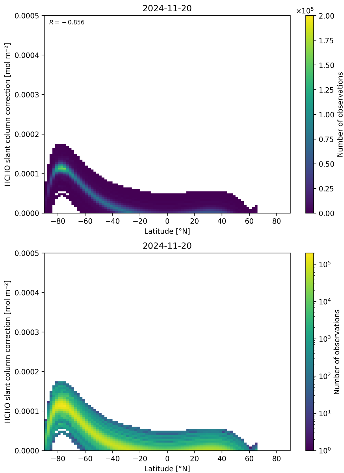
Figure 158: Scatter density plot of “Latitude” against “HCHO slant column correction” for 2024-11-20 to 2024-11-21.
