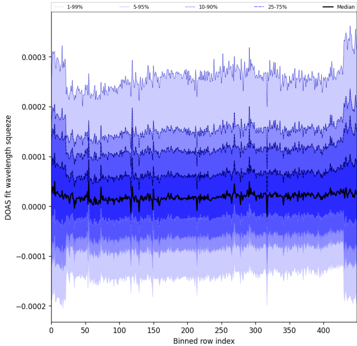
Figure 59: Along track statistics of “DOAS fit wavelength squeeze” for 2024-11-20 to 2024-11-21
