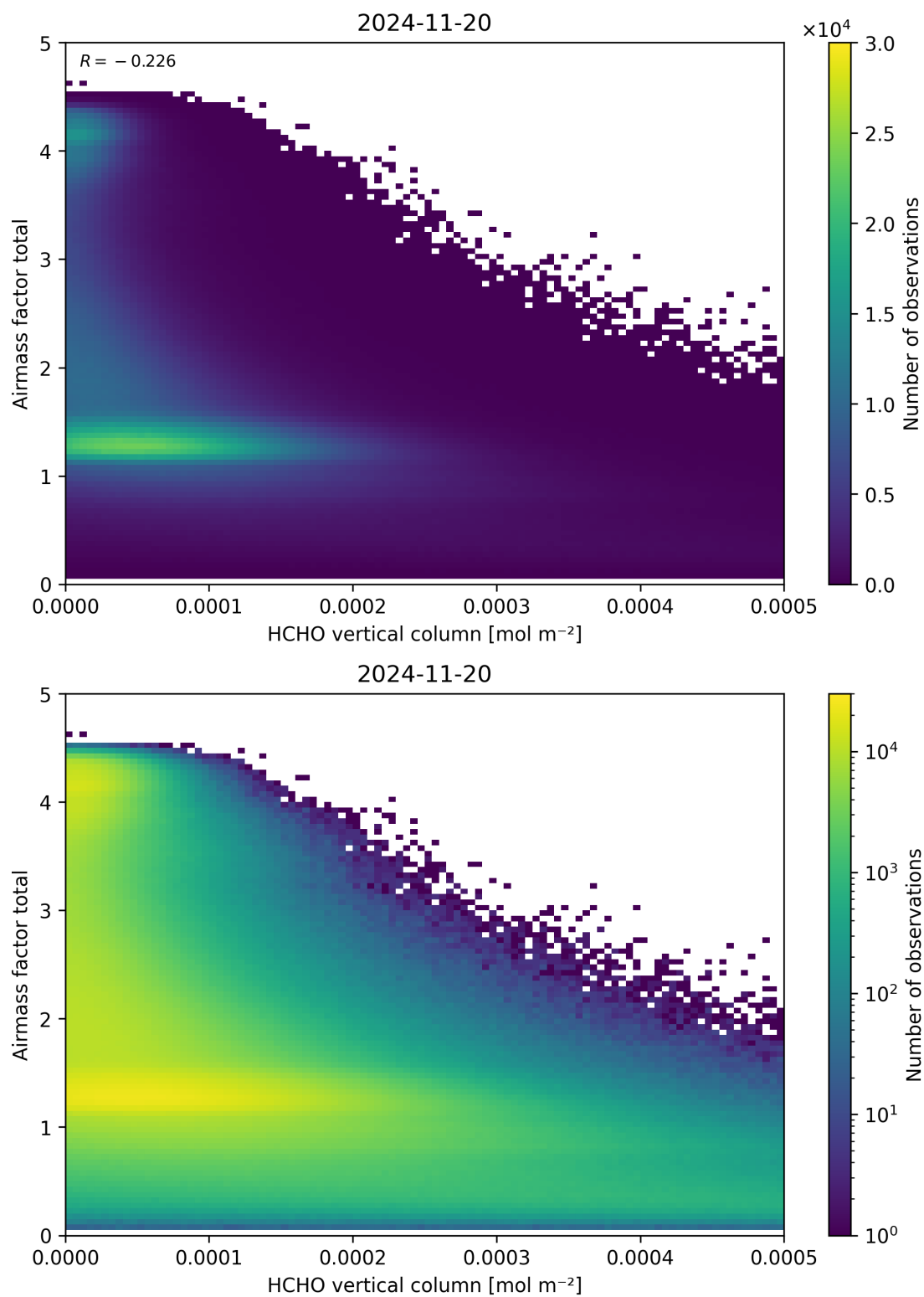
Figure 131: Scatter density plot of “HCHO vertical column” against “Airmass factor total” for 2024-11-20 to 2024-11-21.
