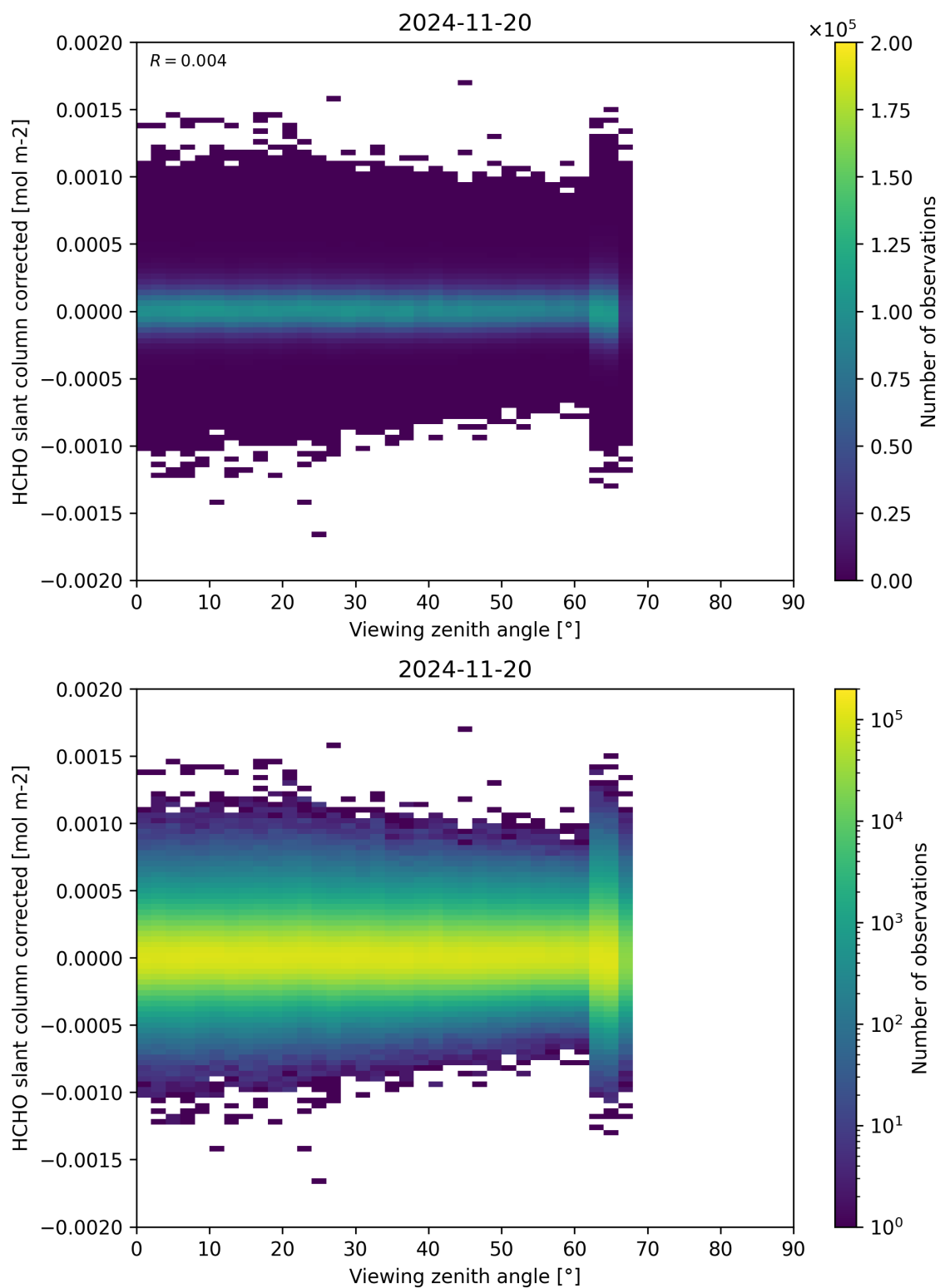
Figure 186: Scatter density plot of “Viewing zenith angle” against “HCHO slant column corrected” for 2024-11-20 to 2024-11-21.
