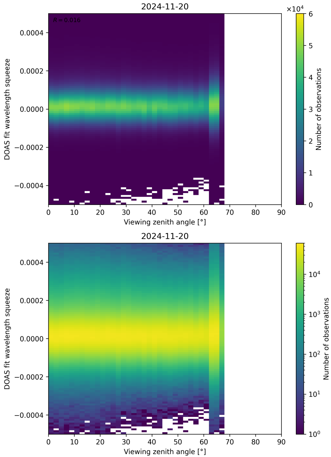
Figure 184: Scatter density plot of “Viewing zenith angle” against “DOAS fit wavelength squeeze” for 2024-11-20 to 2024-11-21.
