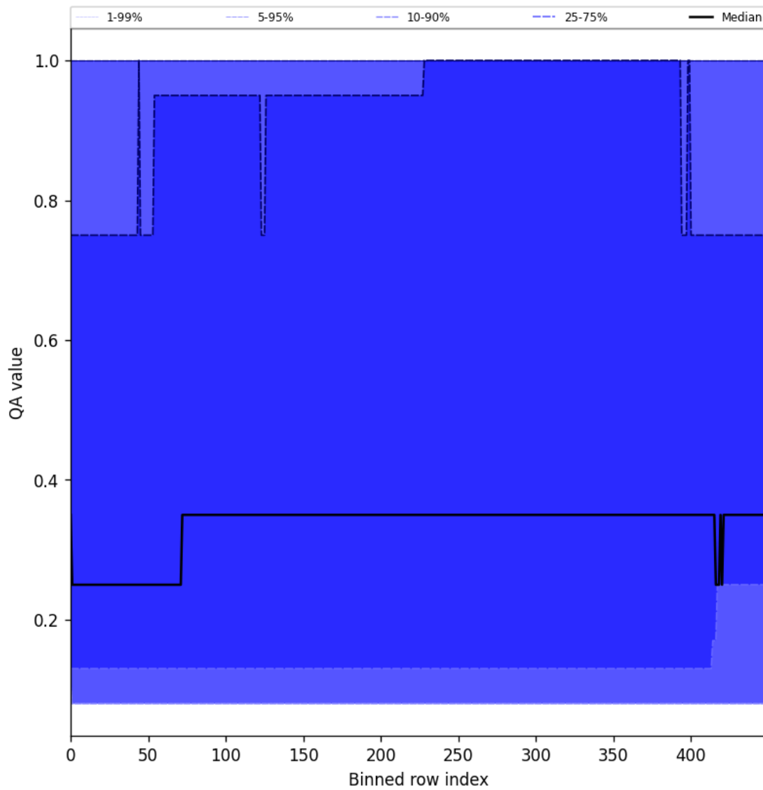
Figure 48: Along track statistics of “QA value” for 2024-11-20 to 2024-11-21
