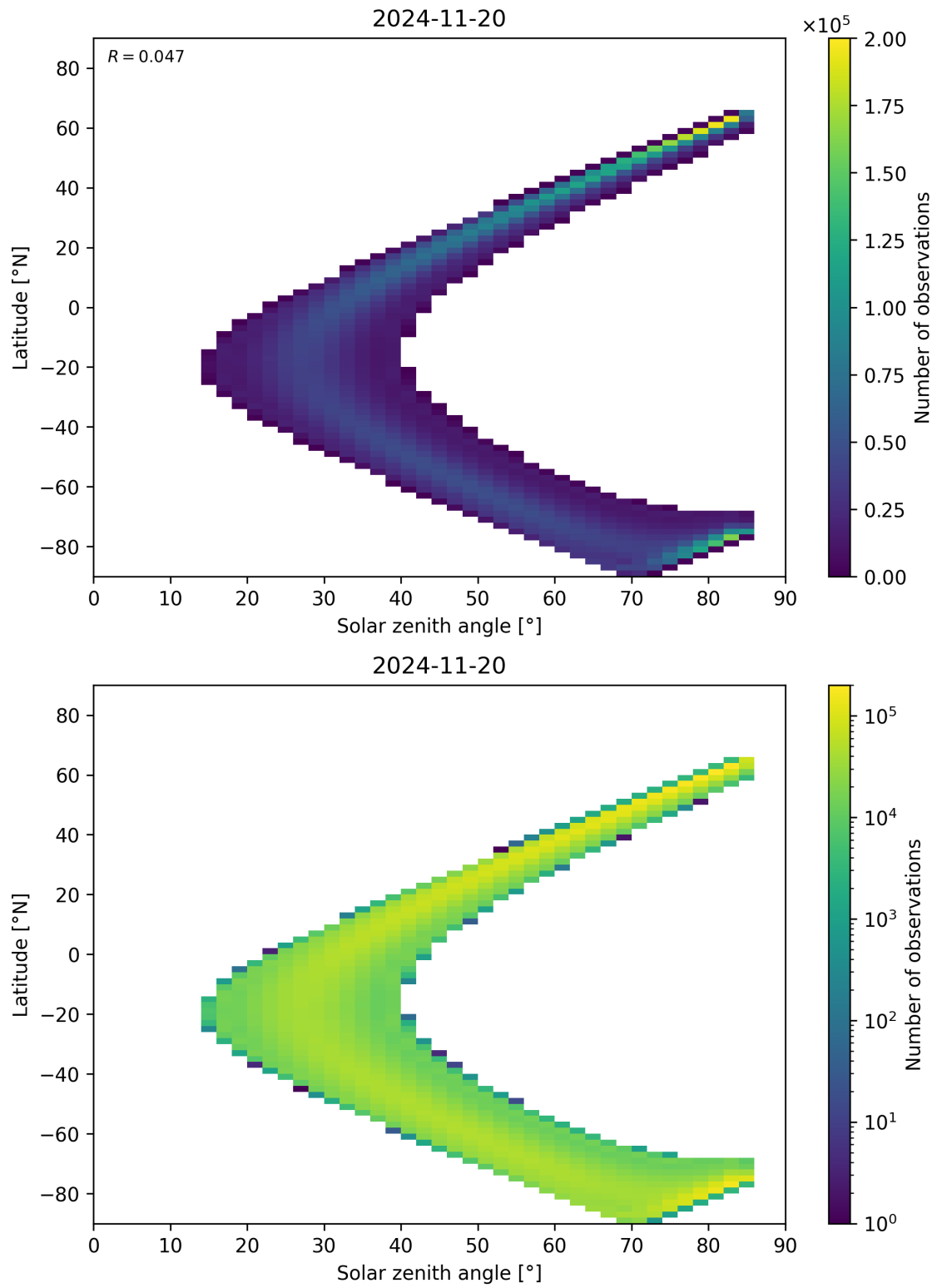
Figure 181: Scatter density plot of “Solar zenith angle” against “Latitude” for 2024-11-20 to 2024-11-21.
