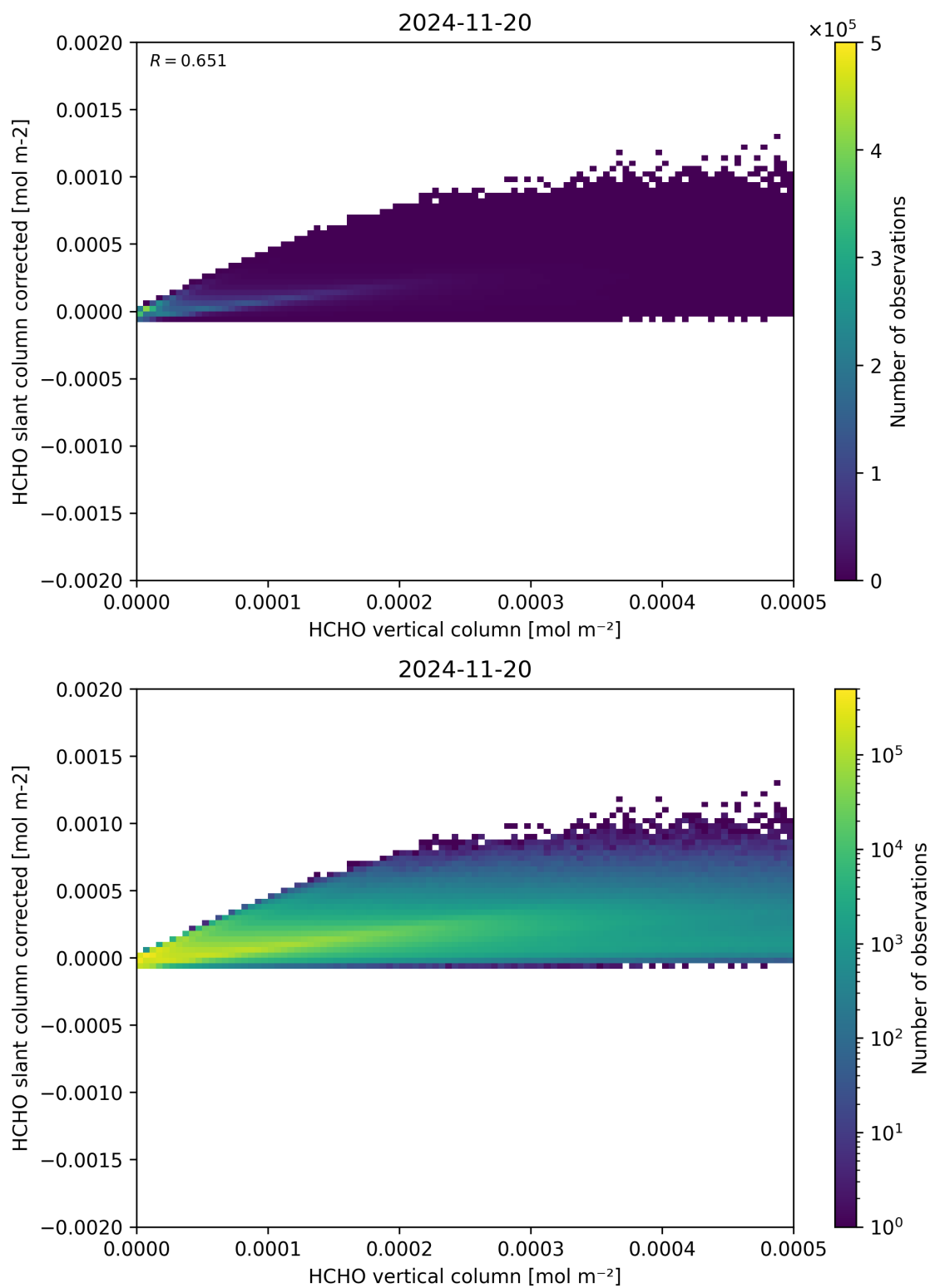
Figure 127: Scatter density plot of “HCHO vertical column” against “HCHO slant column corrected” for 2024-11-20 to 2024-11-21.
