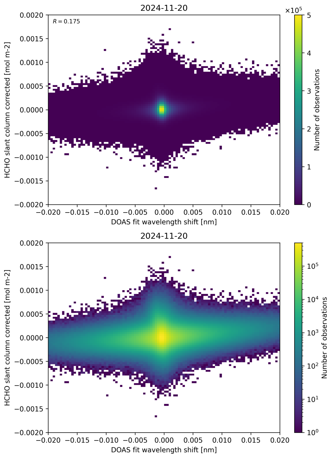
Figure 66: Scatter density plot of “DOAS fit wavelength shift” against “HCHO slant column corrected” for 2024-11-20 to 2024-11-21.
