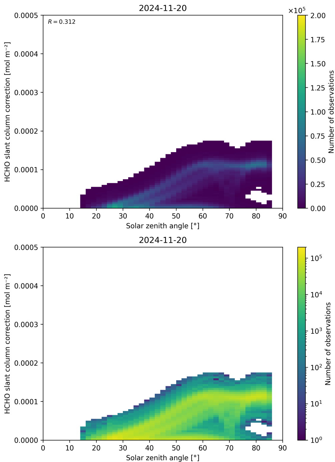
Figure 172: Scatter density plot of “Solar zenith angle” against “HCHO slant column correction” for 2024-11-20 to 2024-11-21.
