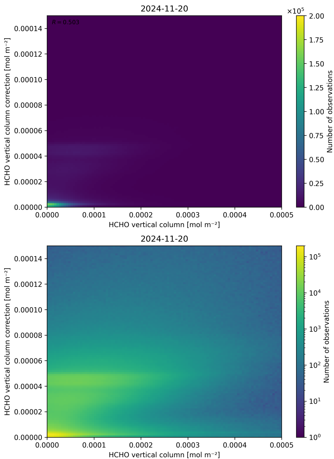
Figure 133: Scatter density plot of “HCHO vertical column” against “HCHO vertical column correction” for 2024-11-20 to 2024-11-21.
