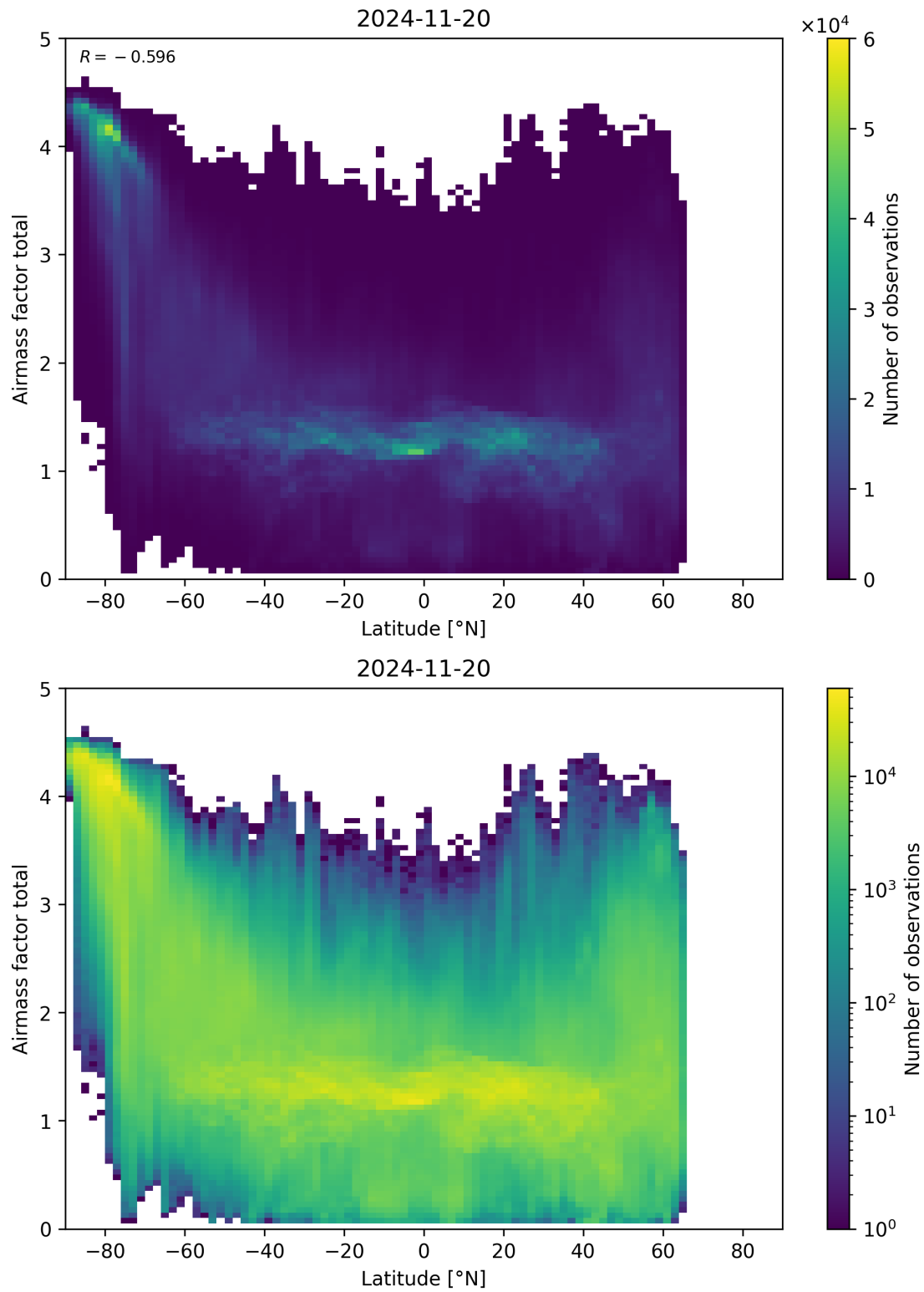
Figure 161: Scatter density plot of “Latitude” against “Airmass factor total” for 2024-11-20 to 2024-11-21.
