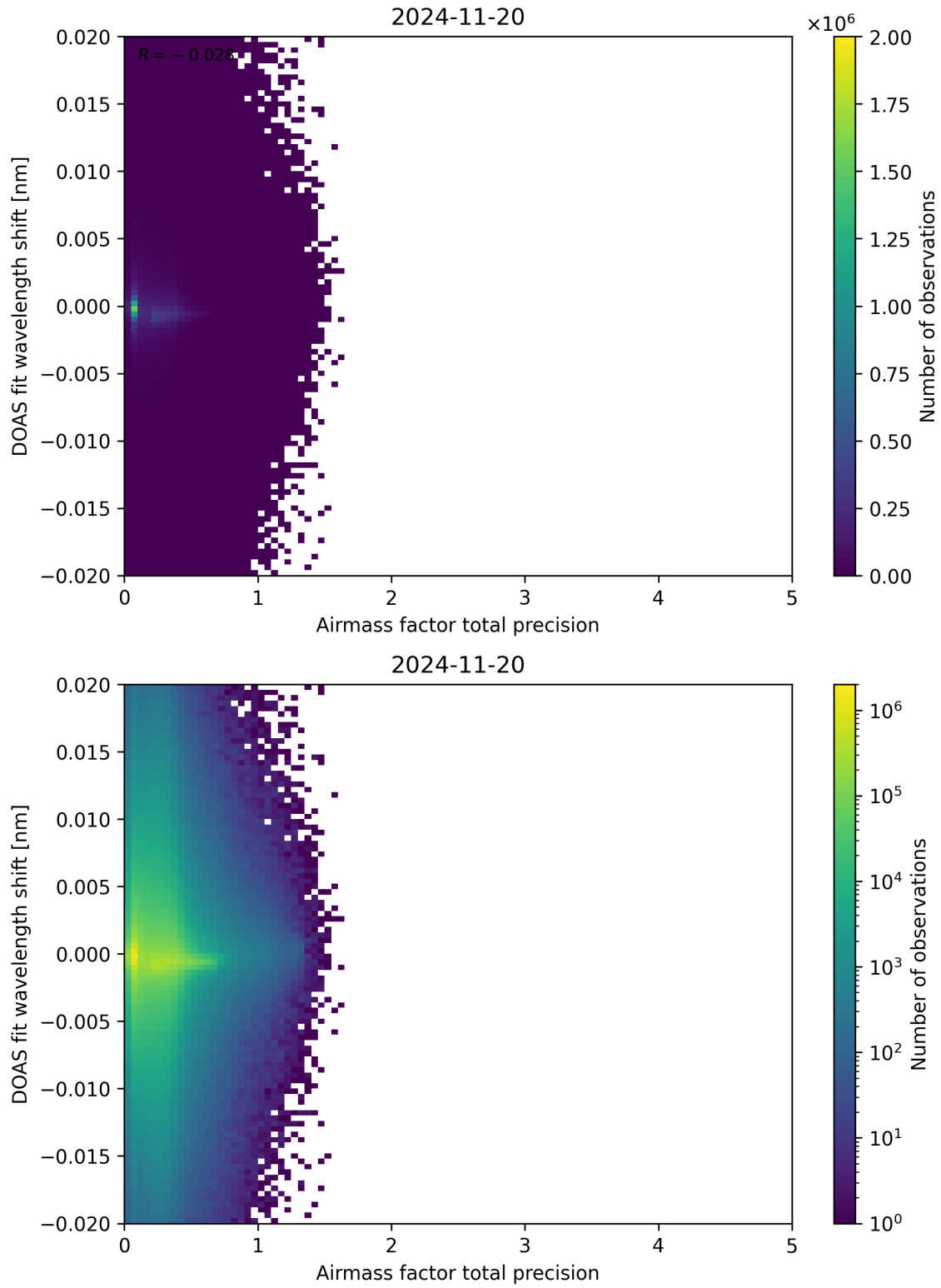
Figure 106: Scatter density plot of “Airmass factor total precision” against “DOAS fit wavelength shift” for 2024-11-20 to 2024-11-21.
