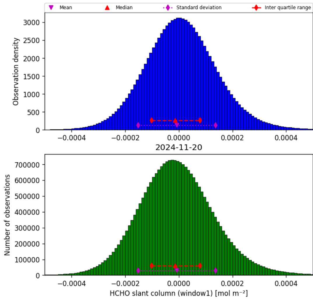
Figure 38: Histogram of “HCHO slant column (window1)” for 2024-11-20 to 2024-11-21
