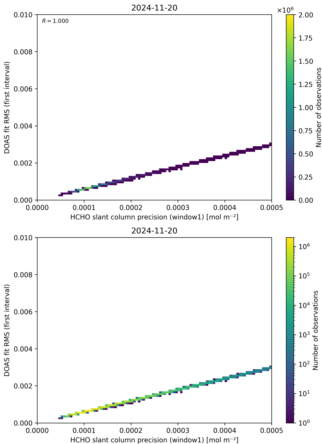
Figure 88: Scatter density plot of “HCHO slant column precision (window1)” against “DOAS fit RMS (first interval)” for 2024-11-20 to 2024-11-21.
