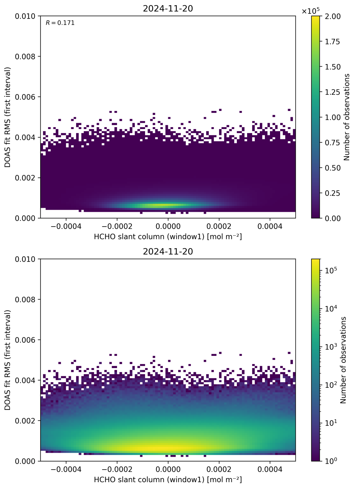
Figure 78: Scatter density plot of “HCHO slant column (window1)” against “DOAS fit RMS (first interval)” for 2024-11-20 to 2024-11-21.
