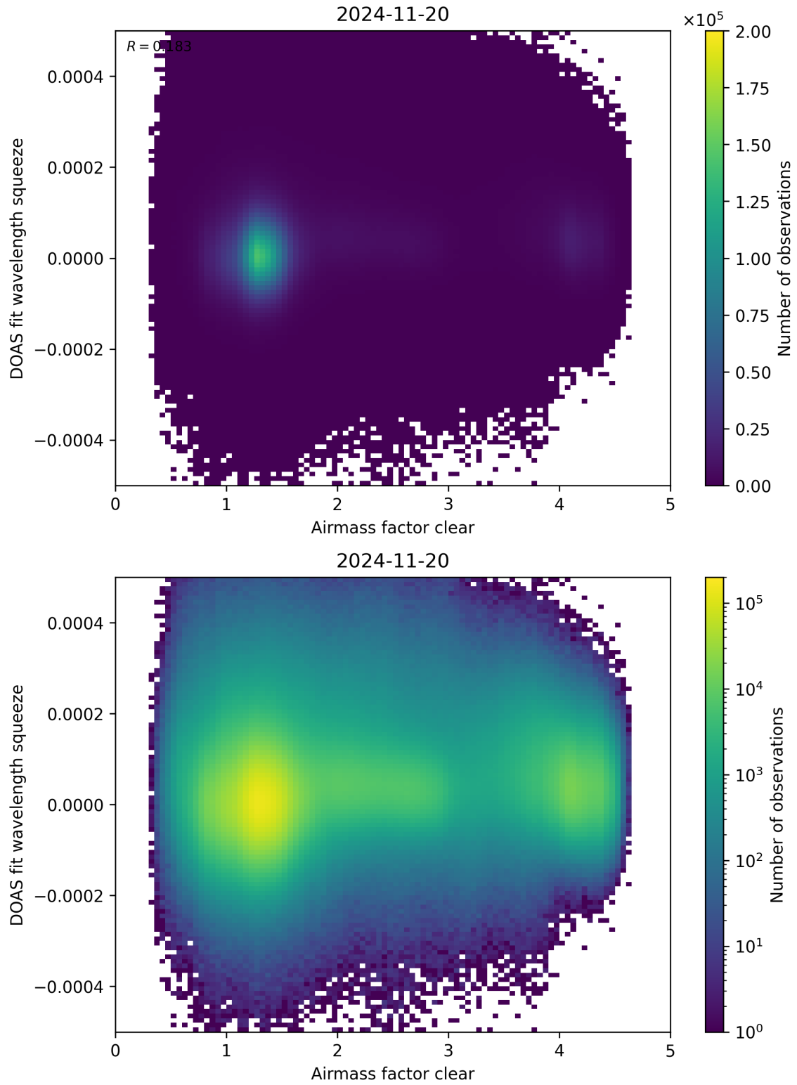
Figure 73: Scatter density plot of “Airmass factor clear” against “DOAS fit wavelength squeeze” for 2024-11-20 to 2024-11-21.
