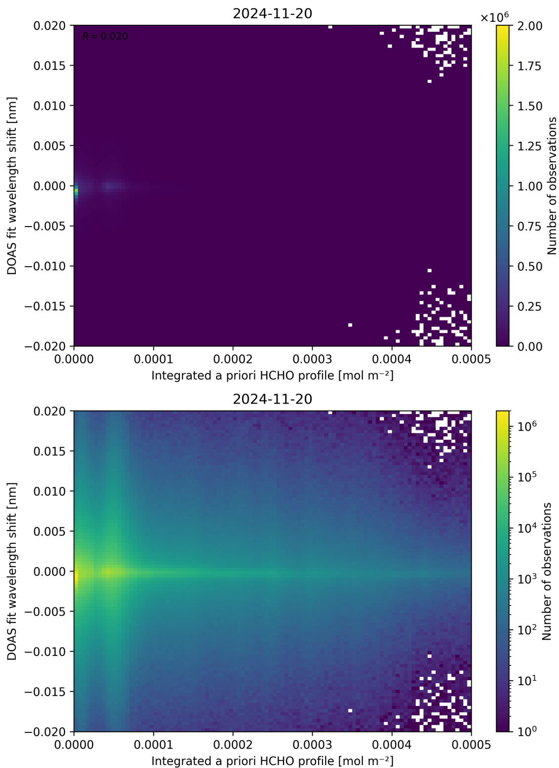
Figure 149: Scatter density plot of “Integrated a priori HCHO profile” against “DOAS fit wavelength shift” for 2024-11-20 to 2024-11-21.
