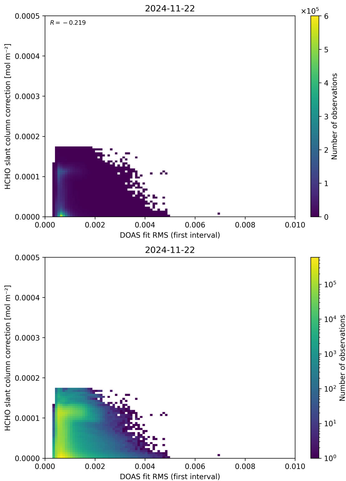
Figure 63: Scatter density plot of “DOAS fit RMS (first interval)” against “HCHO slant column correction” for 2024-11-21 to 2024-11-23.
