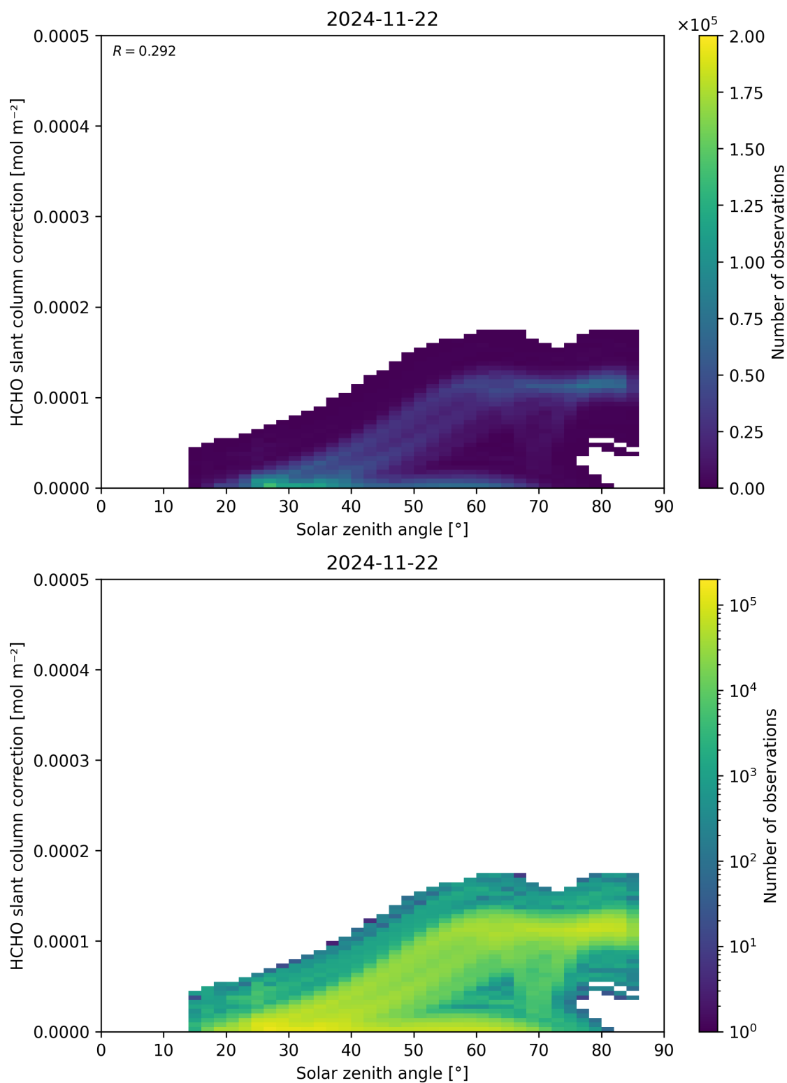
Figure 172: Scatter density plot of “Solar zenith angle” against “HCHO slant column correction” for 2024-11-21 to 2024-11-23.
