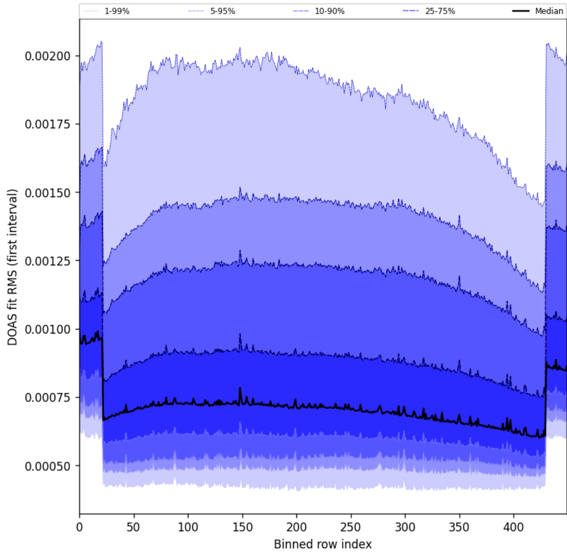
Figure 60: Along track statistics of “DOAS fit RMS (first interval)” for 2024-11-21 to 2024-11-23
