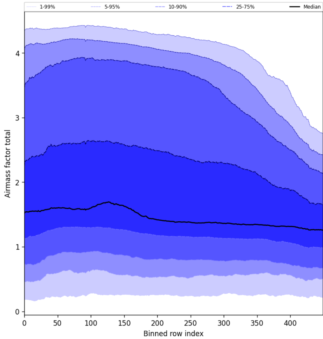
Figure 54: Along track statistics of “Airmass factor total” for 2024-11-21 to 2024-11-23
