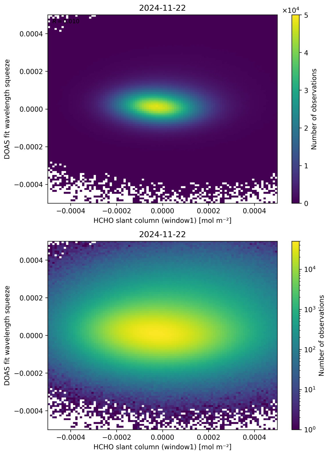
Figure 80: Scatter density plot of “HCHO slant column (window1)” against “DOAS fit wavelength squeeze” for 2024-11-21 to 2024-11-23.
