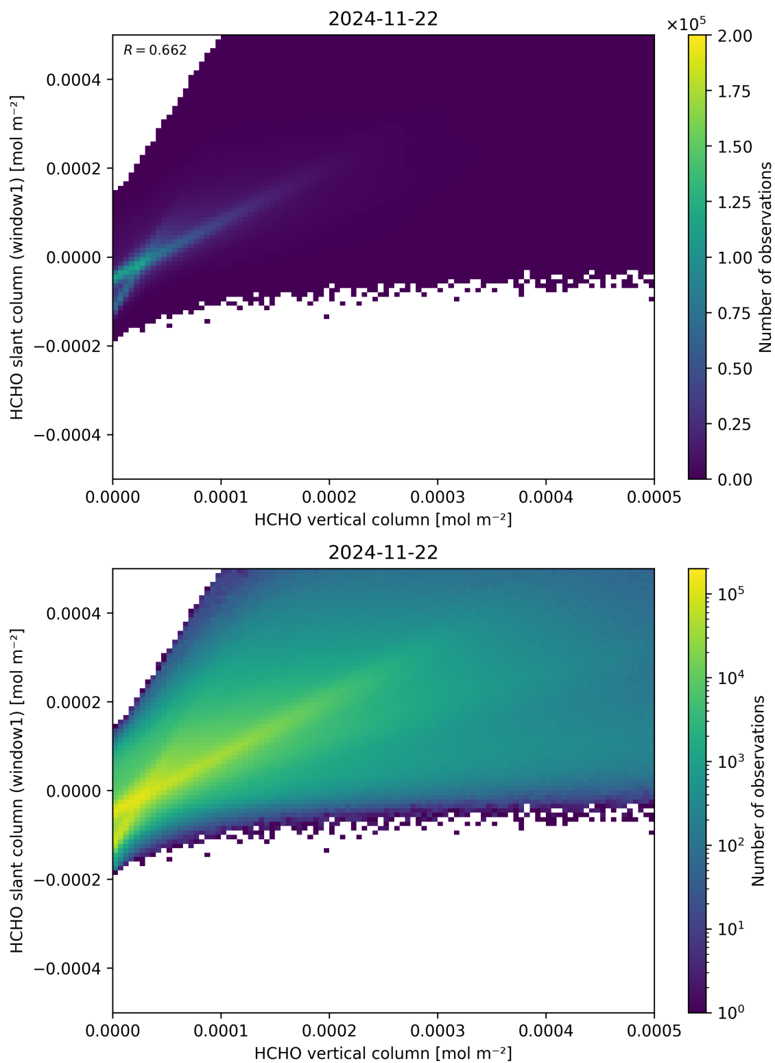
Figure 129: Scatter density plot of “HCHO vertical column” against “HCHO slant column (window1)” for 2024-11-21 to 2024-11-23.
