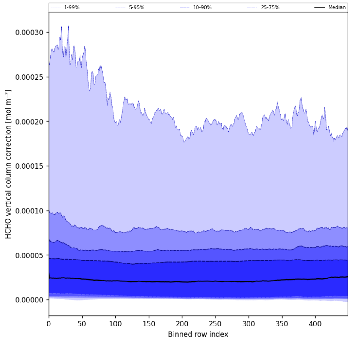
Figure 51: Along track statistics of “HCHO vertical column correction” for 2024-11-21 to 2024-11-23
