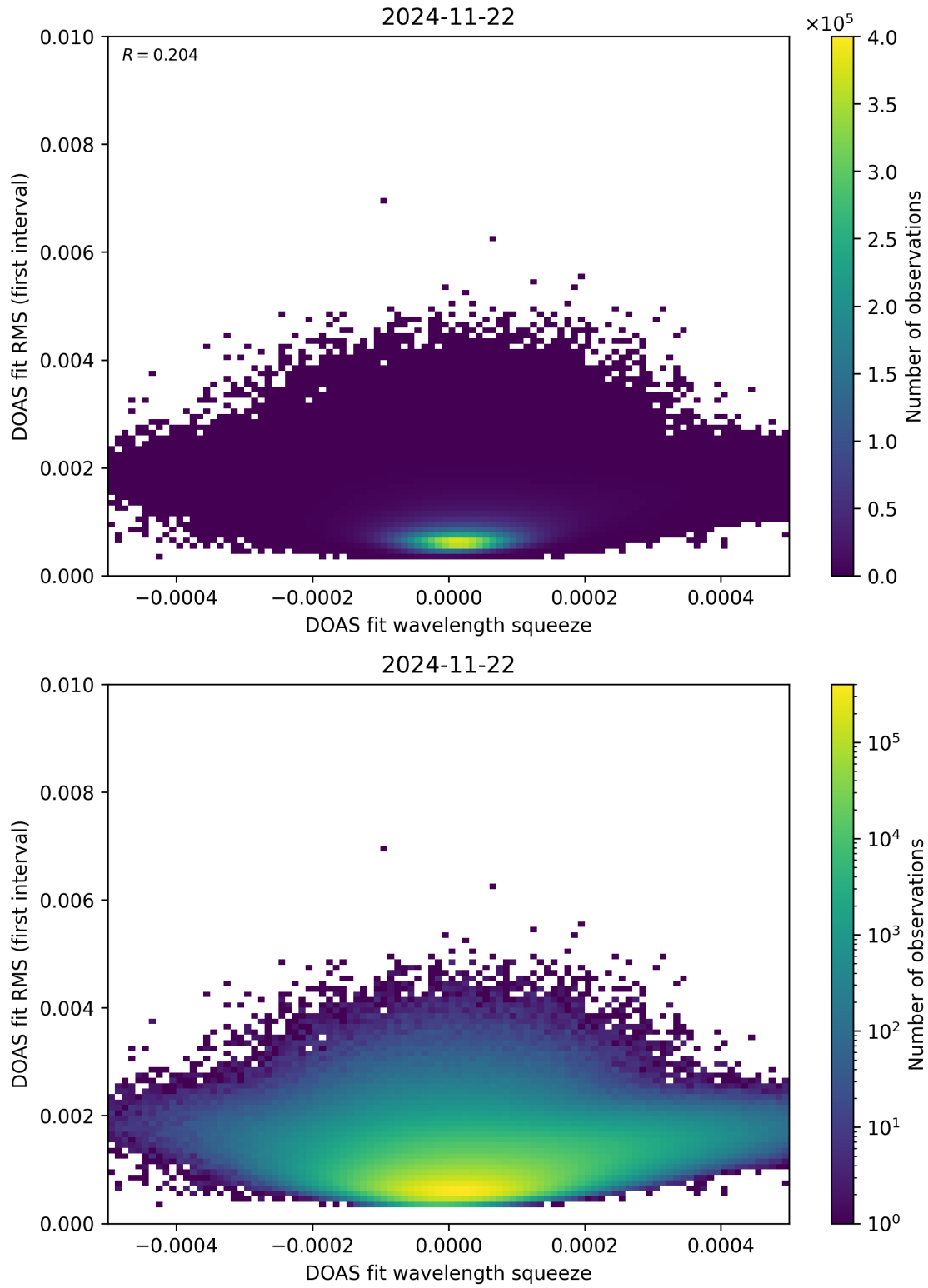
Figure 68: Scatter density plot of “DOAS fit wavelength squeeze” against “DOAS fit RMS (first interval)” for 2024-11-21 to 2024-11-23.
