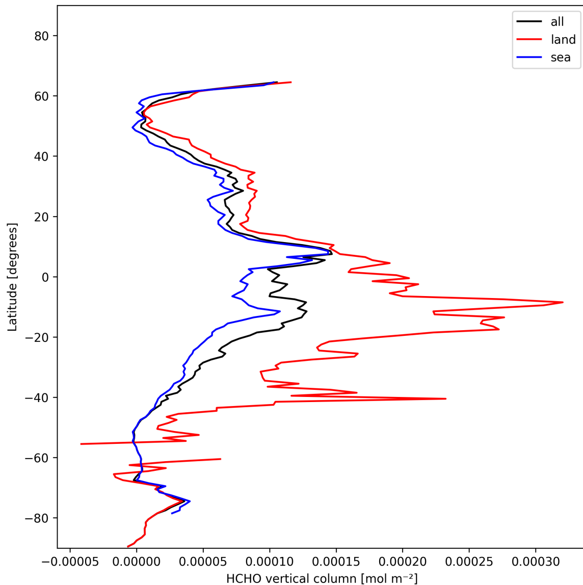
Figure 21: Zonal average of “HCHO vertical column” for 2024-11-21 to 2024-11-23.
