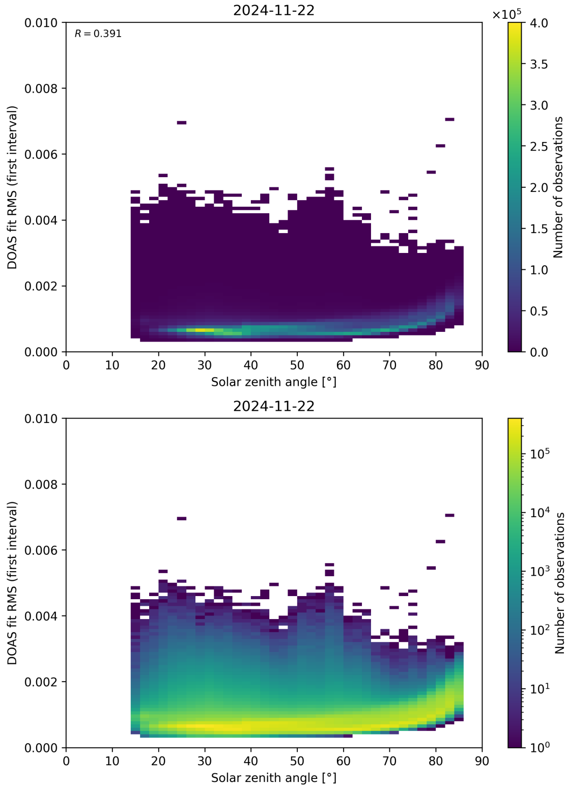
Figure 167: Scatter density plot of “Solar zenith angle” against “DOAS fit RMS (first interval)” for 2024-11-21 to 2024-11-23.
