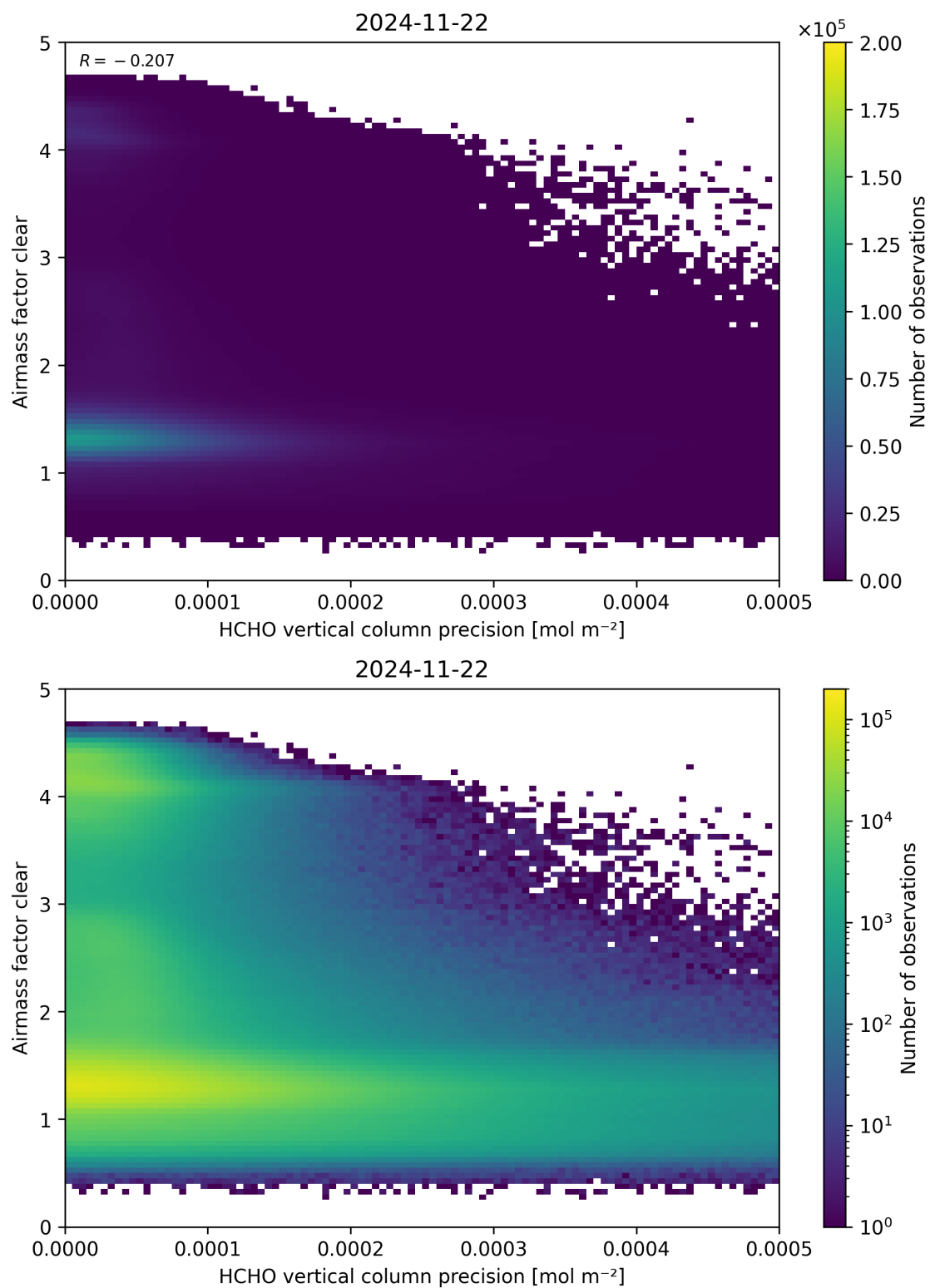
Figure 139: Scatter density plot of “HCHO vertical column precision” against “Airmass factor clear” for 2024-11-21 to 2024-11-23.
