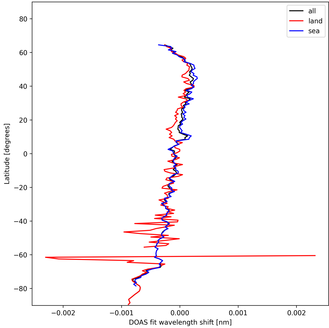
Figure 30: Zonal average of “DOAS fit wavelength shift” for 2024-11-21 to 2024-11-23.
