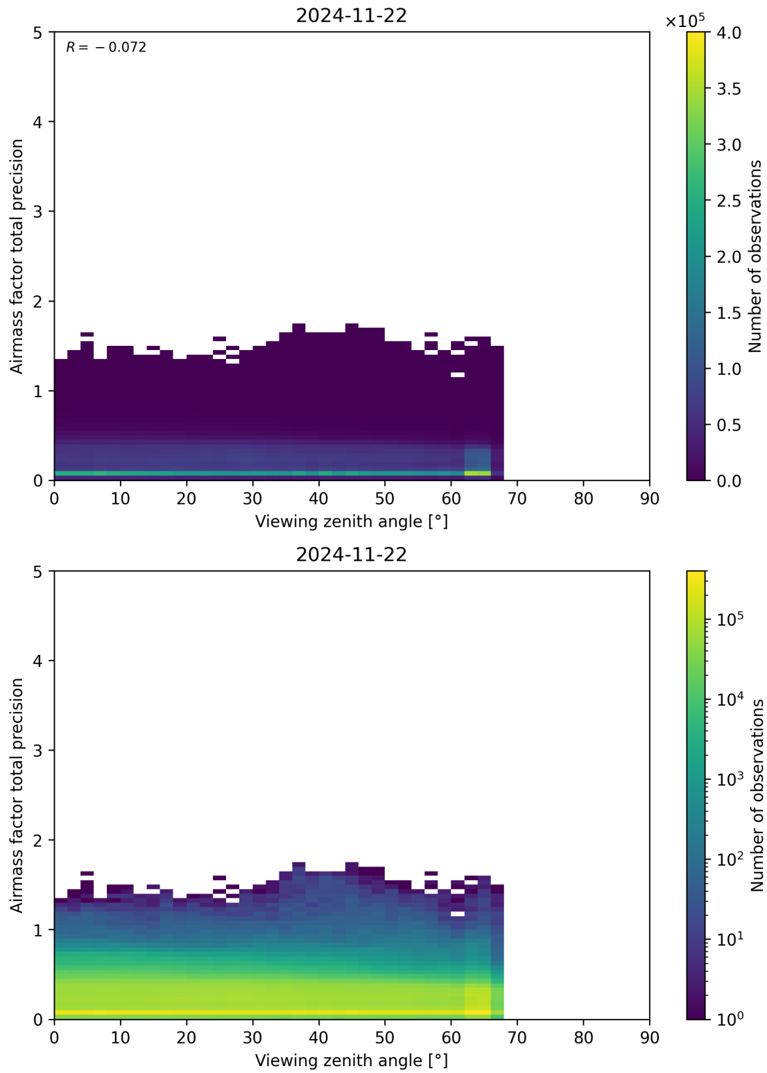
Figure 191: Scatter density plot of “Viewing zenith angle” against “Airmass factor total precision” for 2024-11-21 to 2024-11-23.
