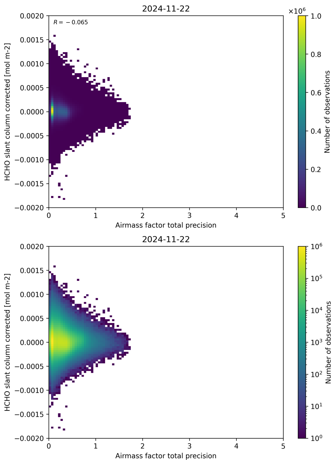
Figure 109: Scatter density plot of “Airmass factor total precision” against “HCHO slant column corrected” for 2024-11-21 to 2024-11-23.
