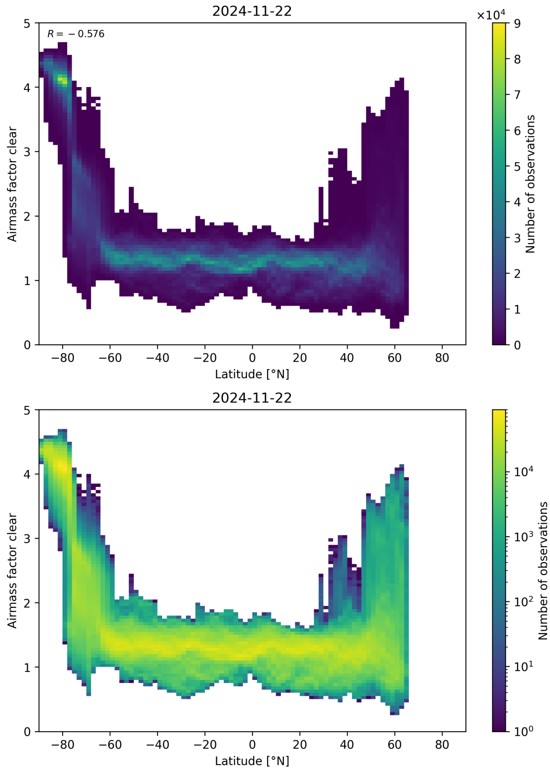
Figure 156: Scatter density plot of “Latitude” against “Airmass factor clear” for 2024-11-21 to 2024-11-23.
