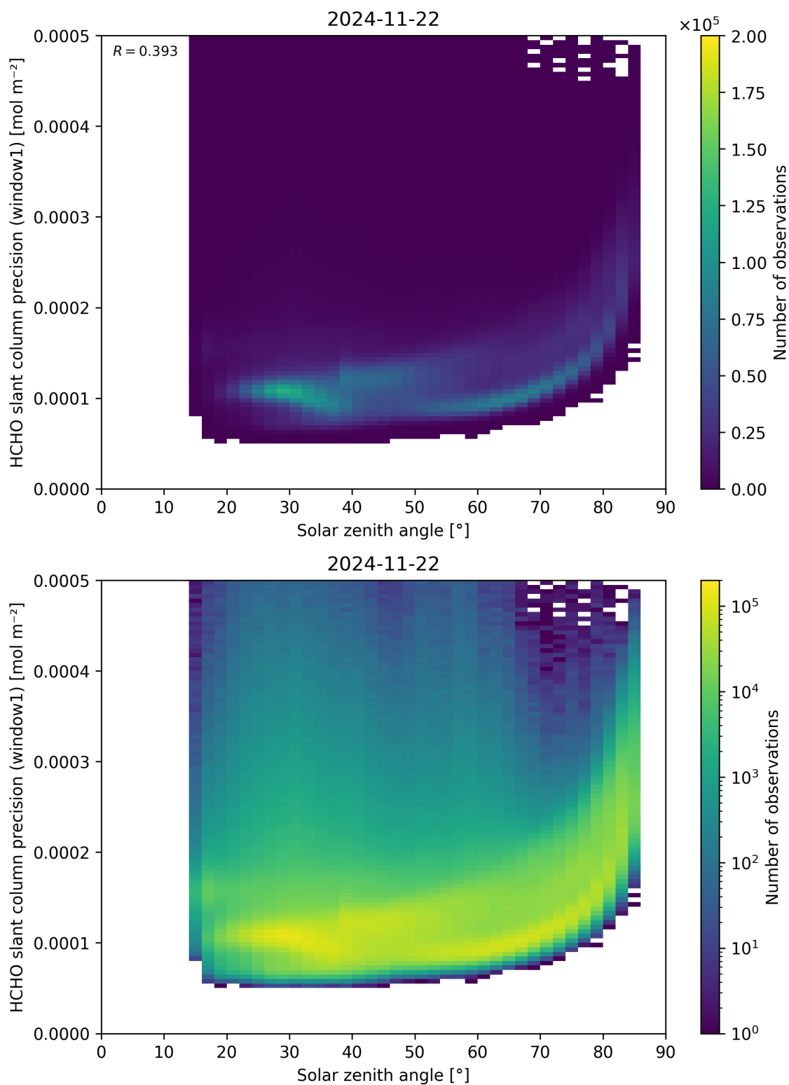
Figure 174: Scatter density plot of “Solar zenith angle” against “HCHO slant column precision (window1)” for 2024-11-21 to 2024-11-23.
