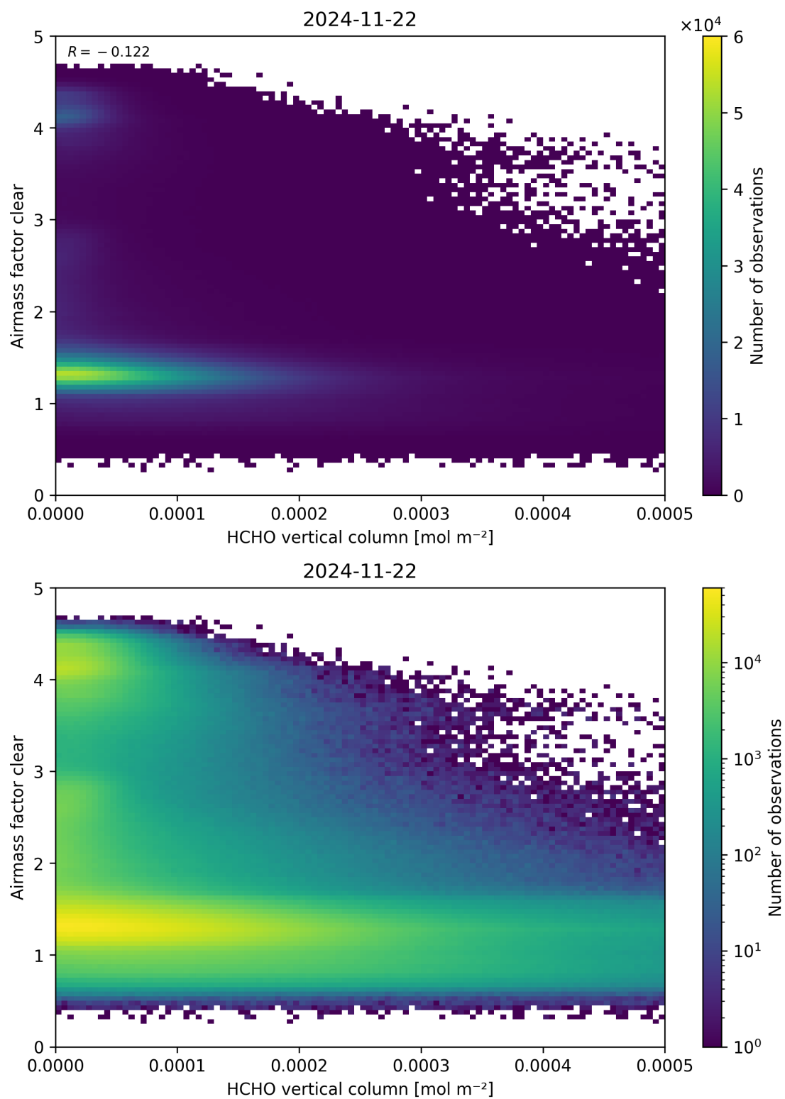
Figure 126: Scatter density plot of “HCHO vertical column” against “Airmass factor clear” for 2024-11-21 to 2024-11-23.
