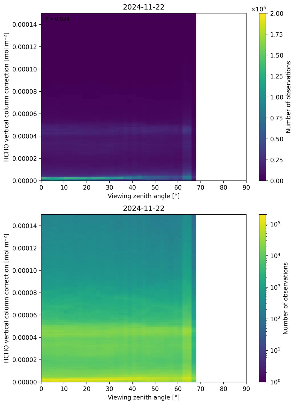
Figure 193: Scatter density plot of “Viewing zenith angle” against “HCHO vertical column correction” for 2024-11-21 to 2024-11-23.
