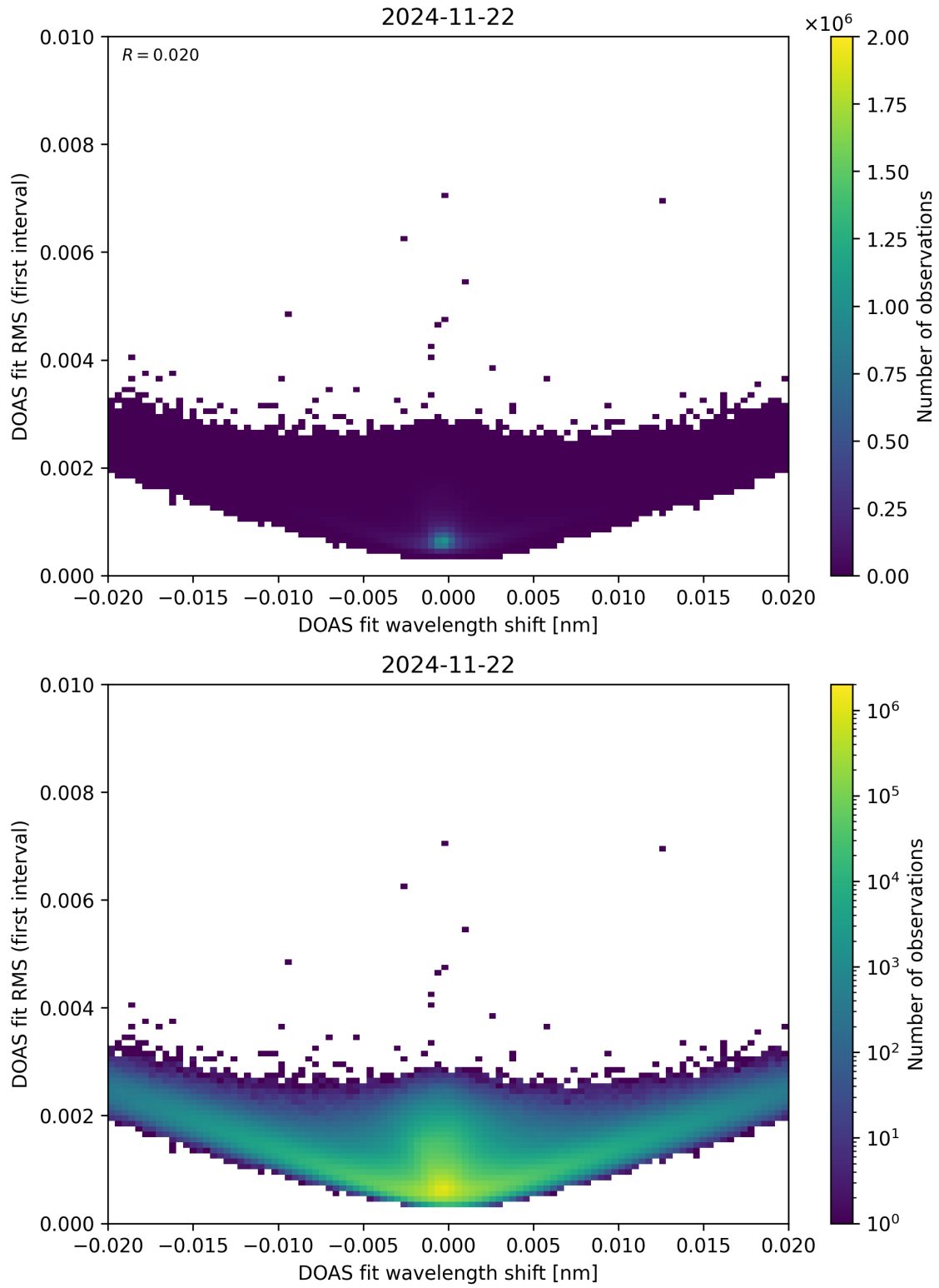
Figure 64: Scatter density plot of “DOAS fit wavelength shift” against “DOAS fit RMS (first interval)” for 2024-11-21 to 2024-11-23.
