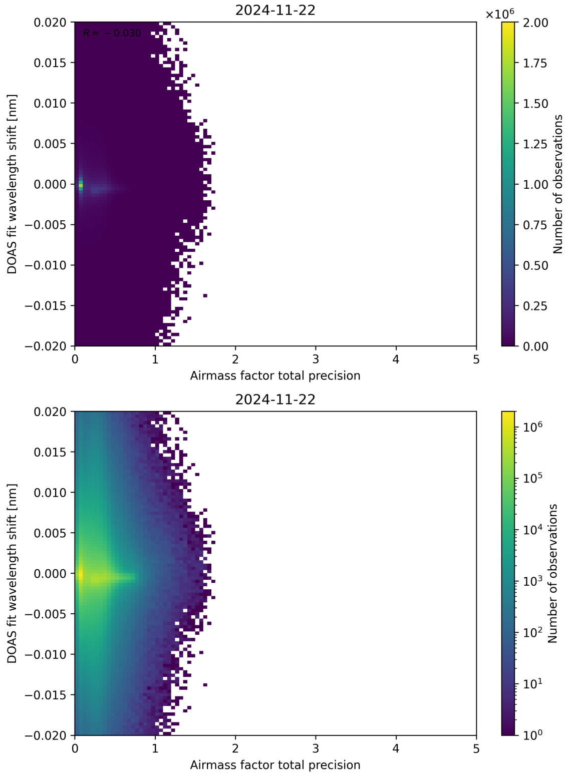
Figure 106: Scatter density plot of “Airmass factor total precision” against “DOAS fit wavelength shift” for 2024-11-21 to 2024-11-23.
