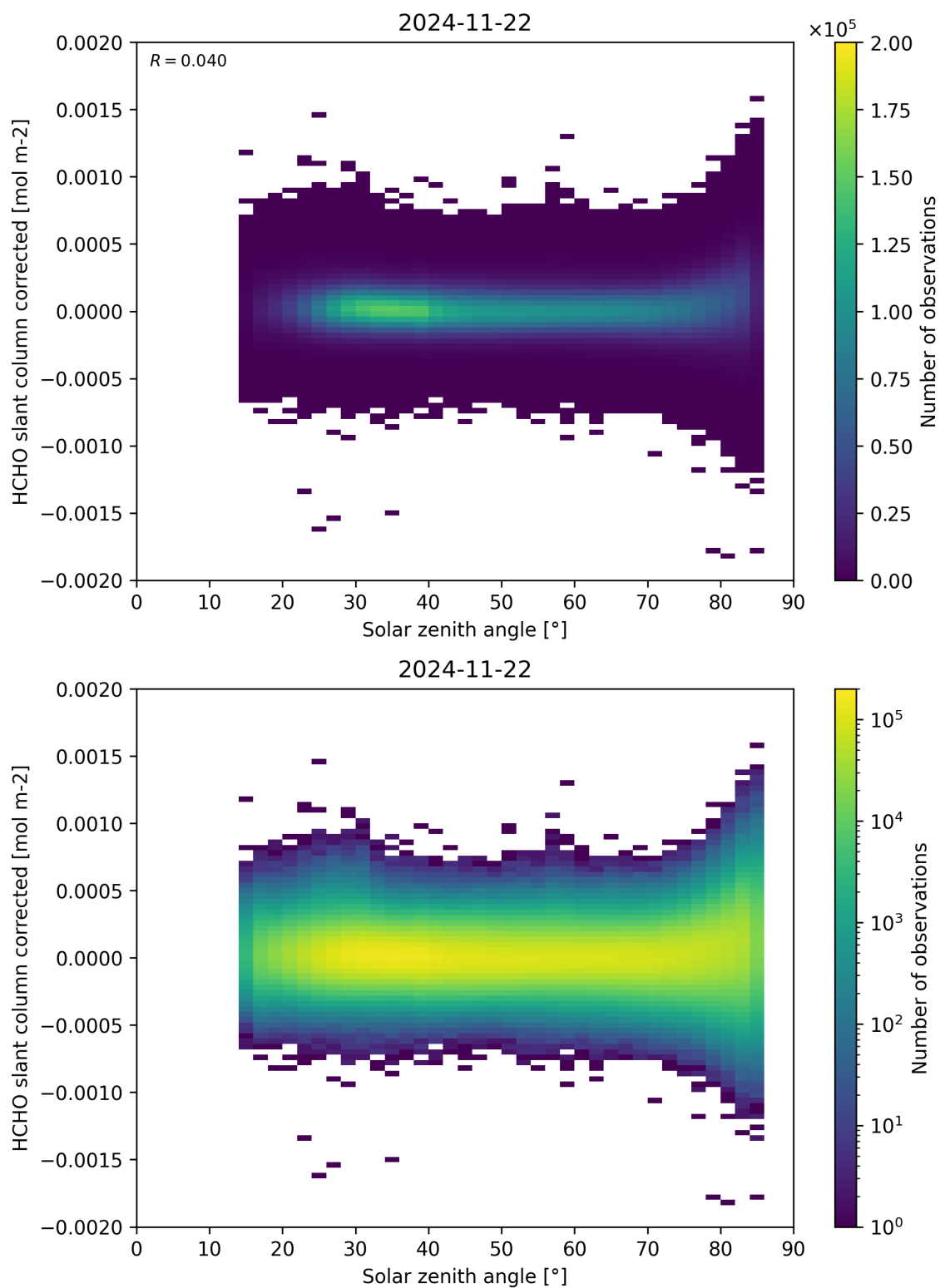
Figure 171: Scatter density plot of “Solar zenith angle” against “HCHO slant column corrected” for 2024-11-21 to 2024-11-23.
