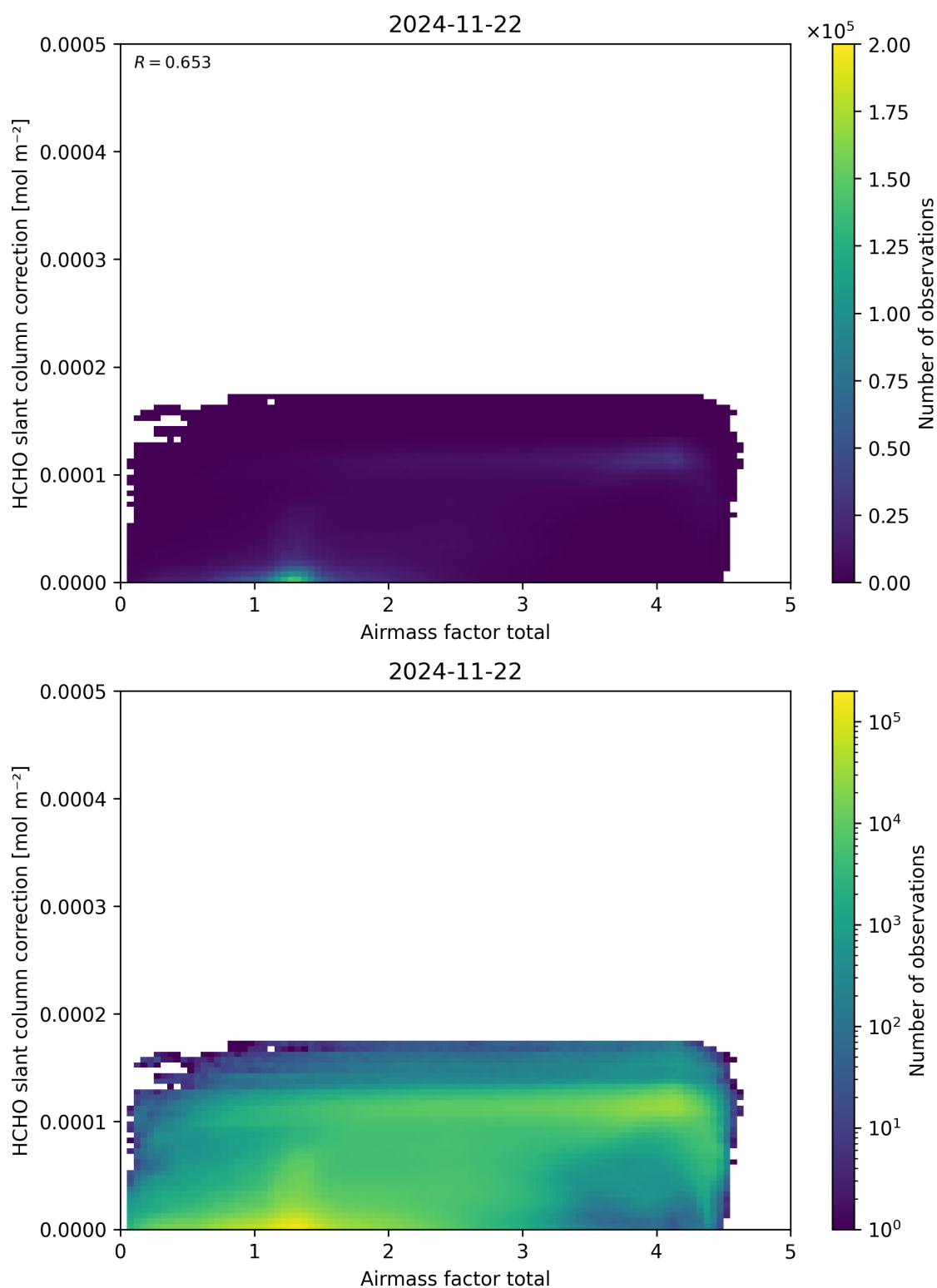
Figure 102: Scatter density plot of “Airmass factor total” against “HCHO slant column correction” for 2024-11-21 to 2024-11-23.
