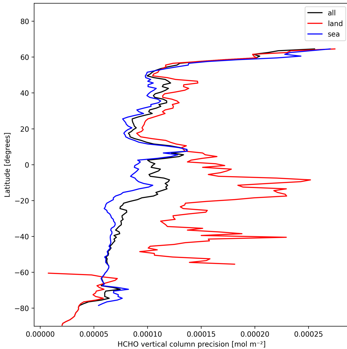
Figure 22: Zonal average of “HCHO vertical column precision” for 2024-11-21 to 2024-11-23.
