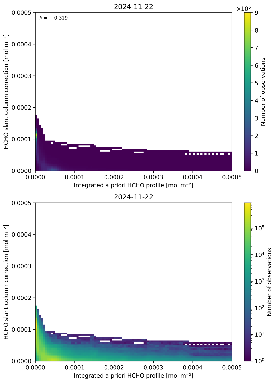
Figure 152: Scatter density plot of “Integrated a priori HCHO profile” against “HCHO slant column correction” for 2024-11-21 to 2024-11-23.
