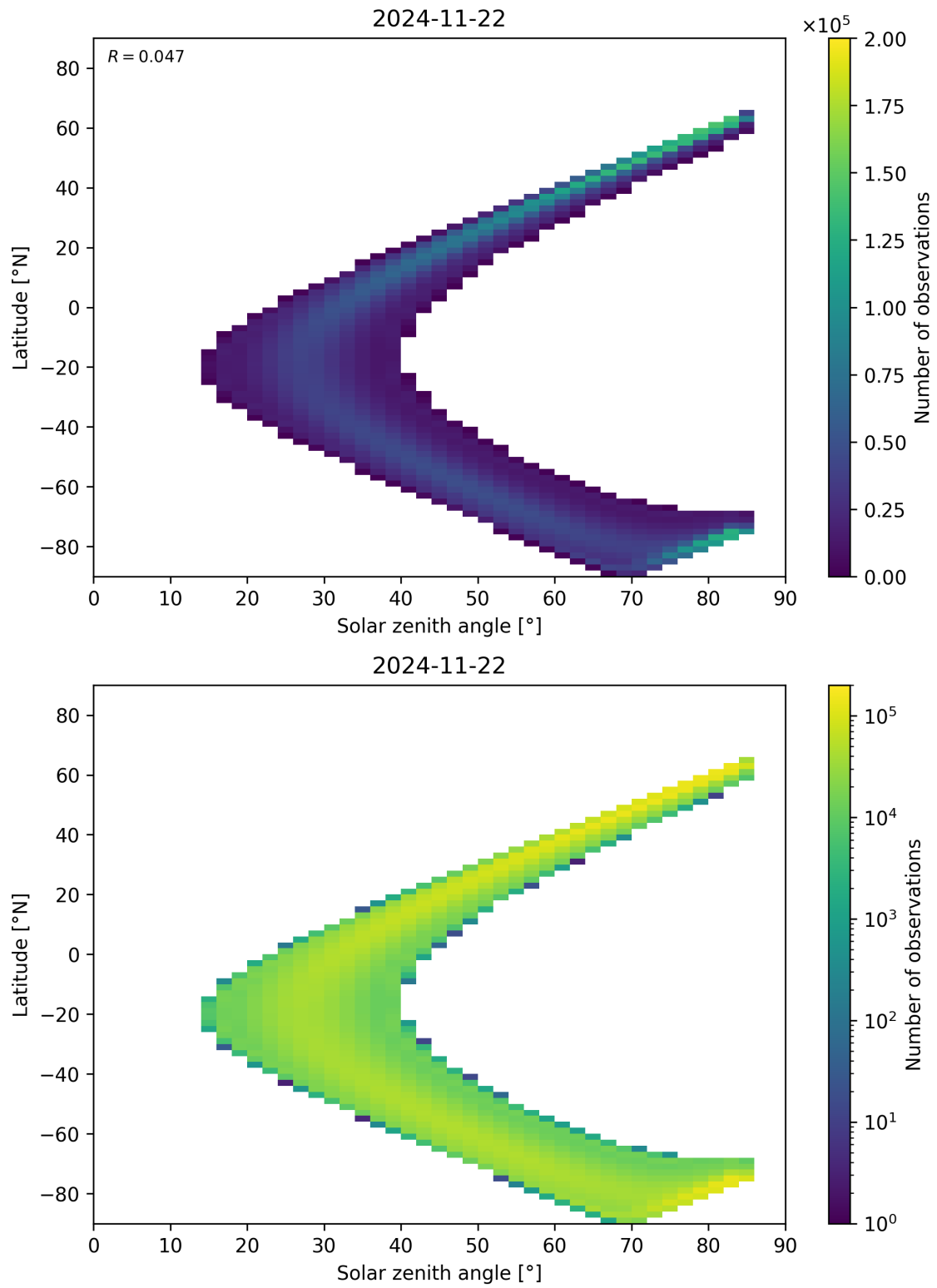
Figure 181: Scatter density plot of “Solar zenith angle” against “Latitude” for 2024-11-21 to 2024-11-23.
