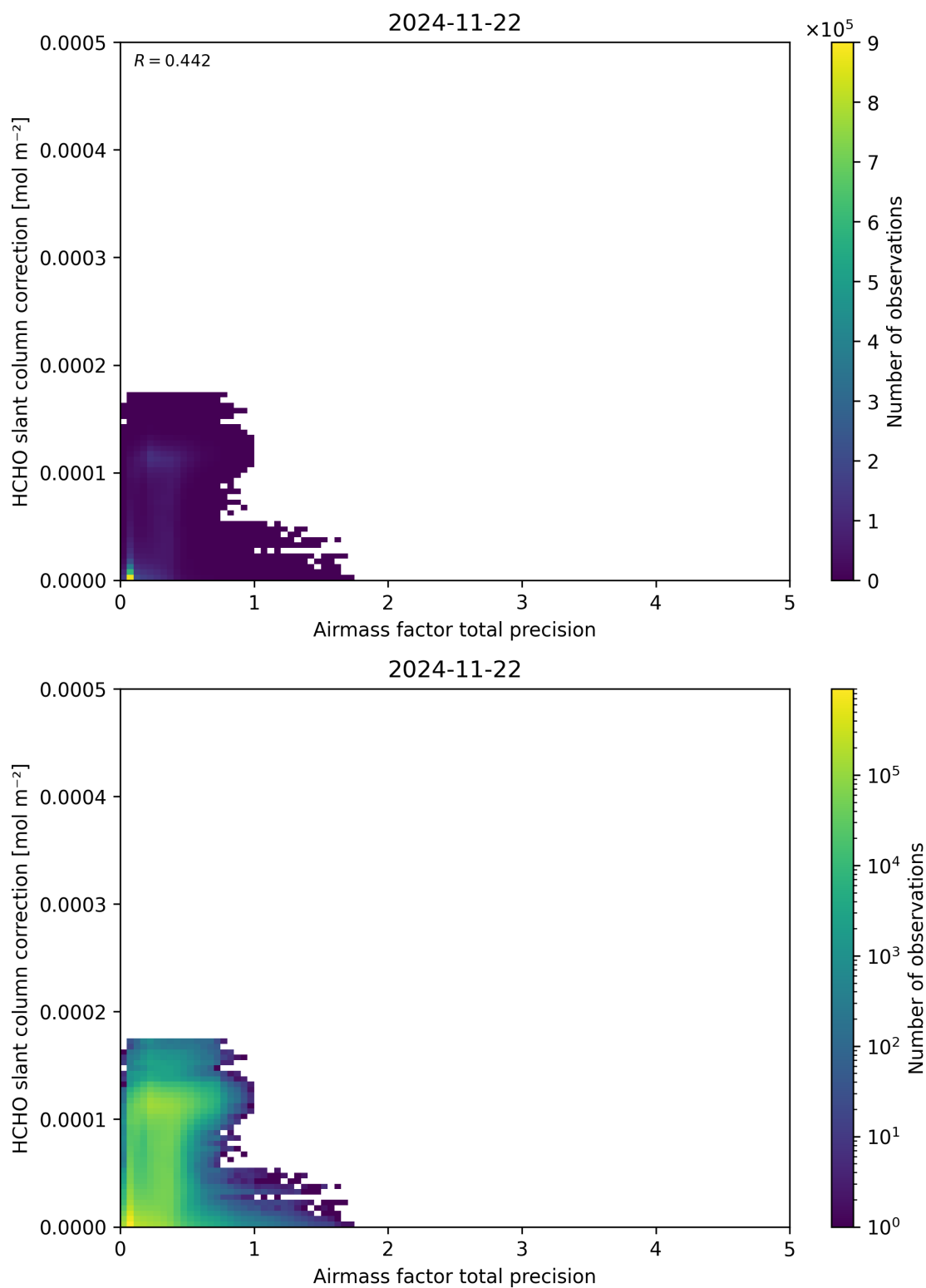
Figure 110: Scatter density plot of “Airmass factor total precision” against “HCHO slant column correction” for 2024-11-21 to 2024-11-23.
