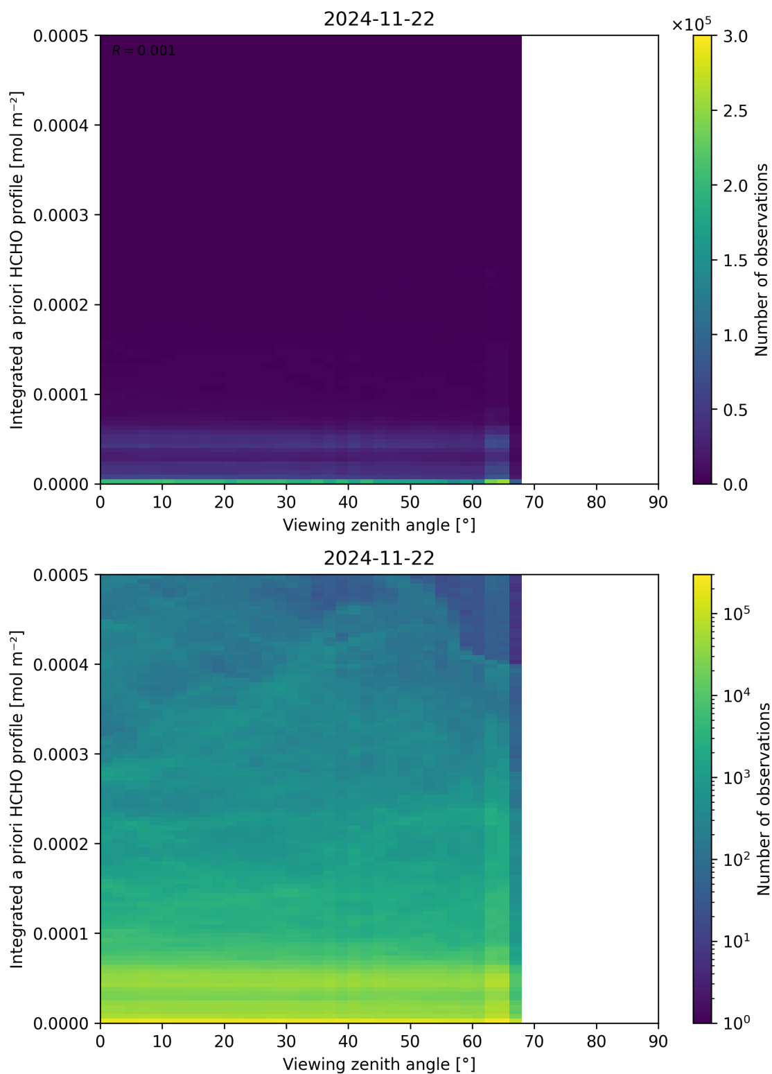
Figure 195: Scatter density plot of “Viewing zenith angle” against “Integrated a priori HCHO profile” for 2024-11-21 to 2024-11-23.
