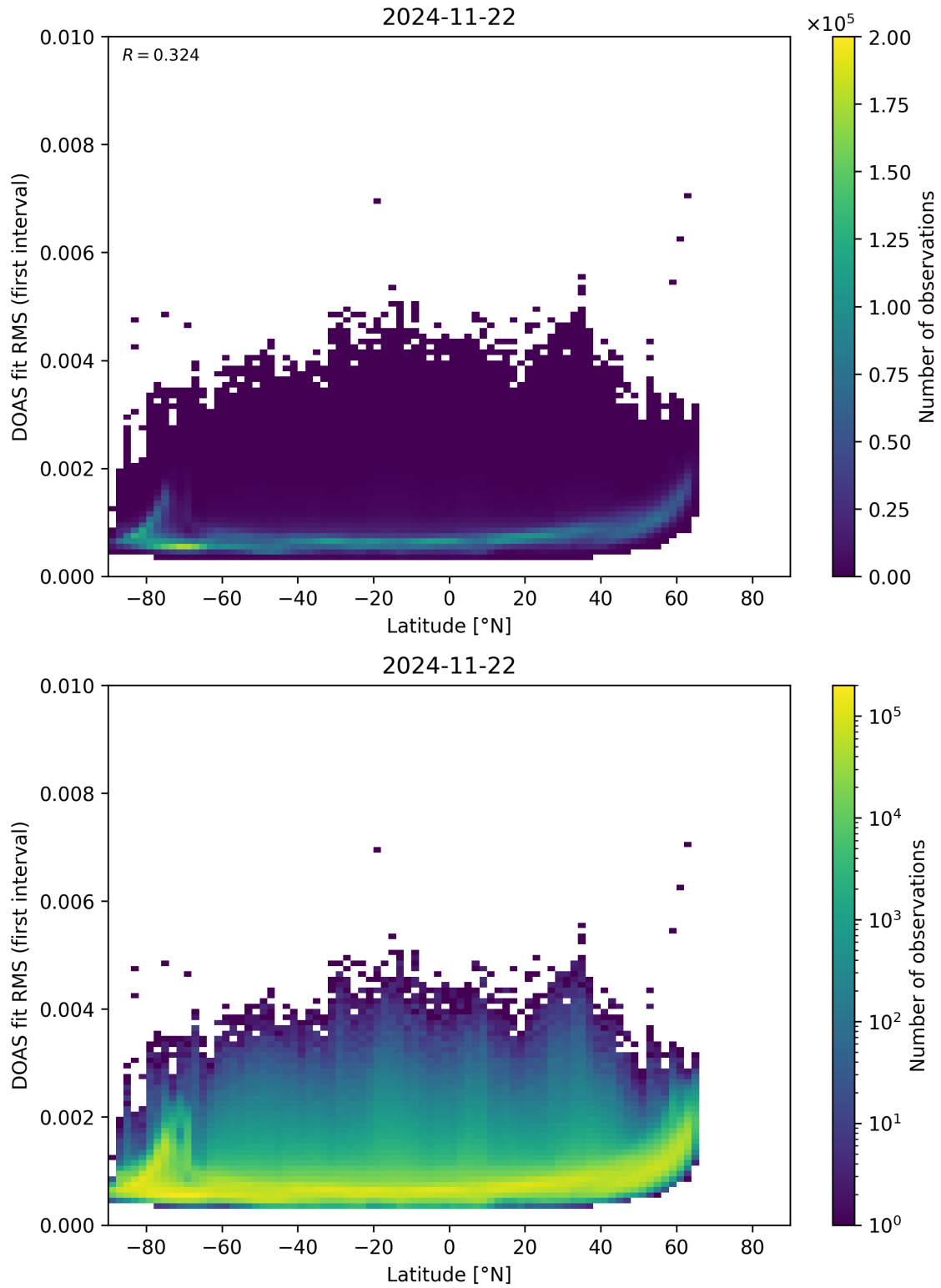
Figure 153: Scatter density plot of “Latitude” against “DOAS fit RMS (first interval)” for 2024-11-21 to 2024-11-23.
