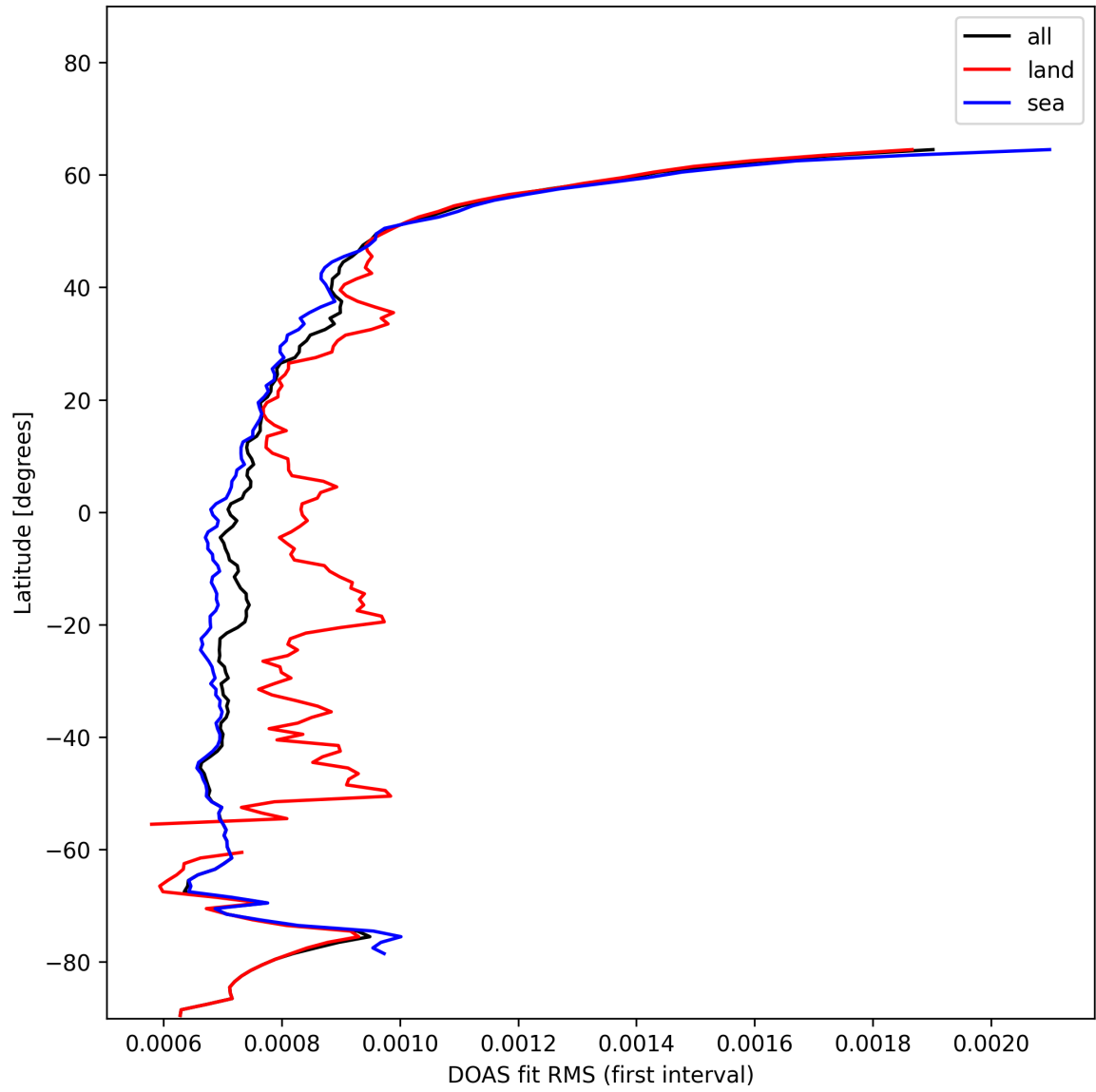
Figure 32: Zonal average of “DOAS fit RMS (first interval)” for 2024-11-21 to 2024-11-23.
