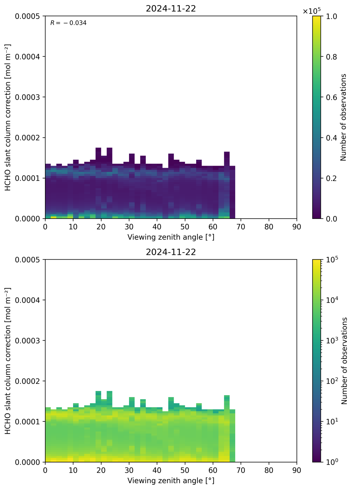
Figure 187: Scatter density plot of “Viewing zenith angle” against “HCHO slant column correction” for 2024-11-21 to 2024-11-23.
