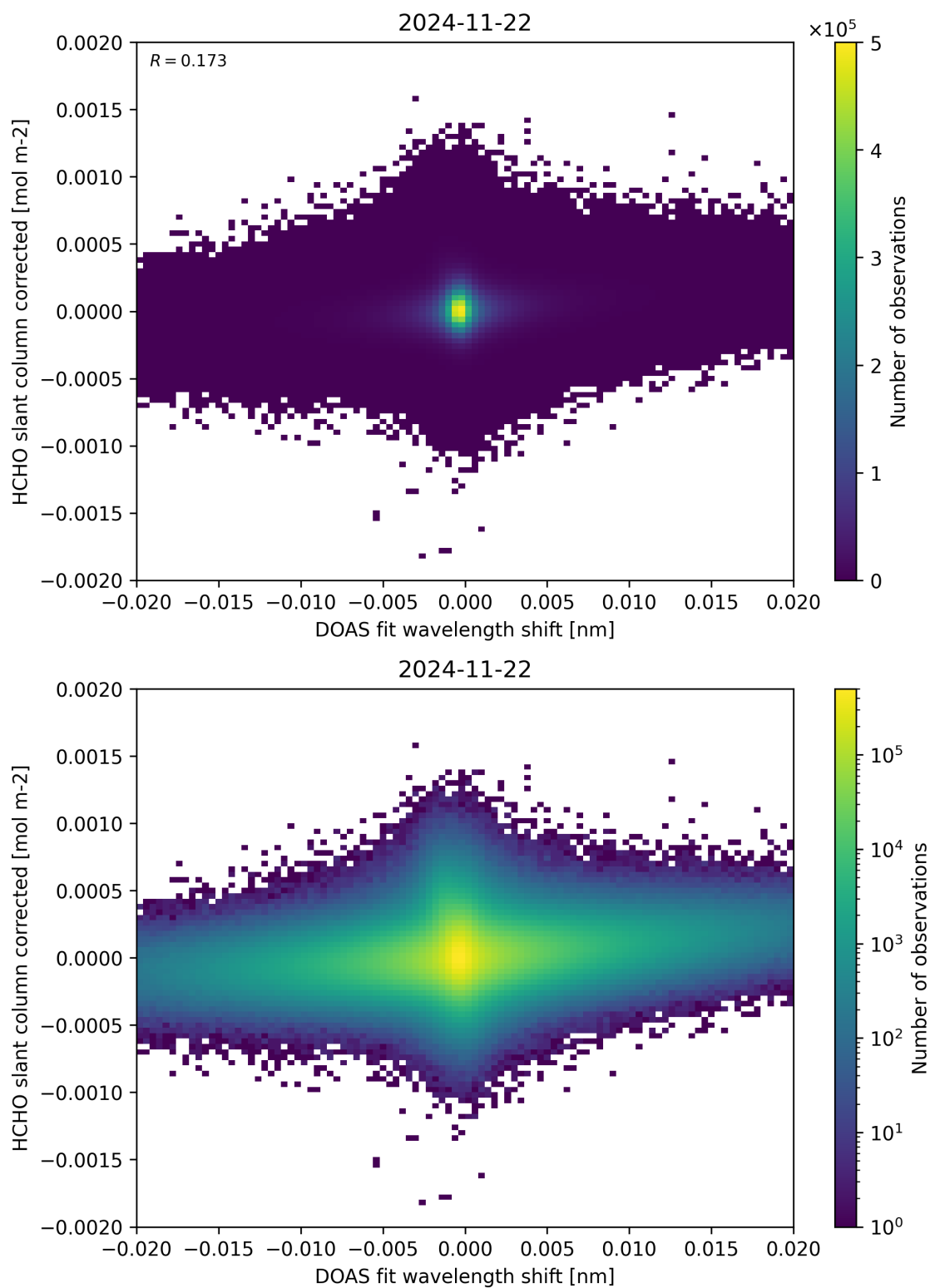
Figure 66: Scatter density plot of “DOAS fit wavelength shift” against “HCHO slant column corrected” for 2024-11-21 to 2024-11-23.
