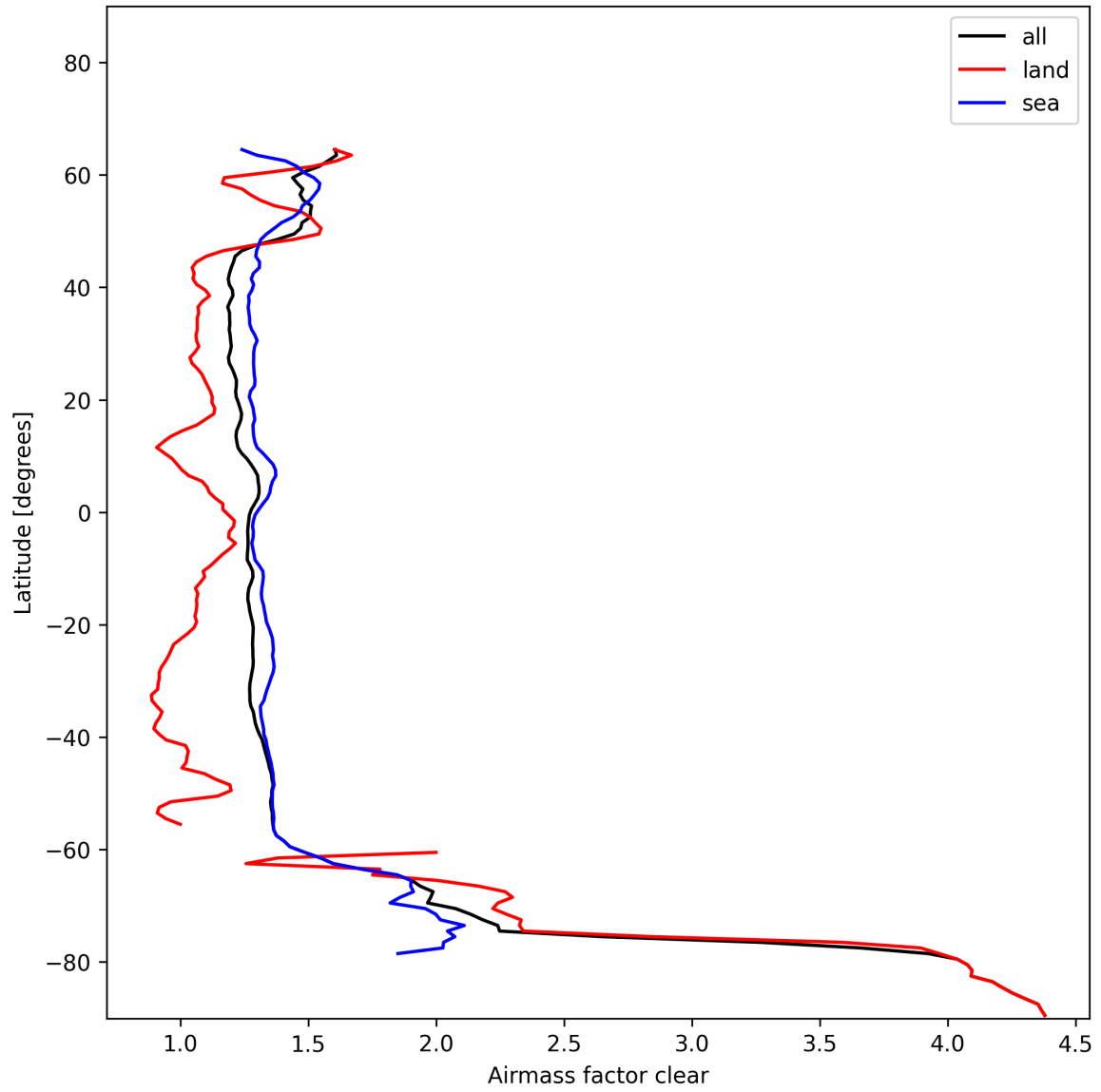
Figure 28: Zonal average of “Airmass factor clear” for 2024-11-21 to 2024-11-23.
