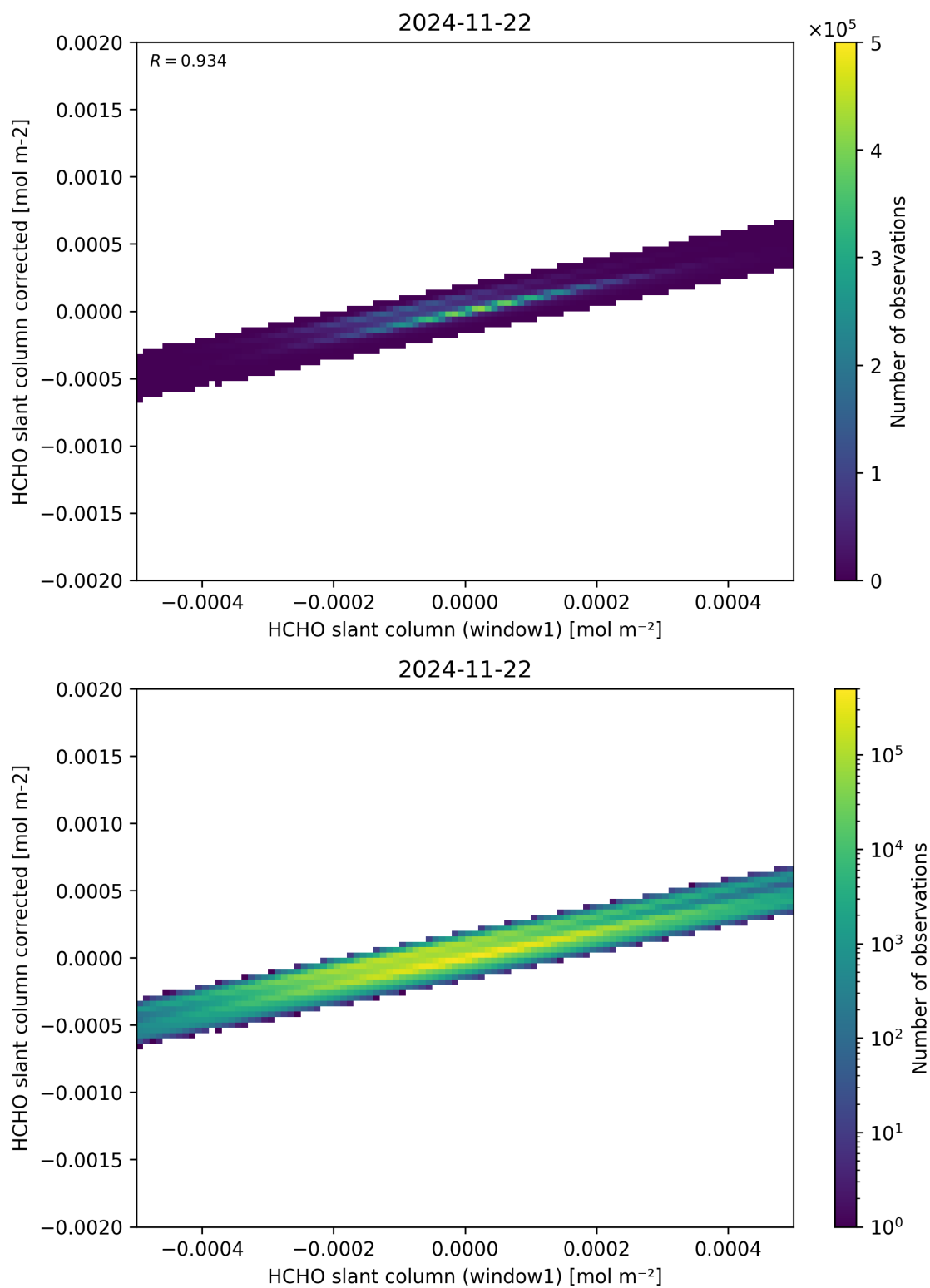
Figure 82: Scatter density plot of “HCHO slant column (window1)” against “HCHO slant column corrected” for 2024-11-21 to 2024-11-23.
