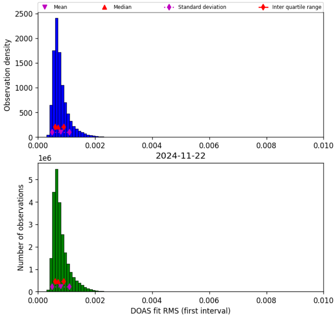
Figure 46: Histogram of “DOAS fit RMS (first interval)” for 2024-11-21 to 2024-11-23
