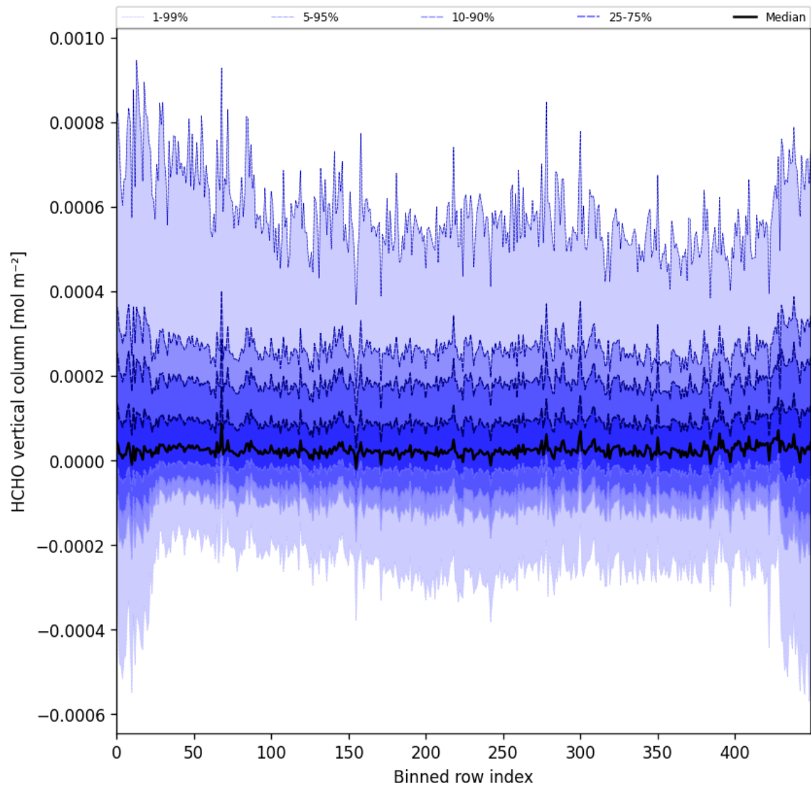
Figure 49: Along track statistics of “HCHO vertical column” for 2024-11-21 to 2024-11-23
