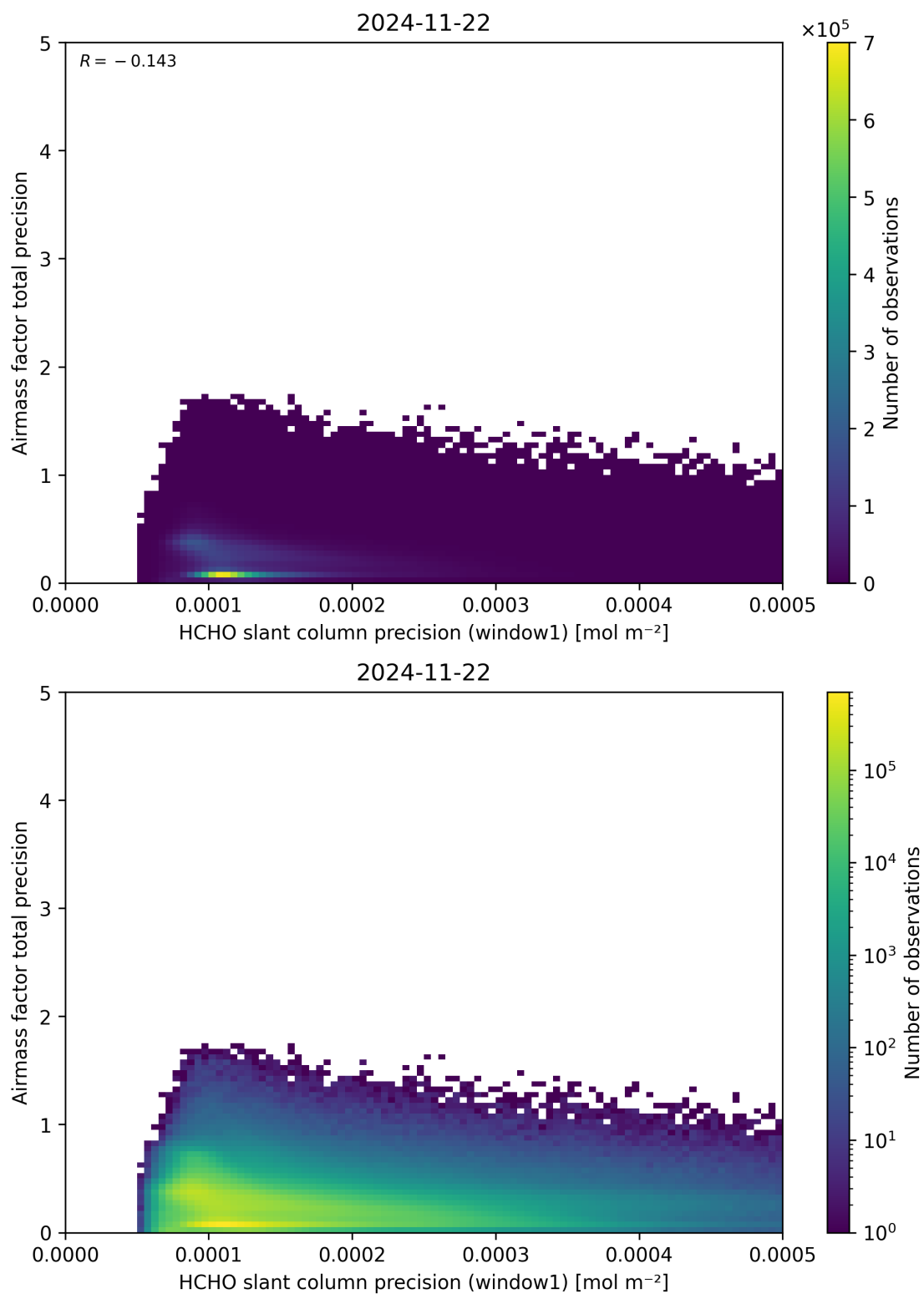
Figure 95: Scatter density plot of “HCHO slant column precision (window1)” against “Airmass factor total precision” for 2024-11-21 to 2024-11-23.
