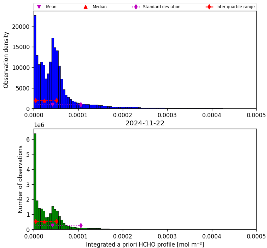
Figure 43: Histogram of “Integrated a priori HCHO profile” for 2024-11-21 to 2024-11-23
