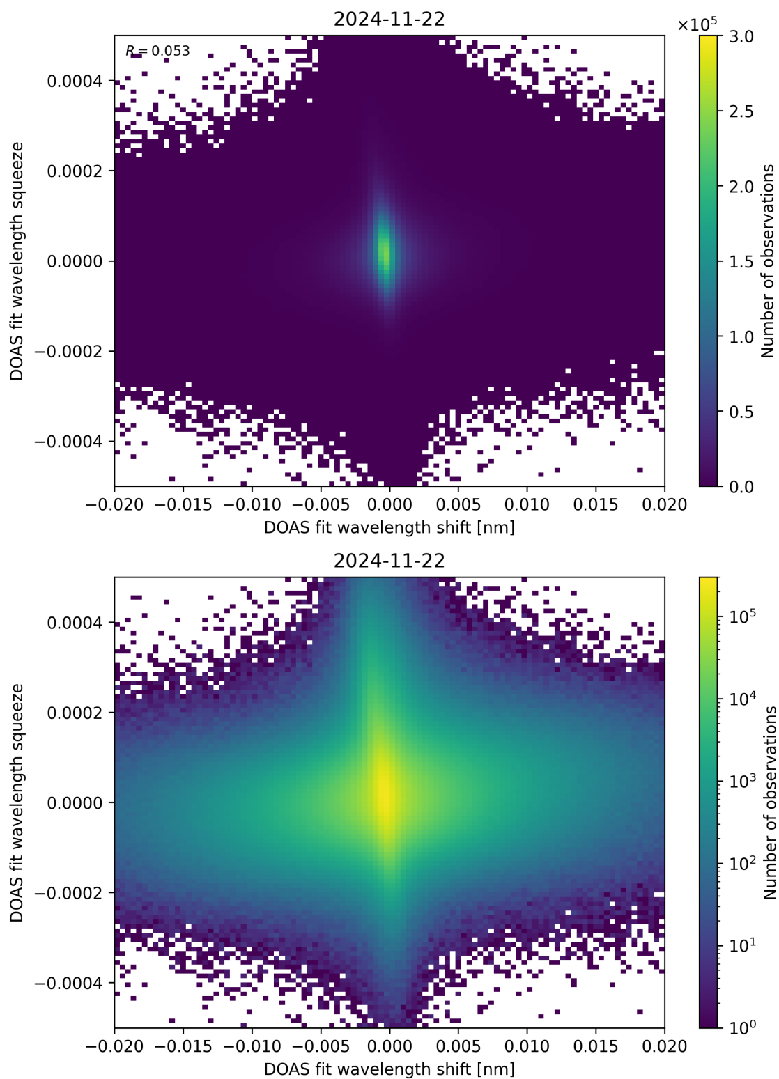
Figure 65: Scatter density plot of “DOAS fit wavelength shift” against “DOAS fit wavelength squeeze” for 2024-11-21 to 2024-11-23.
