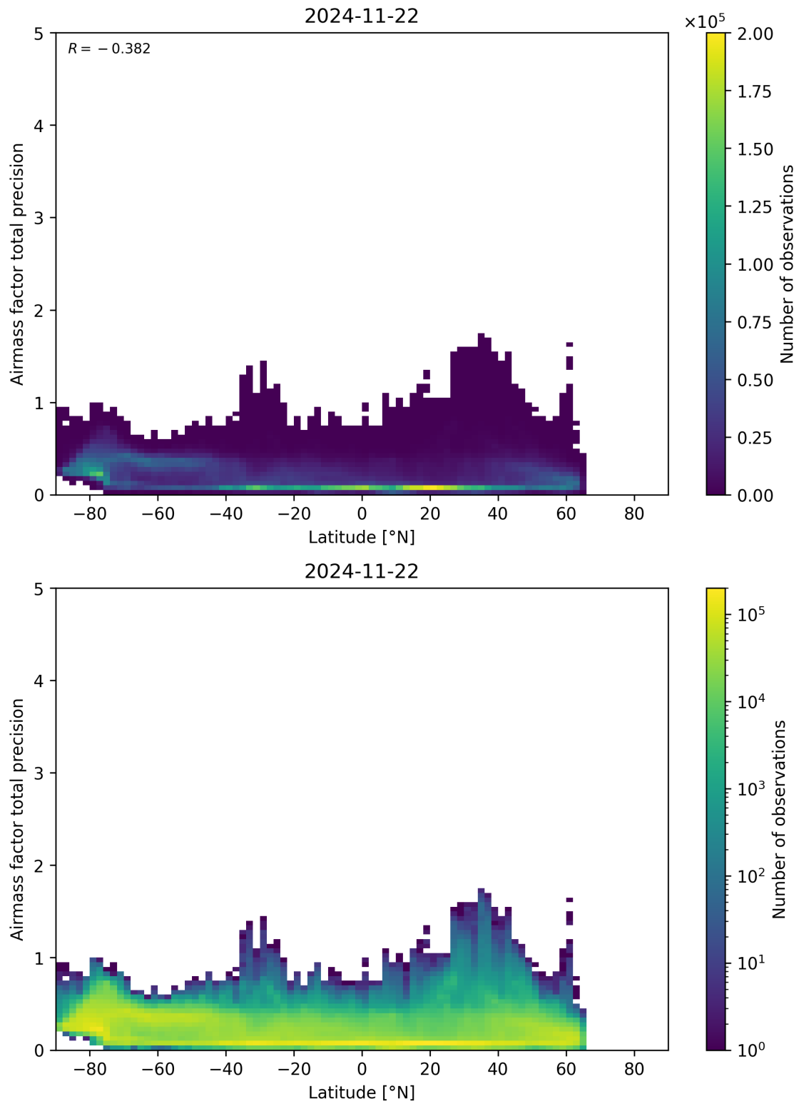
Figure 162: Scatter density plot of “Latitude” against “Airmass factor total precision” for 2024-11-21 to 2024-11-23.
