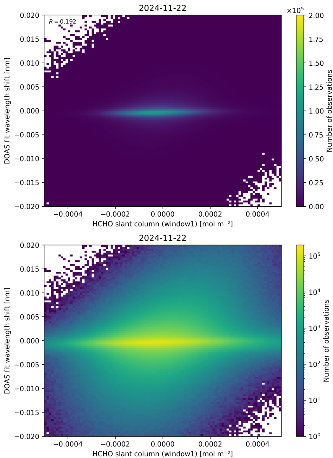
Figure 79: Scatter density plot of “HCHO slant column (window1)” against “DOAS fit wavelength shift” for 2024-11-21 to 2024-11-23.
