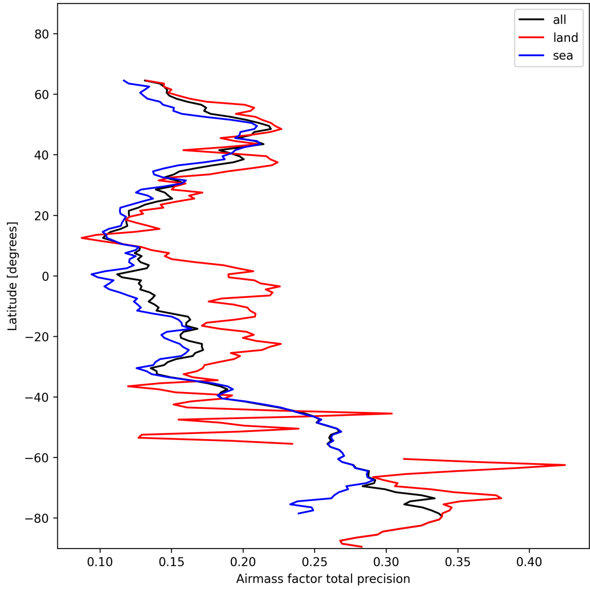
Figure 27: Zonal average of “Airmass factor total precision” for 2024-11-21 to 2024-11-23.
