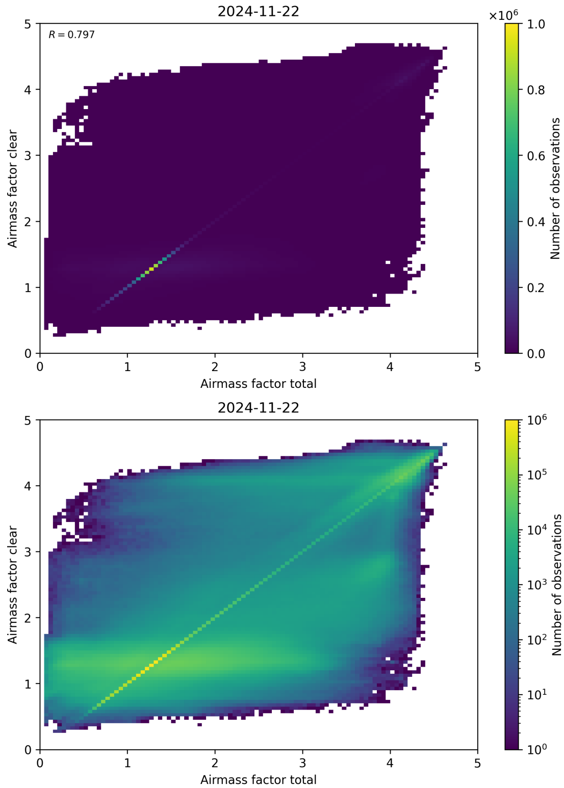
Figure 100: Scatter density plot of “Airmass factor total” against “Airmass factor clear” for 2024-11-21 to 2024-11-23.
