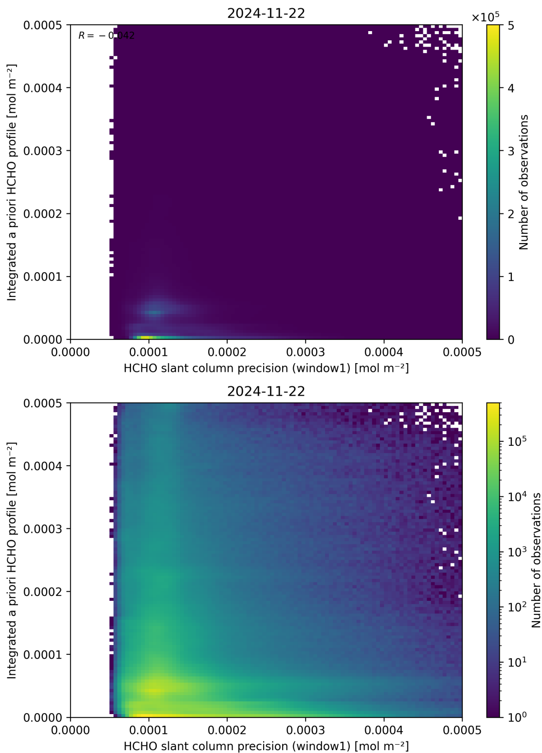
Figure 96: Scatter density plot of “HCHO slant column precision (window1)” against “Integrated a priori HCHO profile” for 2024-11-21 to 2024-11-23.
