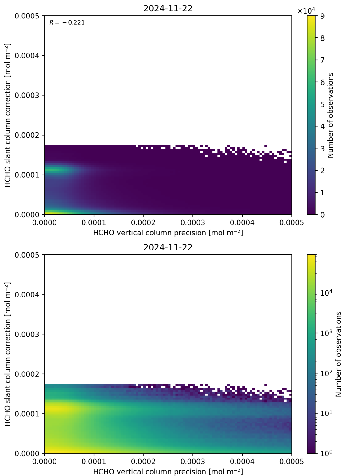
Figure 141: Scatter density plot of “HCHO vertical column precision” against “HCHO slant column correction” for 2024-11-21 to 2024-11-23.
