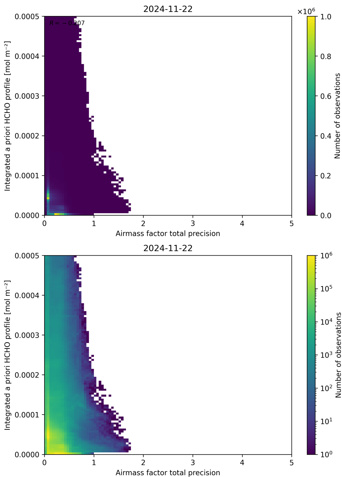
Figure 111: Scatter density plot of “Airmass factor total precision” against “Integrated a priori HCHO profile” for 2024-11-21 to 2024-11-23.
