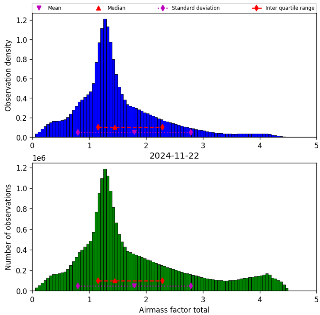
Figure 40: Histogram of “Airmass factor total” for 2024-11-21 to 2024-11-23
