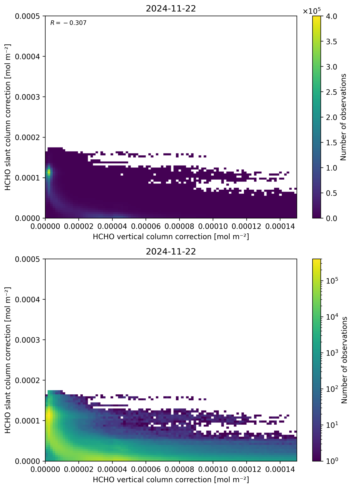
Figure 117: Scatter density plot of “HCHO vertical column correction” against “HCHO slant column correction” for 2024-11-21 to 2024-11-23.
