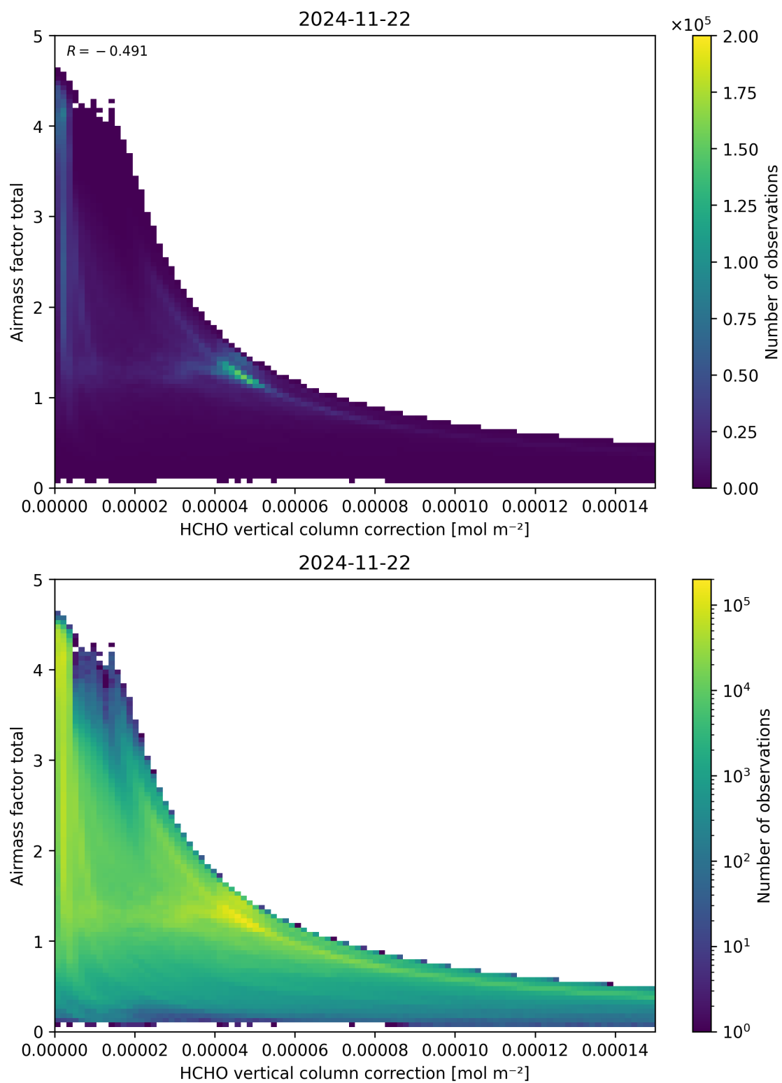
Figure 120: Scatter density plot of “HCHO vertical column correction” against “Airmass factor total” for 2024-11-21 to 2024-11-23.
