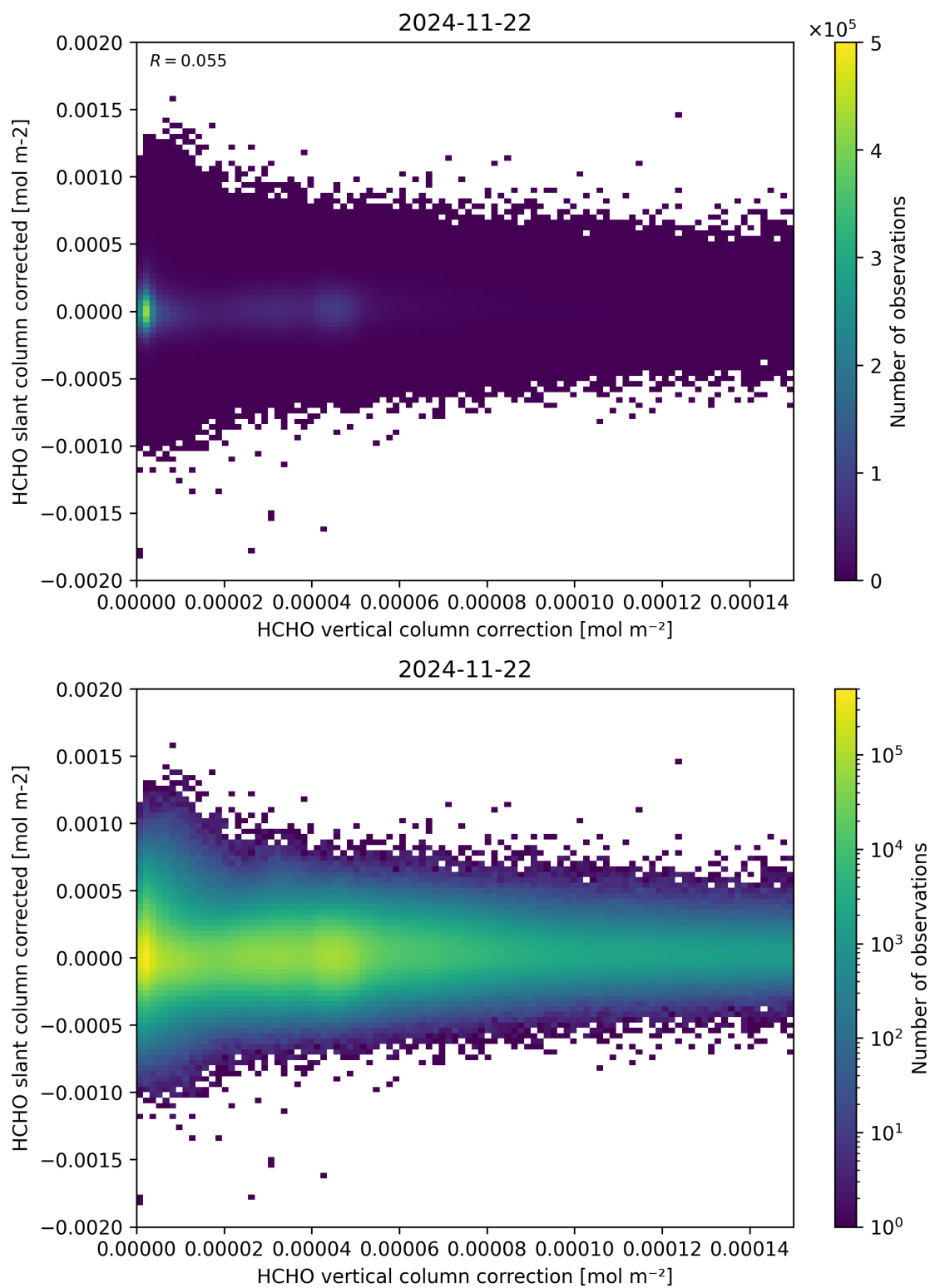
Figure 116: Scatter density plot of “HCHO vertical column correction” against “HCHO slant column corrected” for 2024-11-21 to 2024-11-23.
