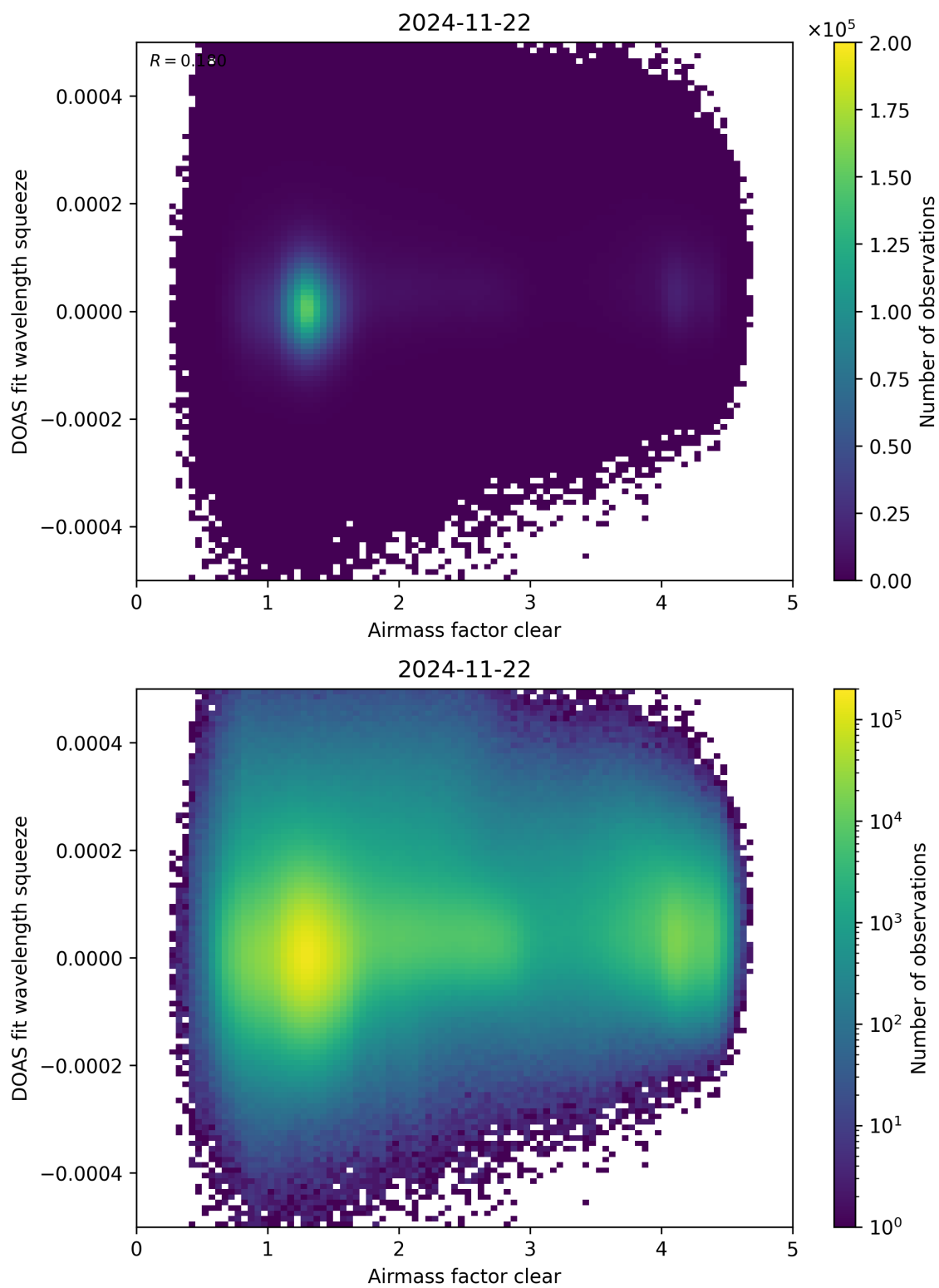
Figure 73: Scatter density plot of “Airmass factor clear” against “DOAS fit wavelength squeeze” for 2024-11-21 to 2024-11-23.
