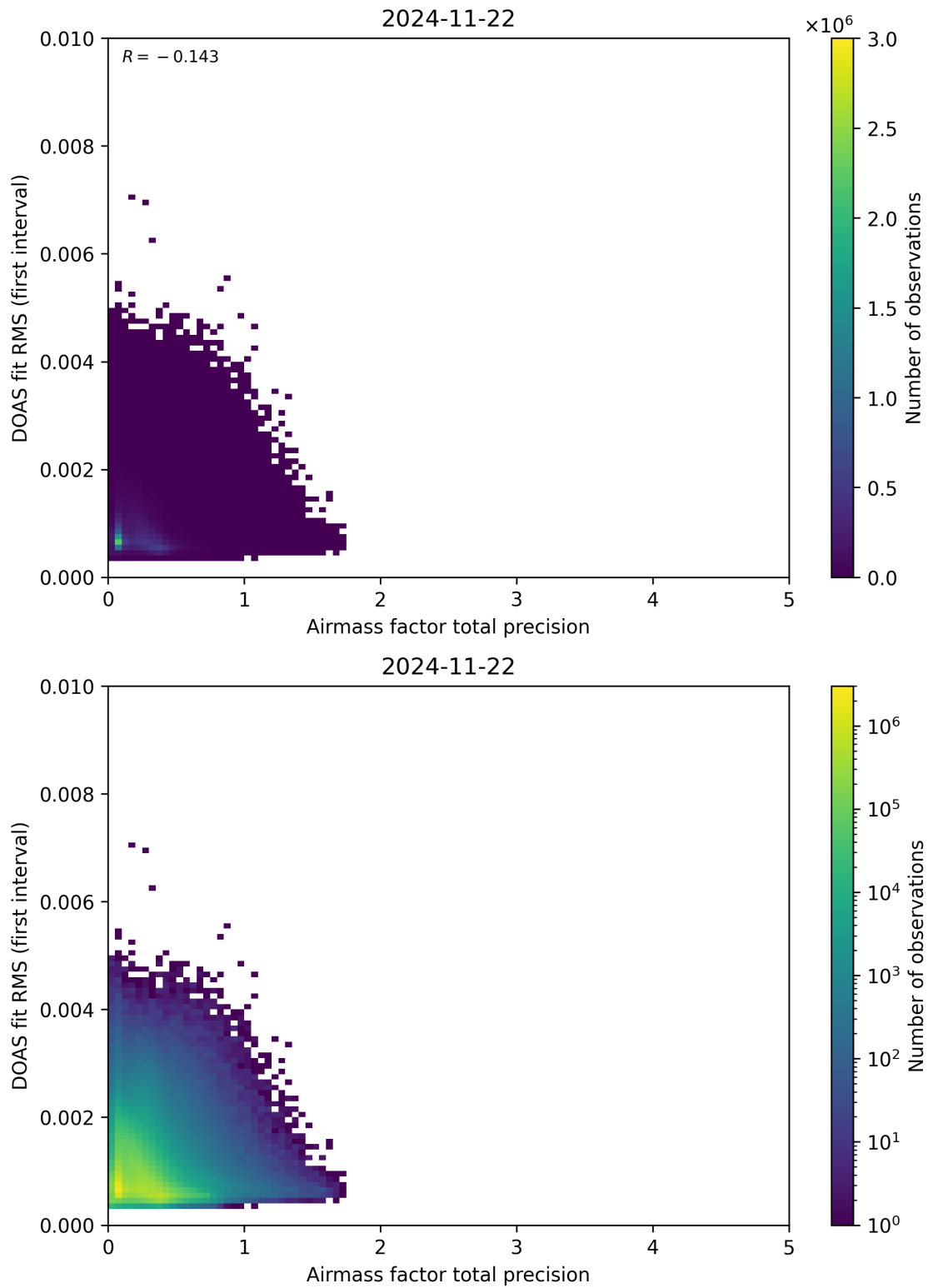
Figure 105: Scatter density plot of “Airmass factor total precision” against “DOAS fit RMS (first interval)” for 2024-11-21 to 2024-11-23.
