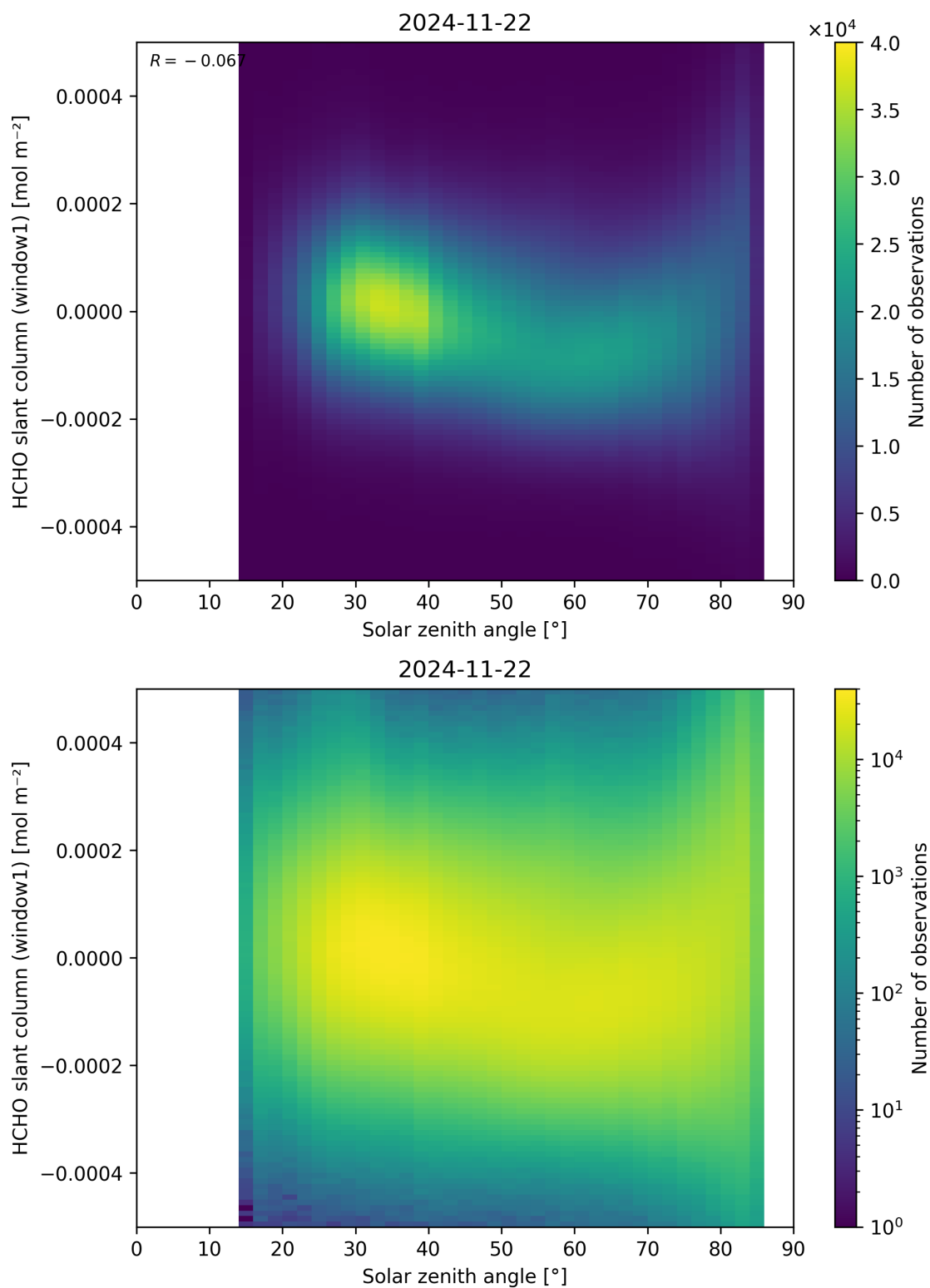
Figure 173: Scatter density plot of “Solar zenith angle” against “HCHO slant column (window1)” for 2024-11-21 to 2024-11-23.
