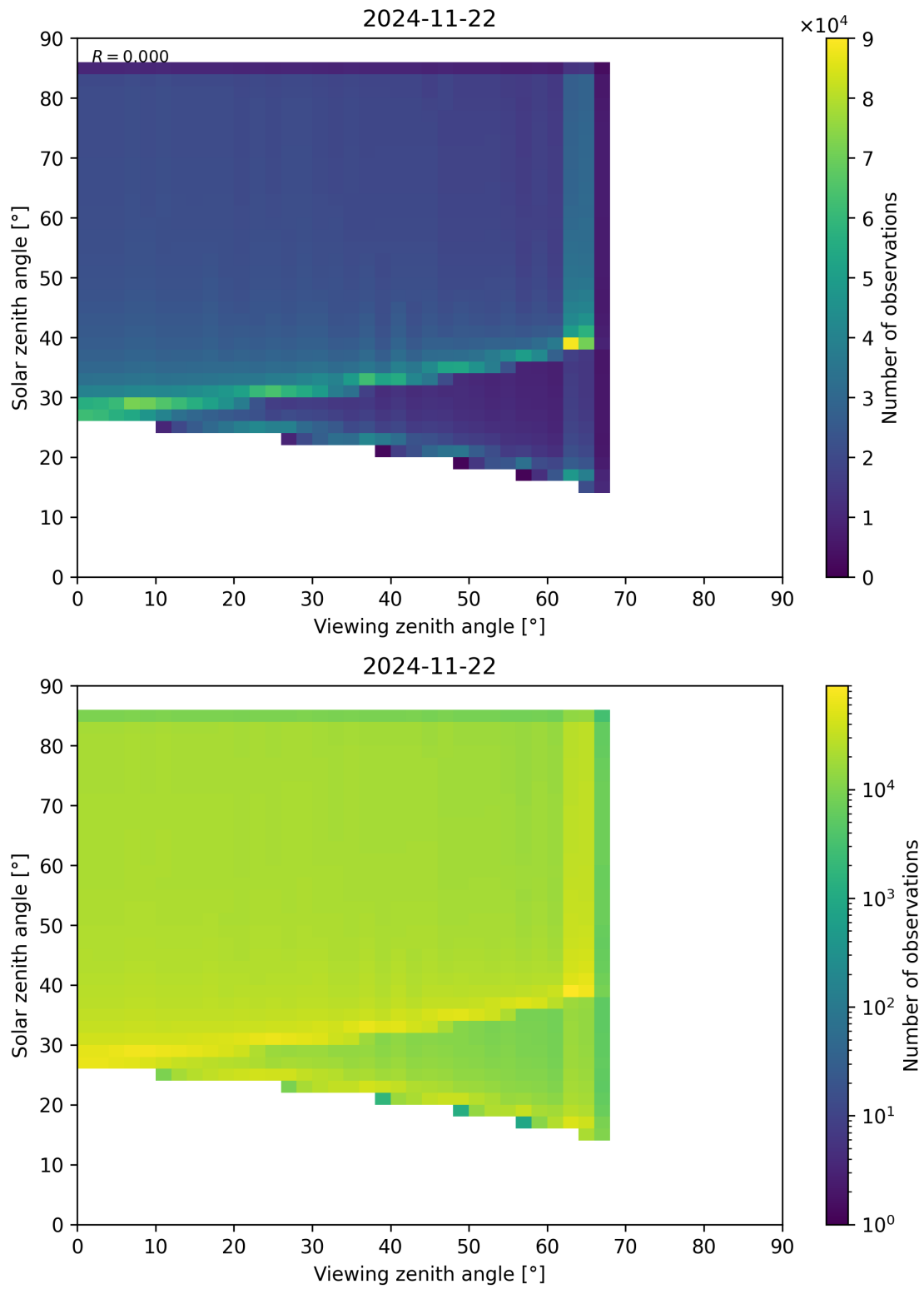
Figure 197: Scatter density plot of “Viewing zenith angle” against “Solar zenith angle” for 2024-11-21 to 2024-11-23.
