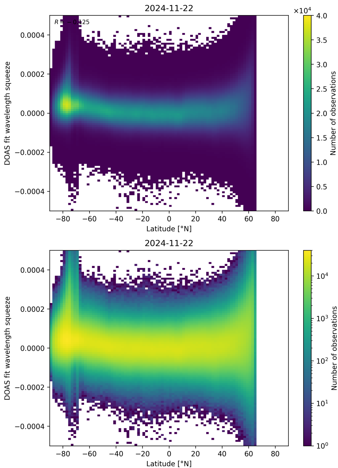
Figure 155: Scatter density plot of “Latitude” against “DOAS fit wavelength squeeze” for 2024-11-21 to 2024-11-23.
