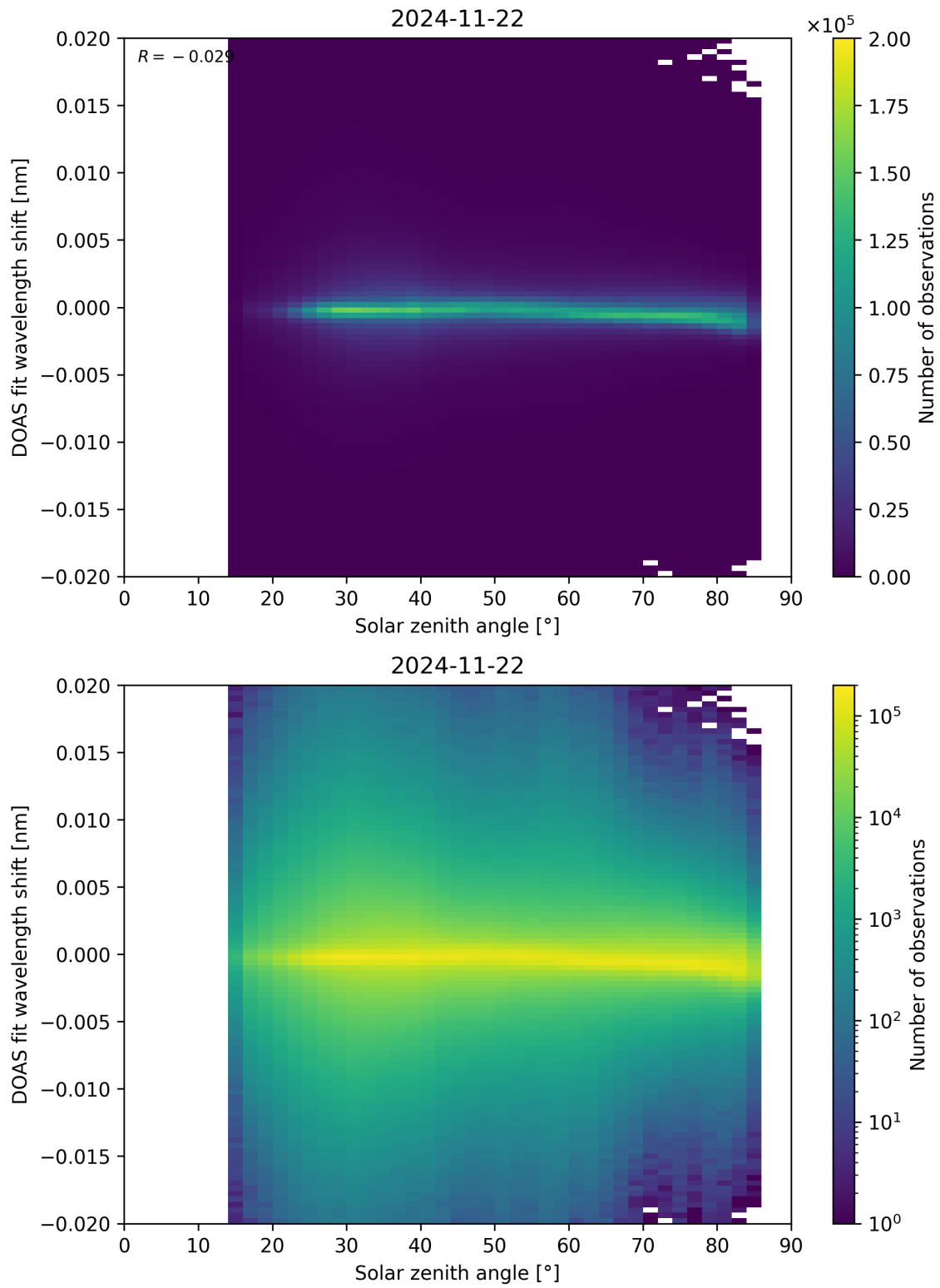
Figure 168: Scatter density plot of “Solar zenith angle” against “DOAS fit wavelength shift” for 2024-11-21 to 2024-11-23.
