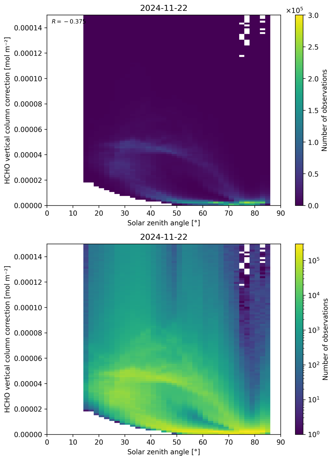
Figure 178: Scatter density plot of “Solar zenith angle” against “HCHO vertical column correction” for 2024-11-21 to 2024-11-23.
