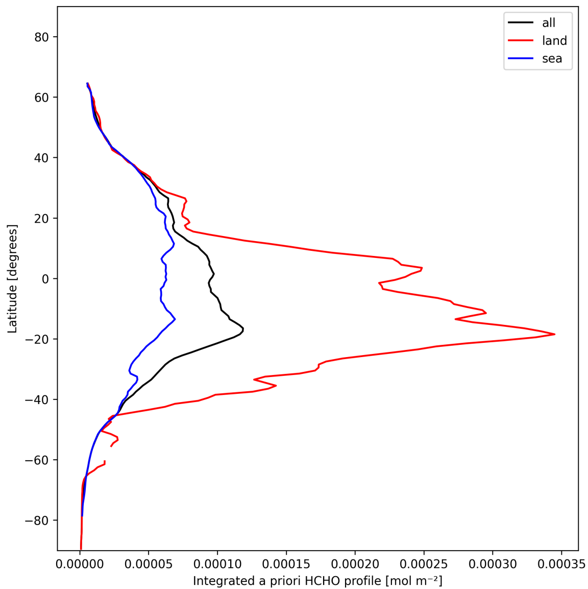
Figure 29: Zonal average of “Integrated a priori HCHO profile” for 2024-11-21 to 2024-11-23.
