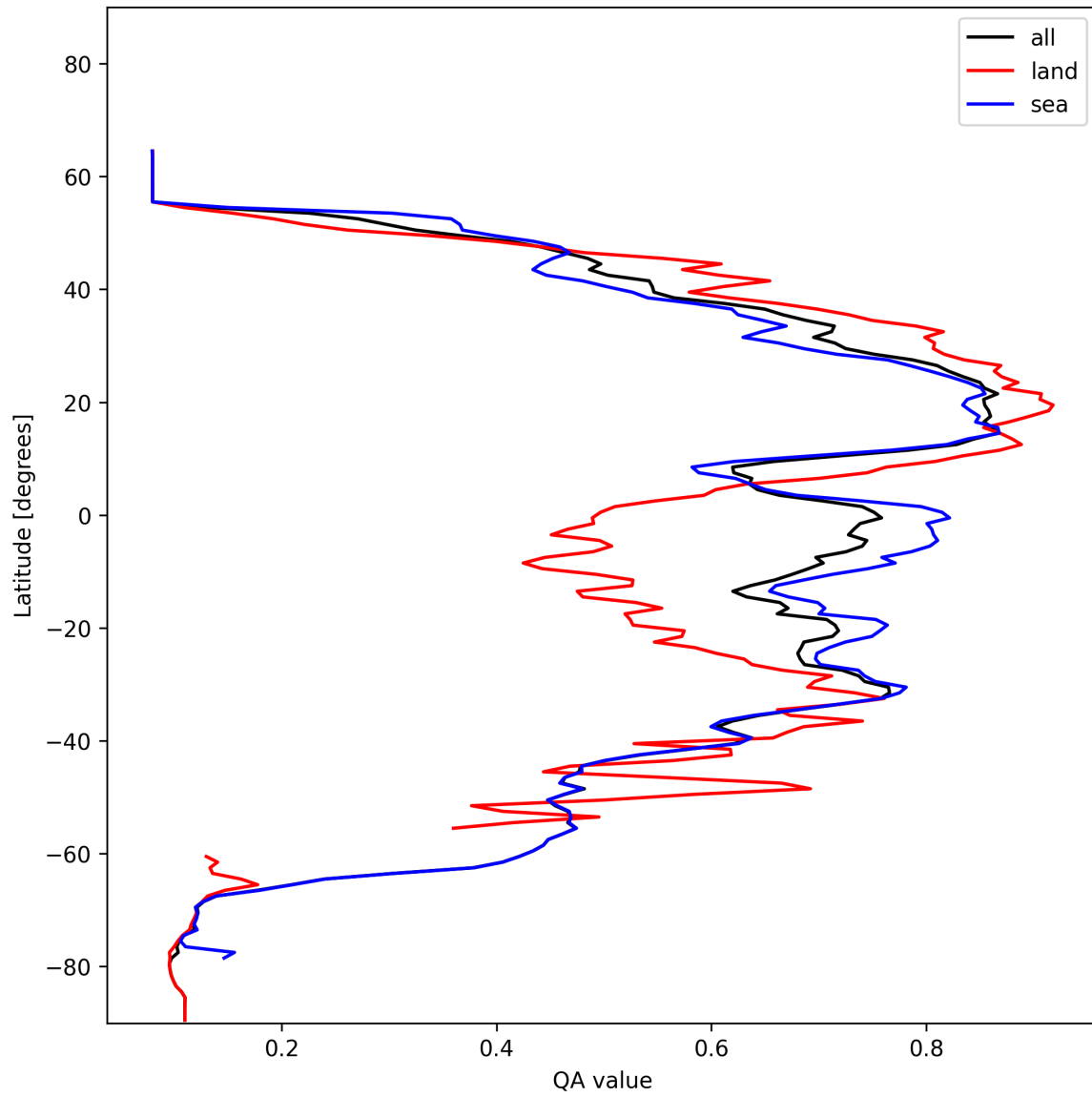
Figure 20: Zonal average of “QA value” for 2024-11-21 to 2024-11-23.
