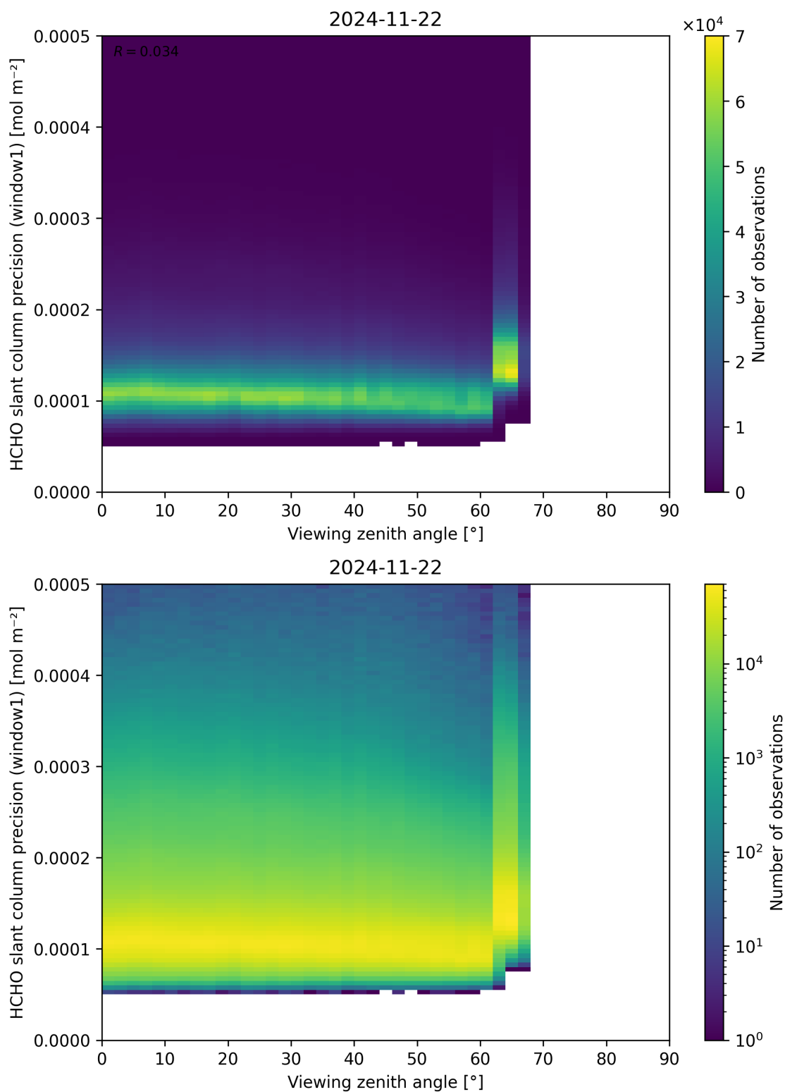
Figure 189: Scatter density plot of “Viewing zenith angle” against “HCHO slant column precision (window1)” for 2024-11-21 to 2024-11-23.
