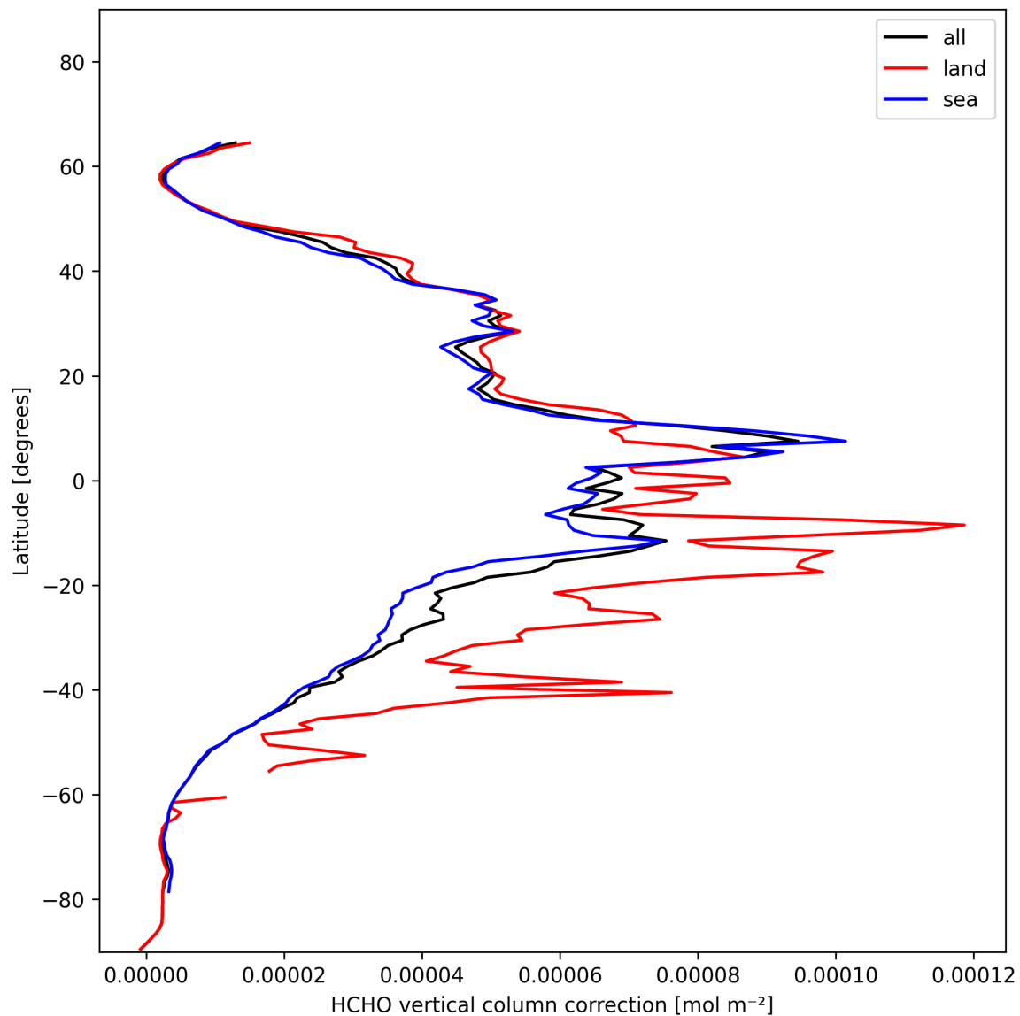
Figure 23: Zonal average of “HCHO vertical column correction” for 2024-11-21 to 2024-11-23.
