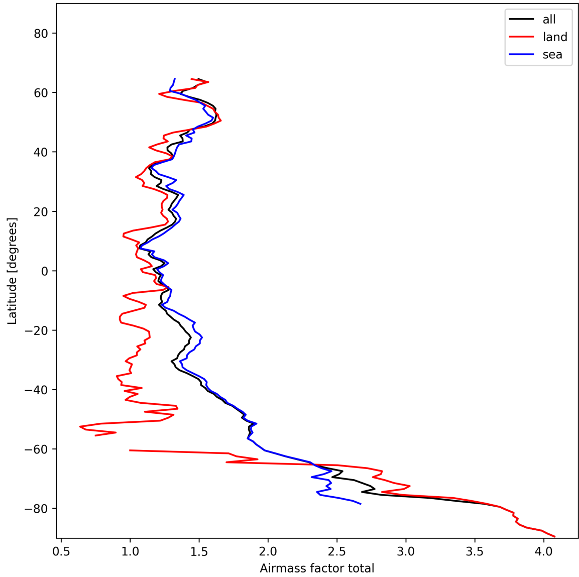
Figure 26: Zonal average of “Airmass factor total” for 2024-11-21 to 2024-11-23.
