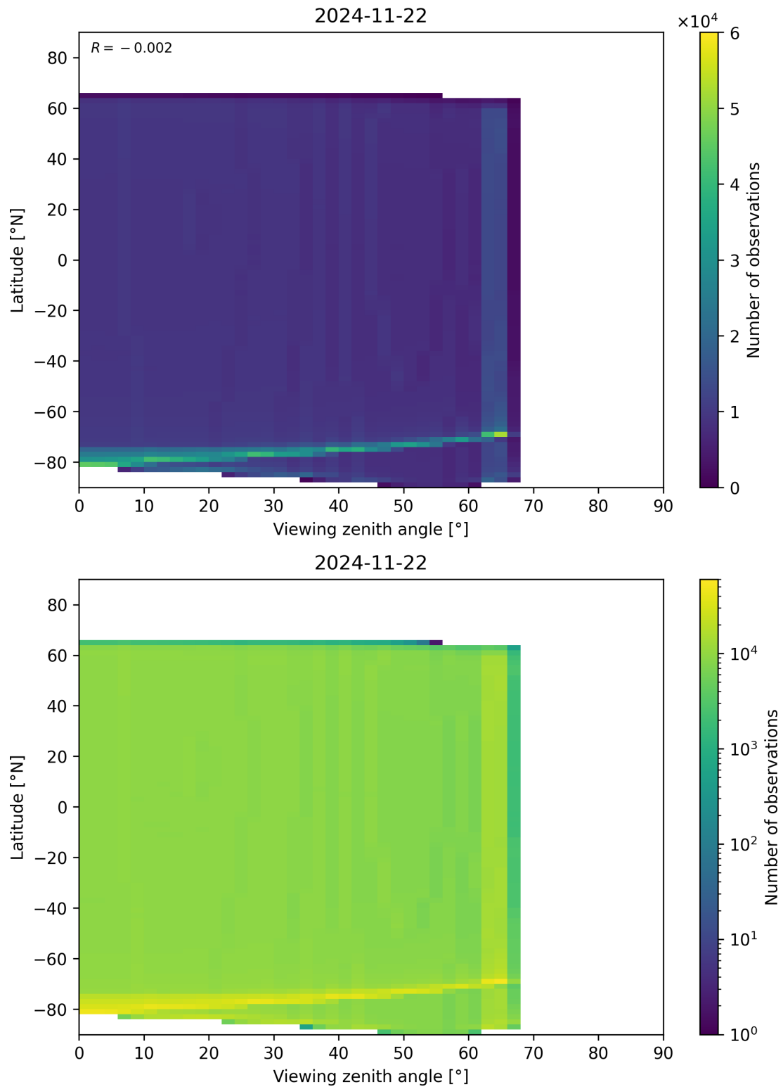
Figure 196: Scatter density plot of “Viewing zenith angle” against “Latitude” for 2024-11-21 to 2024-11-23.
