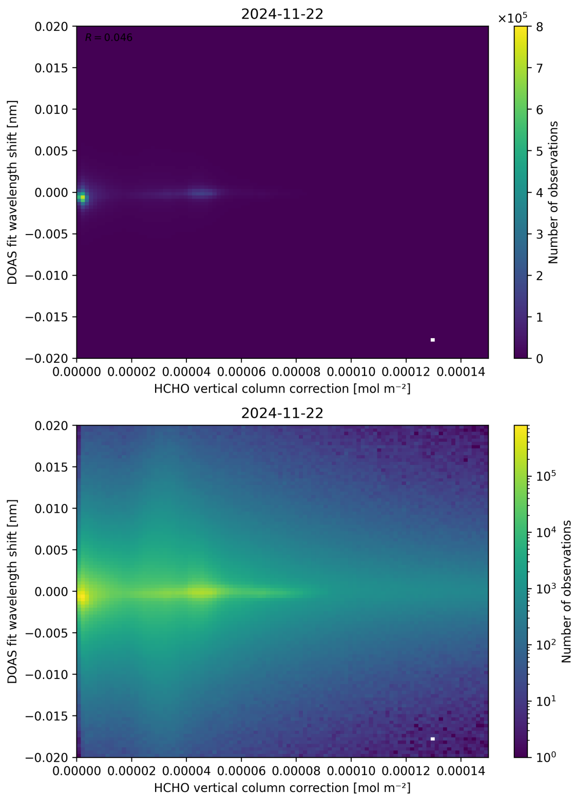
Figure 113: Scatter density plot of “HCHO vertical column correction” against “DOAS fit wavelength shift” for 2024-11-21 to 2024-11-23.
