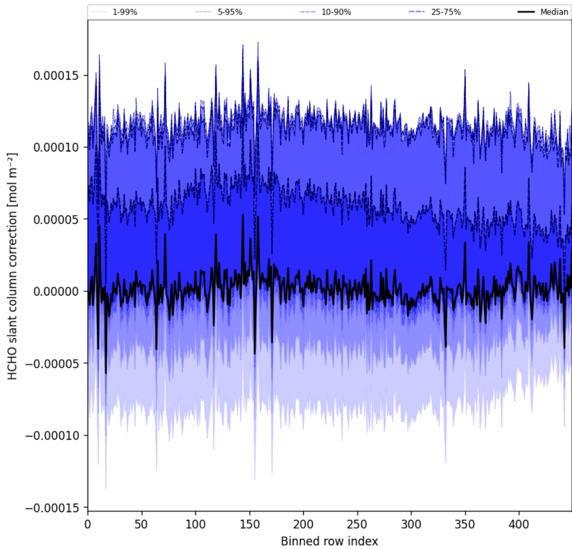
Figure 61: Along track statistics of “HCHO slant column correction” for 2024-11-21 to 2024-11-23
