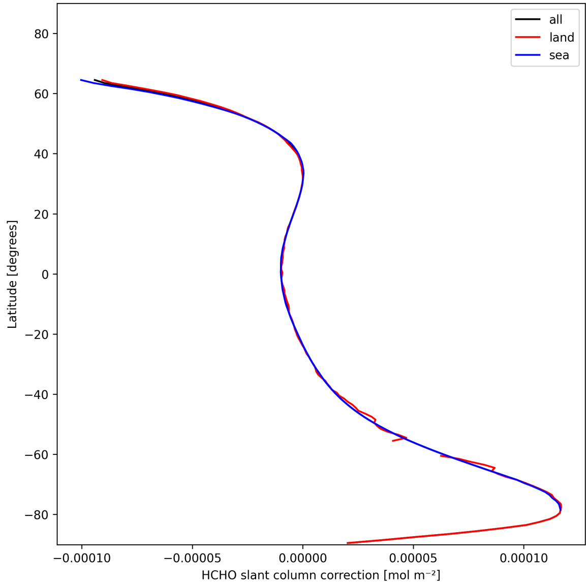
Figure 33: Zonal average of “HCHO slant column correction” for 2024-11-21 to 2024-11-23.
