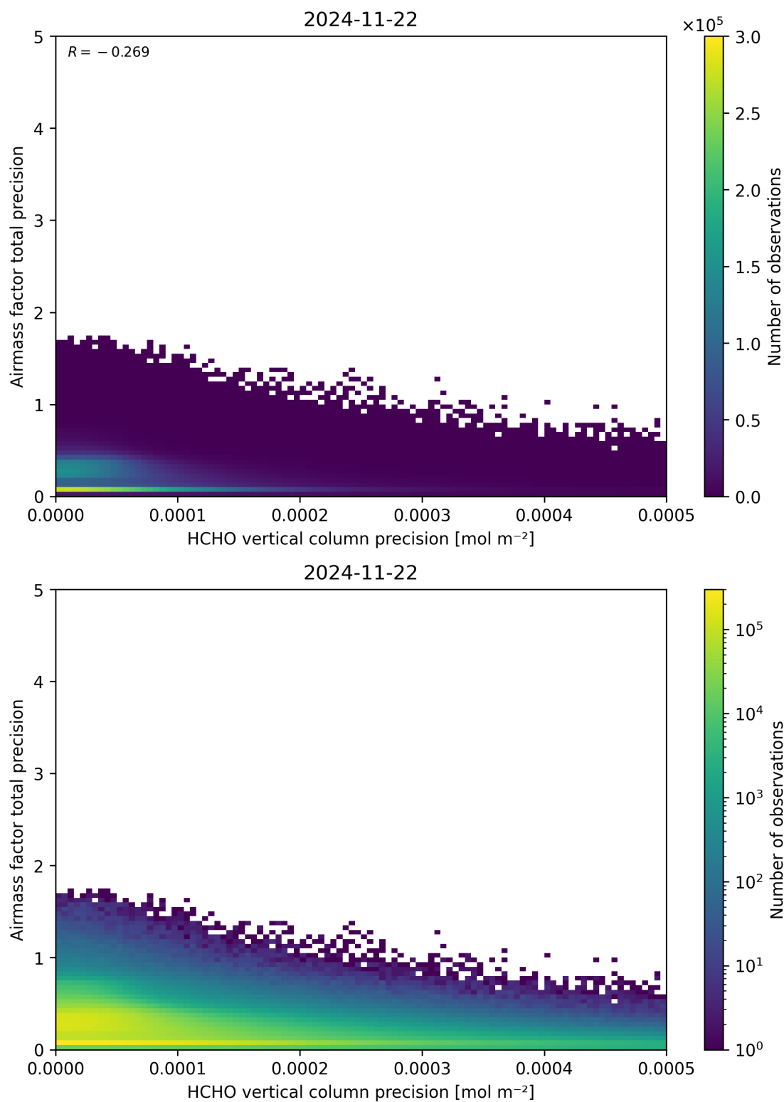
Figure 145: Scatter density plot of “HCHO vertical column precision” against “Airmass factor total precision” for 2024-11-21 to 2024-11-23.
