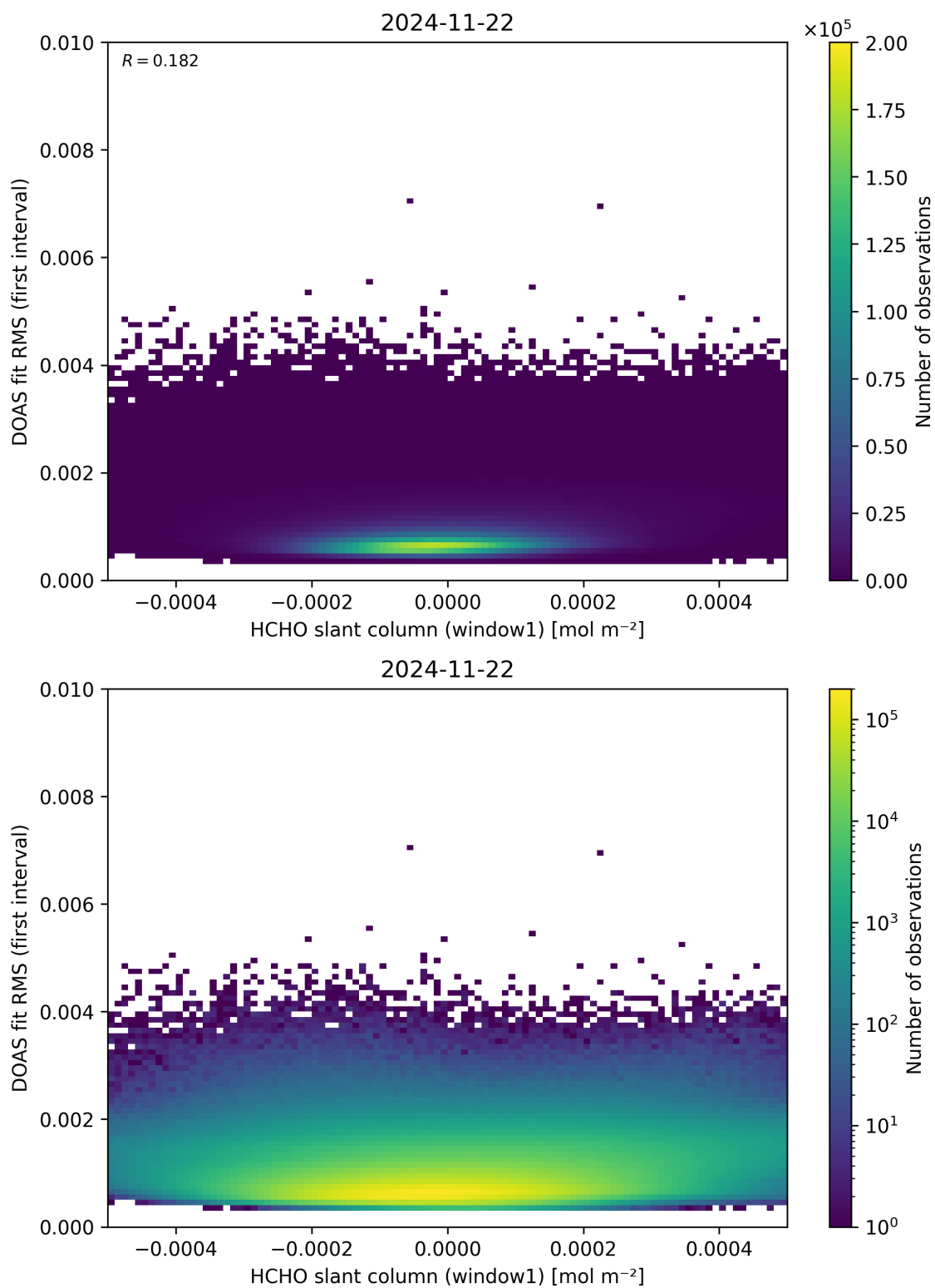
Figure 78: Scatter density plot of “HCHO slant column (window1)” against “DOAS fit RMS (first interval)” for 2024-11-21 to 2024-11-23.
