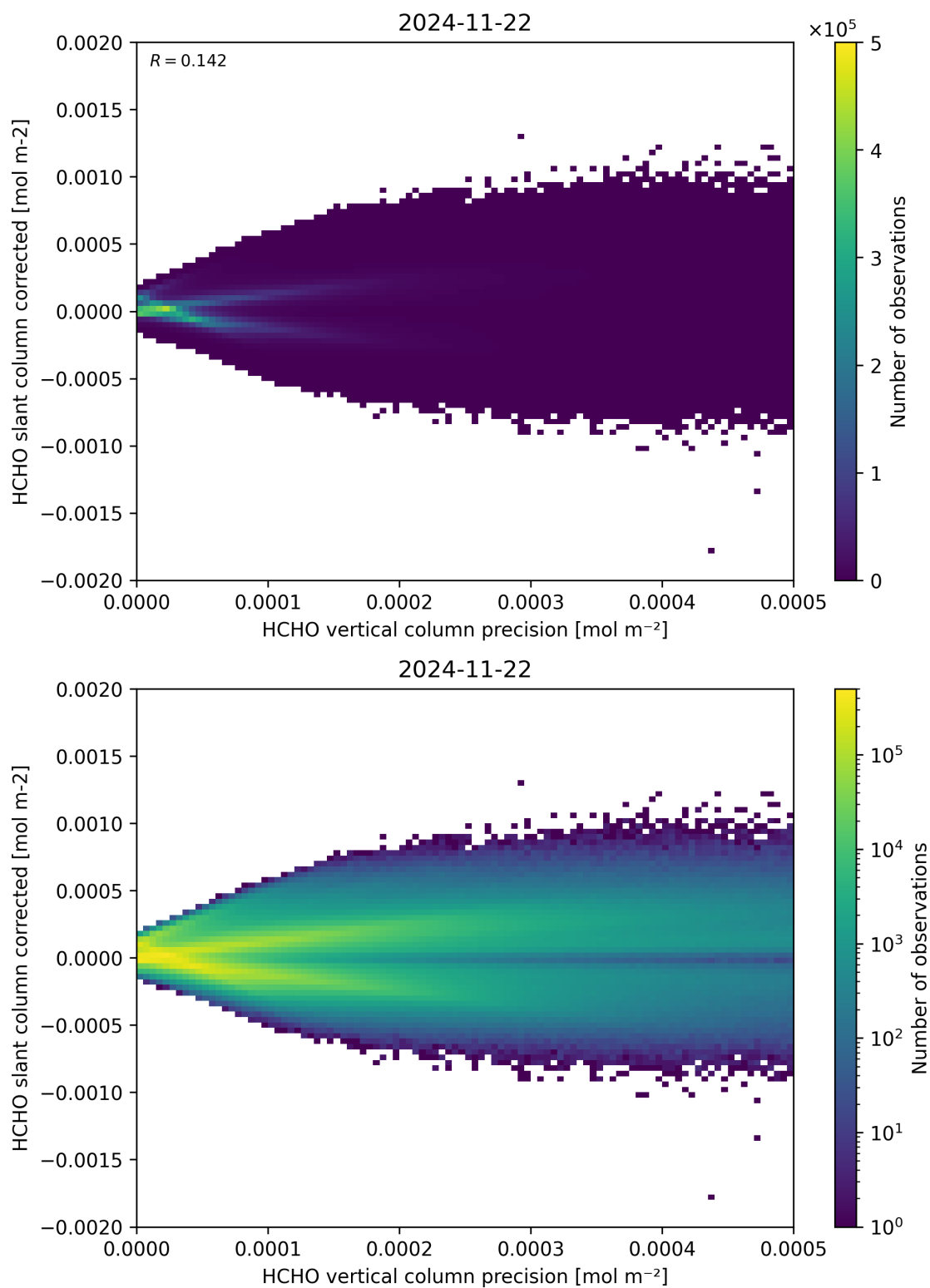
Figure 140: Scatter density plot of “HCHO vertical column precision” against “HCHO slant column corrected” for 2024-11-21 to 2024-11-23.
