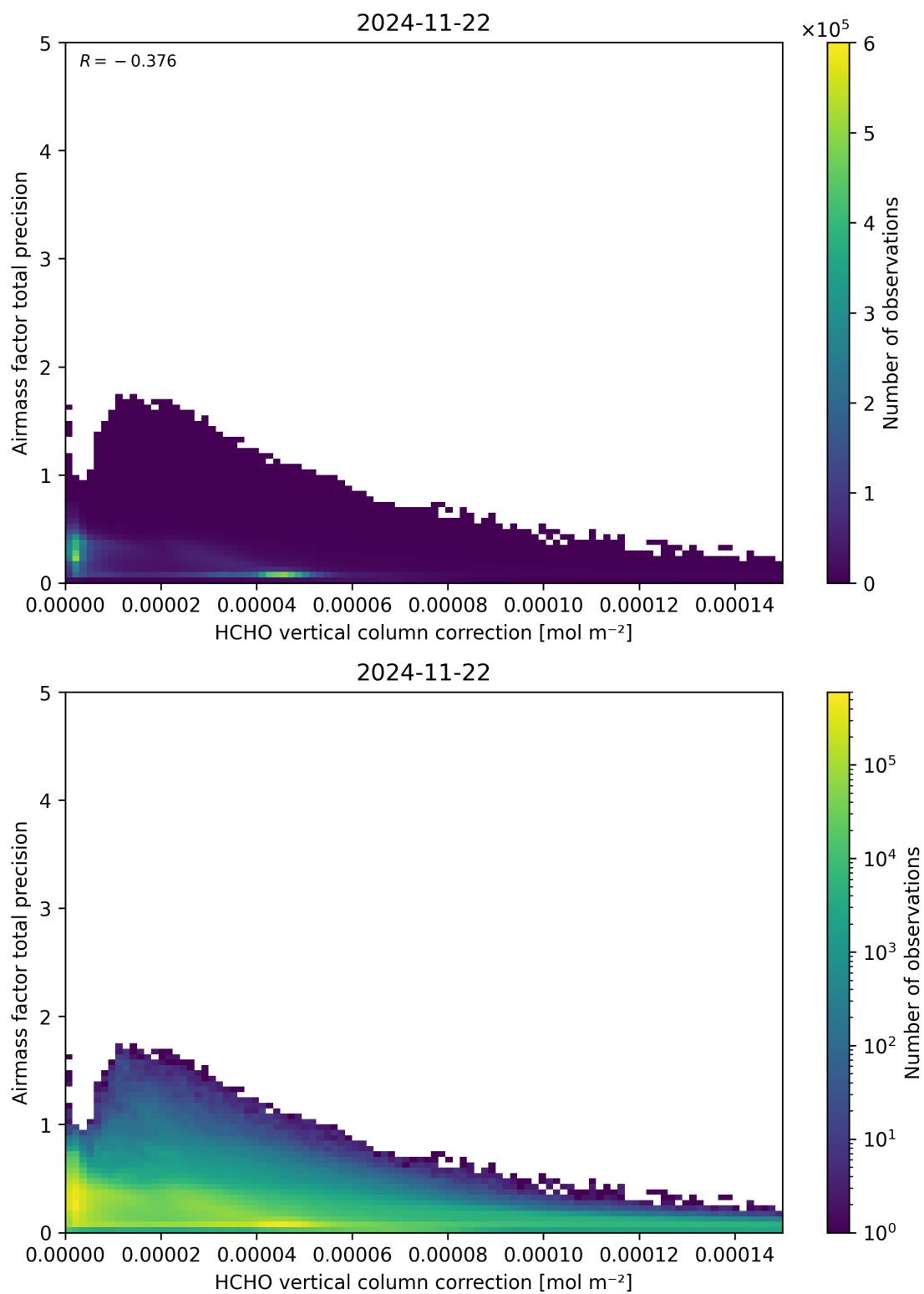
Figure 121: Scatter density plot of “HCHO vertical column correction” against “Airmass factor total precision” for 2024-11-21 to 2024-11-23.
