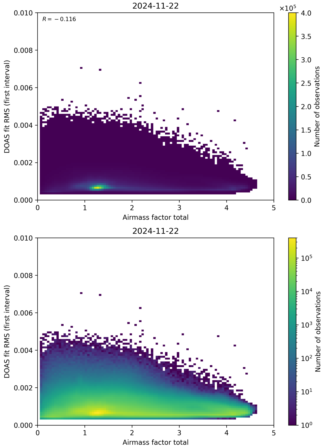
Figure 97: Scatter density plot of “Airmass factor total” against “DOAS fit RMS (first interval)” for 2024-11-21 to 2024-11-23.
