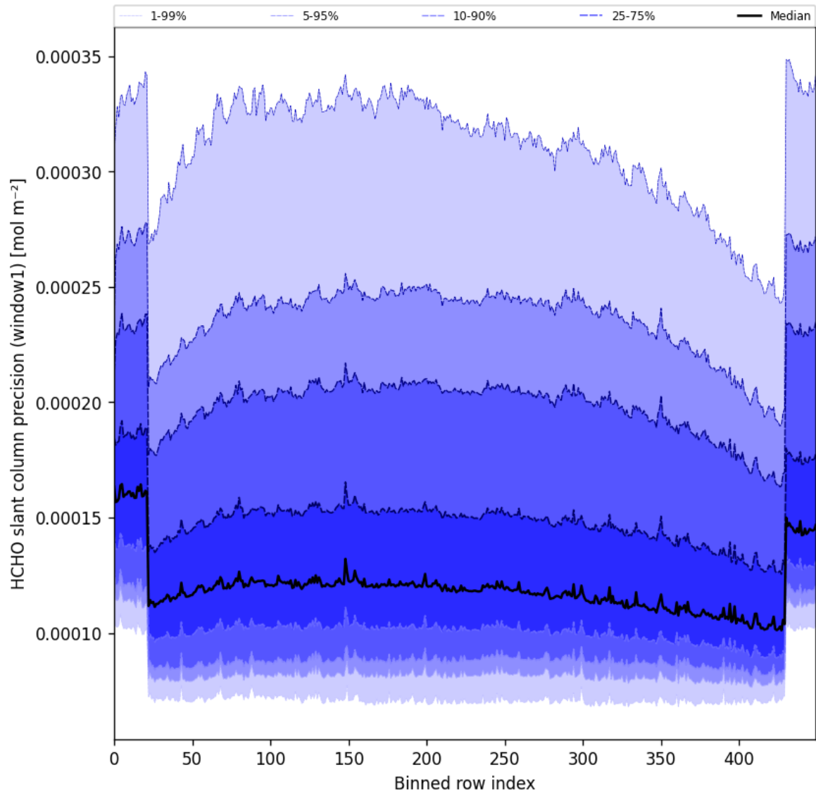
Figure 53: Along track statistics of “HCHO slant column precision (window1)” for 2024-11-21 to 2024-11-23
