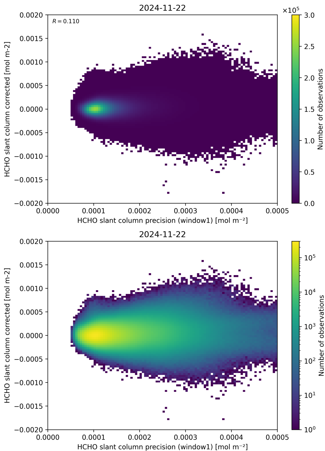
Figure 92: Scatter density plot of “HCHO slant column precision (window1)” against “HCHO slant column corrected” for 2024-11-21 to 2024-11-23.
