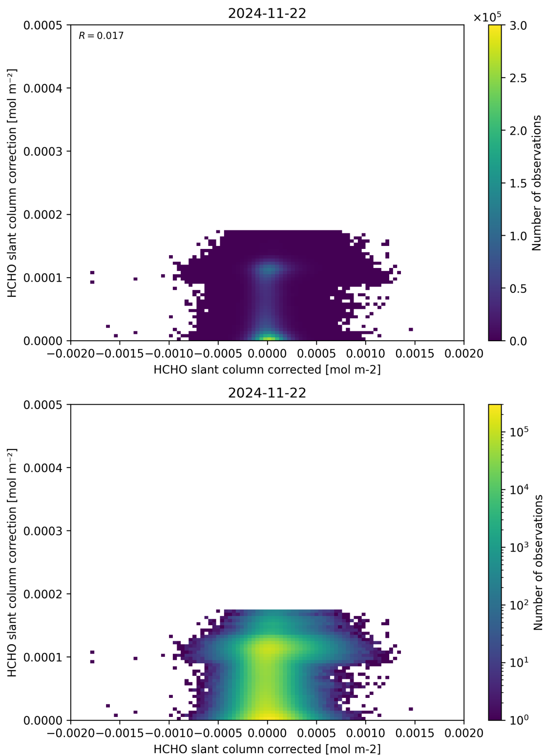
Figure 77: Scatter density plot of “HCHO slant column corrected” against “HCHO slant column correction” for 2024-11-21 to 2024-11-23.
