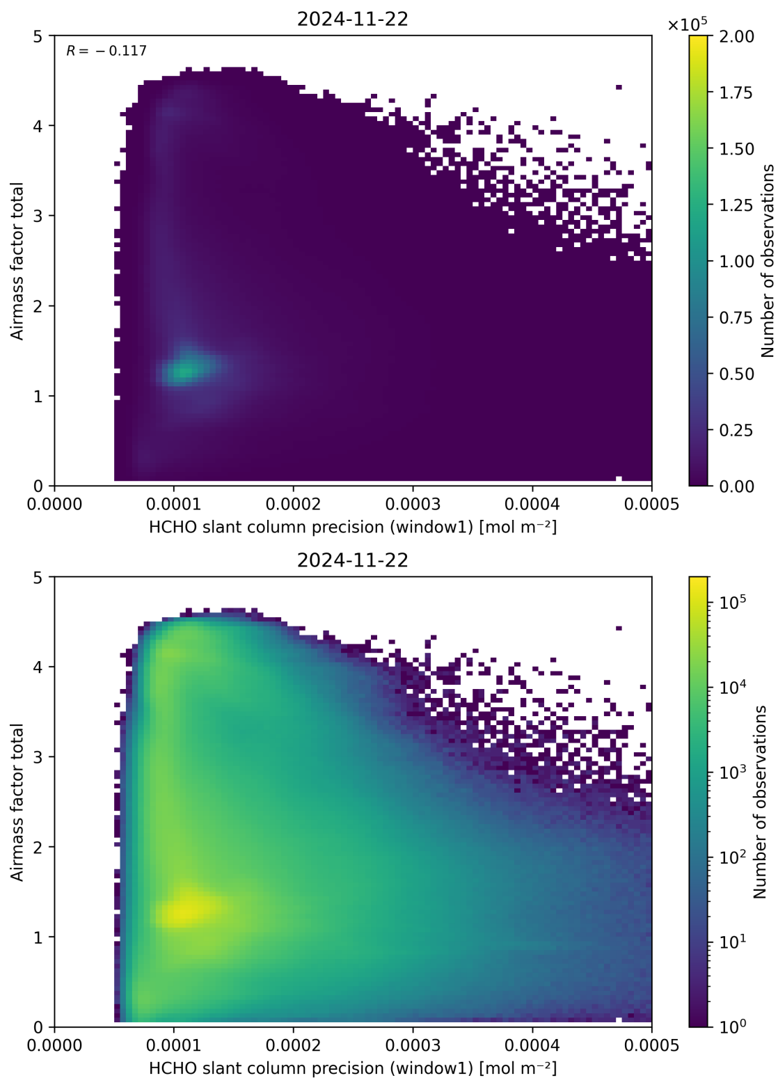
Figure 94: Scatter density plot of “HCHO slant column precision (window1)” against “Airmass factor total” for 2024-11-21 to 2024-11-23.
