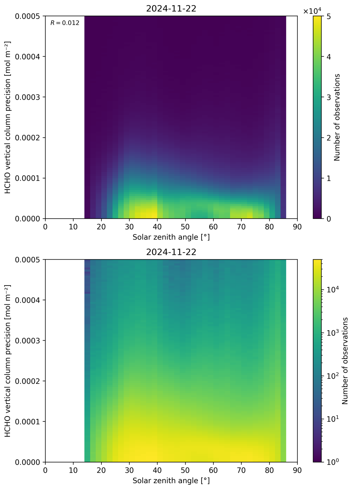
Figure 179: Scatter density plot of “Solar zenith angle” against “HCHO vertical column precision” for 2024-11-21 to 2024-11-23.
