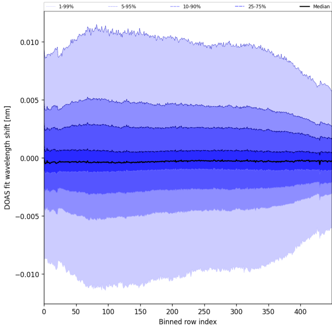
Figure 58: Along track statistics of “DOAS fit wavelength shift” for 2024-11-21 to 2024-11-23
