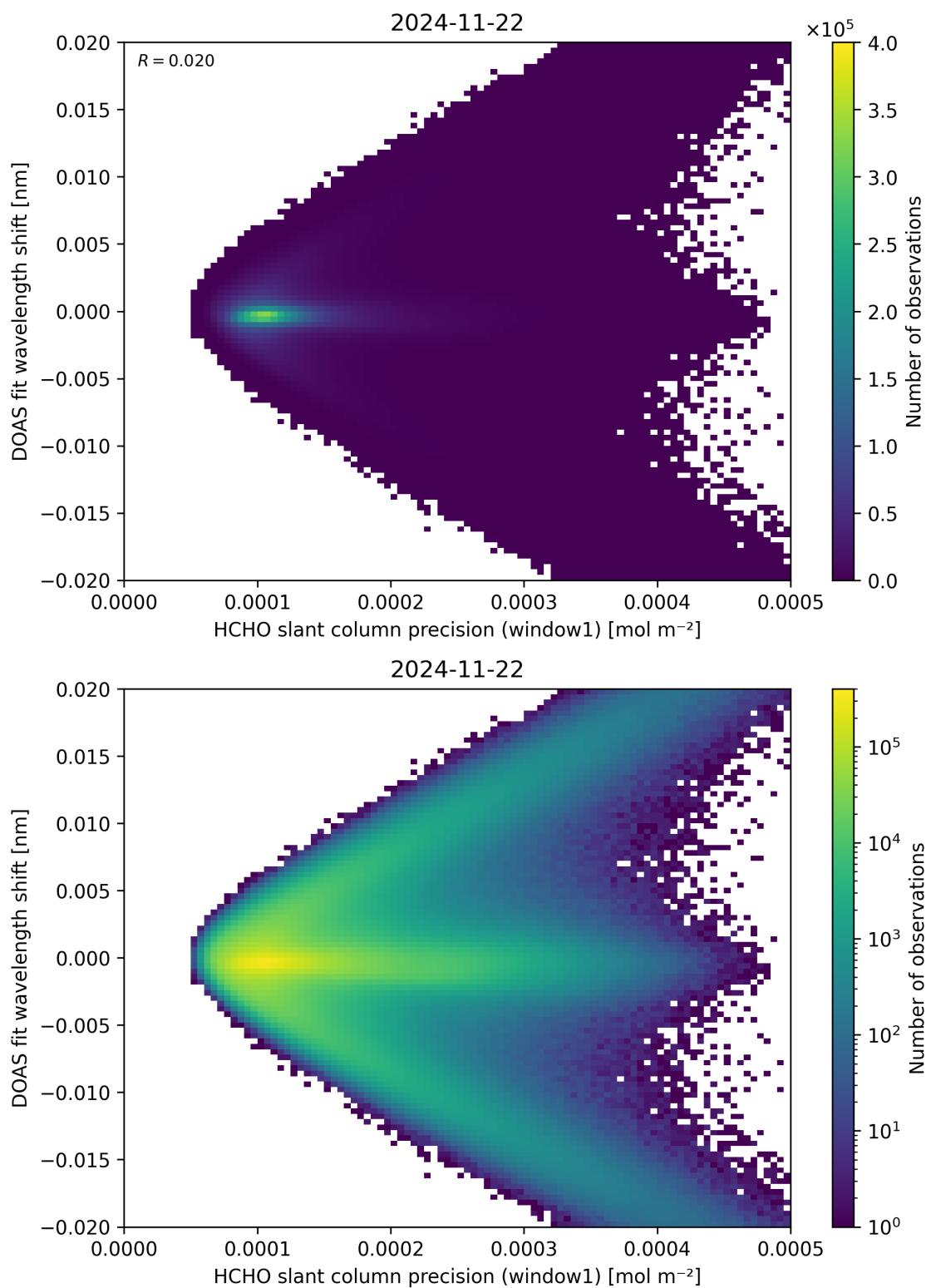
Figure 89: Scatter density plot of “HCHO slant column precision (window1)” against “DOAS fit wavelength shift” for 2024-11-21 to 2024-11-23.
