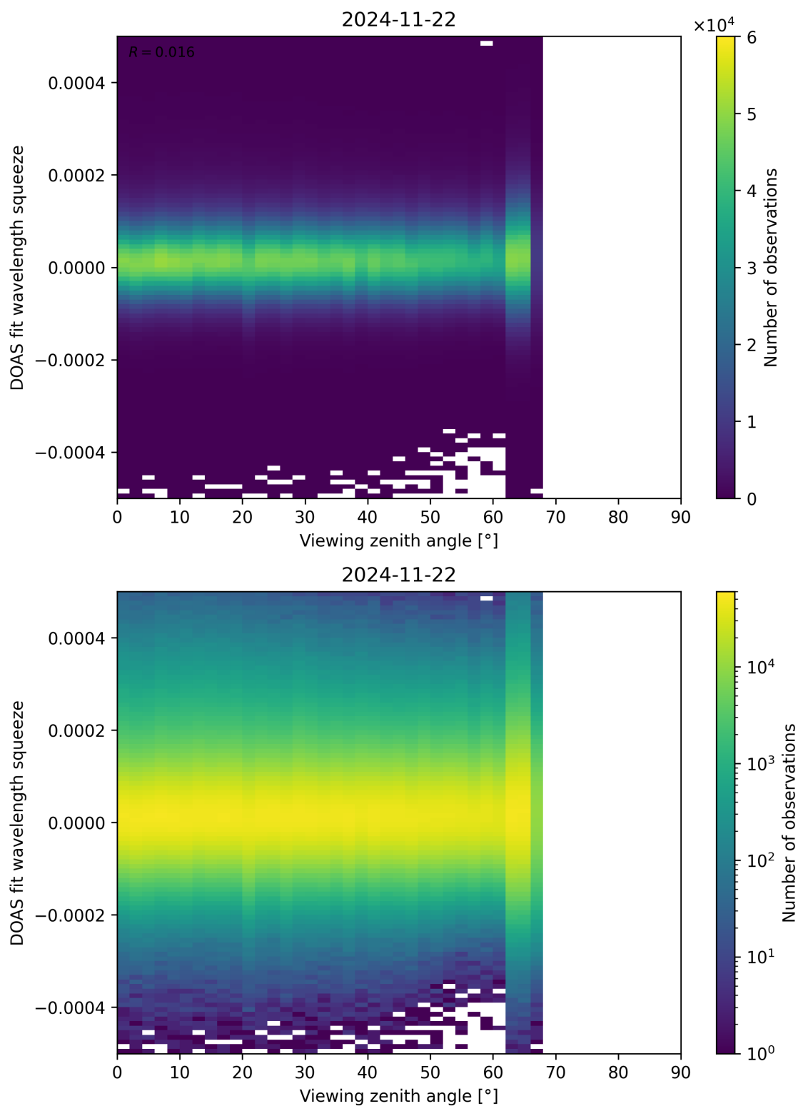
Figure 184: Scatter density plot of “Viewing zenith angle” against “DOAS fit wavelength squeeze” for 2024-11-21 to 2024-11-23.
