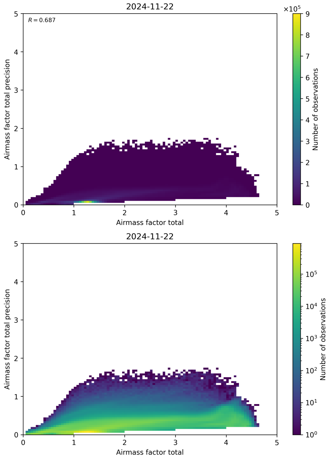
Figure 103: Scatter density plot of “Airmass factor total” against “Airmass factor total precision” for 2024-11-21 to 2024-11-23.
