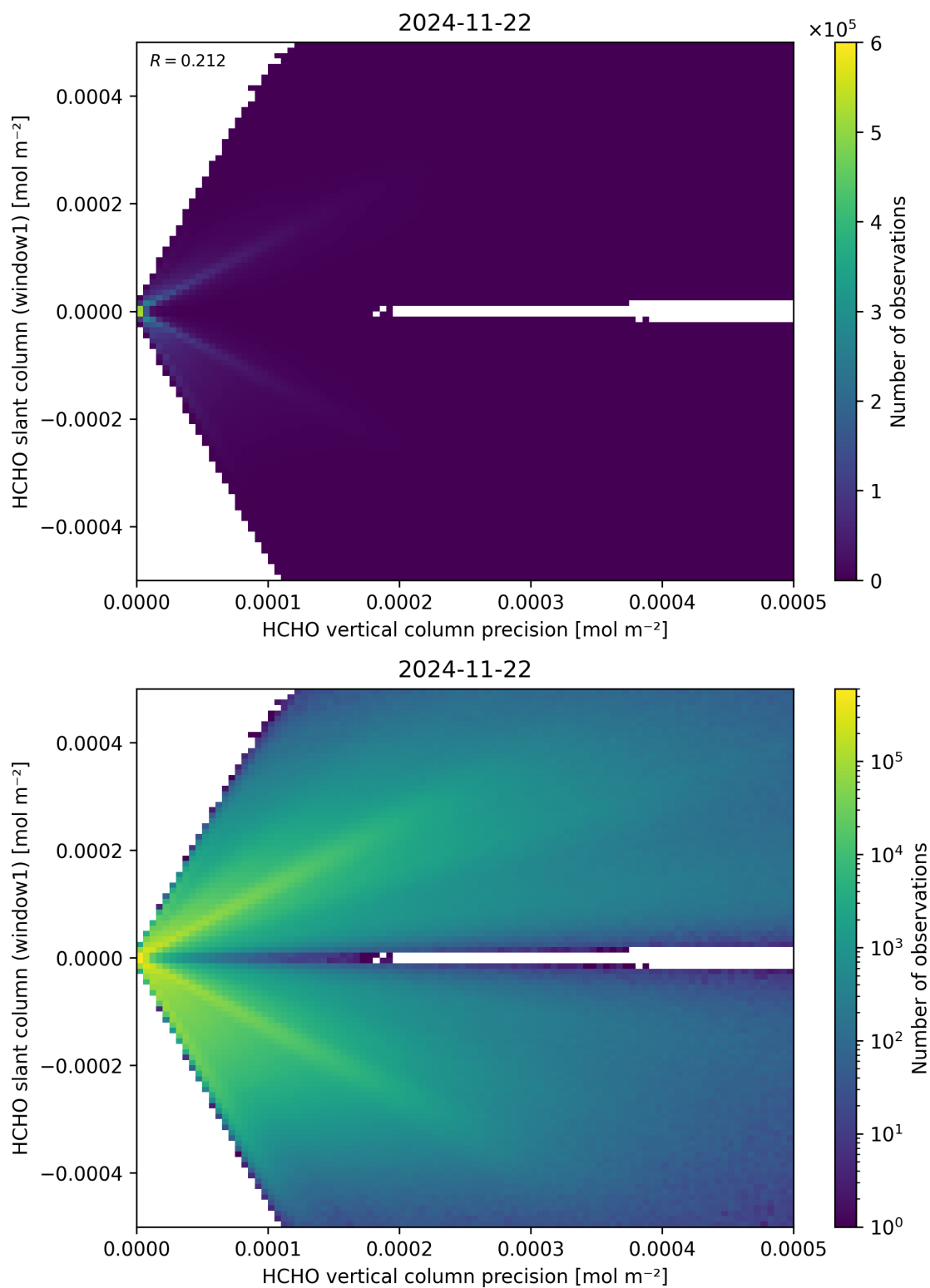
Figure 142: Scatter density plot of “HCHO vertical column precision” against “HCHO slant column (window1)” for 2024-11-21 to 2024-11-23.
