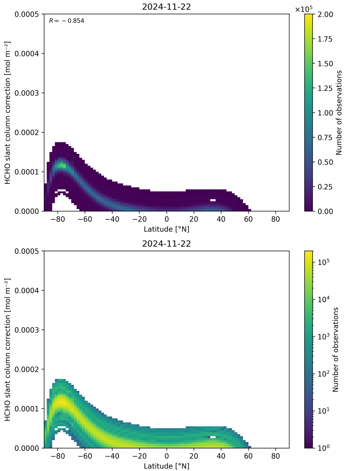
Figure 158: Scatter density plot of “Latitude” against “HCHO slant column correction” for 2024-11-21 to 2024-11-23.
