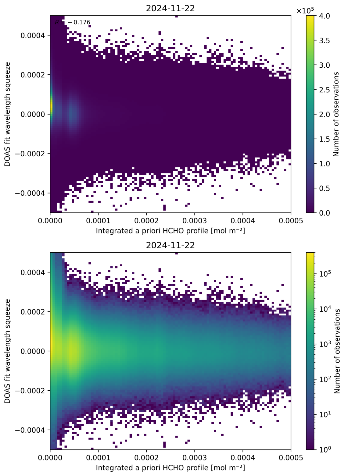
Figure 150: Scatter density plot of “Integrated a priori HCHO profile” against “DOAS fit wavelength squeeze” for 2024-11-21 to 2024-11-23.
