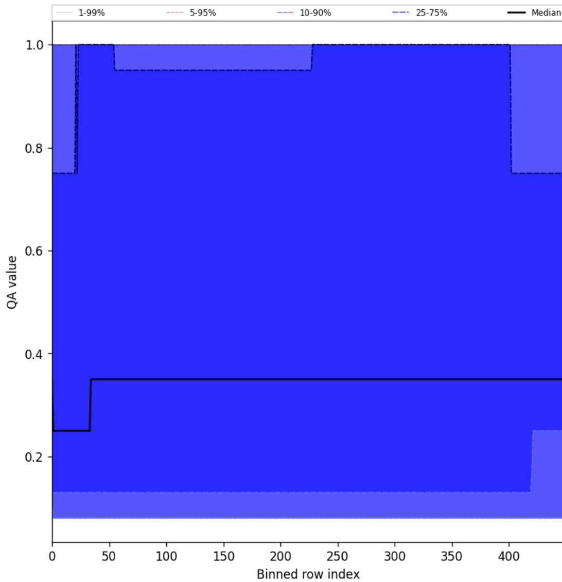
Figure 48: Along track statistics of “QA value” for 2024-11-21 to 2024-11-23
