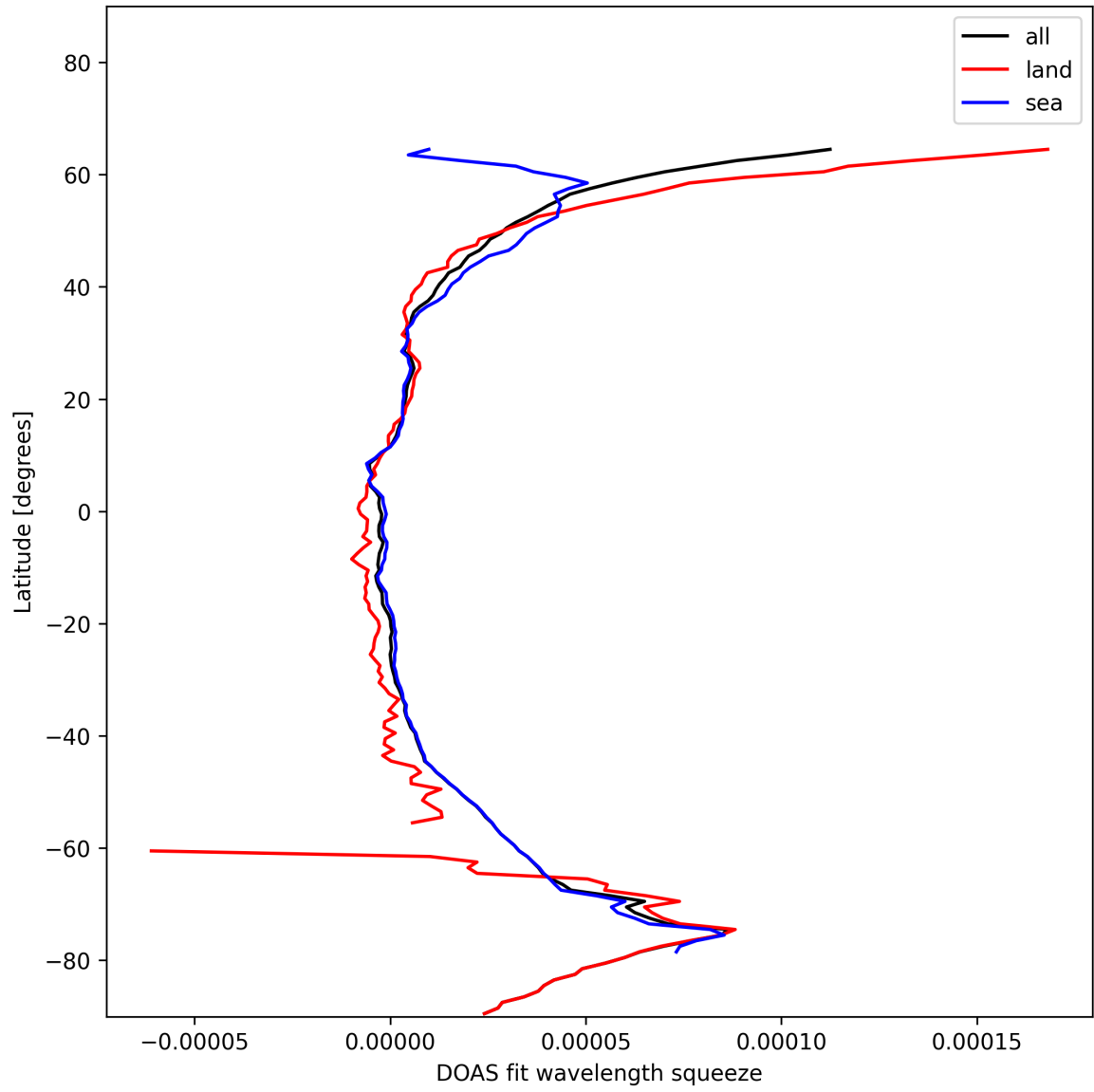
Figure 31: Zonal average of “DOAS fit wavelength squeeze” for 2024-11-21 to 2024-11-23.
