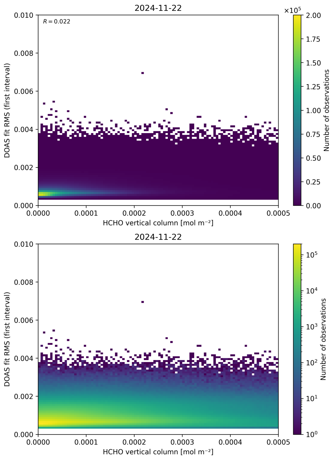
Figure 123: Scatter density plot of “HCHO vertical column” against “DOAS fit RMS (first interval)” for 2024-11-21 to 2024-11-23.
