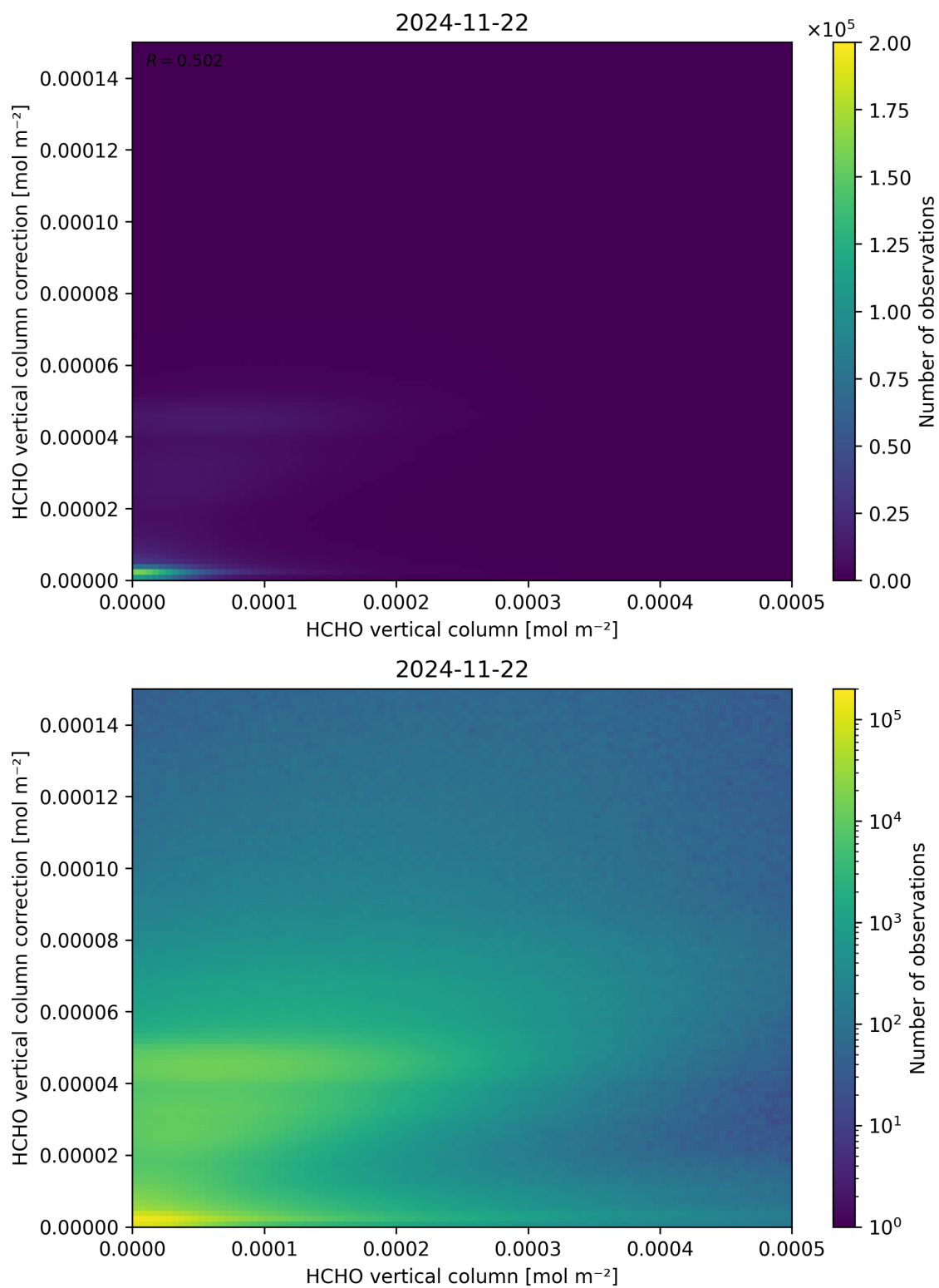
Figure 133: Scatter density plot of “HCHO vertical column” against “HCHO vertical column correction” for 2024-11-21 to 2024-11-23.
