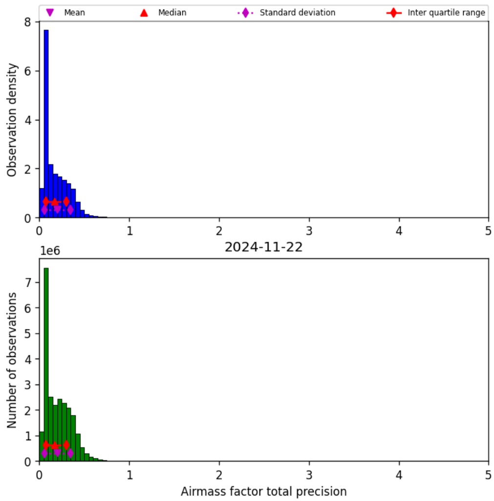
Figure 41: Histogram of “Airmass factor total precision” for 2024-11-21 to 2024-11-23
