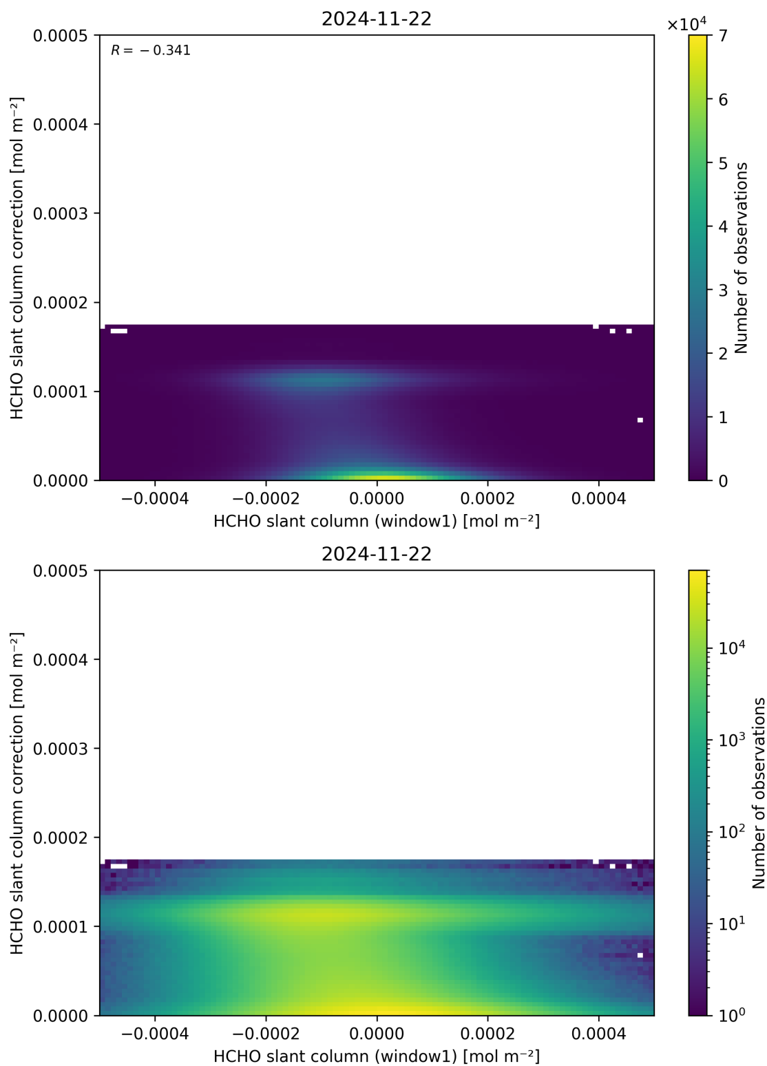
Figure 83: Scatter density plot of “HCHO slant column (window1)” against “HCHO slant column correction” for 2024-11-21 to 2024-11-23.
