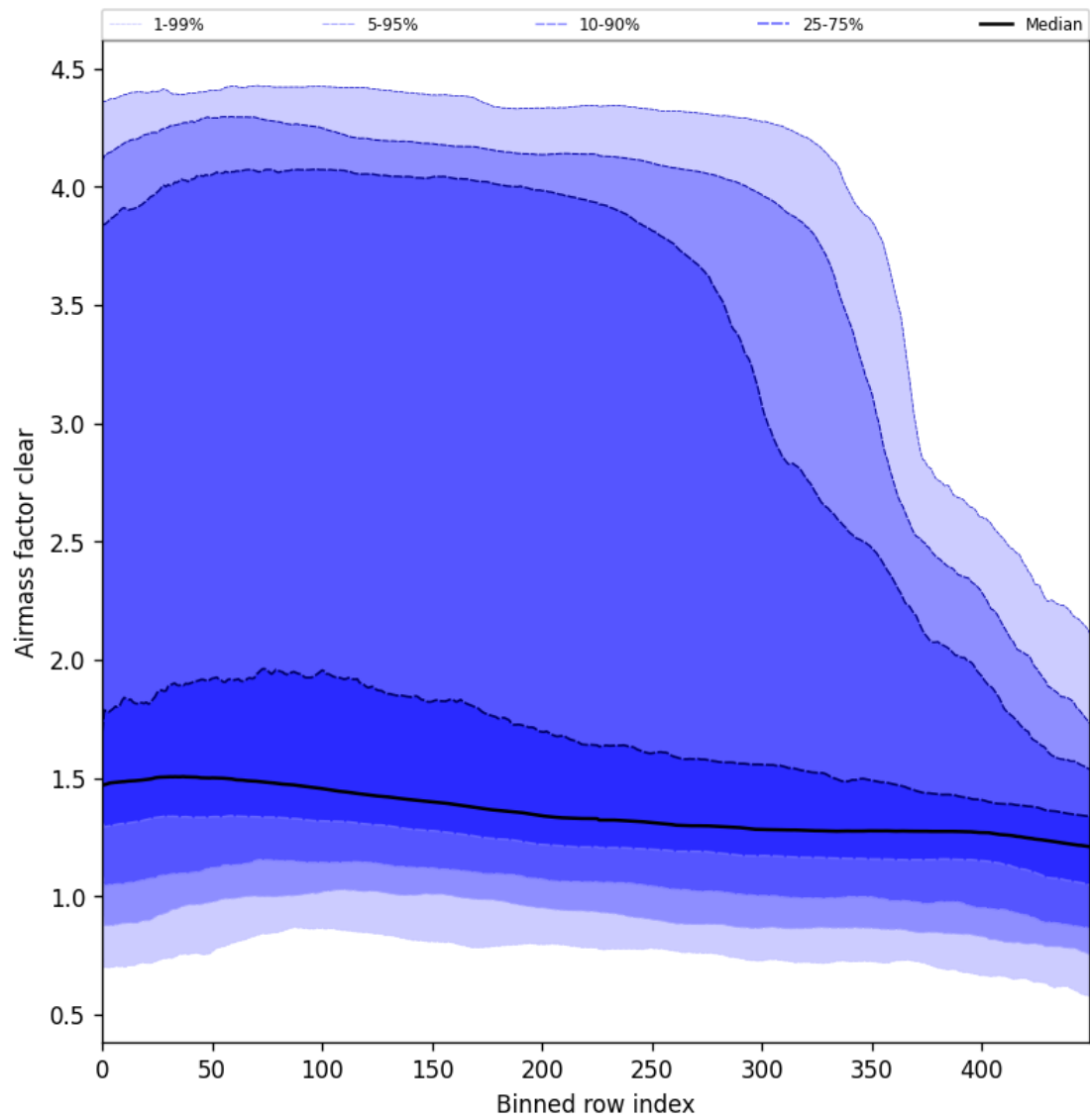
Figure 56: Along track statistics of “Air mass factor clear” for 2024-11-21 to 2024-11-23
