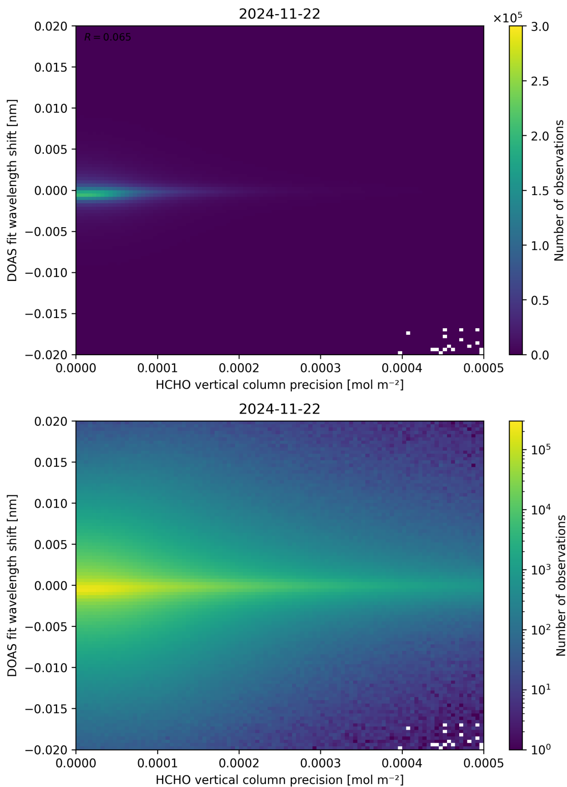
Figure 137: Scatter density plot of “HCHO vertical column precision” against “DOAS fit wavelength shift” for 2024-11-21 to 2024-11-23.
