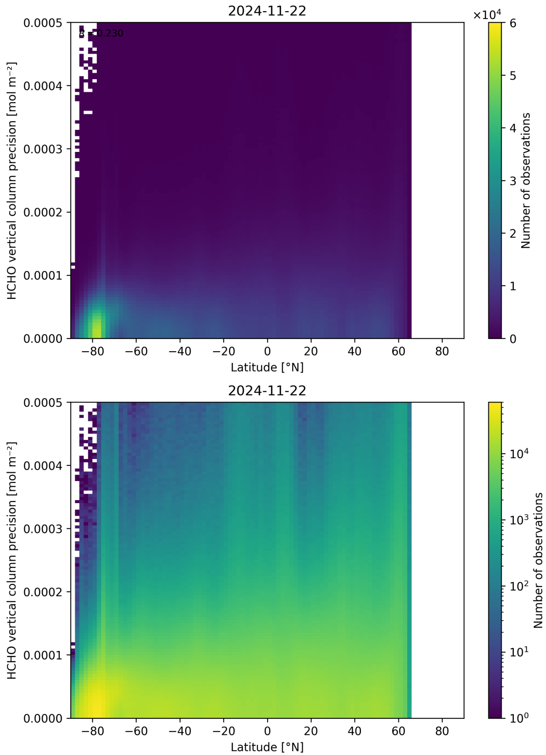
Figure 165: Scatter density plot of “Latitude” against “HCHO vertical column precision” for 2024-11-21 to 2024-11-23.
