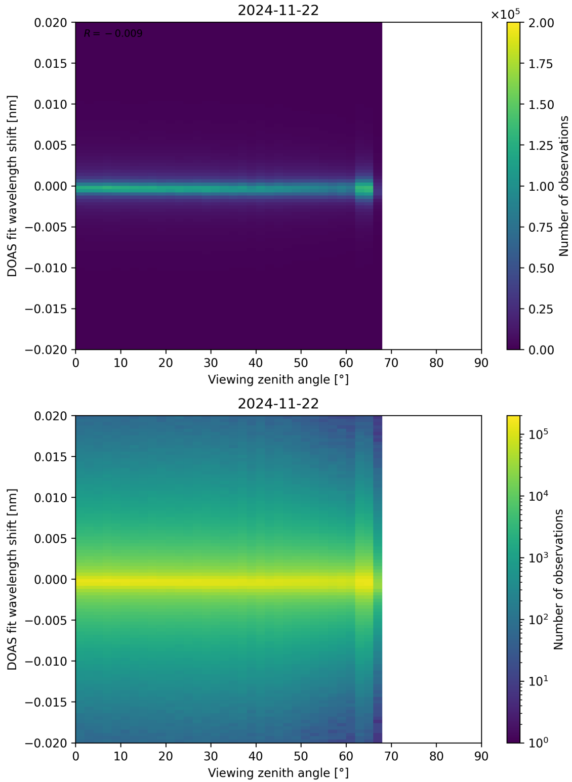
Figure 183: Scatter density plot of “Viewing zenith angle” against “DOAS fit wavelength shift” for 2024-11-21 to 2024-11-23.
