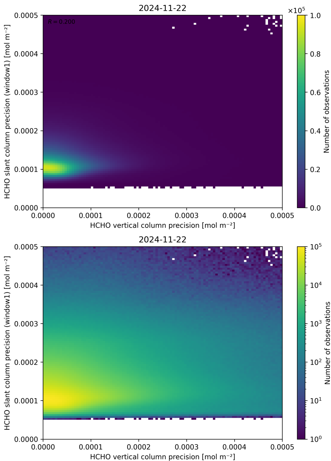
Figure 143: Scatter density plot of “HCHO vertical column precision” against “HCHO slant column precision (window1)” for 2024-11-21 to 2024-11-23.
