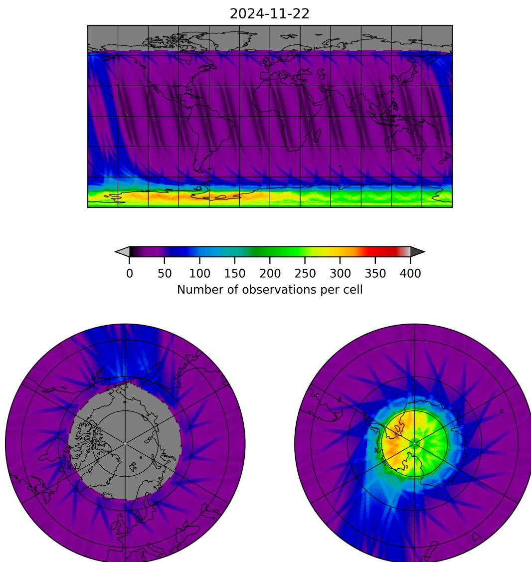
Figure 19: Map of the number of observations for 2024-11-21 to 2024-11-23
