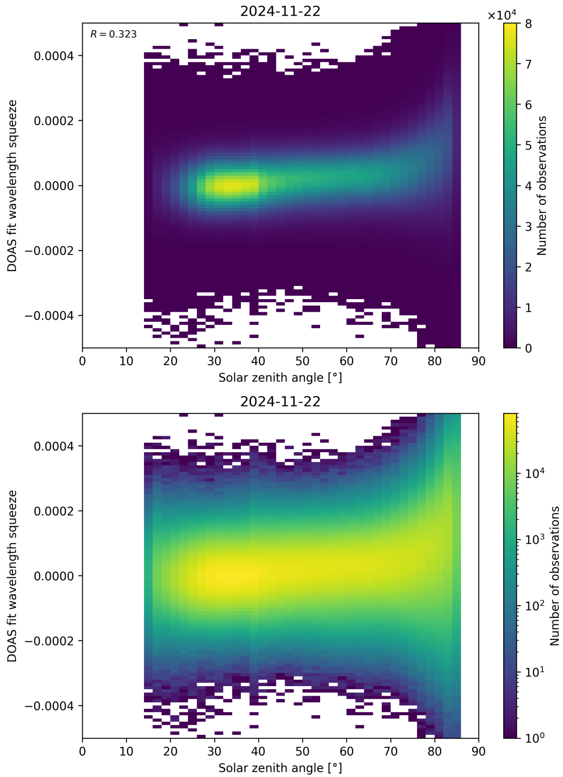
Figure 169: Scatter density plot of “Solar zenith angle” against “DOAS fit wavelength squeeze” for 2024-11-21 to 2024-11-23.
