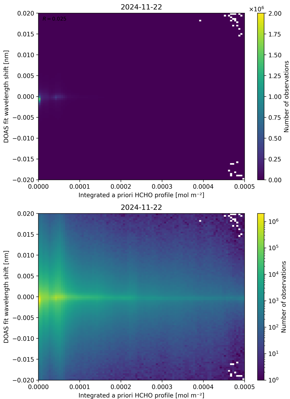
Figure 149: Scatter density plot of “Integrated a priori HCHO profile” against “DOAS fit wavelength shift” for 2024-11-21 to 2024-11-23.
