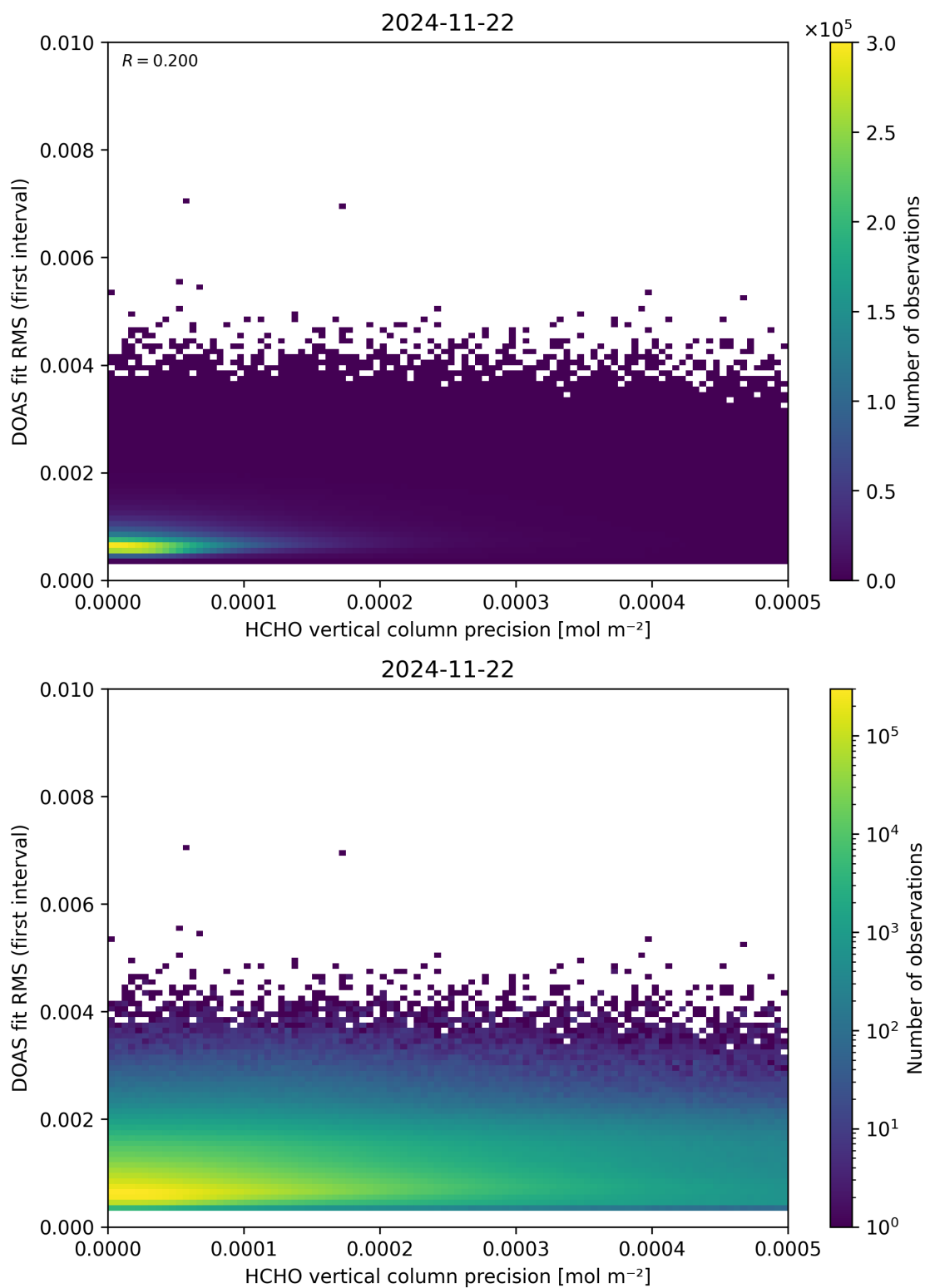
Figure 136: Scatter density plot of “HCHO vertical column precision” against “DOAS fit RMS (first interval)” for 2024-11-21 to 2024-11-23.
