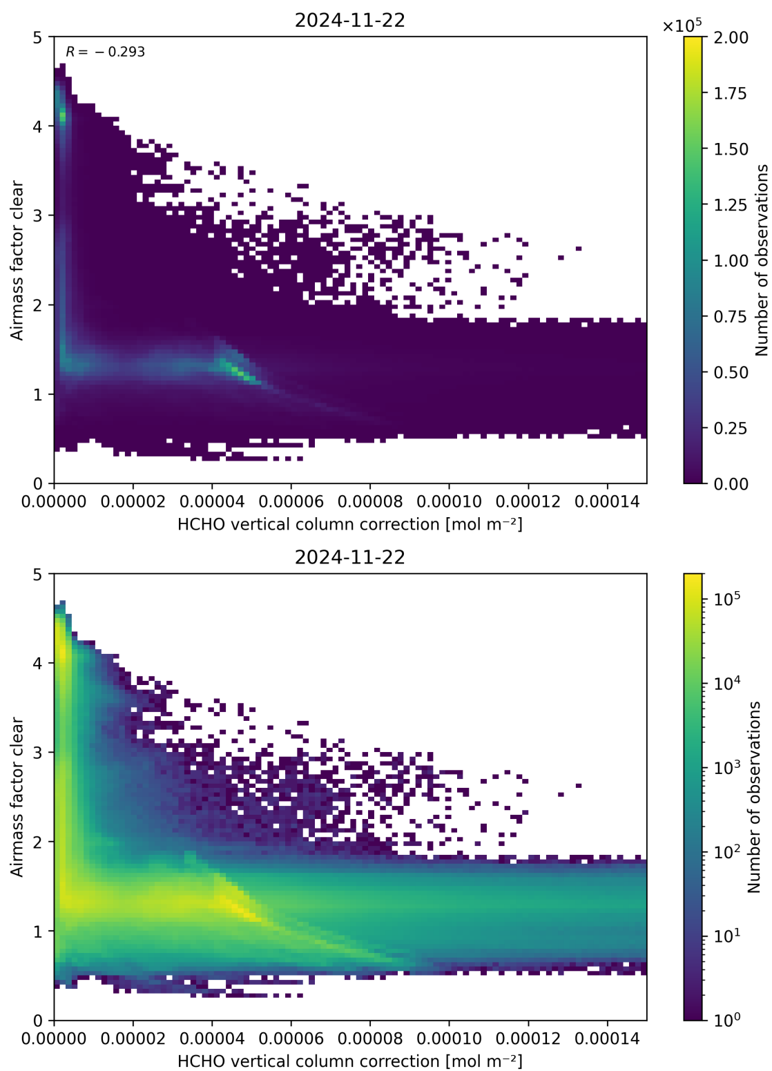
Figure 115: Scatter density plot of “HCHO vertical column correction” against “Airmass factor clear” for 2024-11-21 to 2024-11-23.
