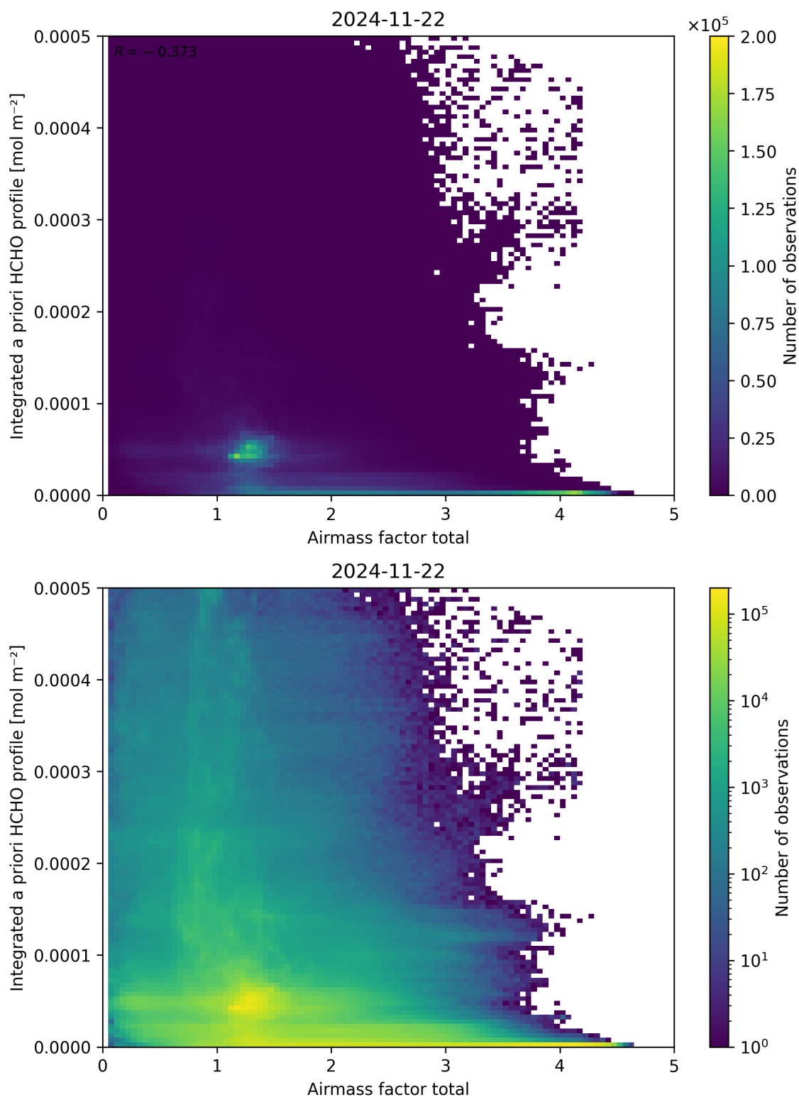
Figure 104: Scatter density plot of “Airmass factor total” against “Integrated a priori HCHO profile” for 2024-11-21 to 2024-11-23.
