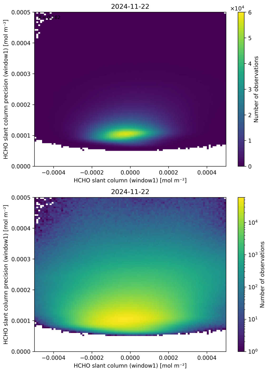
Figure 84: Scatter density plot of “HCHO slant column (window1)” against “HCHO slant column precision (window1)” for 2024-11-21 to 2024-11-23.
