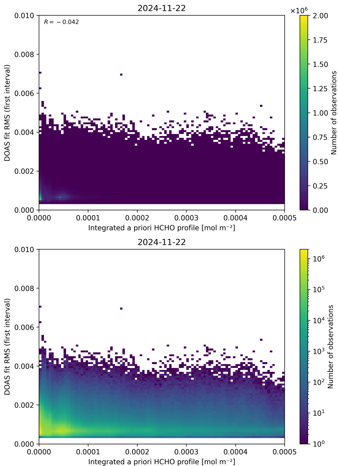
Figure 148: Scatter density plot of “Integrated a priori HCHO profile” against “DOAS fit RMS (first interval)” for 2024-11-21 to 2024-11-23.
