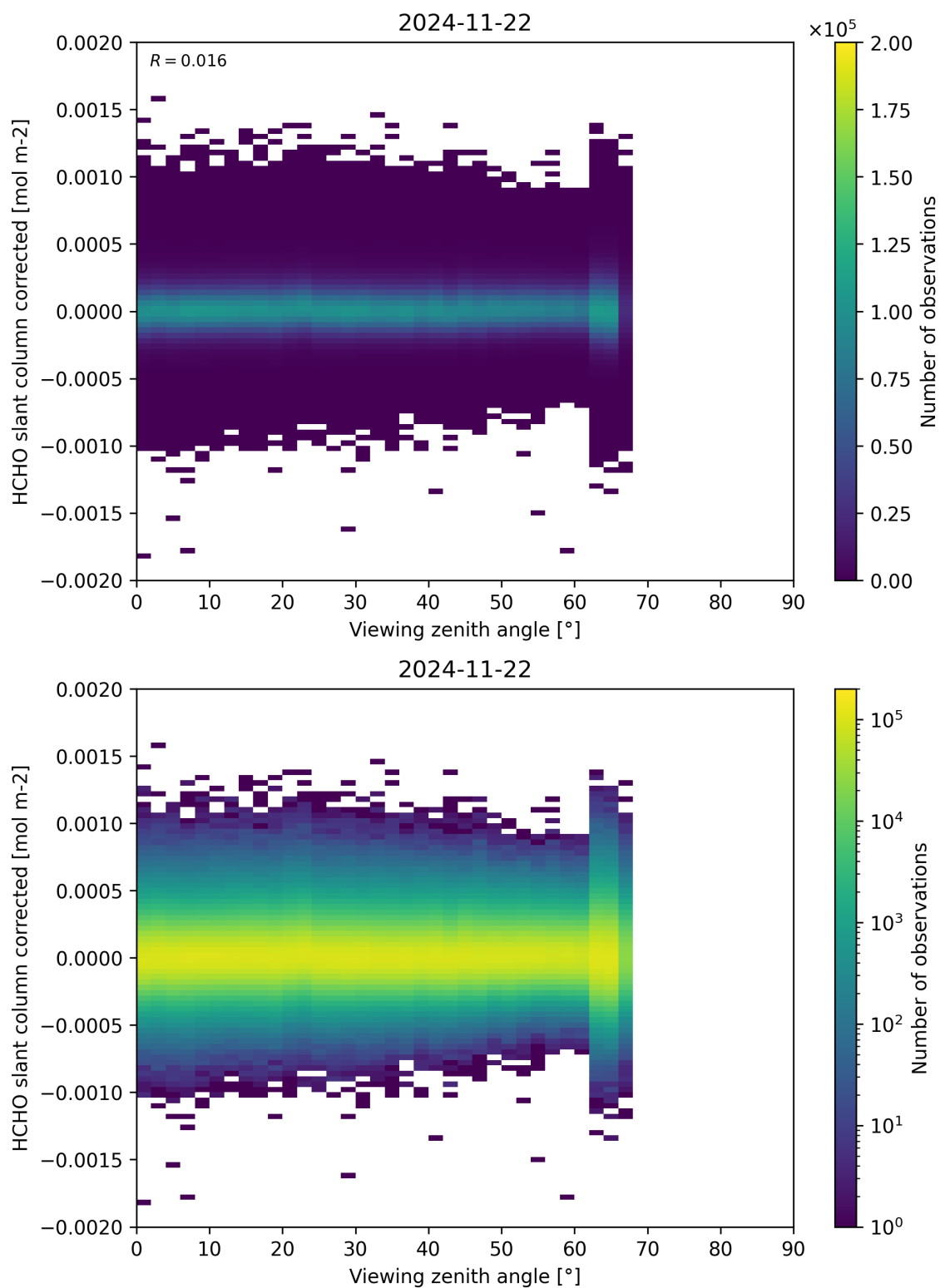
Figure 186: Scatter density plot of “Viewing zenith angle” against “HCHO slant column corrected” for 2024-11-21 to 2024-11-23.
