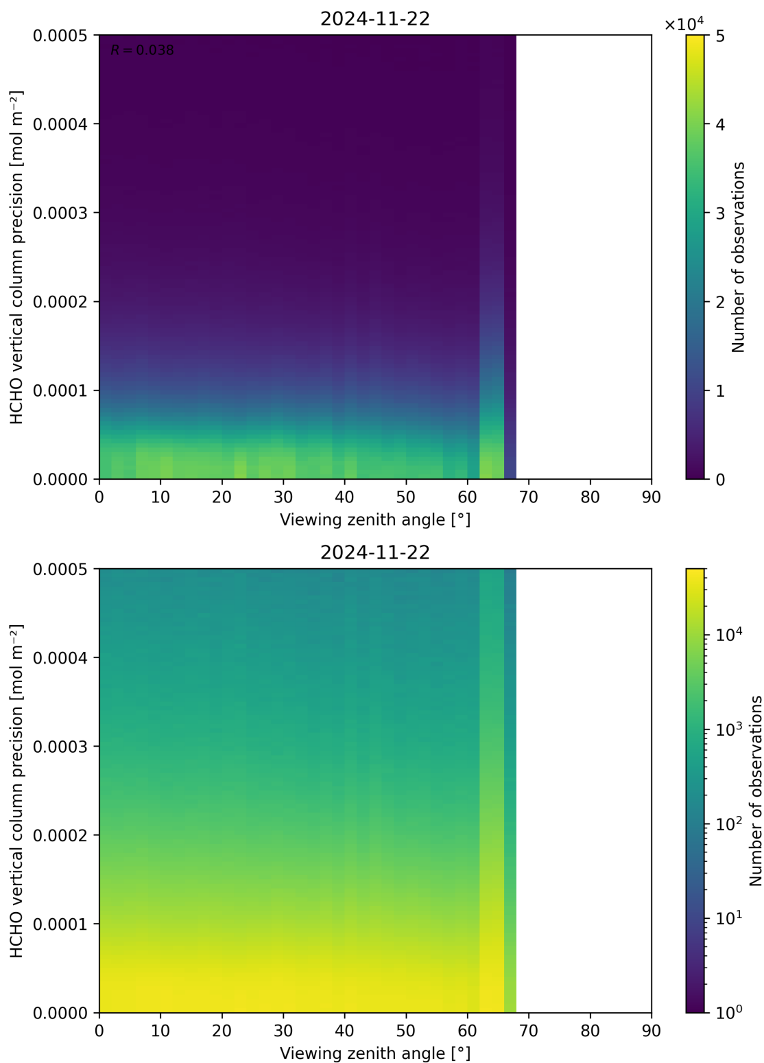
Figure 194: Scatter density plot of “Viewing zenith angle” against “HCHO vertical column precision” for 2024-11-21 to 2024-11-23.
