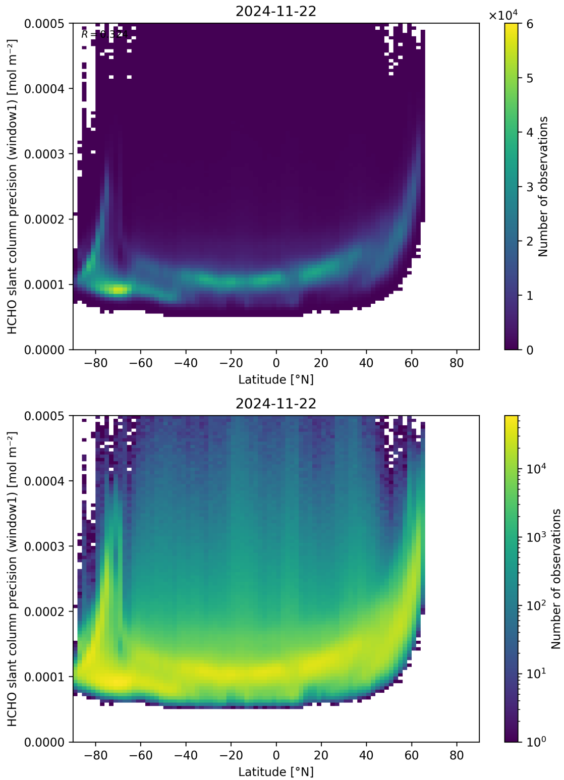
Figure 160: Scatter density plot of “Latitude” against “HCHO slant column precision (window1)” for 2024-11-21 to 2024-11-23.
