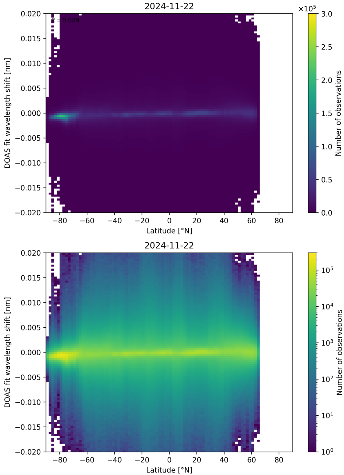
Figure 154: Scatter density plot of “Latitude” against “DOAS fit wavelength shift” for 2024-11-21 to 2024-11-23.
