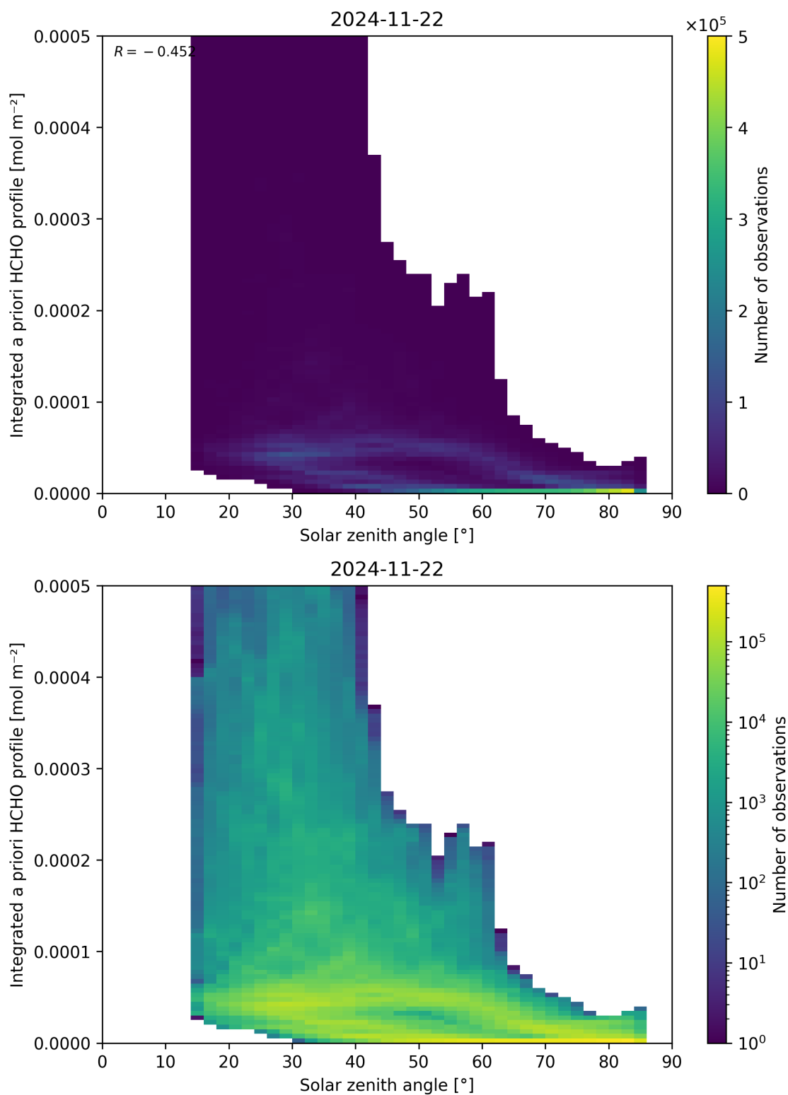
Figure 180: Scatter density plot of “Solar zenith angle” against “Integrated a priori HCHO profile” for 2024-11-21 to 2024-11-23.
