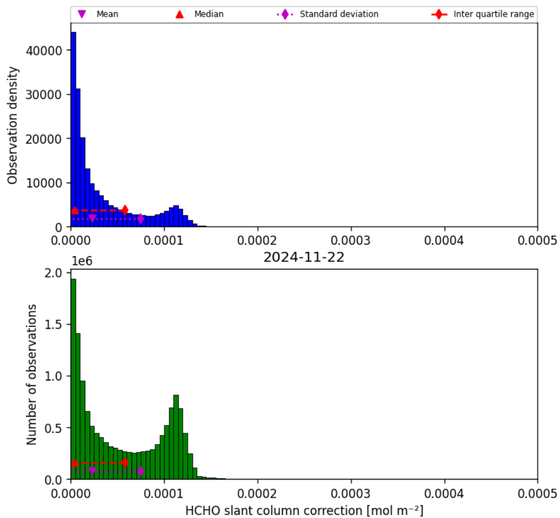
Figure 47: Histogram of “HCHO slant column correction” for 2024-11-21 to 2024-11-23
