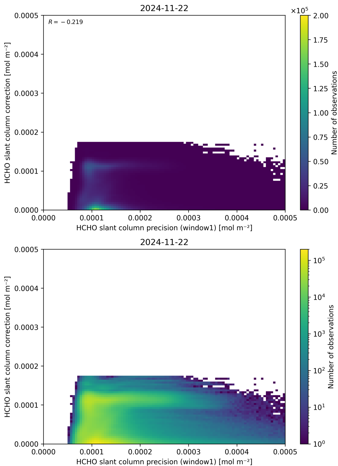
Figure 93: Scatter density plot of “HCHO slant column precision (window1)” against “HCHO slant column correction” for 2024-11-21 to 2024-11-23.
