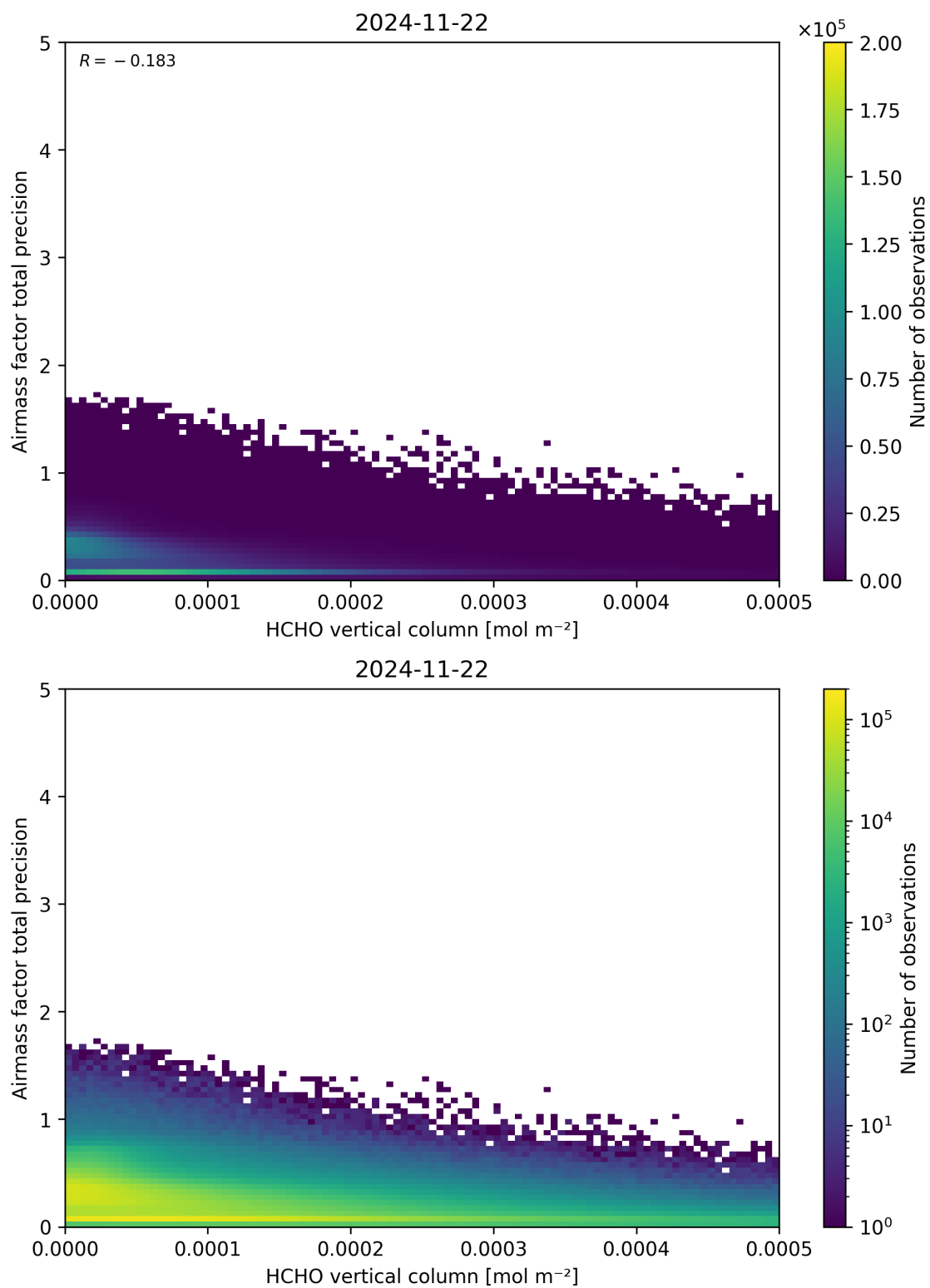
Figure 132: Scatter density plot of “HCHO vertical column” against “Airmass factor total precision” for 2024-11-21 to 2024-11-23.
