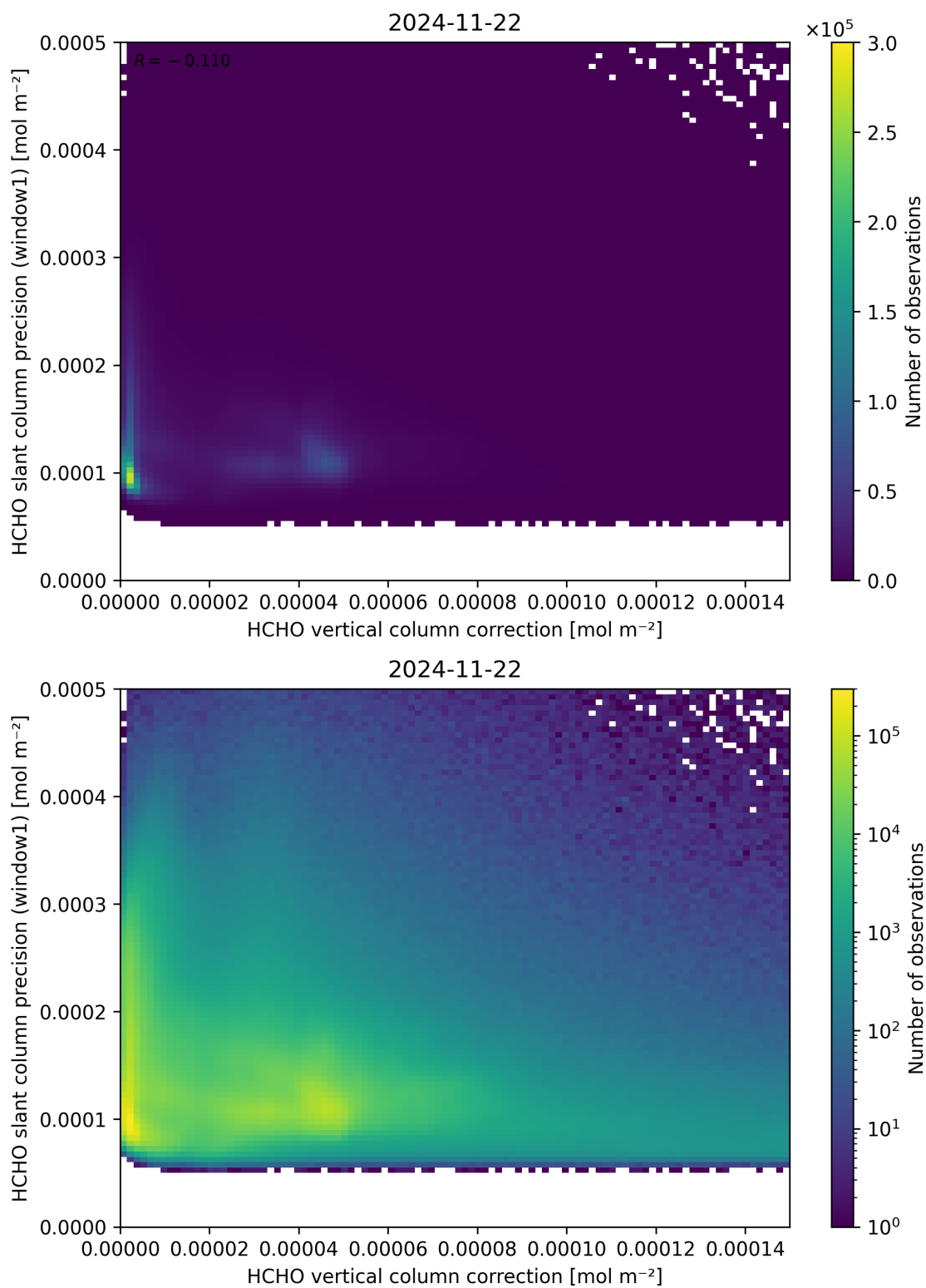
Figure 119: Scatter density plot of “HCHO vertical column correction” against “HCHO slant column precision (window1)” for 2024-11-21 to 2024-11-23.
