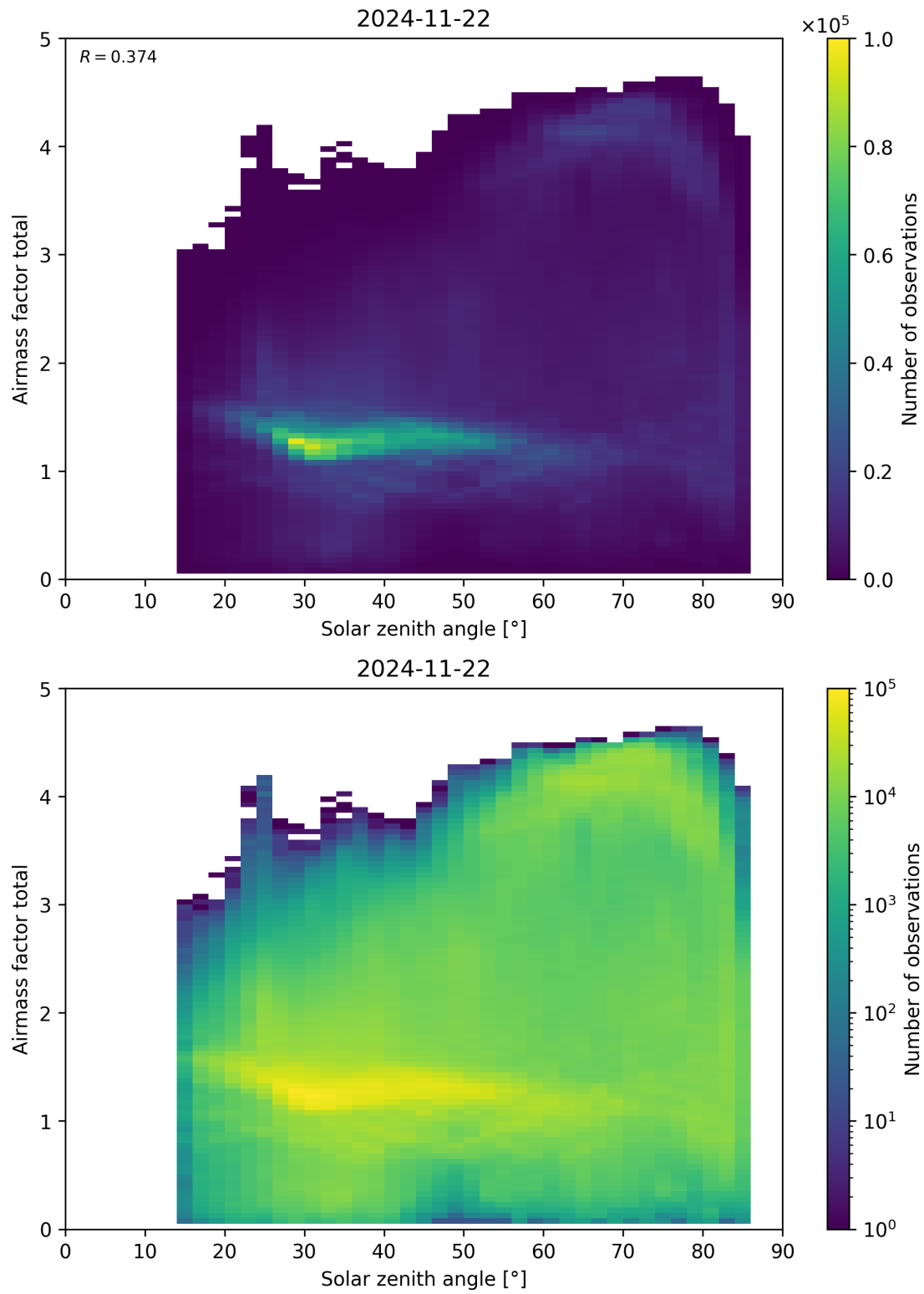
Figure 175: Scatter density plot of “Solar zenith angle” against “Airmass factor total” for 2024-11-21 to 2024-11-23.
