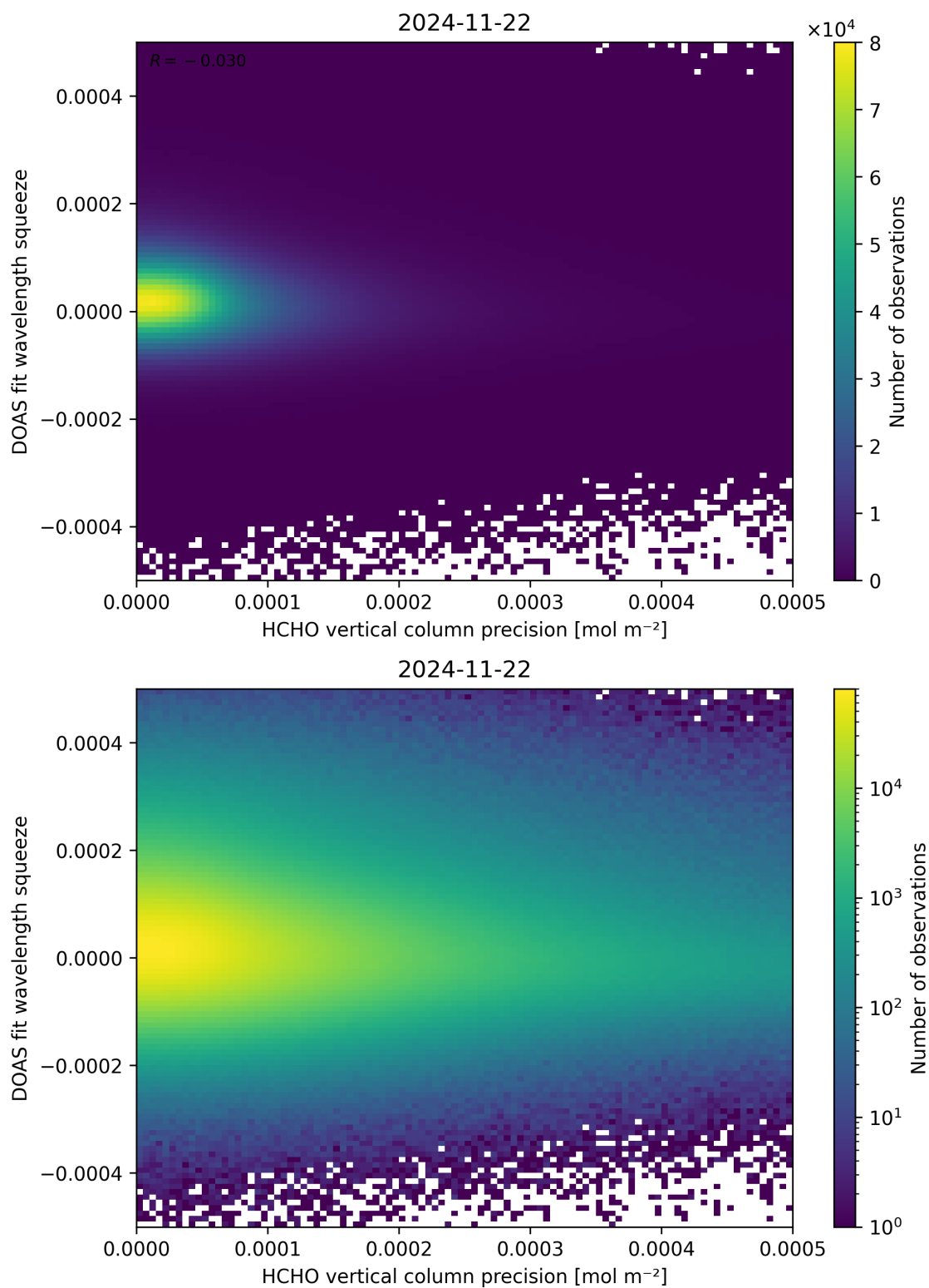
Figure 138: Scatter density plot of “HCHO vertical column precision” against “DOAS fit wavelength squeeze” for 2024-11-21 to 2024-11-23.
