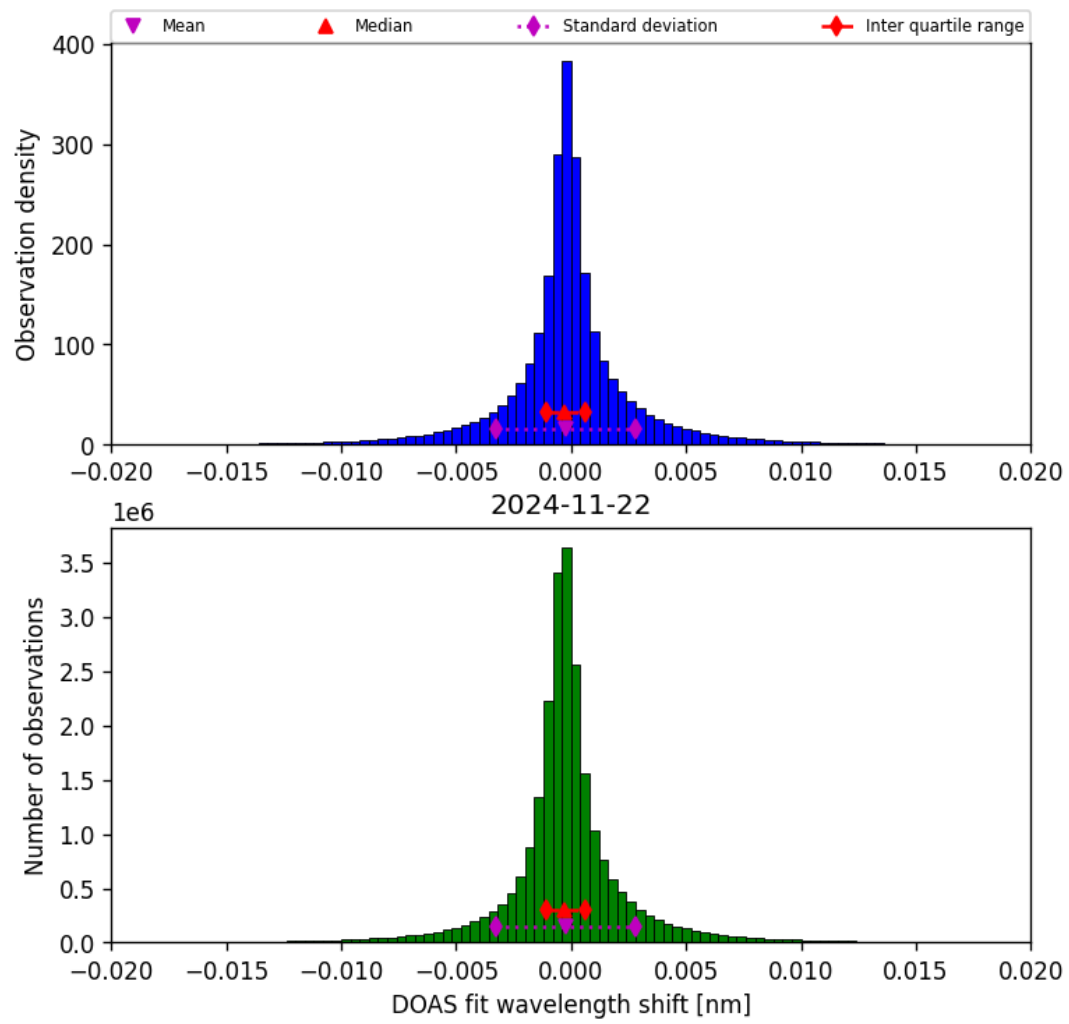
Figure 44: Histogram of “DOAS fit wavelength shift” for 2024-11-21 to 2024-11-23
