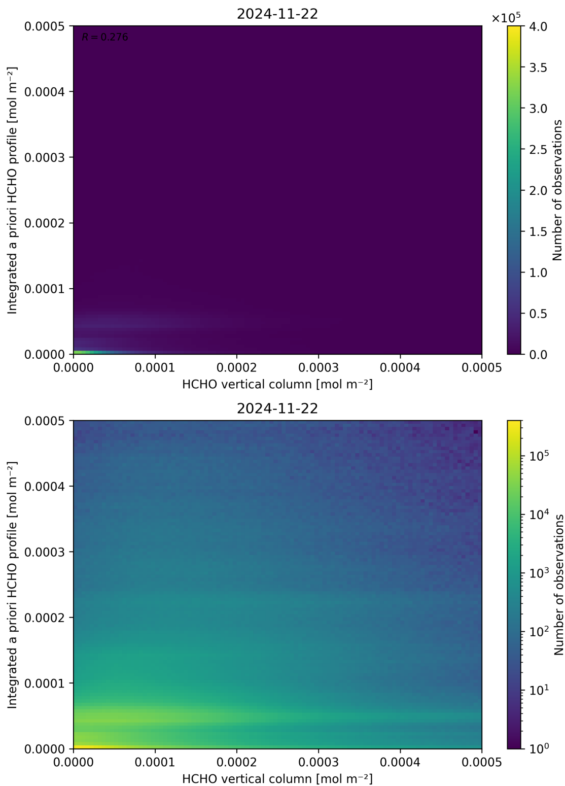
Figure 135: Scatter density plot of “HCHO vertical column” against “Integrated a priori HCHO profile” for 2024-11-21 to 2024-11-23.
