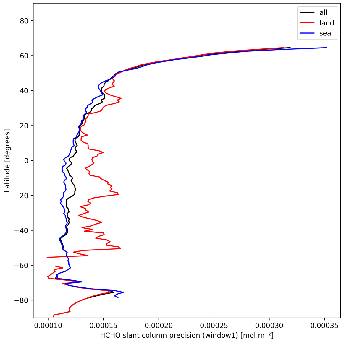
Figure 25: Zonal average of “HCHO slant column precision (window1)” for 2024-11-21 to 2024-11-23.
