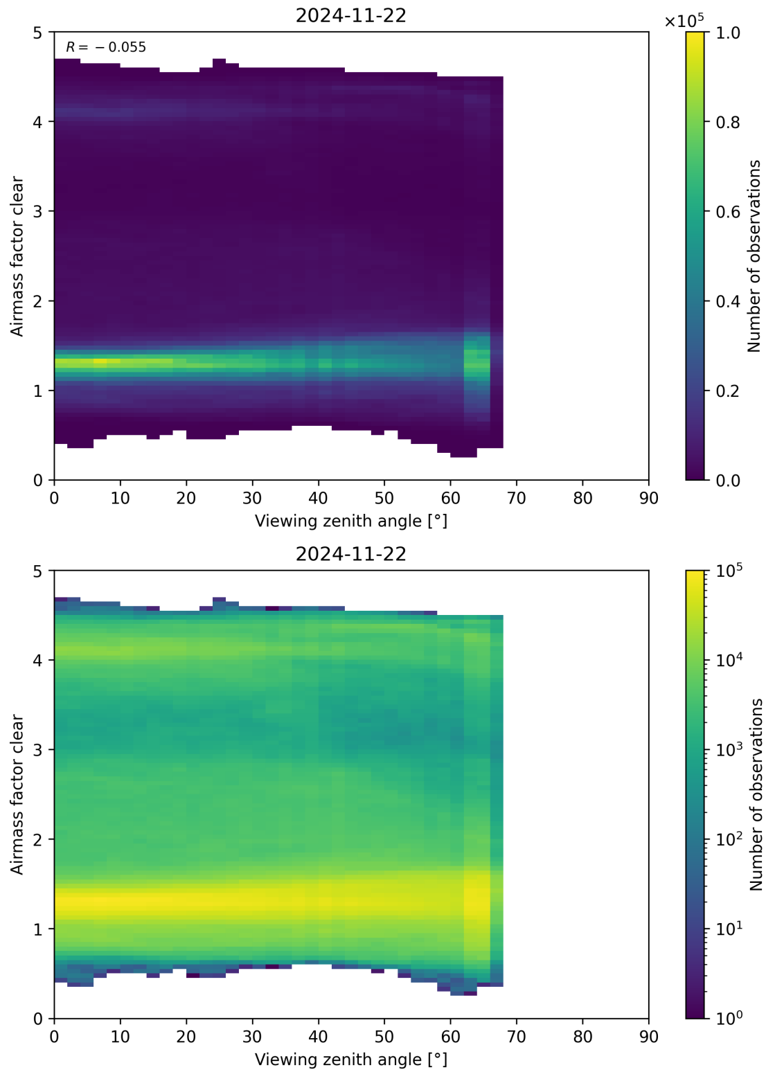
Figure 185: Scatter density plot of “Viewing zenith angle” against “Airmass factor clear” for 2024-11-21 to 2024-11-23.
