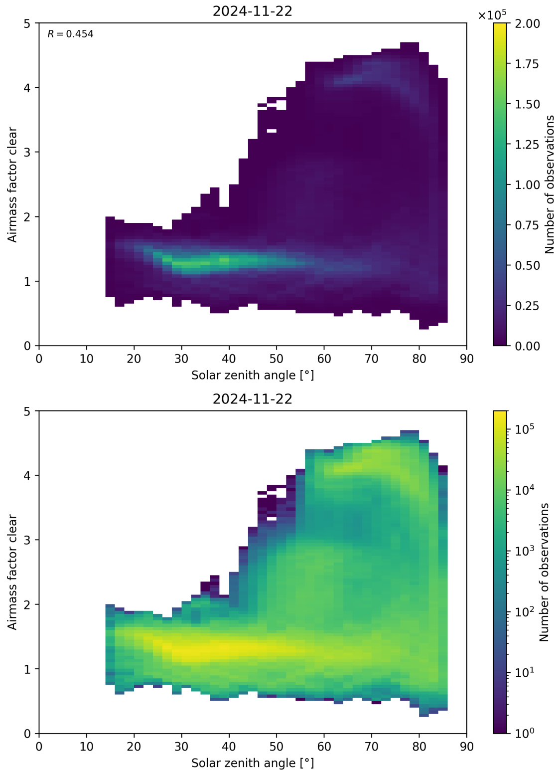
Figure 170: Scatter density plot of “Solar zenith angle” against “Airmass factor clear” for 2024-11-21 to 2024-11-23.
