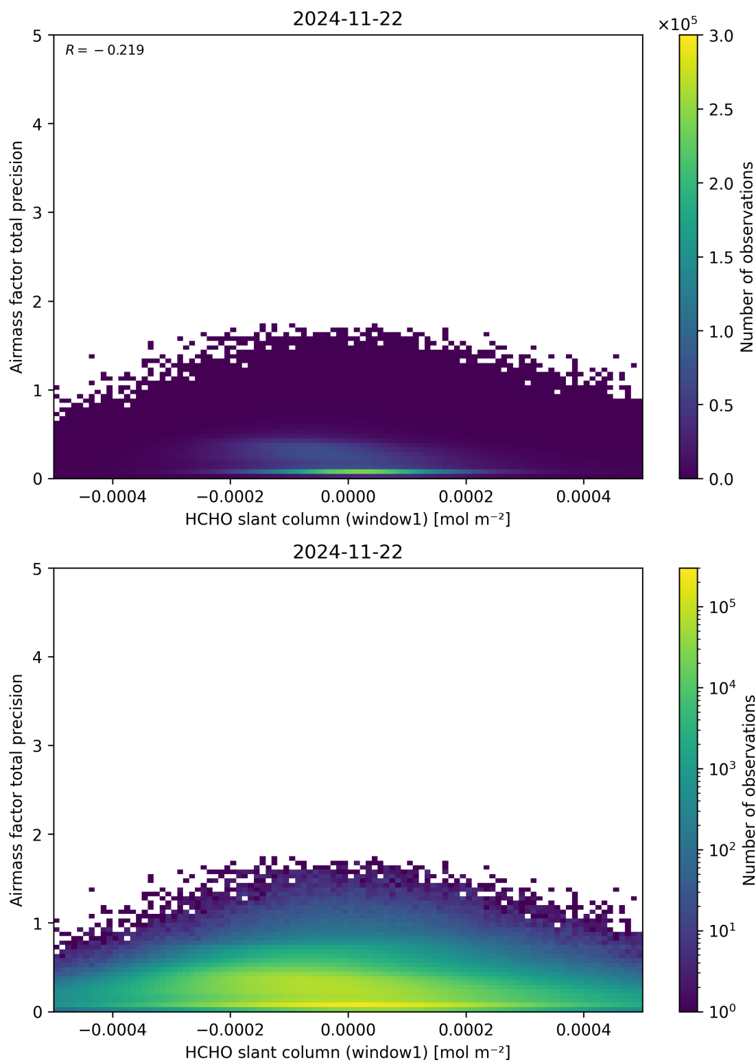
Figure 86: Scatter density plot of “HCHO slant column (window1)” against “Airmass factor total precision” for 2024-11-21 to 2024-11-23.
