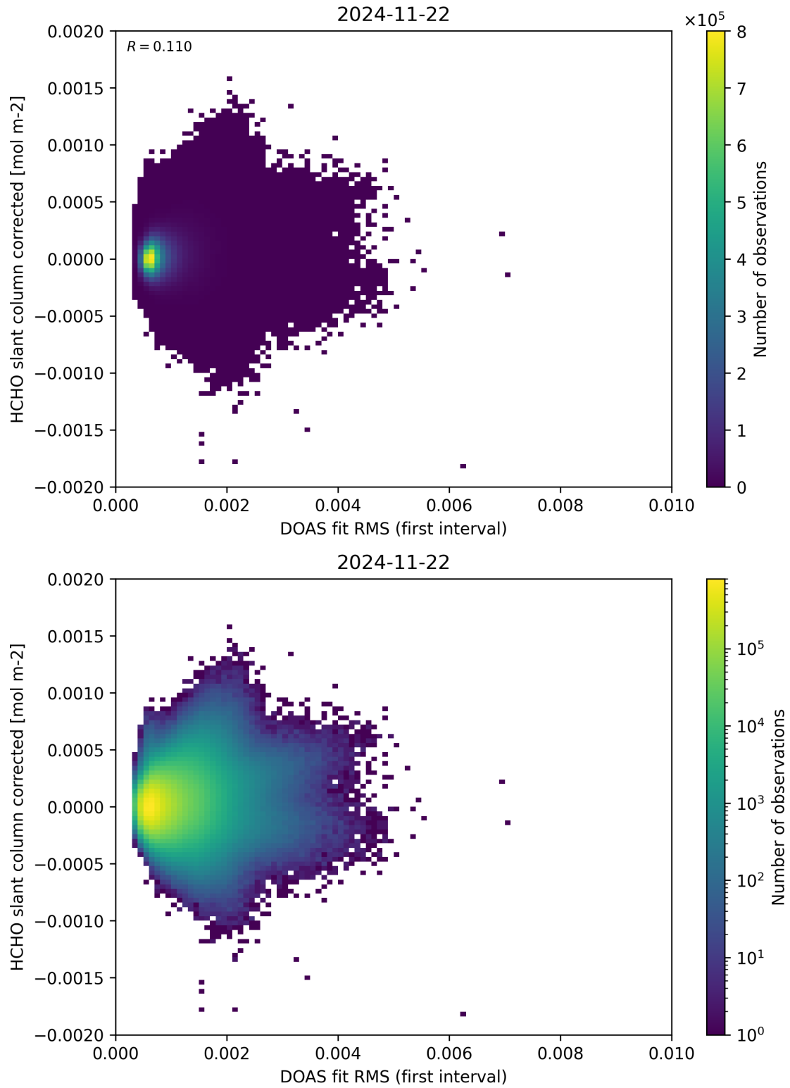
Figure 62: Scatter density plot of “DOAS fit RMS (first interval)” against “HCHO slant column corrected” for 2024-11-21 to 2024-11-23.
