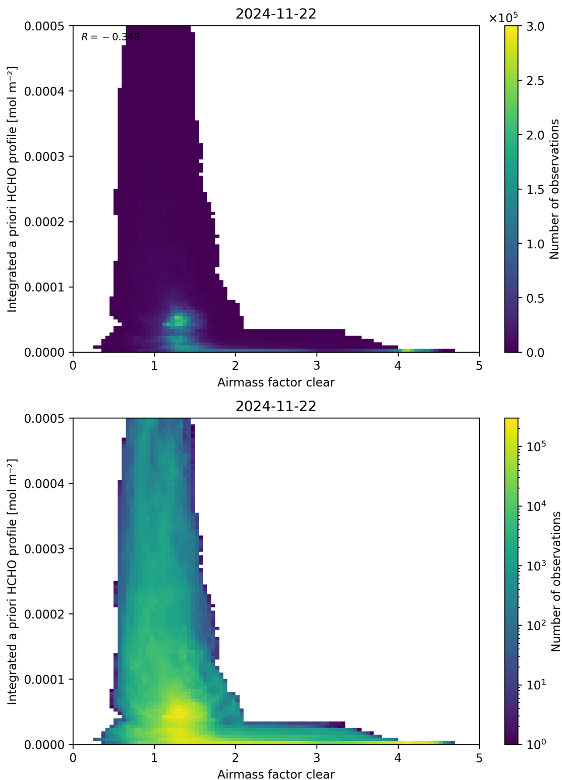
Figure 76: Scatter density plot of “Airmass factor clear” against “Integrated a priori HCHO profile” for 2024-11-21 to 2024-11-23.
