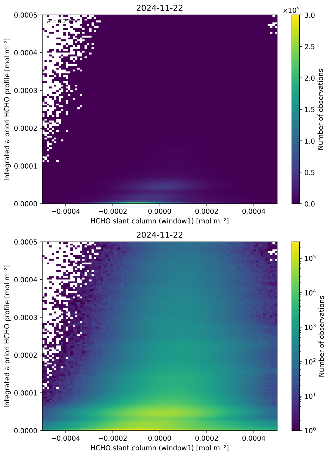
Figure 87: Scatter density plot of “HCHO slant column (window1)” against “Integrated a priori HCHO profile” for 2024-11-21 to 2024-11-23.
