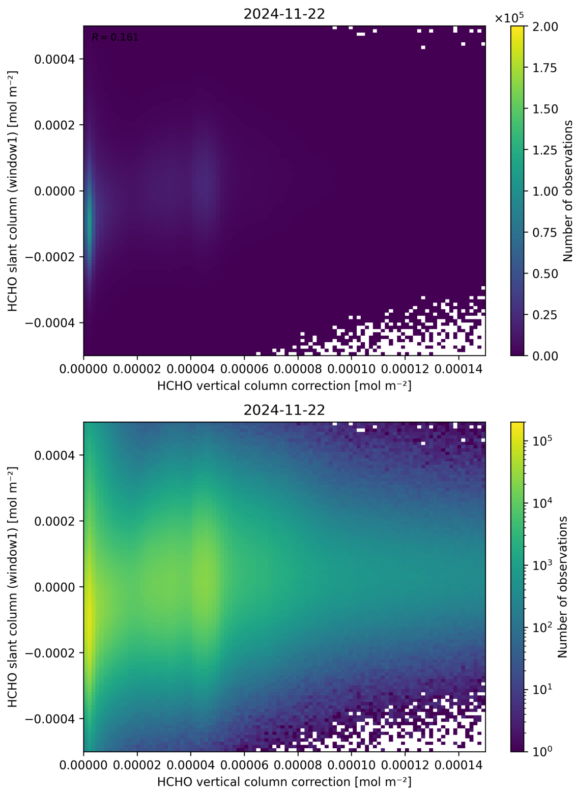
Figure 118: Scatter density plot of “HCHO vertical column correction” against “HCHO slant column (window1)” for 2024-11-21 to 2024-11-23.
