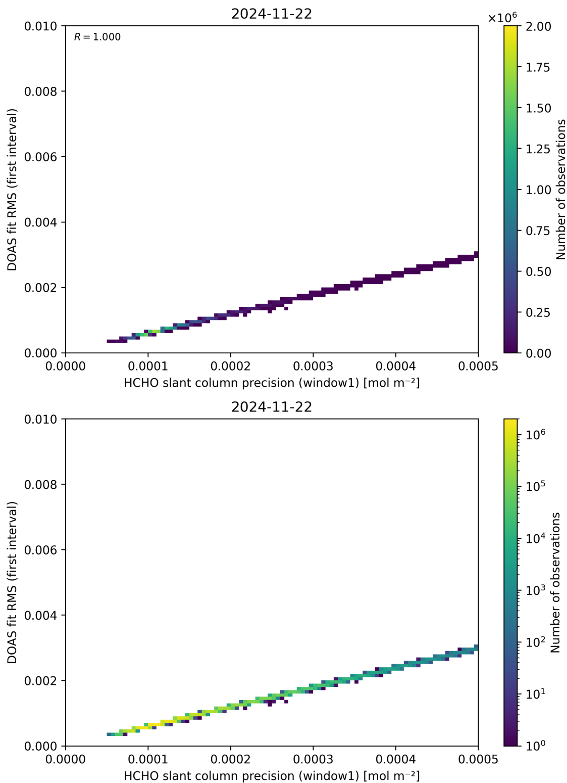
Figure 88: Scatter density plot of “HCHO slant column precision (window1)” against “DOAS fit RMS (first interval)” for 2024-11-21 to 2024-11-23.
