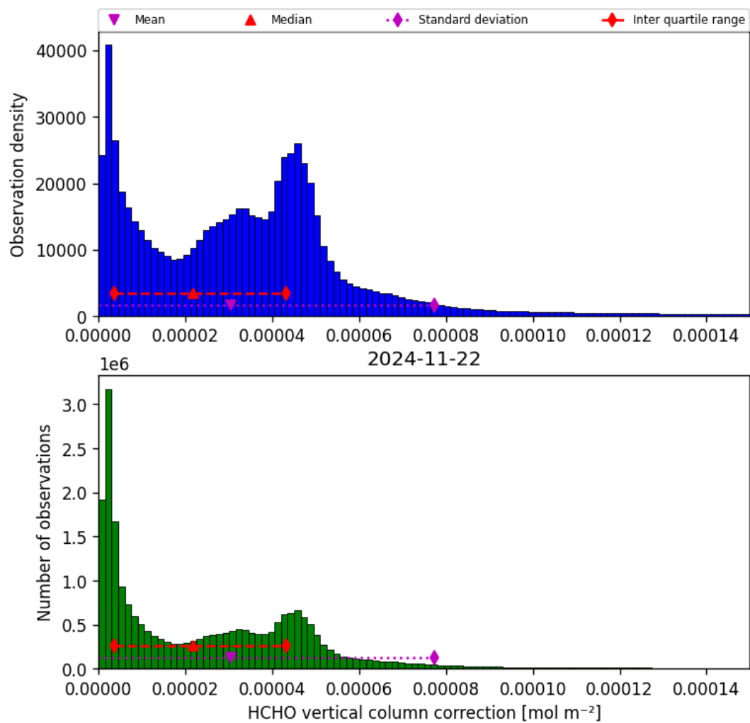
Figure 37: Histogram of “HCHO vertical column correction” for 2024-11-21 to 2024-11-23
