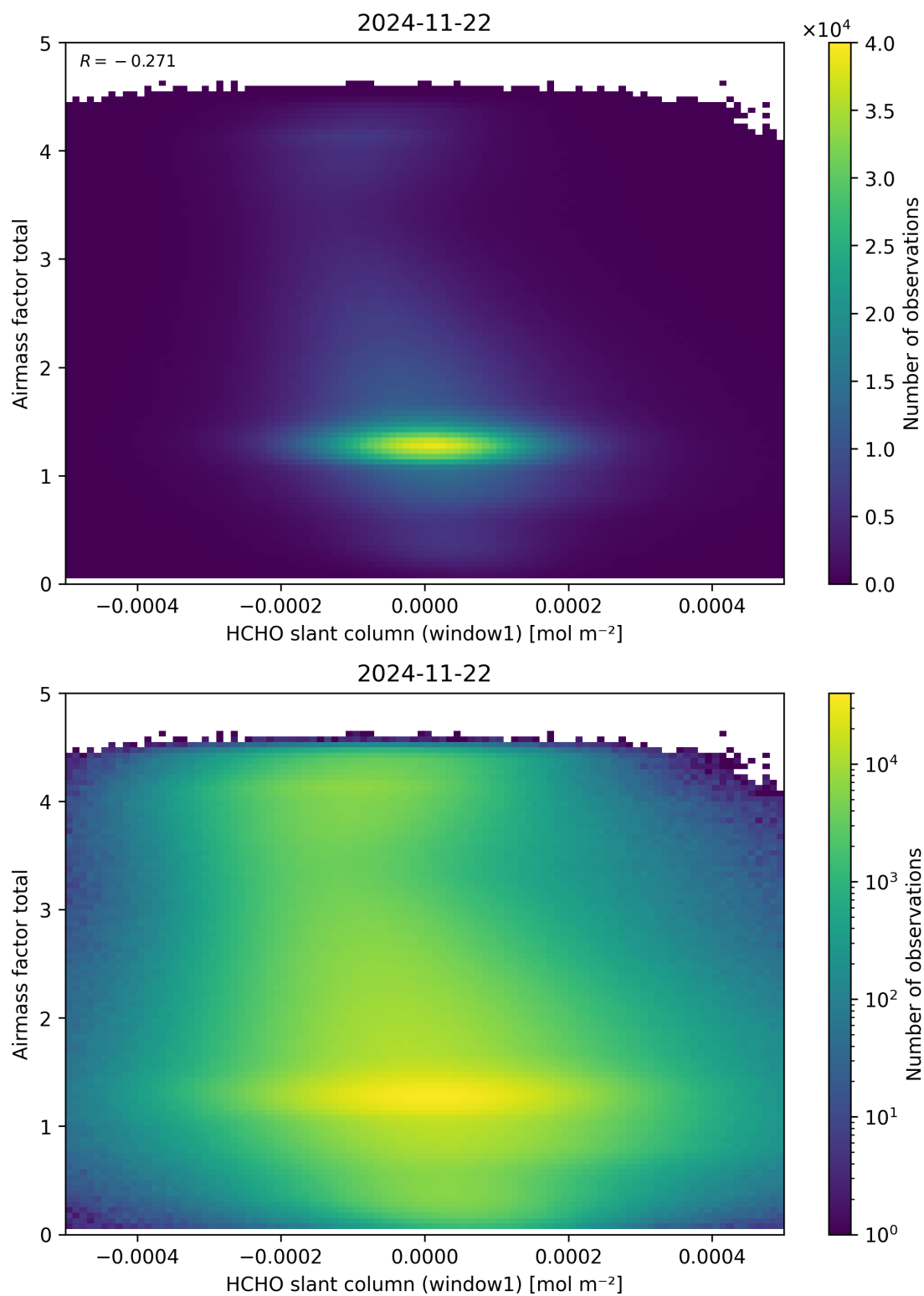
Figure 85: Scatter density plot of “HCHO slant column (window1)” against “Airmass factor total” for 2024-11-21 to 2024-11-23.
