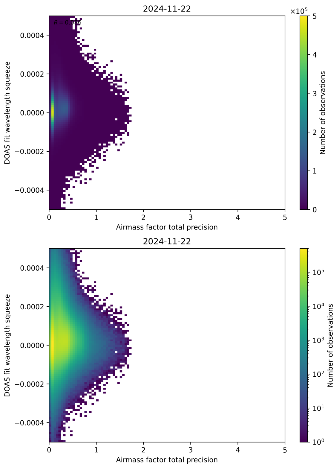
Figure 107: Scatter density plot of “Airmass factor total precision” against “DOAS fit wavelength squeeze” for 2024-11-21 to 2024-11-23.
