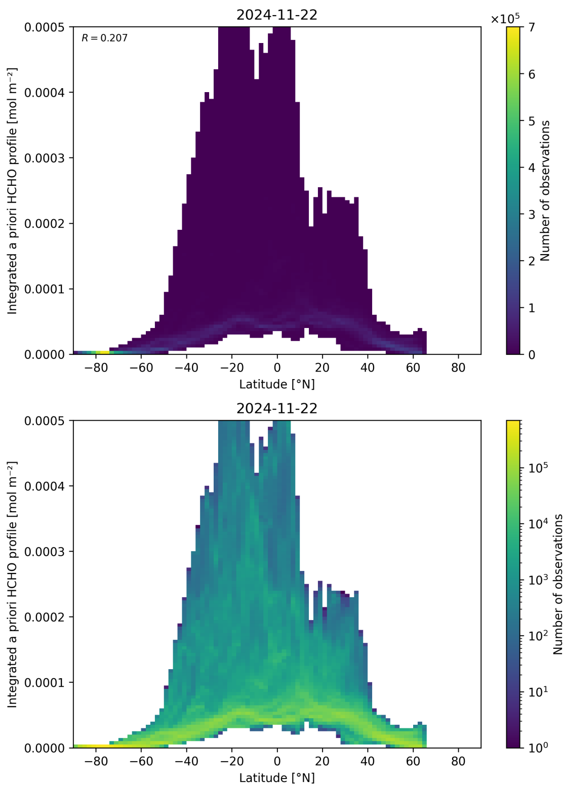
Figure 166: Scatter density plot of “Latitude” against “Integrated a priori HCHO profile” for 2024-11-21 to 2024-11-23.
