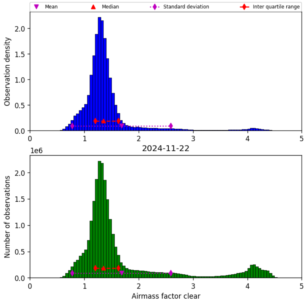
Figure 42: Histogram of “Airmass factor clear” for 2024-11-21 to 2024-11-23
