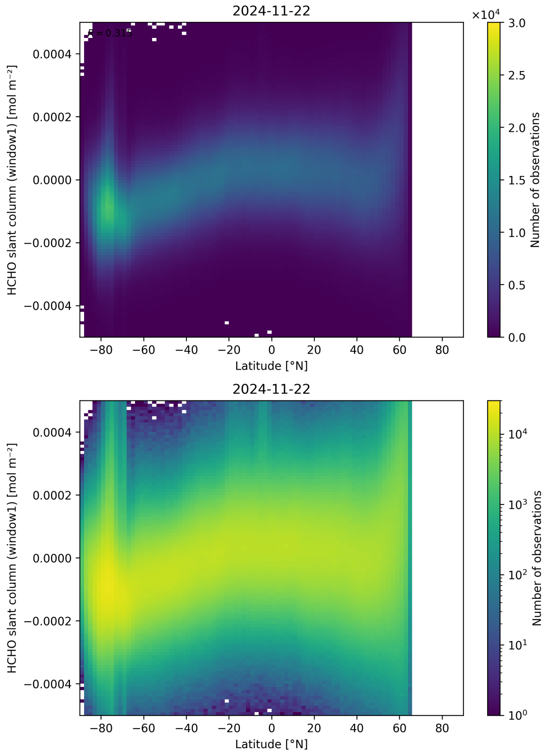
Figure 159: Scatter density plot of “Latitude” against “HCHO slant column (window1)” for 2024-11-21 to 2024-11-23.
