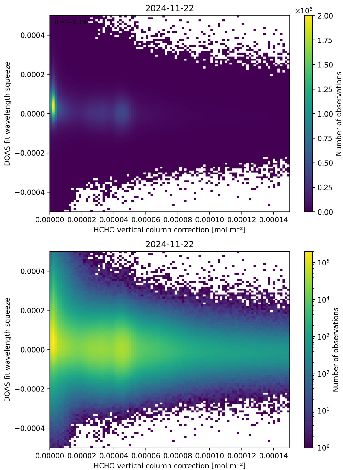
Figure 114: Scatter density plot of “HCHO vertical column correction” against “DOAS fit wavelength squeeze” for 2024-11-21 to 2024-11-23.
