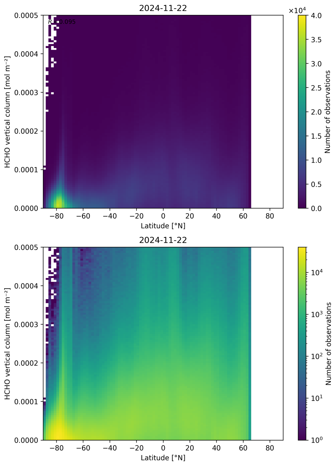
Figure 163: Scatter density plot of “Latitude” against “HCHO vertical column” for 2024-11-21 to 2024-11-23.
