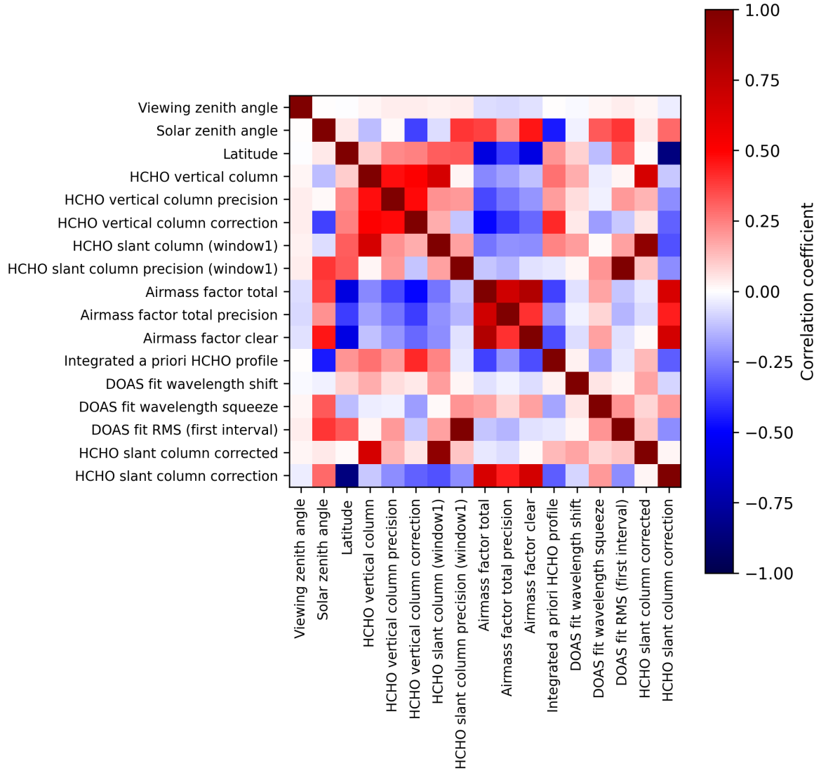
Figure 2: Map of correlation matrix for 2024-11-21 to 2024-11-23.
