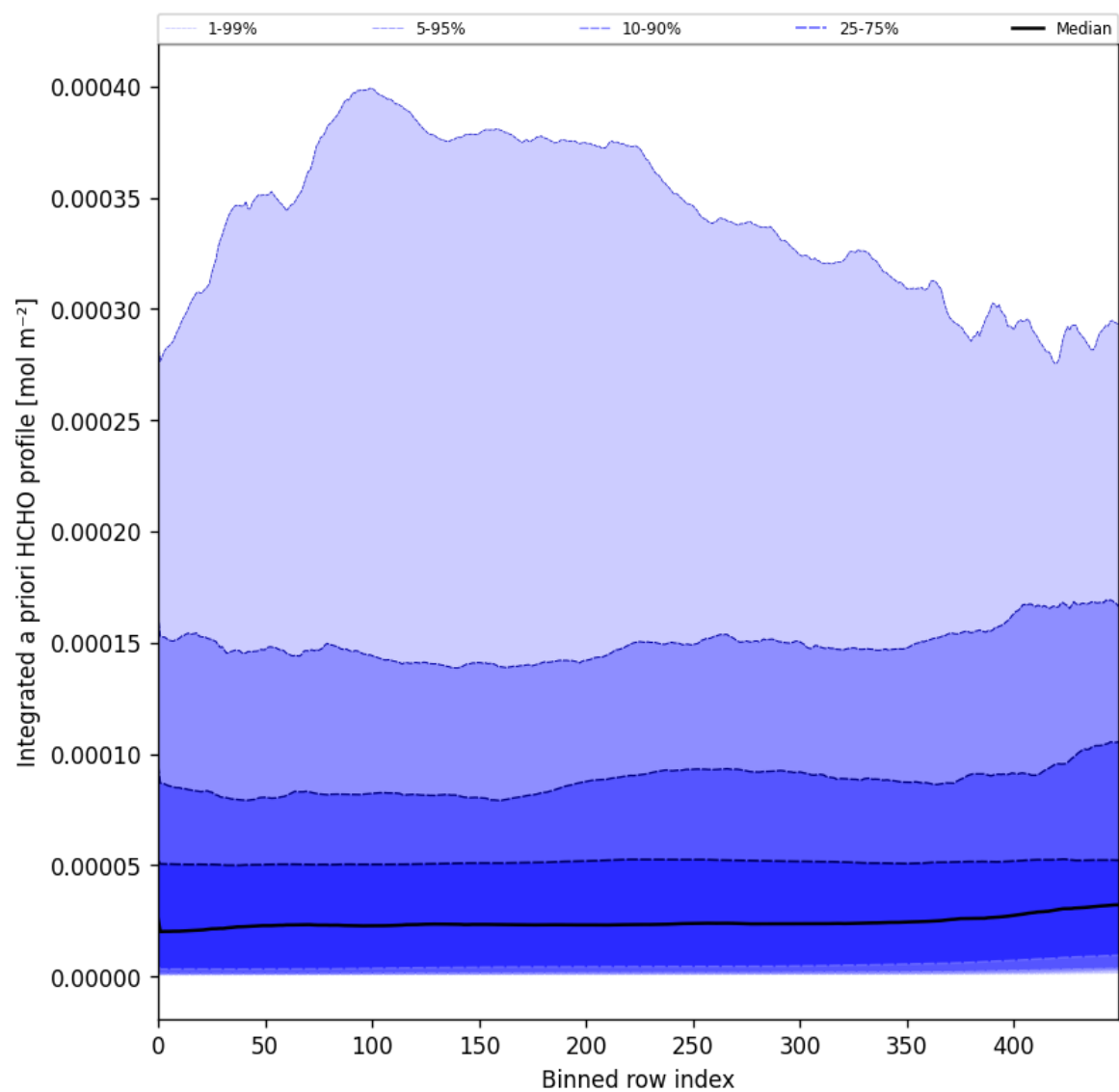
Figure 57: Along track statistics of “Integrated a priori HCHO profile” for 2024-11-21 to 2024-11-23
