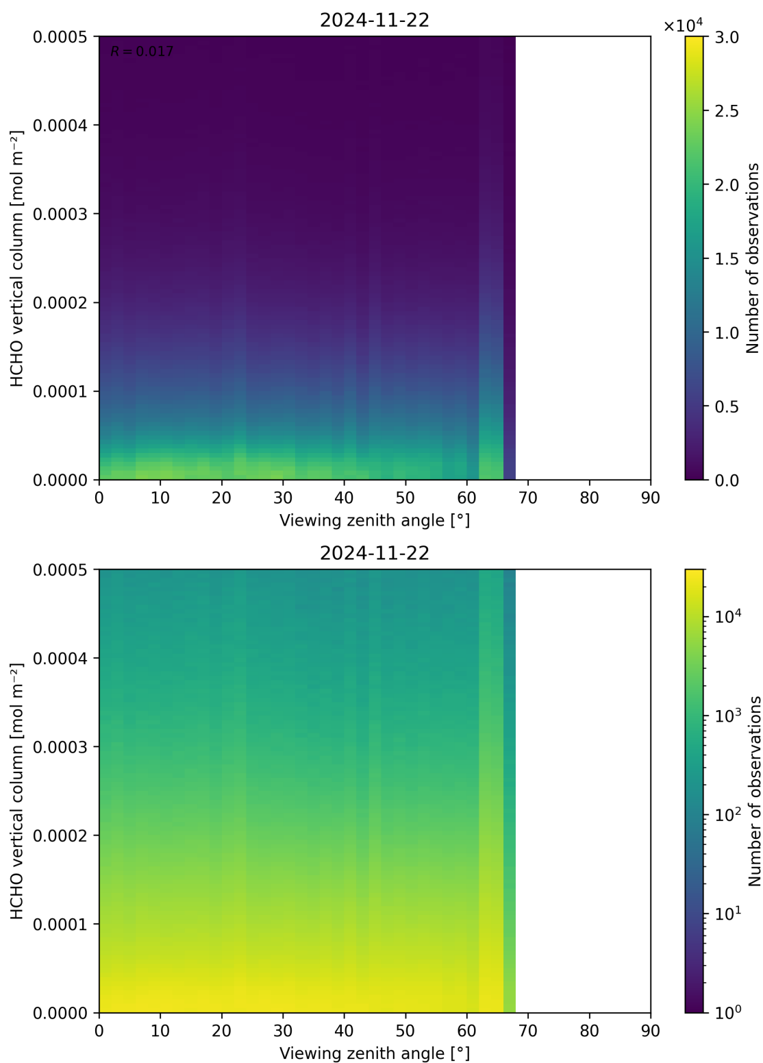
Figure 192: Scatter density plot of “Viewing zenith angle” against “HCHO vertical column” for 2024-11-21 to 2024-11-23.
