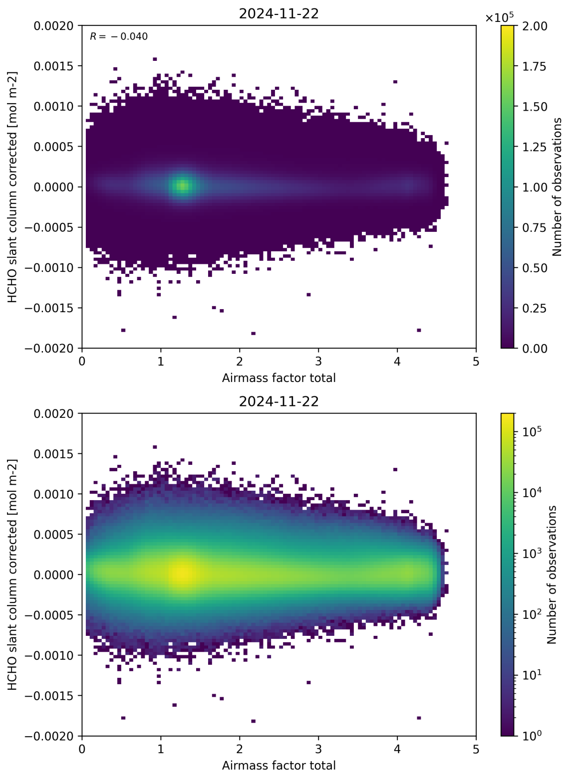
Figure 101: Scatter density plot of “Airmass factor total” against “HCHO slant column corrected” for 2024-11-21 to 2024-11-23.
