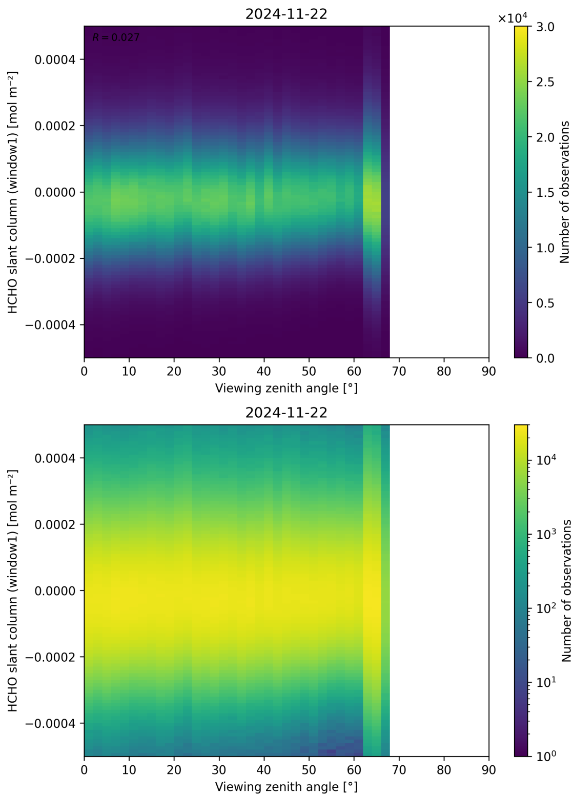
Figure 188: Scatter density plot of “Viewing zenith angle” against “HCHO slant column (window1)” for 2024-11-21 to 2024-11-23.
