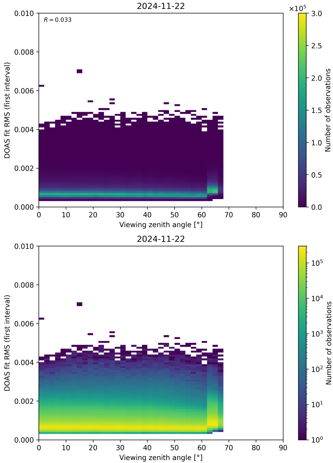
Figure 182: Scatter density plot of “Viewing zenith angle” against “DOAS fit RMS (first interval)” for 2024-11-21 to 2024-11-23.
