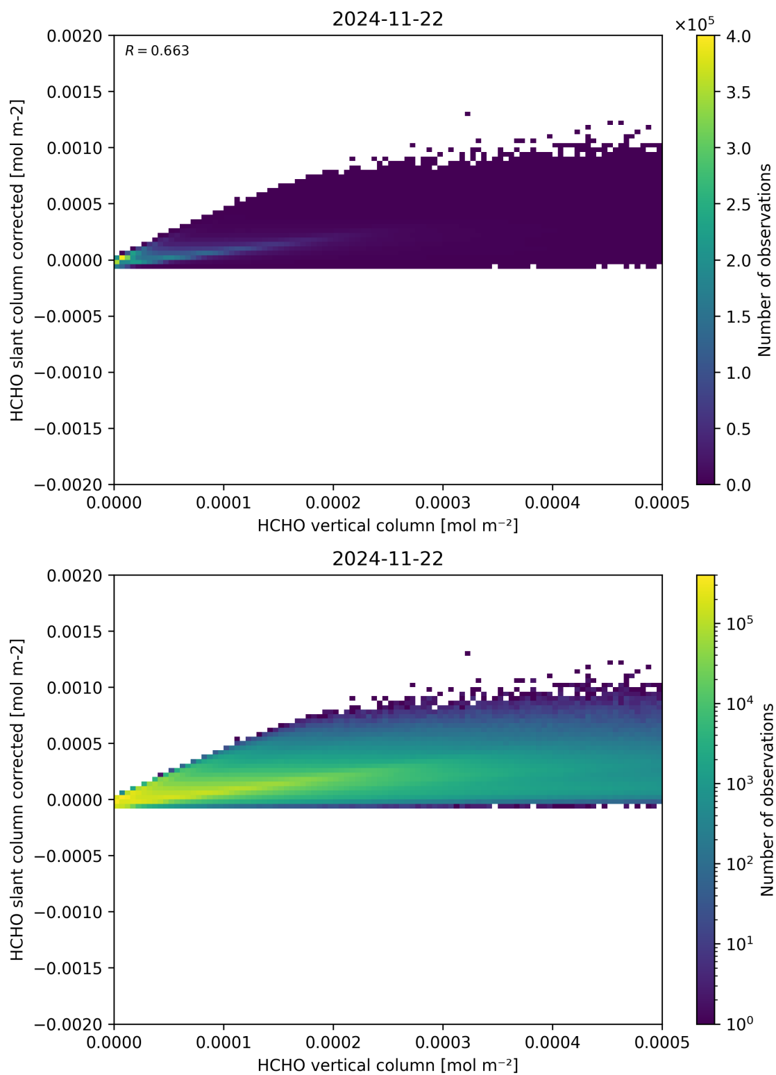
Figure 127: Scatter density plot of “HCHO vertical column” against “HCHO slant column corrected” for 2024-11-21 to 2024-11-23.
