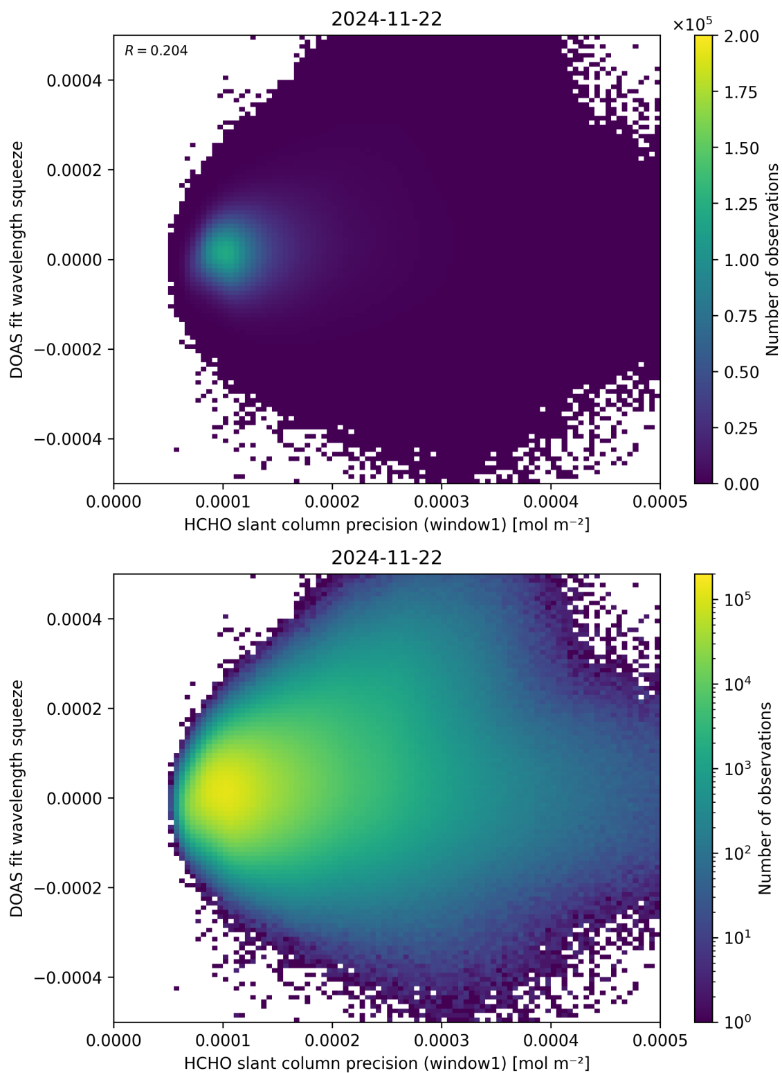
Figure 90: Scatter density plot of “HCHO slant column precision (window1)” against “DOAS fit wavelength squeeze” for 2024-11-21 to 2024-11-23.
