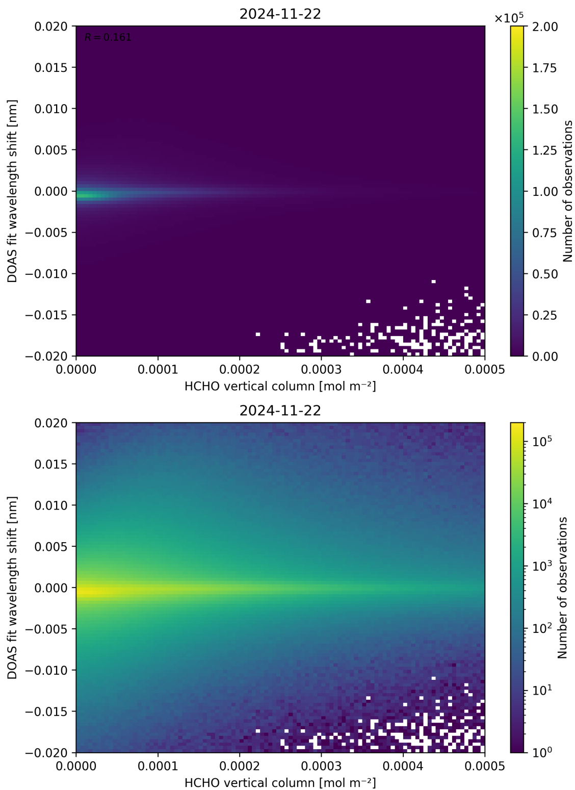
Figure 124: Scatter density plot of “HCHO vertical column” against “DOAS fit wavelength shift” for 2024-11-21 to 2024-11-23.
