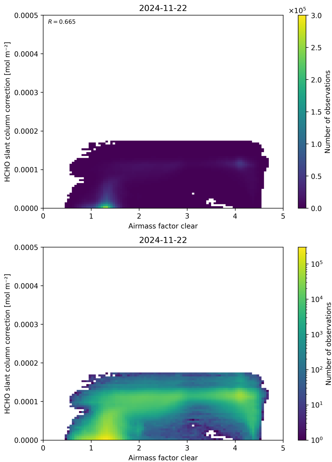
Figure 75: Scatter density plot of “Airmass factor clear” against “HCHO slant column correction” for 2024-11-21 to 2024-11-23.
