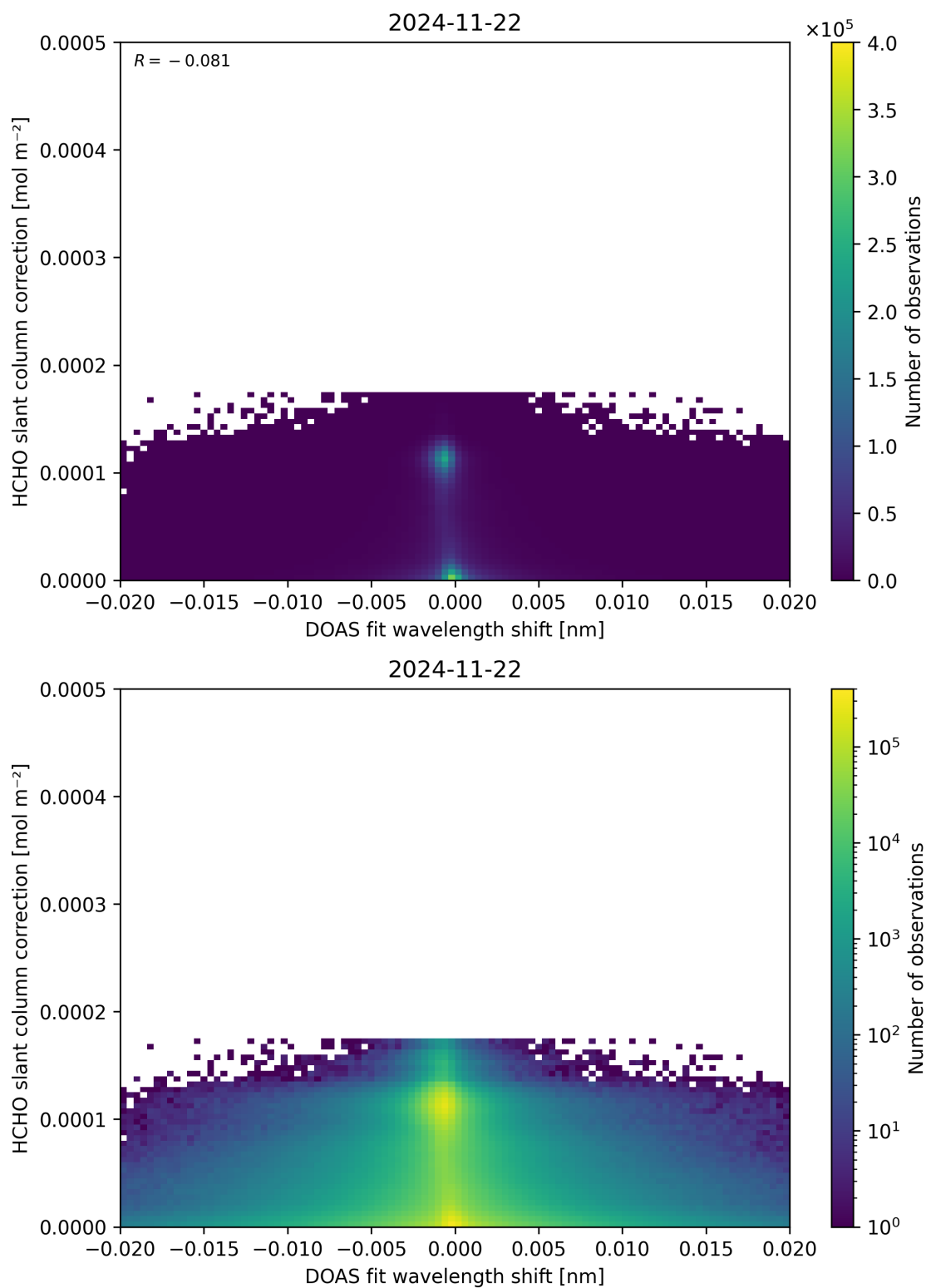
Figure 67: Scatter density plot of “DOAS fit wavelength shift” against “HCHO slant column correction” for 2024-11-21 to 2024-11-23.
