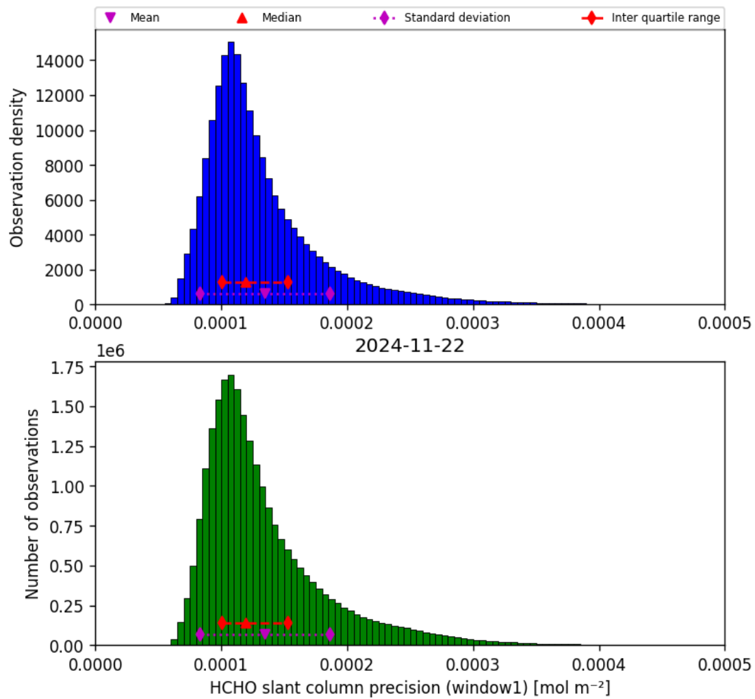
Figure 39: Histogram of “HCHO slant column precision (window1)” for 2024-11-21 to 2024-11-23
