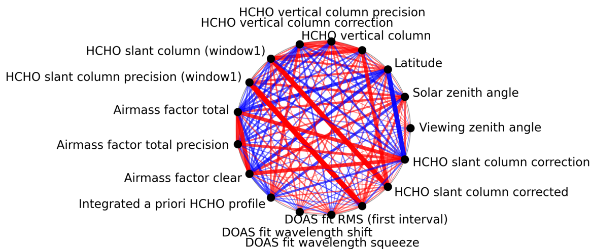
Figure 1: Map of correlation graph for 2024-11-21 to 2024-11-23.
