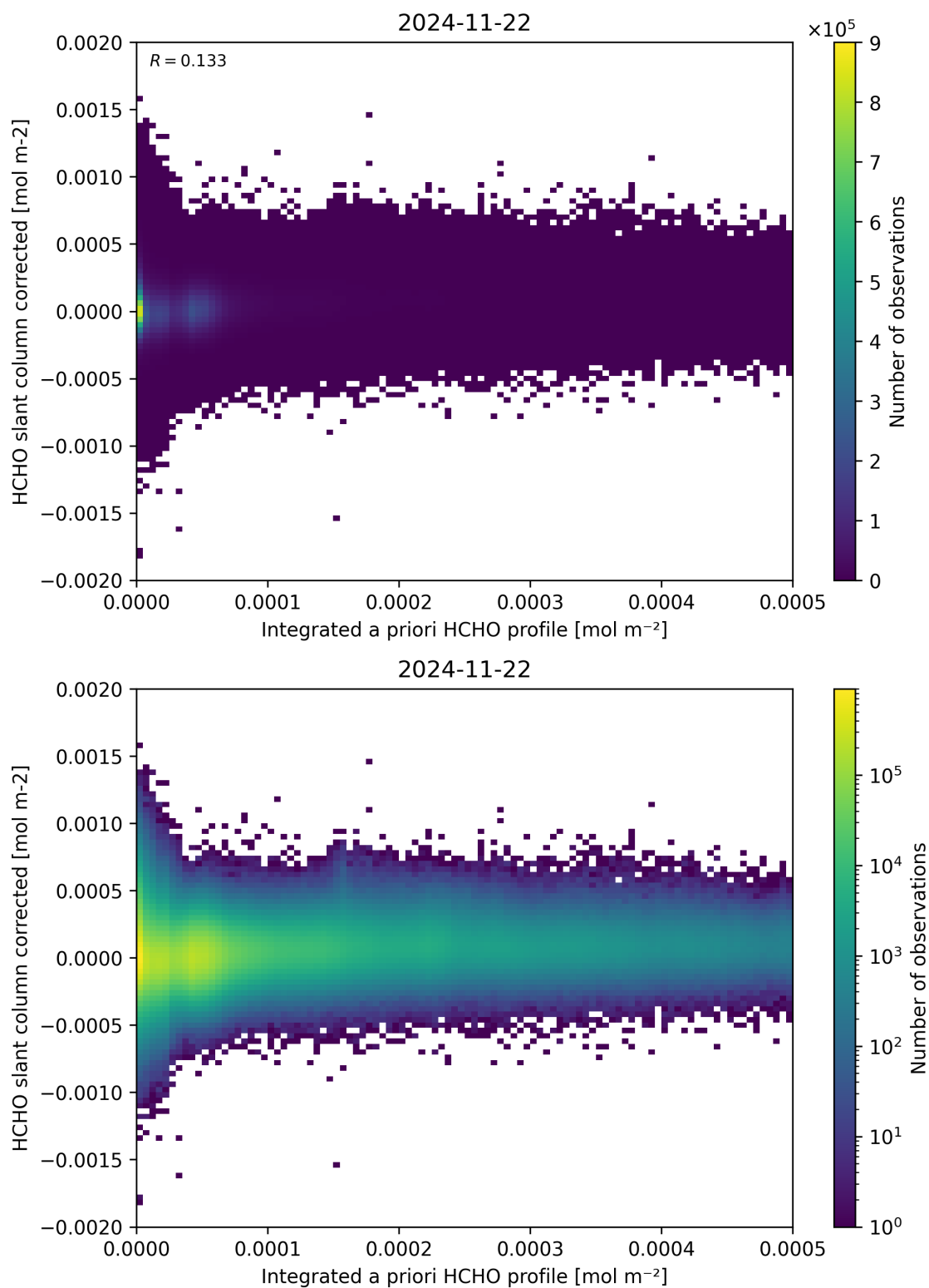
Figure 151: Scatter density plot of “Integrated a priori HCHO profile” against “HCHO slant column corrected” for 2024-11-21 to 2024-11-23.
