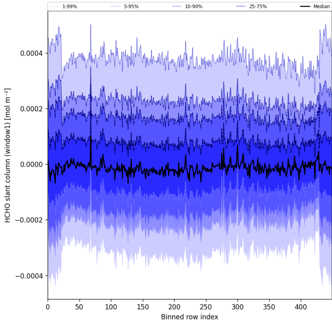
Figure 52: Along track statistics of “HCHO slant column (window1)” for 2024-11-21 to 2024-11-23
