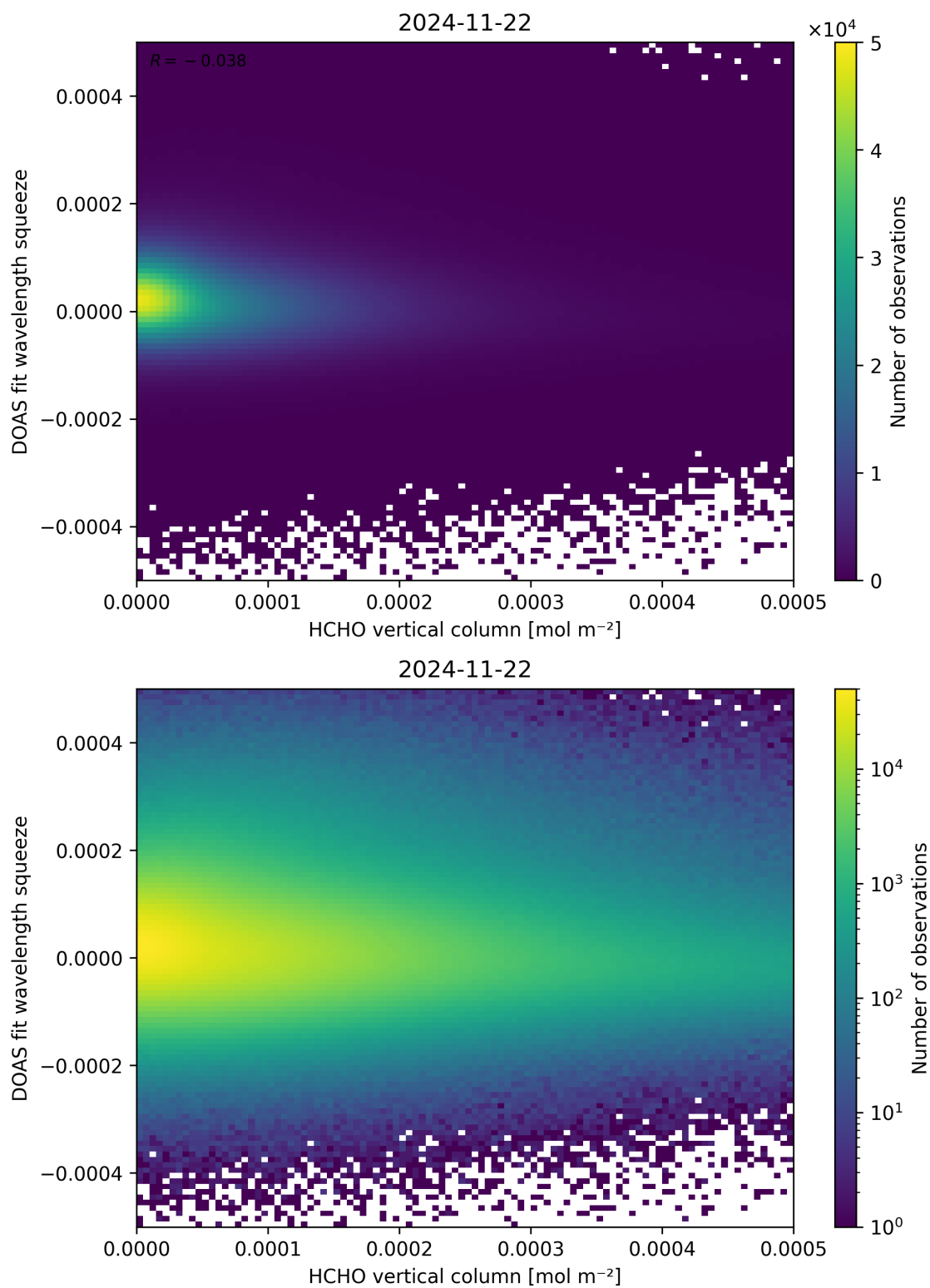
Figure 125: Scatter density plot of “HCHO vertical column” against “DOAS fit wavelength squeeze” for 2024-11-21 to 2024-11-23.
