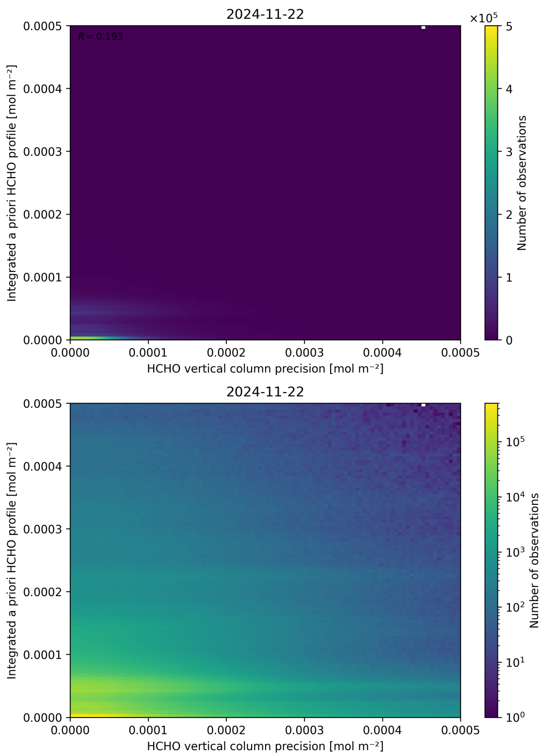
Figure 147: Scatter density plot of “HCHO vertical column precision” against “Integrated a priori HCHO profile” for 2024-11-21 to 2024-11-23.
