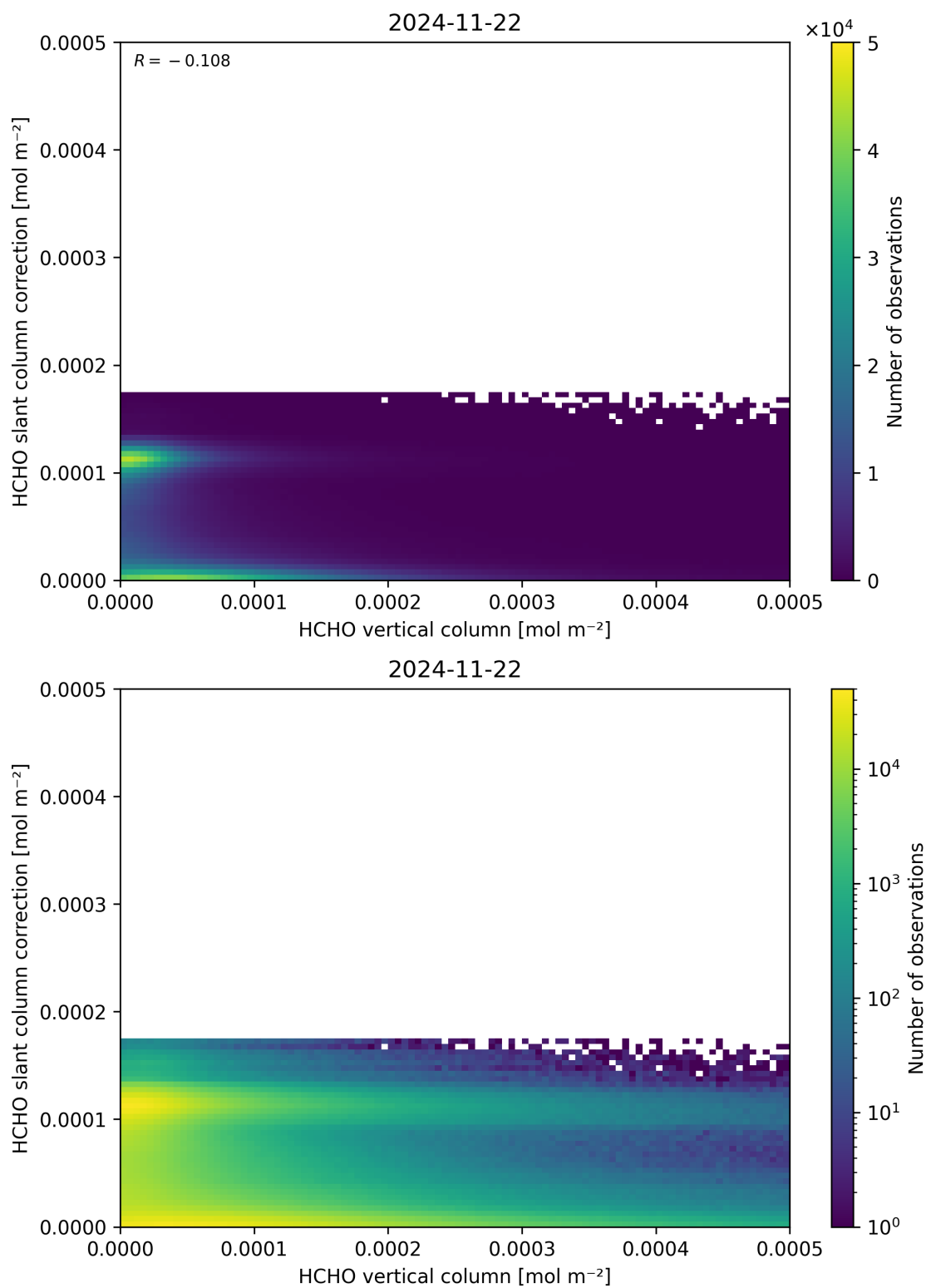
Figure 128: Scatter density plot of “HCHO vertical column” against “HCHO slant column correction” for 2024-11-21 to 2024-11-23.
