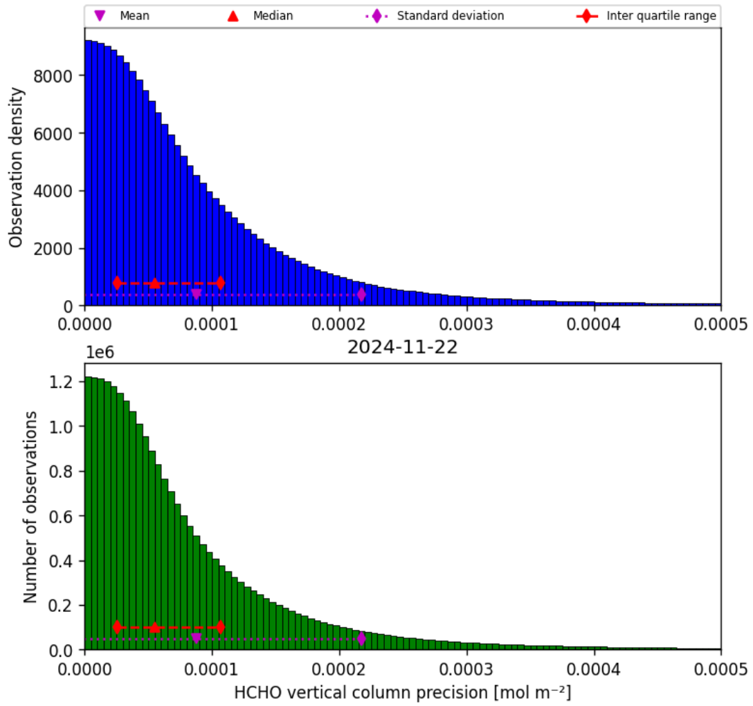
Figure 36: Histogram of “HCHO vertical column precision” for 2024-11-21 to 2024-11-23
