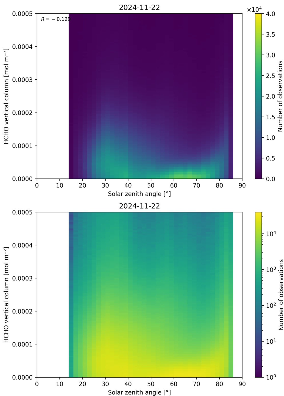
Figure 177: Scatter density plot of “Solar zenith angle” against “HCHO vertical column” for 2024-11-21 to 2024-11-23.
