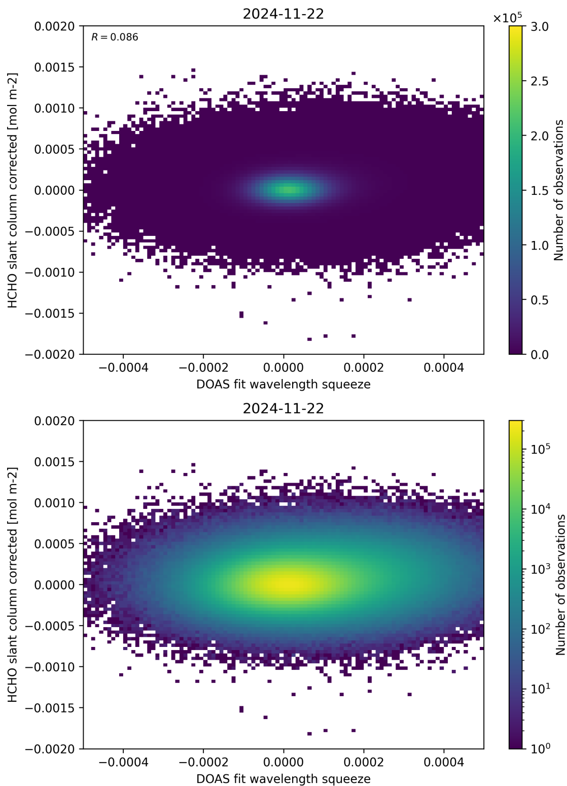
Figure 69: Scatter density plot of “DOAS fit wavelength squeeze” against “HCHO slant column corrected” for 2024-11-21 to 2024-11-23.
