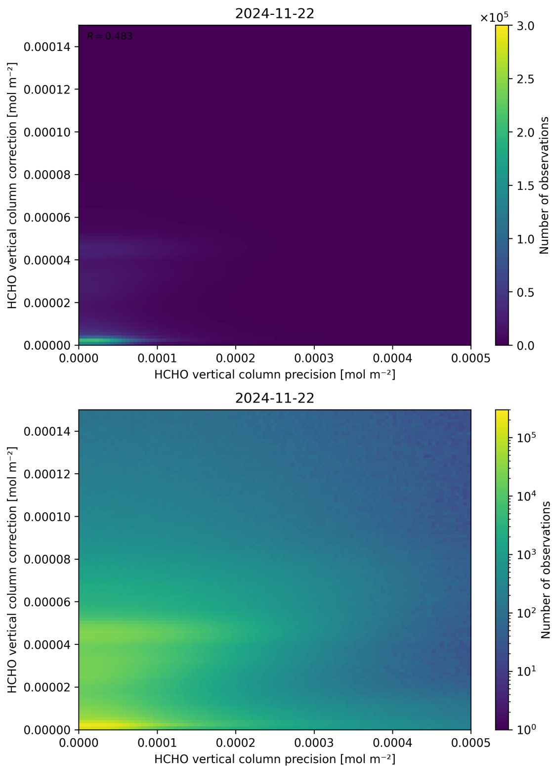
Figure 146: Scatter density plot of “HCHO vertical column precision” against “HCHO vertical column correction” for 2024-11-21 to 2024-11-23.
