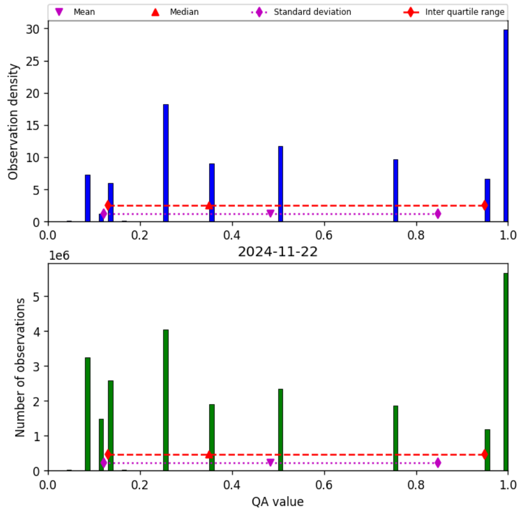
Figure 34: Histogram of “QA value” for 2024-11-21 to 2024-11-23
