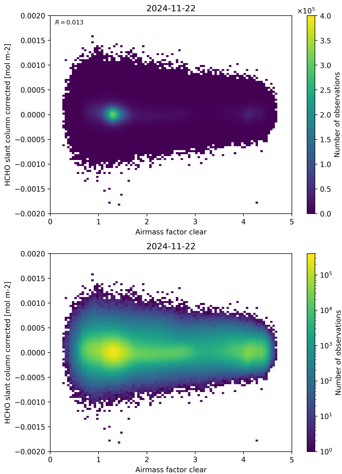
Figure 74: Scatter density plot of “Airmass factor clear” against “HCHO slant column corrected” for 2024-11-21 to 2024-11-23.
