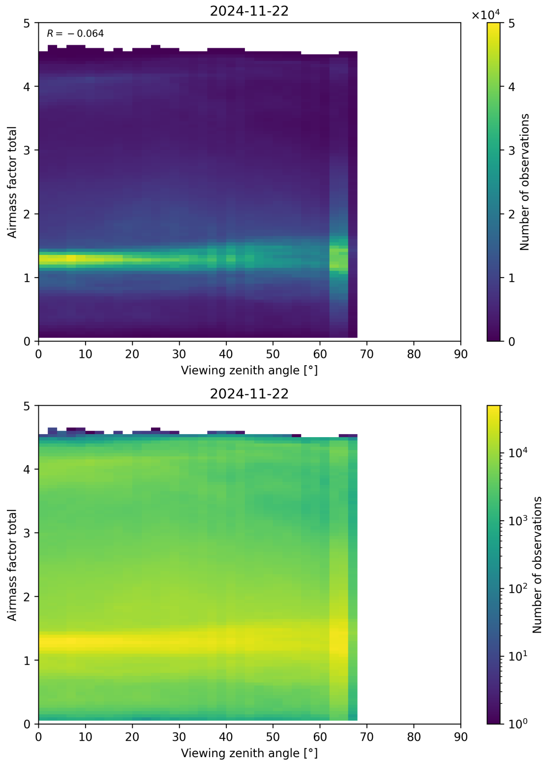
Figure 190: Scatter density plot of “Viewing zenith angle” against “Airmass factor total” for 2024-11-21 to 2024-11-23.
