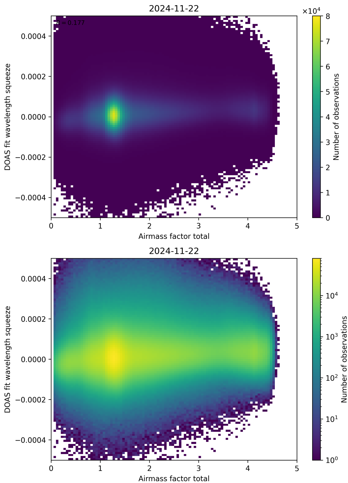
Figure 99: Scatter density plot of “Airmass factor total” against “DOAS fit wavelength squeeze” for 2024-11-21 to 2024-11-23.
