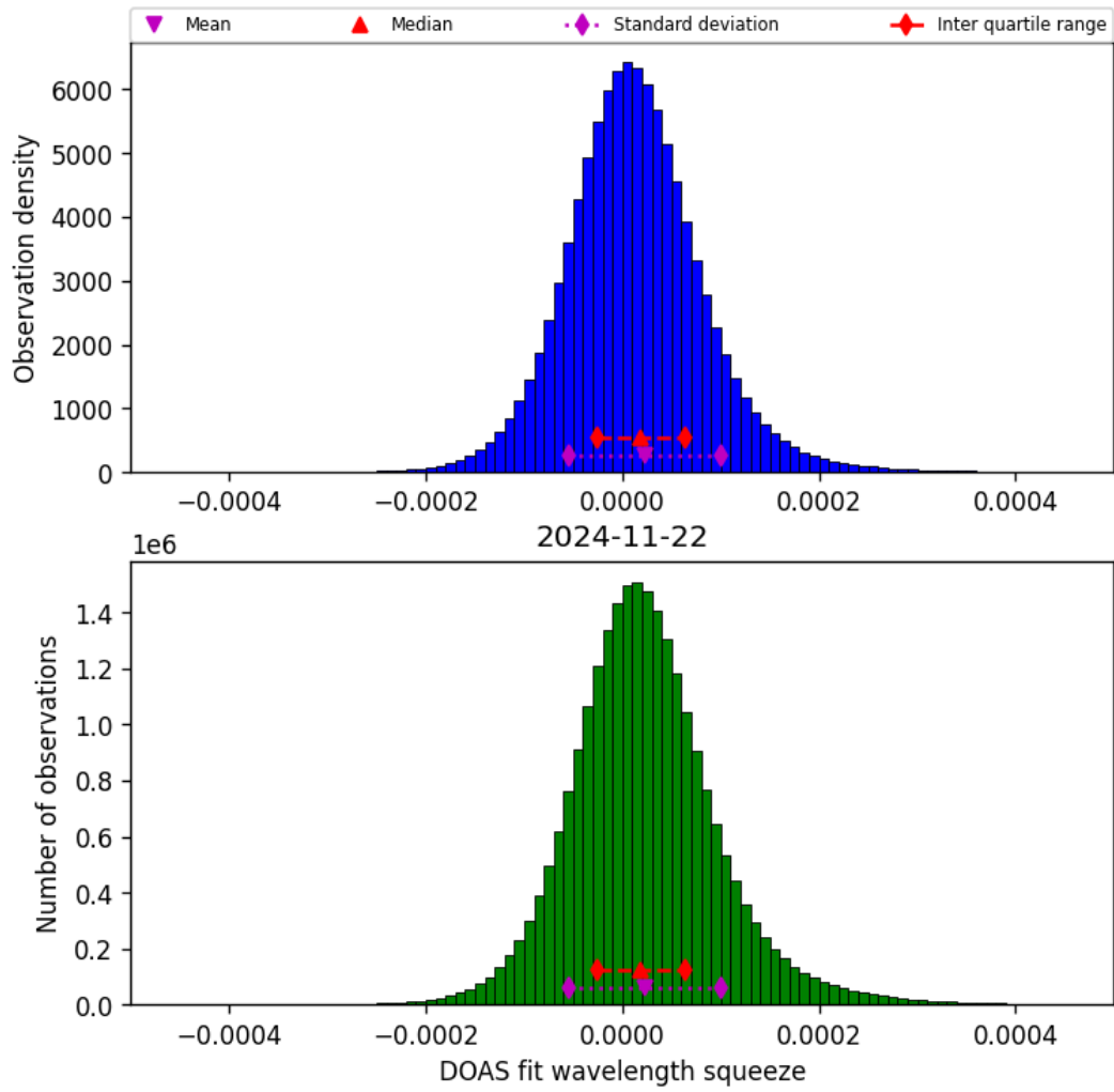
Figure 45: Histogram of “DOAS fit wavelength squeeze” for 2024-11-21 to 2024-11-23
