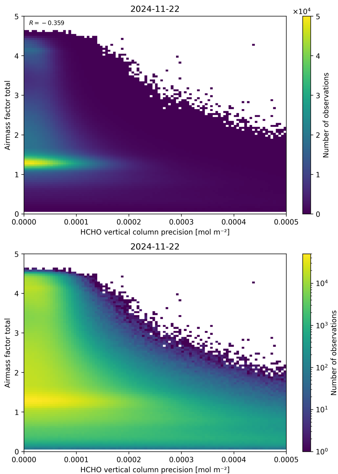
Figure 144: Scatter density plot of “HCHO vertical column precision” against “Airmass factor total” for 2024-11-21 to 2024-11-23.
