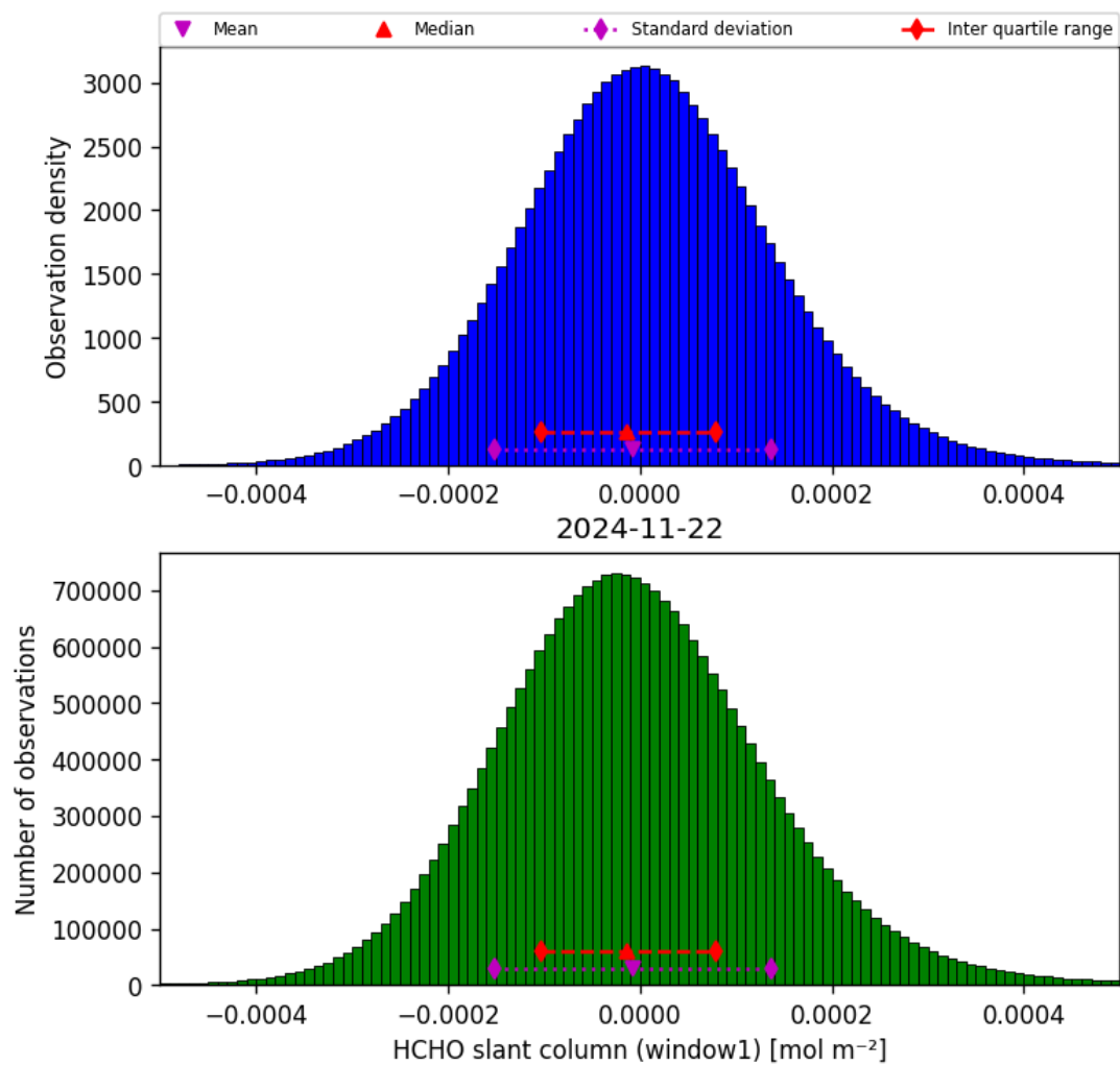
Figure 38: Histogram of “HCHO slant column (window1)” for 2024-11-21 to 2024-11-23
