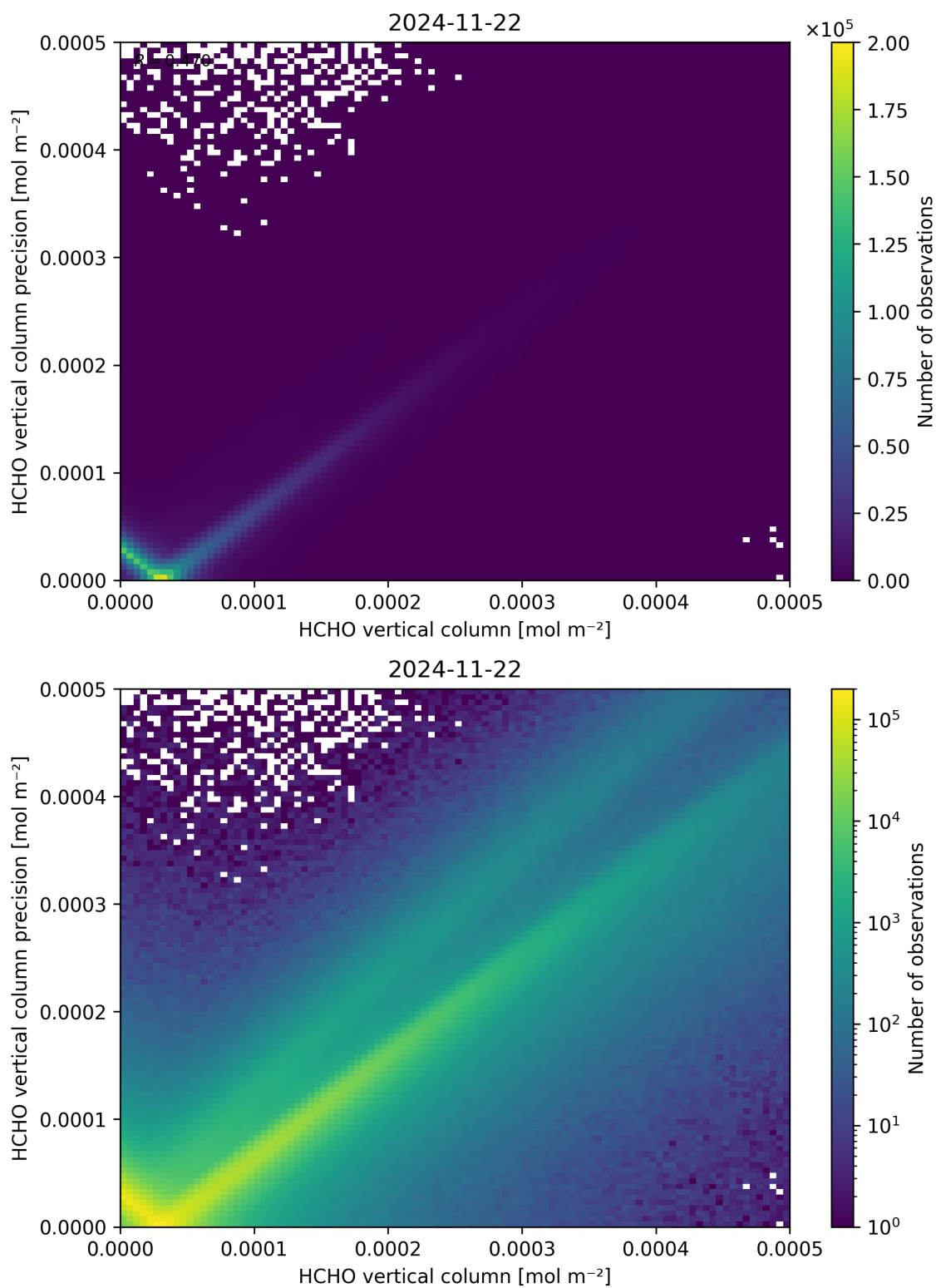
Figure 134: Scatter density plot of “HCHO vertical column” against “HCHO vertical column precision” for 2024-11-21 to 2024-11-23.
