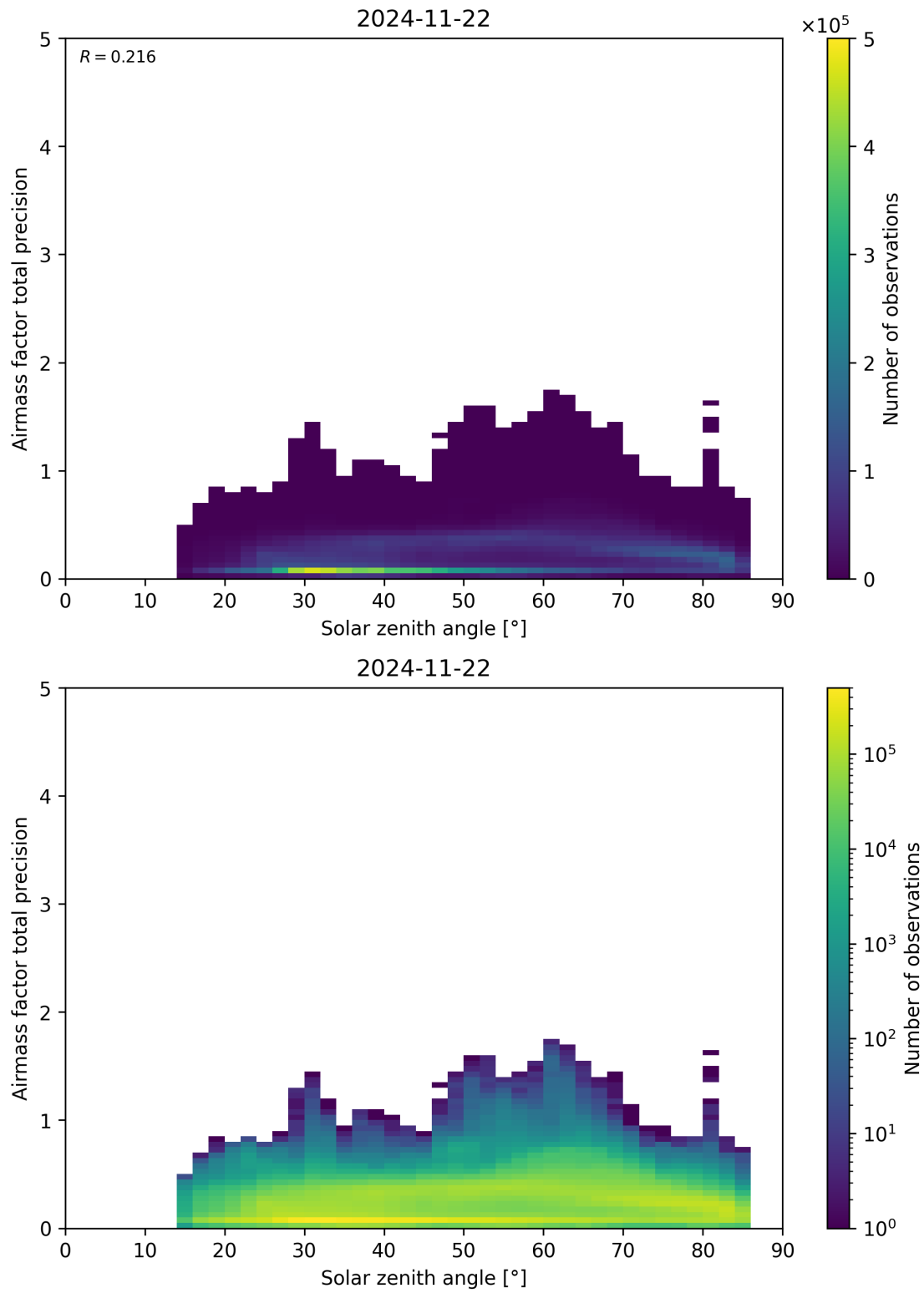
Figure 176: Scatter density plot of “Solar zenith angle” against “Airmass factor total precision” for 2024-11-21 to 2024-11-23.
