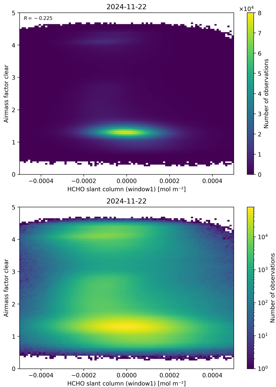
Figure 81: Scatter density plot of “HCHO slant column (window1)” against “Airmass factor clear” for 2024-11-21 to 2024-11-23.
