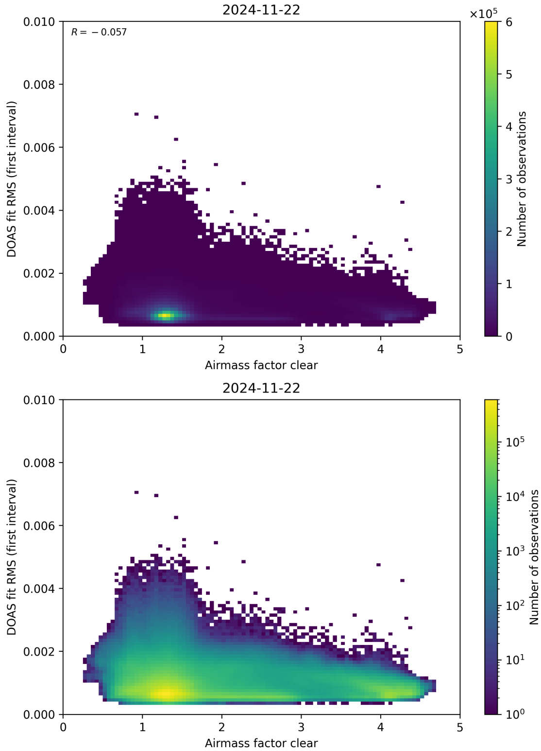
Figure 71: Scatter density plot of “Airmass factor clear” against “DOAS fit RMS (first interval)” for 2024-11-21 to 2024-11-23.
