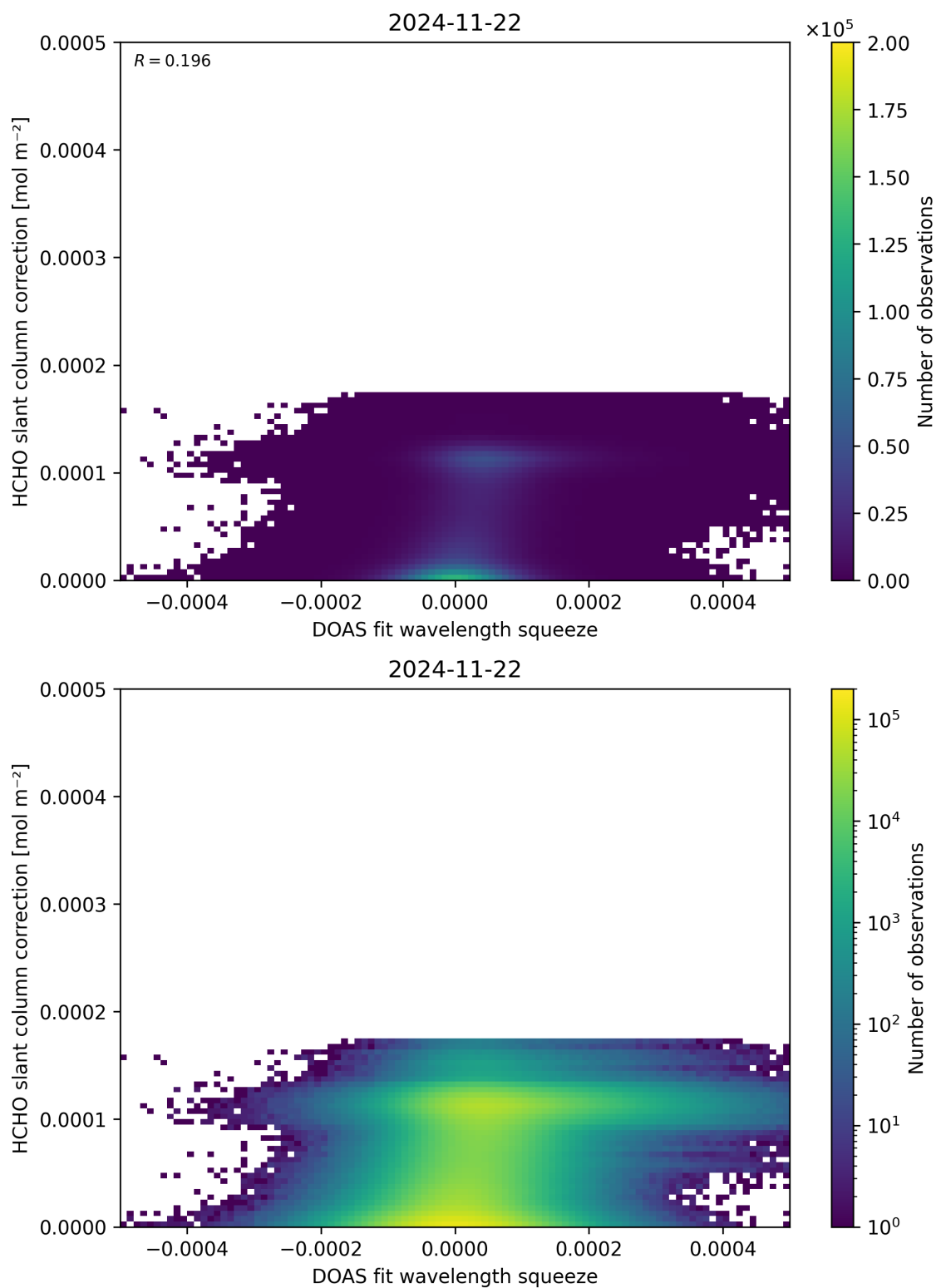
Figure 70: Scatter density plot of “DOAS fit wavelength squeeze” against “HCHO slant column correction” for 2024-11-21 to 2024-11-23.
