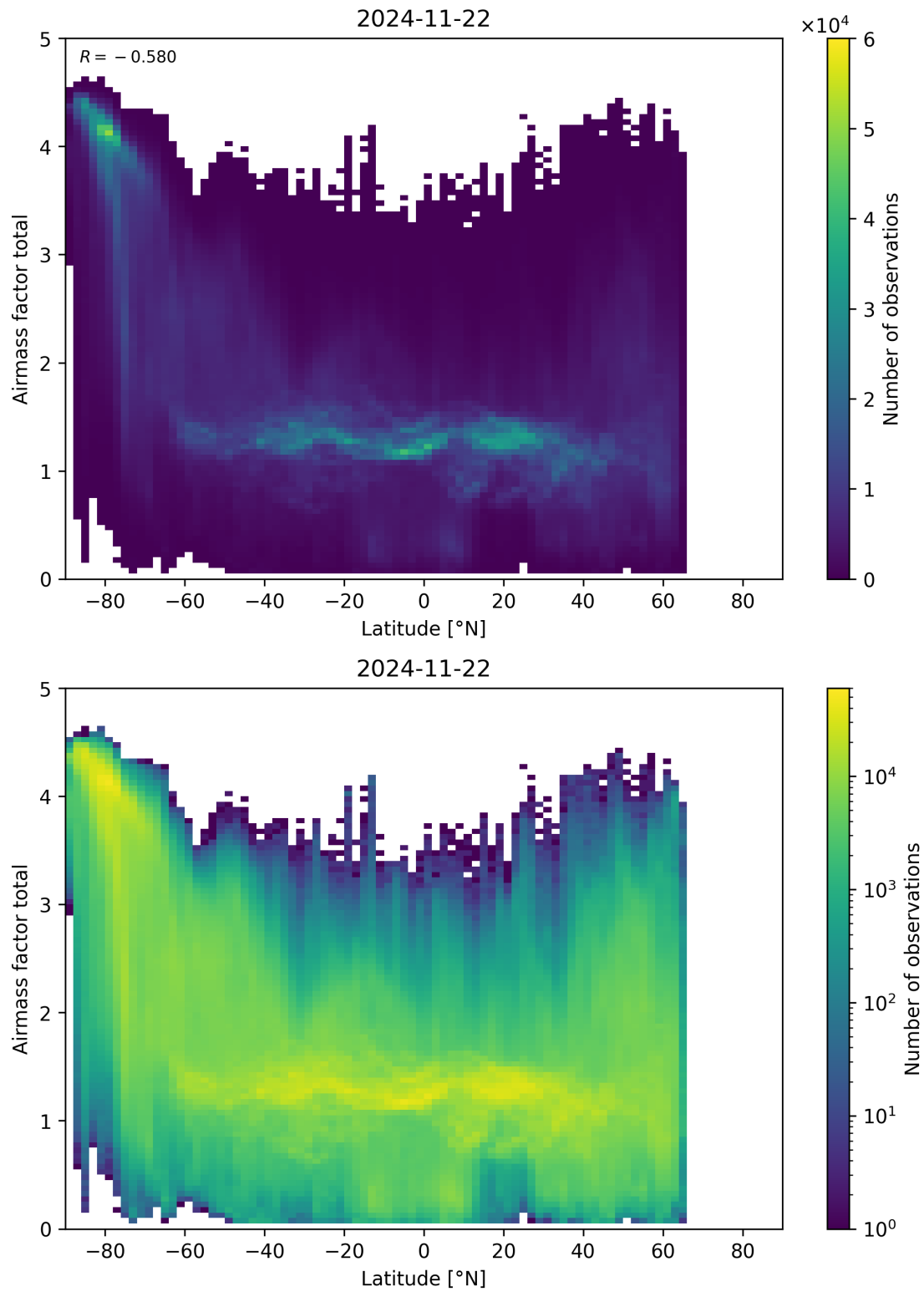
Figure 161: Scatter density plot of “Latitude” against “Airmass factor total” for 2024-11-21 to 2024-11-23.
