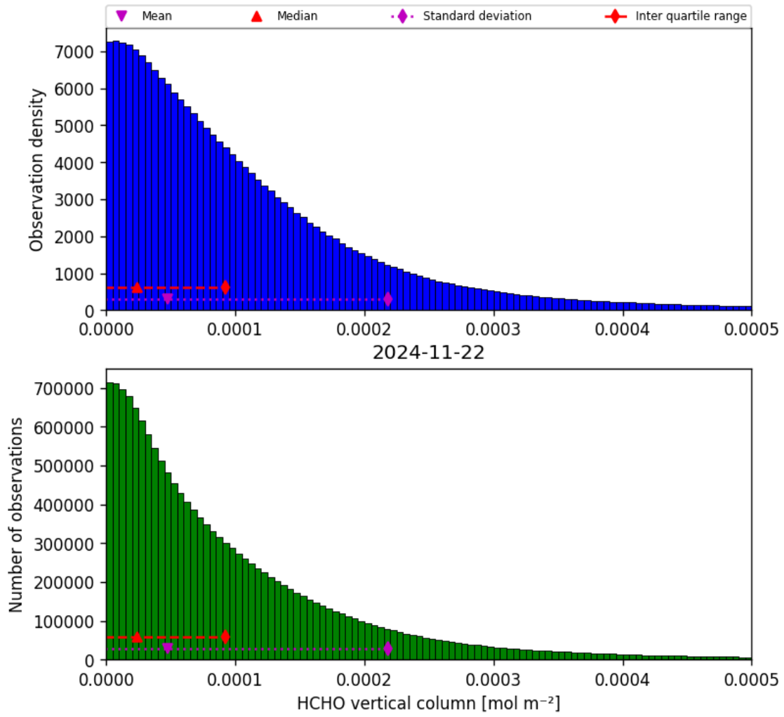
Figure 35: Histogram of “HCHO vertical column” for 2024-11-21 to 2024-11-23
