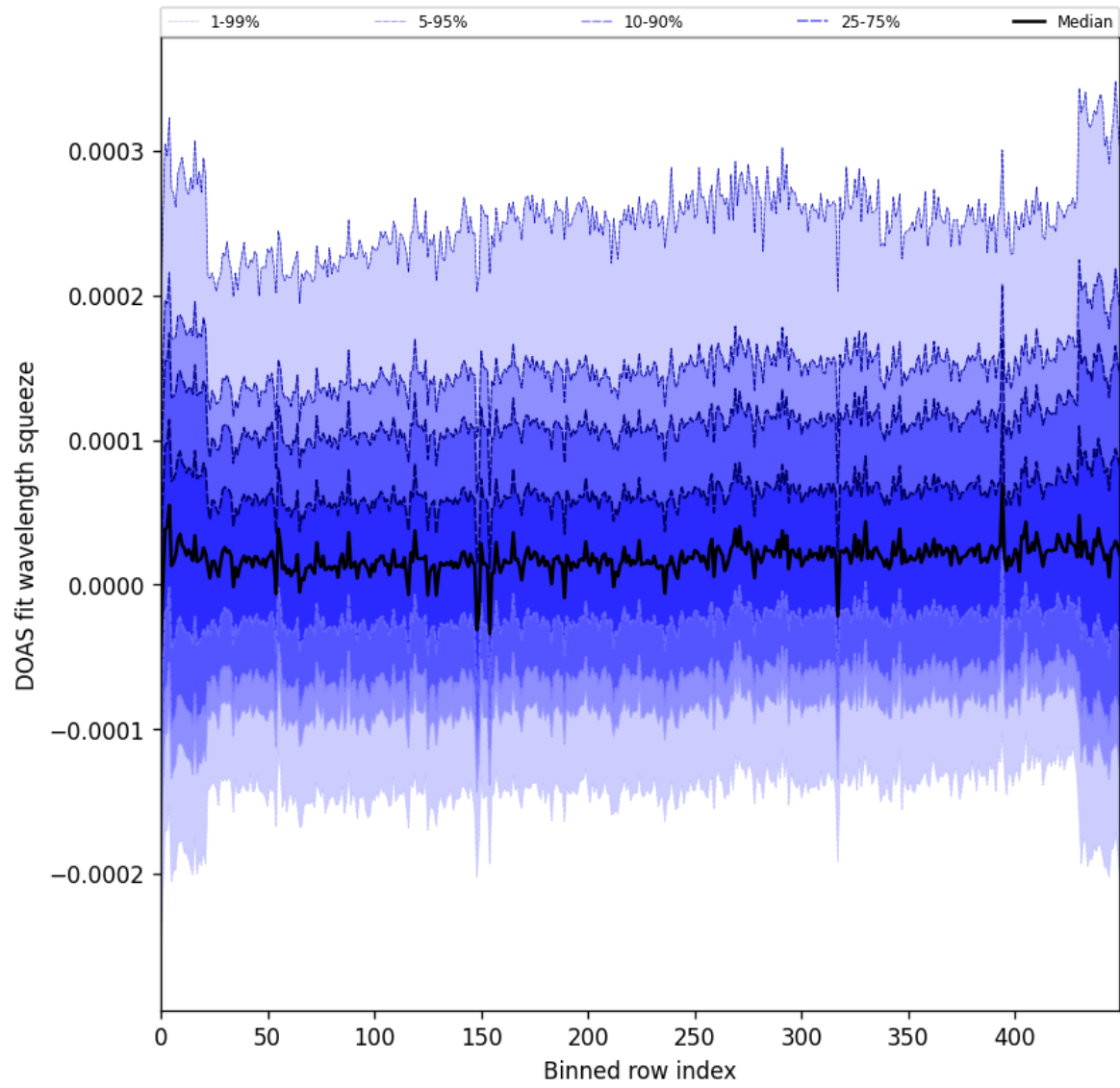
Figure 59: Along track statistics of “DOAS fit wavelength squeeze” for 2024-11-21 to 2024-11-23
