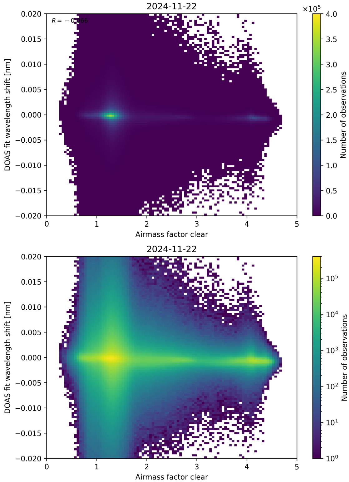
Figure 72: Scatter density plot of “Airmass factor clear” against “DOAS fit wavelength shift” for 2024-11-21 to 2024-11-23.
