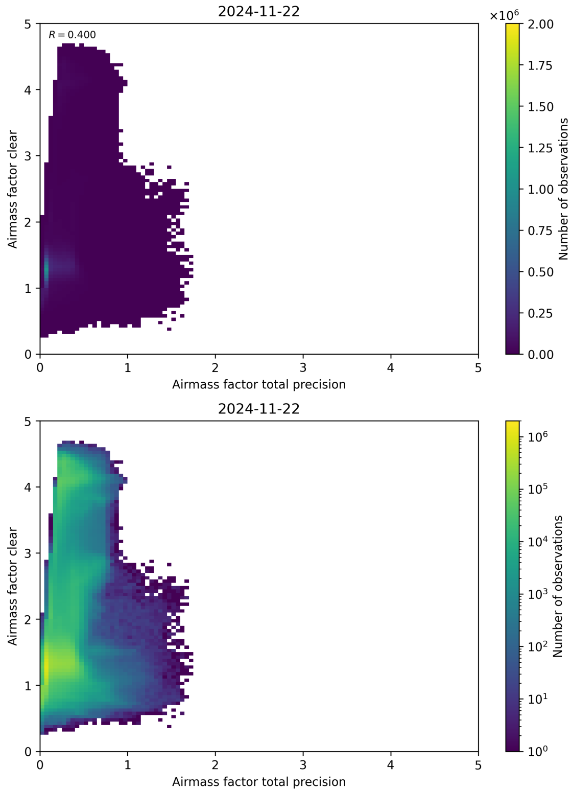
Figure 108: Scatter density plot of “Airmass factor total precision” against “Airmass factor clear” for 2024-11-21 to 2024-11-23.
