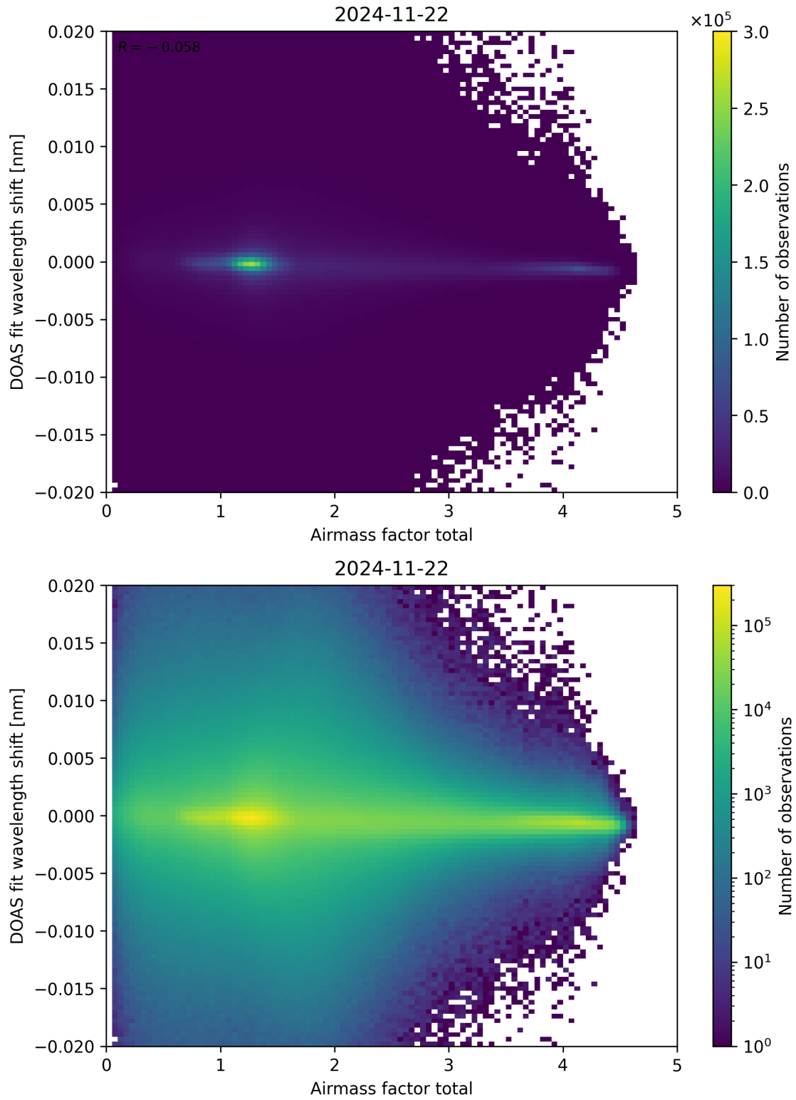
Figure 98: Scatter density plot of “Airmass factor total” against “DOAS fit wavelength shift” for 2024-11-21 to 2024-11-23.
