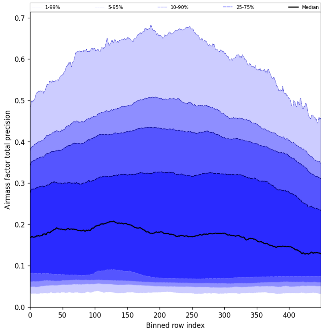
Figure 55: Along track statistics of “Airmass factor total precision” for 2024-11-21 to 2024-11-23
