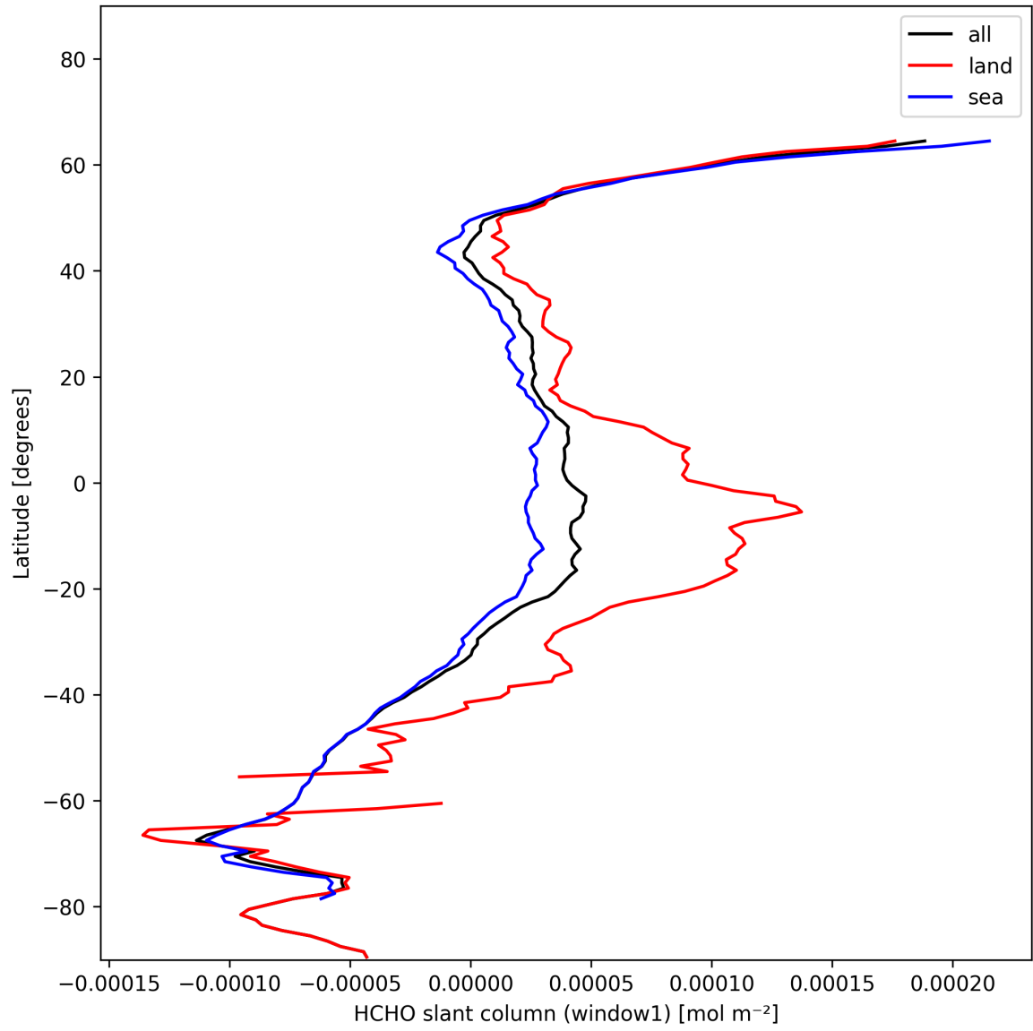
Figure 24: Zonal average of “HCHO slant column (window1)” for 2024-11-21 to 2024-11-23.
