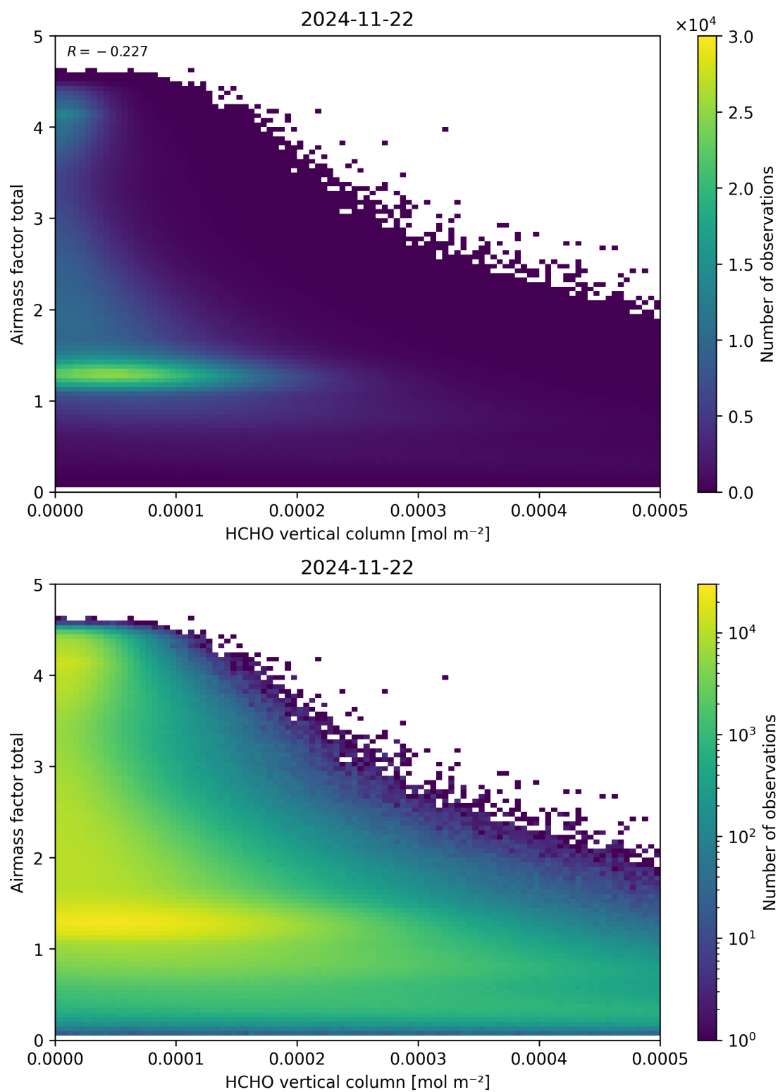
Figure 131: Scatter density plot of “HCHO vertical column” against “Airmass factor total” for 2024-11-21 to 2024-11-23.
