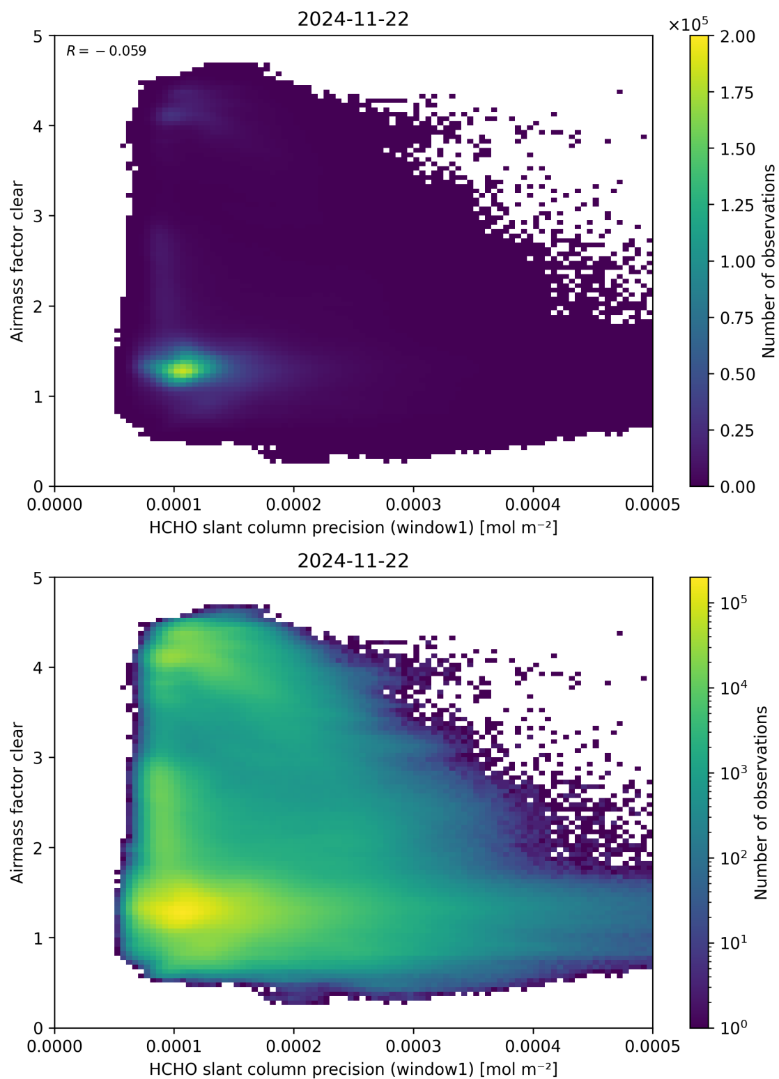
Figure 91: Scatter density plot of “HCHO slant column precision (window1)” against “Airmass factor clear” for 2024-11-21 to 2024-11-23.
