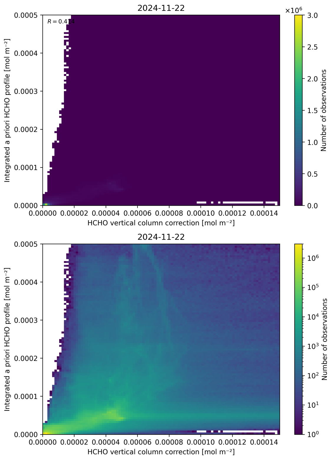
Figure 122: Scatter density plot of “HCHO vertical column correction” against “Integrated a priori HCHO profile” for 2024-11-21 to 2024-11-23.
