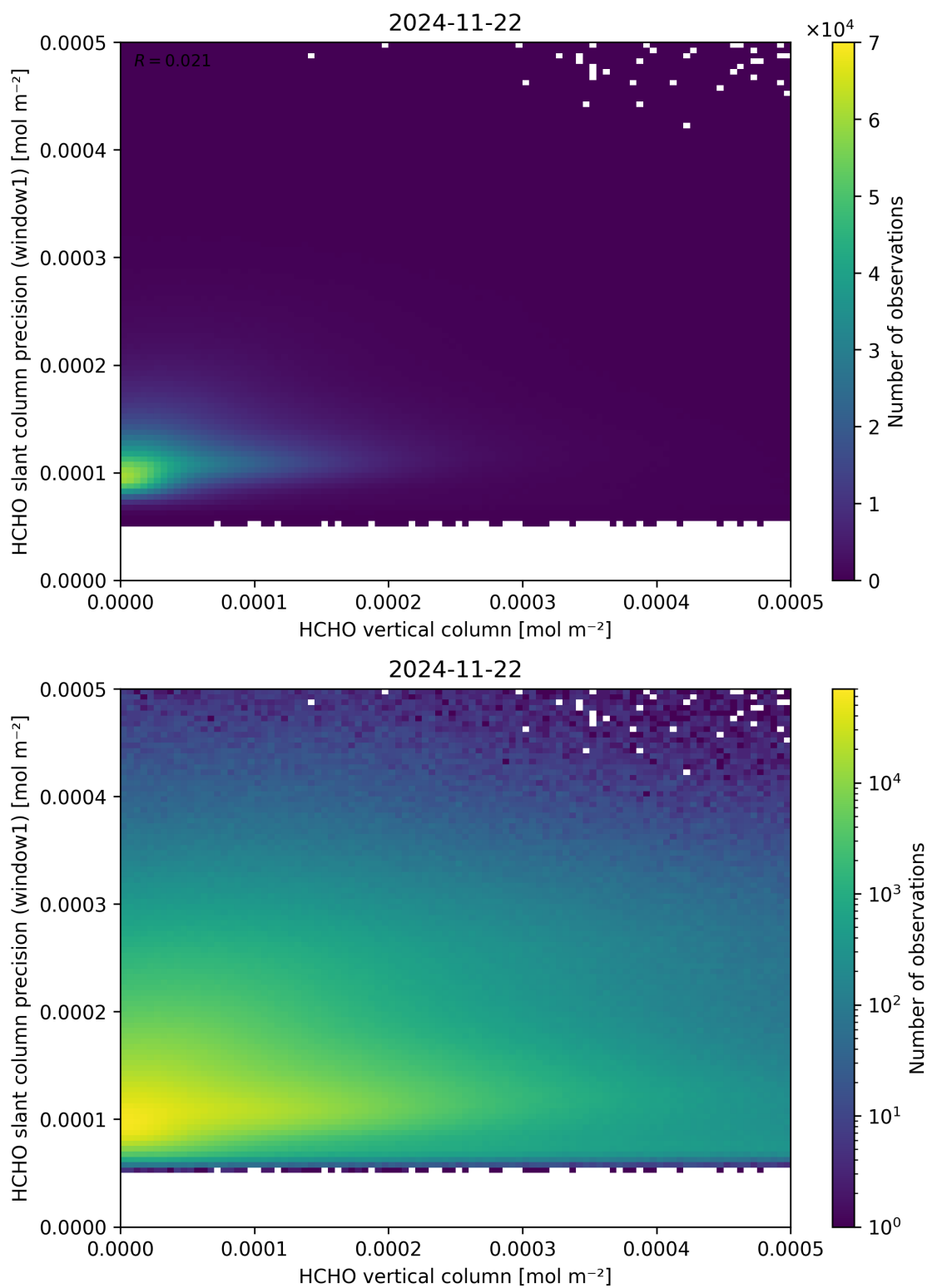
Figure 130: Scatter density plot of “HCHO vertical column” against “HCHO slant column precision (window1)” for 2024-11-21 to 2024-11-23.
