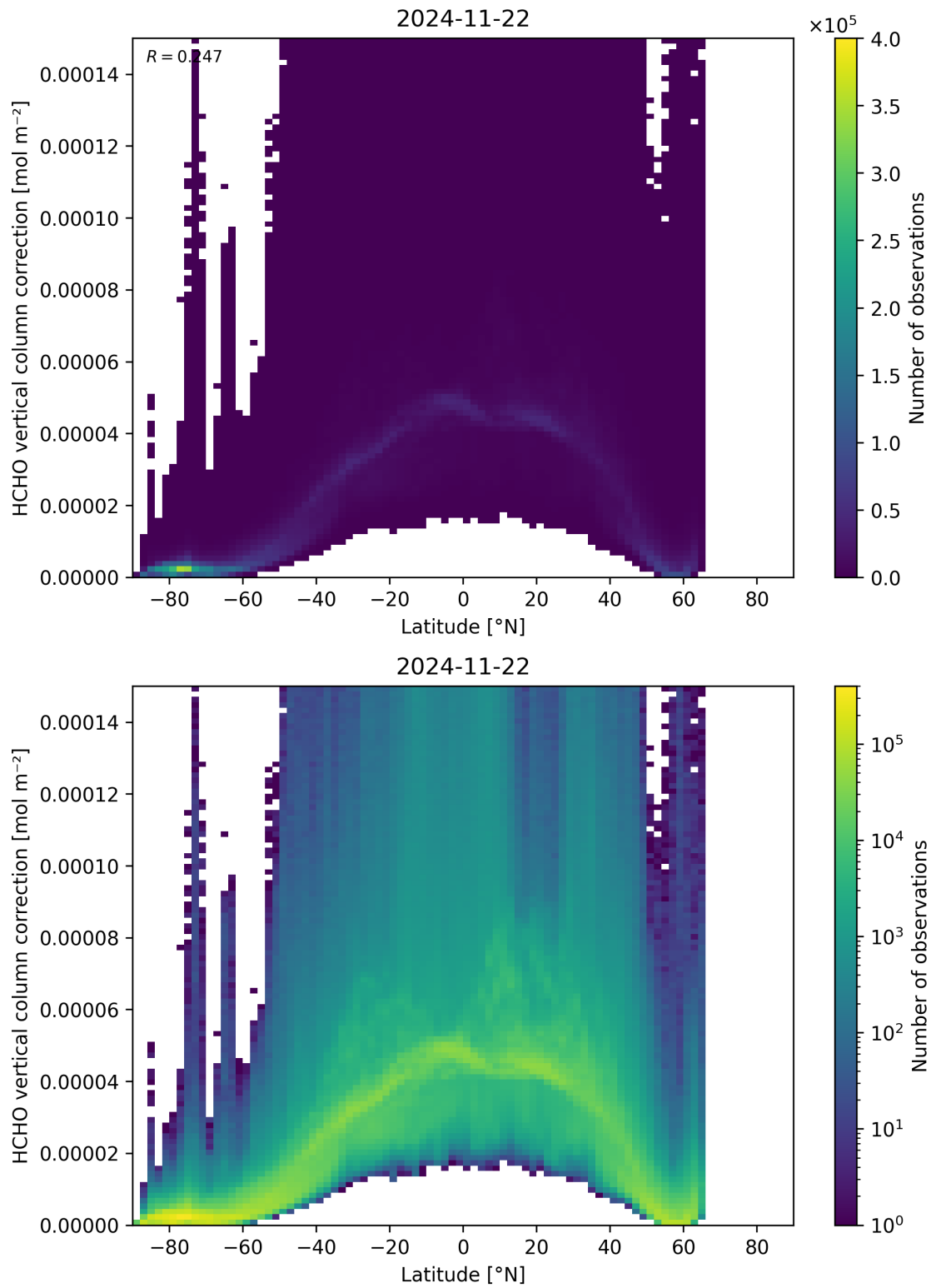
Figure 164: Scatter density plot of “Latitude” against “HCHO vertical column correction” for 2024-11-21 to 2024-11-23.
