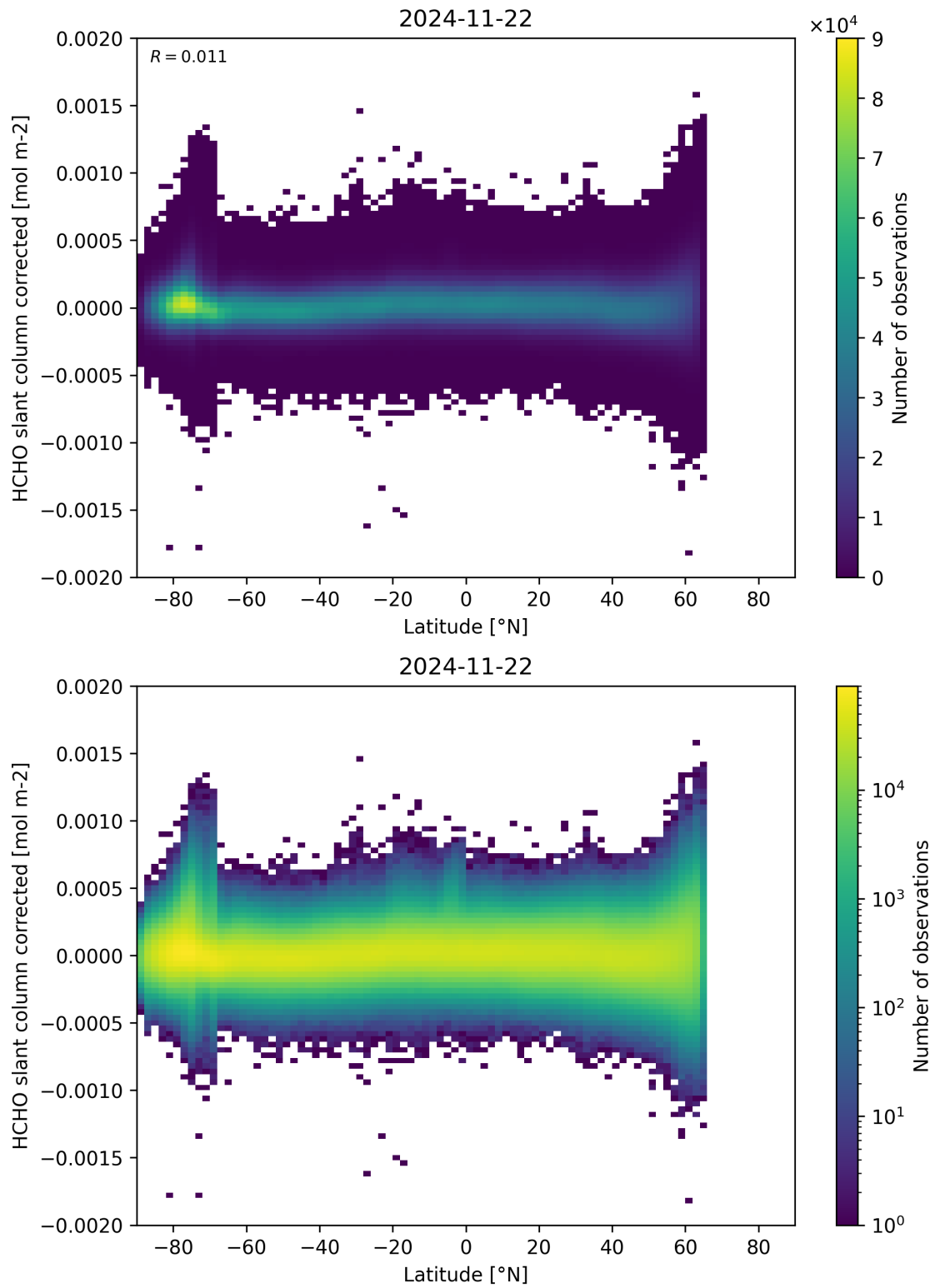
Figure 157: Scatter density plot of “Latitude” against “HCHO slant column corrected” for 2024-11-21 to 2024-11-23.
