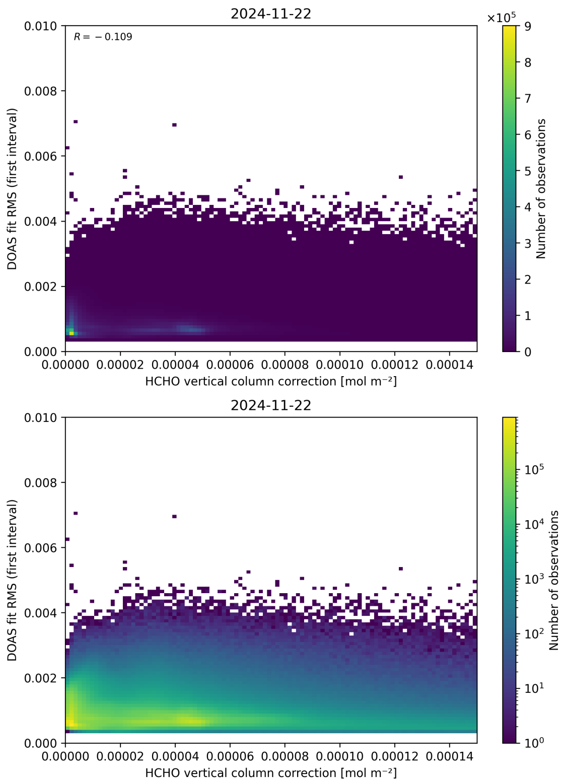
Figure 112: Scatter density plot of “HCHO vertical column correction” against “DOAS fit RMS (first interval)” for 2024-11-21 to 2024-11-23.
