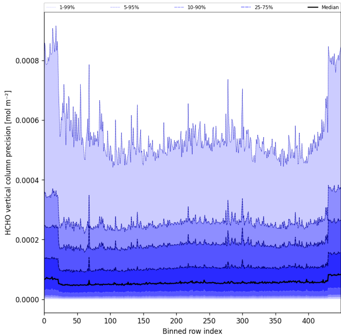
Figure 50: Along track statistics of “HCHO vertical column precision” for 2024-11-21 to 2024-11-23
