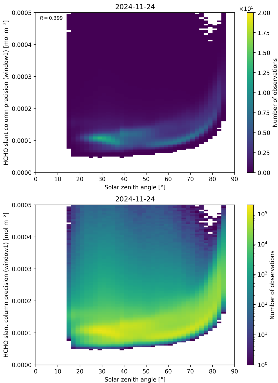
Figure 174: Scatter density plot of “Solar zenith angle” against “HCHO slant column precision (window1)” for 2024-11-23 to 2024-11-25.
