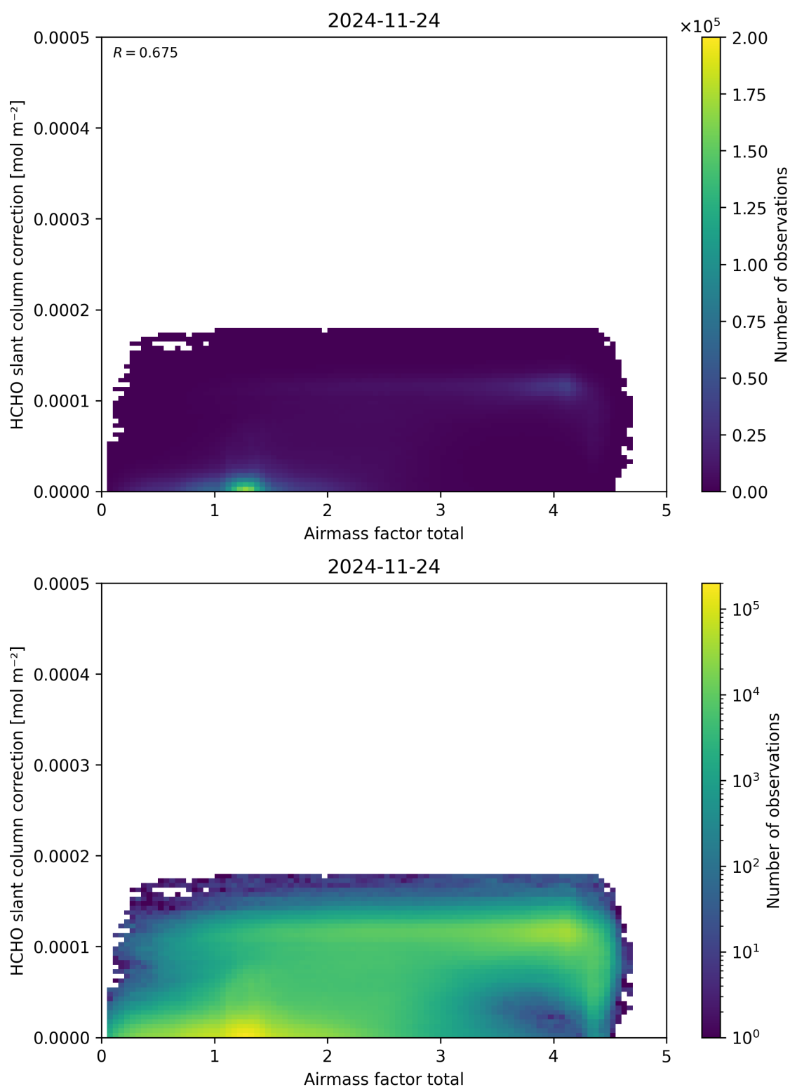
Figure 102: Scatter density plot of “Airmass factor total” against “HCHO slant column correction” for 2024-11-23 to 2024-11-25.
