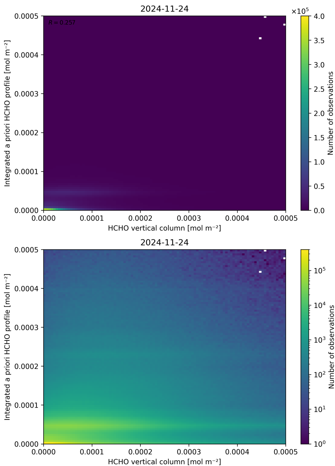
Figure 135: Scatter density plot of “HCHO vertical column” against “Integrated a priori HCHO profile” for 2024-11-23 to 2024-11-25.
