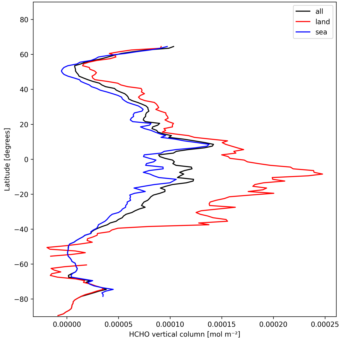
Figure 21: Zonal average of “HCHO vertical column” for 2024-11-23 to 2024-11-25.
