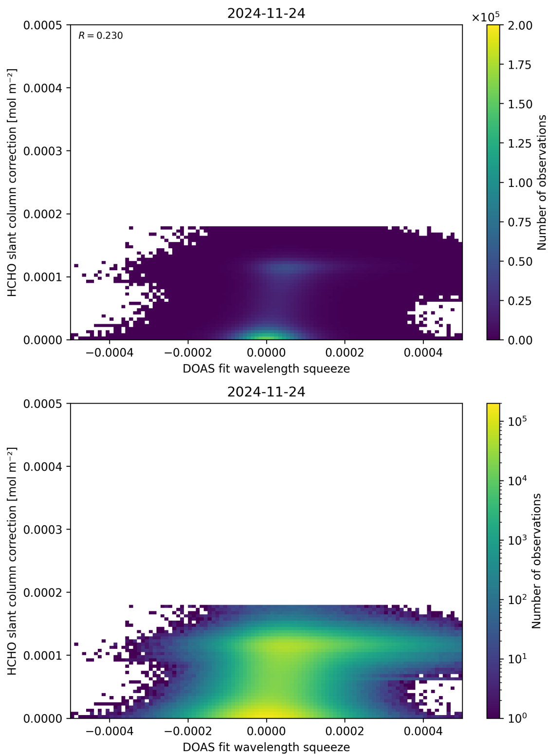
Figure 70: Scatter density plot of “DOAS fit wavelength squeeze” against “HCHO slant column correction” for 2024-11-23 to 2024-11-25.
