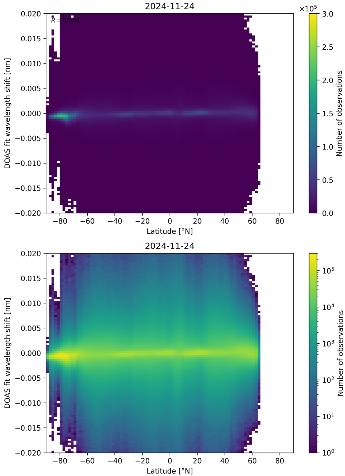
Figure 154: Scatter density plot of “Latitude” against “DOAS fit wavelength shift” for 2024-11-23 to 2024-11-25.
