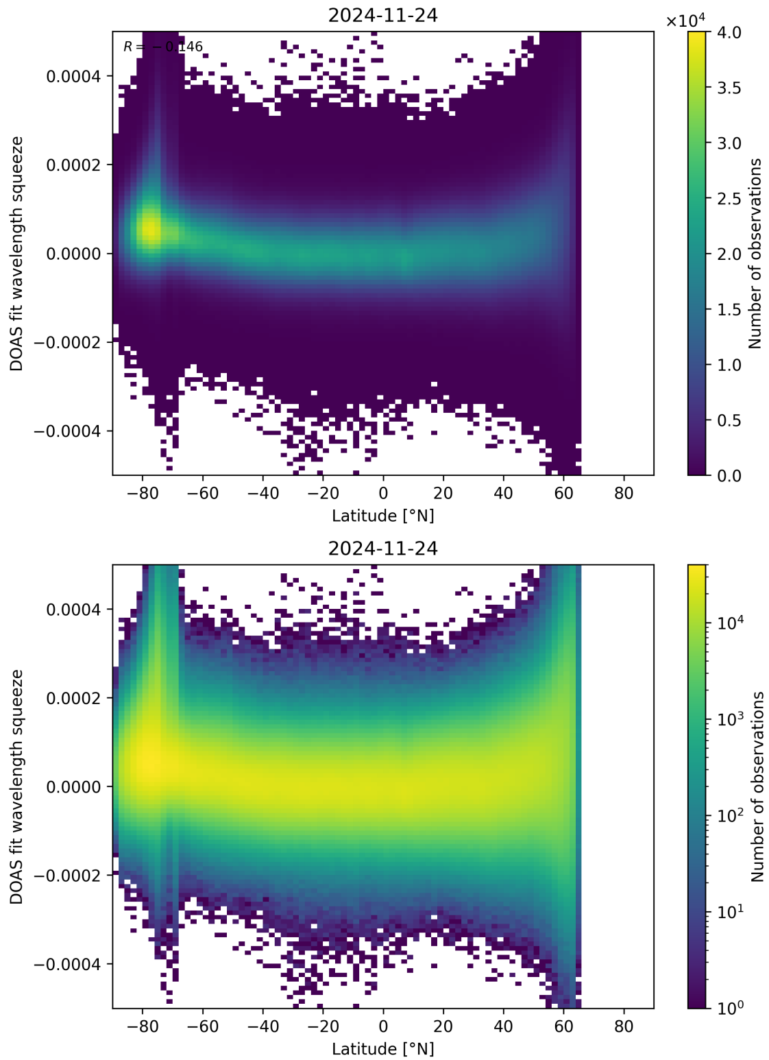
Figure 155: Scatter density plot of “Latitude” against “DOAS fit wavelength squeeze” for 2024-11-23 to 2024-11-25.
