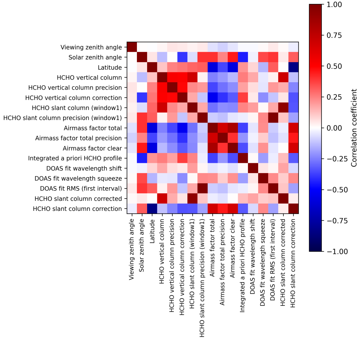
Figure 2: Map of correlation matrix for 2024-11-23 to 2024-11-25.
