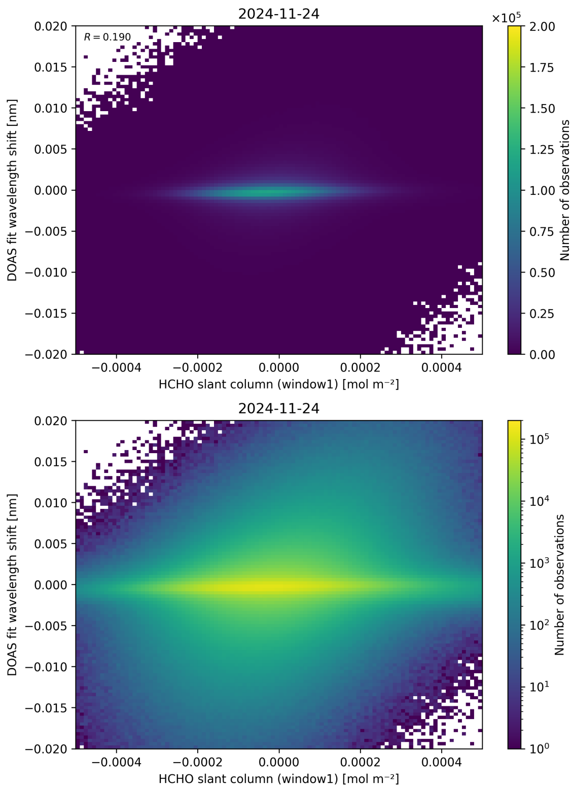
Figure 79: Scatter density plot of “HCHO slant column (window1)” against “DOAS fit wavelength shift” for 2024-11-23 to 2024-11-25.
