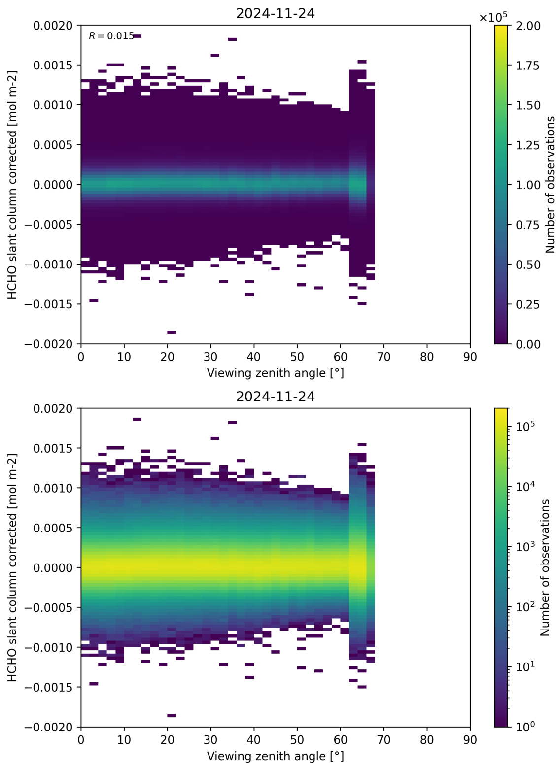
Figure 186: Scatter density plot of “Viewing zenith angle” against “HCHO slant column corrected” for 2024-11-23 to 2024-11-25.
