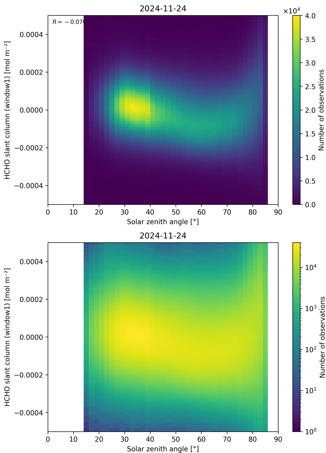
Figure 173: Scatter density plot of “Solar zenith angle” against “HCHO slant column (window1)” for 2024-11-23 to 2024-11-25.
