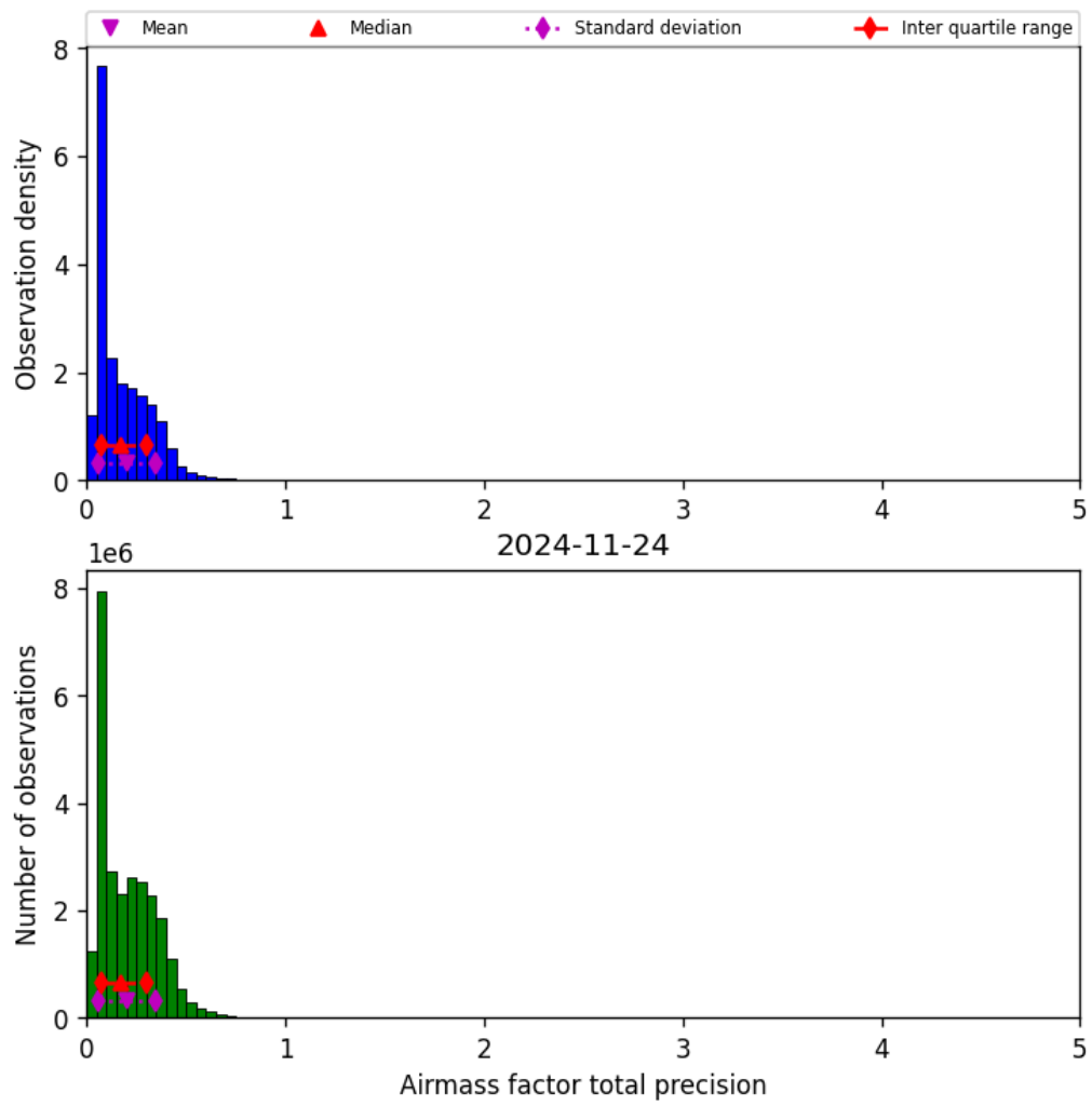
Figure 41: Histogram of “Airmass factor total precision” for 2024-11-23 to 2024-11-25
