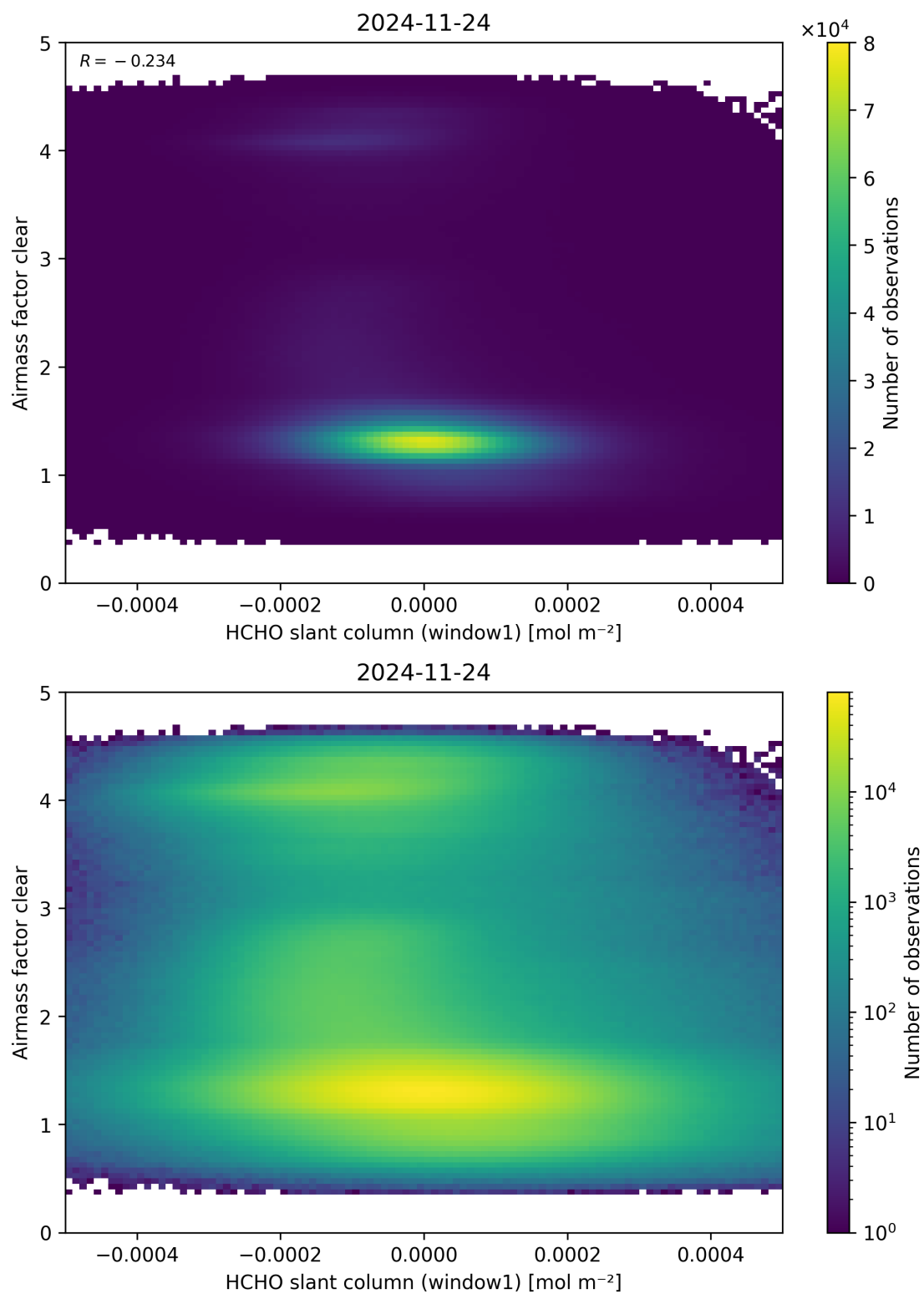
Figure 81: Scatter density plot of “HCHO slant column (window1)” against “Airmass factor clear” for 2024-11-23 to 2024-11-25.
