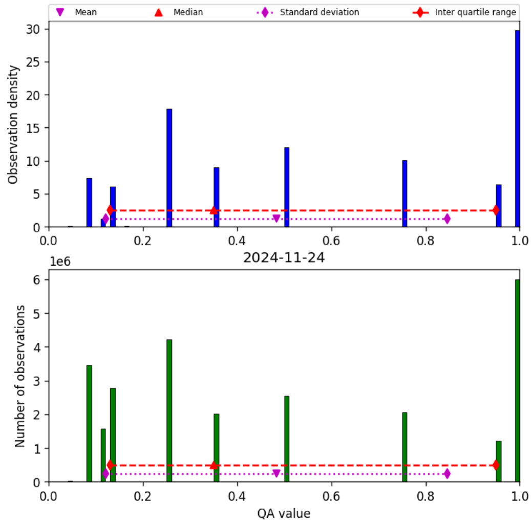
Figure 34: Histogram of “QA value” for 2024-11-23 to 2024-11-25
