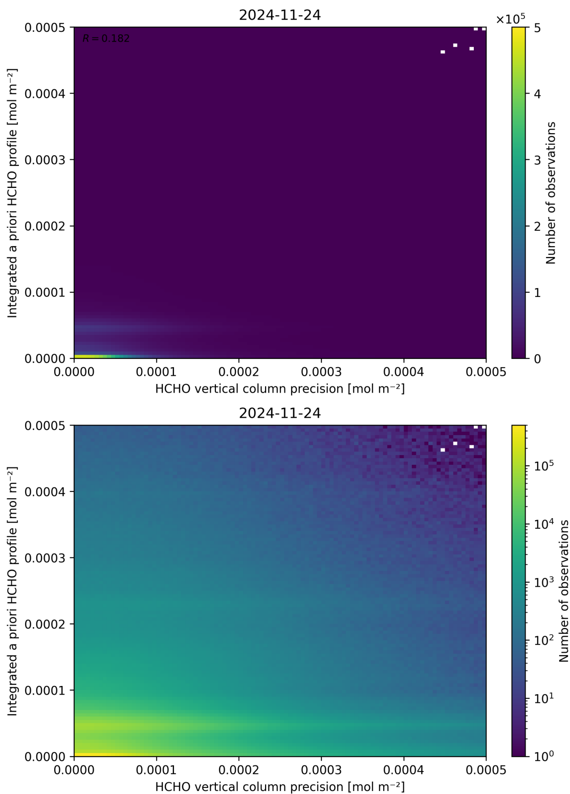
Figure 147: Scatter density plot of “HCHO vertical column precision” against “Integrated a priori HCHO profile” for 2024-11-23 to 2024-11-25.
