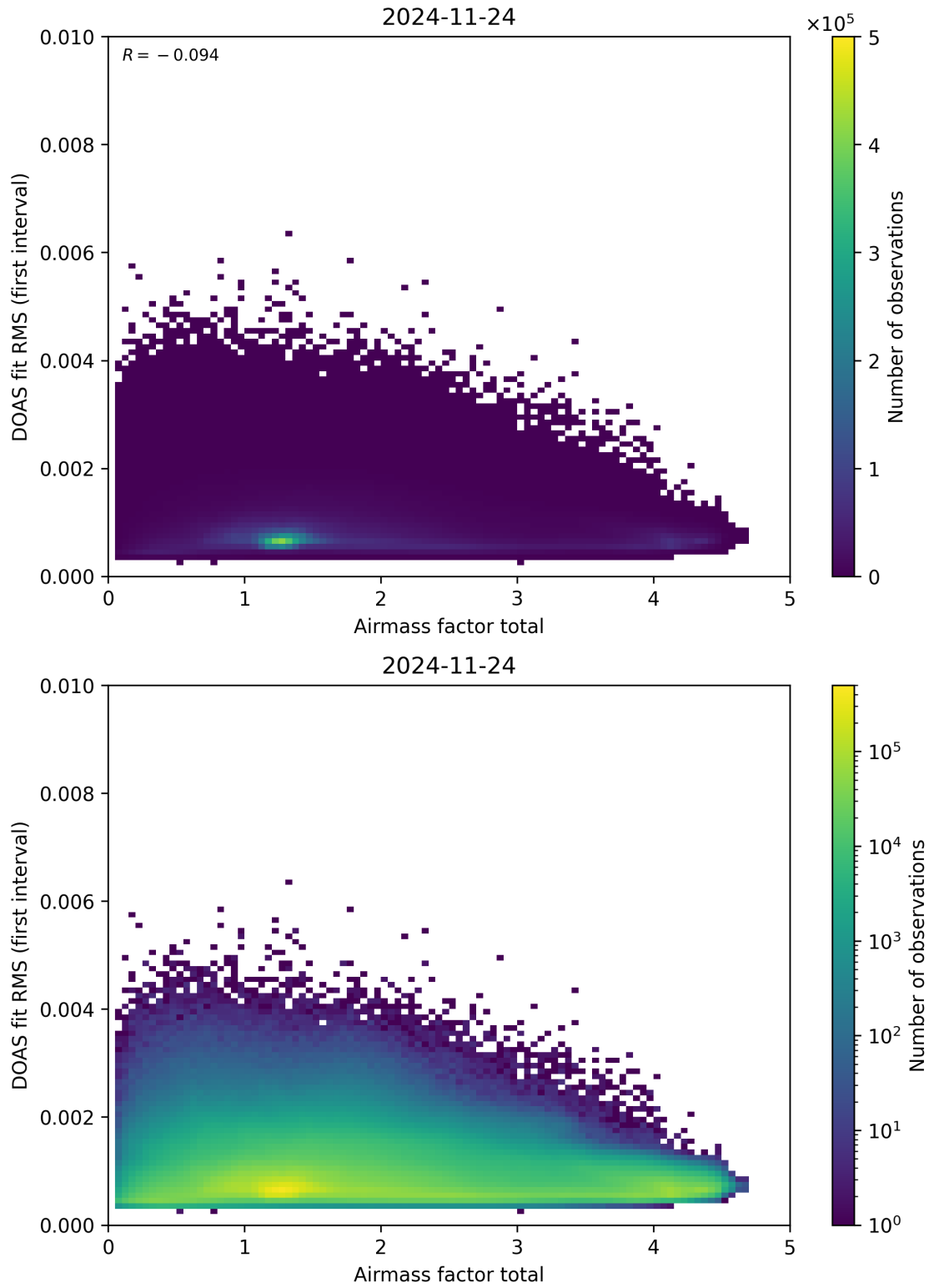
Figure 97: Scatter density plot of “Airmass factor total” against “DOAS fit RMS (first interval)” for 2024-11-23 to 2024-11-25.
