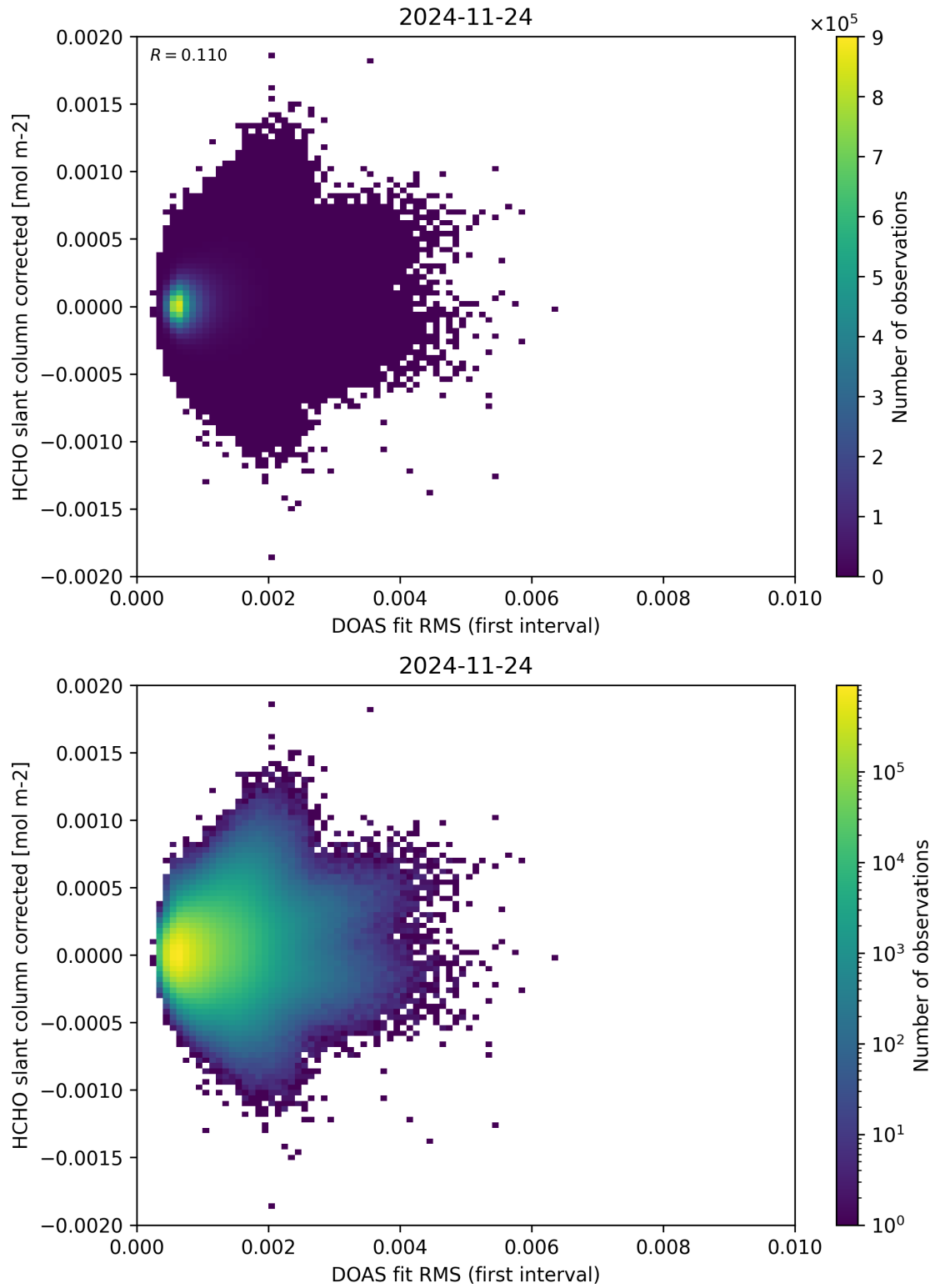
Figure 62: Scatter density plot of “DOAS fit RMS (first interval)” against “HCHO slant column corrected” for 2024-11-23 to 2024-11-25.
