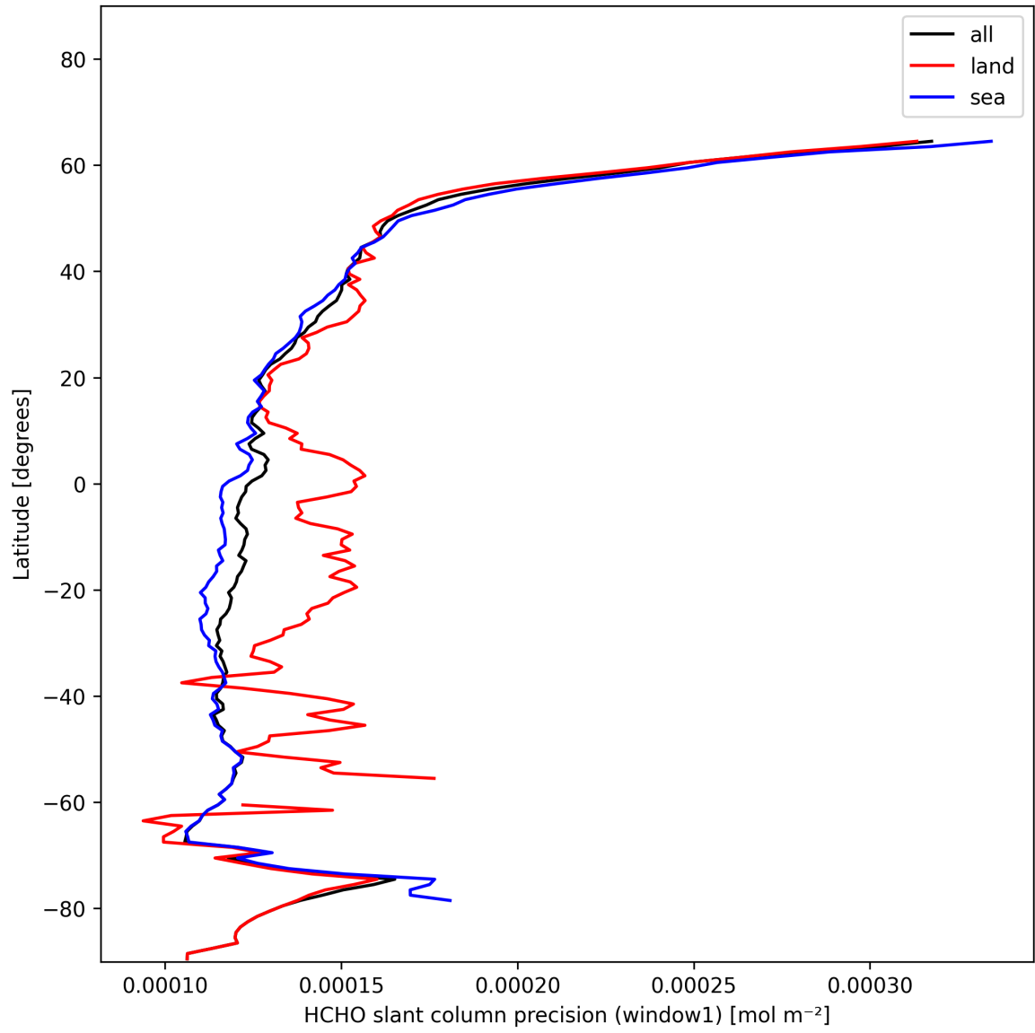
Figure 25: Zonal average of “HCHO slant column precision (window1)” for 2024-11-23 to 2024-11-25.
