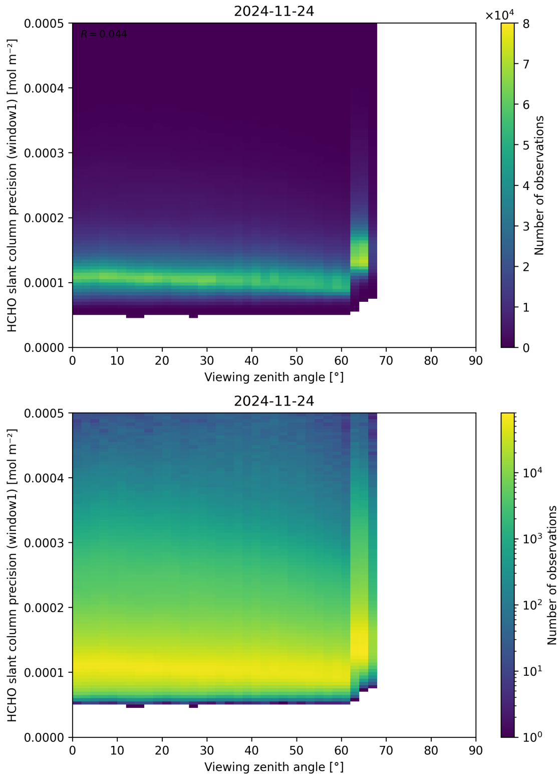
Figure 189: Scatter density plot of “Viewing zenith angle” against “HCHO slant column precision (window1)” for 2024-11-23 to 2024-11-25.
