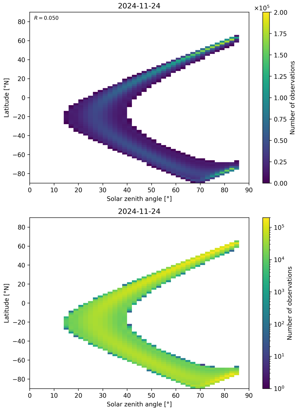
Figure 181: Scatter density plot of “Solar zenith angle” against “Latitude” for 2024-11-23 to 2024-11-25.
