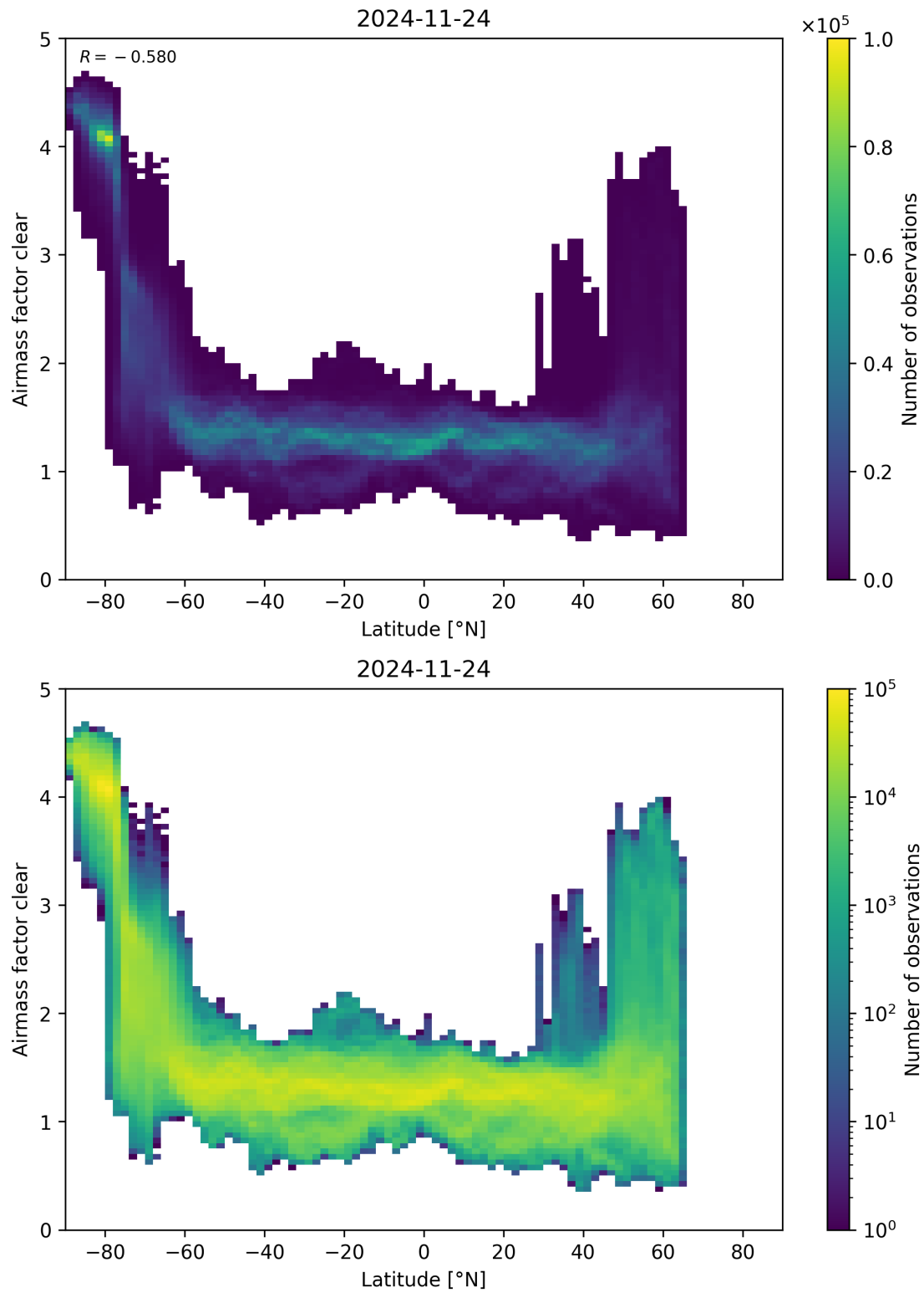
Figure 156: Scatter density plot of “Latitude” against “Airmass factor clear” for 2024-11-23 to 2024-11-25.
