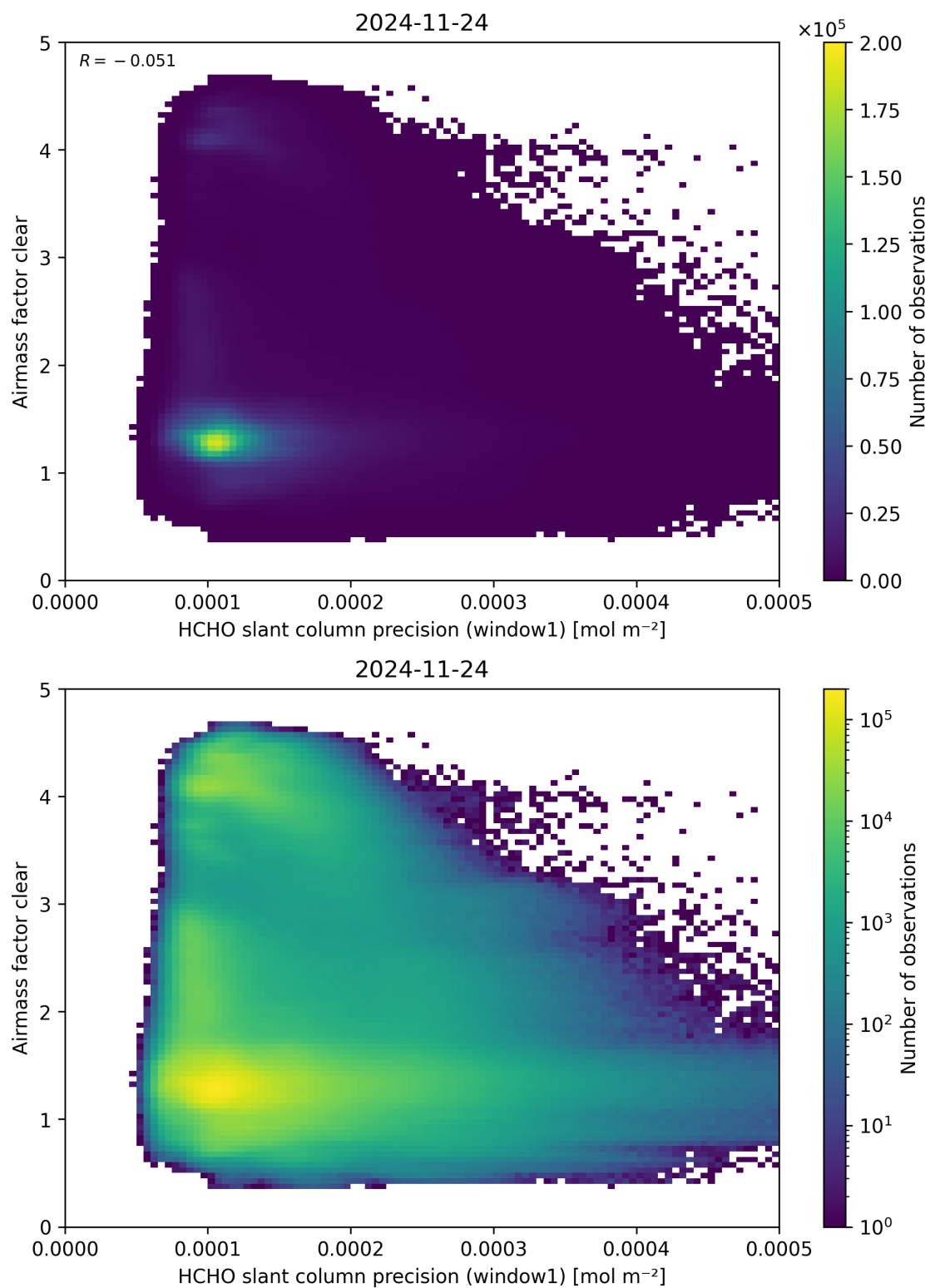
Figure 91: Scatter density plot of “HCHO slant column precision (window1)” against “Airmass factor clear” for 2024-11-23 to 2024-11-25.
