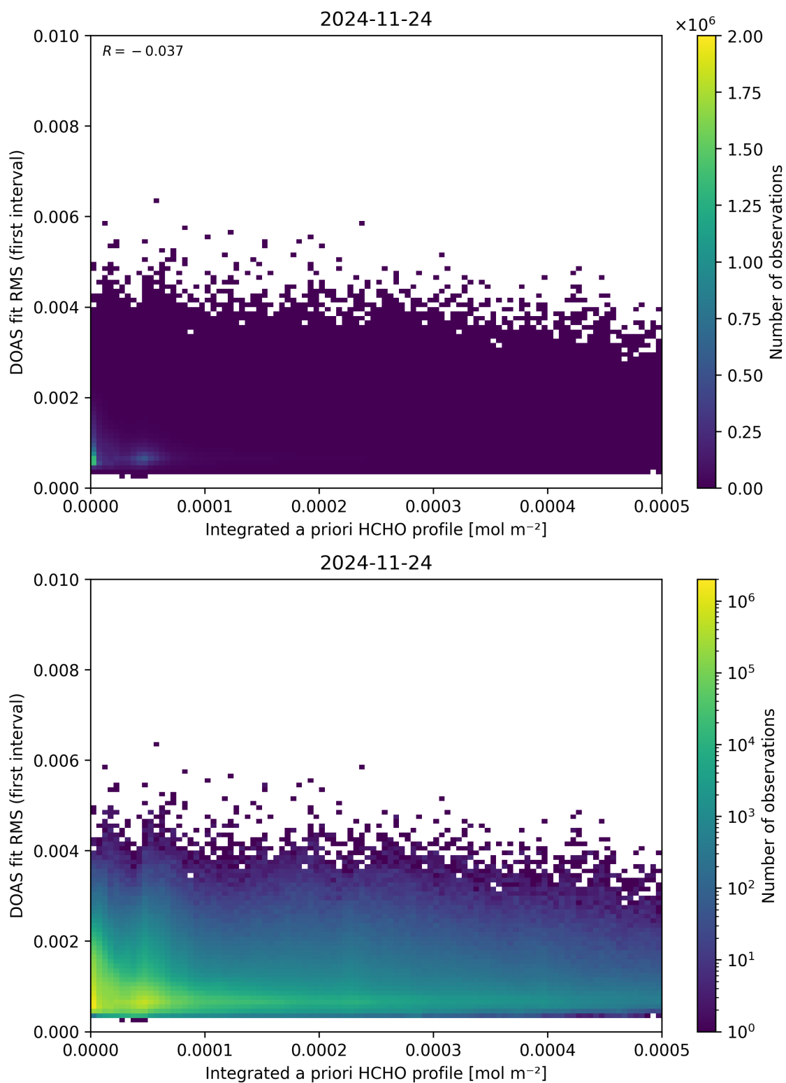
Figure 148: Scatter density plot of “Integrated a priori HCHO profile” against “DOAS fit RMS (first interval)” for 2024-11-23 to 2024-11-25.
