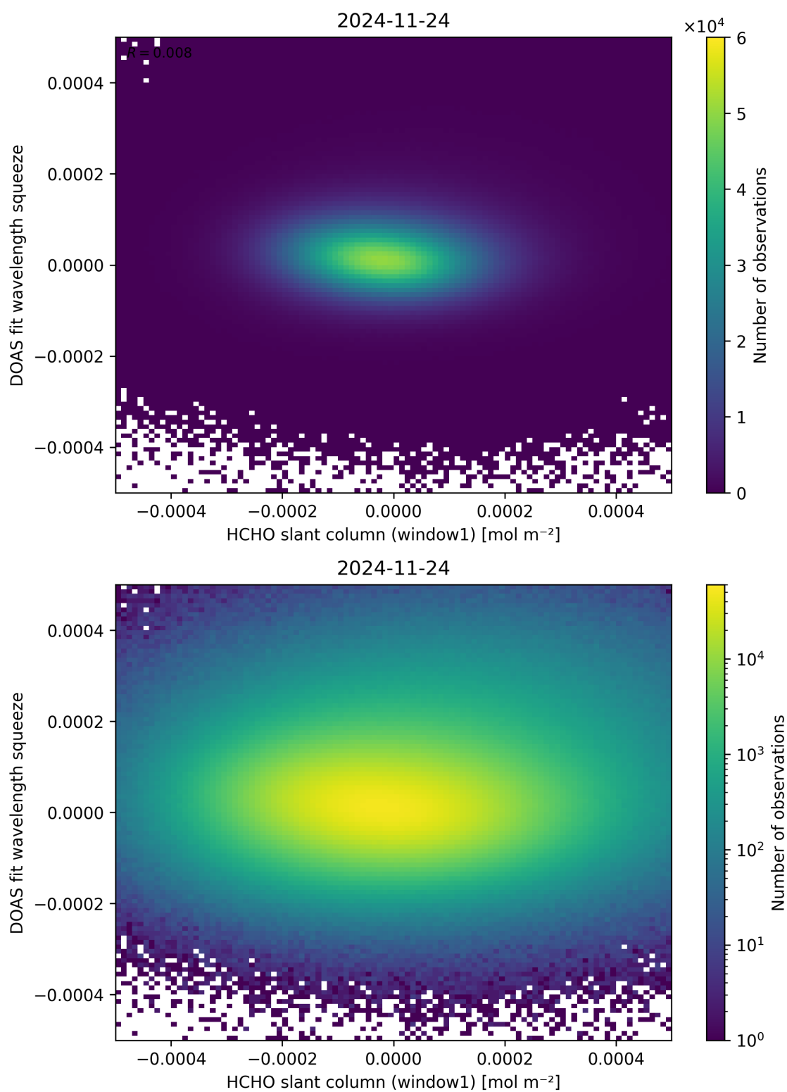
Figure 80: Scatter density plot of “HCHO slant column (window1)” against “DOAS fit wavelength squeeze” for 2024-11-23 to 2024-11-25.
