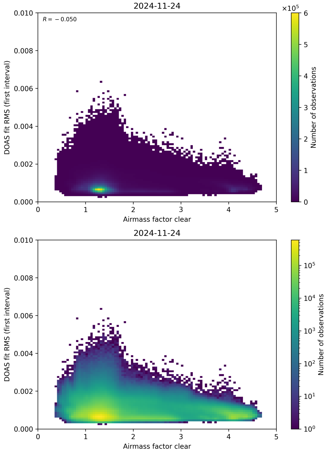
Figure 71: Scatter density plot of “Airmass factor clear” against “DOAS fit RMS (first interval)” for 2024-11-23 to 2024-11-25.
