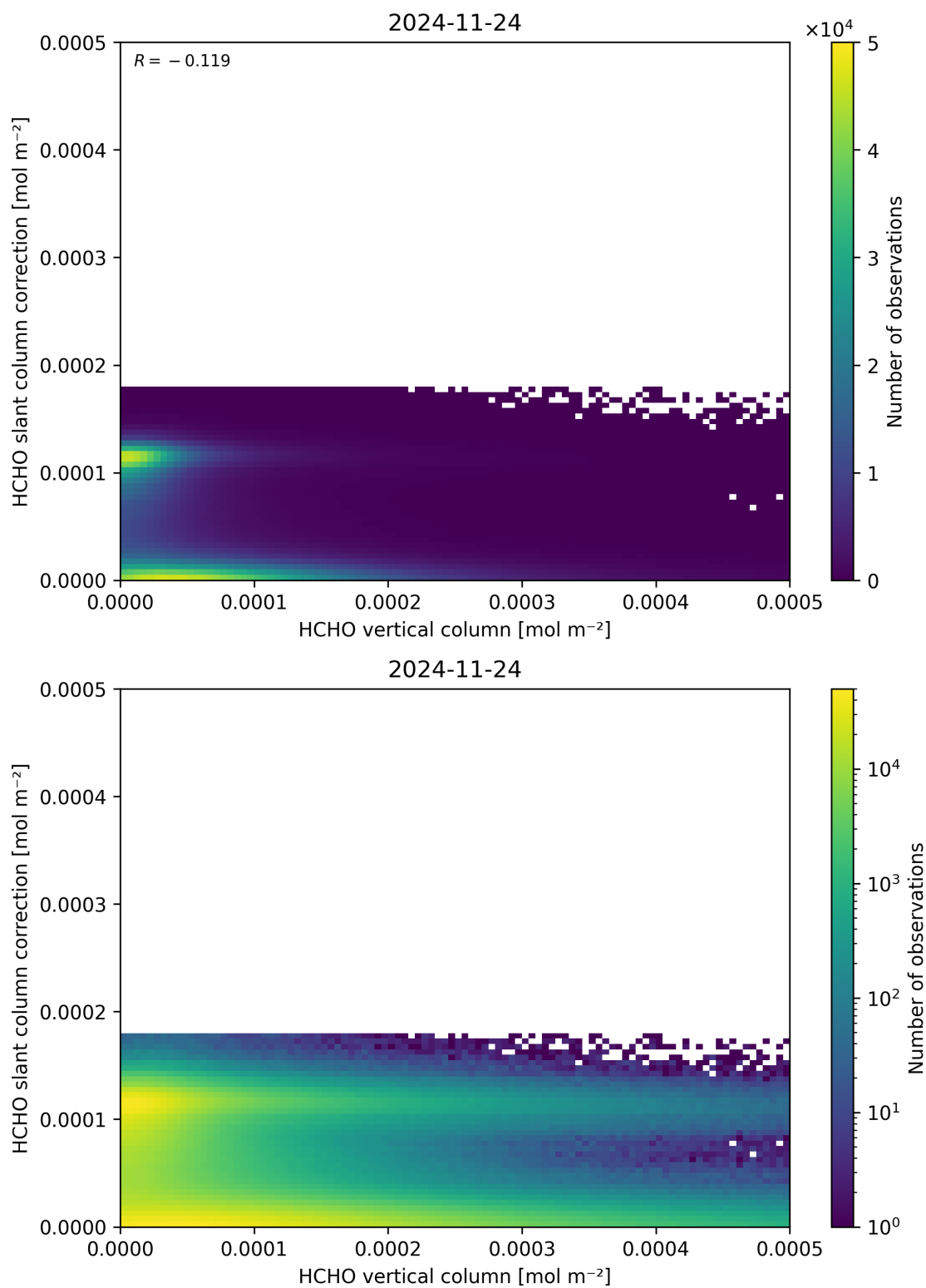
Figure 128: Scatter density plot of “HCHO vertical column” against “HCHO slant column correction” for 2024-11-23 to 2024-11-25.
