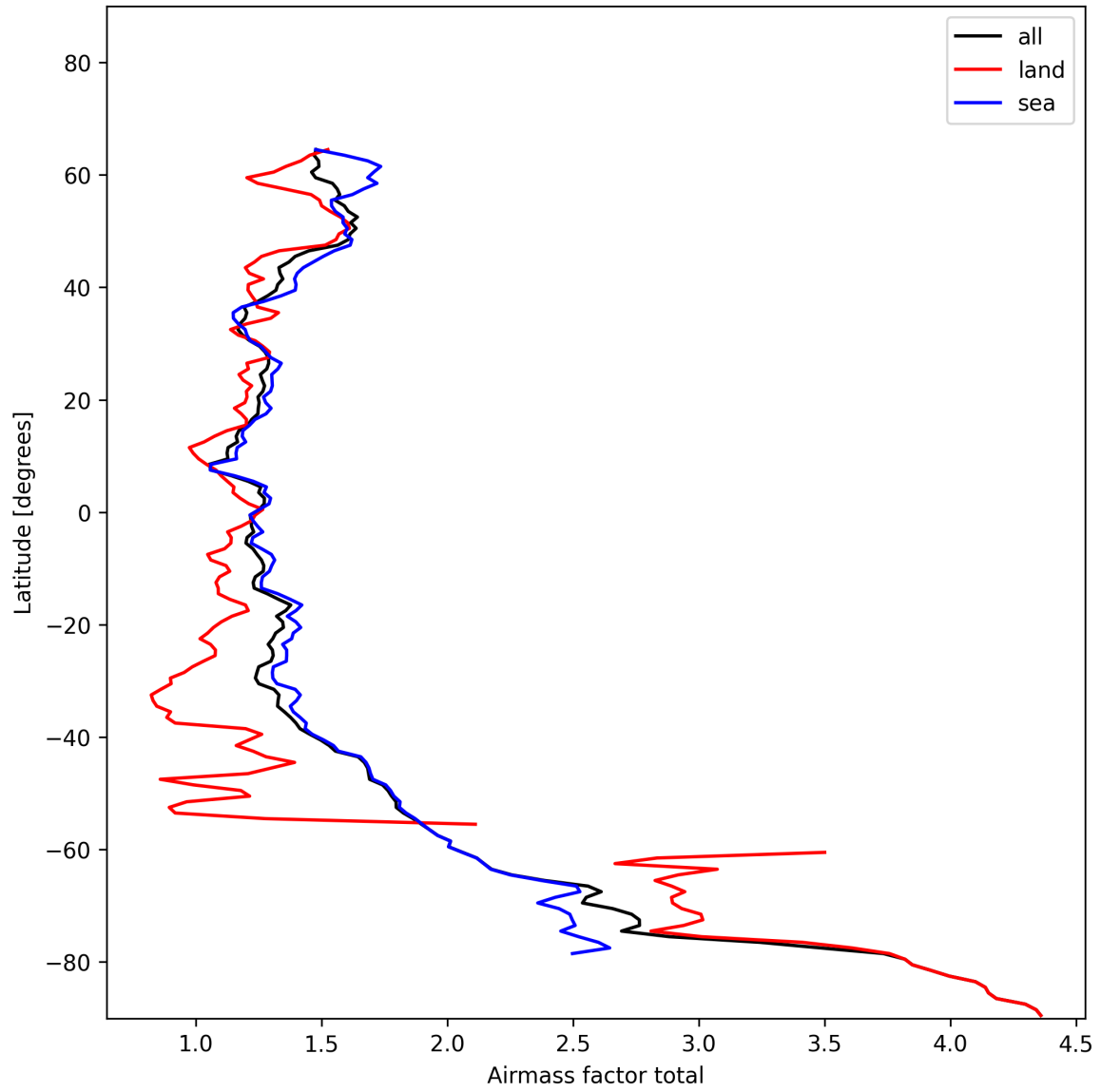
Figure 26: Zonal average of “Airmass factor total” for 2024-11-23 to 2024-11-25.
