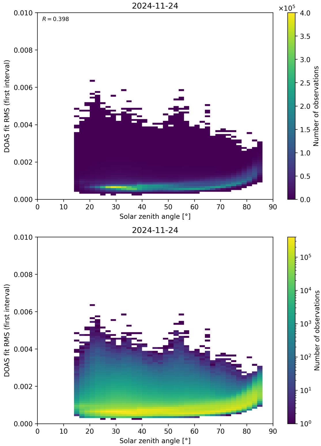
Figure 167: Scatter density plot of “Solar zenith angle” against “DOAS fit RMS (first interval)” for 2024-11-23 to 2024-11-25.
