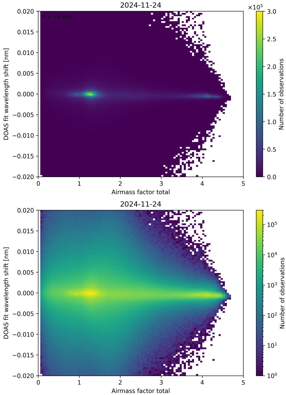
Figure 98: Scatter density plot of “Airmass factor total” against “DOAS fit wavelength shift” for 2024-11-23 to 2024-11-25.
