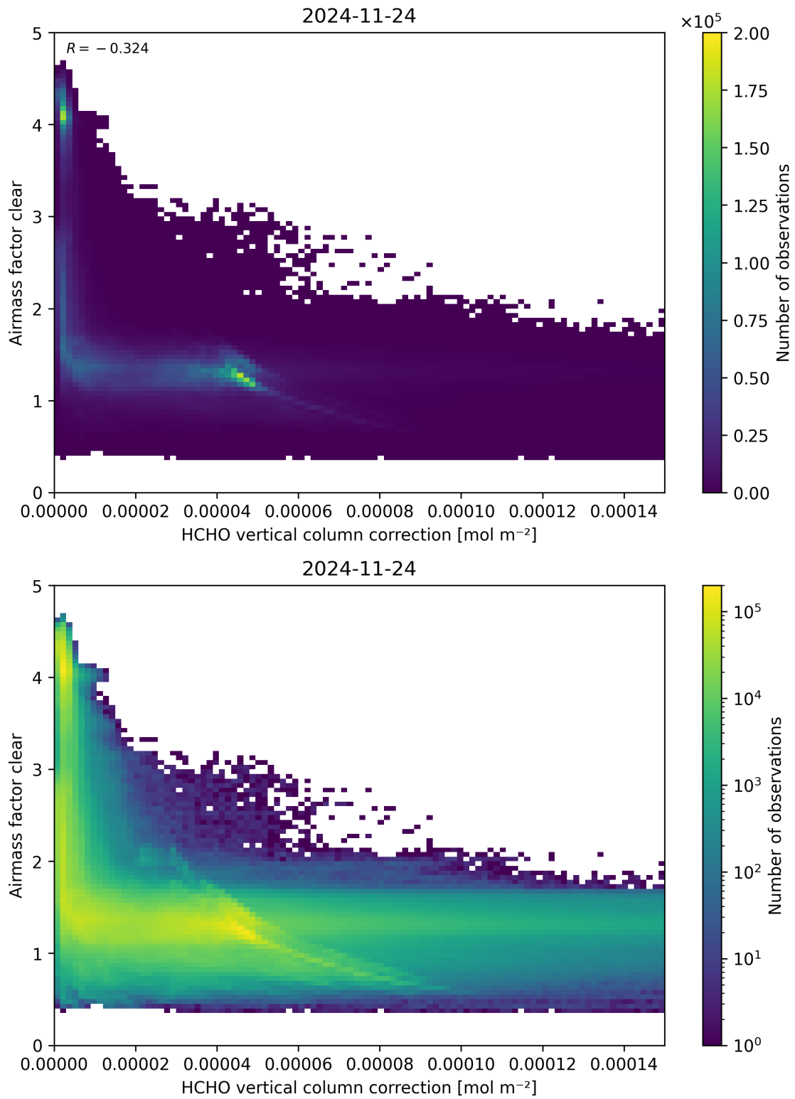
Figure 115: Scatter density plot of “HCHO vertical column correction” against “Airmass factor clear” for 2024-11-23 to 2024-11-25.
