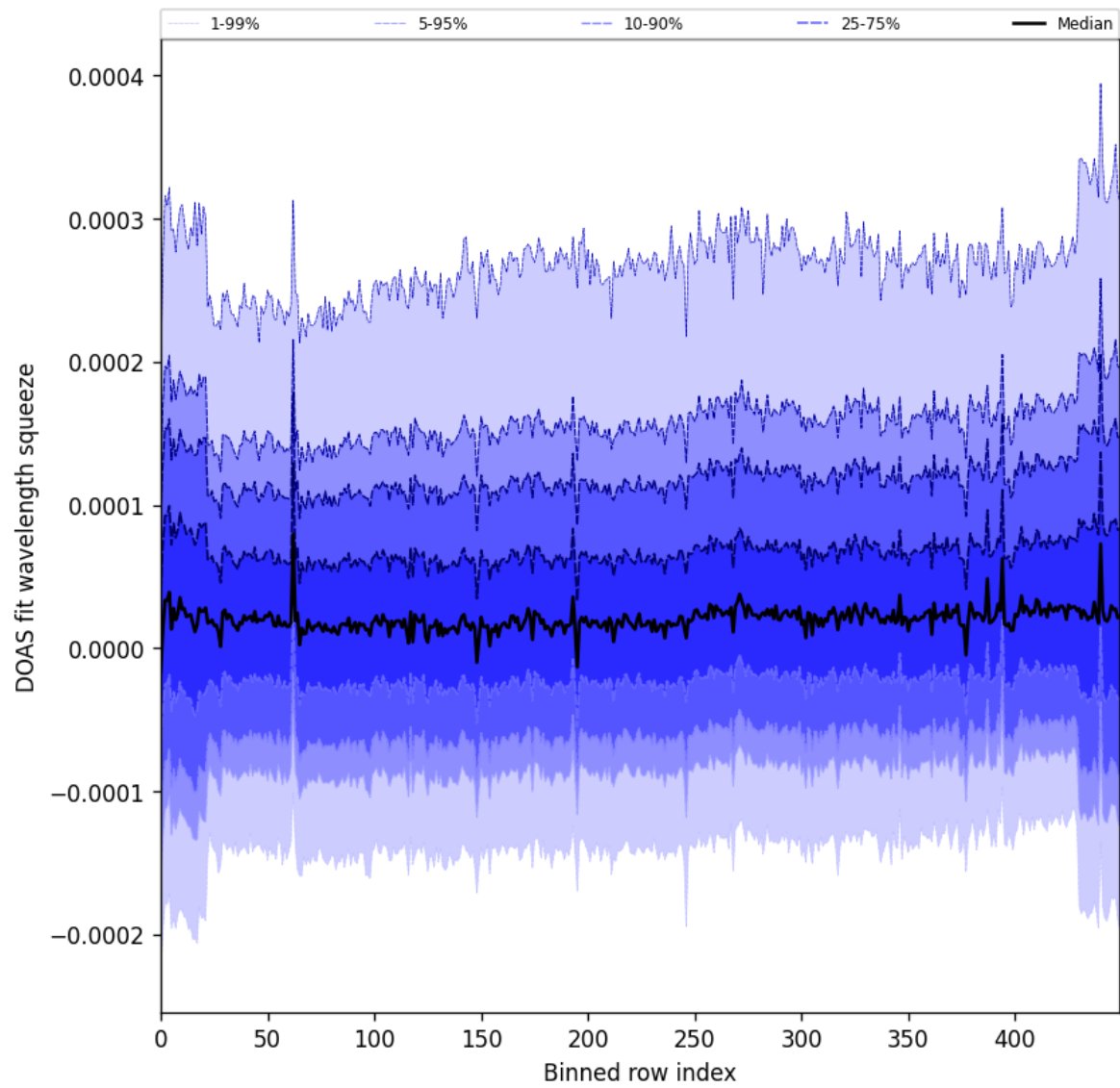
Figure 59: Along track statistics of “DOAS fit wavelength squeeze” for 2024-11-23 to 2024-11-25
