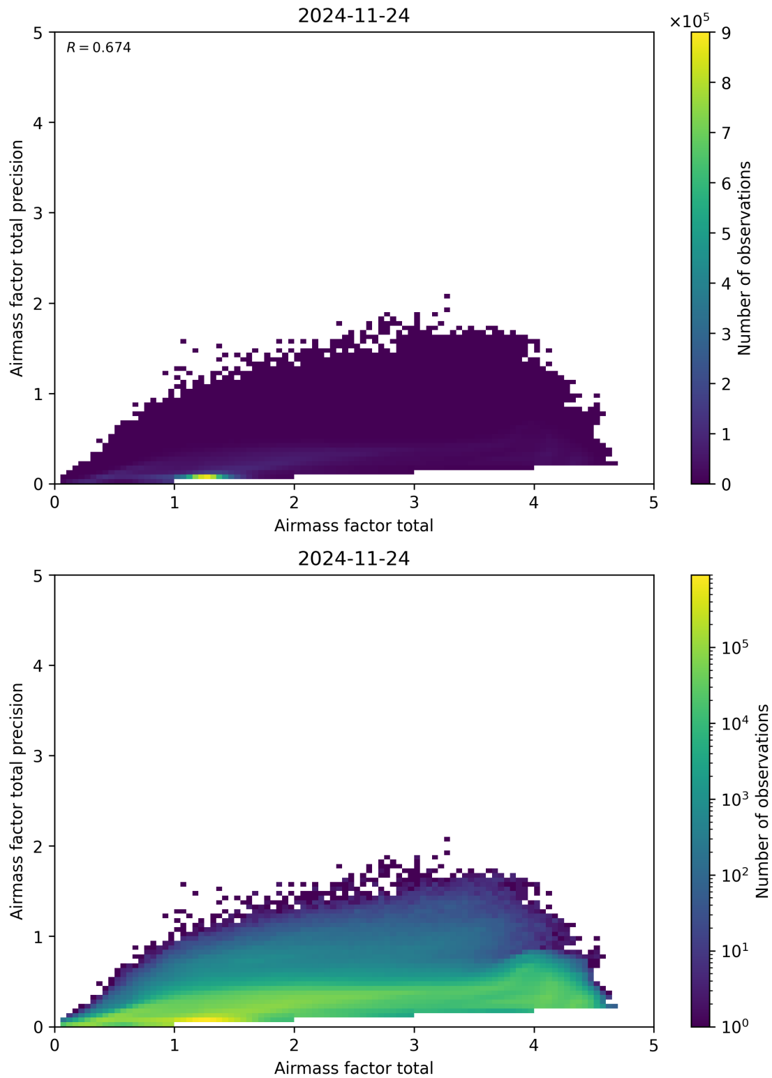
Figure 103: Scatter density plot of “Airmass factor total” against “Airmass factor total precision” for 2024-11-23 to 2024-11-25.
