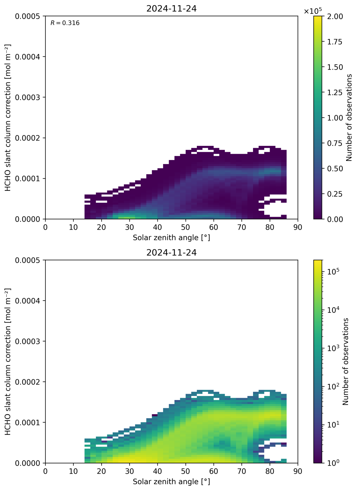
Figure 172: Scatter density plot of “Solar zenith angle” against “HCHO slant column correction” for 2024-11-23 to 2024-11-25.
