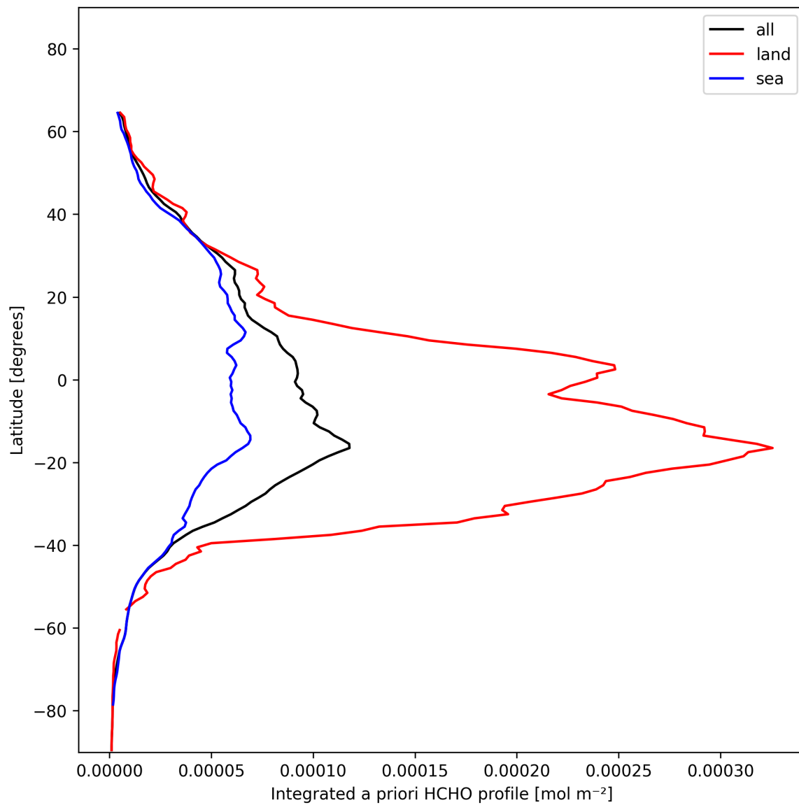
Figure 29: Zonal average of “Integrated a priori HCHO profile” for 2024-11-23 to 2024-11-25.
