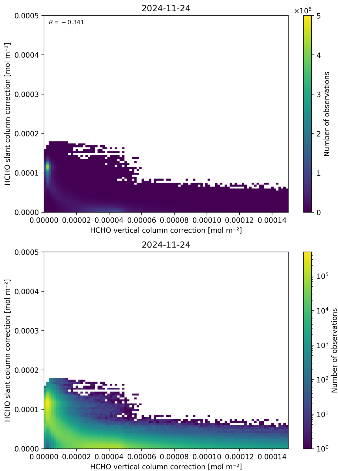
Figure 117: Scatter density plot of “HCHO vertical column correction” against “HCHO slant column correction” for 2024-11-23 to 2024-11-25.
