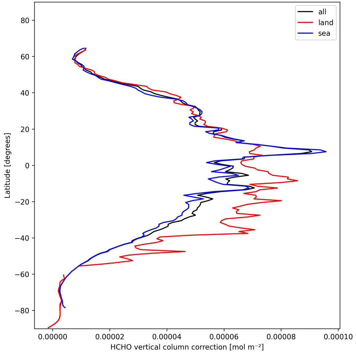
Figure 23: Zonal average of “HCHO vertical column correction” for 2024-11-23 to 2024-11-25.
