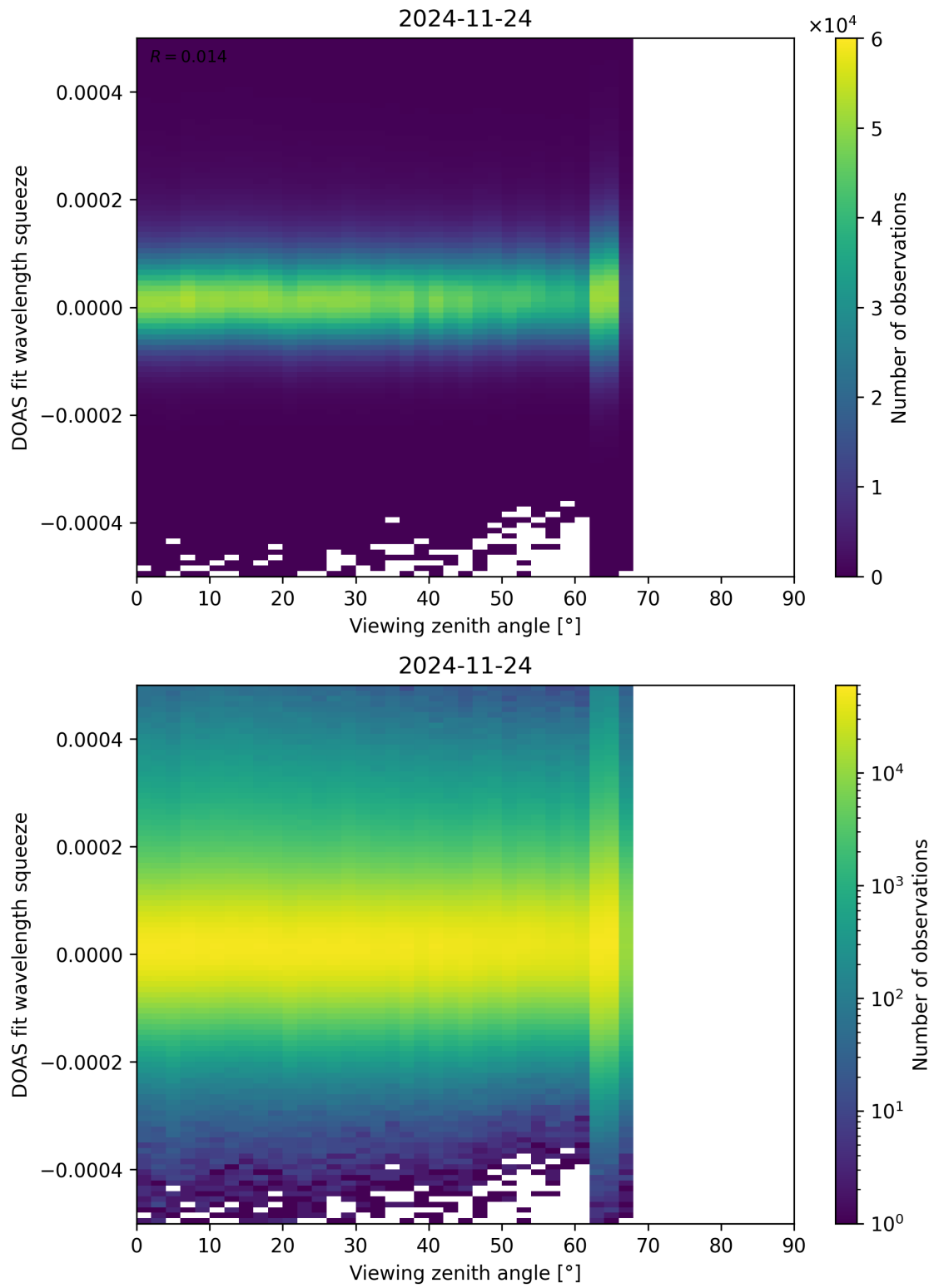
Figure 184: Scatter density plot of “Viewing zenith angle” against “DOAS fit wavelength squeeze” for 2024-11-23 to 2024-11-25.
