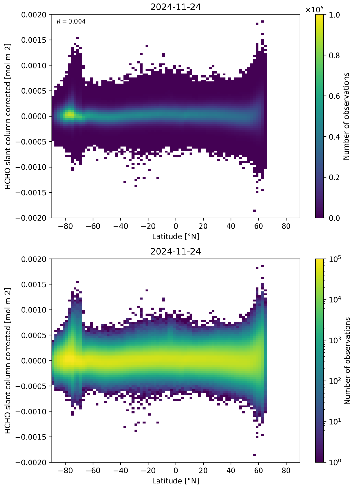
Figure 157: Scatter density plot of “Latitude” against “HCHO slant column corrected” for 2024-11-23 to 2024-11-25.
