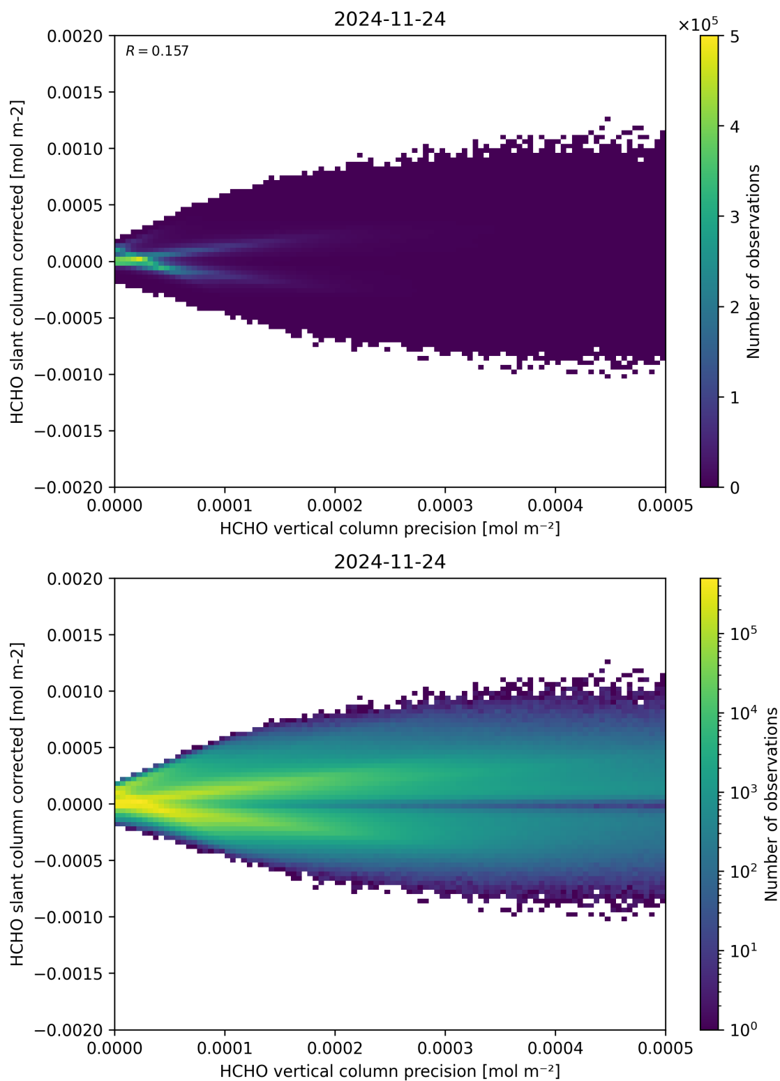
Figure 140: Scatter density plot of “HCHO vertical column precision” against “HCHO slant column corrected” for 2024-11-23 to 2024-11-25.
