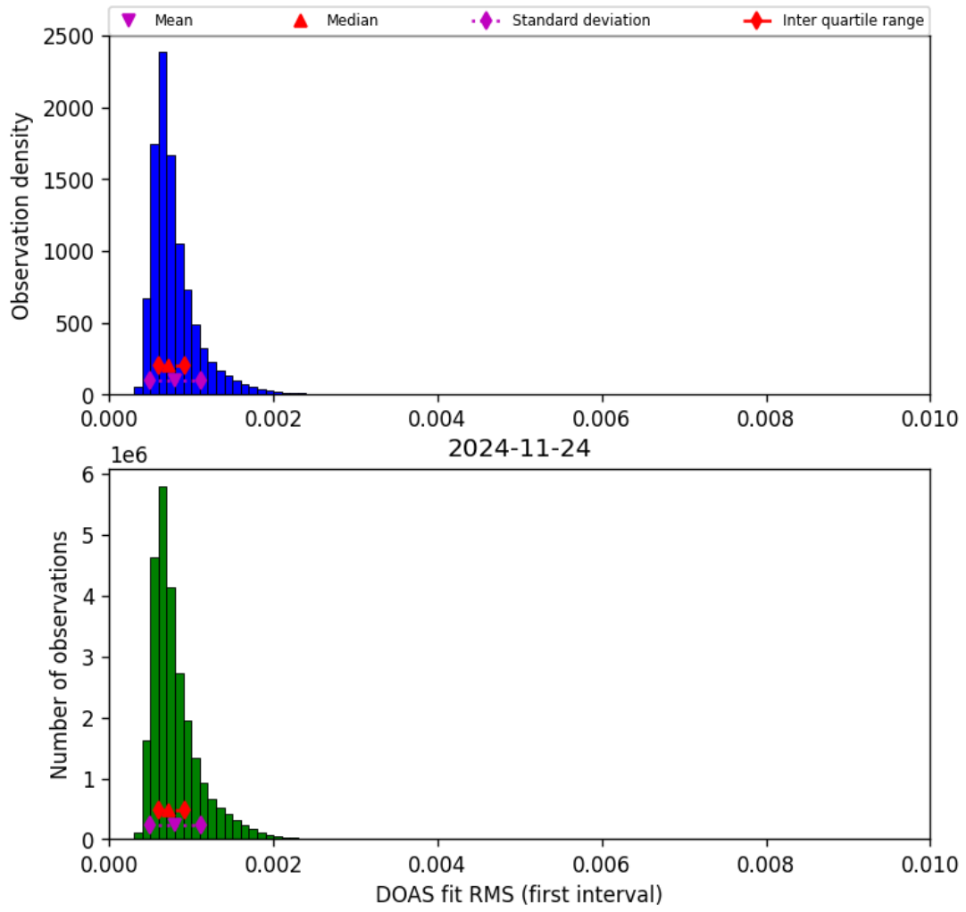
Figure 46: Histogram of “DOAS fit RMS (first interval)” for 2024-11-23 to 2024-11-25
