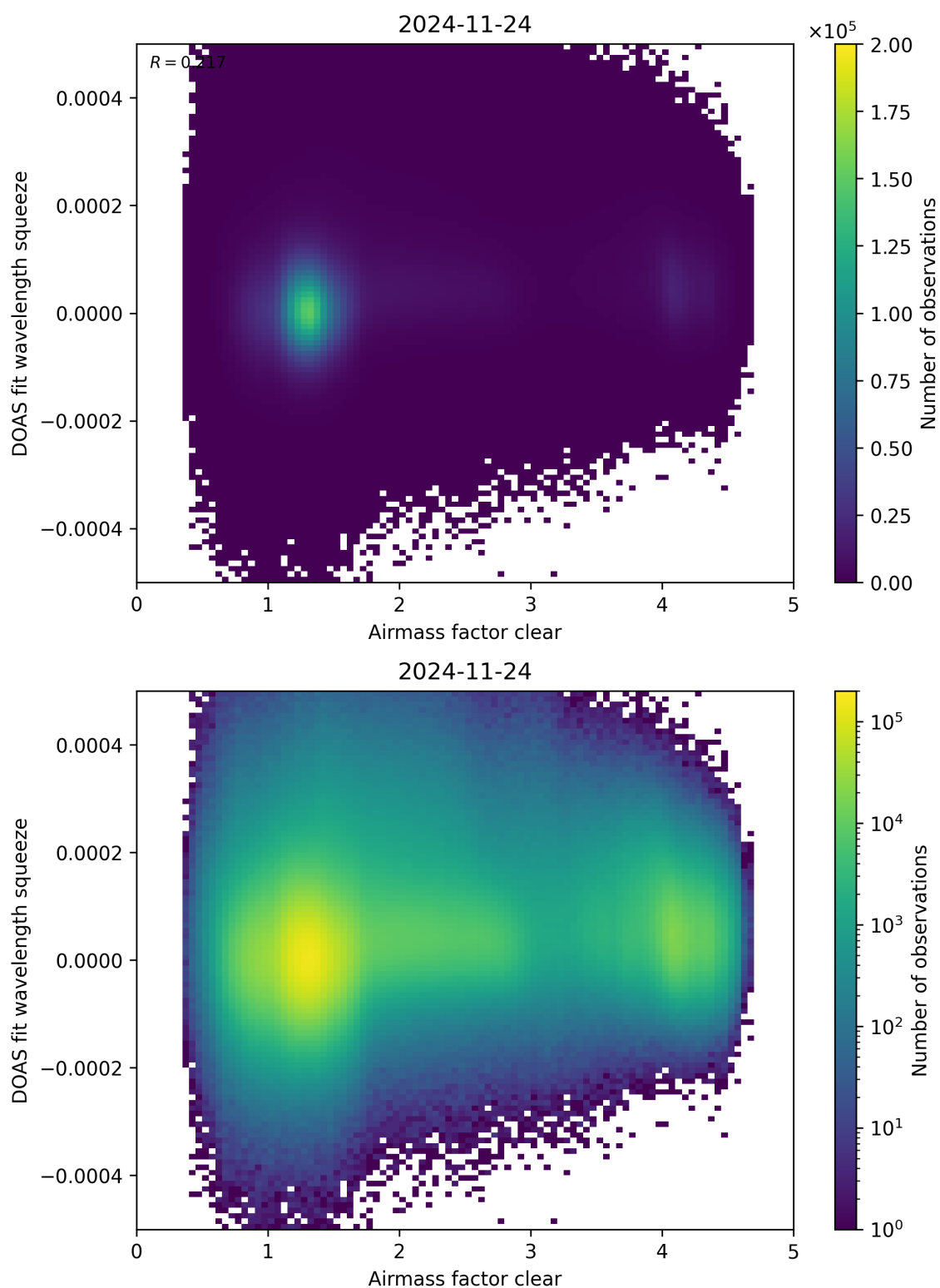
Figure 73: Scatter density plot of “Airmass factor clear” against “DOAS fit wavelength squeeze” for 2024-11-23 to 2024-11-25.
