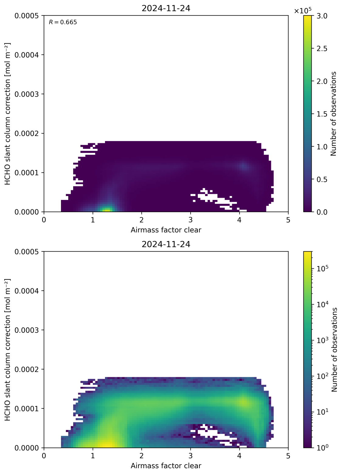
Figure 75: Scatter density plot of “Airmass factor clear” against “HCHO slant column correction” for 2024-11-23 to 2024-11-25.
