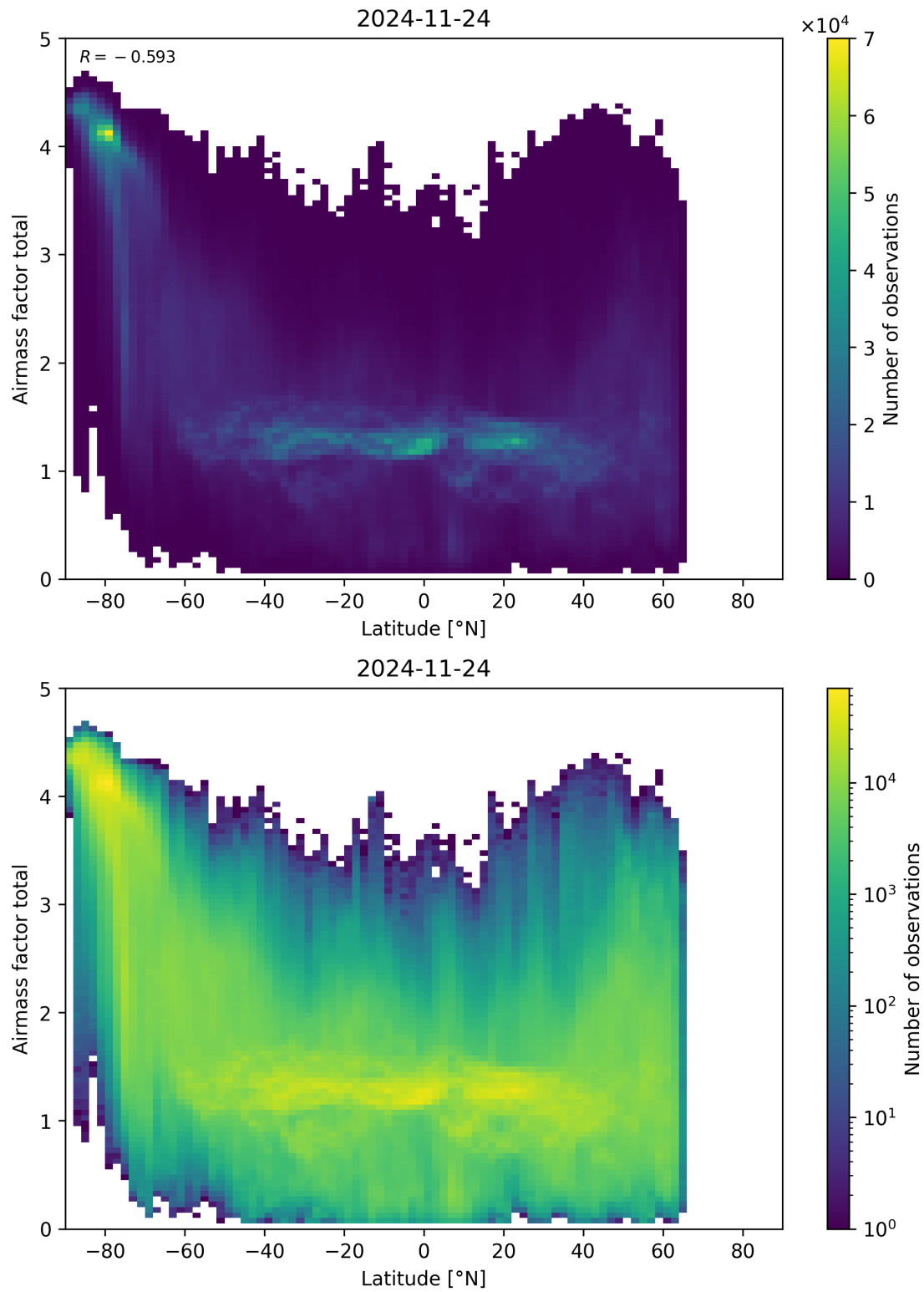
Figure 161: Scatter density plot of “Latitude” against “Airmass factor total” for 2024-11-23 to 2024-11-25.
