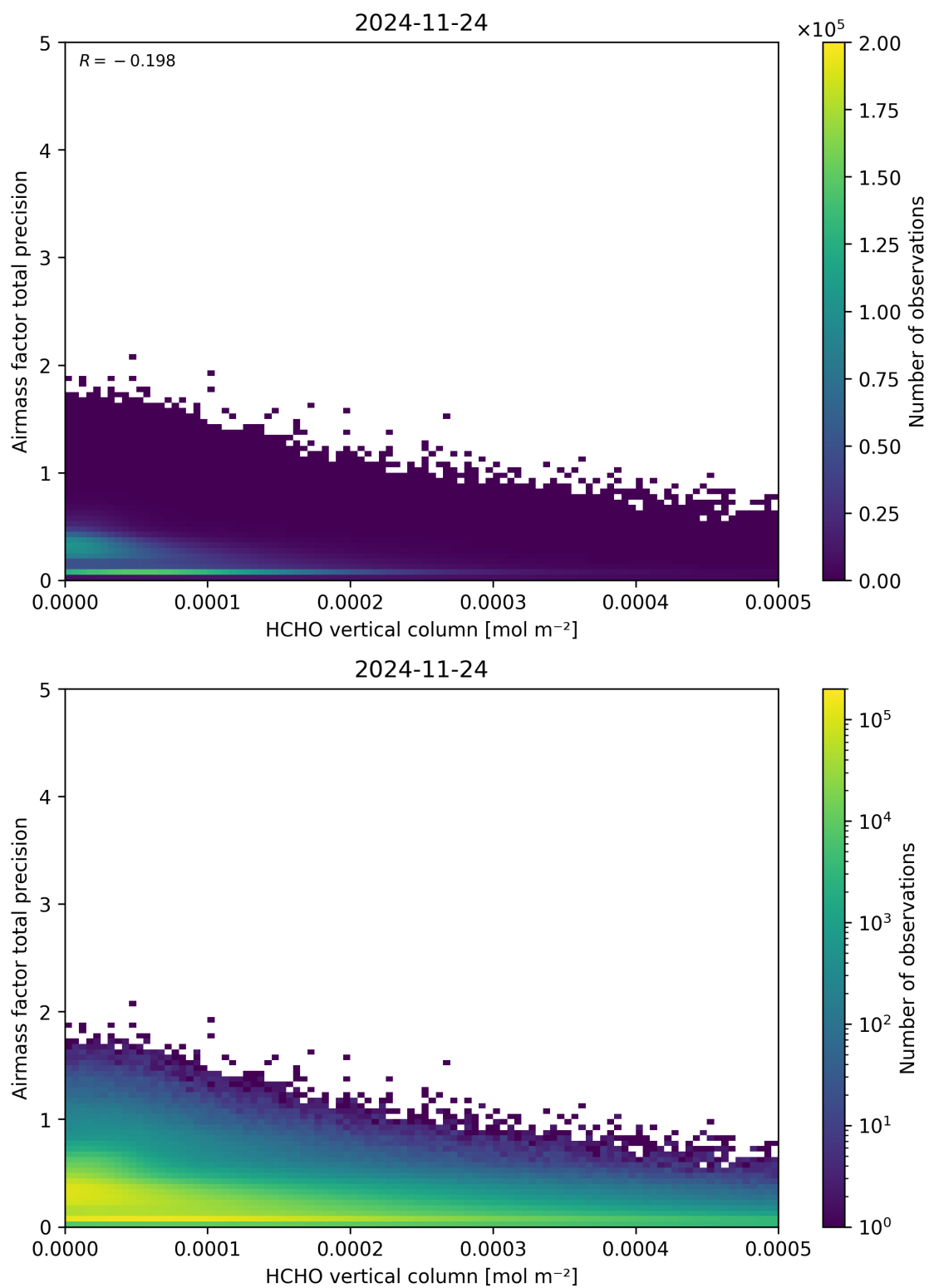
Figure 132: Scatter density plot of “HCHO vertical column” against “Airmass factor total precision” for 2024-11-23 to 2024-11-25.
