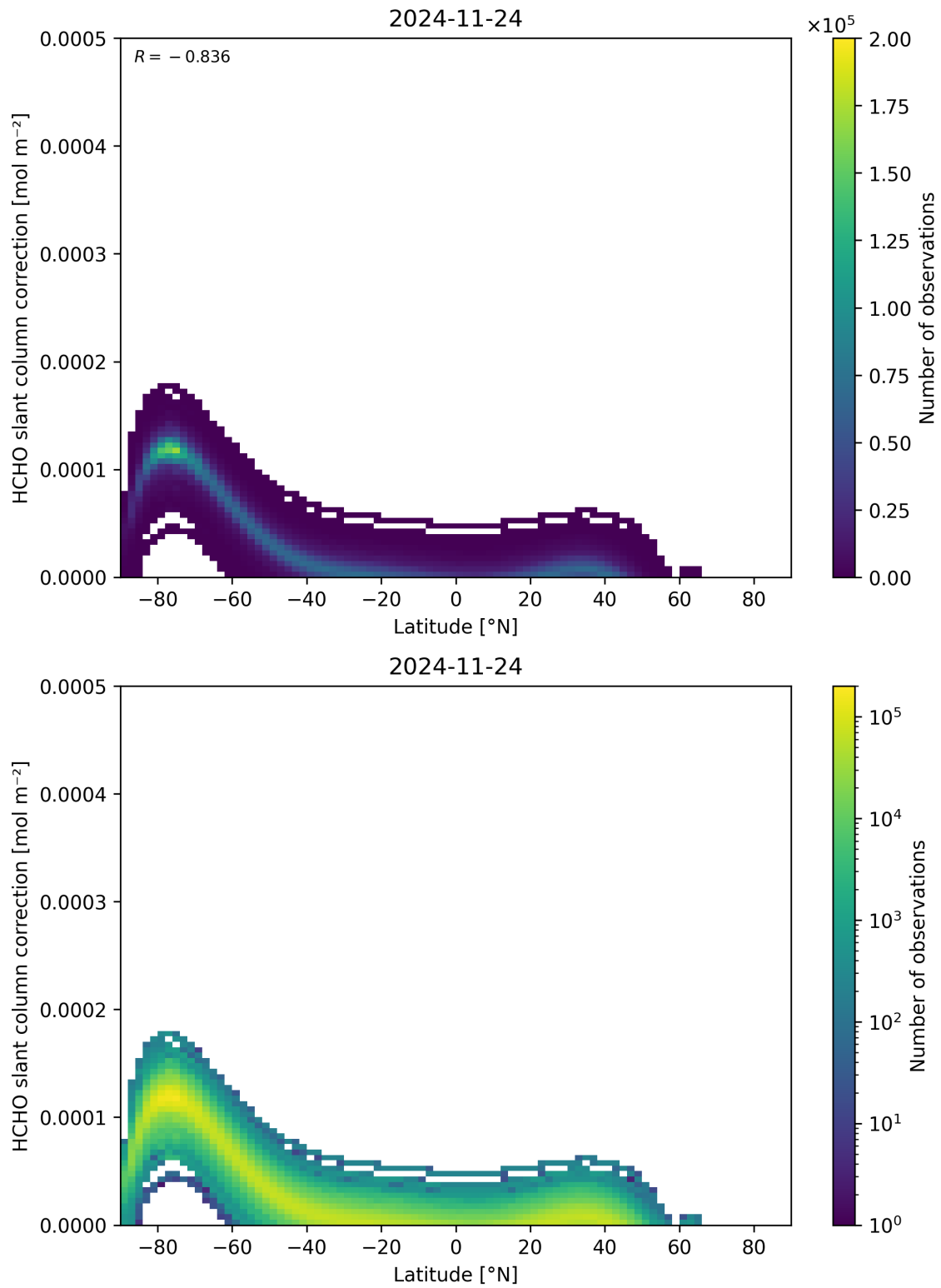
Figure 158: Scatter density plot of “Latitude” against “HCHO slant column correction” for 2024-11-23 to 2024-11-25.
