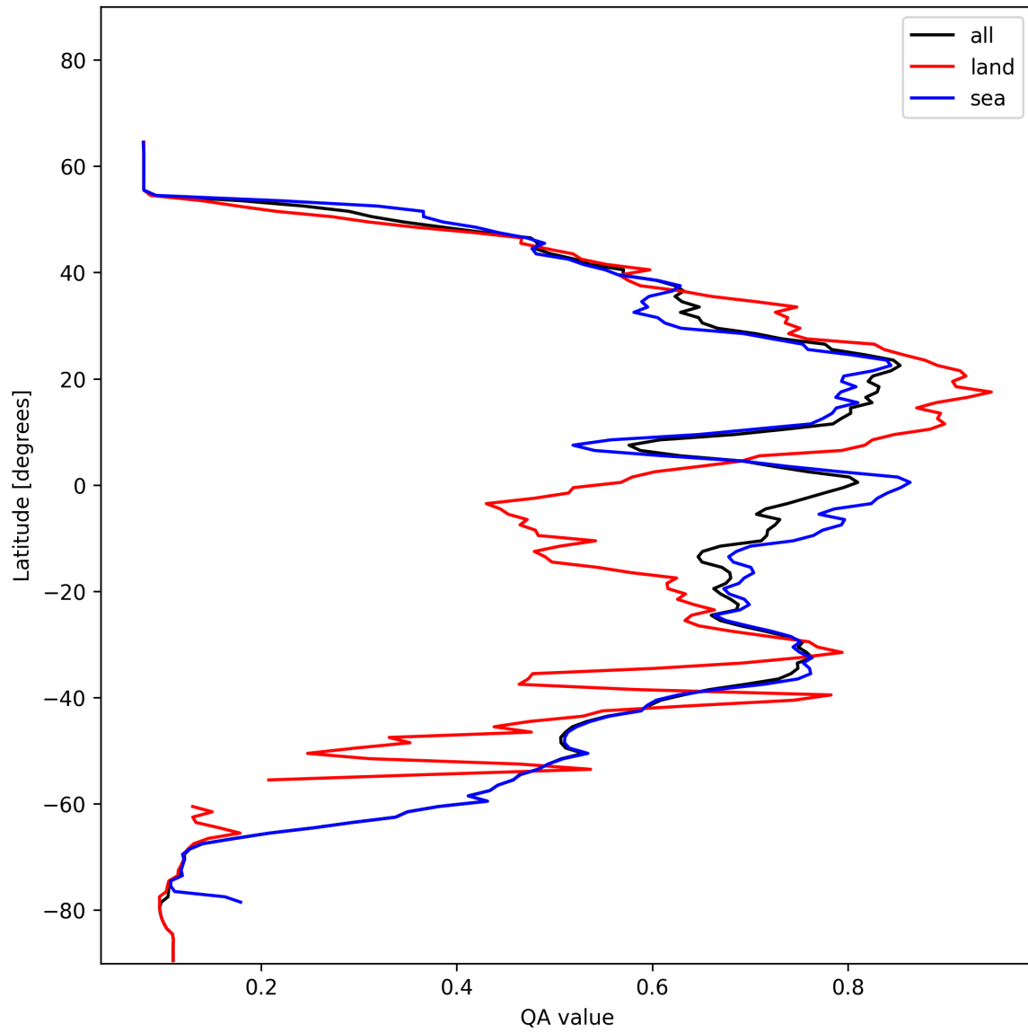
Figure 20: Zonal average of “QA value” for 2024-11-23 to 2024-11-25.
