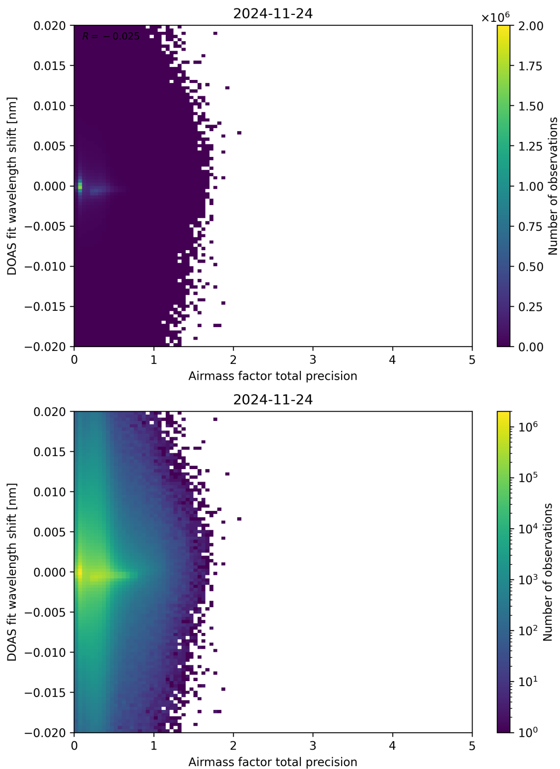
Figure 106: Scatter density plot of “Airmass factor total precision” against “DOAS fit wavelength shift” for 2024-11-23 to 2024-11-25.
