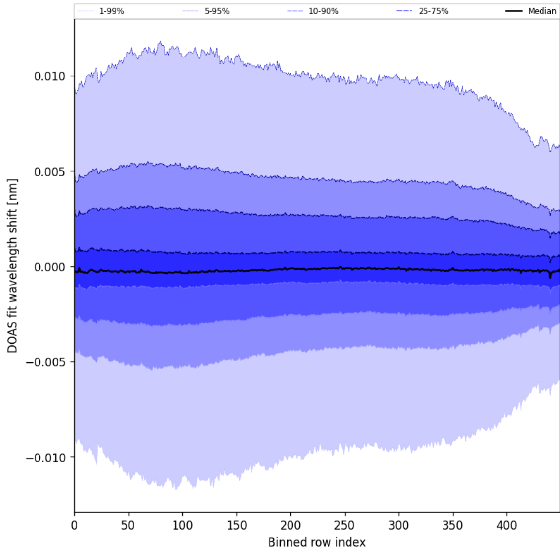
Figure 58: Along track statistics of “DOAS fit wavelength shift” for 2024-11-23 to 2024-11-25
