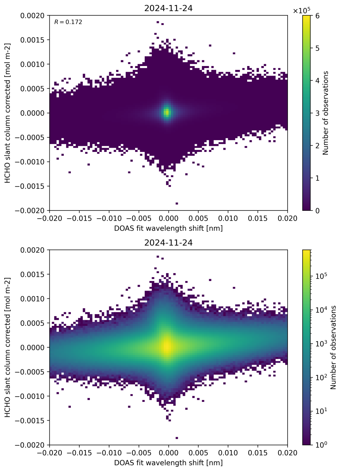
Figure 66: Scatter density plot of “DOAS fit wavelength shift” against “HCHO slant column corrected” for 2024-11-23 to 2024-11-25.
