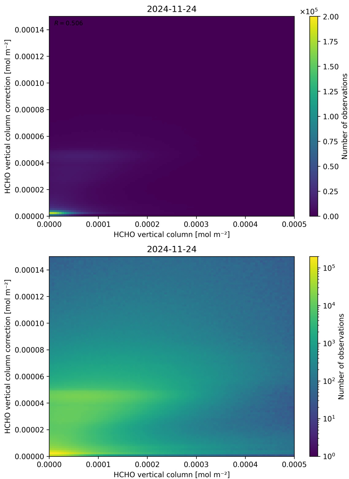
Figure 133: Scatter density plot of “HCHO vertical column” against “HCHO vertical column correction” for 2024-11-23 to 2024-11-25.
