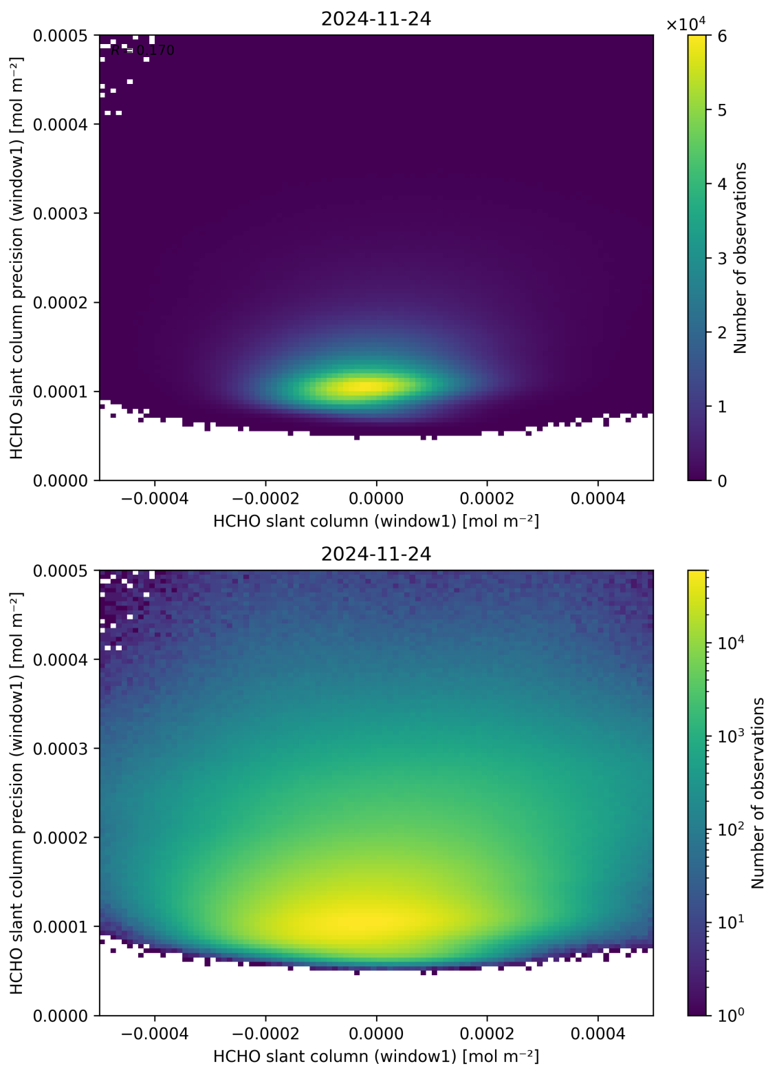
Figure 84: Scatter density plot of “HCHO slant column (window1)” against “HCHO slant column precision (window1)” for 2024-11-23 to 2024-11-25.
