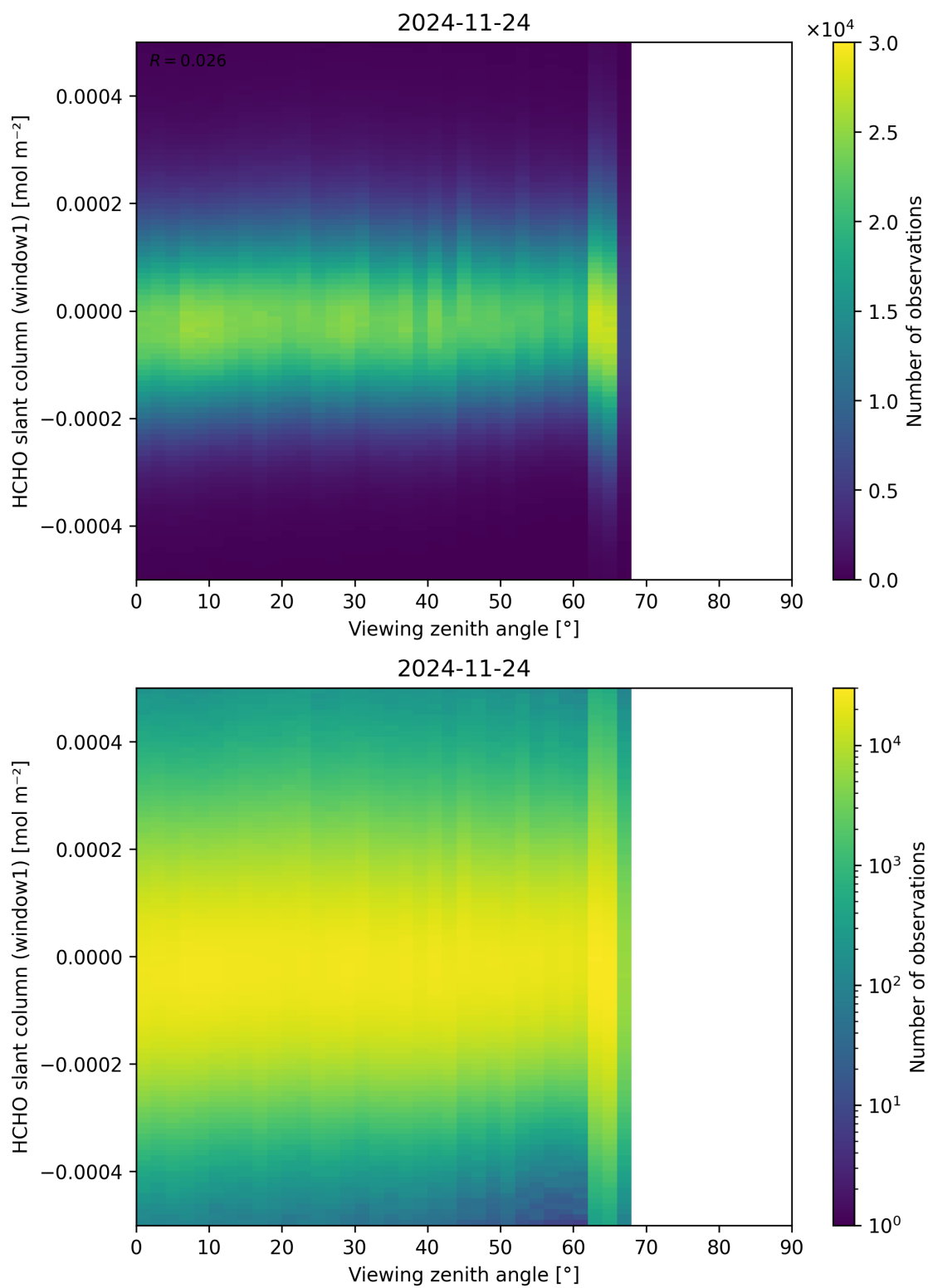
Figure 188: Scatter density plot of “Viewing zenith angle” against “HCHO slant column (window1)” for 2024-11-23 to 2024-11-25.
