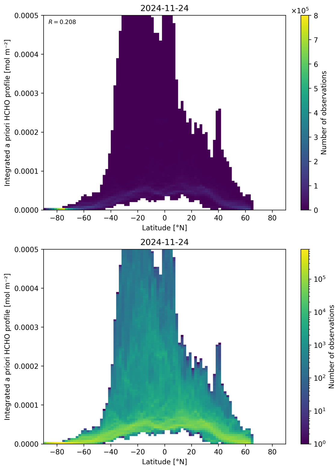
Figure 166: Scatter density plot of “Latitude” against “Integrated a priori HCHO profile” for 2024-11-23 to 2024-11-25.
