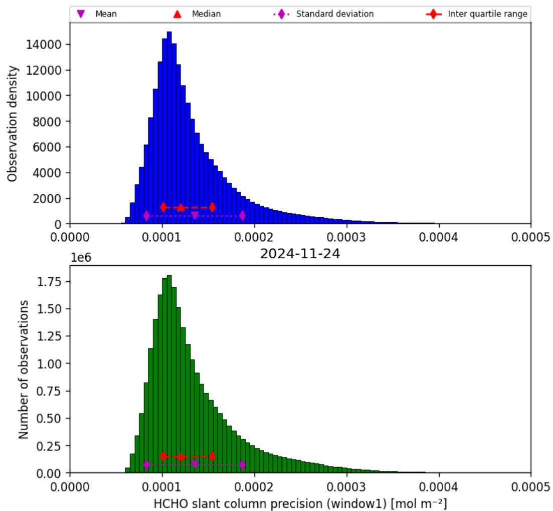
Figure 39: Histogram of “HCHO slant column precision (window1)” for 2024-11-23 to 2024-11-25
