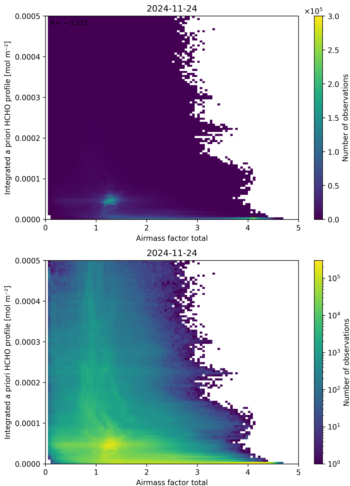
Figure 104: Scatter density plot of “Airmass factor total” against “Integrated a priori HCHO profile” for 2024-11-23 to 2024-11-25.
