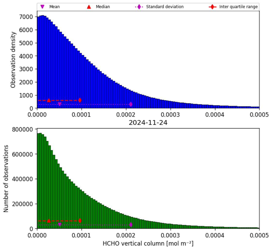
Figure 35: Histogram of “HCHO vertical column” for 2024-11-23 to 2024-11-25
