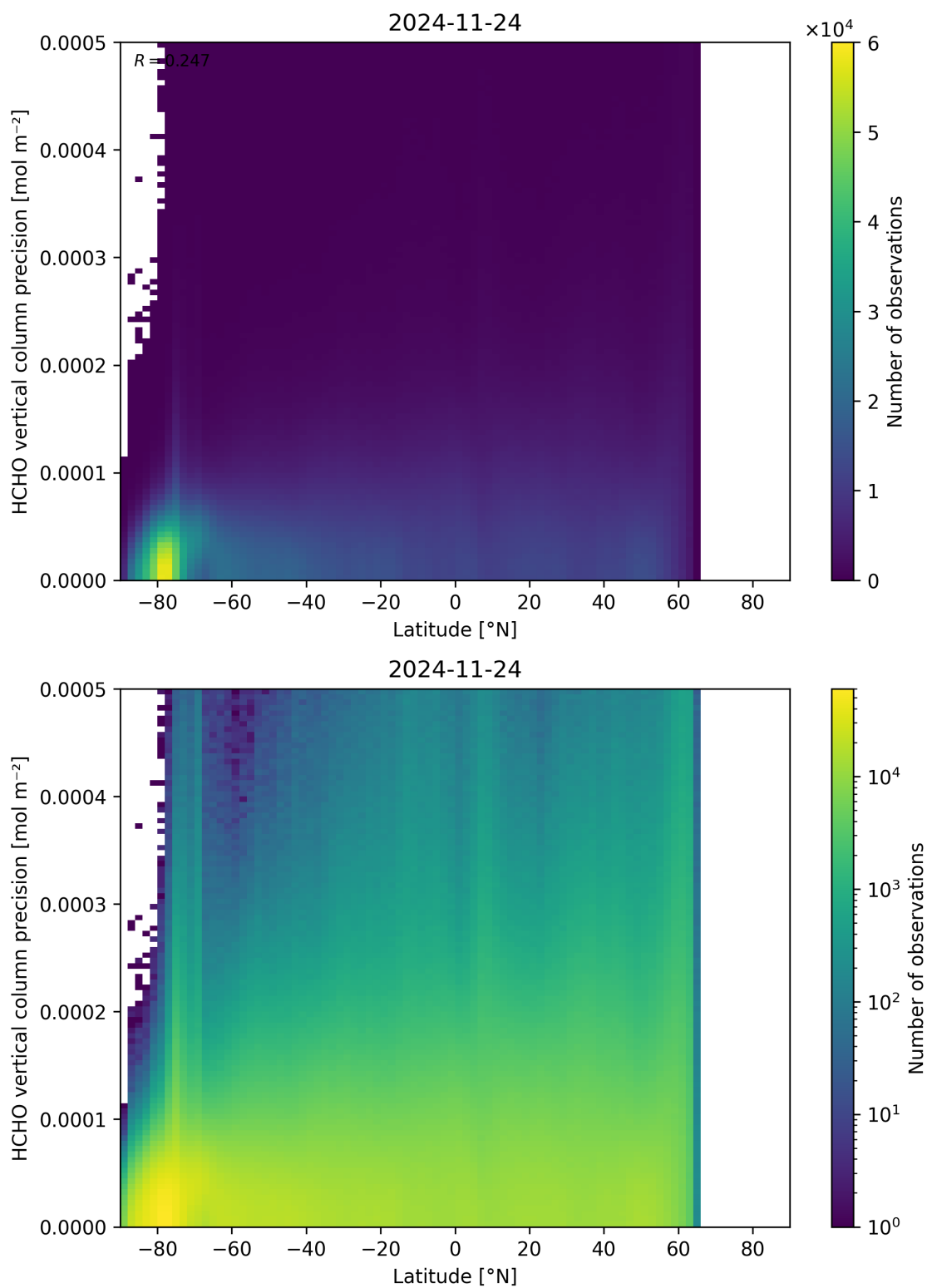
Figure 165: Scatter density plot of “Latitude” against “HCHO vertical column precision” for 2024-11-23 to 2024-11-25.
