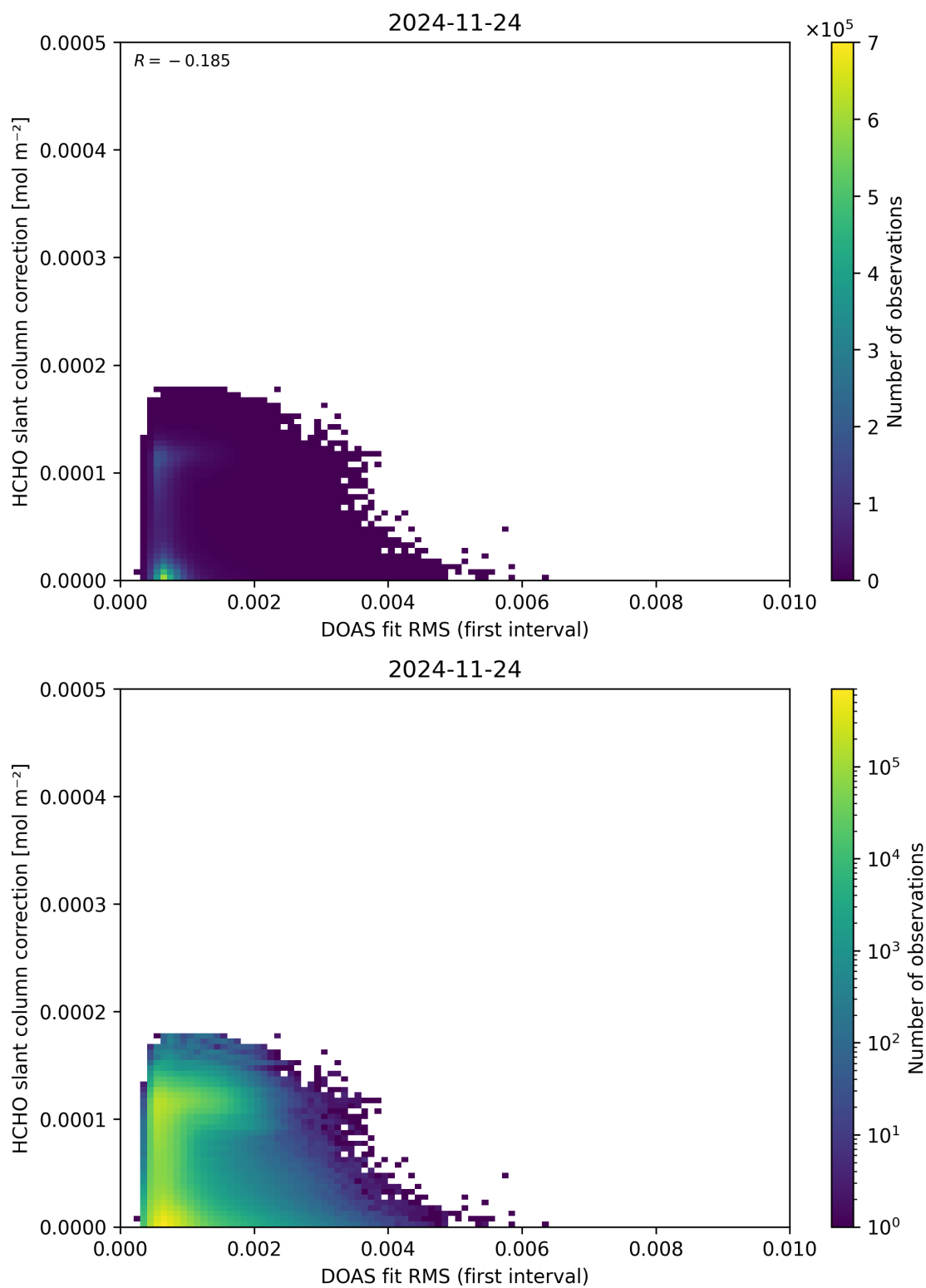
Figure 63: Scatter density plot of “DOAS fit RMS (first interval)” against “HCHO slant column correction” for 2024-11-23 to 2024-11-25.
