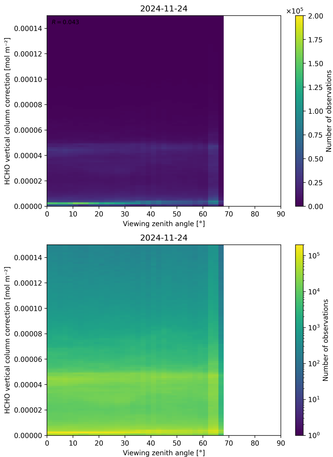
Figure 193: Scatter density plot of “Viewing zenith angle” against “HCHO vertical column correction” for 2024-11-23 to 2024-11-25.
