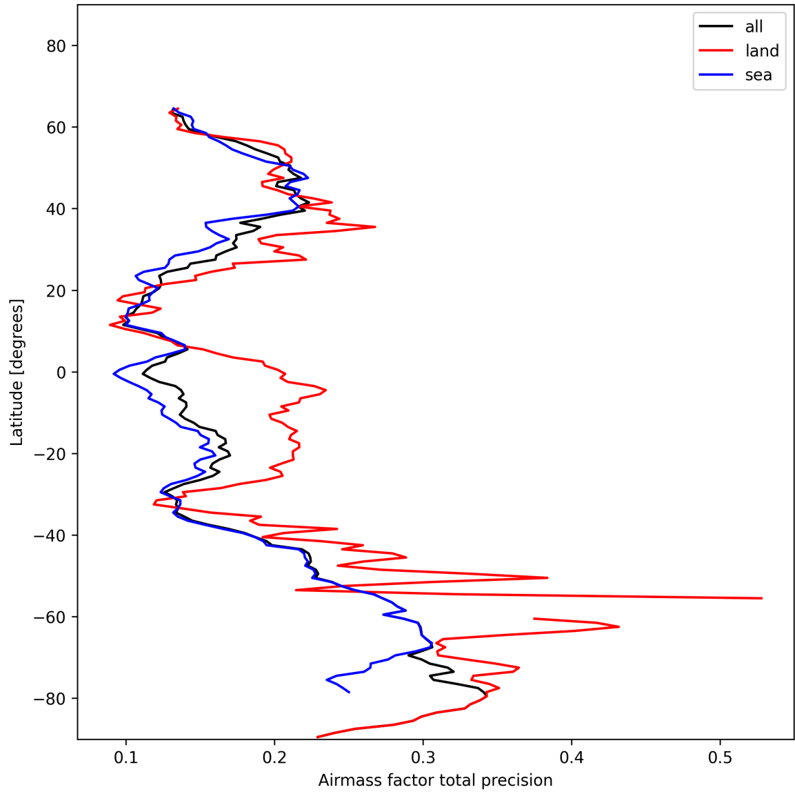
Figure 27: Zonal average of “Airmass factor total precision” for 2024-11-23 to 2024-11-25.
