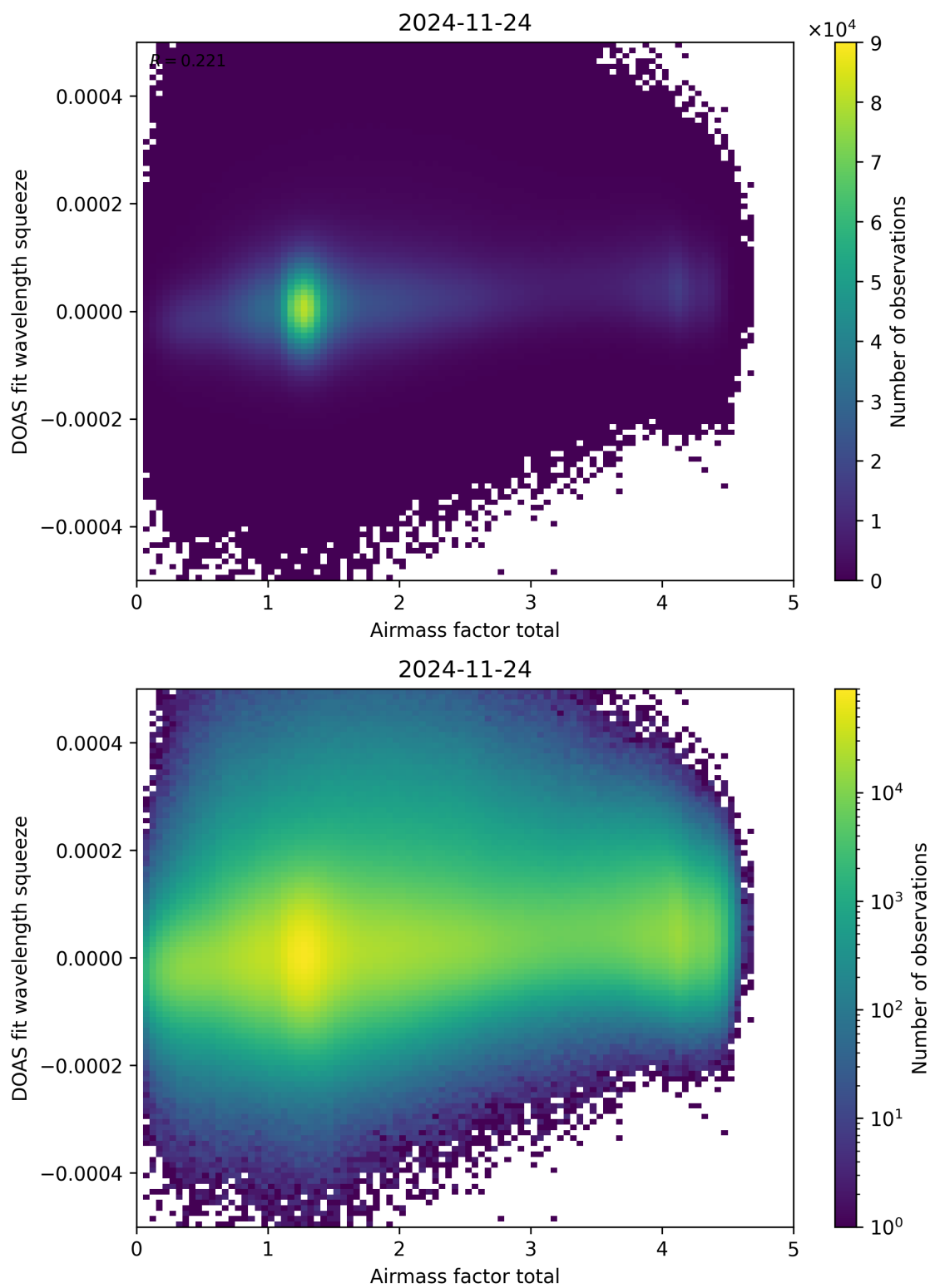
Figure 99: Scatter density plot of “Airmass factor total” against “DOAS fit wavelength squeeze” for 2024-11-23 to 2024-11-25.
