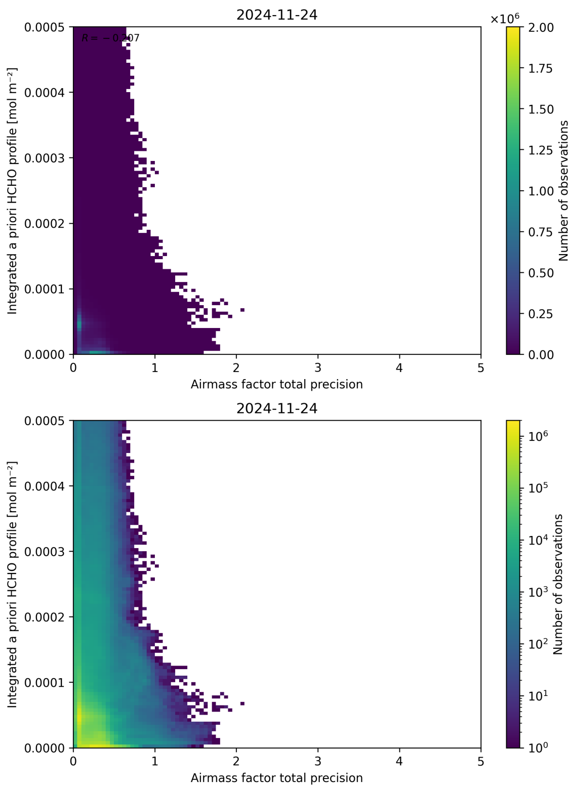
Figure 111: Scatter density plot of “Airmass factor total precision” against “Integrated a priori HCHO profile” for 2024-11-23 to 2024-11-25.
