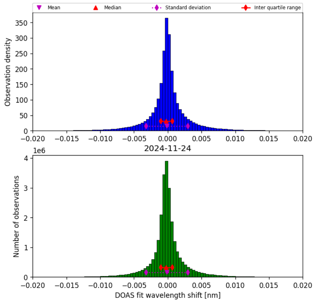
Figure 44: Histogram of “DOAS fit wavelength shift” for 2024-11-23 to 2024-11-25
