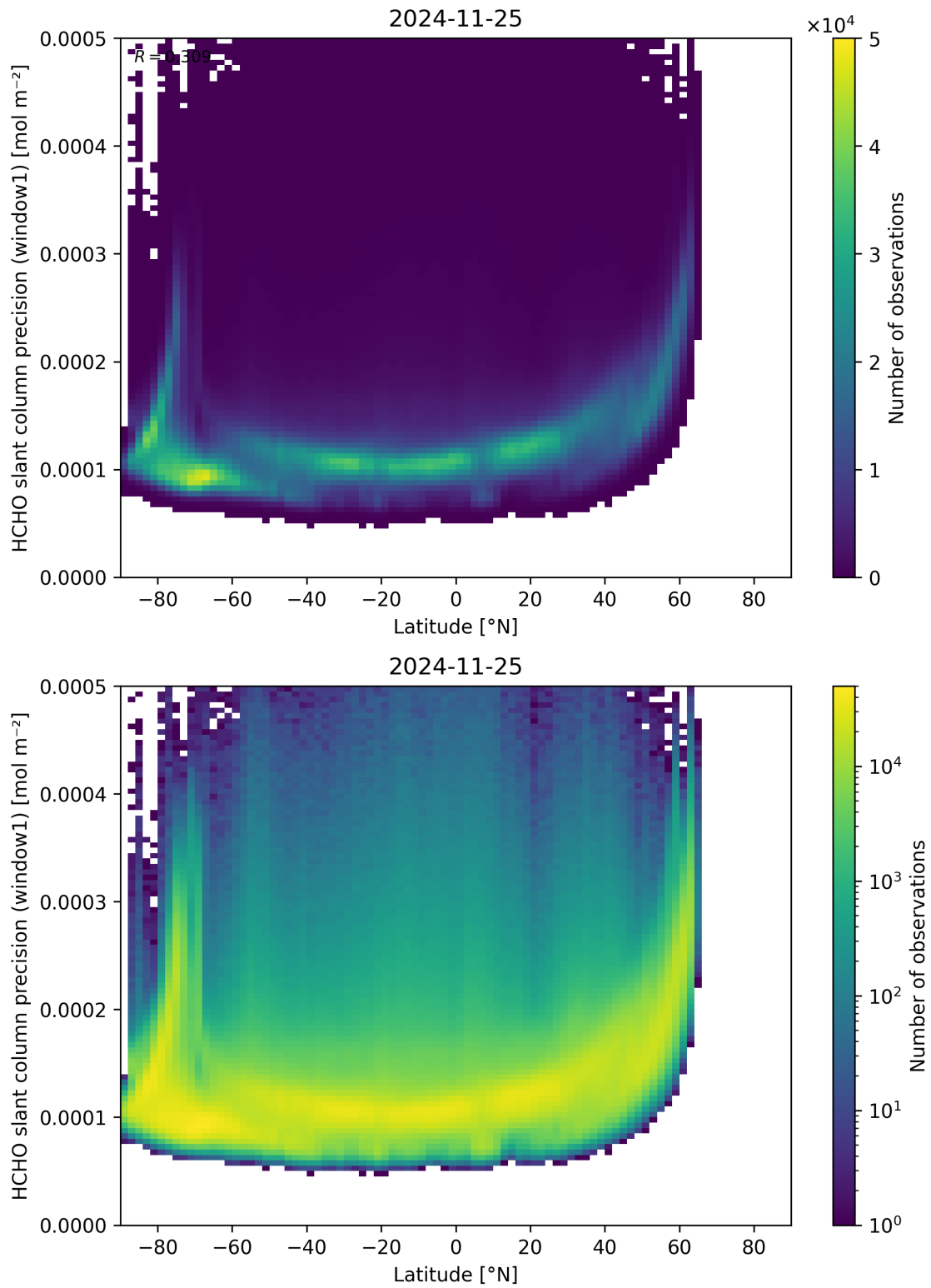
Figure 160: Scatter density plot of “Latitude” against “HCHO slant column precision (window1)” for 2024-11-25 to 2024-11-26.
