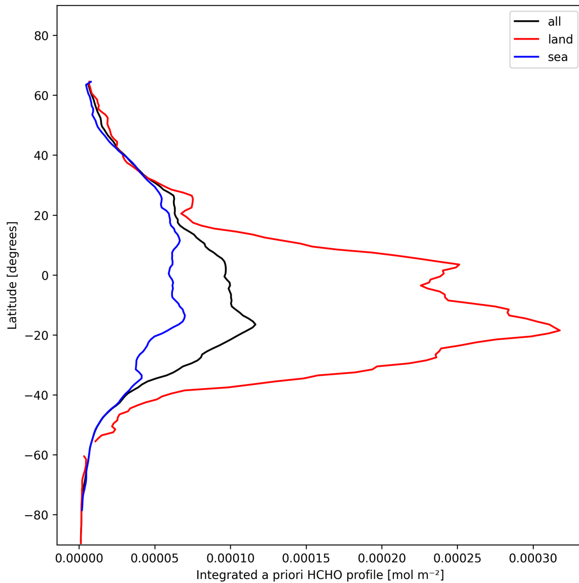
Figure 29: Zonal average of “Integrated a priori HCHO profile” for 2024-11-25 to 2024-11-26.
