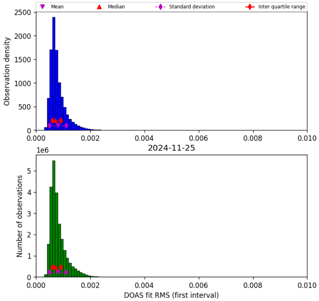
Figure 46: Histogram of “DOAS fit RMS (first interval)” for 2024-11-25 to 2024-11-26
