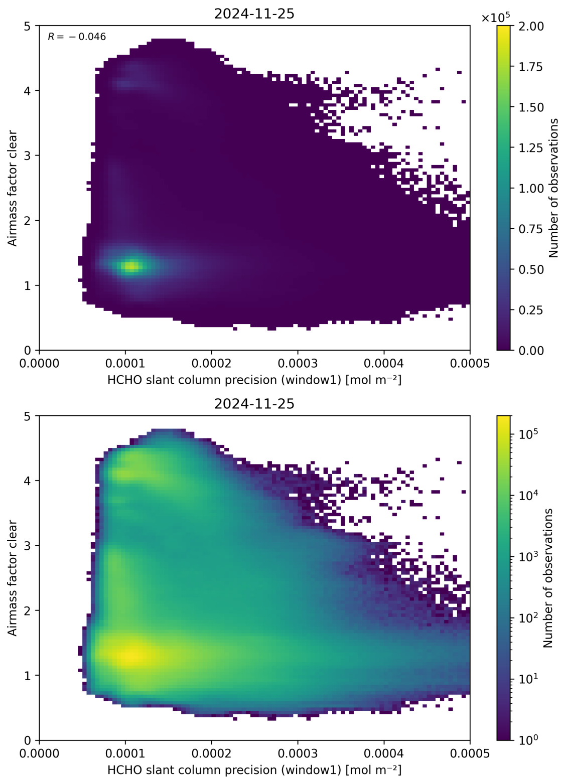
Figure 91: Scatter density plot of “HCHO slant column precision (window1)” against “Airmass factor clear” for 2024-11-25 to 2024-11-26.
