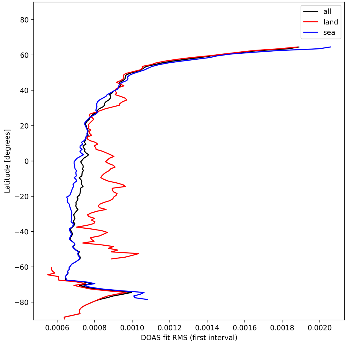
Figure 32: Zonal average of “DOAS fit RMS (first interval)” for 2024-11-25 to 2024-11-26.
