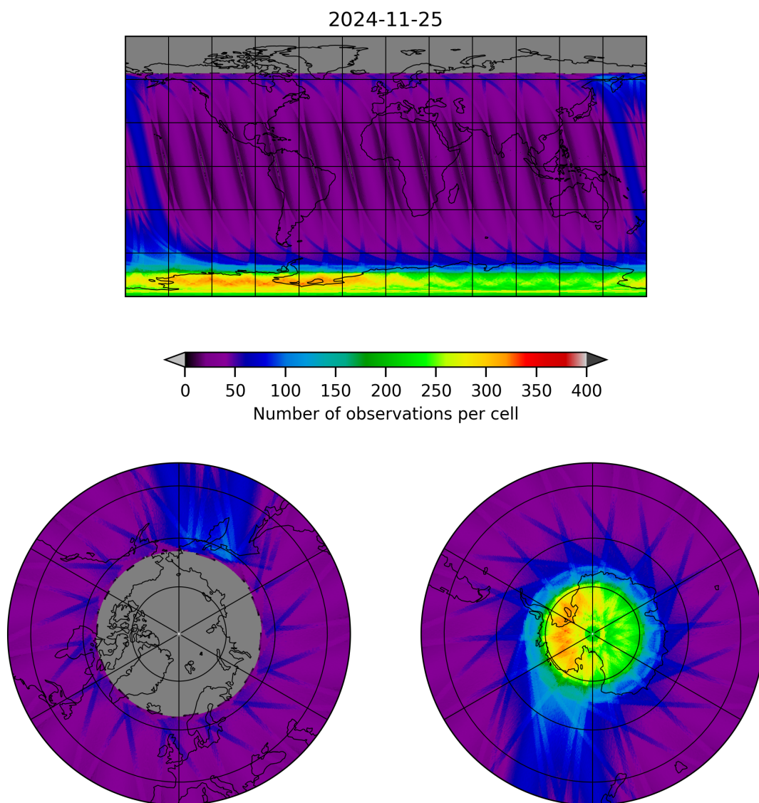
Figure 19: Map of the number of observations for 2024-11-25 to 2024-11-26
