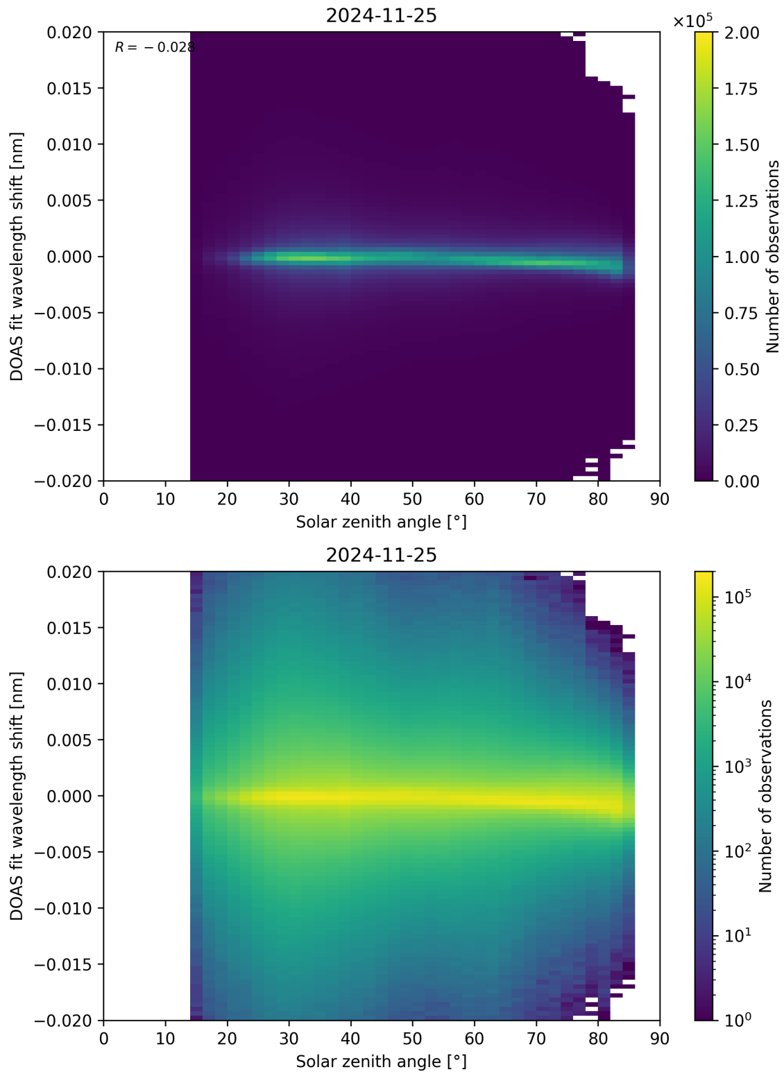
Figure 168: Scatter density plot of “Solar zenith angle” against “DOAS fit wavelength shift” for 2024-11-25 to 2024-11-26.
