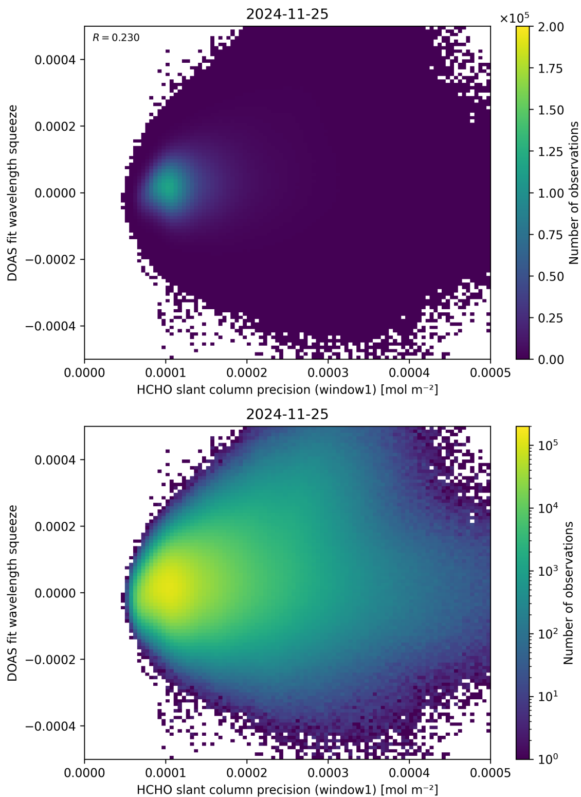
Figure 90: Scatter density plot of “HCHO slant column precision (window1)” against “DOAS fit wavelength squeeze” for 2024-11-25 to 2024-11-26.
