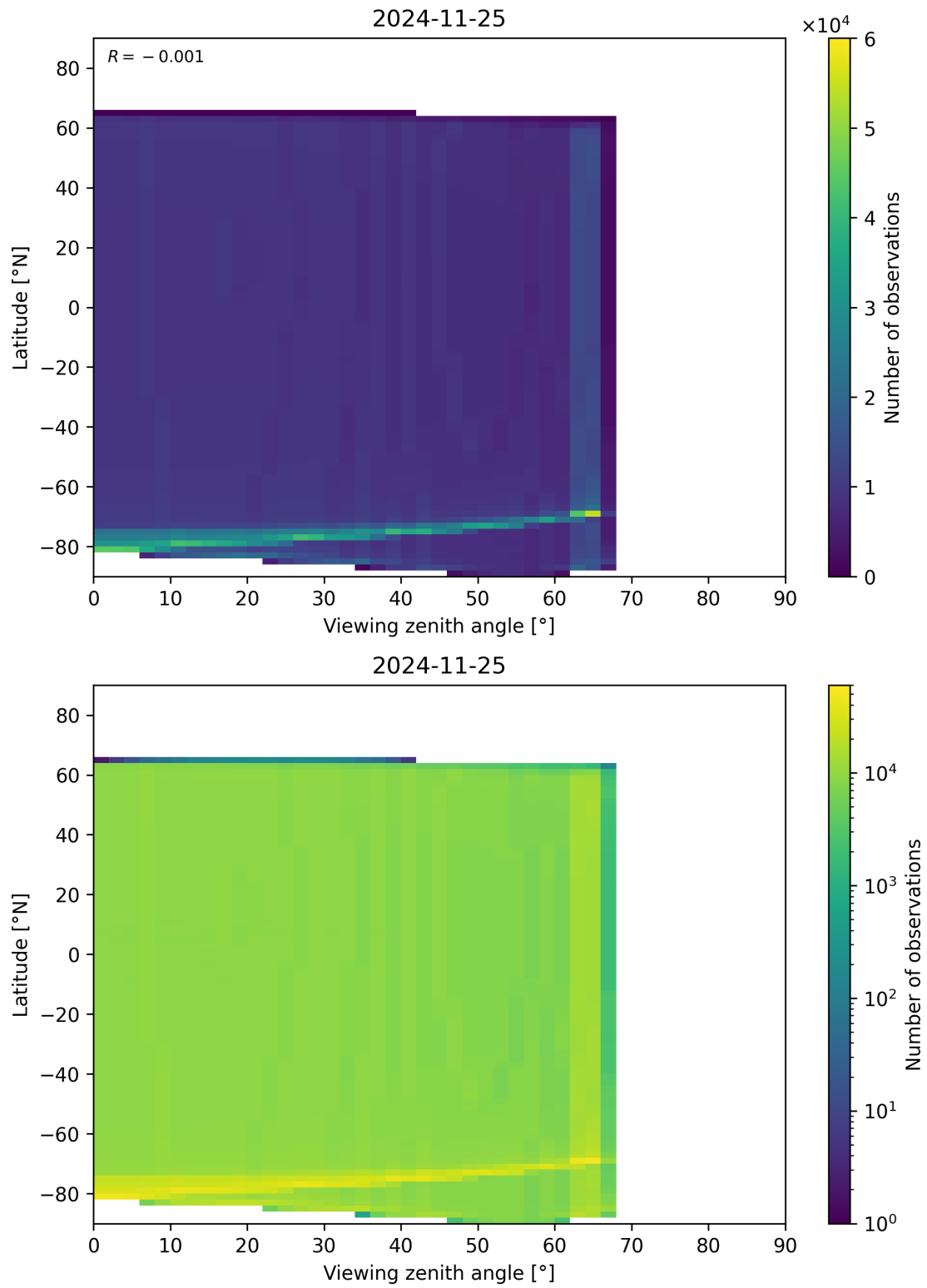
Figure 196: Scatter density plot of “Viewing zenith angle” against “Latitude” for 2024-11-25 to 2024-11-26.
