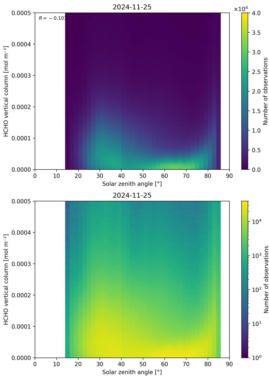
Figure 177: Scatter density plot of “Solar zenith angle” against “HCHO vertical column” for 2024-11-25 to 2024-11-26.
