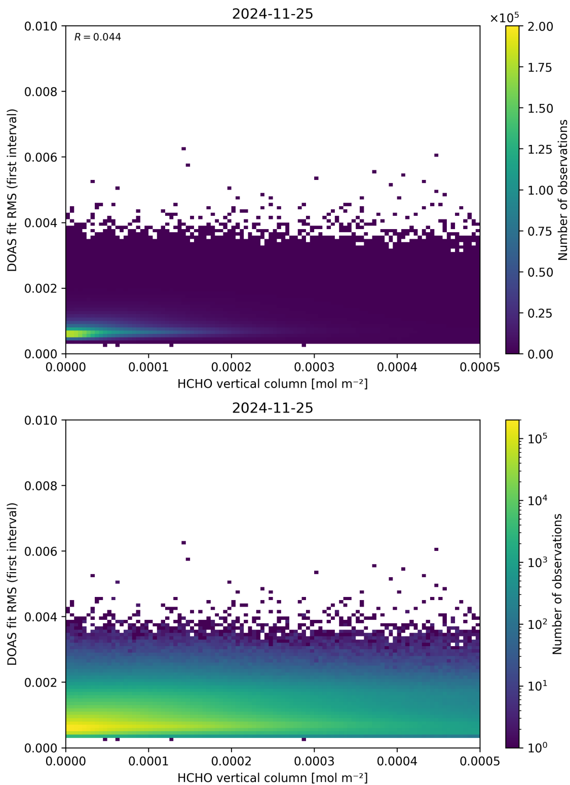
Figure 123: Scatter density plot of “HCHO vertical column” against “DOAS fit RMS (first interval)” for 2024-11-25 to 2024-11-26.
