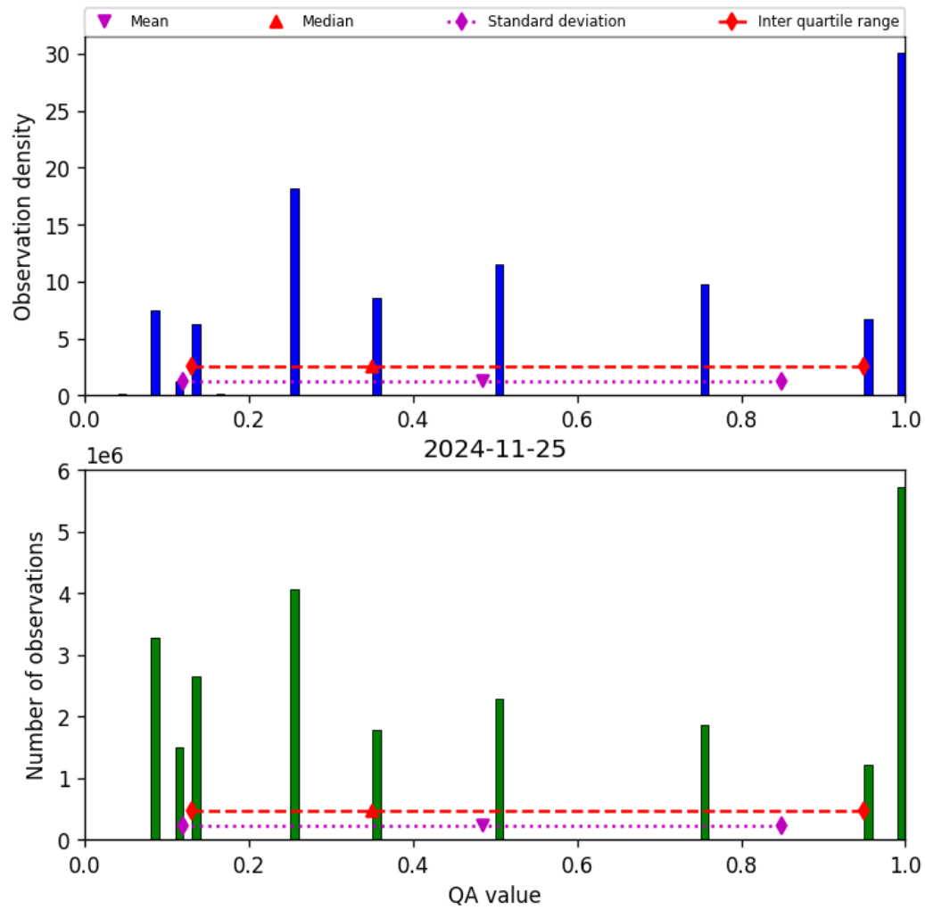
Figure 34: Histogram of “QA value” for 2024-11-25 to 2024-11-26
