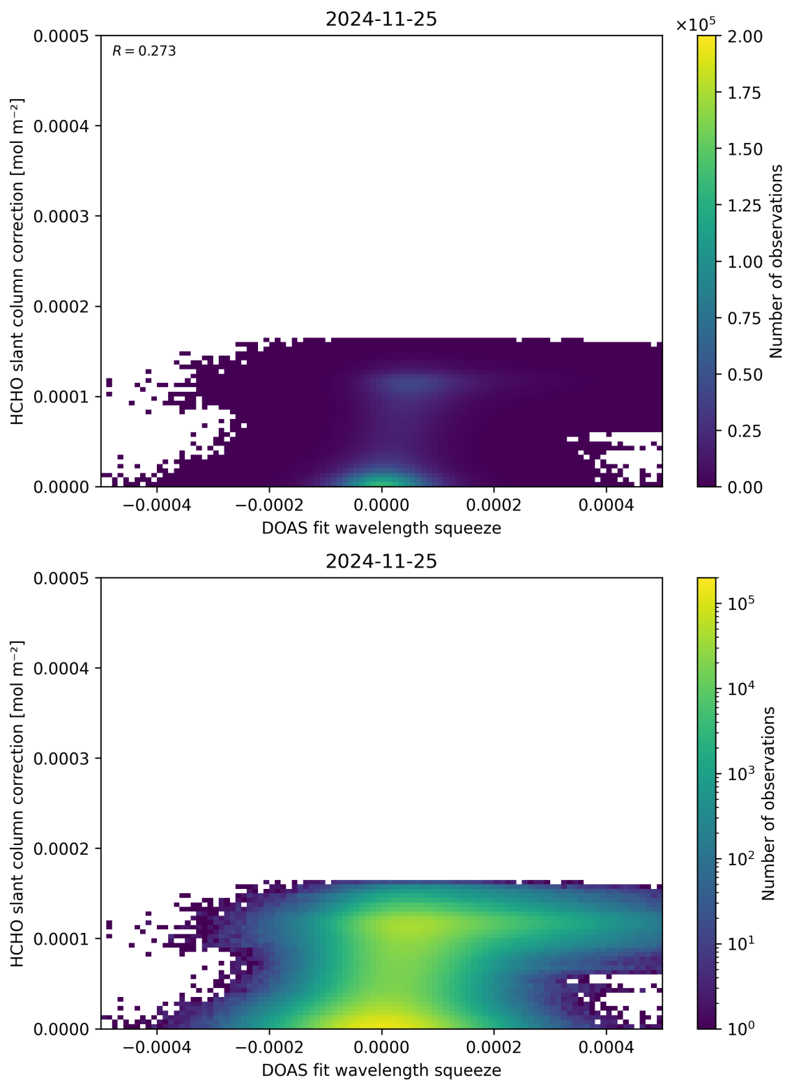
Figure 70: Scatter density plot of “DOAS fit wavelength squeeze” against “HCHO slant column correction” for 2024-11-25 to 2024-11-26.
