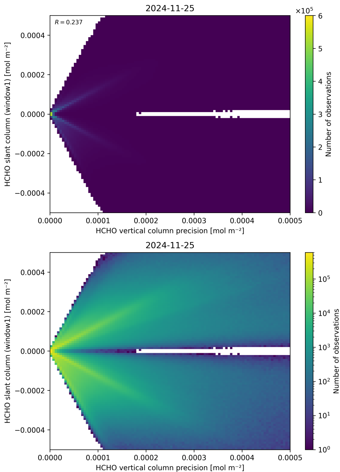
Figure 142: Scatter density plot of “HCHO vertical column precision” against “HCHO slant column (window1)” for 2024-11-25 to 2024-11-26.
