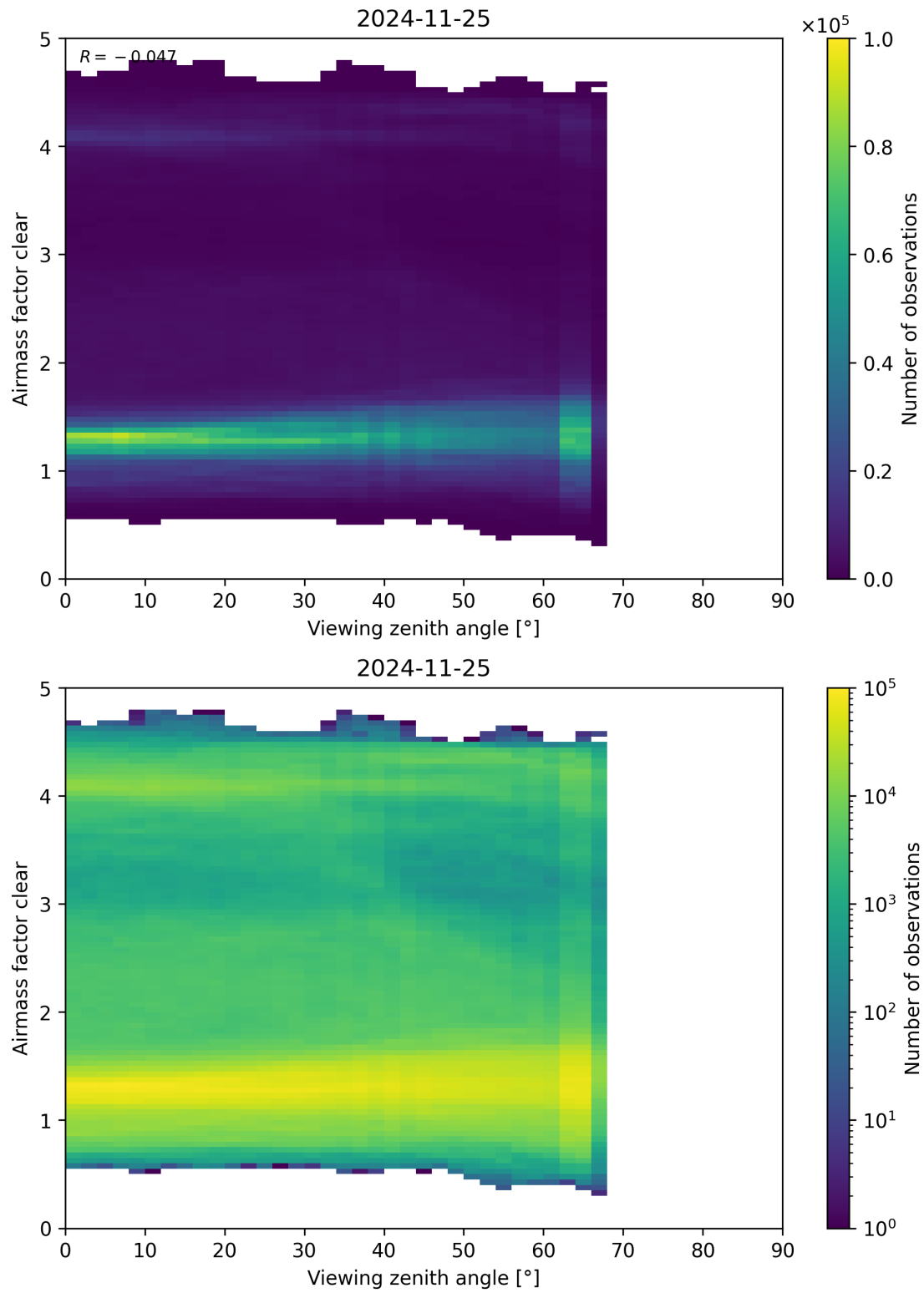
Figure 185: Scatter density plot of “Viewing zenith angle” against “Airmass factor clear” for 2024-11-25 to 2024-11-26.
