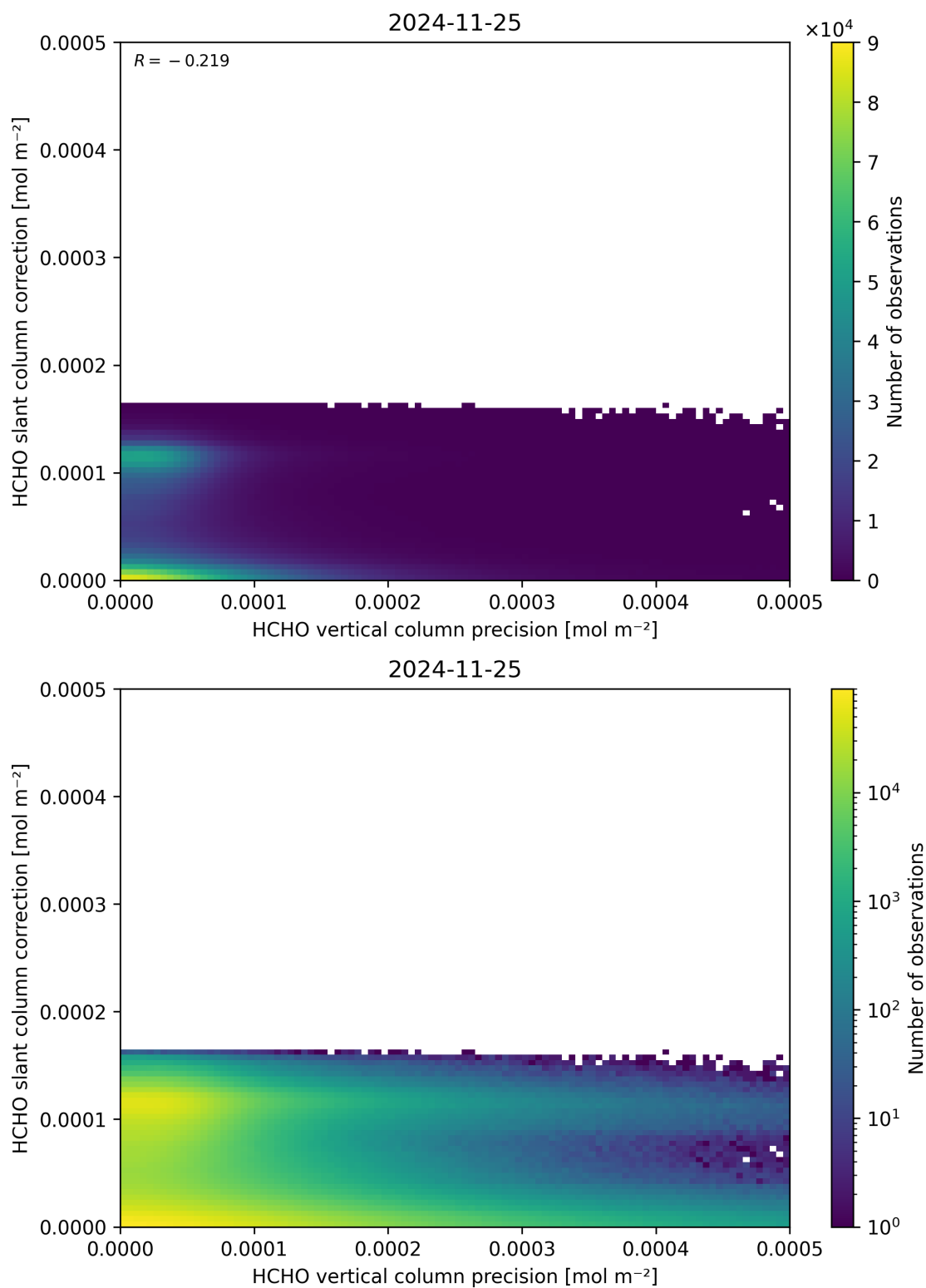
Figure 141: Scatter density plot of “HCHO vertical column precision” against “HCHO slant column correction” for 2024-11-25 to 2024-11-26.
