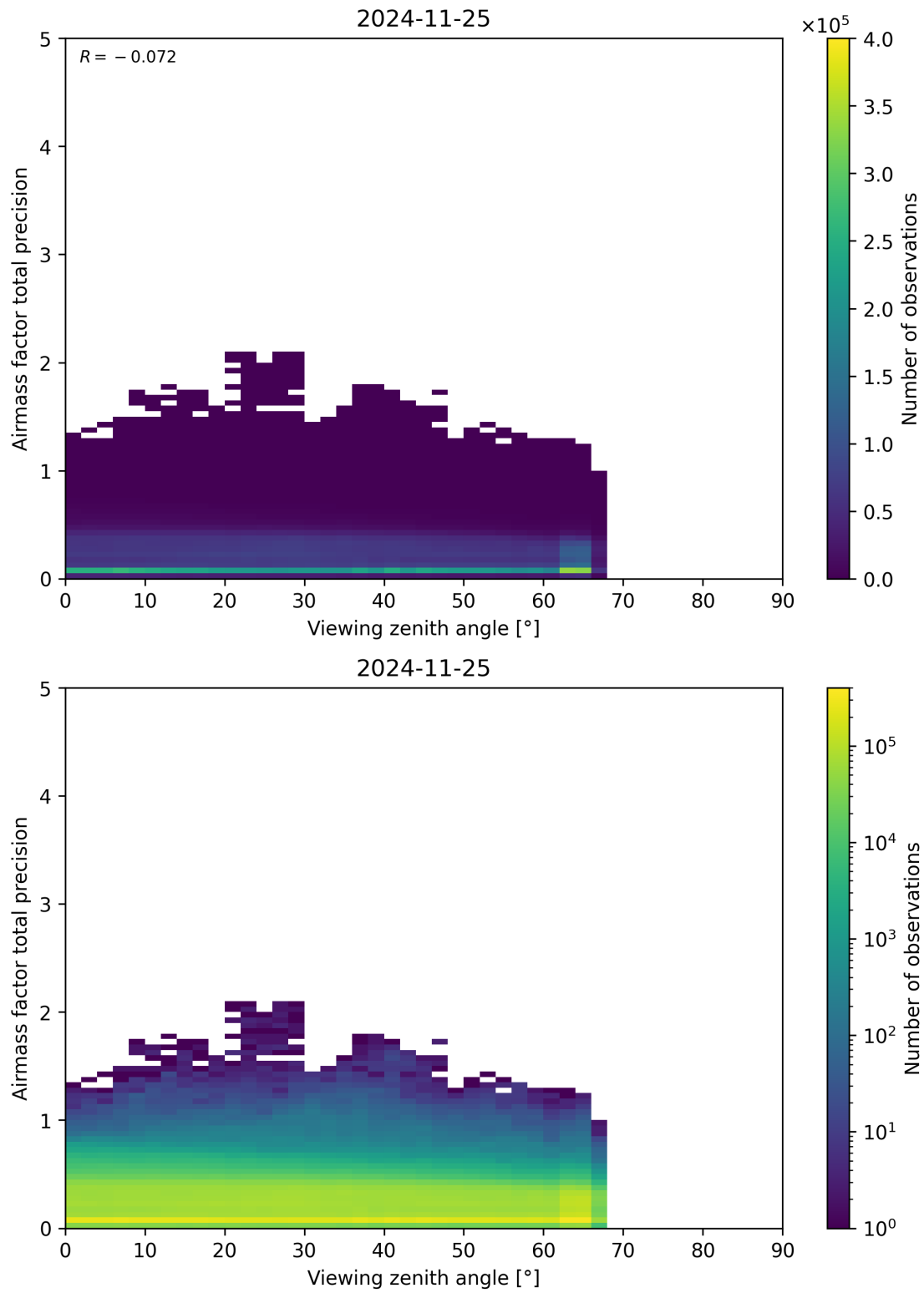
Figure 191: Scatter density plot of “Viewing zenith angle” against “Airmass factor total precision” for 2024-11-25 to 2024-11-26.
