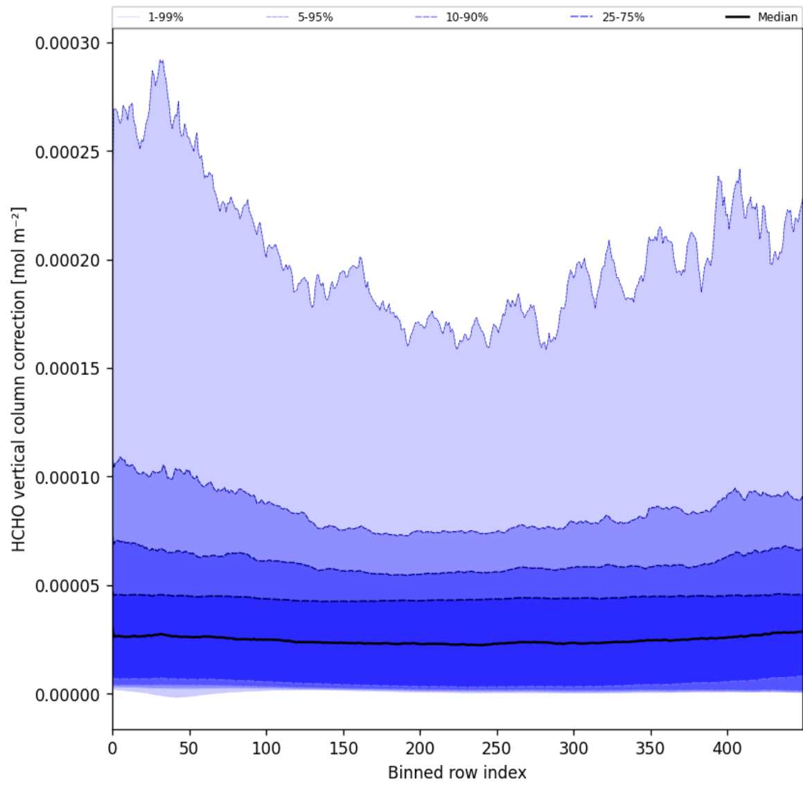
Figure 51: Along track statistics of “HCHO vertical column correction” for 2024-11-25 to 2024-11-26
