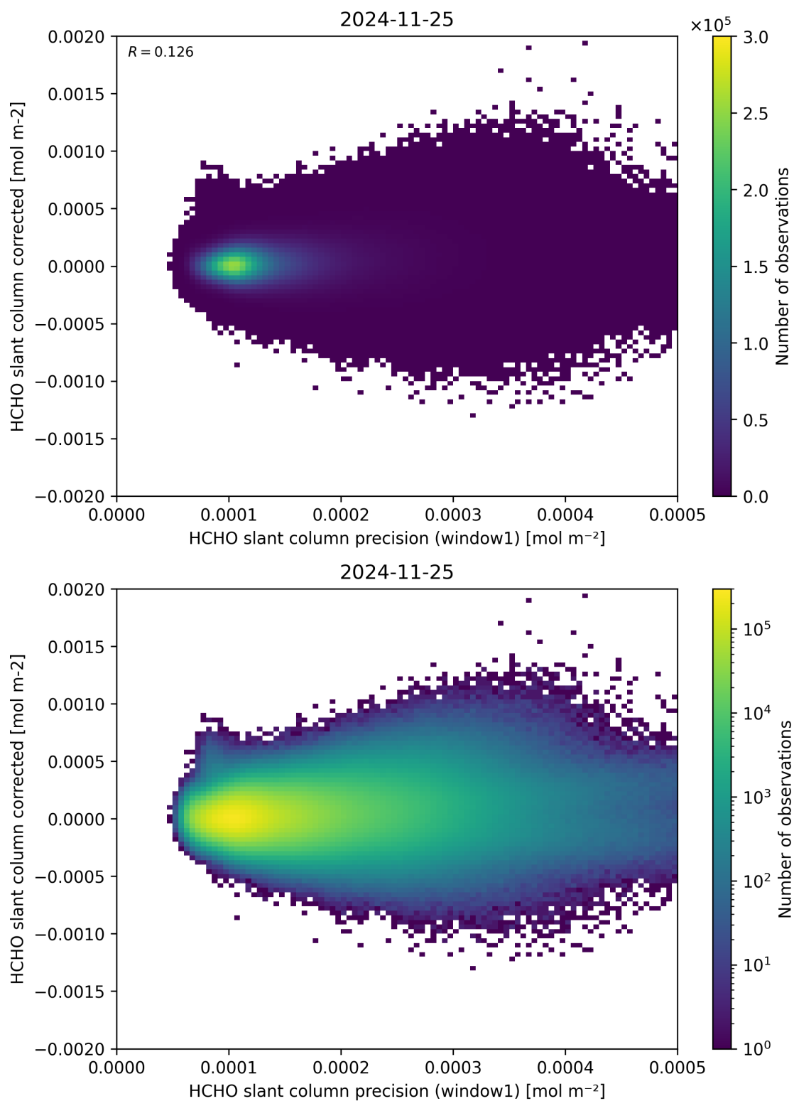
Figure 92: Scatter density plot of “HCHO slant column precision (window1)” against “HCHO slant column corrected” for 2024-11-25 to 2024-11-26.
