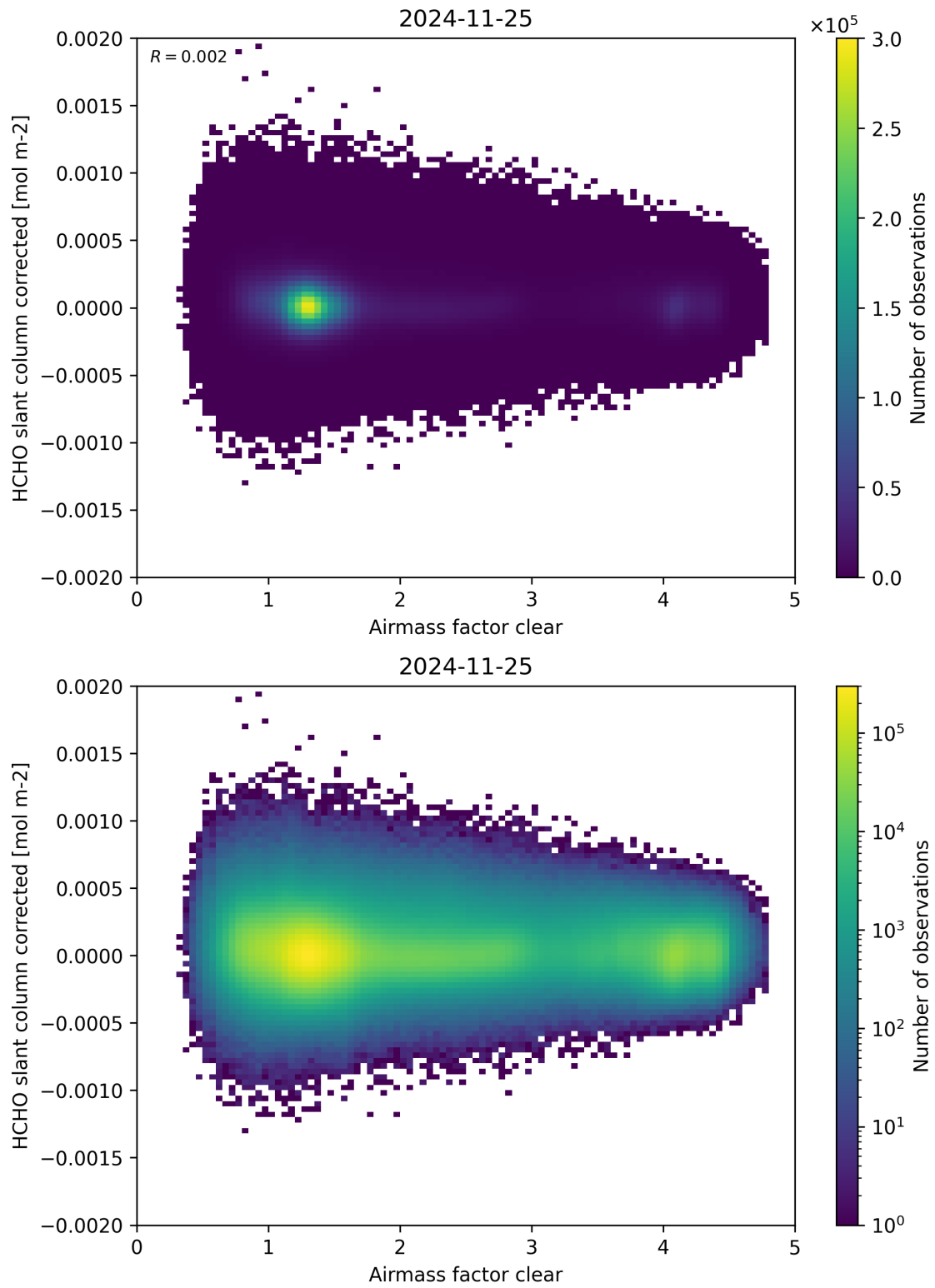
Figure 74: Scatter density plot of “Airmass factor clear” against “HCHO slant column corrected” for 2024-11-25 to 2024-11-26.
