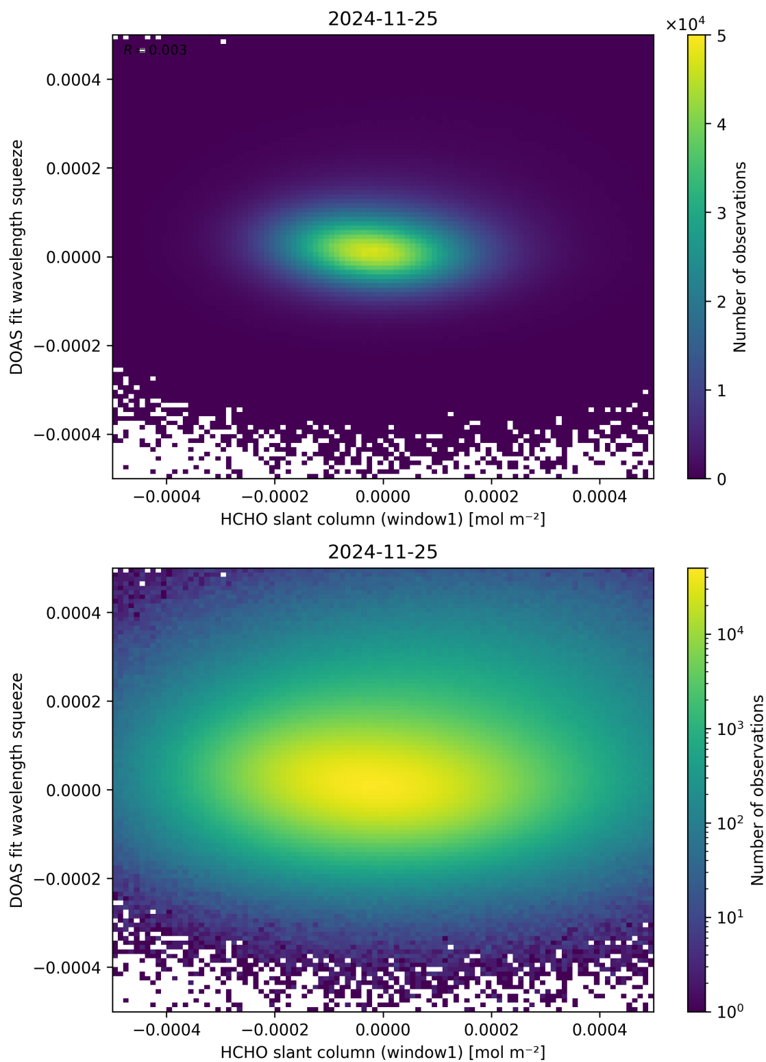
Figure 80: Scatter density plot of “HCHO slant column (window1)” against “DOAS fit wavelength squeeze” for 2024-11-25 to 2024-11-26.
