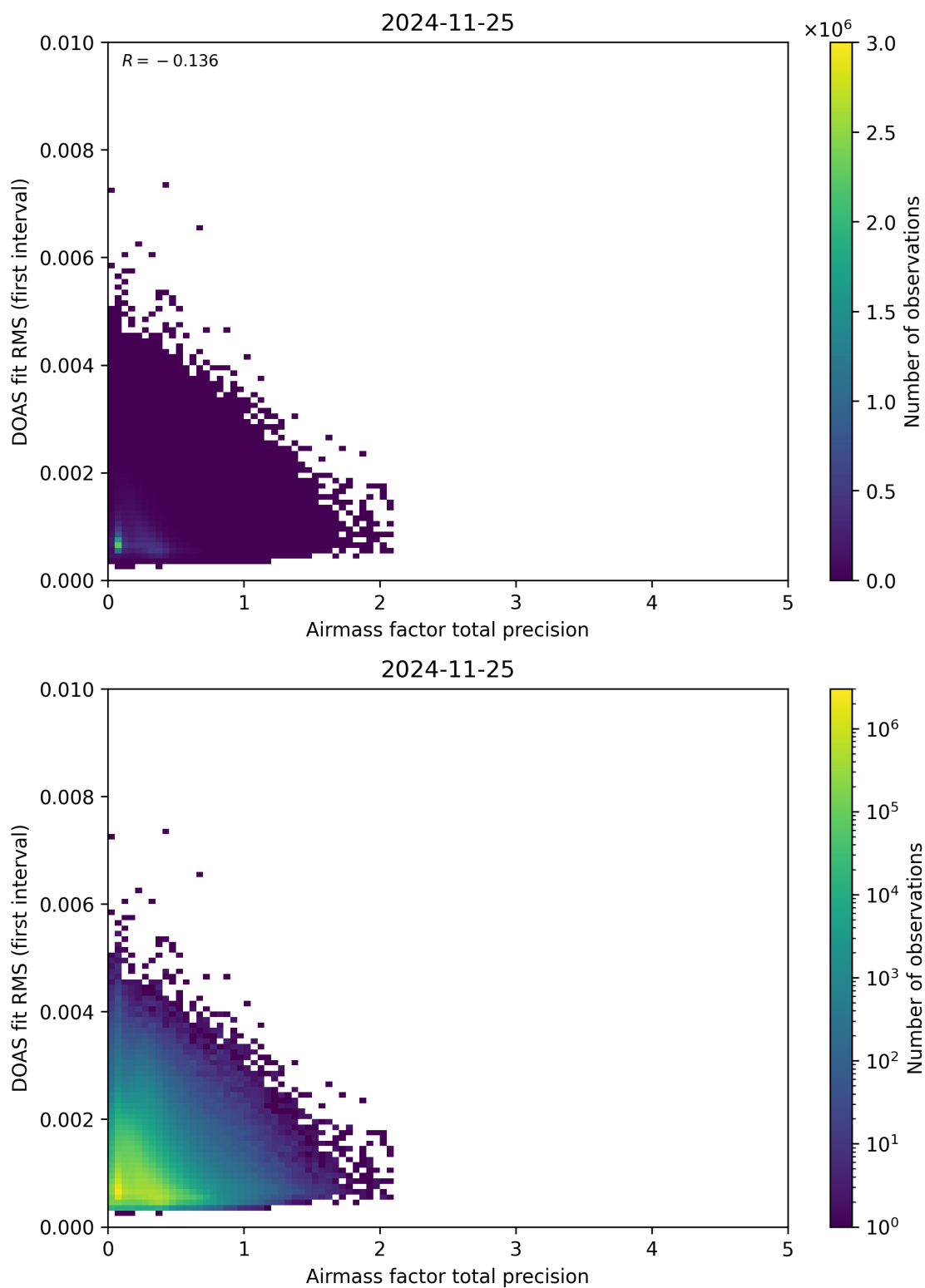
Figure 105: Scatter density plot of “Airmass factor total precision” against “DOAS fit RMS (first interval)” for 2024-11-25 to 2024-11-26.
