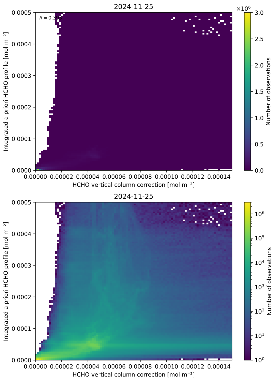
Figure 122: Scatter density plot of “HCHO vertical column correction” against “Integrated a priori HCHO profile” for 2024-11-25 to 2024-11-26.
