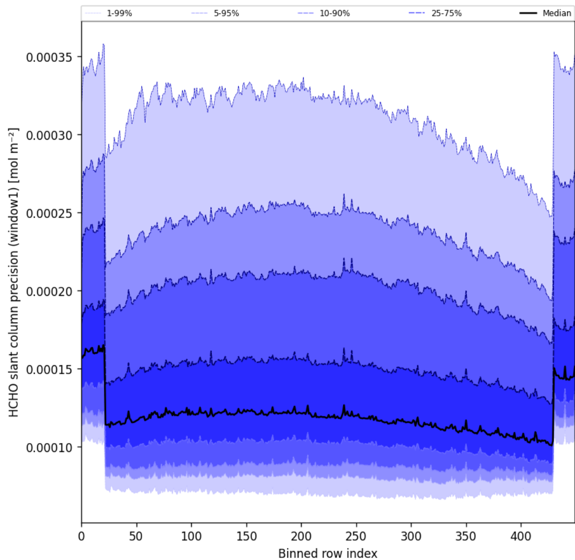
Figure 53: Along track statistics of “HCHO slant column precision (window1)” for 2024-11-25 to 2024-11-26
