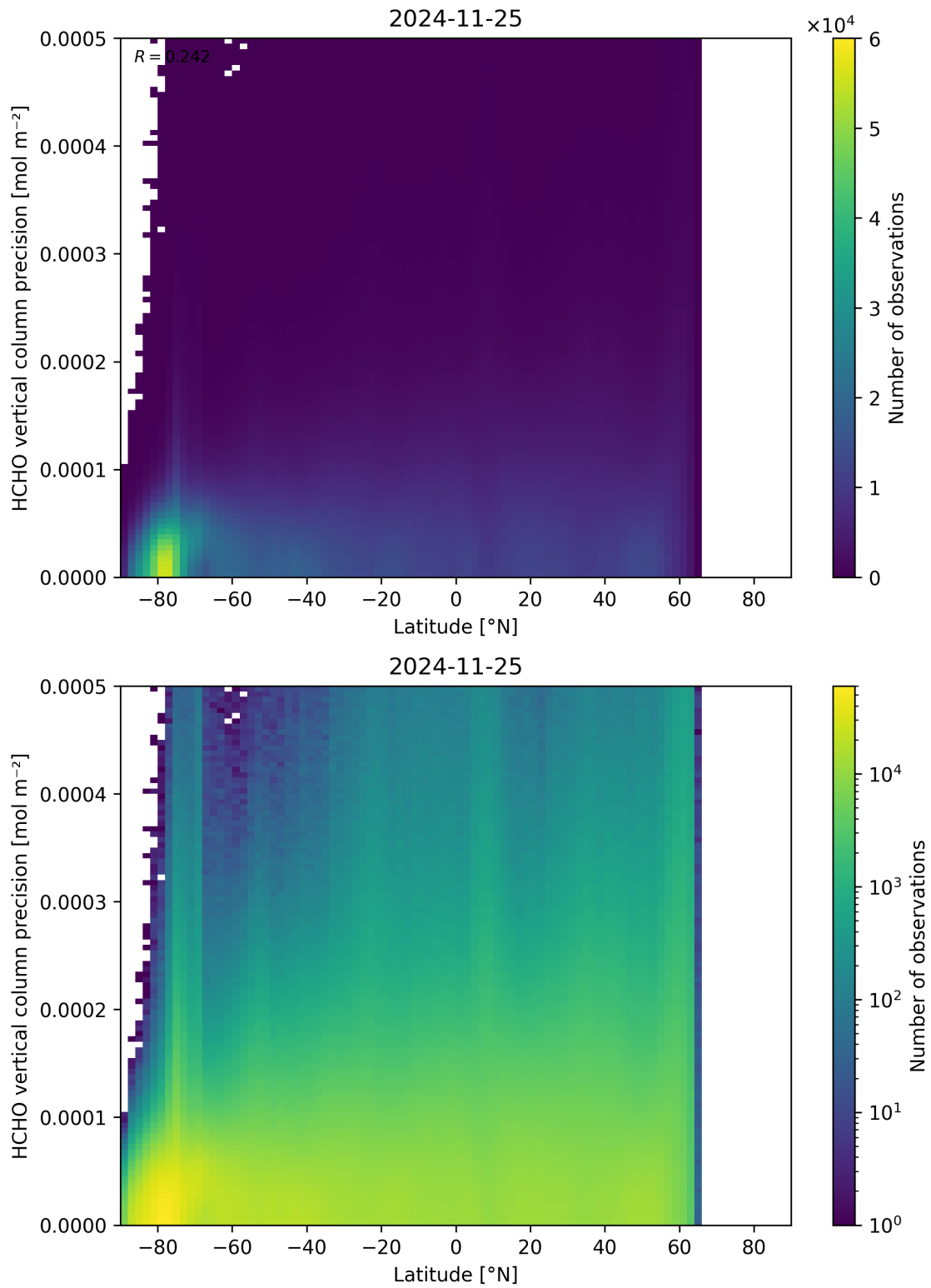
Figure 165: Scatter density plot of “Latitude” against “HCHO vertical column precision” for 2024-11-25 to 2024-11-26.
