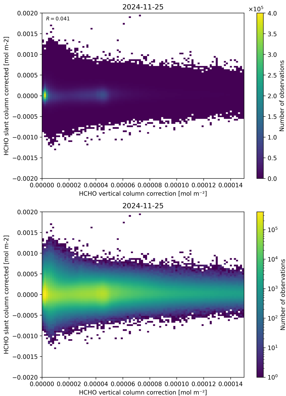
Figure 116: Scatter density plot of “HCHO vertical column correction” against “HCHO slant column corrected” for 2024-11-25 to 2024-11-26.
