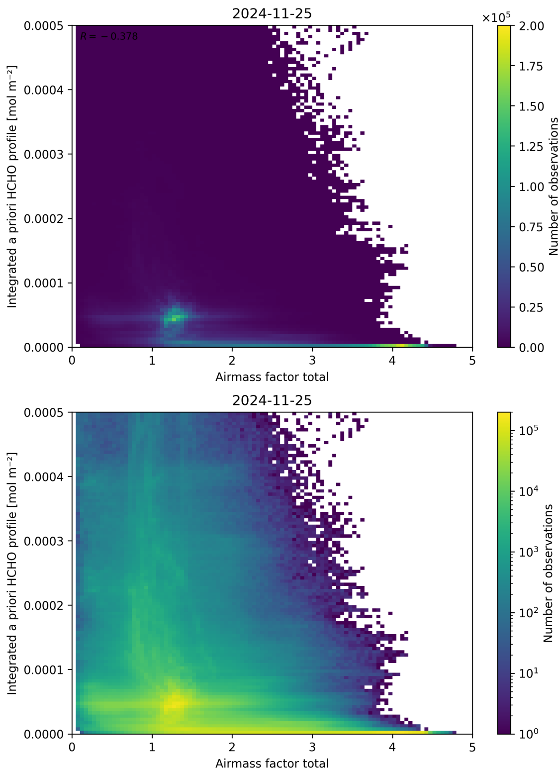
Figure 104: Scatter density plot of “Airmass factor total” against “Integrated a priori HCHO profile” for 2024-11-25 to 2024-11-26.
