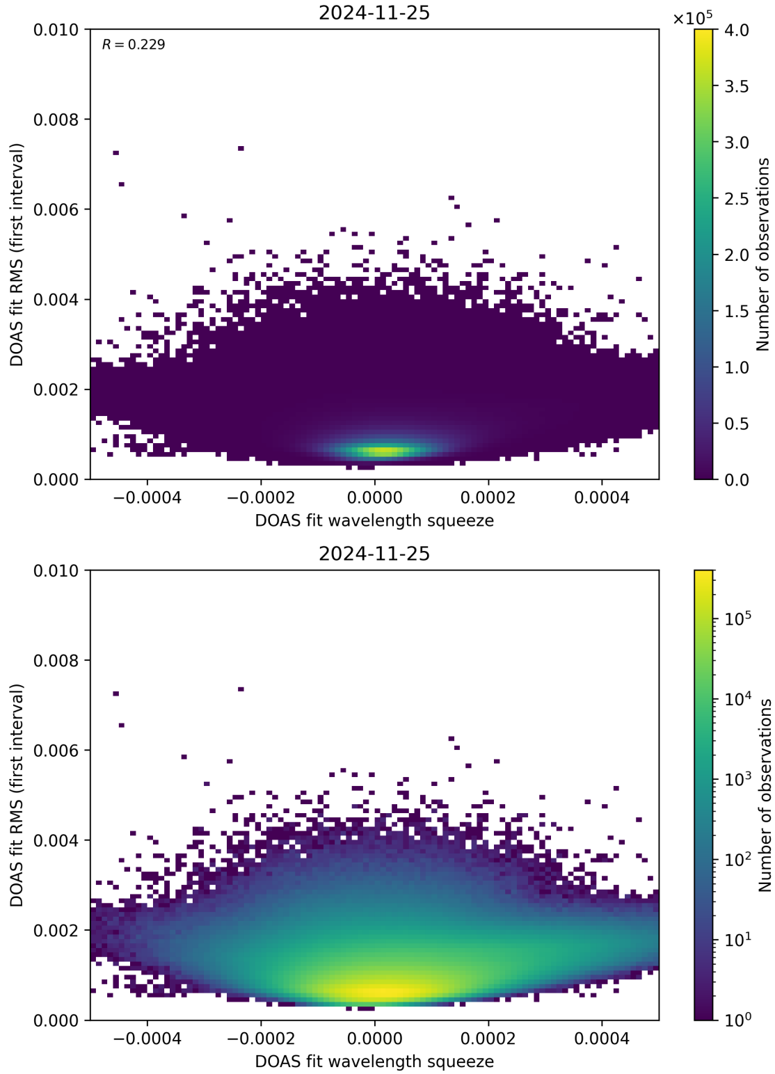
Figure 68: Scatter density plot of “DOAS fit wavelength squeeze” against “DOAS fit RMS (first interval)” for 2024-11-25 to 2024-11-26.
