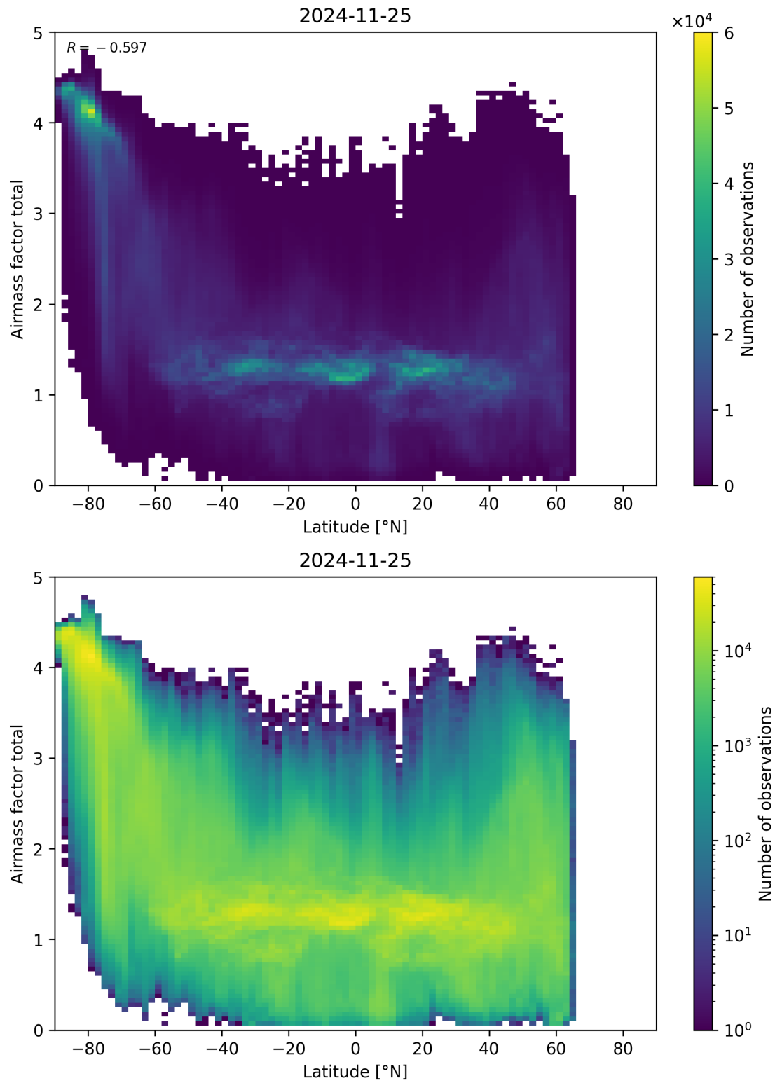
Figure 161: Scatter density plot of “Latitude” against “Airmass factor total” for 2024-11-25 to 2024-11-26.
