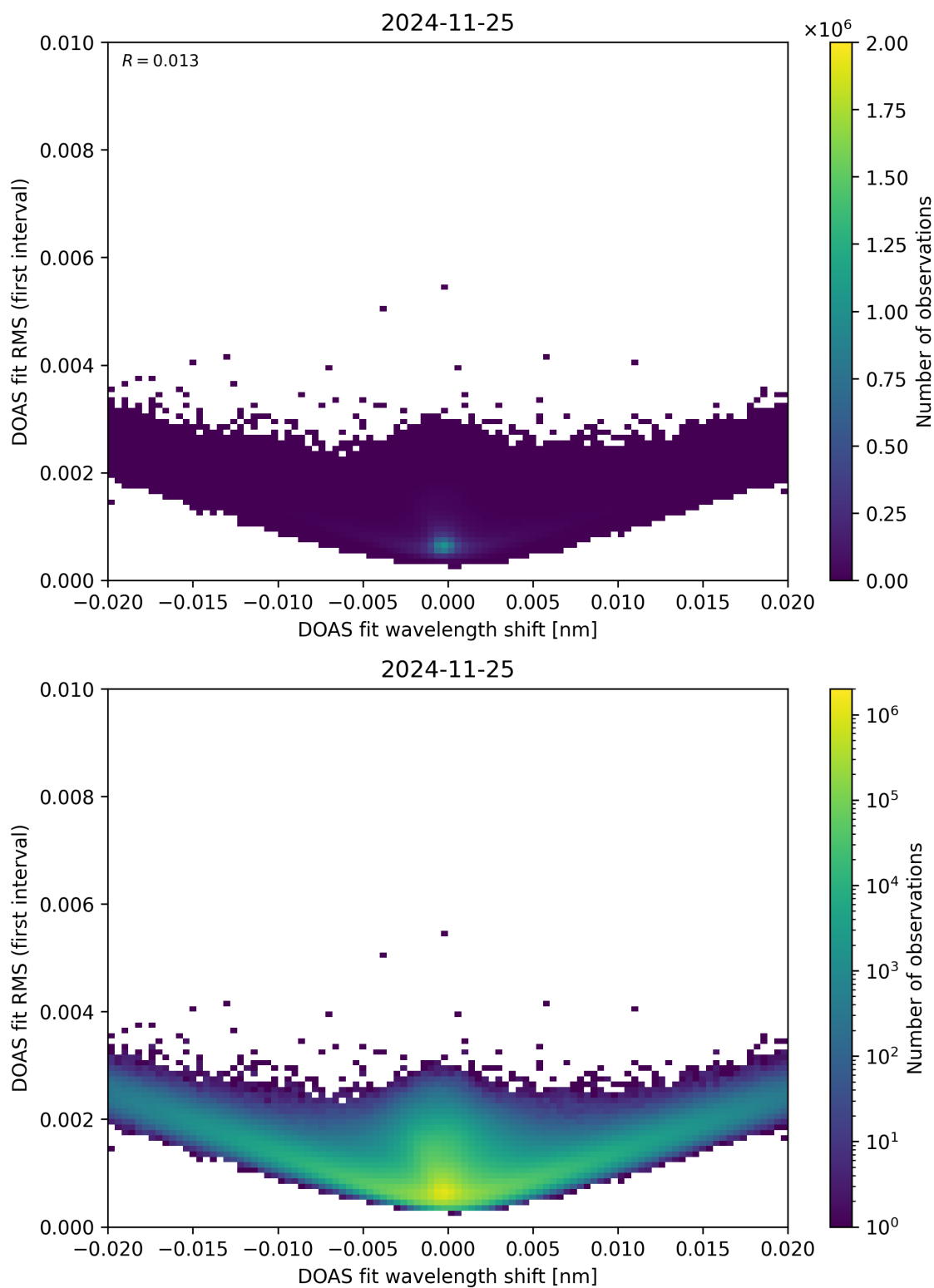
Figure 64: Scatter density plot of “DOAS fit wavelength shift” against “DOAS fit RMS (first interval)” for 2024-11-25 to 2024-11-26.
