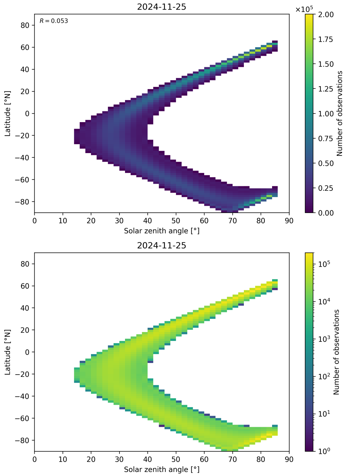
Figure 181: Scatter density plot of “Solar zenith angle” against “Latitude” for 2024-11-25 to 2024-11-26.
