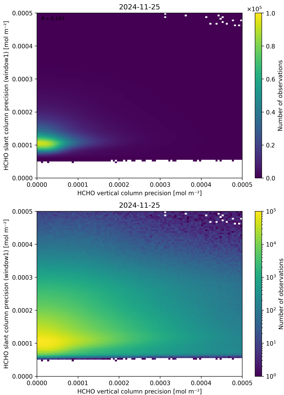
Figure 143: Scatter density plot of “HCHO vertical column precision” against “HCHO slant column precision (window1)” for 2024-11-25 to 2024-11-26.
