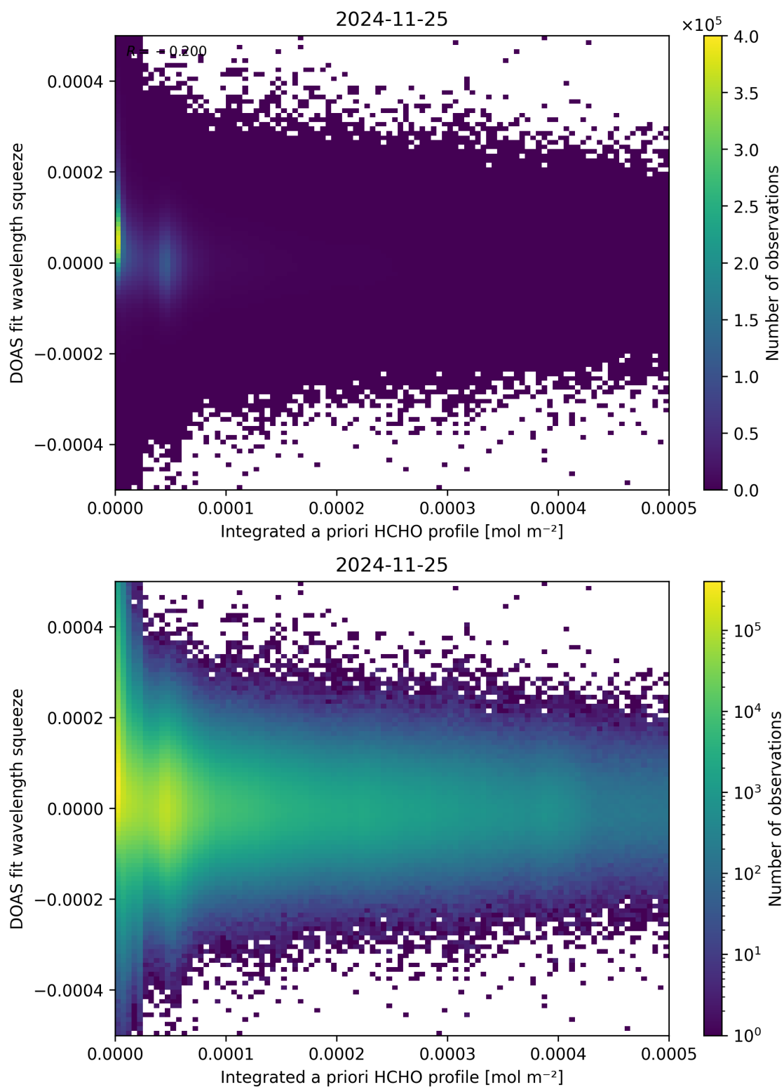
Figure 150: Scatter density plot of “Integrated a priori HCHO profile” against “DOAS fit wavelength squeeze” for 2024-11-25 to 2024-11-26.
