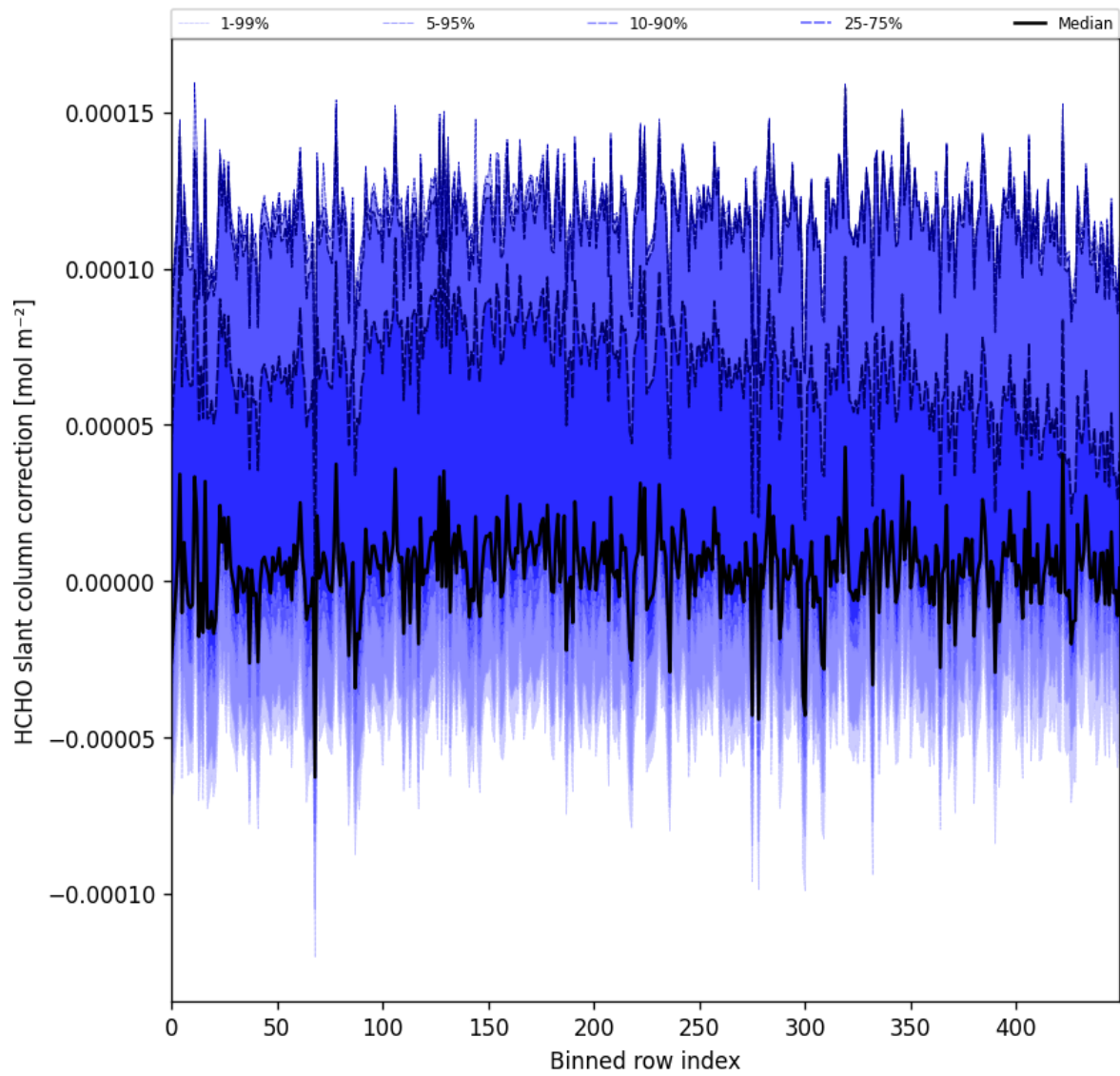
Figure 61: Along track statistics of “HCHO slant column correction” for 2024-11-25 to 2024-11-26
