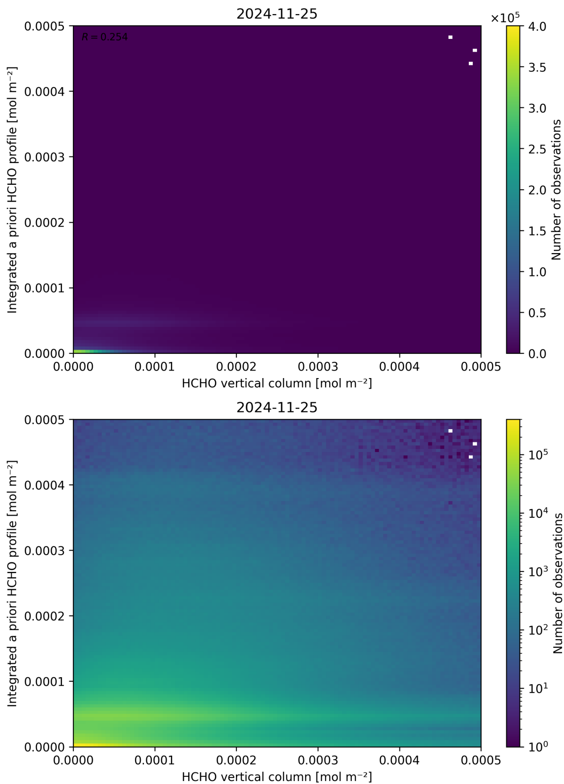
Figure 135: Scatter density plot of “HCHO vertical column” against “Integrated a priori HCHO profile” for 2024-11-25 to 2024-11-26.
