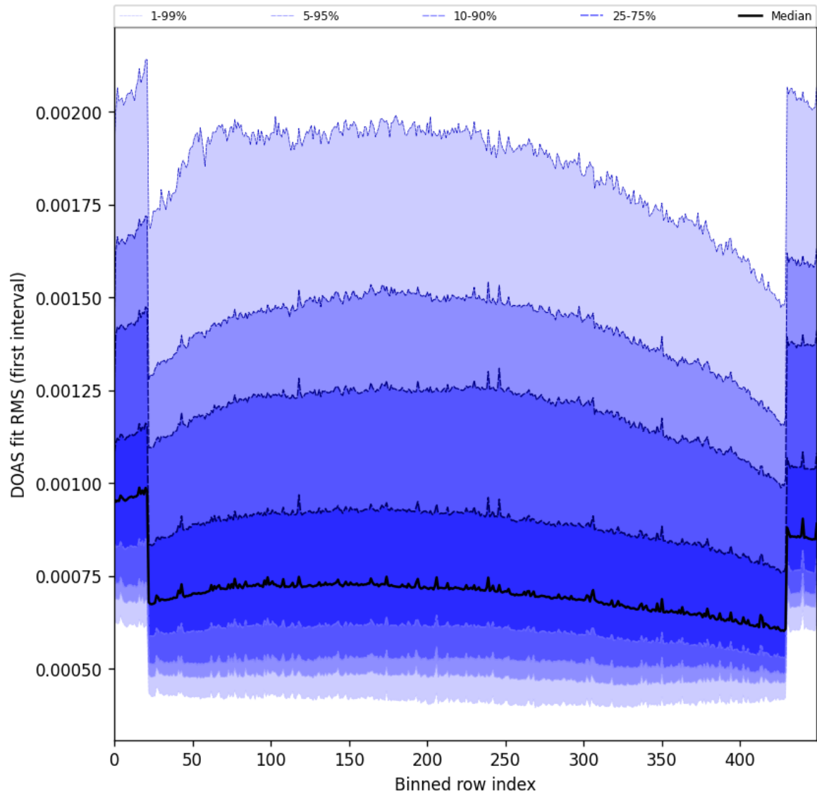
Figure 60: Along track statistics of “DOAS fit RMS (first interval)” for 2024-11-25 to 2024-11-26
