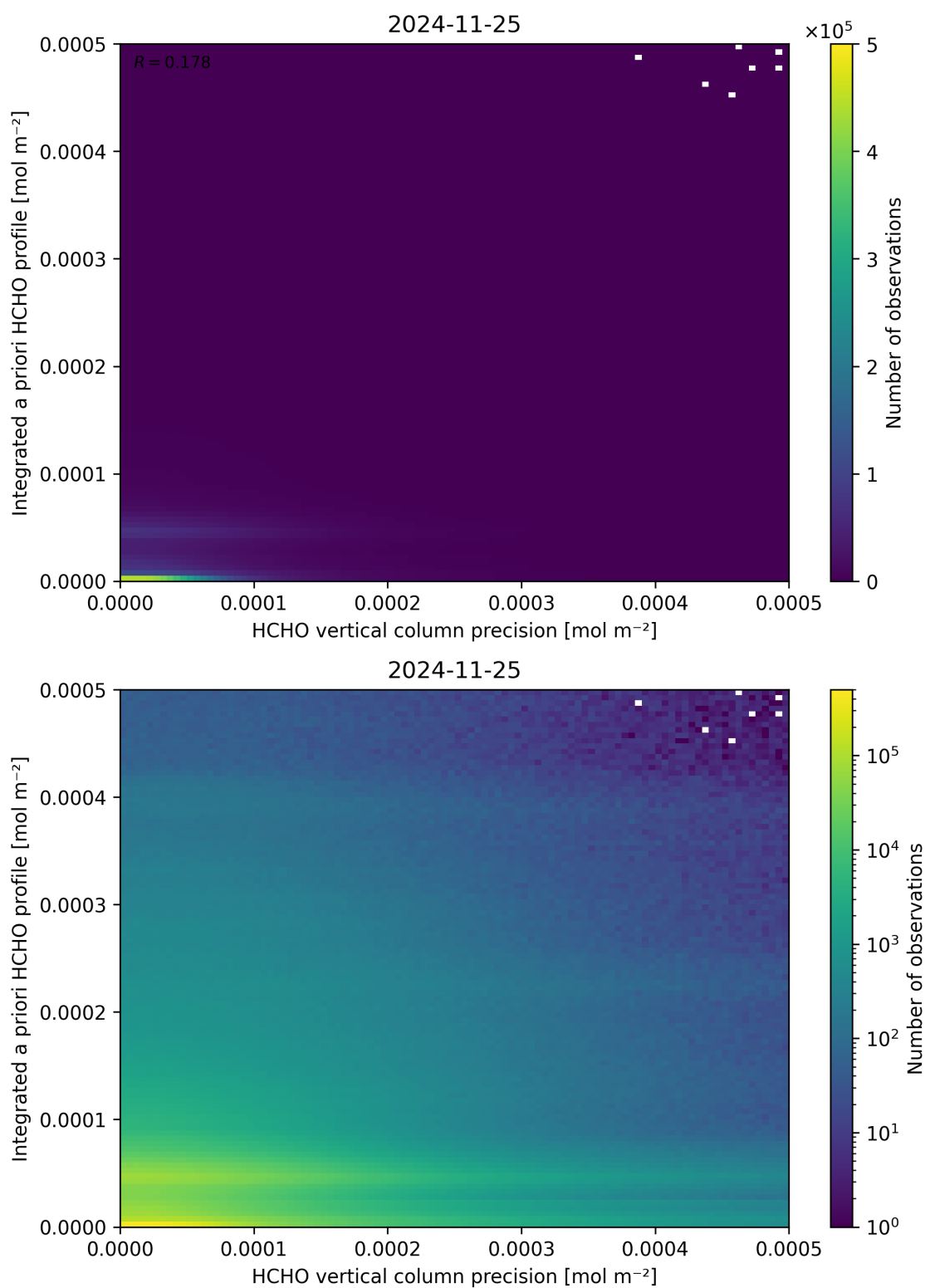
Figure 147: Scatter density plot of “HCHO vertical column precision” against “Integrated a priori HCHO profile” for 2024-11-25 to 2024-11-26.
