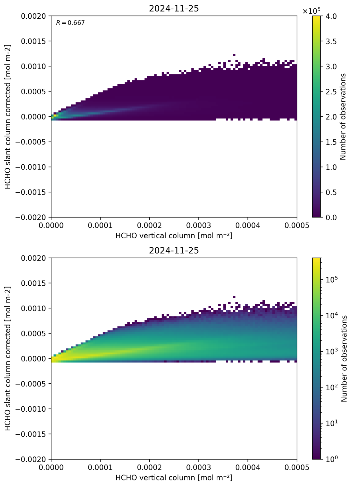
Figure 127: Scatter density plot of “HCHO vertical column” against “HCHO slant column corrected” for 2024-11-25 to 2024-11-26.
