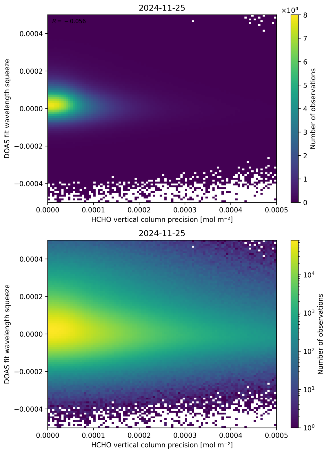
Figure 138: Scatter density plot of “HCHO vertical column precision” against “DOAS fit wavelength squeeze” for 2024-11-25 to 2024-11-26.
