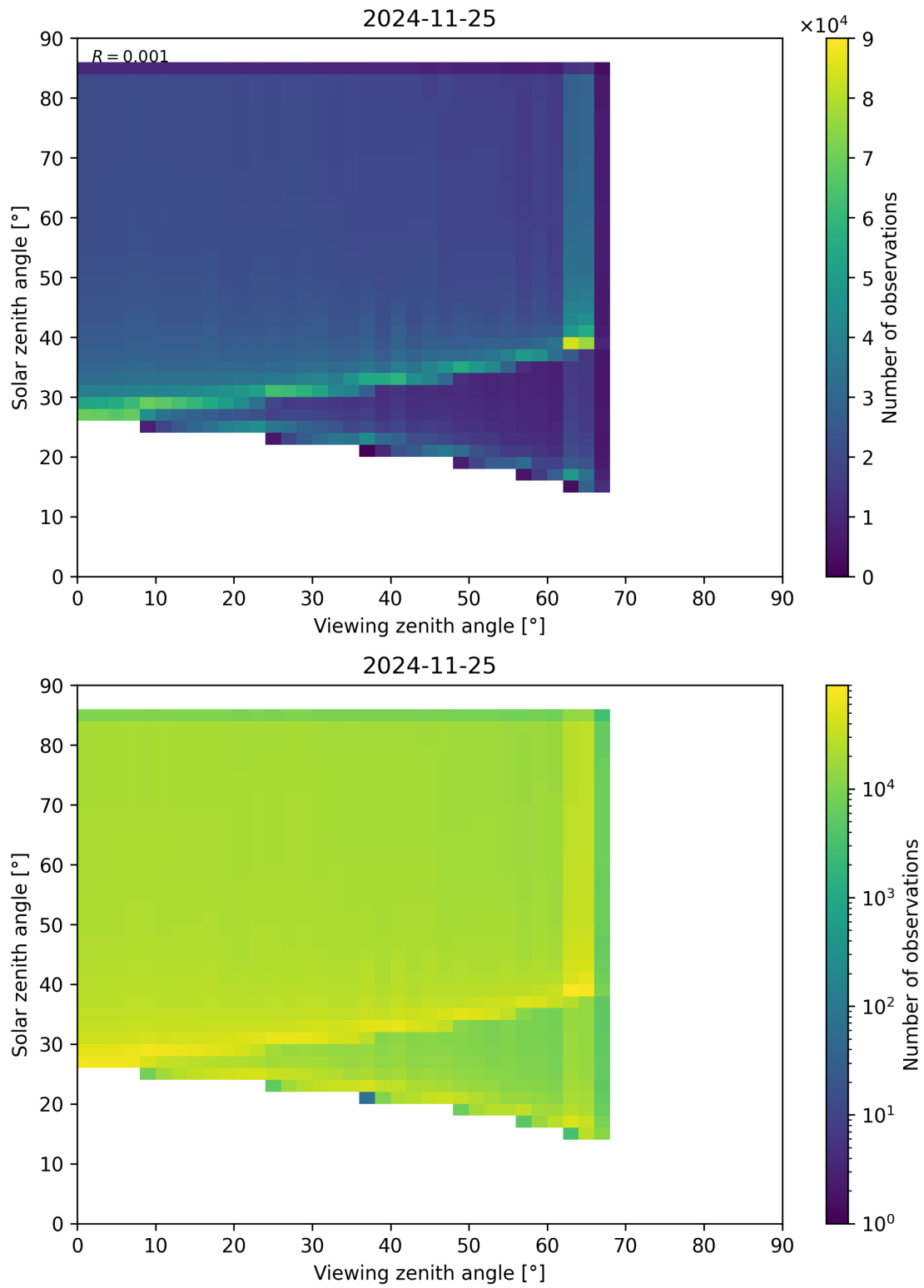
Figure 197: Scatter density plot of “Viewing zenith angle” against “Solar zenith angle” for 2024-11-25 to 2024-11-26.
