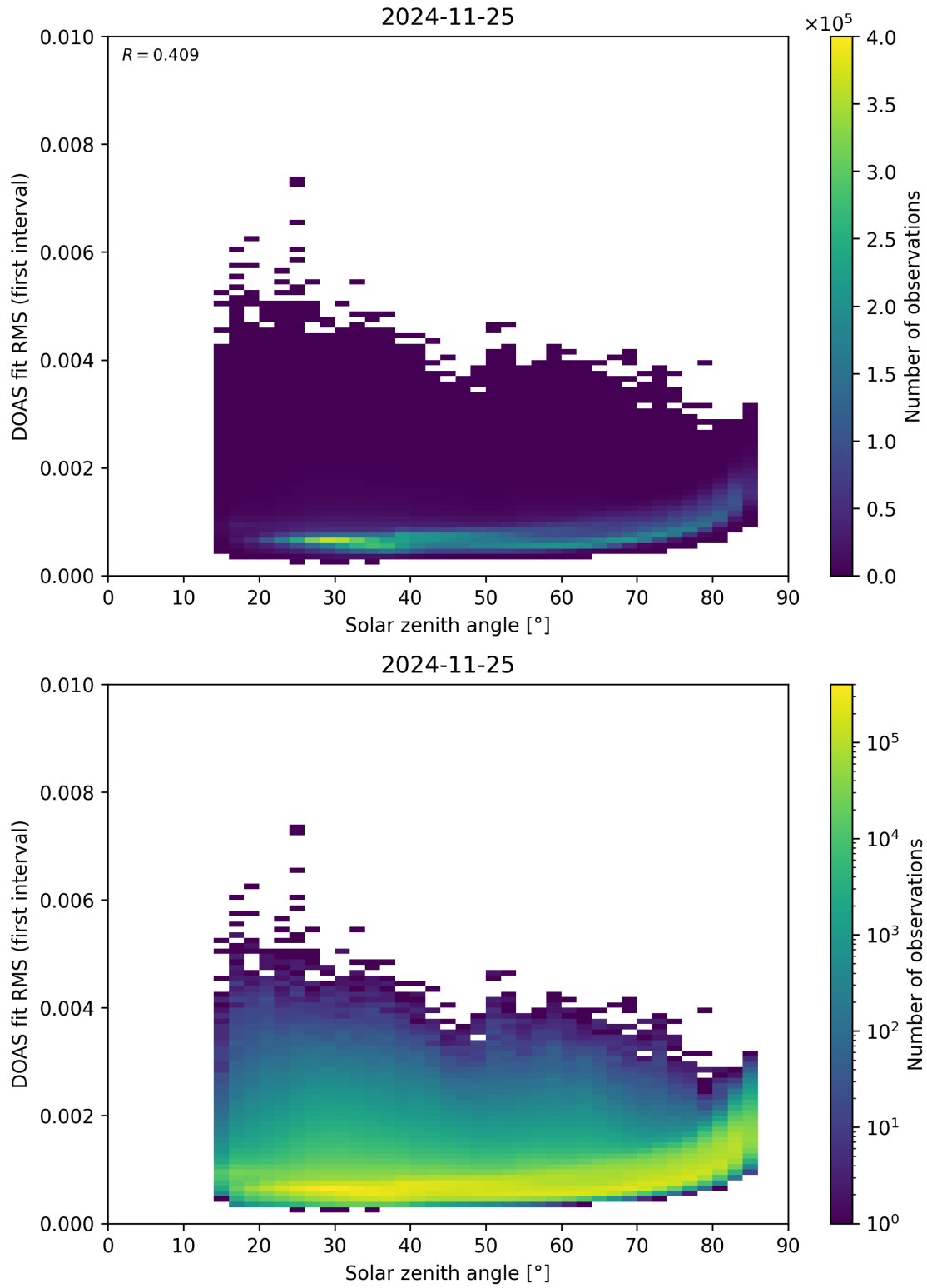
Figure 167: Scatter density plot of “Solar zenith angle” against “DOAS fit RMS (first interval)” for 2024-11-25 to 2024-11-26.
