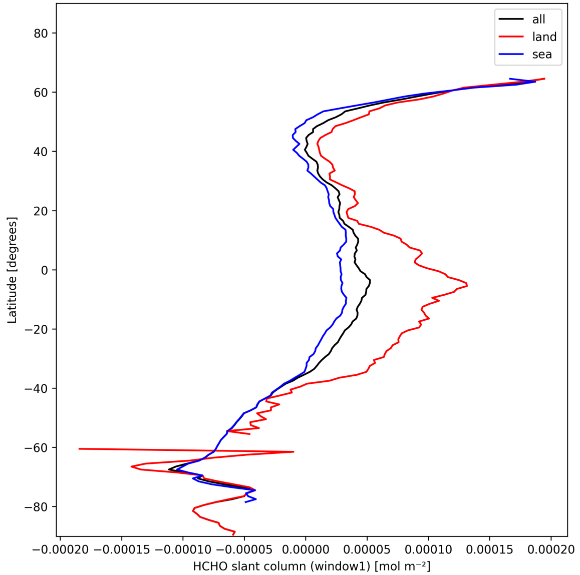
Figure 24: Zonal average of “HCHO slant column (window1)” for 2024-11-25 to 2024-11-26.
