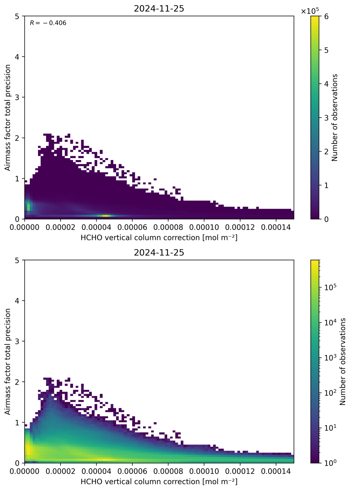
Figure 121: Scatter density plot of “HCHO vertical column correction” against “Airmass factor total precision” for 2024-11-25 to 2024-11-26.
