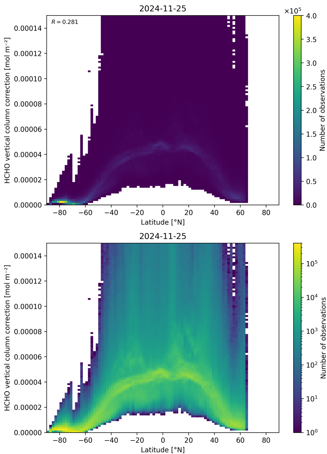
Figure 164: Scatter density plot of “Latitude” against “HCHO vertical column correction” for 2024-11-25 to 2024-11-26.
