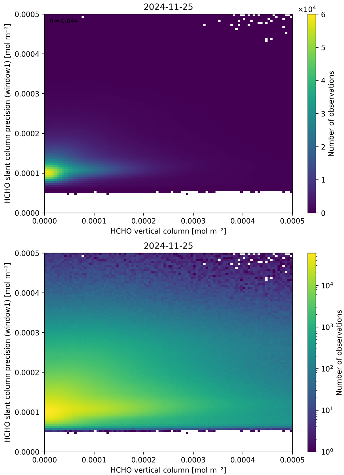
Figure 130: Scatter density plot of “HCHO vertical column” against “HCHO slant column precision (window1)” for 2024-11-25 to 2024-11-26.
