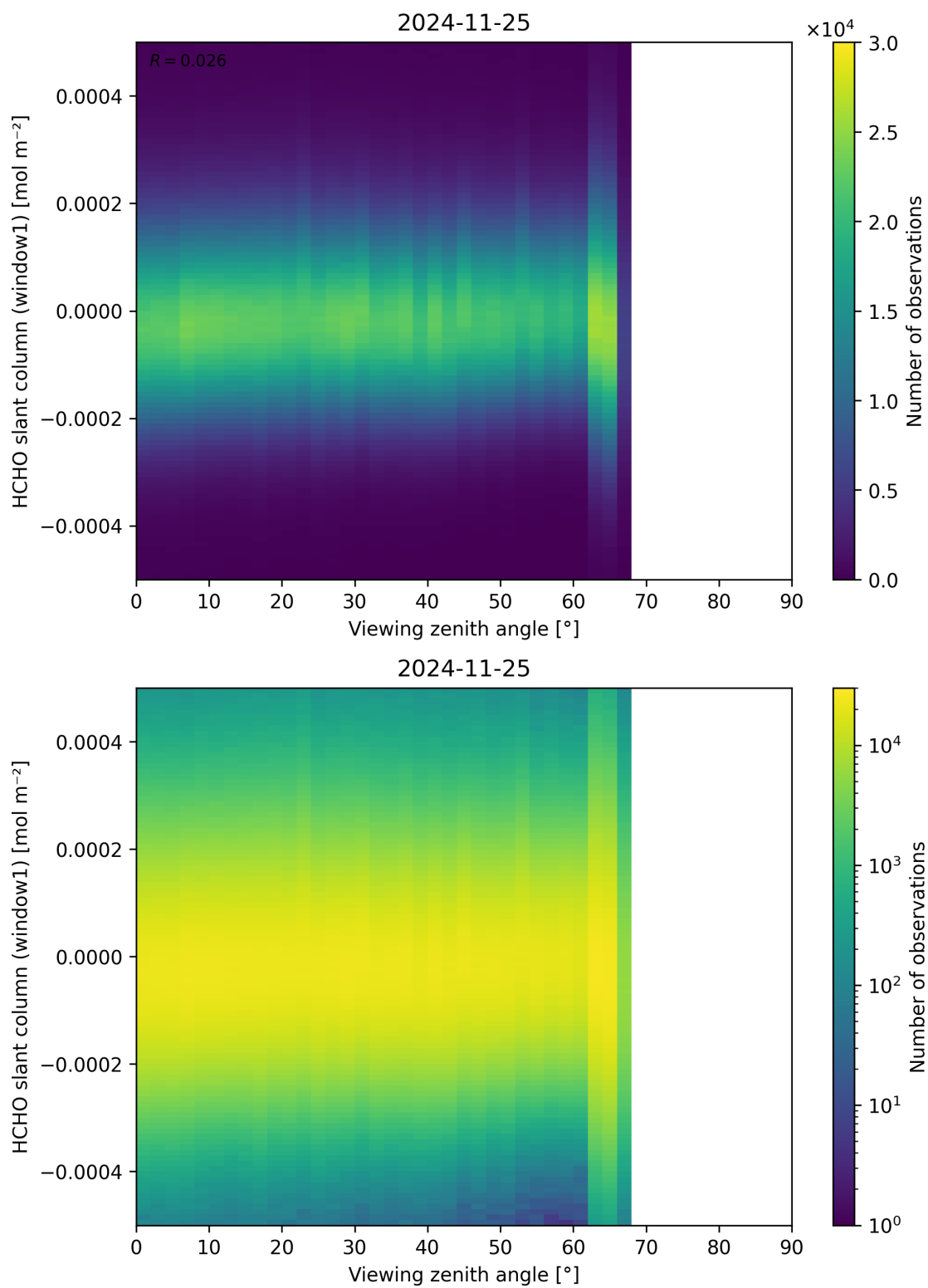
Figure 188: Scatter density plot of “Viewing zenith angle” against “HCHO slant column (window1)” for 2024-11-25 to 2024-11-26.
