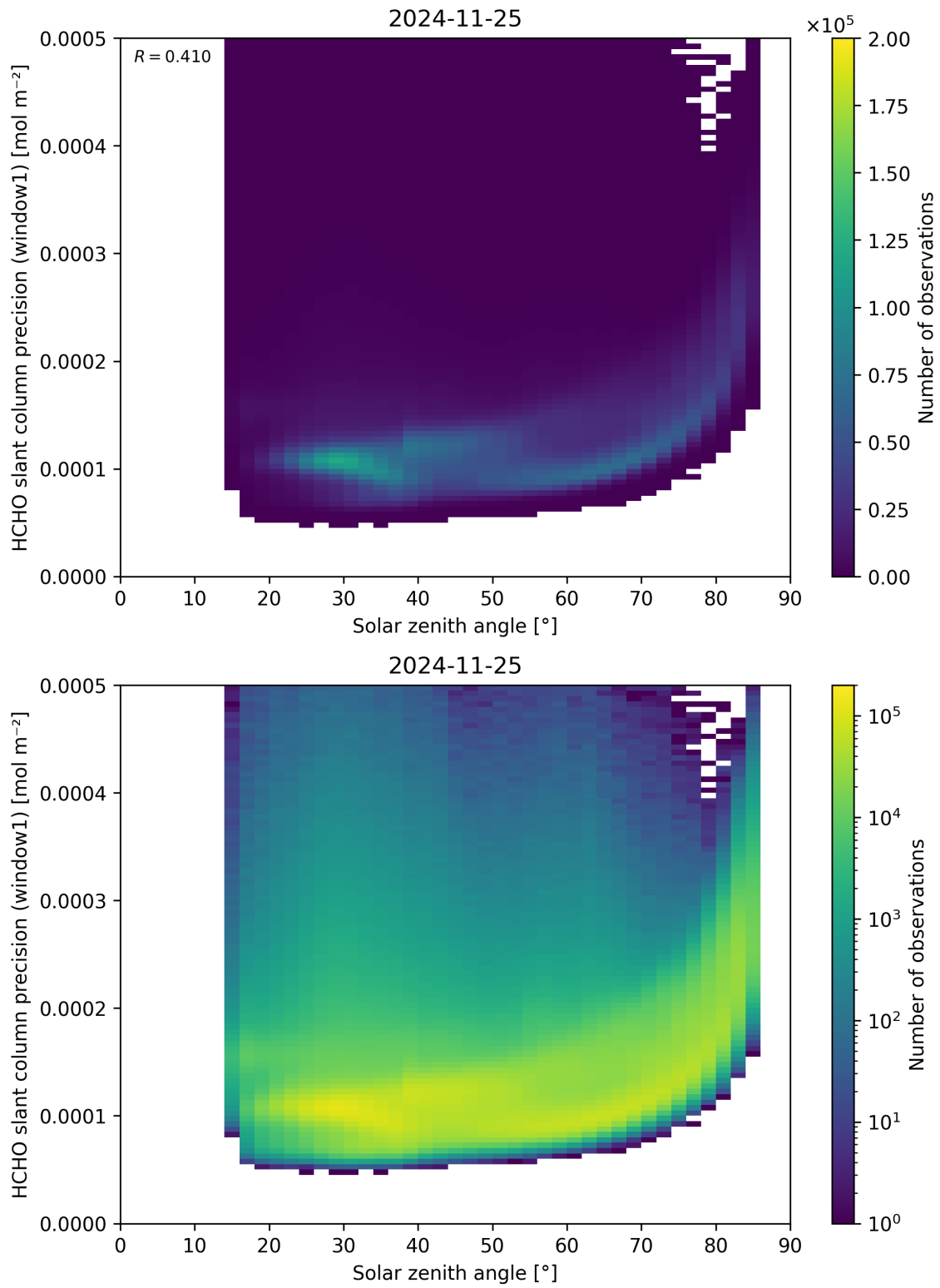
Figure 174: Scatter density plot of “Solar zenith angle” against “HCHO slant column precision (window1)” for 2024-11-25 to 2024-11-26.
