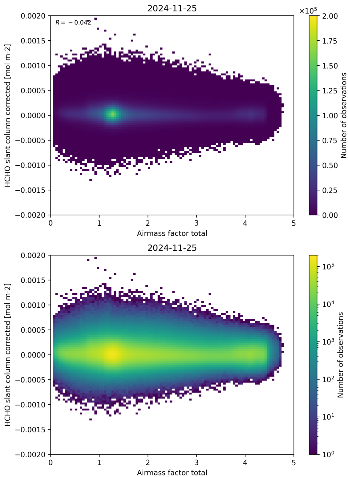
Figure 101: Scatter density plot of “Airmass factor total” against “HCHO slant column corrected” for 2024-11-25 to 2024-11-26.
