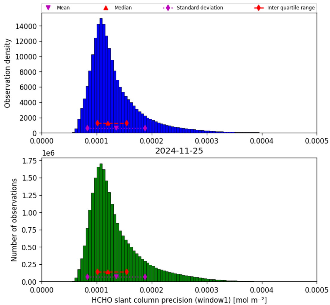
Figure 39: Histogram of “HCHO slant column precision (window1)” for 2024-11-25 to 2024-11-26
