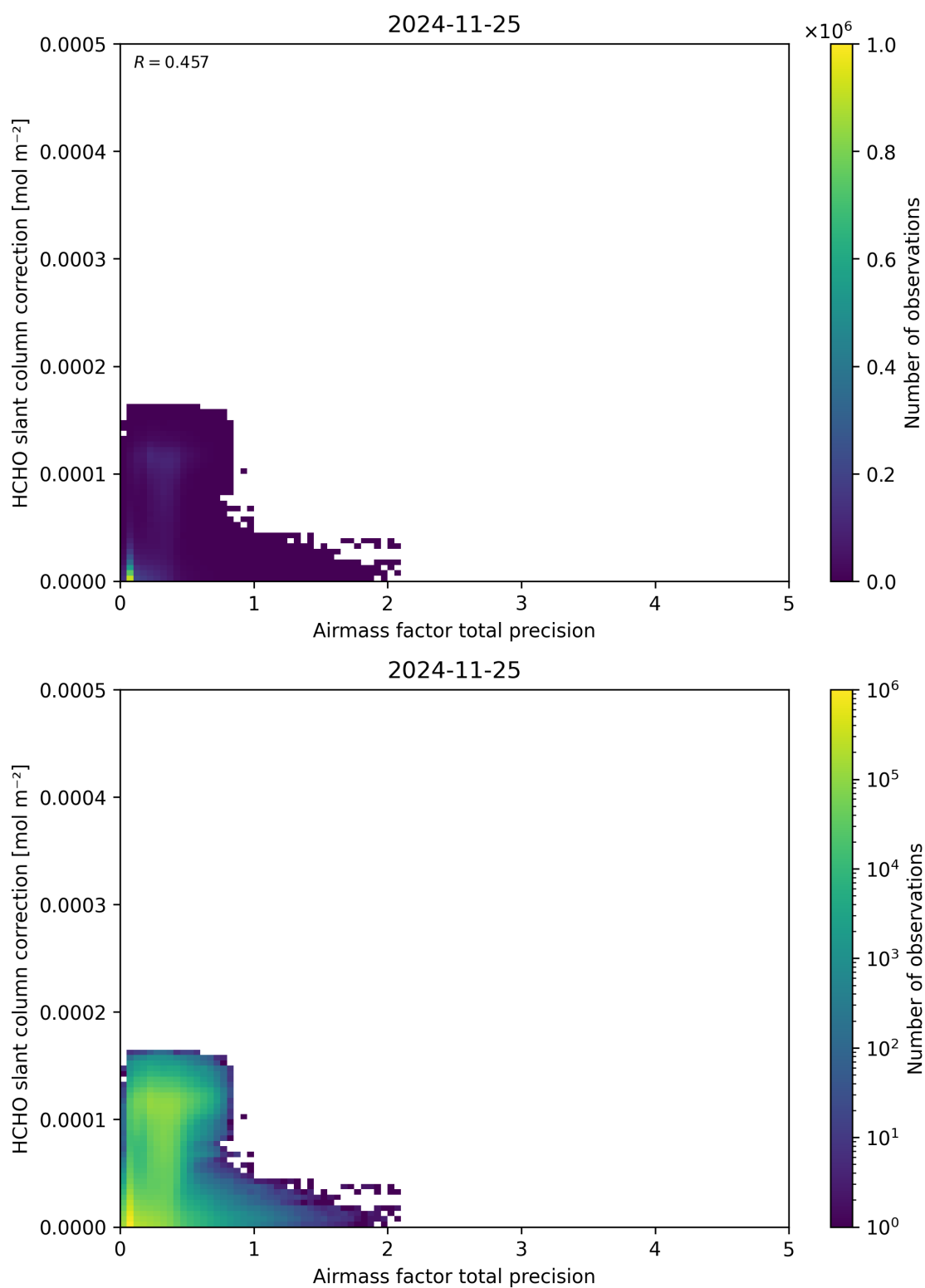
Figure 110: Scatter density plot of “Airmass factor total precision” against “HCHO slant column correction” for 2024-11-25 to 2024-11-26.
