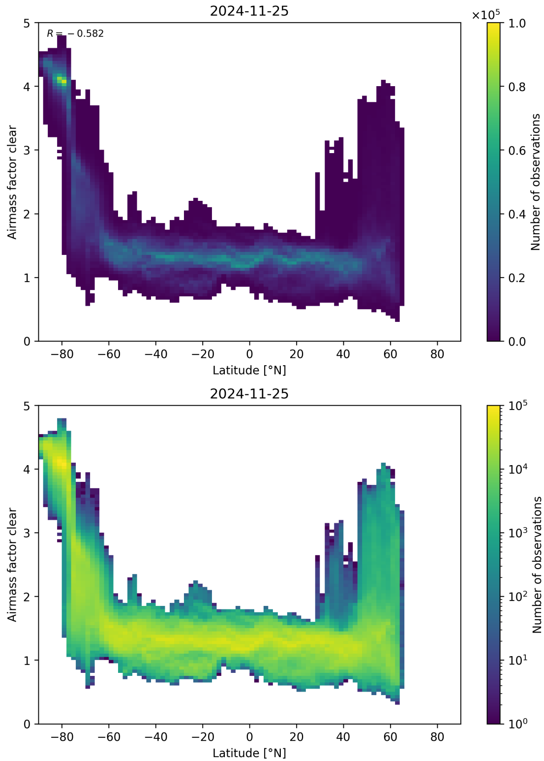
Figure 156: Scatter density plot of “Latitude” against “Airmass factor clear” for 2024-11-25 to 2024-11-26.
