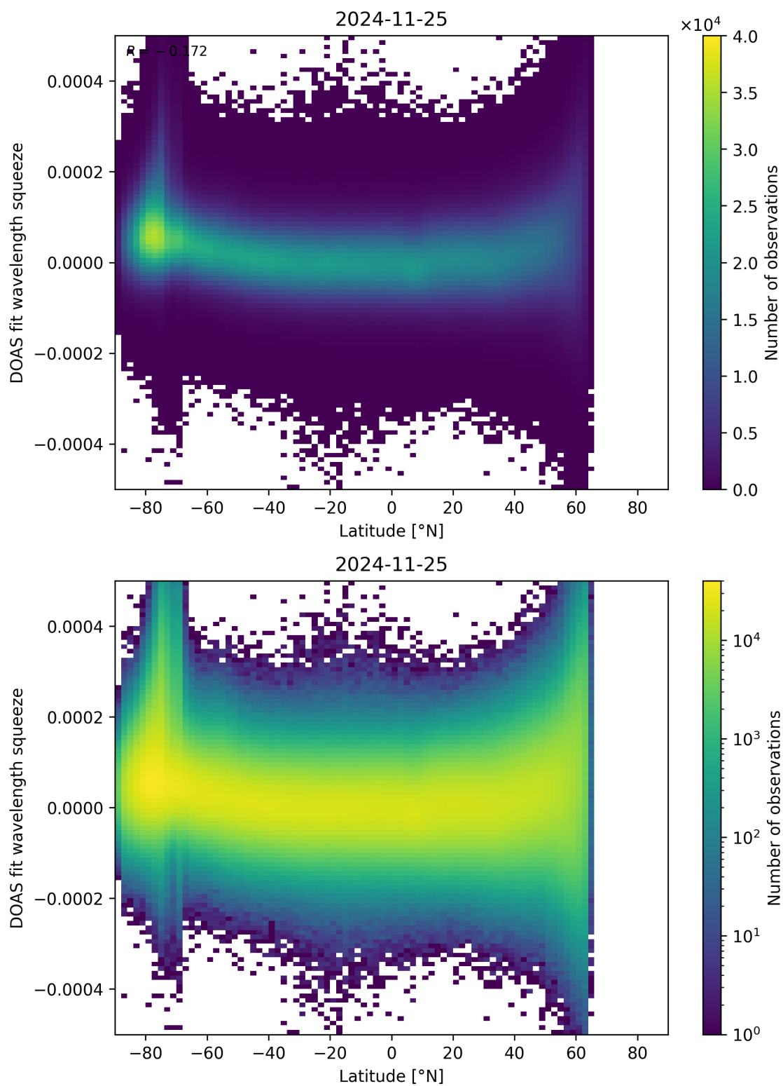
Figure 155: Scatter density plot of “Latitude” against “DOAS fit wavelength squeeze” for 2024-11-25 to 2024-11-26.
