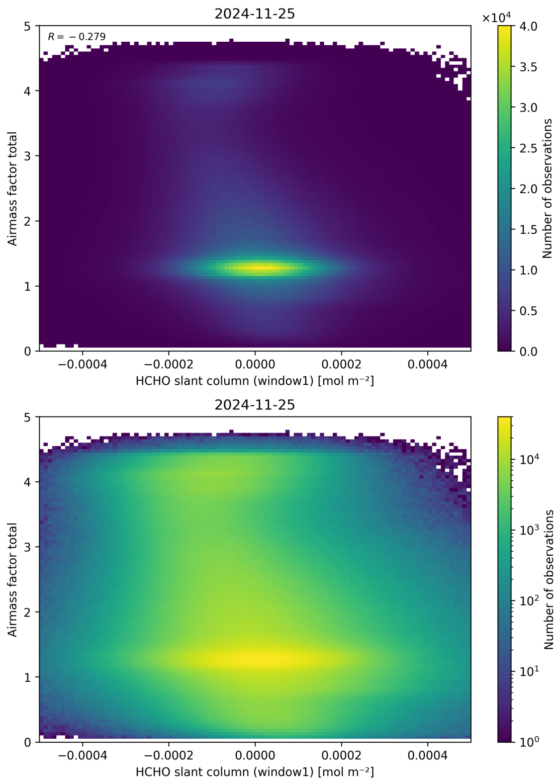
Figure 85: Scatter density plot of “HCHO slant column (window1)” against “Airmass factor total” for 2024-11-25 to 2024-11-26.
