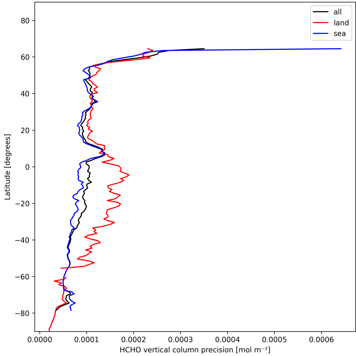
Figure 22: Zonal average of “HCHO vertical column precision” for 2024-11-25 to 2024-11-26.
