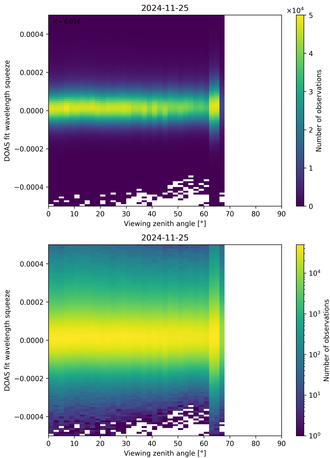
Figure 184: Scatter density plot of “Viewing zenith angle” against “DOAS fit wavelength squeeze” for 2024-11-25 to 2024-11-26.
