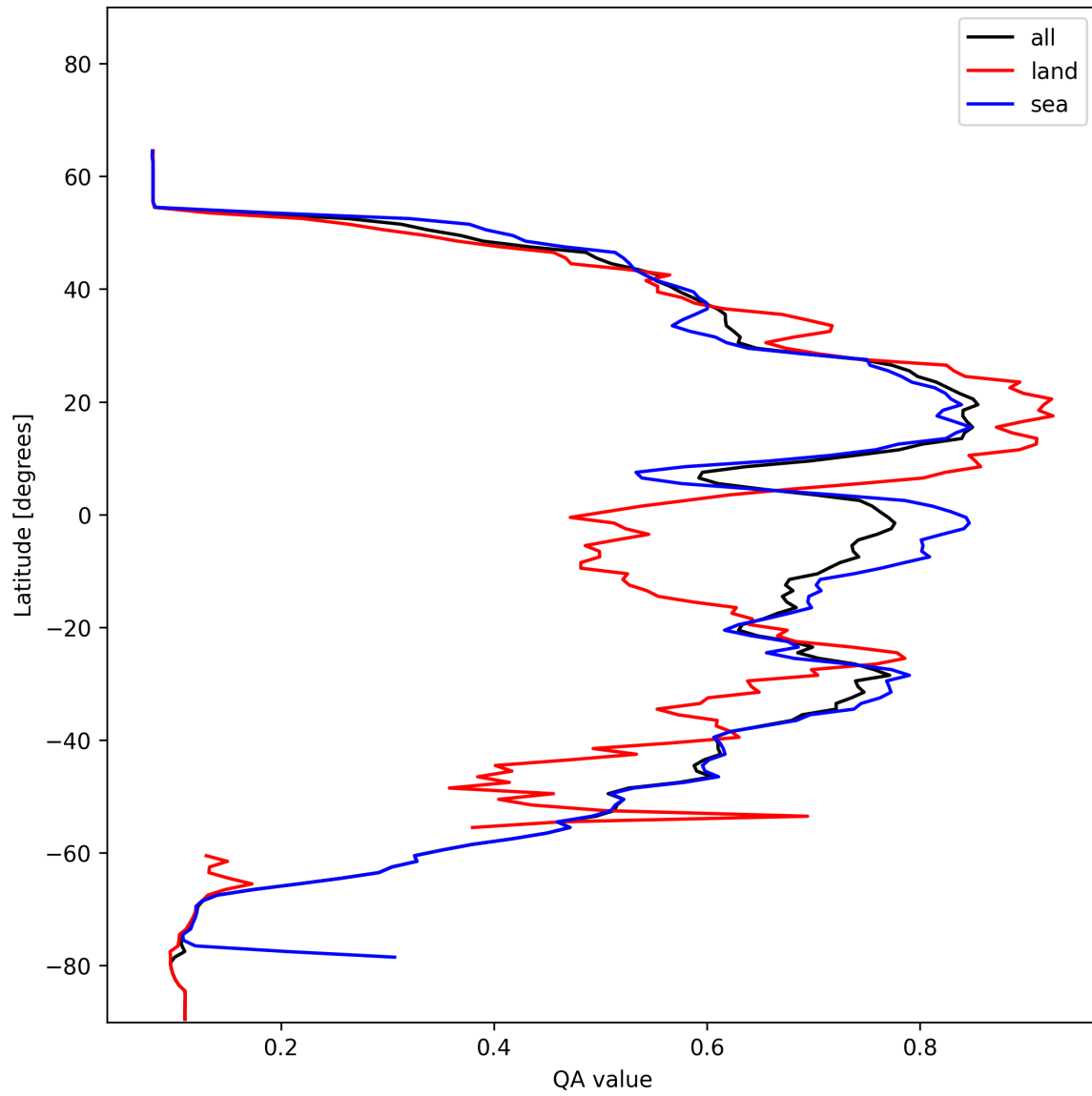
Figure 20: Zonal average of “QA value” for 2024-11-25 to 2024-11-26.
