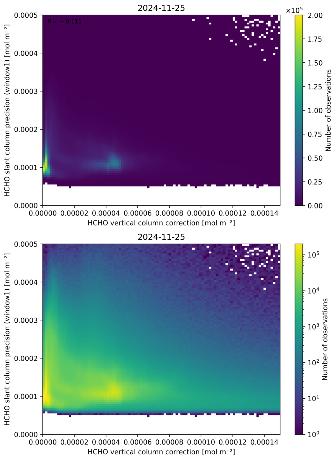
Figure 119: Scatter density plot of “HCHO vertical column correction” against “HCHO slant column precision (window1)” for 2024-11-25 to 2024-11-26.
