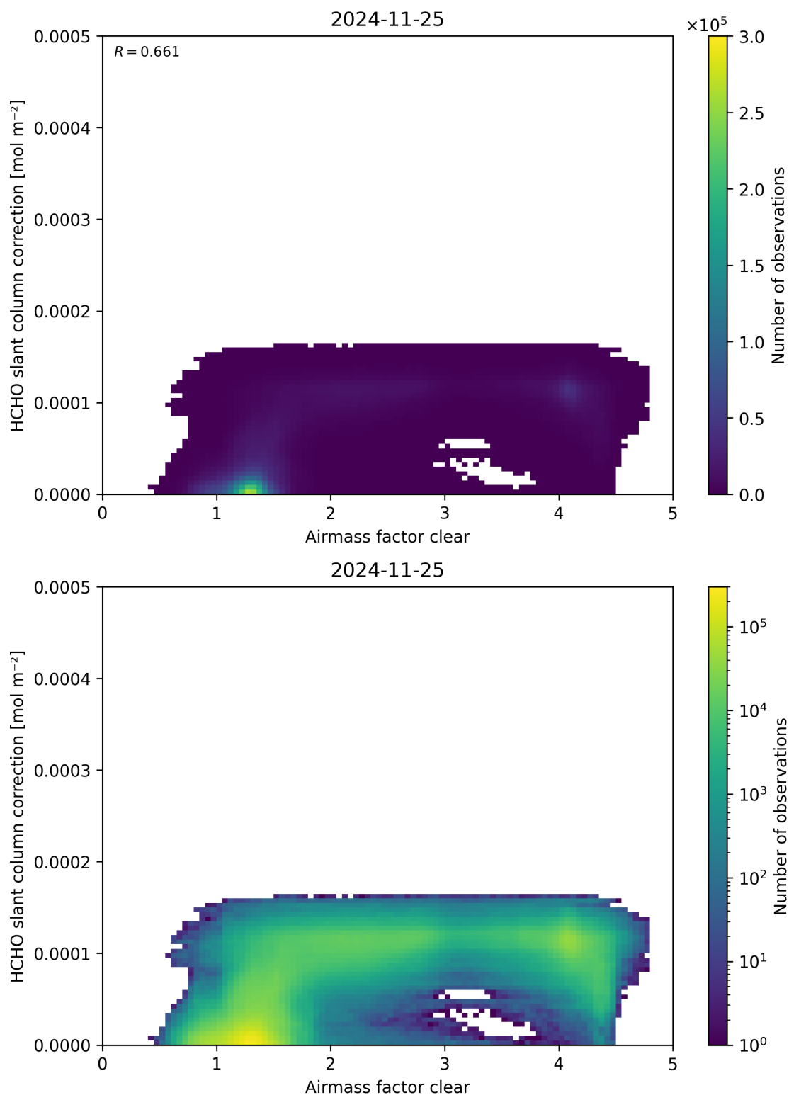
Figure 75: Scatter density plot of “Airmass factor clear” against “HCHO slant column correction” for 2024-11-25 to 2024-11-26.
