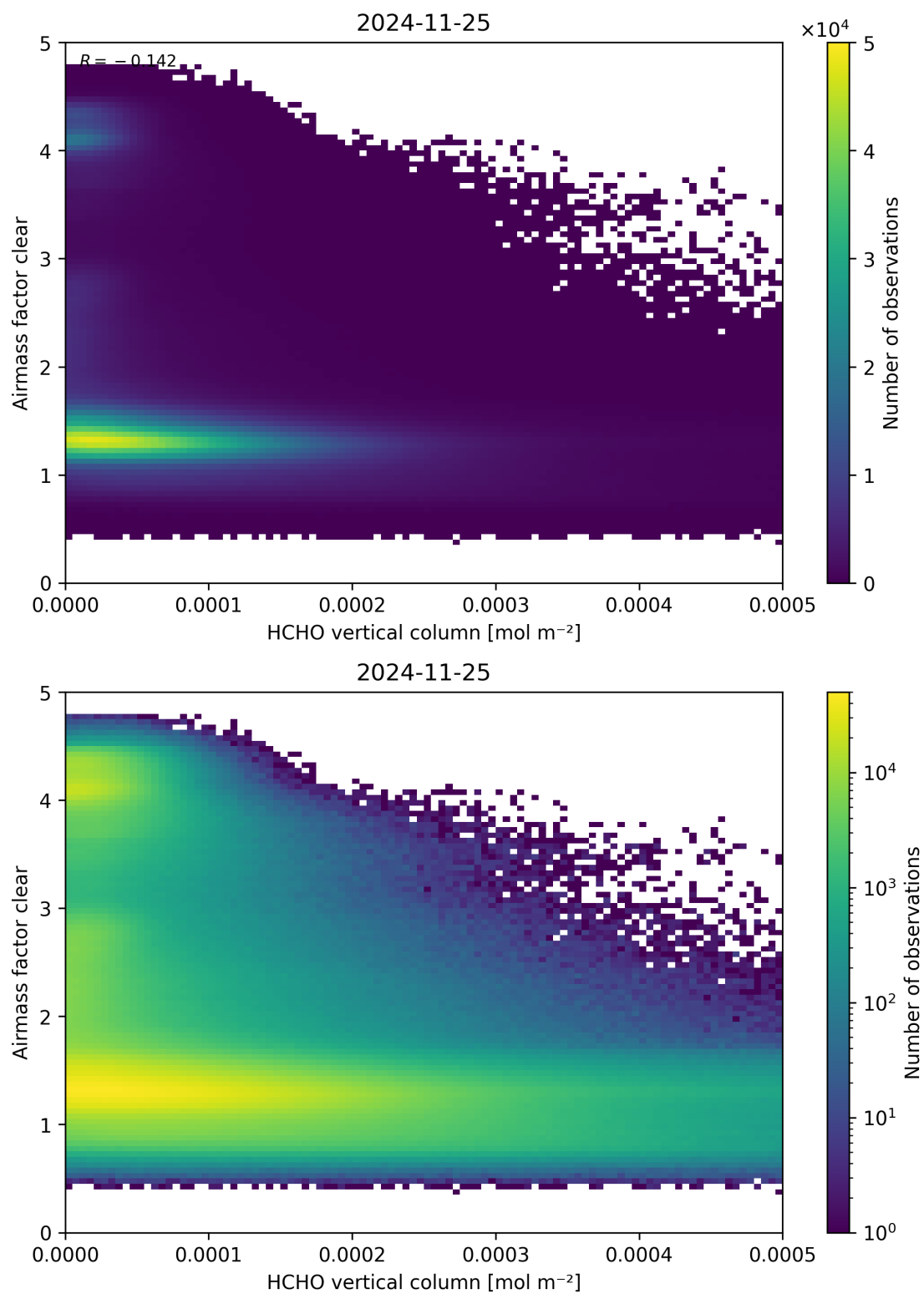
Figure 126: Scatter density plot of “HCHO vertical column” against “Airmass factor clear” for 2024-11-25 to 2024-11-26.
