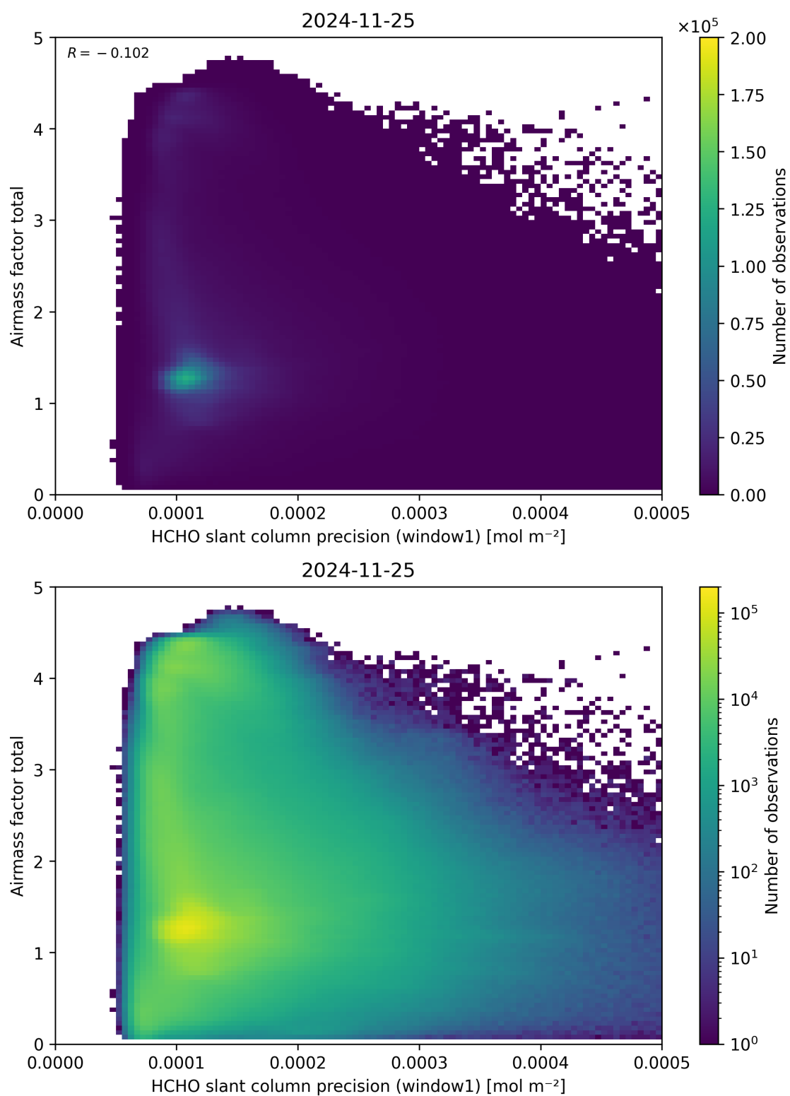
Figure 94: Scatter density plot of “HCHO slant column precision (window1)” against “Airmass factor total” for 2024-11-25 to 2024-11-26.
