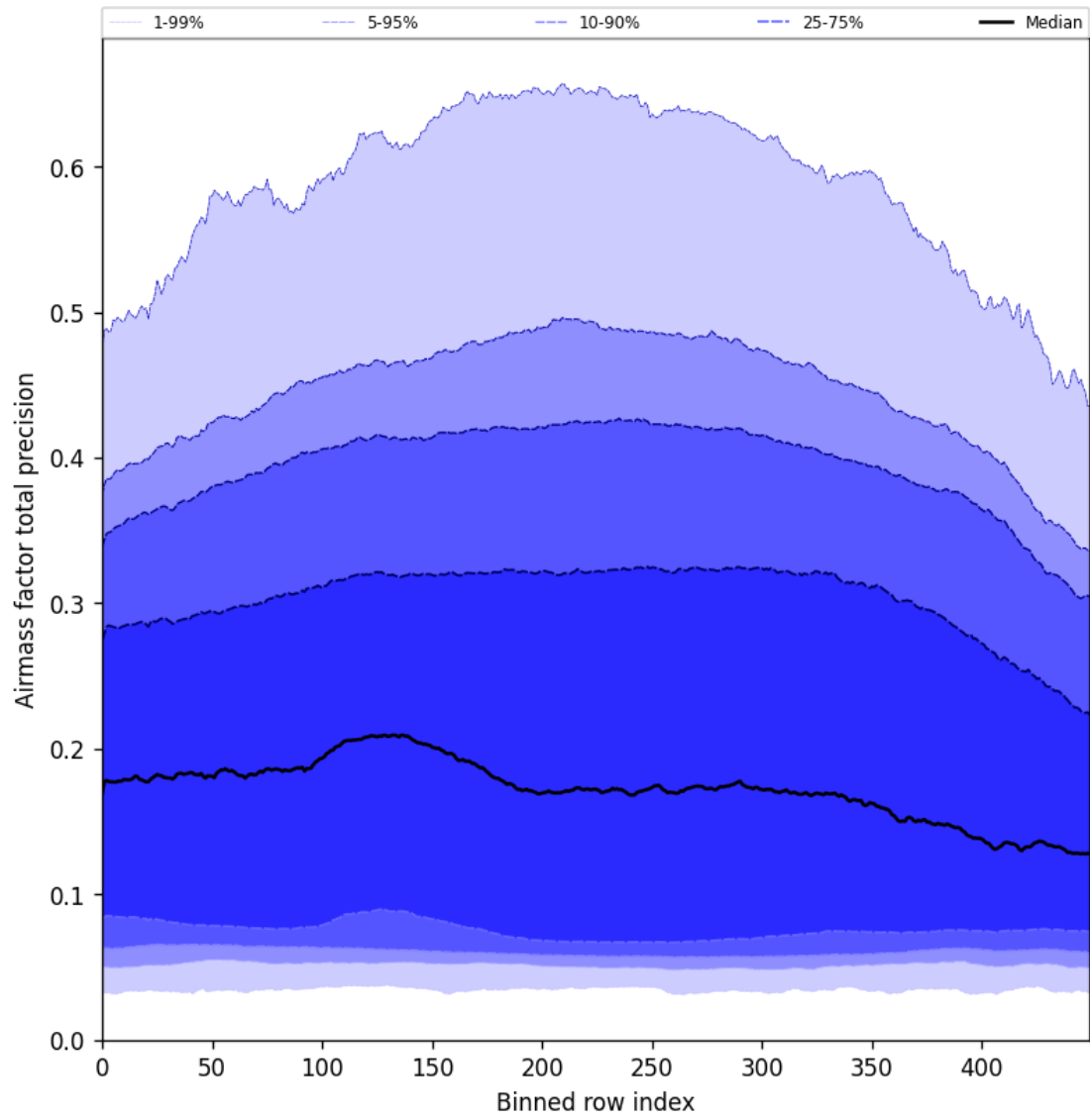
Figure 55: Along track statistics of “Airmass factor total precision” for 2024-11-25 to 2024-11-26
