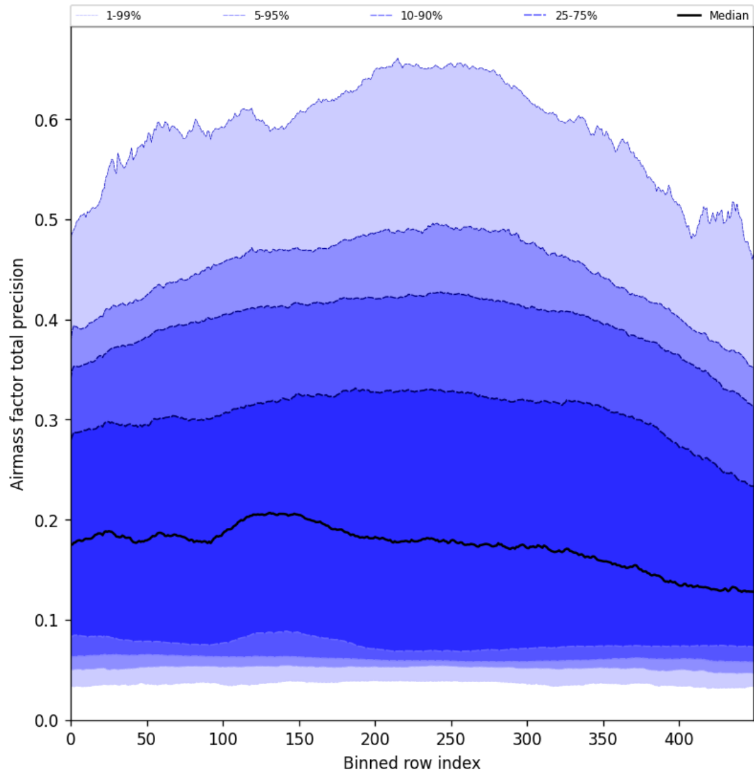
Figure 55: Along track statistics of “Airmass factor total precision” for 2024-11-25 to 2024-11-27
