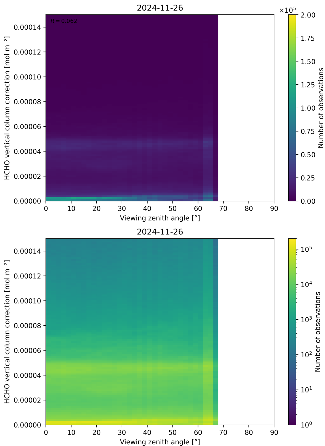
Figure 193: Scatter density plot of “Viewing zenith angle” against “HCHO vertical column correction” for 2024-11-25 to 2024-11-27.
