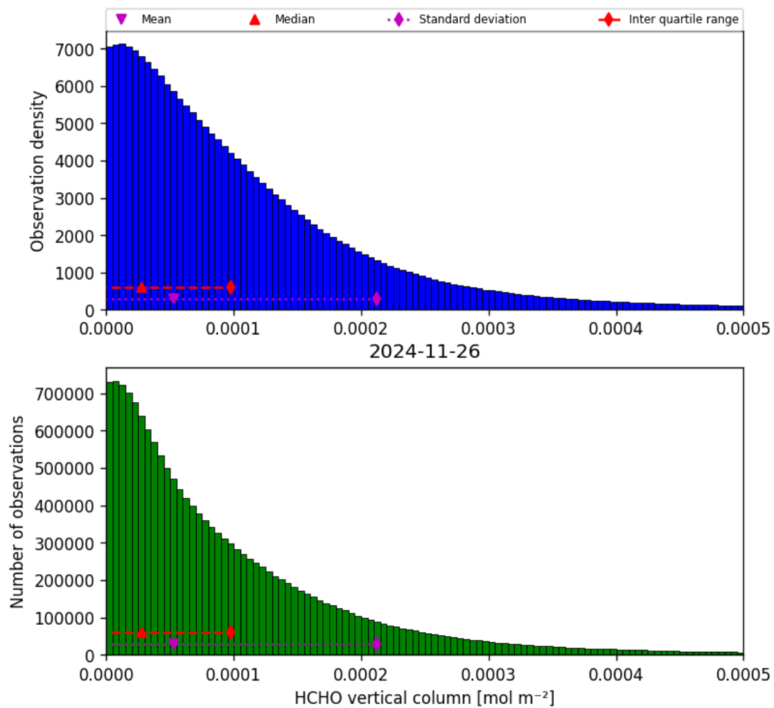
Figure 35: Histogram of “HCHO vertical column” for 2024-11-25 to 2024-11-27
