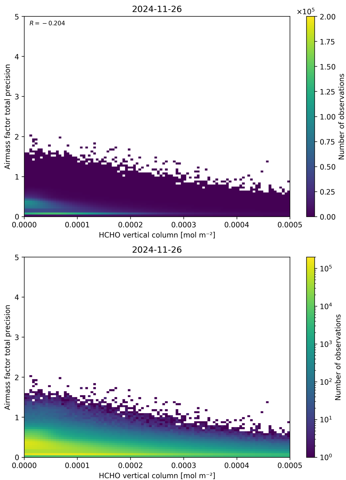
Figure 132: Scatter density plot of “HCHO vertical column” against “Airmass factor total precision” for 2024-11-25 to 2024-11-27.
