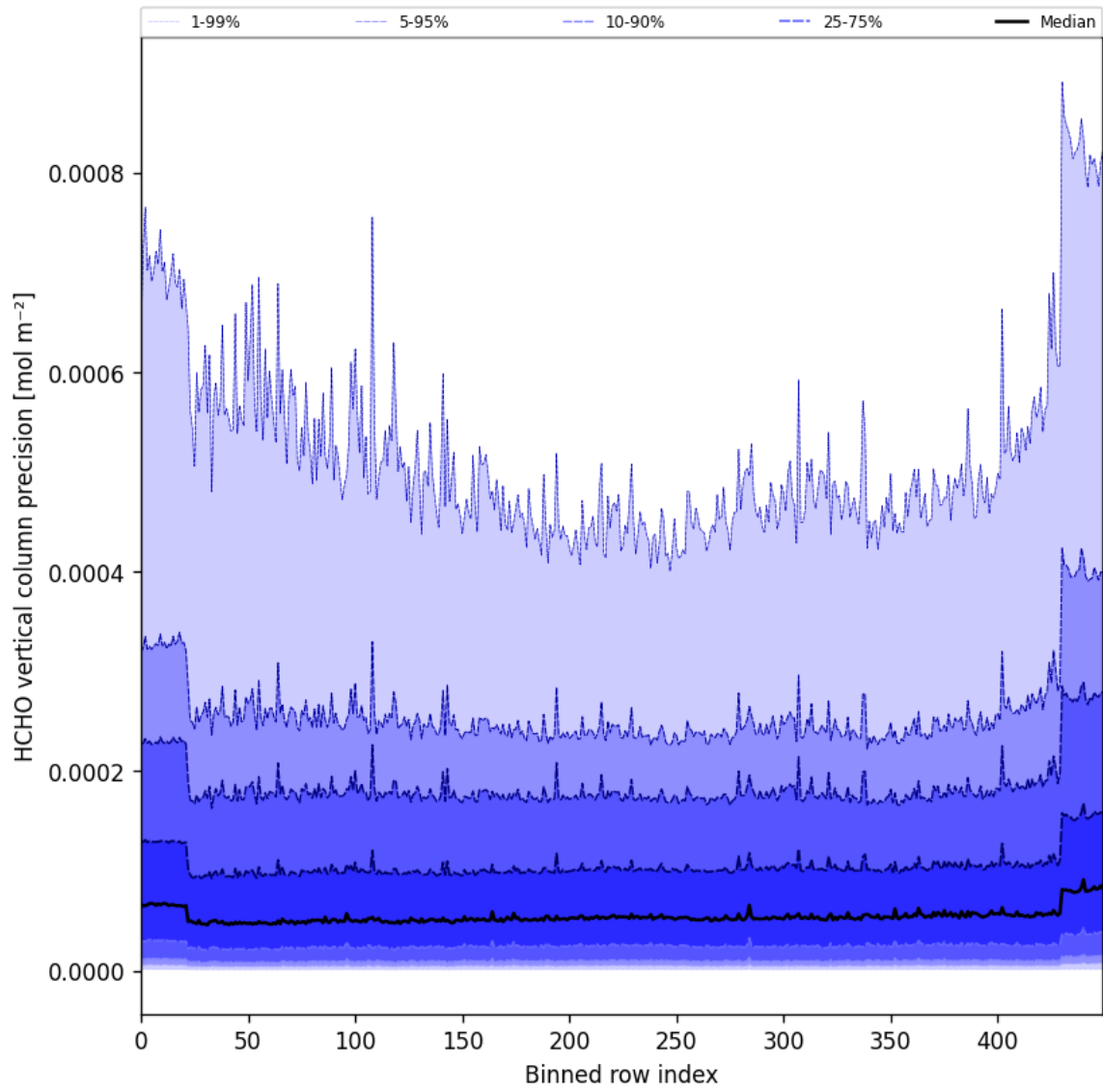
Figure 50: Along track statistics of “HCHO vertical column precision” for 2024-11-25 to 2024-11-27
