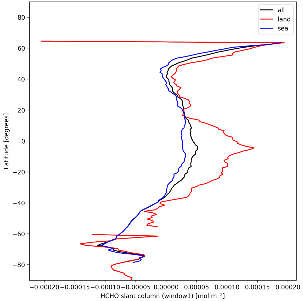
Figure 24: Zonal average of “HCHO slant column (window1)” for 2024-11-25 to 2024-11-27.
