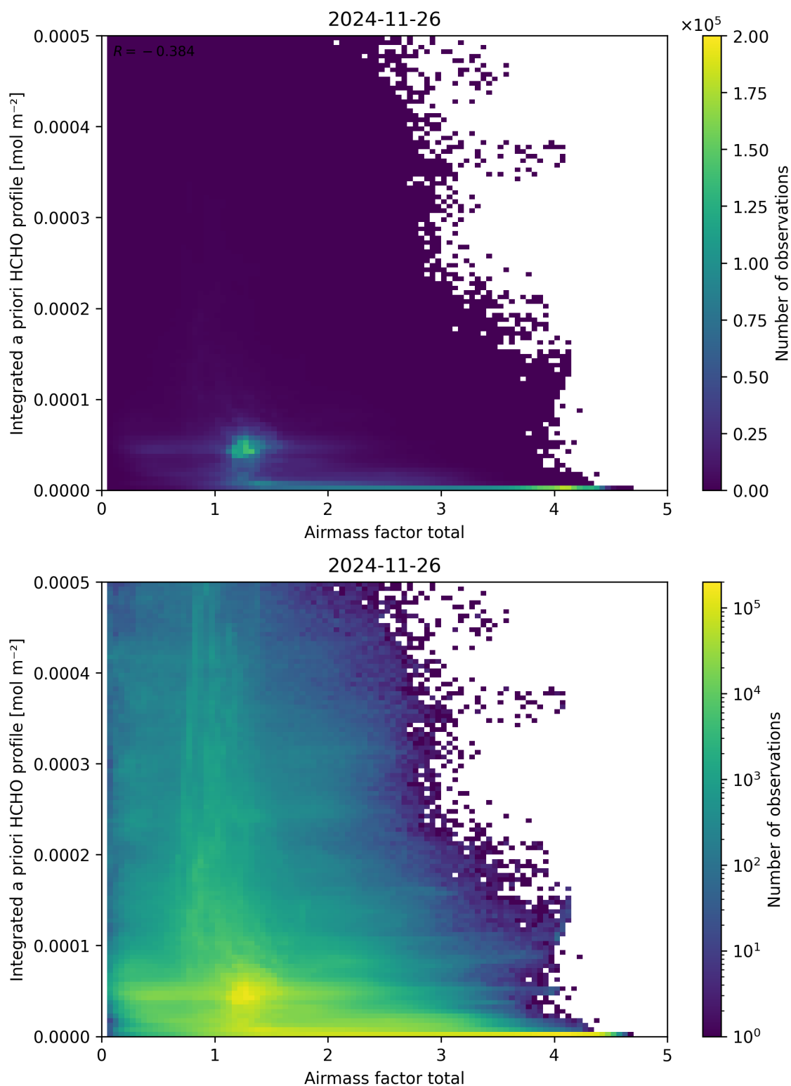
Figure 104: Scatter density plot of “Airmass factor total” against “Integrated a priori HCHO profile” for 2024-11-25 to 2024-11-27.
