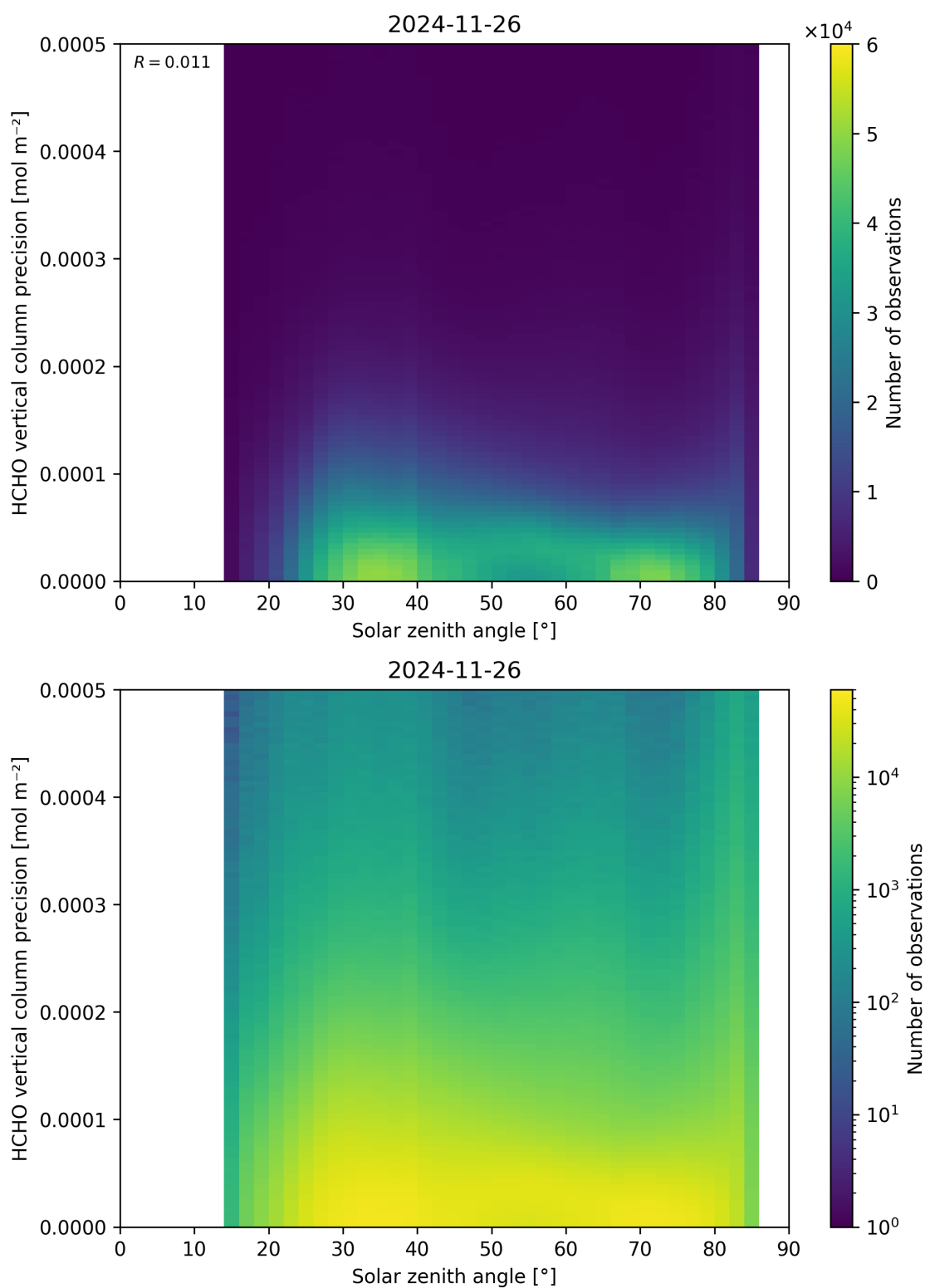
Figure 179: Scatter density plot of “Solar zenith angle” against “HCHO vertical column precision” for 2024-11-25 to 2024-11-27.
