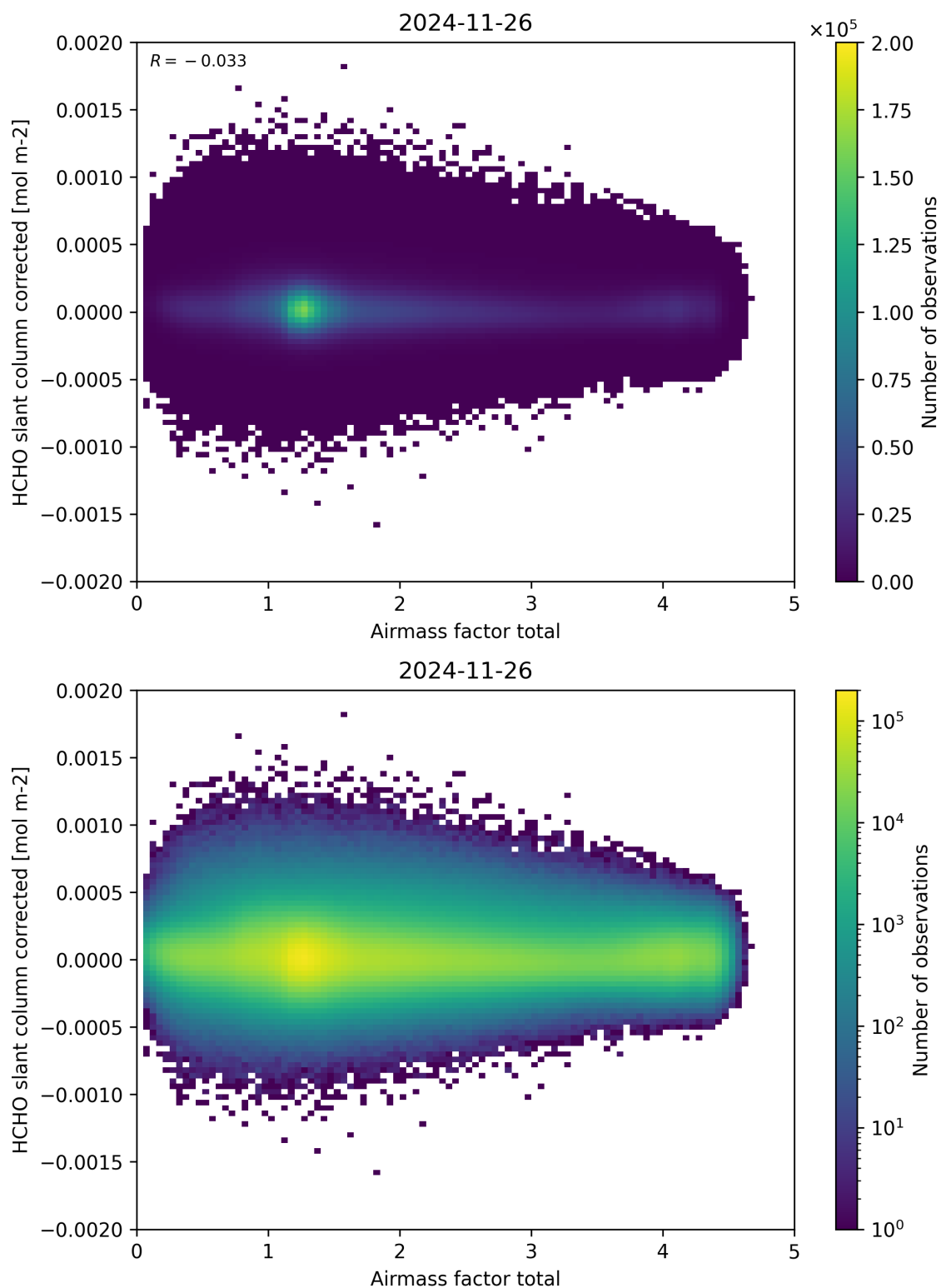
Figure 101: Scatter density plot of “Airmass factor total” against “HCHO slant column corrected” for 2024-11-25 to 2024-11-27.
