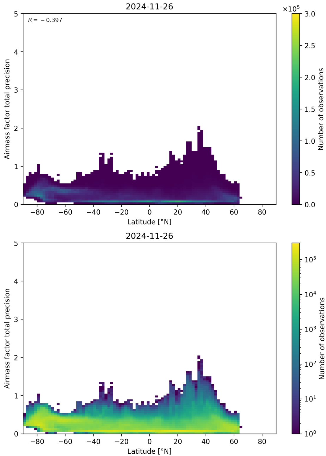
Figure 162: Scatter density plot of “Latitude” against “Airmass factor total precision” for 2024-11-25 to 2024-11-27.
