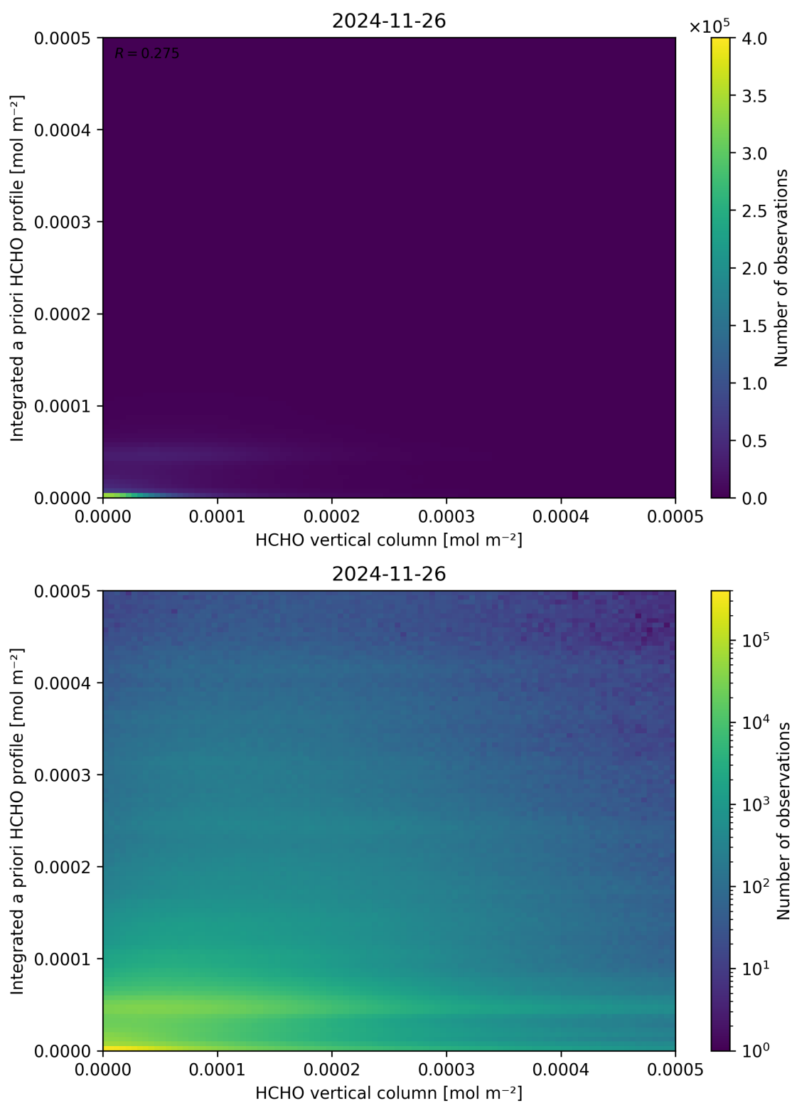
Figure 135: Scatter density plot of “HCHO vertical column” against “Integrated a priori HCHO profile” for 2024-11-25 to 2024-11-27.
