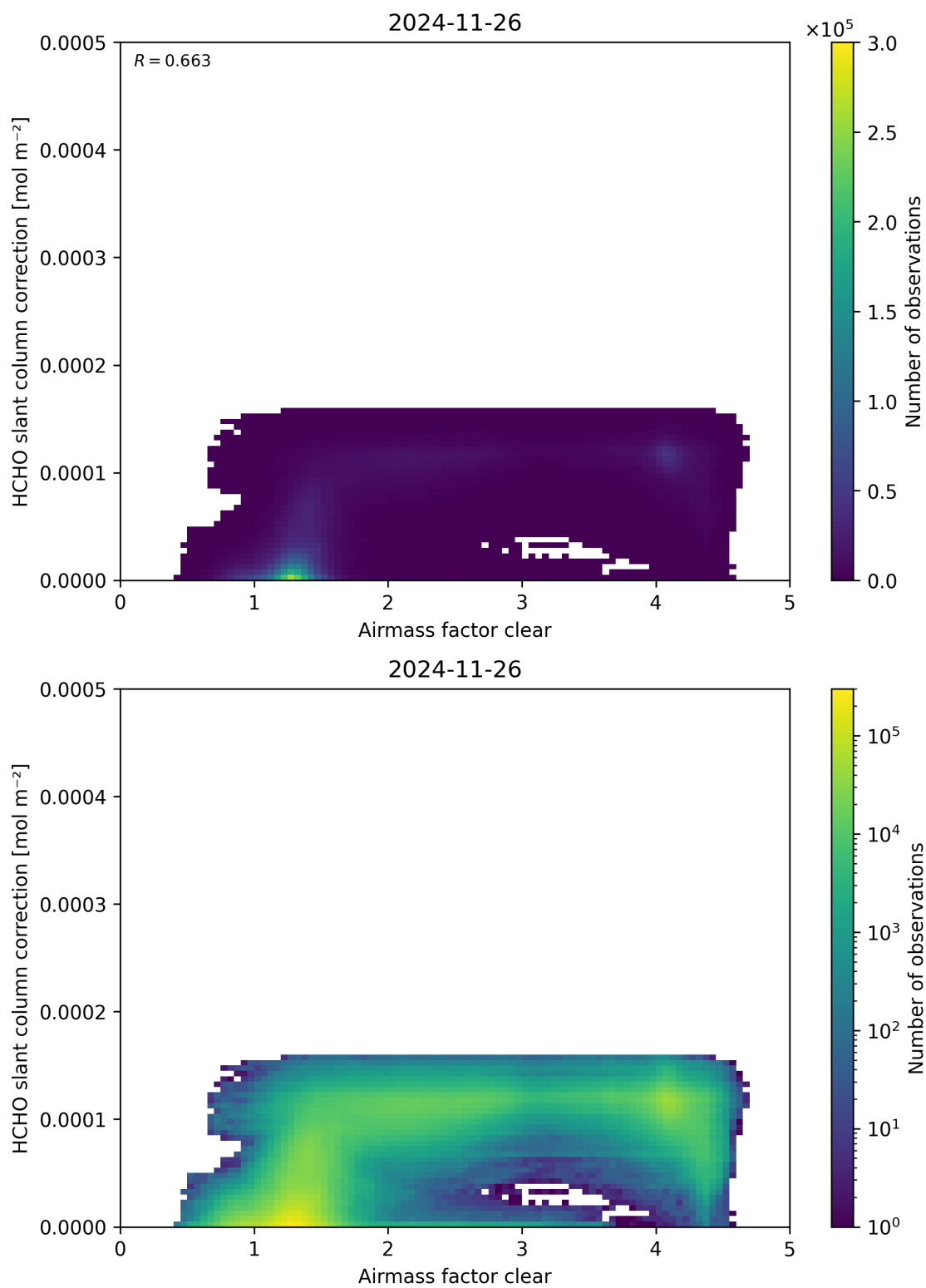
Figure 75: Scatter density plot of “Airmass factor clear” against “HCHO slant column correction” for 2024-11-25 to 2024-11-27.
