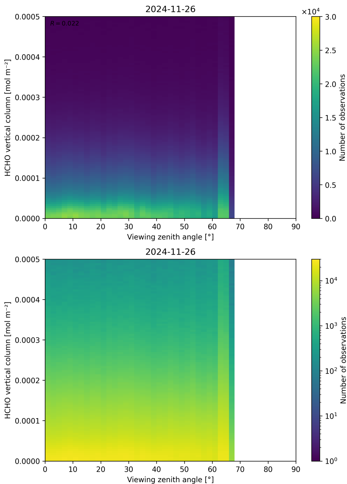
Figure 192: Scatter density plot of “Viewing zenith angle” against “HCHO vertical column” for 2024-11-25 to 2024-11-27.
