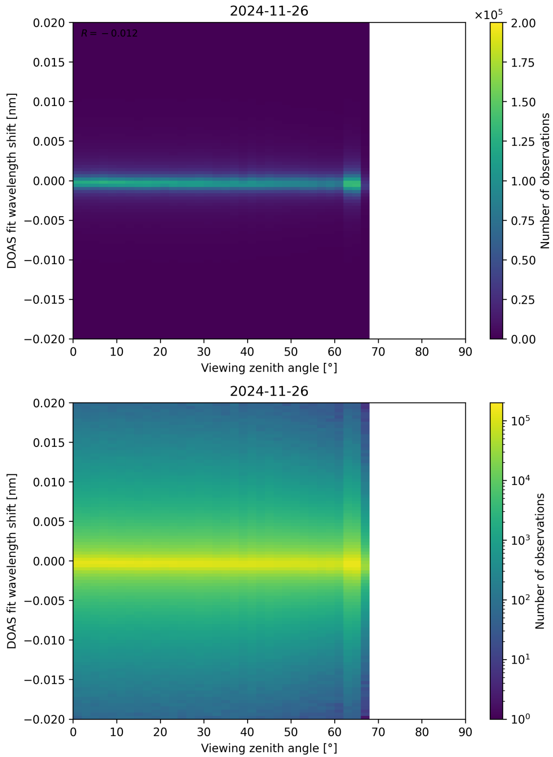
Figure 183: Scatter density plot of “Viewing zenith angle” against “DOAS fit wavelength shift” for 2024-11-25 to 2024-11-27.
