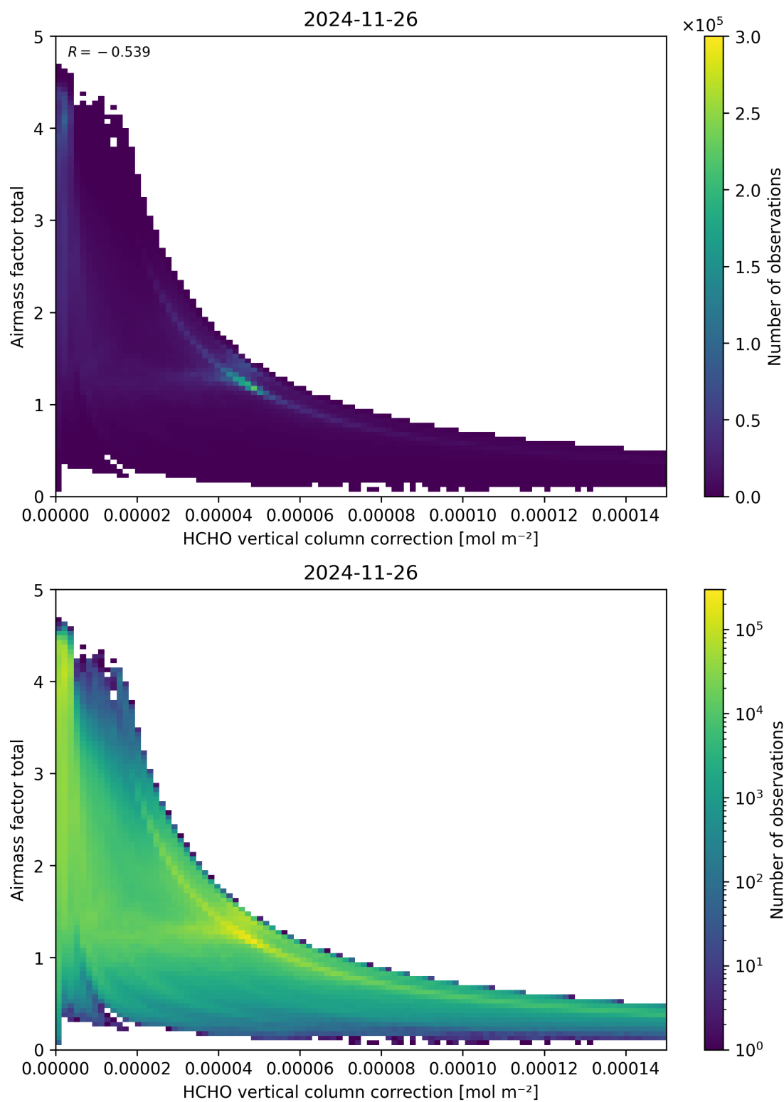
Figure 120: Scatter density plot of “HCHO vertical column correction” against “Airmass factor total” for 2024-11-25 to 2024-11-27.
