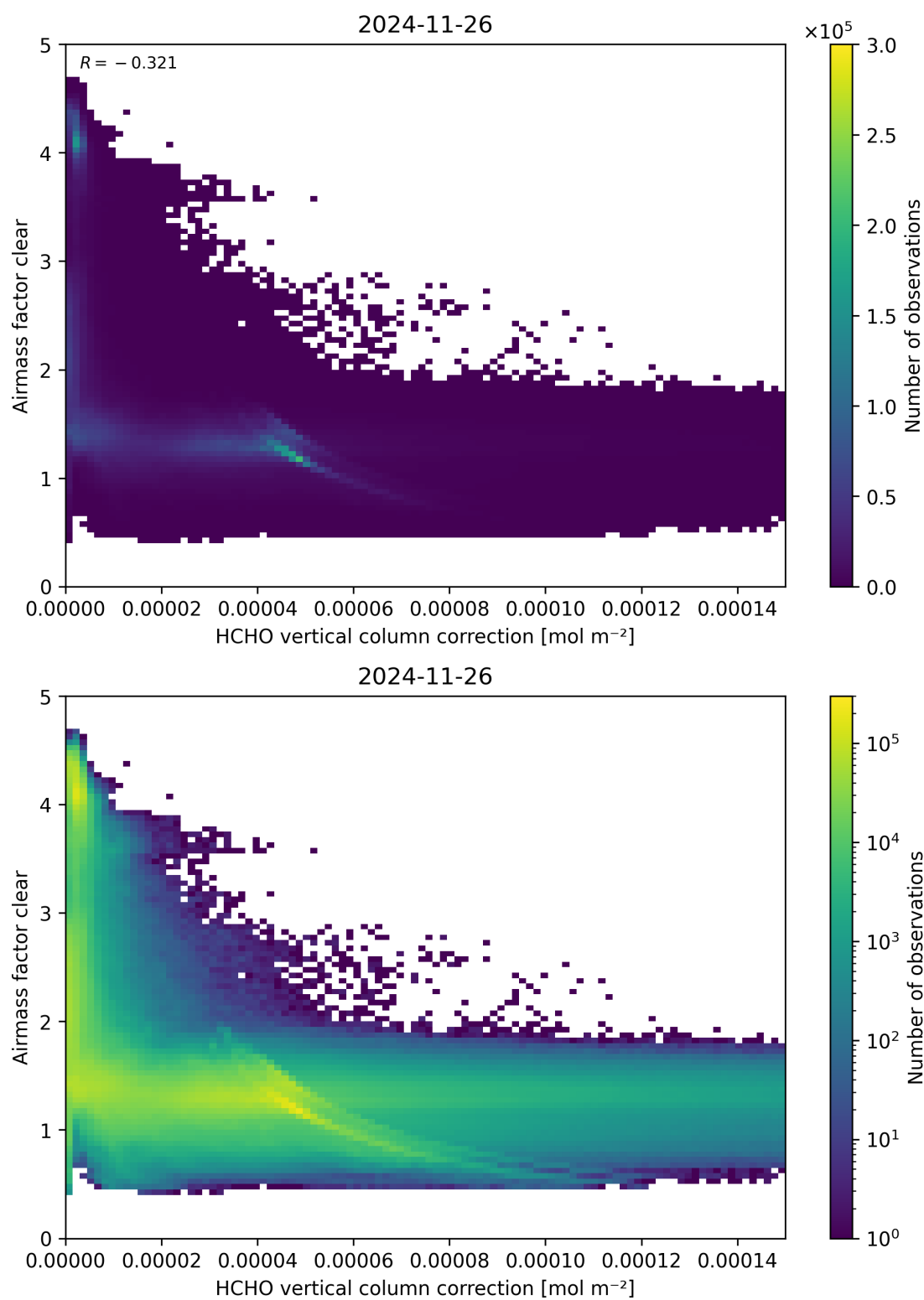
Figure 115: Scatter density plot of “HCHO vertical column correction” against “Airmass factor clear” for 2024-11-25 to 2024-11-27.
