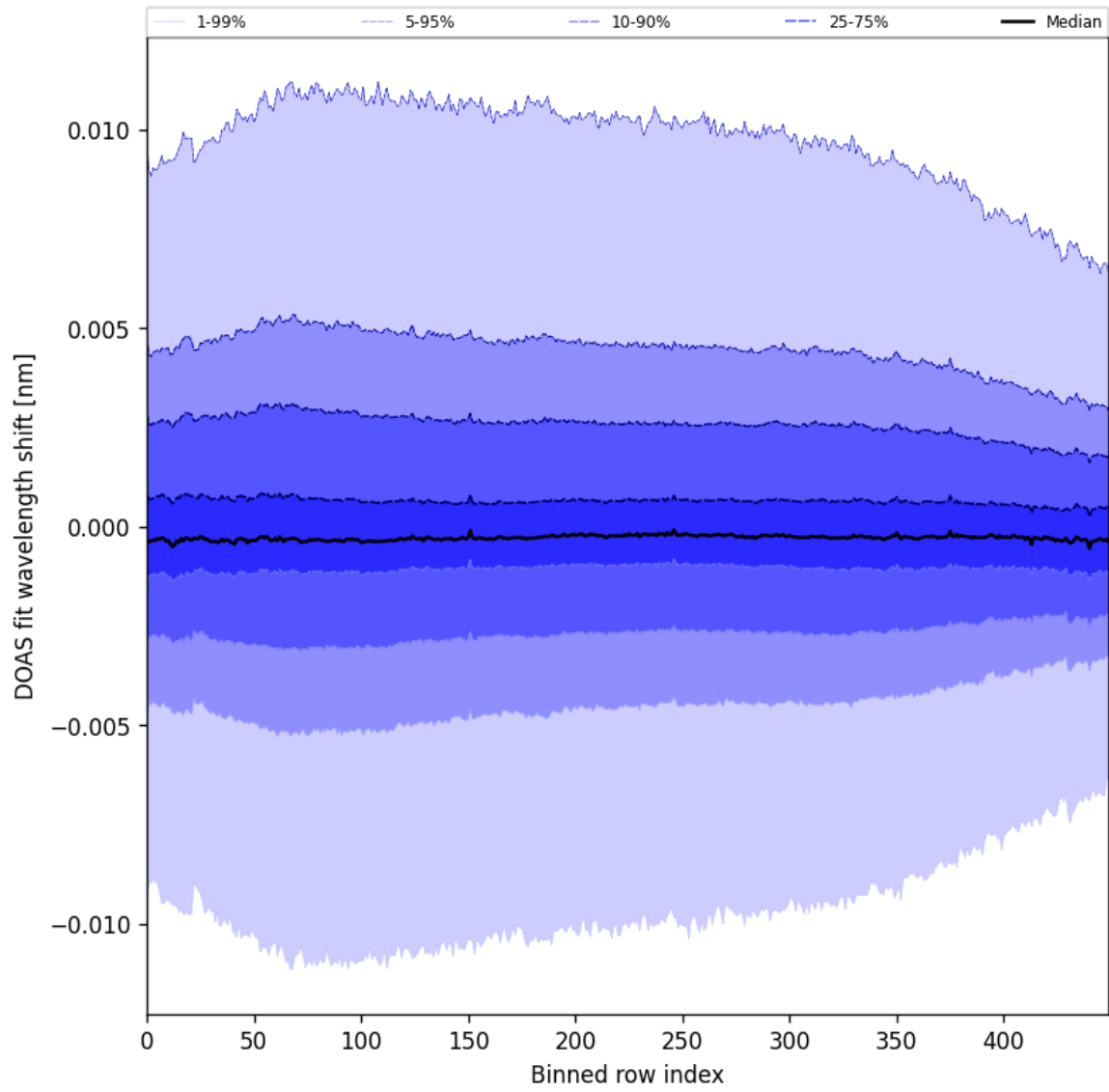
Figure 58: Along track statistics of “DOAS fit wavelength shift” for 2024-11-25 to 2024-11-27
