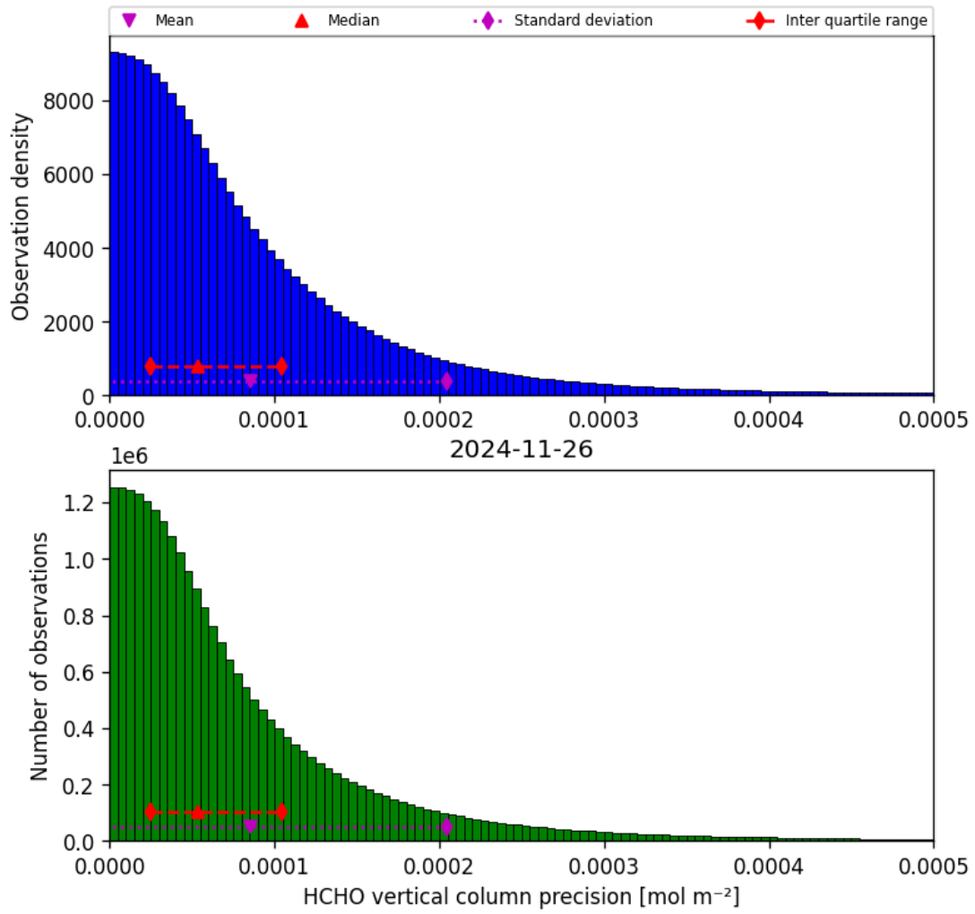
Figure 36: Histogram of “HCHO vertical column precision” for 2024-11-25 to 2024-11-27
