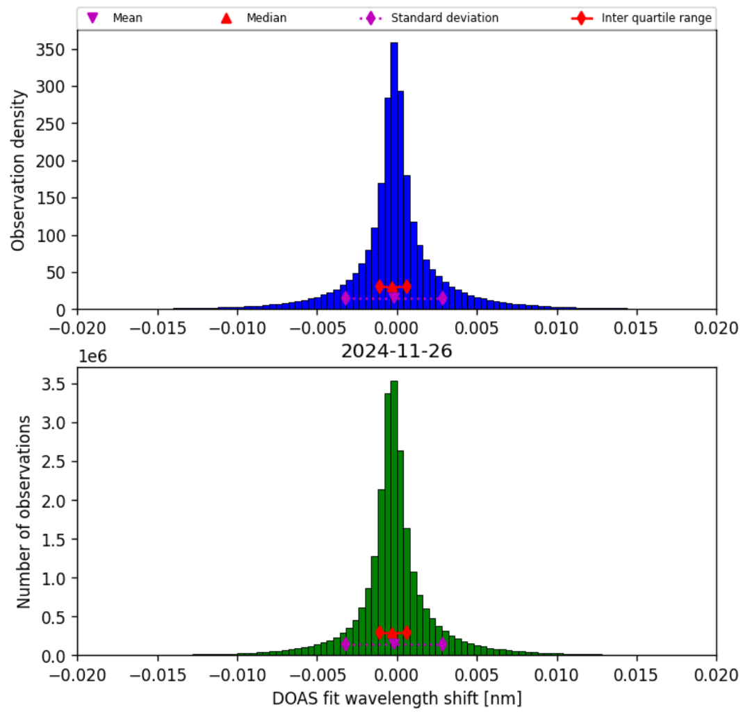
Figure 44: Histogram of “DOAS fit wavelength shift” for 2024-11-25 to 2024-11-27
