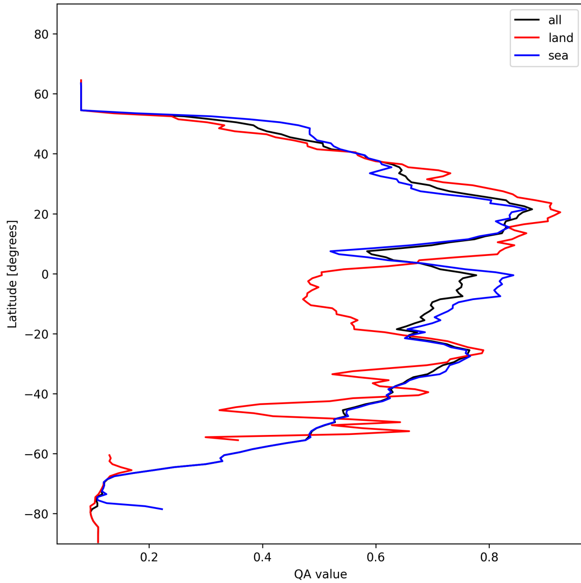
Figure 20: Zonal average of “QA value” for 2024-11-25 to 2024-11-27.
