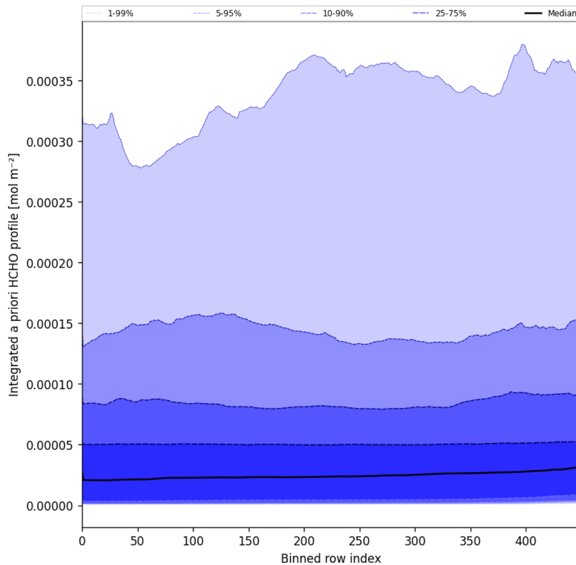
Figure 57: Along track statistics of "Integrated a priori HCHO profile" for 2024-11-25 to 2024-11-27
