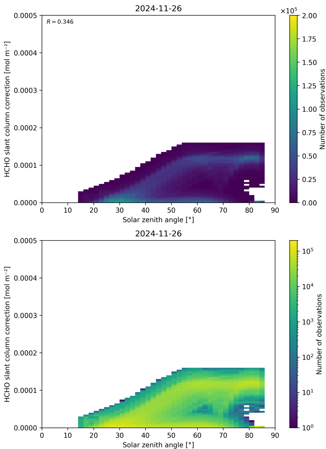
Figure 172: Scatter density plot of “Solar zenith angle” against “HCHO slant column correction” for 2024-11-25 to 2024-11-27.
