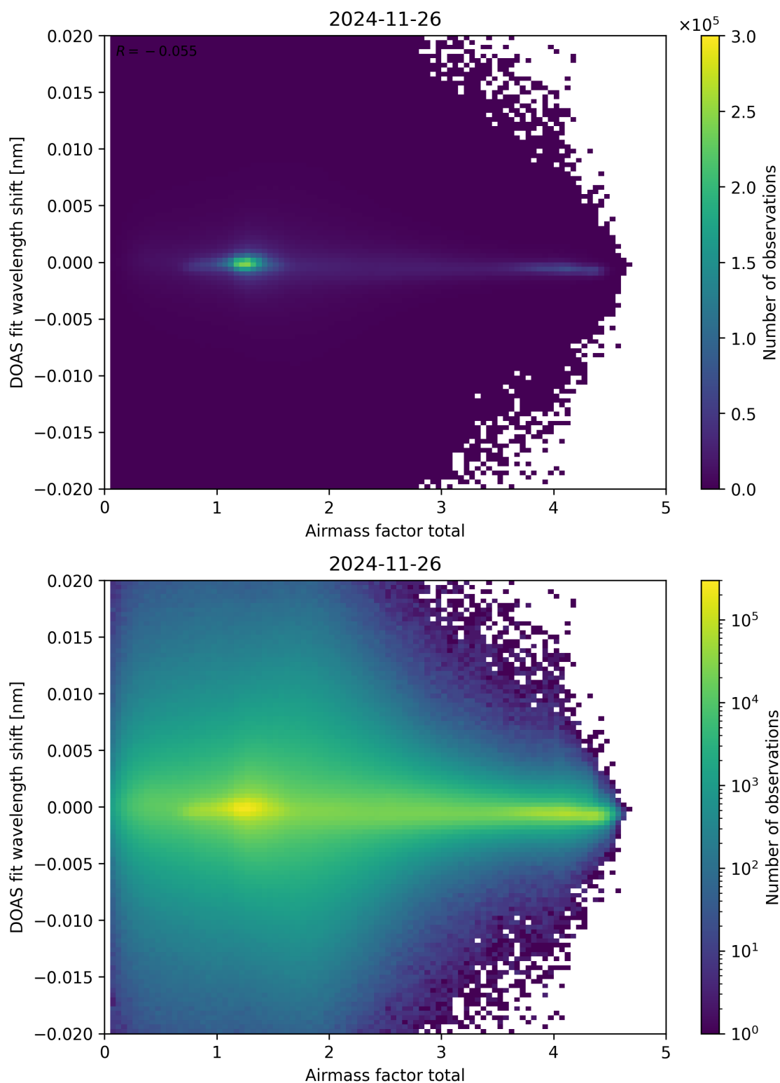
Figure 98: Scatter density plot of “Airmass factor total” against “DOAS fit wavelength shift” for 2024-11-25 to 2024-11-27.
