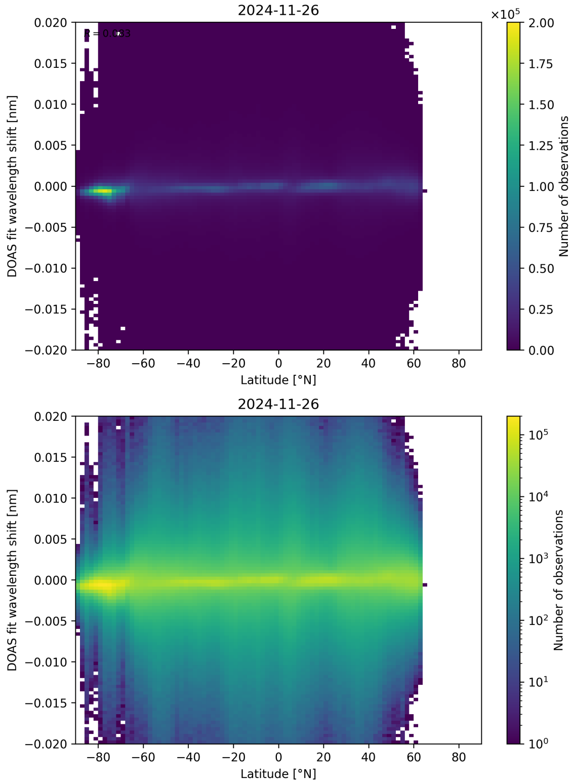
Figure 154: Scatter density plot of “Latitude” against “DOAS fit wavelength shift” for 2024-11-25 to 2024-11-27.
