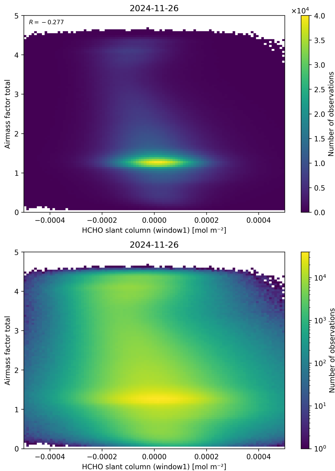
Figure 85: Scatter density plot of “HCHO slant column (window1)” against “Airmass factor total” for 2024-11-25 to 2024-11-27.
