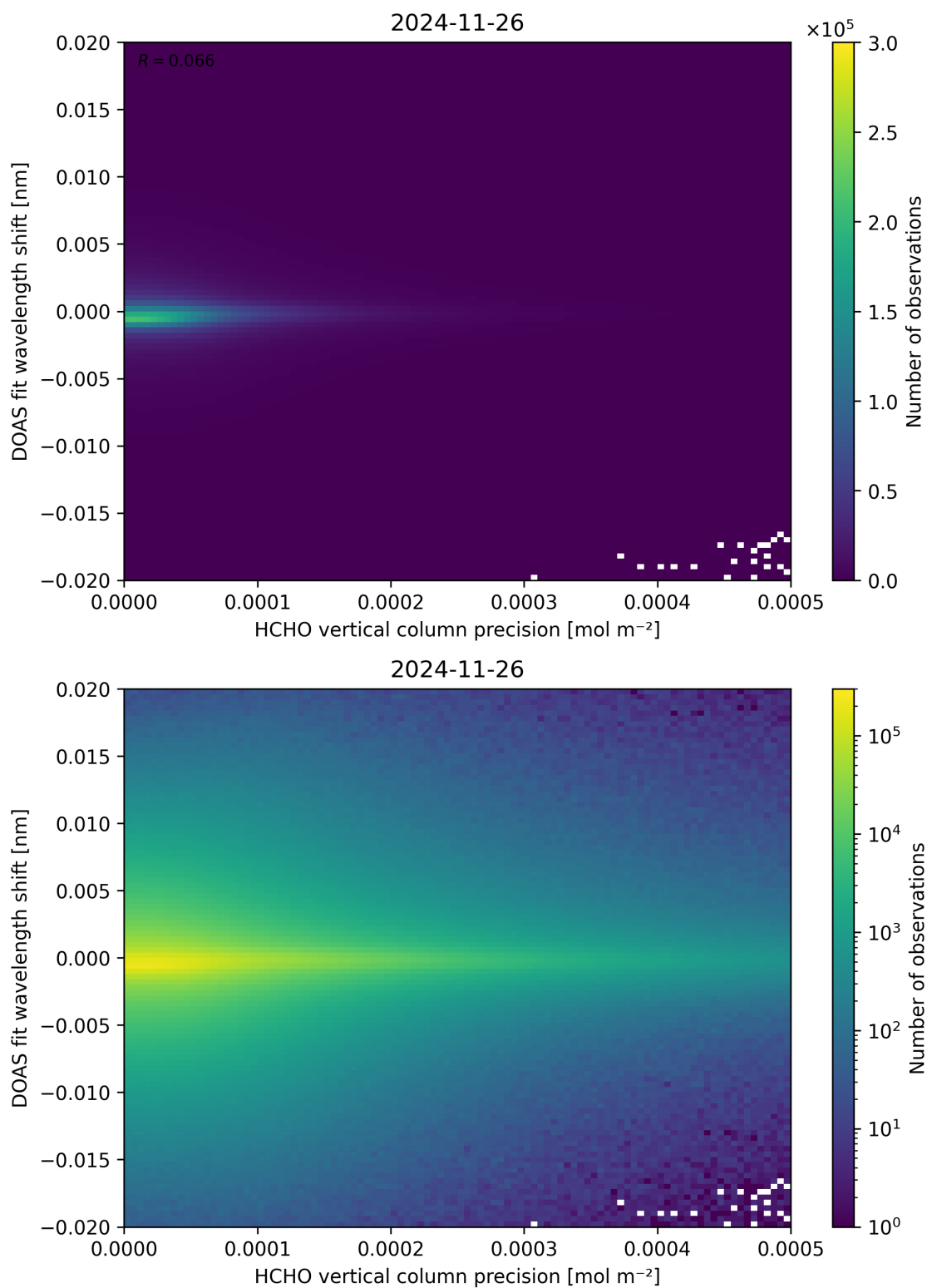
Figure 137: Scatter density plot of “HCHO vertical column precision” against “DOAS fit wavelength shift” for 2024-11-25 to 2024-11-27.
