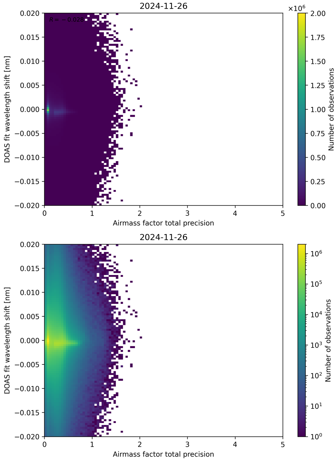
Figure 106: Scatter density plot of “Airmass factor total precision” against “DOAS fit wavelength shift” for 2024-11-25 to 2024-11-27.
