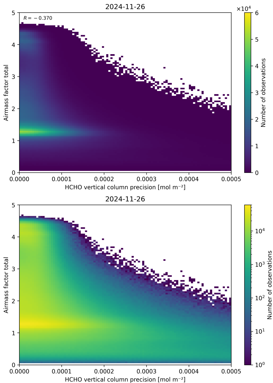
Figure 144: Scatter density plot of “HCHO vertical column precision” against “Airmass factor total” for 2024-11-25 to 2024-11-27.
