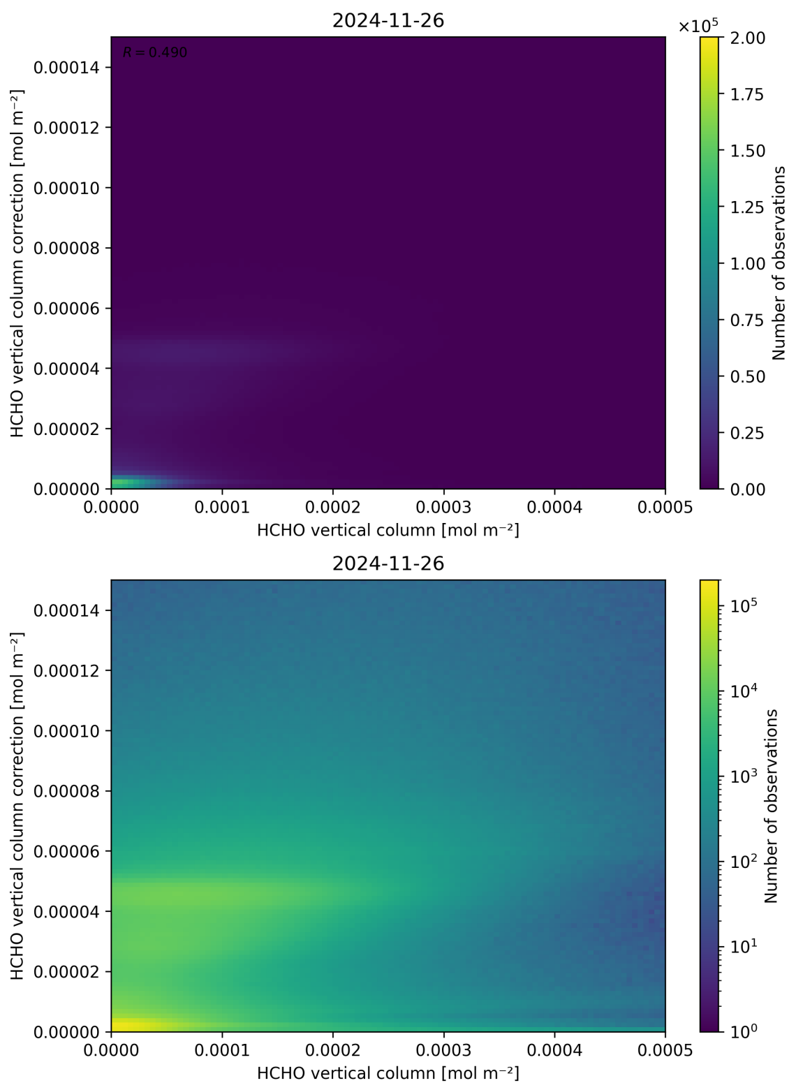
Figure 133: Scatter density plot of “HCHO vertical column” against “HCHO vertical column correction” for 2024-11-25 to 2024-11-27.
