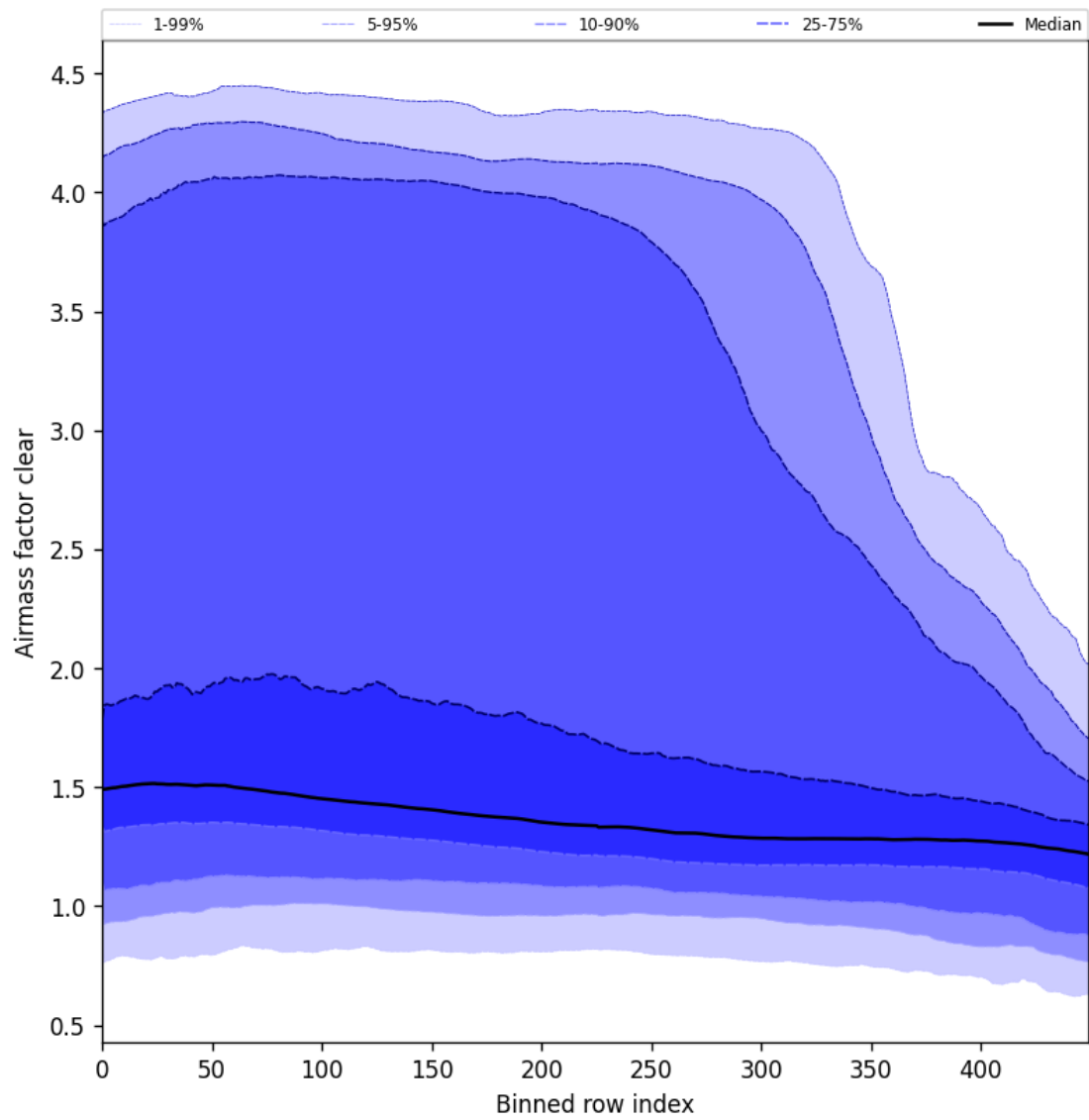
Figure 56: Along track statistics of “Airmass factor clear” for 2024-11-25 to 2024-11-27
