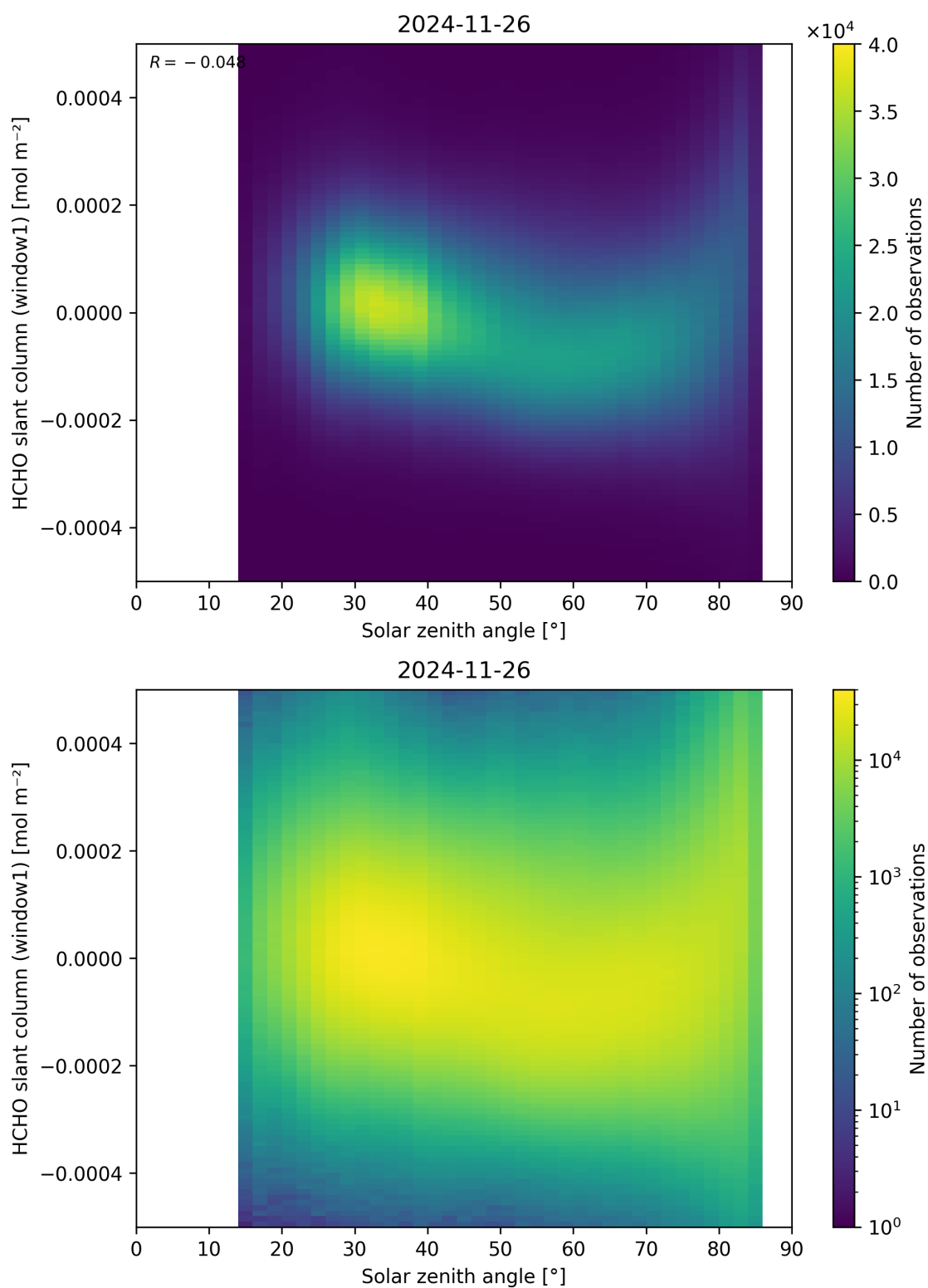
Figure 173: Scatter density plot of “Solar zenith angle” against “HCHO slant column (window1)” for 2024-11-25 to 2024-11-27.
