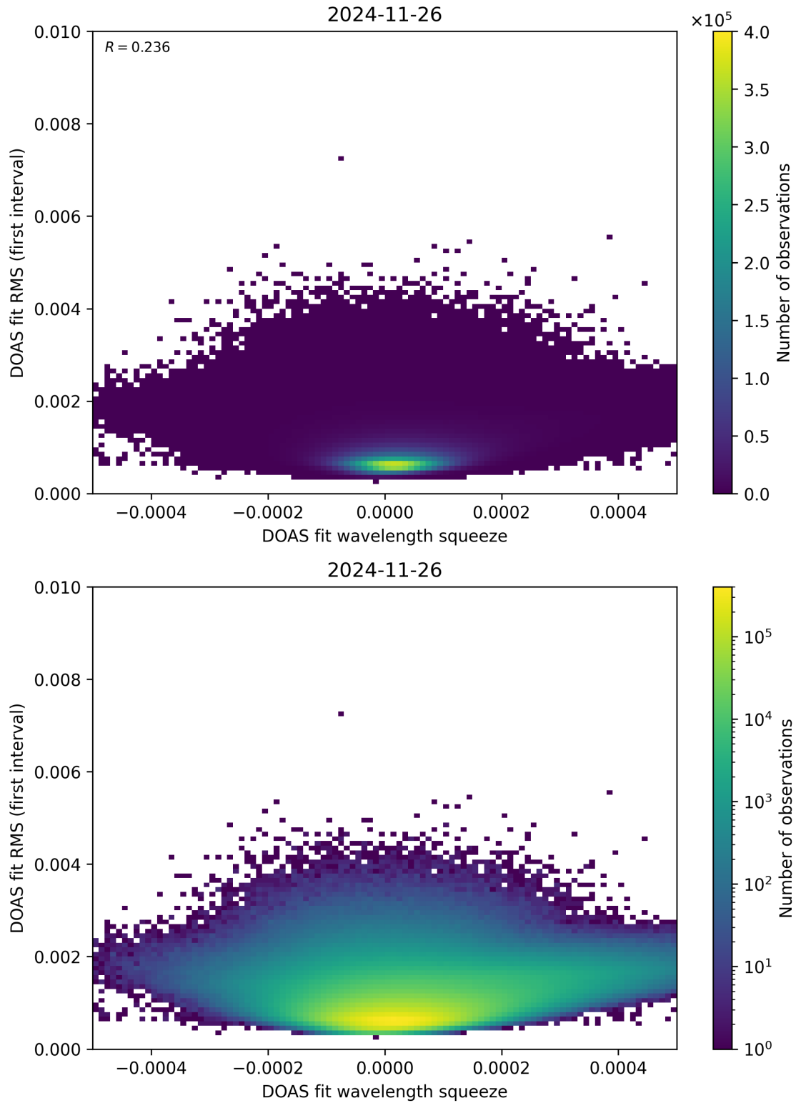
Figure 68: Scatter density plot of “DOAS fit wavelength squeeze” against “DOAS fit RMS (first interval)” for 2024-11-25 to 2024-11-27.
