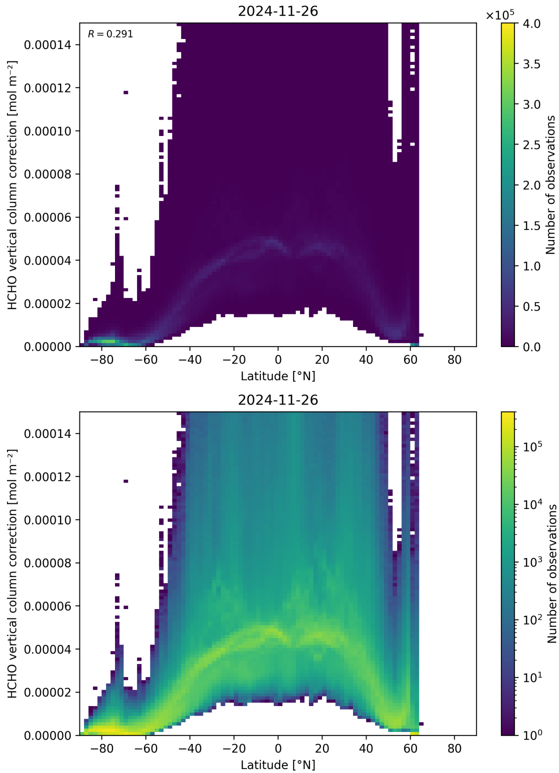
Figure 164: Scatter density plot of “Latitude” against “HCHO vertical column correction” for 2024-11-25 to 2024-11-27.
