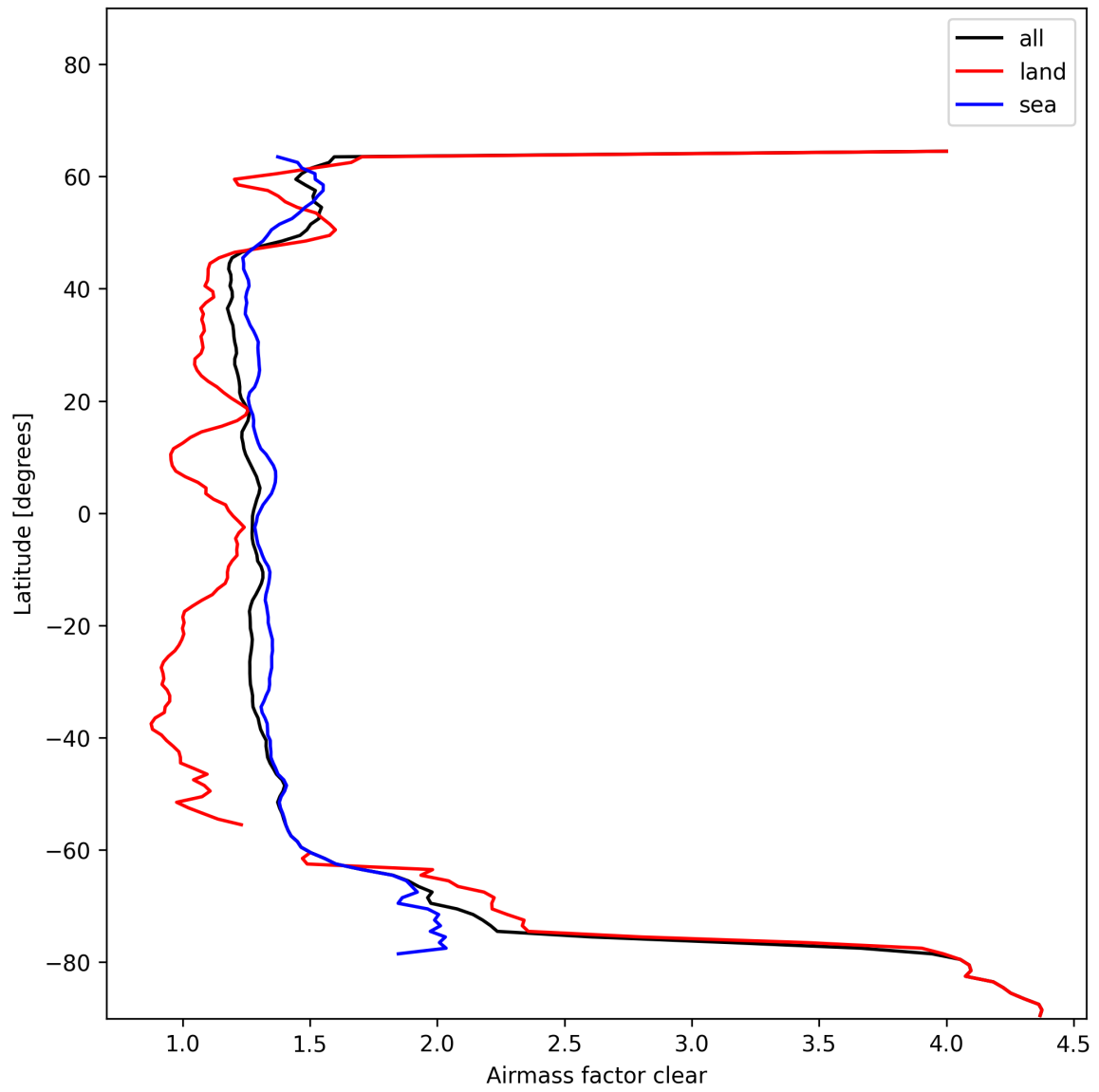
Figure 28: Zonal average of “Airmass factor clear” for 2024-11-25 to 2024-11-27.
