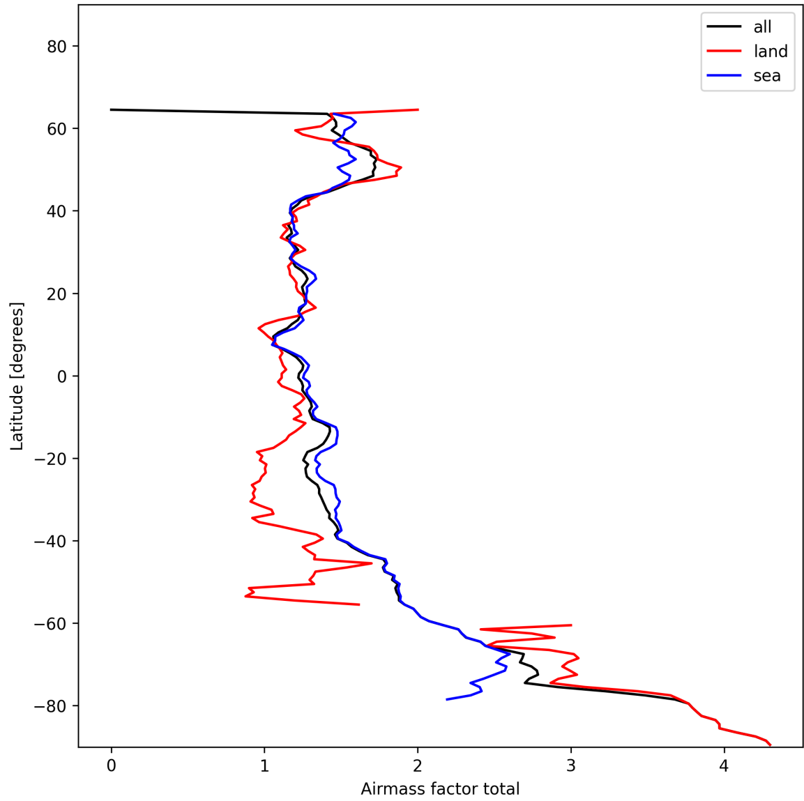
Figure 26: Zonal average of “Airmass factor total” for 2024-11-25 to 2024-11-27.
