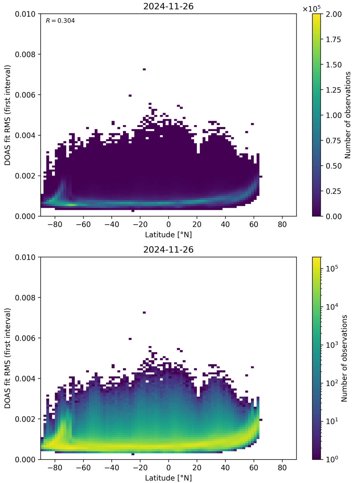
Figure 153: Scatter density plot of “Latitude” against “DOAS fit RMS (first interval)” for 2024-11-25 to 2024-11-27.
