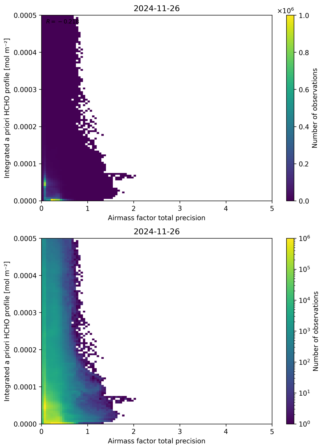
Figure 111: Scatter density plot of “Airmass factor total precision” against “Integrated a priori HCHO profile” for 2024-11-25 to 2024-11-27.
