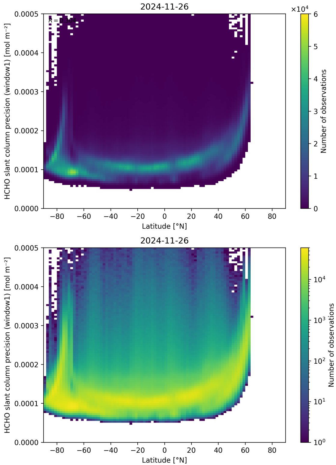
Figure 160: Scatter density plot of “Latitude” against “HCHO slant column precision (window1)” for 2024-11-25 to 2024-11-27.
