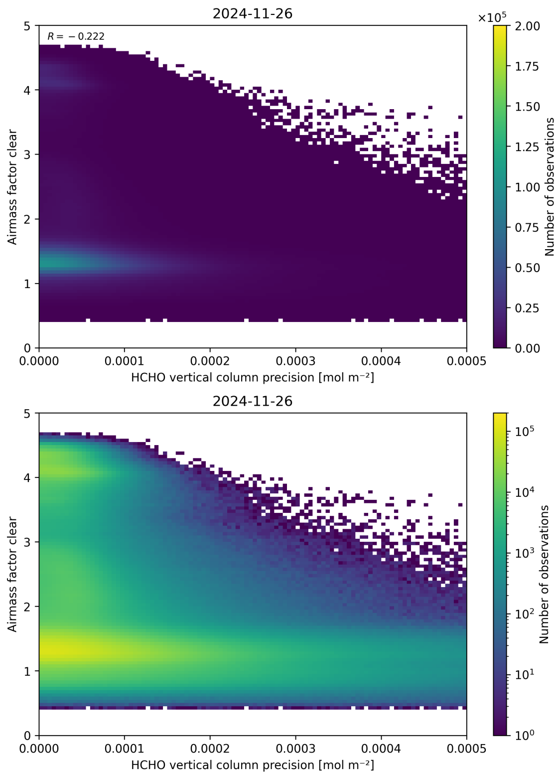
Figure 139: Scatter density plot of “HCHO vertical column precision” against “Airmass factor clear” for 2024-11-25 to 2024-11-27.
