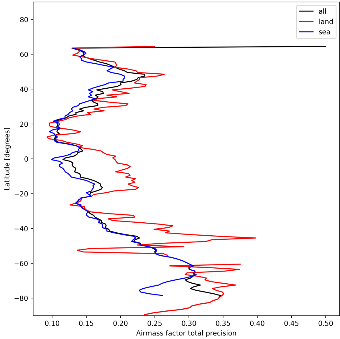
Figure 27: Zonal average of “Airmass factor total precision” for 2024-11-25 to 2024-11-27.
