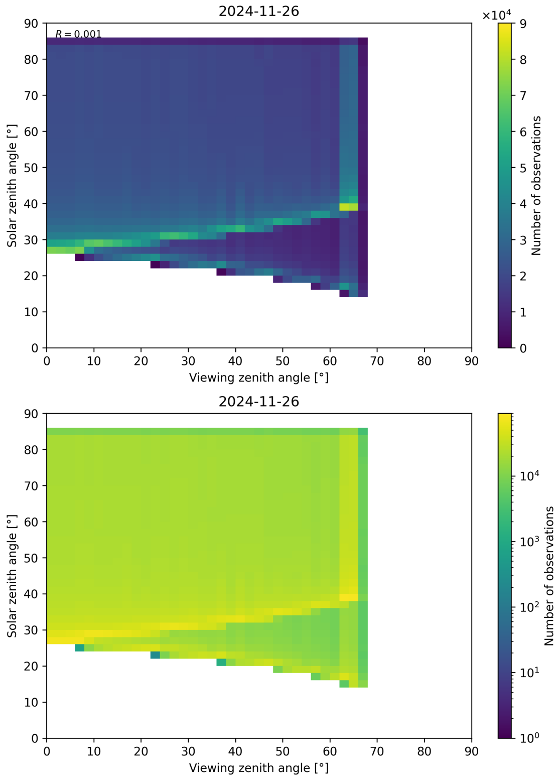
Figure 197: Scatter density plot of “Viewing zenith angle” against “Solar zenith angle” for 2024-11-25 to 2024-11-27.
