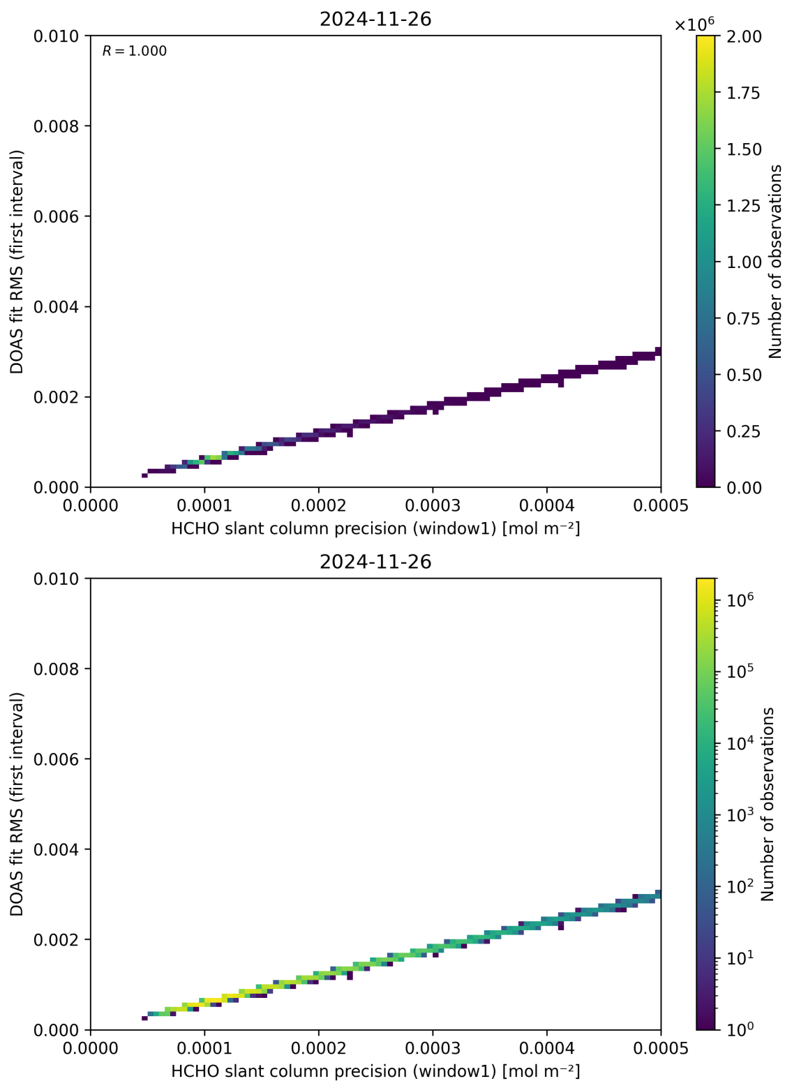
Figure 88: Scatter density plot of “HCHO slant column precision (window1)” against “DOAS fit RMS (first interval)” for 2024-11-25 to 2024-11-27.
