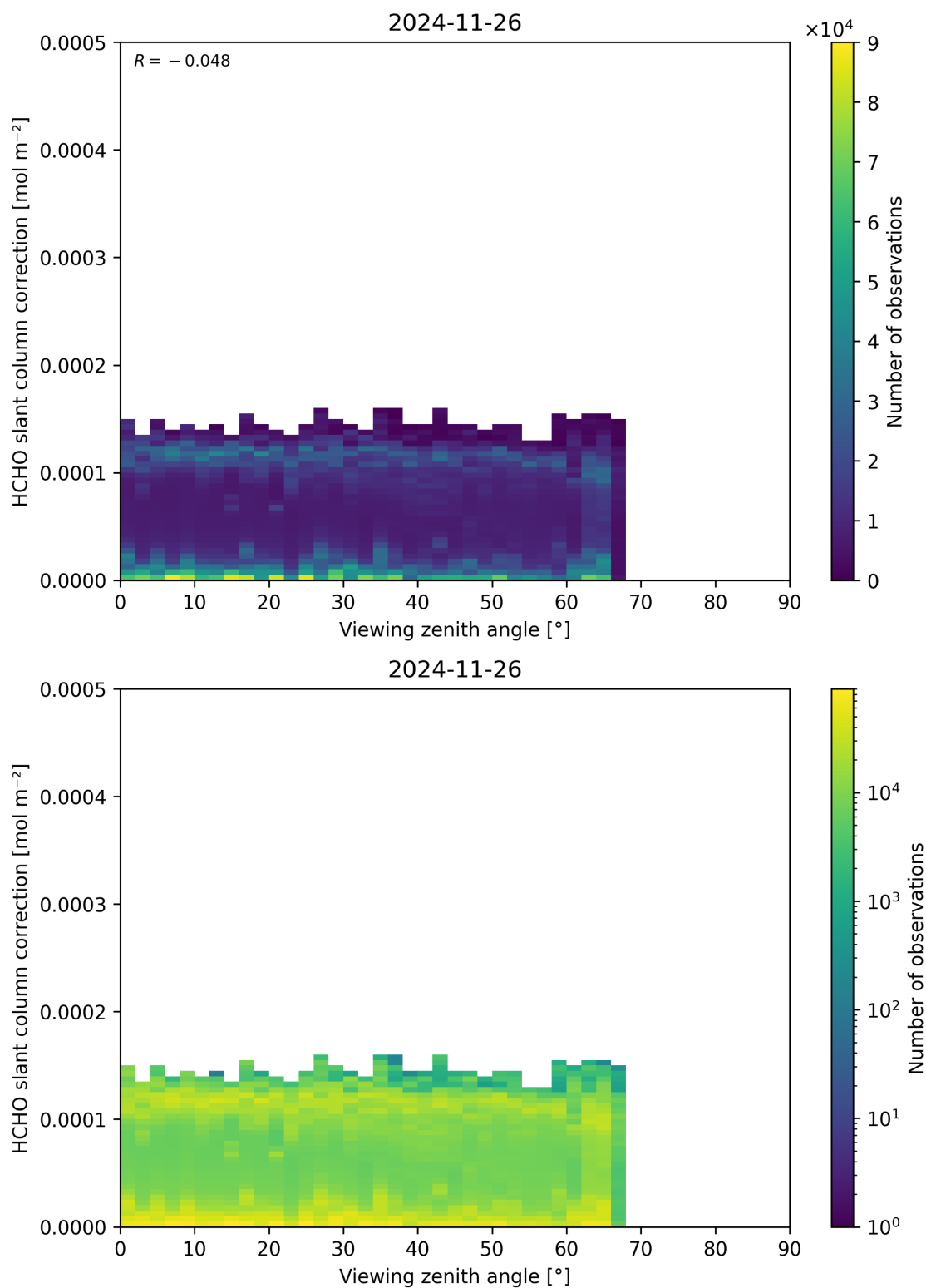
Figure 187: Scatter density plot of “Viewing zenith angle” against “HCHO slant column correction” for 2024-11-25 to 2024-11-27.
