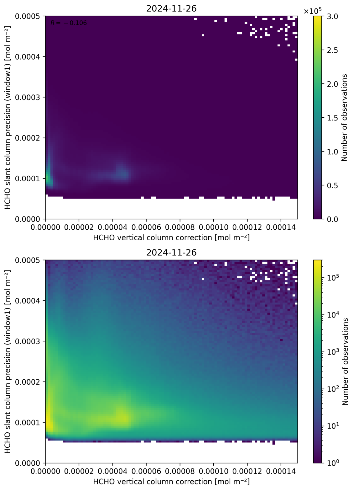
Figure 119: Scatter density plot of “HCHO vertical column correction” against “HCHO slant column precision (window1)” for 2024-11-25 to 2024-11-27.
