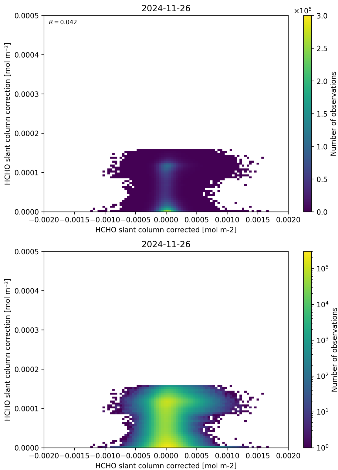
Figure 77: Scatter density plot of “HCHO slant column corrected” against “HCHO slant column correction” for 2024-11-25 to 2024-11-27.
