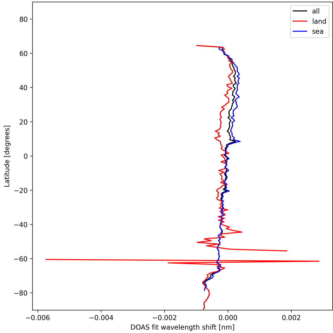
Figure 30: Zonal average of “DOAS fit wavelength shift” for 2024-11-25 to 2024-11-27.
