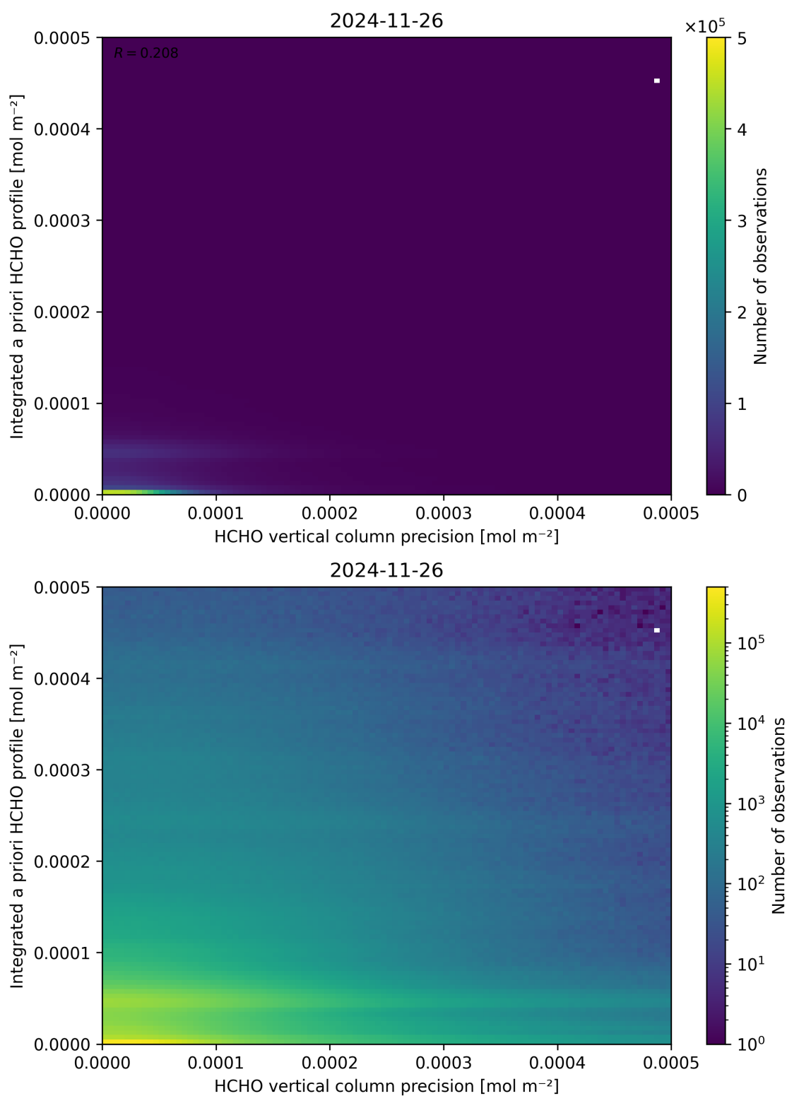
Figure 147: Scatter density plot of “HCHO vertical column precision” against “Integrated a priori HCHO profile” for 2024-11-25 to 2024-11-27.
