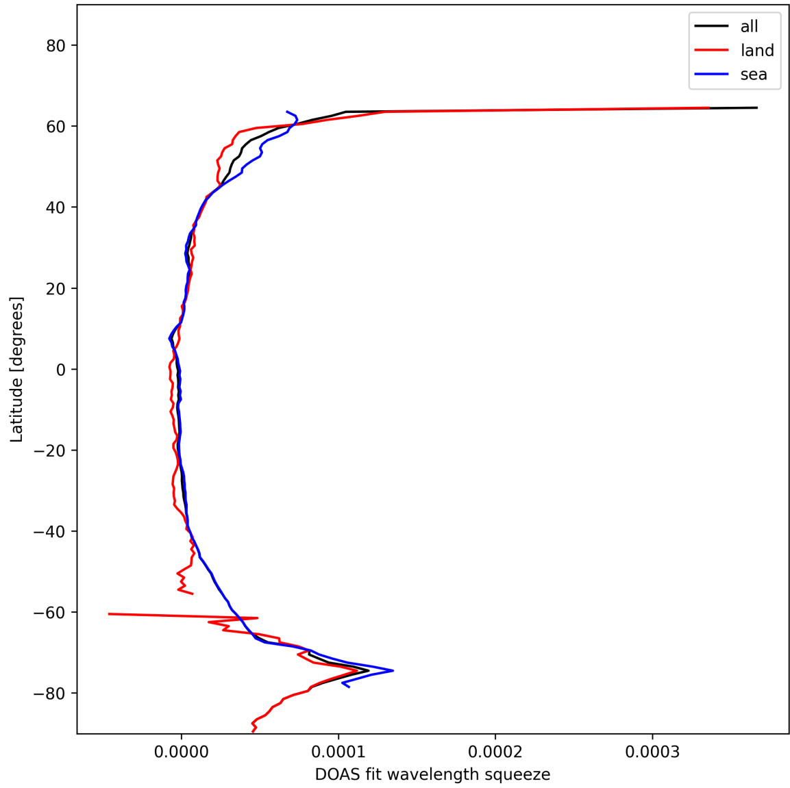
Figure 31: Zonal average of “DOAS fit wavelength squeeze” for 2024-11-25 to 2024-11-27.
