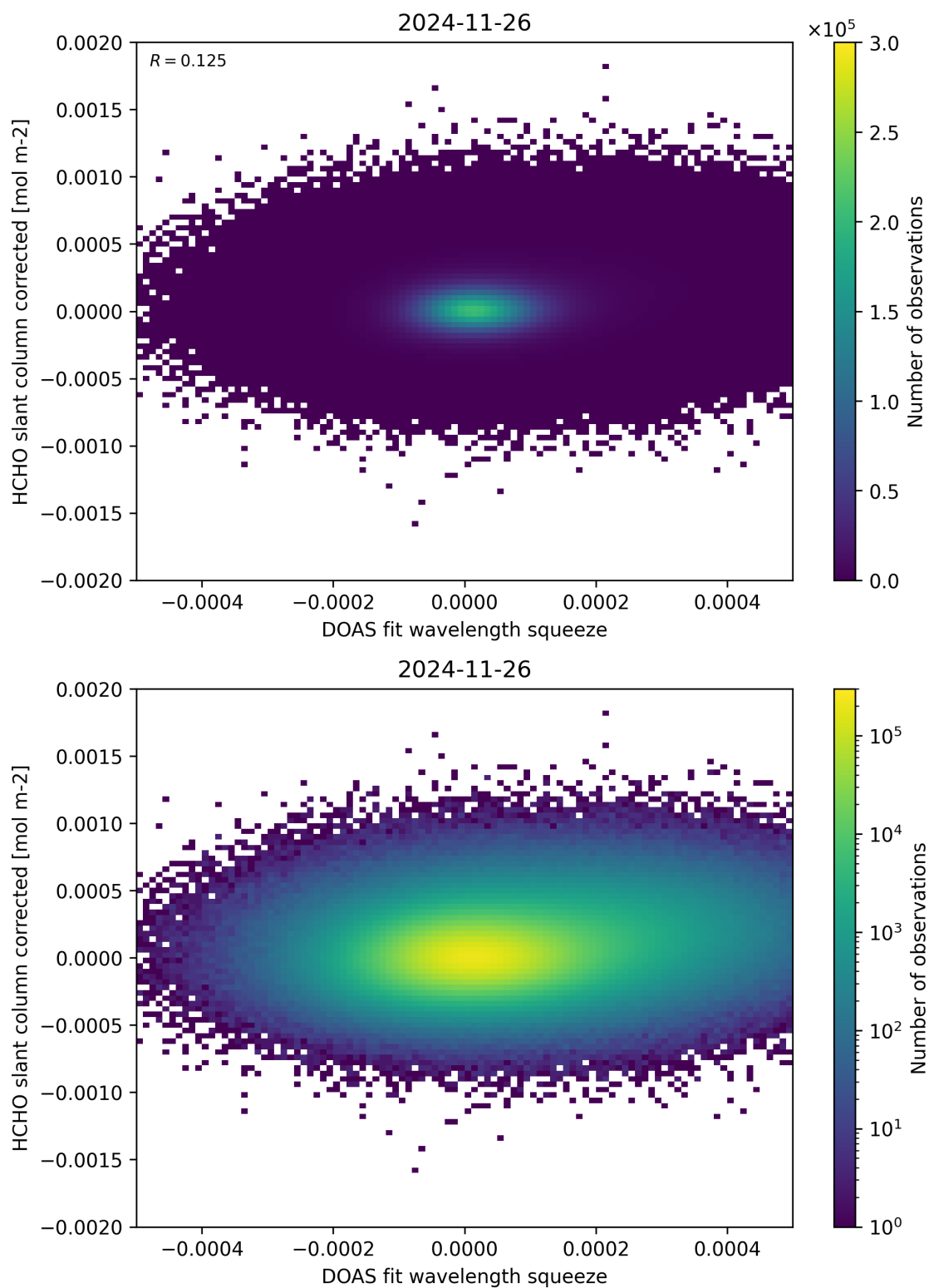
Figure 69: Scatter density plot of “DOAS fit wavelength squeeze” against “HCHO slant column corrected” for 2024-11-25 to 2024-11-27.
