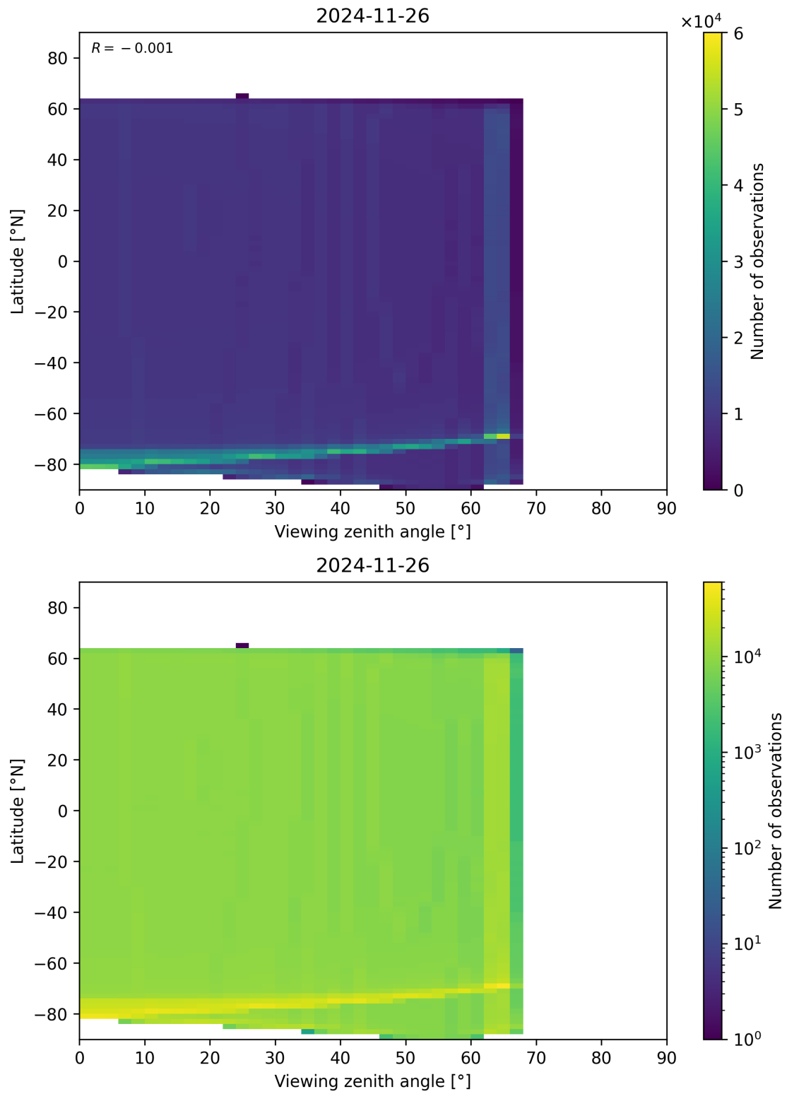
Figure 196: Scatter density plot of “Viewing zenith angle” against “Latitude” for 2024-11-25 to 2024-11-27.
