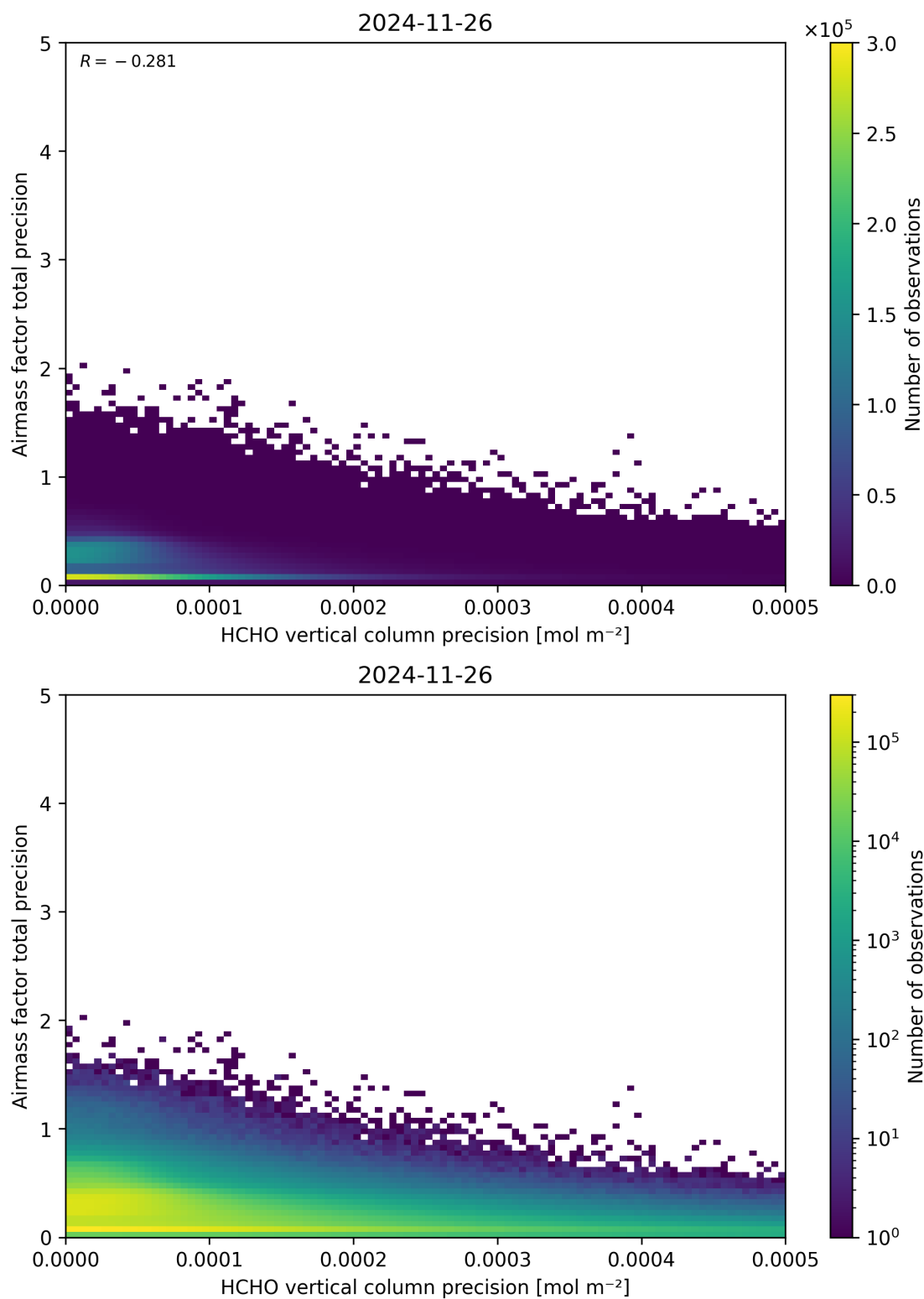
Figure 145: Scatter density plot of “HCHO vertical column precision” against “Airmass factor total precision” for 2024-11-25 to 2024-11-27.
