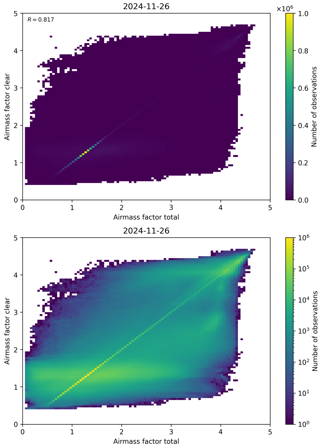
Figure 100: Scatter density plot of “Airmass factor total” against “Airmass factor clear” for 2024-11-25 to 2024-11-27.
