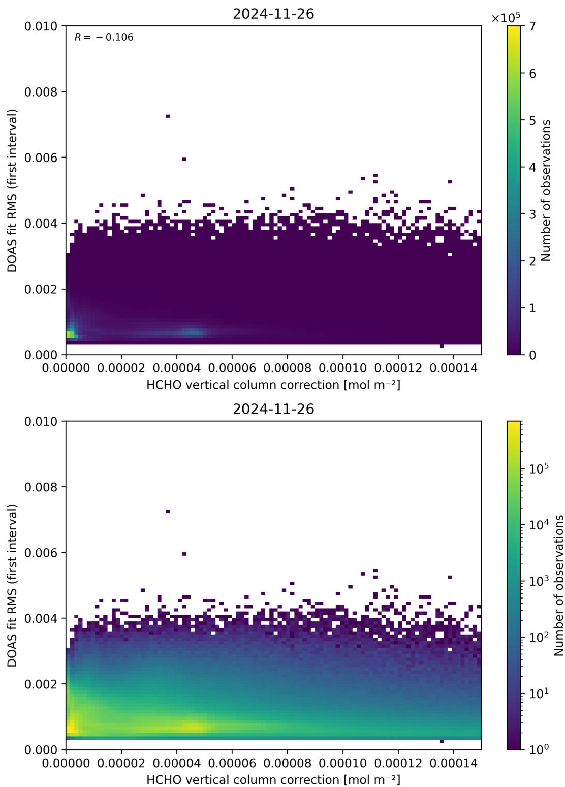
Figure 112: Scatter density plot of “HCHO vertical column correction” against “DOAS fit RMS (first interval)” for 2024-11-25 to 2024-11-27.
