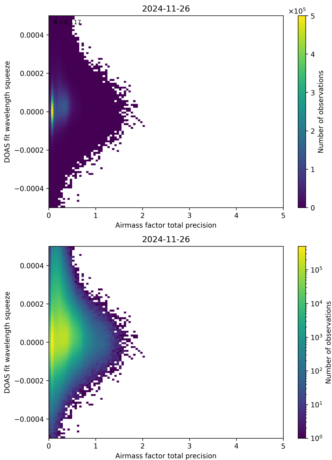
Figure 107: Scatter density plot of “Airmass factor total precision” against “DOAS fit wavelength squeeze” for 2024-11-25 to 2024-11-27.
