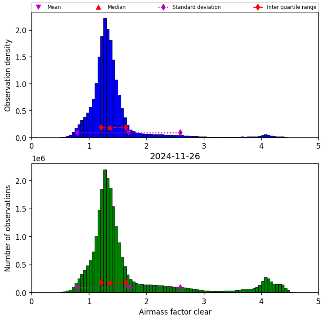
Figure 42: Histogram of “Airmass factor clear” for 2024-11-25 to 2024-11-27
