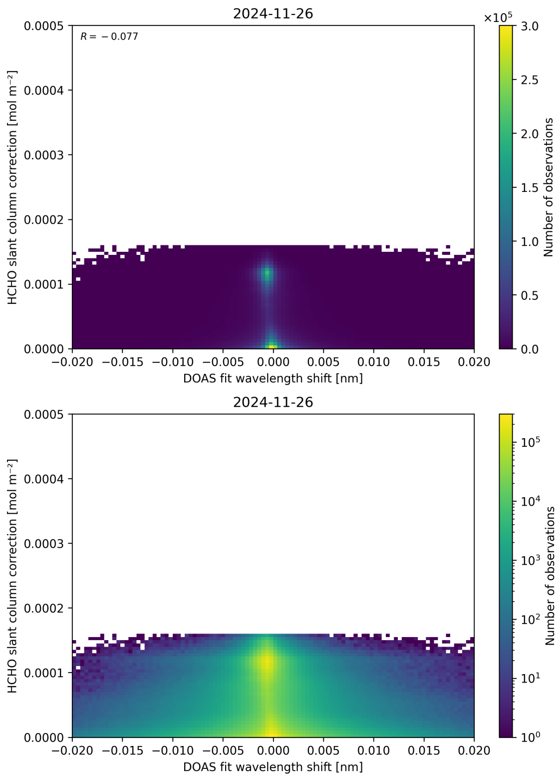
Figure 67: Scatter density plot of “DOAS fit wavelength shift” against “HCHO slant column correction” for 2024-11-25 to 2024-11-27.
