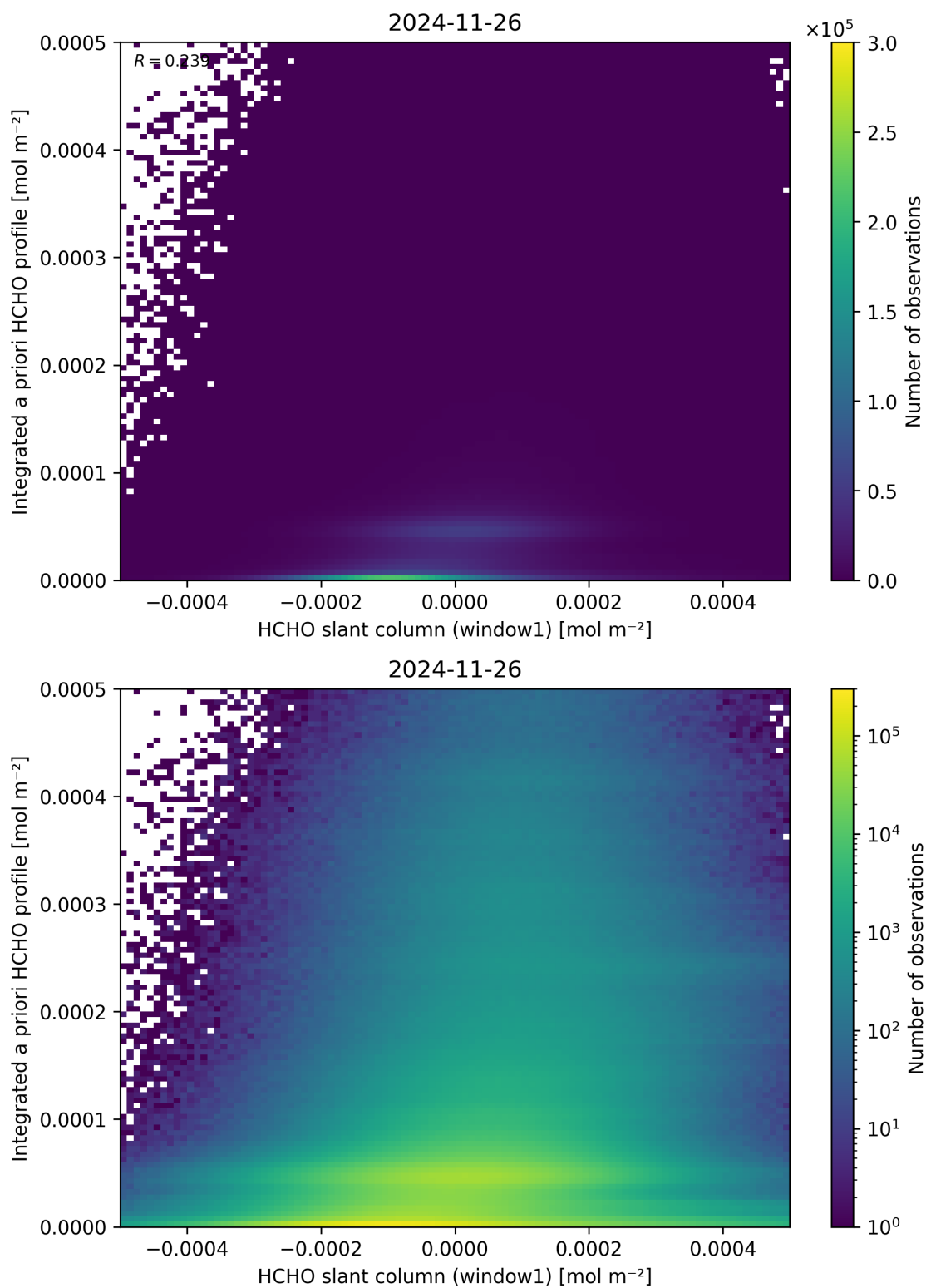
Figure 87: Scatter density plot of “HCHO slant column (window1)” against “Integrated a priori HCHO profile” for 2024-11-25 to 2024-11-27.
