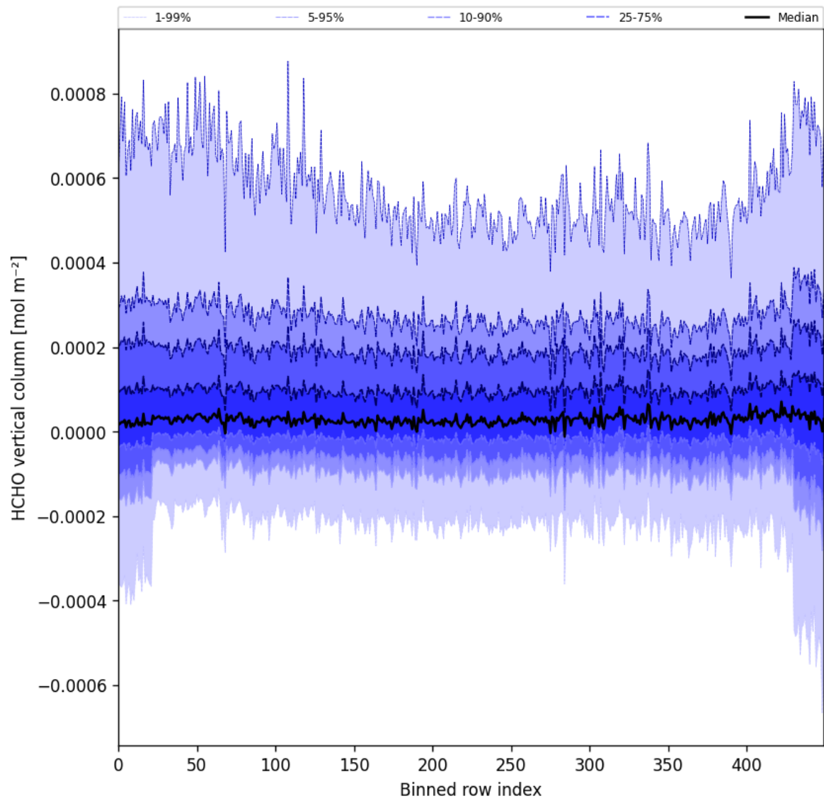
Figure 49: Along track statistics of “HCHO vertical column” for 2024-11-25 to 2024-11-27
