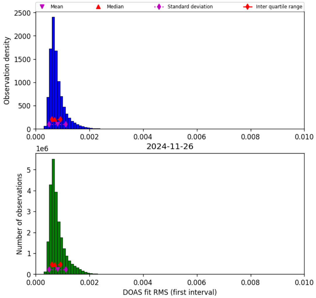
Figure 46: Histogram of “DOAS fit RMS (first interval)” for 2024-11-25 to 2024-11-27
