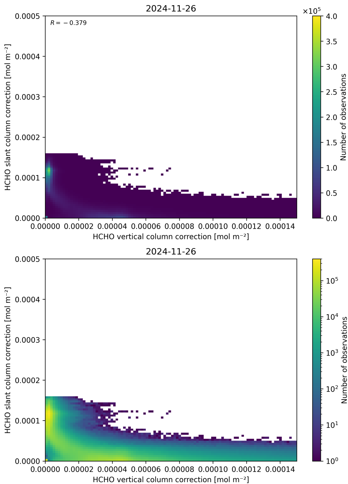
Figure 117: Scatter density plot of “HCHO vertical column correction” against “HCHO slant column correction” for 2024-11-25 to 2024-11-27.
