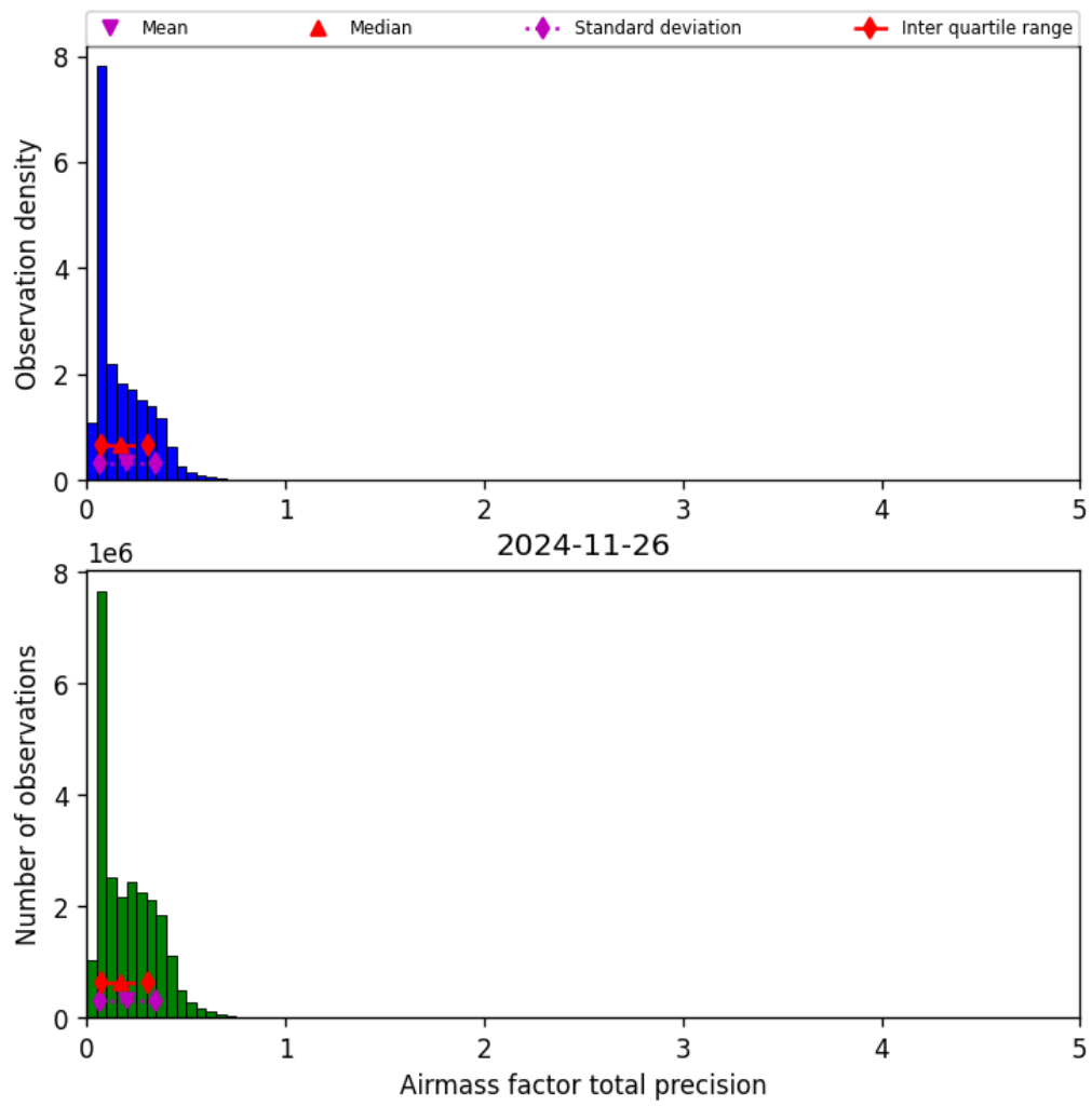
Figure 41: Histogram of “Airmass factor total precision” for 2024-11-25 to 2024-11-27
