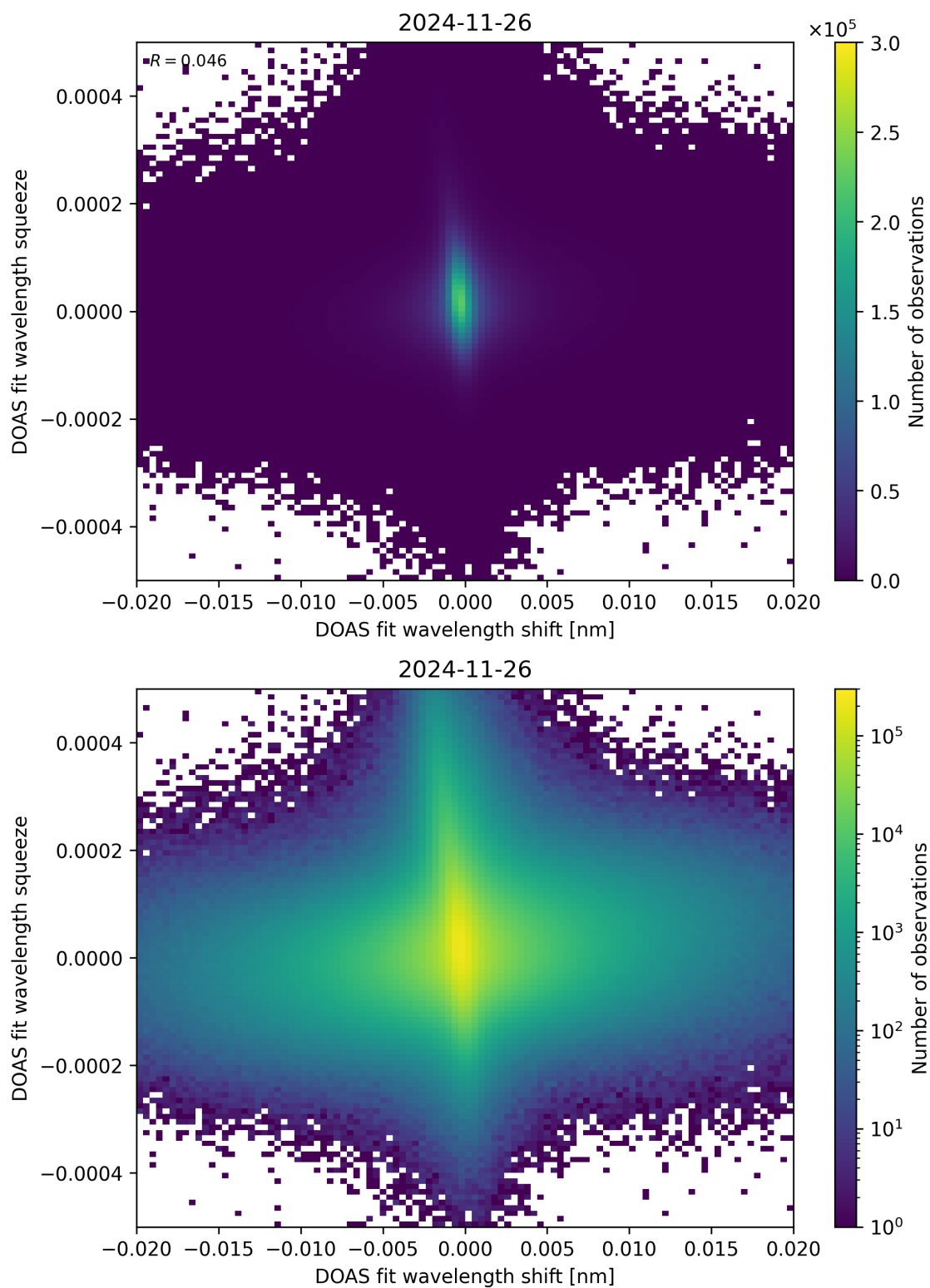
Figure 65: Scatter density plot of “DOAS fit wavelength shift” against “DOAS fit wavelength squeeze” for 2024-11-25 to 2024-11-27.
