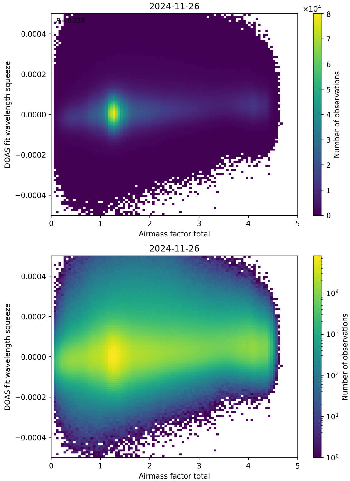
Figure 99: Scatter density plot of “Airmass factor total” against “DOAS fit wavelength squeeze” for 2024-11-25 to 2024-11-27.
