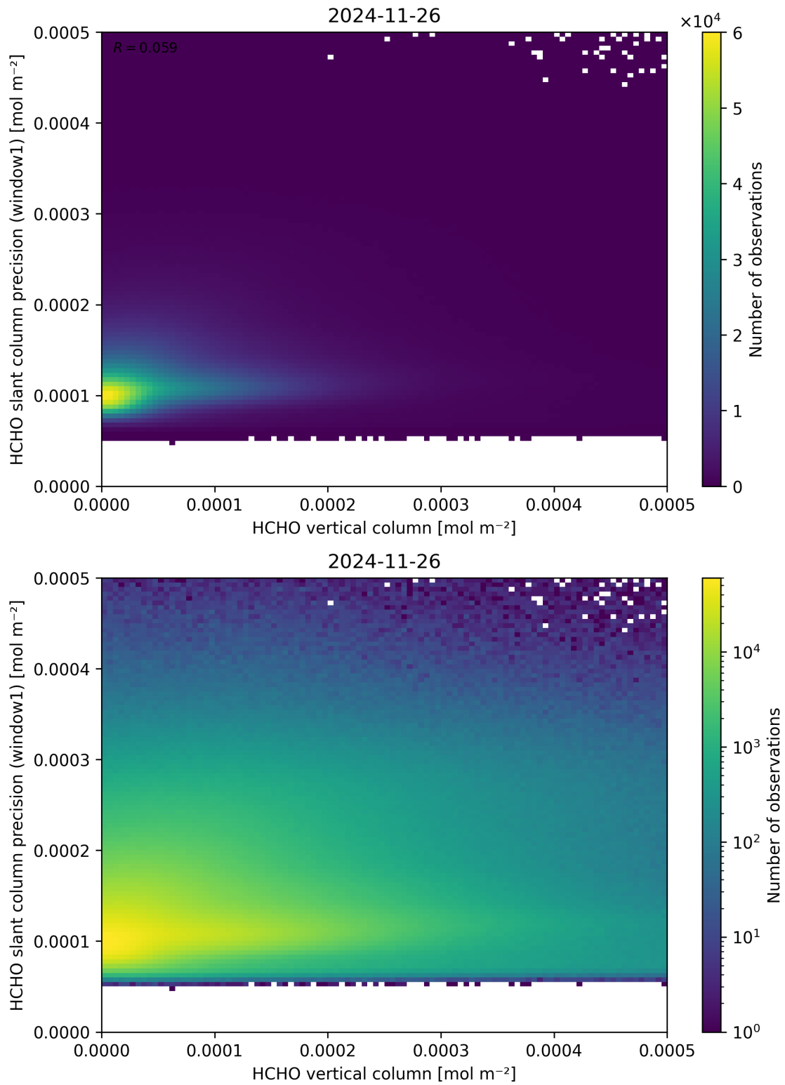
Figure 130: Scatter density plot of “HCHO vertical column” against “HCHO slant column precision (window1)” for 2024-11-25 to 2024-11-27.
