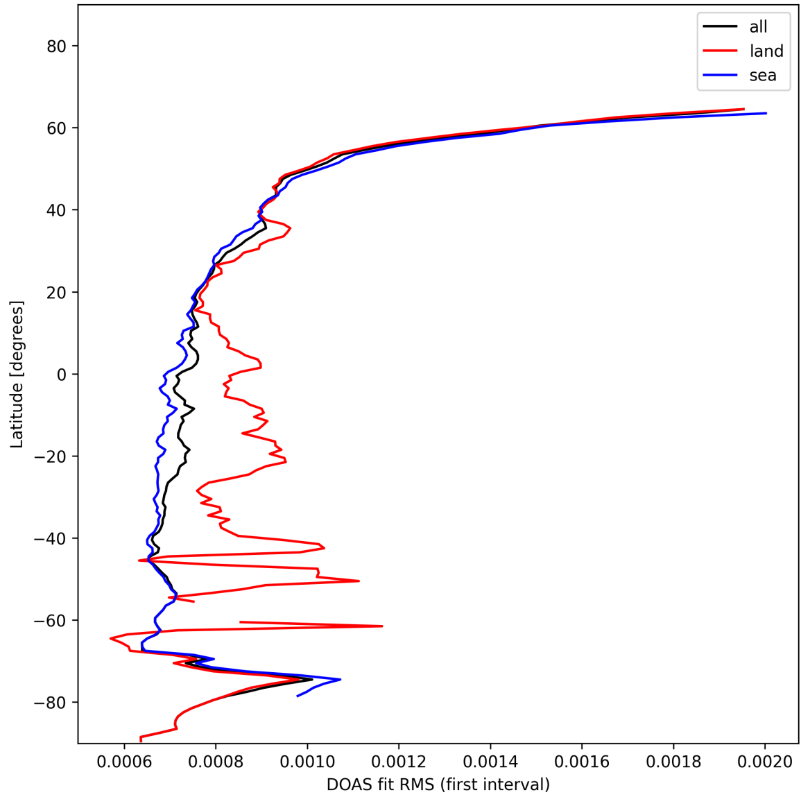
Figure 32: Zonal average of “DOAS fit RMS (first interval)” for 2024-11-25 to 2024-11-27.
