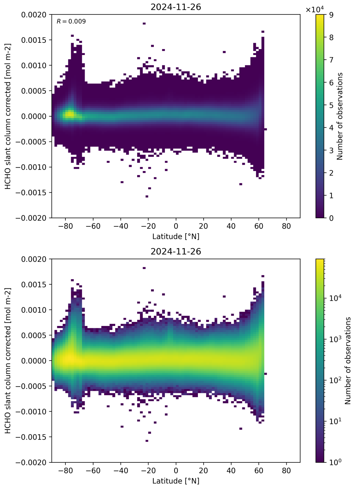
Figure 157: Scatter density plot of “Latitude” against “HCHO slant column corrected” for 2024-11-25 to 2024-11-27.
