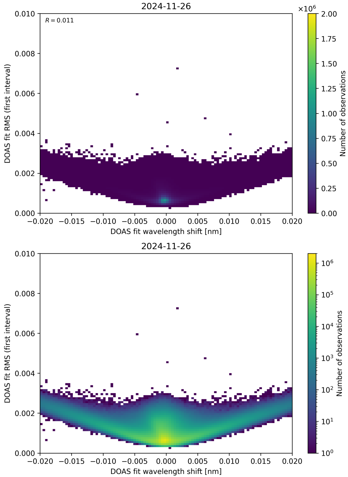
Figure 64: Scatter density plot of “DOAS fit wavelength shift” against “DOAS fit RMS (first interval)” for 2024-11-25 to 2024-11-27.
