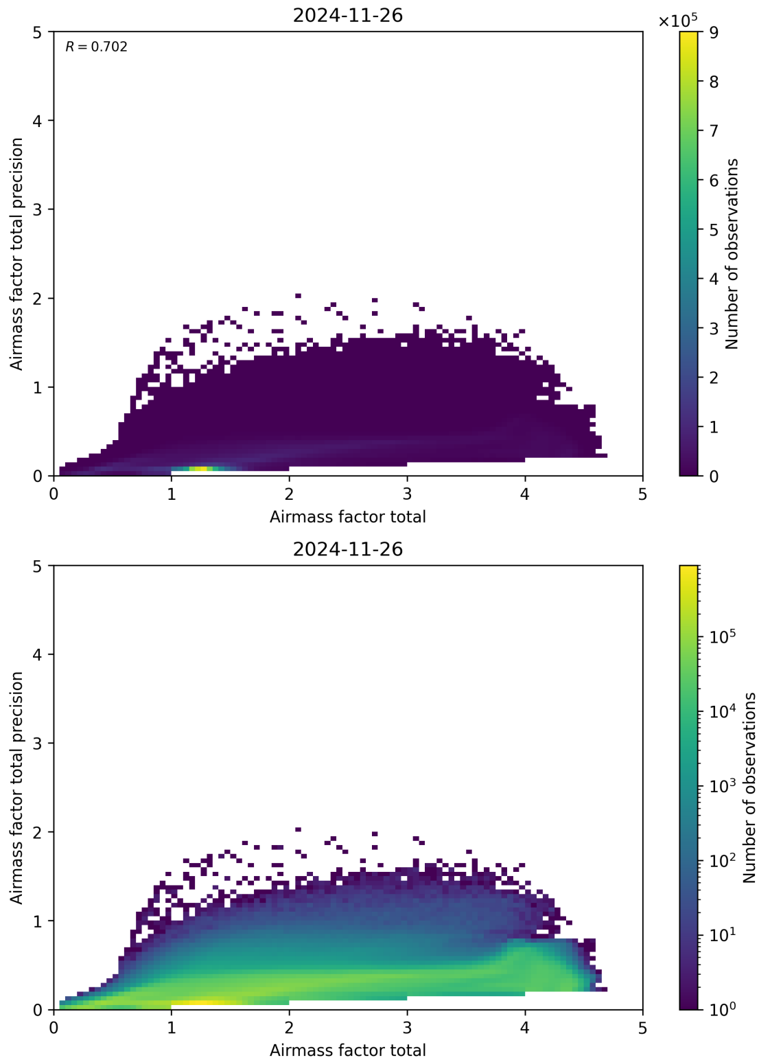
Figure 103: Scatter density plot of “Airmass factor total” against “Airmass factor total precision” for 2024-11-25 to 2024-11-27.
