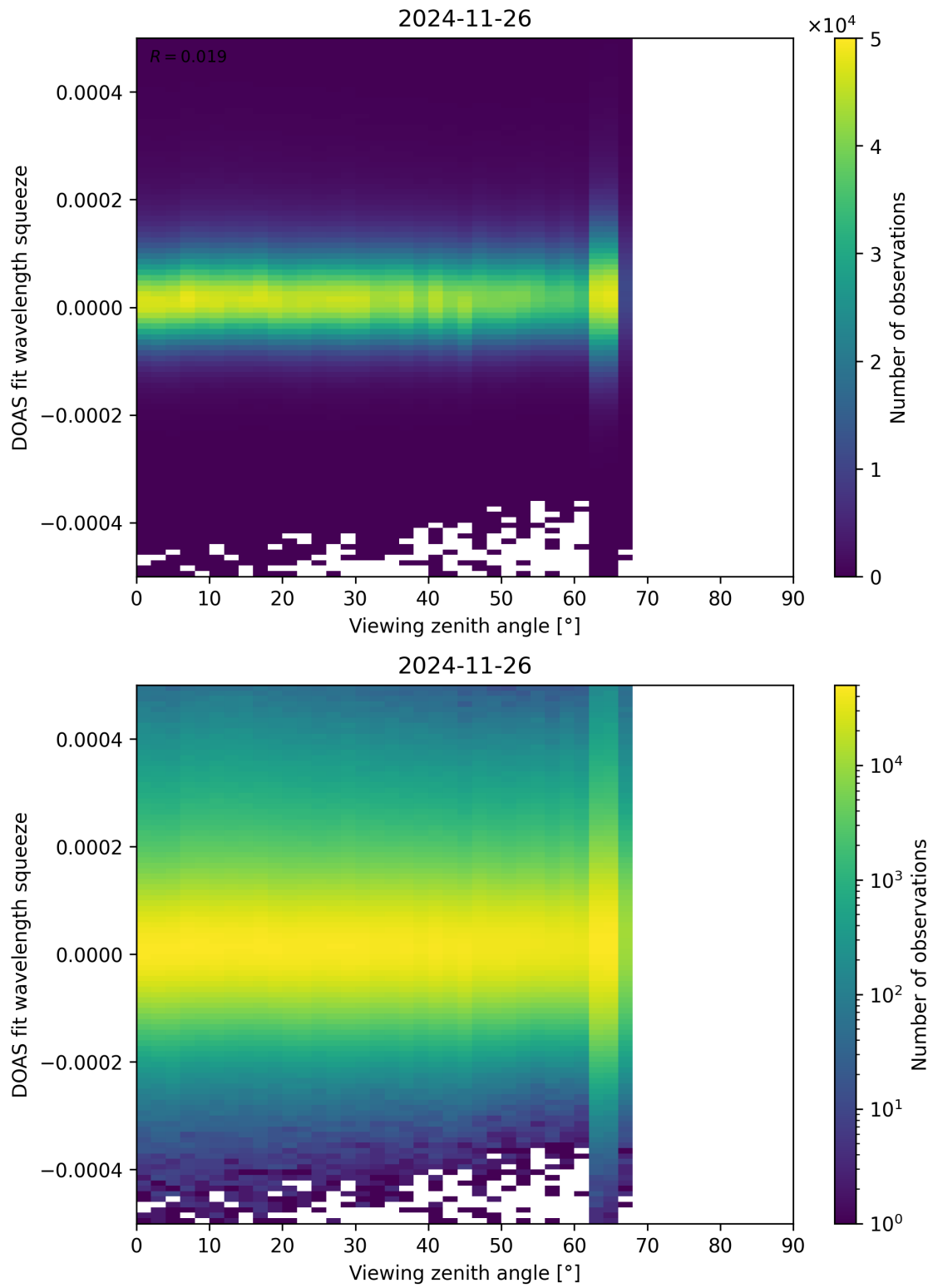
Figure 184: Scatter density plot of “Viewing zenith angle” against “DOAS fit wavelength squeeze” for 2024-11-25 to 2024-11-27.
