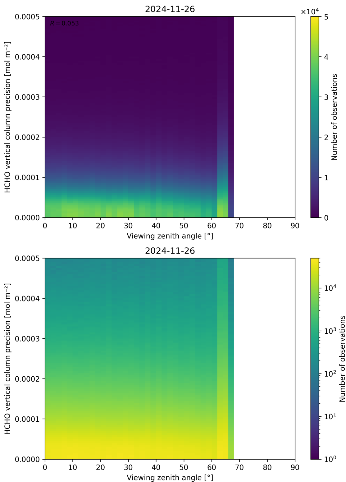
Figure 194: Scatter density plot of “Viewing zenith angle” against “HCHO vertical column precision” for 2024-11-25 to 2024-11-27.
