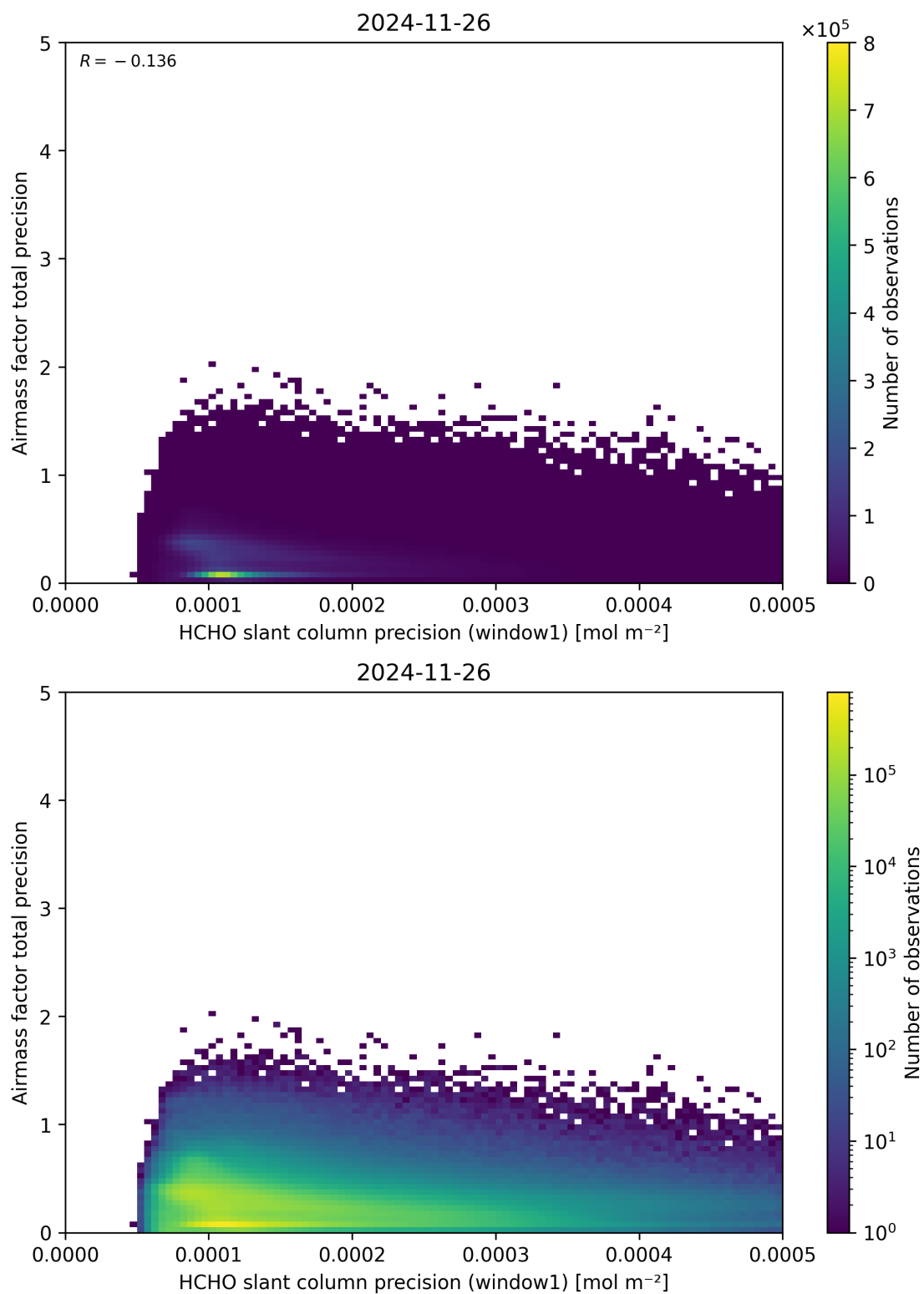
Figure 95: Scatter density plot of “HCHO slant column precision (window1)” against “Airmass factor total precision” for 2024-11-25 to 2024-11-27.
