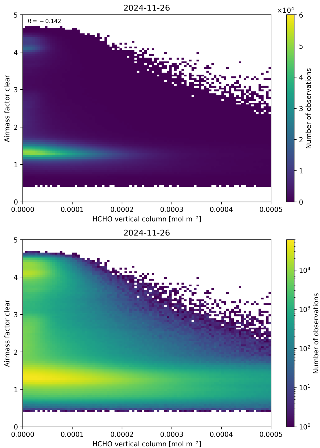
Figure 126: Scatter density plot of “HCHO vertical column” against “Airmass factor clear” for 2024-11-25 to 2024-11-27.
