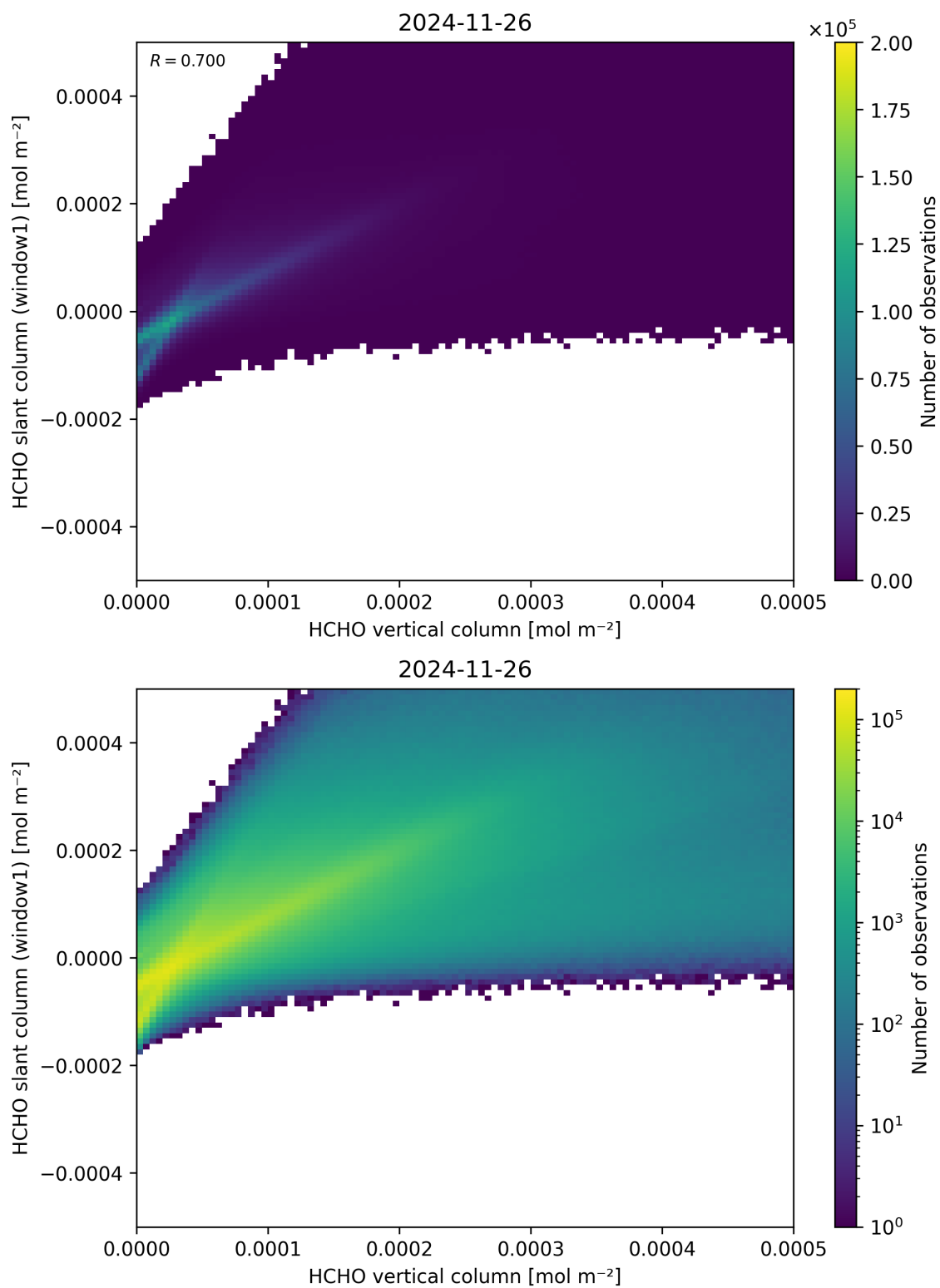
Figure 129: Scatter density plot of “HCHO vertical column” against “HCHO slant column (window1)” for 2024-11-25 to 2024-11-27.
