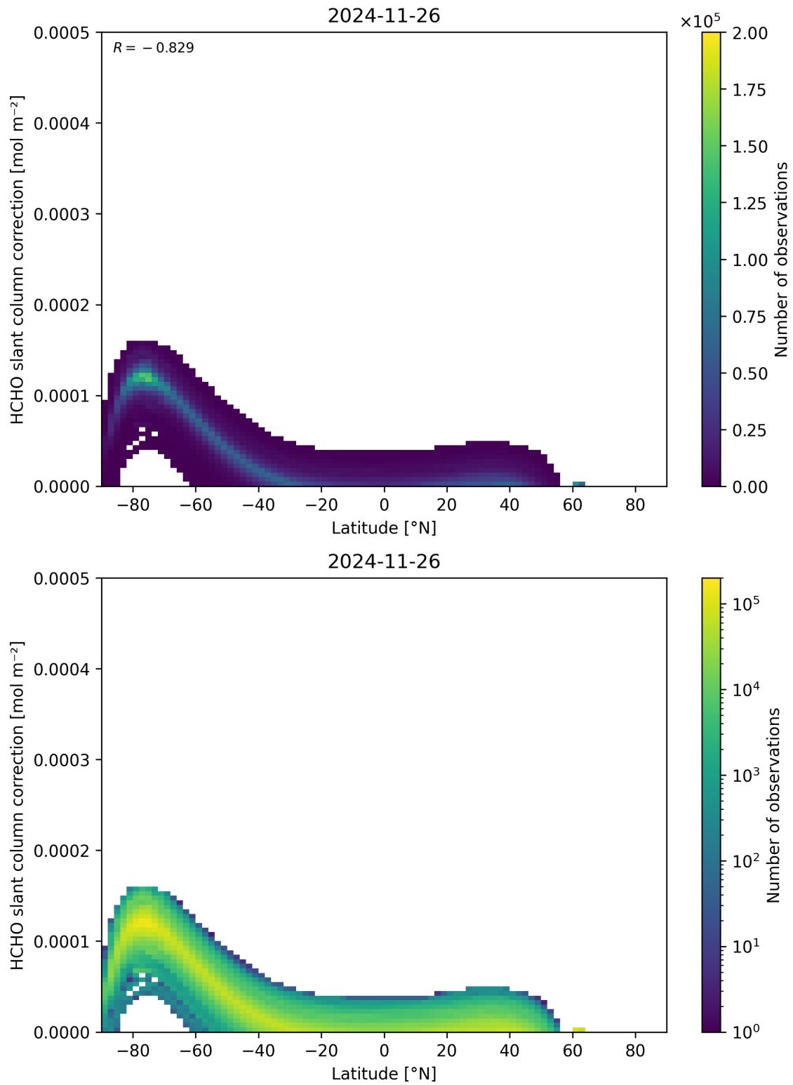
Figure 158: Scatter density plot of “Latitude” against “HCHO slant column correction” for 2024-11-25 to 2024-11-27.
