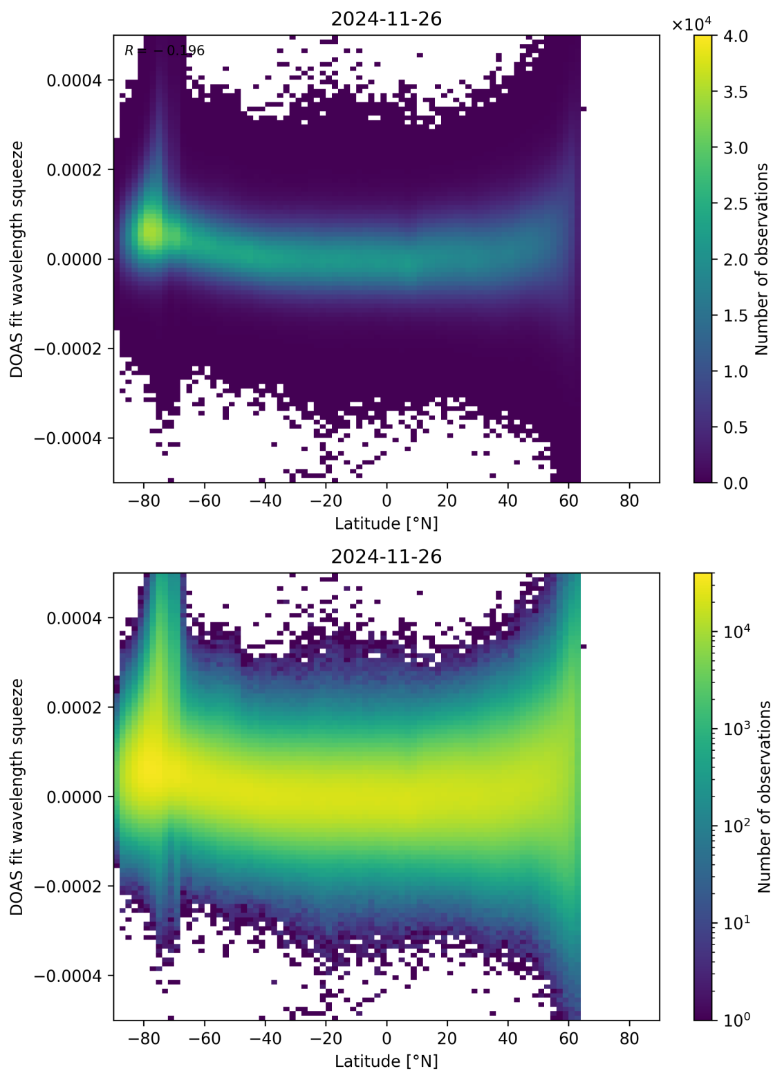
Figure 155: Scatter density plot of “Latitude” against “DOAS fit wavelength squeeze” for 2024-11-25 to 2024-11-27.
