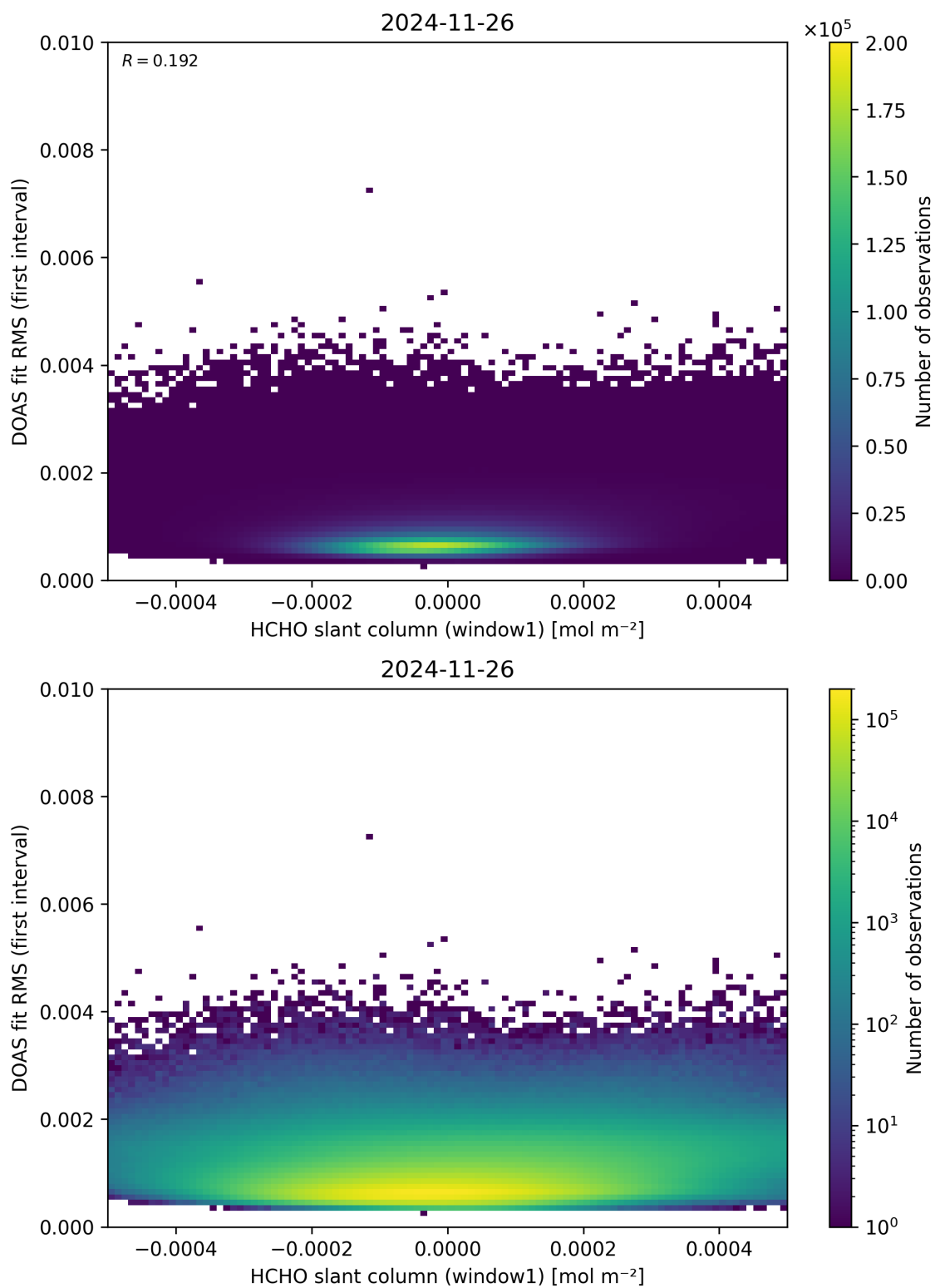
Figure 78: Scatter density plot of “HCHO slant column (window1)” against “DOAS fit RMS (first interval)” for 2024-11-25 to 2024-11-27.
