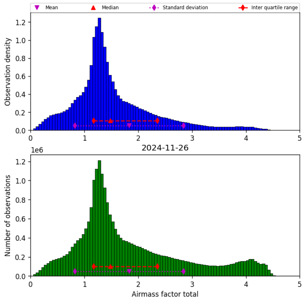
Figure 40: Histogram of “Airmass factor total” for 2024-11-25 to 2024-11-27
