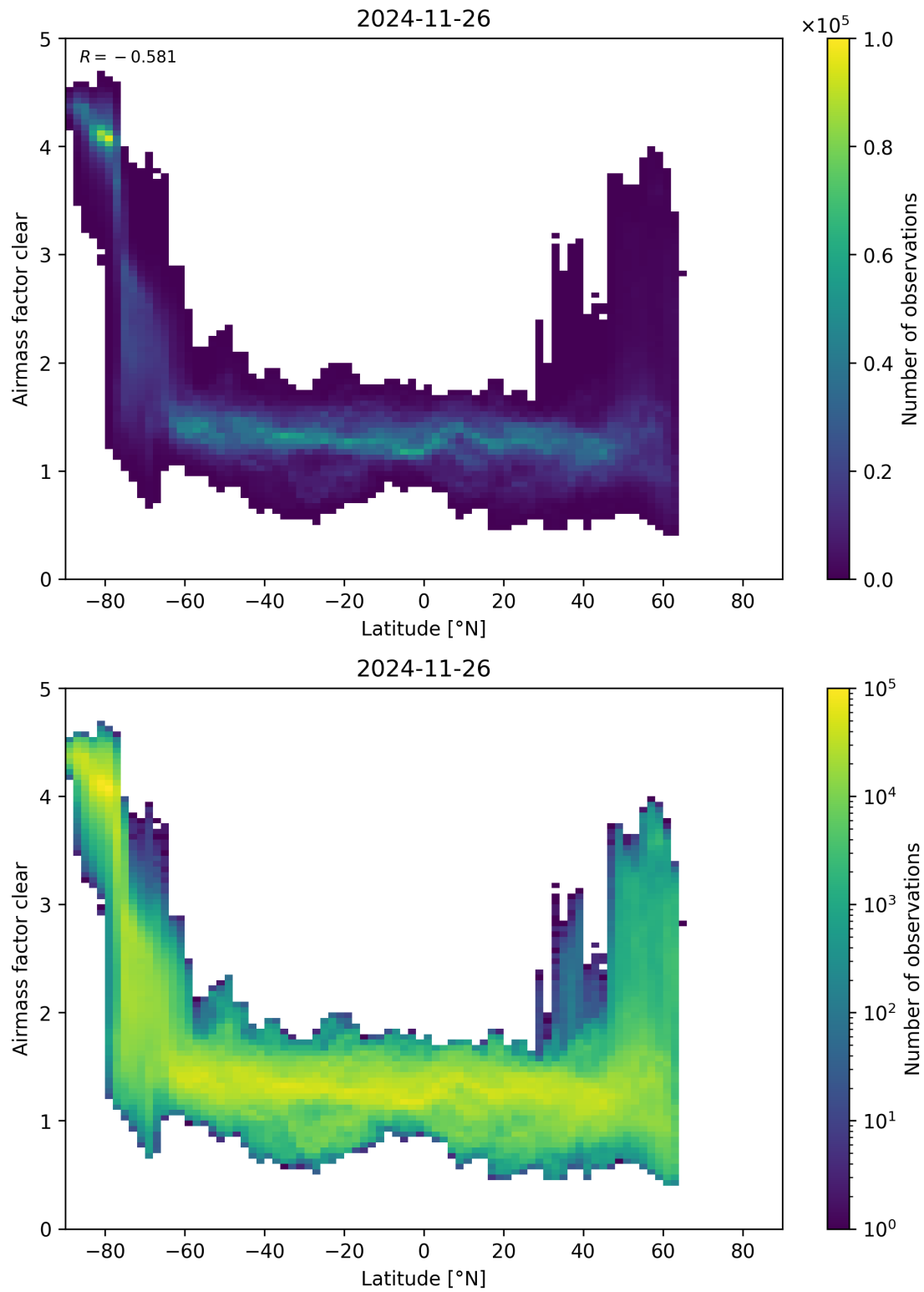
Figure 156: Scatter density plot of “Latitude” against “Airmass factor clear” for 2024-11-25 to 2024-11-27.
