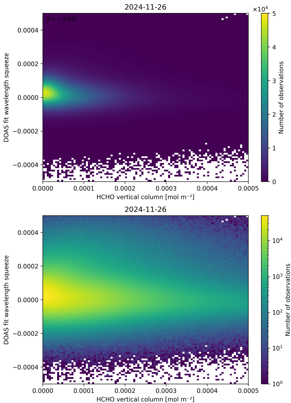
Figure 125: Scatter density plot of “HCHO vertical column” against “DOAS fit wavelength squeeze” for 2024-11-25 to 2024-11-27.
