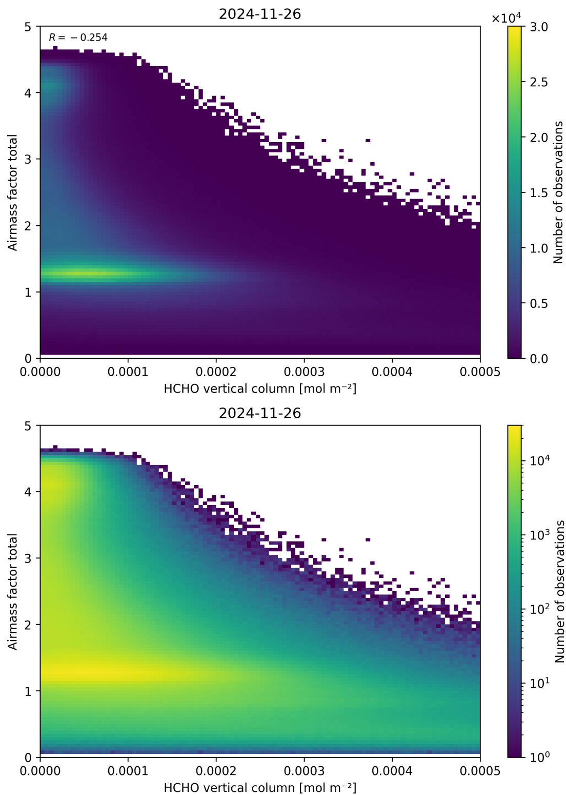
Figure 131: Scatter density plot of “HCHO vertical column” against “Airmass factor total” for 2024-11-25 to 2024-11-27.
