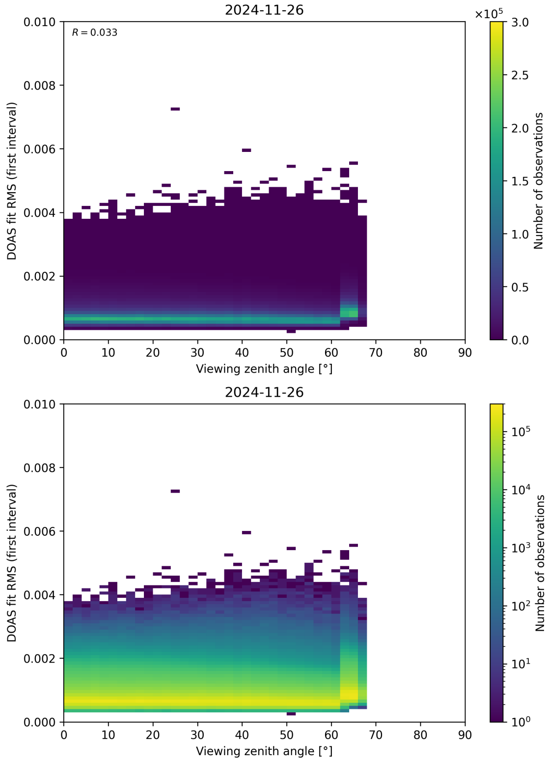
Figure 182: Scatter density plot of “Viewing zenith angle” against “DOAS fit RMS (first interval)” for 2024-11-25 to 2024-11-27.
