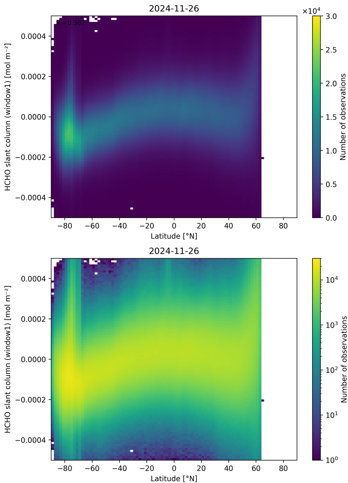
Figure 159: Scatter density plot of “Latitude” against “HCHO slant column (window1)” for 2024-11-25 to 2024-11-27.
