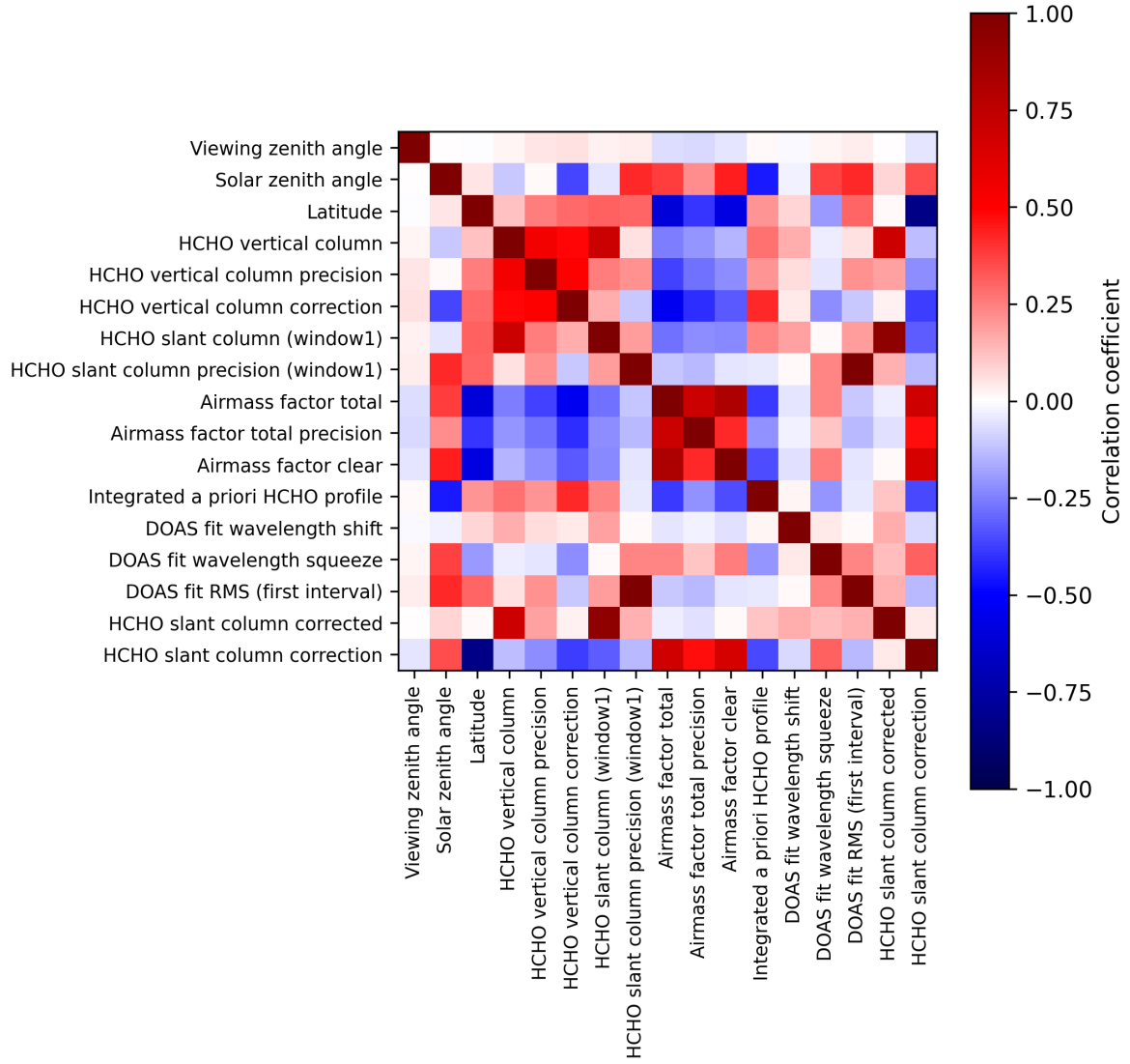
Figure 2: Map of correlation matrix for 2024-11-25 to 2024-11-27.
