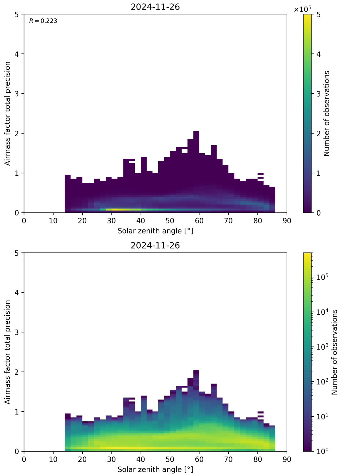
Figure 176: Scatter density plot of “Solar zenith angle” against “Airmass factor total precision” for 2024-11-25 to 2024-11-27.
