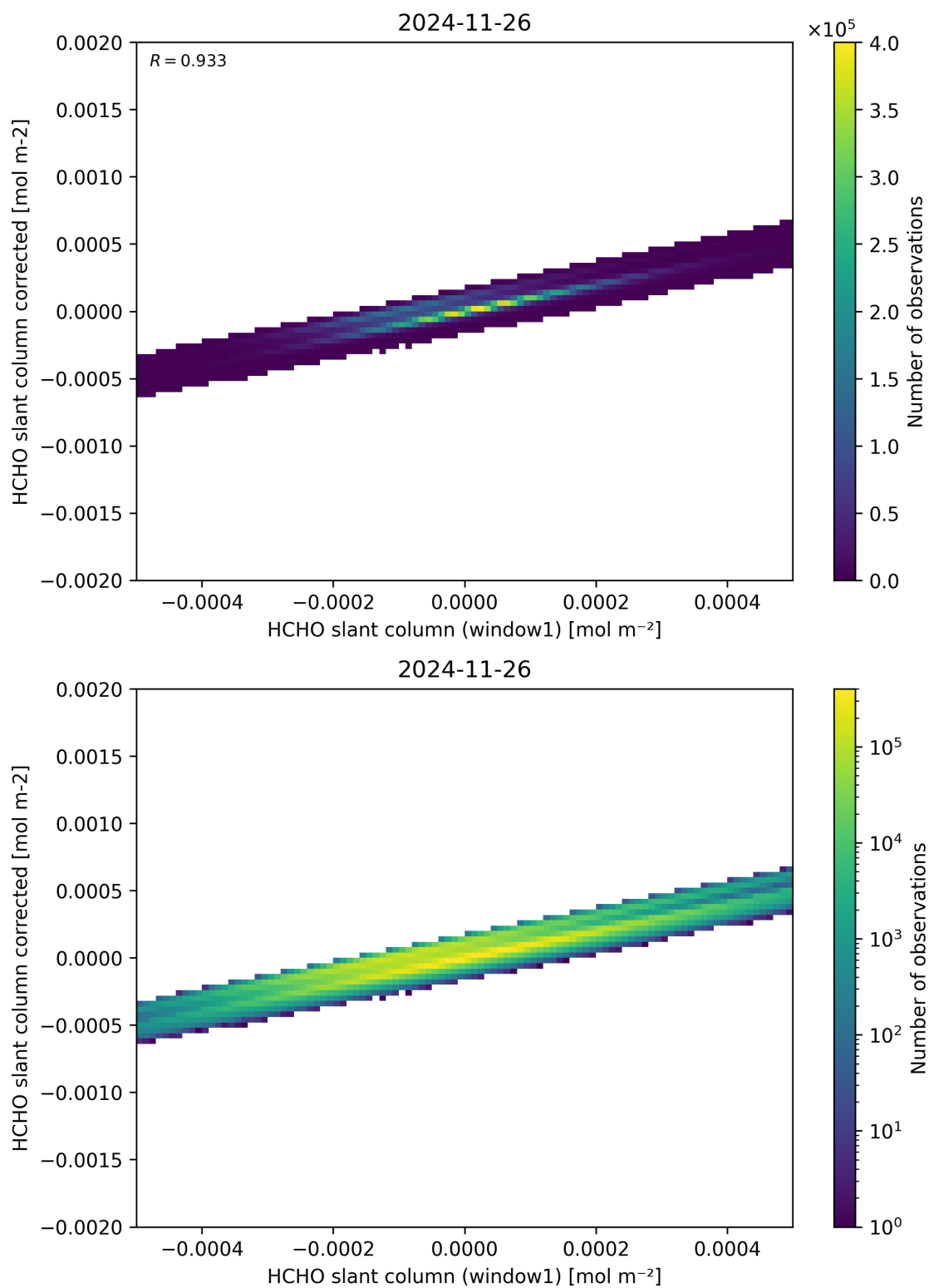
Figure 82: Scatter density plot of “HCHO slant column (window1)” against “HCHO slant column corrected” for 2024-11-25 to 2024-11-27.
