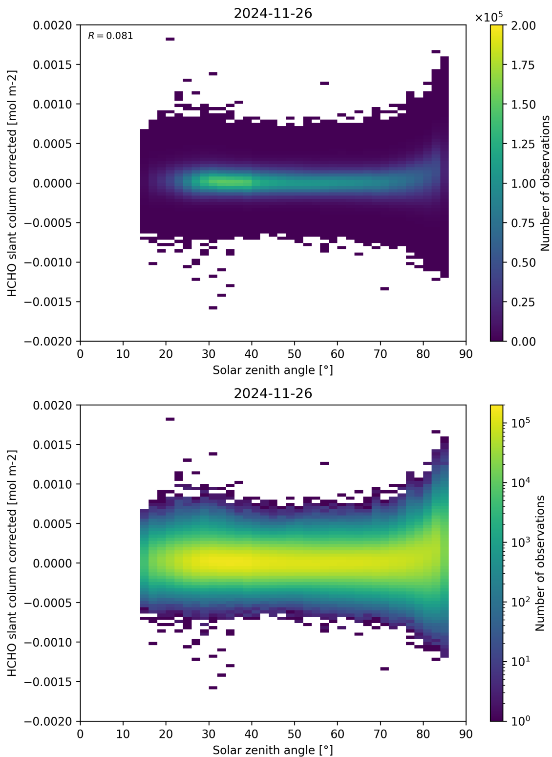
Figure 171: Scatter density plot of “Solar zenith angle” against “HCHO slant column corrected” for 2024-11-25 to 2024-11-27.
