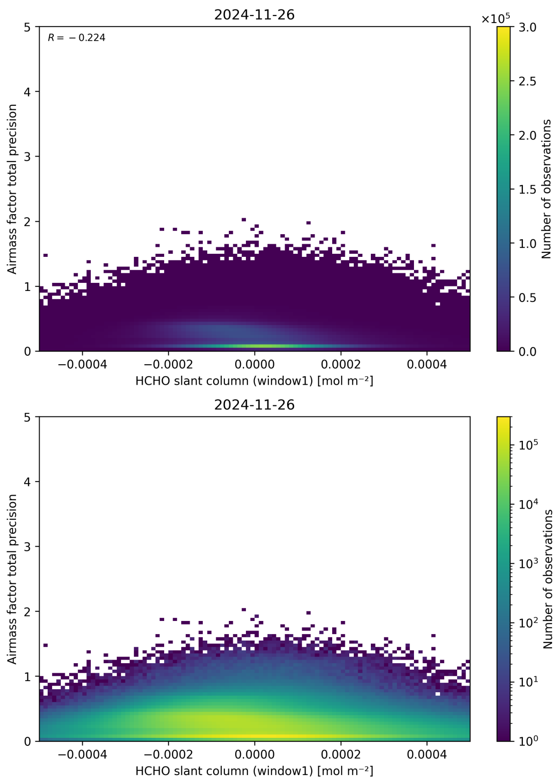
Figure 86: Scatter density plot of “HCHO slant column (window1)” against “Airmass factor total precision” for 2024-11-25 to 2024-11-27.
