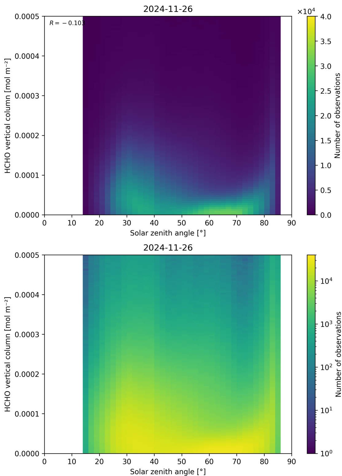
Figure 177: Scatter density plot of “Solar zenith angle” against “HCHO vertical column” for 2024-11-25 to 2024-11-27.
