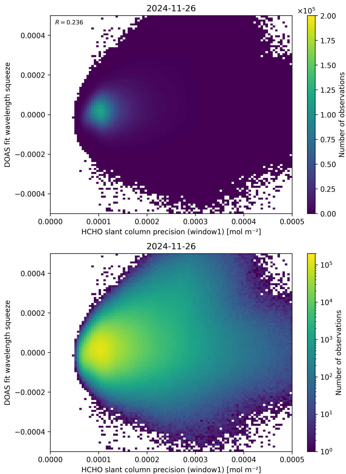
Figure 90: Scatter density plot of “HCHO slant column precision (window1)” against “DOAS fit wavelength squeeze” for 2024-11-25 to 2024-11-27.
