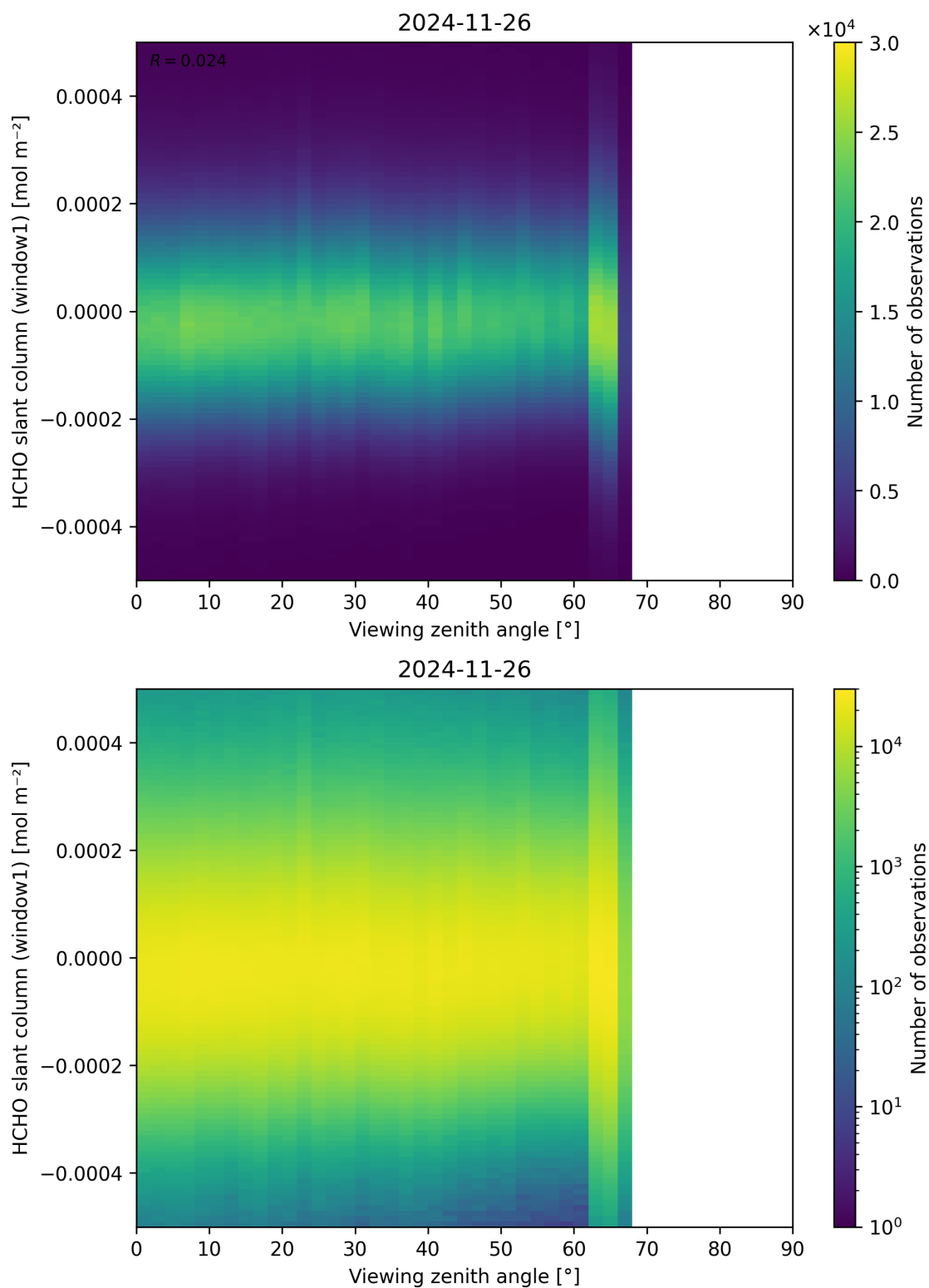
Figure 188: Scatter density plot of “Viewing zenith angle” against “HCHO slant column (window1)” for 2024-11-25 to 2024-11-27.
