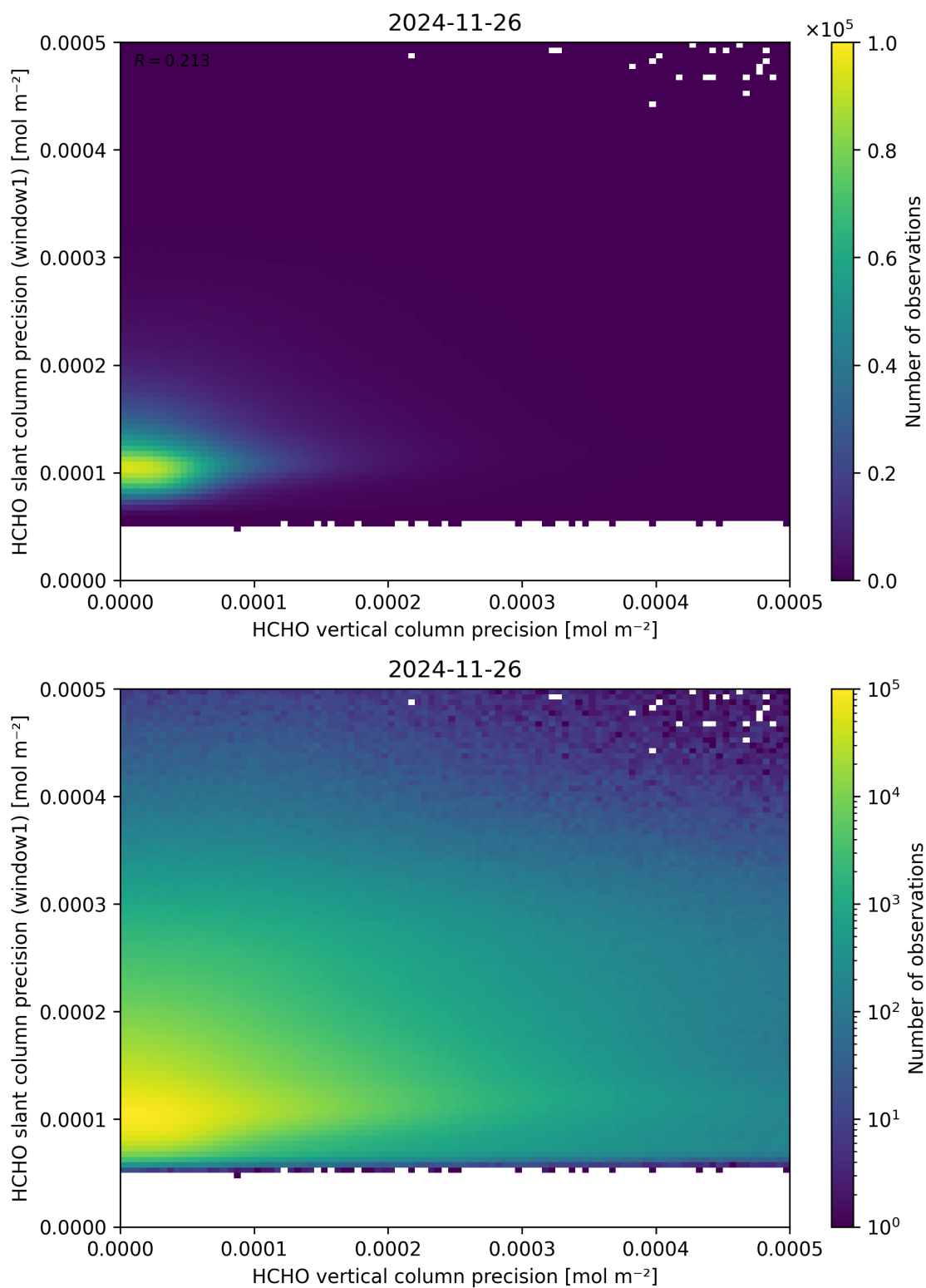
Figure 143: Scatter density plot of “HCHO vertical column precision” against “HCHO slant column precision (window1)” for 2024-11-25 to 2024-11-27.
