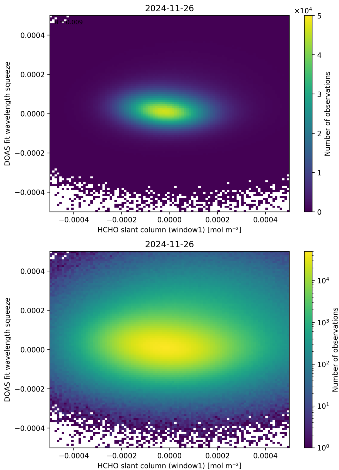
Figure 80: Scatter density plot of “HCHO slant column (window1)” against “DOAS fit wavelength squeeze” for 2024-11-25 to 2024-11-27.
