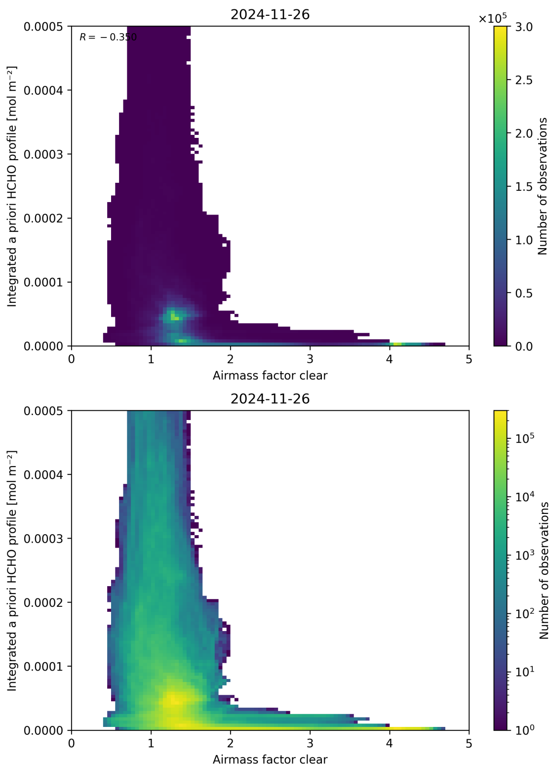
Figure 76: Scatter density plot of “Airmass factor clear” against “Integrated a priori HCHO profile” for 2024-11-25 to 2024-11-27.
