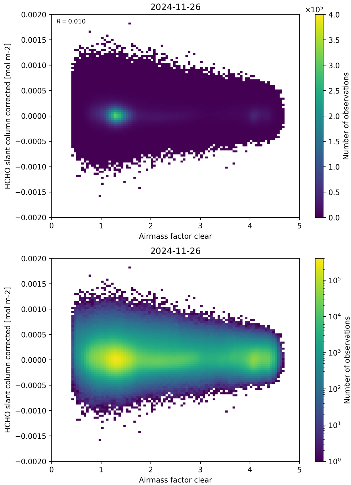
Figure 74: Scatter density plot of “Airmass factor clear” against “HCHO slant column corrected” for 2024-11-25 to 2024-11-27.
