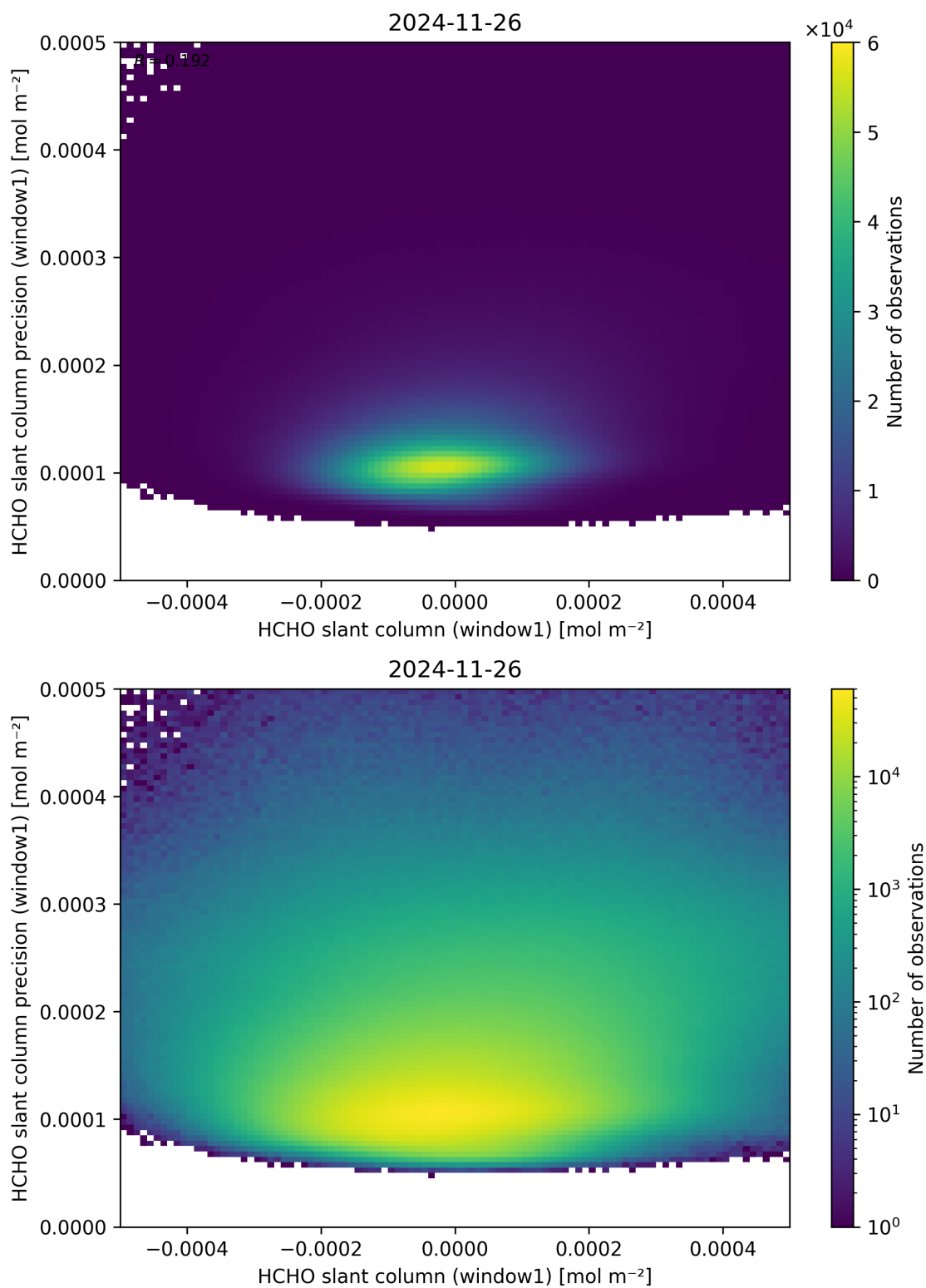
Figure 84: Scatter density plot of “HCHO slant column (window1)” against “HCHO slant column precision (window1)” for 2024-11-25 to 2024-11-27.
