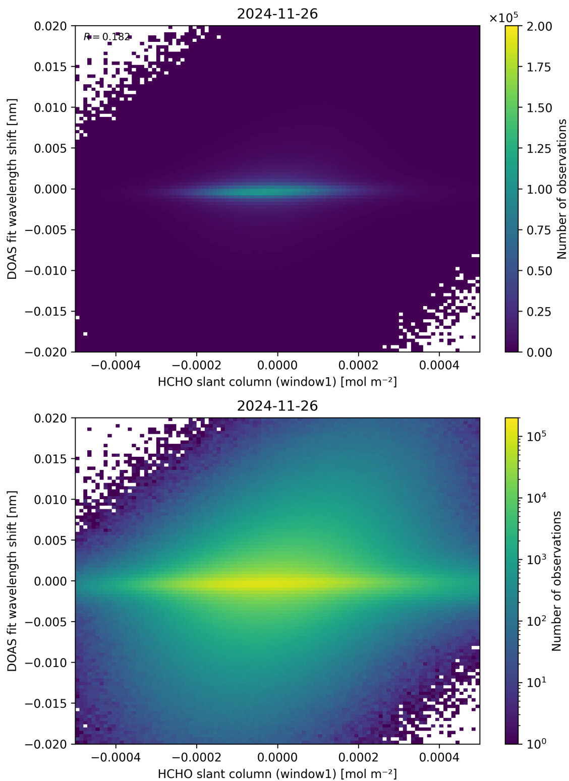
Figure 79: Scatter density plot of “HCHO slant column (window1)” against “DOAS fit wavelength shift” for 2024-11-25 to 2024-11-27.
