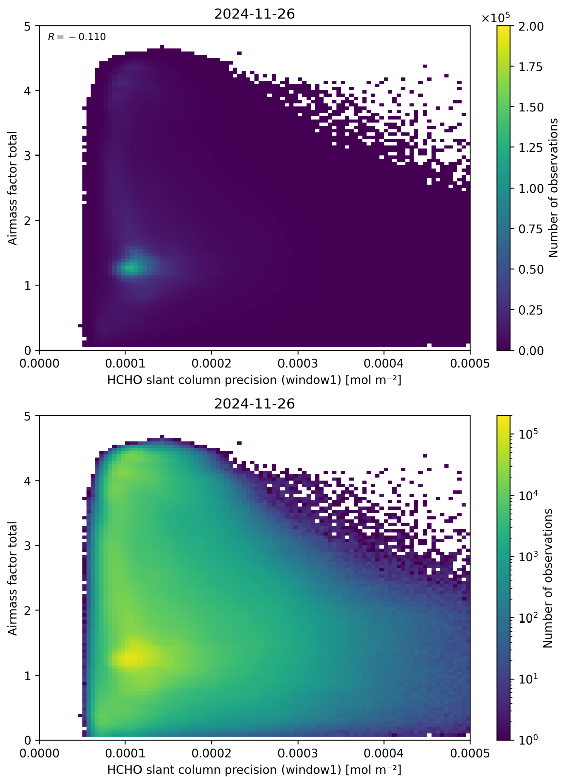
Figure 94: Scatter density plot of “HCHO slant column precision (window1)” against “Airmass factor total” for 2024-11-25 to 2024-11-27.
