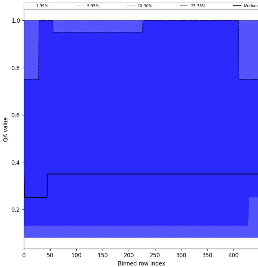
Figure 48: Along track statistics of “QA value” for 2024-11-25 to 2024-11-27
