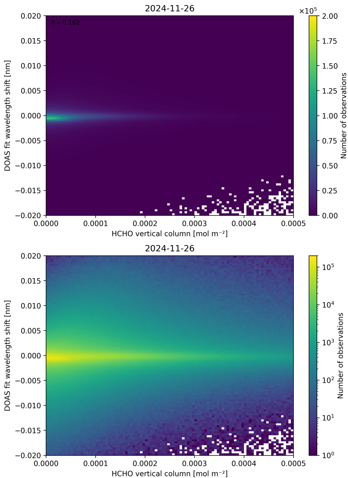
Figure 124: Scatter density plot of “HCHO vertical column” against “DOAS fit wavelength shift” for 2024-11-25 to 2024-11-27.
