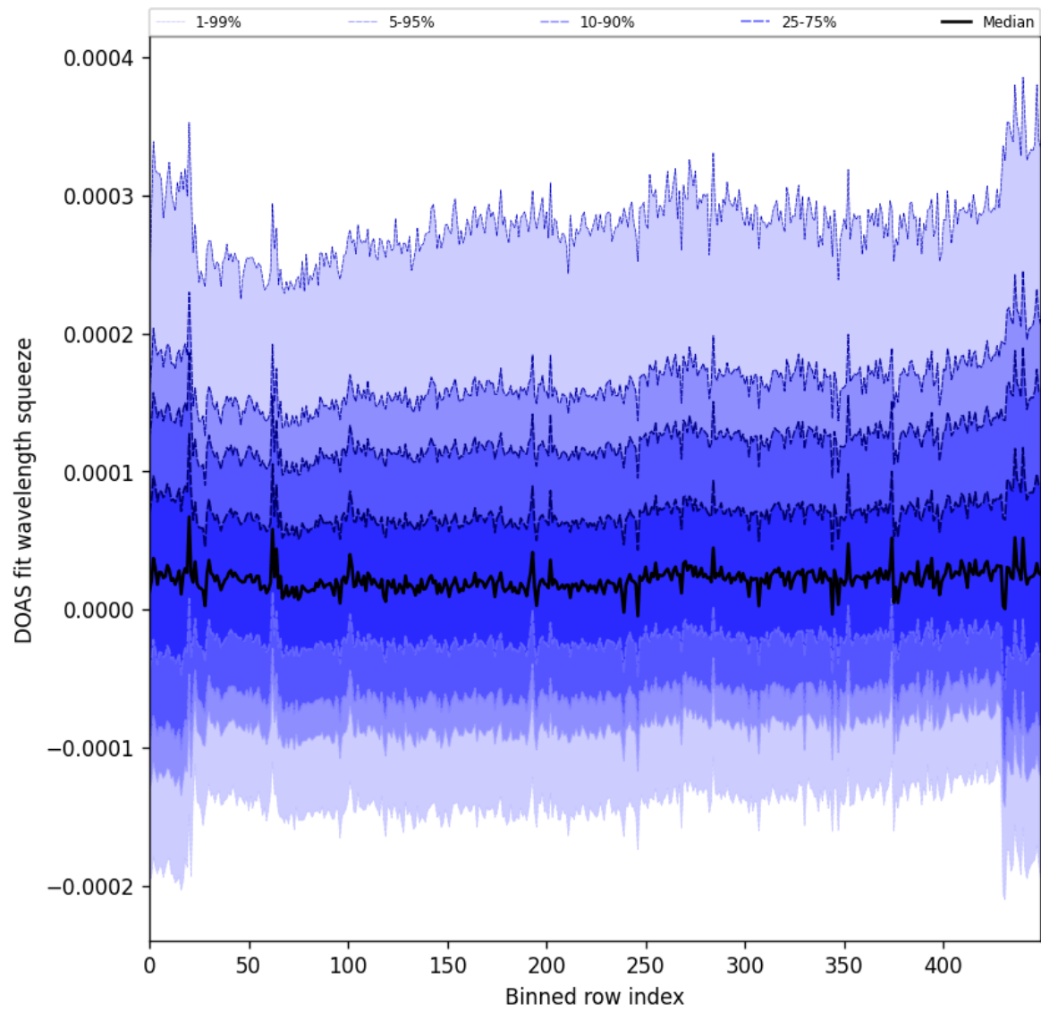
Figure 59: Along track statistics of “DOAS fit wavelength squeeze” for 2024-11-25 to 2024-11-27
