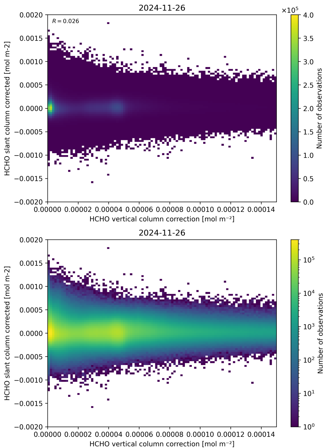
Figure 116: Scatter density plot of “HCHO vertical column correction” against “HCHO slant column corrected” for 2024-11-25 to 2024-11-27.
