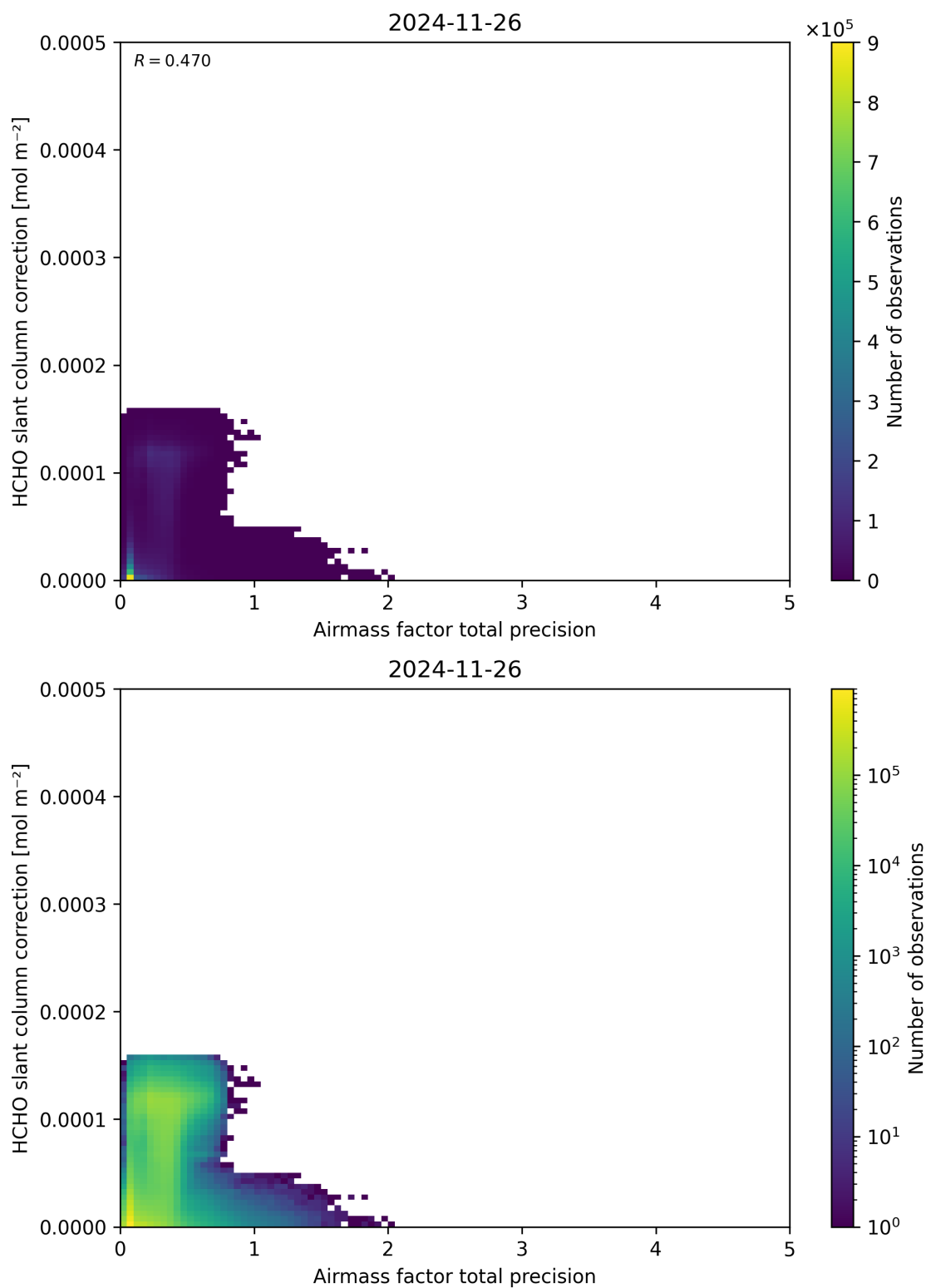
Figure 110: Scatter density plot of “Airmass factor total precision” against “HCHO slant column correction” for 2024-11-25 to 2024-11-27.
