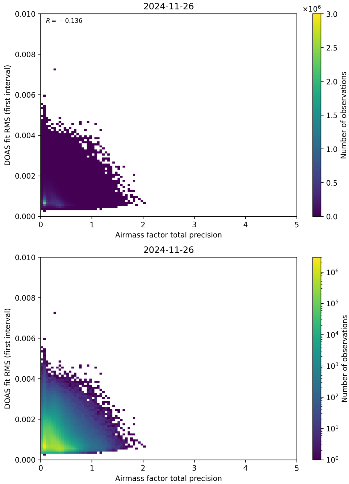
Figure 105: Scatter density plot of “Airmass factor total precision” against “DOAS fit RMS (first interval)” for 2024-11-25 to 2024-11-27.
