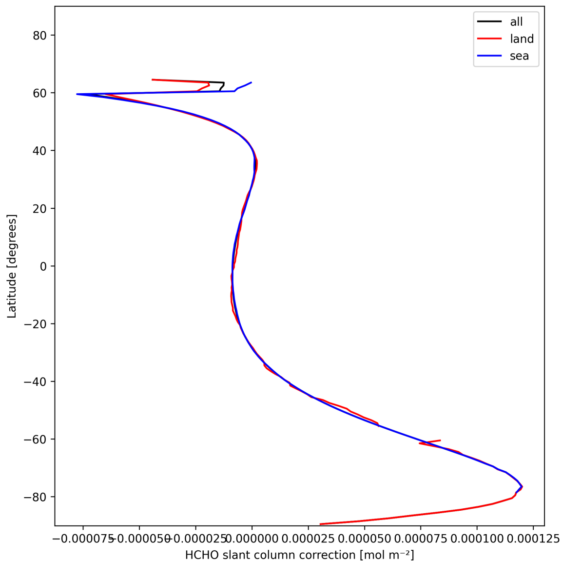
Figure 33: Zonal average of “HCHO slant column correction” for 2024-11-25 to 2024-11-27.
