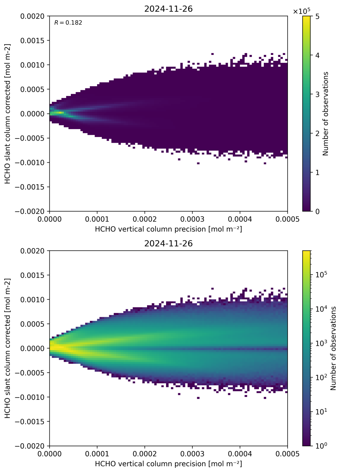
Figure 140: Scatter density plot of “HCHO vertical column precision” against “HCHO slant column corrected” for 2024-11-25 to 2024-11-27.
