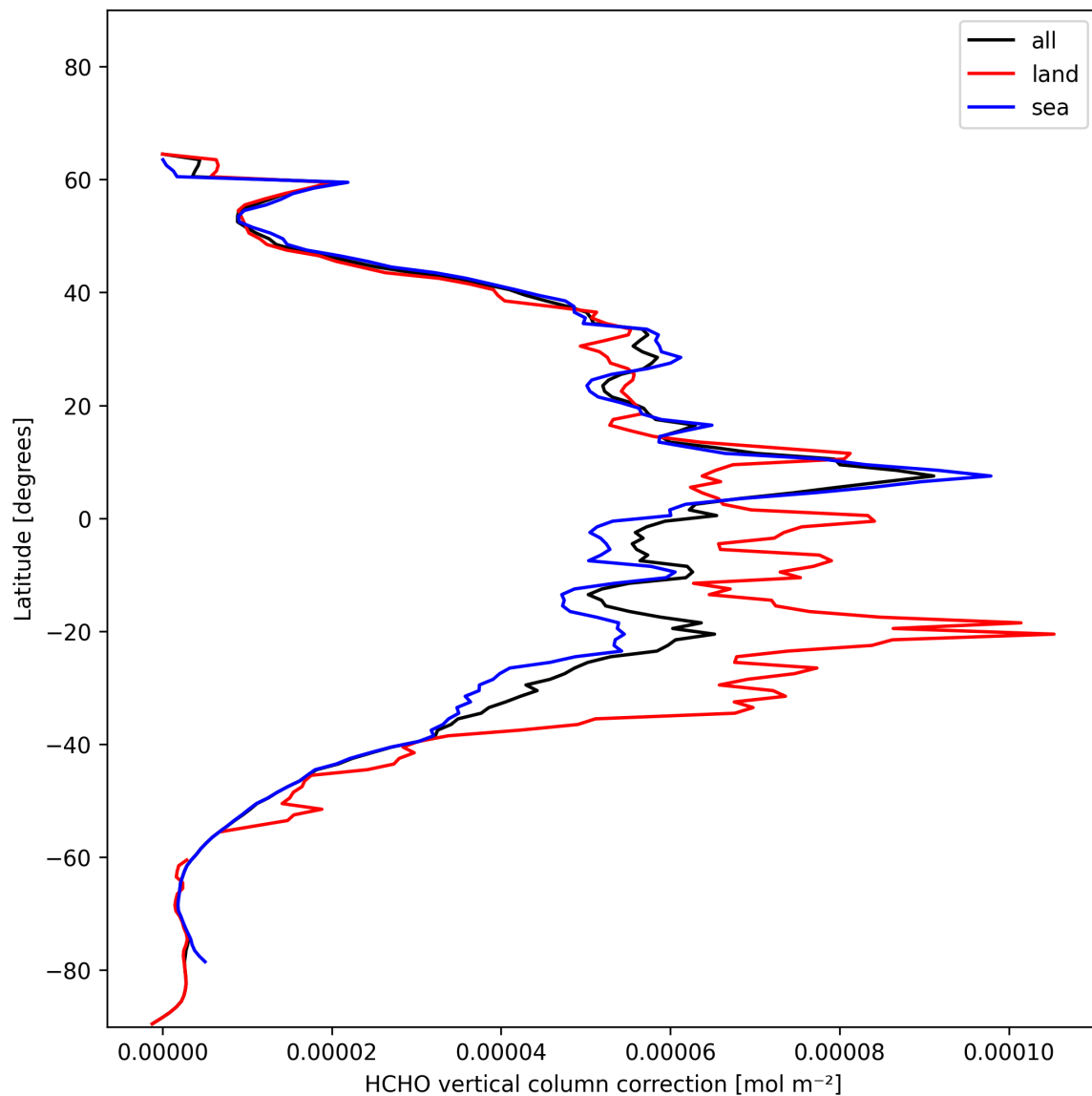
Figure 23: Zonal average of “HCHO vertical column correction” for 2024-11-25 to 2024-11-27.
