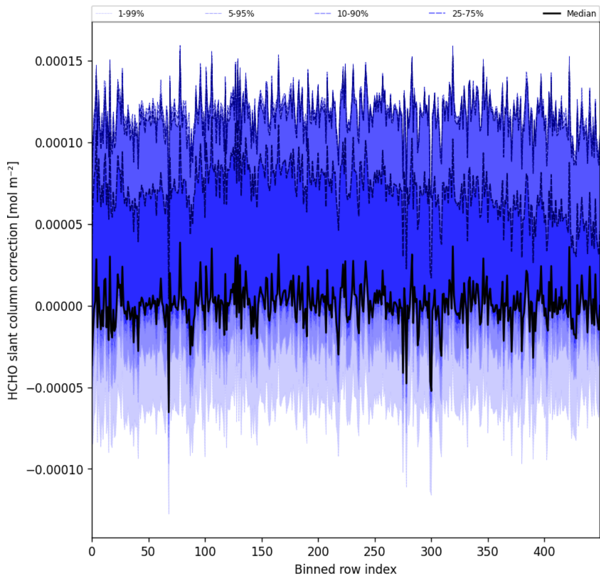
Figure 61: Along track statistics of “HCHO slant column correction” for 2024-11-25 to 2024-11-27
