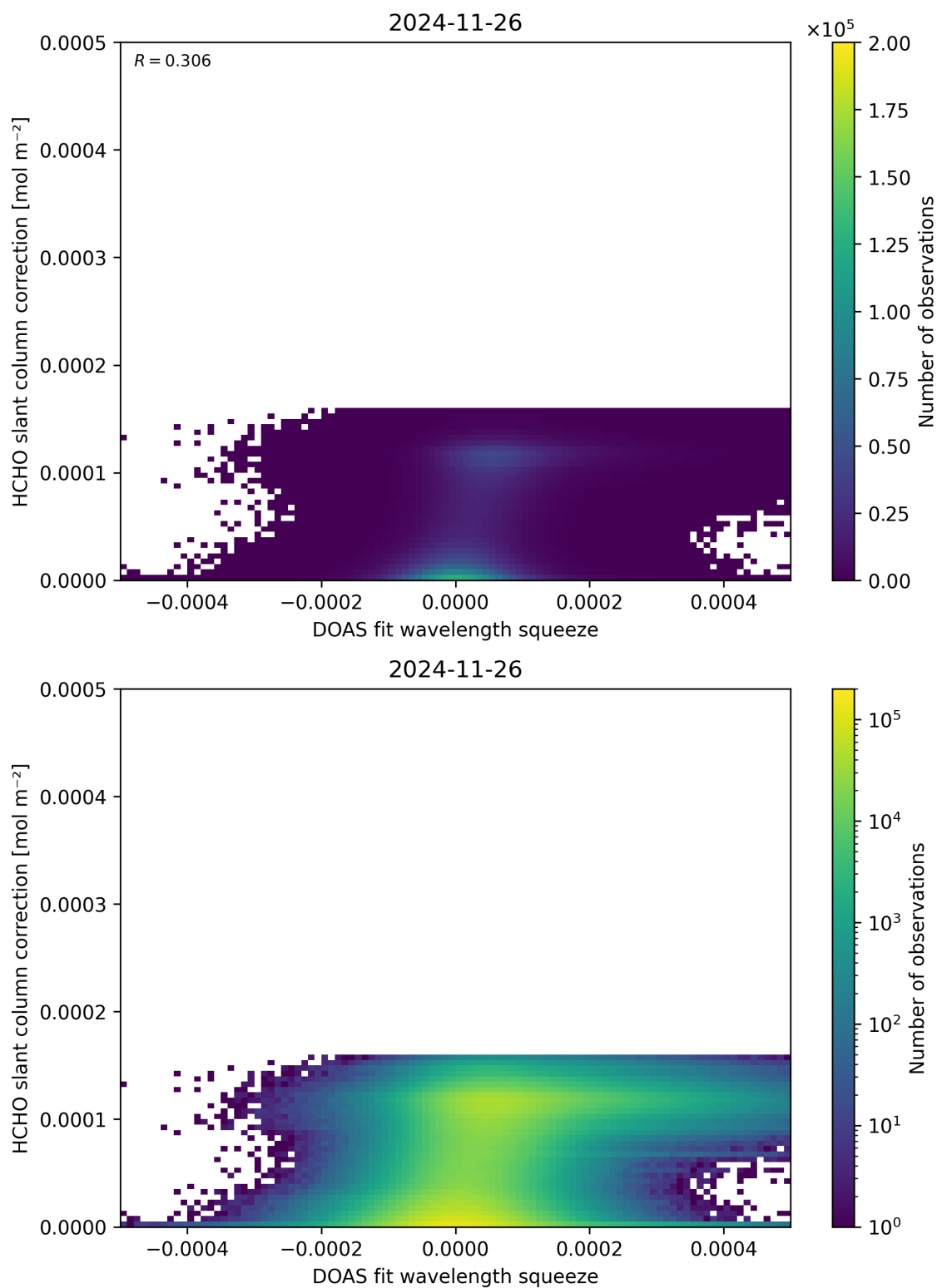
Figure 70: Scatter density plot of “DOAS fit wavelength squeeze” against “HCHO slant column correction” for 2024-11-25 to 2024-11-27.
