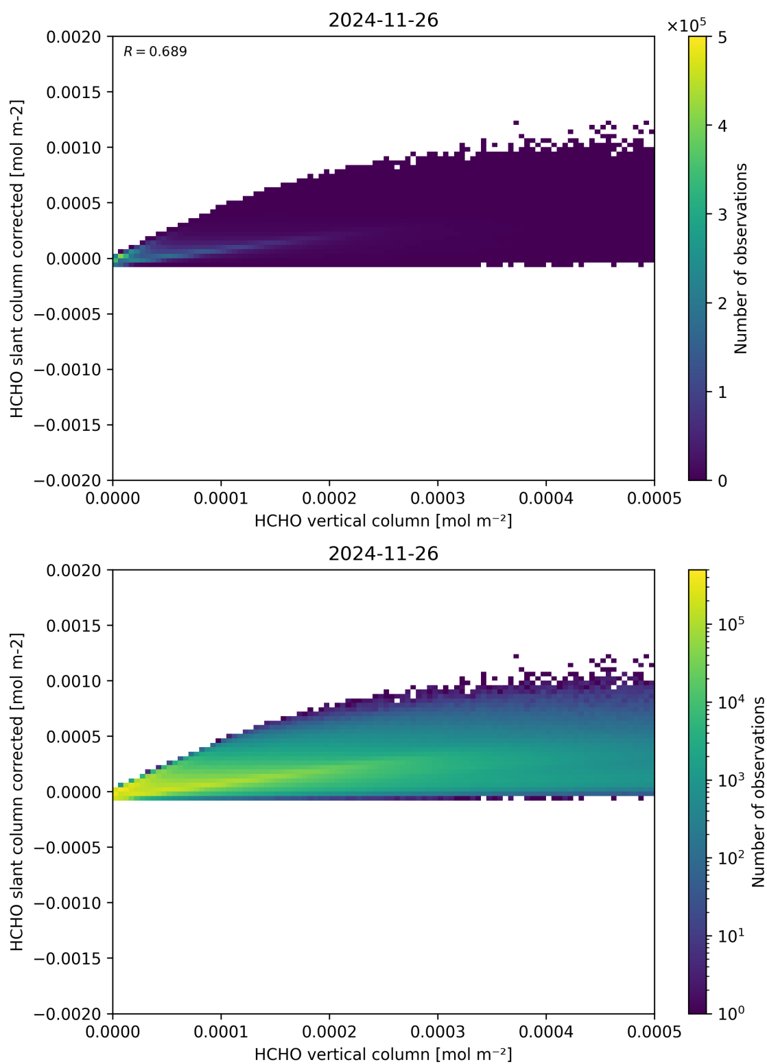
Figure 127: Scatter density plot of “HCHO vertical column” against “HCHO slant column corrected” for 2024-11-25 to 2024-11-27.
