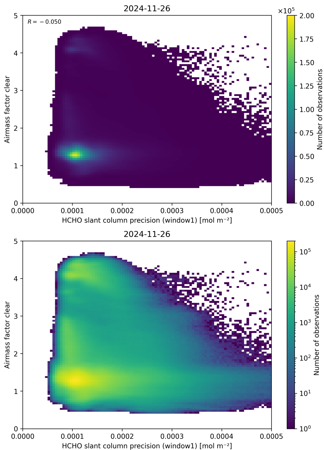
Figure 91: Scatter density plot of “HCHO slant column precision (window1)” against “Airmass factor clear” for 2024-11-25 to 2024-11-27.
