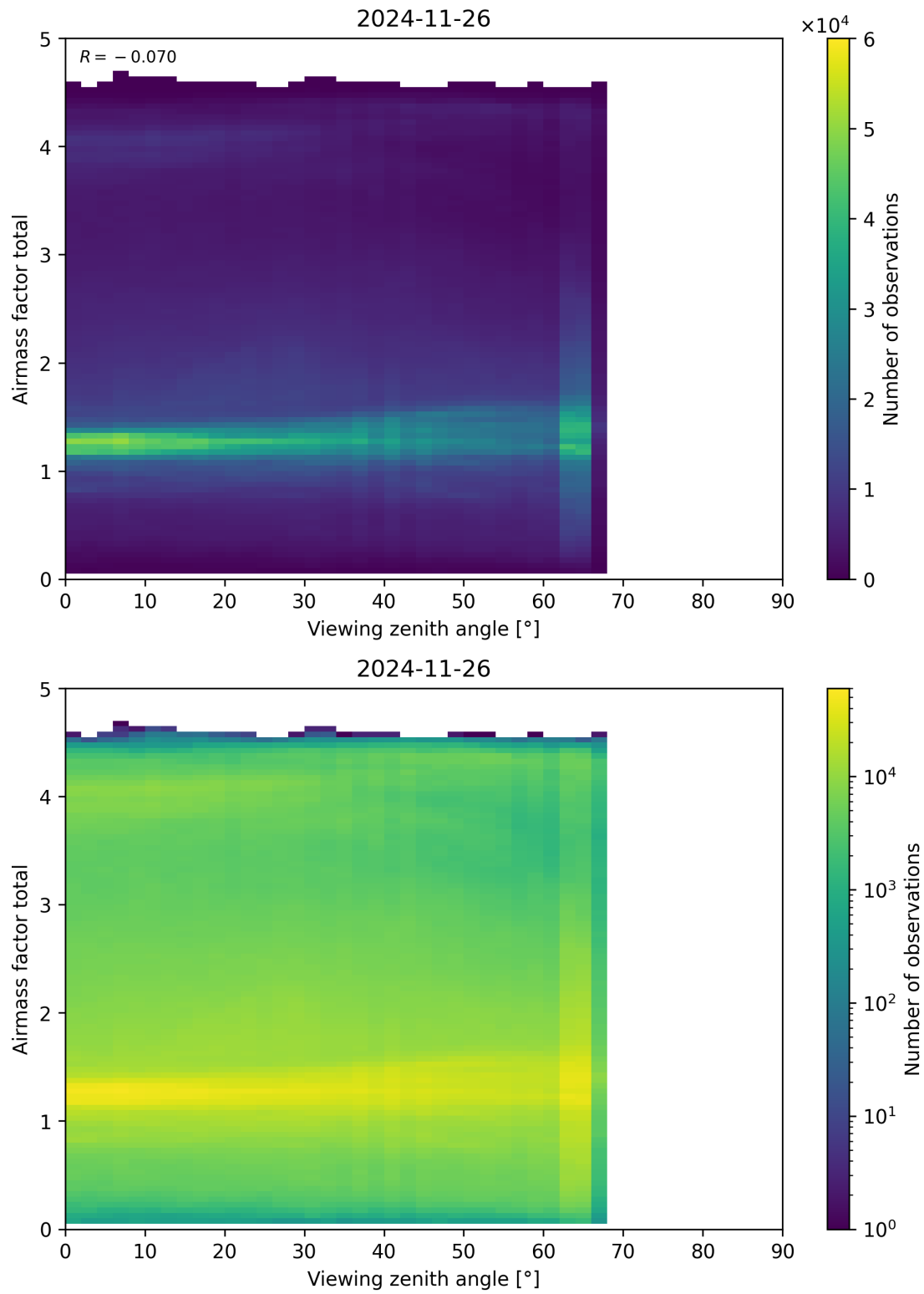
Figure 190: Scatter density plot of “Viewing zenith angle” against “Airmass factor total” for 2024-11-25 to 2024-11-27.
