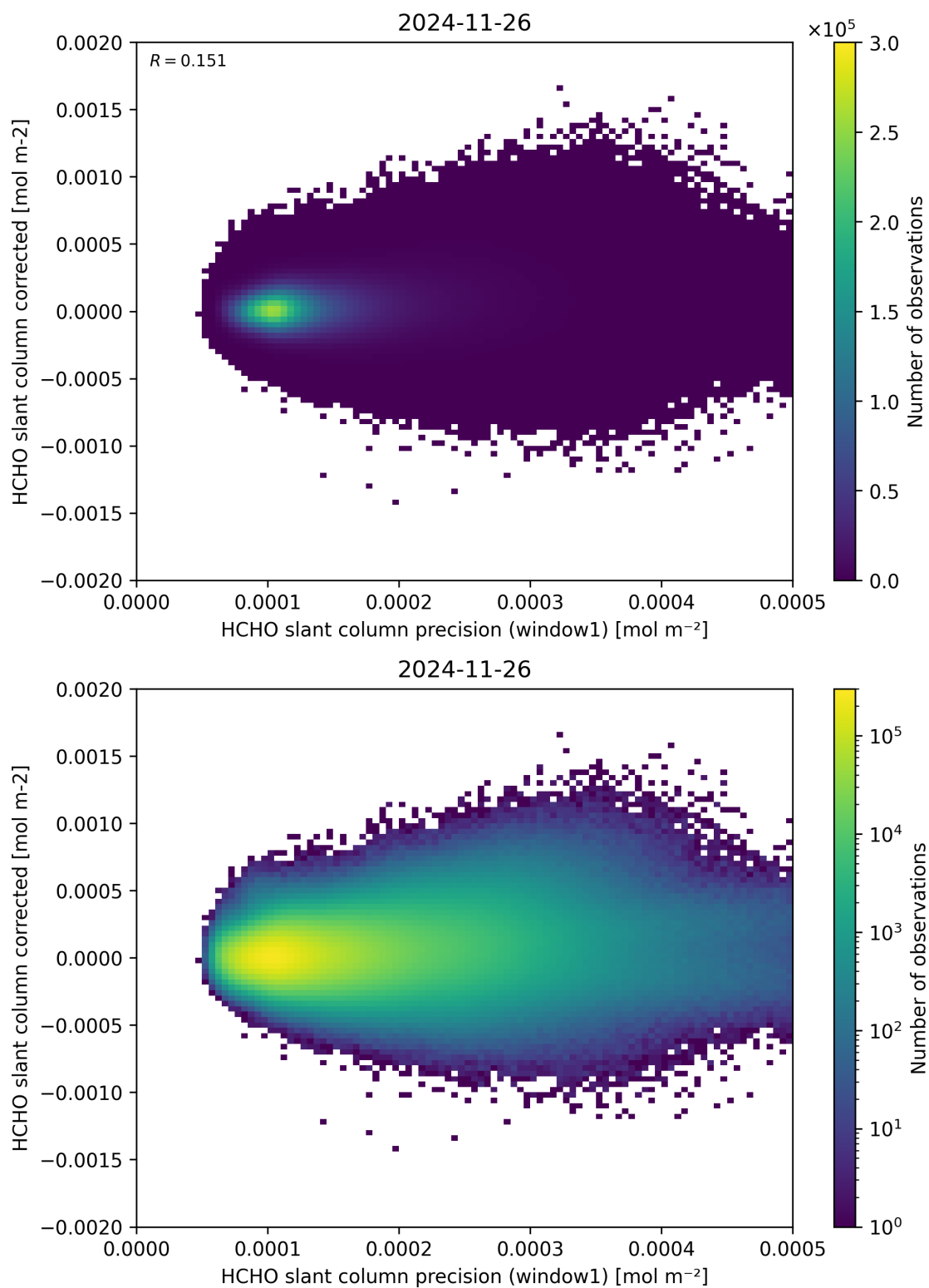
Figure 92: Scatter density plot of “HCHO slant column precision (window1)” against “HCHO slant column corrected” for 2024-11-25 to 2024-11-27.
