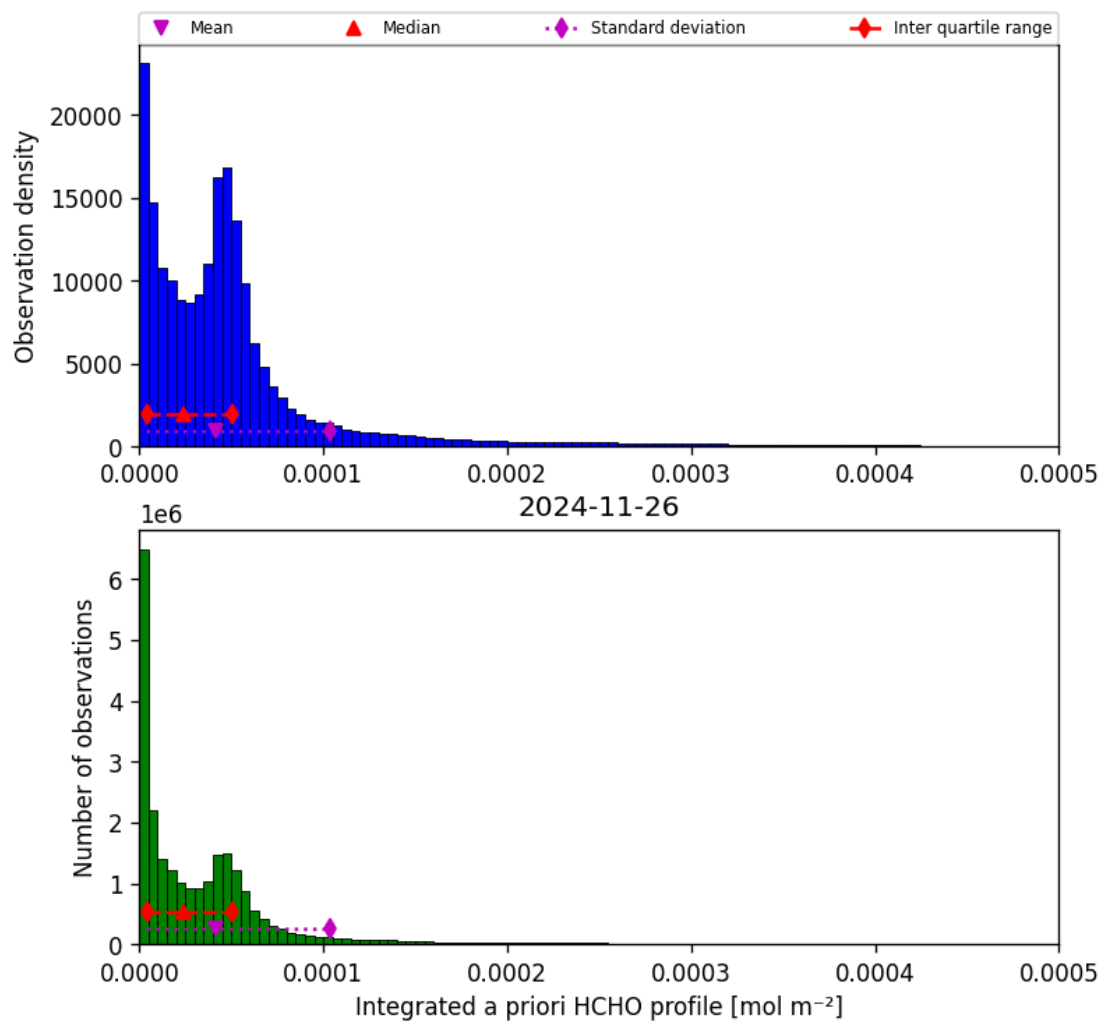
Figure 43: Histogram of “Integrated a priori HCHO profile” for 2024-11-25 to 2024-11-27
