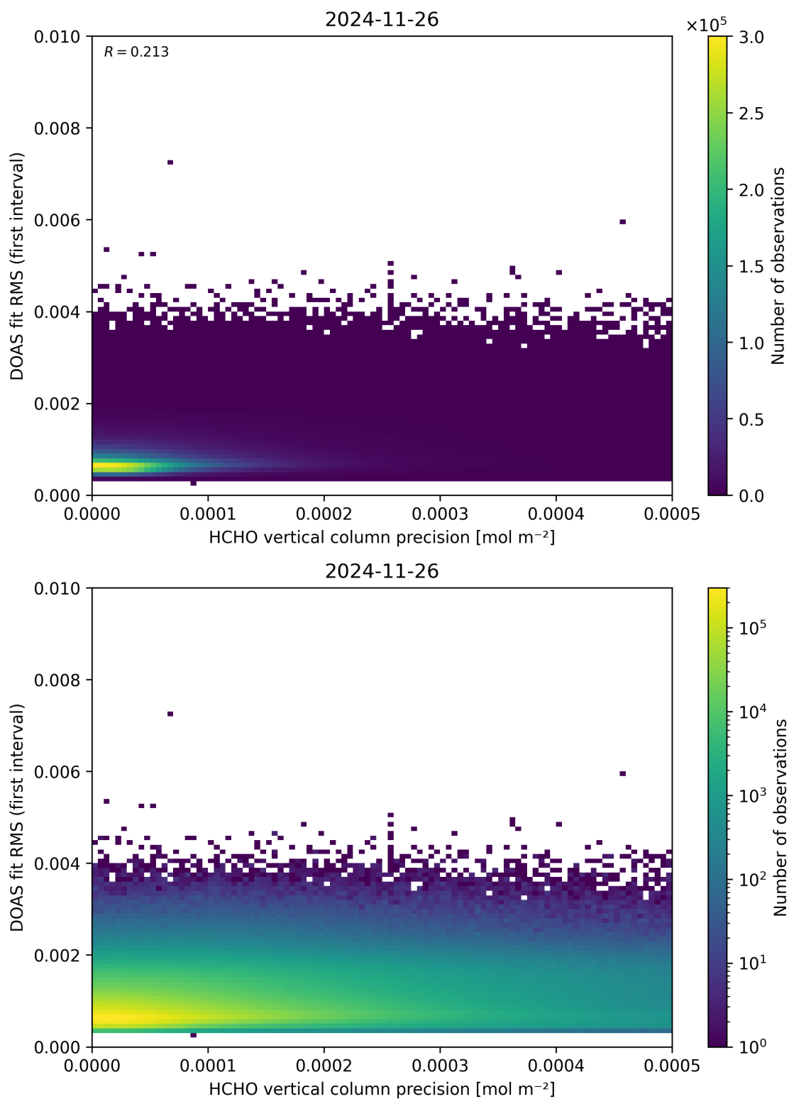
Figure 136: Scatter density plot of “HCHO vertical column precision” against “DOAS fit RMS (first interval)” for 2024-11-25 to 2024-11-27.
