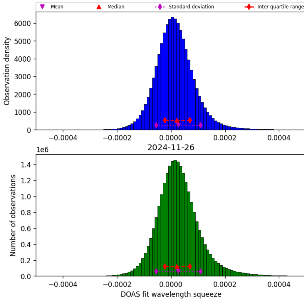
Figure 45: Histogram of “DOAS fit wavelength squeeze” for 2024-11-25 to 2024-11-27
