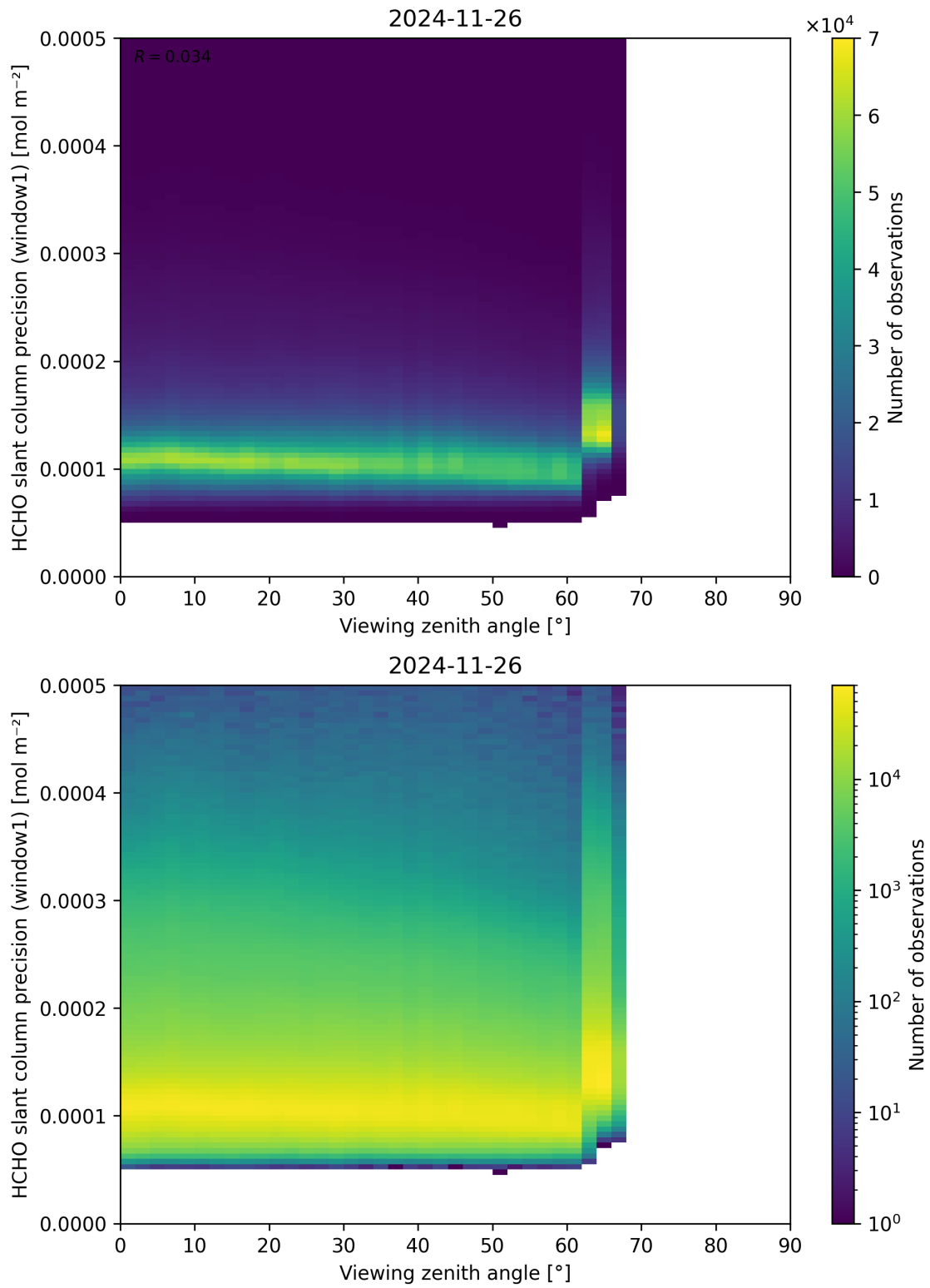
Figure 189: Scatter density plot of “Viewing zenith angle” against “HCHO slant column precision (window1)” for 2024-11-25 to 2024-11-27.
