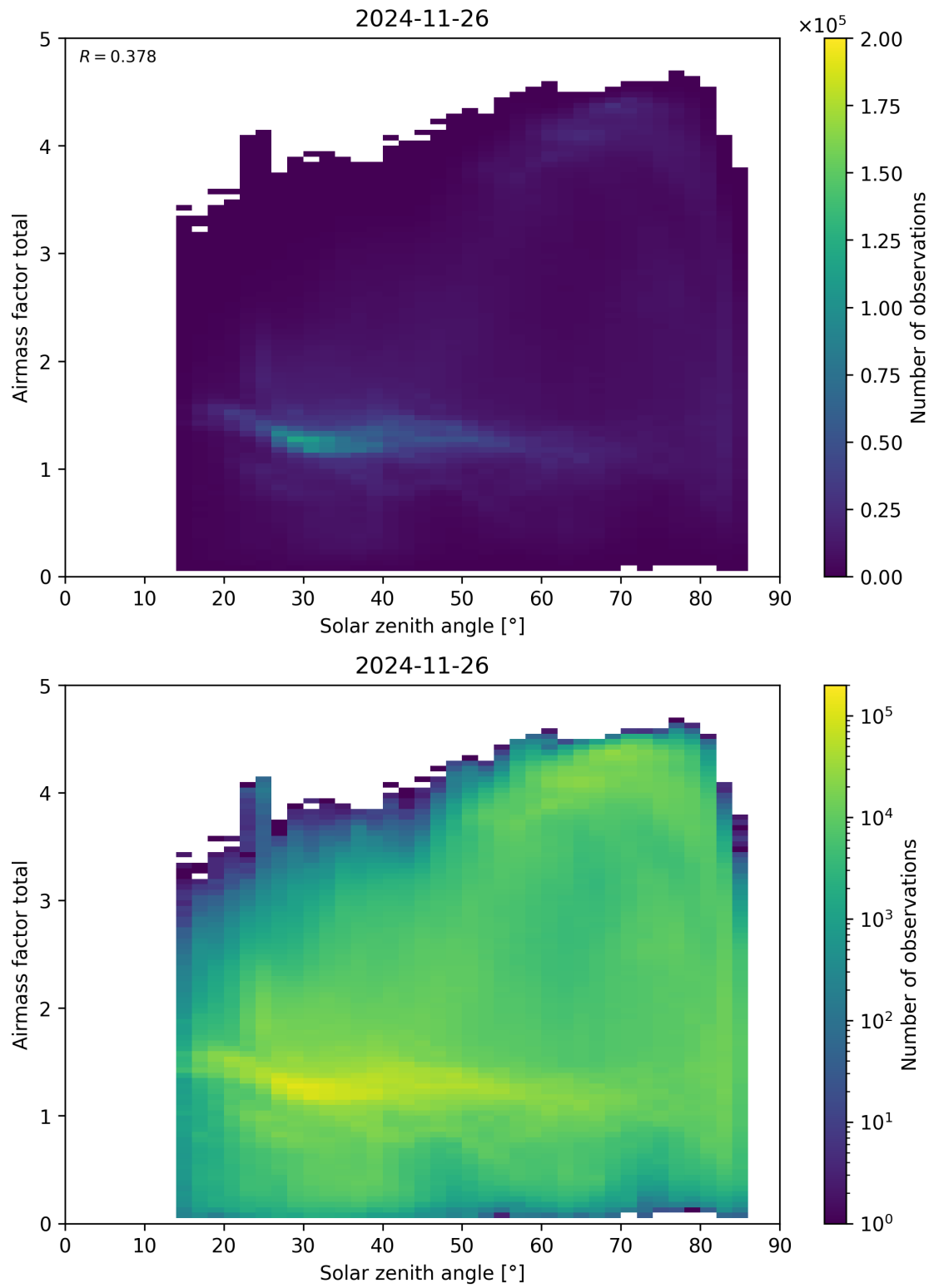
Figure 175: Scatter density plot of “Solar zenith angle” against “Airmass factor total” for 2024-11-25 to 2024-11-27.
