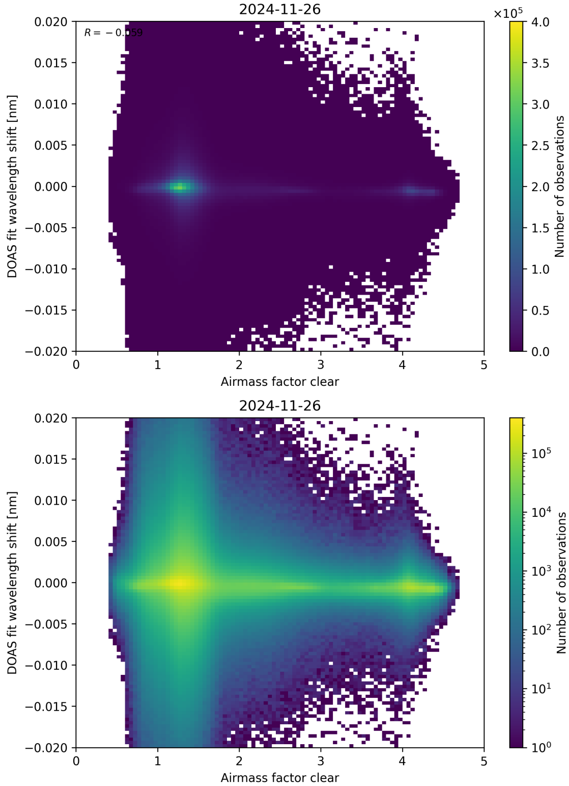
Figure 72: Scatter density plot of “Airmass factor clear” against “DOAS fit wavelength shift” for 2024-11-25 to 2024-11-27.
