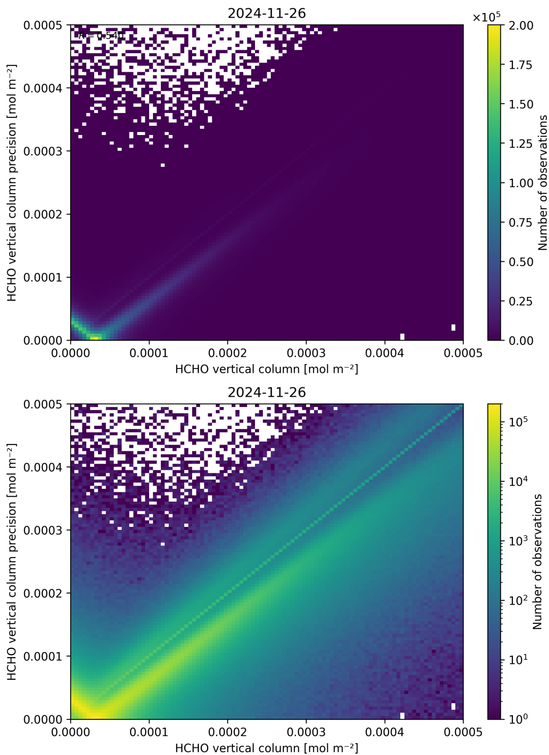
Figure 134: Scatter density plot of “HCHO vertical column” against “HCHO vertical column precision” for 2024-11-25 to 2024-11-27.
