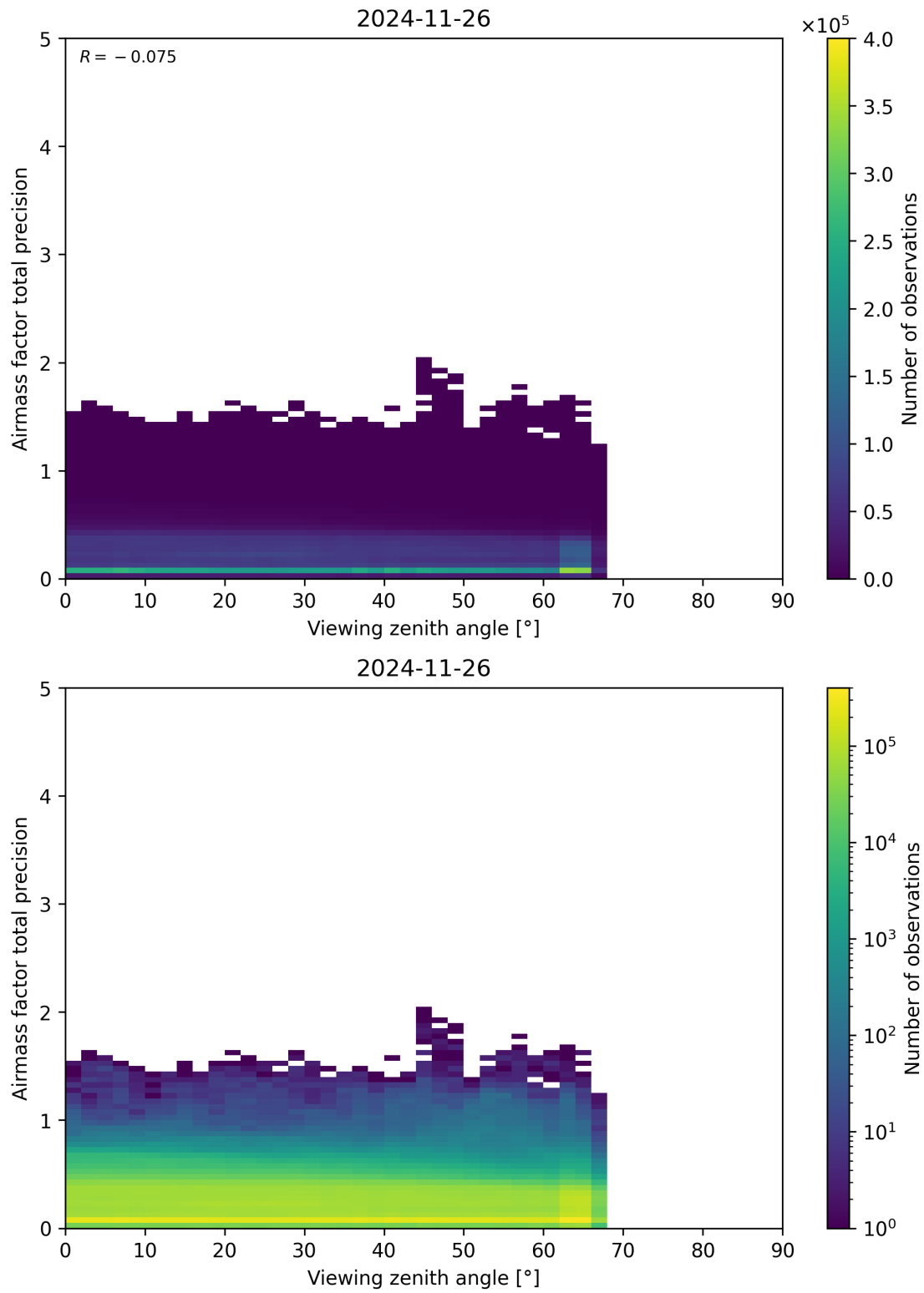
Figure 191: Scatter density plot of “Viewing zenith angle” against “Airmass factor total precision” for 2024-11-25 to 2024-11-27.
