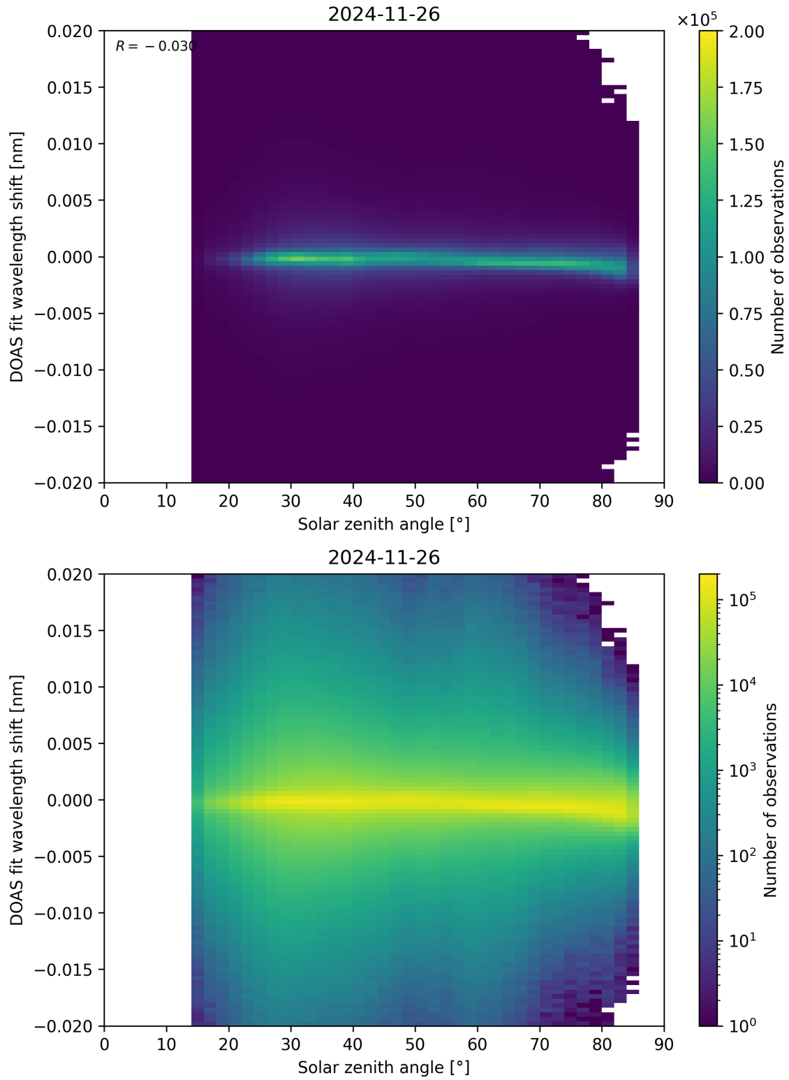
Figure 168: Scatter density plot of “Solar zenith angle” against “DOAS fit wavelength shift” for 2024-11-25 to 2024-11-27.
