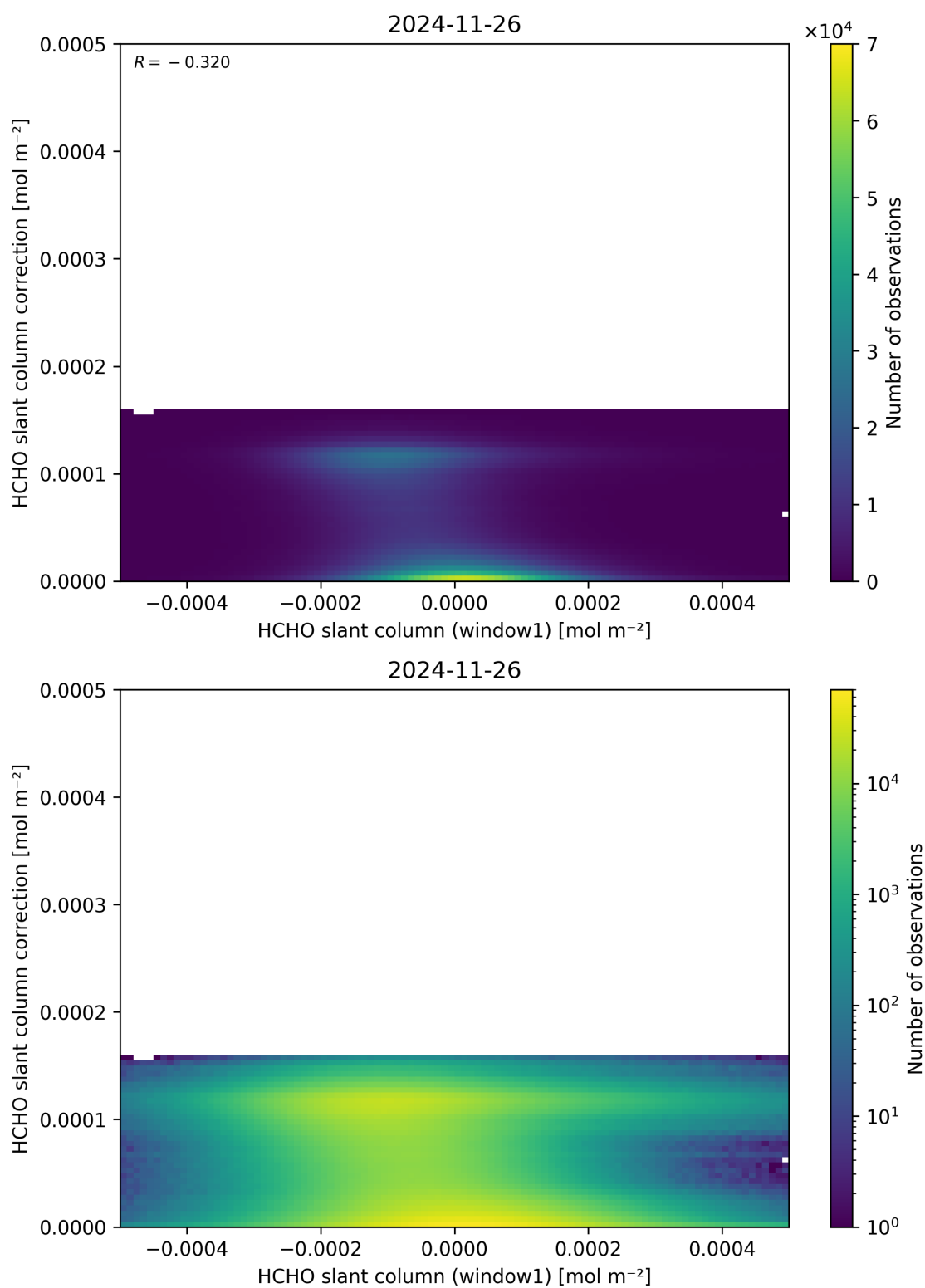
Figure 83: Scatter density plot of “HCHO slant column (window1)” against “HCHO slant column correction” for 2024-11-25 to 2024-11-27.
