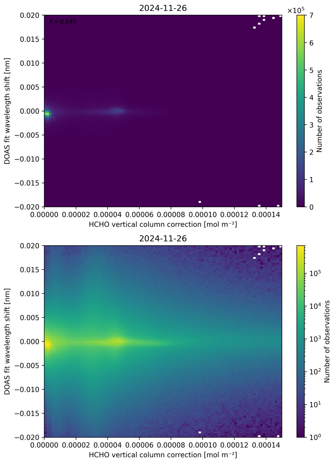
Figure 113: Scatter density plot of “HCHO vertical column correction” against “DOAS fit wavelength shift” for 2024-11-25 to 2024-11-27.
