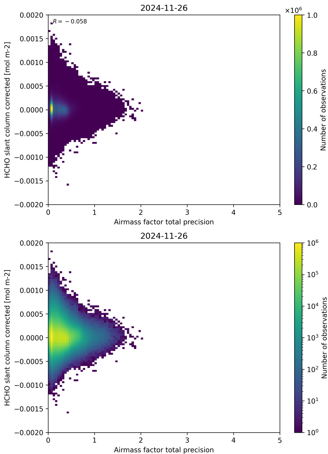
Figure 109: Scatter density plot of “Airmass factor total precision” against “HCHO slant column corrected” for 2024-11-25 to 2024-11-27.
