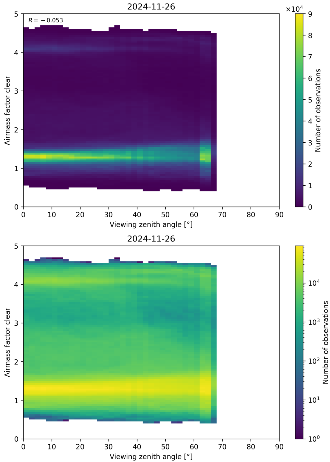
Figure 185: Scatter density plot of “Viewing zenith angle” against “Airmass factor clear” for 2024-11-25 to 2024-11-27.
