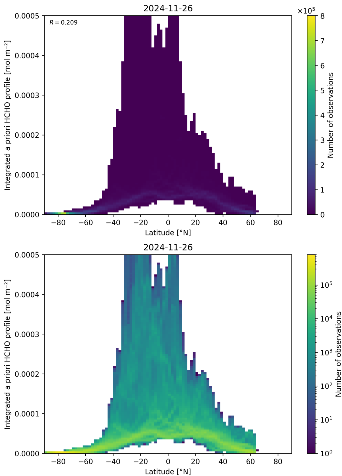
Figure 166: Scatter density plot of “Latitude” against “Integrated a priori HCHO profile” for 2024-11-25 to 2024-11-27.
