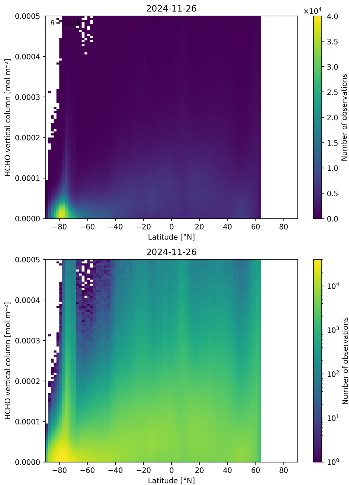
Figure 163: Scatter density plot of “Latitude” against “HCHO vertical column” for 2024-11-25 to 2024-11-27.
