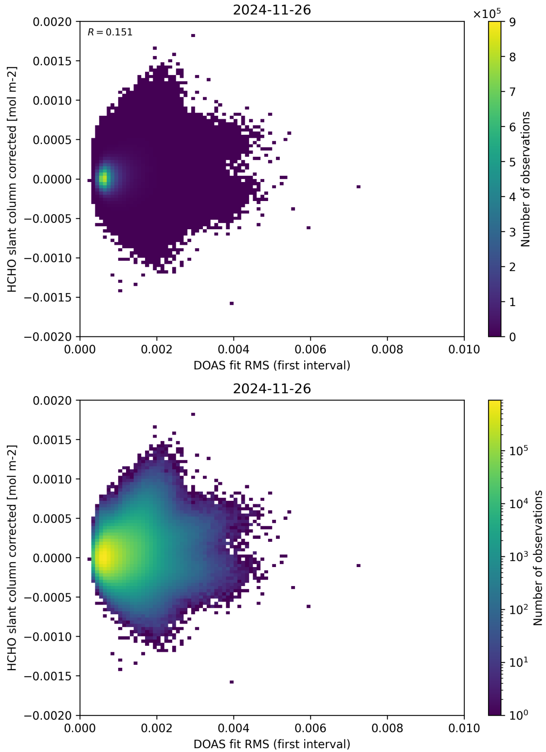
Figure 62: Scatter density plot of “DOAS fit RMS (first interval)” against “HCHO slant column corrected” for 2024-11-25 to 2024-11-27.
