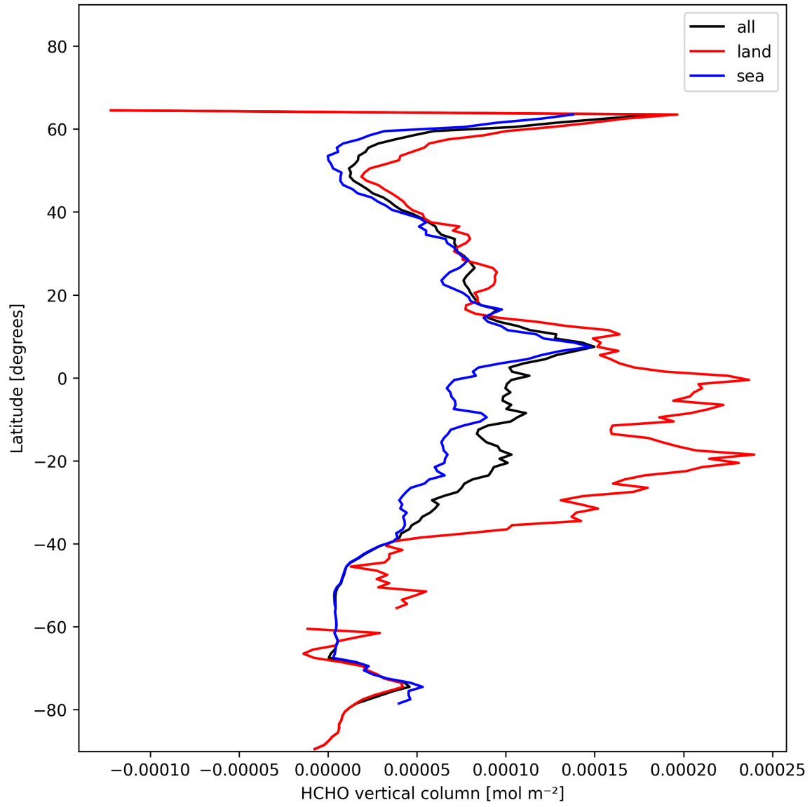
Figure 21: Zonal average of “HCHO vertical column” for 2024-11-25 to 2024-11-27.
