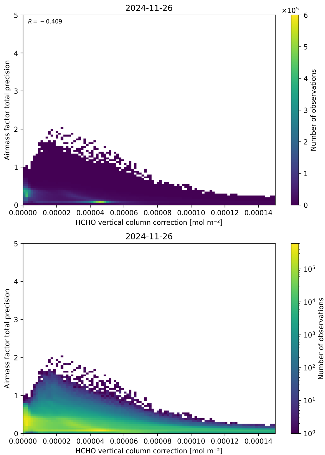
Figure 121: Scatter density plot of “HCHO vertical column correction” against “Airmass factor total precision” for 2024-11-25 to 2024-11-27.
