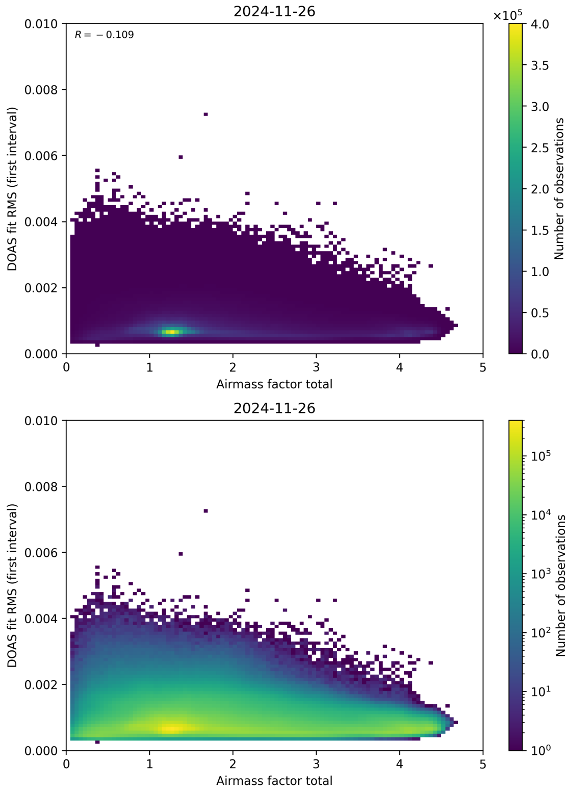
Figure 97: Scatter density plot of “Airmass factor total” against “DOAS fit RMS (first interval)” for 2024-11-25 to 2024-11-27.
