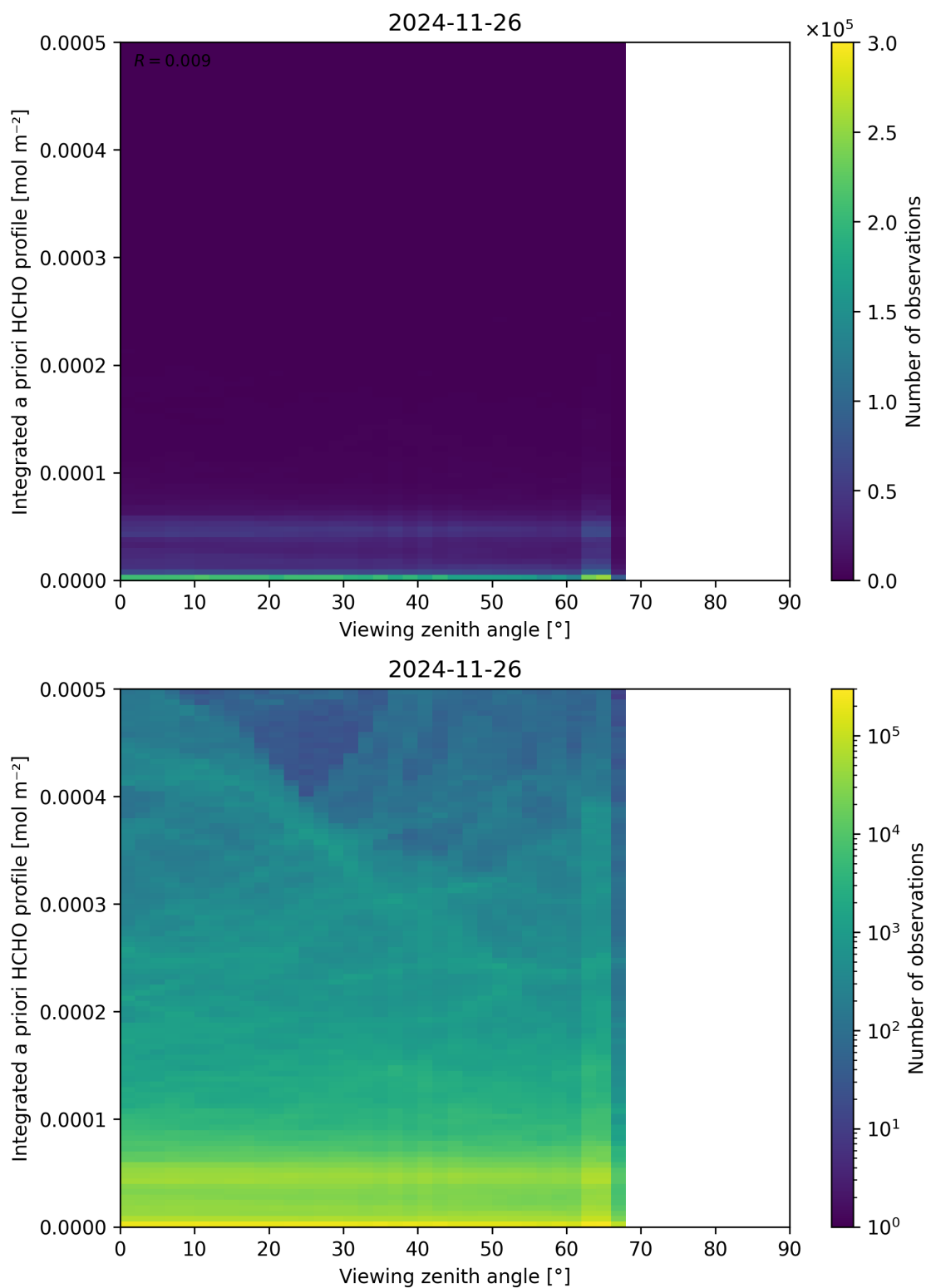
Figure 195: Scatter density plot of “Viewing zenith angle” against “Integrated a priori HCHO profile” for 2024-11-25 to 2024-11-27.
