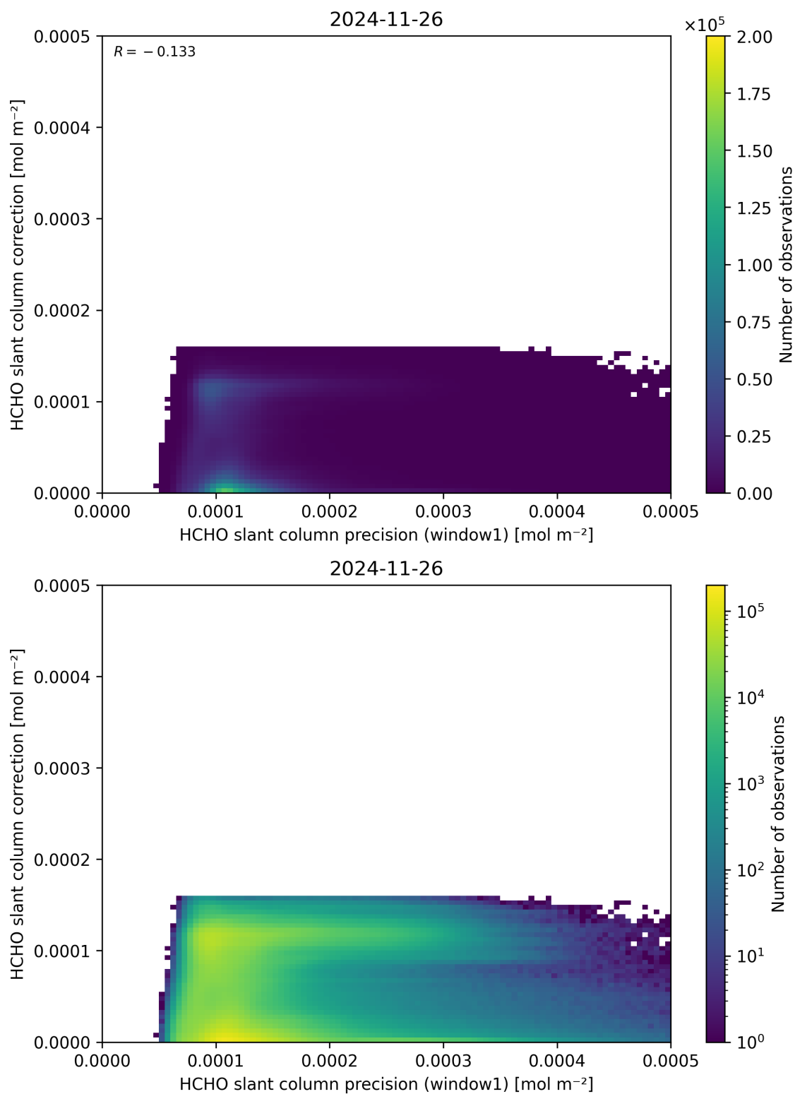
Figure 93: Scatter density plot of “HCHO slant column precision (window1)” against “HCHO slant column correction” for 2024-11-25 to 2024-11-27.
