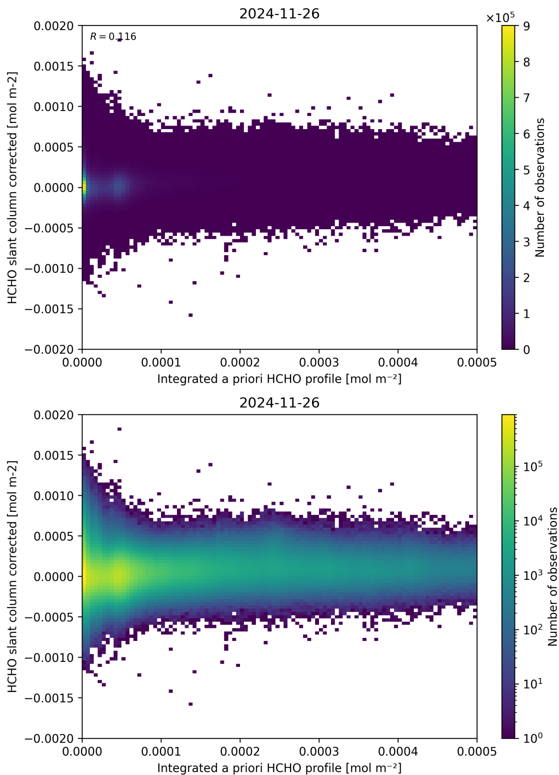
Figure 151: Scatter density plot of “Integrated a priori HCHO profile” against “HCHO slant column corrected” for 2024-11-25 to 2024-11-27.
