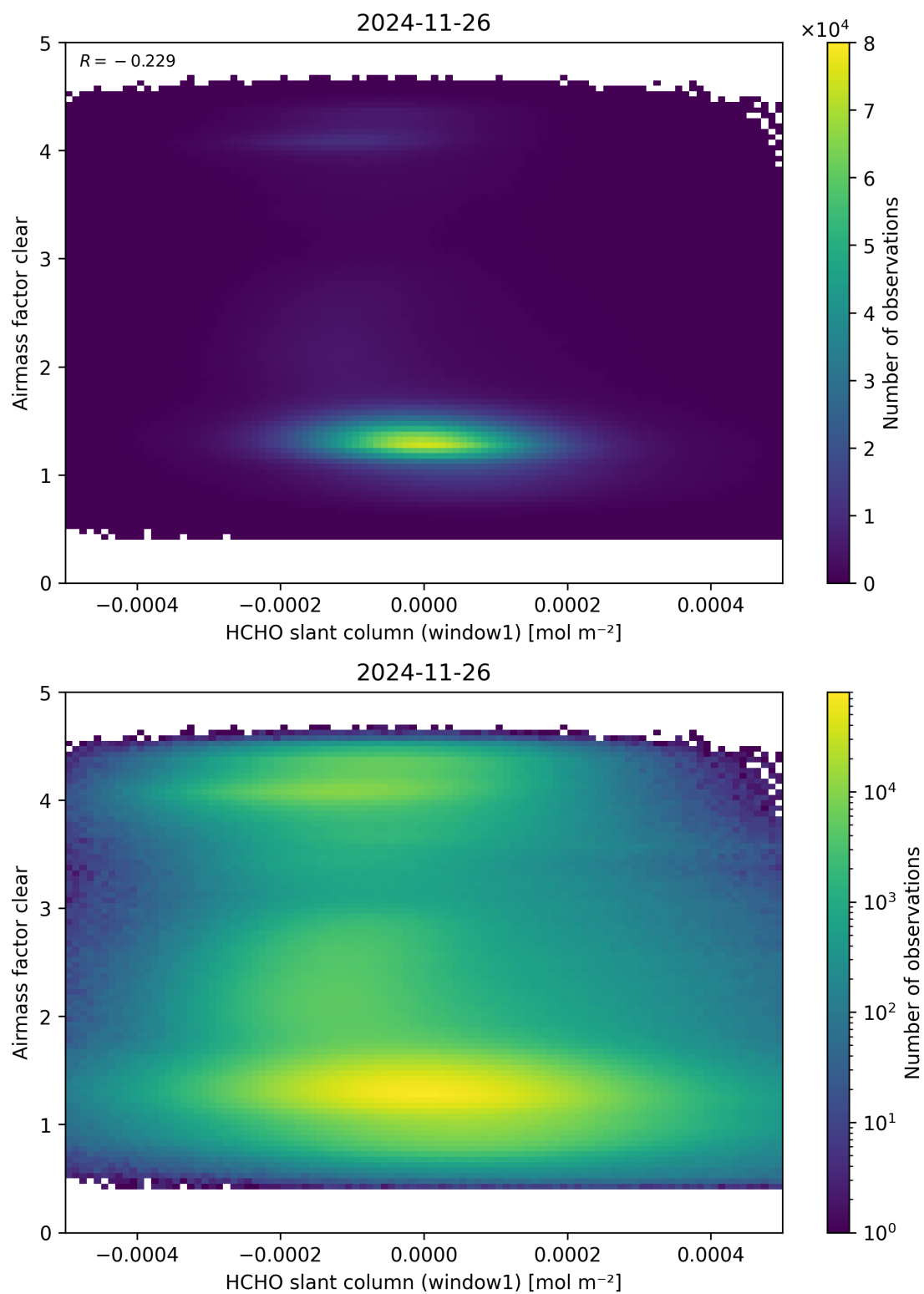
Figure 81: Scatter density plot of “HCHO slant column (window1)” against “Airmass factor clear” for 2024-11-25 to 2024-11-27.
