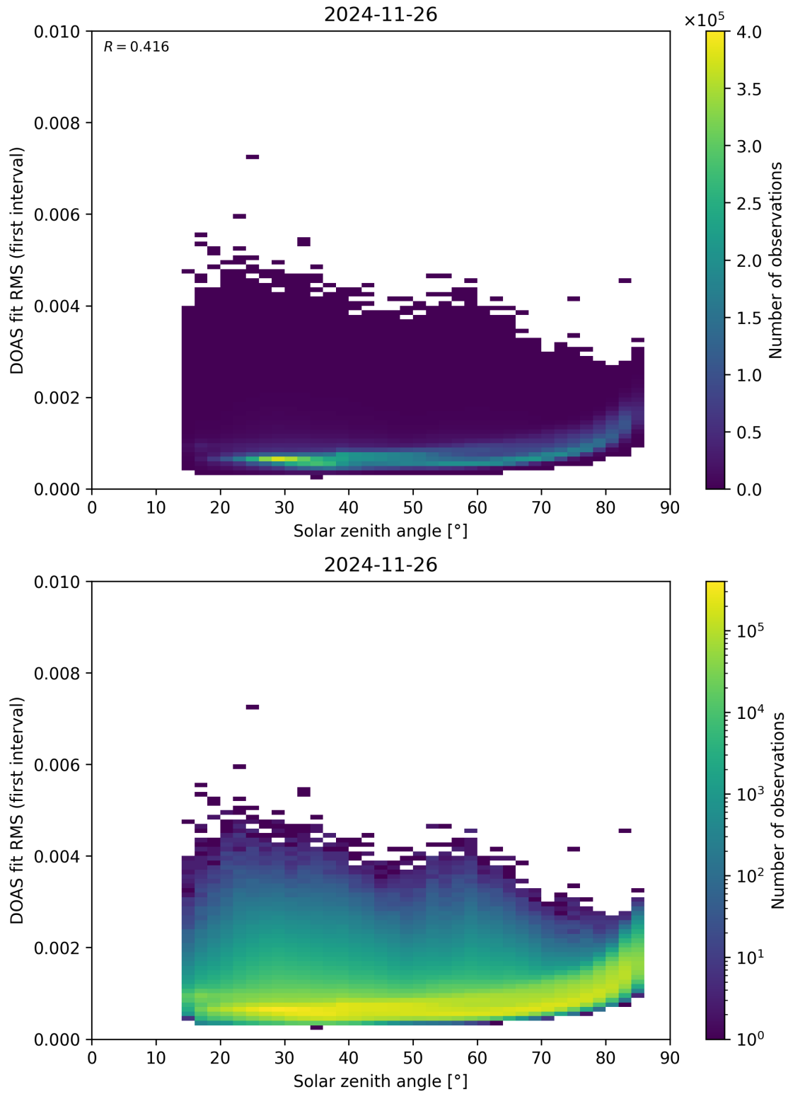
Figure 167: Scatter density plot of “Solar zenith angle” against “DOAS fit RMS (first interval)” for 2024-11-25 to 2024-11-27.
