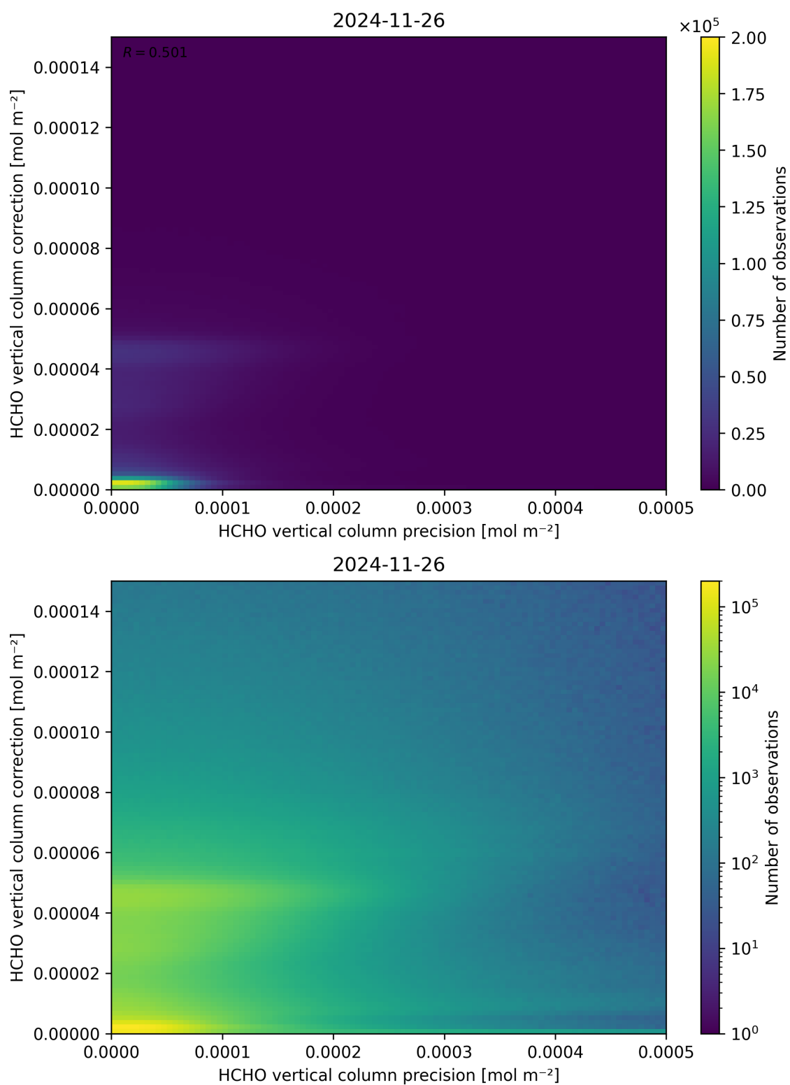
Figure 146: Scatter density plot of “HCHO vertical column precision” against “HCHO vertical column correction” for 2024-11-25 to 2024-11-27.
