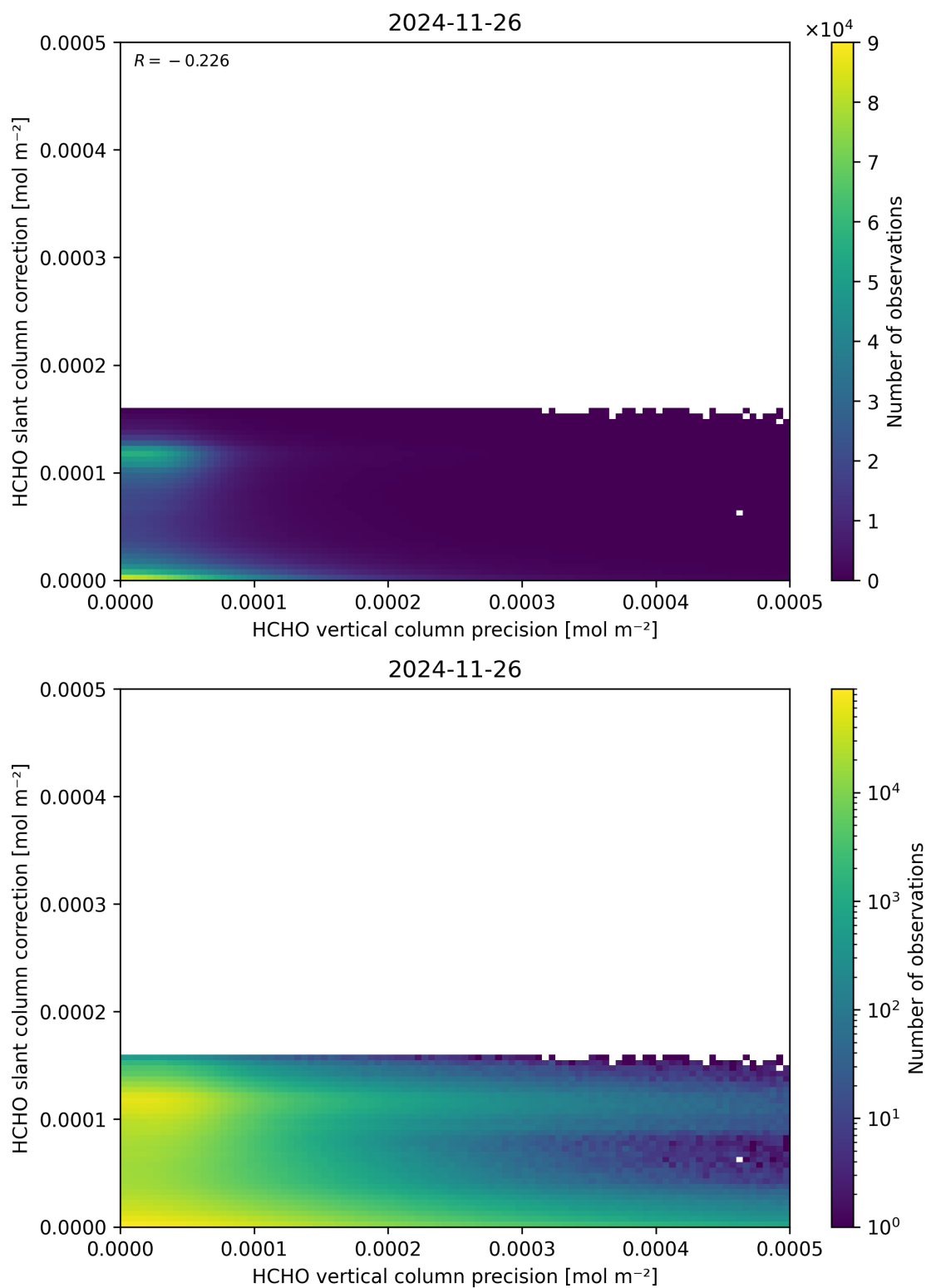
Figure 141: Scatter density plot of “HCHO vertical column precision” against “HCHO slant column correction” for 2024-11-25 to 2024-11-27.
