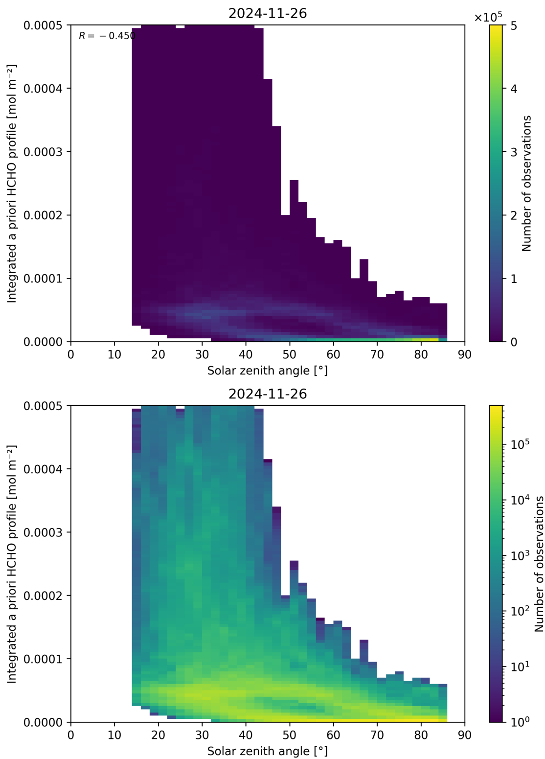
Figure 180: Scatter density plot of “Solar zenith angle” against “Integrated a priori HCHO profile” for 2024-11-25 to 2024-11-27.
