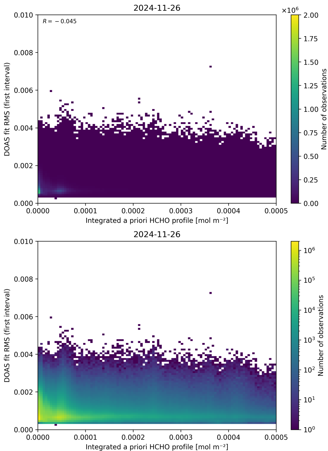
Figure 148: Scatter density plot of “Integrated a priori HCHO profile” against “DOAS fit RMS (first interval)” for 2024-11-25 to 2024-11-27.
