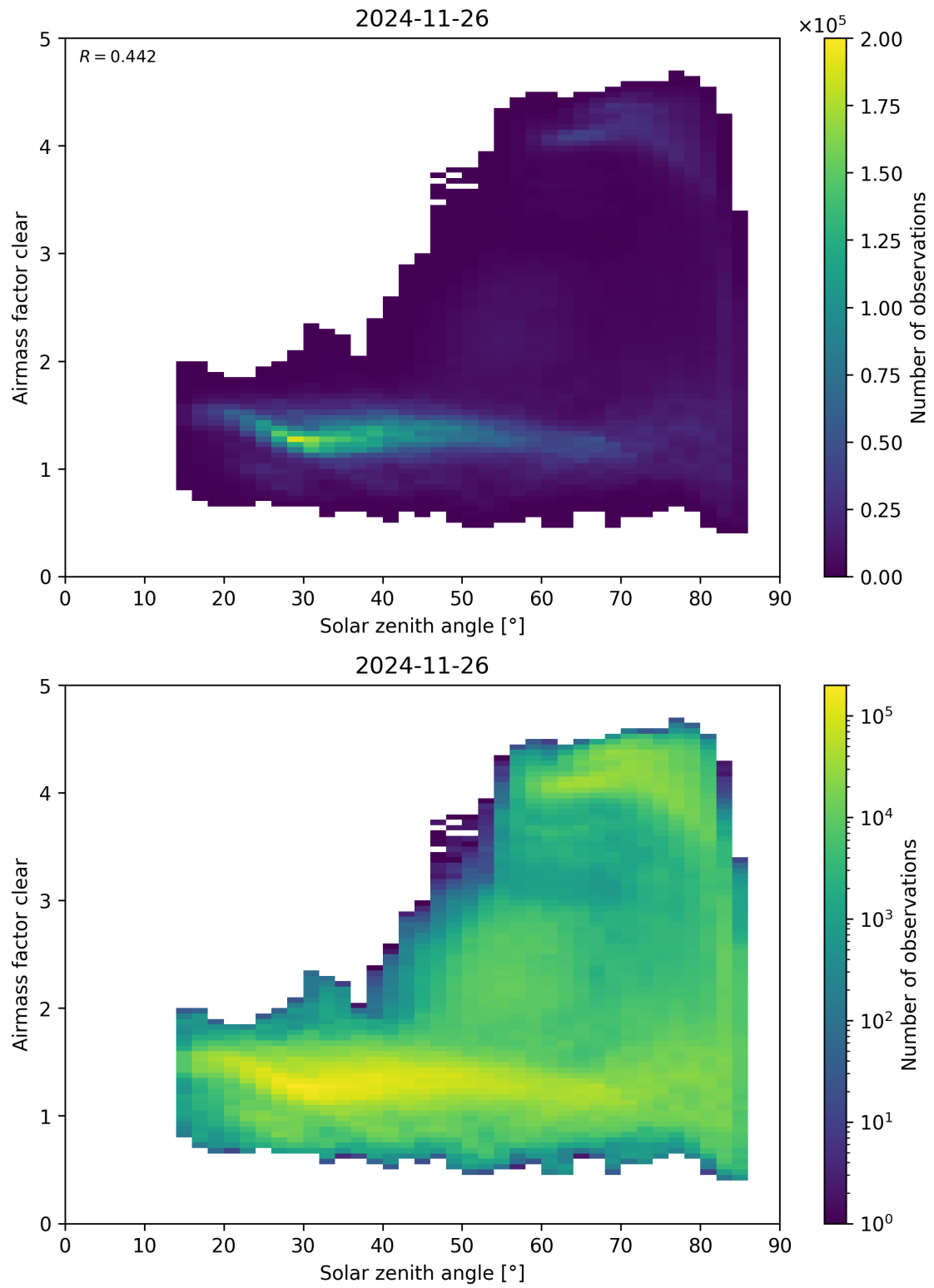
Figure 170: Scatter density plot of “Solar zenith angle” against “Airmass factor clear” for 2024-11-25 to 2024-11-27.
