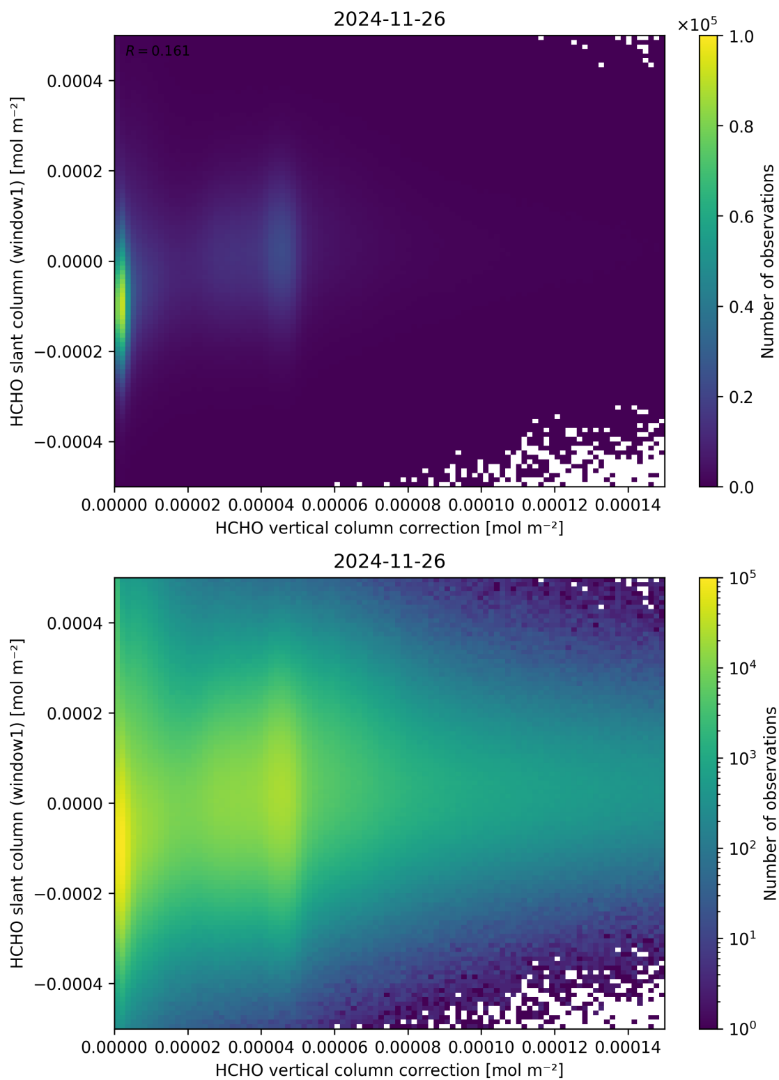
Figure 118: Scatter density plot of “HCHO vertical column correction” against “HCHO slant column (window1)” for 2024-11-25 to 2024-11-27.
