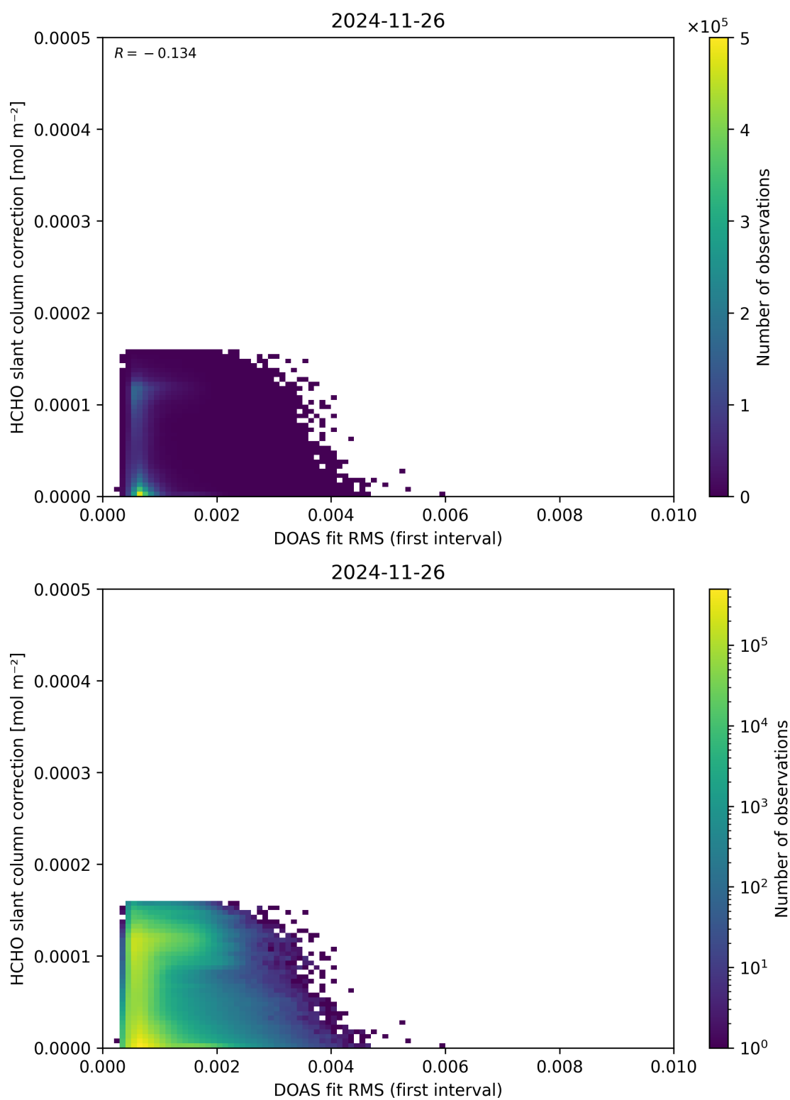
Figure 63: Scatter density plot of “DOAS fit RMS (first interval)” against “HCHO slant column correction” for 2024-11-25 to 2024-11-27.
