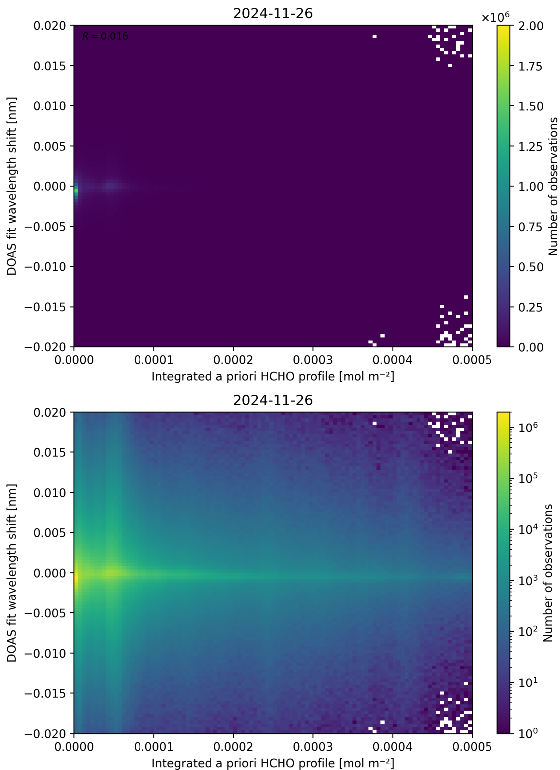
Figure 149: Scatter density plot of “Integrated a priori HCHO profile” against “DOAS fit wavelength shift” for 2024-11-25 to 2024-11-27.
