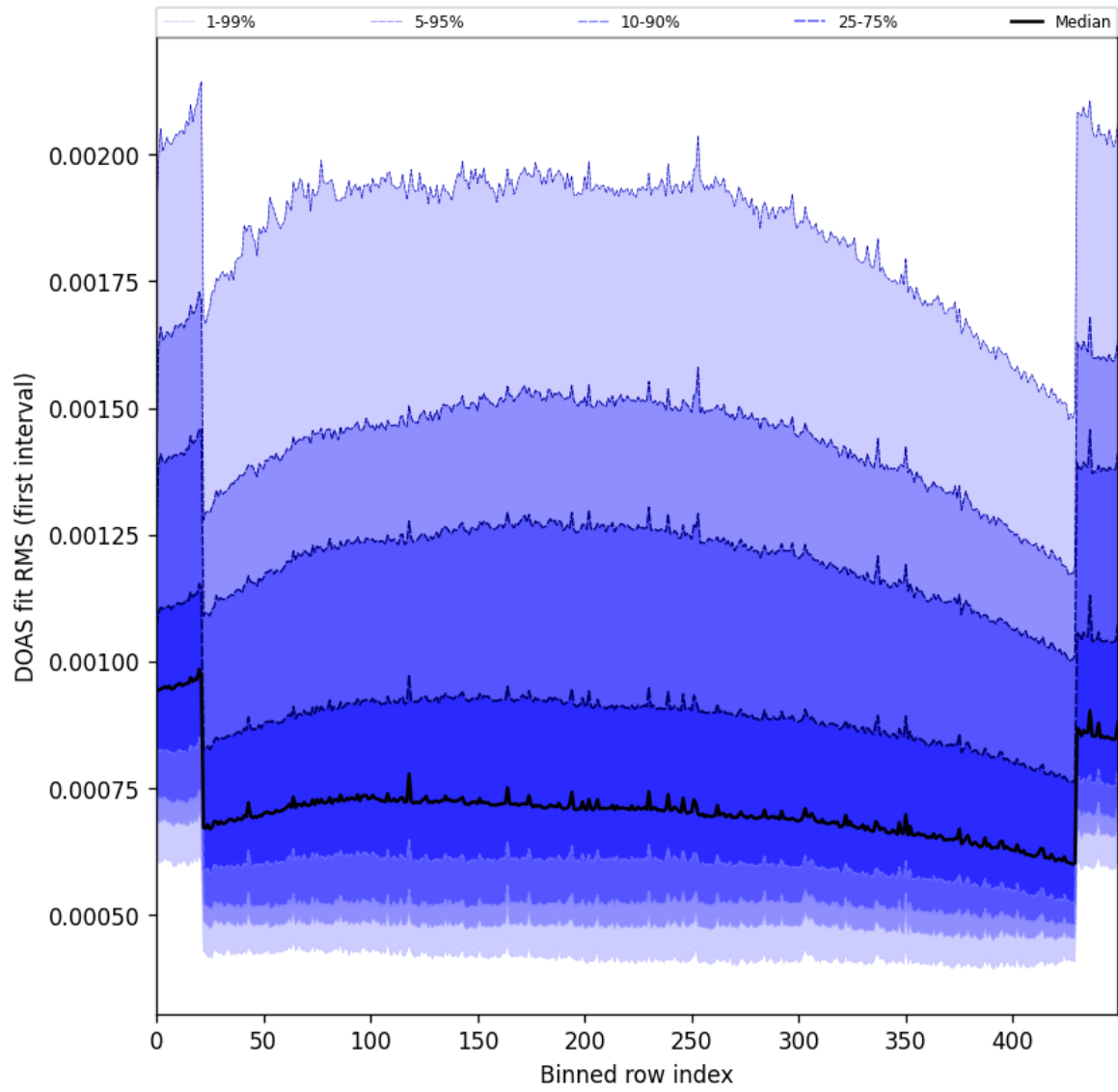
Figure 60: Along track statistics of “DOAS fit RMS (first interval)” for 2024-11-25 to 2024-11-27
