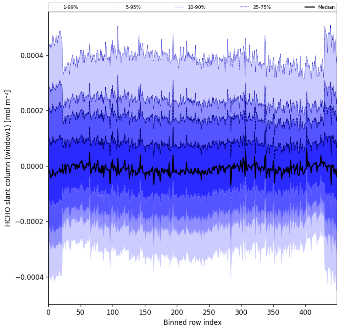
Figure 52: Along track statistics of “HCHO slant column (window1)” for 2024-11-25 to 2024-11-27
