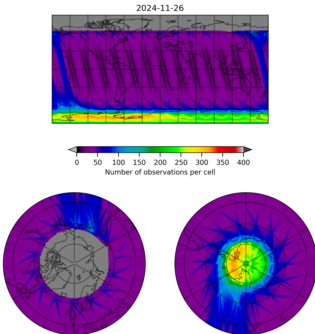
Figure 19: Map of the number of observations for 2024-11-25 to 2024-11-27
