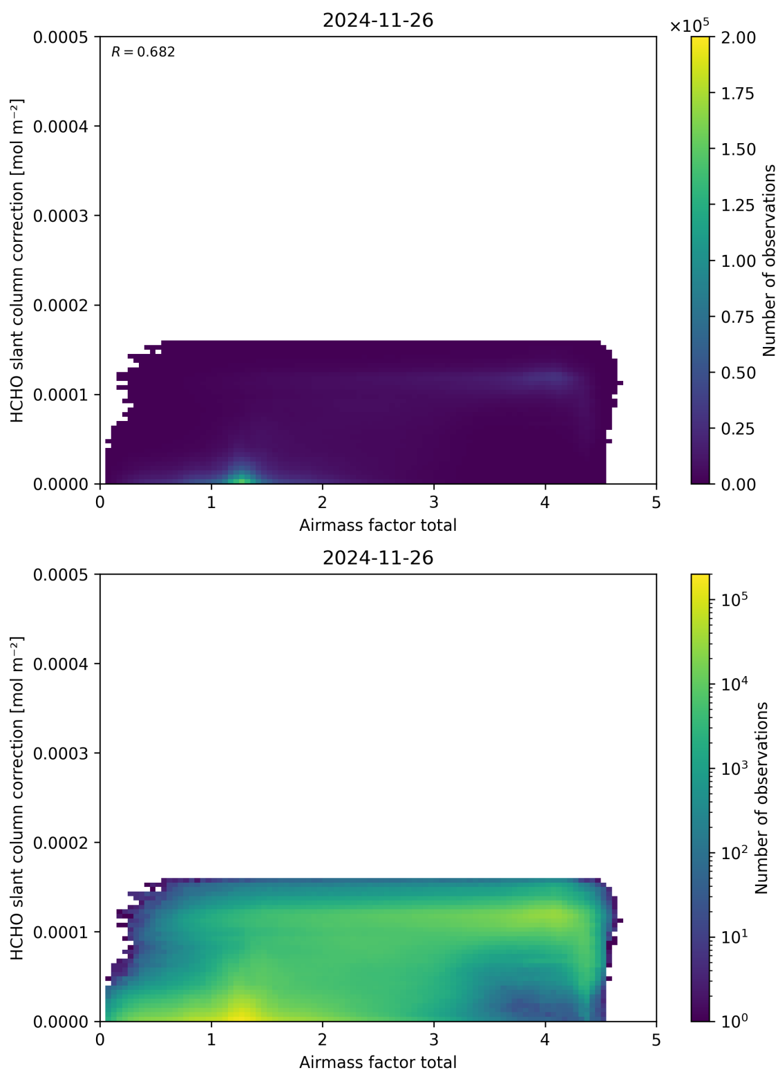
Figure 102: Scatter density plot of “Airmass factor total” against “HCHO slant column correction” for 2024-11-25 to 2024-11-27.
