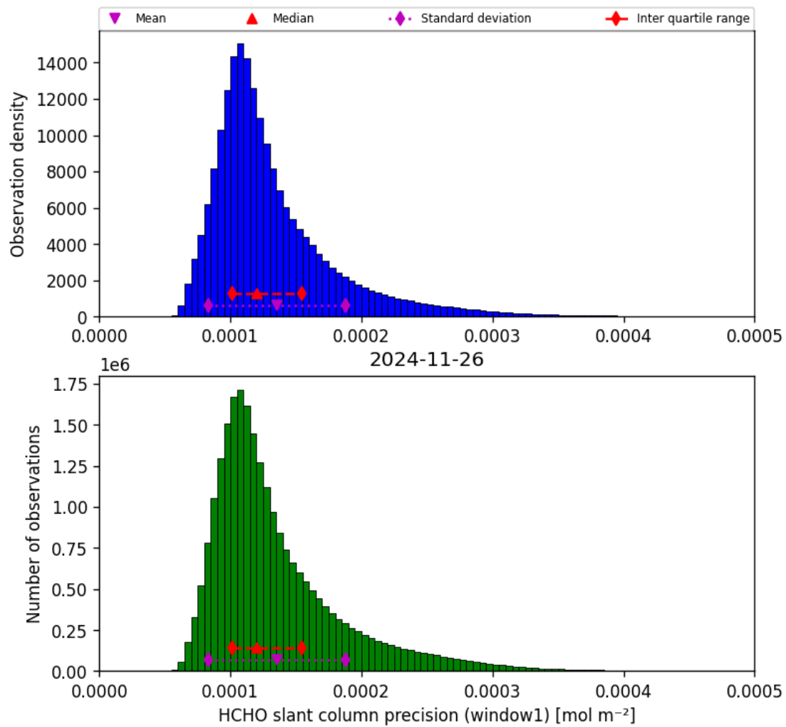
Figure 39: Histogram of “HCHO slant column precision (window1)” for 2024-11-25 to 2024-11-27
