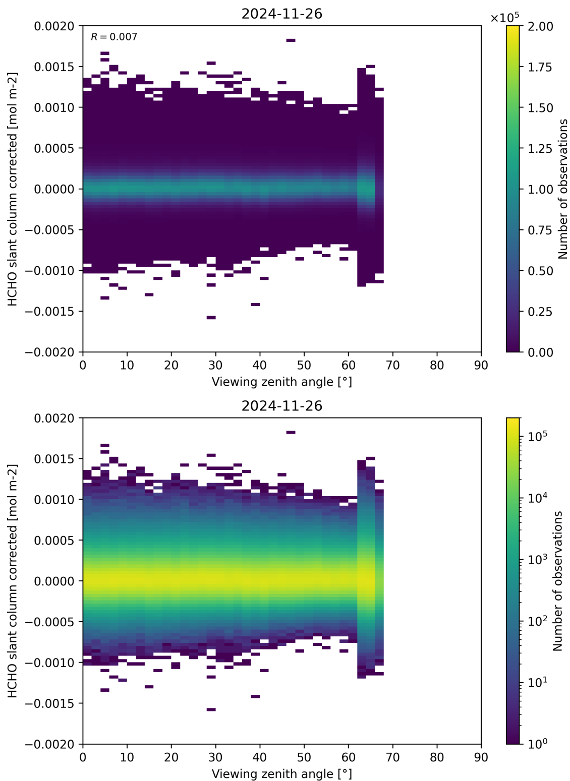
Figure 186: Scatter density plot of “Viewing zenith angle” against “HCHO slant column corrected” for 2024-11-25 to 2024-11-27.
