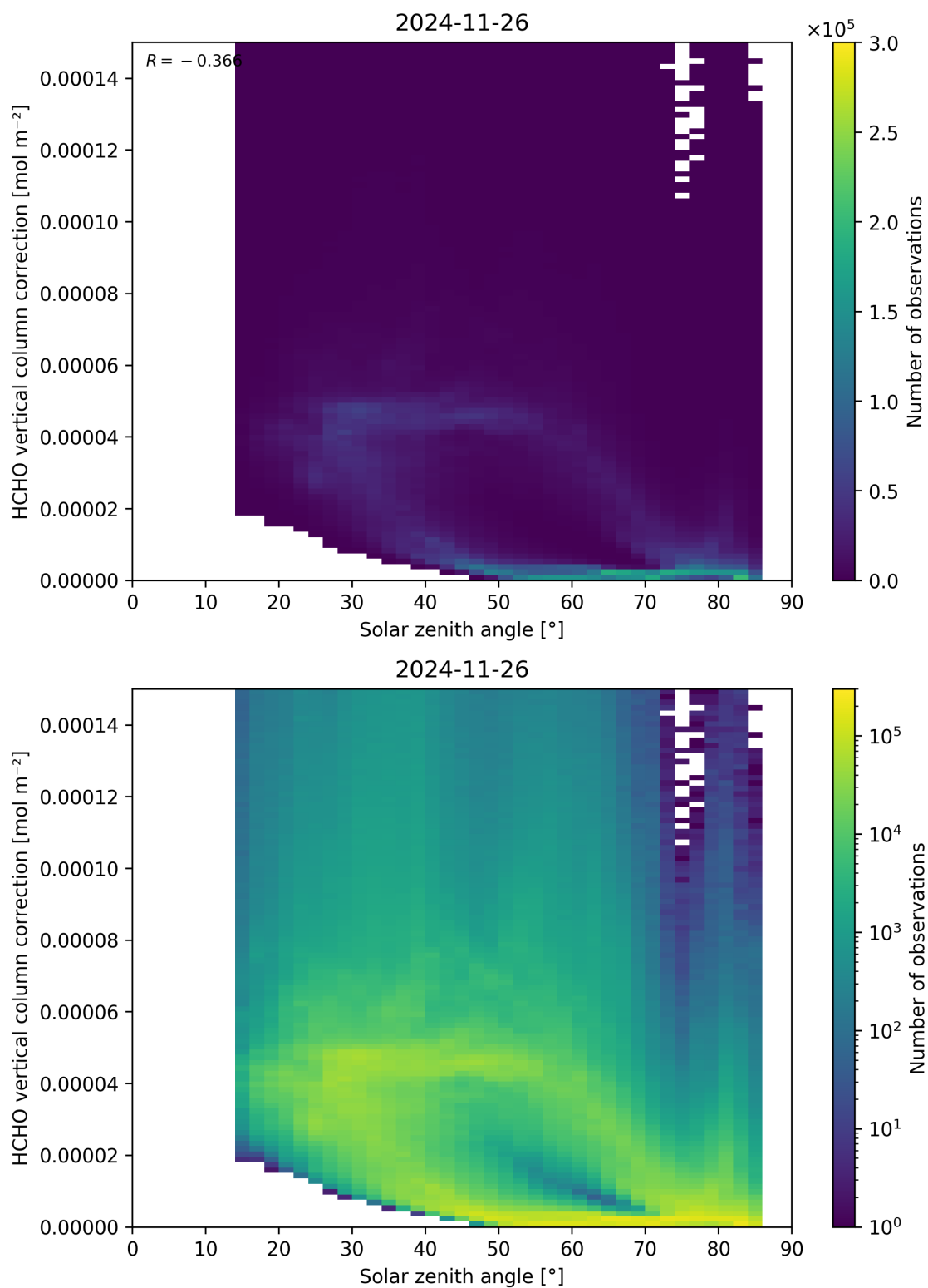
Figure 178: Scatter density plot of “Solar zenith angle” against “HCHO vertical column correction” for 2024-11-25 to 2024-11-27.
