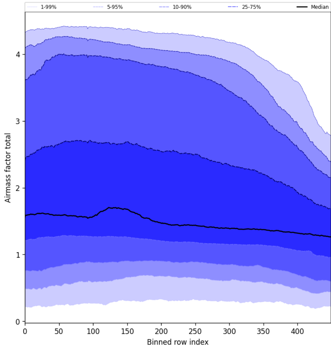
Figure 54: Along track statistics of “Airmass factor total” for 2024-11-25 to 2024-11-27
