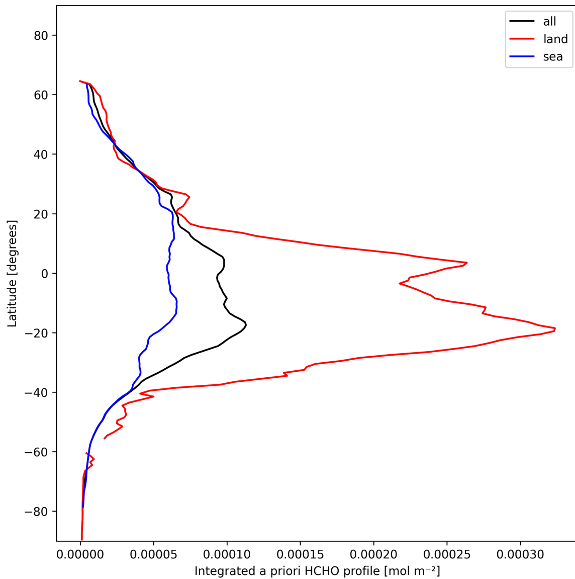
Figure 29: Zonal average of “Integrated a priori HCHO profile” for 2024-11-25 to 2024-11-27.
