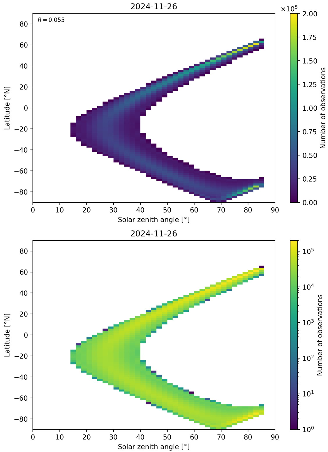
Figure 181: Scatter density plot of “Solar zenith angle” against “Latitude” for 2024-11-25 to 2024-11-27.
