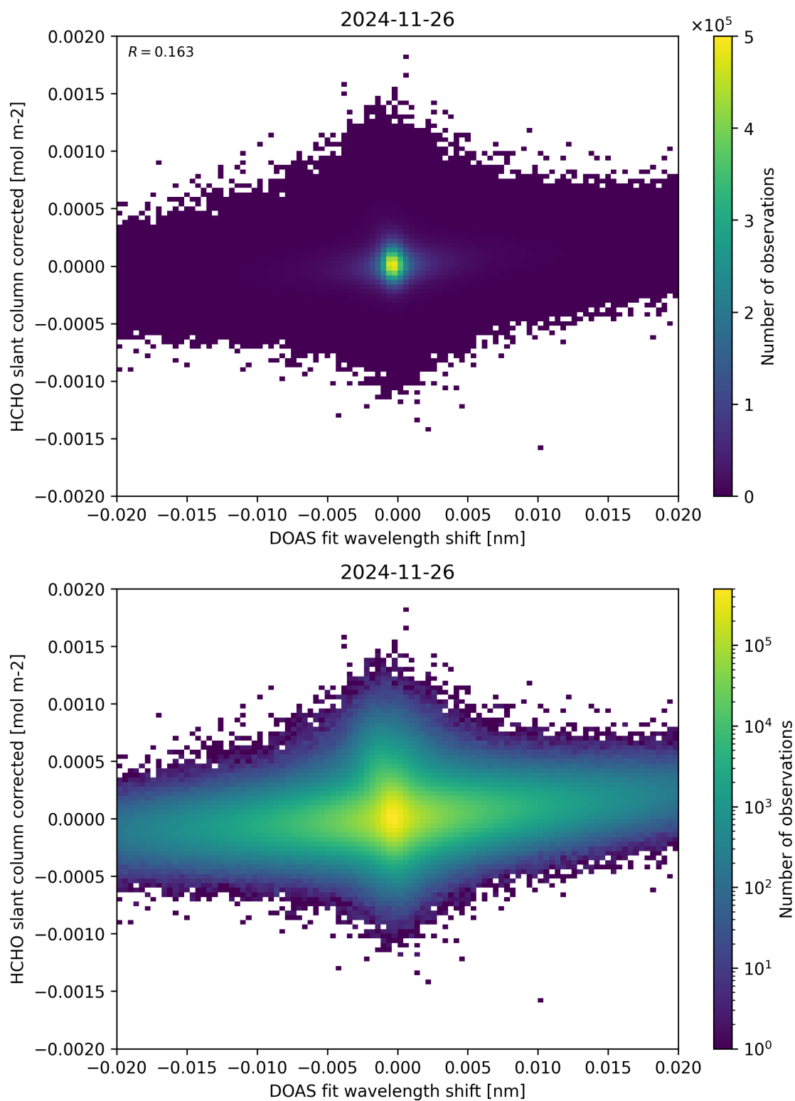
Figure 66: Scatter density plot of “DOAS fit wavelength shift” against “HCHO slant column corrected” for 2024-11-25 to 2024-11-27.
