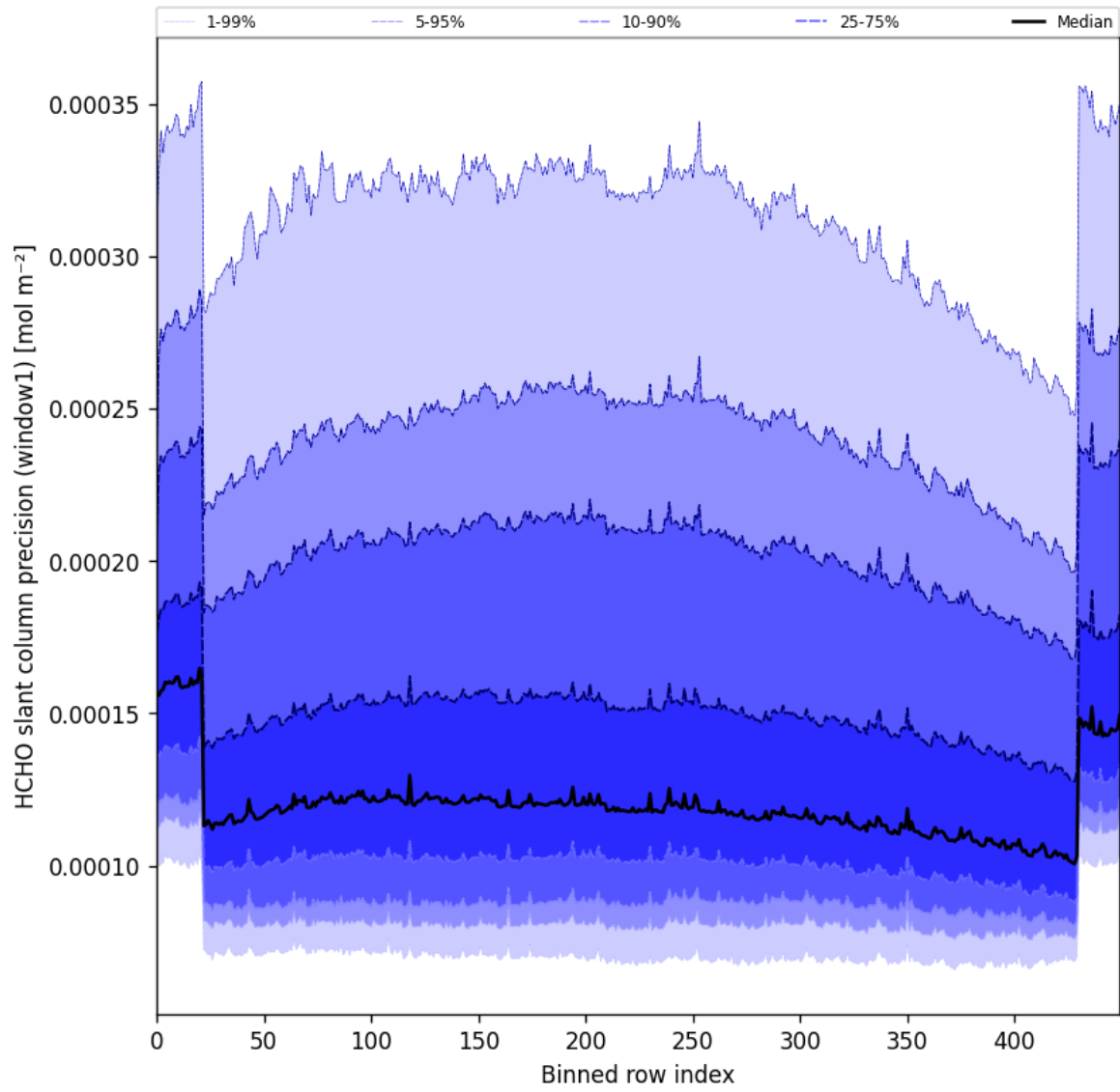
Figure 53: Along track statistics of “HCHO slant column precision (window1)” for 2024-11-25 to 2024-11-27
