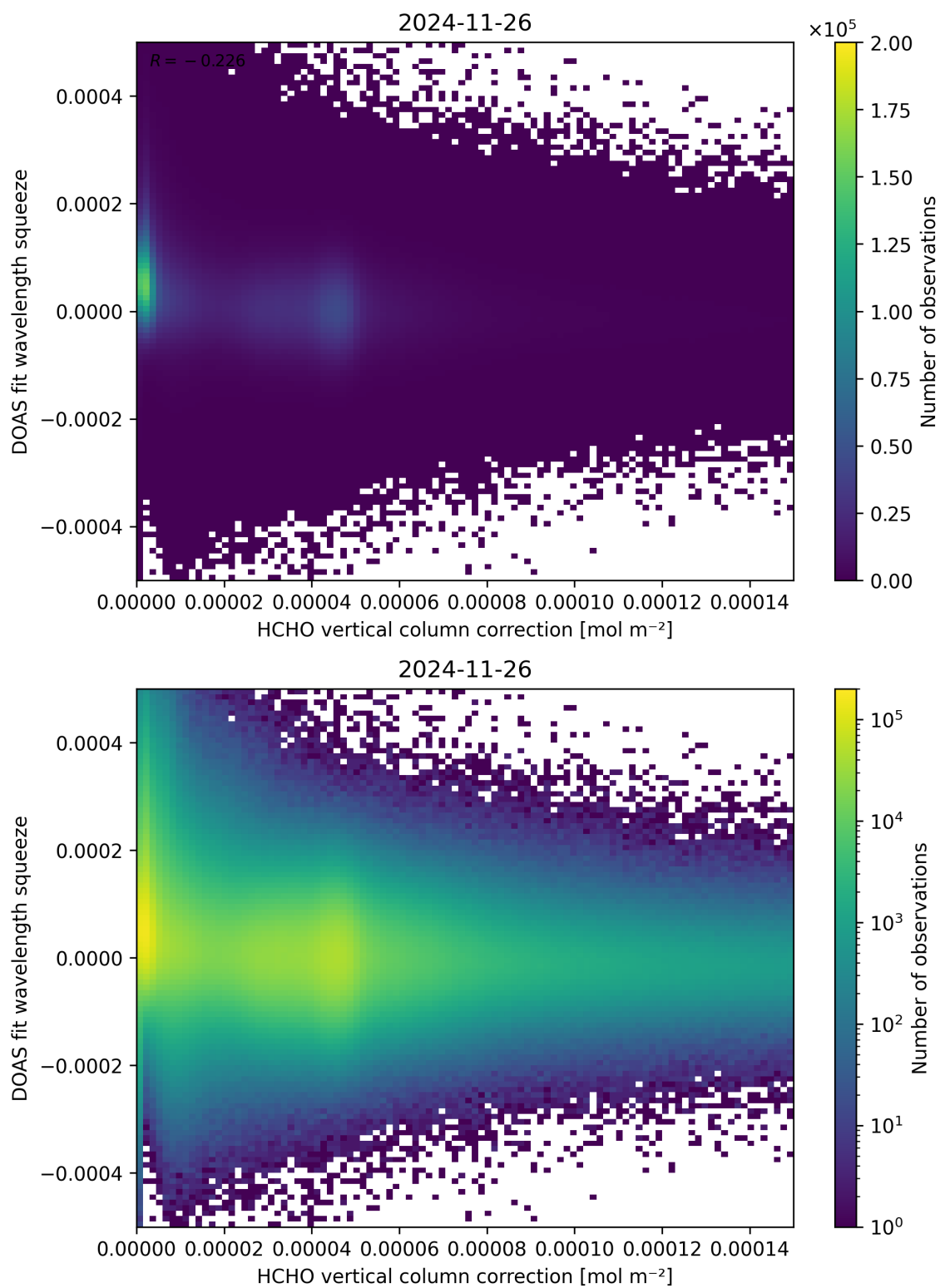
Figure 114: Scatter density plot of “HCHO vertical column correction” against “DOAS fit wavelength squeeze” for 2024-11-25 to 2024-11-27.
