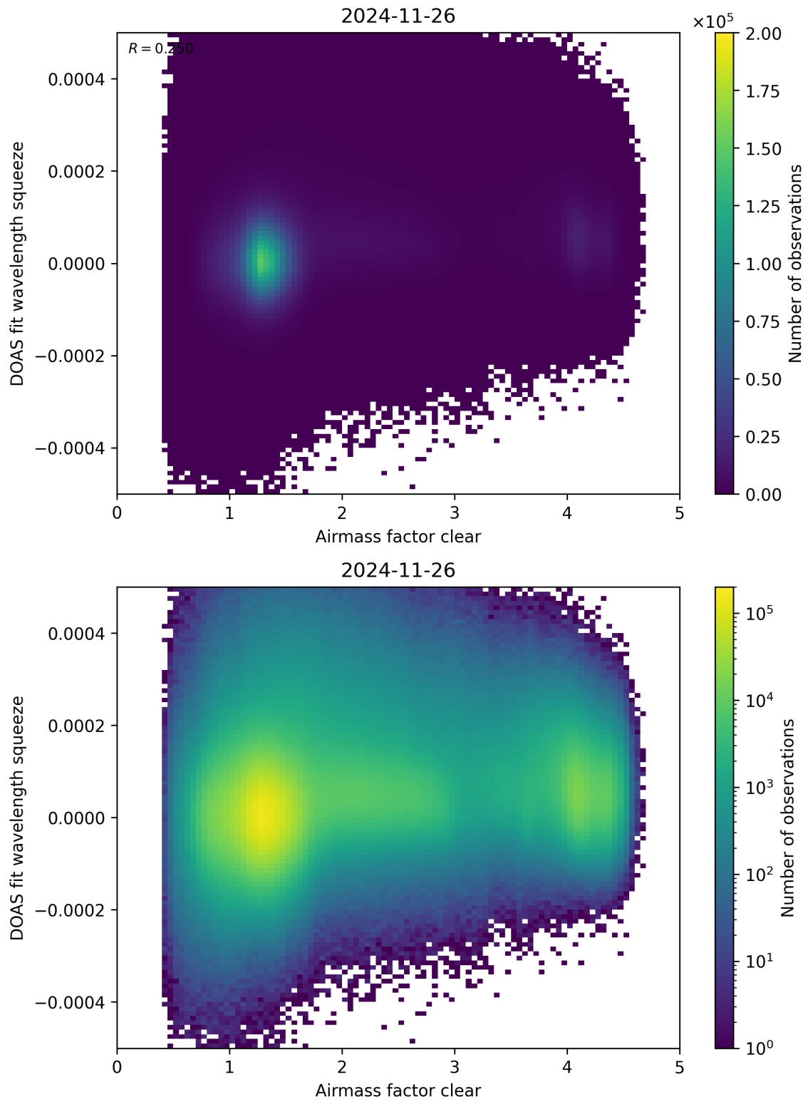
Figure 73: Scatter density plot of “Airmass factor clear” against “DOAS fit wavelength squeeze” for 2024-11-25 to 2024-11-27.
