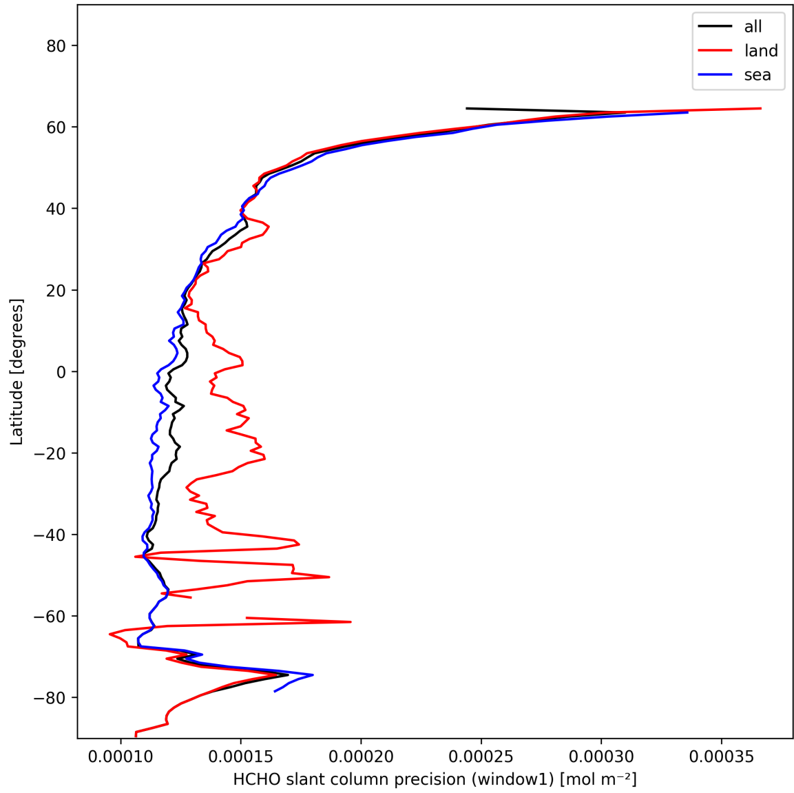
Figure 25: Zonal average of “HCHO slant column precision (window1)” for 2024-11-25 to 2024-11-27.
