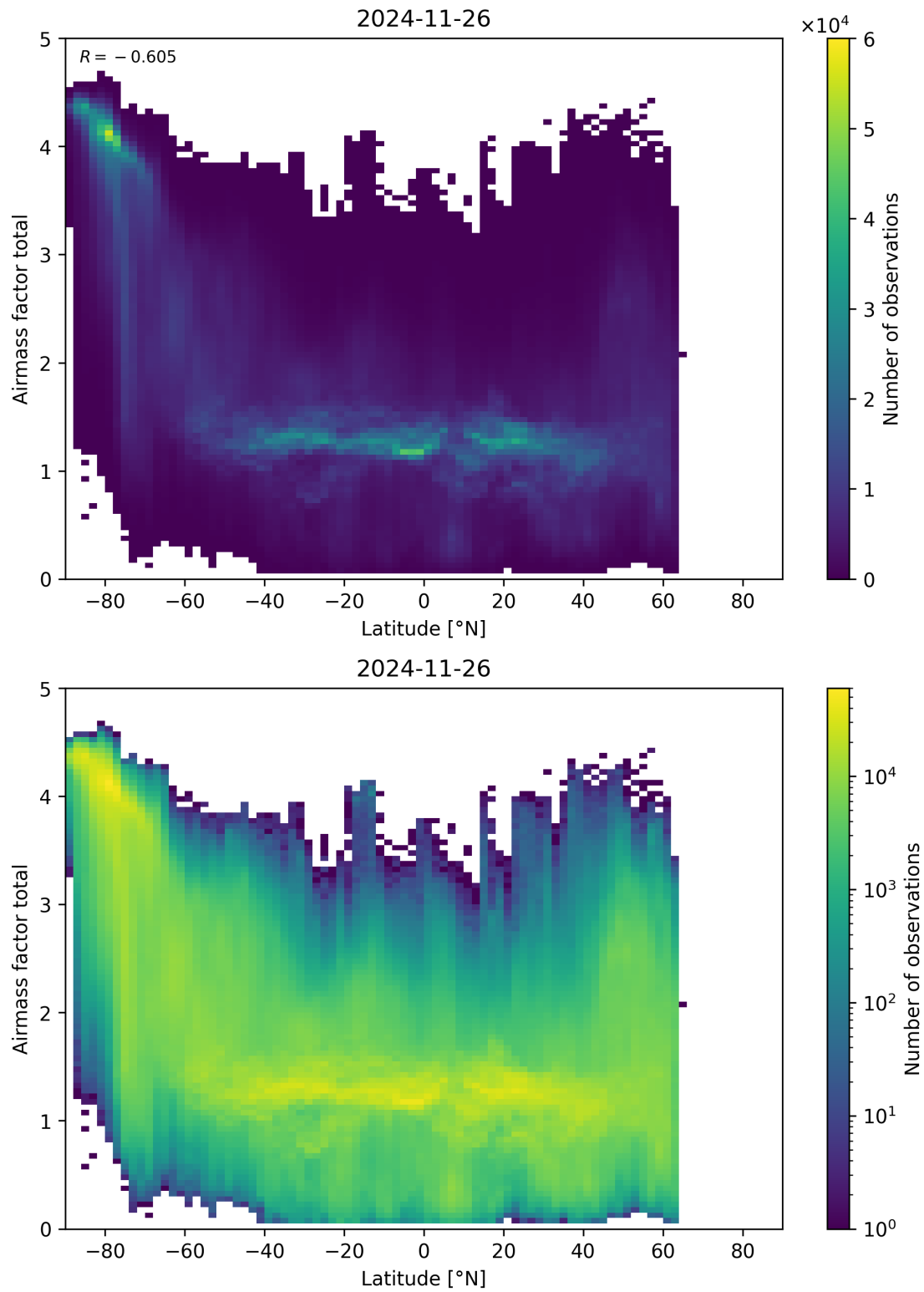
Figure 161: Scatter density plot of “Latitude” against “Airmass factor total” for 2024-11-25 to 2024-11-27.
