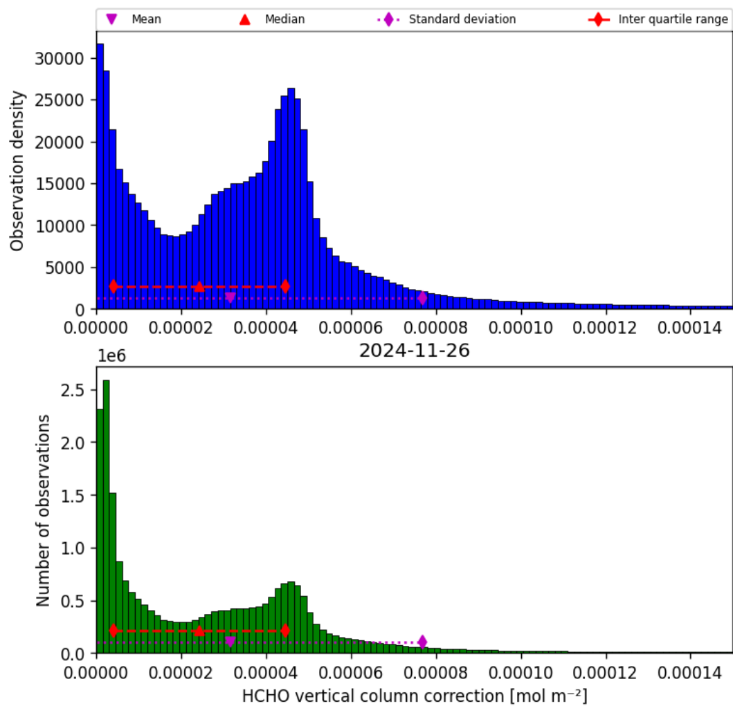
Figure 37: Histogram of “HCHO vertical column correction” for 2024-11-25 to 2024-11-27
