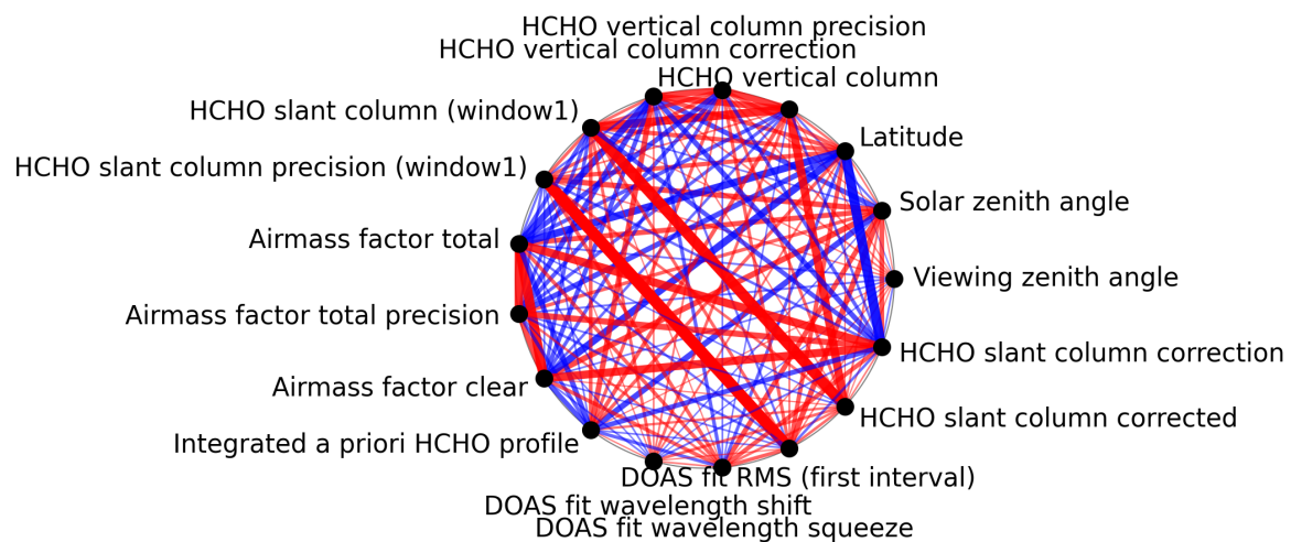
Figure 1: Map of correlation graph for 2024-11-25 to 2024-11-27.
