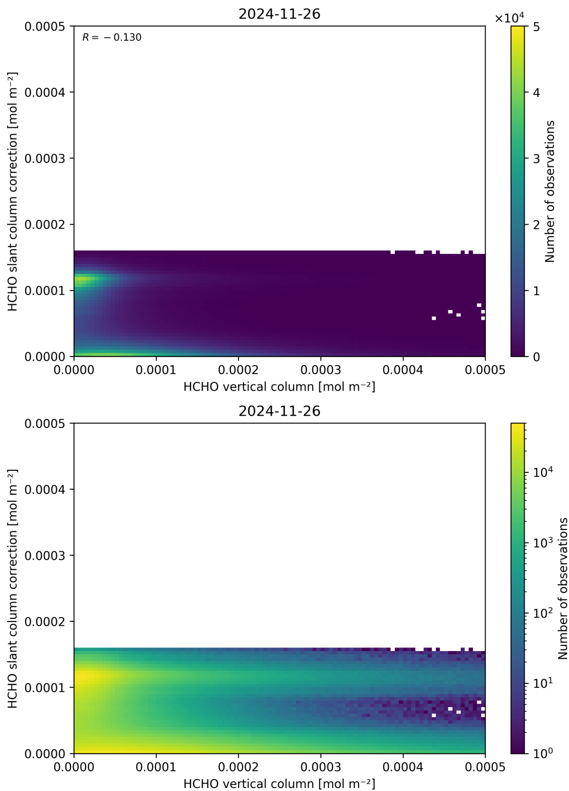
Figure 128: Scatter density plot of “HCHO vertical column” against “HCHO slant column correction” for 2024-11-25 to 2024-11-27.
