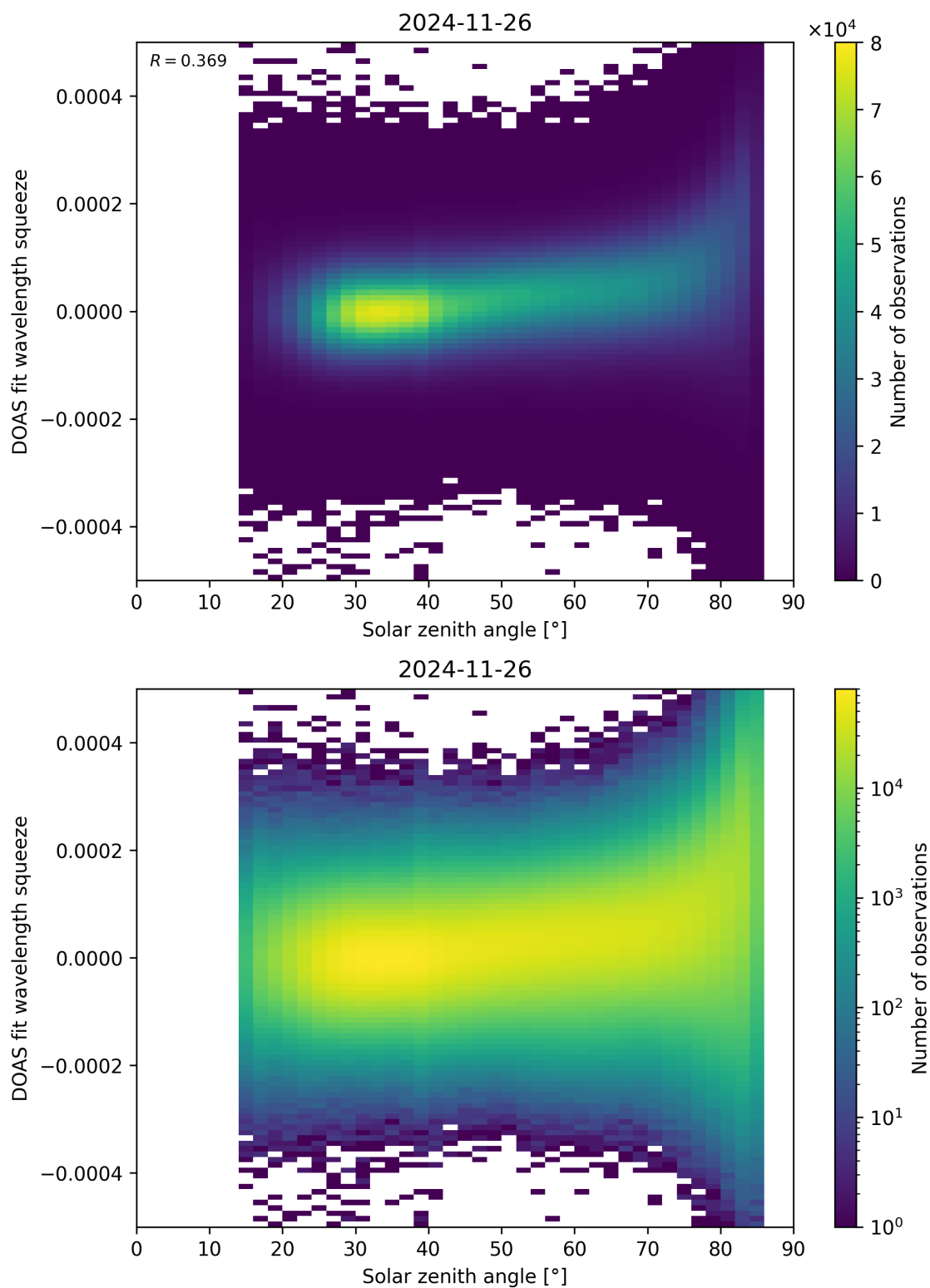
Figure 169: Scatter density plot of “Solar zenith angle” against “DOAS fit wavelength squeeze” for 2024-11-25 to 2024-11-27.
