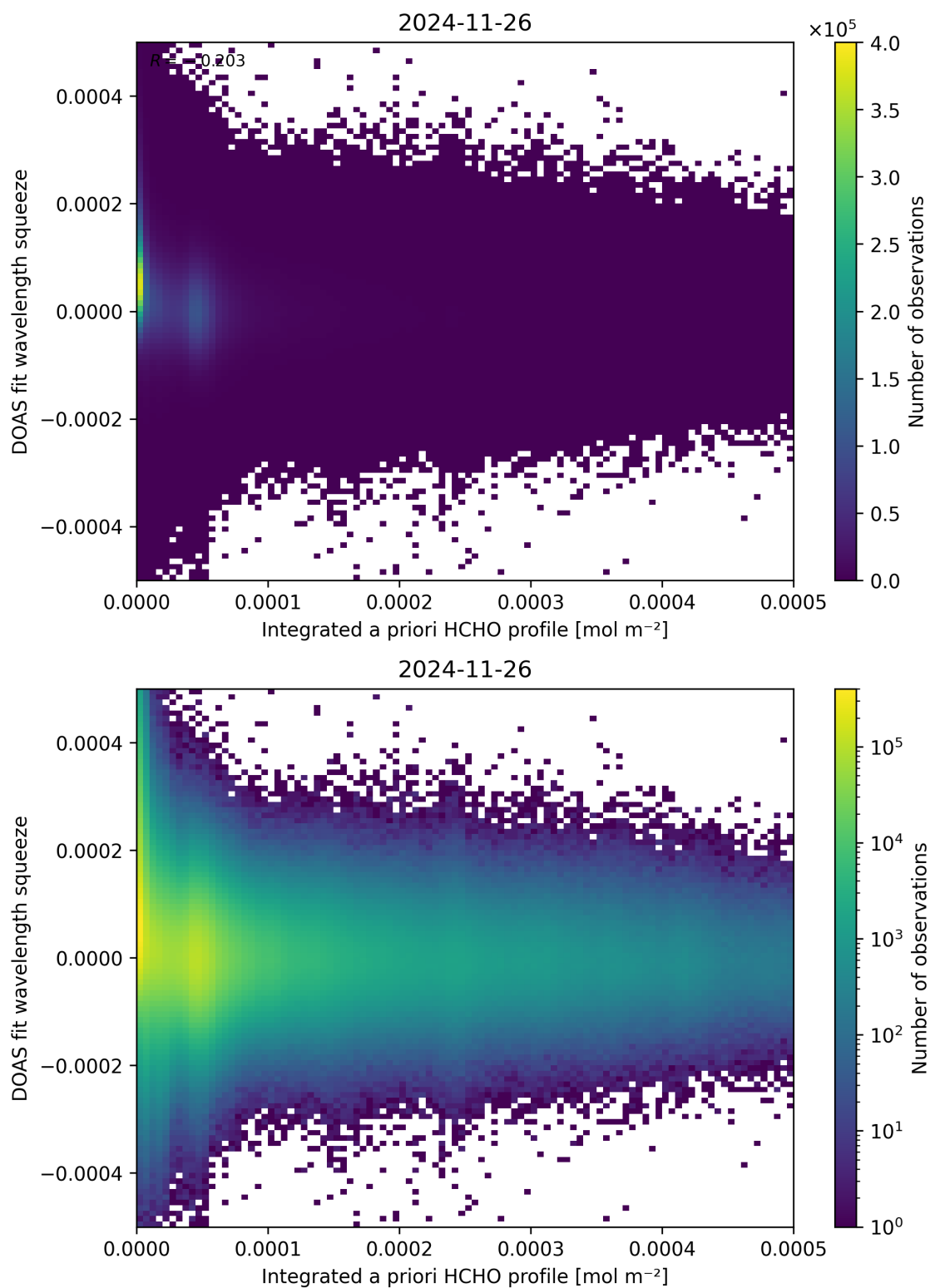
Figure 150: Scatter density plot of “Integrated a priori HCHO profile” against “DOAS fit wavelength squeeze” for 2024-11-25 to 2024-11-27.
