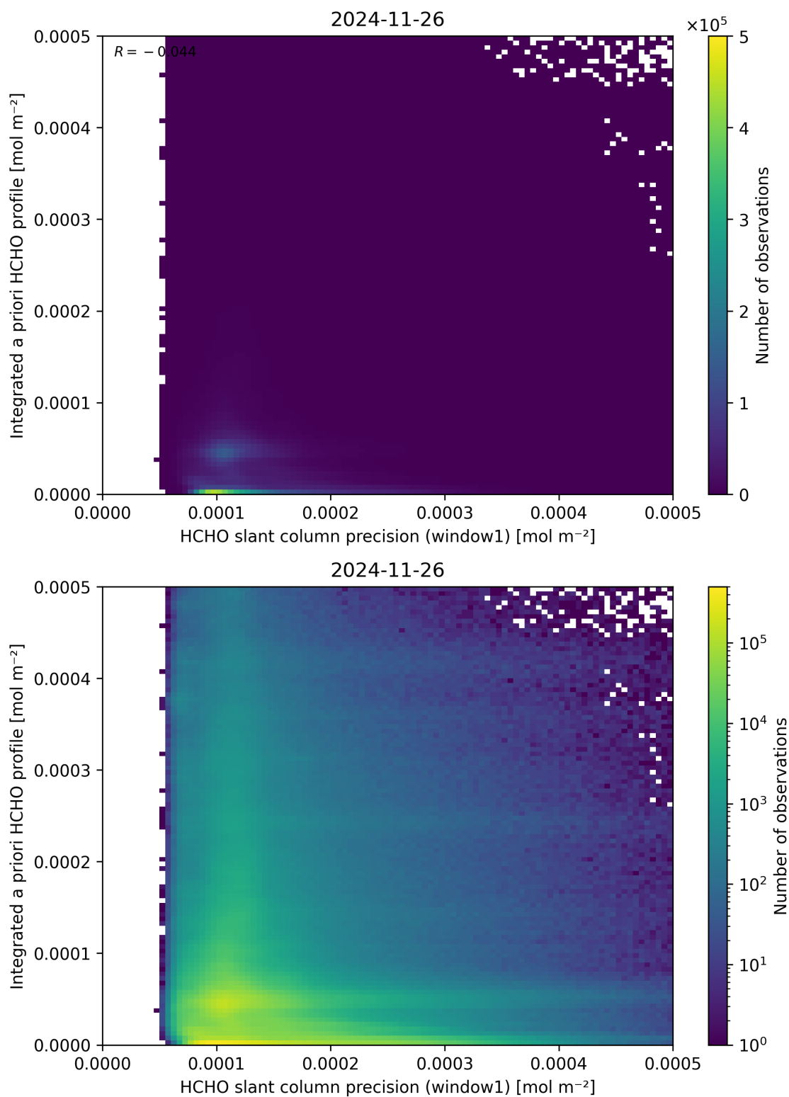
Figure 96: Scatter density plot of “HCHO slant column precision (window1)” against “Integrated a priori HCHO profile” for 2024-11-25 to 2024-11-27.
