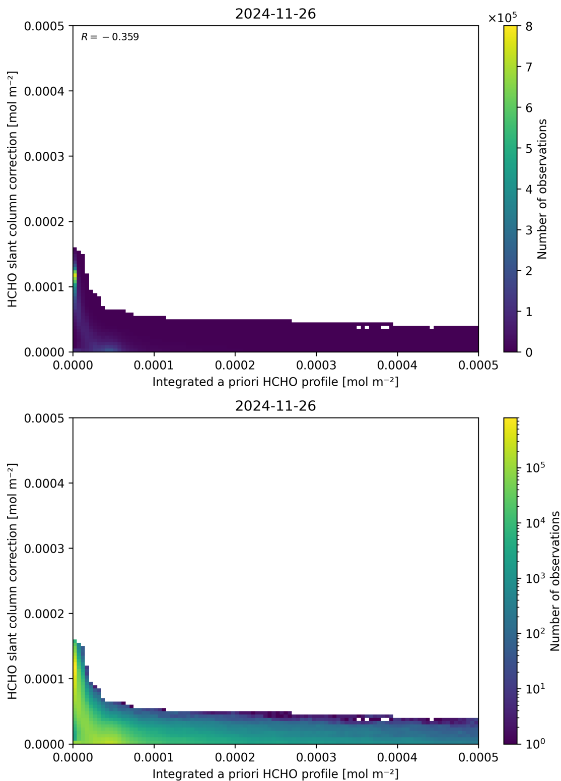
Figure 152: Scatter density plot of “Integrated a priori HCHO profile” against “HCHO slant column correction” for 2024-11-25 to 2024-11-27.
