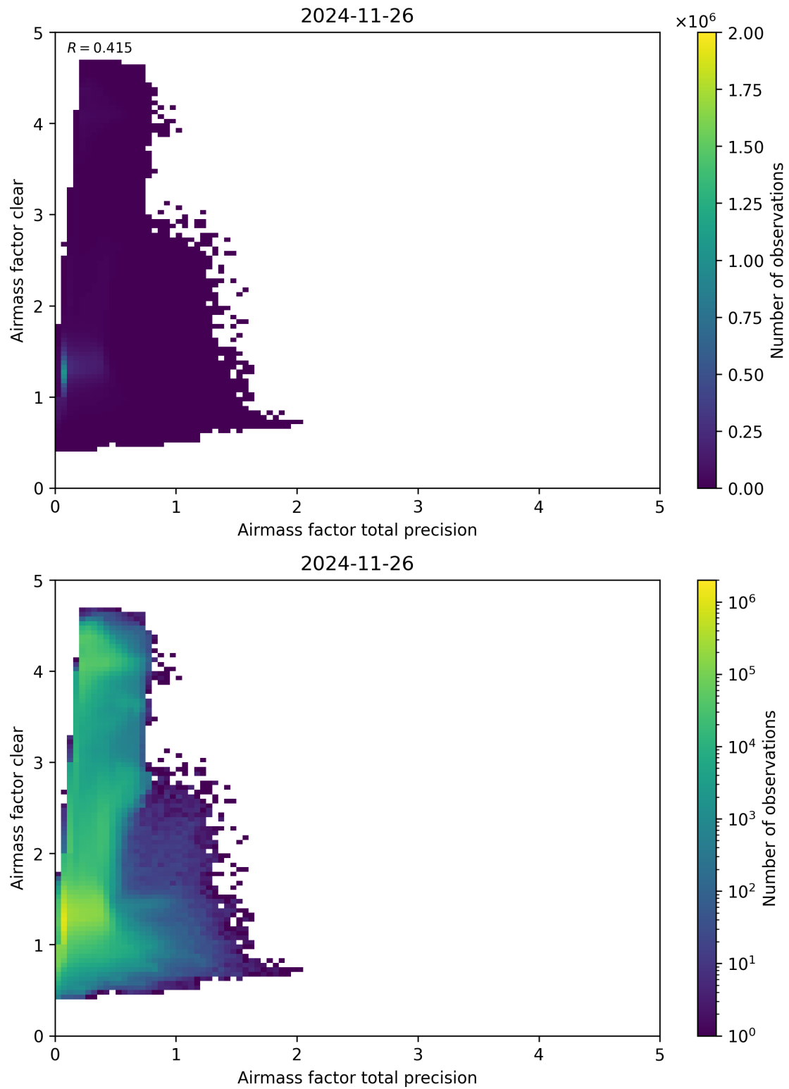
Figure 108: Scatter density plot of “Airmass factor total precision” against “Airmass factor clear” for 2024-11-25 to 2024-11-27.
