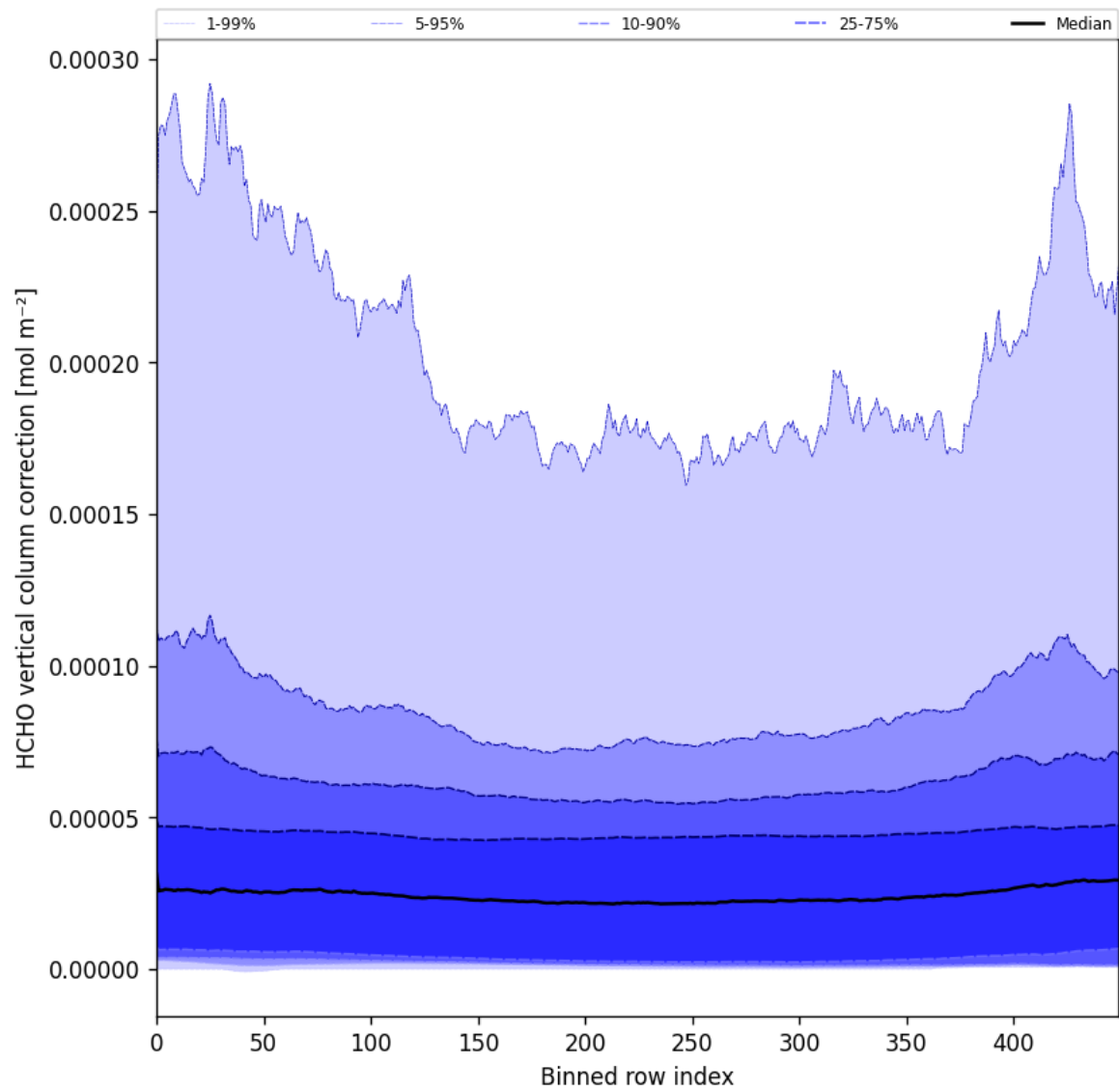
Figure 51: Along track statistics of “HCHO vertical column correction” for 2024-11-25 to 2024-11-27
