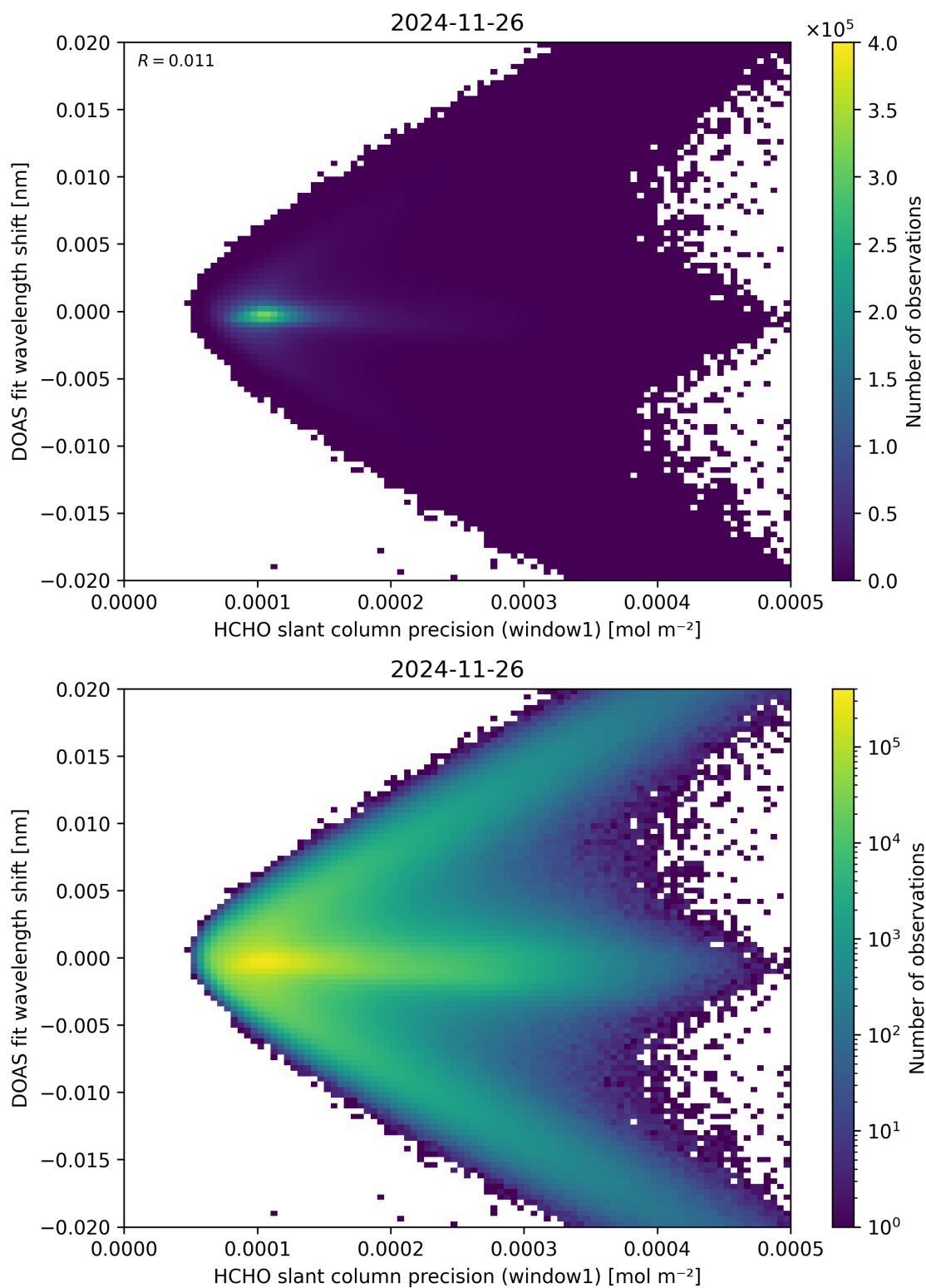
Figure 89: Scatter density plot of “HCHO slant column precision (window1)” against “DOAS fit wavelength shift” for 2024-11-25 to 2024-11-27.
