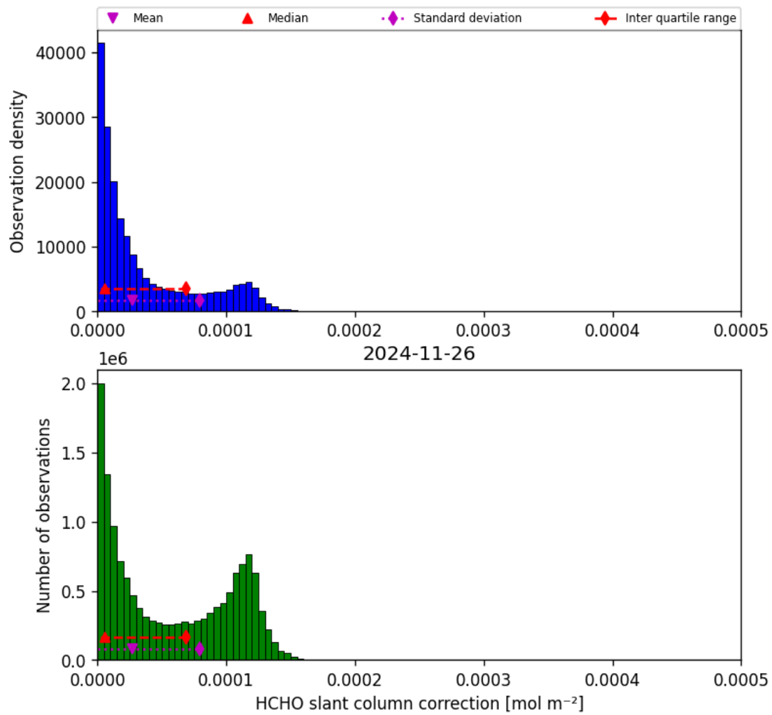
Figure 47: Histogram of “HCHO slant column correction” for 2024-11-25 to 2024-11-27
