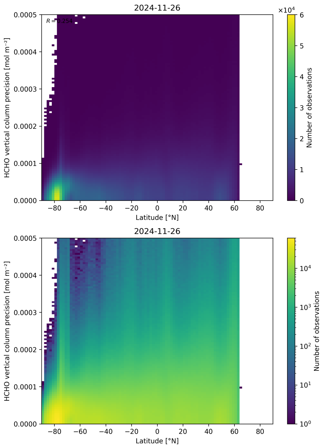
Figure 165: Scatter density plot of “Latitude” against “HCHO vertical column precision” for 2024-11-25 to 2024-11-27.
