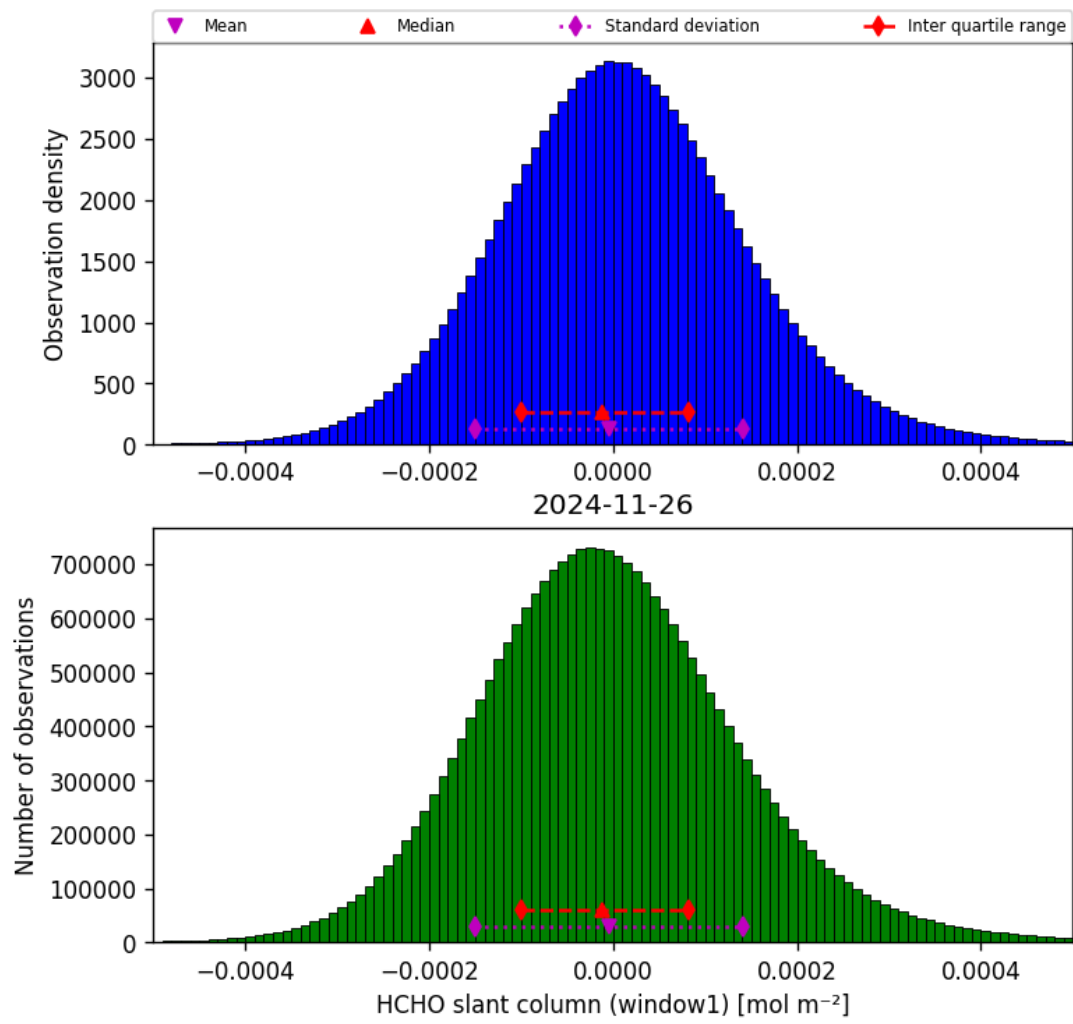
Figure 38: Histogram of “HCHO slant column (window1)” for 2024-11-25 to 2024-11-27
