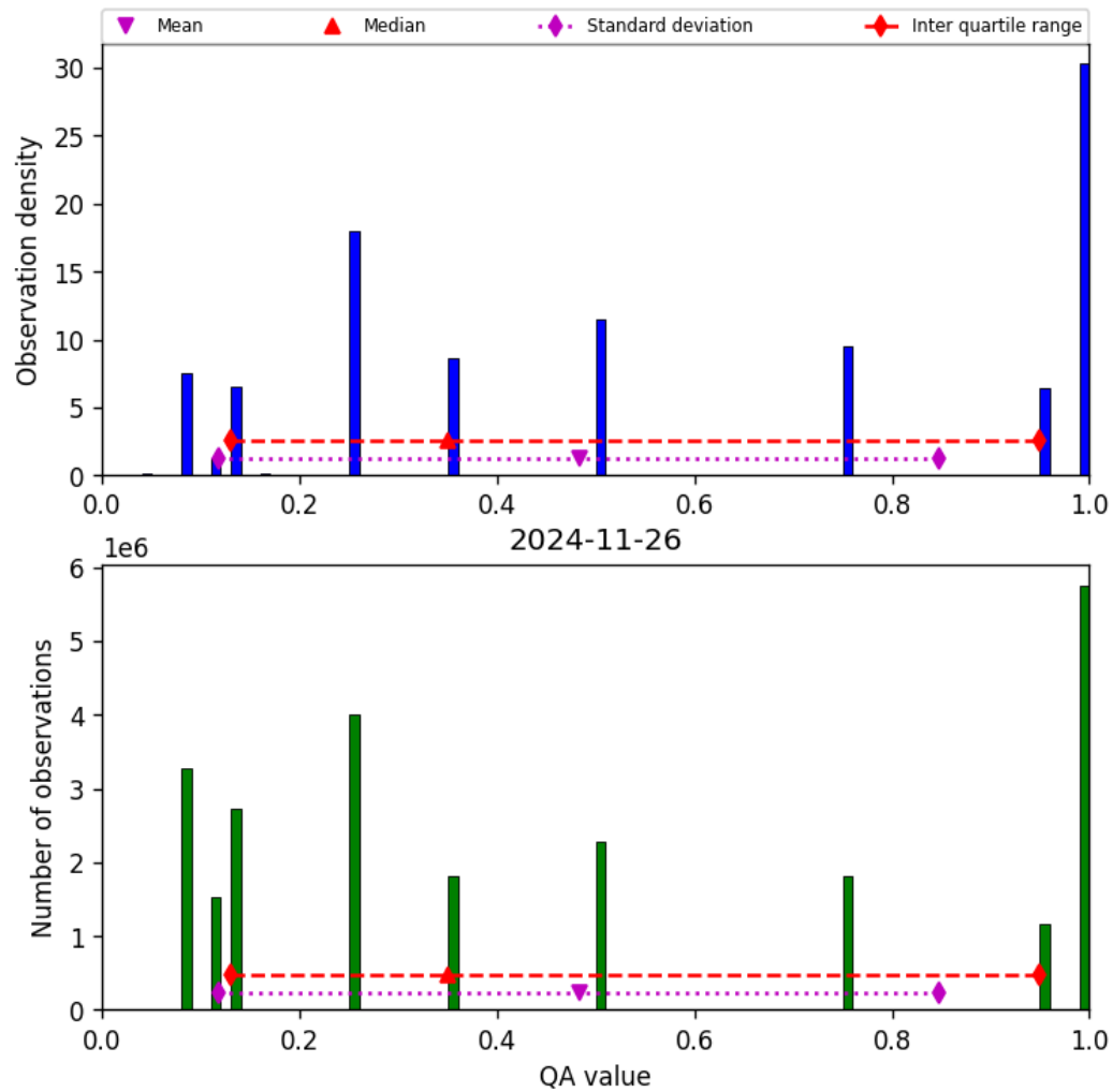
Figure 34: Histogram of “QA value” for 2024-11-25 to 2024-11-27
