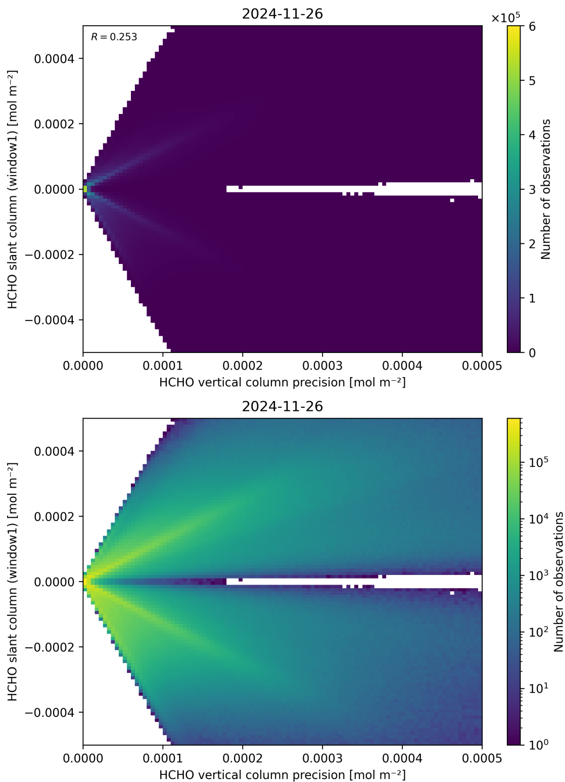
Figure 142: Scatter density plot of “HCHO vertical column precision” against “HCHO slant column (window1)” for 2024-11-25 to 2024-11-27.
