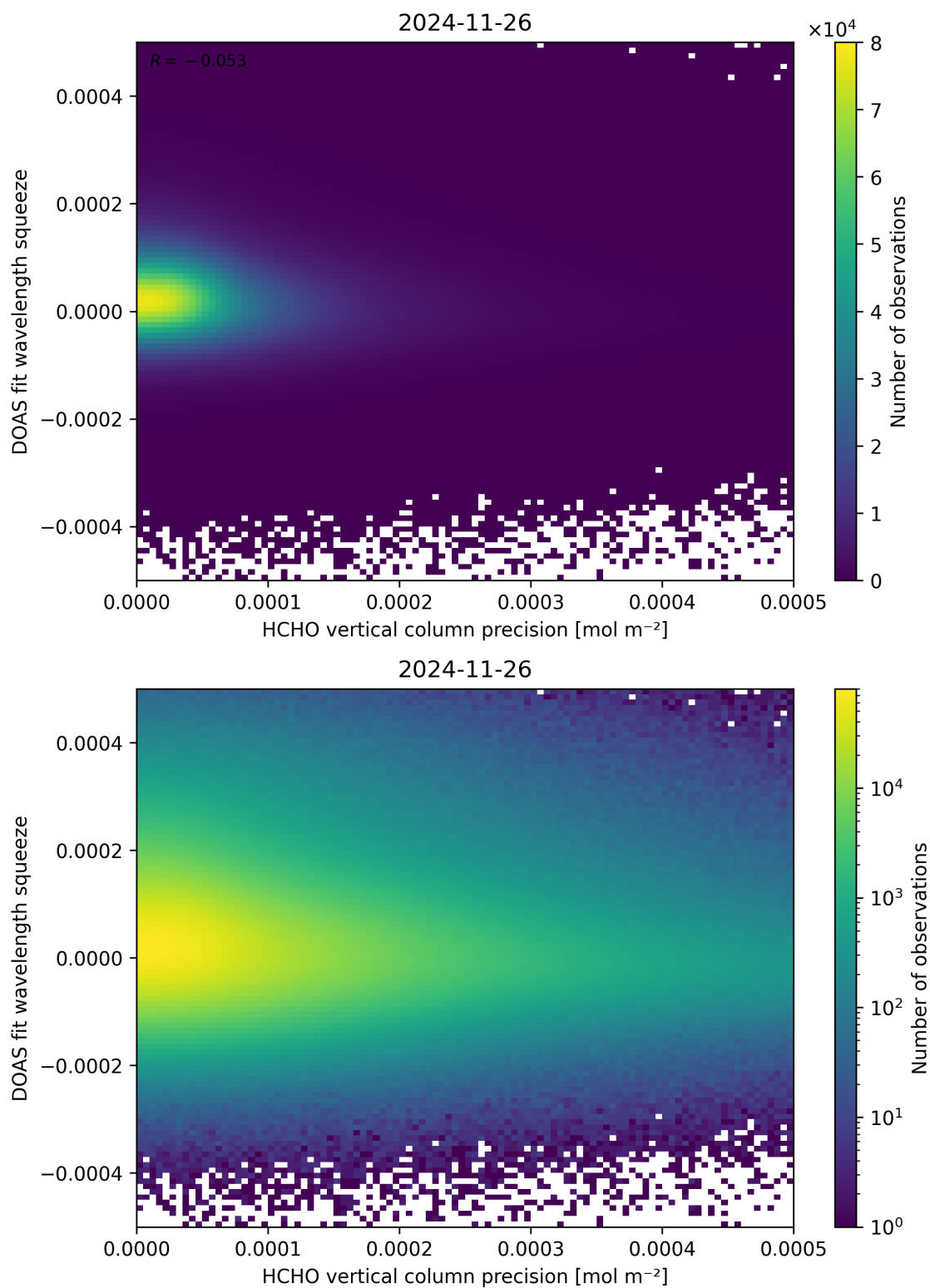
Figure 138: Scatter density plot of “HCHO vertical column precision” against “DOAS fit wavelength squeeze” for 2024-11-25 to 2024-11-27.
