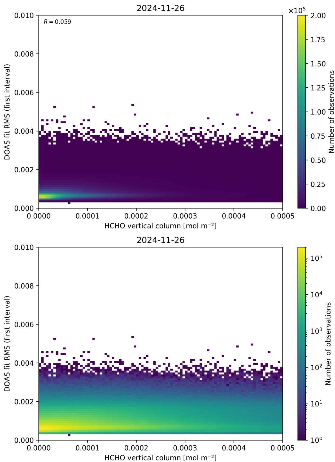
Figure 123: Scatter density plot of “HCHO vertical column” against “DOAS fit RMS (first interval)” for 2024-11-25 to 2024-11-27.
