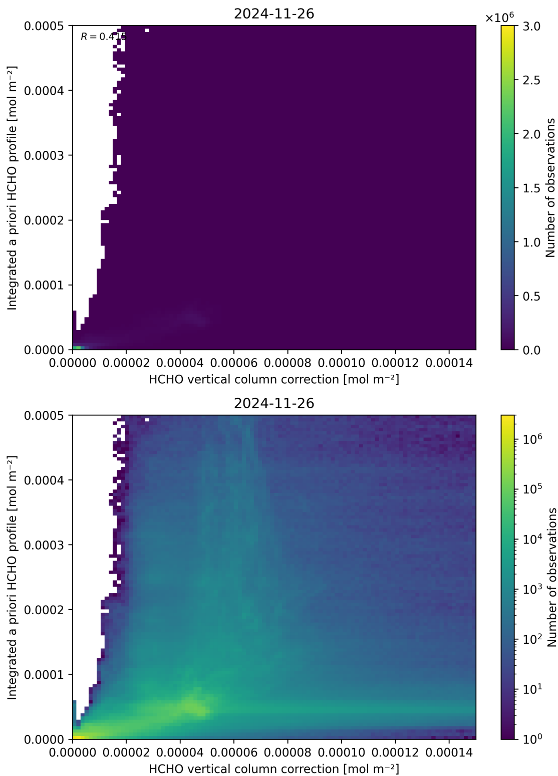
Figure 122: Scatter density plot of “HCHO vertical column correction” against “Integrated a priori HCHO profile” for 2024-11-25 to 2024-11-27.
