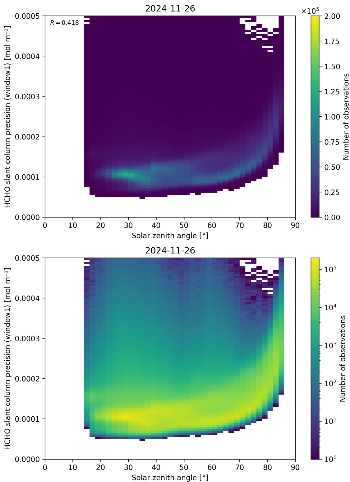
Figure 174: Scatter density plot of “Solar zenith angle” against “HCHO slant column precision (window1)” for 2024-11-25 to 2024-11-27.
