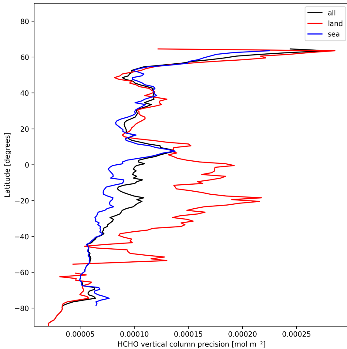
Figure 22: Zonal average of “HCHO vertical column precision” for 2024-11-25 to 2024-11-27.
