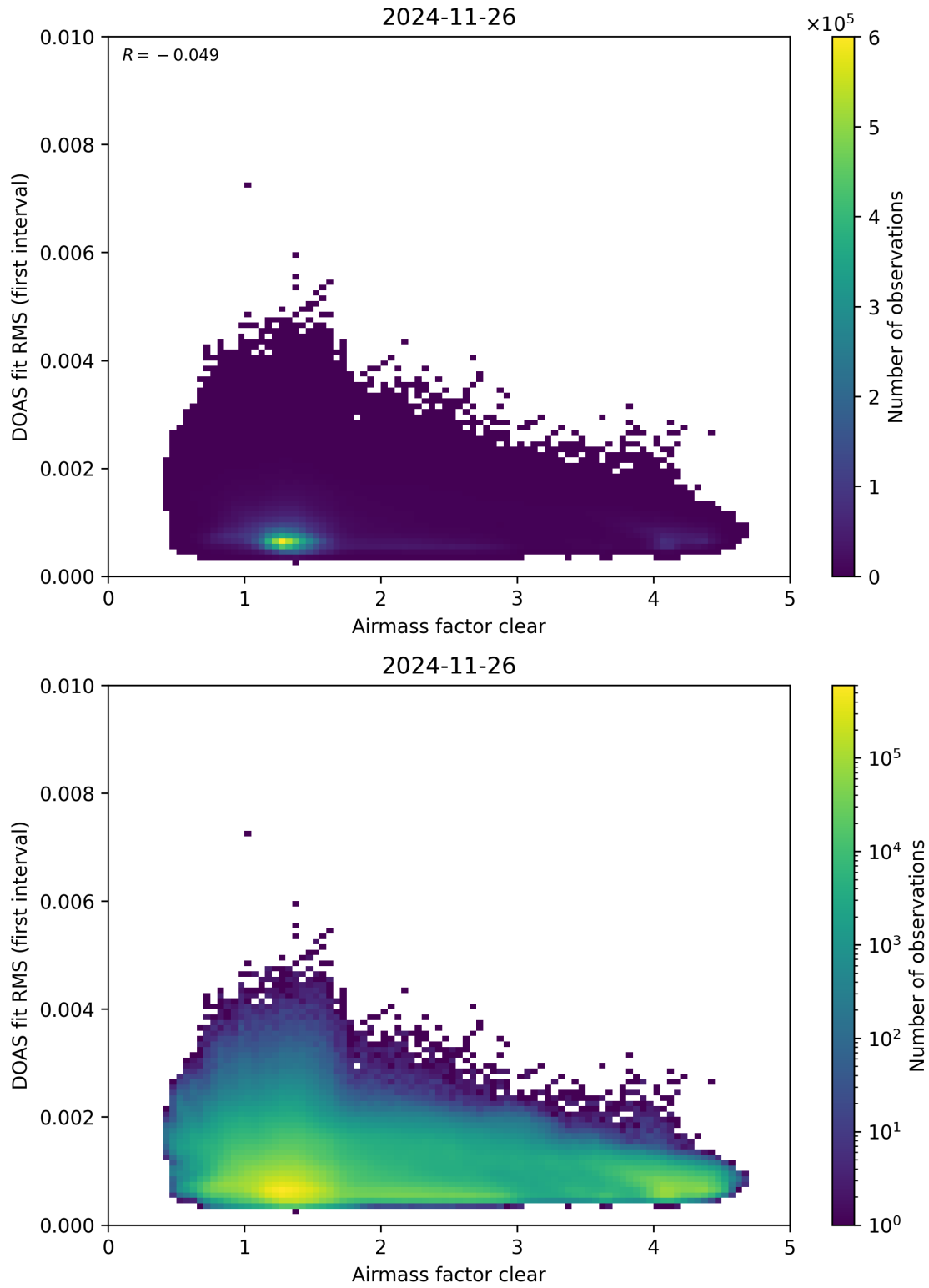
Figure 71: Scatter density plot of “Airmass factor clear” against “DOAS fit RMS (first interval)” for 2024-11-25 to 2024-11-27.
