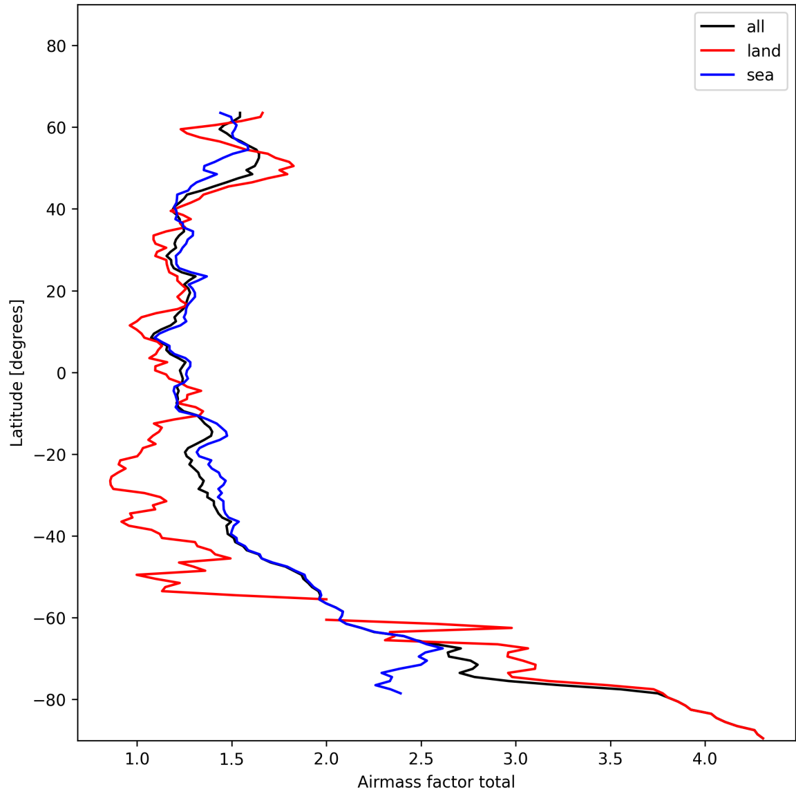
Figure 26: Zonal average of “Airmass factor total” for 2024-11-26 to 2024-11-28.
