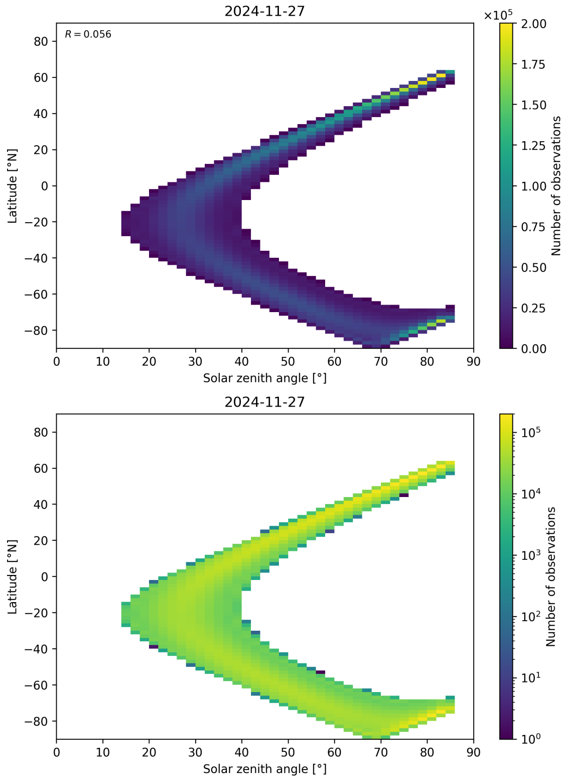
Figure 181: Scatter density plot of “Solar zenith angle” against “Latitude” for 2024-11-26 to 2024-11-28.
