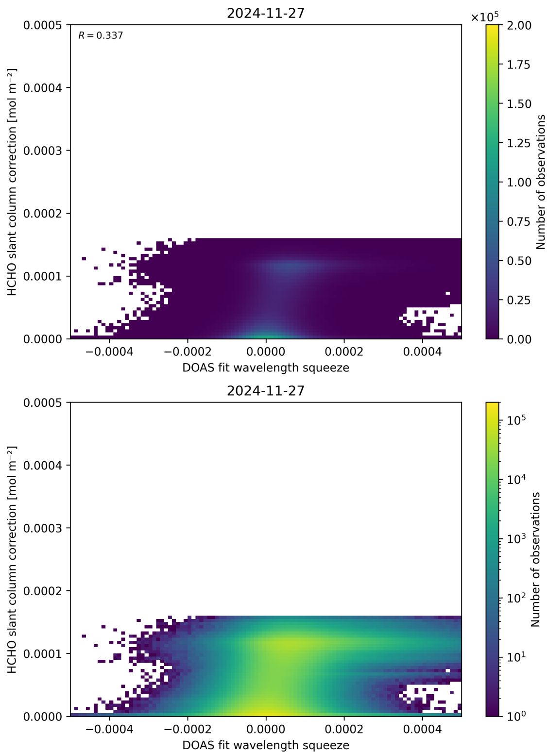
Figure 70: Scatter density plot of “DOAS fit wavelength squeeze” against “HCHO slant column correction” for 2024-11-26 to 2024-11-28.
