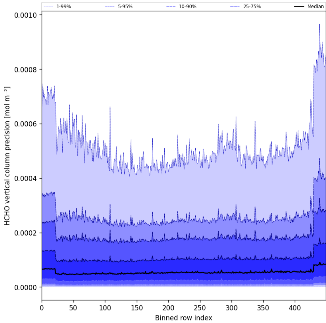
Figure 50: Along track statistics of “HCHO vertical column precision” for 2024-11-26 to 2024-11-28
