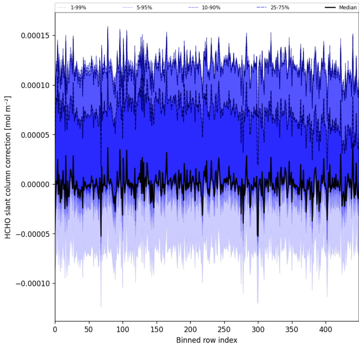
Figure 61: Along track statistics of “HCHO slant column correction” for 2024-11-26 to 2024-11-28
