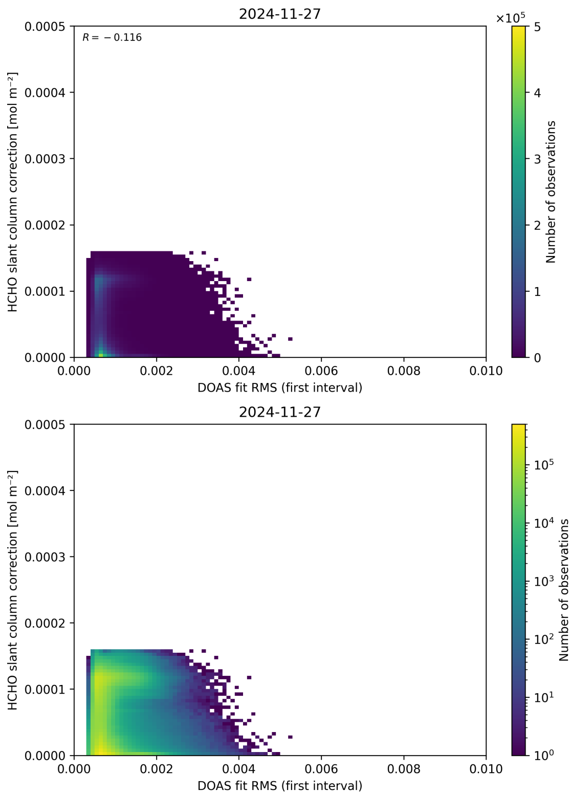
Figure 63: Scatter density plot of “DOAS fit RMS (first interval)” against “HCHO slant column correction” for 2024-11-26 to 2024-11-28.
