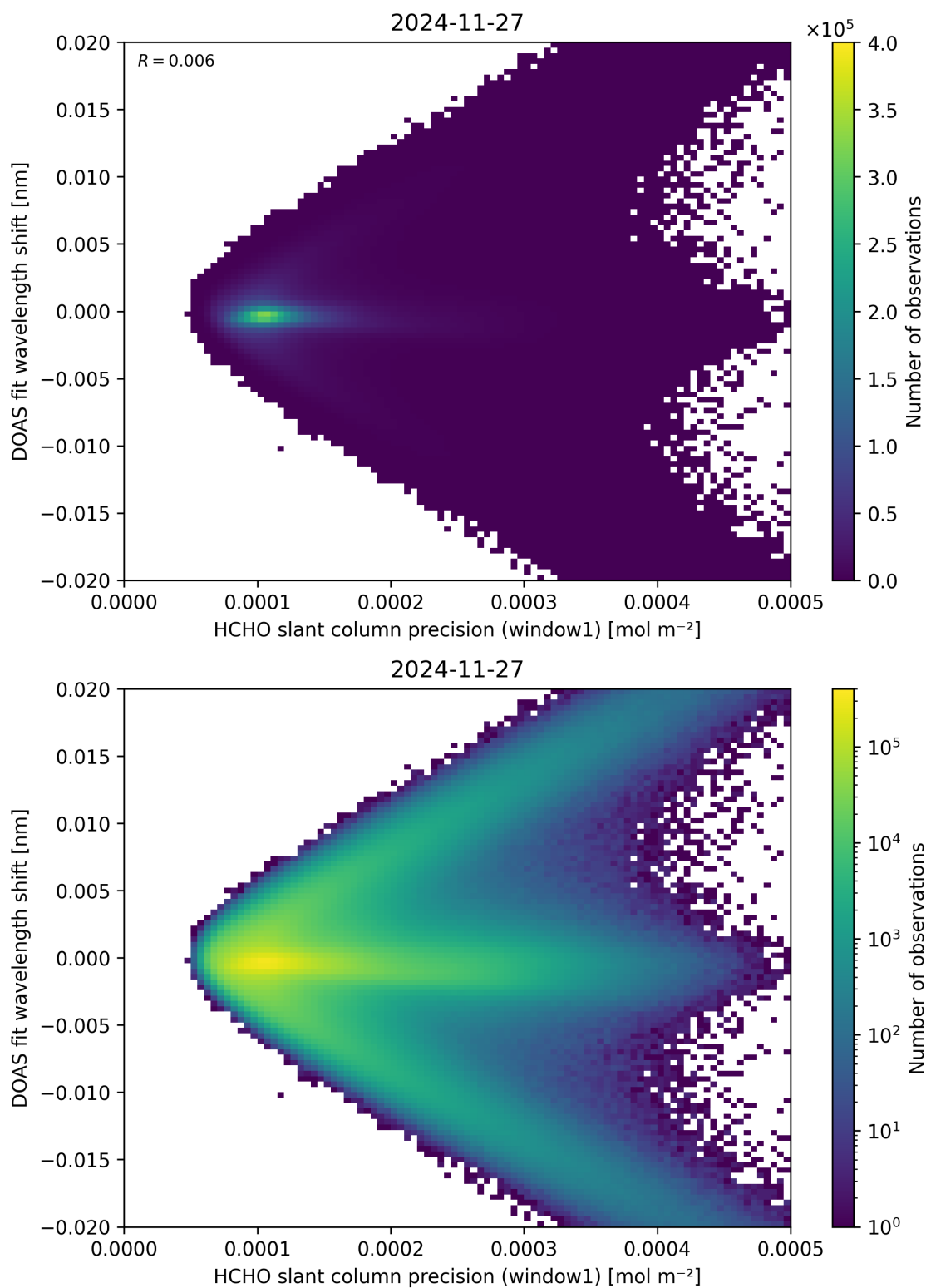
Figure 89: Scatter density plot of “HCHO slant column precision (window1)” against “DOAS fit wavelength shift” for 2024-11-26 to 2024-11-28.
