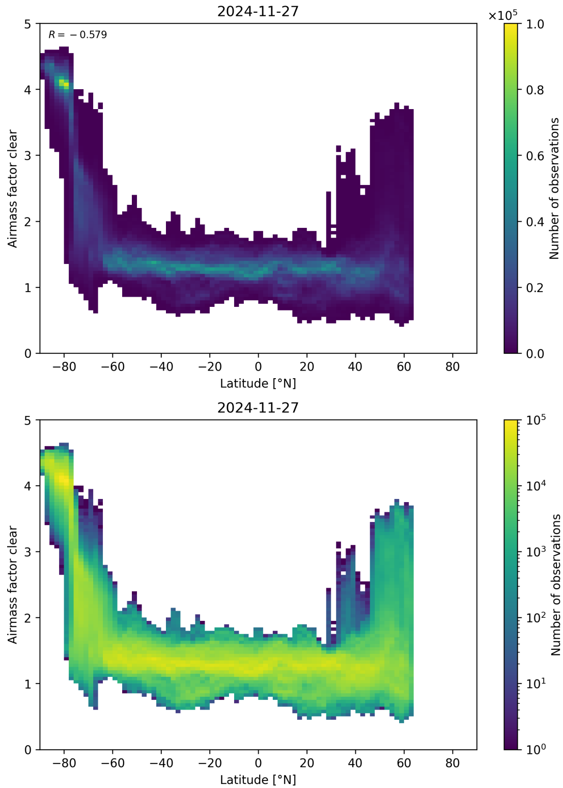
Figure 156: Scatter density plot of “Latitude” against “Airmass factor clear” for 2024-11-26 to 2024-11-28.
