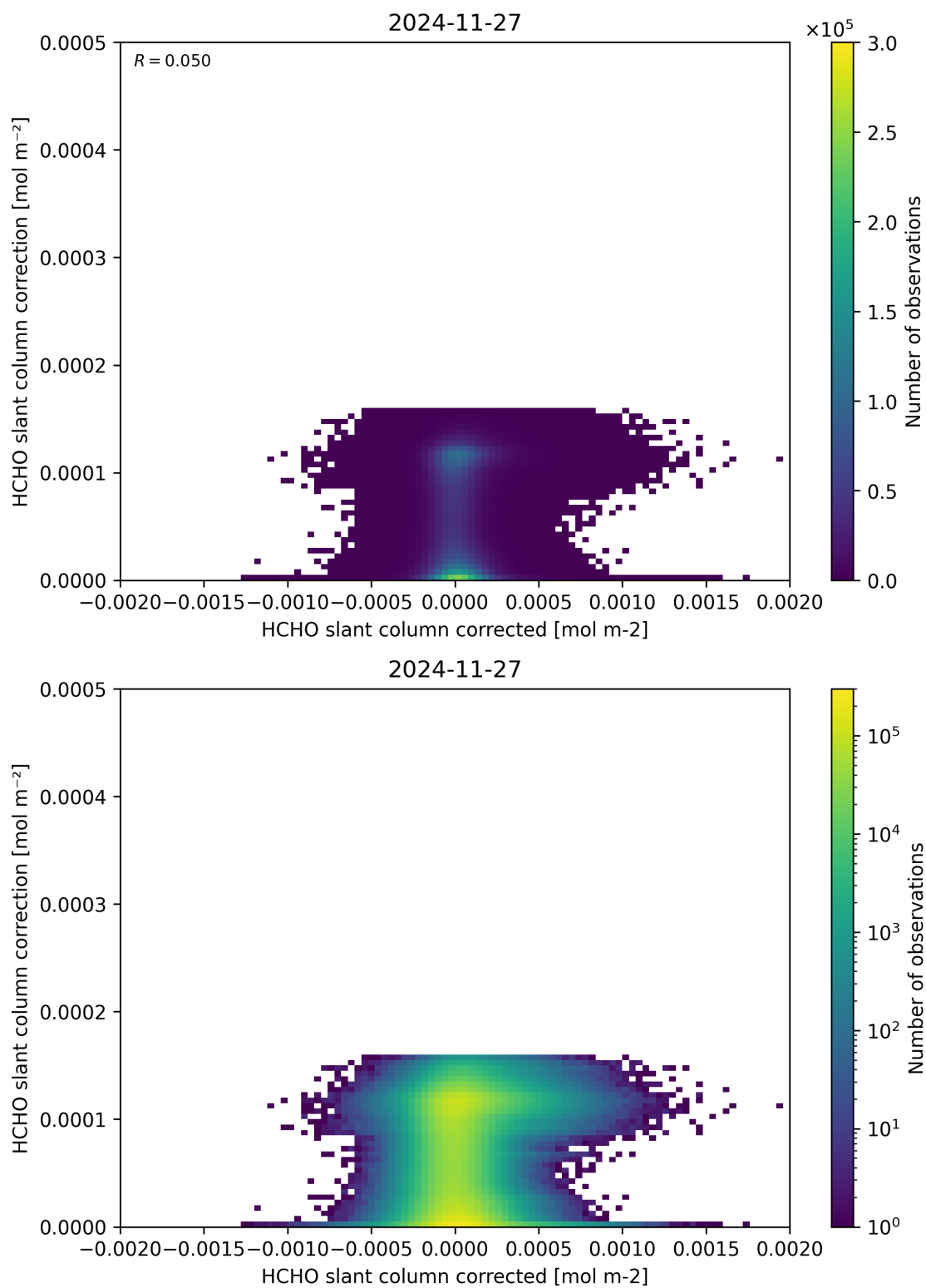
Figure 77: Scatter density plot of “HCHO slant column corrected” against “HCHO slant column correction” for 2024-11-26 to 2024-11-28.
