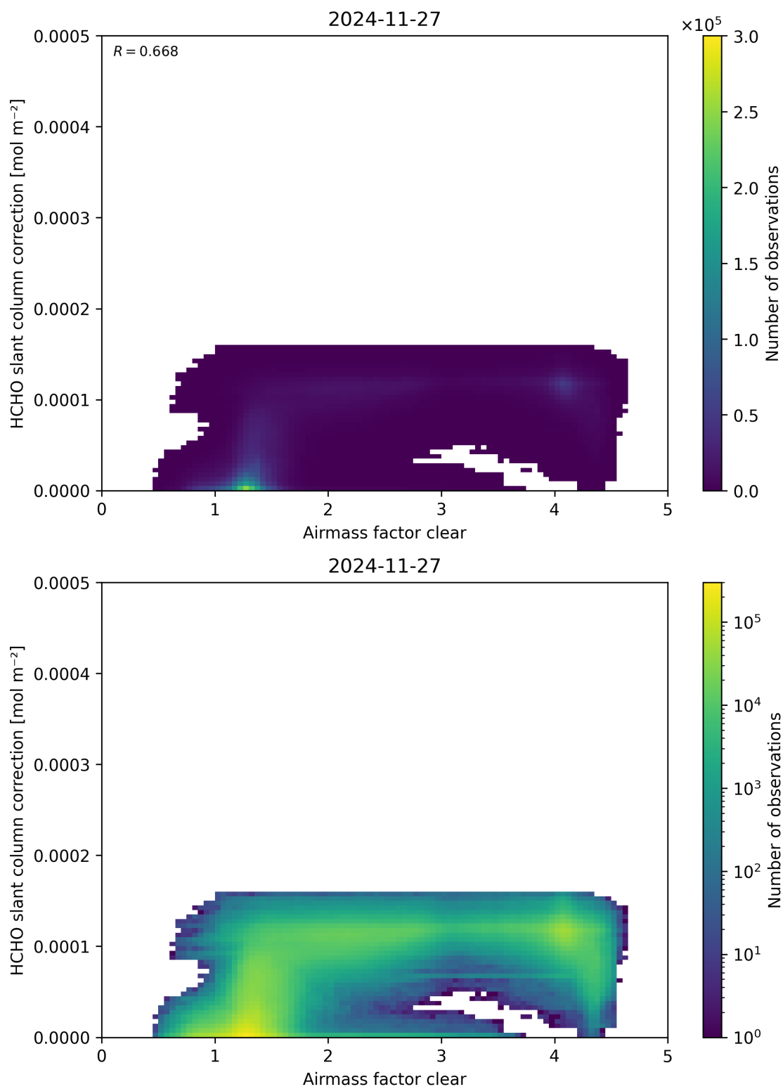
Figure 75: Scatter density plot of “Airmass factor clear” against “HCHO slant column correction” for 2024-11-26 to 2024-11-28.
