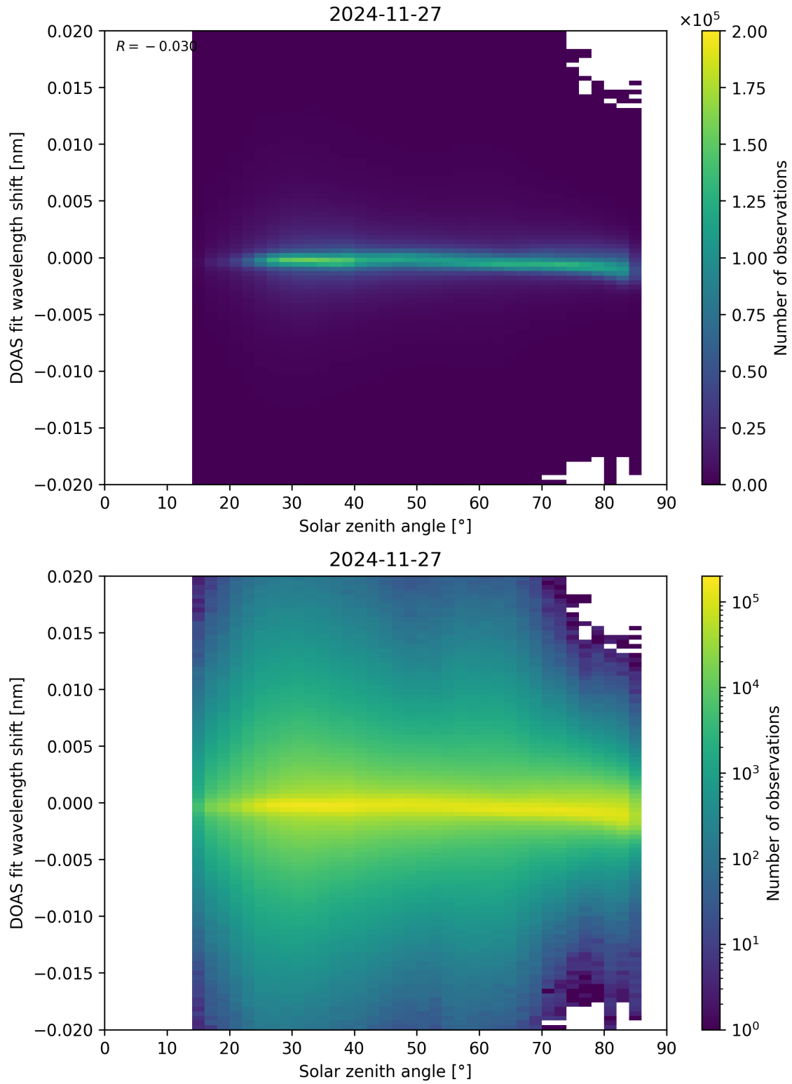
Figure 168: Scatter density plot of “Solar zenith angle” against “DOAS fit wavelength shift” for 2024-11-26 to 2024-11-28.
