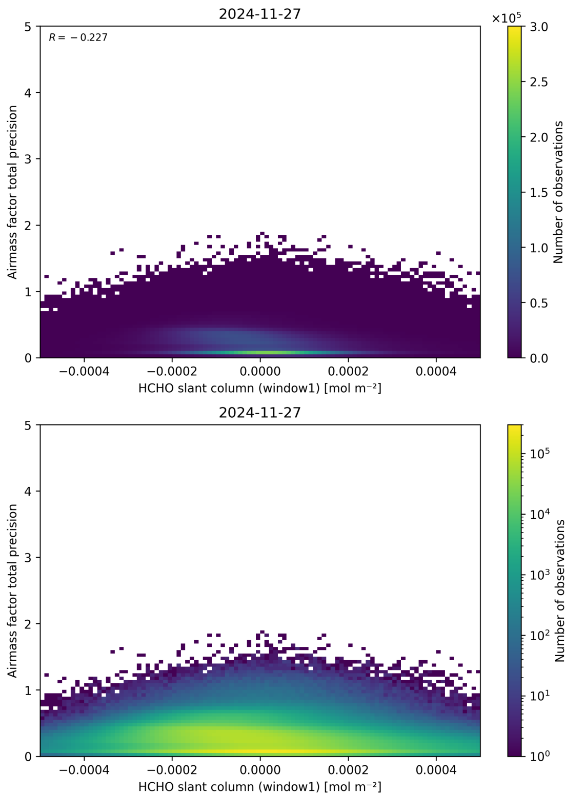
Figure 86: Scatter density plot of “HCHO slant column (window1)” against “Airmass factor total precision” for 2024-11-26 to 2024-11-28.
