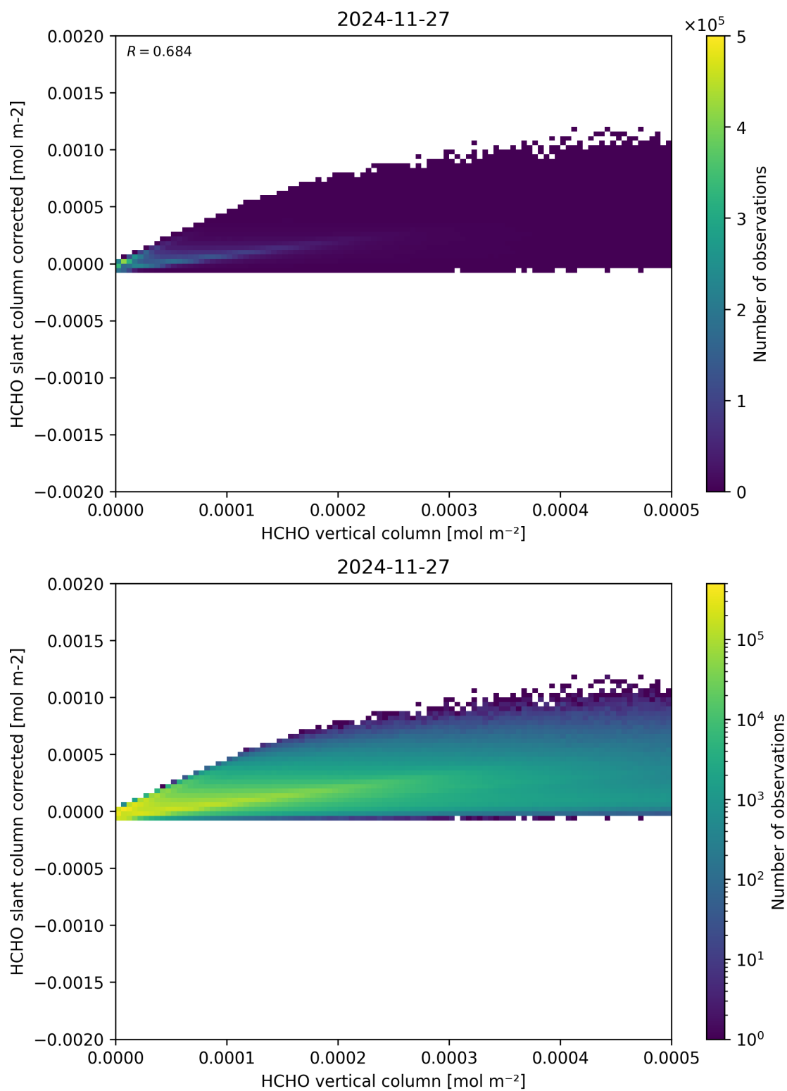
Figure 127: Scatter density plot of “HCHO vertical column” against “HCHO slant column corrected” for 2024-11-26 to 2024-11-28.
