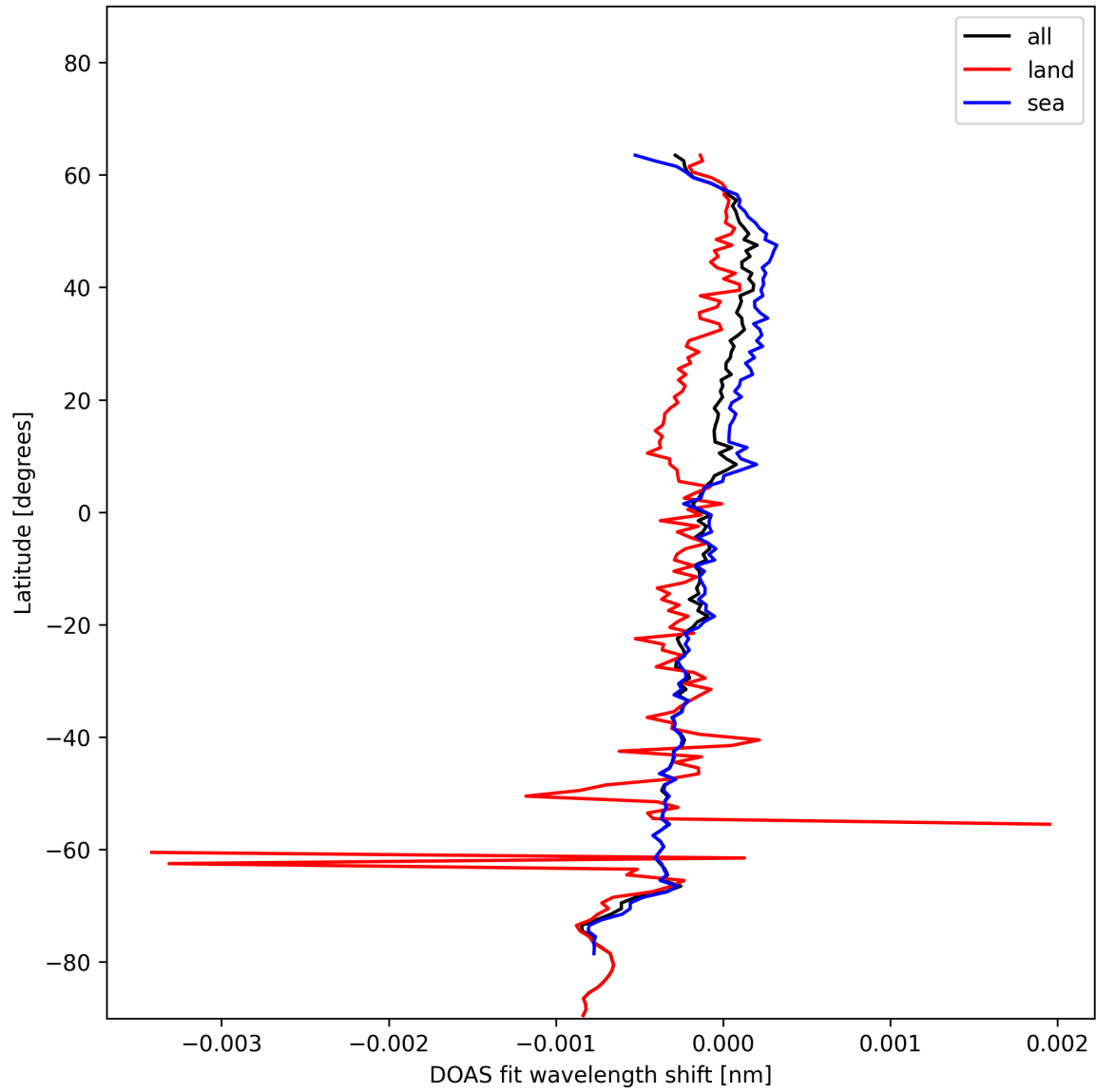
Figure 30: Zonal average of “DOAS fit wavelength shift” for 2024-11-26 to 2024-11-28.
