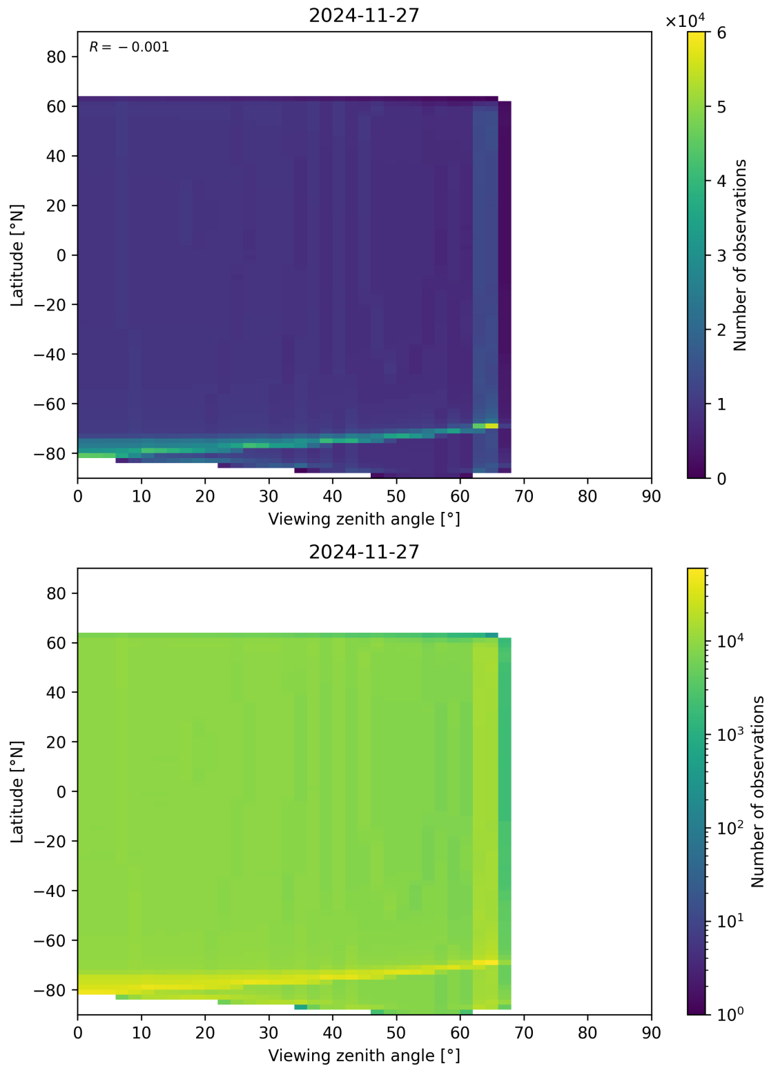
Figure 196: Scatter density plot of “Viewing zenith angle” against “Latitude” for 2024-11-26 to 2024-11-28.
