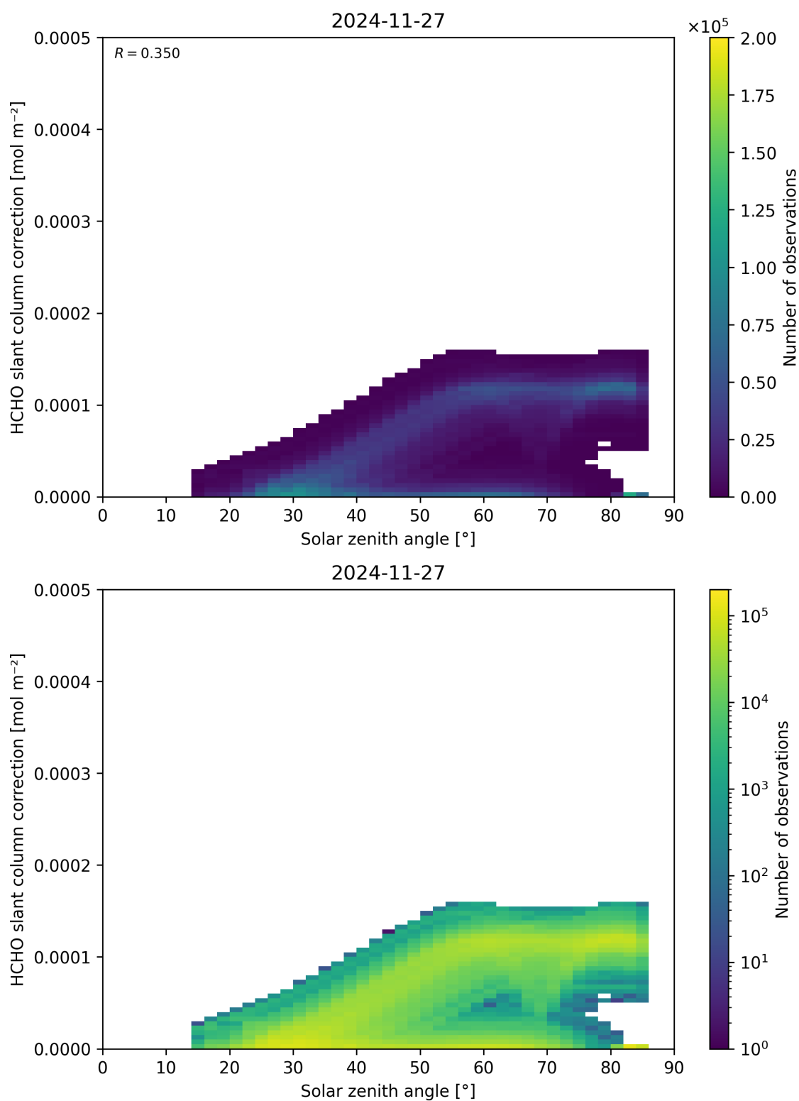
Figure 172: Scatter density plot of “Solar zenith angle” against “HCHO slant column correction” for 2024-11-26 to 2024-11-28.
