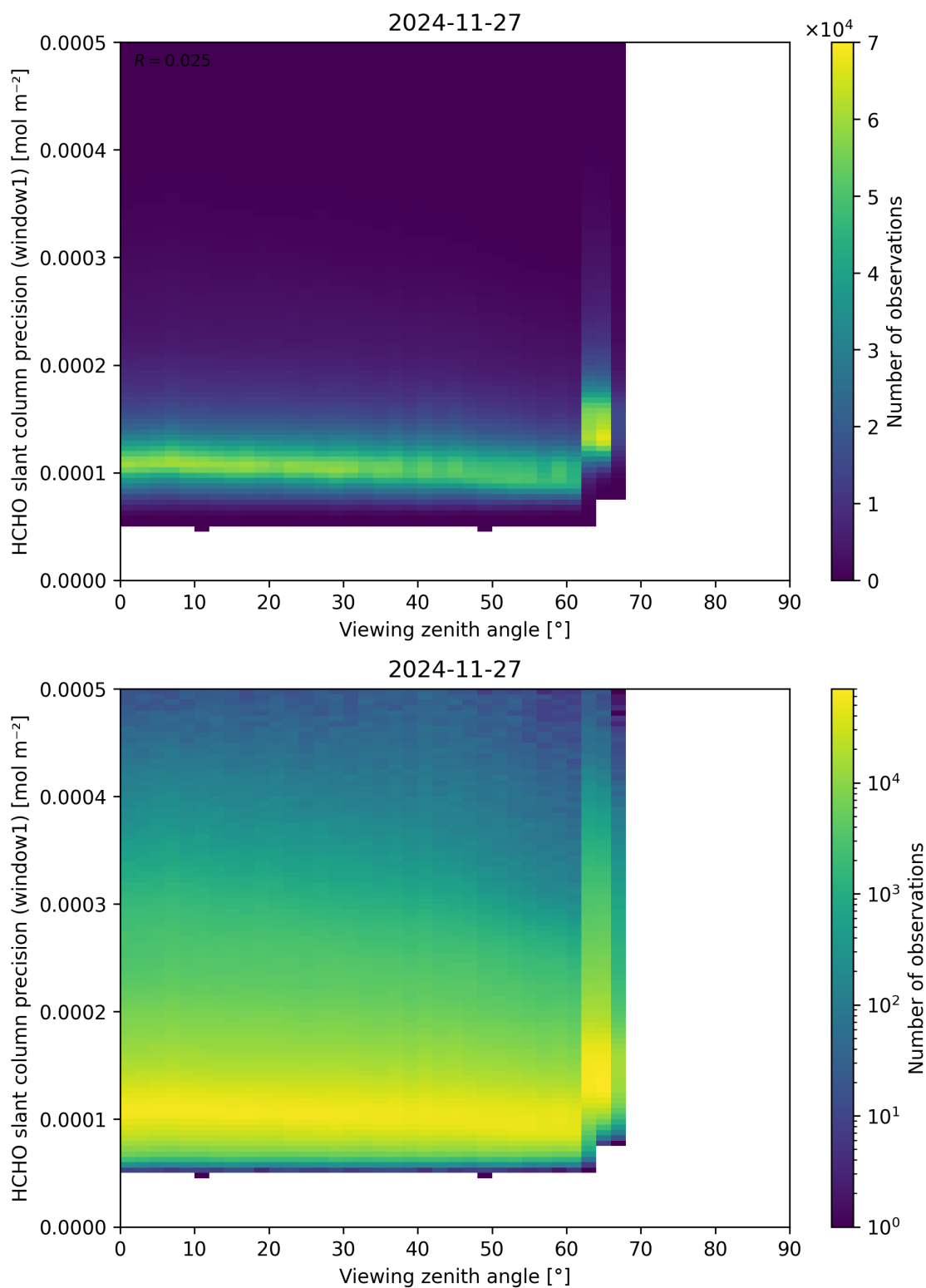
Figure 189: Scatter density plot of “Viewing zenith angle” against “HCHO slant column precision (window1)” for 2024-11-26 to 2024-11-28.
