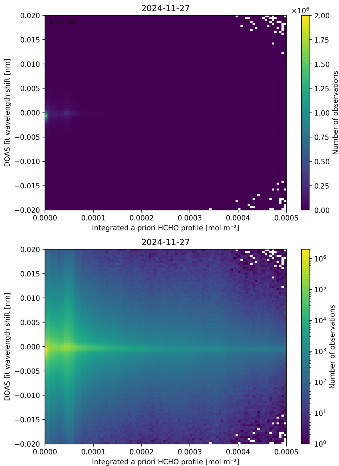
Figure 149: Scatter density plot of “Integrated a priori HCHO profile” against “DOAS fit wavelength shift” for 2024-11-26 to 2024-11-28.
