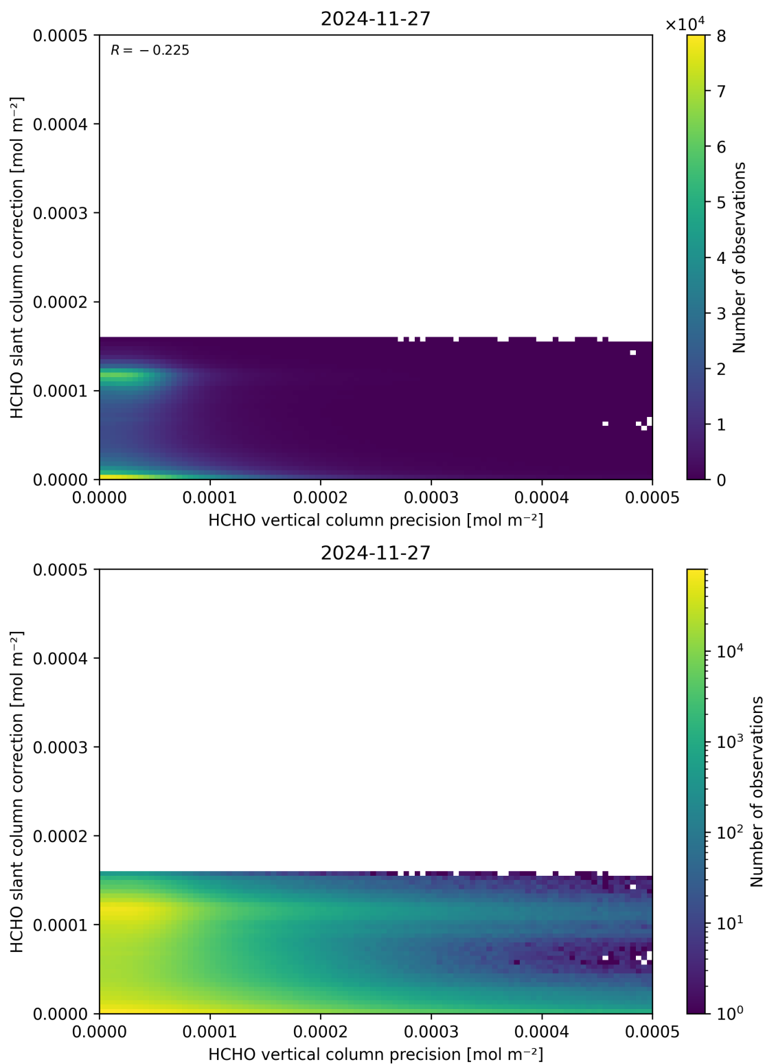
Figure 141: Scatter density plot of “HCHO vertical column precision” against “HCHO slant column correction” for 2024-11-26 to 2024-11-28.
