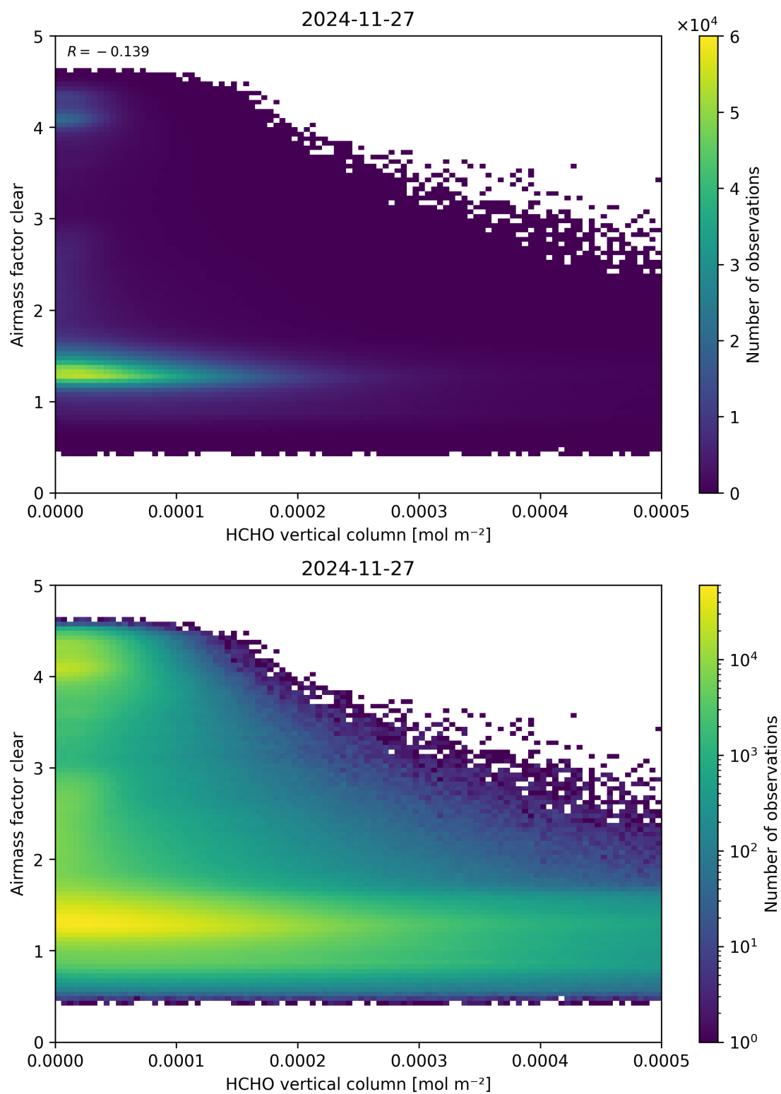
Figure 126: Scatter density plot of “HCHO vertical column” against “Airmass factor clear” for 2024-11-26 to 2024-11-28.
