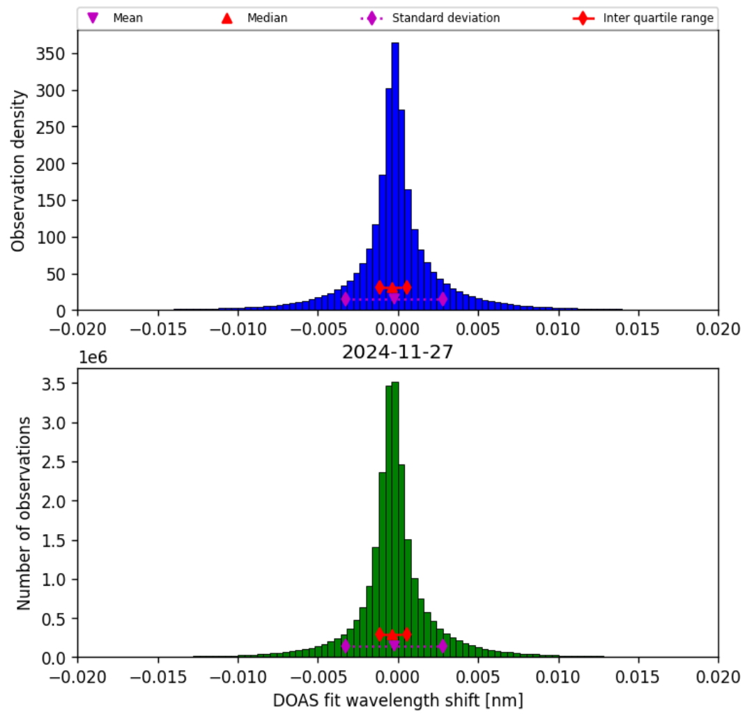
Figure 44: Histogram of “DOAS fit wavelength shift” for 2024-11-26 to 2024-11-28
