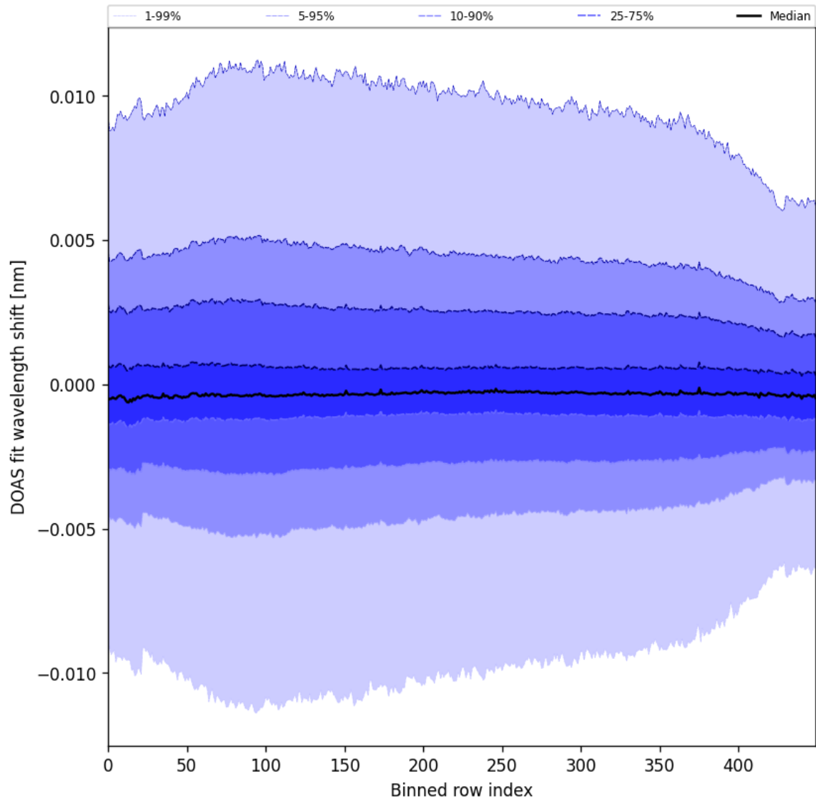
Figure 58: Along track statistics of “DOAS fit wavelength shift” for 2024-11-26 to 2024-11-28
