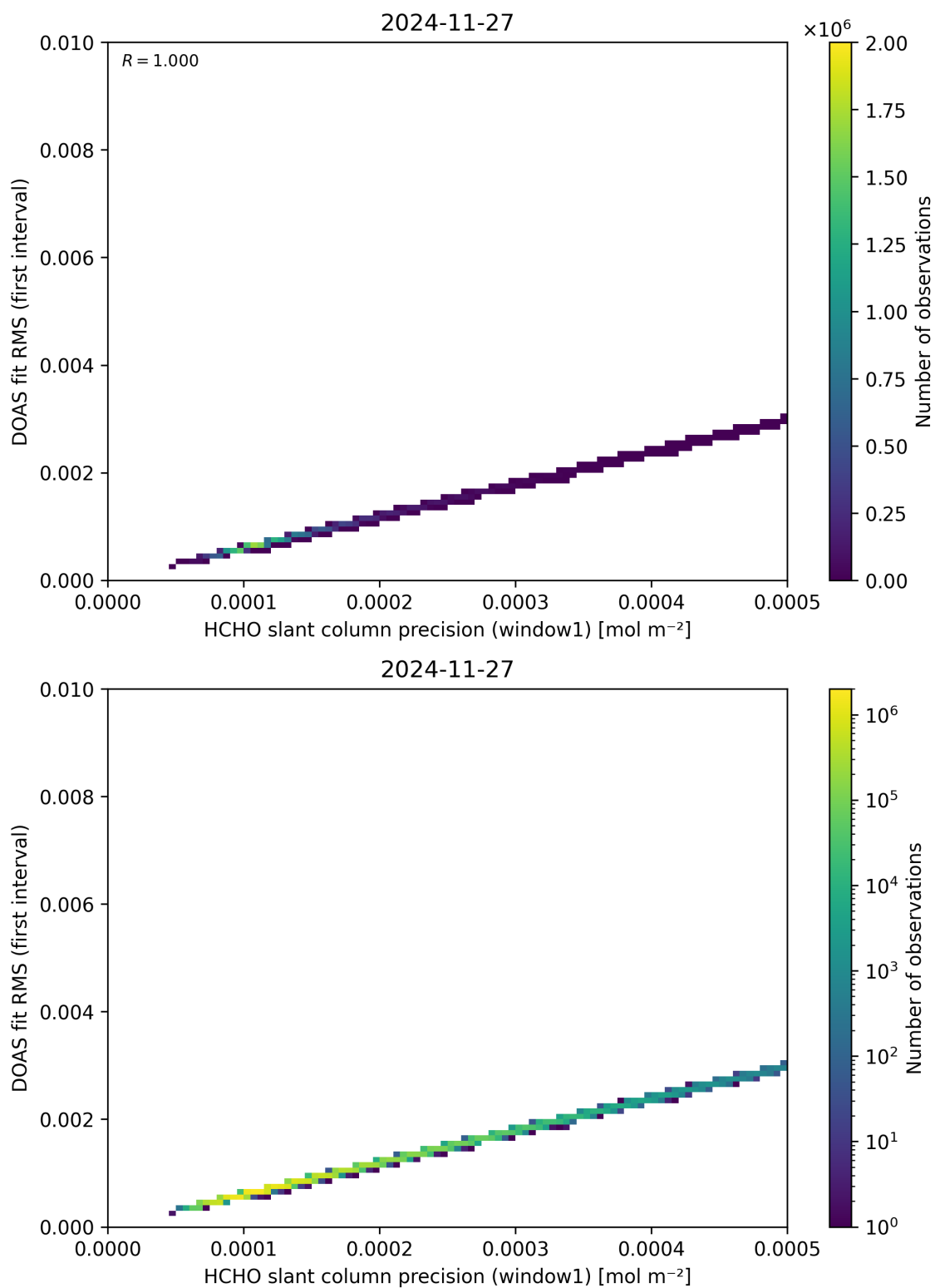
Figure 88: Scatter density plot of “HCHO slant column precision (window1)” against “DOAS fit RMS (first interval)” for 2024-11-26 to 2024-11-28.
