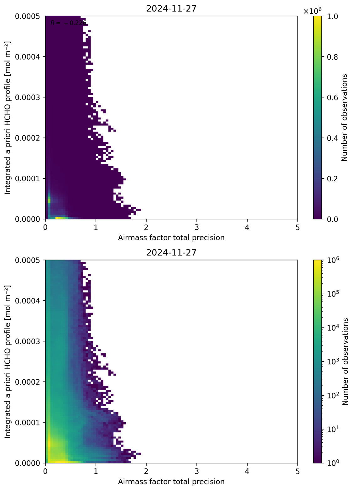
Figure 111: Scatter density plot of “Airmass factor total precision” against “Integrated a priori HCHO profile” for 2024-11-26 to 2024-11-28.
