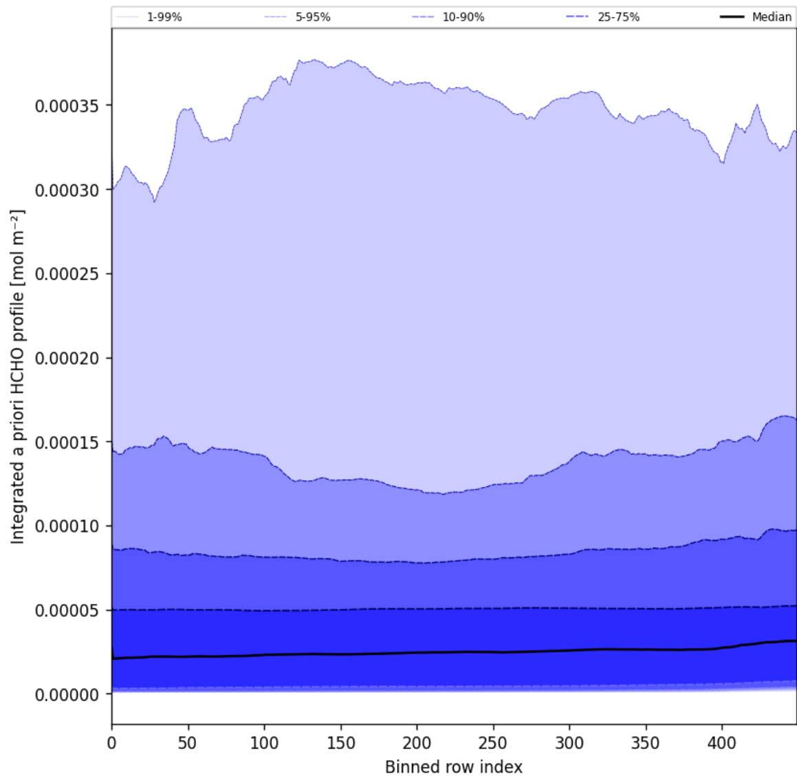
Figure 57: Along track statistics of "Integrated a priori HCHO profile" for 2024-11-26 to 2024-11-28
