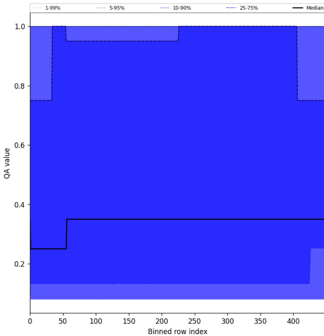
Figure 48: Along track statistics of “QA value” for 2024-11-26 to 2024-11-28
