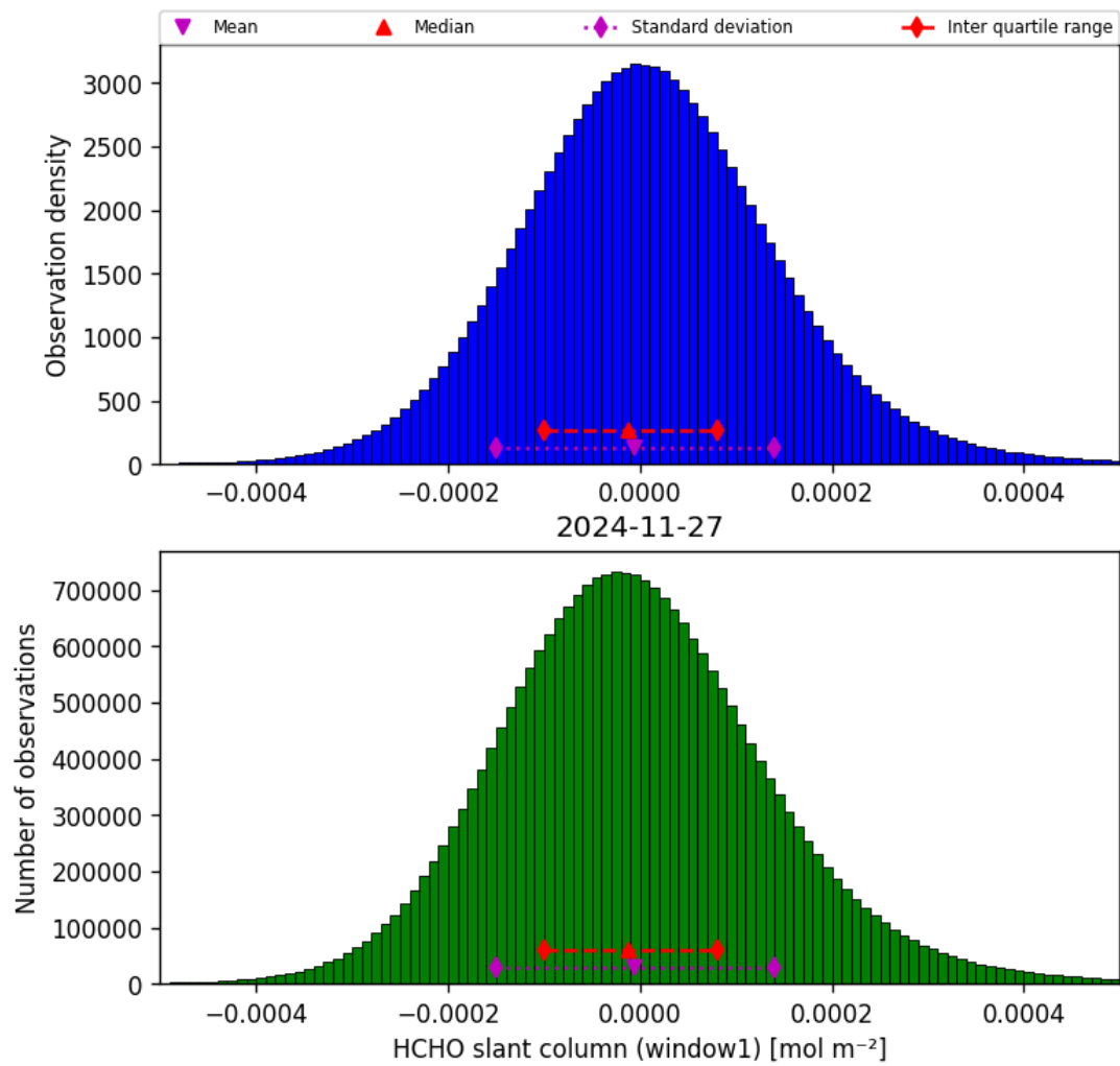
Figure 38: Histogram of “HCHO slant column (window1)” for 2024-11-26 to 2024-11-28
