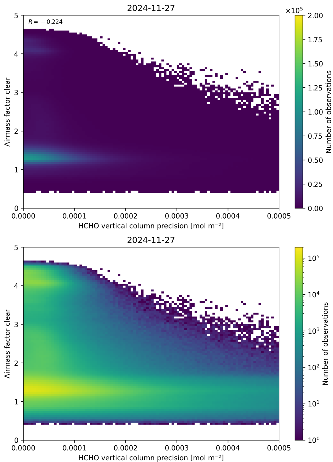
Figure 139: Scatter density plot of “HCHO vertical column precision” against “Airmass factor clear” for 2024-11-26 to 2024-11-28.
