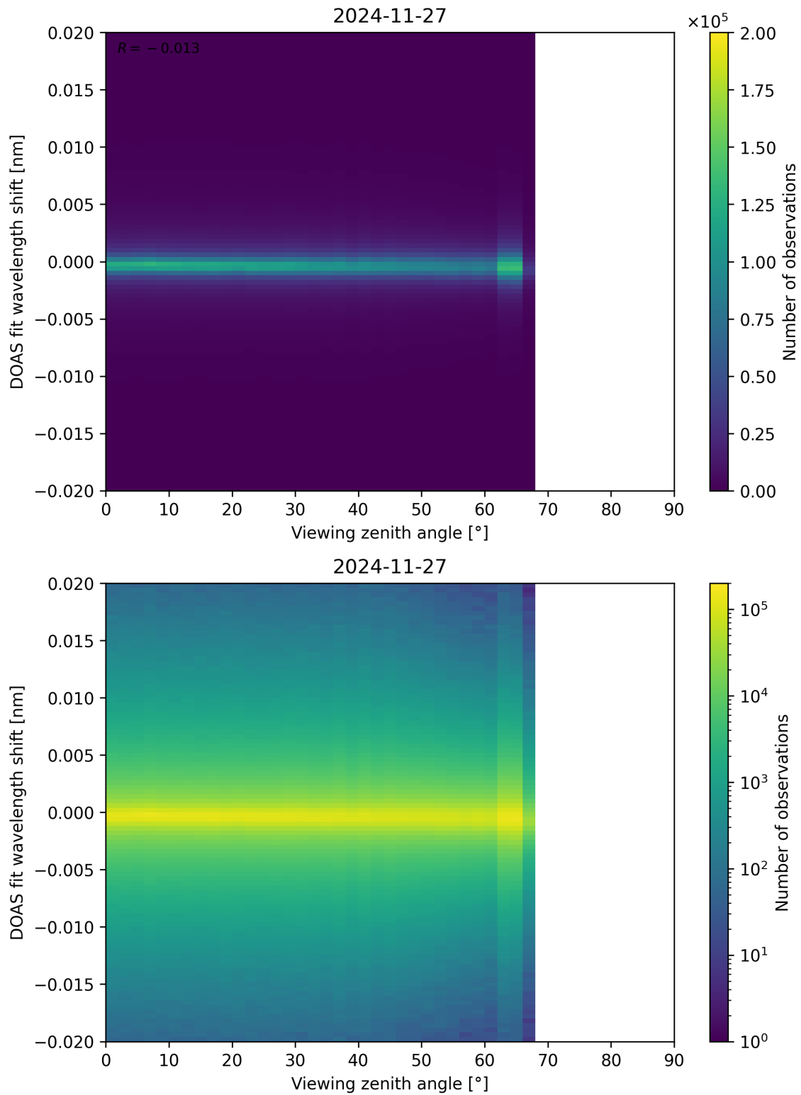
Figure 183: Scatter density plot of “Viewing zenith angle” against “DOAS fit wavelength shift” for 2024-11-26 to 2024-11-28.
