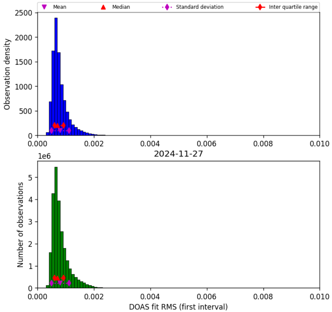
Figure 46: Histogram of “DOAS fit RMS (first interval)” for 2024-11-26 to 2024-11-28
