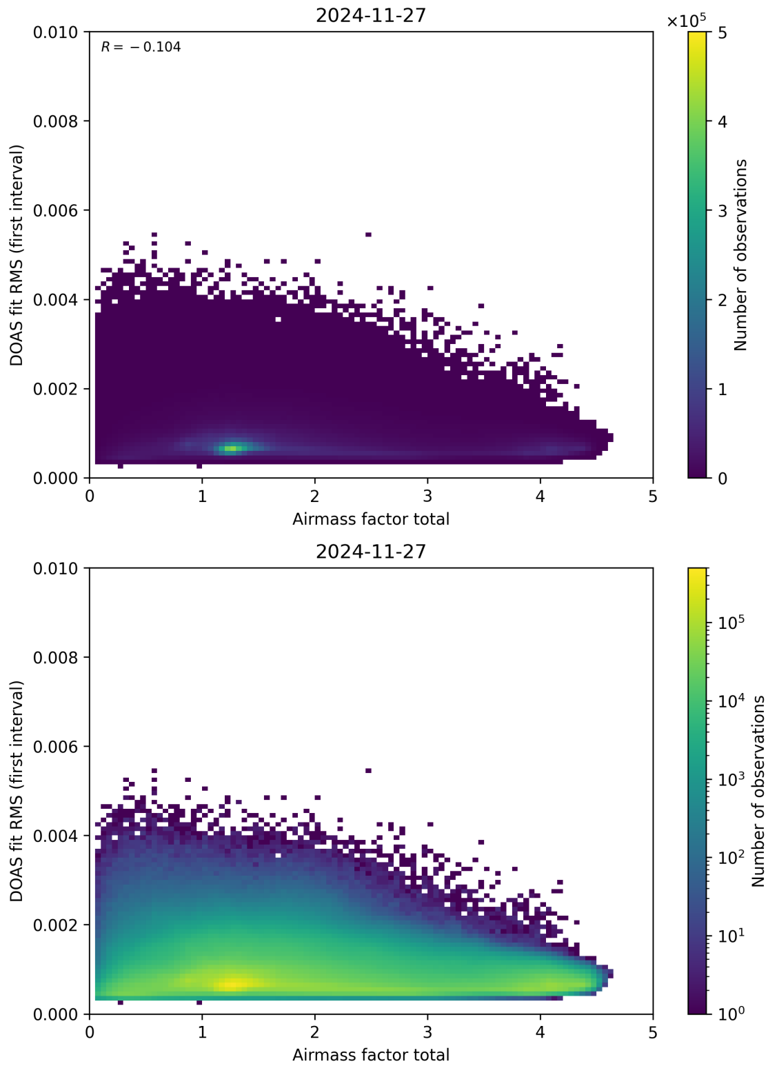
Figure 97: Scatter density plot of “Airmass factor total” against “DOAS fit RMS (first interval)” for 2024-11-26 to 2024-11-28.
