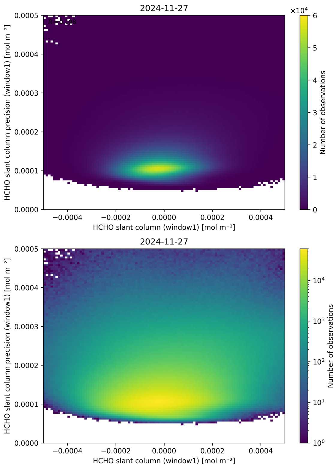
Figure 84: Scatter density plot of “HCHO slant column (window1)” against “HCHO slant column precision (window1)” for 2024-11-26 to 2024-11-28.
