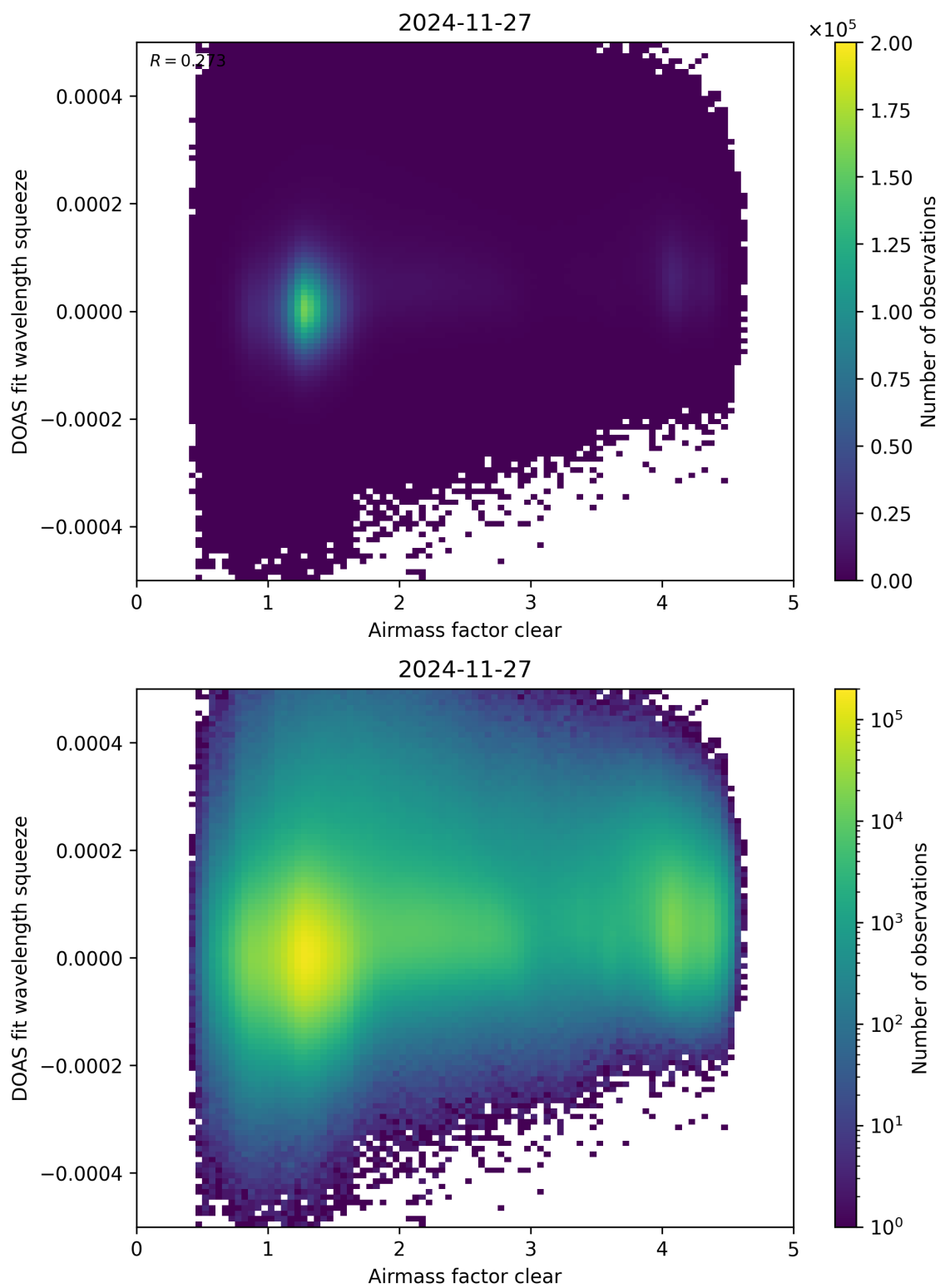
Figure 73: Scatter density plot of “Airmass factor clear” against “DOAS fit wavelength squeeze” for 2024-11-26 to 2024-11-28.
