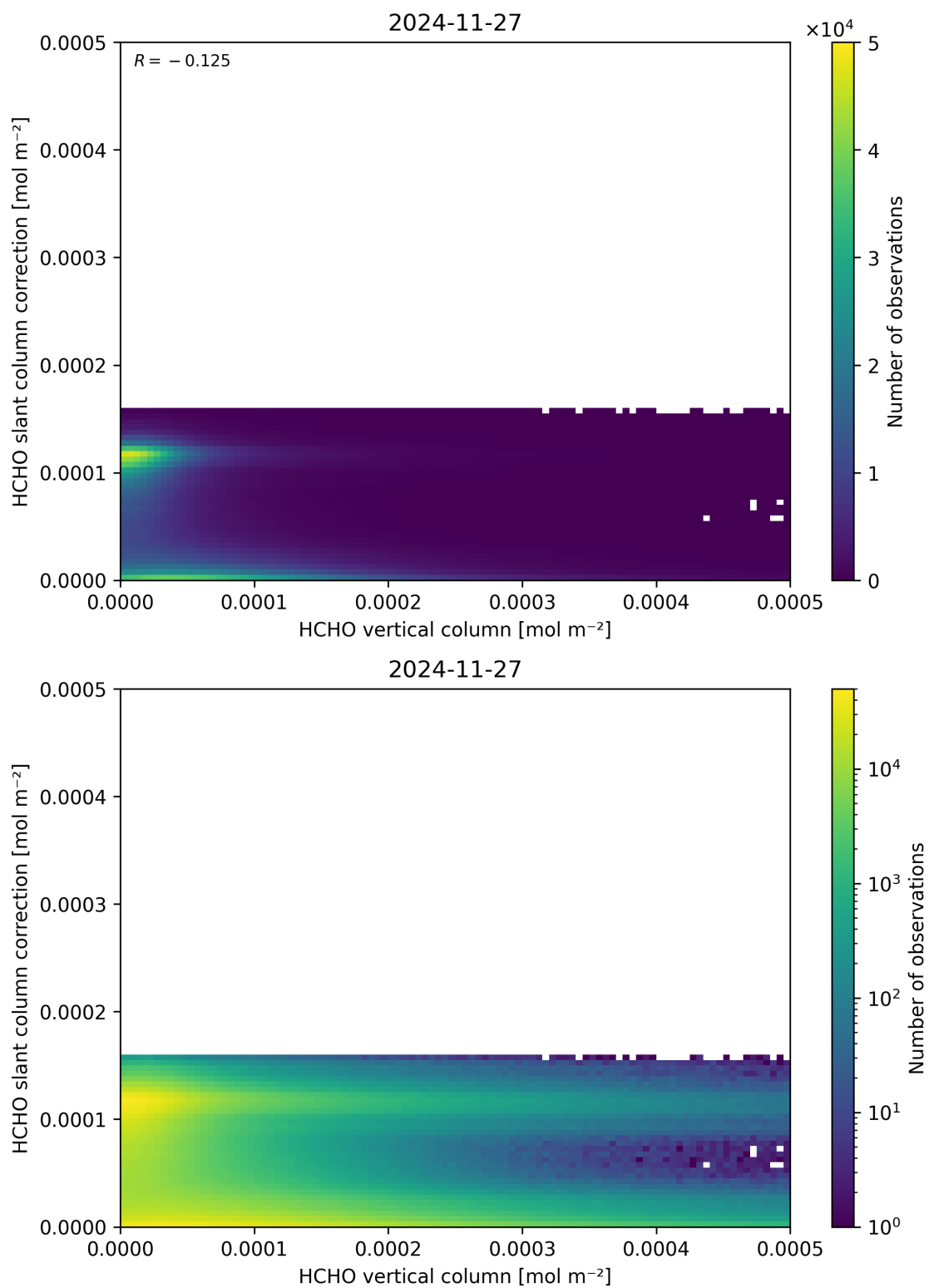
Figure 128: Scatter density plot of “HCHO vertical column” against “HCHO slant column correction” for 2024-11-26 to 2024-11-28.
