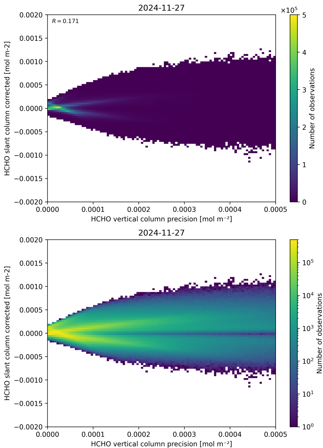
Figure 140: Scatter density plot of “HCHO vertical column precision” against “HCHO slant column corrected” for 2024-11-26 to 2024-11-28.
