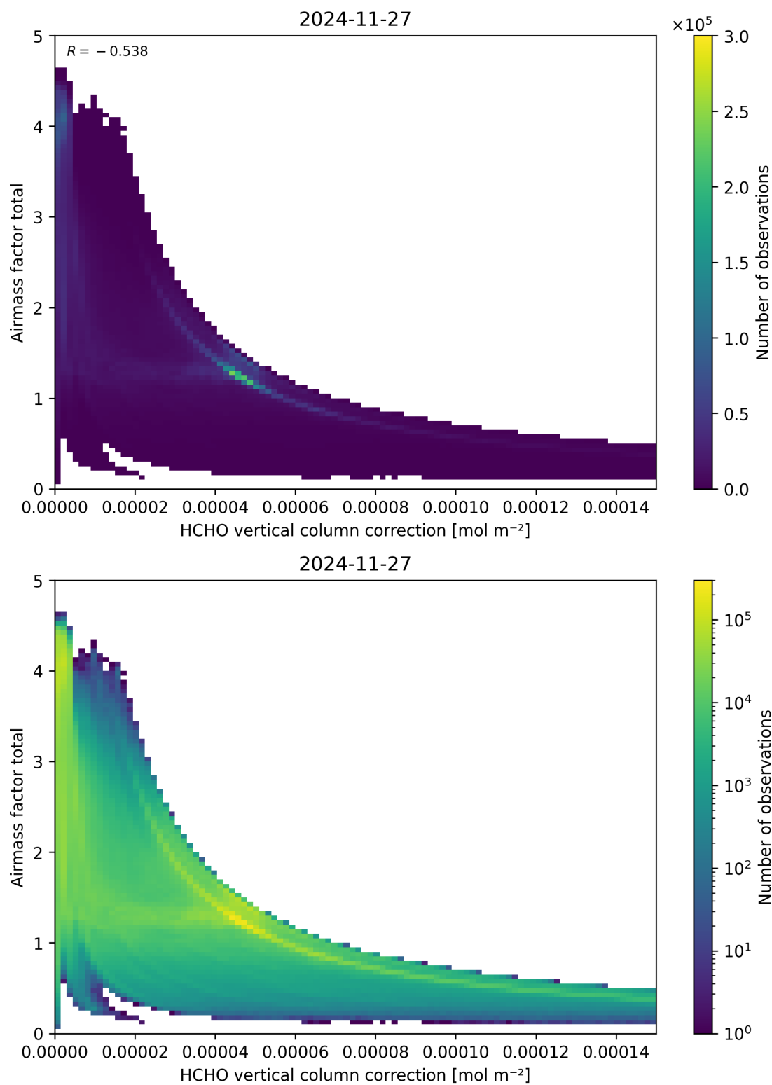
Figure 120: Scatter density plot of “HCHO vertical column correction” against “Airmass factor total” for 2024-11-26 to 2024-11-28.
