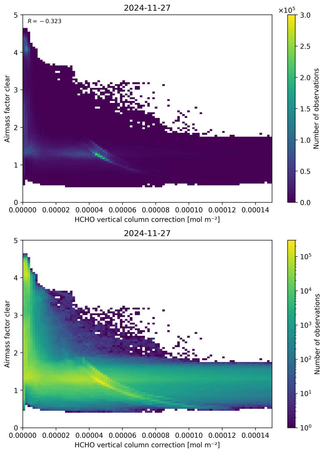
Figure 115: Scatter density plot of “HCHO vertical column correction” against “Airmass factor clear” for 2024-11-26 to 2024-11-28.
