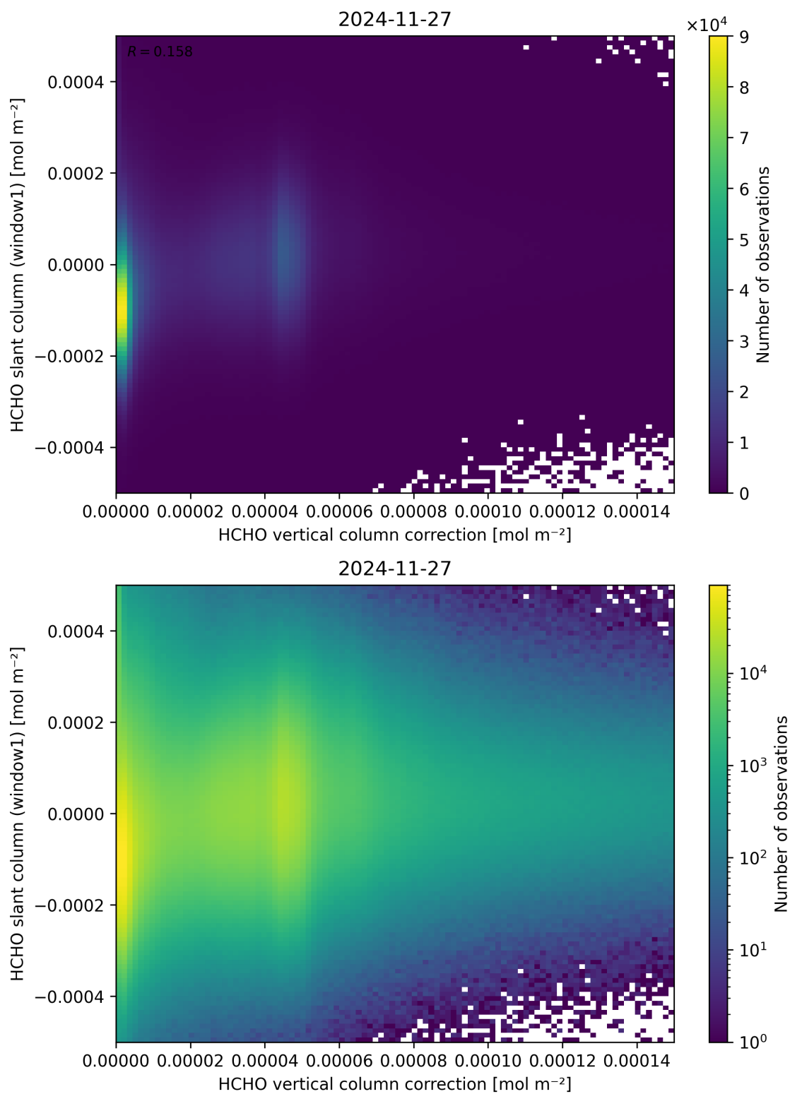
Figure 118: Scatter density plot of “HCHO vertical column correction” against “HCHO slant column (window1)” for 2024-11-26 to 2024-11-28.
