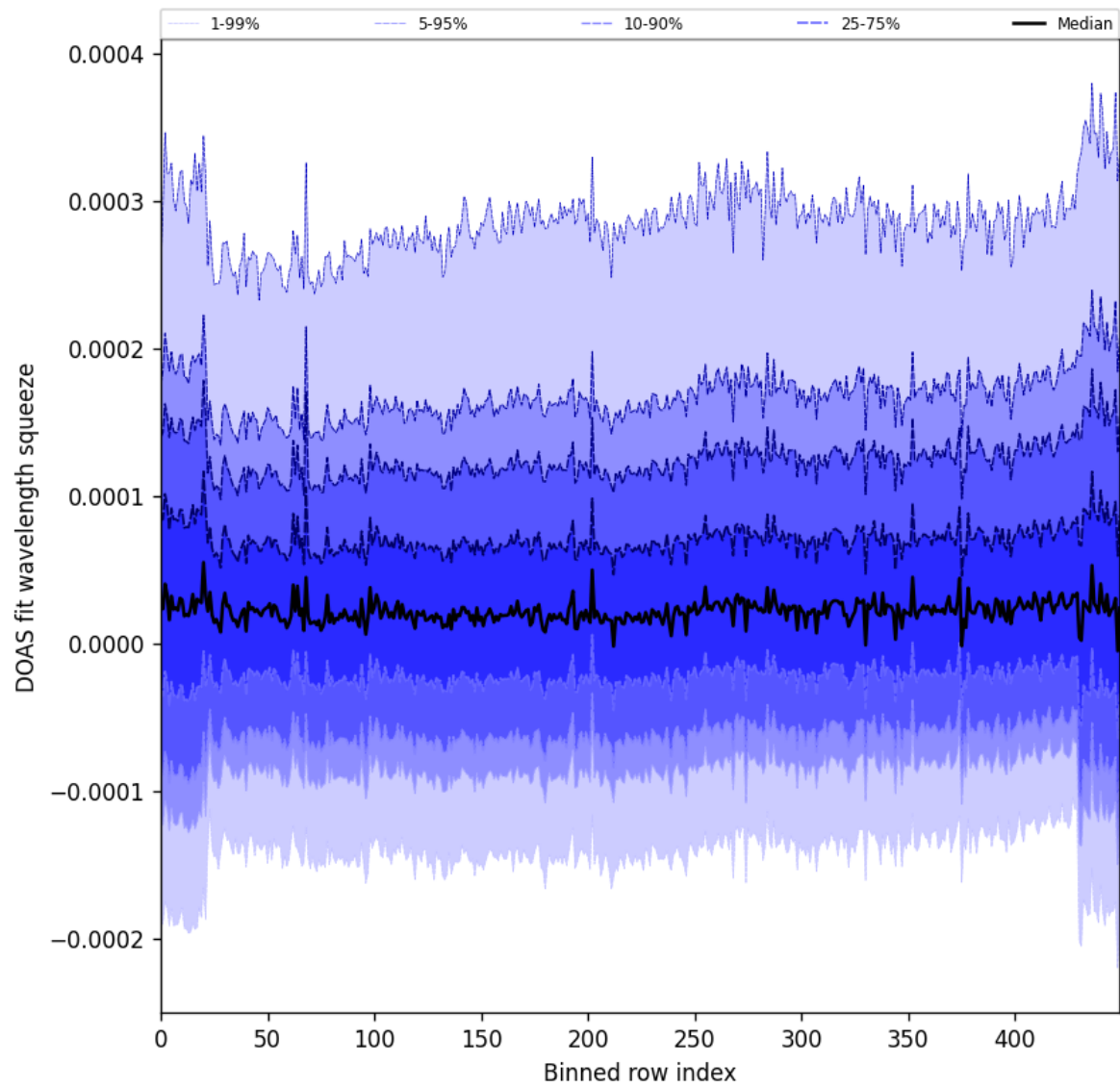
Figure 59: Along track statistics of “DOAS fit wavelength squeeze” for 2024-11-26 to 2024-11-28
