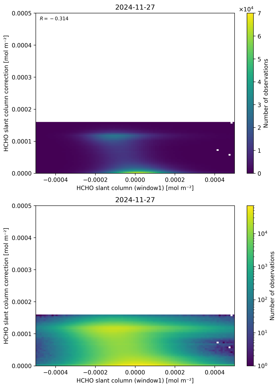
Figure 83: Scatter density plot of “HCHO slant column (window1)” against “HCHO slant column correction” for 2024-11-26 to 2024-11-28.
