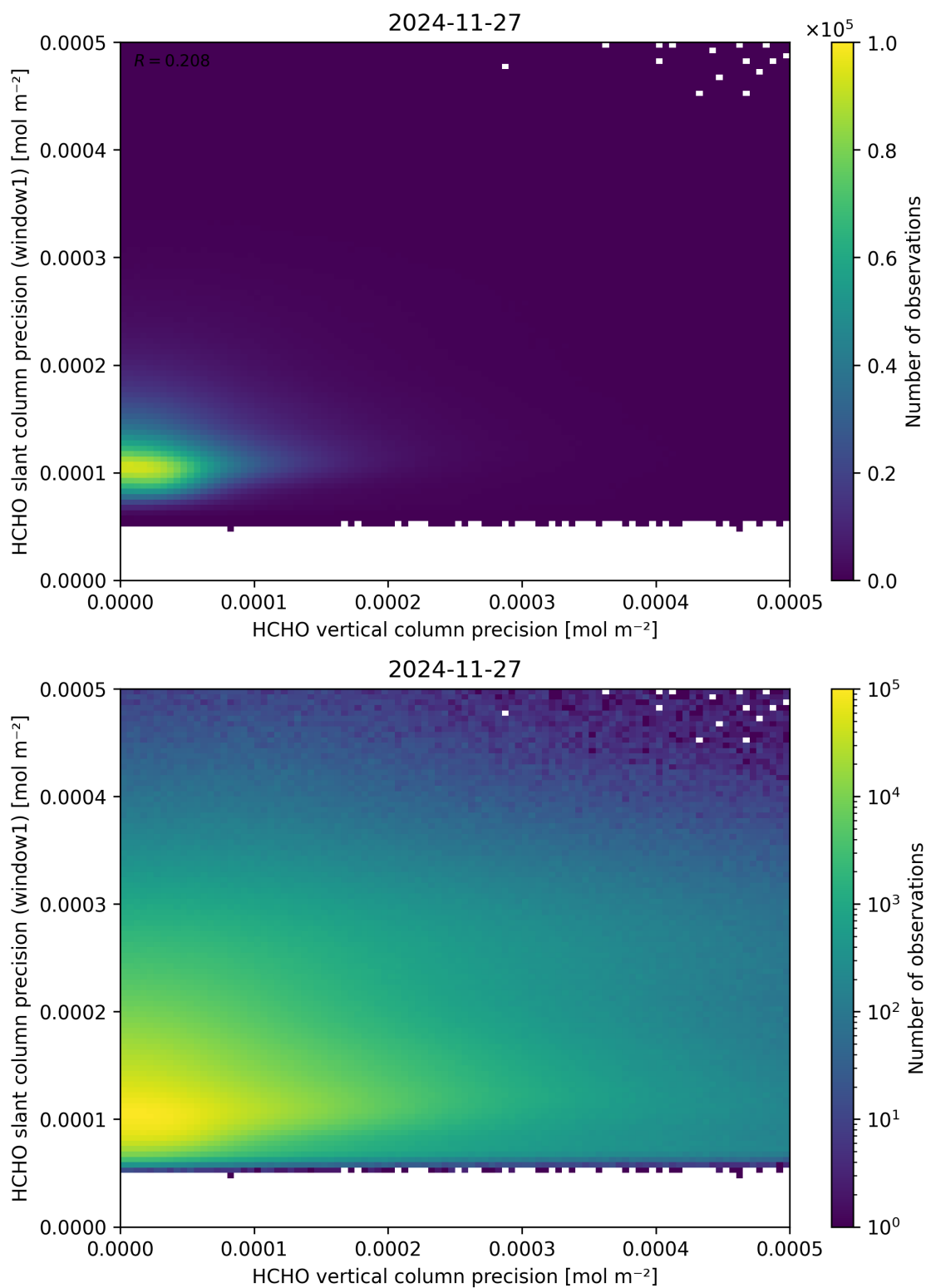
Figure 143: Scatter density plot of “HCHO vertical column precision” against “HCHO slant column precision (window1)” for 2024-11-26 to 2024-11-28.
