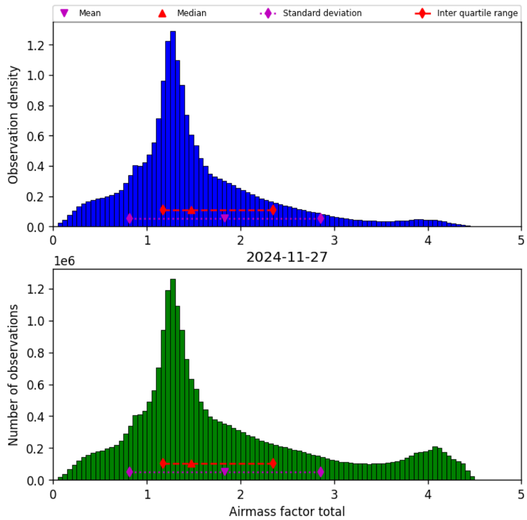
Figure 40: Histogram of “Airmass factor total” for 2024-11-26 to 2024-11-28
