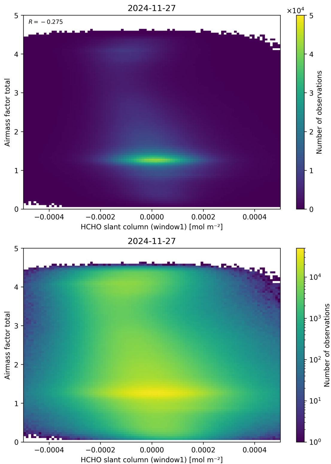
Figure 85: Scatter density plot of “HCHO slant column (window1)” against “Airmass factor total” for 2024-11-26 to 2024-11-28.
