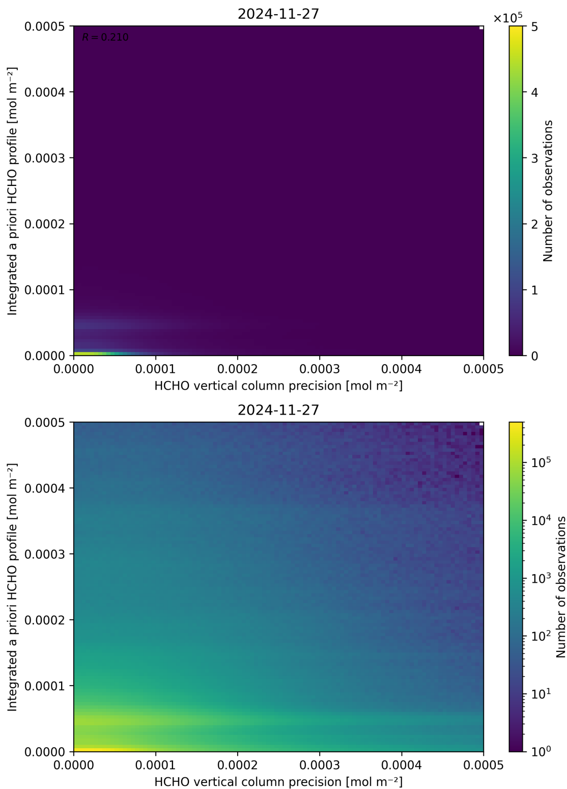
Figure 147: Scatter density plot of “HCHO vertical column precision” against “Integrated a priori HCHO profile” for 2024-11-26 to 2024-11-28.
