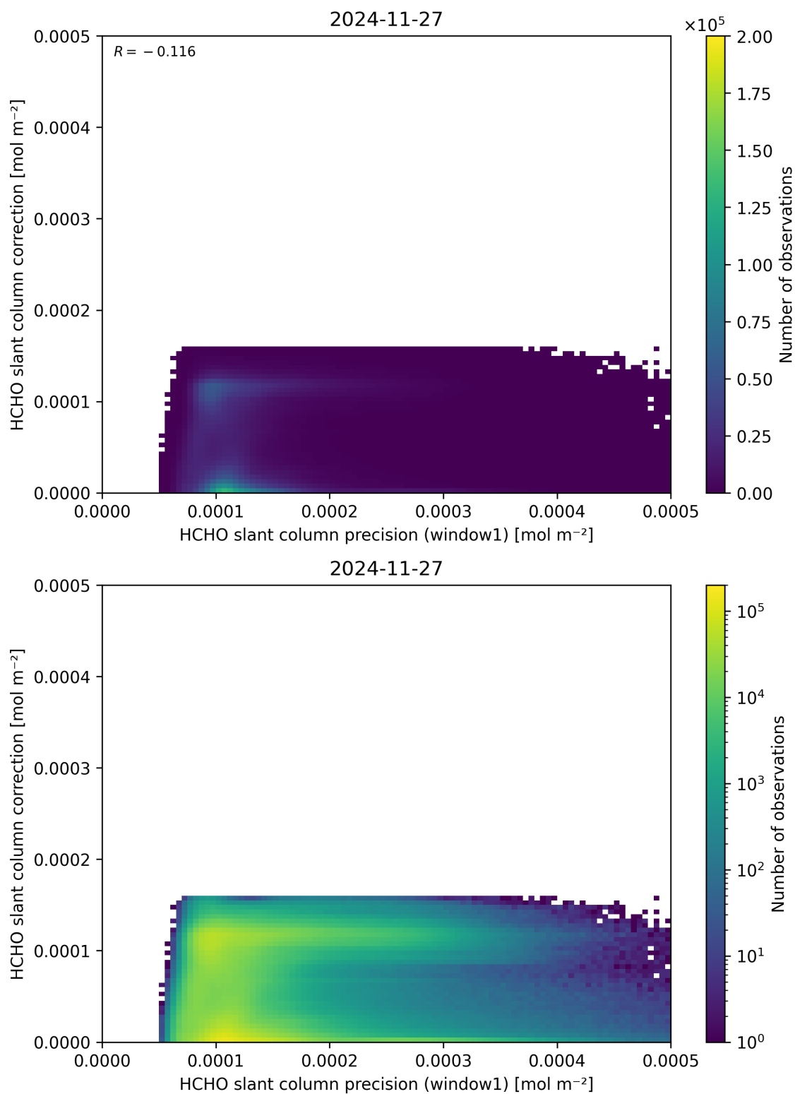
Figure 93: Scatter density plot of “HCHO slant column precision (window1)” against “HCHO slant column correction” for 2024-11-26 to 2024-11-28.
