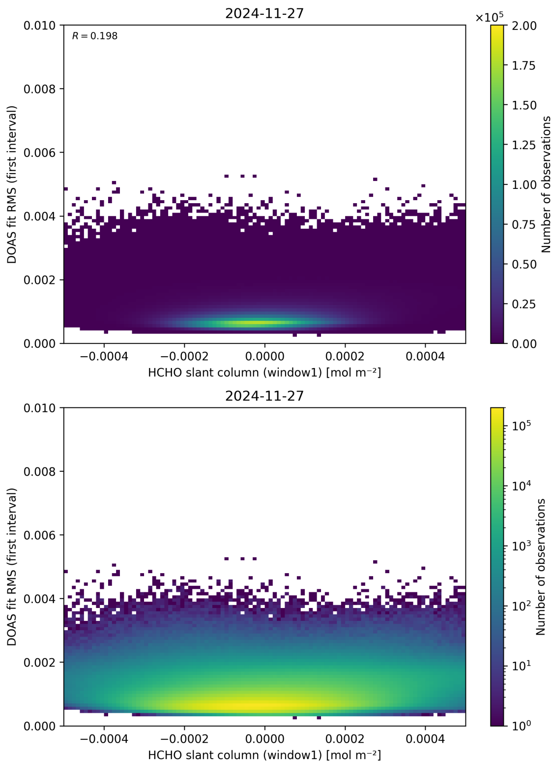
Figure 78: Scatter density plot of “HCHO slant column (window1)” against “DOAS fit RMS (first interval)” for 2024-11-26 to 2024-11-28.
