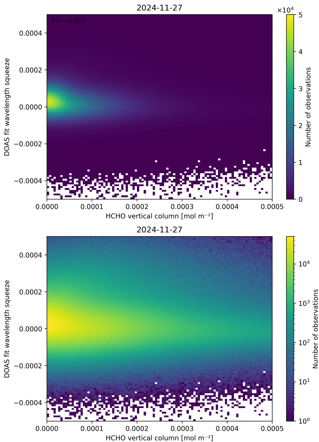
Figure 125: Scatter density plot of “HCHO vertical column” against “DOAS fit wavelength squeeze” for 2024-11-26 to 2024-11-28.
