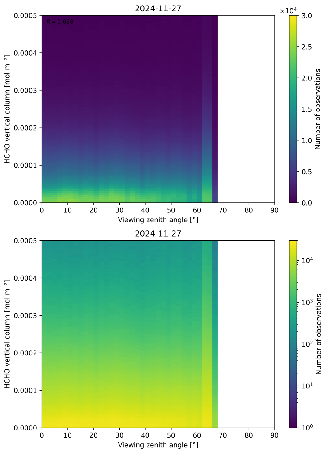
Figure 192: Scatter density plot of “Viewing zenith angle” against “HCHO vertical column” for 2024-11-26 to 2024-11-28.
