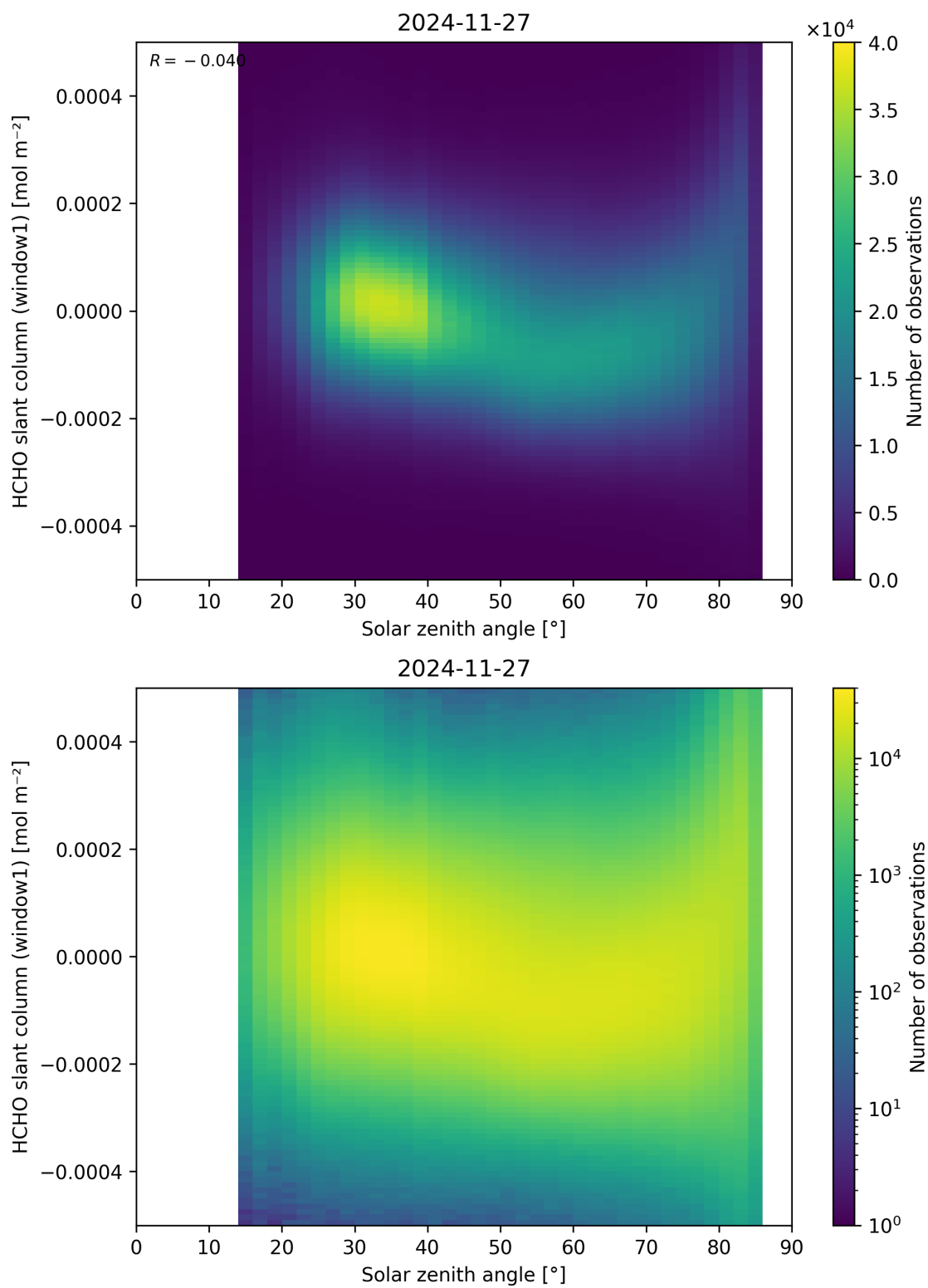
Figure 173: Scatter density plot of “Solar zenith angle” against “HCHO slant column (window1)” for 2024-11-26 to 2024-11-28.
