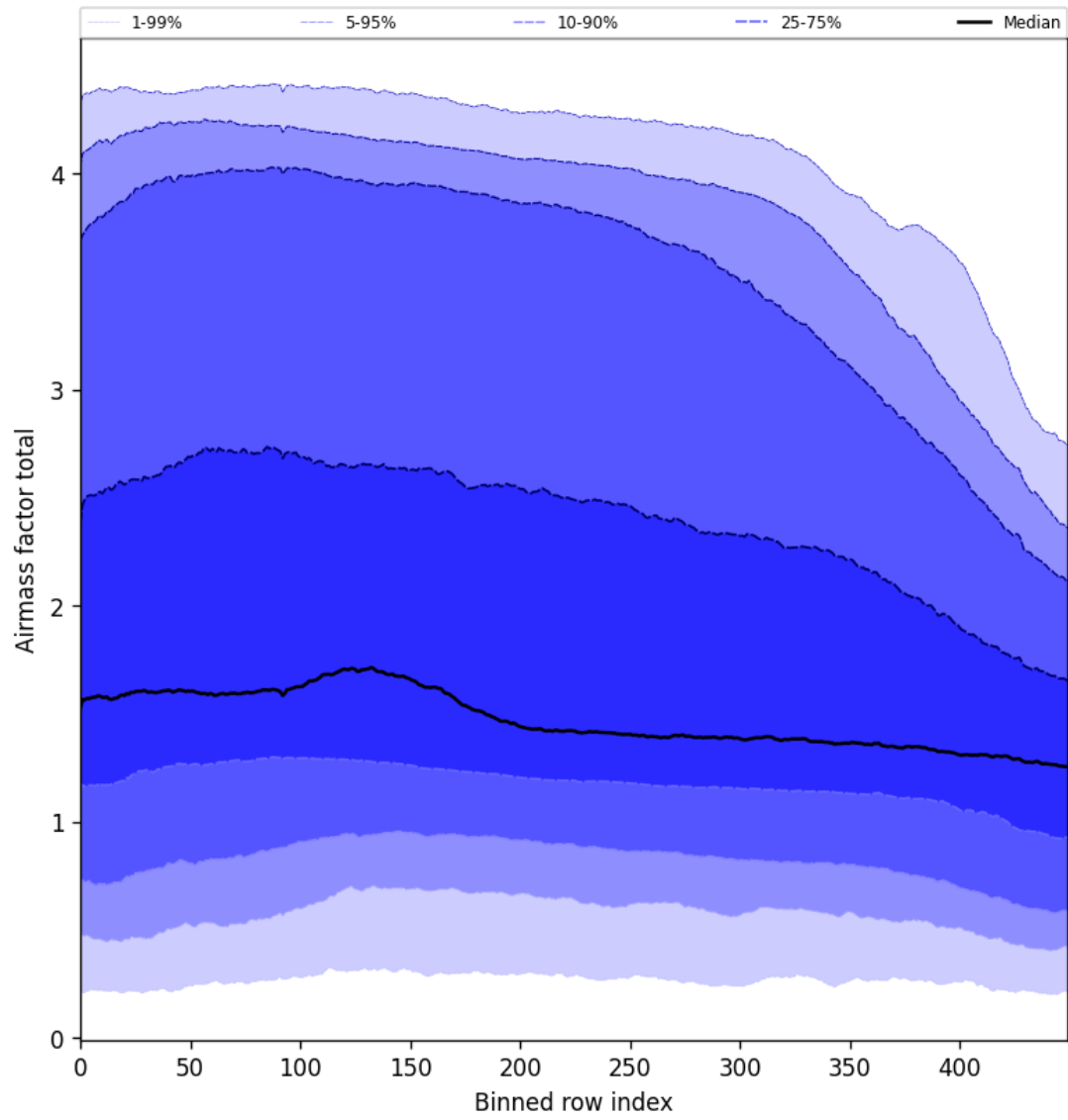
Figure 54: Along track statistics of “Airmass factor total” for 2024-11-26 to 2024-11-28
