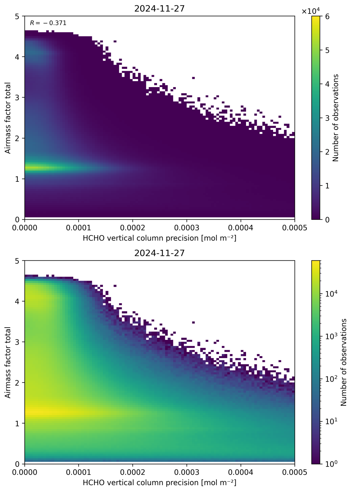
Figure 144: Scatter density plot of “HCHO vertical column precision” against “Airmass factor total” for 2024-11-26 to 2024-11-28.
