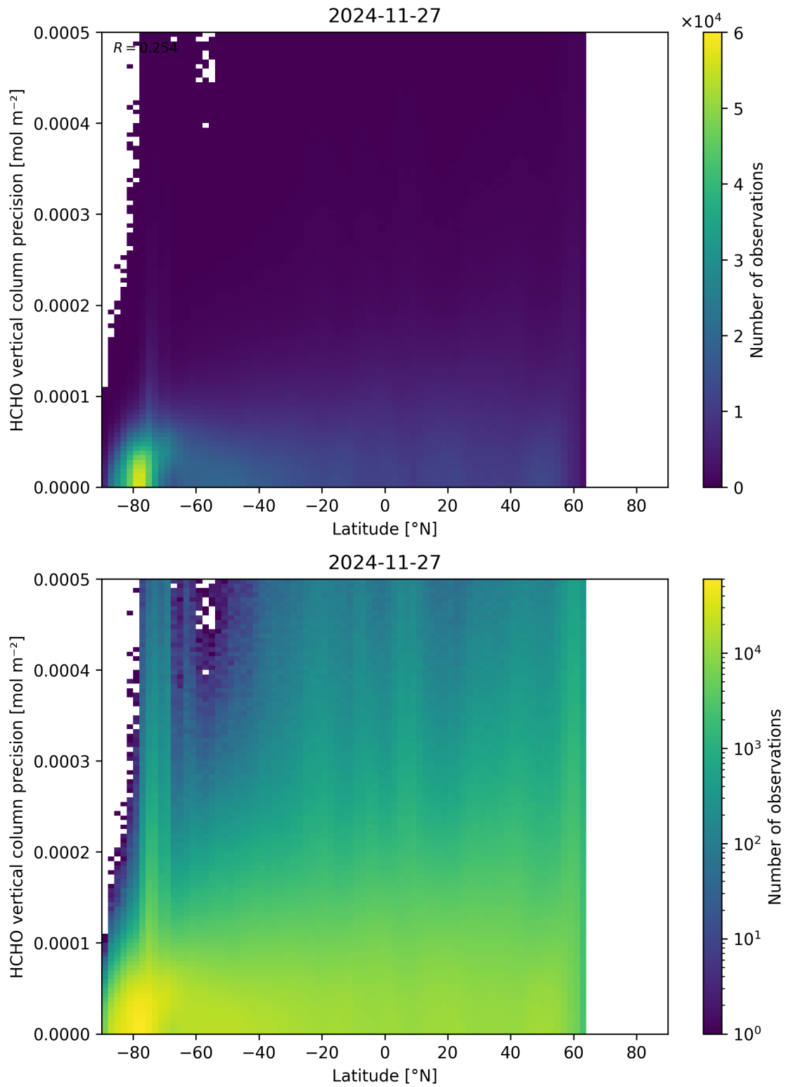
Figure 165: Scatter density plot of “Latitude” against “HCHO vertical column precision” for 2024-11-26 to 2024-11-28.
