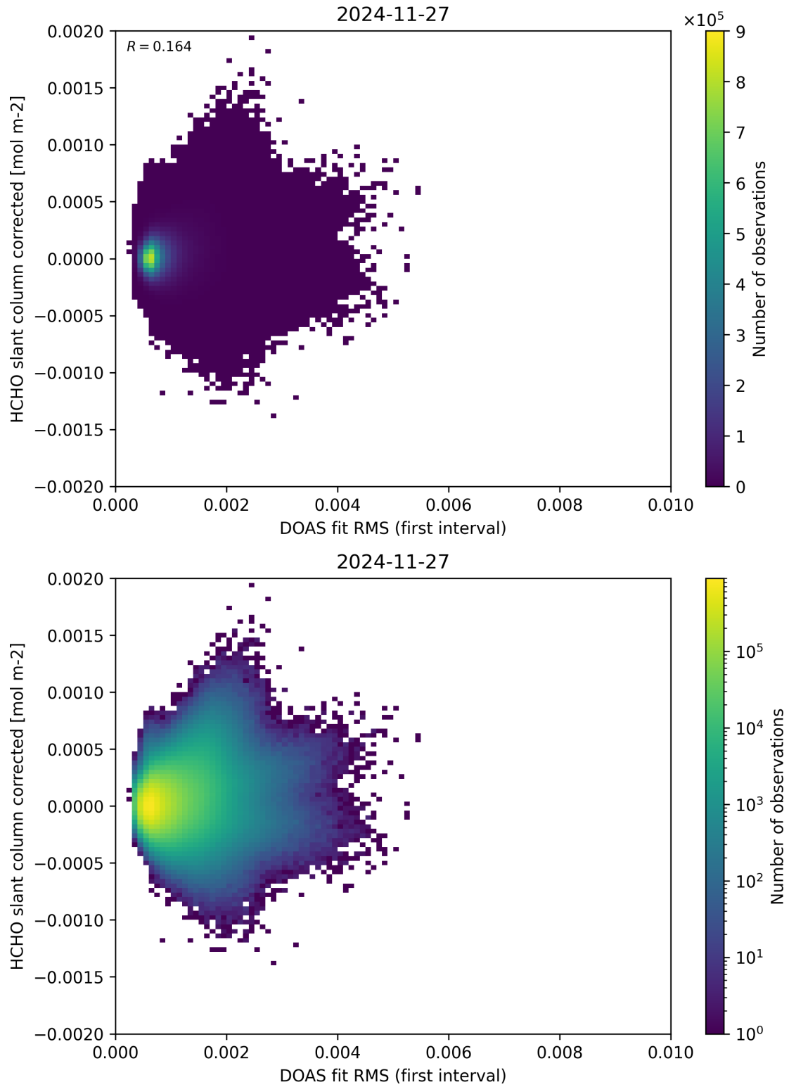
Figure 62: Scatter density plot of “DOAS fit RMS (first interval)” against “HCHO slant column corrected” for 2024-11-26 to 2024-11-28.
