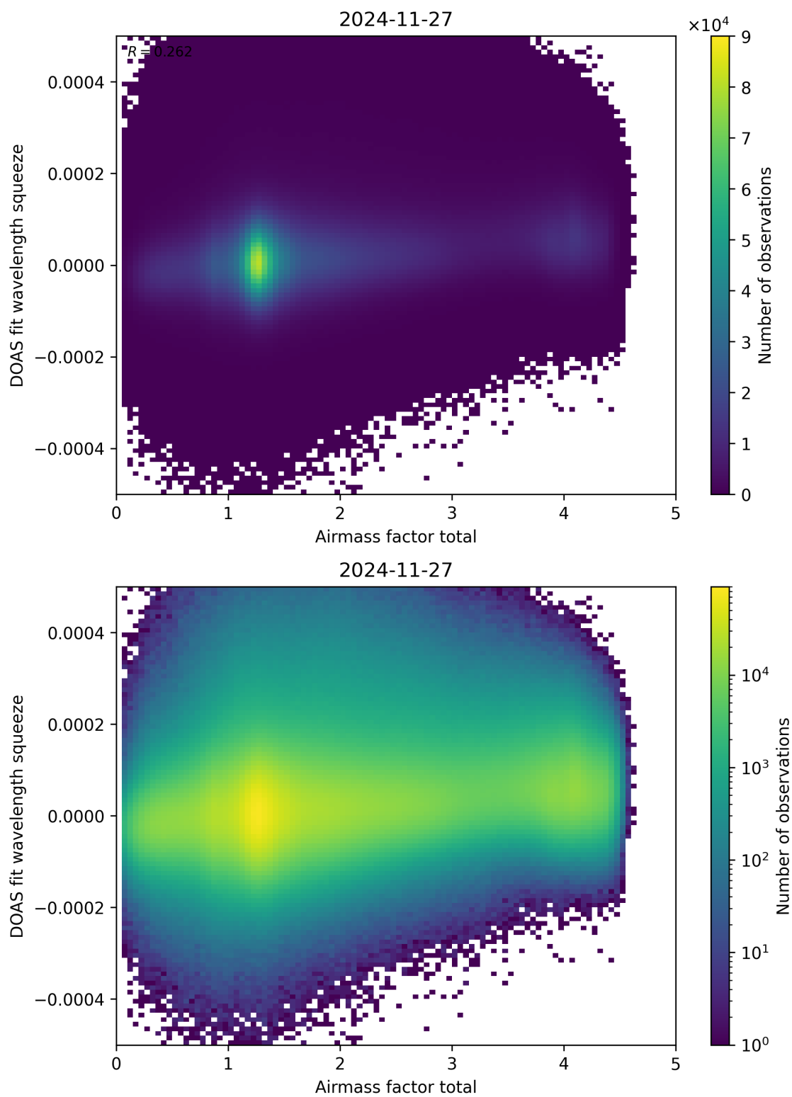
Figure 99: Scatter density plot of “Airmass factor total” against “DOAS fit wavelength squeeze” for 2024-11-26 to 2024-11-28.
