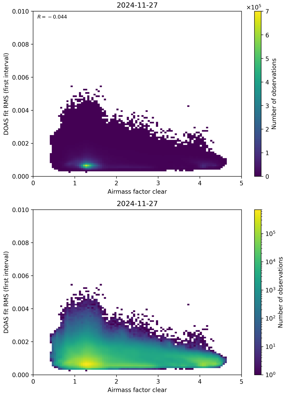
Figure 71: Scatter density plot of “Airmass factor clear” against “DOAS fit RMS (first interval)” for 2024-11-26 to 2024-11-28.
