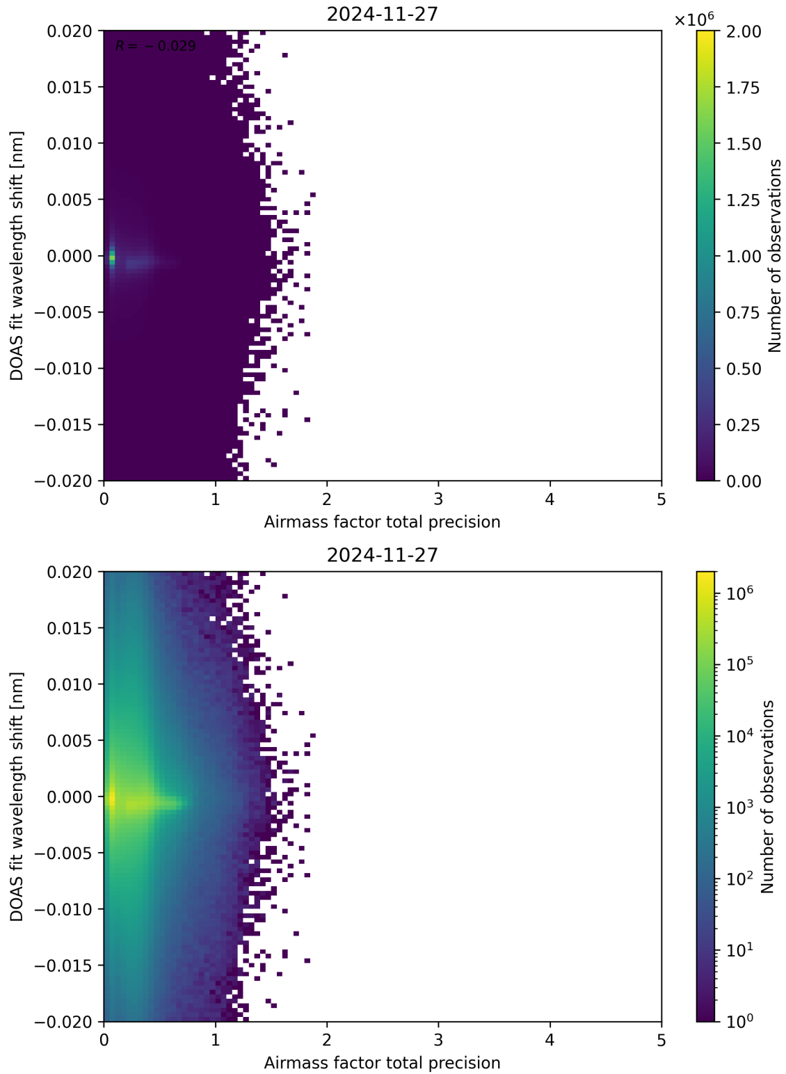
Figure 106: Scatter density plot of “Airmass factor total precision” against “DOAS fit wavelength shift” for 2024-11-26 to 2024-11-28.
