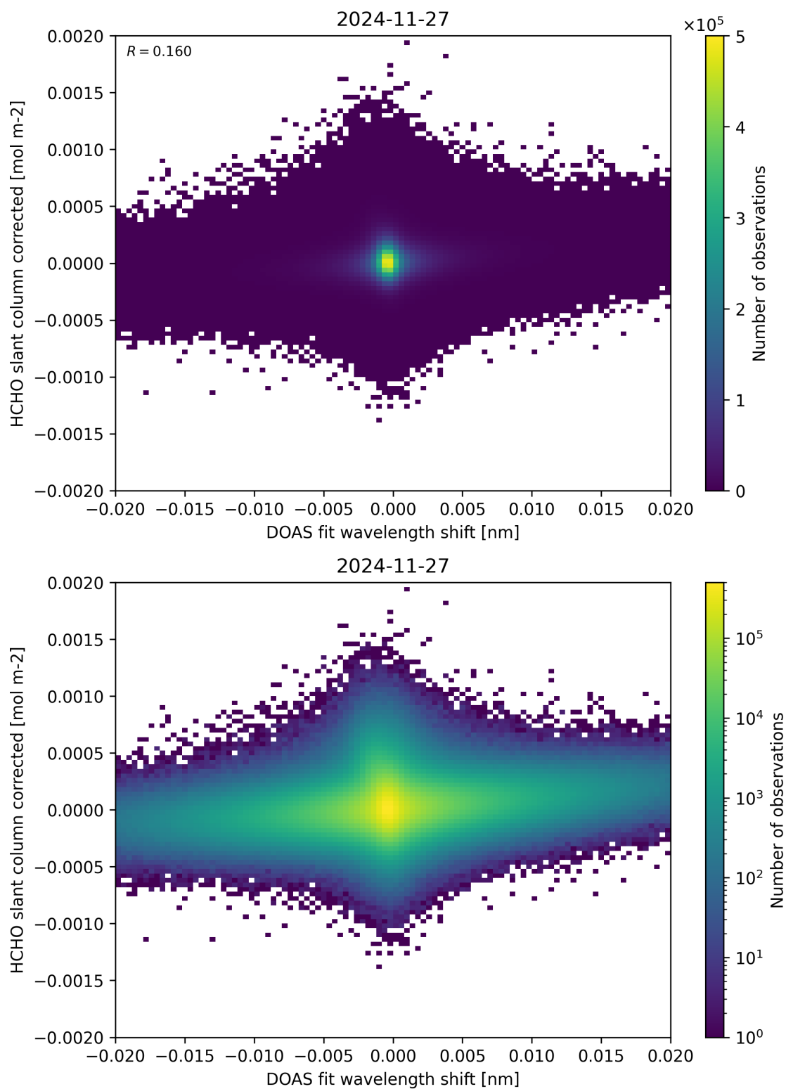
Figure 66: Scatter density plot of “DOAS fit wavelength shift” against “HCHO slant column corrected” for 2024-11-26 to 2024-11-28.
