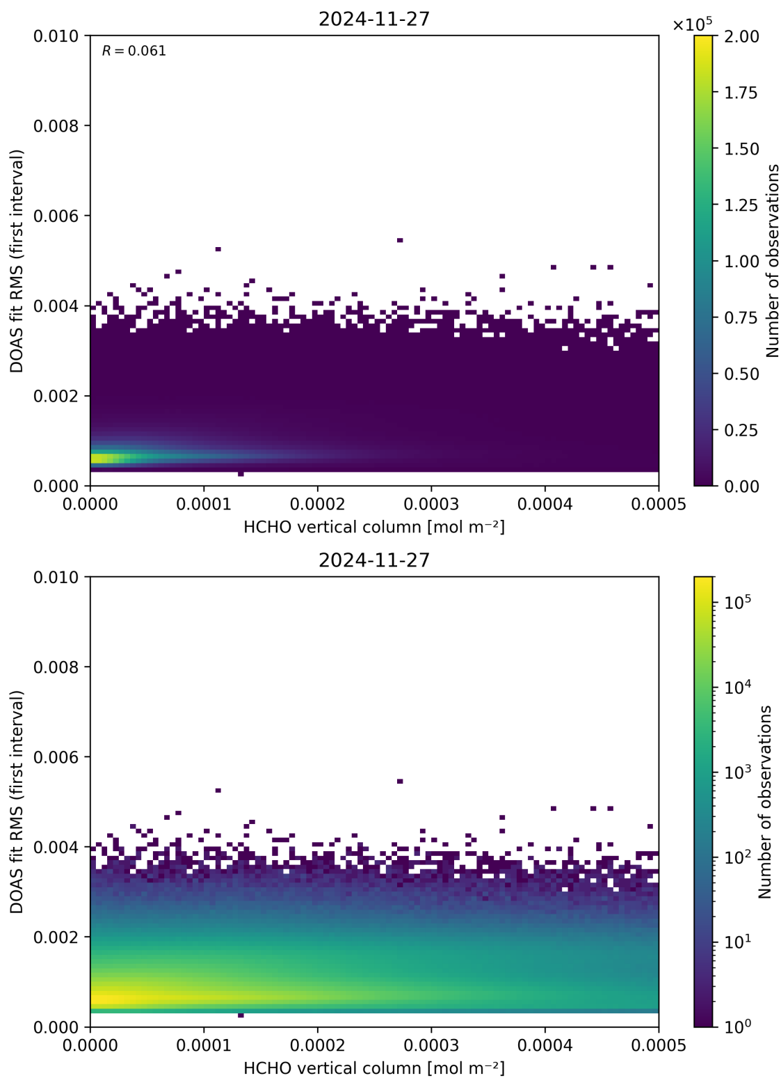
Figure 123: Scatter density plot of “HCHO vertical column” against “DOAS fit RMS (first interval)” for 2024-11-26 to 2024-11-28.
