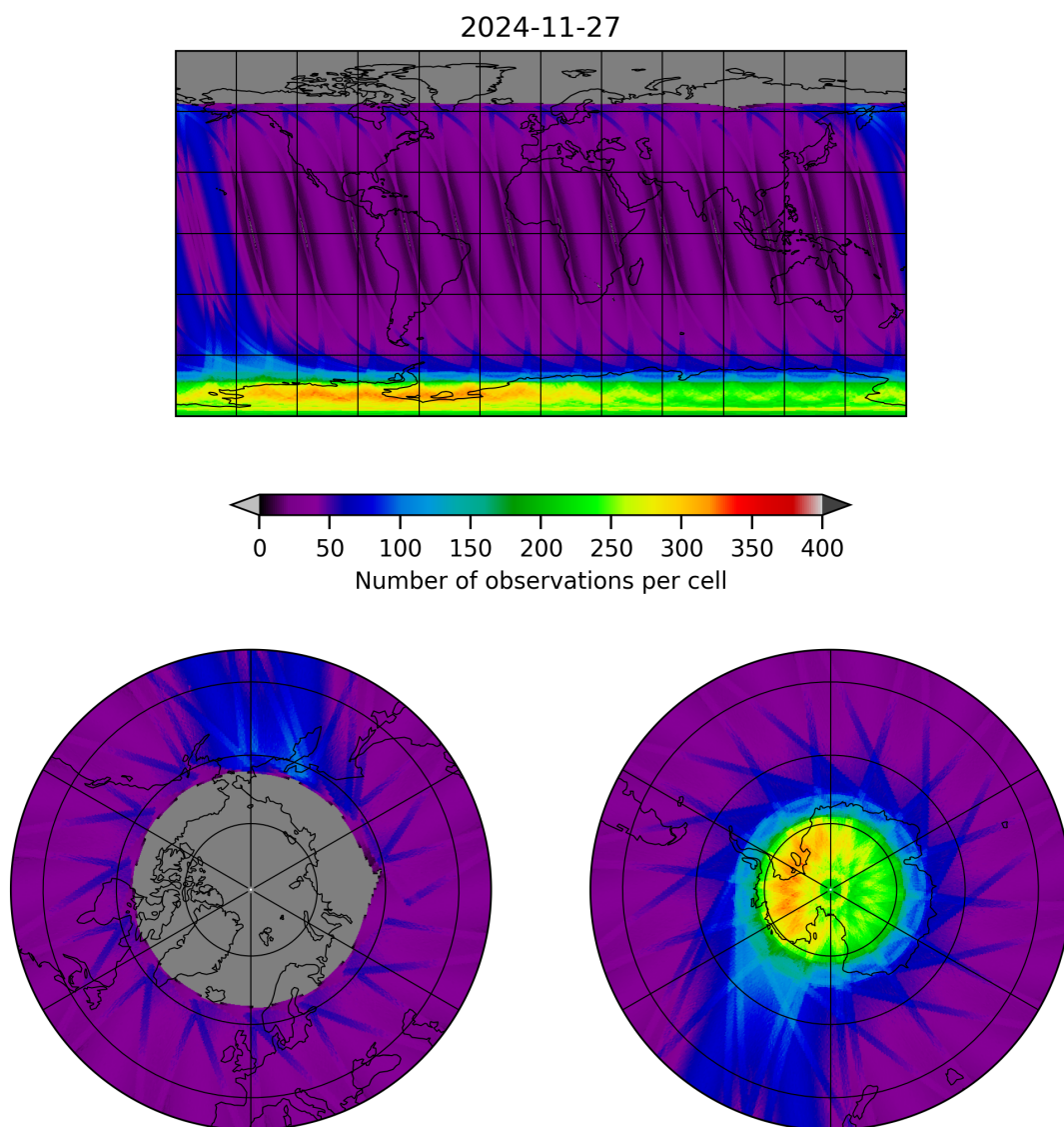
Figure 19: Map of the number of observations for 2024-11-26 to 2024-11-28
