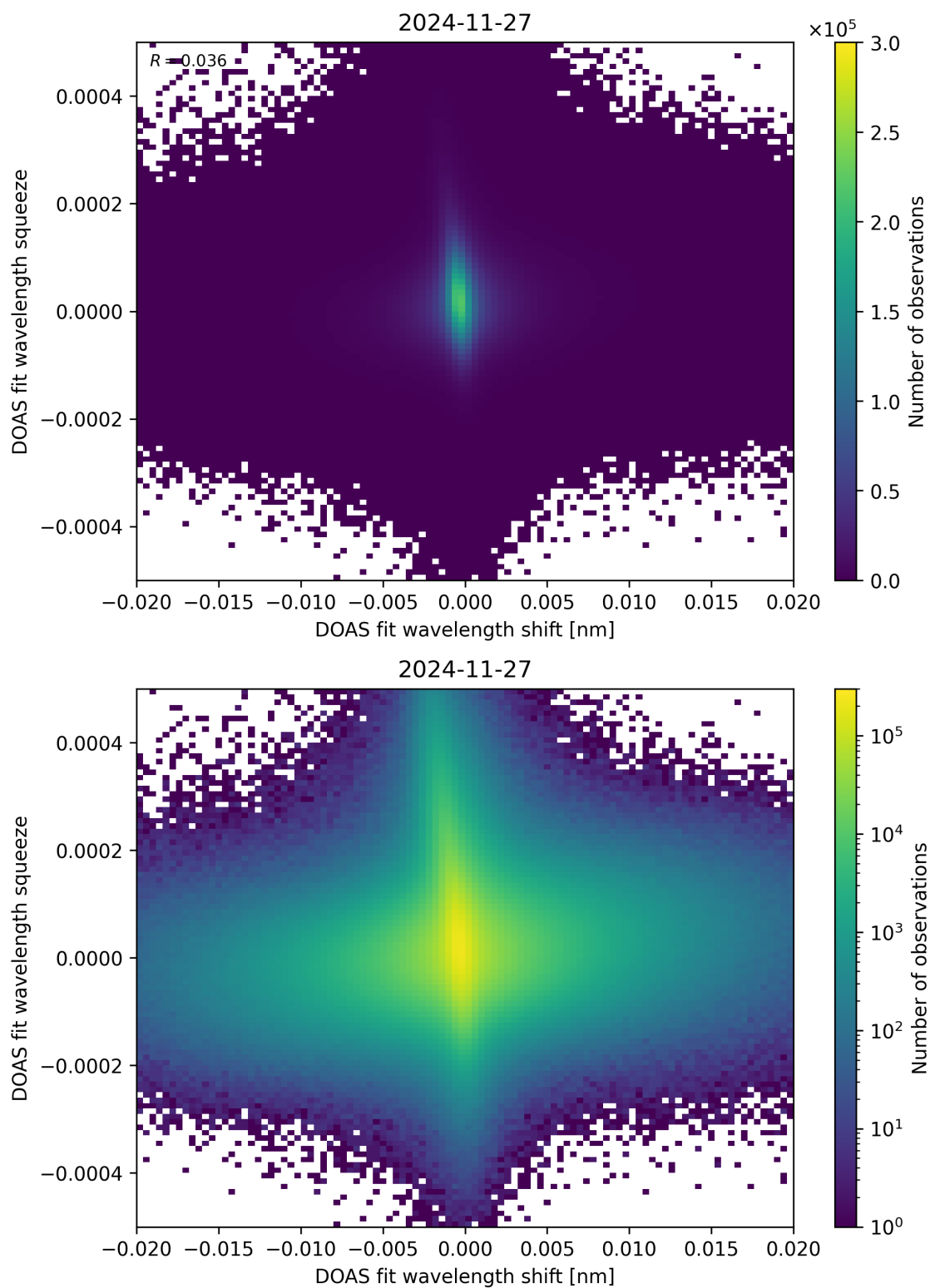
Figure 65: Scatter density plot of “DOAS fit wavelength shift” against “DOAS fit wavelength squeeze” for 2024-11-26 to 2024-11-28.
