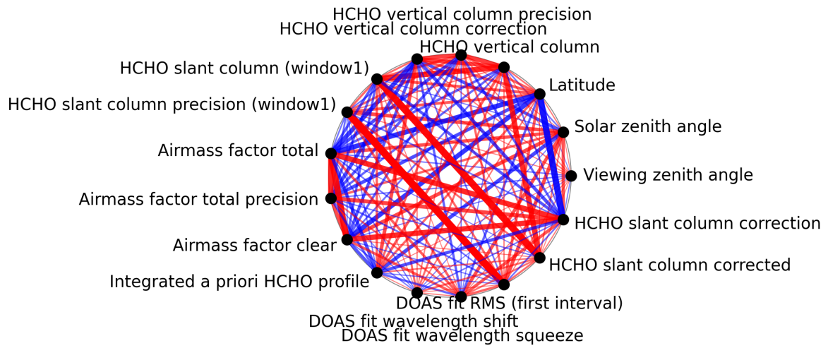
Figure 1: Map of correlation graph for 2024-11-26 to 2024-11-28.
