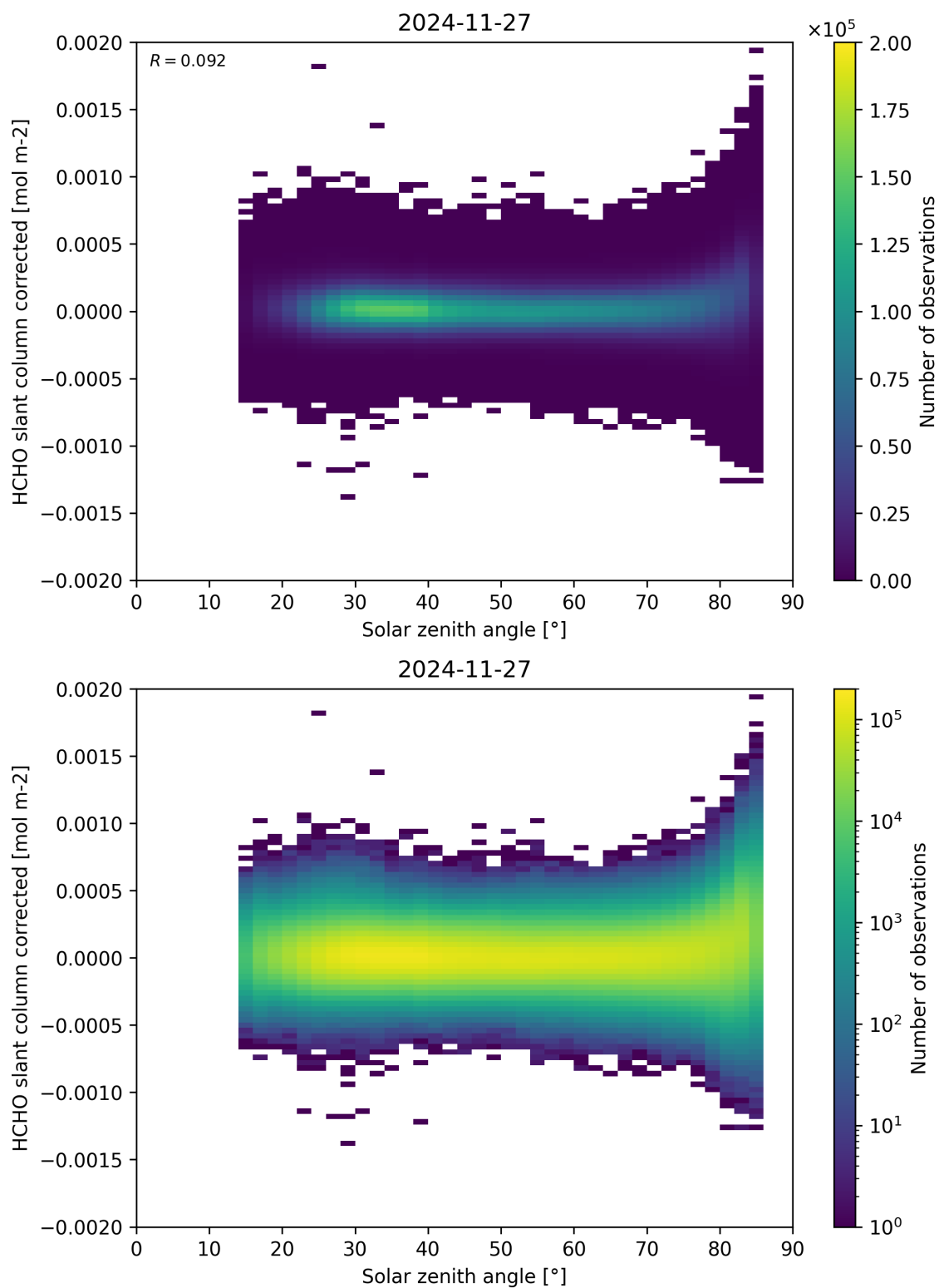
Figure 171: Scatter density plot of “Solar zenith angle” against “HCHO slant column corrected” for 2024-11-26 to 2024-11-28.
