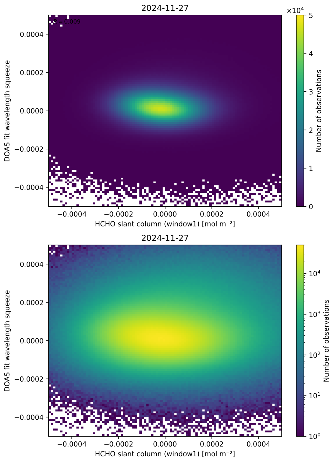
Figure 80: Scatter density plot of “HCHO slant column (window1)” against “DOAS fit wavelength squeeze” for 2024-11-26 to 2024-11-28.
