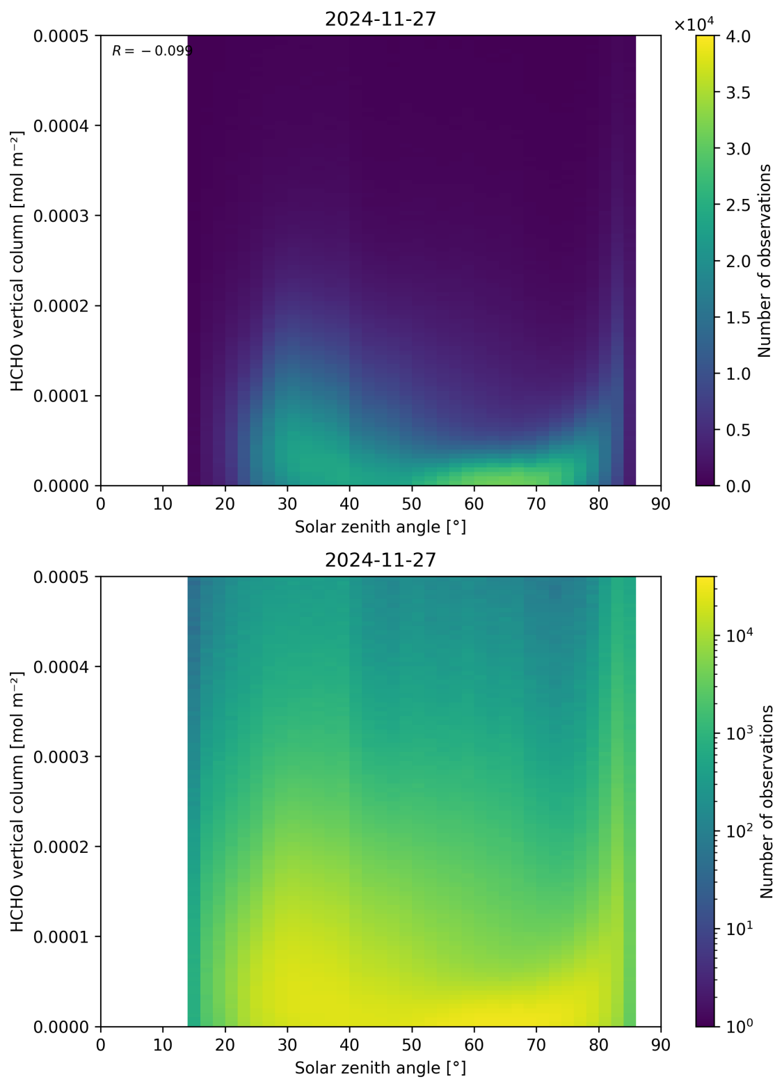
Figure 177: Scatter density plot of “Solar zenith angle” against “HCHO vertical column” for 2024-11-26 to 2024-11-28.
