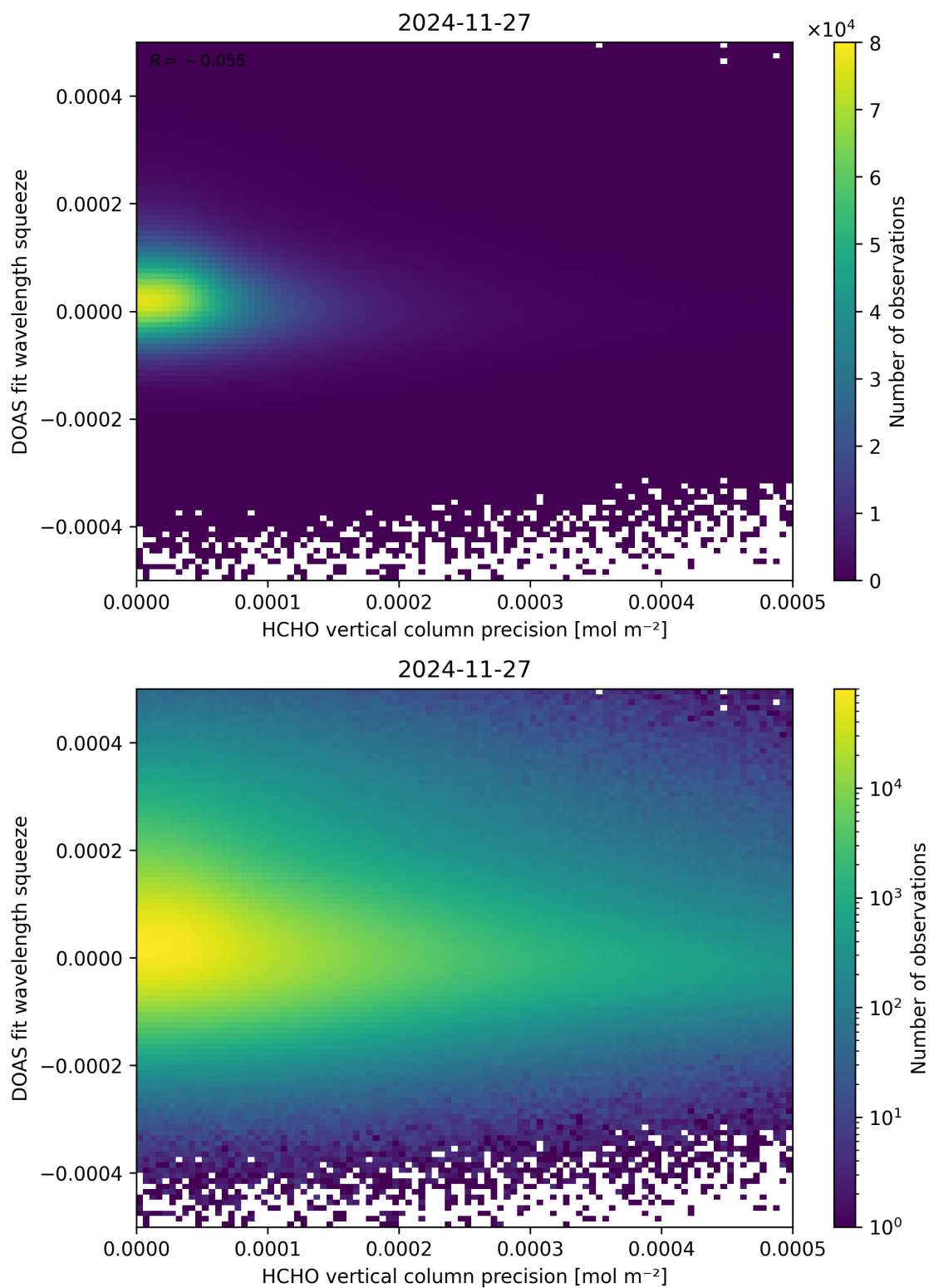
Figure 138: Scatter density plot of “HCHO vertical column precision” against “DOAS fit wavelength squeeze” for 2024-11-26 to 2024-11-28.
