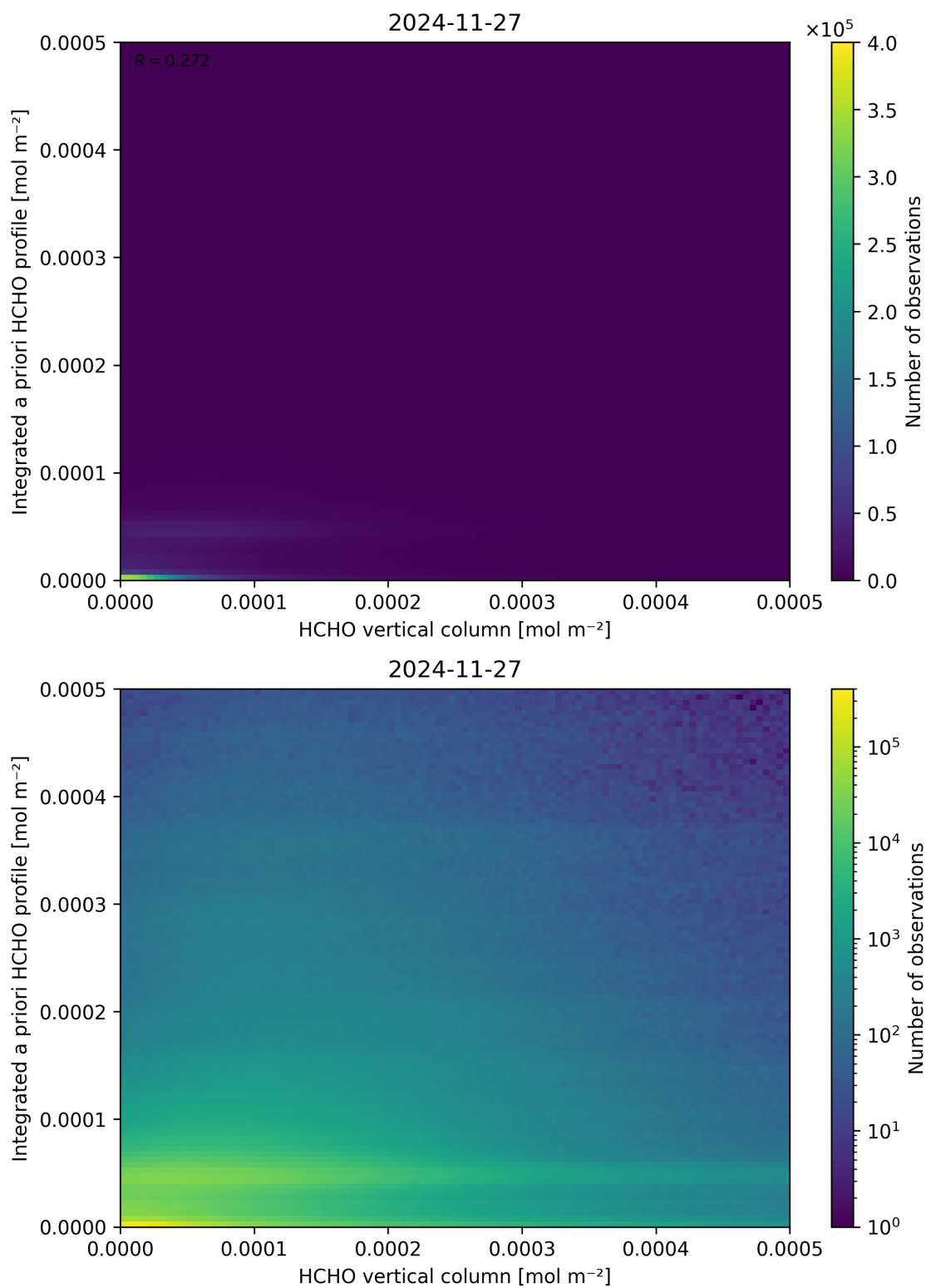
Figure 135: Scatter density plot of “HCHO vertical column” against “Integrated a priori HCHO profile” for 2024-11-26 to 2024-11-28.
