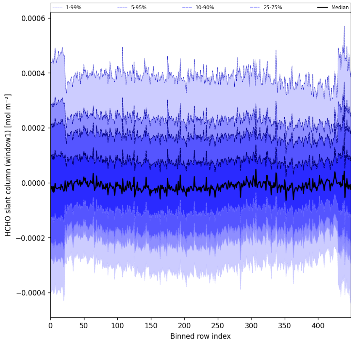
Figure 52: Along track statistics of “HCHO slant column (window1)” for 2024-11-26 to 2024-11-28
