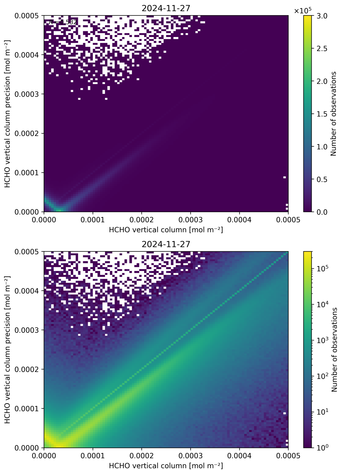
Figure 134: Scatter density plot of “HCHO vertical column” against “HCHO vertical column precision” for 2024-11-26 to 2024-11-28.
