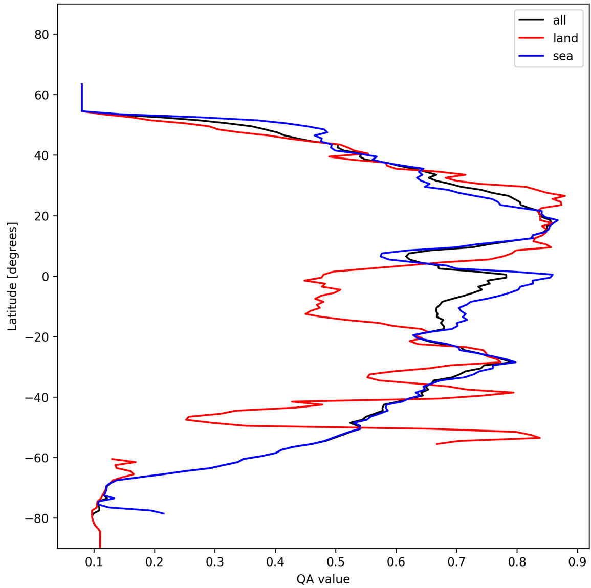
Figure 20: Zonal average of “QA value” for 2024-11-26 to 2024-11-28.
