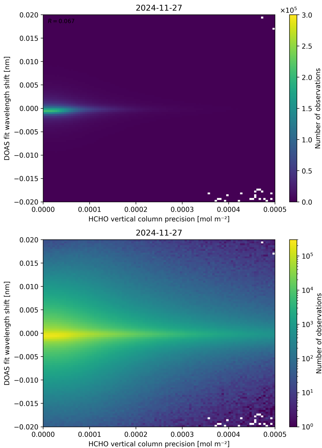
Figure 137: Scatter density plot of “HCHO vertical column precision” against “DOAS fit wavelength shift” for 2024-11-26 to 2024-11-28.
