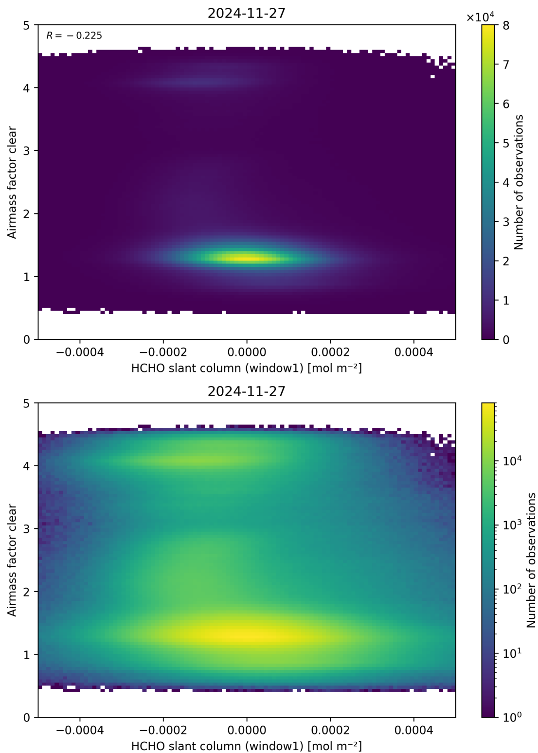
Figure 81: Scatter density plot of “HCHO slant column (window1)” against “Airmass factor clear” for 2024-11-26 to 2024-11-28.
