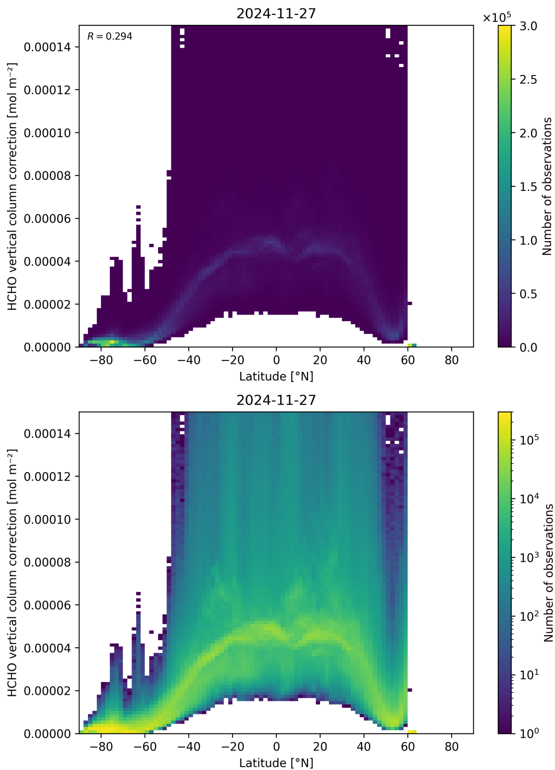
Figure 164: Scatter density plot of “Latitude” against “HCHO vertical column correction” for 2024-11-26 to 2024-11-28.
