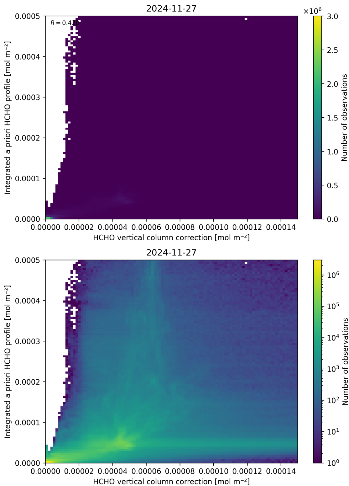
Figure 122: Scatter density plot of “HCHO vertical column correction” against “Integrated a priori HCHO profile” for 2024-11-26 to 2024-11-28.
