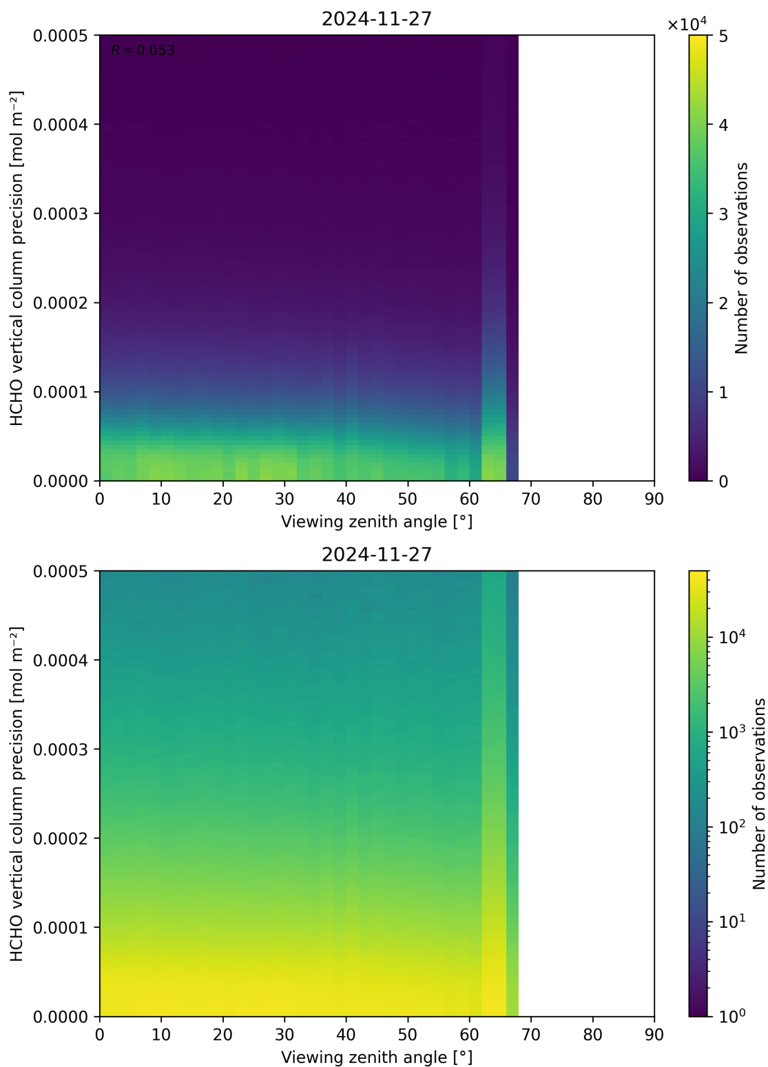
Figure 194: Scatter density plot of “Viewing zenith angle” against “HCHO vertical column precision” for 2024-11-26 to 2024-11-28.
