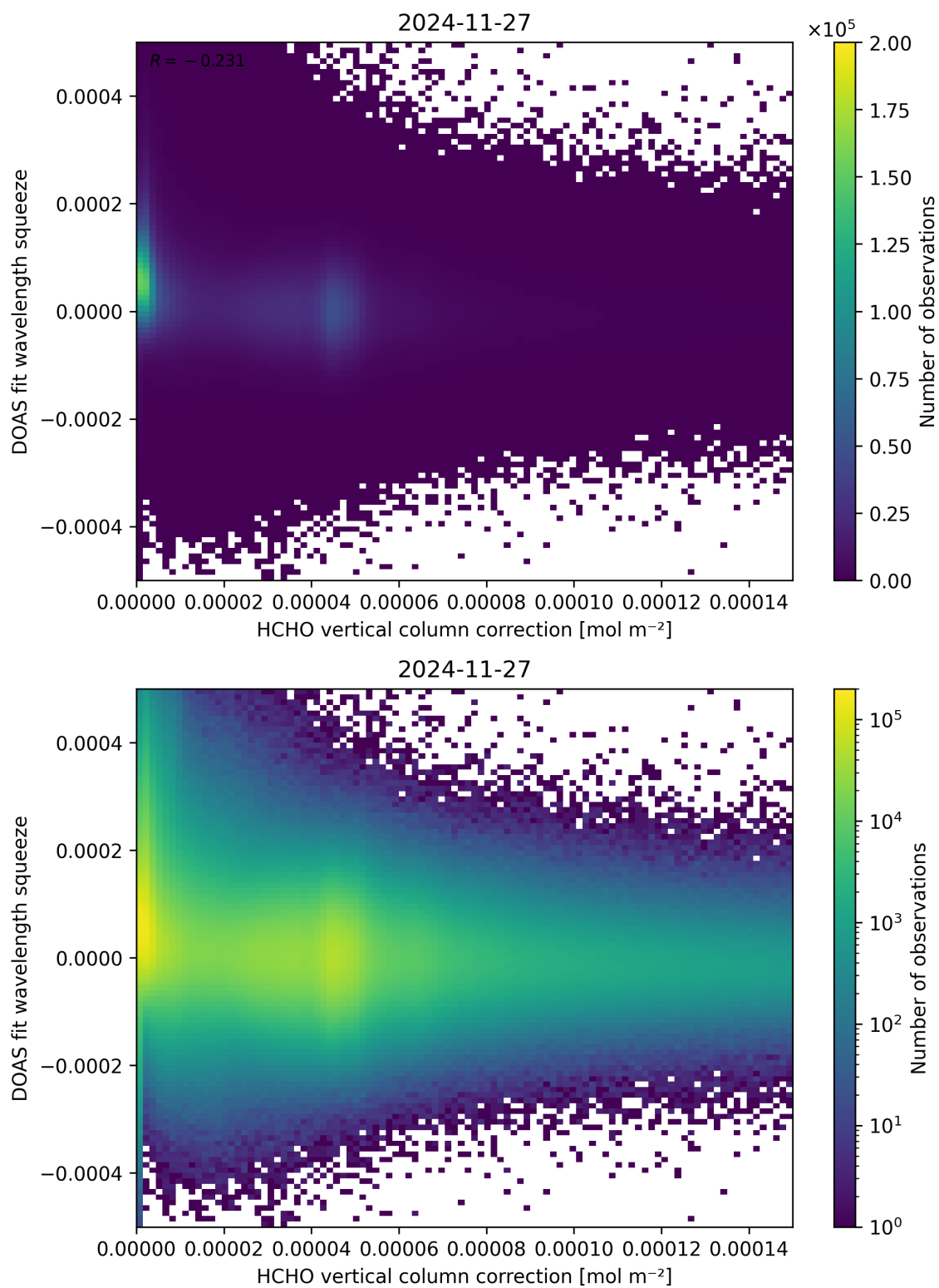
Figure 114: Scatter density plot of “HCHO vertical column correction” against “DOAS fit wavelength squeeze” for 2024-11-26 to 2024-11-28.
