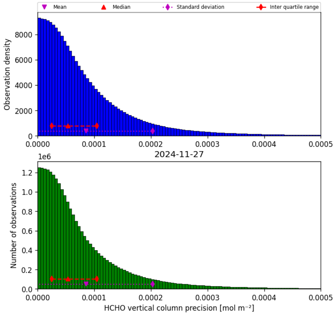
Figure 36: Histogram of “HCHO vertical column precision” for 2024-11-26 to 2024-11-28
