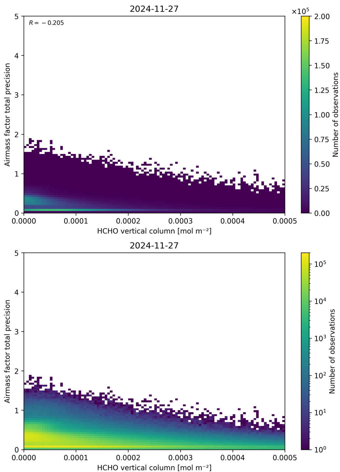
Figure 132: Scatter density plot of “HCHO vertical column” against “Airmass factor total precision” for 2024-11-26 to 2024-11-28.
