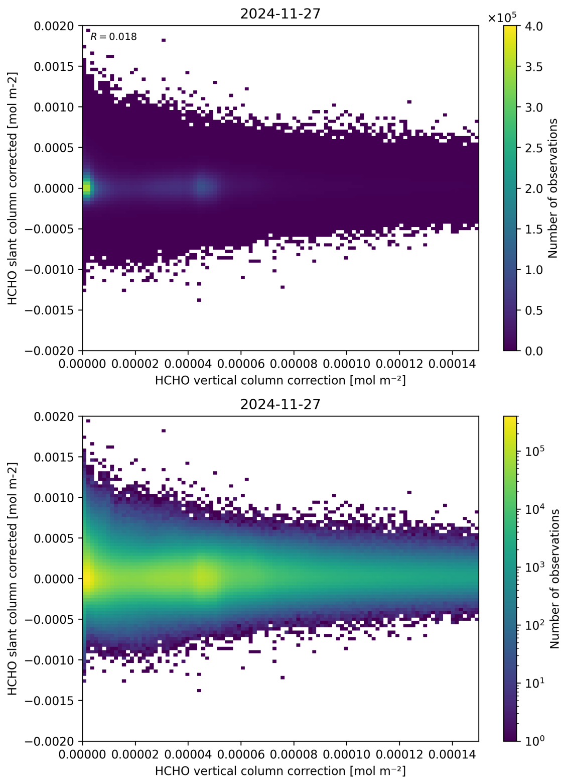
Figure 116: Scatter density plot of “HCHO vertical column correction” against “HCHO slant column corrected” for 2024-11-26 to 2024-11-28.
