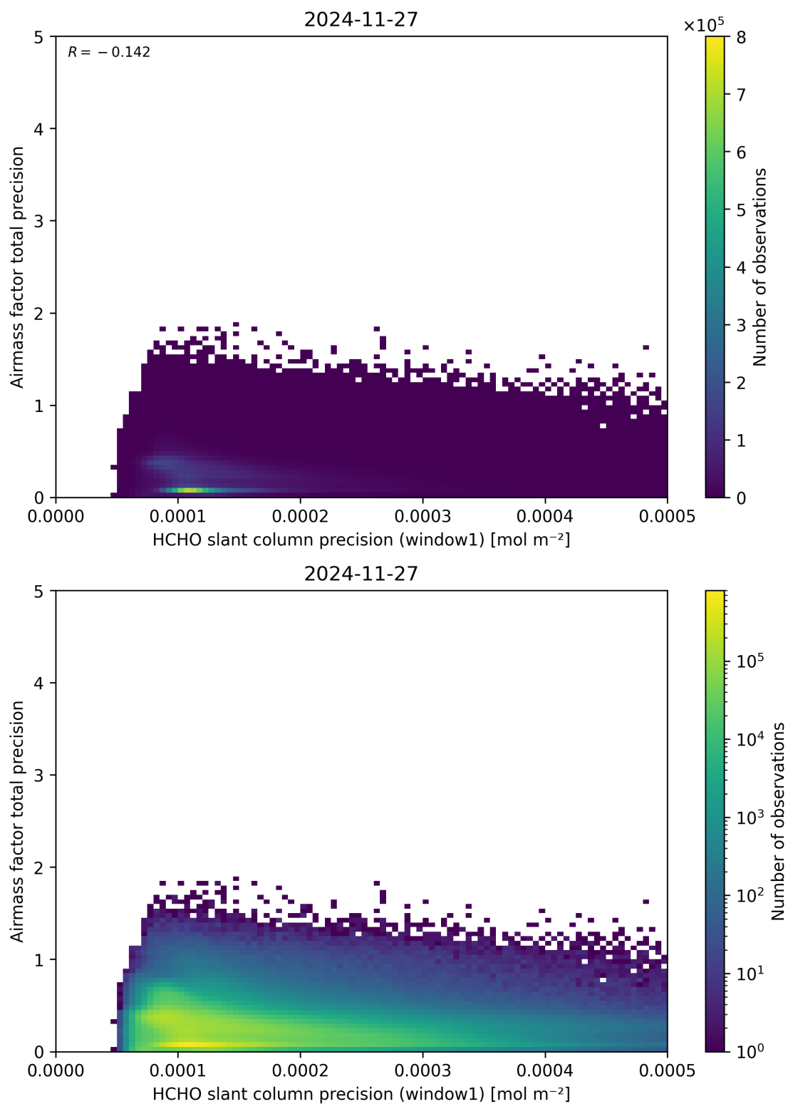
Figure 95: Scatter density plot of “HCHO slant column precision (window1)” against “Airmass factor total precision” for 2024-11-26 to 2024-11-28.
