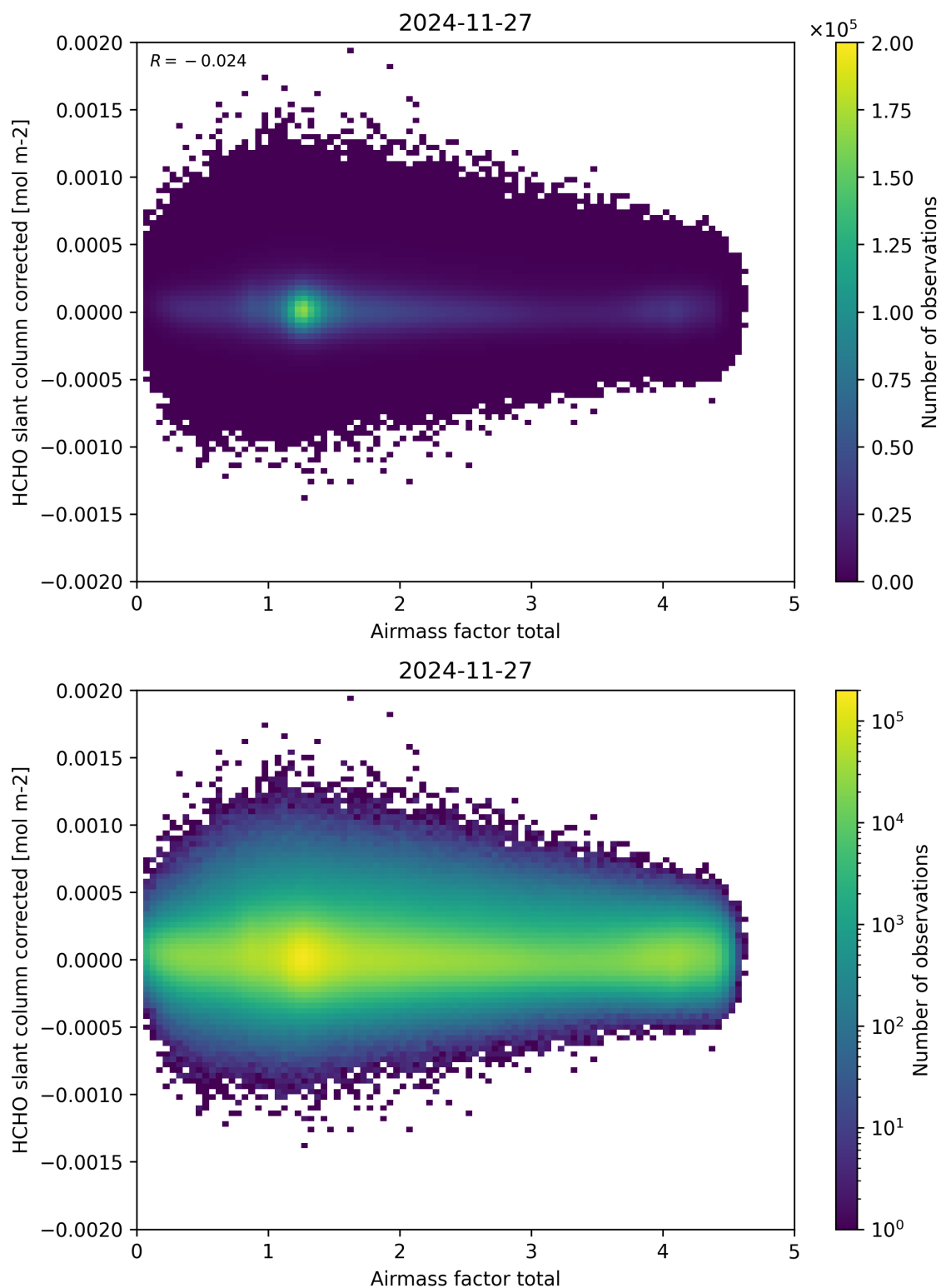
Figure 101: Scatter density plot of “Airmass factor total” against “HCHO slant column corrected” for 2024-11-26 to 2024-11-28.
