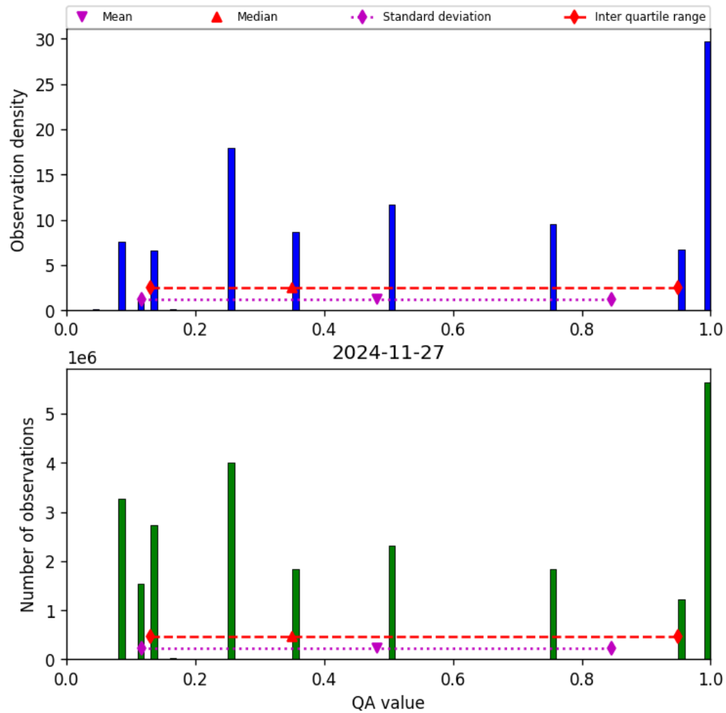
Figure 34: Histogram of “QA value” for 2024-11-26 to 2024-11-28
