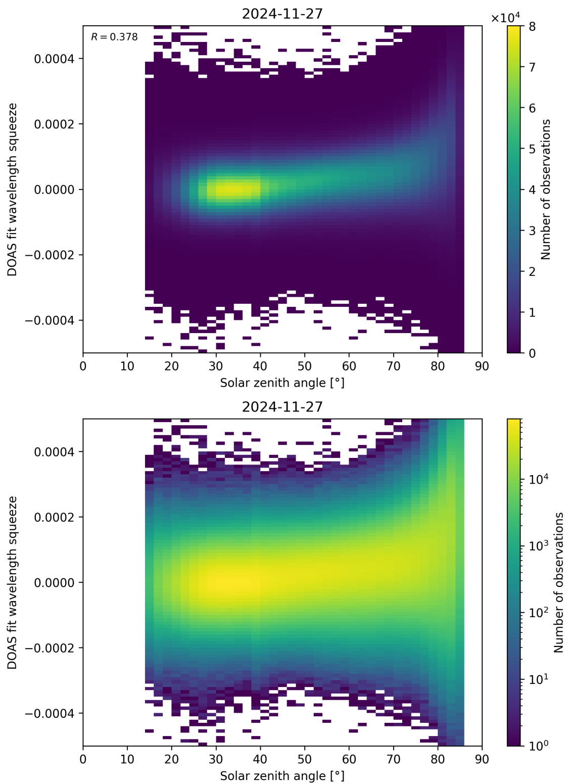
Figure 169: Scatter density plot of “Solar zenith angle” against “DOAS fit wavelength squeeze” for 2024-11-26 to 2024-11-28.
