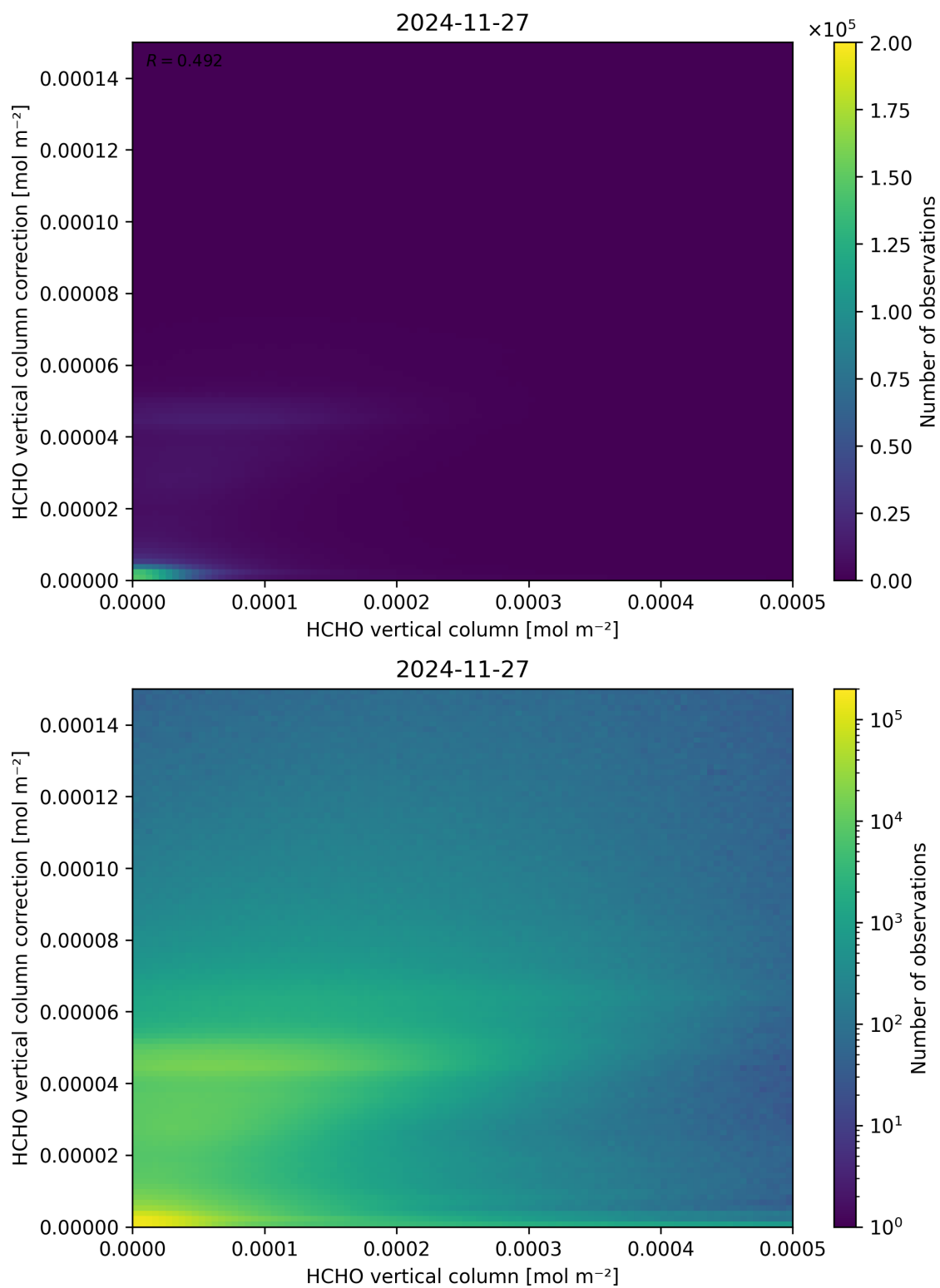
Figure 133: Scatter density plot of “HCHO vertical column” against “HCHO vertical column correction” for 2024-11-26 to 2024-11-28.
