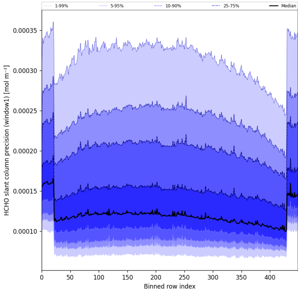
Figure 53: Along track statistics of “HCHO slant column precision (window1)” for 2024-11-26 to 2024-11-28
