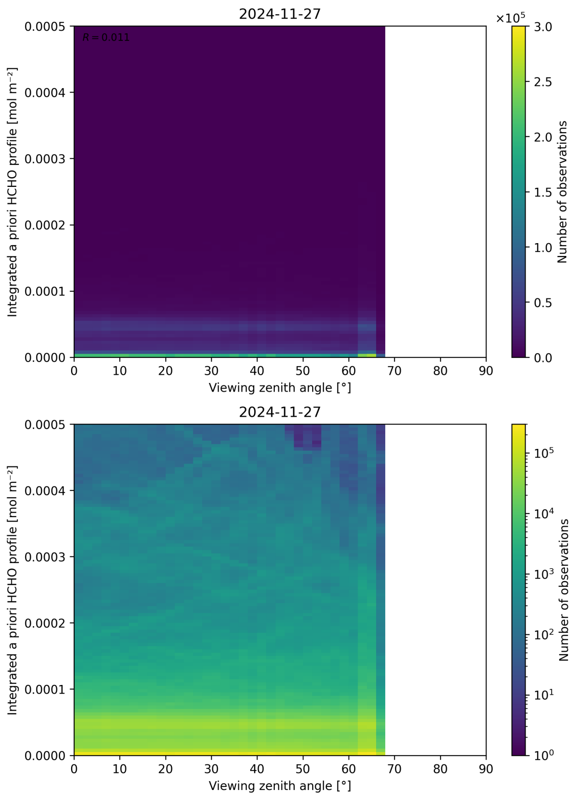
Figure 195: Scatter density plot of “Viewing zenith angle” against “Integrated a priori HCHO profile” for 2024-11-26 to 2024-11-28.
