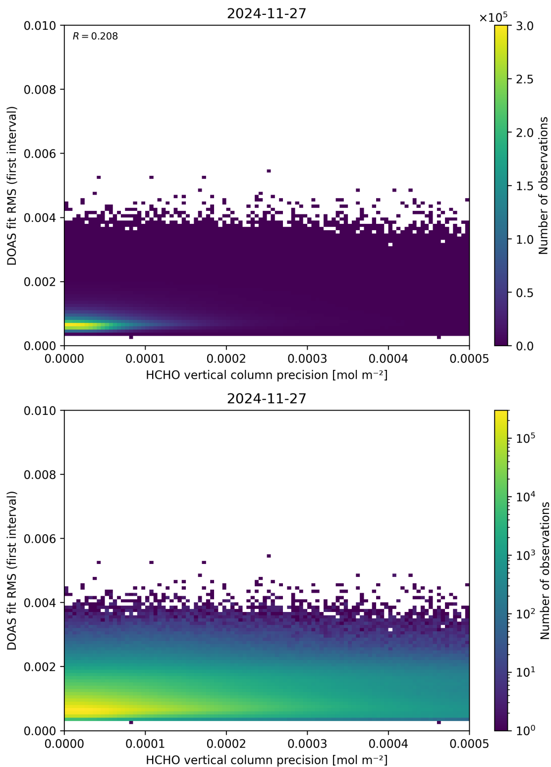
Figure 136: Scatter density plot of “HCHO vertical column precision” against “DOAS fit RMS (first interval)” for 2024-11-26 to 2024-11-28.
