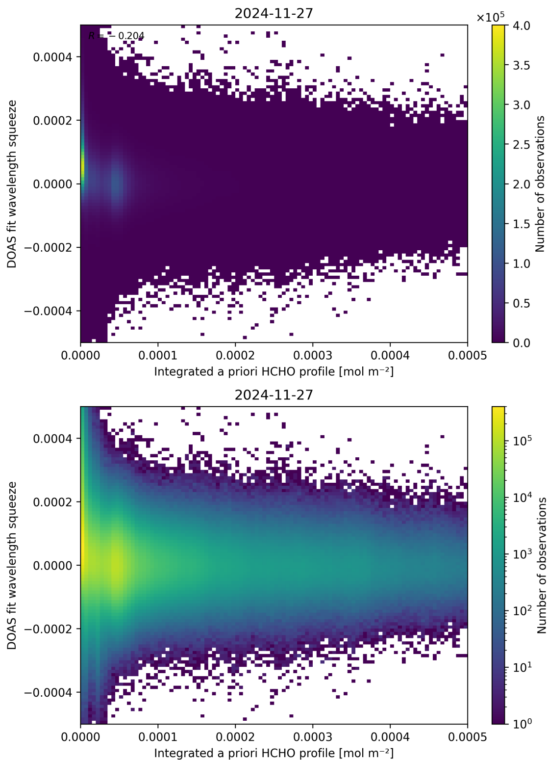
Figure 150: Scatter density plot of “Integrated a priori HCHO profile” against “DOAS fit wavelength squeeze” for 2024-11-26 to 2024-11-28.
