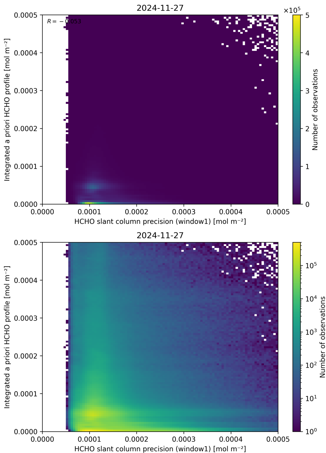
Figure 96: Scatter density plot of “HCHO slant column precision (window1)” against “Integrated a priori HCHO profile” for 2024-11-26 to 2024-11-28.
