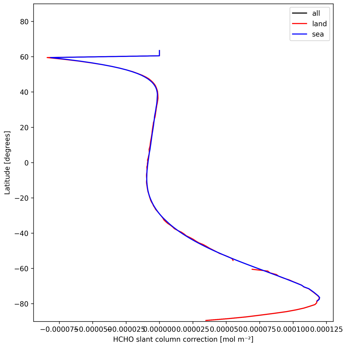
Figure 33: Zonal average of “HCHO slant column correction” for 2024-11-26 to 2024-11-28.
