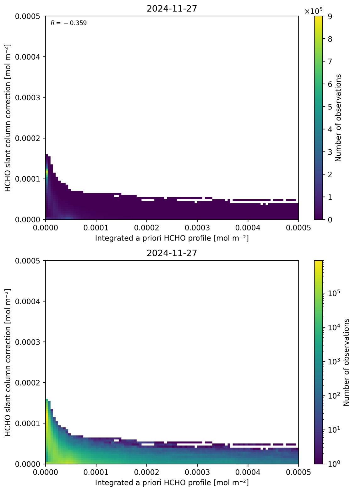
Figure 152: Scatter density plot of “Integrated a priori HCHO profile” against “HCHO slant column correction” for 2024-11-26 to 2024-11-28.
