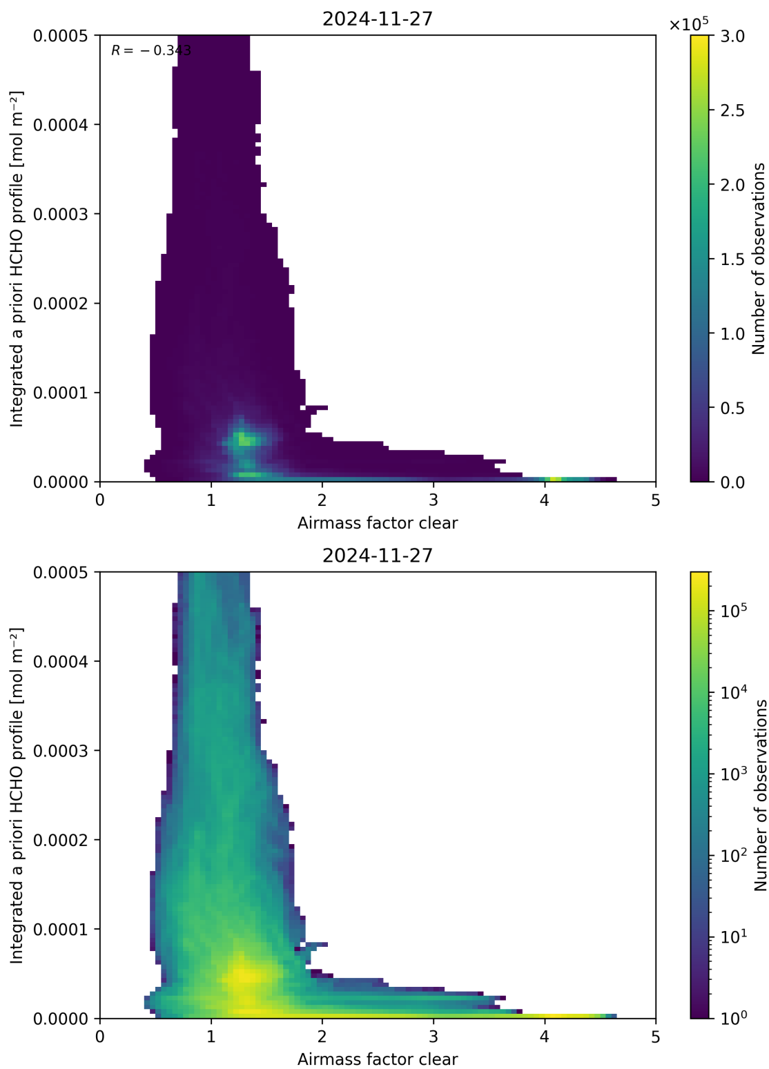
Figure 76: Scatter density plot of “Airmass factor clear” against “Integrated a priori HCHO profile” for 2024-11-26 to 2024-11-28.
