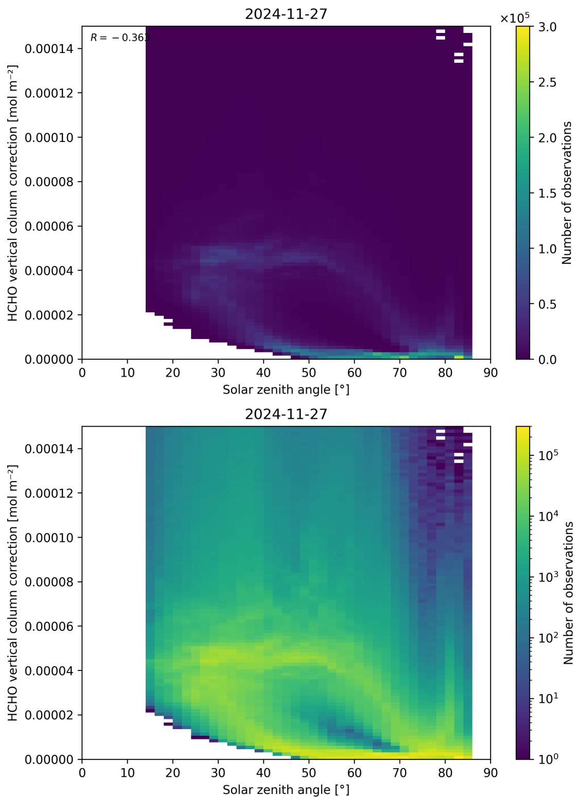
Figure 178: Scatter density plot of “Solar zenith angle” against “HCHO vertical column correction” for 2024-11-26 to 2024-11-28.
