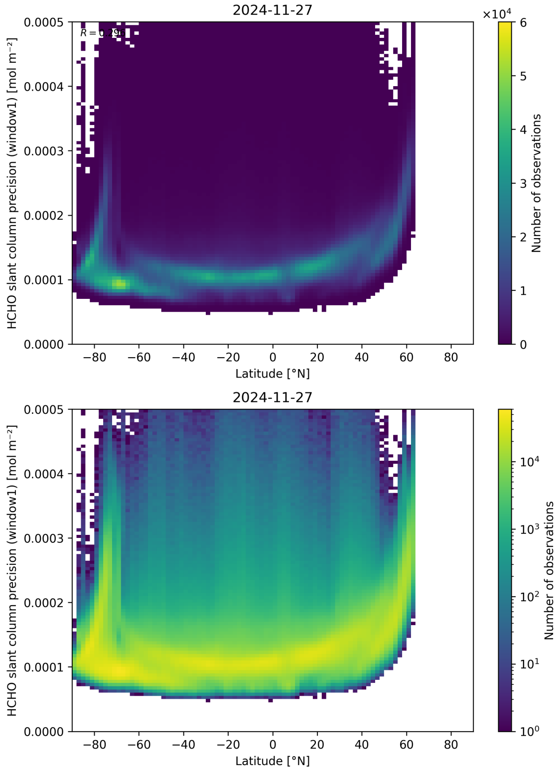
Figure 160: Scatter density plot of “Latitude” against “HCHO slant column precision (window1)” for 2024-11-26 to 2024-11-28.
