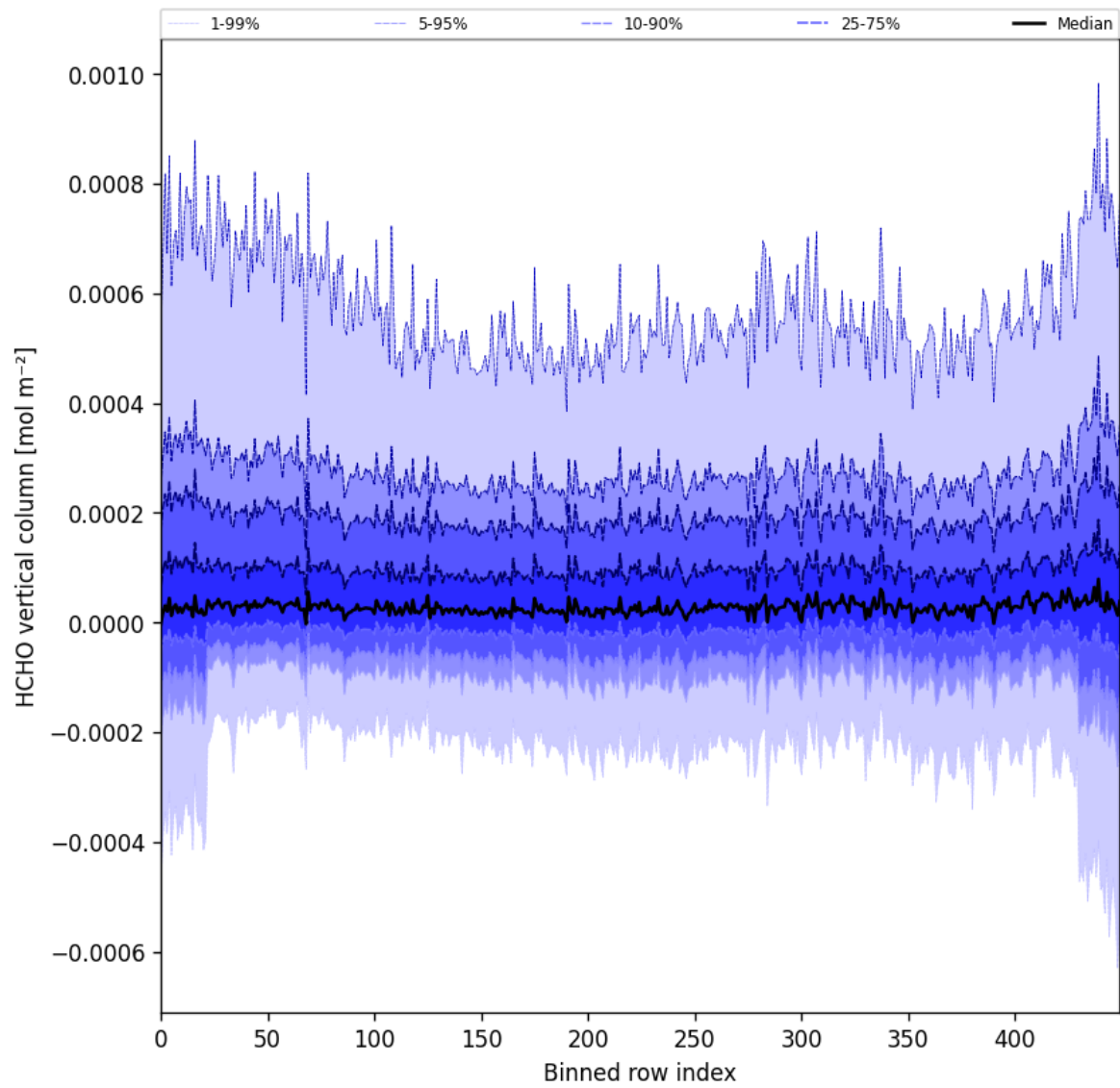
Figure 49: Along track statistics of “HCHO vertical column” for 2024-11-26 to 2024-11-28
