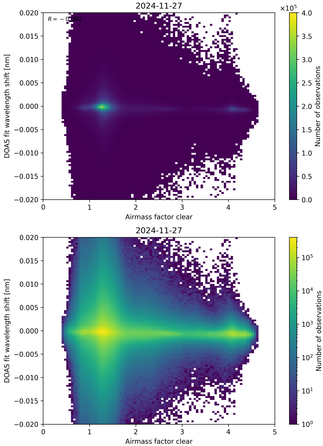
Figure 72: Scatter density plot of “Airmass factor clear” against “DOAS fit wavelength shift” for 2024-11-26 to 2024-11-28.
