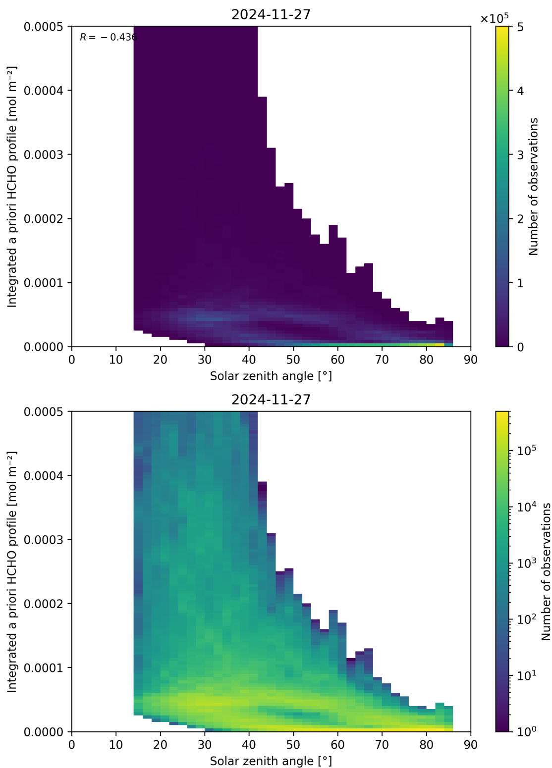
Figure 180: Scatter density plot of “Solar zenith angle” against “Integrated a priori HCHO profile” for 2024-11-26 to 2024-11-28.
