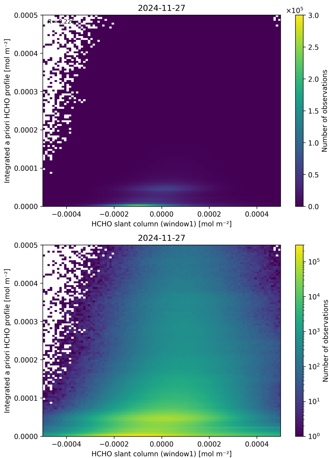
Figure 87: Scatter density plot of “HCHO slant column (window1)” against “Integrated a priori HCHO profile” for 2024-11-26 to 2024-11-28.
