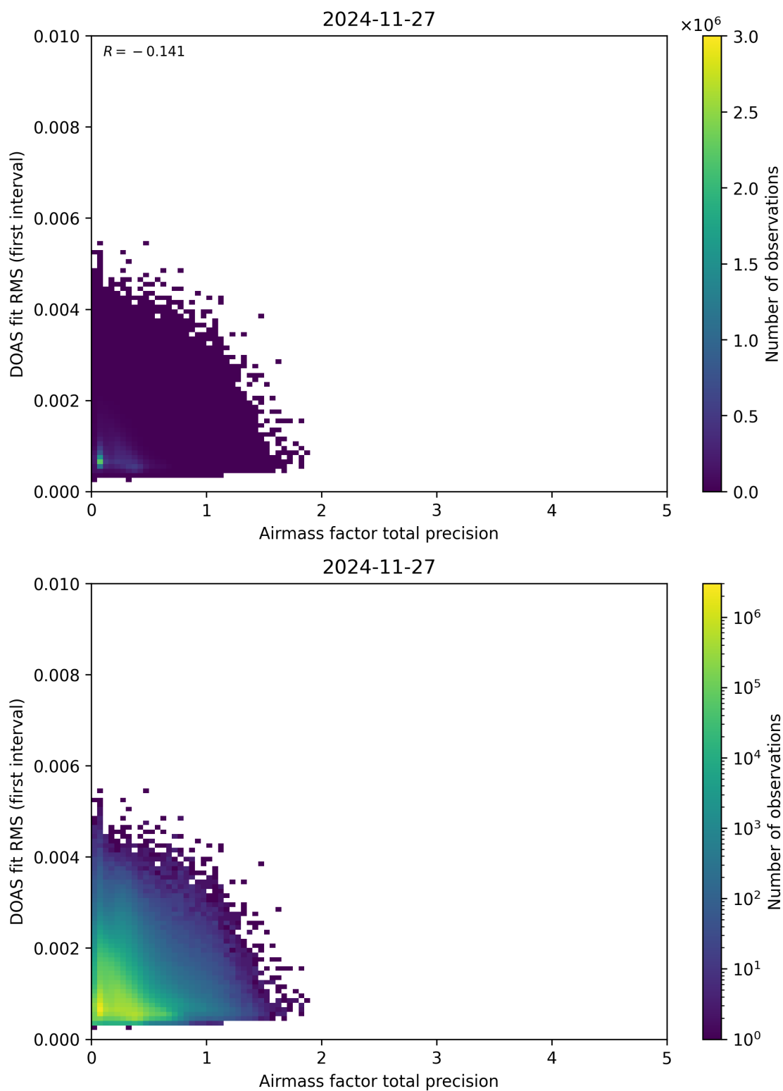
Figure 105: Scatter density plot of “Airmass factor total precision” against “DOAS fit RMS (first interval)” for 2024-11-26 to 2024-11-28.
