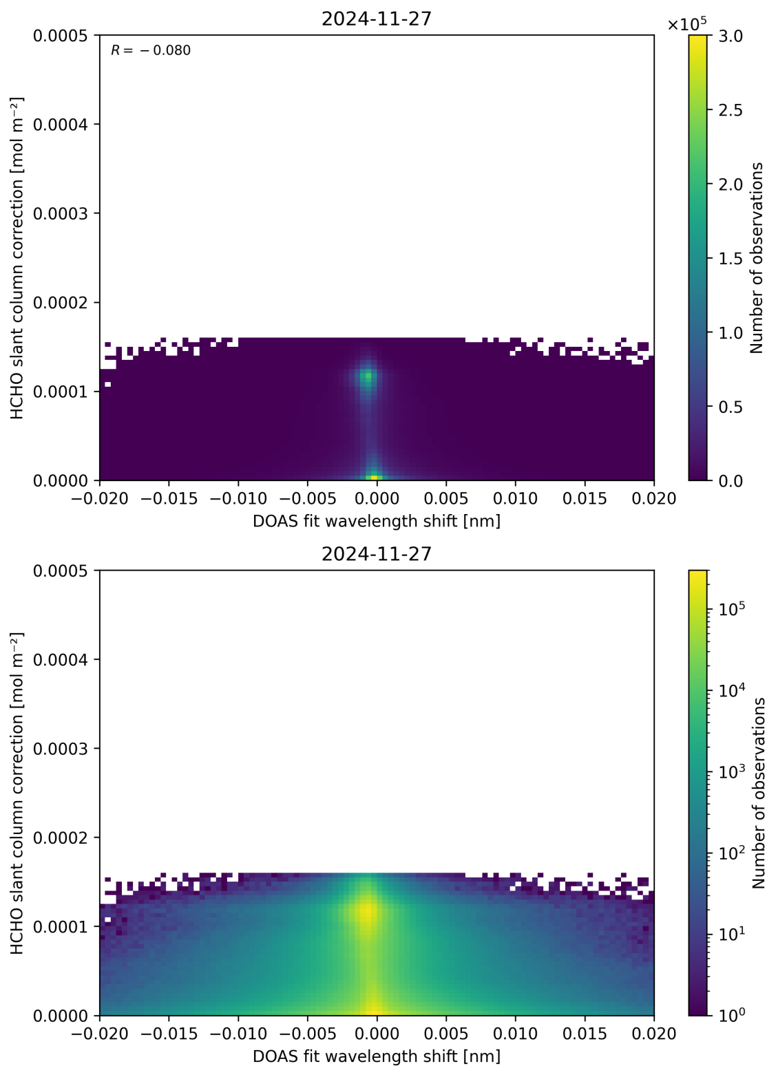
Figure 67: Scatter density plot of “DOAS fit wavelength shift” against “HCHO slant column correction” for 2024-11-26 to 2024-11-28.
