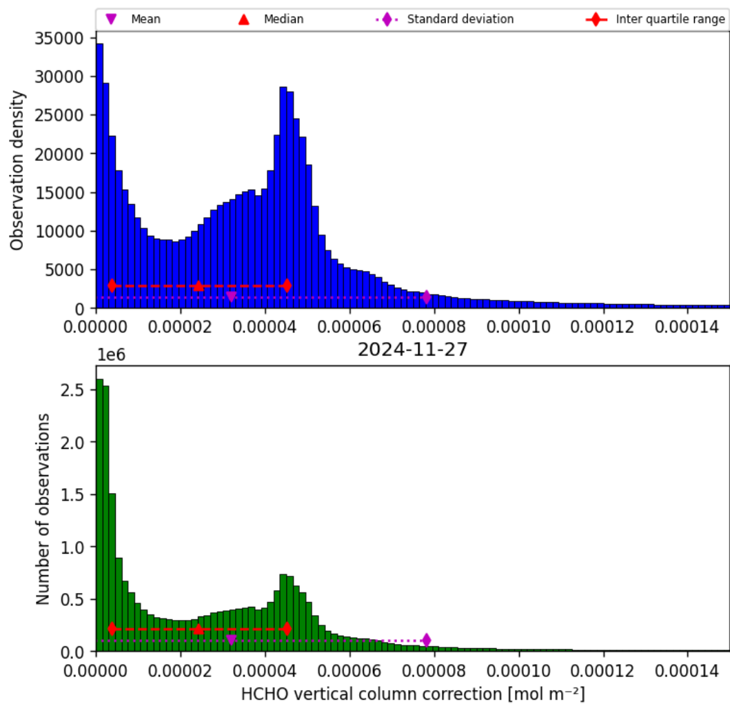
Figure 37: Histogram of “HCHO vertical column correction” for 2024-11-26 to 2024-11-28
