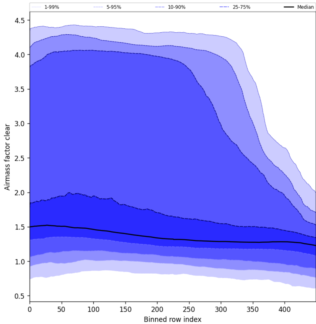
Figure 56: Along track statistics of “Air mass factor clear” for 2024-11-26 to 2024-11-28
