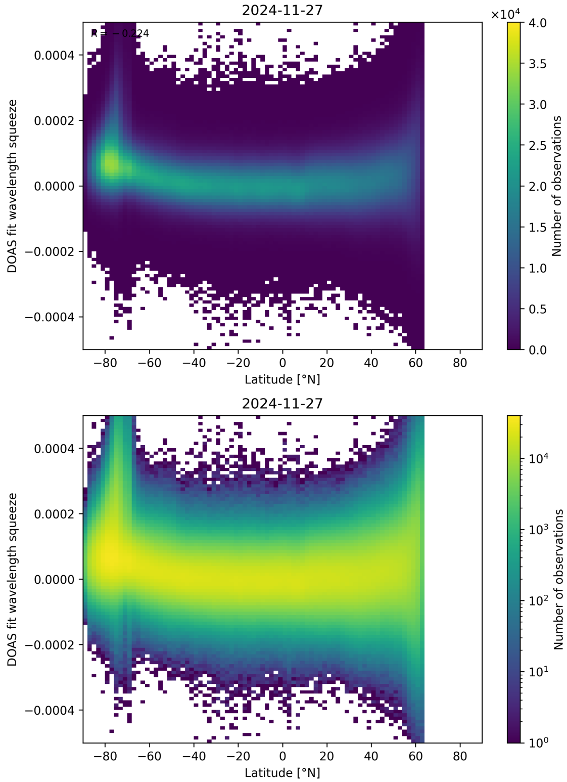
Figure 155: Scatter density plot of “Latitude” against “DOAS fit wavelength squeeze” for 2024-11-26 to 2024-11-28.
