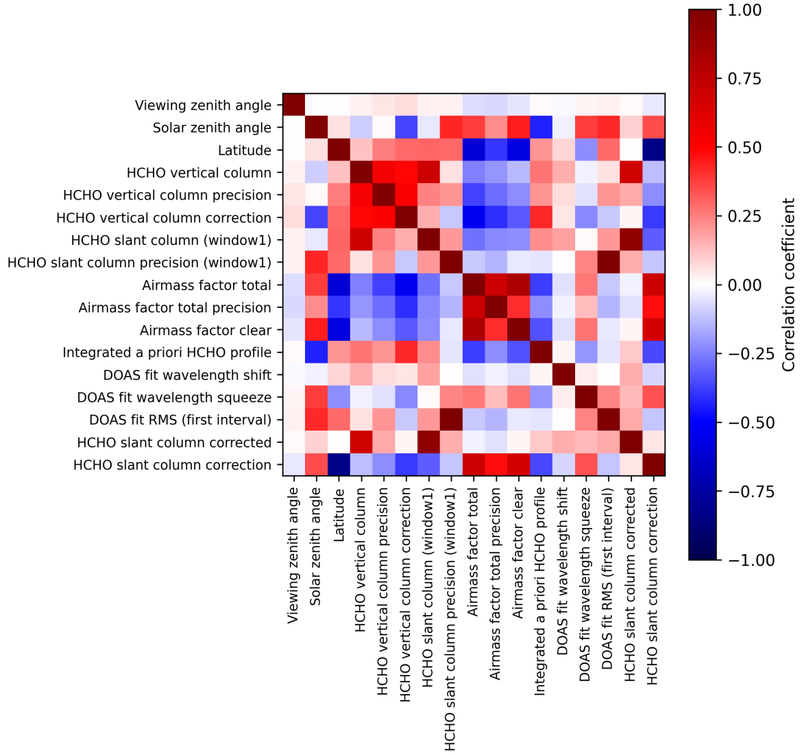
Figure 2: Map of correlation matrix for 2024-11-26 to 2024-11-28.
