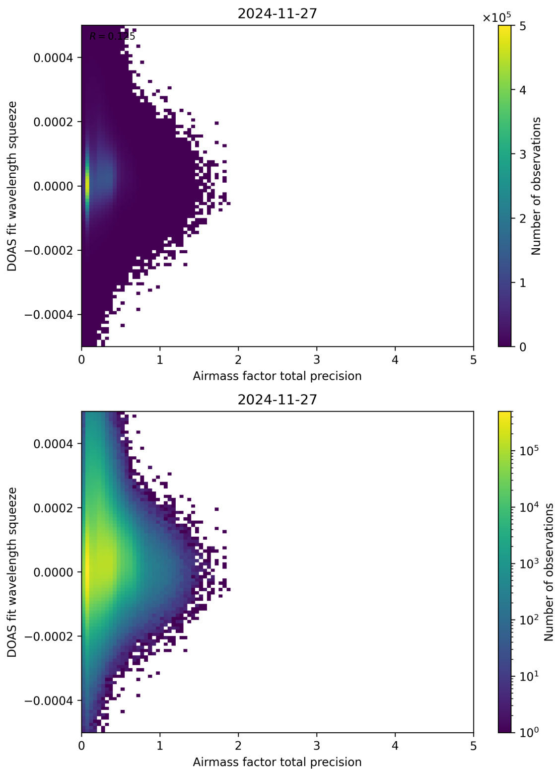
Figure 107: Scatter density plot of “Airmass factor total precision” against “DOAS fit wavelength squeeze” for 2024-11-26 to 2024-11-28.
