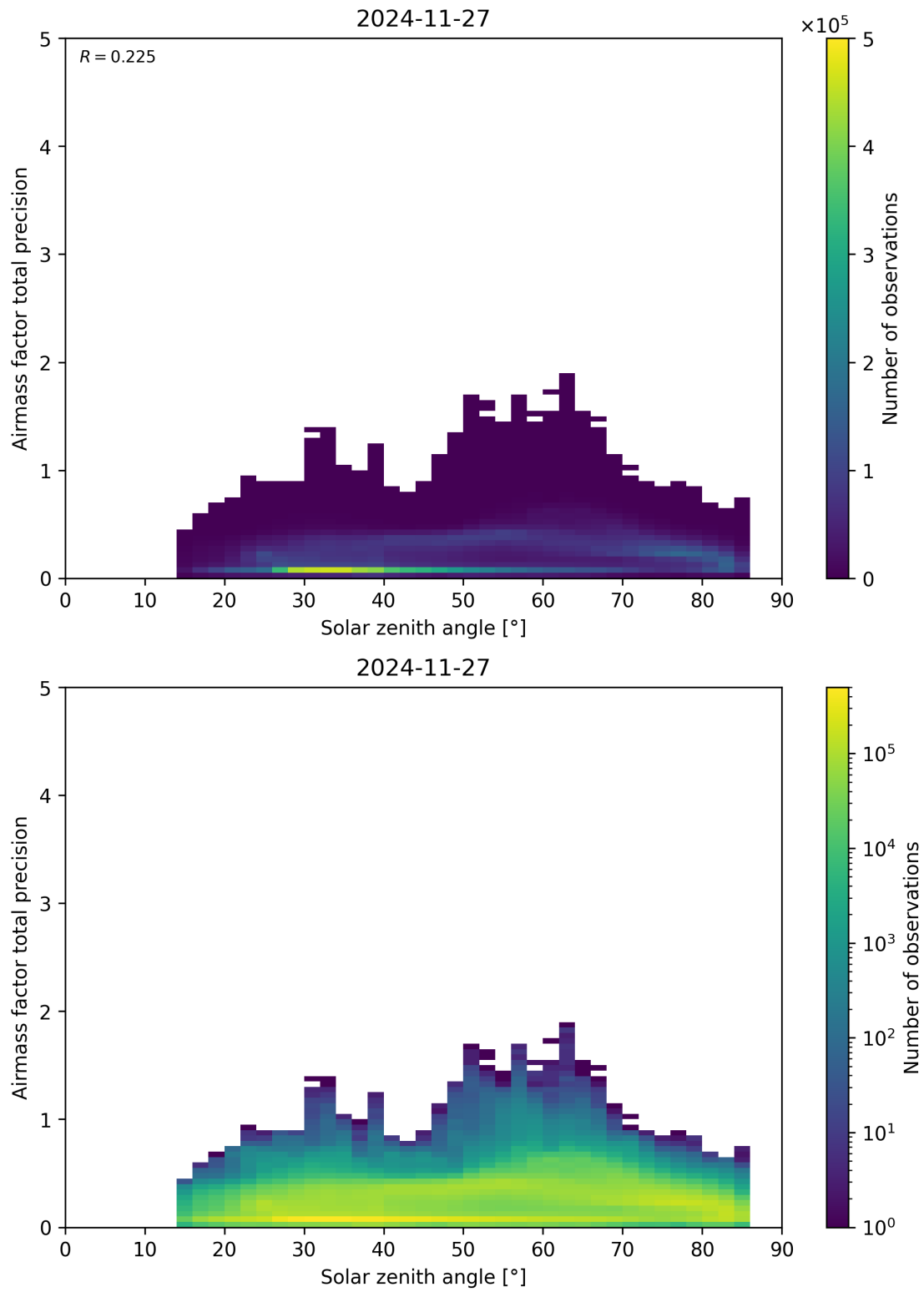
Figure 176: Scatter density plot of “Solar zenith angle” against “Airmass factor total precision” for 2024-11-26 to 2024-11-28.
