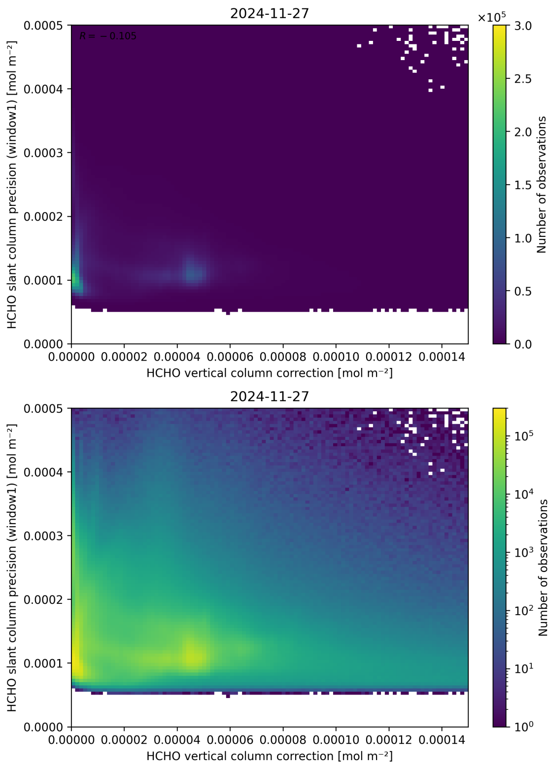
Figure 119: Scatter density plot of “HCHO vertical column correction” against “HCHO slant column precision (window1)” for 2024-11-26 to 2024-11-28.
