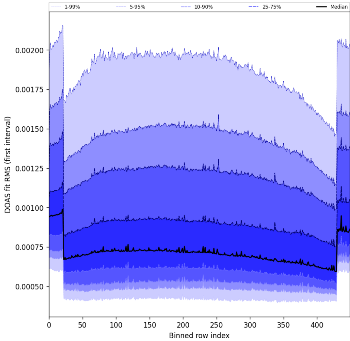
Figure 60: Along track statistics of “DOAS fit RMS (first interval)” for 2024-11-26 to 2024-11-28
