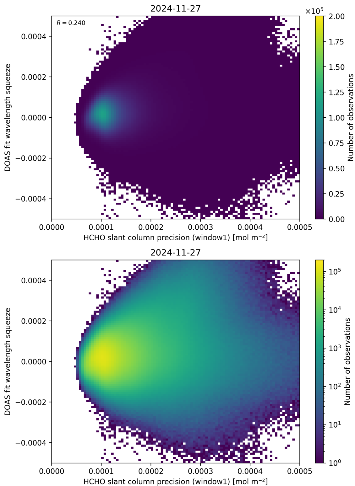
Figure 90: Scatter density plot of “HCHO slant column precision (window1)” against “DOAS fit wavelength squeeze” for 2024-11-26 to 2024-11-28.
