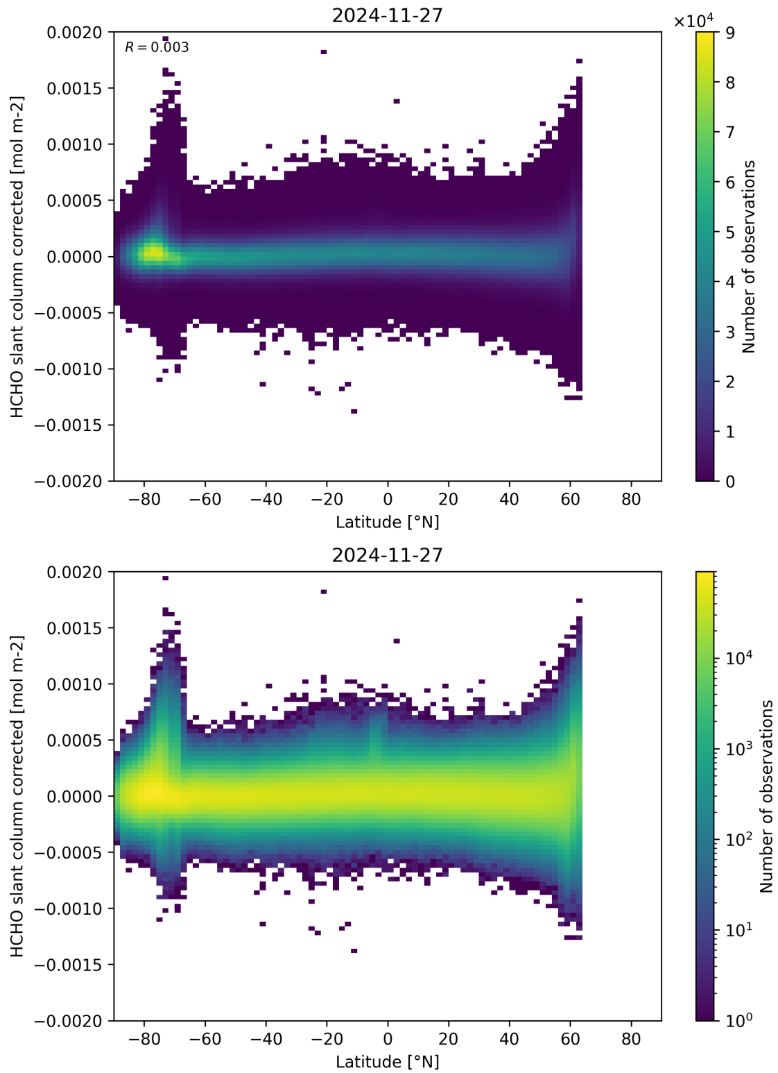
Figure 157: Scatter density plot of “Latitude” against “HCHO slant column corrected” for 2024-11-26 to 2024-11-28.
