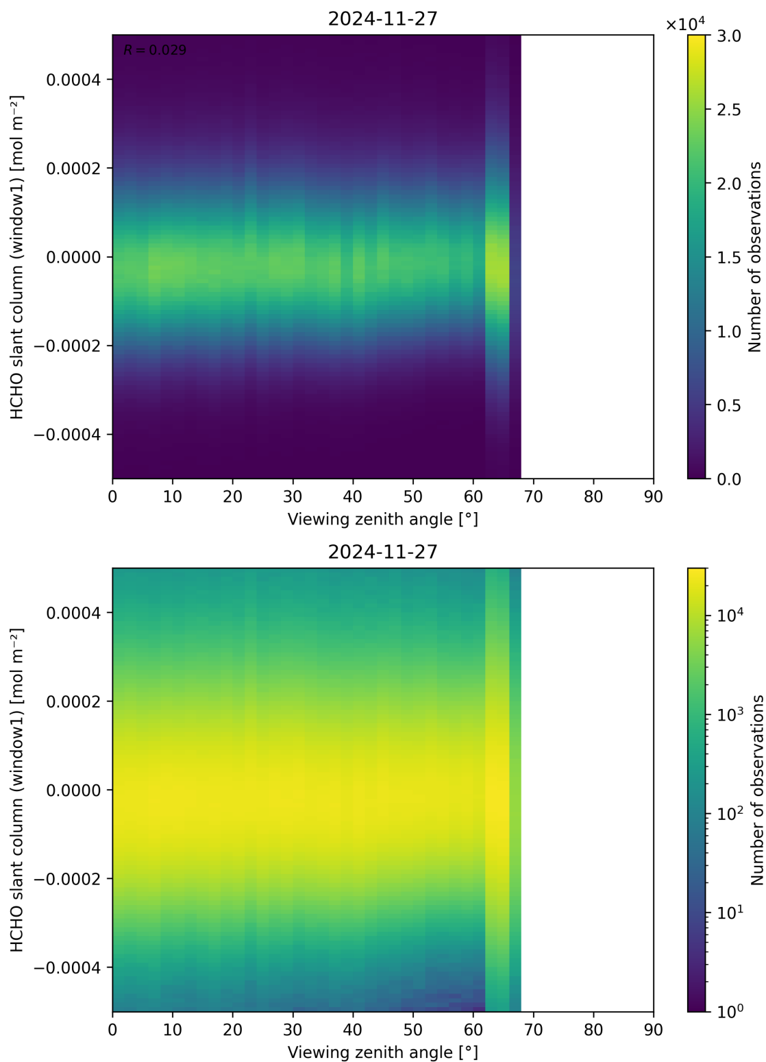
Figure 188: Scatter density plot of “Viewing zenith angle” against “HCHO slant column (window1)” for 2024-11-26 to 2024-11-28.
