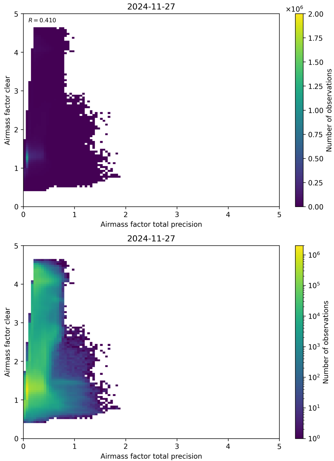
Figure 108: Scatter density plot of “Airmass factor total precision” against “Airmass factor clear” for 2024-11-26 to 2024-11-28.
