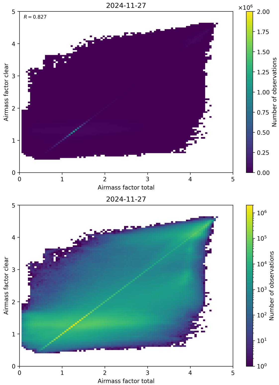
Figure 100: Scatter density plot of “Airmass factor total” against “Airmass factor clear” for 2024-11-26 to 2024-11-28.
