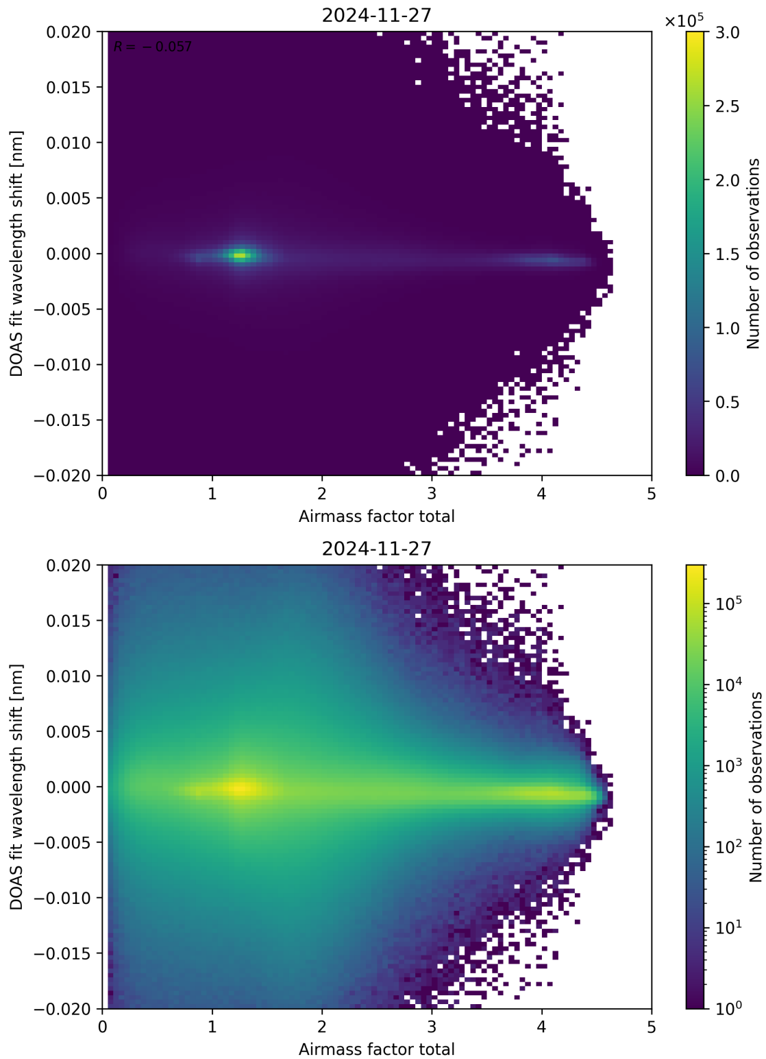
Figure 98: Scatter density plot of “Airmass factor total” against “DOAS fit wavelength shift” for 2024-11-26 to 2024-11-28.
