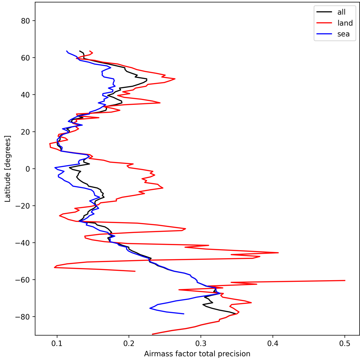
Figure 27: Zonal average of “Airmass factor total precision” for 2024-11-26 to 2024-11-28.
