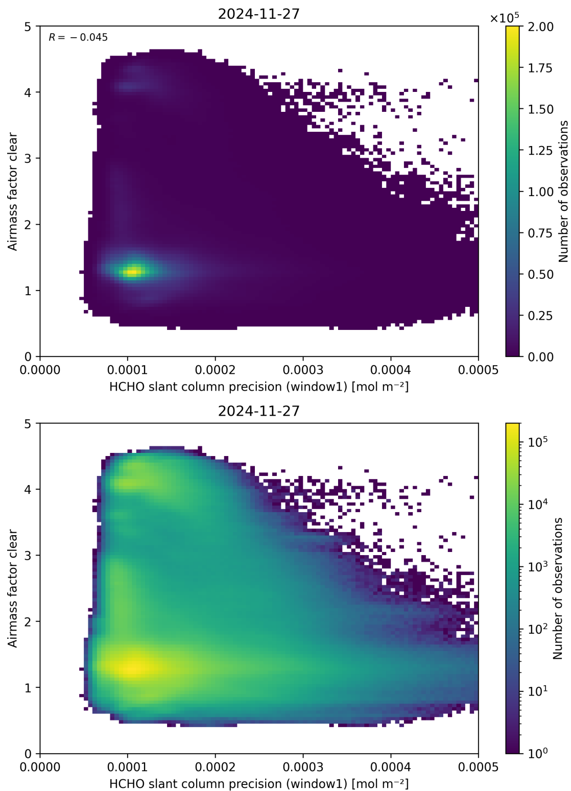
Figure 91: Scatter density plot of “HCHO slant column precision (window1)” against “Airmass factor clear” for 2024-11-26 to 2024-11-28.
