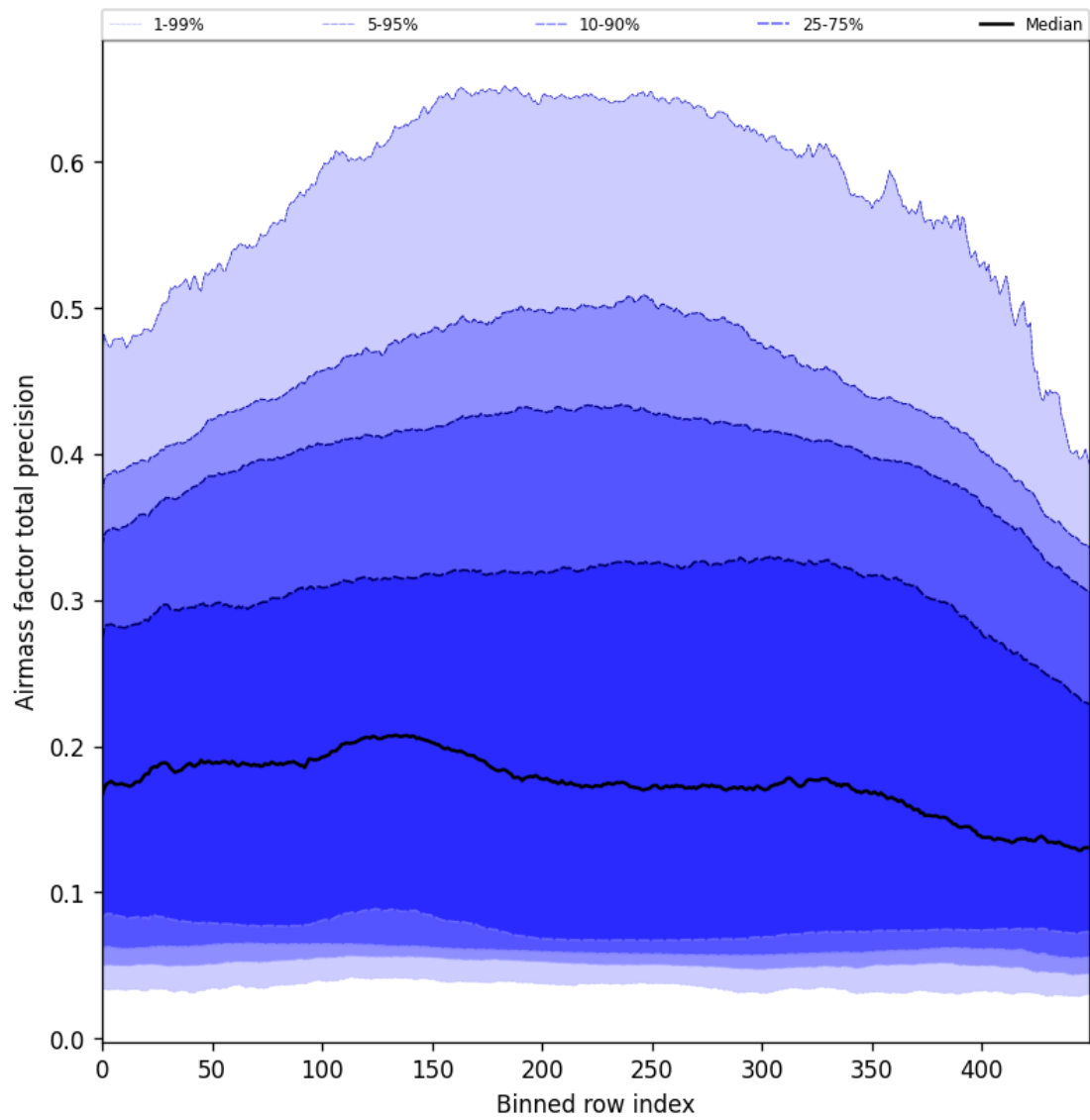
Figure 55: Along track statistics of “Airmass factor total precision” for 2024-11-26 to 2024-11-28
