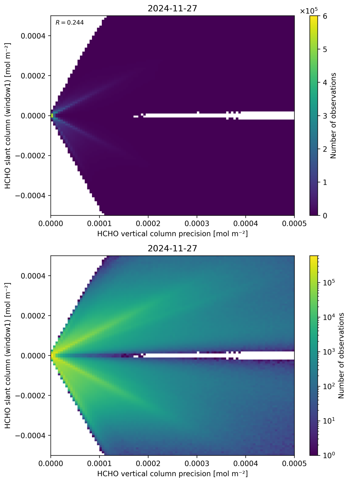
Figure 142: Scatter density plot of “HCHO vertical column precision” against “HCHO slant column (window1)” for 2024-11-26 to 2024-11-28.
