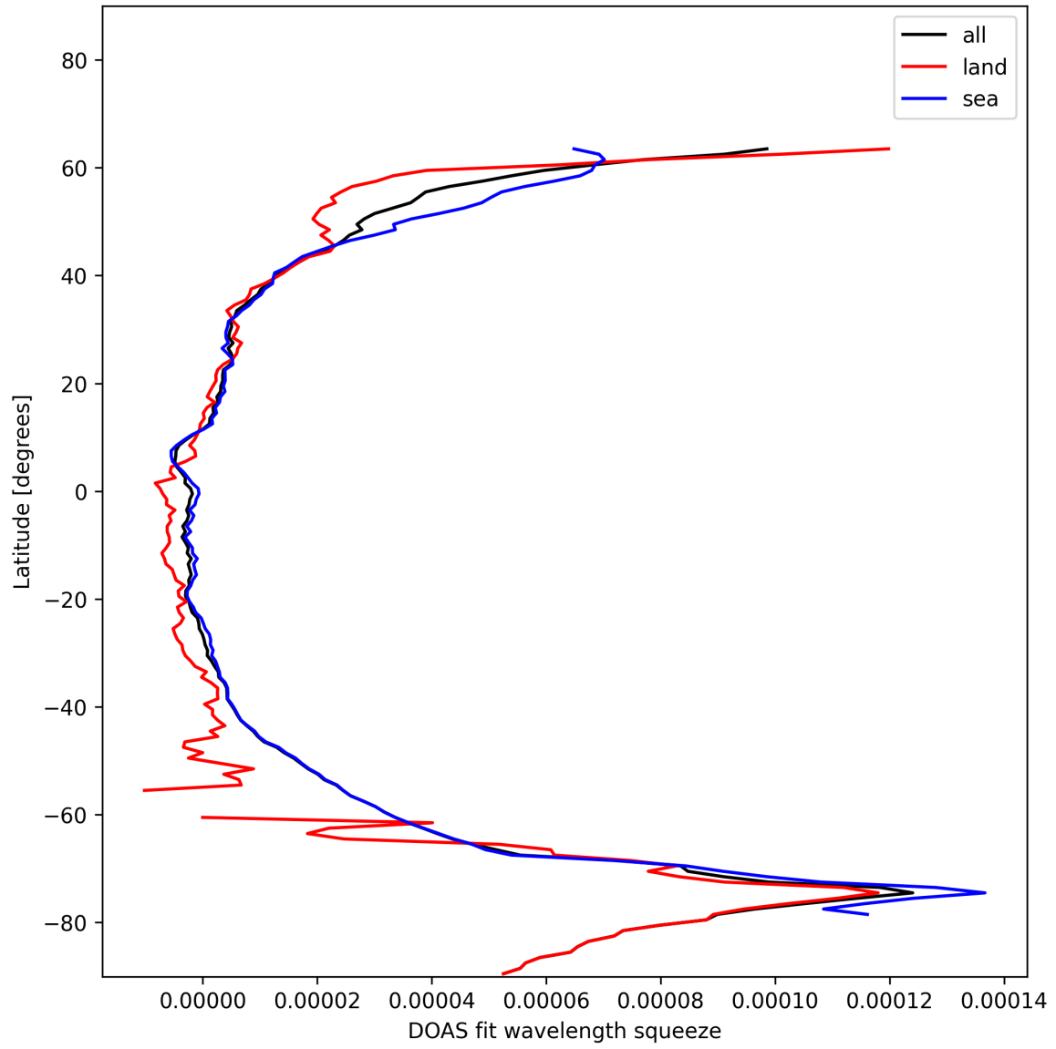
Figure 31: Zonal average of “DOAS fit wavelength squeeze” for 2024-11-26 to 2024-11-28.
