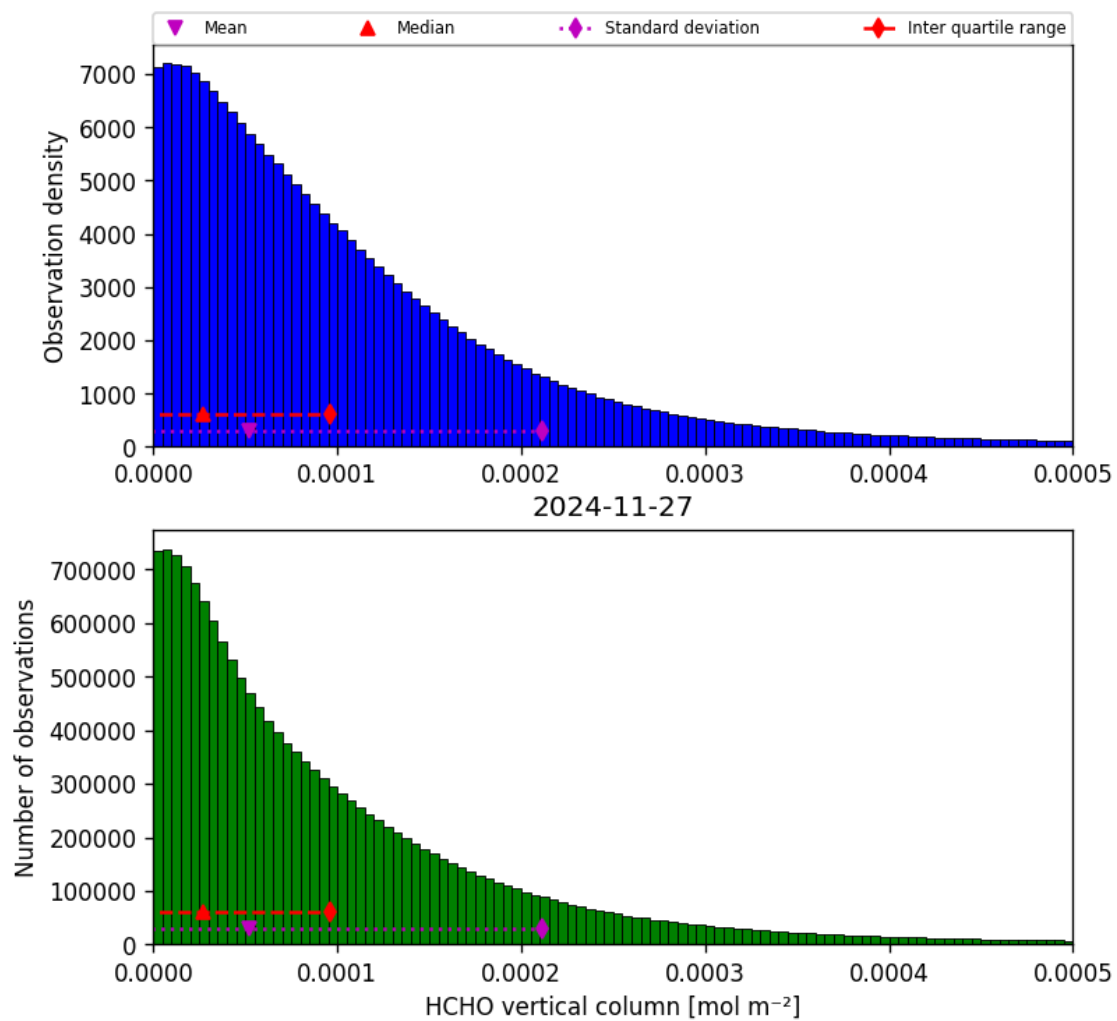
Figure 35: Histogram of “HCHO vertical column” for 2024-11-26 to 2024-11-28
