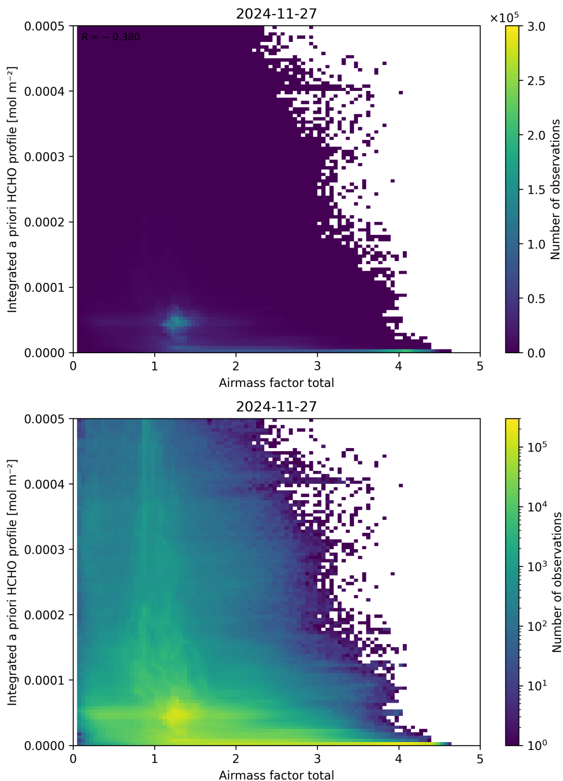
Figure 104: Scatter density plot of “Airmass factor total” against “Integrated a priori HCHO profile” for 2024-11-26 to 2024-11-28.
