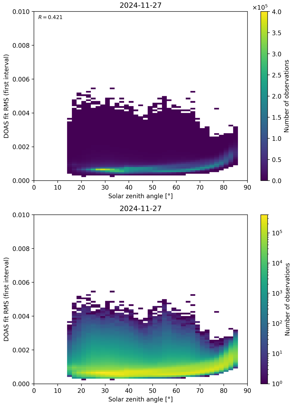
Figure 167: Scatter density plot of “Solar zenith angle” against “DOAS fit RMS (first interval)” for 2024-11-26 to 2024-11-28.
