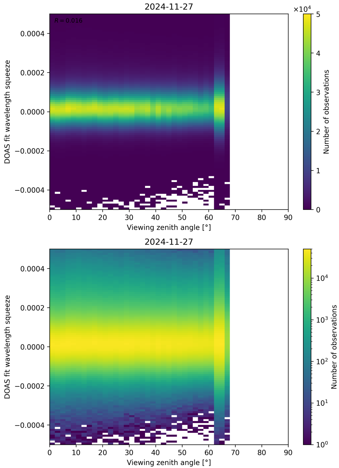
Figure 184: Scatter density plot of “Viewing zenith angle” against “DOAS fit wavelength squeeze” for 2024-11-26 to 2024-11-28.
