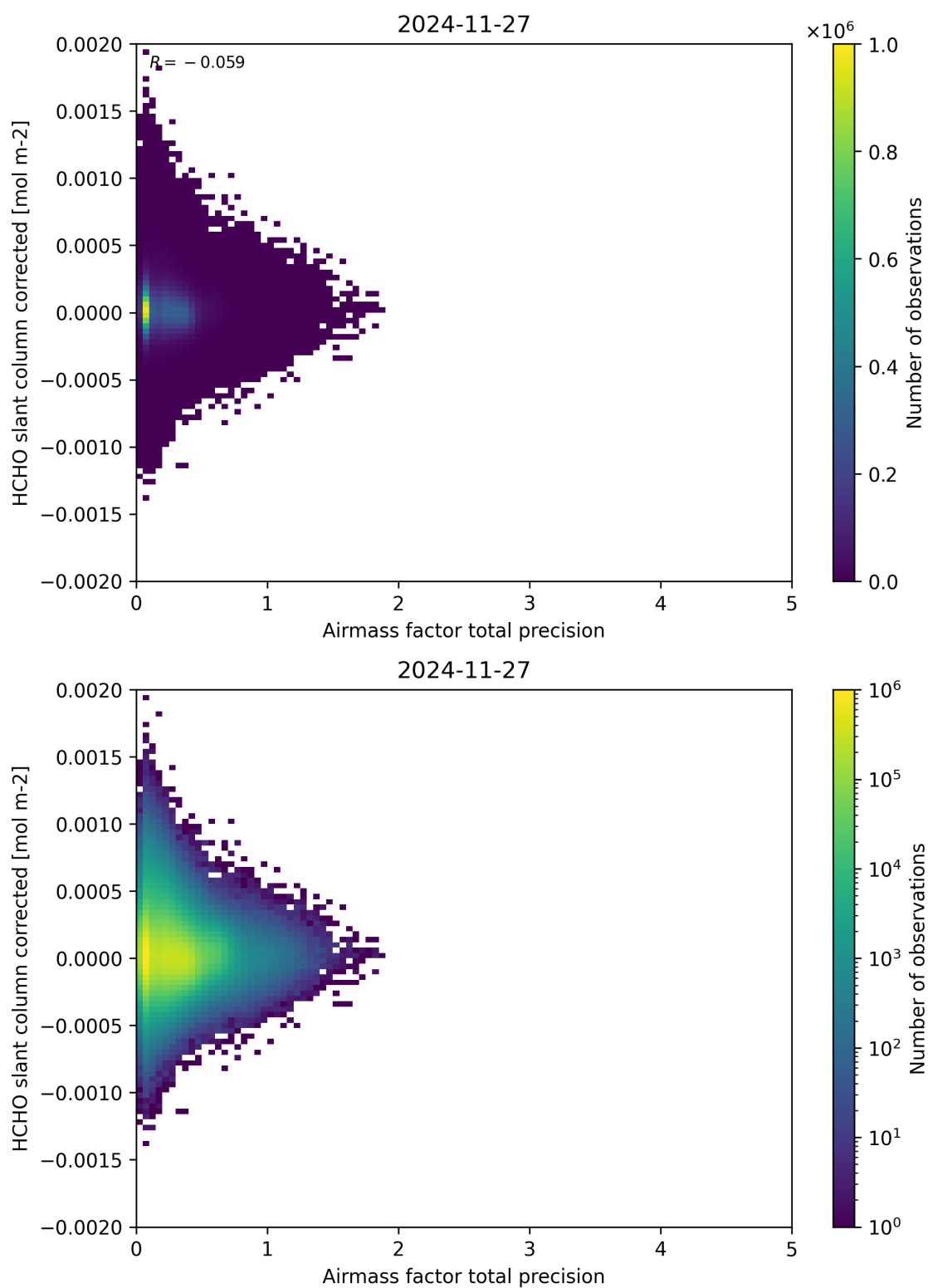
Figure 109: Scatter density plot of “Airmass factor total precision” against “HCHO slant column corrected” for 2024-11-26 to 2024-11-28.
