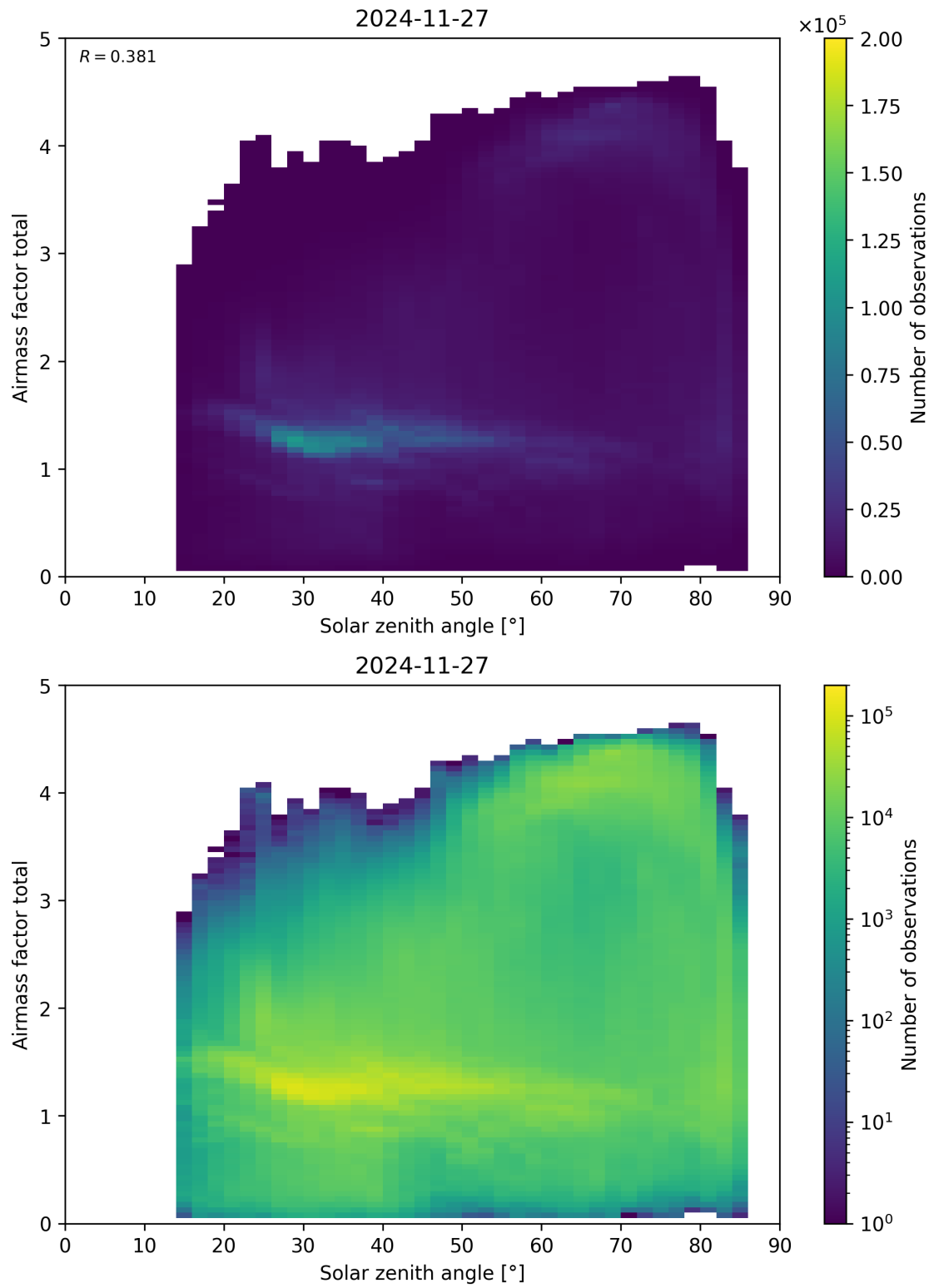
Figure 175: Scatter density plot of “Solar zenith angle” against “Airmass factor total” for 2024-11-26 to 2024-11-28.
