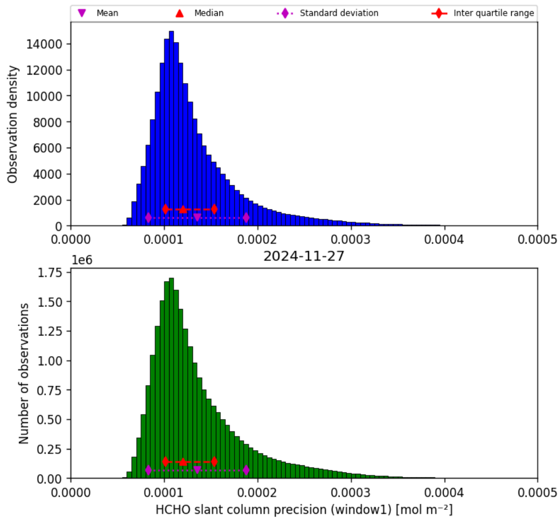
Figure 39: Histogram of “HCHO slant column precision (window1)” for 2024-11-26 to 2024-11-28
