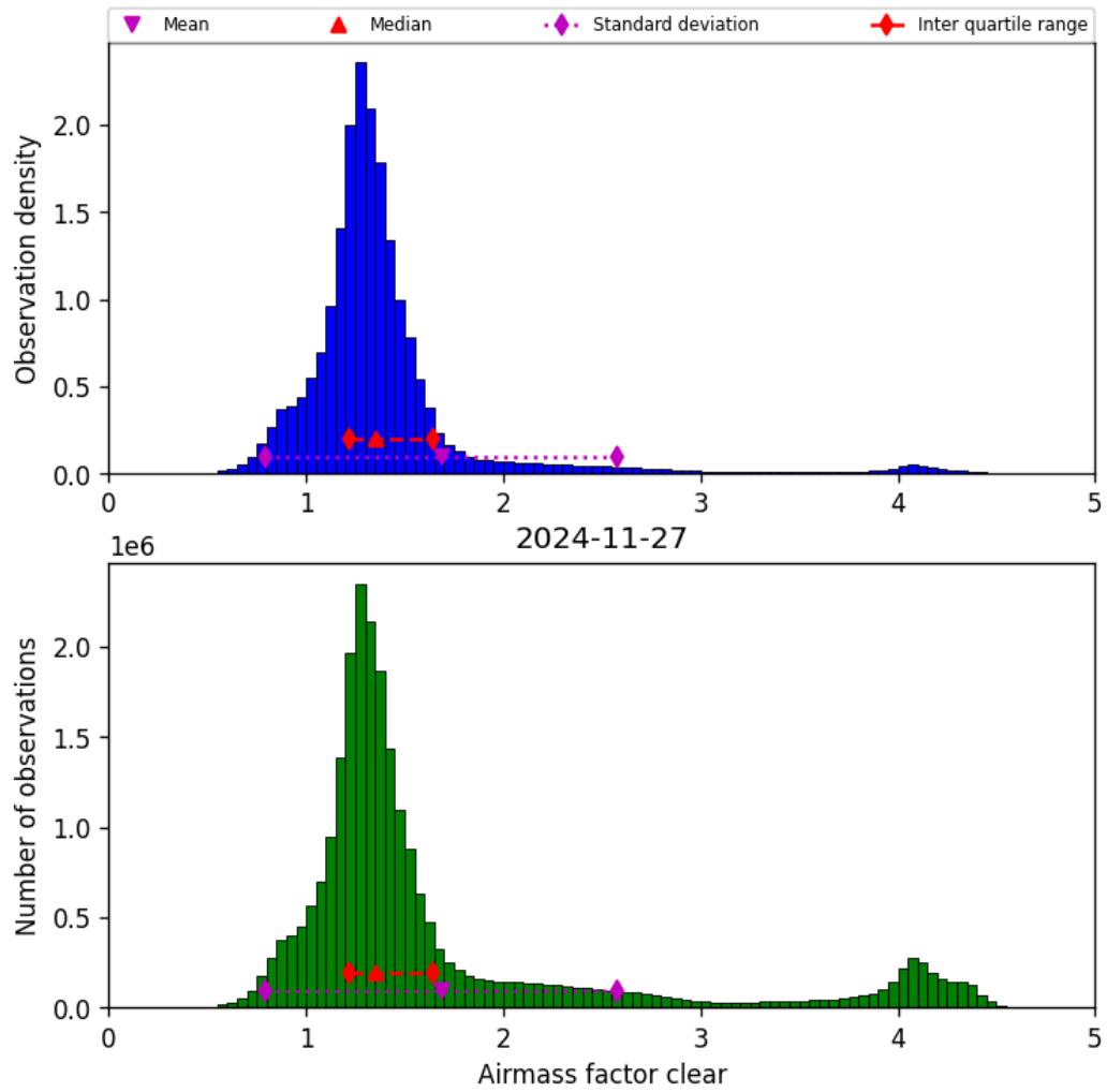
Figure 42: Histogram of “Airmass factor clear” for 2024-11-26 to 2024-11-28
