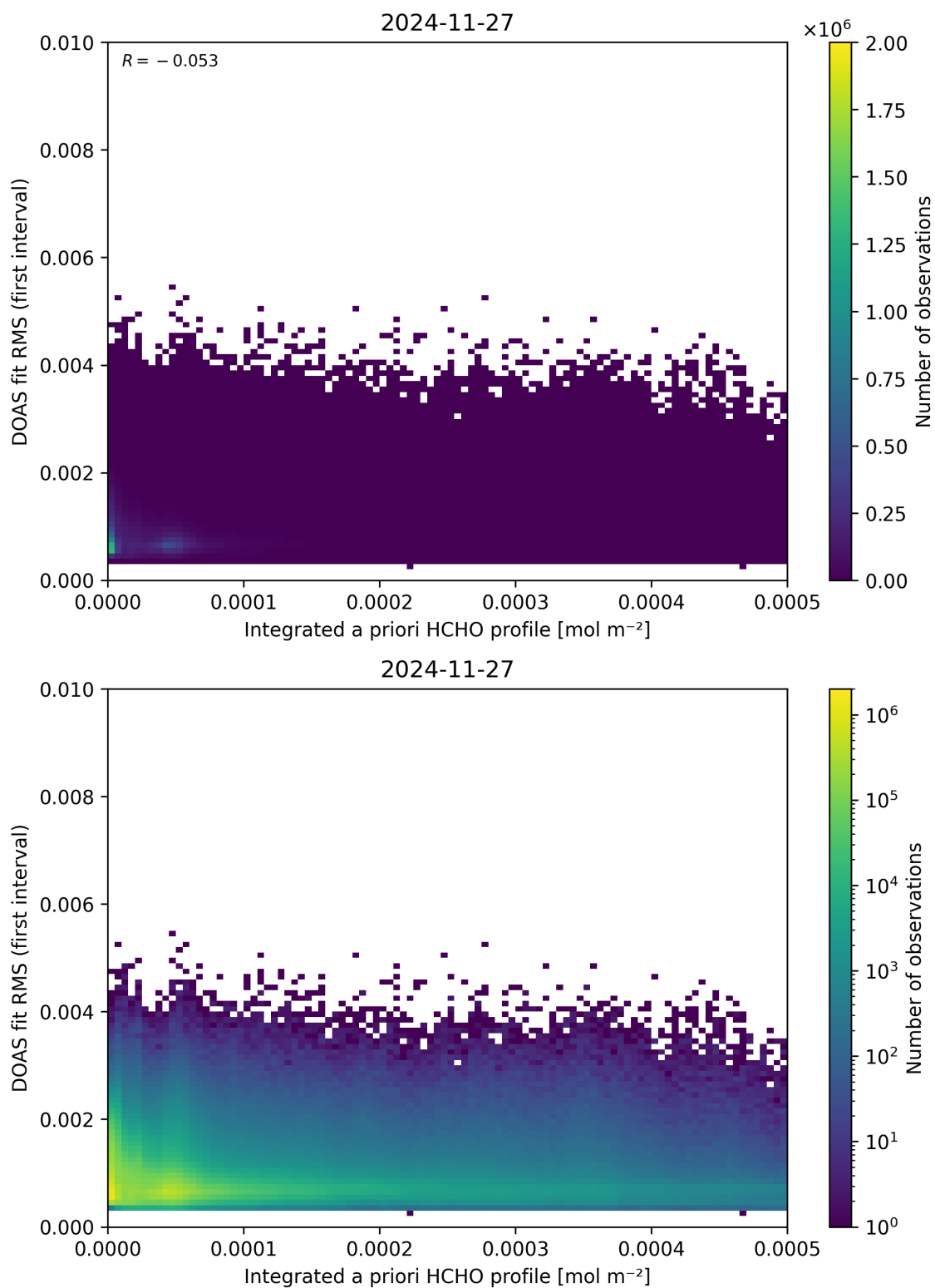
Figure 148: Scatter density plot of “Integrated a priori HCHO profile” against “DOAS fit RMS (first interval)” for 2024-11-26 to 2024-11-28.
