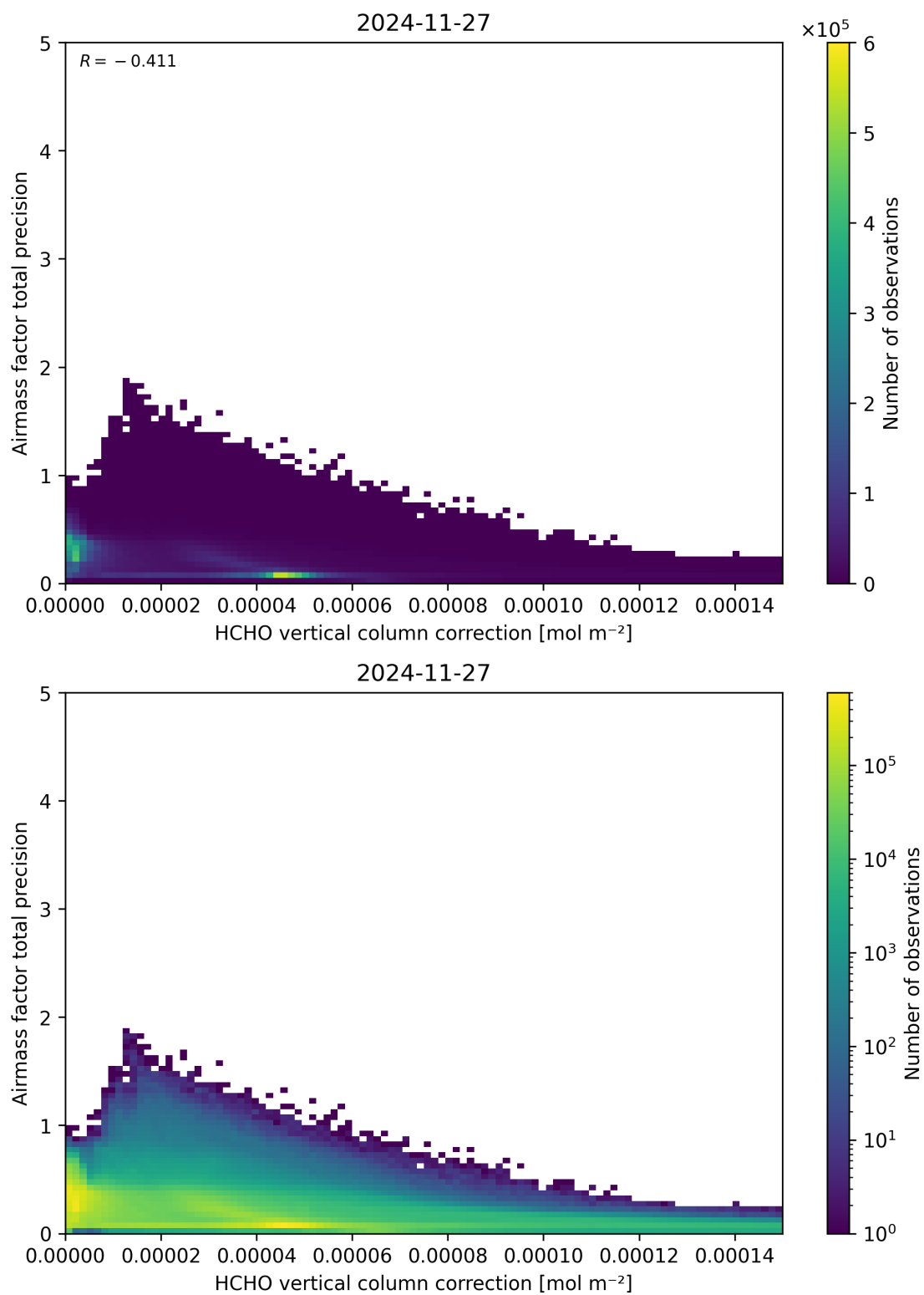
Figure 121: Scatter density plot of “HCHO vertical column correction” against “Airmass factor total precision” for 2024-11-26 to 2024-11-28.
