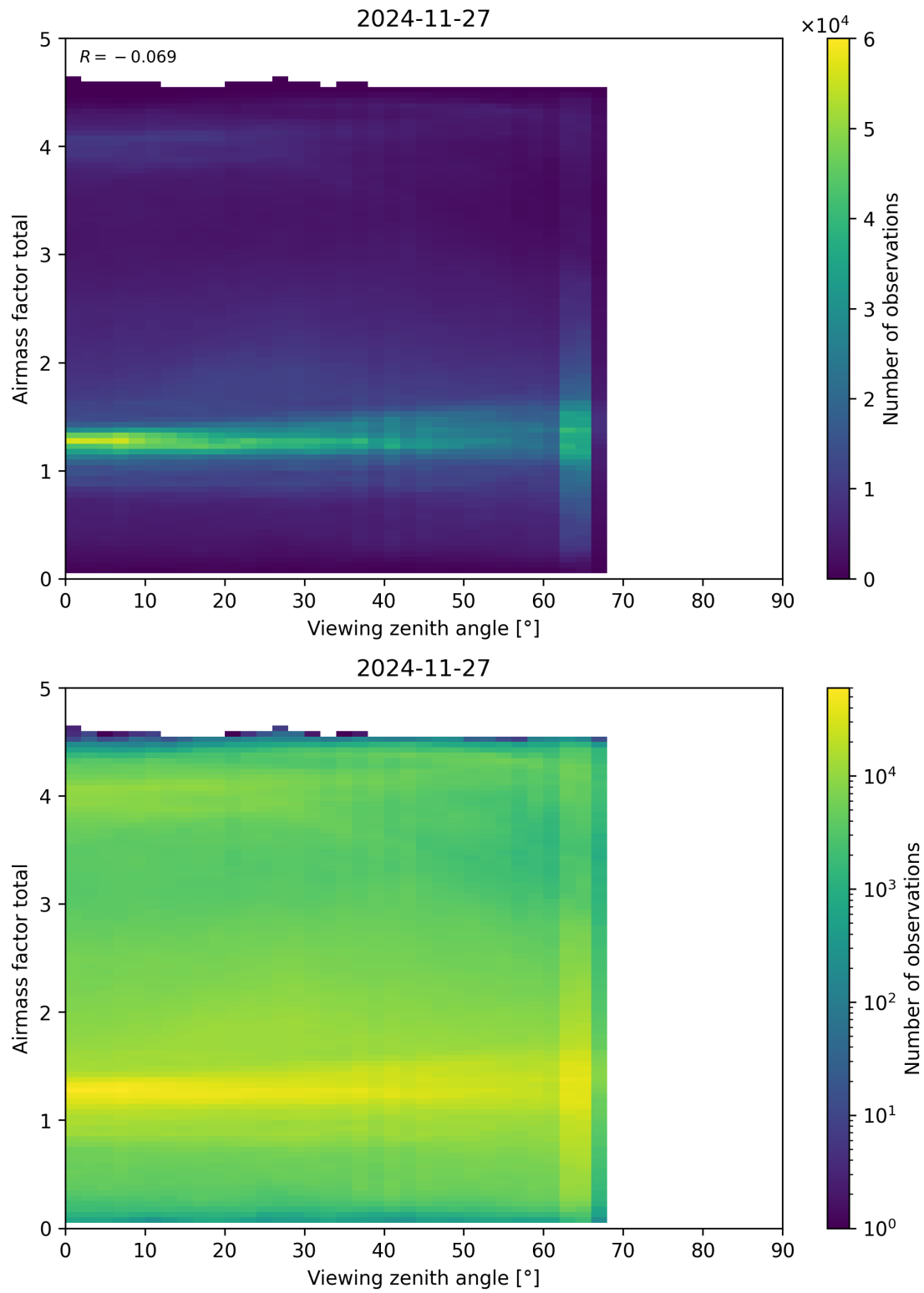
Figure 190: Scatter density plot of “Viewing zenith angle” against “Airmass factor total” for 2024-11-26 to 2024-11-28.
