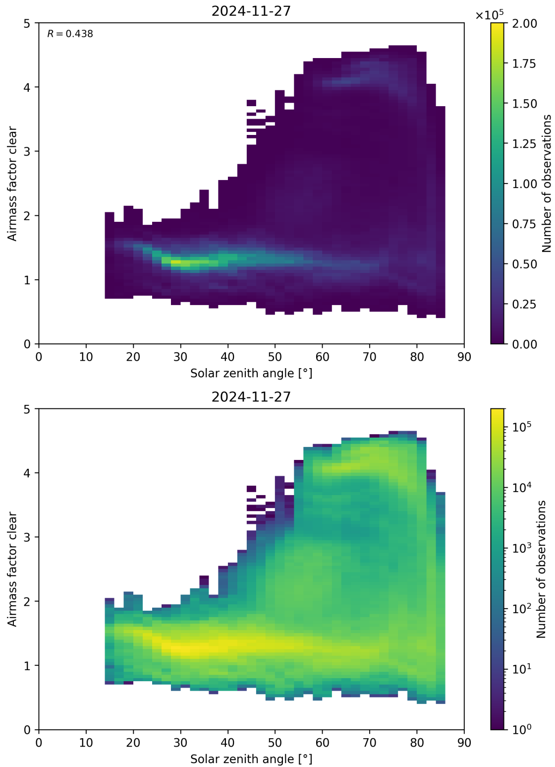
Figure 170: Scatter density plot of “Solar zenith angle” against “Airmass factor clear” for 2024-11-26 to 2024-11-28.
