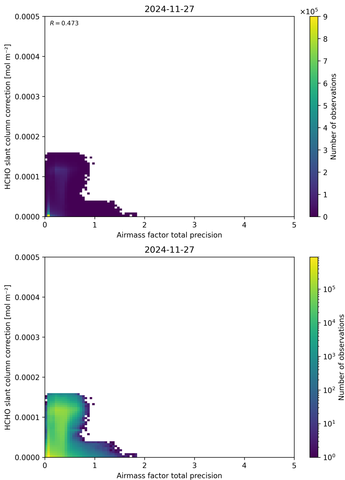
Figure 110: Scatter density plot of “Airmass factor total precision” against “HCHO slant column correction” for 2024-11-26 to 2024-11-28.
