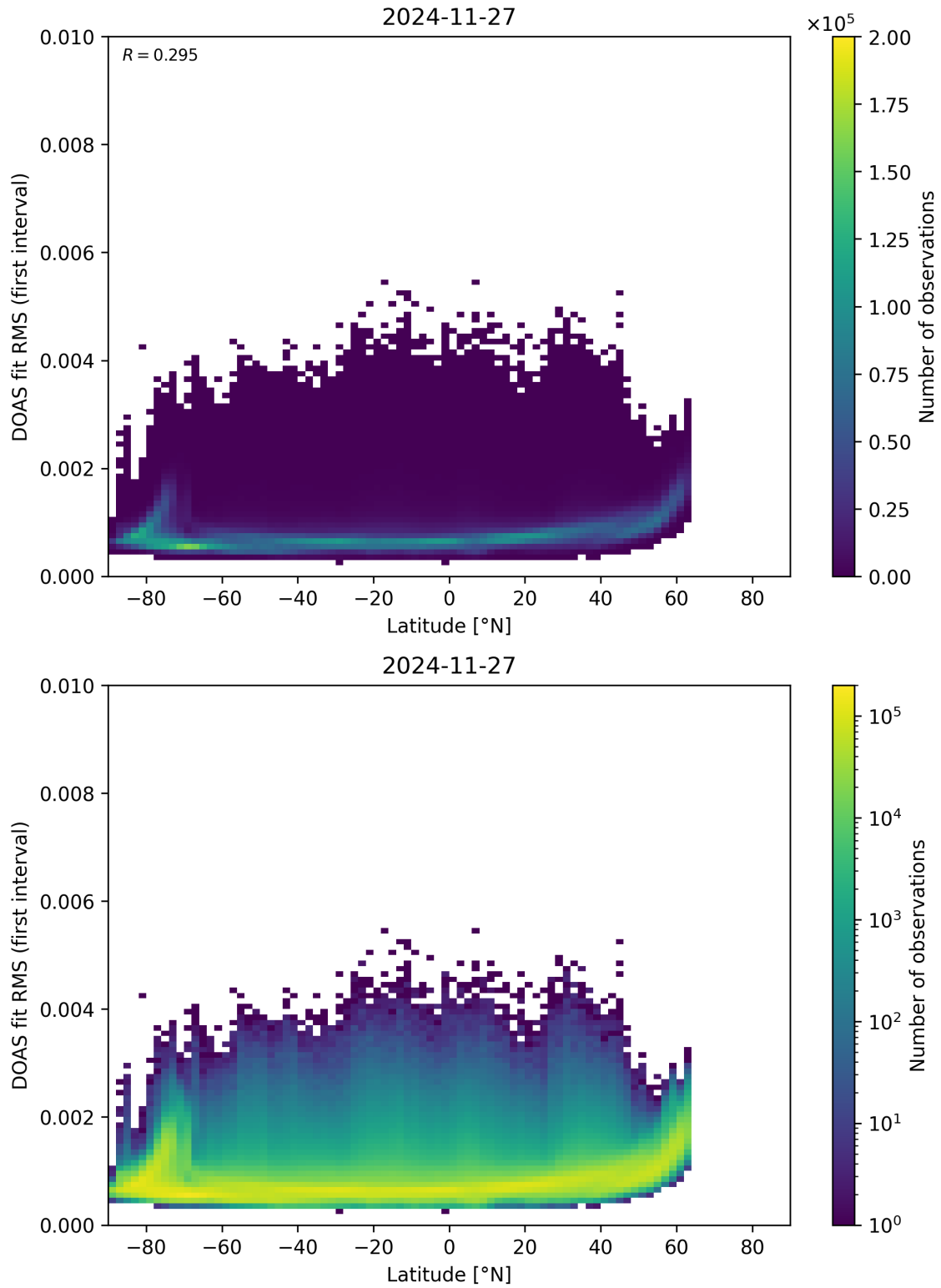
Figure 153: Scatter density plot of “Latitude” against “DOAS fit RMS (first interval)” for 2024-11-26 to 2024-11-28.
