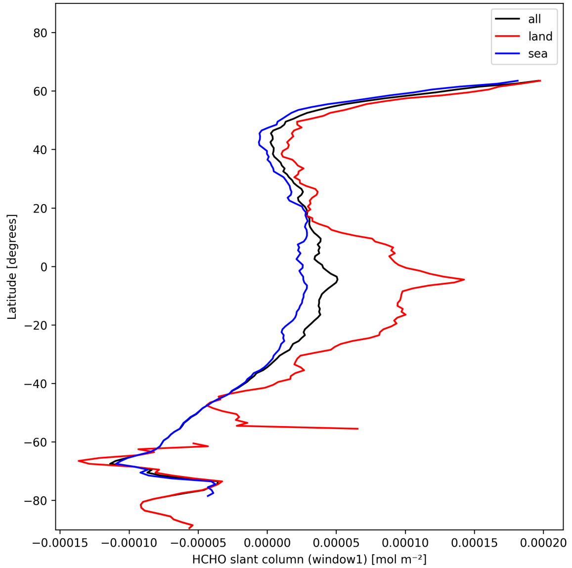
Figure 24: Zonal average of “HCHO slant column (window1)” for 2024-11-26 to 2024-11-28.
