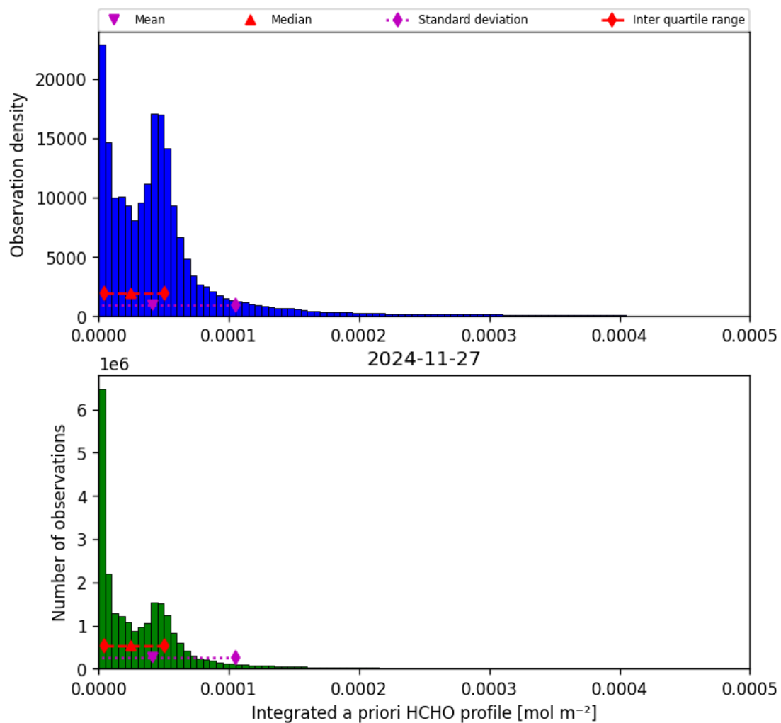
Figure 43: Histogram of “Integrated a priori HCHO profile” for 2024-11-26 to 2024-11-28
