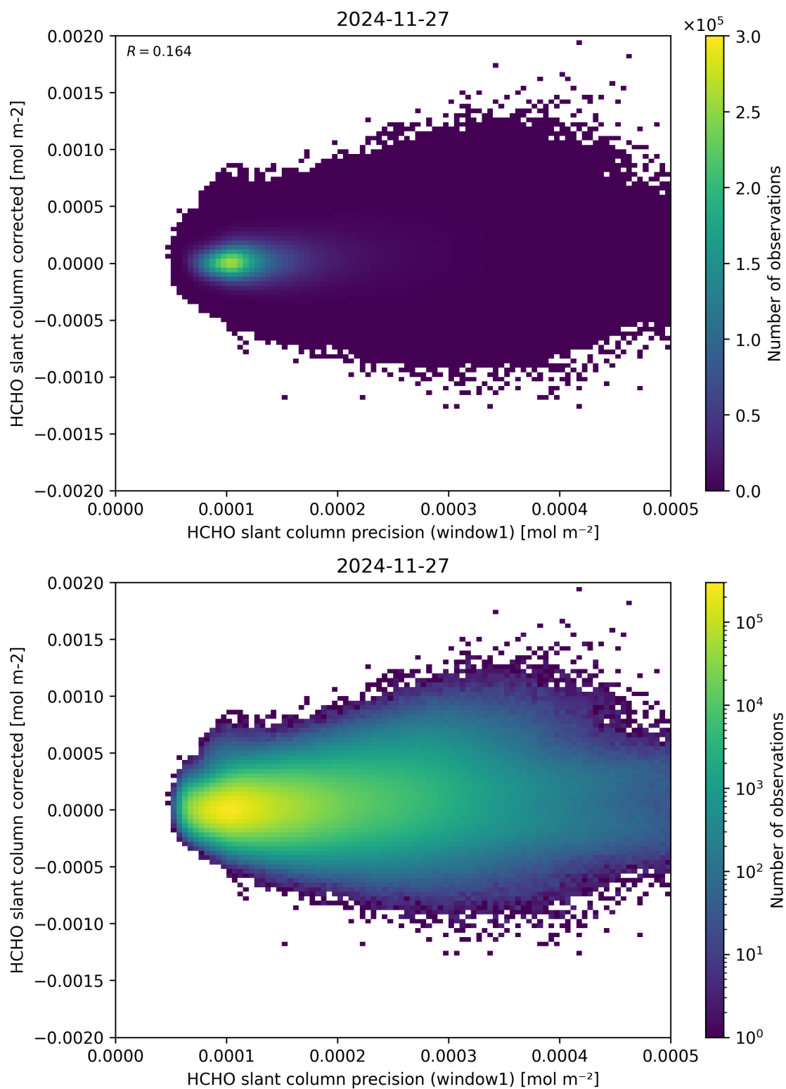
Figure 92: Scatter density plot of “HCHO slant column precision (window1)” against “HCHO slant column corrected” for 2024-11-26 to 2024-11-28.
