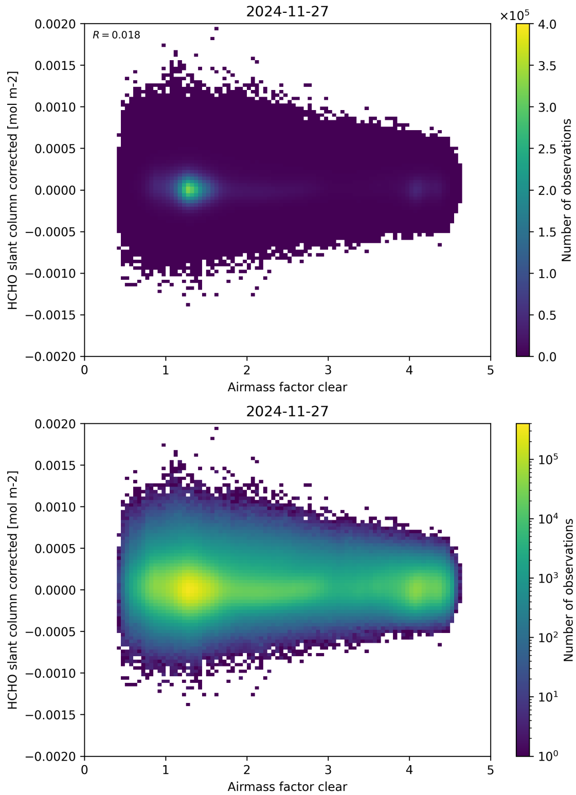
Figure 74: Scatter density plot of “Airmass factor clear” against “HCHO slant column corrected” for 2024-11-26 to 2024-11-28.
