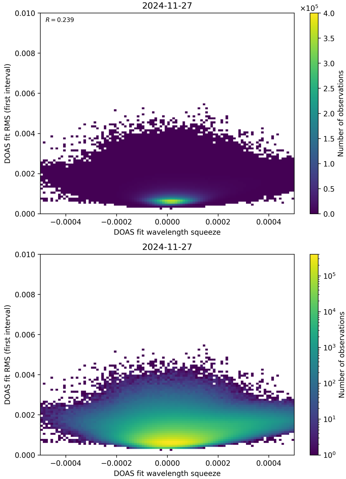
Figure 68: Scatter density plot of “DOAS fit wavelength squeeze” against “DOAS fit RMS (first interval)” for 2024-11-26 to 2024-11-28.
