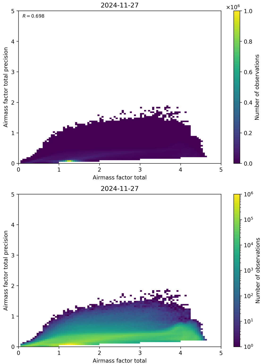
Figure 103: Scatter density plot of “Airmass factor total” against “Airmass factor total precision” for 2024-11-26 to 2024-11-28.
