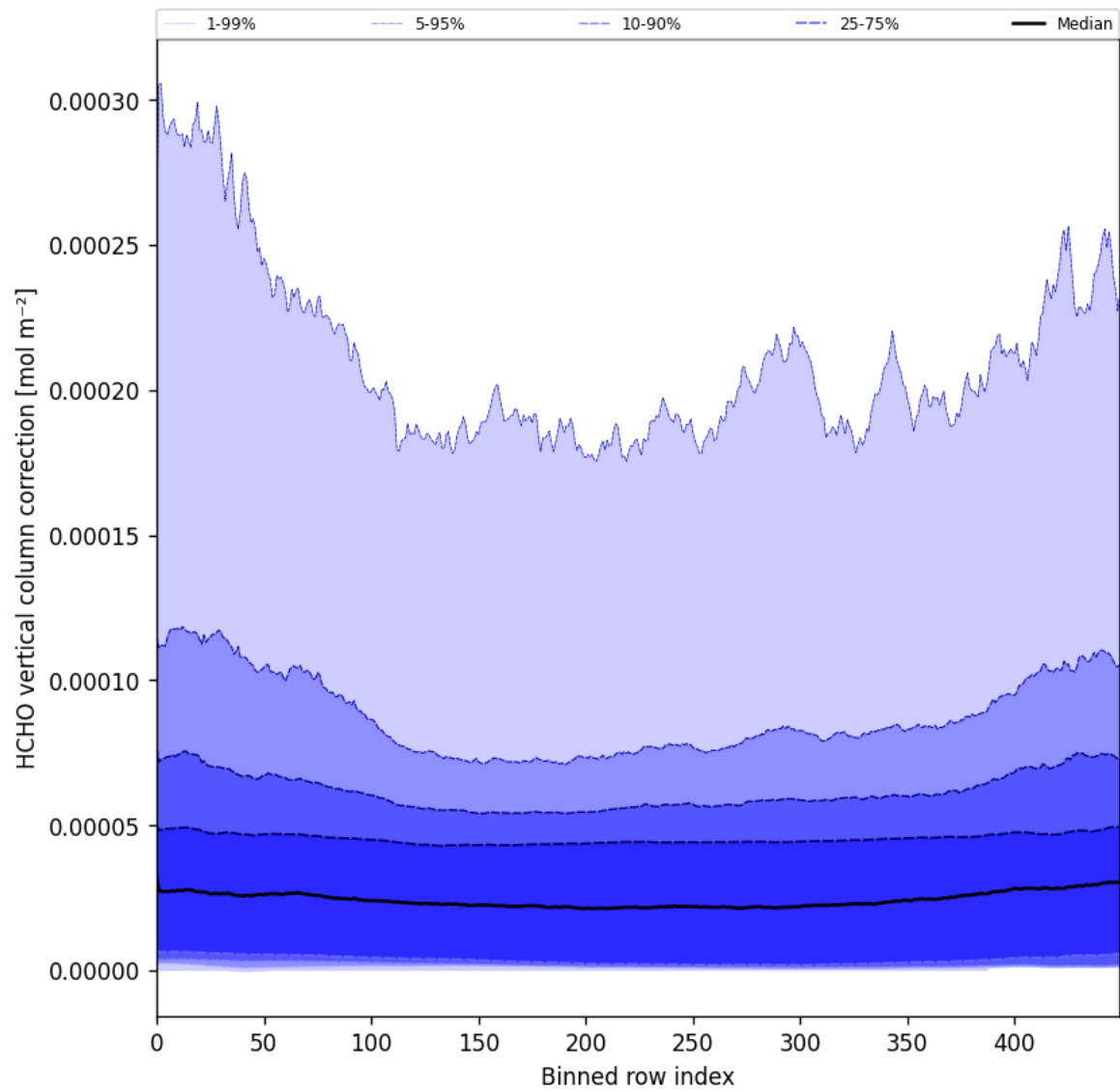
Figure 51: Along track statistics of “HCHO vertical column correction” for 2024-11-26 to 2024-11-28
