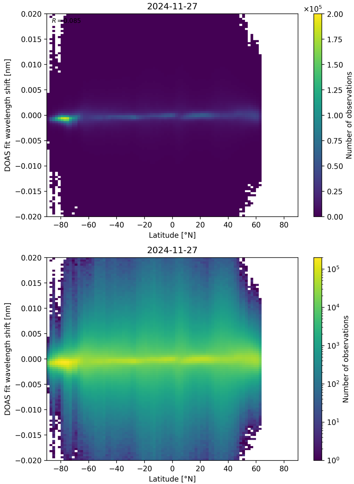
Figure 154: Scatter density plot of “Latitude” against “DOAS fit wavelength shift” for 2024-11-26 to 2024-11-28.
