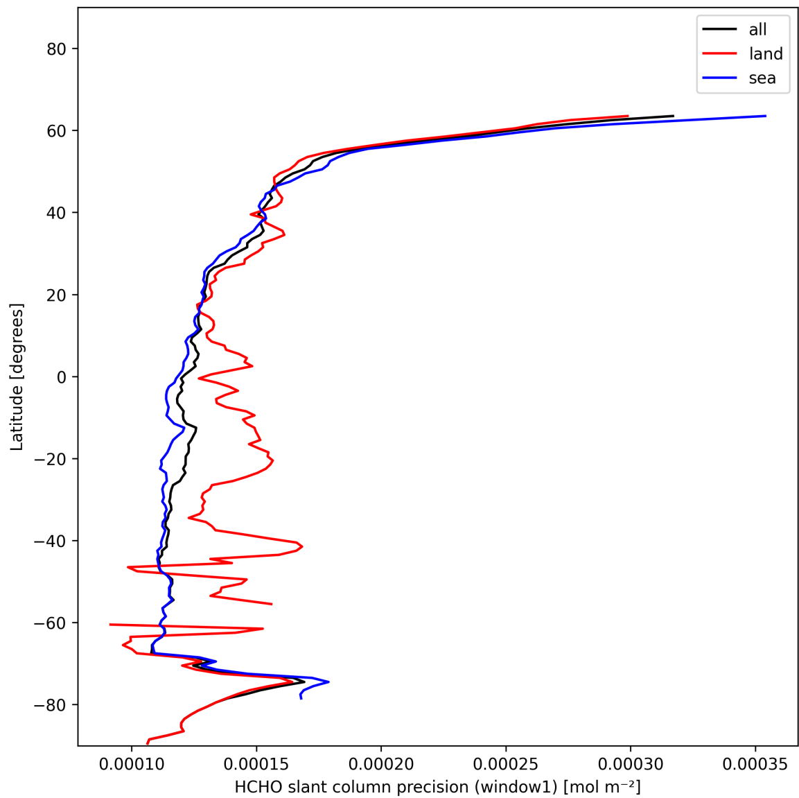
Figure 25: Zonal average of “HCHO slant column precision (window1)” for 2024-11-26 to 2024-11-28.
