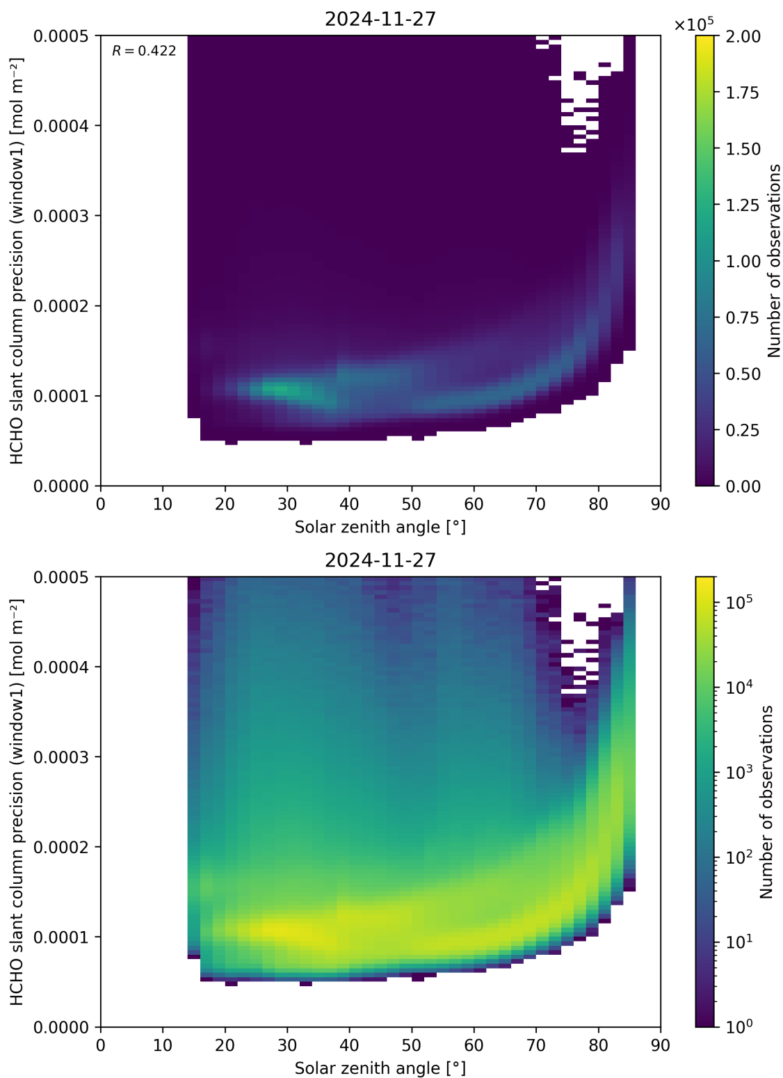
Figure 174: Scatter density plot of “Solar zenith angle” against “HCHO slant column precision (window1)” for 2024-11-26 to 2024-11-28.
