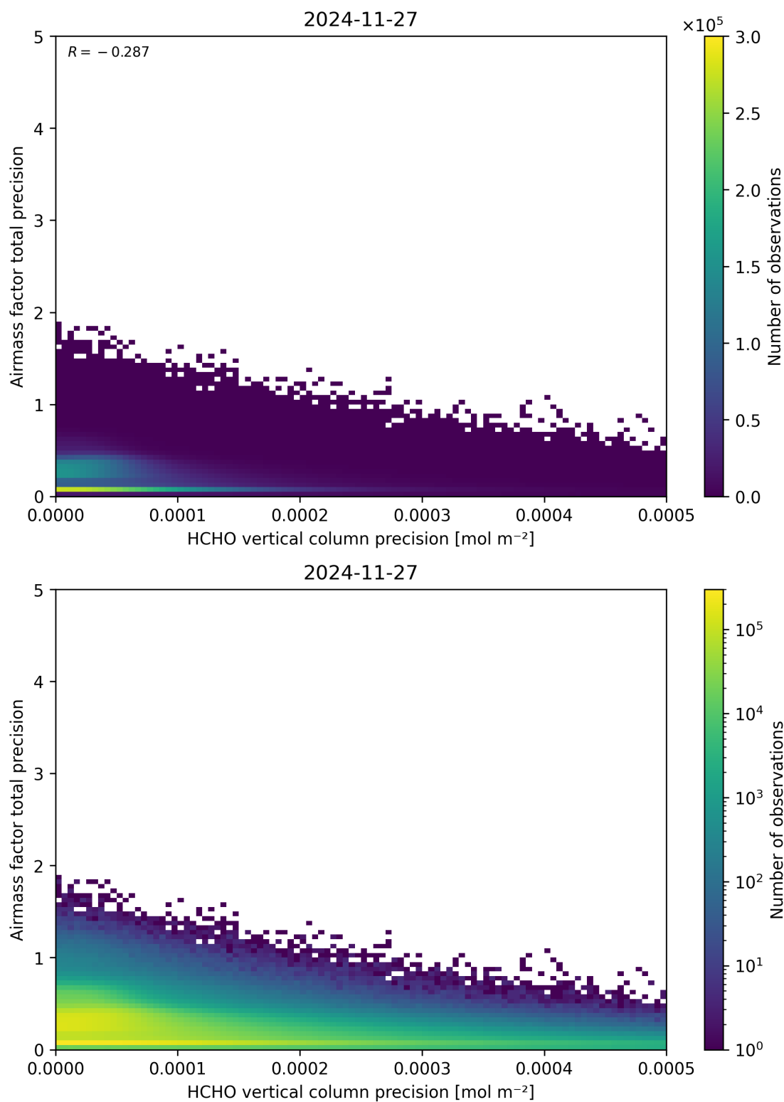
Figure 145: Scatter density plot of “HCHO vertical column precision” against “Airmass factor total precision” for 2024-11-26 to 2024-11-28.
