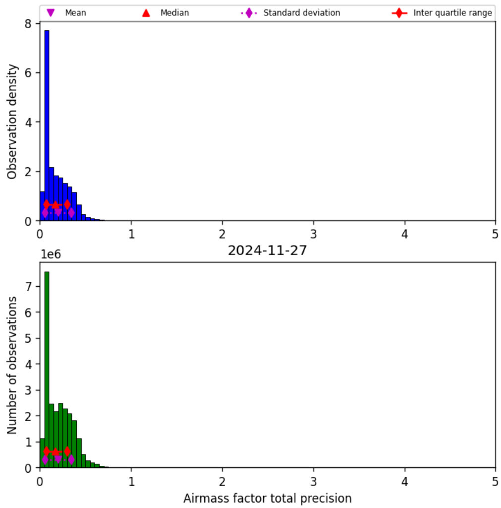
Figure 41: Histogram of “Airmass factor total precision” for 2024-11-26 to 2024-11-28
