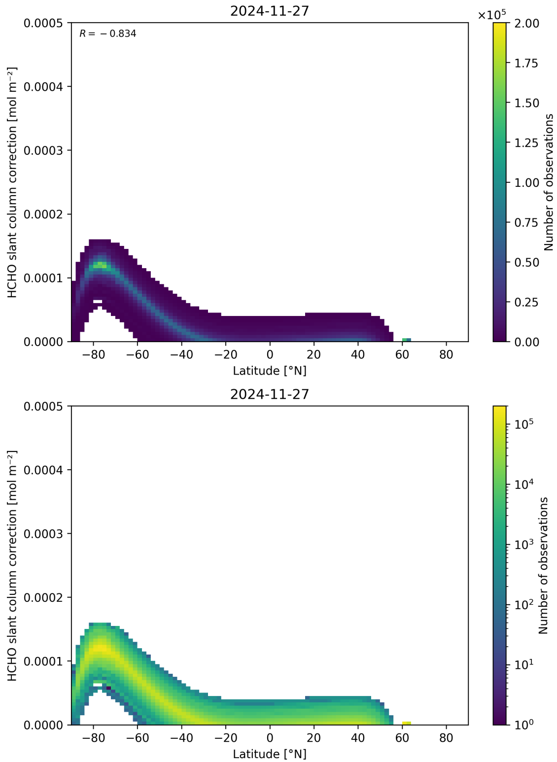
Figure 158: Scatter density plot of “Latitude” against “HCHO slant column correction” for 2024-11-26 to 2024-11-28.
