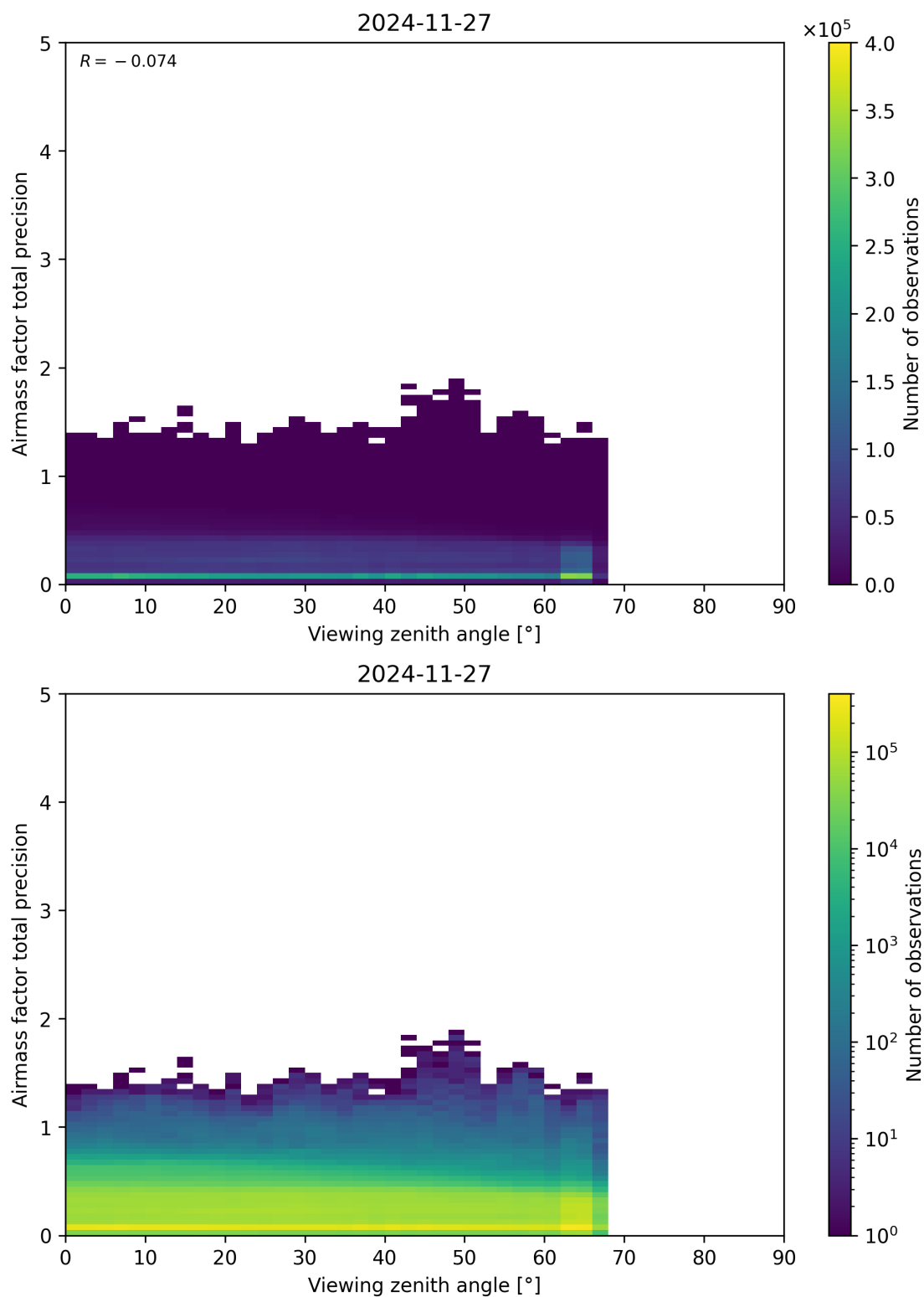
Figure 191: Scatter density plot of “Viewing zenith angle” against “Airmass factor total precision” for 2024-11-26 to 2024-11-28.
