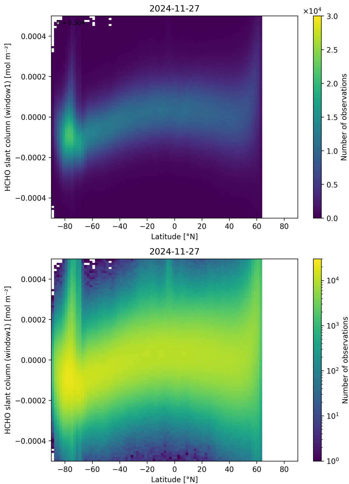
Figure 159: Scatter density plot of “Latitude” against “HCHO slant column (window1)” for 2024-11-26 to 2024-11-28.
