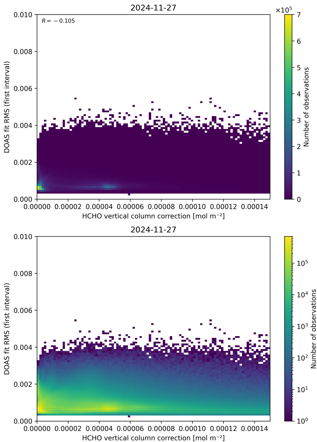
Figure 112: Scatter density plot of “HCHO vertical column correction” against “DOAS fit RMS (first interval)” for 2024-11-26 to 2024-11-28.
