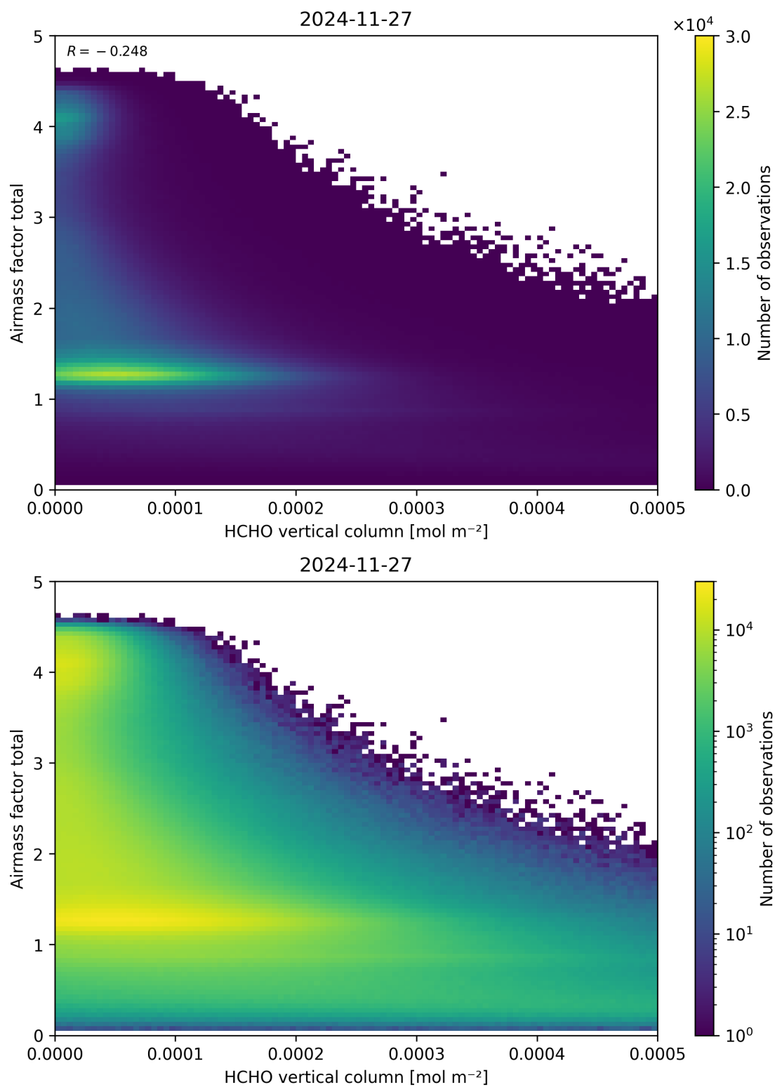
Figure 131: Scatter density plot of “HCHO vertical column” against “Airmass factor total” for 2024-11-26 to 2024-11-28.
