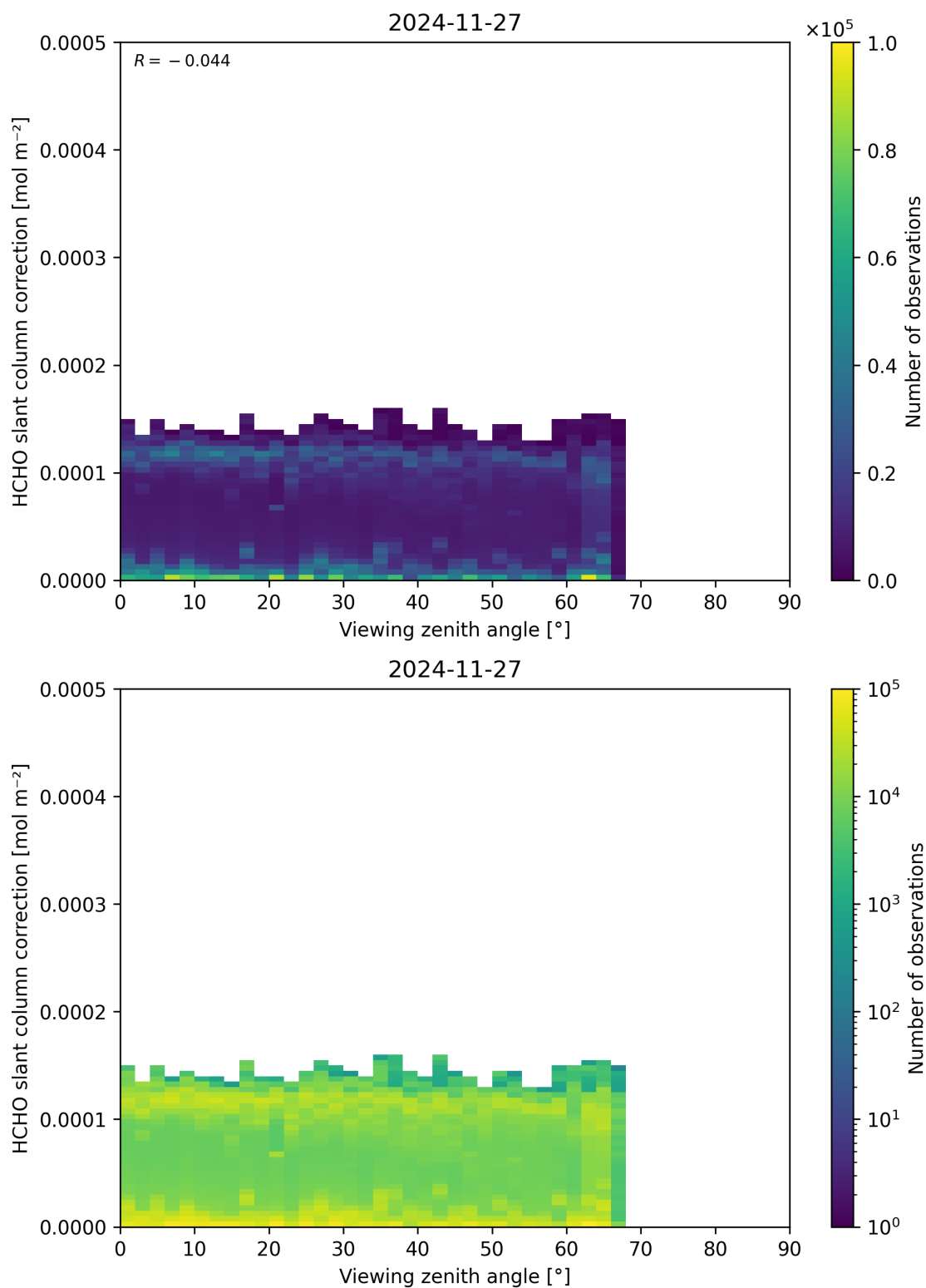
Figure 187: Scatter density plot of “Viewing zenith angle” against “HCHO slant column correction” for 2024-11-26 to 2024-11-28.
