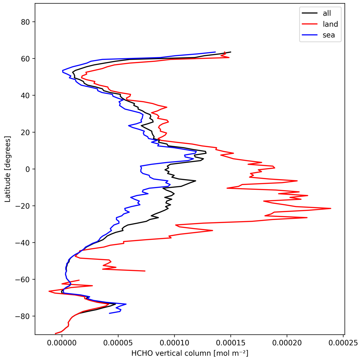
Figure 21: Zonal average of “HCHO vertical column” for 2024-11-26 to 2024-11-28.
