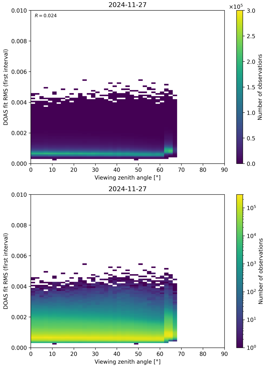
Figure 182: Scatter density plot of “Viewing zenith angle” against “DOAS fit RMS (first interval)” for 2024-11-26 to 2024-11-28.
