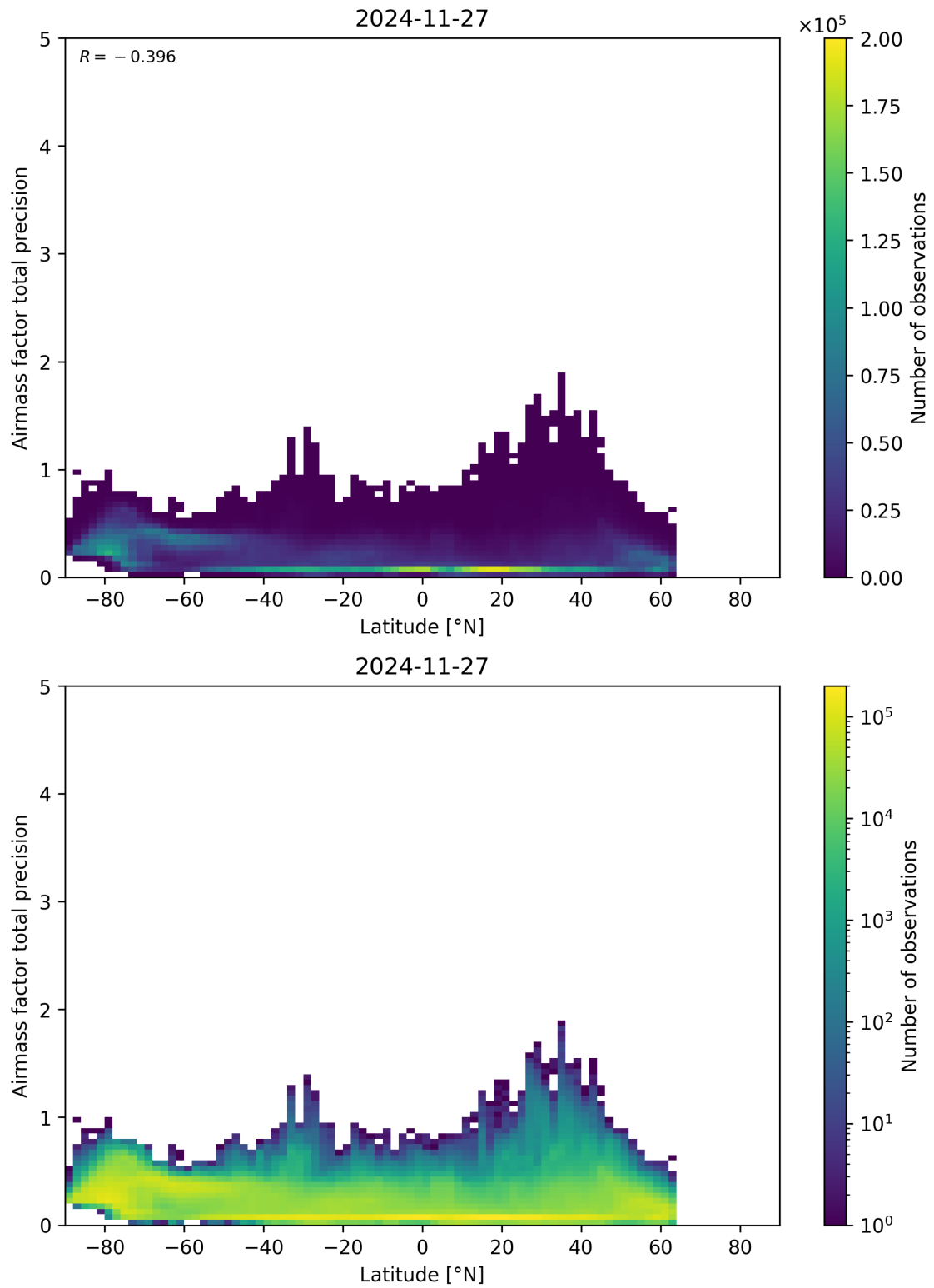
Figure 162: Scatter density plot of “Latitude” against “Airmass factor total precision” for 2024-11-26 to 2024-11-28.
