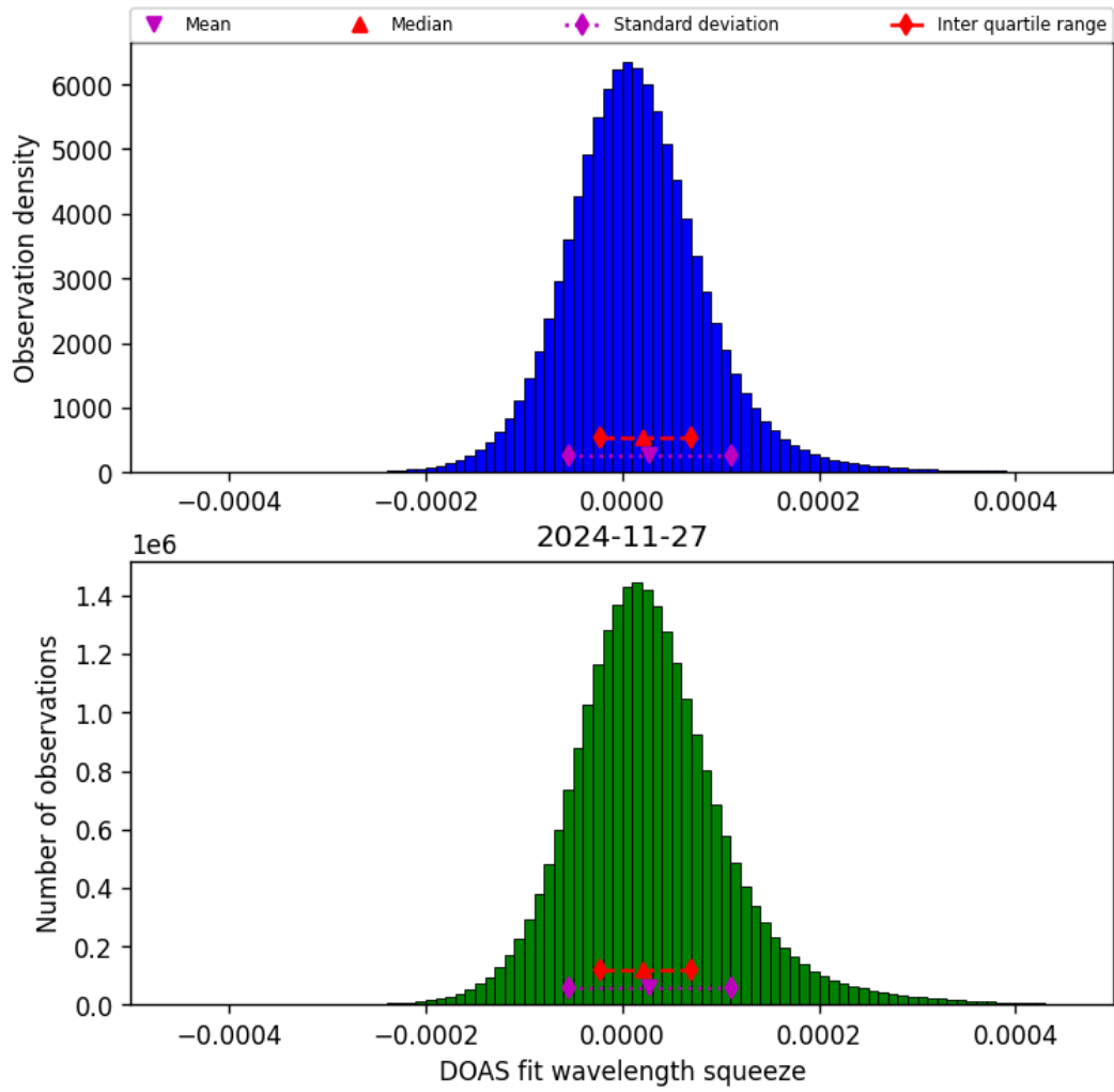
Figure 45: Histogram of “DOAS fit wavelength squeeze” for 2024-11-26 to 2024-11-28
