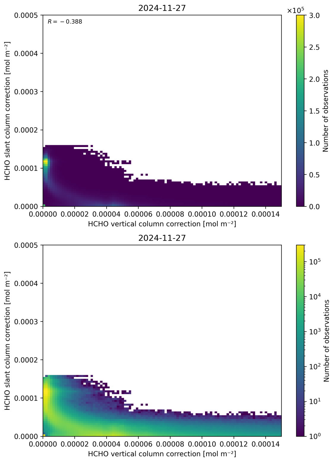
Figure 117: Scatter density plot of “HCHO vertical column correction” against “HCHO slant column correction” for 2024-11-26 to 2024-11-28.
