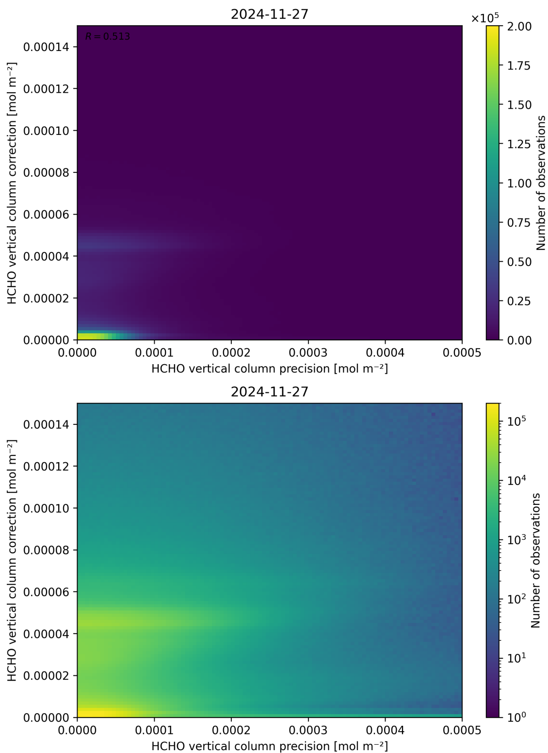
Figure 146: Scatter density plot of “HCHO vertical column precision” against “HCHO vertical column correction” for 2024-11-26 to 2024-11-28.
