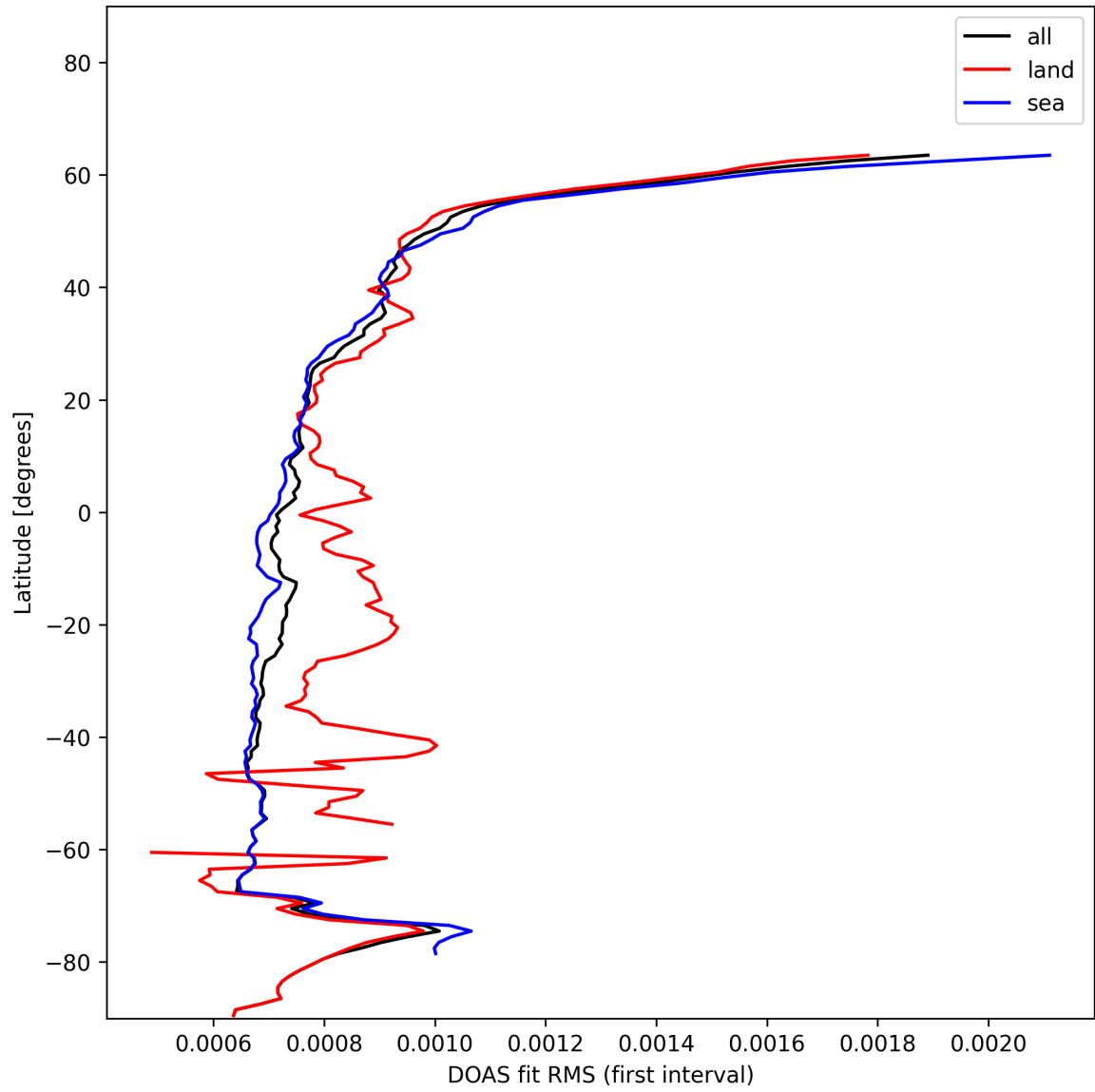
Figure 32: Zonal average of "DOAS fit RMS (first interval)" for 2024-11-26 to 2024-11-28.
