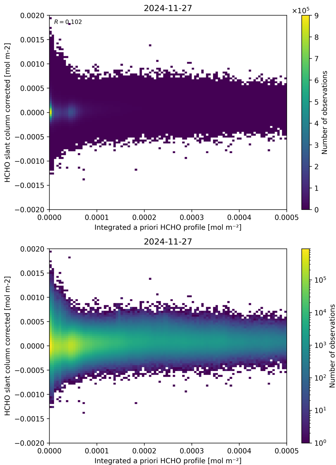
Figure 151: Scatter density plot of “Integrated a priori HCHO profile” against “HCHO slant column corrected” for 2024-11-26 to 2024-11-28.
