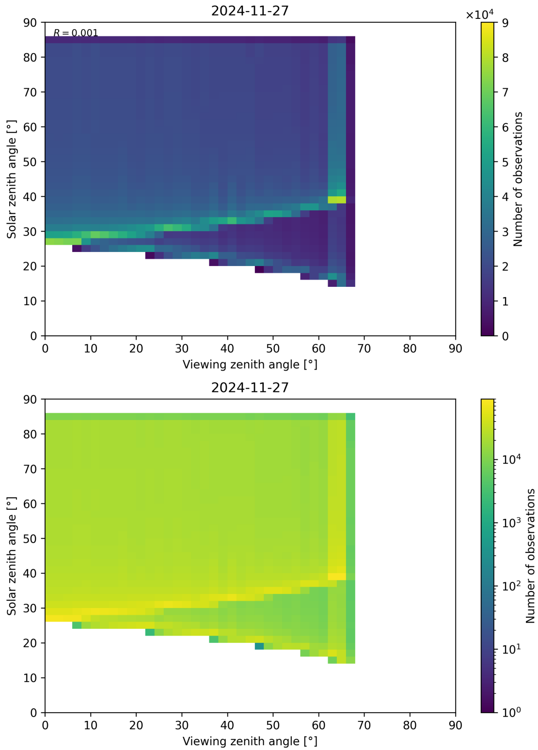
Figure 197: Scatter density plot of “Viewing zenith angle” against “Solar zenith angle” for 2024-11-26 to 2024-11-28.
