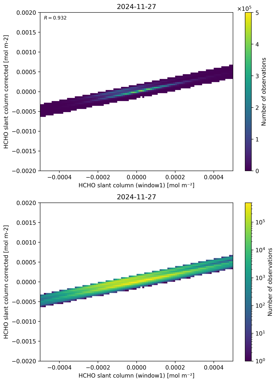
Figure 82: Scatter density plot of “HCHO slant column (window1)” against “HCHO slant column corrected” for 2024-11-26 to 2024-11-28.
