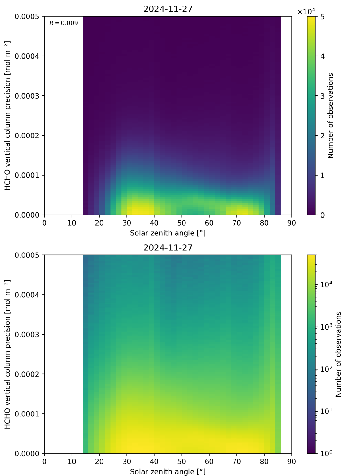
Figure 179: Scatter density plot of “Solar zenith angle” against “HCHO vertical column precision” for 2024-11-26 to 2024-11-28.
