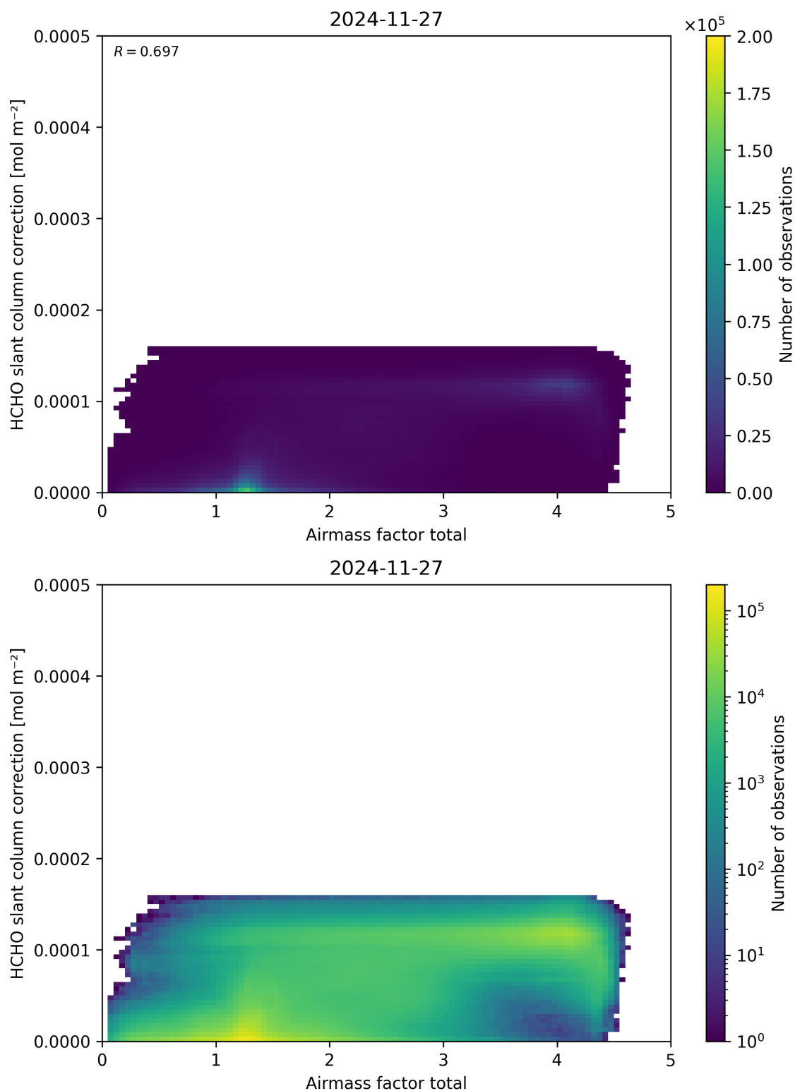
Figure 102: Scatter density plot of “Airmass factor total” against “HCHO slant column correction” for 2024-11-26 to 2024-11-28.
