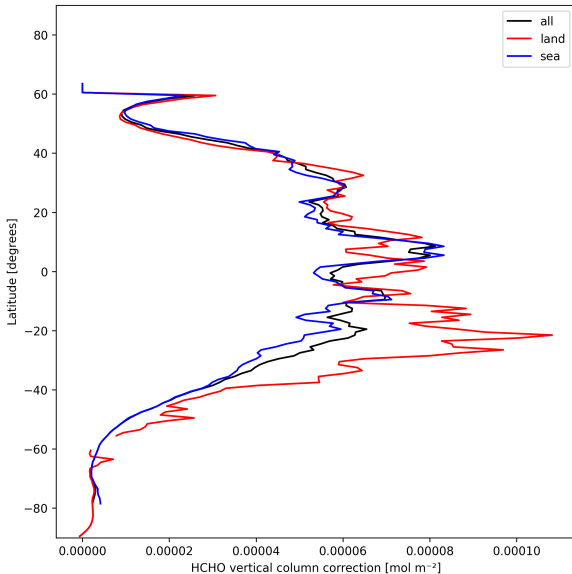
Figure 23: Zonal average of “HCHO vertical column correction” for 2024-11-26 to 2024-11-28.
