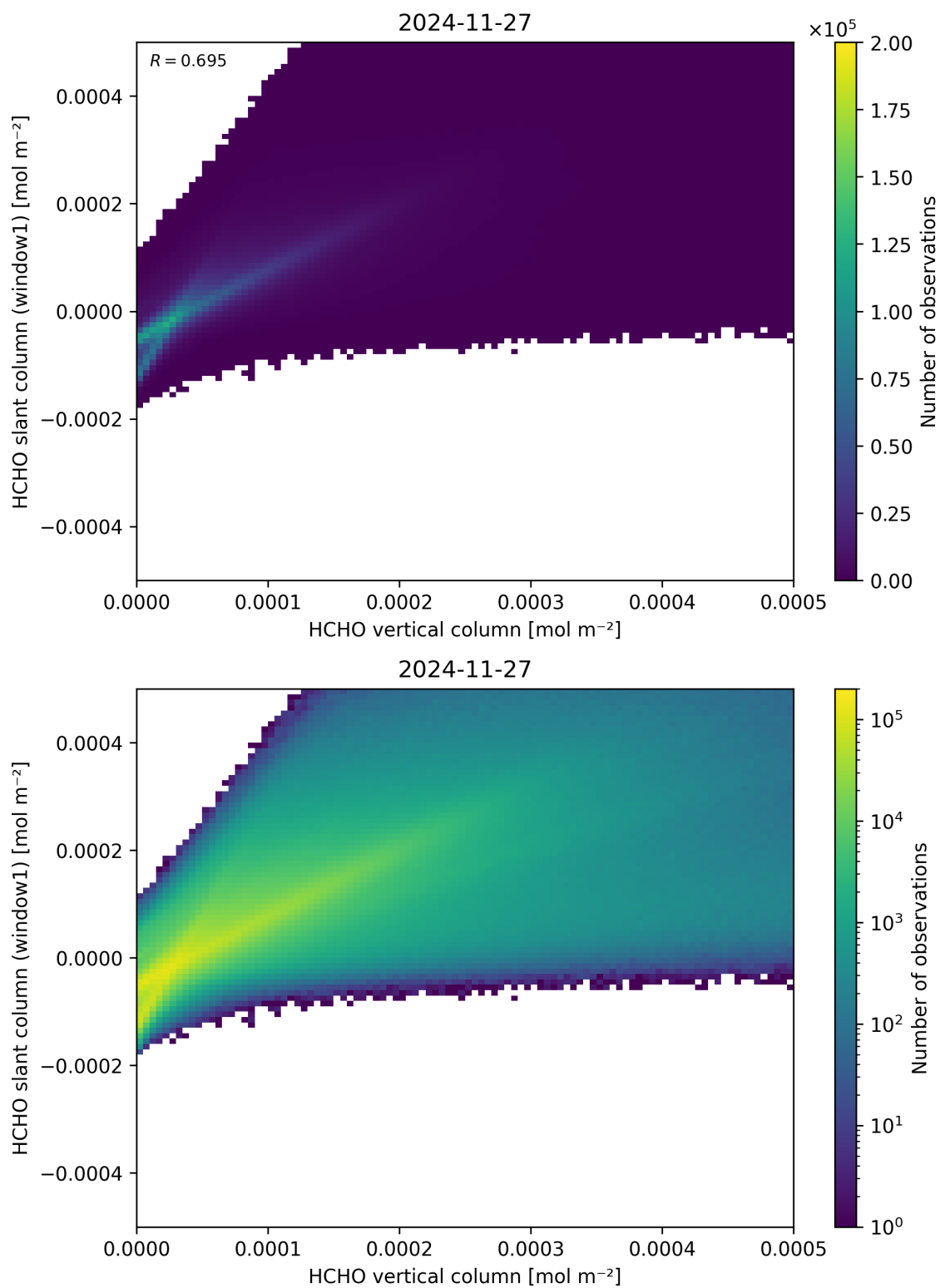
Figure 129: Scatter density plot of “HCHO vertical column” against “HCHO slant column (window1)” for 2024-11-26 to 2024-11-28.
