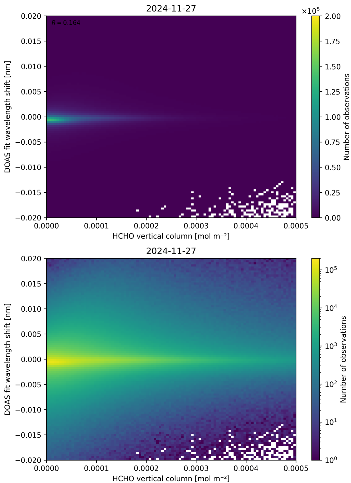
Figure 124: Scatter density plot of “HCHO vertical column” against “DOAS fit wavelength shift” for 2024-11-26 to 2024-11-28.
