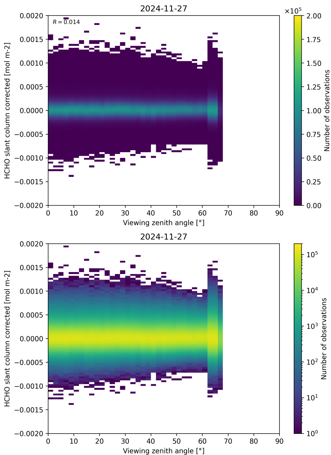
Figure 186: Scatter density plot of “Viewing zenith angle” against “HCHO slant column corrected” for 2024-11-26 to 2024-11-28.
