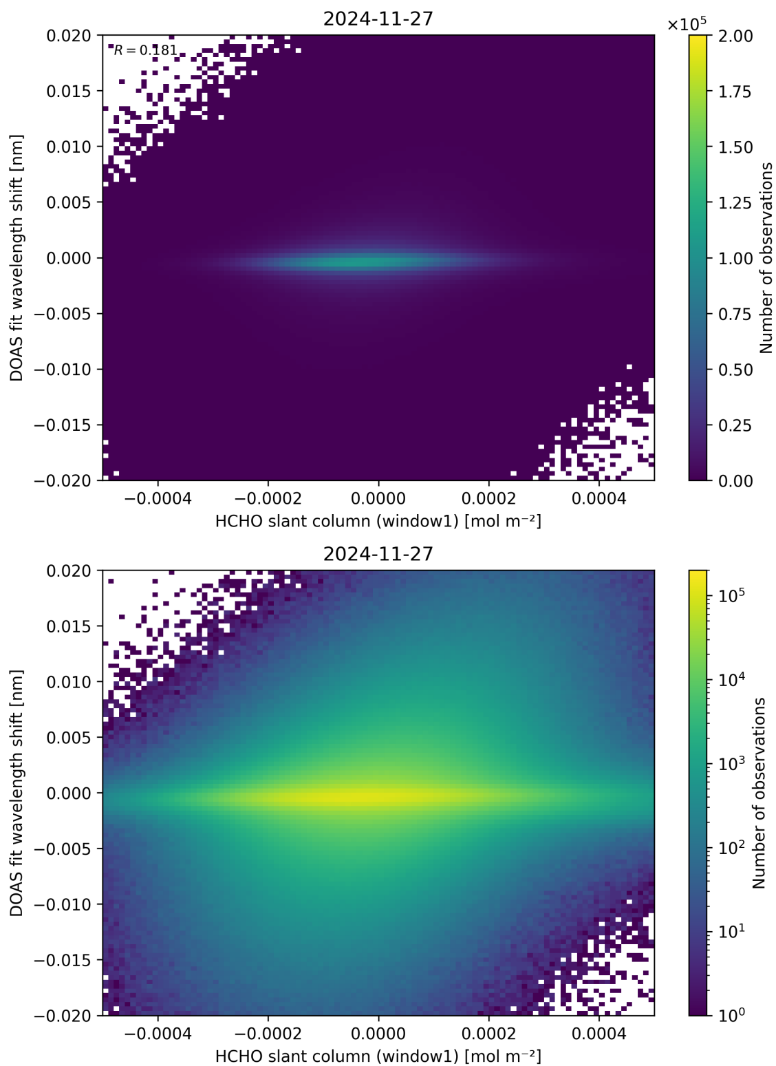
Figure 79: Scatter density plot of “HCHO slant column (window1)” against “DOAS fit wavelength shift” for 2024-11-26 to 2024-11-28.
