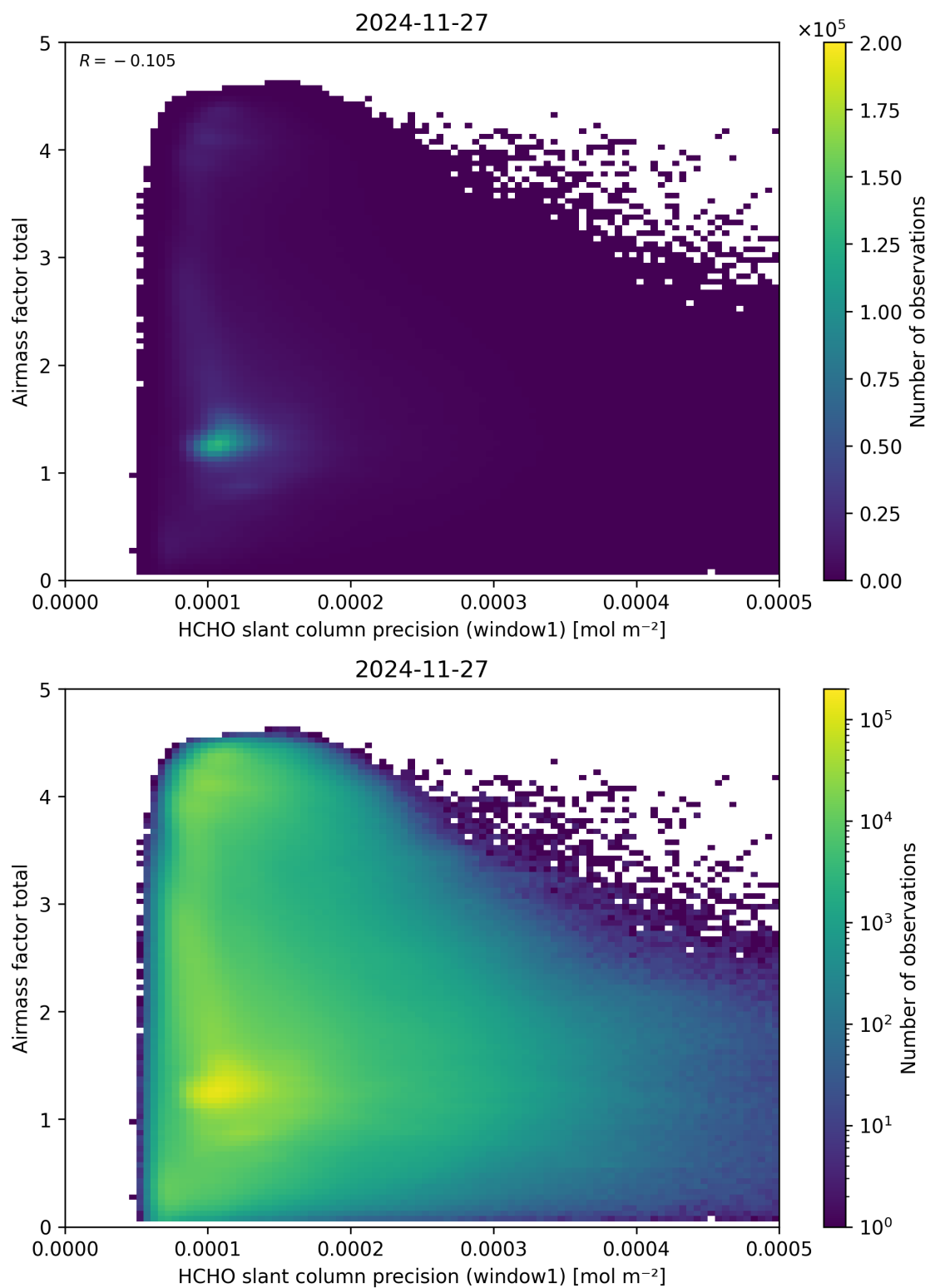
Figure 94: Scatter density plot of “HCHO slant column precision (window1)” against “Airmass factor total” for 2024-11-26 to 2024-11-28.
