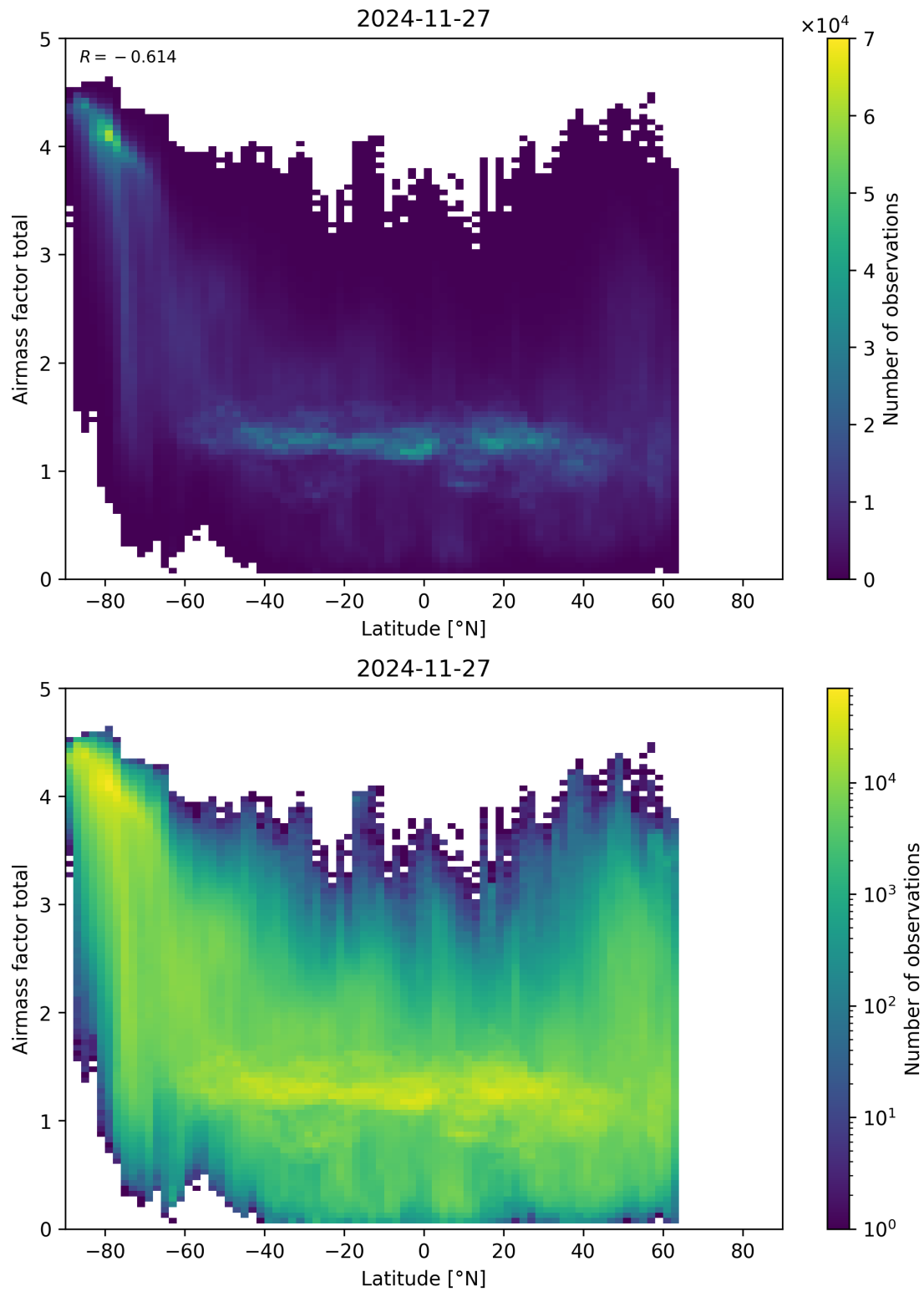
Figure 161: Scatter density plot of “Latitude” against “Airmass factor total” for 2024-11-26 to 2024-11-28.
