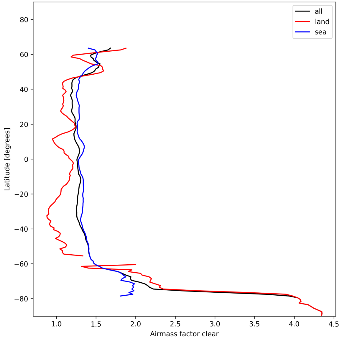
Figure 28: Zonal average of “Airmass factor clear” for 2024-11-26 to 2024-11-28.
