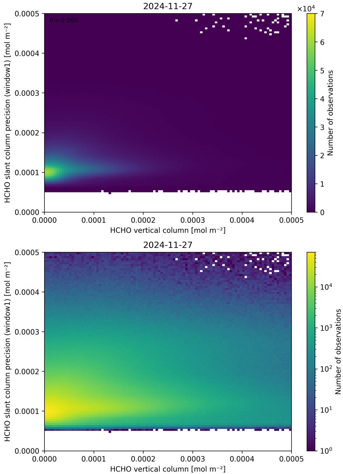
Figure 130: Scatter density plot of “HCHO vertical column” against “HCHO slant column precision (window1)” for 2024-11-26 to 2024-11-28.
