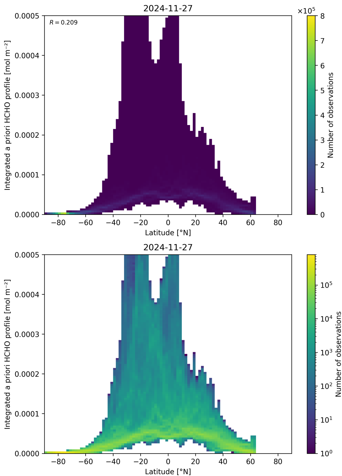
Figure 166: Scatter density plot of “Latitude” against “Integrated a priori HCHO profile” for 2024-11-26 to 2024-11-28.
