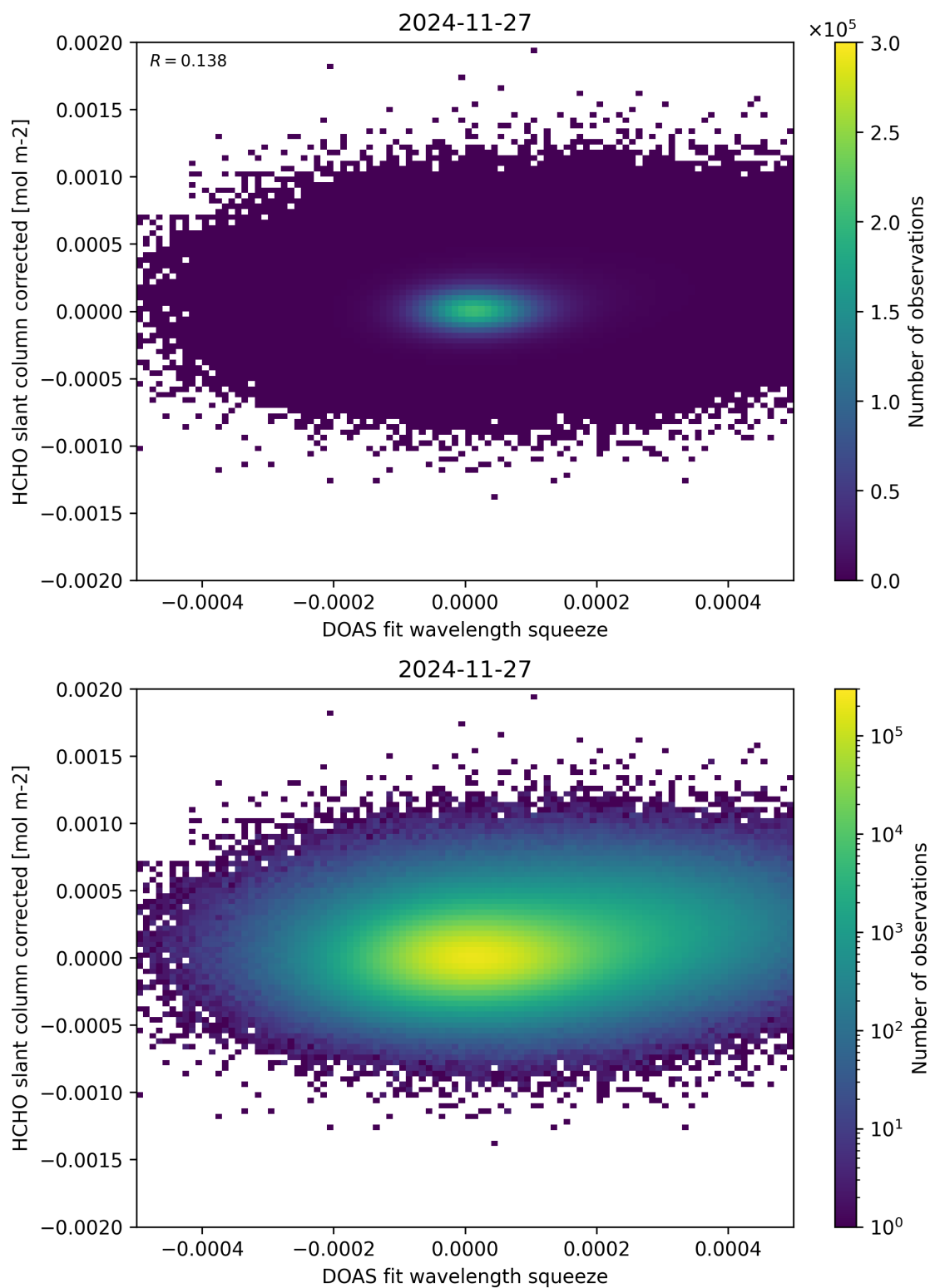
Figure 69: Scatter density plot of “DOAS fit wavelength squeeze” against “HCHO slant column corrected” for 2024-11-26 to 2024-11-28.
