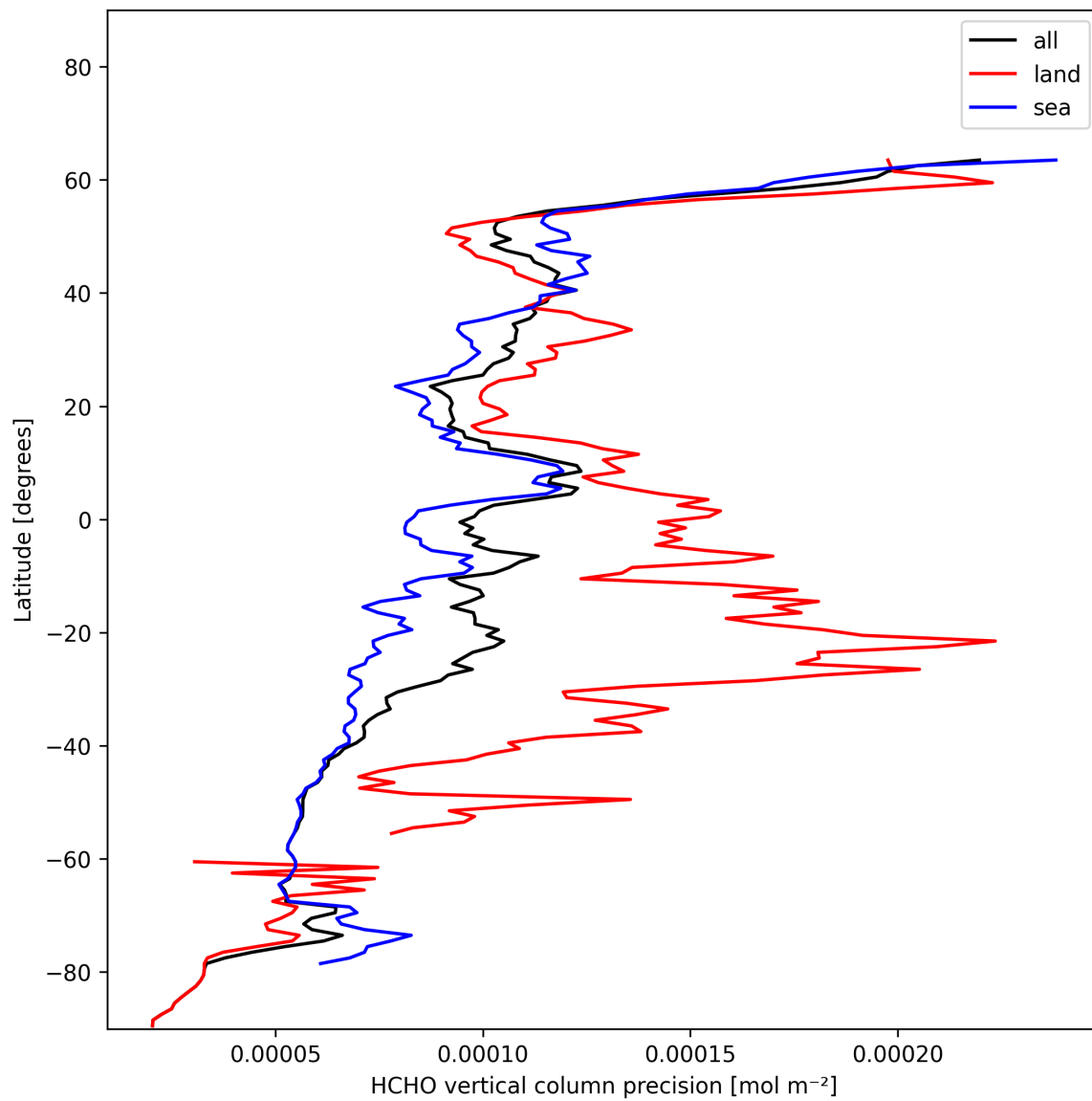
Figure 22: Zonal average of “HCHO vertical column precision” for 2024-11-26 to 2024-11-28.
