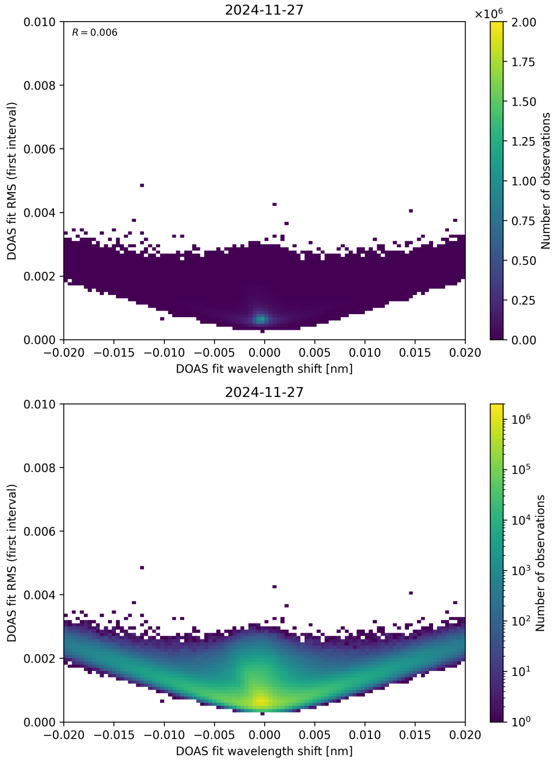
Figure 64: Scatter density plot of “DOAS fit wavelength shift” against “DOAS fit RMS (first interval)” for 2024-11-26 to 2024-11-28.
