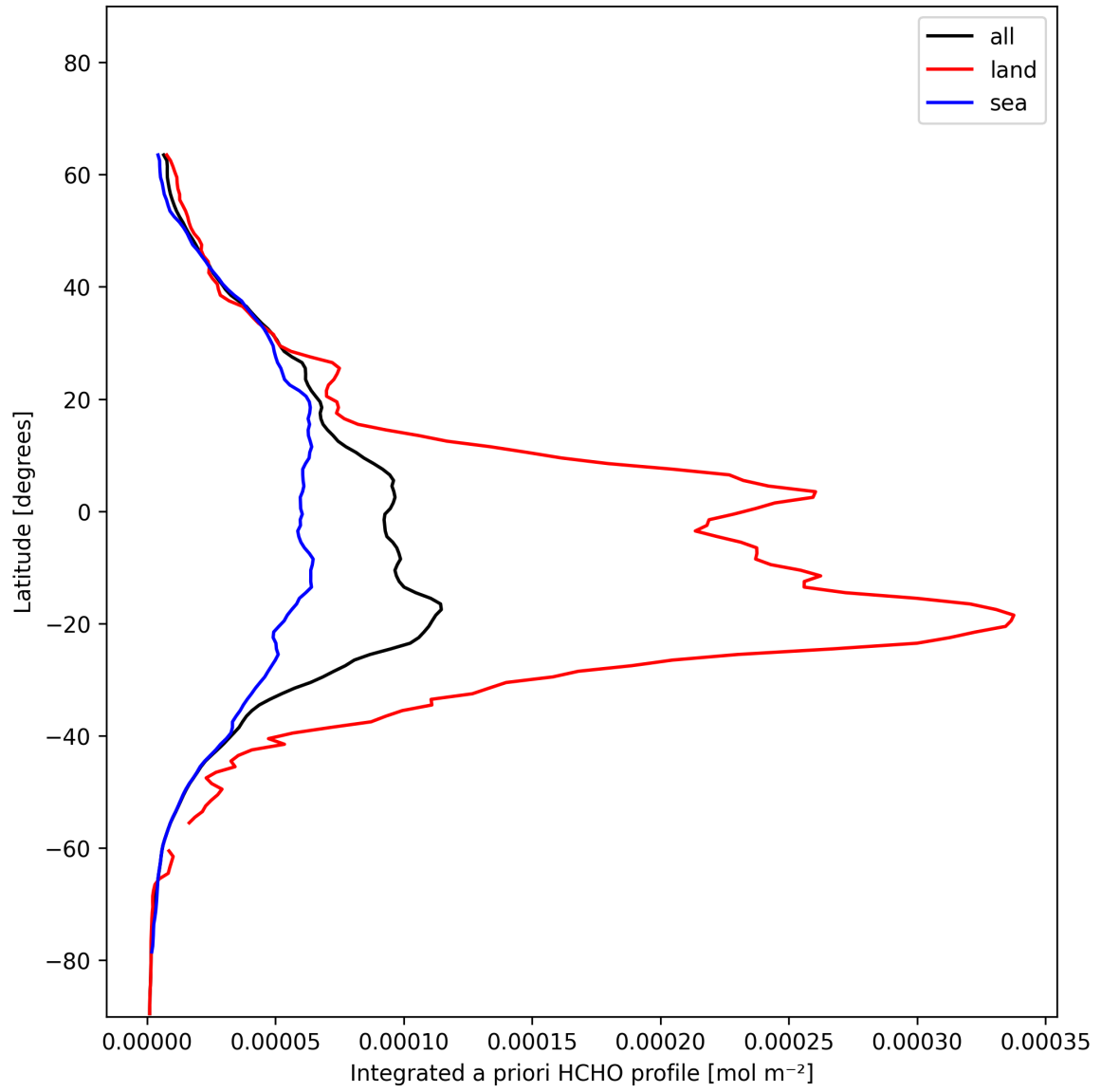
Figure 29: Zonal average of “Integrated a priori HCHO profile” for 2024-11-26 to 2024-11-28.
