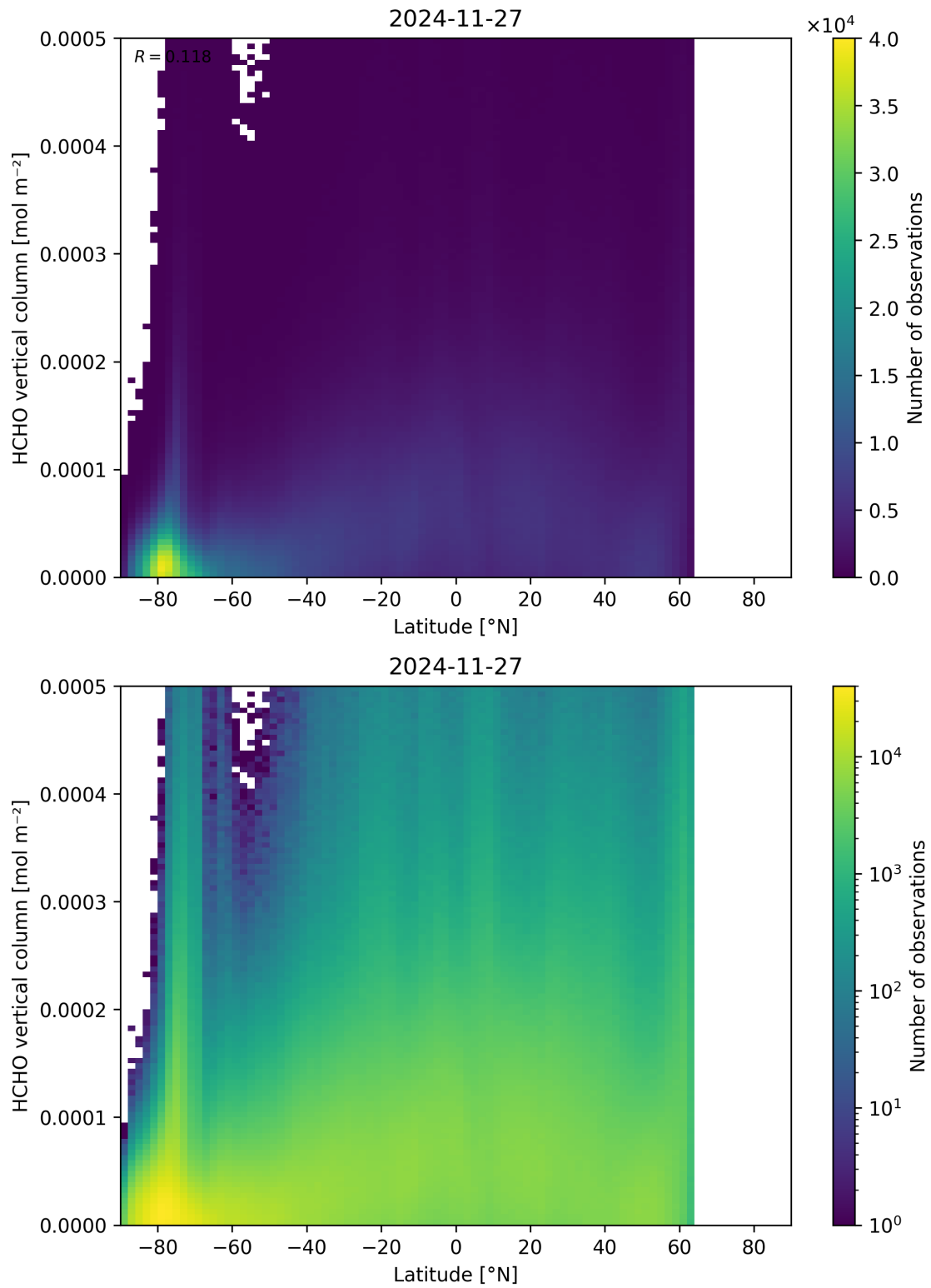
Figure 163: Scatter density plot of “Latitude” against “HCHO vertical column” for 2024-11-26 to 2024-11-28.
