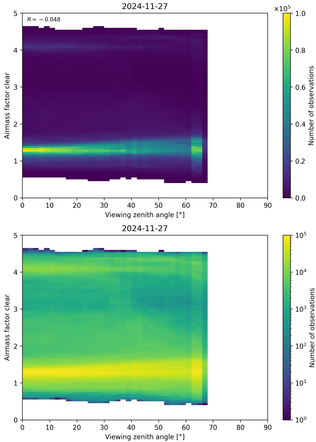
Figure 185: Scatter density plot of “Viewing zenith angle” against “Airmass factor clear” for 2024-11-26 to 2024-11-28.
