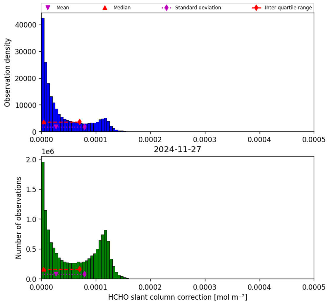
Figure 47: Histogram of “HCHO slant column correction” for 2024-11-26 to 2024-11-28
