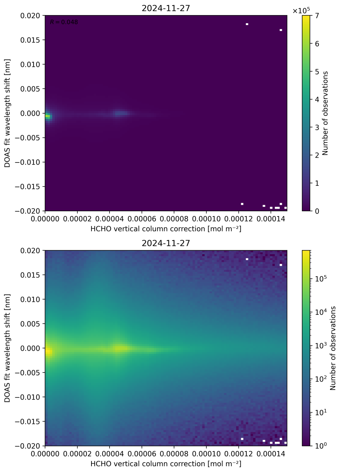
Figure 113: Scatter density plot of “HCHO vertical column correction” against “DOAS fit wavelength shift” for 2024-11-26 to 2024-11-28.
