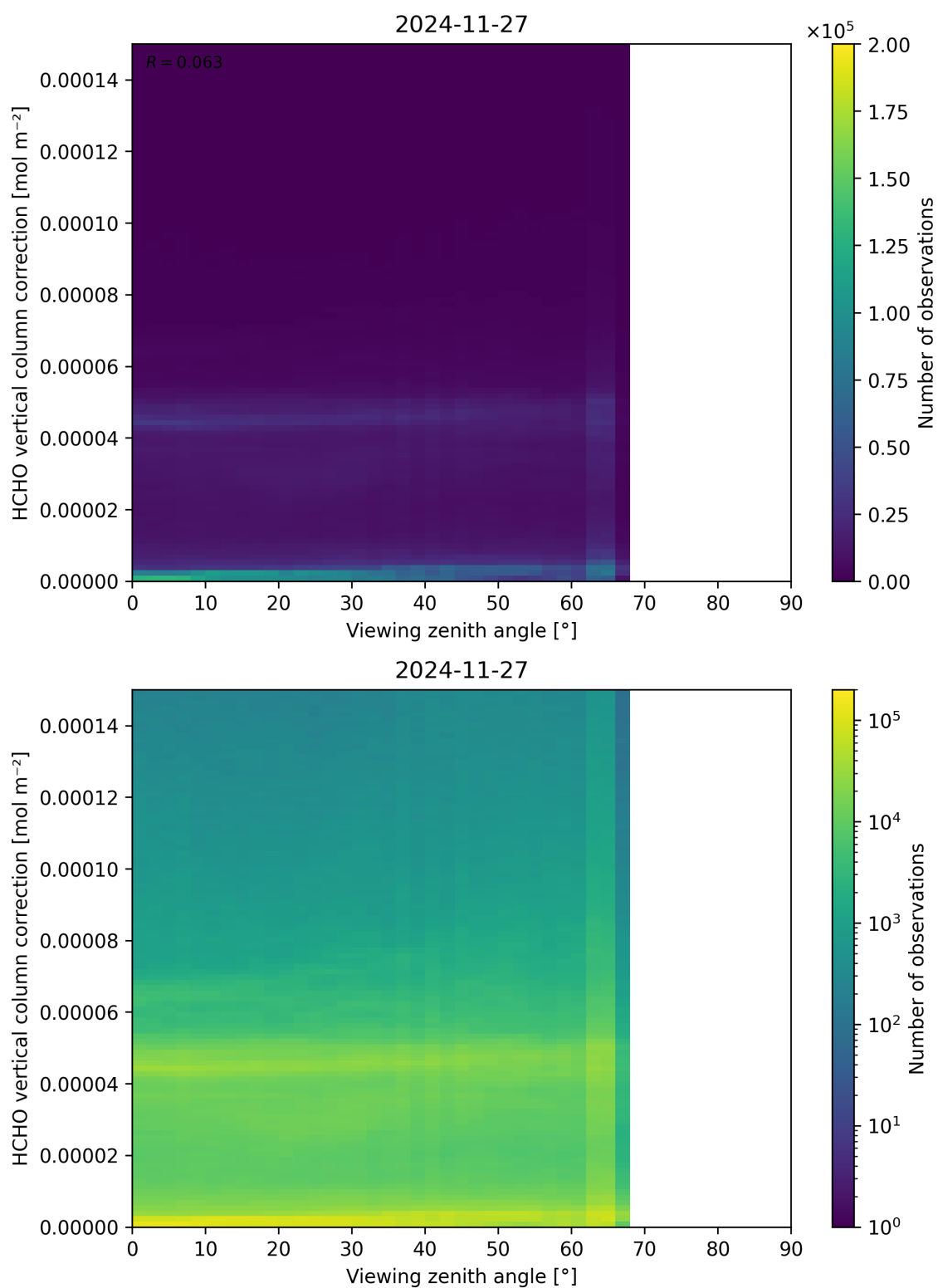
Figure 193: Scatter density plot of “Viewing zenith angle” against “HCHO vertical column correction” for 2024-11-26 to 2024-11-28.
