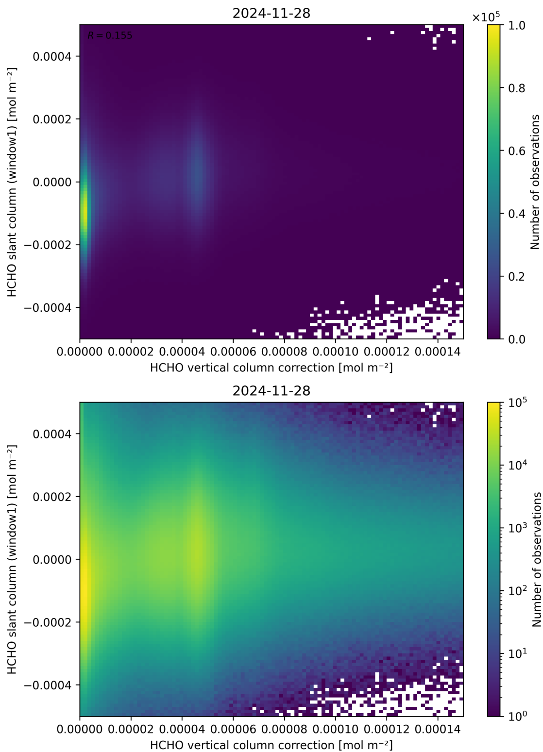
Figure 118: Scatter density plot of “HCHO vertical column correction” against “HCHO slant column (window1)” for 2024-11-27 to 2024-11-29.
