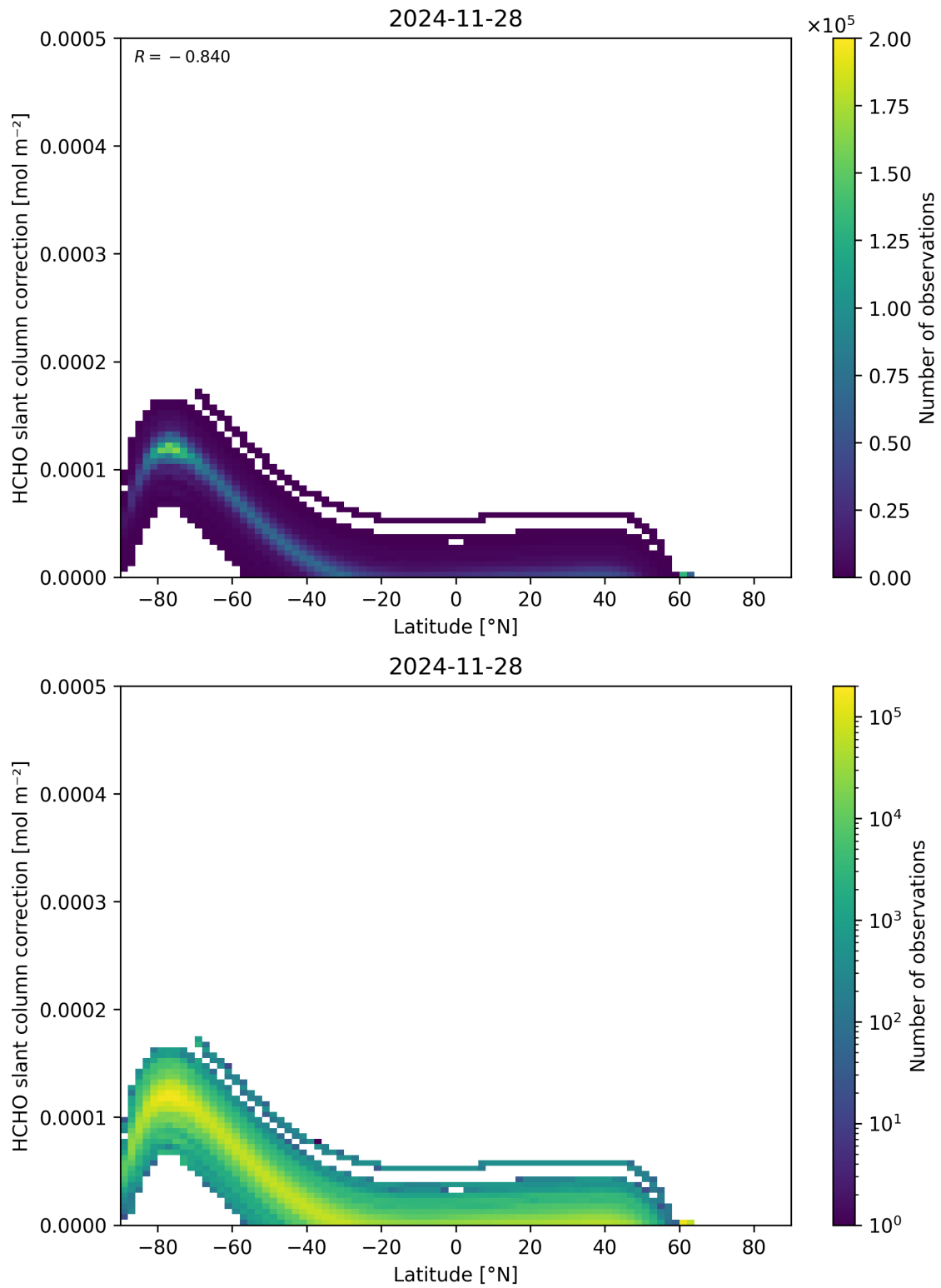
Figure 158: Scatter density plot of “Latitude” against “HCHO slant column correction” for 2024-11-27 to 2024-11-29.
