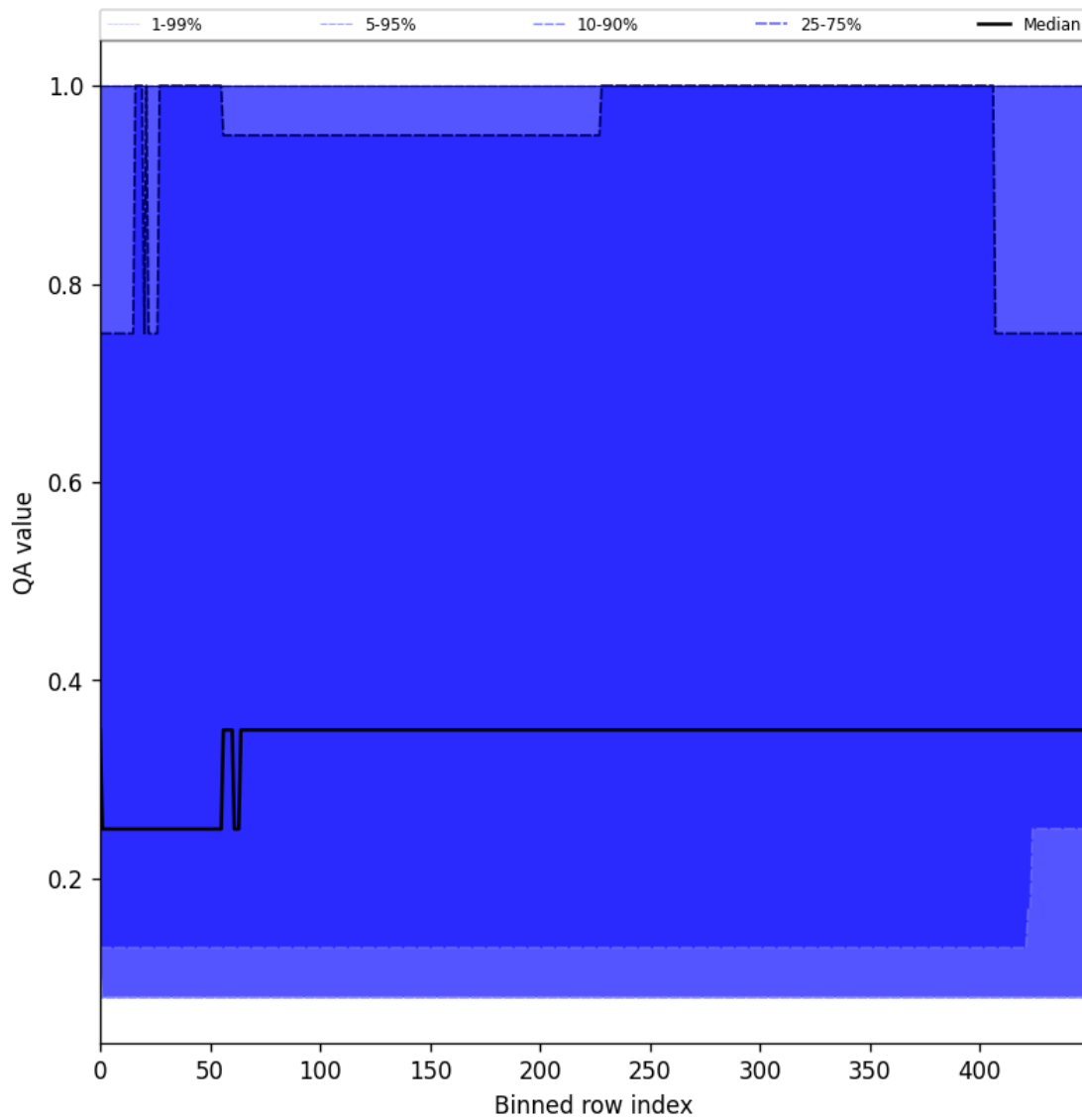
Figure 48: Along track statistics of “QA value” for 2024-11-27 to 2024-11-29
