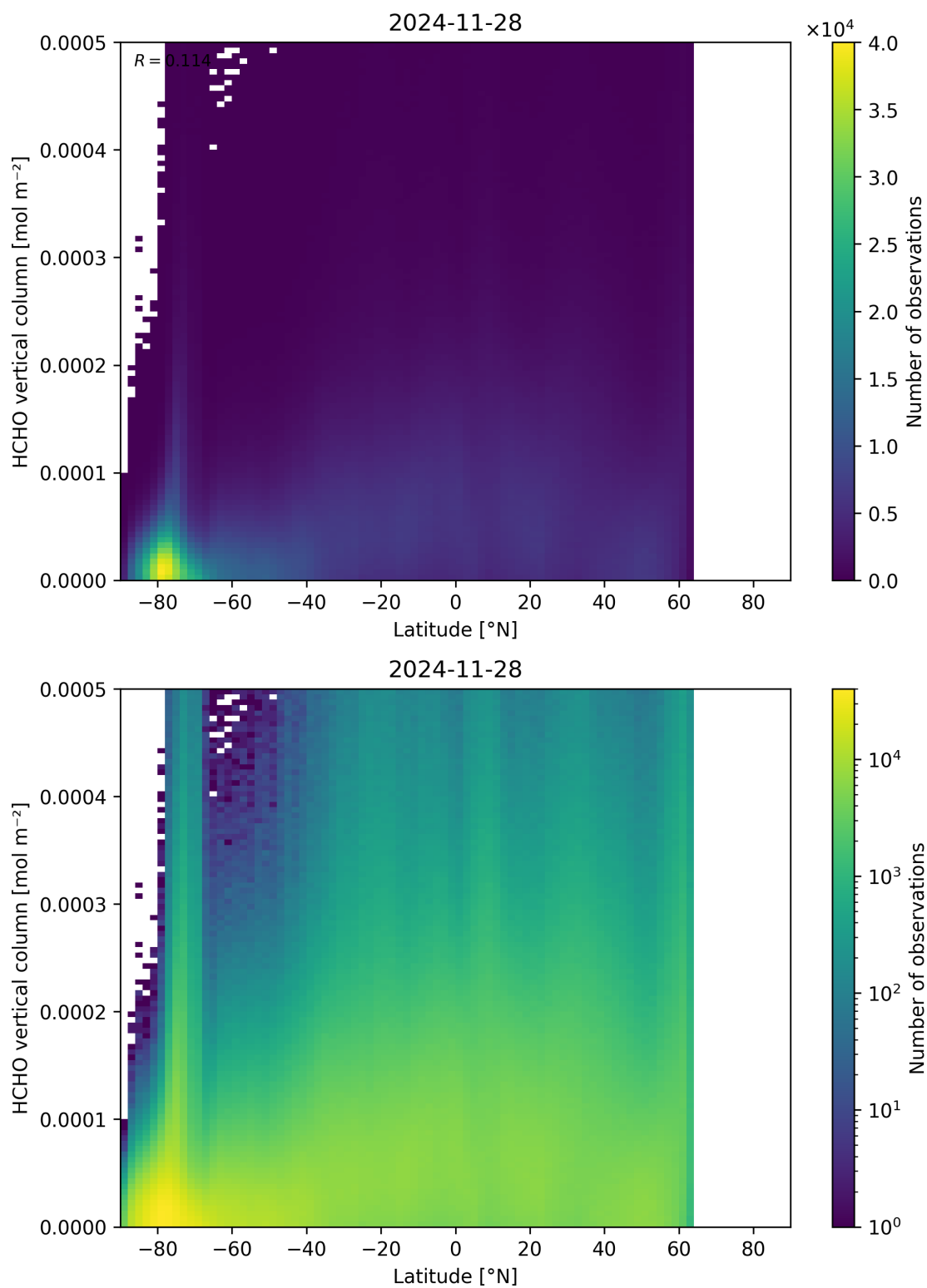
Figure 163: Scatter density plot of “Latitude” against “HCHO vertical column” for 2024-11-27 to 2024-11-29.
