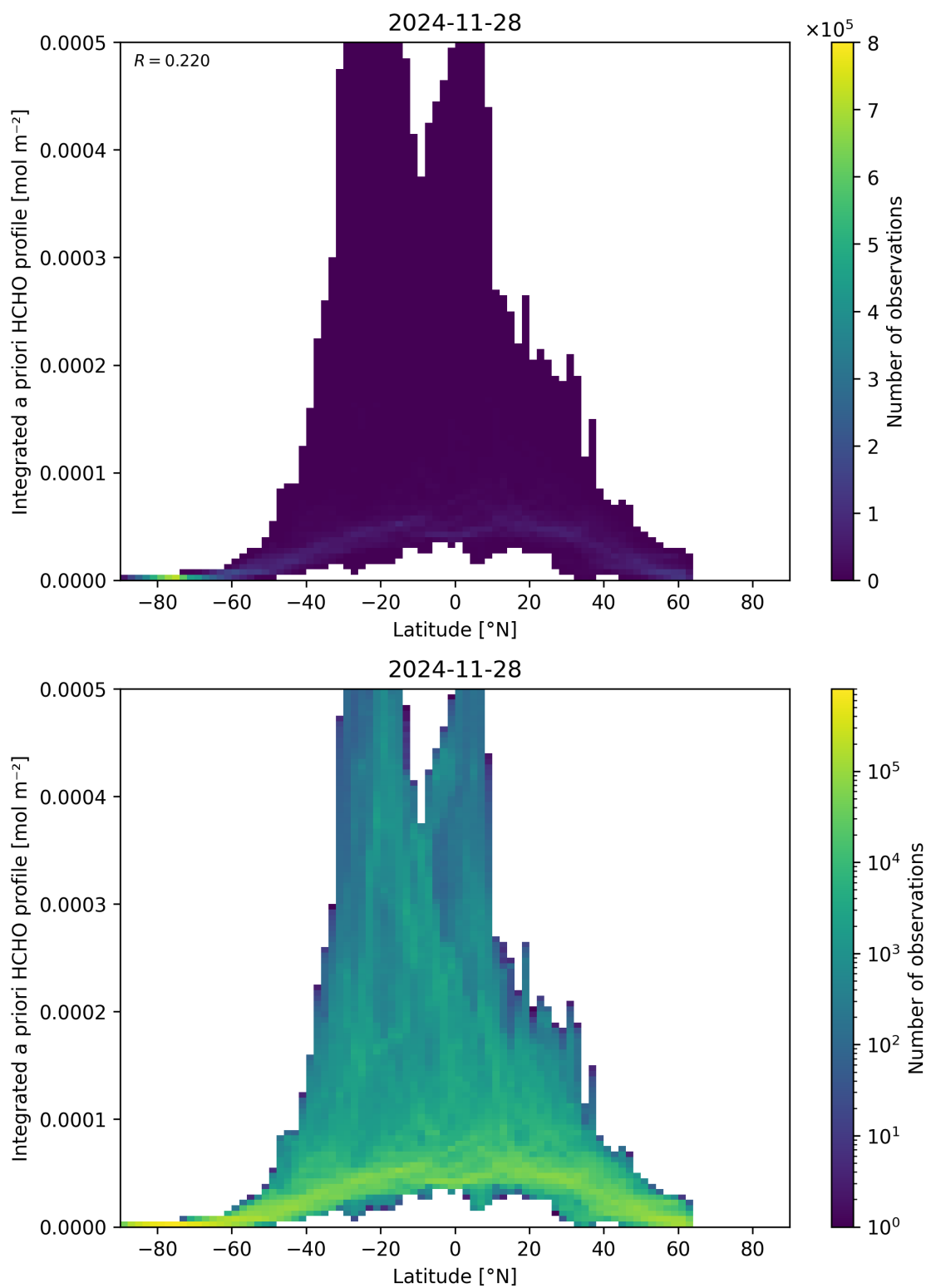
Figure 166: Scatter density plot of “Latitude” against “Integrated a priori HCHO profile” for 2024-11-27 to 2024-11-29.
