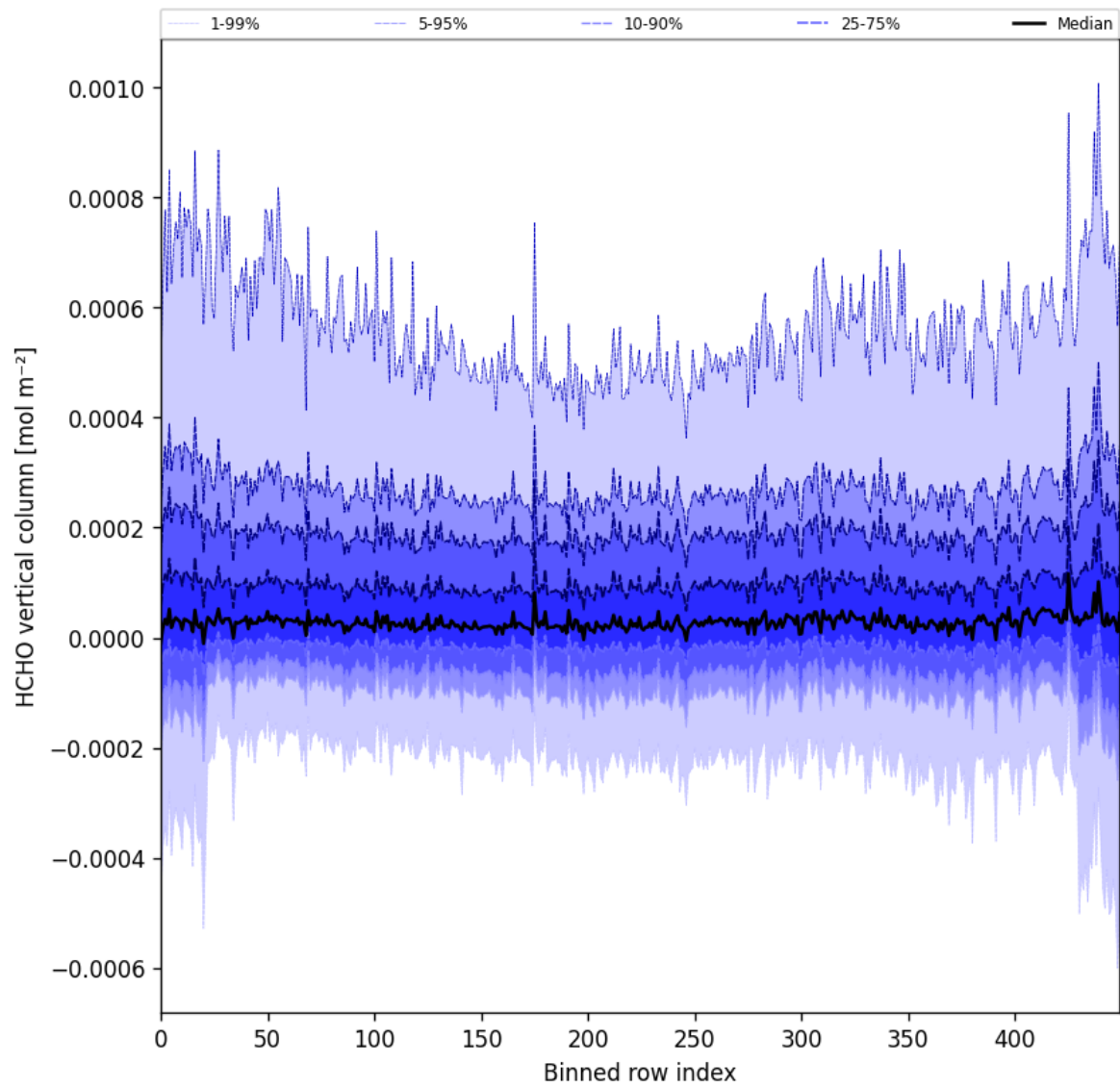
Figure 49: Along track statistics of “HCHO vertical column” for 2024-11-27 to 2024-11-29
