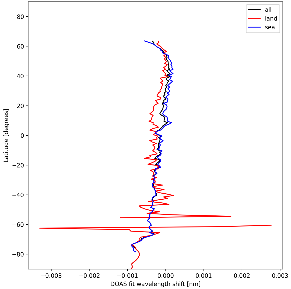
Figure 30: Zonal average of “DOAS fit wavelength shift” for 2024-11-27 to 2024-11-29.
