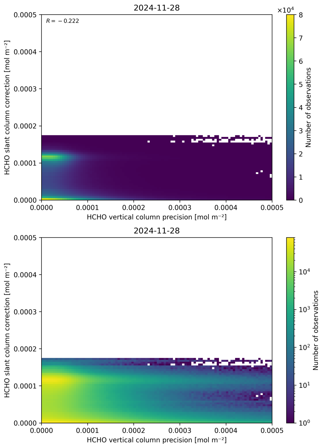
Figure 141: Scatter density plot of “HCHO vertical column precision” against “HCHO slant column correction” for 2024-11-27 to 2024-11-29.
