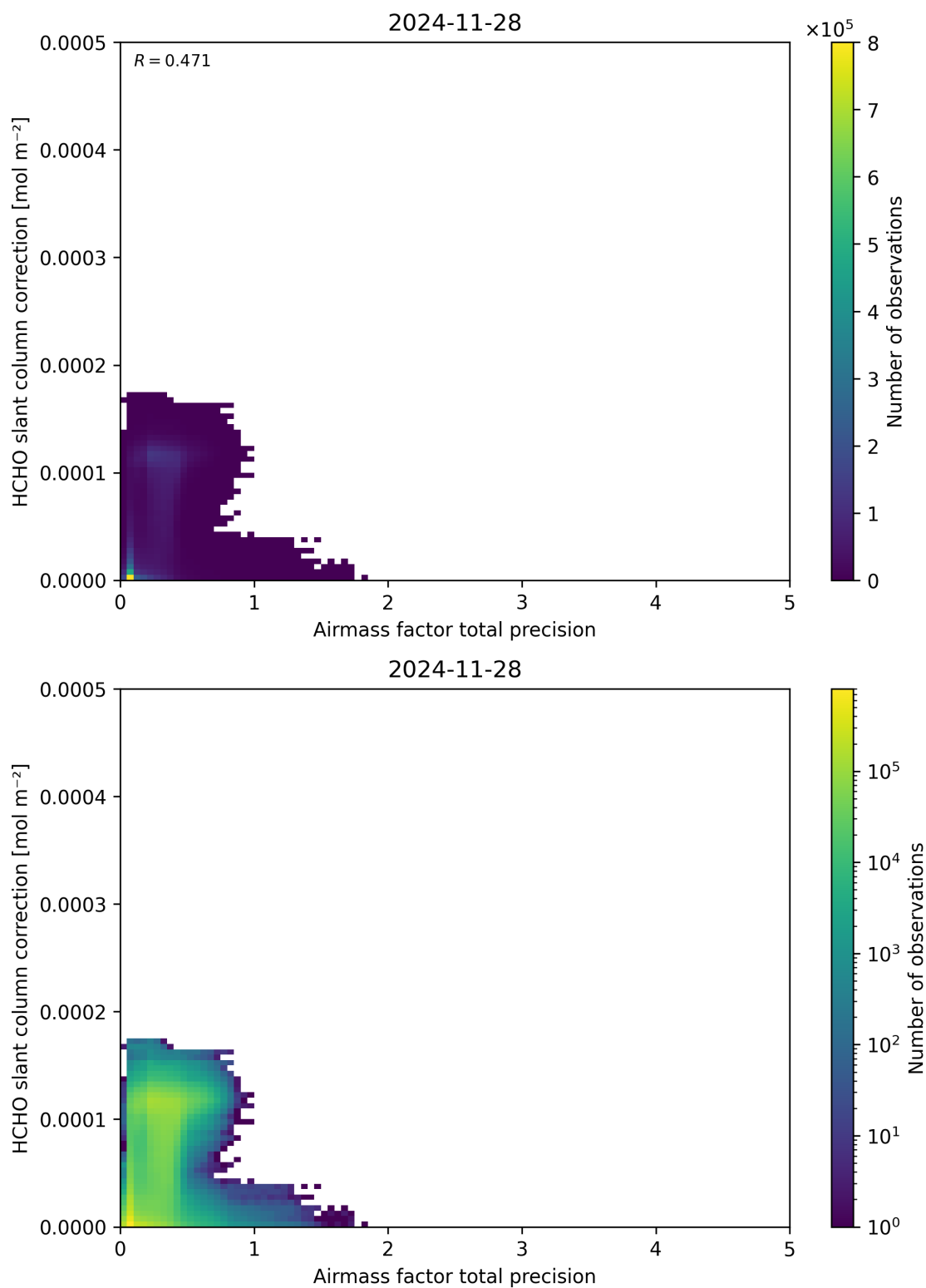
Figure 110: Scatter density plot of “Airmass factor total precision” against “HCHO slant column correction” for 2024-11-27 to 2024-11-29.
