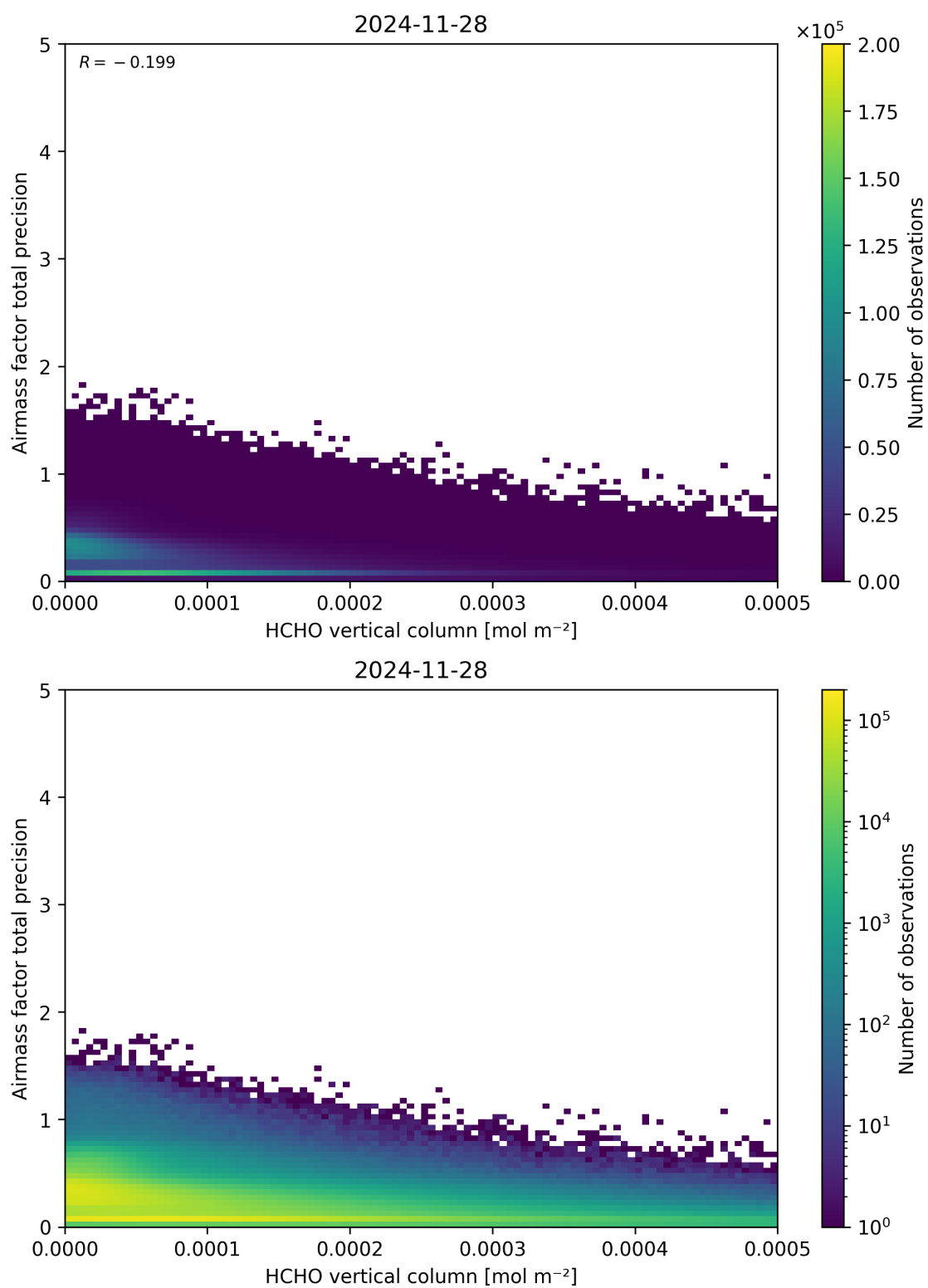
Figure 132: Scatter density plot of “HCHO vertical column” against “Airmass factor total precision” for 2024-11-27 to 2024-11-29.
