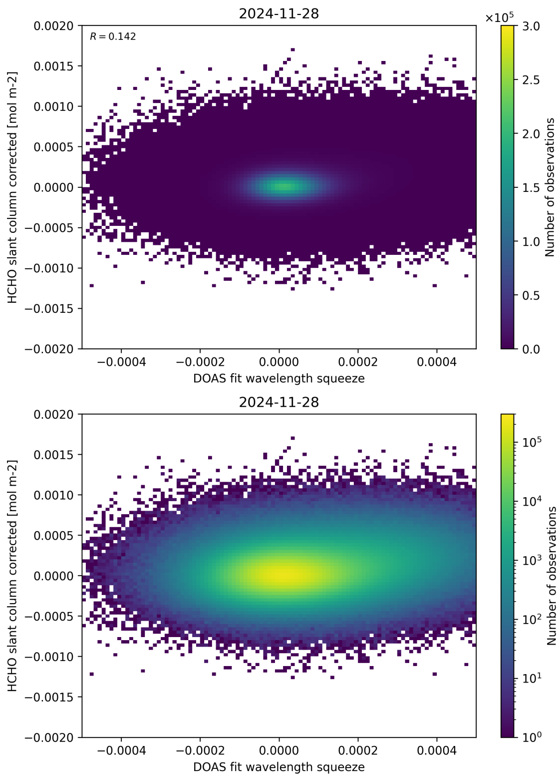
Figure 69: Scatter density plot of “DOAS fit wavelength squeeze” against “HCHO slant column corrected” for 2024-11-27 to 2024-11-29.
