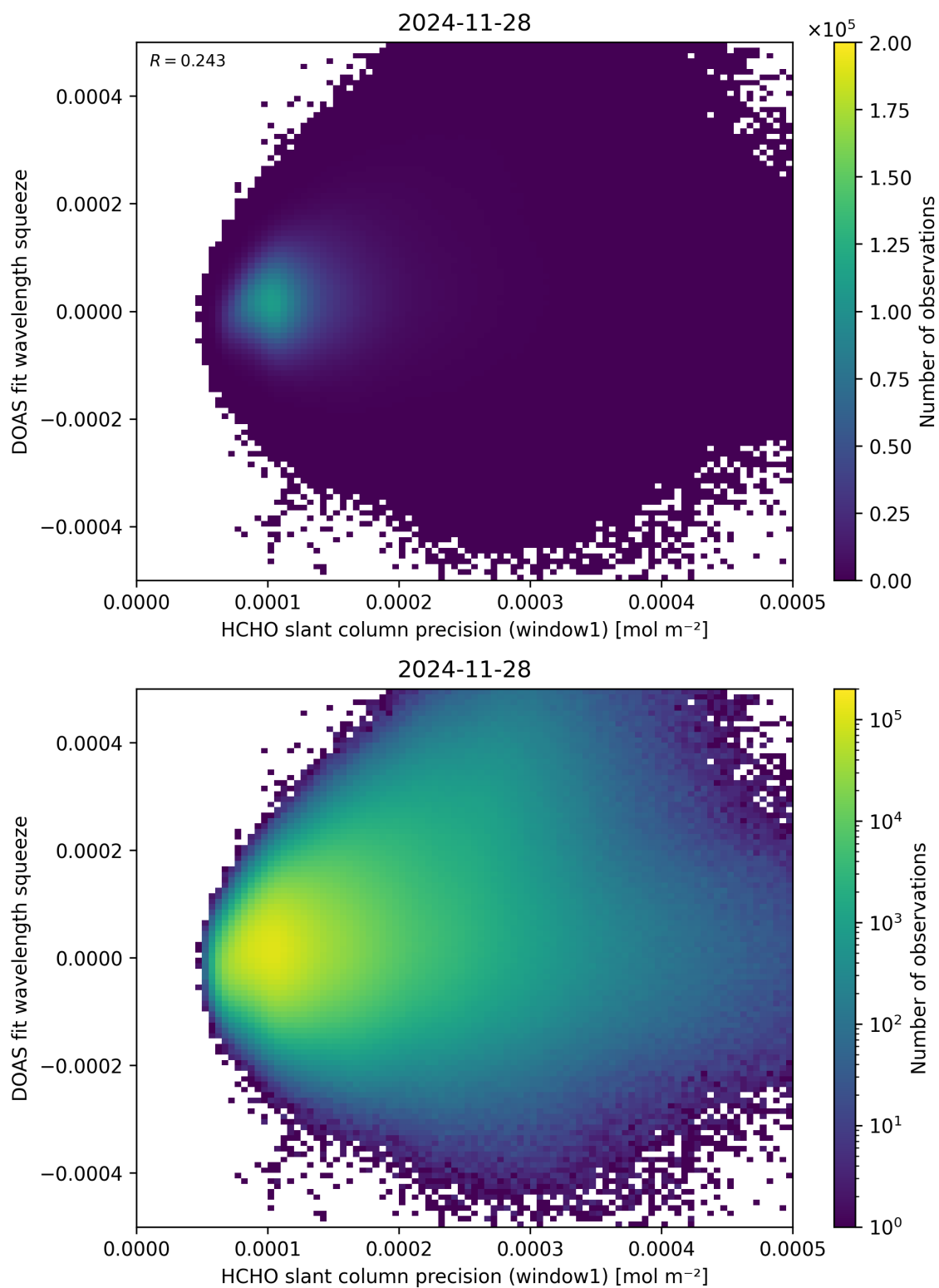
Figure 90: Scatter density plot of “HCHO slant column precision (window1)” against “DOAS fit wavelength squeeze” for 2024-11-27 to 2024-11-29.
