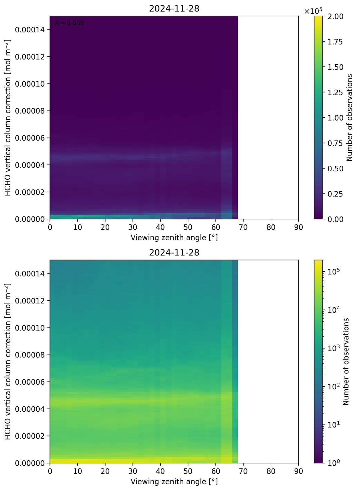
Figure 193: Scatter density plot of “Viewing zenith angle” against “HCHO vertical column correction” for 2024-11-27 to 2024-11-29.
