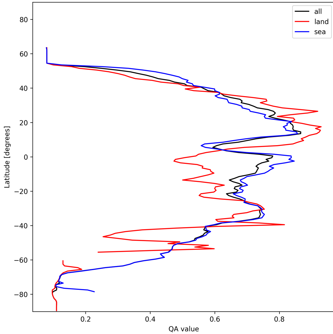
Figure 20: Zonal average of “QA value” for 2024-11-27 to 2024-11-29.
