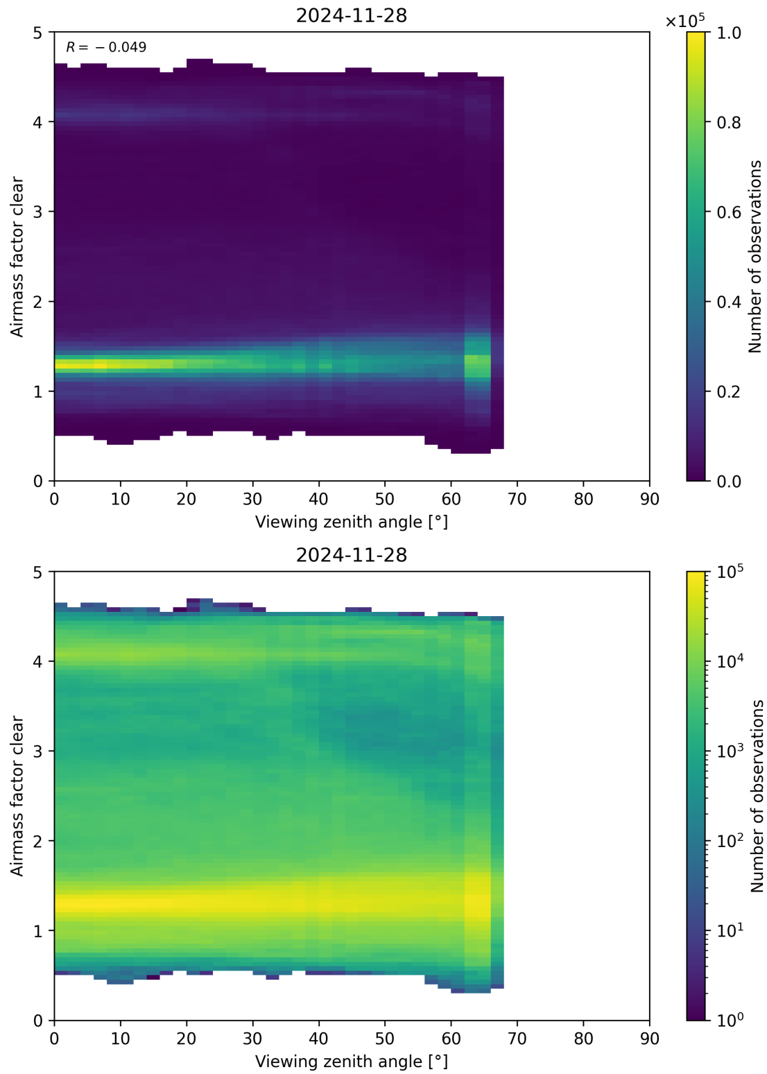
Figure 185: Scatter density plot of “Viewing zenith angle” against “Airmass factor clear” for 2024-11-27 to 2024-11-29.
