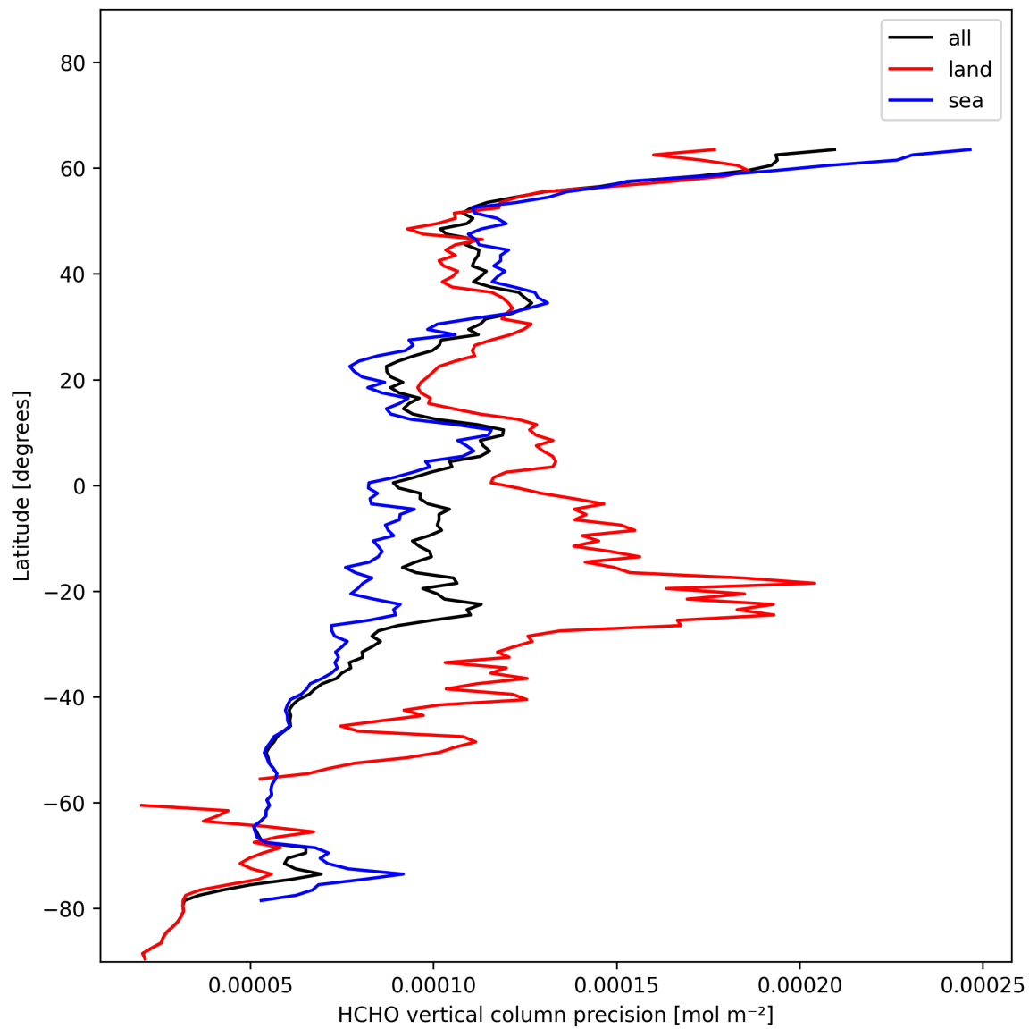
Figure 22: Zonal average of “HCHO vertical column precision” for 2024-11-27 to 2024-11-29.
