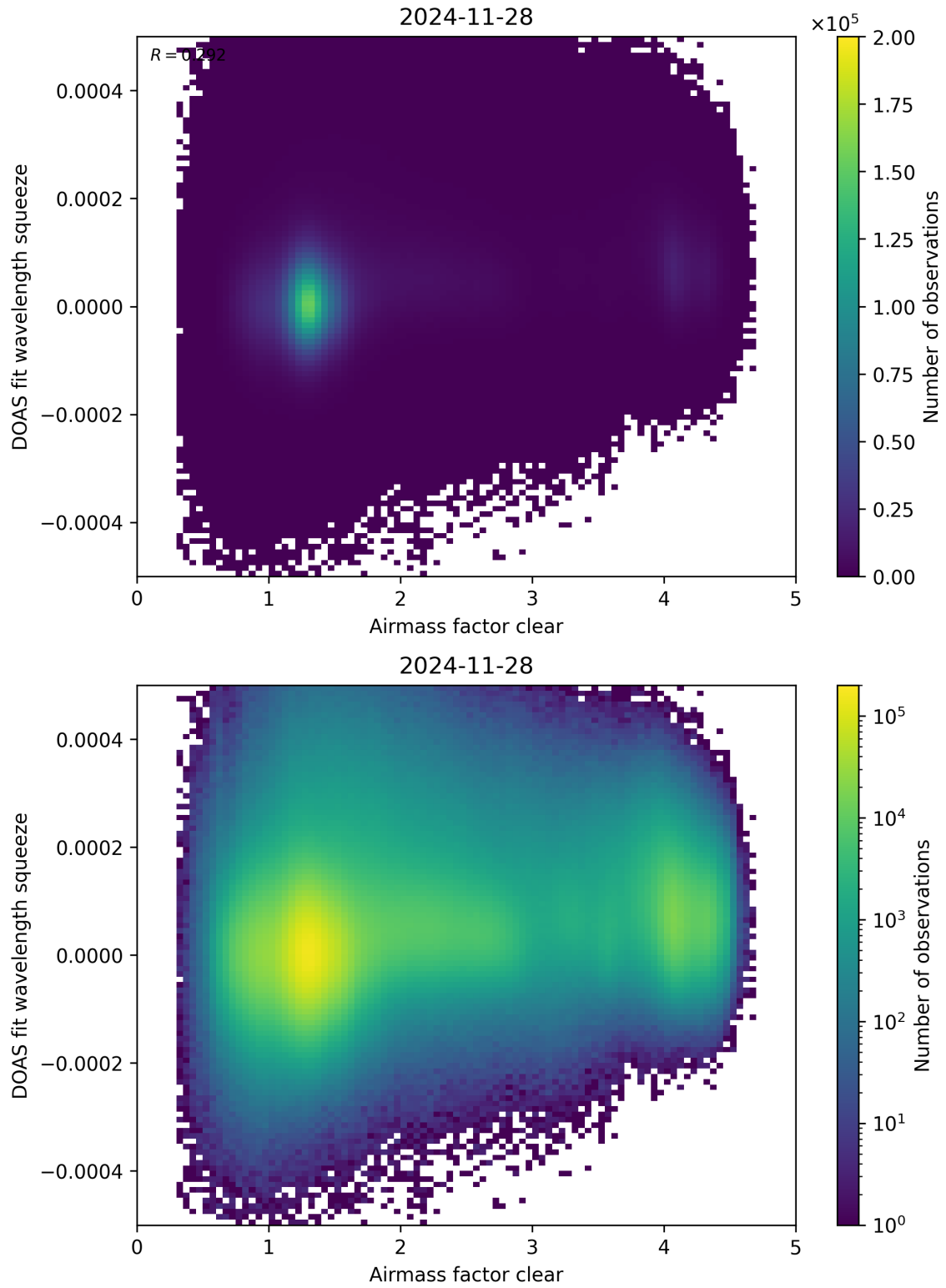
Figure 73: Scatter density plot of “Airmass factor clear” against “DOAS fit wavelength squeeze” for 2024-11-27 to 2024-11-29.
