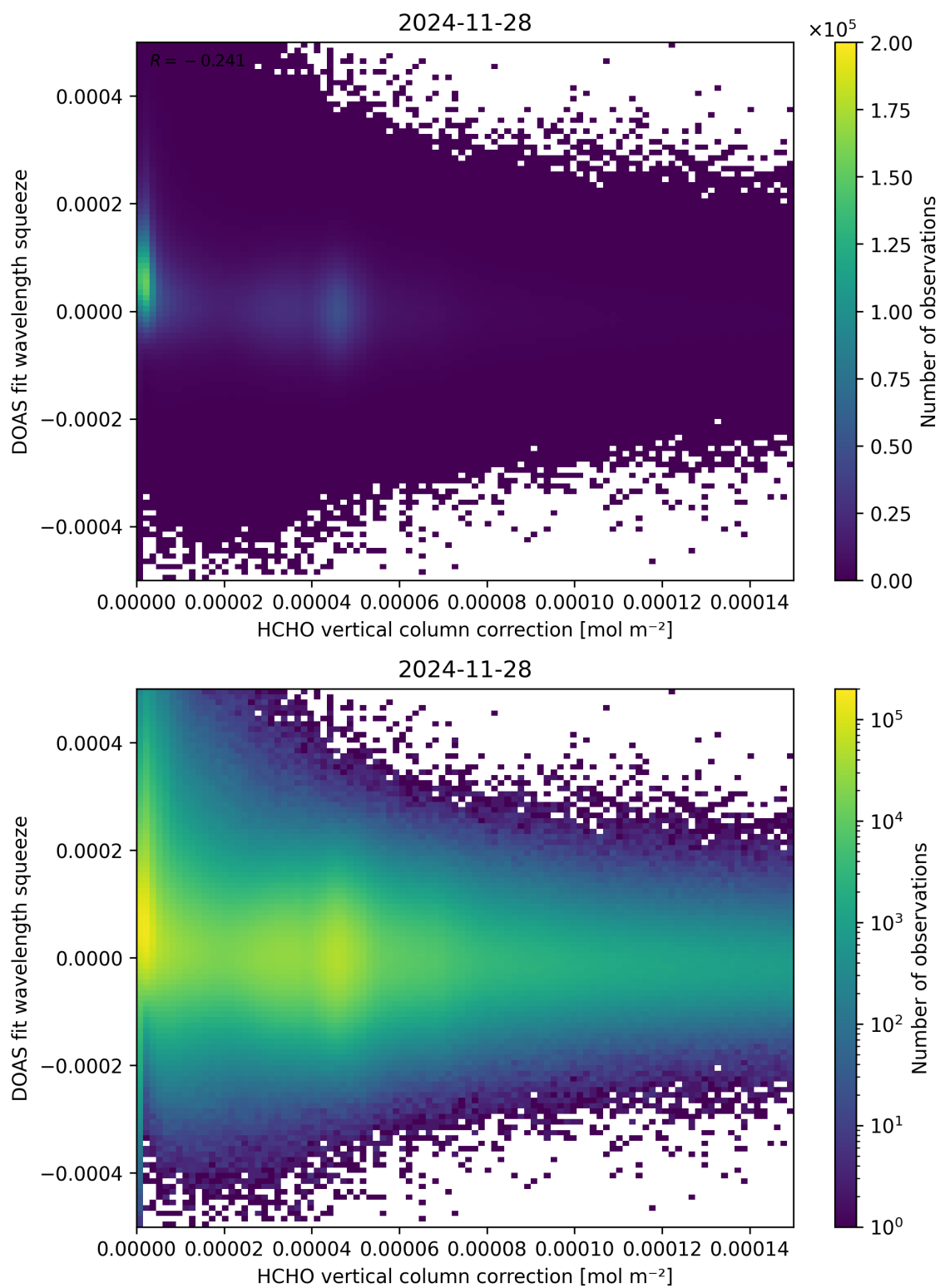
Figure 114: Scatter density plot of “HCHO vertical column correction” against “DOAS fit wavelength squeeze” for 2024-11-27 to 2024-11-29.
