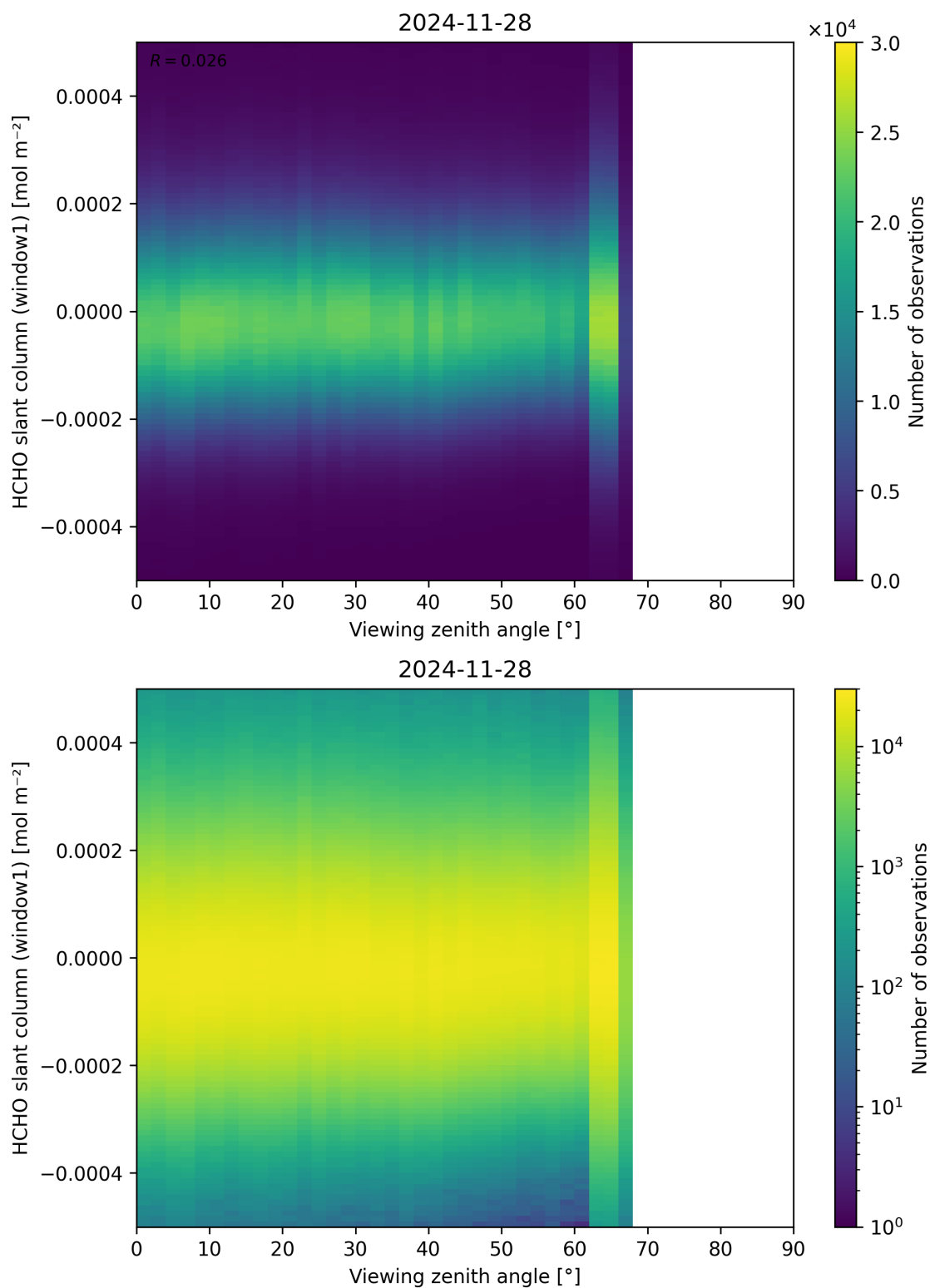
Figure 188: Scatter density plot of “Viewing zenith angle” against “HCHO slant column (window1)” for 2024-11-27 to 2024-11-29.
