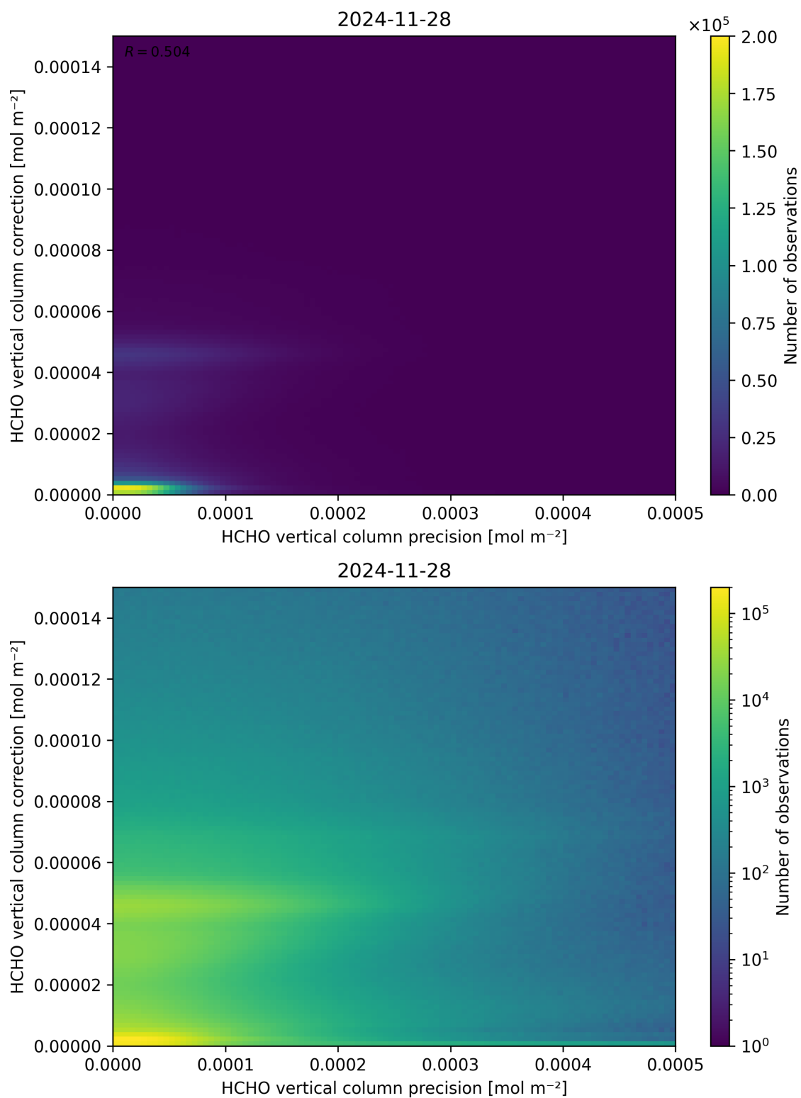
Figure 146: Scatter density plot of “HCHO vertical column precision” against “HCHO vertical column correction” for 2024-11-27 to 2024-11-29.
