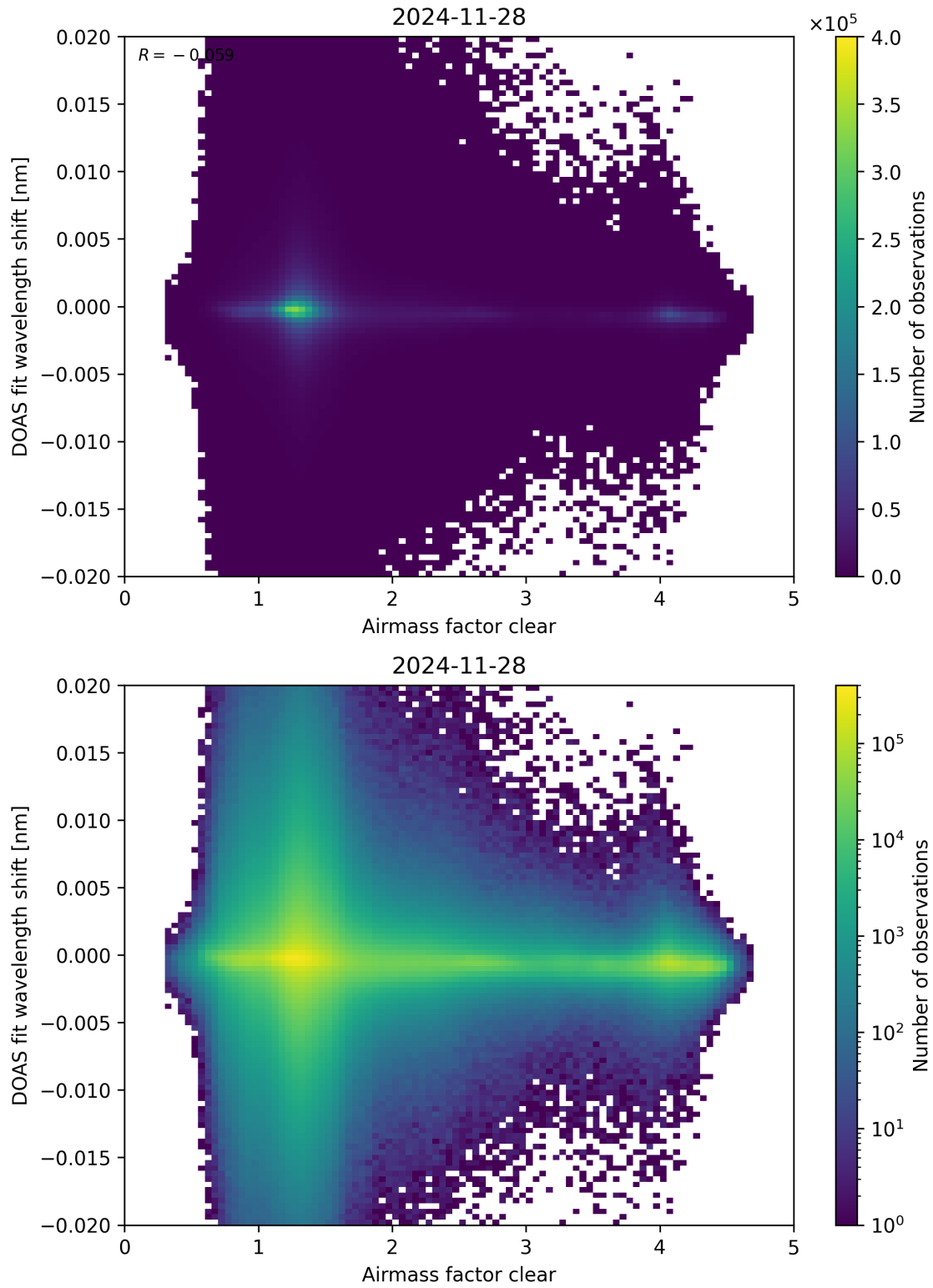
Figure 72: Scatter density plot of “Airmass factor clear” against “DOAS fit wavelength shift” for 2024-11-27 to 2024-11-29.
