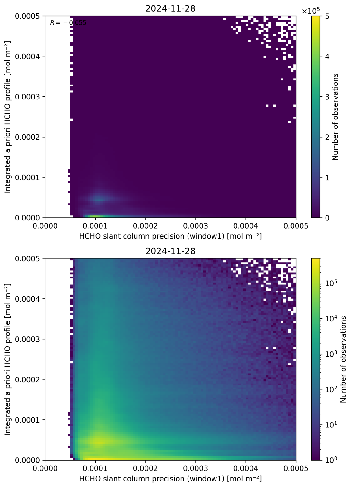
Figure 96: Scatter density plot of “HCHO slant column precision (window1)” against “Integrated a priori HCHO profile” for 2024-11-27 to 2024-11-29.
