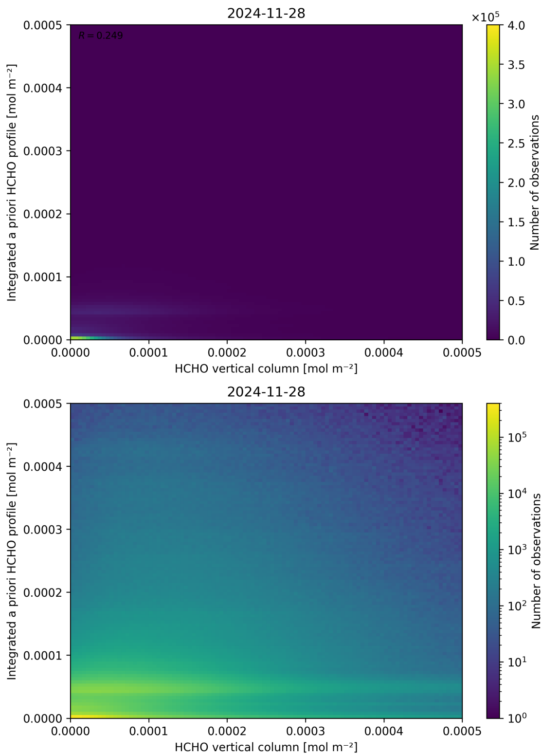
Figure 135: Scatter density plot of “HCHO vertical column” against “Integrated a priori HCHO profile” for 2024-11-27 to 2024-11-29.
