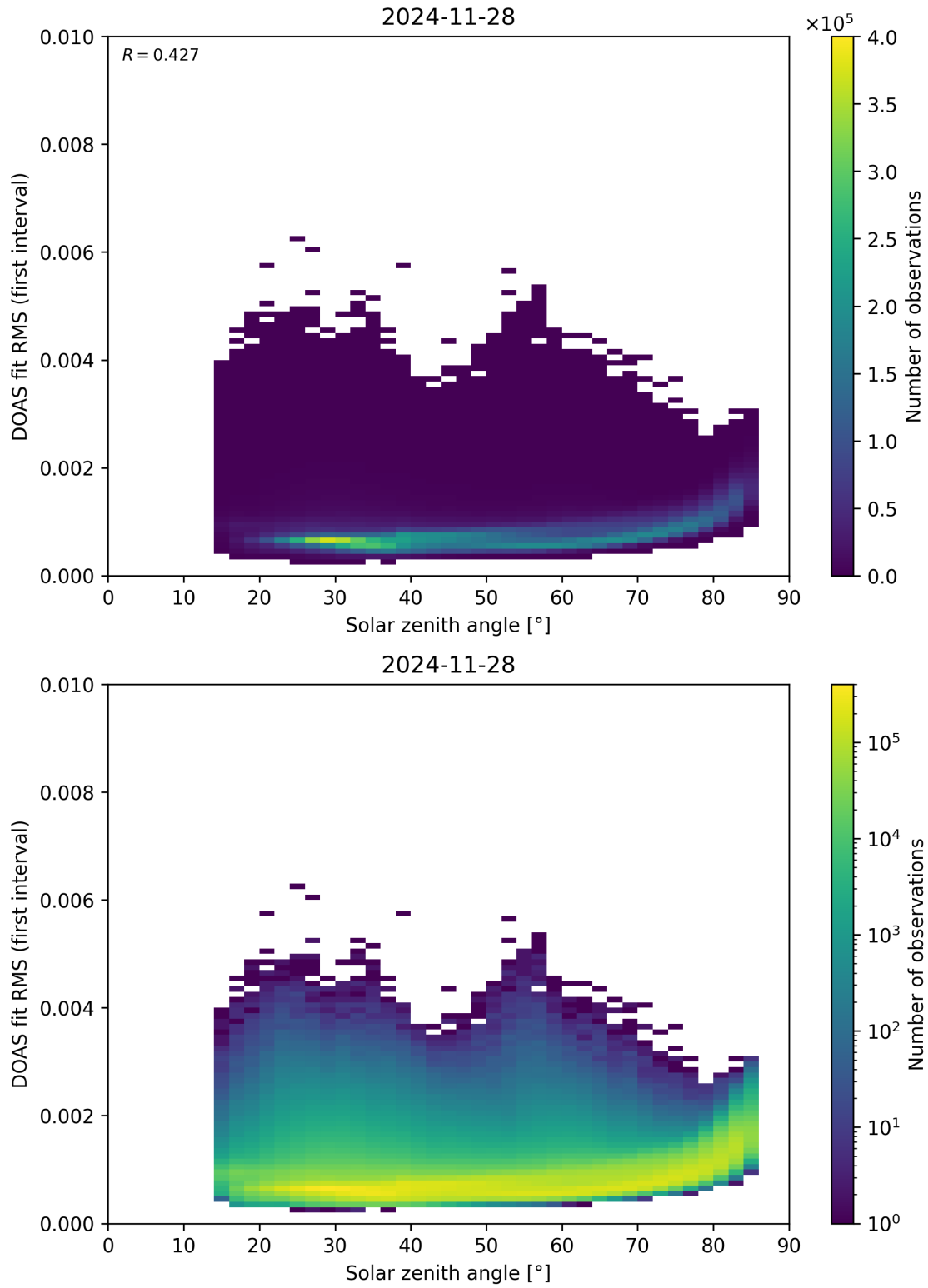
Figure 167: Scatter density plot of “Solar zenith angle” against “DOAS fit RMS (first interval)” for 2024-11-27 to 2024-11-29.
