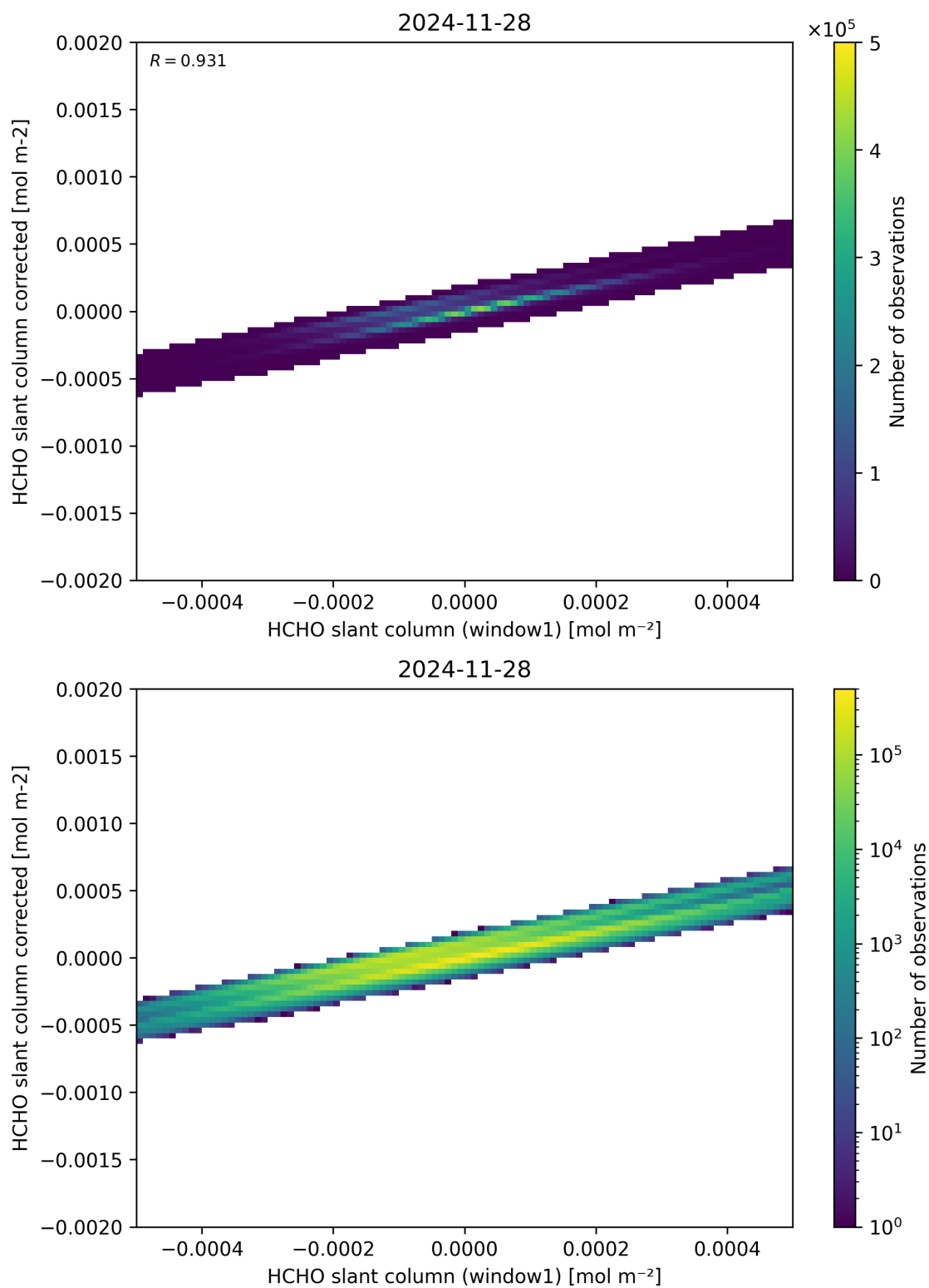
Figure 82: Scatter density plot of “HCHO slant column (window1)” against “HCHO slant column corrected” for 2024-11-27 to 2024-11-29.
