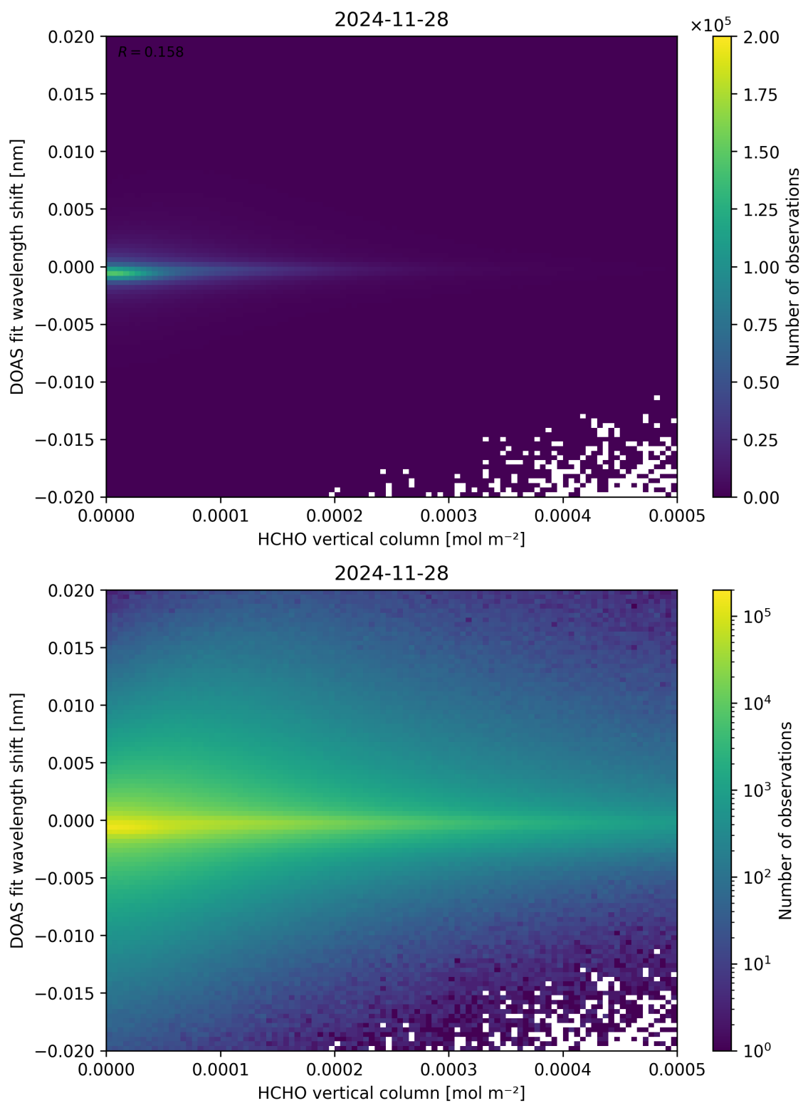
Figure 124: Scatter density plot of “HCHO vertical column” against “DOAS fit wavelength shift” for 2024-11-27 to 2024-11-29.
