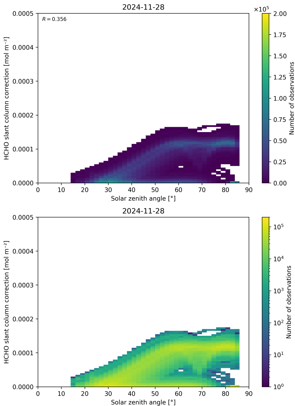
Figure 172: Scatter density plot of “Solar zenith angle” against “HCHO slant column correction” for 2024-11-27 to 2024-11-29.
