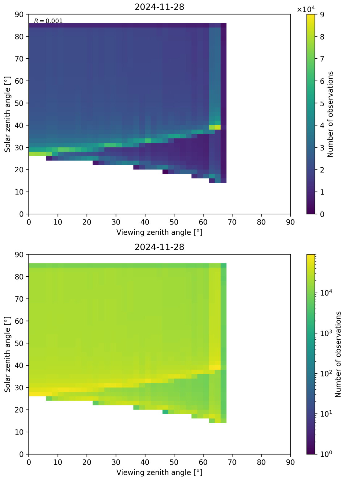
Figure 197: Scatter density plot of “Viewing zenith angle” against “Solar zenith angle” for 2024-11-27 to 2024-11-29.
