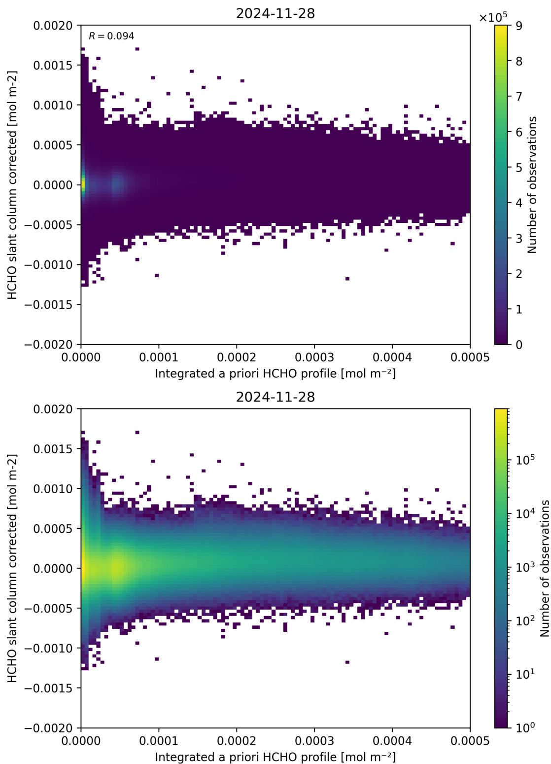
Figure 151: Scatter density plot of “Integrated a priori HCHO profile” against “HCHO slant column corrected” for 2024-11-27 to 2024-11-29.
