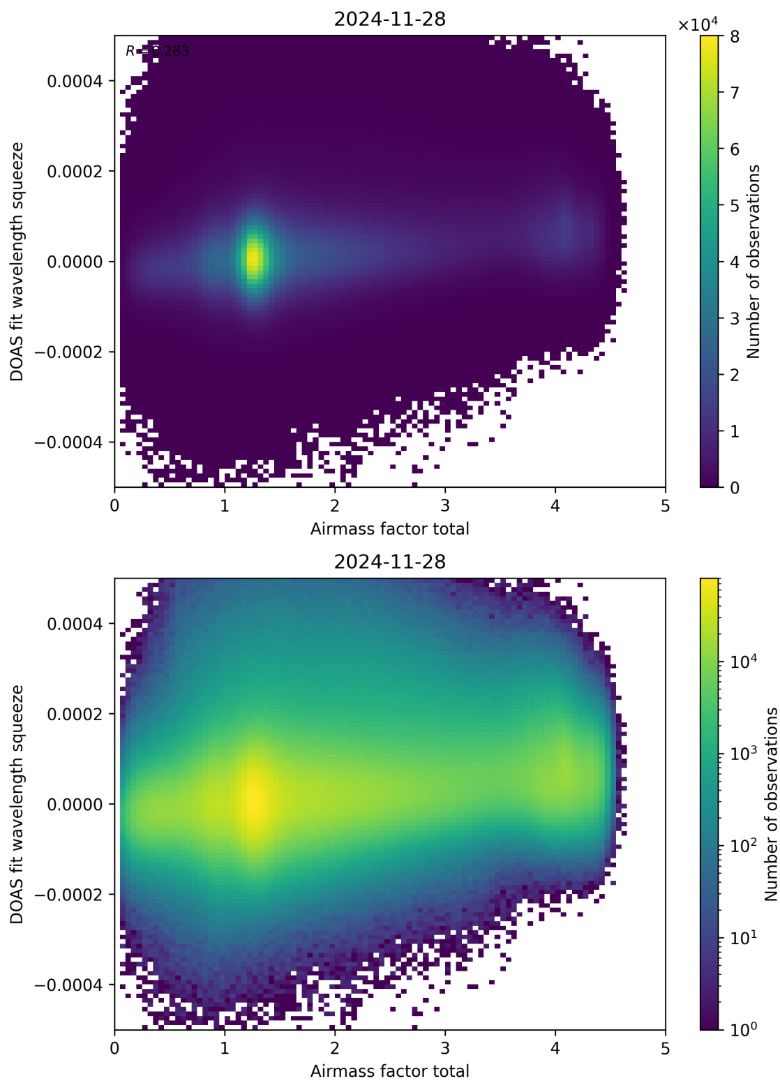
Figure 99: Scatter density plot of “Airmass factor total” against “DOAS fit wavelength squeeze” for 2024-11-27 to 2024-11-29.
