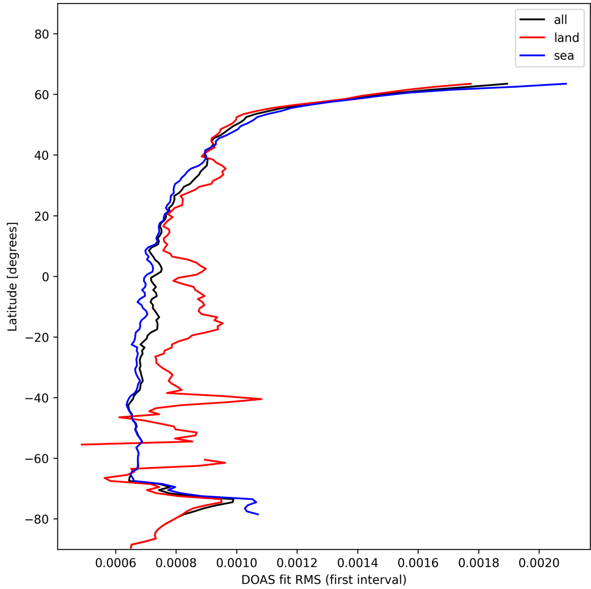
Figure 32: Zonal average of “DOAS fit RMS (first interval)” for 2024-11-27 to 2024-11-29.
