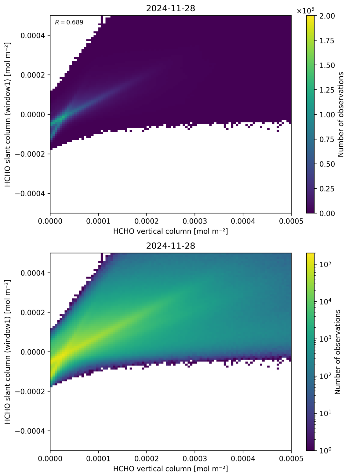
Figure 129: Scatter density plot of “HCHO vertical column” against “HCHO slant column (window1)” for 2024-11-27 to 2024-11-29.
