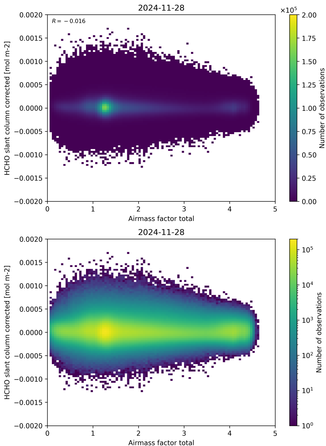
Figure 101: Scatter density plot of “Airmass factor total” against “HCHO slant column corrected” for 2024-11-27 to 2024-11-29.
