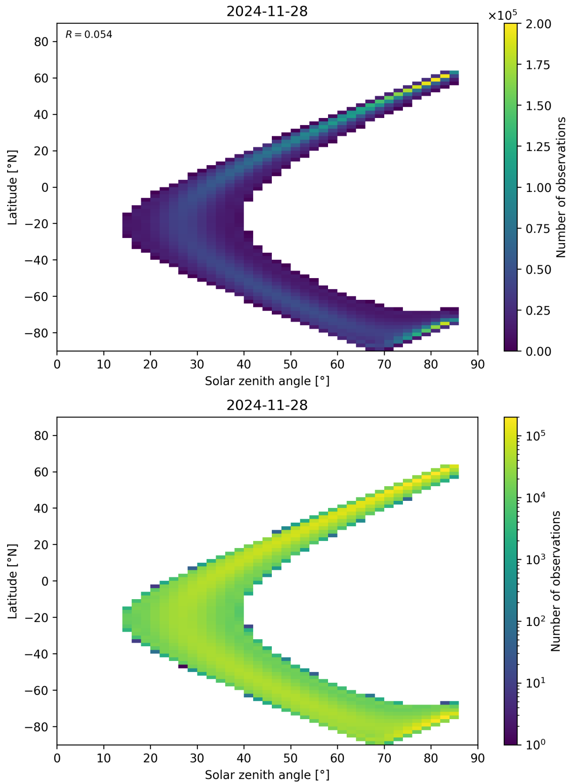
Figure 181: Scatter density plot of “Solar zenith angle” against “Latitude” for 2024-11-27 to 2024-11-29.
