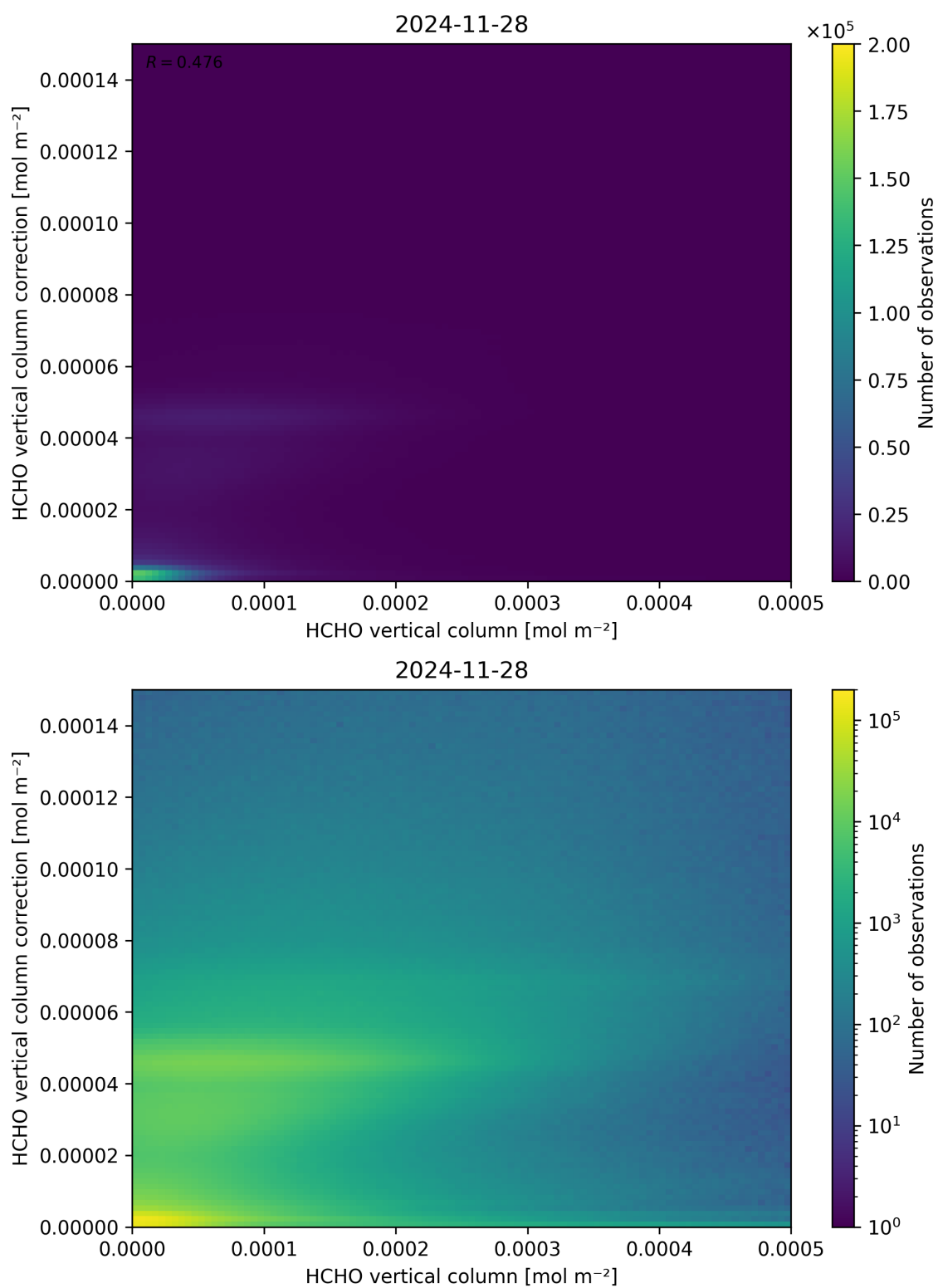
Figure 133: Scatter density plot of “HCHO vertical column” against “HCHO vertical column correction” for 2024-11-27 to 2024-11-29.
