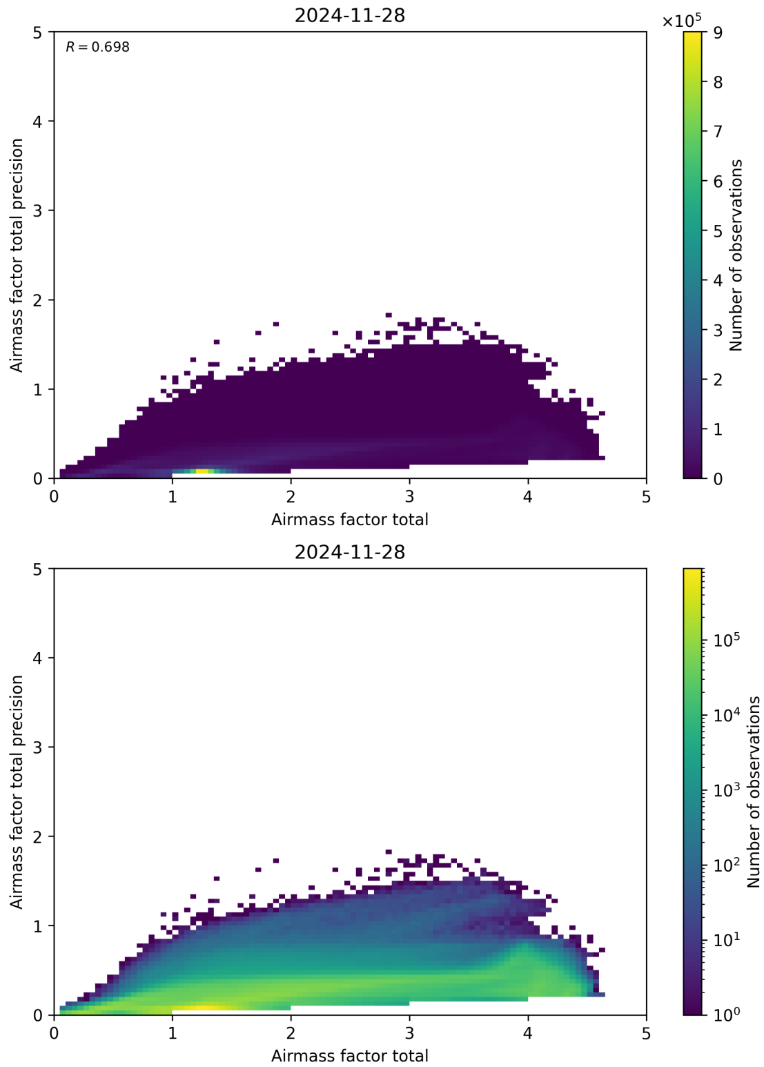
Figure 103: Scatter density plot of “Airmass factor total” against “Airmass factor total precision” for 2024-11-27 to 2024-11-29.
