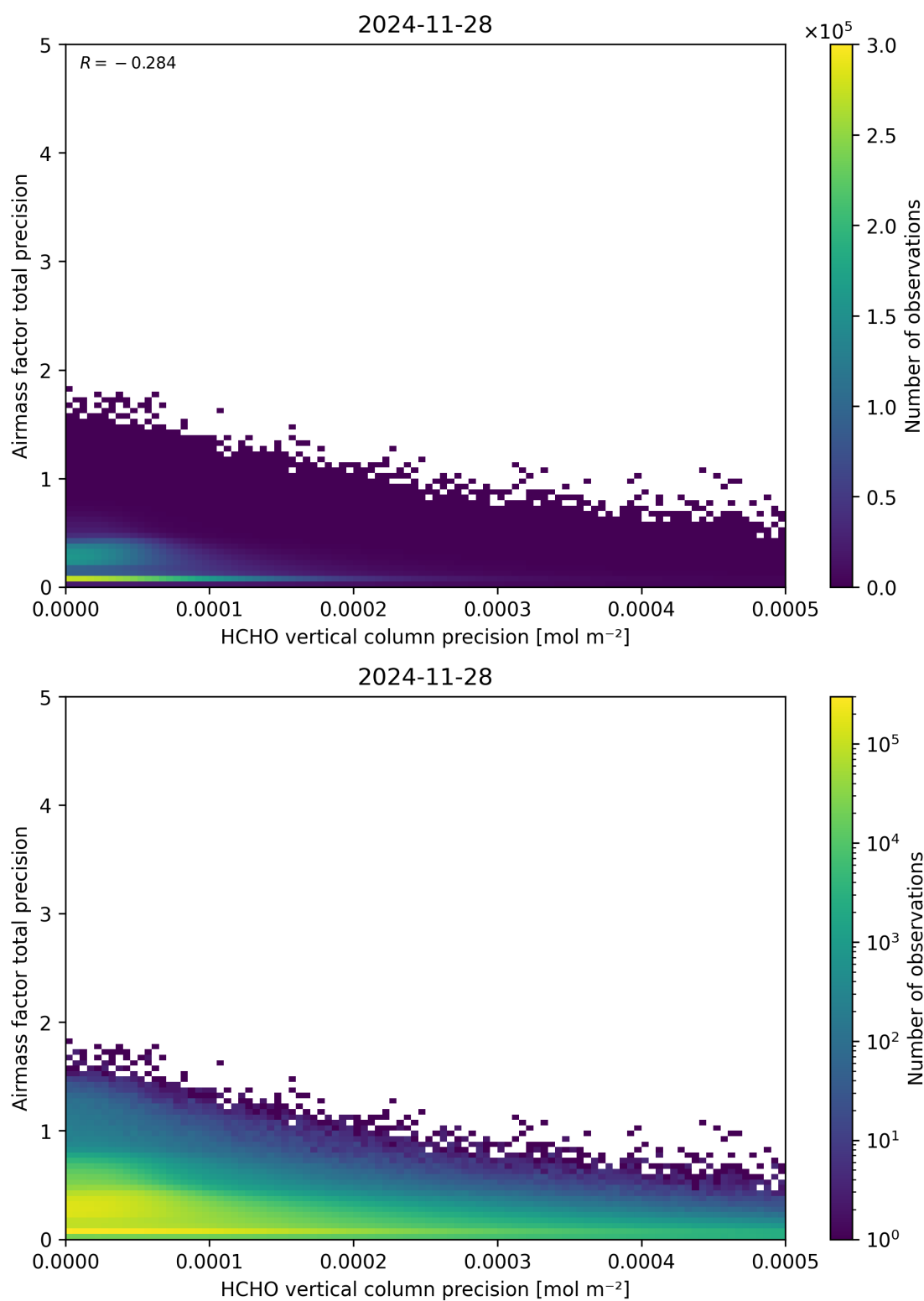
Figure 145: Scatter density plot of “HCHO vertical column precision” against “Airmass factor total precision” for 2024-11-27 to 2024-11-29.
