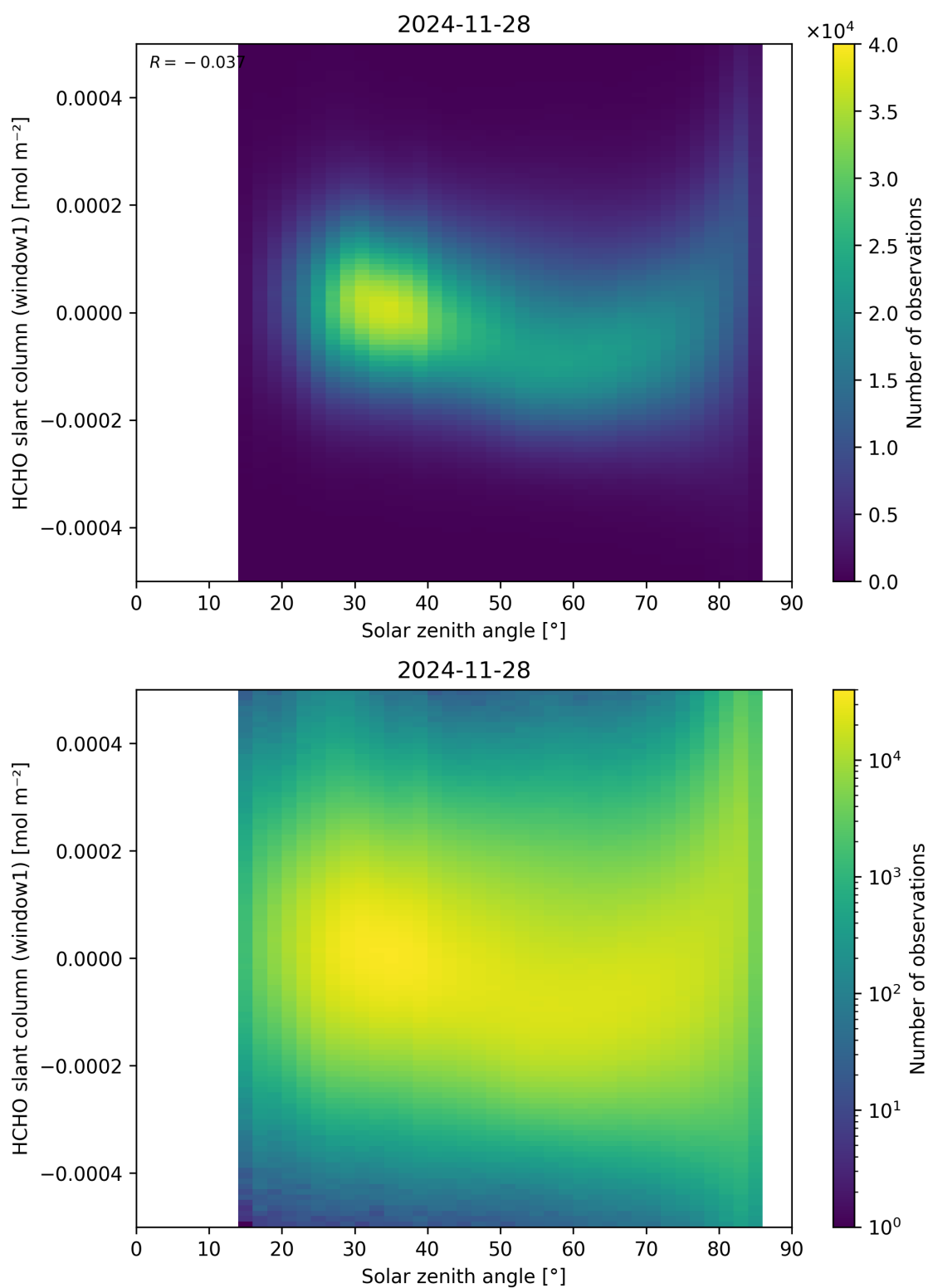
Figure 173: Scatter density plot of “Solar zenith angle” against “HCHO slant column (window1)” for 2024-11-27 to 2024-11-29.
