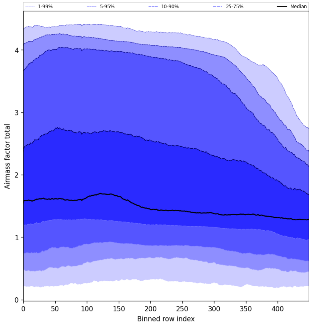
Figure 54: Along track statistics of “Airmass factor total” for 2024-11-27 to 2024-11-29
