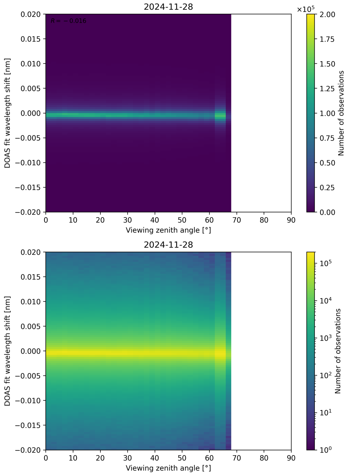
Figure 183: Scatter density plot of “Viewing zenith angle” against “DOAS fit wavelength shift” for 2024-11-27 to 2024-11-29.
