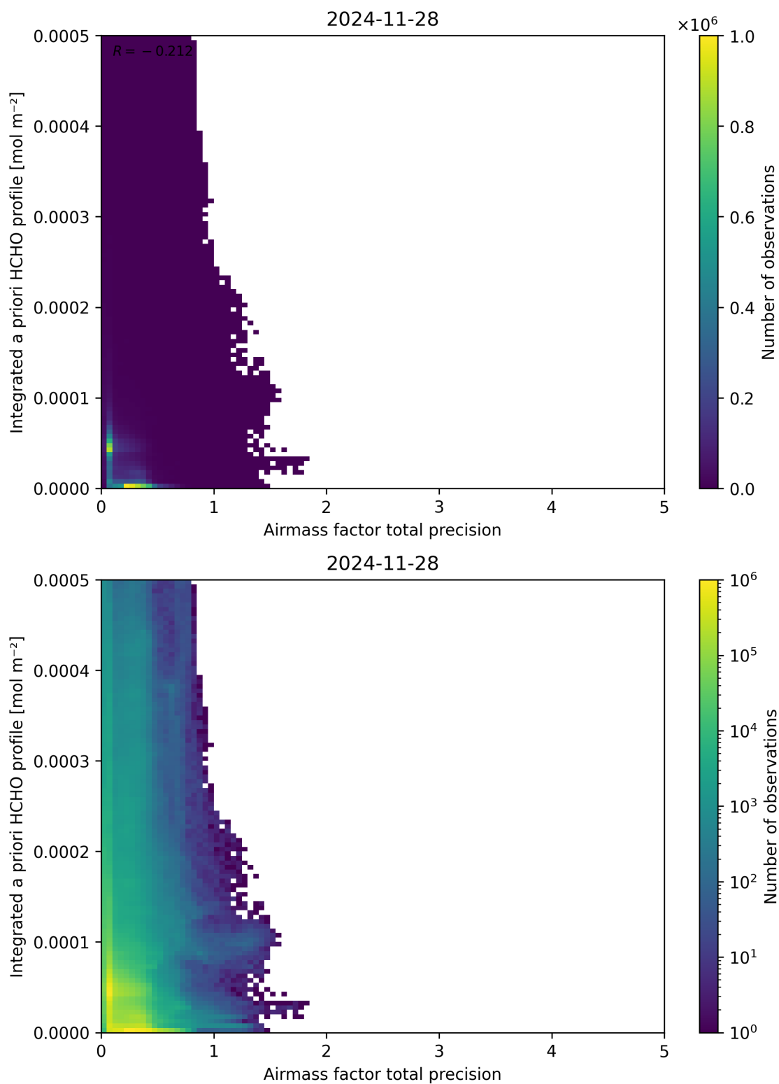
Figure 111: Scatter density plot of “Airmass factor total precision” against “Integrated a priori HCHO profile” for 2024-11-27 to 2024-11-29.
