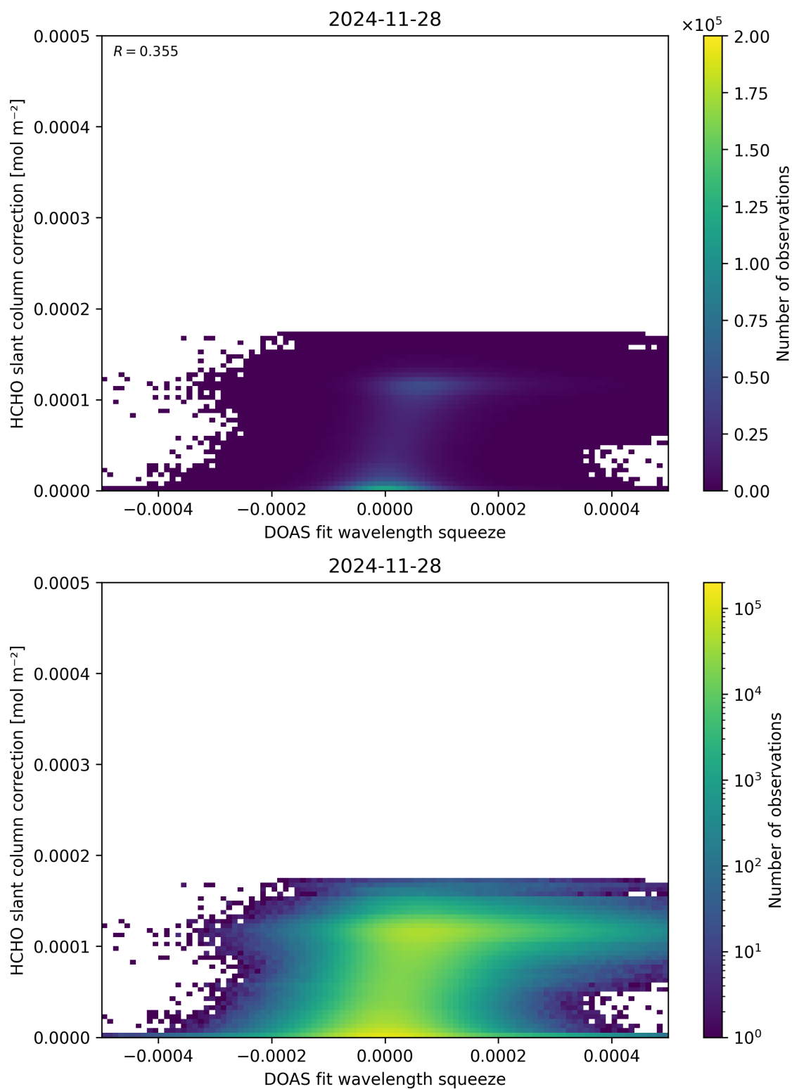
Figure 70: Scatter density plot of “DOAS fit wavelength squeeze” against “HCHO slant column correction” for 2024-11-27 to 2024-11-29.
