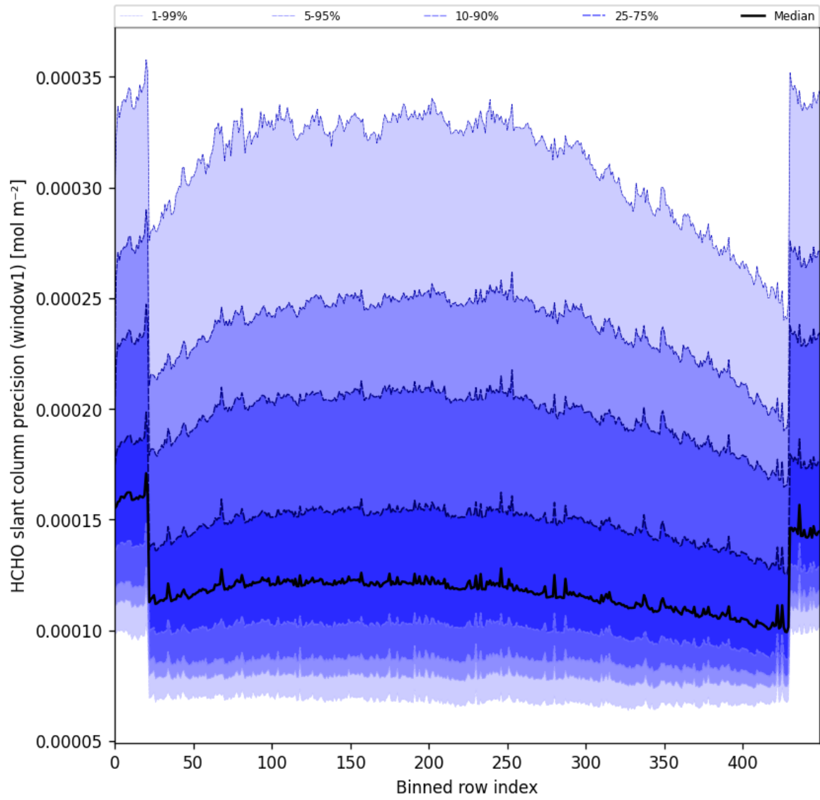
Figure 53: Along track statistics of “HCHO slant column precision (window1)” for 2024-11-27 to 2024-11-29
