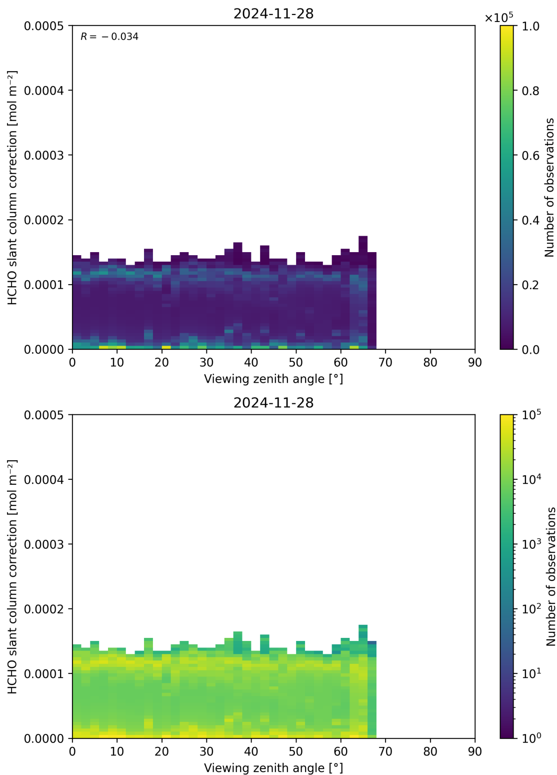
Figure 187: Scatter density plot of “Viewing zenith angle” against “HCHO slant column correction” for 2024-11-27 to 2024-11-29.
