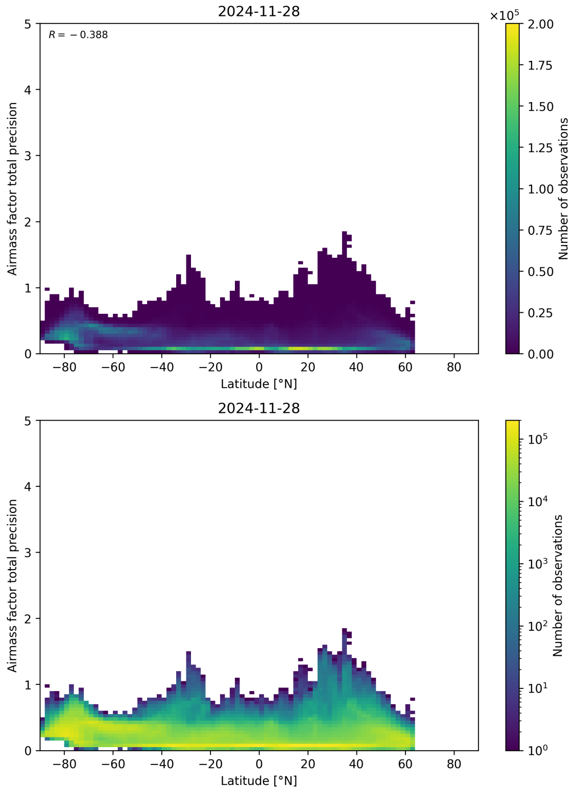
Figure 162: Scatter density plot of “Latitude” against “Airmass factor total precision” for 2024-11-27 to 2024-11-29.
