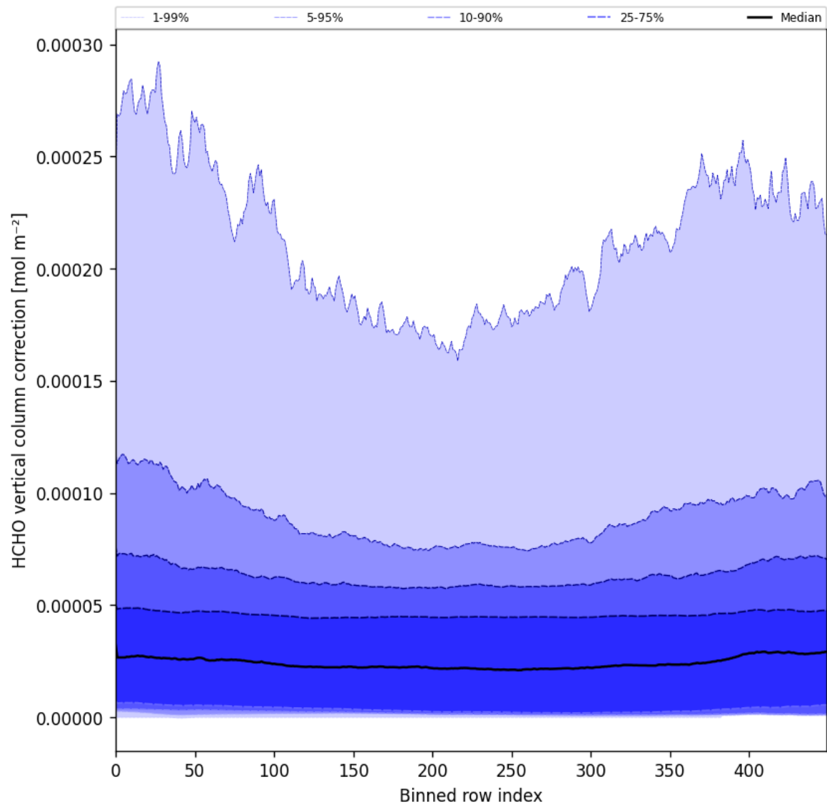
Figure 51: Along track statistics of “HCHO vertical column correction” for 2024-11-27 to 2024-11-29
