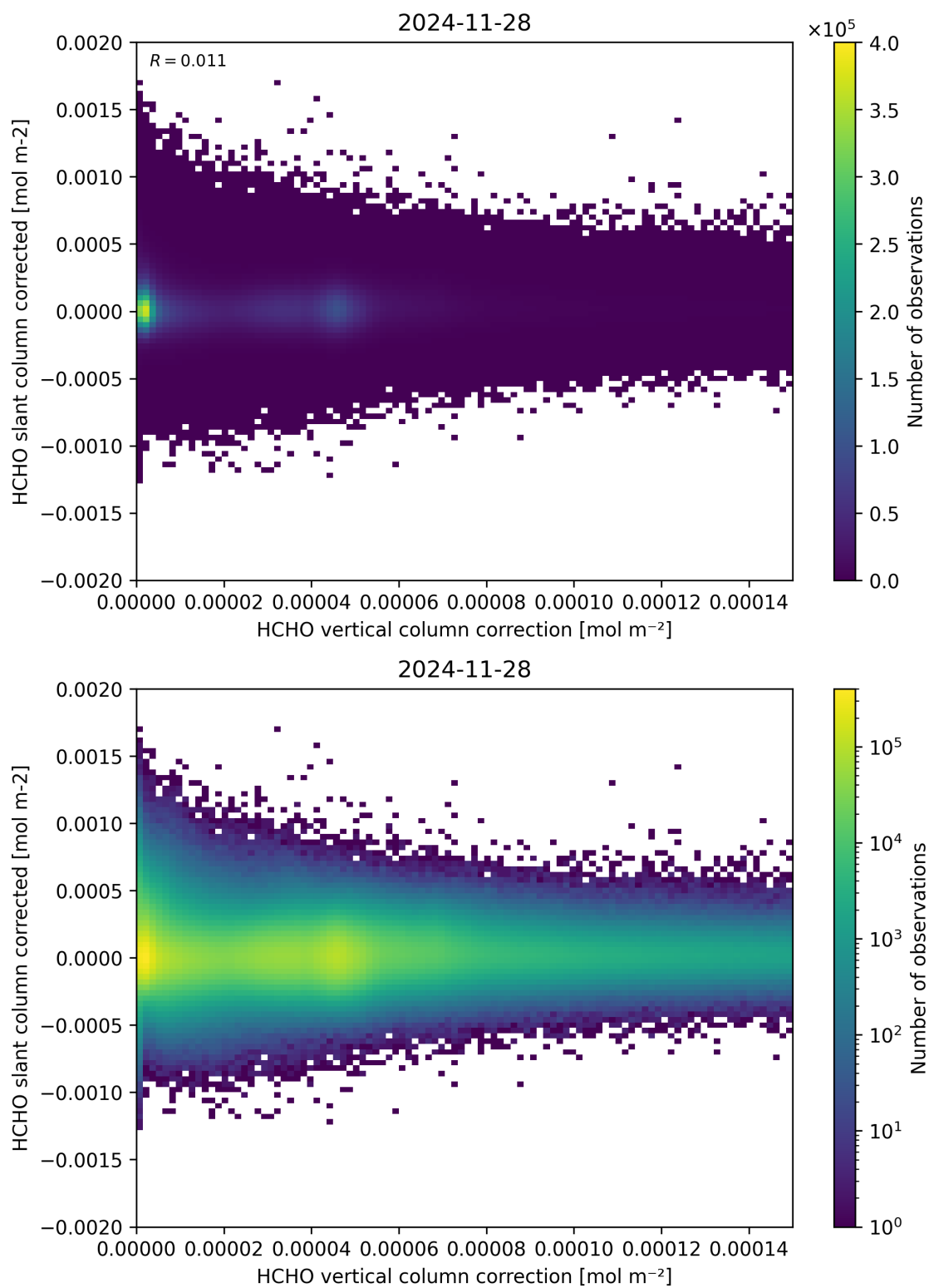
Figure 116: Scatter density plot of “HCHO vertical column correction” against “HCHO slant column corrected” for 2024-11-27 to 2024-11-29.
