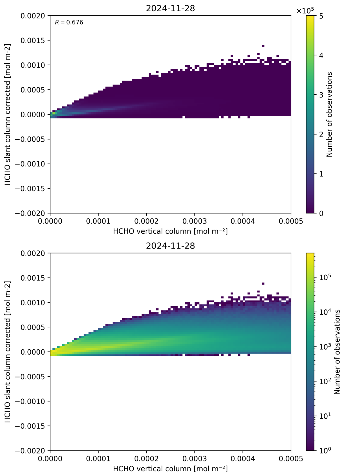
Figure 127: Scatter density plot of “HCHO vertical column” against “HCHO slant column corrected” for 2024-11-27 to 2024-11-29.
