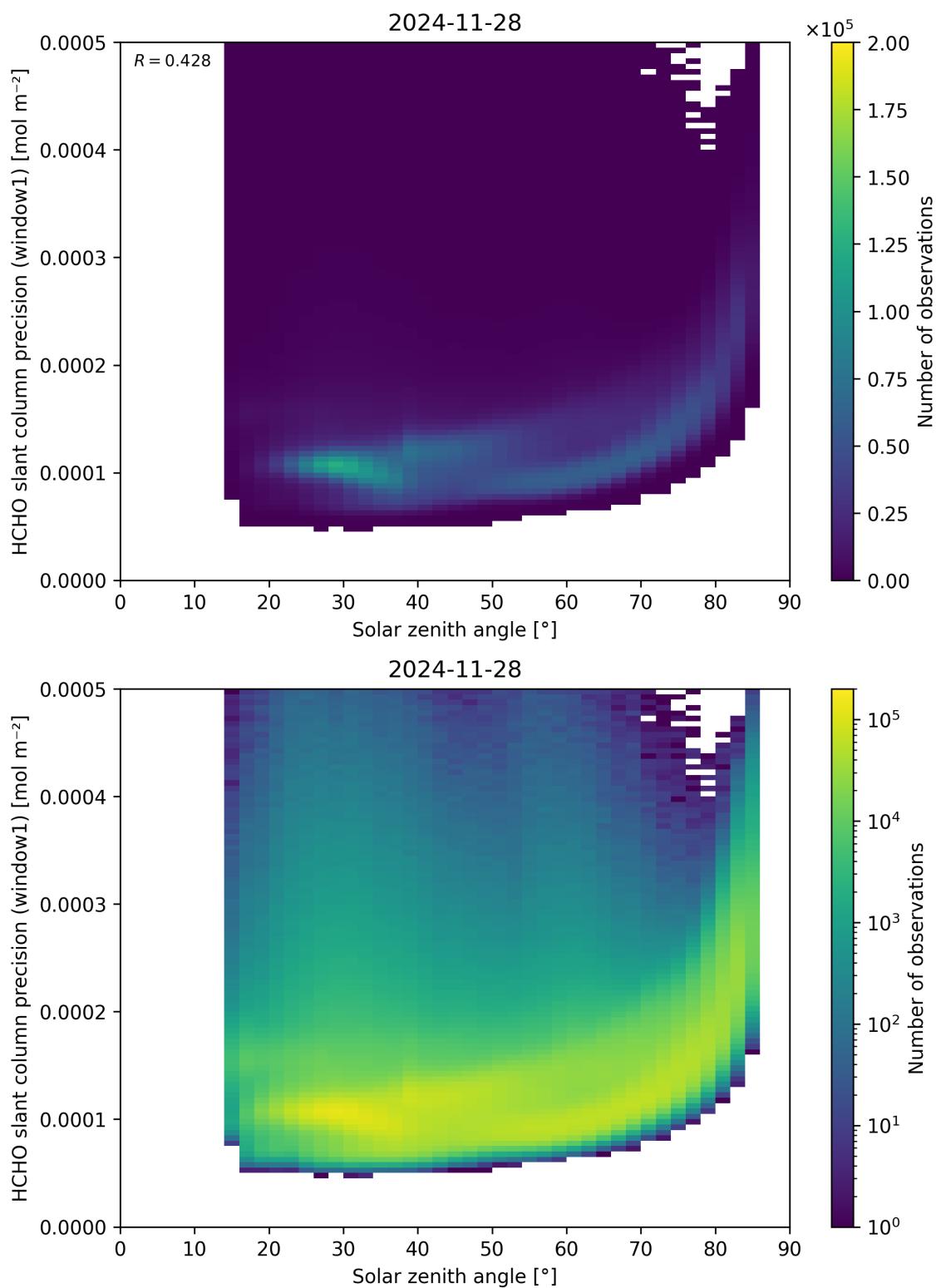
Figure 174: Scatter density plot of “Solar zenith angle” against “HCHO slant column precision (window1)” for 2024-11-27 to 2024-11-29.
