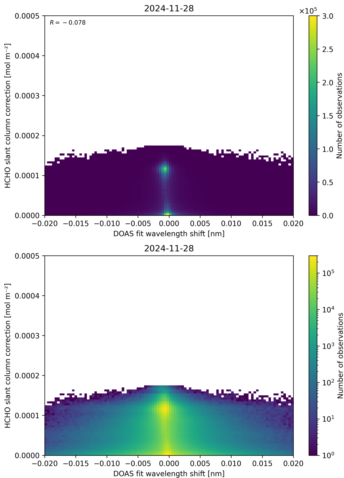
Figure 67: Scatter density plot of “DOAS fit wavelength shift” against “HCHO slant column correction” for 2024-11-27 to 2024-11-29.
