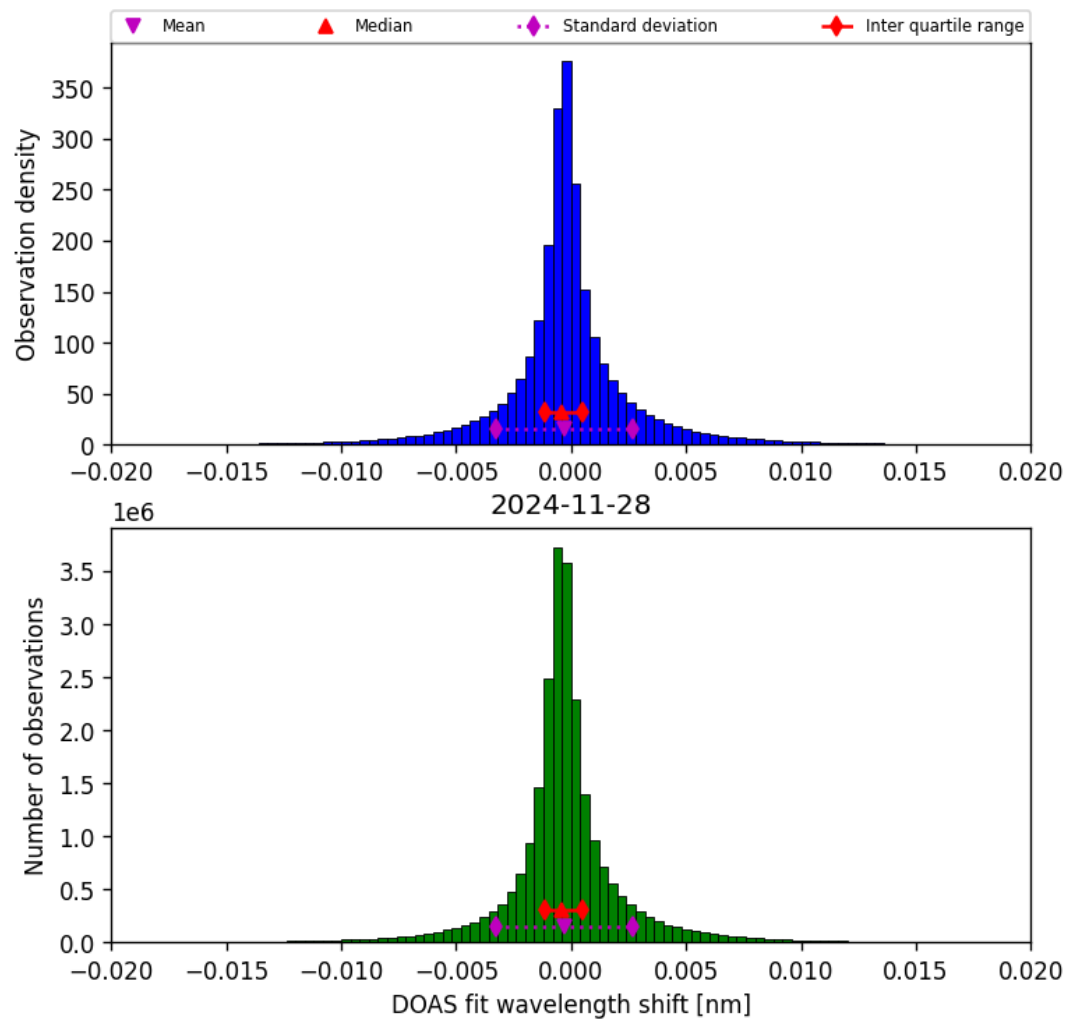
Figure 44: Histogram of “DOAS fit wavelength shift” for 2024-11-27 to 2024-11-29
