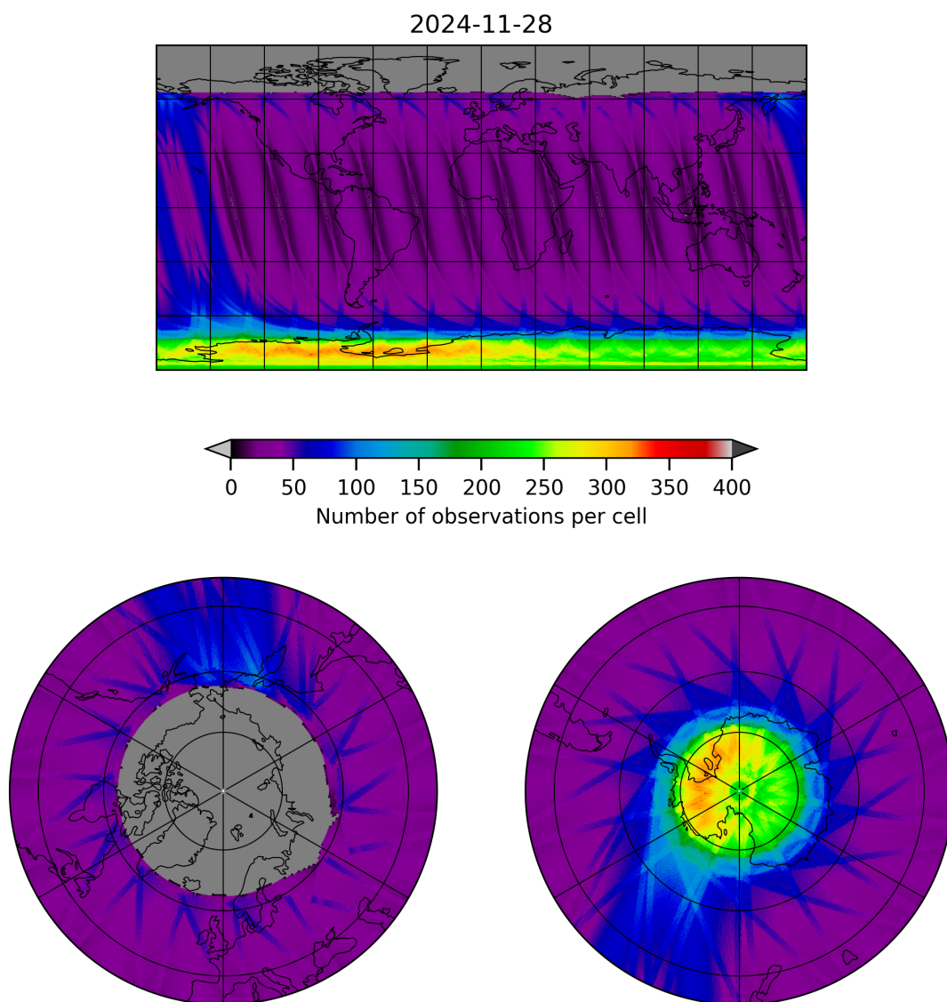
Figure 19: Map of the number of observations for 2024-11-27 to 2024-11-29
