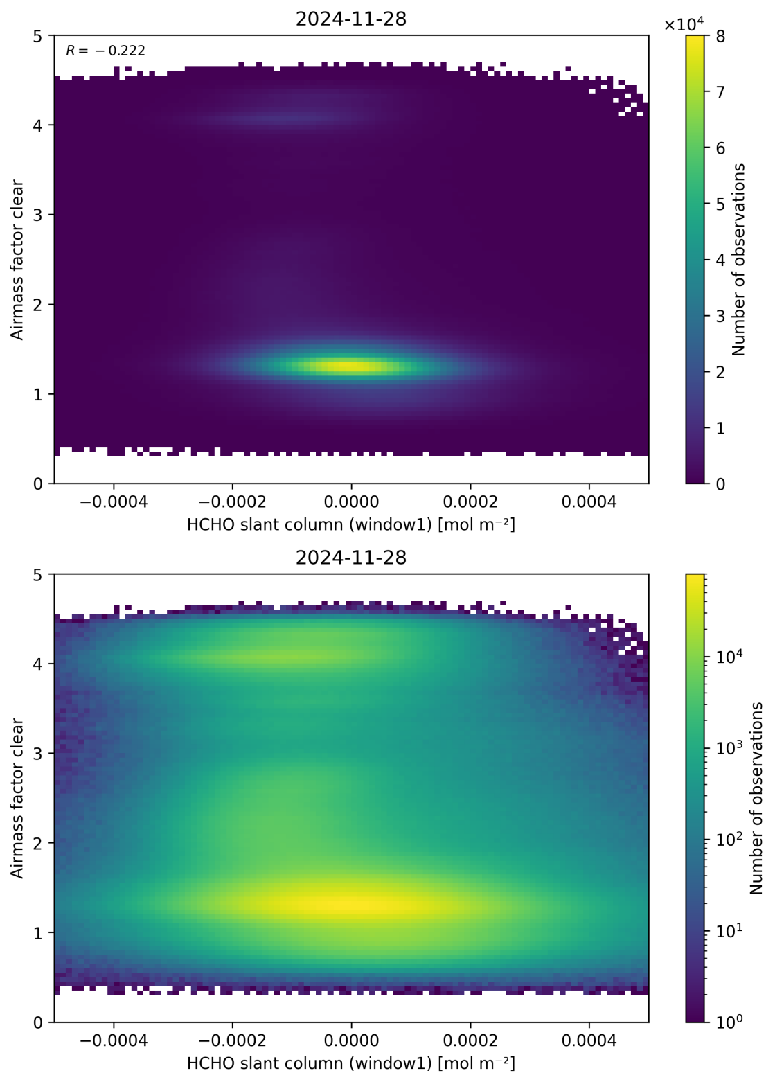
Figure 81: Scatter density plot of “HCHO slant column (window1)” against “Airmass factor clear” for 2024-11-27 to 2024-11-29.
