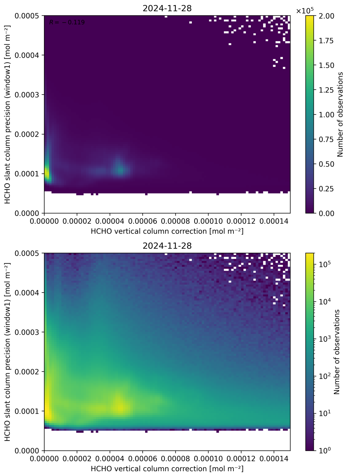
Figure 119: Scatter density plot of “HCHO vertical column correction” against “HCHO slant column precision (window1)” for 2024-11-27 to 2024-11-29.
