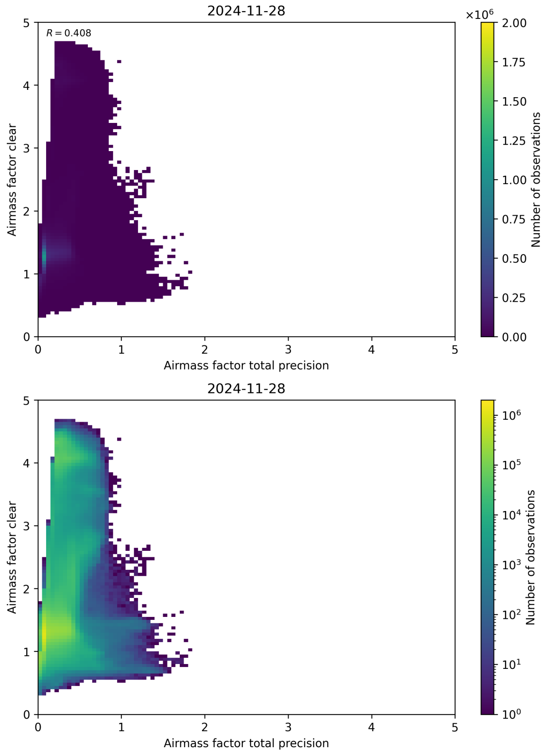
Figure 108: Scatter density plot of “Airmass factor total precision” against “Airmass factor clear” for 2024-11-27 to 2024-11-29.
