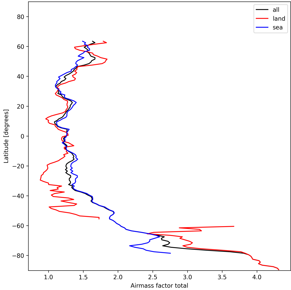
Figure 26: Zonal average of “Airmass factor total” for 2024-11-27 to 2024-11-29.
