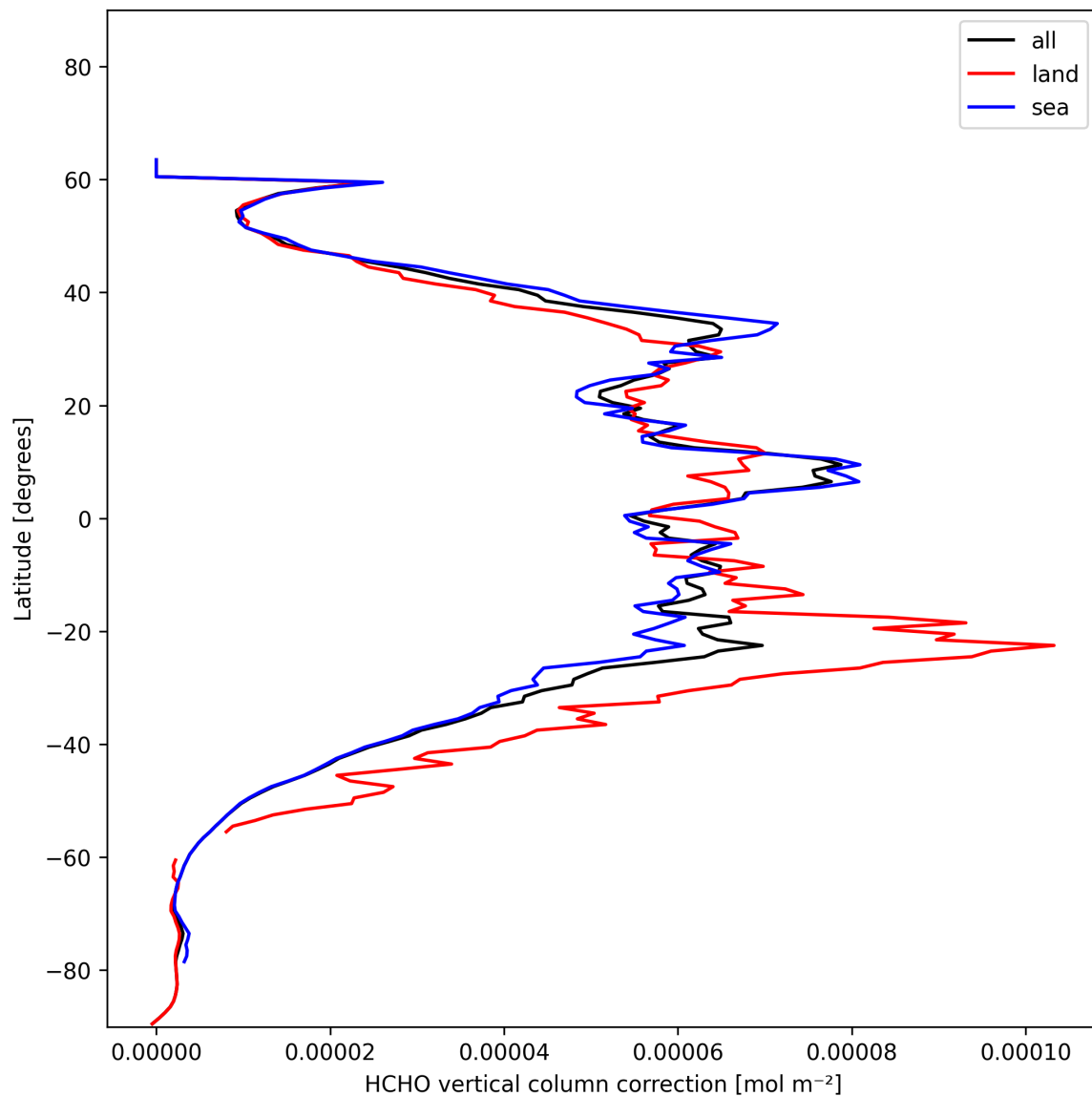
Figure 23: Zonal average of “HCHO vertical column correction” for 2024-11-27 to 2024-11-29.
