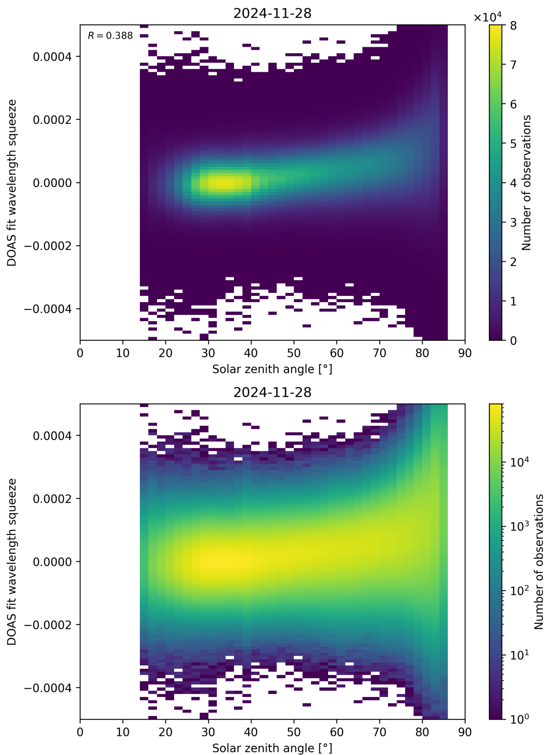
Figure 169: Scatter density plot of “Solar zenith angle” against “DOAS fit wavelength squeeze” for 2024-11-27 to 2024-11-29.
