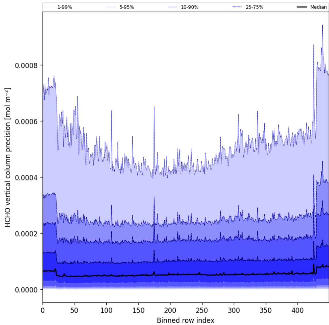
Figure 50: Along track statistics of “HCHO vertical column precision” for 2024-11-27 to 2024-11-29
