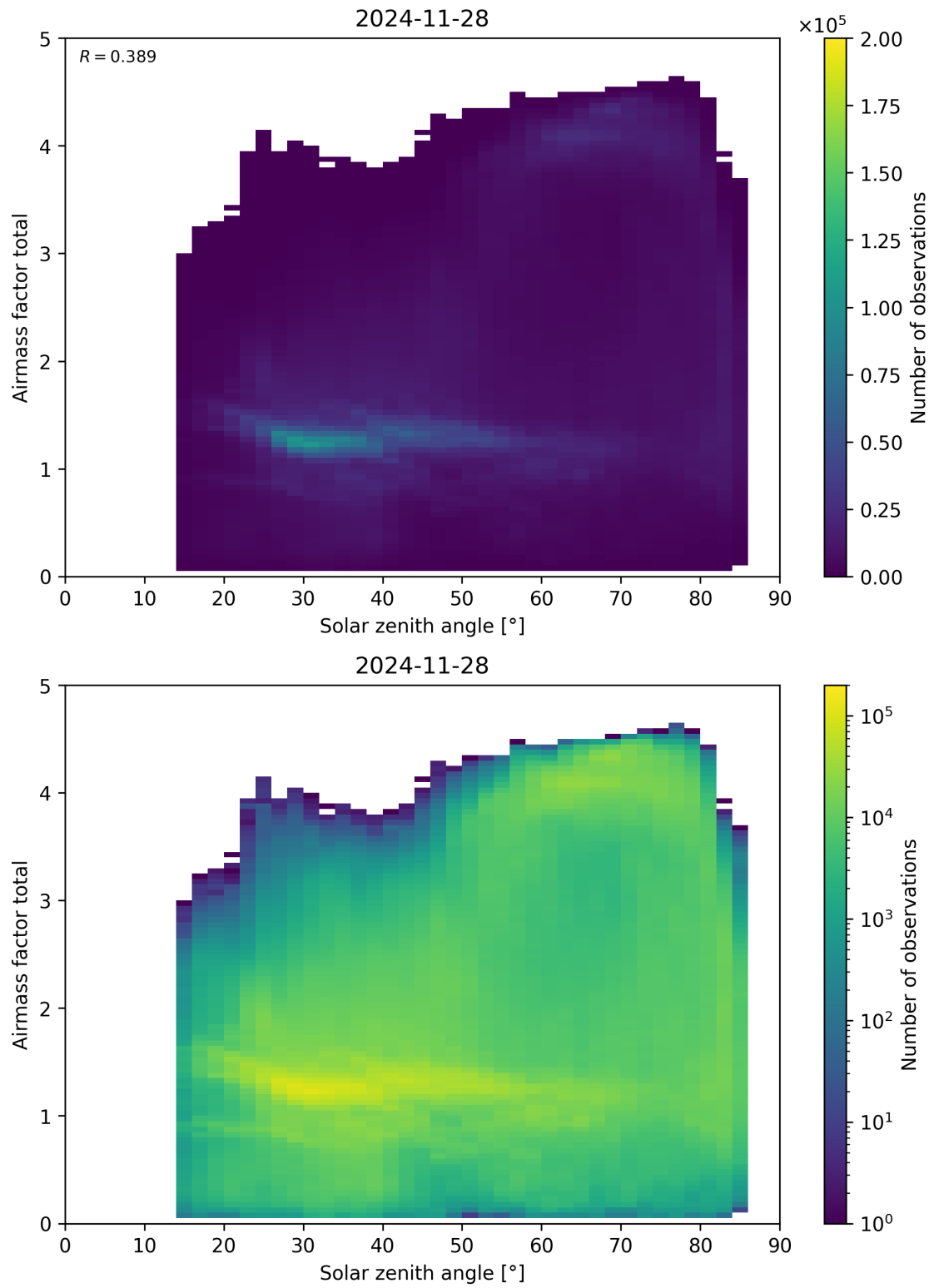
Figure 175: Scatter density plot of “Solar zenith angle” against “Airmass factor total” for 2024-11-27 to 2024-11-29.
