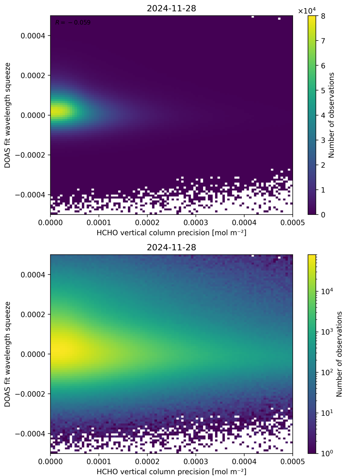
Figure 138: Scatter density plot of “HCHO vertical column precision” against “DOAS fit wavelength squeeze” for 2024-11-27 to 2024-11-29.
