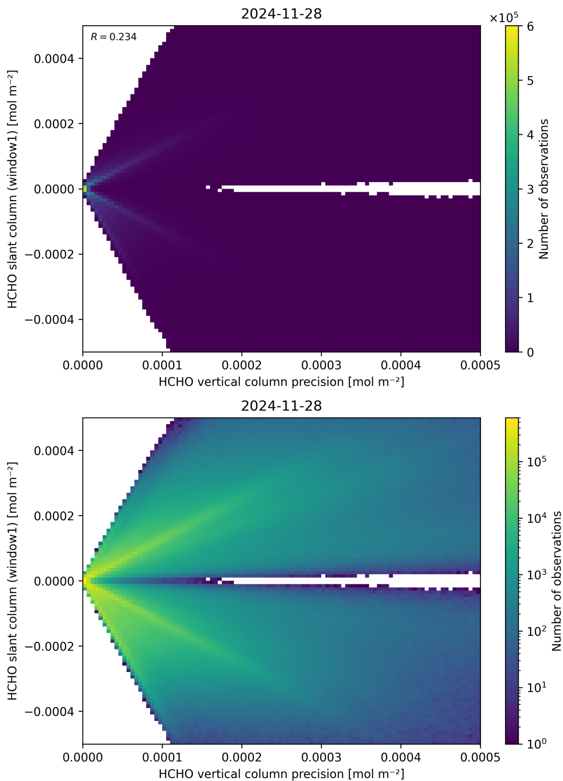
Figure 142: Scatter density plot of “HCHO vertical column precision” against “HCHO slant column (window1)” for 2024-11-27 to 2024-11-29.
