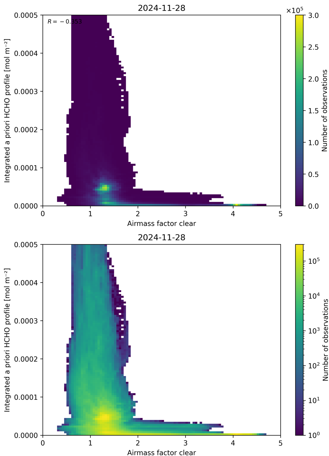
Figure 76: Scatter density plot of “Airmass factor clear” against “Integrated a priori HCHO profile” for 2024-11-27 to 2024-11-29.
