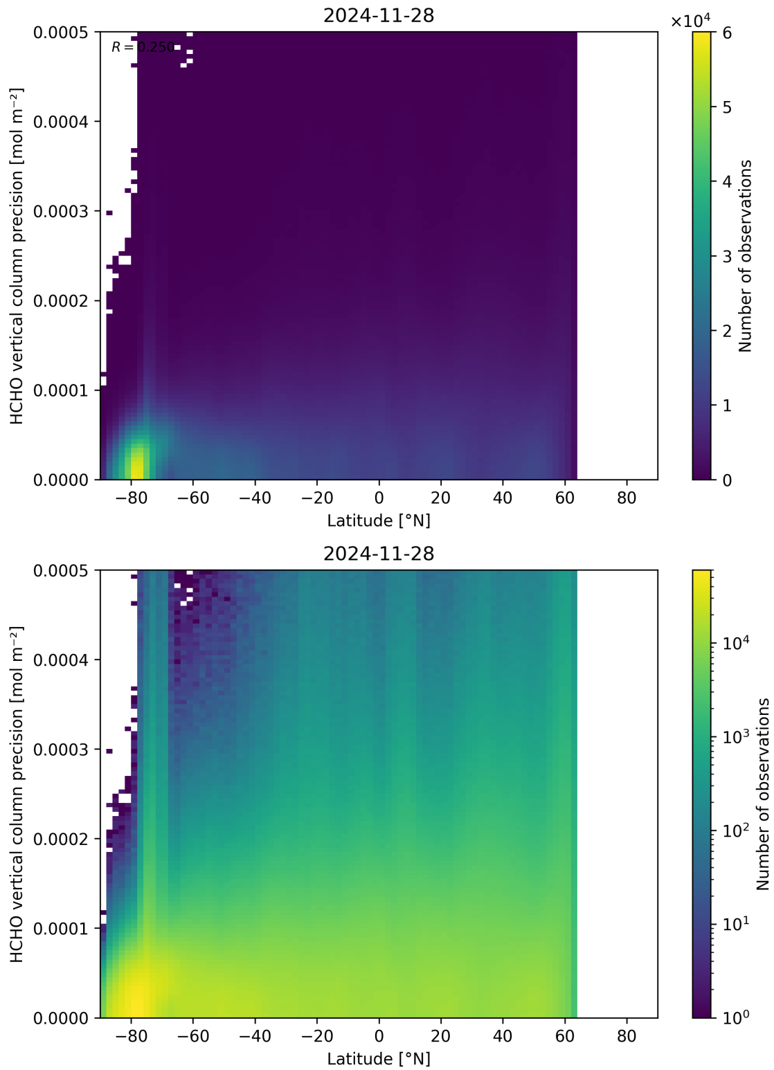
Figure 165: Scatter density plot of “Latitude” against “HCHO vertical column precision” for 2024-11-27 to 2024-11-29.
