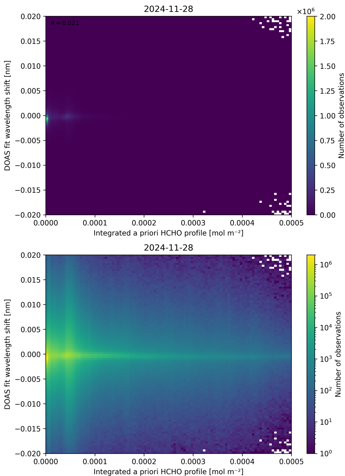
Figure 149: Scatter density plot of “Integrated a priori HCHO profile” against “DOAS fit wavelength shift” for 2024-11-27 to 2024-11-29.
