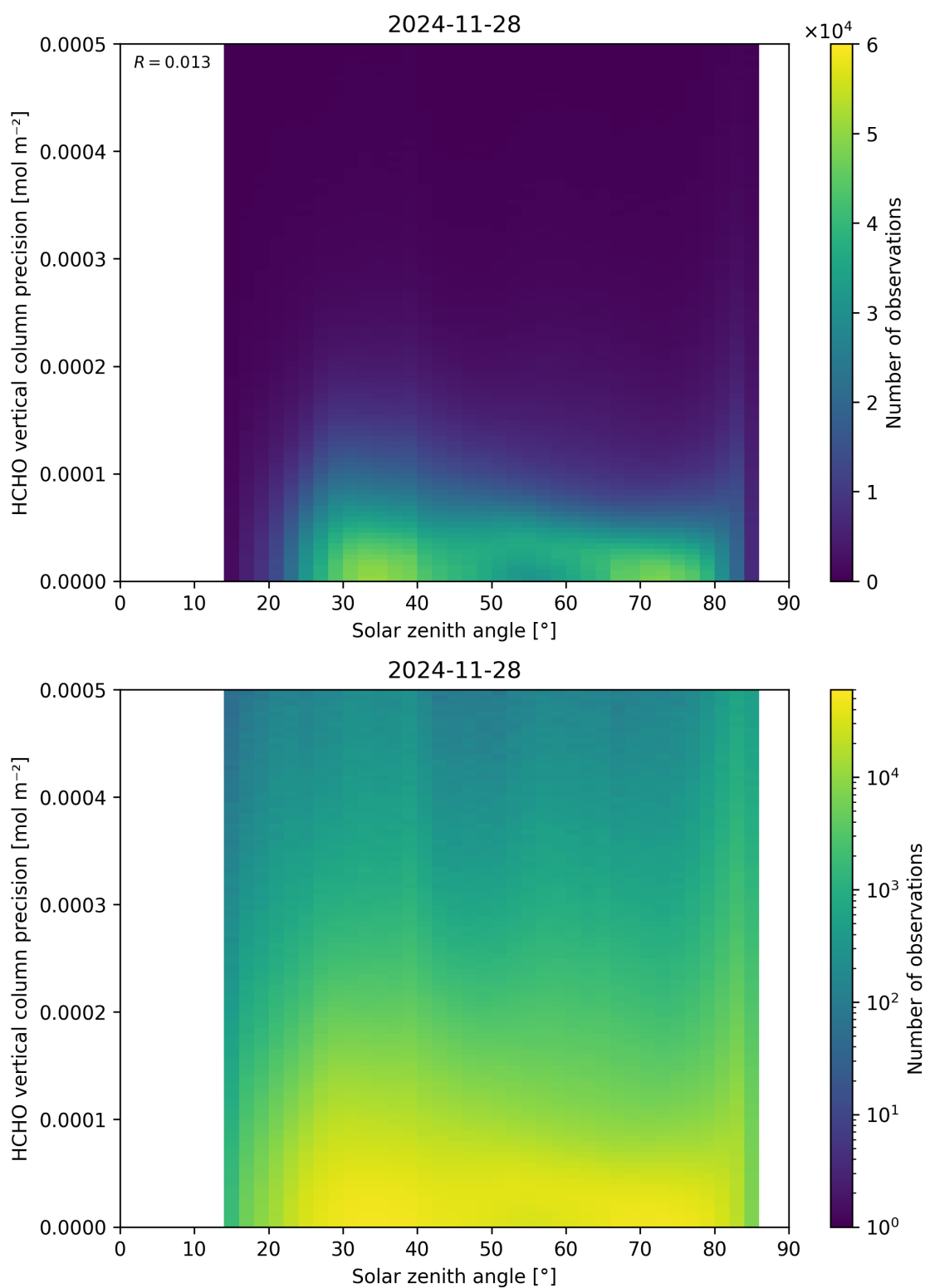
Figure 179: Scatter density plot of “Solar zenith angle” against “HCHO vertical column precision” for 2024-11-27 to 2024-11-29.
