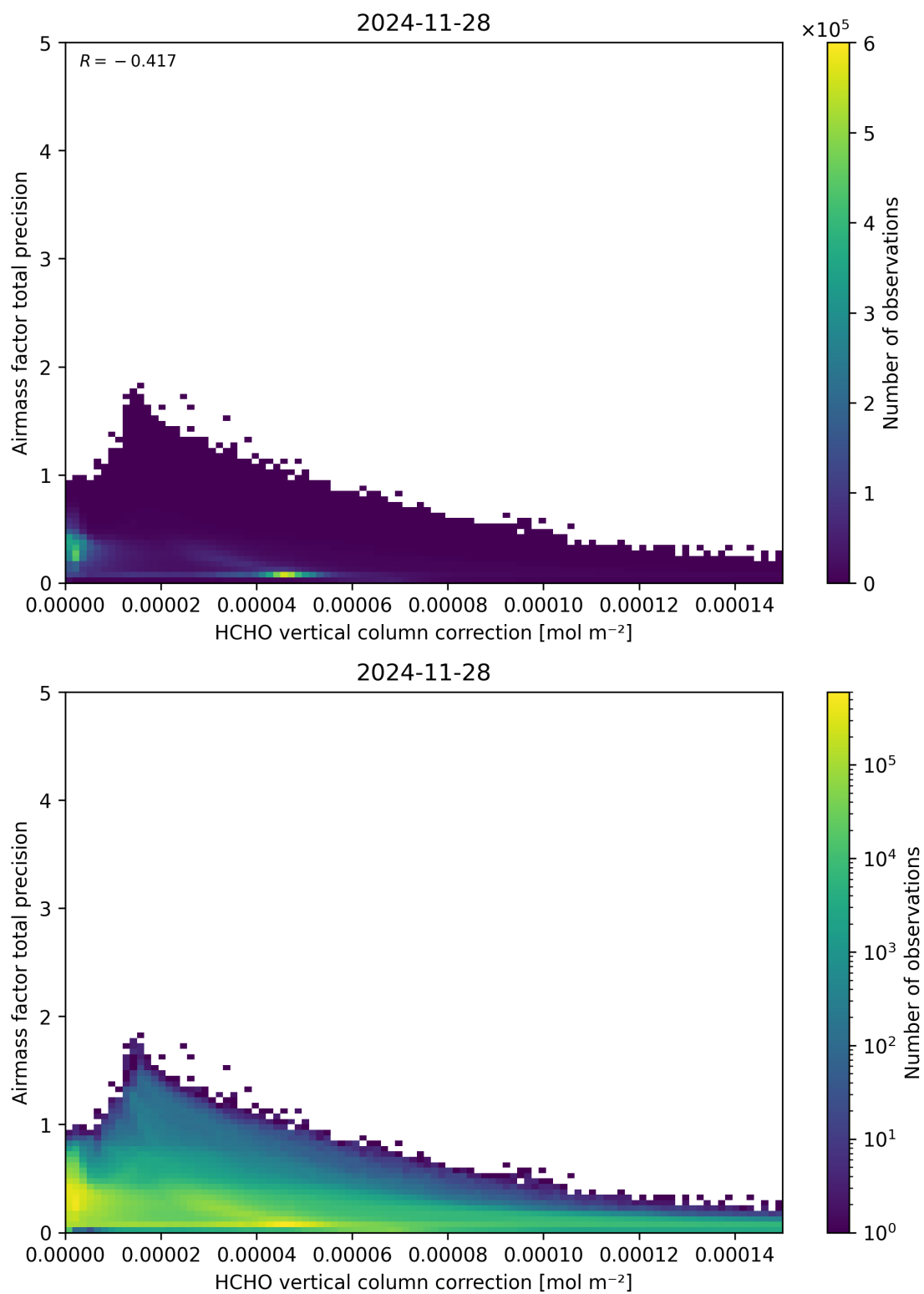
Figure 121: Scatter density plot of “HCHO vertical column correction” against “Airmass factor total precision” for 2024-11-27 to 2024-11-29.
