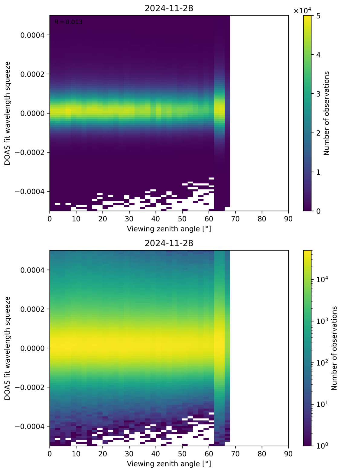
Figure 184: Scatter density plot of “Viewing zenith angle” against “DOAS fit wavelength squeeze” for 2024-11-27 to 2024-11-29.
