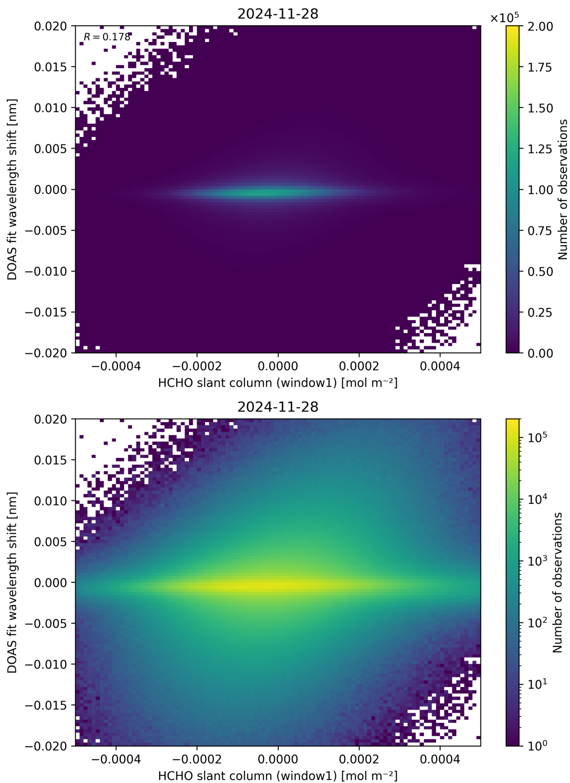
Figure 79: Scatter density plot of “HCHO slant column (window1)” against “DOAS fit wavelength shift” for 2024-11-27 to 2024-11-29.
