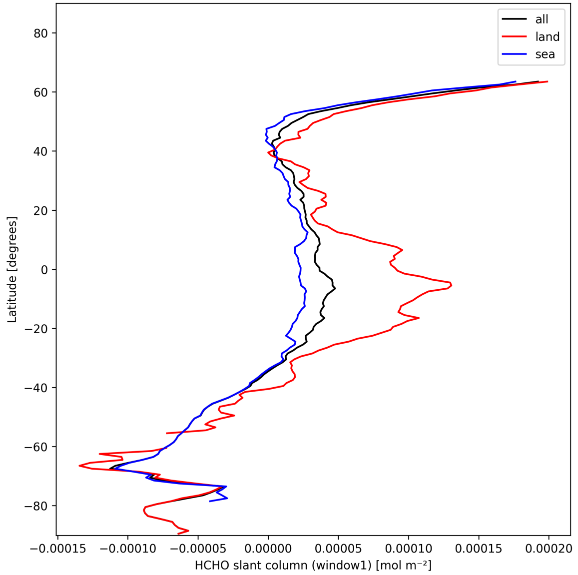
Figure 24: Zonal average of “HCHO slant column (window1)” for 2024-11-27 to 2024-11-29.
