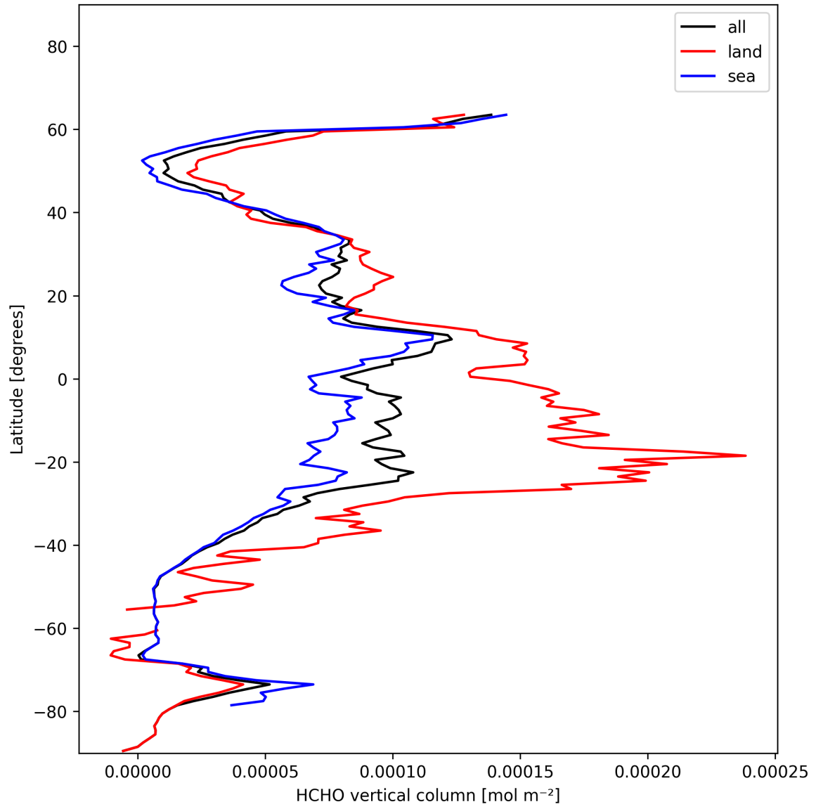
Figure 21: Zonal average of “HCHO vertical column” for 2024-11-27 to 2024-11-29.
