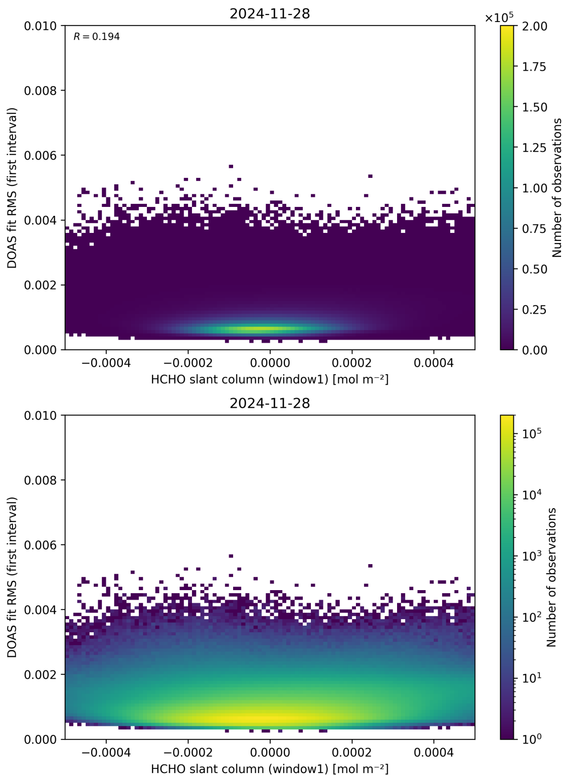
Figure 78: Scatter density plot of “HCHO slant column (window1)” against “DOAS fit RMS (first interval)” for 2024-11-27 to 2024-11-29.
