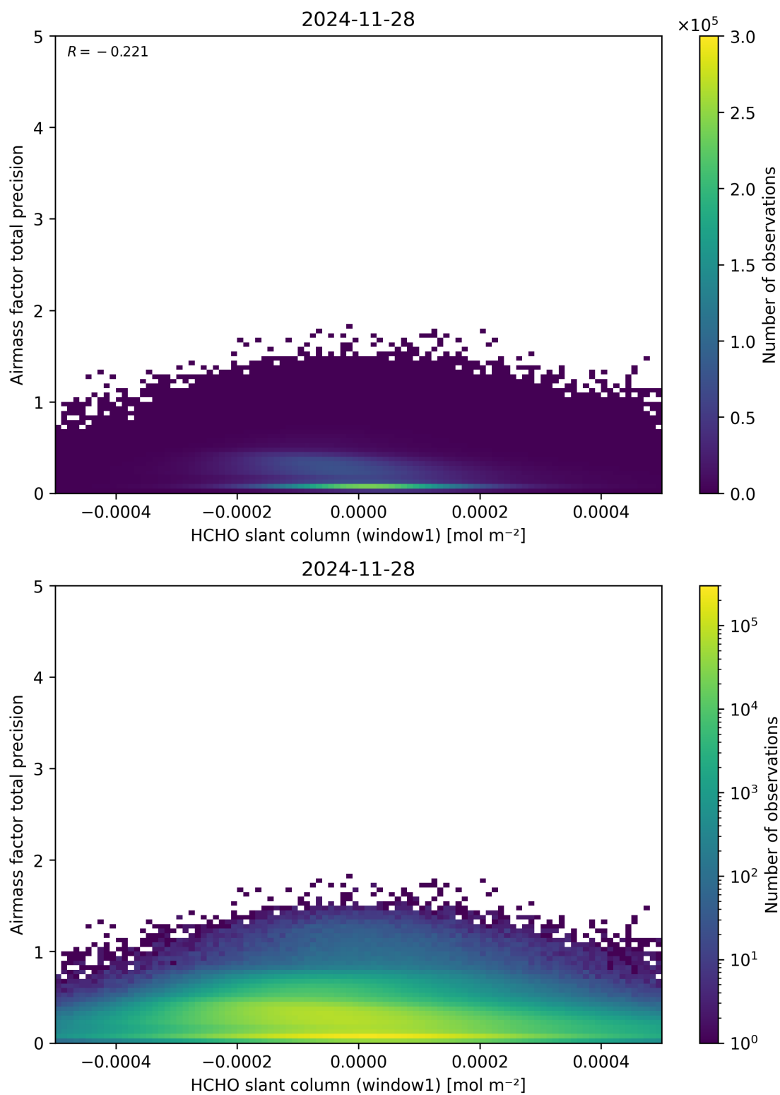
Figure 86: Scatter density plot of “HCHO slant column (window1)” against “Airmass factor total precision” for 2024-11-27 to 2024-11-29.
