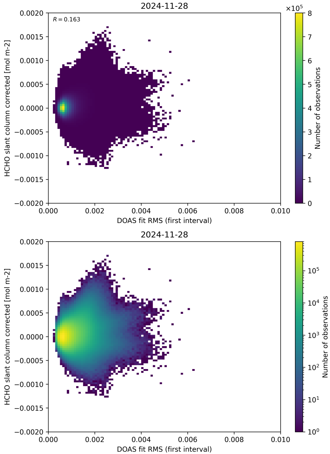
Figure 62: Scatter density plot of “DOAS fit RMS (first interval)” against “HCHO slant column corrected” for 2024-11-27 to 2024-11-29.
