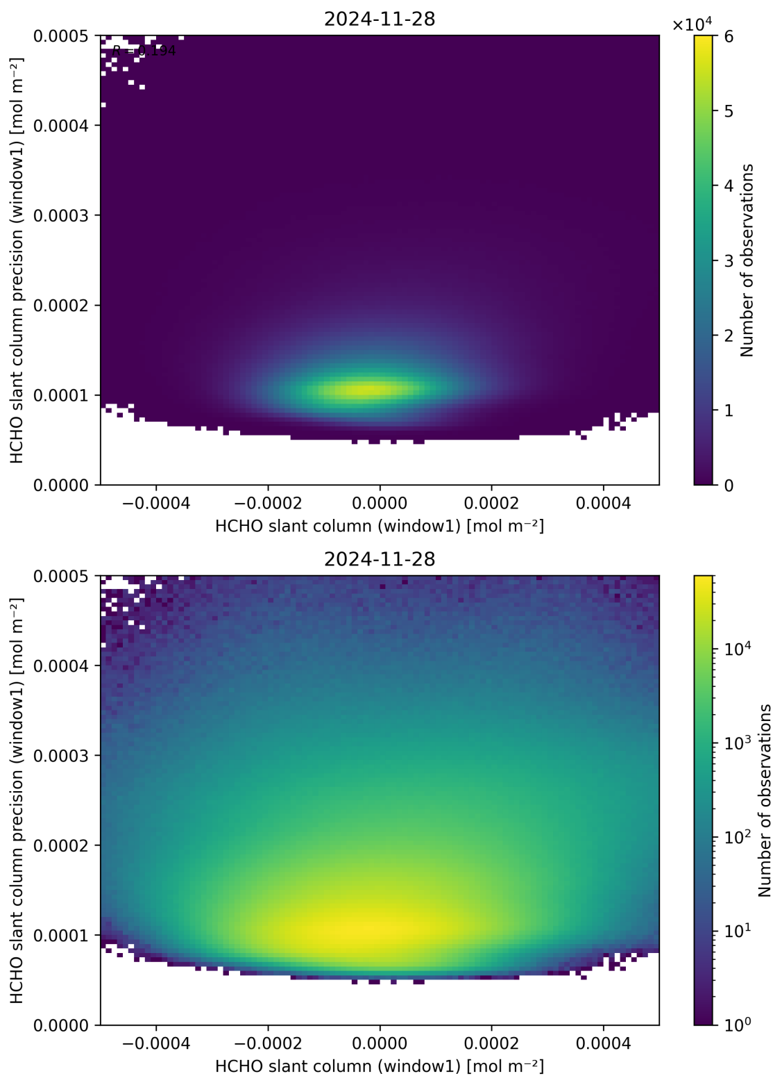
Figure 84: Scatter density plot of “HCHO slant column (window1)” against “HCHO slant column precision (window1)” for 2024-11-27 to 2024-11-29.
