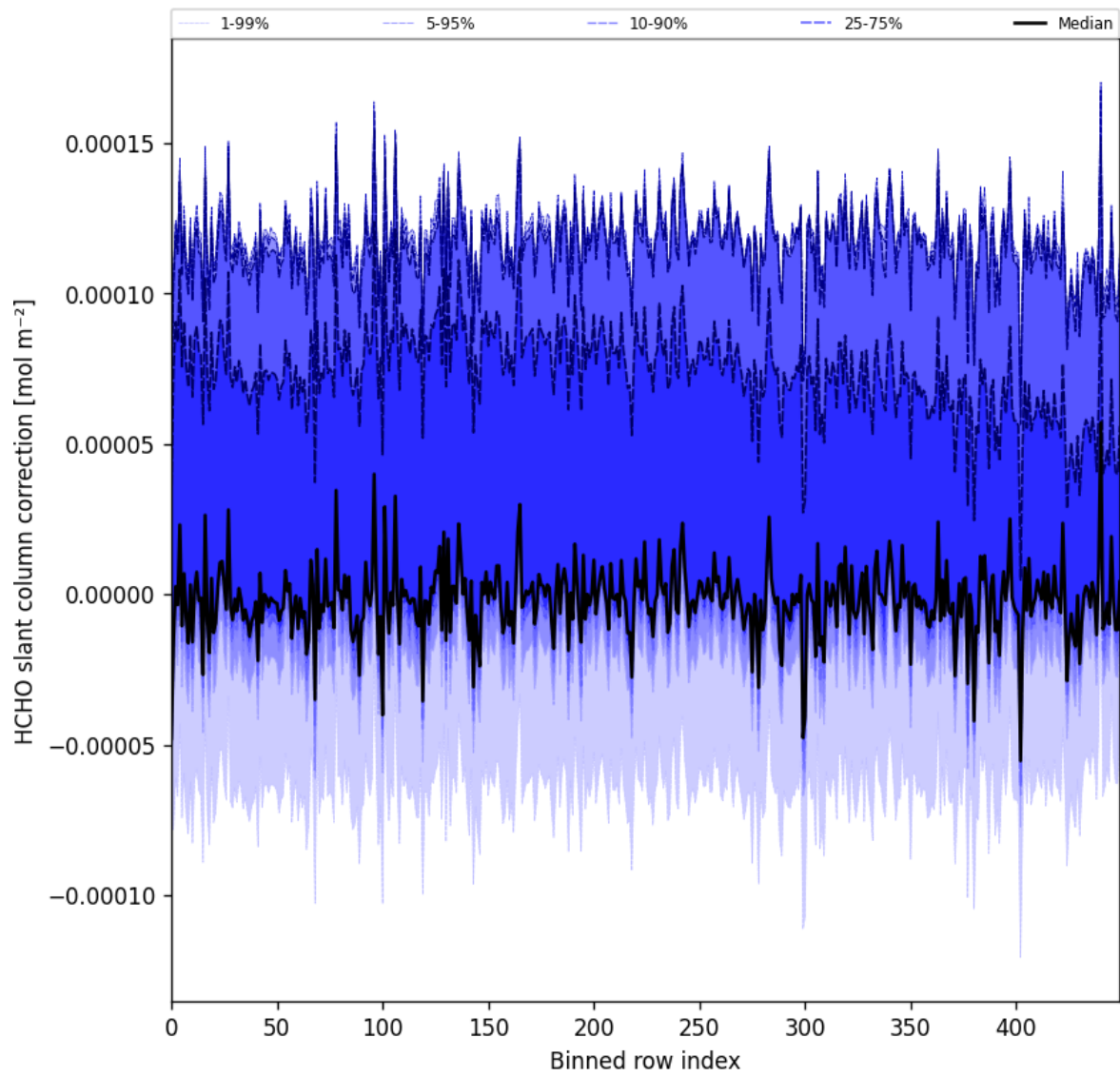
Figure 61: Along track statistics of “HCHO slant column correction” for 2024-11-27 to 2024-11-29
