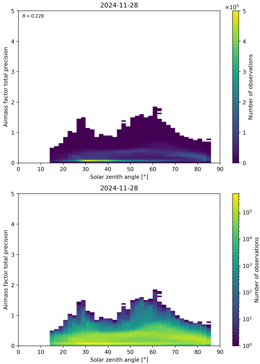
Figure 176: Scatter density plot of “Solar zenith angle” against “Airmass factor total precision” for 2024-11-27 to 2024-11-29.
