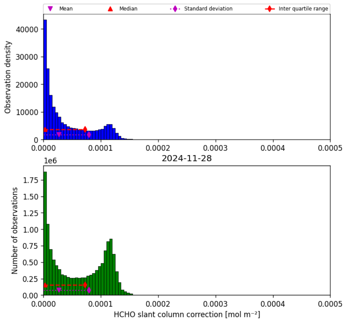
Figure 47: Histogram of “HCHO slant column correction” for 2024-11-27 to 2024-11-29
