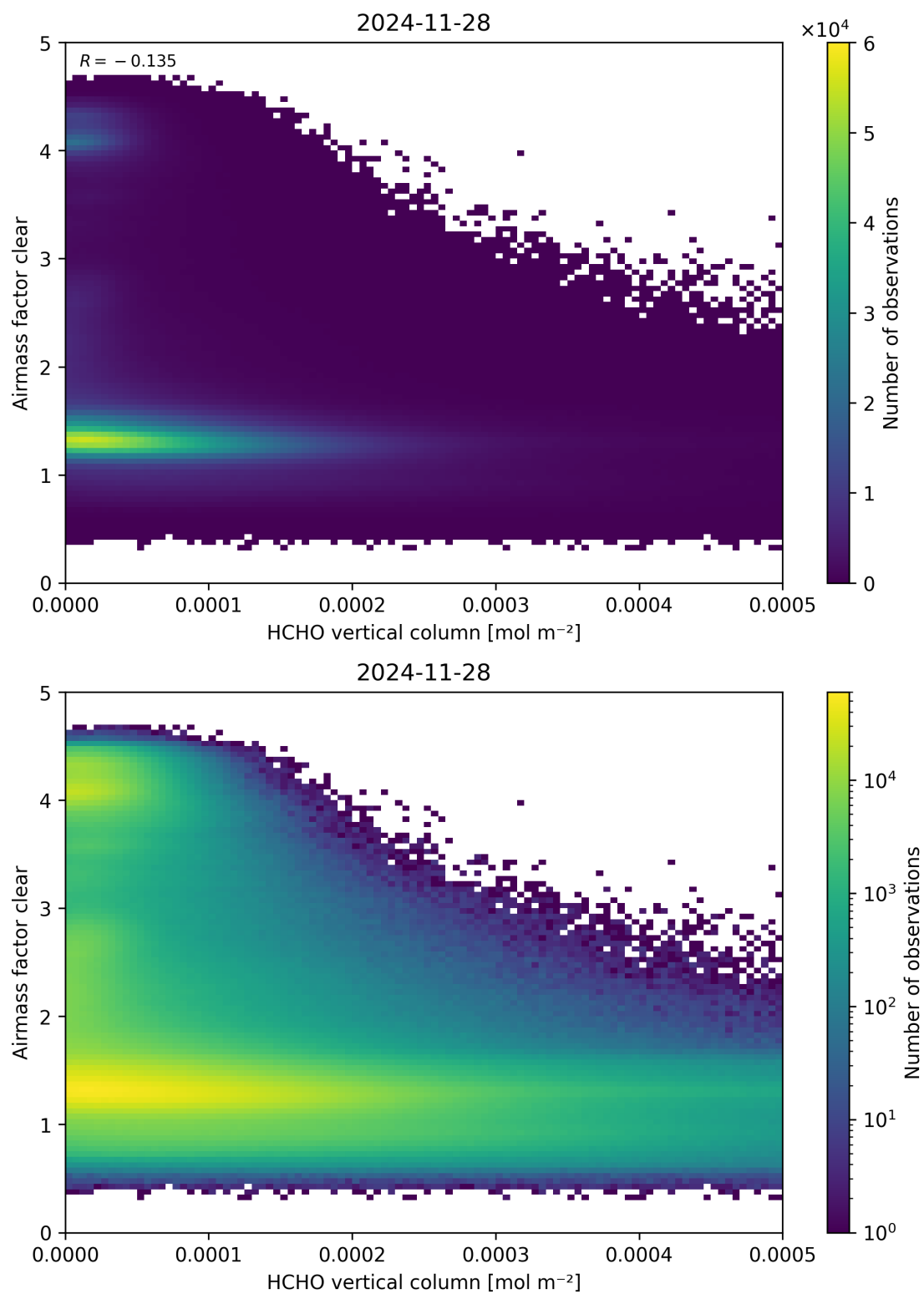
Figure 126: Scatter density plot of “HCHO vertical column” against “Airmass factor clear” for 2024-11-27 to 2024-11-29.
