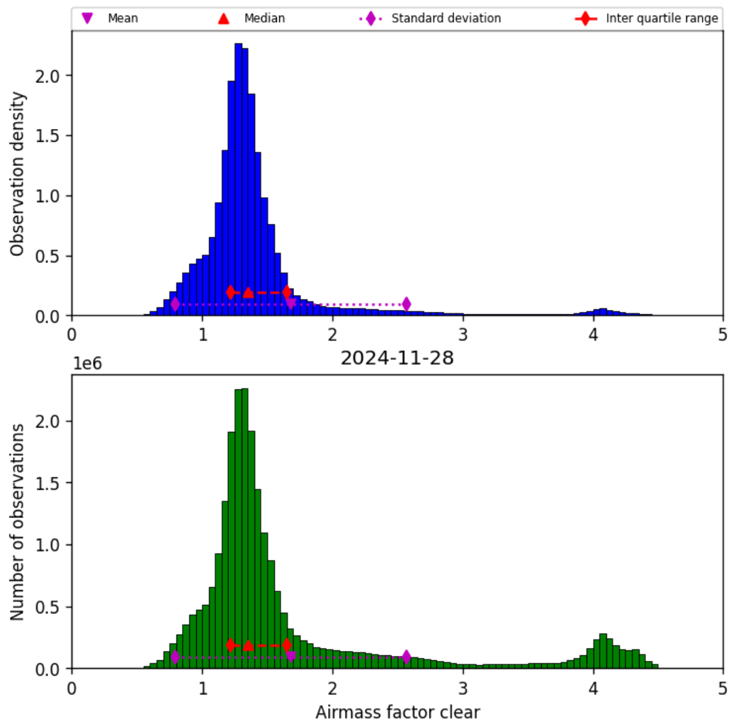
Figure 42: Histogram of “Airmass factor clear” for 2024-11-27 to 2024-11-29
