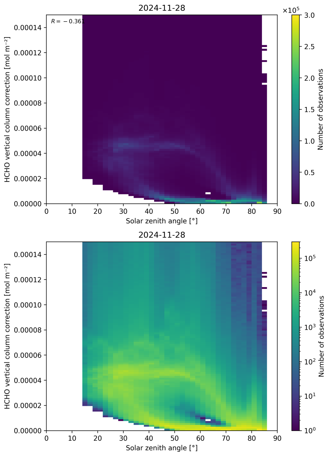
Figure 178: Scatter density plot of “Solar zenith angle” against “HCHO vertical column correction” for 2024-11-27 to 2024-11-29.
