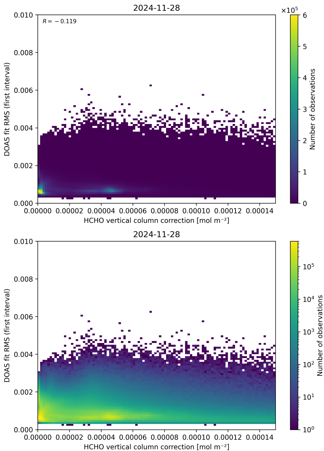
Figure 112: Scatter density plot of “HCHO vertical column correction” against “DOAS fit RMS (first interval)” for 2024-11-27 to 2024-11-29.
