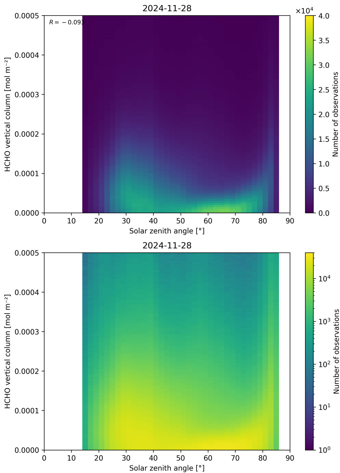
Figure 177: Scatter density plot of “Solar zenith angle” against “HCHO vertical column” for 2024-11-27 to 2024-11-29.
