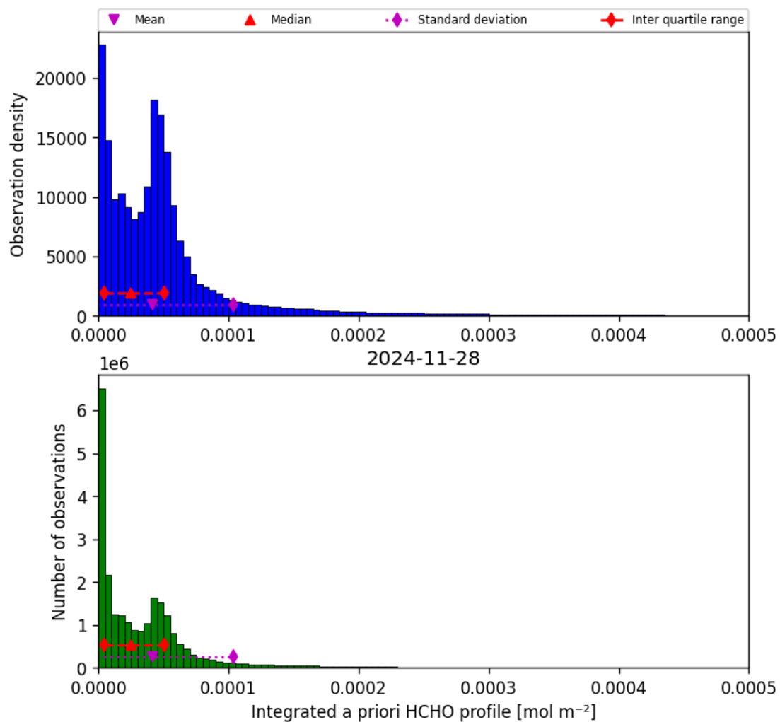
Figure 43: Histogram of “Integrated a priori HCHO profile” for 2024-11-27 to 2024-11-29
