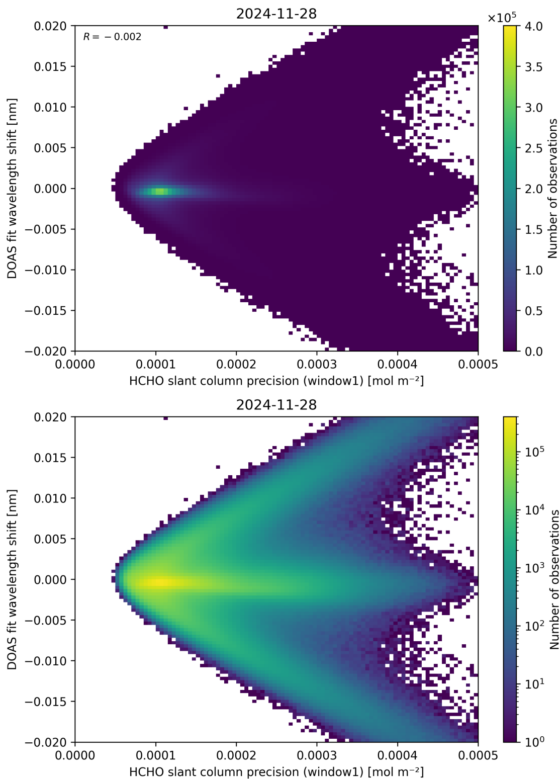
Figure 89: Scatter density plot of “HCHO slant column precision (window1)” against “DOAS fit wavelength shift” for 2024-11-27 to 2024-11-29.
