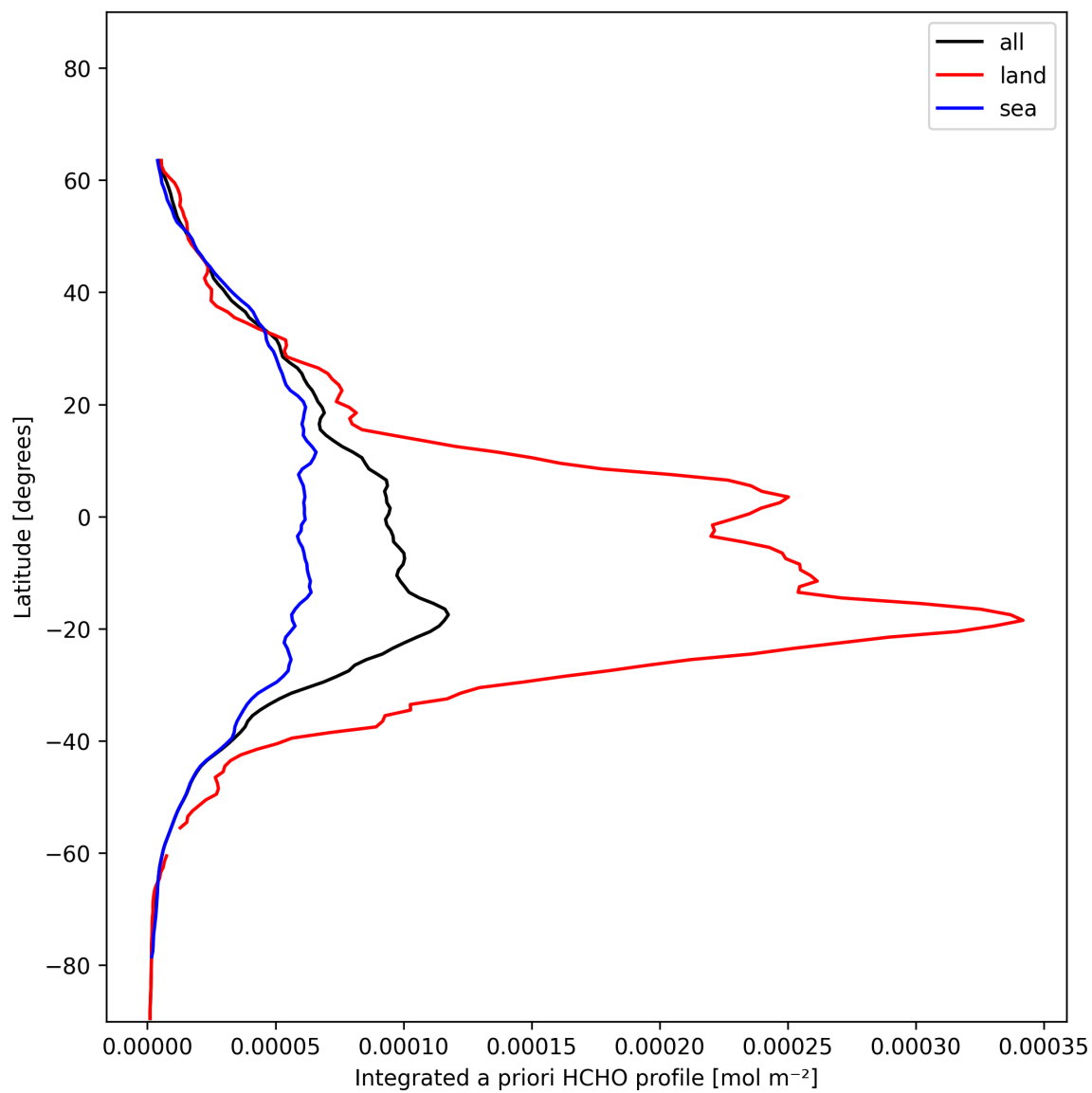
Figure 29: Zonal average of “Integrated a priori HCHO profile” for 2024-11-27 to 2024-11-29.
