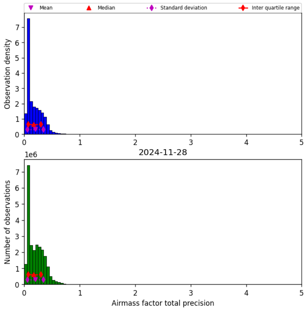
Figure 41: Histogram of “Airmass factor total precision” for 2024-11-27 to 2024-11-29
