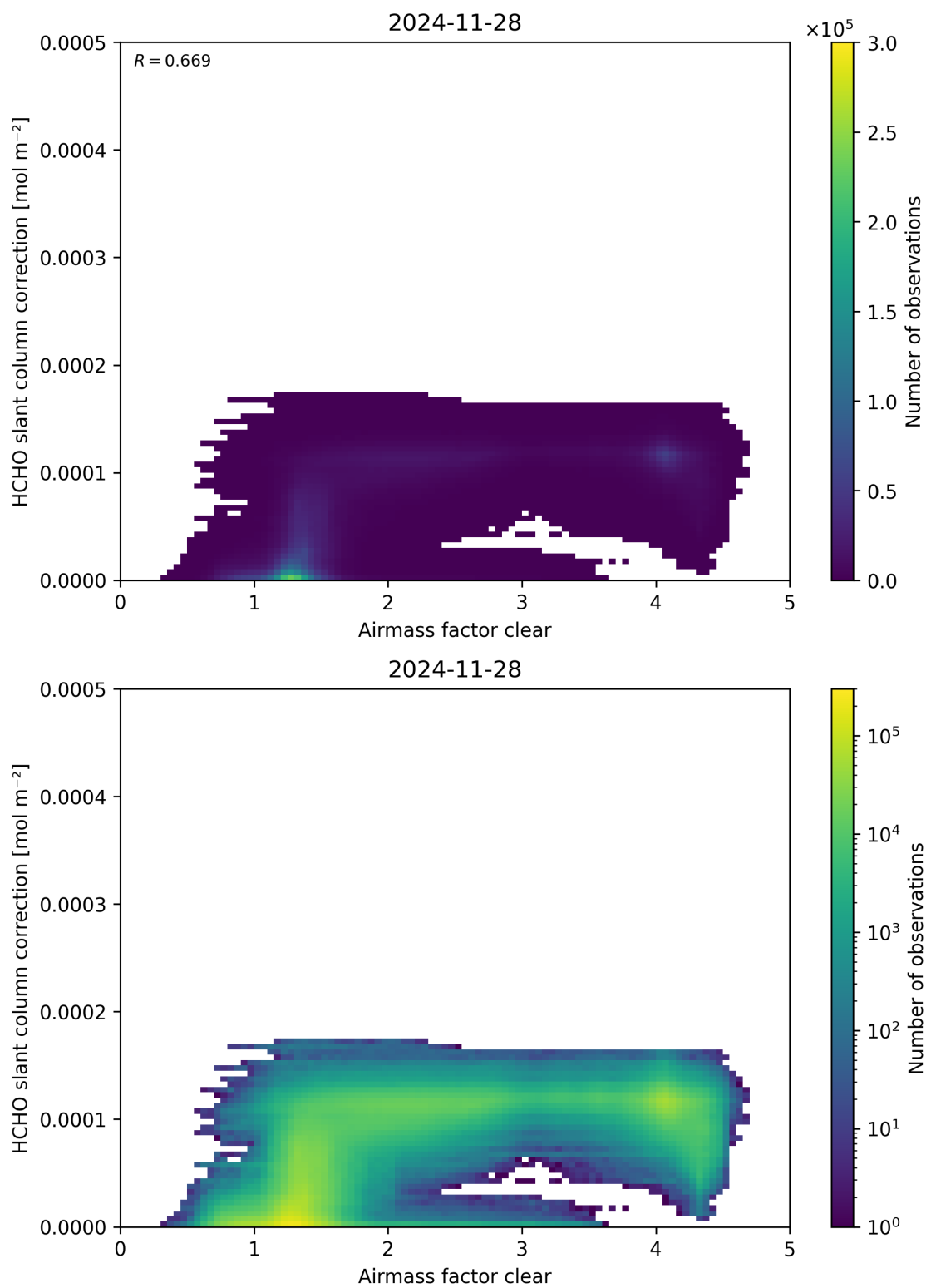
Figure 75: Scatter density plot of “Airmass factor clear” against “HCHO slant column correction” for 2024-11-27 to 2024-11-29.
