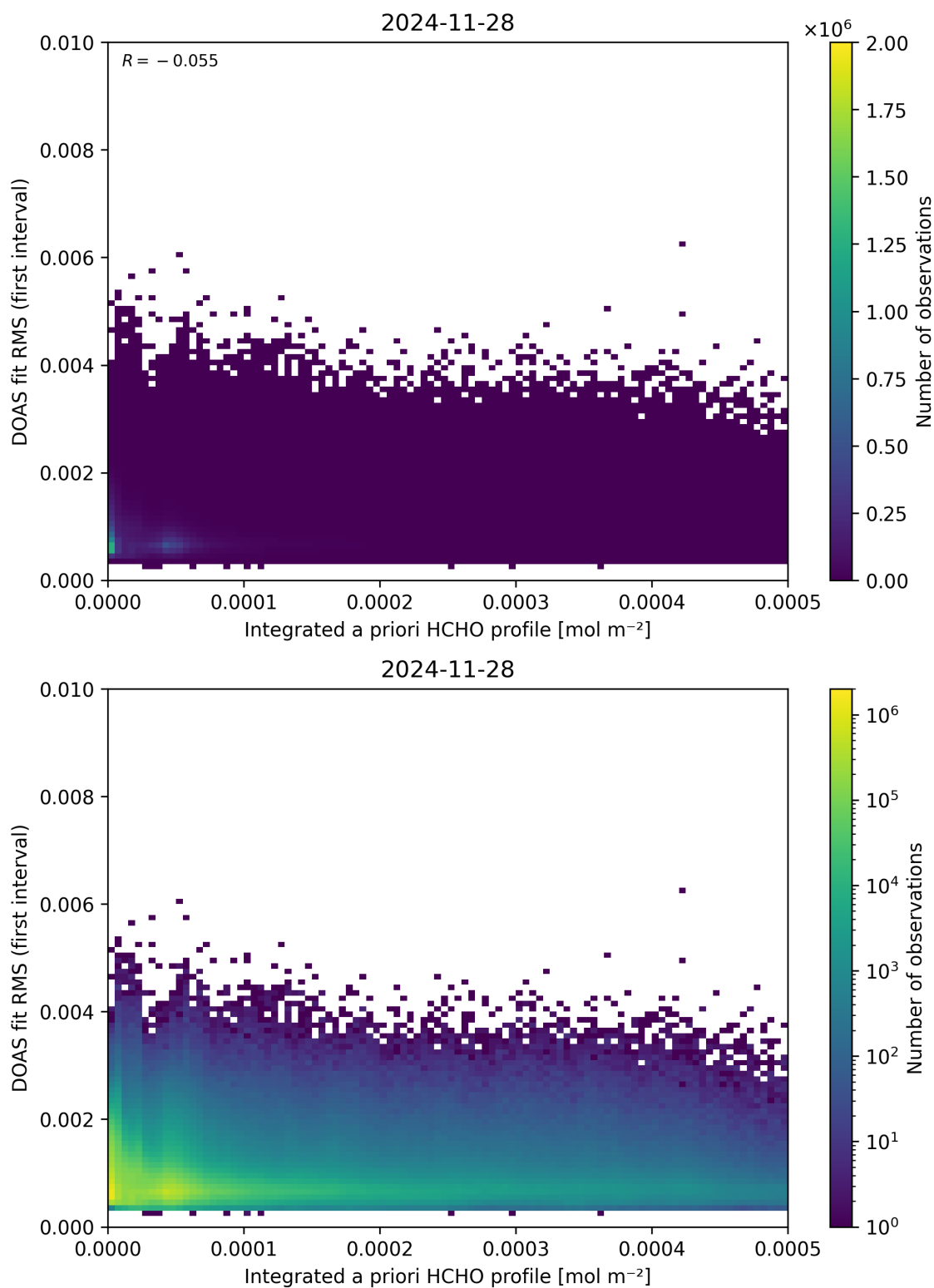
Figure 148: Scatter density plot of “Integrated a priori HCHO profile” against “DOAS fit RMS (first interval)” for 2024-11-27 to 2024-11-29.
