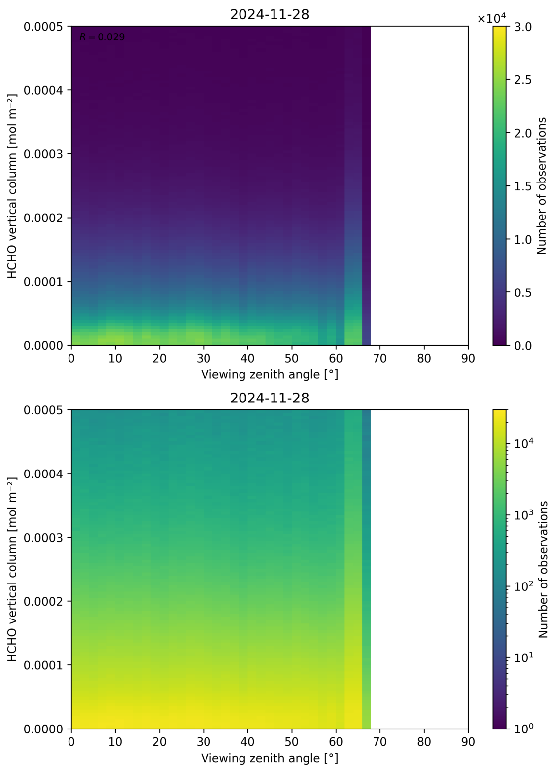
Figure 192: Scatter density plot of “Viewing zenith angle” against “HCHO vertical column” for 2024-11-27 to 2024-11-29.
