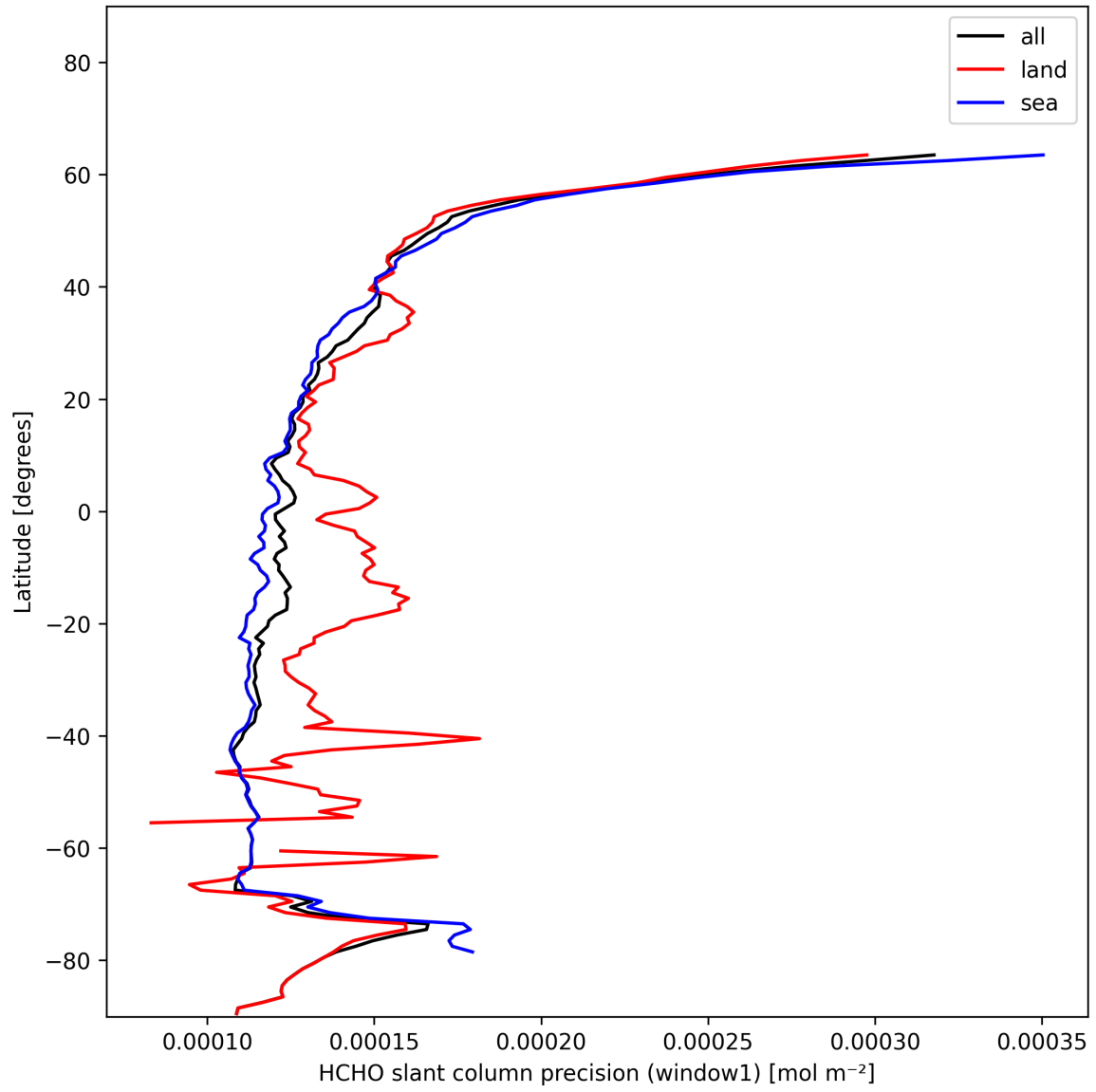
Figure 25: Zonal average of “HCHO slant column precision (window1)” for 2024-11-27 to 2024-11-29.
