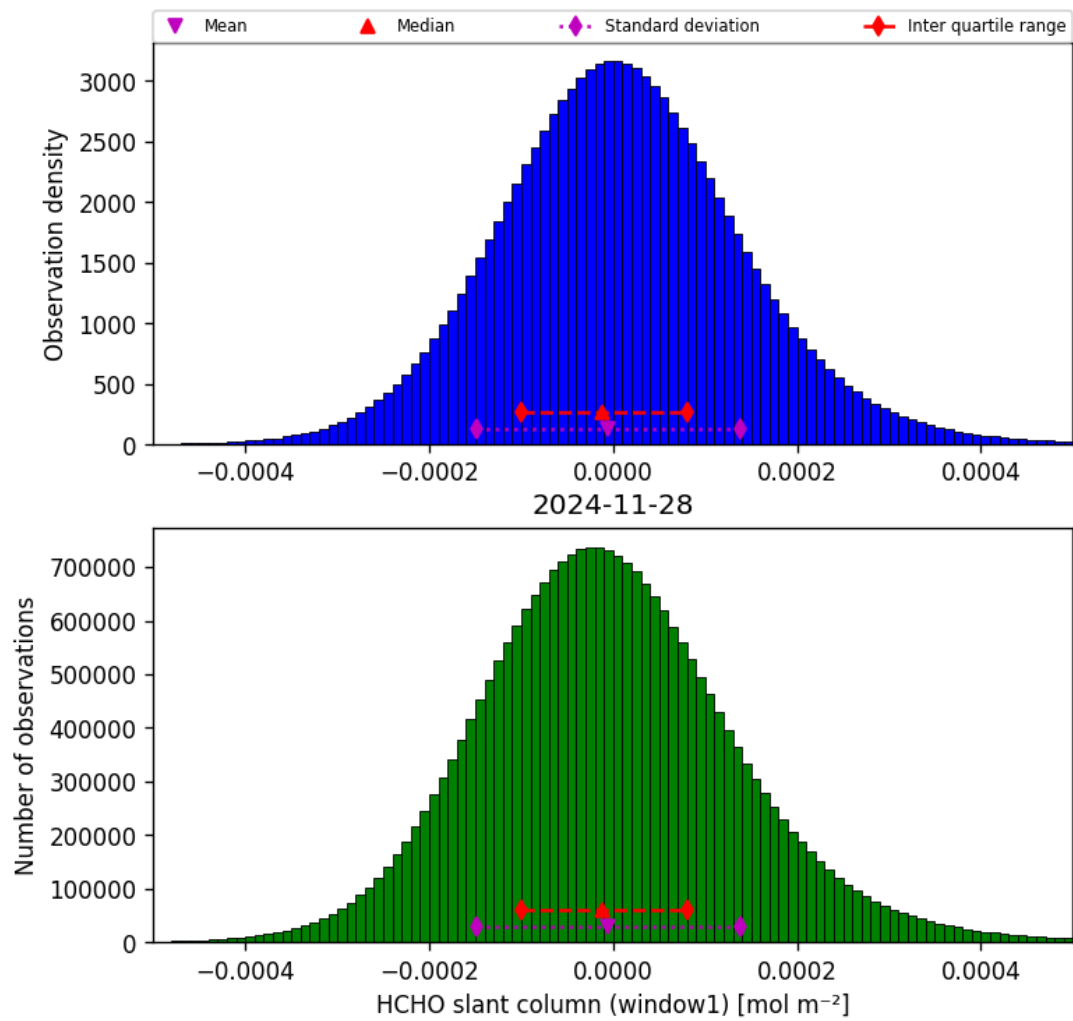
Figure 38: Histogram of “HCHO slant column (window1)” for 2024-11-27 to 2024-11-29
