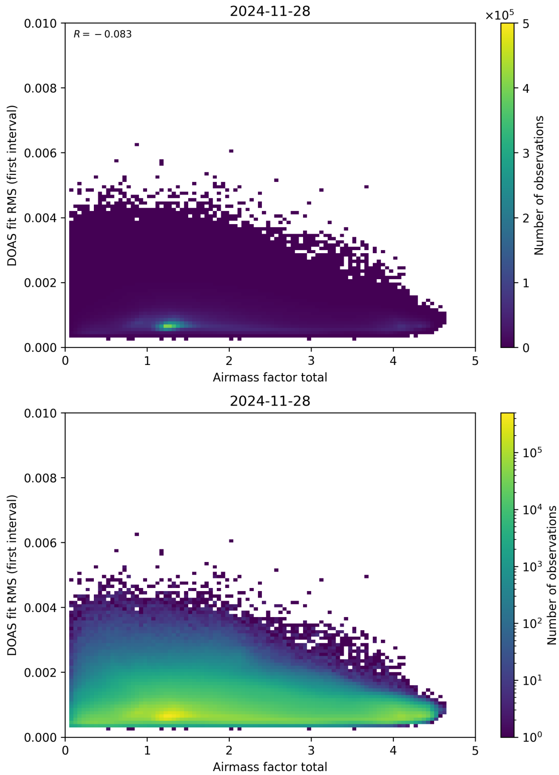
Figure 97: Scatter density plot of “Airmass factor total” against “DOAS fit RMS (first interval)” for 2024-11-27 to 2024-11-29.
