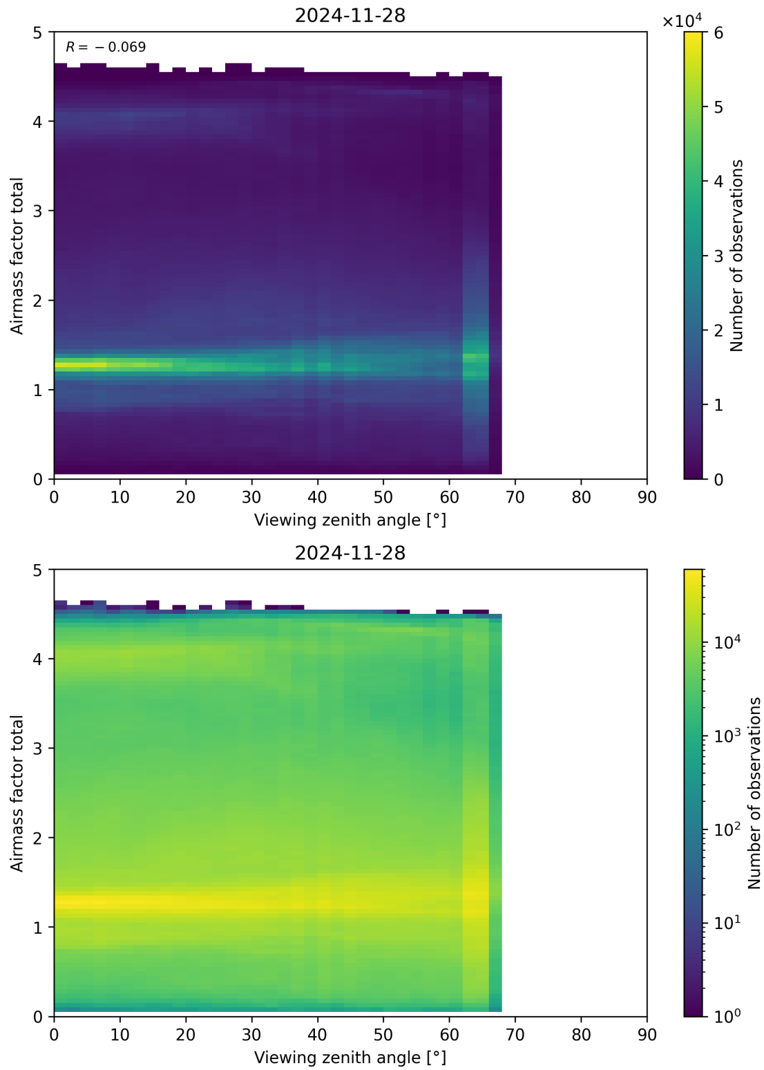
Figure 190: Scatter density plot of “Viewing zenith angle” against “Airmass factor total” for 2024-11-27 to 2024-11-29.
