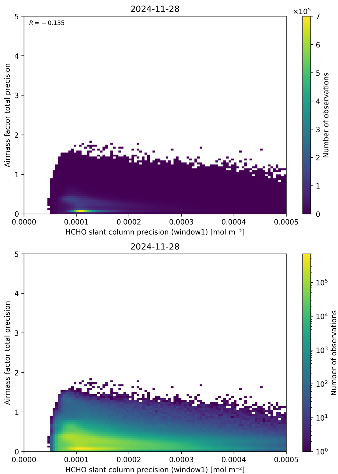
Figure 95: Scatter density plot of “HCHO slant column precision (window1)” against “Airmass factor total precision” for 2024-11-27 to 2024-11-29.
