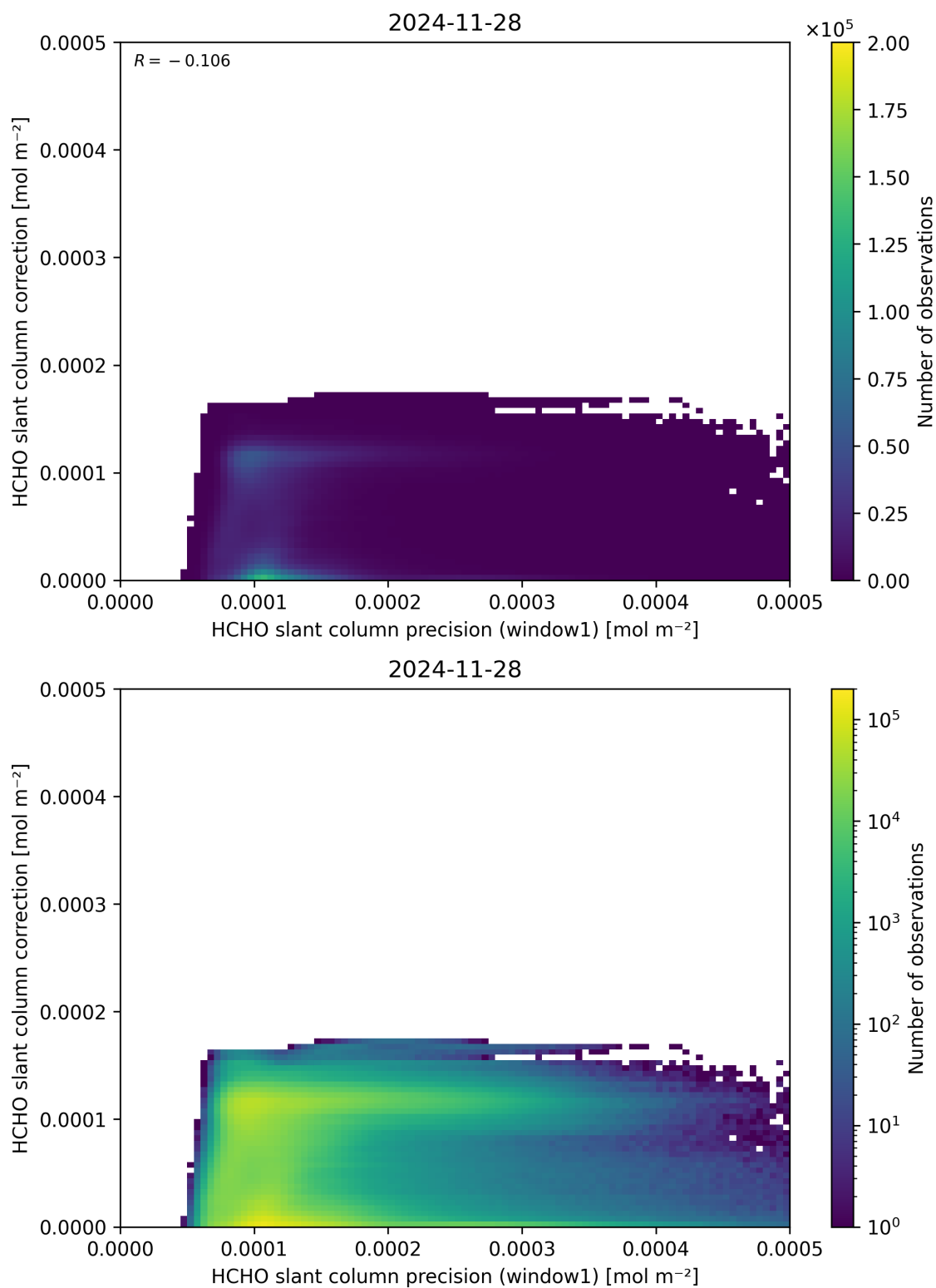
Figure 93: Scatter density plot of “HCHO slant column precision (window1)” against “HCHO slant column correction” for 2024-11-27 to 2024-11-29.
