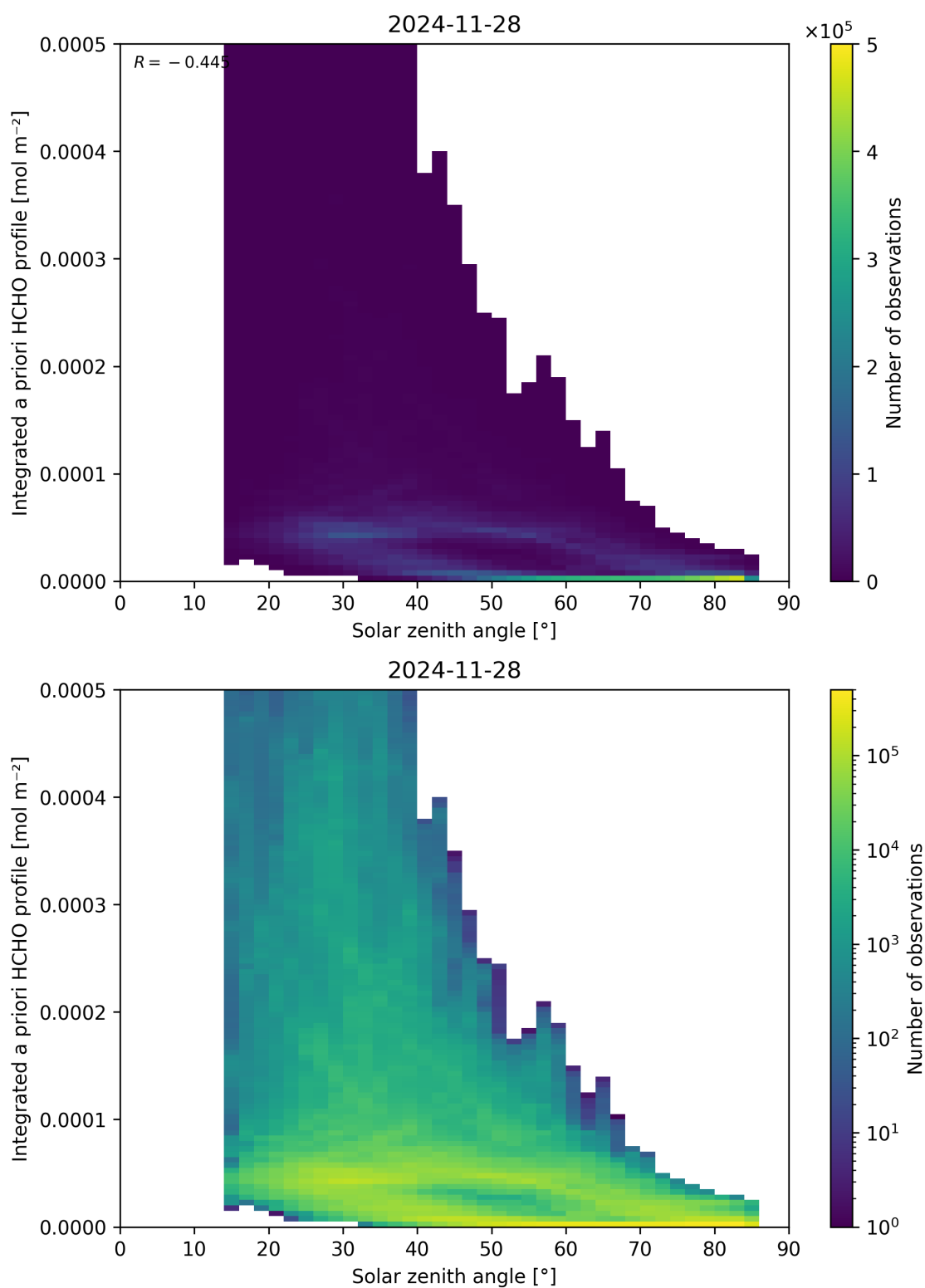
Figure 180: Scatter density plot of “Solar zenith angle” against “Integrated a priori HCHO profile” for 2024-11-27 to 2024-11-29.
