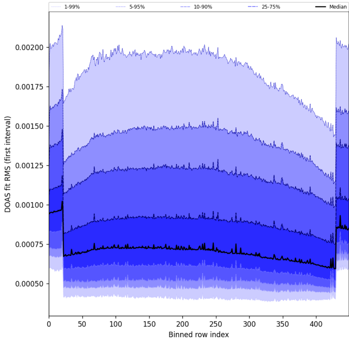
Figure 60: Along track statistics of “DOAS fit RMS (first interval)” for 2024-11-27 to 2024-11-29
