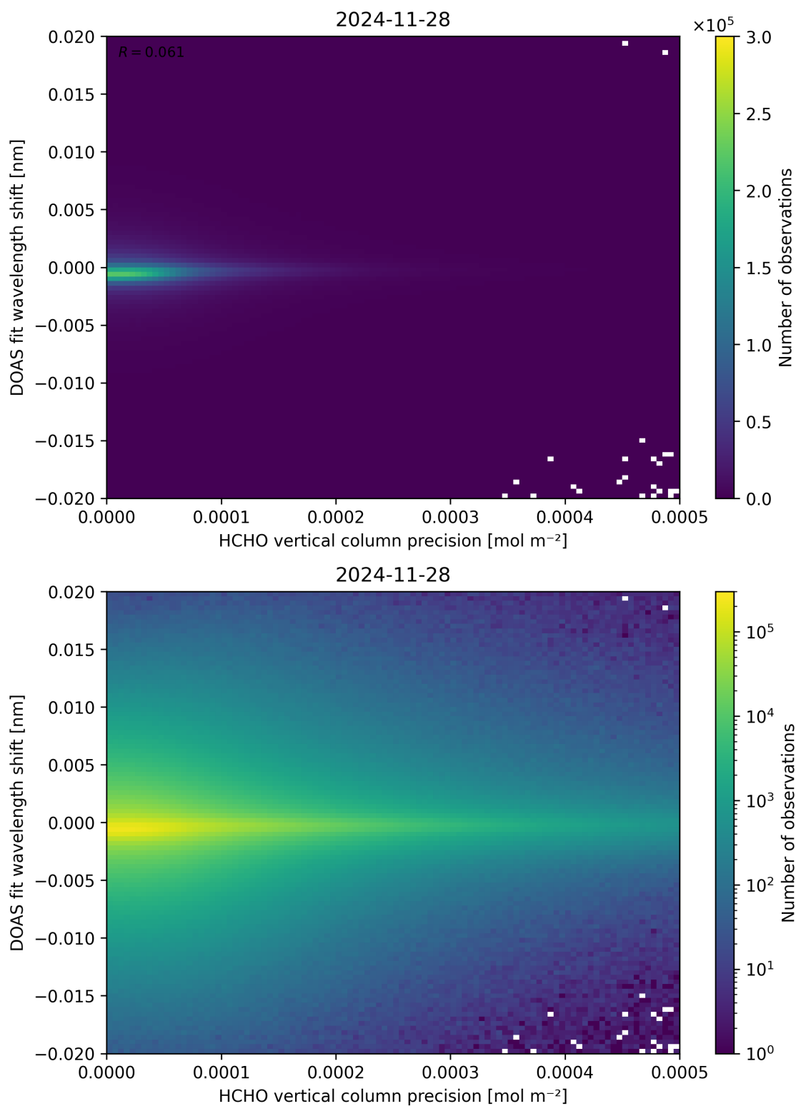
Figure 137: Scatter density plot of “HCHO vertical column precision” against “DOAS fit wavelength shift” for 2024-11-27 to 2024-11-29.
