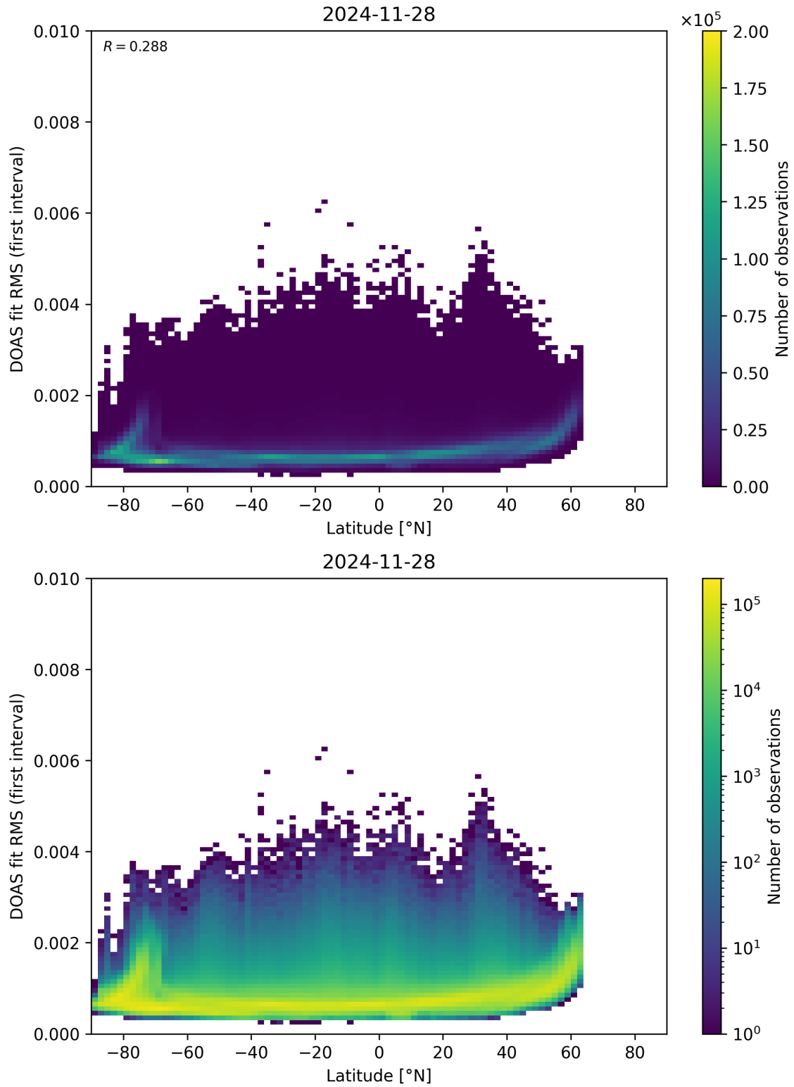
Figure 153: Scatter density plot of “Latitude” against “DOAS fit RMS (first interval)” for 2024-11-27 to 2024-11-29.
