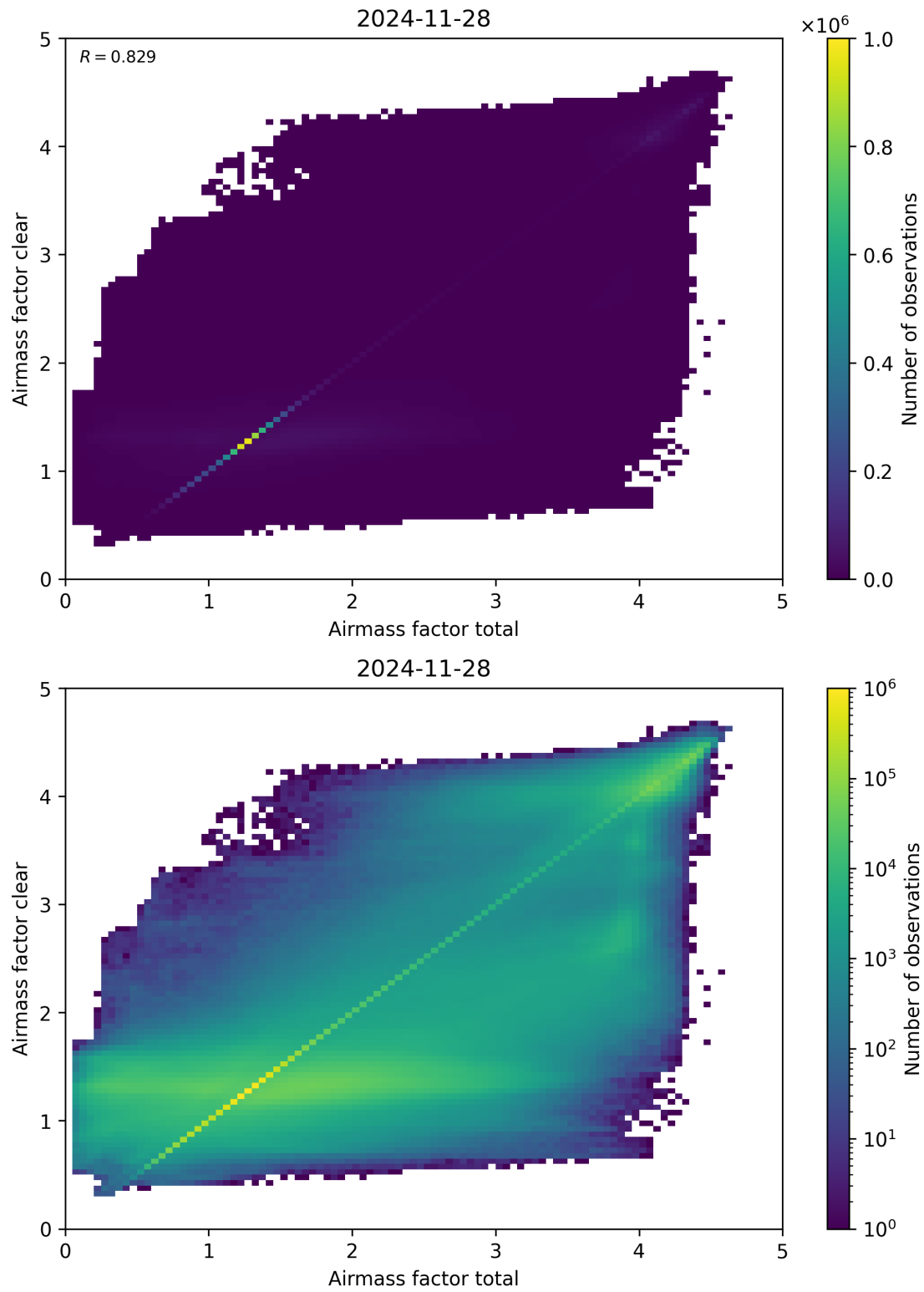
Figure 100: Scatter density plot of “Airmass factor total” against “Airmass factor clear” for 2024-11-27 to 2024-11-29.
