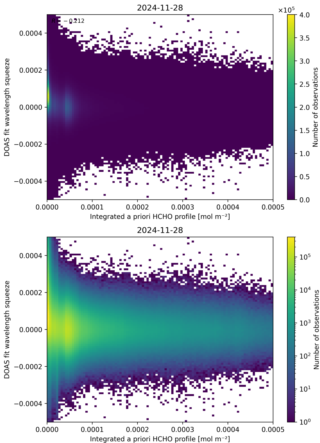
Figure 150: Scatter density plot of “Integrated a priori HCHO profile” against “DOAS fit wavelength squeeze” for 2024-11-27 to 2024-11-29.
