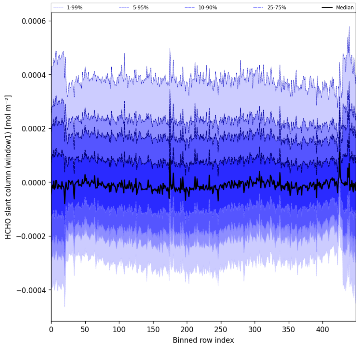
Figure 52: Along track statistics of “HCHO slant column (window1)” for 2024-11-27 to 2024-11-29
