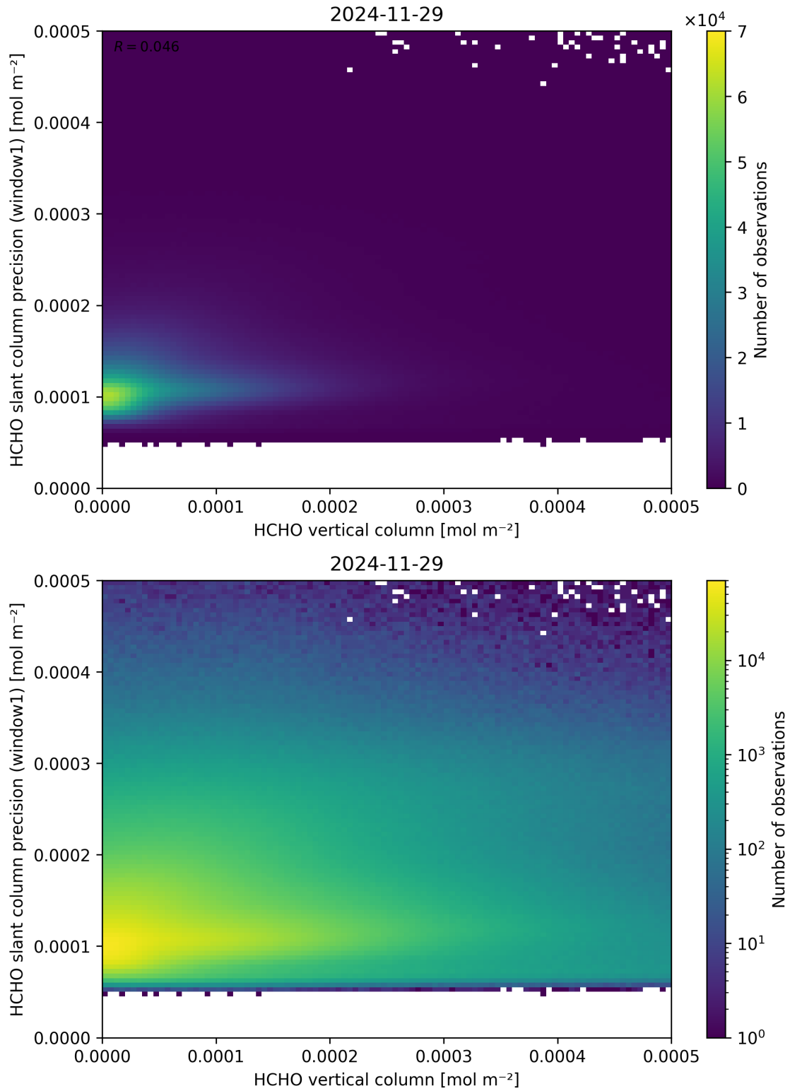
Figure 130: Scatter density plot of “HCHO vertical column” against “HCHO slant column precision (window1)” for 2024-11-28 to 2024-11-30.
