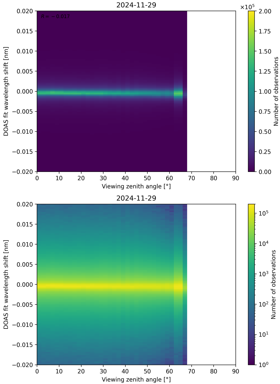
Figure 183: Scatter density plot of “Viewing zenith angle” against “DOAS fit wavelength shift” for 2024-11-28 to 2024-11-30.
