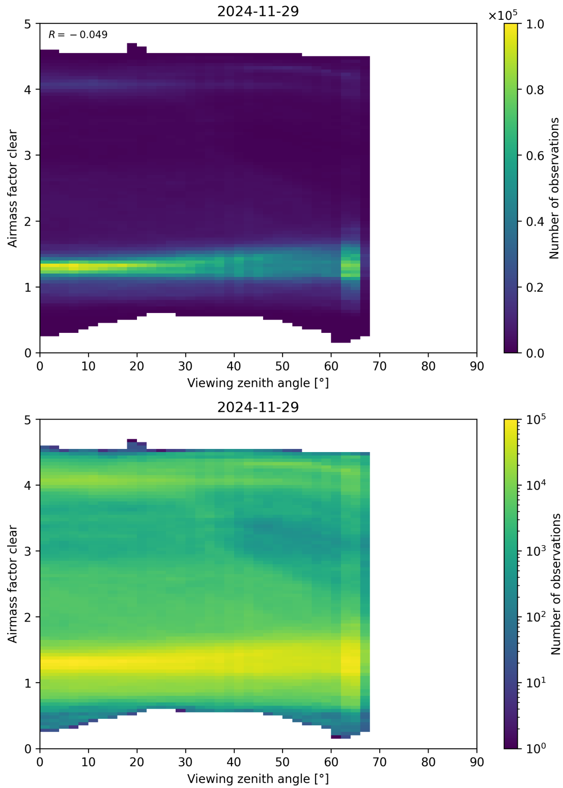
Figure 185: Scatter density plot of “Viewing zenith angle” against “Airmass factor clear” for 2024-11-28 to 2024-11-30.
