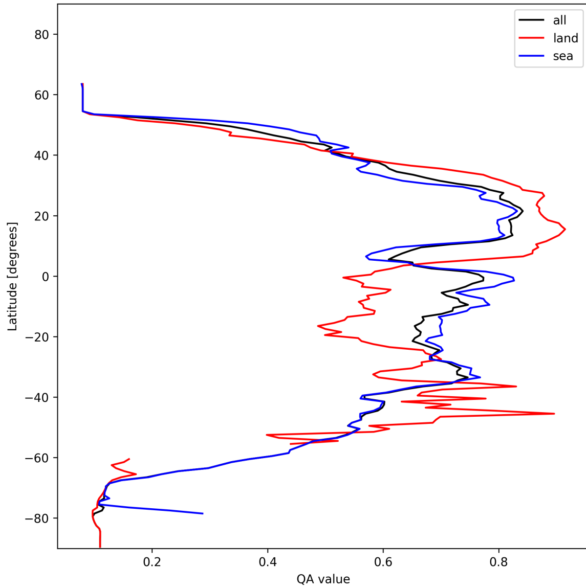
Figure 20: Zonal average of “QA value” for 2024-11-28 to 2024-11-30.
