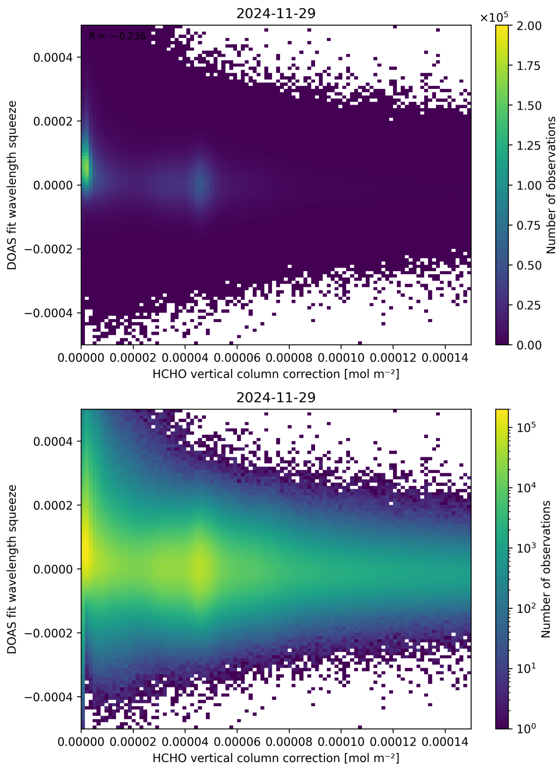
Figure 114: Scatter density plot of “HCHO vertical column correction” against “DOAS fit wavelength squeeze” for 2024-11-28 to 2024-11-30.
