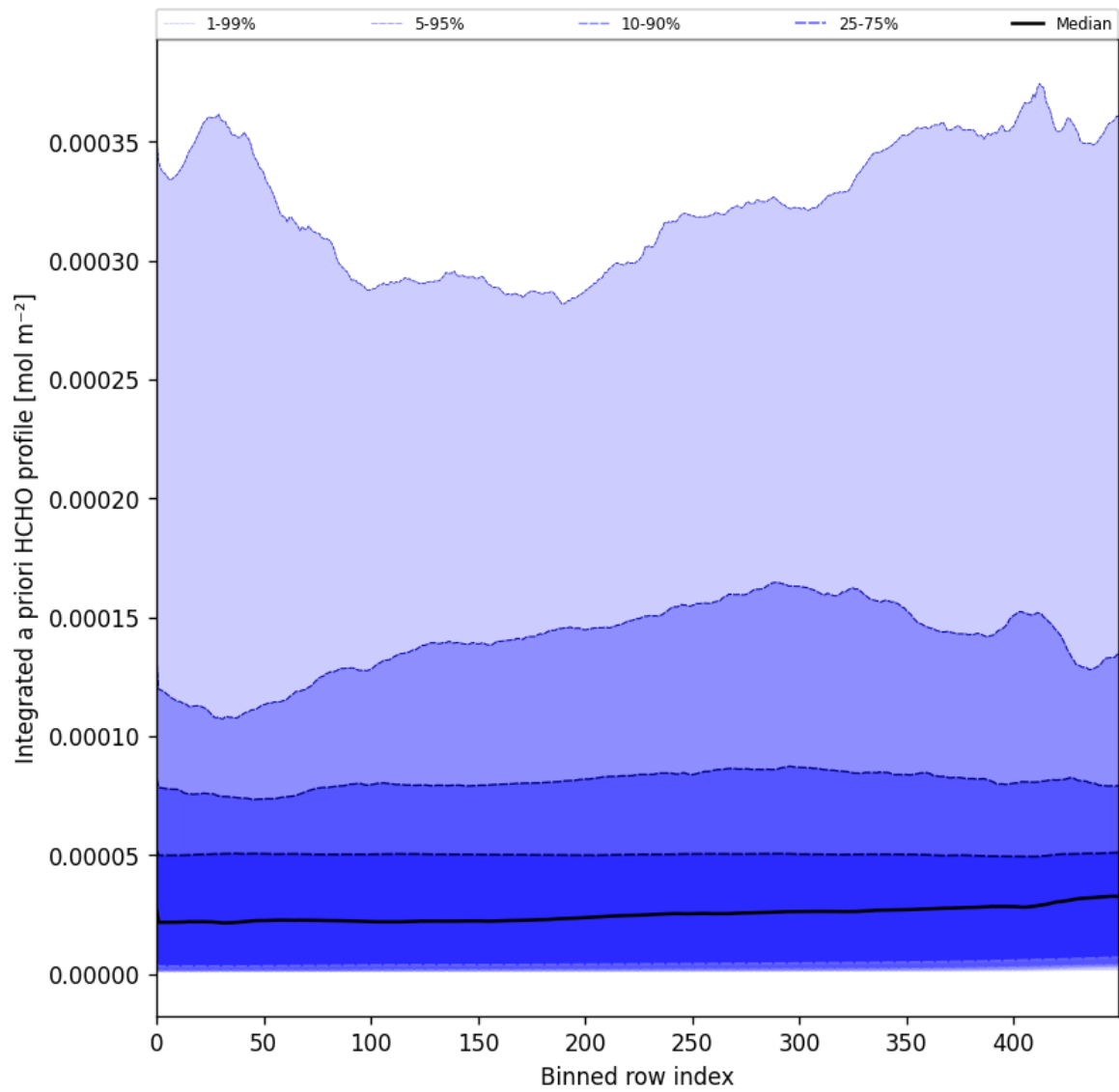
Figure 57: Along track statistics of “Integrated a priori HCHO profile” for 2024-11-28 to 2024-11-30
