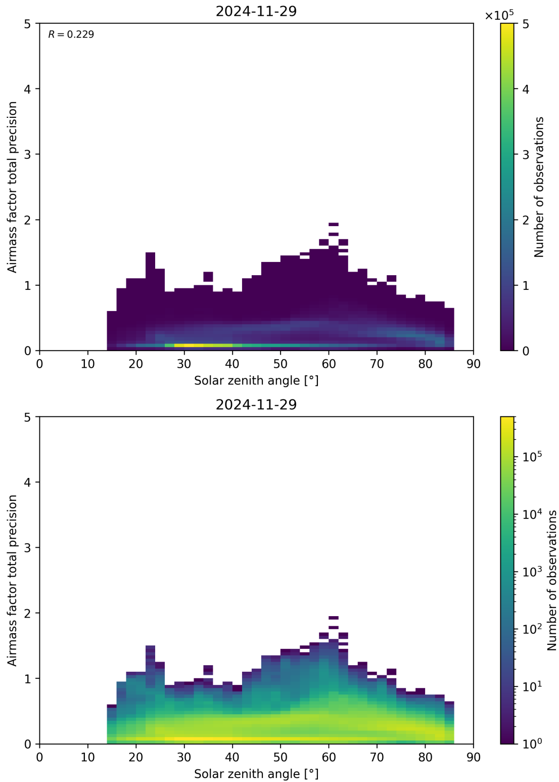
Figure 176: Scatter density plot of “Solar zenith angle” against “Airmass factor total precision” for 2024-11-28 to 2024-11-30.
