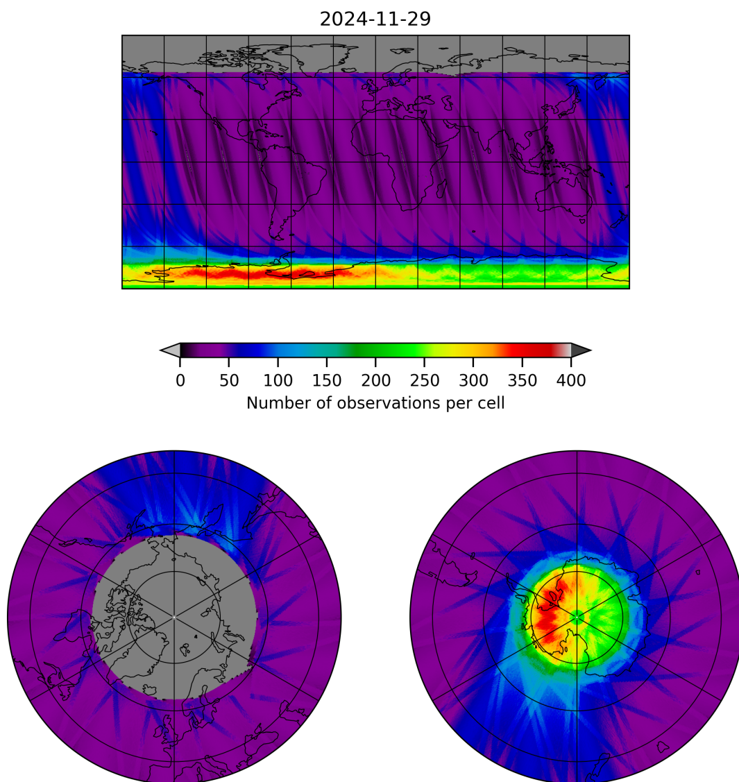
Figure 19: Map of the number of observations for 2024-11-28 to 2024-11-30
