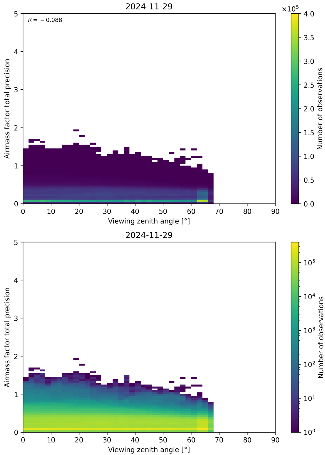
Figure 191: Scatter density plot of “Viewing zenith angle” against “Airmass factor total precision” for 2024-11-28 to 2024-11-30.
