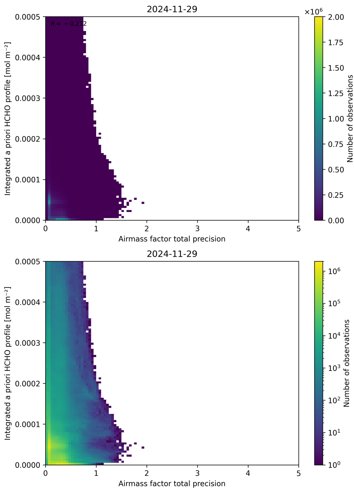
Figure 111: Scatter density plot of “Airmass factor total precision” against “Integrated a priori HCHO profile” for 2024-11-28 to 2024-11-30.
