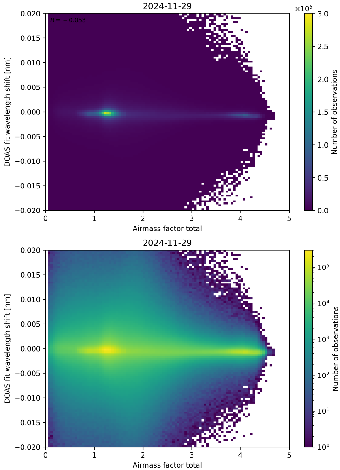
Figure 98: Scatter density plot of “Airmass factor total” against “DOAS fit wavelength shift” for 2024-11-28 to 2024-11-30.
