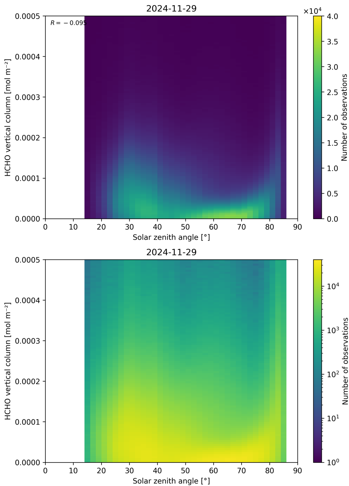
Figure 177: Scatter density plot of “Solar zenith angle” against “HCHO vertical column” for 2024-11-28 to 2024-11-30.
