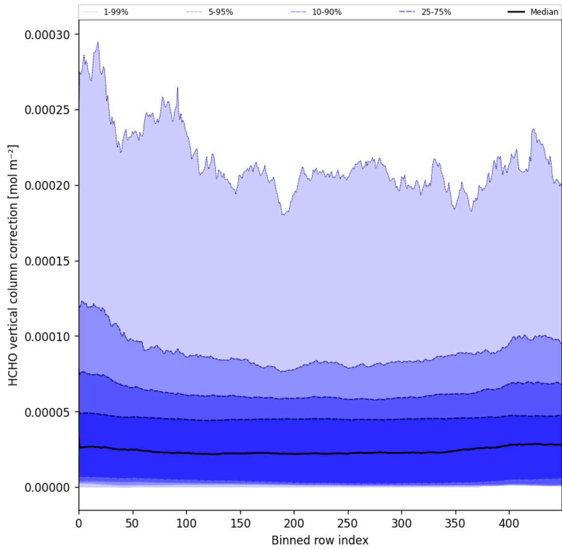
Figure 51: Along track statistics of “HCHO vertical column correction” for 2024-11-28 to 2024-11-30
