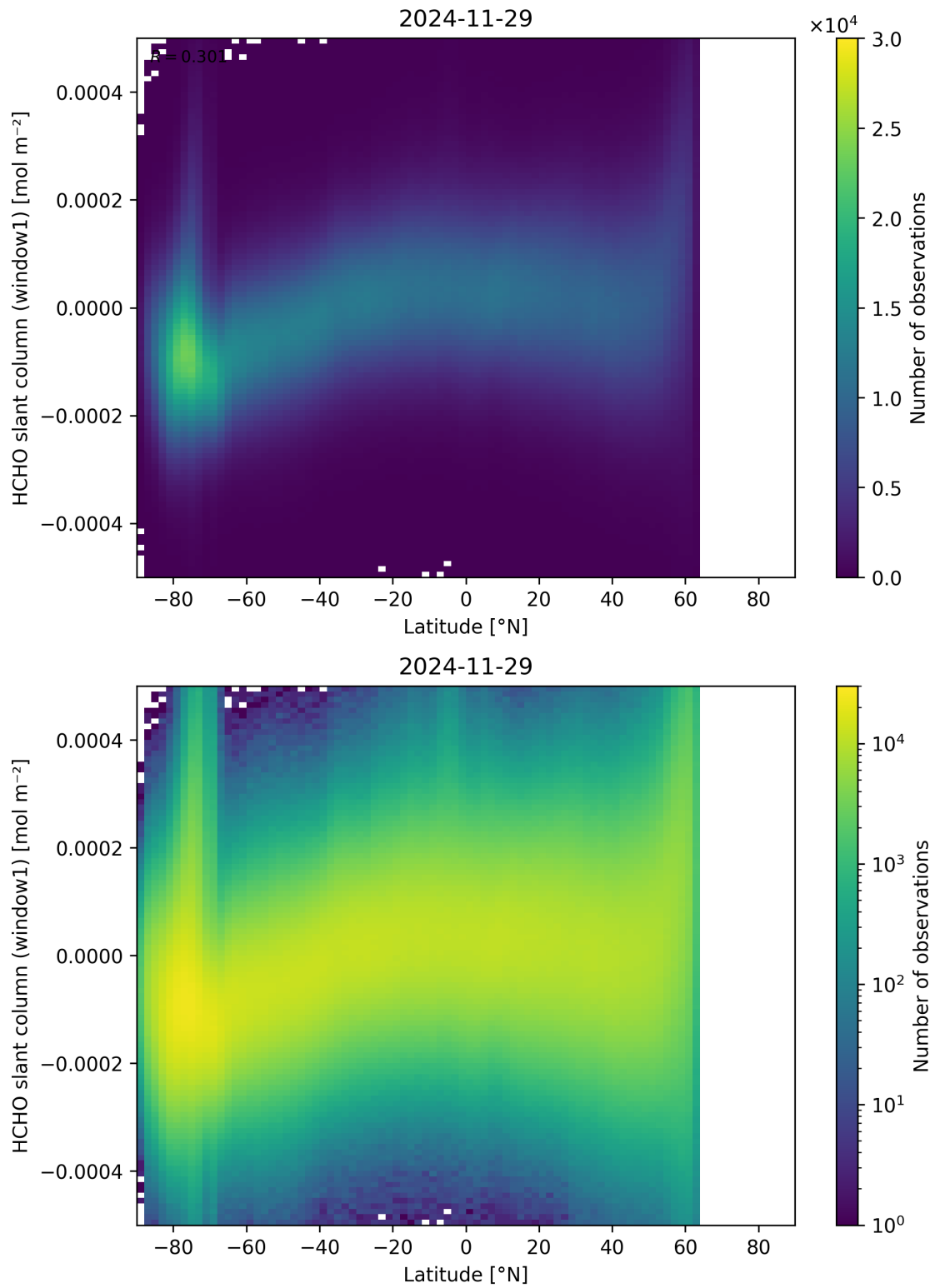
Figure 159: Scatter density plot of “Latitude” against “HCHO slant column (window1)” for 2024-11-28 to 2024-11-30.
