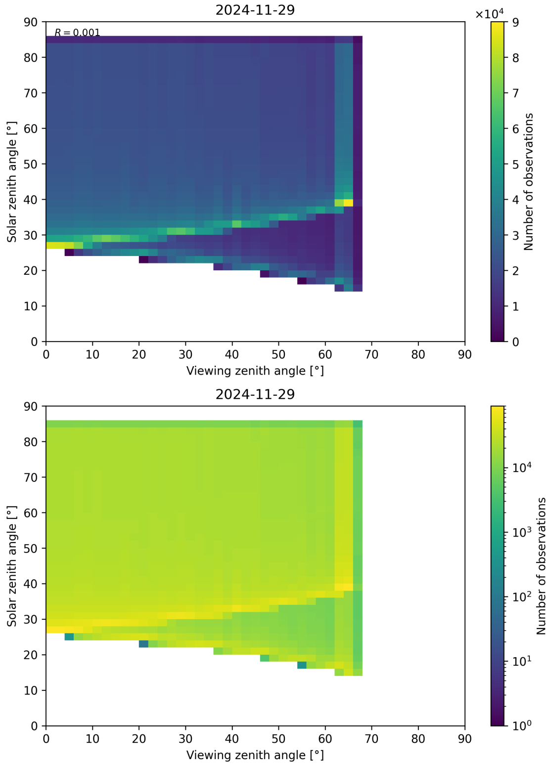
Figure 197: Scatter density plot of “Viewing zenith angle” against “Solar zenith angle” for 2024-11-28 to 2024-11-30.
