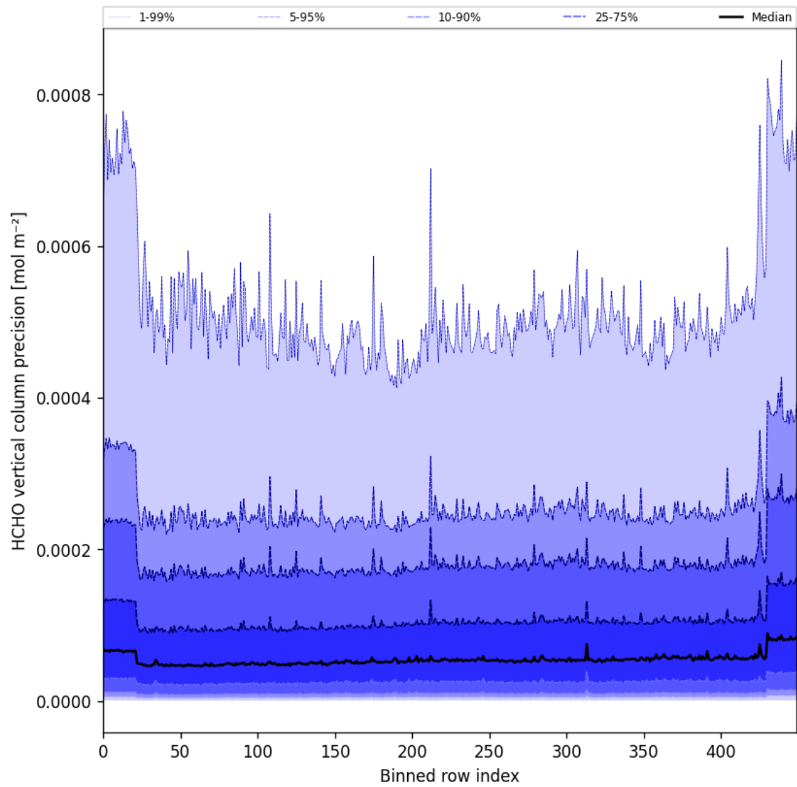
Figure 50: Along track statistics of “HCHO vertical column precision” for 2024-11-28 to 2024-11-30
