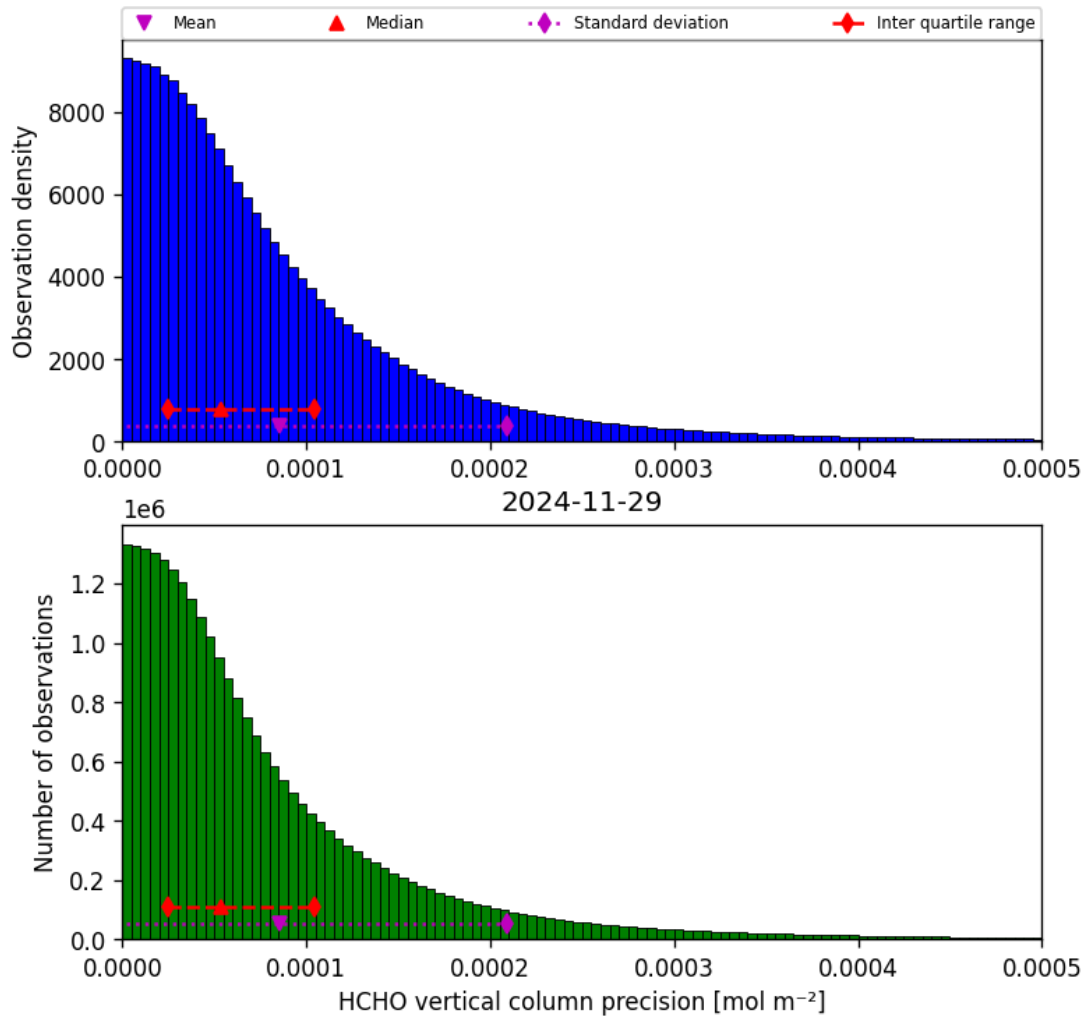
Figure 36: Histogram of “HCHO vertical column precision” for 2024-11-28 to 2024-11-30
