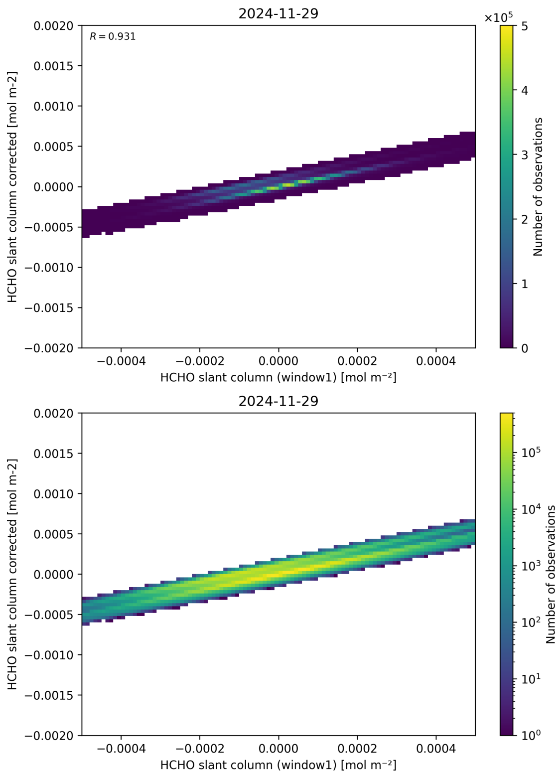
Figure 82: Scatter density plot of “HCHO slant column (window1)” against “HCHO slant column corrected” for 2024-11-28 to 2024-11-30.
