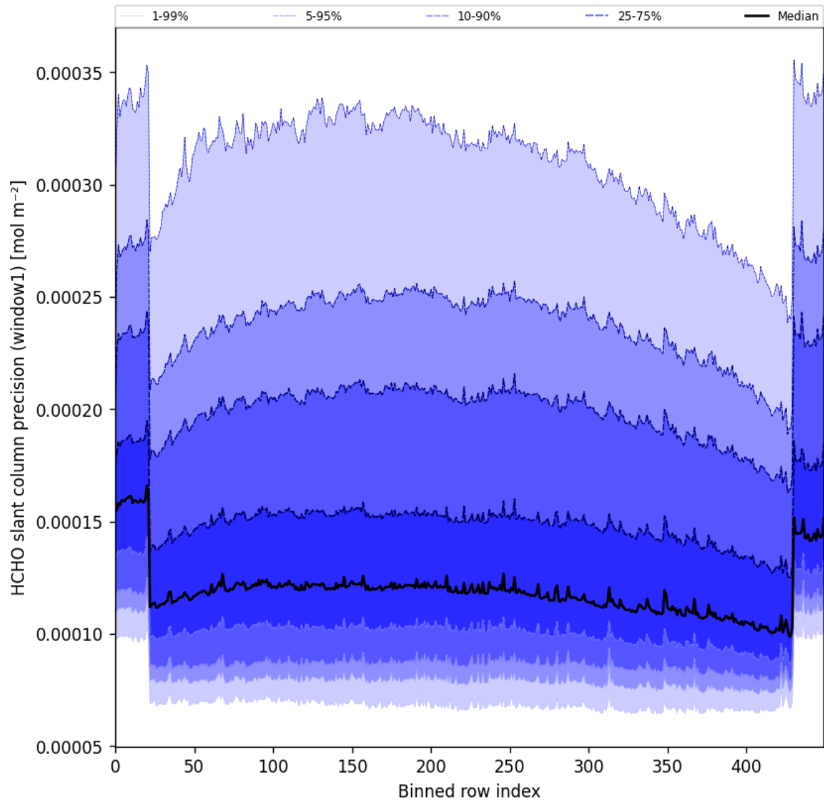
Figure 53: Along track statistics of “HCHO slant column precision (window1)” for 2024-11-28 to 2024-11-30
