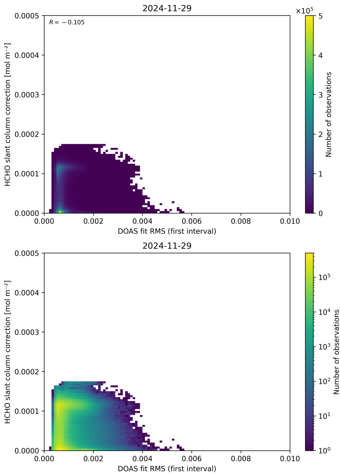
Figure 63: Scatter density plot of “DOAS fit RMS (first interval)” against “HCHO slant column correction” for 2024-11-28 to 2024-11-30.
