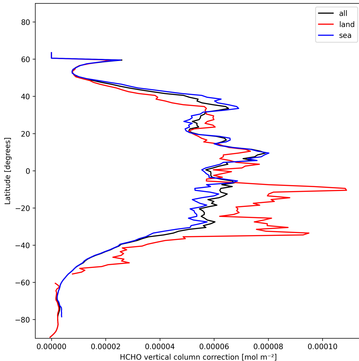
Figure 23: Zonal average of “HCHO vertical column correction” for 2024-11-28 to 2024-11-30.
