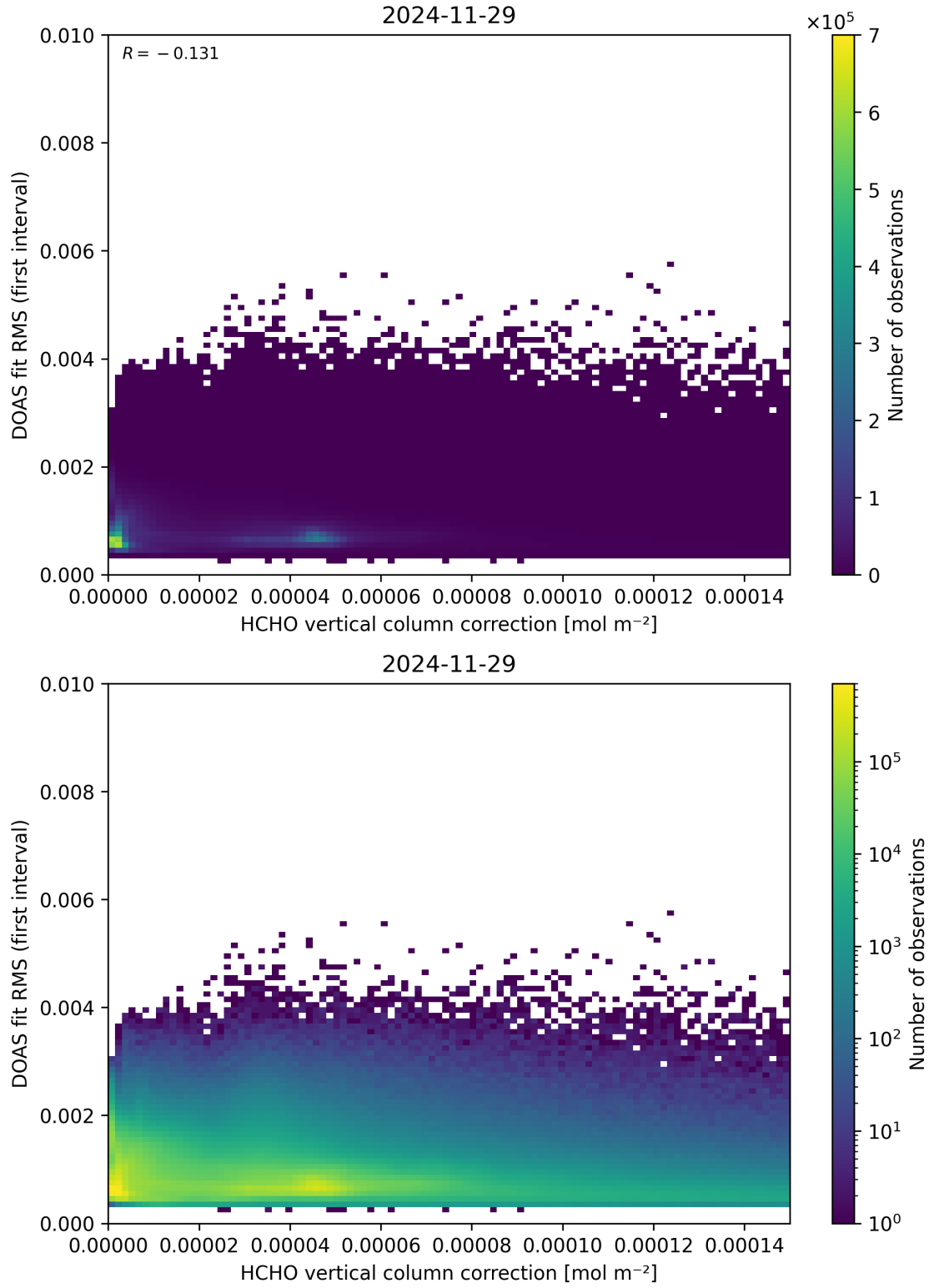
Figure 112: Scatter density plot of “HCHO vertical column correction” against “DOAS fit RMS (first interval)” for 2024-11-28 to 2024-11-30.
