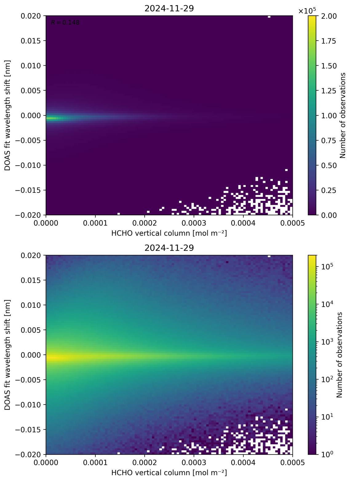
Figure 124: Scatter density plot of “HCHO vertical column” against “DOAS fit wavelength shift” for 2024-11-28 to 2024-11-30.
