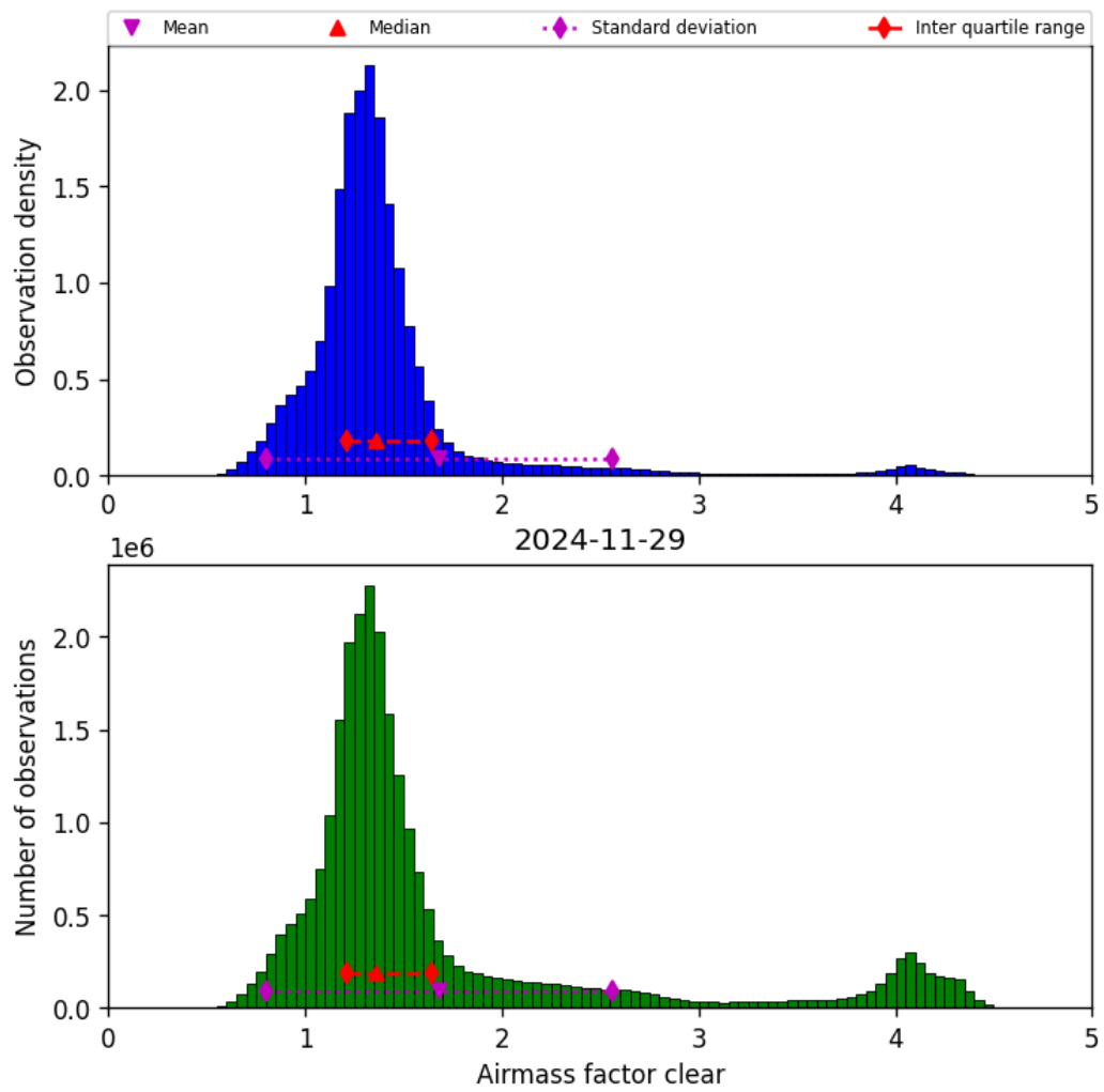
Figure 42: Histogram of “Airmass factor clear” for 2024-11-28 to 2024-11-30
