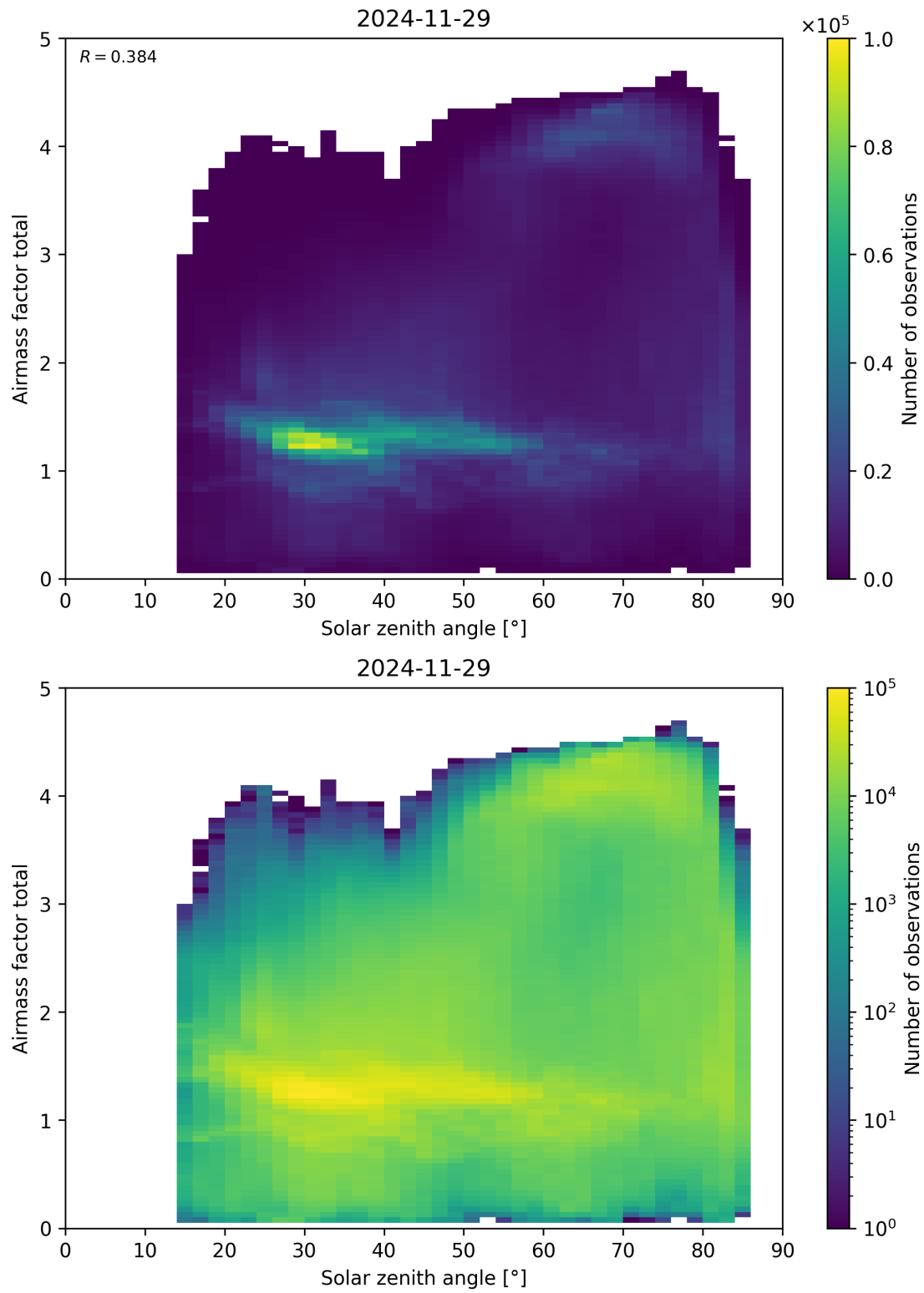
Figure 175: Scatter density plot of “Solar zenith angle” against “Airmass factor total” for 2024-11-28 to 2024-11-30.
