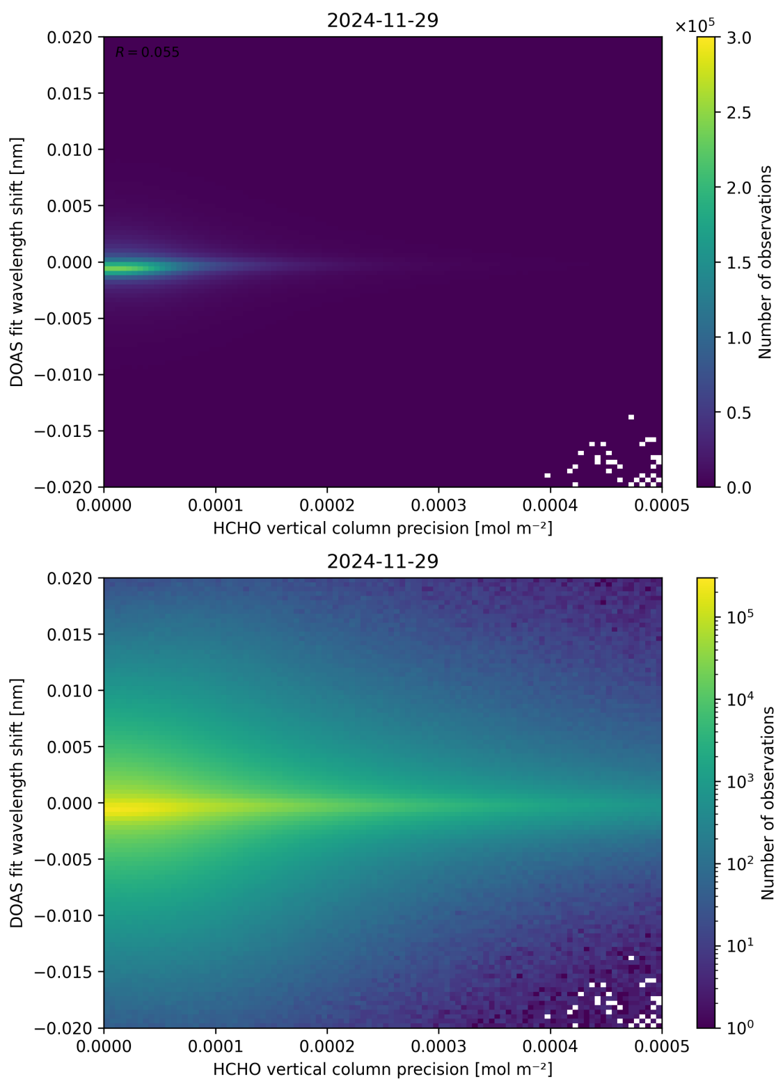
Figure 137: Scatter density plot of “HCHO vertical column precision” against “DOAS fit wavelength shift” for 2024-11-28 to 2024-11-30.
