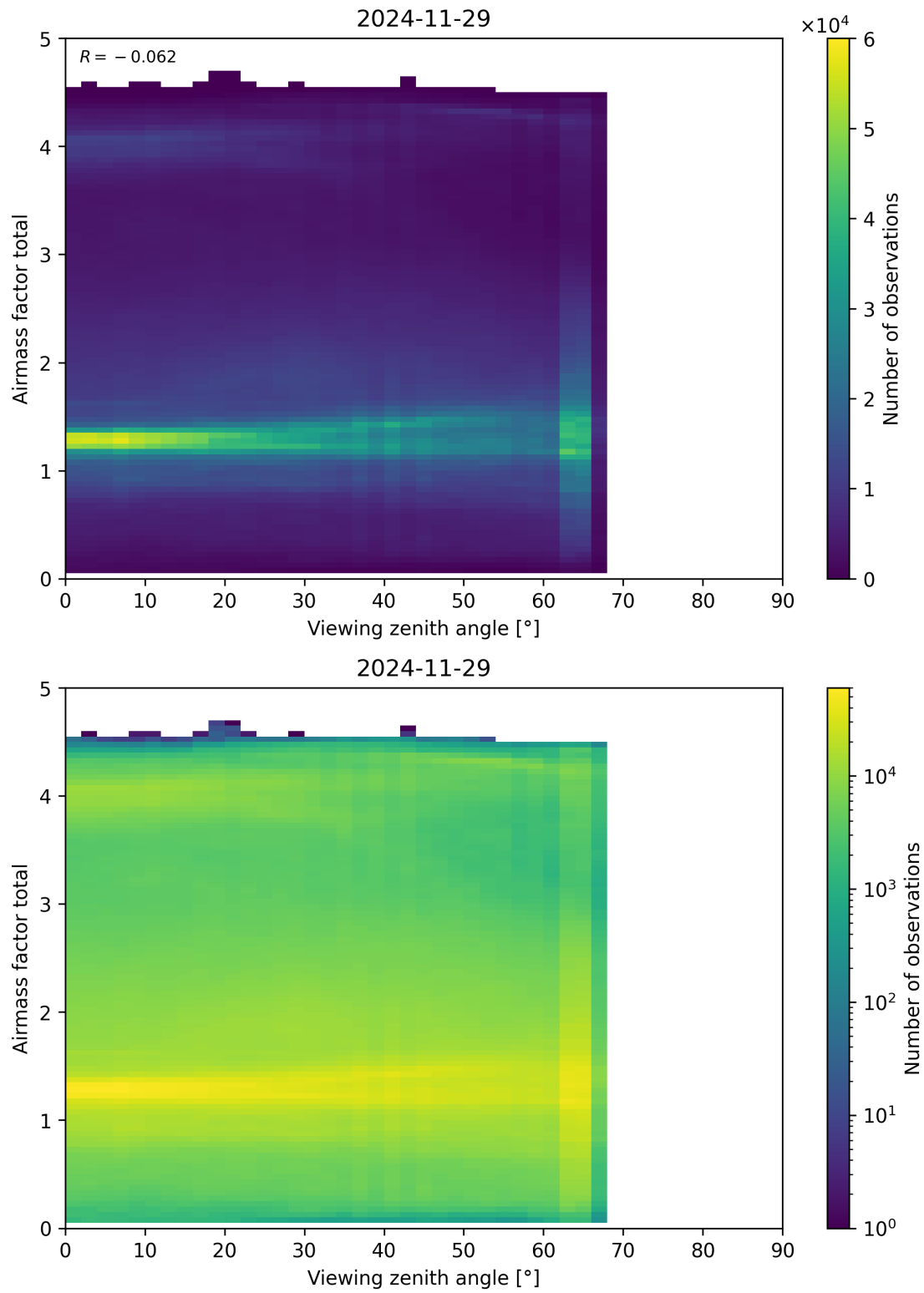
Figure 190: Scatter density plot of “Viewing zenith angle” against “Airmass factor total” for 2024-11-28 to 2024-11-30.
