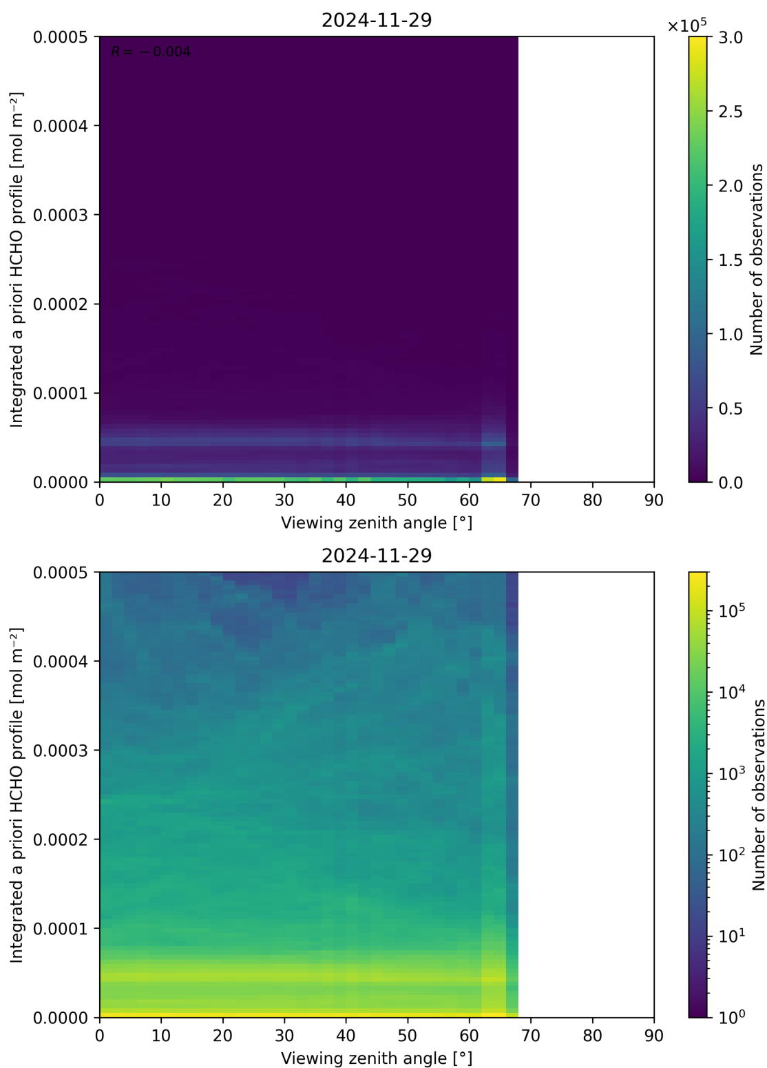
Figure 195: Scatter density plot of “Viewing zenith angle” against “Integrated a priori HCHO profile” for 2024-11-28 to 2024-11-30.
