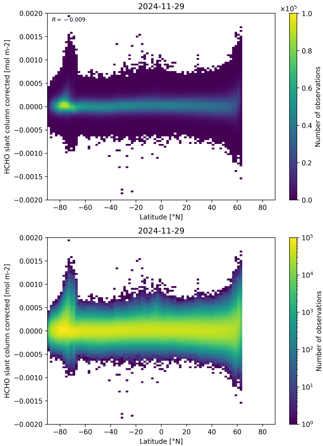
Figure 157: Scatter density plot of “Latitude” against “HCHO slant column corrected” for 2024-11-28 to 2024-11-30.
