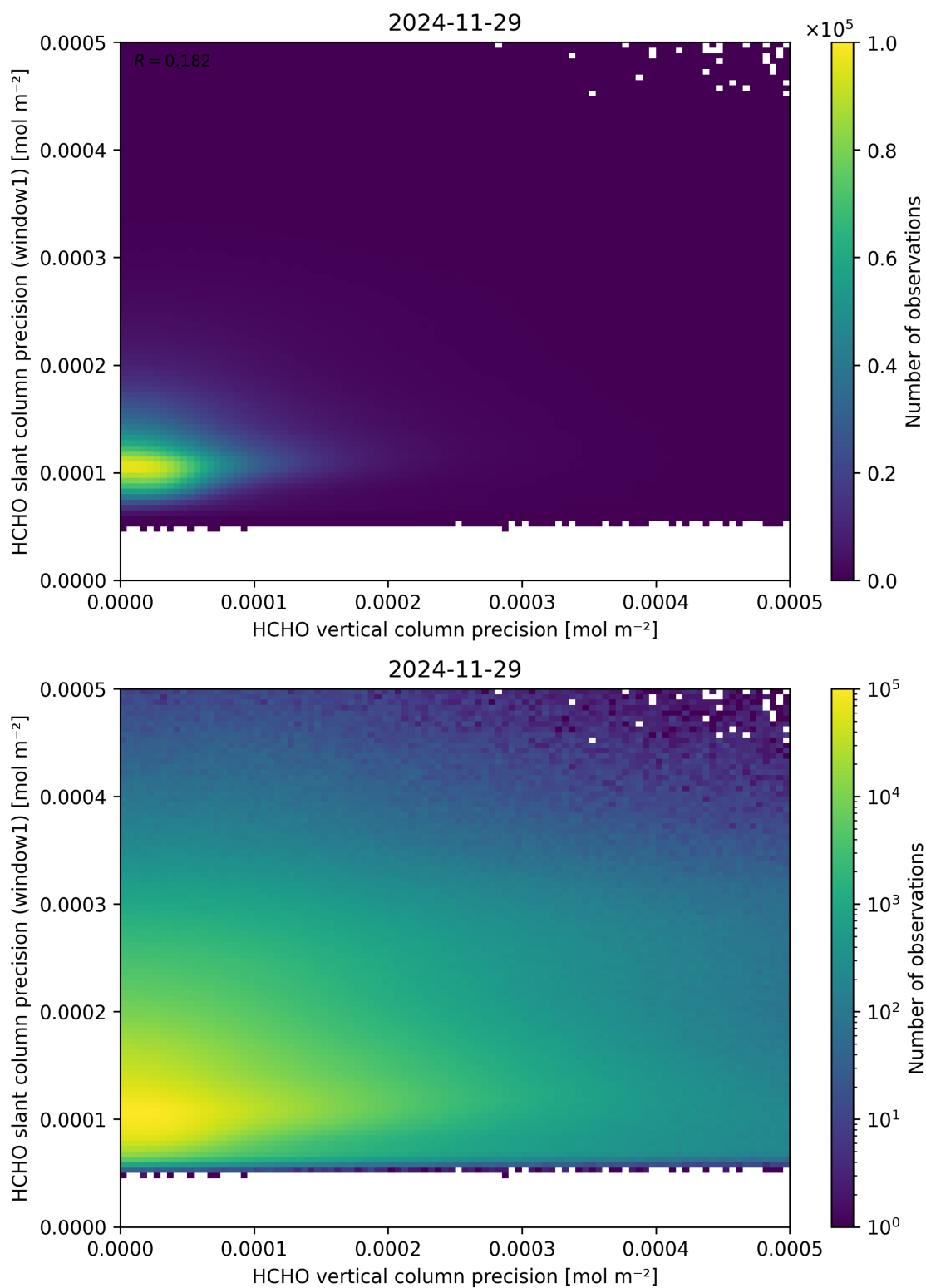
Figure 143: Scatter density plot of “HCHO vertical column precision” against “HCHO slant column precision (window1)” for 2024-11-28 to 2024-11-30.
