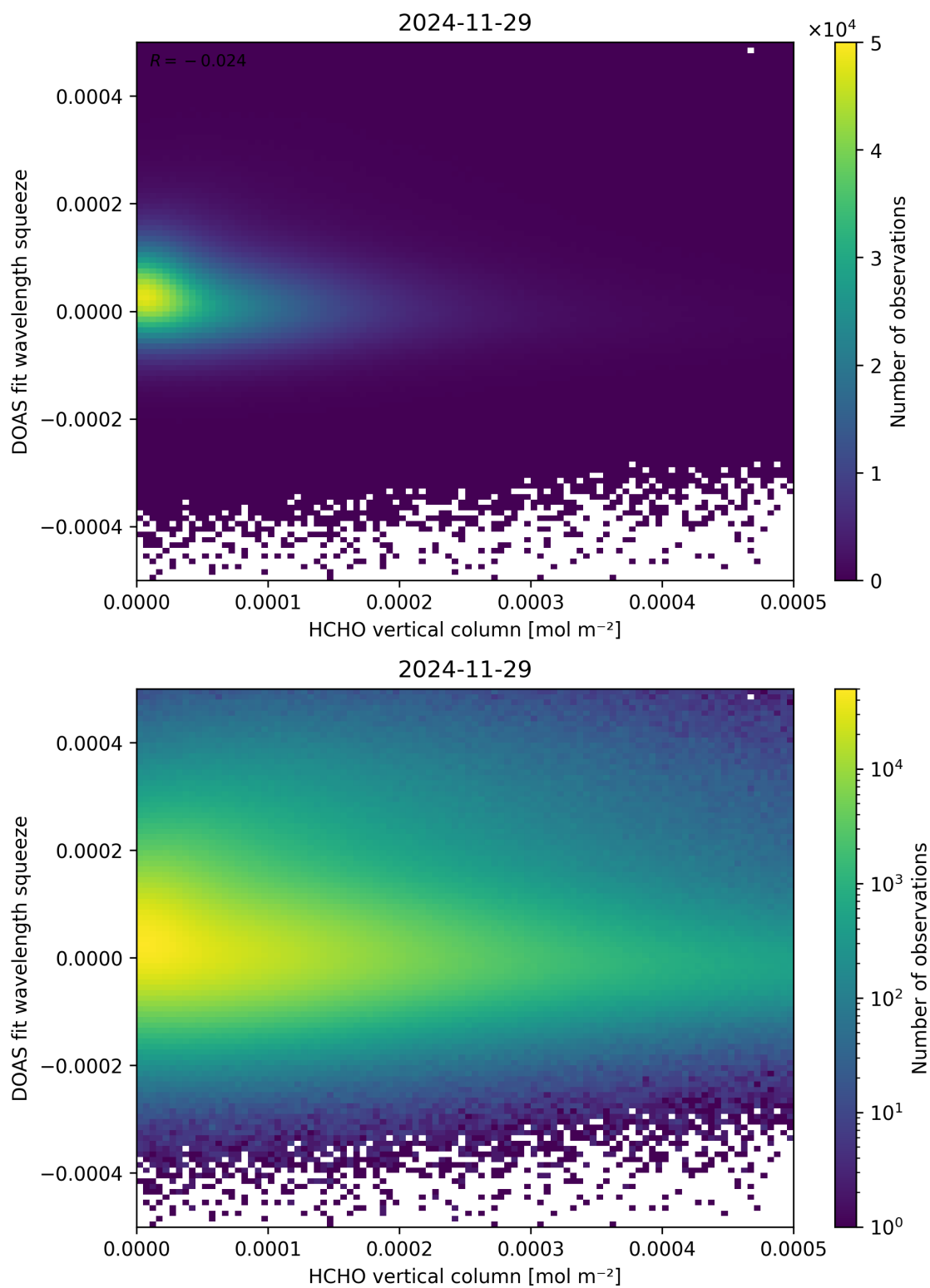
Figure 125: Scatter density plot of “HCHO vertical column” against “DOAS fit wavelength squeeze” for 2024-11-28 to 2024-11-30.
