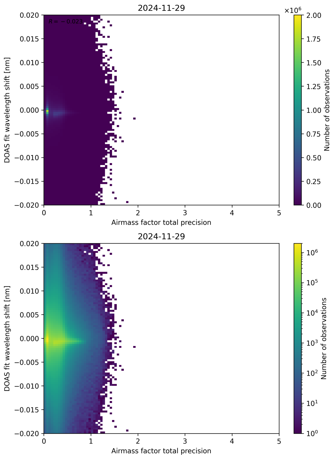
Figure 106: Scatter density plot of “Airmass factor total precision” against “DOAS fit wavelength shift” for 2024-11-28 to 2024-11-30.
