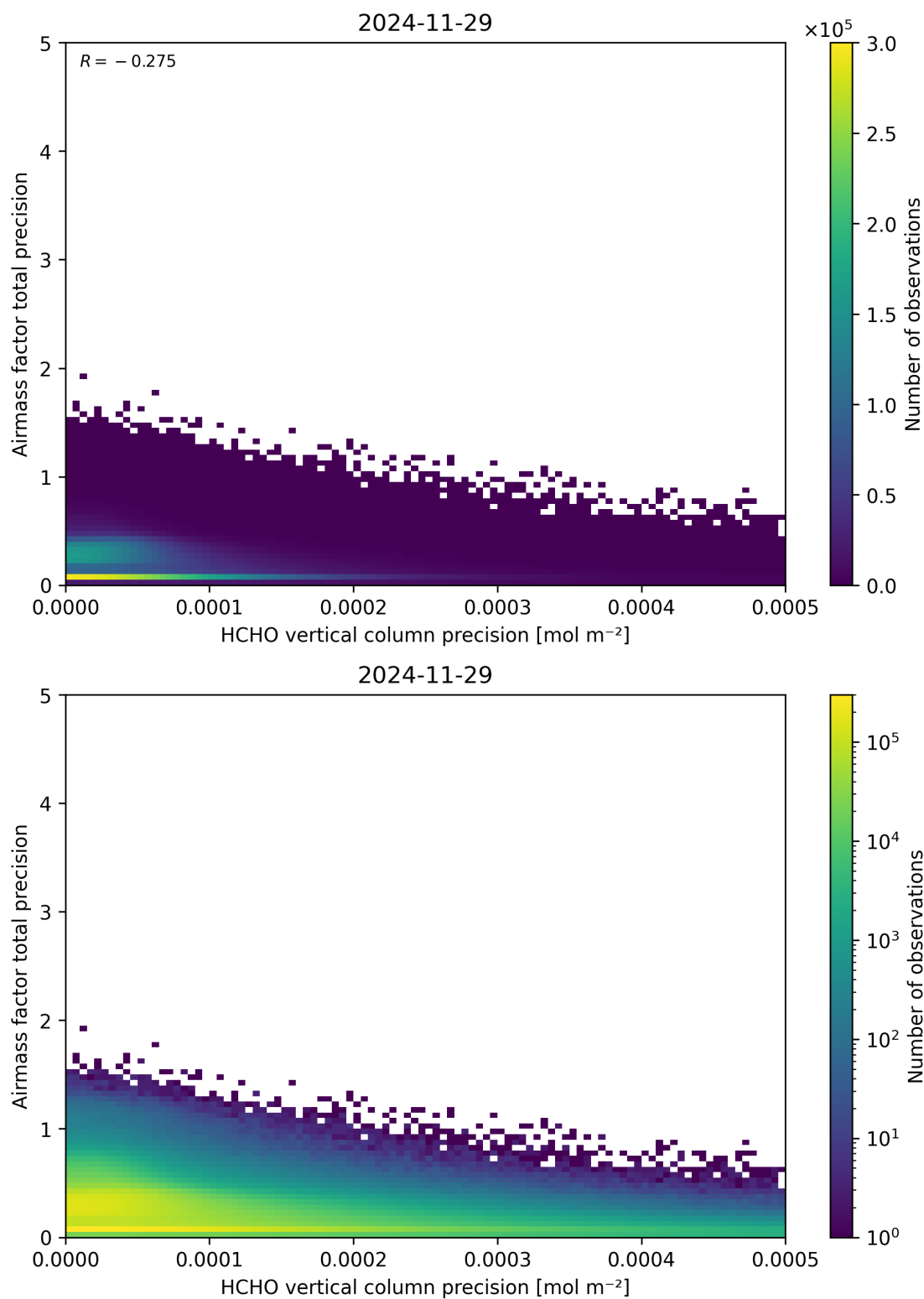
Figure 145: Scatter density plot of “HCHO vertical column precision” against “Airmass factor total precision” for 2024-11-28 to 2024-11-30.
