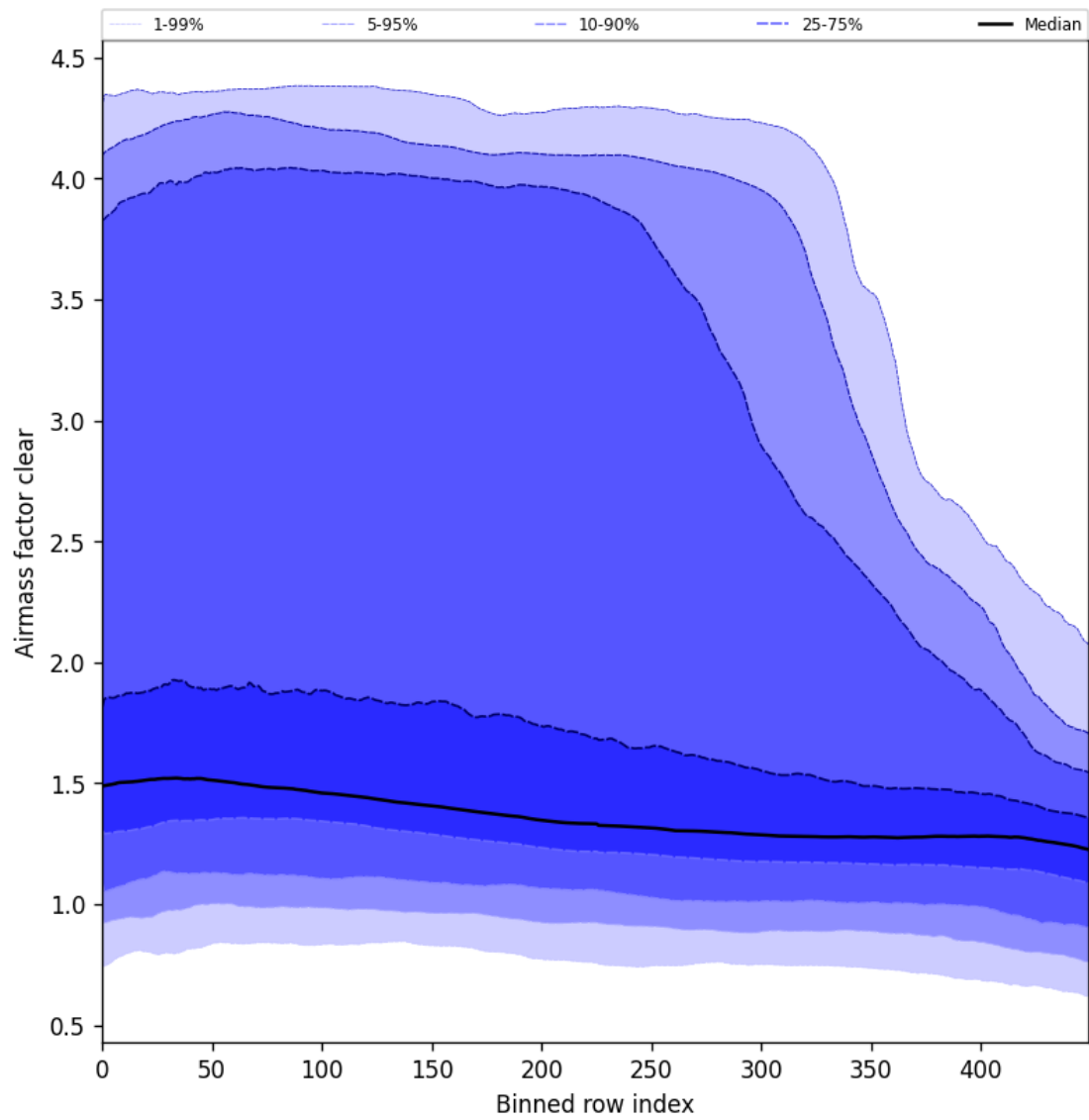
Figure 56: Along track statistics of “Air mass factor clear” for 2024-11-28 to 2024-11-30
