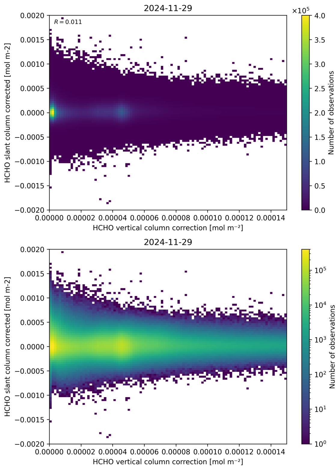
Figure 116: Scatter density plot of “HCHO vertical column correction” against “HCHO slant column corrected” for 2024-11-28 to 2024-11-30.
