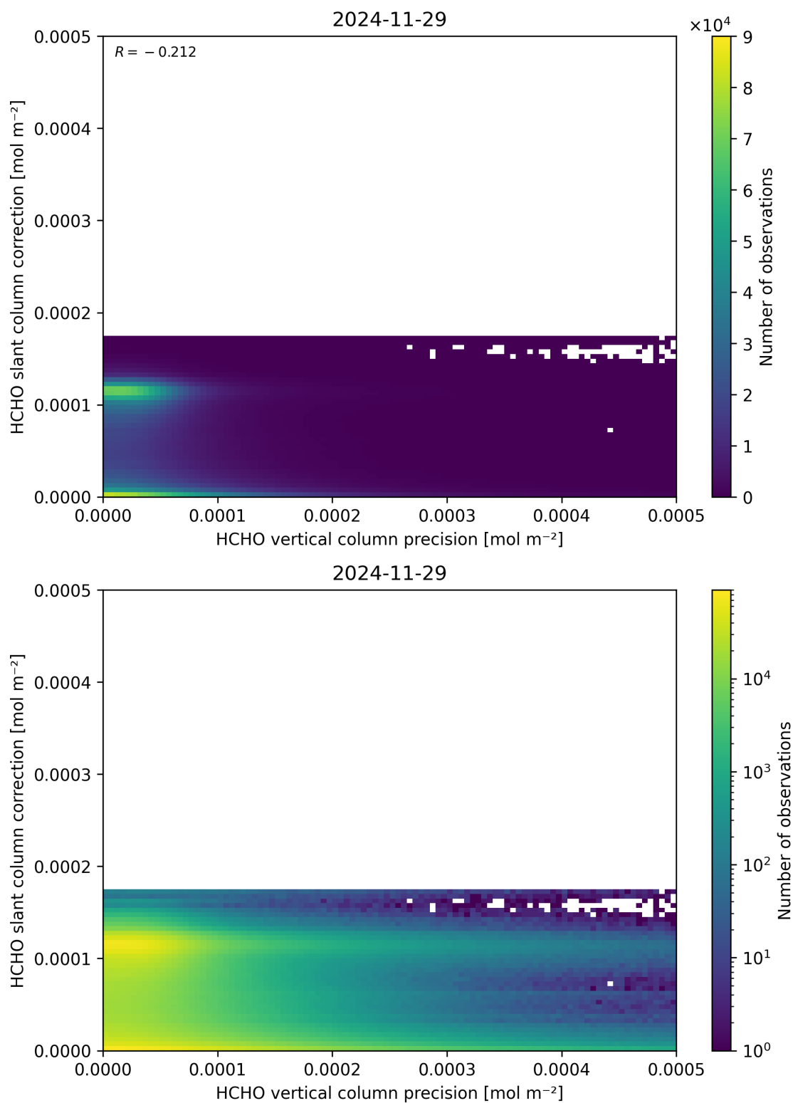
Figure 141: Scatter density plot of “HCHO vertical column precision” against “HCHO slant column correction” for 2024-11-28 to 2024-11-30.
