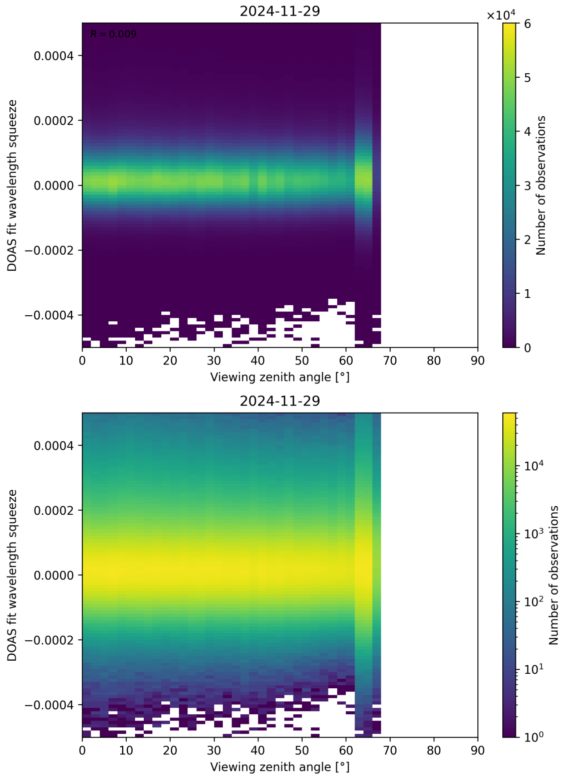
Figure 184: Scatter density plot of “Viewing zenith angle” against “DOAS fit wavelength squeeze” for 2024-11-28 to 2024-11-30.
