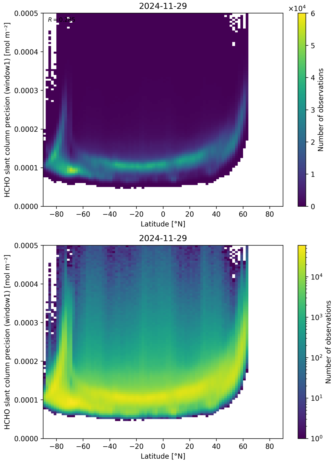
Figure 160: Scatter density plot of “Latitude” against “HCHO slant column precision (window1)” for 2024-11-28 to 2024-11-30.
