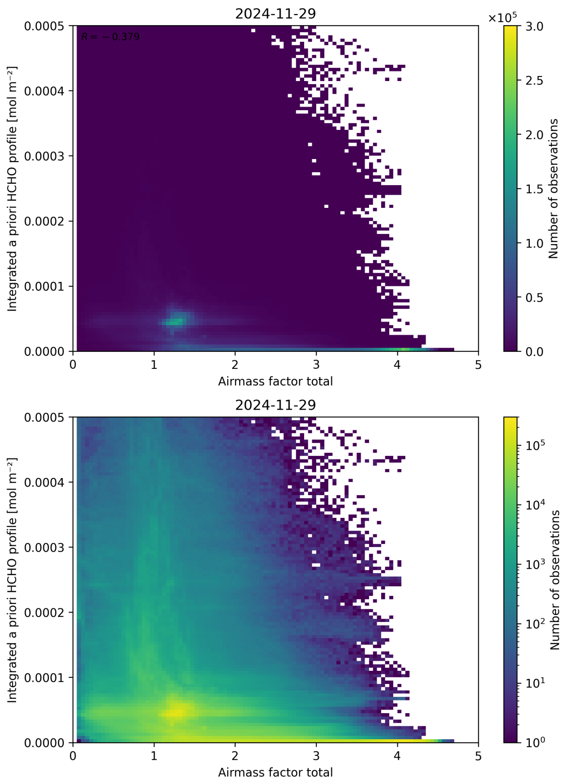
Figure 104: Scatter density plot of “Airmass factor total” against “Integrated a priori HCHO profile” for 2024-11-28 to 2024-11-30.
