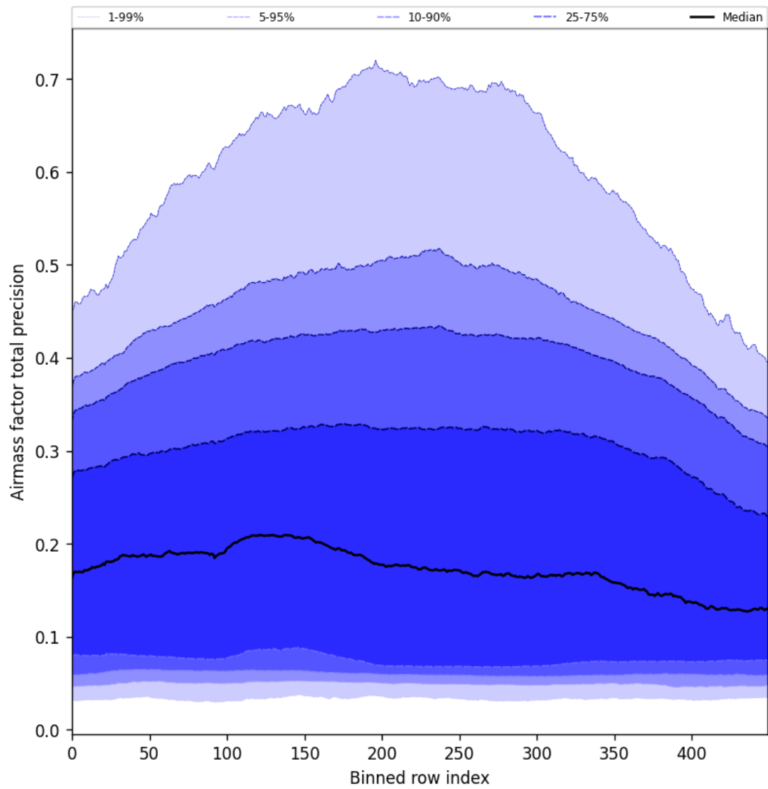
Figure 55: Along track statistics of “Airmass factor total precision” for 2024-11-28 to 2024-11-30
