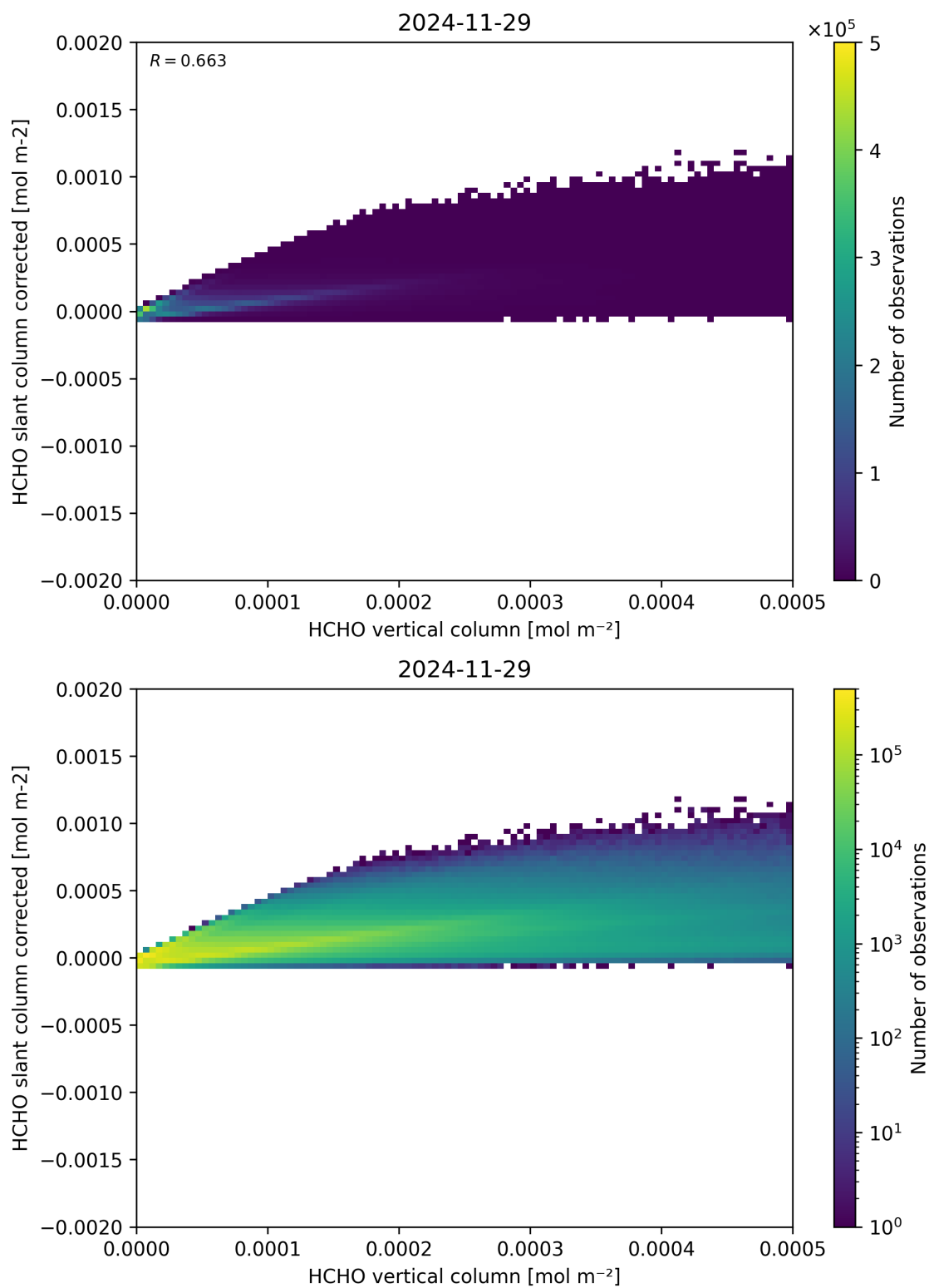
Figure 127: Scatter density plot of “HCHO vertical column” against “HCHO slant column corrected” for 2024-11-28 to 2024-11-30.
