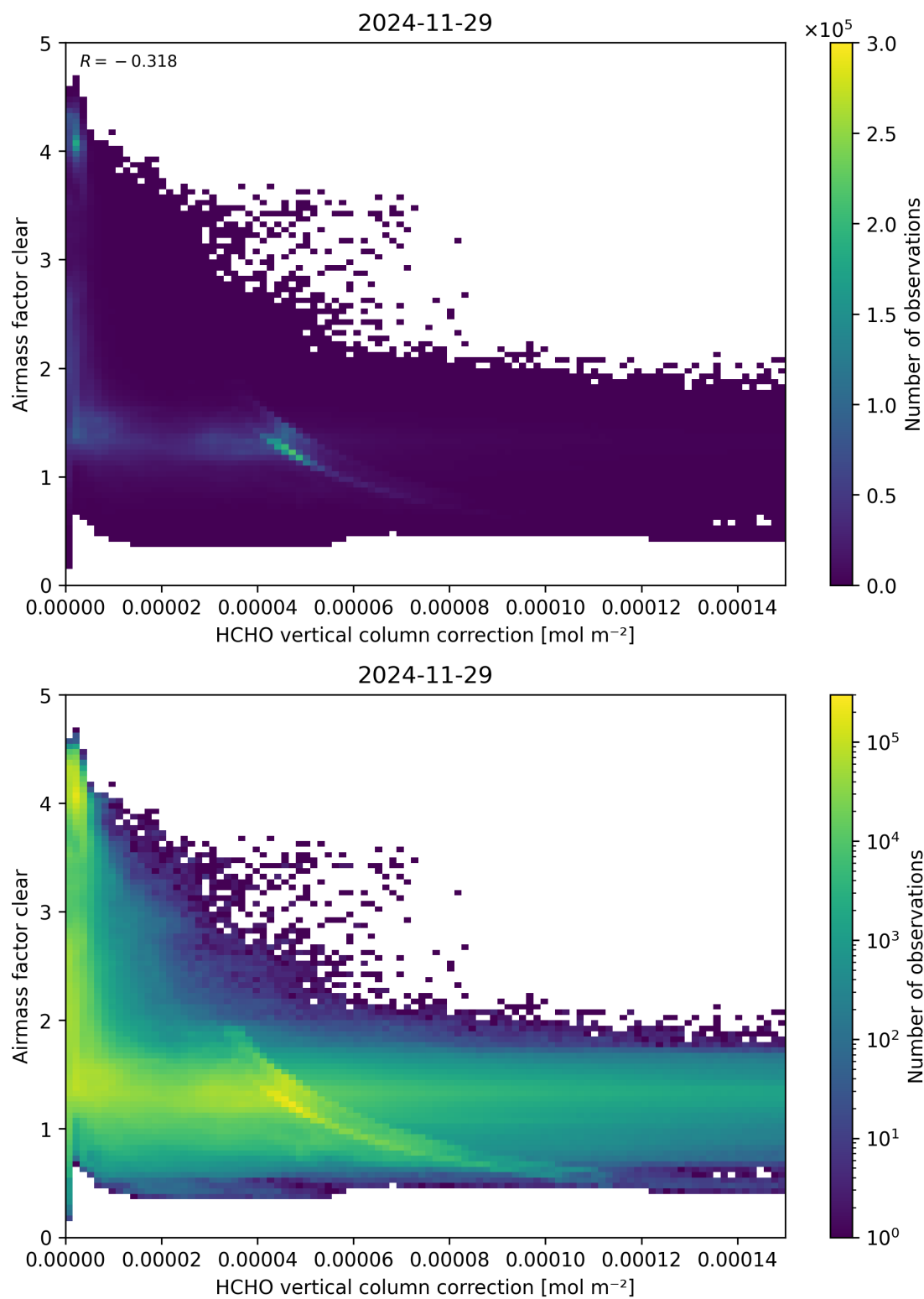
Figure 115: Scatter density plot of “HCHO vertical column correction” against “Airmass factor clear” for 2024-11-28 to 2024-11-30.
