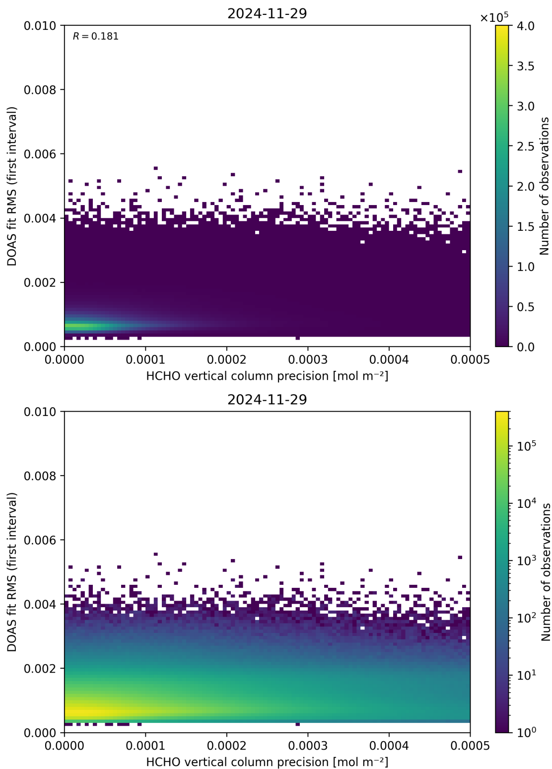
Figure 136: Scatter density plot of “HCHO vertical column precision” against “DOAS fit RMS (first interval)” for 2024-11-28 to 2024-11-30.
