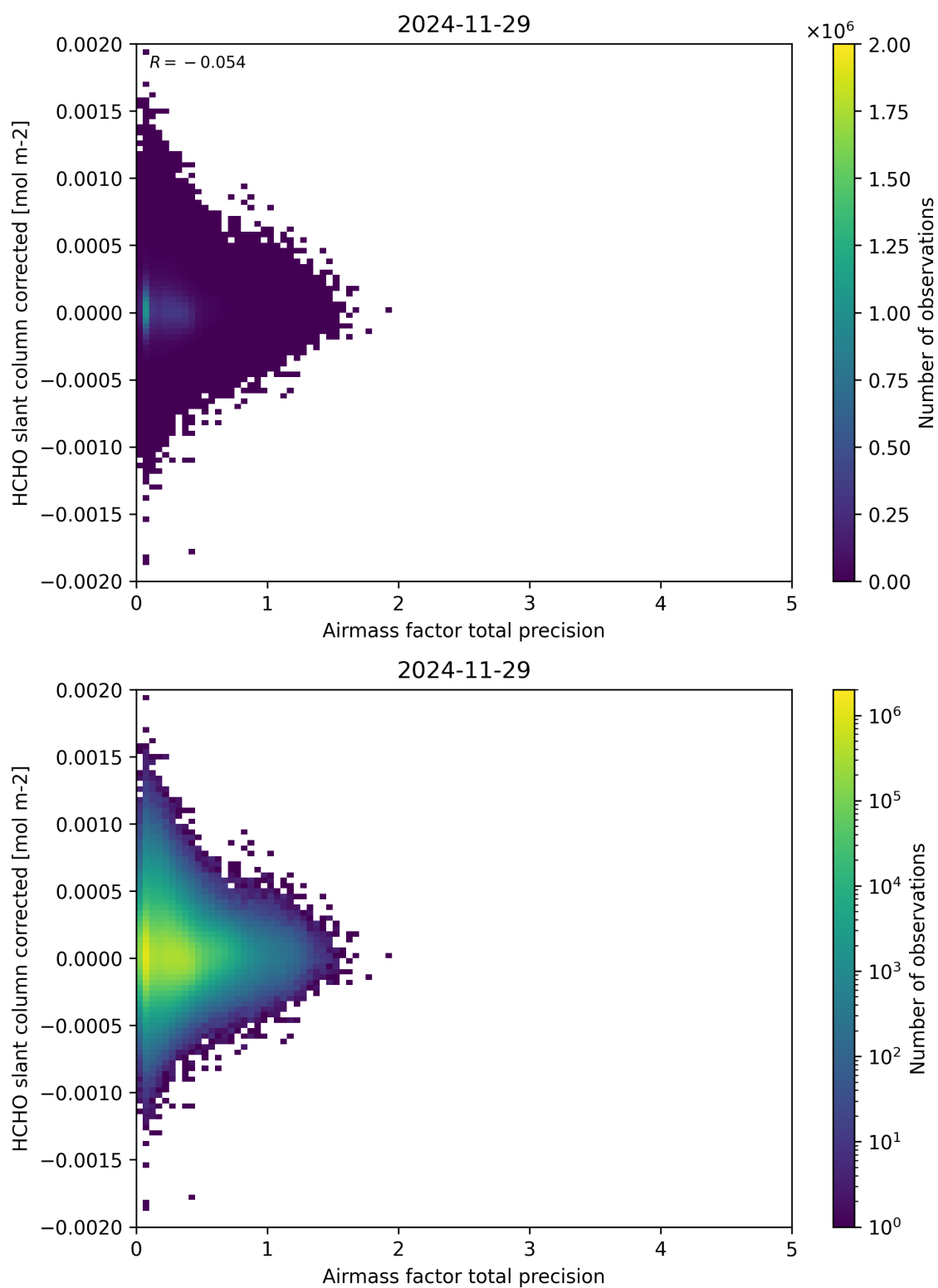
Figure 109: Scatter density plot of “Airmass factor total precision” against “HCHO slant column corrected” for 2024-11-28 to 2024-11-30.
