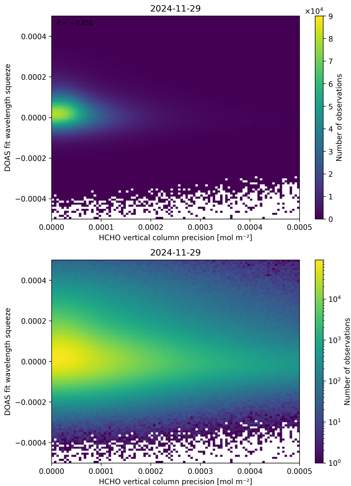
Figure 138: Scatter density plot of “HCHO vertical column precision” against “DOAS fit wavelength squeeze” for 2024-11-28 to 2024-11-30.
