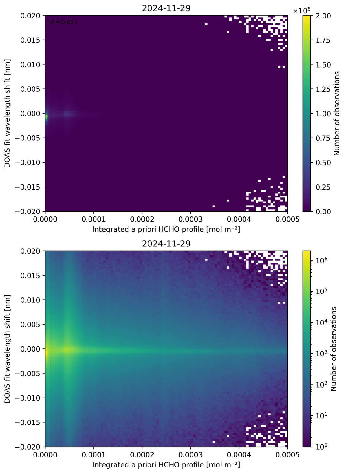
Figure 149: Scatter density plot of “Integrated a priori HCHO profile” against “DOAS fit wavelength shift” for 2024-11-28 to 2024-11-30.
