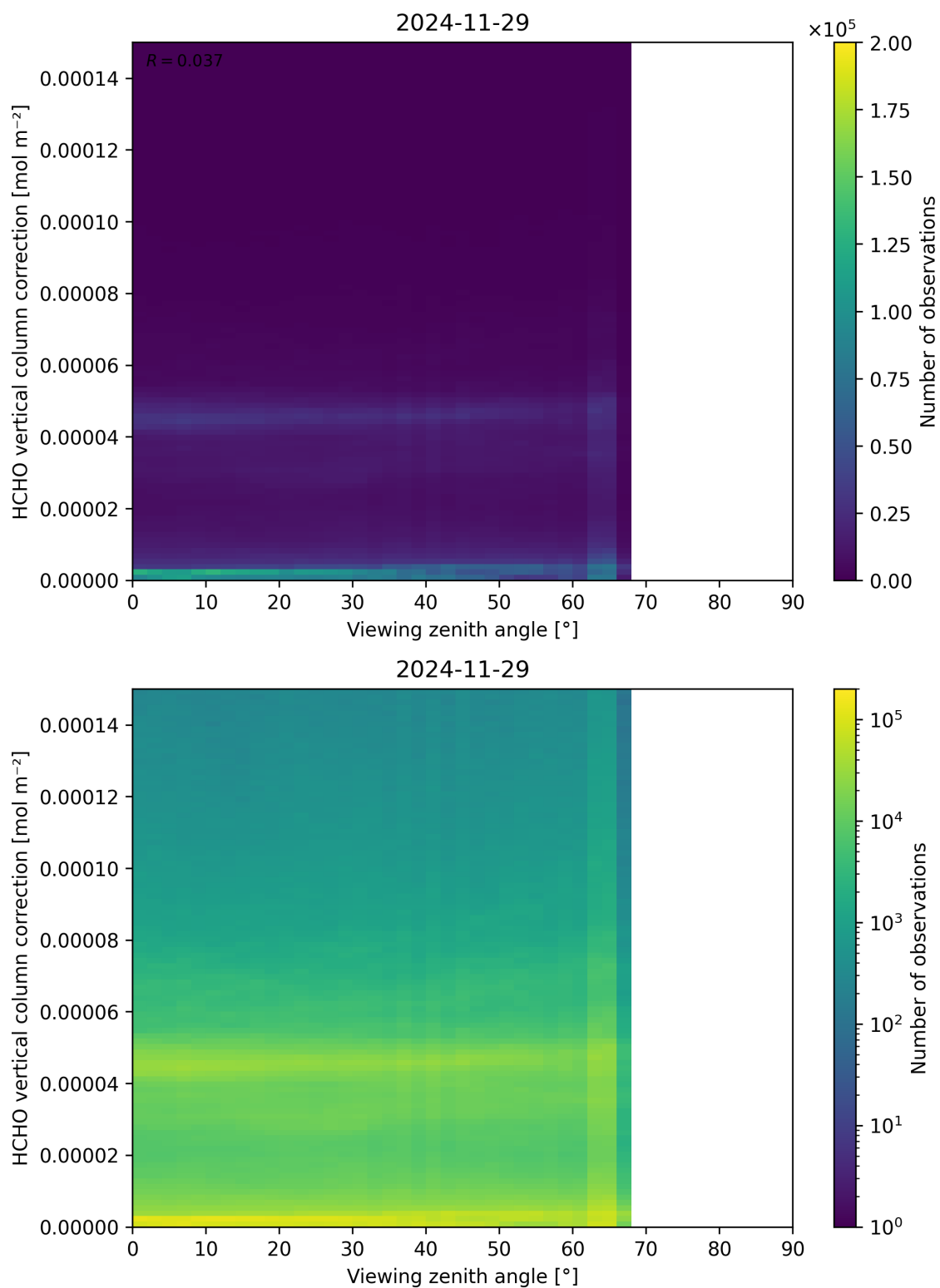
Figure 193: Scatter density plot of “Viewing zenith angle” against “HCHO vertical column correction” for 2024-11-28 to 2024-11-30.
