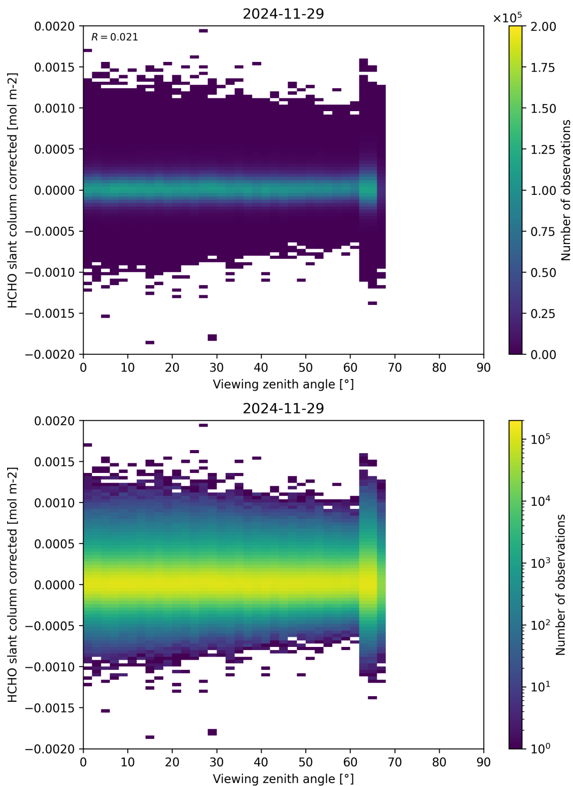
Figure 186: Scatter density plot of “Viewing zenith angle” against “HCHO slant column corrected” for 2024-11-28 to 2024-11-30.
