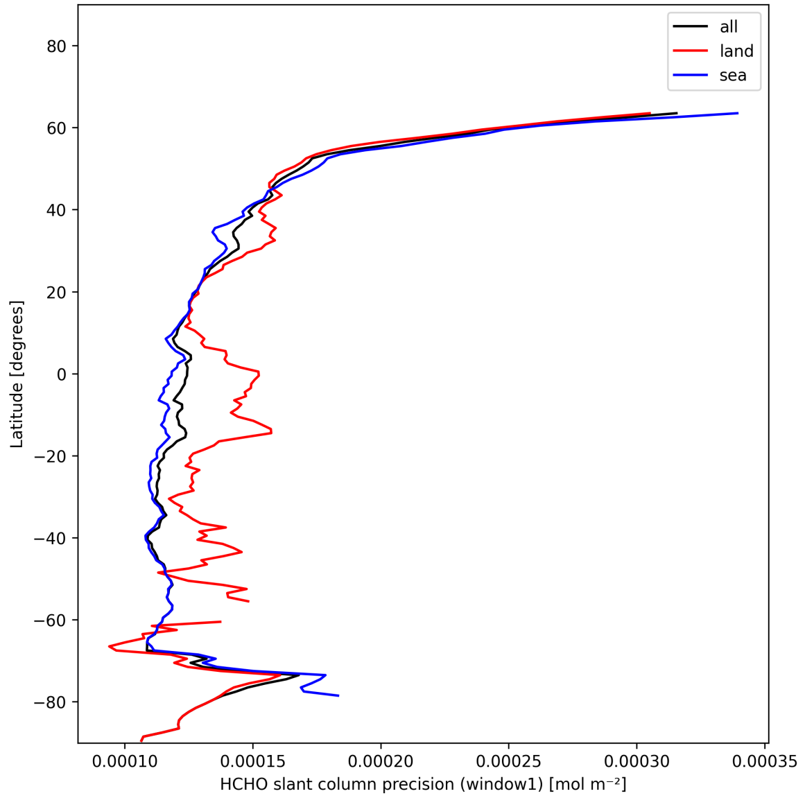
Figure 25: Zonal average of “HCHO slant column precision (window1)” for 2024-11-28 to 2024-11-30.
