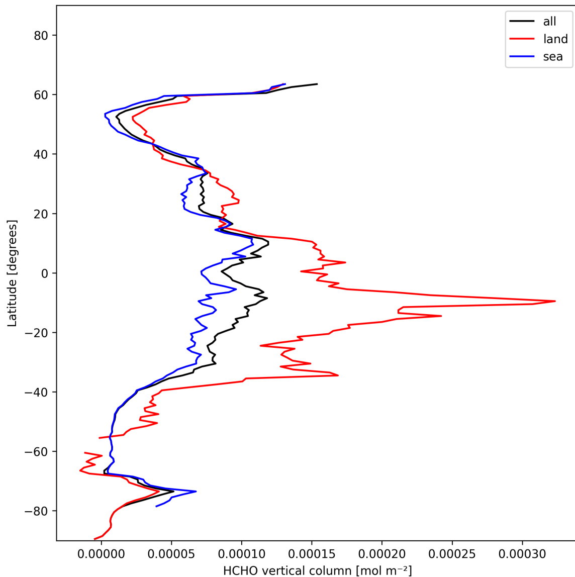
Figure 21: Zonal average of “HCHO vertical column” for 2024-11-28 to 2024-11-30.
