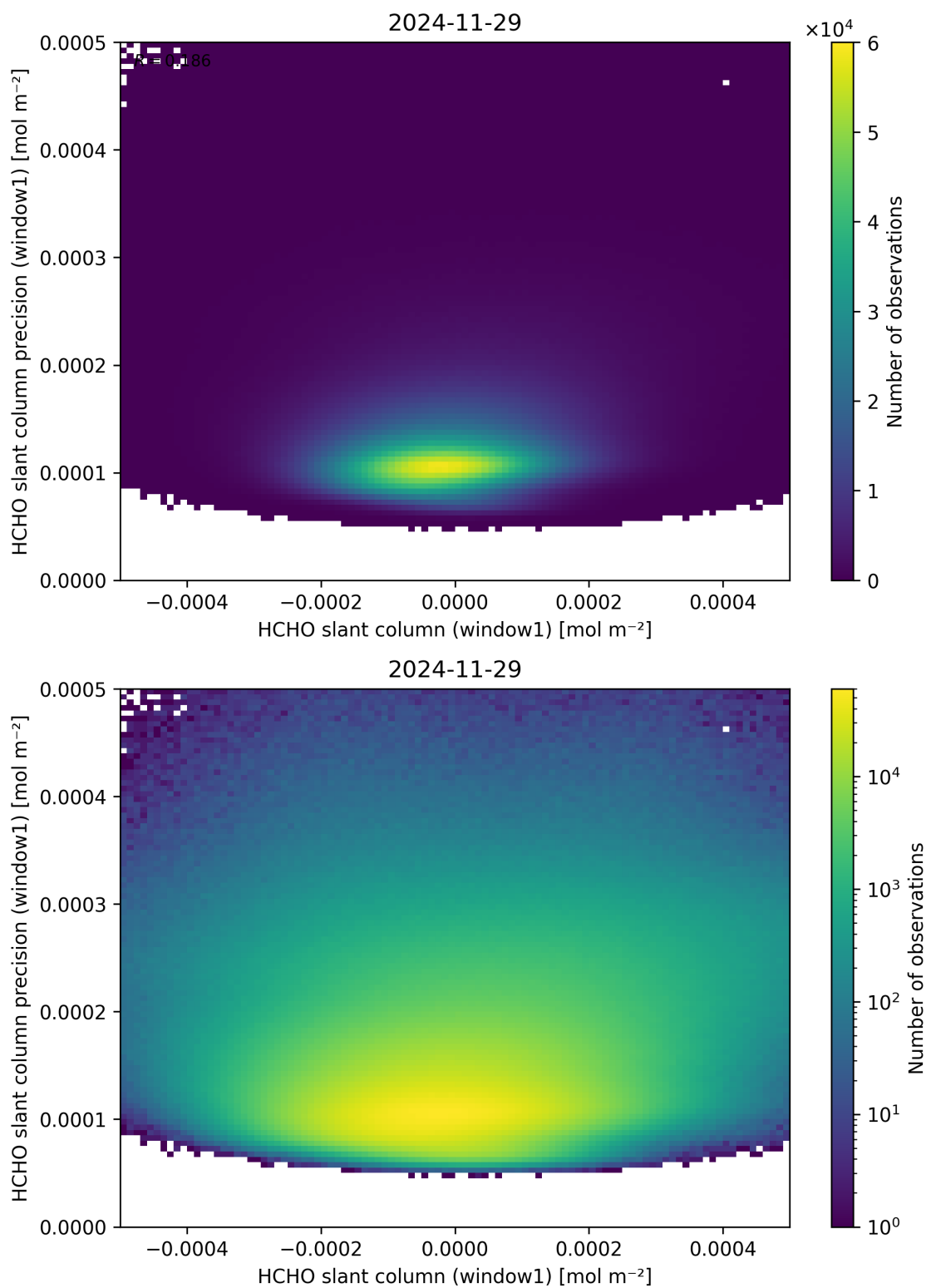
Figure 84: Scatter density plot of “HCHO slant column (window1)” against “HCHO slant column precision (window1)” for 2024-11-28 to 2024-11-30.
