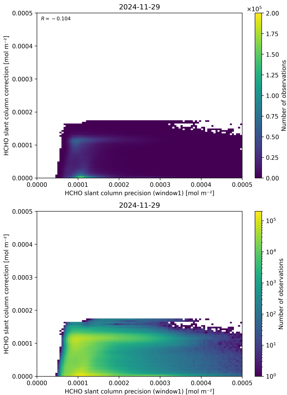
Figure 93: Scatter density plot of “HCHO slant column precision (window1)” against “HCHO slant column correction” for 2024-11-28 to 2024-11-30.
