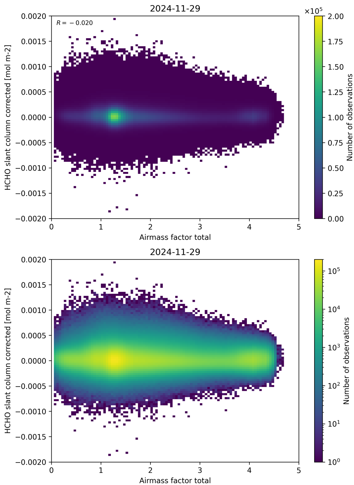
Figure 101: Scatter density plot of “Airmass factor total” against “HCHO slant column corrected” for 2024-11-28 to 2024-11-30.
