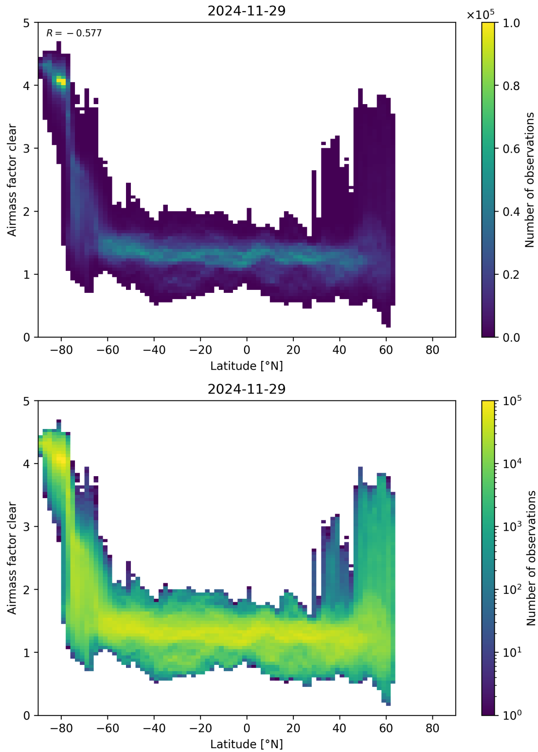
Figure 156: Scatter density plot of “Latitude” against “Airmass factor clear” for 2024-11-28 to 2024-11-30.
