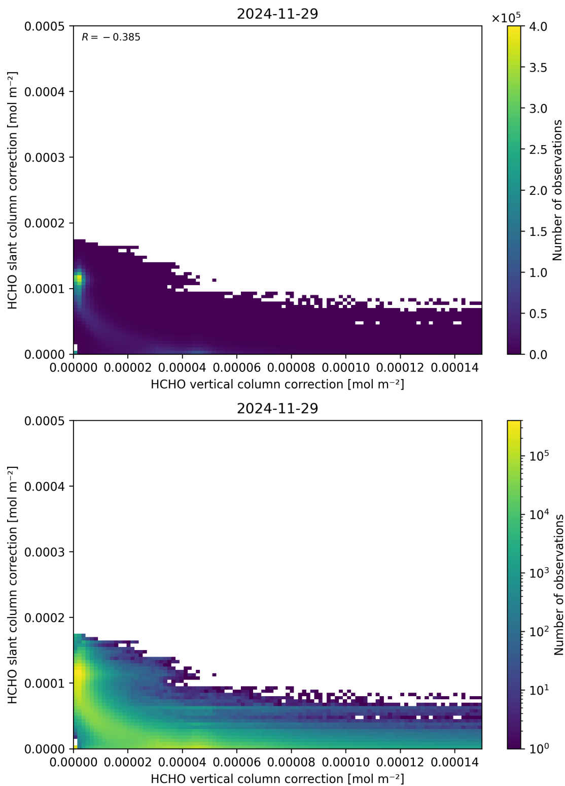
Figure 117: Scatter density plot of “HCHO vertical column correction” against “HCHO slant column correction” for 2024-11-28 to 2024-11-30.
