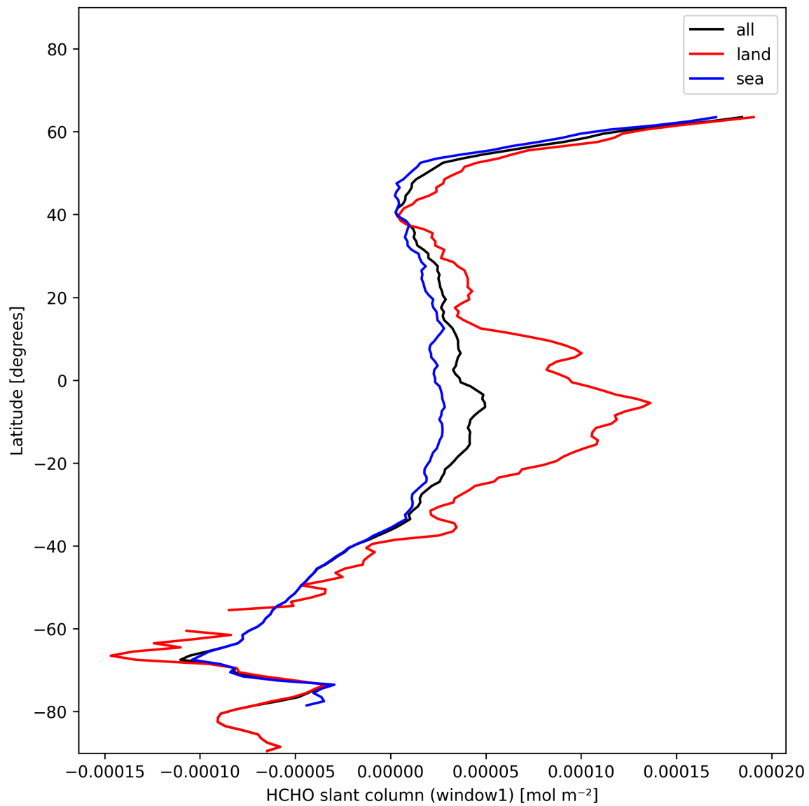
Figure 24: Zonal average of “HCHO slant column (window1)” for 2024-11-28 to 2024-11-30.
