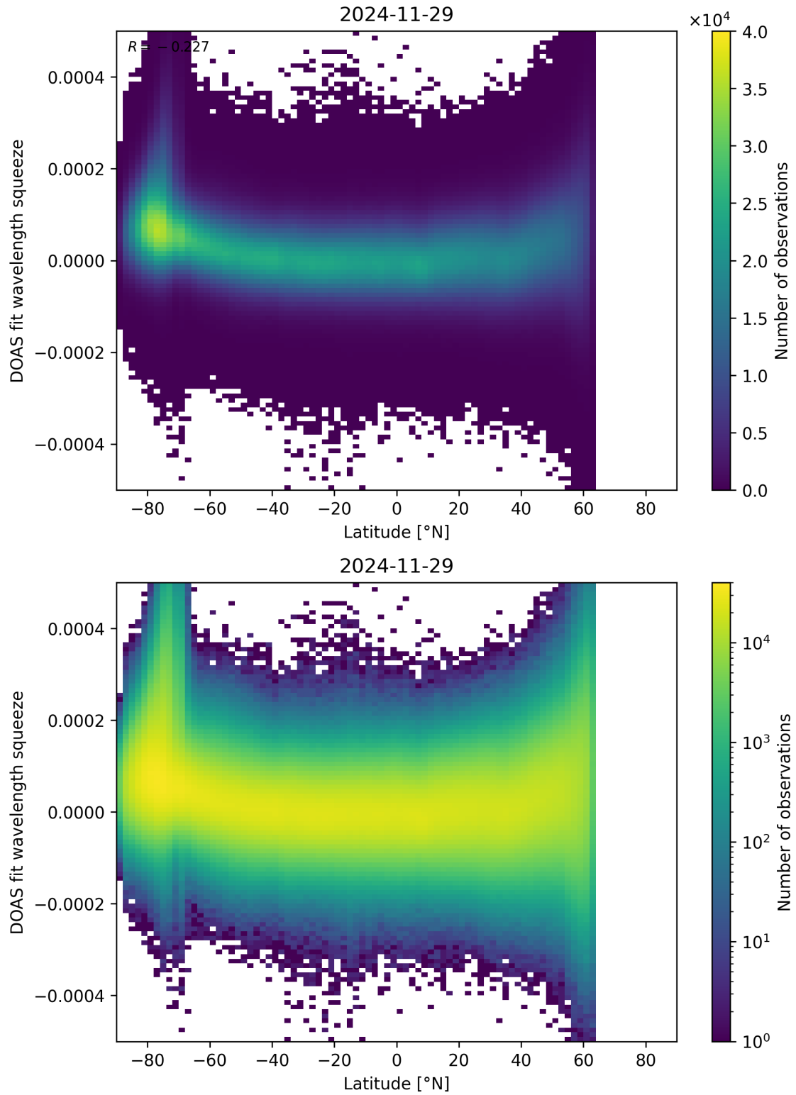
Figure 155: Scatter density plot of “Latitude” against “DOAS fit wavelength squeeze” for 2024-11-28 to 2024-11-30.
