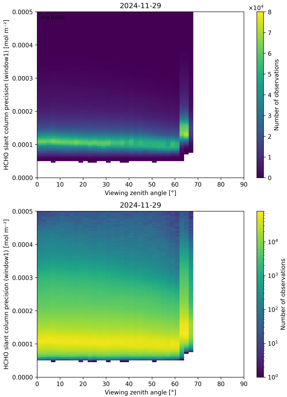
Figure 189: Scatter density plot of “Viewing zenith angle” against “HCHO slant column precision (window1)” for 2024-11-28 to 2024-11-30.
