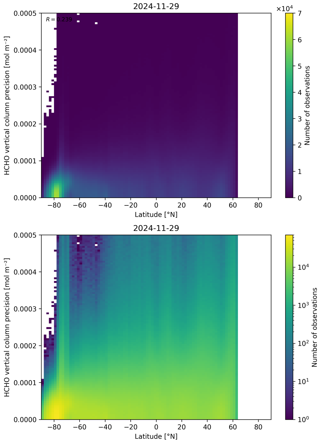
Figure 165: Scatter density plot of “Latitude” against “HCHO vertical column precision” for 2024-11-28 to 2024-11-30.
