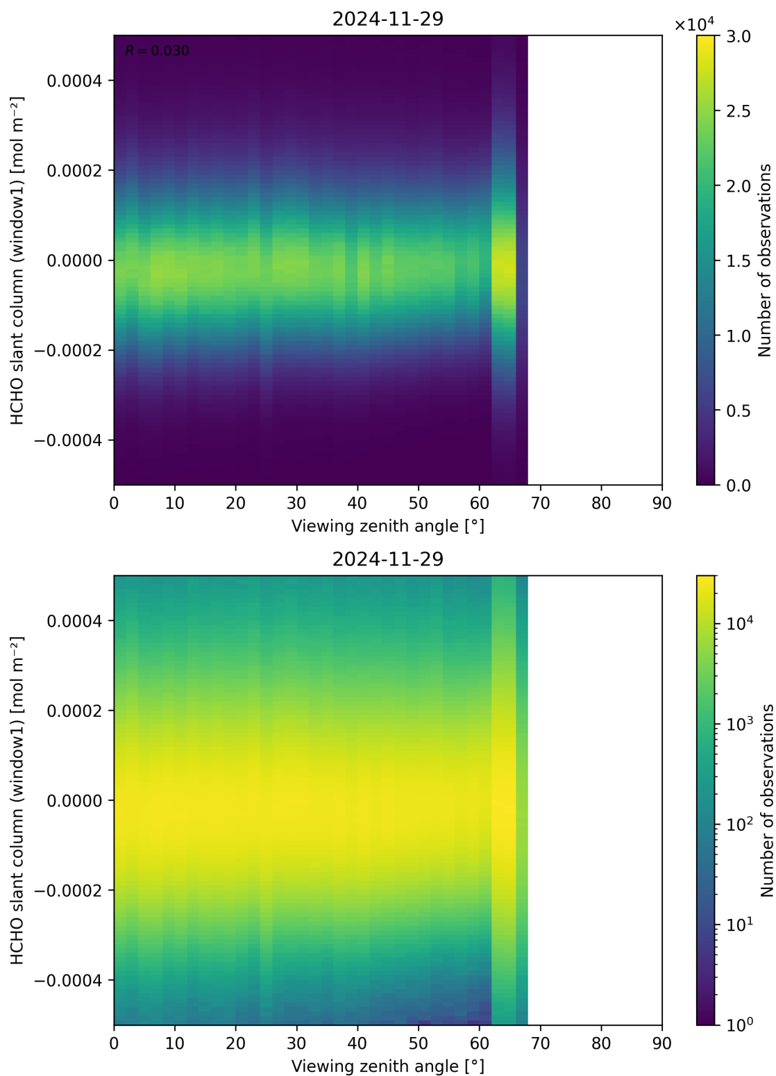
Figure 188: Scatter density plot of “Viewing zenith angle” against “HCHO slant column (window1)” for 2024-11-28 to 2024-11-30.
