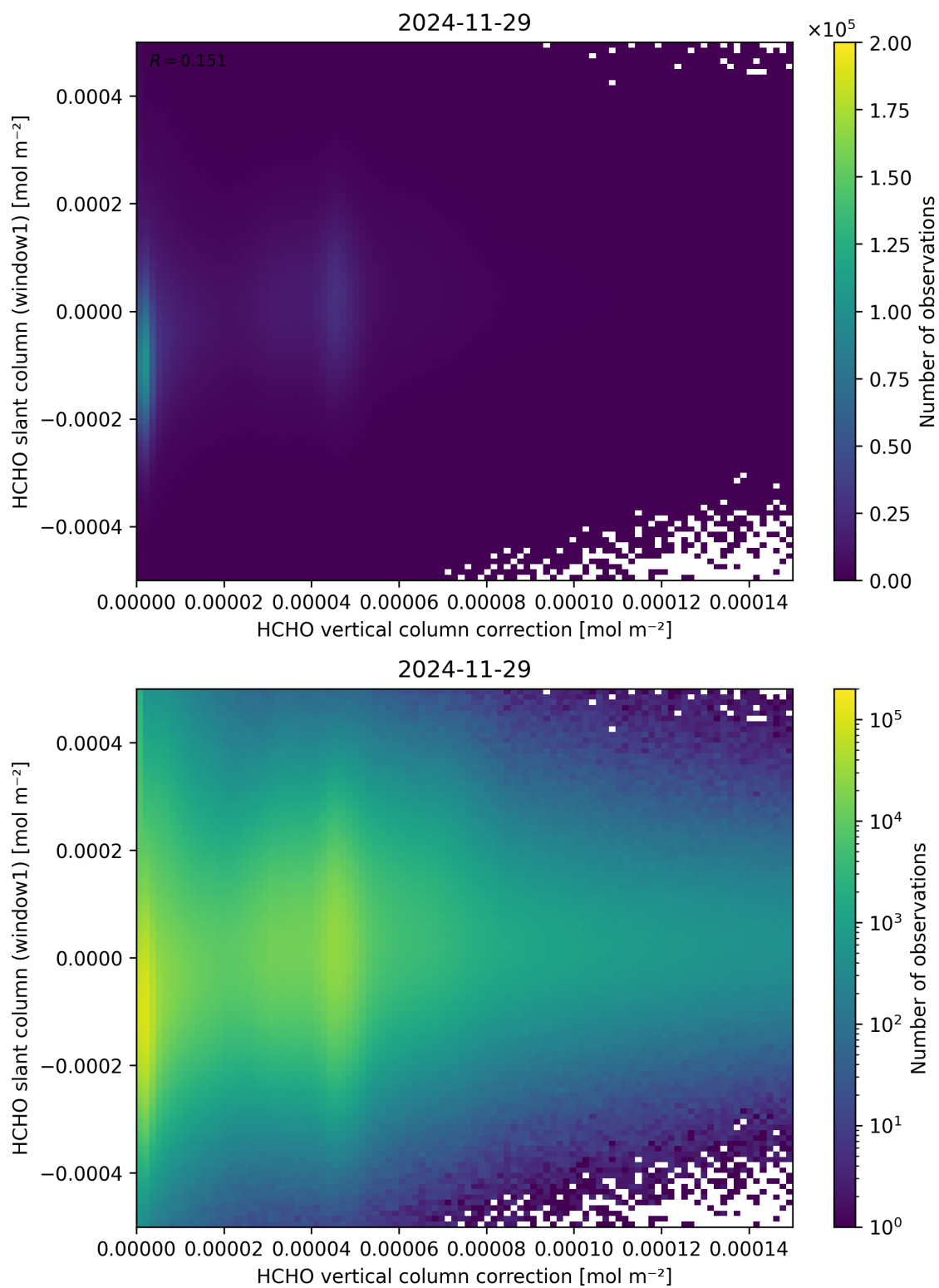
Figure 118: Scatter density plot of “HCHO vertical column correction” against “HCHO slant column (window1)” for 2024-11-28 to 2024-11-30.
