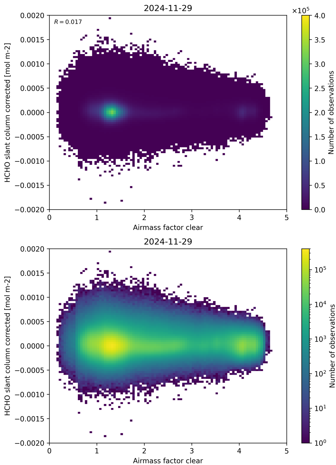
Figure 74: Scatter density plot of “Airmass factor clear” against “HCHO slant column corrected” for 2024-11-28 to 2024-11-30.
