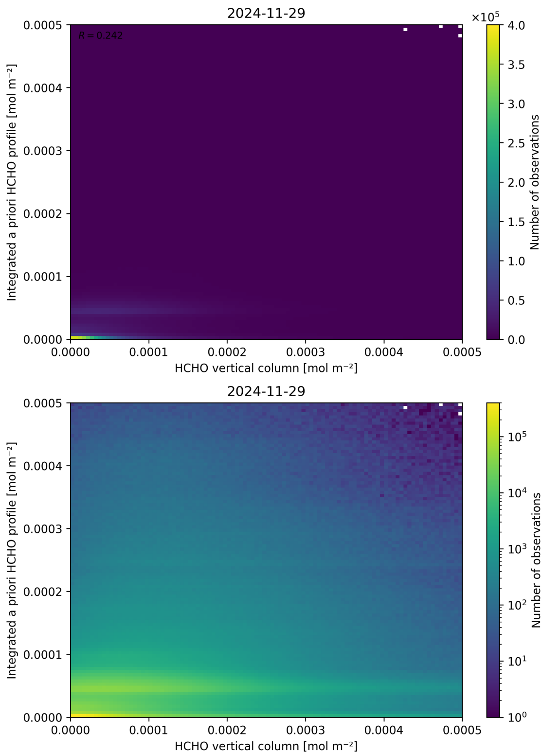
Figure 135: Scatter density plot of “HCHO vertical column” against “Integrated a priori HCHO profile” for 2024-11-28 to 2024-11-30.
