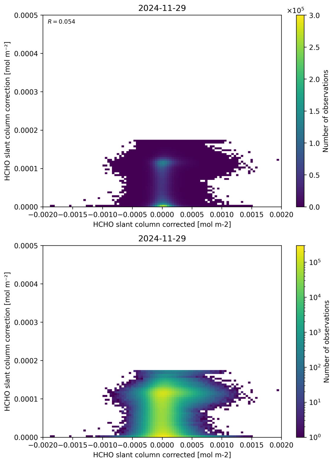
Figure 77: Scatter density plot of “HCHO slant column corrected” against “HCHO slant column correction” for 2024-11-28 to 2024-11-30.
