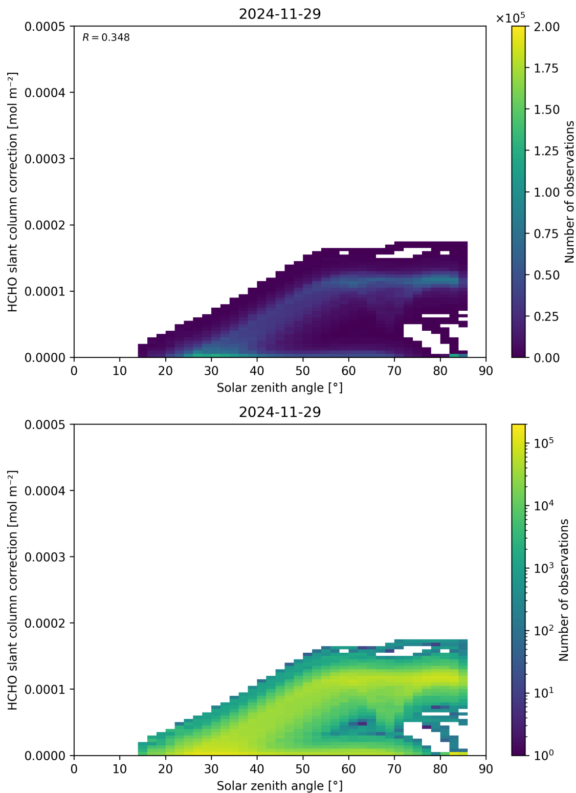
Figure 172: Scatter density plot of “Solar zenith angle” against “HCHO slant column correction” for 2024-11-28 to 2024-11-30.
