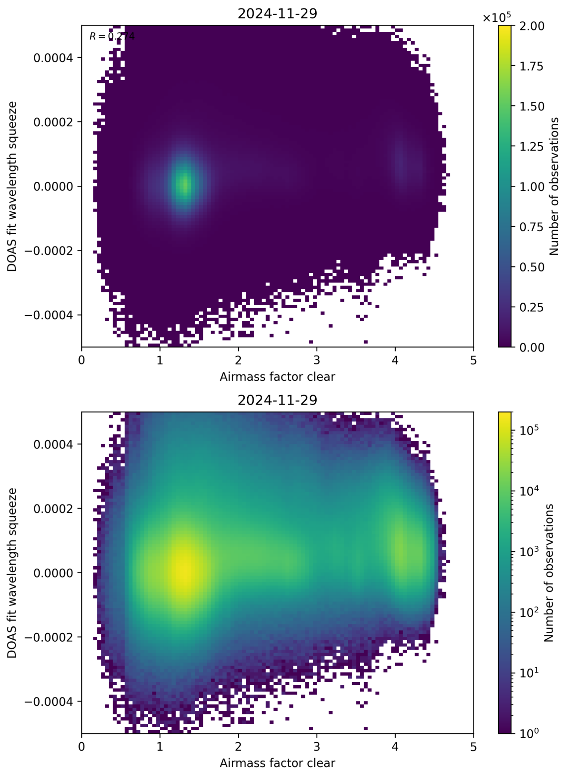
Figure 73: Scatter density plot of “Airmass factor clear” against “DOAS fit wavelength squeeze” for 2024-11-28 to 2024-11-30.
