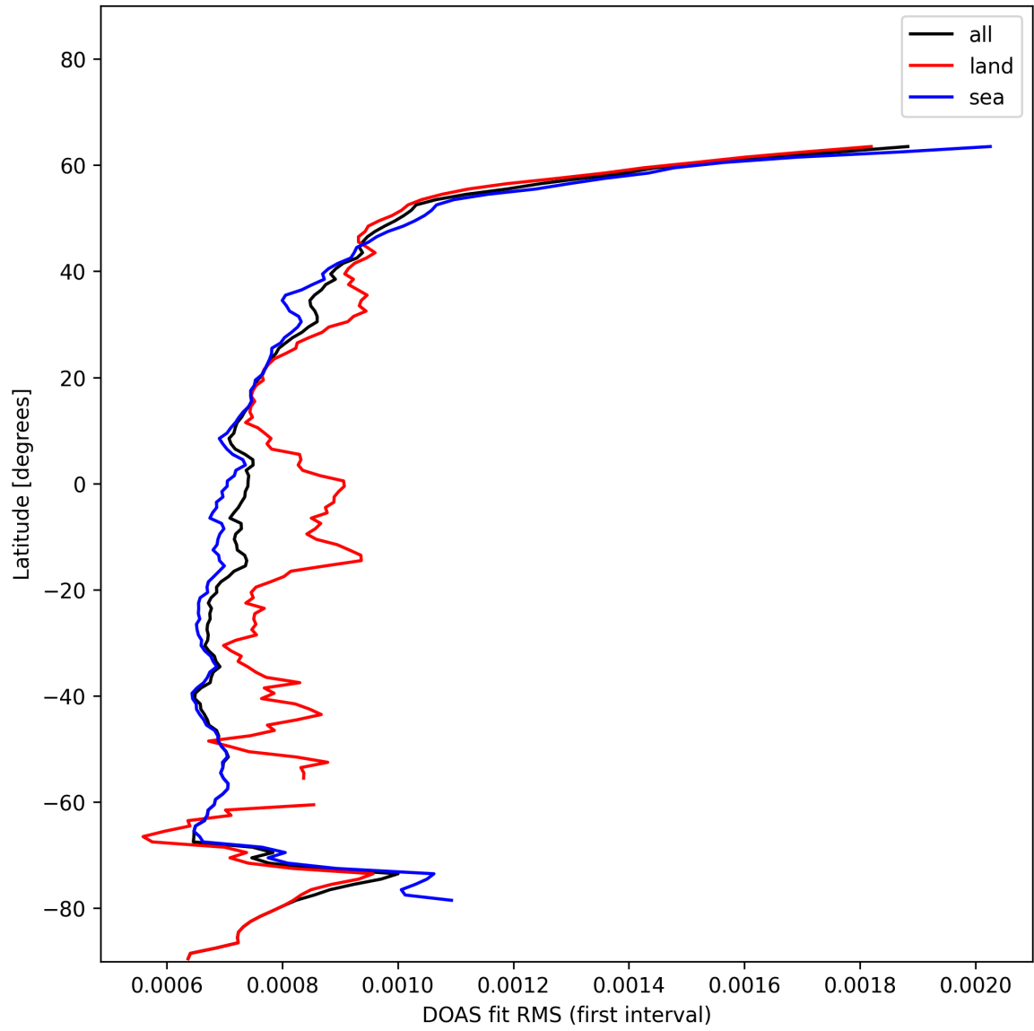
Figure 32: Zonal average of “DOAS fit RMS (first interval)” for 2024-11-28 to 2024-11-30.
