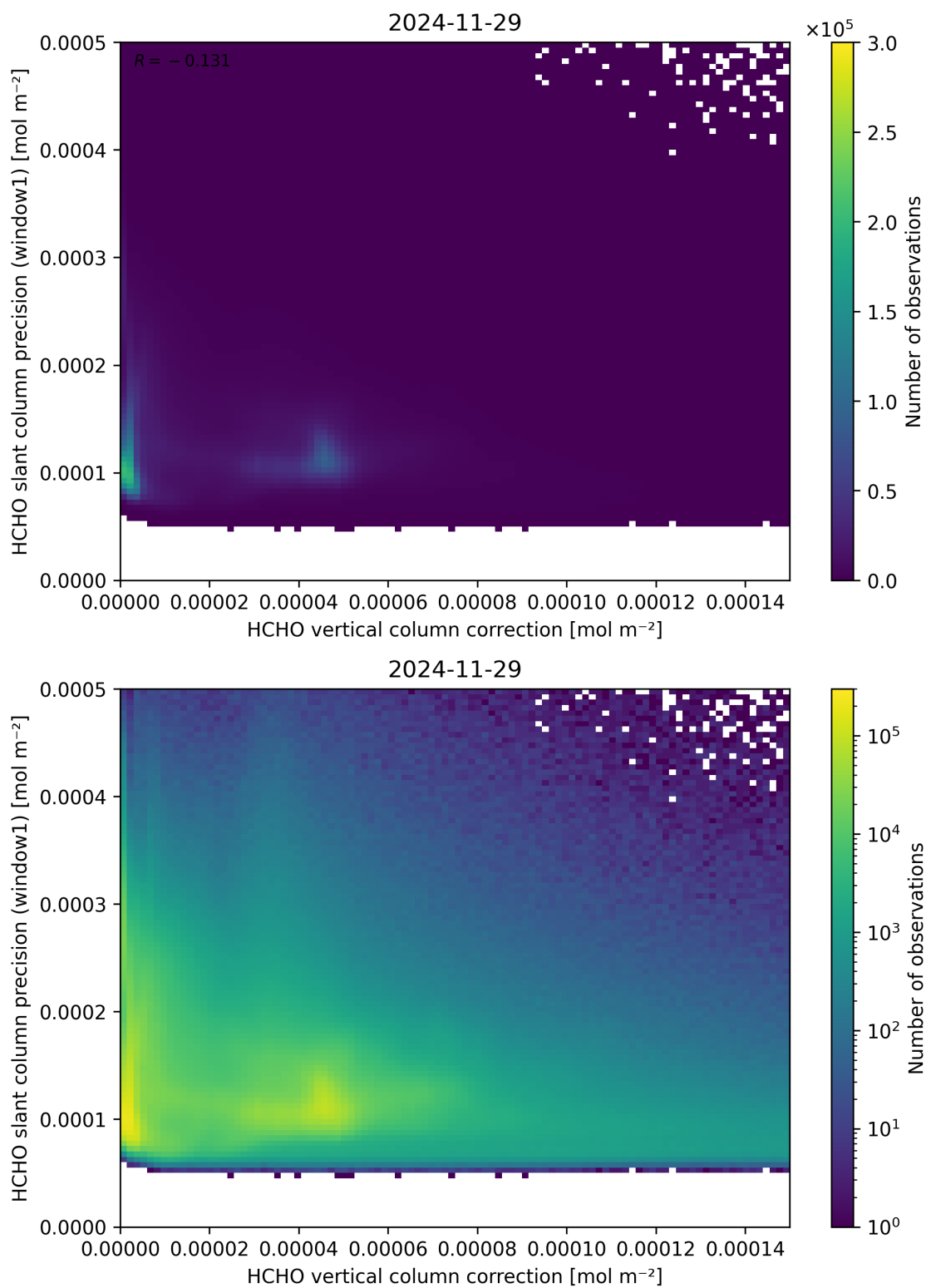
Figure 119: Scatter density plot of “HCHO vertical column correction” against “HCHO slant column precision (window1)” for 2024-11-28 to 2024-11-30.
