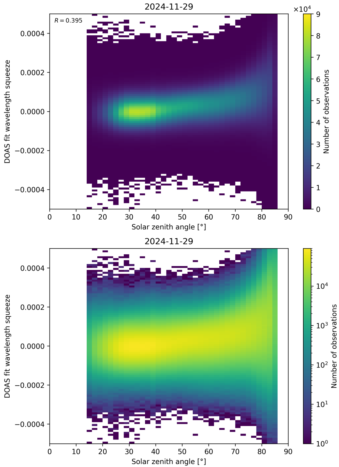
Figure 169: Scatter density plot of “Solar zenith angle” against “DOAS fit wavelength squeeze” for 2024-11-28 to 2024-11-30.
