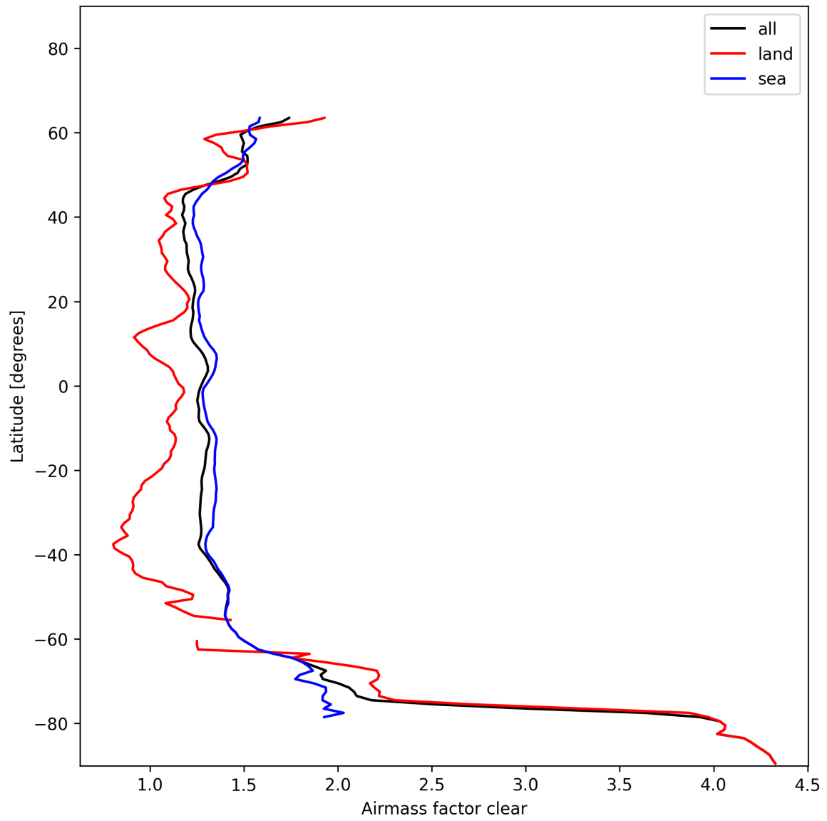
Figure 28: Zonal average of “Airmass factor clear” for 2024-11-28 to 2024-11-30.
