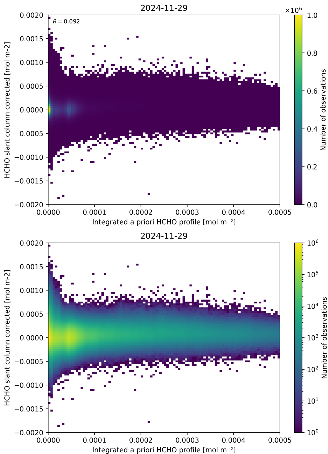
Figure 151: Scatter density plot of “Integrated a priori HCHO profile” against “HCHO slant column corrected” for 2024-11-28 to 2024-11-30.
