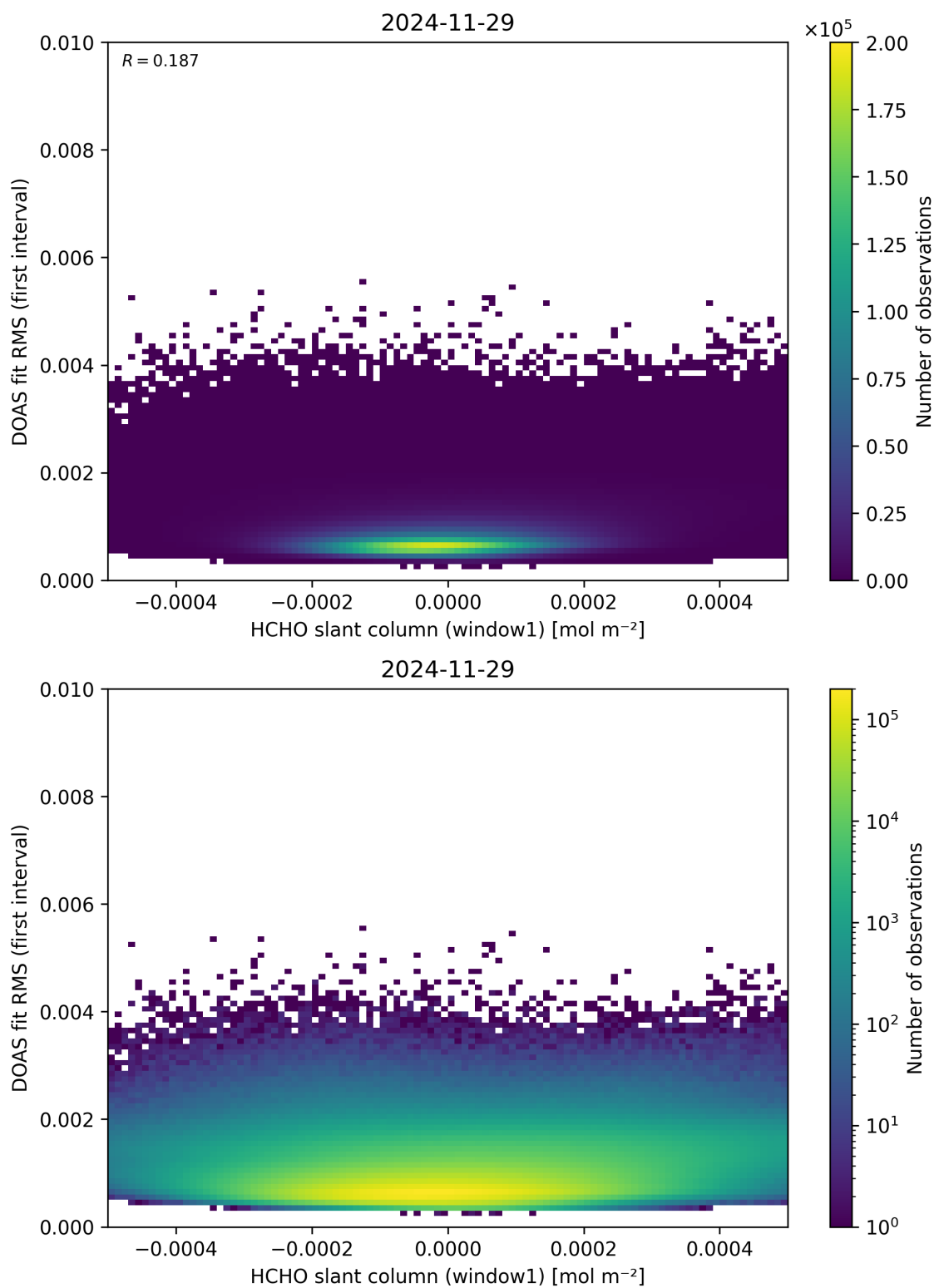
Figure 78: Scatter density plot of “HCHO slant column (window1)” against “DOAS fit RMS (first interval)” for 2024-11-28 to 2024-11-30.
