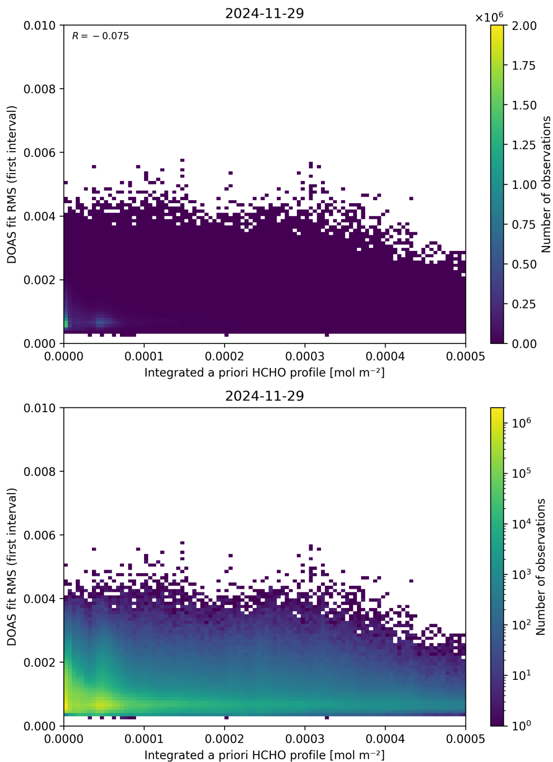
Figure 148: Scatter density plot of “Integrated a priori HCHO profile” against “DOAS fit RMS (first interval)” for 2024-11-28 to 2024-11-30.
