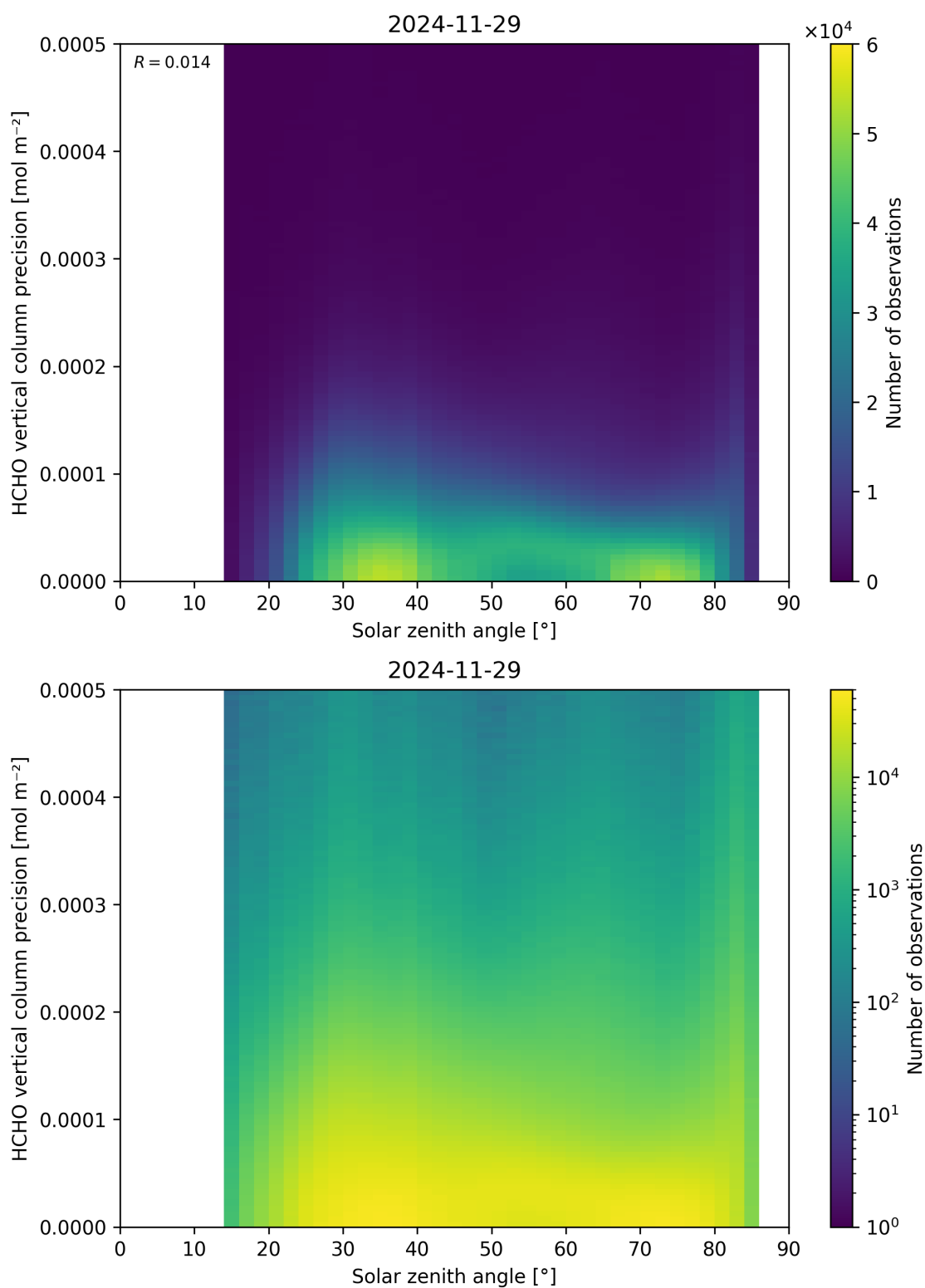
Figure 179: Scatter density plot of “Solar zenith angle” against “HCHO vertical column precision” for 2024-11-28 to 2024-11-30.
