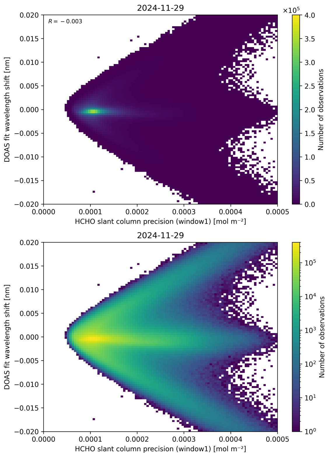
Figure 89: Scatter density plot of “HCHO slant column precision (window1)” against “DOAS fit wavelength shift” for 2024-11-28 to 2024-11-30.
