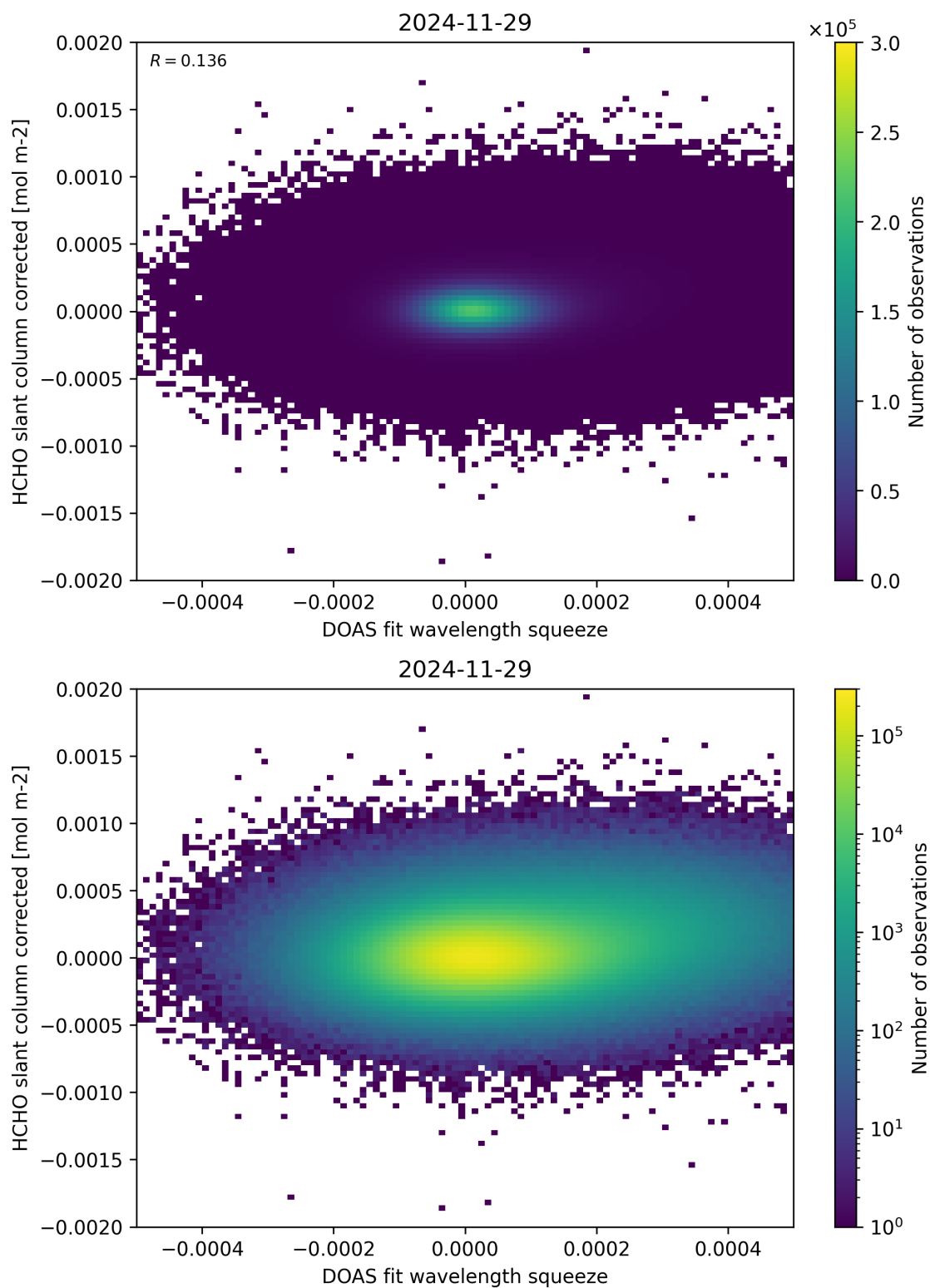
Figure 69: Scatter density plot of “DOAS fit wavelength squeeze” against “HCHO slant column corrected” for 2024-11-28 to 2024-11-30.
