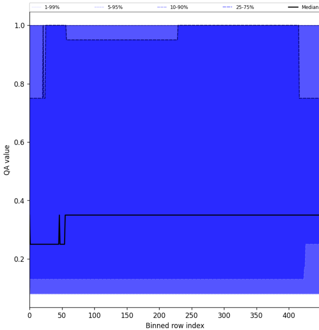
Figure 48: Along track statistics of “QA value” for 2024-11-28 to 2024-11-30
