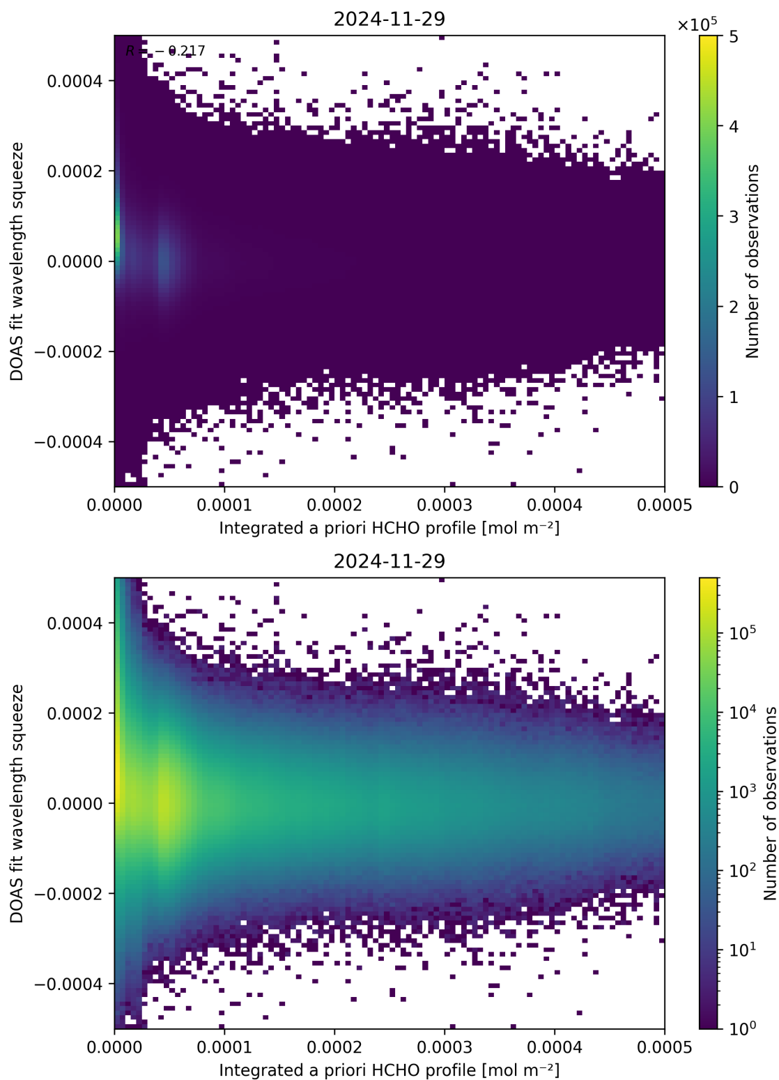
Figure 150: Scatter density plot of “Integrated a priori HCHO profile” against “DOAS fit wavelength squeeze” for 2024-11-28 to 2024-11-30.
