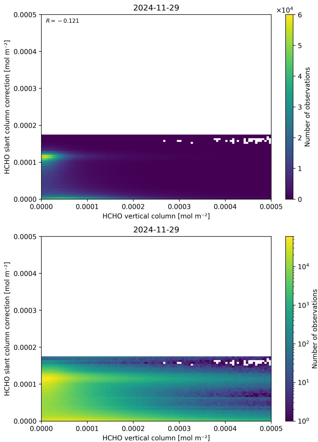
Figure 128: Scatter density plot of “HCHO vertical column” against “HCHO slant column correction” for 2024-11-28 to 2024-11-30.
