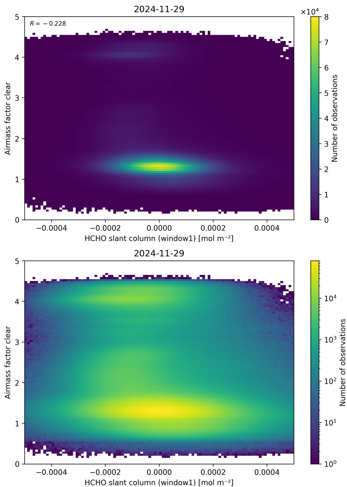
Figure 81: Scatter density plot of “HCHO slant column (window1)” against “Airmass factor clear” for 2024-11-28 to 2024-11-30.
