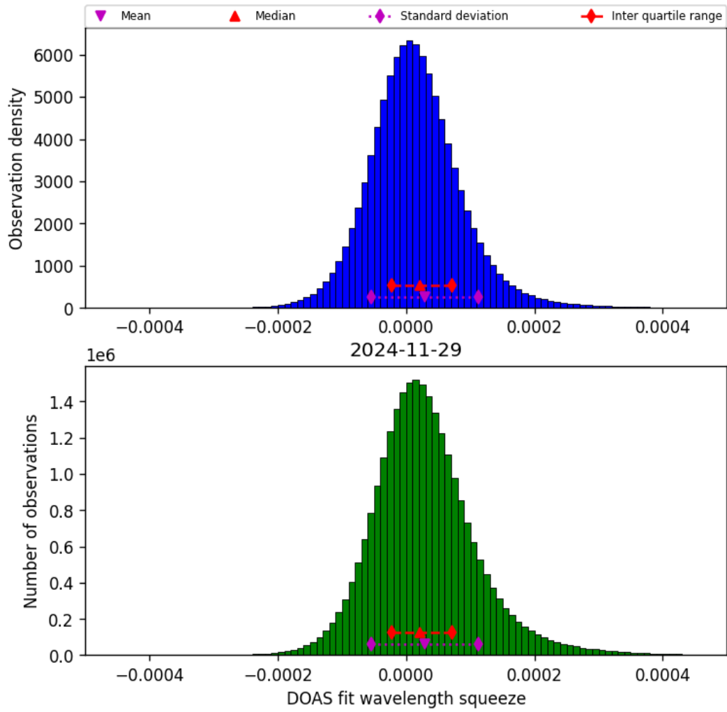
Figure 45: Histogram of “DOAS fit wavelength squeeze” for 2024-11-28 to 2024-11-30
