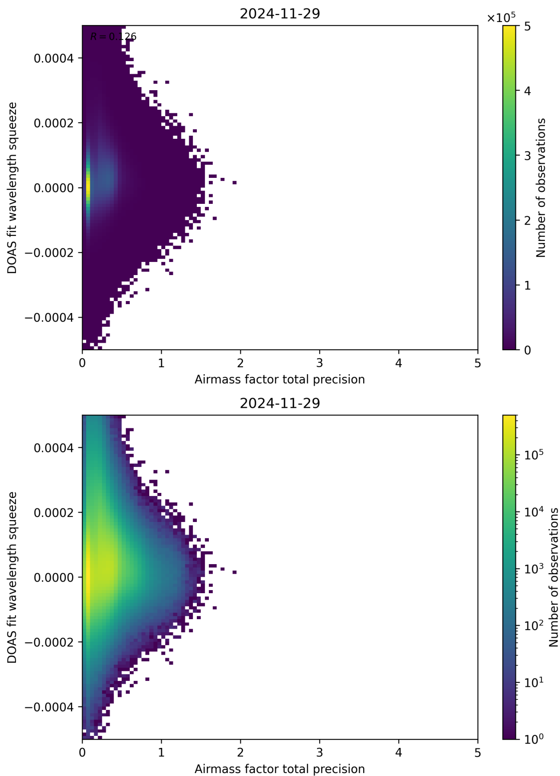
Figure 107: Scatter density plot of “Airmass factor total precision” against “DOAS fit wavelength squeeze” for 2024-11-28 to 2024-11-30.
