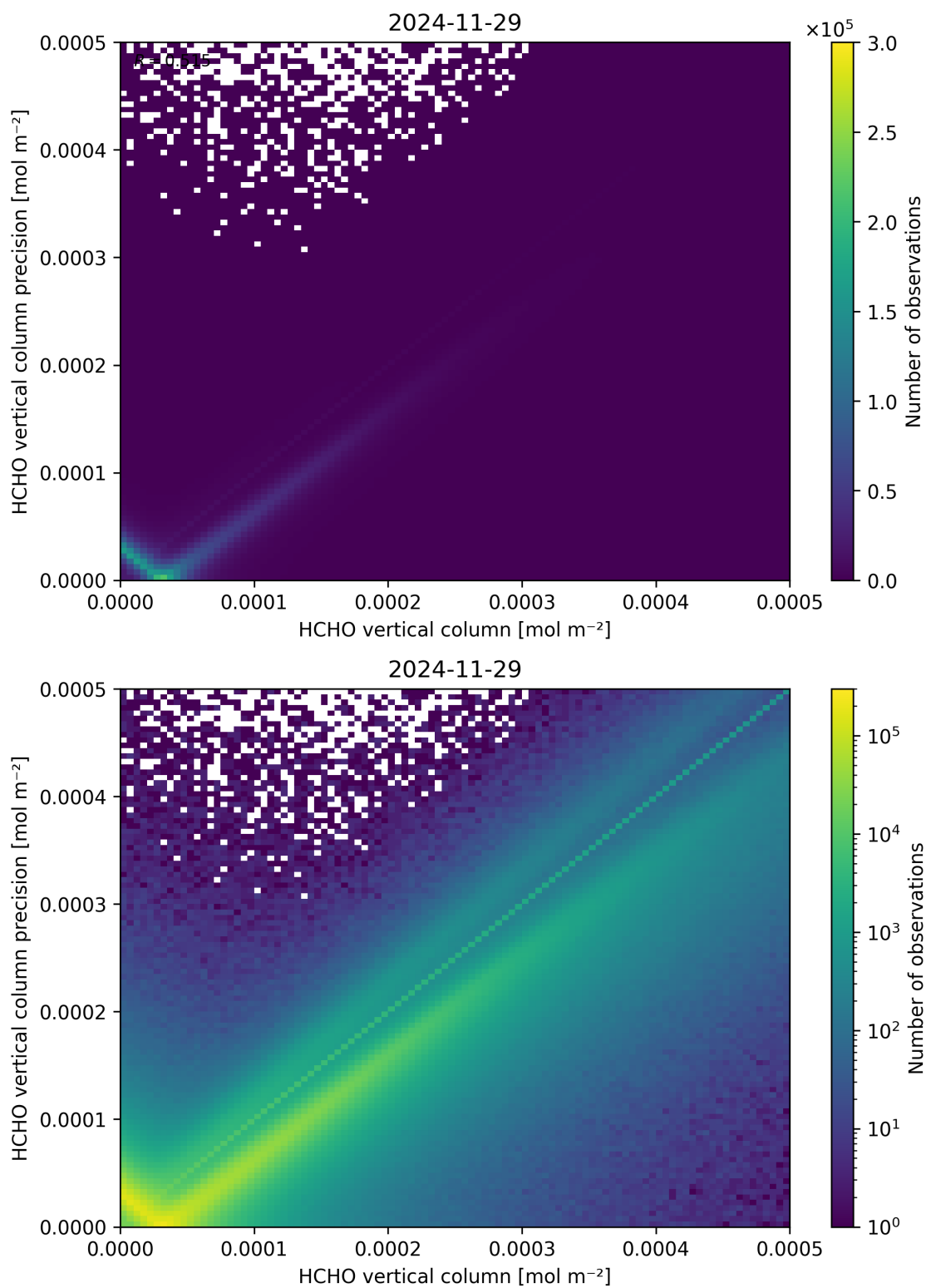
Figure 134: Scatter density plot of “HCHO vertical column” against “HCHO vertical column precision” for 2024-11-28 to 2024-11-30.
