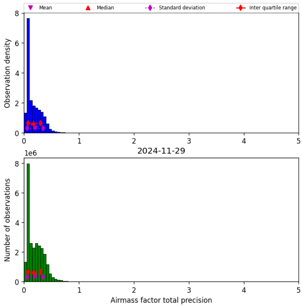
Figure 41: Histogram of “Airmass factor total precision” for 2024-11-28 to 2024-11-30
