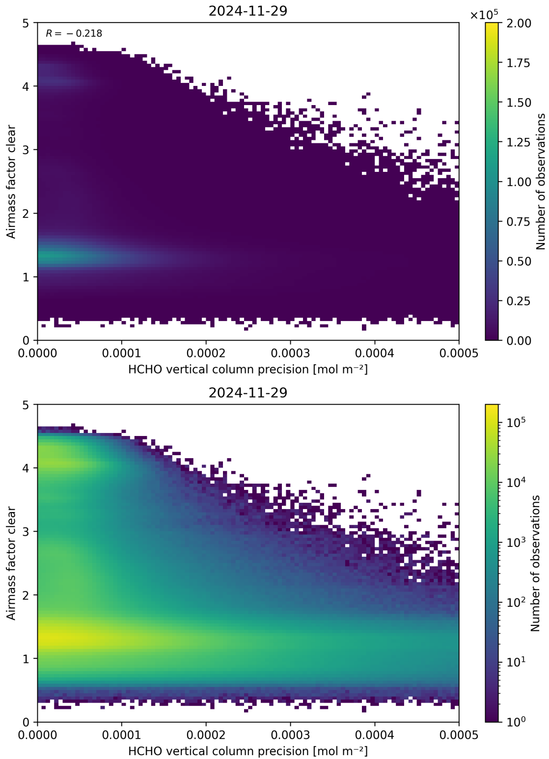
Figure 139: Scatter density plot of “HCHO vertical column precision” against “Airmass factor clear” for 2024-11-28 to 2024-11-30.
