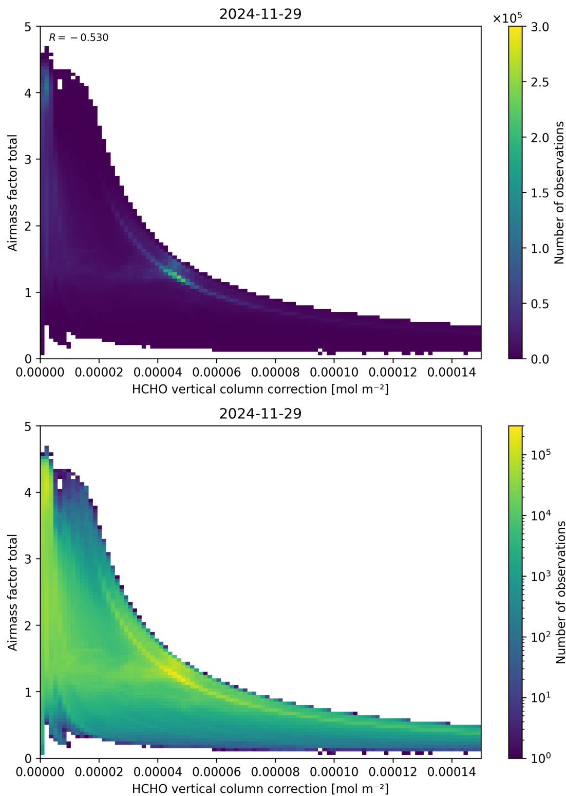
Figure 120: Scatter density plot of “HCHO vertical column correction” against “Airmass factor total” for 2024-11-28 to 2024-11-30.
