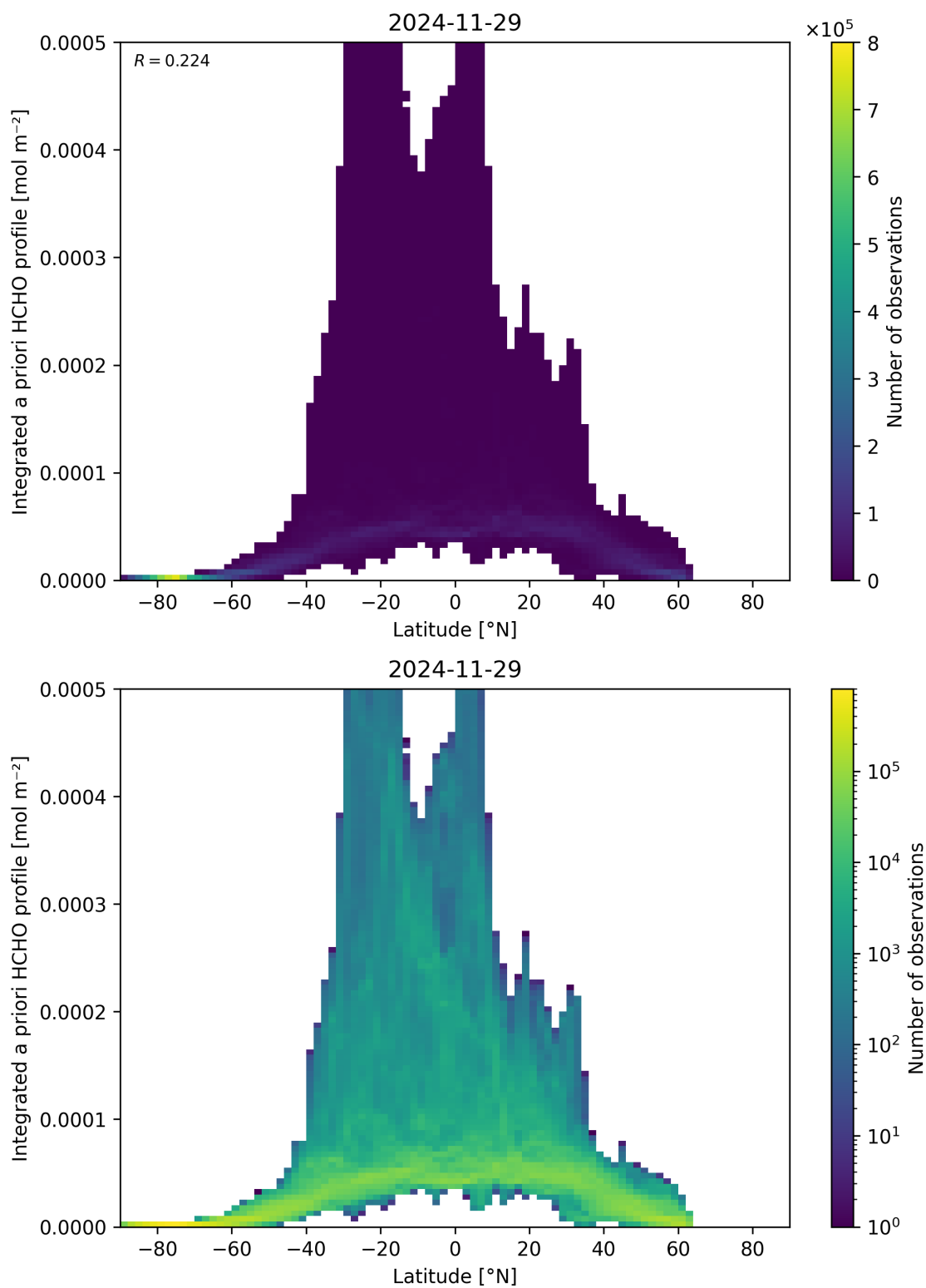
Figure 166: Scatter density plot of “Latitude” against “Integrated a priori HCHO profile” for 2024-11-28 to 2024-11-30.
