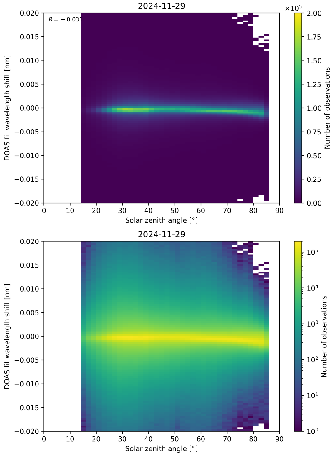
Figure 168: Scatter density plot of “Solar zenith angle” against “DOAS fit wavelength shift” for 2024-11-28 to 2024-11-30.
