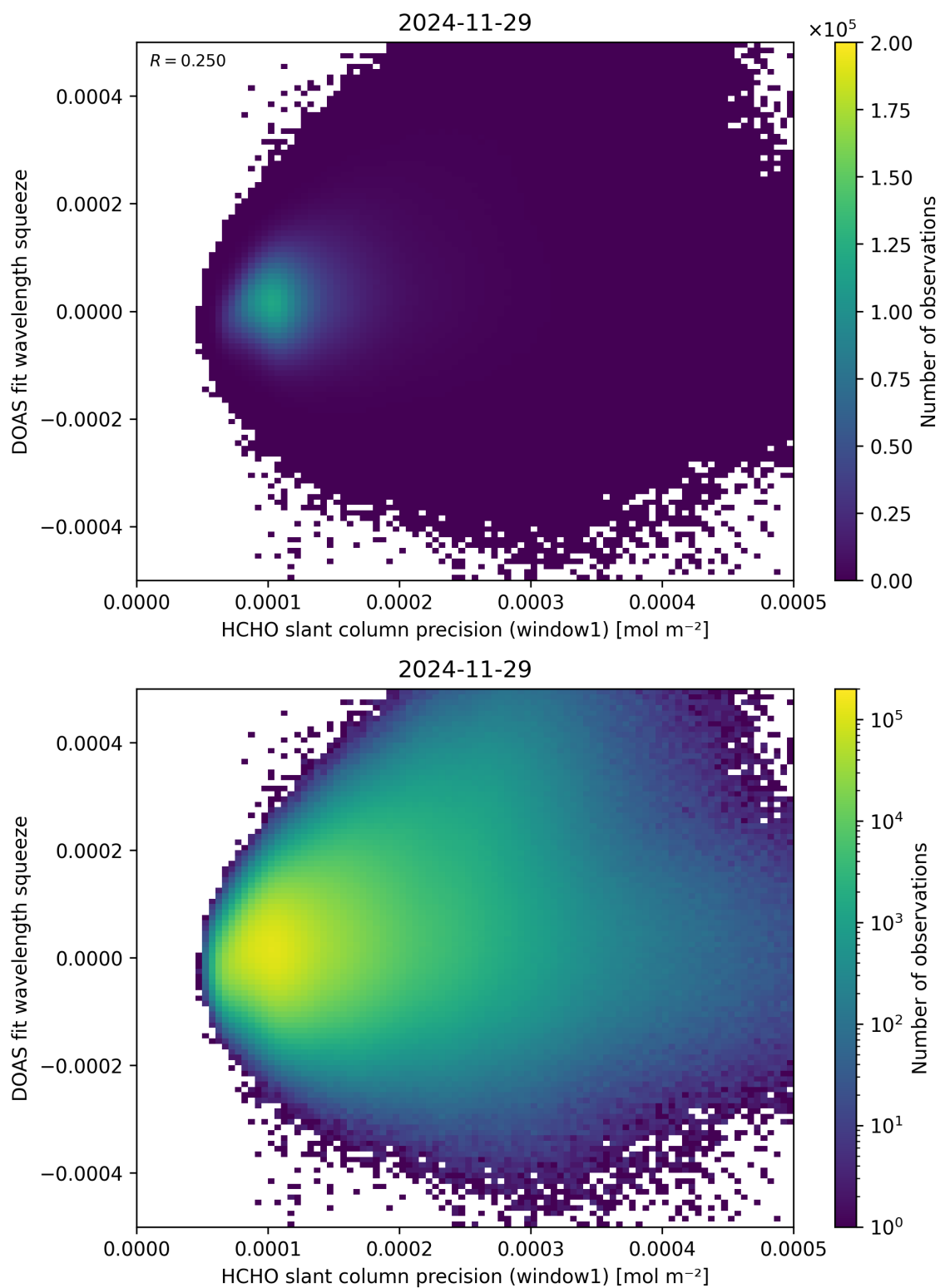
Figure 90: Scatter density plot of “HCHO slant column precision (window1)” against “DOAS fit wavelength squeeze” for 2024-11-28 to 2024-11-30.
