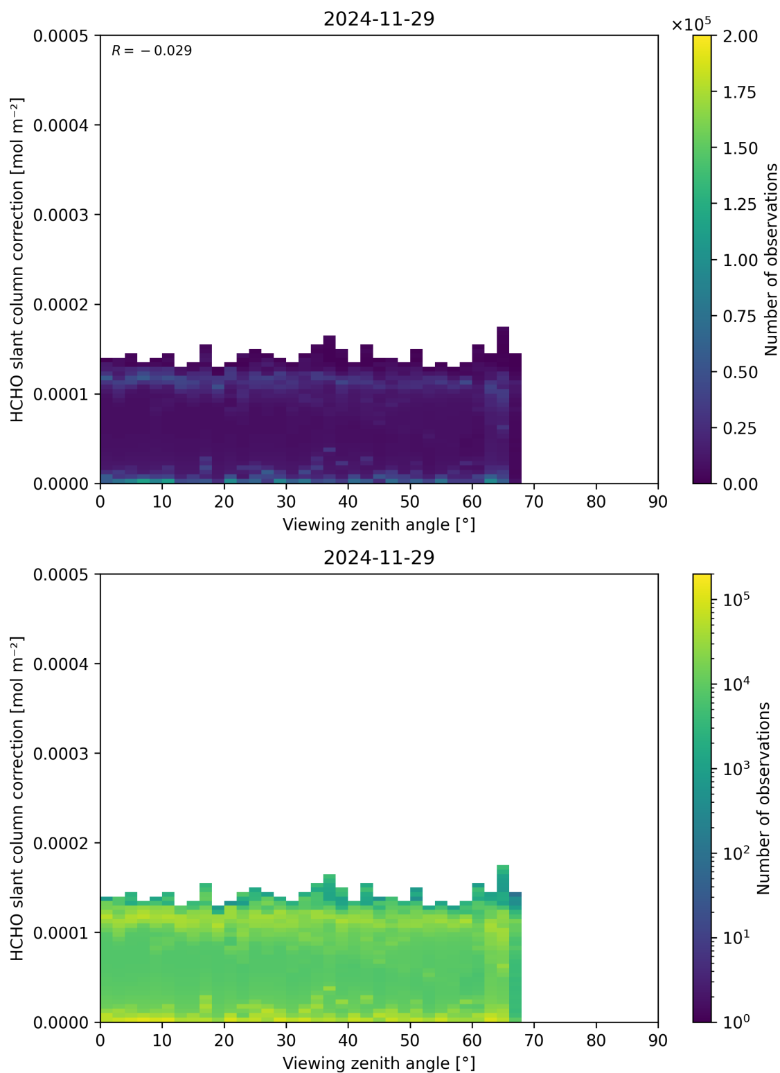
Figure 187: Scatter density plot of “Viewing zenith angle” against “HCHO slant column correction” for 2024-11-28 to 2024-11-30.
