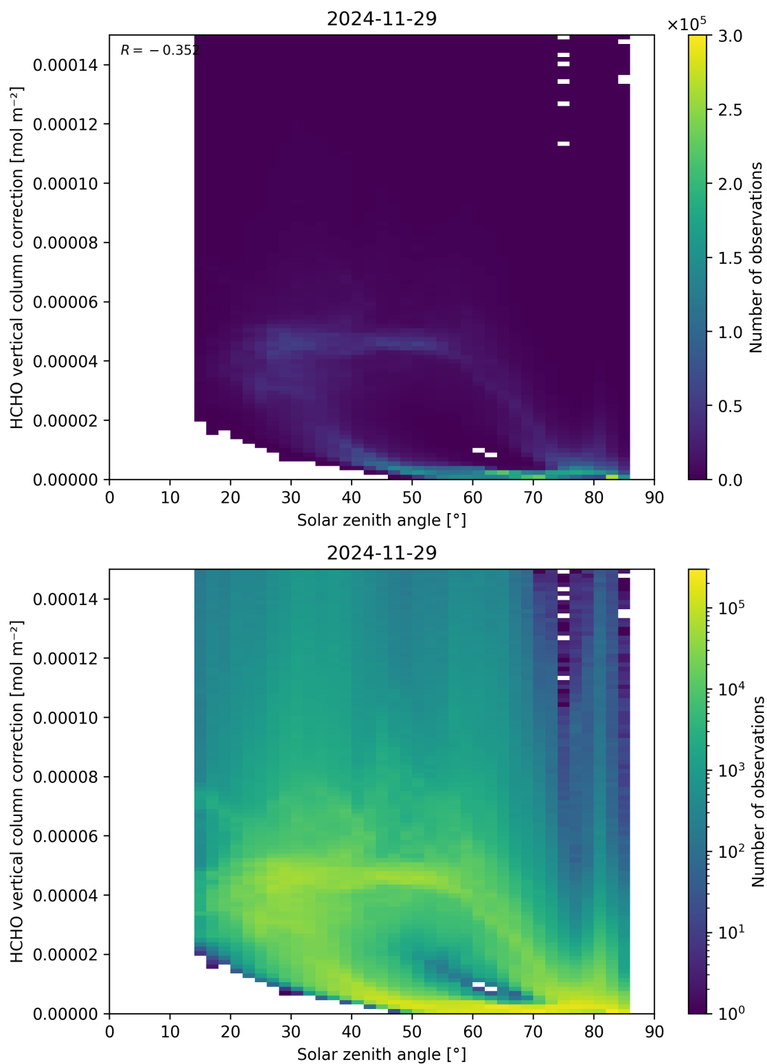
Figure 178: Scatter density plot of “Solar zenith angle” against “HCHO vertical column correction” for 2024-11-28 to 2024-11-30.
