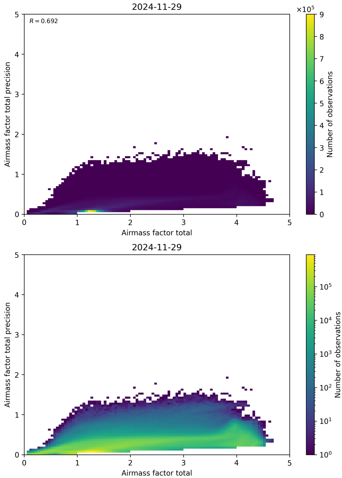
Figure 103: Scatter density plot of “Airmass factor total” against “Airmass factor total precision” for 2024-11-28 to 2024-11-30.
