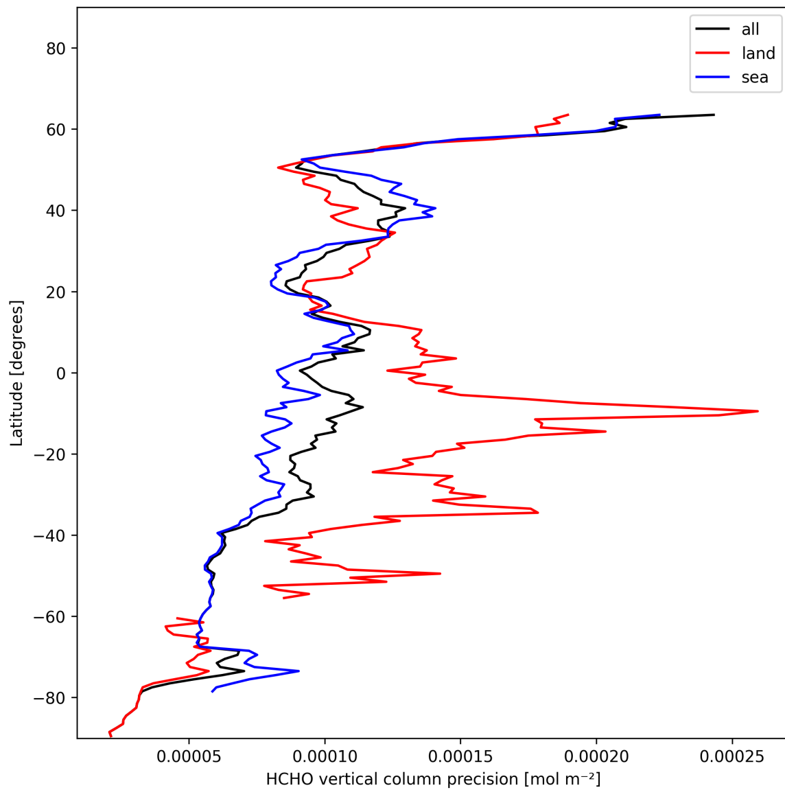
Figure 22: Zonal average of “HCHO vertical column precision” for 2024-11-28 to 2024-11-30.
