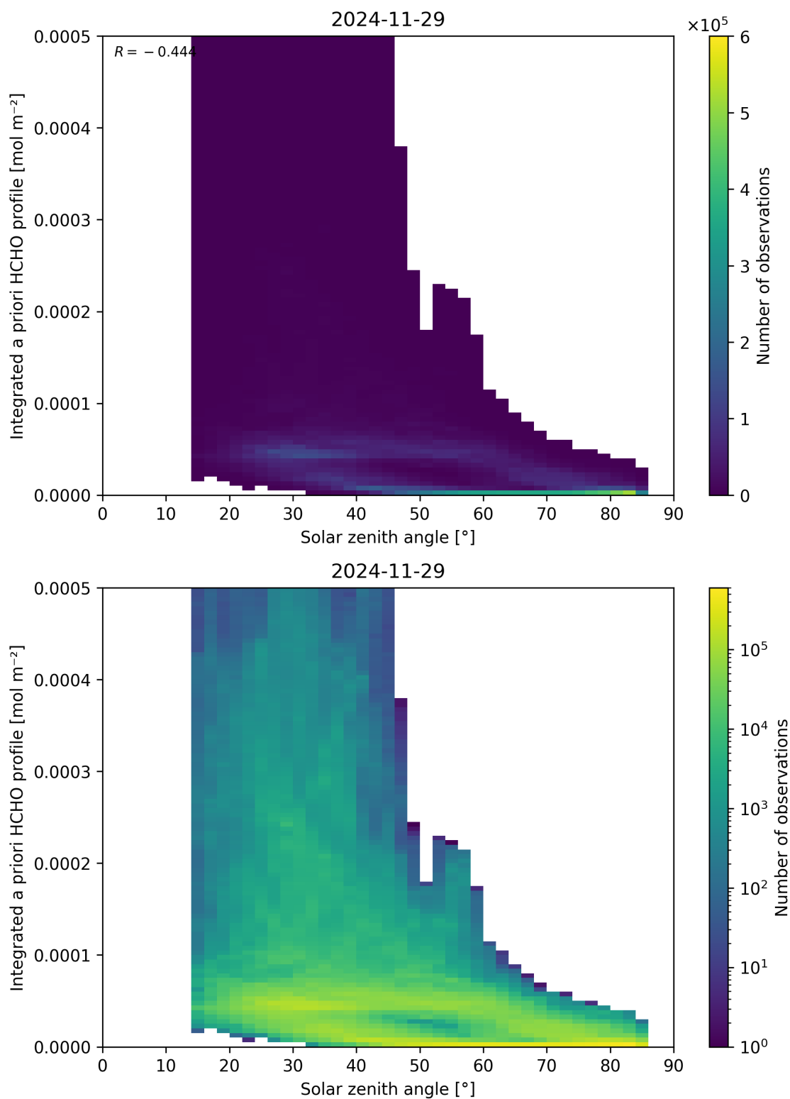
Figure 180: Scatter density plot of “Solar zenith angle” against “Integrated a priori HCHO profile” for 2024-11-28 to 2024-11-30.
