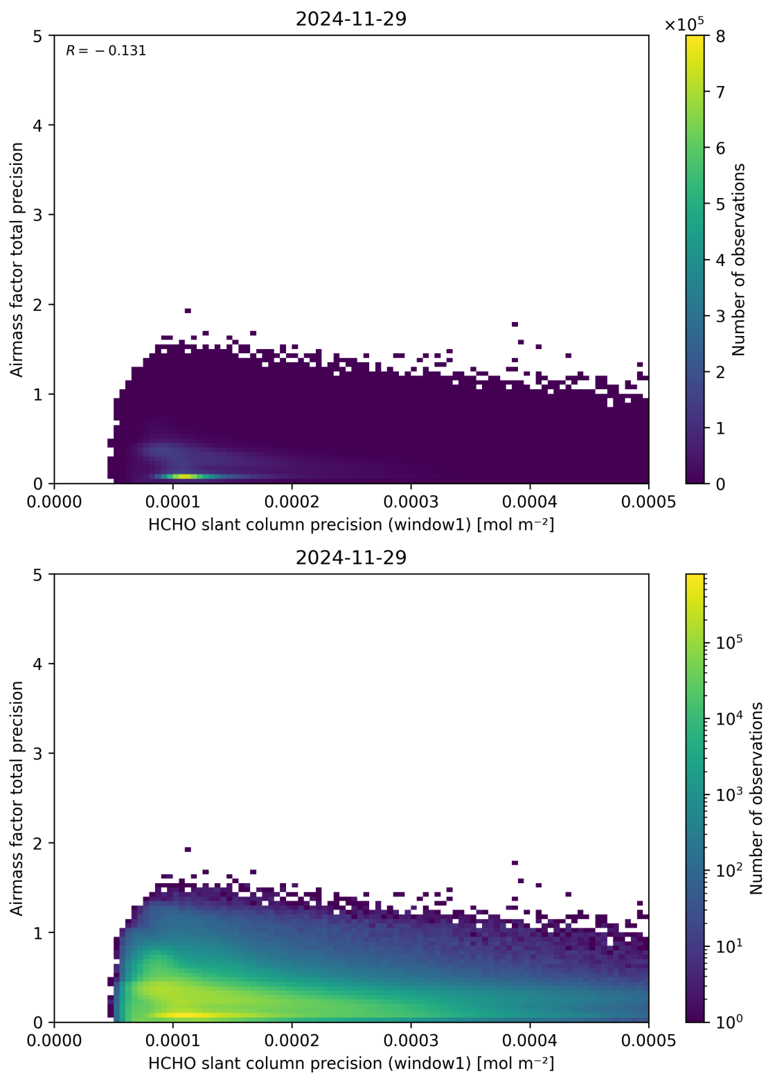
Figure 95: Scatter density plot of “HCHO slant column precision (window1)” against “Airmass factor total precision” for 2024-11-28 to 2024-11-30.
