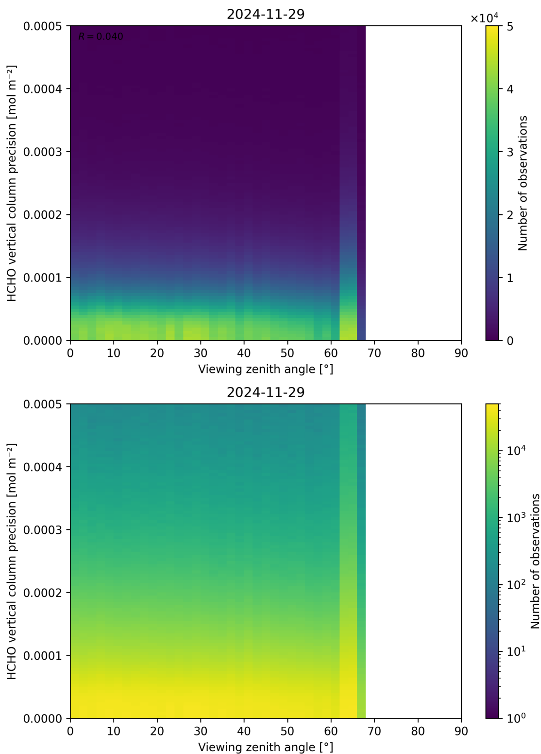
Figure 194: Scatter density plot of “Viewing zenith angle” against “HCHO vertical column precision” for 2024-11-28 to 2024-11-30.
