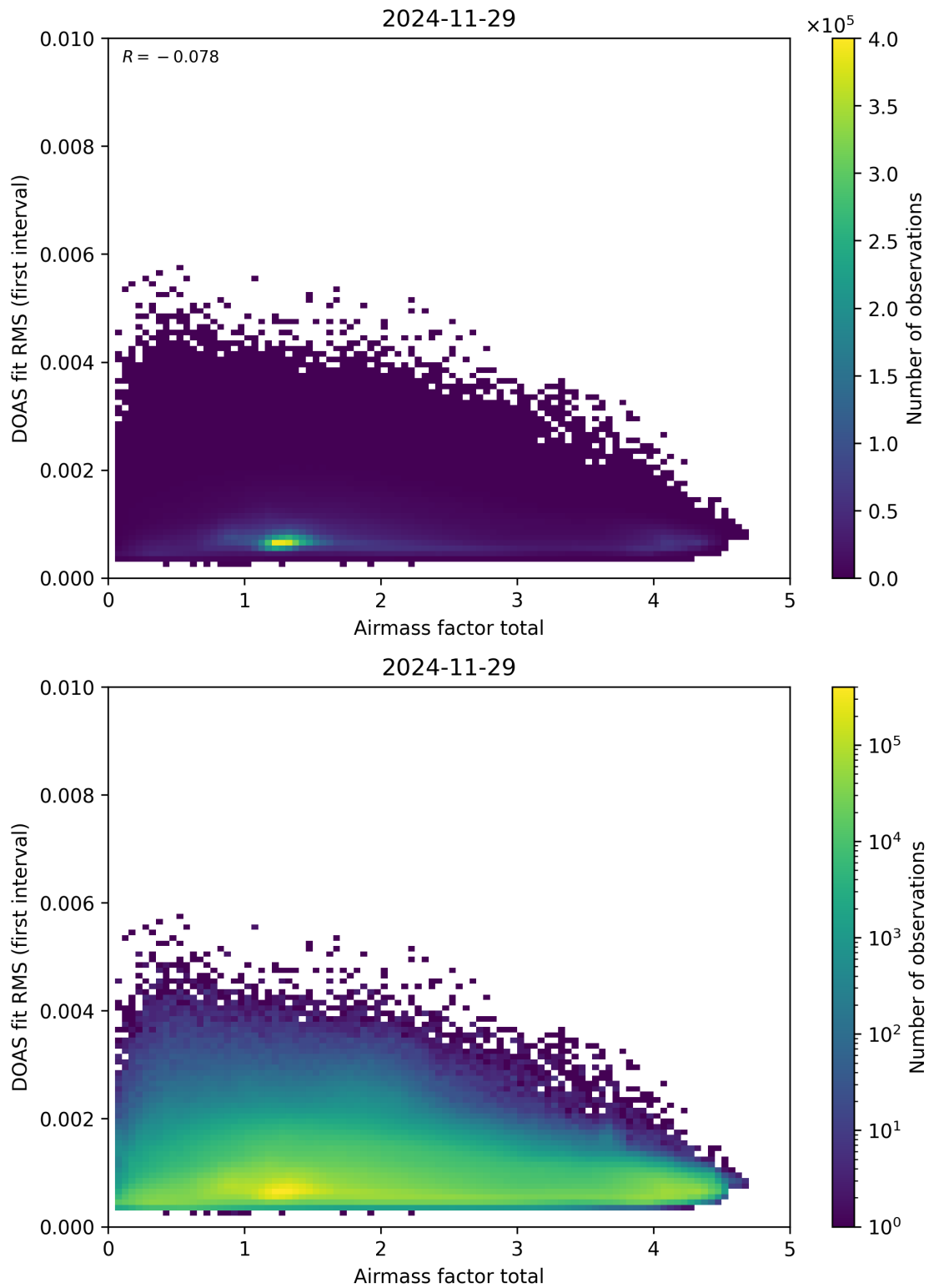
Figure 97: Scatter density plot of “Airmass factor total” against “DOAS fit RMS (first interval)” for 2024-11-28 to 2024-11-30.
