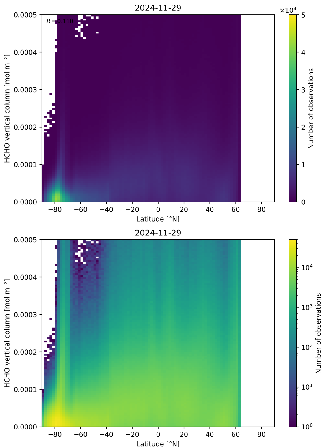
Figure 163: Scatter density plot of “Latitude” against “HCHO vertical column” for 2024-11-28 to 2024-11-30.
