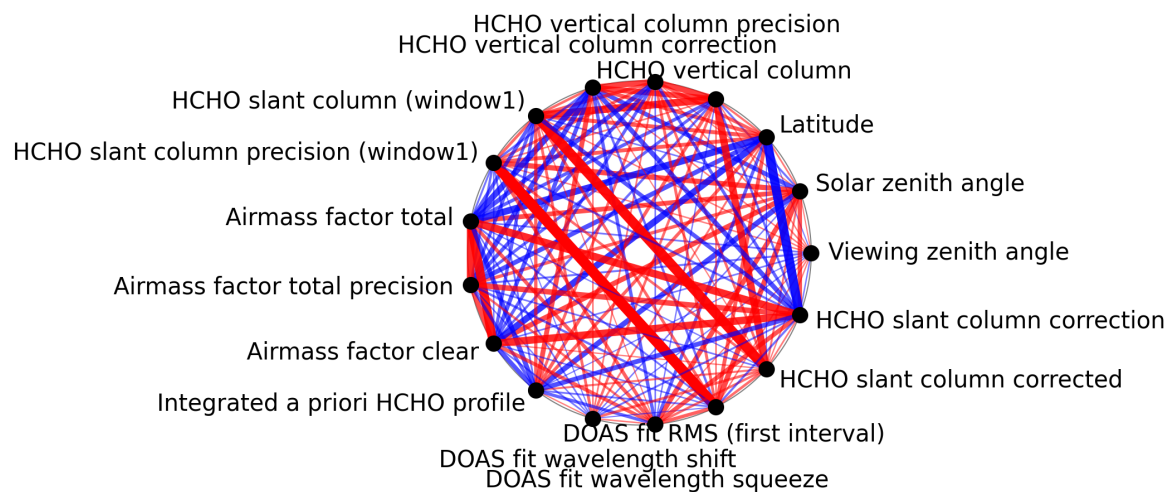
Figure 1: Map of correlation graph for 2024-11-28 to 2024-11-30.
