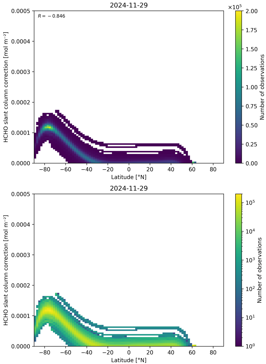
Figure 158: Scatter density plot of “Latitude” against “HCHO slant column correction” for 2024-11-28 to 2024-11-30.
