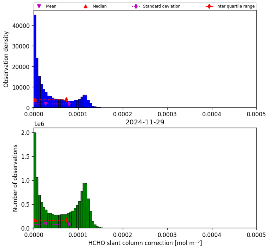
Figure 47: Histogram of “HCHO slant column correction” for 2024-11-28 to 2024-11-30
