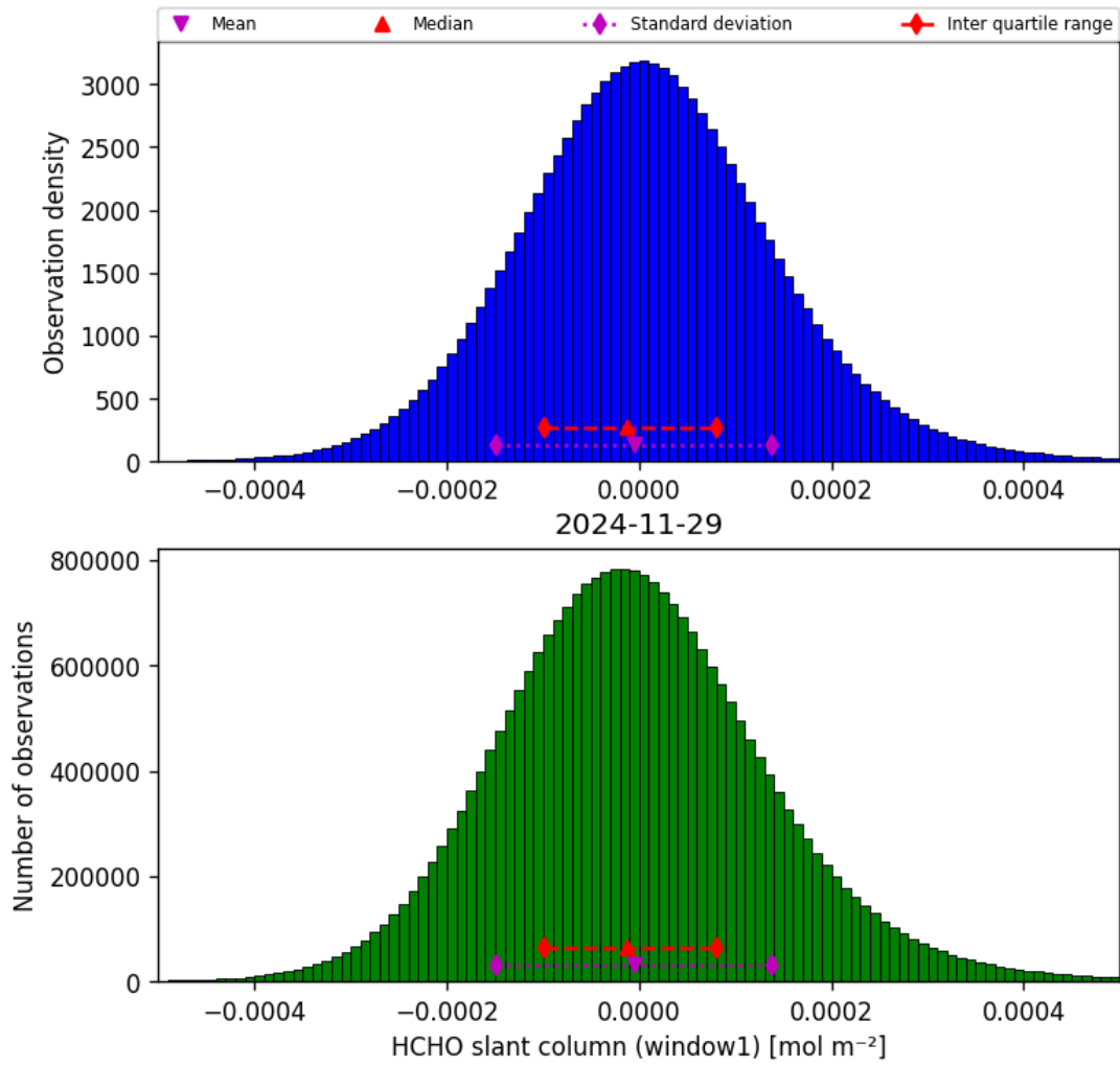
Figure 38: Histogram of “HCHO slant column (window1)” for 2024-11-28 to 2024-11-30
