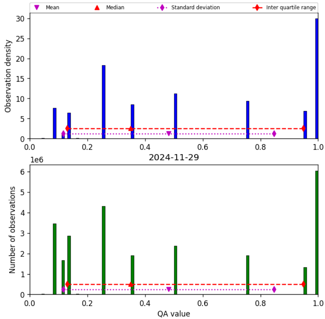
Figure 34: Histogram of “QA value” for 2024-11-28 to 2024-11-30
