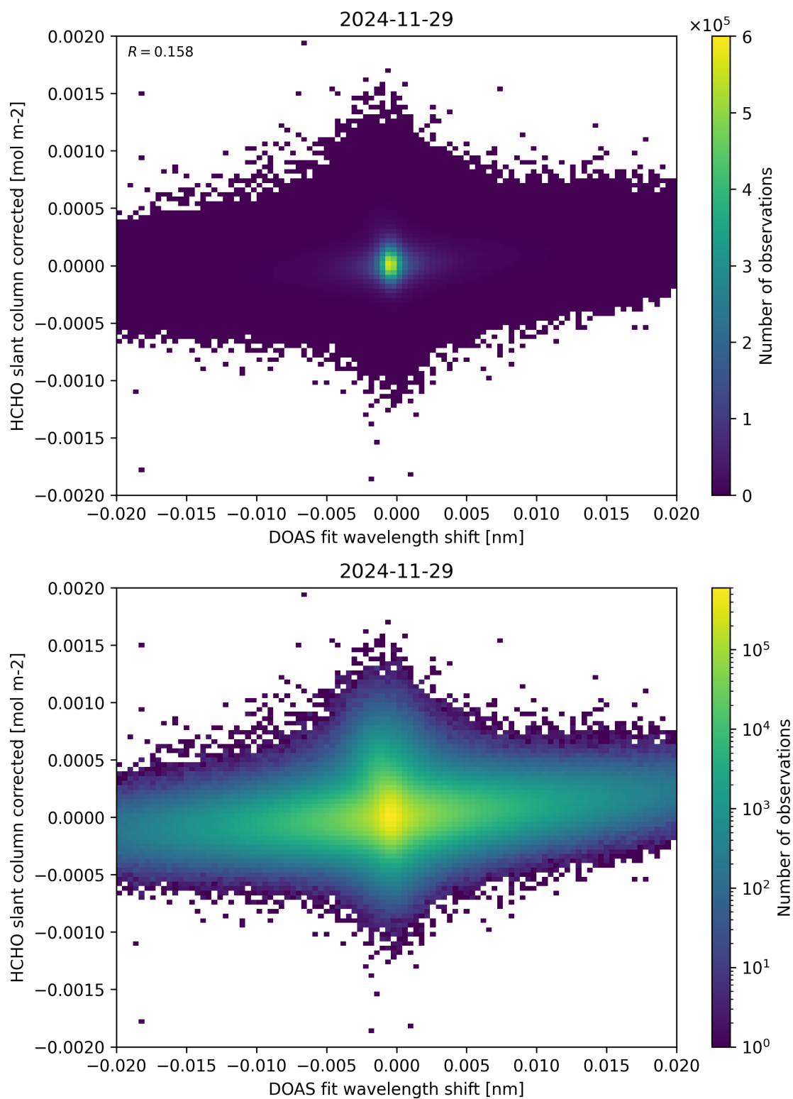
Figure 66: Scatter density plot of “DOAS fit wavelength shift” against “HCHO slant column corrected” for 2024-11-28 to 2024-11-30.
