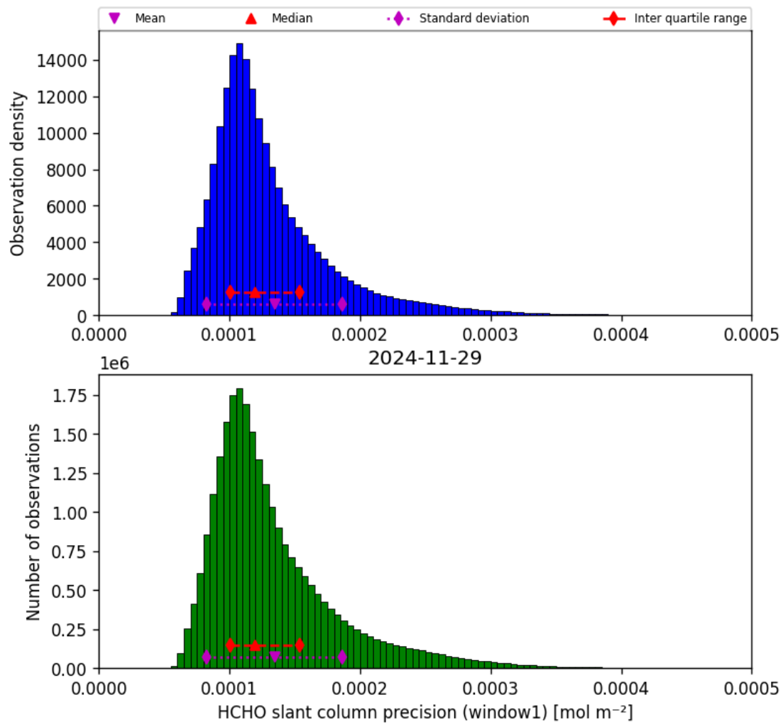
Figure 39: Histogram of “HCHO slant column precision (window1)” for 2024-11-28 to 2024-11-30
