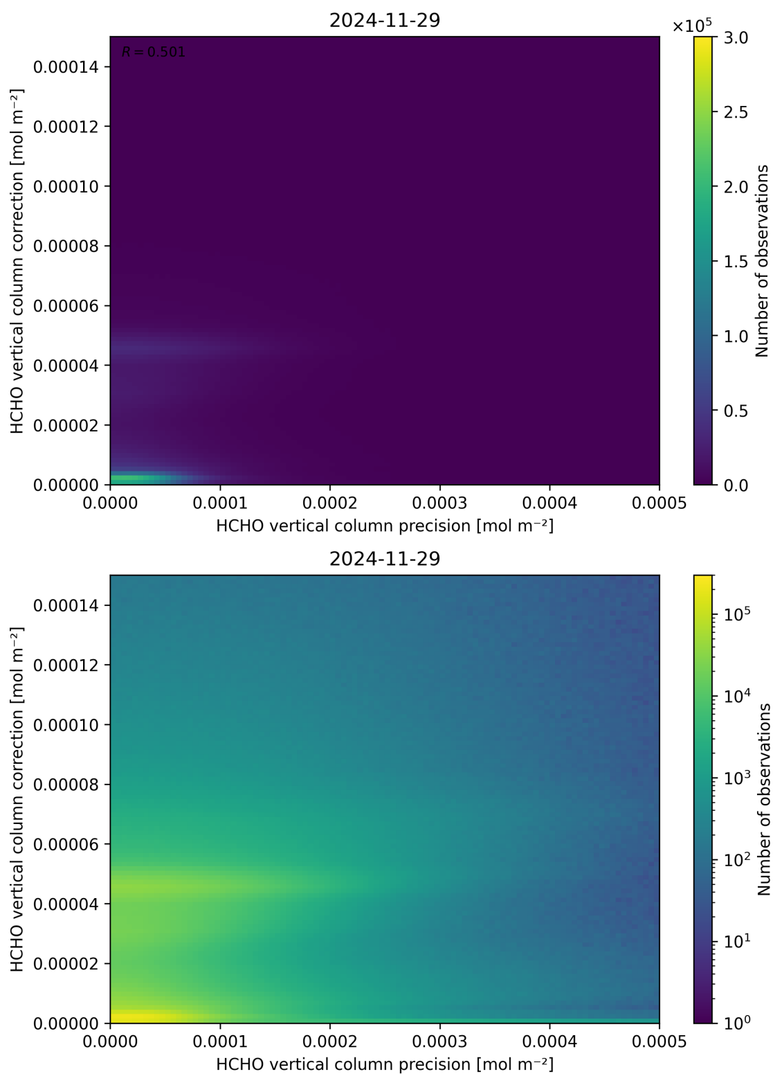
Figure 146: Scatter density plot of “HCHO vertical column precision” against “HCHO vertical column correction” for 2024-11-28 to 2024-11-30.
