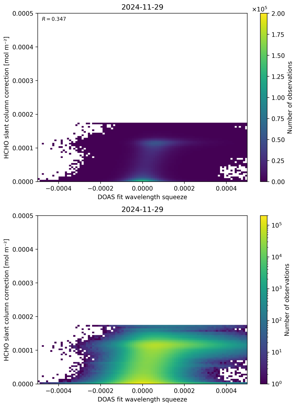
Figure 70: Scatter density plot of “DOAS fit wavelength squeeze” against “HCHO slant column correction” for 2024-11-28 to 2024-11-30.
