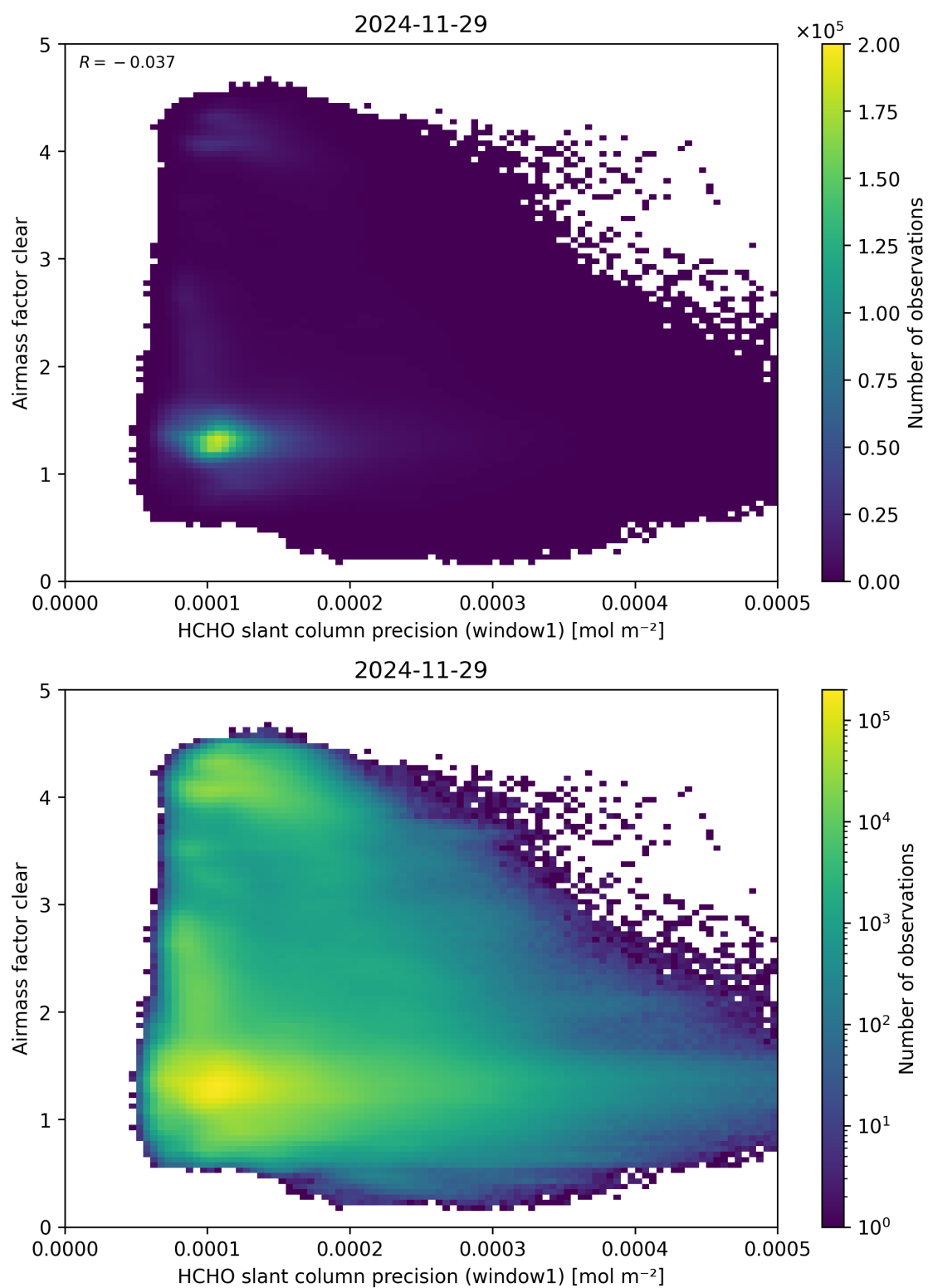
Figure 91: Scatter density plot of “HCHO slant column precision (window1)” against “Airmass factor clear” for 2024-11-28 to 2024-11-30.
