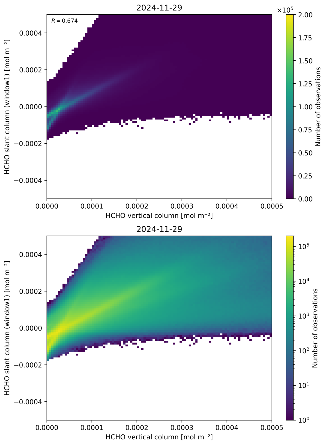
Figure 129: Scatter density plot of “HCHO vertical column” against “HCHO slant column (window1)” for 2024-11-28 to 2024-11-30.
