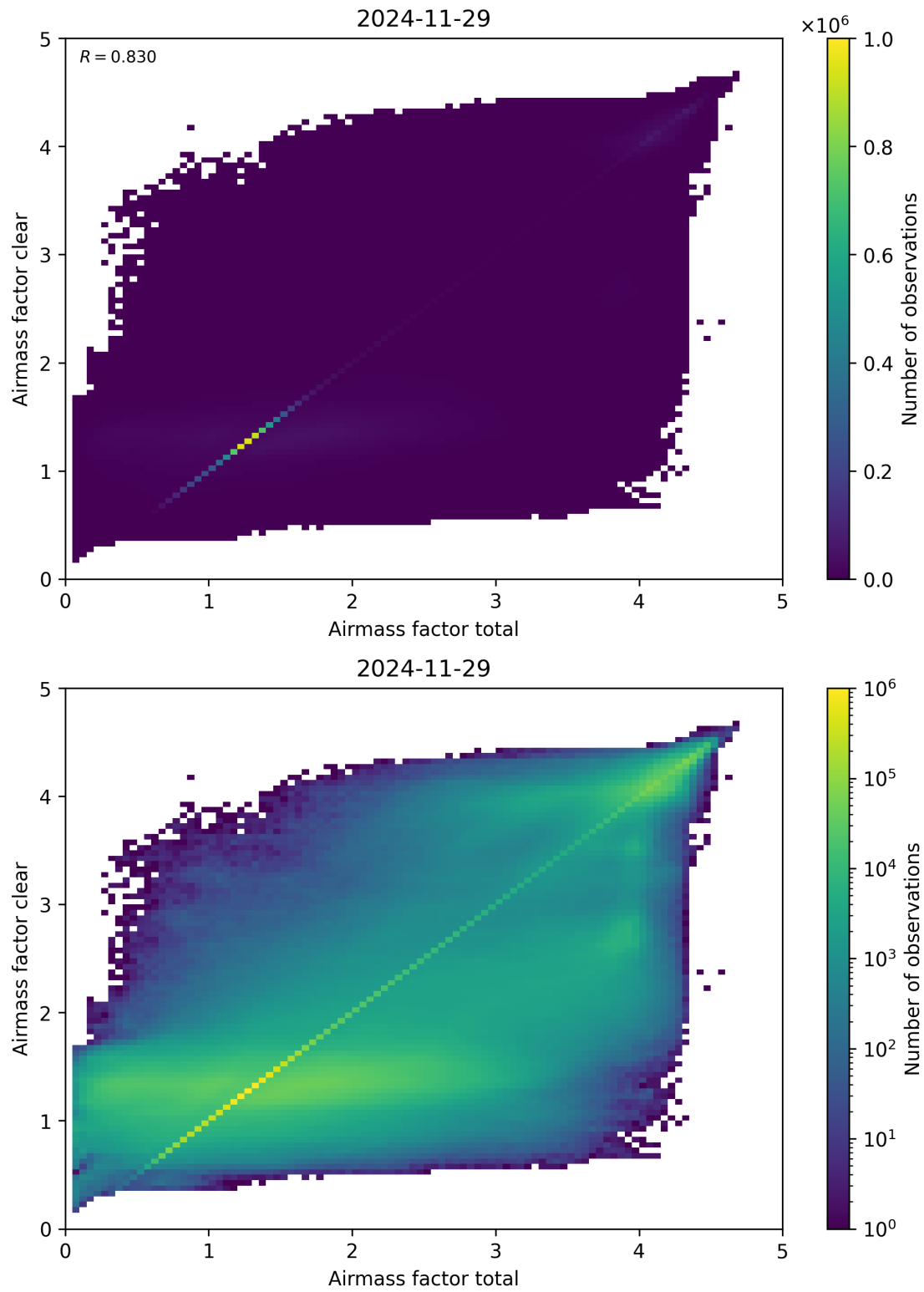
Figure 100: Scatter density plot of “Airmass factor total” against “Airmass factor clear” for 2024-11-28 to 2024-11-30.
