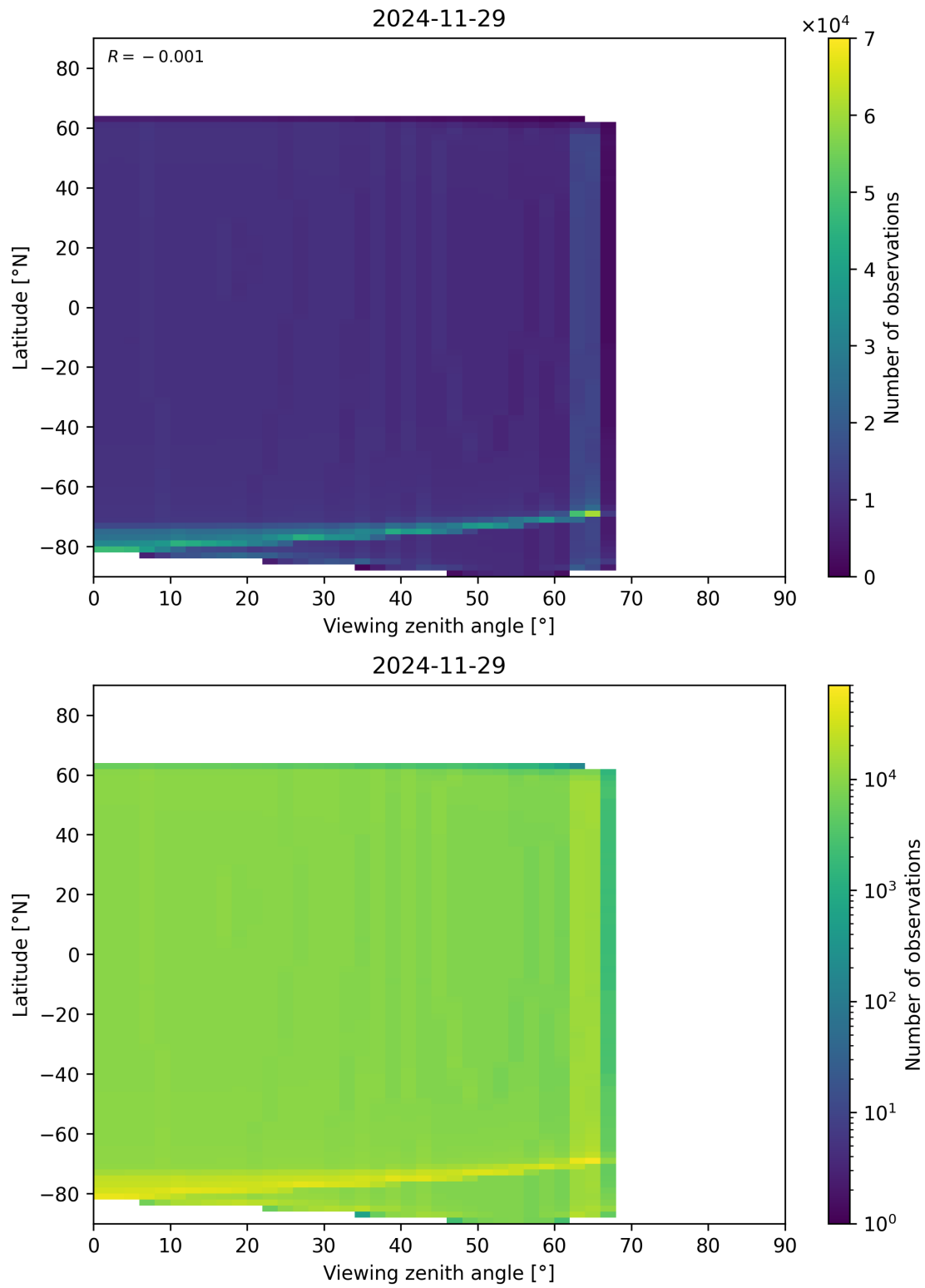
Figure 196: Scatter density plot of “Viewing zenith angle” against “Latitude” for 2024-11-28 to 2024-11-30.
