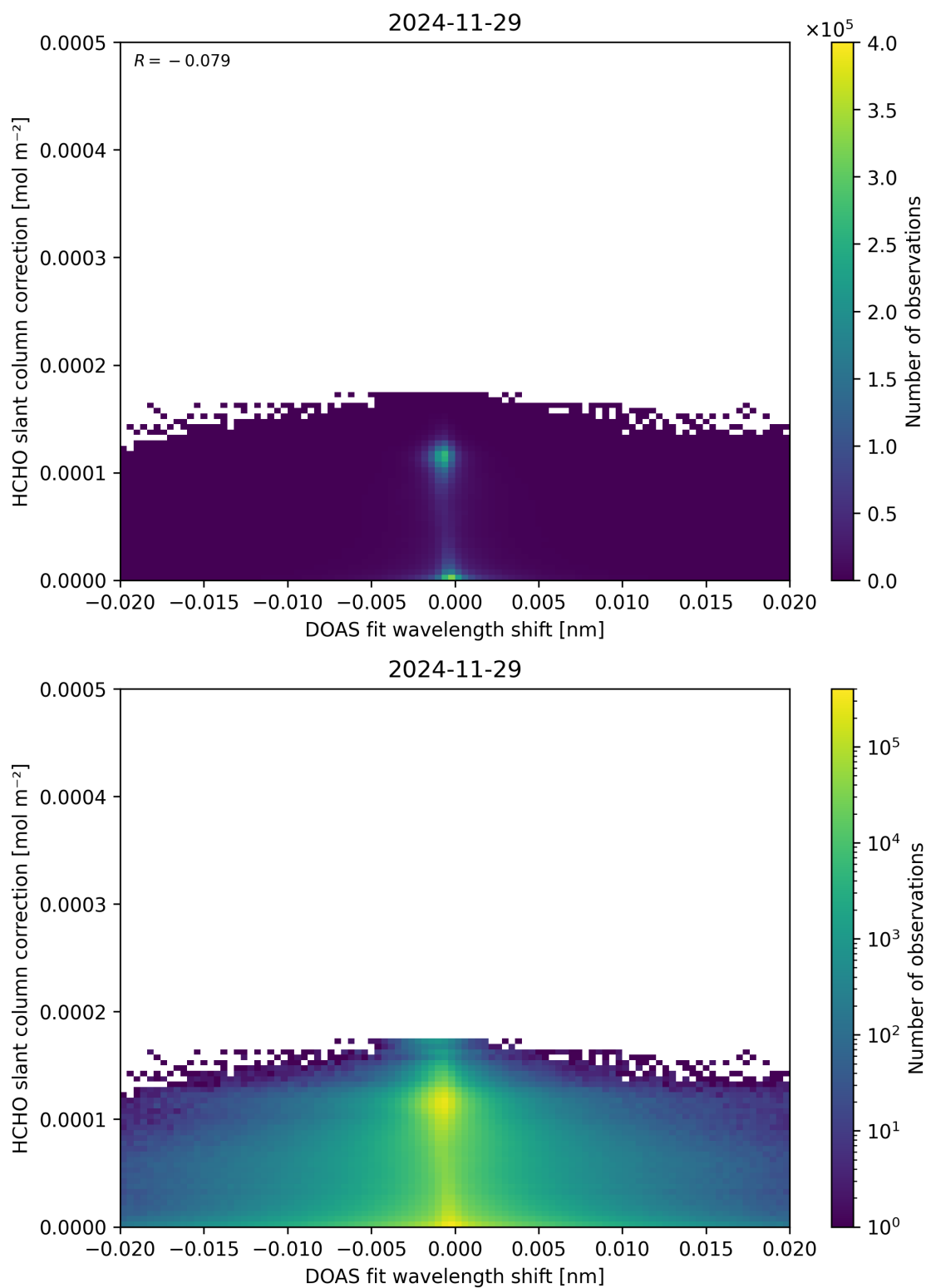
Figure 67: Scatter density plot of “DOAS fit wavelength shift” against “HCHO slant column correction” for 2024-11-28 to 2024-11-30.
