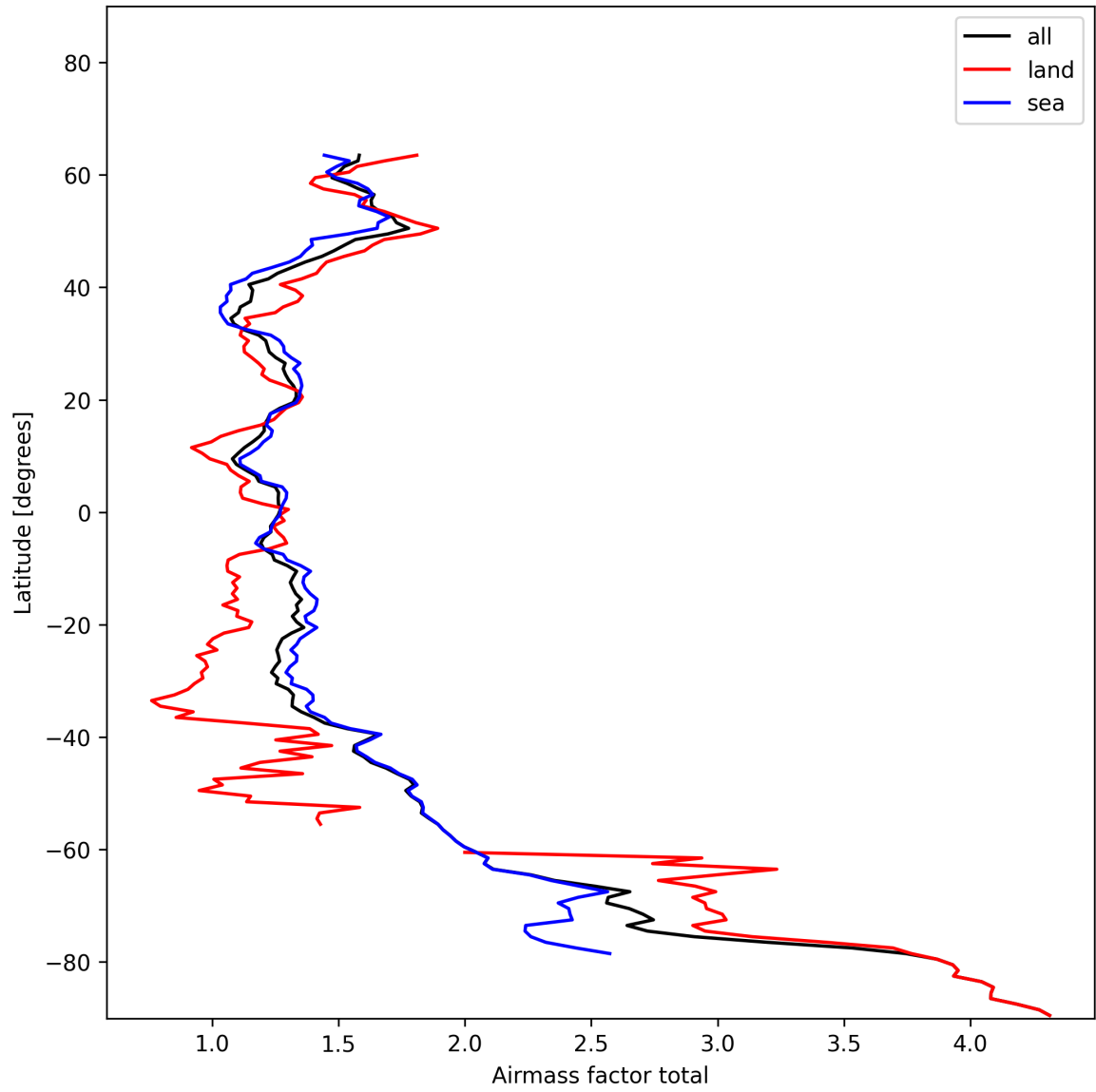
Figure 26: Zonal average of “Airmass factor total” for 2024-11-28 to 2024-11-30.
