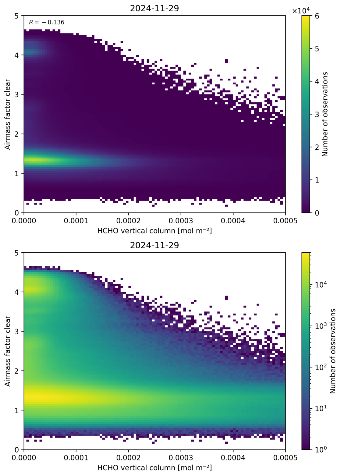
Figure 126: Scatter density plot of “HCHO vertical column” against “Airmass factor clear” for 2024-11-28 to 2024-11-30.
