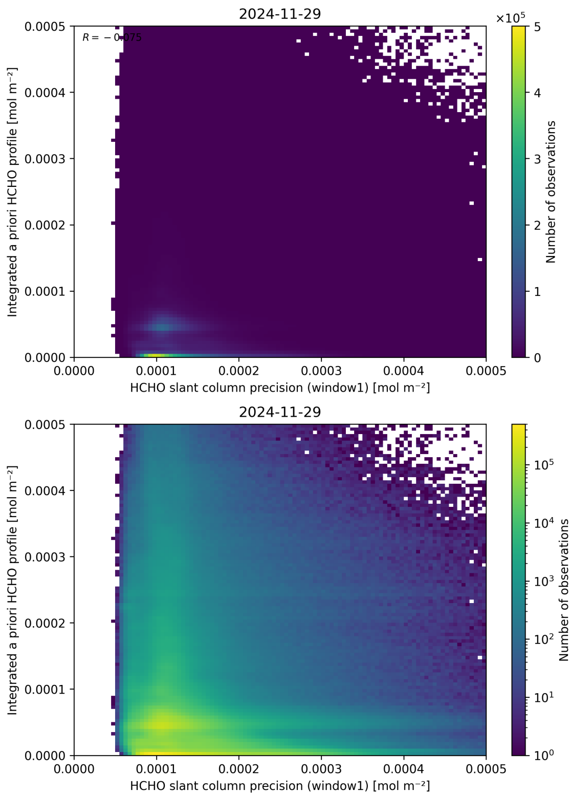
Figure 96: Scatter density plot of “HCHO slant column precision (window1)” against “Integrated a priori HCHO profile” for 2024-11-28 to 2024-11-30.
