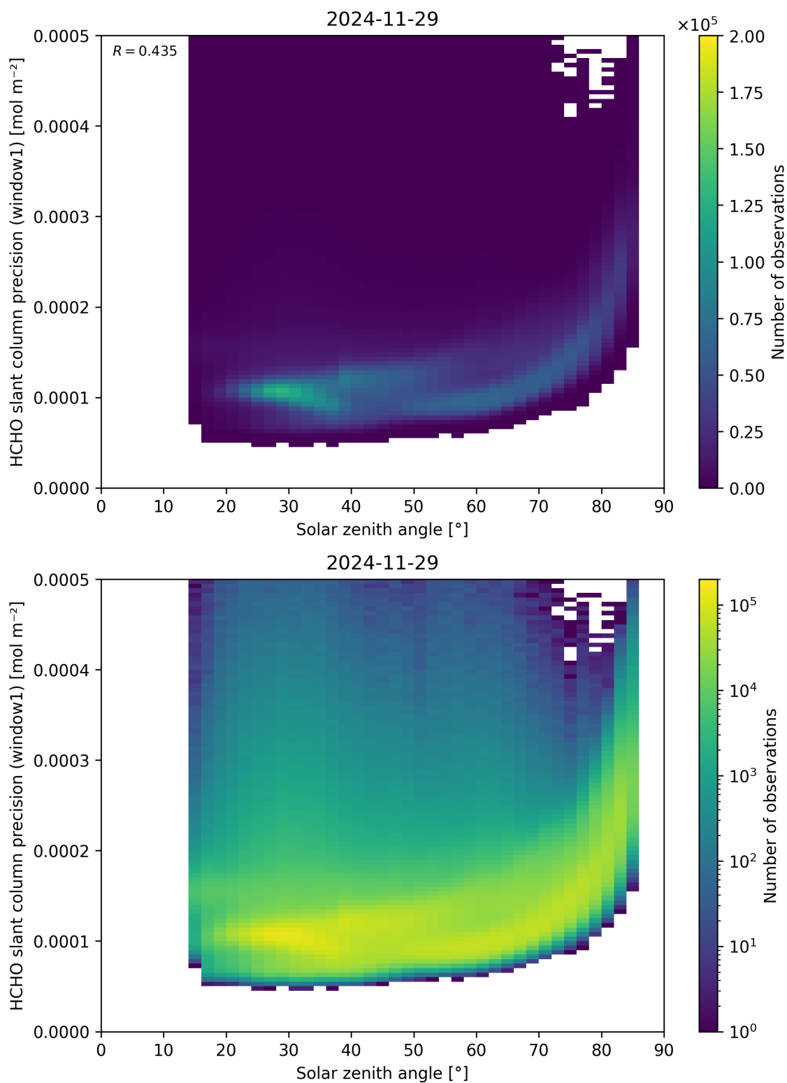
Figure 174: Scatter density plot of “Solar zenith angle” against “HCHO slant column precision (window1)” for 2024-11-28 to 2024-11-30.
