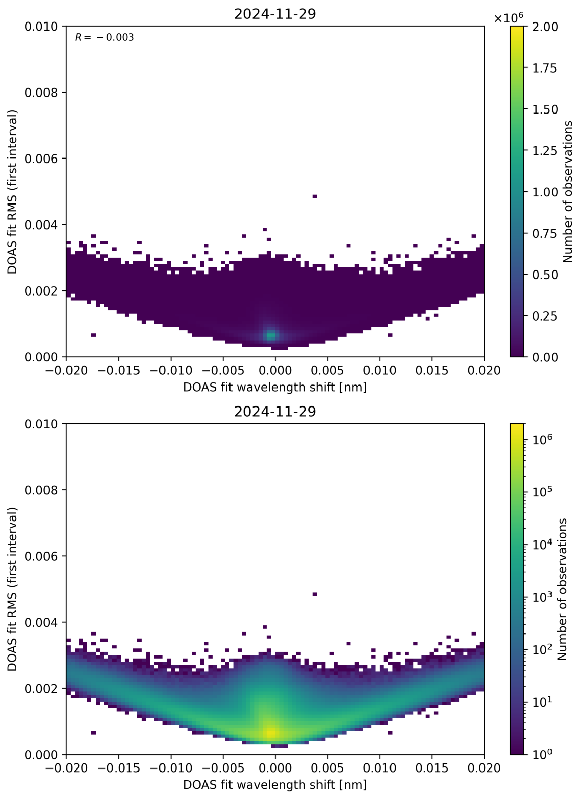
Figure 64: Scatter density plot of “DOAS fit wavelength shift” against “DOAS fit RMS (first interval)” for 2024-11-28 to 2024-11-30.
