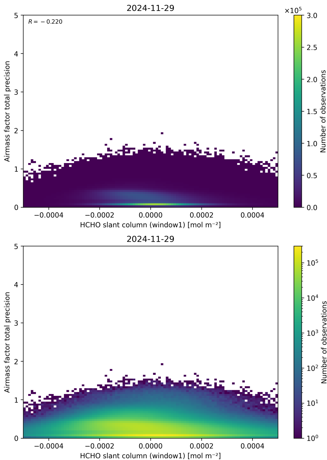
Figure 86: Scatter density plot of “HCHO slant column (window1)” against “Airmass factor total precision” for 2024-11-28 to 2024-11-30.
