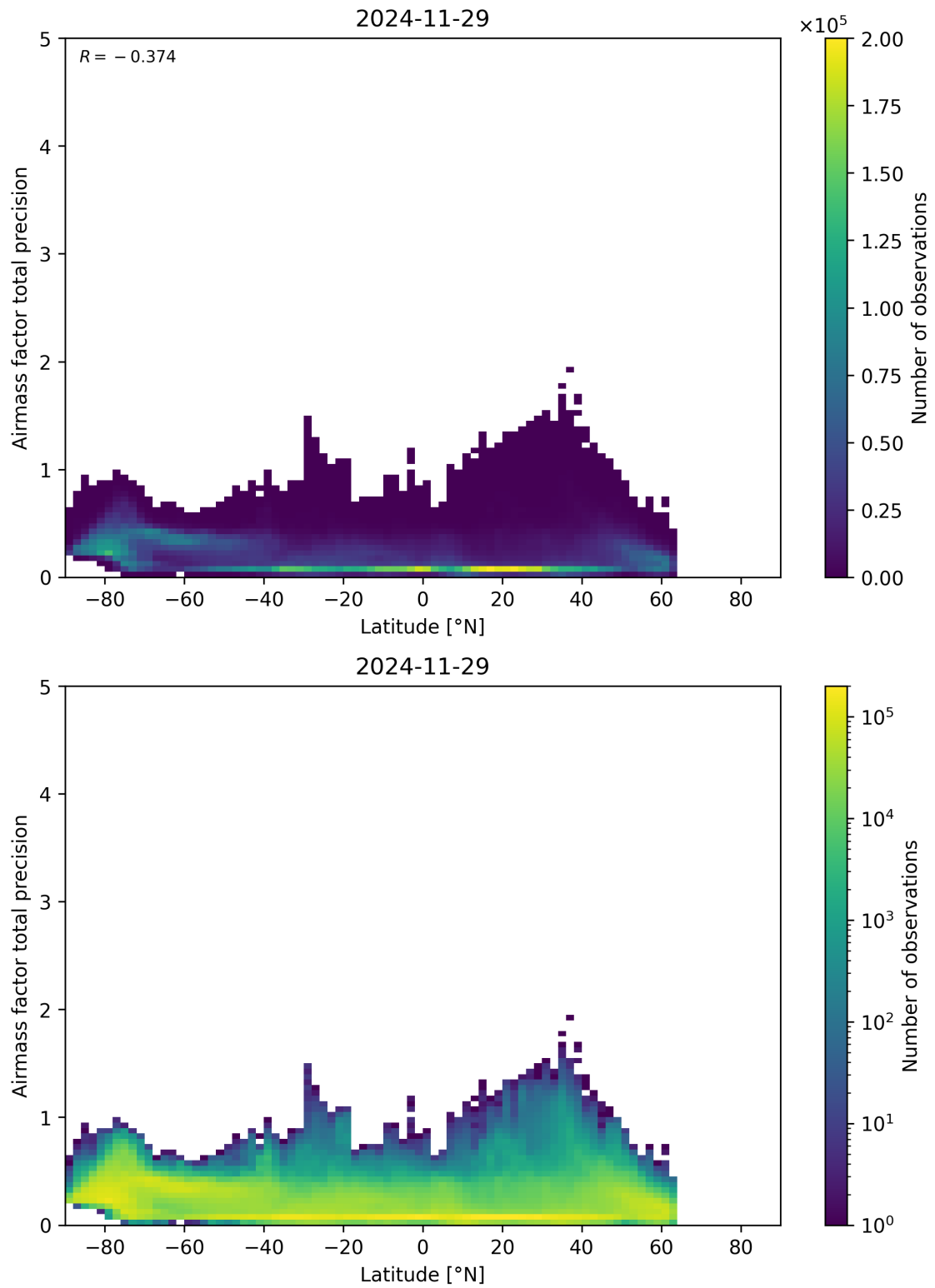
Figure 162: Scatter density plot of “Latitude” against “Airmass factor total precision” for 2024-11-28 to 2024-11-30.
