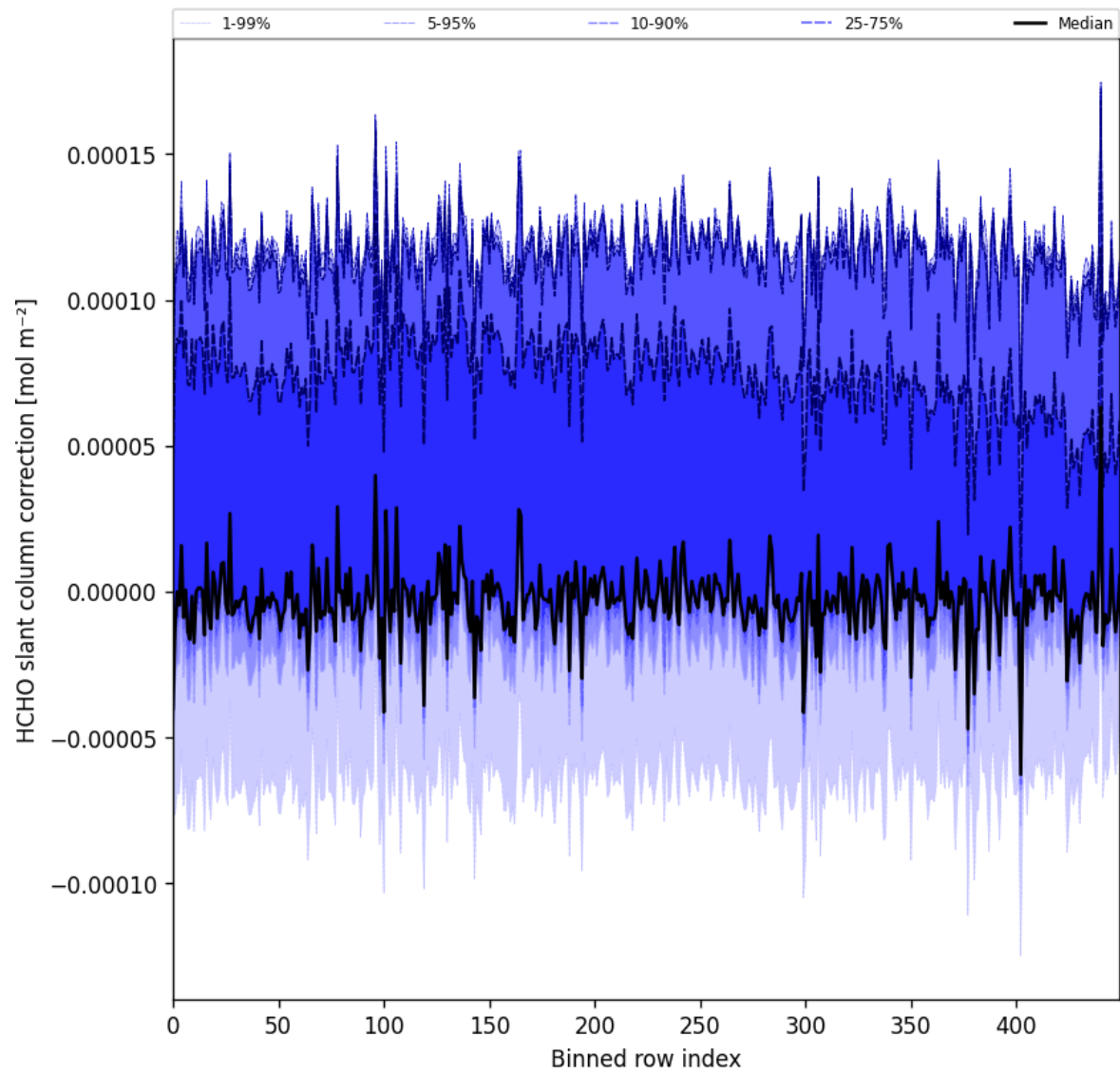
Figure 61: Along track statistics of “HCHO slant column correction” for 2024-11-28 to 2024-11-30
