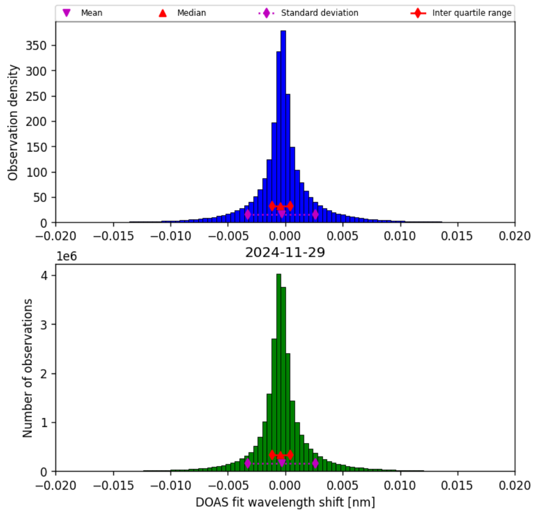
Figure 44: Histogram of “DOAS fit wavelength shift” for 2024-11-28 to 2024-11-30
