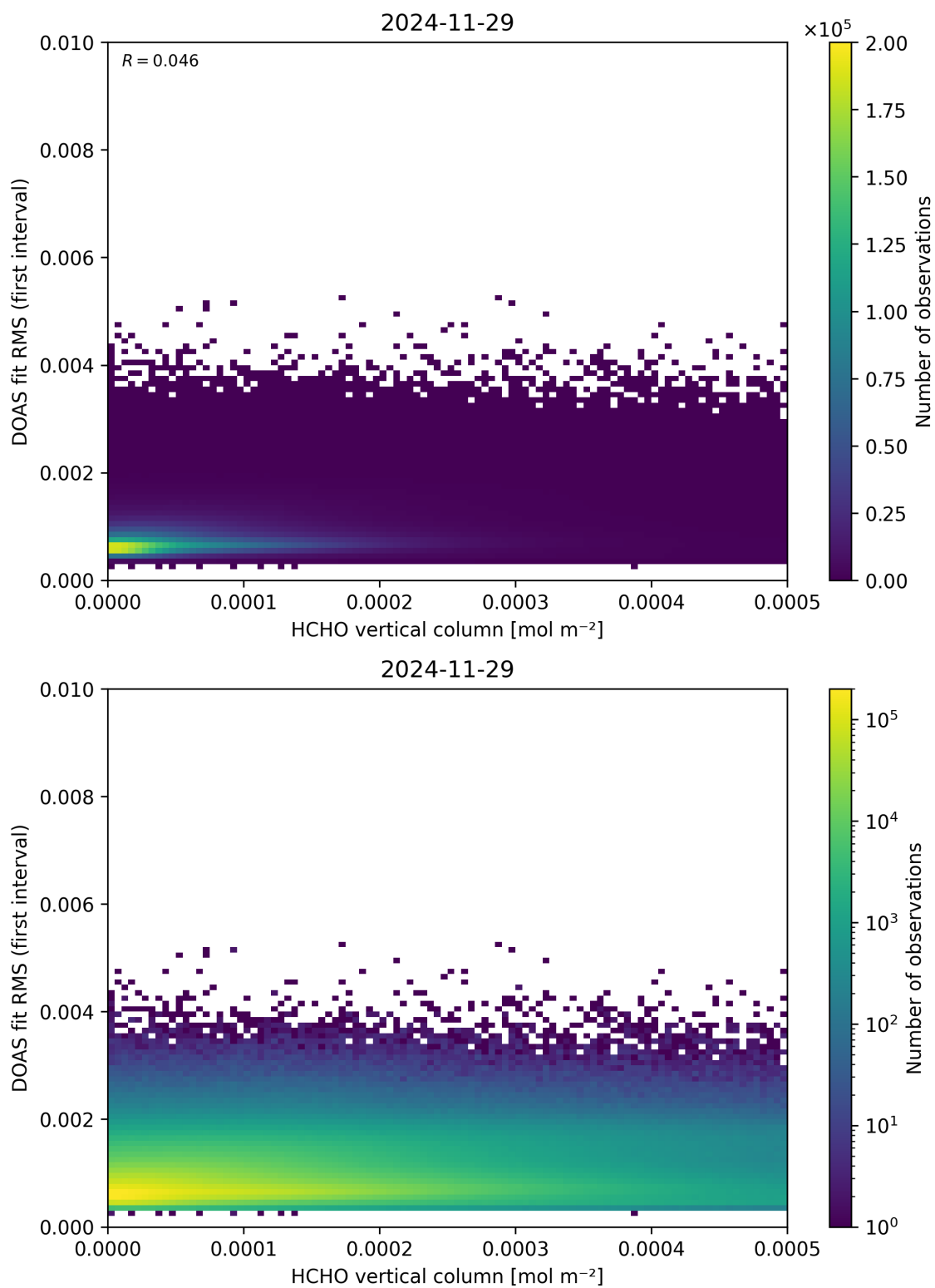
Figure 123: Scatter density plot of “HCHO vertical column” against “DOAS fit RMS (first interval)” for 2024-11-28 to 2024-11-30.
