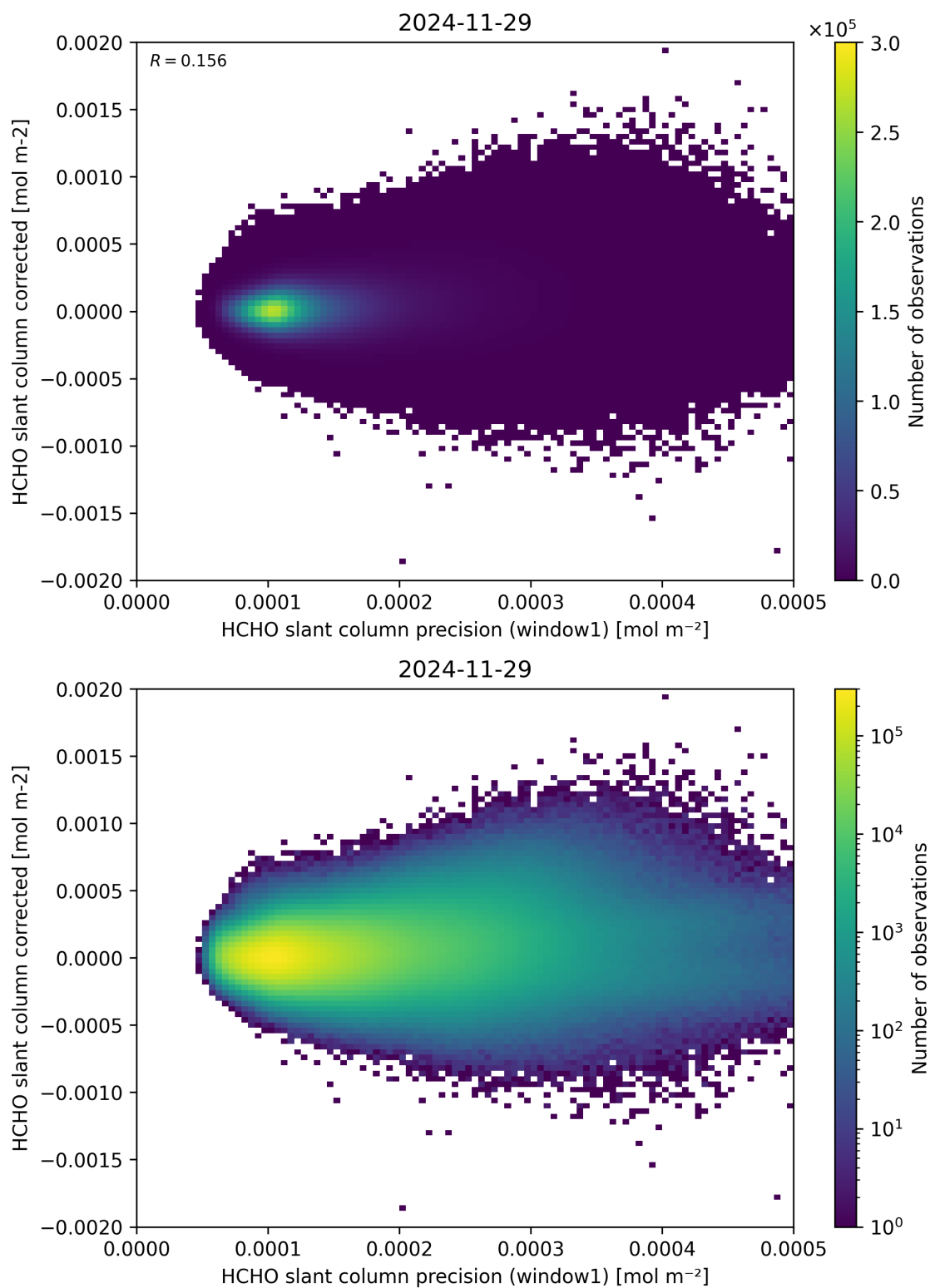
Figure 92: Scatter density plot of “HCHO slant column precision (window1)” against “HCHO slant column corrected” for 2024-11-28 to 2024-11-30.
