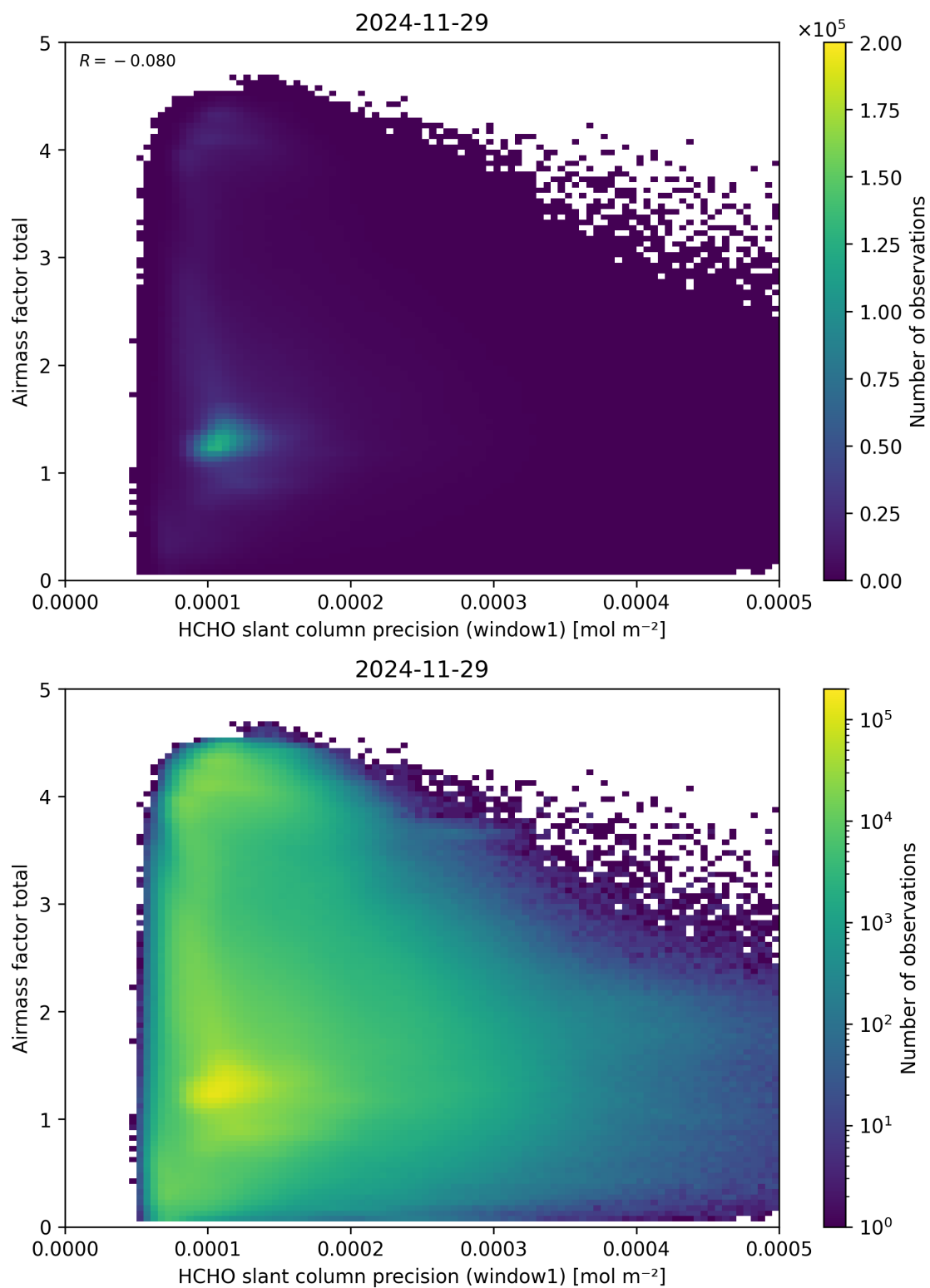
Figure 94: Scatter density plot of “HCHO slant column precision (window1)” against “Airmass factor total” for 2024-11-28 to 2024-11-30.
