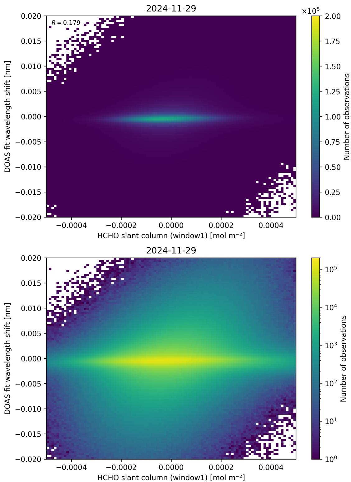
Figure 79: Scatter density plot of “HCHO slant column (window1)” against “DOAS fit wavelength shift” for 2024-11-28 to 2024-11-30.
