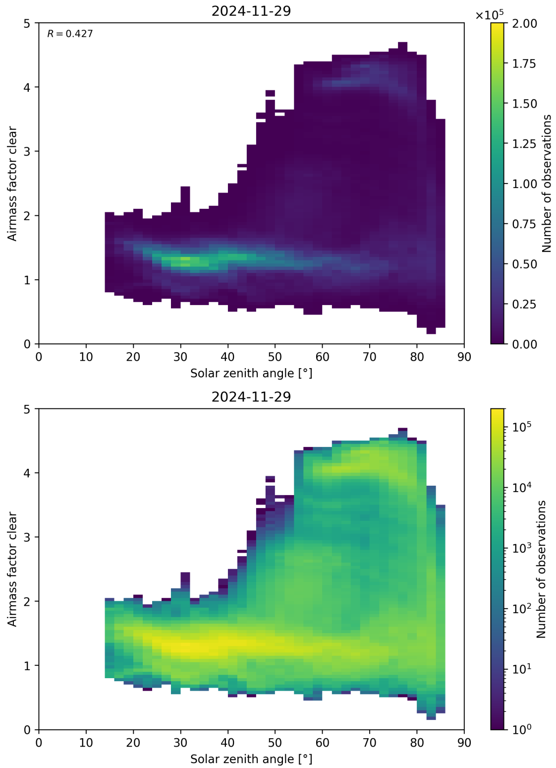
Figure 170: Scatter density plot of “Solar zenith angle” against “Airmass factor clear” for 2024-11-28 to 2024-11-30.
