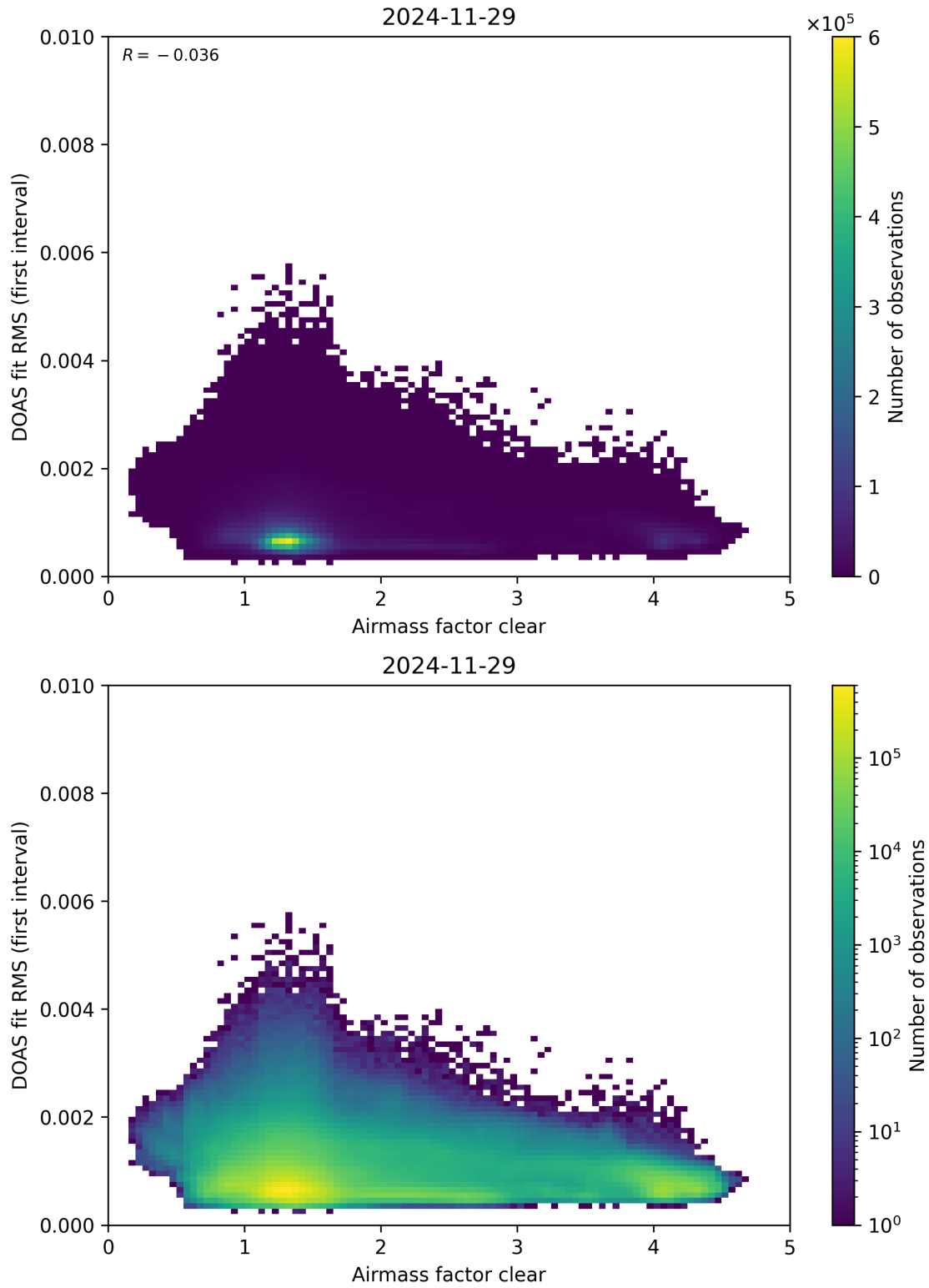
Figure 71: Scatter density plot of “Airmass factor clear” against “DOAS fit RMS (first interval)” for 2024-11-28 to 2024-11-30.
