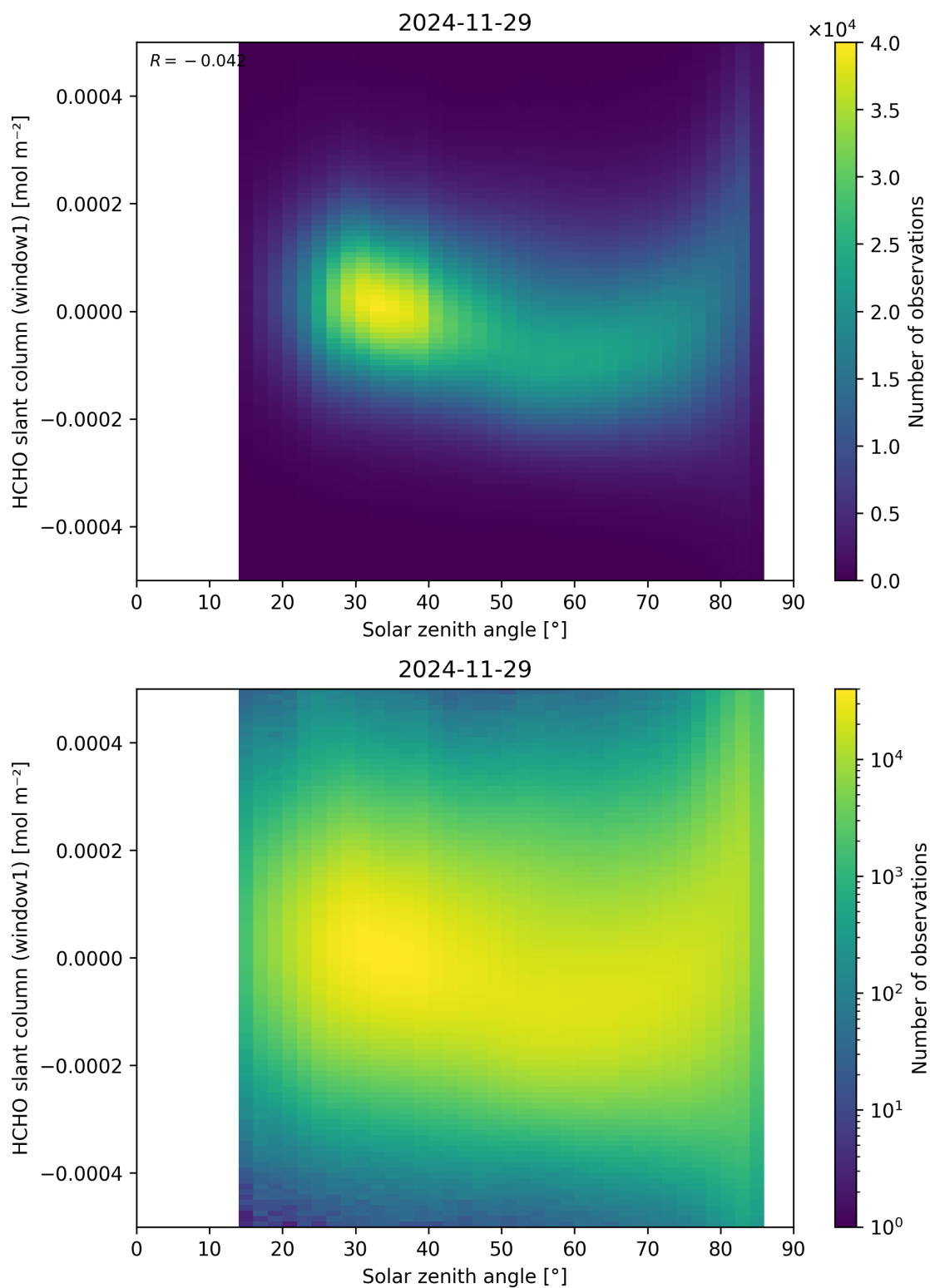
Figure 173: Scatter density plot of “Solar zenith angle” against “HCHO slant column (window1)” for 2024-11-28 to 2024-11-30.
