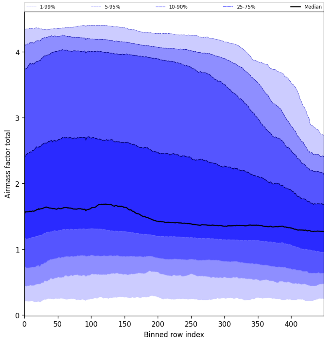
Figure 54: Along track statistics of “Airmass factor total” for 2024-11-28 to 2024-11-30
