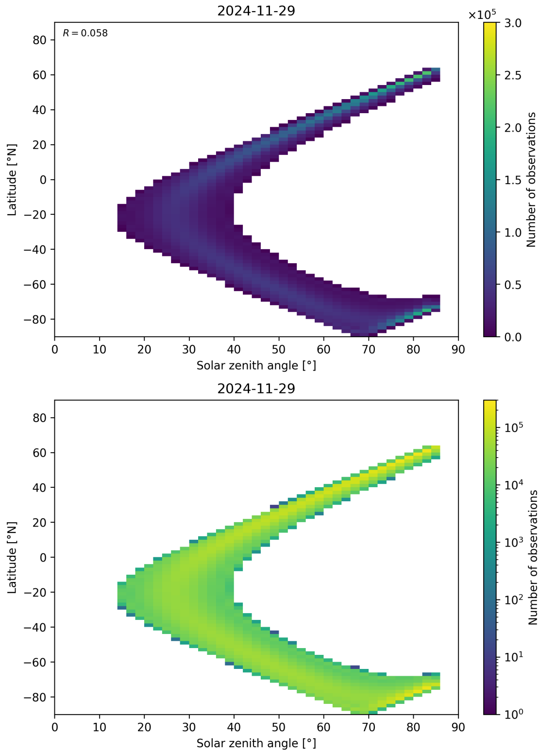
Figure 181: Scatter density plot of “Solar zenith angle” against “Latitude” for 2024-11-28 to 2024-11-30.
