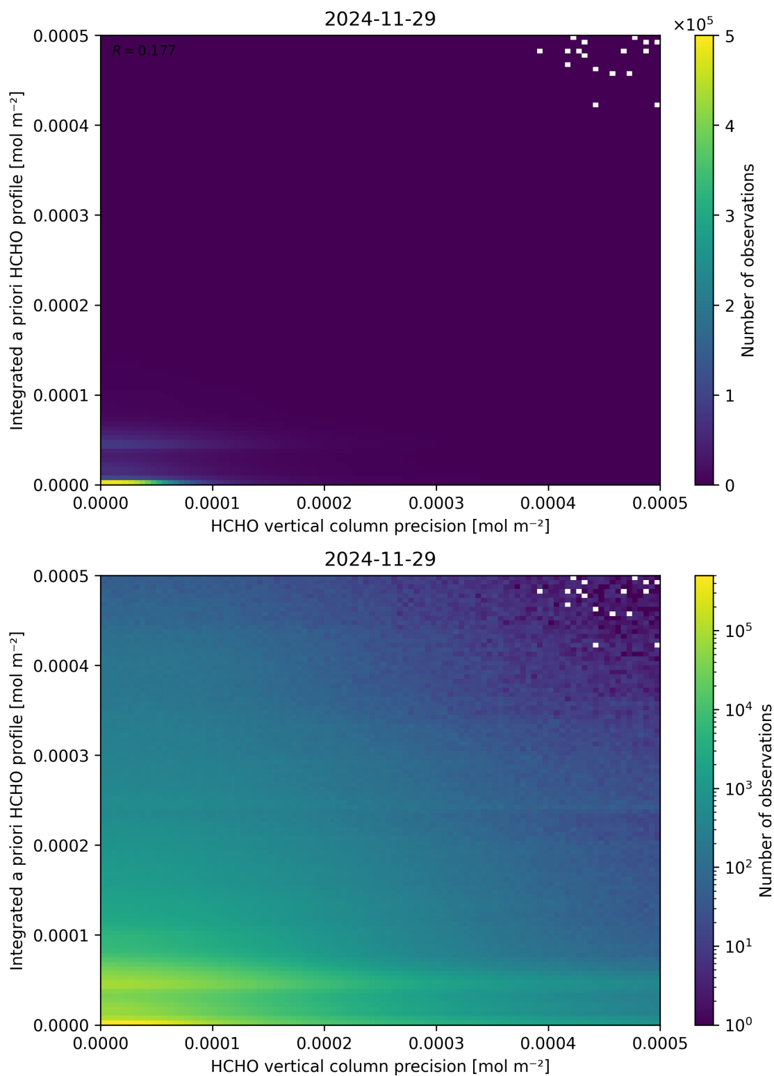
Figure 147: Scatter density plot of “HCHO vertical column precision” against “Integrated a priori HCHO profile” for 2024-11-28 to 2024-11-30.
