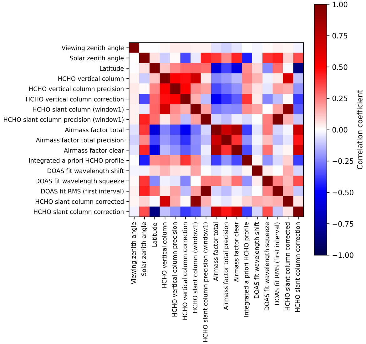
Figure 2: Map of correlation matrix for 2024-11-28 to 2024-11-30.
