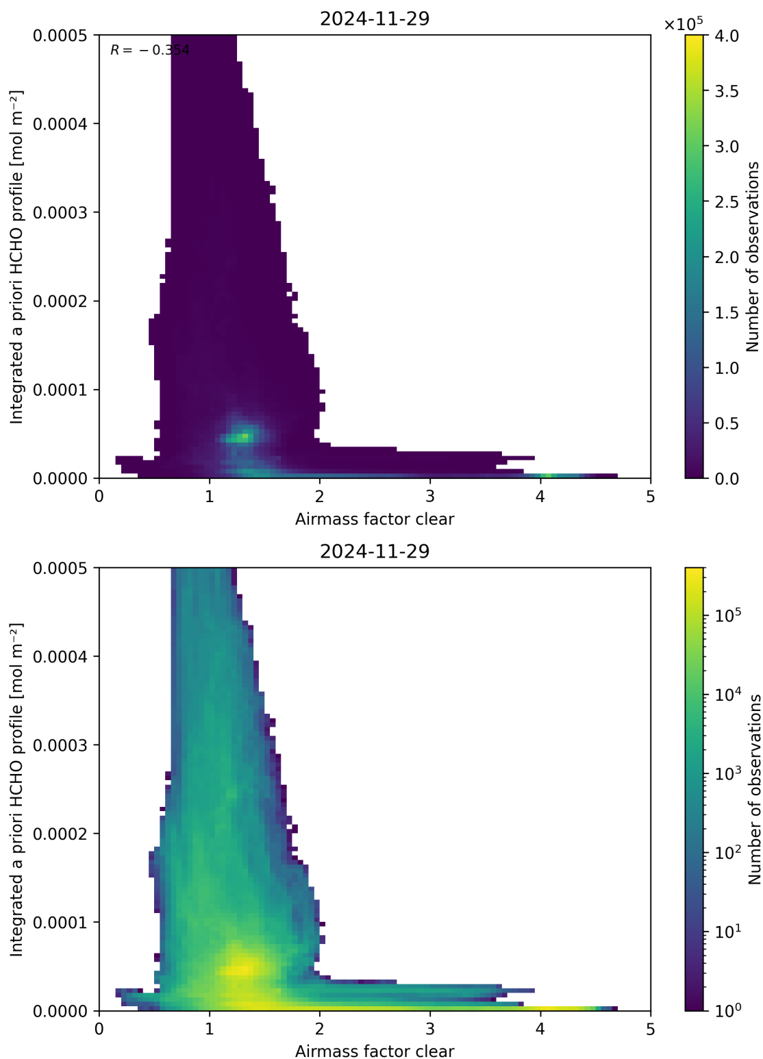
Figure 76: Scatter density plot of “Airmass factor clear” against “Integrated a priori HCHO profile” for 2024-11-28 to 2024-11-30.
