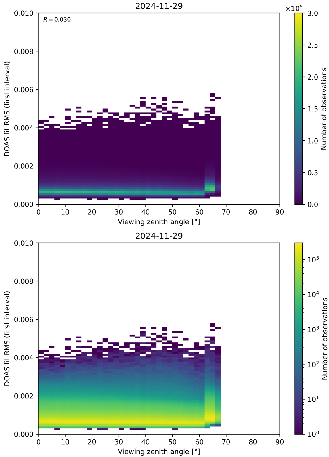
Figure 182: Scatter density plot of “Viewing zenith angle” against “DOAS fit RMS (first interval)” for 2024-11-28 to 2024-11-30.
