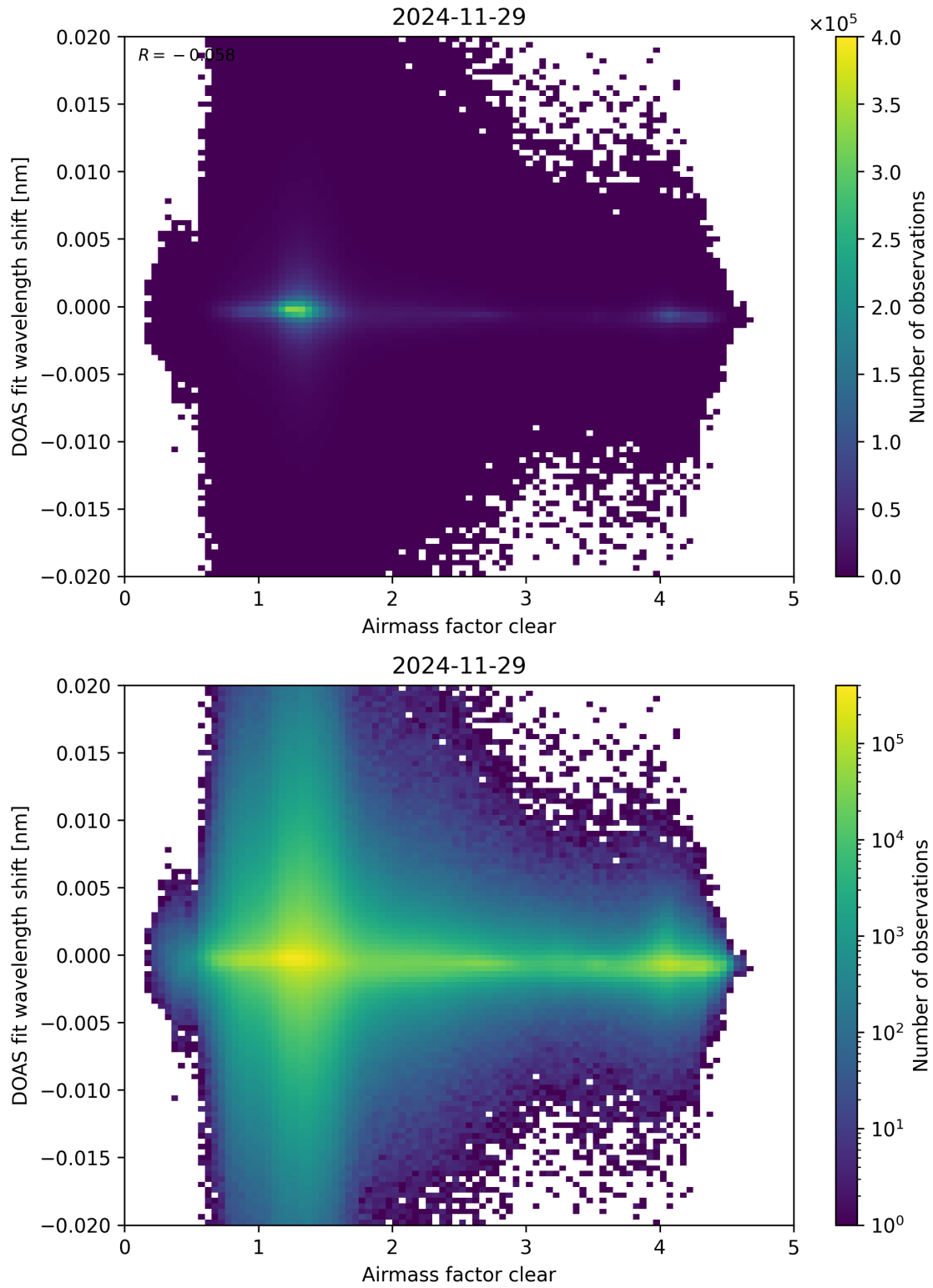
Figure 72: Scatter density plot of “Airmass factor clear” against “DOAS fit wavelength shift” for 2024-11-28 to 2024-11-30.
