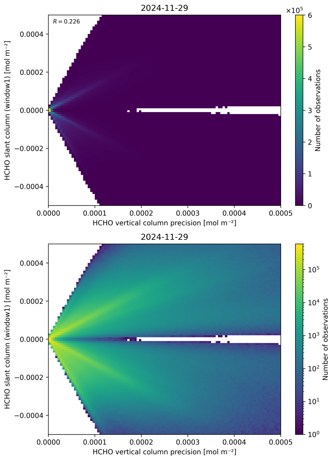
Figure 142: Scatter density plot of “HCHO vertical column precision” against “HCHO slant column (window1)” for 2024-11-28 to 2024-11-30.
