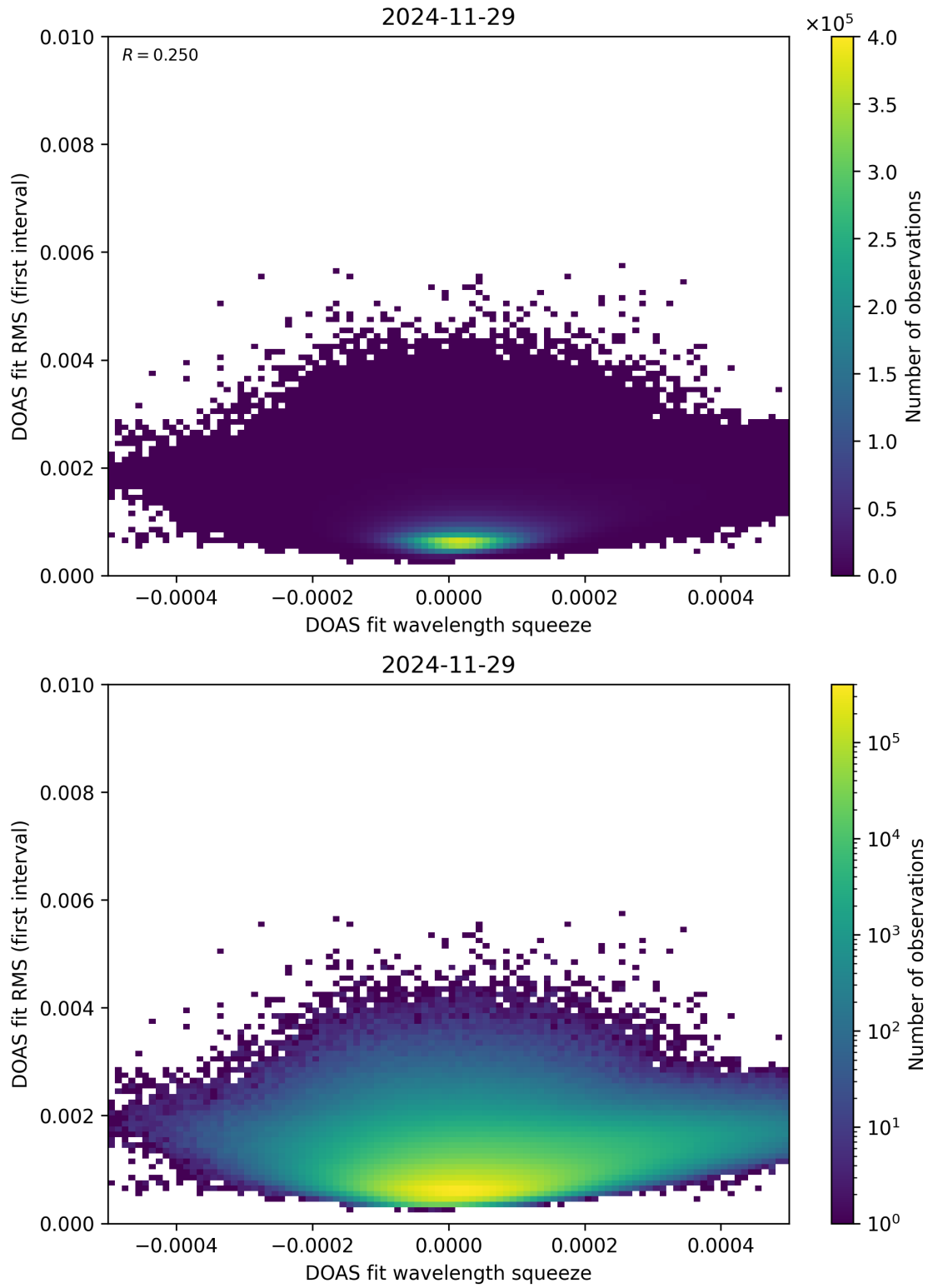
Figure 68: Scatter density plot of “DOAS fit wavelength squeeze” against “DOAS fit RMS (first interval)” for 2024-11-28 to 2024-11-30.
