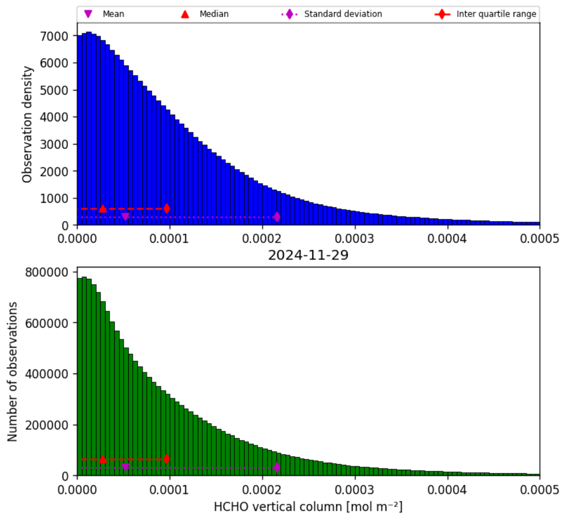
Figure 35: Histogram of “HCHO vertical column” for 2024-11-28 to 2024-11-30
