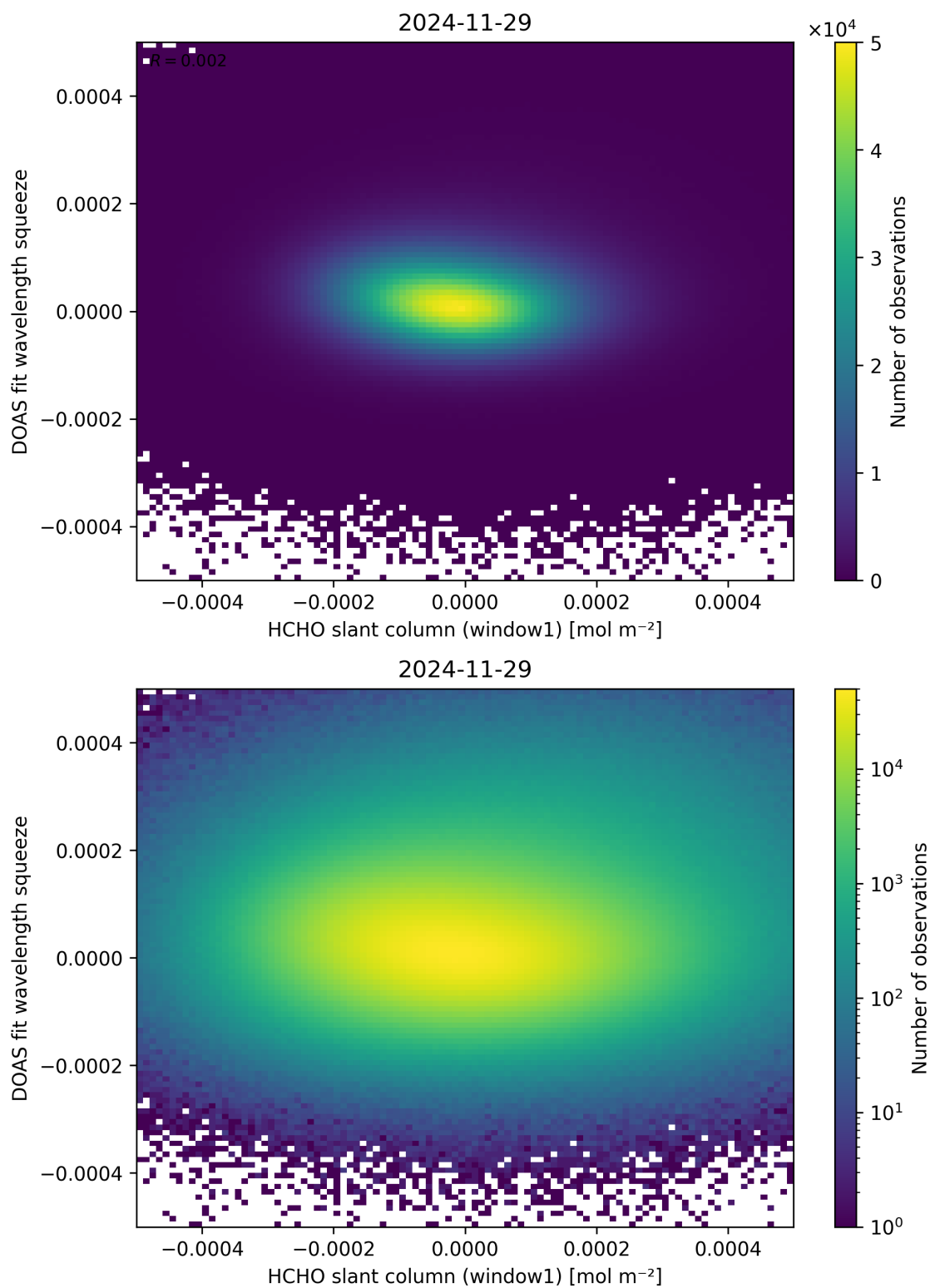
Figure 80: Scatter density plot of “HCHO slant column (window1)” against “DOAS fit wavelength squeeze” for 2024-11-28 to 2024-11-30.
