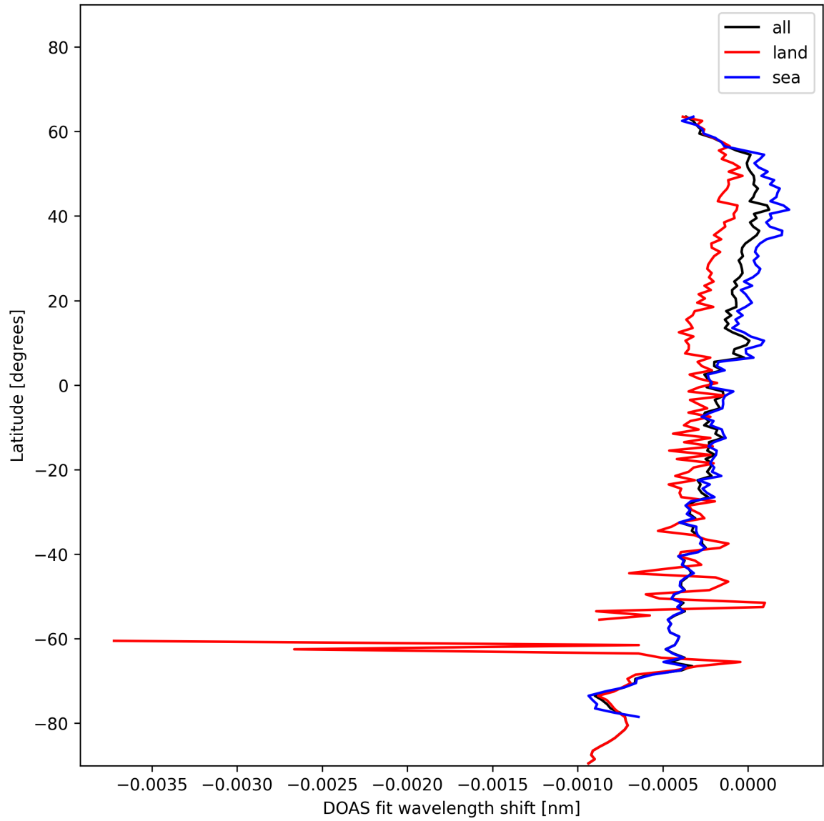
Figure 30: Zonal average of “DOAS fit wavelength shift” for 2024-11-28 to 2024-11-30.
