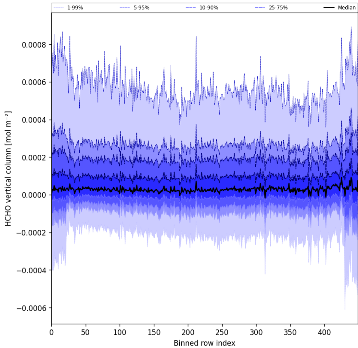
Figure 49: Along track statistics of “HCHO vertical column” for 2024-11-28 to 2024-11-30
