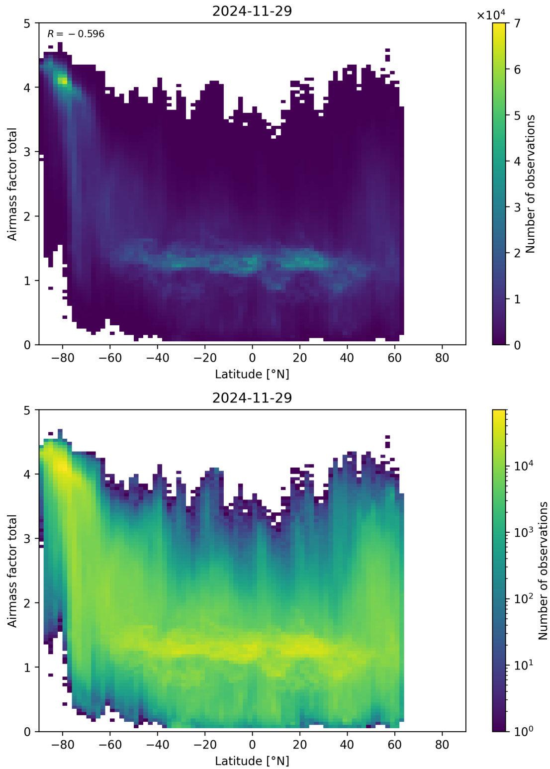
Figure 161: Scatter density plot of “Latitude” against “Airmass factor total” for 2024-11-28 to 2024-11-30.
