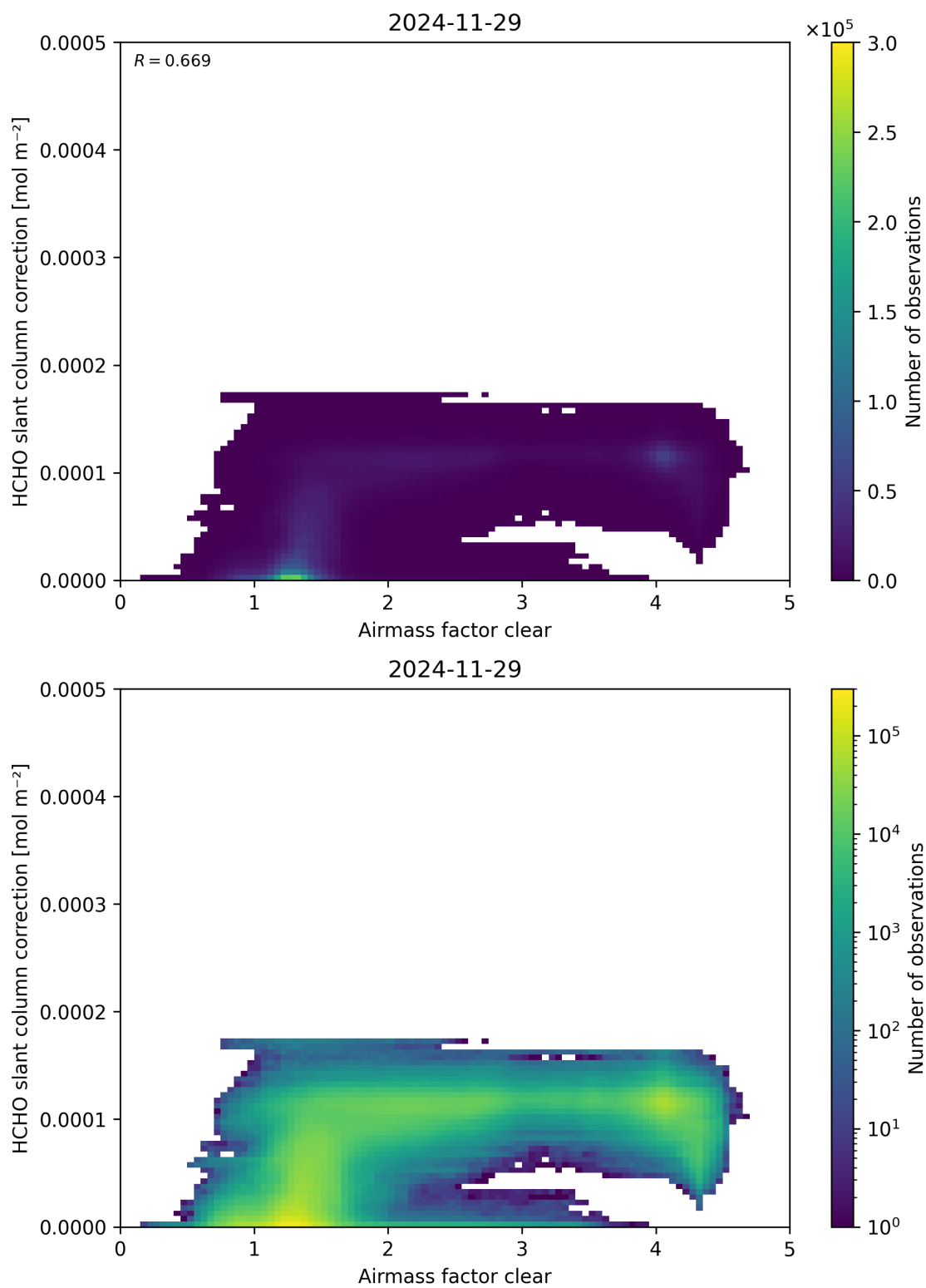
Figure 75: Scatter density plot of “Airmass factor clear” against “HCHO slant column correction” for 2024-11-28 to 2024-11-30.
