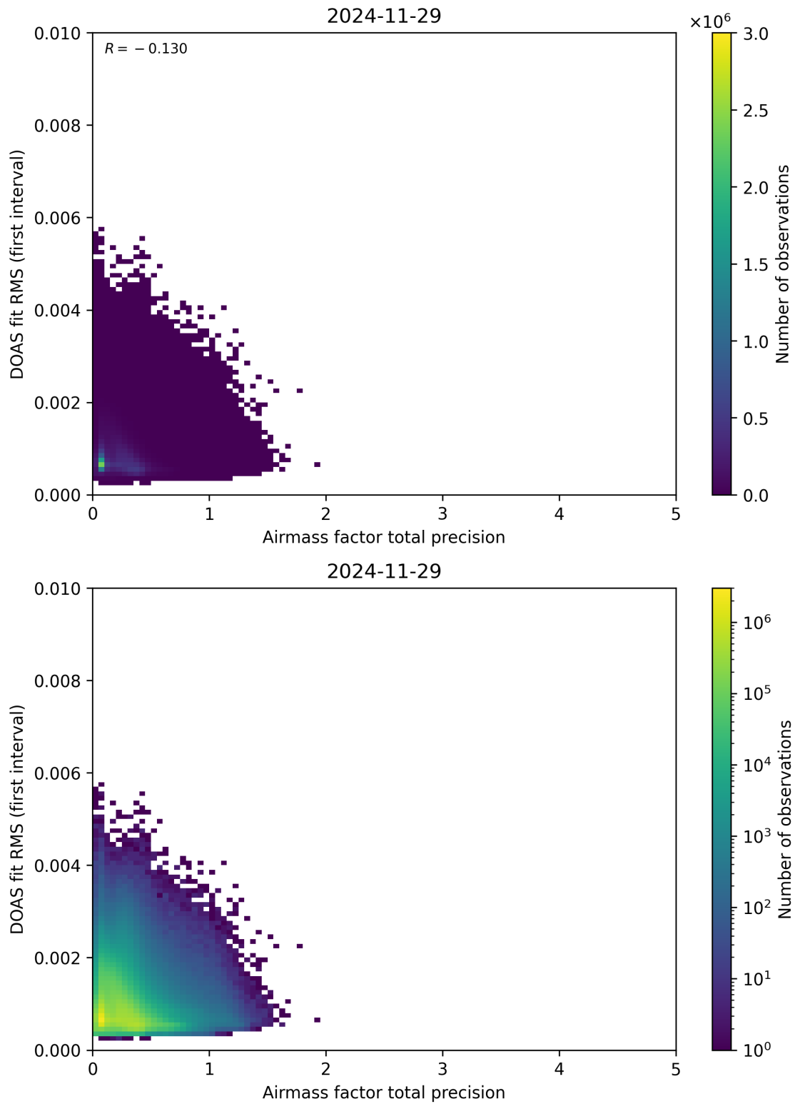
Figure 105: Scatter density plot of “Airmass factor total precision” against “DOAS fit RMS (first interval)” for 2024-11-28 to 2024-11-30.
