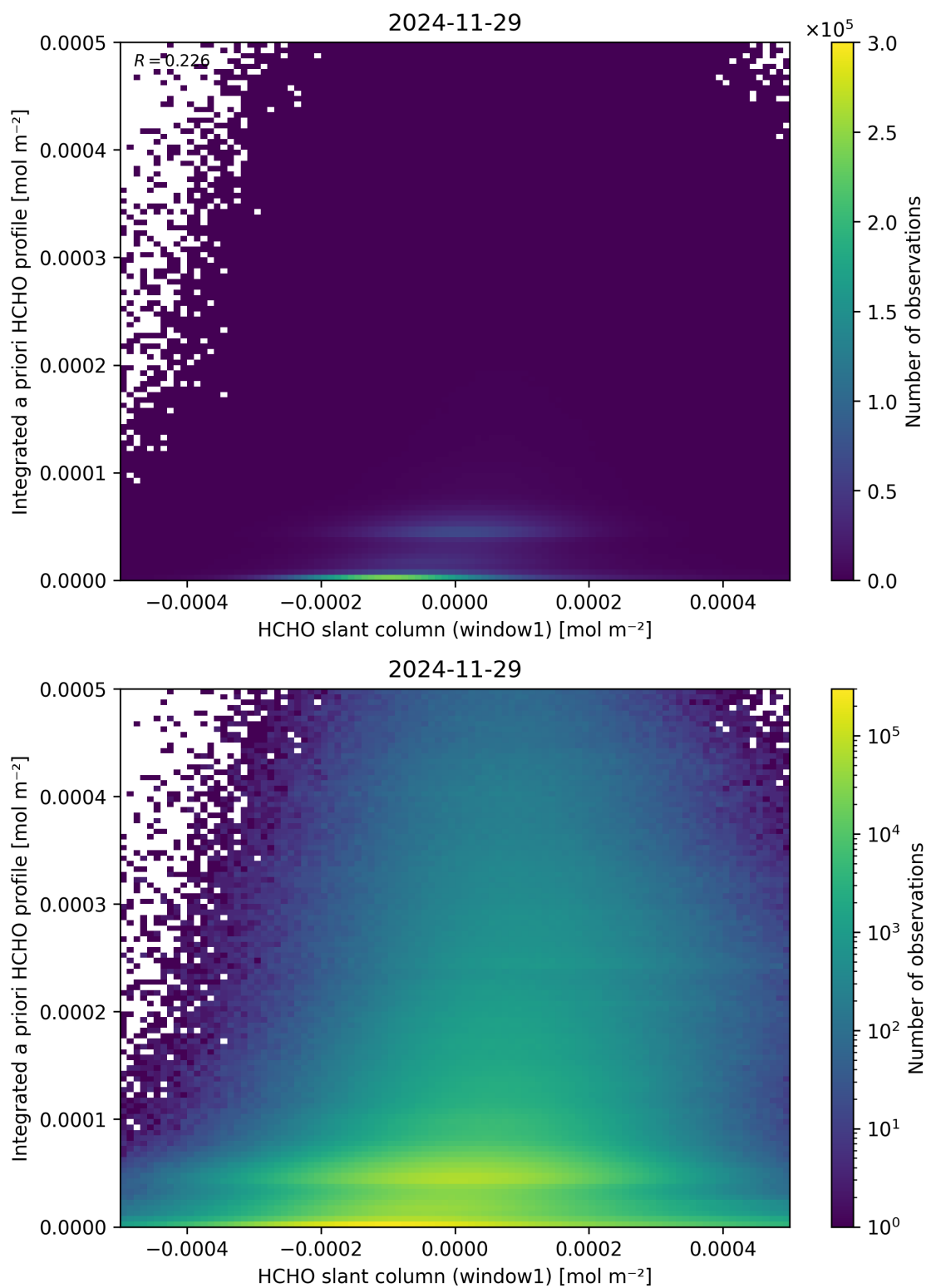
Figure 87: Scatter density plot of “HCHO slant column (window1)” against “Integrated a priori HCHO profile” for 2024-11-28 to 2024-11-30.
