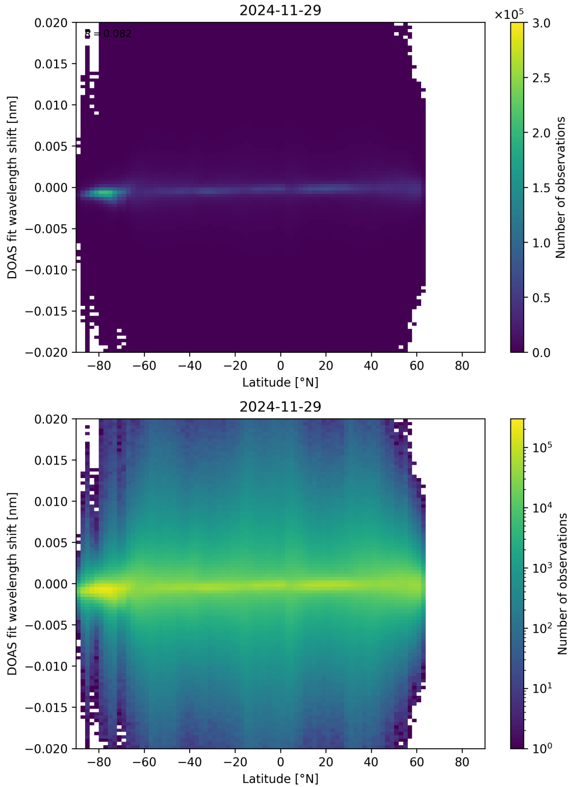
Figure 154: Scatter density plot of “Latitude” against “DOAS fit wavelength shift” for 2024-11-28 to 2024-11-30.
