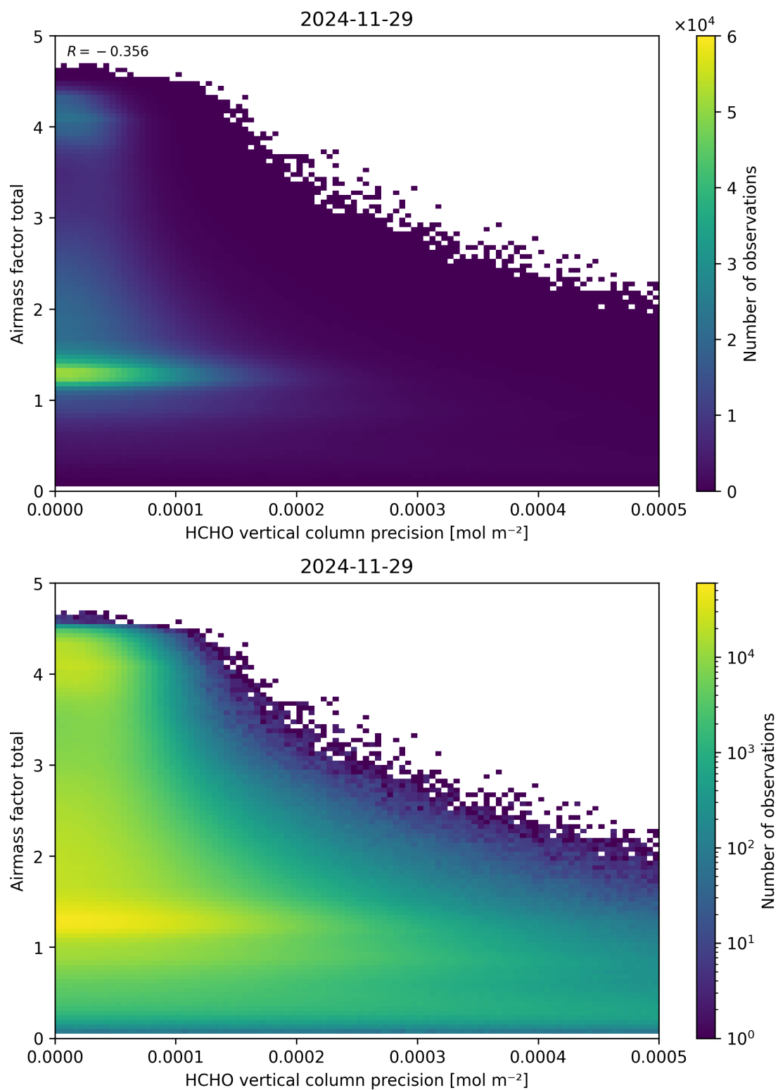
Figure 144: Scatter density plot of “HCHO vertical column precision” against “Airmass factor total” for 2024-11-28 to 2024-11-30.
