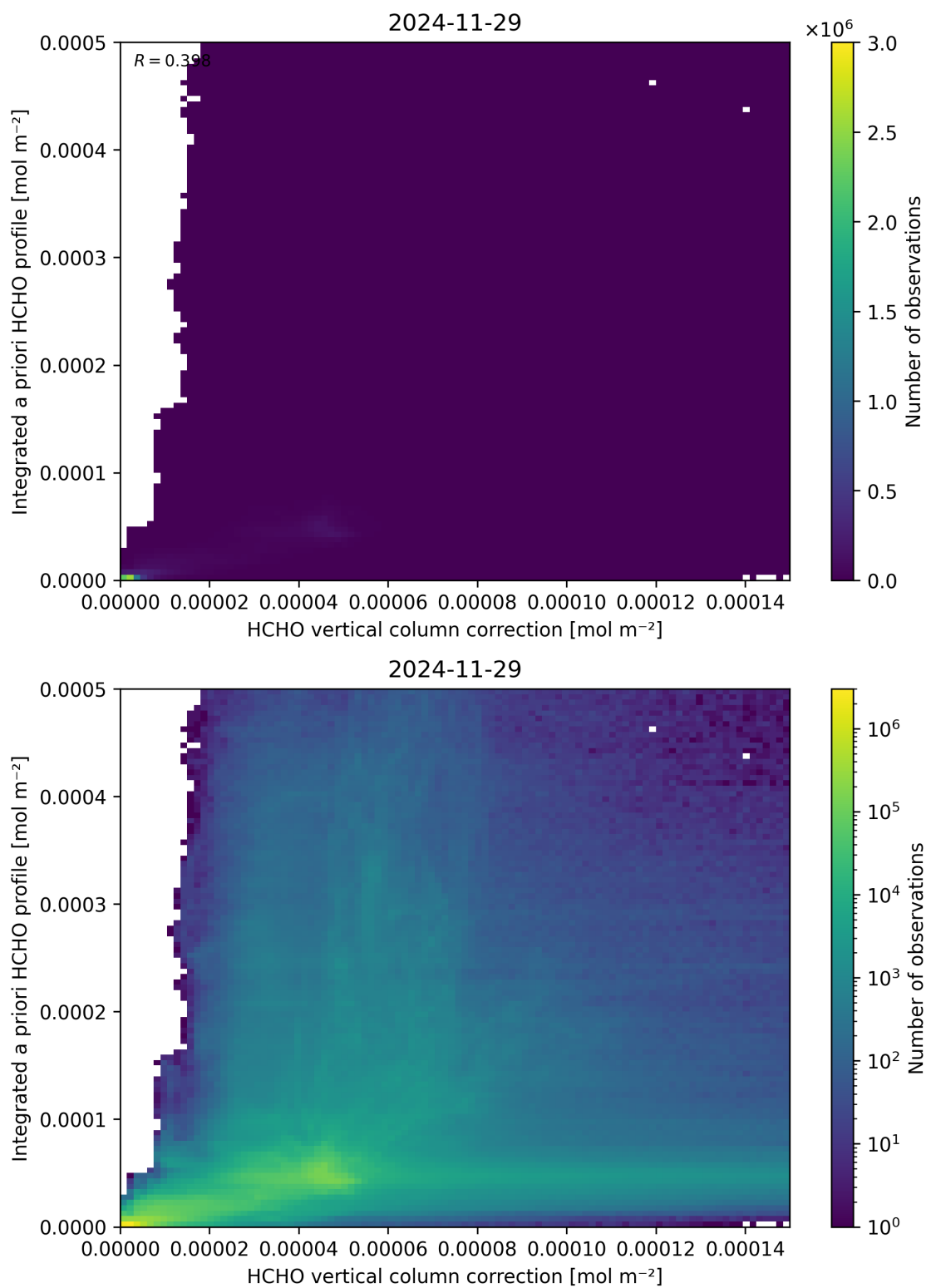
Figure 122: Scatter density plot of “HCHO vertical column correction” against “Integrated a priori HCHO profile” for 2024-11-28 to 2024-11-30.
