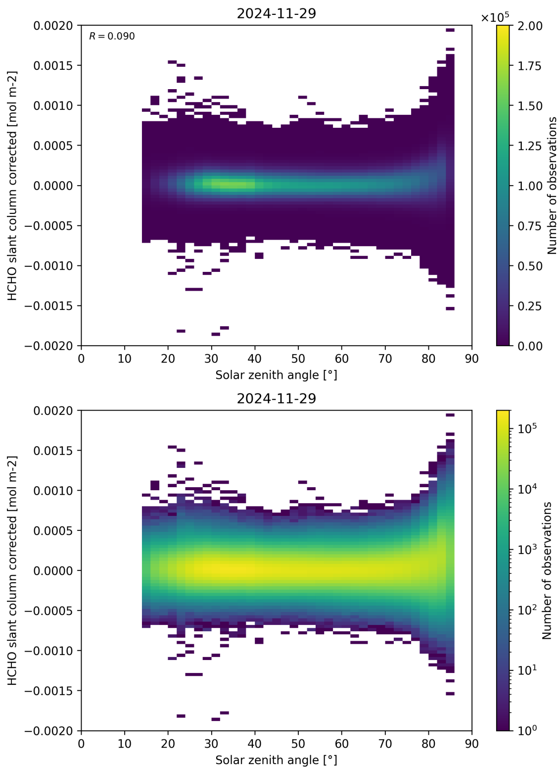
Figure 171: Scatter density plot of “Solar zenith angle” against “HCHO slant column corrected” for 2024-11-28 to 2024-11-30.
