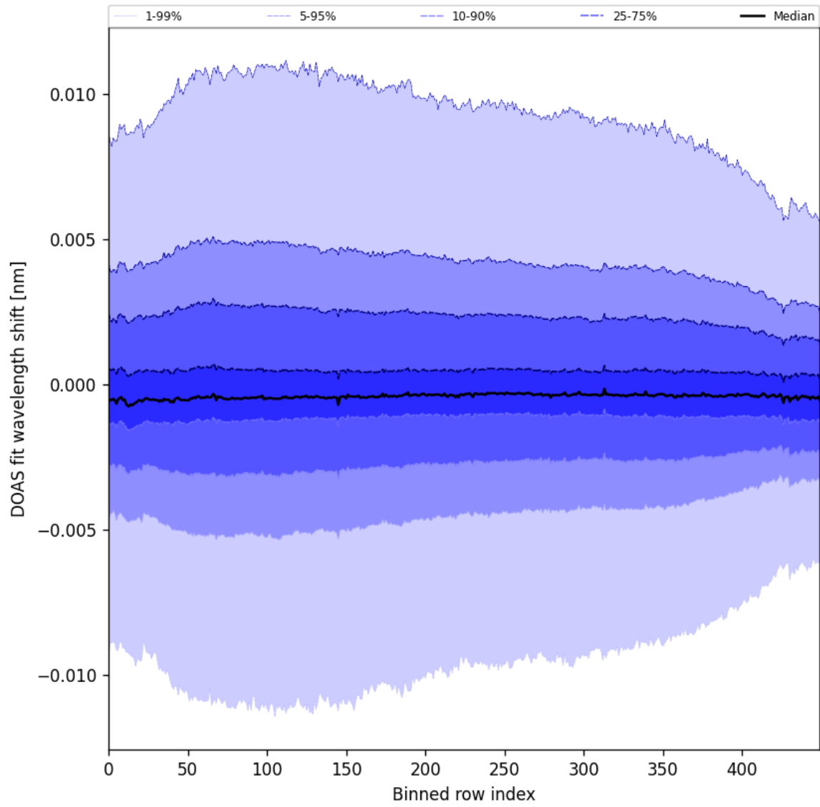
Figure 58: Along track statistics of “DOAS fit wavelength shift” for 2024-11-28 to 2024-11-30
