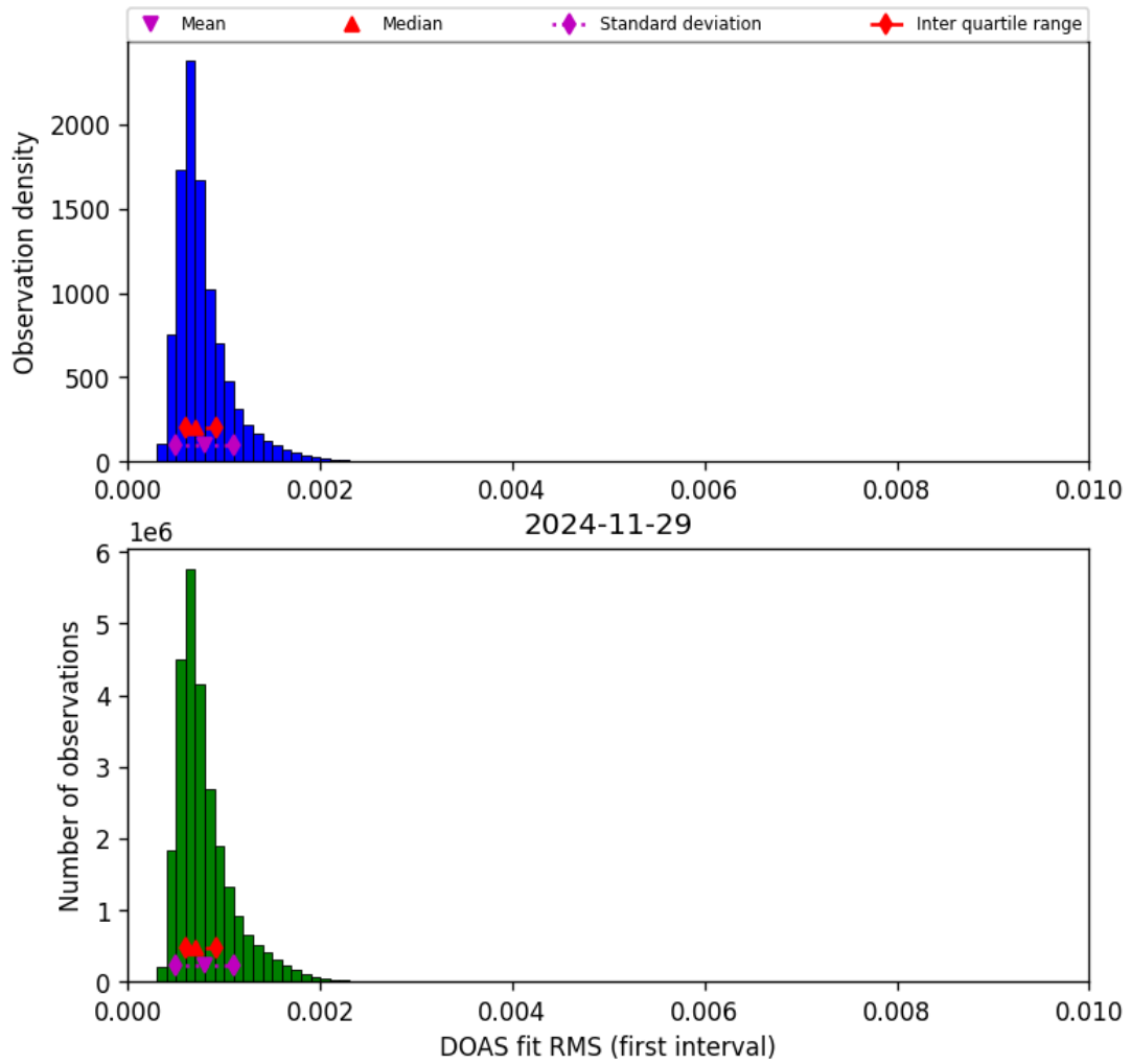
Figure 46: Histogram of “DOAS fit RMS (first interval)” for 2024-11-28 to 2024-11-30
