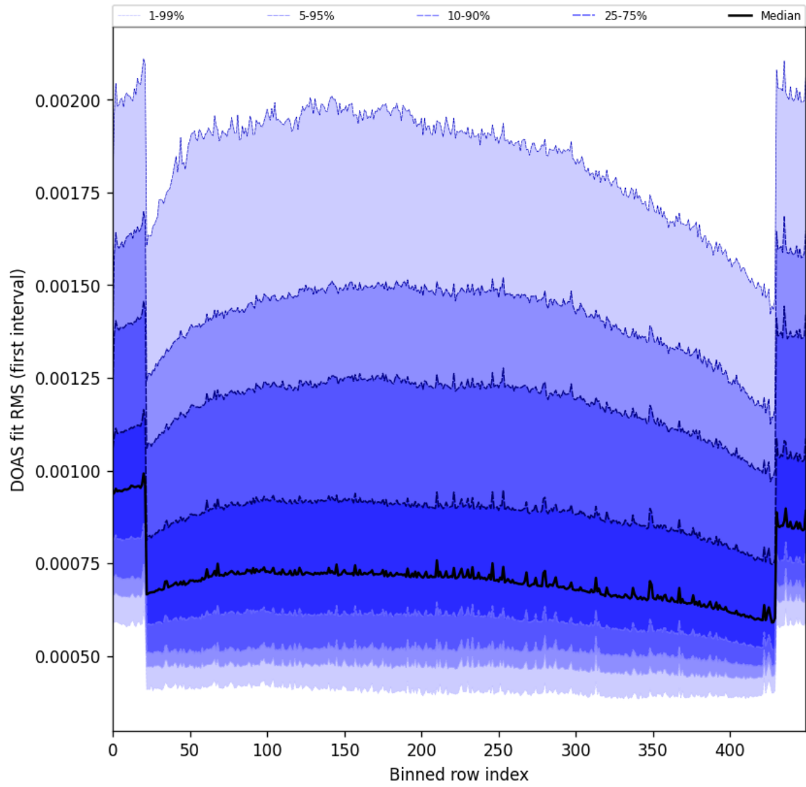
Figure 60: Along track statistics of “DOAS fit RMS (first interval)” for 2024-11-28 to 2024-11-30
