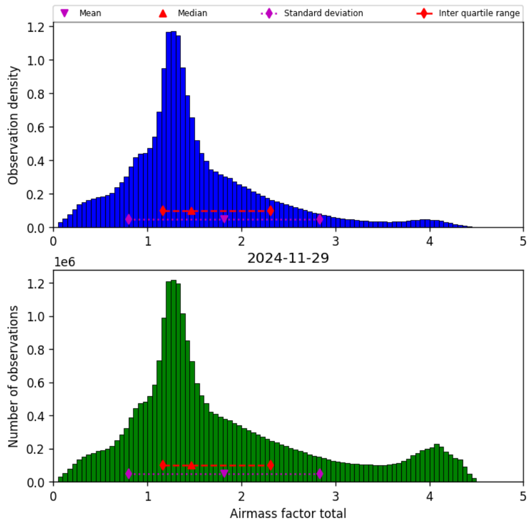
Figure 40: Histogram of “Airmass factor total” for 2024-11-28 to 2024-11-30
