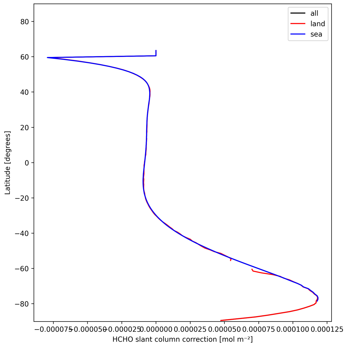
Figure 33: Zonal average of “HCHO slant column correction” for 2024-11-28 to 2024-11-30.
