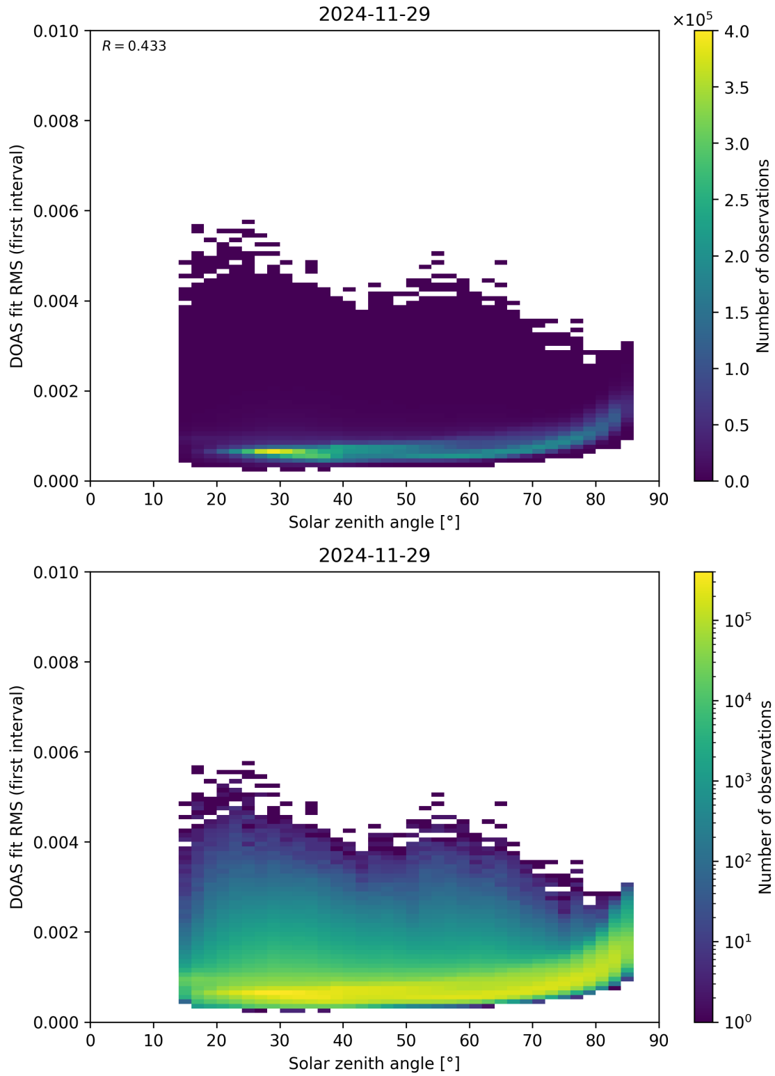
Figure 167: Scatter density plot of “Solar zenith angle” against “DOAS fit RMS (first interval)” for 2024-11-28 to 2024-11-30.
