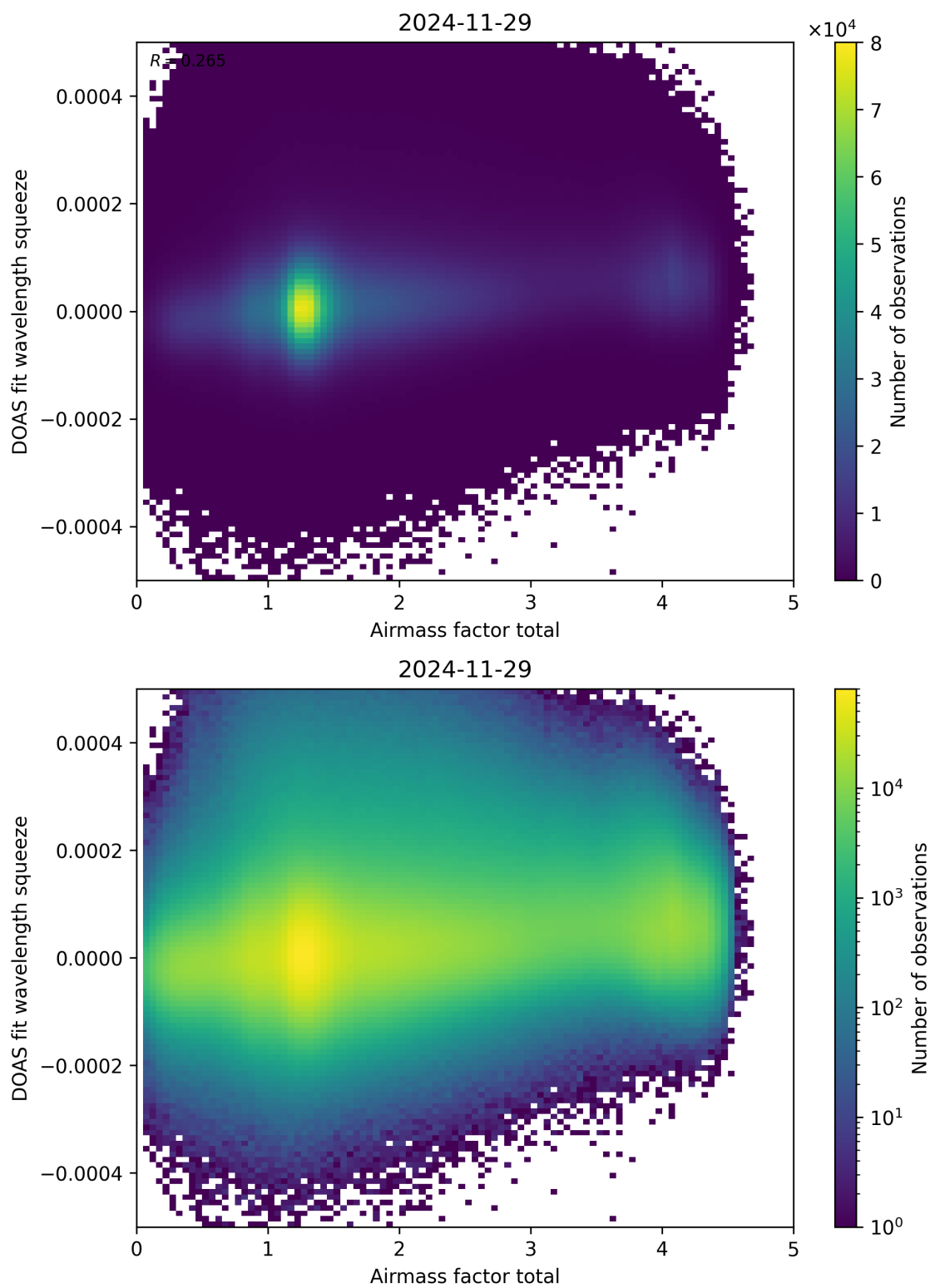
Figure 99: Scatter density plot of “Airmass factor total” against “DOAS fit wavelength squeeze” for 2024-11-28 to 2024-11-30.
