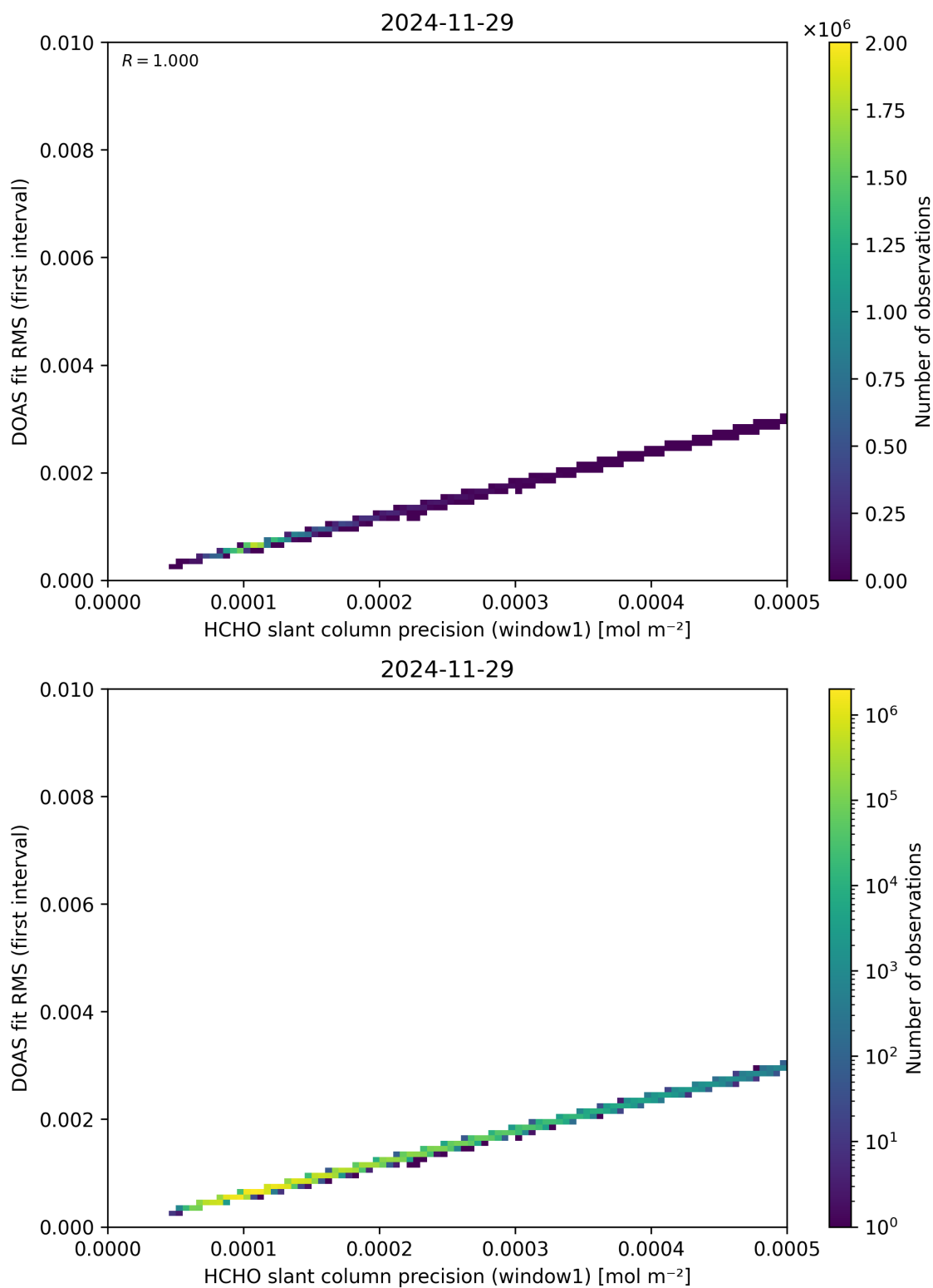
Figure 88: Scatter density plot of “HCHO slant column precision (window1)” against “DOAS fit RMS (first interval)” for 2024-11-28 to 2024-11-30.
