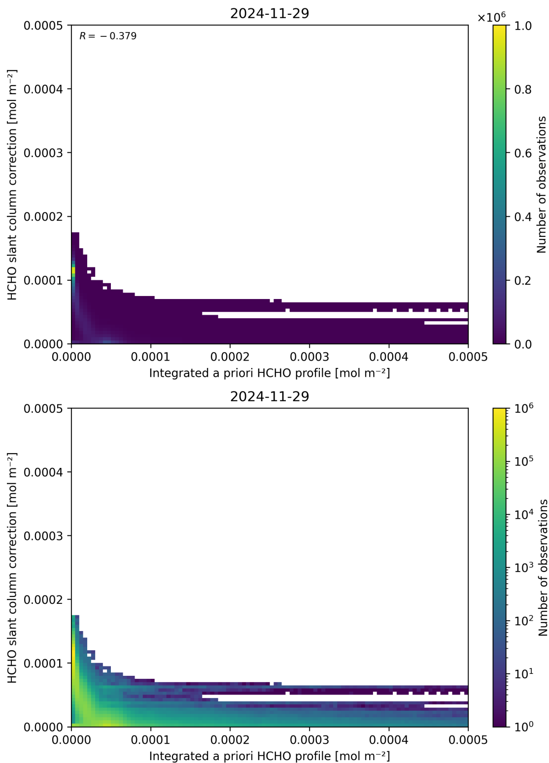
Figure 152: Scatter density plot of “Integrated a priori HCHO profile” against “HCHO slant column correction” for 2024-11-28 to 2024-11-30.
