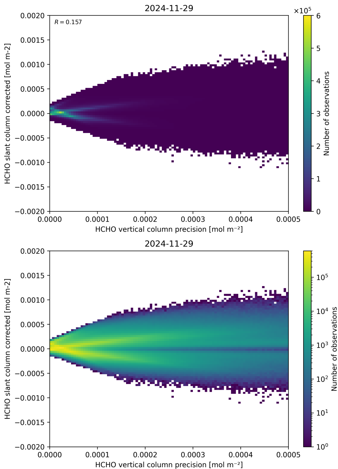
Figure 140: Scatter density plot of “HCHO vertical column precision” against “HCHO slant column corrected” for 2024-11-28 to 2024-11-30.
