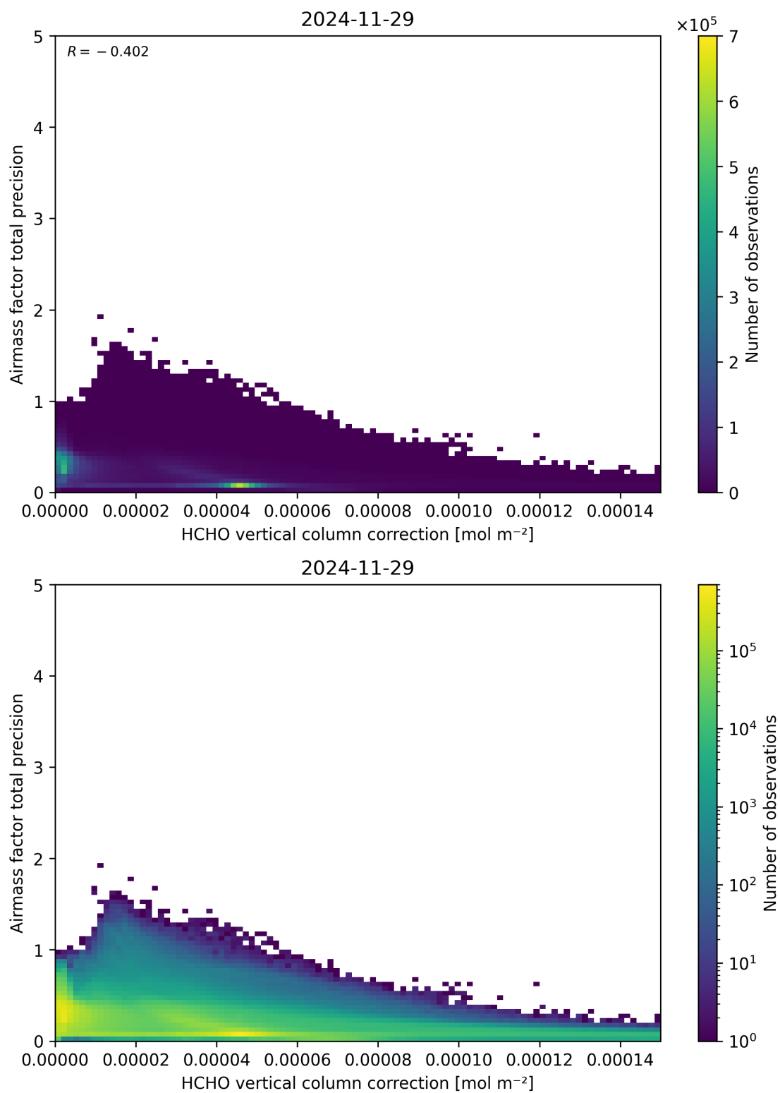
Figure 121: Scatter density plot of “HCHO vertical column correction” against “Airmass factor total precision” for 2024-11-28 to 2024-11-30.
