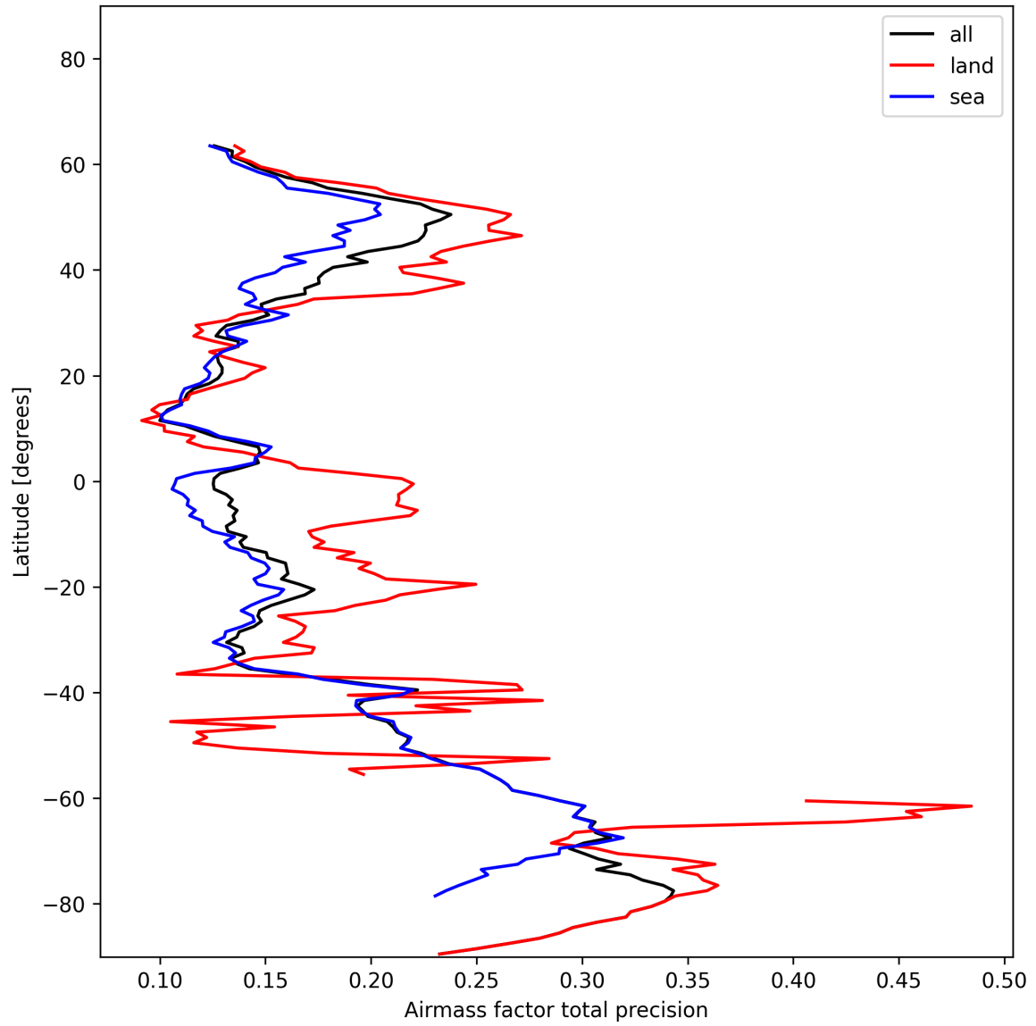
Figure 27: Zonal average of “Airmass factor total precision” for 2024-11-28 to 2024-11-30.
