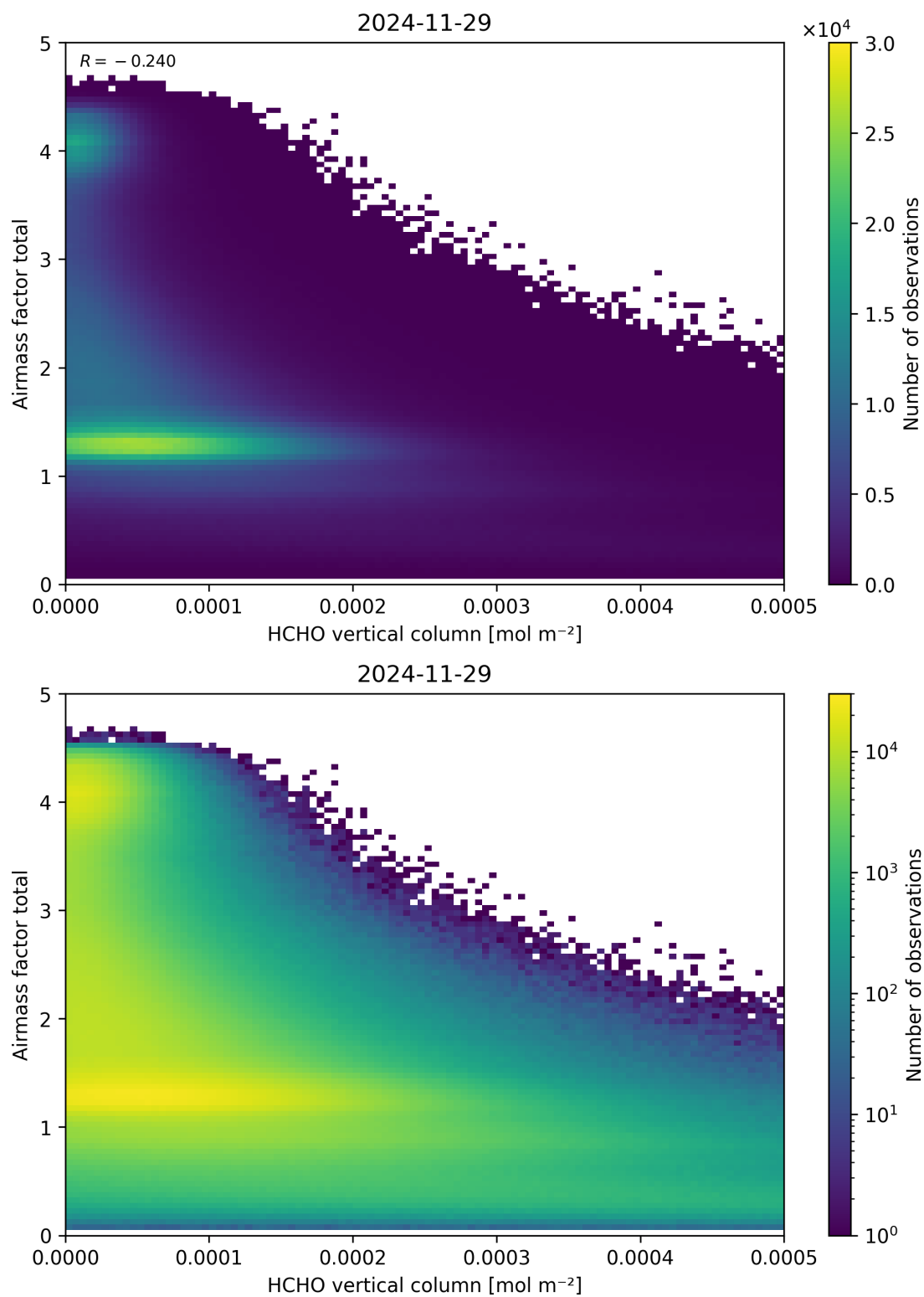
Figure 131: Scatter density plot of “HCHO vertical column” against “Airmass factor total” for 2024-11-28 to 2024-11-30.
