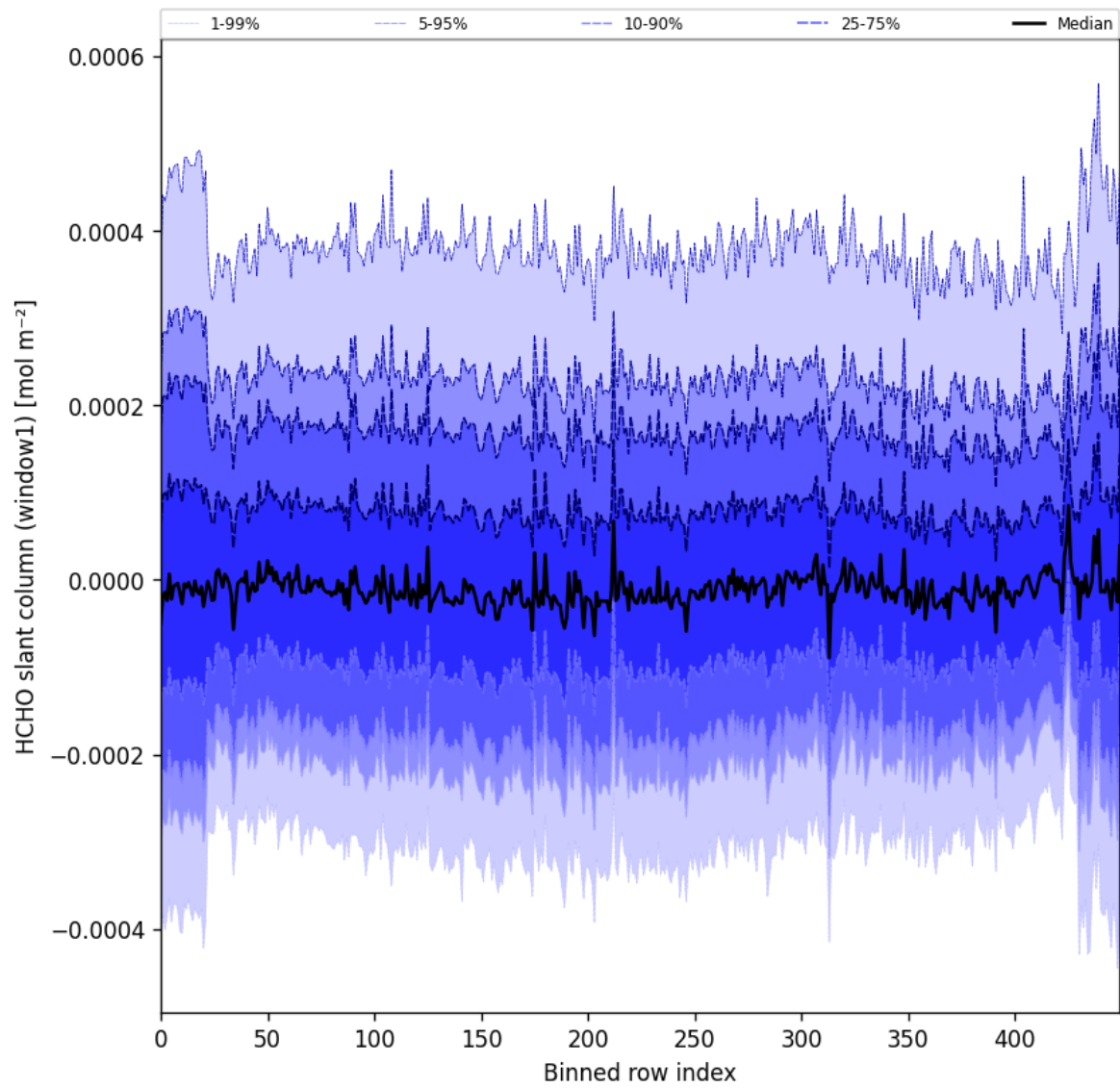
Figure 52: Along track statistics of “HCHO slant column (window1)” for 2024-11-28 to 2024-11-30
