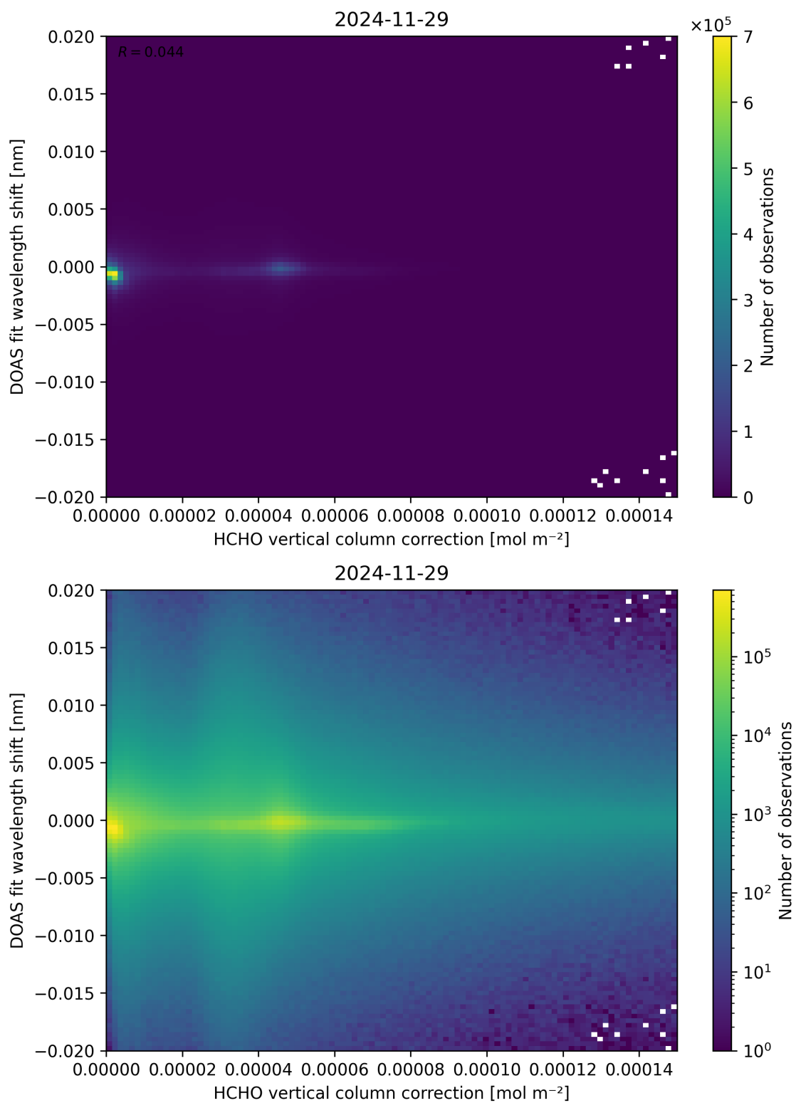
Figure 113: Scatter density plot of “HCHO vertical column correction” against “DOAS fit wavelength shift” for 2024-11-28 to 2024-11-30.
