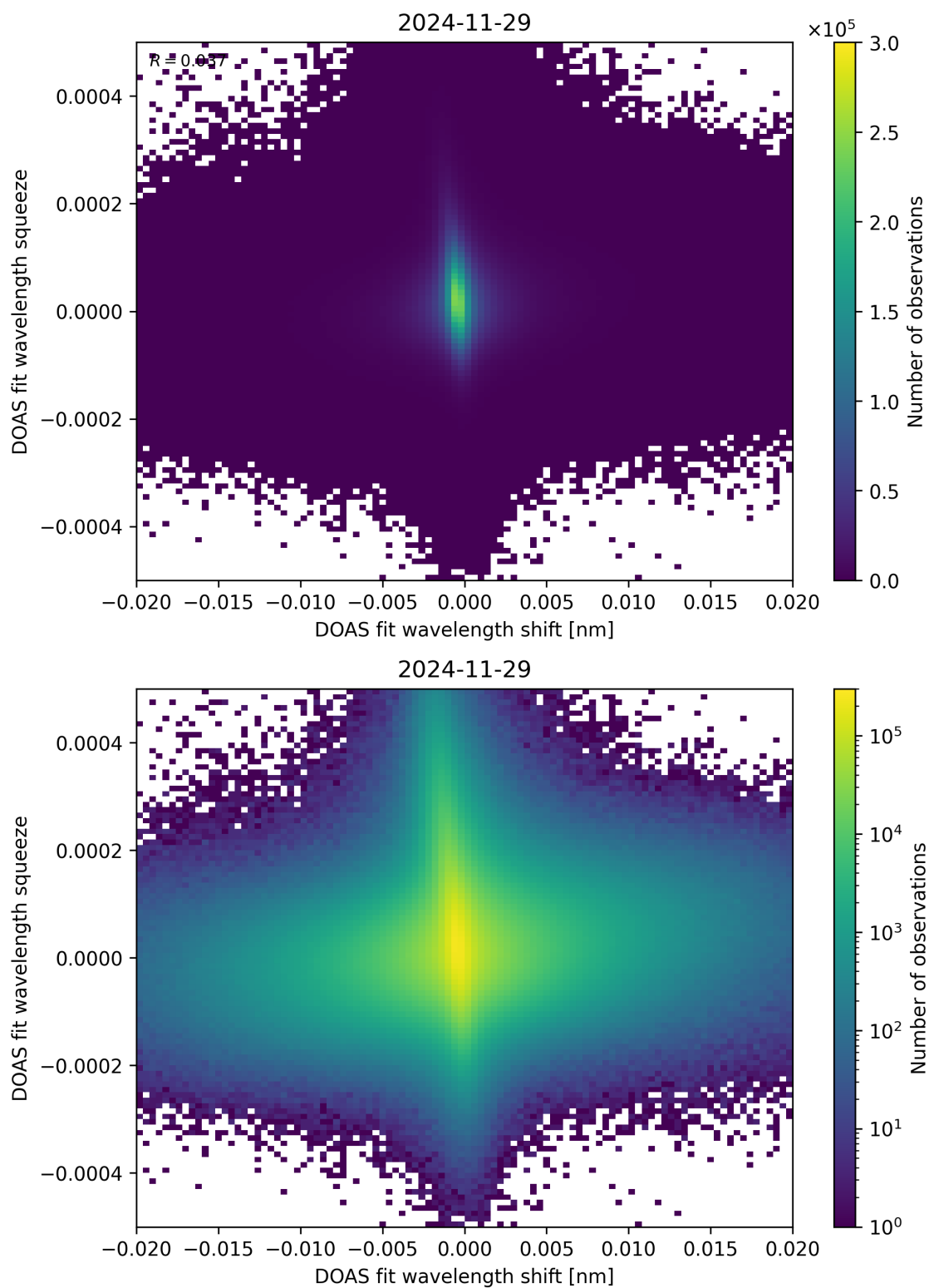
Figure 65: Scatter density plot of “DOAS fit wavelength shift” against “DOAS fit wavelength squeeze” for 2024-11-28 to 2024-11-30.
