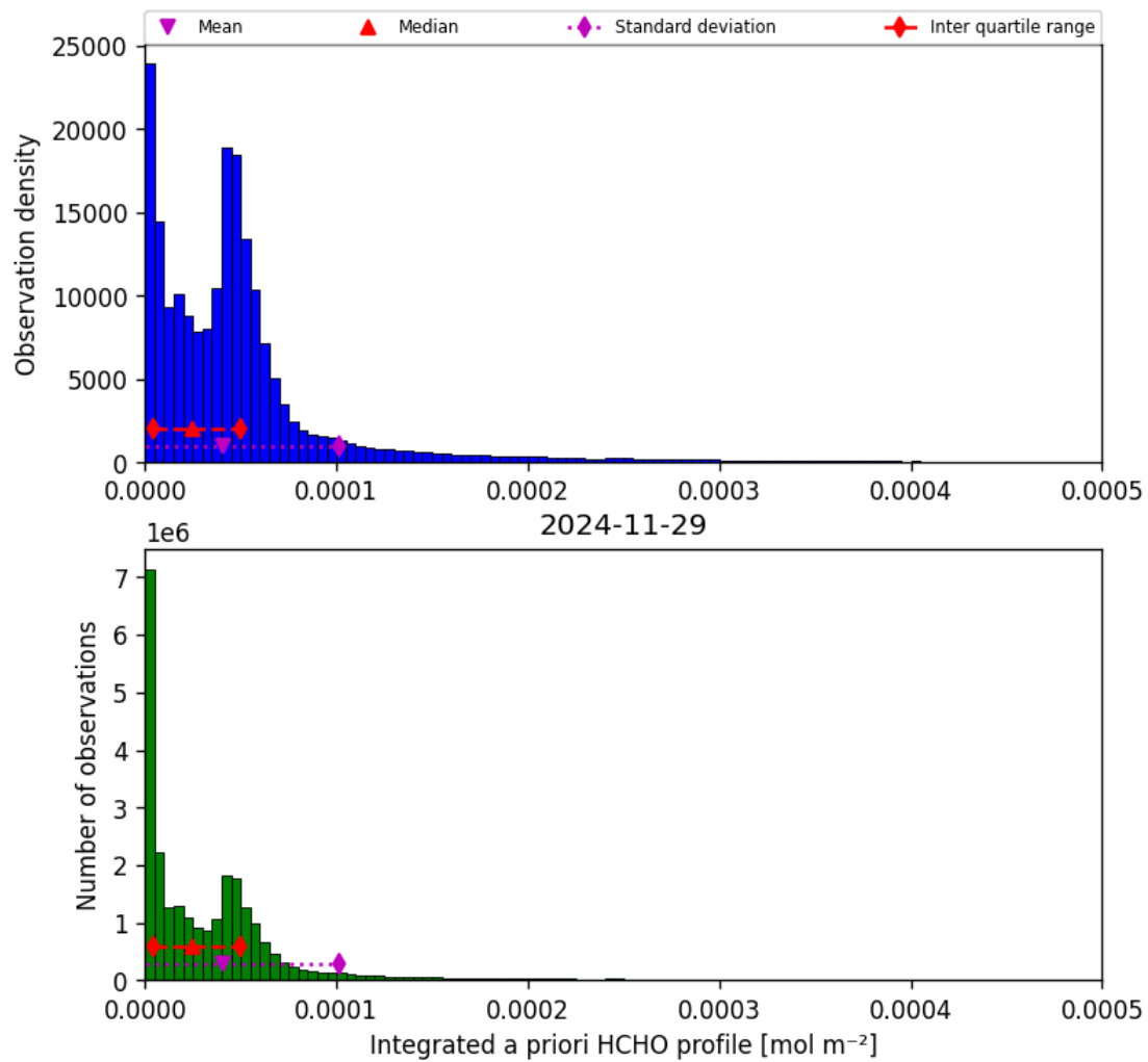
Figure 43: Histogram of “Integrated a priori HCHO profile” for 2024-11-28 to 2024-11-30
