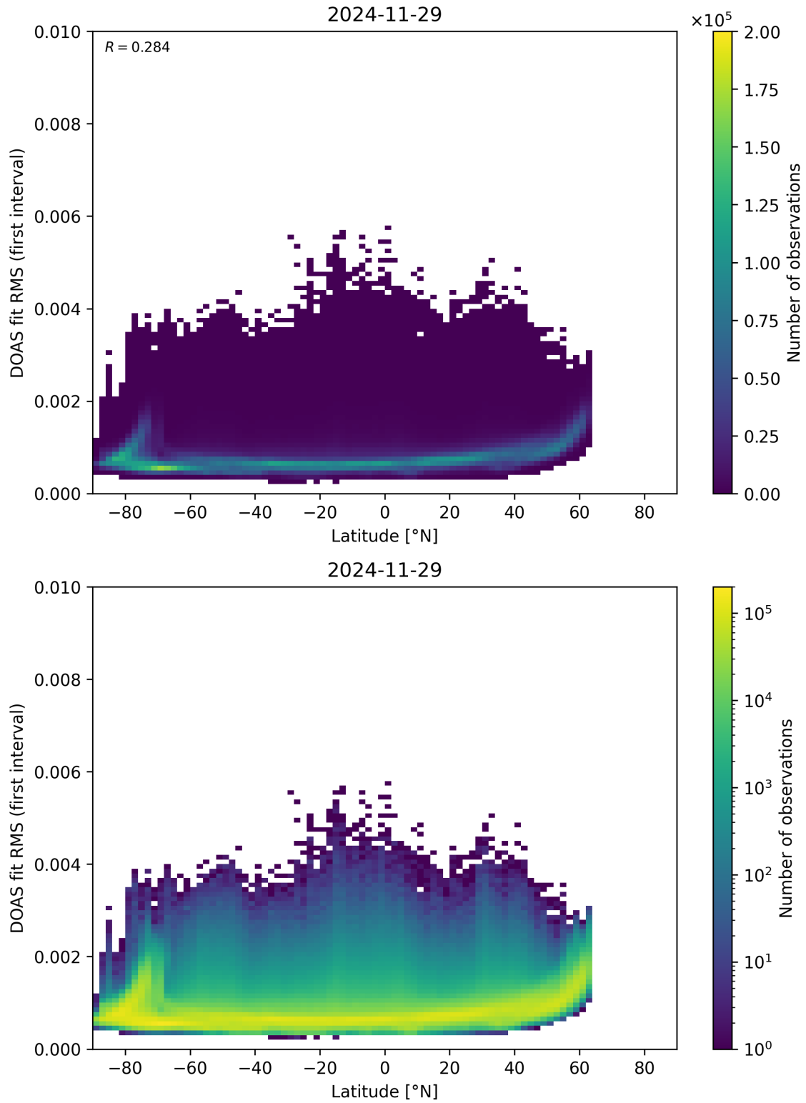
Figure 153: Scatter density plot of “Latitude” against “DOAS fit RMS (first interval)” for 2024-11-28 to 2024-11-30.
