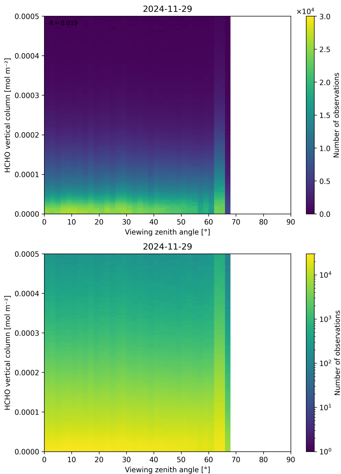
Figure 192: Scatter density plot of “Viewing zenith angle” against “HCHO vertical column” for 2024-11-28 to 2024-11-30.
