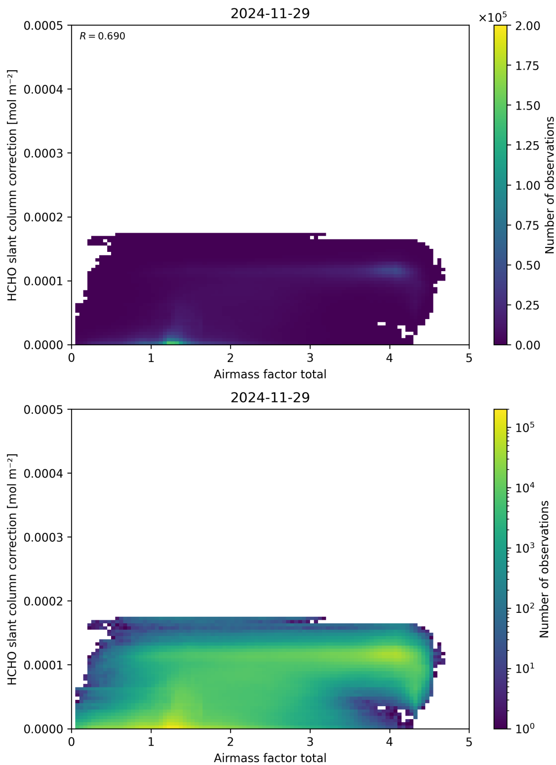
Figure 102: Scatter density plot of “Airmass factor total” against “HCHO slant column correction” for 2024-11-28 to 2024-11-30.
