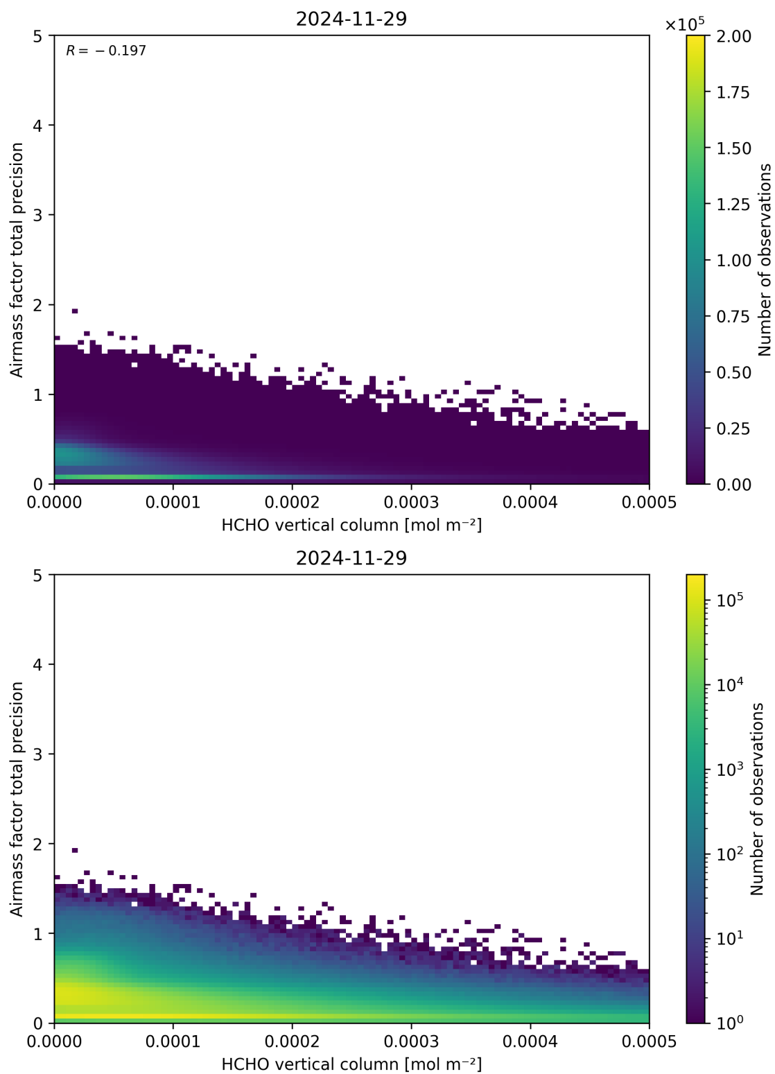
Figure 132: Scatter density plot of “HCHO vertical column” against “Airmass factor total precision” for 2024-11-28 to 2024-11-30.
