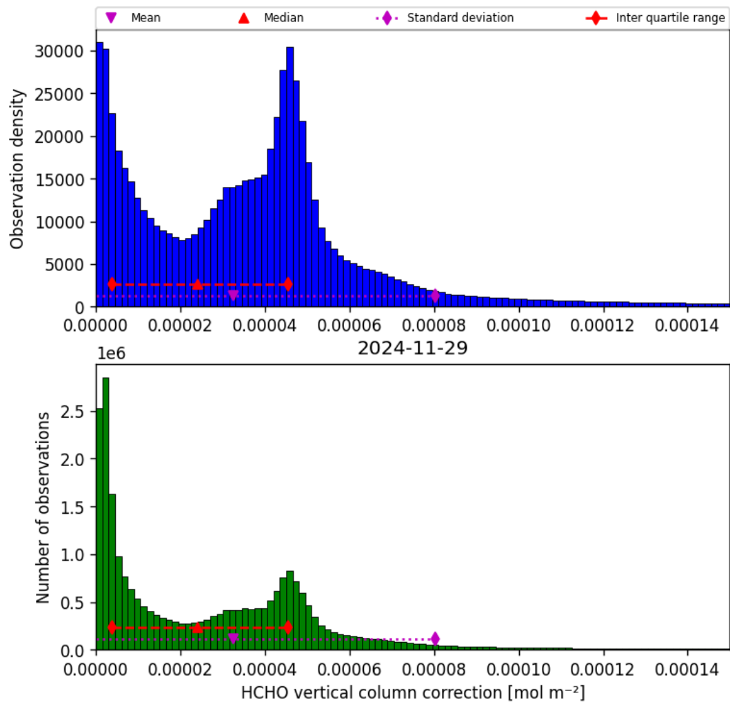
Figure 37: Histogram of “HCHO vertical column correction” for 2024-11-28 to 2024-11-30
