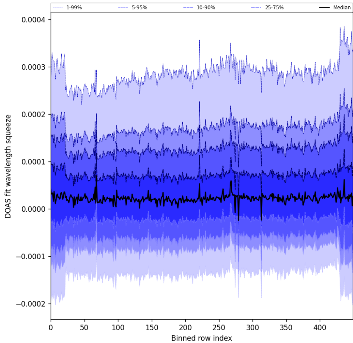
Figure 59: Along track statistics of “DOAS fit wavelength squeeze” for 2024-11-28 to 2024-11-30
