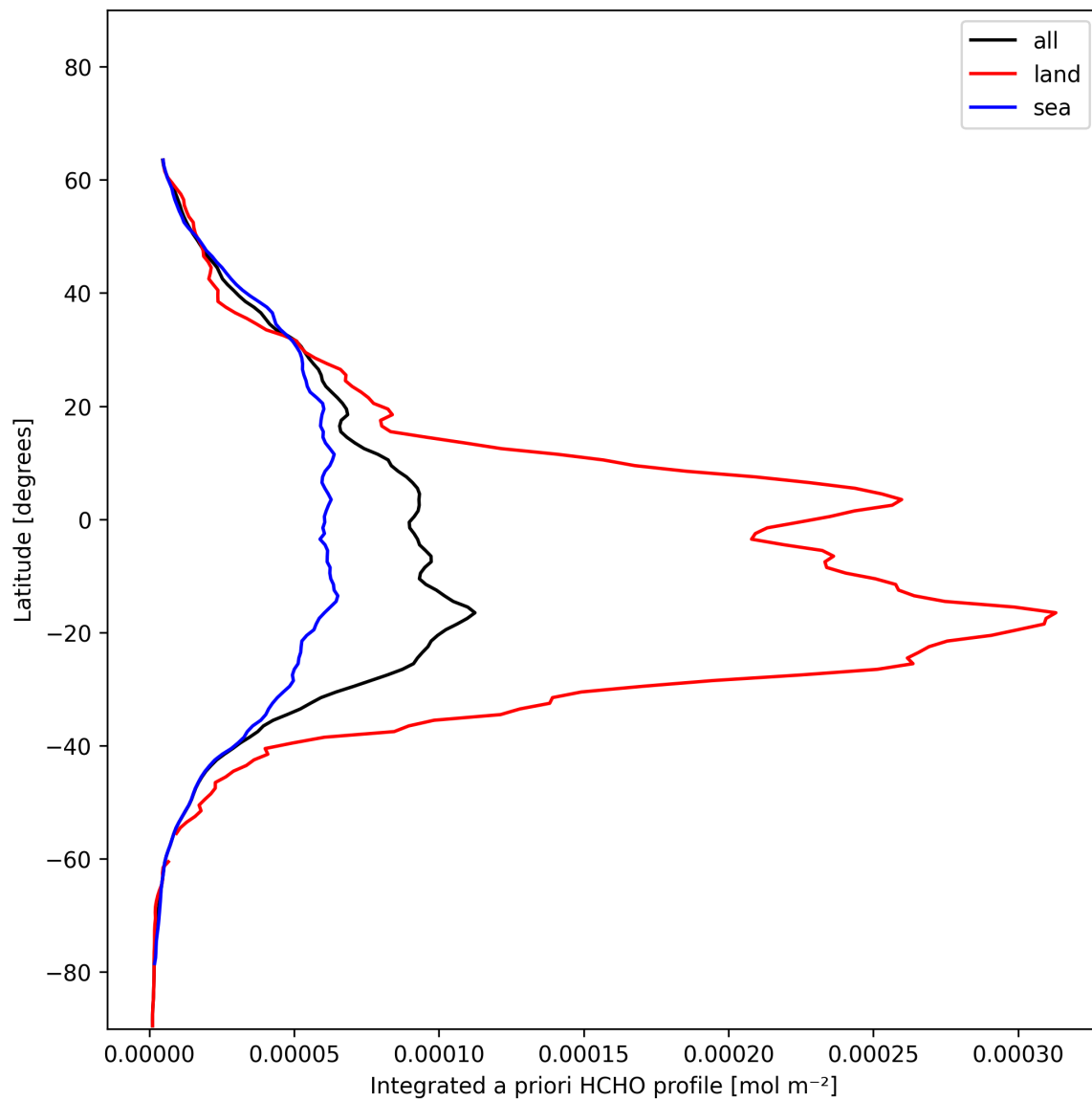
Figure 29: Zonal average of “Integrated a priori HCHO profile” for 2024-11-28 to 2024-11-30.
