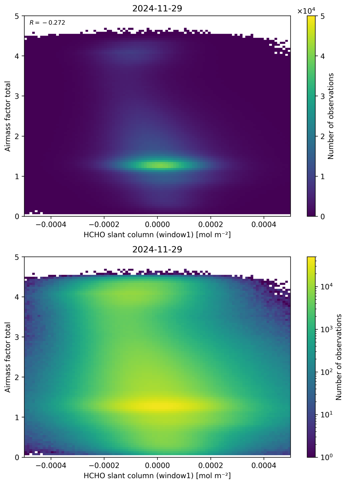
Figure 85: Scatter density plot of “HCHO slant column (window1)” against “Airmass factor total” for 2024-11-28 to 2024-11-30.
