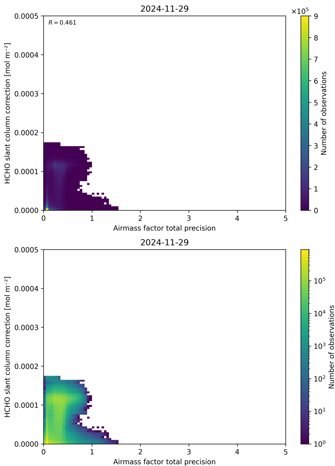
Figure 110: Scatter density plot of “Airmass factor total precision” against “HCHO slant column correction” for 2024-11-28 to 2024-11-30.
