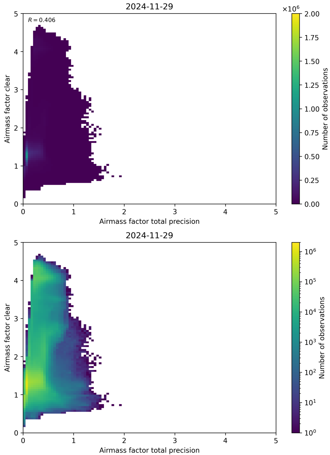
Figure 108: Scatter density plot of “Airmass factor total precision” against “Airmass factor clear” for 2024-11-28 to 2024-11-30.
