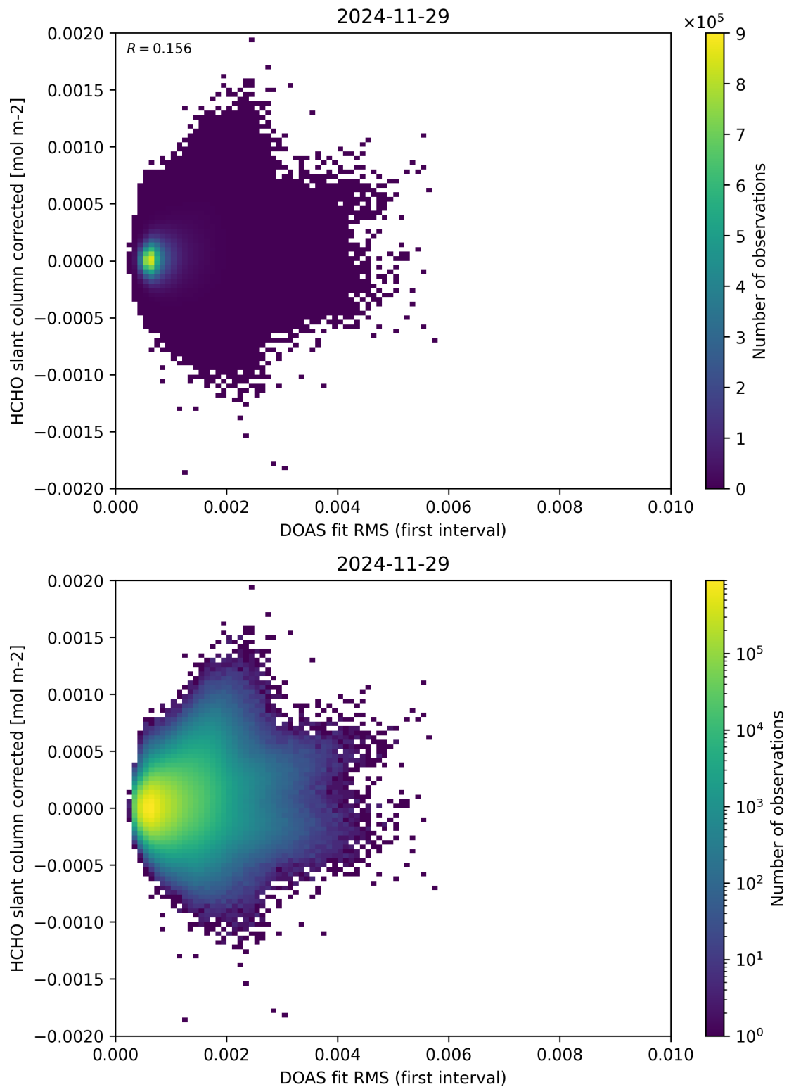
Figure 62: Scatter density plot of “DOAS fit RMS (first interval)” against “HCHO slant column corrected” for 2024-11-28 to 2024-11-30.
