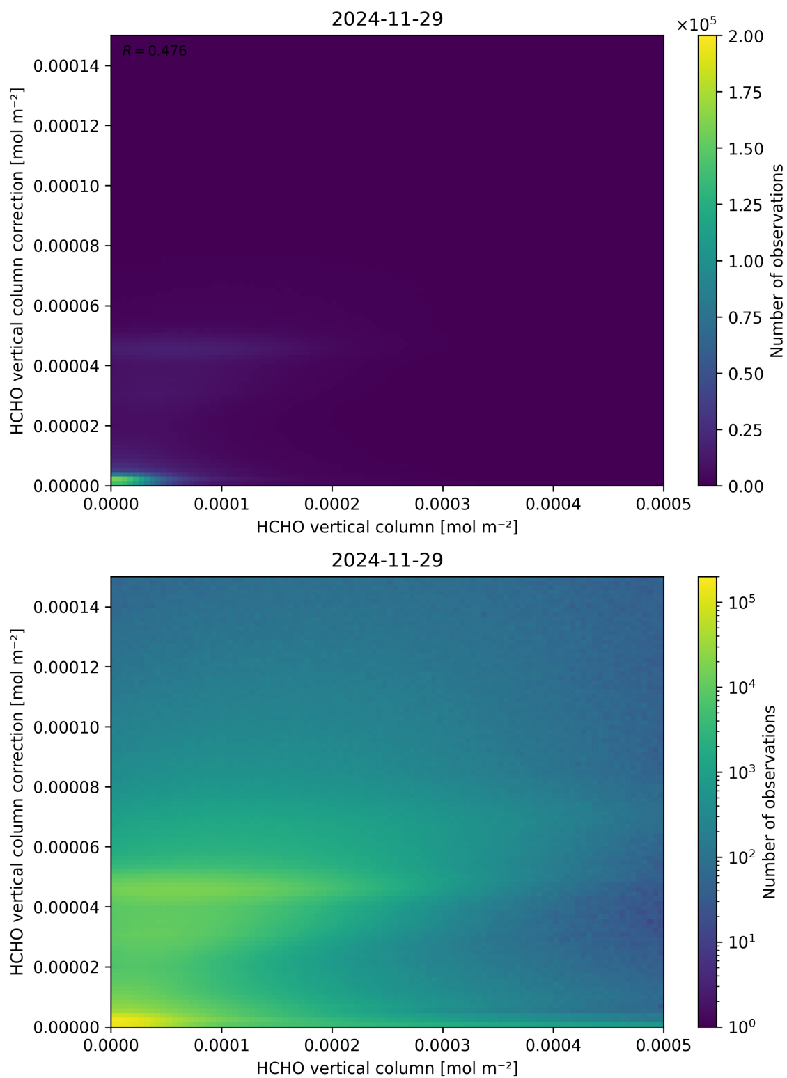
Figure 133: Scatter density plot of “HCHO vertical column” against “HCHO vertical column correction” for 2024-11-28 to 2024-11-30.
