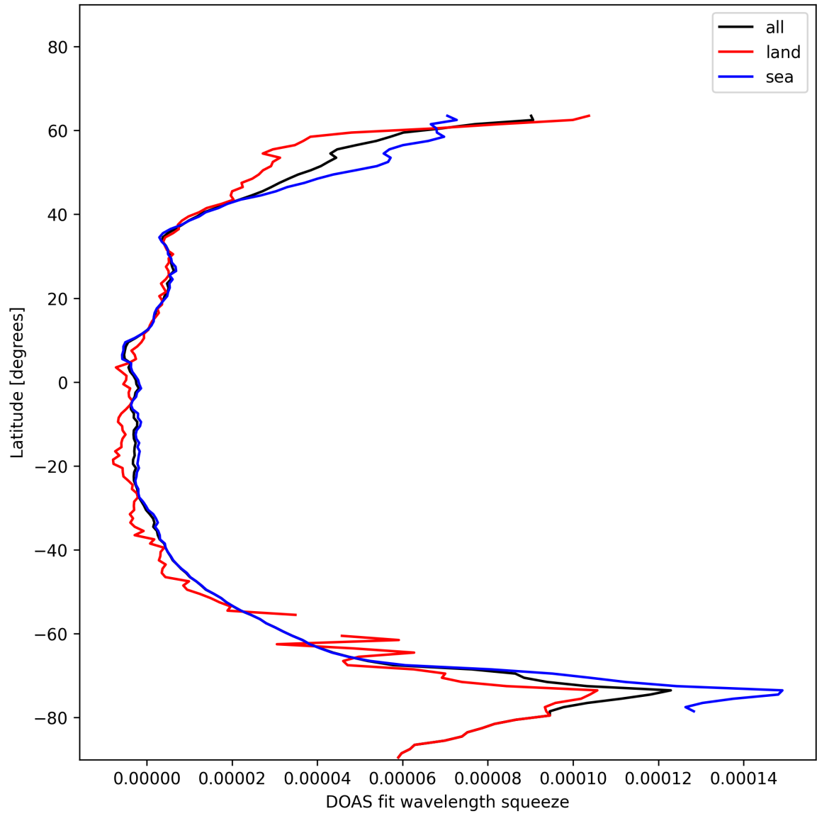
Figure 31: Zonal average of “DOAS fit wavelength squeeze” for 2024-11-28 to 2024-11-30.
