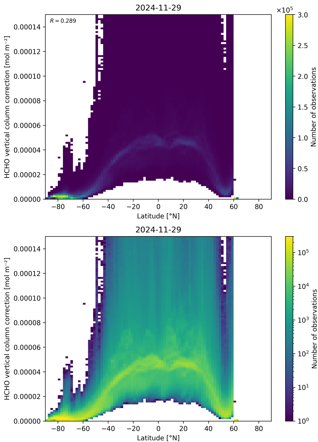
Figure 164: Scatter density plot of “Latitude” against “HCHO vertical column correction” for 2024-11-28 to 2024-11-30.
