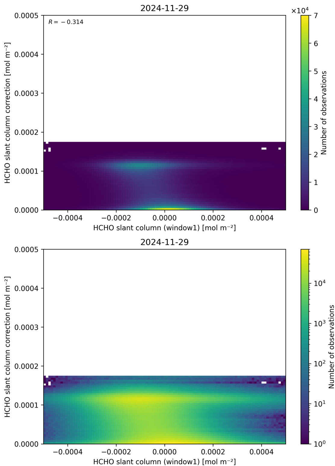
Figure 83: Scatter density plot of “HCHO slant column (window1)” against “HCHO slant column correction” for 2024-11-28 to 2024-11-30.
