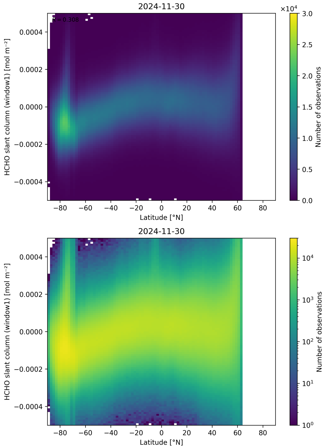
Figure 159: Scatter density plot of “Latitude” against “HCHO slant column (window1)” for 2024-11-30 to 2024-12-01.
