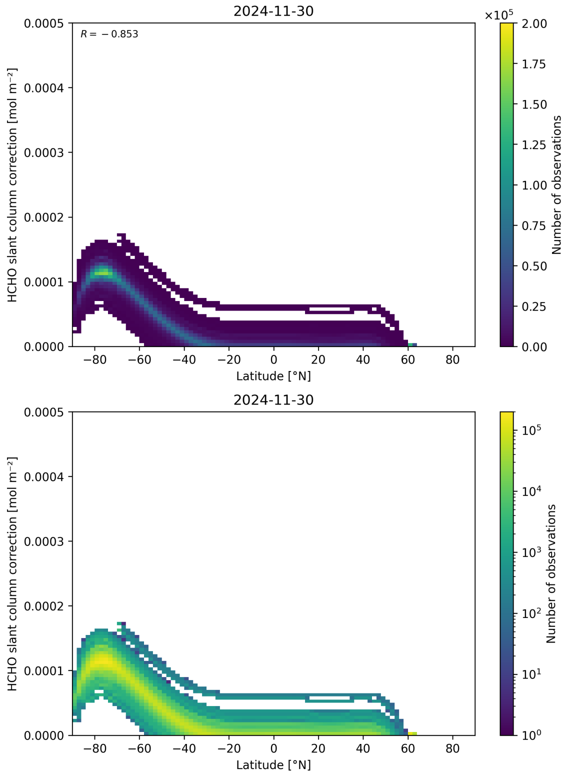
Figure 158: Scatter density plot of “Latitude” against “HCHO slant column correction” for 2024-11-30 to 2024-12-01.
