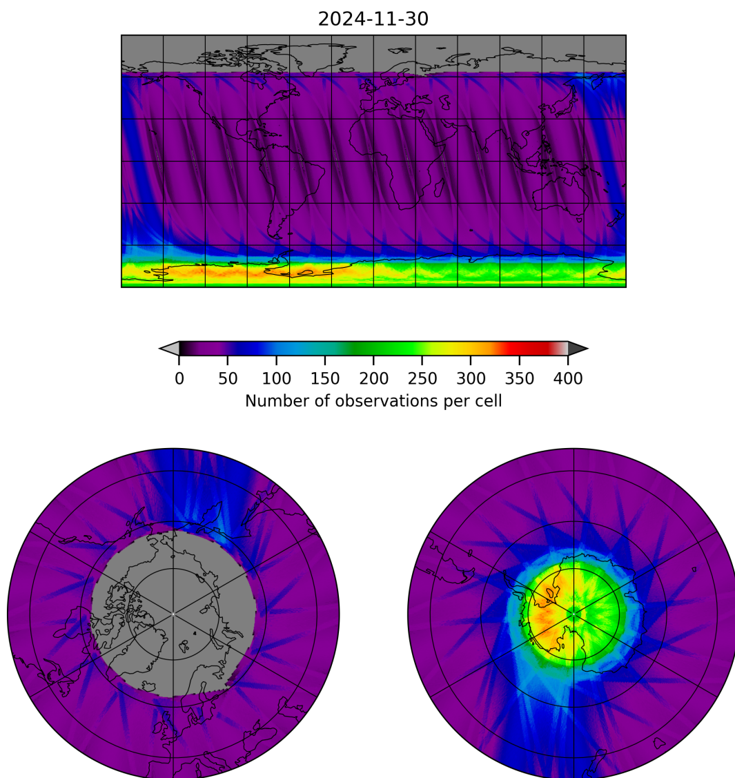
Figure 19: Map of the number of observations for 2024-11-30 to 2024-12-01
