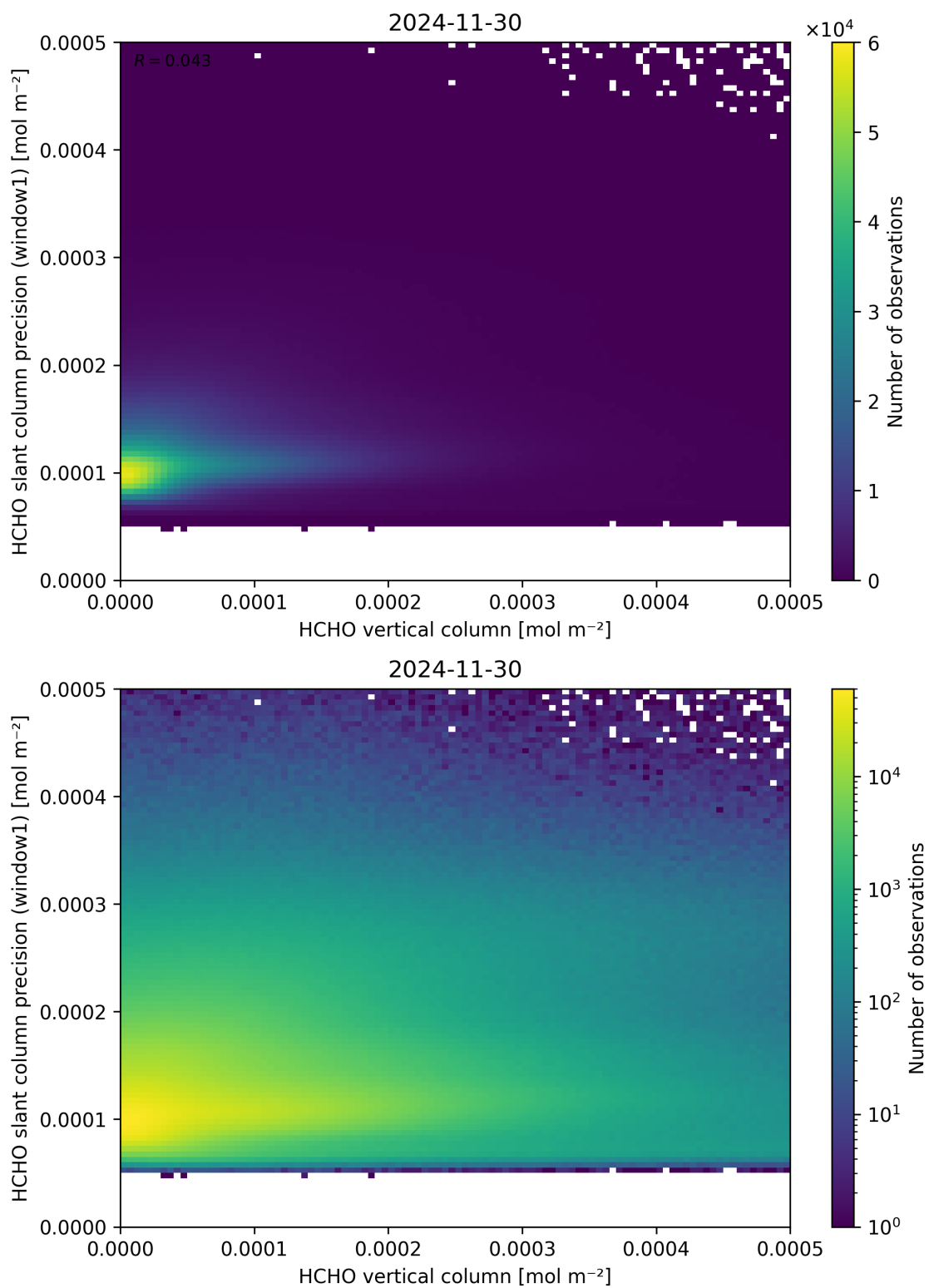
Figure 130: Scatter density plot of “HCHO vertical column” against “HCHO slant column precision (window1)” for 2024-11-30 to 2024-12-01.
