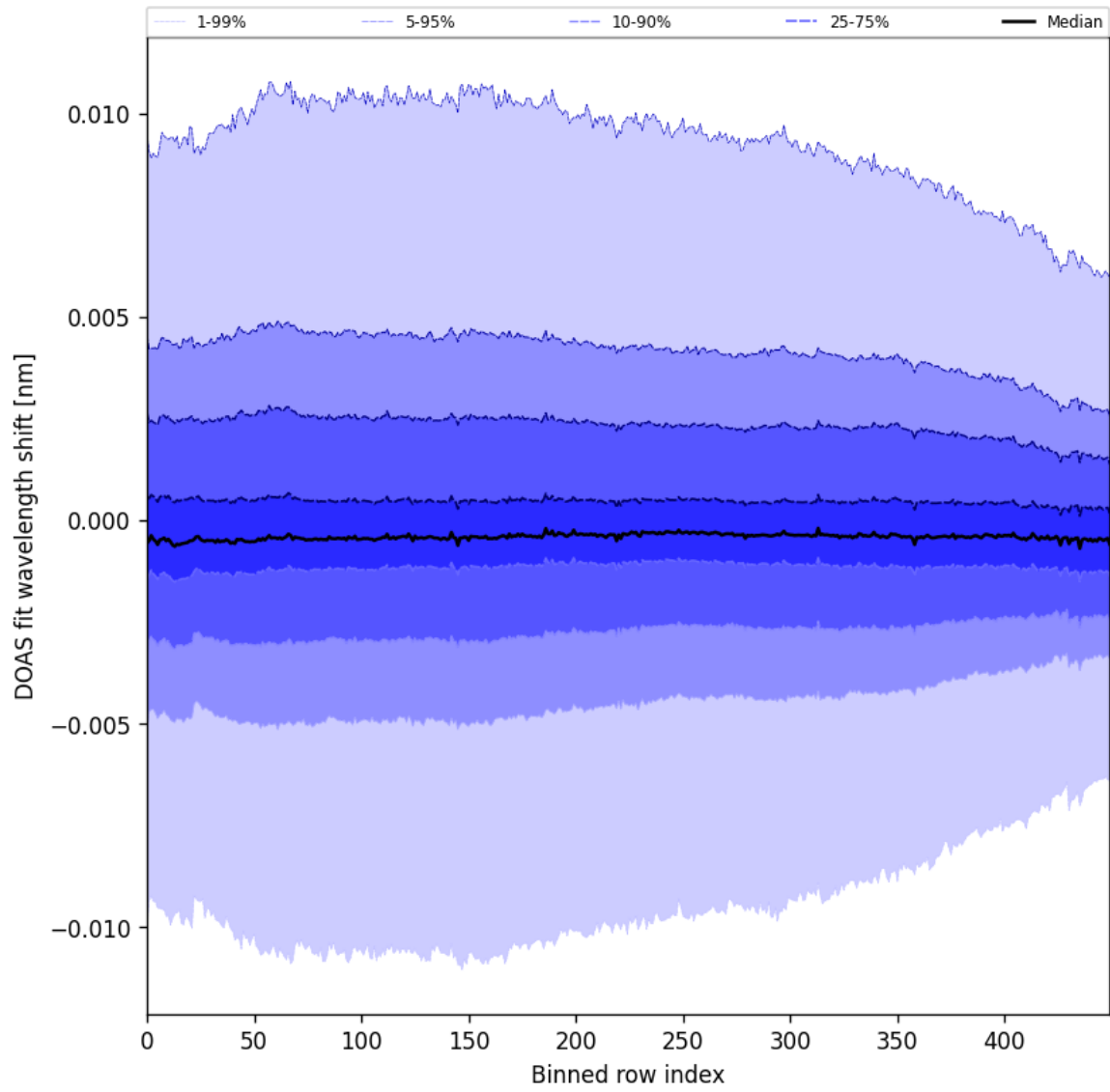
Figure 58: Along track statistics of “DOAS fit wavelength shift” for 2024-11-30 to 2024-12-01
