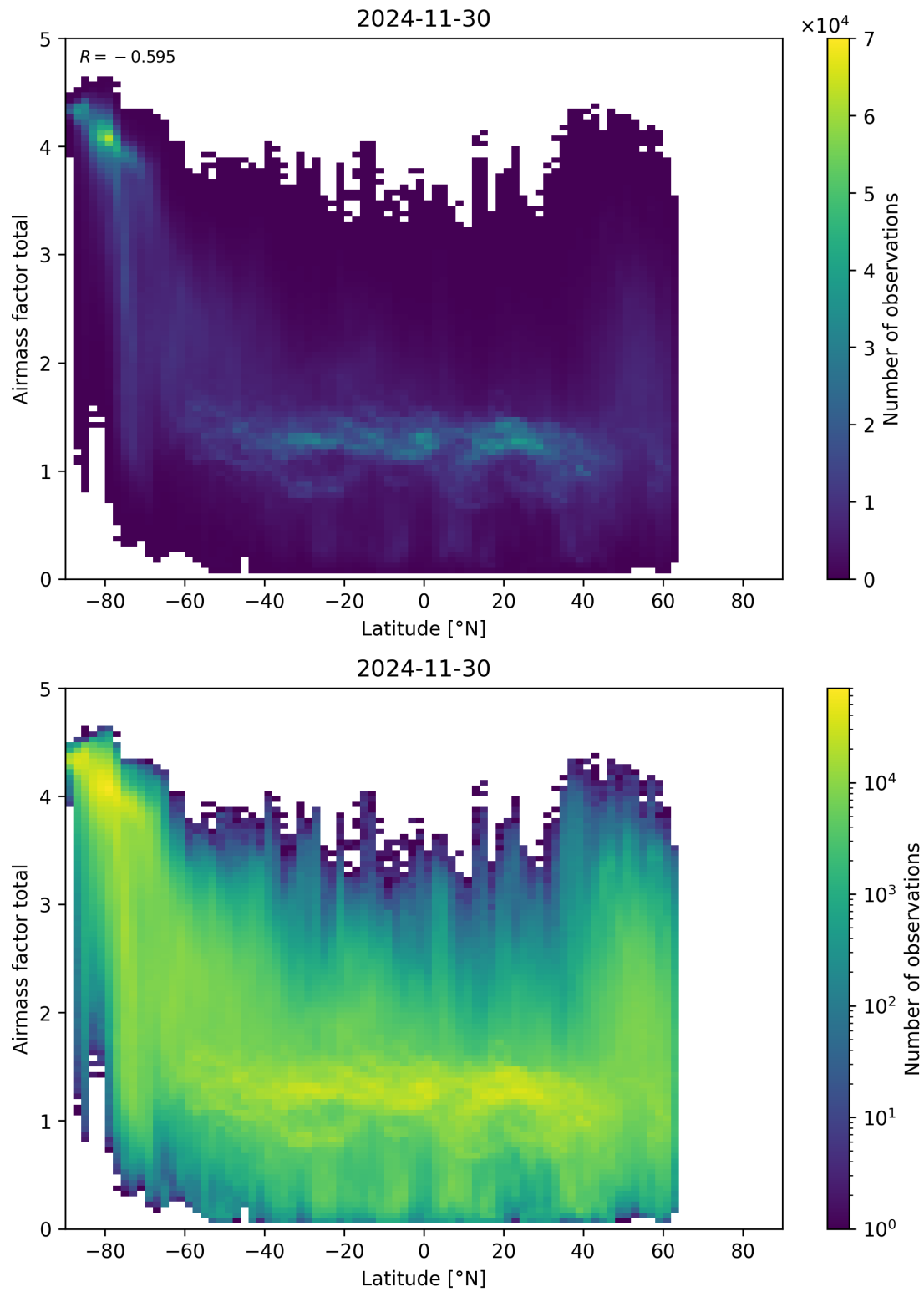
Figure 161: Scatter density plot of “Latitude” against “Airmass factor total” for 2024-11-30 to 2024-12-01.
