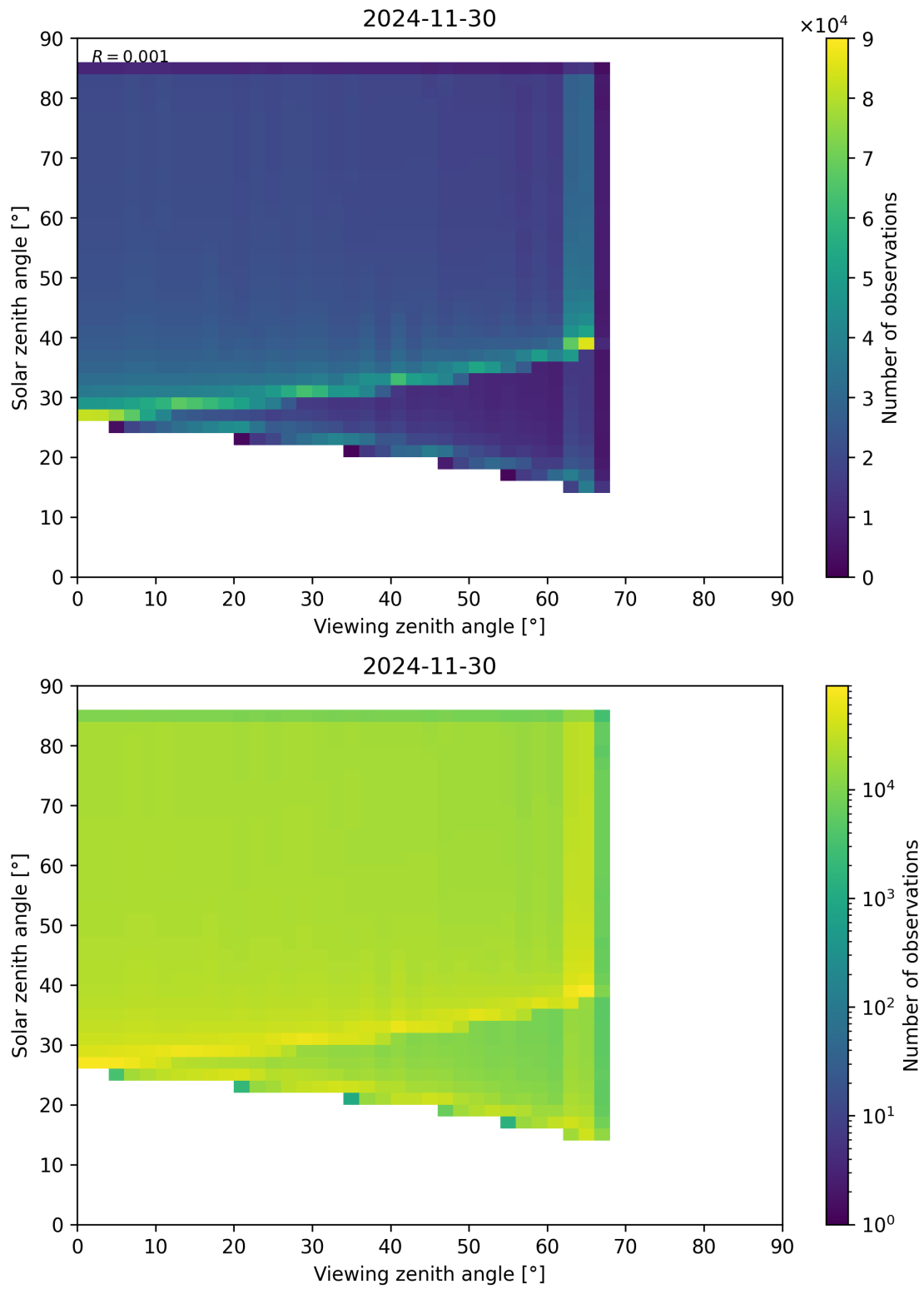
Figure 197: Scatter density plot of “Viewing zenith angle” against “Solar zenith angle” for 2024-11-30 to 2024-12-01.
