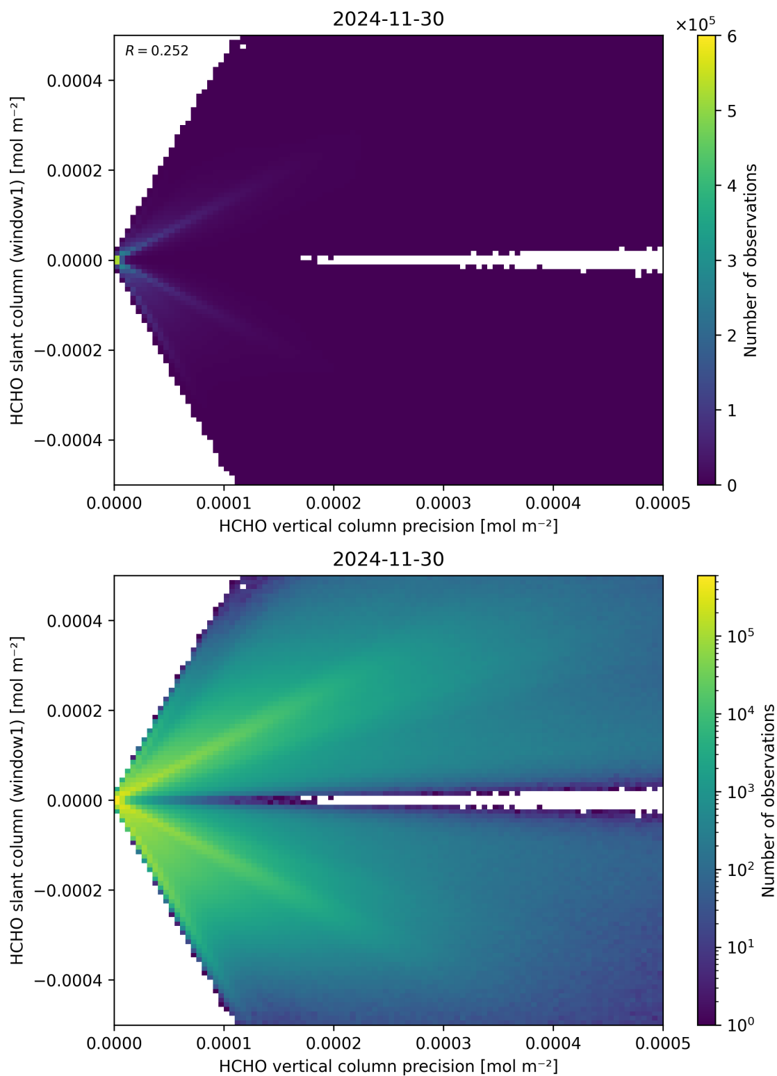
Figure 142: Scatter density plot of “HCHO vertical column precision” against “HCHO slant column (window1)” for 2024-11-30 to 2024-12-01.
