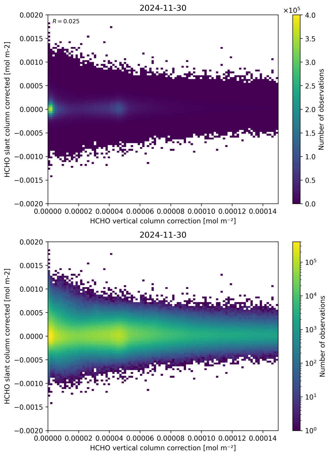
Figure 116: Scatter density plot of “HCHO vertical column correction” against “HCHO slant column corrected” for 2024-11-30 to 2024-12-01.
