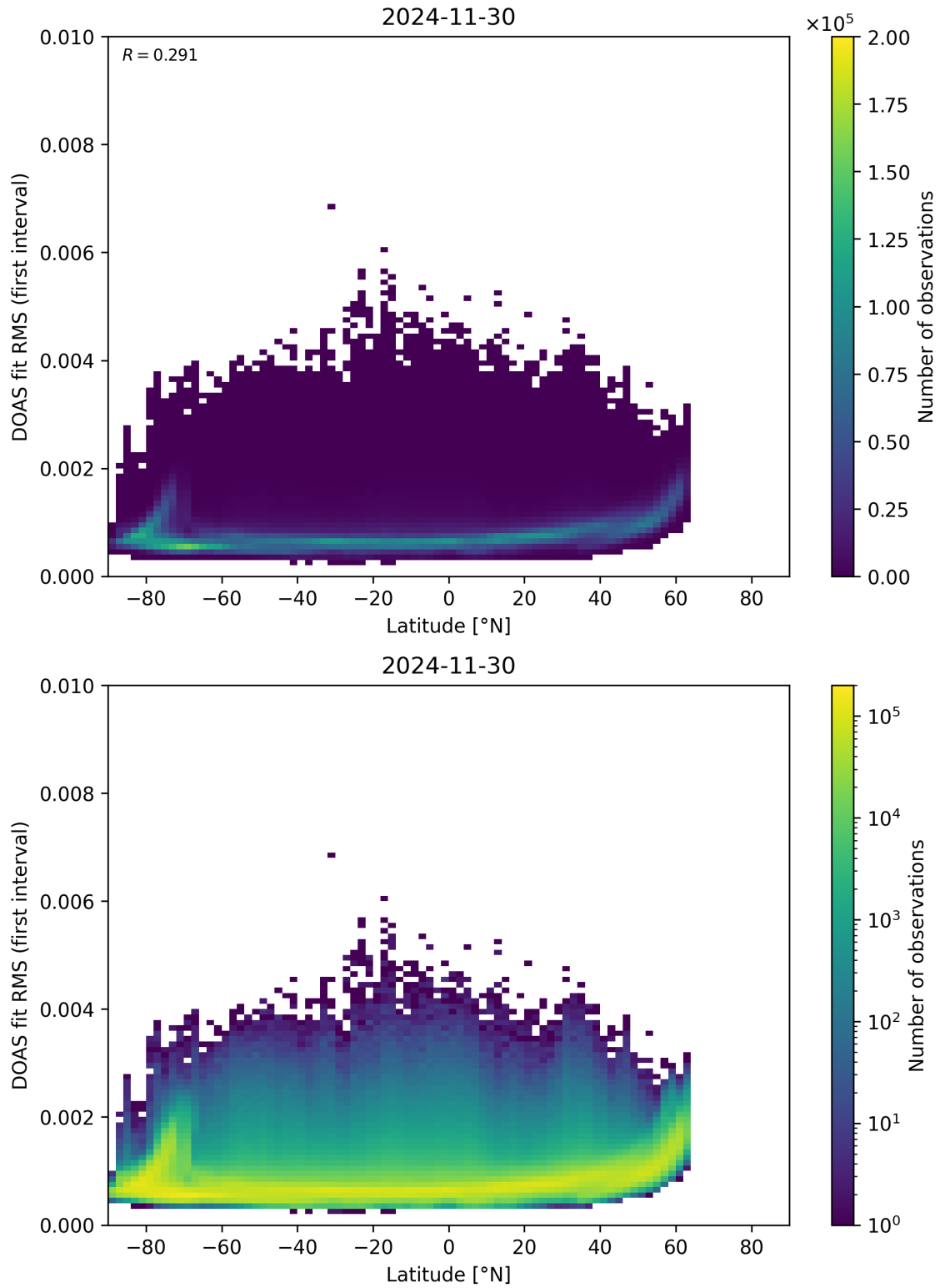
Figure 153: Scatter density plot of “Latitude” against “DOAS fit RMS (first interval)” for 2024-11-30 to 2024-12-01.
