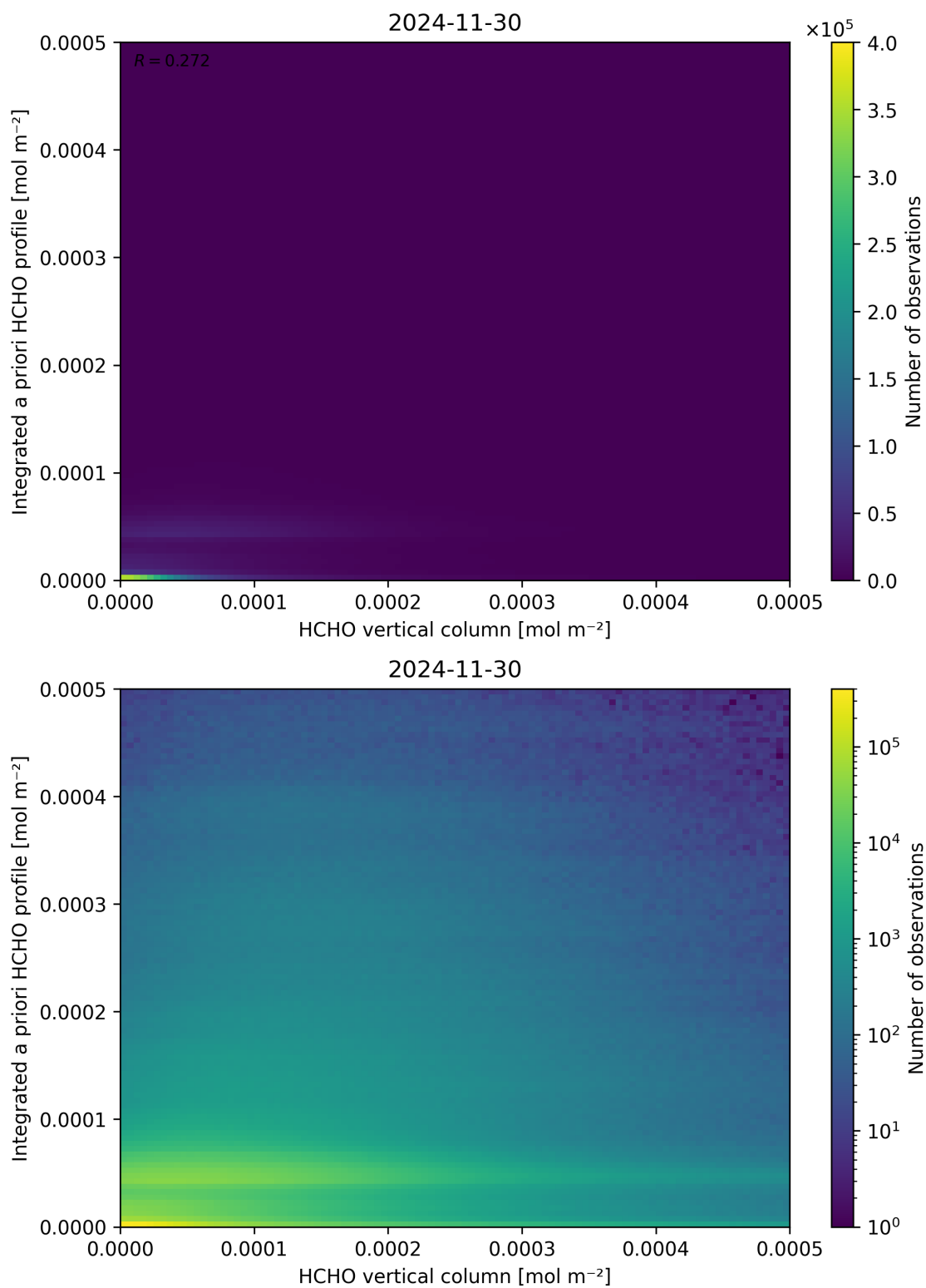
Figure 135: Scatter density plot of “HCHO vertical column” against “Integrated a priori HCHO profile” for 2024-11-30 to 2024-12-01.
