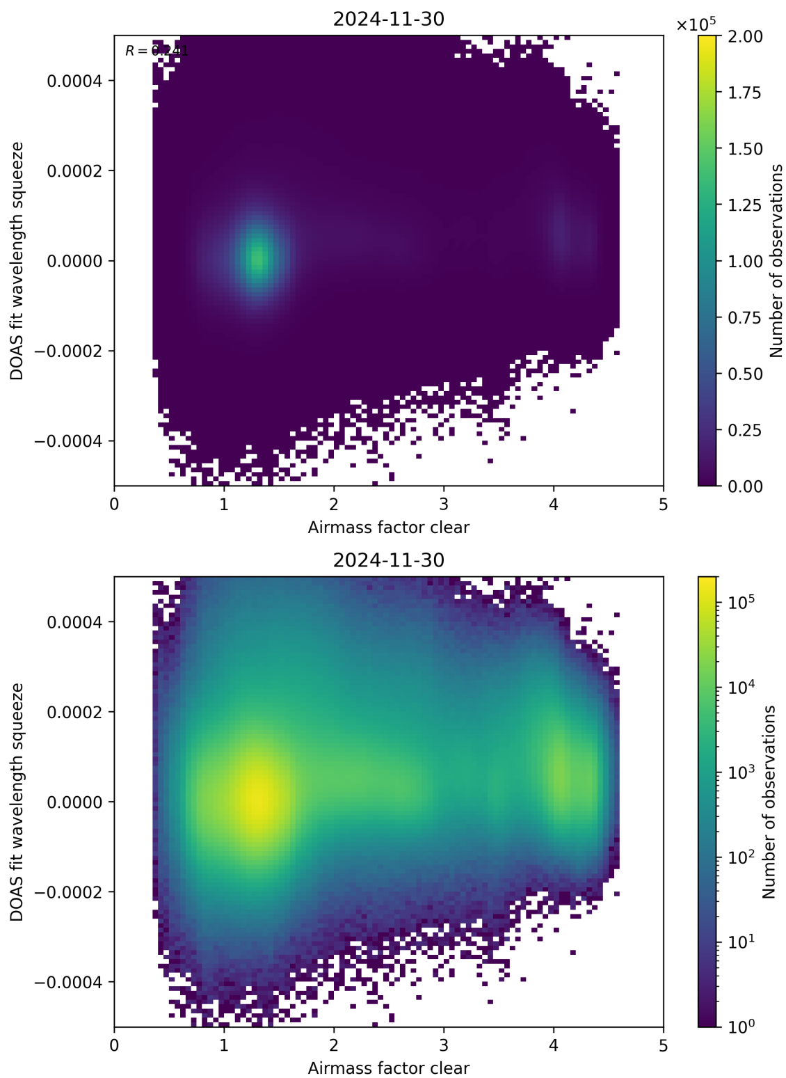
Figure 73: Scatter density plot of “Airmass factor clear” against “DOAS fit wavelength squeeze” for 2024-11-30 to 2024-12-01.
