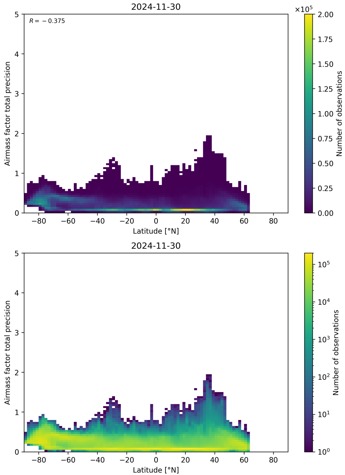
Figure 162: Scatter density plot of “Latitude” against “Airmass factor total precision” for 2024-11-30 to 2024-12-01.
