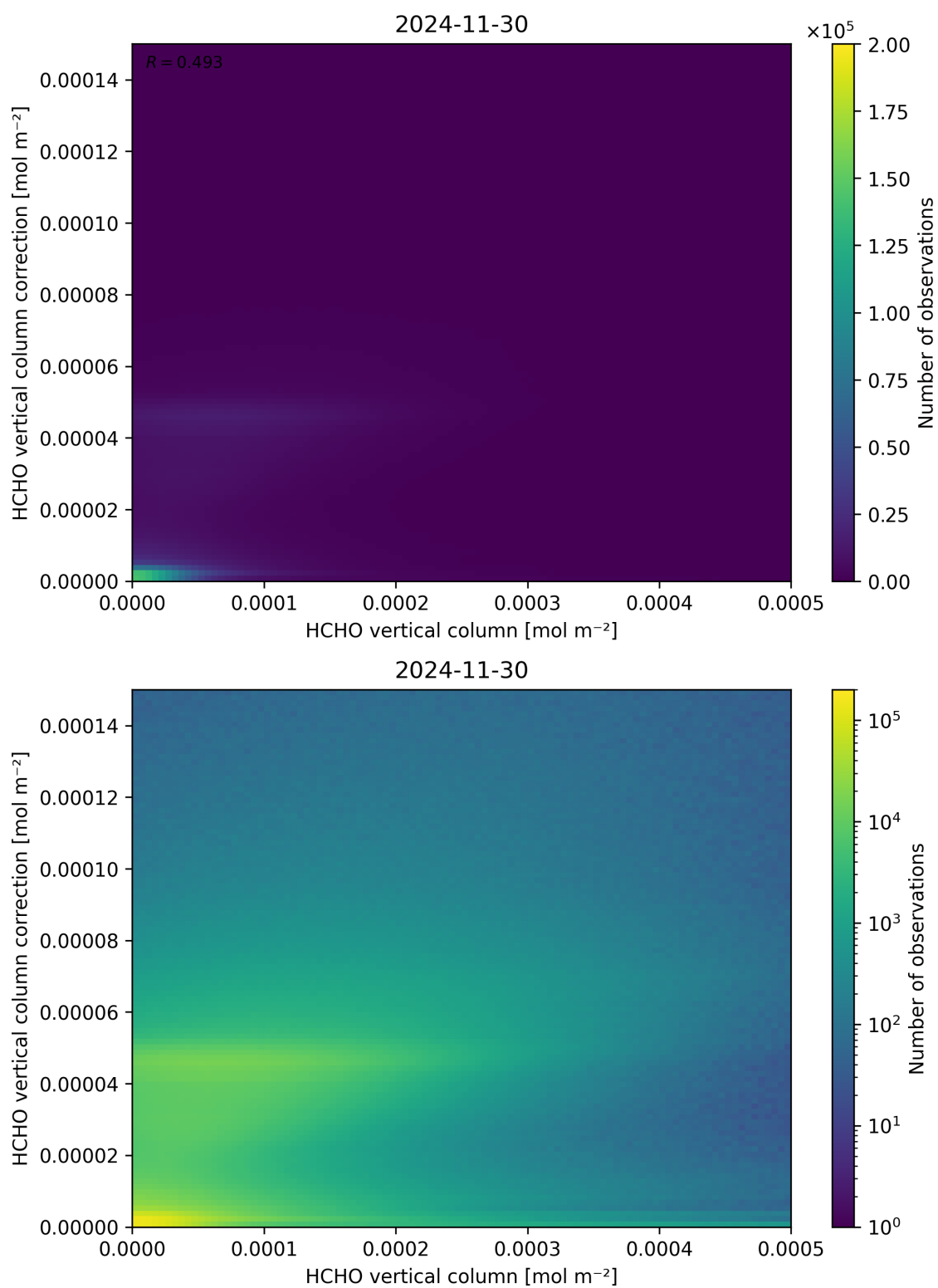
Figure 133: Scatter density plot of “HCHO vertical column” against “HCHO vertical column correction” for 2024-11-30 to 2024-12-01.
