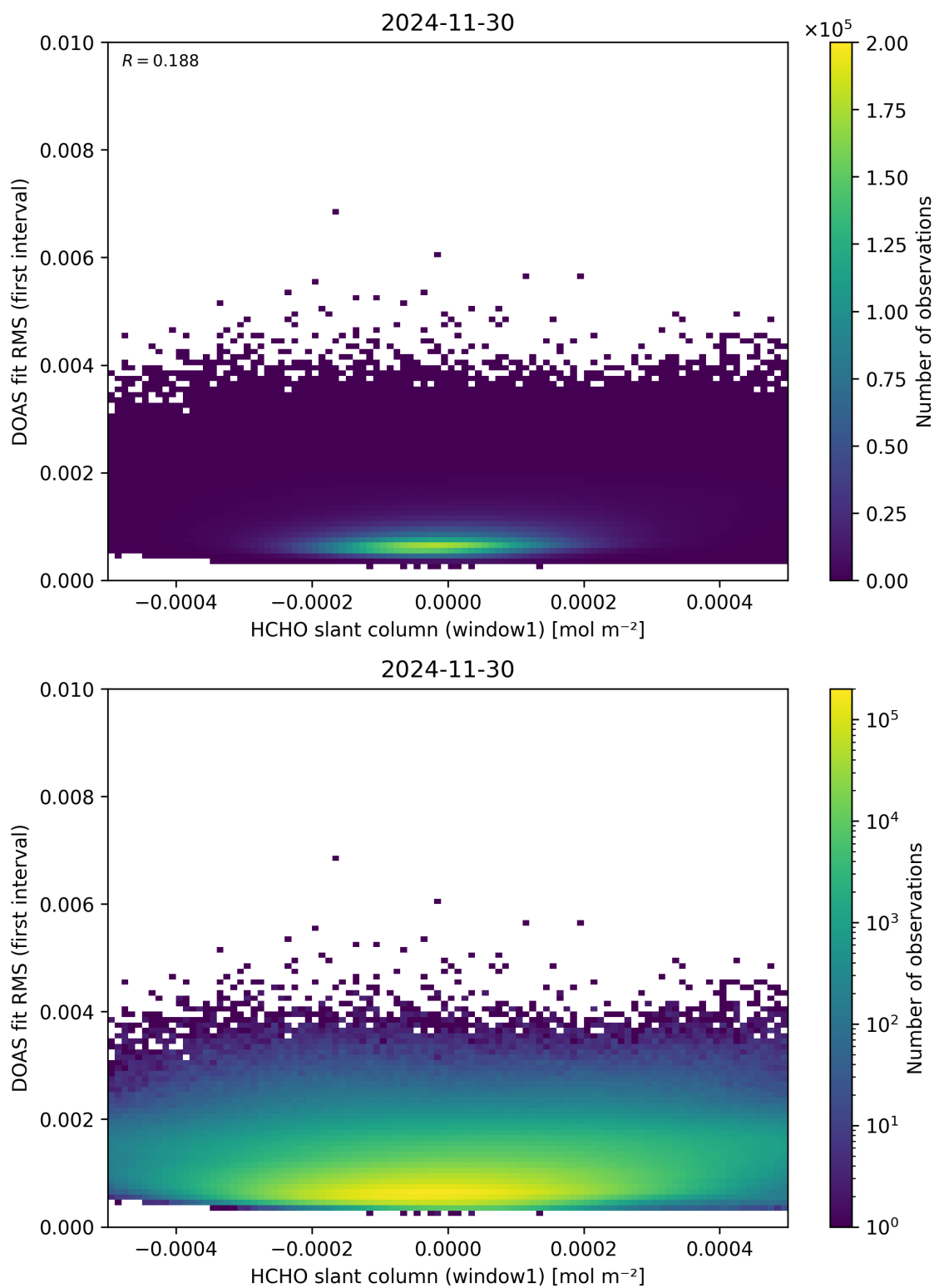
Figure 78: Scatter density plot of “HCHO slant column (window1)” against “DOAS fit RMS (first interval)” for 2024-11-30 to 2024-12-01.
