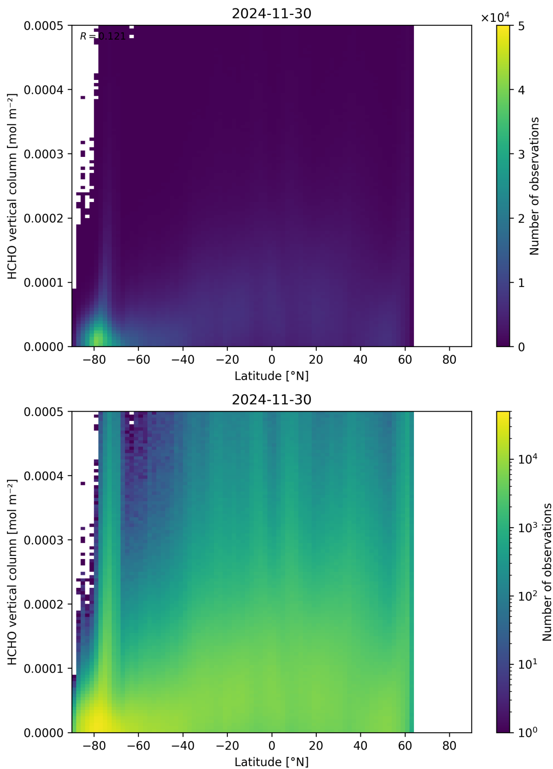
Figure 163: Scatter density plot of “Latitude” against “HCHO vertical column” for 2024-11-30 to 2024-12-01.
