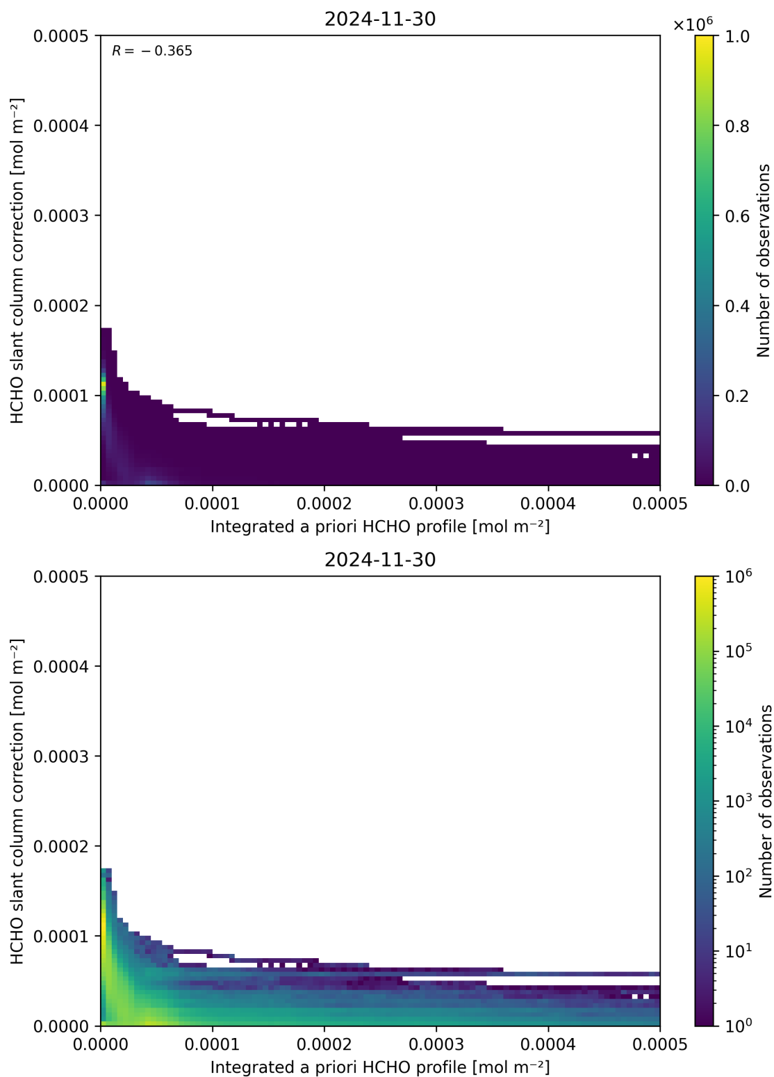
Figure 152: Scatter density plot of “Integrated a priori HCHO profile” against “HCHO slant column correction” for 2024-11-30 to 2024-12-01.
