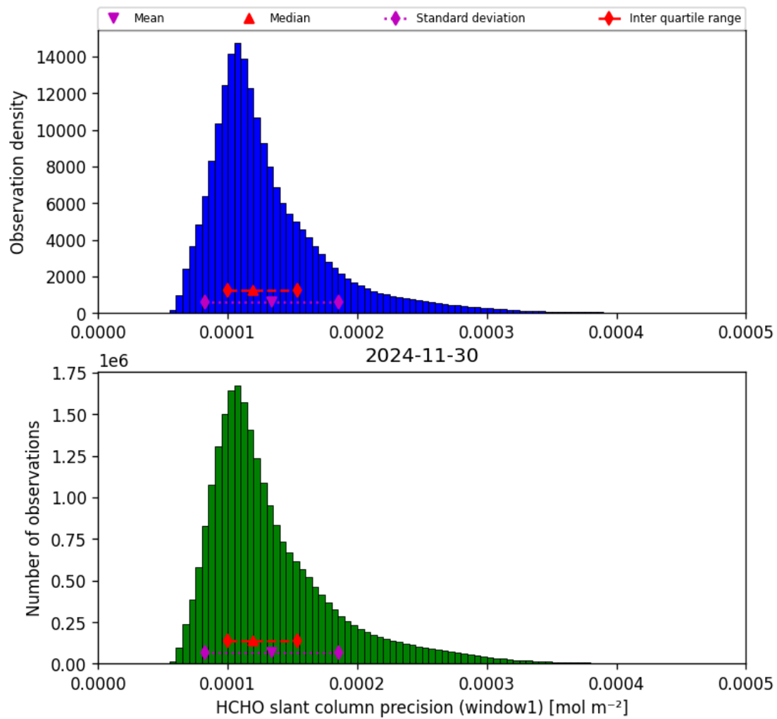
Figure 39: Histogram of “HCHO slant column precision (window1)” for 2024-11-30 to 2024-12-01
