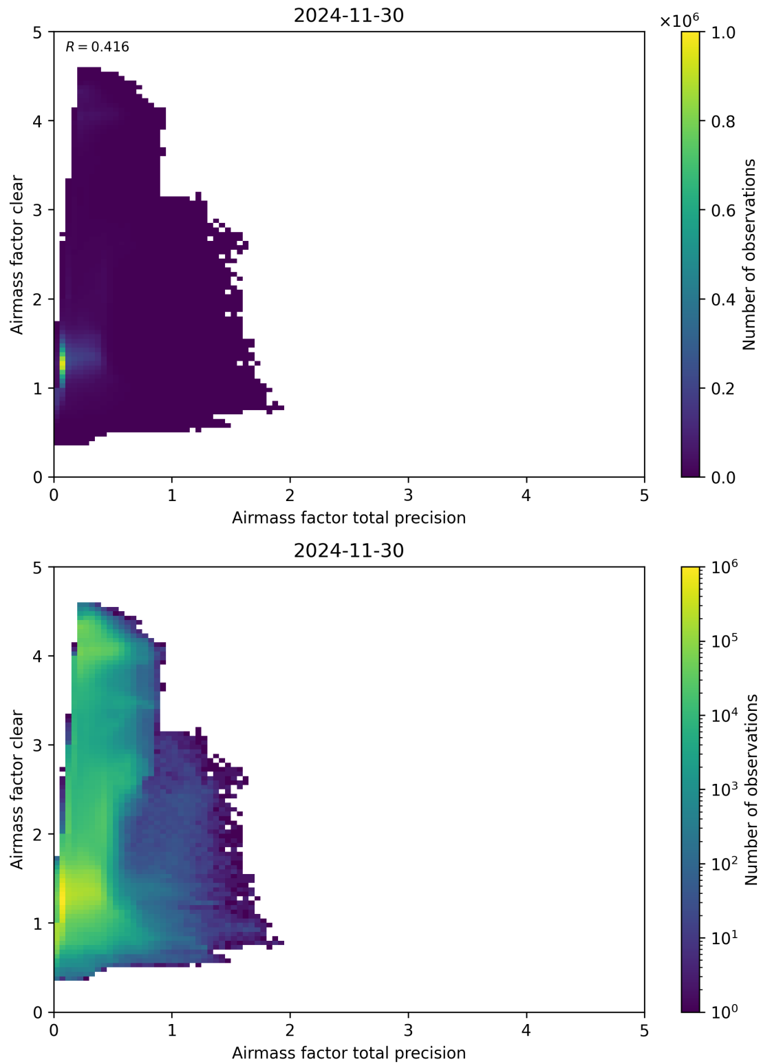
Figure 108: Scatter density plot of “Airmass factor total precision” against “Airmass factor clear” for 2024-11-30 to 2024-12-01.
