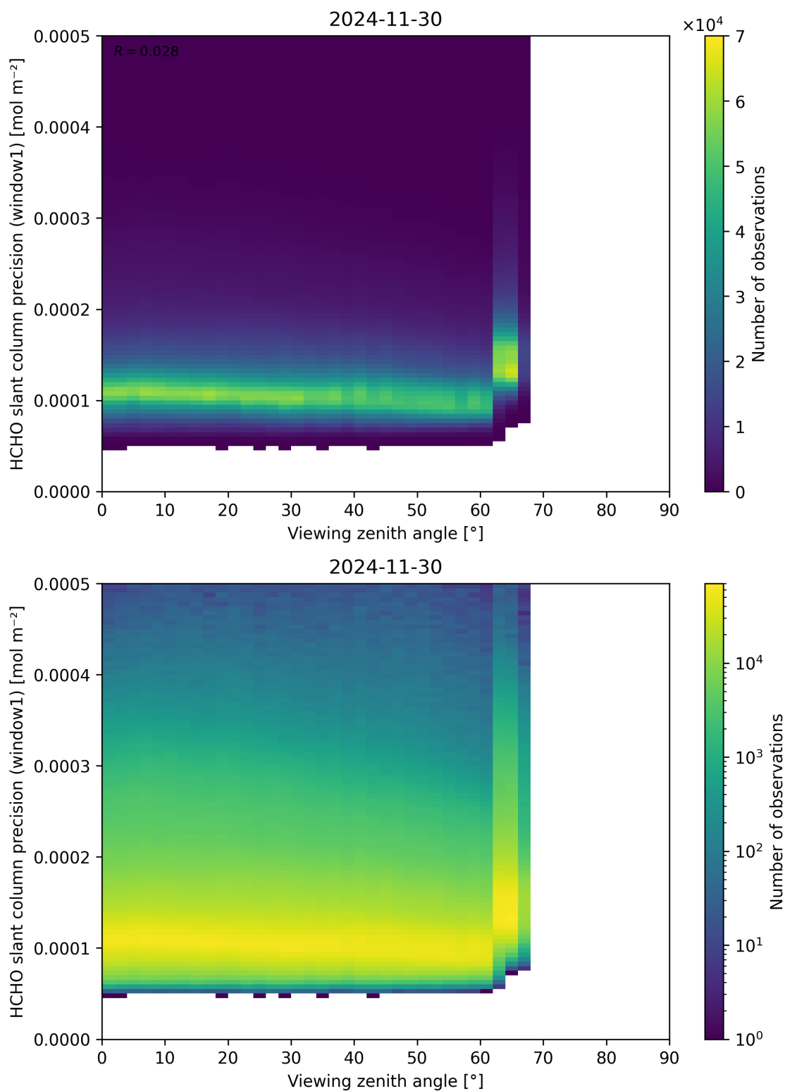
Figure 189: Scatter density plot of “Viewing zenith angle” against “HCHO slant column precision (window1)” for 2024-11-30 to 2024-12-01.
