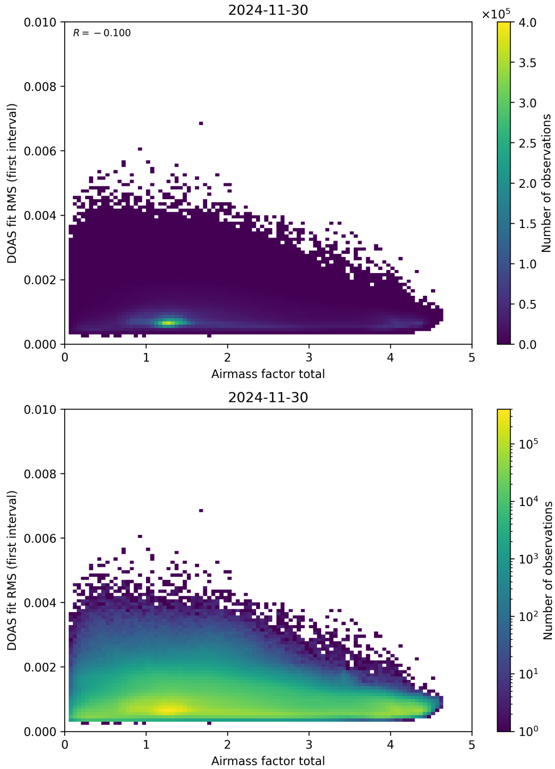
Figure 97: Scatter density plot of “Airmass factor total” against “DOAS fit RMS (first interval)” for 2024-11-30 to 2024-12-01.
