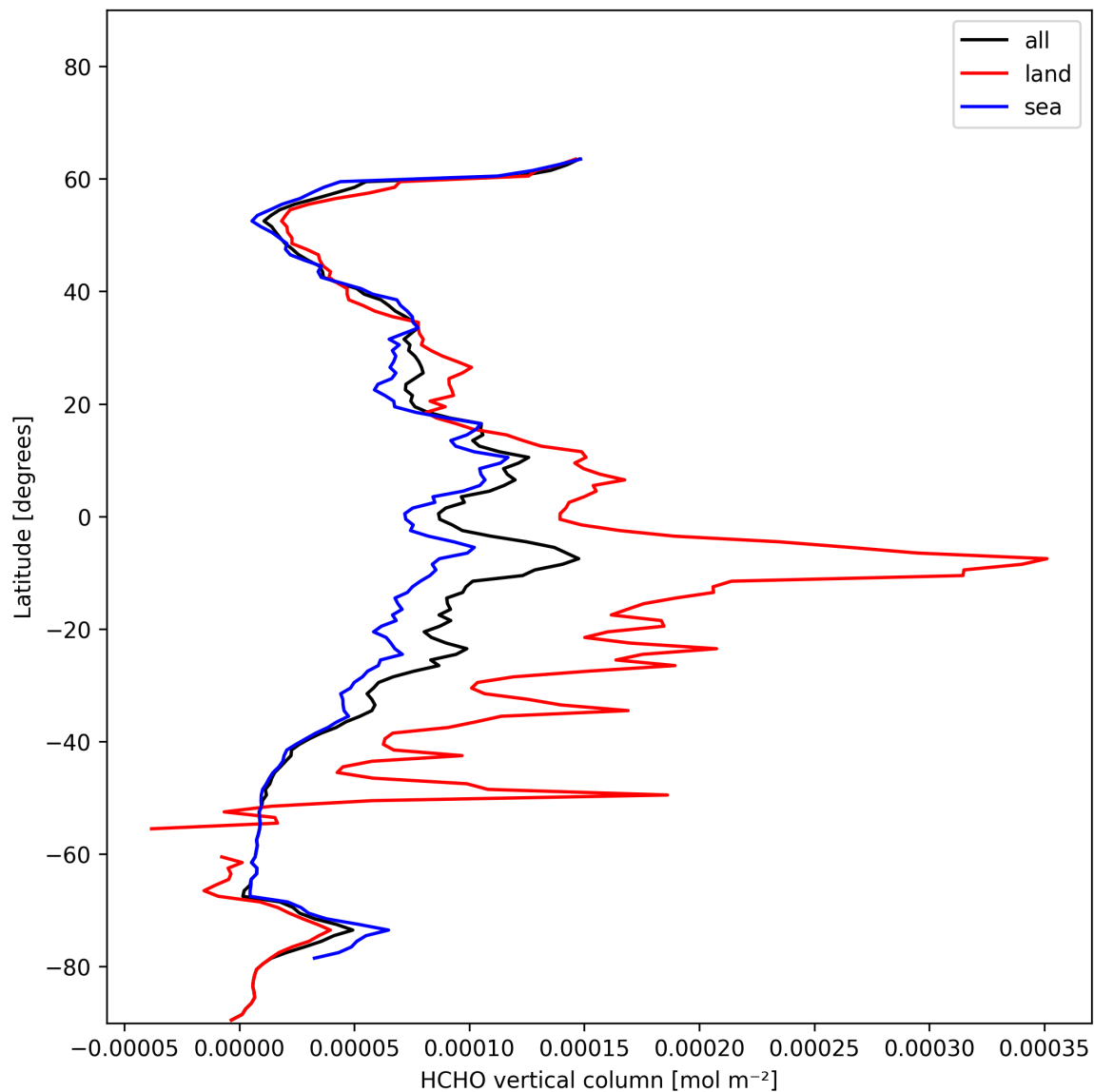
Figure 21: Zonal average of “HCHO vertical column” for 2024-11-30 to 2024-12-01.
