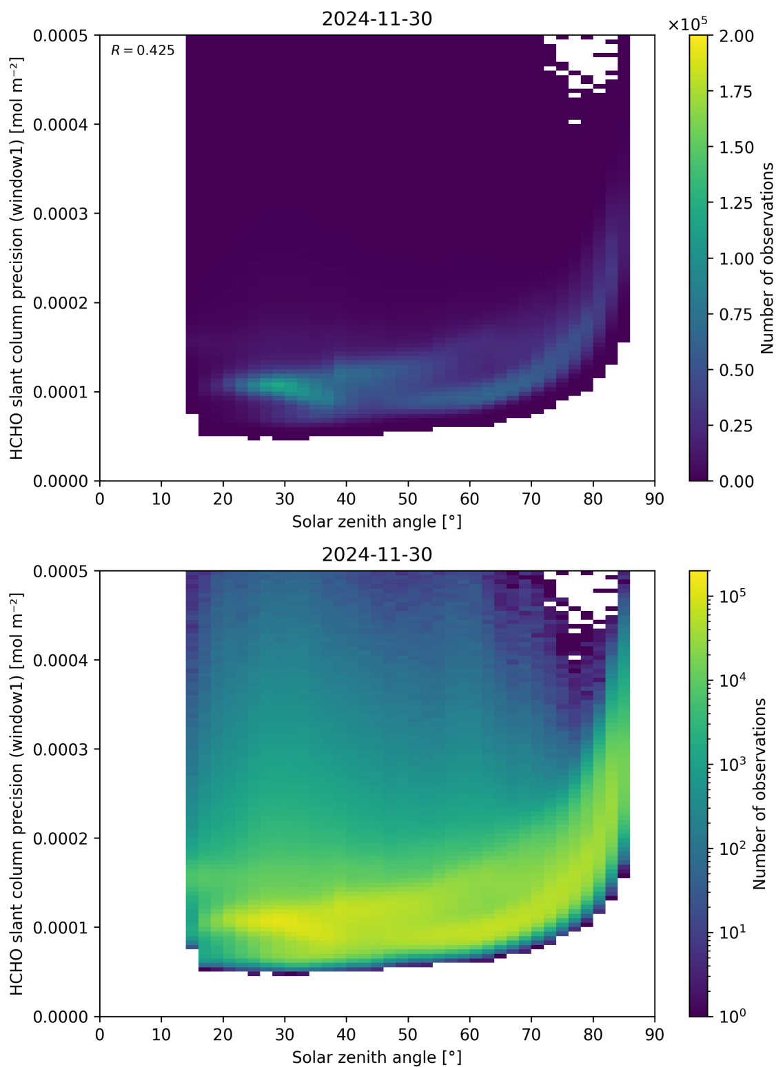
Figure 174: Scatter density plot of “Solar zenith angle” against “HCHO slant column precision (window1)” for 2024-11-30 to 2024-12-01.
