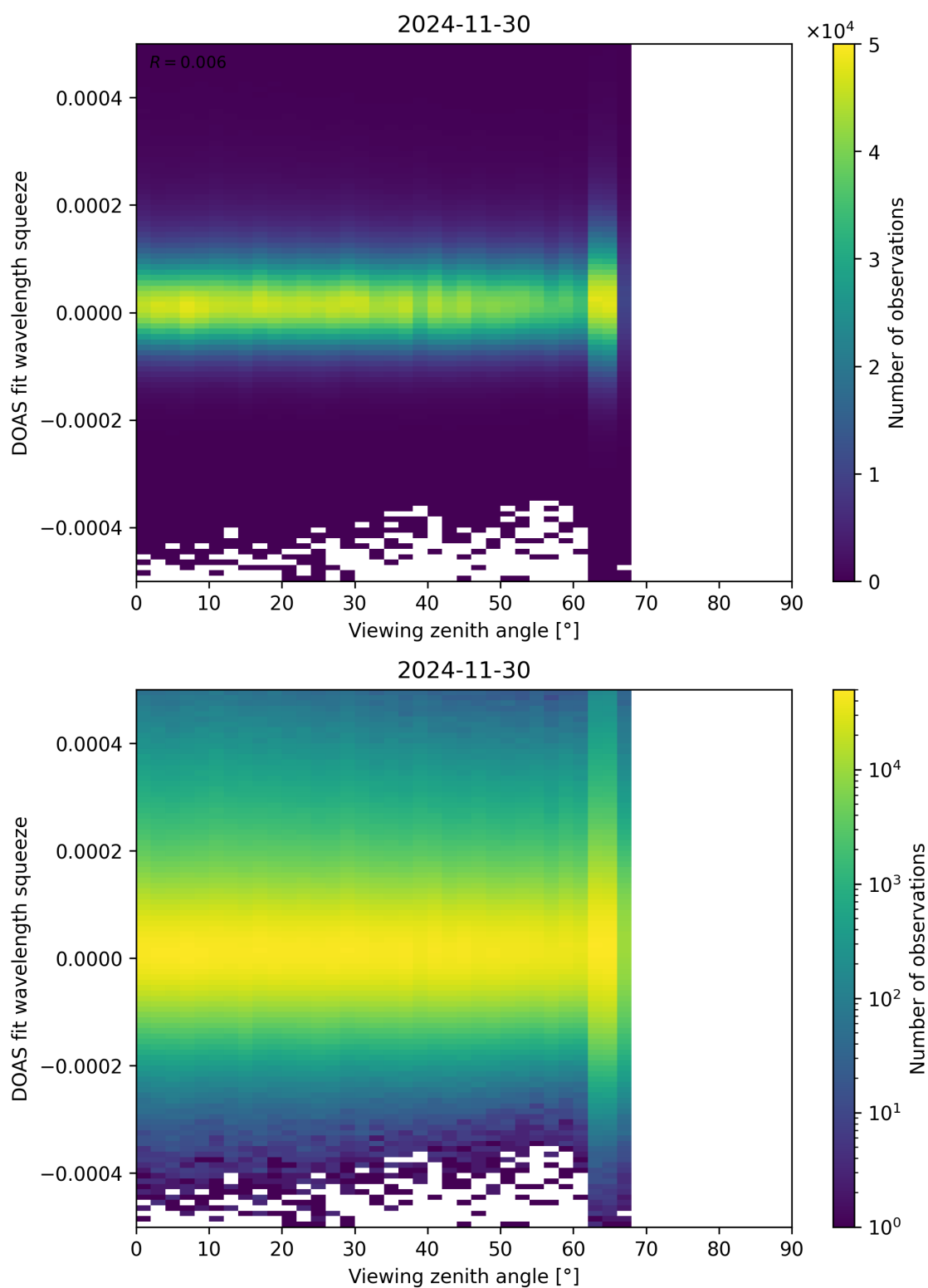
Figure 184: Scatter density plot of “Viewing zenith angle” against “DOAS fit wavelength squeeze” for 2024-11-30 to 2024-12-01.
