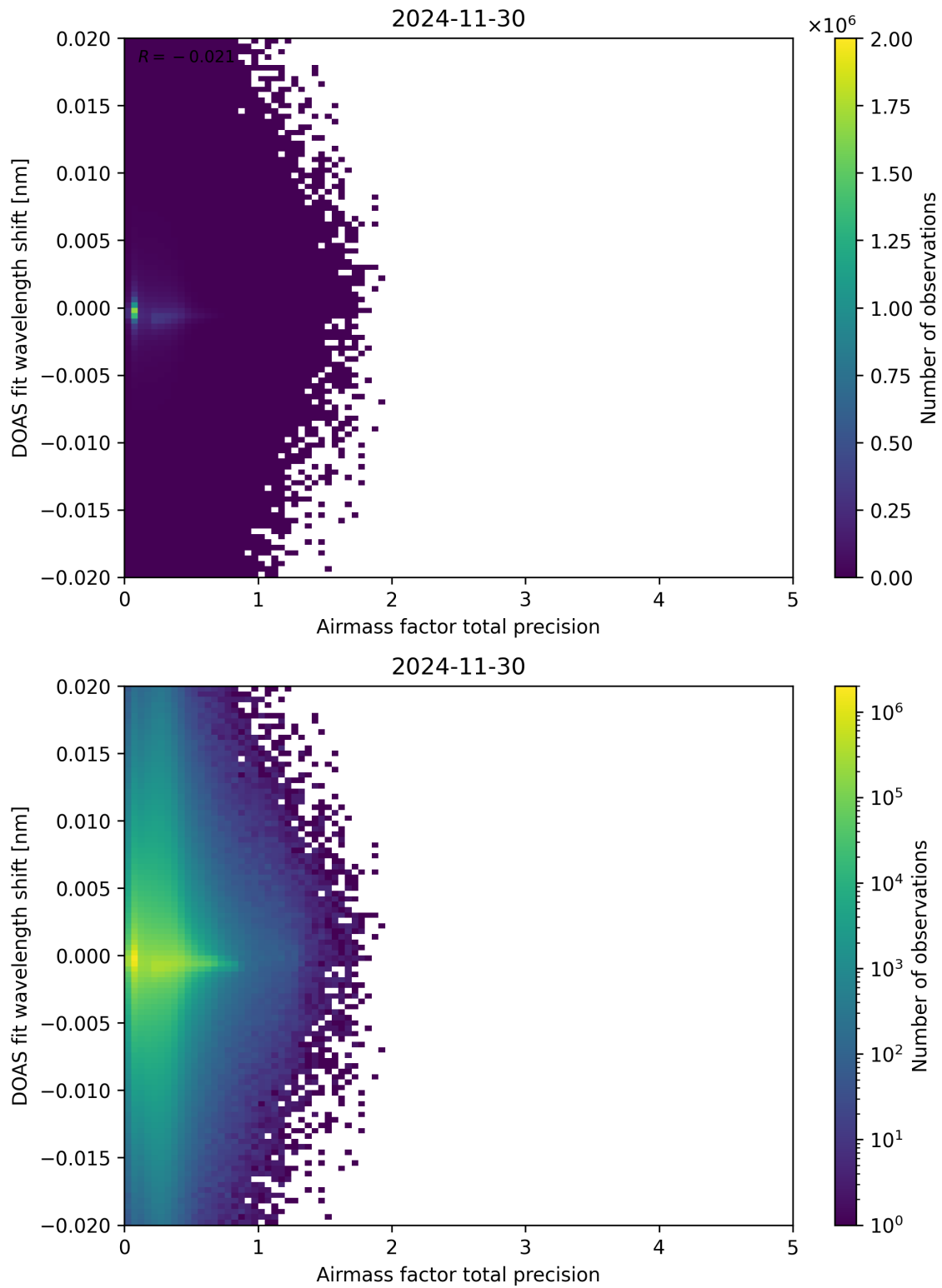
Figure 106: Scatter density plot of “Airmass factor total precision” against “DOAS fit wavelength shift” for 2024-11-30 to 2024-12-01.
