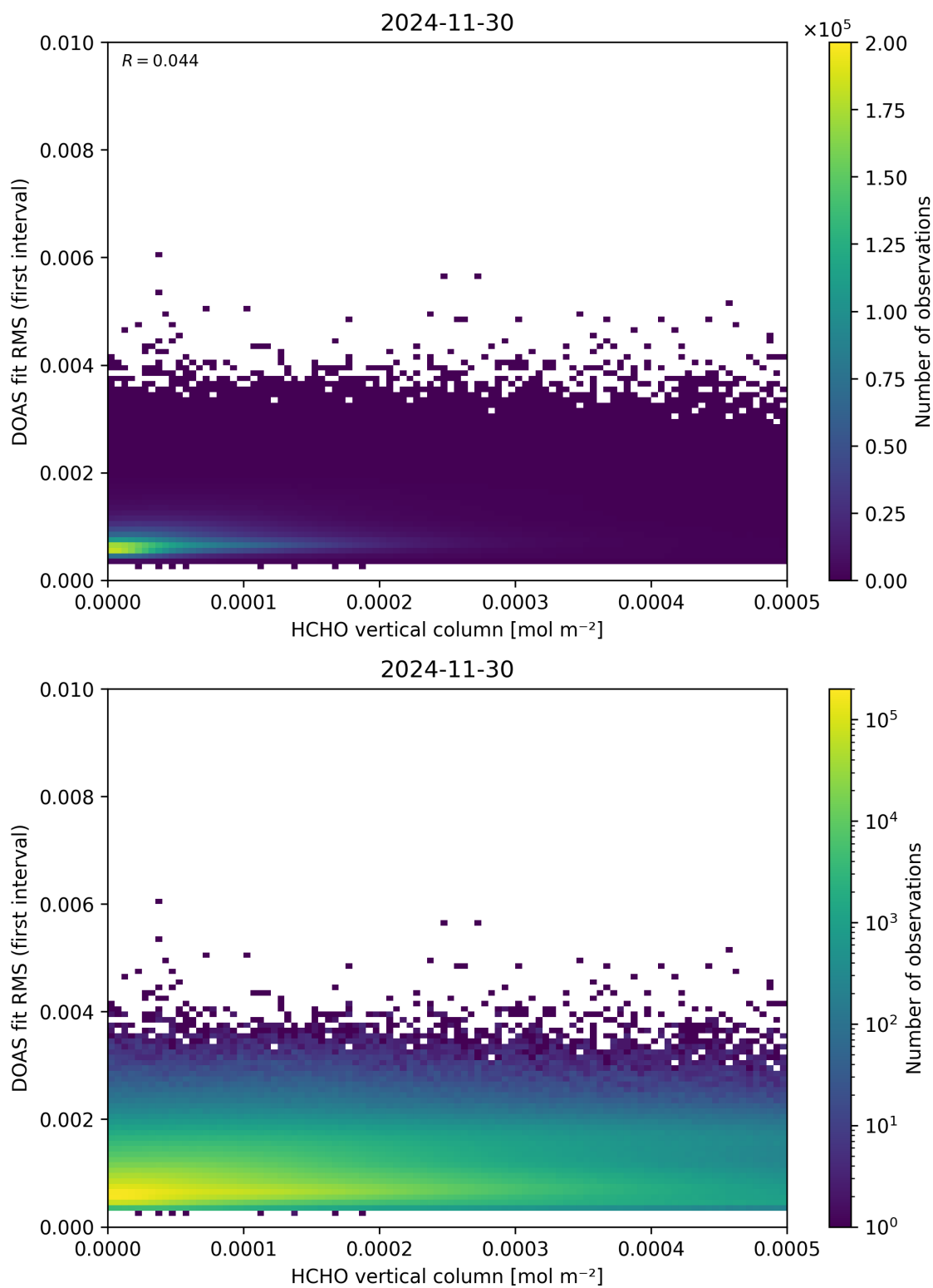
Figure 123: Scatter density plot of “HCHO vertical column” against “DOAS fit RMS (first interval)” for 2024-11-30 to 2024-12-01.
