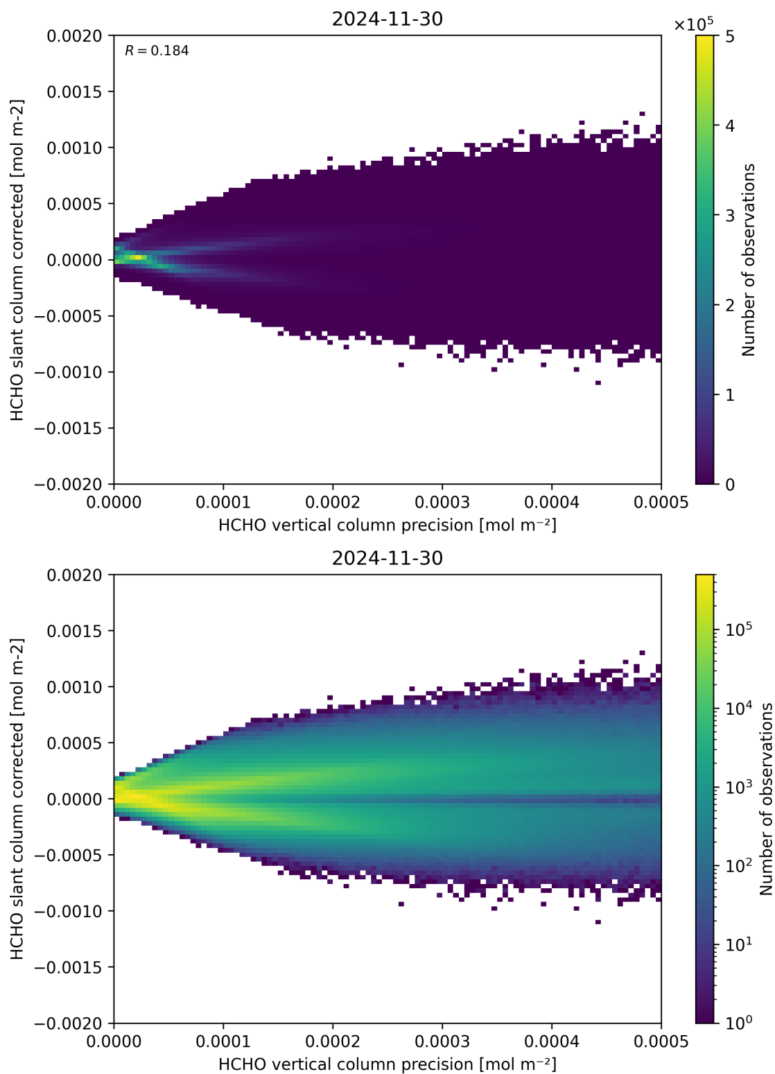
Figure 140: Scatter density plot of “HCHO vertical column precision” against “HCHO slant column corrected” for 2024-11-30 to 2024-12-01.
