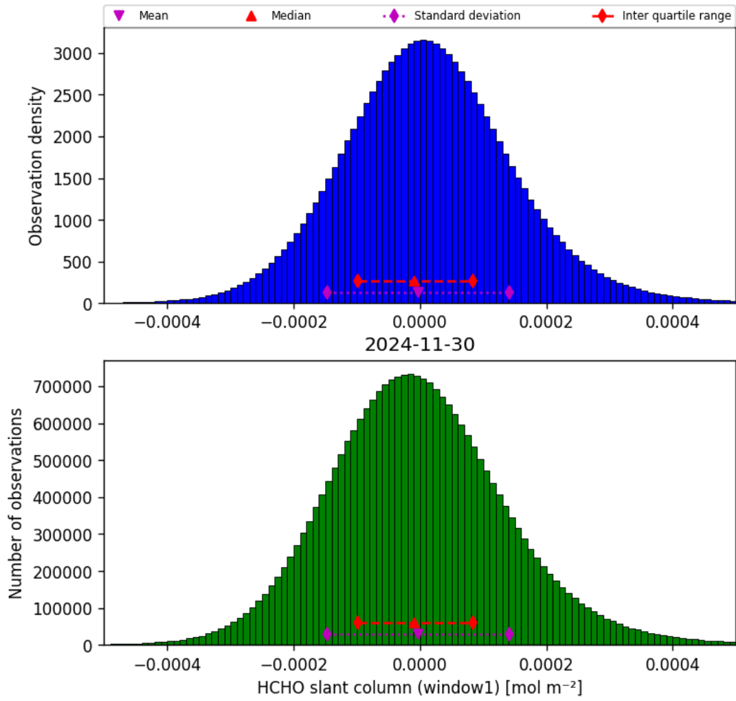
Figure 38: Histogram of “HCHO slant column (window1)” for 2024-11-30 to 2024-12-01
