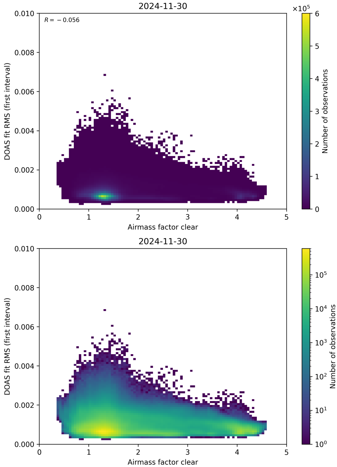
Figure 71: Scatter density plot of “Airmass factor clear” against “DOAS fit RMS (first interval)” for 2024-11-30 to 2024-12-01.
