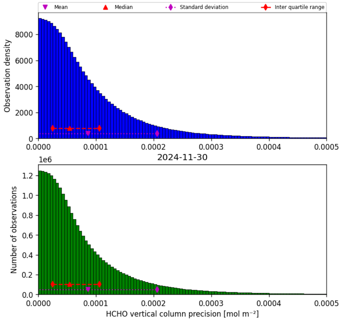
Figure 36: Histogram of “HCHO vertical column precision” for 2024-11-30 to 2024-12-01
