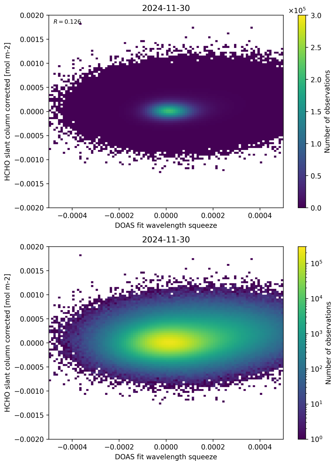
Figure 69: Scatter density plot of “DOAS fit wavelength squeeze” against “HCHO slant column corrected” for 2024-11-30 to 2024-12-01.
