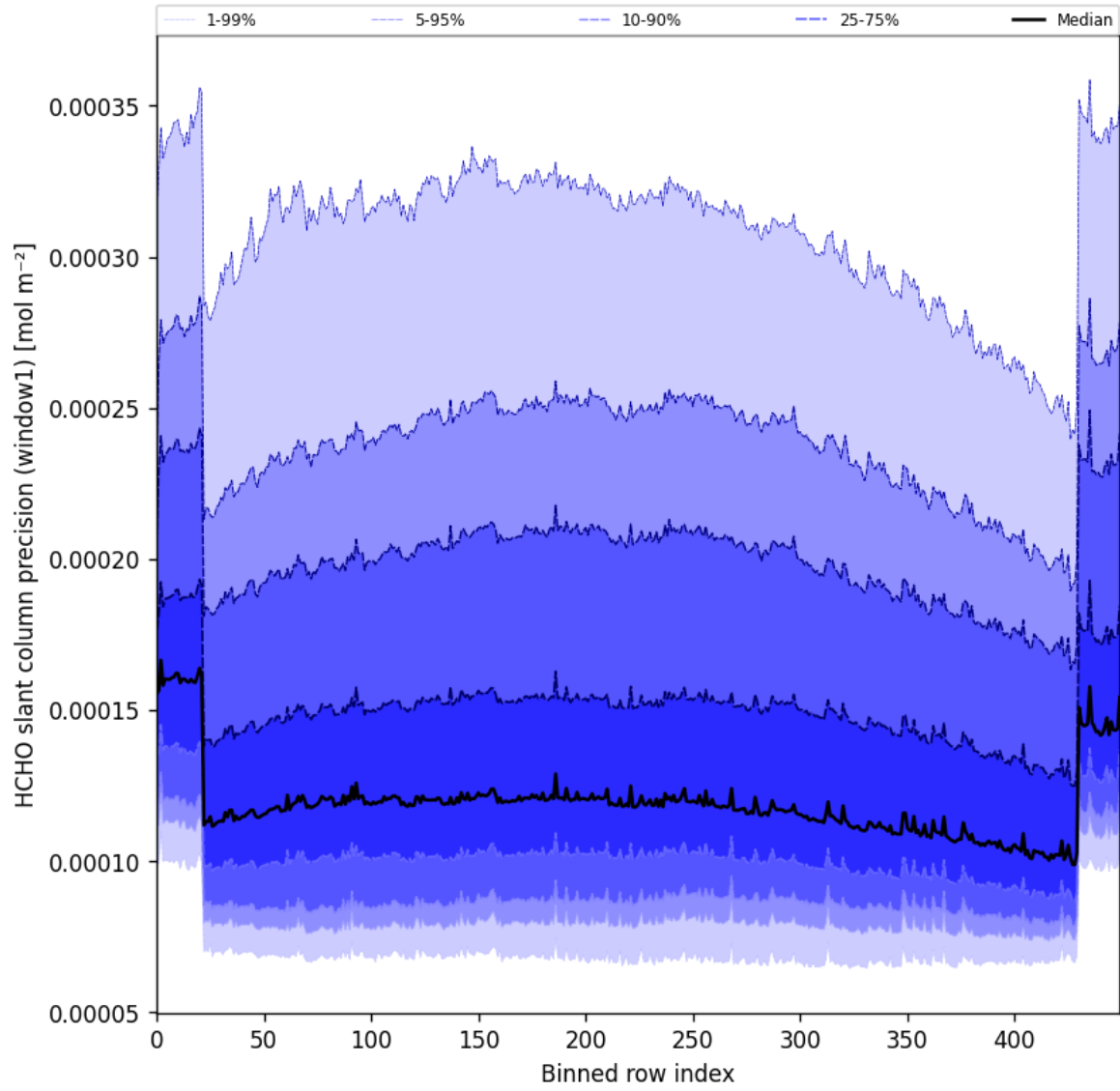
Figure 53: Along track statistics of “HCHO slant column precision (window1)” for 2024-11-30 to 2024-12-01
