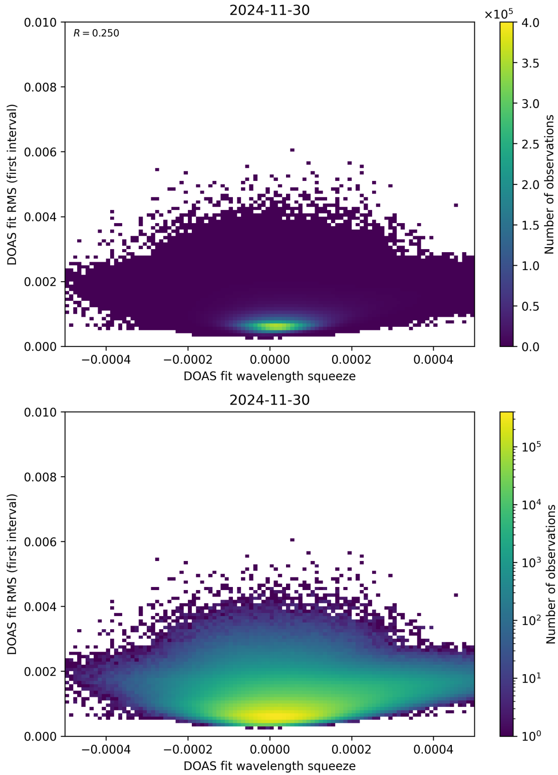
Figure 68: Scatter density plot of “DOAS fit wavelength squeeze” against “DOAS fit RMS (first interval)” for 2024-11-30 to 2024-12-01.
