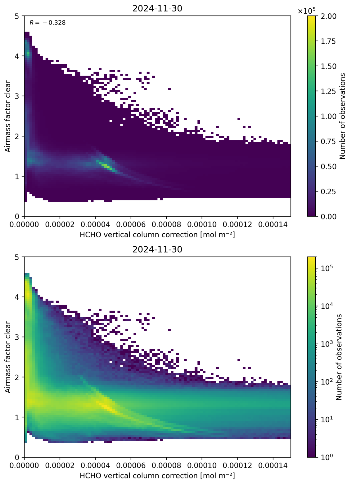
Figure 115: Scatter density plot of “HCHO vertical column correction” against “Airmass factor clear” for 2024-11-30 to 2024-12-01.
