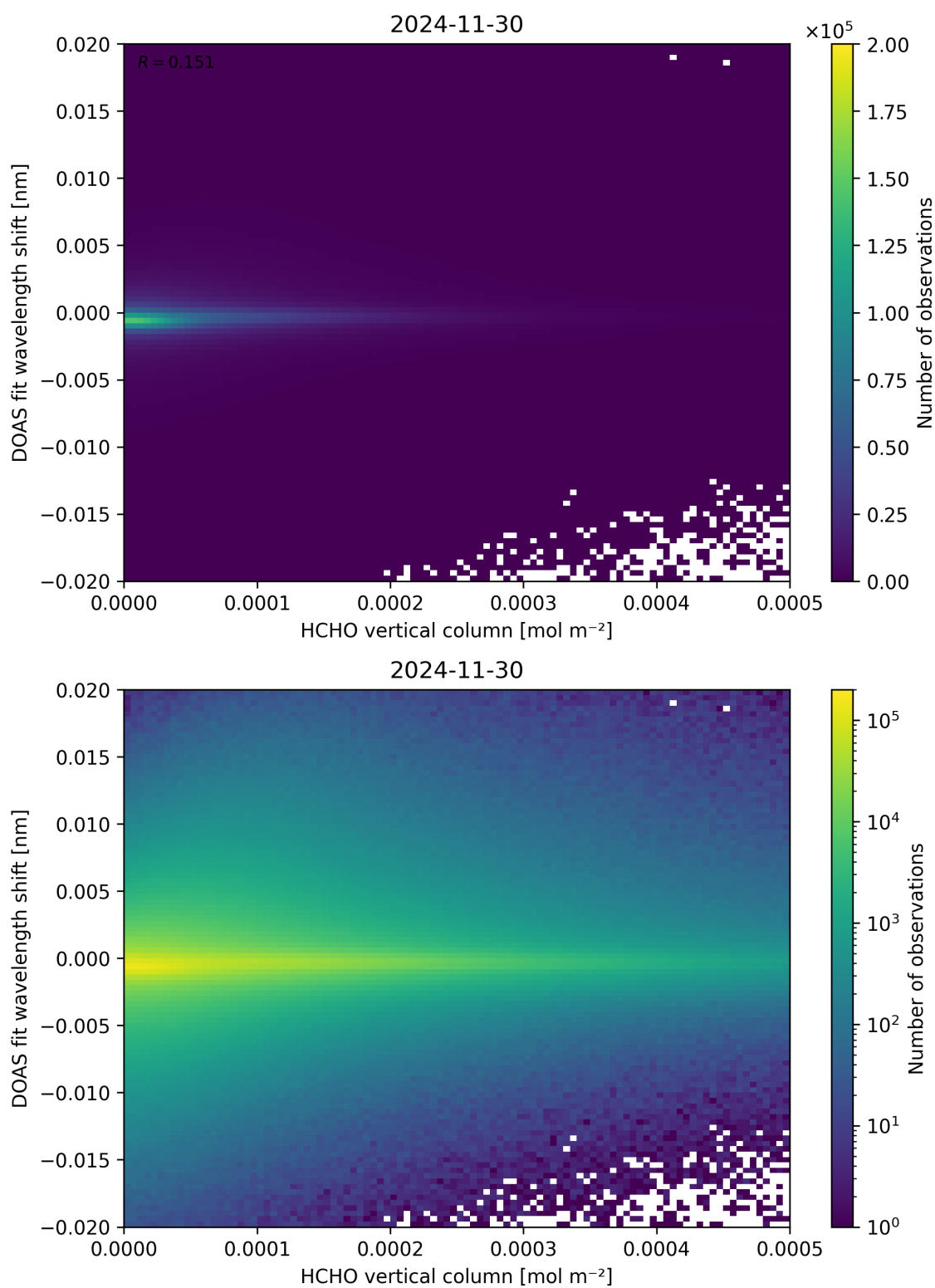
Figure 124: Scatter density plot of “HCHO vertical column” against “DOAS fit wavelength shift” for 2024-11-30 to 2024-12-01.
