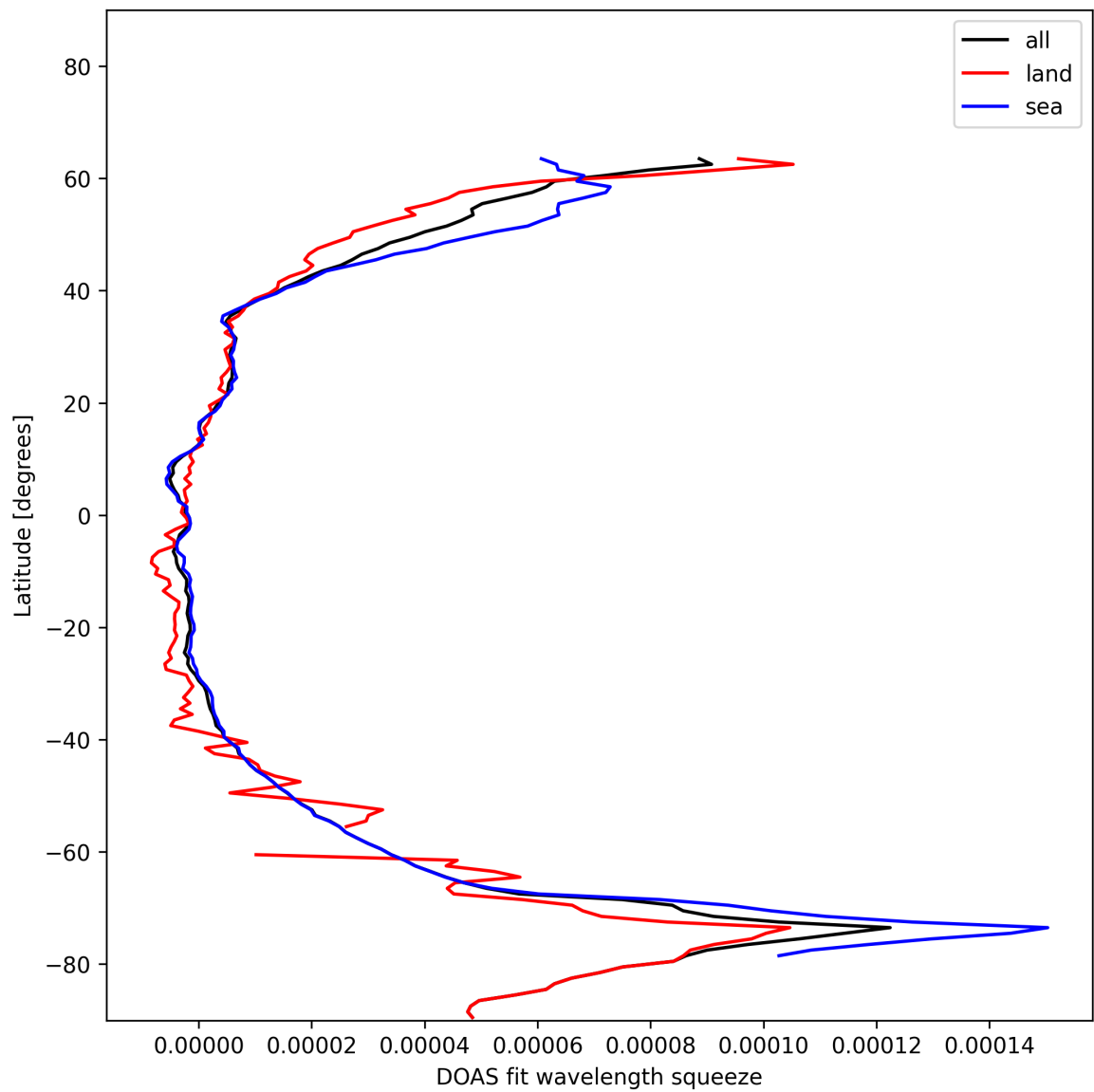
Figure 31: Zonal average of “DOAS fit wavelength squeeze” for 2024-11-30 to 2024-12-01.
