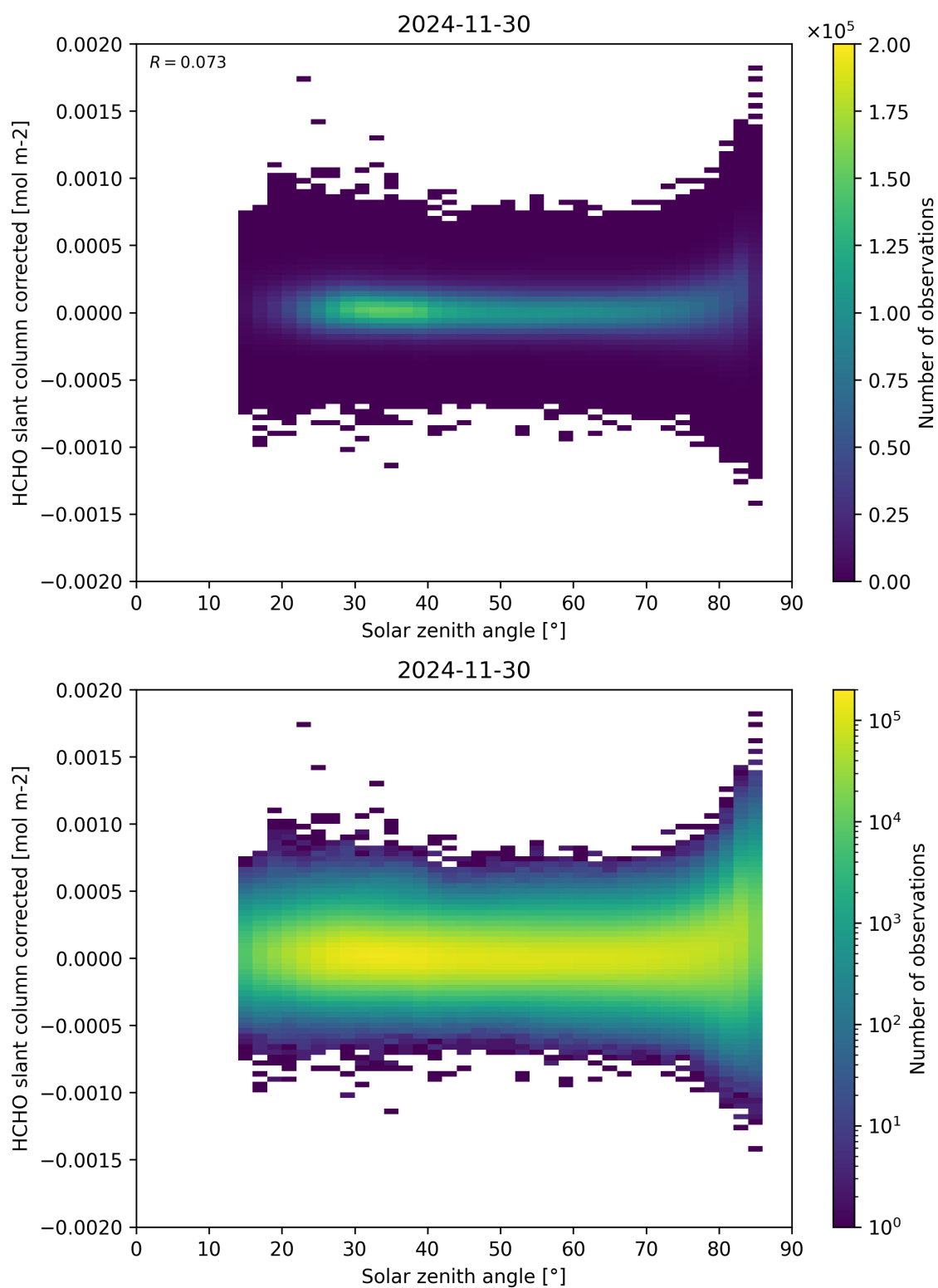
Figure 171: Scatter density plot of “Solar zenith angle” against “HCHO slant column corrected” for 2024-11-30 to 2024-12-01.
