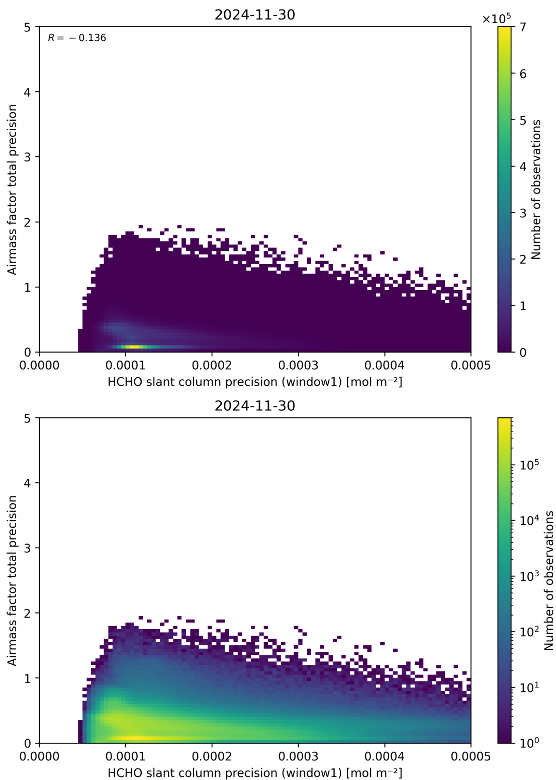
Figure 95: Scatter density plot of “HCHO slant column precision (window1)” against “Airmass factor total precision” for 2024-11-30 to 2024-12-01.
