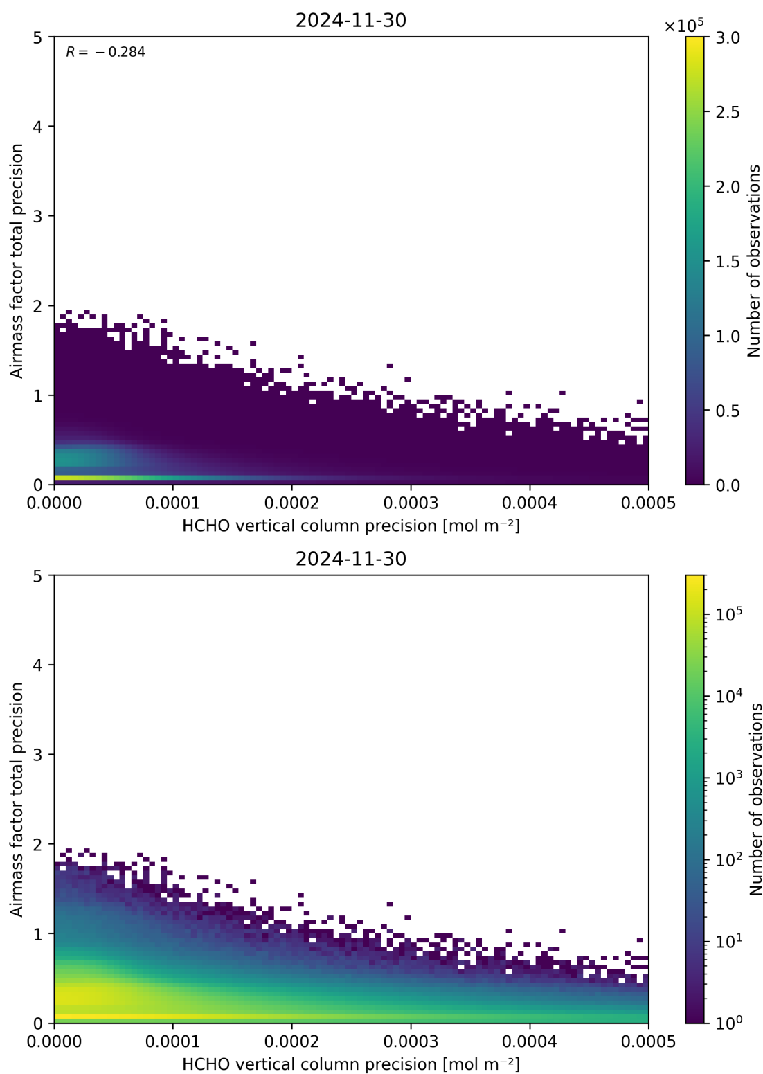
Figure 145: Scatter density plot of “HCHO vertical column precision” against “Airmass factor total precision” for 2024-11-30 to 2024-12-01.
