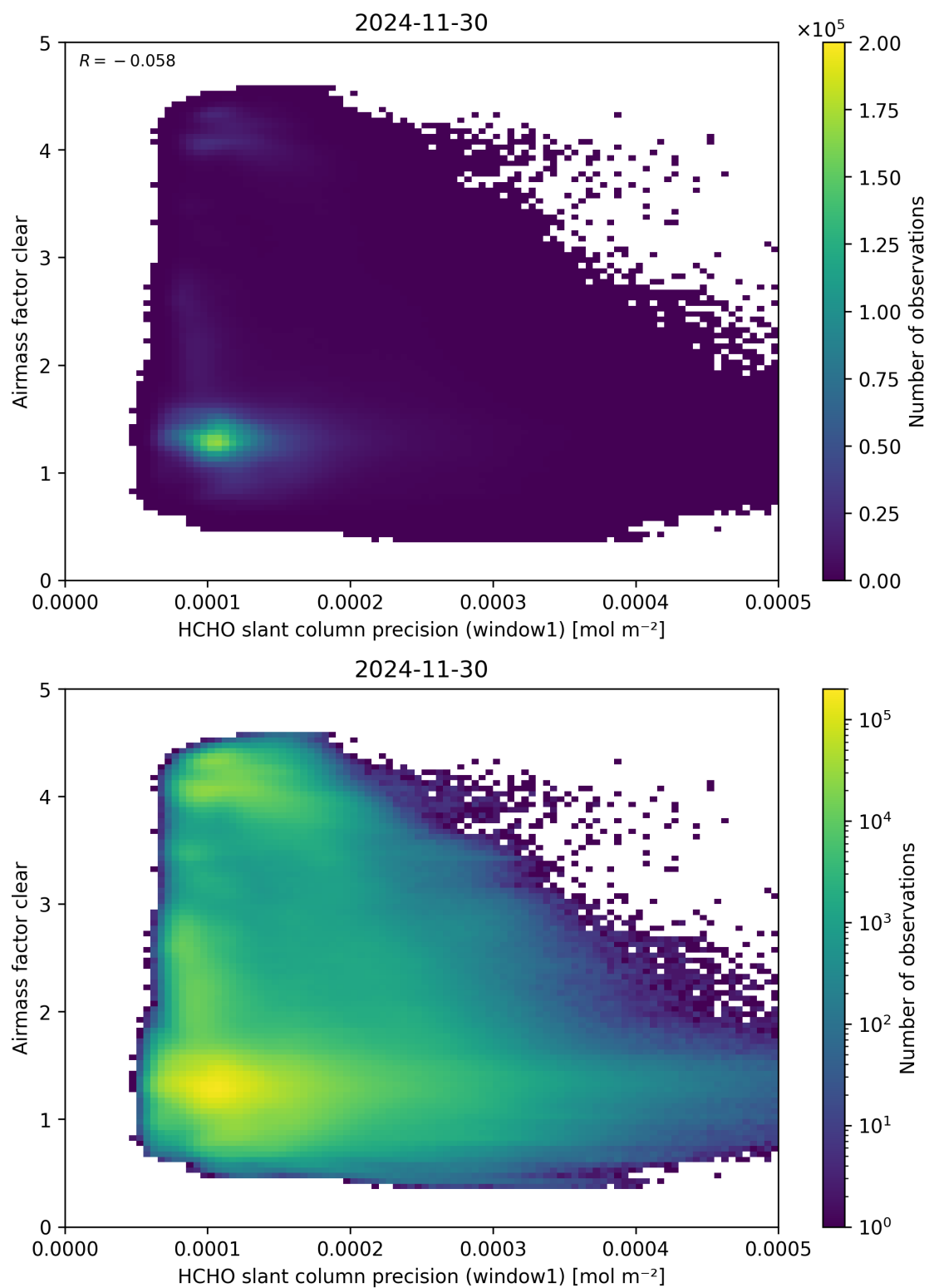
Figure 91: Scatter density plot of “HCHO slant column precision (window1)” against “Airmass factor clear” for 2024-11-30 to 2024-12-01.
