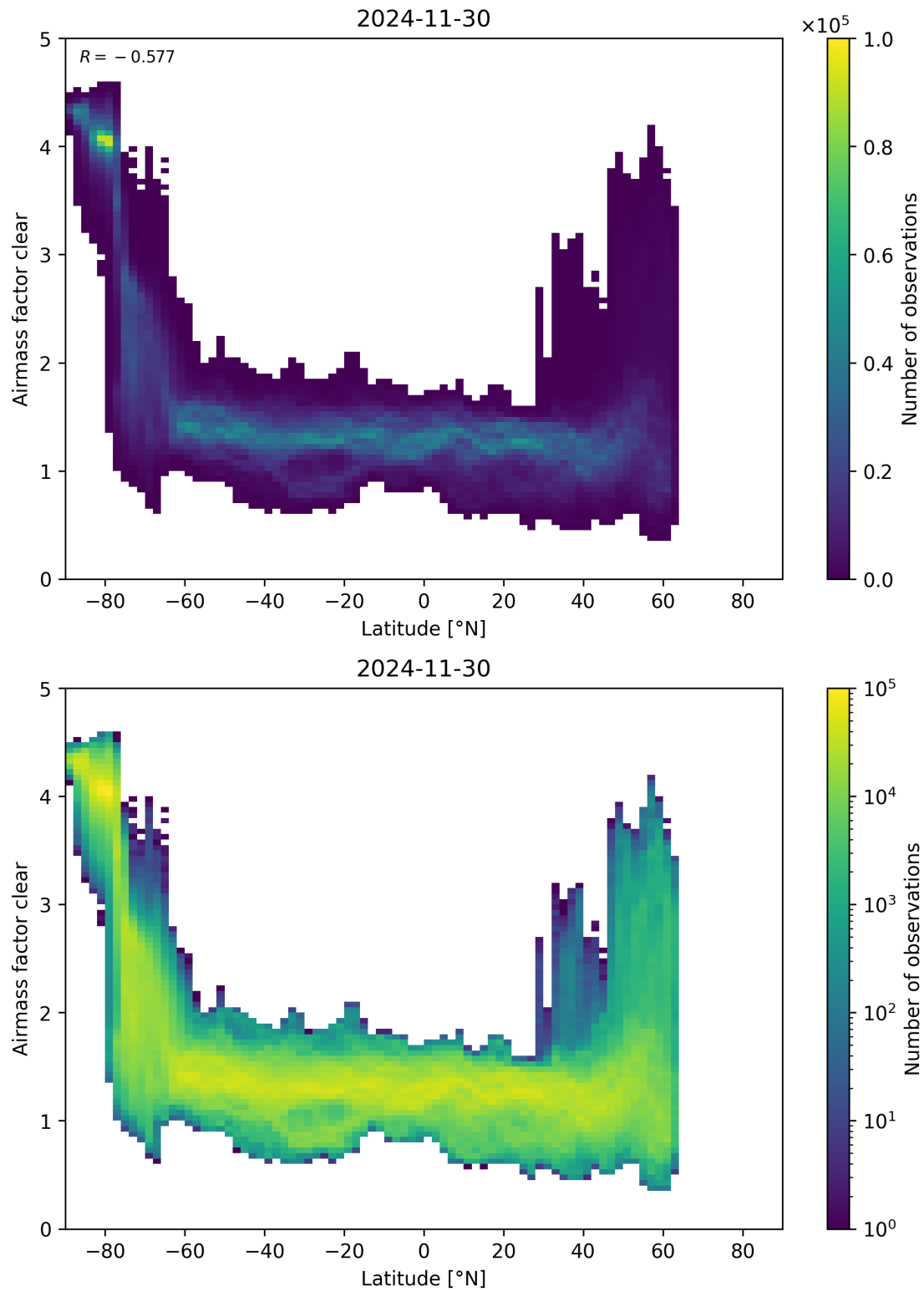
Figure 156: Scatter density plot of “Latitude” against “Airmass factor clear” for 2024-11-30 to 2024-12-01.
