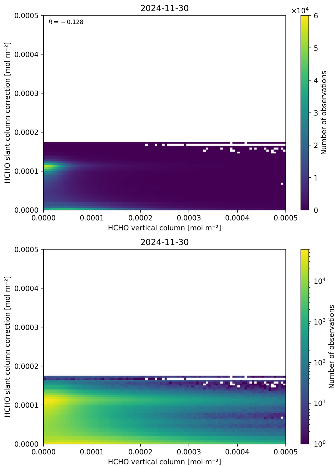
Figure 128: Scatter density plot of “HCHO vertical column” against “HCHO slant column correction” for 2024-11-30 to 2024-12-01.
