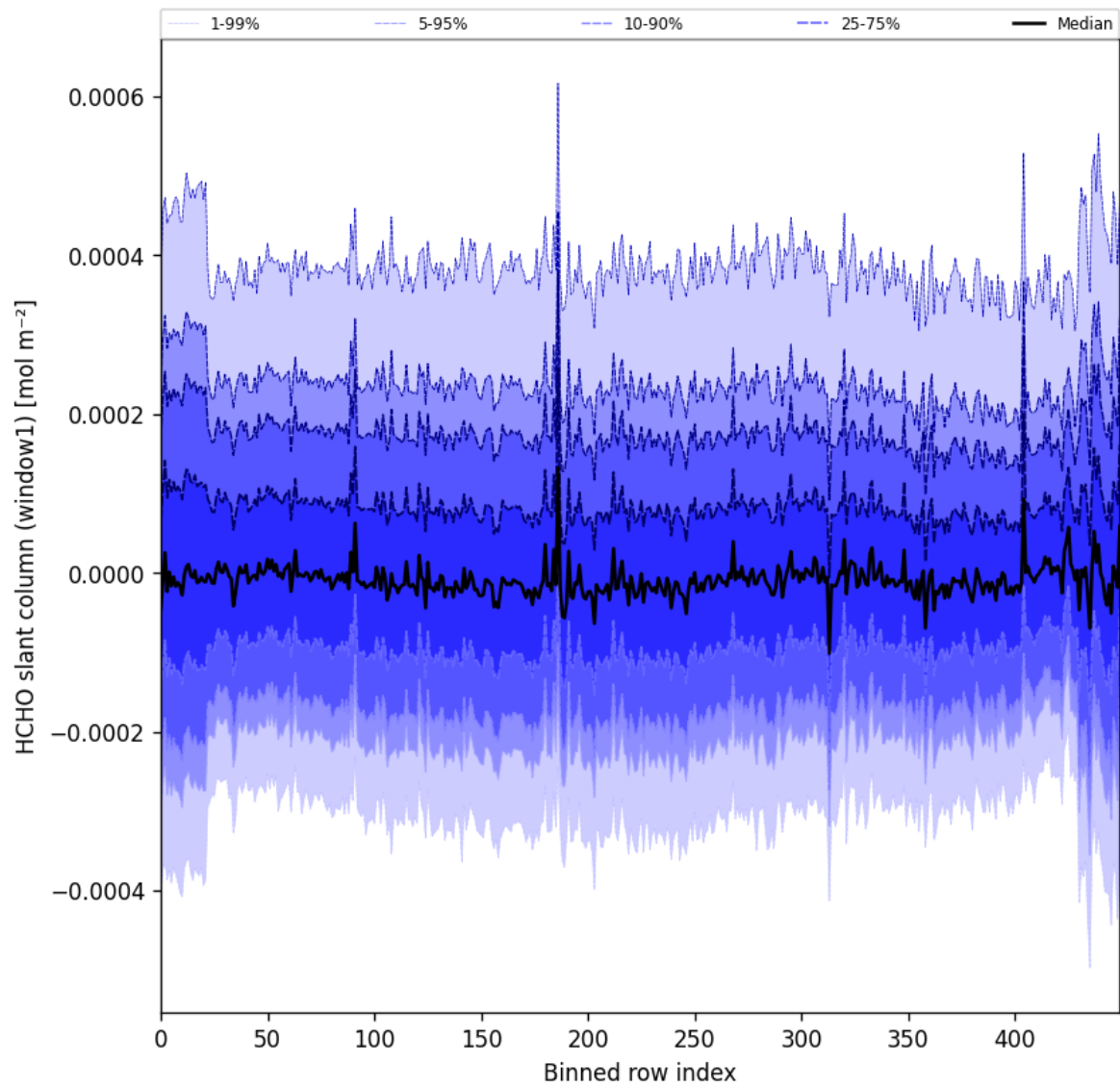
Figure 52: Along track statistics of “HCHO slant column (window1)” for 2024-11-30 to 2024-12-01
