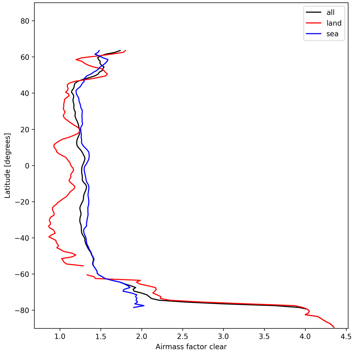
Figure 28: Zonal average of “Airmass factor clear” for 2024-11-30 to 2024-12-01.
