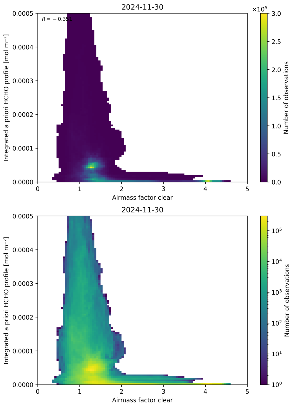
Figure 76: Scatter density plot of “Airmass factor clear” against “Integrated a priori HCHO profile” for 2024-11-30 to 2024-12-01.
