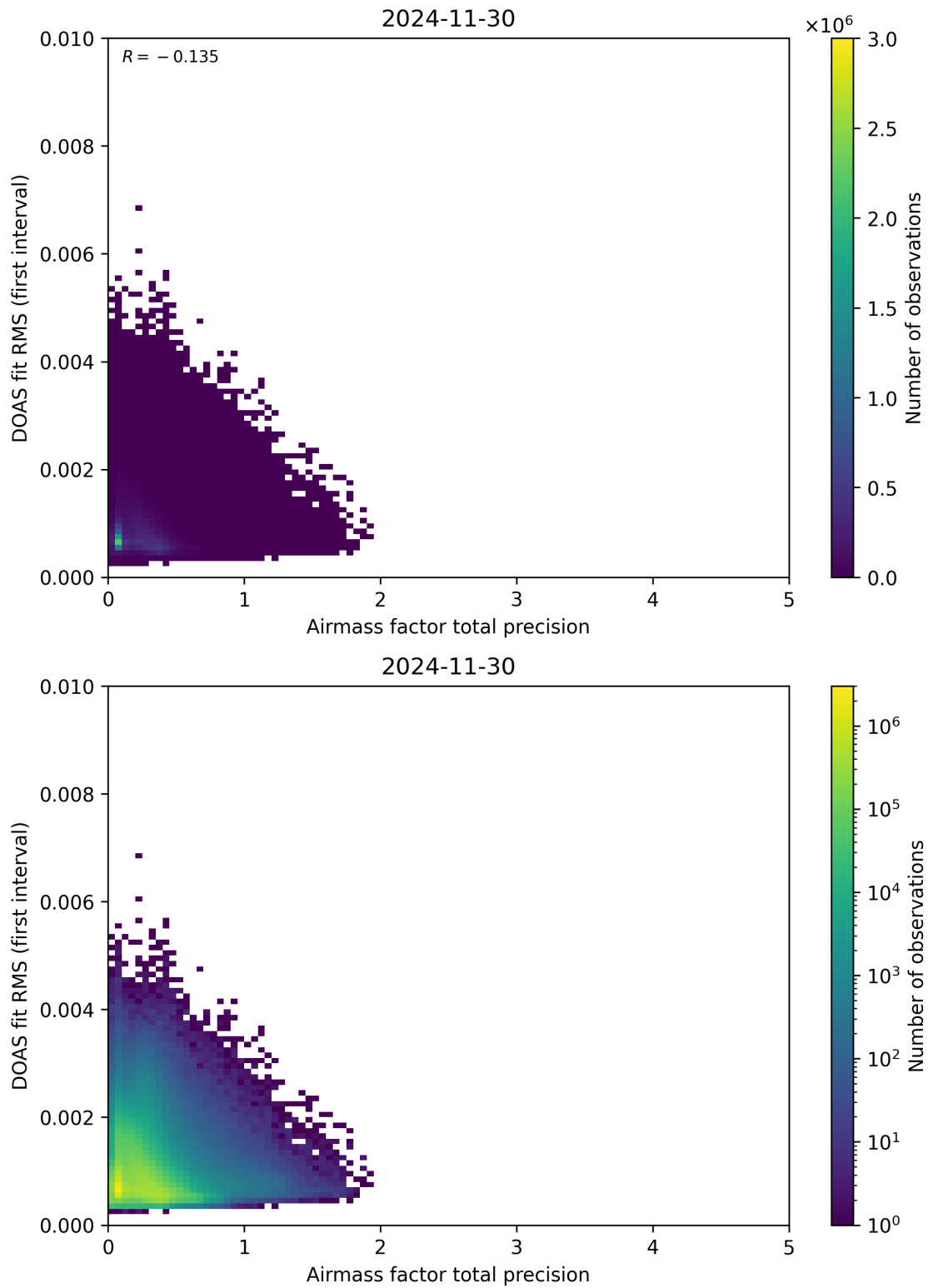
Figure 105: Scatter density plot of “Airmass factor total precision” against “DOAS fit RMS (first interval)” for 2024-11-30 to 2024-12-01.
