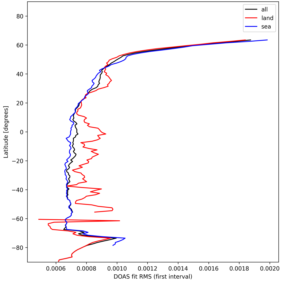
Figure 32: Zonal average of “DOAS fit RMS (first interval)” for 2024-11-30 to 2024-12-01.
