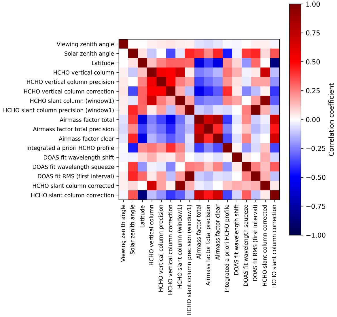
Figure 2: Map of correlation matrix for 2024-11-30 to 2024-12-01.
