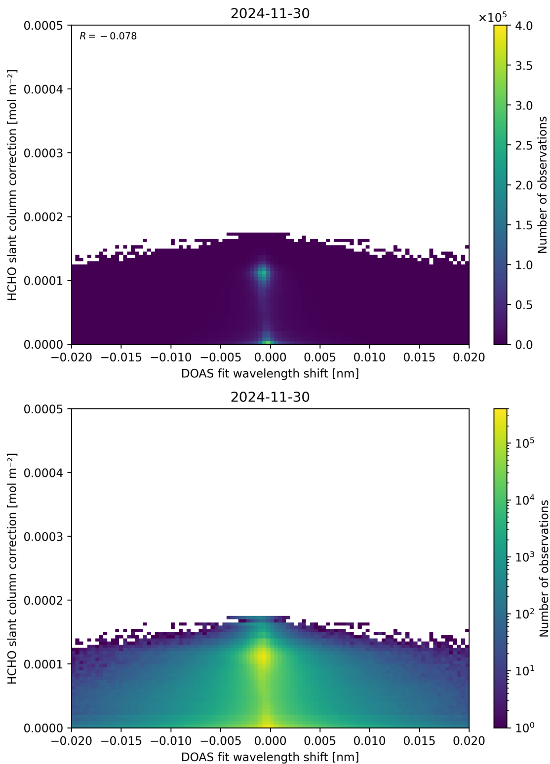
Figure 67: Scatter density plot of “DOAS fit wavelength shift” against “HCHO slant column correction” for 2024-11-30 to 2024-12-01.
