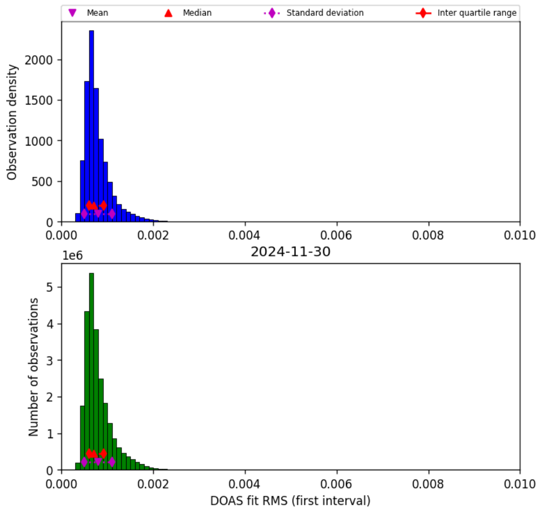
Figure 46: Histogram of “DOAS fit RMS (first interval)” for 2024-11-30 to 2024-12-01
