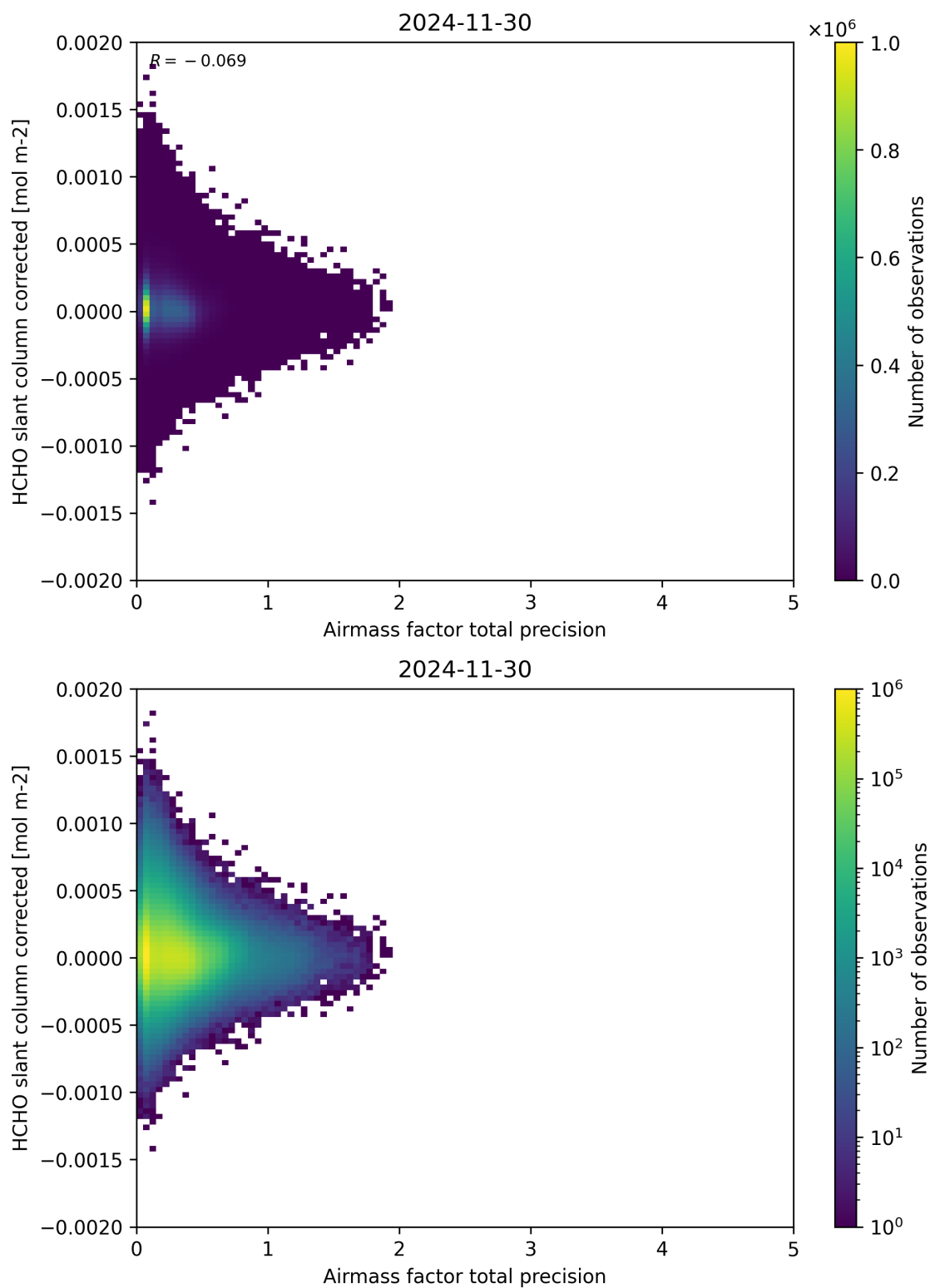
Figure 109: Scatter density plot of “Airmass factor total precision” against “HCHO slant column corrected” for 2024-11-30 to 2024-12-01.
