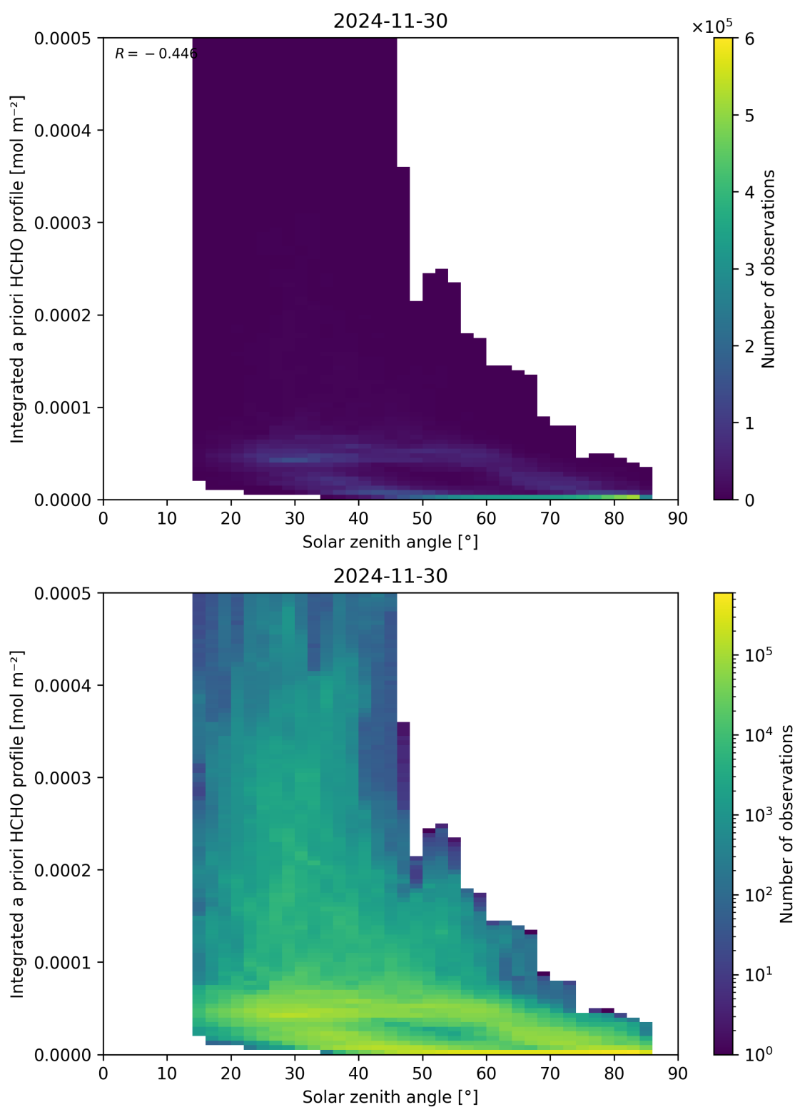
Figure 180: Scatter density plot of “Solar zenith angle” against “Integrated a priori HCHO profile” for 2024-11-30 to 2024-12-01.
