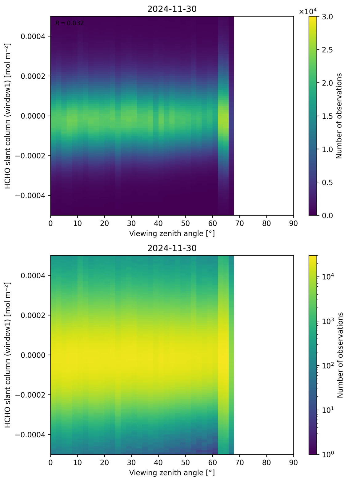
Figure 188: Scatter density plot of “Viewing zenith angle” against “HCHO slant column (window1)” for 2024-11-30 to 2024-12-01.
