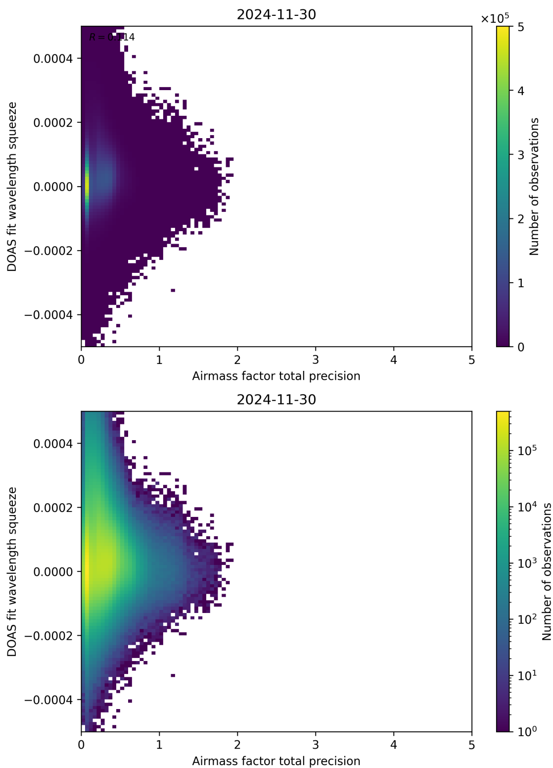
Figure 107: Scatter density plot of “Airmass factor total precision” against “DOAS fit wavelength squeeze” for 2024-11-30 to 2024-12-01.
