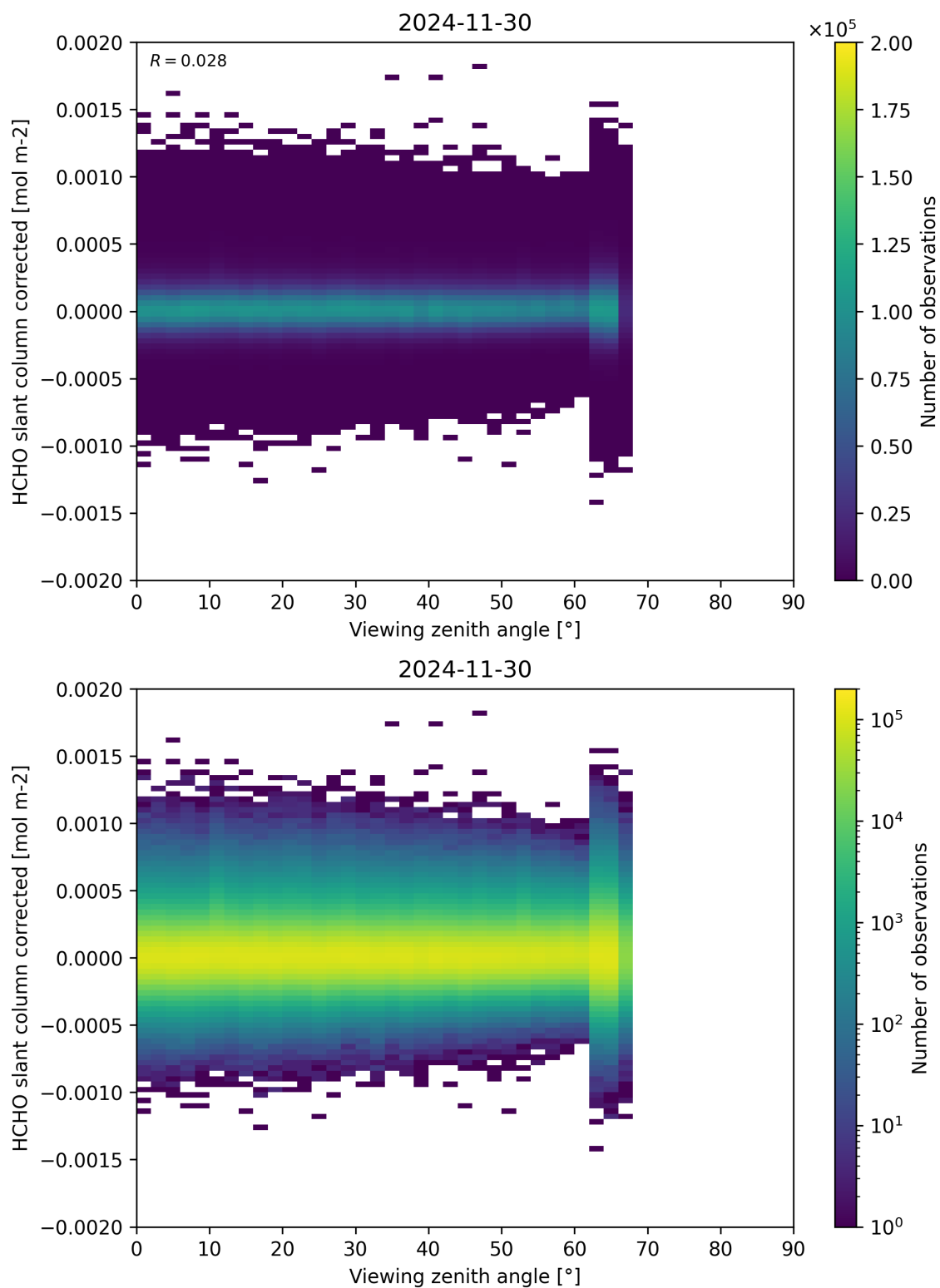
Figure 186: Scatter density plot of “Viewing zenith angle” against “HCHO slant column corrected” for 2024-11-30 to 2024-12-01.
