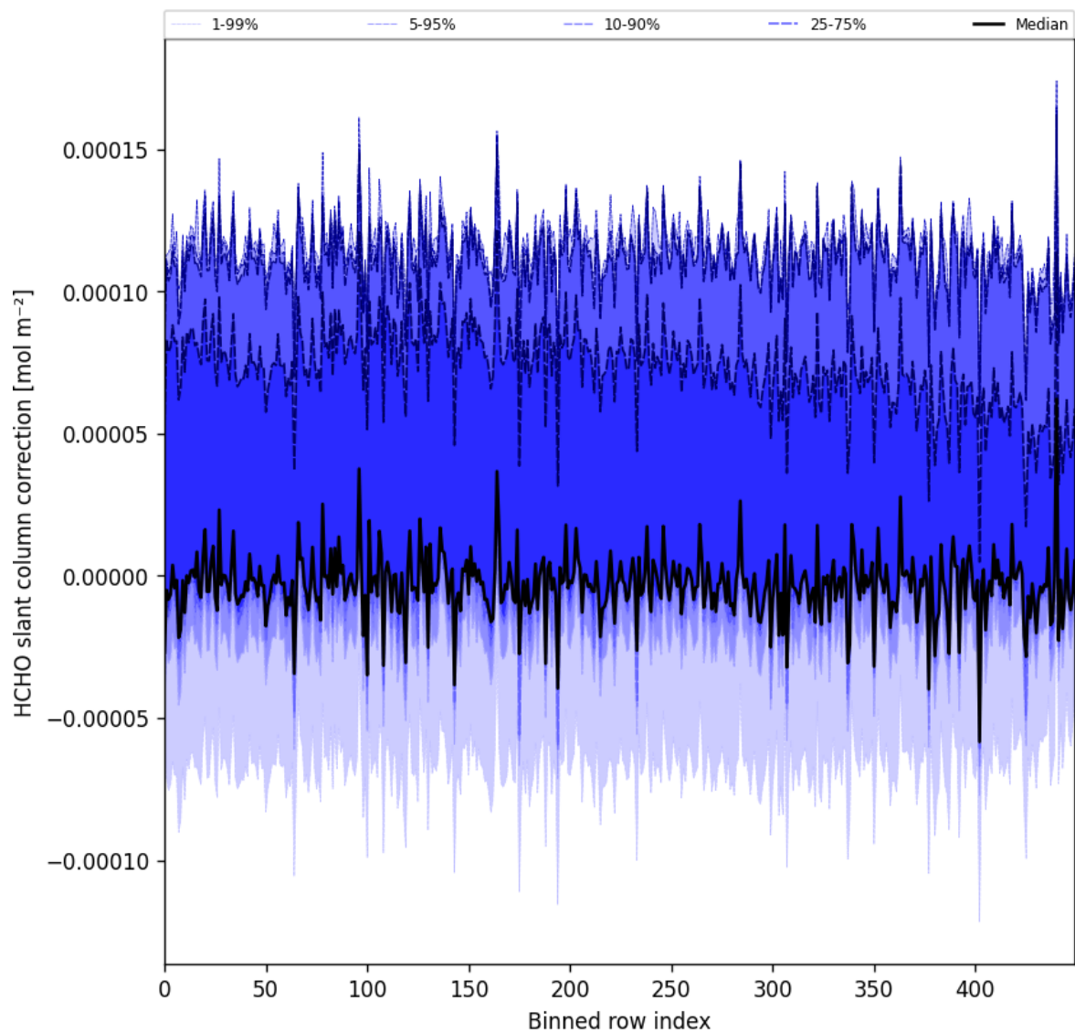
Figure 61: Along track statistics of “HCHO slant column correction” for 2024-11-30 to 2024-12-01
