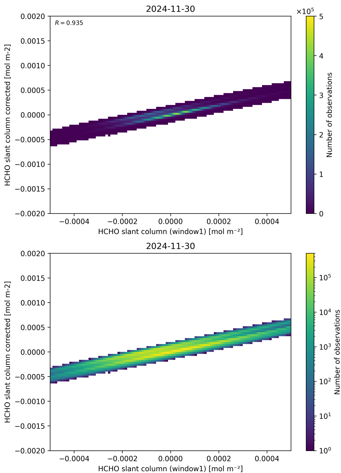
Figure 82: Scatter density plot of “HCHO slant column (window1)” against “HCHO slant column corrected” for 2024-11-30 to 2024-12-01.
