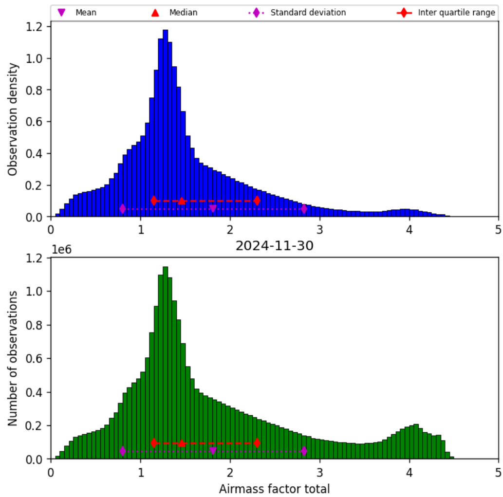
Figure 40: Histogram of “Airmass factor total” for 2024-11-30 to 2024-12-01
