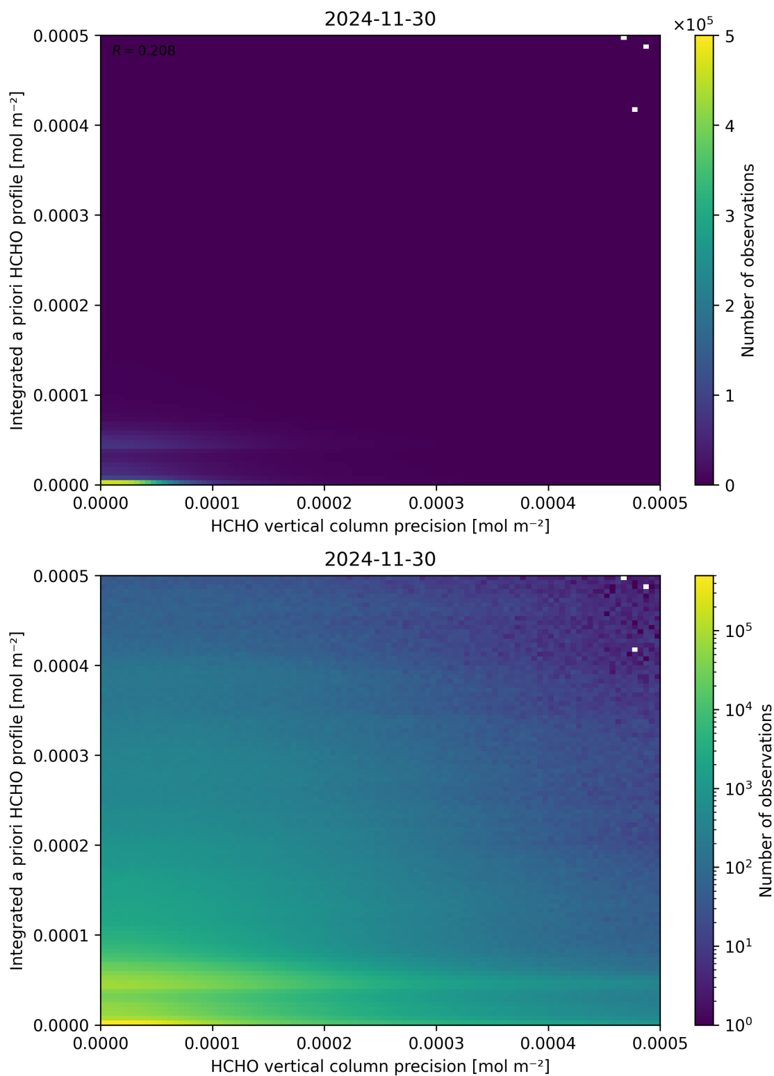
Figure 147: Scatter density plot of “HCHO vertical column precision” against “Integrated a priori HCHO profile” for 2024-11-30 to 2024-12-01.
