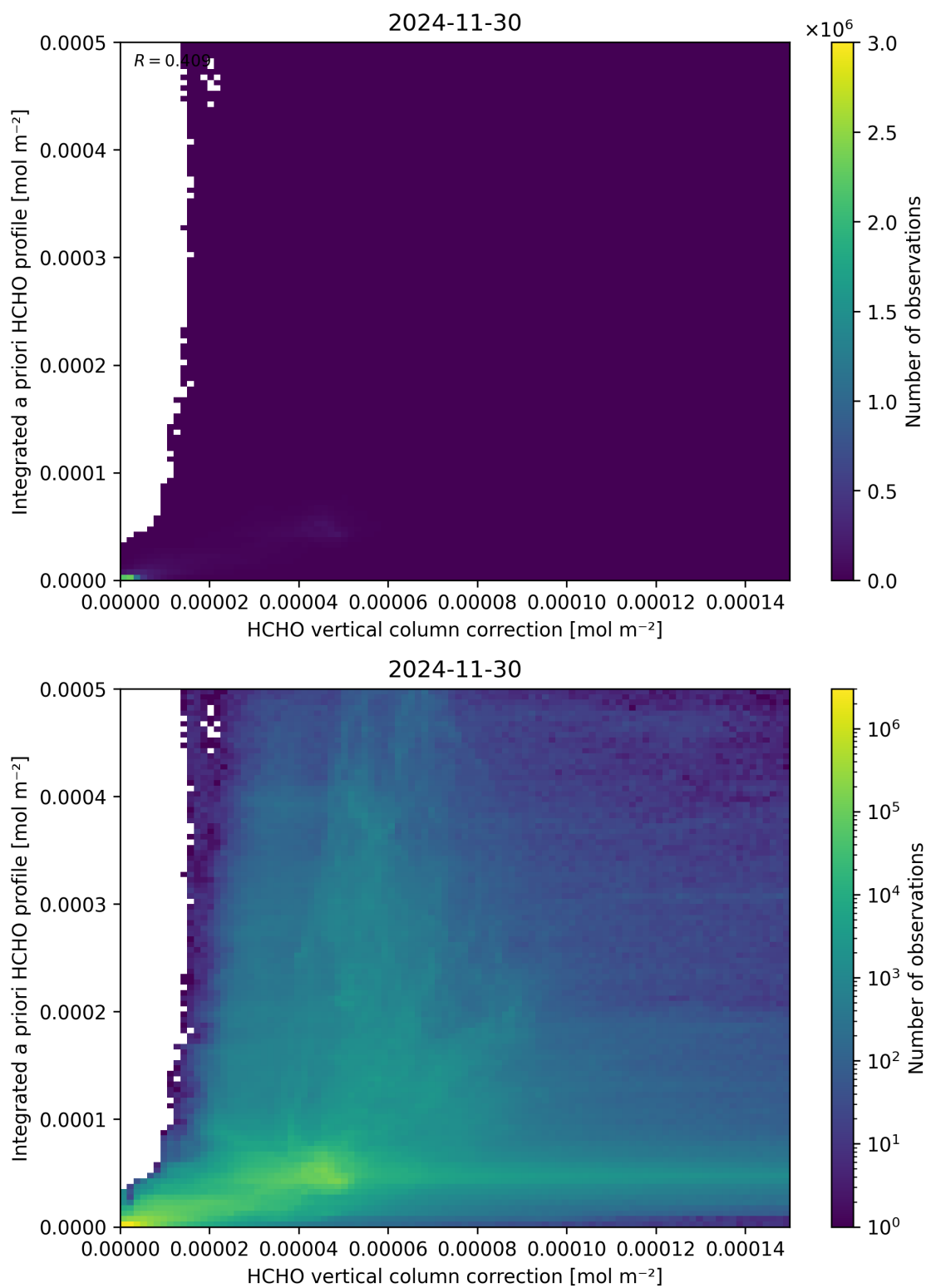
Figure 122: Scatter density plot of “HCHO vertical column correction” against “Integrated a priori HCHO profile” for 2024-11-30 to 2024-12-01.
