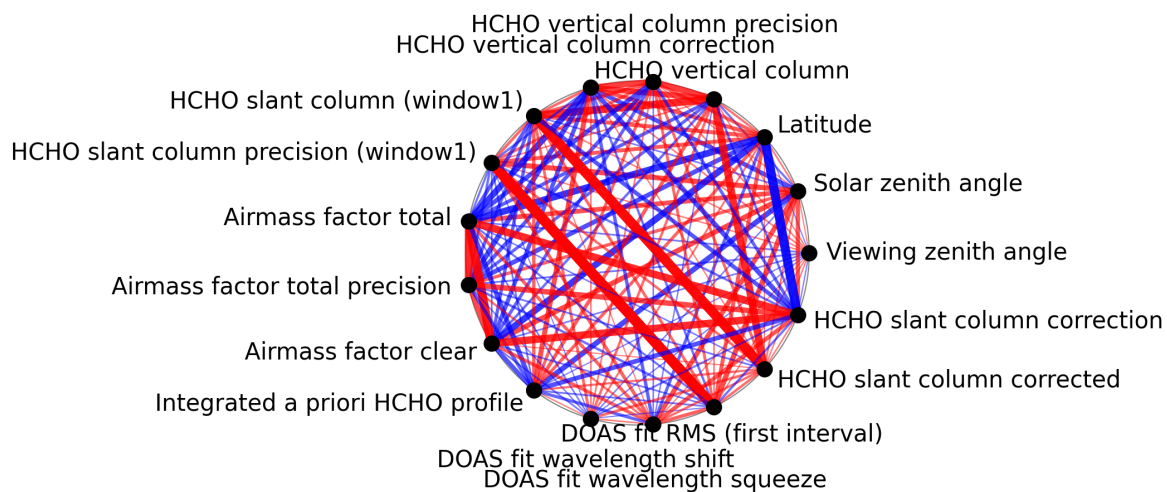
Figure 1: Map of correlation graph for 2024-11-30 to 2024-12-01.
