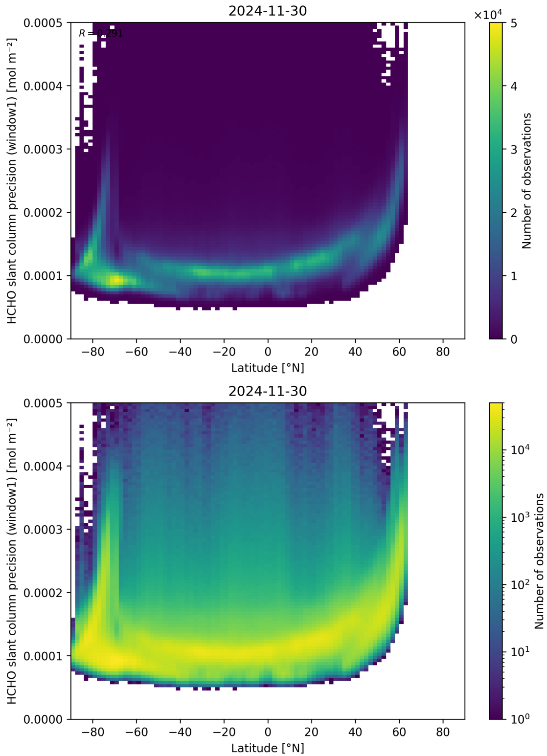
Figure 160: Scatter density plot of “Latitude” against “HCHO slant column precision (window1)” for 2024-11-30 to 2024-12-01.
