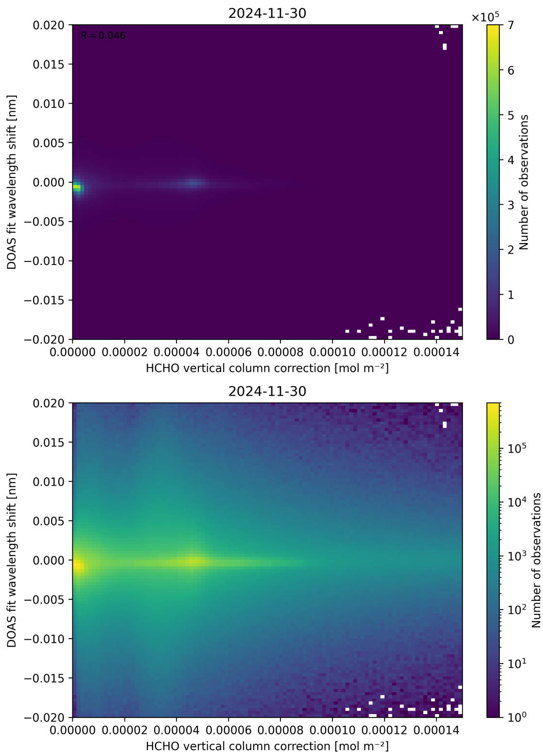
Figure 113: Scatter density plot of “HCHO vertical column correction” against “DOAS fit wavelength shift” for 2024-11-30 to 2024-12-01.
