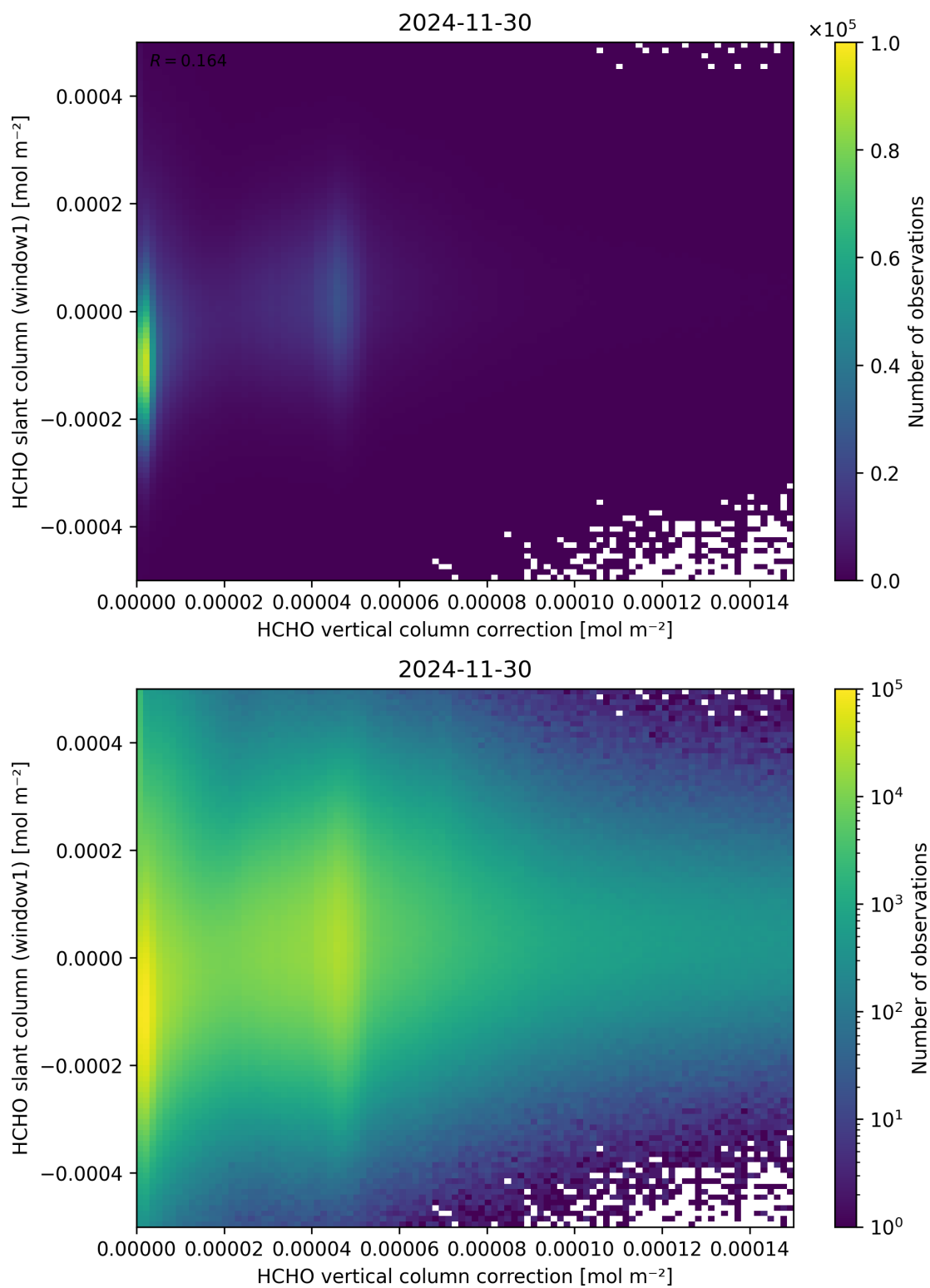
Figure 118: Scatter density plot of “HCHO vertical column correction” against “HCHO slant column (window1)” for 2024-11-30 to 2024-12-01.
