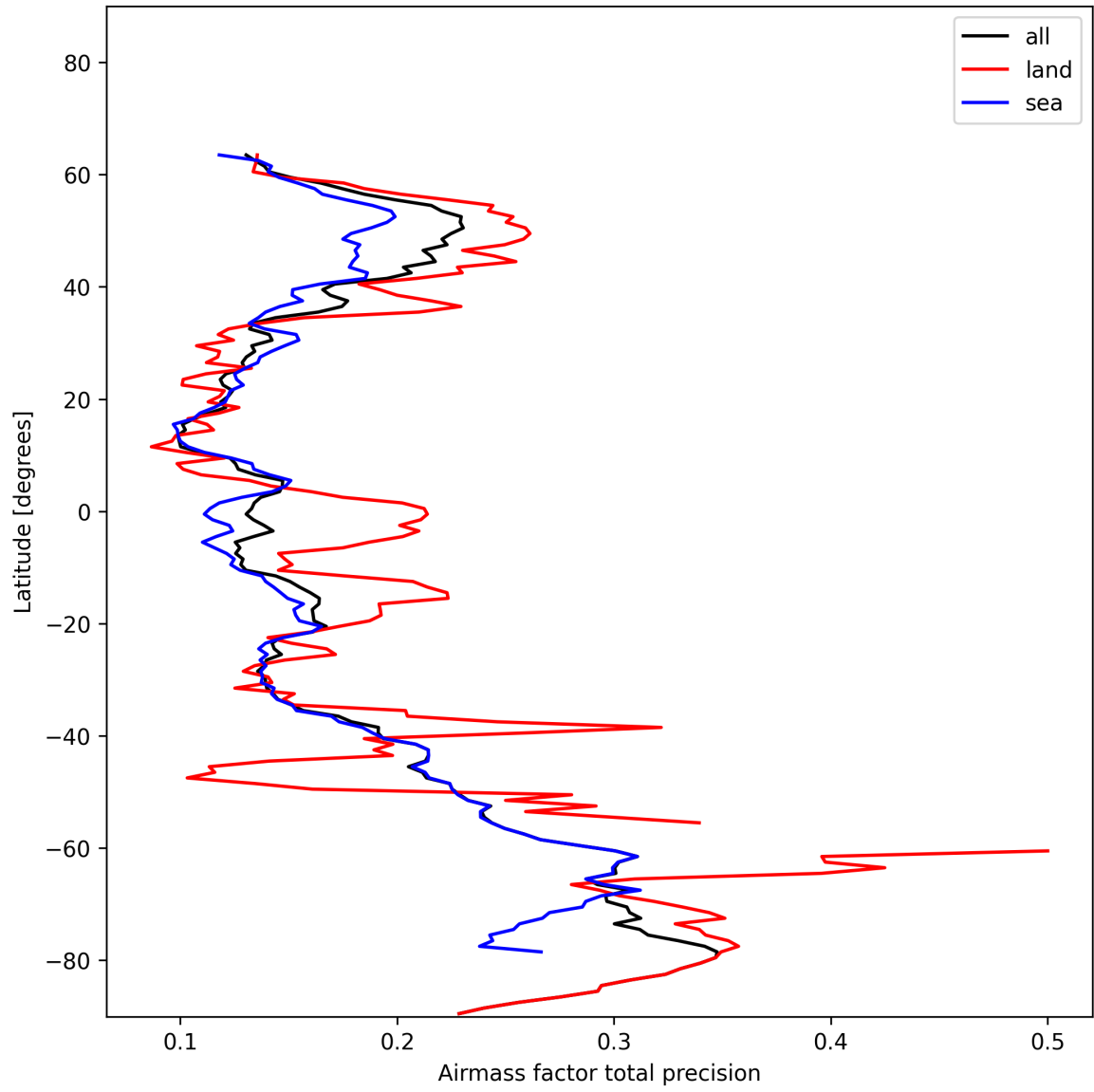
Figure 27: Zonal average of “Airmass factor total precision” for 2024-11-30 to 2024-12-01.
