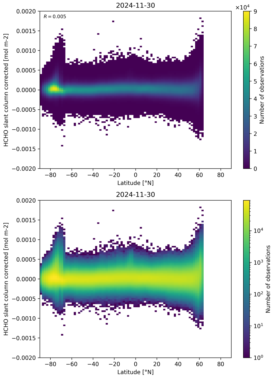
Figure 157: Scatter density plot of “Latitude” against “HCHO slant column corrected” for 2024-11-30 to 2024-12-01.
