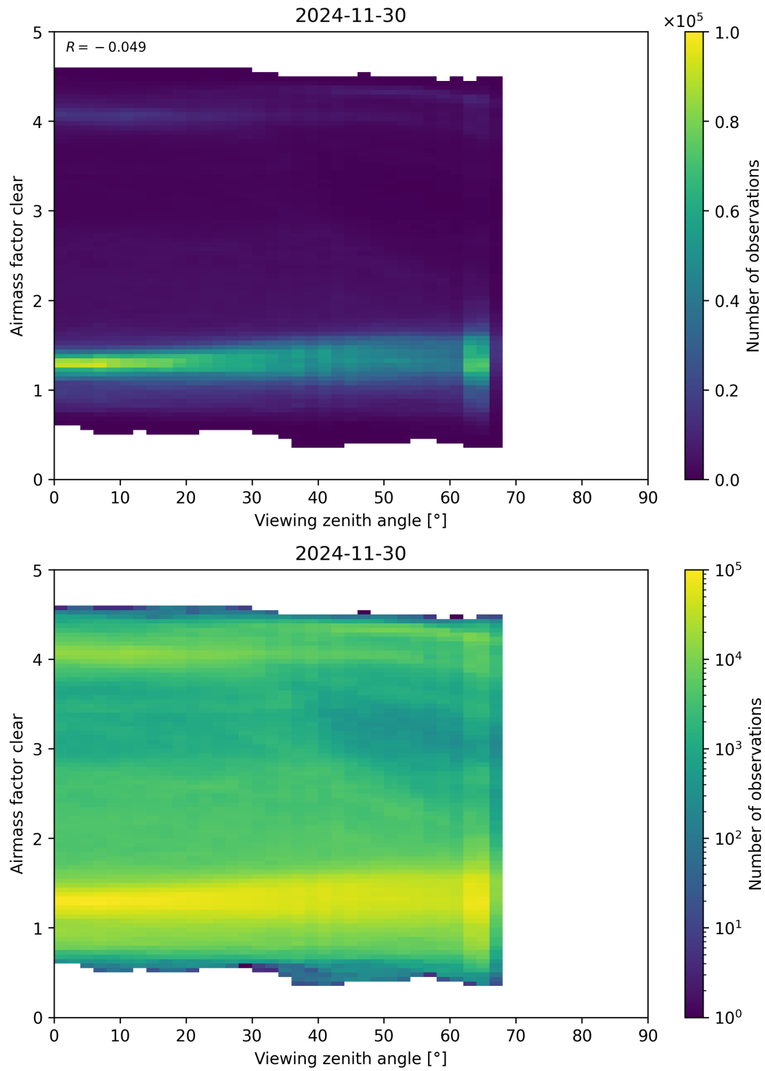
Figure 185: Scatter density plot of “Viewing zenith angle” against “Airmass factor clear” for 2024-11-30 to 2024-12-01.
