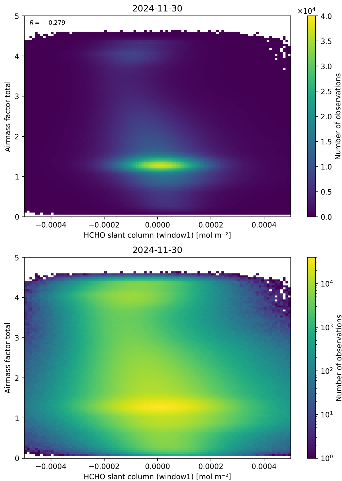
Figure 85: Scatter density plot of “HCHO slant column (window1)” against “Airmass factor total” for 2024-11-30 to 2024-12-01.
