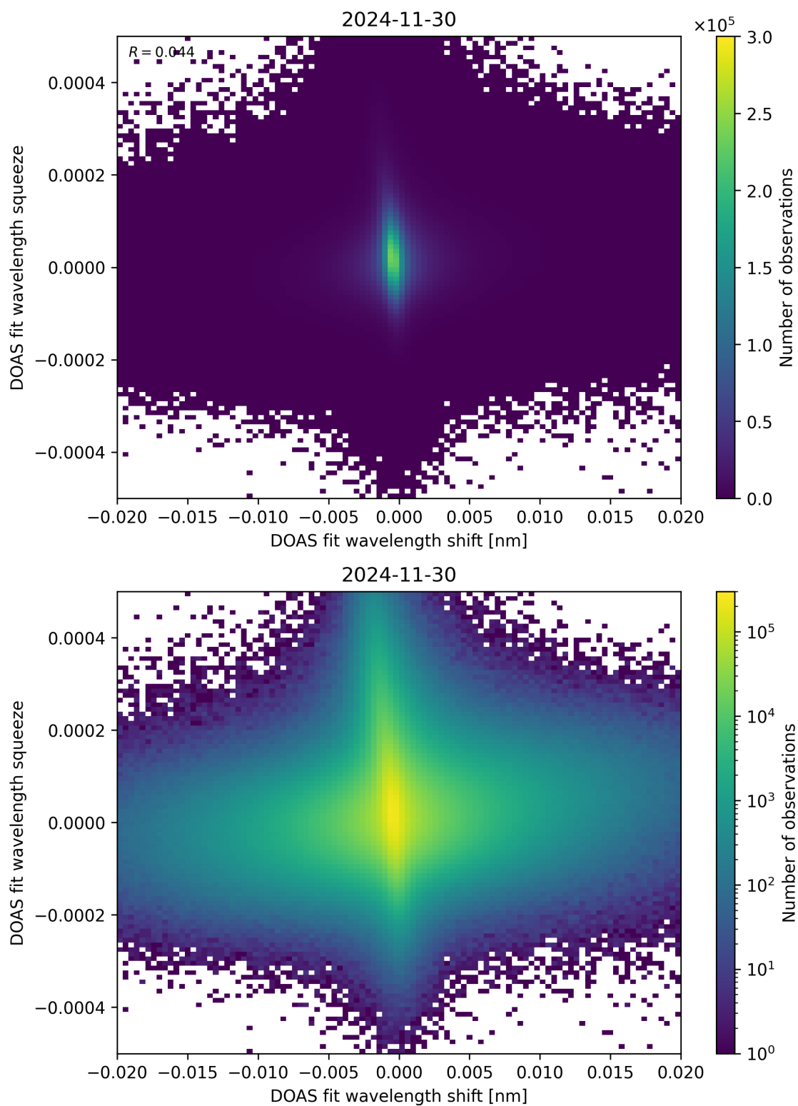
Figure 65: Scatter density plot of “DOAS fit wavelength shift” against “DOAS fit wavelength squeeze” for 2024-11-30 to 2024-12-01.
