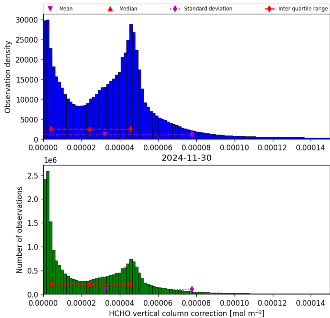
Figure 37: Histogram of “HCHO vertical column correction” for 2024-11-30 to 2024-12-01
