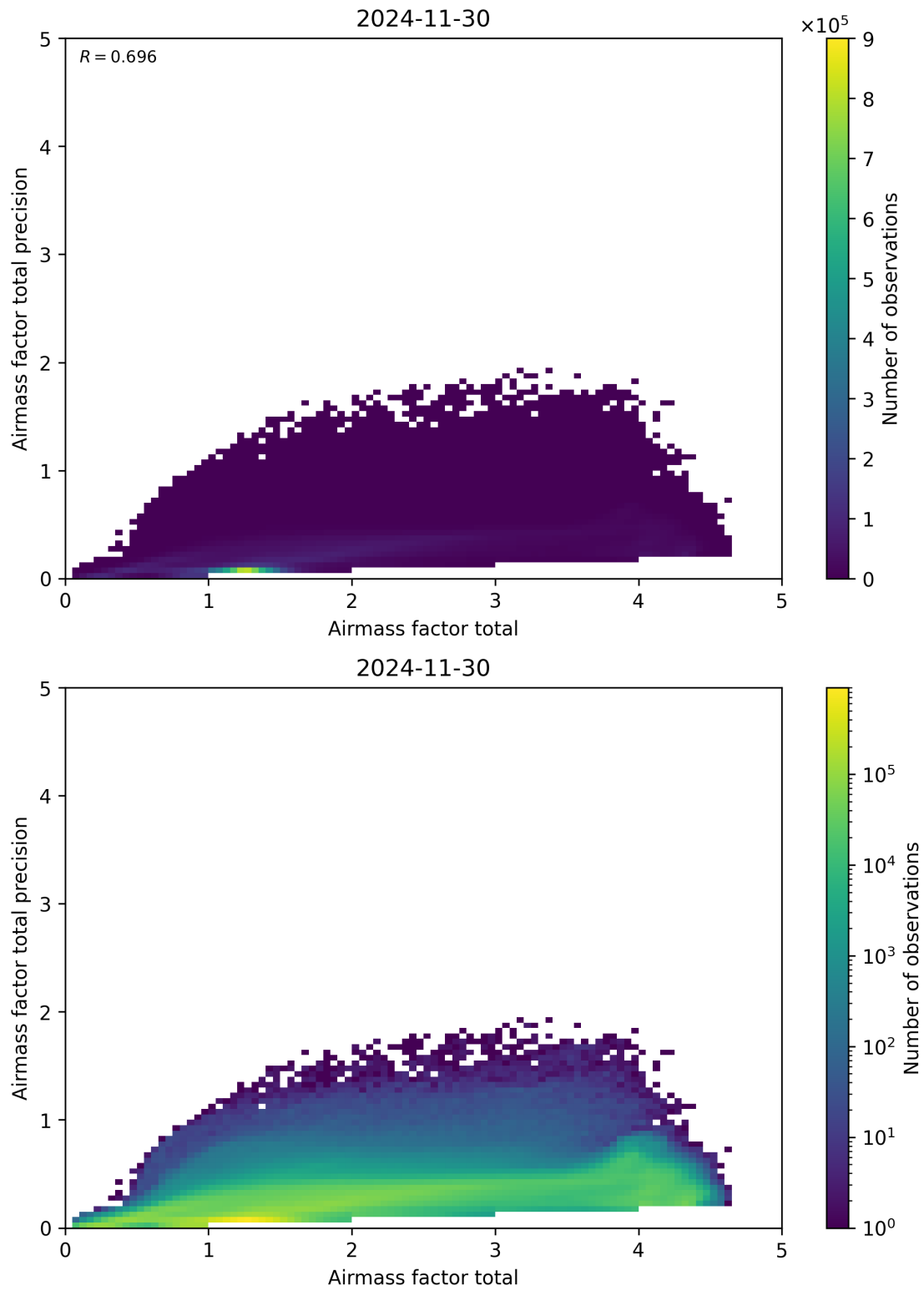
Figure 103: Scatter density plot of “Airmass factor total” against “Airmass factor total precision” for 2024-11-30 to 2024-12-01.
