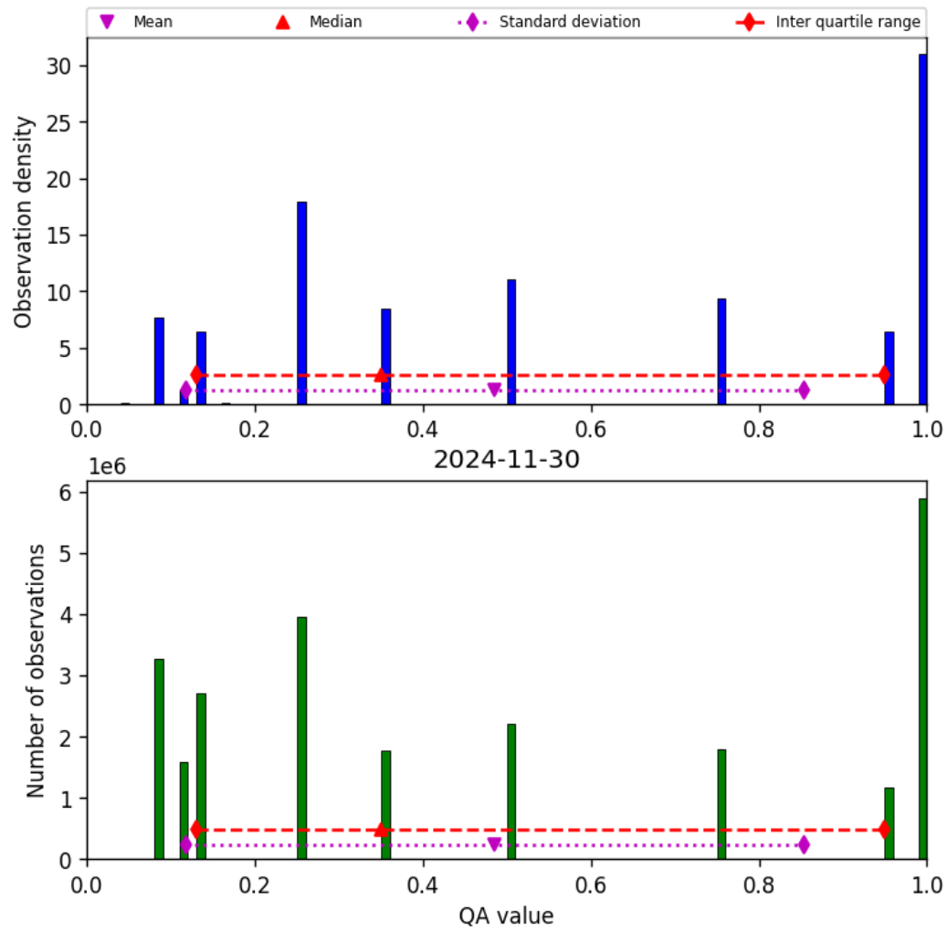
Figure 34: Histogram of “QA value” for 2024-11-30 to 2024-12-01
