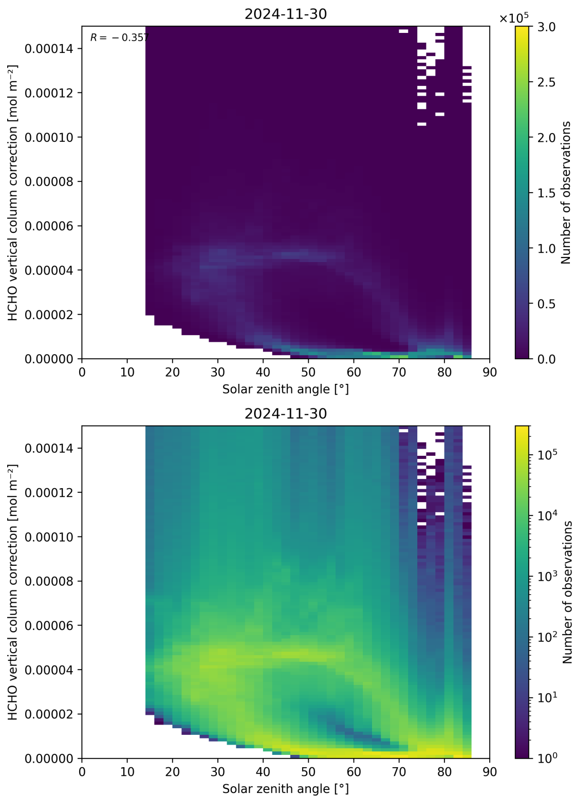
Figure 178: Scatter density plot of “Solar zenith angle” against “HCHO vertical column correction” for 2024-11-30 to 2024-12-01.
