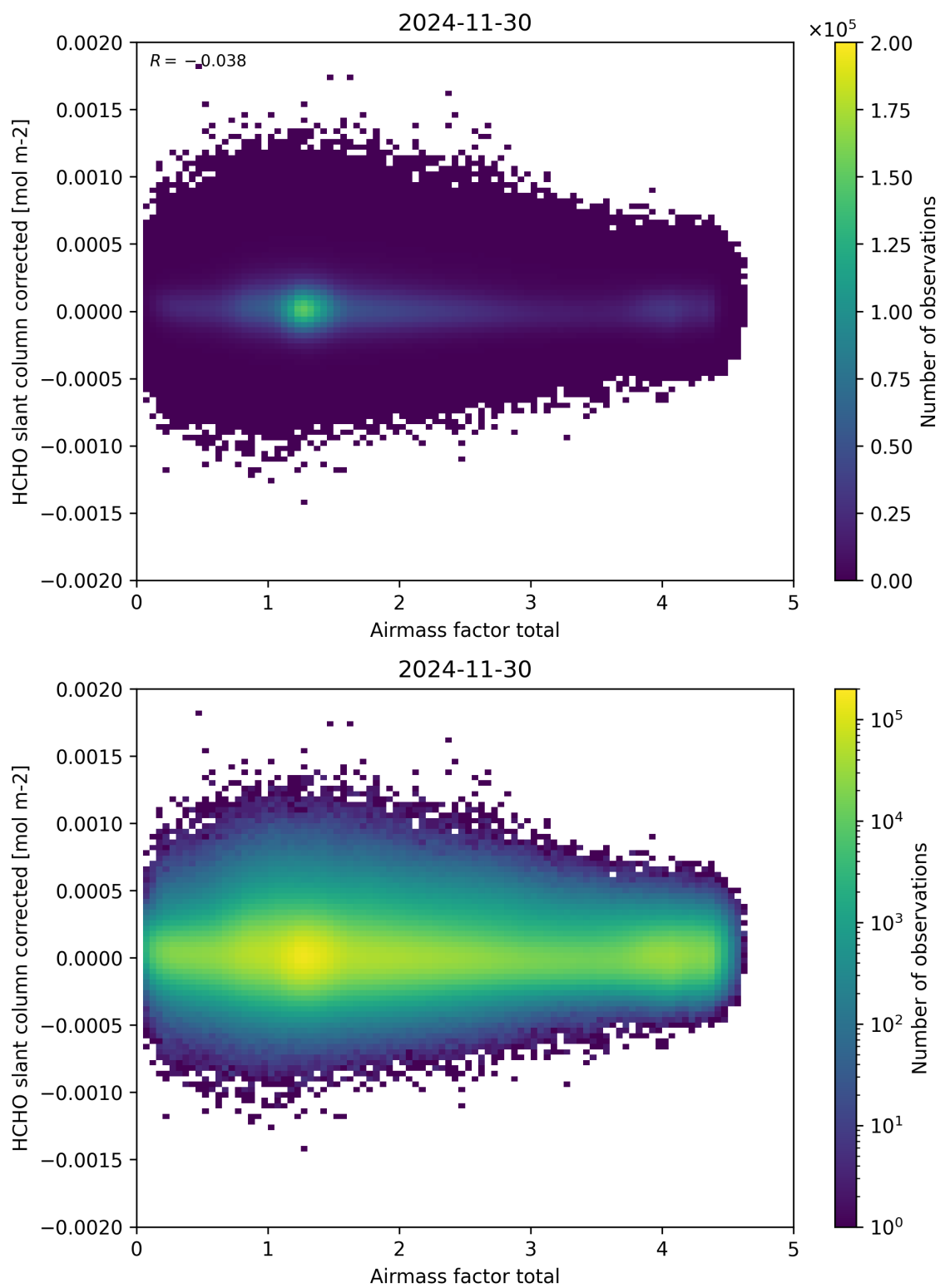
Figure 101: Scatter density plot of “Airmass factor total” against “HCHO slant column corrected” for 2024-11-30 to 2024-12-01.
