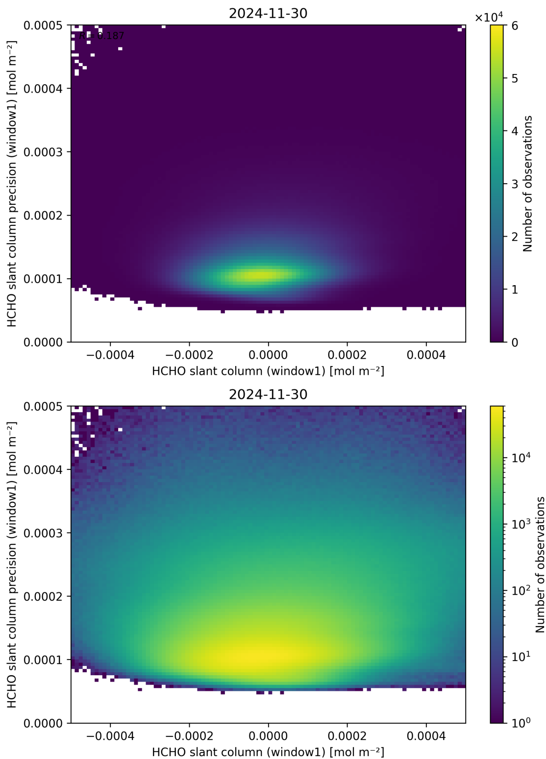
Figure 84: Scatter density plot of “HCHO slant column (window1)” against “HCHO slant column precision (window1)” for 2024-11-30 to 2024-12-01.
