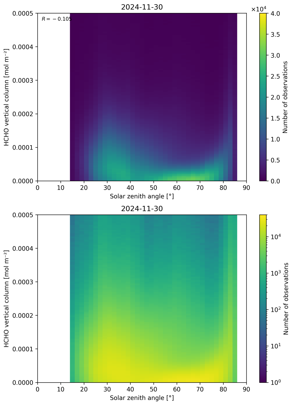
Figure 177: Scatter density plot of “Solar zenith angle” against “HCHO vertical column” for 2024-11-30 to 2024-12-01.
