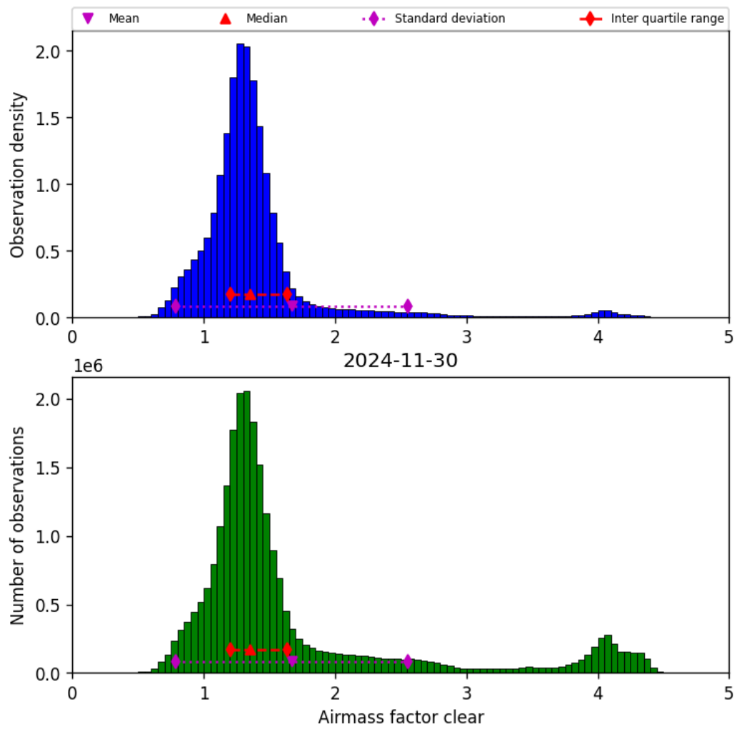
Figure 42: Histogram of “Airmass factor clear” for 2024-11-30 to 2024-12-01
