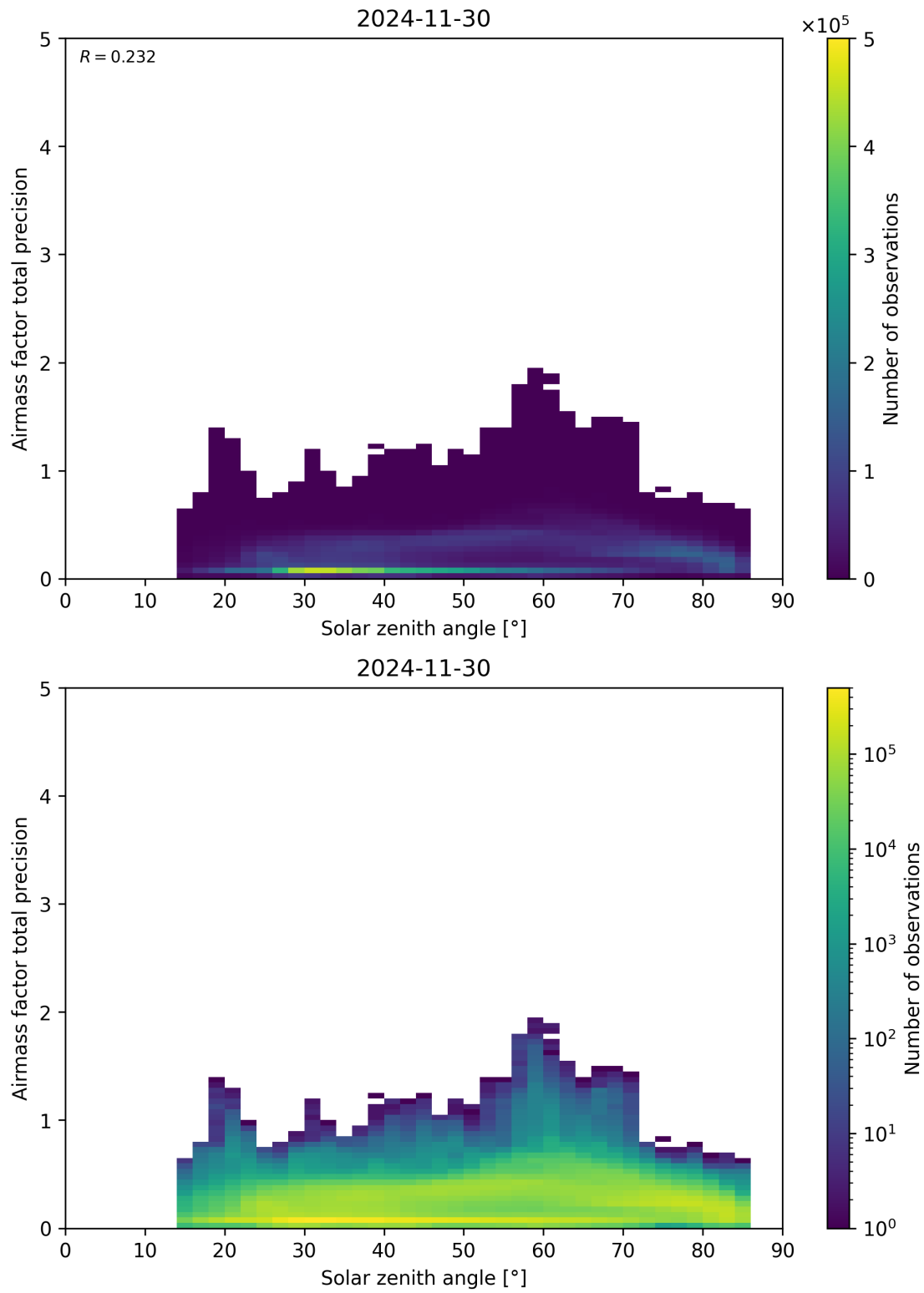
Figure 176: Scatter density plot of “Solar zenith angle” against “Airmass factor total precision” for 2024-11-30 to 2024-12-01.
