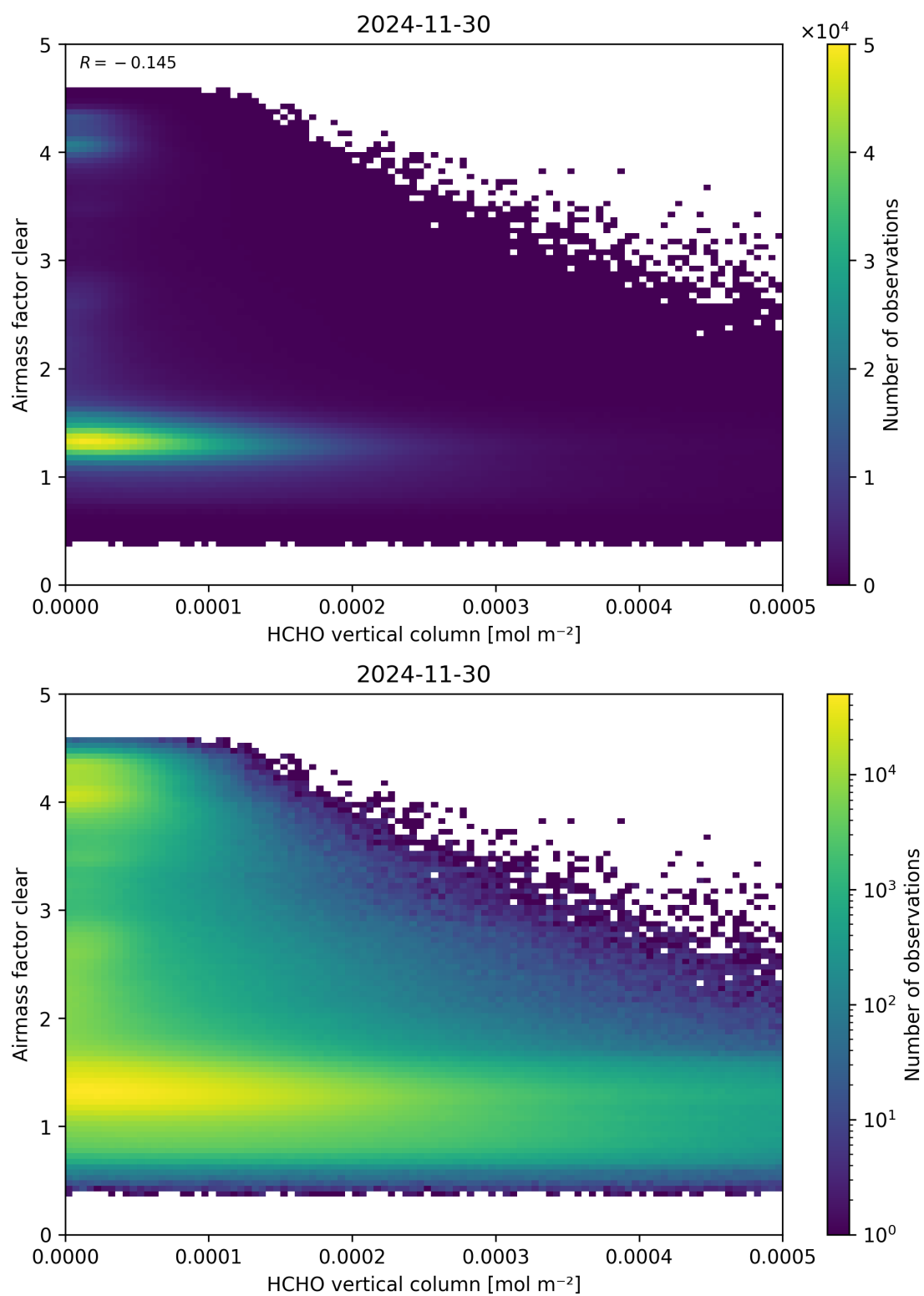
Figure 126: Scatter density plot of “HCHO vertical column” against “Airmass factor clear” for 2024-11-30 to 2024-12-01.
