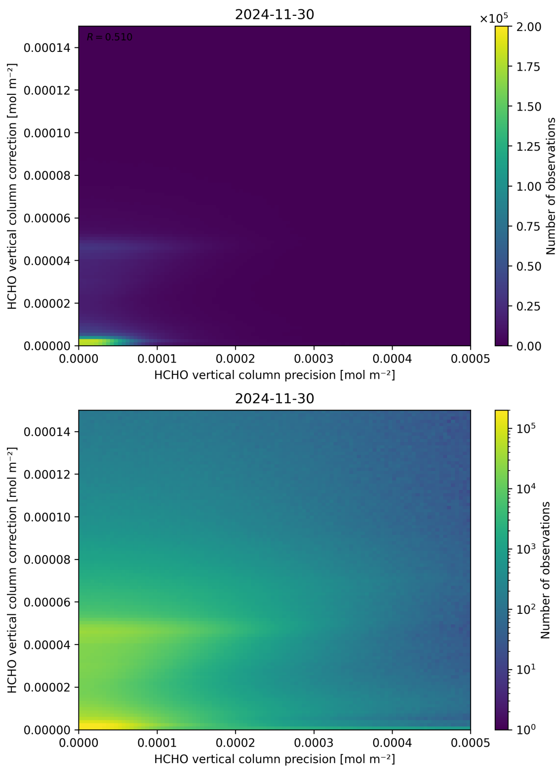
Figure 146: Scatter density plot of “HCHO vertical column precision” against “HCHO vertical column correction” for 2024-11-30 to 2024-12-01.
