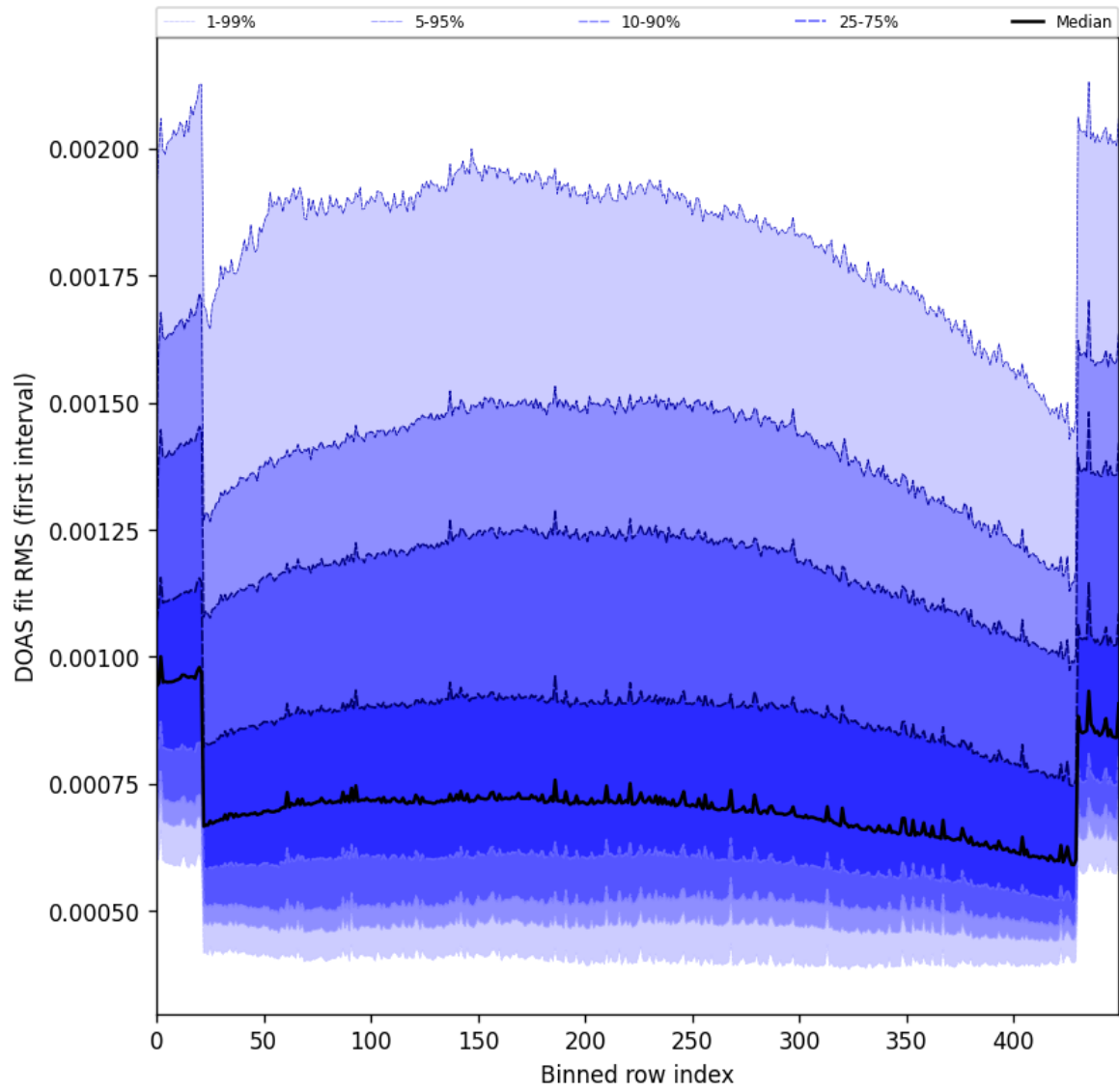
Figure 60: Along track statistics of “DOAS fit RMS (first interval)” for 2024-11-30 to 2024-12-01
