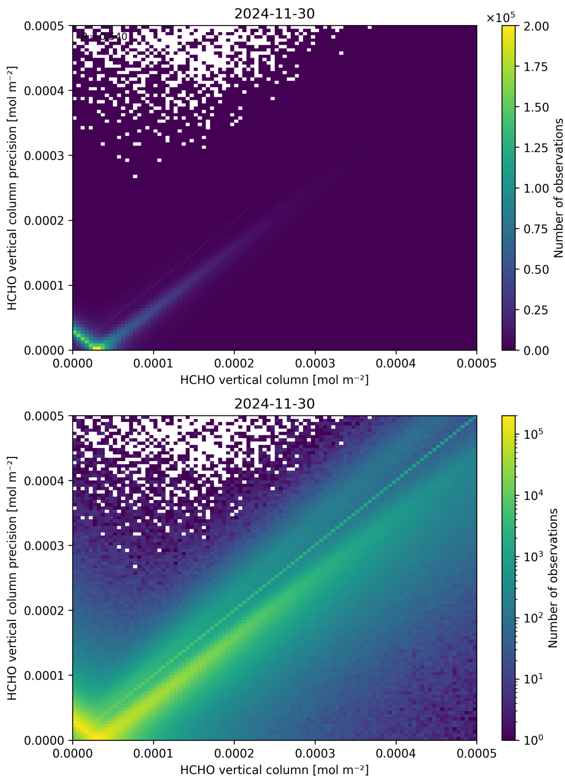
Figure 134: Scatter density plot of “HCHO vertical column” against “HCHO vertical column precision” for 2024-11-30 to 2024-12-01.
