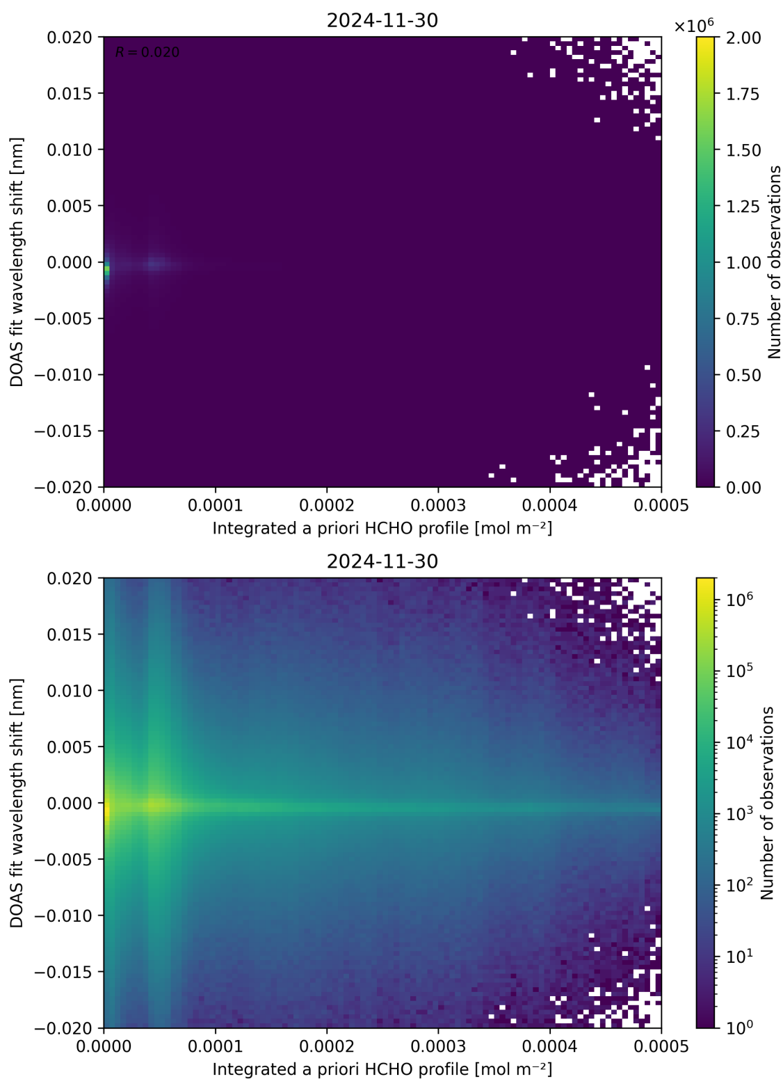
Figure 149: Scatter density plot of “Integrated a priori HCHO profile” against “DOAS fit wavelength shift” for 2024-11-30 to 2024-12-01.
