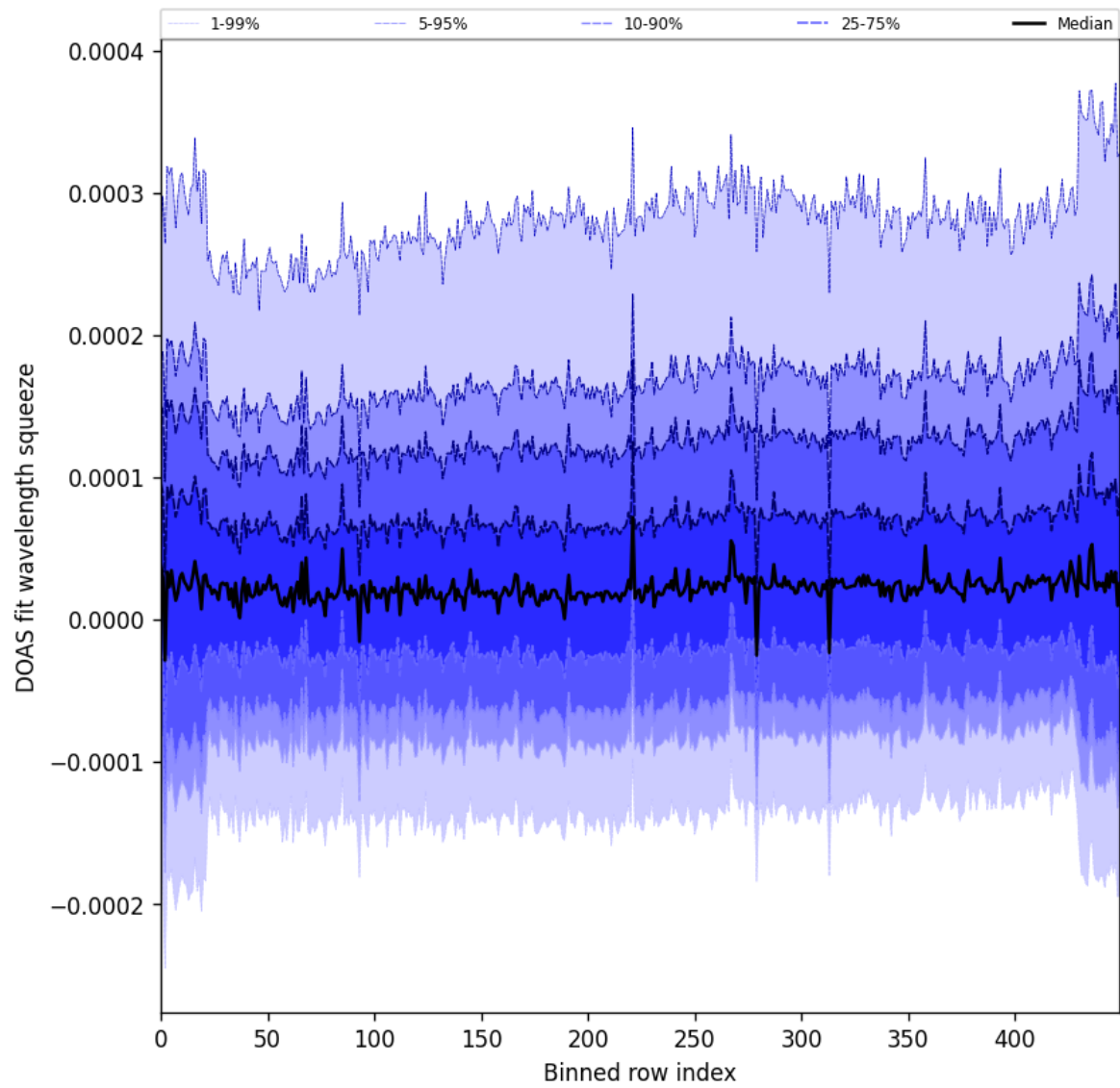
Figure 59: Along track statistics of “DOAS fit wavelength squeeze” for 2024-11-30 to 2024-12-01
