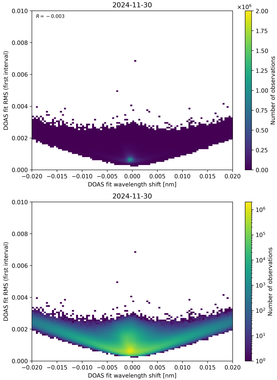
Figure 64: Scatter density plot of “DOAS fit wavelength shift” against “DOAS fit RMS (first interval)” for 2024-11-30 to 2024-12-01.
