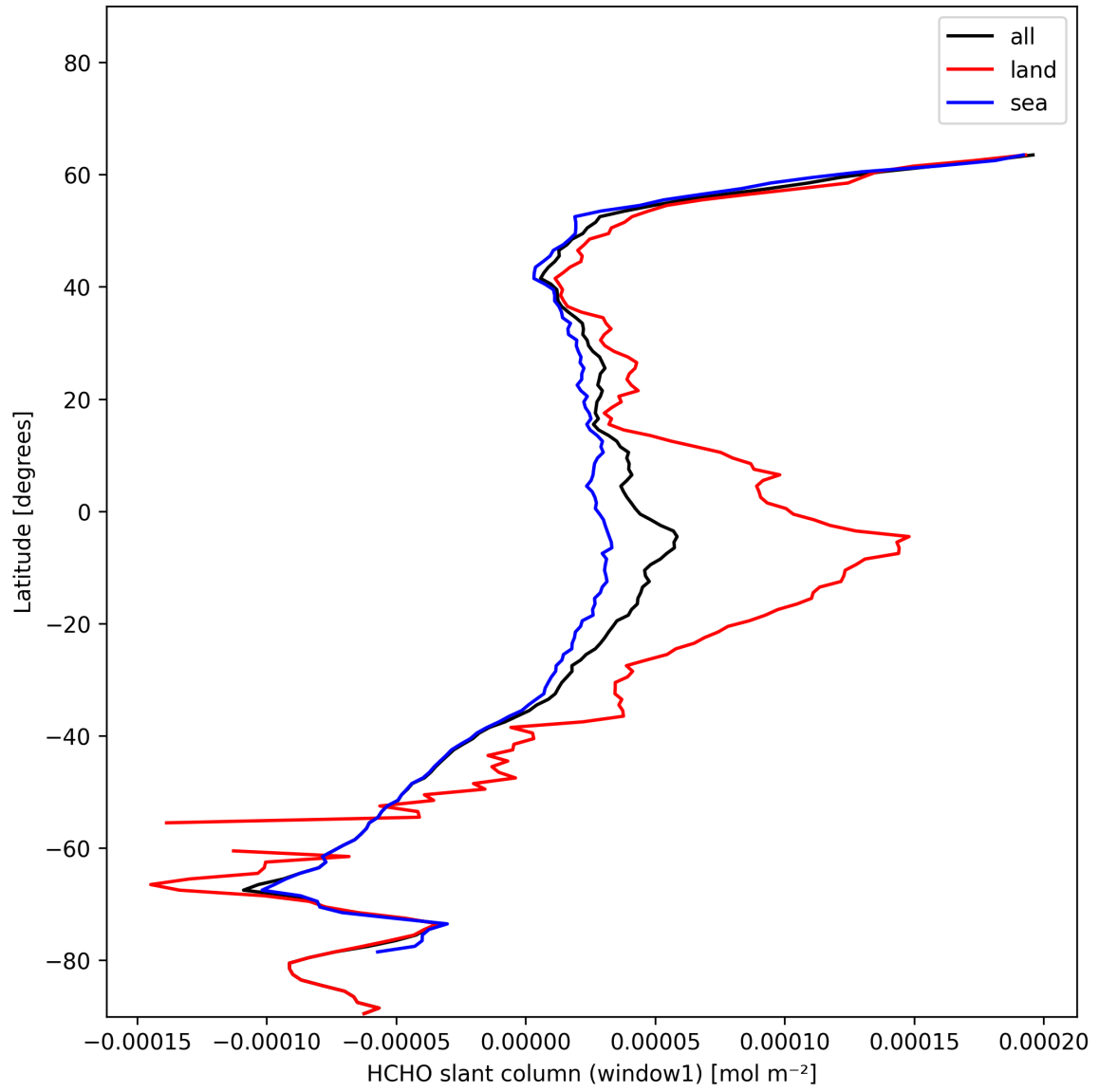
Figure 24: Zonal average of “HCHO slant column (window1)” for 2024-11-30 to 2024-12-01.
