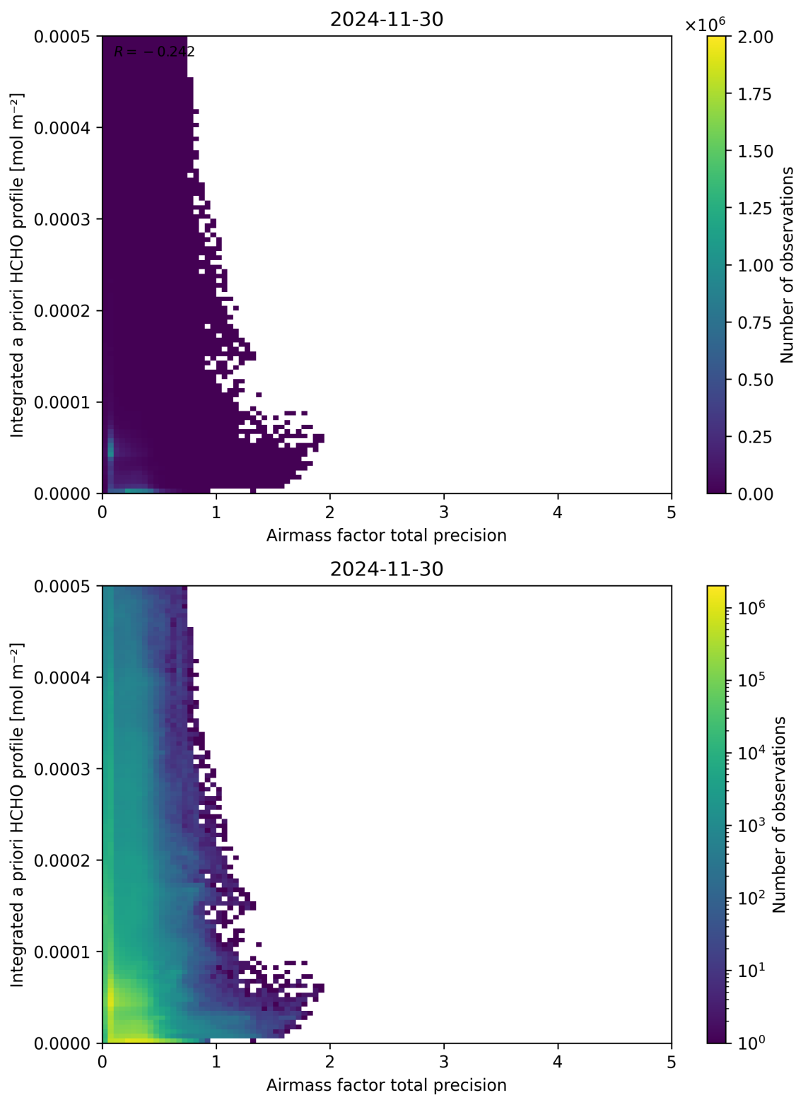
Figure 111: Scatter density plot of “Airmass factor total precision” against “Integrated a priori HCHO profile” for 2024-11-30 to 2024-12-01.
