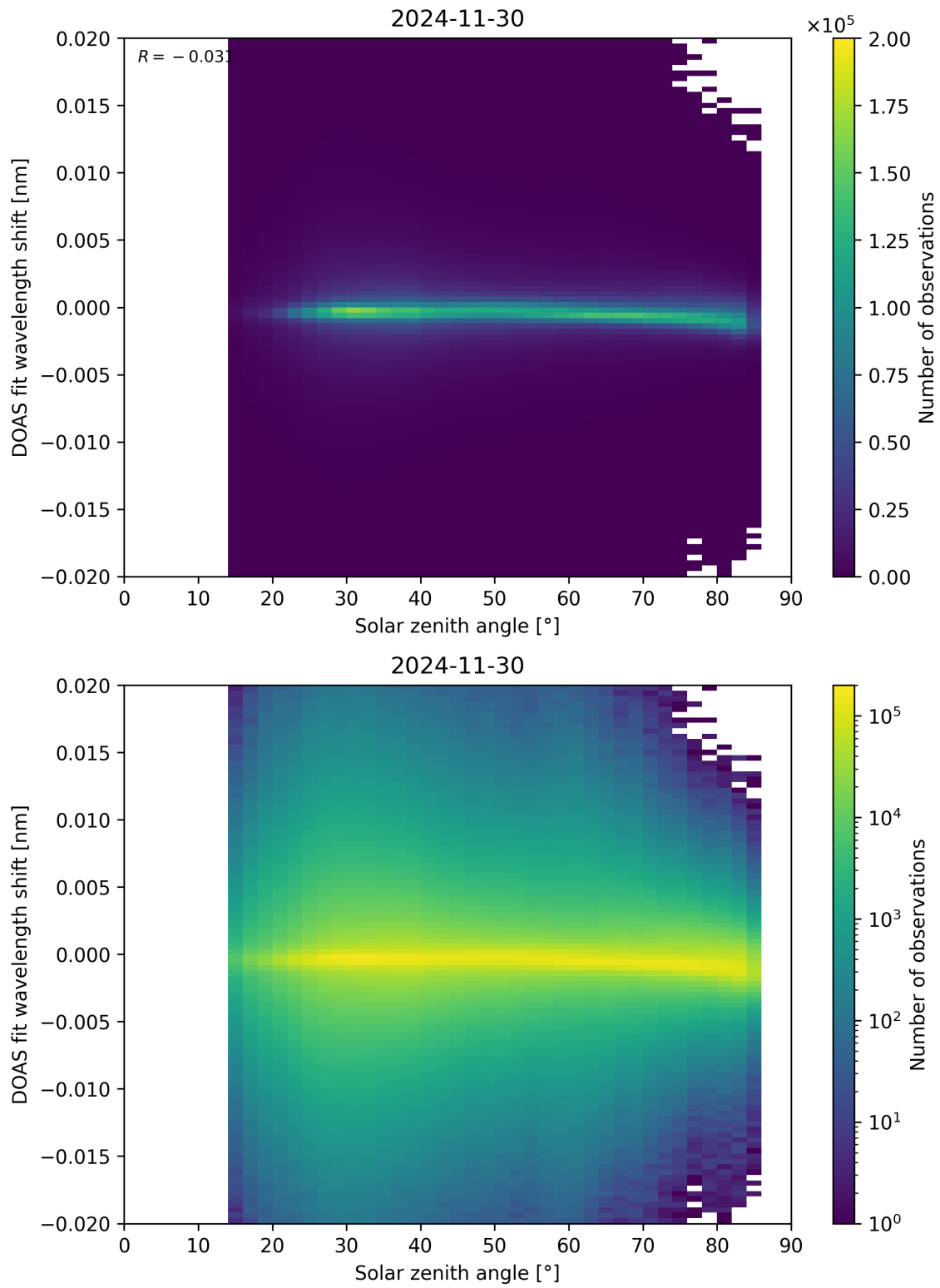
Figure 168: Scatter density plot of “Solar zenith angle” against “DOAS fit wavelength shift” for 2024-11-30 to 2024-12-01.
