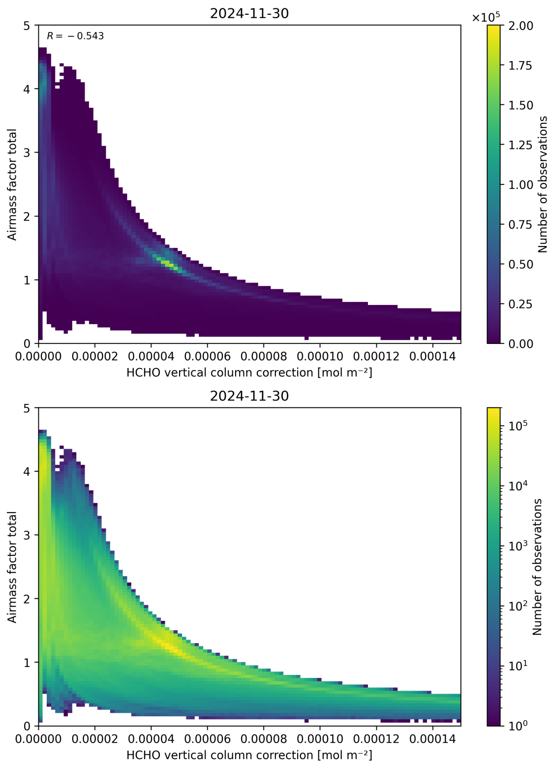
Figure 120: Scatter density plot of “HCHO vertical column correction” against “Airmass factor total” for 2024-11-30 to 2024-12-01.
