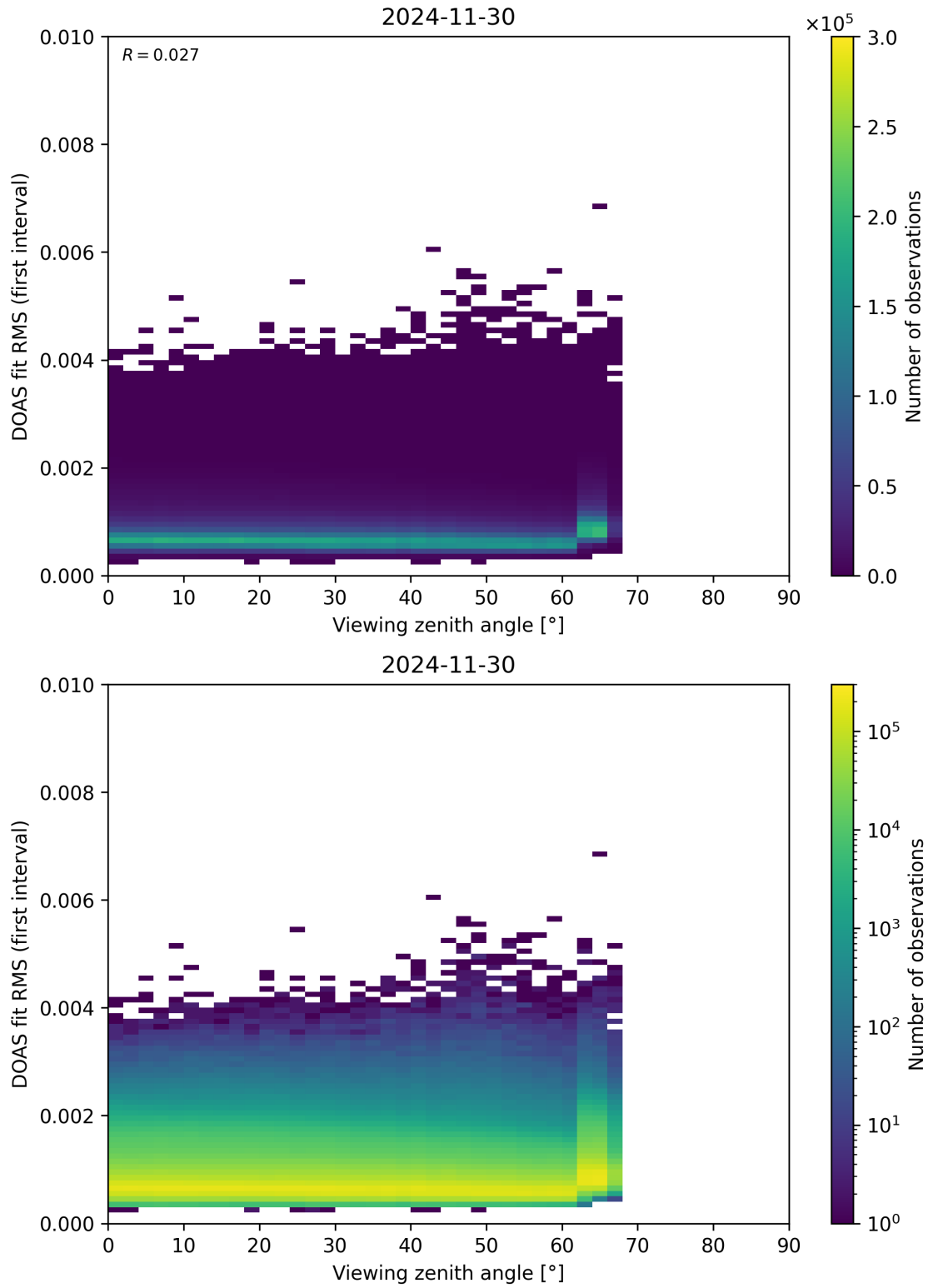
Figure 182: Scatter density plot of “Viewing zenith angle” against “DOAS fit RMS (first interval)” for 2024-11-30 to 2024-12-01.
