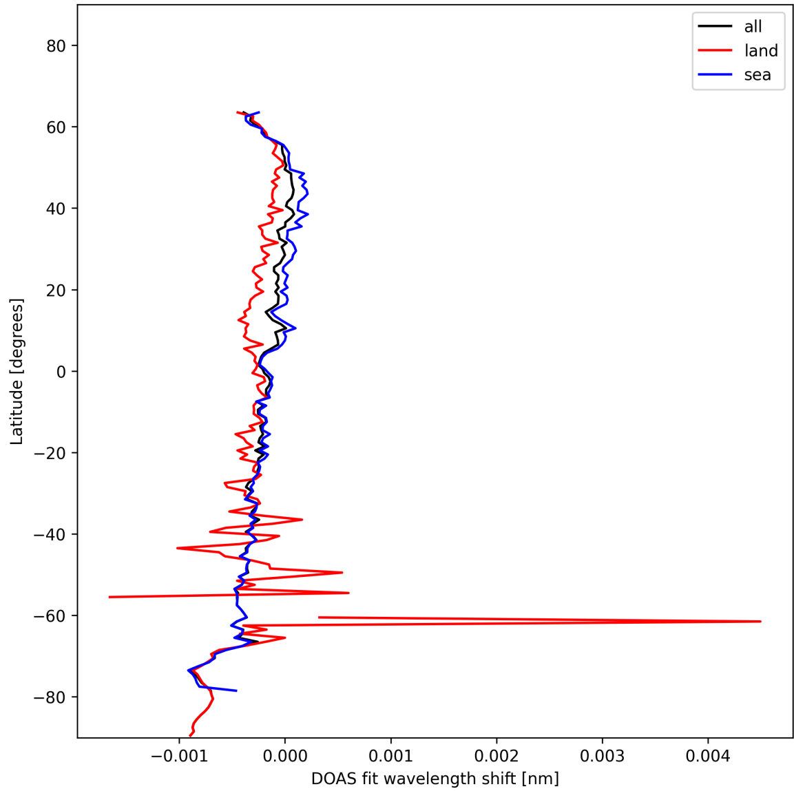
Figure 30: Zonal average of “DOAS fit wavelength shift” for 2024-11-30 to 2024-12-01.
