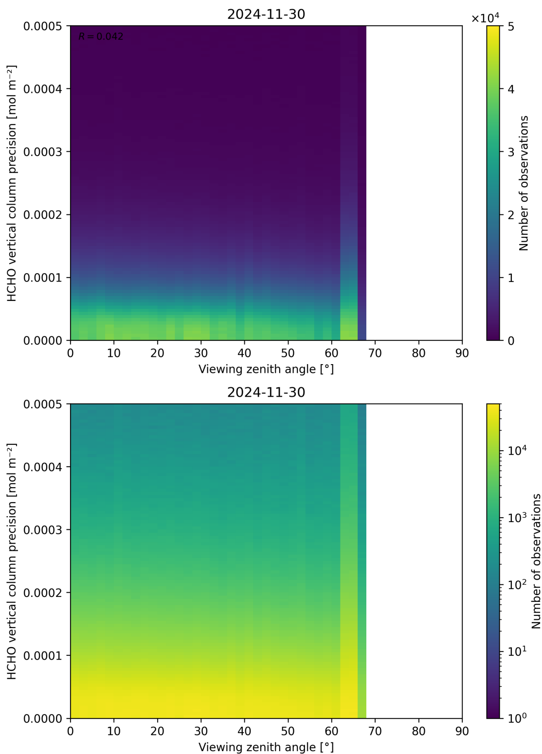
Figure 194: Scatter density plot of “Viewing zenith angle” against “HCHO vertical column precision” for 2024-11-30 to 2024-12-01.
