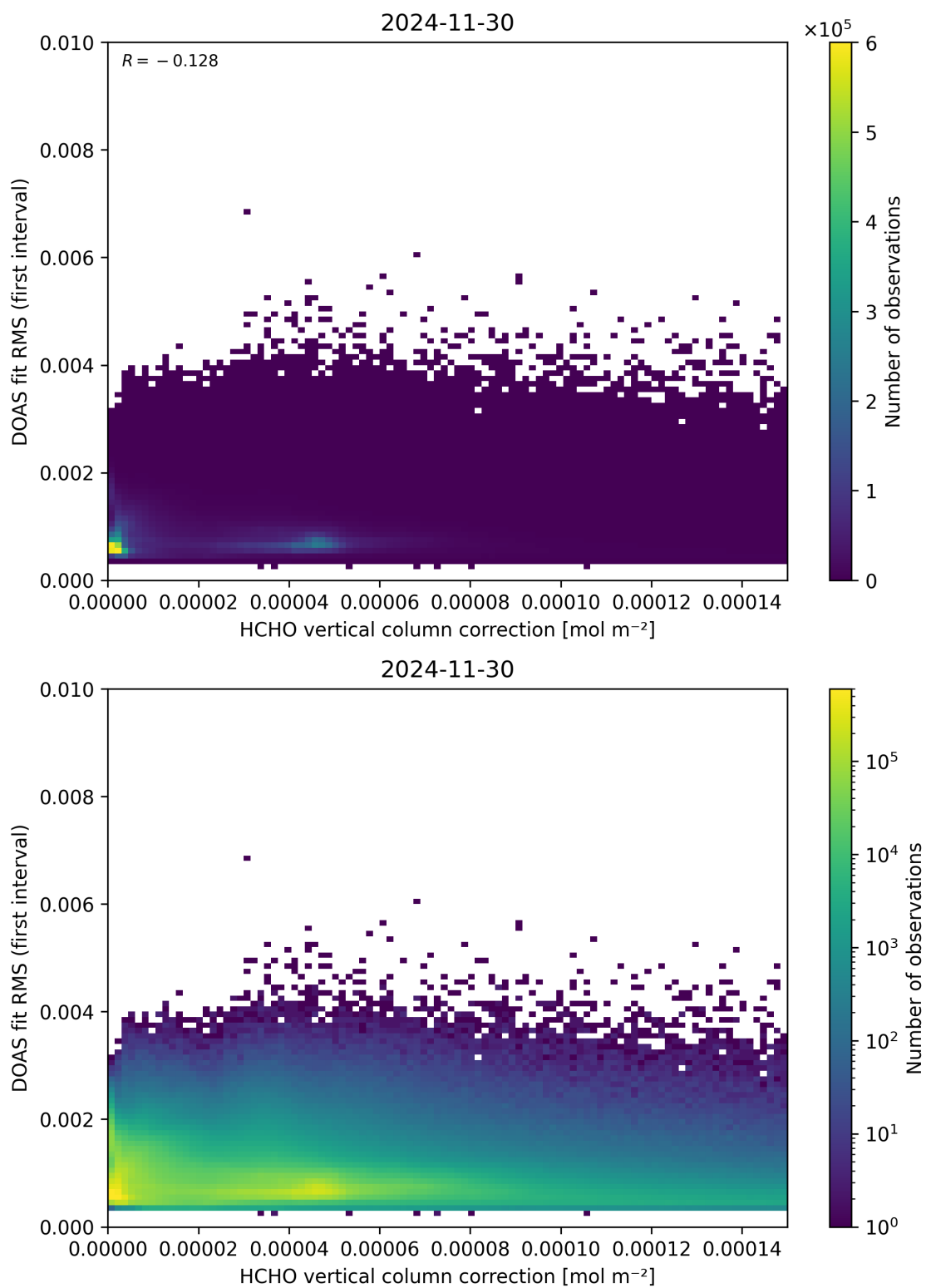
Figure 112: Scatter density plot of “HCHO vertical column correction” against “DOAS fit RMS (first interval)” for 2024-11-30 to 2024-12-01.
