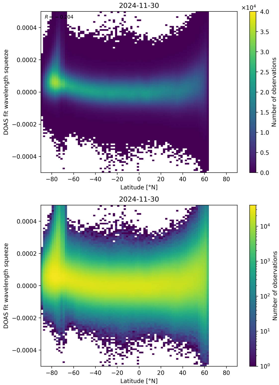
Figure 155: Scatter density plot of “Latitude” against “DOAS fit wavelength squeeze” for 2024-11-30 to 2024-12-01.
