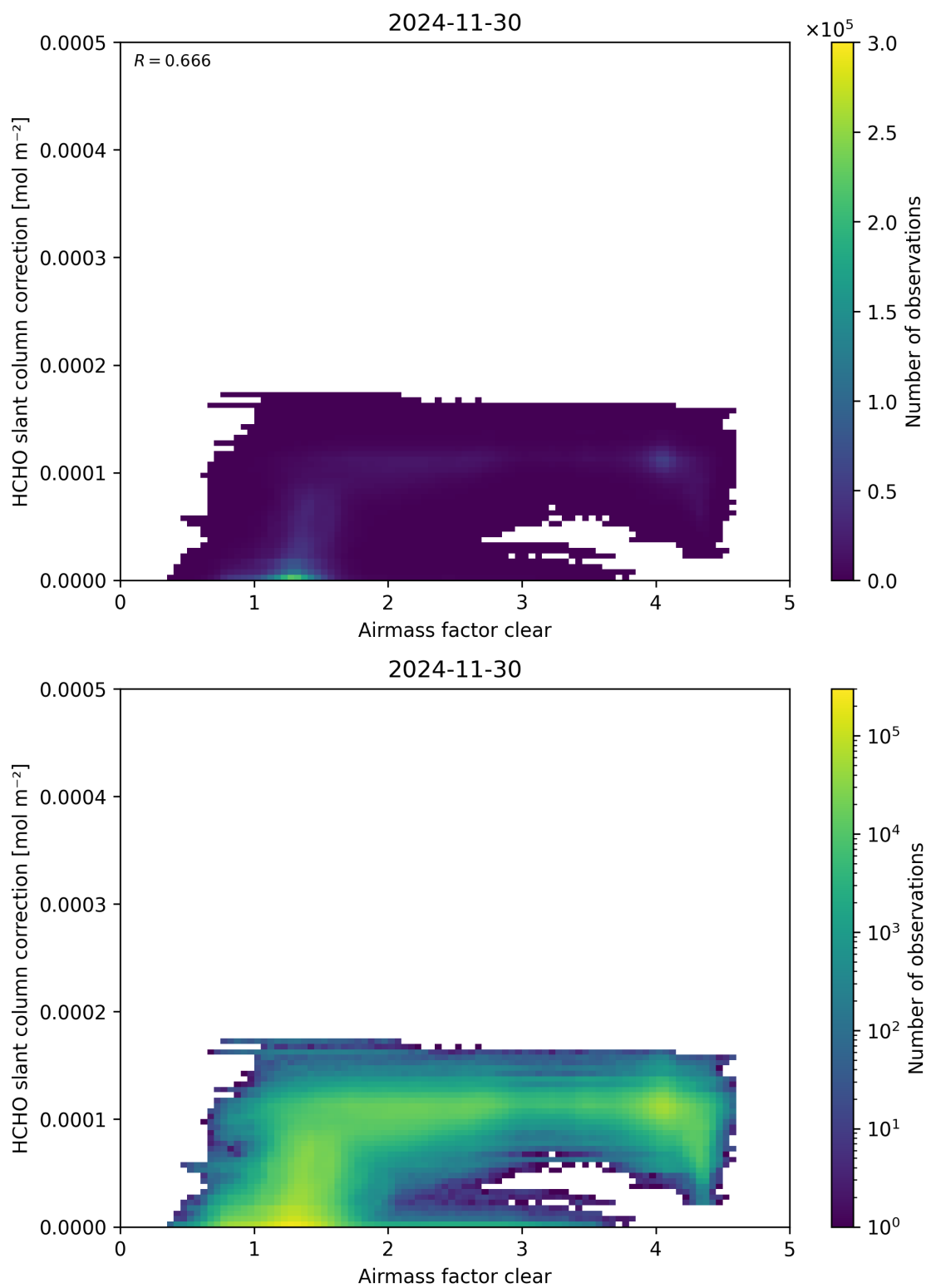
Figure 75: Scatter density plot of “Airmass factor clear” against “HCHO slant column correction” for 2024-11-30 to 2024-12-01.
