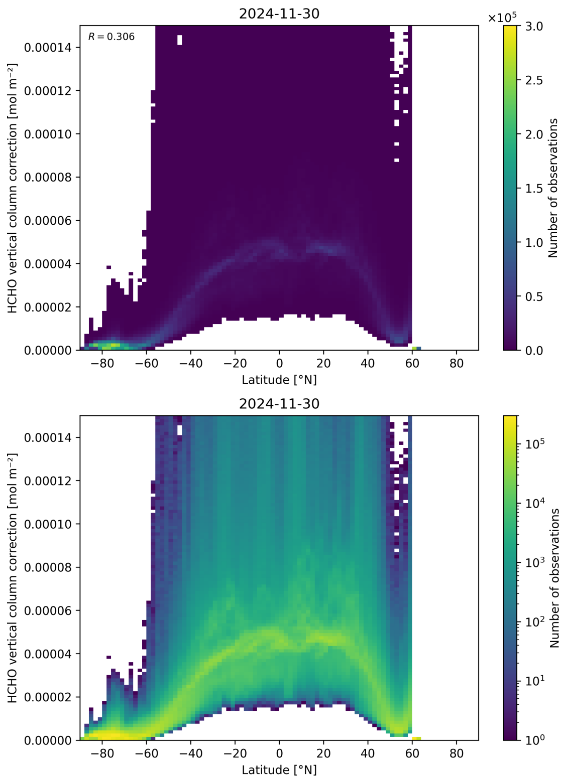
Figure 164: Scatter density plot of “Latitude” against “HCHO vertical column correction” for 2024-11-30 to 2024-12-01.
