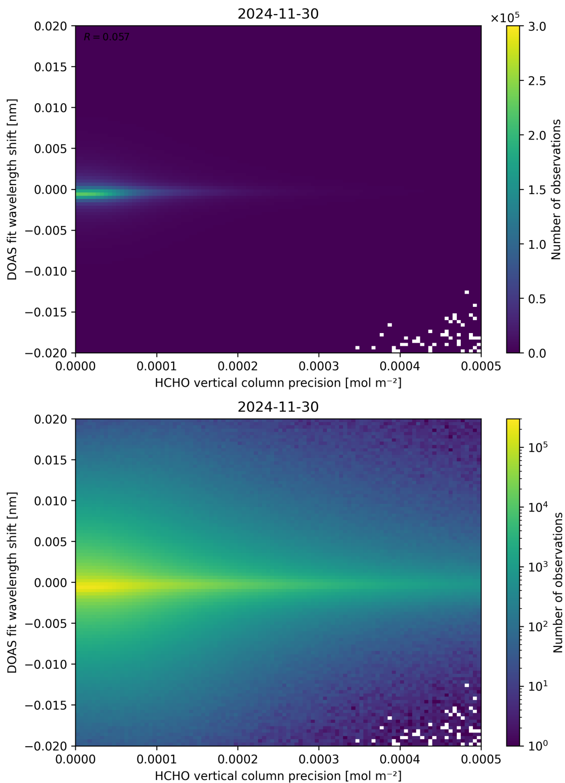
Figure 137: Scatter density plot of “HCHO vertical column precision” against “DOAS fit wavelength shift” for 2024-11-30 to 2024-12-01.
