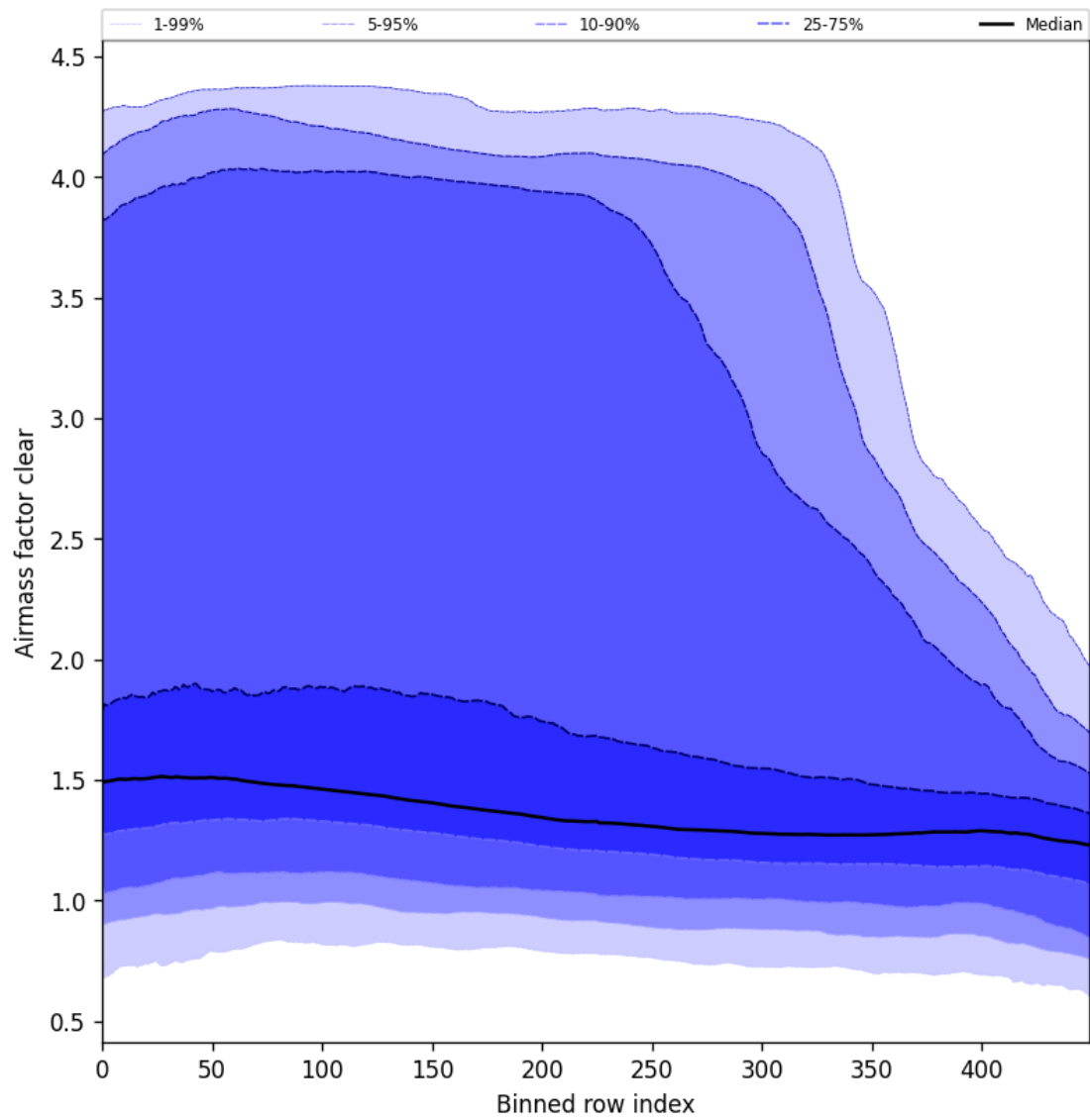
Figure 56: Along track statistics of “Air mass factor clear” for 2024-11-30 to 2024-12-01
