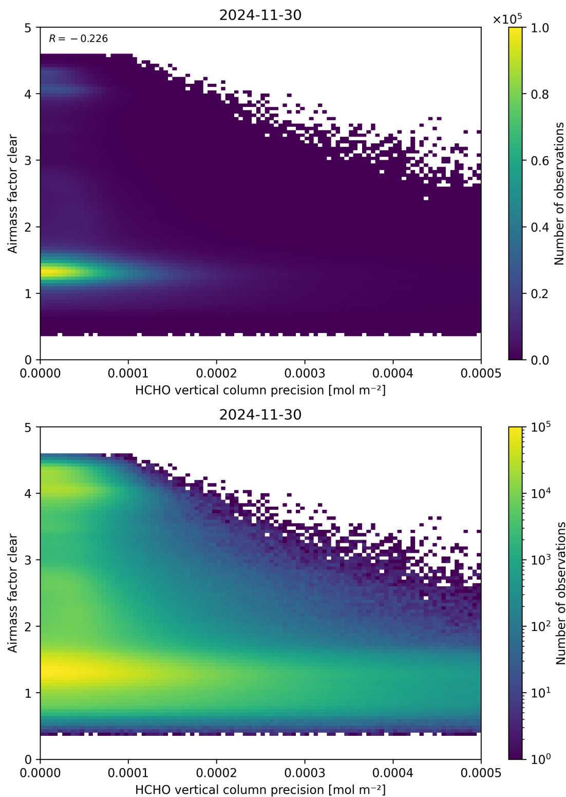
Figure 139: Scatter density plot of “HCHO vertical column precision” against “Airmass factor clear” for 2024-11-30 to 2024-12-01.
