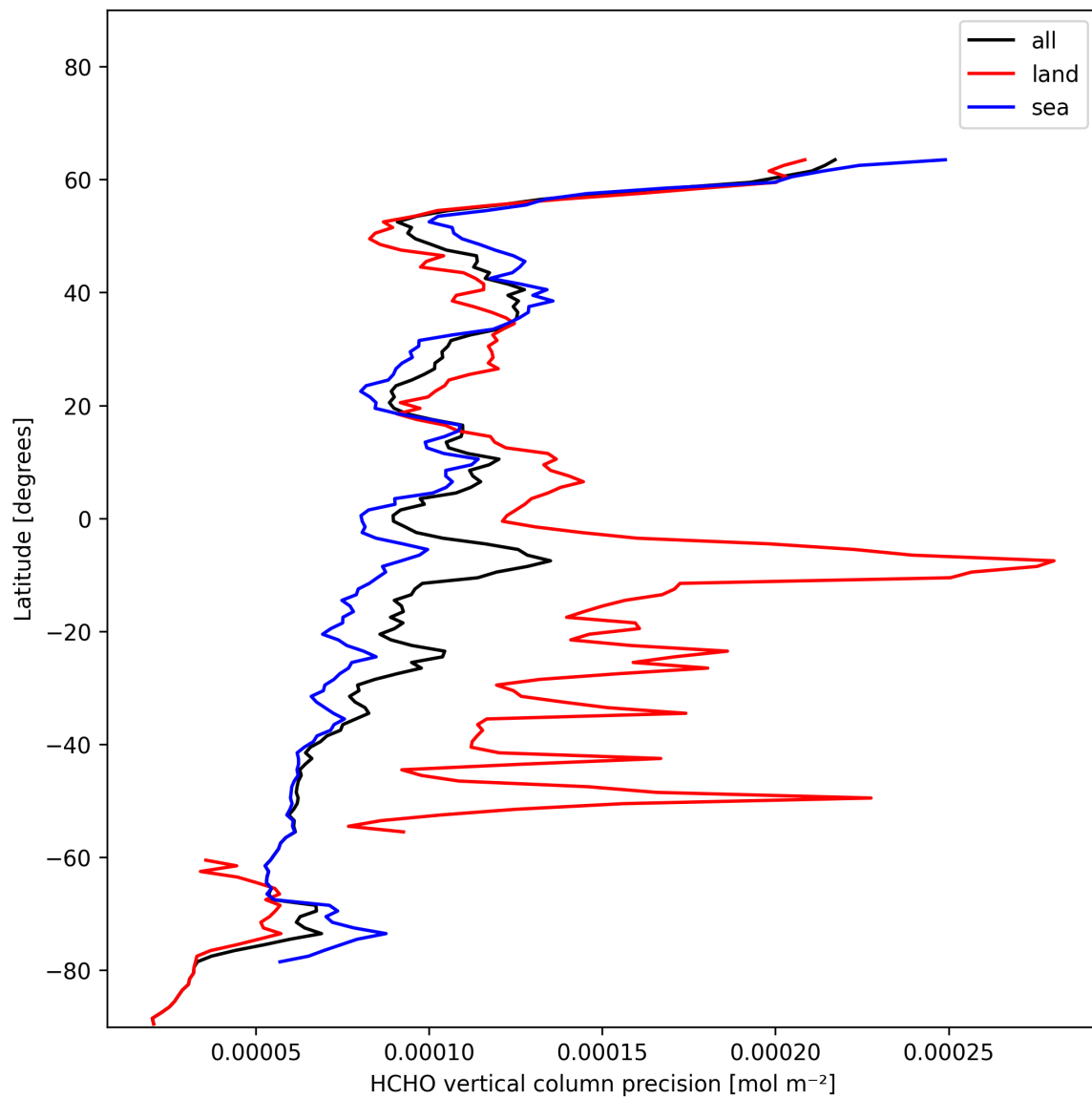
Figure 22: Zonal average of “HCHO vertical column precision” for 2024-11-30 to 2024-12-01.
