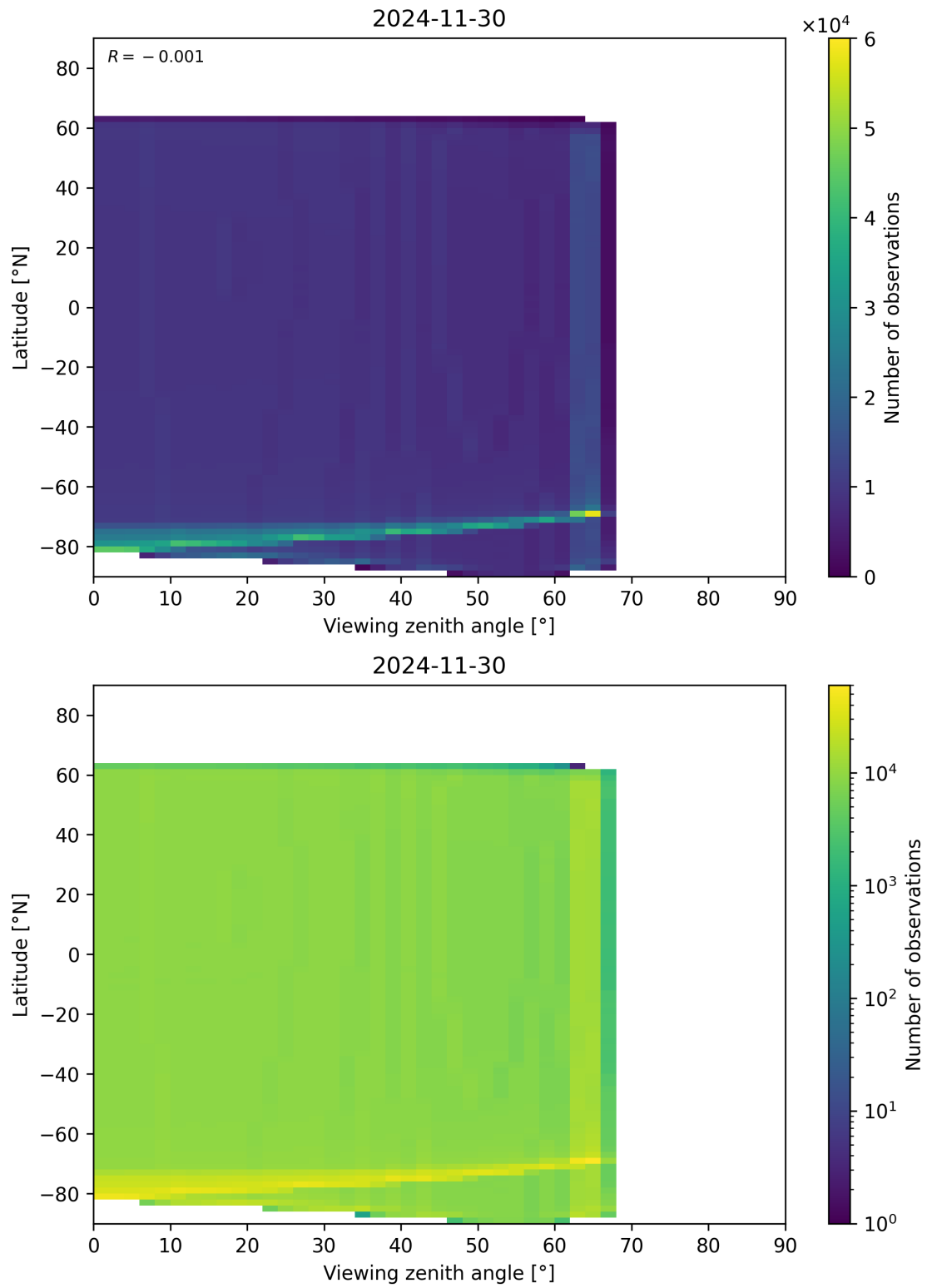
Figure 196: Scatter density plot of “Viewing zenith angle” against “Latitude” for 2024-11-30 to 2024-12-01.
