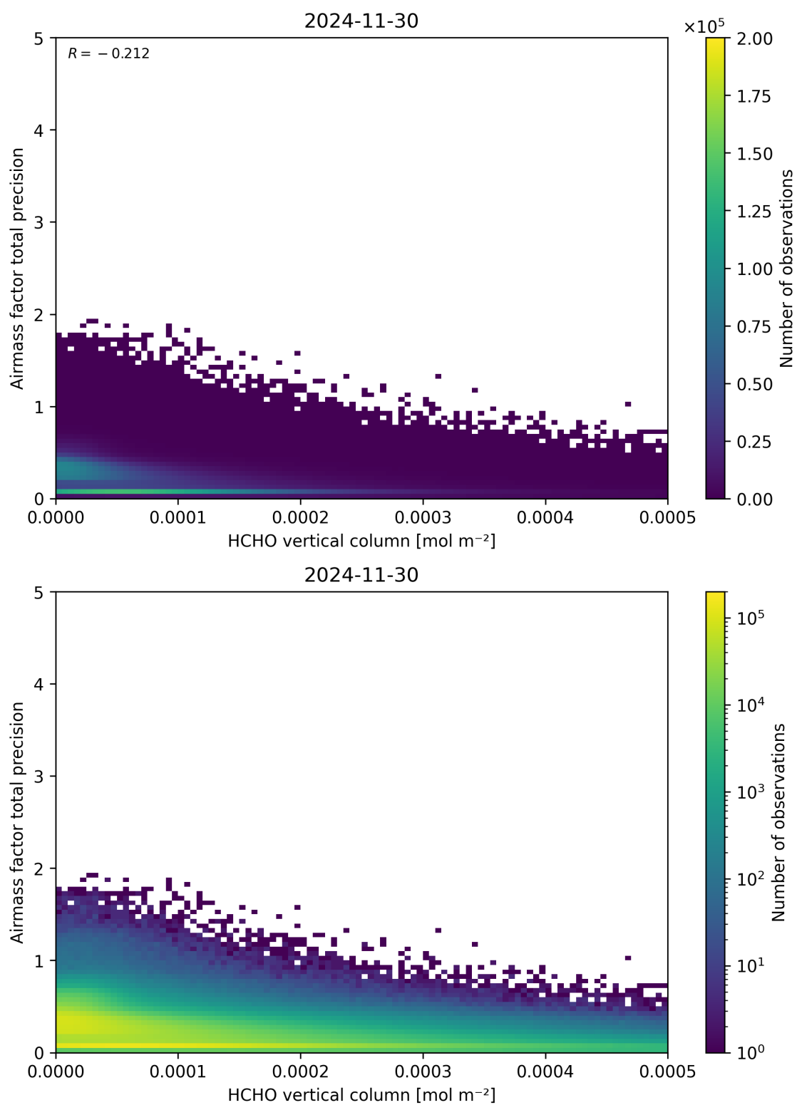
Figure 132: Scatter density plot of “HCHO vertical column” against “Airmass factor total precision” for 2024-11-30 to 2024-12-01.
