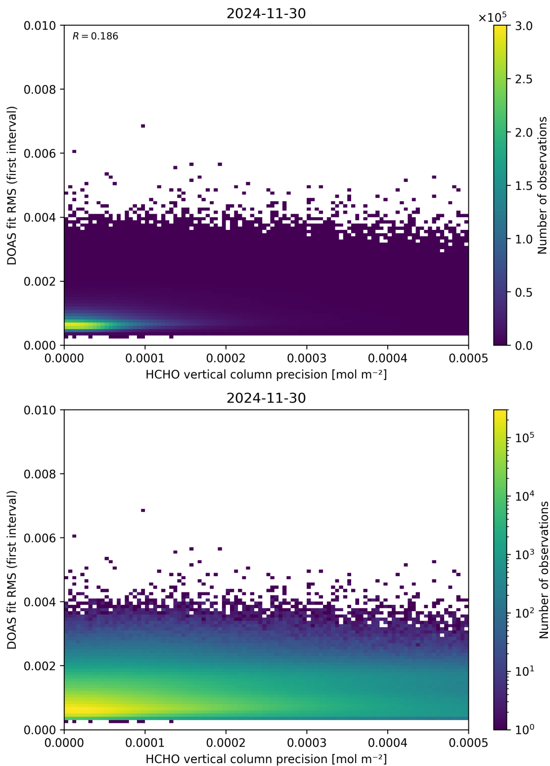
Figure 136: Scatter density plot of “HCHO vertical column precision” against “DOAS fit RMS (first interval)” for 2024-11-30 to 2024-12-01.
