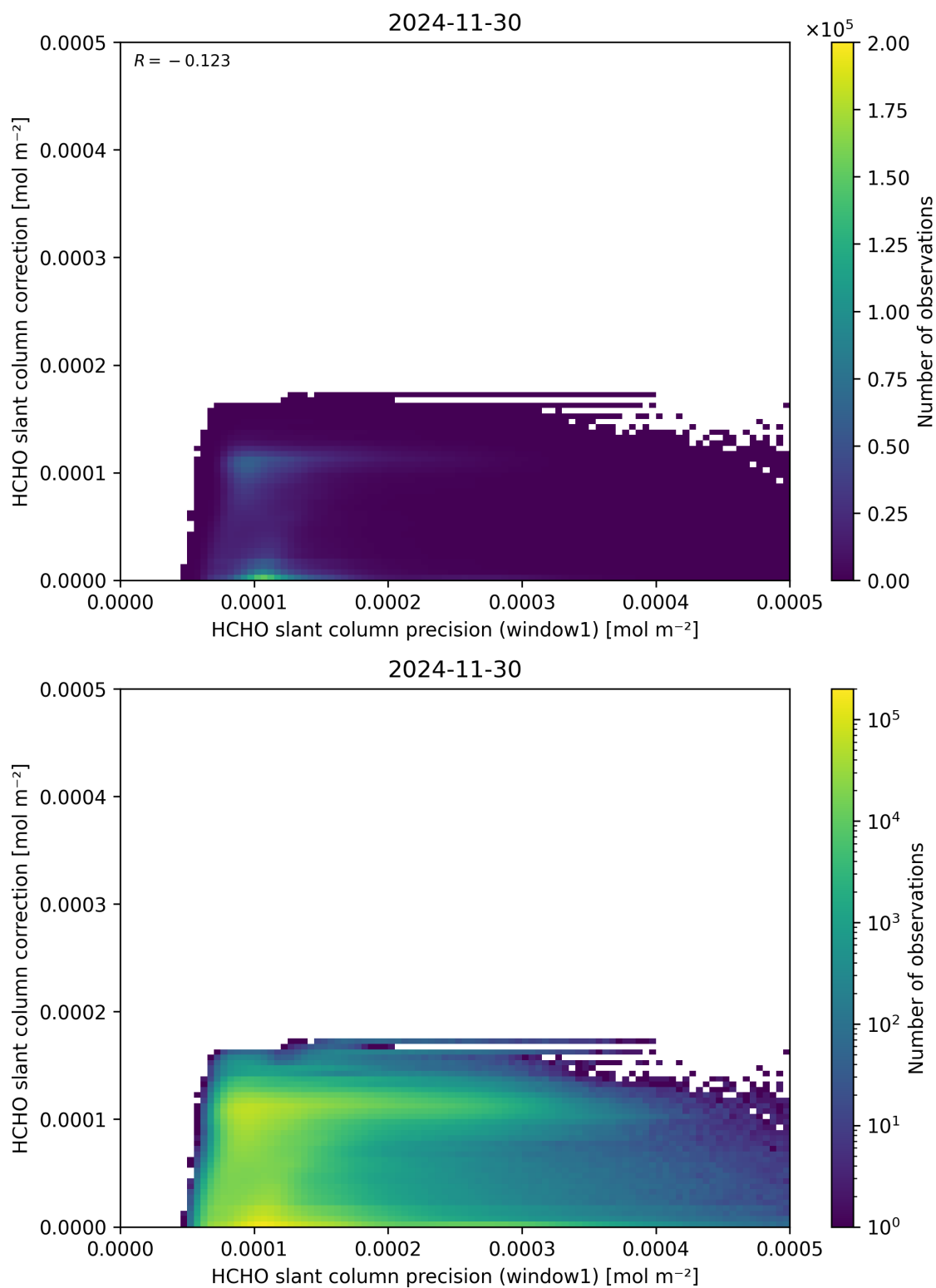
Figure 93: Scatter density plot of “HCHO slant column precision (window1)” against “HCHO slant column correction” for 2024-11-30 to 2024-12-01.
