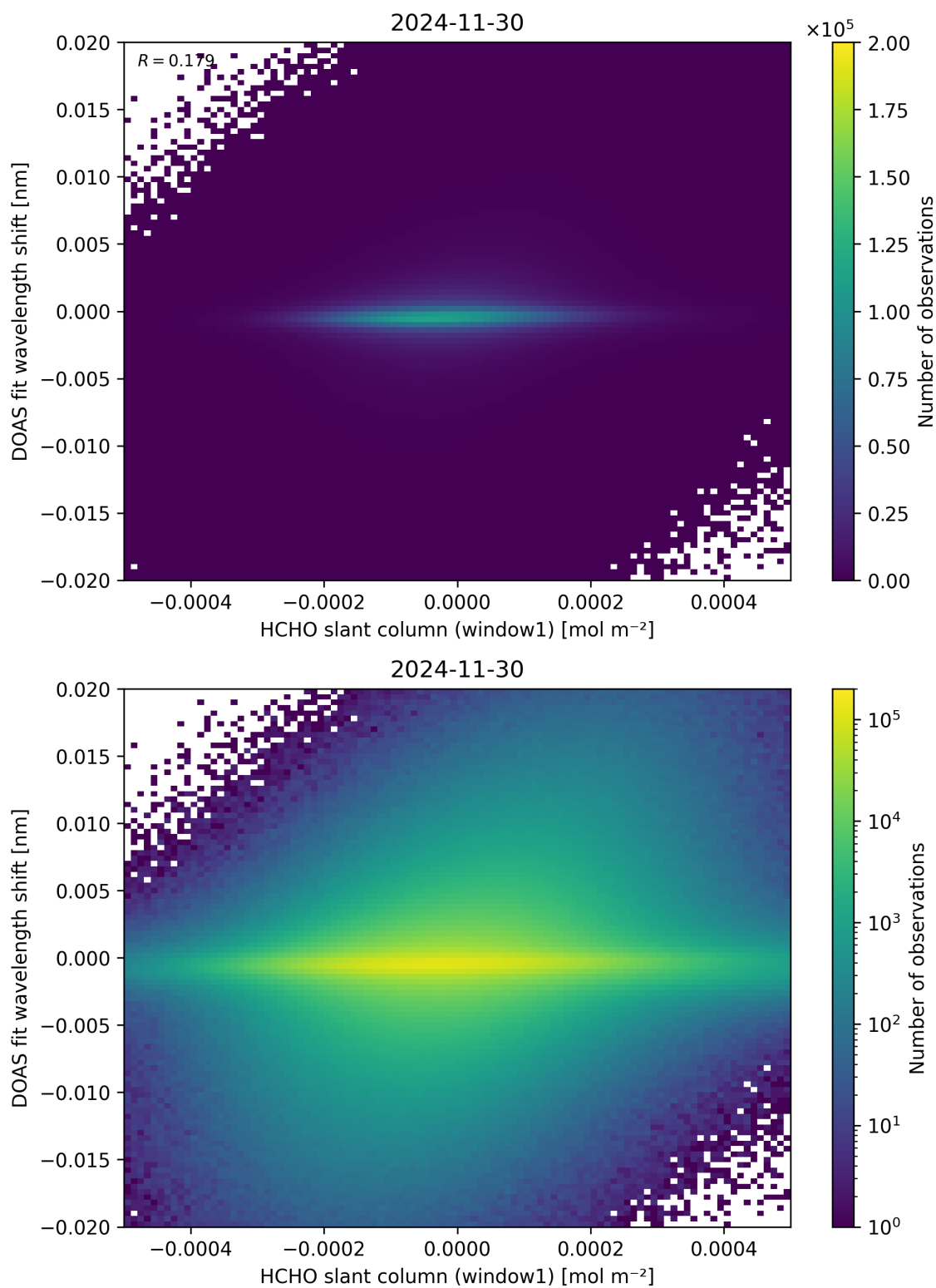
Figure 79: Scatter density plot of “HCHO slant column (window1)” against “DOAS fit wavelength shift” for 2024-11-30 to 2024-12-01.
