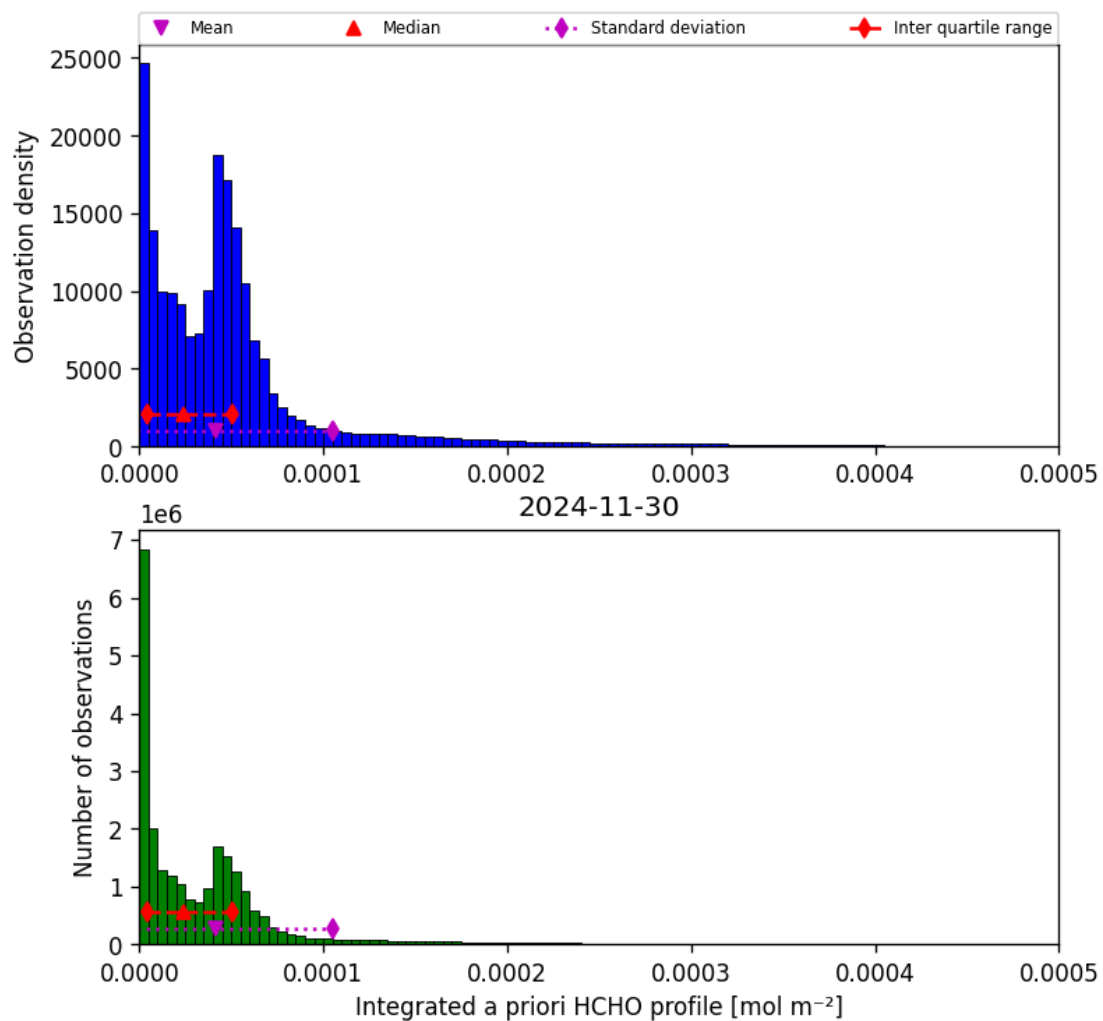
Figure 43: Histogram of “Integrated a priori HCHO profile” for 2024-11-30 to 2024-12-01
