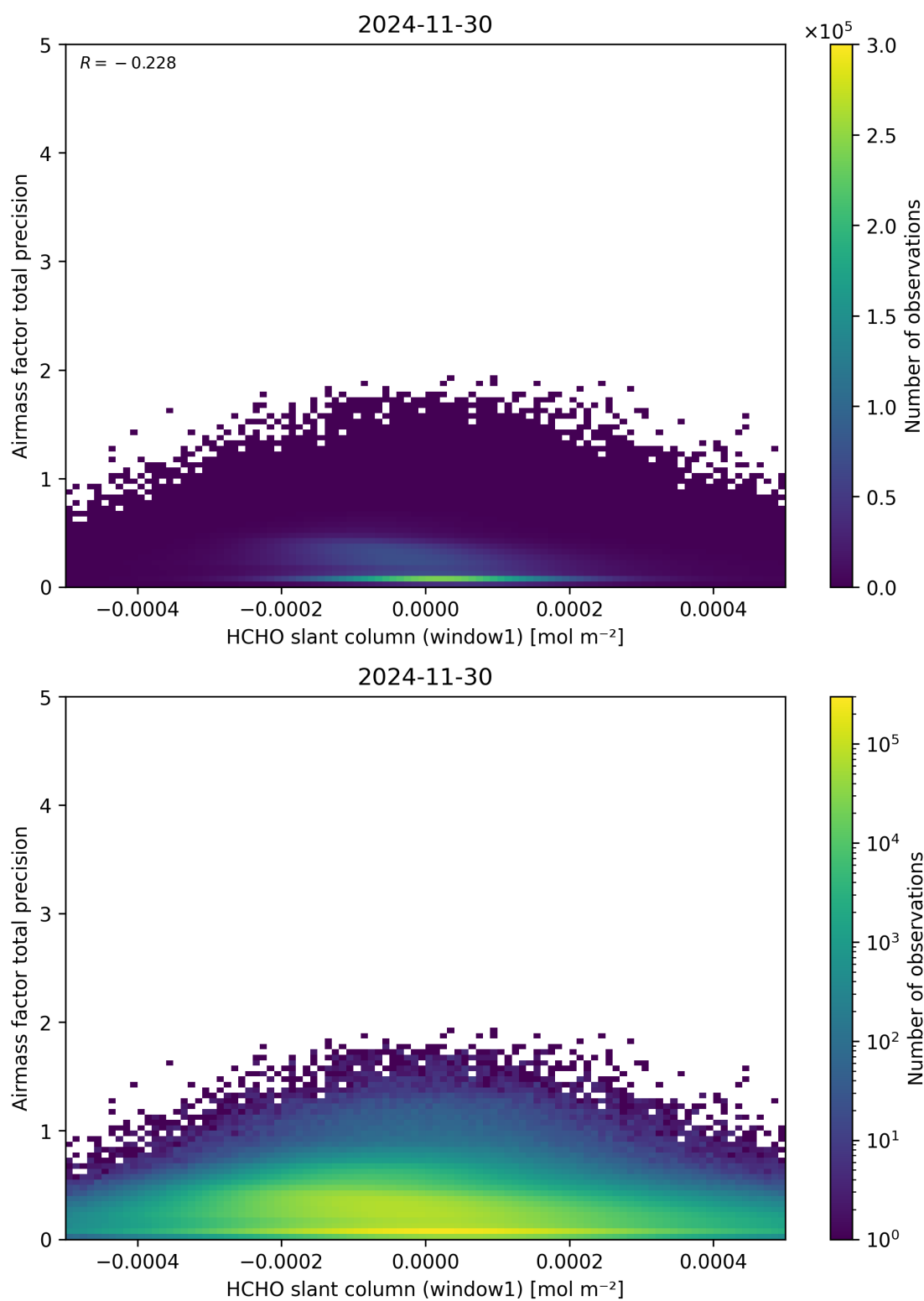
Figure 86: Scatter density plot of “HCHO slant column (window1)” against “Airmass factor total precision” for 2024-11-30 to 2024-12-01.
