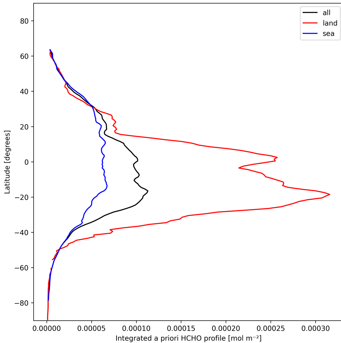
Figure 29: Zonal average of “Integrated a priori HCHO profile” for 2024-11-30 to 2024-12-01.
