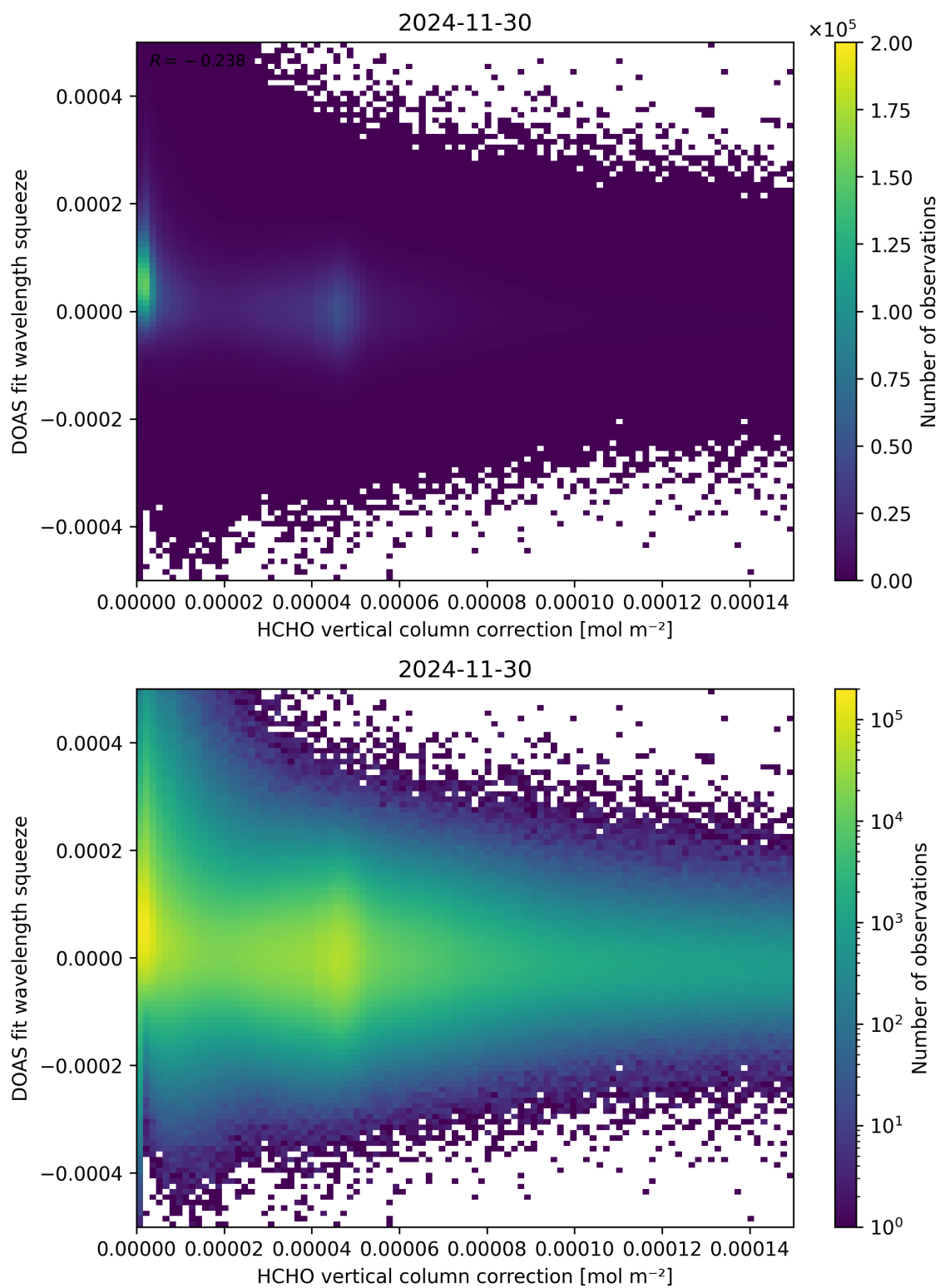
Figure 114: Scatter density plot of “HCHO vertical column correction” against “DOAS fit wavelength squeeze” for 2024-11-30 to 2024-12-01.
