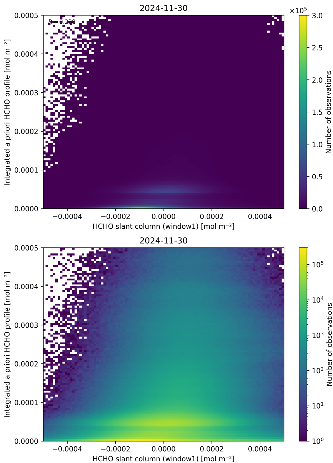
Figure 87: Scatter density plot of “HCHO slant column (window1)” against “Integrated a priori HCHO profile” for 2024-11-30 to 2024-12-01.
