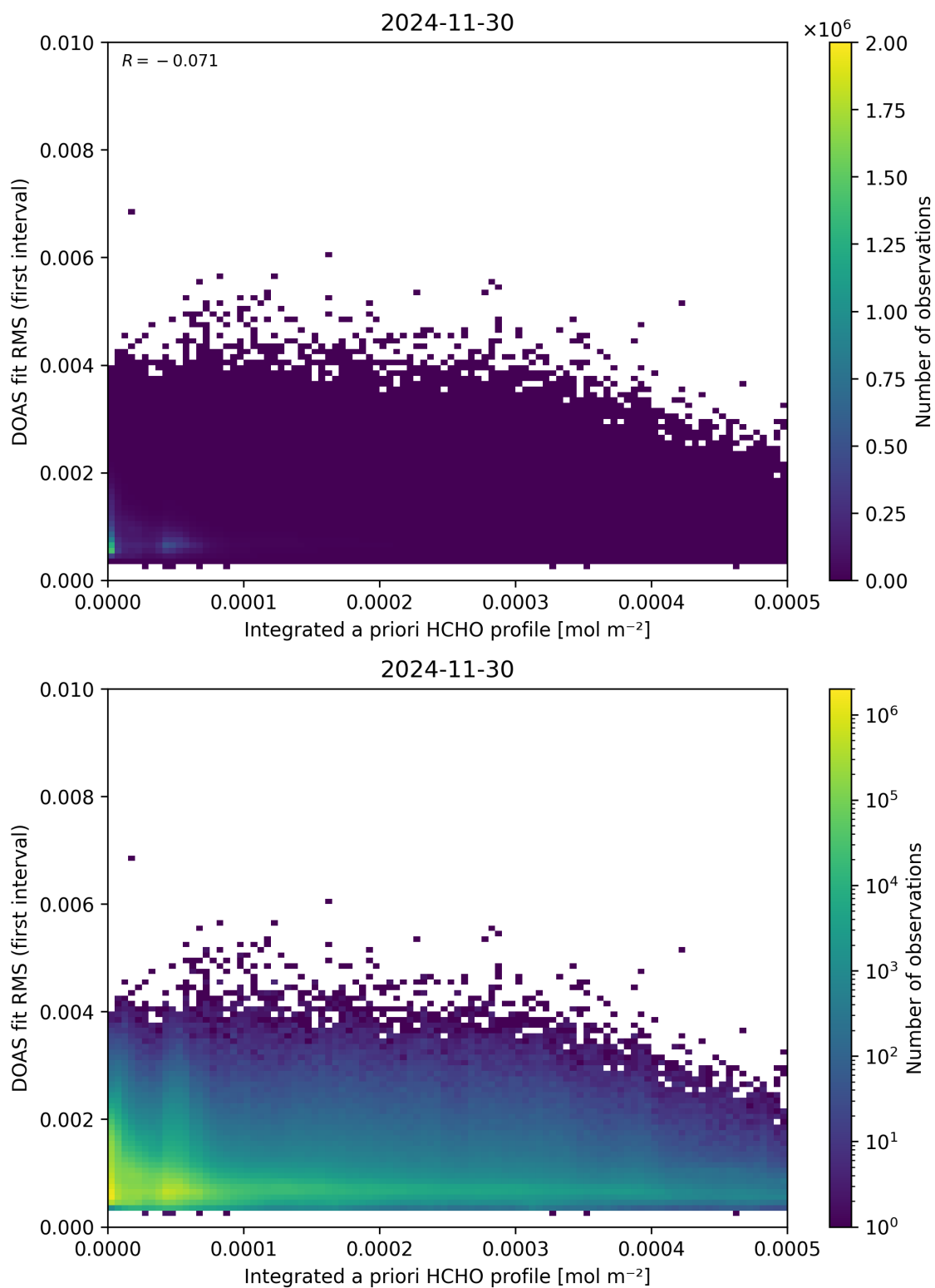
Figure 148: Scatter density plot of “Integrated a priori HCHO profile” against “DOAS fit RMS (first interval)” for 2024-11-30 to 2024-12-01.
