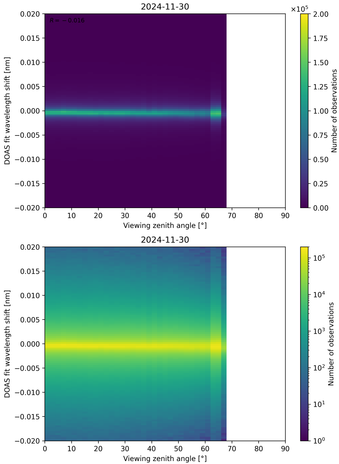
Figure 183: Scatter density plot of “Viewing zenith angle” against “DOAS fit wavelength shift” for 2024-11-30 to 2024-12-01.
