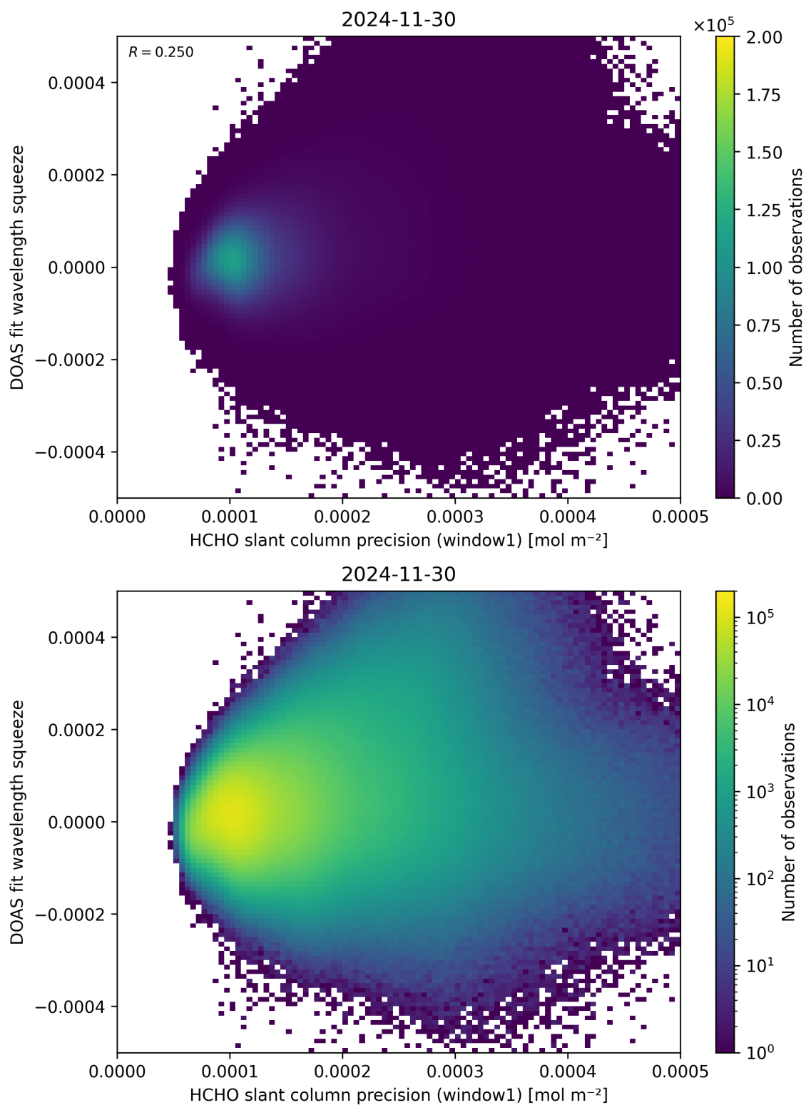
Figure 90: Scatter density plot of “HCHO slant column precision (window1)” against “DOAS fit wavelength squeeze” for 2024-11-30 to 2024-12-01.
