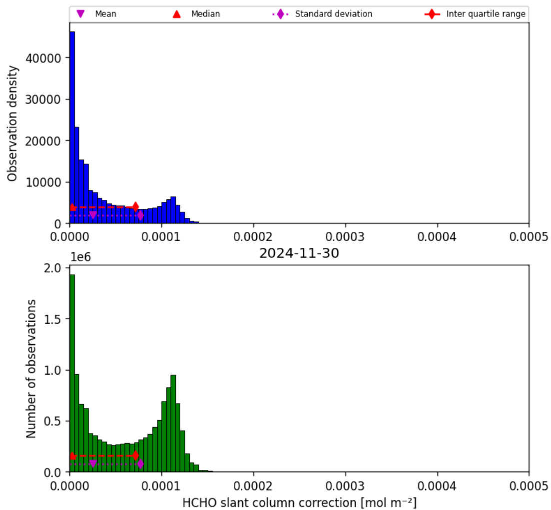
Figure 47: Histogram of “HCHO slant column correction” for 2024-11-30 to 2024-12-01
