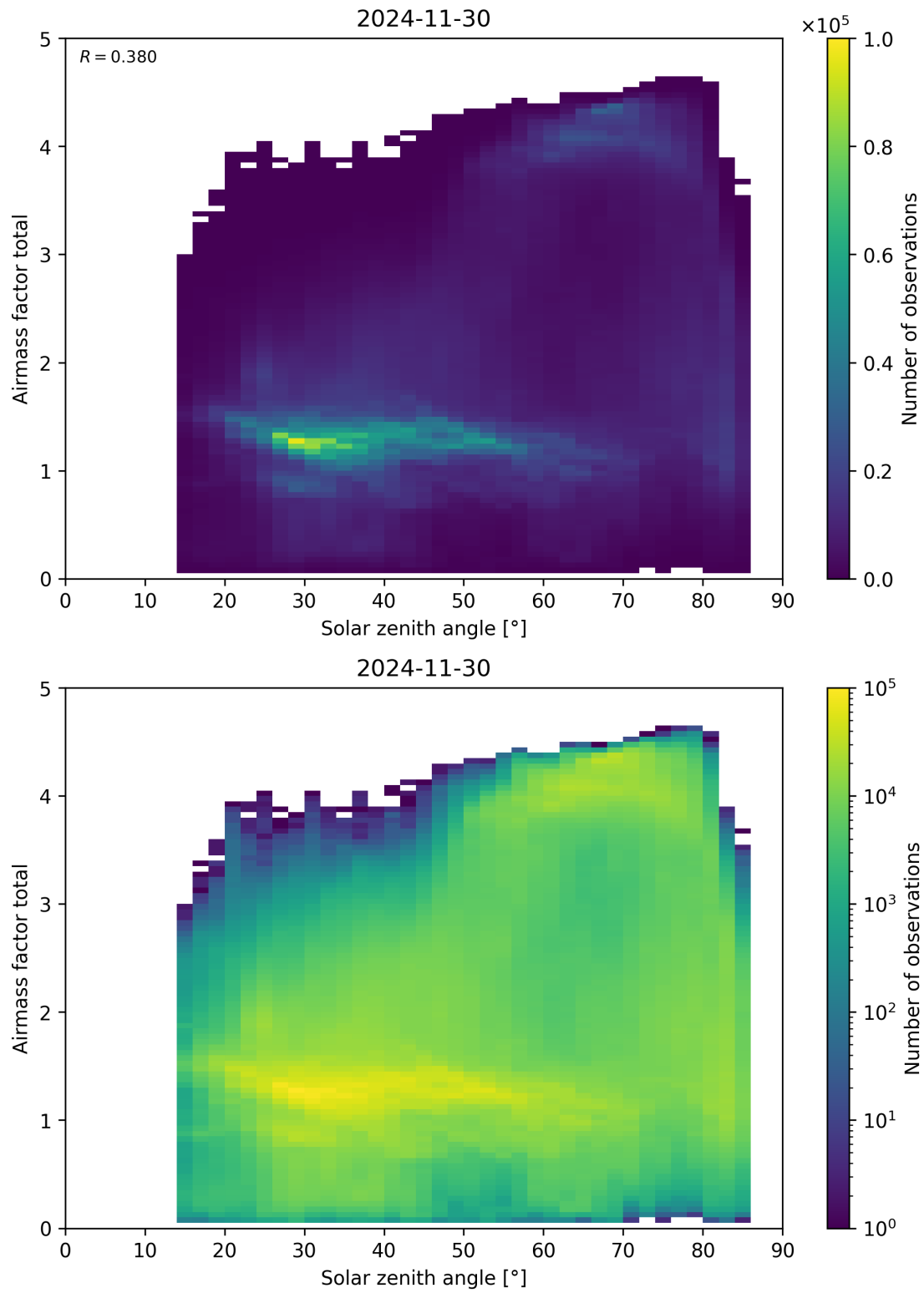
Figure 175: Scatter density plot of “Solar zenith angle” against “Airmass factor total” for 2024-11-30 to 2024-12-01.
