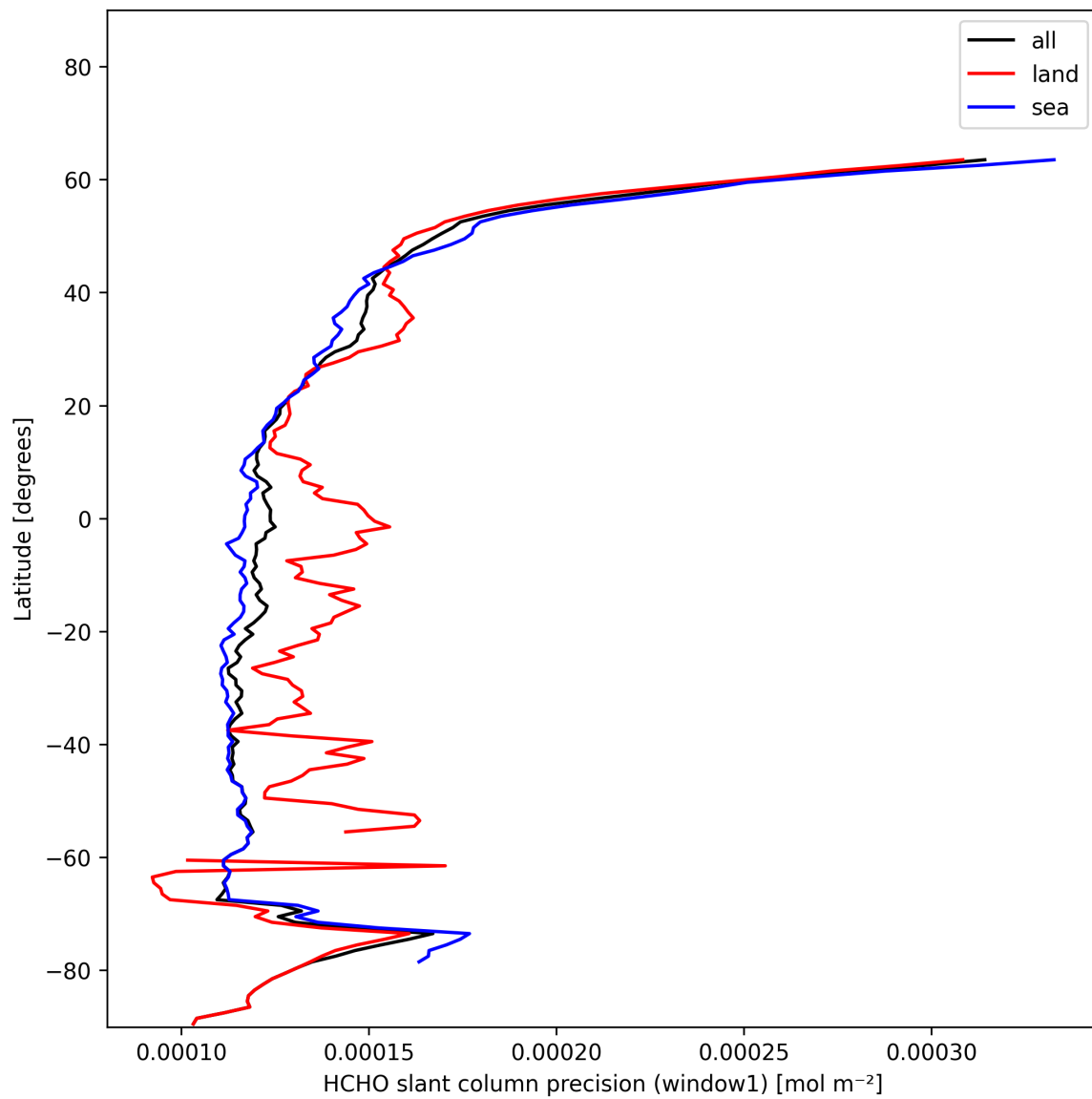
Figure 25: Zonal average of “HCHO slant column precision (window1)” for 2024-11-30 to 2024-12-01.
