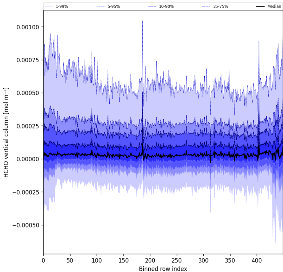
Figure 49: Along track statistics of “HCHO vertical column” for 2024-11-30 to 2024-12-01
