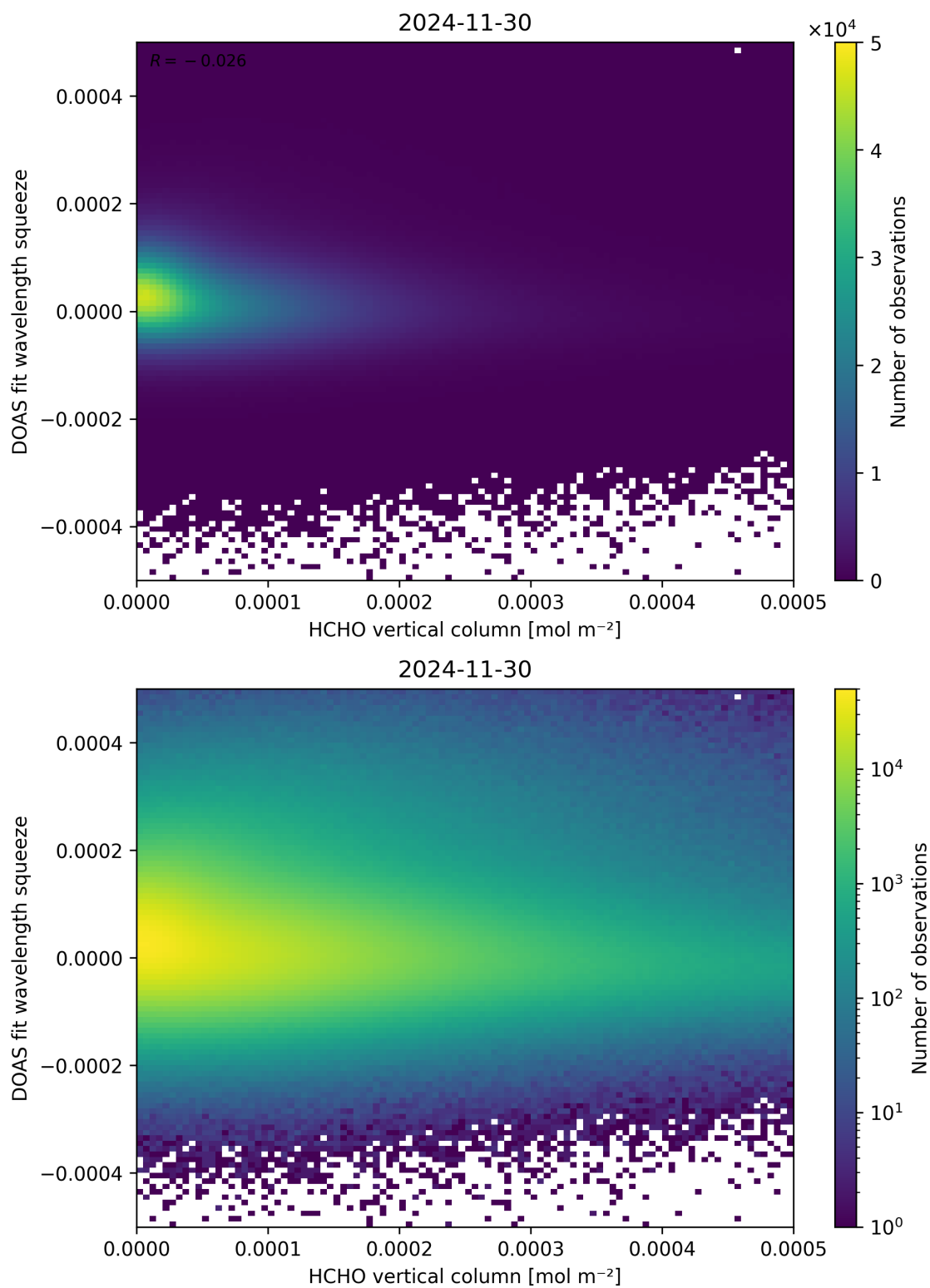
Figure 125: Scatter density plot of “HCHO vertical column” against “DOAS fit wavelength squeeze” for 2024-11-30 to 2024-12-01.
