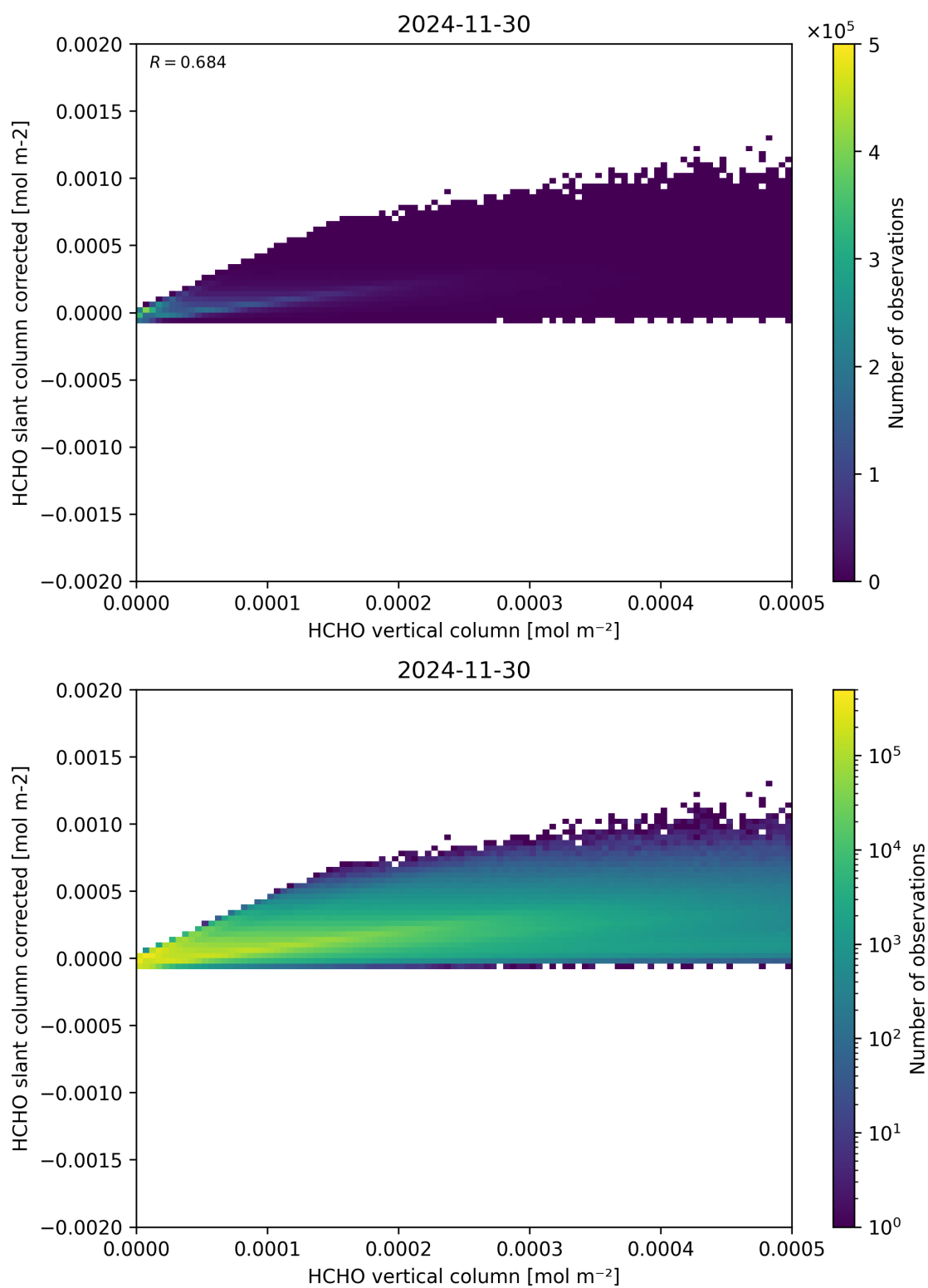
Figure 127: Scatter density plot of “HCHO vertical column” against “HCHO slant column corrected” for 2024-11-30 to 2024-12-01.
