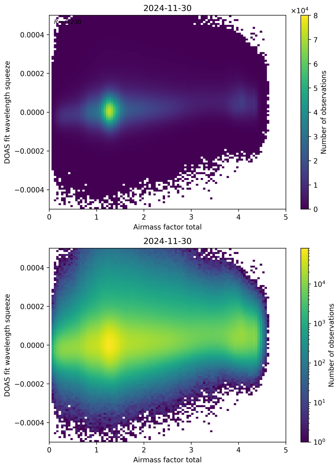
Figure 99: Scatter density plot of “Airmass factor total” against “DOAS fit wavelength squeeze” for 2024-11-30 to 2024-12-01.
