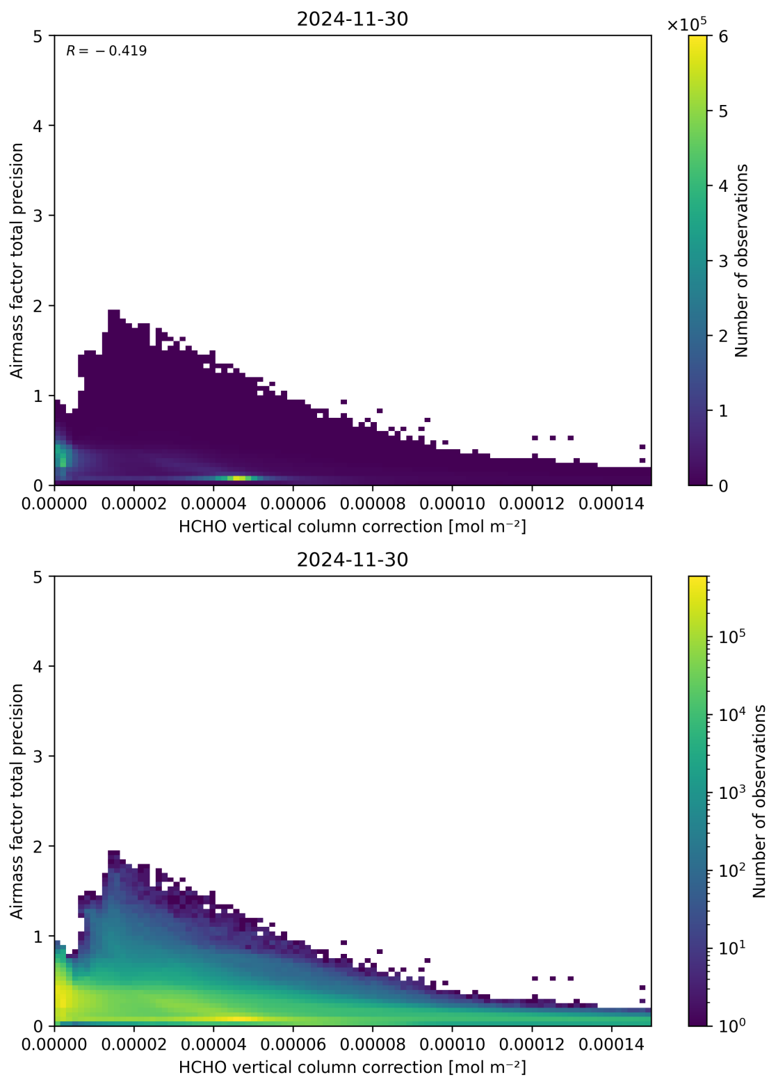
Figure 121: Scatter density plot of “HCHO vertical column correction” against “Airmass factor total precision” for 2024-11-30 to 2024-12-01.
