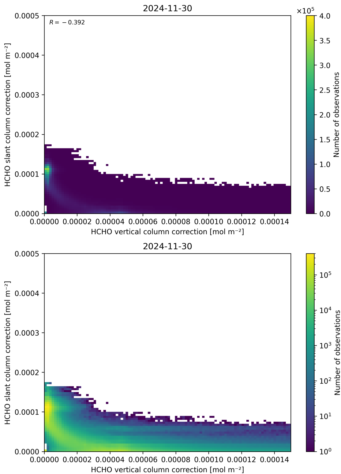
Figure 117: Scatter density plot of “HCHO vertical column correction” against “HCHO slant column correction” for 2024-11-30 to 2024-12-01.
