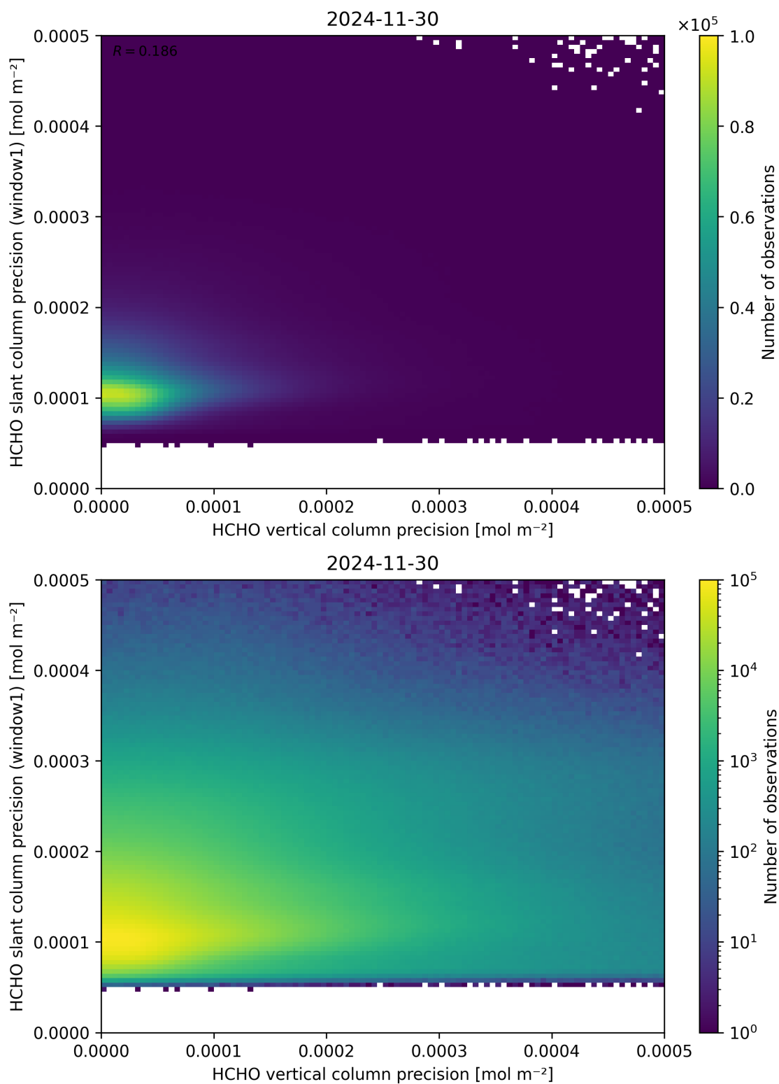
Figure 143: Scatter density plot of “HCHO vertical column precision” against “HCHO slant column precision (window1)” for 2024-11-30 to 2024-12-01.
