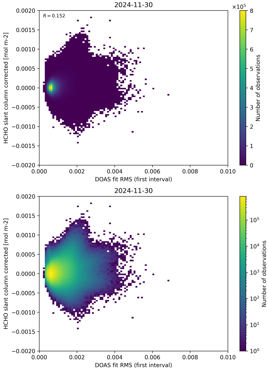
Figure 62: Scatter density plot of “DOAS fit RMS (first interval)” against “HCHO slant column corrected” for 2024-11-30 to 2024-12-01.
