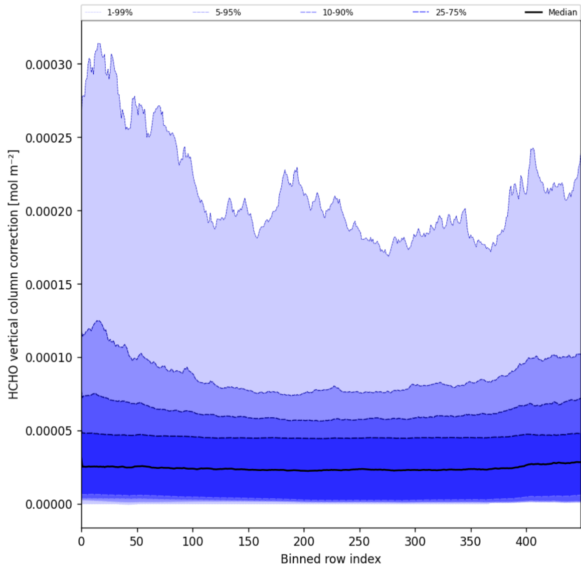
Figure 51: Along track statistics of “HCHO vertical column correction” for 2024-11-30 to 2024-12-01
