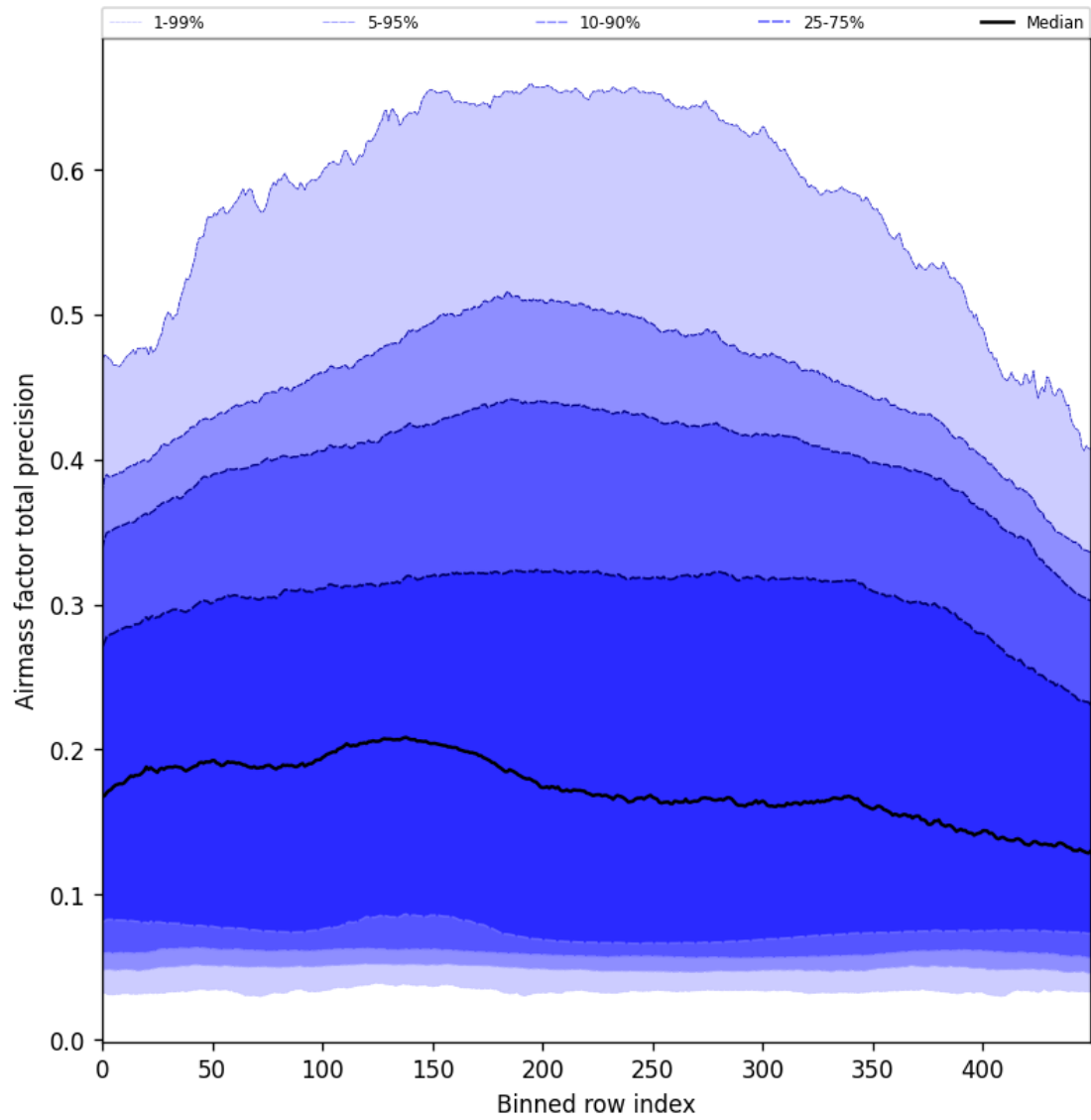
Figure 55: Along track statistics of “Airmass factor total precision” for 2024-11-30 to 2024-12-01
