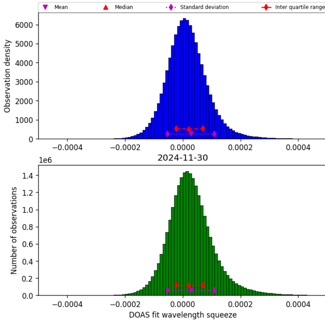
Figure 45: Histogram of “DOAS fit wavelength squeeze” for 2024-11-30 to 2024-12-01
