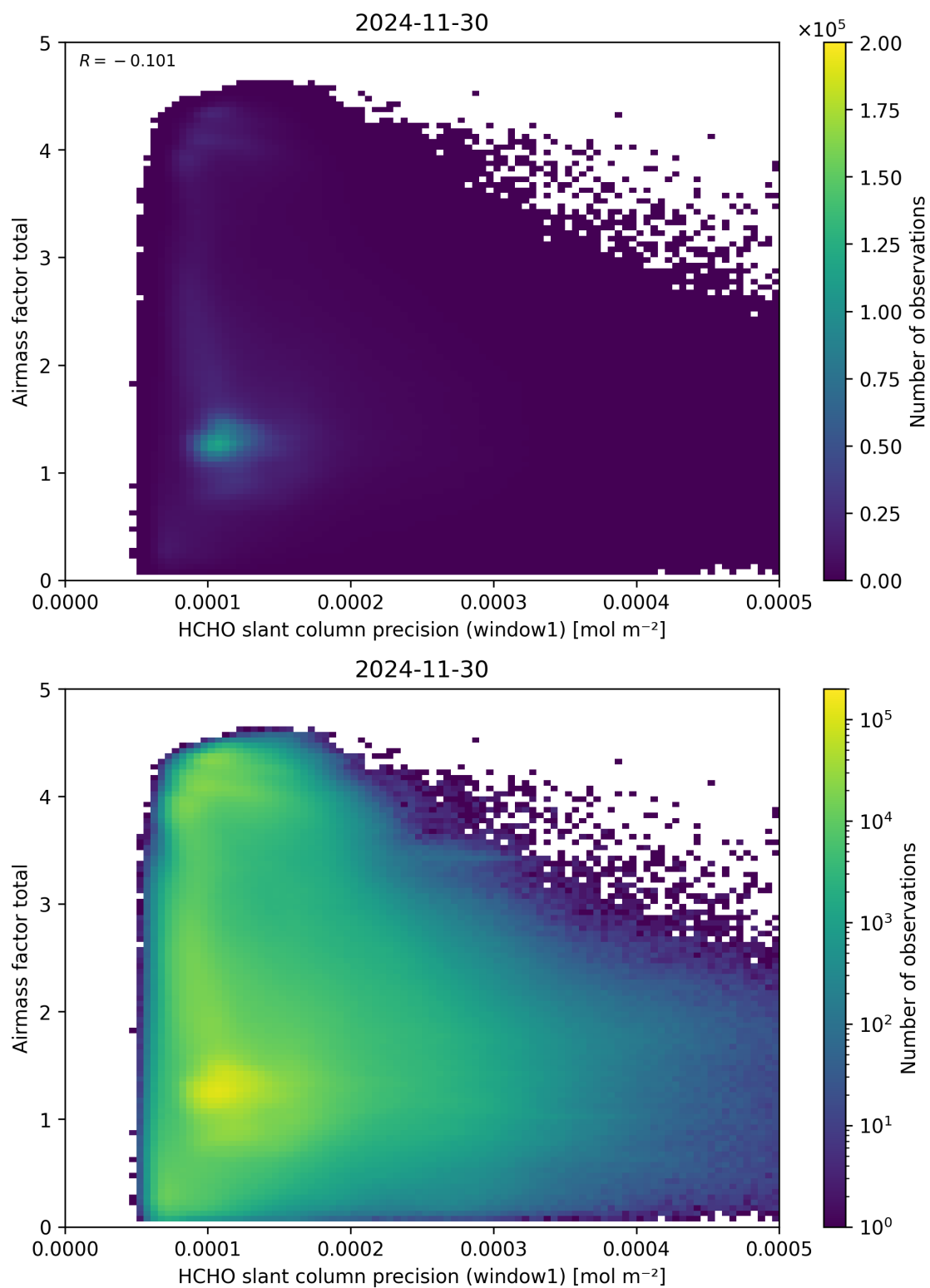
Figure 94: Scatter density plot of “HCHO slant column precision (window1)” against “Airmass factor total” for 2024-11-30 to 2024-12-01.
