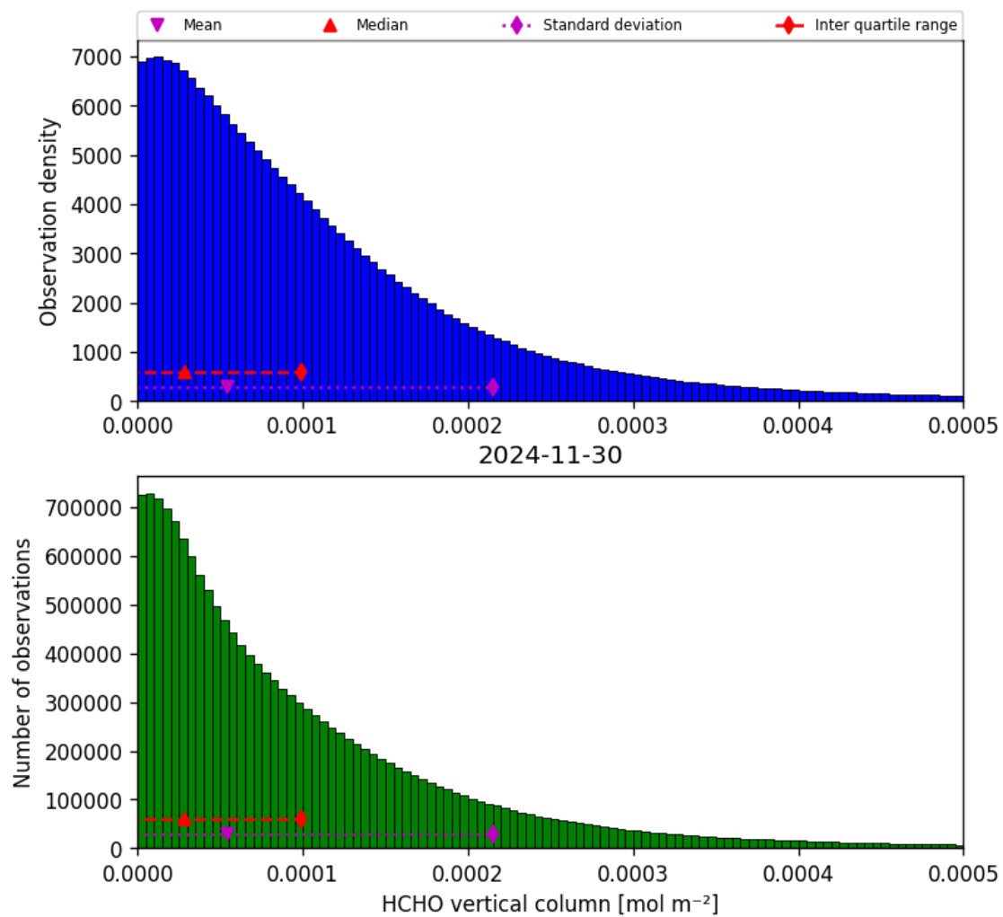
Figure 35: Histogram of “HCHO vertical column” for 2024-11-30 to 2024-12-01
