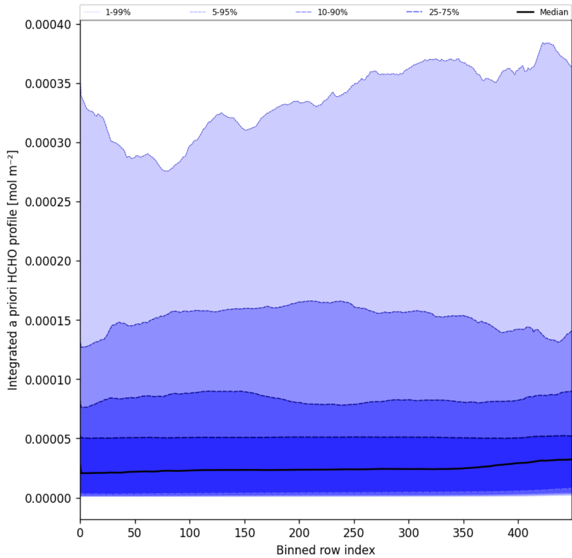
Figure 57: Along track statistics of “Integrated a priori HCHO profile” for 2024-11-30 to 2024-12-01
