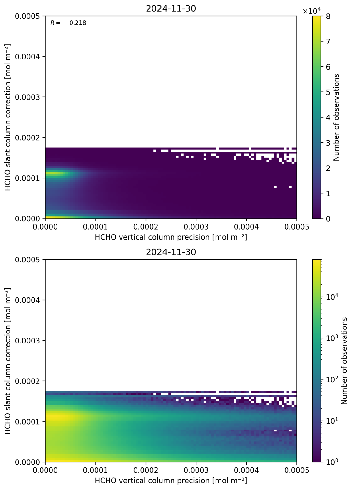
Figure 141: Scatter density plot of “HCHO vertical column precision” against “HCHO slant column correction” for 2024-11-30 to 2024-12-01.
