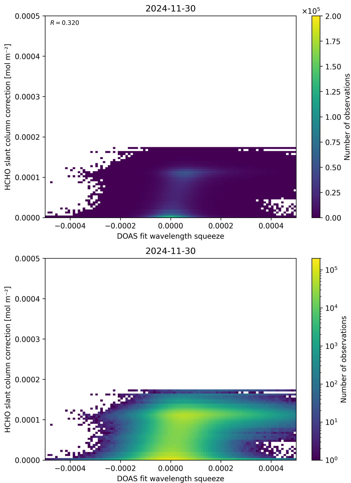
Figure 70: Scatter density plot of “DOAS fit wavelength squeeze” against “HCHO slant column correction” for 2024-11-30 to 2024-12-01.
