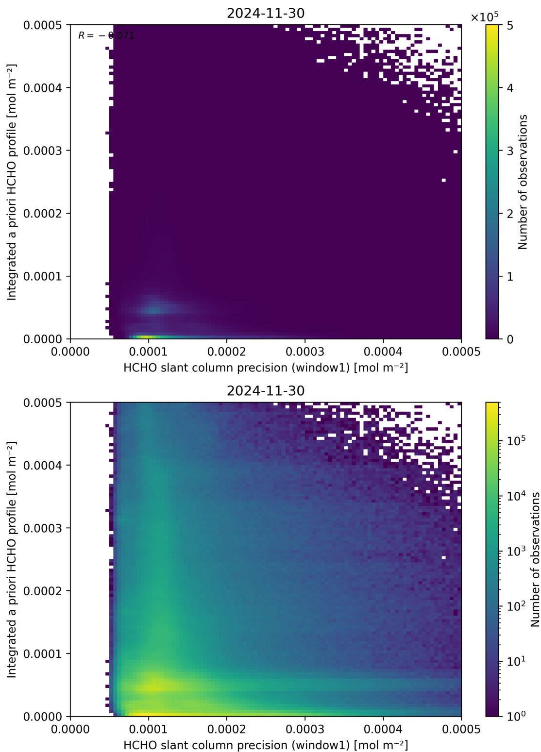
Figure 96: Scatter density plot of “HCHO slant column precision (window1)” against “Integrated a priori HCHO profile” for 2024-11-30 to 2024-12-01.
