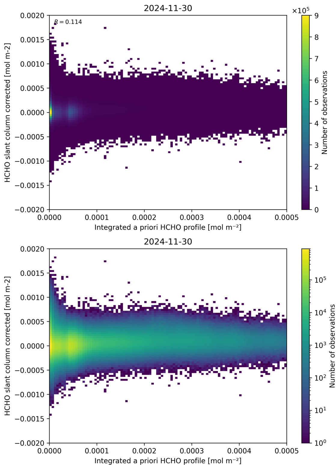
Figure 151: Scatter density plot of “Integrated a priori HCHO profile” against “HCHO slant column corrected” for 2024-11-30 to 2024-12-01.
