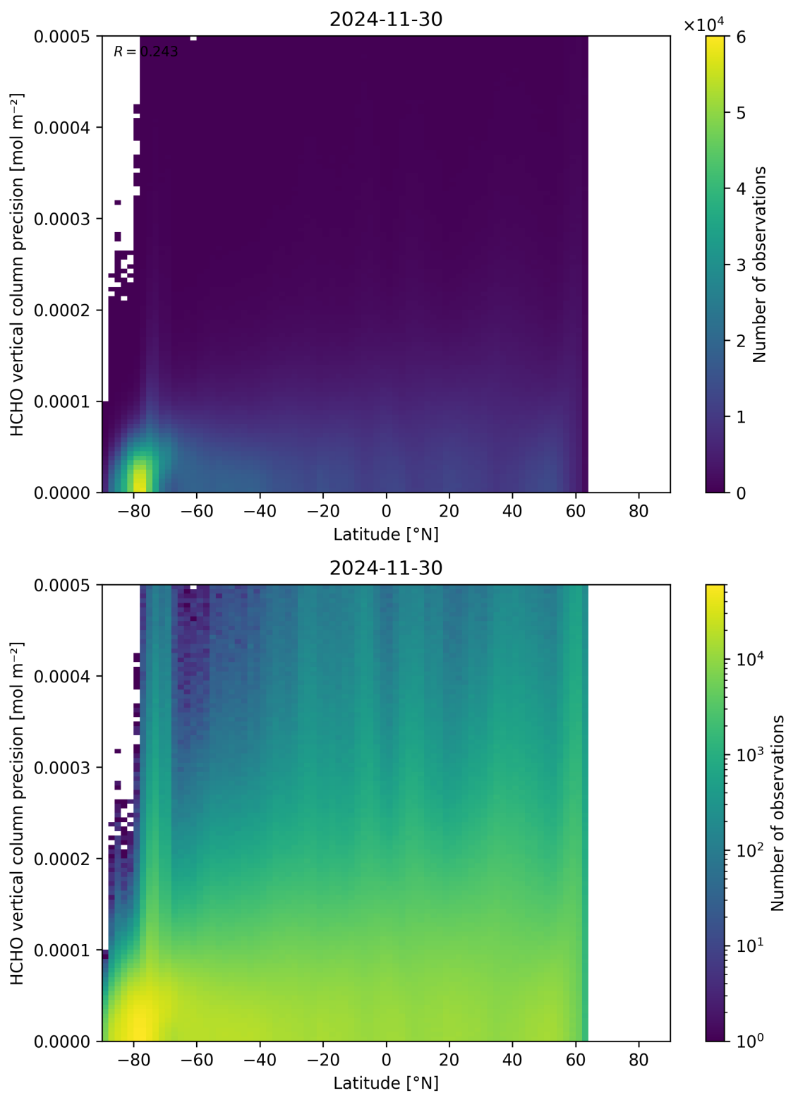
Figure 165: Scatter density plot of “Latitude” against “HCHO vertical column precision” for 2024-11-30 to 2024-12-01.
