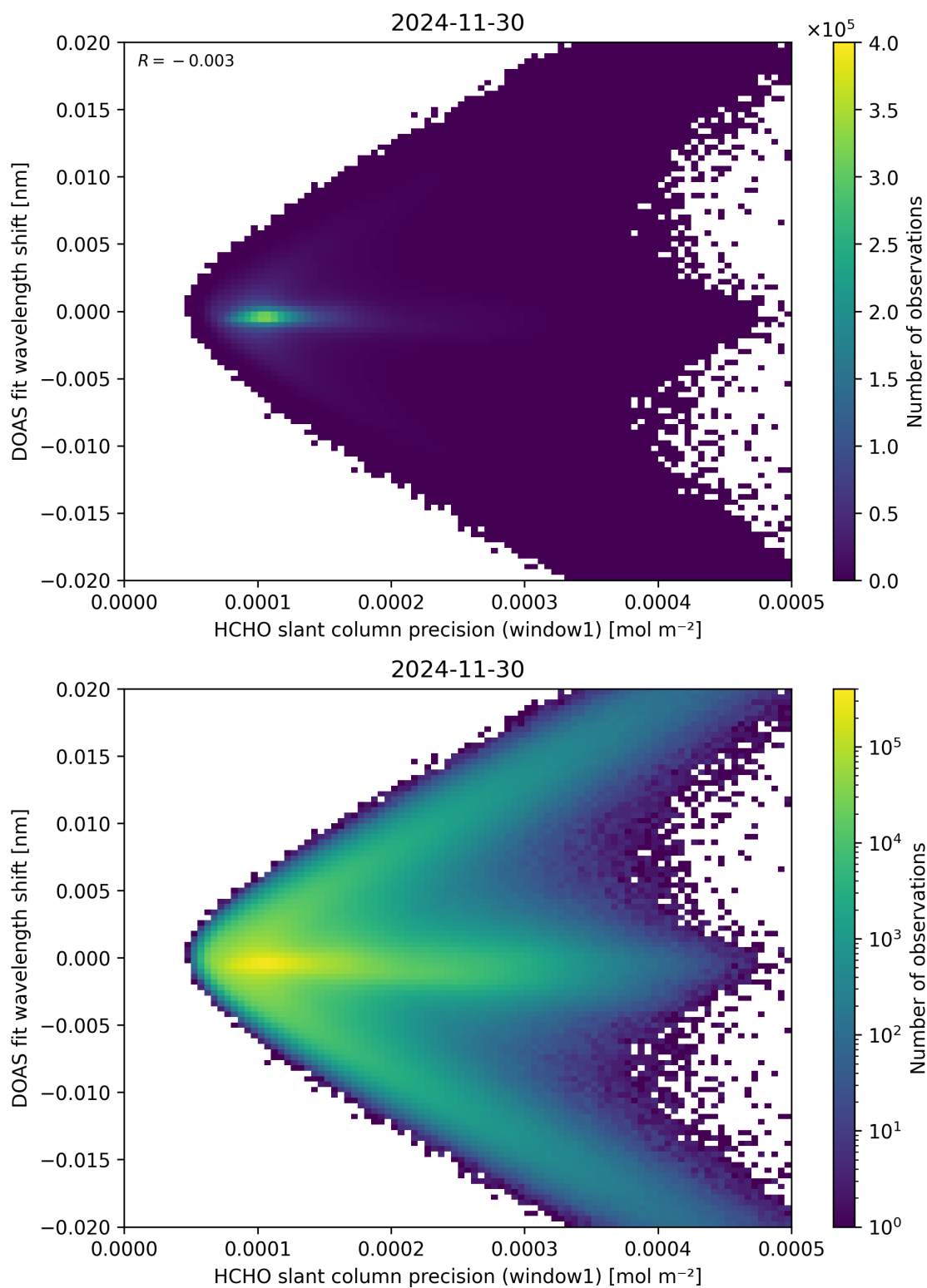
Figure 89: Scatter density plot of “HCHO slant column precision (window1)” against “DOAS fit wavelength shift” for 2024-11-30 to 2024-12-01.
