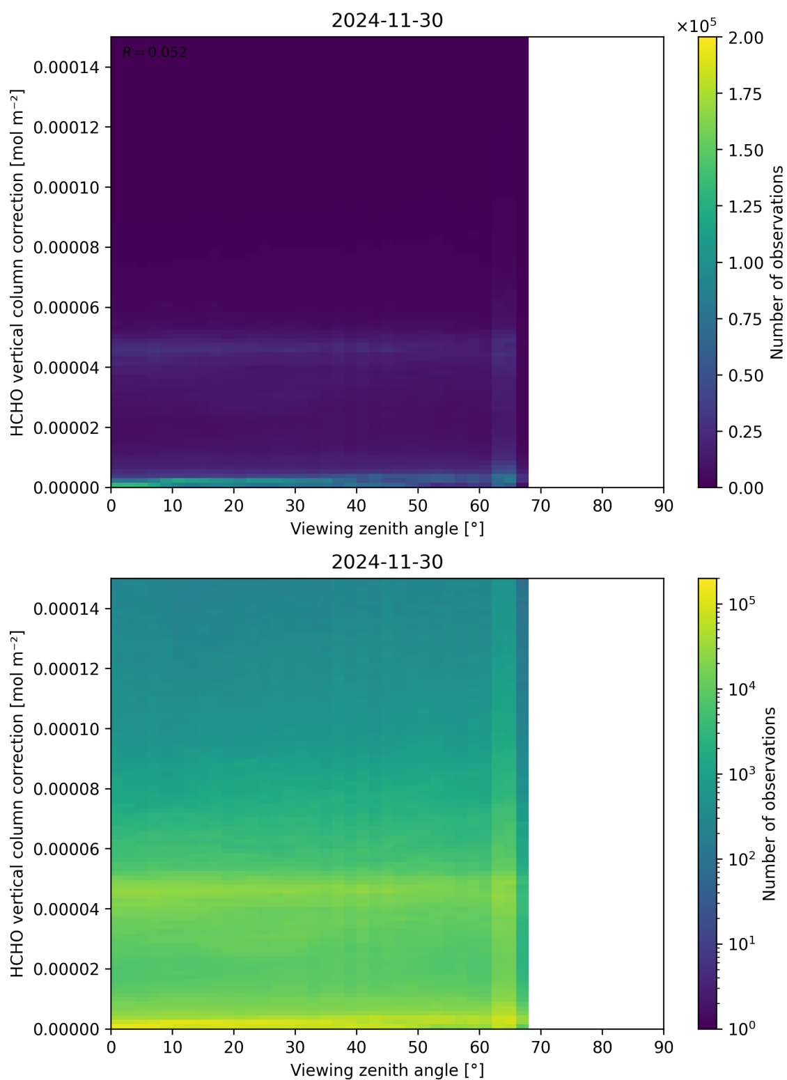
Figure 193: Scatter density plot of “Viewing zenith angle” against “HCHO vertical column correction” for 2024-11-30 to 2024-12-01.
