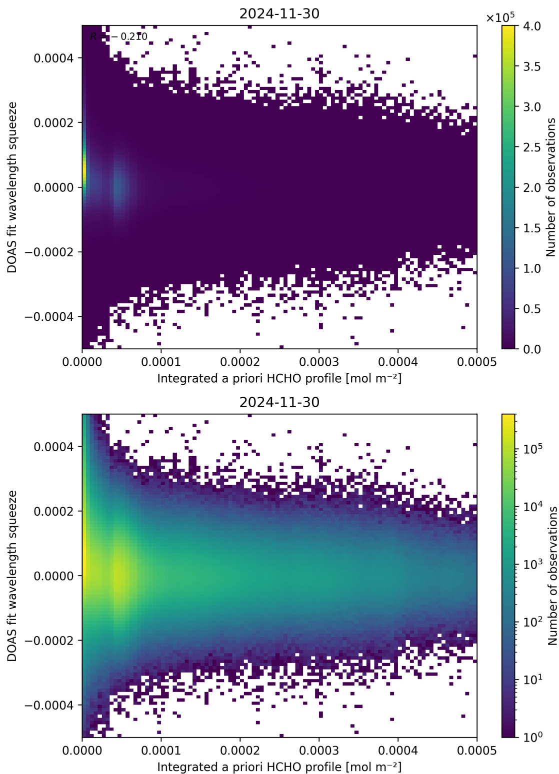
Figure 150: Scatter density plot of “Integrated a priori HCHO profile” against “DOAS fit wavelength squeeze” for 2024-11-30 to 2024-12-01.
