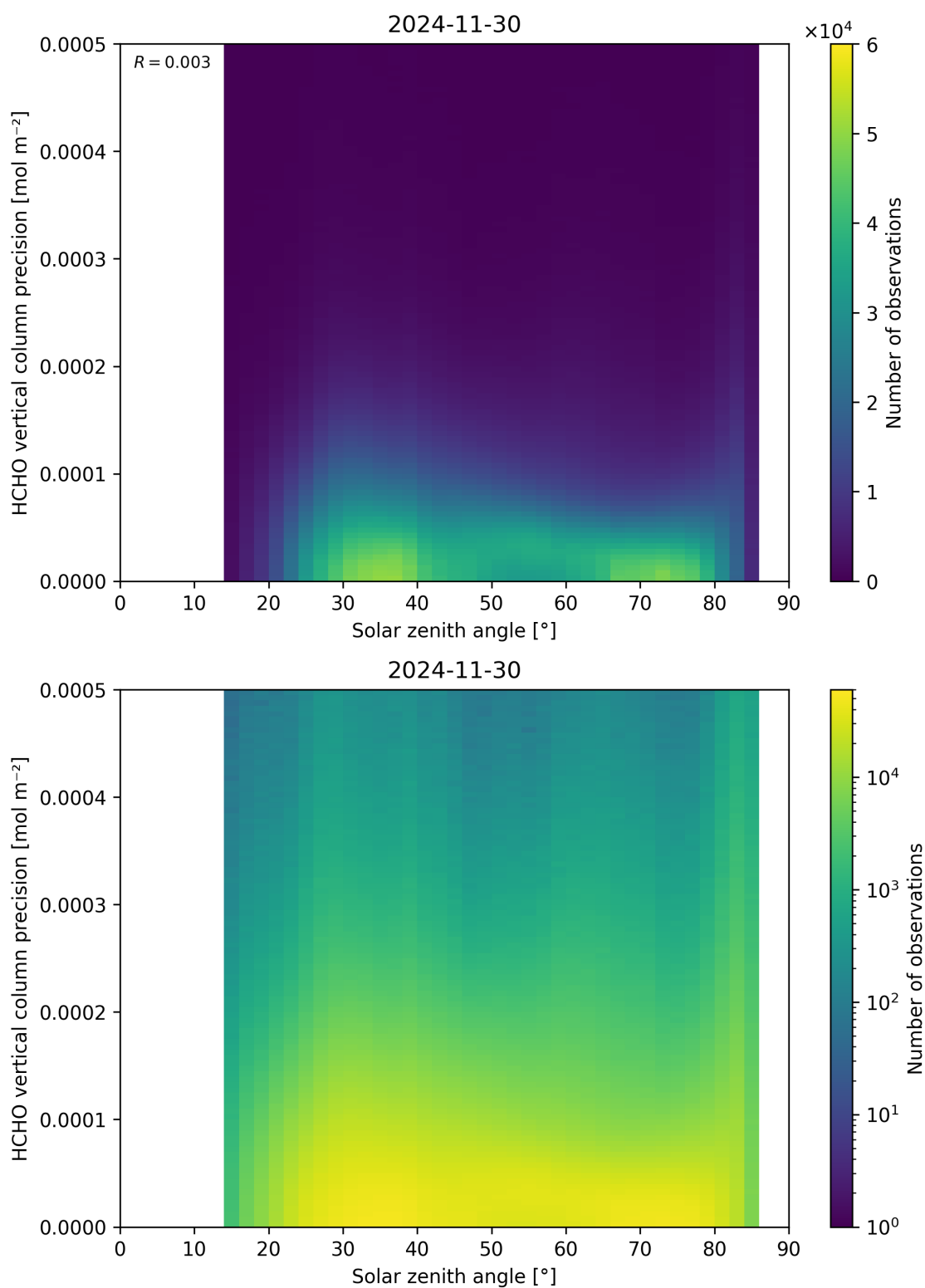
Figure 179: Scatter density plot of “Solar zenith angle” against “HCHO vertical column precision” for 2024-11-30 to 2024-12-01.
