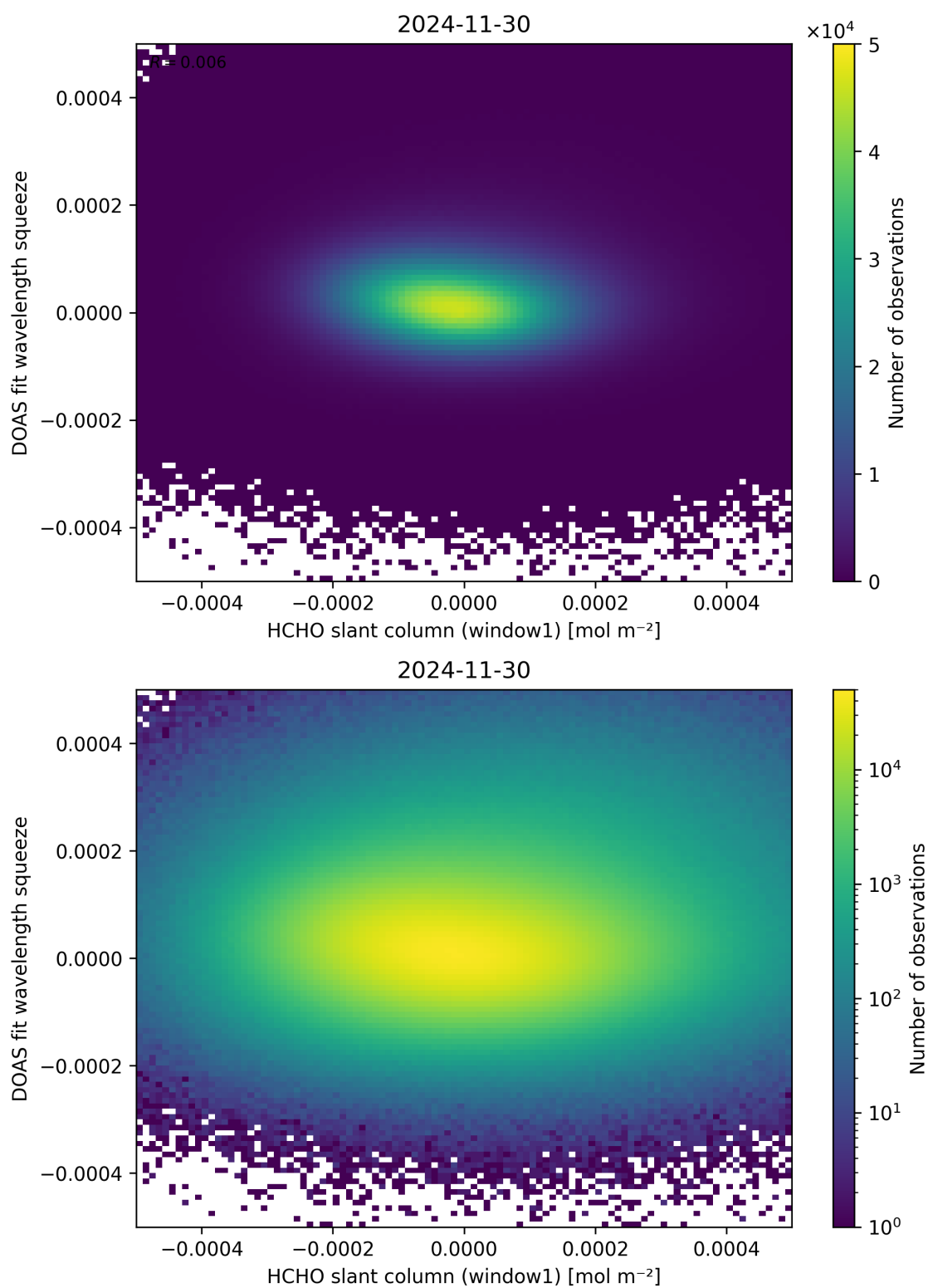
Figure 80: Scatter density plot of “HCHO slant column (window1)” against “DOAS fit wavelength squeeze” for 2024-11-30 to 2024-12-01.
