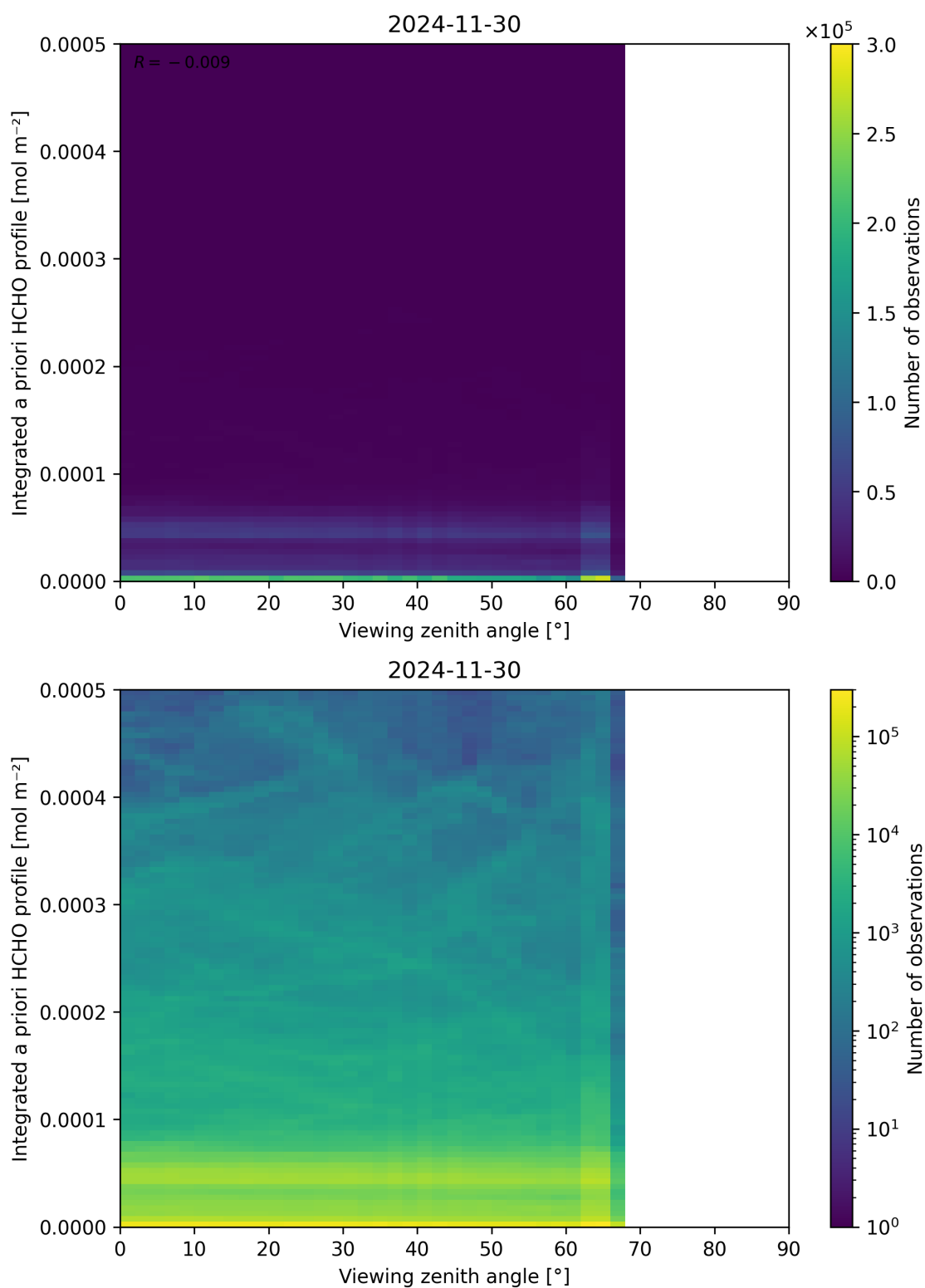
Figure 195: Scatter density plot of “Viewing zenith angle” against “Integrated a priori HCHO profile” for 2024-11-30 to 2024-12-01.
