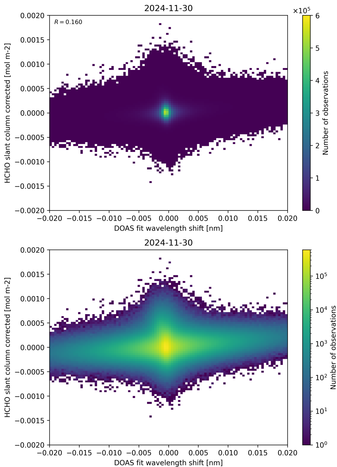
Figure 66: Scatter density plot of “DOAS fit wavelength shift” against “HCHO slant column corrected” for 2024-11-30 to 2024-12-01.
