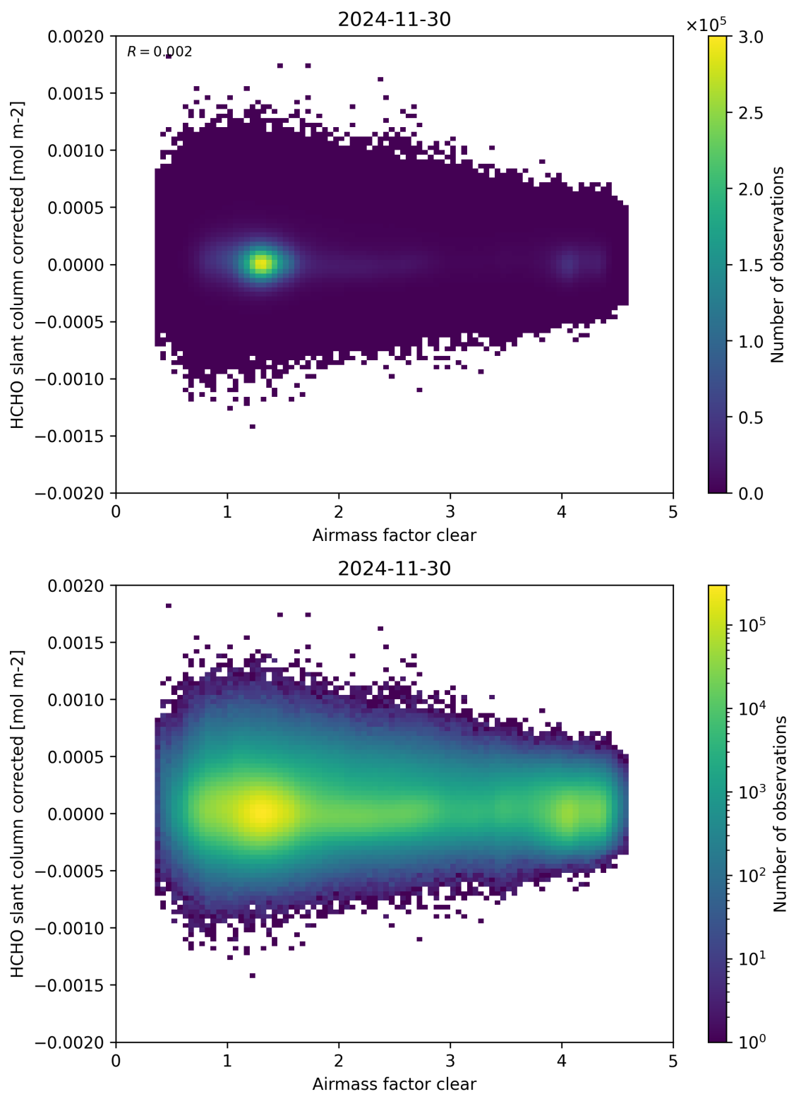
Figure 74: Scatter density plot of “Airmass factor clear” against “HCHO slant column corrected” for 2024-11-30 to 2024-12-01.
