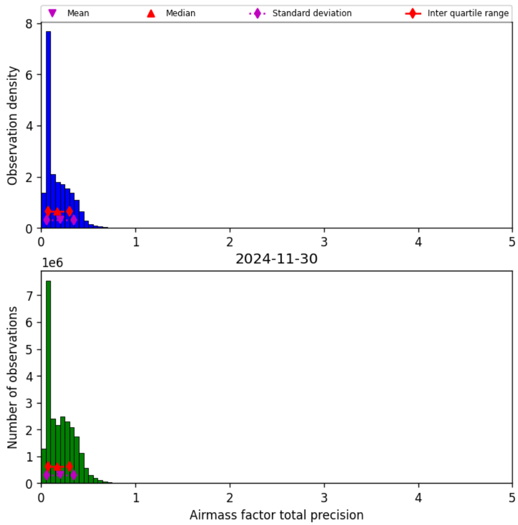
Figure 41: Histogram of “Airmass factor total precision” for 2024-11-30 to 2024-12-01
