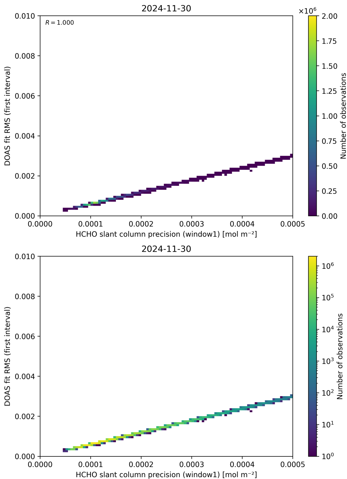
Figure 88: Scatter density plot of “HCHO slant column precision (window1)” against “DOAS fit RMS (first interval)” for 2024-11-30 to 2024-12-01.
