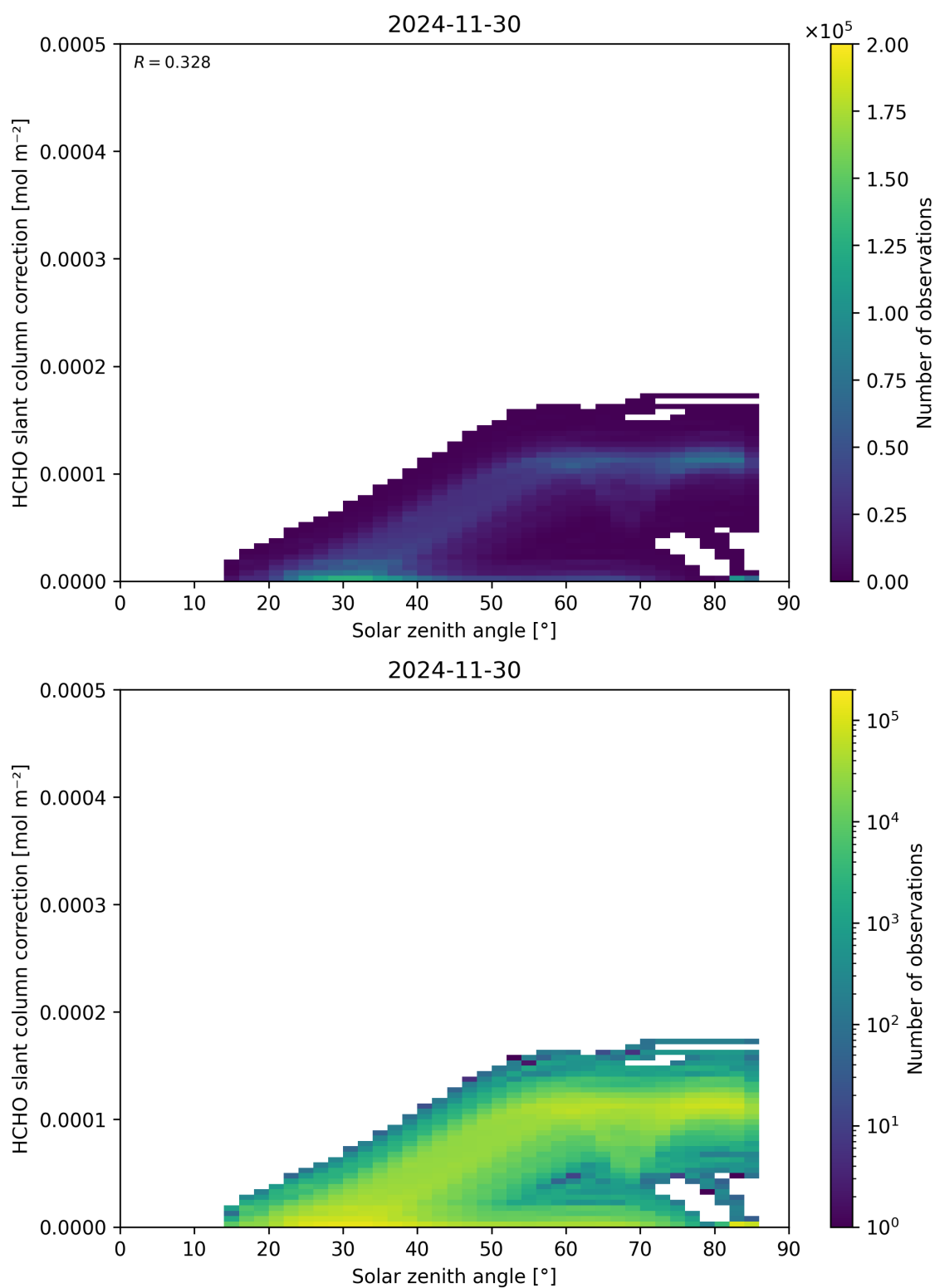
Figure 172: Scatter density plot of “Solar zenith angle” against “HCHO slant column correction” for 2024-11-30 to 2024-12-01.
