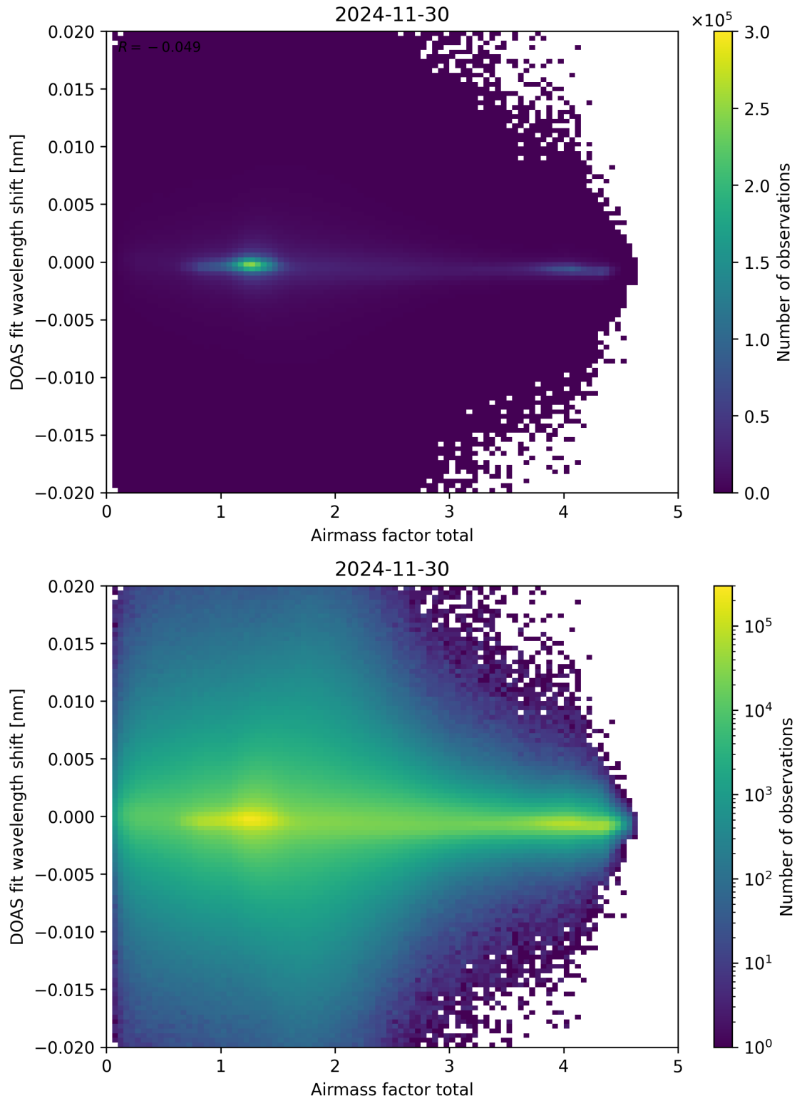
Figure 98: Scatter density plot of “Airmass factor total” against “DOAS fit wavelength shift” for 2024-11-30 to 2024-12-01.
