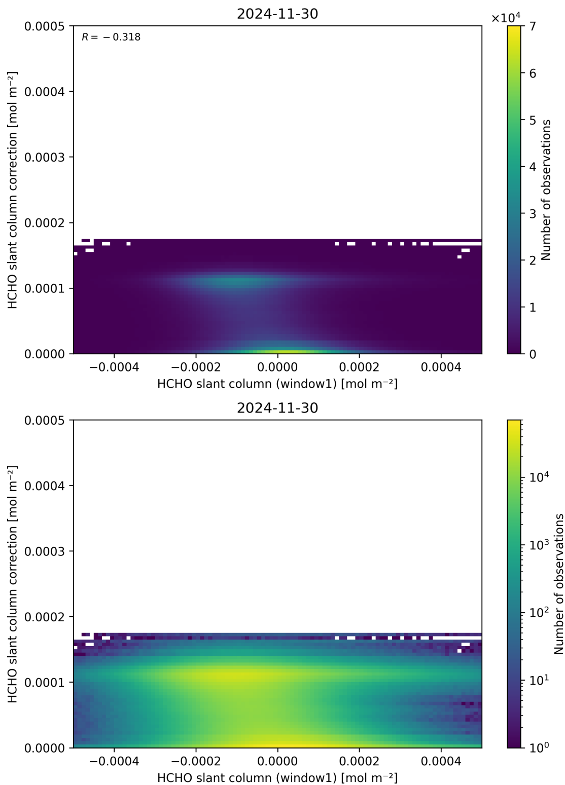
Figure 83: Scatter density plot of “HCHO slant column (window1)” against “HCHO slant column correction” for 2024-11-30 to 2024-12-01.
