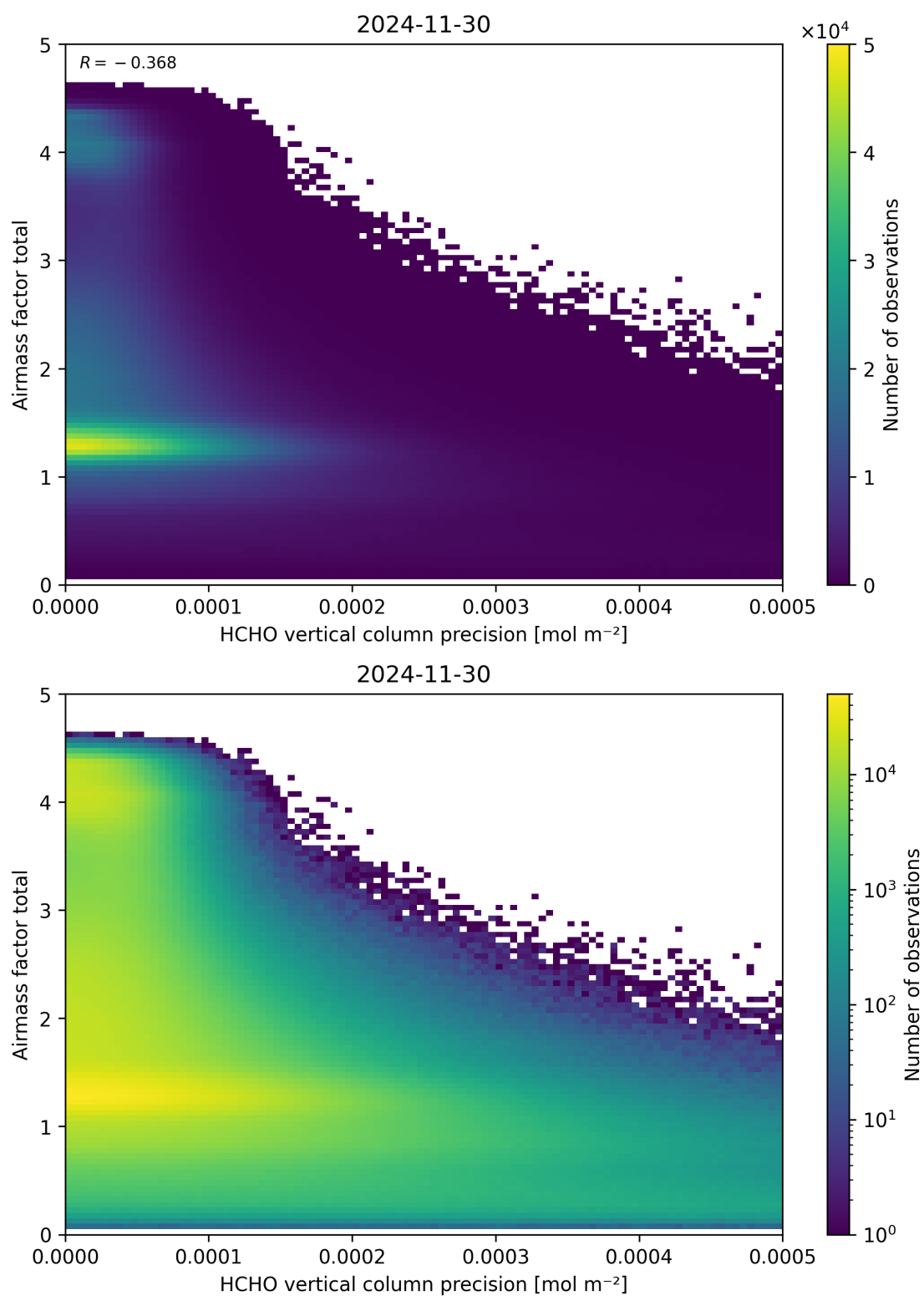
Figure 144: Scatter density plot of “HCHO vertical column precision” against “Airmass factor total” for 2024-11-30 to 2024-12-01.
