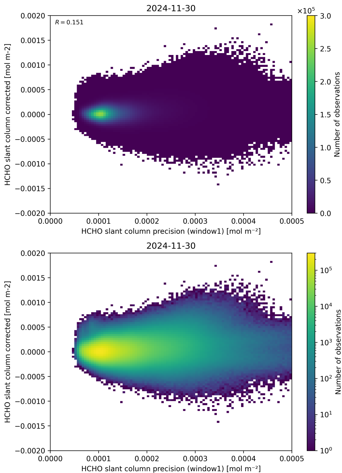
Figure 92: Scatter density plot of “HCHO slant column precision (window1)” against “HCHO slant column corrected” for 2024-11-30 to 2024-12-01.
