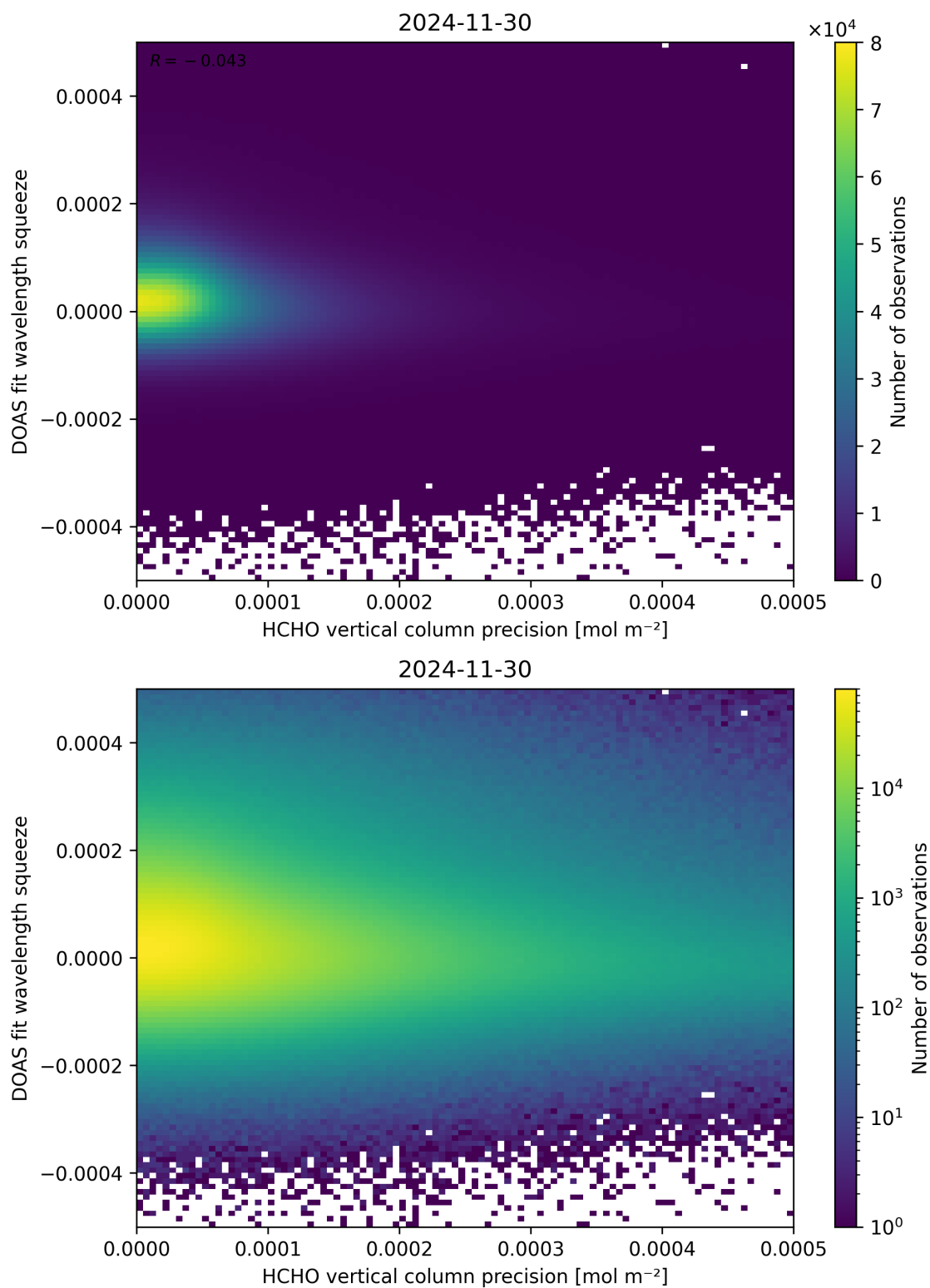
Figure 138: Scatter density plot of “HCHO vertical column precision” against “DOAS fit wavelength squeeze” for 2024-11-30 to 2024-12-01.
