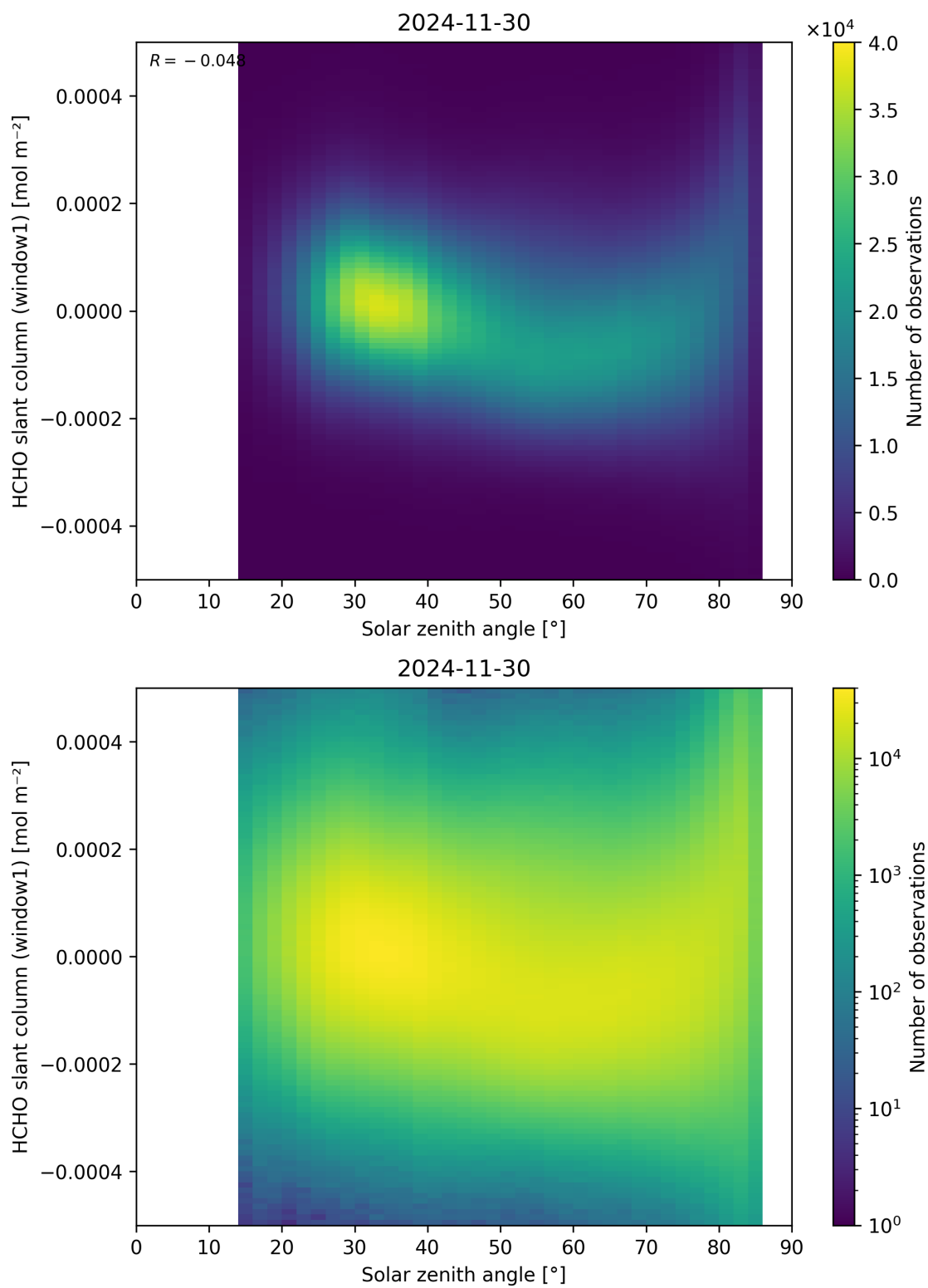
Figure 173: Scatter density plot of “Solar zenith angle” against “HCHO slant column (window1)” for 2024-11-30 to 2024-12-01.
