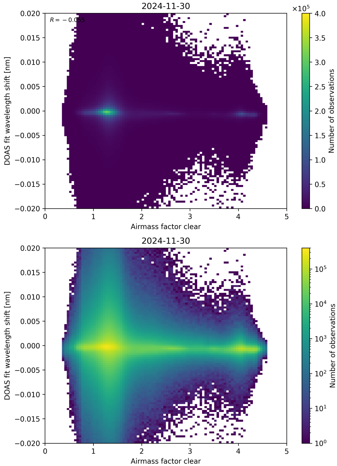
Figure 72: Scatter density plot of “Airmass factor clear” against “DOAS fit wavelength shift” for 2024-11-30 to 2024-12-01.
