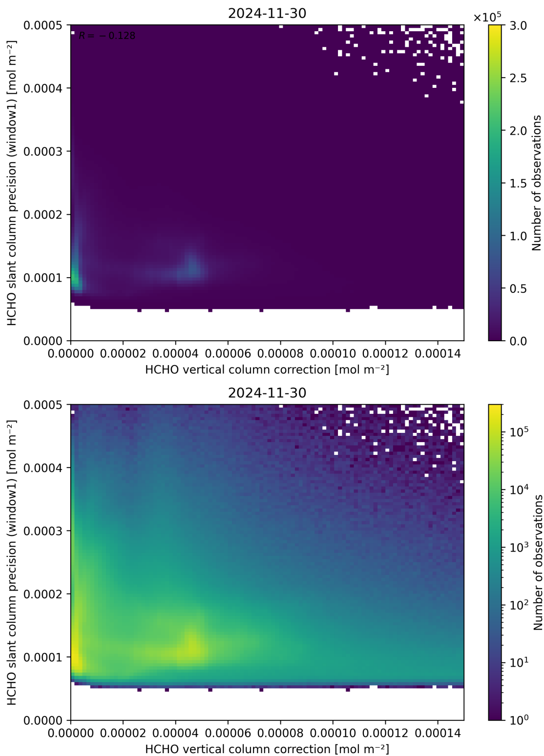
Figure 119: Scatter density plot of “HCHO vertical column correction” against “HCHO slant column precision (window1)” for 2024-11-30 to 2024-12-01.
