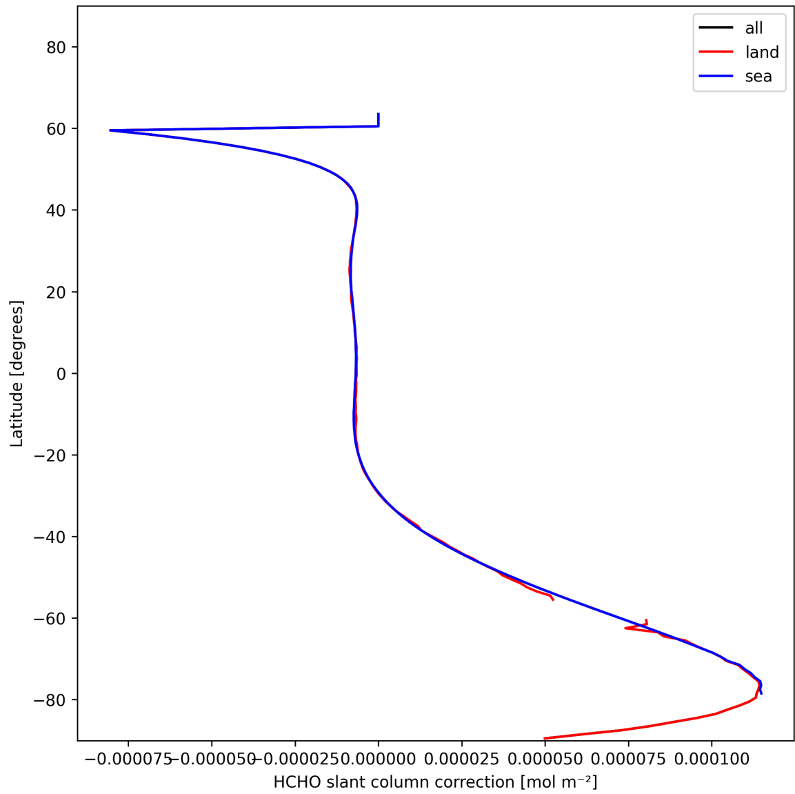
Figure 33: Zonal average of “HCHO slant column correction” for 2024-11-30 to 2024-12-01.
