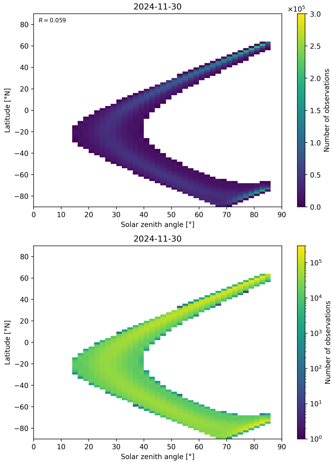
Figure 181: Scatter density plot of “Solar zenith angle” against “Latitude” for 2024-11-30 to 2024-12-01.
