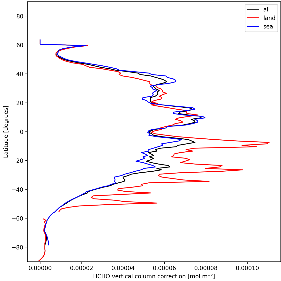
Figure 23: Zonal average of “HCHO vertical column correction” for 2024-11-30 to 2024-12-01.
