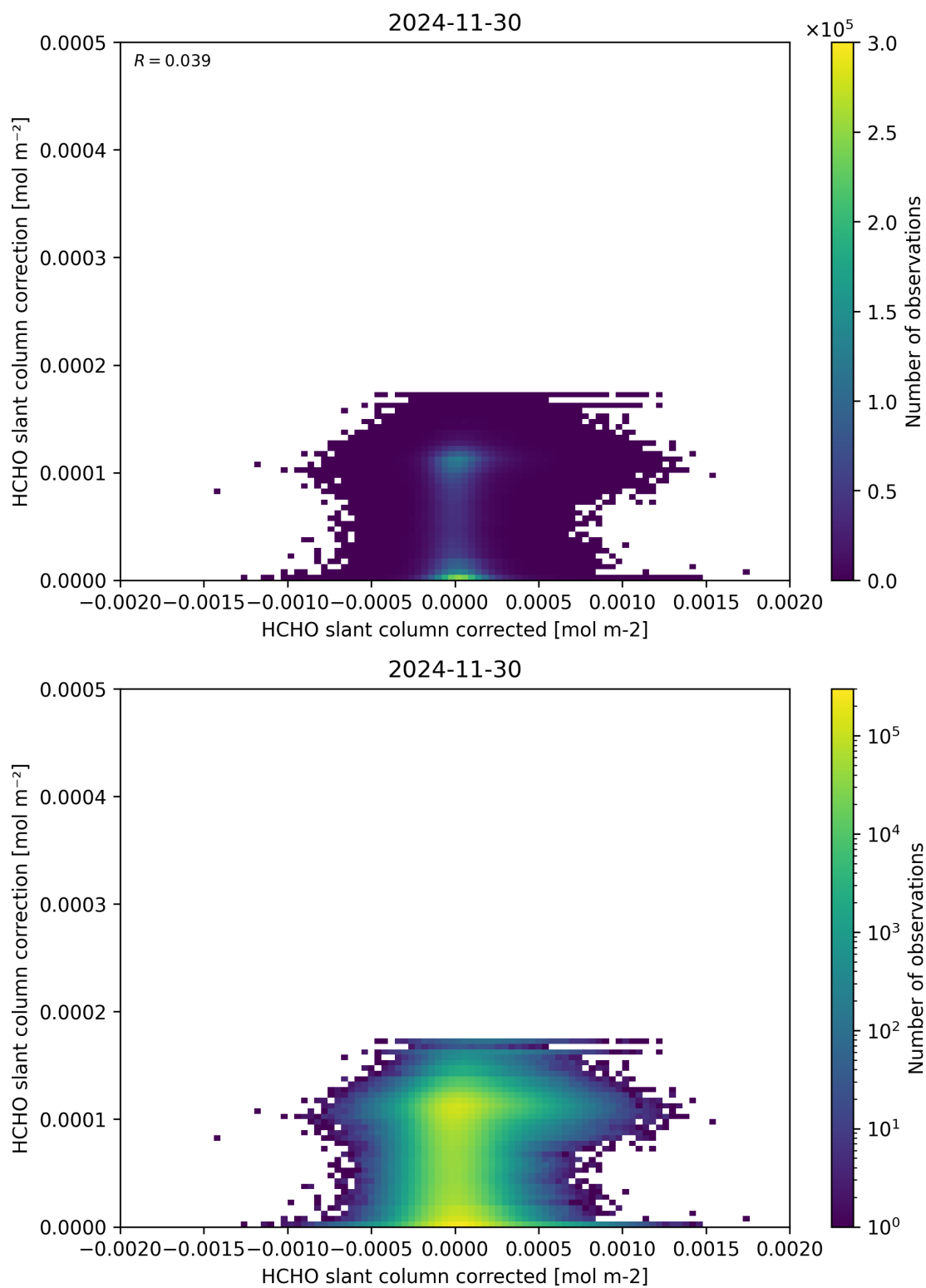
Figure 77: Scatter density plot of “HCHO slant column corrected” against “HCHO slant column correction” for 2024-11-30 to 2024-12-01.
