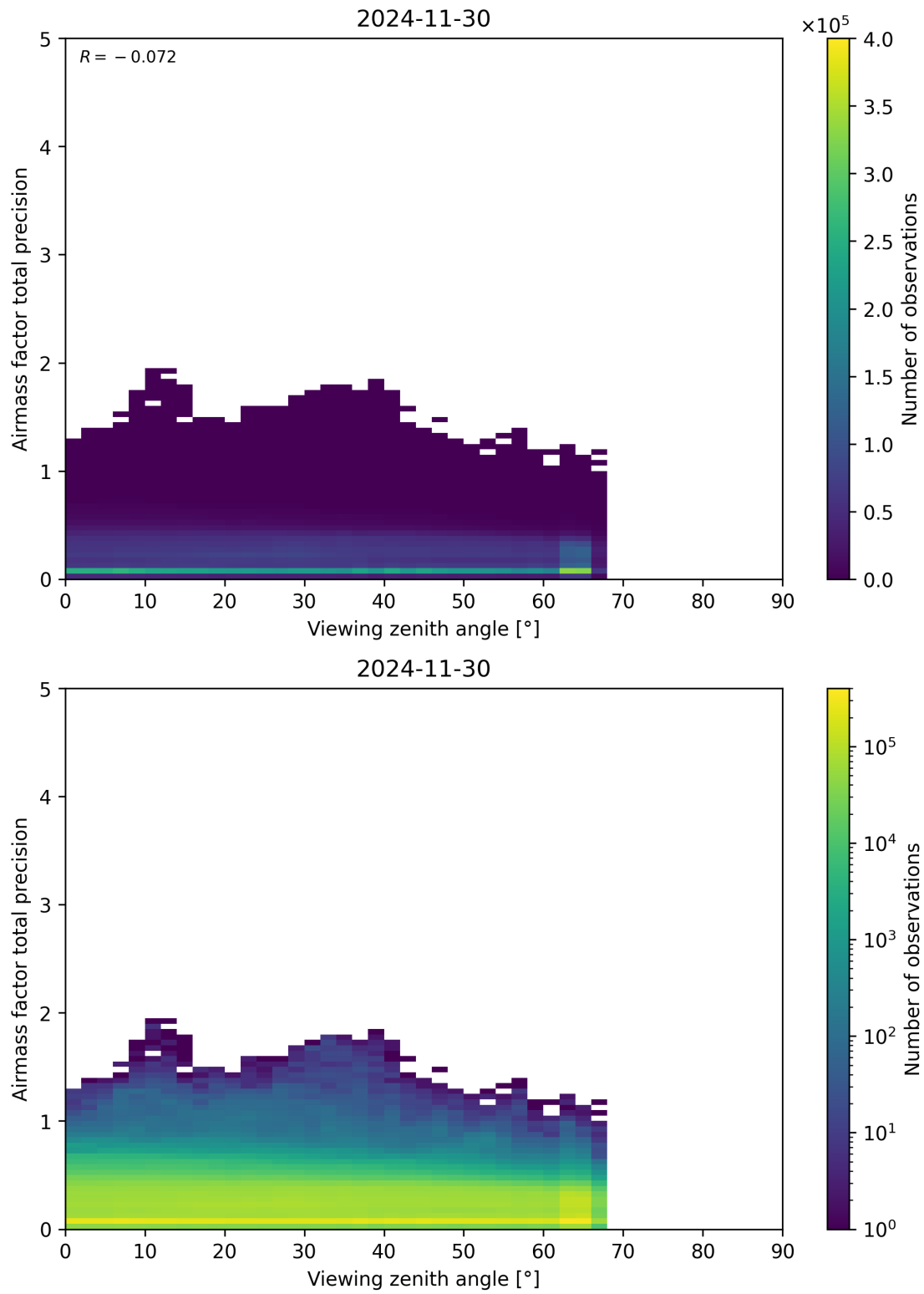
Figure 191: Scatter density plot of “Viewing zenith angle” against “Airmass factor total precision” for 2024-11-30 to 2024-12-01.
