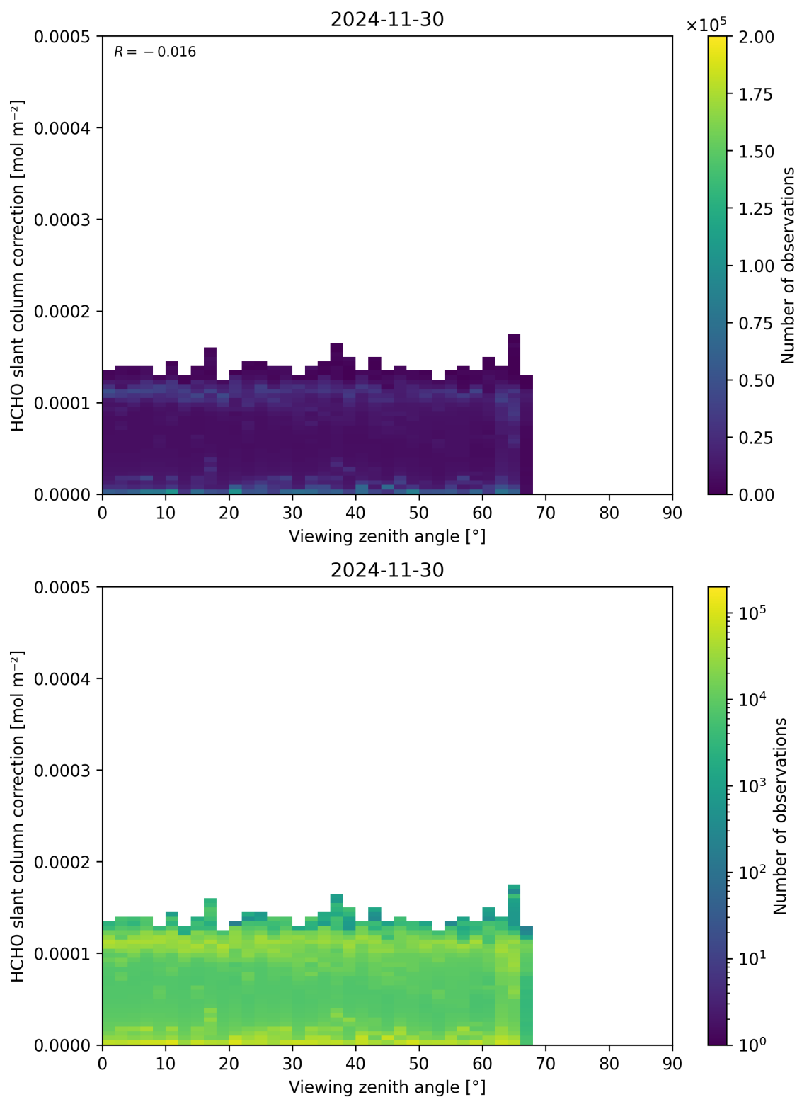
Figure 187: Scatter density plot of “Viewing zenith angle” against “HCHO slant column correction” for 2024-11-30 to 2024-12-01.
