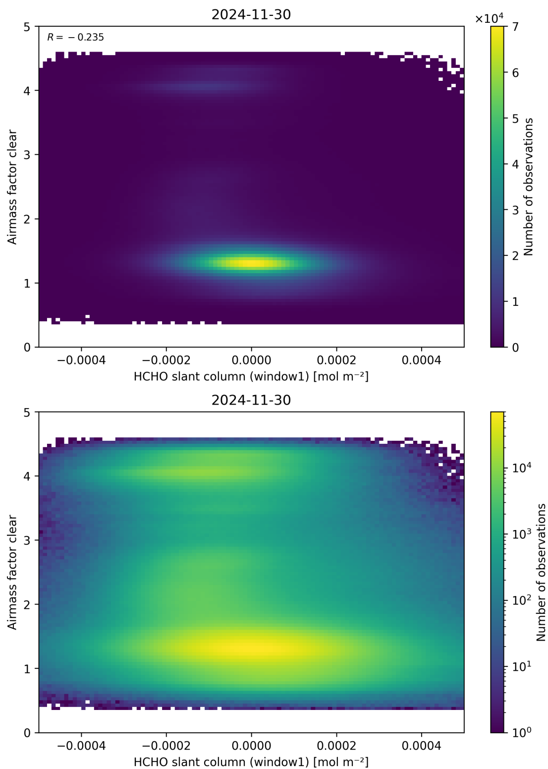
Figure 81: Scatter density plot of “HCHO slant column (window1)” against “Airmass factor clear” for 2024-11-30 to 2024-12-01.
