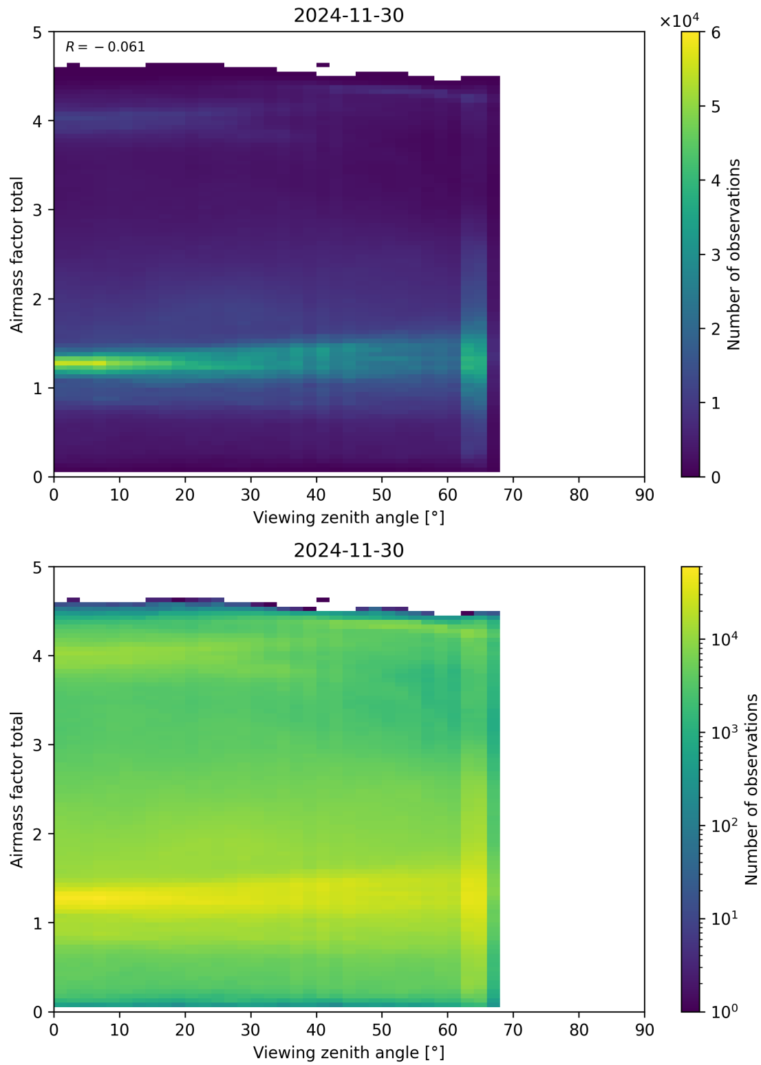
Figure 190: Scatter density plot of “Viewing zenith angle” against “Airmass factor total” for 2024-11-30 to 2024-12-01.
