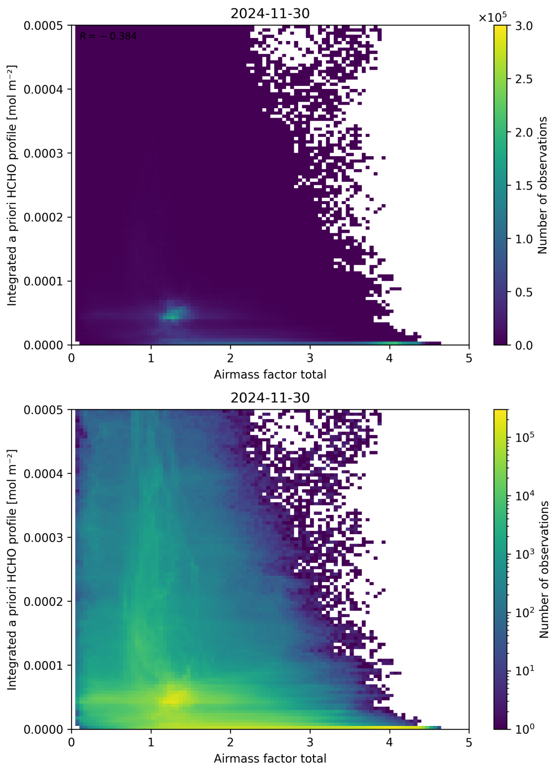
Figure 104: Scatter density plot of “Airmass factor total” against “Integrated a priori HCHO profile” for 2024-11-30 to 2024-12-01.
