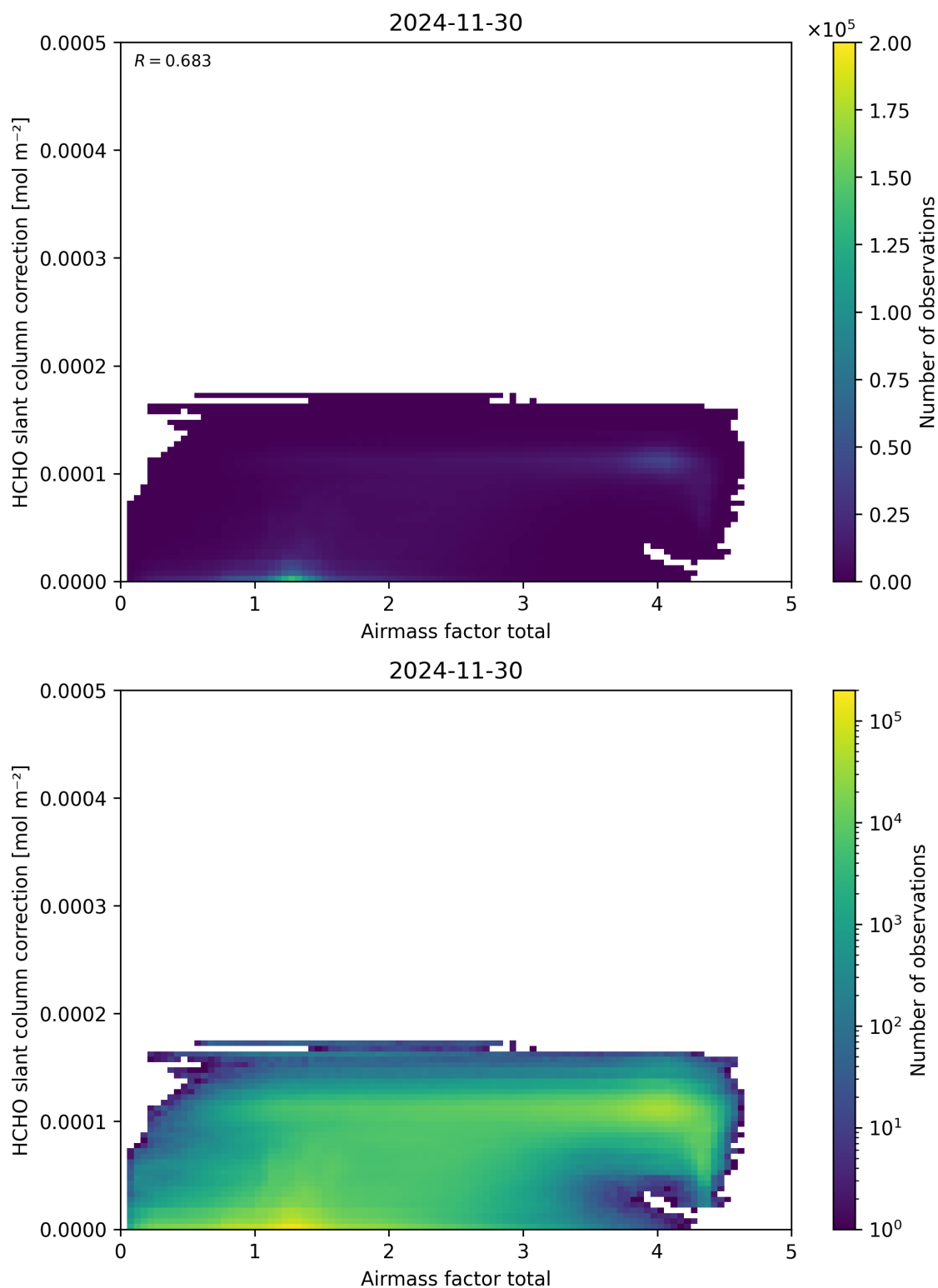
Figure 102: Scatter density plot of “Airmass factor total” against “HCHO slant column correction” for 2024-11-30 to 2024-12-01.
