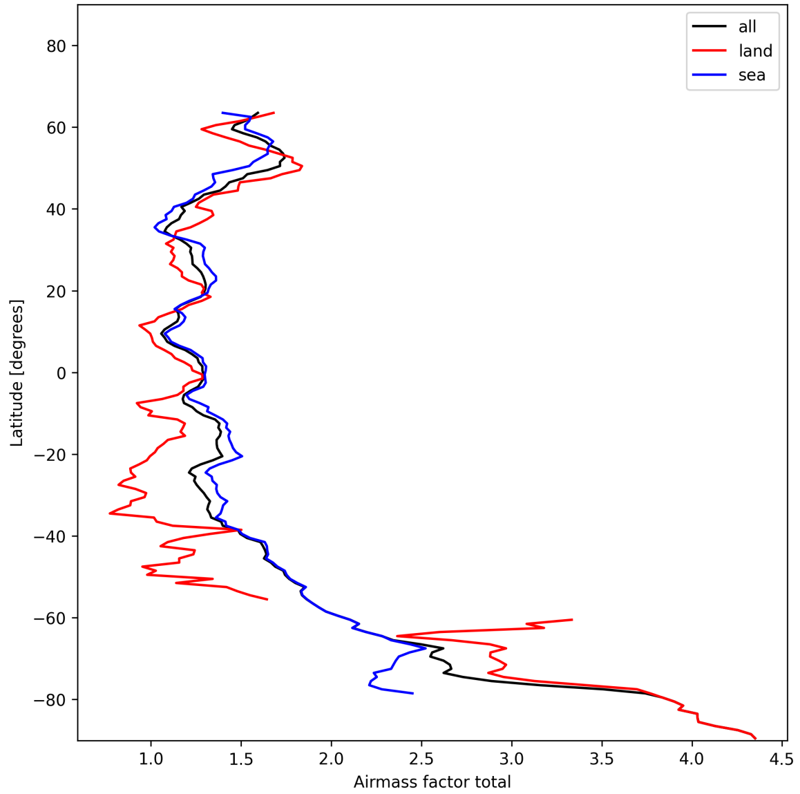
Figure 26: Zonal average of “Airmass factor total” for 2024-11-30 to 2024-12-01.
