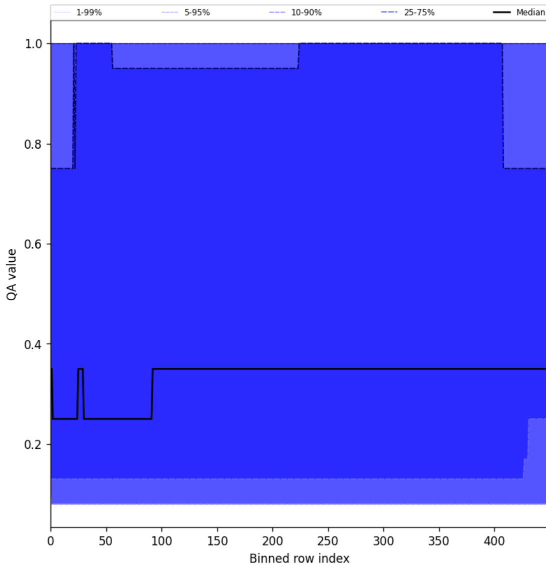
Figure 48: Along track statistics of “QA value” for 2024-11-30 to 2024-12-01
