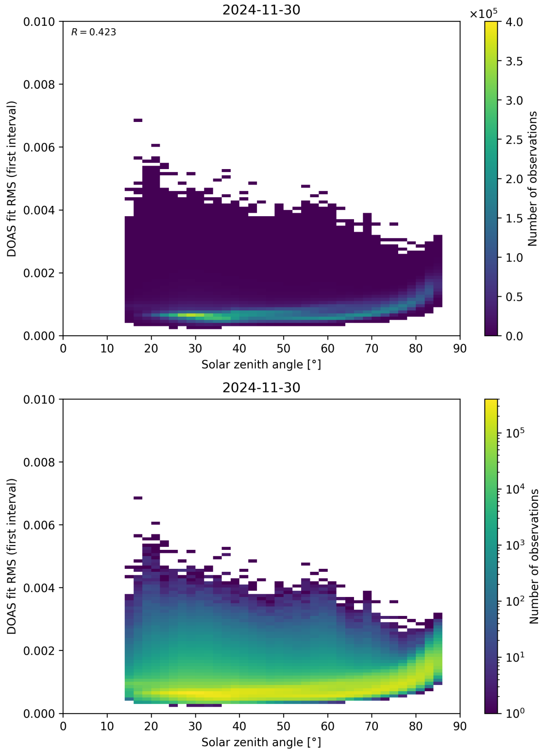
Figure 167: Scatter density plot of “Solar zenith angle” against “DOAS fit RMS (first interval)” for 2024-11-30 to 2024-12-01.
