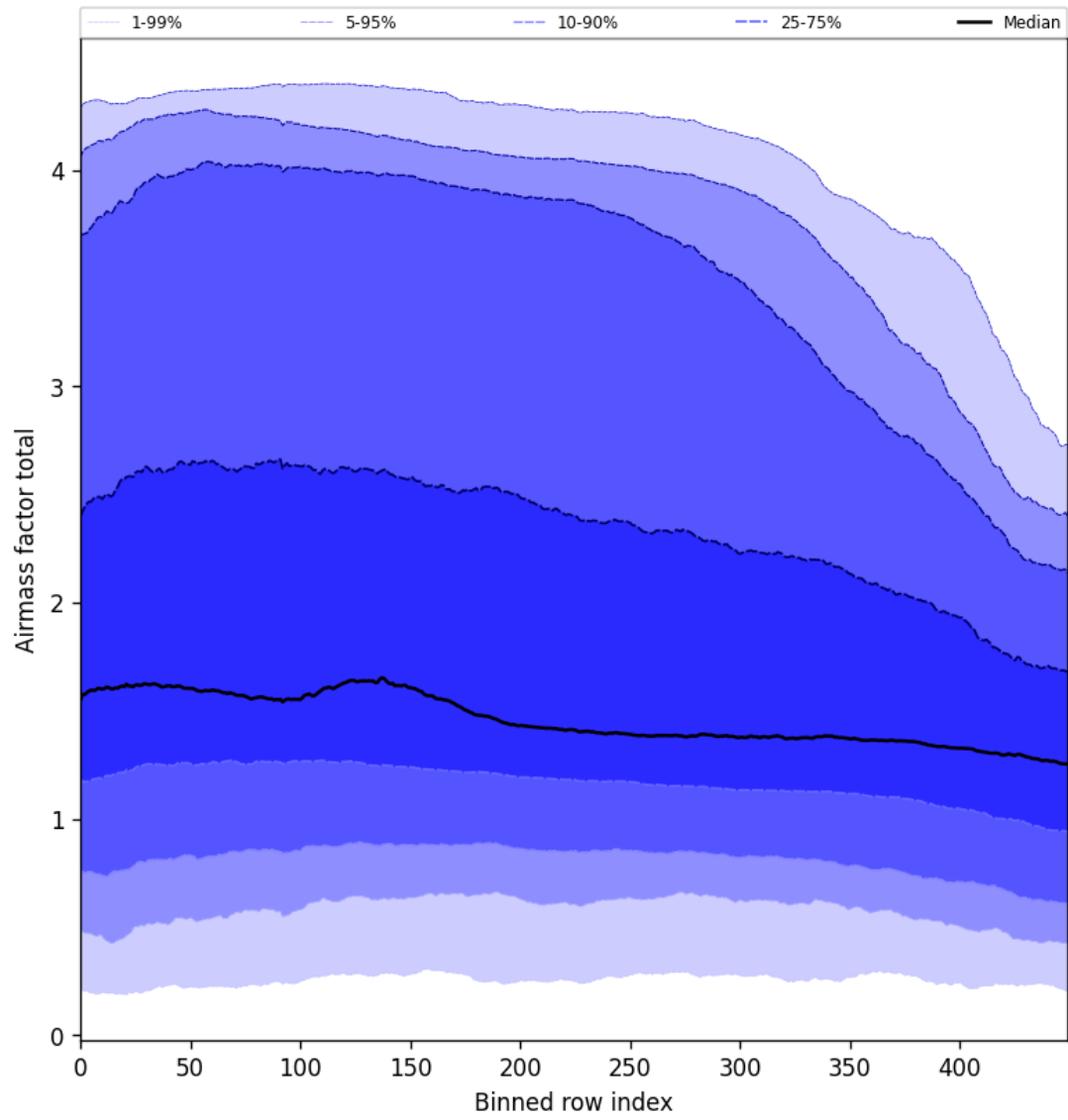
Figure 54: Along track statistics of “Airmass factor total” for 2024-11-30 to 2024-12-01
