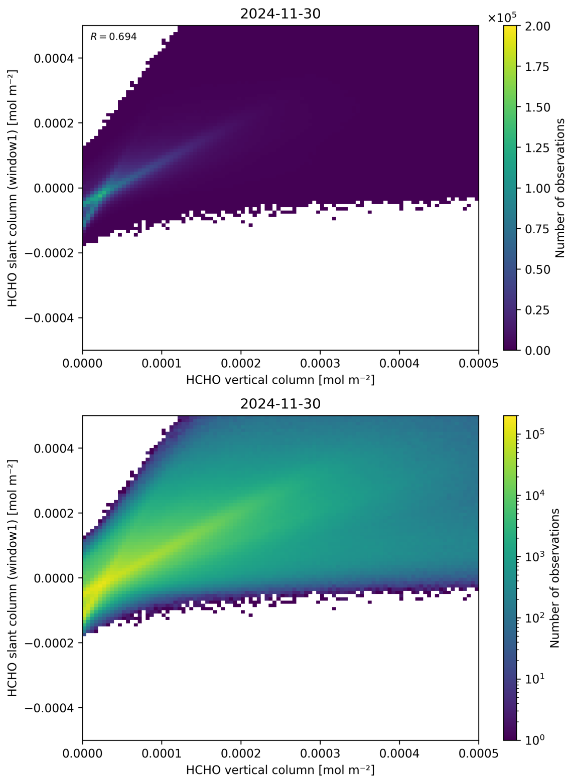
Figure 129: Scatter density plot of “HCHO vertical column” against “HCHO slant column (window1)” for 2024-11-30 to 2024-12-01.
