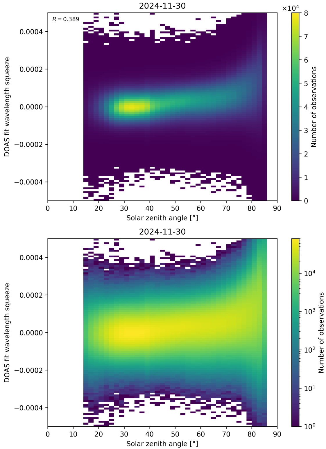
Figure 169: Scatter density plot of “Solar zenith angle” against “DOAS fit wavelength squeeze” for 2024-11-30 to 2024-12-01.
