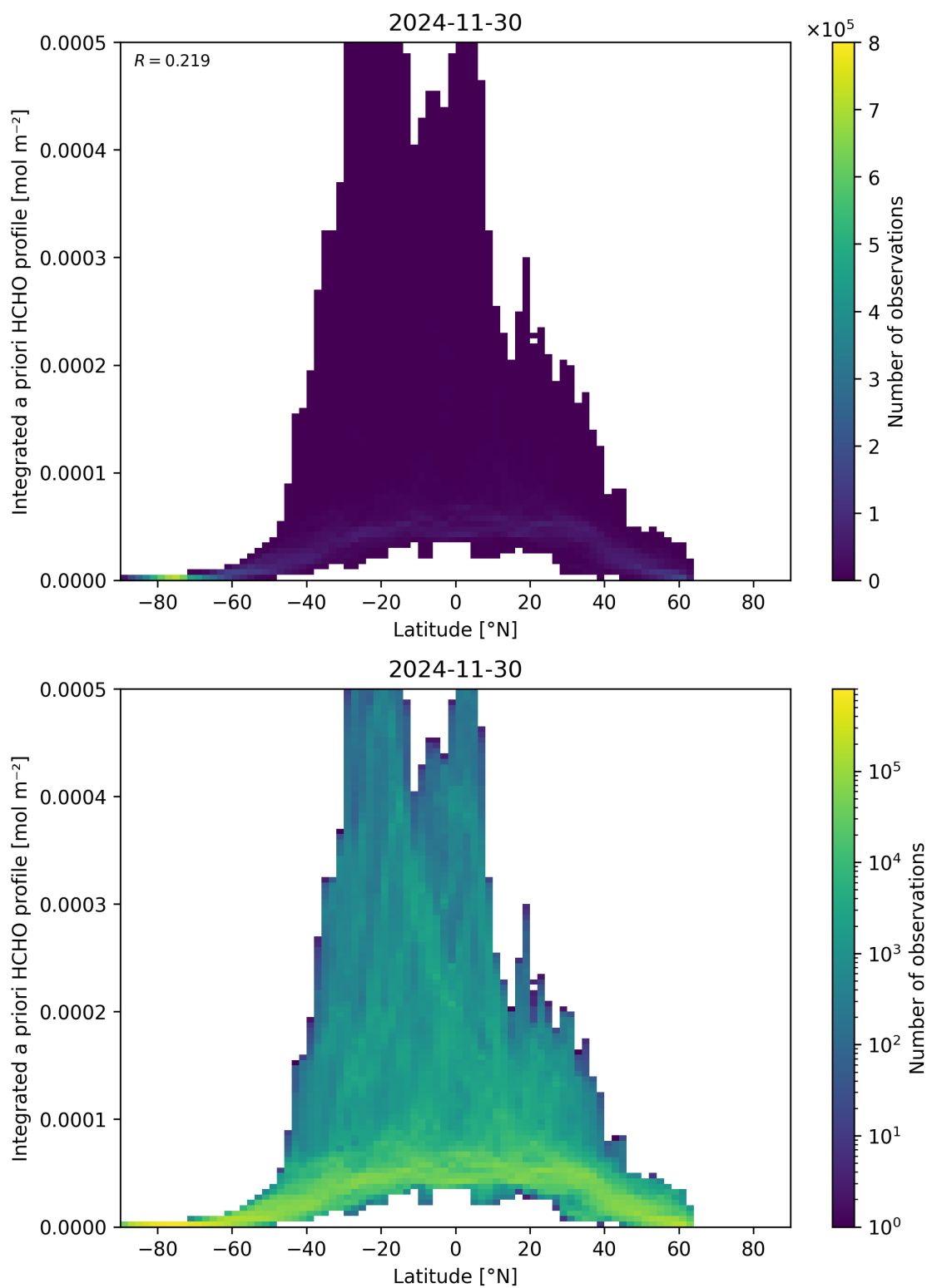
Figure 166: Scatter density plot of “Latitude” against “Integrated a priori HCHO profile” for 2024-11-30 to 2024-12-01.
