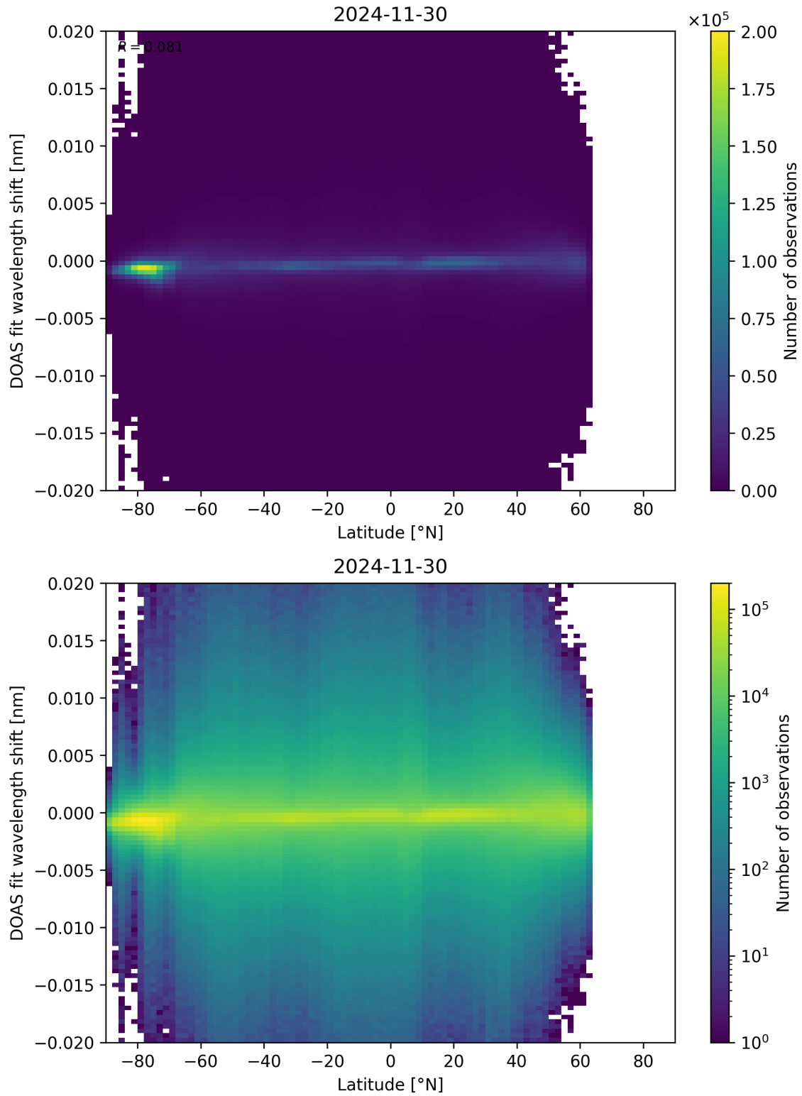
Figure 154: Scatter density plot of “Latitude” against “DOAS fit wavelength shift” for 2024-11-30 to 2024-12-01.
