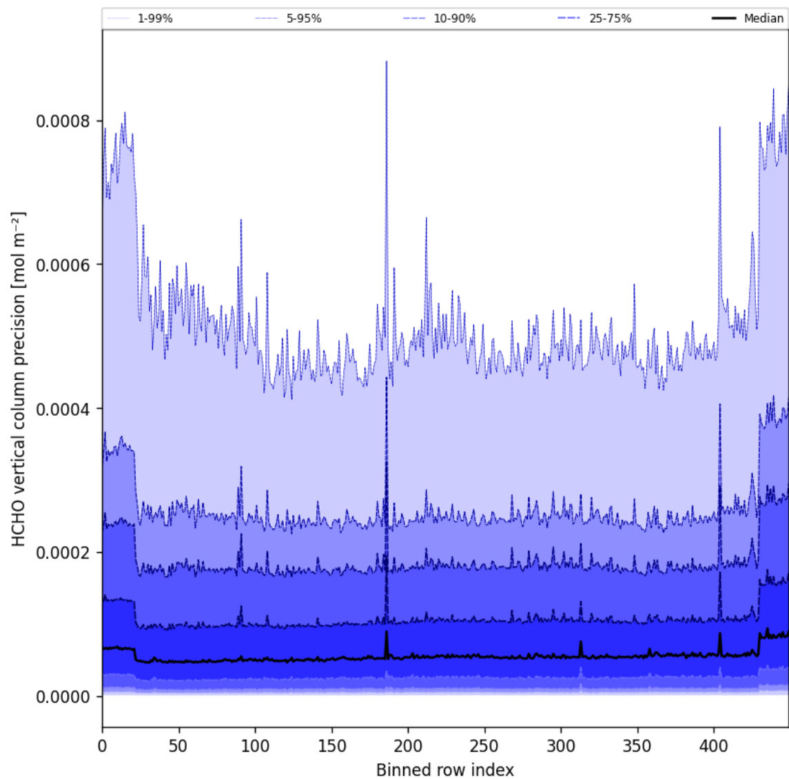
Figure 50: Along track statistics of “HCHO vertical column precision” for 2024-11-30 to 2024-12-01
