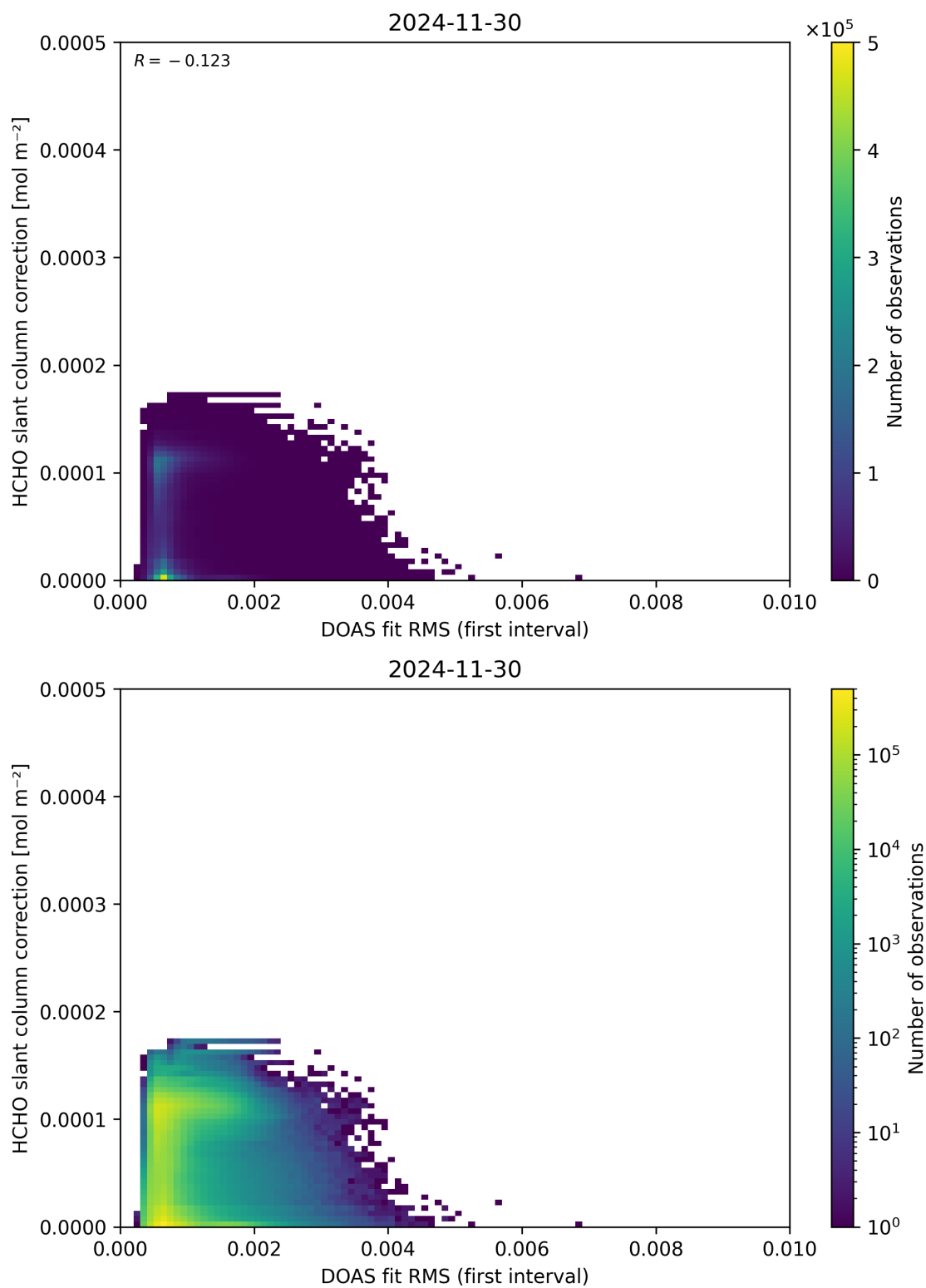
Figure 63: Scatter density plot of “DOAS fit RMS (first interval)” against “HCHO slant column correction” for 2024-11-30 to 2024-12-01.
