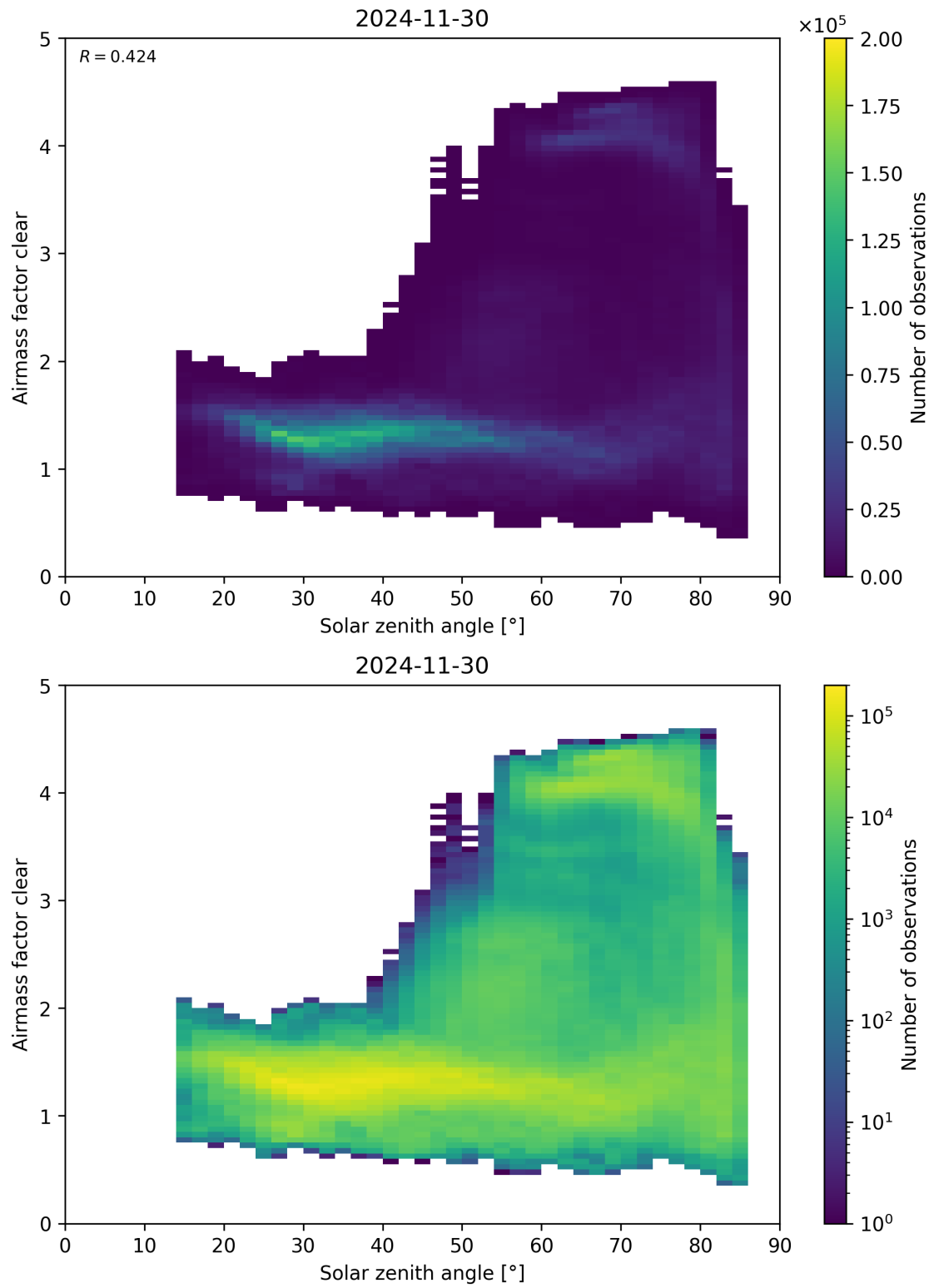
Figure 170: Scatter density plot of “Solar zenith angle” against “Airmass factor clear” for 2024-11-30 to 2024-12-01.
