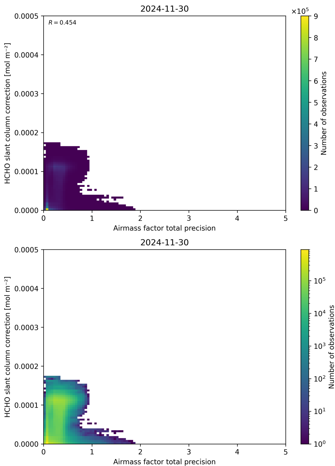
Figure 110: Scatter density plot of “Airmass factor total precision” against “HCHO slant column correction” for 2024-11-30 to 2024-12-01.
