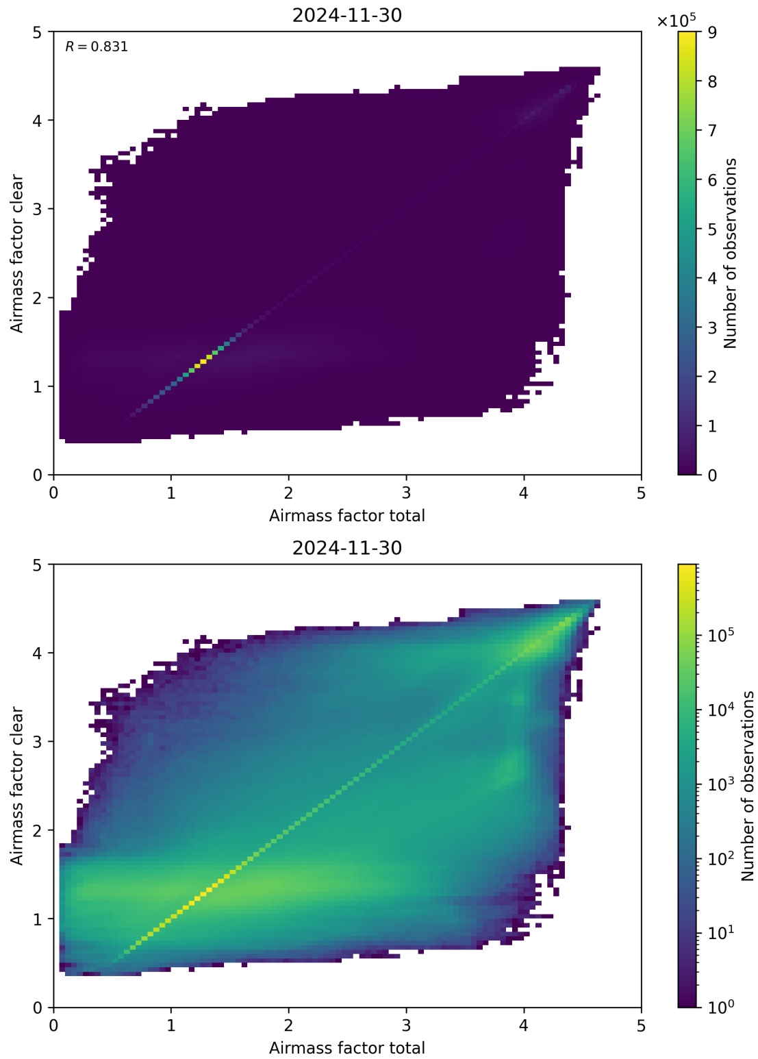
Figure 100: Scatter density plot of “Airmass factor total” against “Airmass factor clear” for 2024-11-30 to 2024-12-01.
