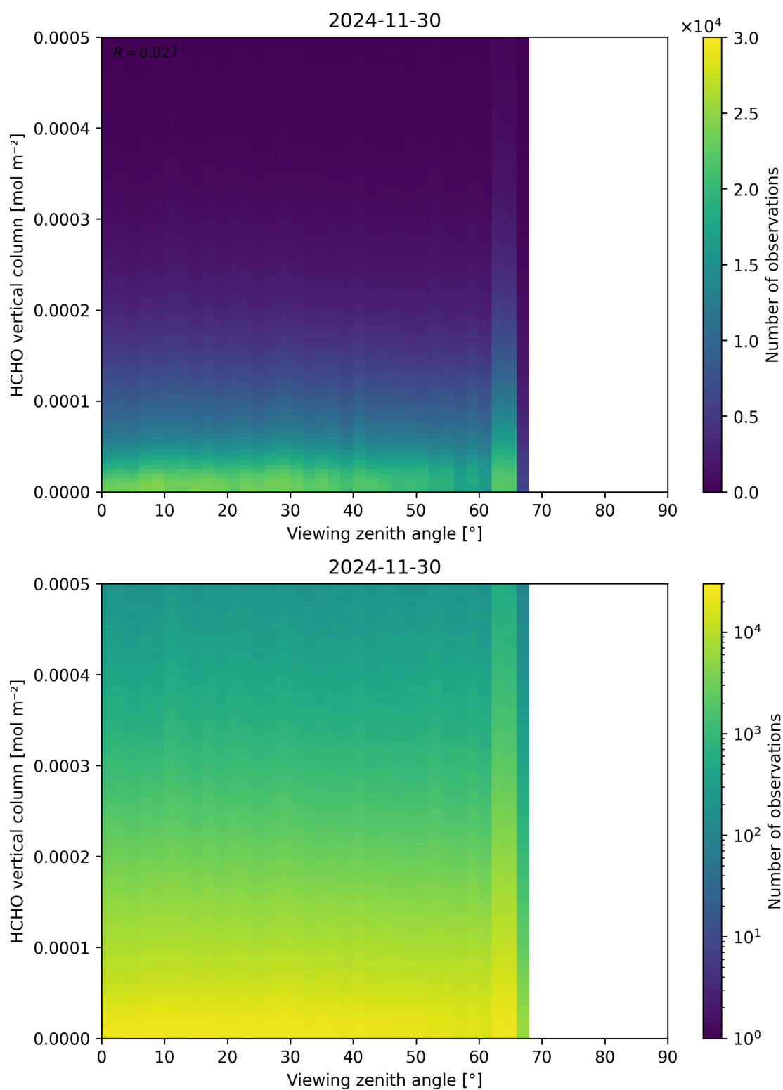
Figure 192: Scatter density plot of “Viewing zenith angle” against “HCHO vertical column” for 2024-11-30 to 2024-12-01.
