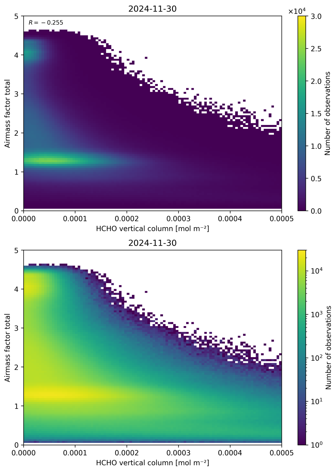
Figure 131: Scatter density plot of “HCHO vertical column” against “Airmass factor total” for 2024-11-30 to 2024-12-01.
