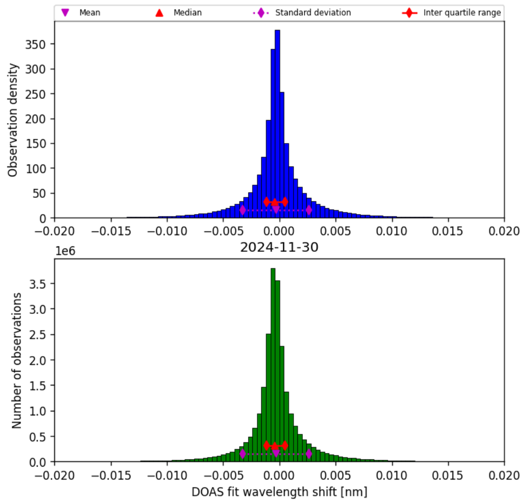
Figure 44: Histogram of “DOAS fit wavelength shift” for 2024-11-30 to 2024-12-01
