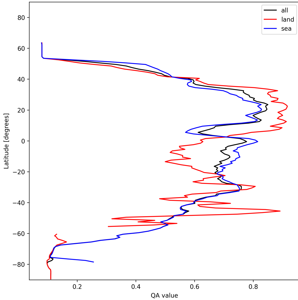
Figure 20: Zonal average of “QA value” for 2024-11-30 to 2024-12-01.
