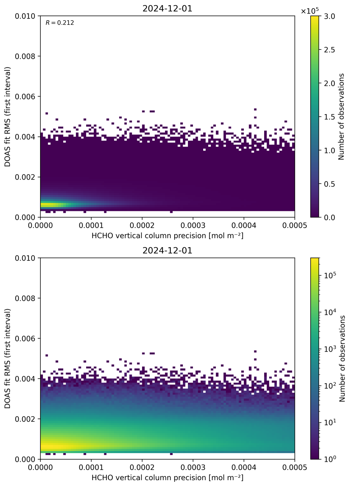
Figure 136: Scatter density plot of “HCHO vertical column precision” against “DOAS fit RMS (first interval)” for 2024-11-30 to 2024-12-02.
