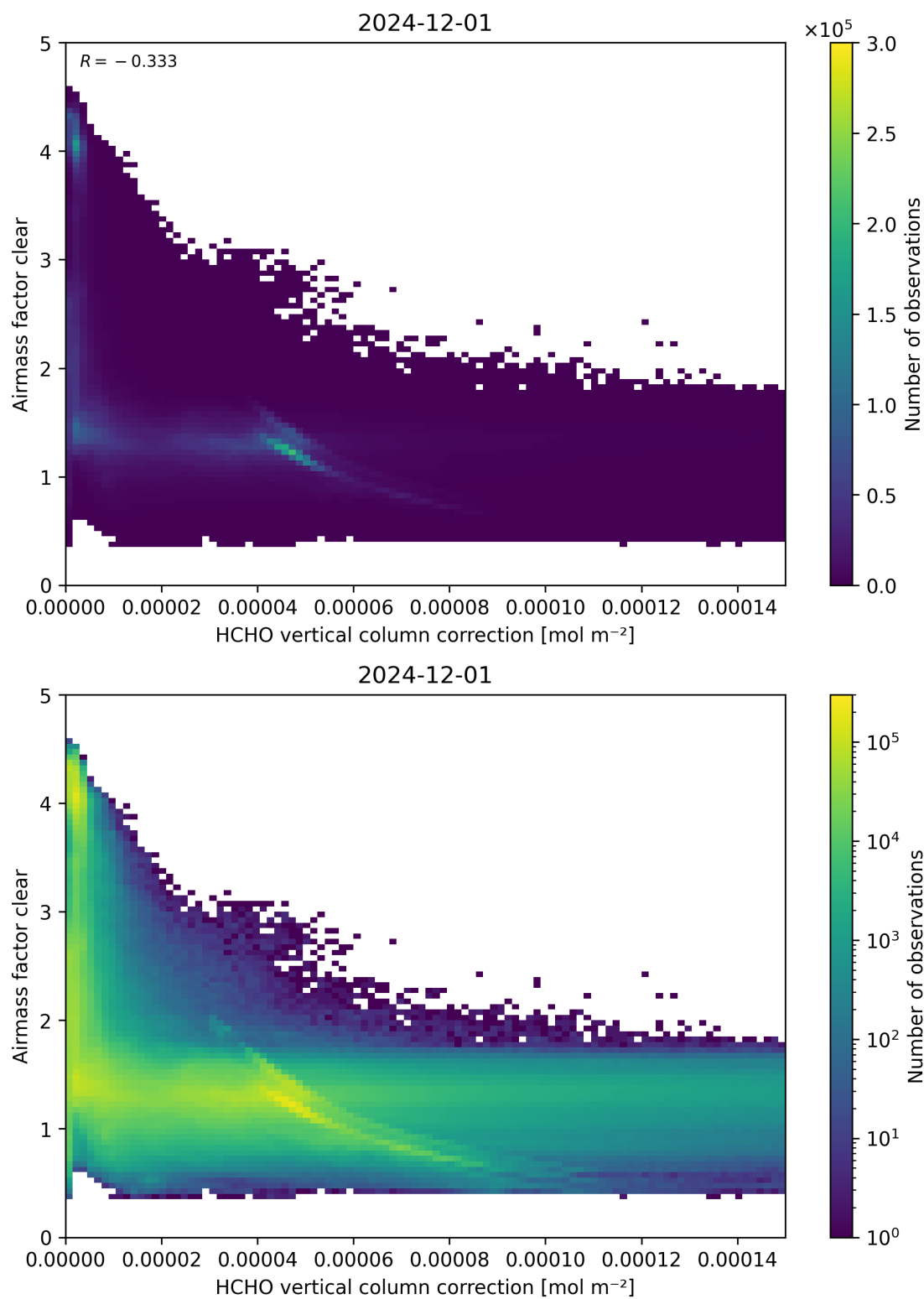
Figure 115: Scatter density plot of “HCHO vertical column correction” against “Airmass factor clear” for 2024-11-30 to 2024-12-02.
