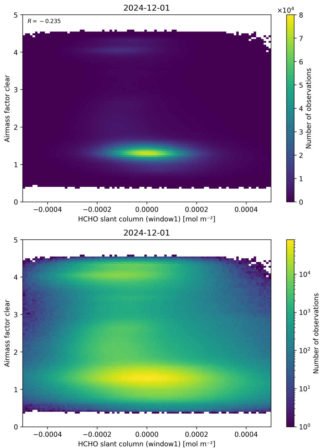
Figure 81: Scatter density plot of “HCHO slant column (window1)” against “Airmass factor clear” for 2024-11-30 to 2024-12-02.
