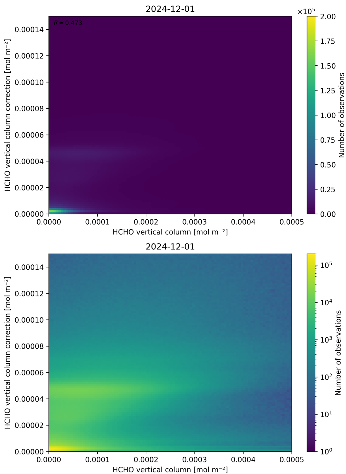
Figure 133: Scatter density plot of “HCHO vertical column” against “HCHO vertical column correction” for 2024-11-30 to 2024-12-02.
