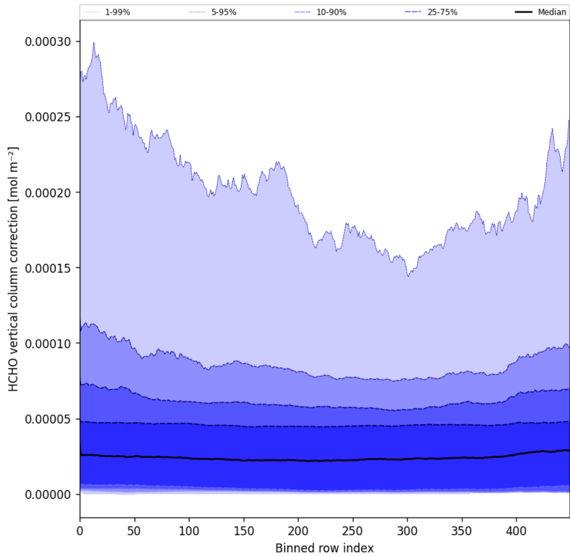
Figure 51: Along track statistics of “HCHO vertical column correction” for 2024-11-30 to 2024-12-02
