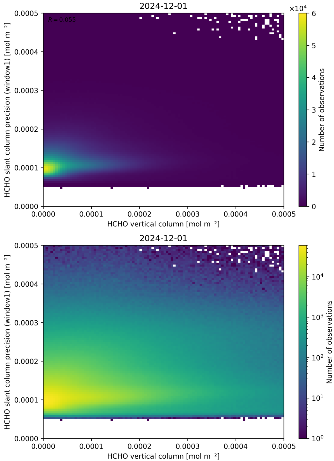
Figure 130: Scatter density plot of “HCHO vertical column” against “HCHO slant column precision (window1)” for 2024-11-30 to 2024-12-02.
