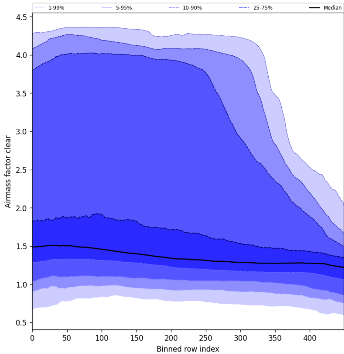
Figure 56: Along track statistics of “Airmass factor clear” for 2024-11-30 to 2024-12-02
