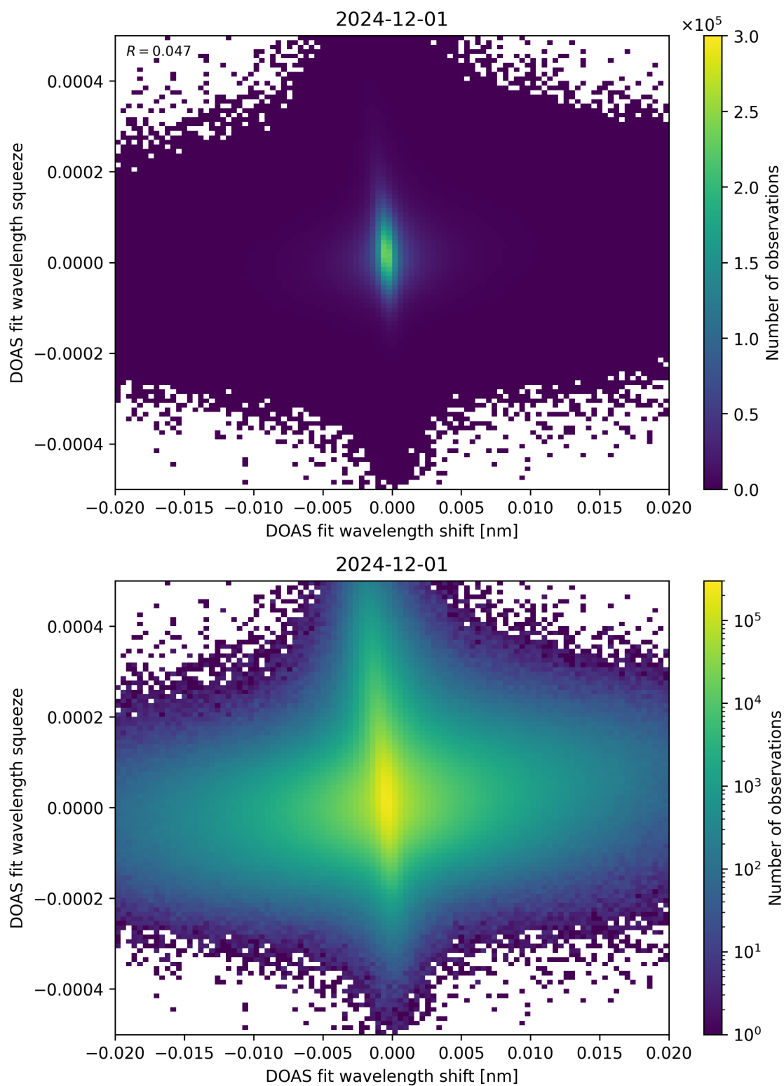
Figure 65: Scatter density plot of “DOAS fit wavelength shift” against “DOAS fit wavelength squeeze” for 2024-11-30 to 2024-12-02.
