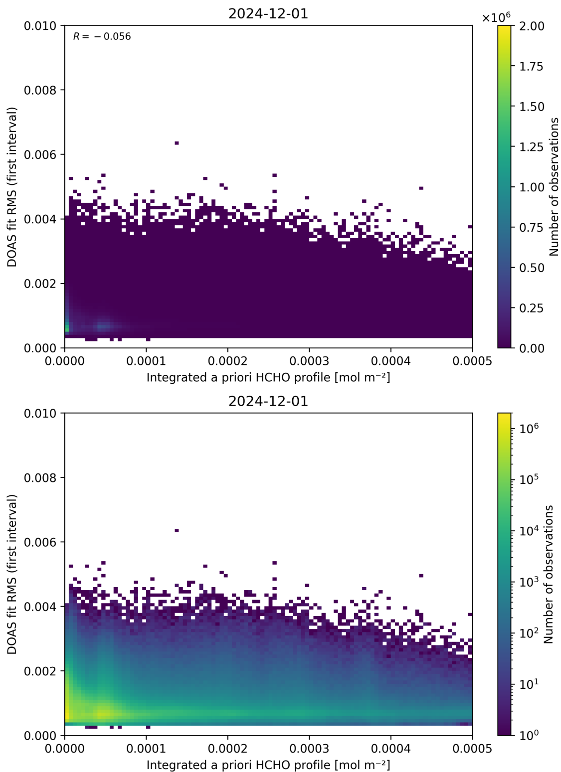
Figure 148: Scatter density plot of “Integrated a priori HCHO profile” against “DOAS fit RMS (first interval)” for 2024-11-30 to 2024-12-02.
