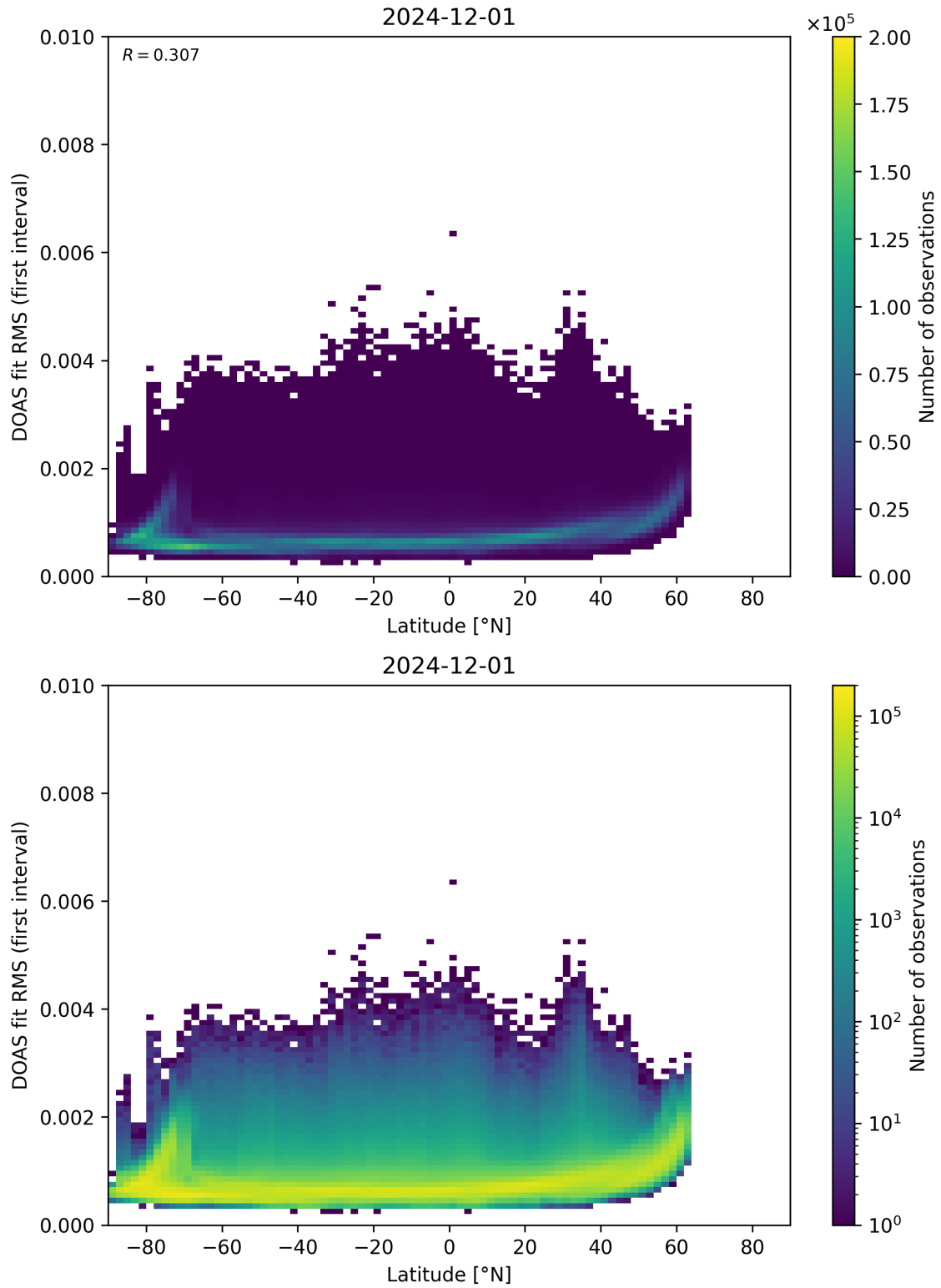
Figure 153: Scatter density plot of “Latitude” against “DOAS fit RMS (first interval)” for 2024-11-30 to 2024-12-02.
