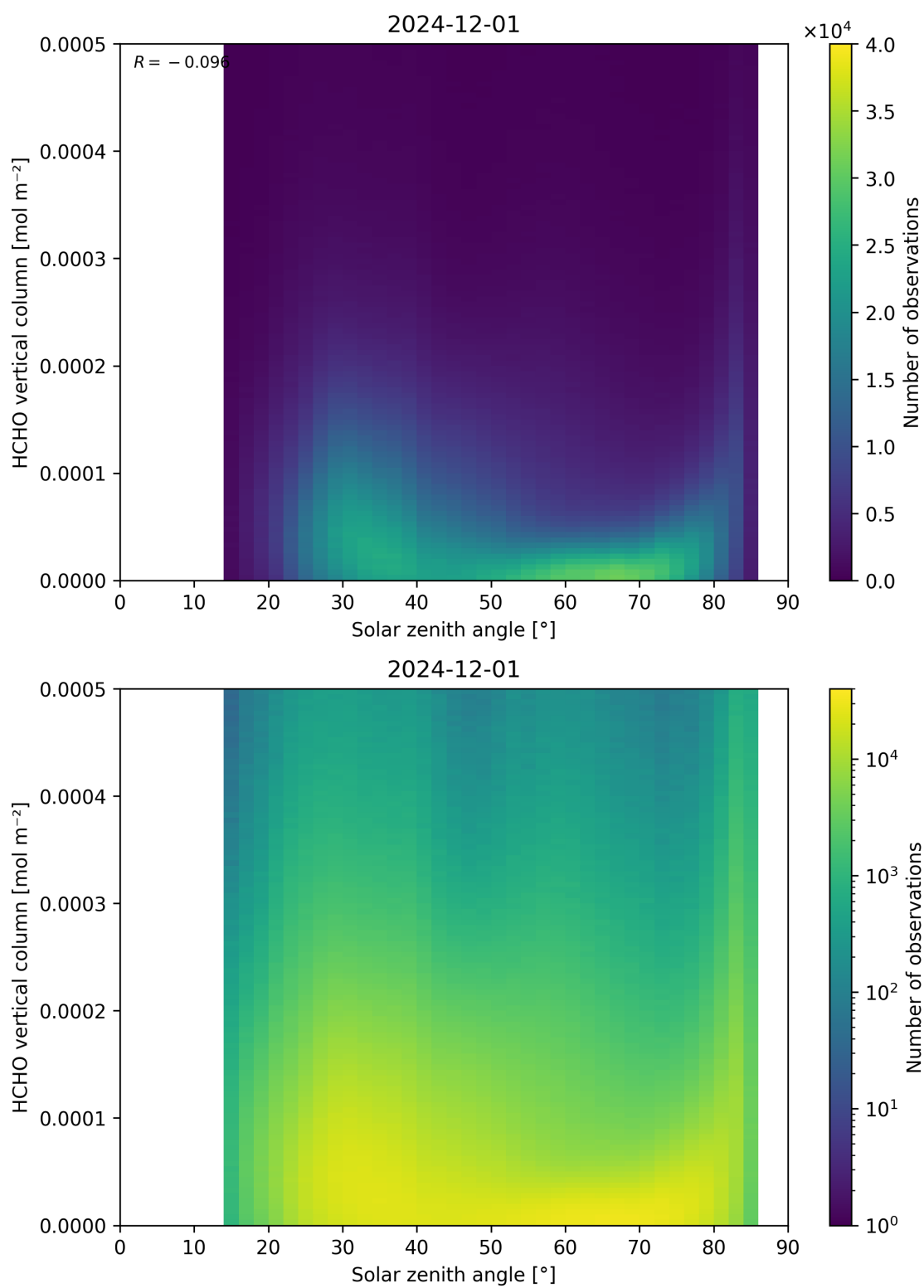
Figure 177: Scatter density plot of “Solar zenith angle” against “HCHO vertical column” for 2024-11-30 to 2024-12-02.
