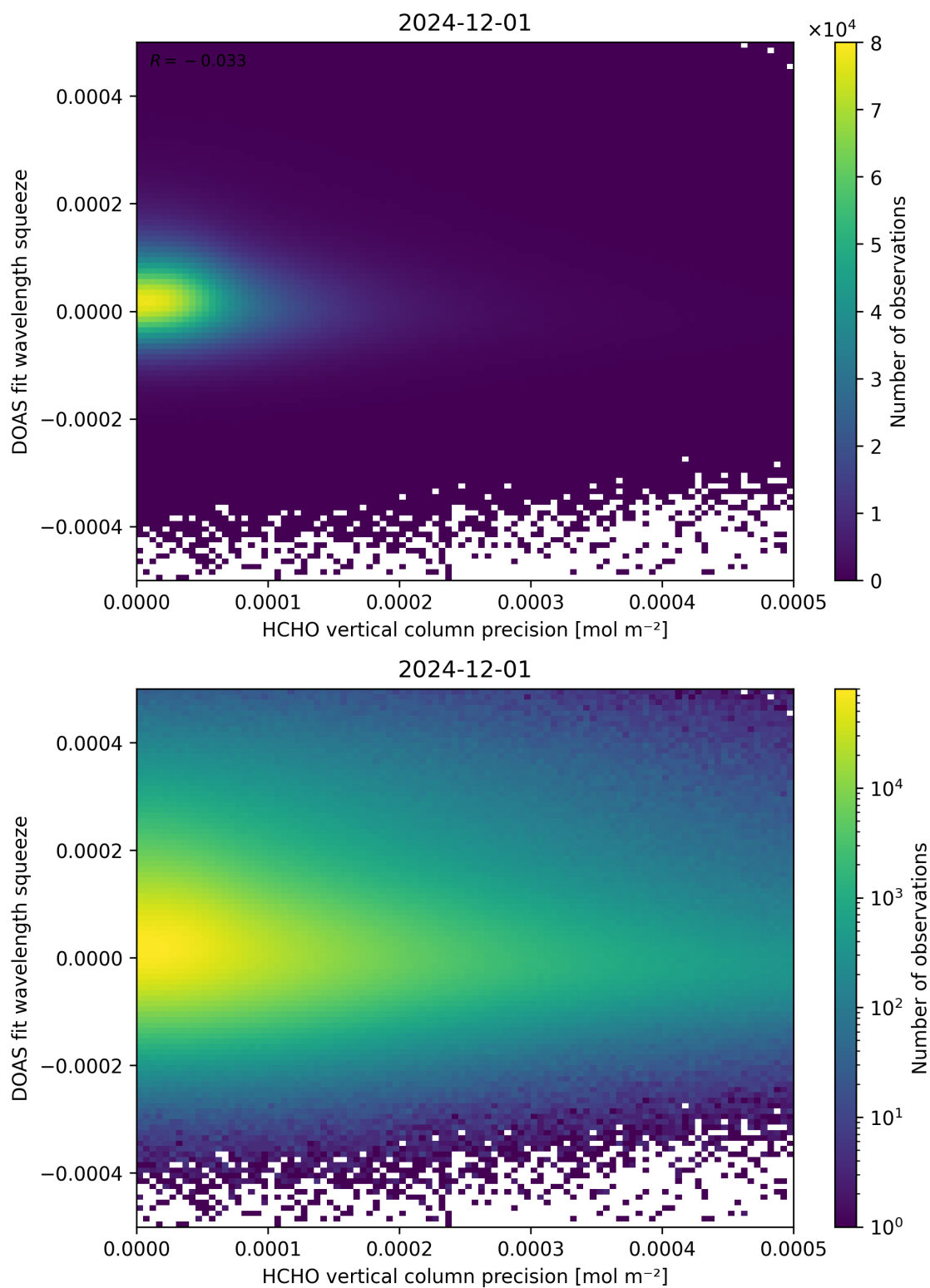
Figure 138: Scatter density plot of “HCHO vertical column precision” against “DOAS fit wavelength squeeze” for 2024-11-30 to 2024-12-02.
