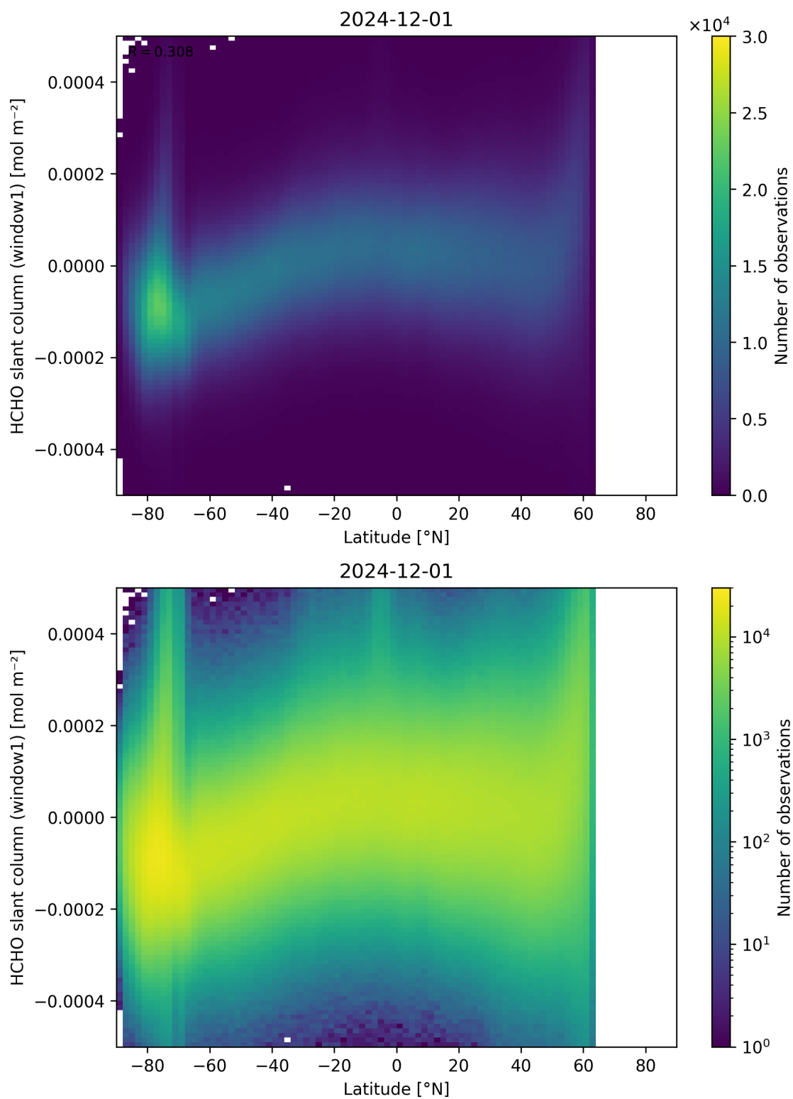
Figure 159: Scatter density plot of “Latitude” against “HCHO slant column (window1)” for 2024-11-30 to 2024-12-02.
