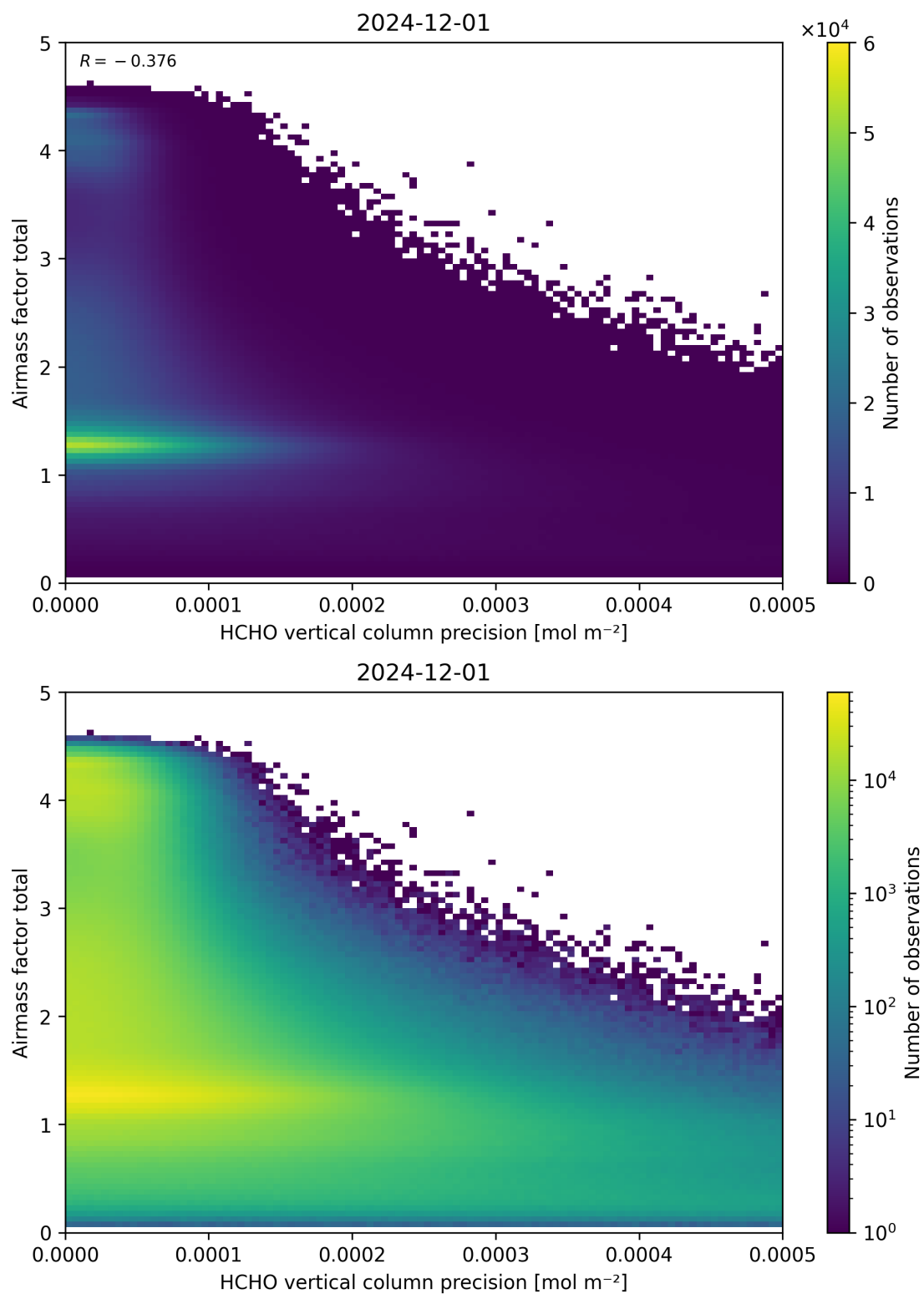
Figure 144: Scatter density plot of “HCHO vertical column precision” against “Airmass factor total” for 2024-11-30 to 2024-12-02.
