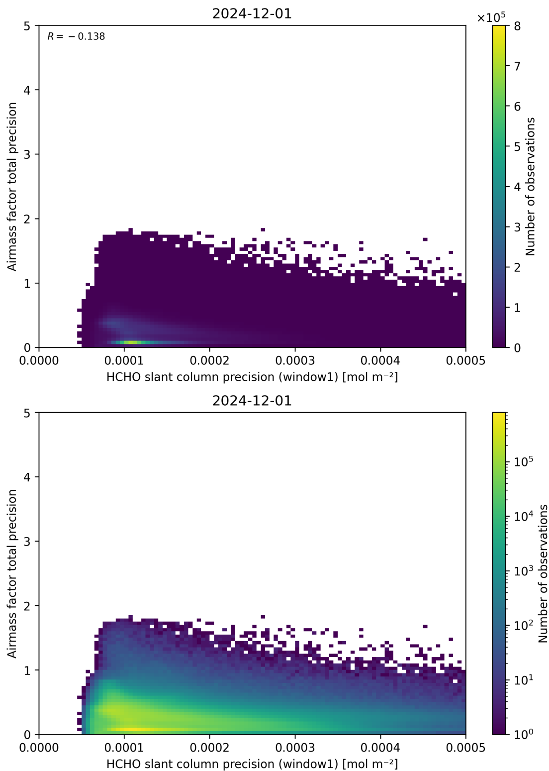
Figure 95: Scatter density plot of “HCHO slant column precision (window1)” against “Airmass factor total precision” for 2024-11-30 to 2024-12-02.
