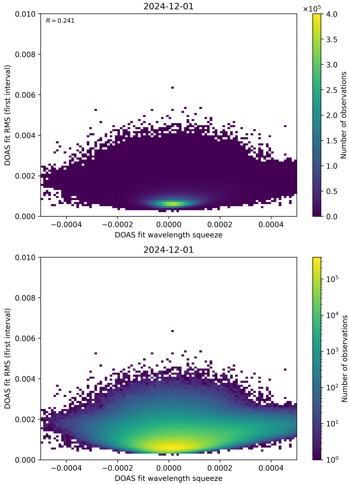
Figure 68: Scatter density plot of “DOAS fit wavelength squeeze” against “DOAS fit RMS (first interval)” for 2024-11-30 to 2024-12-02.
