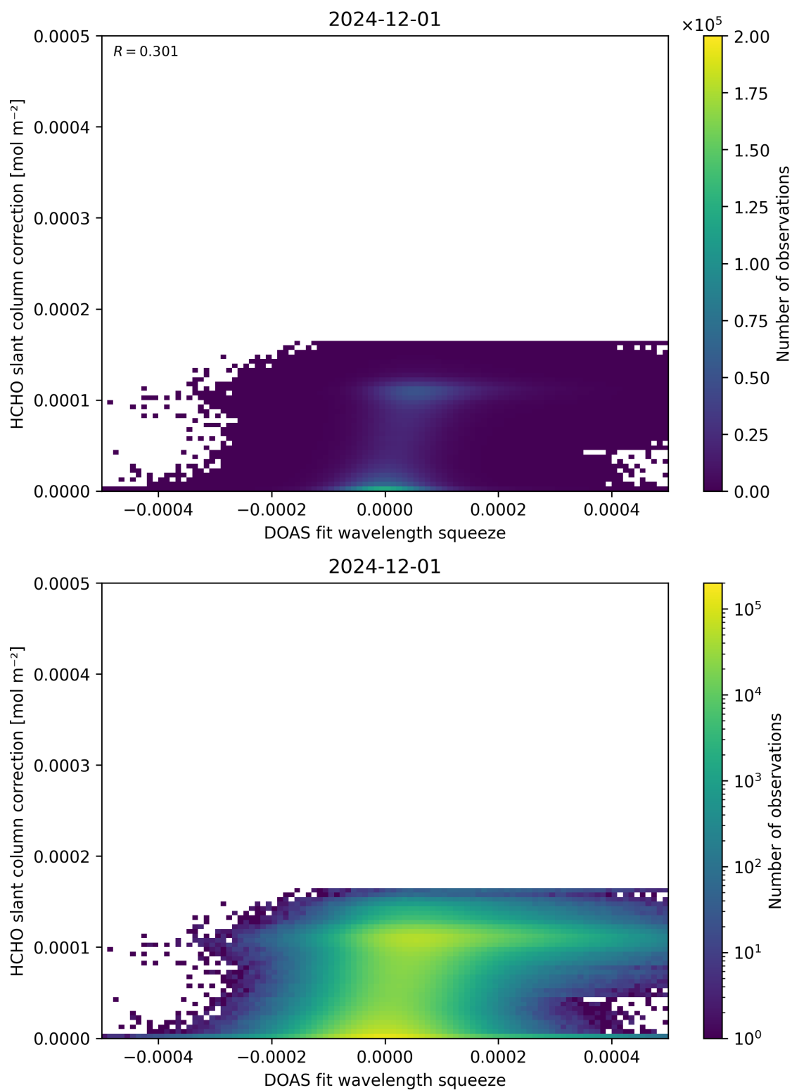
Figure 70: Scatter density plot of “DOAS fit wavelength squeeze” against “HCHO slant column correction” for 2024-11-30 to 2024-12-02.
