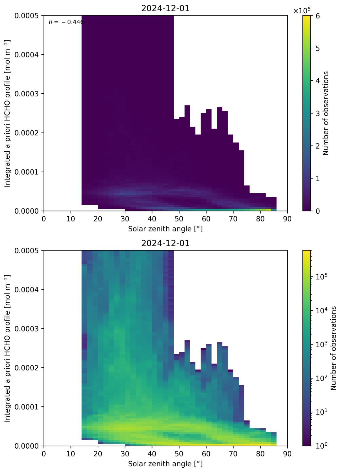
Figure 180: Scatter density plot of “Solar zenith angle” against “Integrated a priori HCHO profile” for 2024-11-30 to 2024-12-02.
