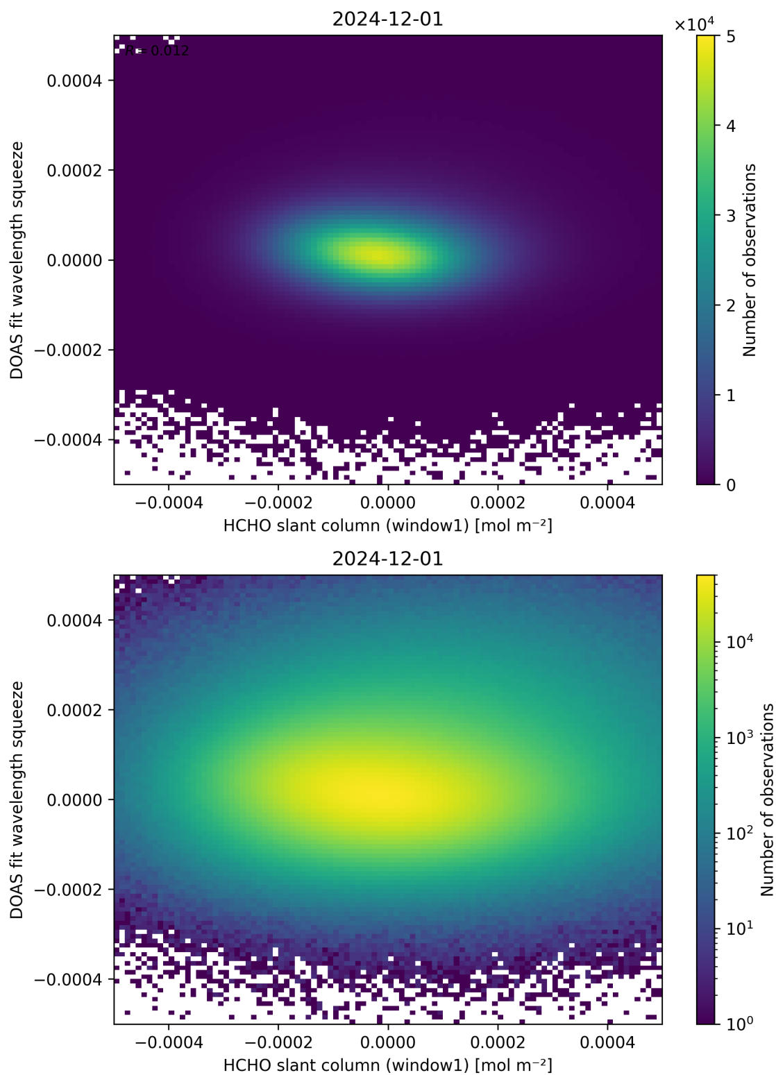
Figure 80: Scatter density plot of “HCHO slant column (window1)” against “DOAS fit wavelength squeeze” for 2024-11-30 to 2024-12-02.
