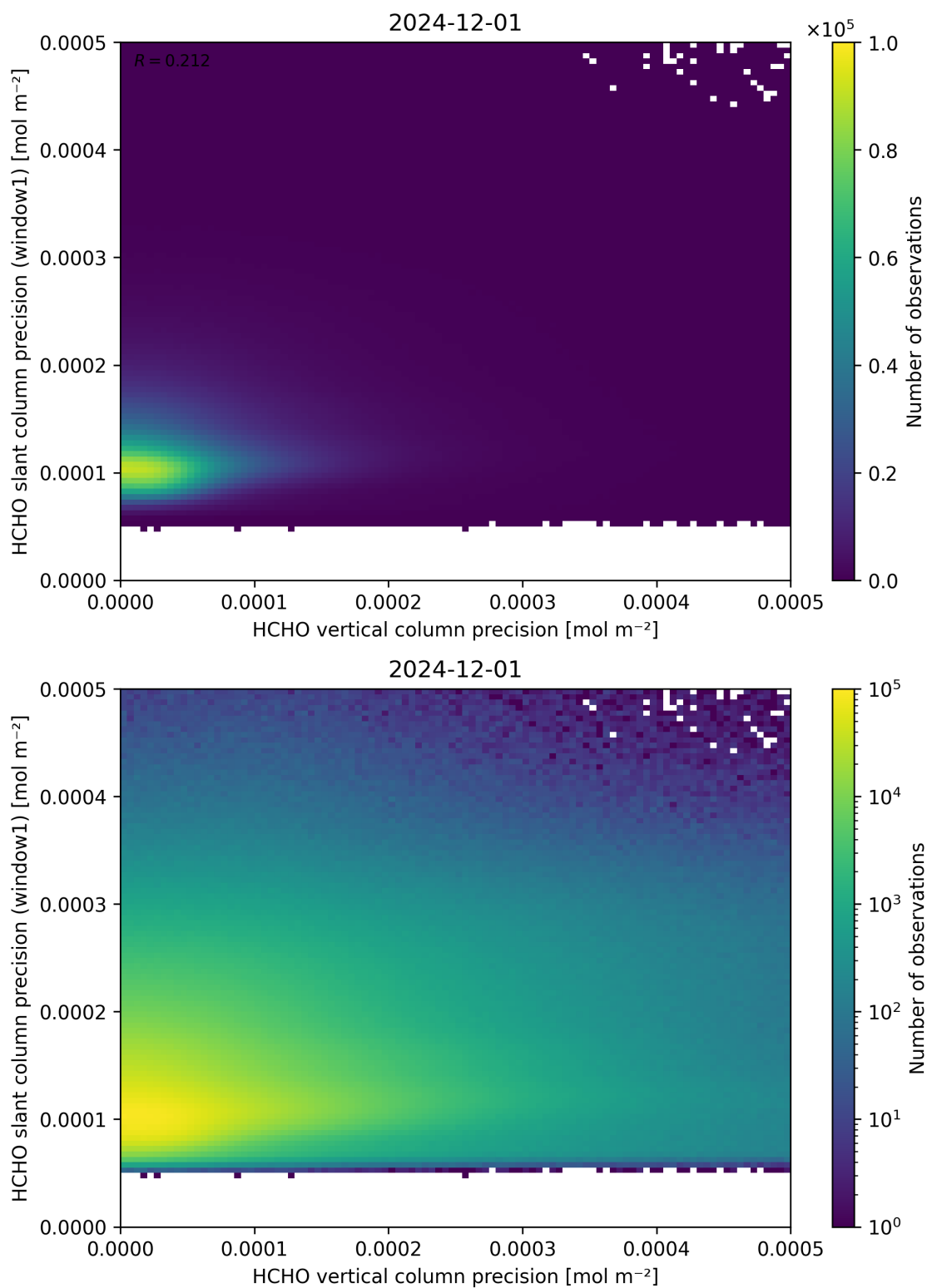
Figure 143: Scatter density plot of “HCHO vertical column precision” against “HCHO slant column precision (window1)” for 2024-11-30 to 2024-12-02.
