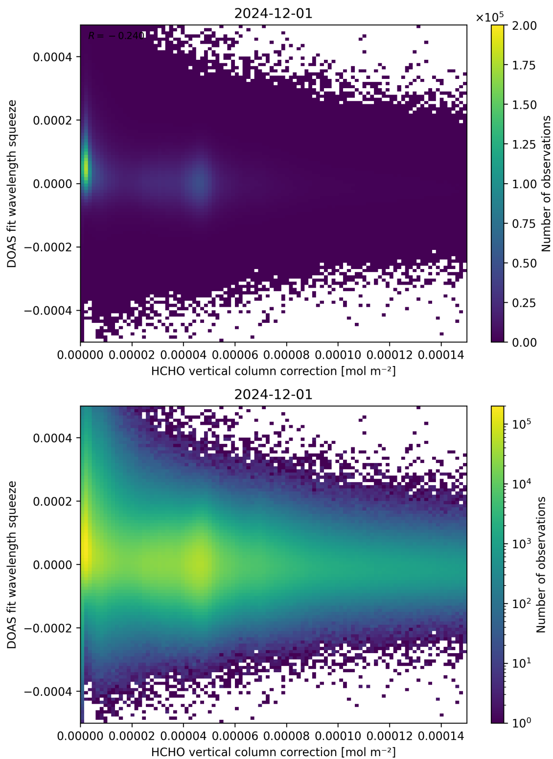
Figure 114: Scatter density plot of “HCHO vertical column correction” against “DOAS fit wavelength squeeze” for 2024-11-30 to 2024-12-02.
