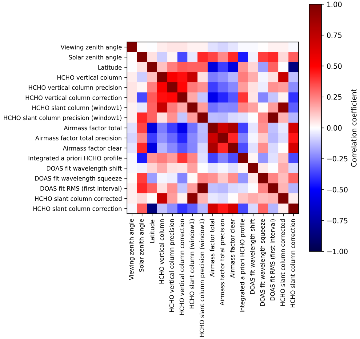
Figure 2: Map of correlation matrix for 2024-11-30 to 2024-12-02.
