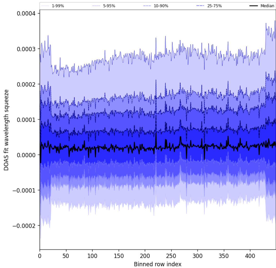
Figure 59: Along track statistics of “DOAS fit wavelength squeeze” for 2024-11-30 to 2024-12-02
