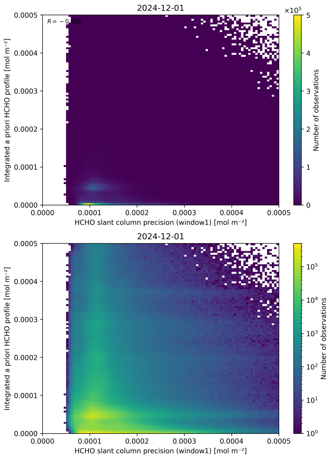
Figure 96: Scatter density plot of “HCHO slant column precision (window1)” against “Integrated a priori HCHO profile” for 2024-11-30 to 2024-12-02.
