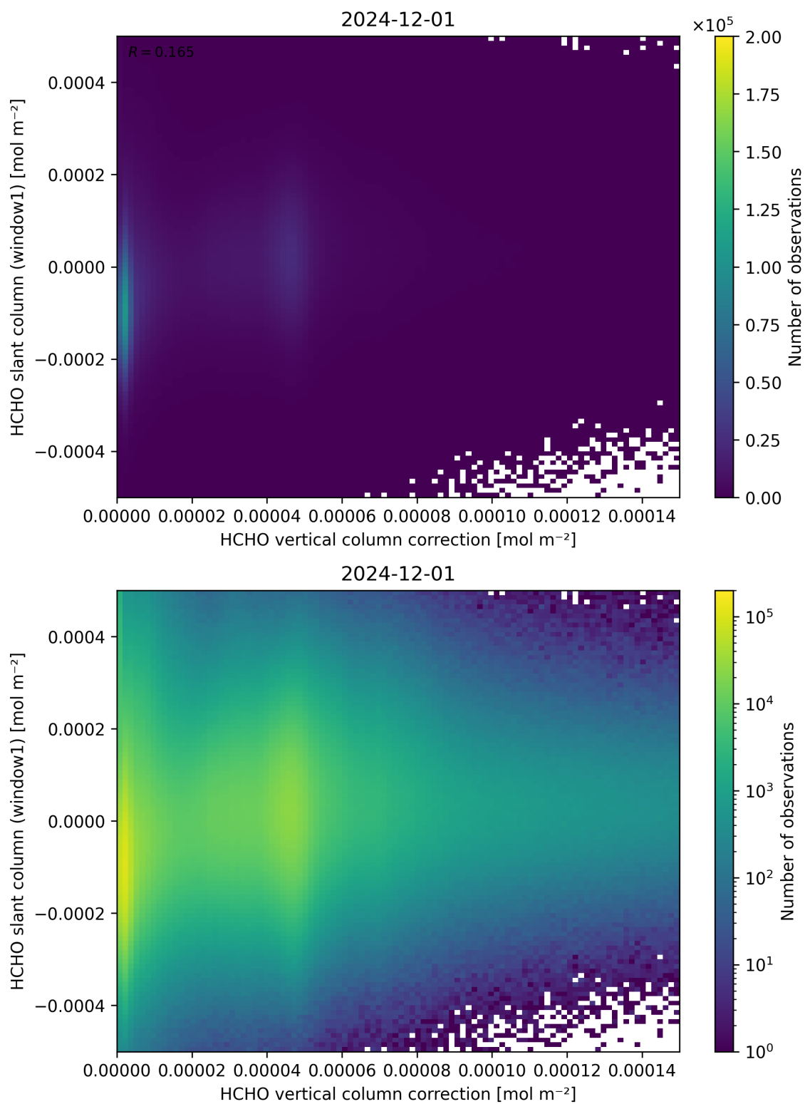
Figure 118: Scatter density plot of “HCHO vertical column correction” against “HCHO slant column (window1)” for 2024-11-30 to 2024-12-02.
