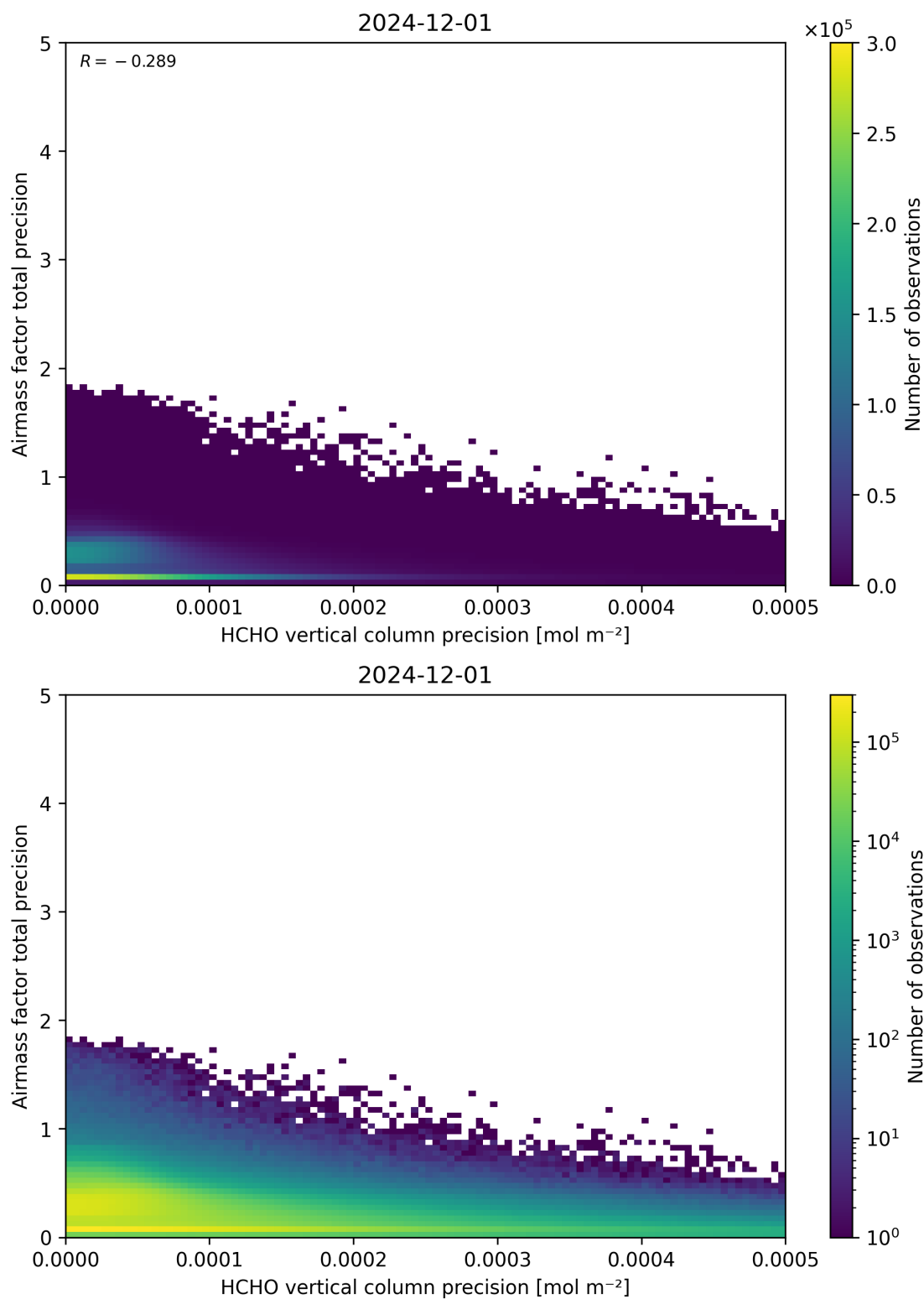
Figure 145: Scatter density plot of “HCHO vertical column precision” against “Airmass factor total precision” for 2024-11-30 to 2024-12-02.
