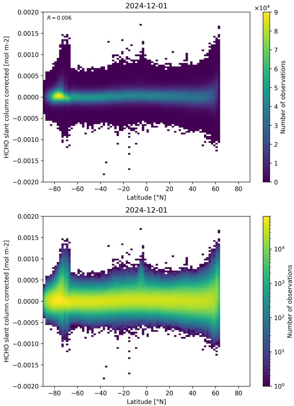
Figure 157: Scatter density plot of “Latitude” against “HCHO slant column corrected” for 2024-11-30 to 2024-12-02.
