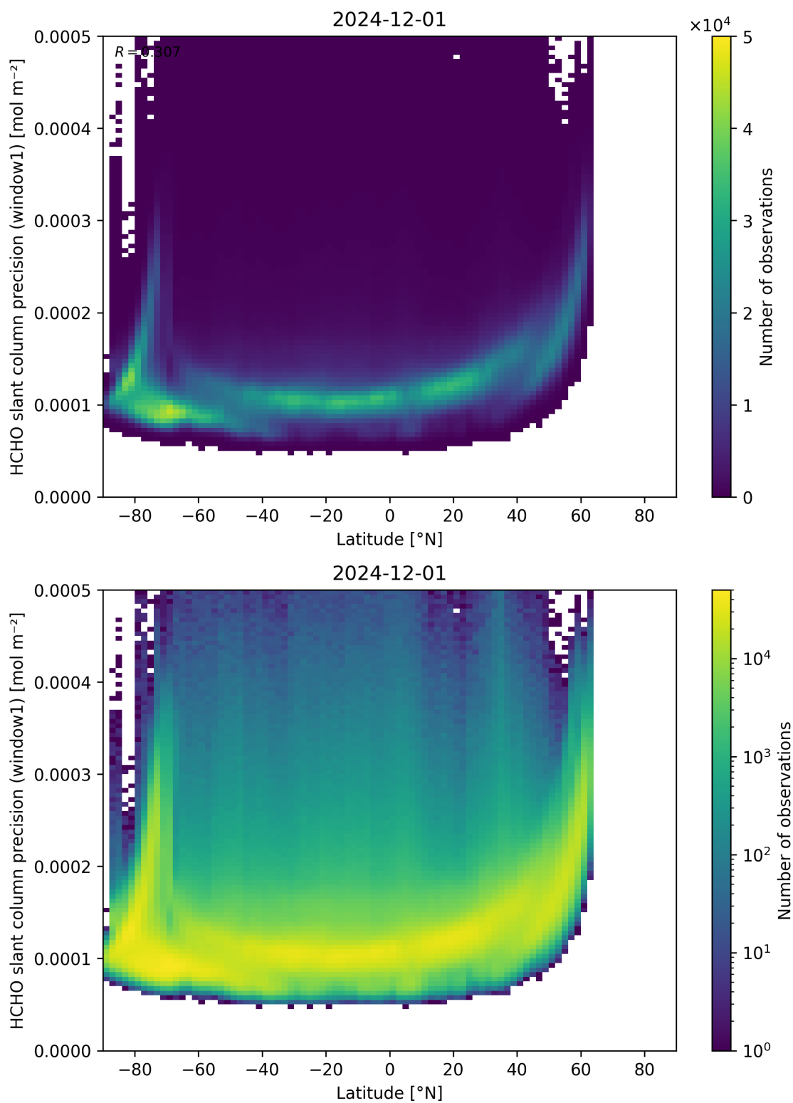
Figure 160: Scatter density plot of “Latitude” against “HCHO slant column precision (window1)” for 2024-11-30 to 2024-12-02.
