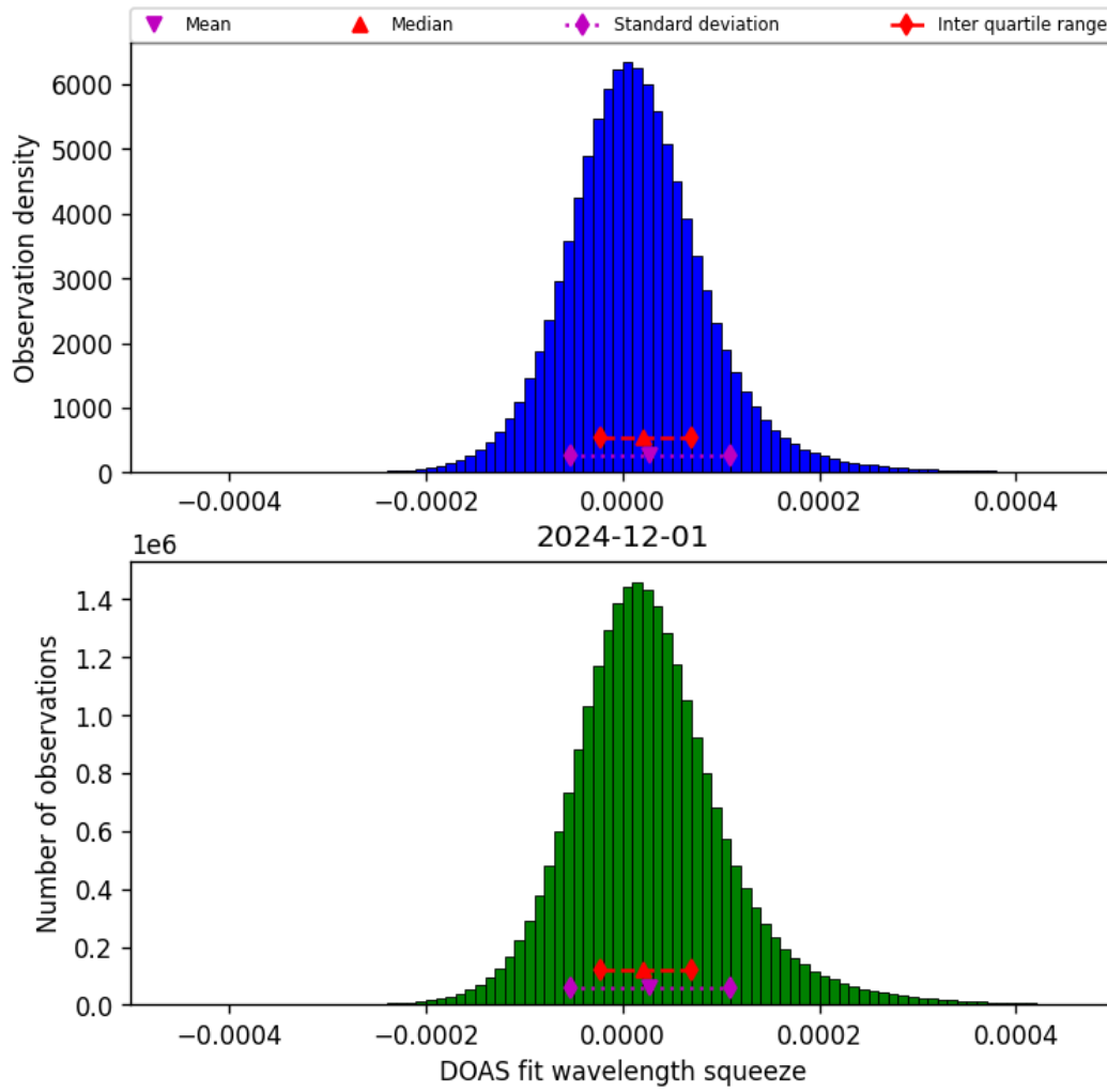
Figure 45: Histogram of “DOAS fit wavelength squeeze” for 2024-11-30 to 2024-12-02
