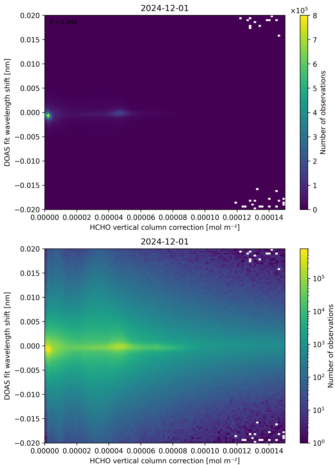
Figure 113: Scatter density plot of “HCHO vertical column correction” against “DOAS fit wavelength shift” for 2024-11-30 to 2024-12-02.
