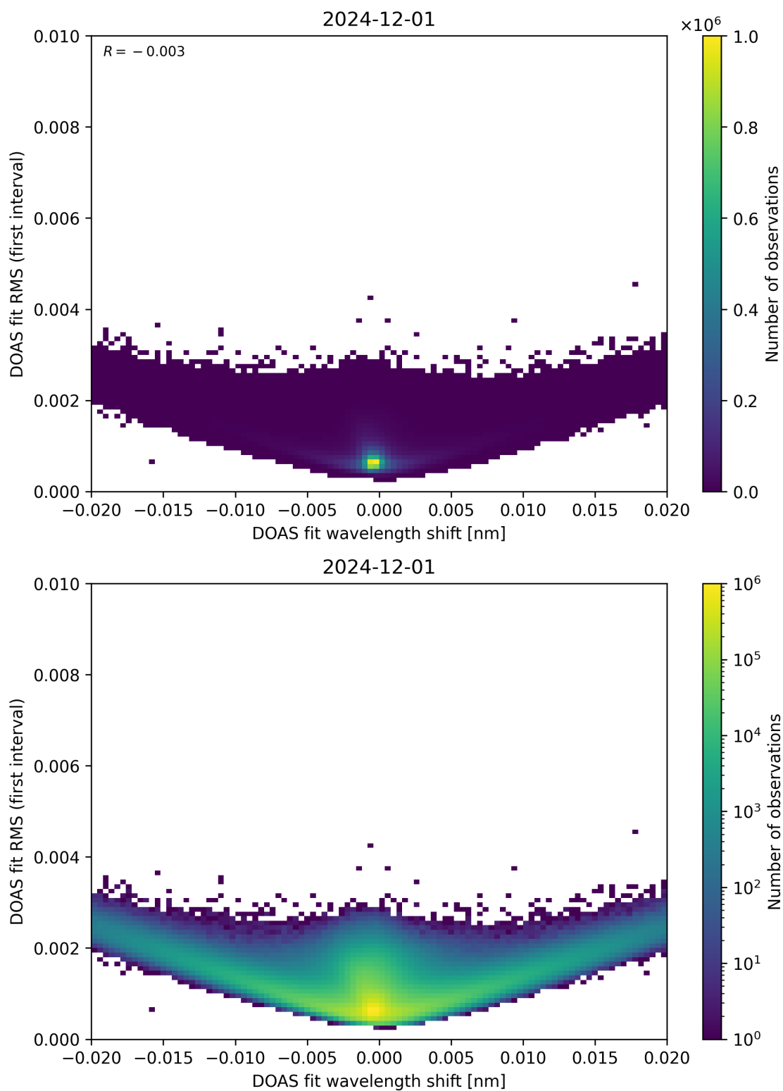
Figure 64: Scatter density plot of “DOAS fit wavelength shift” against “DOAS fit RMS (first interval)” for 2024-11-30 to 2024-12-02.
