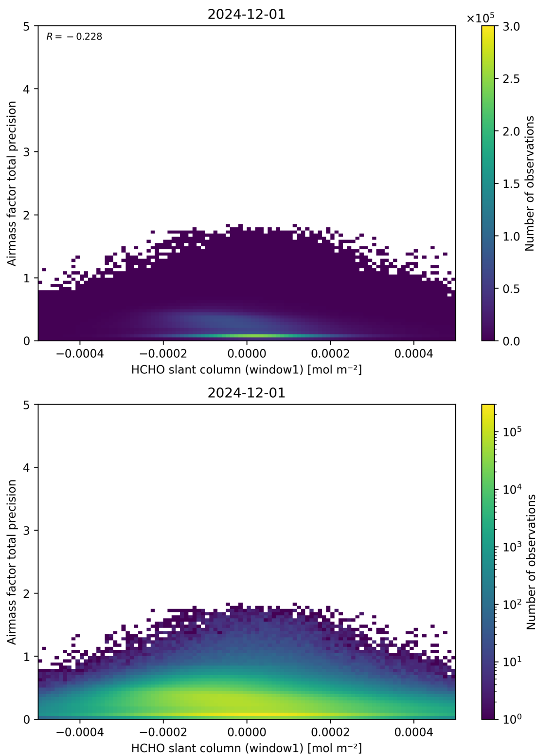
Figure 86: Scatter density plot of “HCHO slant column (window1)” against “Airmass factor total precision” for 2024-11-30 to 2024-12-02.
