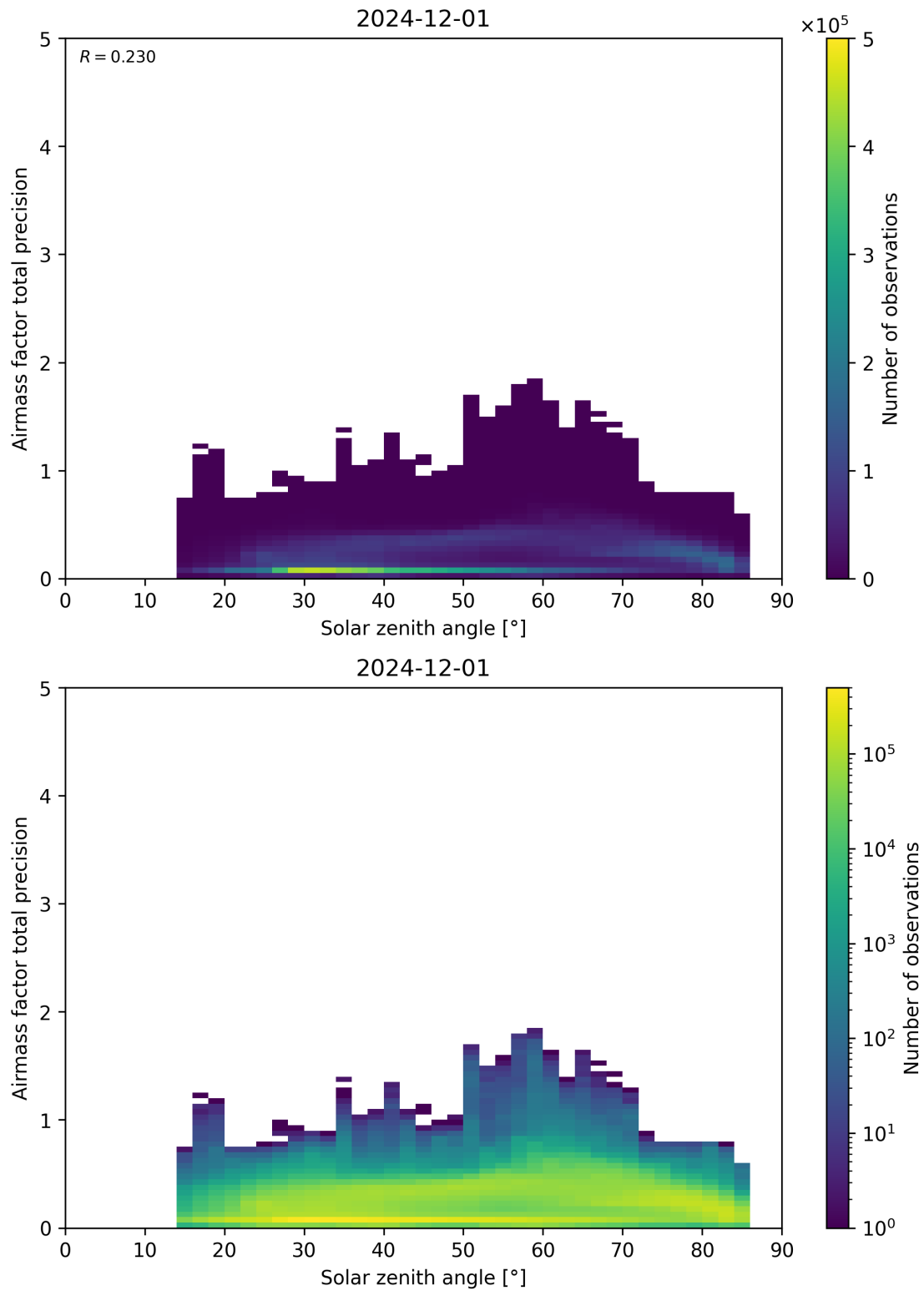
Figure 176: Scatter density plot of “Solar zenith angle” against “Airmass factor total precision” for 2024-11-30 to 2024-12-02.
