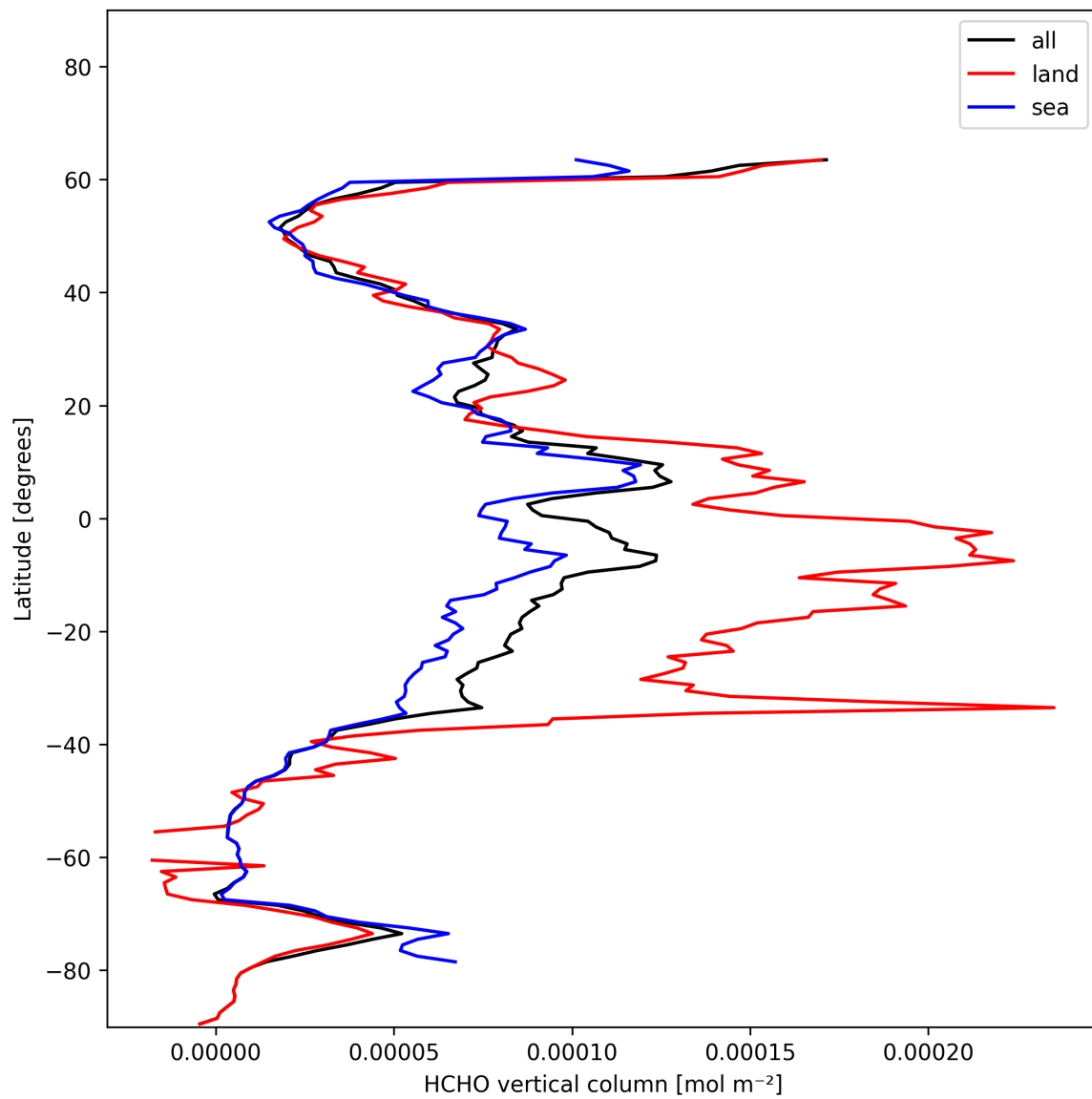
Figure 21: Zonal average of “HCHO vertical column” for 2024-11-30 to 2024-12-02.
