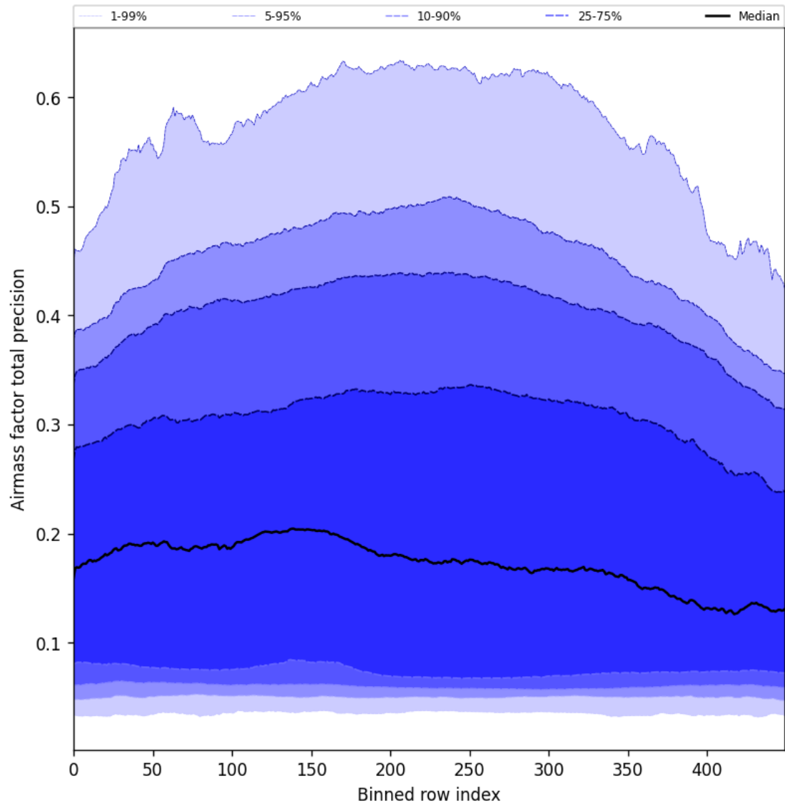
Figure 55: Along track statistics of “Airmass factor total precision” for 2024-11-30 to 2024-12-02
