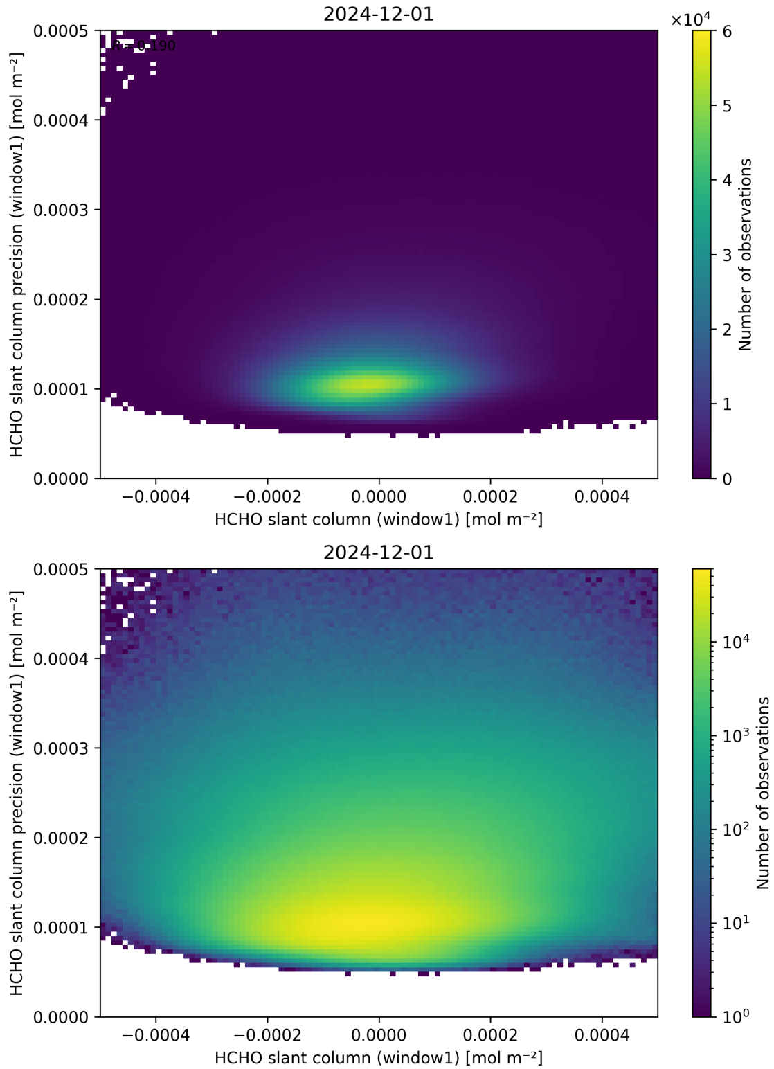
Figure 84: Scatter density plot of “HCHO slant column (window1)” against “HCHO slant column precision (window1)” for 2024-11-30 to 2024-12-02.
