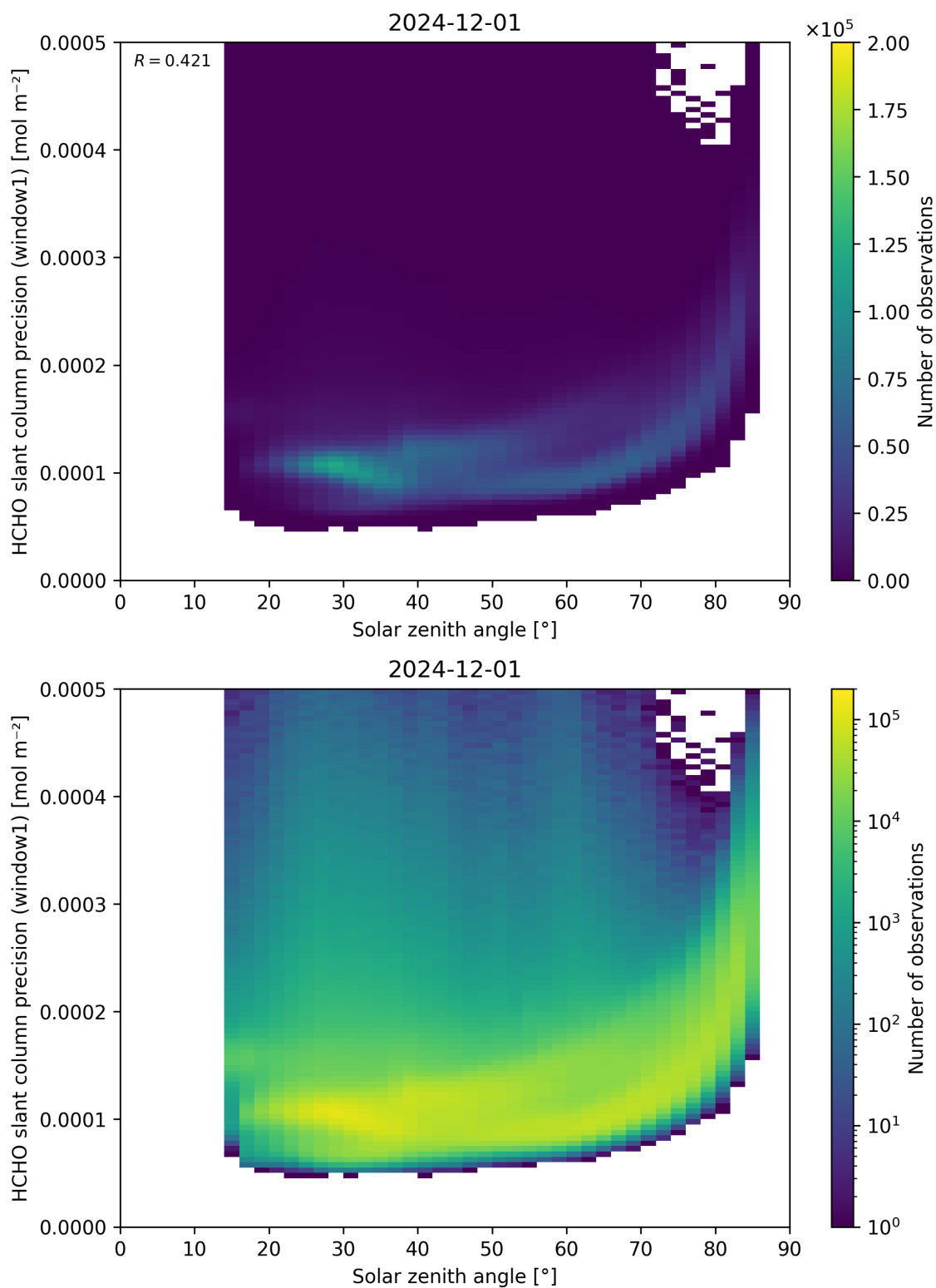
Figure 174: Scatter density plot of “Solar zenith angle” against “HCHO slant column precision (window1)” for 2024-11-30 to 2024-12-02.
