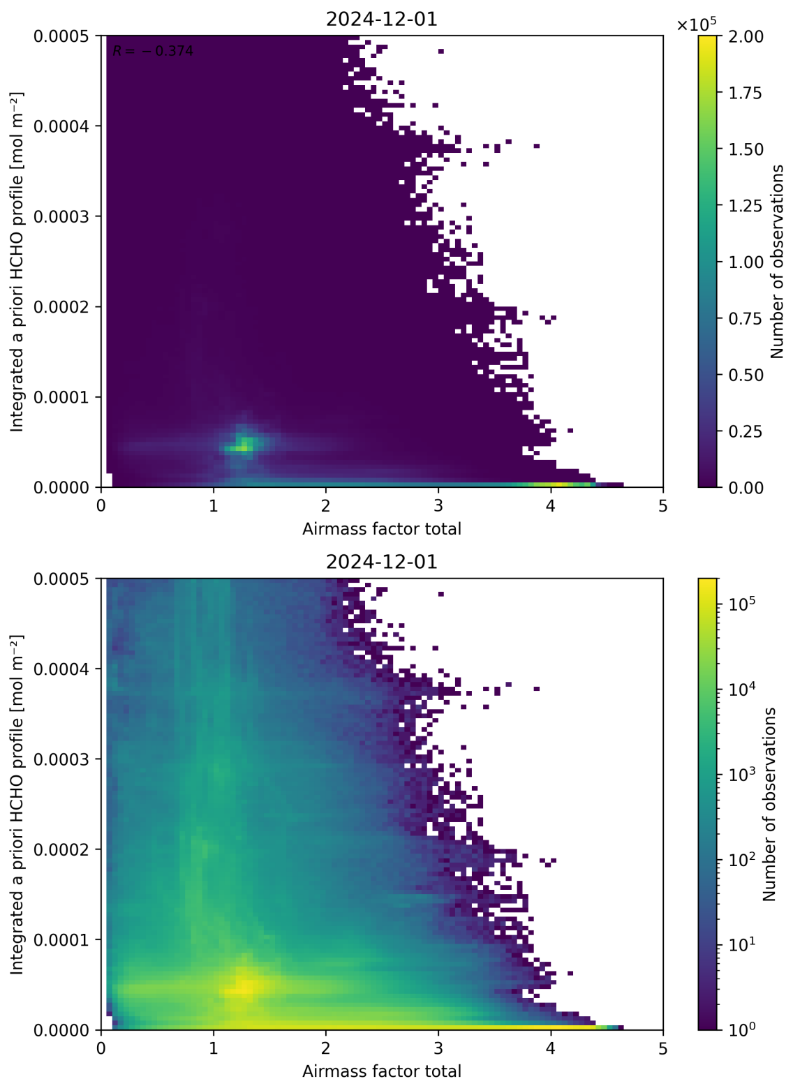
Figure 104: Scatter density plot of “Airmass factor total” against “Integrated a priori HCHO profile” for 2024-11-30 to 2024-12-02.
