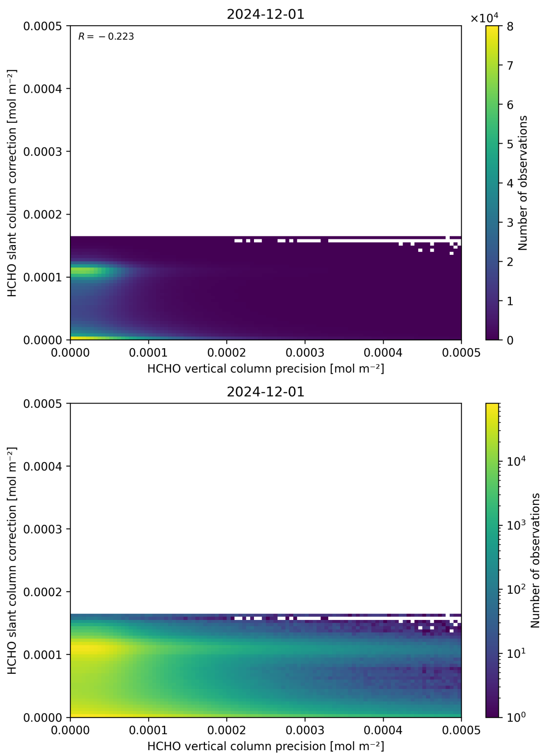
Figure 141: Scatter density plot of “HCHO vertical column precision” against “HCHO slant column correction” for 2024-11-30 to 2024-12-02.
