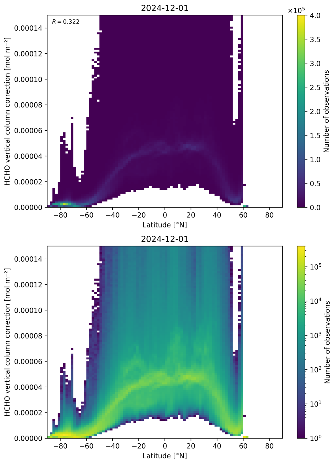
Figure 164: Scatter density plot of “Latitude” against “HCHO vertical column correction” for 2024-11-30 to 2024-12-02.
