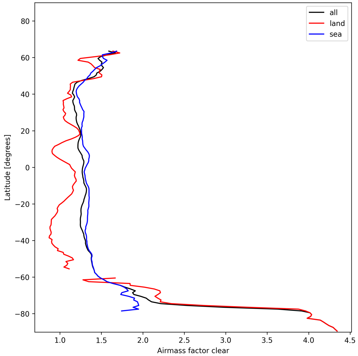
Figure 28: Zonal average of “Airmass factor clear” for 2024-11-30 to 2024-12-02.
