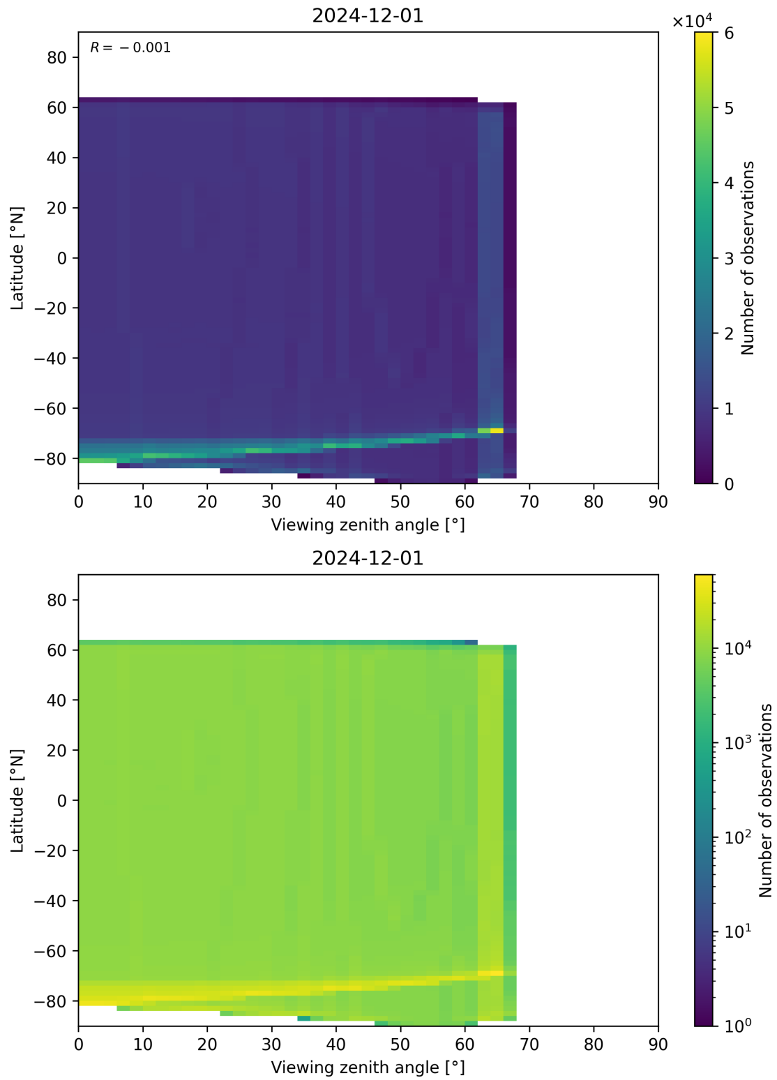
Figure 196: Scatter density plot of “Viewing zenith angle” against “Latitude” for 2024-11-30 to 2024-12-02.
