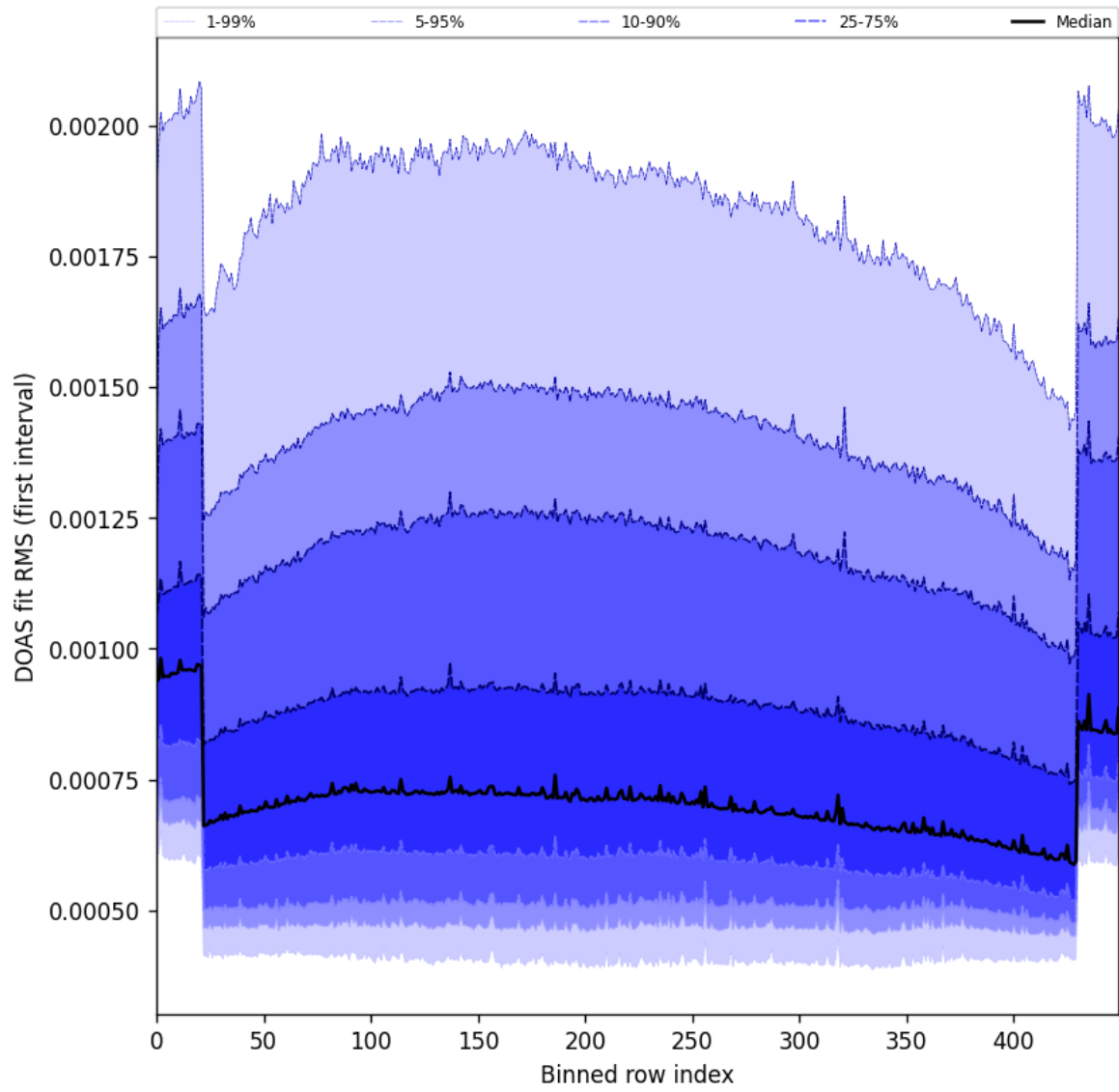
Figure 60: Along track statistics of “DOAS fit RMS (first interval)” for 2024-11-30 to 2024-12-02
