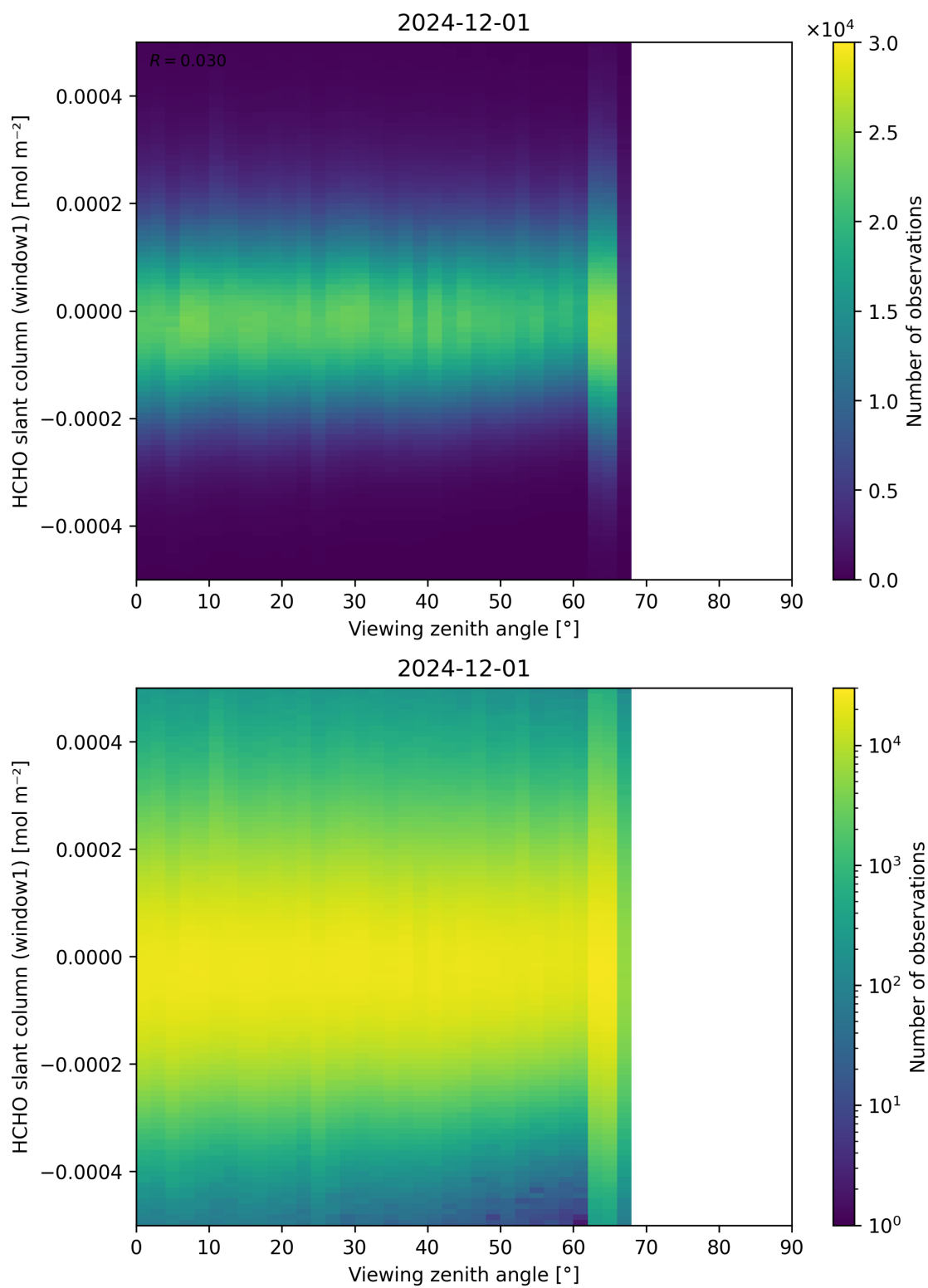
Figure 188: Scatter density plot of “Viewing zenith angle” against “HCHO slant column (window1)” for 2024-11-30 to 2024-12-02.
