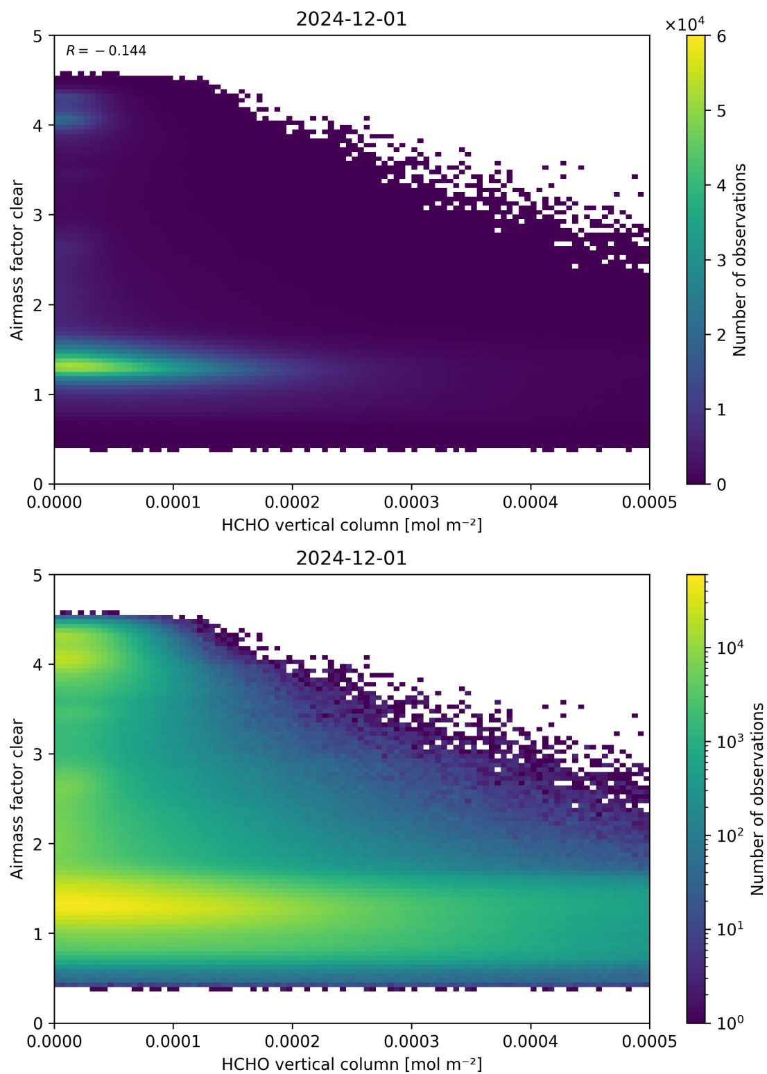
Figure 126: Scatter density plot of “HCHO vertical column” against “Airmass factor clear” for 2024-11-30 to 2024-12-02.
