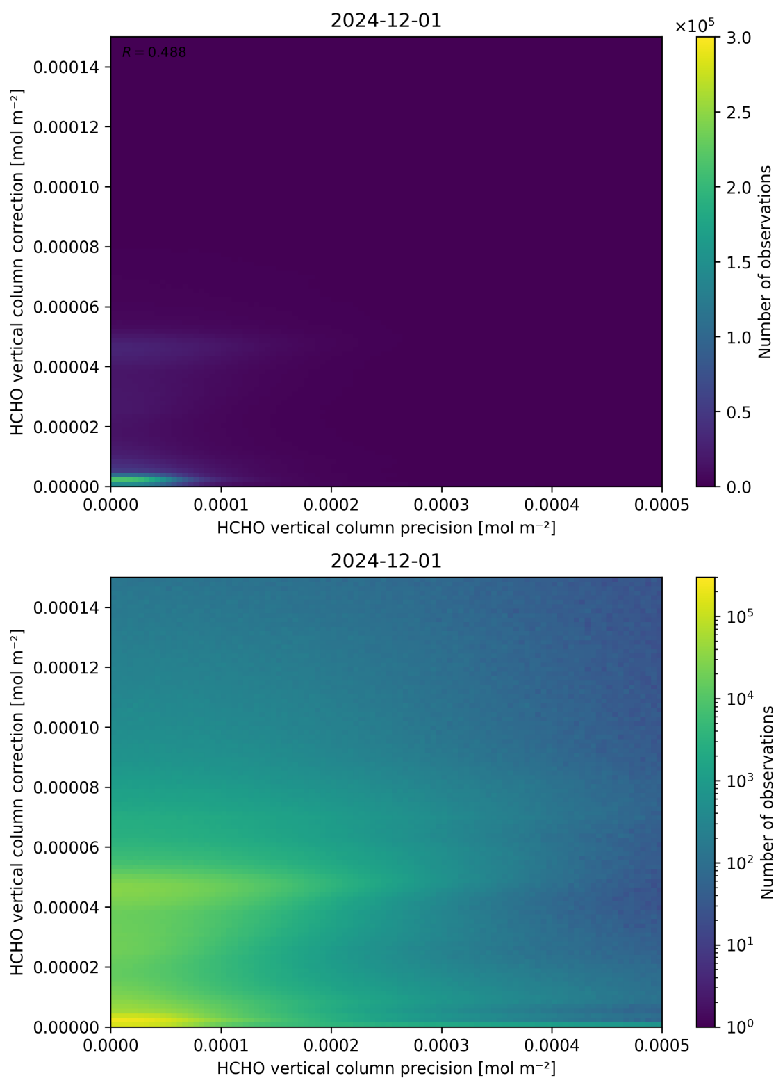
Figure 146: Scatter density plot of “HCHO vertical column precision” against “HCHO vertical column correction” for 2024-11-30 to 2024-12-02.
