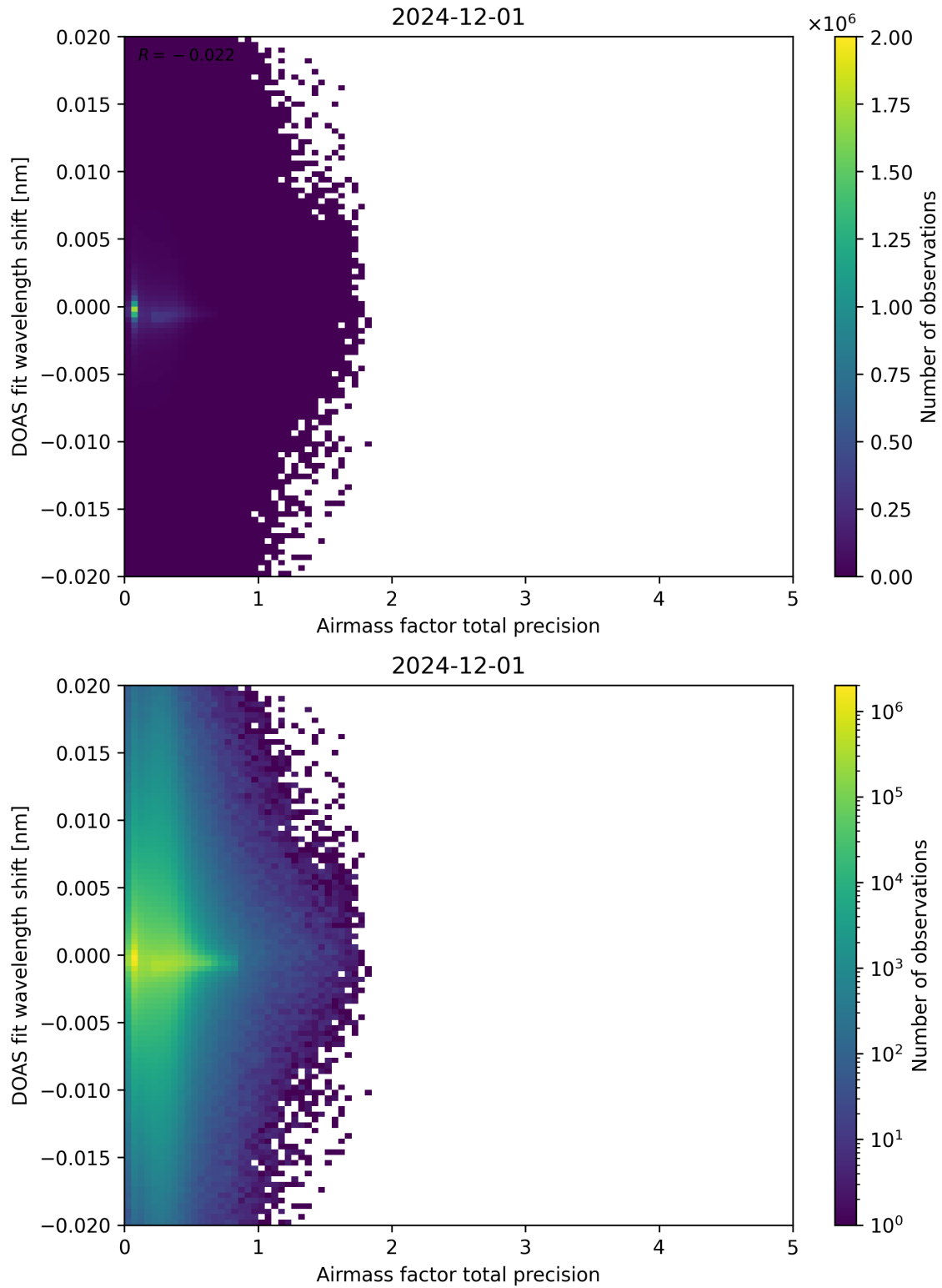
Figure 106: Scatter density plot of “Airmass factor total precision” against “DOAS fit wavelength shift” for 2024-11-30 to 2024-12-02.
