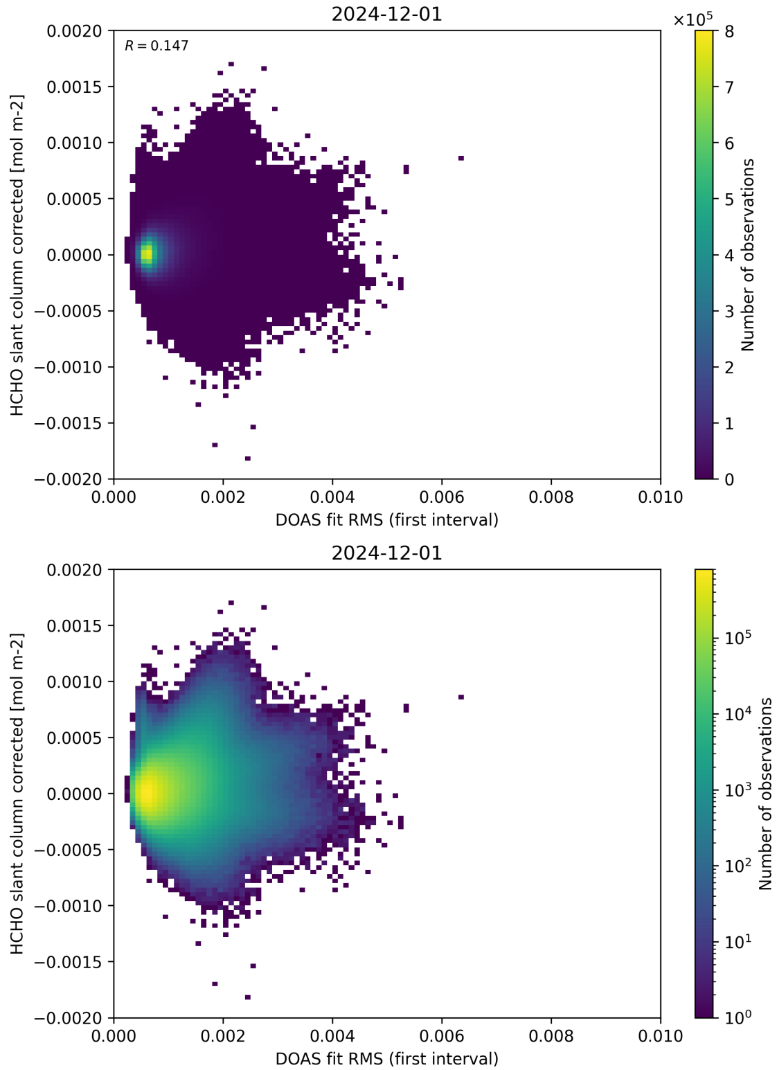
Figure 62: Scatter density plot of “DOAS fit RMS (first interval)” against “HCHO slant column corrected” for 2024-11-30 to 2024-12-02.
