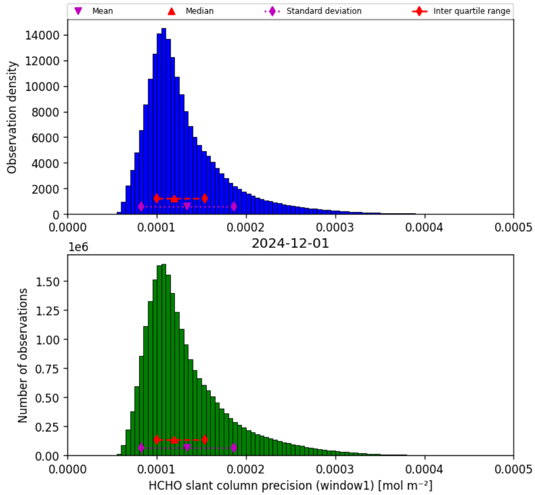
Figure 39: Histogram of “HCHO slant column precision (window1)” for 2024-11-30 to 2024-12-02
