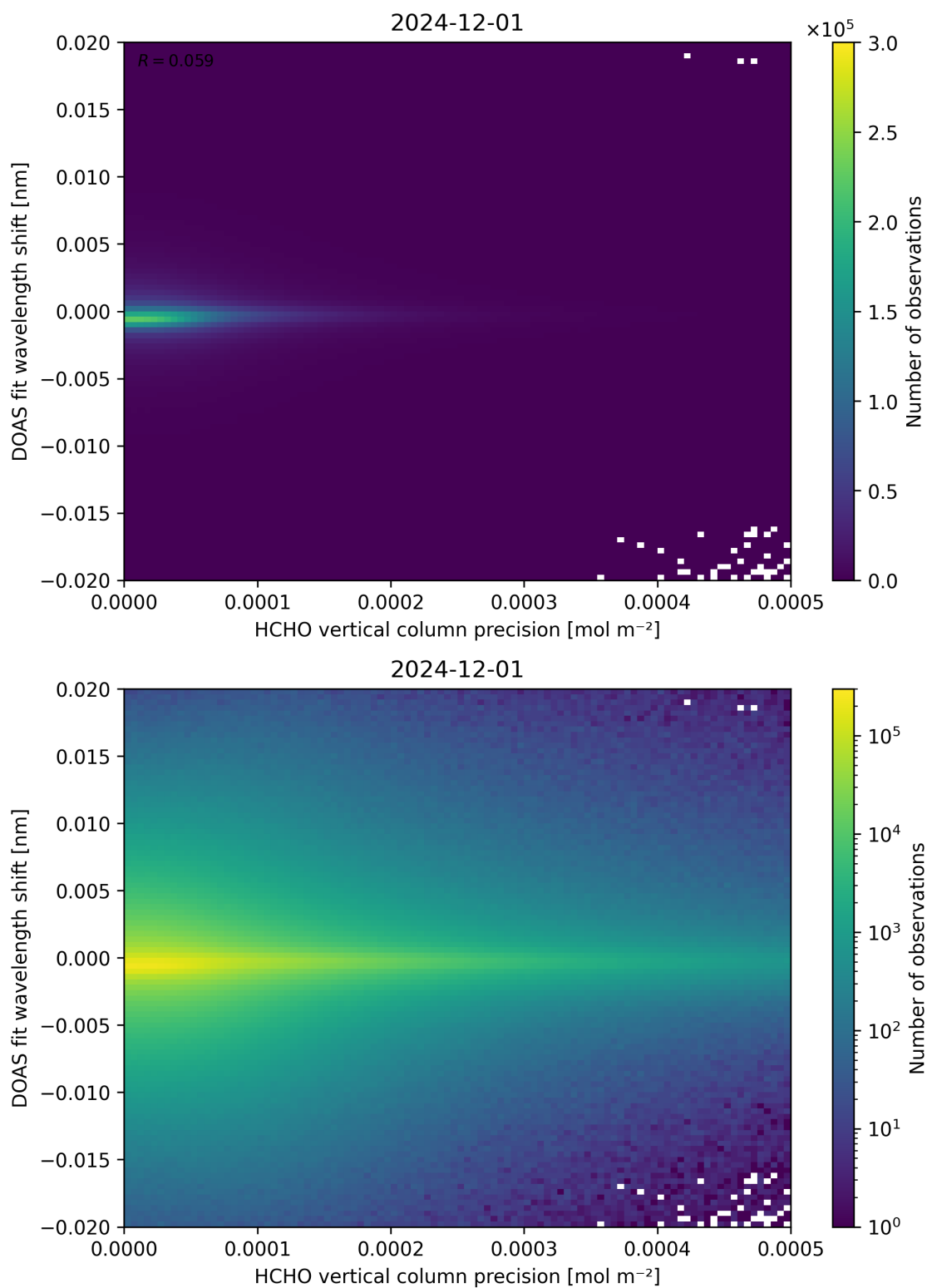
Figure 137: Scatter density plot of “HCHO vertical column precision” against “DOAS fit wavelength shift” for 2024-11-30 to 2024-12-02.
