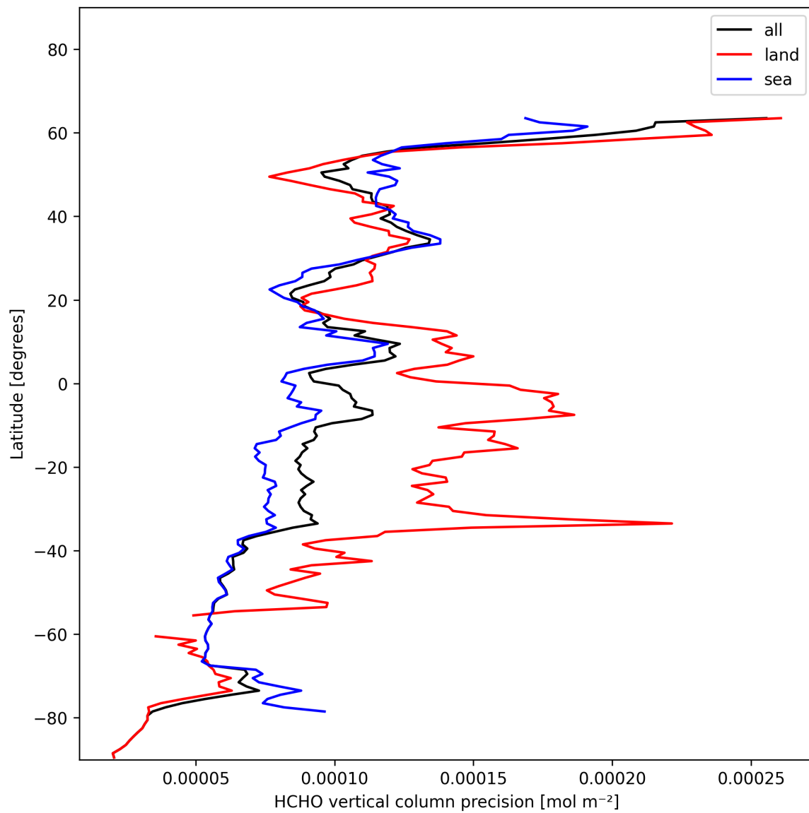
Figure 22: Zonal average of “HCHO vertical column precision” for 2024-11-30 to 2024-12-02.
