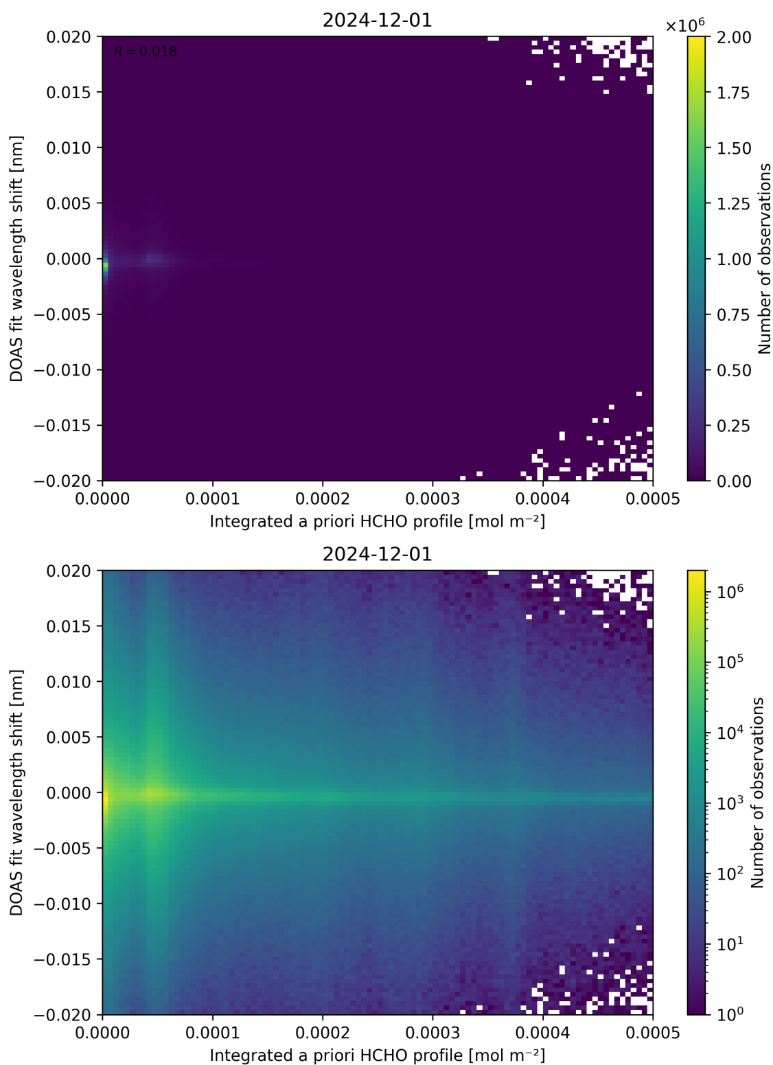
Figure 149: Scatter density plot of “Integrated a priori HCHO profile” against “DOAS fit wavelength shift” for 2024-11-30 to 2024-12-02.
