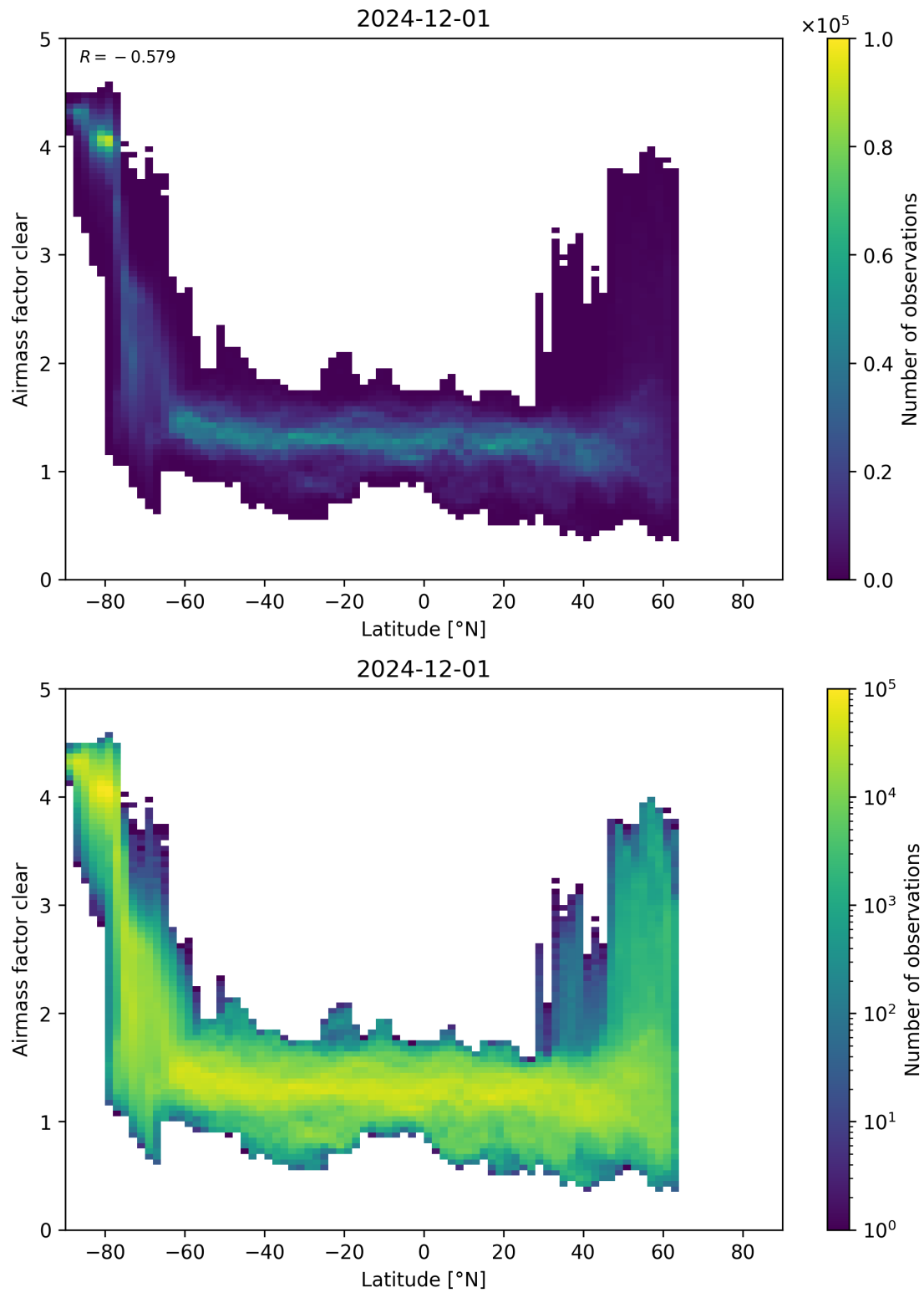
Figure 156: Scatter density plot of “Latitude” against “Airmass factor clear” for 2024-11-30 to 2024-12-02.
