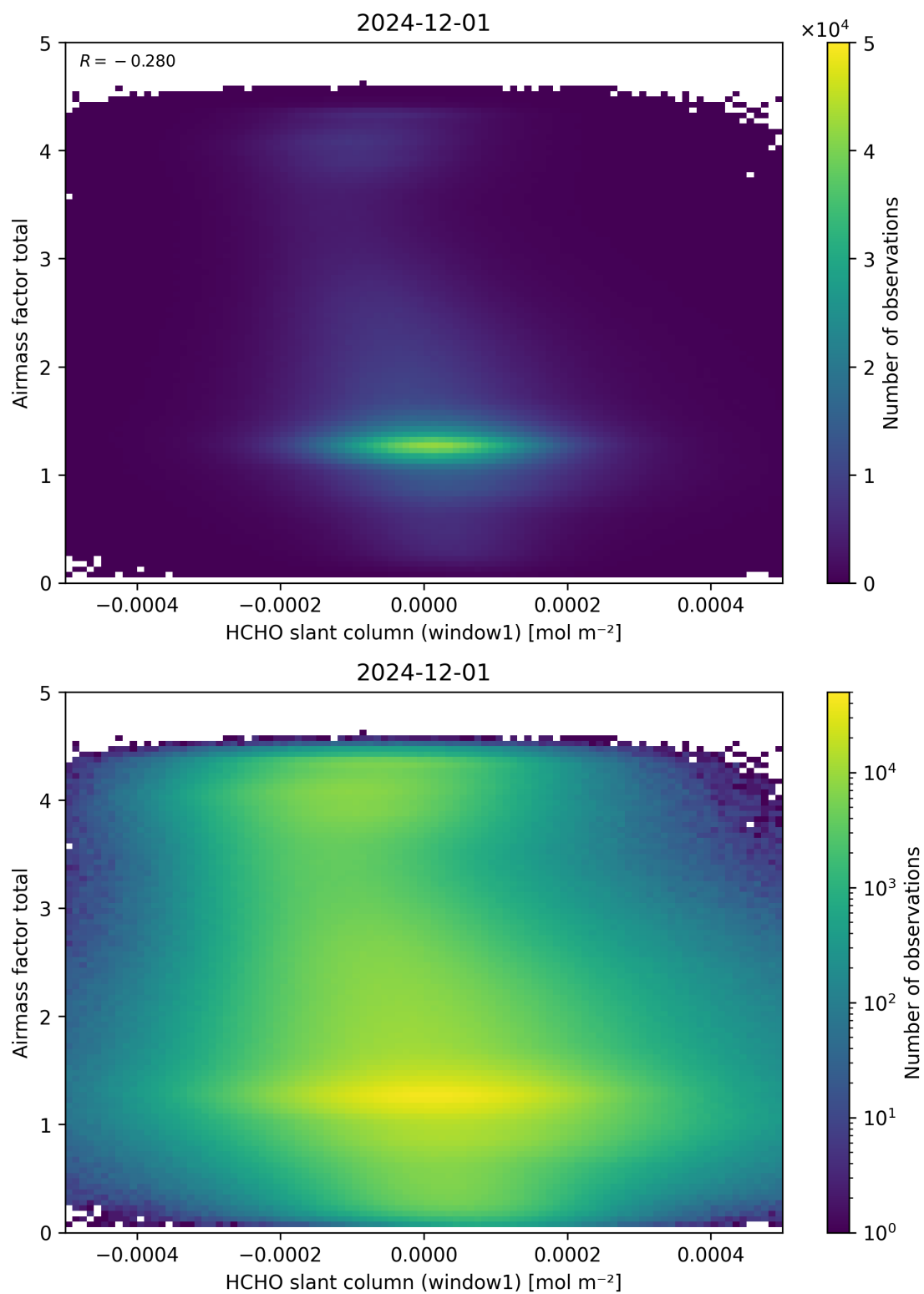
Figure 85: Scatter density plot of “HCHO slant column (window1)” against “Airmass factor total” for 2024-11-30 to 2024-12-02.
