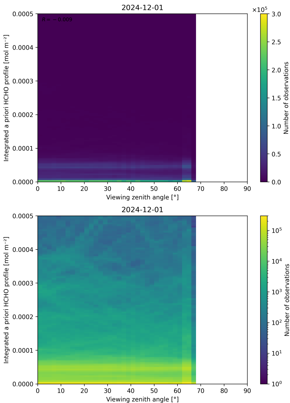
Figure 195: Scatter density plot of “Viewing zenith angle” against “Integrated a priori HCHO profile” for 2024-11-30 to 2024-12-02.
