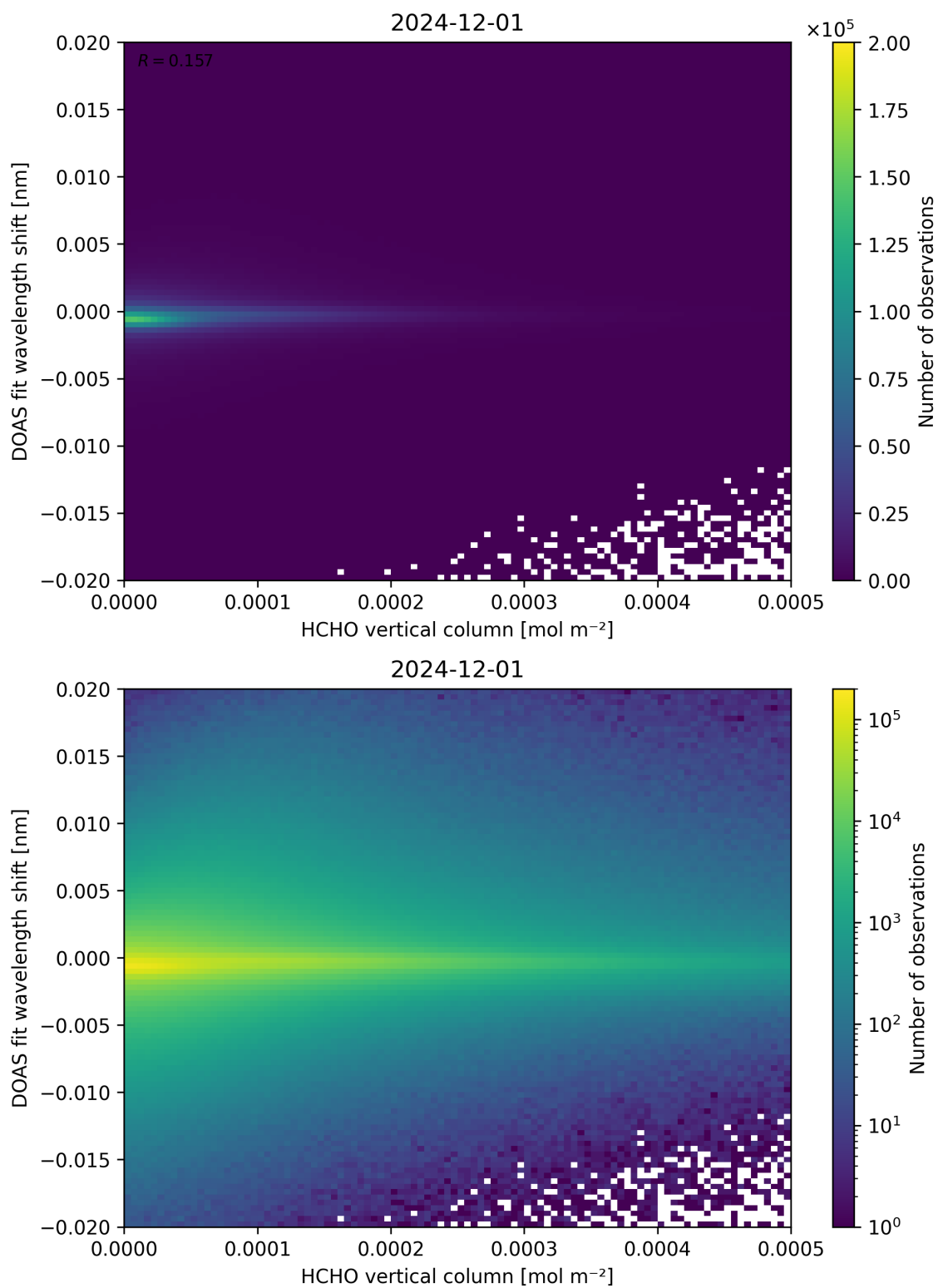
Figure 124: Scatter density plot of “HCHO vertical column” against “DOAS fit wavelength shift” for 2024-11-30 to 2024-12-02.
