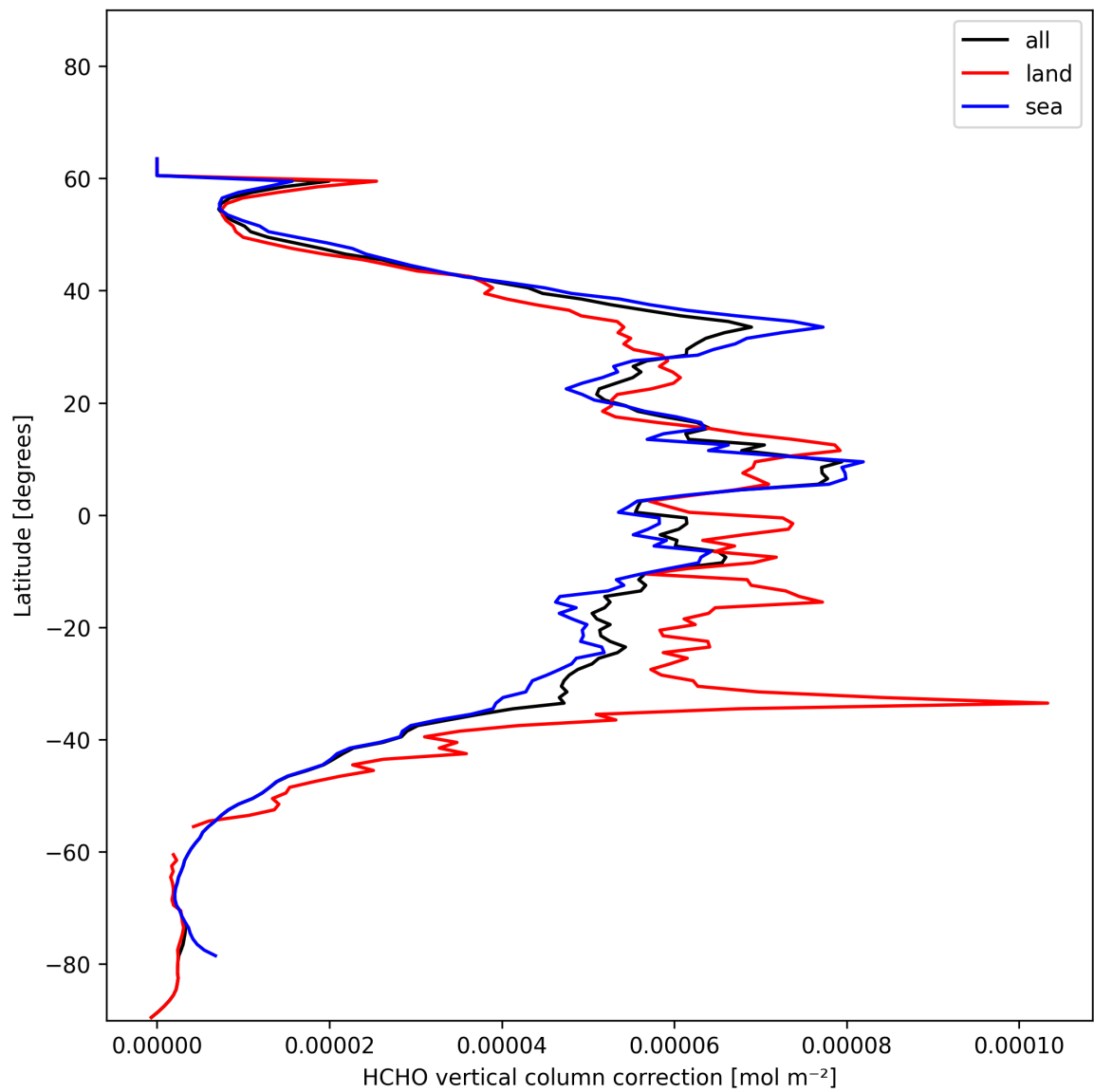
Figure 23: Zonal average of “HCHO vertical column correction” for 2024-11-30 to 2024-12-02.
