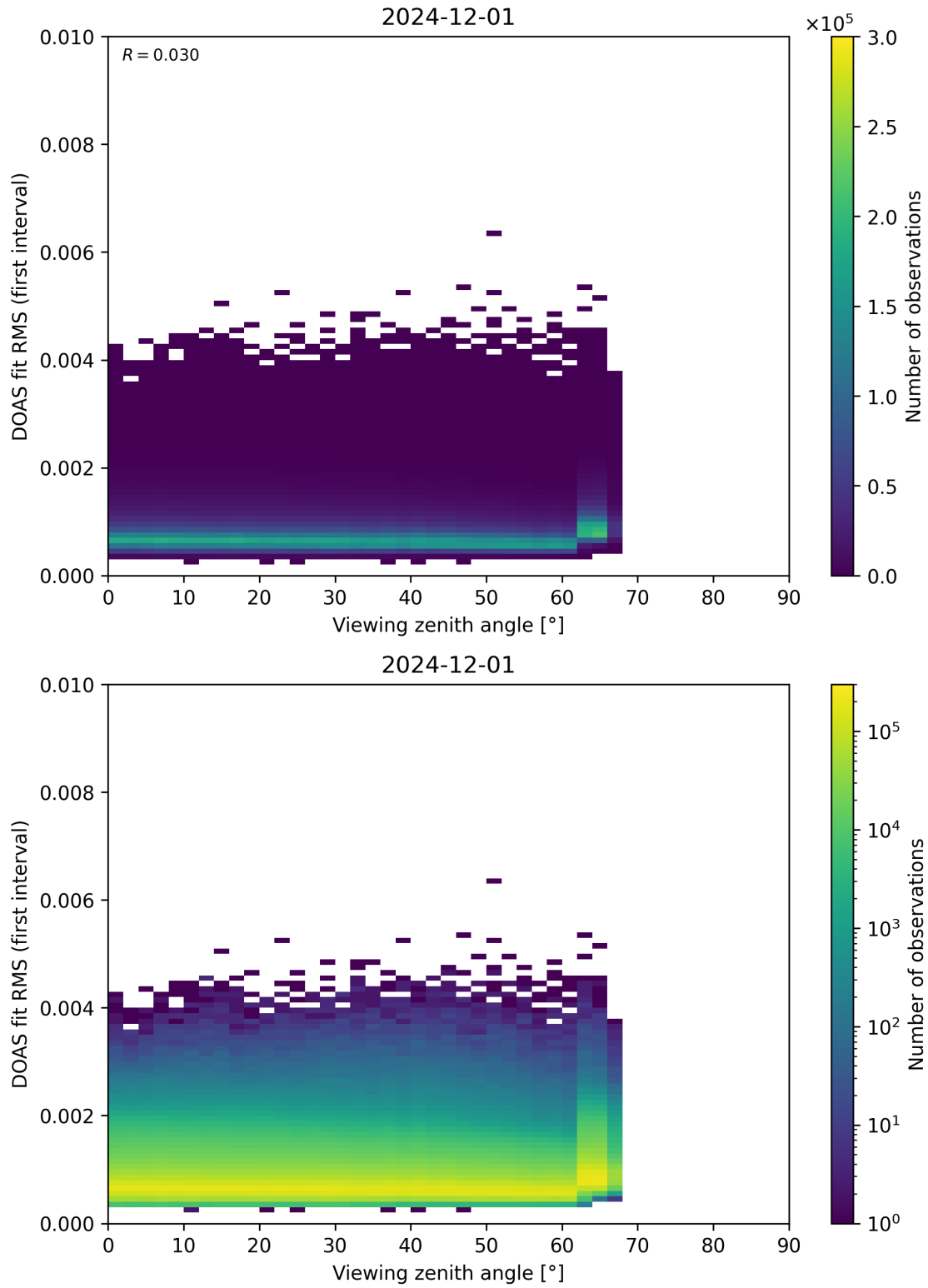
Figure 182: Scatter density plot of “Viewing zenith angle” against “DOAS fit RMS (first interval)” for 2024-11-30 to 2024-12-02.
