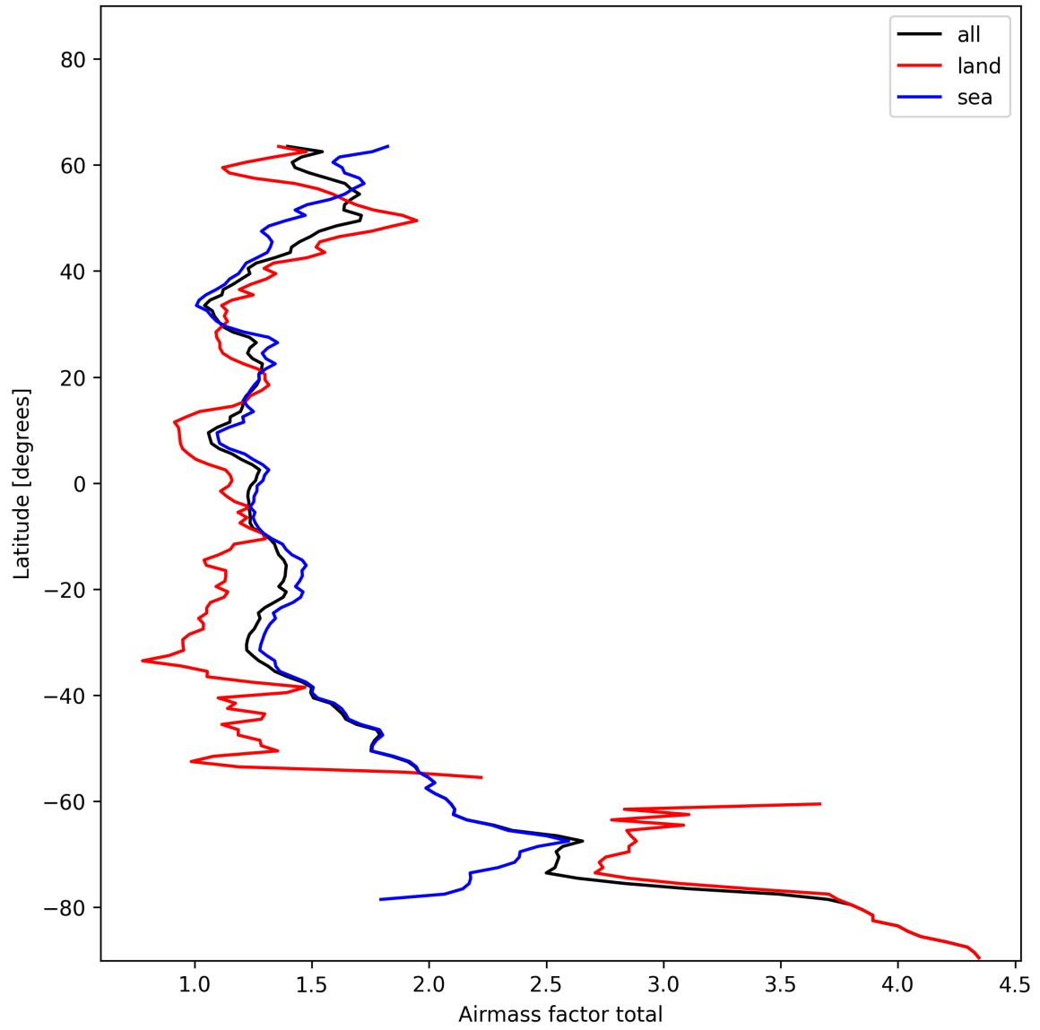
Figure 26: Zonal average of “Airmass factor total” for 2024-11-30 to 2024-12-02.
