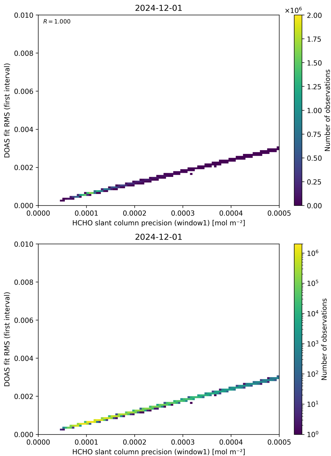
Figure 88: Scatter density plot of “HCHO slant column precision (window1)” against “DOAS fit RMS (first interval)” for 2024-11-30 to 2024-12-02.
