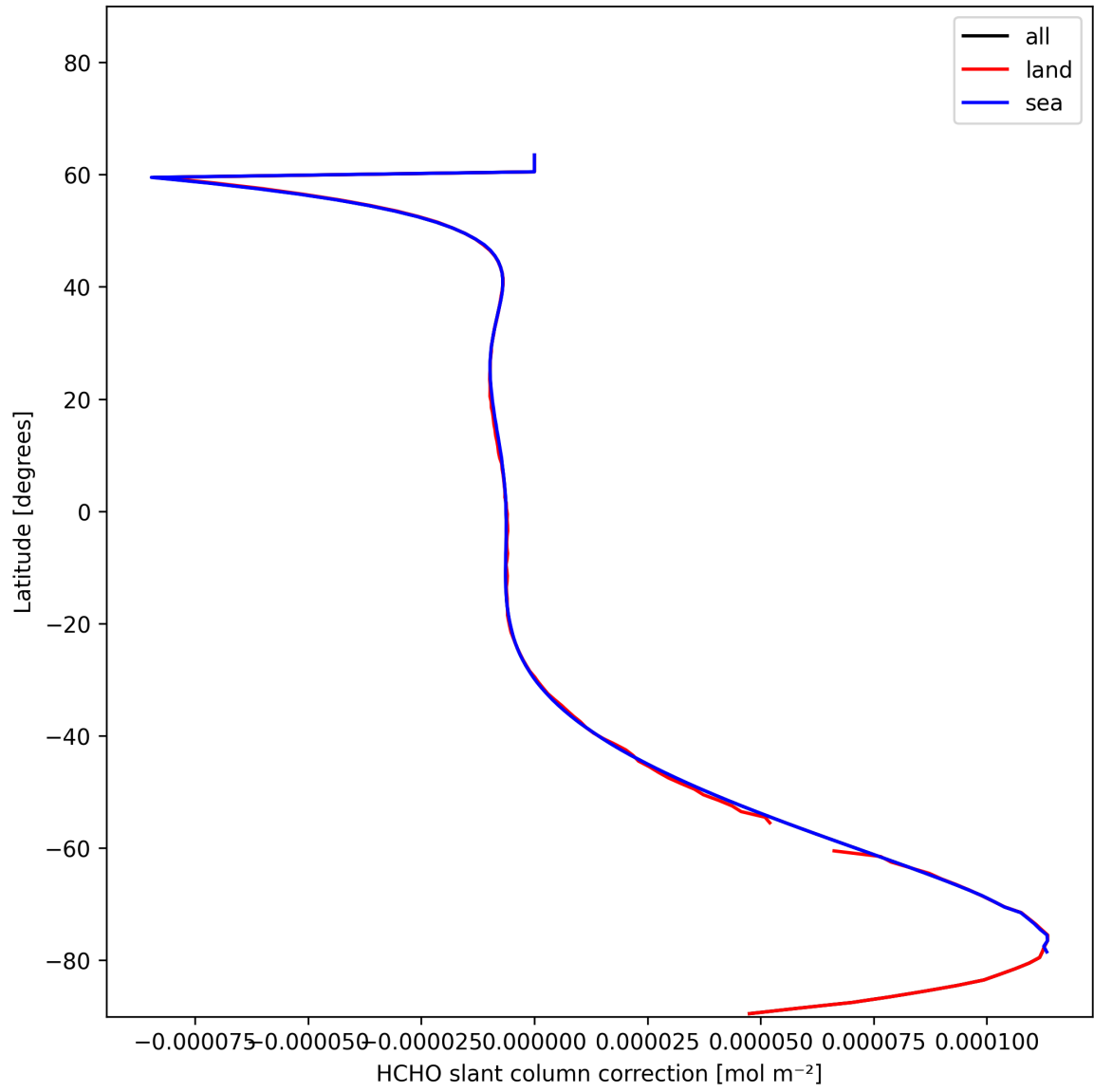
Figure 33: Zonal average of “HCHO slant column correction” for 2024-11-30 to 2024-12-02.
