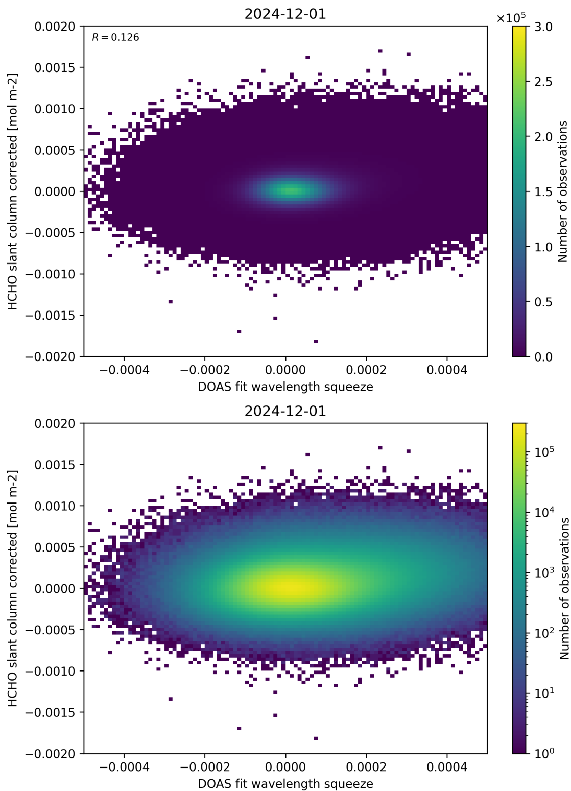
Figure 69: Scatter density plot of “DOAS fit wavelength squeeze” against “HCHO slant column corrected” for 2024-11-30 to 2024-12-02.
