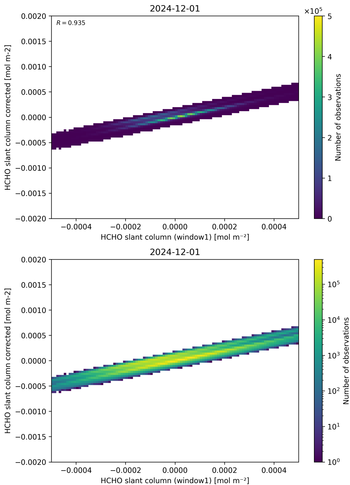
Figure 82: Scatter density plot of “HCHO slant column (window1)” against “HCHO slant column corrected” for 2024-11-30 to 2024-12-02.
