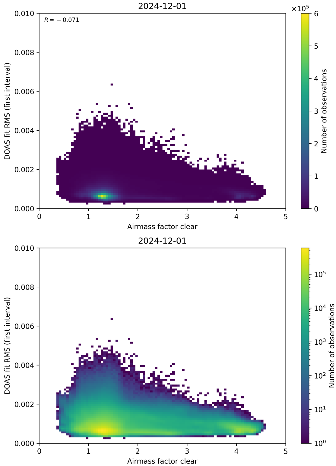
Figure 71: Scatter density plot of “Airmass factor clear” against “DOAS fit RMS (first interval)” for 2024-11-30 to 2024-12-02.
