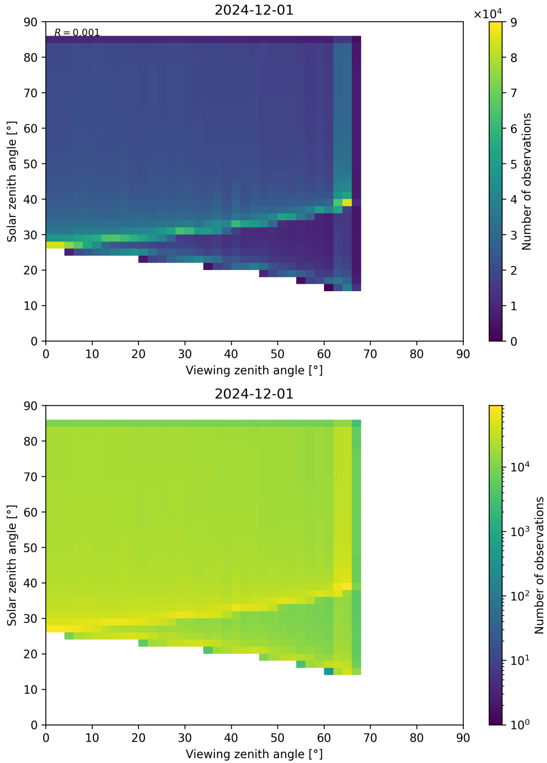
Figure 197: Scatter density plot of “Viewing zenith angle” against “Solar zenith angle” for 2024-11-30 to 2024-12-02.
