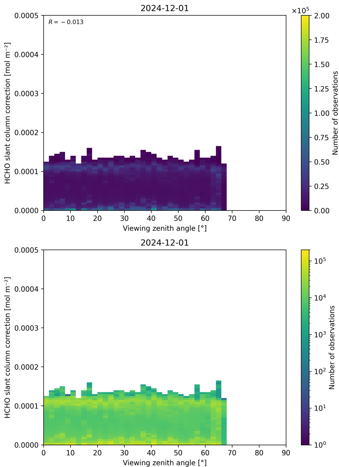
Figure 187: Scatter density plot of “Viewing zenith angle” against “HCHO slant column correction” for 2024-11-30 to 2024-12-02.
