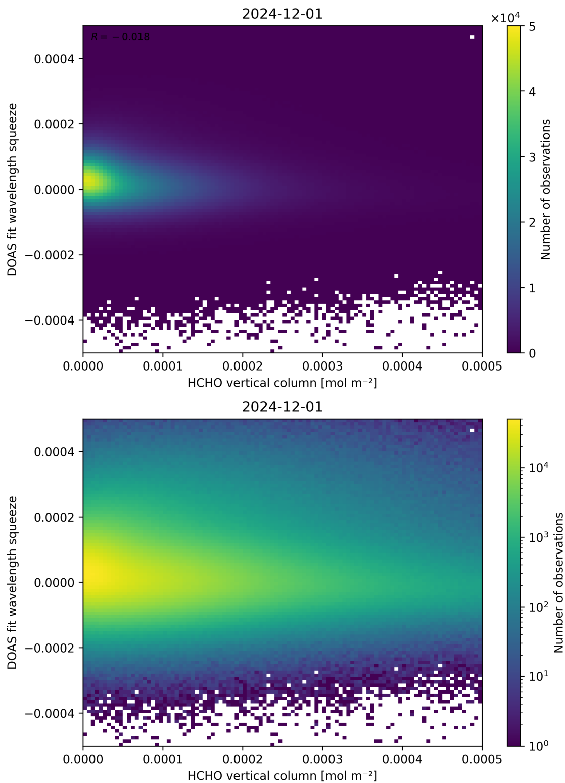
Figure 125: Scatter density plot of “HCHO vertical column” against “DOAS fit wavelength squeeze” for 2024-11-30 to 2024-12-02.
