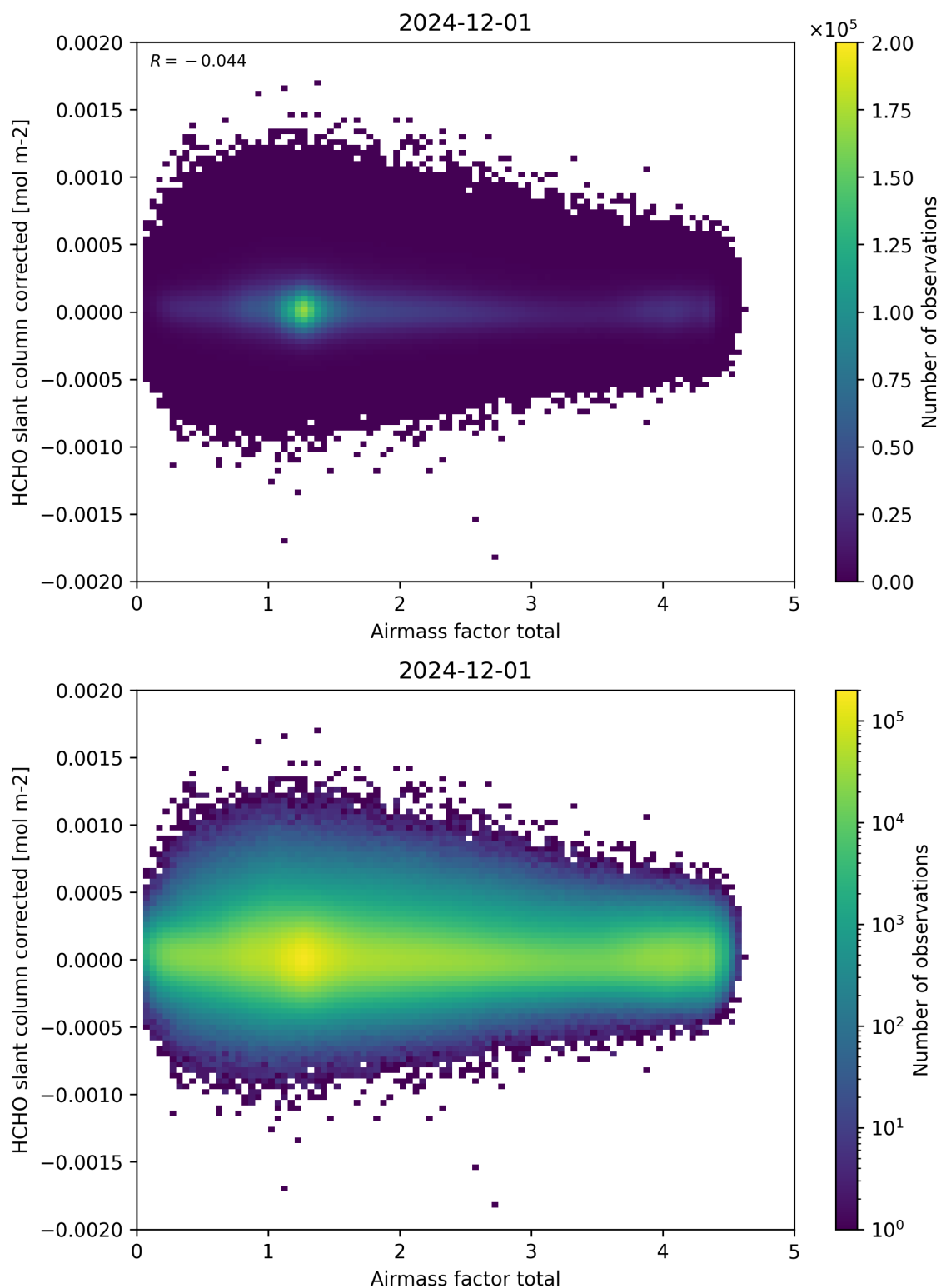
Figure 101: Scatter density plot of “Airmass factor total” against “HCHO slant column corrected” for 2024-11-30 to 2024-12-02.
