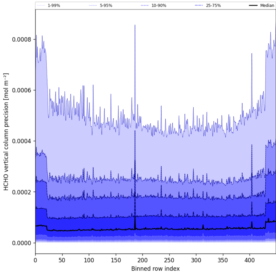
Figure 50: Along track statistics of “HCHO vertical column precision” for 2024-11-30 to 2024-12-02
