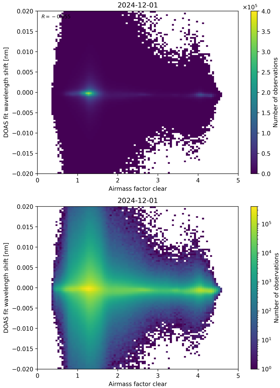
Figure 72: Scatter density plot of “Airmass factor clear” against “DOAS fit wavelength shift” for 2024-11-30 to 2024-12-02.
