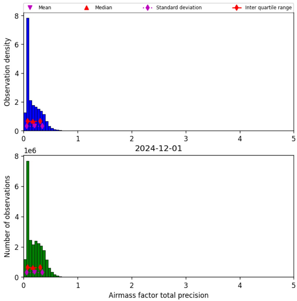
Figure 41: Histogram of “Airmass factor total precision” for 2024-11-30 to 2024-12-02
