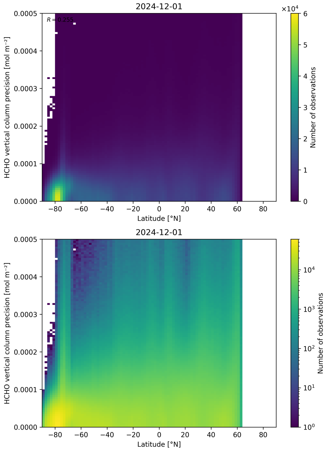
Figure 165: Scatter density plot of “Latitude” against “HCHO vertical column precision” for 2024-11-30 to 2024-12-02.
