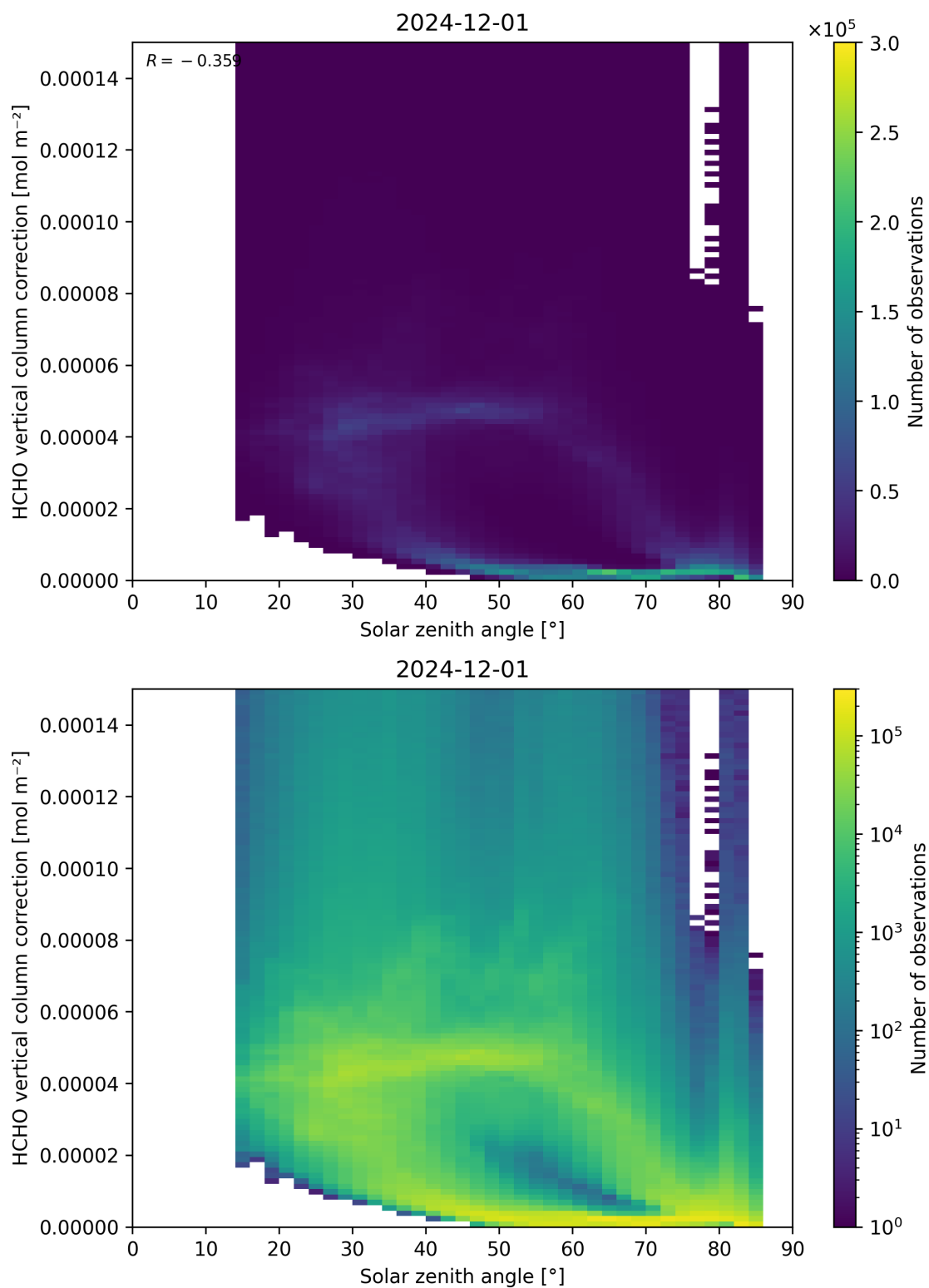
Figure 178: Scatter density plot of “Solar zenith angle” against “HCHO vertical column correction” for 2024-11-30 to 2024-12-02.
