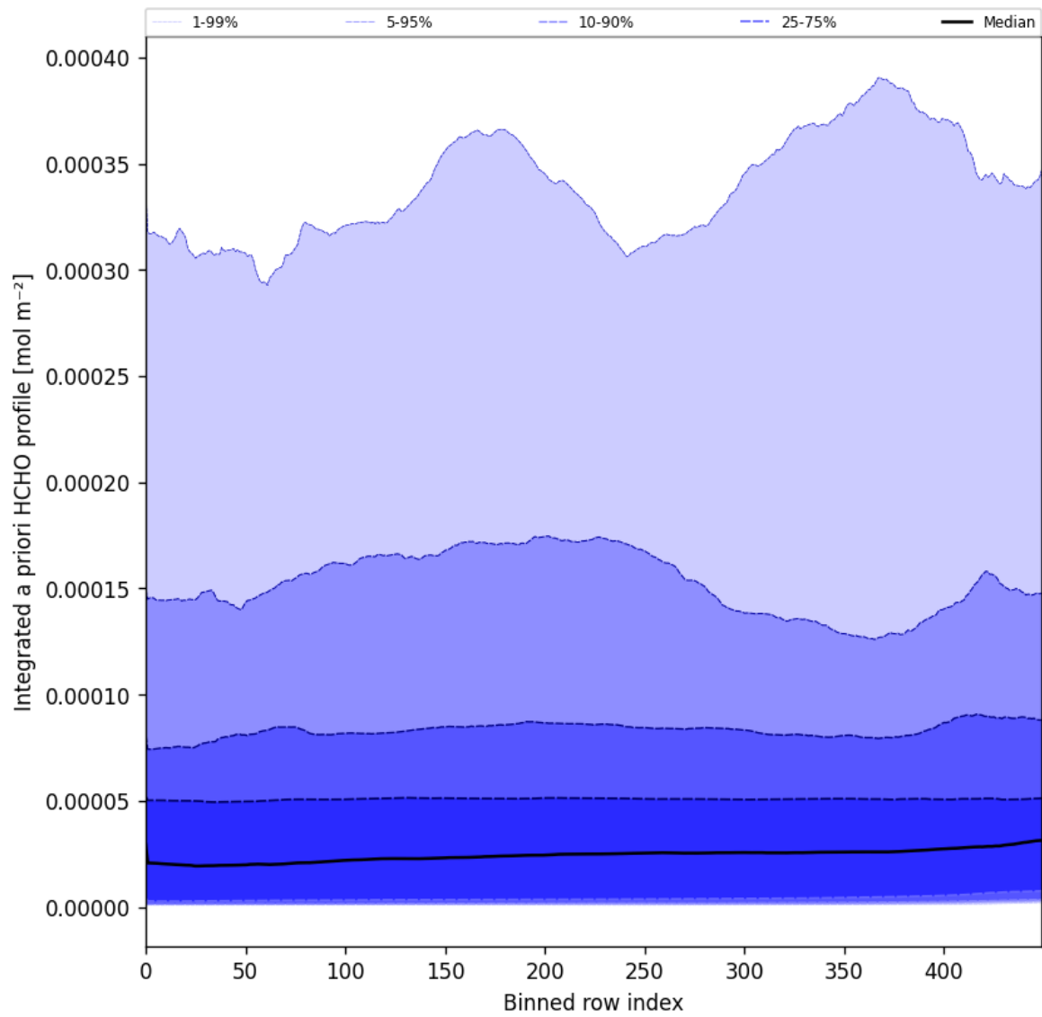
Figure 57: Along track statistics of “Integrated a priori HCHO profile” for 2024-11-30 to 2024-12-02
