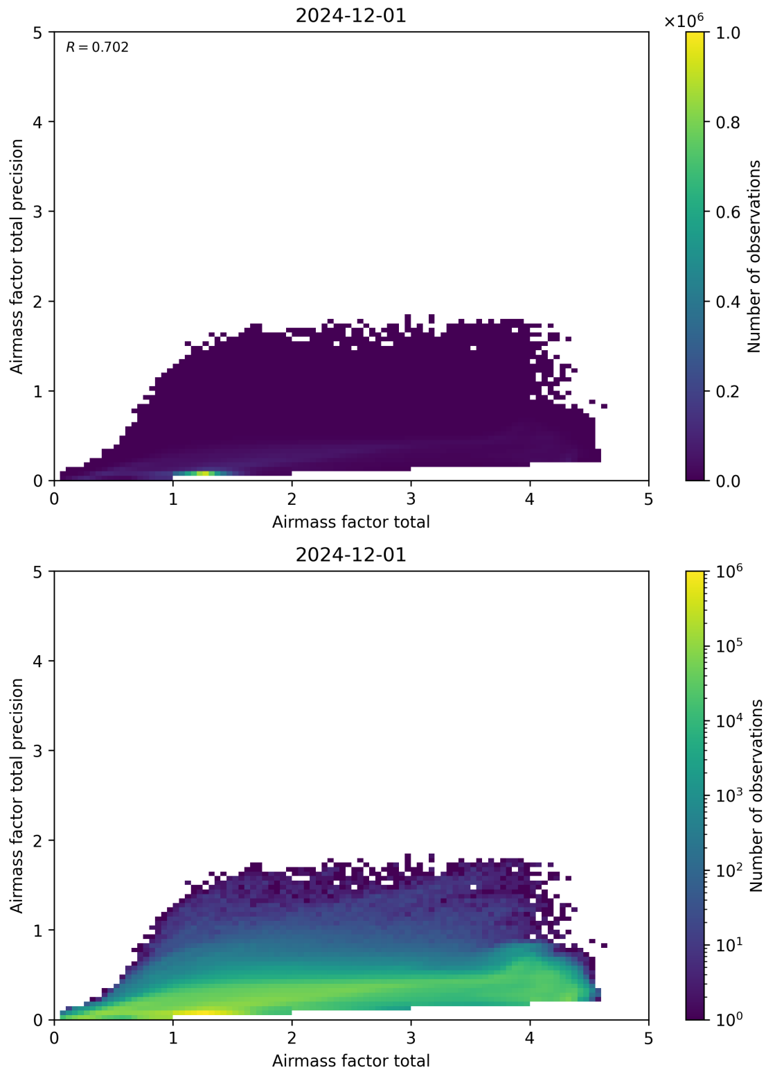
Figure 103: Scatter density plot of “Airmass factor total” against “Airmass factor total precision” for 2024-11-30 to 2024-12-02.
