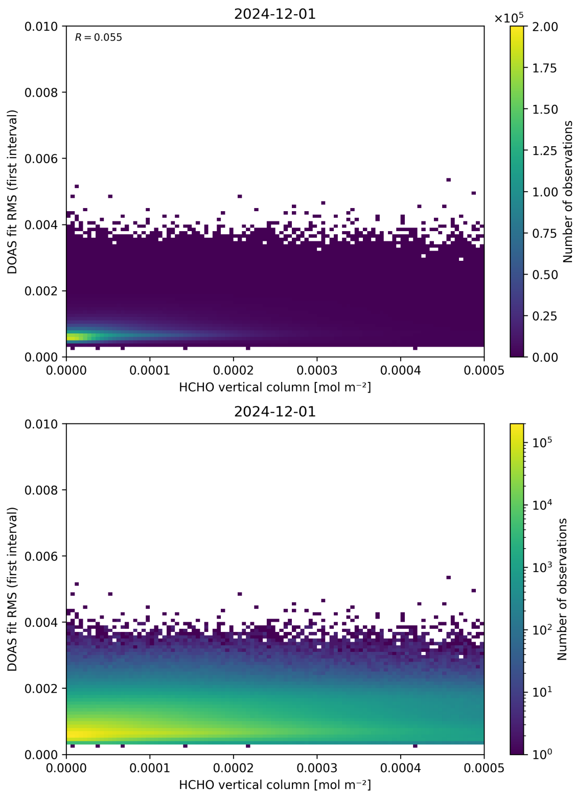
Figure 123: Scatter density plot of “HCHO vertical column” against “DOAS fit RMS (first interval)” for 2024-11-30 to 2024-12-02.
