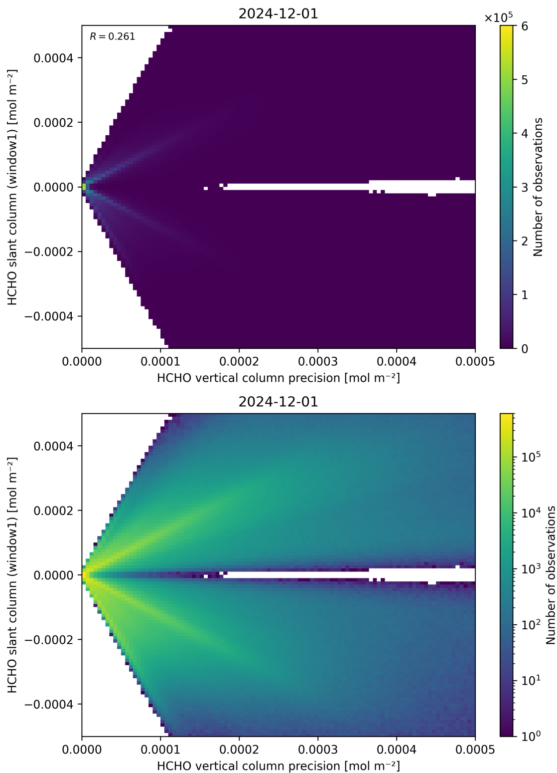
Figure 142: Scatter density plot of “HCHO vertical column precision” against “HCHO slant column (window1)” for 2024-11-30 to 2024-12-02.
