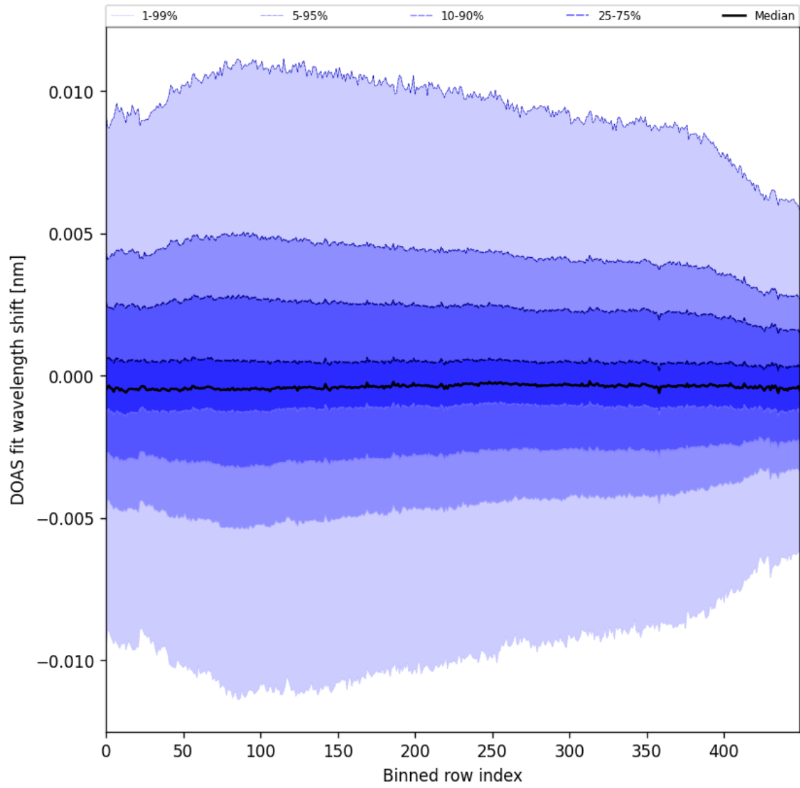
Figure 58: Along track statistics of “DOAS fit wavelength shift” for 2024-11-30 to 2024-12-02
