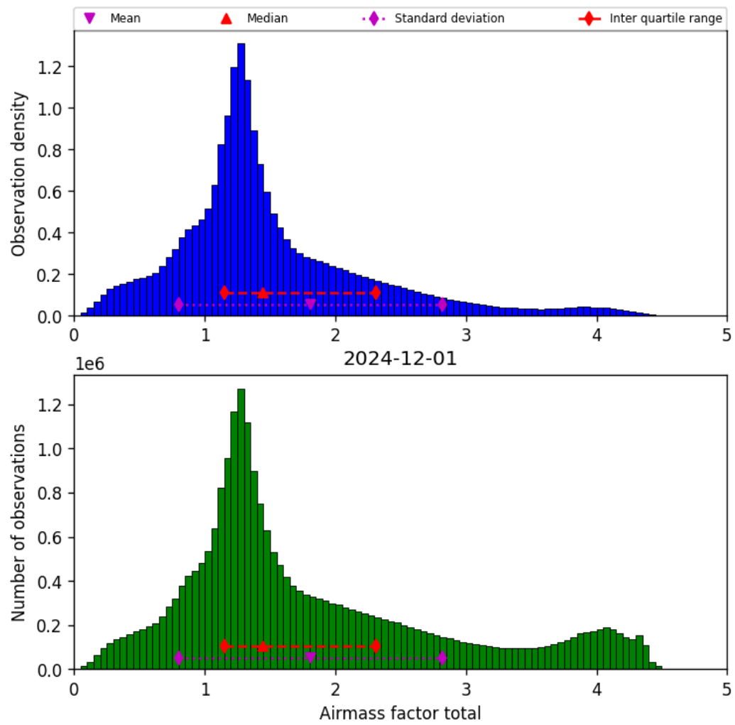
Figure 40: Histogram of “Airmass factor total” for 2024-11-30 to 2024-12-02
