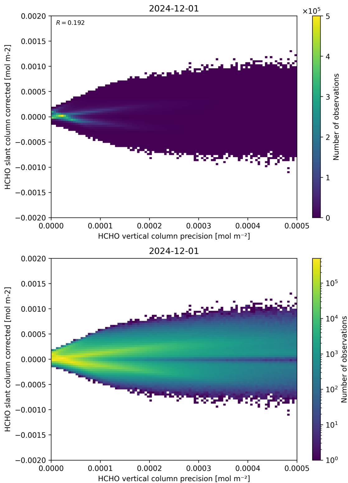
Figure 140: Scatter density plot of “HCHO vertical column precision” against “HCHO slant column corrected” for 2024-11-30 to 2024-12-02.
