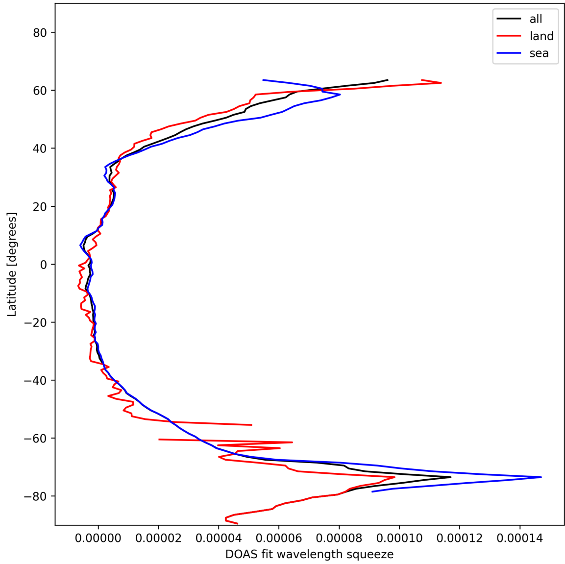
Figure 31: Zonal average of “DOAS fit wavelength squeeze” for 2024-11-30 to 2024-12-02.
