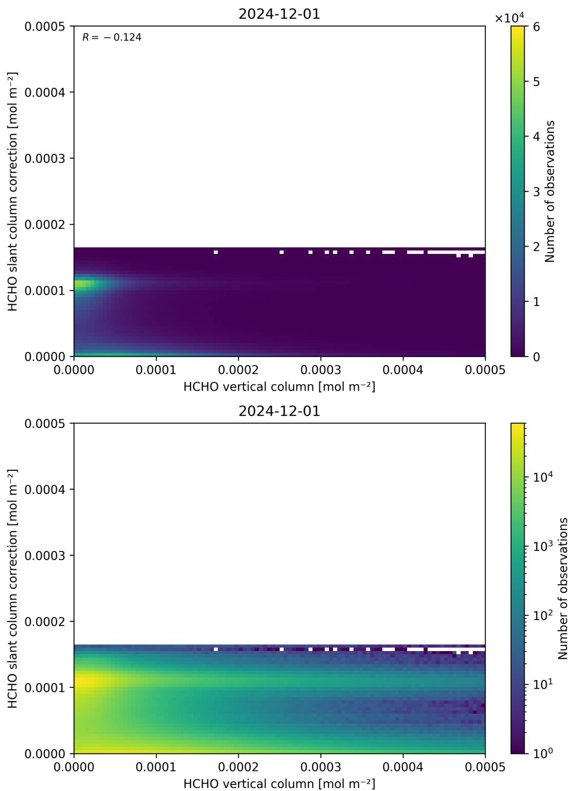
Figure 128: Scatter density plot of “HCHO vertical column” against “HCHO slant column correction” for 2024-11-30 to 2024-12-02.
