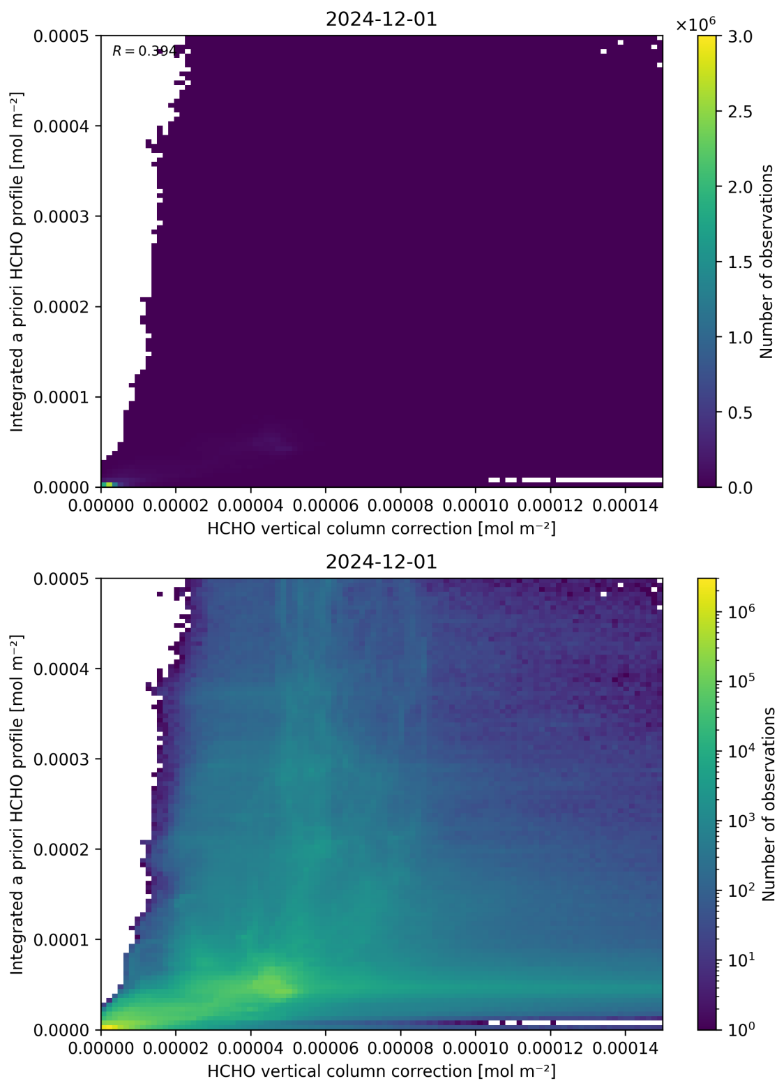
Figure 122: Scatter density plot of “HCHO vertical column correction” against “Integrated a priori HCHO profile” for 2024-11-30 to 2024-12-02.
