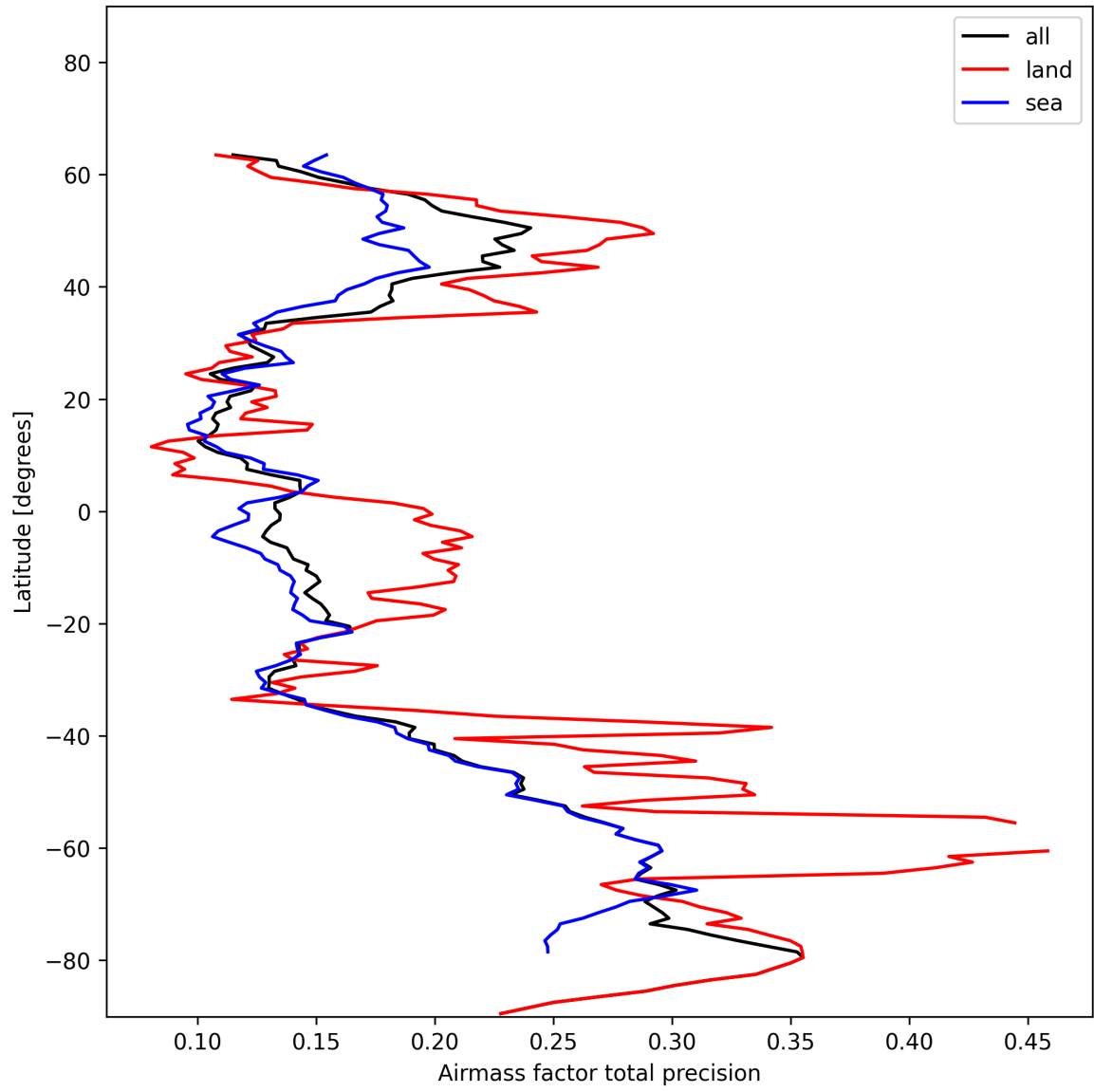
Figure 27: Zonal average of “Airmass factor total precision” for 2024-11-30 to 2024-12-02.
