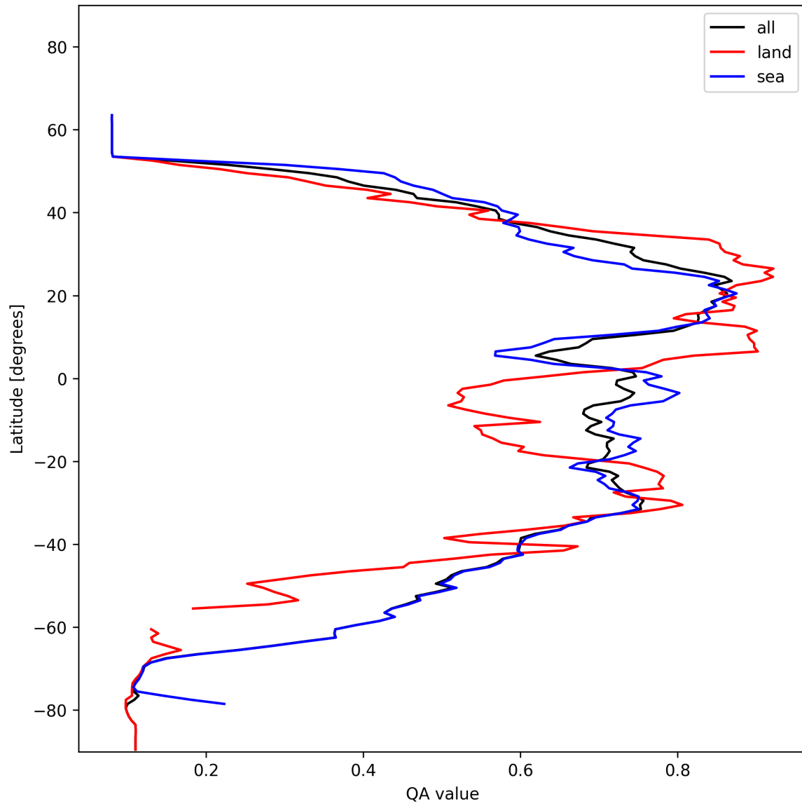
Figure 20: Zonal average of “QA value” for 2024-11-30 to 2024-12-02.
