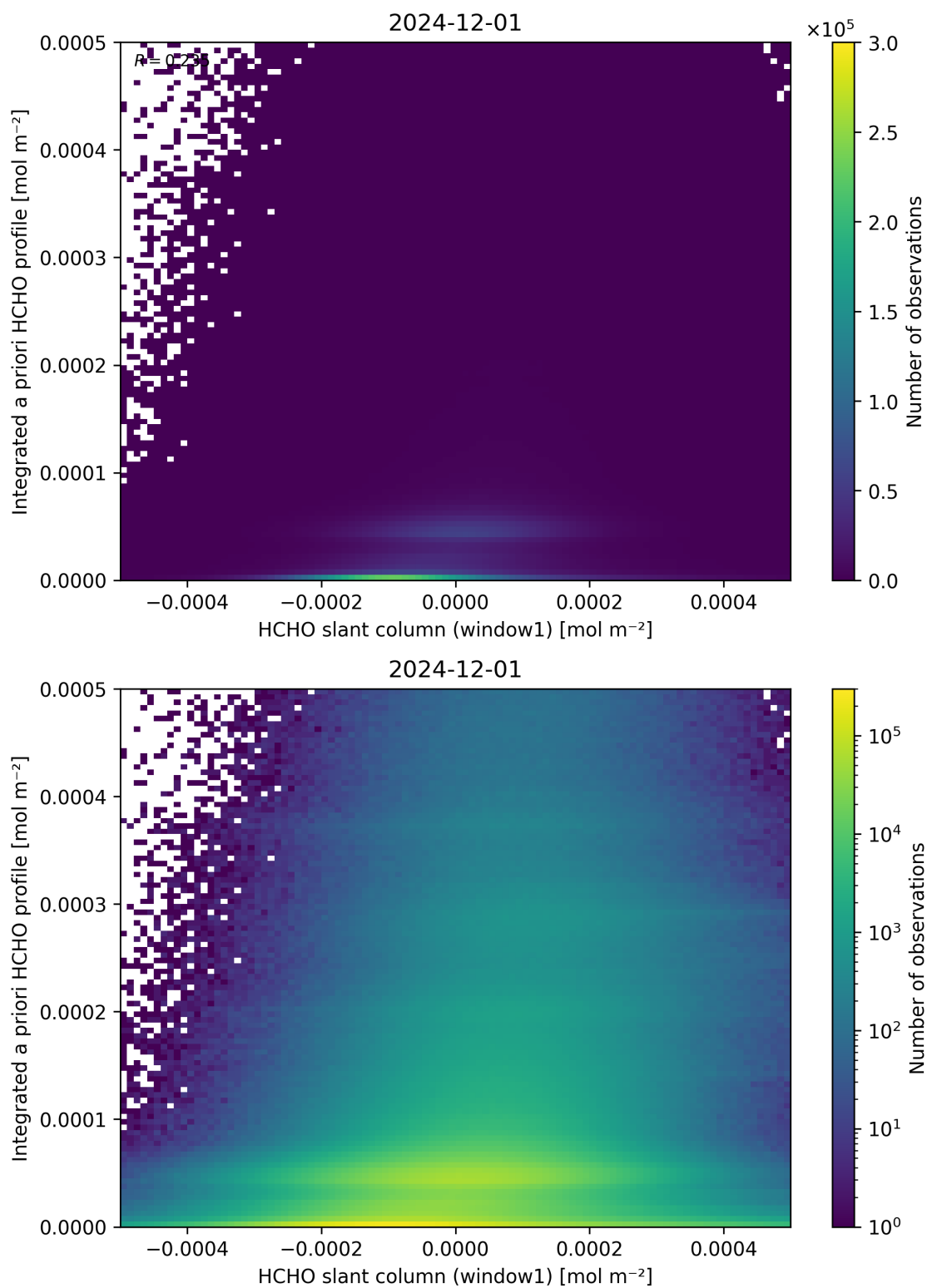
Figure 87: Scatter density plot of “HCHO slant column (window1)” against “Integrated a priori HCHO profile” for 2024-11-30 to 2024-12-02.
