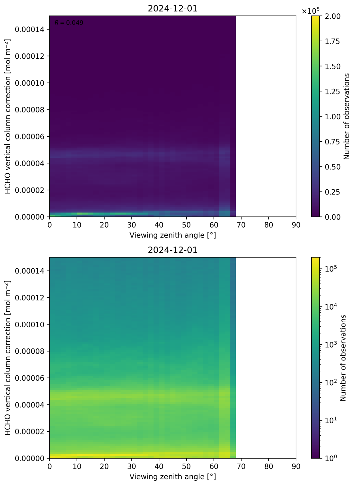
Figure 193: Scatter density plot of “Viewing zenith angle” against “HCHO vertical column correction” for 2024-11-30 to 2024-12-02.
