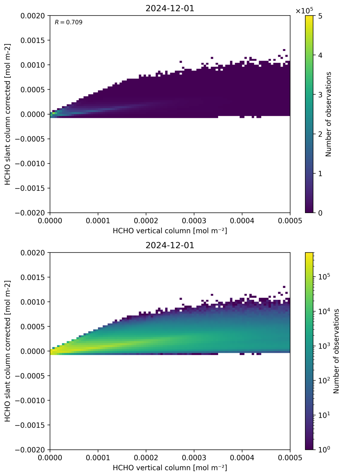
Figure 127: Scatter density plot of “HCHO vertical column” against “HCHO slant column corrected” for 2024-11-30 to 2024-12-02.
