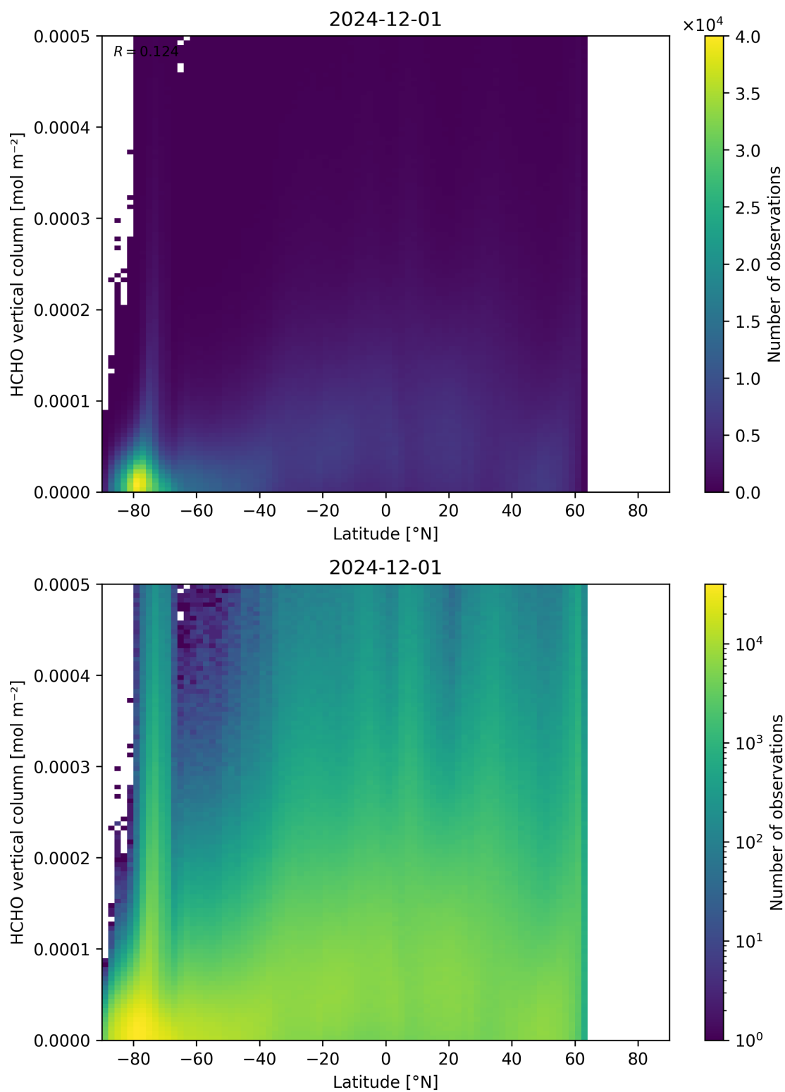
Figure 163: Scatter density plot of “Latitude” against “HCHO vertical column” for 2024-11-30 to 2024-12-02.
