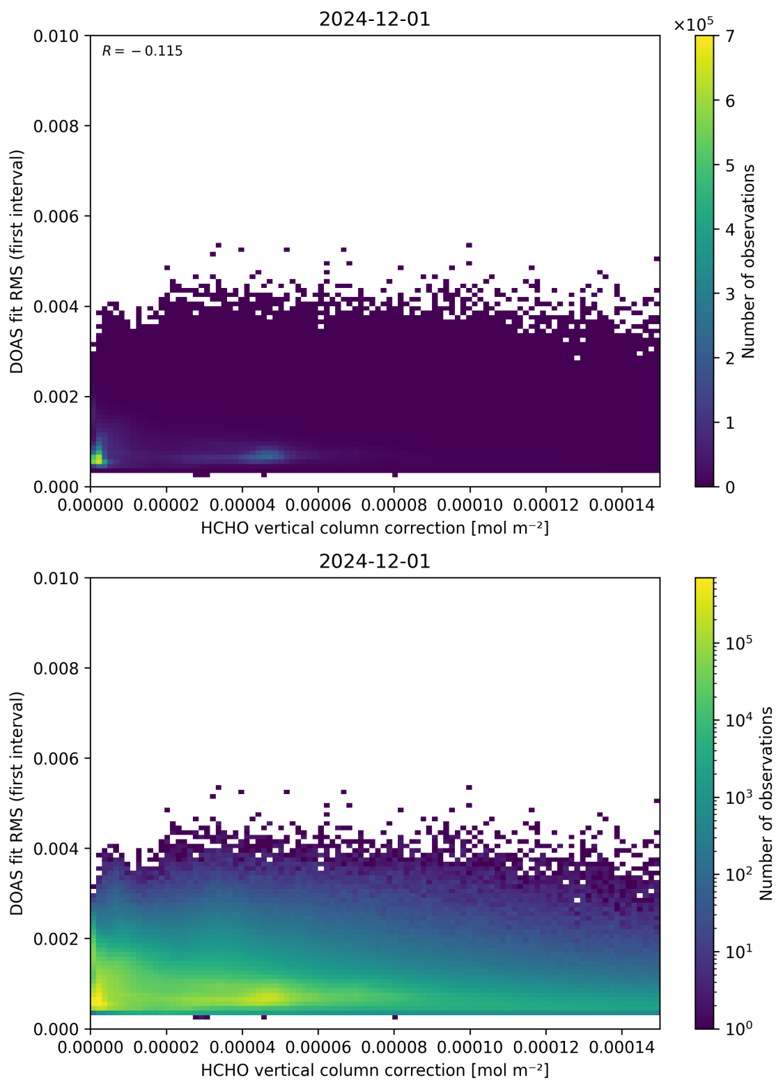
Figure 112: Scatter density plot of “HCHO vertical column correction” against “DOAS fit RMS (first interval)” for 2024-11-30 to 2024-12-02.
