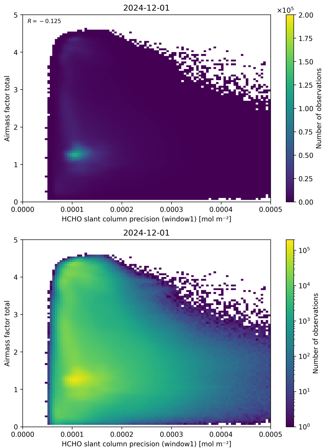
Figure 94: Scatter density plot of “HCHO slant column precision (window1)” against “Airmass factor total” for 2024-11-30 to 2024-12-02.
