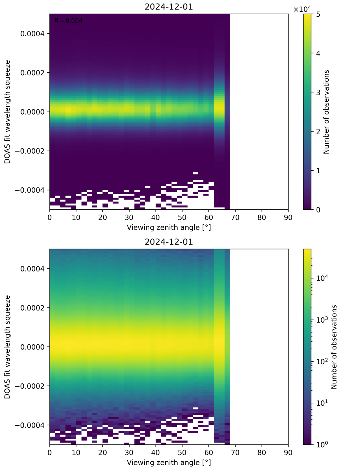
Figure 184: Scatter density plot of “Viewing zenith angle” against “DOAS fit wavelength squeeze” for 2024-11-30 to 2024-12-02.
