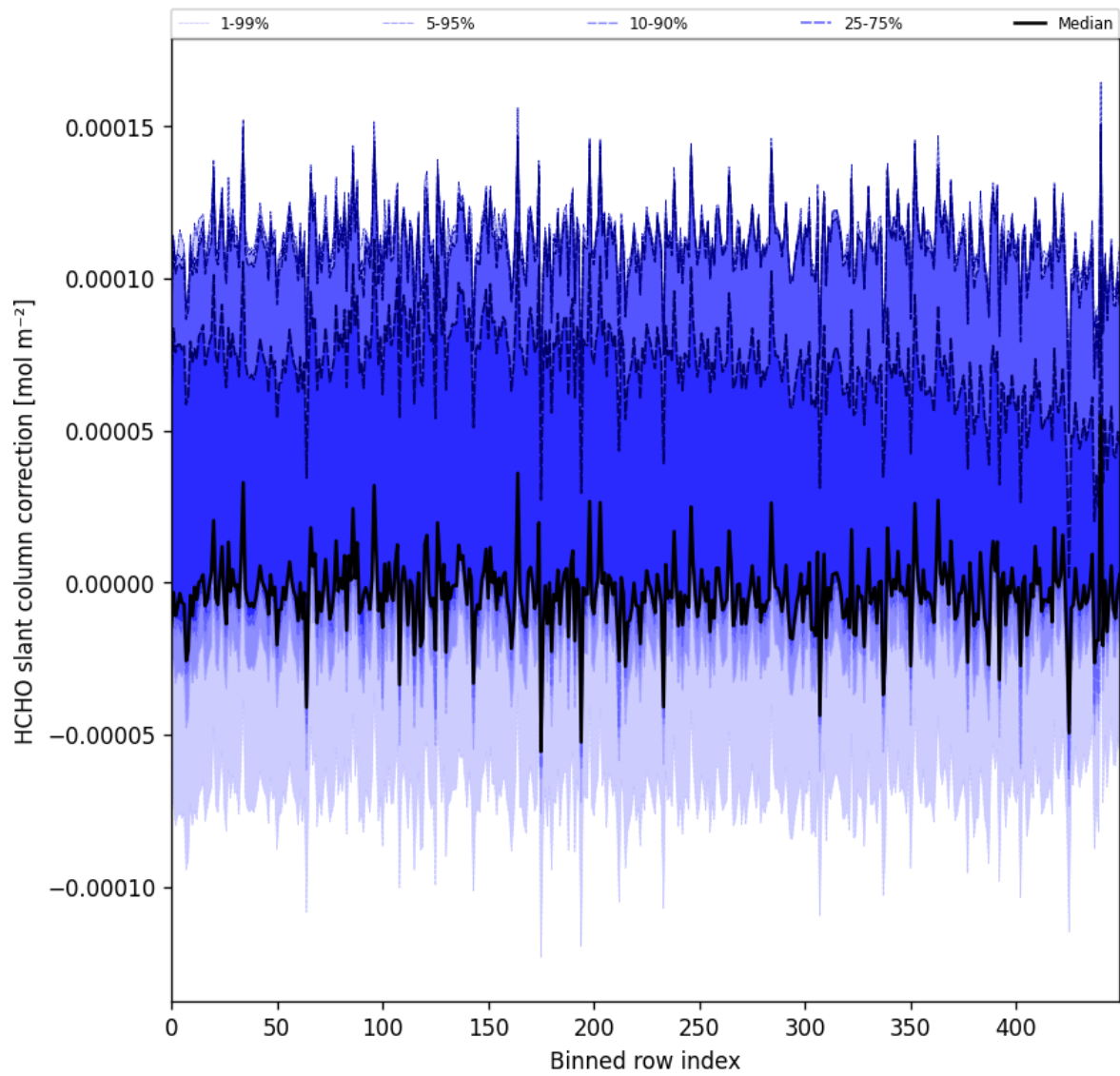
Figure 61: Along track statistics of “HCHO slant column correction” for 2024-11-30 to 2024-12-02
