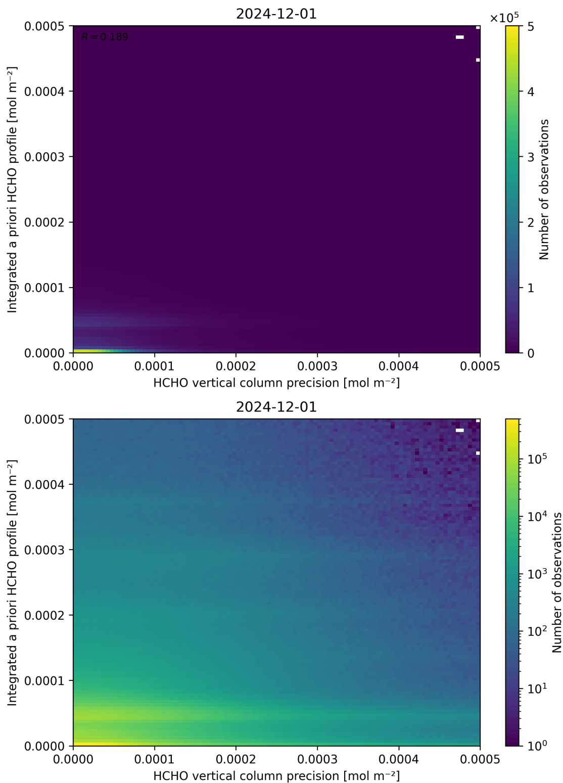
Figure 147: Scatter density plot of “HCHO vertical column precision” against “Integrated a priori HCHO profile” for 2024-11-30 to 2024-12-02.
