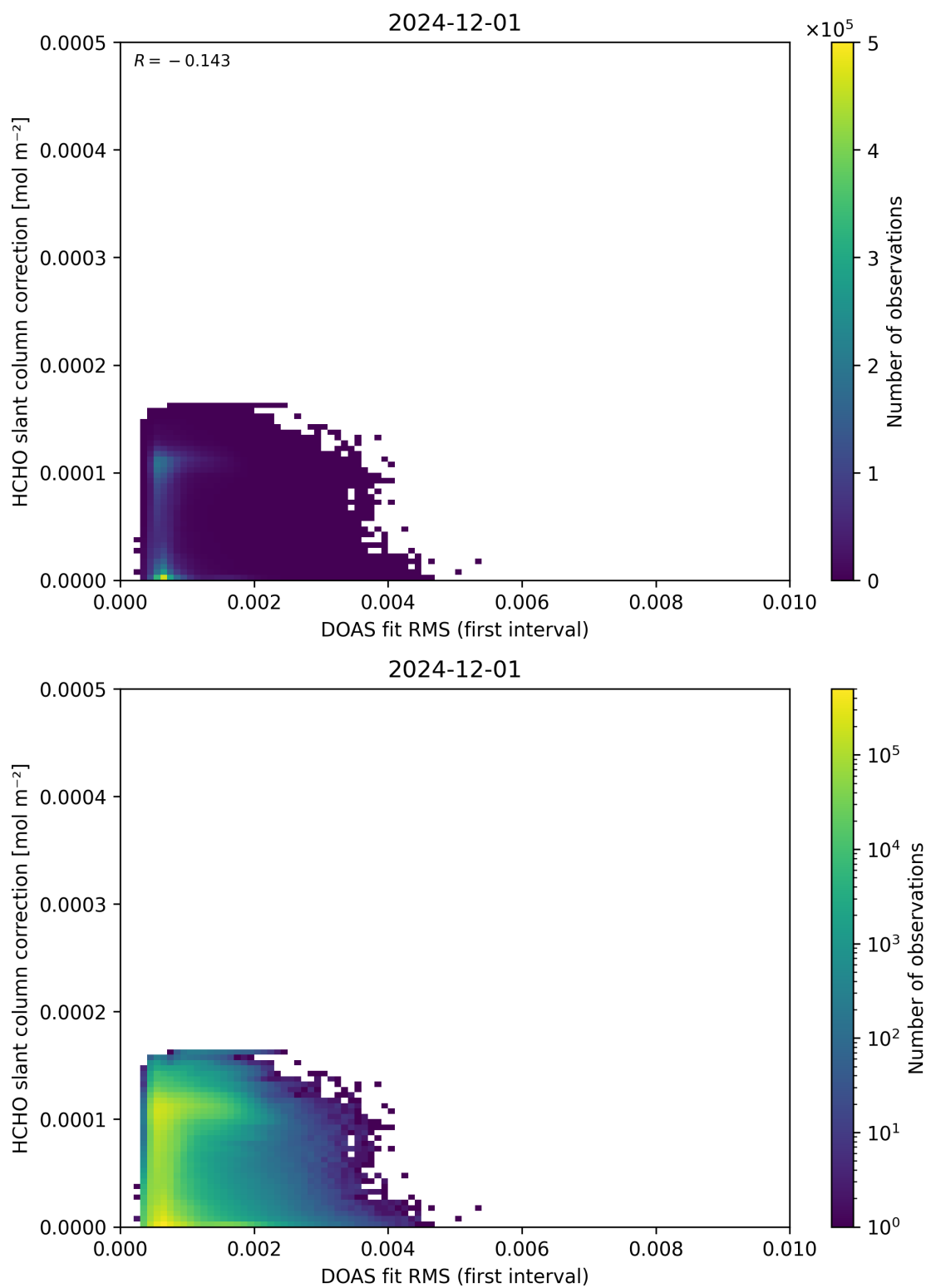
Figure 63: Scatter density plot of “DOAS fit RMS (first interval)” against “HCHO slant column correction” for 2024-11-30 to 2024-12-02.
