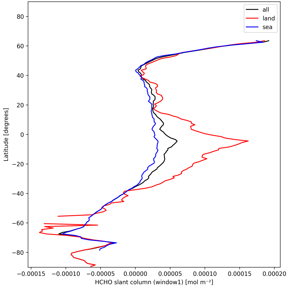
Figure 24: Zonal average of “HCHO slant column (window1)” for 2024-11-30 to 2024-12-02.
