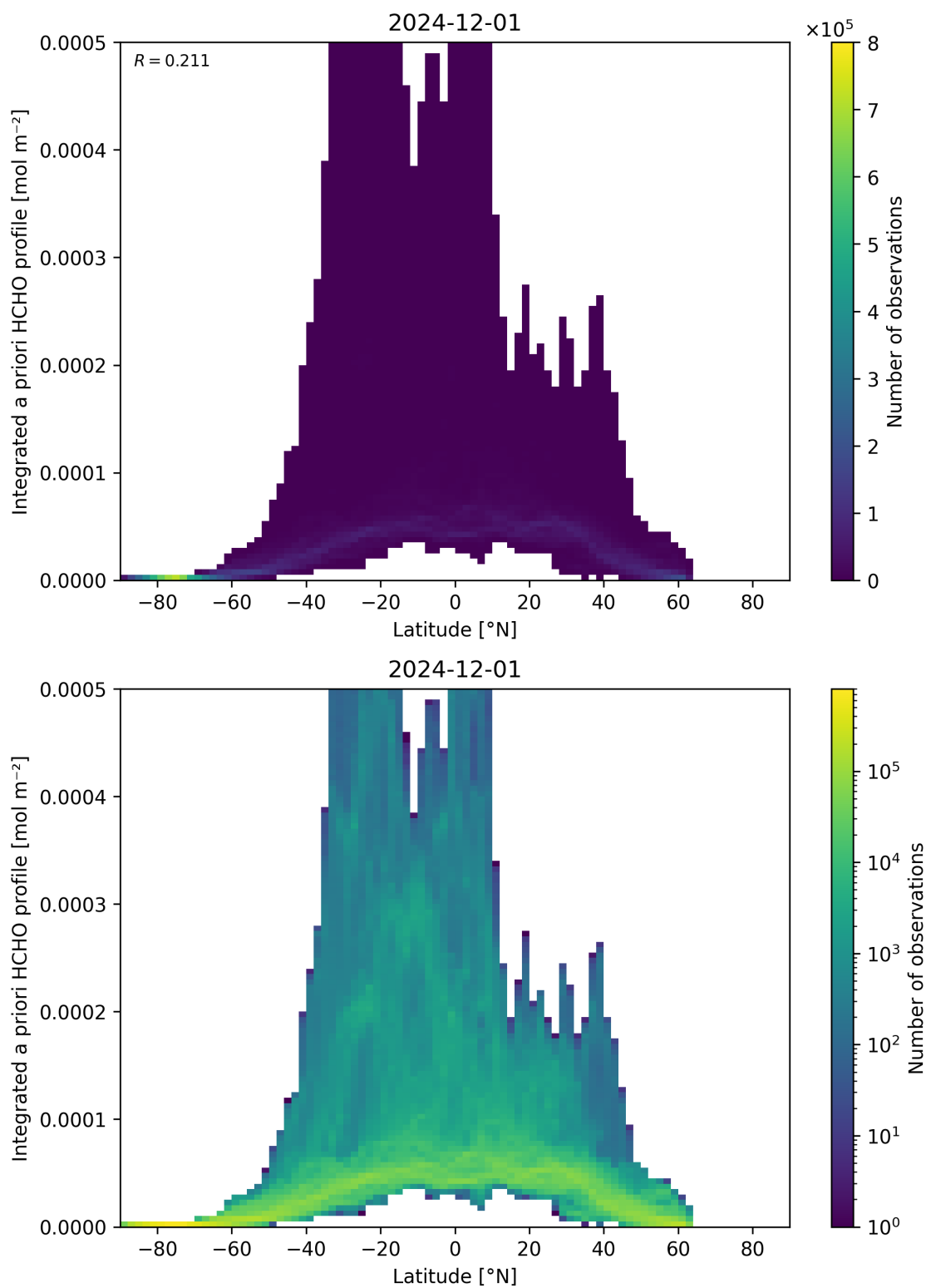
Figure 166: Scatter density plot of “Latitude” against “Integrated a priori HCHO profile” for 2024-11-30 to 2024-12-02.
