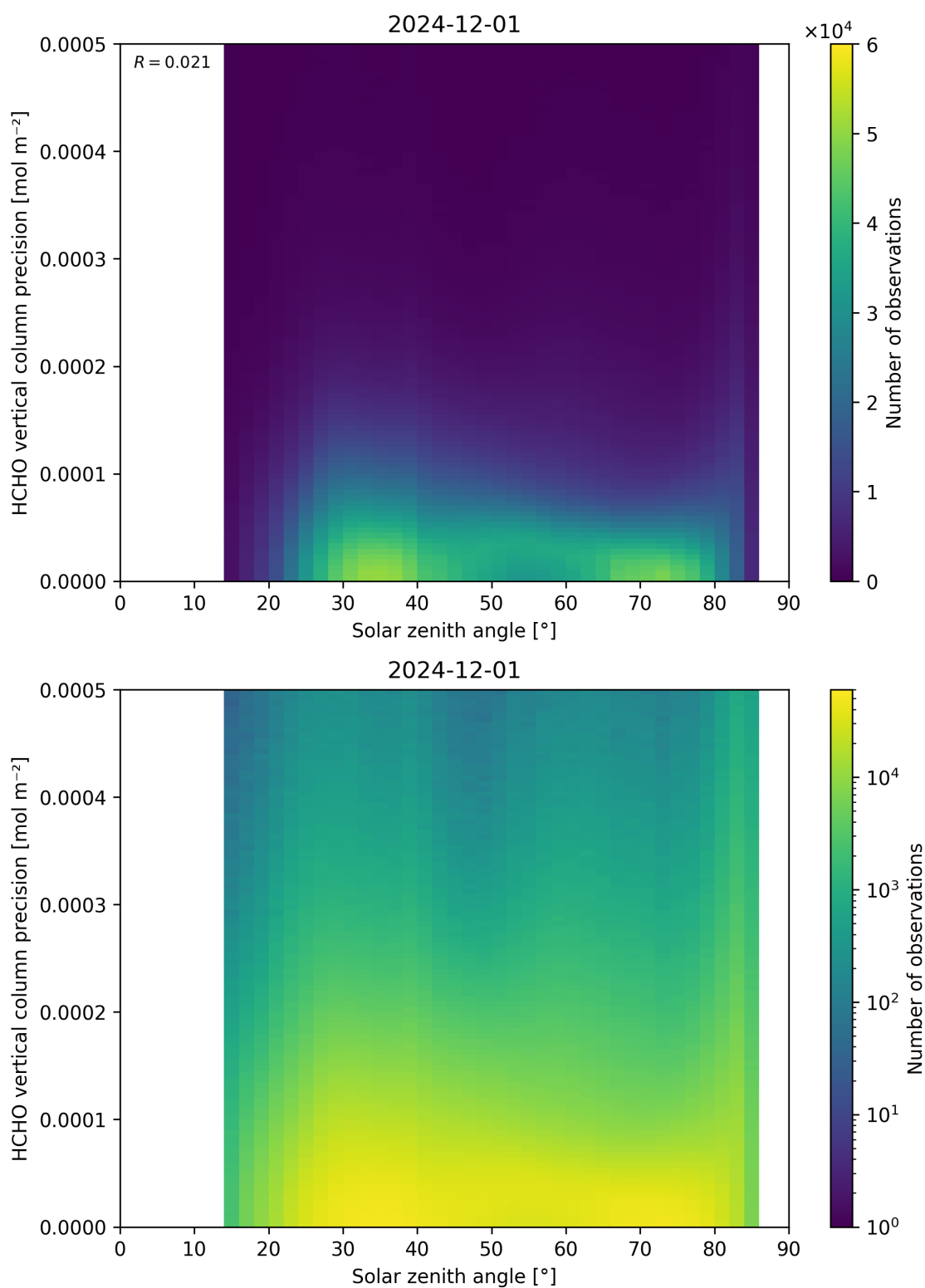
Figure 179: Scatter density plot of “Solar zenith angle” against “HCHO vertical column precision” for 2024-11-30 to 2024-12-02.
