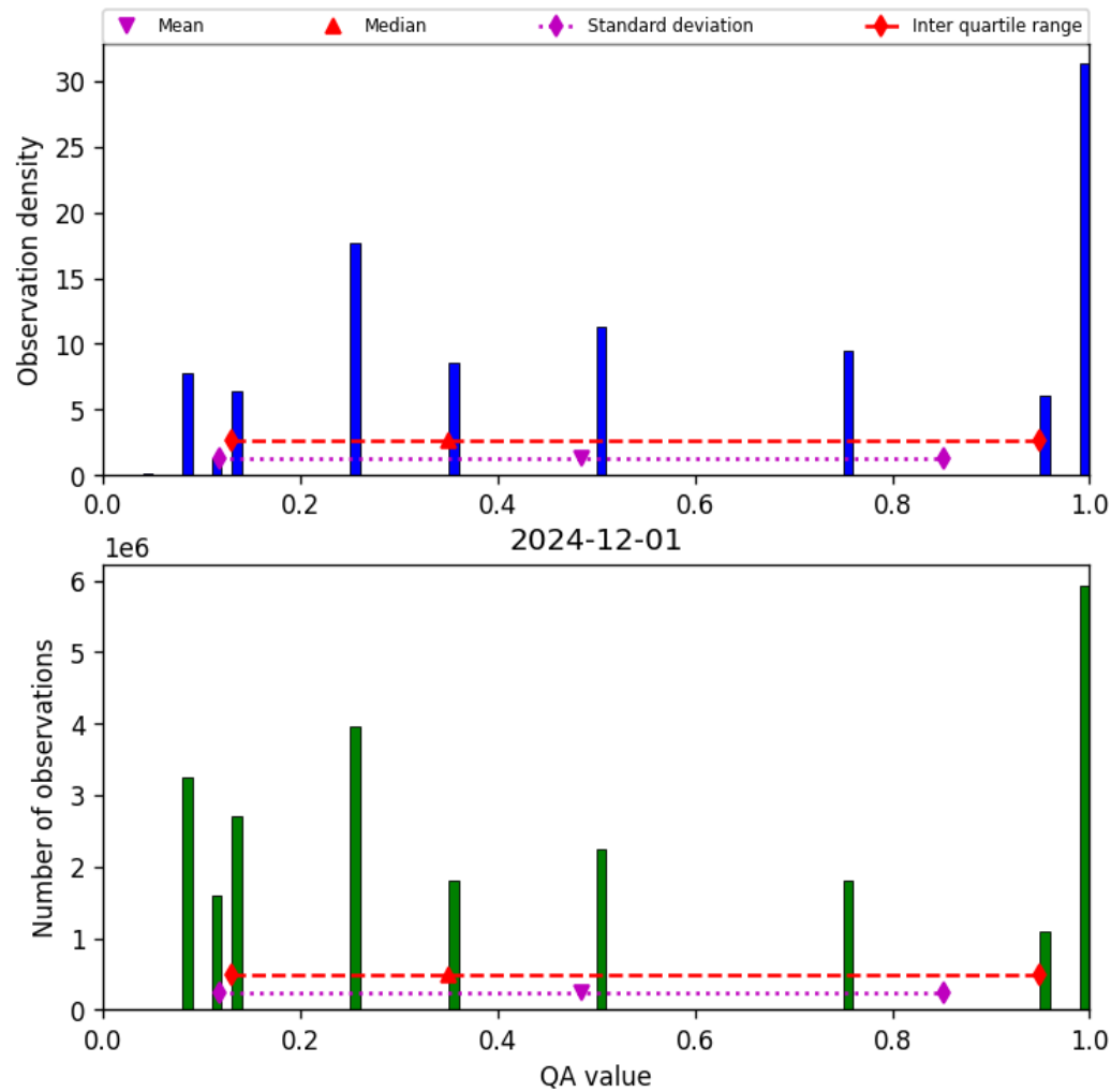
Figure 34: Histogram of “QA value” for 2024-11-30 to 2024-12-02
