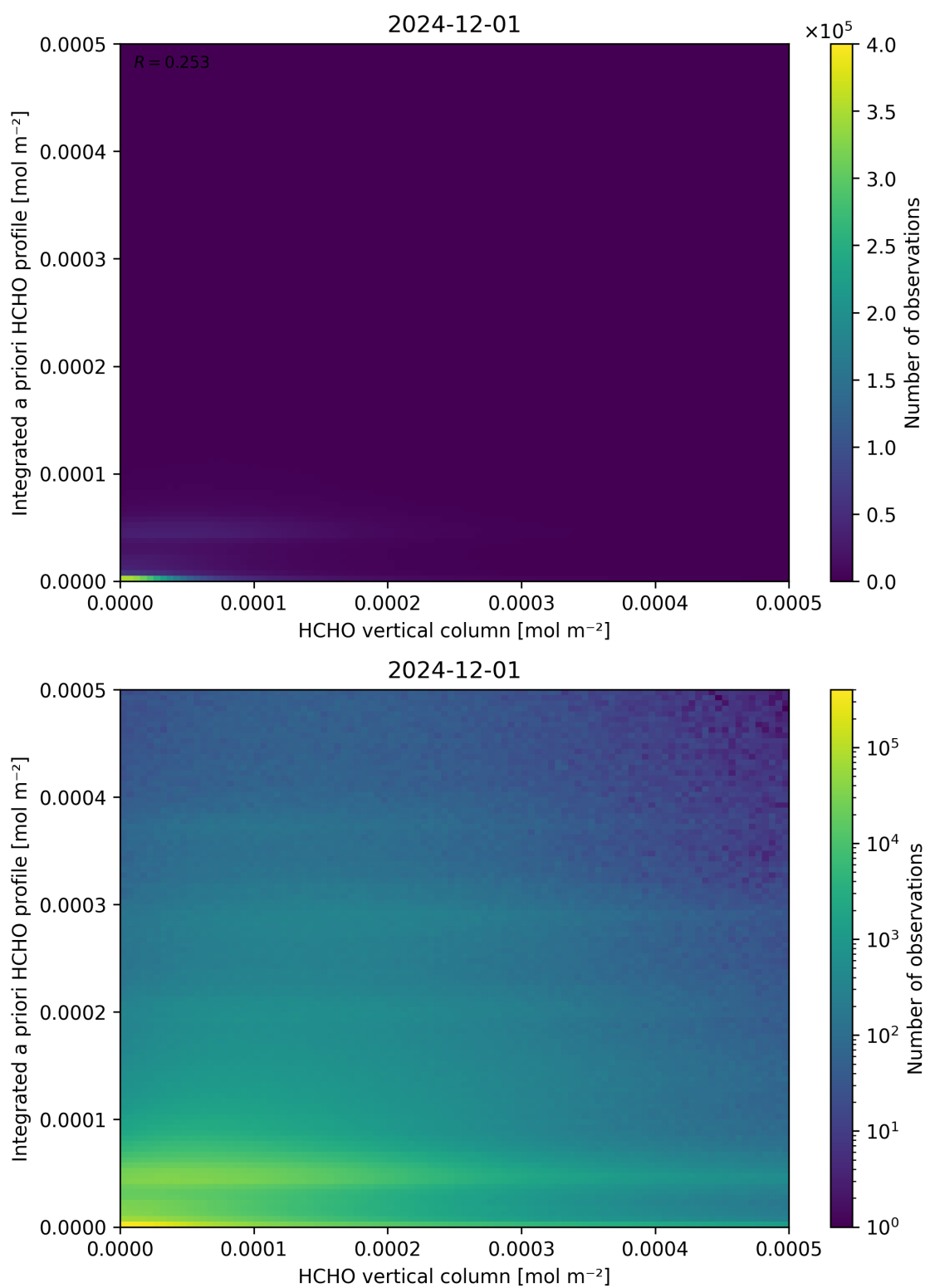
Figure 135: Scatter density plot of “HCHO vertical column” against “Integrated a priori HCHO profile” for 2024-11-30 to 2024-12-02.
