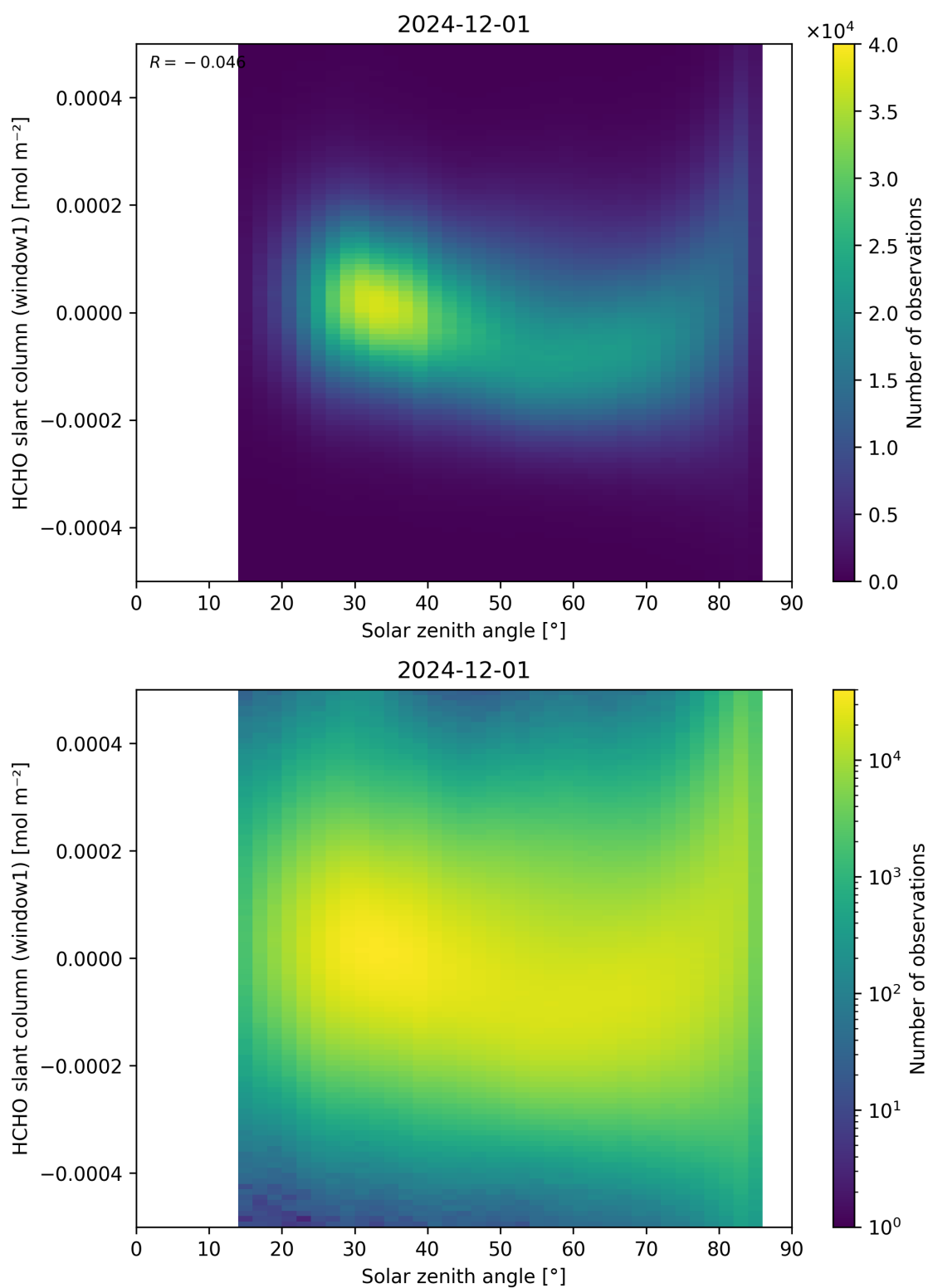
Figure 173: Scatter density plot of “Solar zenith angle” against “HCHO slant column (window1)” for 2024-11-30 to 2024-12-02.
