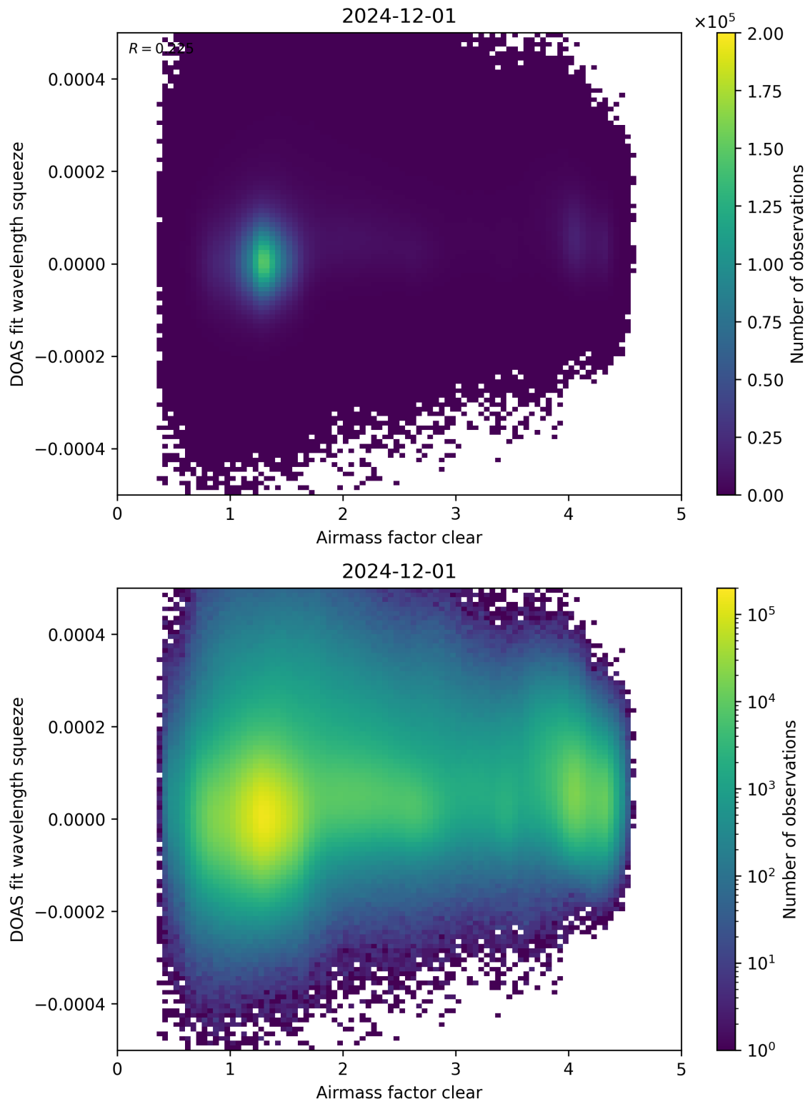
Figure 73: Scatter density plot of “Airmass factor clear” against “DOAS fit wavelength squeeze” for 2024-11-30 to 2024-12-02.
