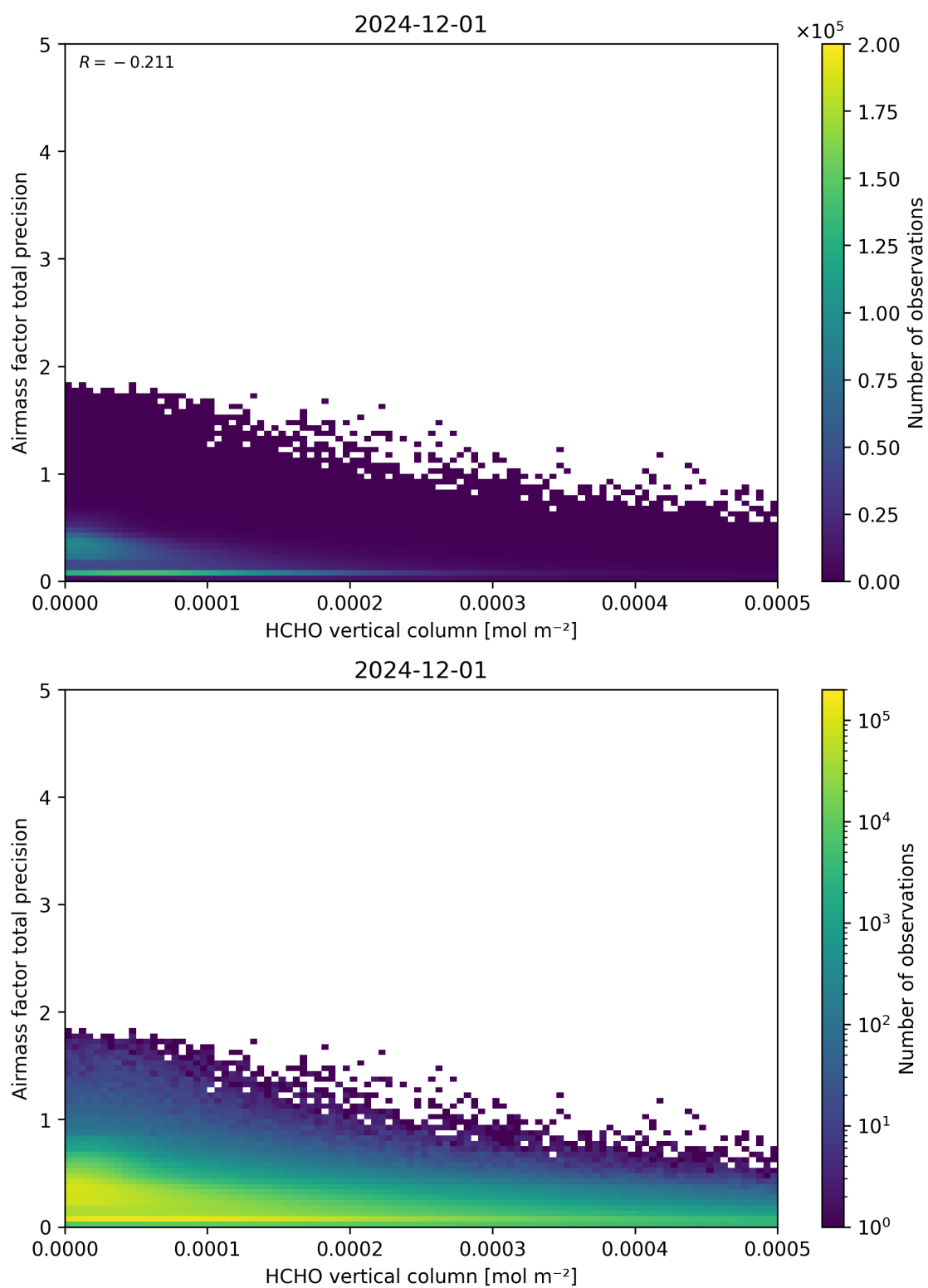
Figure 132: Scatter density plot of “HCHO vertical column” against “Airmass factor total precision” for 2024-11-30 to 2024-12-02.
