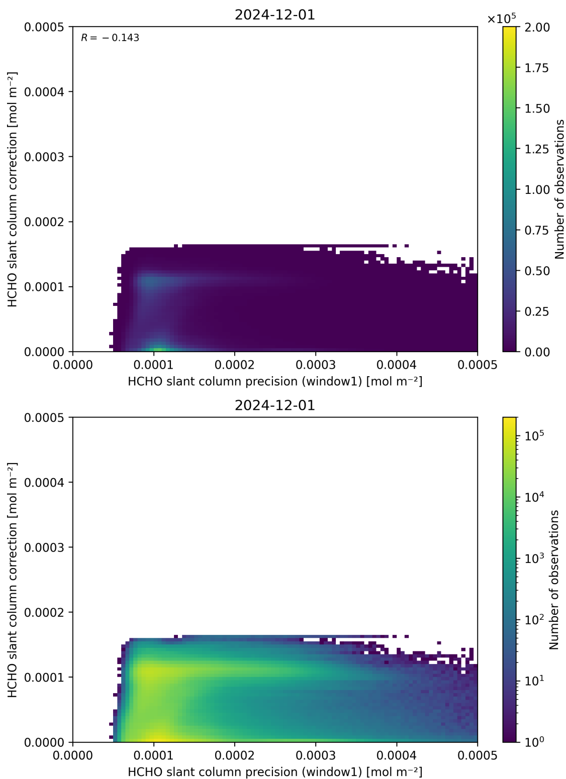
Figure 93: Scatter density plot of “HCHO slant column precision (window1)” against “HCHO slant column correction” for 2024-11-30 to 2024-12-02.
