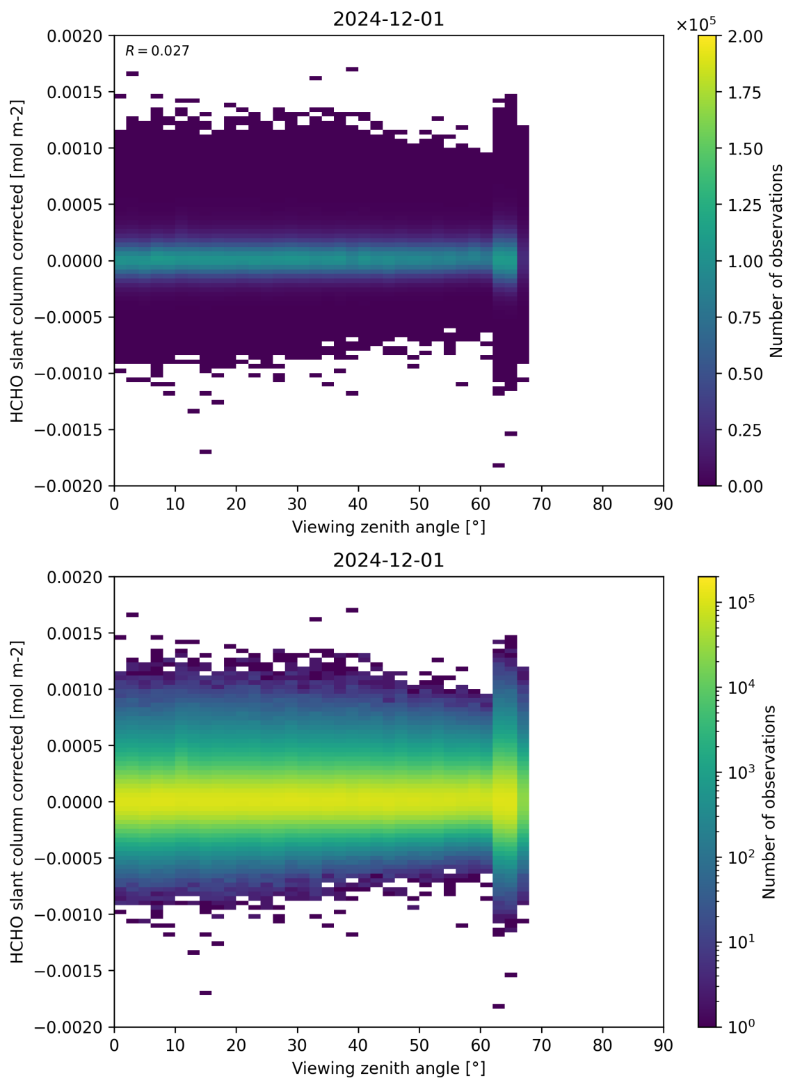
Figure 186: Scatter density plot of “Viewing zenith angle” against “HCHO slant column corrected” for 2024-11-30 to 2024-12-02.
