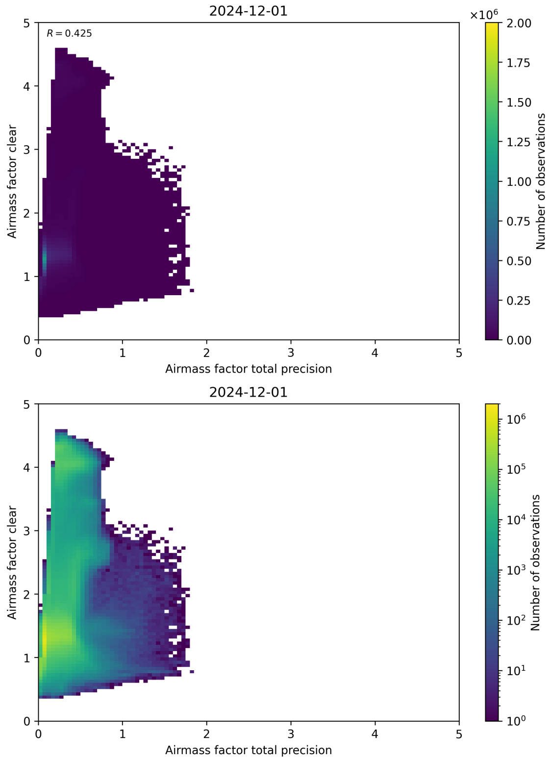
Figure 108: Scatter density plot of “Airmass factor total precision” against “Airmass factor clear” for 2024-11-30 to 2024-12-02.
