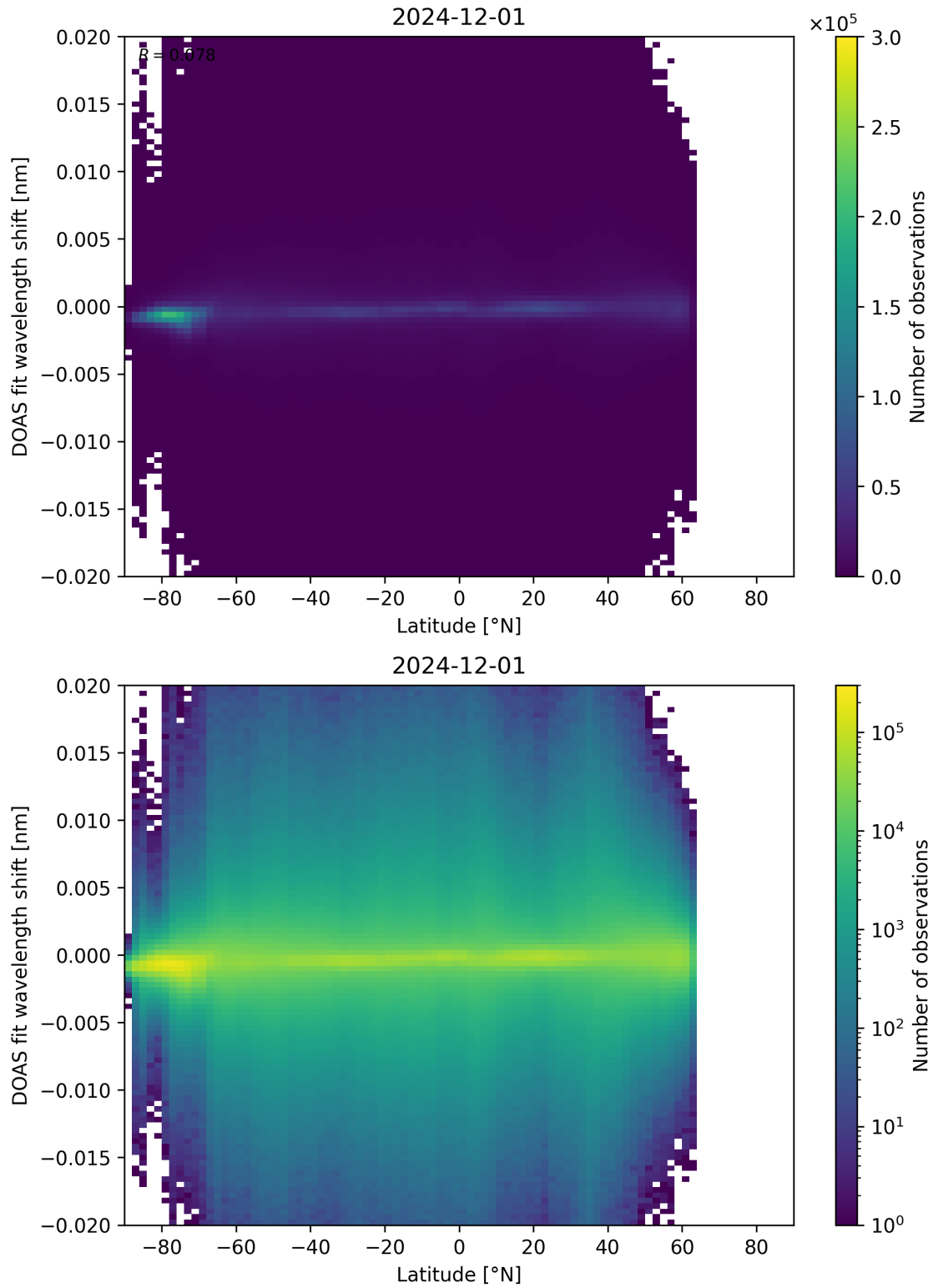
Figure 154: Scatter density plot of “Latitude” against “DOAS fit wavelength shift” for 2024-11-30 to 2024-12-02.
