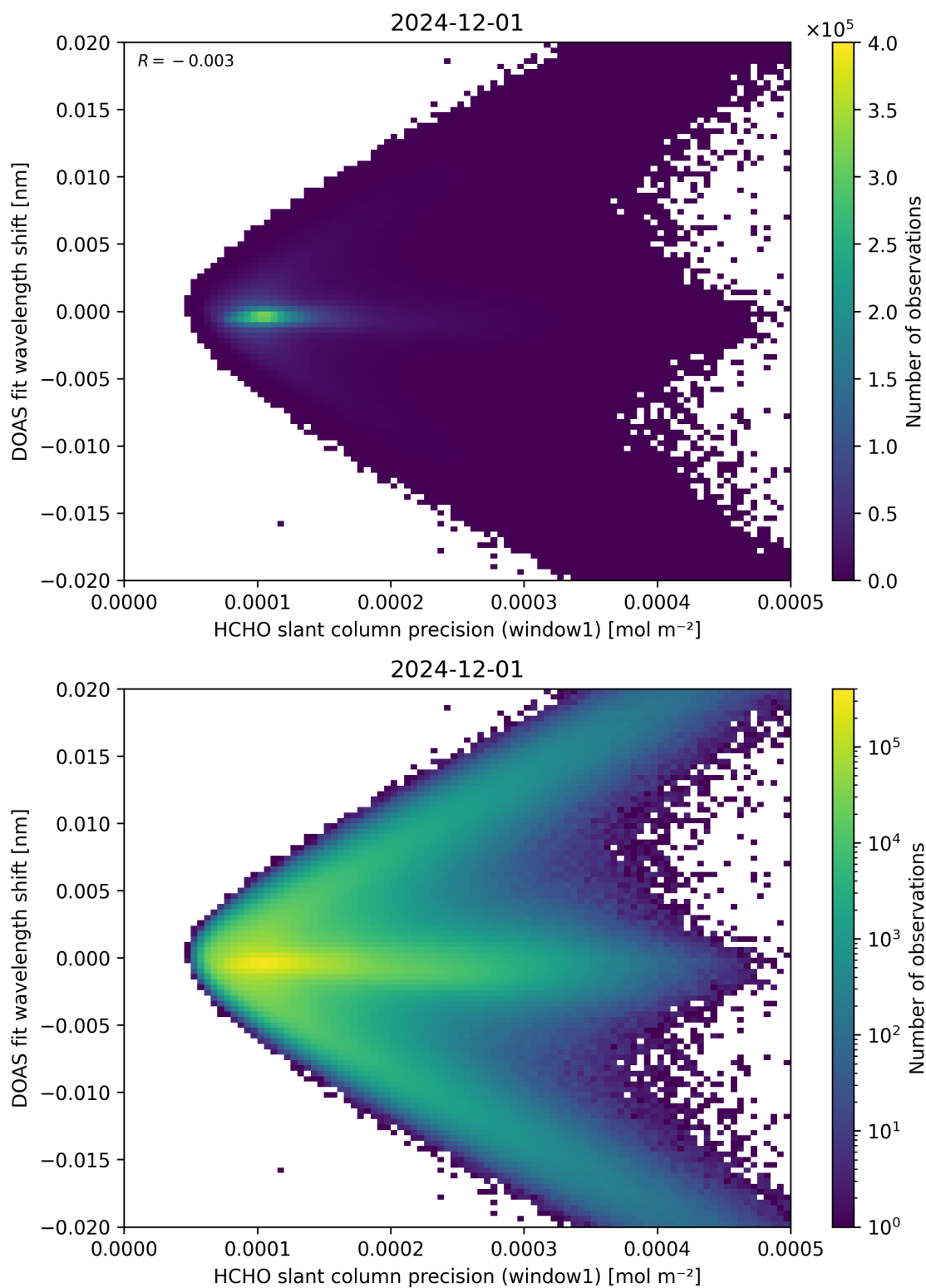
Figure 89: Scatter density plot of “HCHO slant column precision (window1)” against “DOAS fit wavelength shift” for 2024-11-30 to 2024-12-02.
