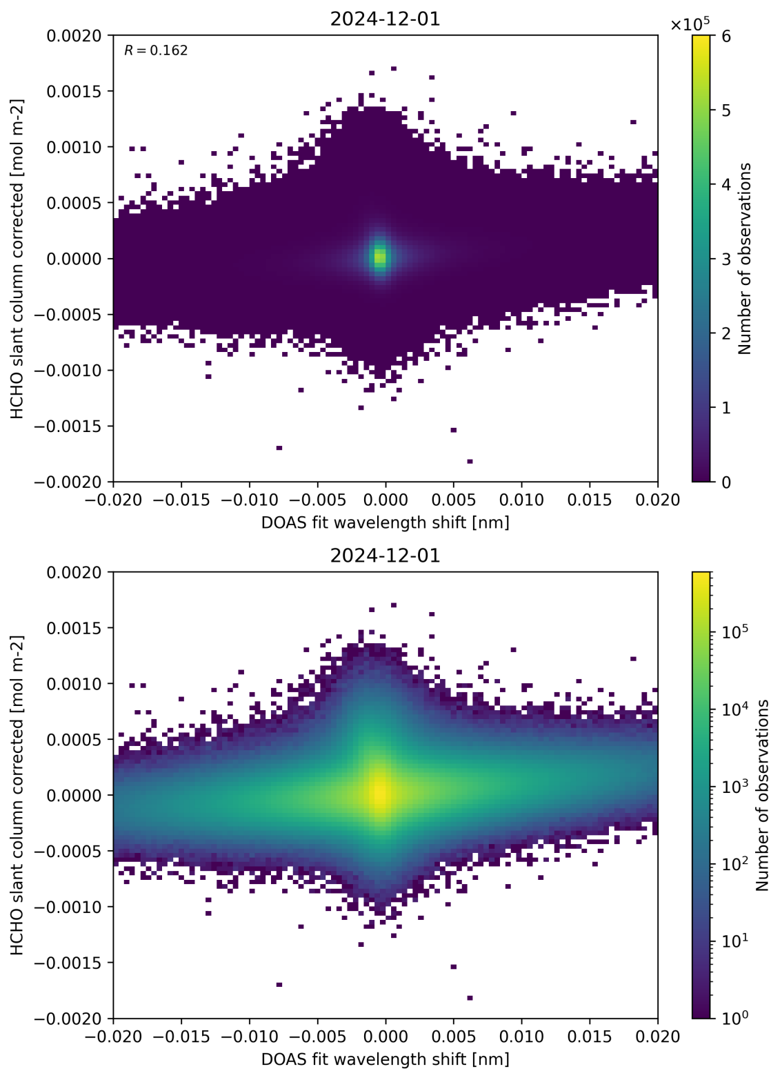
Figure 66: Scatter density plot of “DOAS fit wavelength shift” against “HCHO slant column corrected” for 2024-11-30 to 2024-12-02.
