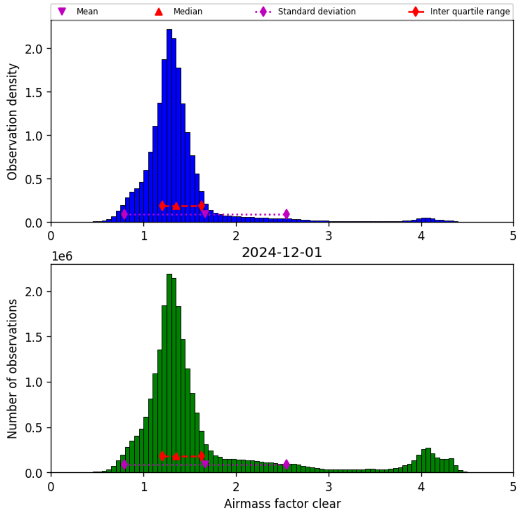
Figure 42: Histogram of “Airmass factor clear” for 2024-11-30 to 2024-12-02
