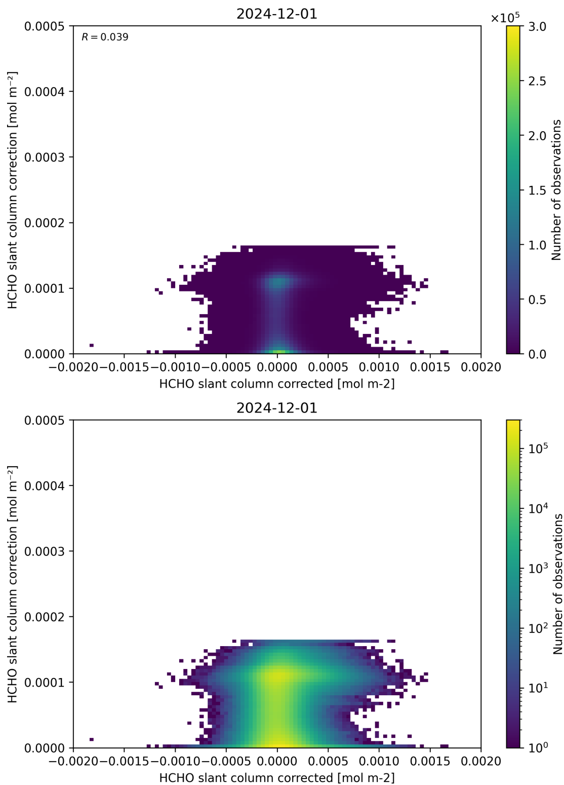
Figure 77: Scatter density plot of “HCHO slant column corrected” against “HCHO slant column correction” for 2024-11-30 to 2024-12-02.
