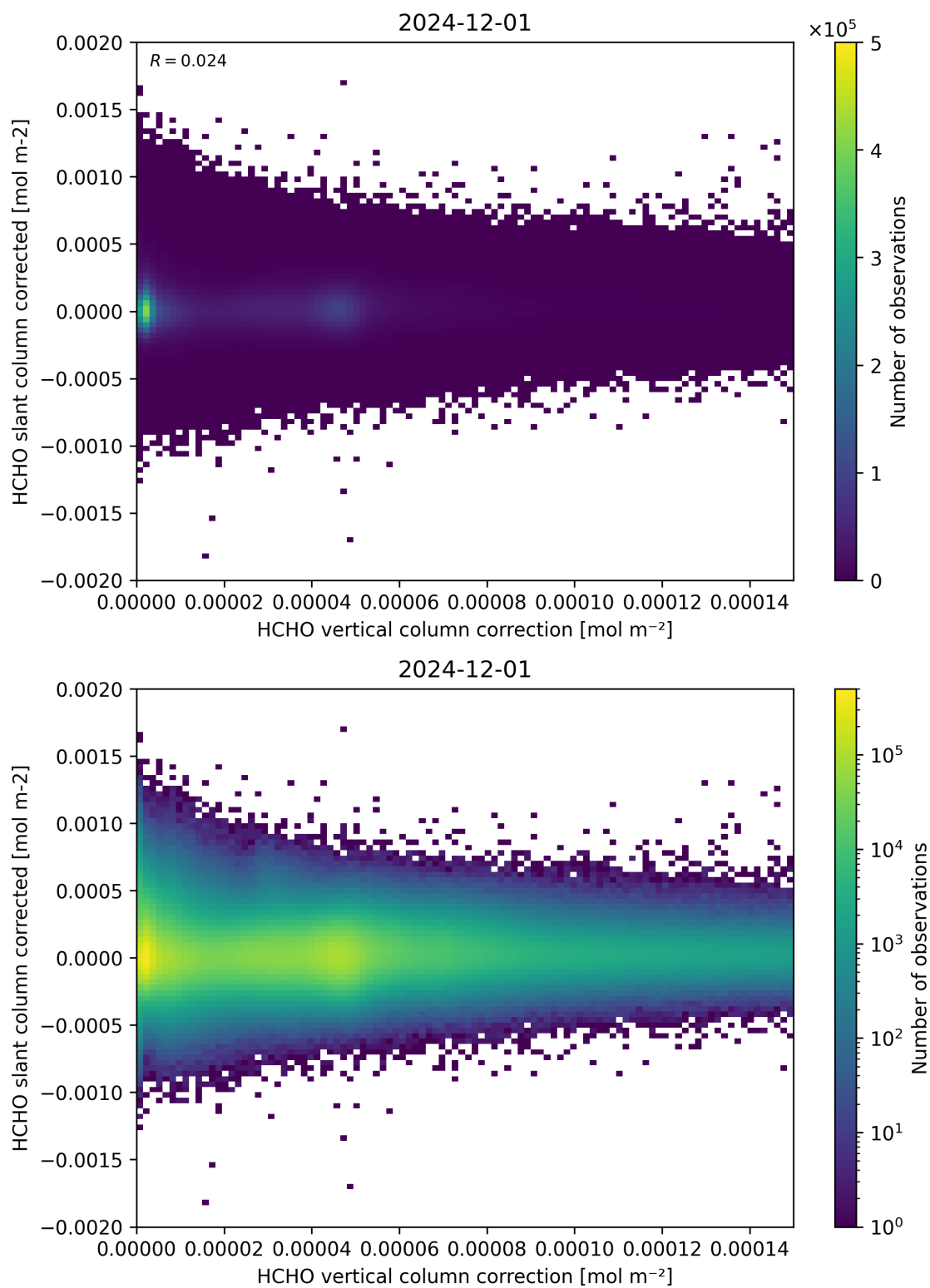
Figure 116: Scatter density plot of “HCHO vertical column correction” against “HCHO slant column corrected” for 2024-11-30 to 2024-12-02.
