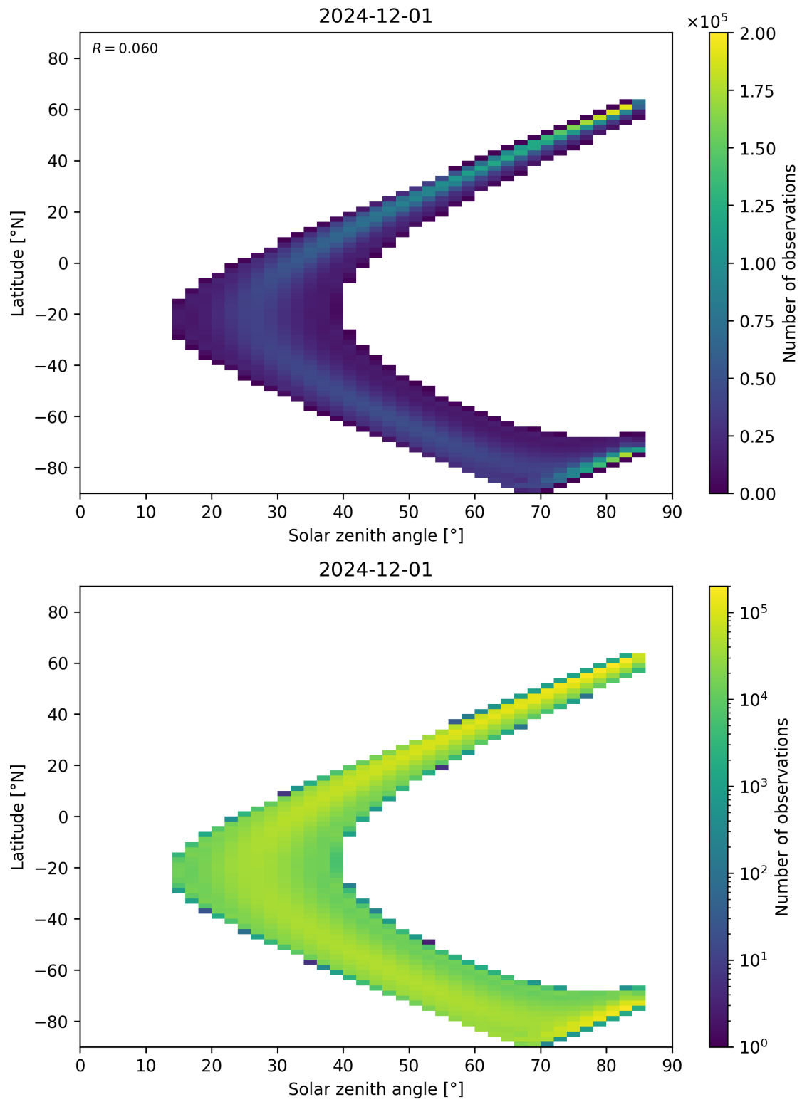
Figure 181: Scatter density plot of “Solar zenith angle” against “Latitude” for 2024-11-30 to 2024-12-02.
