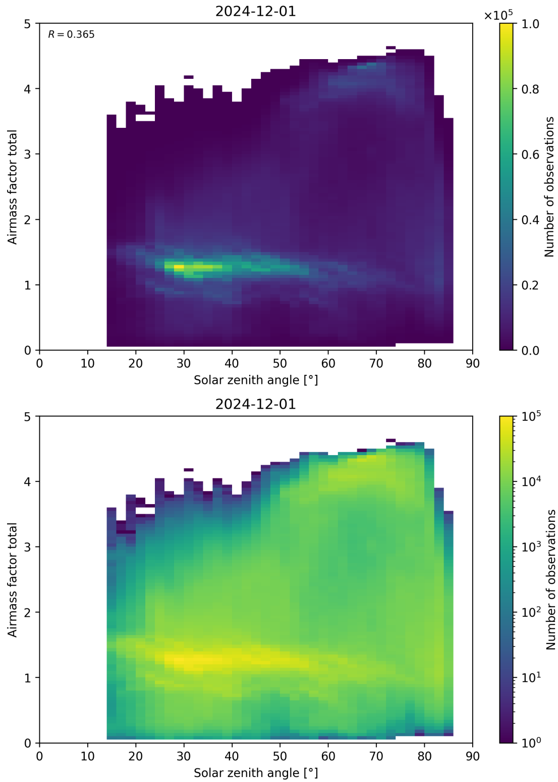
Figure 175: Scatter density plot of “Solar zenith angle” against “Airmass factor total” for 2024-11-30 to 2024-12-02.
