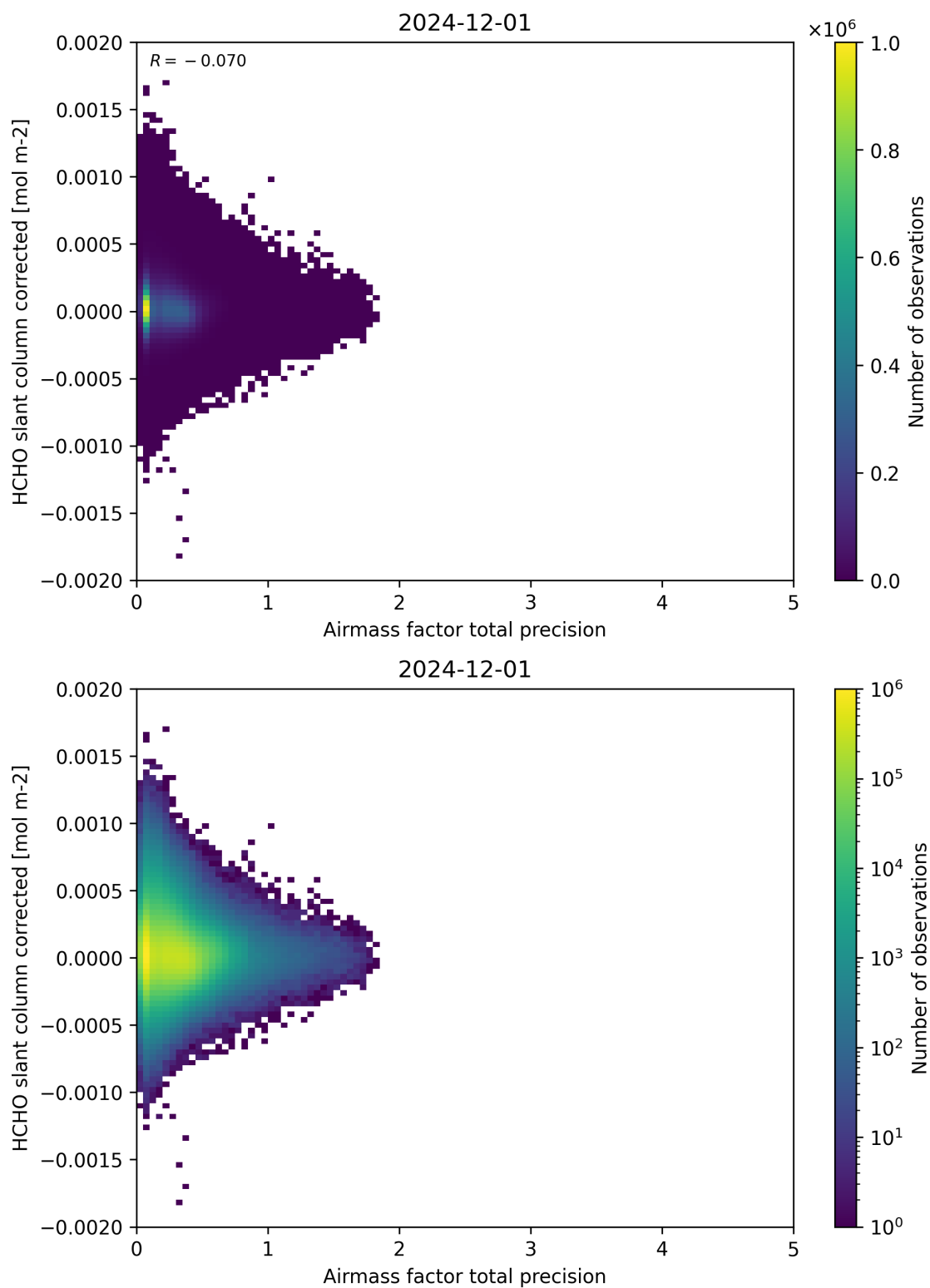
Figure 109: Scatter density plot of “Airmass factor total precision” against “HCHO slant column corrected” for 2024-11-30 to 2024-12-02.
