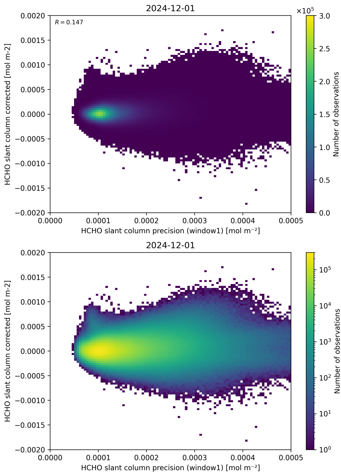
Figure 92: Scatter density plot of “HCHO slant column precision (window1)” against “HCHO slant column corrected” for 2024-11-30 to 2024-12-02.
