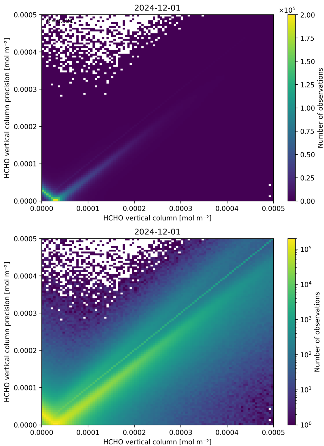
Figure 134: Scatter density plot of “HCHO vertical column” against “HCHO vertical column precision” for 2024-11-30 to 2024-12-02.
