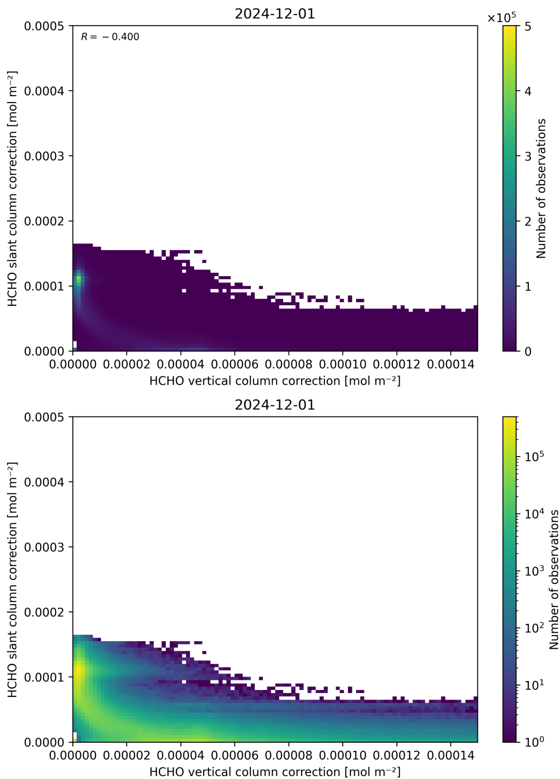
Figure 117: Scatter density plot of “HCHO vertical column correction” against “HCHO slant column correction” for 2024-11-30 to 2024-12-02.
