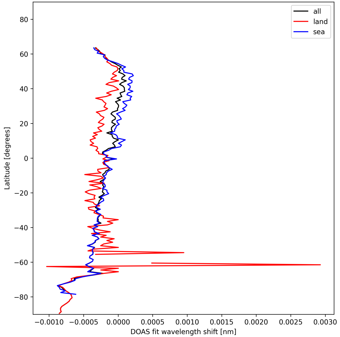
Figure 30: Zonal average of “DOAS fit wavelength shift” for 2024-11-30 to 2024-12-02.
