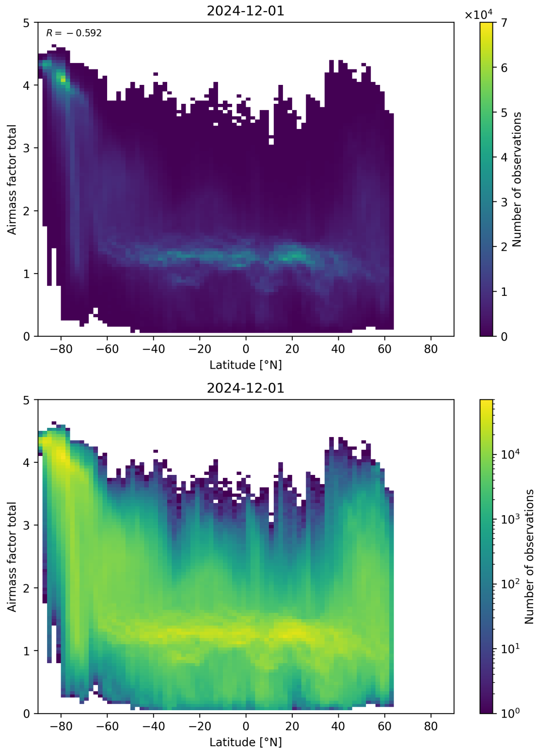
Figure 161: Scatter density plot of “Latitude” against “Airmass factor total” for 2024-11-30 to 2024-12-02.
