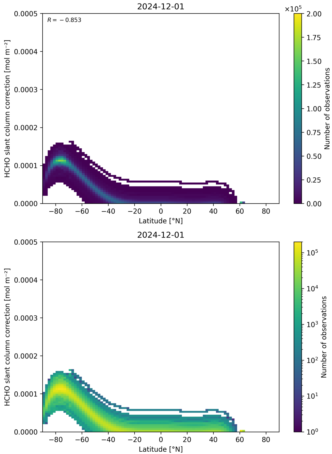
Figure 158: Scatter density plot of “Latitude” against “HCHO slant column correction” for 2024-11-30 to 2024-12-02.
