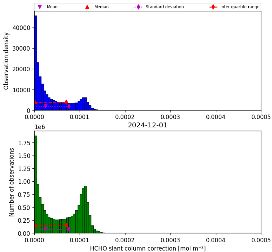
Figure 47: Histogram of “HCHO slant column correction” for 2024-11-30 to 2024-12-02
