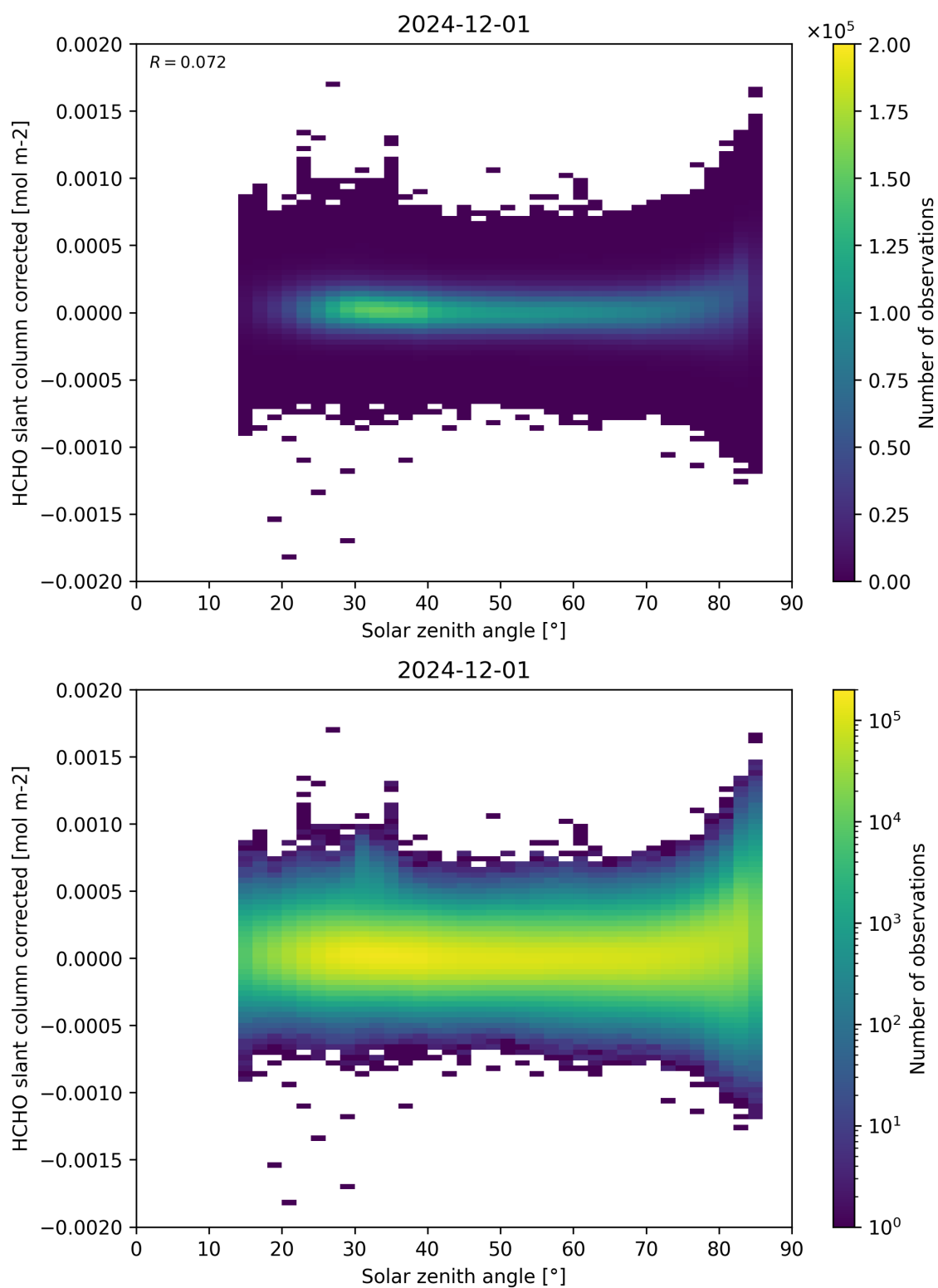
Figure 171: Scatter density plot of “Solar zenith angle” against “HCHO slant column corrected” for 2024-11-30 to 2024-12-02.
