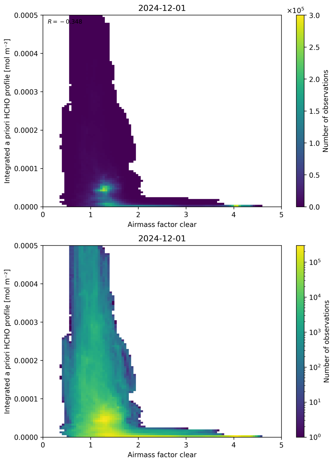
Figure 76: Scatter density plot of “Airmass factor clear” against “Integrated a priori HCHO profile” for 2024-11-30 to 2024-12-02.
