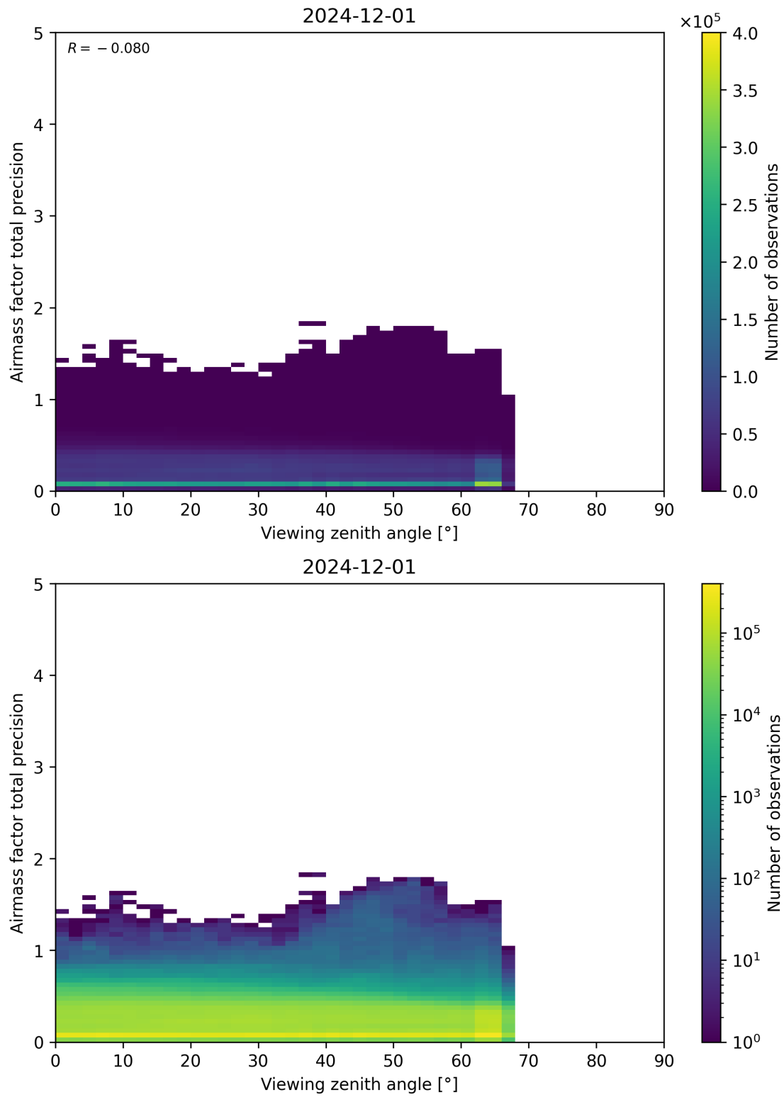
Figure 191: Scatter density plot of “Viewing zenith angle” against “Airmass factor total precision” for 2024-11-30 to 2024-12-02.
