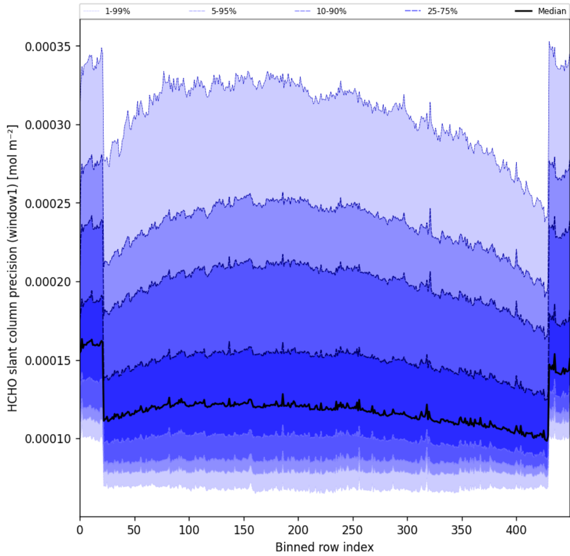
Figure 53: Along track statistics of “HCHO slant column precision (window1)” for 2024-11-30 to 2024-12-02
