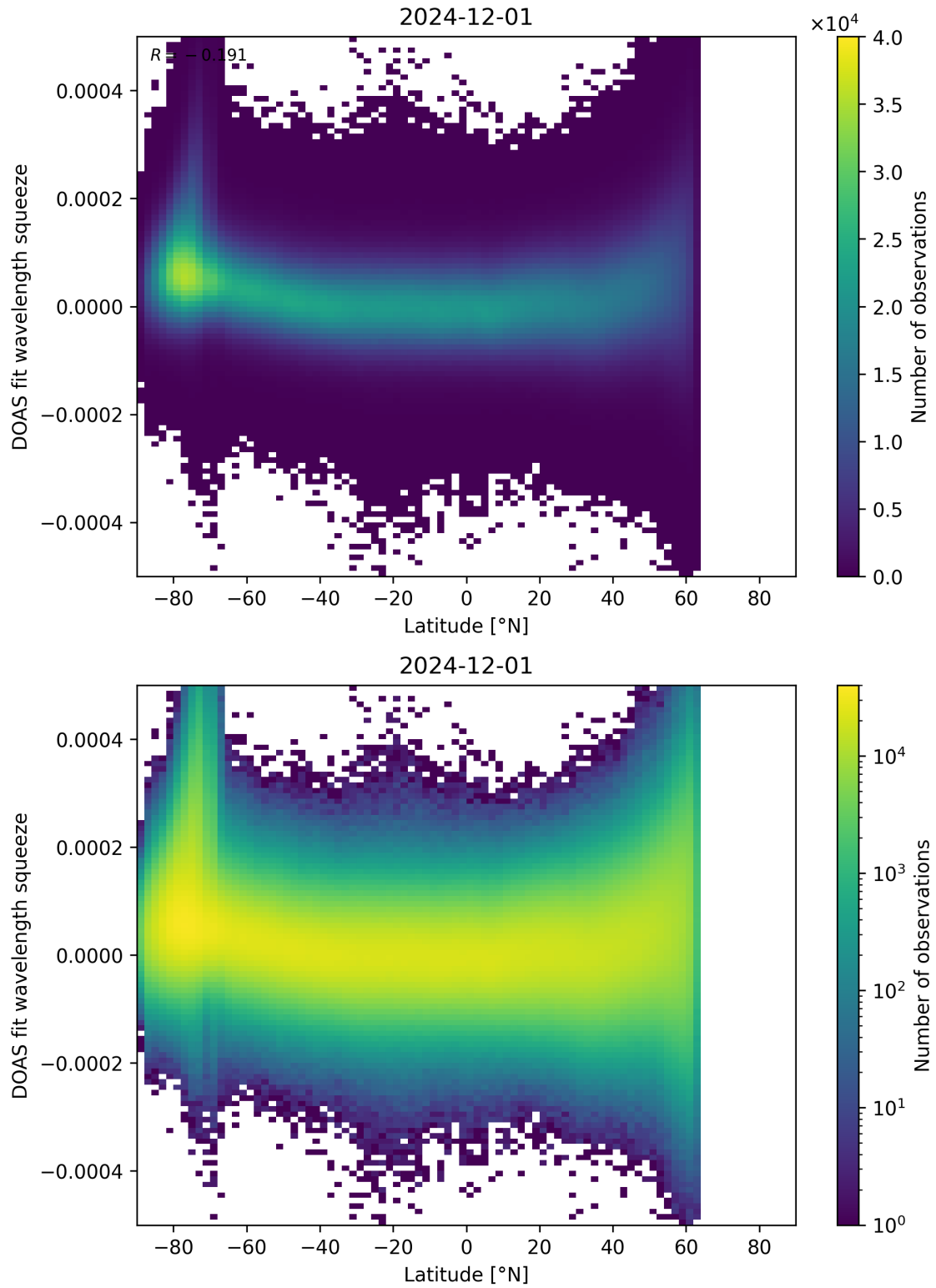
Figure 155: Scatter density plot of “Latitude” against “DOAS fit wavelength squeeze” for 2024-11-30 to 2024-12-02.
