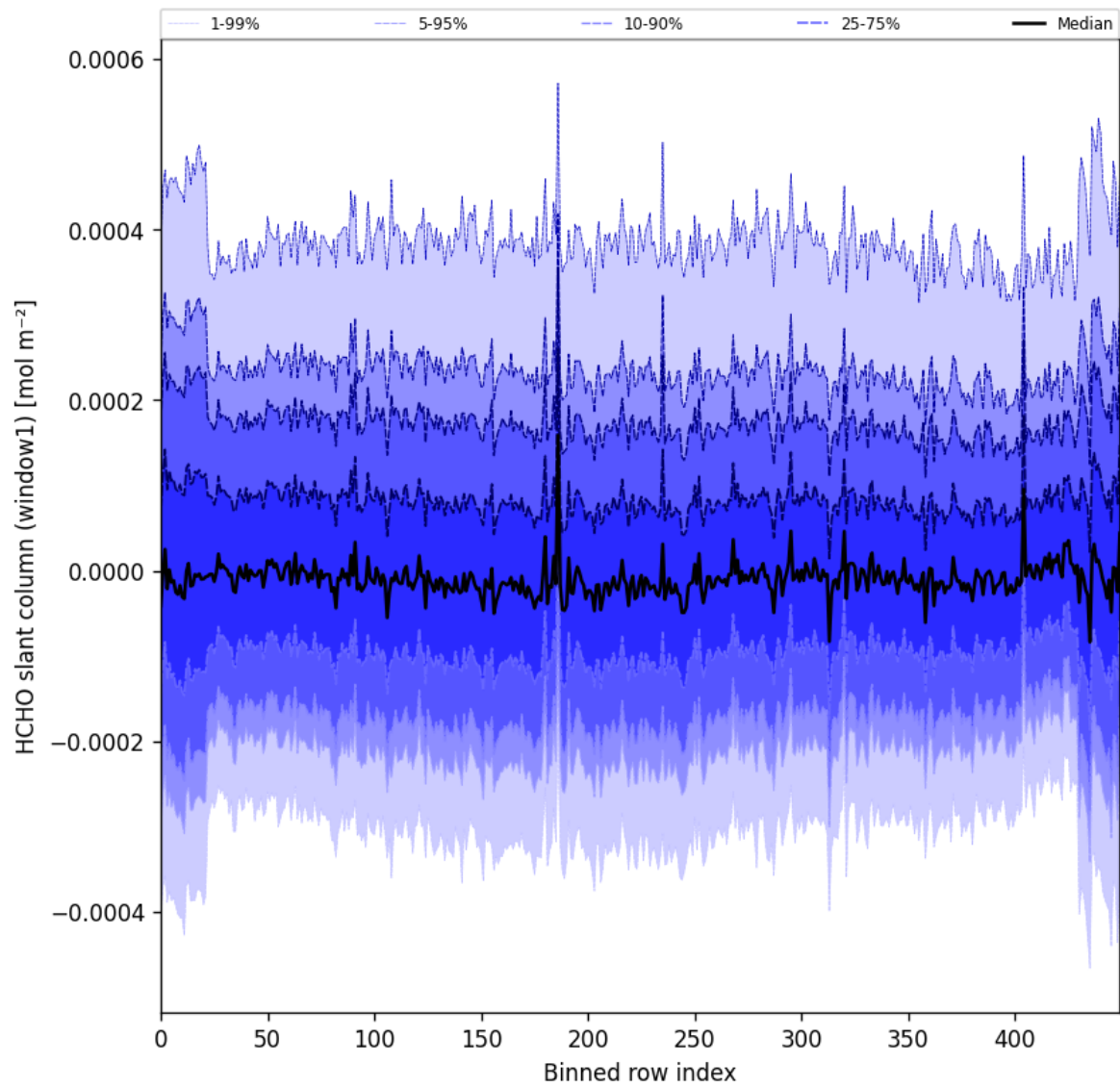
Figure 52: Along track statistics of “HCHO slant column (window1)” for 2024-11-30 to 2024-12-02
