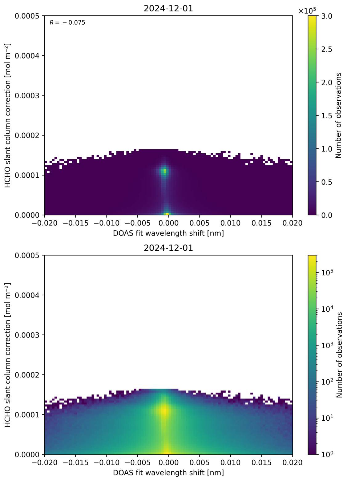
Figure 67: Scatter density plot of “DOAS fit wavelength shift” against “HCHO slant column correction” for 2024-11-30 to 2024-12-02.
