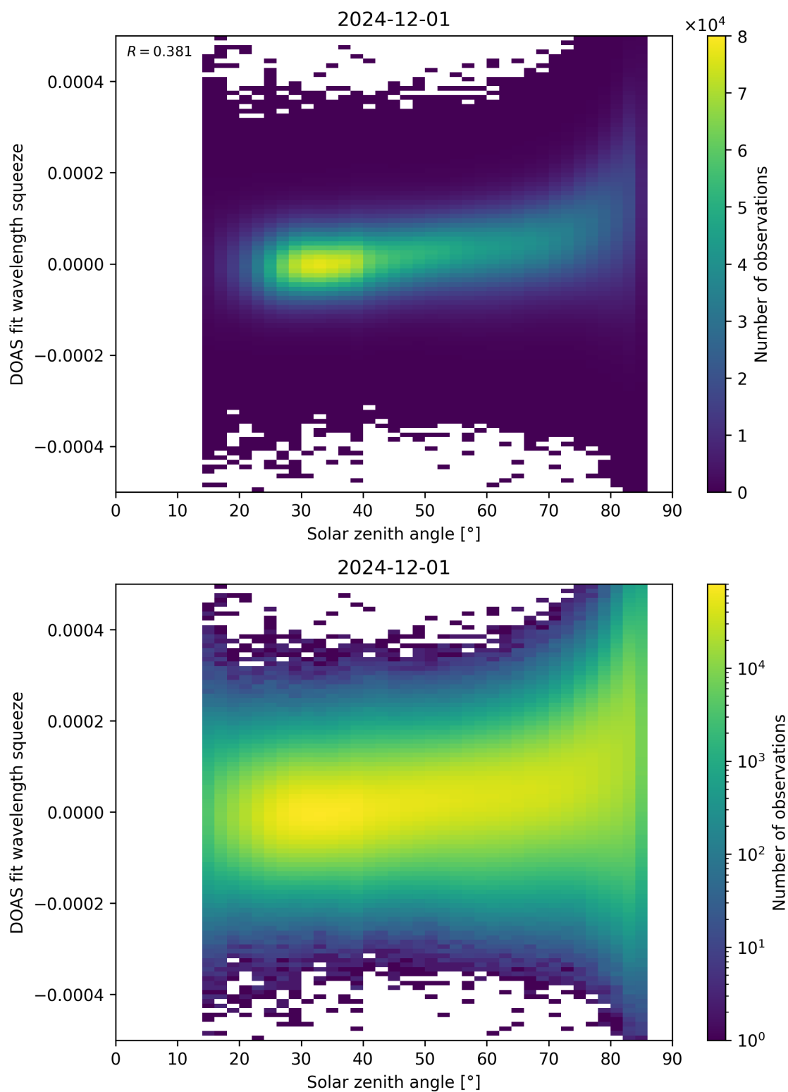
Figure 169: Scatter density plot of “Solar zenith angle” against “DOAS fit wavelength squeeze” for 2024-11-30 to 2024-12-02.
