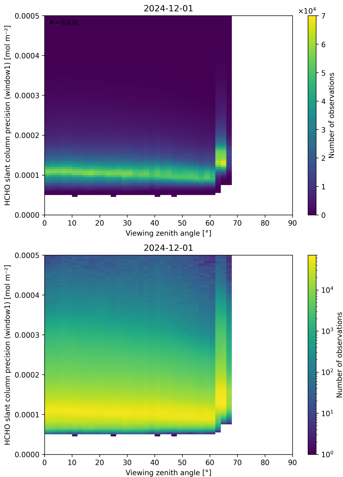
Figure 189: Scatter density plot of “Viewing zenith angle” against “HCHO slant column precision (window1)” for 2024-11-30 to 2024-12-02.
