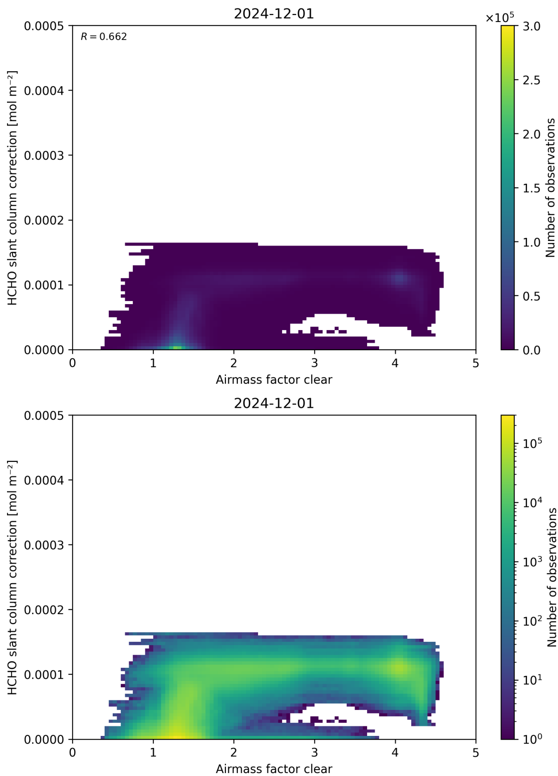
Figure 75: Scatter density plot of “Airmass factor clear” against “HCHO slant column correction” for 2024-11-30 to 2024-12-02.
