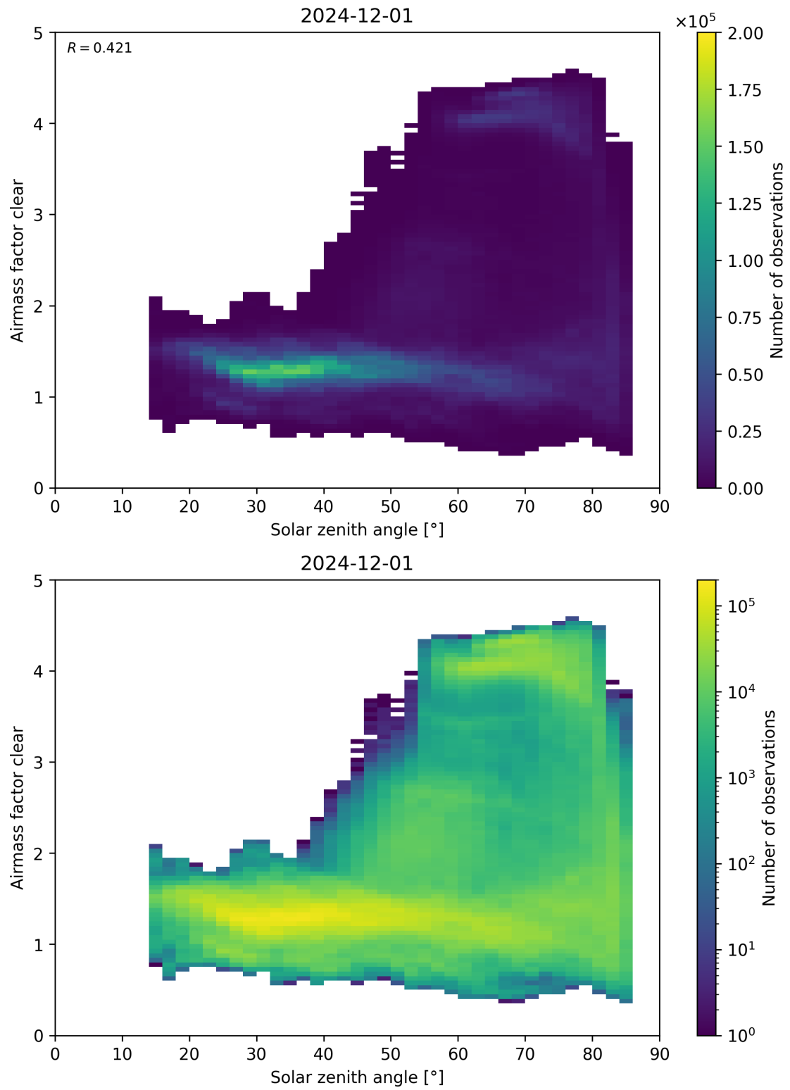
Figure 170: Scatter density plot of “Solar zenith angle” against “Airmass factor clear” for 2024-11-30 to 2024-12-02.
