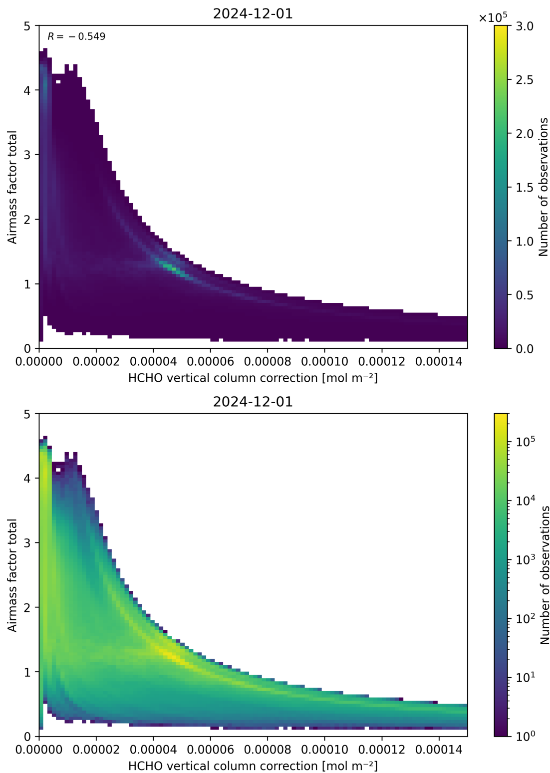
Figure 120: Scatter density plot of “HCHO vertical column correction” against “Airmass factor total” for 2024-11-30 to 2024-12-02.
