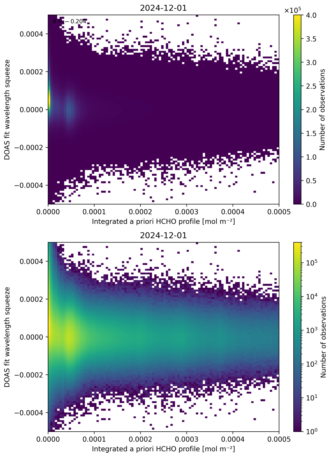
Figure 150: Scatter density plot of “Integrated a priori HCHO profile” against “DOAS fit wavelength squeeze” for 2024-11-30 to 2024-12-02.
