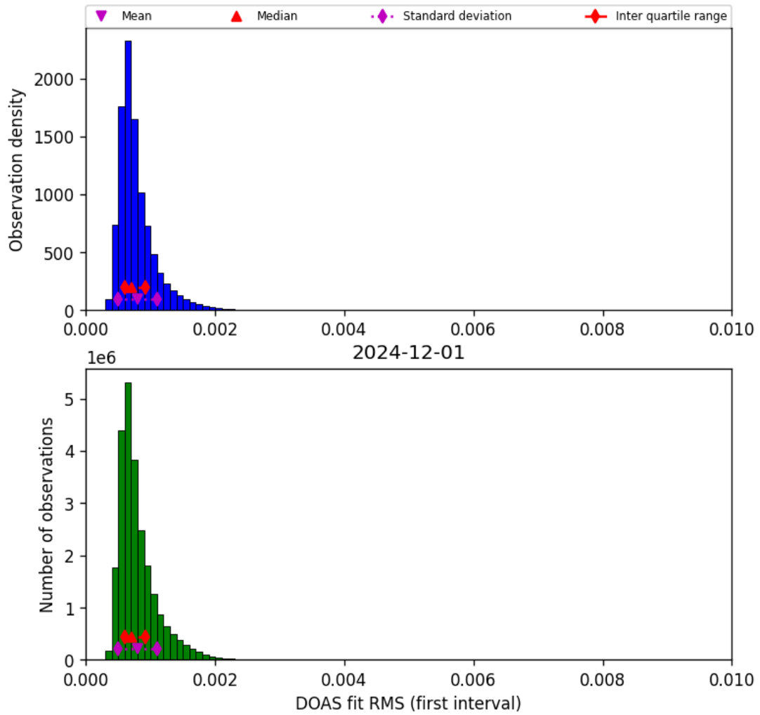
Figure 46: Histogram of “DOAS fit RMS (first interval)” for 2024-11-30 to 2024-12-02
