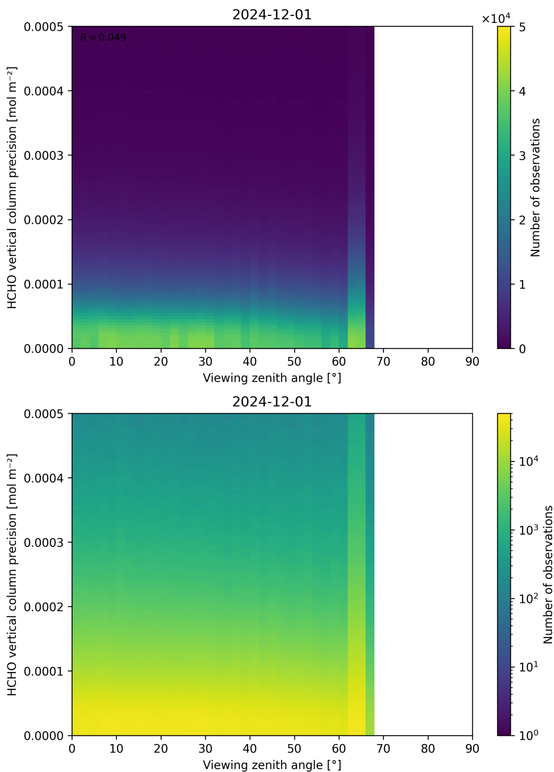
Figure 194: Scatter density plot of “Viewing zenith angle” against “HCHO vertical column precision” for 2024-11-30 to 2024-12-02.
