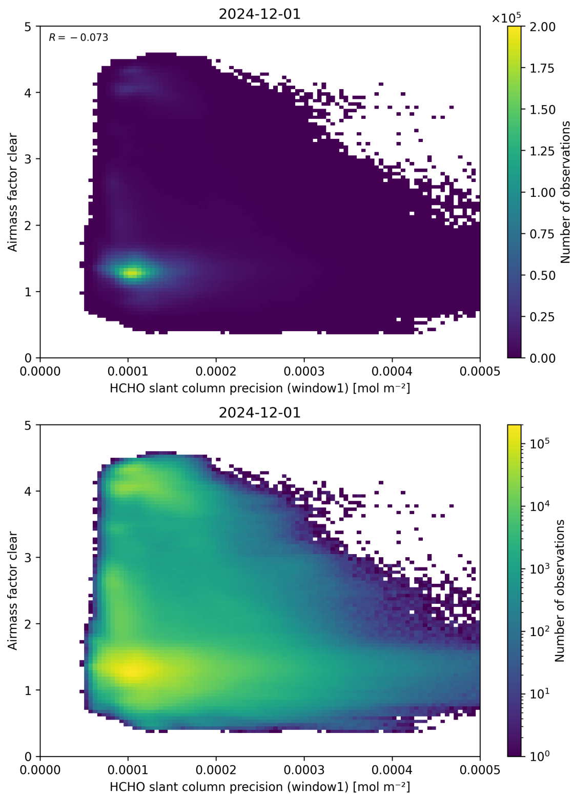
Figure 91: Scatter density plot of “HCHO slant column precision (window1)” against “Airmass factor clear” for 2024-11-30 to 2024-12-02.
