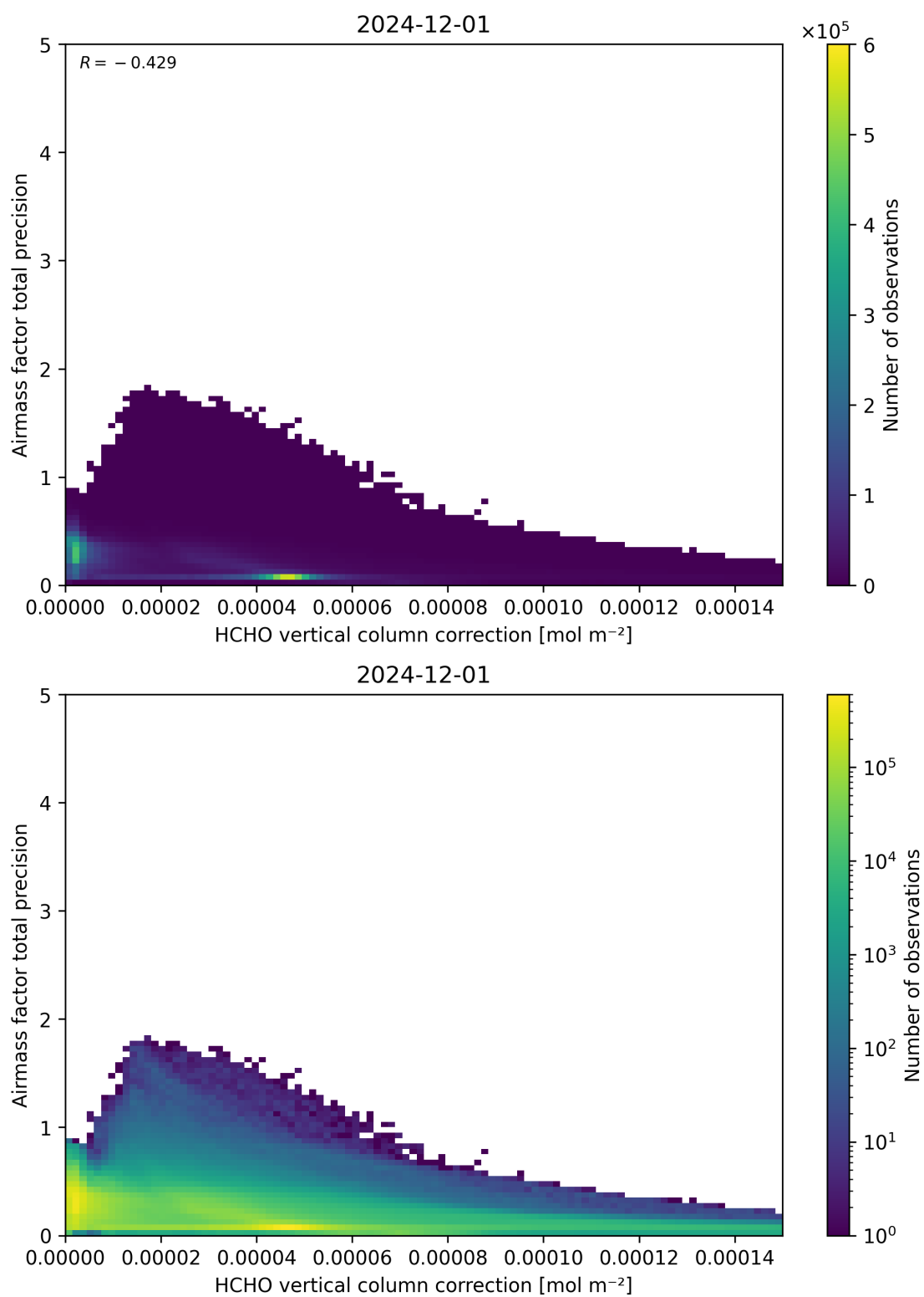
Figure 121: Scatter density plot of “HCHO vertical column correction” against “Airmass factor total precision” for 2024-11-30 to 2024-12-02.
