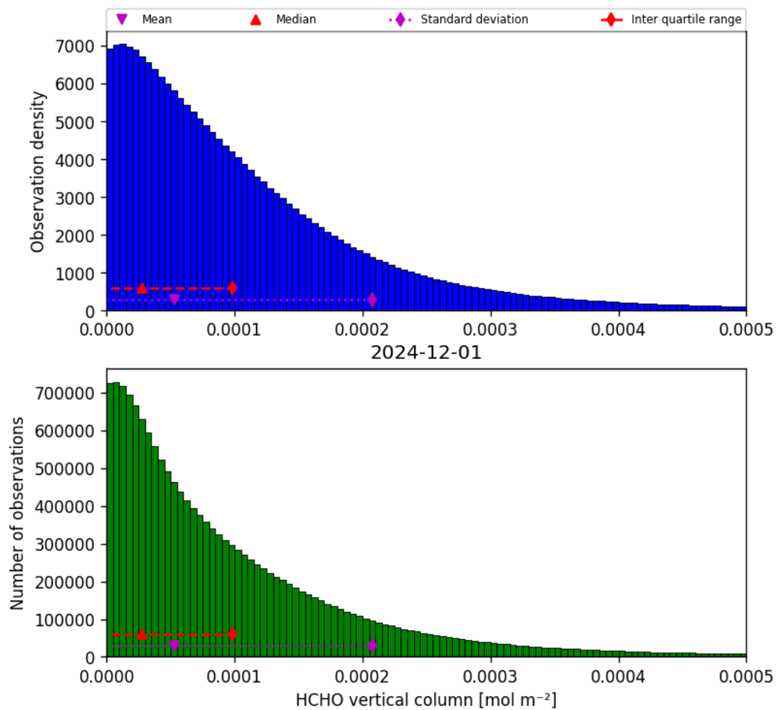
Figure 35: Histogram of “HCHO vertical column” for 2024-11-30 to 2024-12-02
