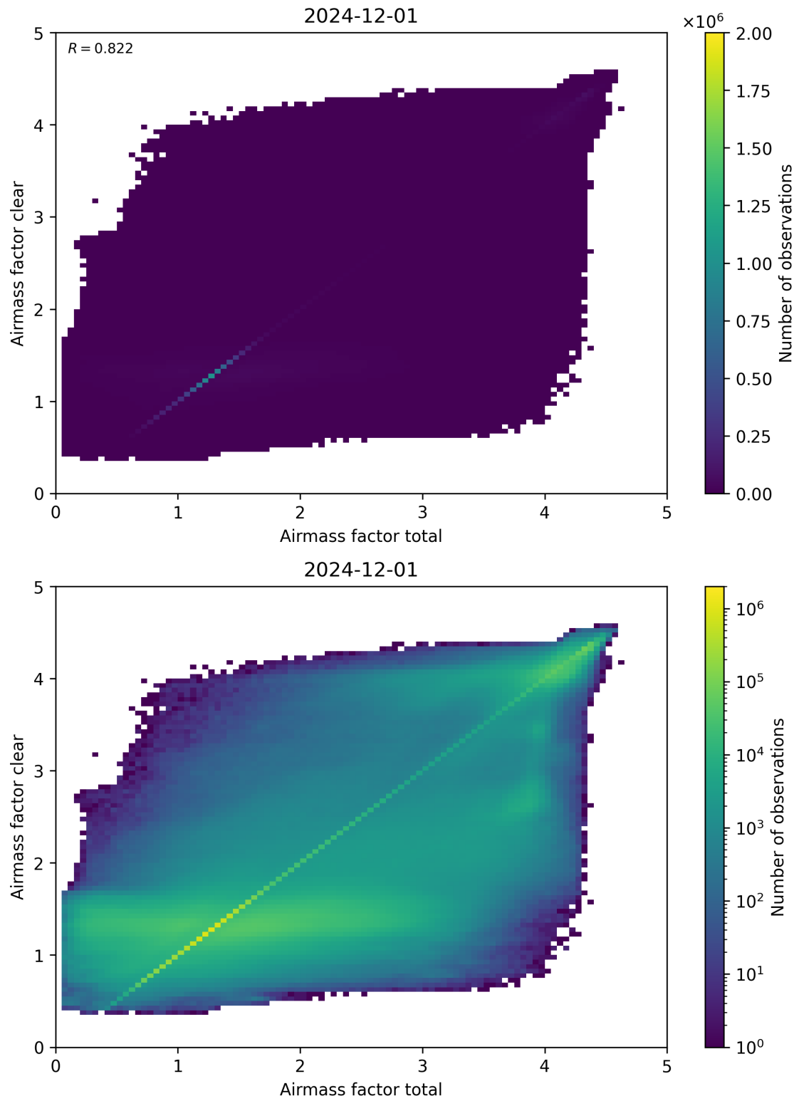
Figure 100: Scatter density plot of “Airmass factor total” against “Airmass factor clear” for 2024-11-30 to 2024-12-02.
