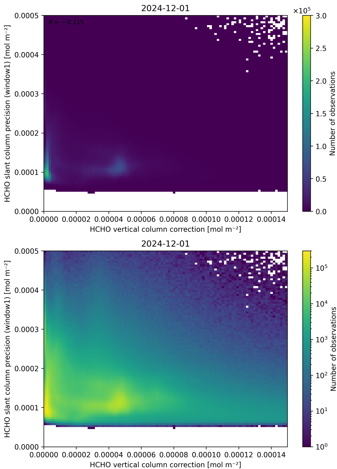
Figure 119: Scatter density plot of “HCHO vertical column correction” against “HCHO slant column precision (window1)” for 2024-11-30 to 2024-12-02.
