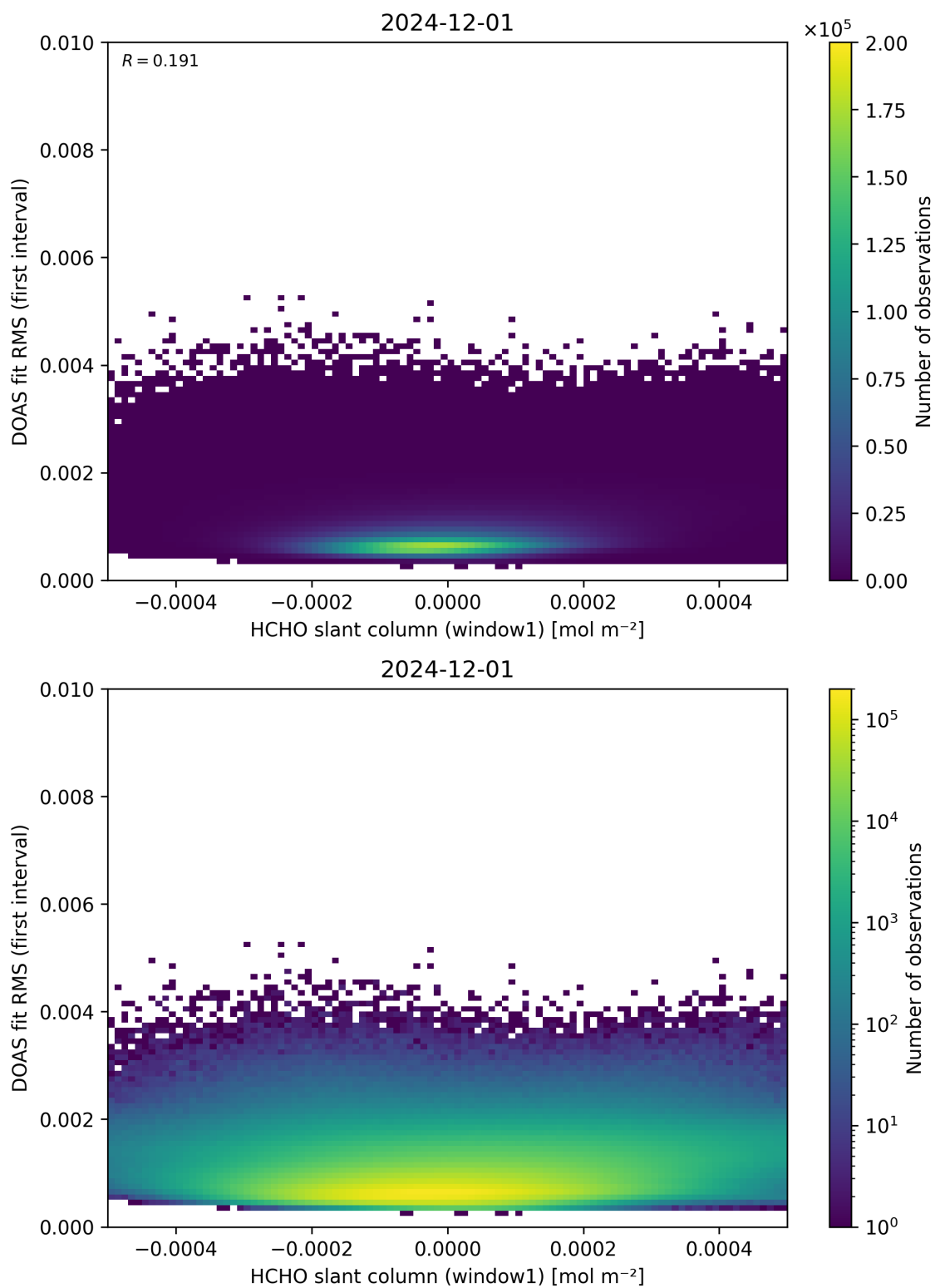
Figure 78: Scatter density plot of “HCHO slant column (window1)” against “DOAS fit RMS (first interval)” for 2024-11-30 to 2024-12-02.
