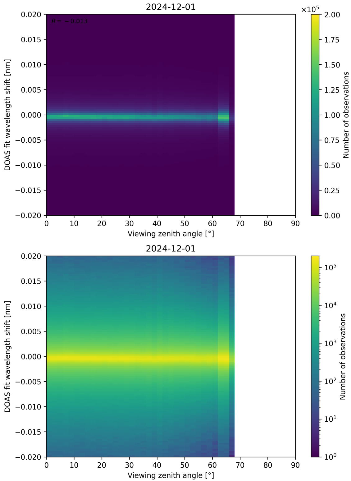
Figure 183: Scatter density plot of “Viewing zenith angle” against “DOAS fit wavelength shift” for 2024-11-30 to 2024-12-02.
