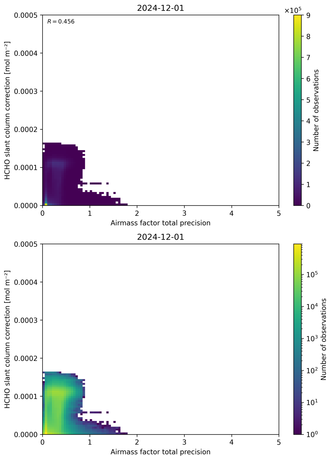
Figure 110: Scatter density plot of “Airmass factor total precision” against “HCHO slant column correction” for 2024-11-30 to 2024-12-02.
