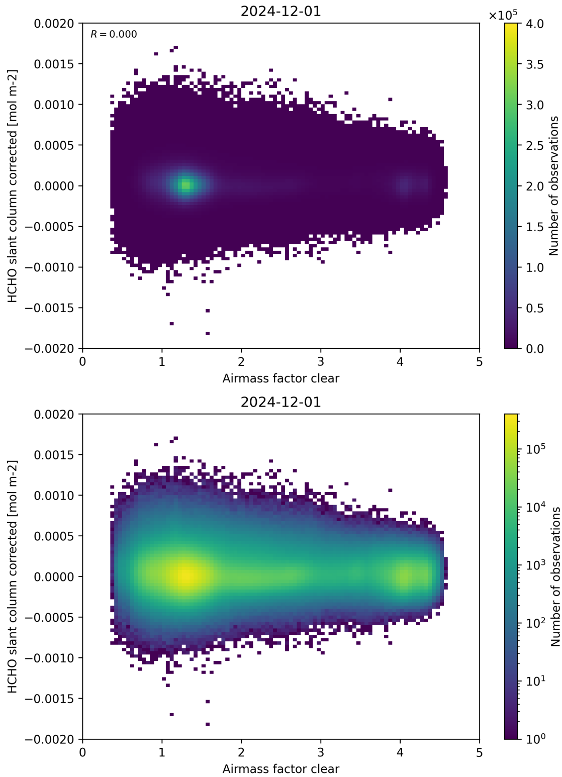
Figure 74: Scatter density plot of “Airmass factor clear” against “HCHO slant column corrected” for 2024-11-30 to 2024-12-02.
