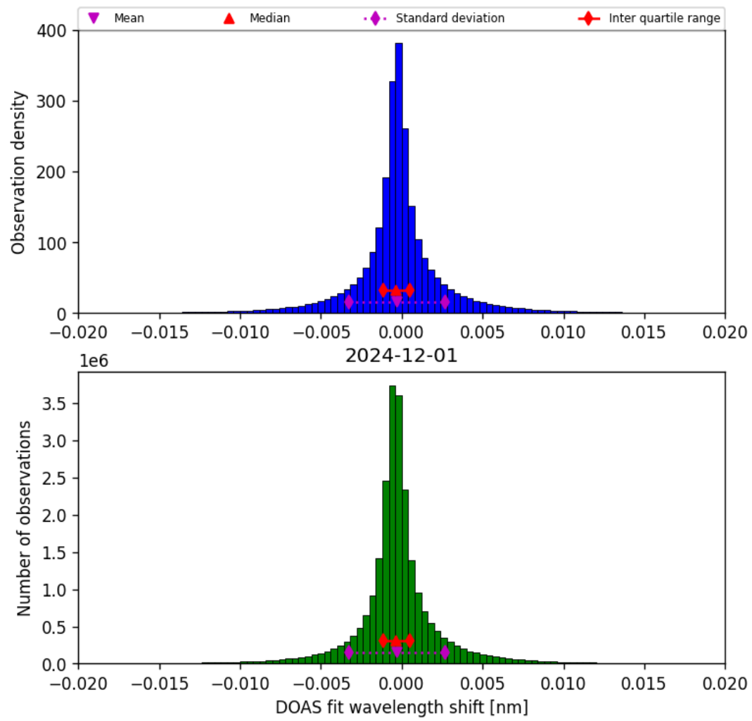
Figure 44: Histogram of “DOAS fit wavelength shift” for 2024-11-30 to 2024-12-02
