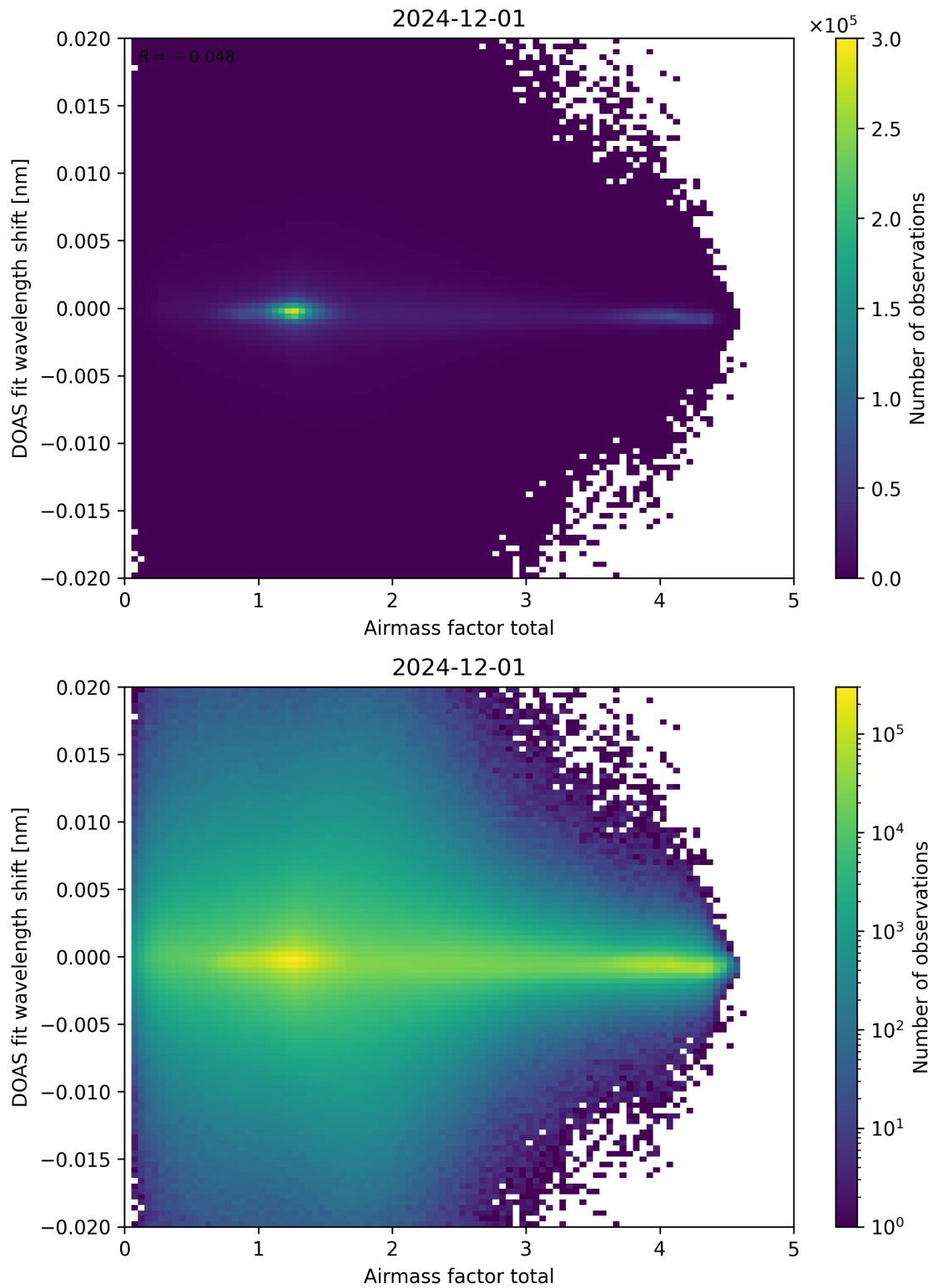
Figure 98: Scatter density plot of “Airmass factor total” against “DOAS fit wavelength shift” for 2024-11-30 to 2024-12-02.
