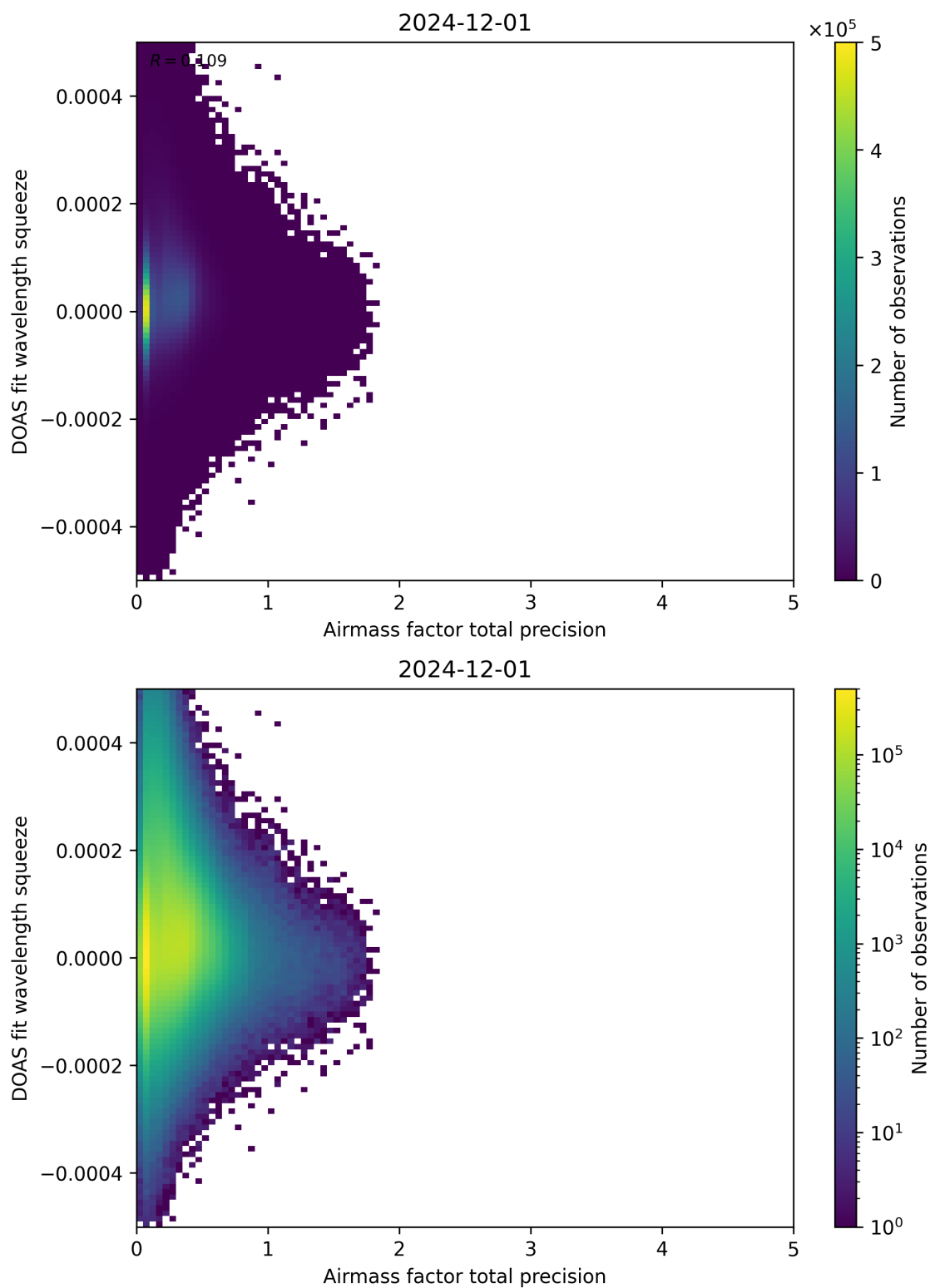
Figure 107: Scatter density plot of “Airmass factor total precision” against “DOAS fit wavelength squeeze” for 2024-11-30 to 2024-12-02.
