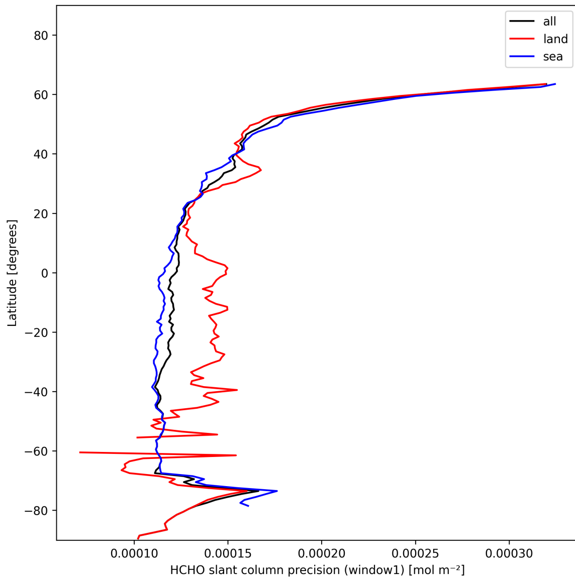
Figure 25: Zonal average of “HCHO slant column precision (window1)” for 2024-11-30 to 2024-12-02.
