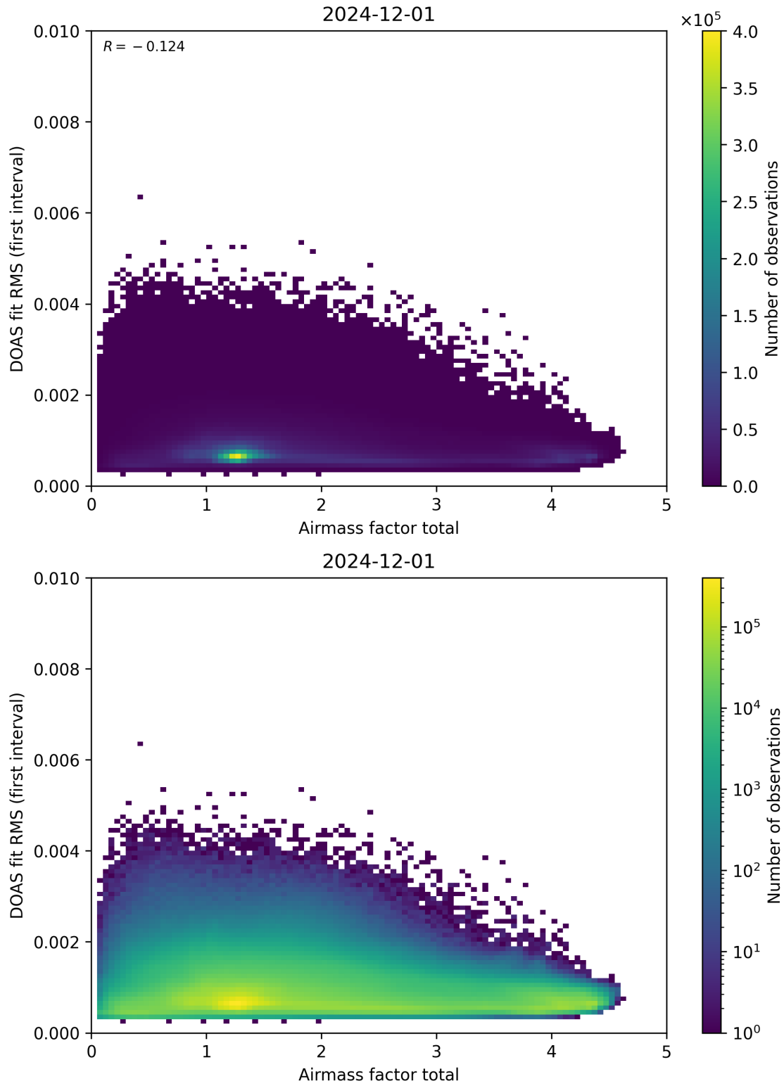
Figure 97: Scatter density plot of “Airmass factor total” against “DOAS fit RMS (first interval)” for 2024-11-30 to 2024-12-02.
