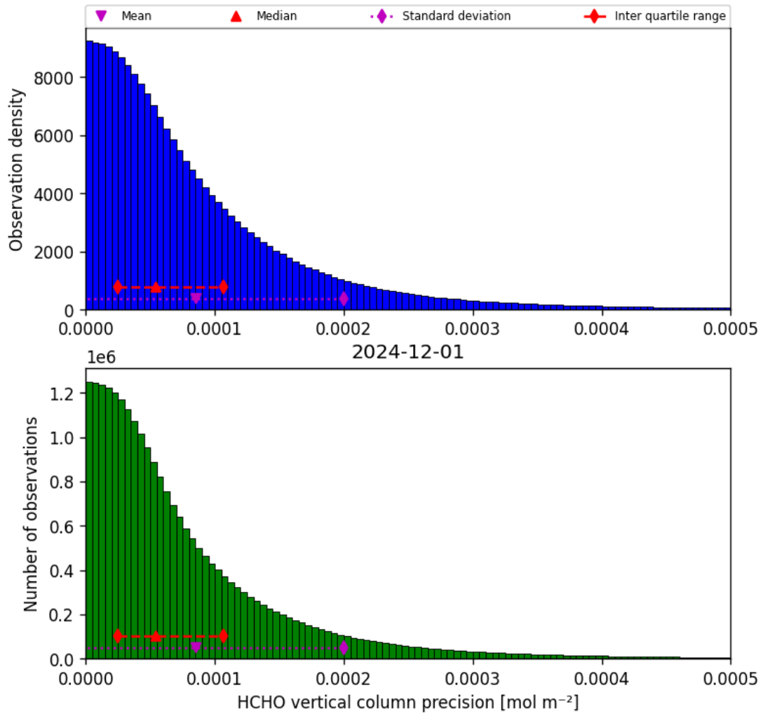
Figure 36: Histogram of “HCHO vertical column precision” for 2024-11-30 to 2024-12-02
