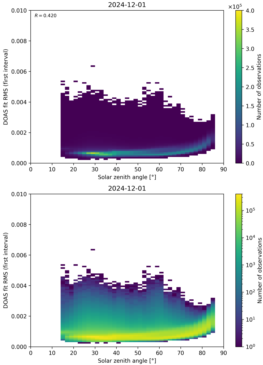
Figure 167: Scatter density plot of “Solar zenith angle” against “DOAS fit RMS (first interval)” for 2024-11-30 to 2024-12-02.
