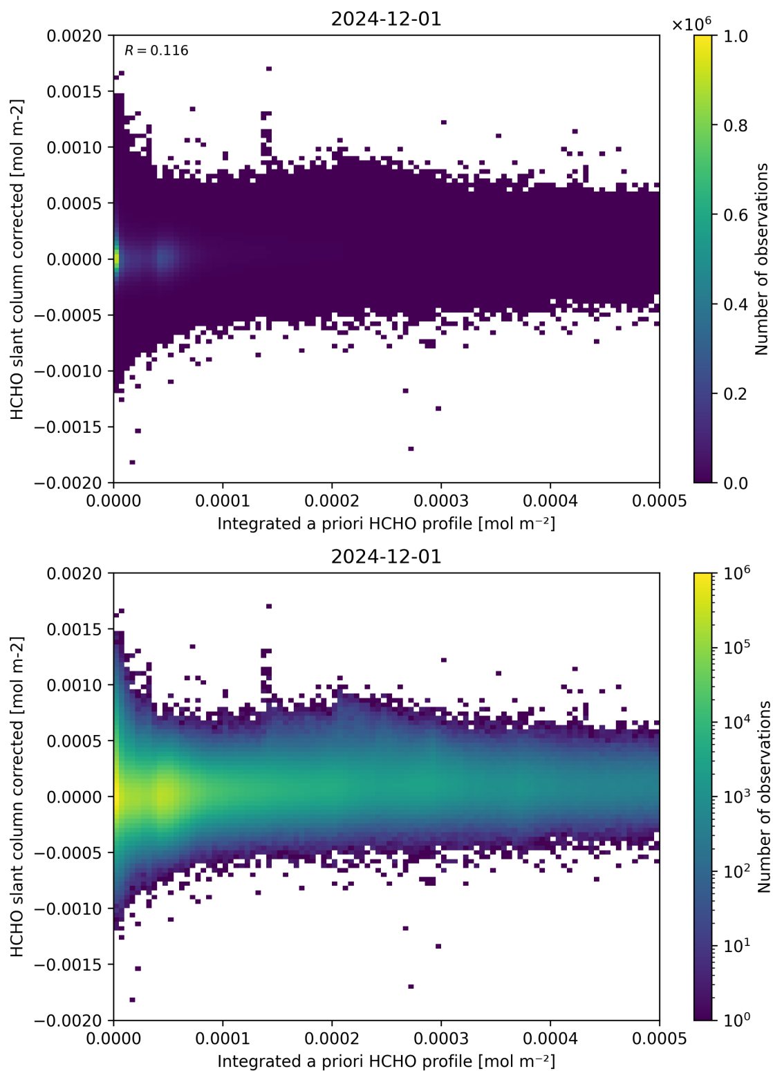
Figure 151: Scatter density plot of “Integrated a priori HCHO profile” against “HCHO slant column corrected” for 2024-11-30 to 2024-12-02.
