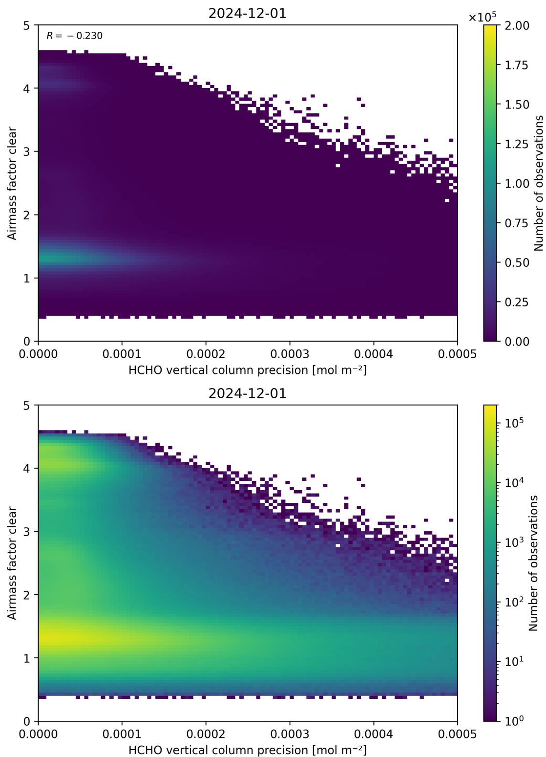
Figure 139: Scatter density plot of “HCHO vertical column precision” against “Airmass factor clear” for 2024-11-30 to 2024-12-02.
