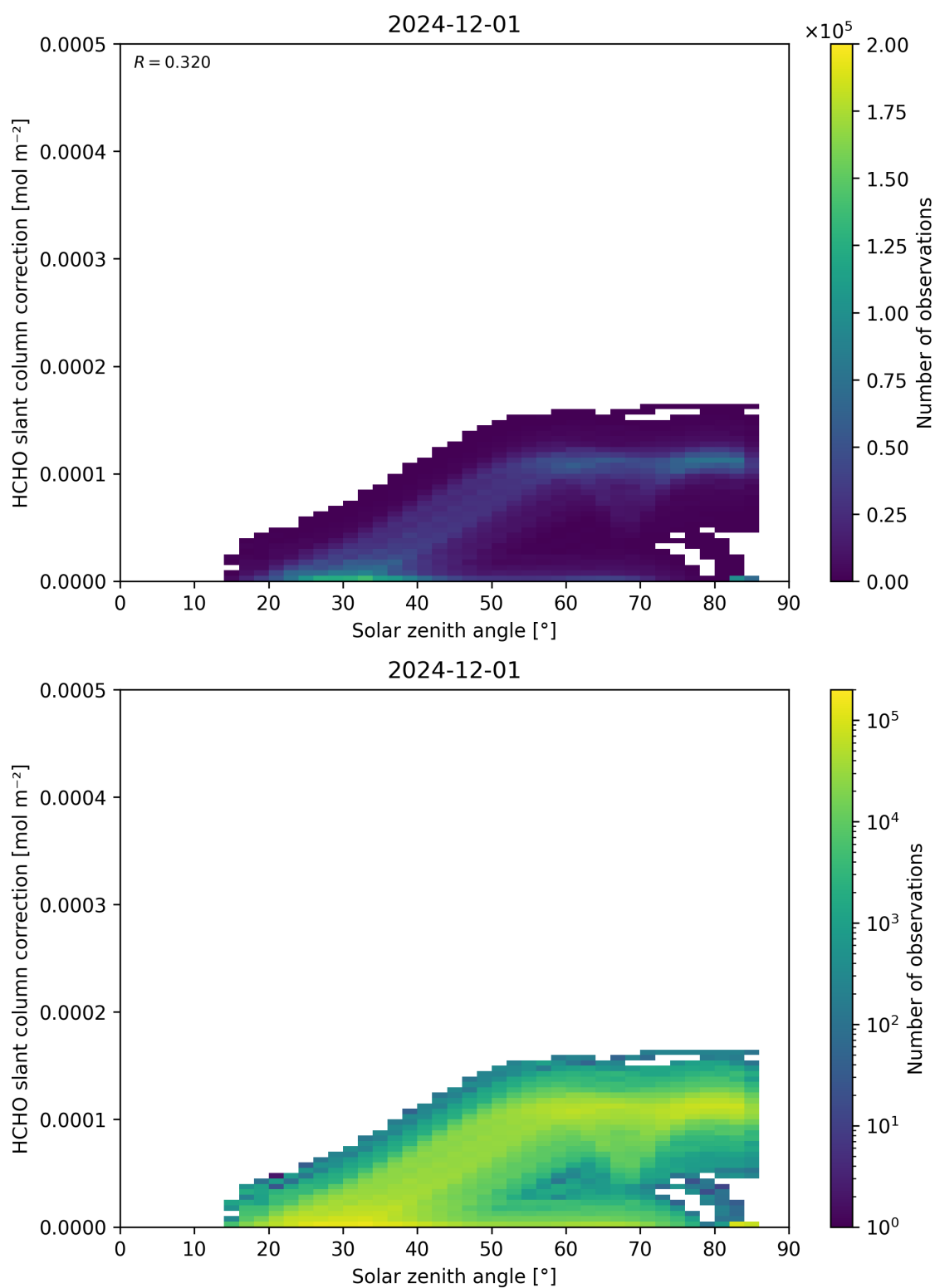
Figure 172: Scatter density plot of “Solar zenith angle” against “HCHO slant column correction” for 2024-11-30 to 2024-12-02.
