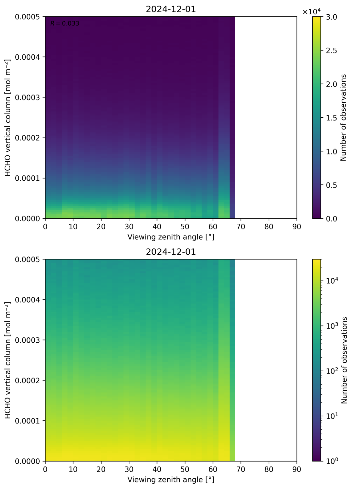
Figure 192: Scatter density plot of “Viewing zenith angle” against “HCHO vertical column” for 2024-11-30 to 2024-12-02.
