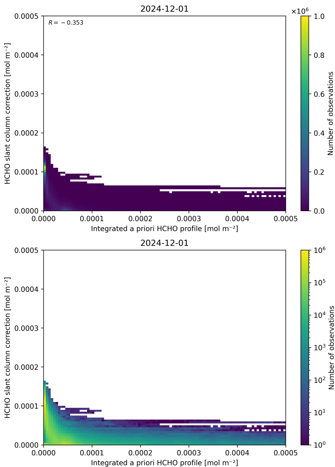
Figure 152: Scatter density plot of “Integrated a priori HCHO profile” against “HCHO slant column correction” for 2024-11-30 to 2024-12-02.
