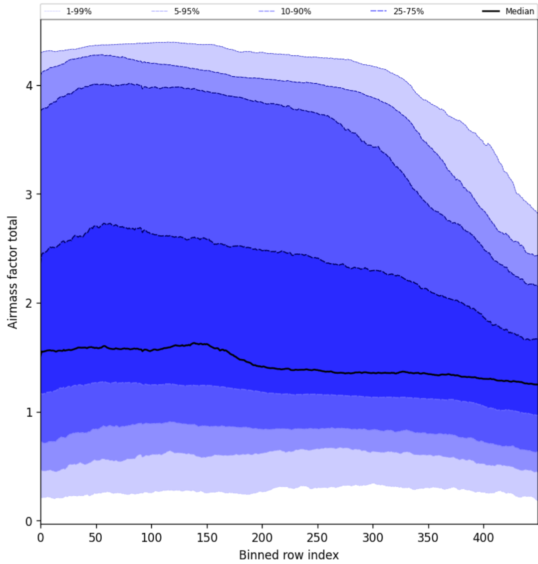
Figure 54: Along track statistics of “Airmass factor total” for 2024-11-30 to 2024-12-02
