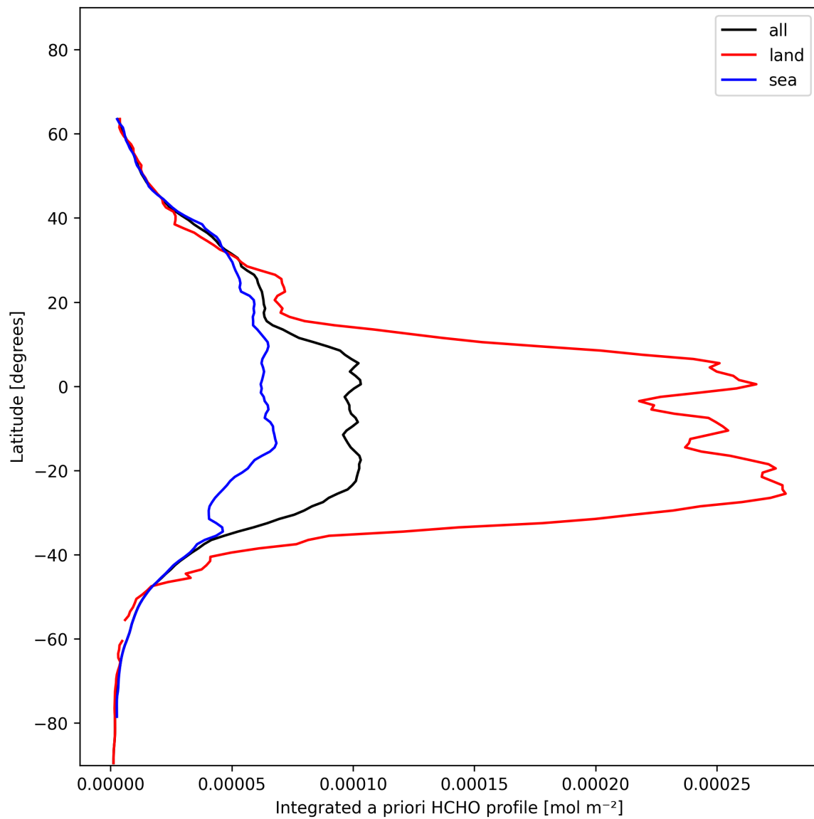
Figure 29: Zonal average of “Integrated a priori HCHO profile” for 2024-11-30 to 2024-12-02.
