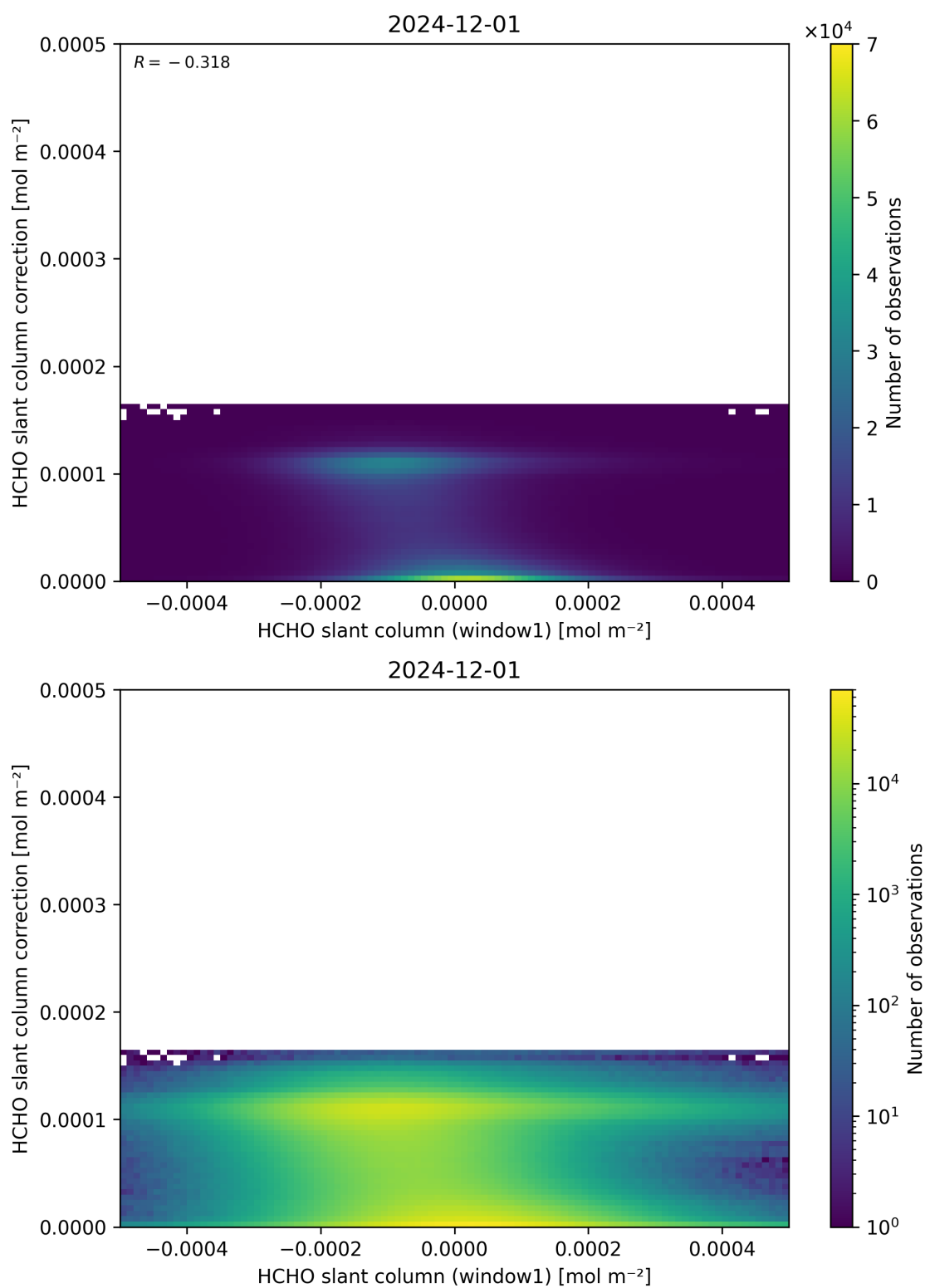
Figure 83: Scatter density plot of “HCHO slant column (window1)” against “HCHO slant column correction” for 2024-11-30 to 2024-12-02.
