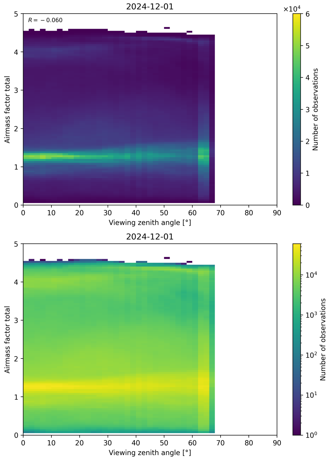
Figure 190: Scatter density plot of “Viewing zenith angle” against “Airmass factor total” for 2024-11-30 to 2024-12-02.
