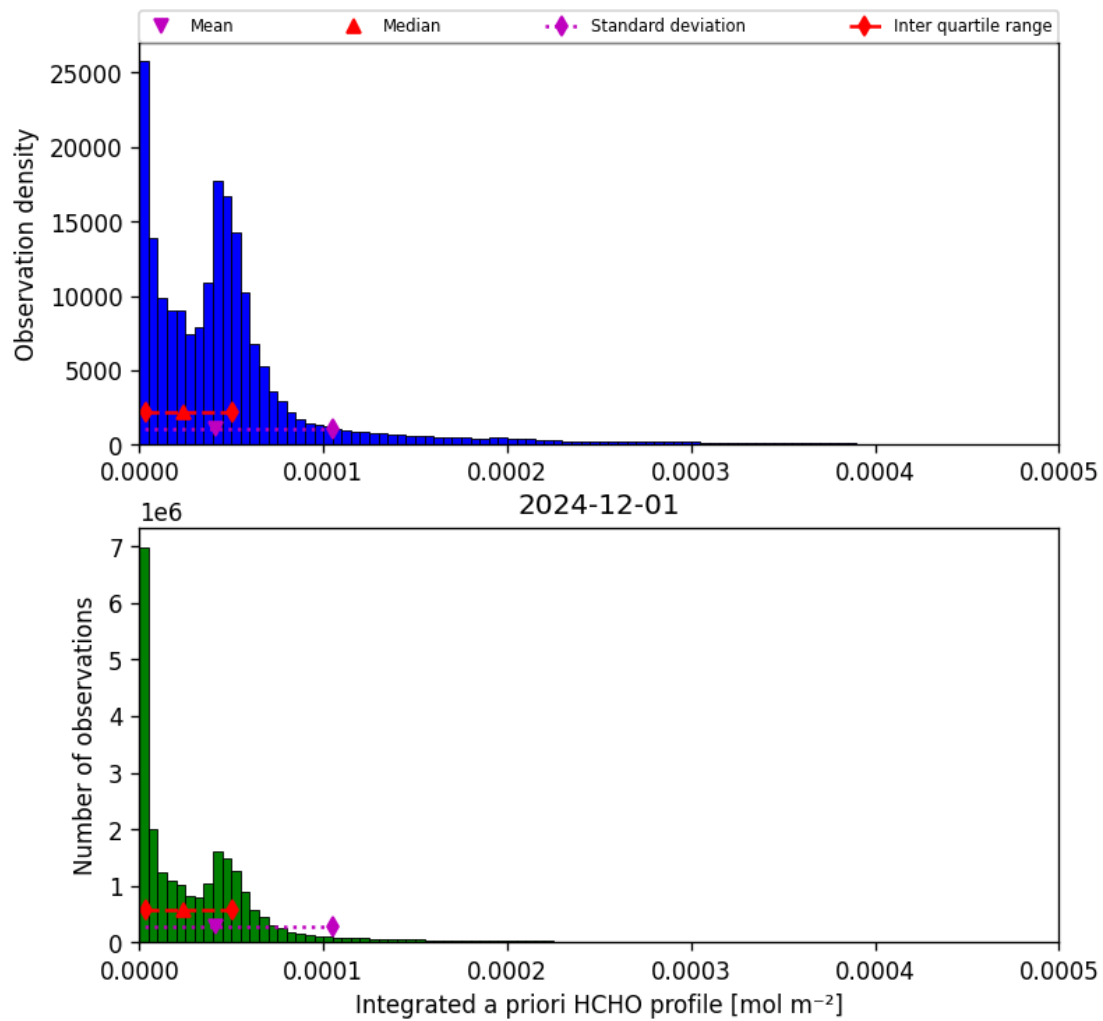
Figure 43: Histogram of “Integrated a priori HCHO profile” for 2024-11-30 to 2024-12-02
