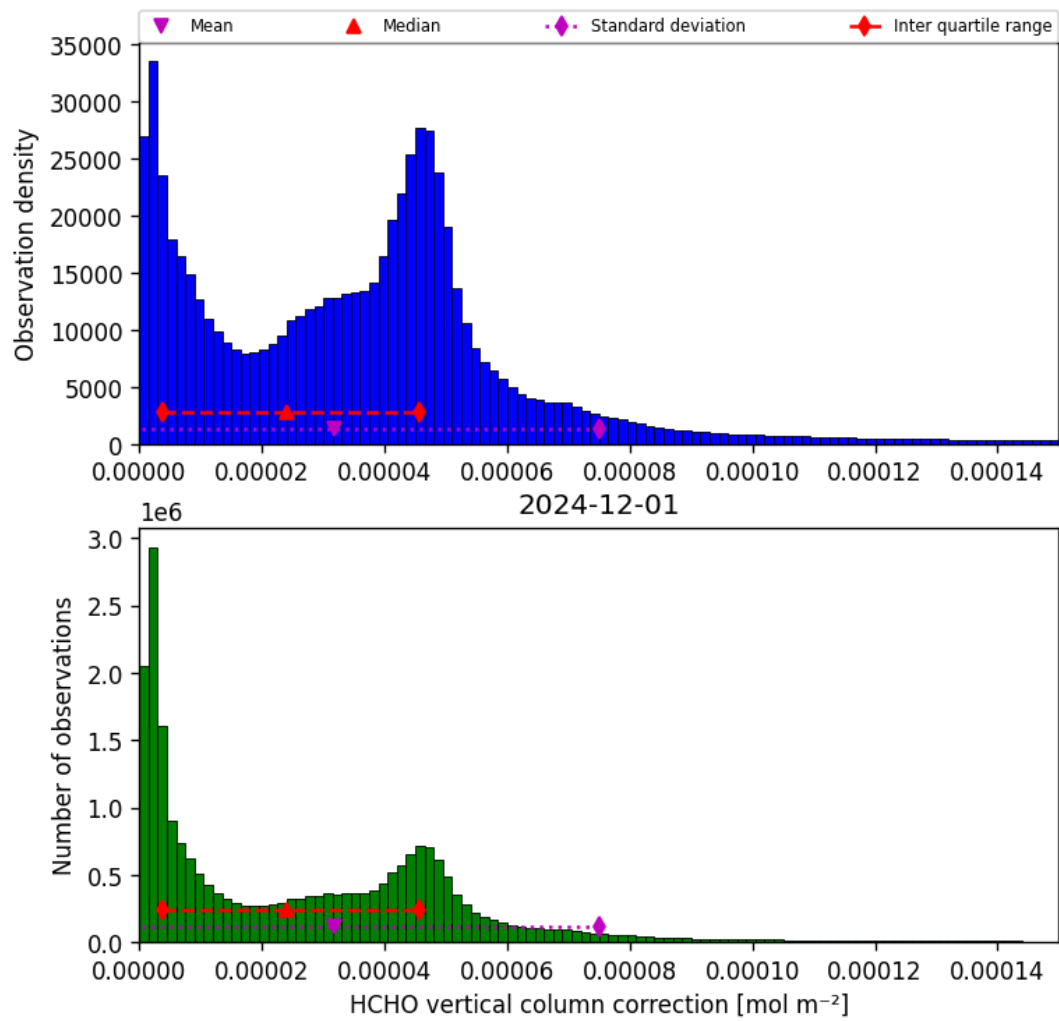
Figure 37: Histogram of “HCHO vertical column correction” for 2024-11-30 to 2024-12-02
