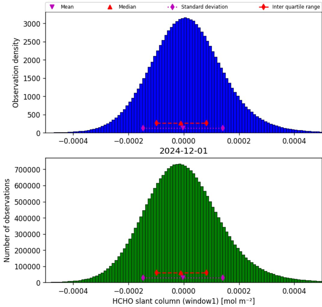
Figure 38: Histogram of “HCHO slant column (window1)” for 2024-11-30 to 2024-12-02
