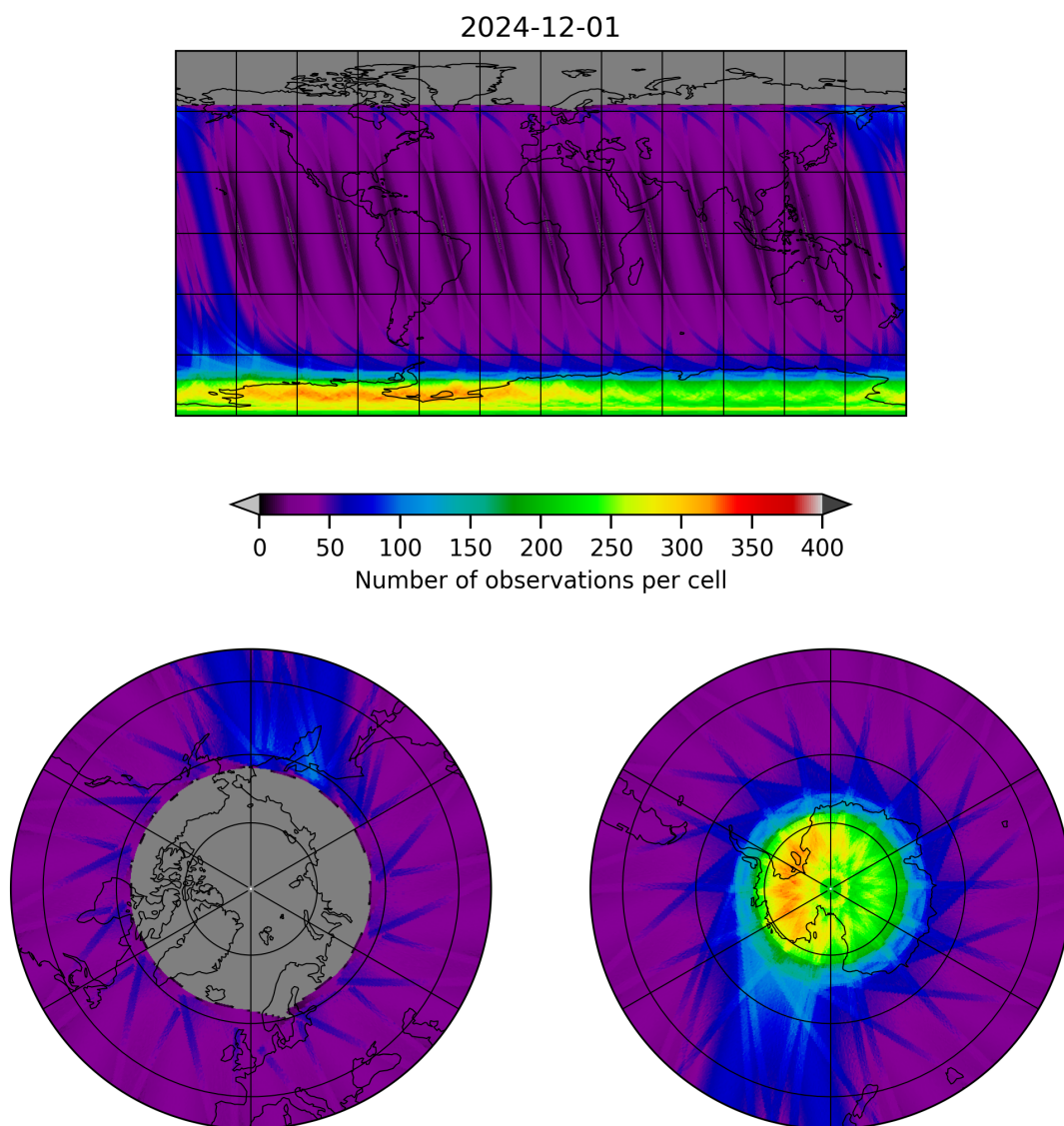
Figure 19: Map of the number of observations for 2024-11-30 to 2024-12-02
