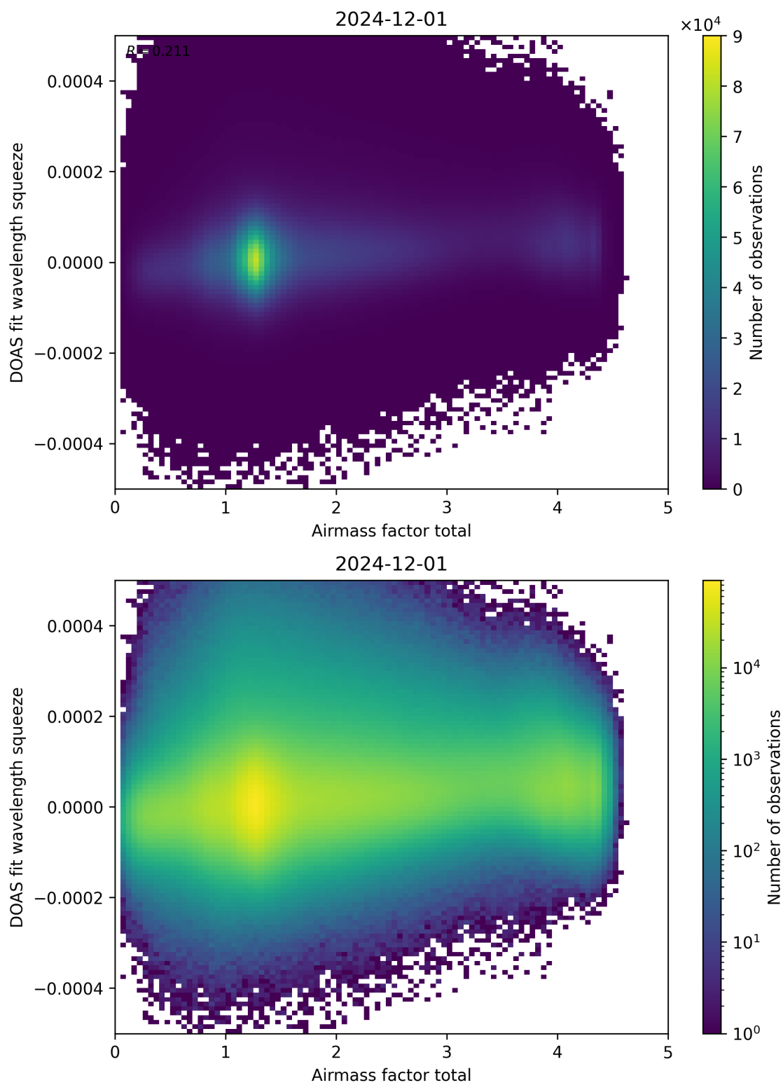
Figure 99: Scatter density plot of “Airmass factor total” against “DOAS fit wavelength squeeze” for 2024-11-30 to 2024-12-02.
