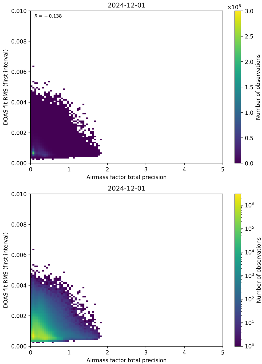
Figure 105: Scatter density plot of “Airmass factor total precision” against “DOAS fit RMS (first interval)” for 2024-11-30 to 2024-12-02.
