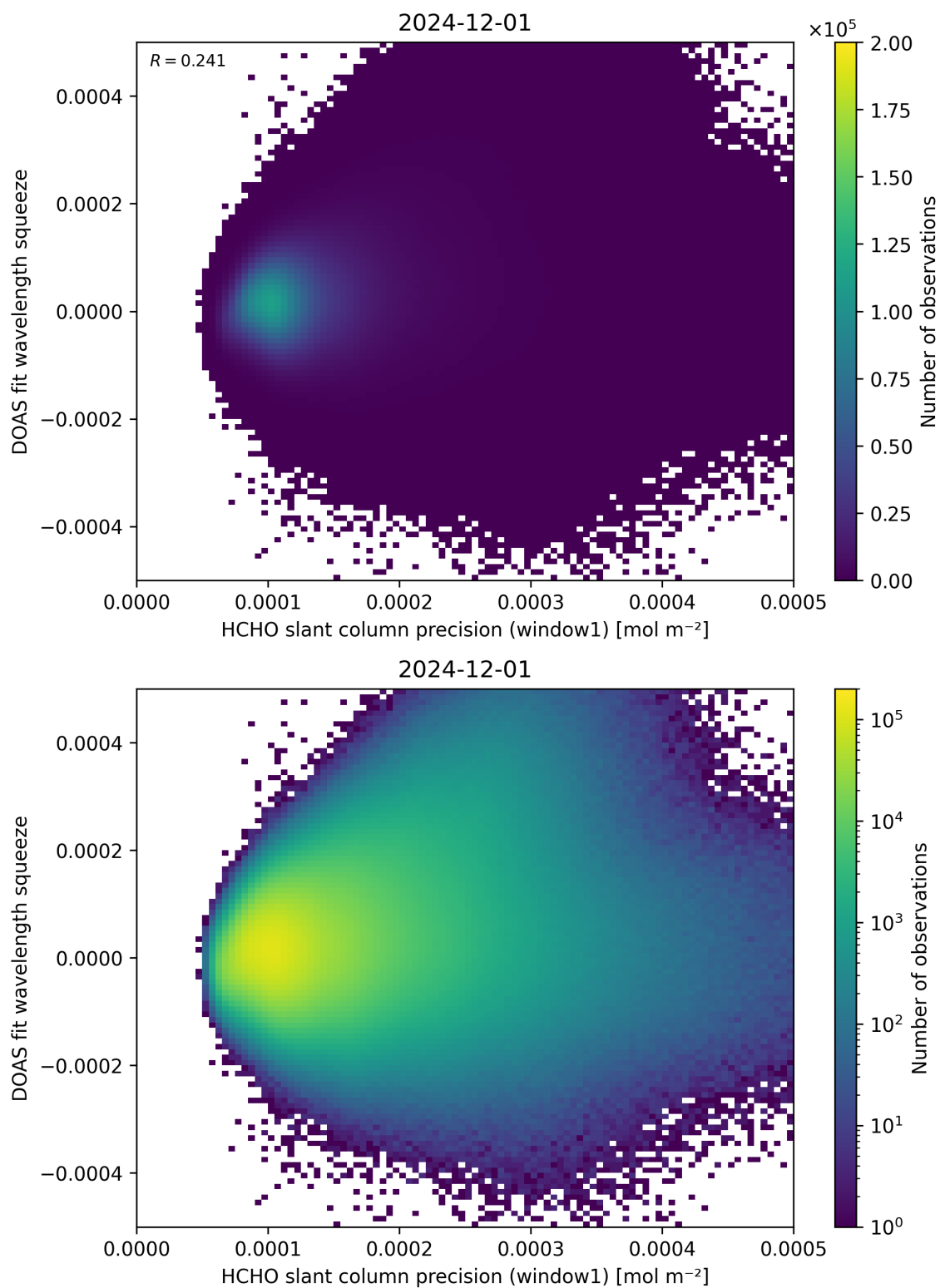
Figure 90: Scatter density plot of “HCHO slant column precision (window1)” against “DOAS fit wavelength squeeze” for 2024-11-30 to 2024-12-02.
