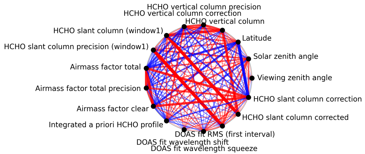
Figure 1: Map of correlation graph for 2024-11-30 to 2024-12-02.
