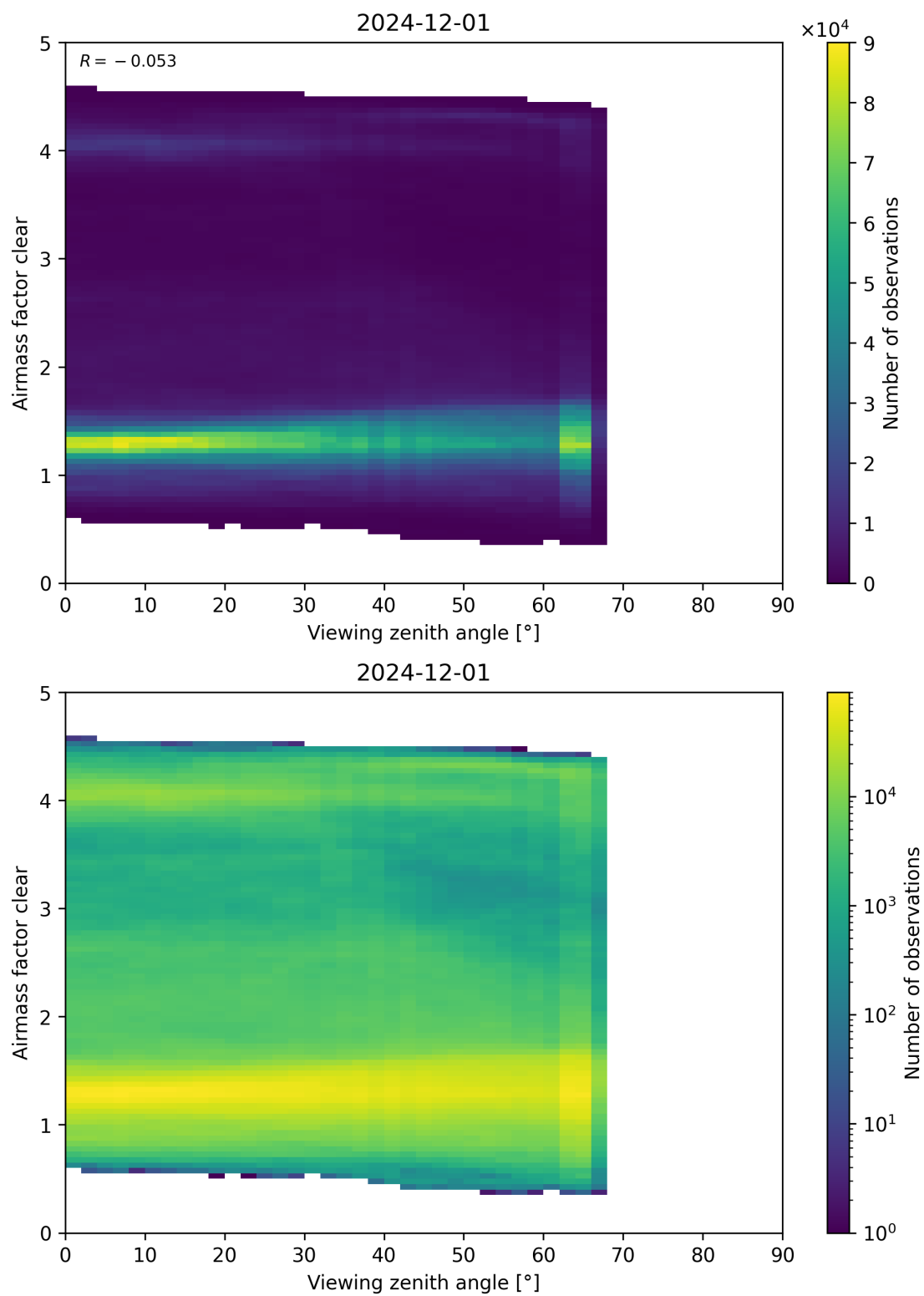
Figure 185: Scatter density plot of “Viewing zenith angle” against “Airmass factor clear” for 2024-11-30 to 2024-12-02.
