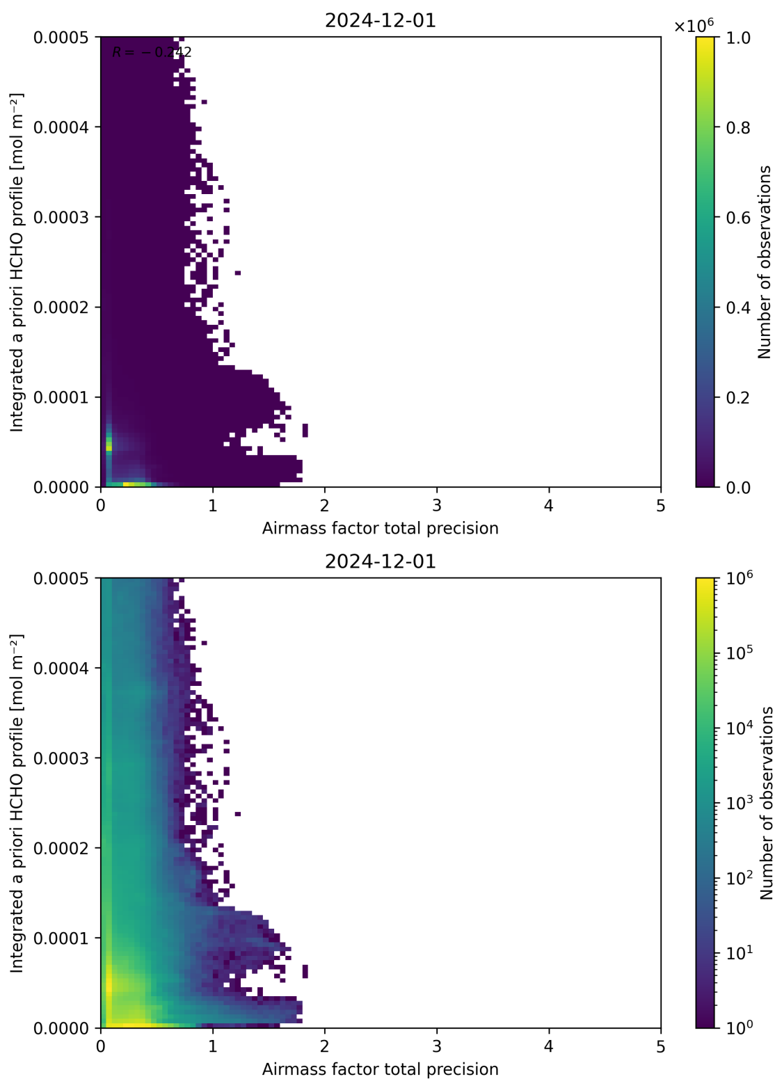
Figure 111: Scatter density plot of “Airmass factor total precision” against “Integrated a priori HCHO profile” for 2024-11-30 to 2024-12-02.
