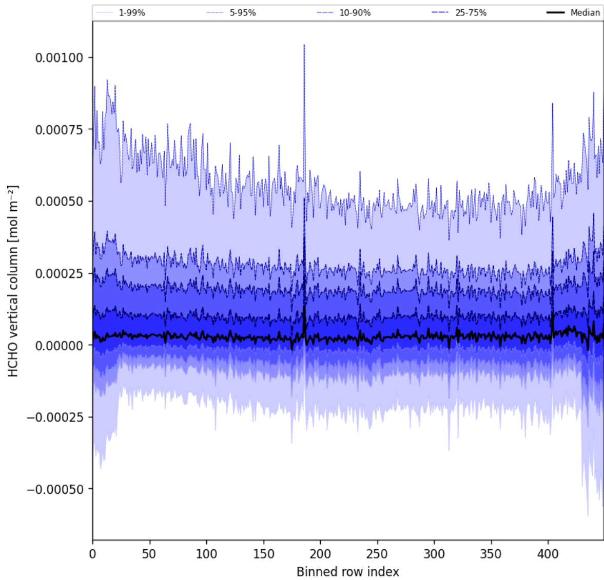
Figure 49: Along track statistics of “HCHO vertical column” for 2024-11-30 to 2024-12-02
