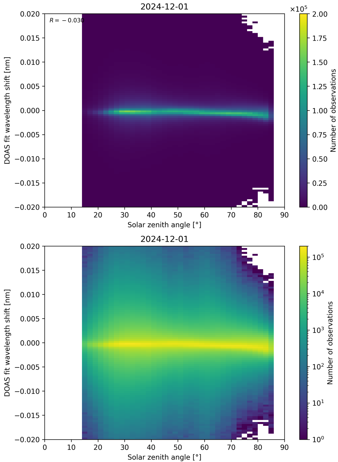
Figure 168: Scatter density plot of “Solar zenith angle” against “DOAS fit wavelength shift” for 2024-11-30 to 2024-12-02.
