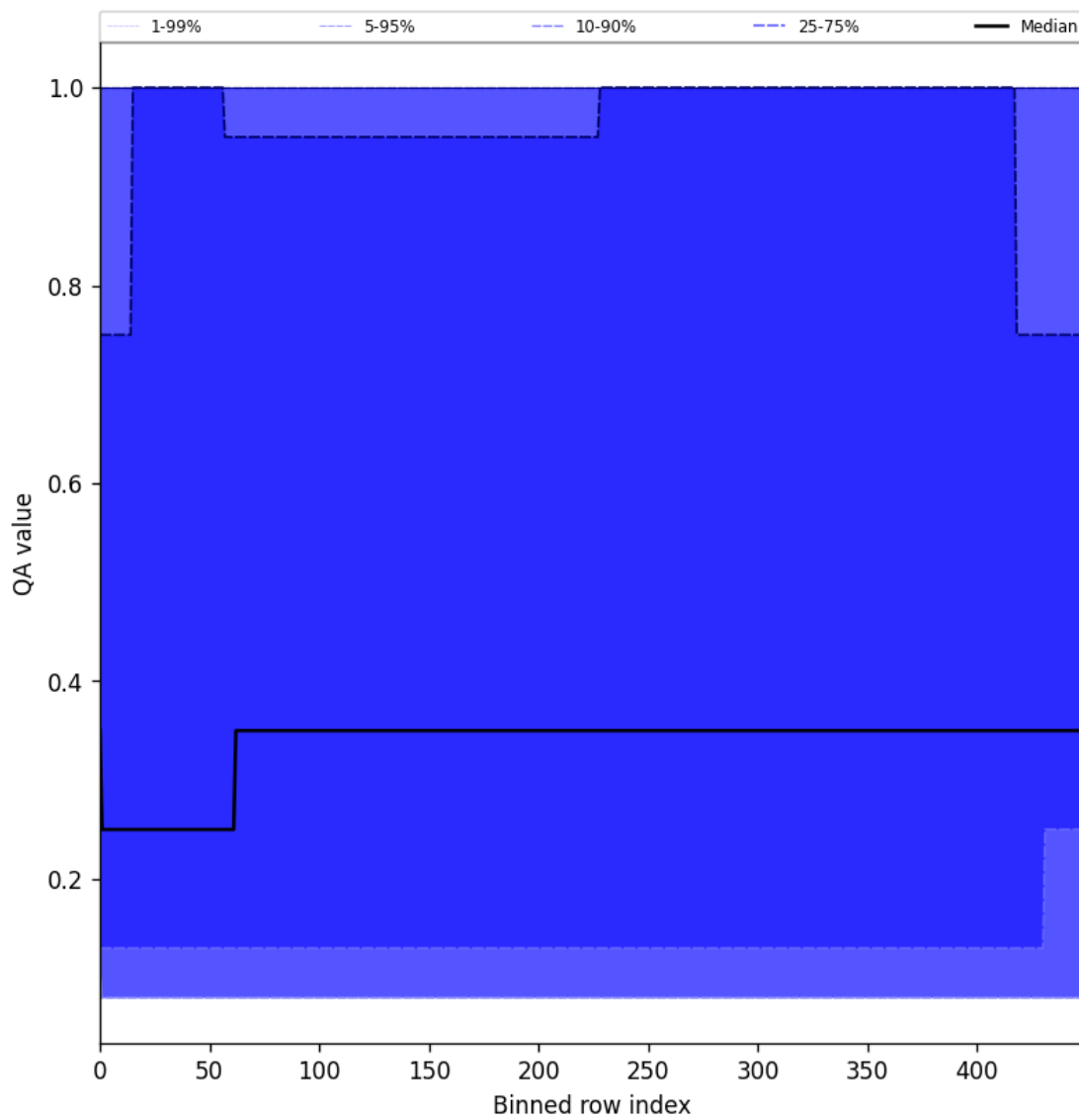
Figure 48: Along track statistics of “QA value” for 2024-11-30 to 2024-12-02
