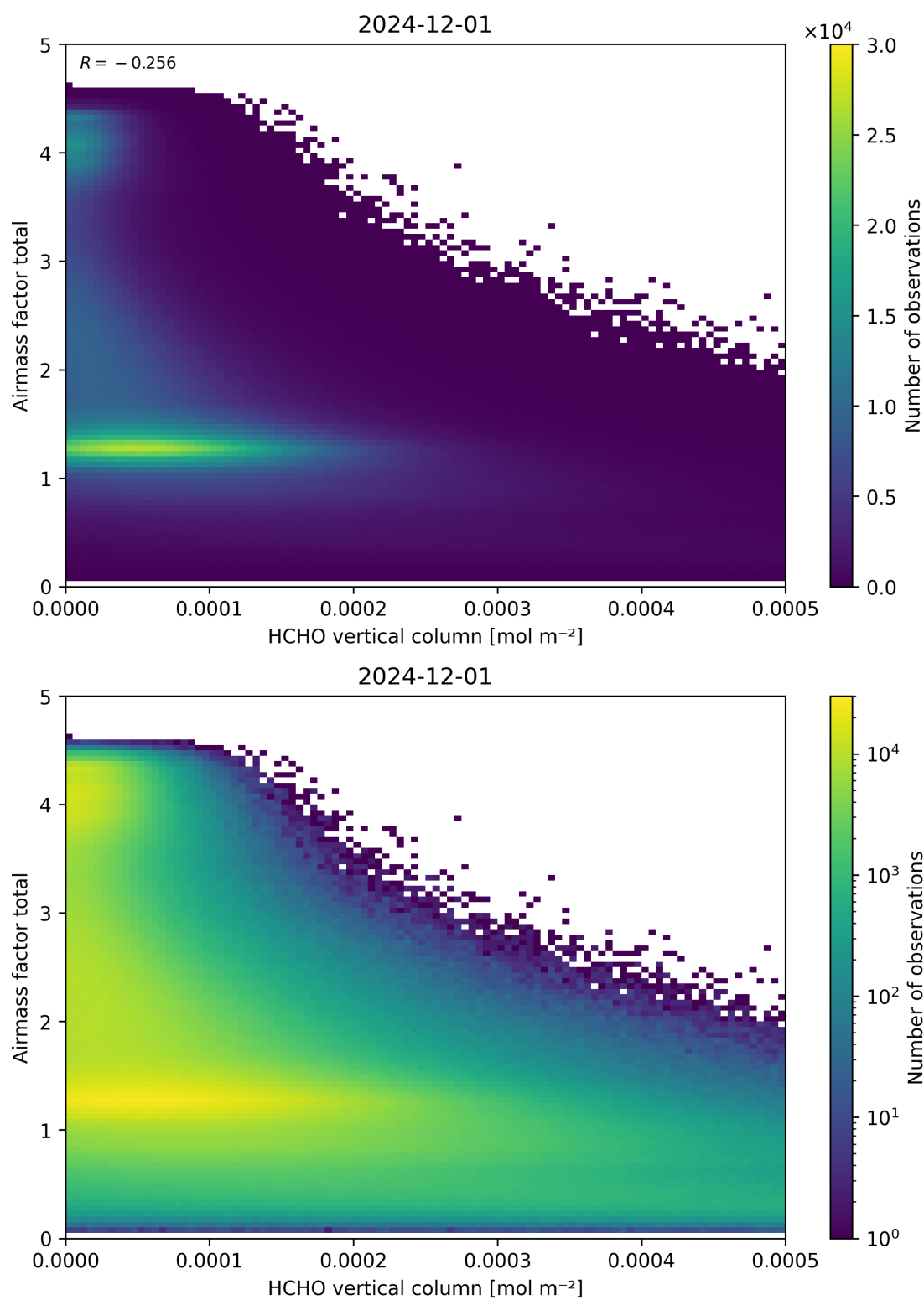
Figure 131: Scatter density plot of “HCHO vertical column” against “Airmass factor total” for 2024-11-30 to 2024-12-02.
