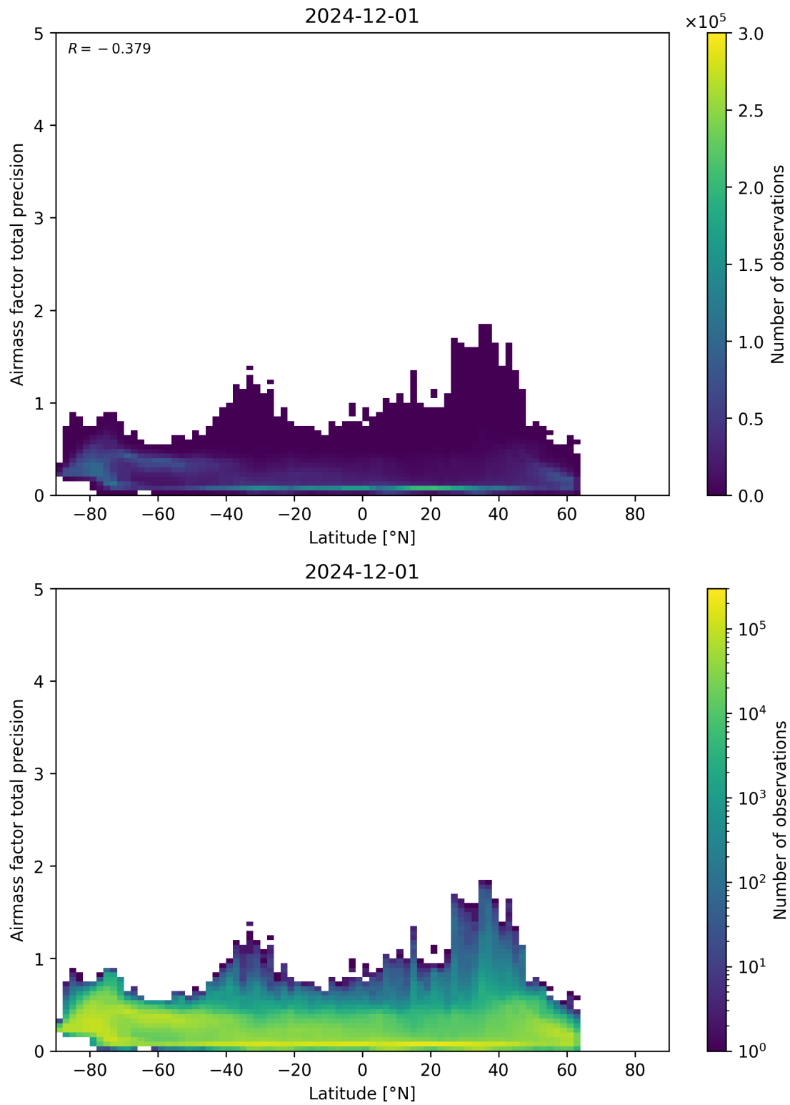
Figure 162: Scatter density plot of “Latitude” against “Airmass factor total precision” for 2024-11-30 to 2024-12-02.
