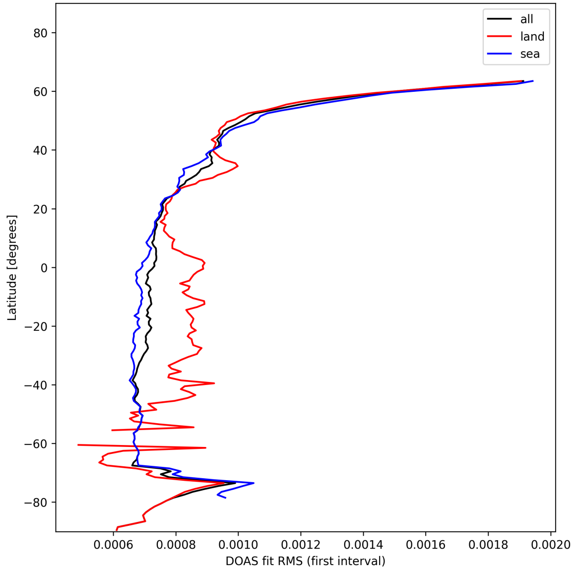
Figure 32: Zonal average of “DOAS fit RMS (first interval)” for 2024-11-30 to 2024-12-02.
