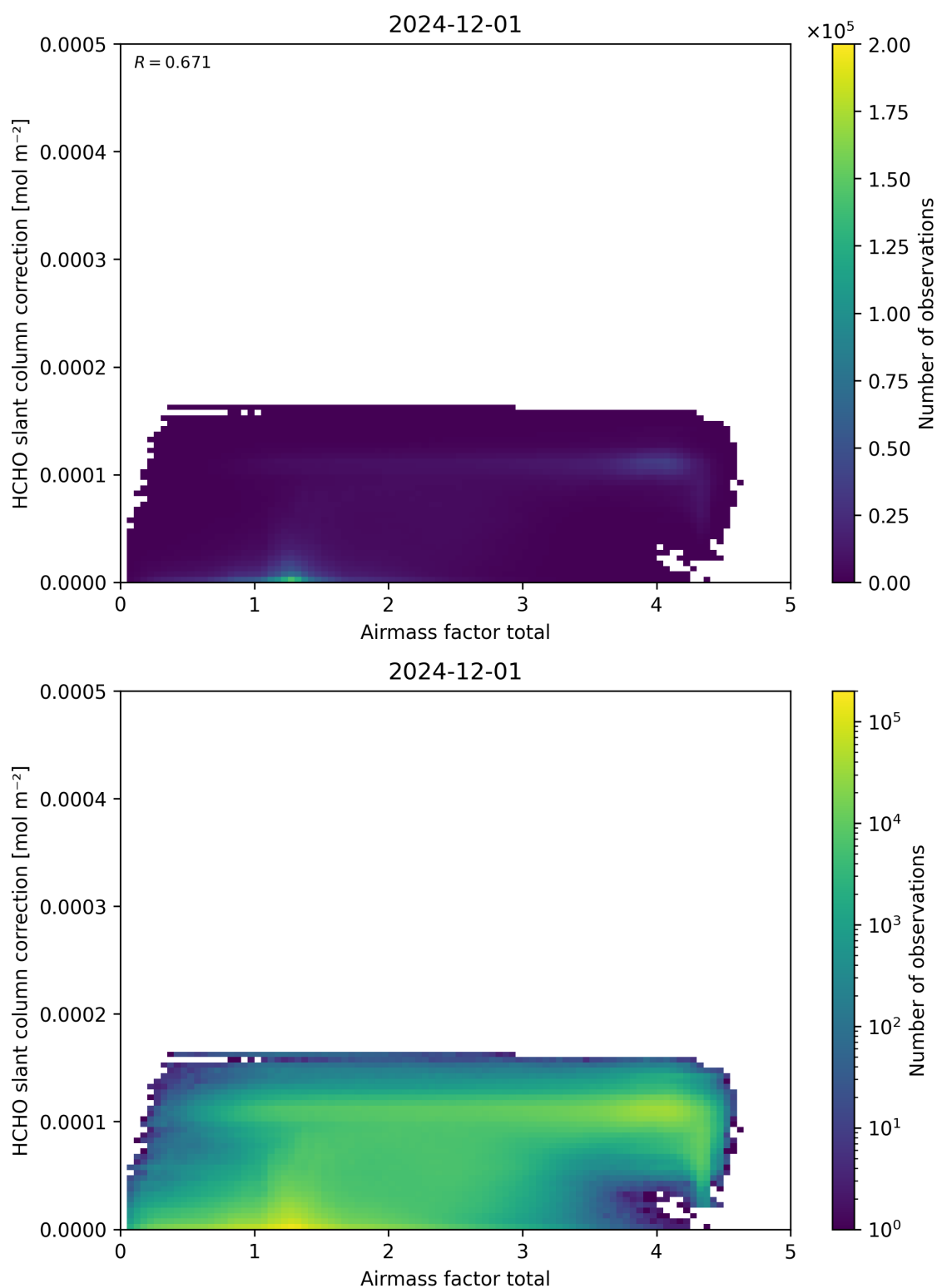
Figure 102: Scatter density plot of “Airmass factor total” against “HCHO slant column correction” for 2024-11-30 to 2024-12-02.
