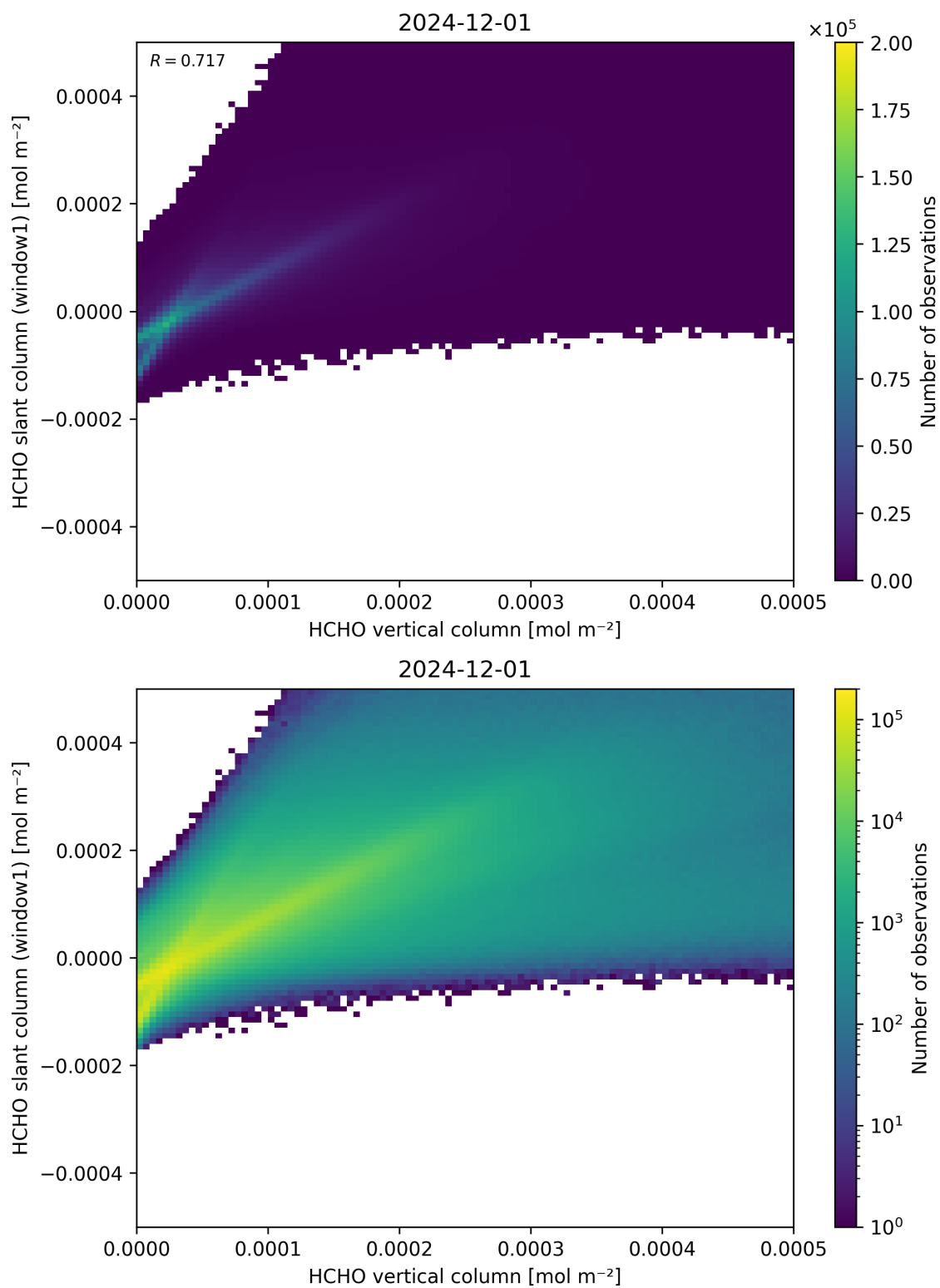
Figure 129: Scatter density plot of “HCHO vertical column” against “HCHO slant column (window1)” for 2024-11-30 to 2024-12-02.
