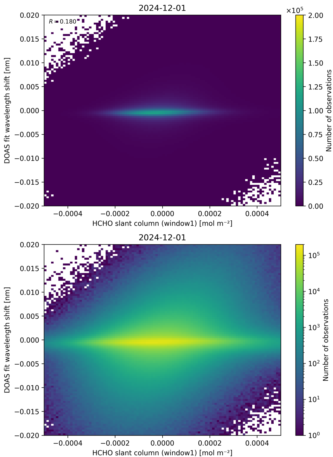
Figure 79: Scatter density plot of “HCHO slant column (window1)” against “DOAS fit wavelength shift” for 2024-11-30 to 2024-12-02.
