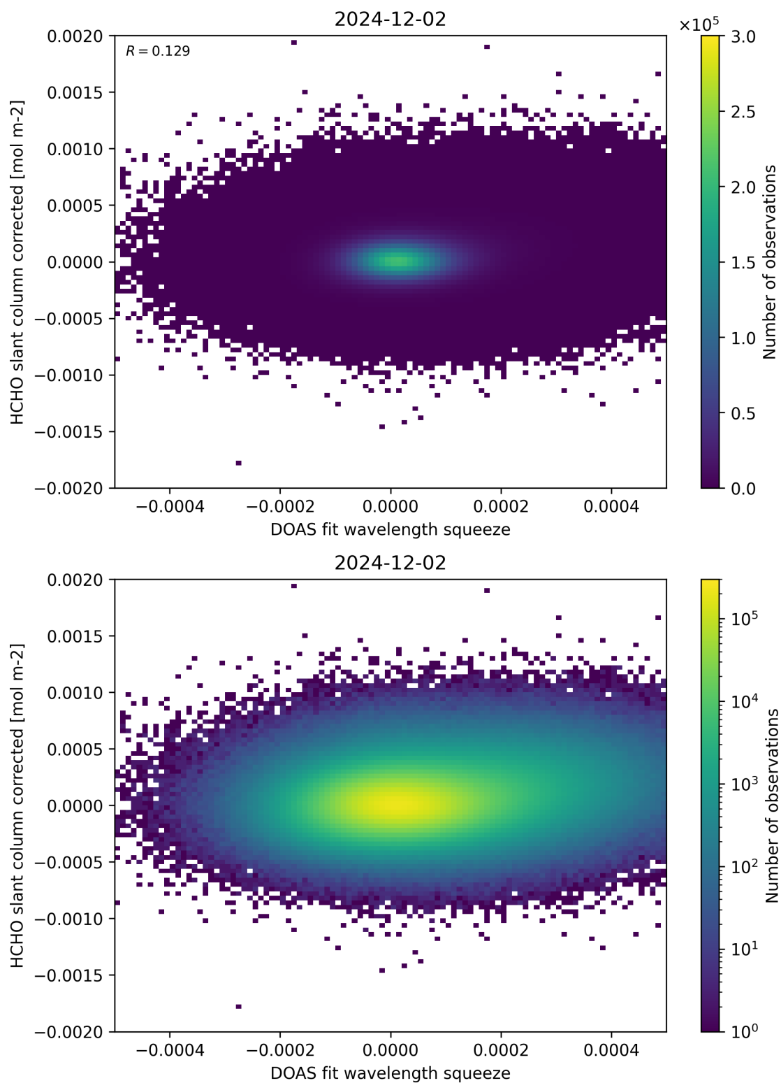
Figure 69: Scatter density plot of “DOAS fit wavelength squeeze” against “HCHO slant column corrected” for 2024-12-01 to 2024-12-03.
