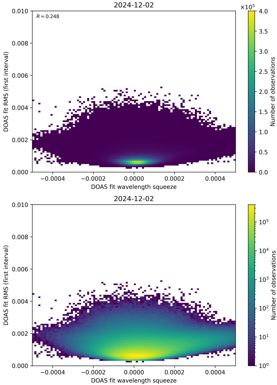
Figure 68: Scatter density plot of “DOAS fit wavelength squeeze” against “DOAS fit RMS (first interval)” for 2024-12-01 to 2024-12-03.
