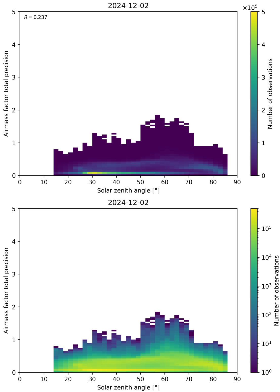
Figure 176: Scatter density plot of “Solar zenith angle” against “Airmass factor total precision” for 2024-12-01 to 2024-12-03.
