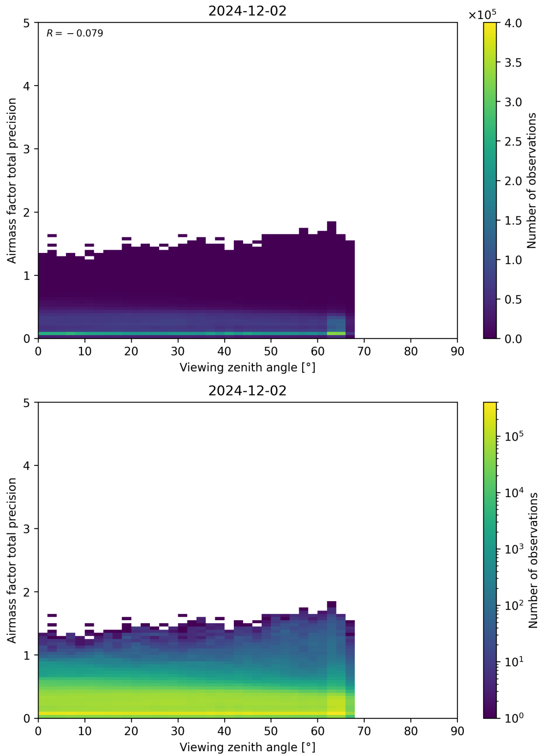
Figure 191: Scatter density plot of “Viewing zenith angle” against “Airmass factor total precision” for 2024-12-01 to 2024-12-03.
