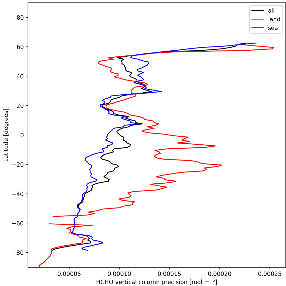
Figure 22: Zonal average of “HCHO vertical column precision” for 2024-12-01 to 2024-12-03.
