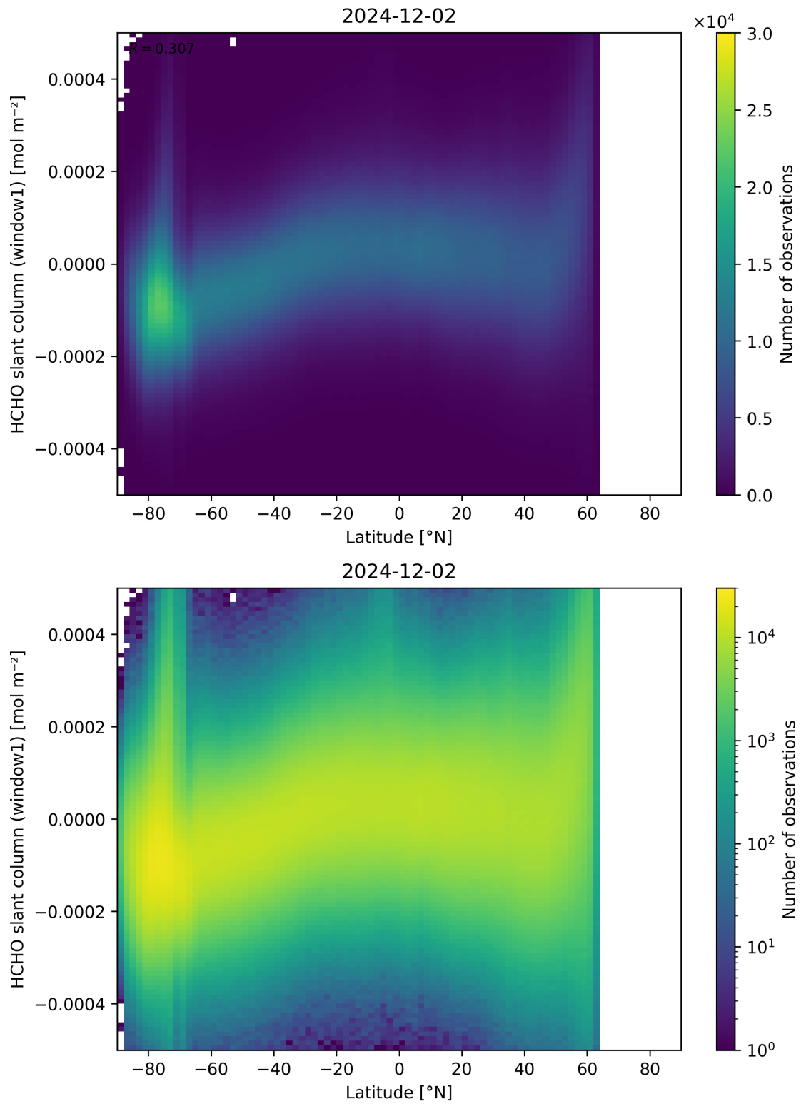
Figure 159: Scatter density plot of “Latitude” against “HCHO slant column (window1)” for 2024-12-01 to 2024-12-03.
