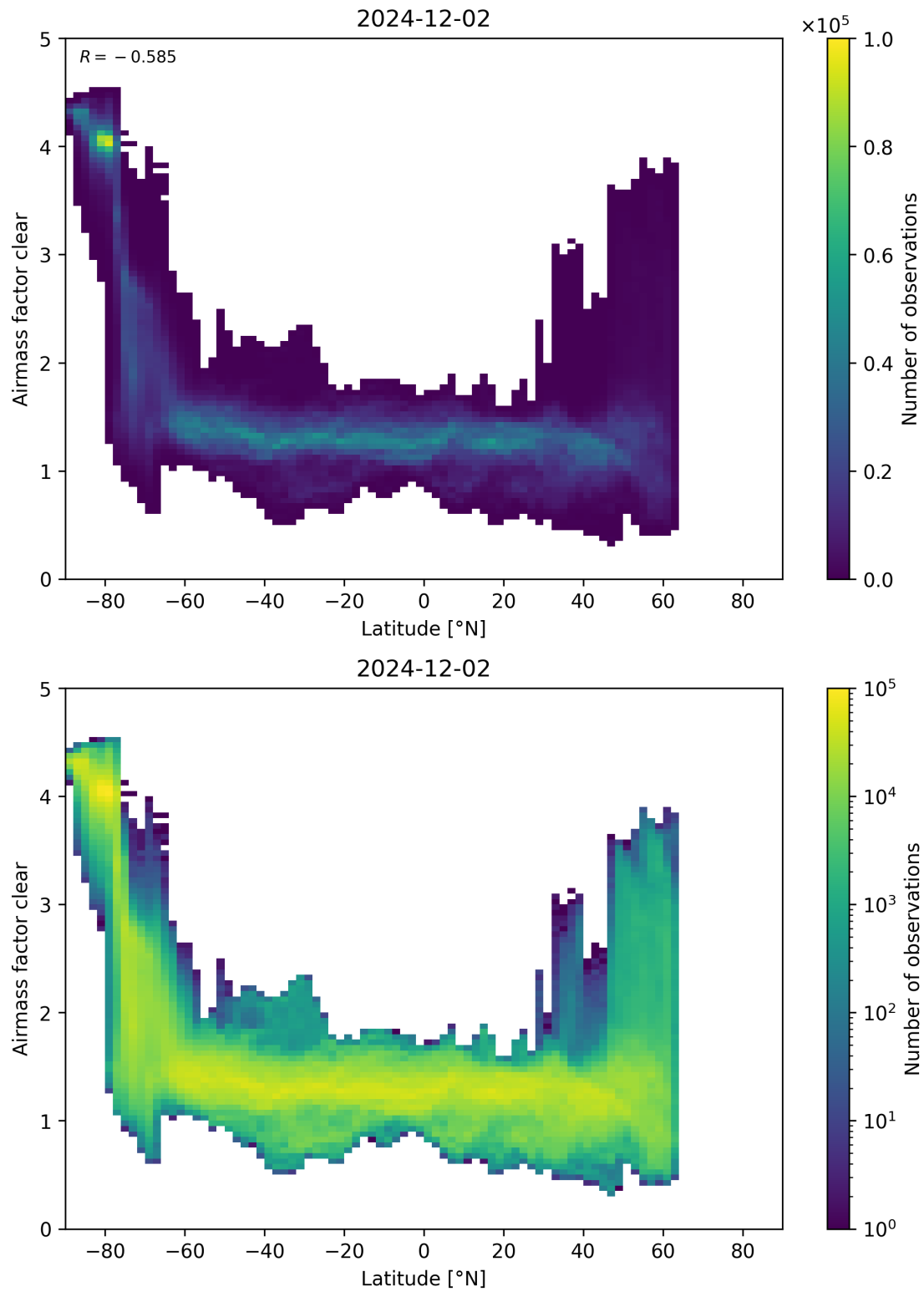
Figure 156: Scatter density plot of “Latitude” against “Airmass factor clear” for 2024-12-01 to 2024-12-03.
