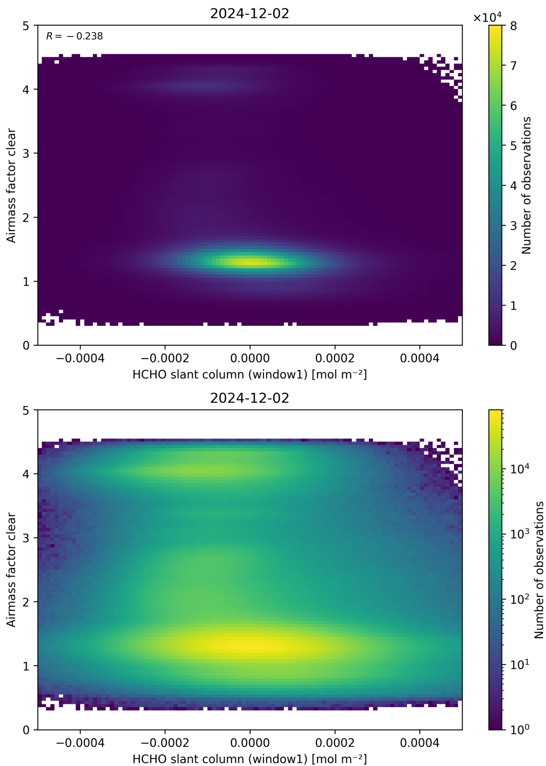
Figure 81: Scatter density plot of “HCHO slant column (window1)” against “Airmass factor clear” for 2024-12-01 to 2024-12-03.
