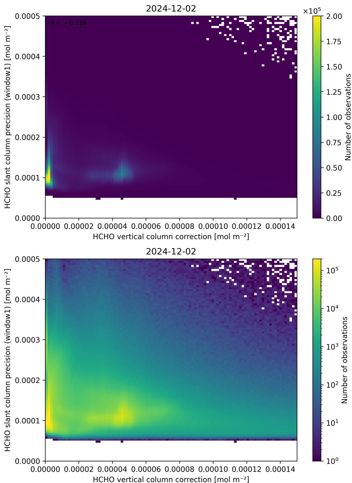
Figure 119: Scatter density plot of “HCHO vertical column correction” against “HCHO slant column precision (window1)” for 2024-12-01 to 2024-12-03.
