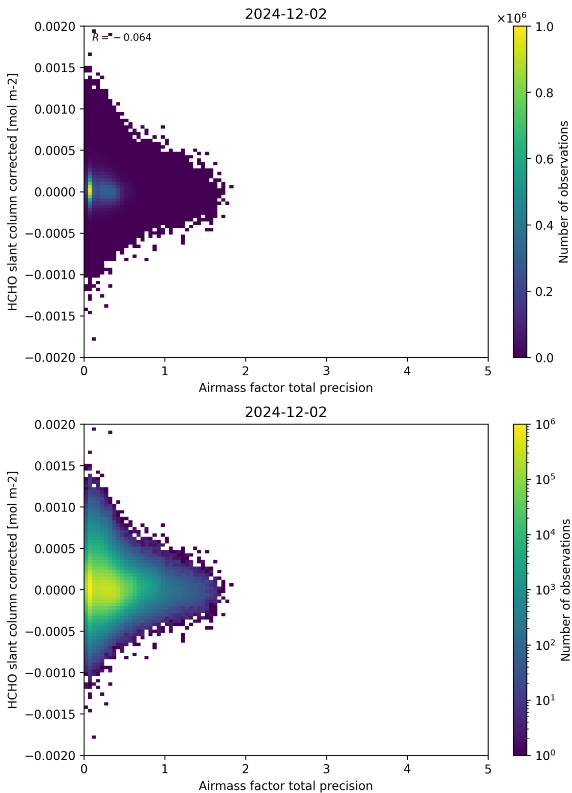
Figure 109: Scatter density plot of “Airmass factor total precision” against “HCHO slant column corrected” for 2024-12-01 to 2024-12-03.
