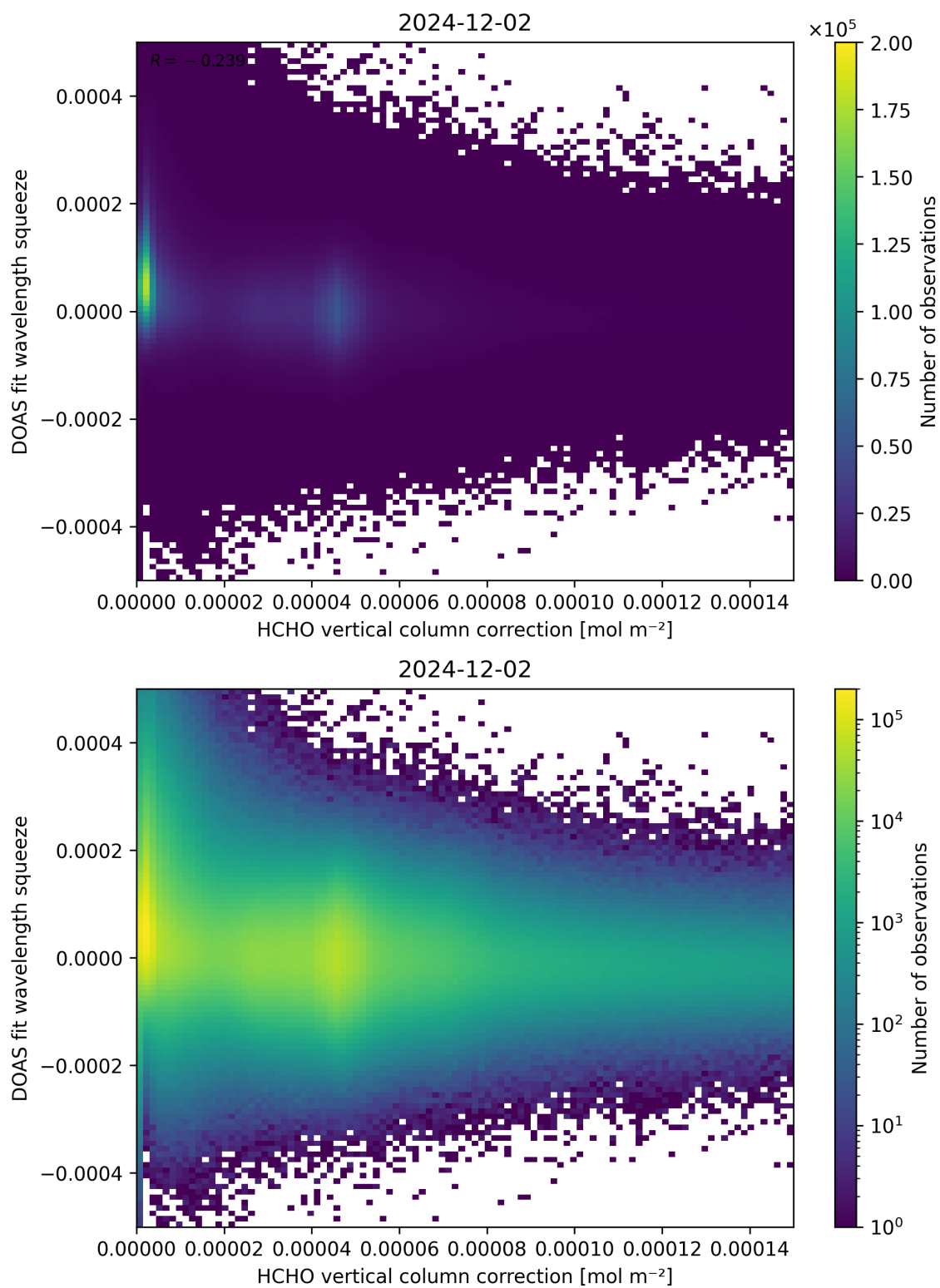
Figure 114: Scatter density plot of “HCHO vertical column correction” against “DOAS fit wavelength squeeze” for 2024-12-01 to 2024-12-03.
