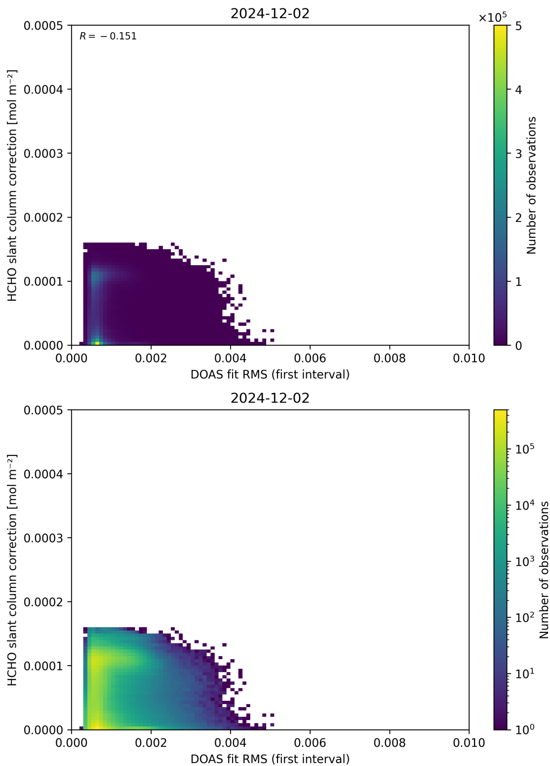
Figure 63: Scatter density plot of “DOAS fit RMS (first interval)” against “HCHO slant column correction” for 2024-12-01 to 2024-12-03.
