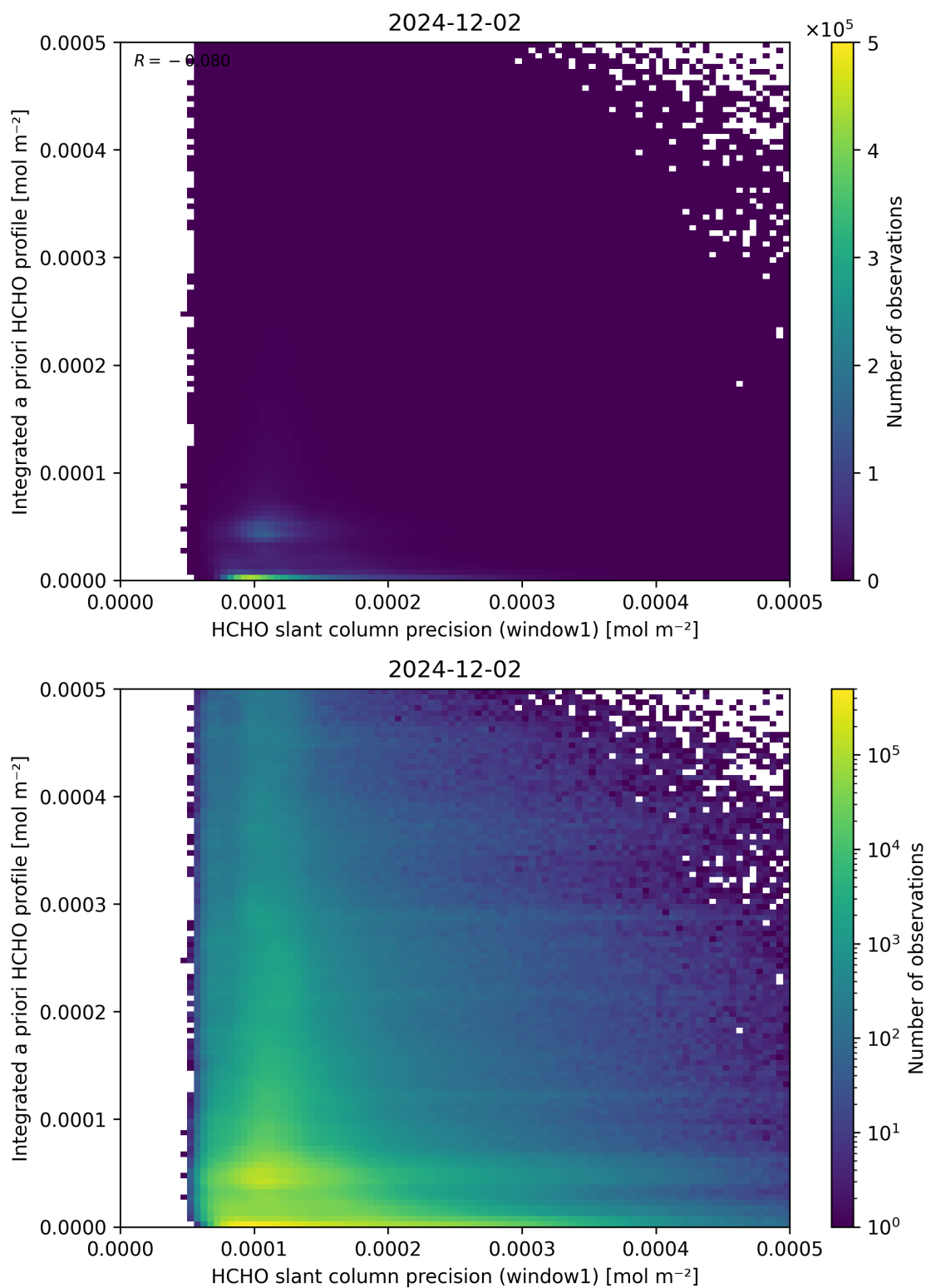
Figure 96: Scatter density plot of “HCHO slant column precision (window1)” against “Integrated a priori HCHO profile” for 2024-12-01 to 2024-12-03.
