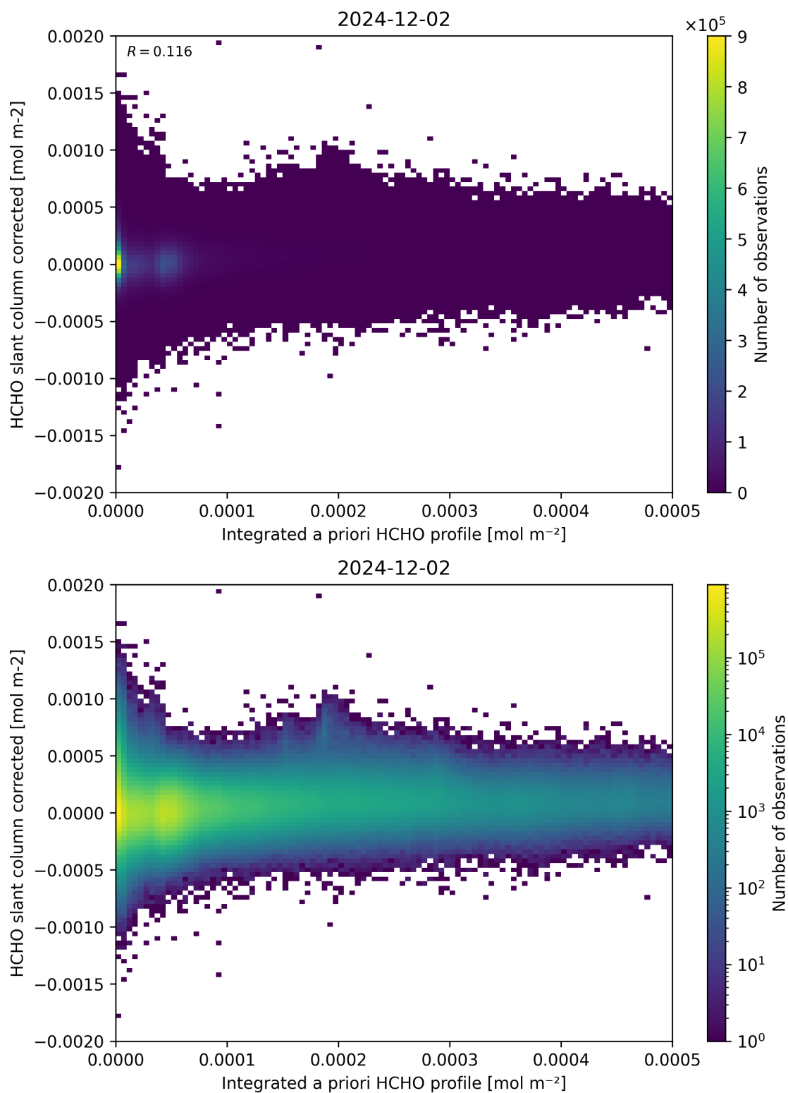
Figure 151: Scatter density plot of “Integrated a priori HCHO profile” against “HCHO slant column corrected” for 2024-12-01 to 2024-12-03.
