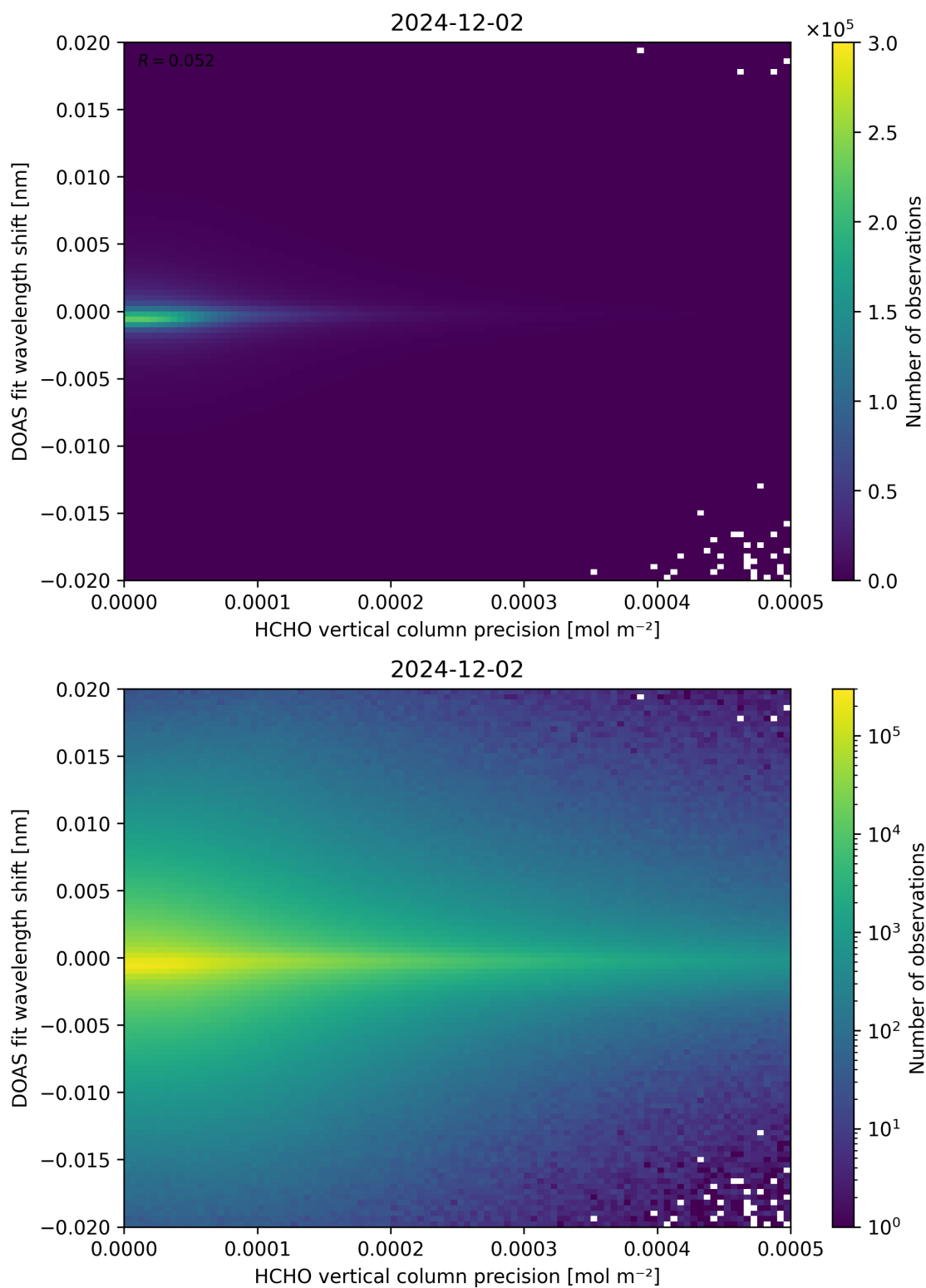
Figure 137: Scatter density plot of “HCHO vertical column precision” against “DOAS fit wavelength shift” for 2024-12-01 to 2024-12-03.
