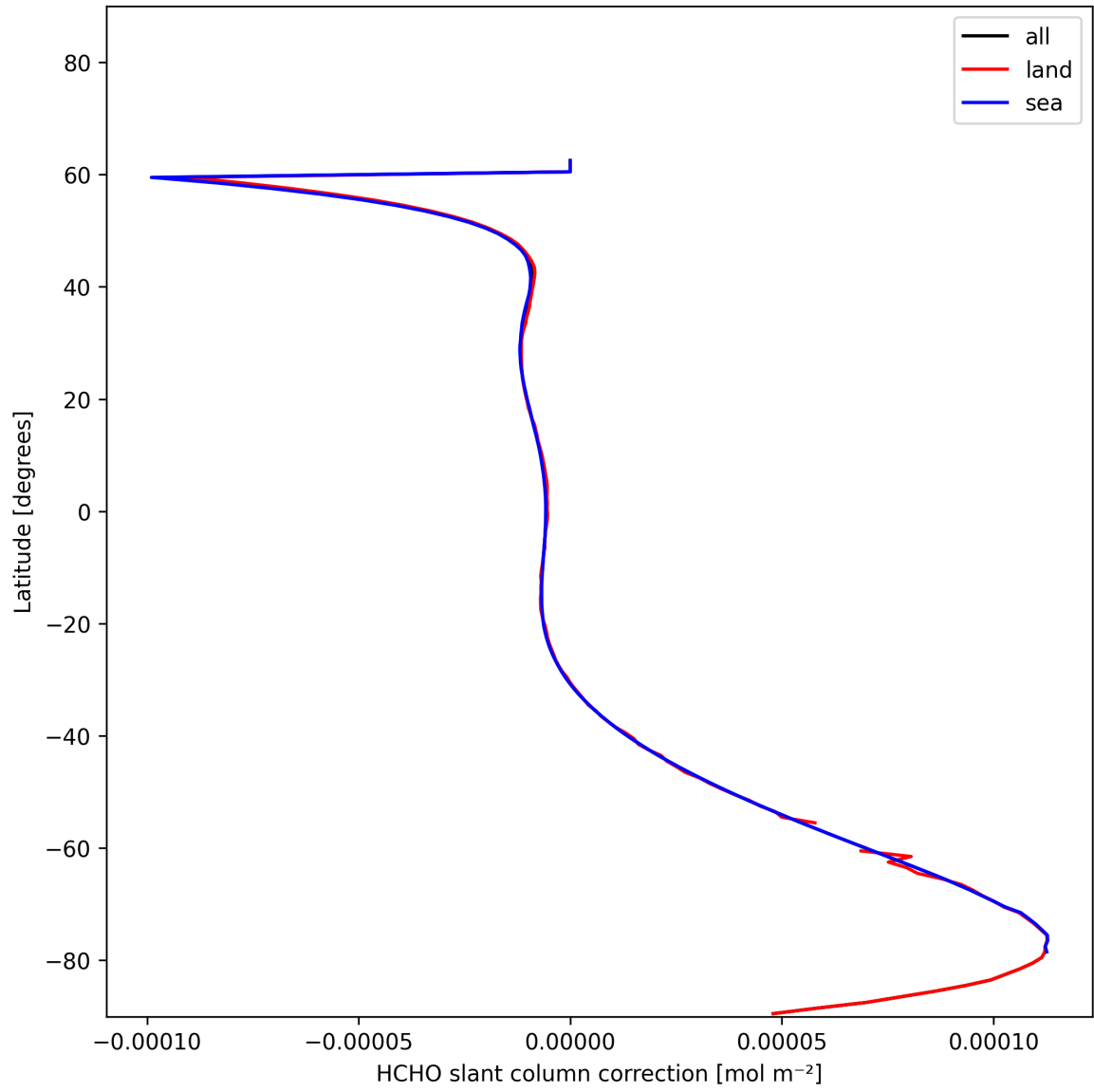
Figure 33: Zonal average of “HCHO slant column correction” for 2024-12-01 to 2024-12-03.
