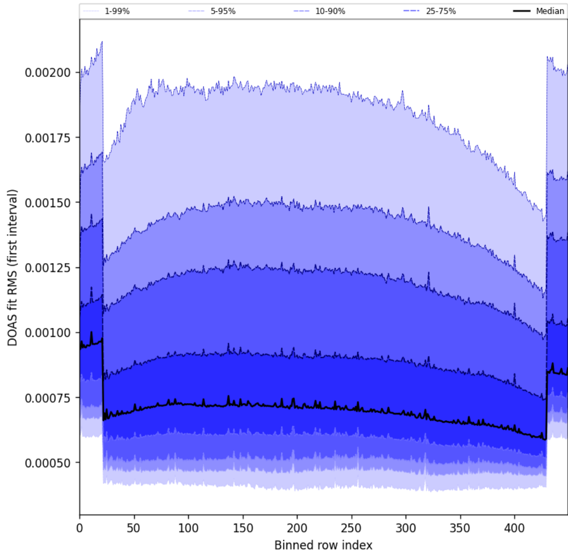
Figure 60: Along track statistics of “DOAS fit RMS (first interval)” for 2024-12-01 to 2024-12-03
