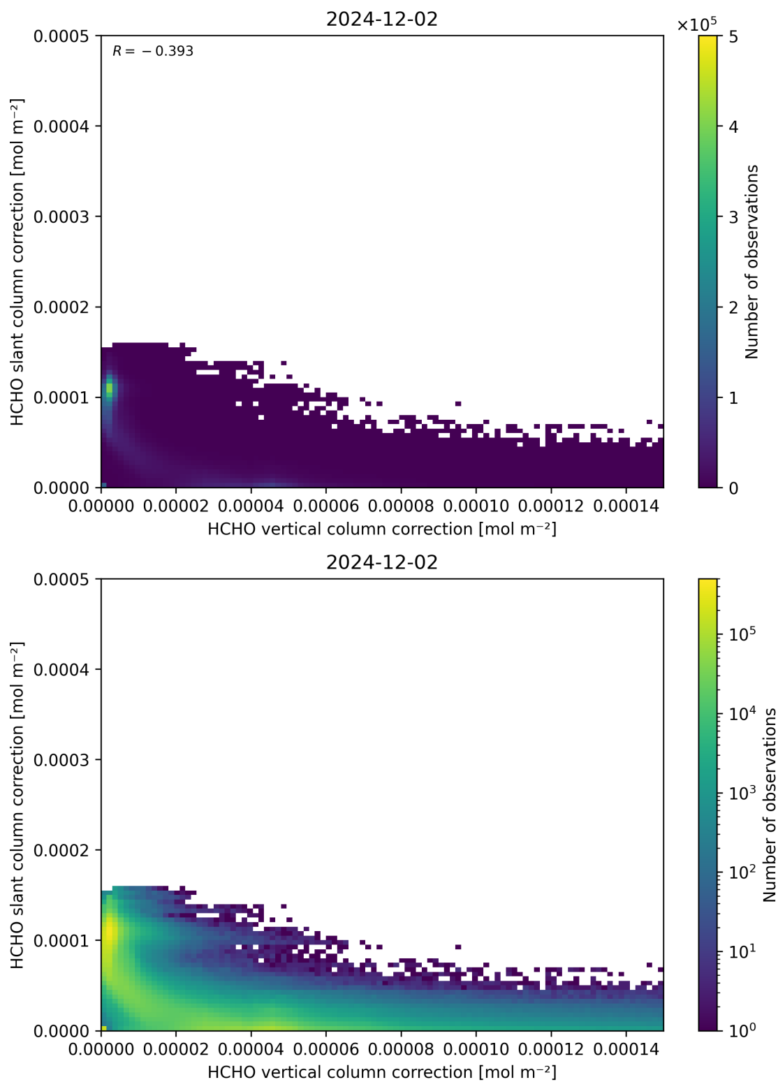
Figure 117: Scatter density plot of “HCHO vertical column correction” against “HCHO slant column correction” for 2024-12-01 to 2024-12-03.
