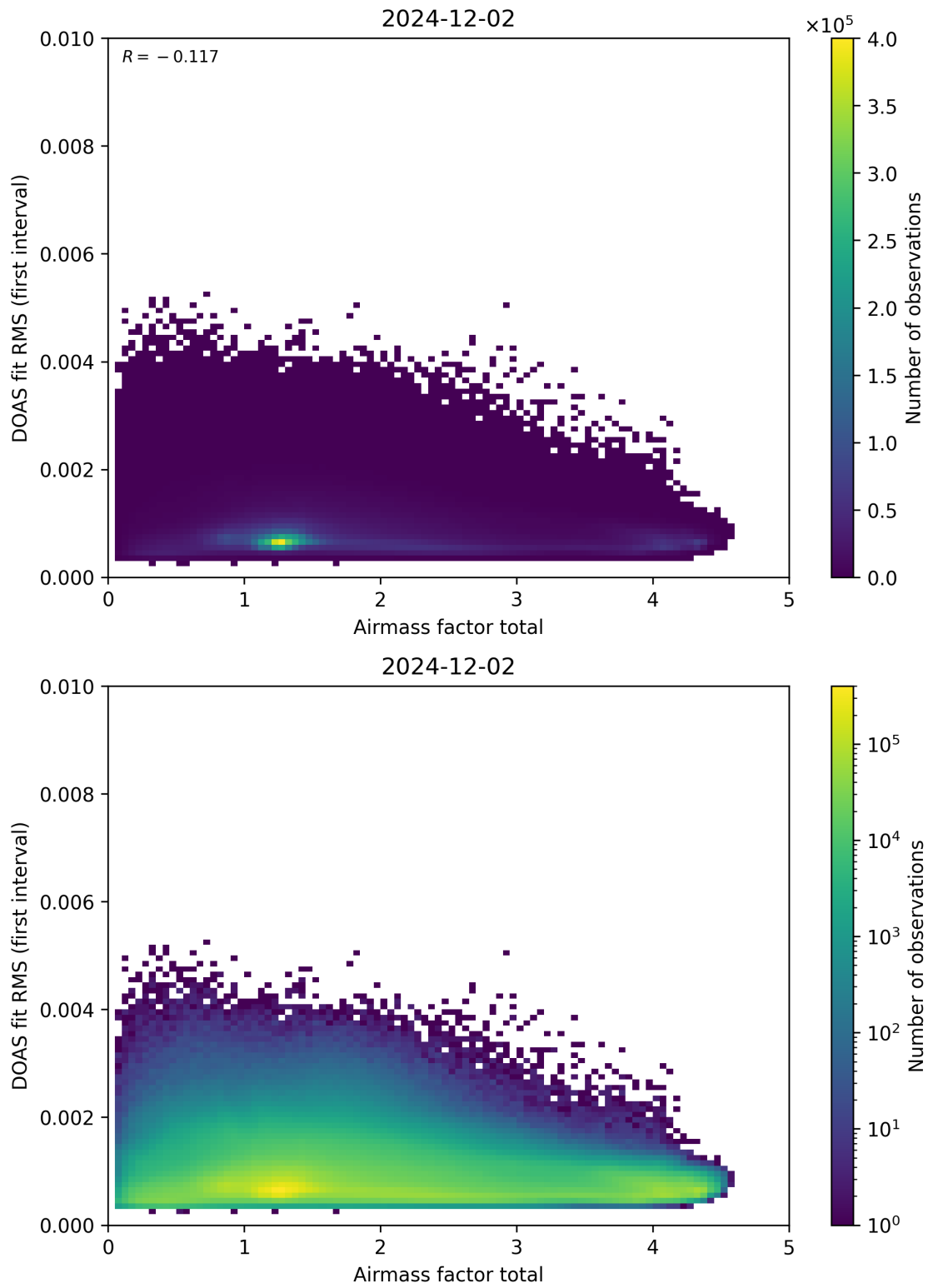
Figure 97: Scatter density plot of “Airmass factor total” against “DOAS fit RMS (first interval)” for 2024-12-01 to 2024-12-03.
