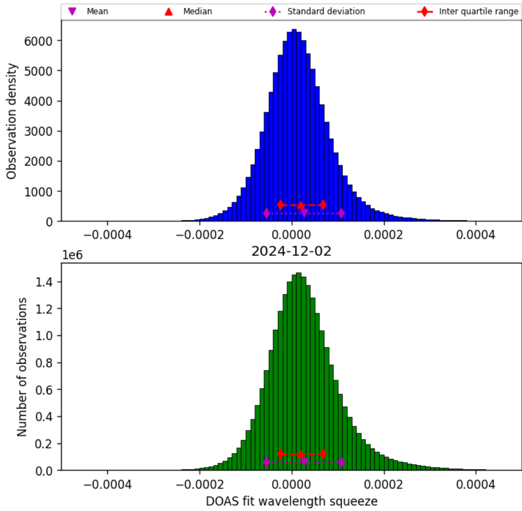
Figure 45: Histogram of “DOAS fit wavelength squeeze” for 2024-12-01 to 2024-12-03
