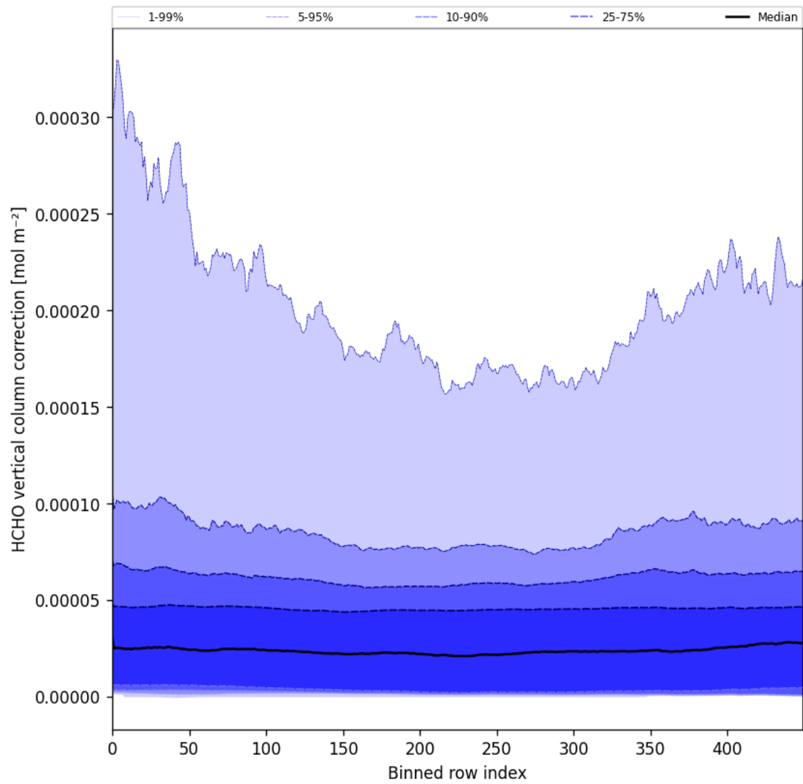
Figure 51: Along track statistics of “HCHO vertical column correction” for 2024-12-01 to 2024-12-03
