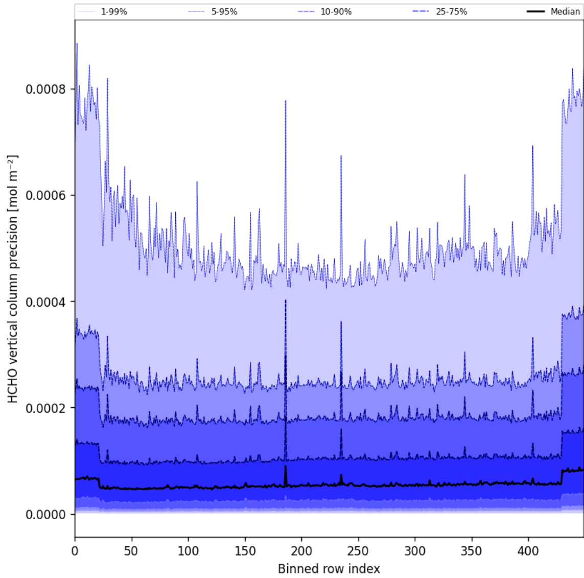
Figure 50: Along track statistics of “HCHO vertical column precision” for 2024-12-01 to 2024-12-03
