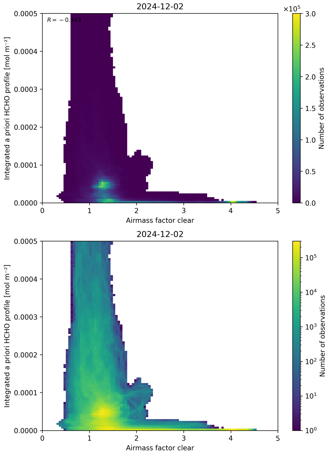
Figure 76: Scatter density plot of “Airmass factor clear” against “Integrated a priori HCHO profile” for 2024-12-01 to 2024-12-03.
