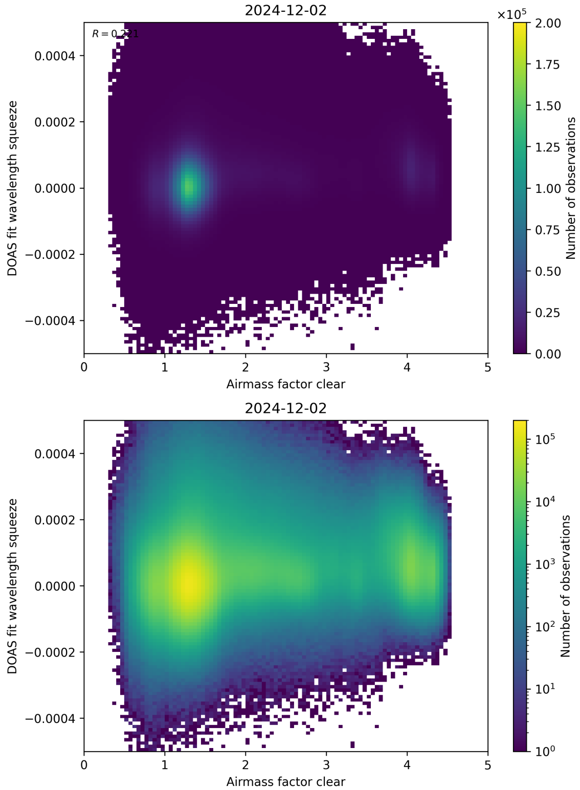
Figure 73: Scatter density plot of “Airmass factor clear” against “DOAS fit wavelength squeeze” for 2024-12-01 to 2024-12-03.
