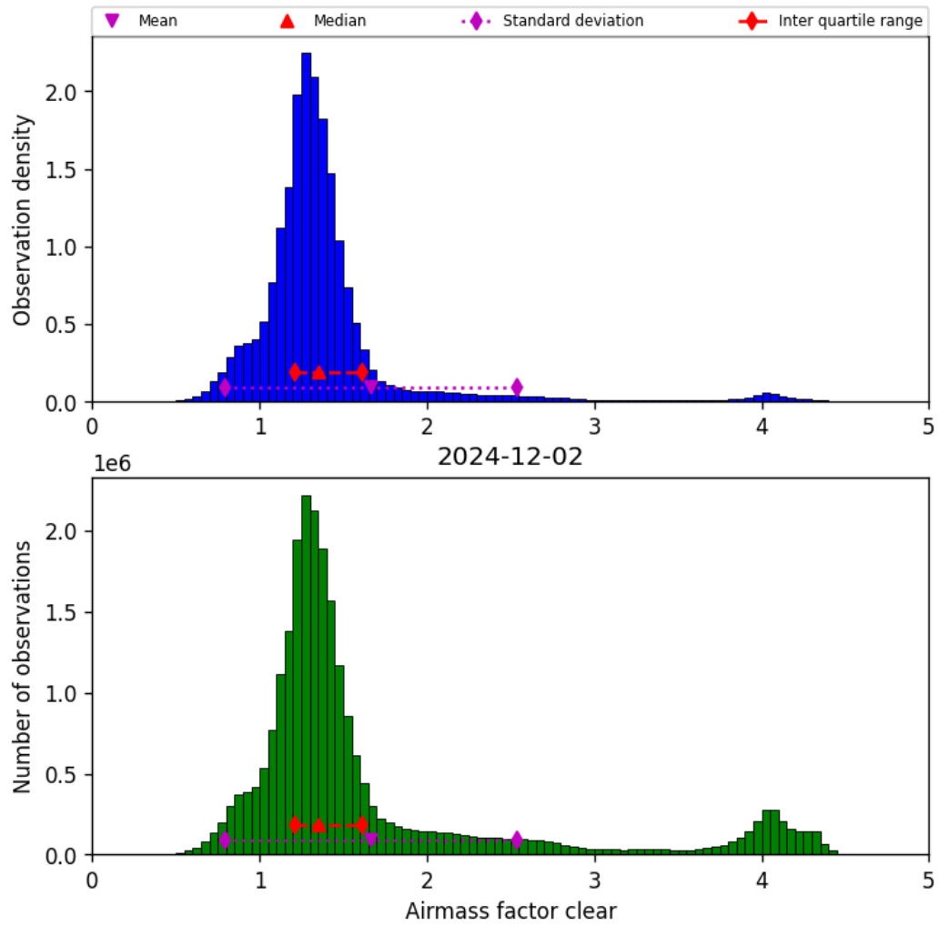
Figure 42: Histogram of “Airmass factor clear” for 2024-12-01 to 2024-12-03
