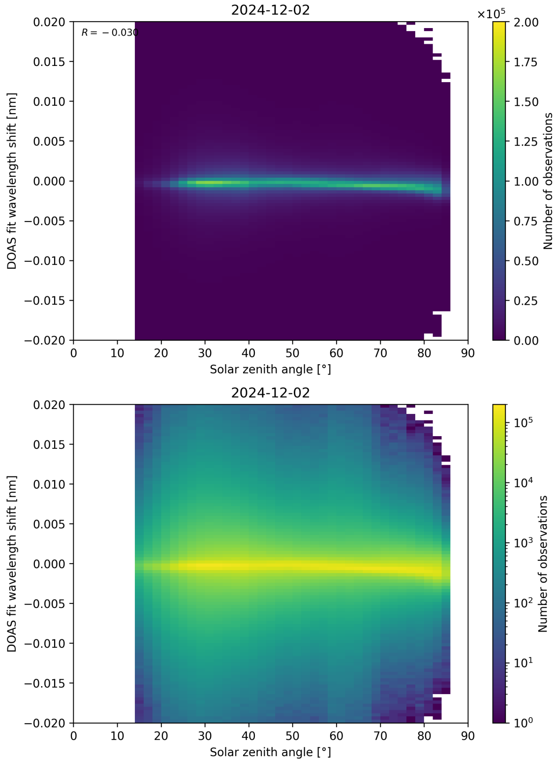
Figure 168: Scatter density plot of “Solar zenith angle” against “DOAS fit wavelength shift” for 2024-12-01 to 2024-12-03.
