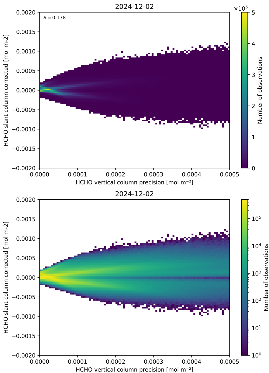
Figure 140: Scatter density plot of “HCHO vertical column precision” against “HCHO slant column corrected” for 2024-12-01 to 2024-12-03.
