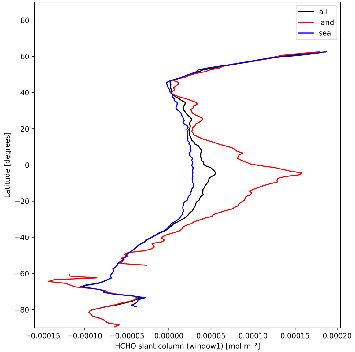
Figure 24: Zonal average of “HCHO slant column (window1)” for 2024-12-01 to 2024-12-03.
