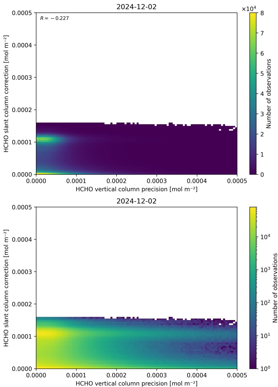
Figure 141: Scatter density plot of “HCHO vertical column precision” against “HCHO slant column correction” for 2024-12-01 to 2024-12-03.
