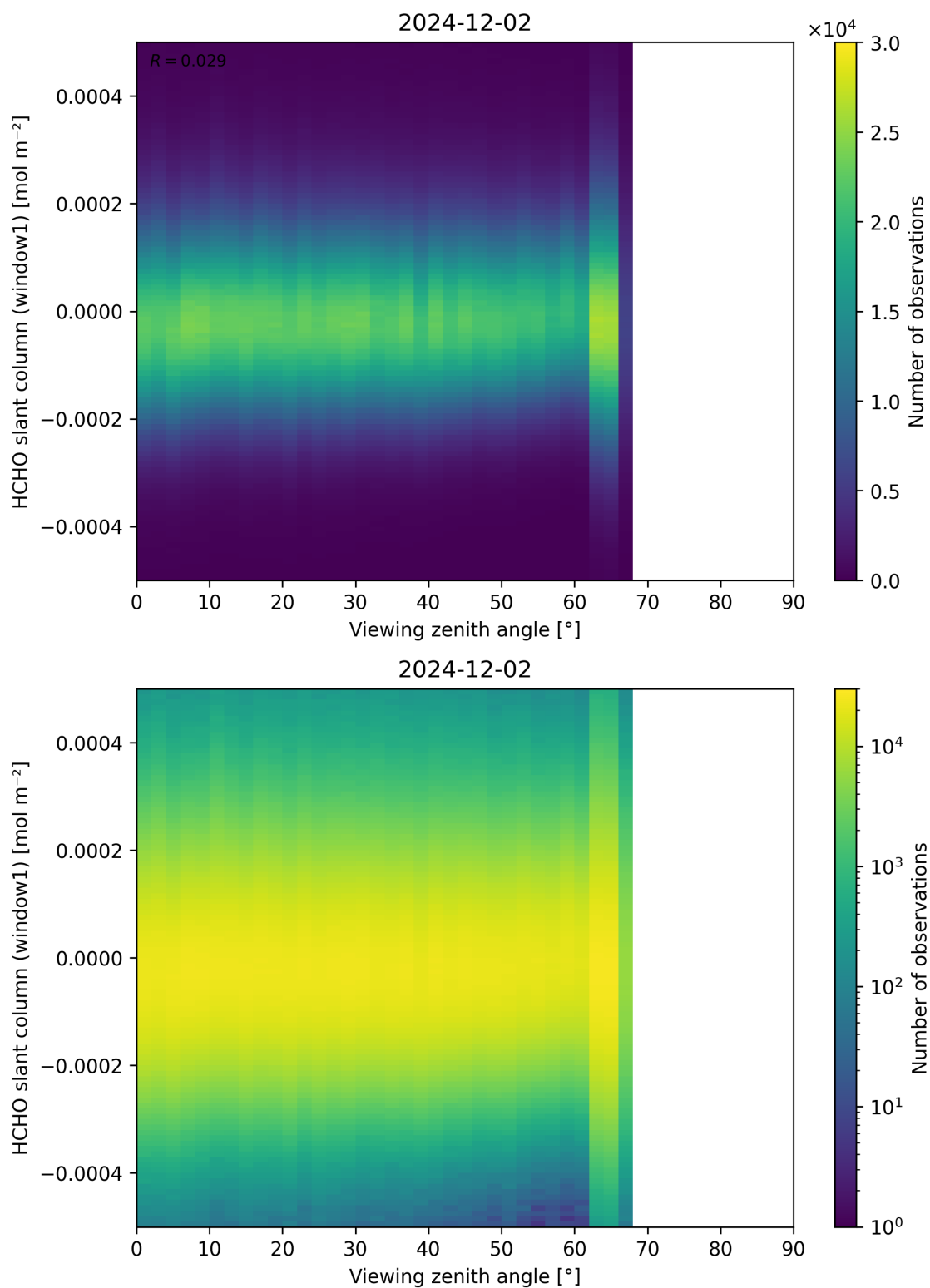
Figure 188: Scatter density plot of “Viewing zenith angle” against “HCHO slant column (window1)” for 2024-12-01 to 2024-12-03.
