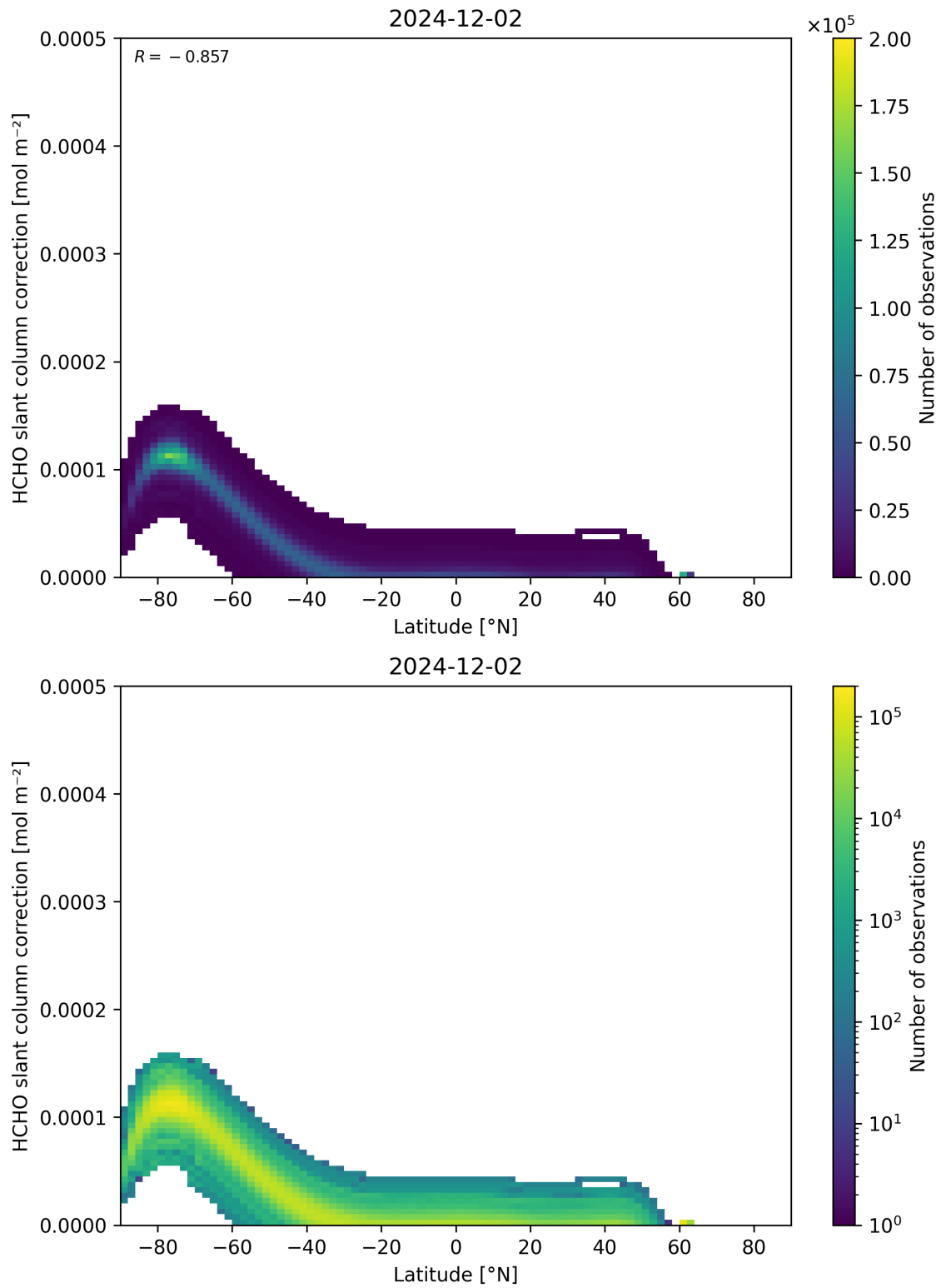
Figure 158: Scatter density plot of “Latitude” against “HCHO slant column correction” for 2024-12-01 to 2024-12-03.
