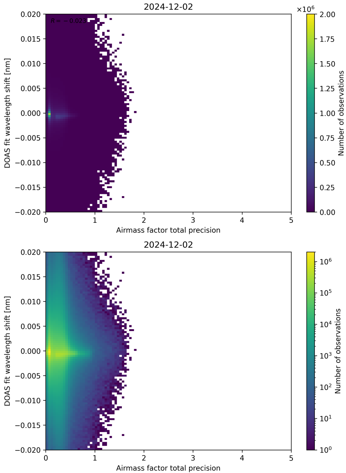
Figure 106: Scatter density plot of “Airmass factor total precision” against “DOAS fit wavelength shift” for 2024-12-01 to 2024-12-03.
