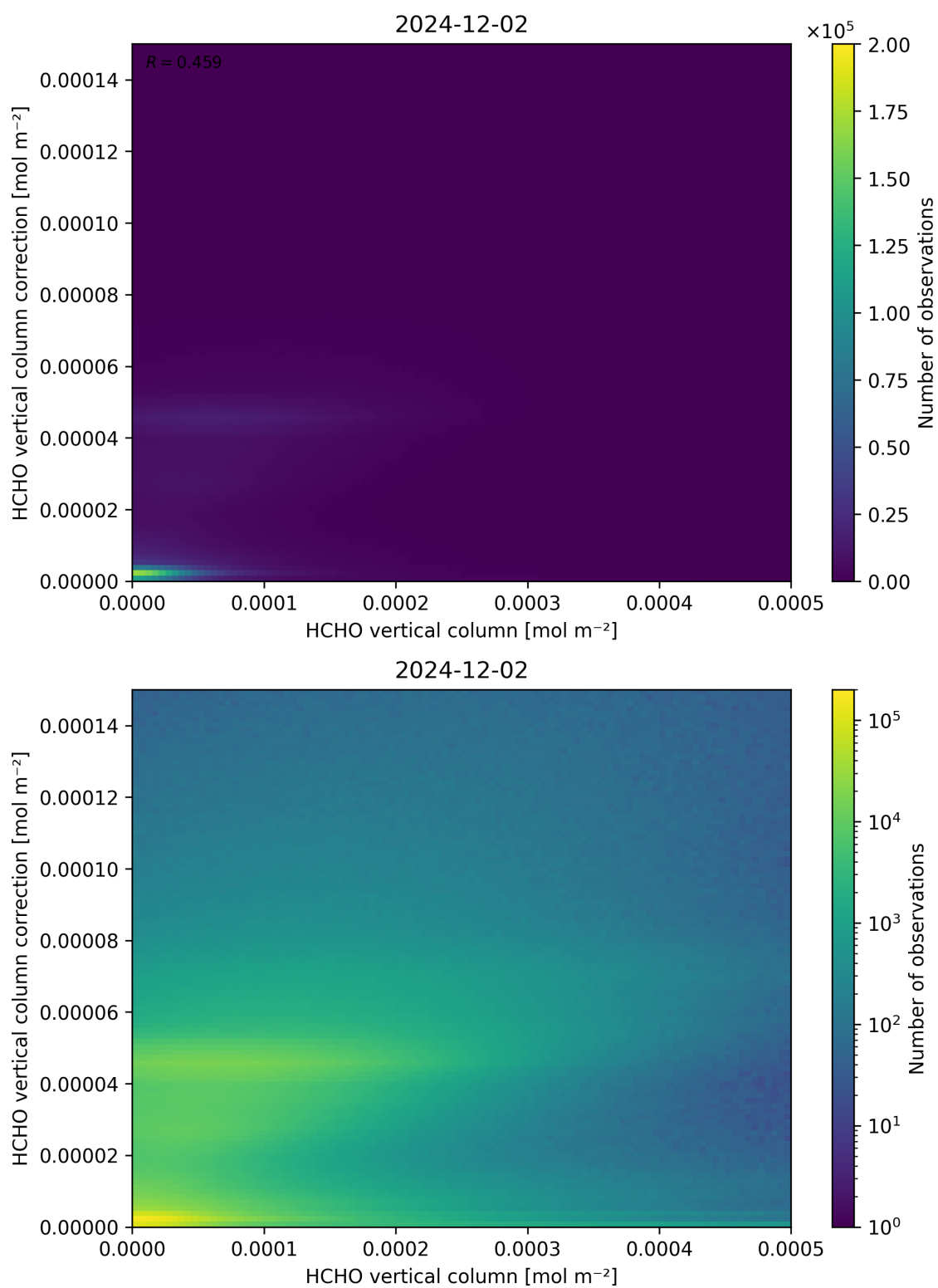
Figure 133: Scatter density plot of “HCHO vertical column” against “HCHO vertical column correction” for 2024-12-01 to 2024-12-03.
