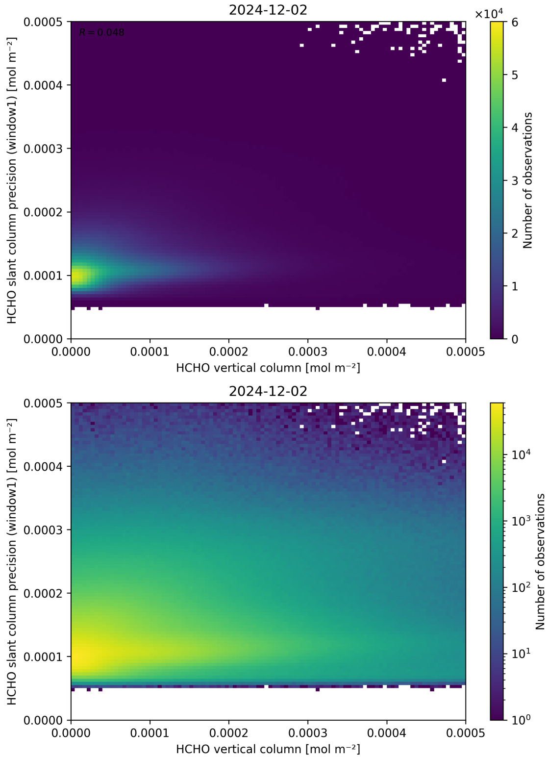
Figure 130: Scatter density plot of “HCHO vertical column” against “HCHO slant column precision (window1)” for 2024-12-01 to 2024-12-03.
