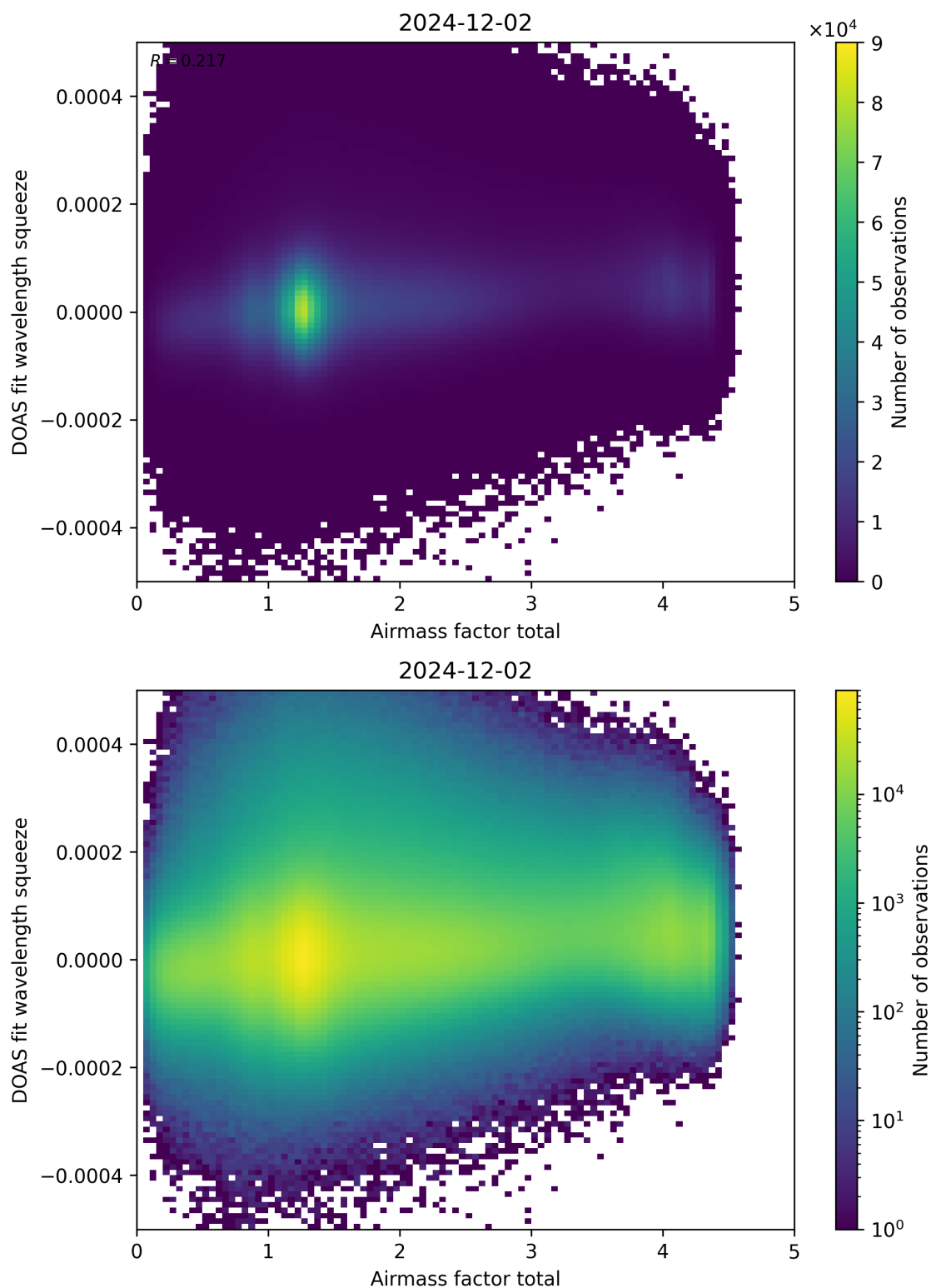
Figure 99: Scatter density plot of “Airmass factor total” against “DOAS fit wavelength squeeze” for 2024-12-01 to 2024-12-03.
