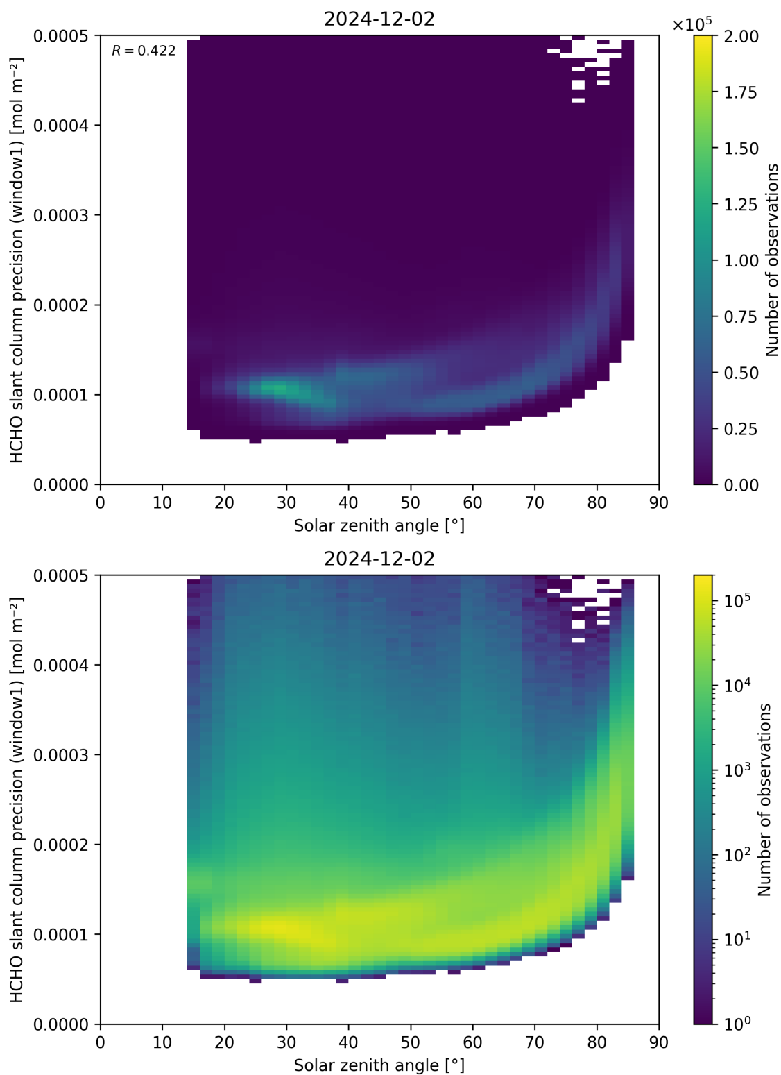
Figure 174: Scatter density plot of “Solar zenith angle” against “HCHO slant column precision (window1)” for 2024-12-01 to 2024-12-03.
