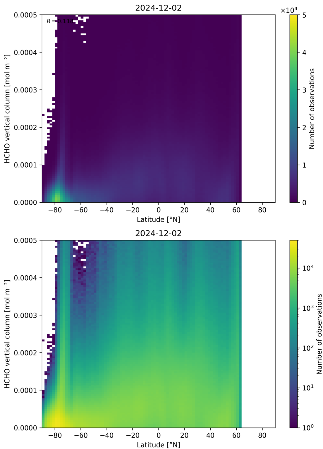
Figure 163: Scatter density plot of “Latitude” against “HCHO vertical column” for 2024-12-01 to 2024-12-03.
