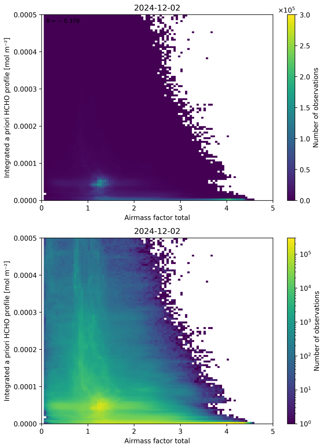
Figure 104: Scatter density plot of “Airmass factor total” against “Integrated a priori HCHO profile” for 2024-12-01 to 2024-12-03.
