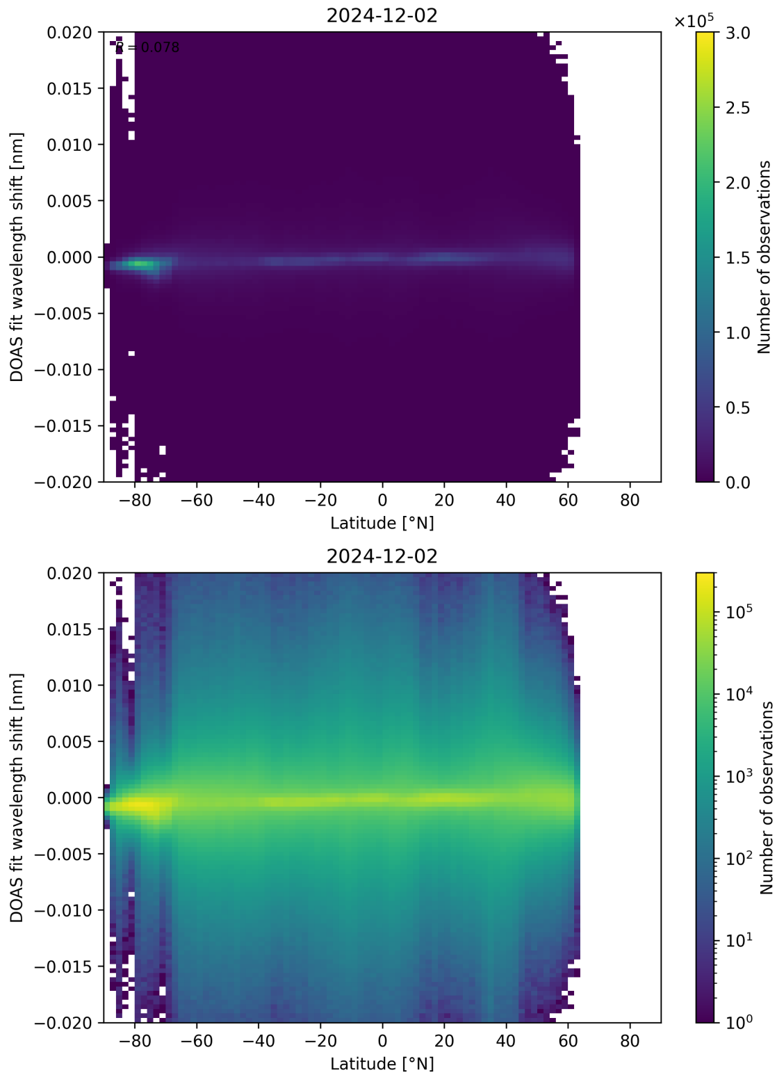
Figure 154: Scatter density plot of “Latitude” against “DOAS fit wavelength shift” for 2024-12-01 to 2024-12-03.
