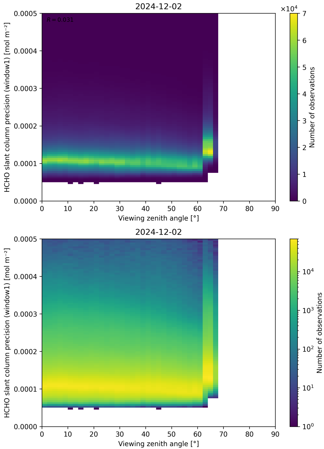
Figure 189: Scatter density plot of “Viewing zenith angle” against “HCHO slant column precision (window1)” for 2024-12-01 to 2024-12-03.
