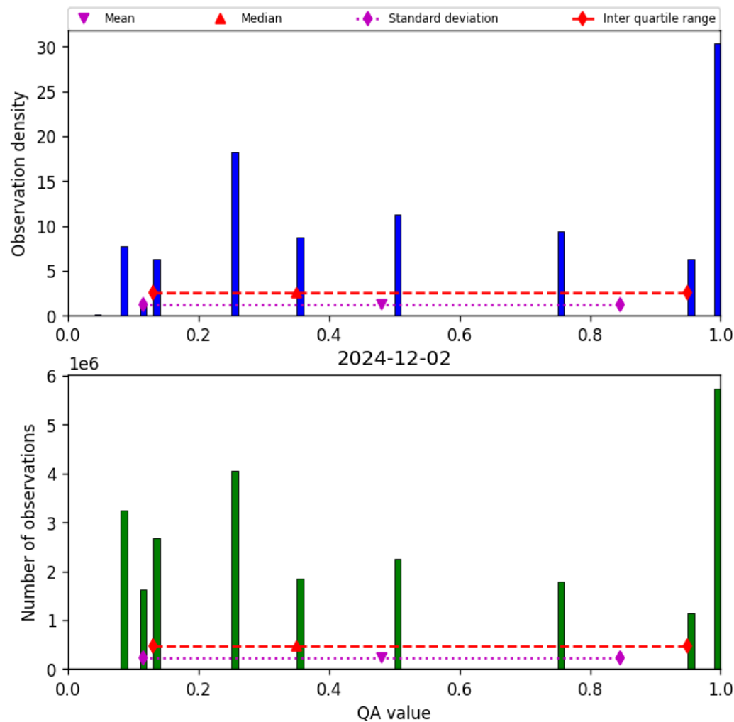
Figure 34: Histogram of “QA value” for 2024-12-01 to 2024-12-03
