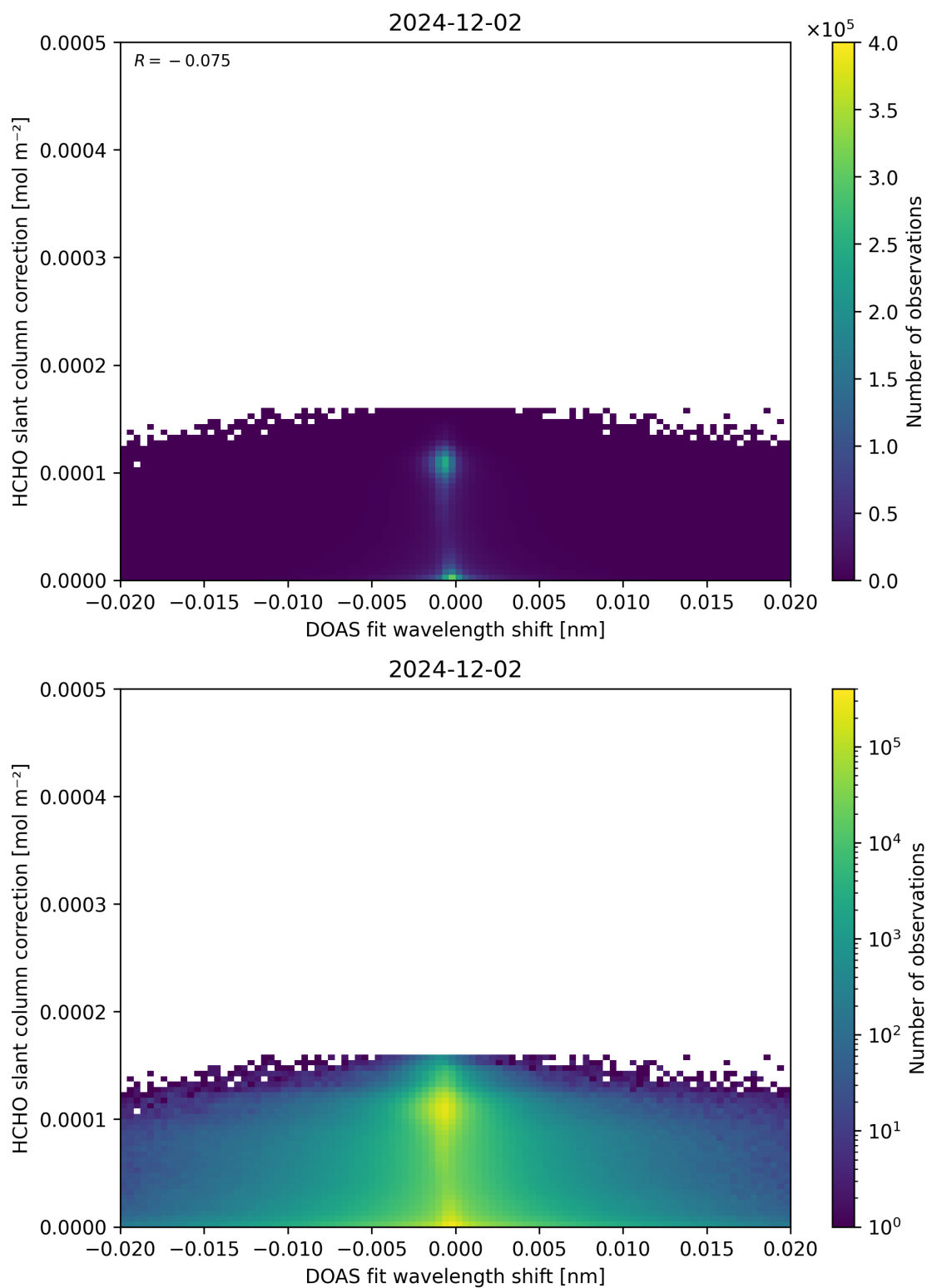
Figure 67: Scatter density plot of “DOAS fit wavelength shift” against “HCHO slant column correction” for 2024-12-01 to 2024-12-03.
