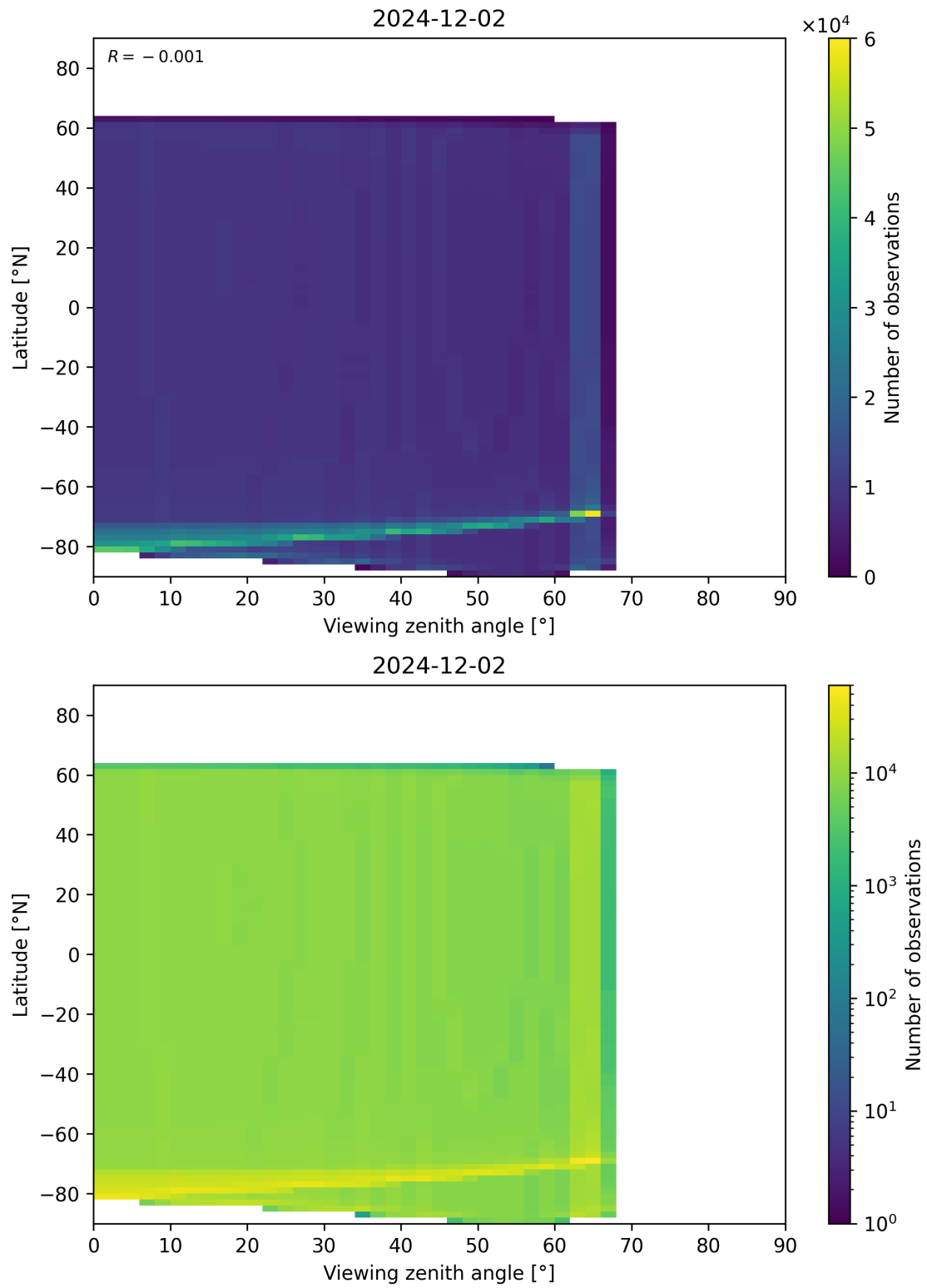
Figure 196: Scatter density plot of “Viewing zenith angle” against “Latitude” for 2024-12-01 to 2024-12-03.
