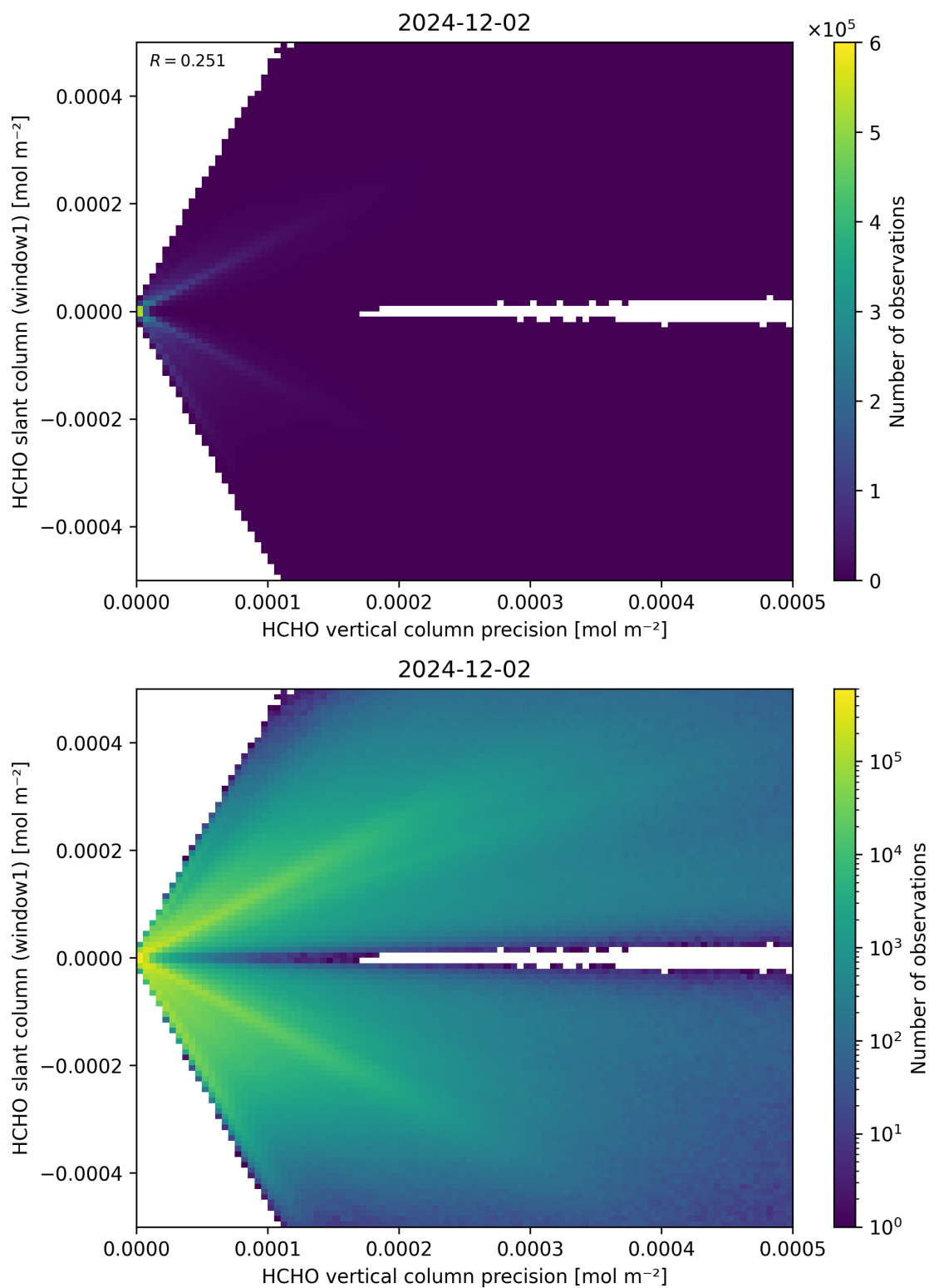
Figure 142: Scatter density plot of “HCHO vertical column precision” against “HCHO slant column (window1)” for 2024-12-01 to 2024-12-03.
