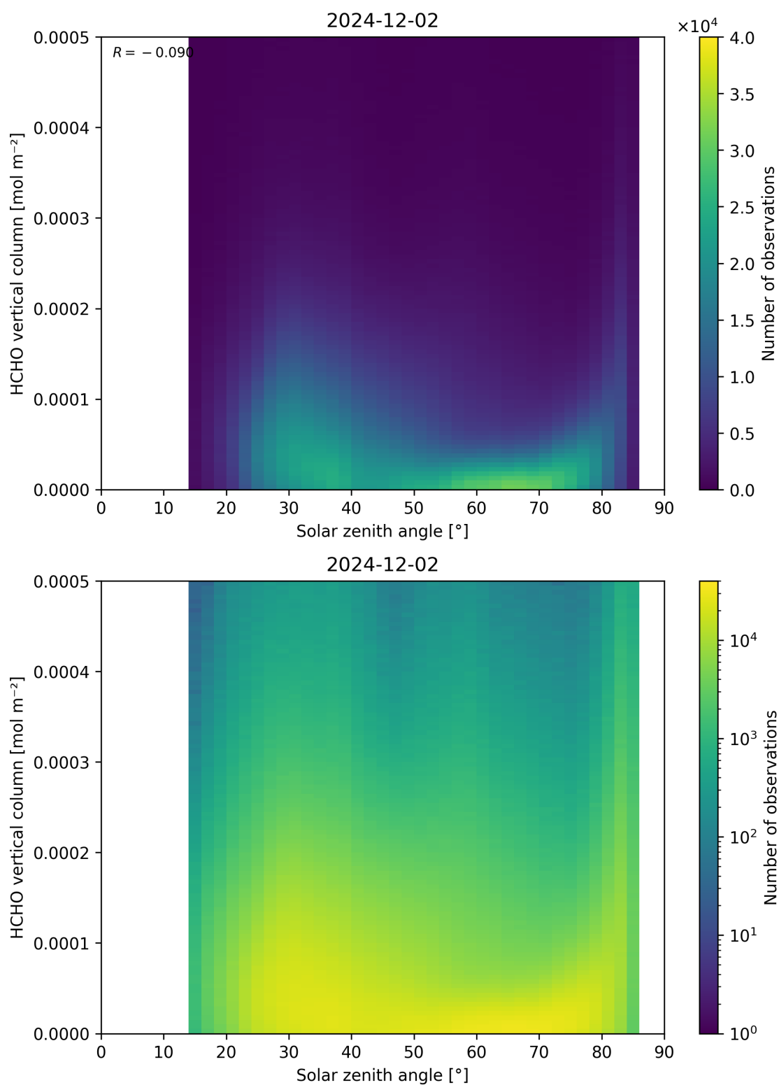
Figure 177: Scatter density plot of “Solar zenith angle” against “HCHO vertical column” for 2024-12-01 to 2024-12-03.
