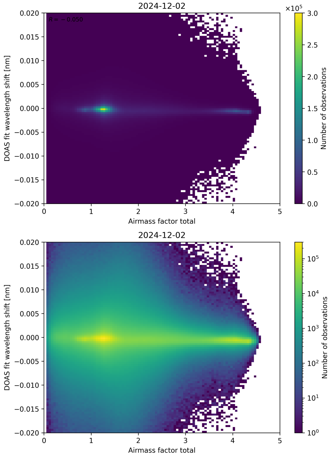
Figure 98: Scatter density plot of “Airmass factor total” against “DOAS fit wavelength shift” for 2024-12-01 to 2024-12-03.
