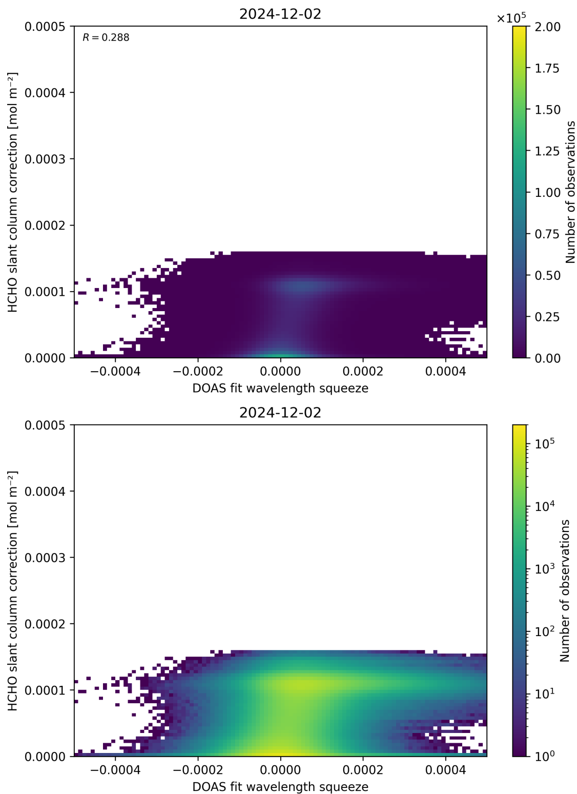
Figure 70: Scatter density plot of “DOAS fit wavelength squeeze” against “HCHO slant column correction” for 2024-12-01 to 2024-12-03.
