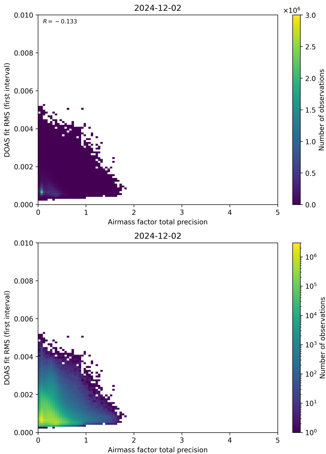
Figure 105: Scatter density plot of “Airmass factor total precision” against “DOAS fit RMS (first interval)” for 2024-12-01 to 2024-12-03.
