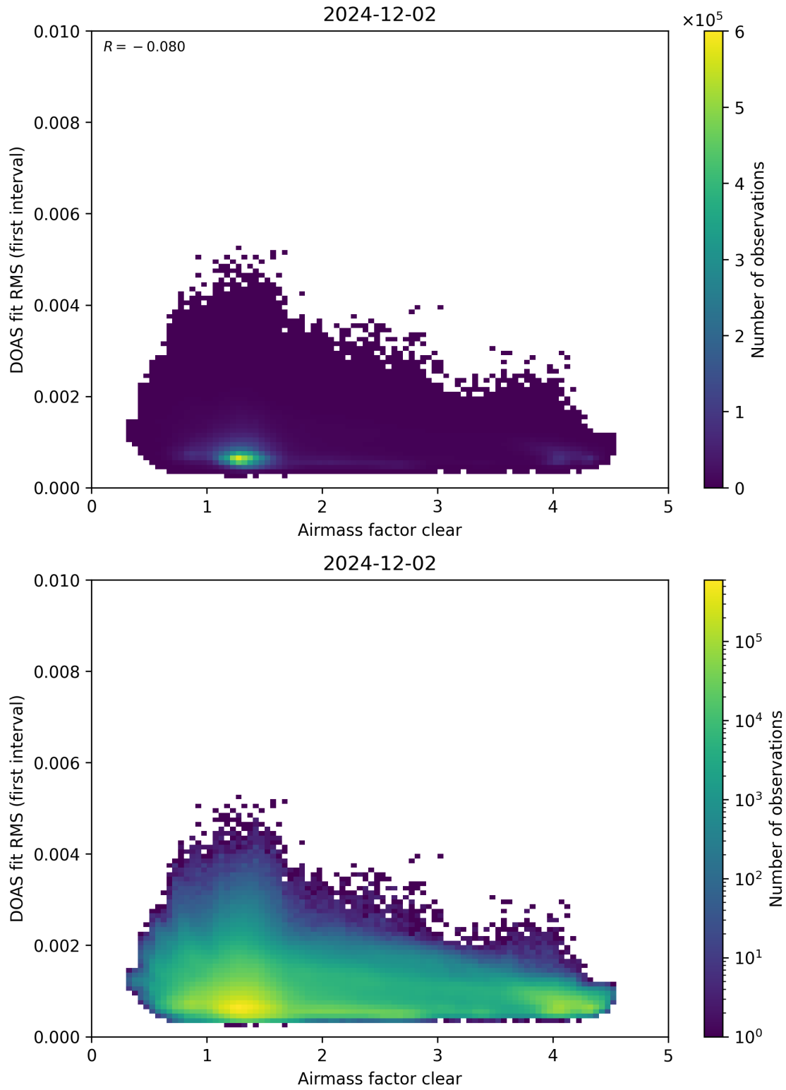
Figure 71: Scatter density plot of “Airmass factor clear” against “DOAS fit RMS (first interval)” for 2024-12-01 to 2024-12-03.
