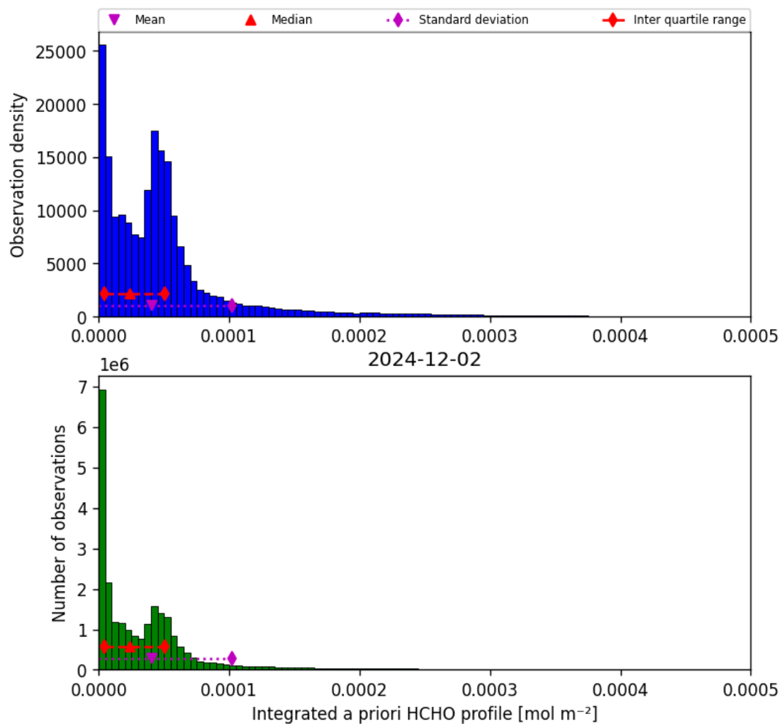
Figure 43: Histogram of “Integrated a priori HCHO profile” for 2024-12-01 to 2024-12-03
