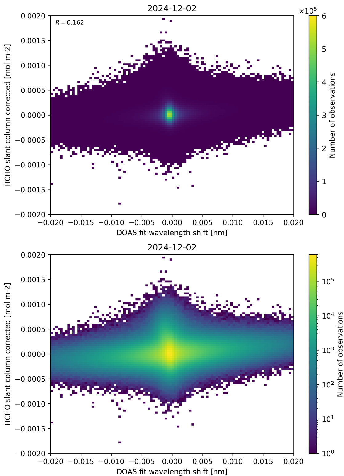
Figure 66: Scatter density plot of “DOAS fit wavelength shift” against “HCHO slant column corrected” for 2024-12-01 to 2024-12-03.
