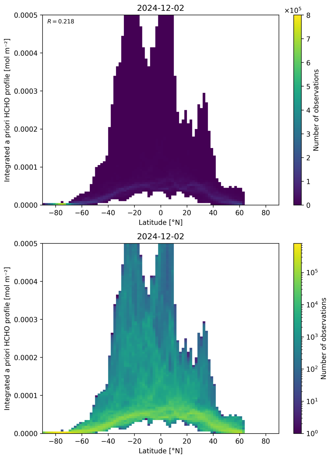
Figure 166: Scatter density plot of “Latitude” against “Integrated a priori HCHO profile” for 2024-12-01 to 2024-12-03.
