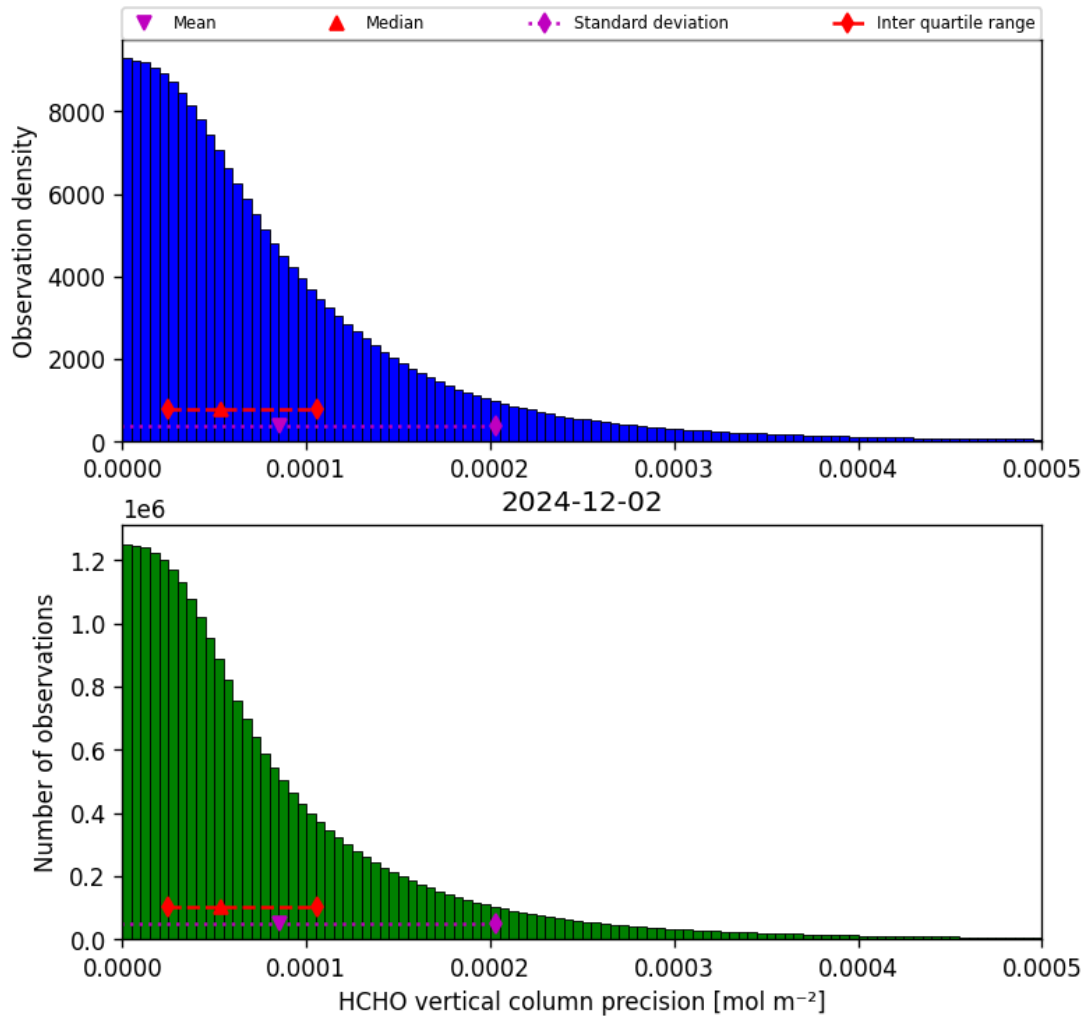
Figure 36: Histogram of “HCHO vertical column precision” for 2024-12-01 to 2024-12-03
