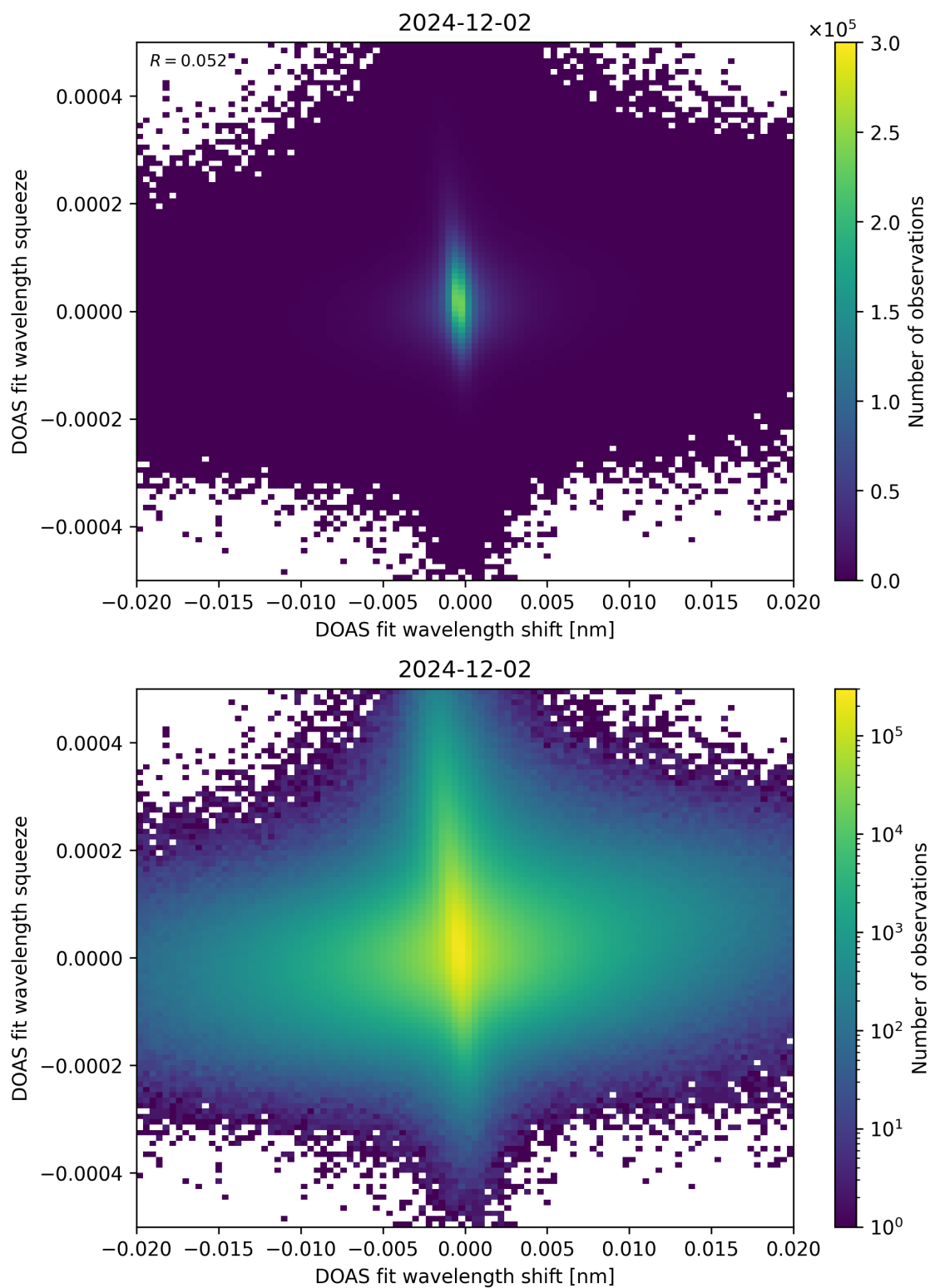
Figure 65: Scatter density plot of “DOAS fit wavelength shift” against “DOAS fit wavelength squeeze” for 2024-12-01 to 2024-12-03.
