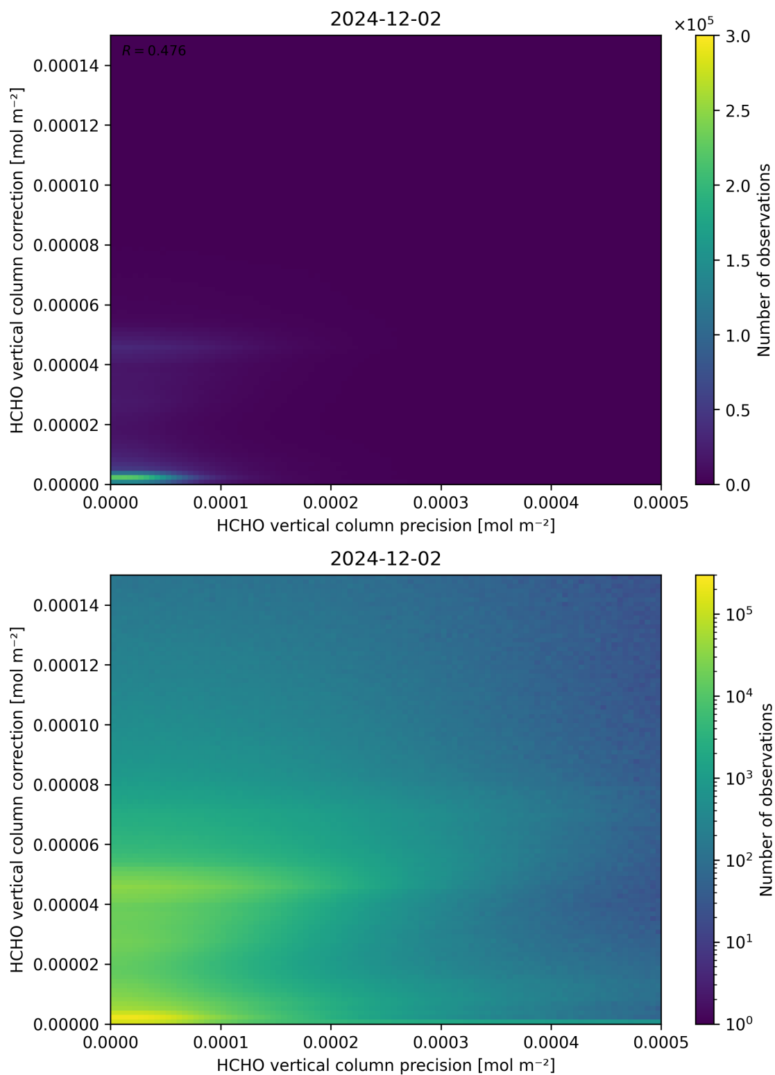
Figure 146: Scatter density plot of “HCHO vertical column precision” against “HCHO vertical column correction” for 2024-12-01 to 2024-12-03.
