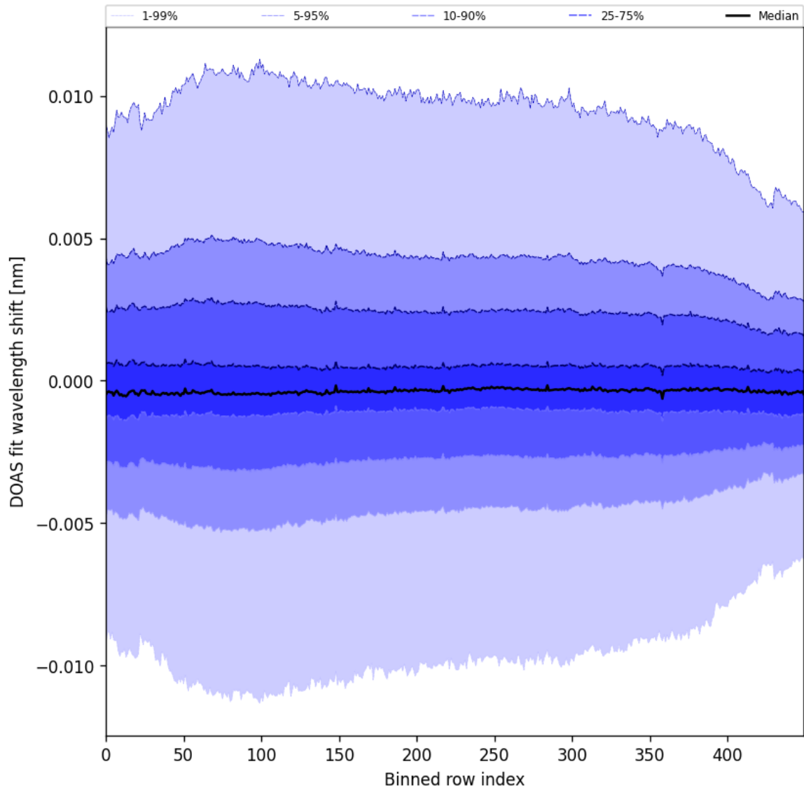
Figure 58: Along track statistics of “DOAS fit wavelength shift” for 2024-12-01 to 2024-12-03
