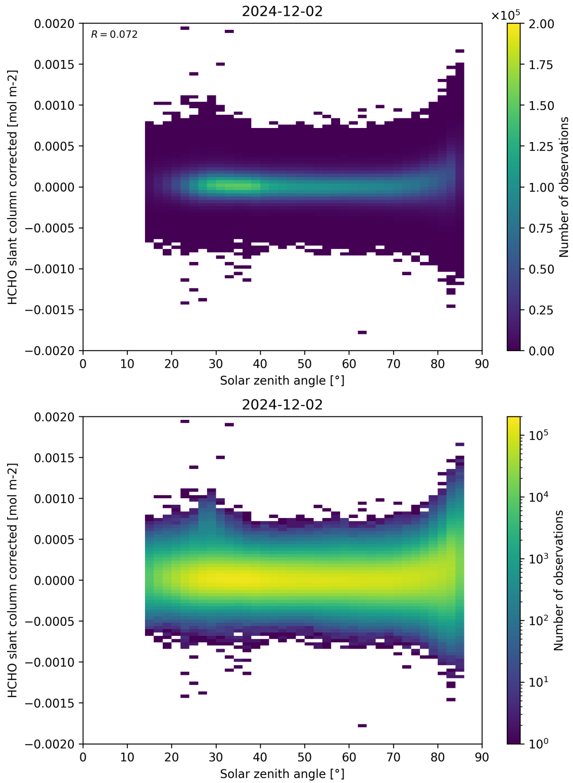
Figure 171: Scatter density plot of “Solar zenith angle” against “HCHO slant column corrected” for 2024-12-01 to 2024-12-03.
