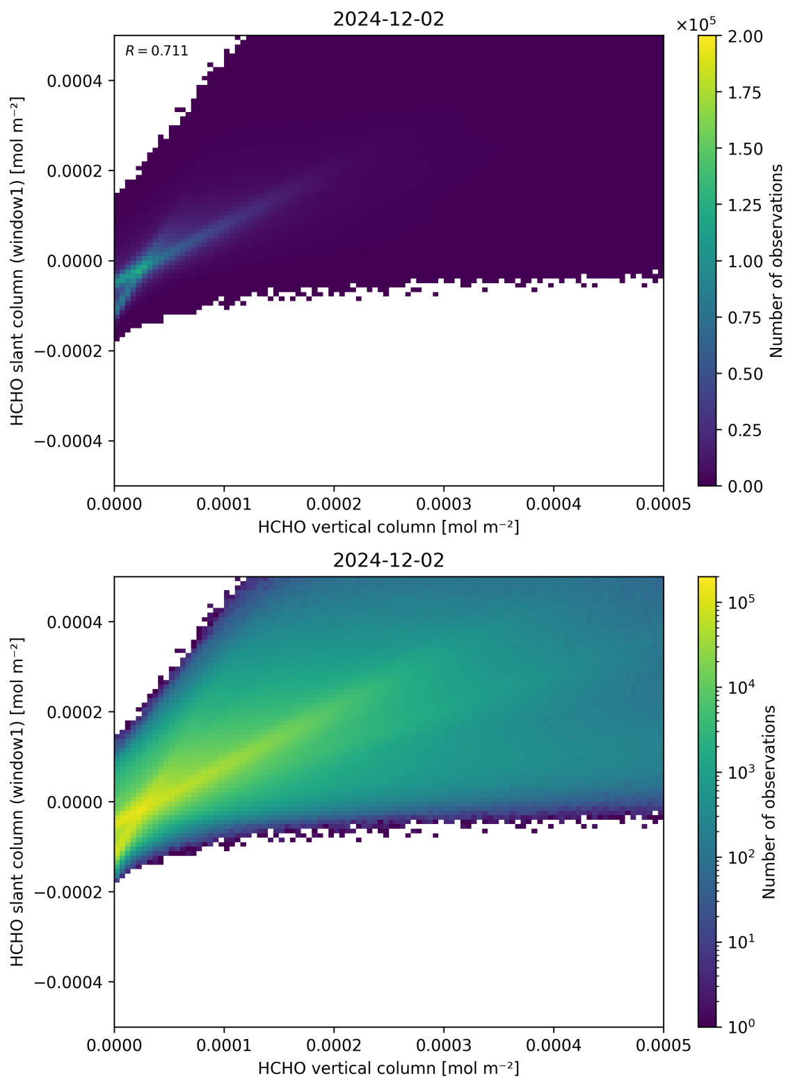
Figure 129: Scatter density plot of “HCHO vertical column” against “HCHO slant column (window1)” for 2024-12-01 to 2024-12-03.
