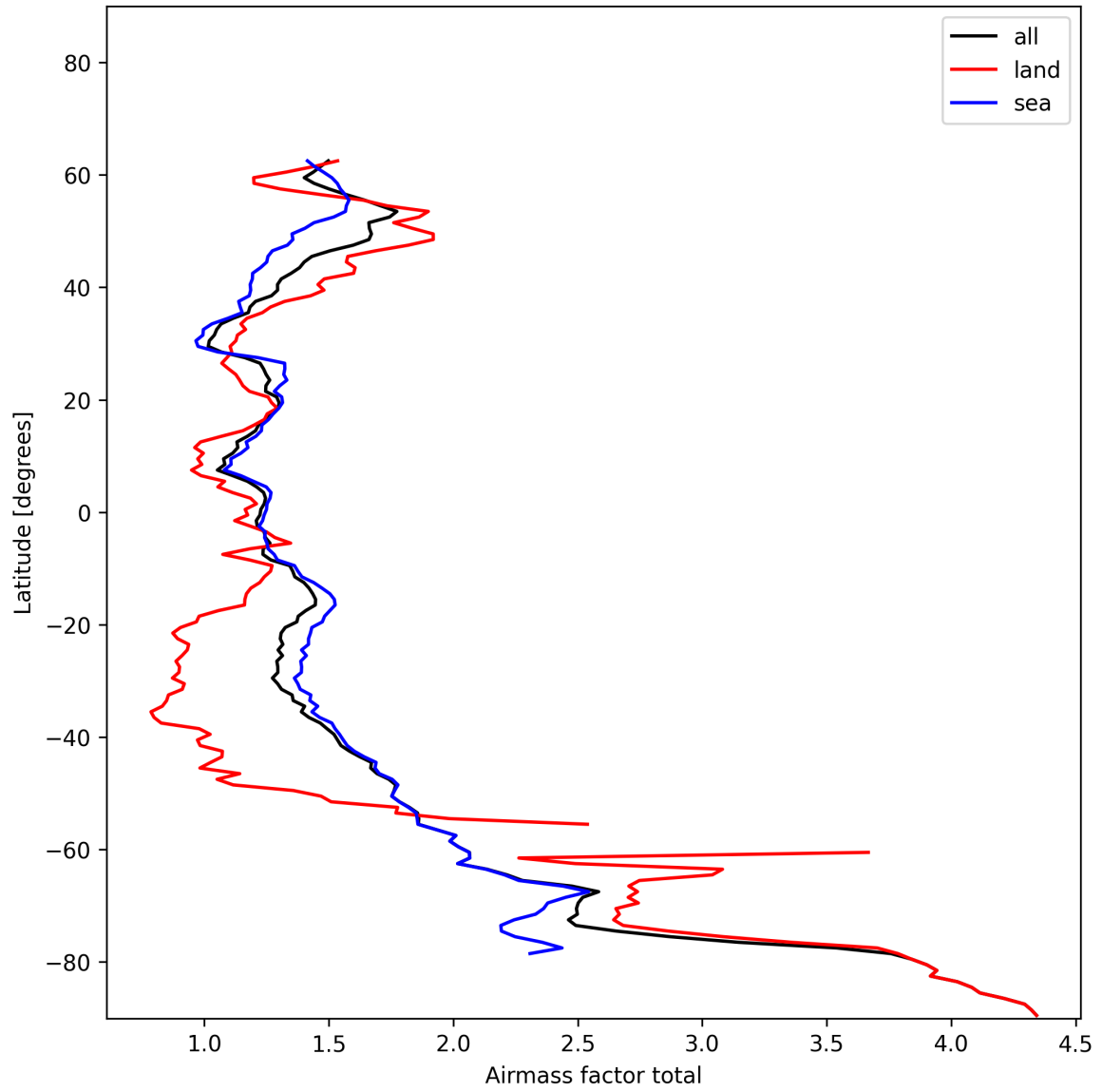
Figure 26: Zonal average of “Airmass factor total” for 2024-12-01 to 2024-12-03.
