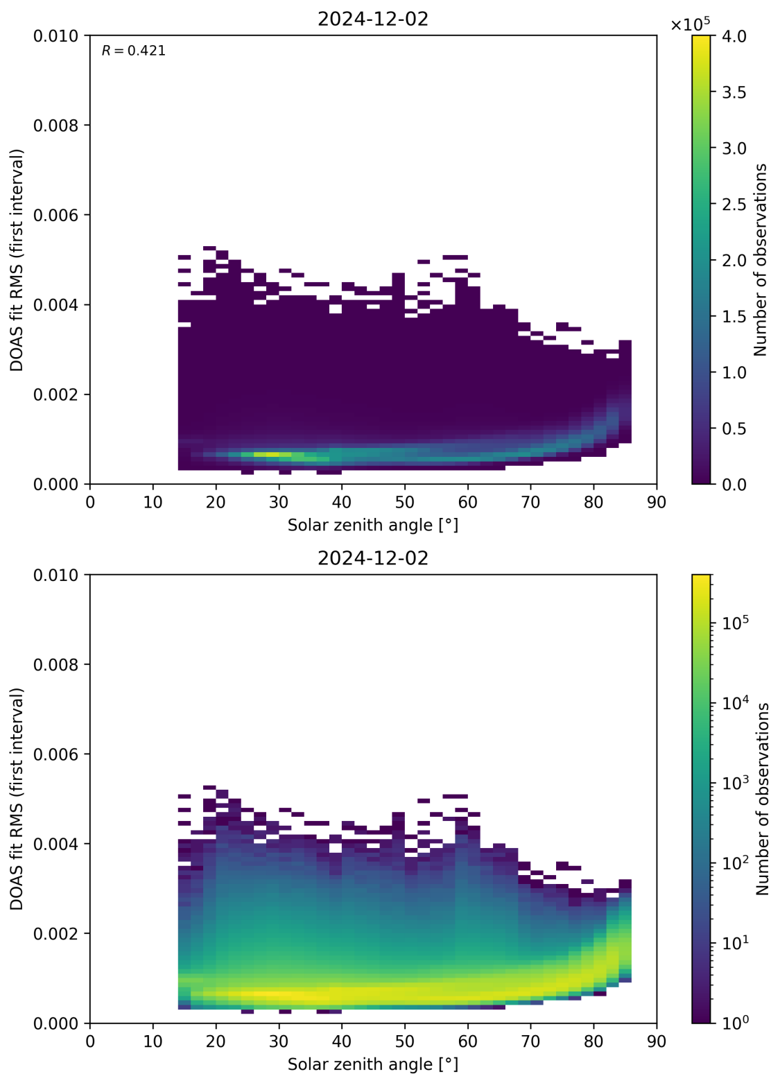
Figure 167: Scatter density plot of “Solar zenith angle” against “DOAS fit RMS (first interval)” for 2024-12-01 to 2024-12-03.
