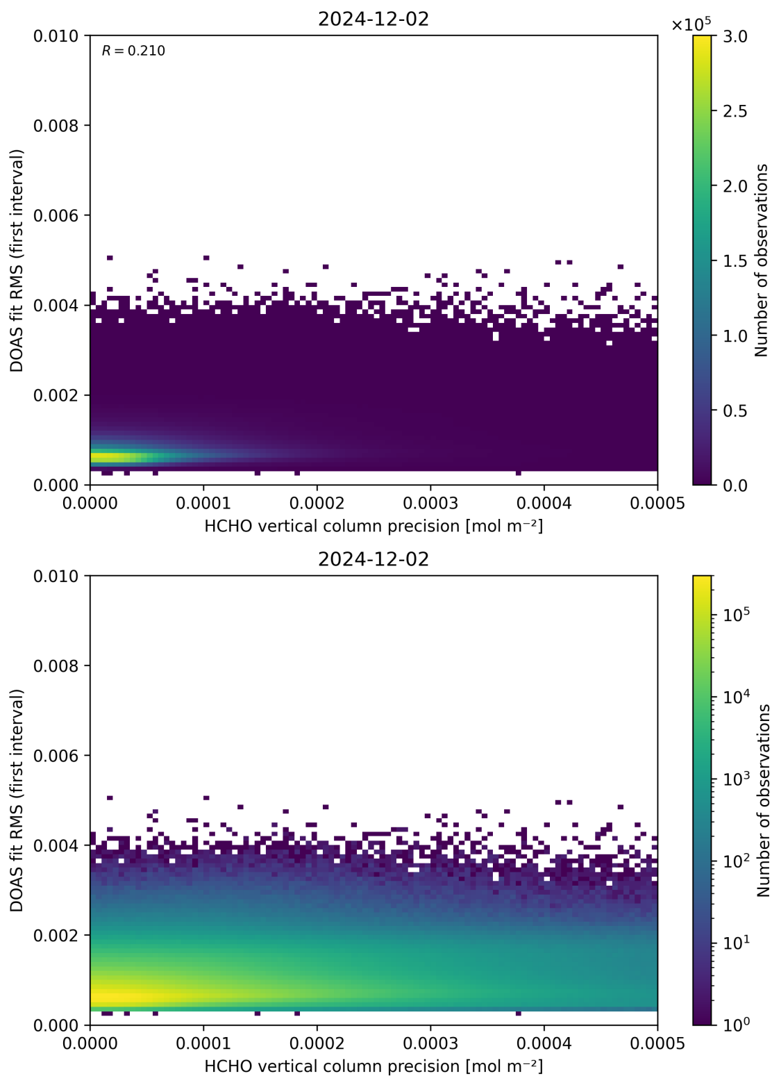
Figure 136: Scatter density plot of “HCHO vertical column precision” against “DOAS fit RMS (first interval)” for 2024-12-01 to 2024-12-03.
