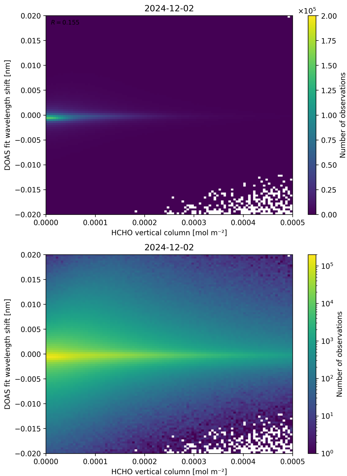
Figure 124: Scatter density plot of “HCHO vertical column” against “DOAS fit wavelength shift” for 2024-12-01 to 2024-12-03.
