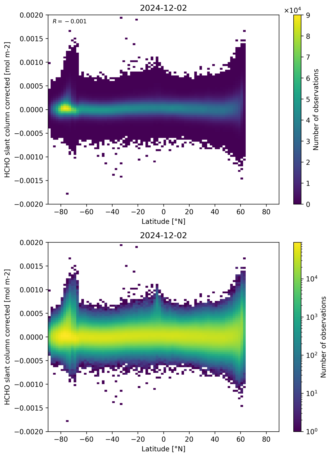
Figure 157: Scatter density plot of “Latitude” against “HCHO slant column corrected” for 2024-12-01 to 2024-12-03.
