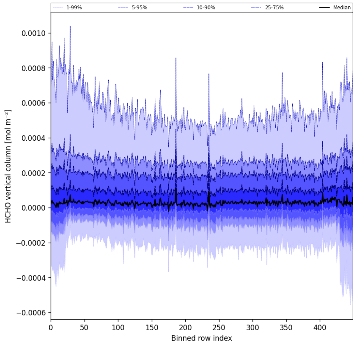
Figure 49: Along track statistics of “HCHO vertical column” for 2024-12-01 to 2024-12-03
