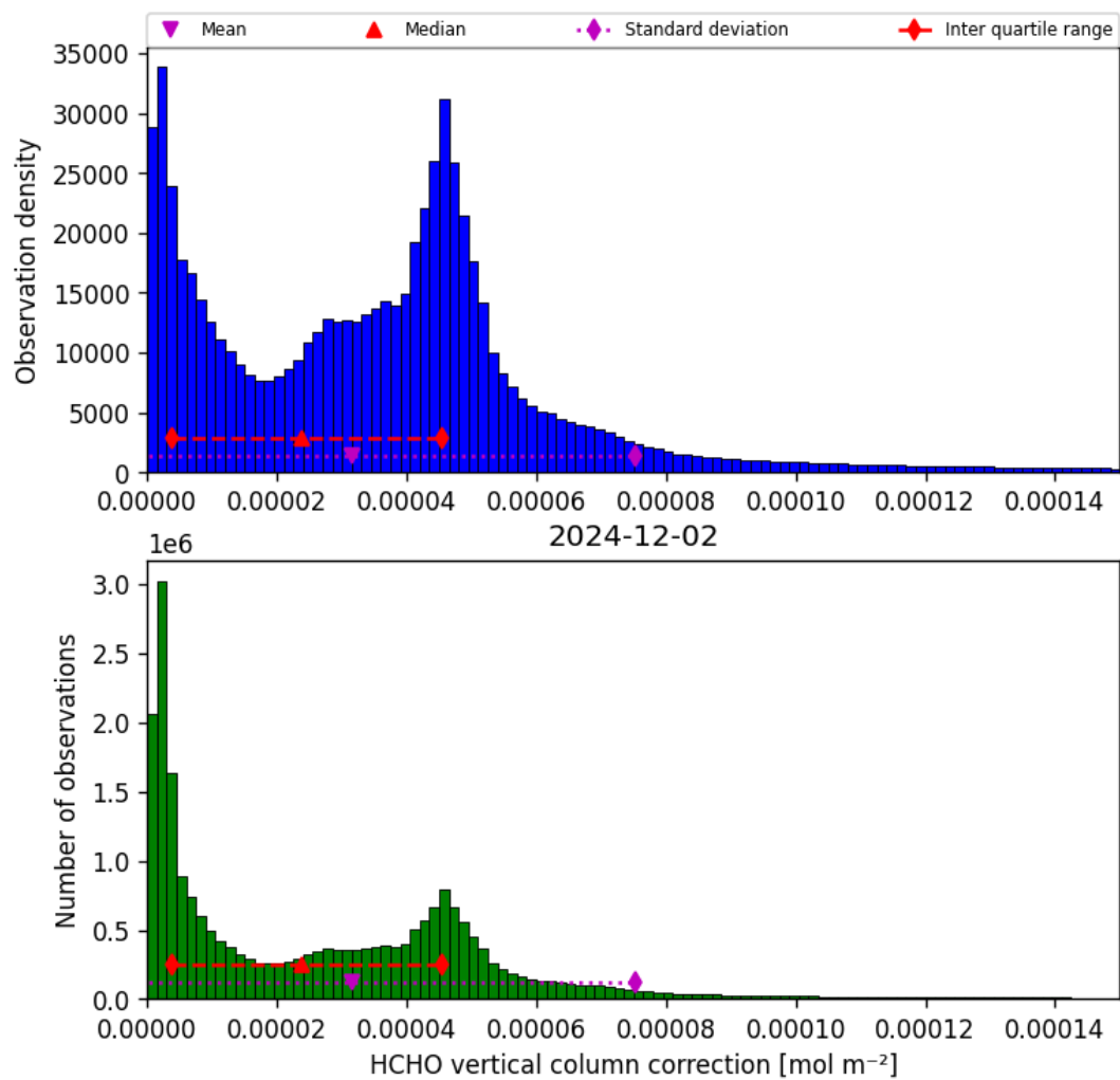
Figure 37: Histogram of “HCHO vertical column correction” for 2024-12-01 to 2024-12-03
