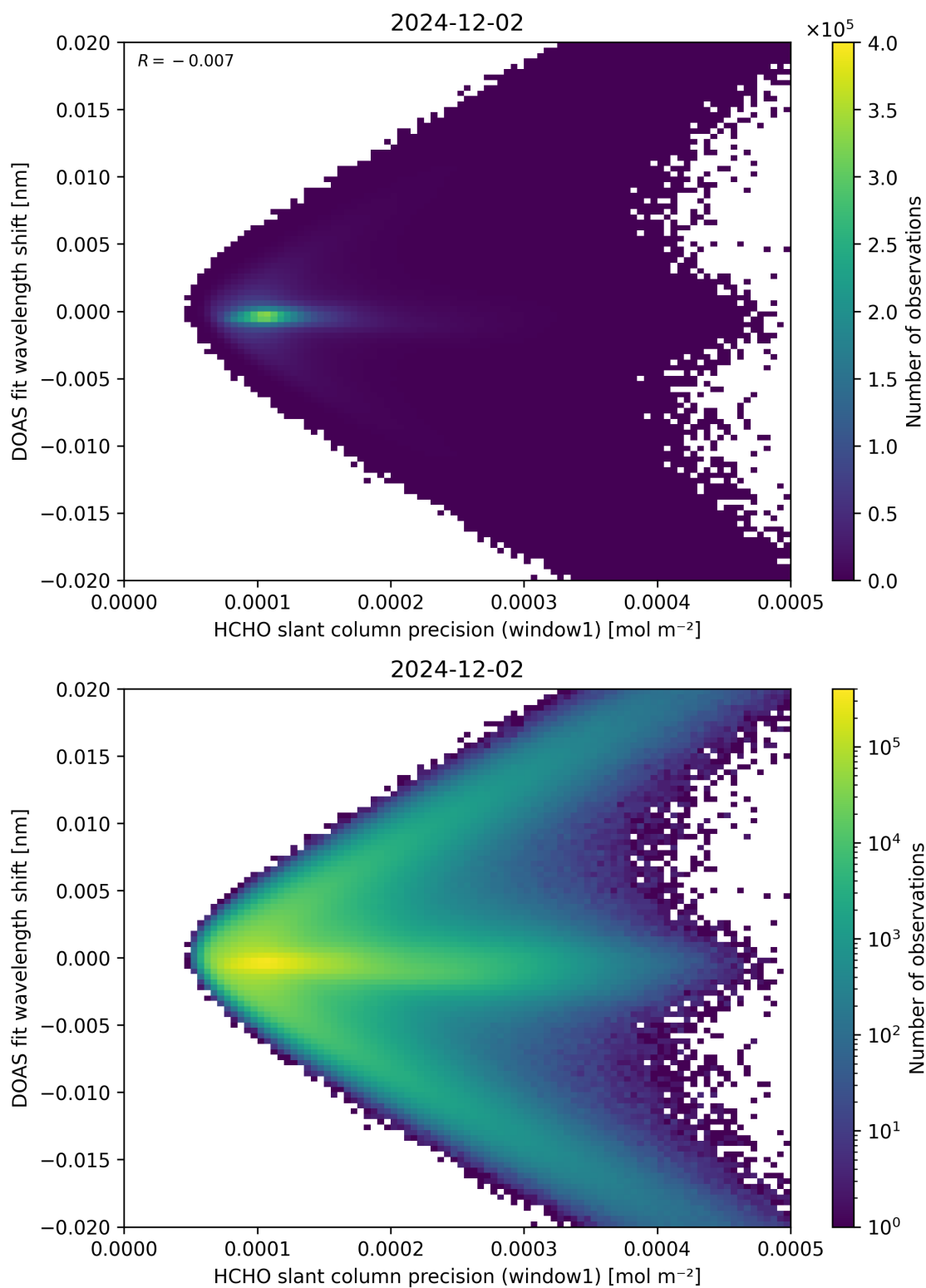
Figure 89: Scatter density plot of “HCHO slant column precision (window1)” against “DOAS fit wavelength shift” for 2024-12-01 to 2024-12-03.
