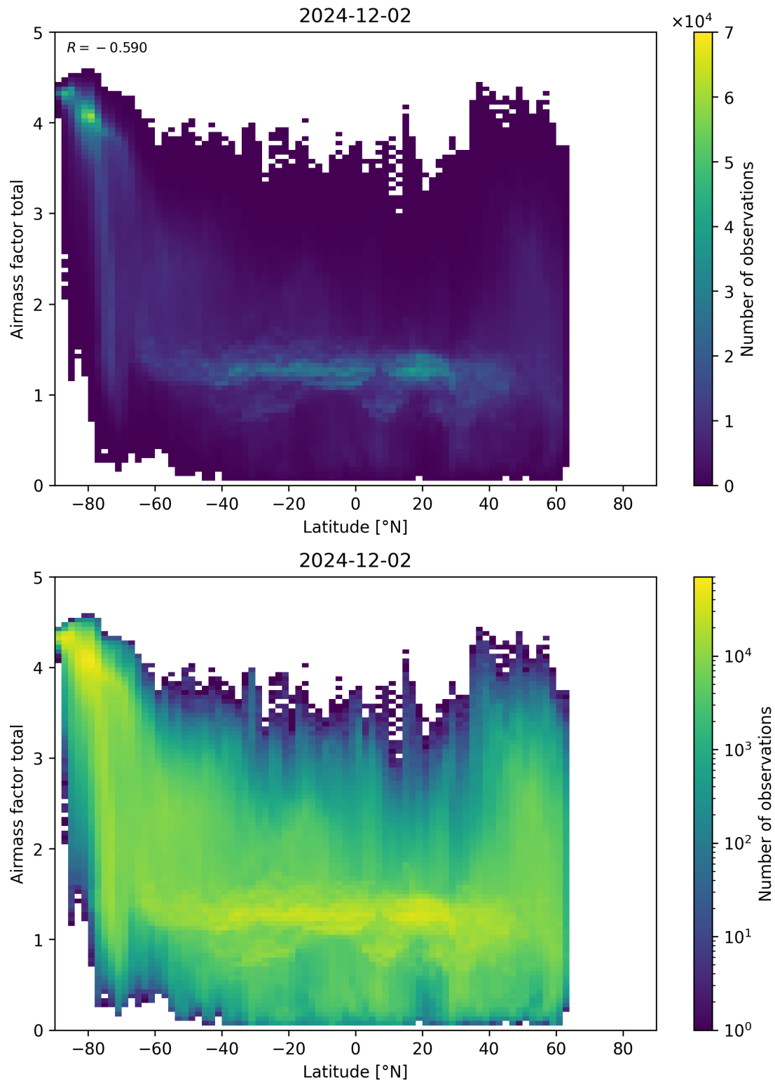
Figure 161: Scatter density plot of “Latitude” against “Airmass factor total” for 2024-12-01 to 2024-12-03.
