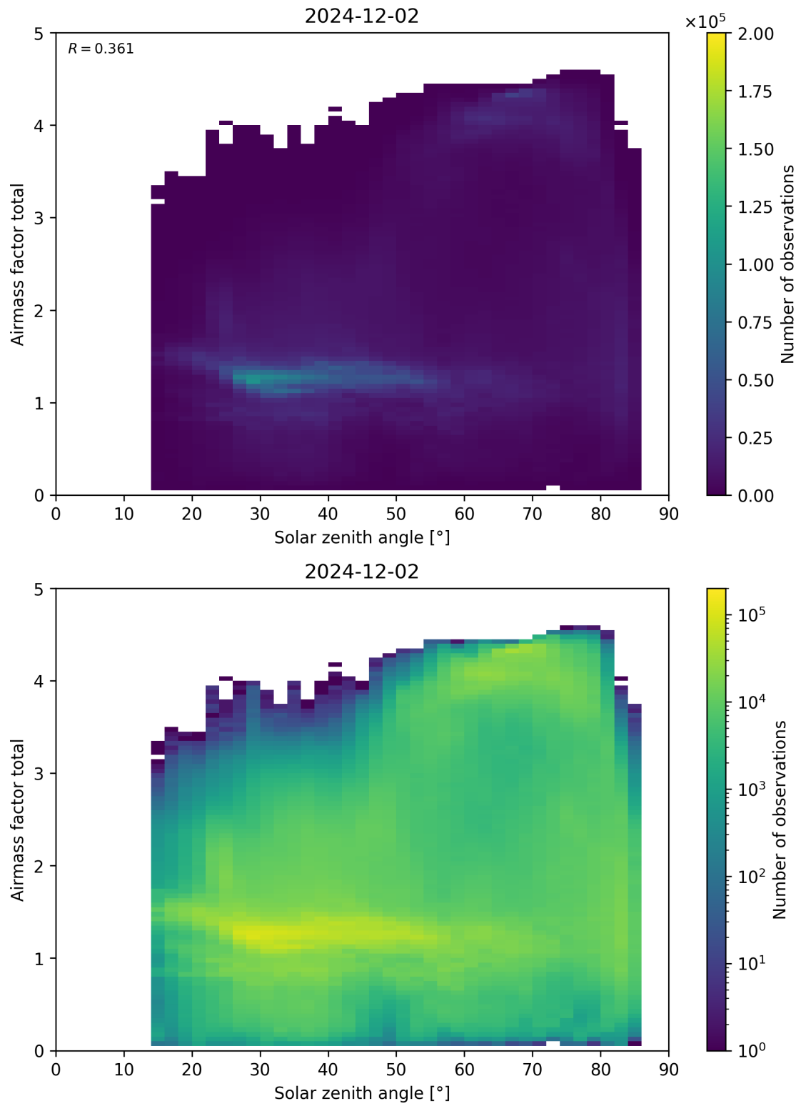
Figure 175: Scatter density plot of “Solar zenith angle” against “Airmass factor total” for 2024-12-01 to 2024-12-03.
