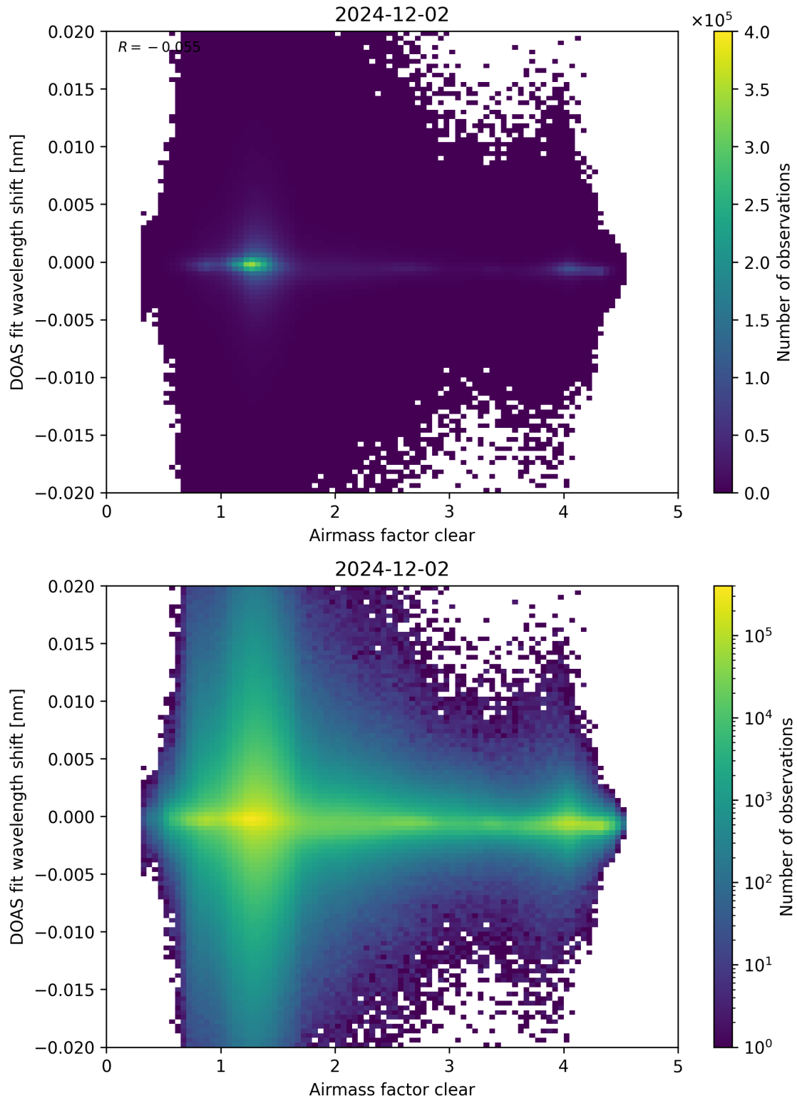
Figure 72: Scatter density plot of “Airmass factor clear” against “DOAS fit wavelength shift” for 2024-12-01 to 2024-12-03.
