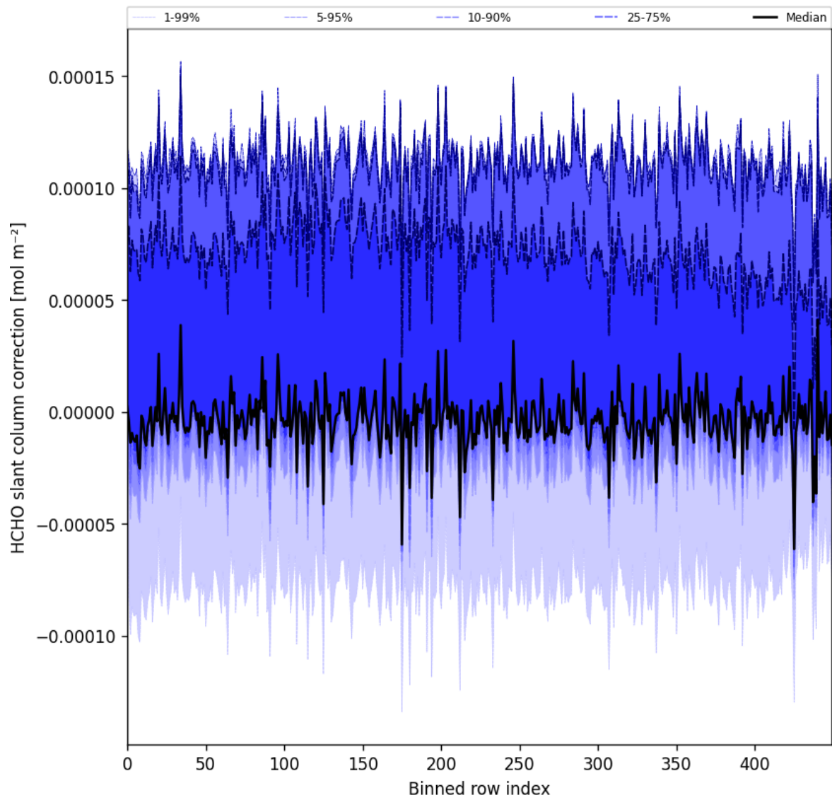
Figure 61: Along track statistics of “HCHO slant column correction” for 2024-12-01 to 2024-12-03
