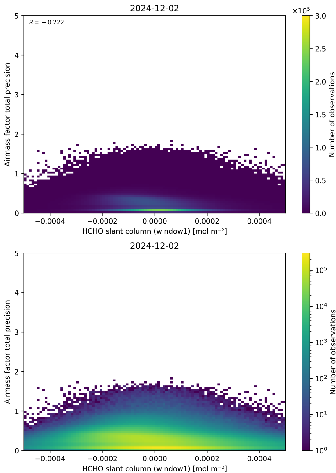
Figure 86: Scatter density plot of “HCHO slant column (window1)” against “Airmass factor total precision” for 2024-12-01 to 2024-12-03.
