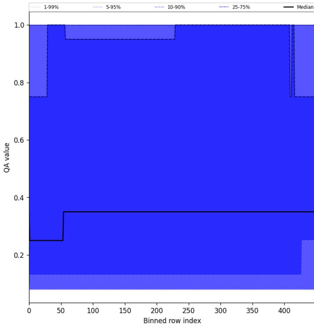
Figure 48: Along track statistics of “QA value” for 2024-12-01 to 2024-12-03
