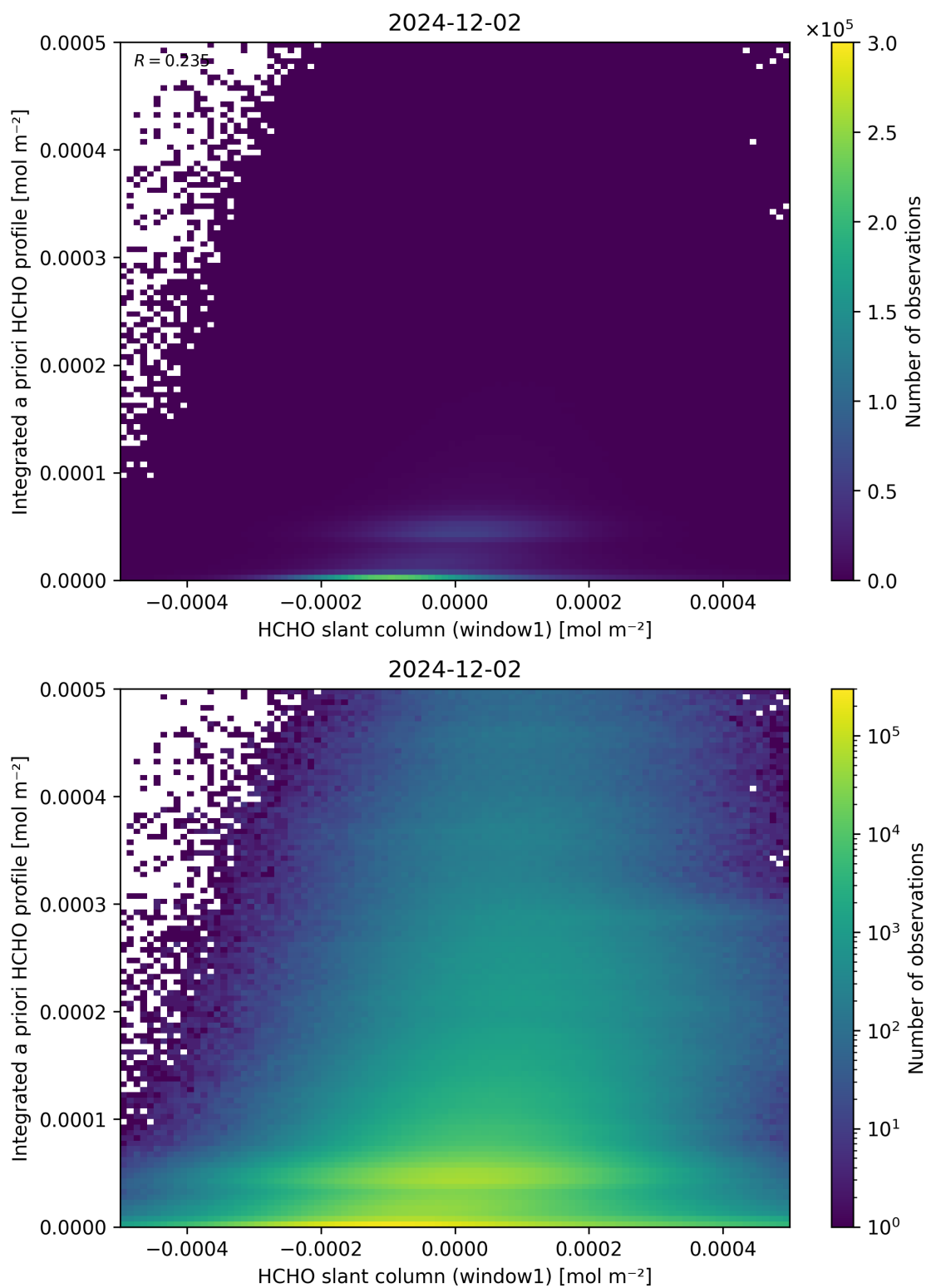
Figure 87: Scatter density plot of “HCHO slant column (window1)” against “Integrated a priori HCHO profile” for 2024-12-01 to 2024-12-03.
