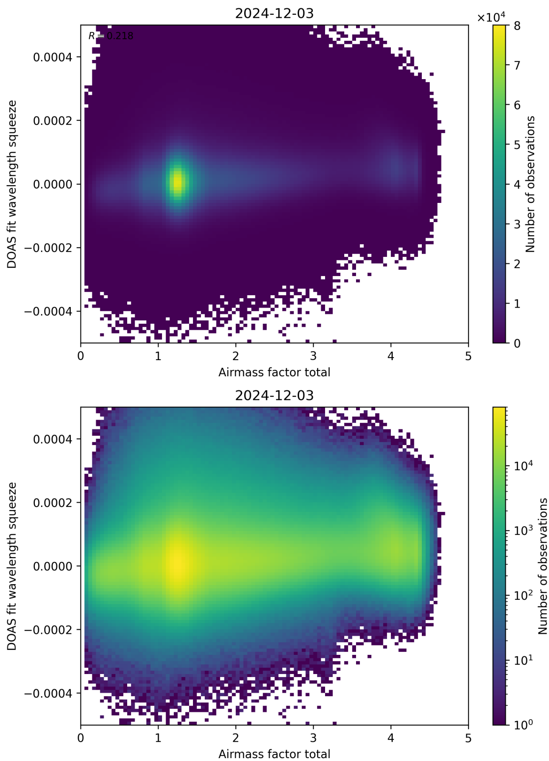
Figure 99: Scatter density plot of “Airmass factor total” against “DOAS fit wavelength squeeze” for 2024-12-02 to 2024-12-04.
