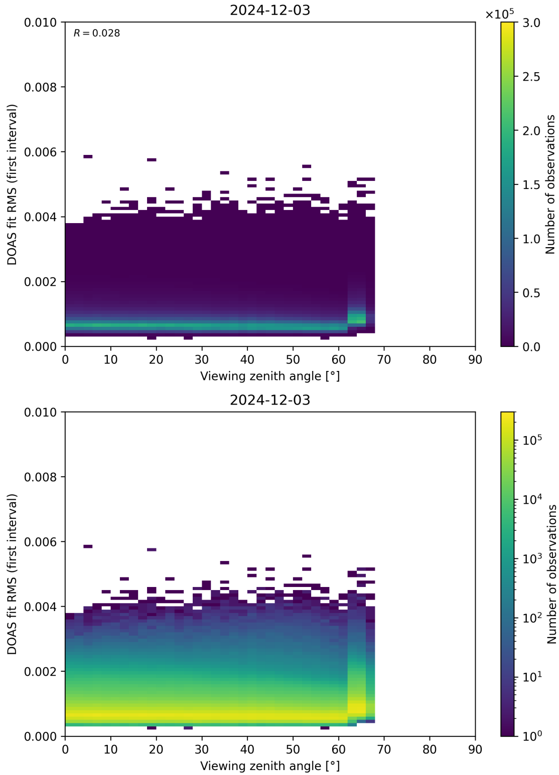
Figure 182: Scatter density plot of “Viewing zenith angle” against “DOAS fit RMS (first interval)” for 2024-12-02 to 2024-12-04.
