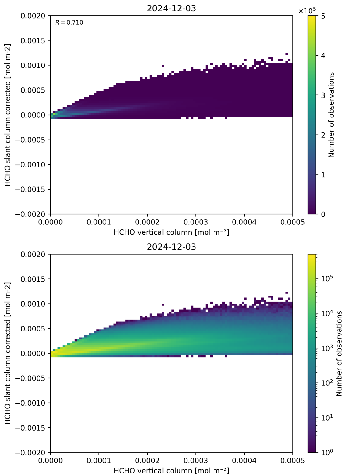
Figure 127: Scatter density plot of “HCHO vertical column” against “HCHO slant column corrected” for 2024-12-02 to 2024-12-04.
