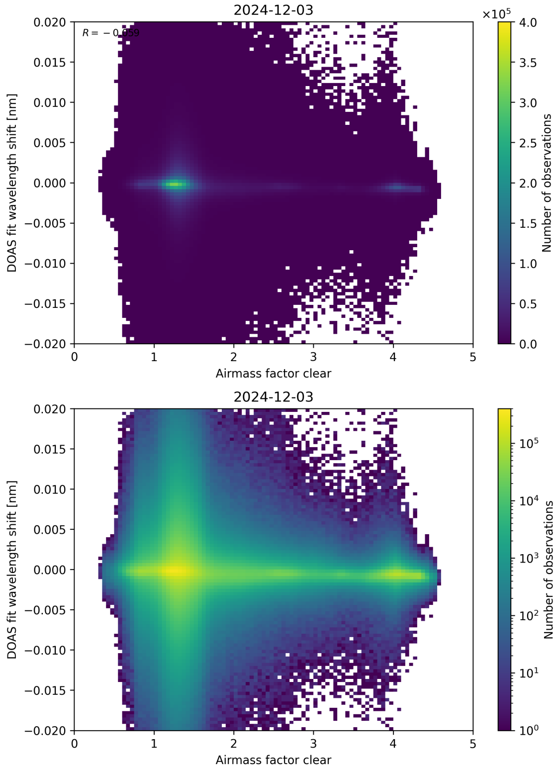
Figure 72: Scatter density plot of “Airmass factor clear” against “DOAS fit wavelength shift” for 2024-12-02 to 2024-12-04.
