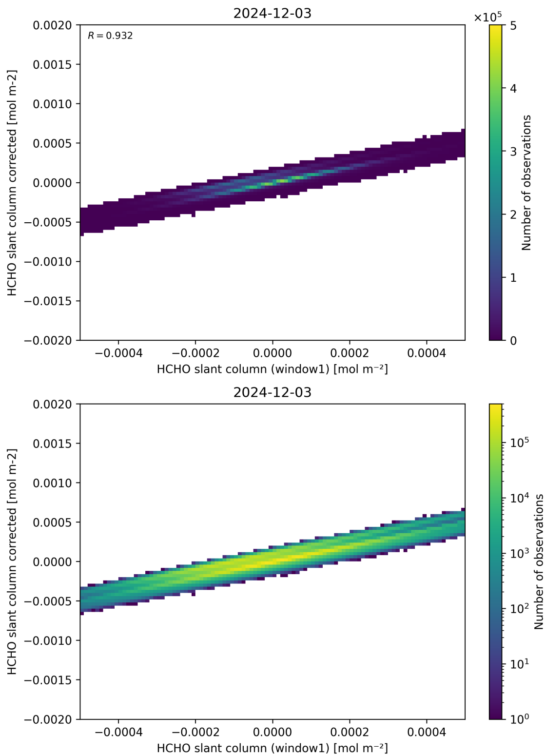
Figure 82: Scatter density plot of “HCHO slant column (window1)” against “HCHO slant column corrected” for 2024-12-02 to 2024-12-04.
