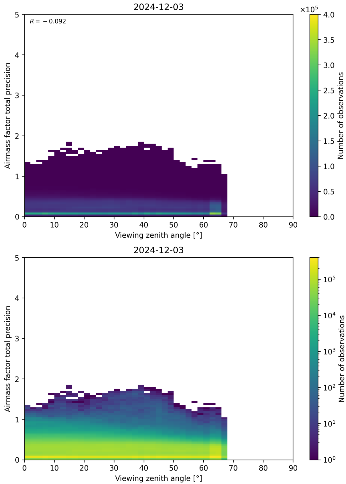
Figure 191: Scatter density plot of “Viewing zenith angle” against “Airmass factor total precision” for 2024-12-02 to 2024-12-04.
