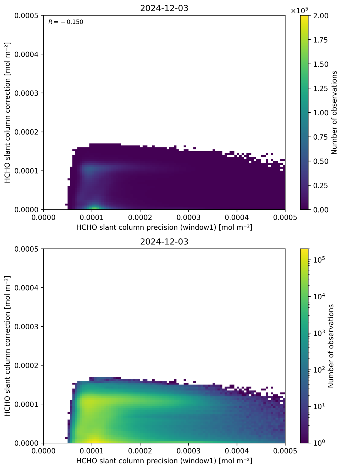
Figure 93: Scatter density plot of “HCHO slant column precision (window1)” against “HCHO slant column correction” for 2024-12-02 to 2024-12-04.
