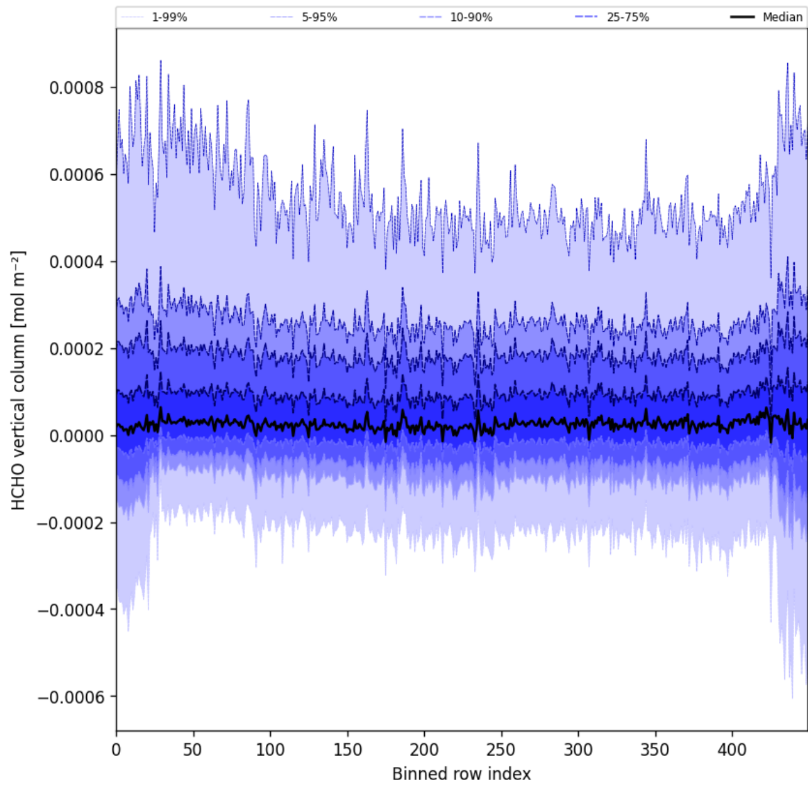
Figure 49: Along track statistics of “HCHO vertical column” for 2024-12-02 to 2024-12-04
