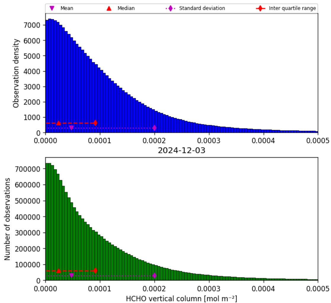
Figure 35: Histogram of “HCHO vertical column” for 2024-12-02 to 2024-12-04
