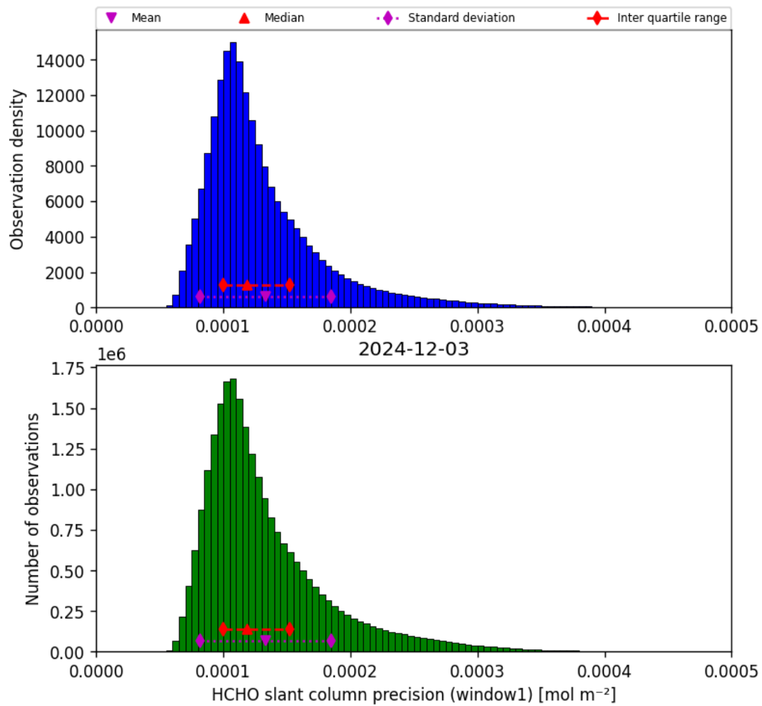
Figure 39: Histogram of “HCHO slant column precision (window1)” for 2024-12-02 to 2024-12-04
