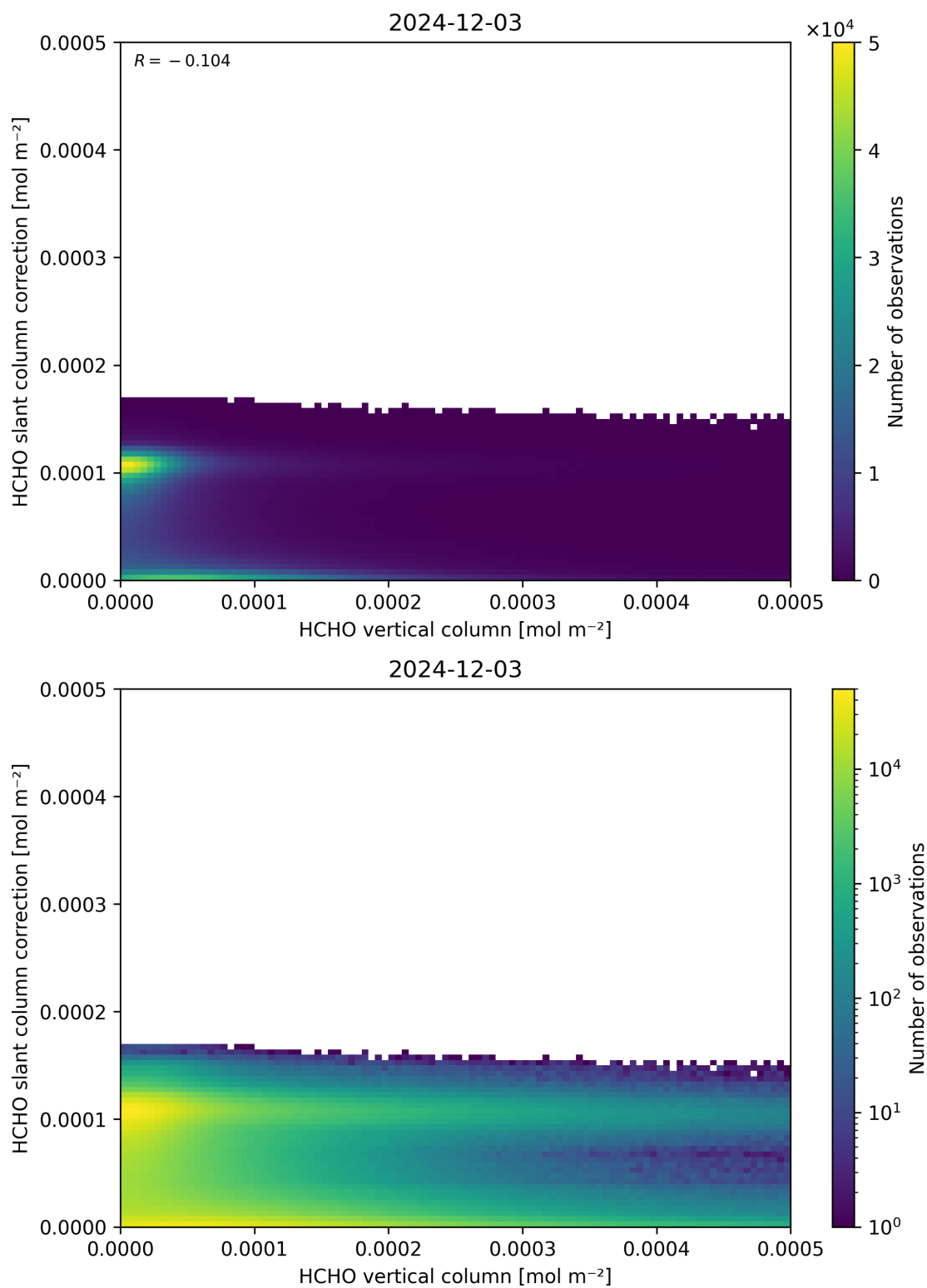
Figure 128: Scatter density plot of “HCHO vertical column” against “HCHO slant column correction” for 2024-12-02 to 2024-12-04.
