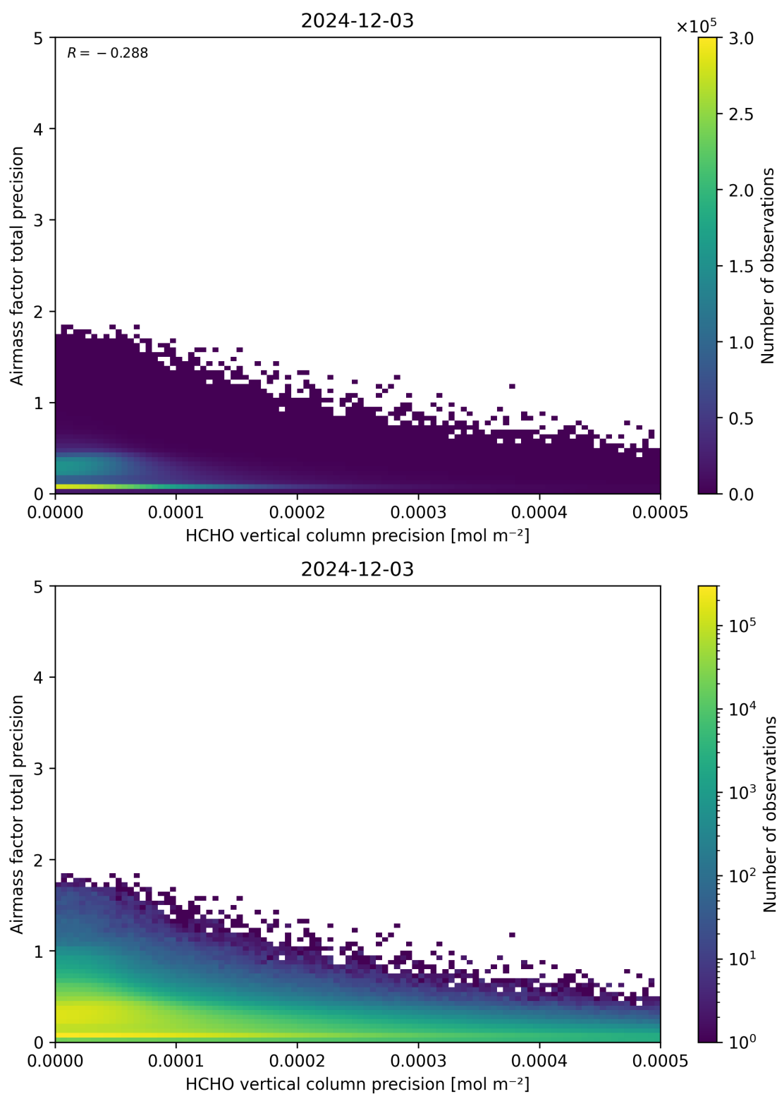
Figure 145: Scatter density plot of “HCHO vertical column precision” against “Airmass factor total precision” for 2024-12-02 to 2024-12-04.
