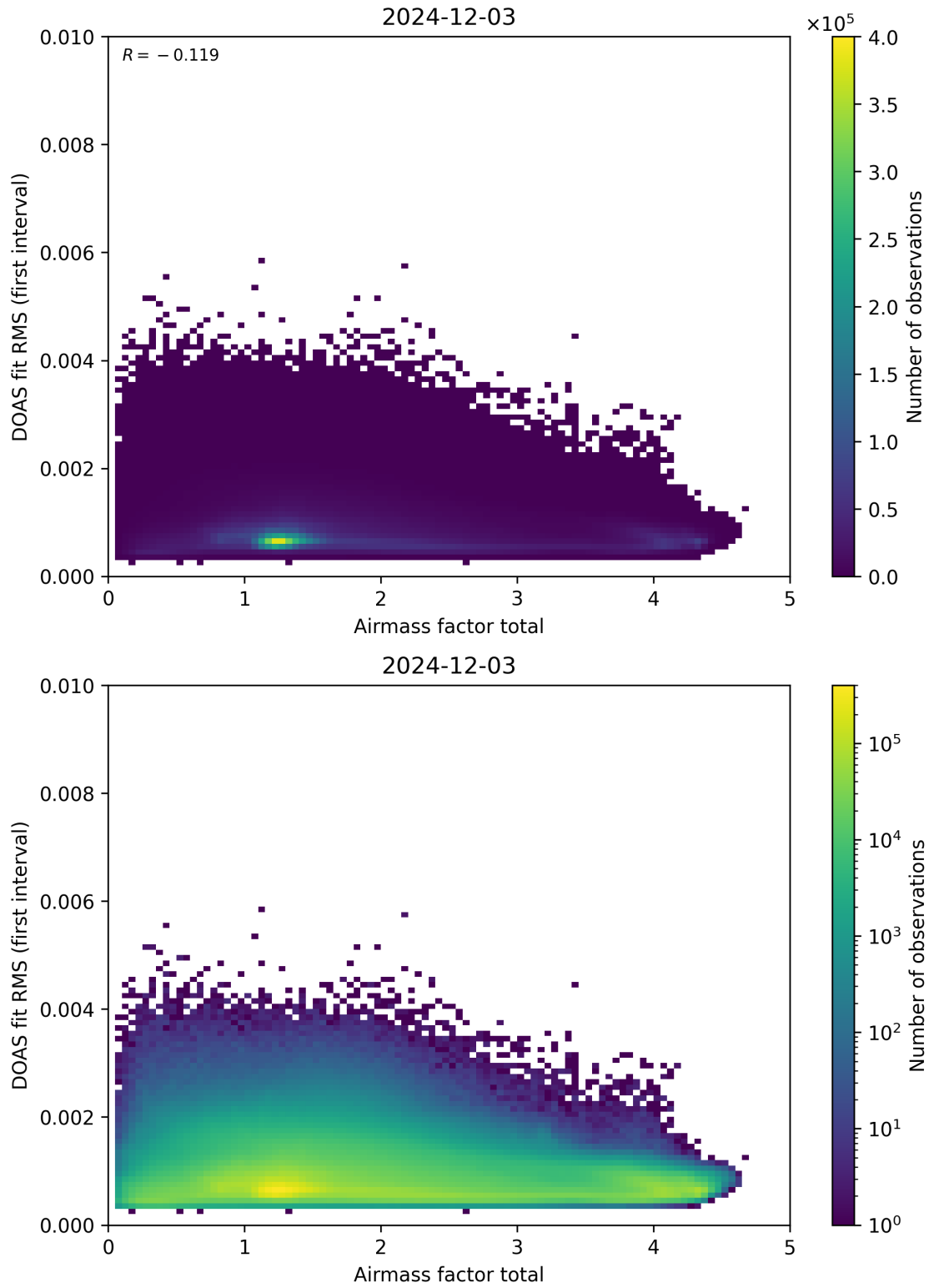
Figure 97: Scatter density plot of “Airmass factor total” against “DOAS fit RMS (first interval)” for 2024-12-02 to 2024-12-04.
