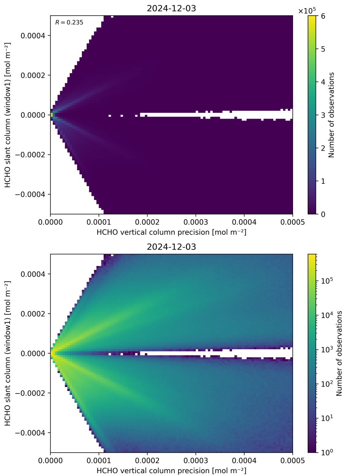
Figure 142: Scatter density plot of “HCHO vertical column precision” against “HCHO slant column (window1)” for 2024-12-02 to 2024-12-04.
