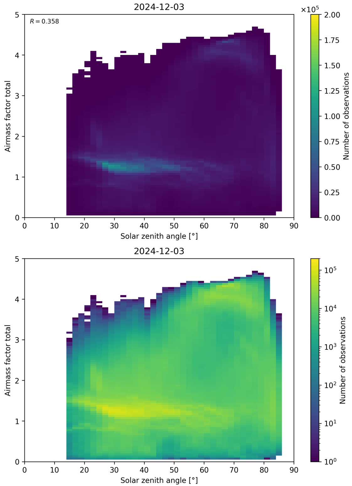
Figure 175: Scatter density plot of “Solar zenith angle” against “Airmass factor total” for 2024-12-02 to 2024-12-04.
