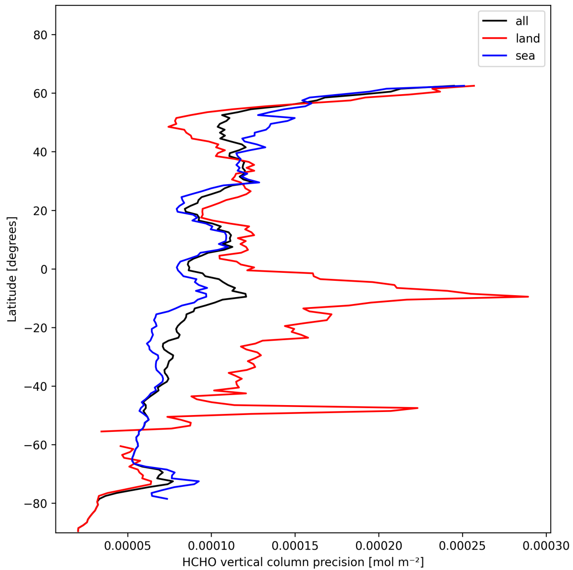
Figure 22: Zonal average of “HCHO vertical column precision” for 2024-12-02 to 2024-12-04.
