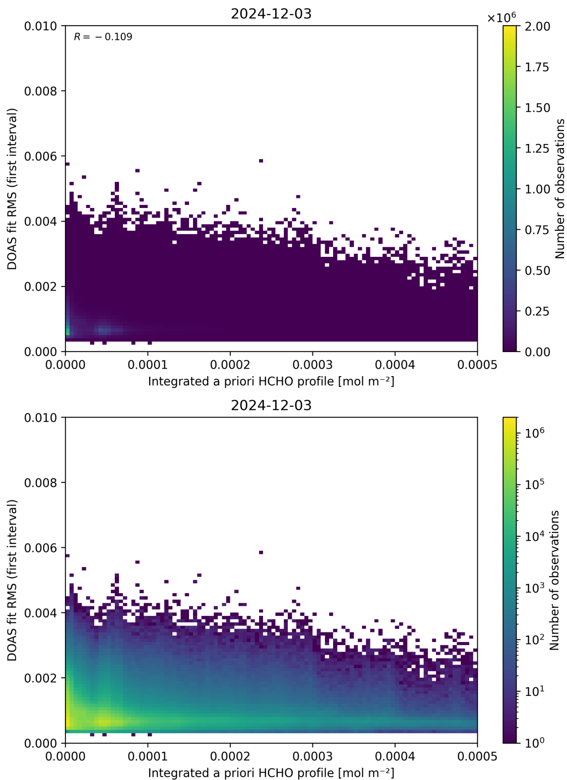
Figure 148: Scatter density plot of “Integrated a priori HCHO profile” against “DOAS fit RMS (first interval)” for 2024-12-02 to 2024-12-04.
