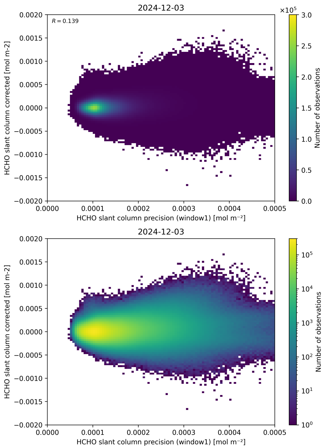
Figure 92: Scatter density plot of “HCHO slant column precision (window1)” against “HCHO slant column corrected” for 2024-12-02 to 2024-12-04.
