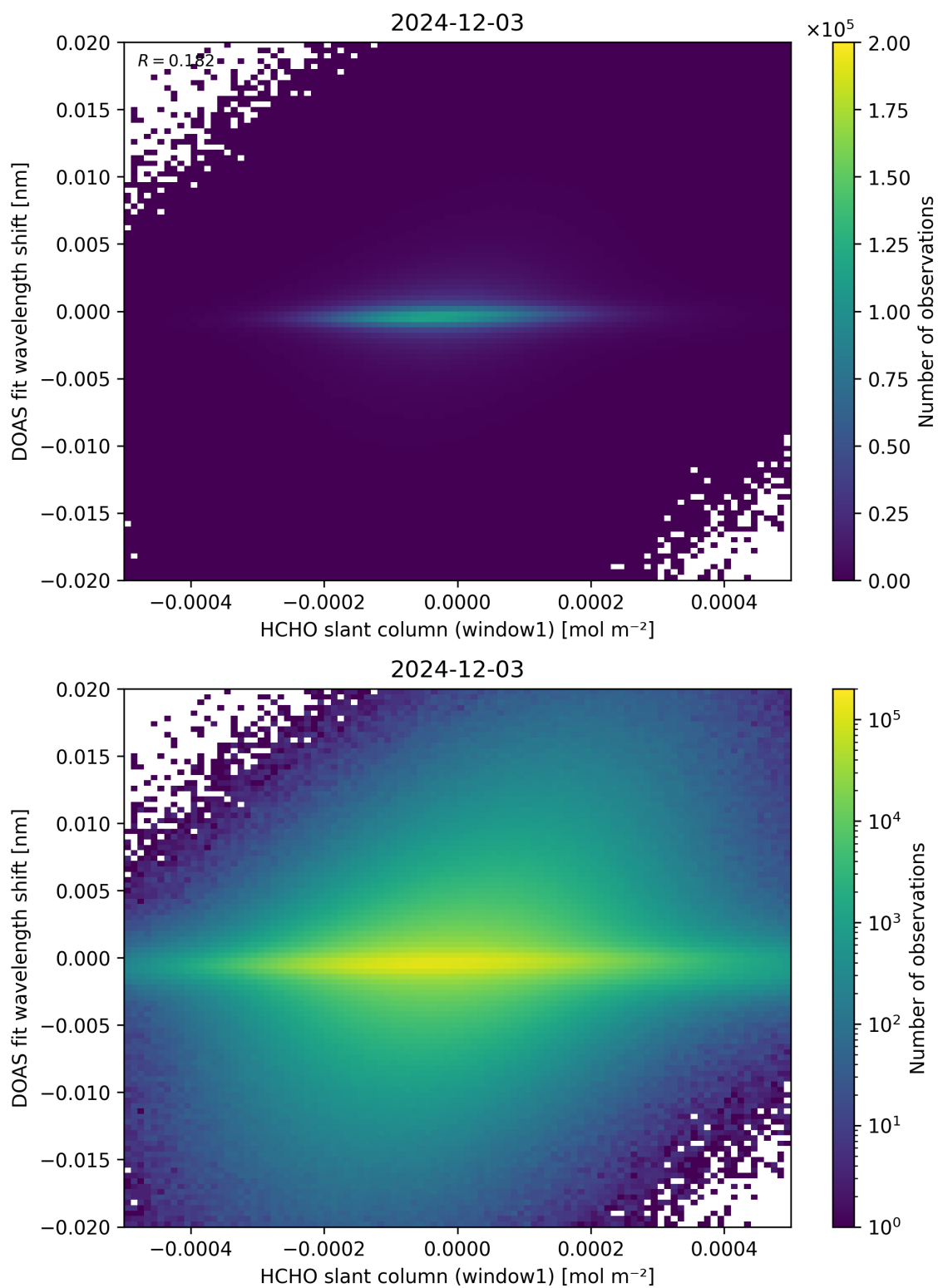
Figure 79: Scatter density plot of “HCHO slant column (window1)” against “DOAS fit wavelength shift” for 2024-12-02 to 2024-12-04.
