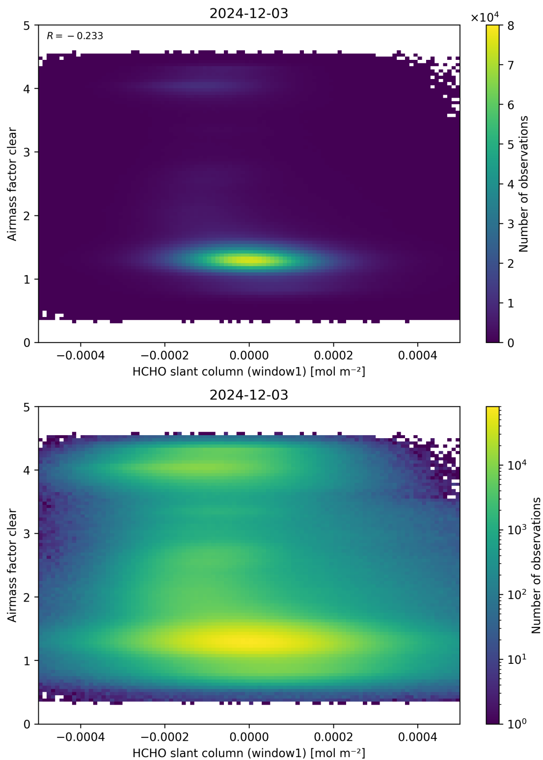
Figure 81: Scatter density plot of “HCHO slant column (window1)” against “Airmass factor clear” for 2024-12-02 to 2024-12-04.
