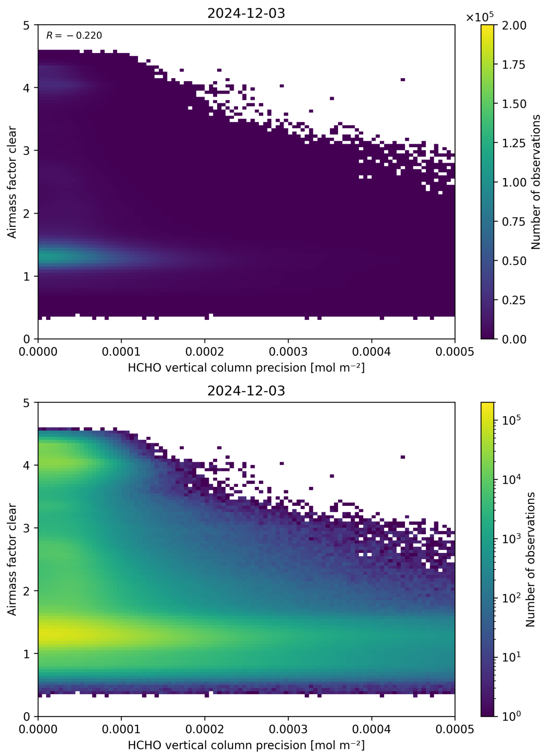
Figure 139: Scatter density plot of “HCHO vertical column precision” against “Airmass factor clear” for 2024-12-02 to 2024-12-04.
