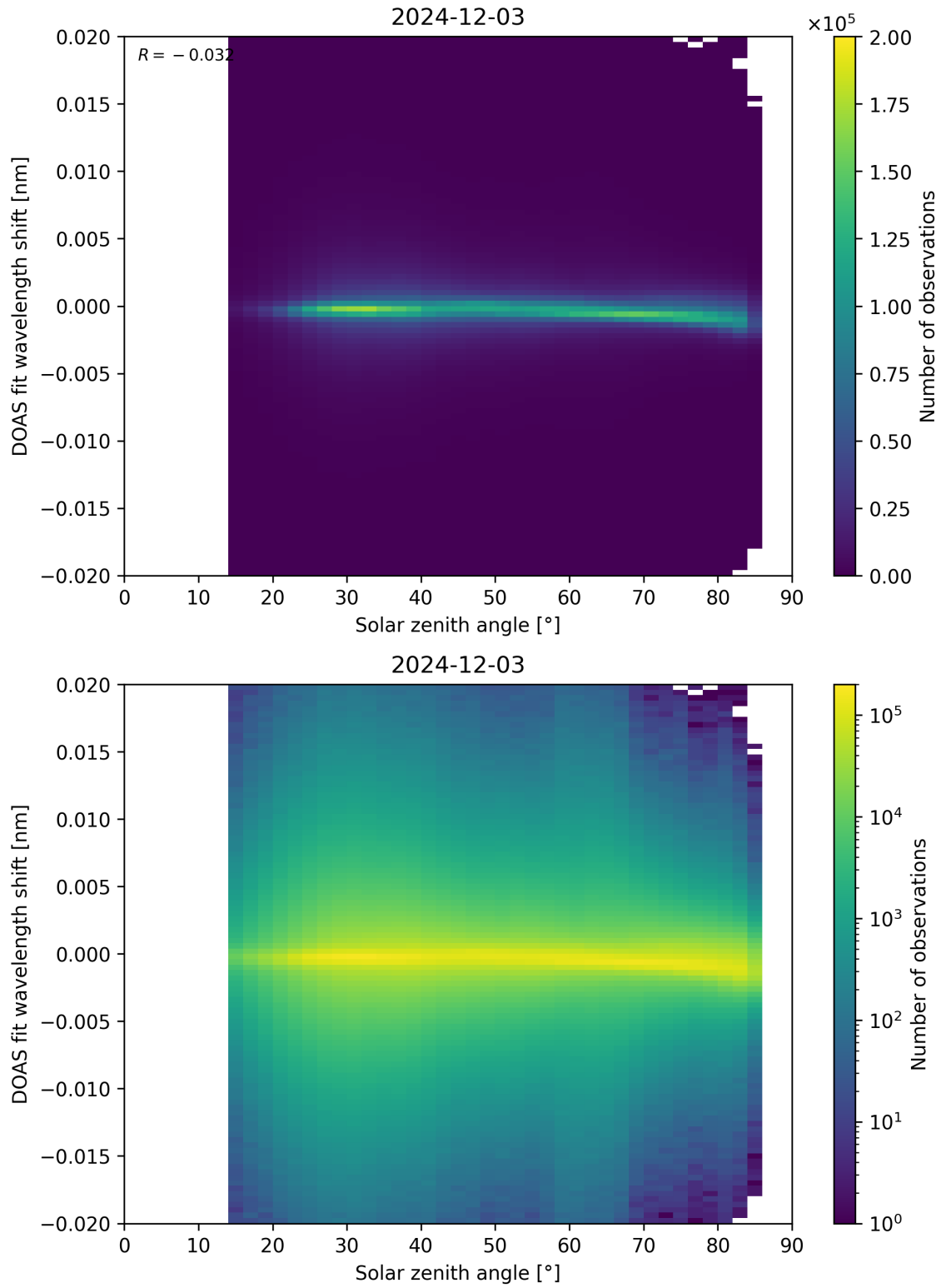
Figure 168: Scatter density plot of “Solar zenith angle” against “DOAS fit wavelength shift” for 2024-12-02 to 2024-12-04.
