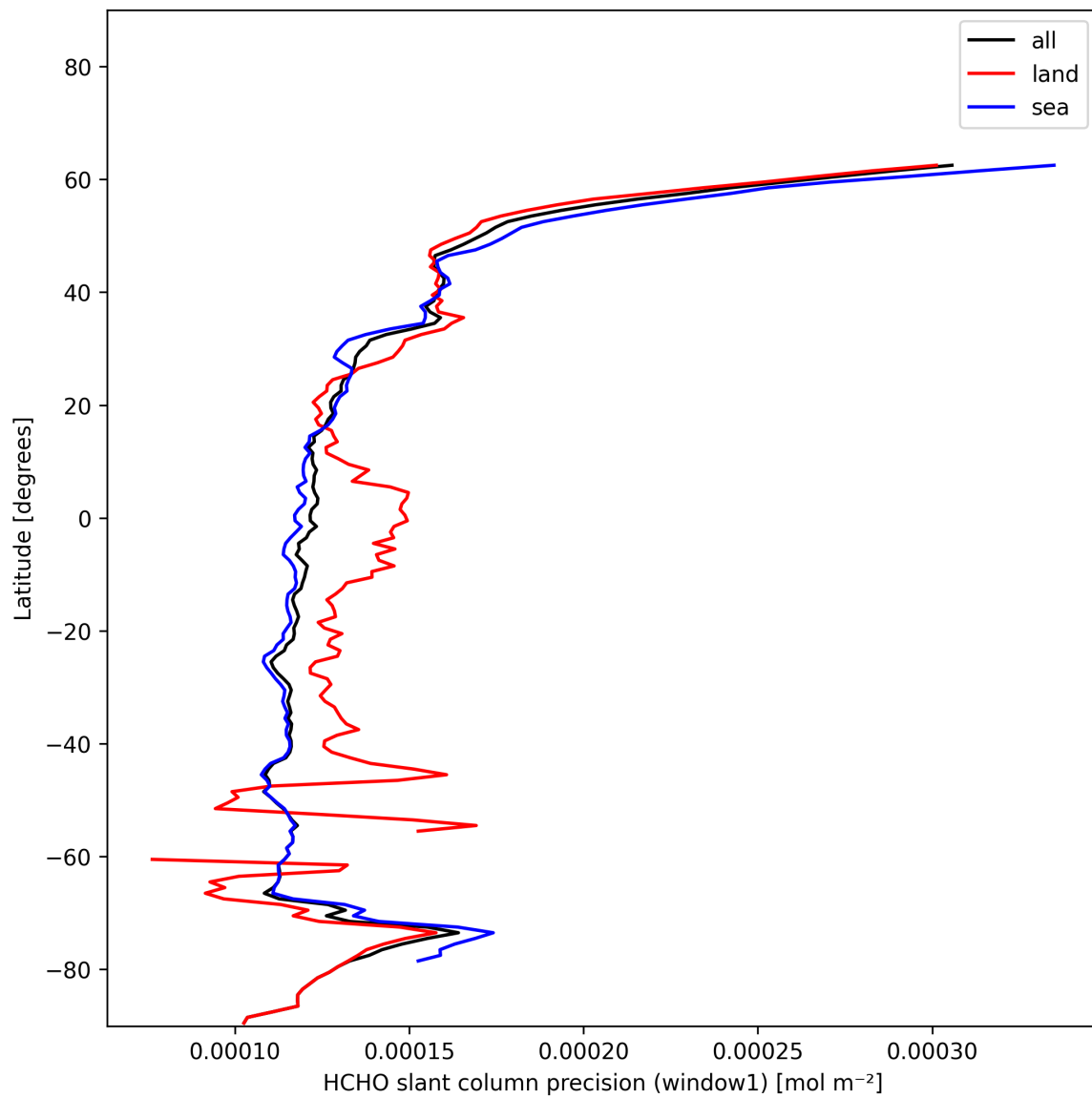
Figure 25: Zonal average of “HCHO slant column precision (window1)” for 2024-12-02 to 2024-12-04.
