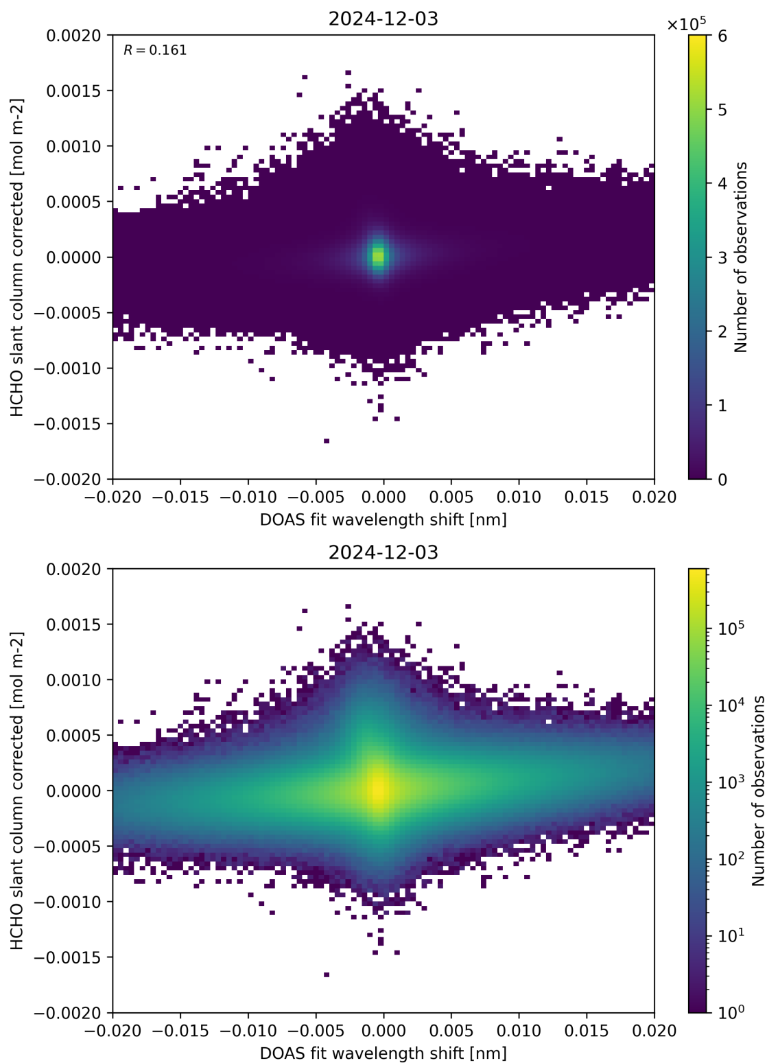
Figure 66: Scatter density plot of “DOAS fit wavelength shift” against “HCHO slant column corrected” for 2024-12-02 to 2024-12-04.
