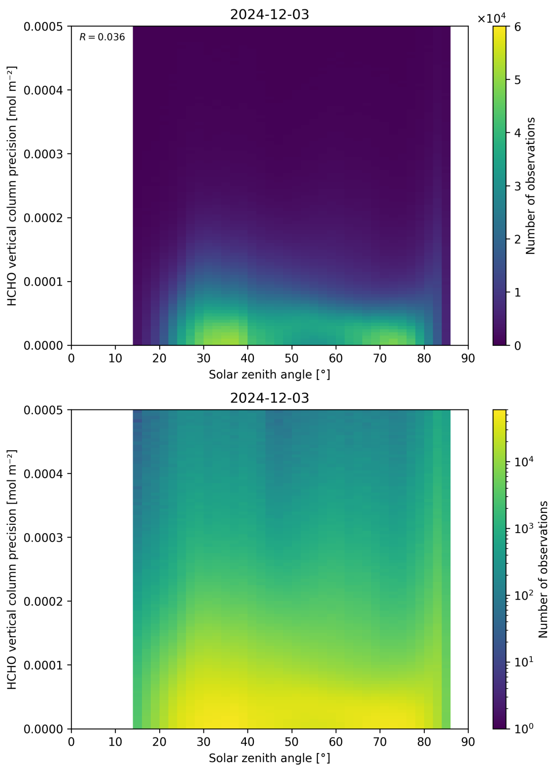
Figure 179: Scatter density plot of “Solar zenith angle” against “HCHO vertical column precision” for 2024-12-02 to 2024-12-04.
