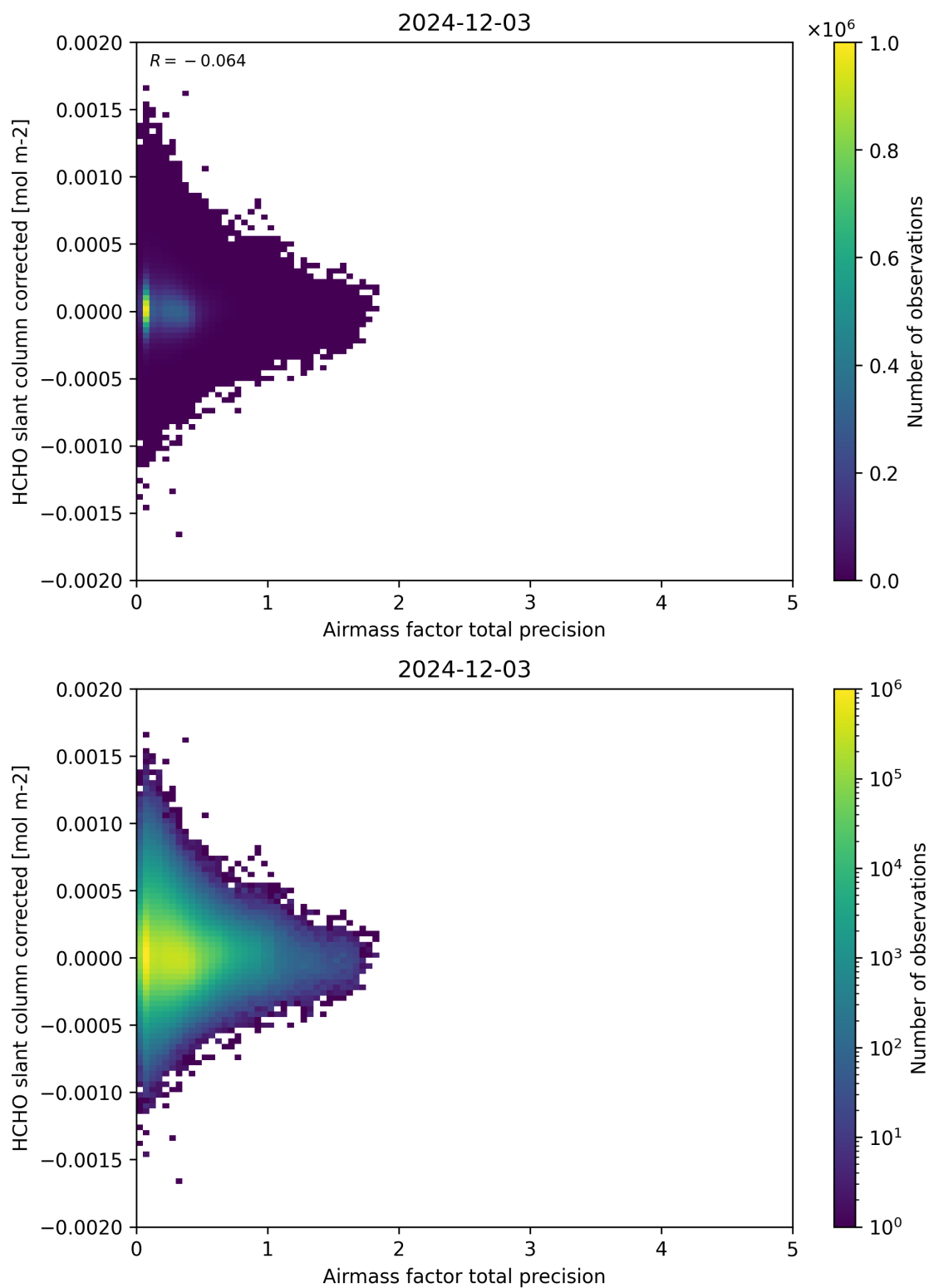
Figure 109: Scatter density plot of “Airmass factor total precision” against “HCHO slant column corrected” for 2024-12-02 to 2024-12-04.
