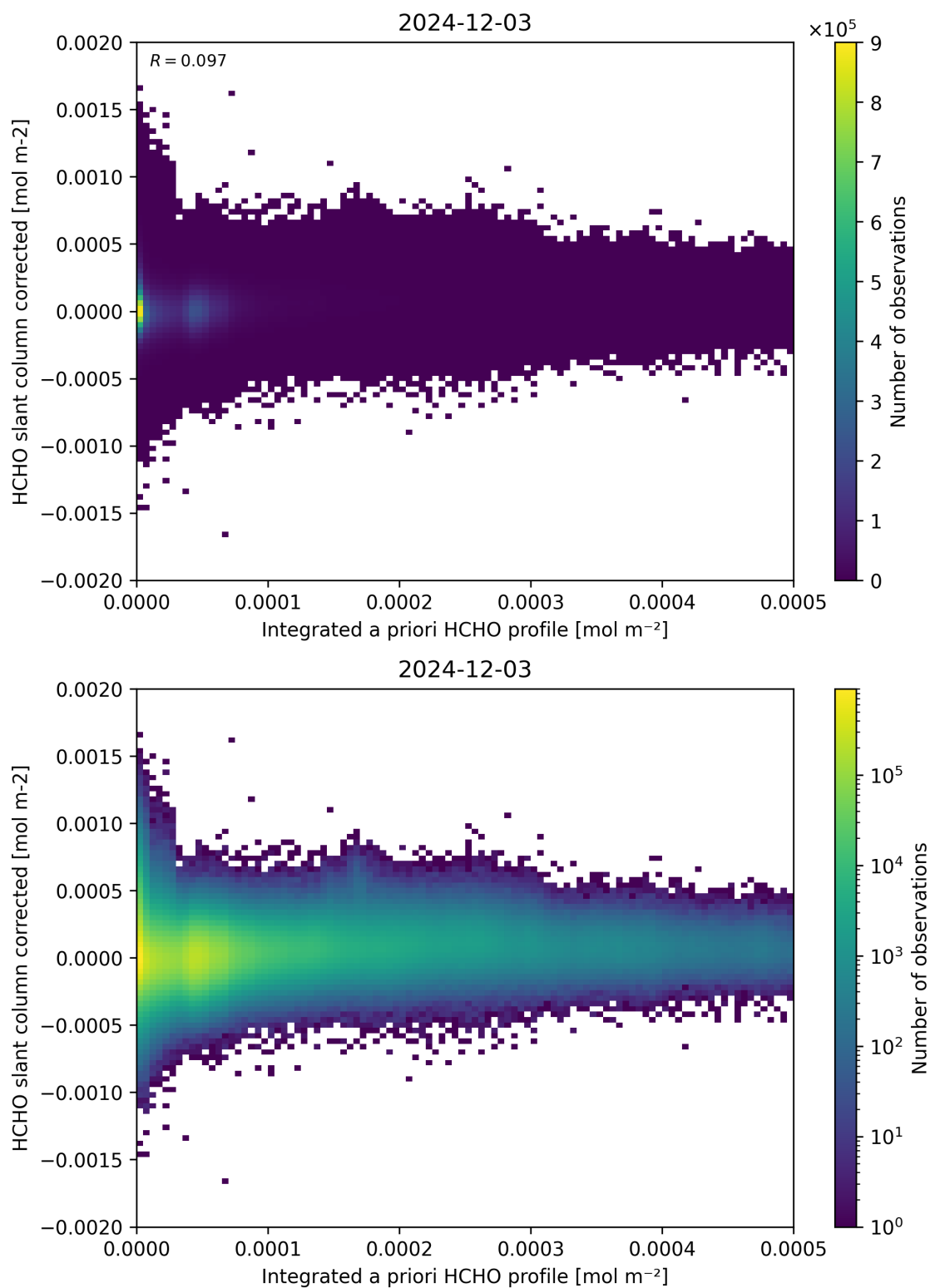
Figure 151: Scatter density plot of “Integrated a priori HCHO profile” against “HCHO slant column corrected” for 2024-12-02 to 2024-12-04.
