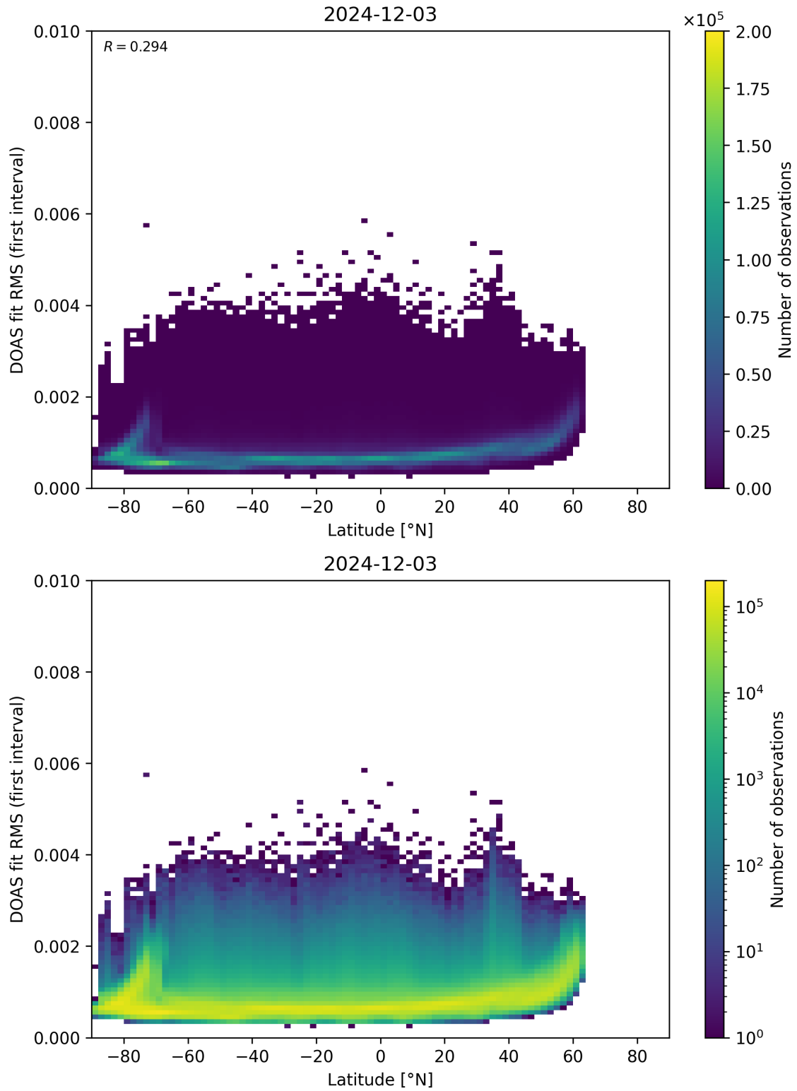
Figure 153: Scatter density plot of “Latitude” against “DOAS fit RMS (first interval)” for 2024-12-02 to 2024-12-04.
