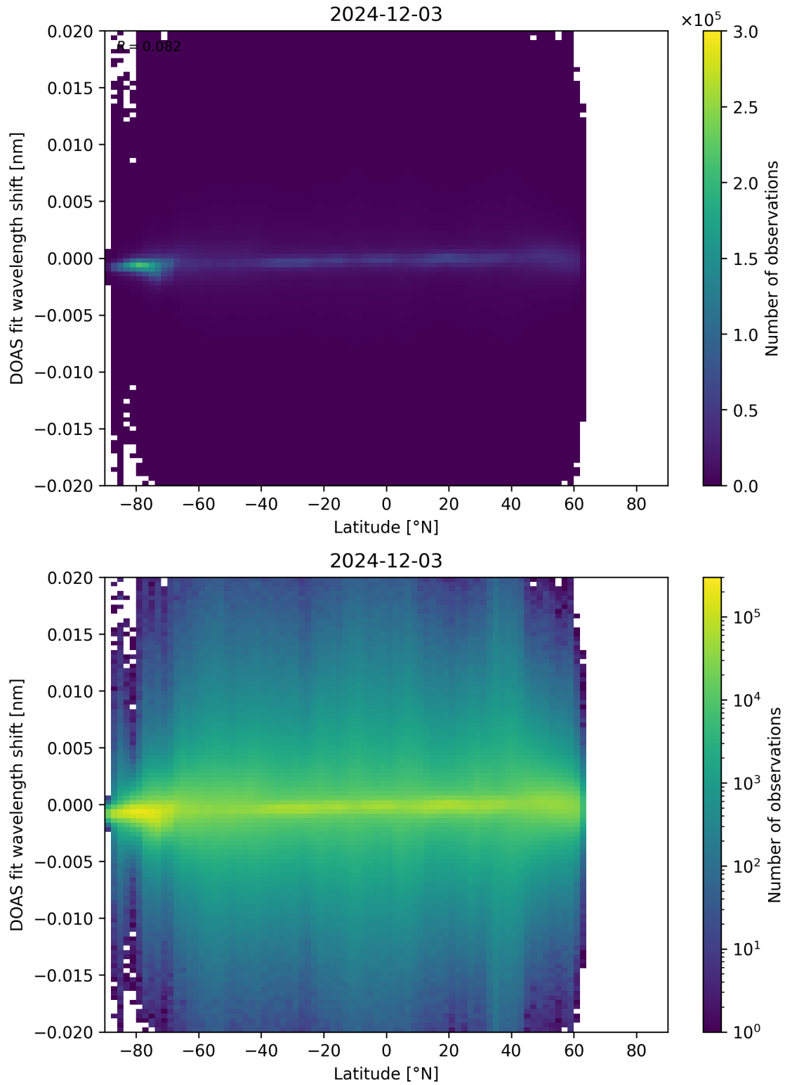
Figure 154: Scatter density plot of “Latitude” against “DOAS fit wavelength shift” for 2024-12-02 to 2024-12-04.
