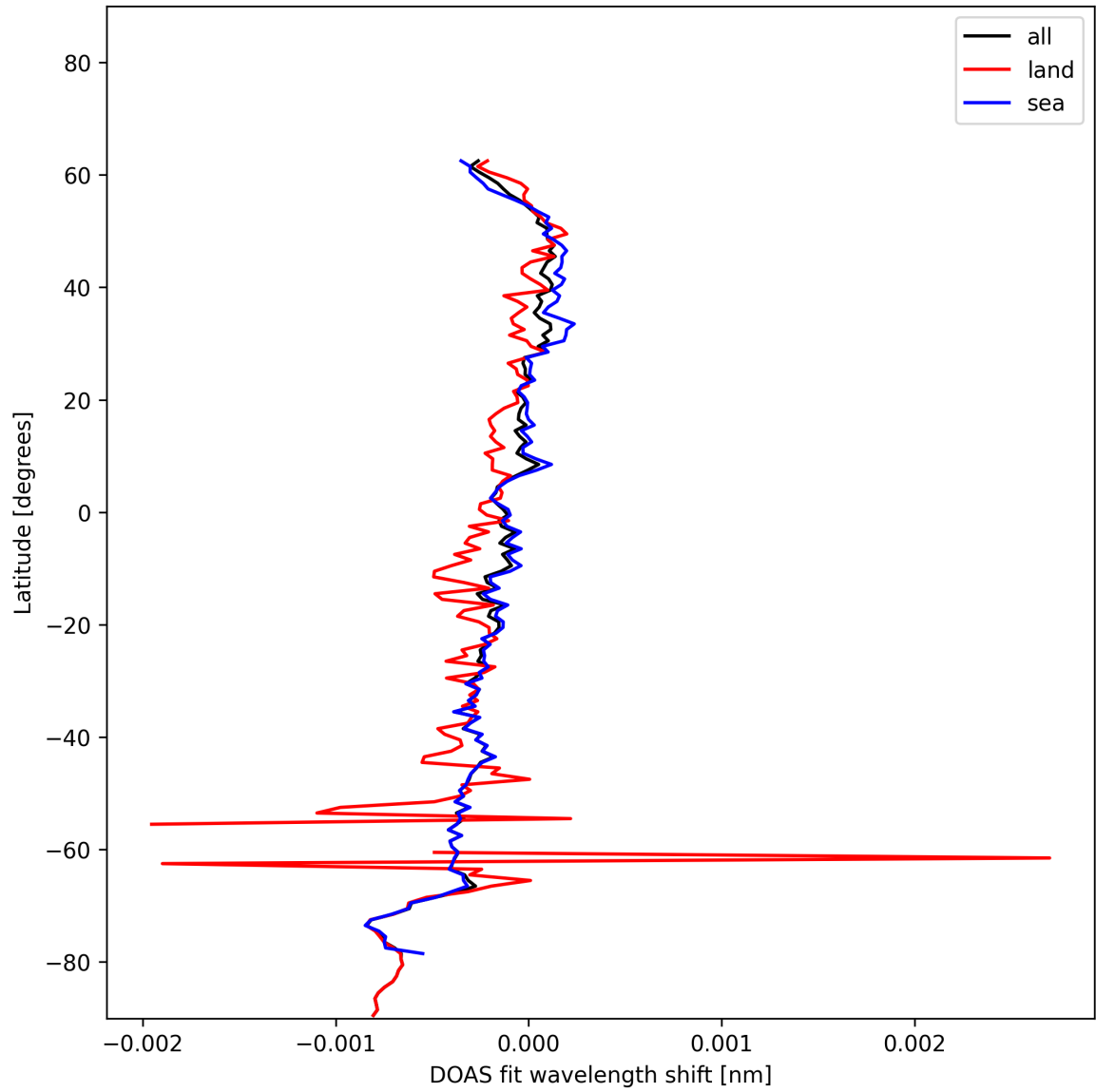
Figure 30: Zonal average of “DOAS fit wavelength shift” for 2024-12-02 to 2024-12-04.
