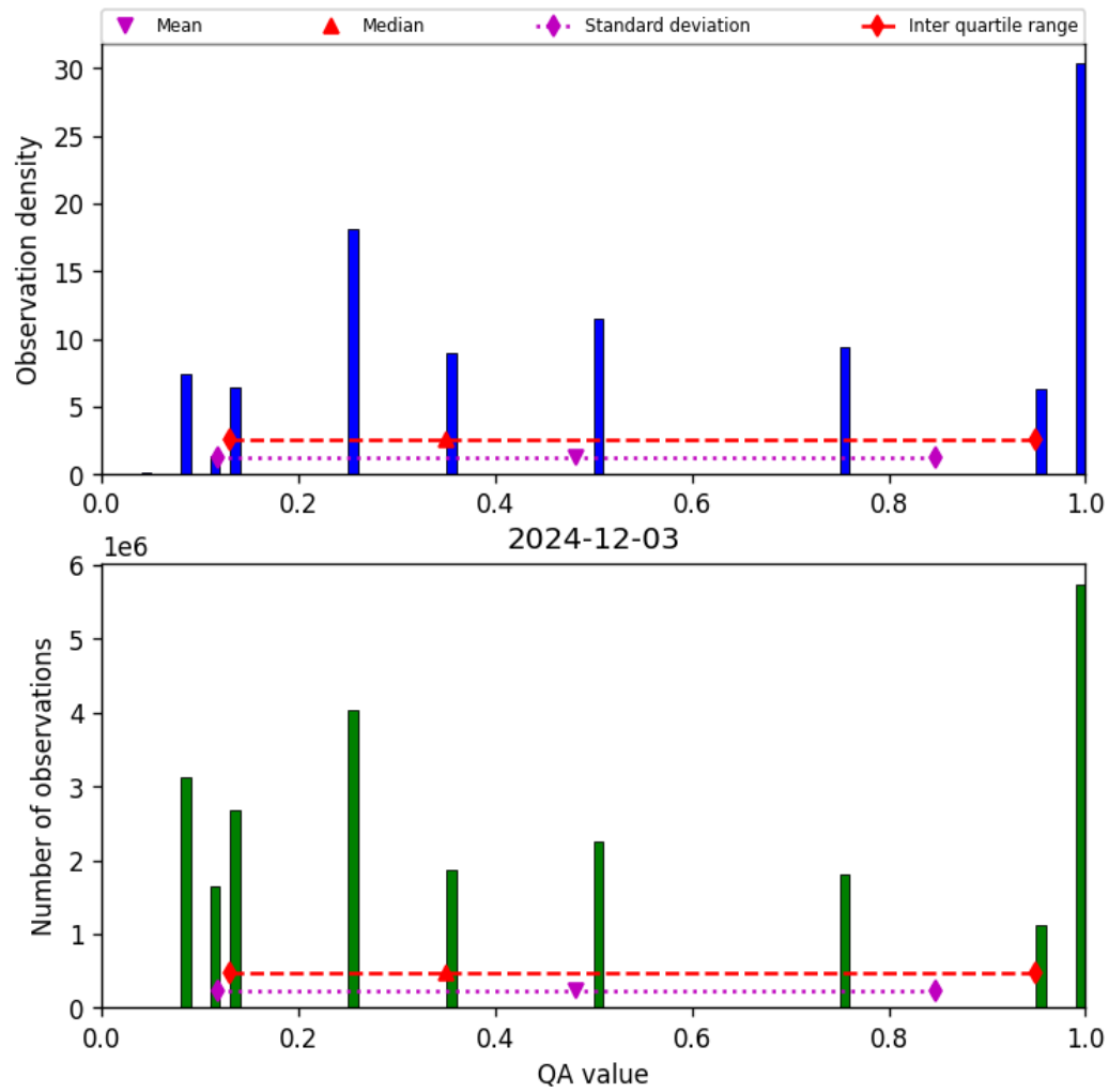
Figure 34: Histogram of “QA value” for 2024-12-02 to 2024-12-04
