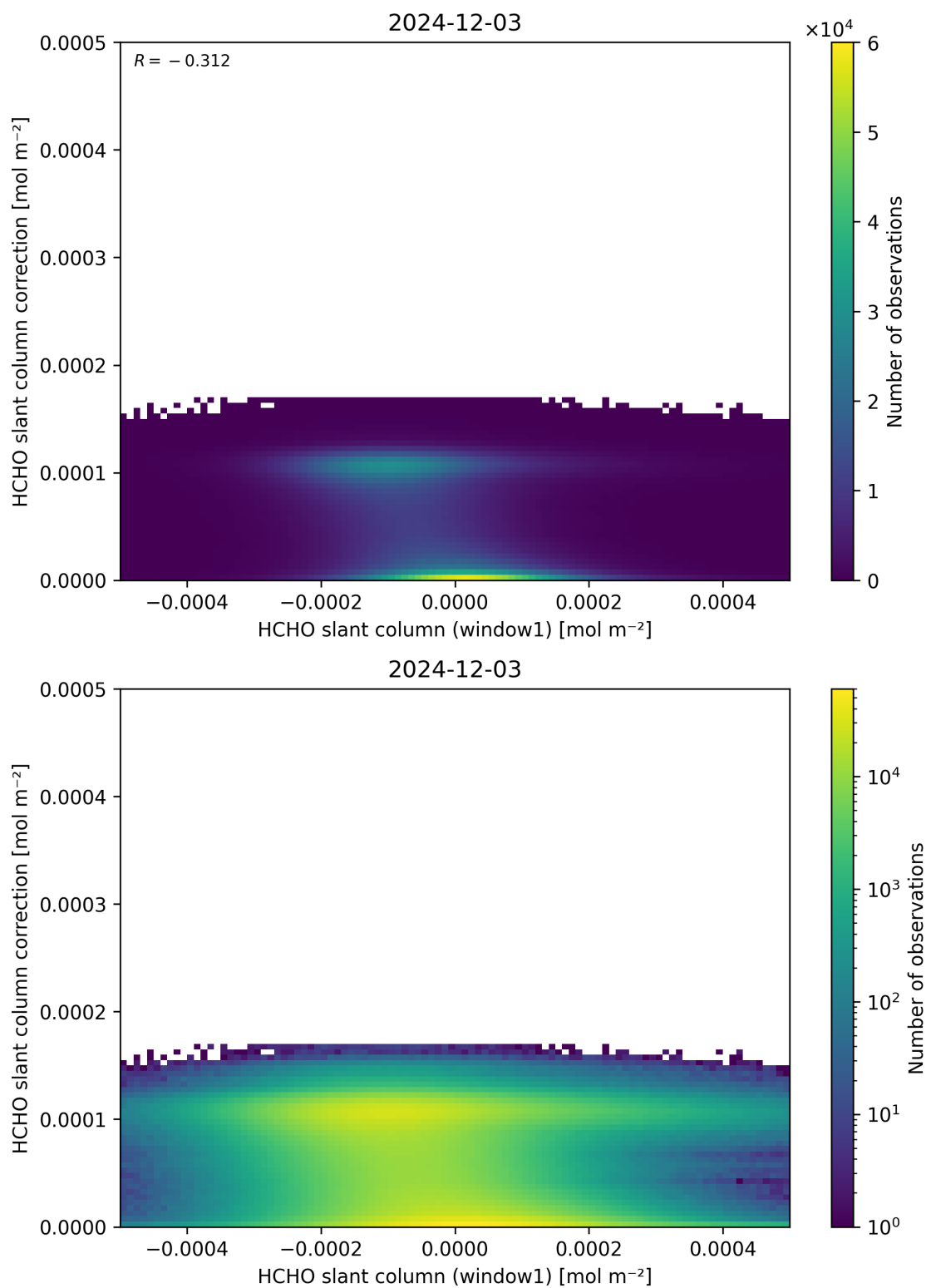
Figure 83: Scatter density plot of “HCHO slant column (window1)” against “HCHO slant column correction” for 2024-12-02 to 2024-12-04.
