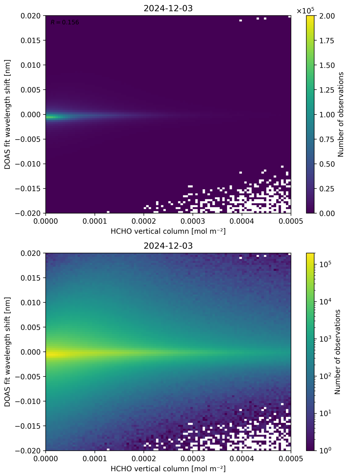
Figure 124: Scatter density plot of “HCHO vertical column” against “DOAS fit wavelength shift” for 2024-12-02 to 2024-12-04.
