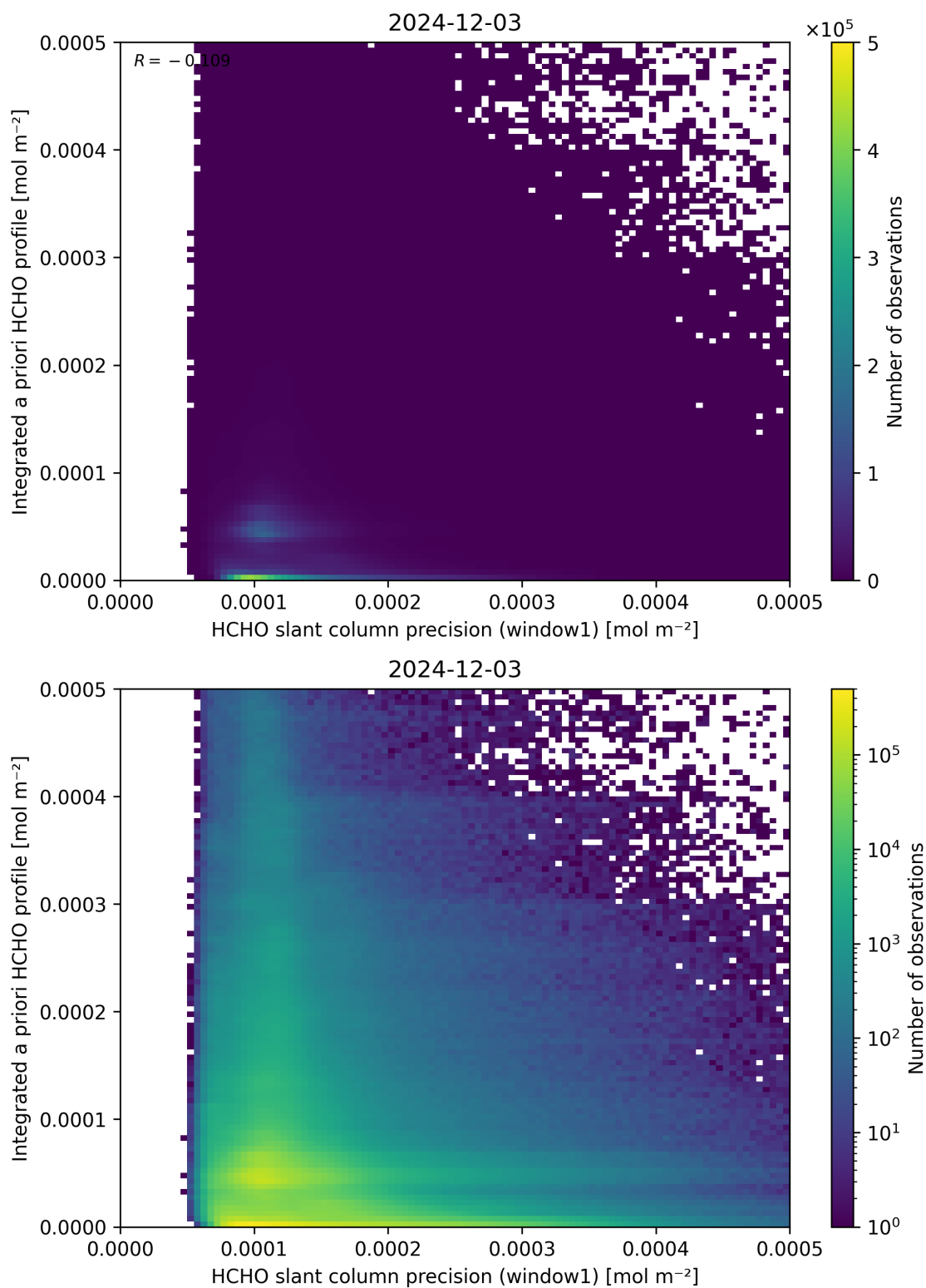
Figure 96: Scatter density plot of “HCHO slant column precision (window1)” against “Integrated a priori HCHO profile” for 2024-12-02 to 2024-12-04.
