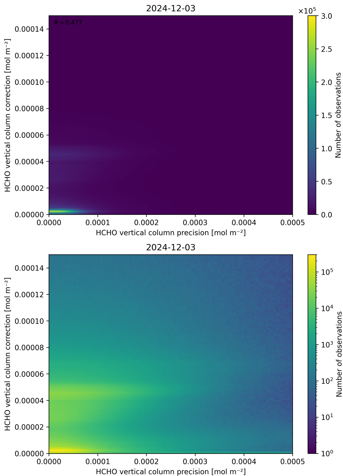
Figure 146: Scatter density plot of “HCHO vertical column precision” against “HCHO vertical column correction” for 2024-12-02 to 2024-12-04.
