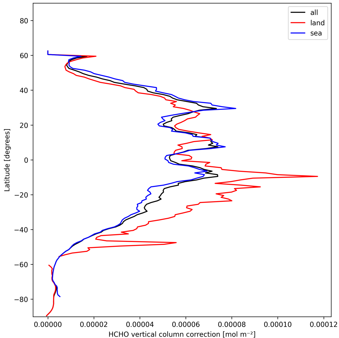
Figure 23: Zonal average of “HCHO vertical column correction” for 2024-12-02 to 2024-12-04.
