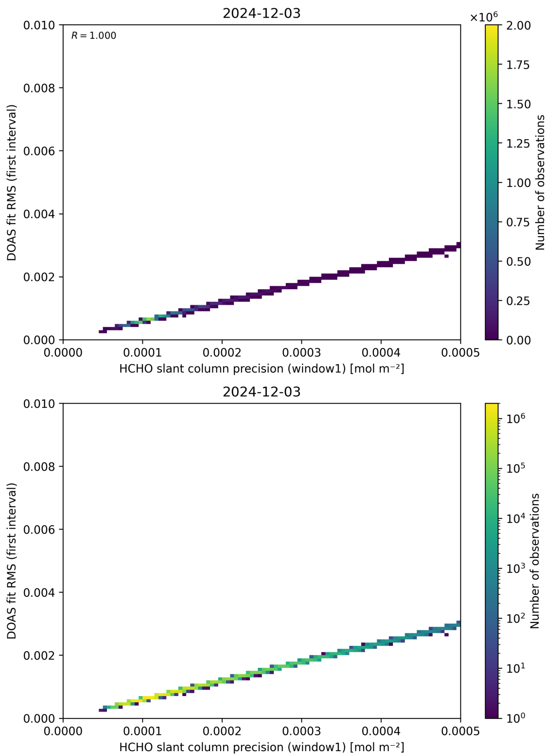
Figure 88: Scatter density plot of “HCHO slant column precision (window1)” against “DOAS fit RMS (first interval)” for 2024-12-02 to 2024-12-04.
