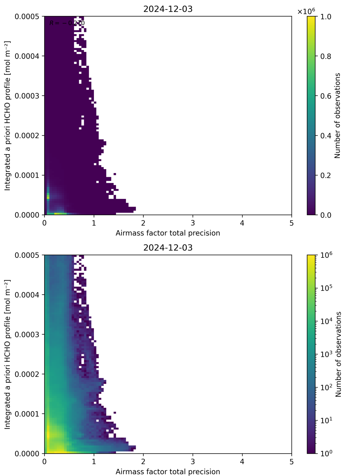
Figure 111: Scatter density plot of “Airmass factor total precision” against “Integrated a priori HCHO profile” for 2024-12-02 to 2024-12-04.
