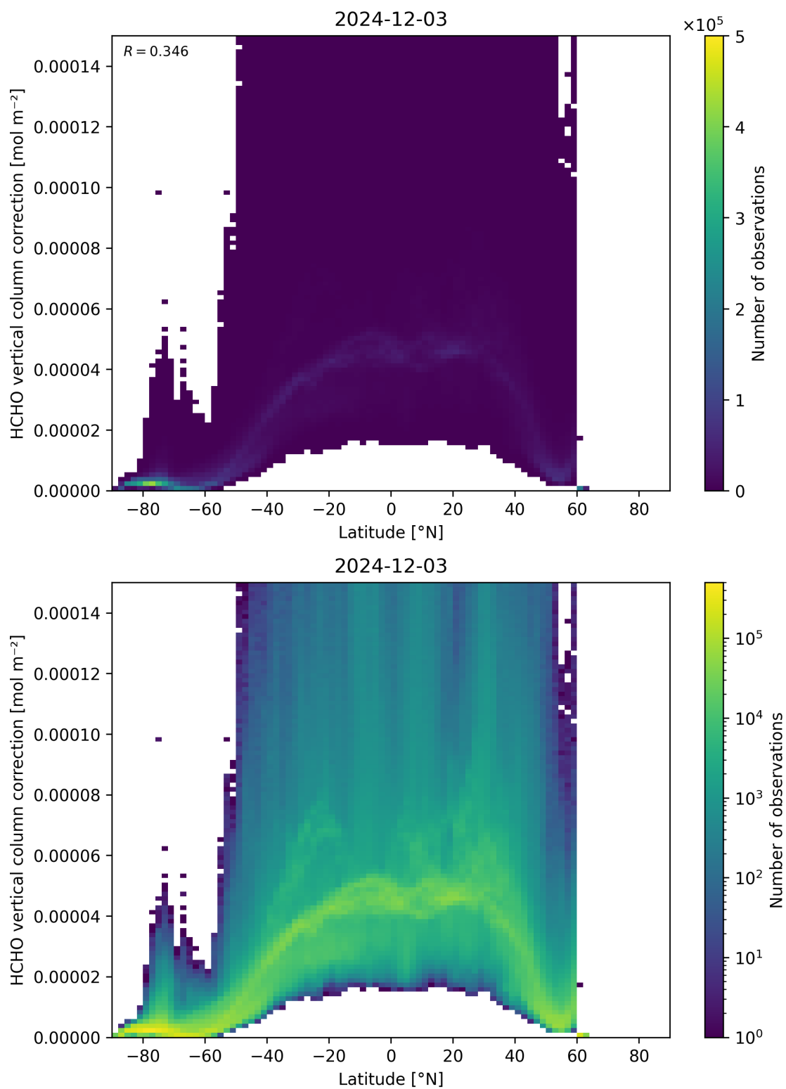
Figure 164: Scatter density plot of “Latitude” against “HCHO vertical column correction” for 2024-12-02 to 2024-12-04.
