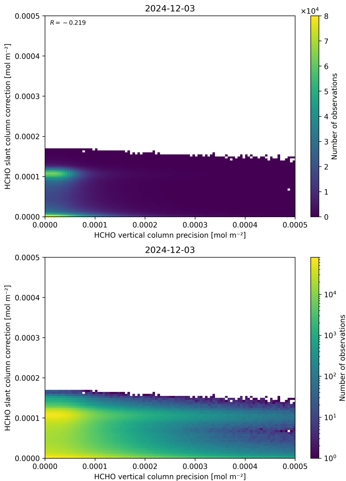
Figure 141: Scatter density plot of “HCHO vertical column precision” against “HCHO slant column correction” for 2024-12-02 to 2024-12-04.
