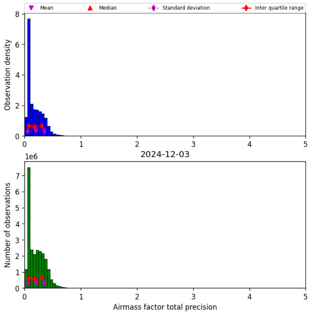
Figure 41: Histogram of “Airmass factor total precision” for 2024-12-02 to 2024-12-04
