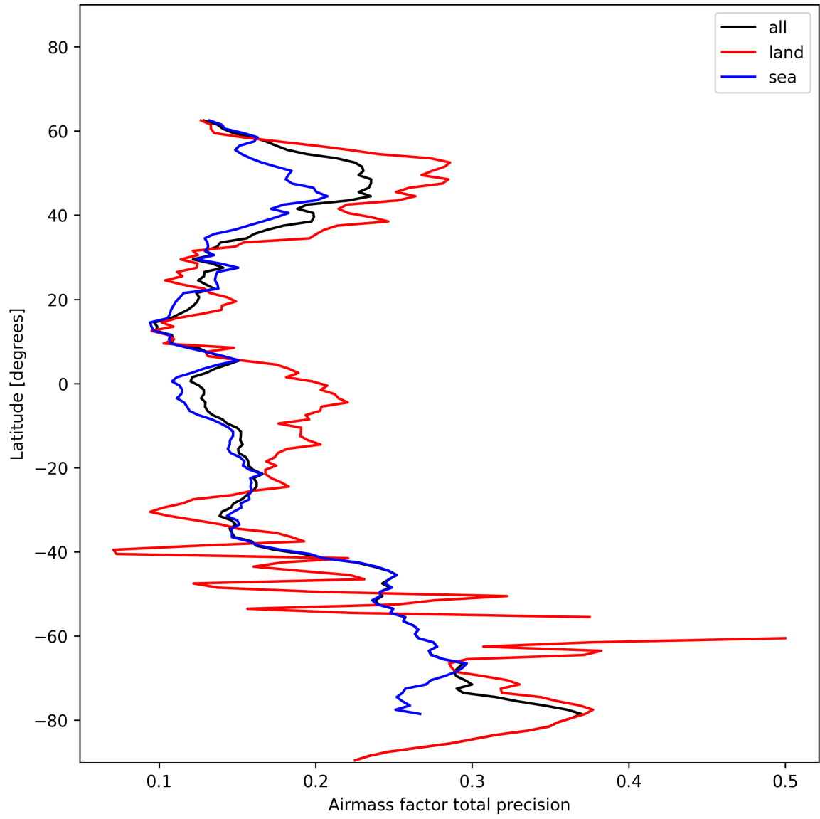
Figure 27: Zonal average of “Airmass factor total precision” for 2024-12-02 to 2024-12-04.
