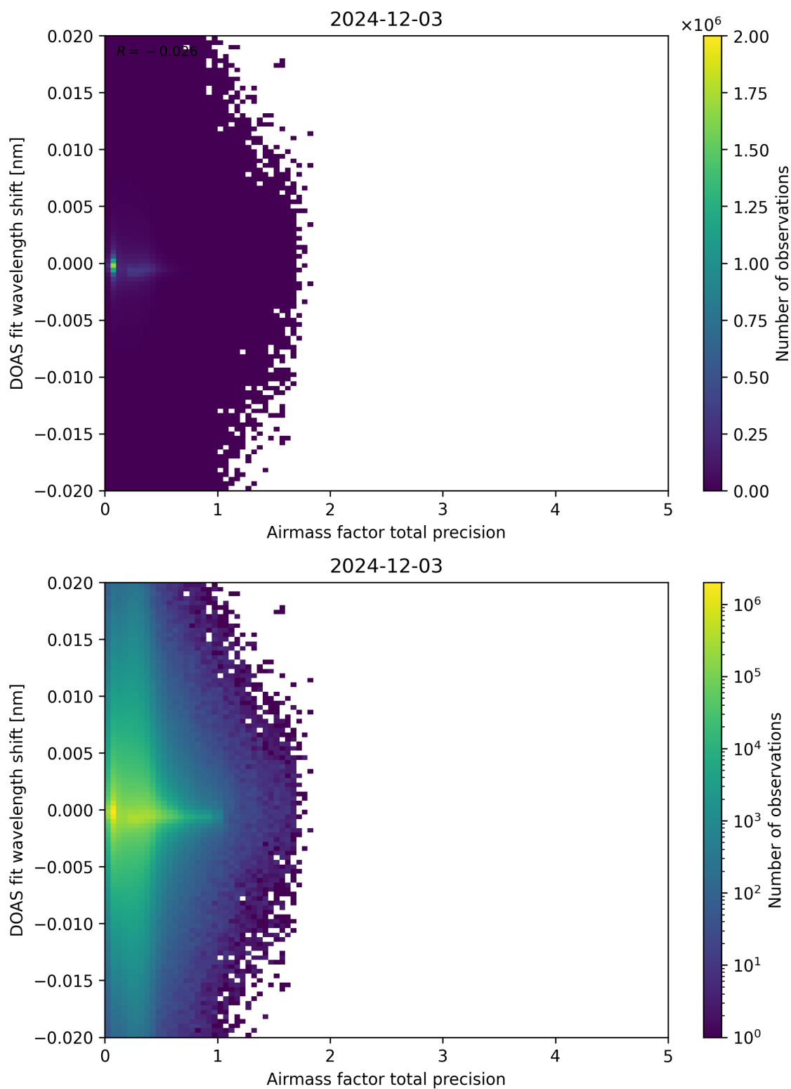
Figure 106: Scatter density plot of “Airmass factor total precision” against “DOAS fit wavelength shift” for 2024-12-02 to 2024-12-04.
