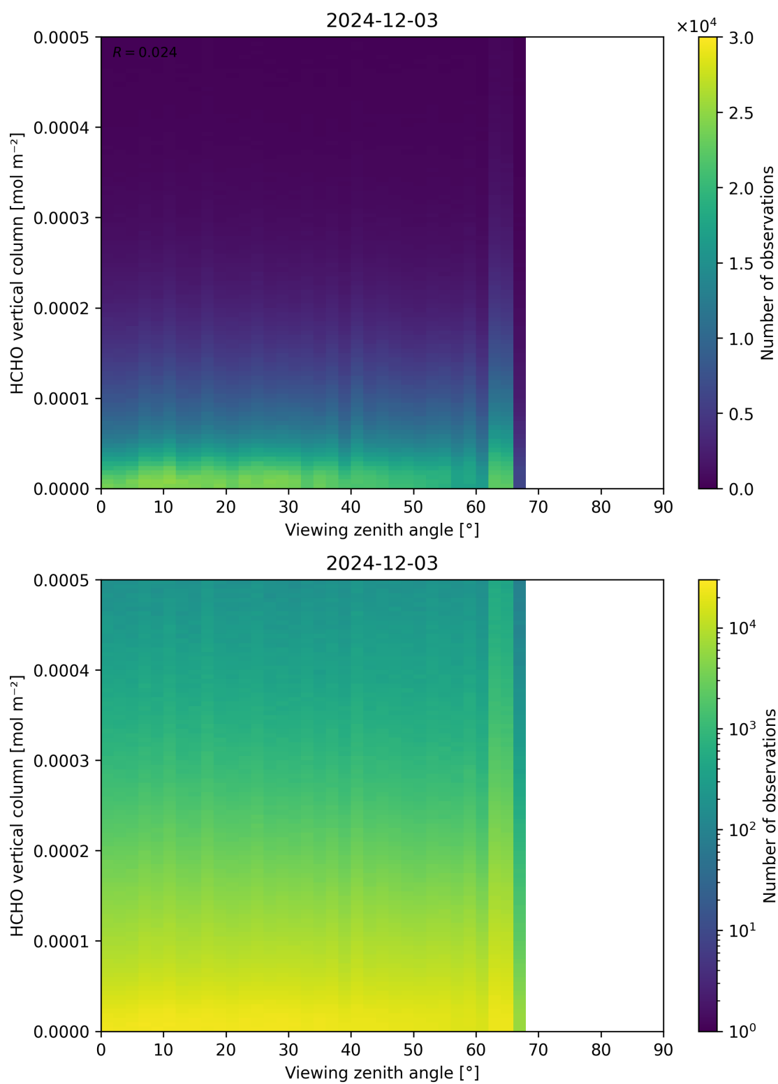
Figure 192: Scatter density plot of “Viewing zenith angle” against “HCHO vertical column” for 2024-12-02 to 2024-12-04.
