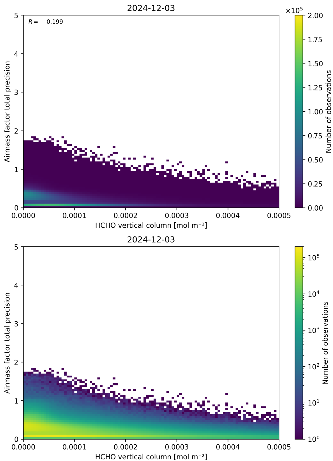
Figure 132: Scatter density plot of “HCHO vertical column” against “Airmass factor total precision” for 2024-12-02 to 2024-12-04.
