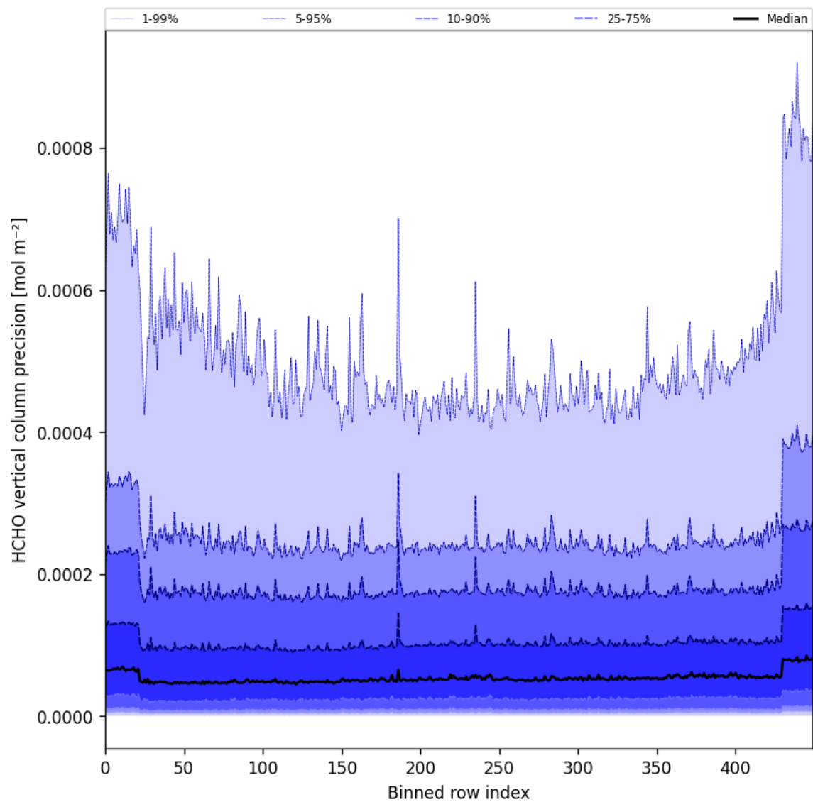
Figure 50: Along track statistics of “HCHO vertical column precision” for 2024-12-02 to 2024-12-04
