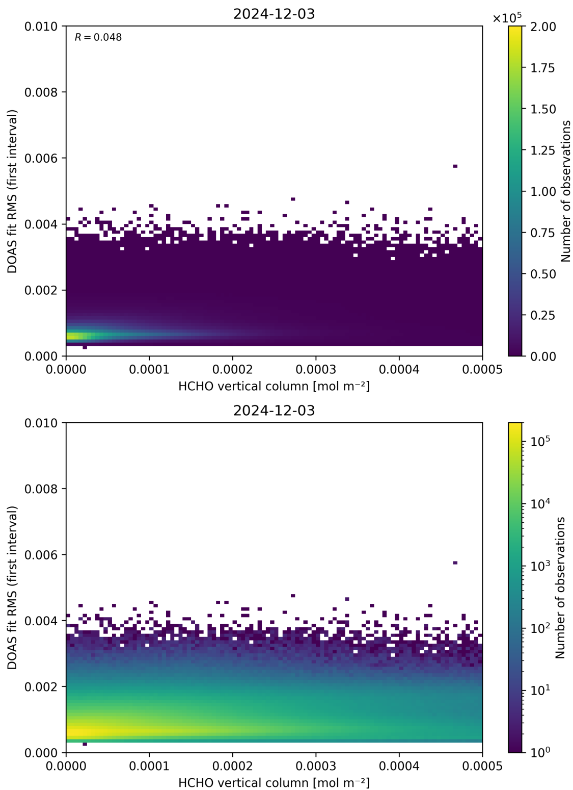
Figure 123: Scatter density plot of “HCHO vertical column” against “DOAS fit RMS (first interval)” for 2024-12-02 to 2024-12-04.
