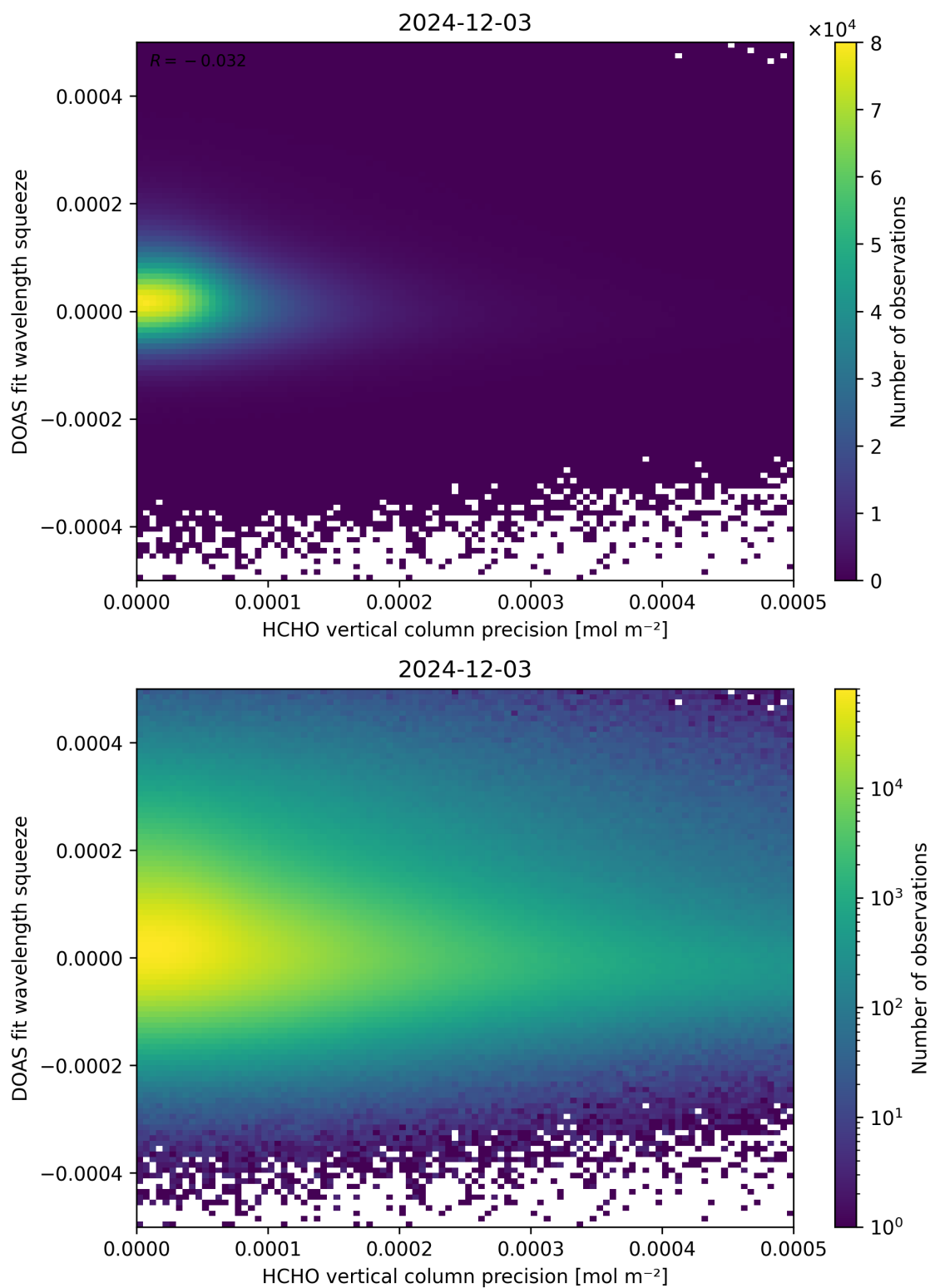
Figure 138: Scatter density plot of “HCHO vertical column precision” against “DOAS fit wavelength squeeze” for 2024-12-02 to 2024-12-04.
