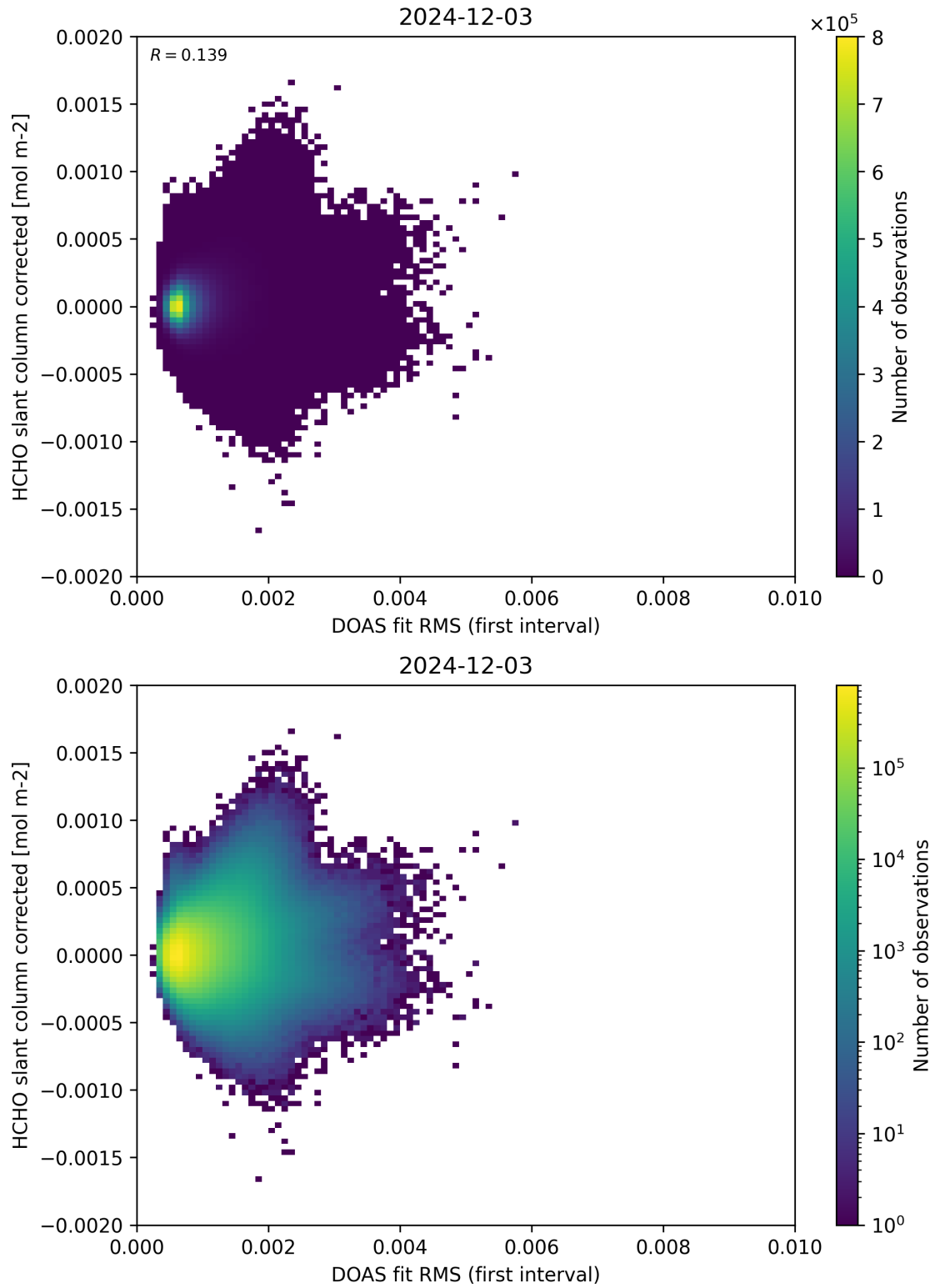
Figure 62: Scatter density plot of “DOAS fit RMS (first interval)” against “HCHO slant column corrected” for 2024-12-02 to 2024-12-04.
