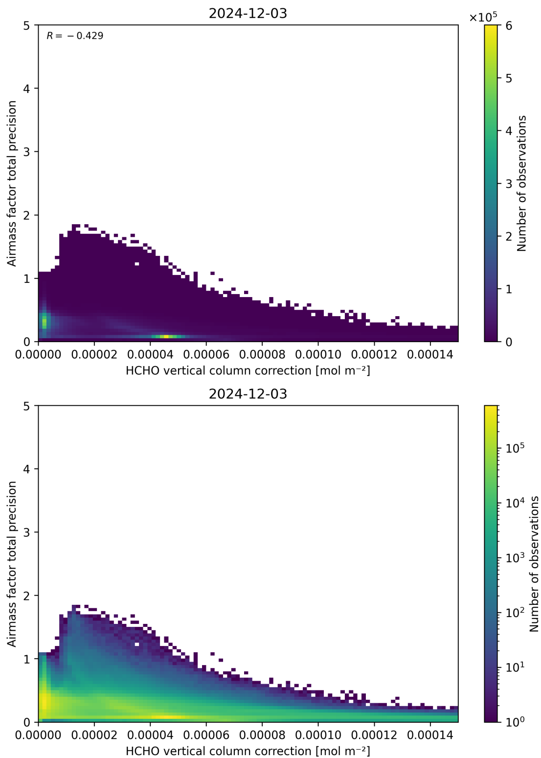
Figure 121: Scatter density plot of “HCHO vertical column correction” against “Airmass factor total precision” for 2024-12-02 to 2024-12-04.
