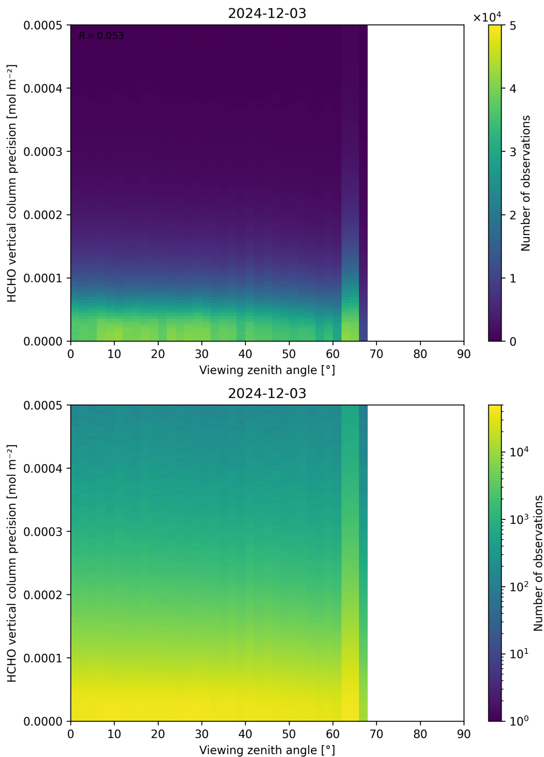
Figure 194: Scatter density plot of “Viewing zenith angle” against “HCHO vertical column precision” for 2024-12-02 to 2024-12-04.
