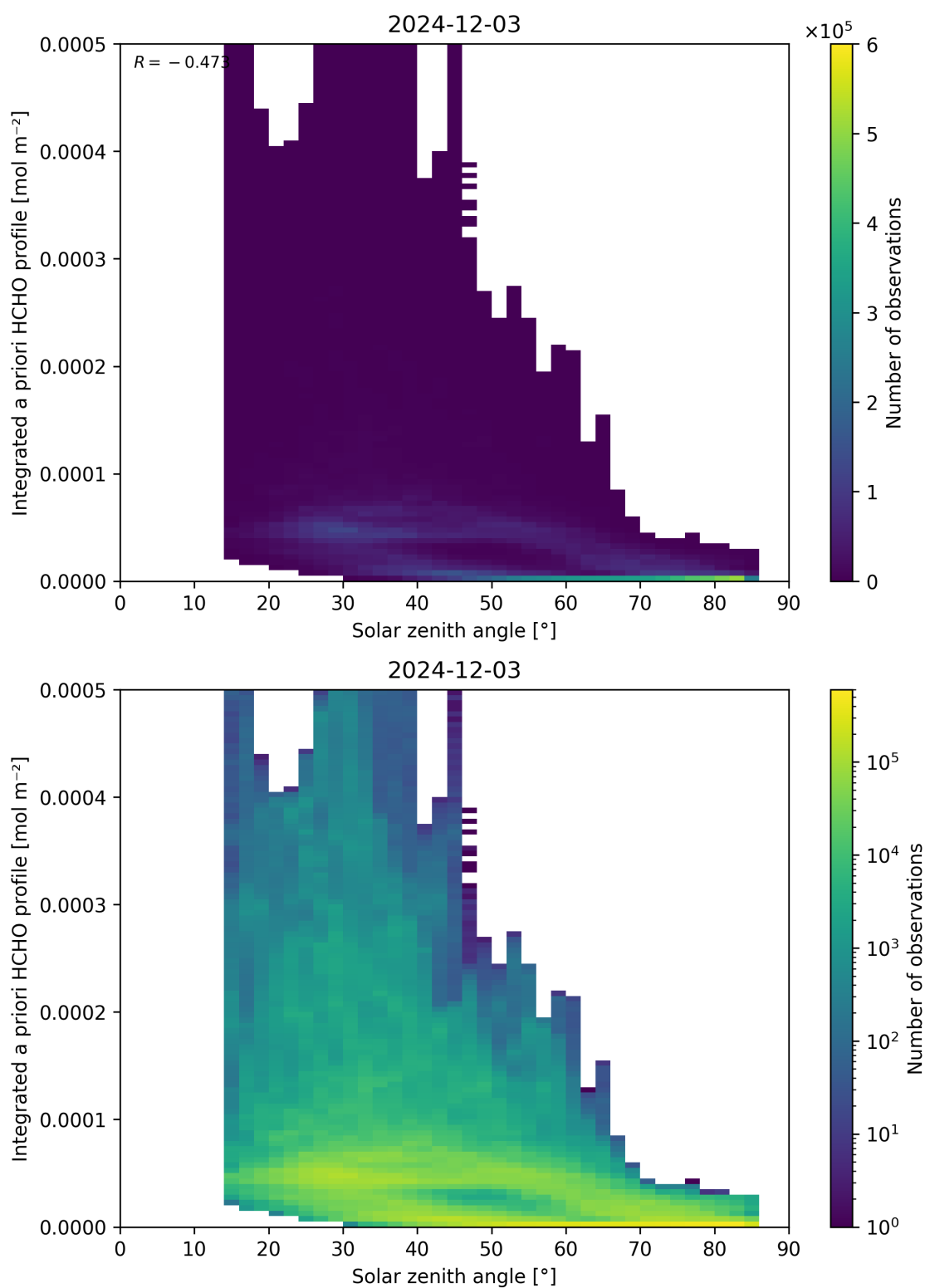
Figure 180: Scatter density plot of “Solar zenith angle” against “Integrated a priori HCHO profile” for 2024-12-02 to 2024-12-04.
