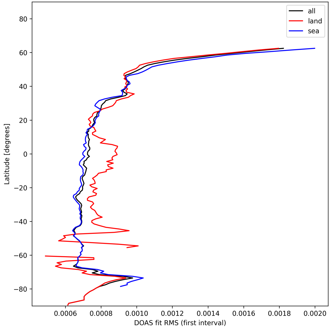
Figure 32: Zonal average of “DOAS fit RMS (first interval)” for 2024-12-02 to 2024-12-04.
