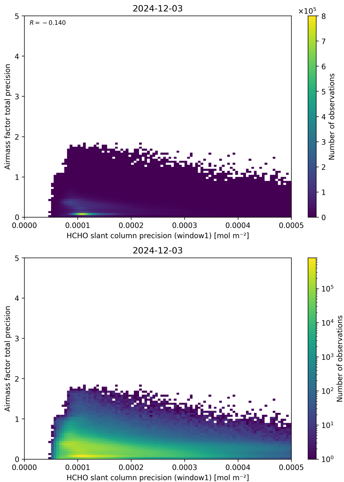
Figure 95: Scatter density plot of “HCHO slant column precision (window1)” against “Airmass factor total precision” for 2024-12-02 to 2024-12-04.
