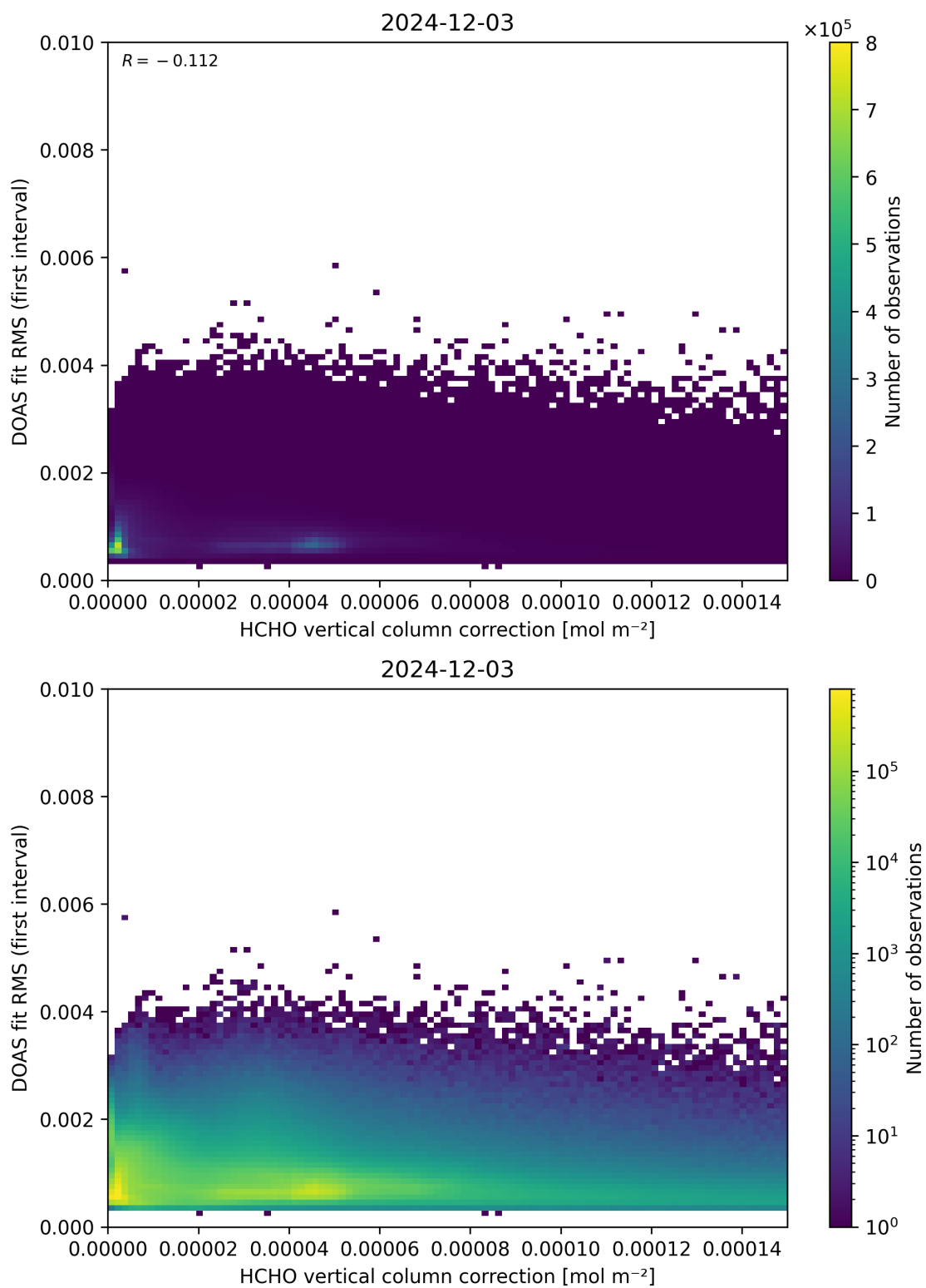
Figure 112: Scatter density plot of “HCHO vertical column correction” against “DOAS fit RMS (first interval)” for 2024-12-02 to 2024-12-04.
