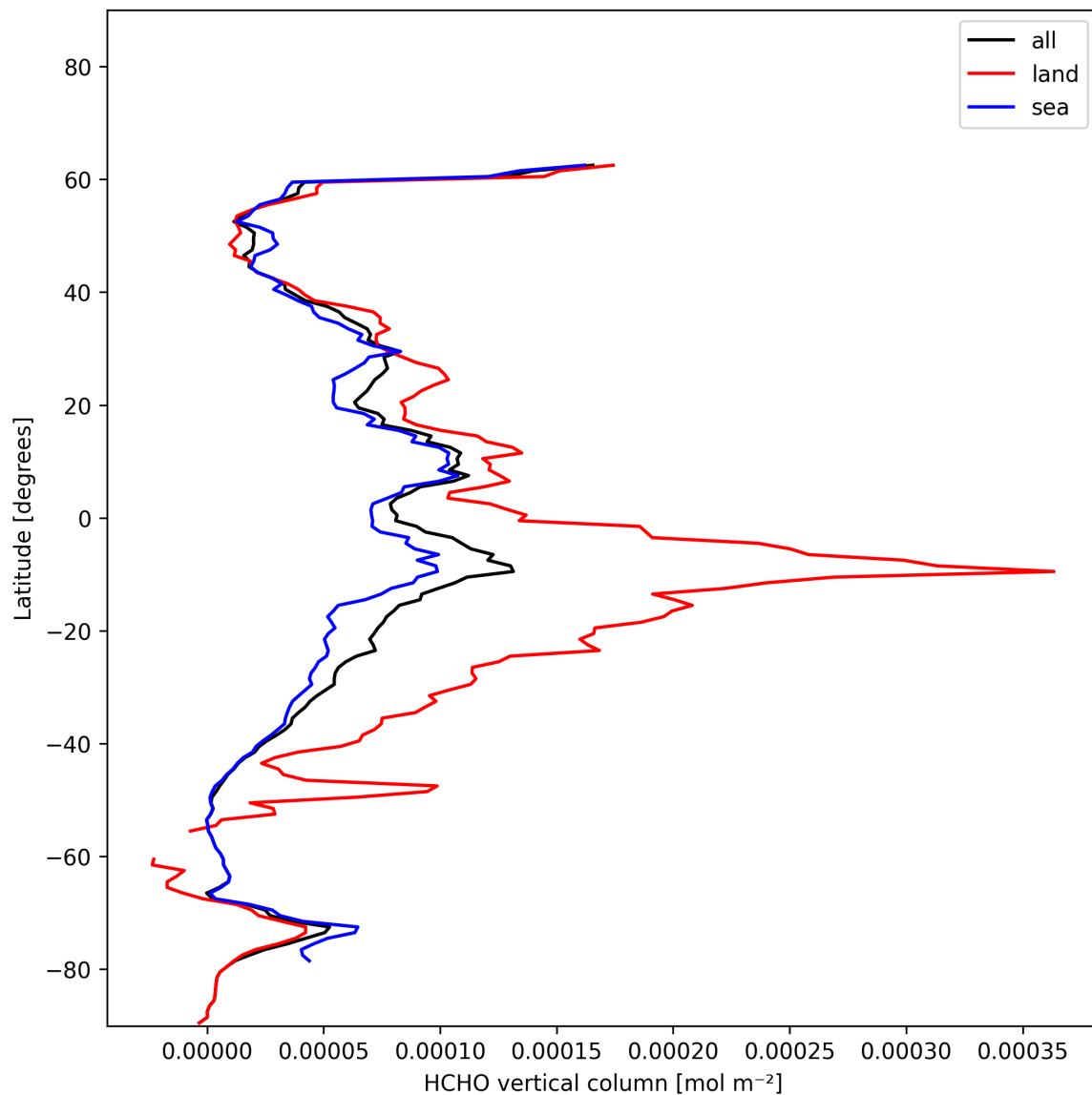
Figure 21: Zonal average of “HCHO vertical column” for 2024-12-02 to 2024-12-04.
