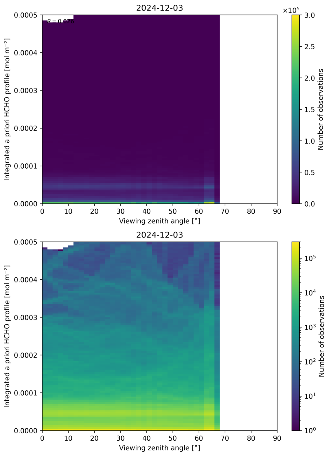
Figure 195: Scatter density plot of “Viewing zenith angle” against “Integrated a priori HCHO profile” for 2024-12-02 to 2024-12-04.
