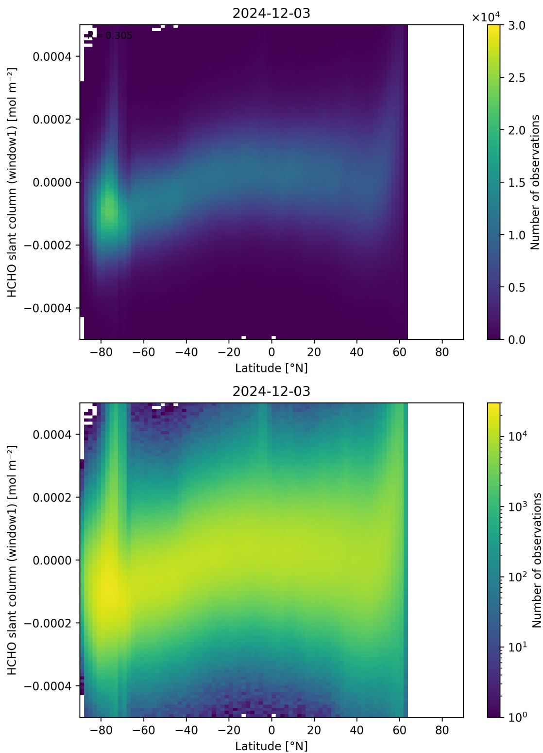
Figure 159: Scatter density plot of “Latitude” against “HCHO slant column (window1)” for 2024-12-02 to 2024-12-04.
