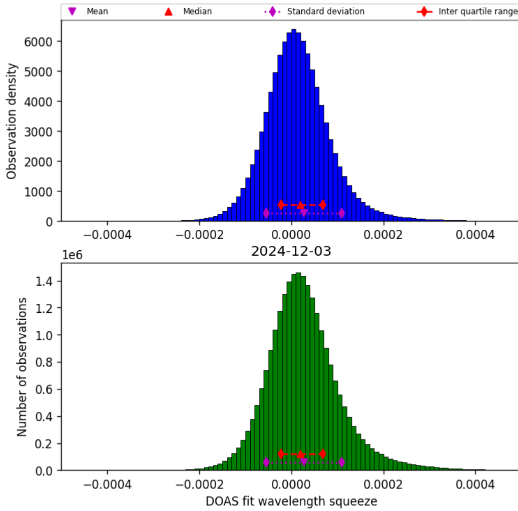
Figure 45: Histogram of “DOAS fit wavelength squeeze” for 2024-12-02 to 2024-12-04
