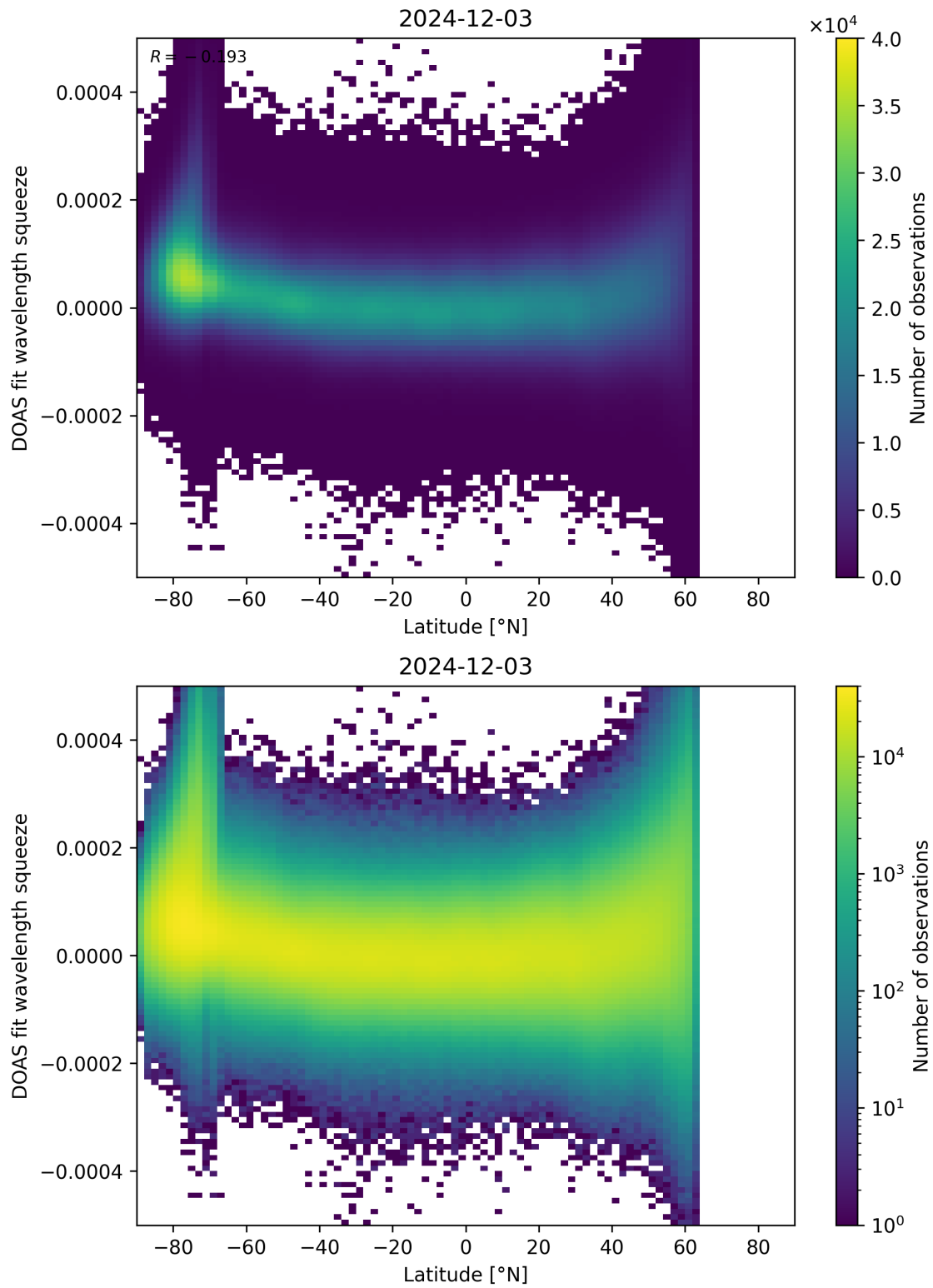
Figure 155: Scatter density plot of “Latitude” against “DOAS fit wavelength squeeze” for 2024-12-02 to 2024-12-04.
