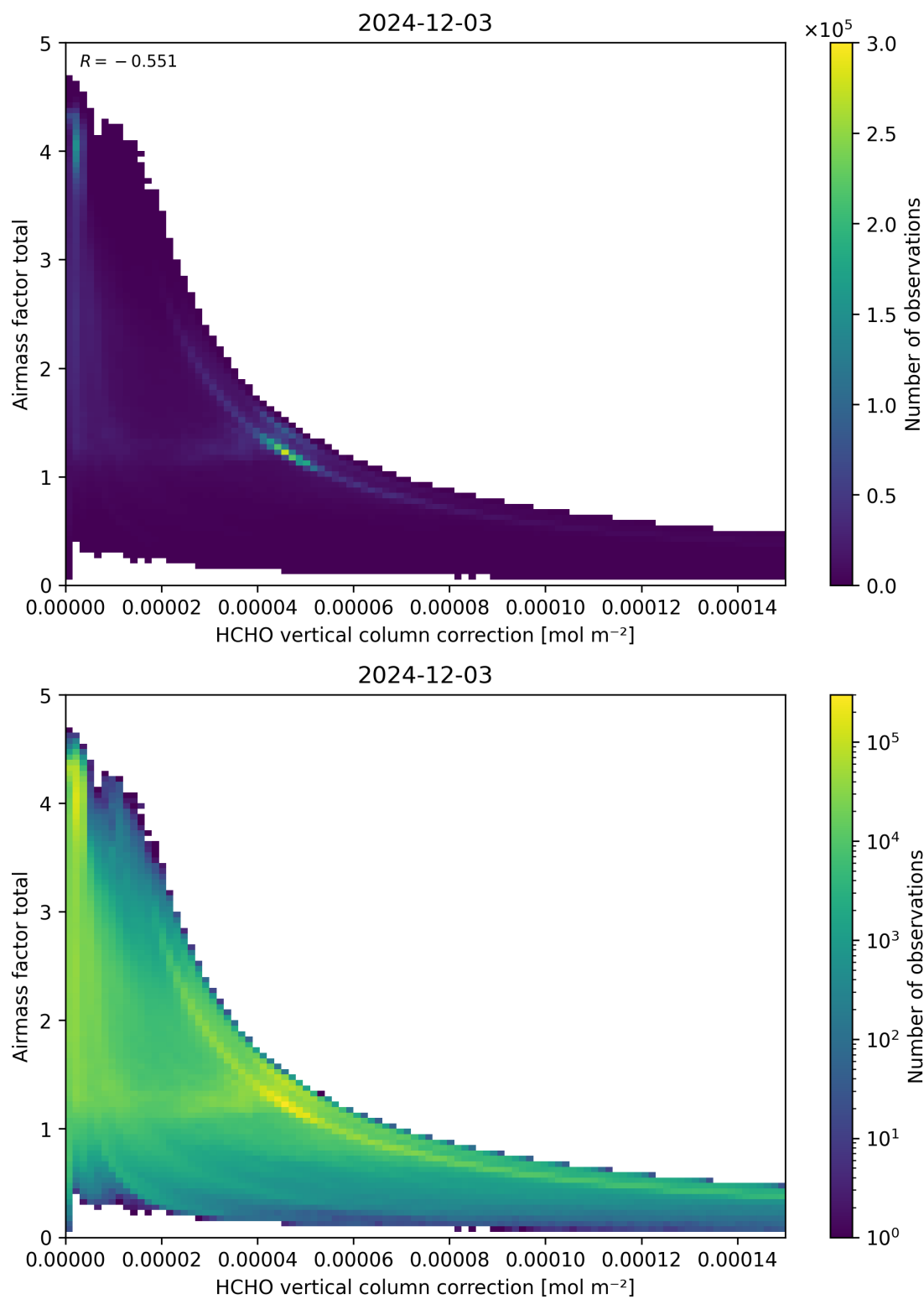
Figure 120: Scatter density plot of “HCHO vertical column correction” against “Airmass factor total” for 2024-12-02 to 2024-12-04.
