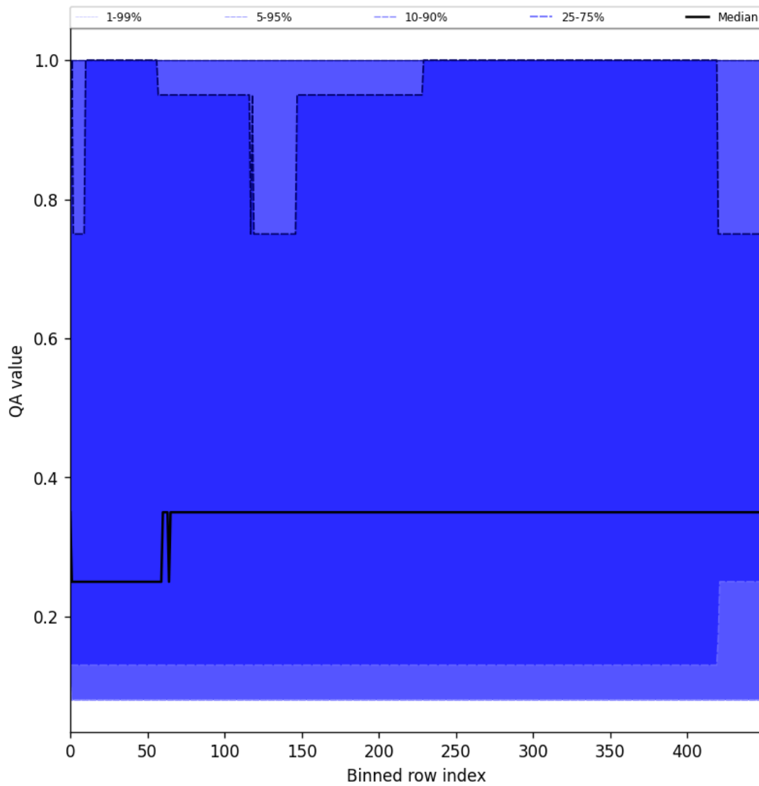
Figure 48: Along track statistics of “QA value” for 2024-12-02 to 2024-12-04
