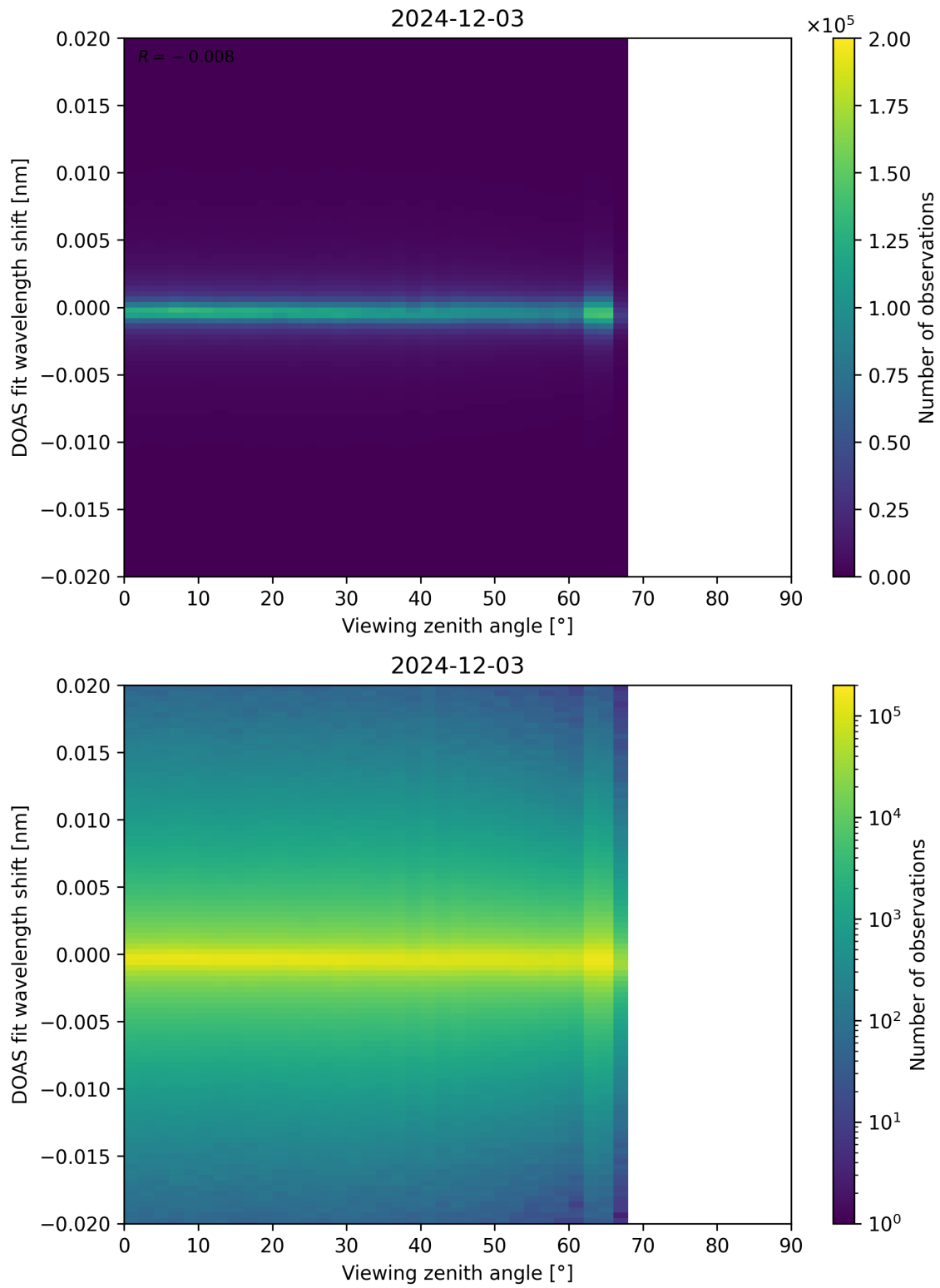
Figure 183: Scatter density plot of “Viewing zenith angle” against “DOAS fit wavelength shift” for 2024-12-02 to 2024-12-04.
