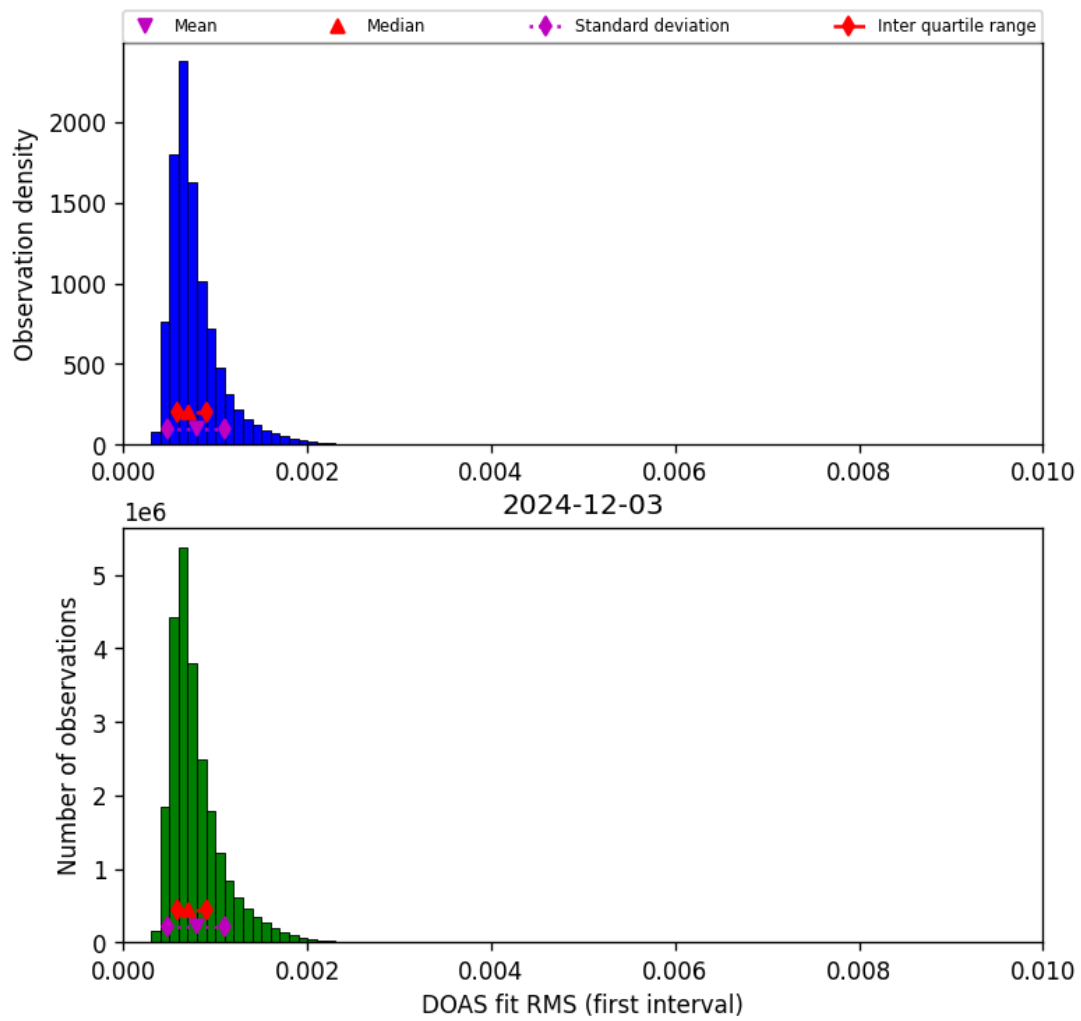
Figure 46: Histogram of “DOAS fit RMS (first interval)” for 2024-12-02 to 2024-12-04
