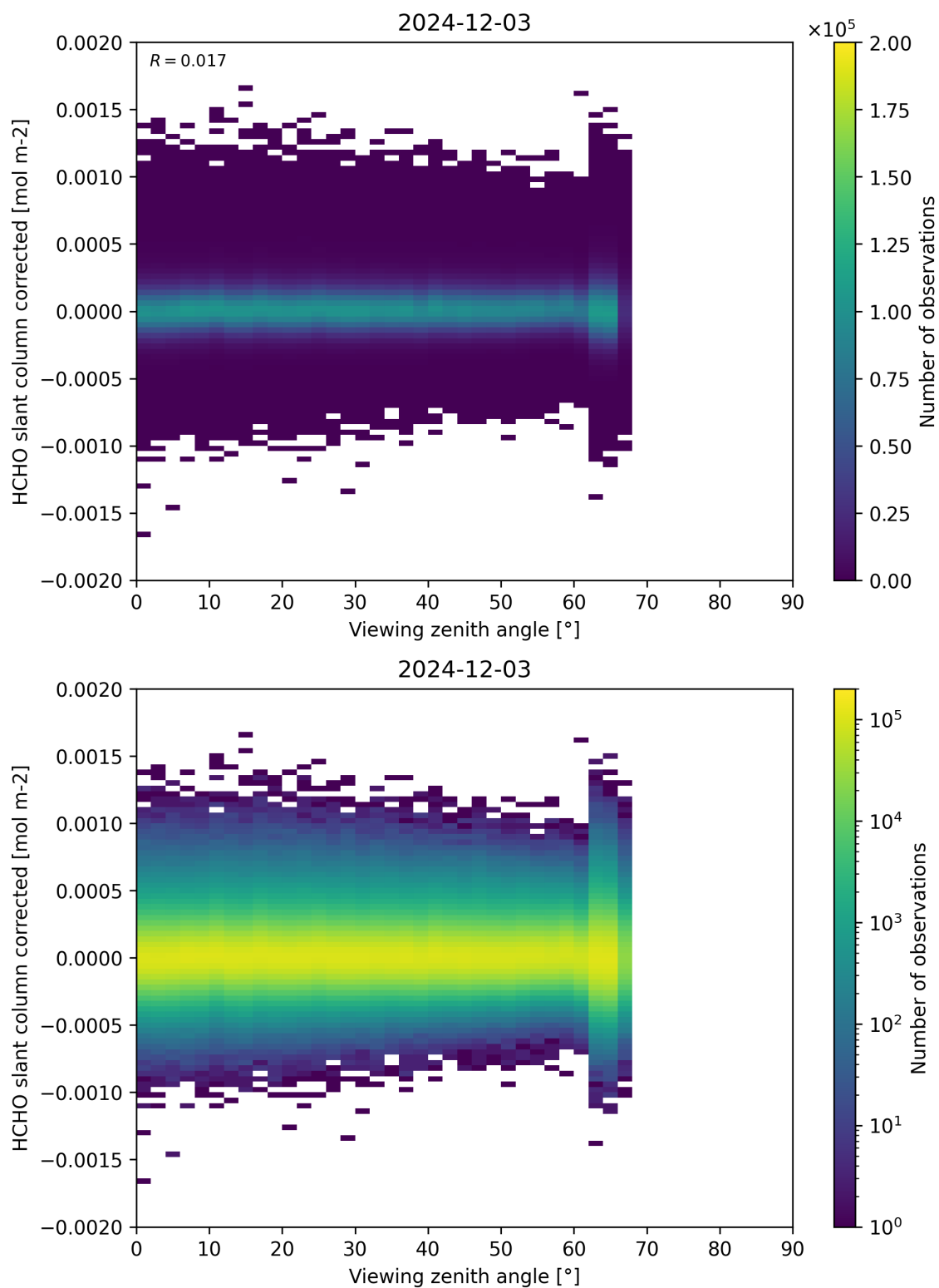
Figure 186: Scatter density plot of “Viewing zenith angle” against “HCHO slant column corrected” for 2024-12-02 to 2024-12-04.
