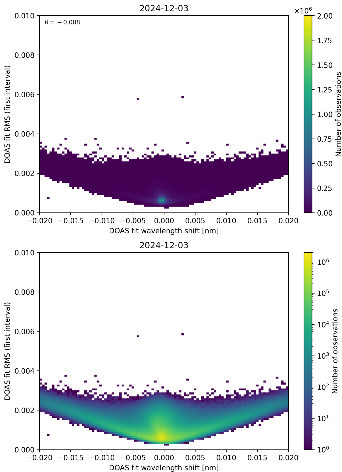
Figure 64: Scatter density plot of “DOAS fit wavelength shift” against “DOAS fit RMS (first interval)” for 2024-12-02 to 2024-12-04.
