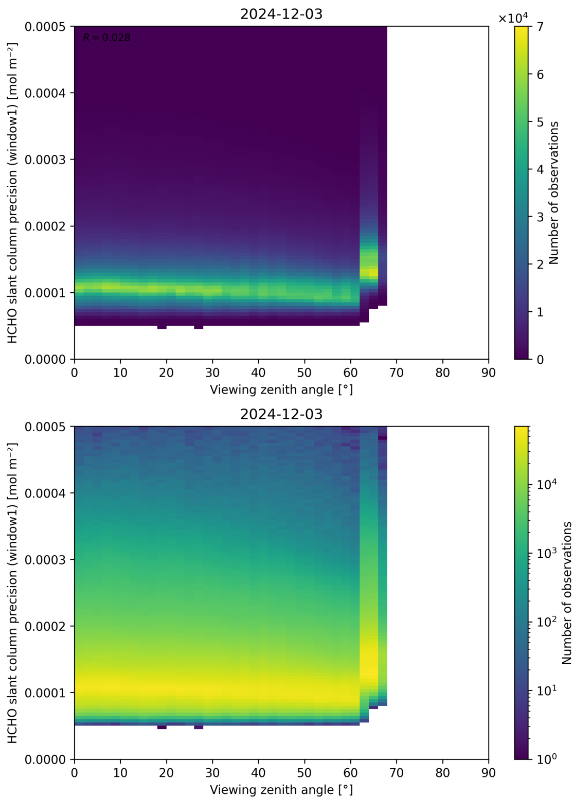
Figure 189: Scatter density plot of “Viewing zenith angle” against “HCHO slant column precision (window1)” for 2024-12-02 to 2024-12-04.
