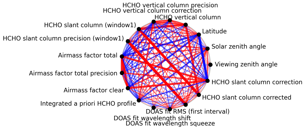
Figure 1: Map of correlation graph for 2024-12-02 to 2024-12-04.
