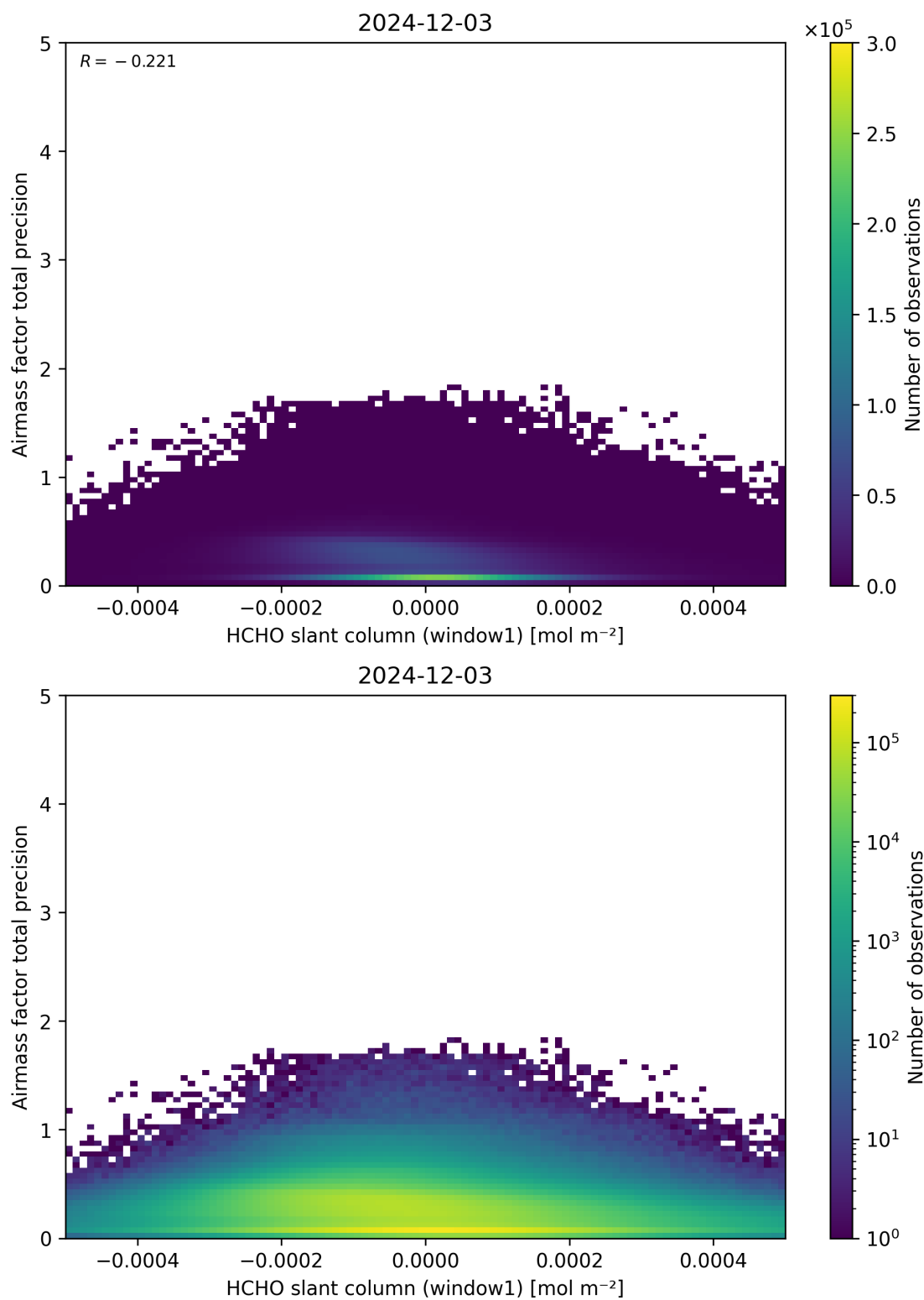
Figure 86: Scatter density plot of “HCHO slant column (window1)” against “Airmass factor total precision” for 2024-12-02 to 2024-12-04.
