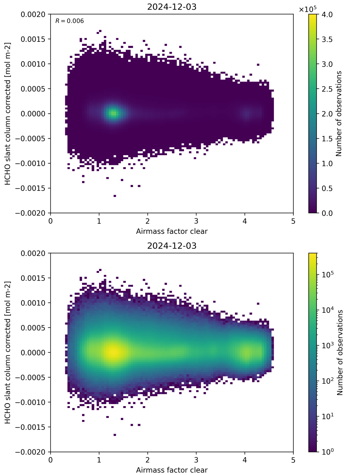
Figure 74: Scatter density plot of “Airmass factor clear” against “HCHO slant column corrected” for 2024-12-02 to 2024-12-04.
