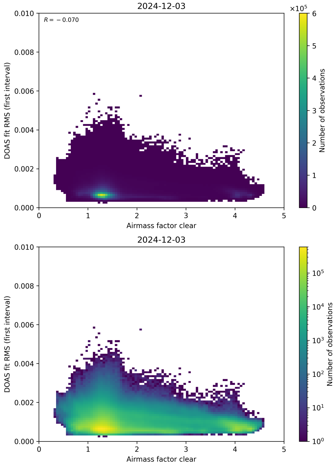
Figure 71: Scatter density plot of “Airmass factor clear” against “DOAS fit RMS (first interval)” for 2024-12-02 to 2024-12-04.
