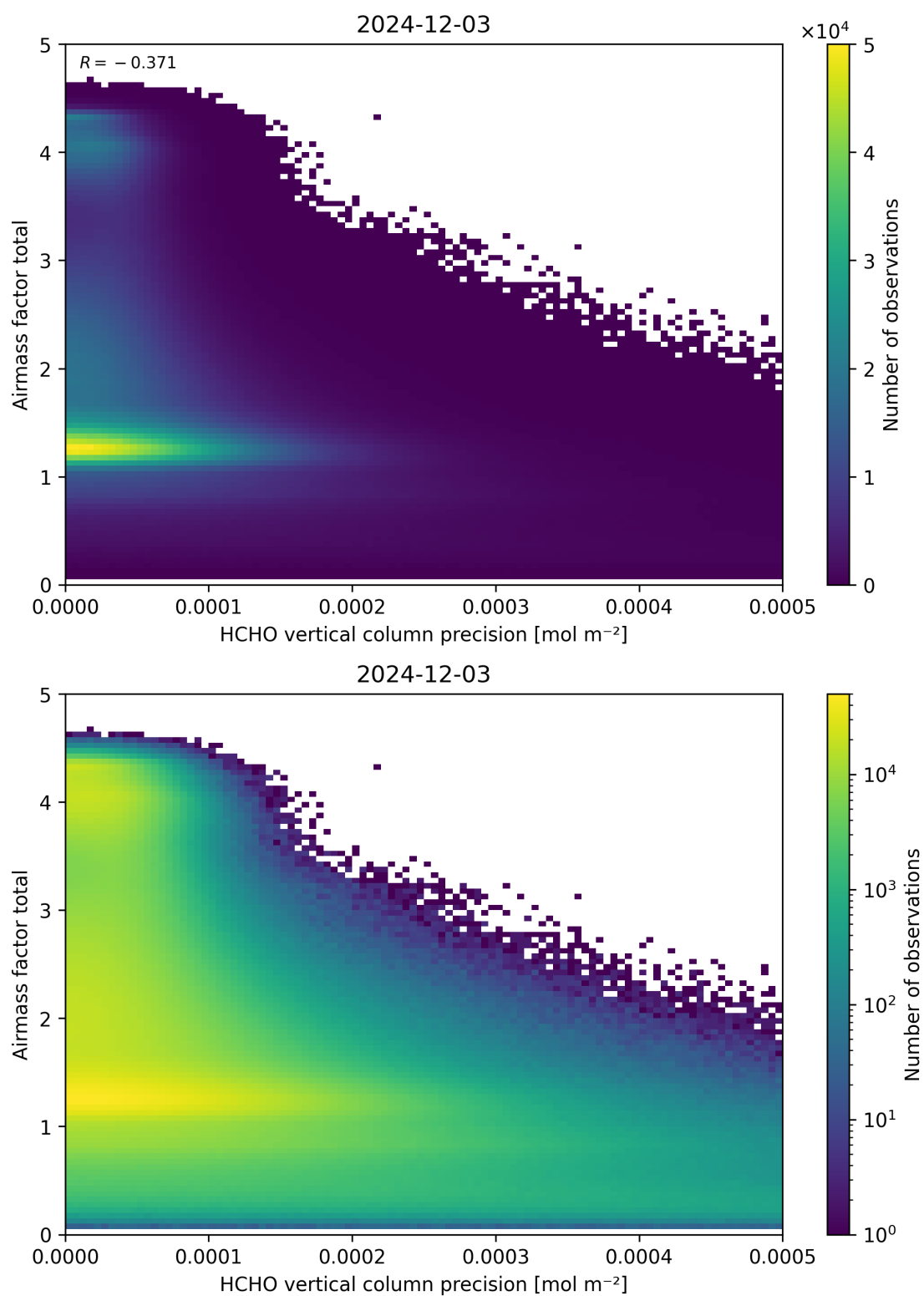
Figure 144: Scatter density plot of “HCHO vertical column precision” against “Airmass factor total” for 2024-12-02 to 2024-12-04.
