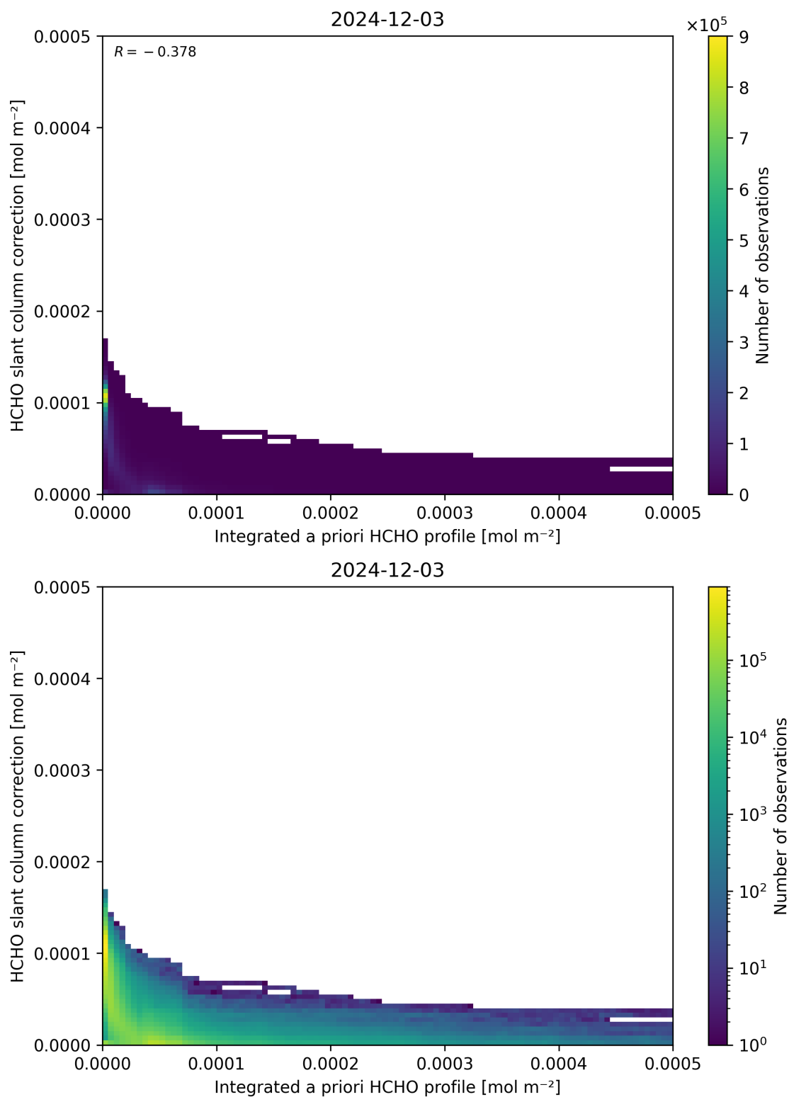
Figure 152: Scatter density plot of “Integrated a priori HCHO profile” against “HCHO slant column correction” for 2024-12-02 to 2024-12-04.
