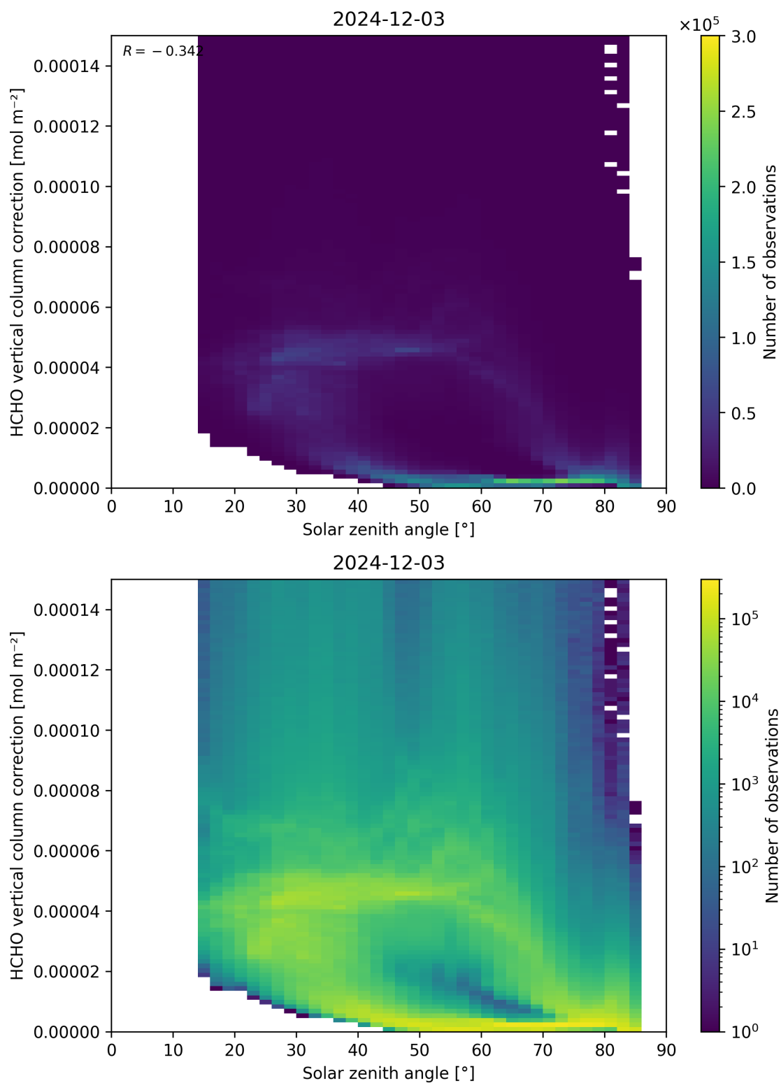
Figure 178: Scatter density plot of “Solar zenith angle” against “HCHO vertical column correction” for 2024-12-02 to 2024-12-04.
