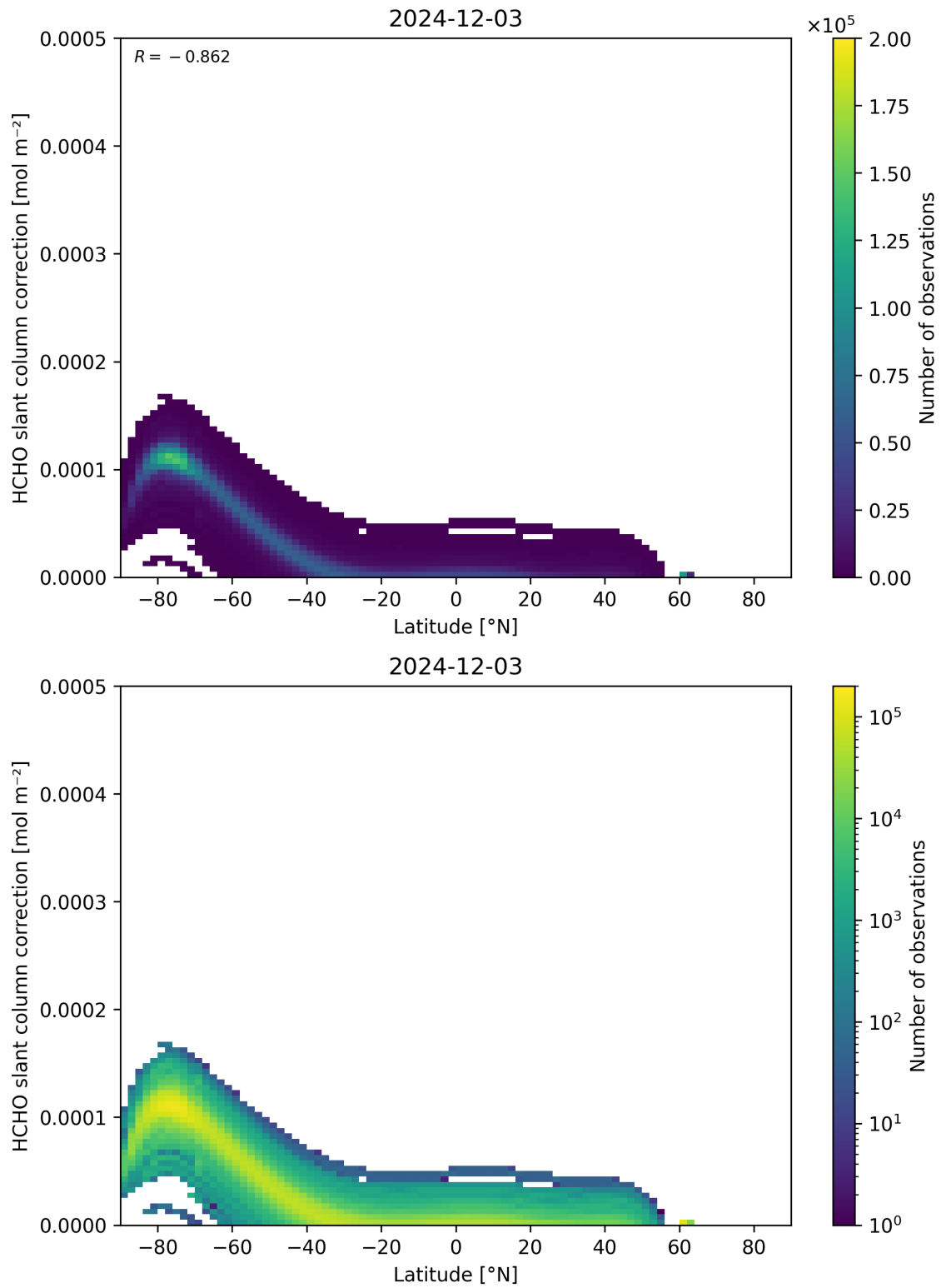
Figure 158: Scatter density plot of “Latitude” against “HCHO slant column correction” for 2024-12-02 to 2024-12-04.
