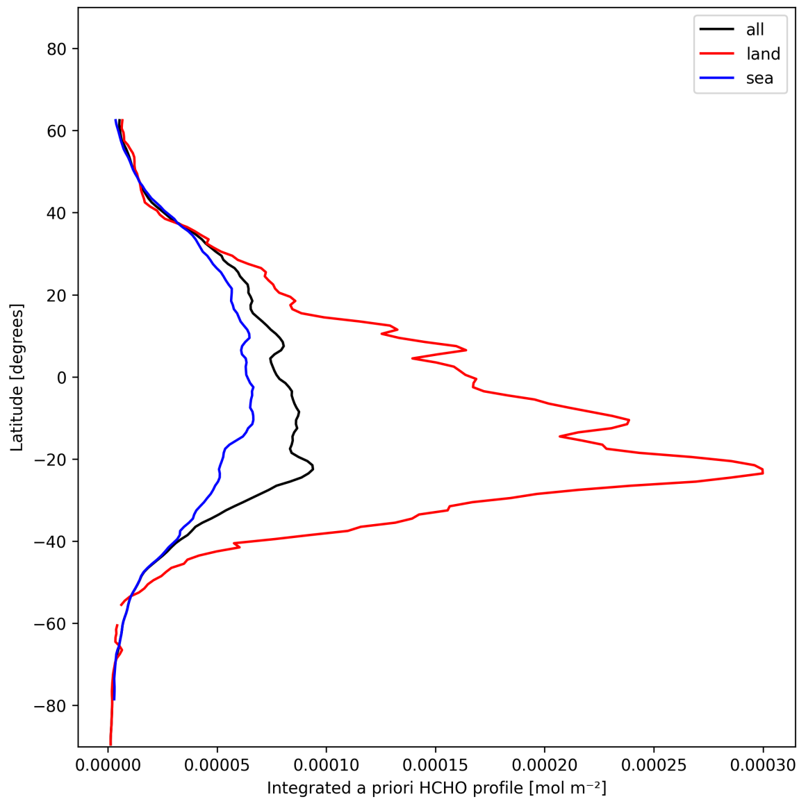
Figure 29: Zonal average of “Integrated a priori HCHO profile” for 2024-12-02 to 2024-12-04.
