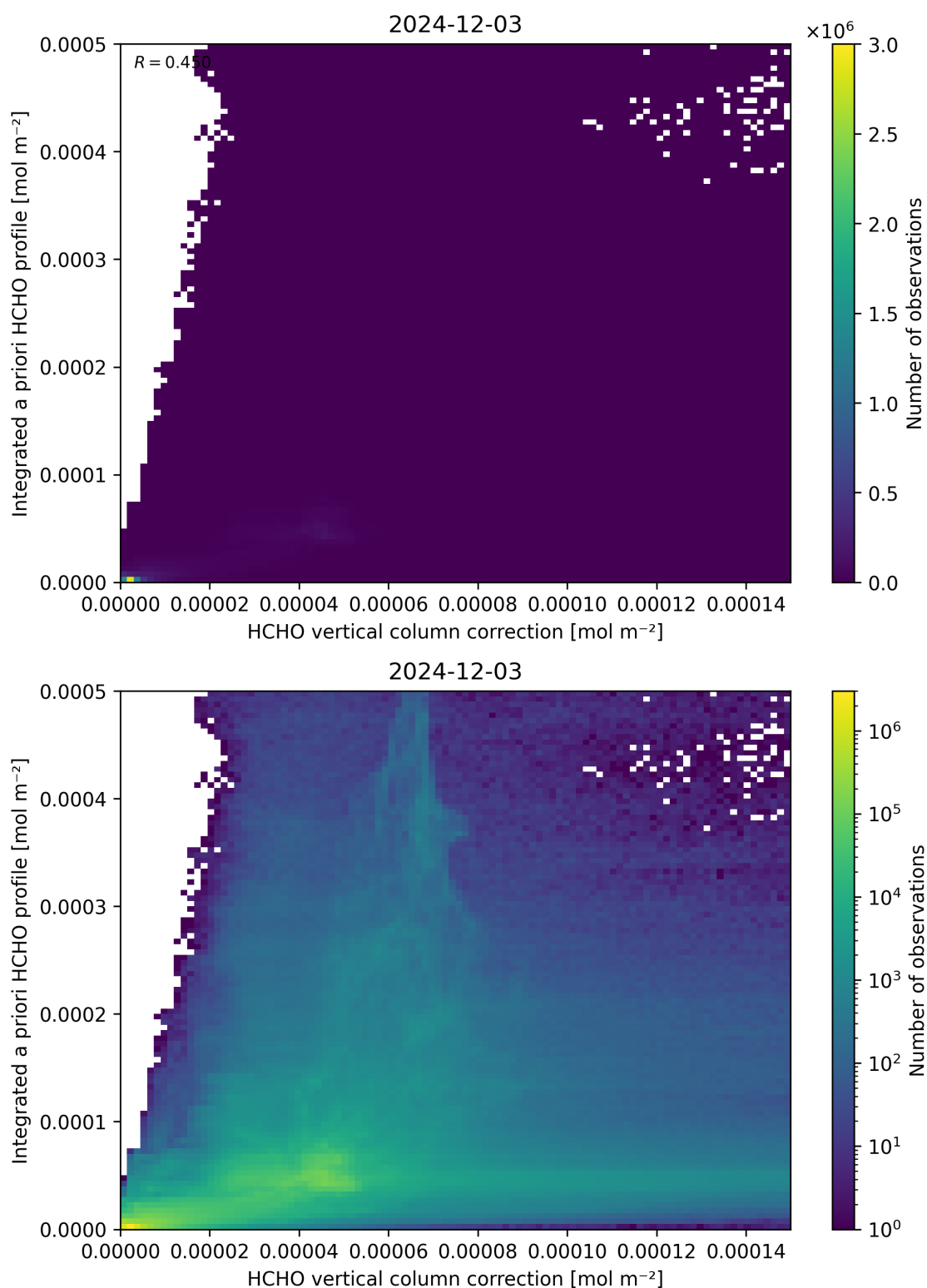
Figure 122: Scatter density plot of “HCHO vertical column correction” against “Integrated a priori HCHO profile” for 2024-12-02 to 2024-12-04.
