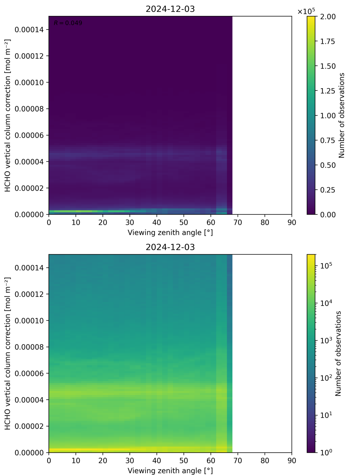
Figure 193: Scatter density plot of “Viewing zenith angle” against “HCHO vertical column correction” for 2024-12-02 to 2024-12-04.
