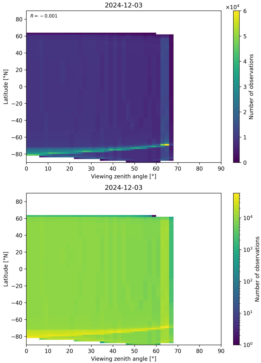
Figure 196: Scatter density plot of “Viewing zenith angle” against “Latitude” for 2024-12-02 to 2024-12-04.
