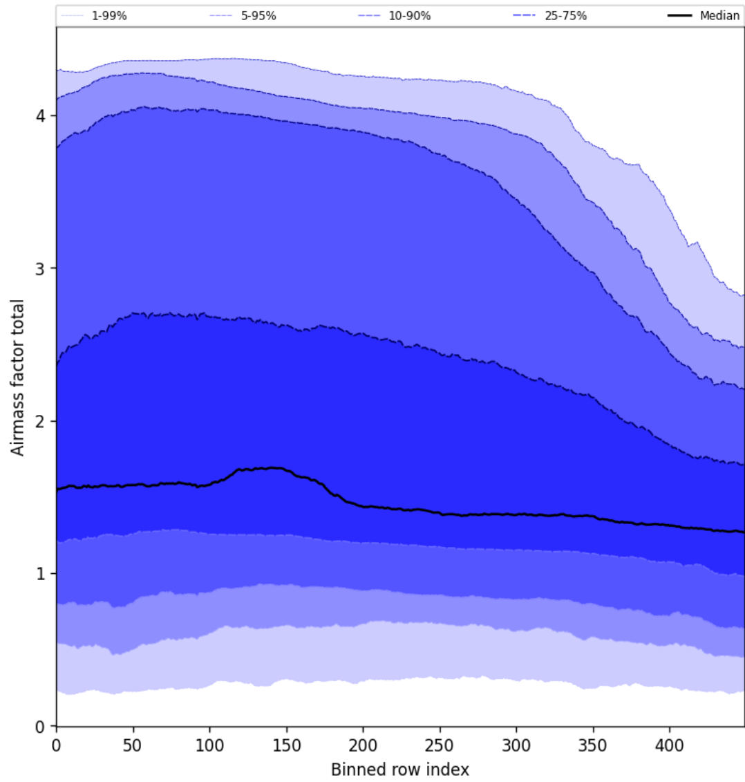
Figure 54: Along track statistics of “Airmass factor total” for 2024-12-02 to 2024-12-04
