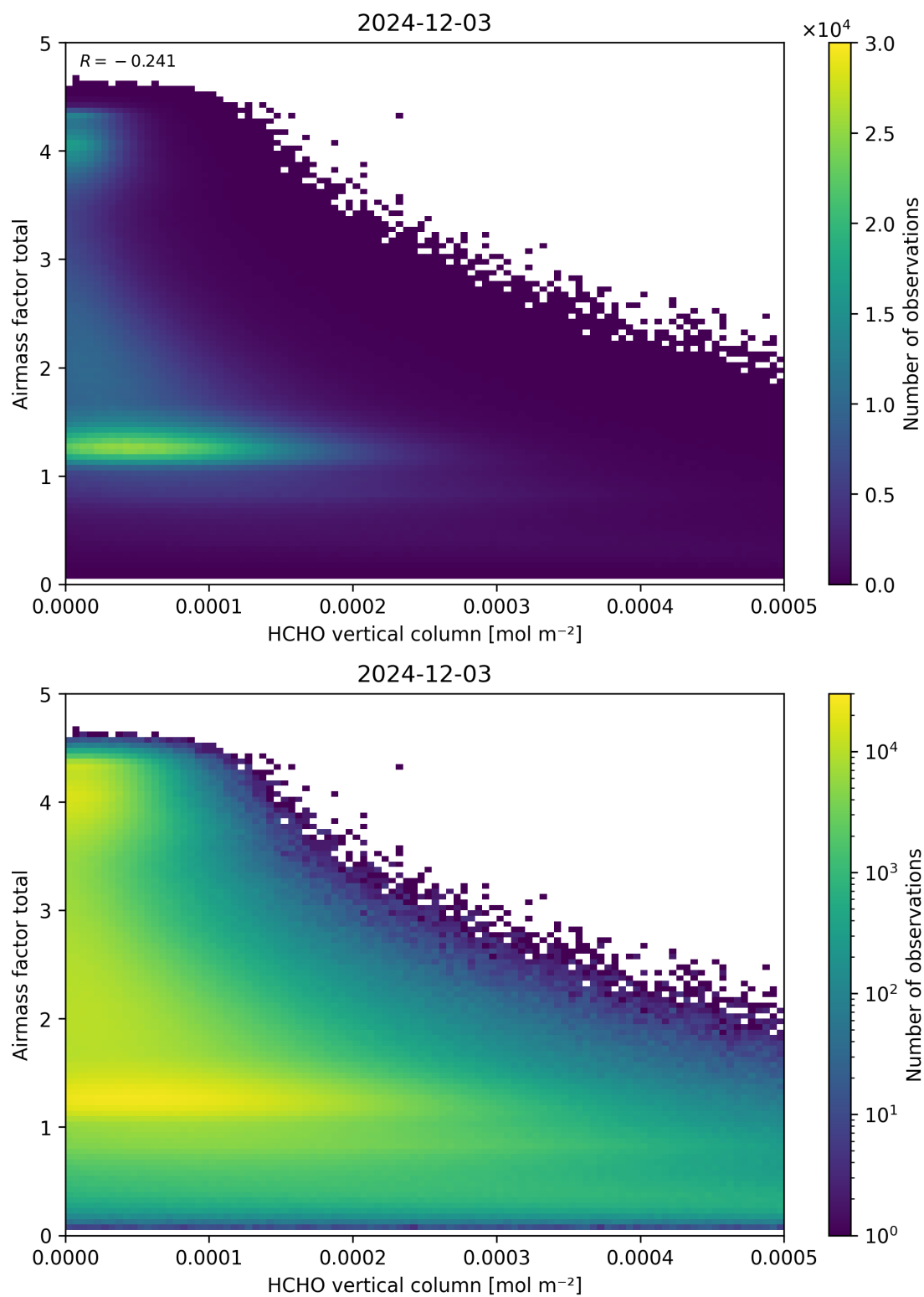
Figure 131: Scatter density plot of “HCHO vertical column” against “Airmass factor total” for 2024-12-02 to 2024-12-04.
