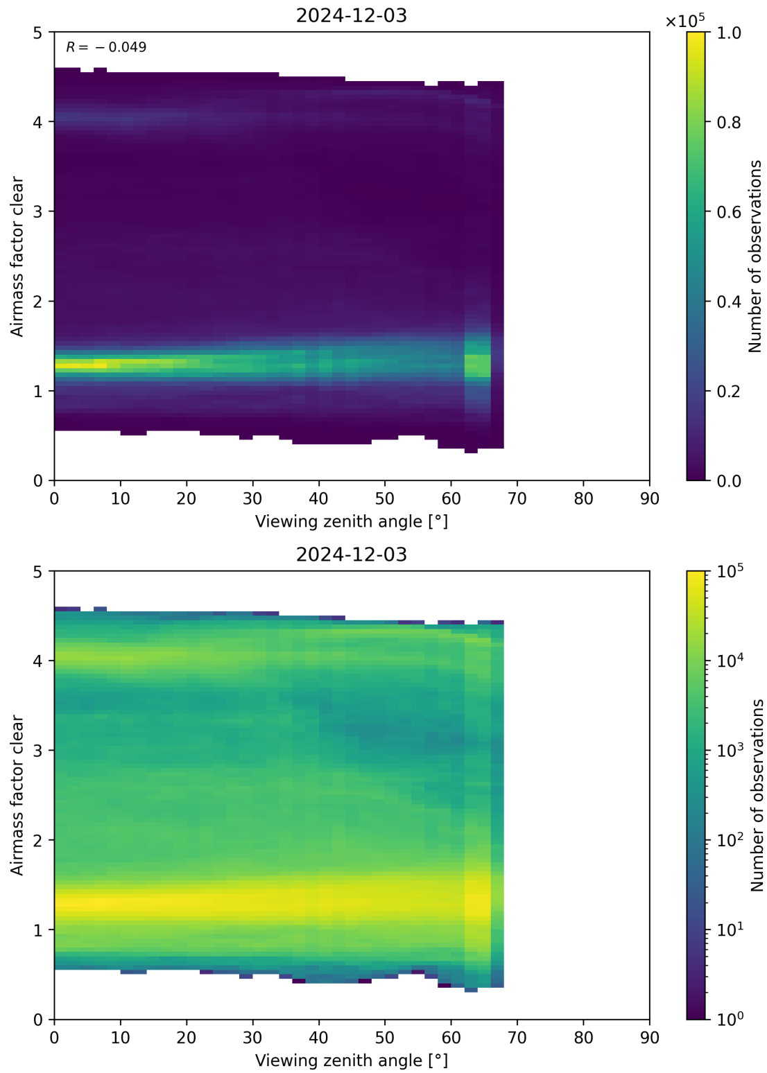
Figure 185: Scatter density plot of “Viewing zenith angle” against “Airmass factor clear” for 2024-12-02 to 2024-12-04.
