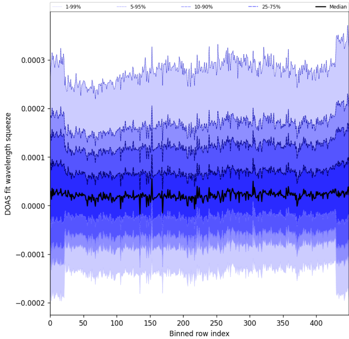
Figure 59: Along track statistics of “DOAS fit wavelength squeeze” for 2024-12-02 to 2024-12-04
