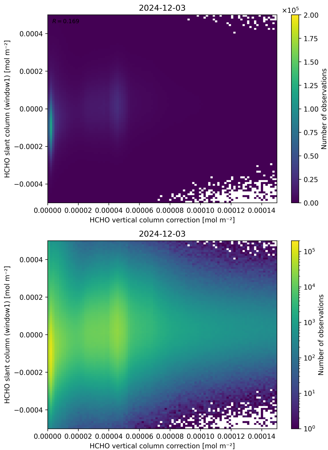
Figure 118: Scatter density plot of “HCHO vertical column correction” against “HCHO slant column (window1)” for 2024-12-02 to 2024-12-04.
