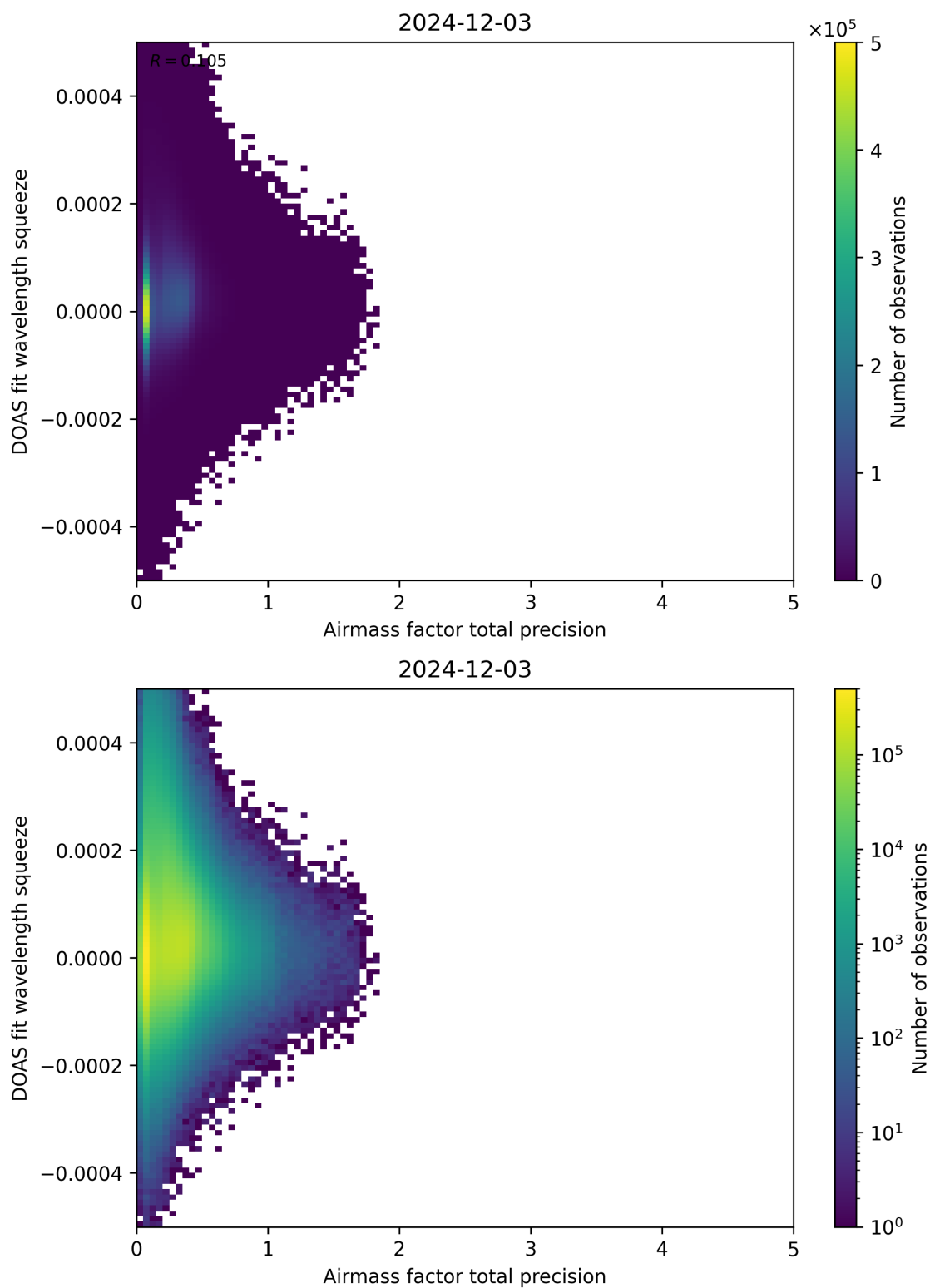
Figure 107: Scatter density plot of “Airmass factor total precision” against “DOAS fit wavelength squeeze” for 2024-12-02 to 2024-12-04.
