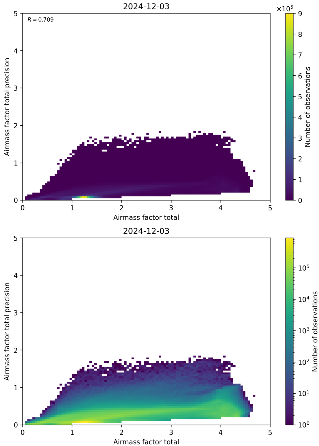
Figure 103: Scatter density plot of “Airmass factor total” against “Airmass factor total precision” for 2024-12-02 to 2024-12-04.
