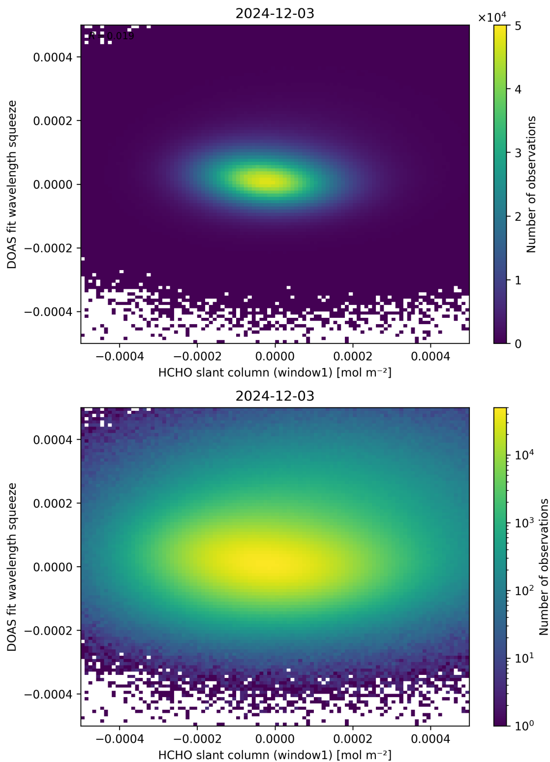
Figure 80: Scatter density plot of “HCHO slant column (window1)” against “DOAS fit wavelength squeeze” for 2024-12-02 to 2024-12-04.
