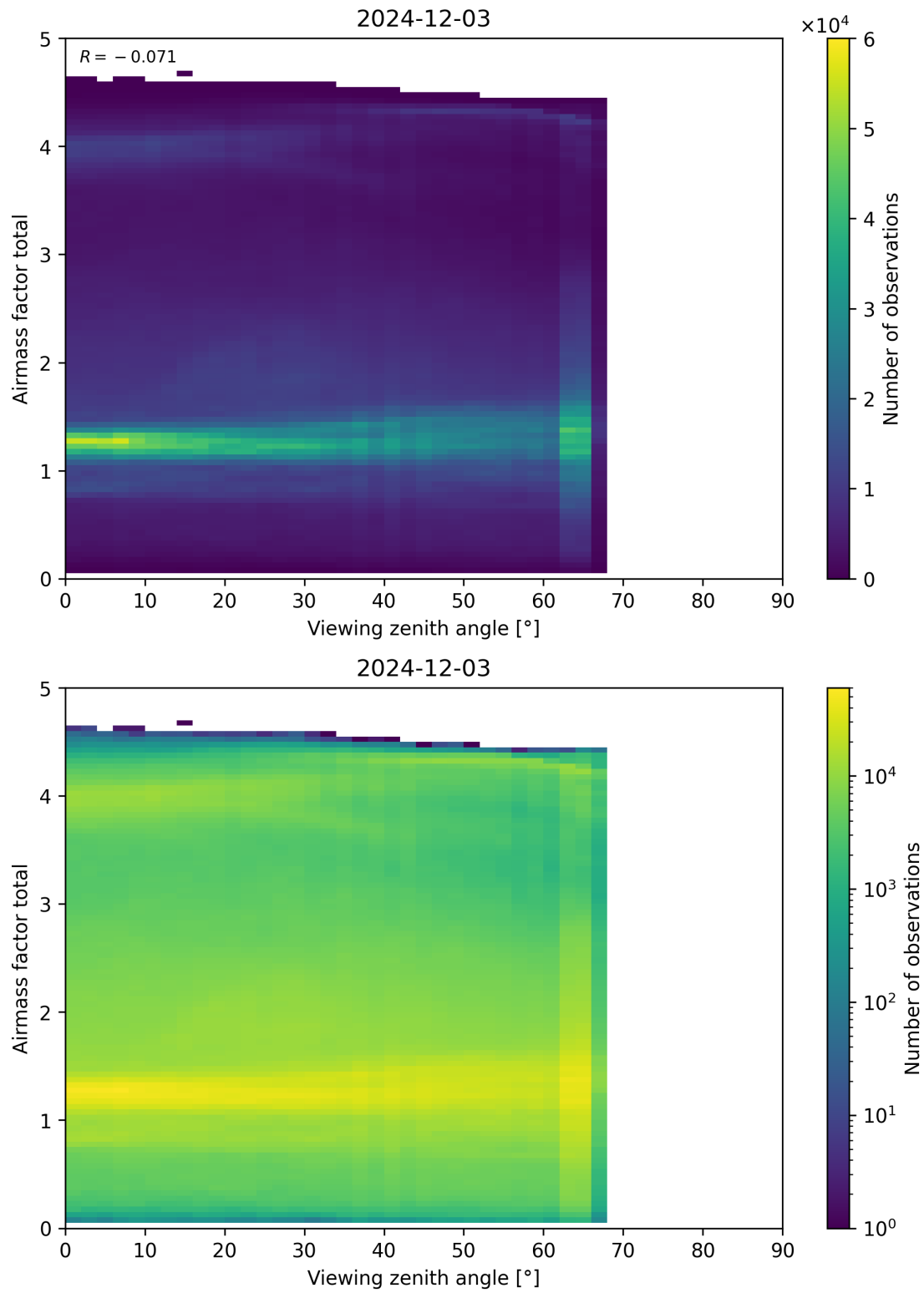
Figure 190: Scatter density plot of “Viewing zenith angle” against “Airmass factor total” for 2024-12-02 to 2024-12-04.
