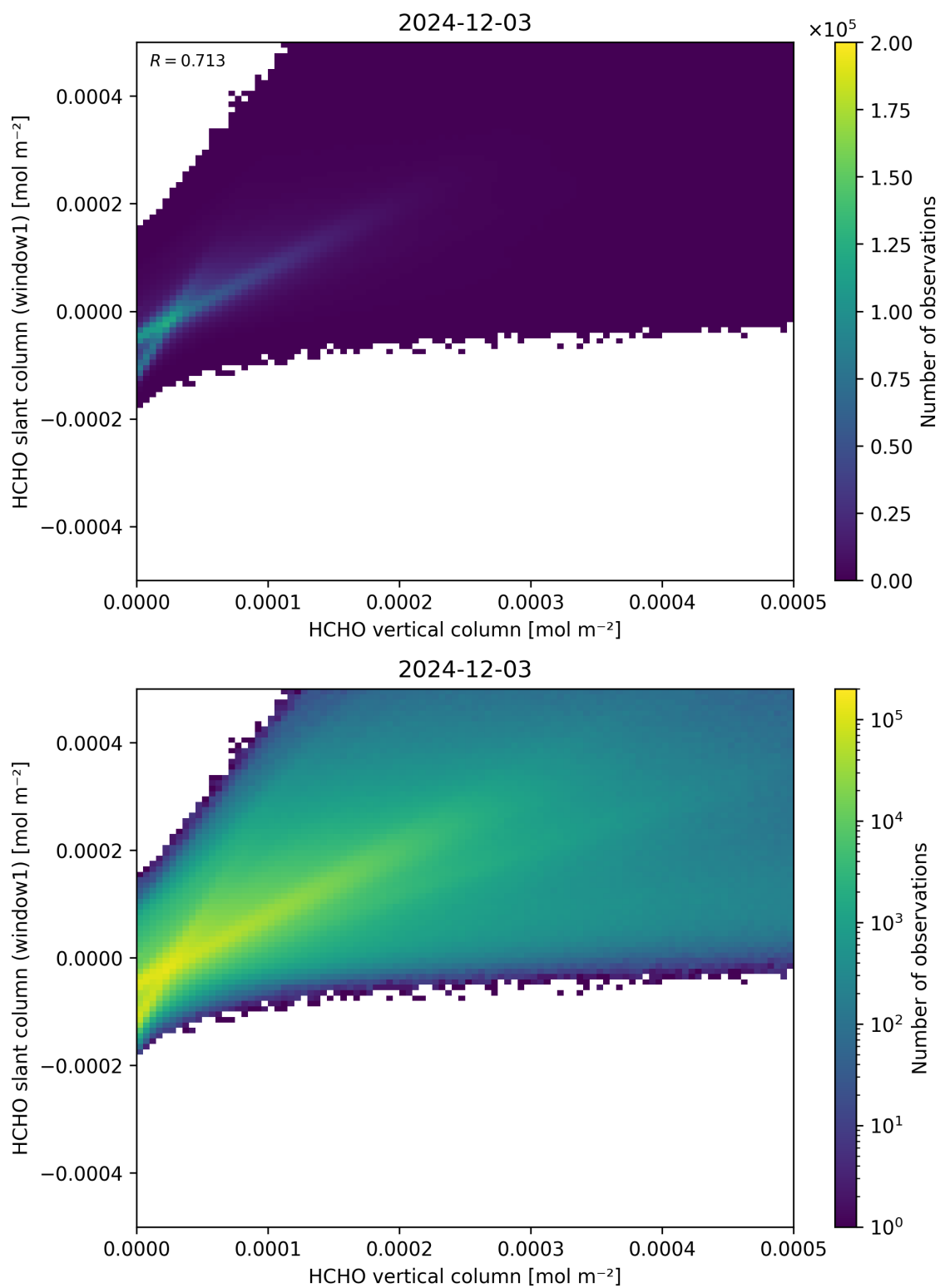
Figure 129: Scatter density plot of “HCHO vertical column” against “HCHO slant column (window1)” for 2024-12-02 to 2024-12-04.
