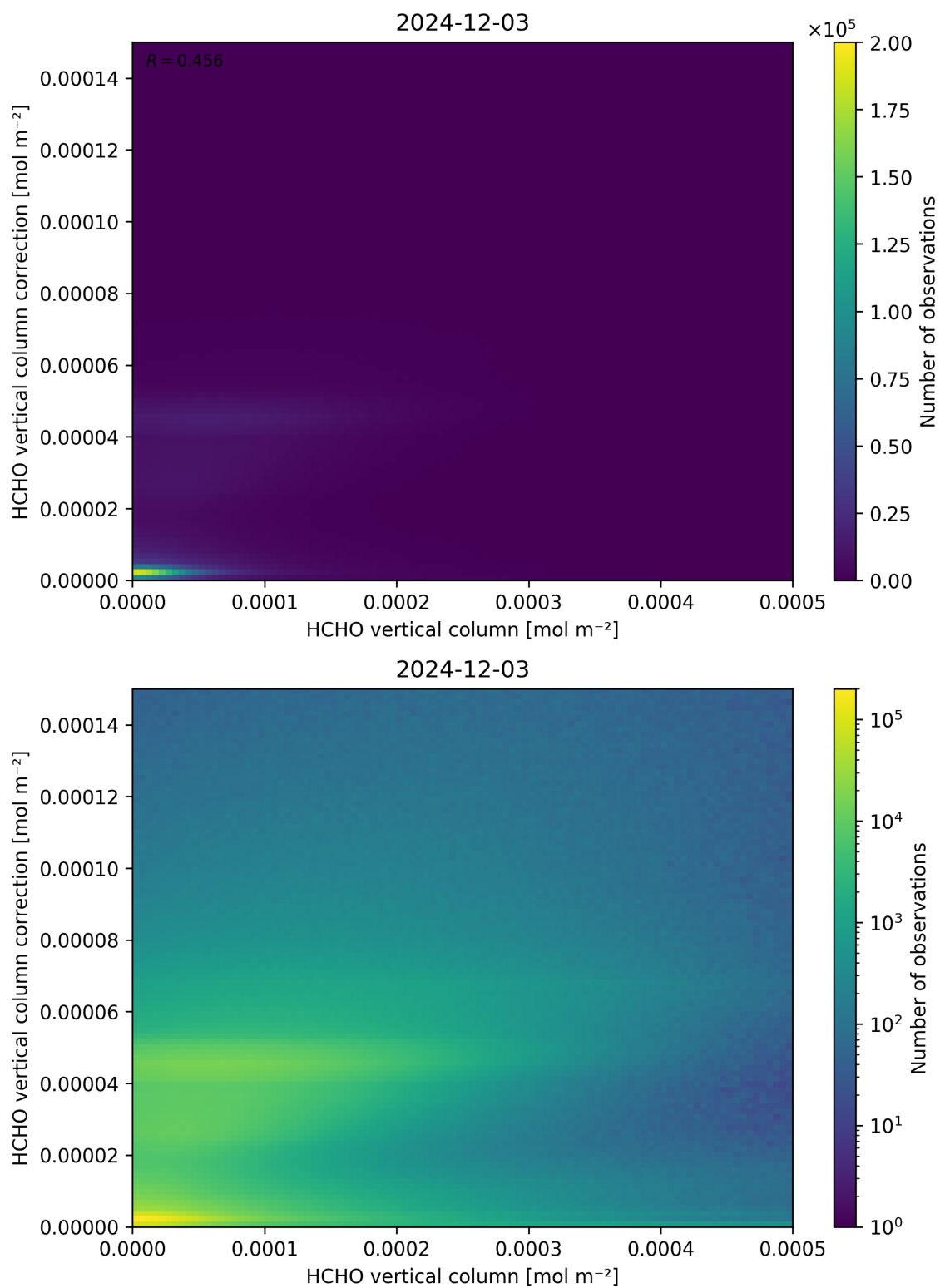
Figure 133: Scatter density plot of “HCHO vertical column” against “HCHO vertical column correction” for 2024-12-02 to 2024-12-04.
