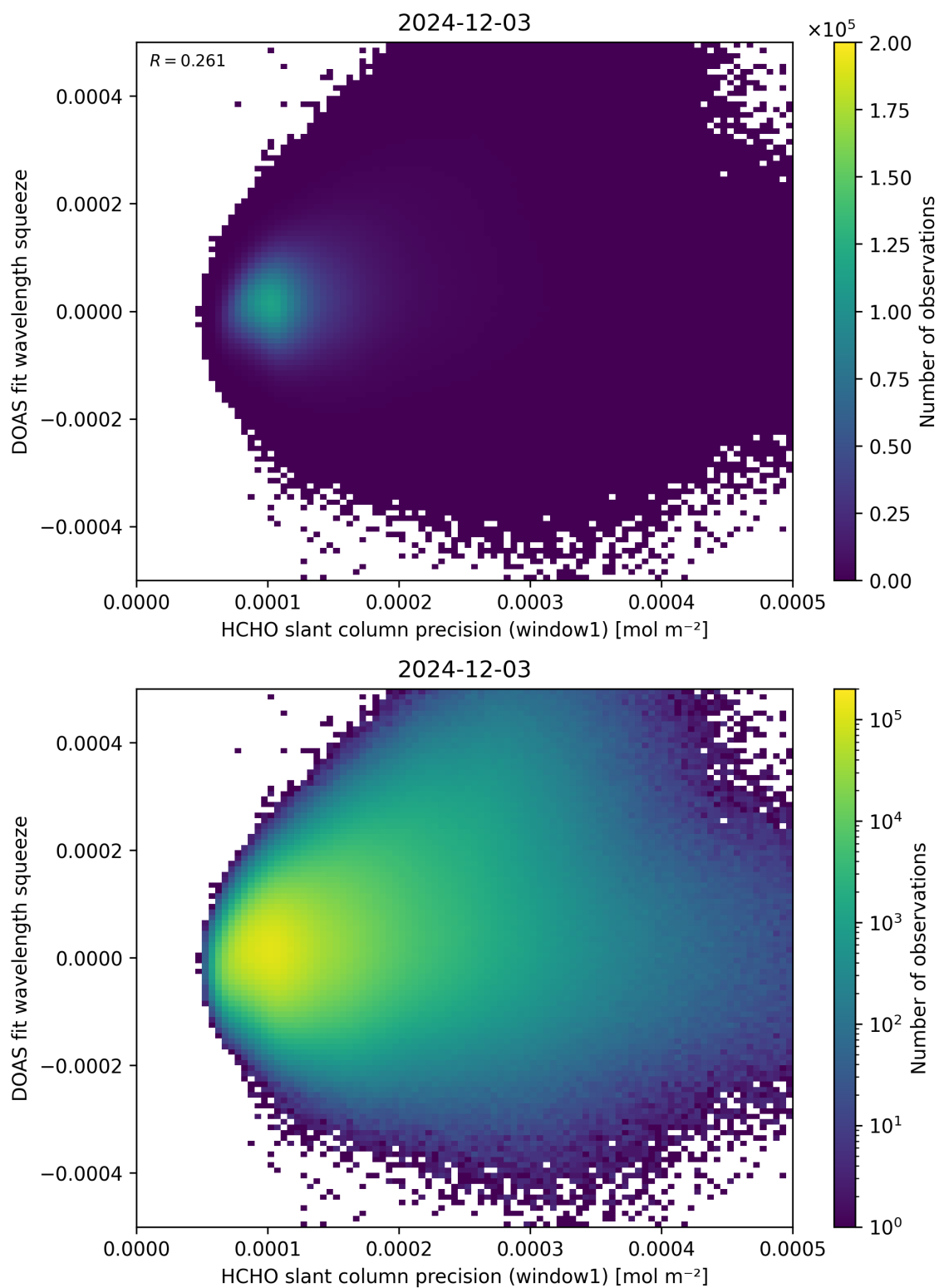
Figure 90: Scatter density plot of “HCHO slant column precision (window1)” against “DOAS fit wavelength squeeze” for 2024-12-02 to 2024-12-04.
