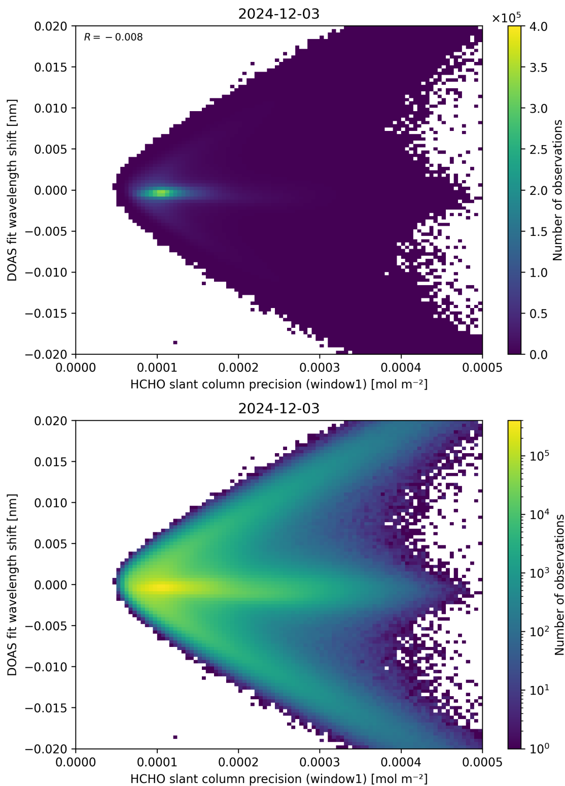
Figure 89: Scatter density plot of “HCHO slant column precision (window1)” against “DOAS fit wavelength shift” for 2024-12-02 to 2024-12-04.
