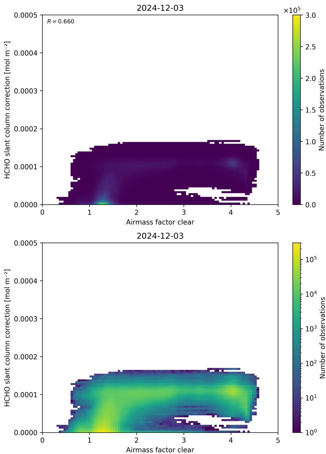
Figure 75: Scatter density plot of “Airmass factor clear” against “HCHO slant column correction” for 2024-12-02 to 2024-12-04.
