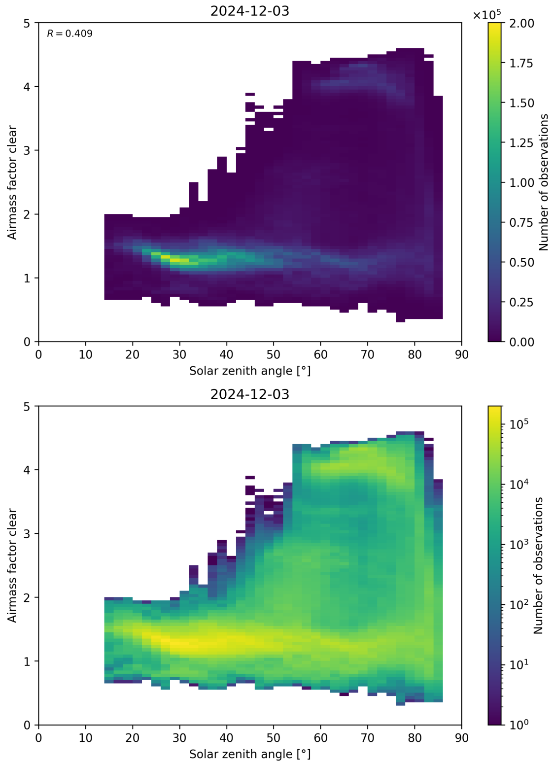
Figure 170: Scatter density plot of “Solar zenith angle” against “Airmass factor clear” for 2024-12-02 to 2024-12-04.
