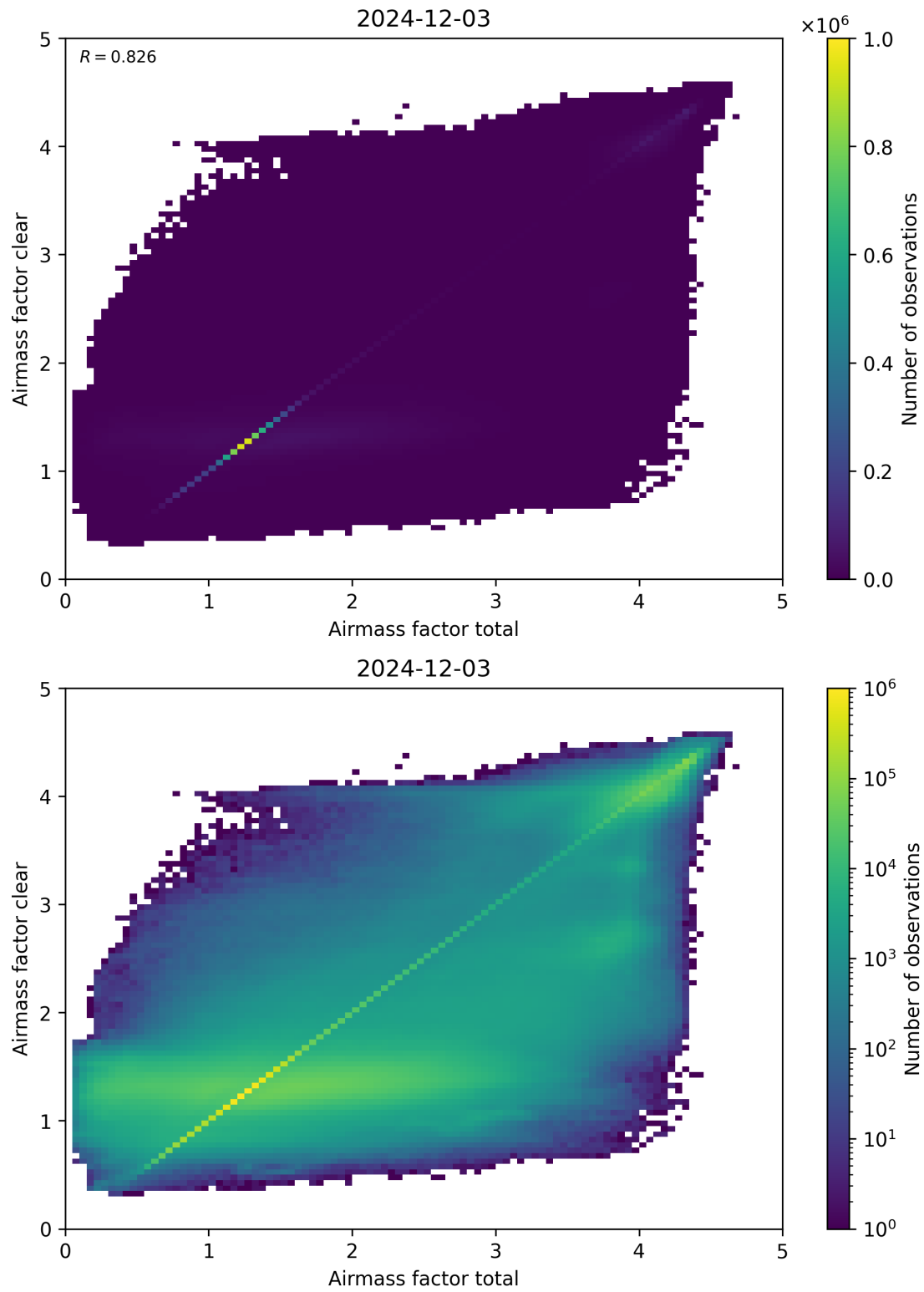
Figure 100: Scatter density plot of “Airmass factor total” against “Airmass factor clear” for 2024-12-02 to 2024-12-04.
