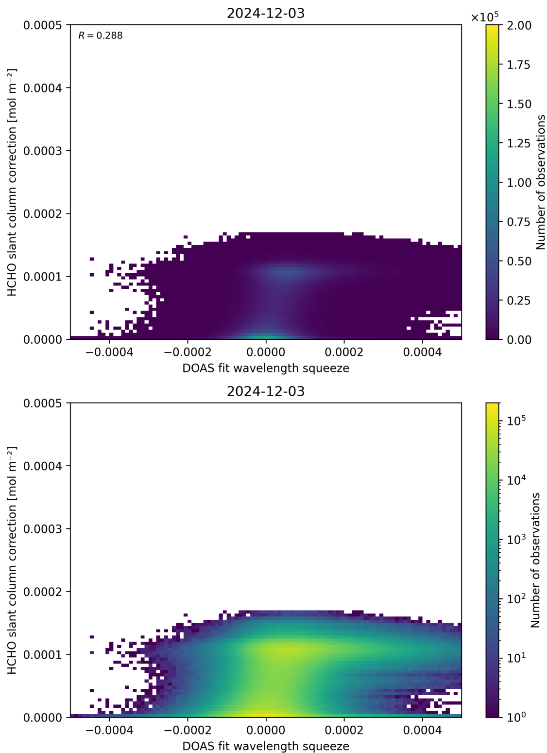
Figure 70: Scatter density plot of “DOAS fit wavelength squeeze” against “HCHO slant column correction” for 2024-12-02 to 2024-12-04.
