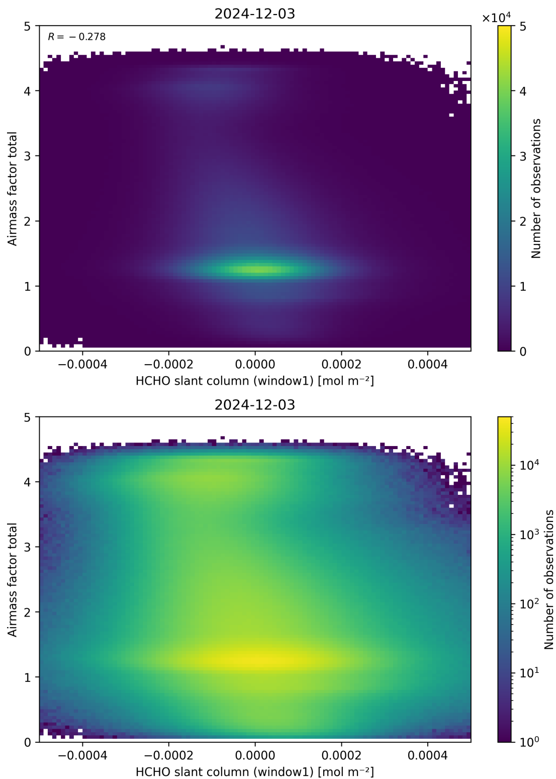
Figure 85: Scatter density plot of “HCHO slant column (window1)” against “Airmass factor total” for 2024-12-02 to 2024-12-04.
