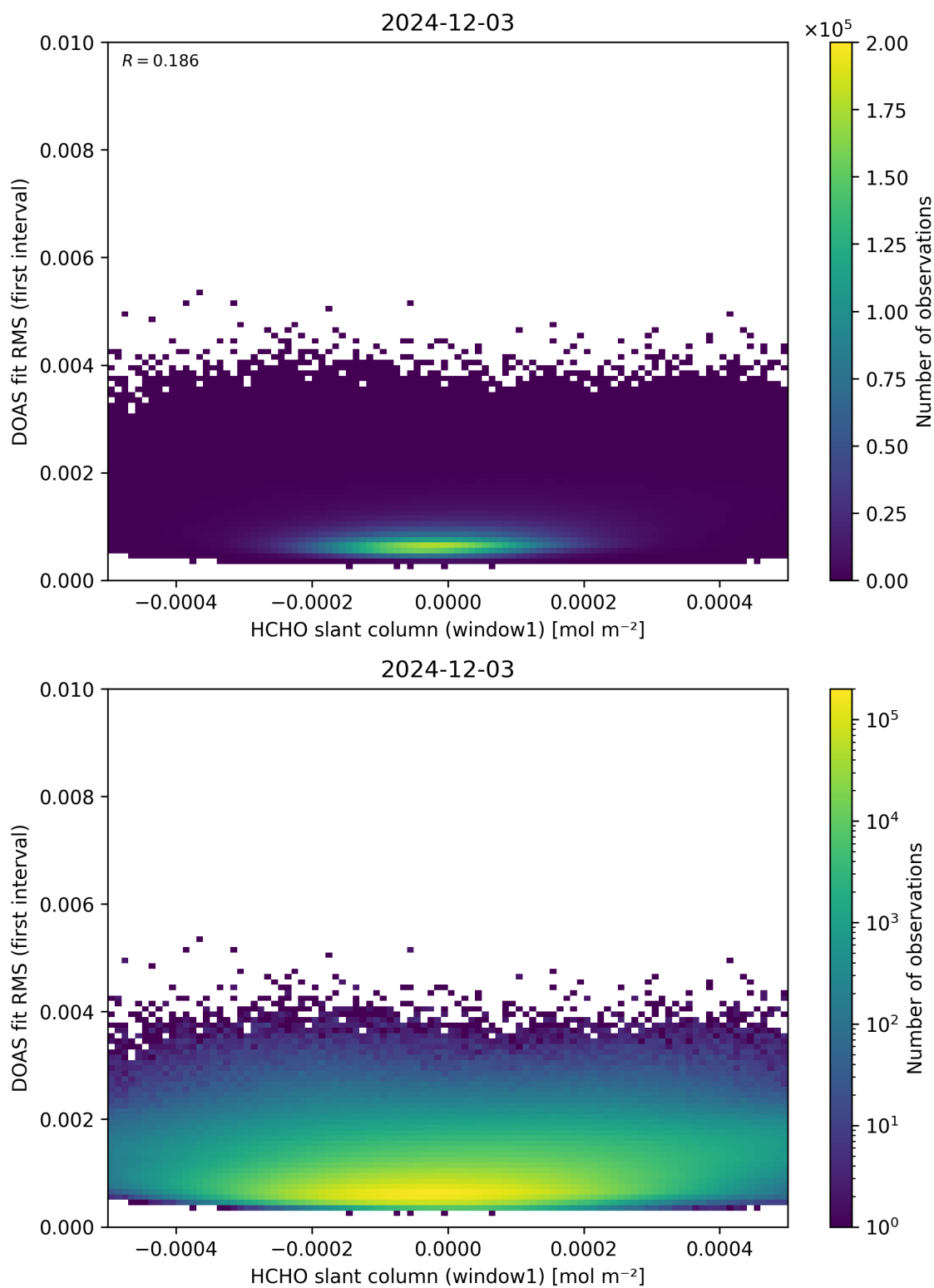
Figure 78: Scatter density plot of “HCHO slant column (window1)” against “DOAS fit RMS (first interval)” for 2024-12-02 to 2024-12-04.
