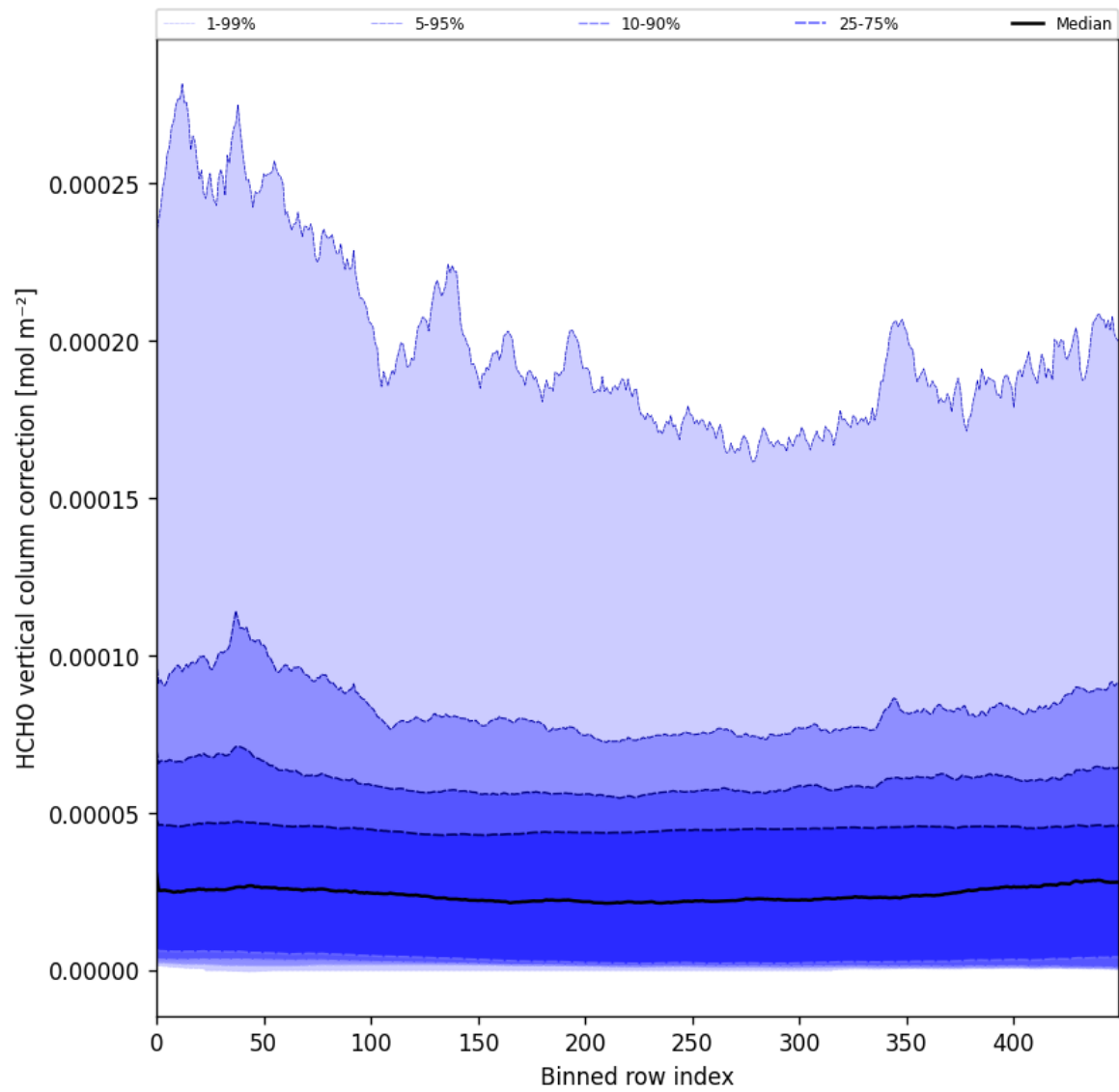
Figure 51: Along track statistics of "HCHO vertical column correction" for 2024-12-02 to 2024-12-04
