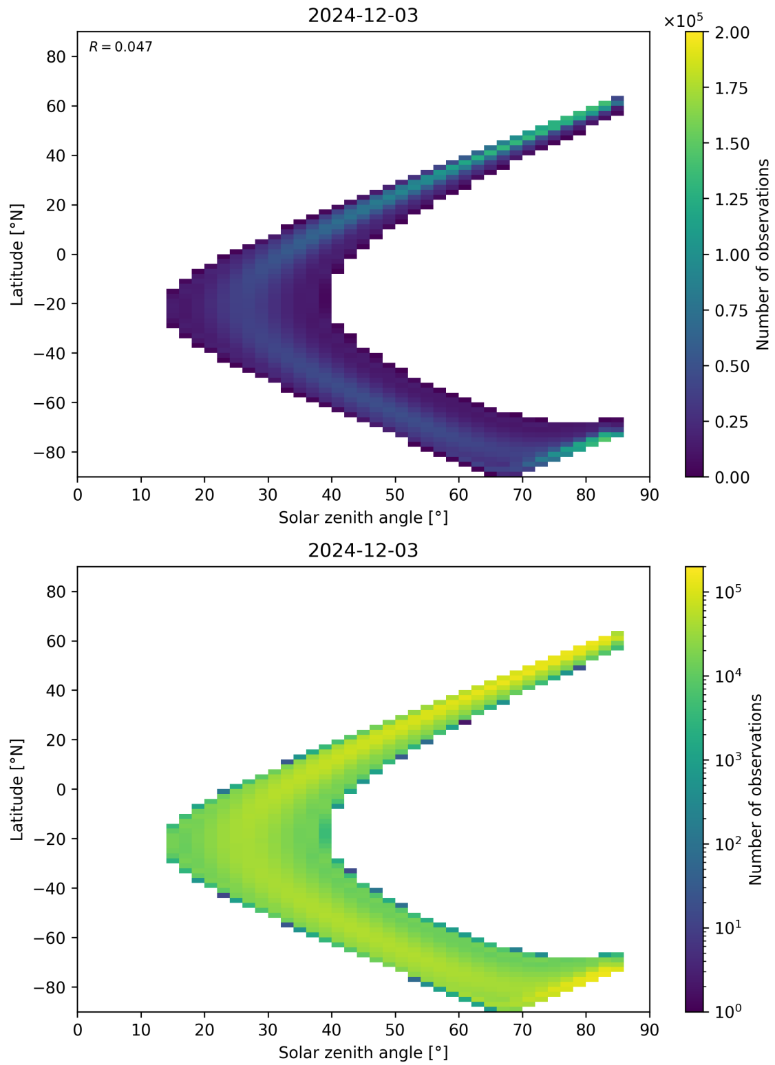
Figure 181: Scatter density plot of “Solar zenith angle” against “Latitude” for 2024-12-02 to 2024-12-04.
