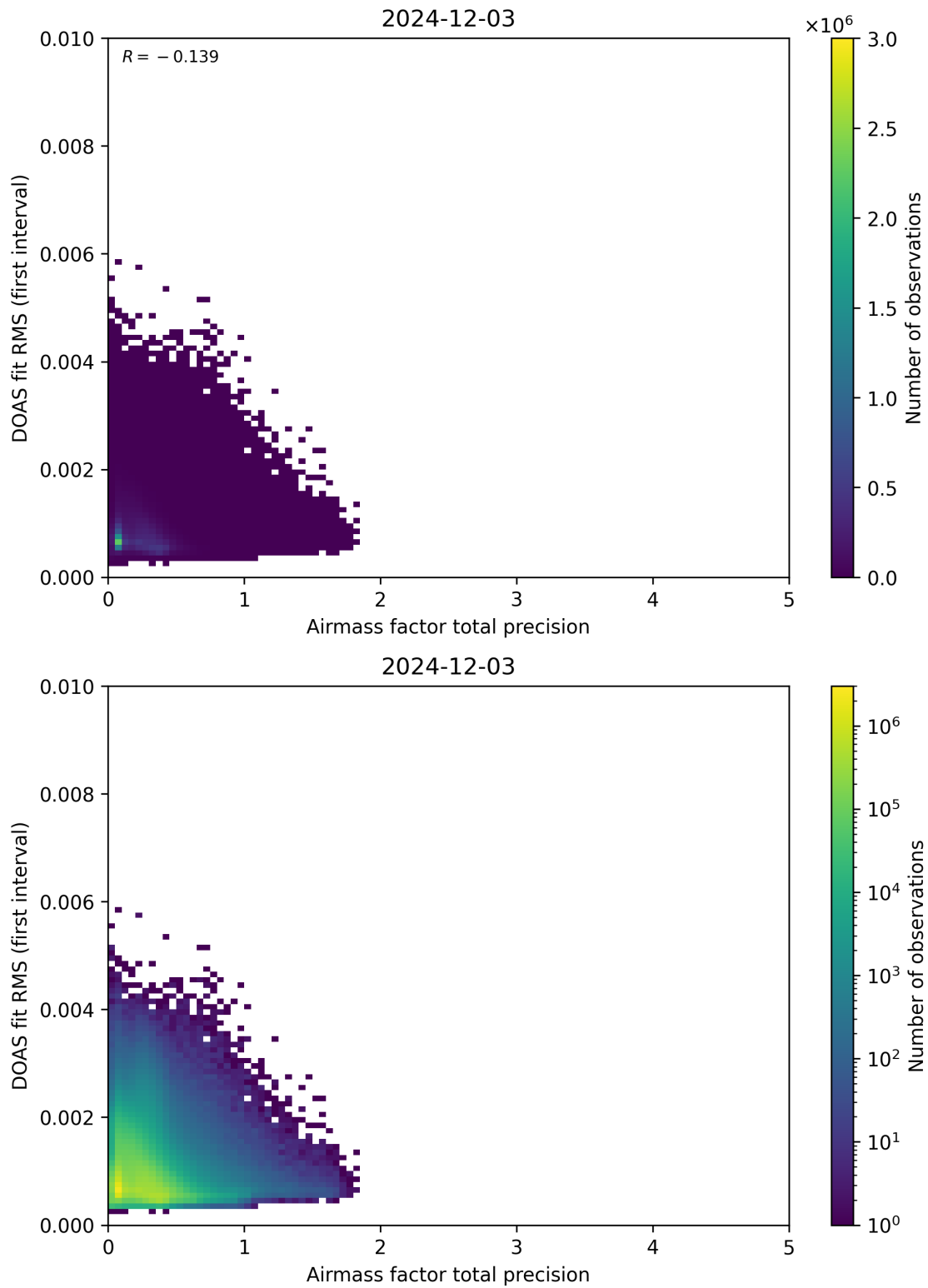
Figure 105: Scatter density plot of “Airmass factor total precision” against “DOAS fit RMS (first interval)” for 2024-12-02 to 2024-12-04.
