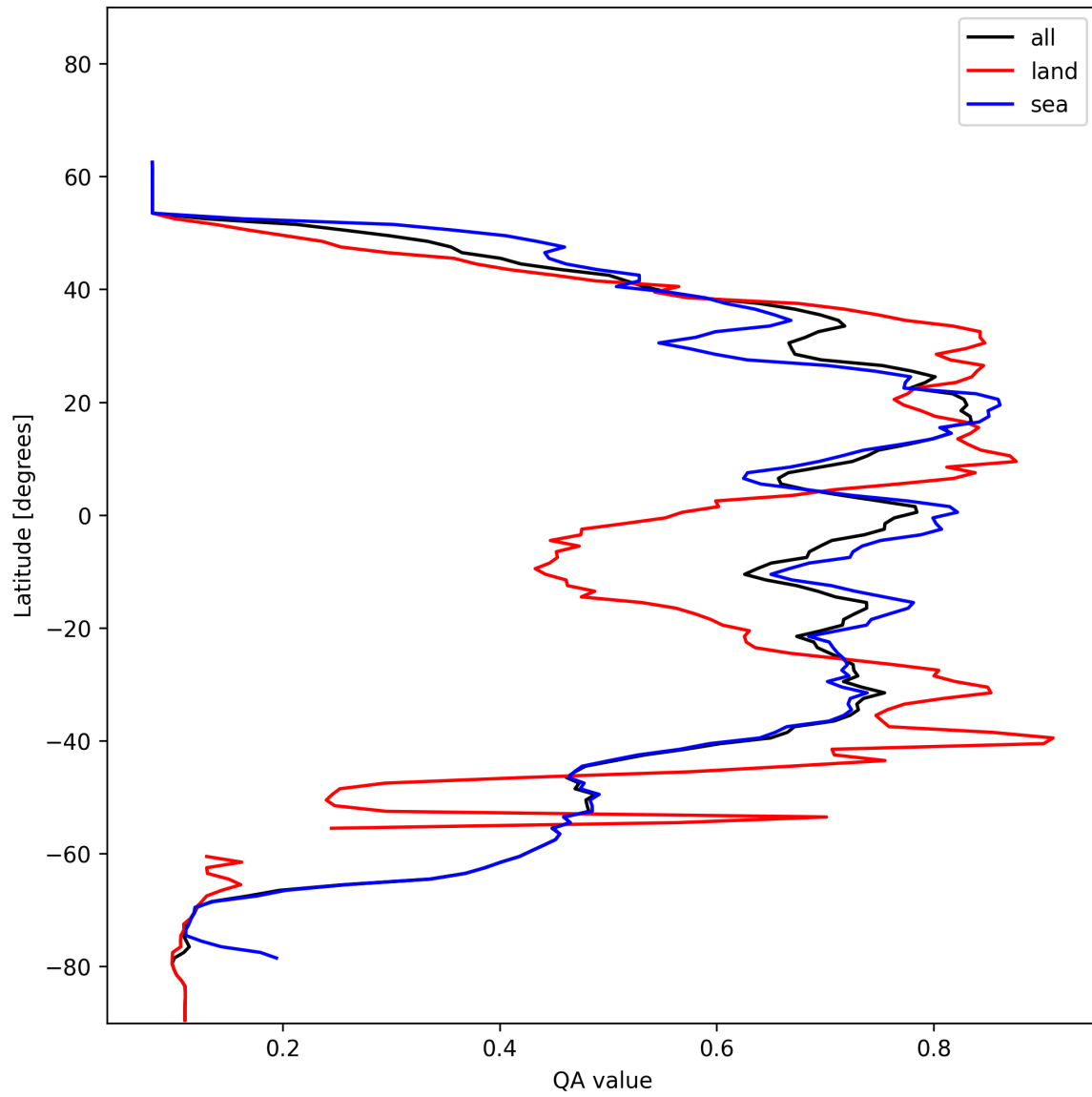
Figure 20: Zonal average of “QA value” for 2024-12-02 to 2024-12-04.
