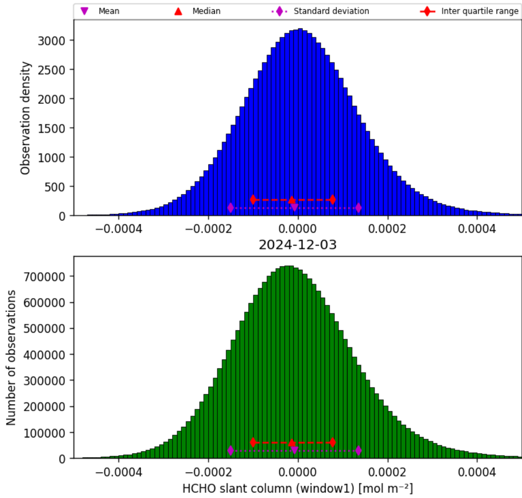
Figure 38: Histogram of “HCHO slant column (window1)” for 2024-12-02 to 2024-12-04
