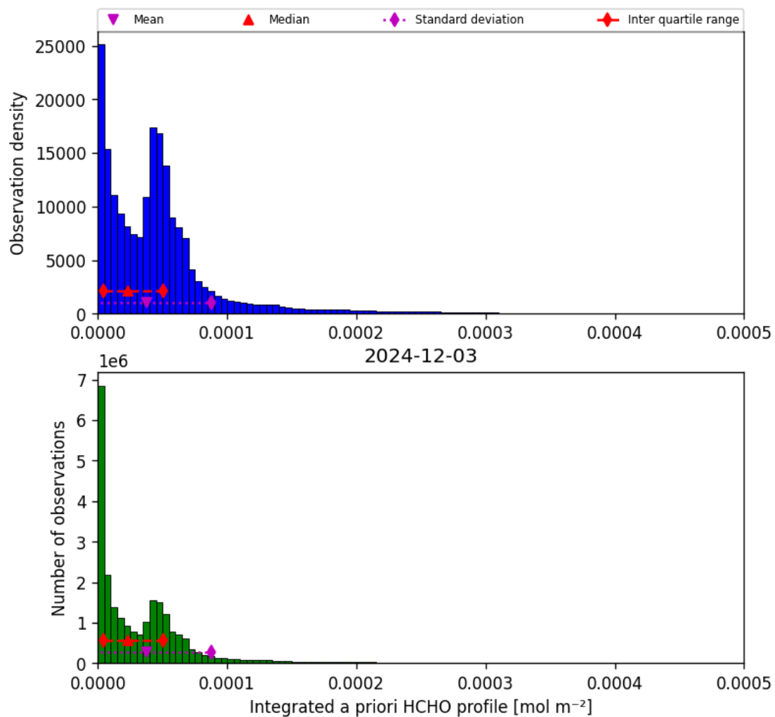
Figure 43: Histogram of “Integrated a priori HCHO profile” for 2024-12-02 to 2024-12-04
