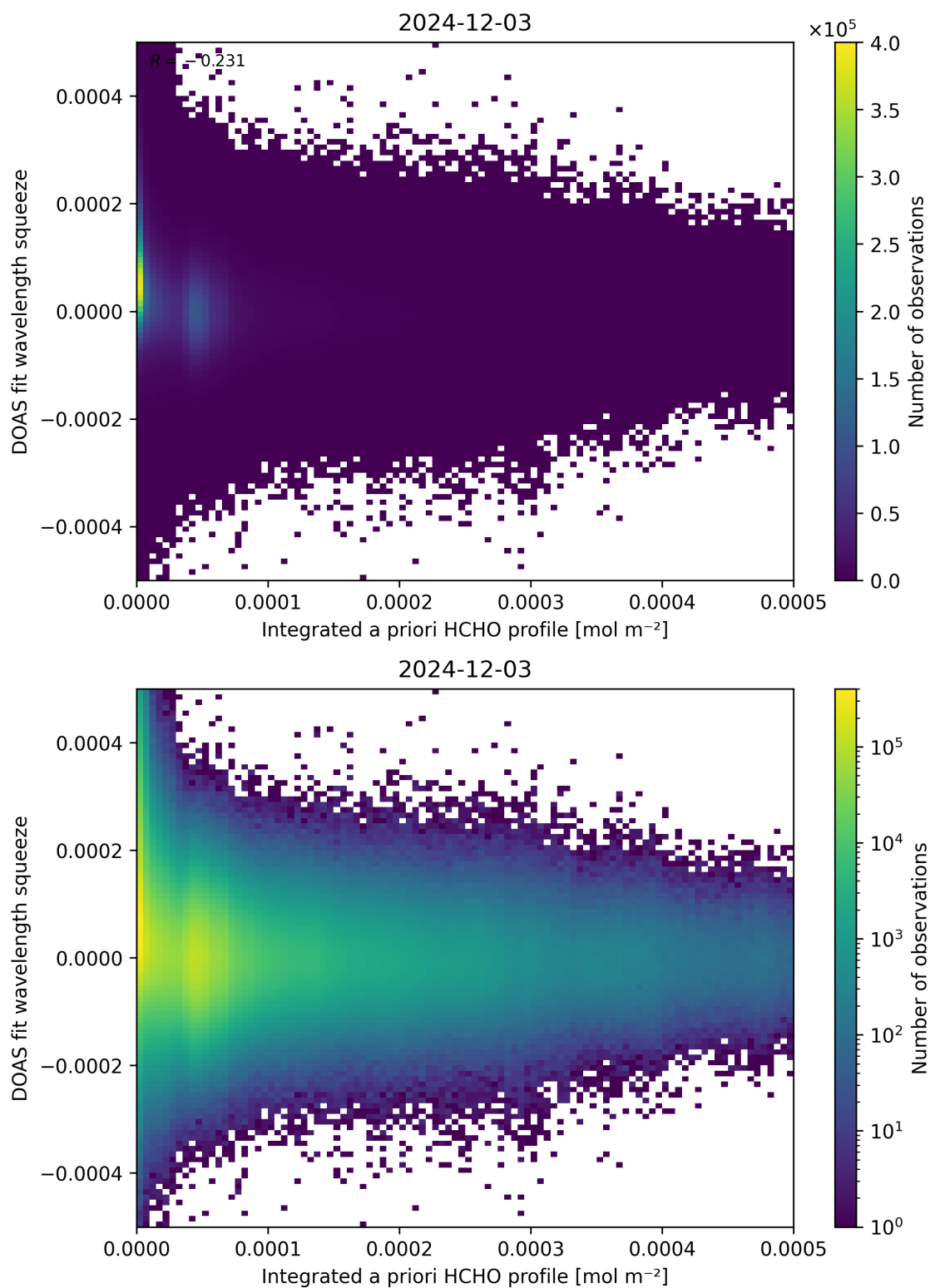
Figure 150: Scatter density plot of “Integrated a priori HCHO profile” against “DOAS fit wavelength squeeze” for 2024-12-02 to 2024-12-04.
