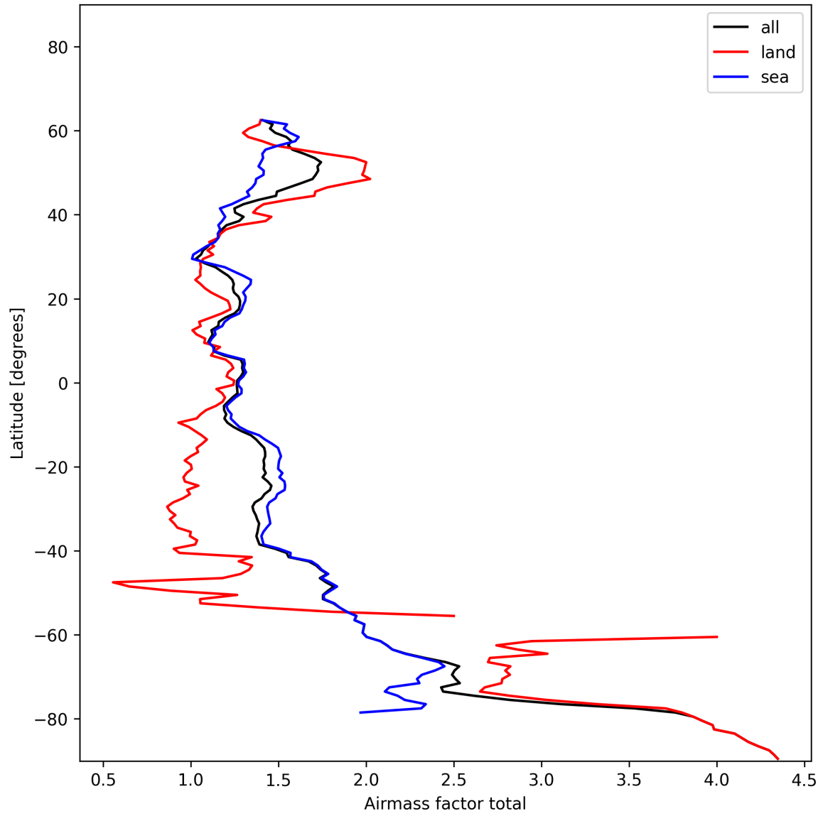
Figure 26: Zonal average of “Airmass factor total” for 2024-12-02 to 2024-12-04.
