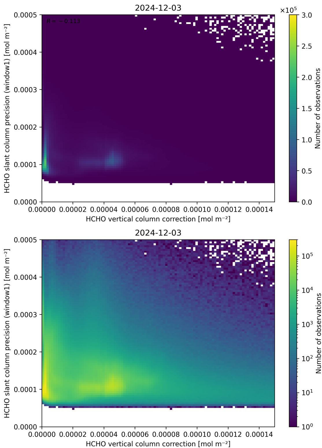
Figure 119: Scatter density plot of “HCHO vertical column correction” against “HCHO slant column precision (window1)” for 2024-12-02 to 2024-12-04.
