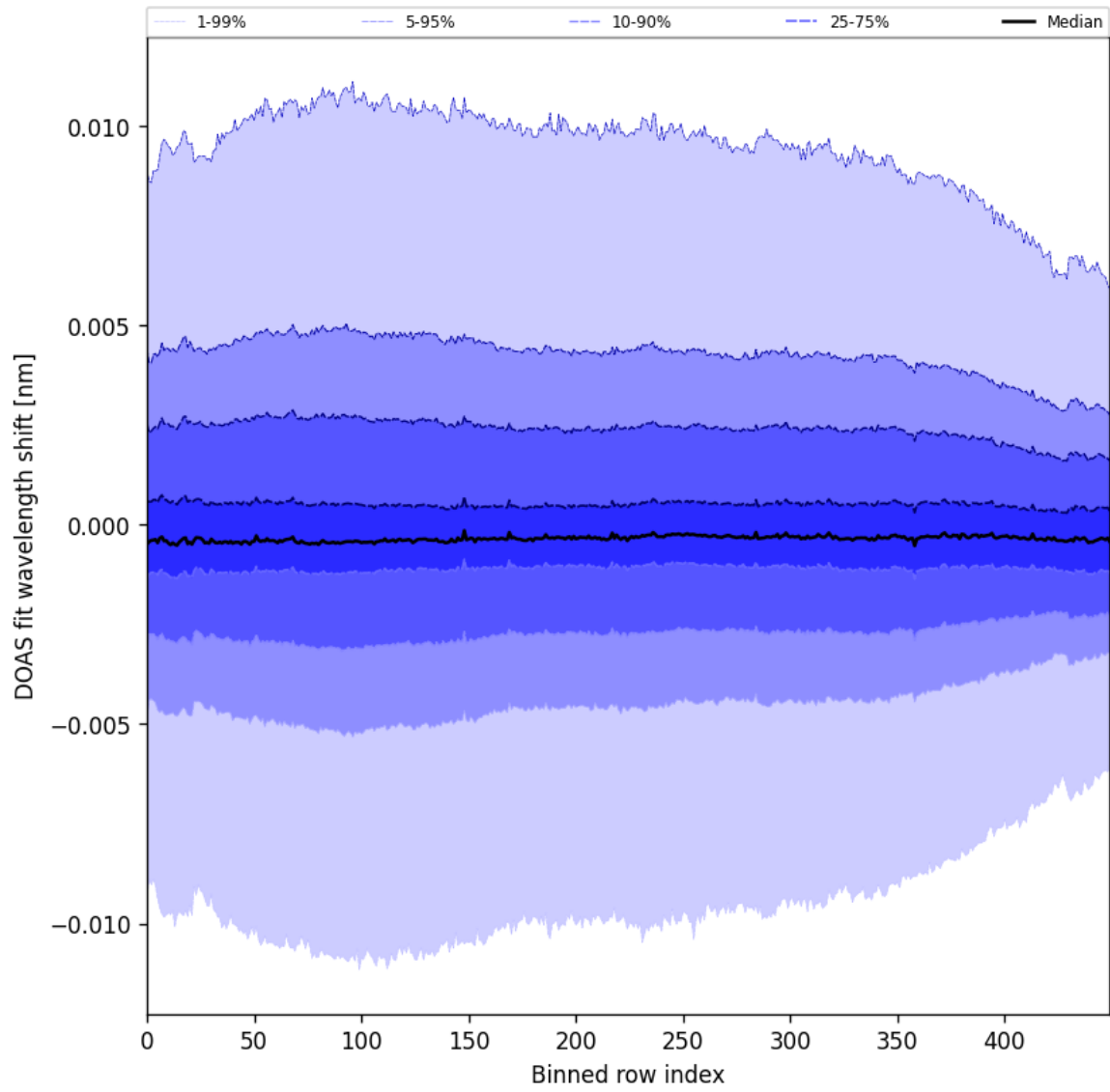
Figure 58: Along track statistics of “DOAS fit wavelength shift” for 2024-12-02 to 2024-12-04
