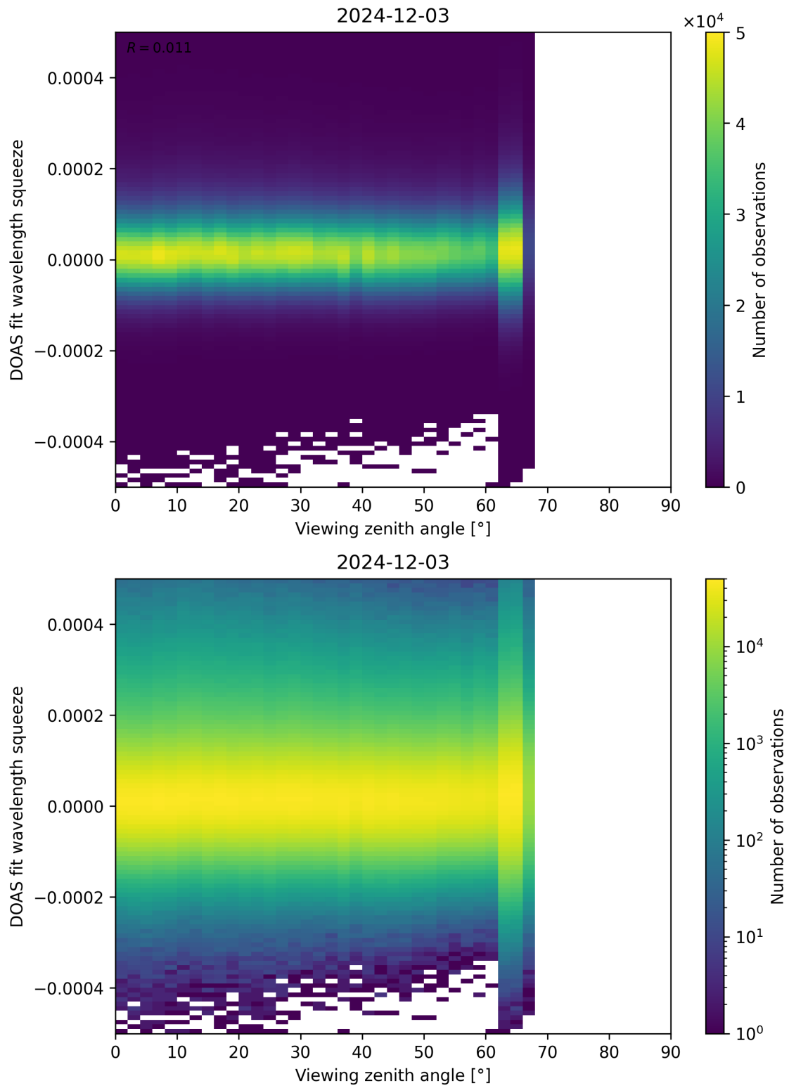
Figure 184: Scatter density plot of “Viewing zenith angle” against “DOAS fit wavelength squeeze” for 2024-12-02 to 2024-12-04.
