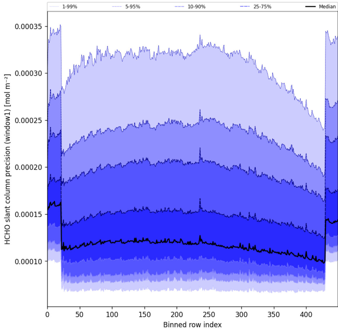
Figure 53: Along track statistics of “HCHO slant column precision (window1)” for 2024-12-02 to 2024-12-04
