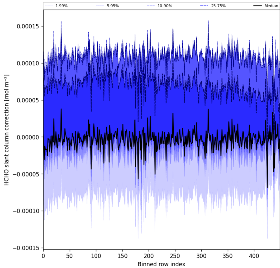
Figure 61: Along track statistics of “HCHO slant column correction” for 2024-12-02 to 2024-12-04
