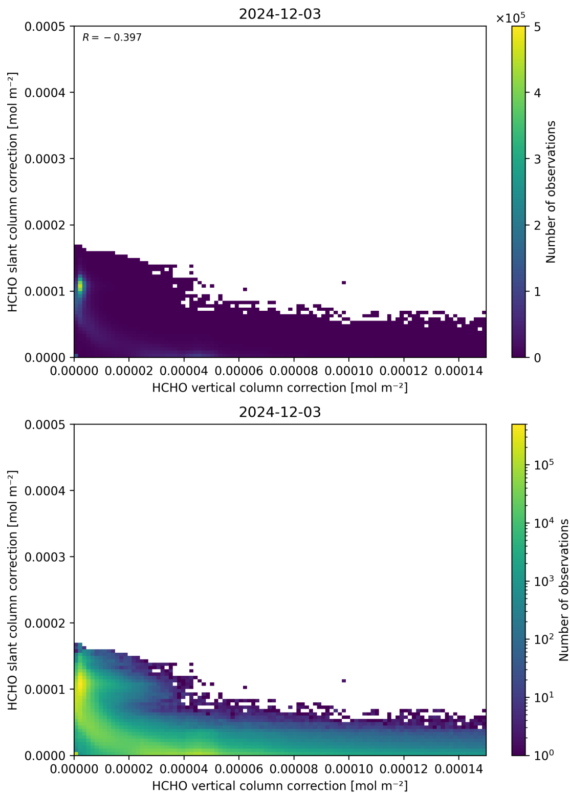
Figure 117: Scatter density plot of “HCHO vertical column correction” against “HCHO slant column correction” for 2024-12-02 to 2024-12-04.
