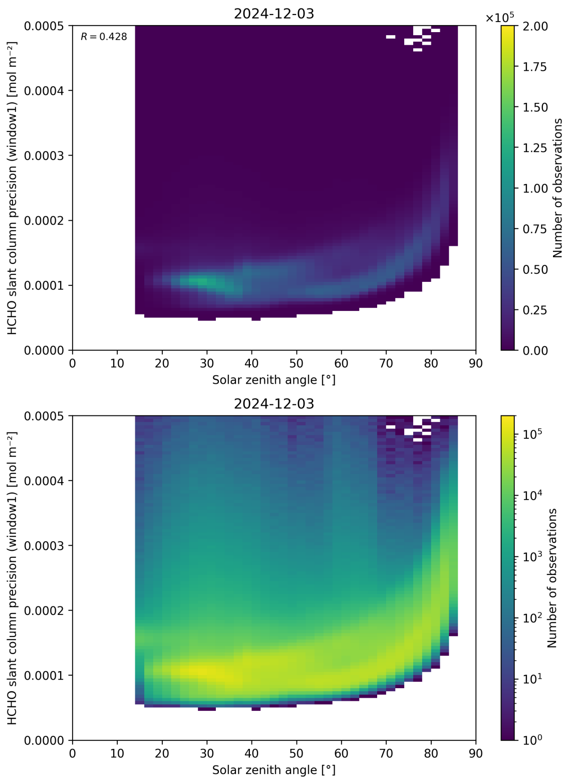
Figure 174: Scatter density plot of “Solar zenith angle” against “HCHO slant column precision (window1)” for 2024-12-02 to 2024-12-04.
