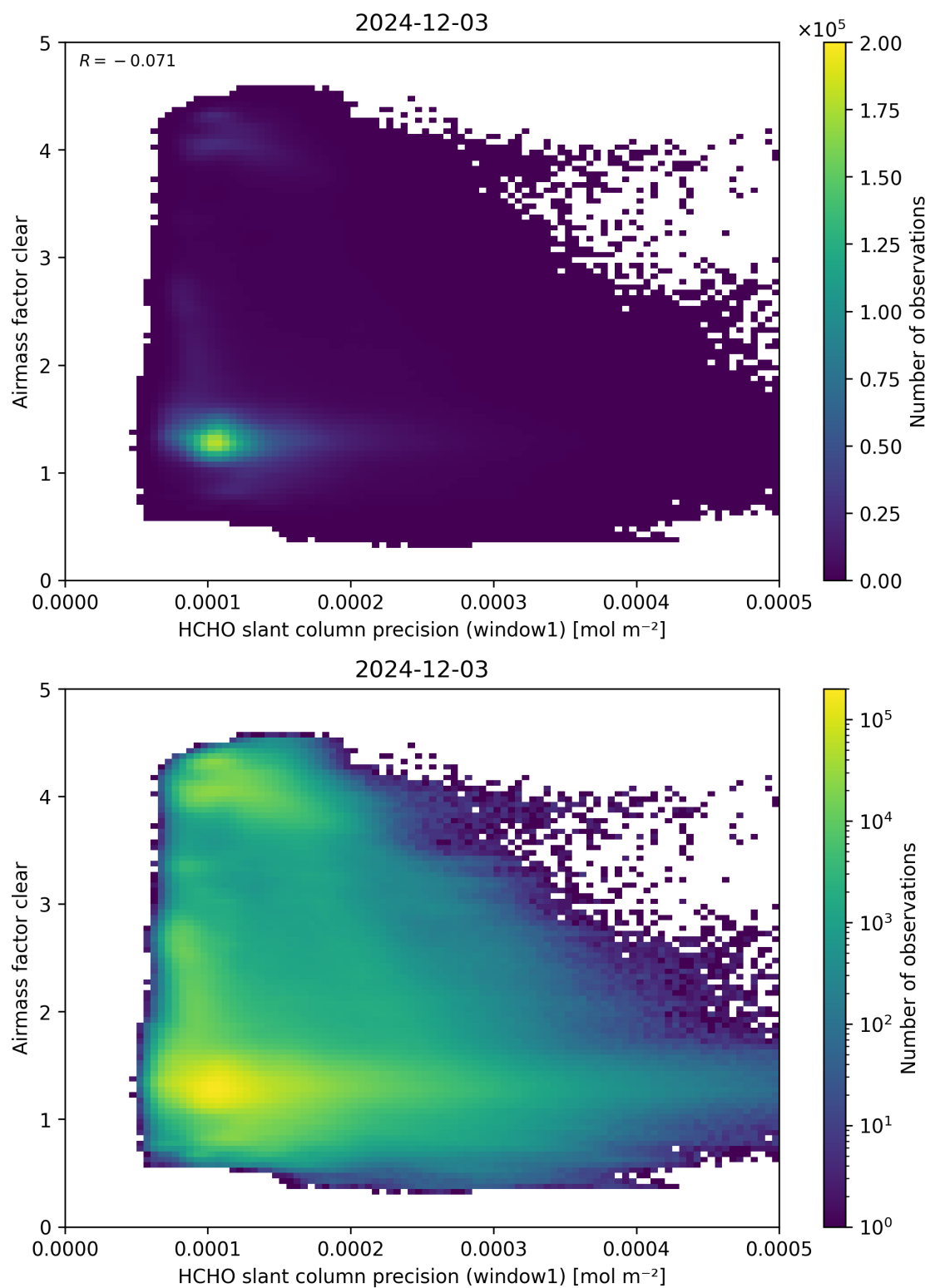
Figure 91: Scatter density plot of “HCHO slant column precision (window1)” against “Airmass factor clear” for 2024-12-02 to 2024-12-04.
