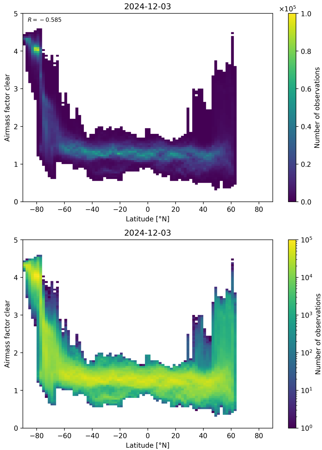
Figure 156: Scatter density plot of “Latitude” against “Airmass factor clear” for 2024-12-02 to 2024-12-04.
