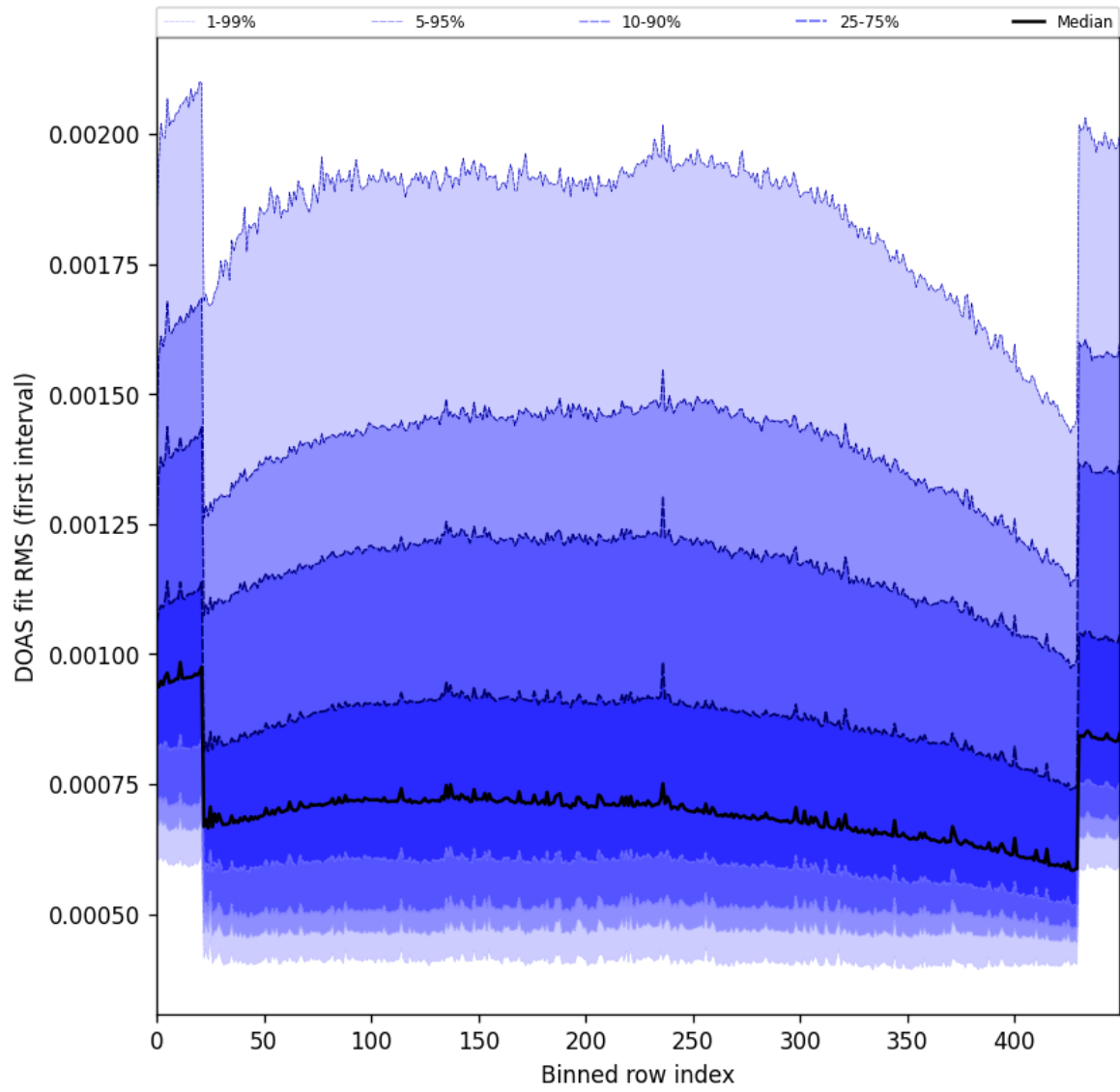
Figure 60: Along track statistics of “DOAS fit RMS (first interval)” for 2024-12-02 to 2024-12-04
