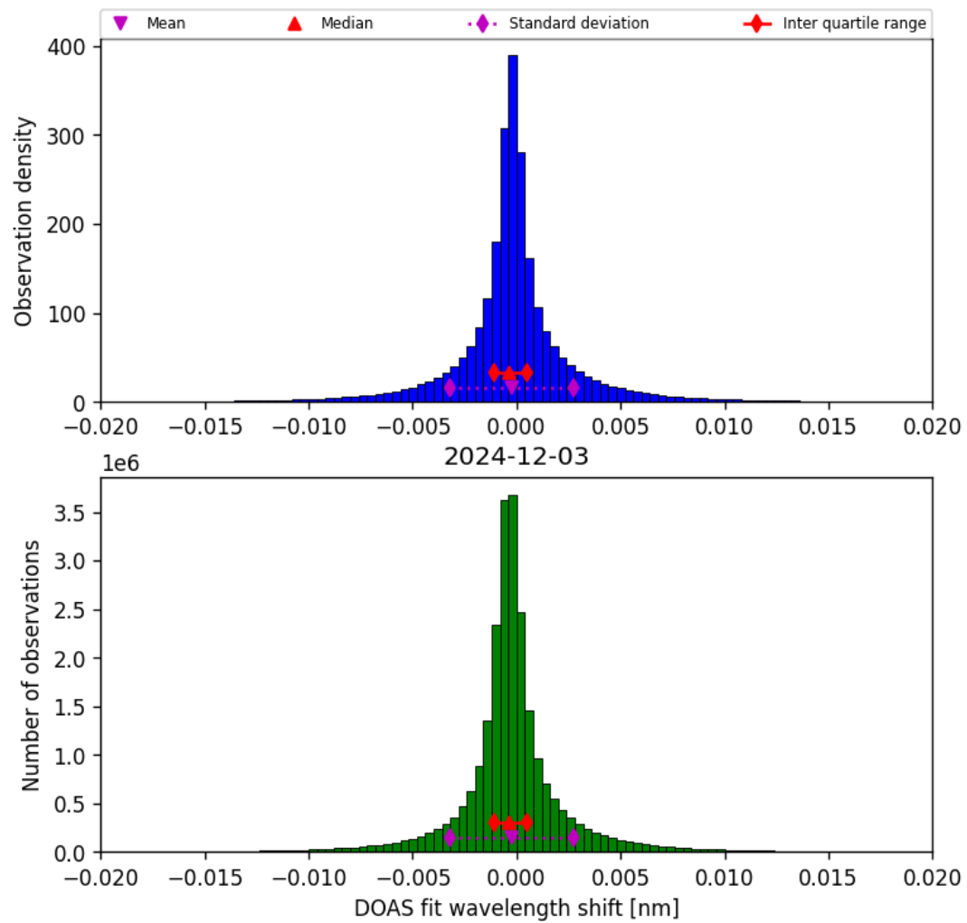
Figure 44: Histogram of “DOAS fit wavelength shift” for 2024-12-02 to 2024-12-04
