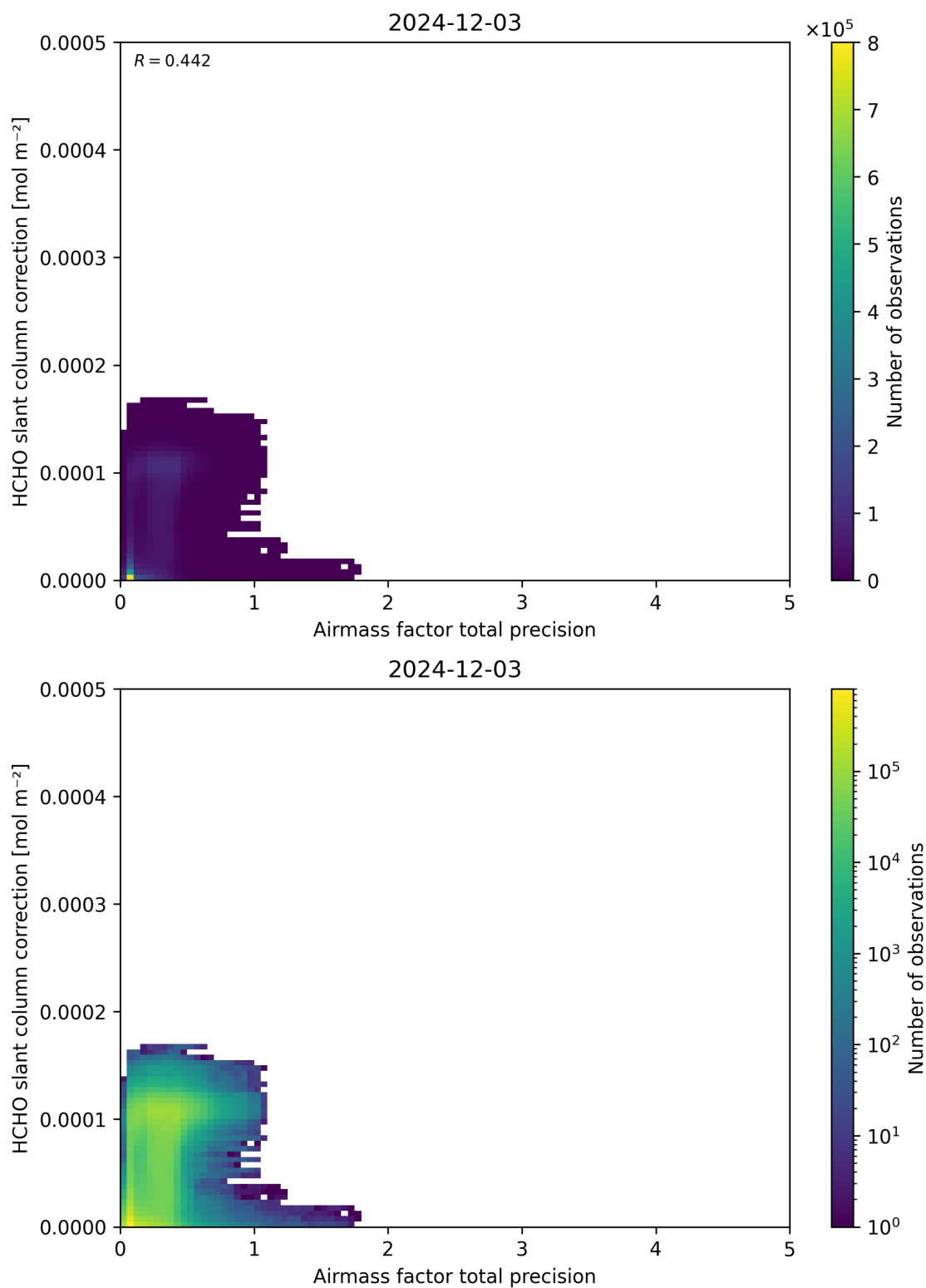
Figure 110: Scatter density plot of “Airmass factor total precision” against “HCHO slant column correction” for 2024-12-02 to 2024-12-04.
