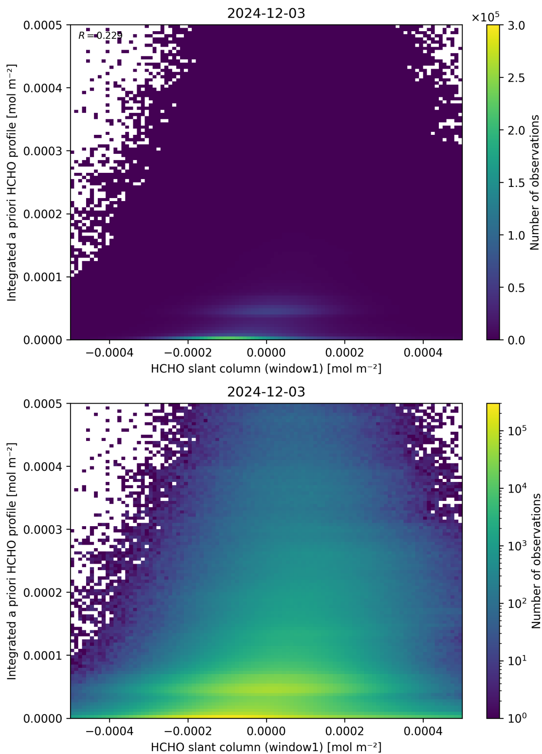
Figure 87: Scatter density plot of “HCHO slant column (window1)” against “Integrated a priori HCHO profile” for 2024-12-02 to 2024-12-04.
