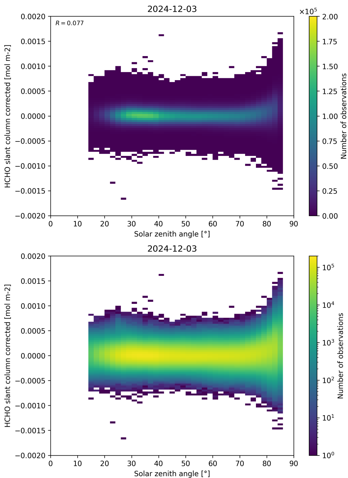
Figure 171: Scatter density plot of “Solar zenith angle” against “HCHO slant column corrected” for 2024-12-02 to 2024-12-04.
