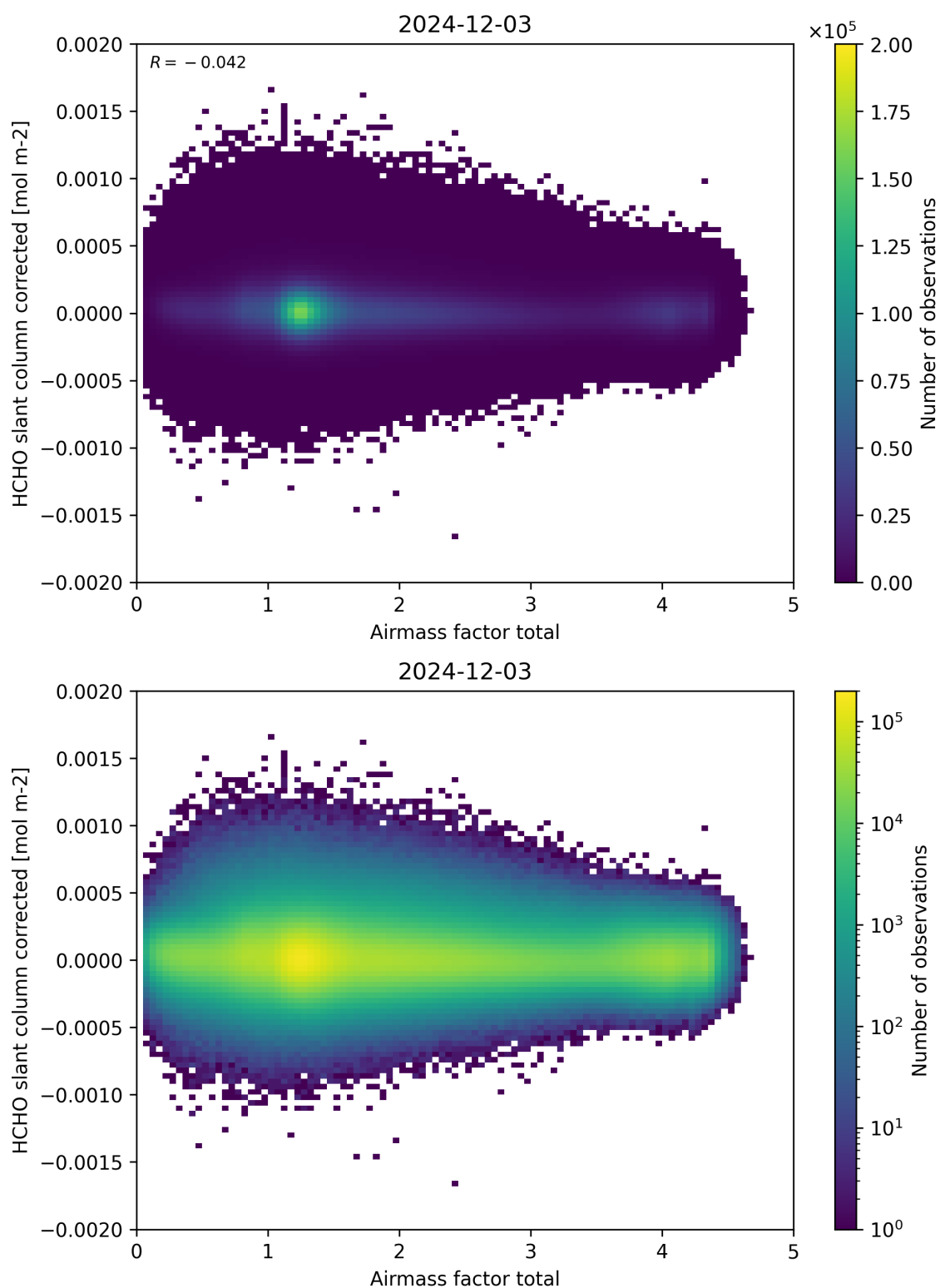
Figure 101: Scatter density plot of “Airmass factor total” against “HCHO slant column corrected” for 2024-12-02 to 2024-12-04.
