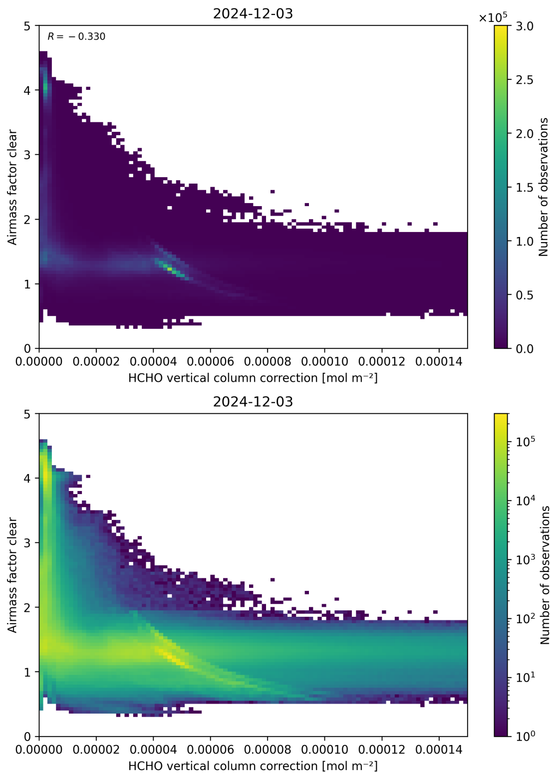
Figure 115: Scatter density plot of “HCHO vertical column correction” against “Airmass factor clear” for 2024-12-02 to 2024-12-04.
