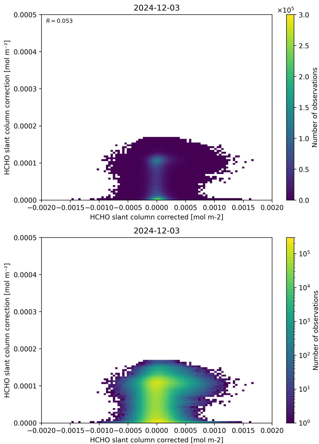
Figure 77: Scatter density plot of “HCHO slant column corrected” against “HCHO slant column correction” for 2024-12-02 to 2024-12-04.
