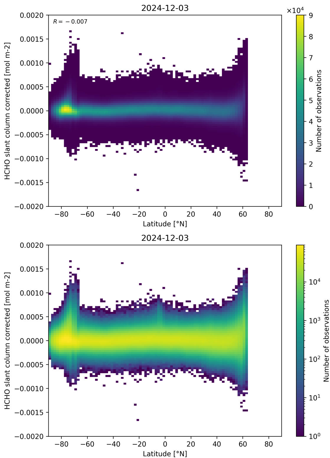
Figure 157: Scatter density plot of “Latitude” against “HCHO slant column corrected” for 2024-12-02 to 2024-12-04.
