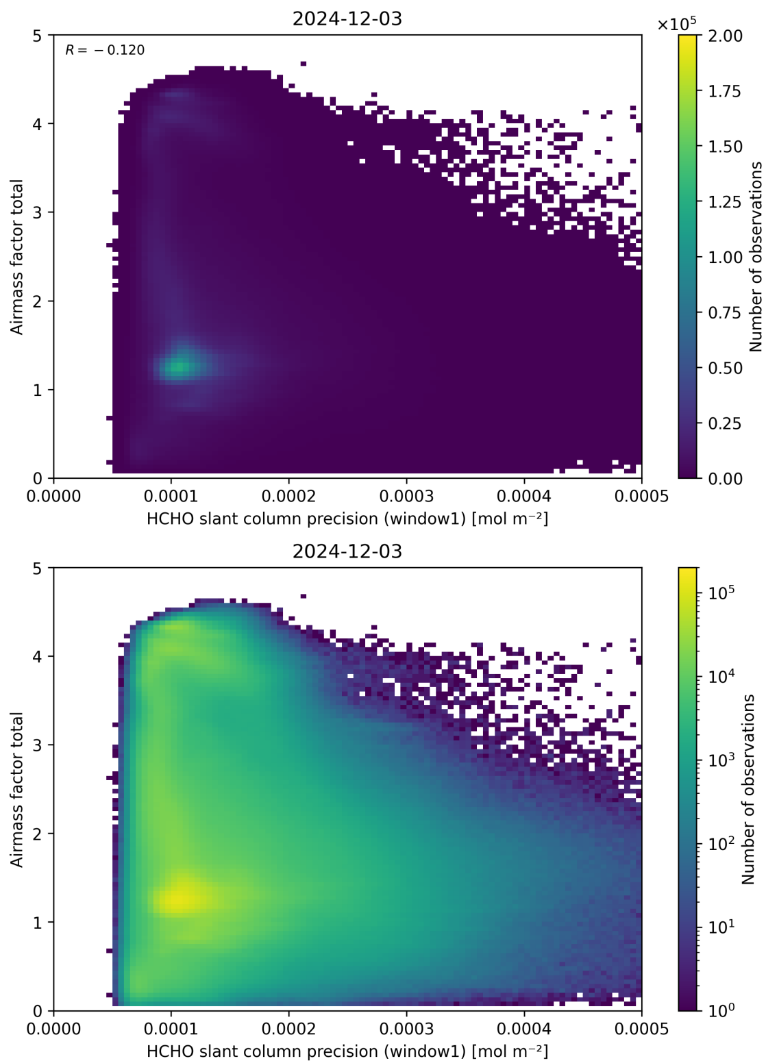
Figure 94: Scatter density plot of “HCHO slant column precision (window1)” against “Airmass factor total” for 2024-12-02 to 2024-12-04.
