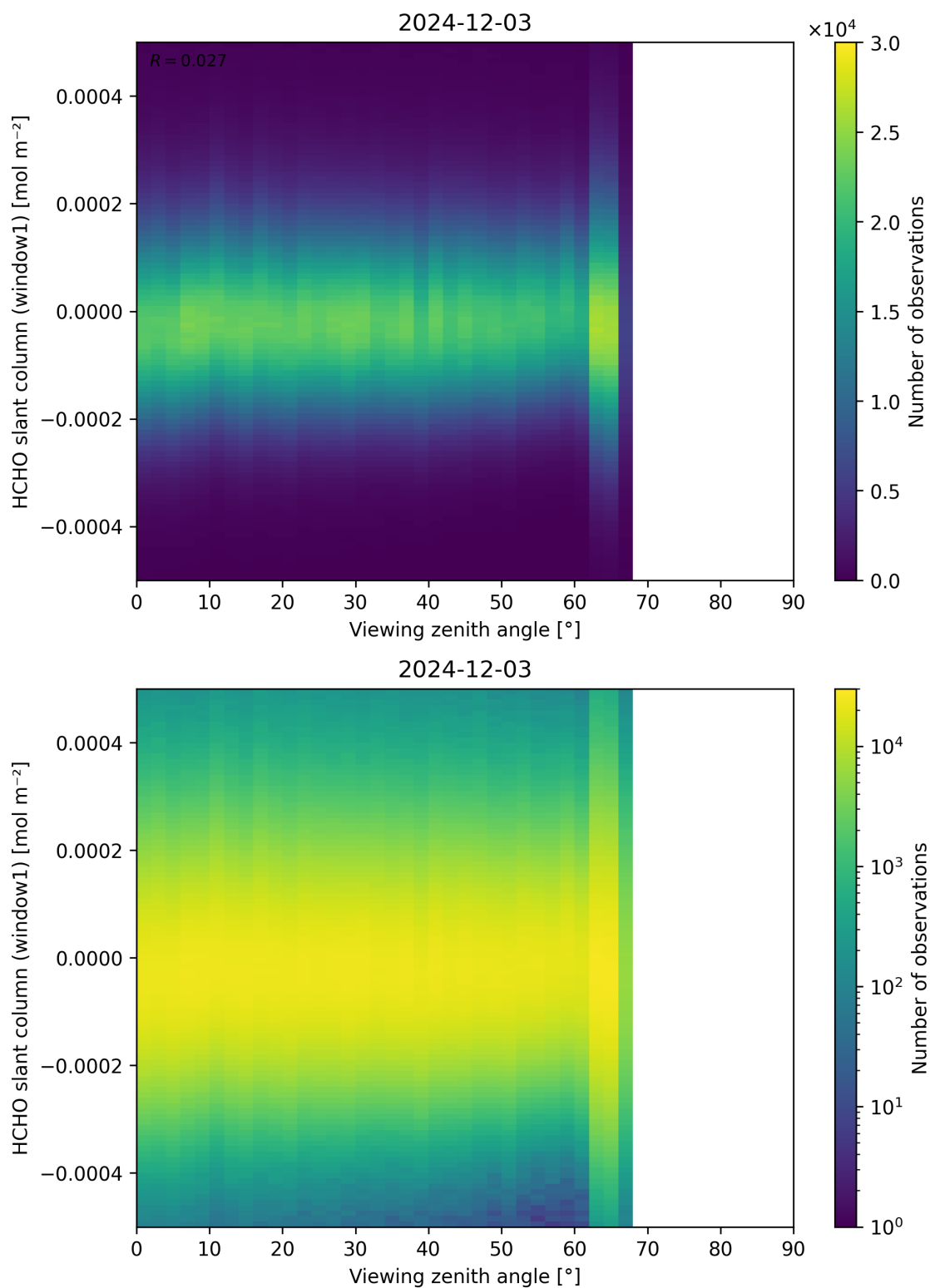
Figure 188: Scatter density plot of “Viewing zenith angle” against “HCHO slant column (window1)” for 2024-12-02 to 2024-12-04.
