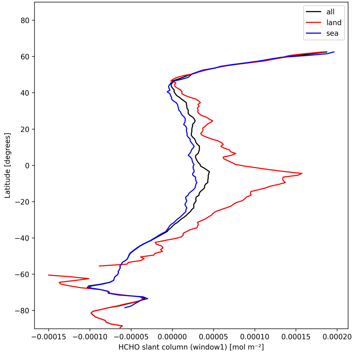
Figure 24: Zonal average of “HCHO slant column (window1)” for 2024-12-02 to 2024-12-04.
