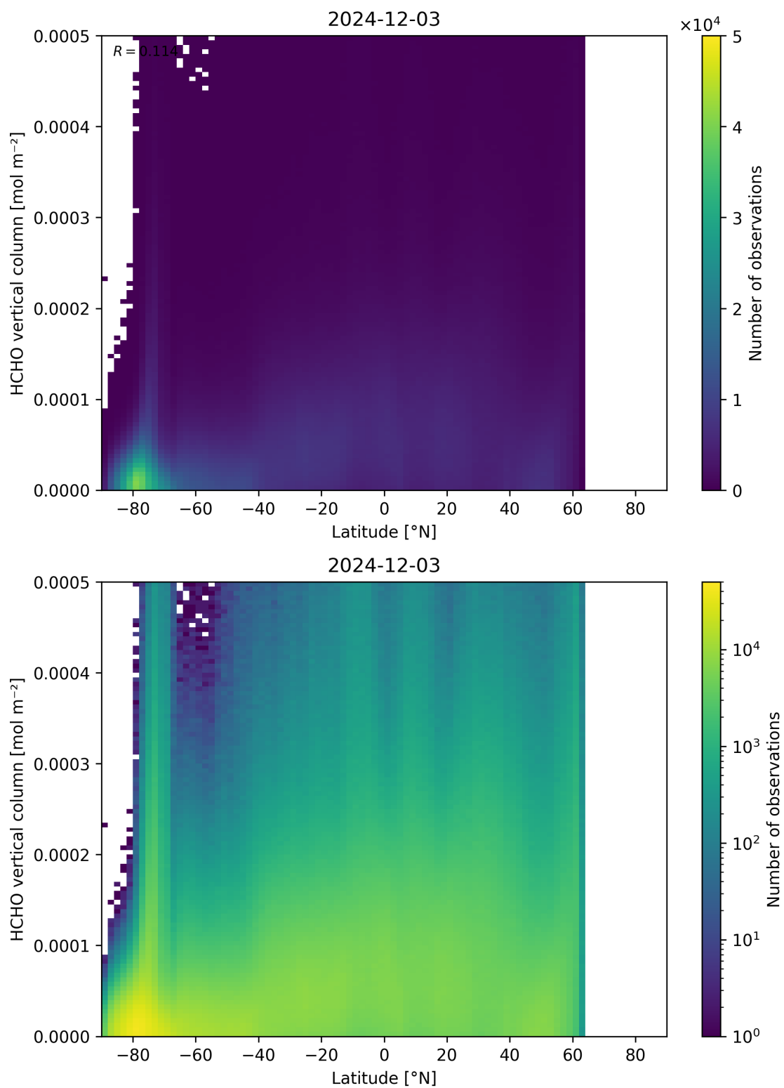
Figure 163: Scatter density plot of “Latitude” against “HCHO vertical column” for 2024-12-02 to 2024-12-04.
