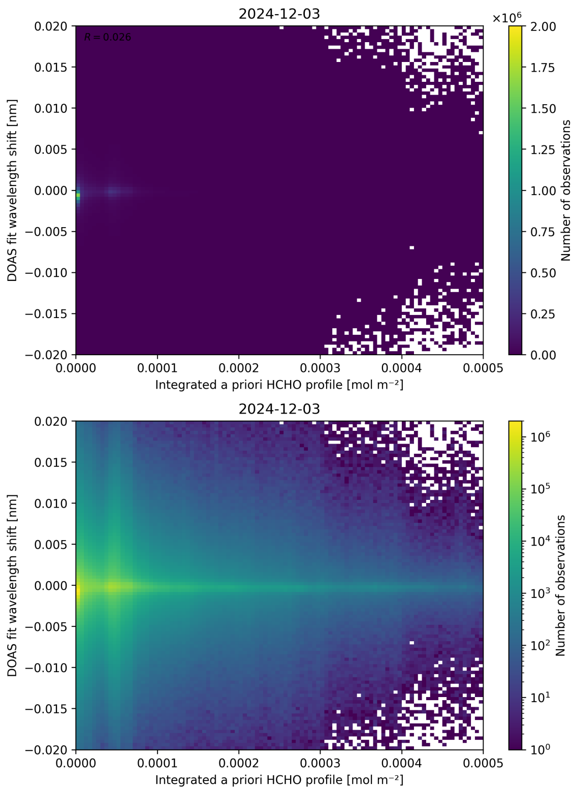
Figure 149: Scatter density plot of “Integrated a priori HCHO profile” against “DOAS fit wavelength shift” for 2024-12-02 to 2024-12-04.
