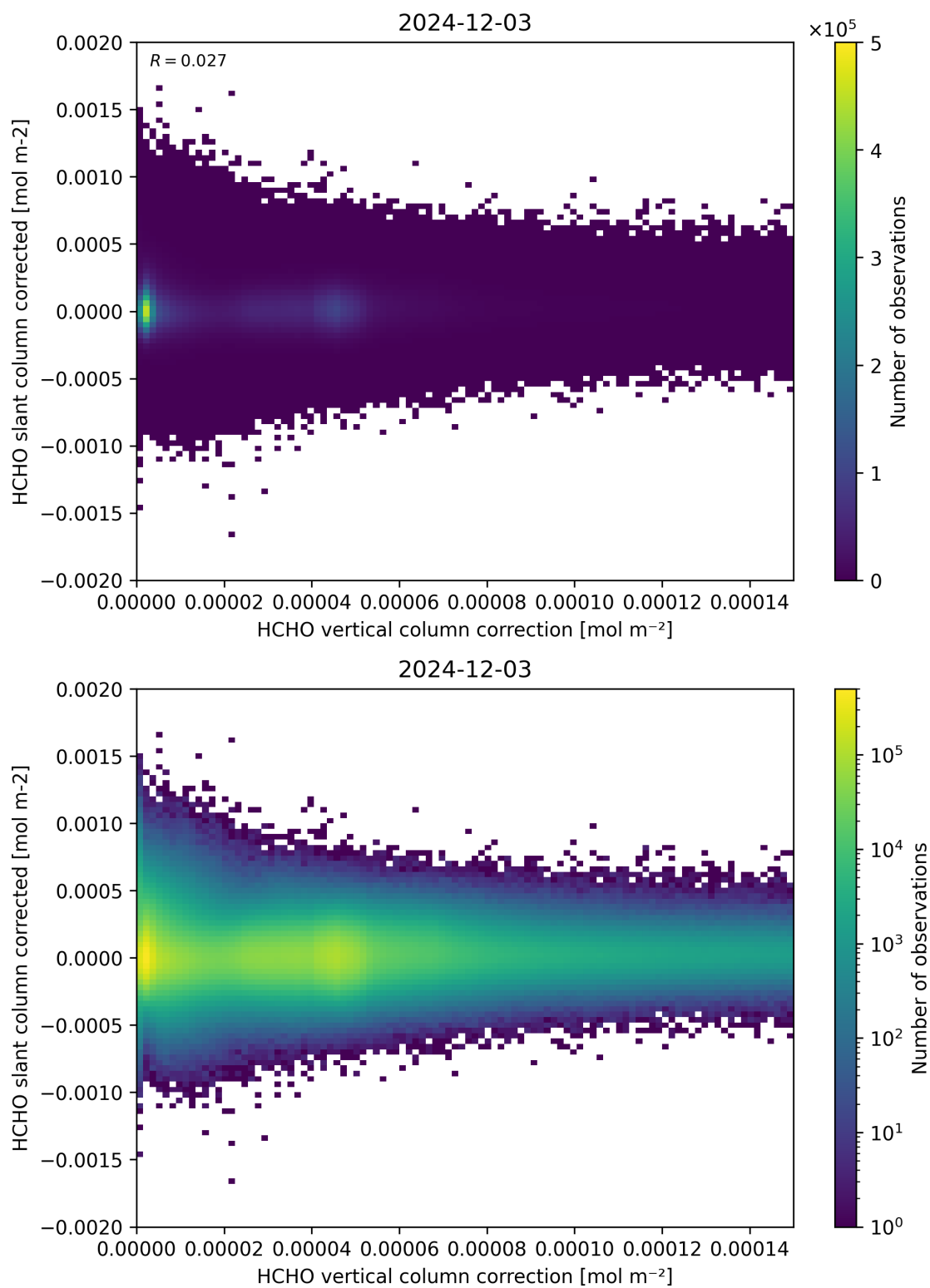
Figure 116: Scatter density plot of “HCHO vertical column correction” against “HCHO slant column corrected” for 2024-12-02 to 2024-12-04.
