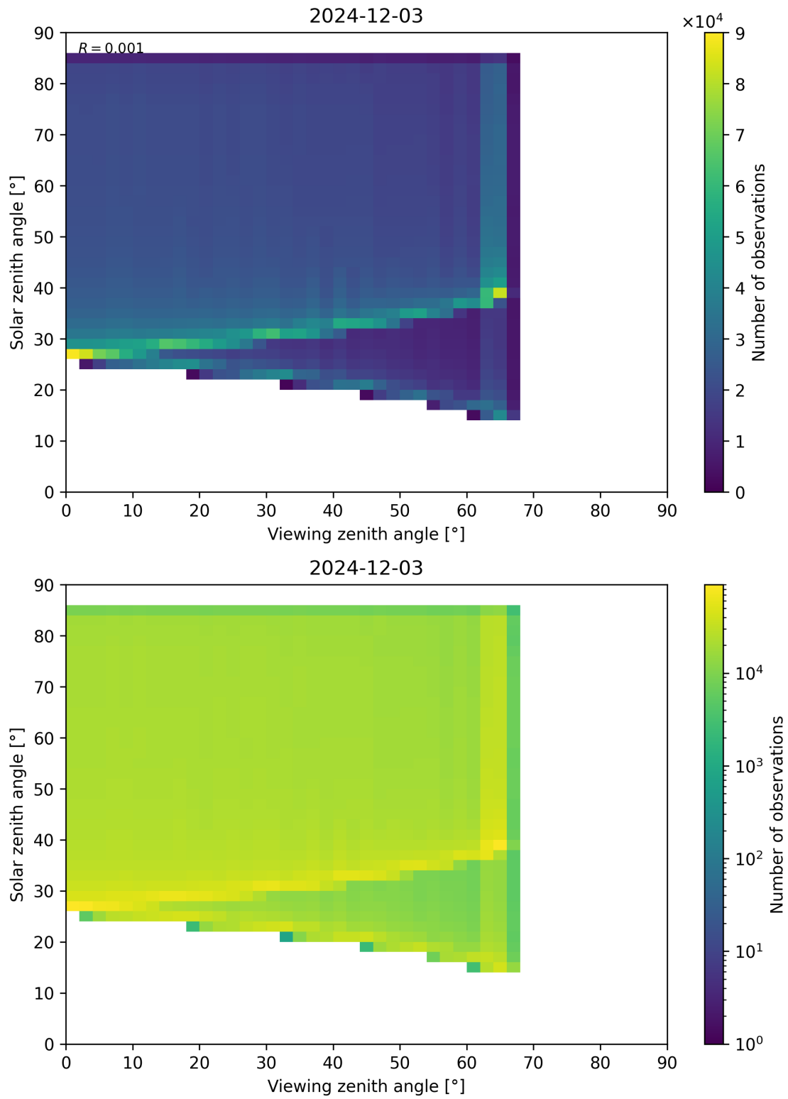
Figure 197: Scatter density plot of “Viewing zenith angle” against “Solar zenith angle” for 2024-12-02 to 2024-12-04.
