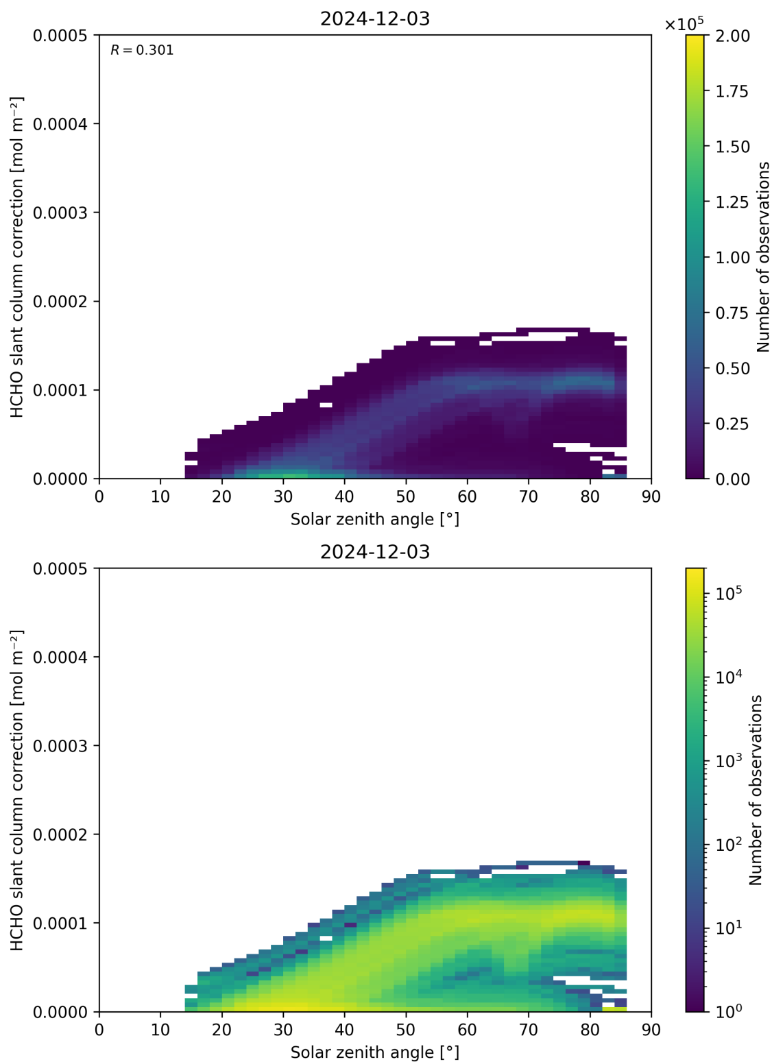
Figure 172: Scatter density plot of “Solar zenith angle” against “HCHO slant column correction” for 2024-12-02 to 2024-12-04.
