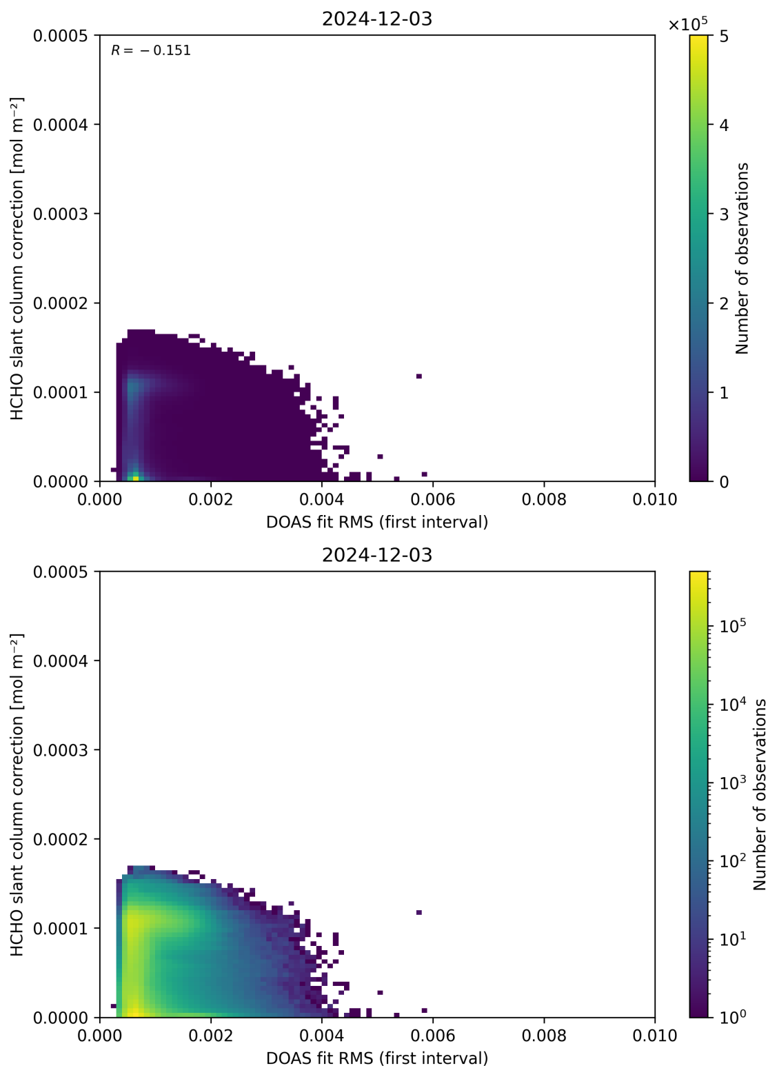
Figure 63: Scatter density plot of “DOAS fit RMS (first interval)” against “HCHO slant column correction” for 2024-12-02 to 2024-12-04.
