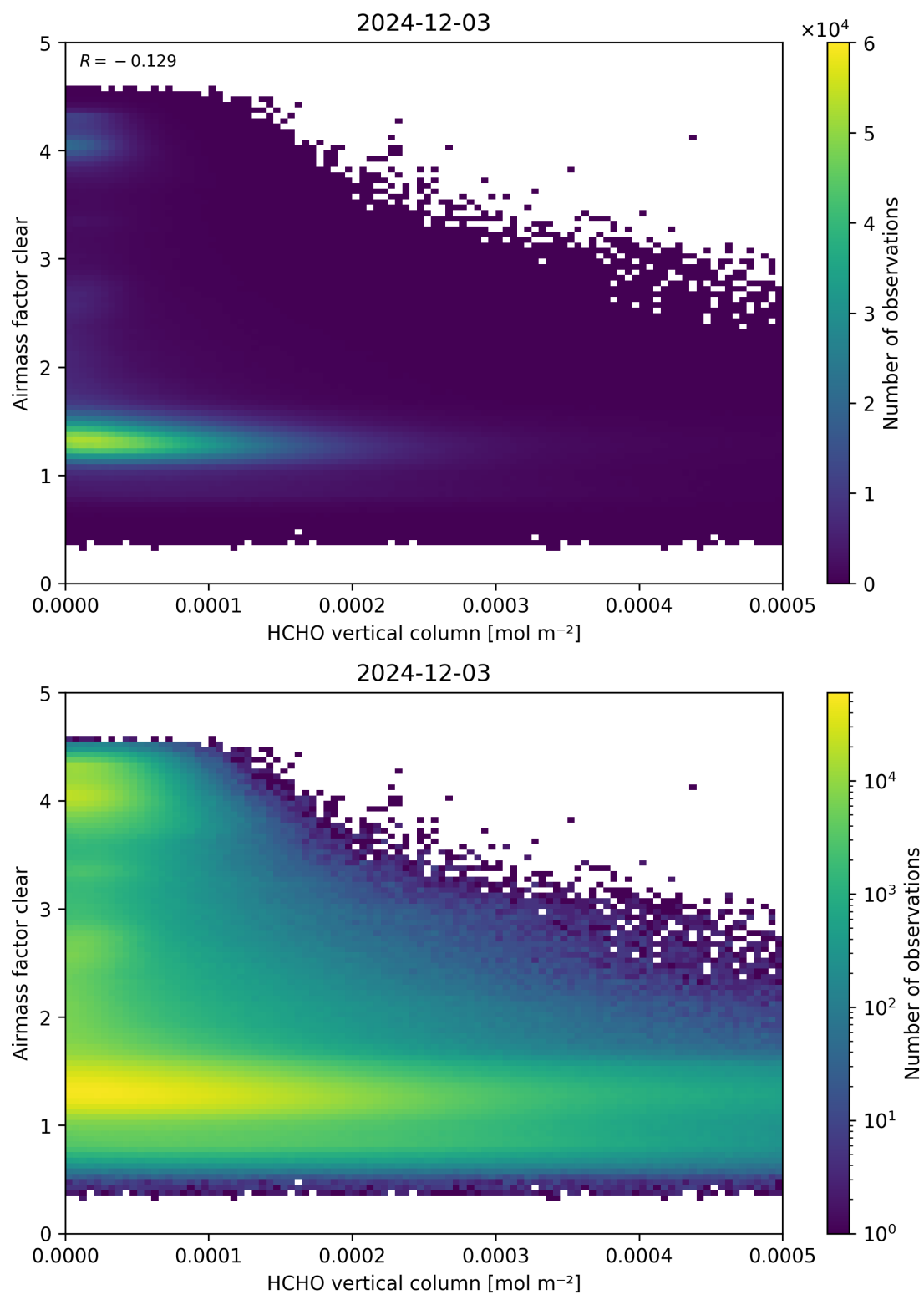
Figure 126: Scatter density plot of “HCHO vertical column” against “Airmass factor clear” for 2024-12-02 to 2024-12-04.
