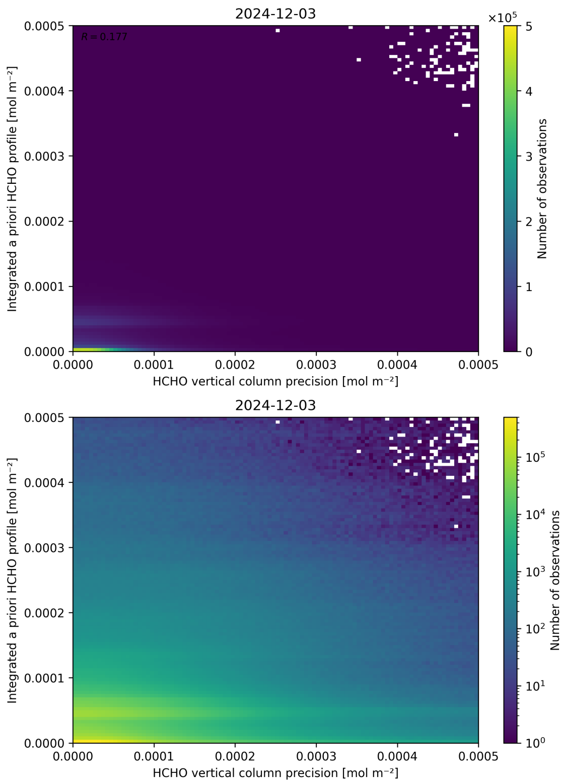
Figure 147: Scatter density plot of “HCHO vertical column precision” against “Integrated a priori HCHO profile” for 2024-12-02 to 2024-12-04.
