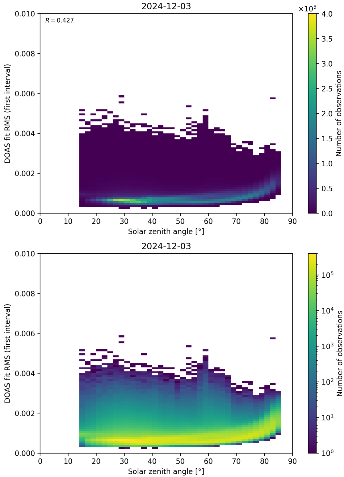
Figure 167: Scatter density plot of “Solar zenith angle” against “DOAS fit RMS (first interval)” for 2024-12-02 to 2024-12-04.
