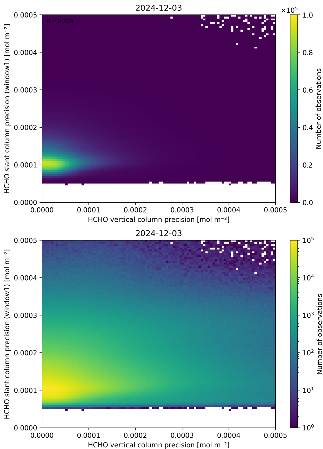
Figure 143: Scatter density plot of “HCHO vertical column precision” against “HCHO slant column precision (window1)” for 2024-12-02 to 2024-12-04.
