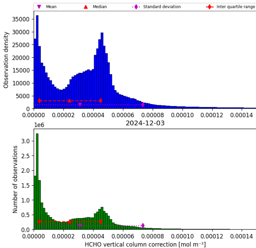
Figure 37: Histogram of “HCHO vertical column correction” for 2024-12-02 to 2024-12-04
