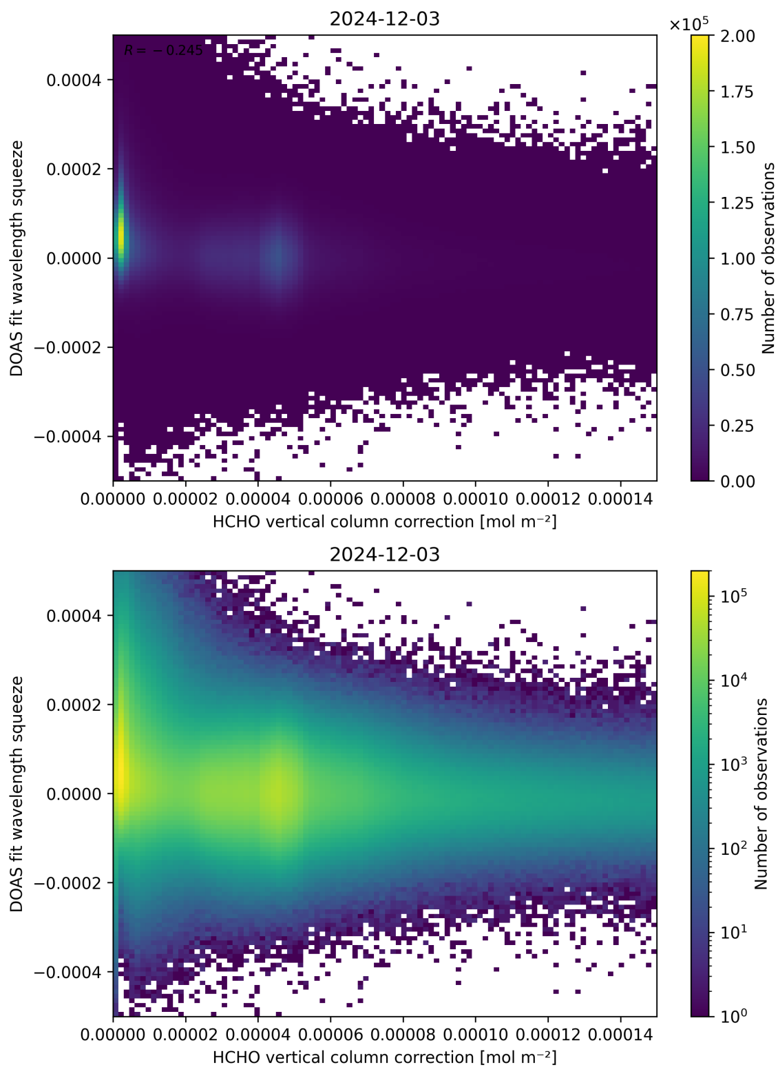
Figure 114: Scatter density plot of “HCHO vertical column correction” against “DOAS fit wavelength squeeze” for 2024-12-02 to 2024-12-04.
