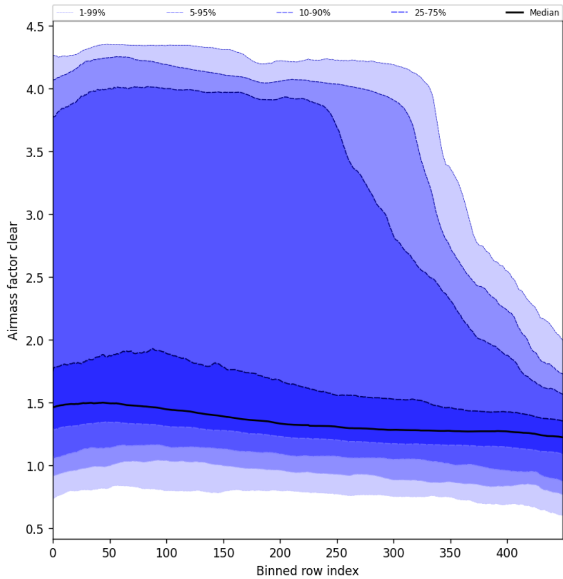
Figure 56: Along track statistics of “Air mass factor clear” for 2024-12-02 to 2024-12-04
