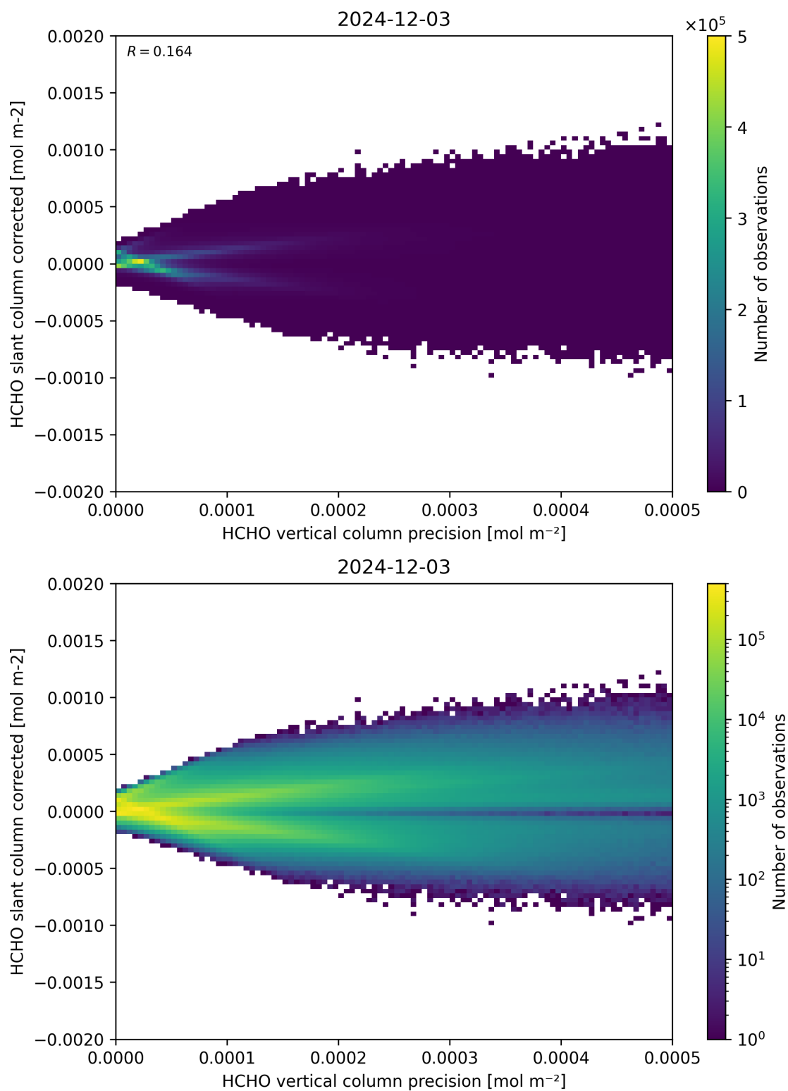
Figure 140: Scatter density plot of “HCHO vertical column precision” against “HCHO slant column corrected” for 2024-12-02 to 2024-12-04.
