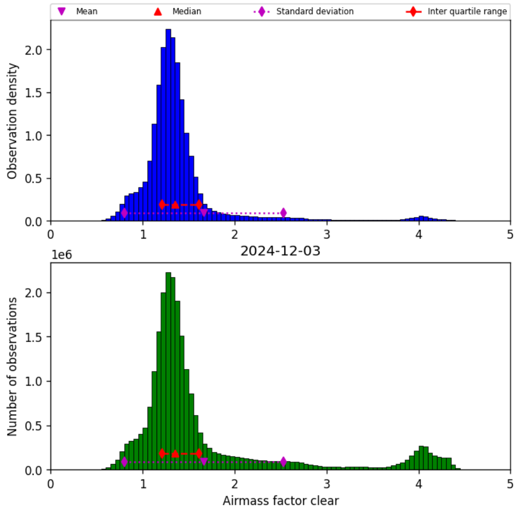
Figure 42: Histogram of “Airmass factor clear” for 2024-12-02 to 2024-12-04
