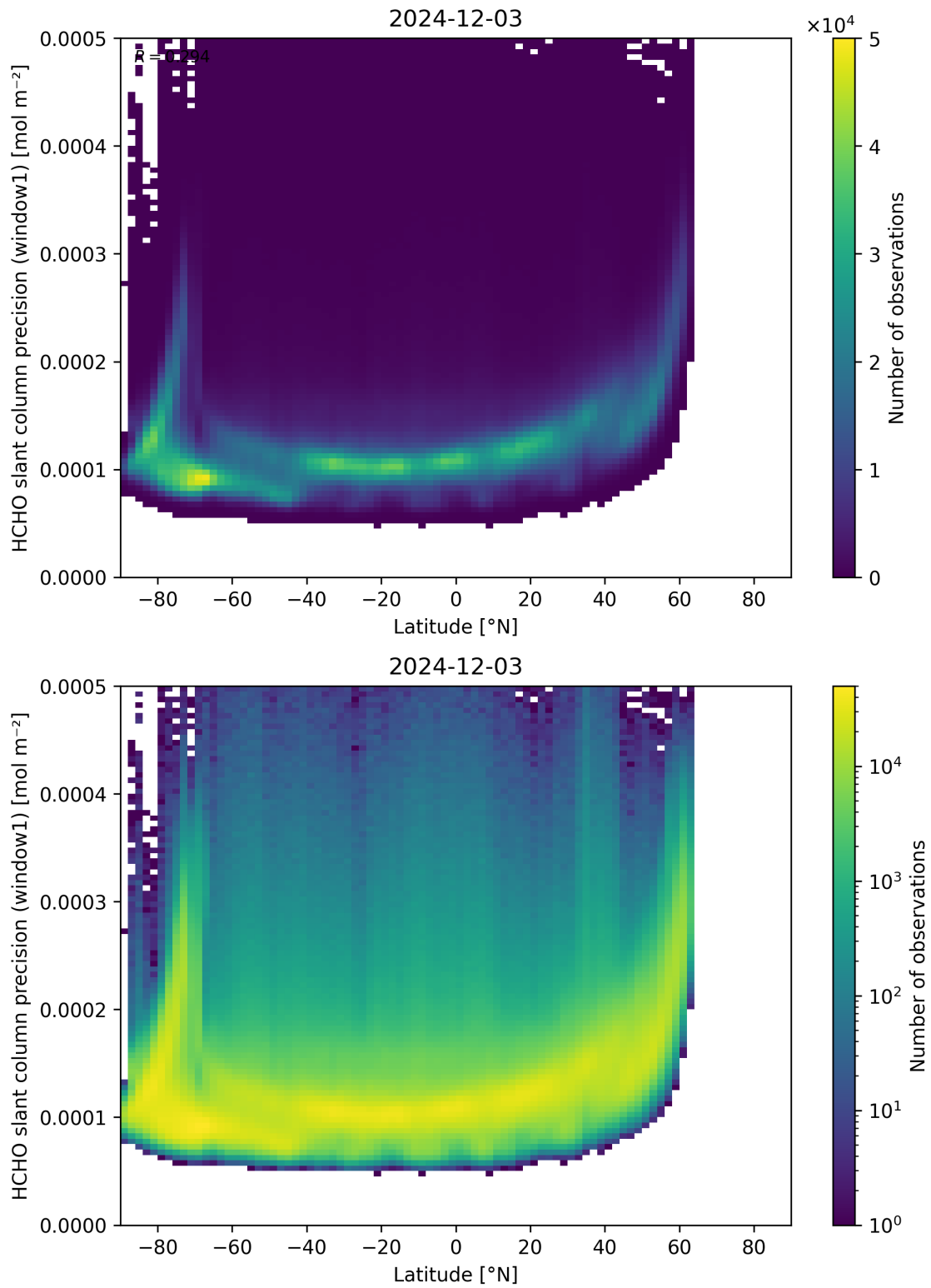
Figure 160: Scatter density plot of “Latitude” against “HCHO slant column precision (window1)” for 2024-12-02 to 2024-12-04.
