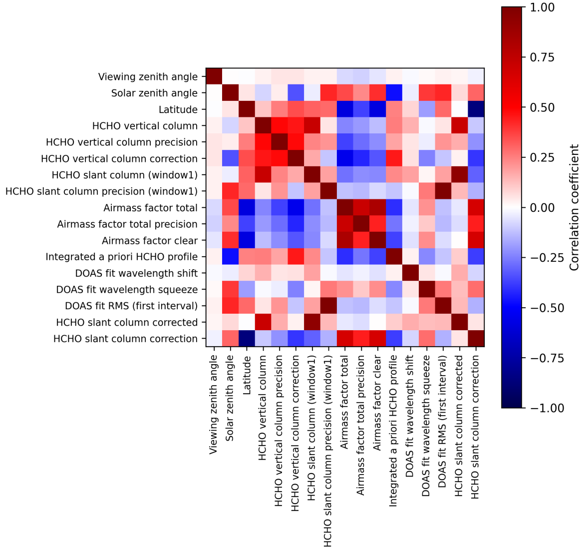
Figure 2: Map of correlation matrix for 2024-12-02 to 2024-12-04.
