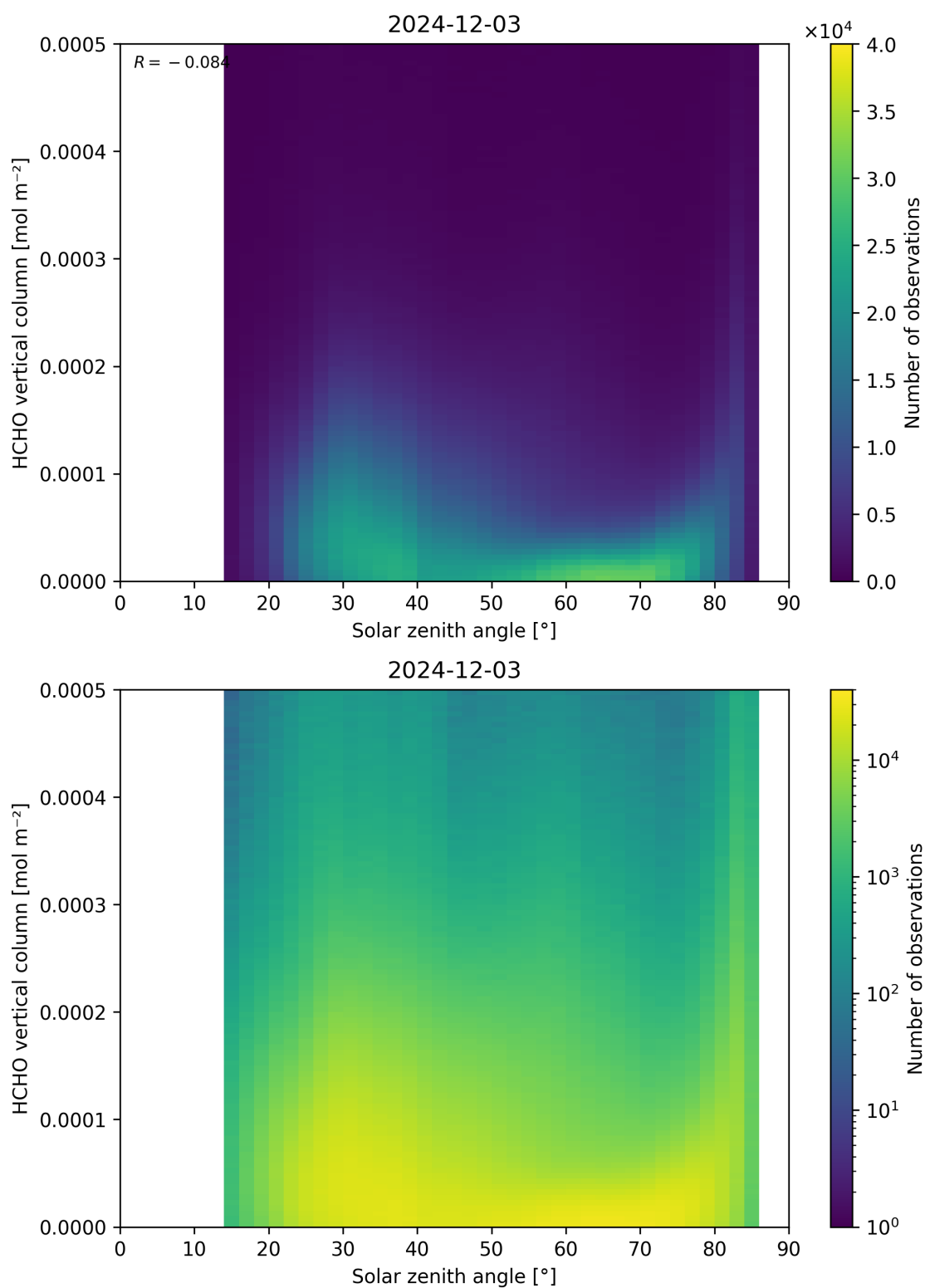
Figure 177: Scatter density plot of “Solar zenith angle” against “HCHO vertical column” for 2024-12-02 to 2024-12-04.
