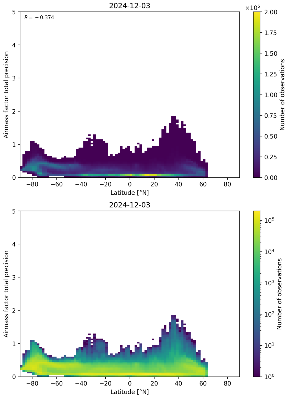
Figure 162: Scatter density plot of “Latitude” against “Airmass factor total precision” for 2024-12-02 to 2024-12-04.
