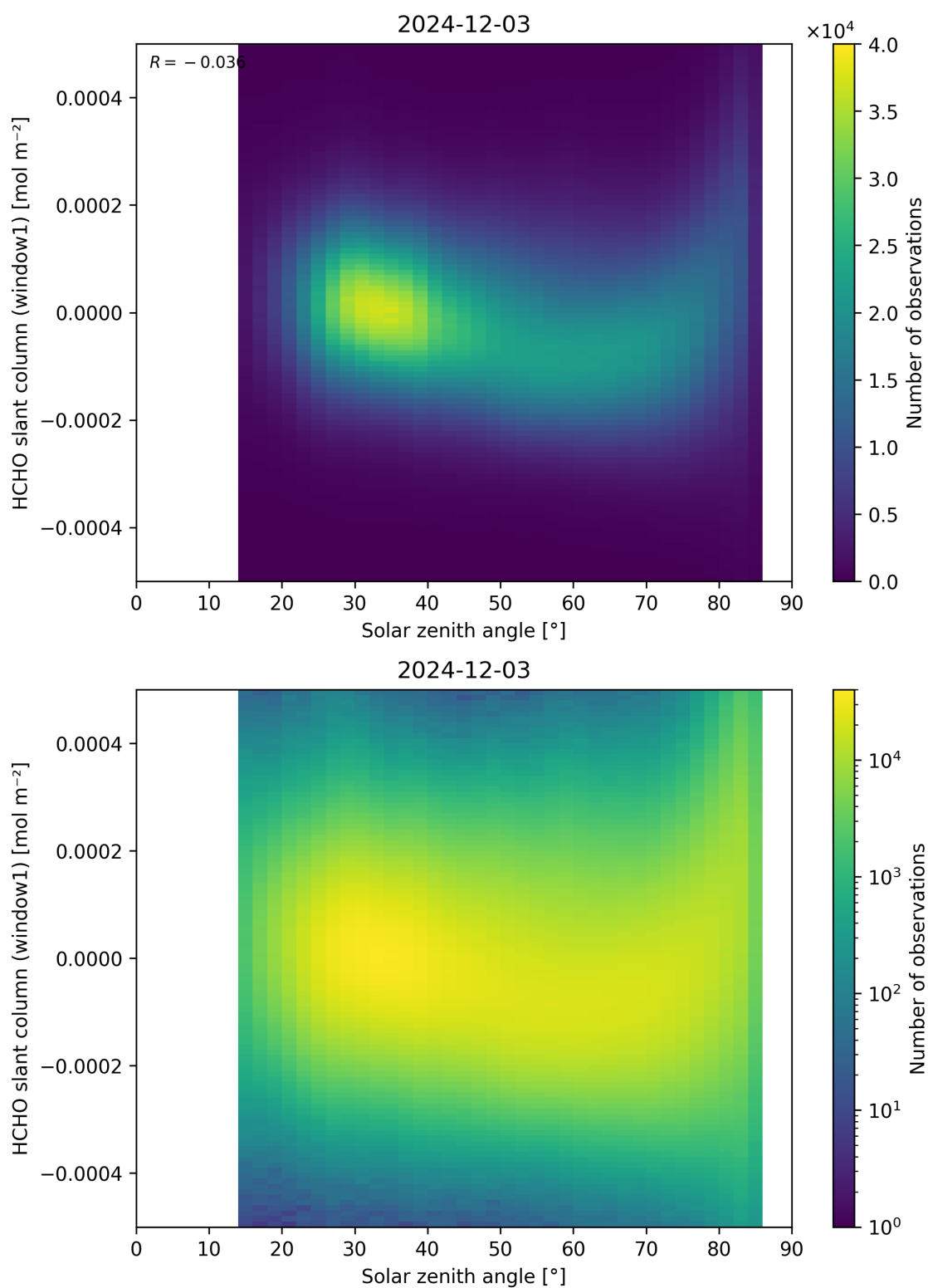
Figure 173: Scatter density plot of “Solar zenith angle” against “HCHO slant column (window1)” for 2024-12-02 to 2024-12-04.
