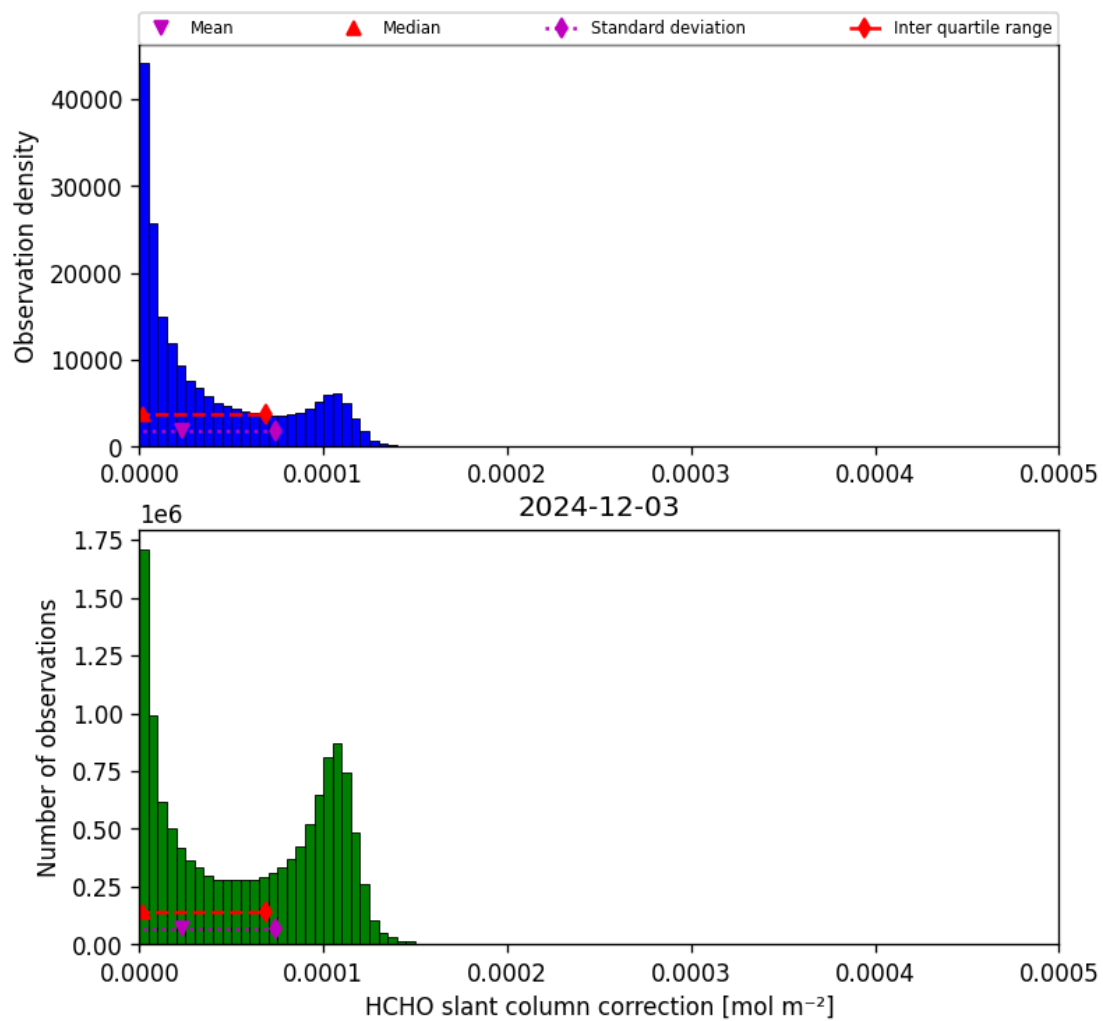
Figure 47: Histogram of “HCHO slant column correction” for 2024-12-02 to 2024-12-04
