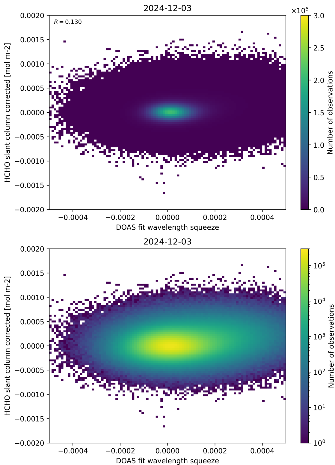
Figure 69: Scatter density plot of “DOAS fit wavelength squeeze” against “HCHO slant column corrected” for 2024-12-02 to 2024-12-04.
