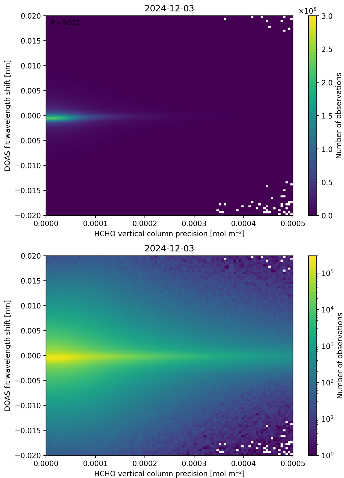
Figure 137: Scatter density plot of “HCHO vertical column precision” against “DOAS fit wavelength shift” for 2024-12-02 to 2024-12-04.
