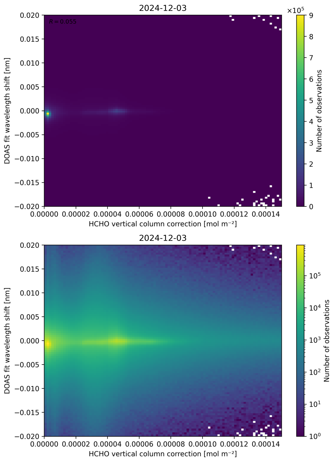
Figure 113: Scatter density plot of “HCHO vertical column correction” against “DOAS fit wavelength shift” for 2024-12-02 to 2024-12-04.
