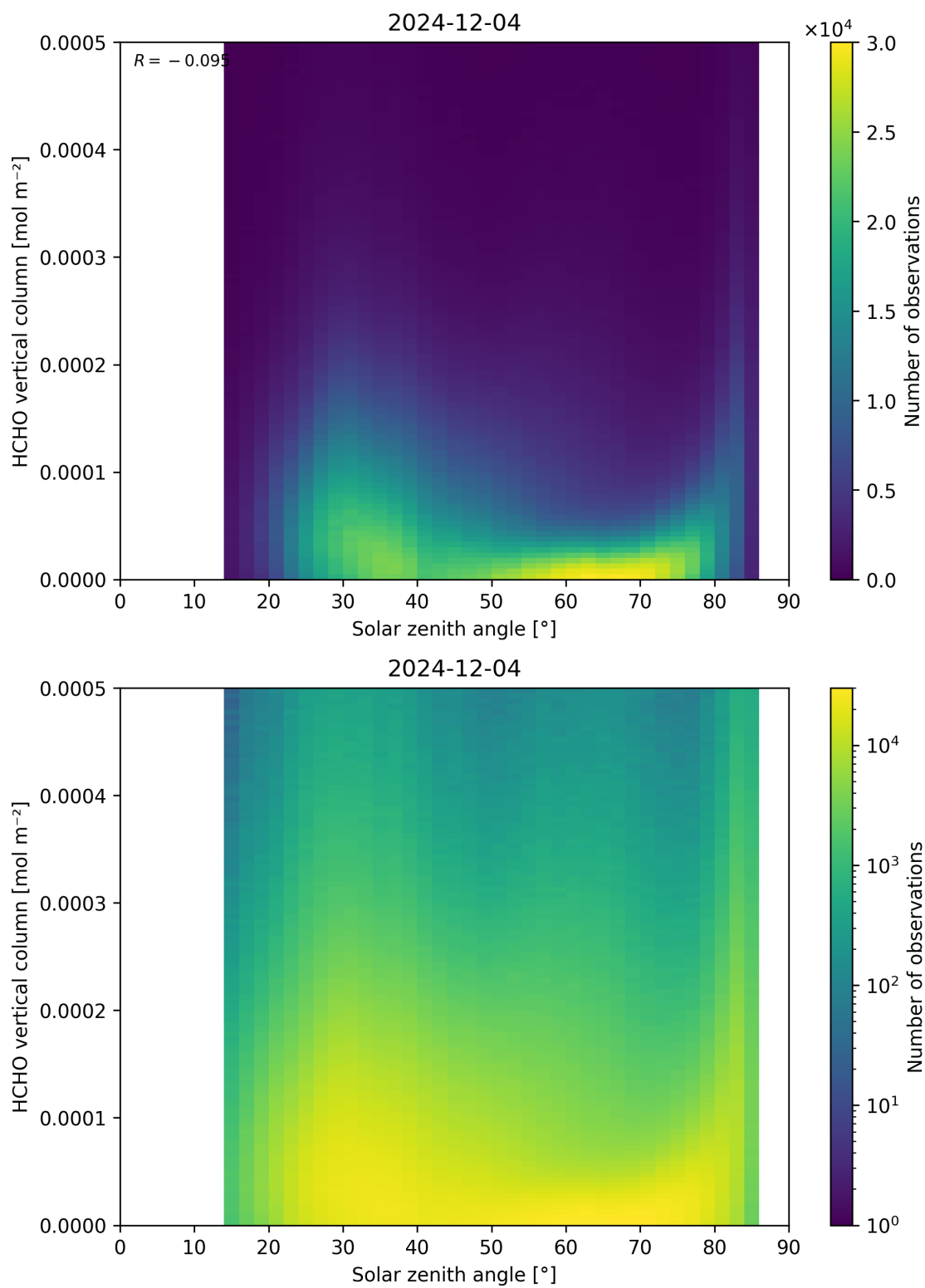
Figure 177: Scatter density plot of “Solar zenith angle” against “HCHO vertical column” for 2024-12-03 to 2024-12-05.
