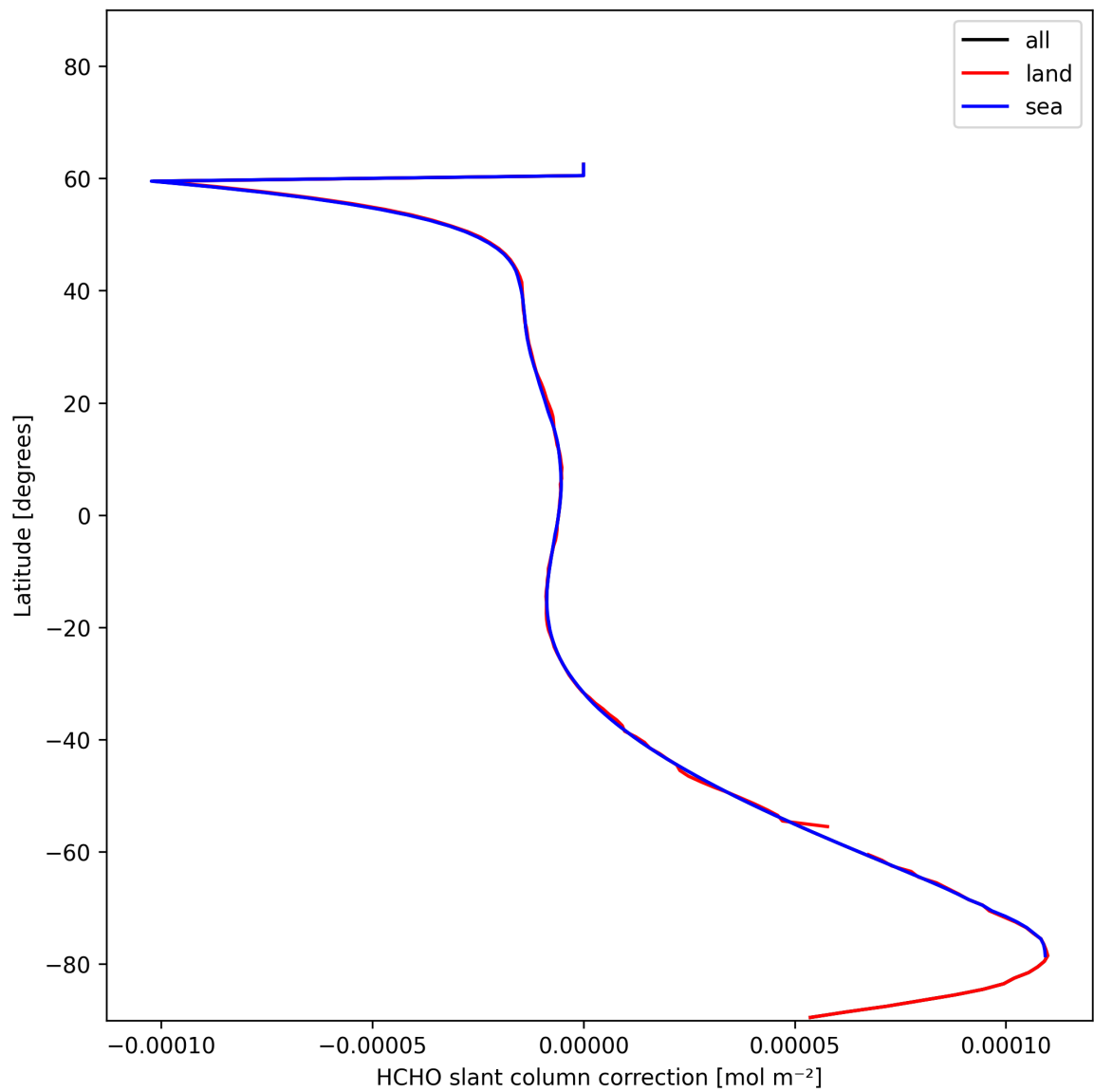
Figure 33: Zonal average of “HCHO slant column correction” for 2024-12-03 to 2024-12-05.
