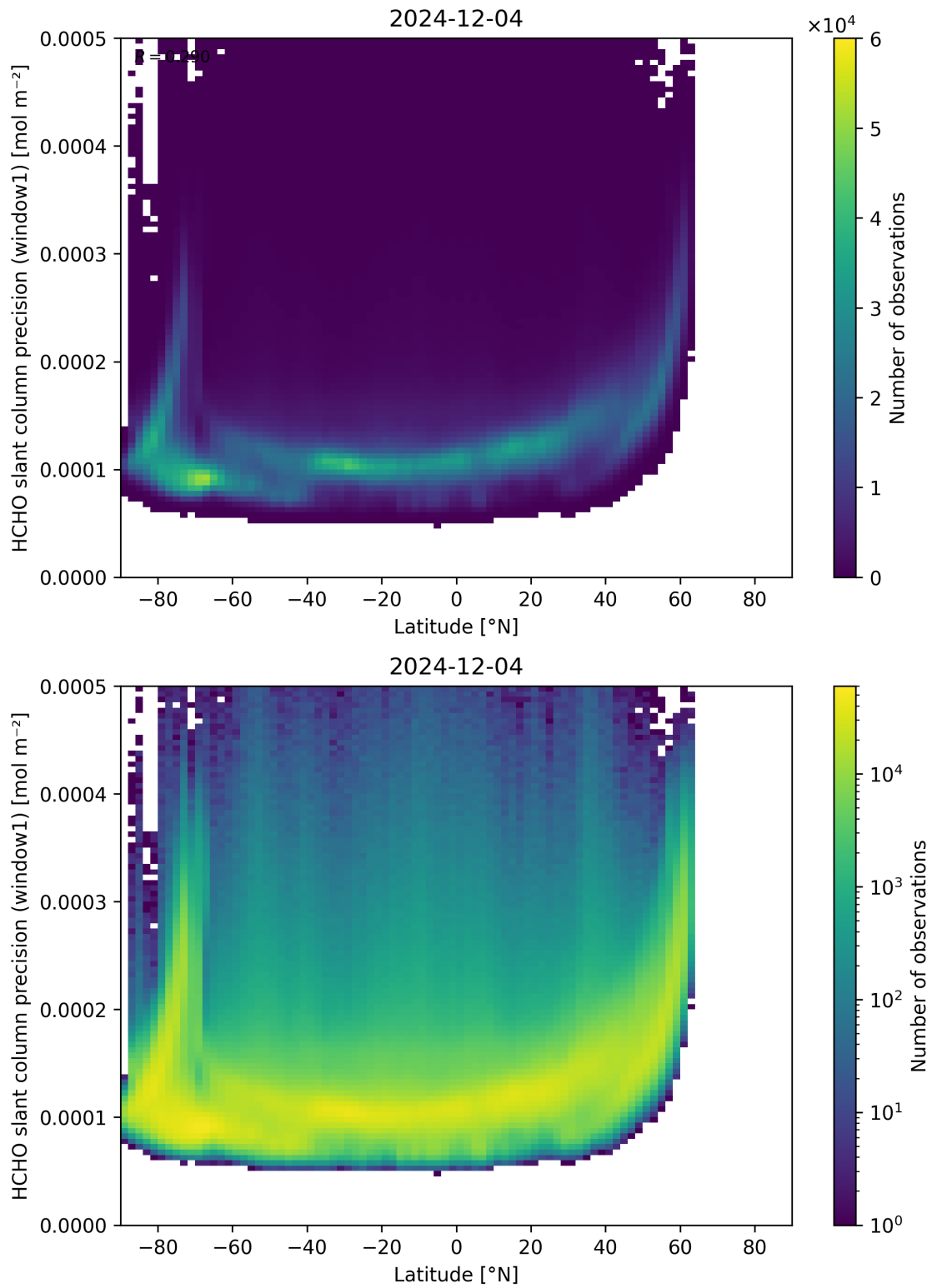
Figure 160: Scatter density plot of “Latitude” against “HCHO slant column precision (window1)” for 2024-12-03 to 2024-12-05.
