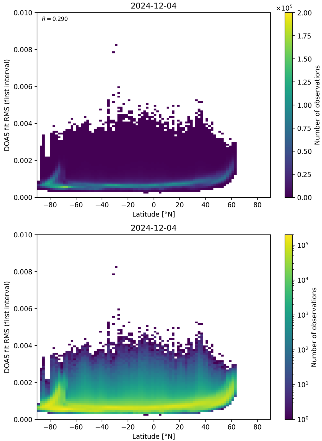
Figure 153: Scatter density plot of “Latitude” against “DOAS fit RMS (first interval)” for 2024-12-03 to 2024-12-05.
