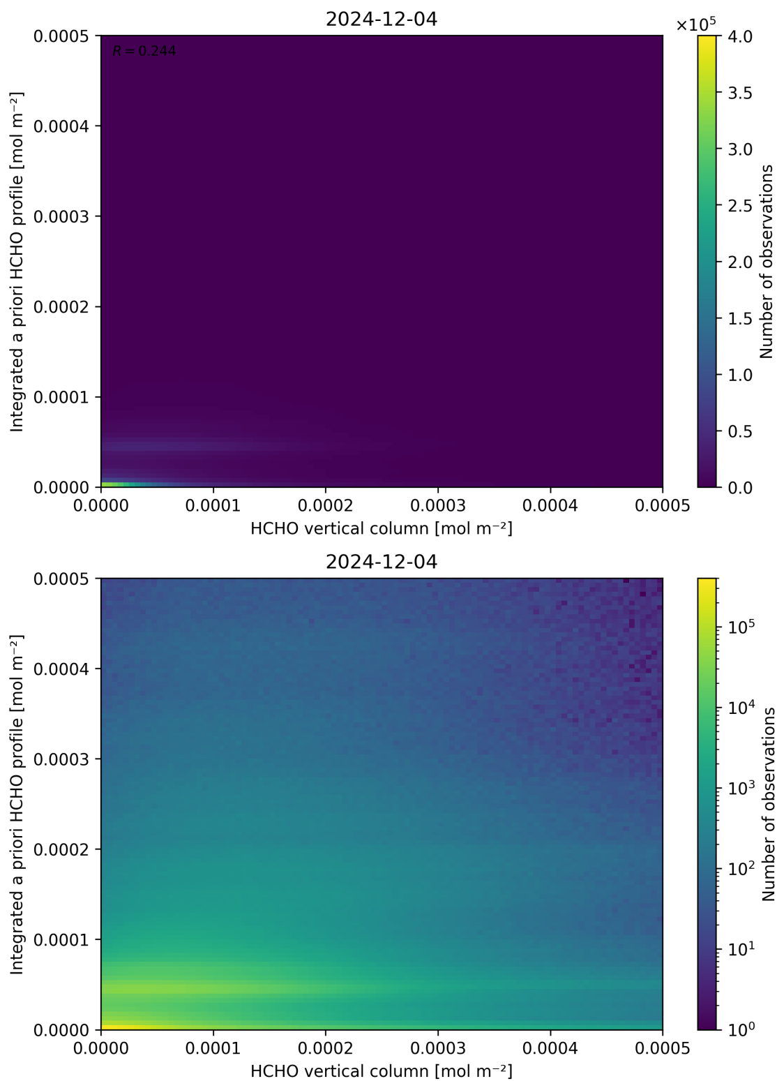
Figure 135: Scatter density plot of “HCHO vertical column” against “Integrated a priori HCHO profile” for 2024-12-03 to 2024-12-05.
