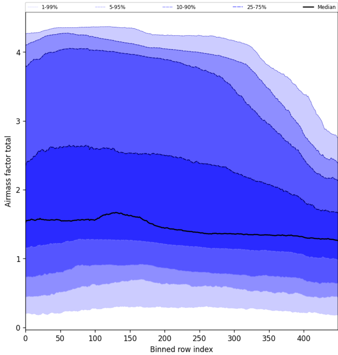
Figure 54: Along track statistics of “Airmass factor total” for 2024-12-03 to 2024-12-05
