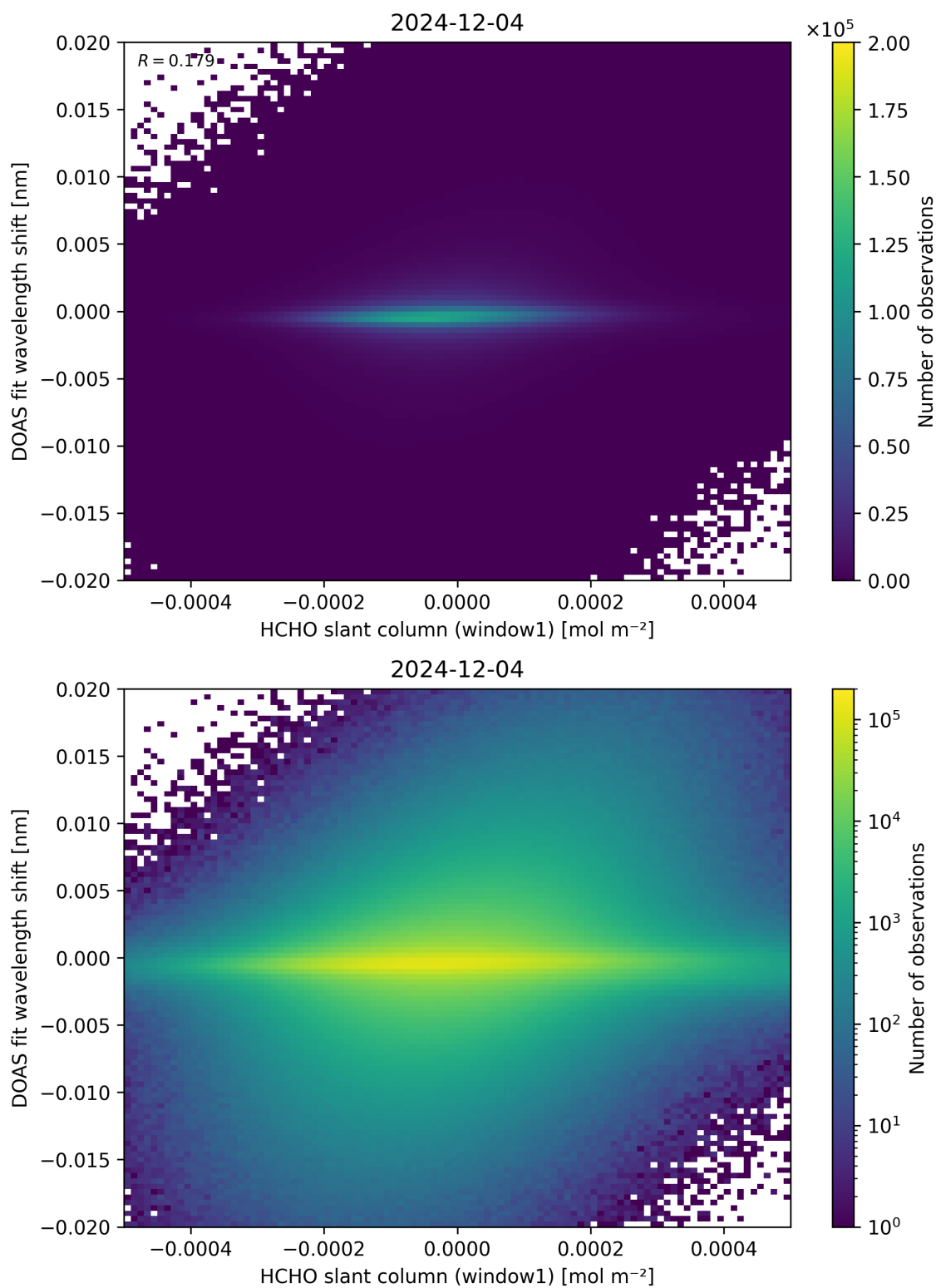
Figure 79: Scatter density plot of “HCHO slant column (window1)” against “DOAS fit wavelength shift” for 2024-12-03 to 2024-12-05.
