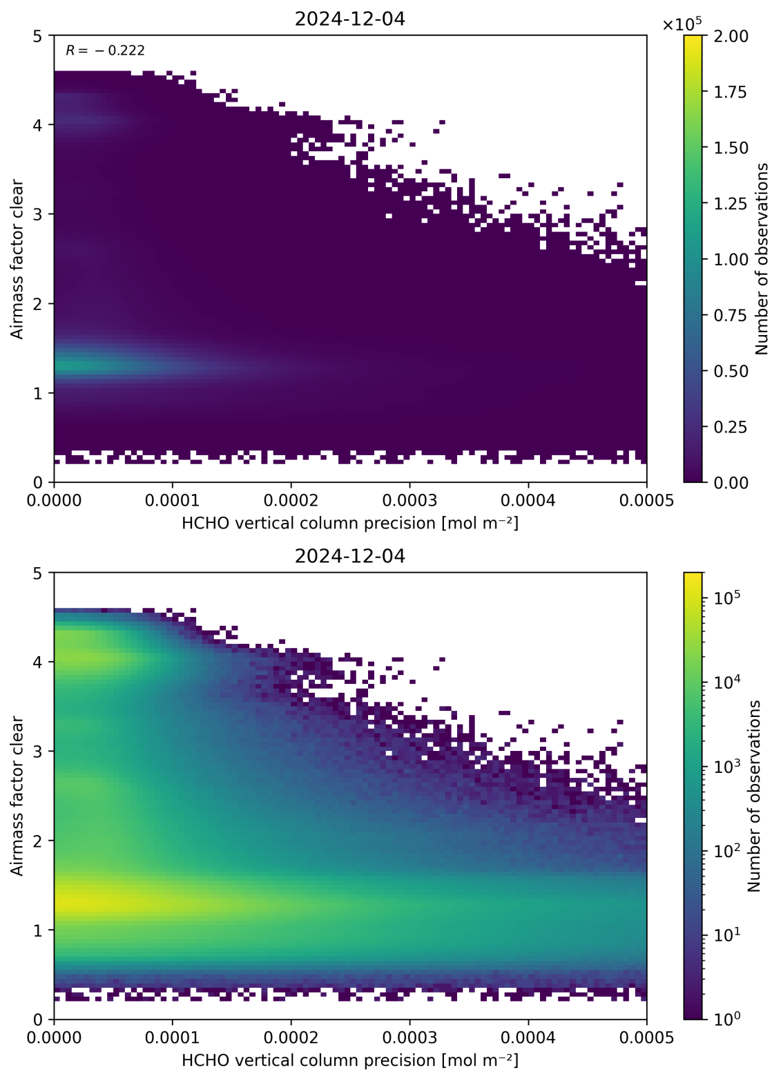
Figure 139: Scatter density plot of “HCHO vertical column precision” against “Airmass factor clear” for 2024-12-03 to 2024-12-05.
