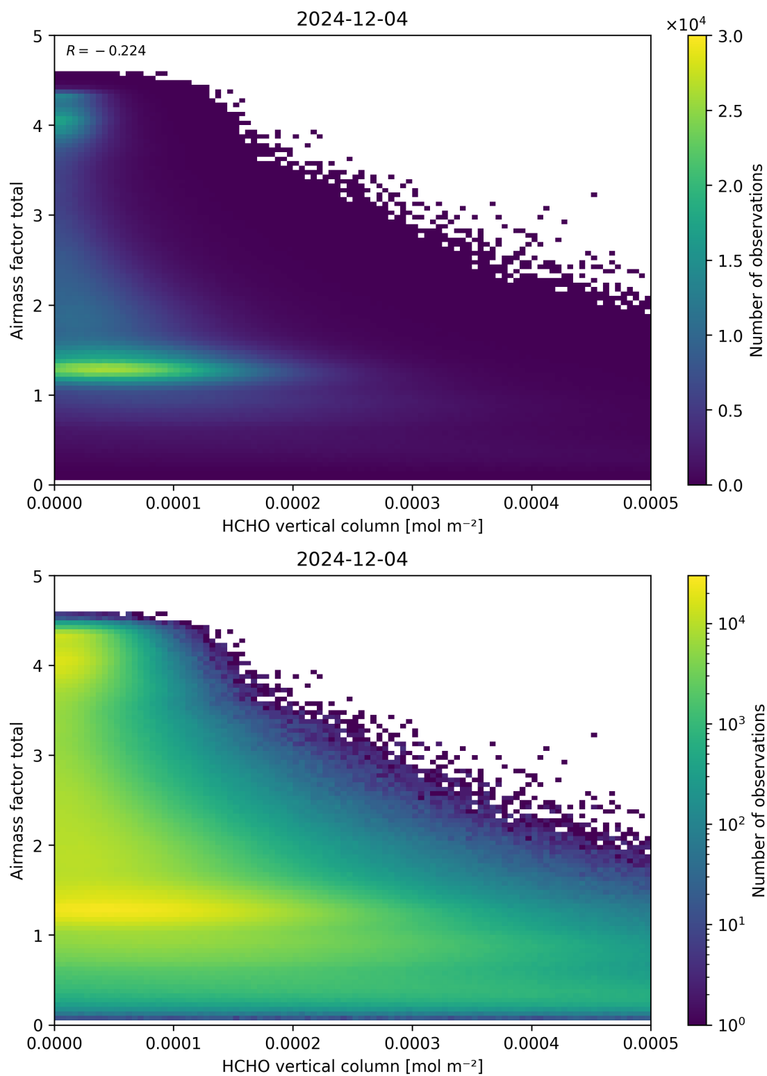
Figure 131: Scatter density plot of “HCHO vertical column” against “Airmass factor total” for 2024-12-03 to 2024-12-05.
