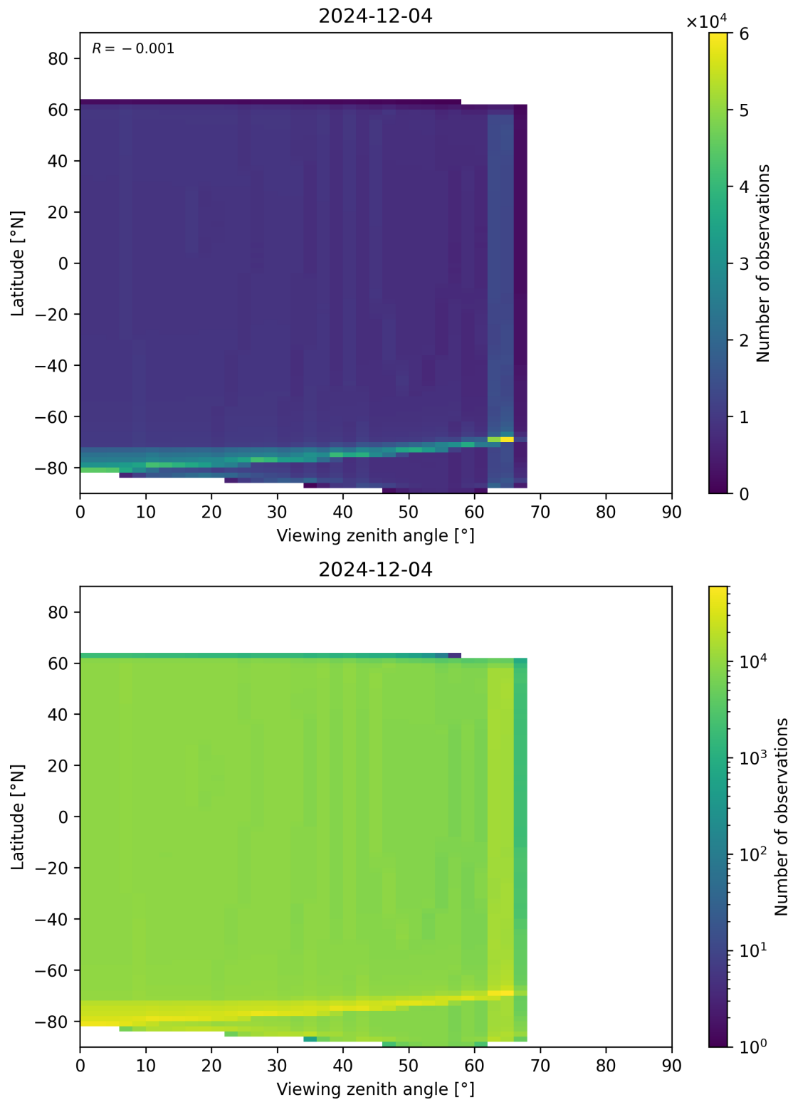
Figure 196: Scatter density plot of “Viewing zenith angle” against “Latitude” for 2024-12-03 to 2024-12-05.
