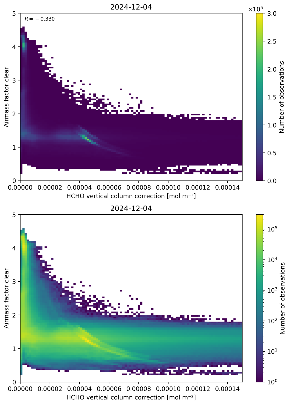
Figure 115: Scatter density plot of “HCHO vertical column correction” against “Airmass factor clear” for 2024-12-03 to 2024-12-05.
