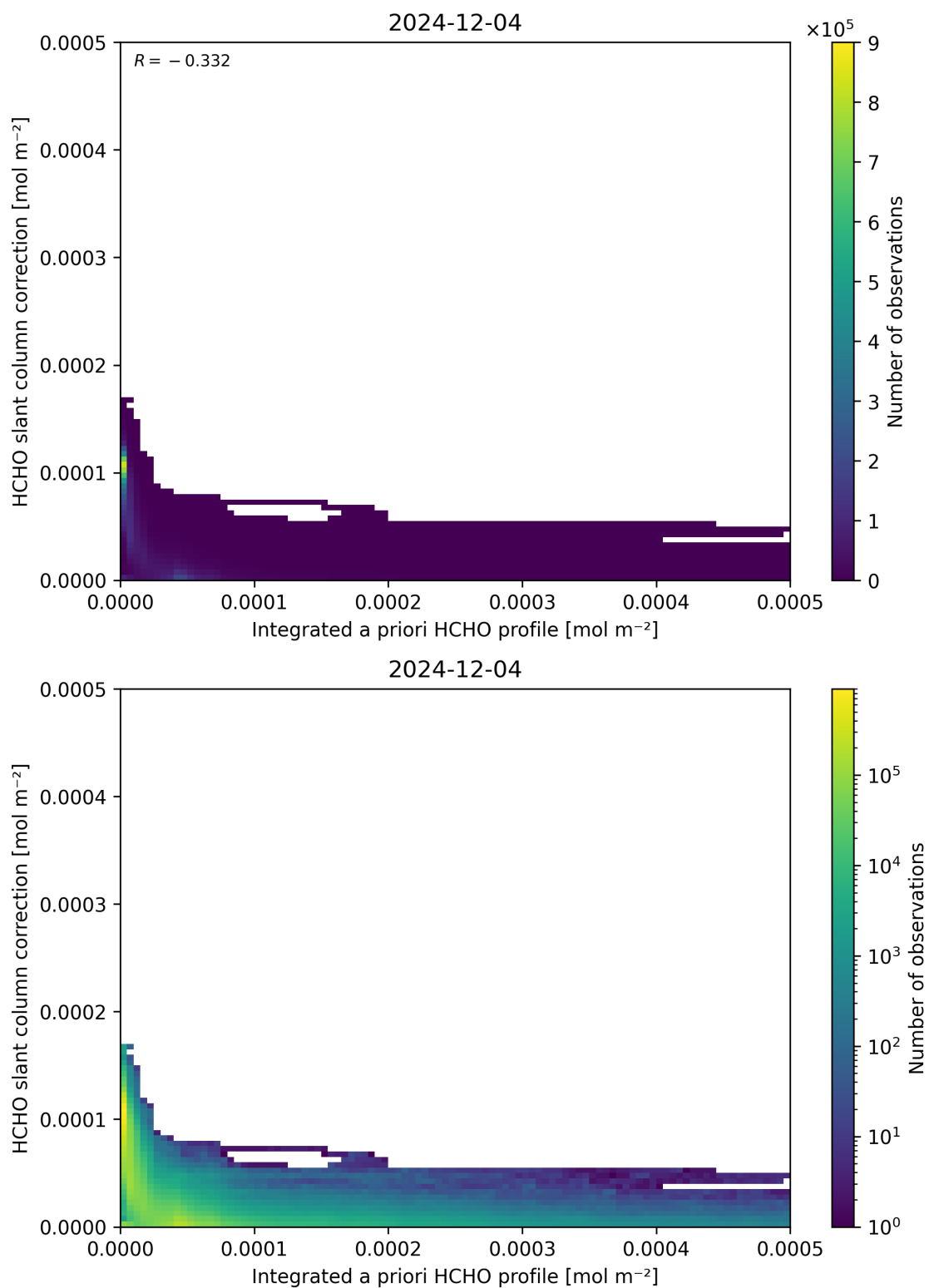
Figure 152: Scatter density plot of “Integrated a priori HCHO profile” against “HCHO slant column correction” for 2024-12-03 to 2024-12-05.
