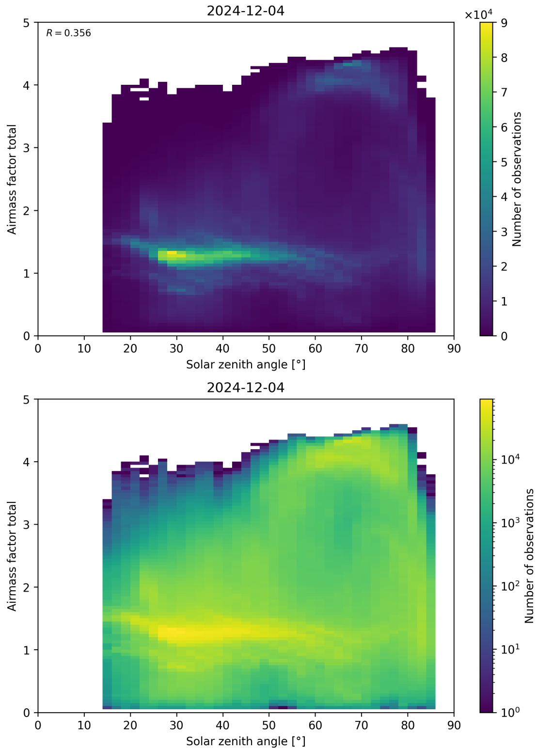
Figure 175: Scatter density plot of “Solar zenith angle” against “Airmass factor total” for 2024-12-03 to 2024-12-05.
