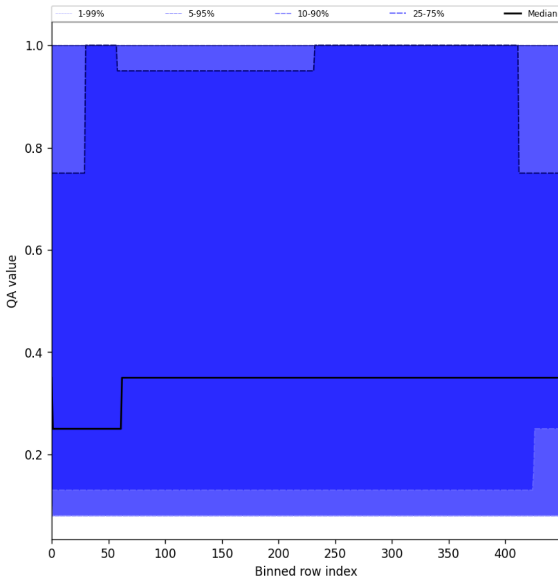
Figure 48: Along track statistics of “QA value” for 2024-12-03 to 2024-12-05
