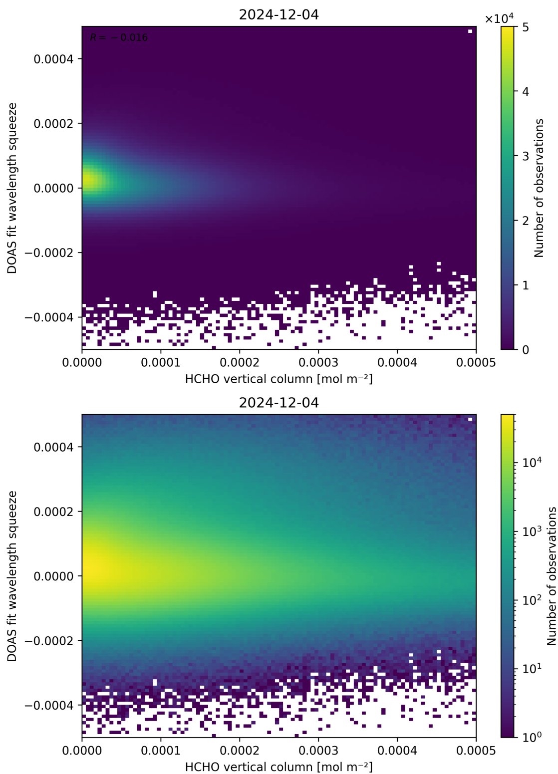
Figure 125: Scatter density plot of “HCHO vertical column” against “DOAS fit wavelength squeeze” for 2024-12-03 to 2024-12-05.
