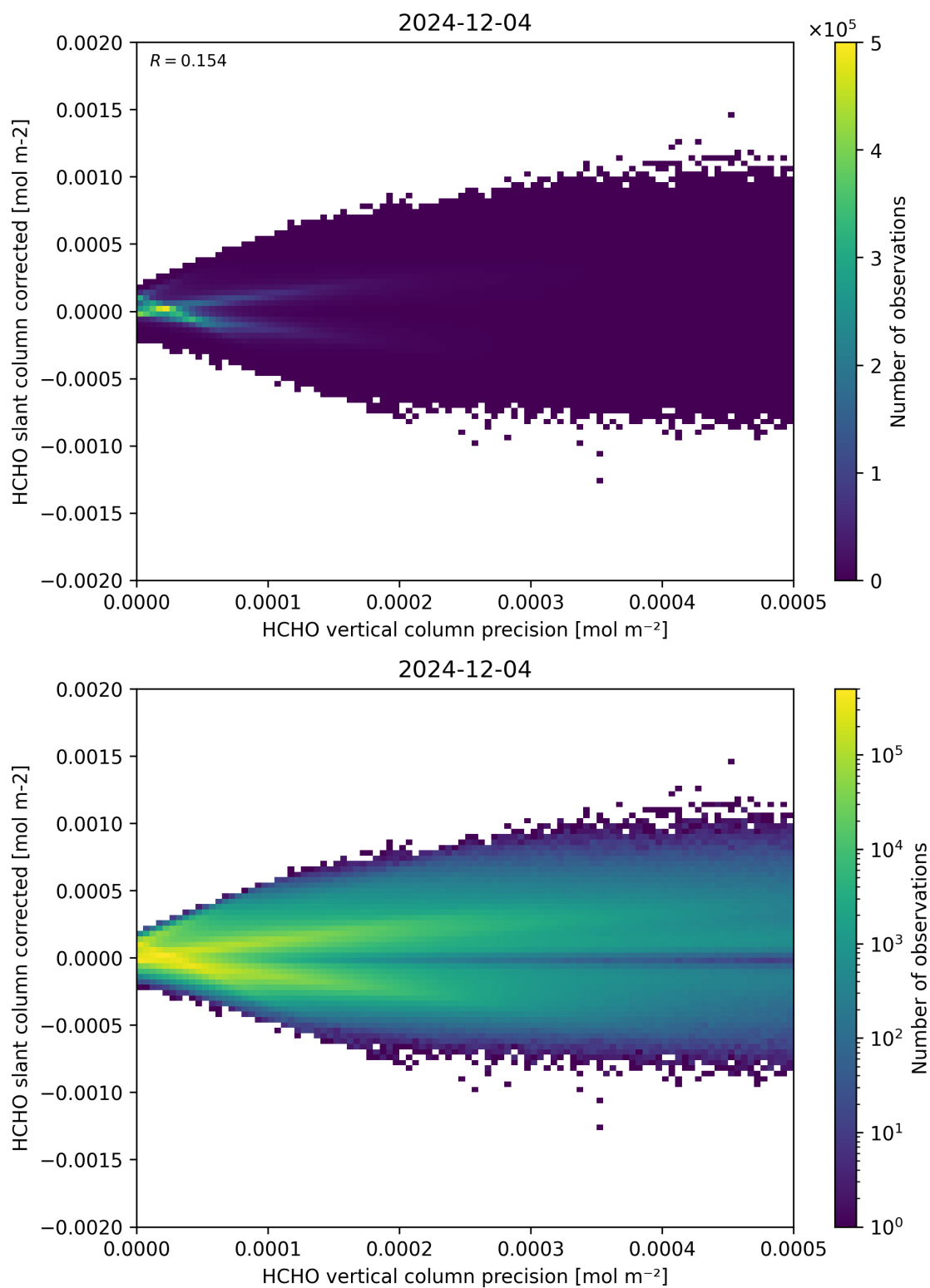
Figure 140: Scatter density plot of “HCHO vertical column precision” against “HCHO slant column corrected” for 2024-12-03 to 2024-12-05.
