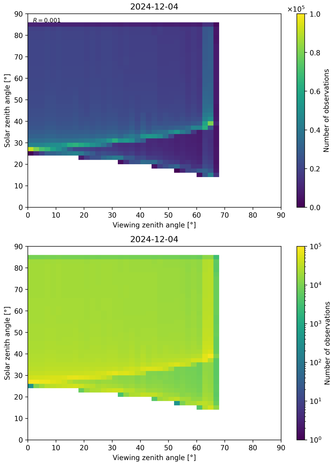
Figure 197: Scatter density plot of “Viewing zenith angle” against “Solar zenith angle” for 2024-12-03 to 2024-12-05.
