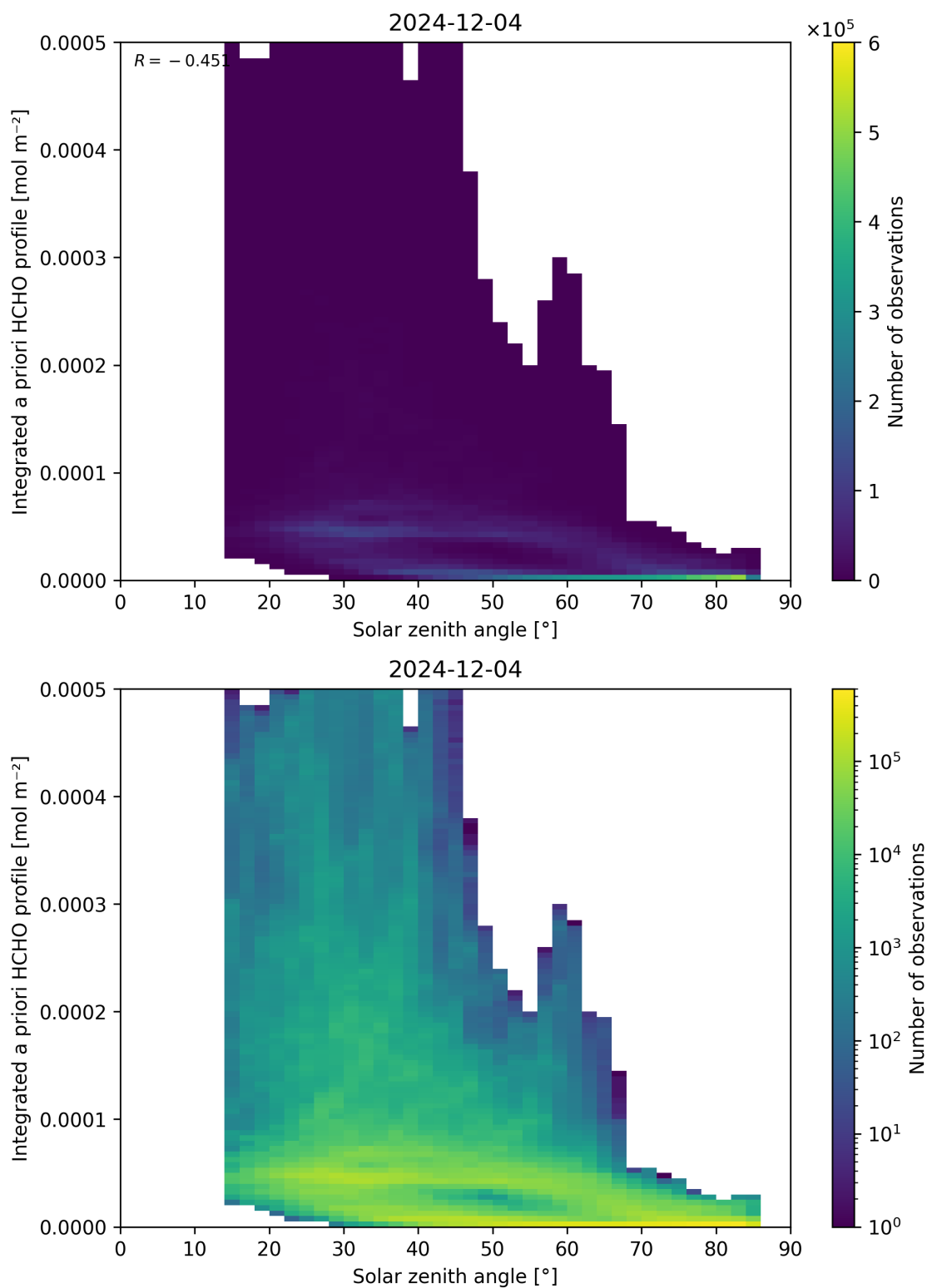
Figure 180: Scatter density plot of “Solar zenith angle” against “Integrated a priori HCHO profile” for 2024-12-03 to 2024-12-05.
