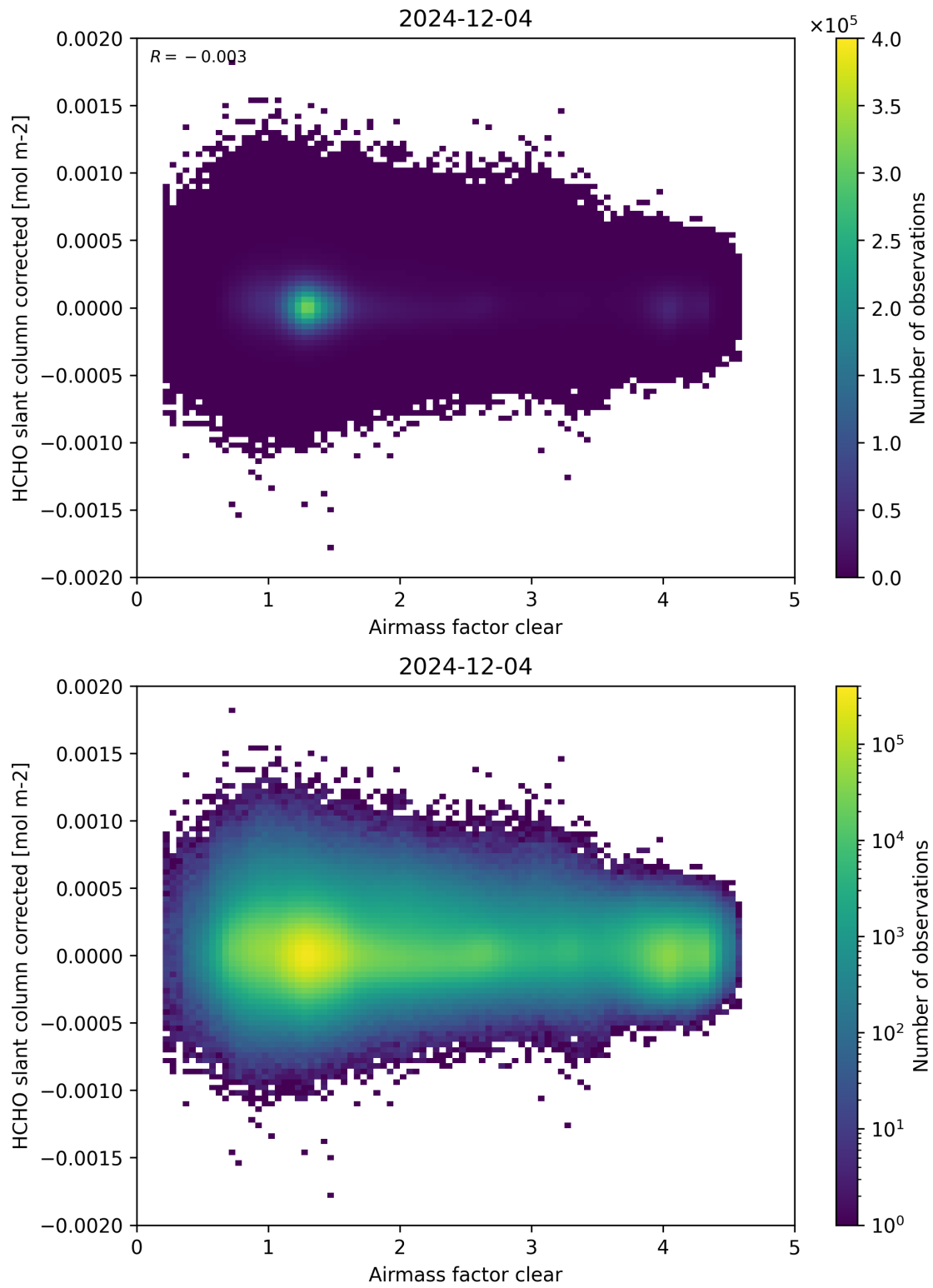
Figure 74: Scatter density plot of “Airmass factor clear” against “HCHO slant column corrected” for 2024-12-03 to 2024-12-05.
