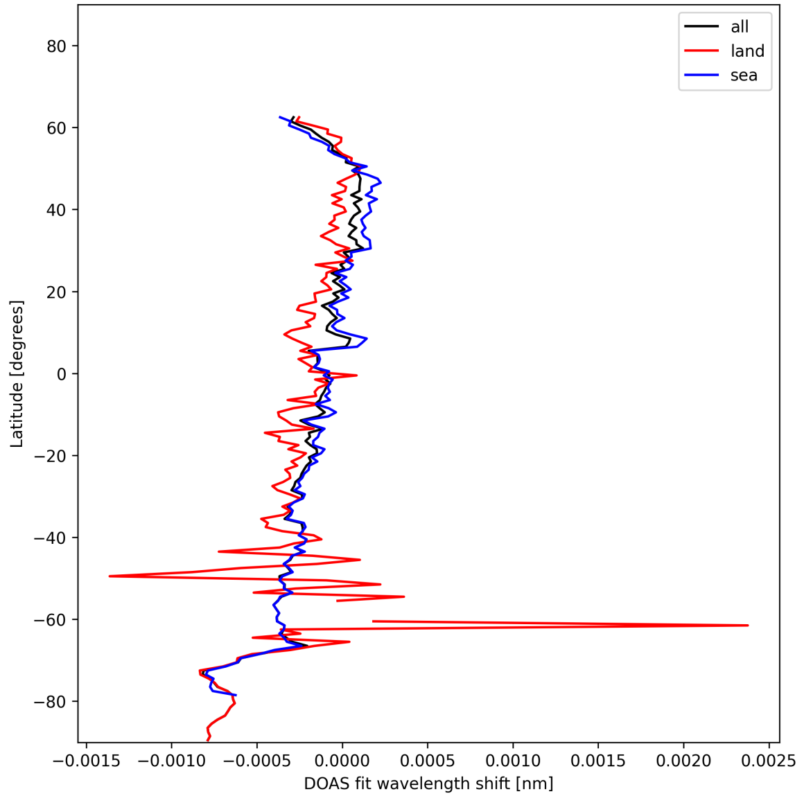
Figure 30: Zonal average of "DOAS fit wavelength shift" for 2024-12-03 to 2024-12-05.
