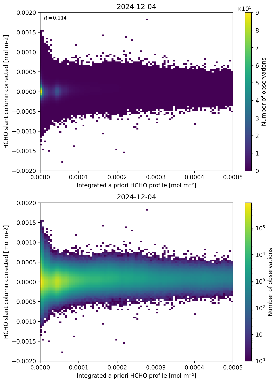
Figure 151: Scatter density plot of “Integrated a priori HCHO profile” against “HCHO slant column corrected” for 2024-12-03 to 2024-12-05.
