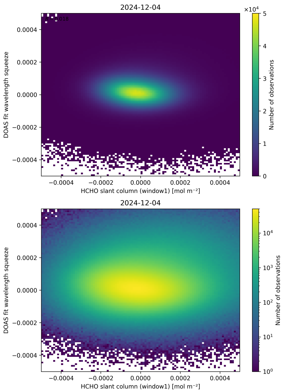
Figure 80: Scatter density plot of “HCHO slant column (window1)” against “DOAS fit wavelength squeeze” for 2024-12-03 to 2024-12-05.
