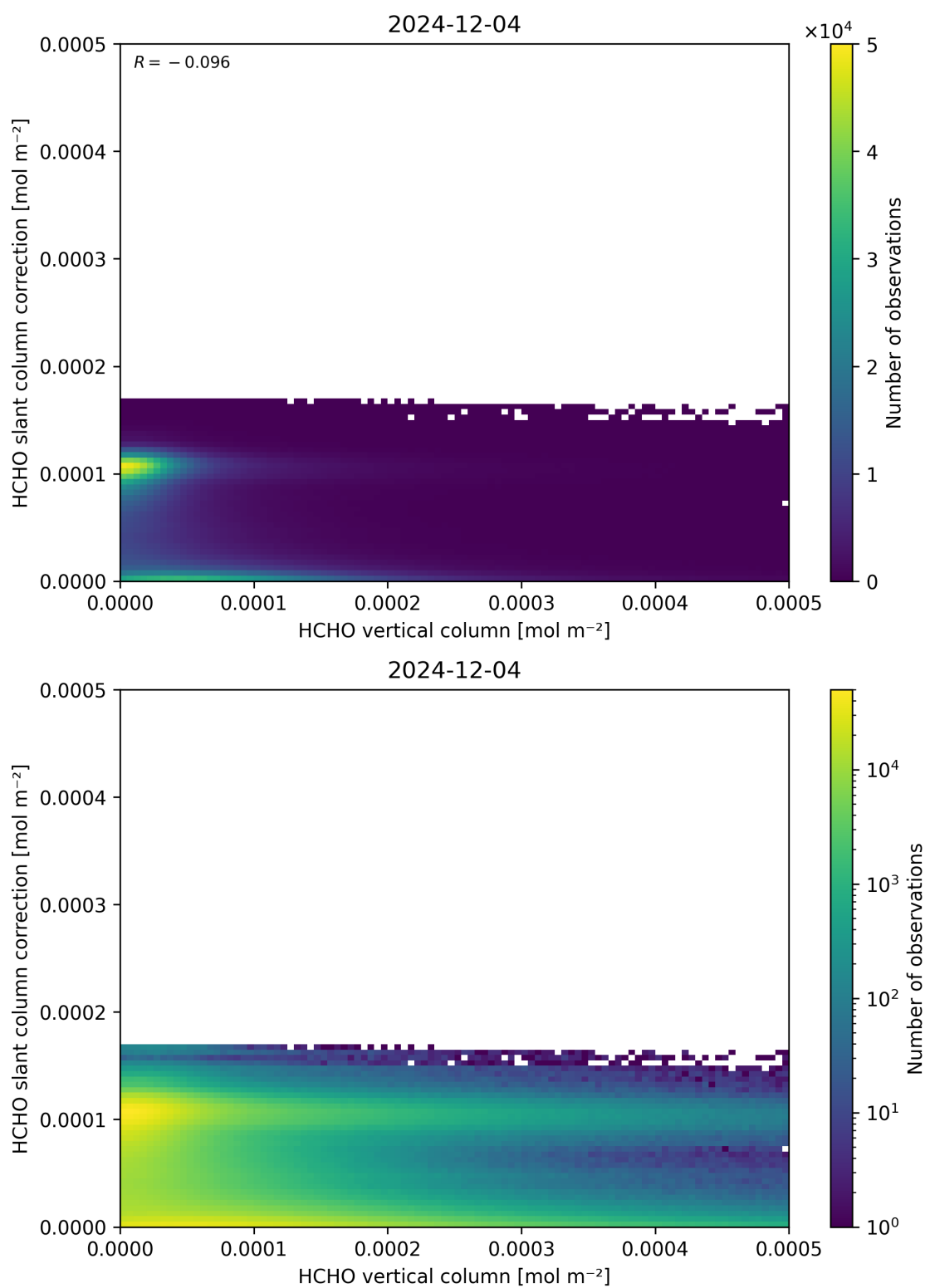
Figure 128: Scatter density plot of “HCHO vertical column” against “HCHO slant column correction” for 2024-12-03 to 2024-12-05.
