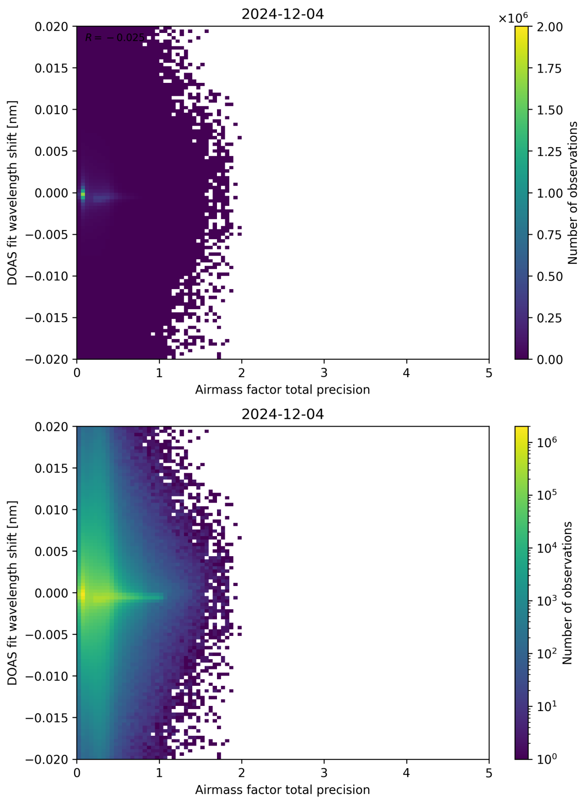
Figure 106: Scatter density plot of “Airmass factor total precision” against “DOAS fit wavelength shift” for 2024-12-03 to 2024-12-05.
