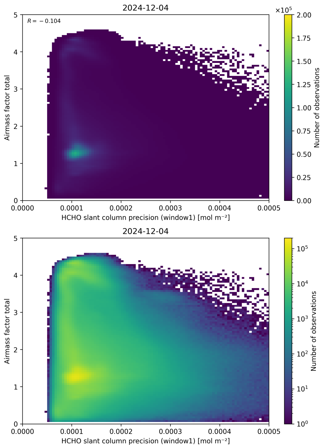
Figure 94: Scatter density plot of “HCHO slant column precision (window1)” against “Airmass factor total” for 2024-12-03 to 2024-12-05.
