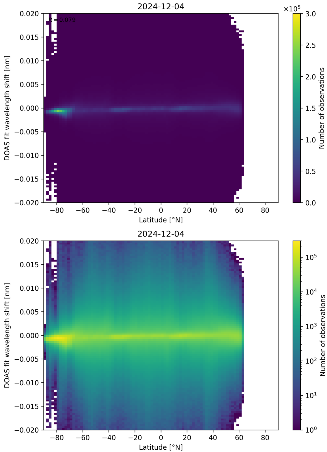
Figure 154: Scatter density plot of “Latitude” against “DOAS fit wavelength shift” for 2024-12-03 to 2024-12-05.
