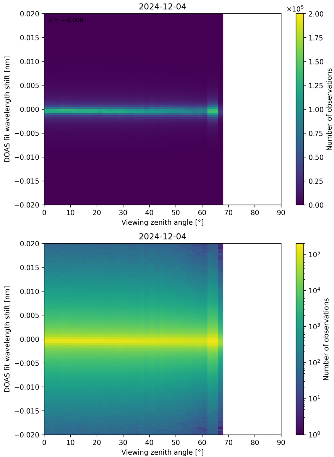
Figure 183: Scatter density plot of “Viewing zenith angle” against “DOAS fit wavelength shift” for 2024-12-03 to 2024-12-05.
