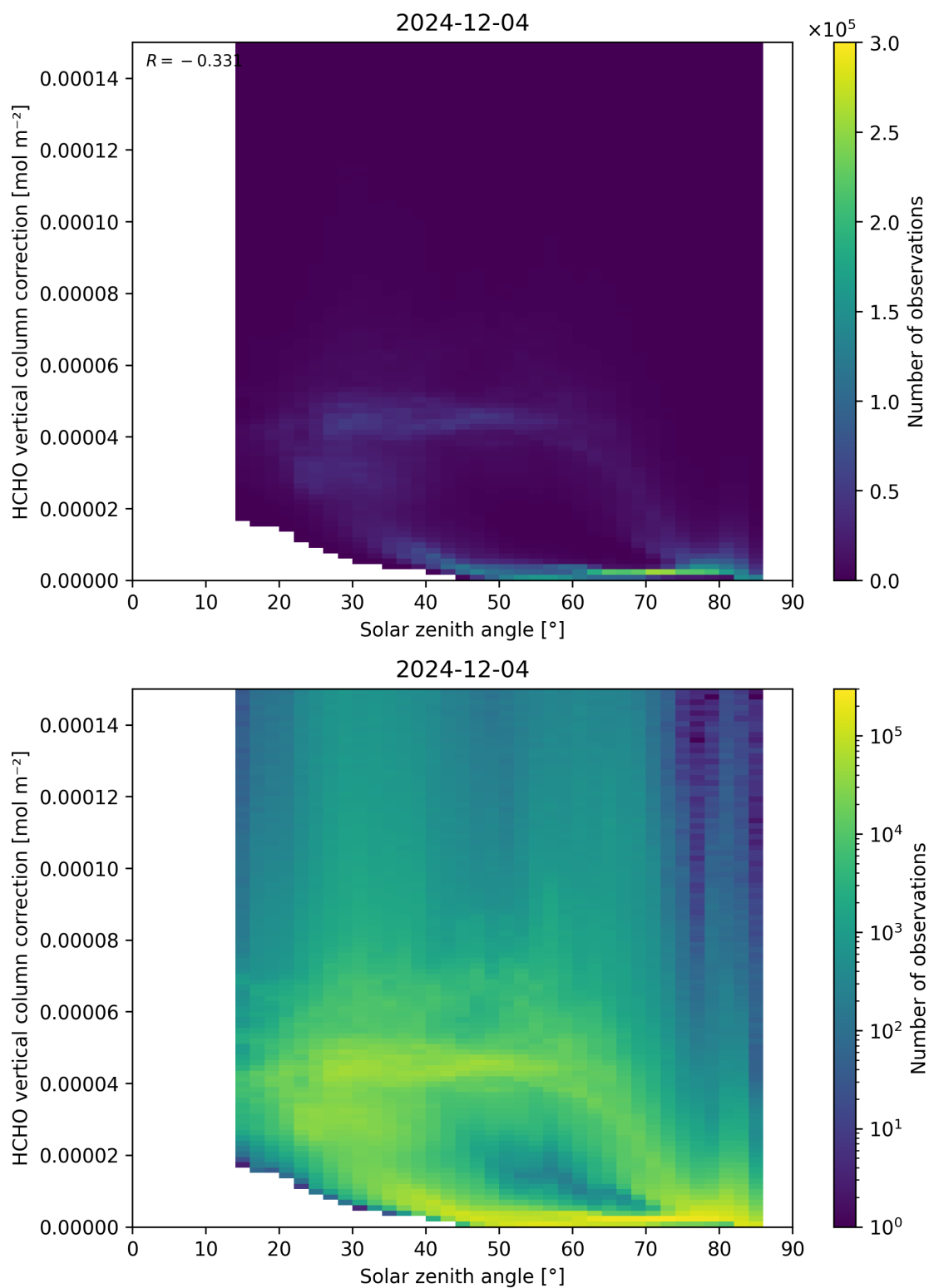
Figure 178: Scatter density plot of “Solar zenith angle” against “HCHO vertical column correction” for 2024-12-03 to 2024-12-05.
