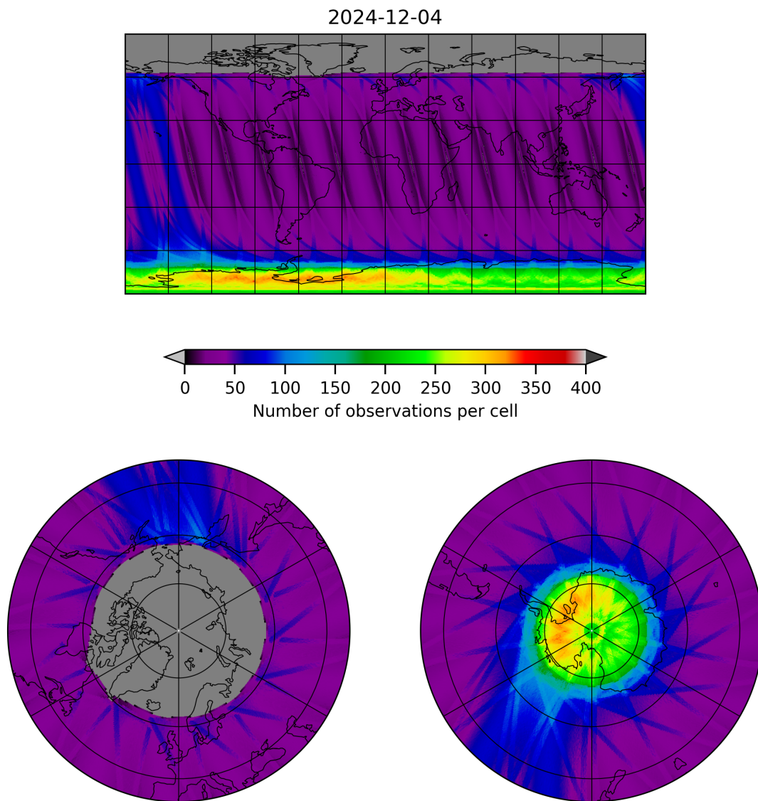
Figure 19: Map of the number of observations for 2024-12-03 to 2024-12-05
