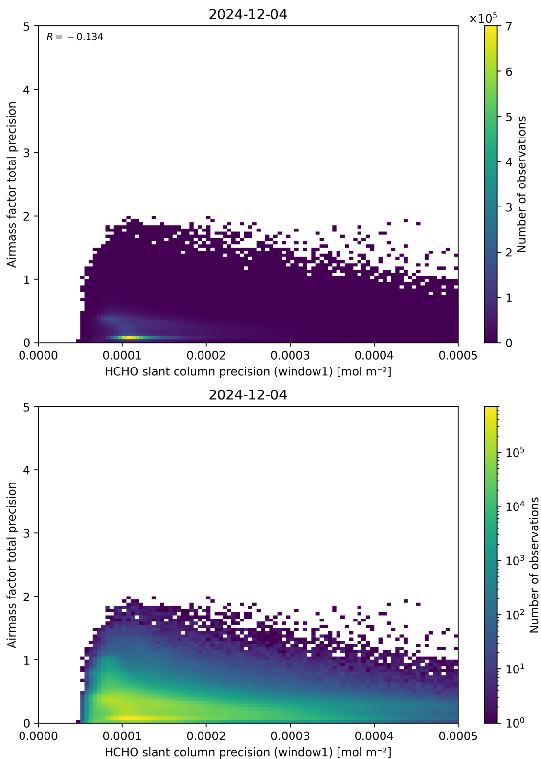
Figure 95: Scatter density plot of “HCHO slant column precision (window1)” against “Airmass factor total precision” for 2024-12-03 to 2024-12-05.
