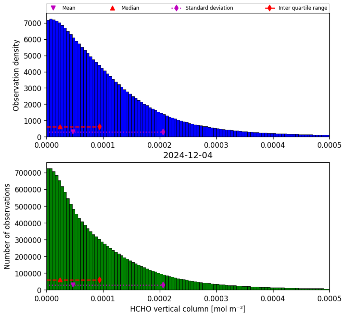
Figure 35: Histogram of “HCHO vertical column” for 2024-12-03 to 2024-12-05
