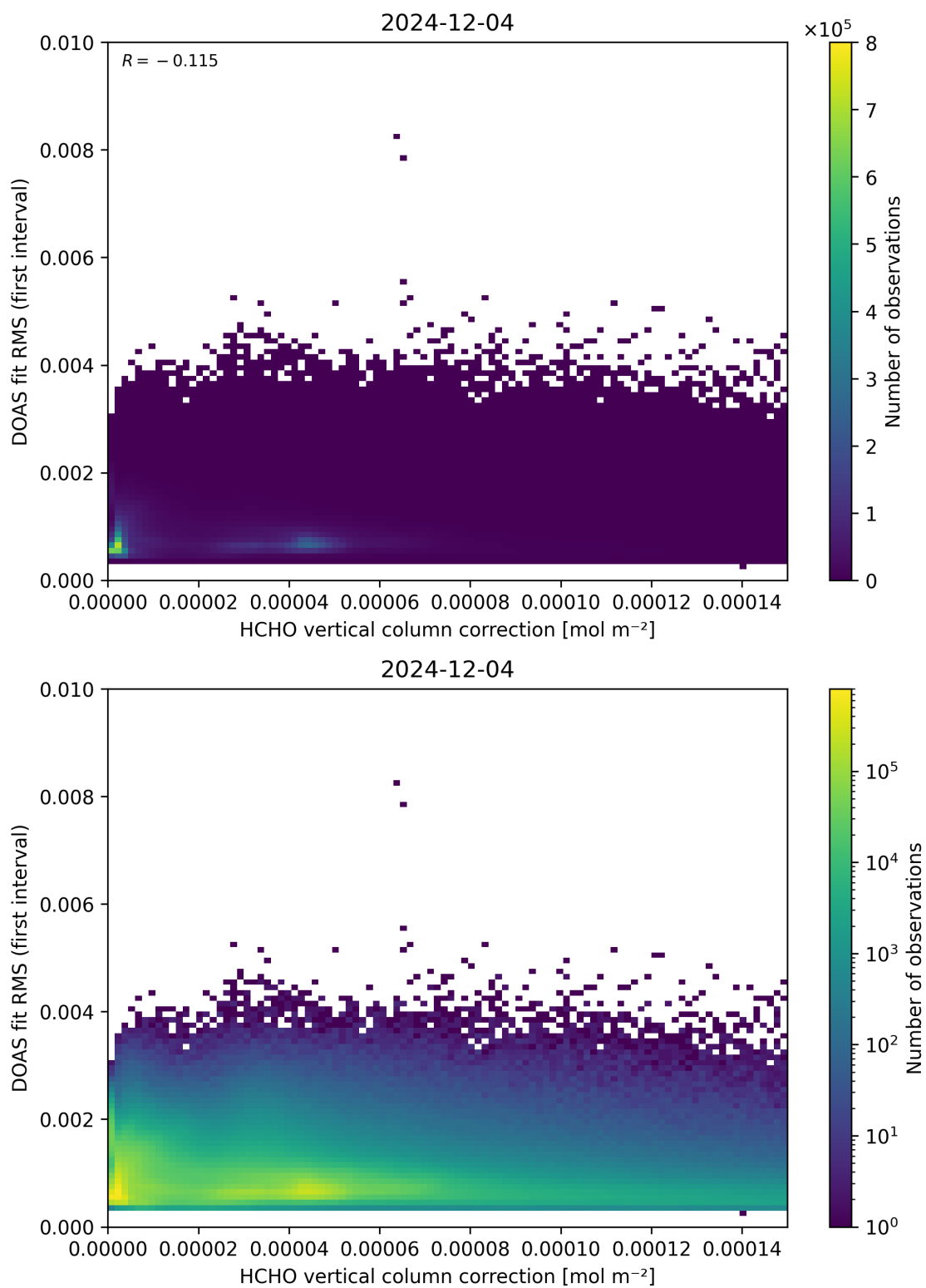
Figure 112: Scatter density plot of “HCHO vertical column correction” against “DOAS fit RMS (first interval)” for 2024-12-03 to 2024-12-05.
