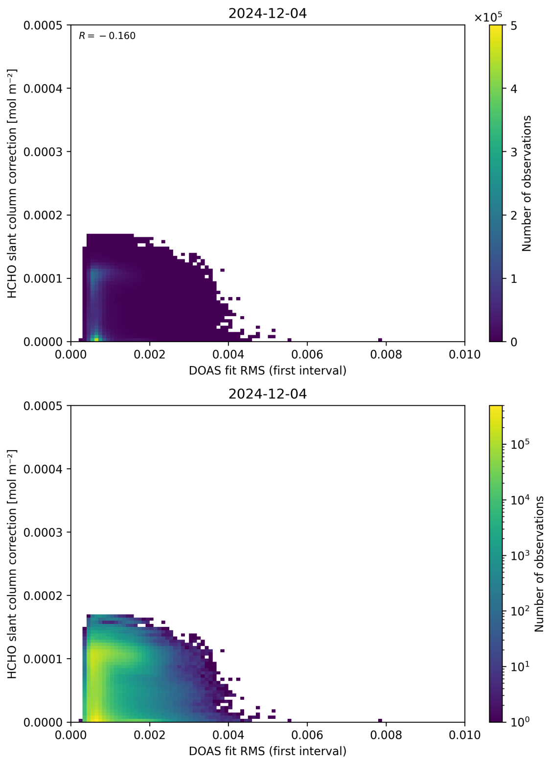
Figure 63: Scatter density plot of “DOAS fit RMS (first interval)” against “HCHO slant column correction” for 2024-12-03 to 2024-12-05.
