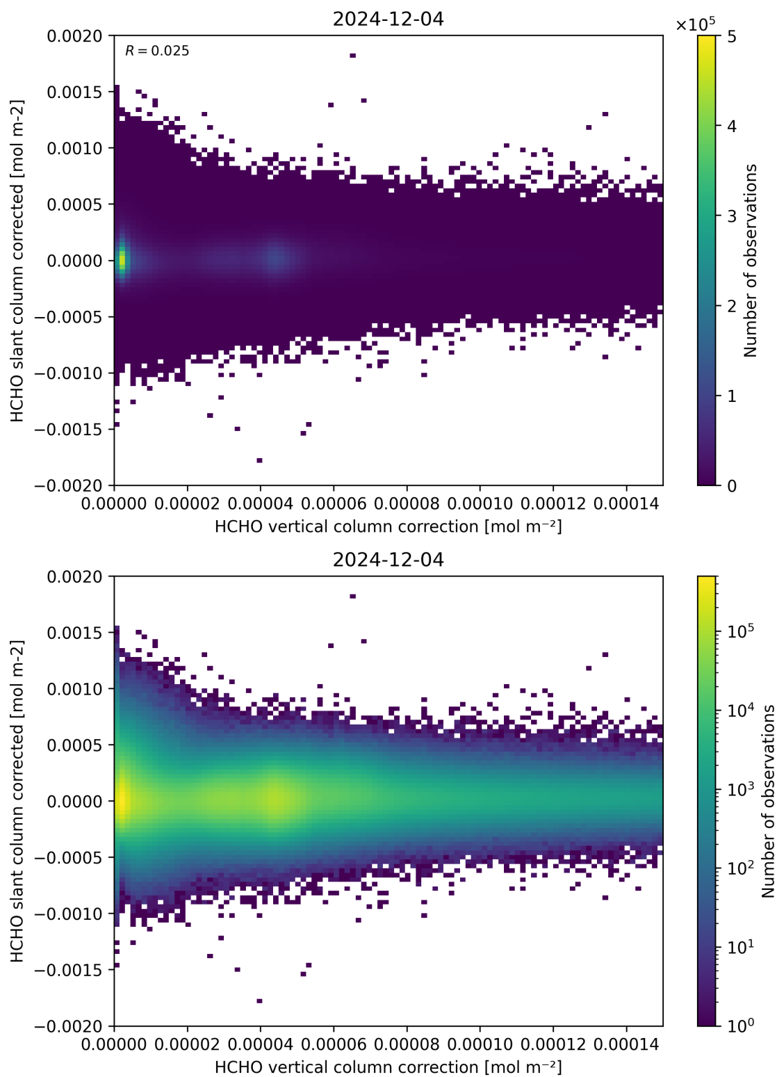
Figure 116: Scatter density plot of “HCHO vertical column correction” against “HCHO slant column corrected” for 2024-12-03 to 2024-12-05.
