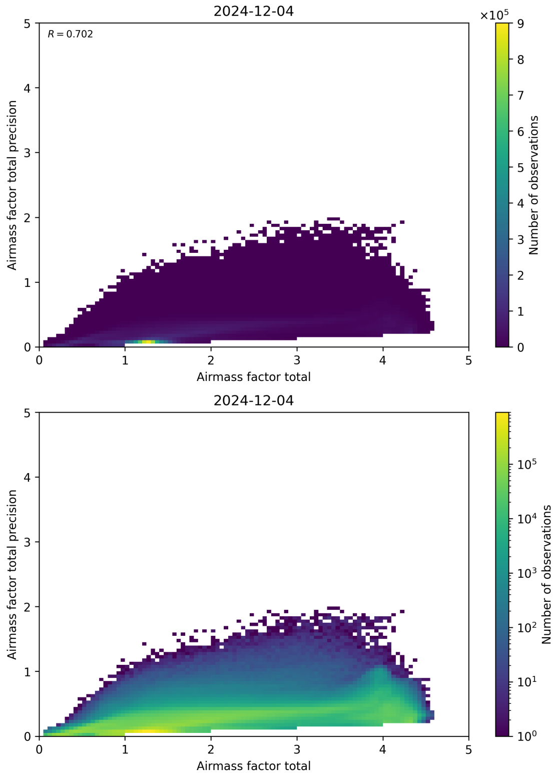
Figure 103: Scatter density plot of “Airmass factor total” against “Airmass factor total precision” for 2024-12-03 to 2024-12-05.
