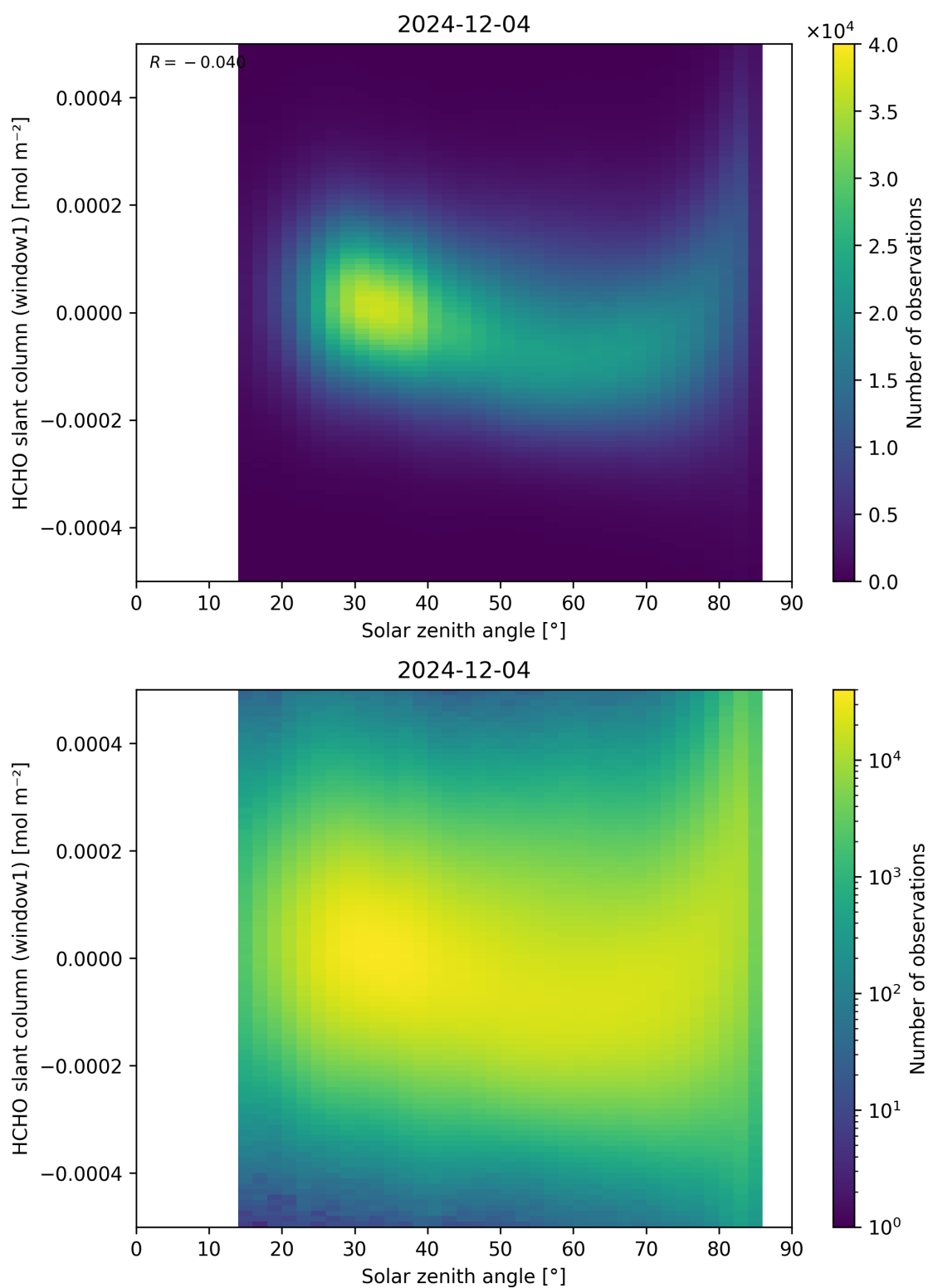
Figure 173: Scatter density plot of “Solar zenith angle” against “HCHO slant column (window1)” for 2024-12-03 to 2024-12-05.
