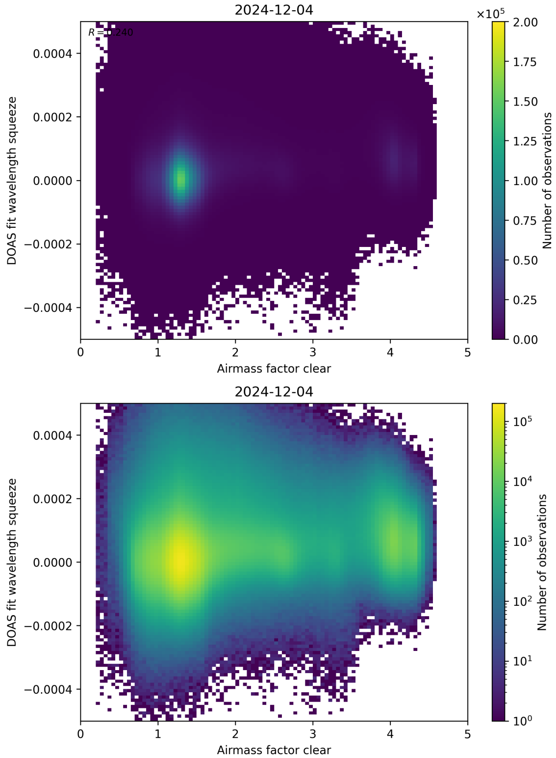
Figure 73: Scatter density plot of “Airmass factor clear” against “DOAS fit wavelength squeeze” for 2024-12-03 to 2024-12-05.
