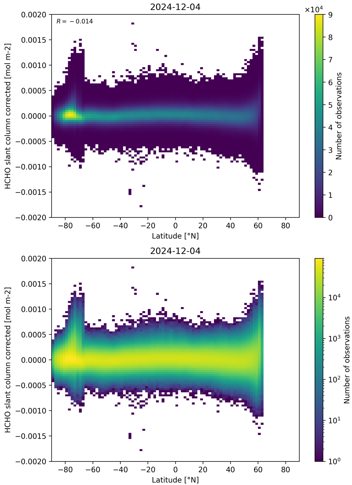
Figure 157: Scatter density plot of “Latitude” against “HCHO slant column corrected” for 2024-12-03 to 2024-12-05.
