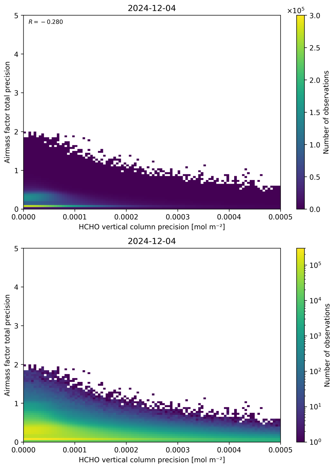
Figure 145: Scatter density plot of “HCHO vertical column precision” against “Airmass factor total precision” for 2024-12-03 to 2024-12-05.
