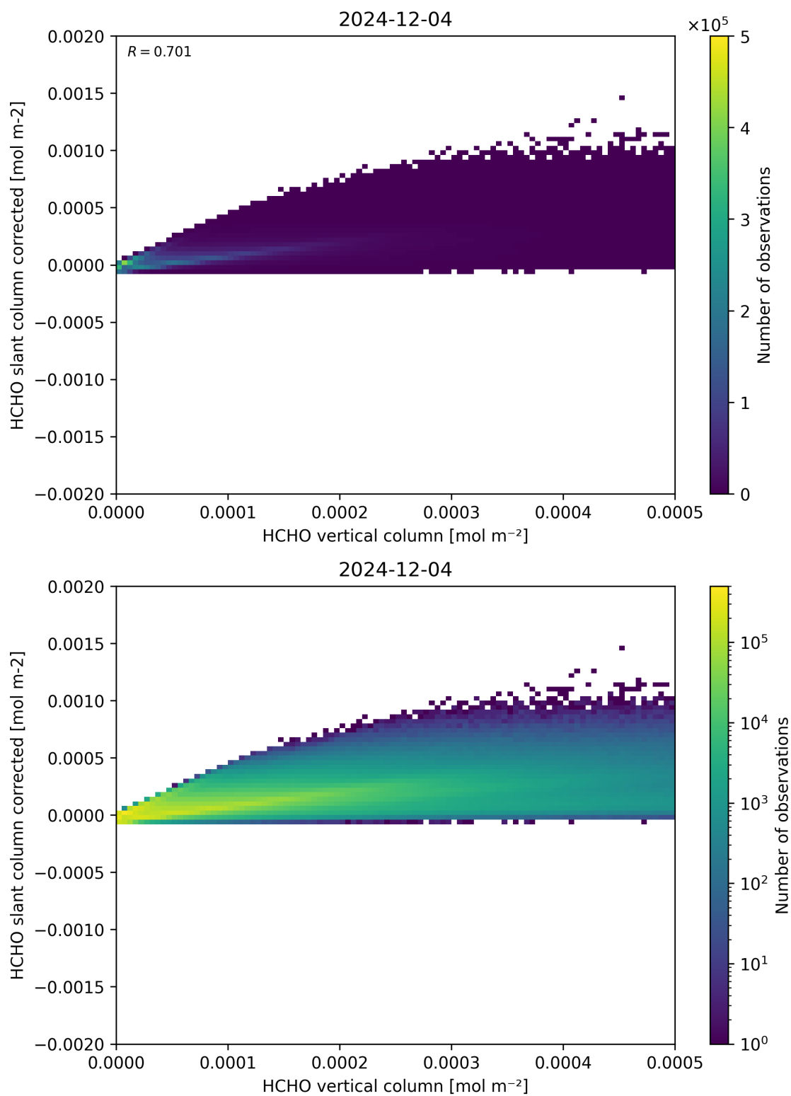
Figure 127: Scatter density plot of “HCHO vertical column” against “HCHO slant column corrected” for 2024-12-03 to 2024-12-05.
