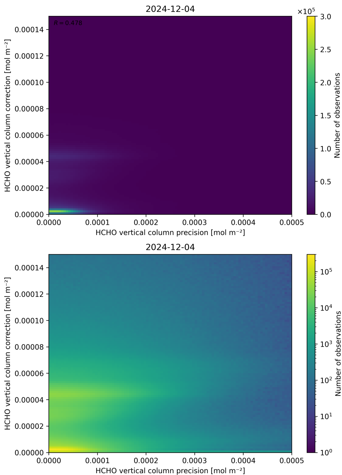
Figure 146: Scatter density plot of “HCHO vertical column precision” against “HCHO vertical column correction” for 2024-12-03 to 2024-12-05.
