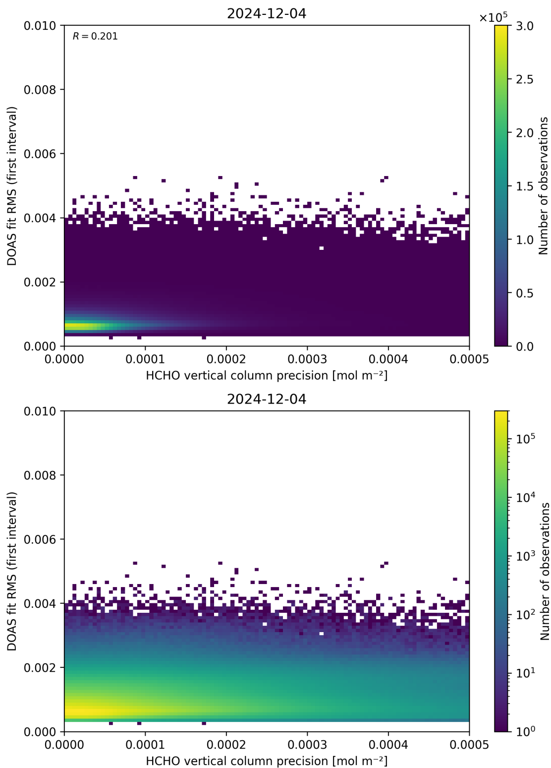
Figure 136: Scatter density plot of “HCHO vertical column precision” against “DOAS fit RMS (first interval)” for 2024-12-03 to 2024-12-05.
