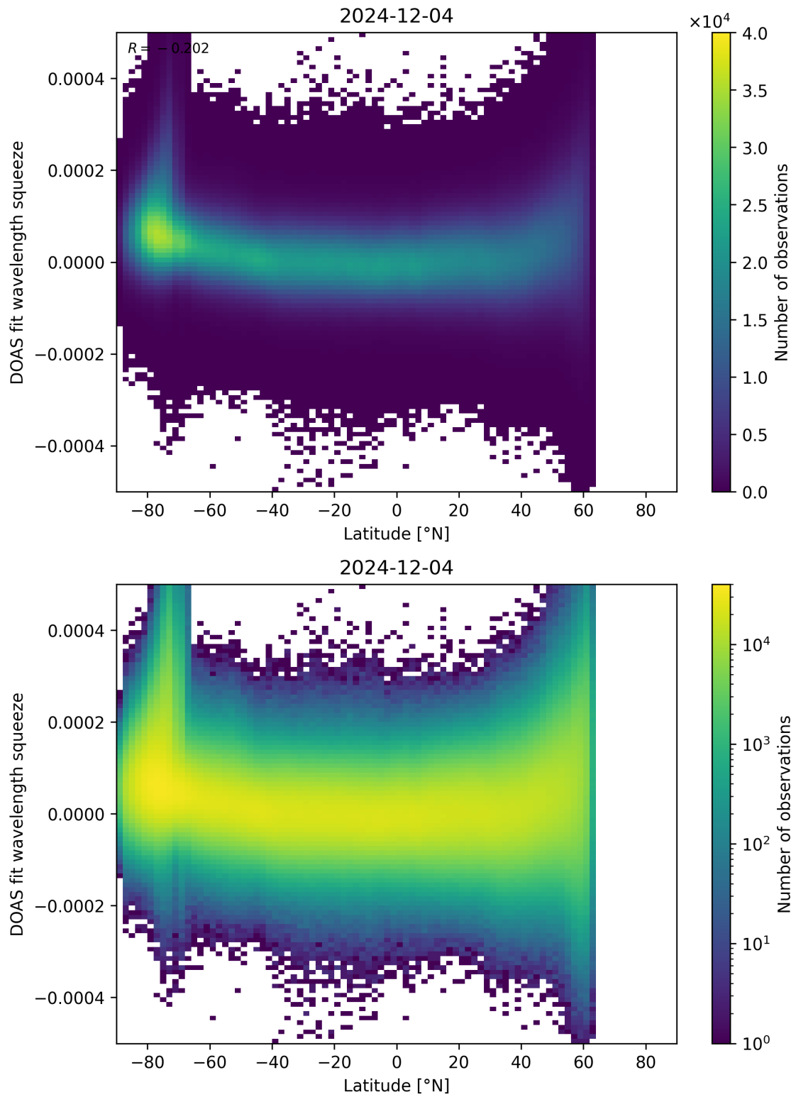
Figure 155: Scatter density plot of “Latitude” against “DOAS fit wavelength squeeze” for 2024-12-03 to 2024-12-05.
