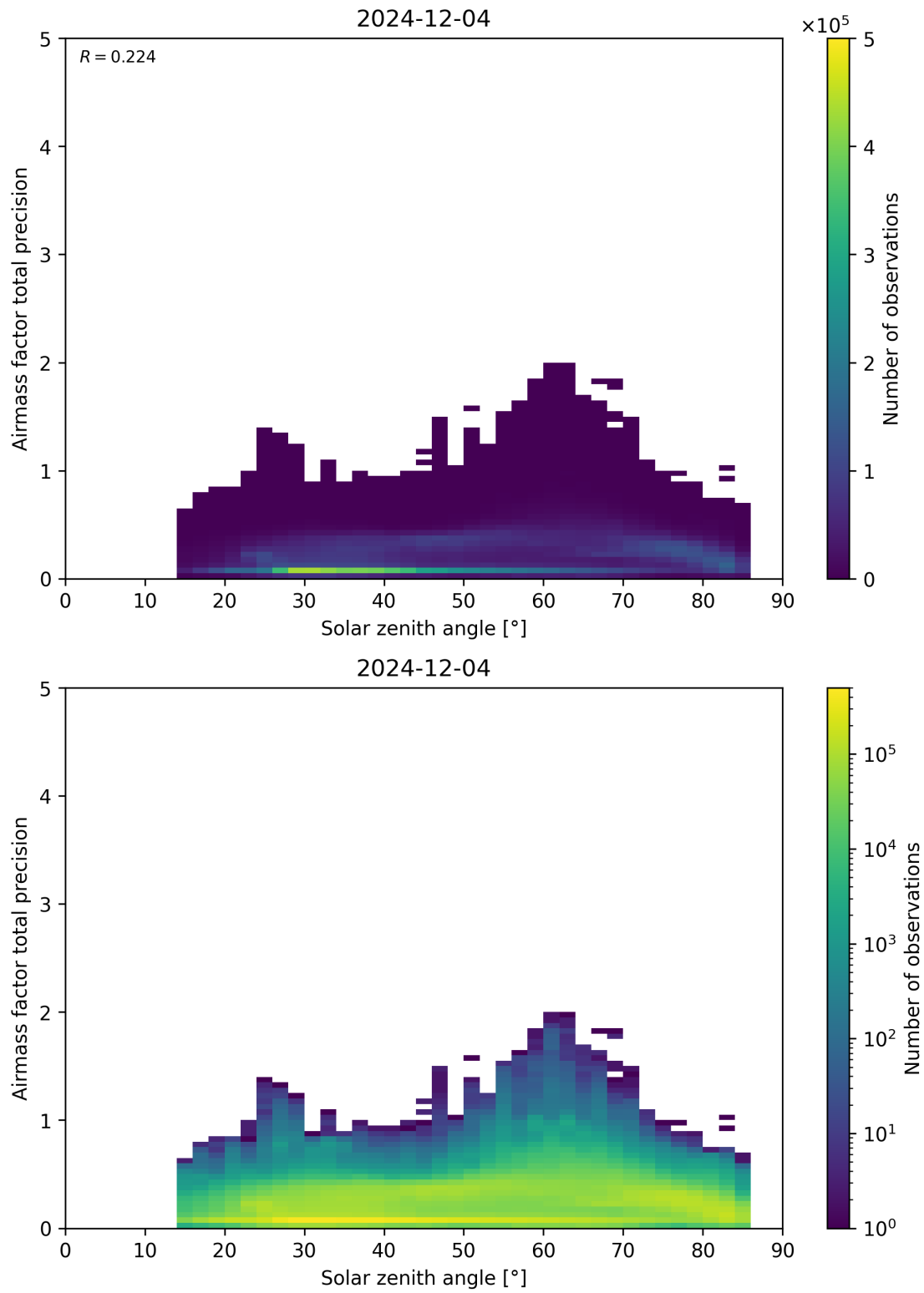
Figure 176: Scatter density plot of “Solar zenith angle” against “Airmass factor total precision” for 2024-12-03 to 2024-12-05.
