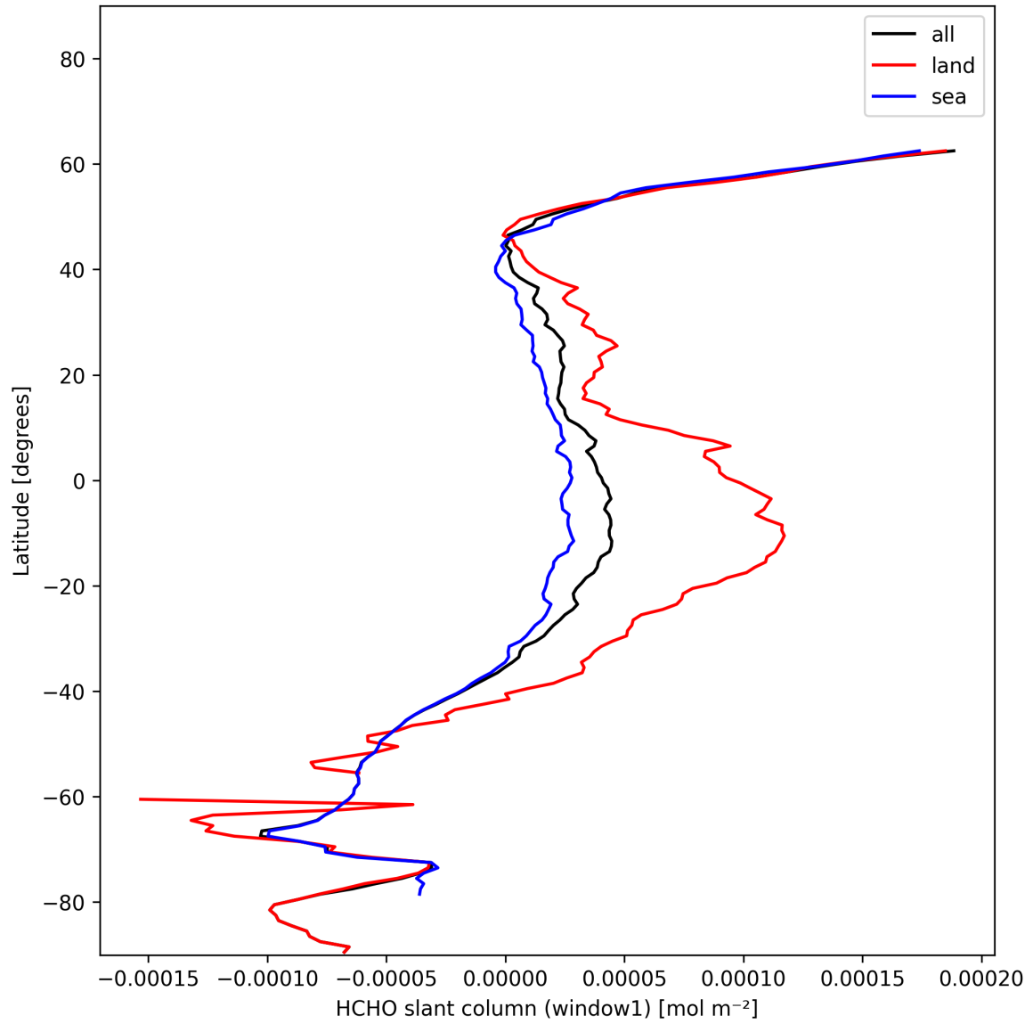
Figure 24: Zonal average of “HCHO slant column (window1)” for 2024-12-03 to 2024-12-05.
