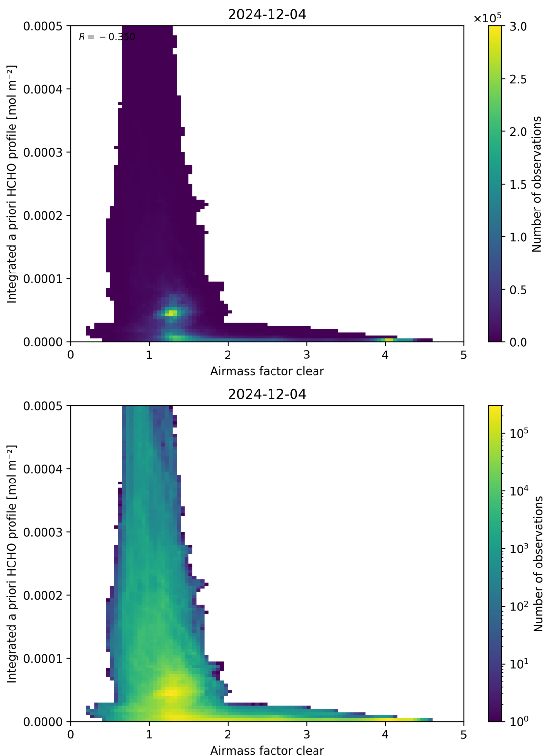
Figure 76: Scatter density plot of “Airmass factor clear” against “Integrated a priori HCHO profile” for 2024-12-03 to 2024-12-05.
