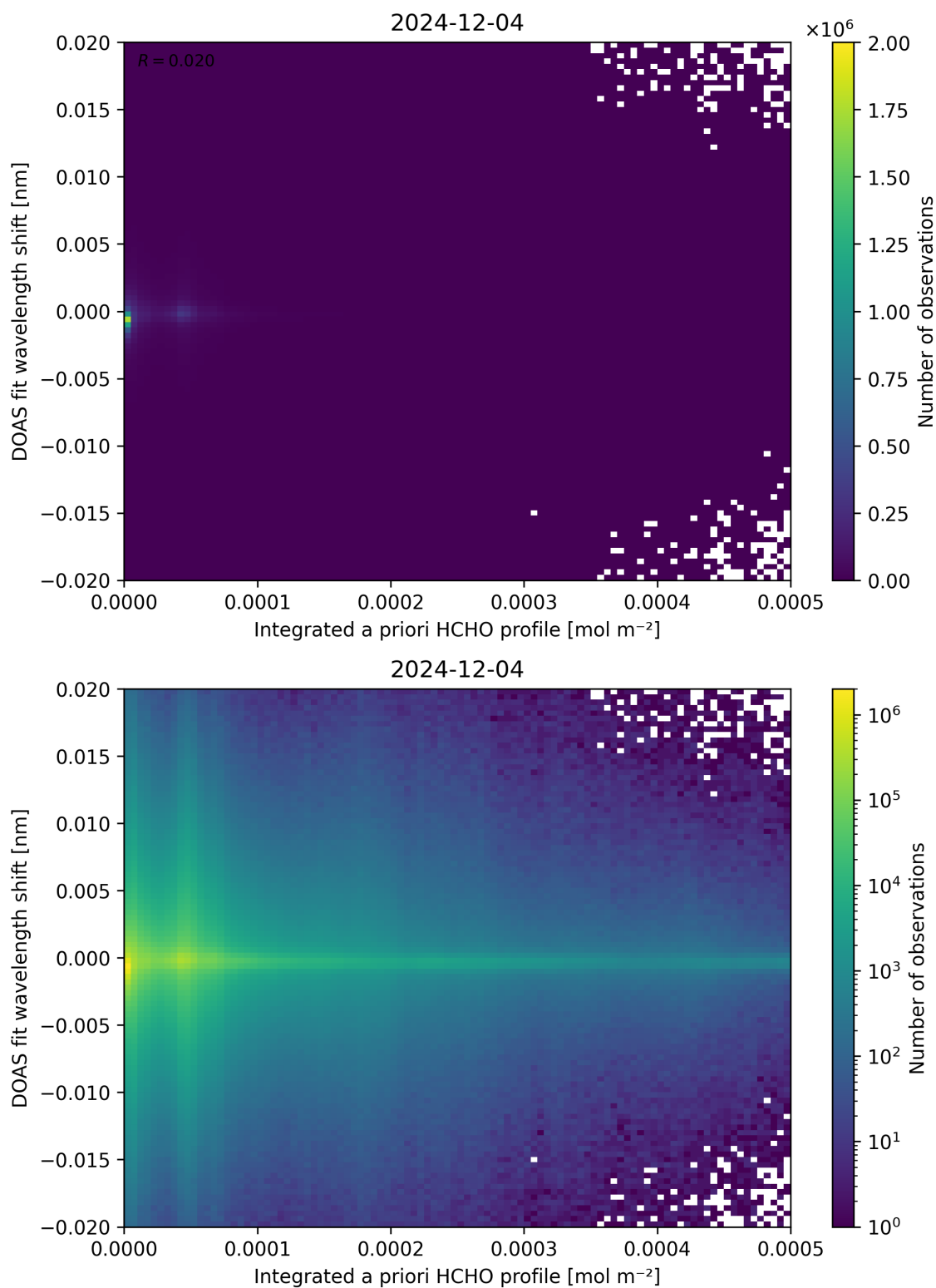
Figure 149: Scatter density plot of “Integrated a priori HCHO profile” against “DOAS fit wavelength shift” for 2024-12-03 to 2024-12-05.
