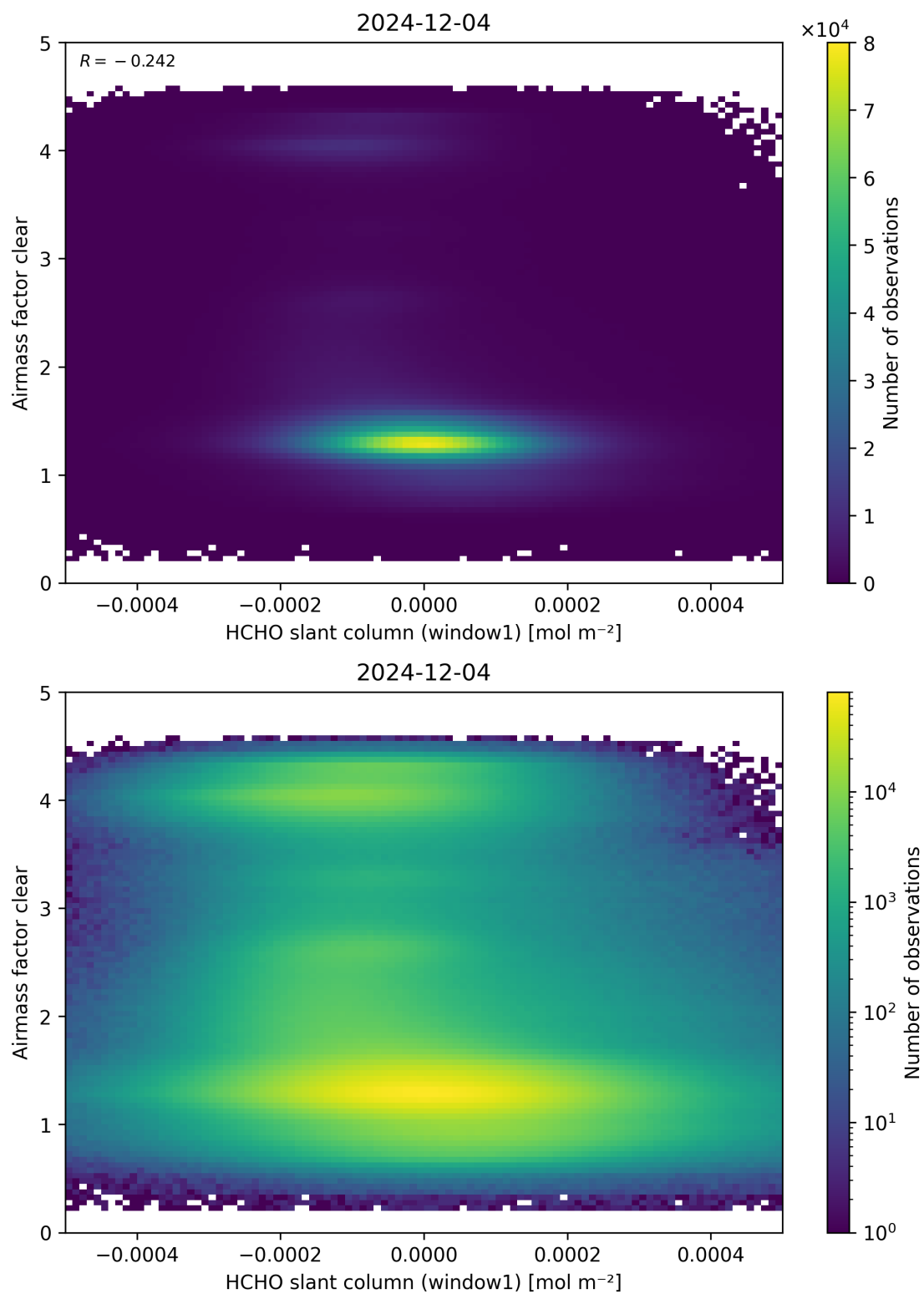
Figure 81: Scatter density plot of “HCHO slant column (window1)” against “Airmass factor clear” for 2024-12-03 to 2024-12-05.
