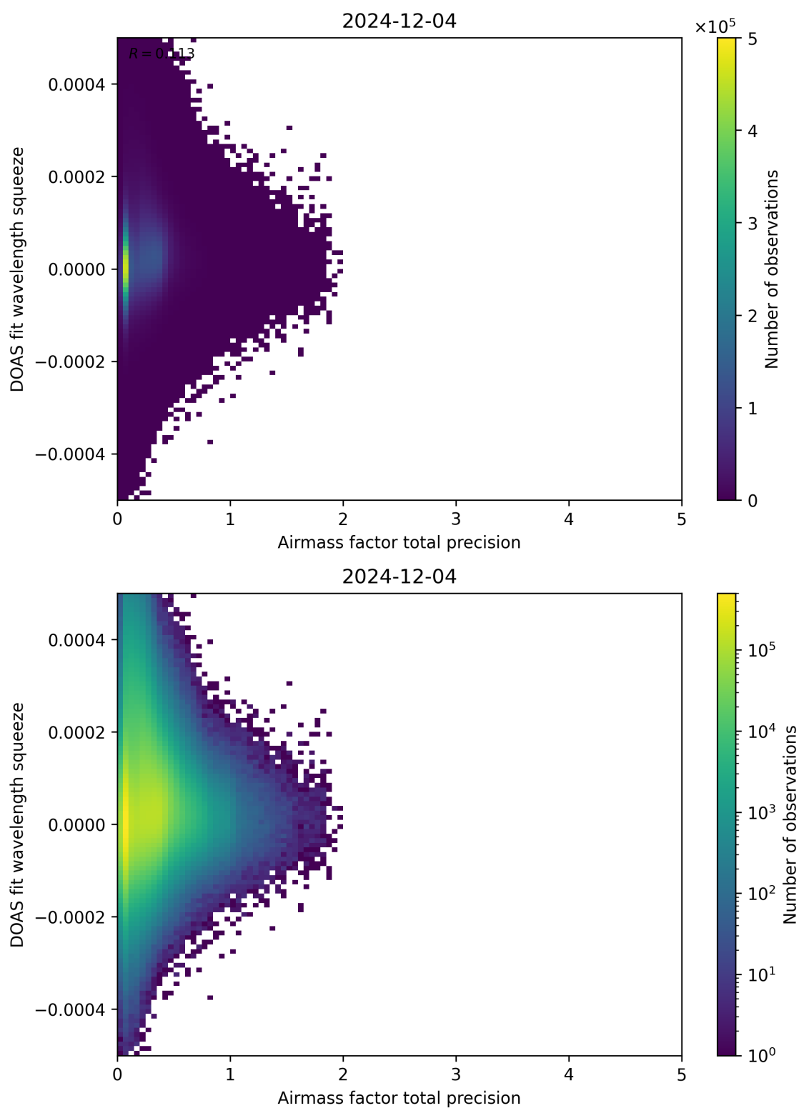
Figure 107: Scatter density plot of “Airmass factor total precision” against “DOAS fit wavelength squeeze” for 2024-12-03 to 2024-12-05.
