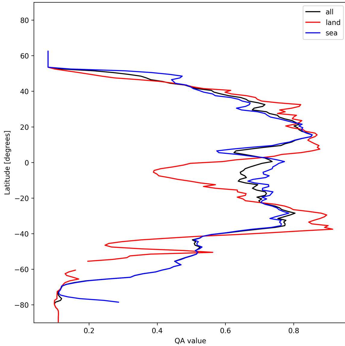
Figure 20: Zonal average of “QA value” for 2024-12-03 to 2024-12-05.
