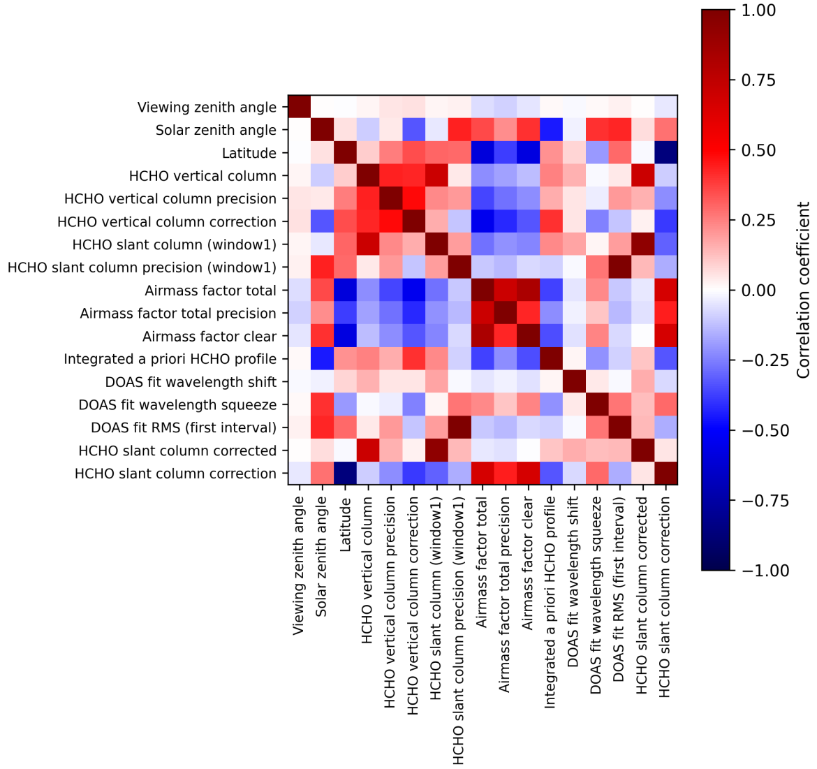
Figure 2: Map of correlation matrix for 2024-12-03 to 2024-12-05.
