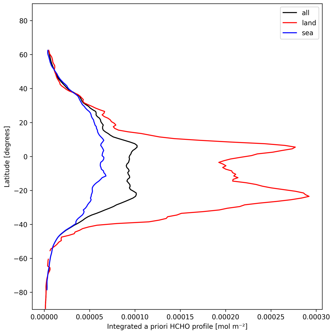
Figure 29: Zonal average of “Integrated a priori HCHO profile” for 2024-12-03 to 2024-12-05.
