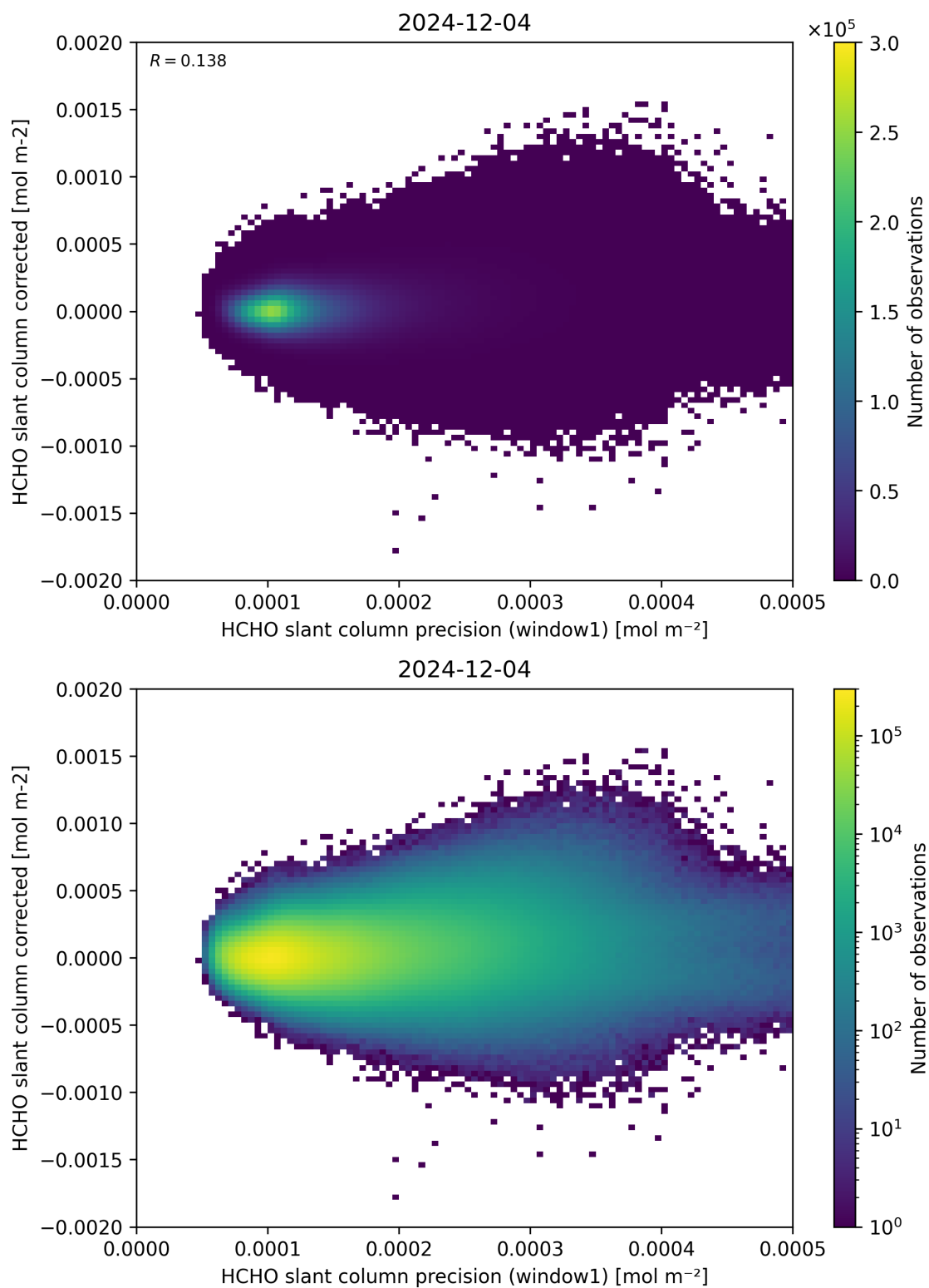
Figure 92: Scatter density plot of “HCHO slant column precision (window1)” against “HCHO slant column corrected” for 2024-12-03 to 2024-12-05.
