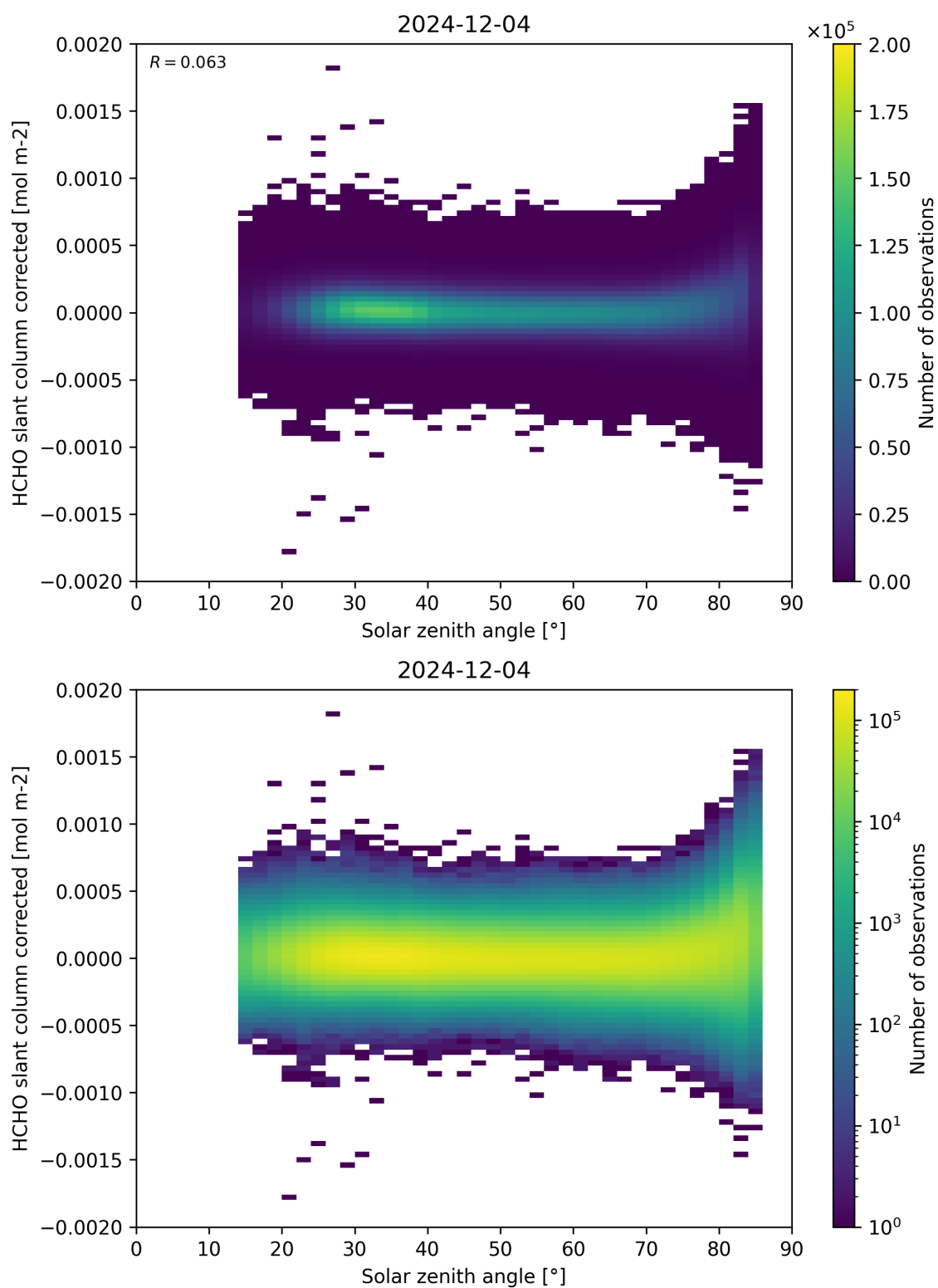
Figure 171: Scatter density plot of “Solar zenith angle” against “HCHO slant column corrected” for 2024-12-03 to 2024-12-05.
