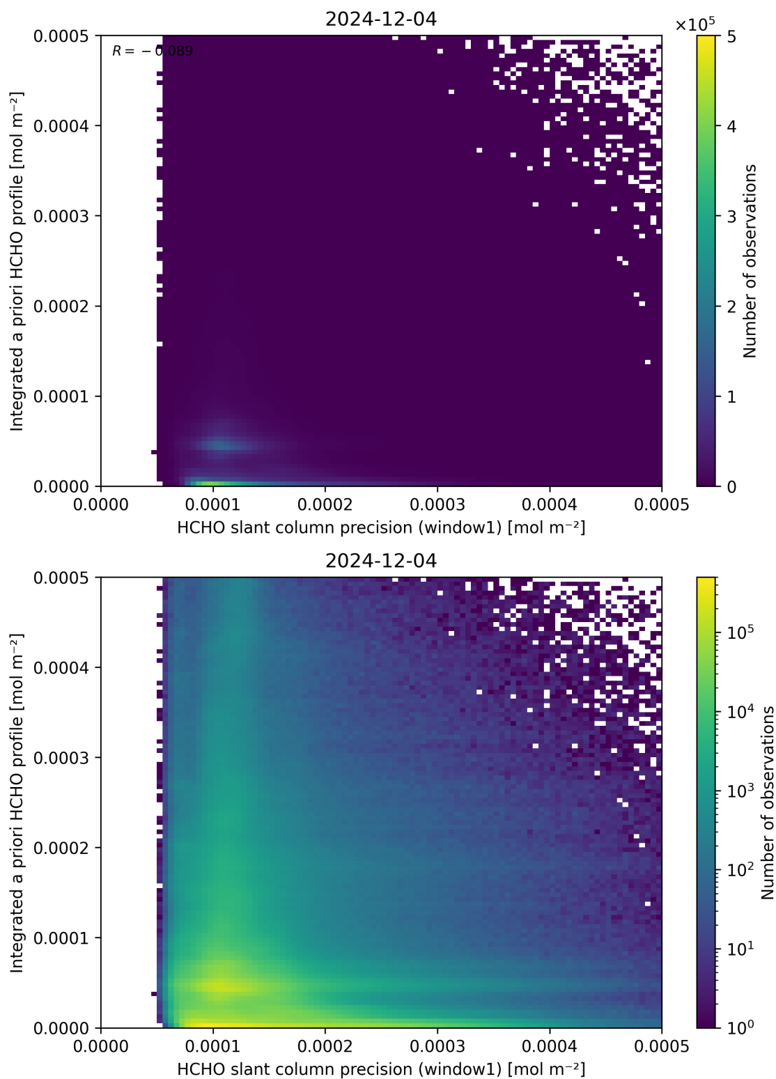
Figure 96: Scatter density plot of “HCHO slant column precision (window1)” against “Integrated a priori HCHO profile” for 2024-12-03 to 2024-12-05.
