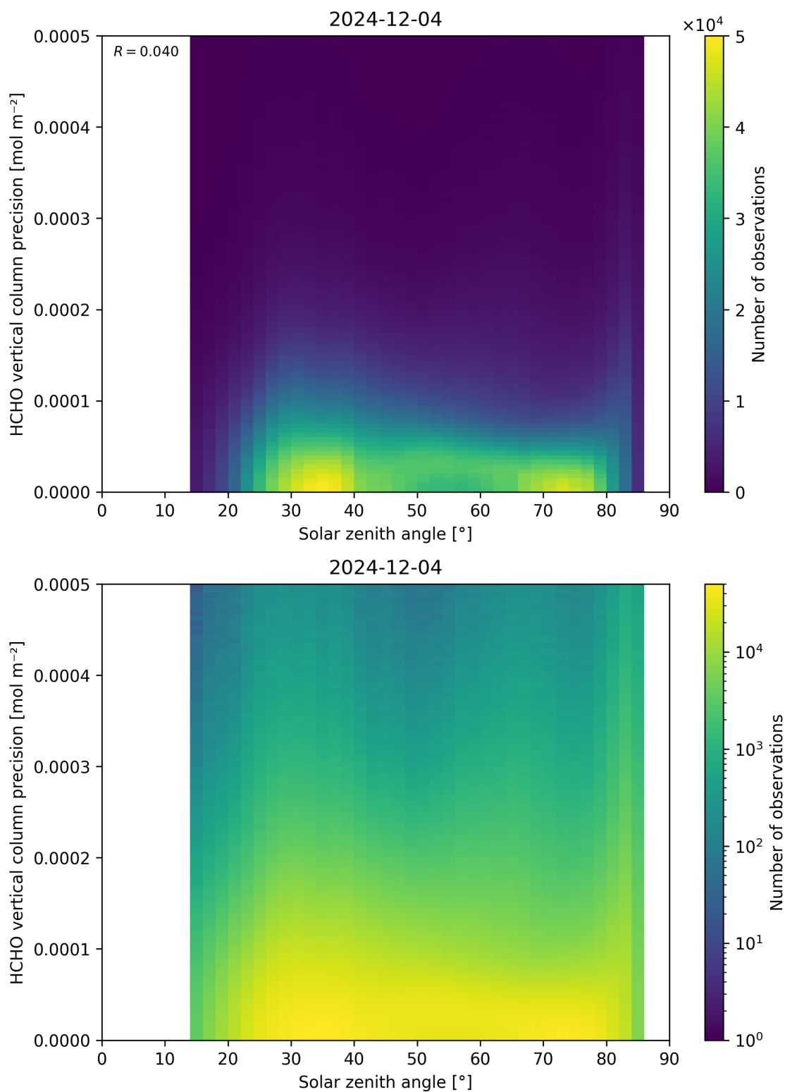
Figure 179: Scatter density plot of “Solar zenith angle” against “HCHO vertical column precision” for 2024-12-03 to 2024-12-05.
