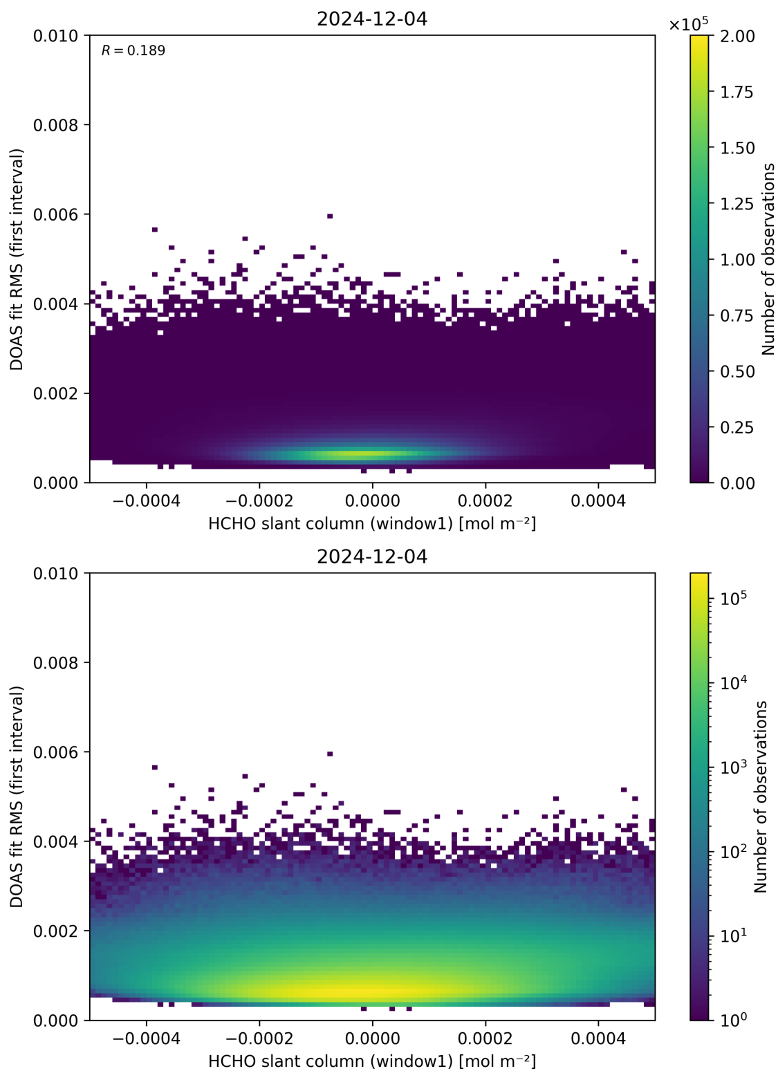
Figure 78: Scatter density plot of “HCHO slant column (window1)” against “DOAS fit RMS (first interval)” for 2024-12-03 to 2024-12-05.
