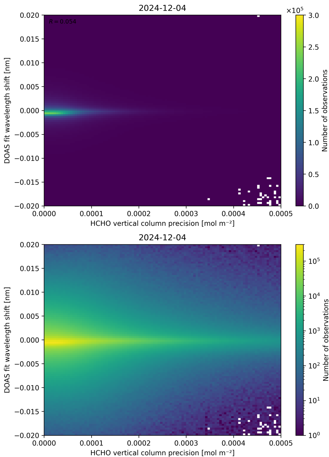
Figure 137: Scatter density plot of “HCHO vertical column precision” against “DOAS fit wavelength shift” for 2024-12-03 to 2024-12-05.
