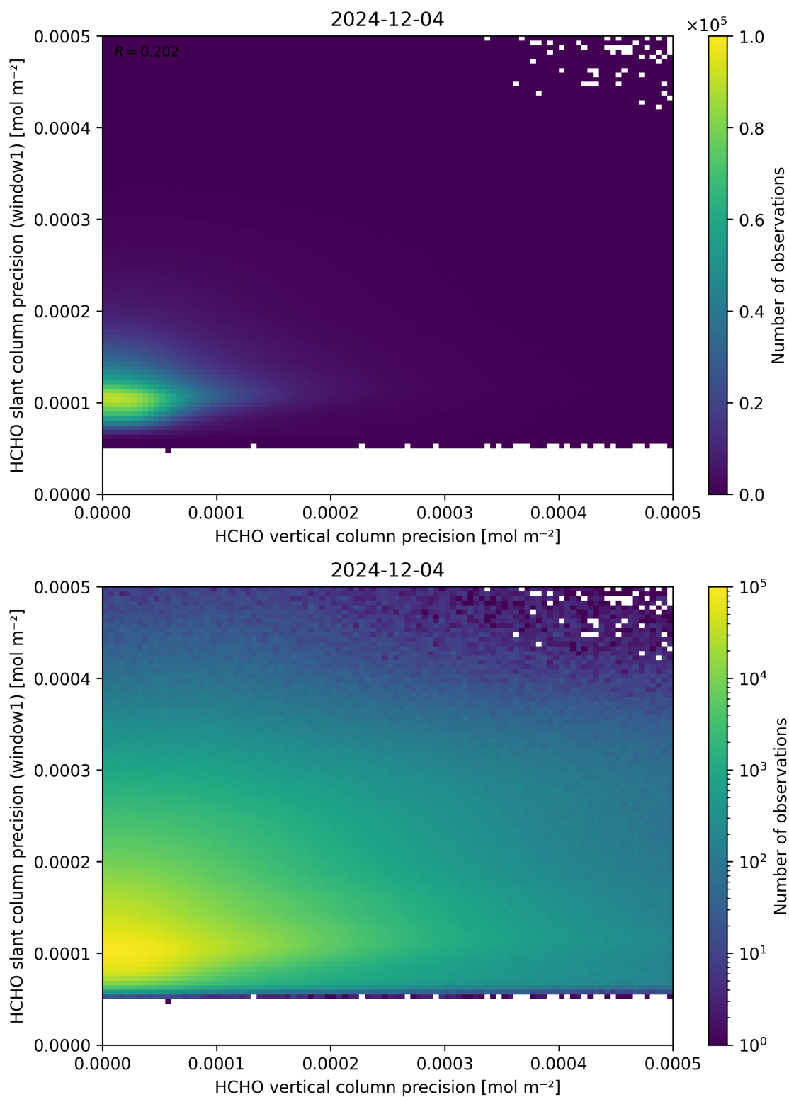
Figure 143: Scatter density plot of “HCHO vertical column precision” against “HCHO slant column precision (window1)” for 2024-12-03 to 2024-12-05.
