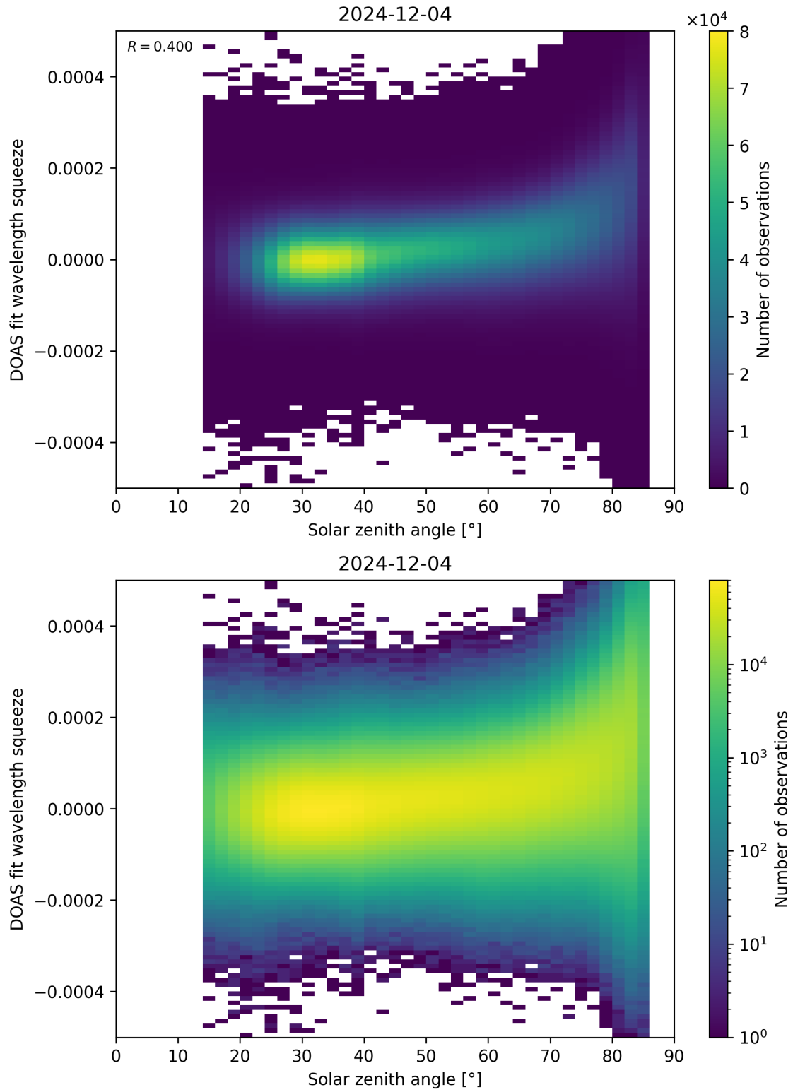
Figure 169: Scatter density plot of “Solar zenith angle” against “DOAS fit wavelength squeeze” for 2024-12-03 to 2024-12-05.
