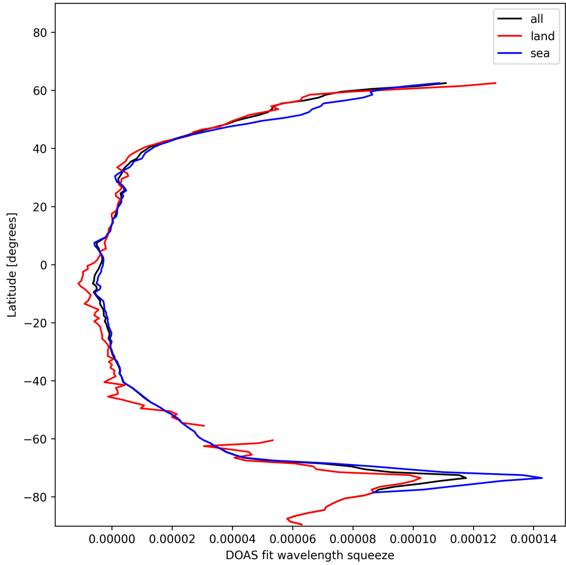
Figure 31: Zonal average of “DOAS fit wavelength squeeze” for 2024-12-03 to 2024-12-05.
