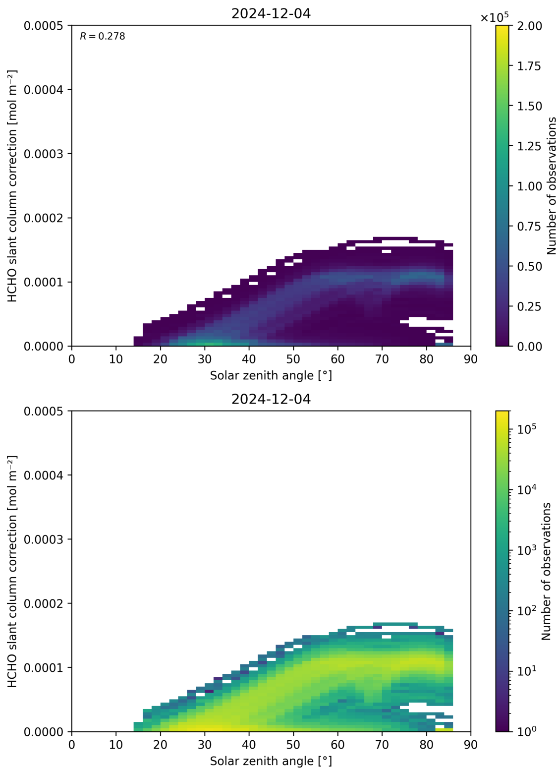
Figure 172: Scatter density plot of “Solar zenith angle” against “HCHO slant column correction” for 2024-12-03 to 2024-12-05.
