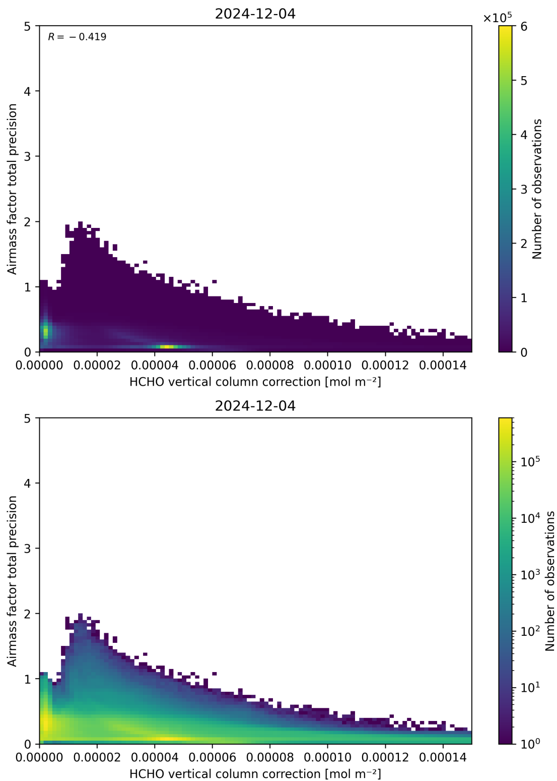
Figure 121: Scatter density plot of “HCHO vertical column correction” against “Airmass factor total precision” for 2024-12-03 to 2024-12-05.
