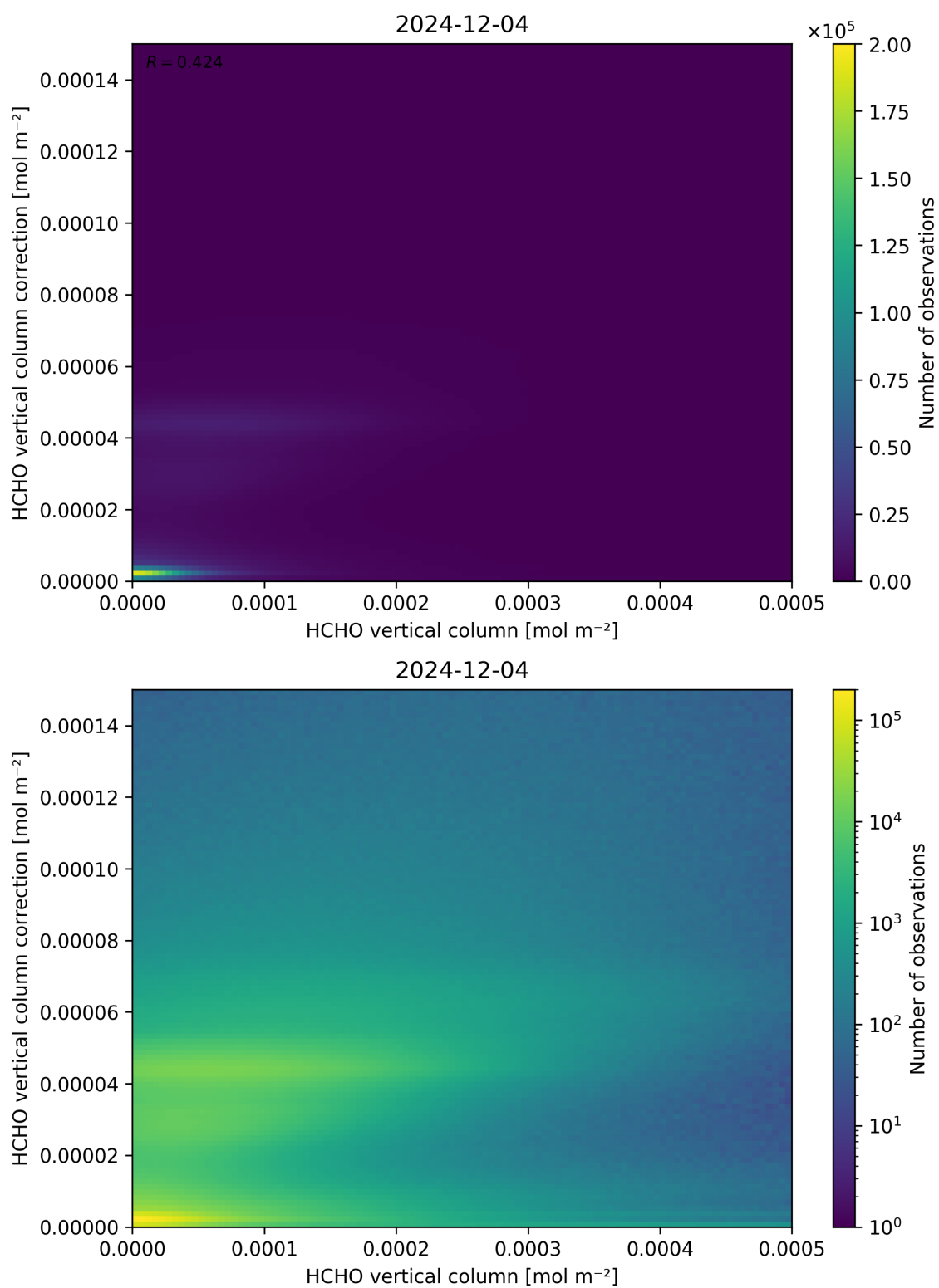
Figure 133: Scatter density plot of “HCHO vertical column” against “HCHO vertical column correction” for 2024-12-03 to 2024-12-05.
