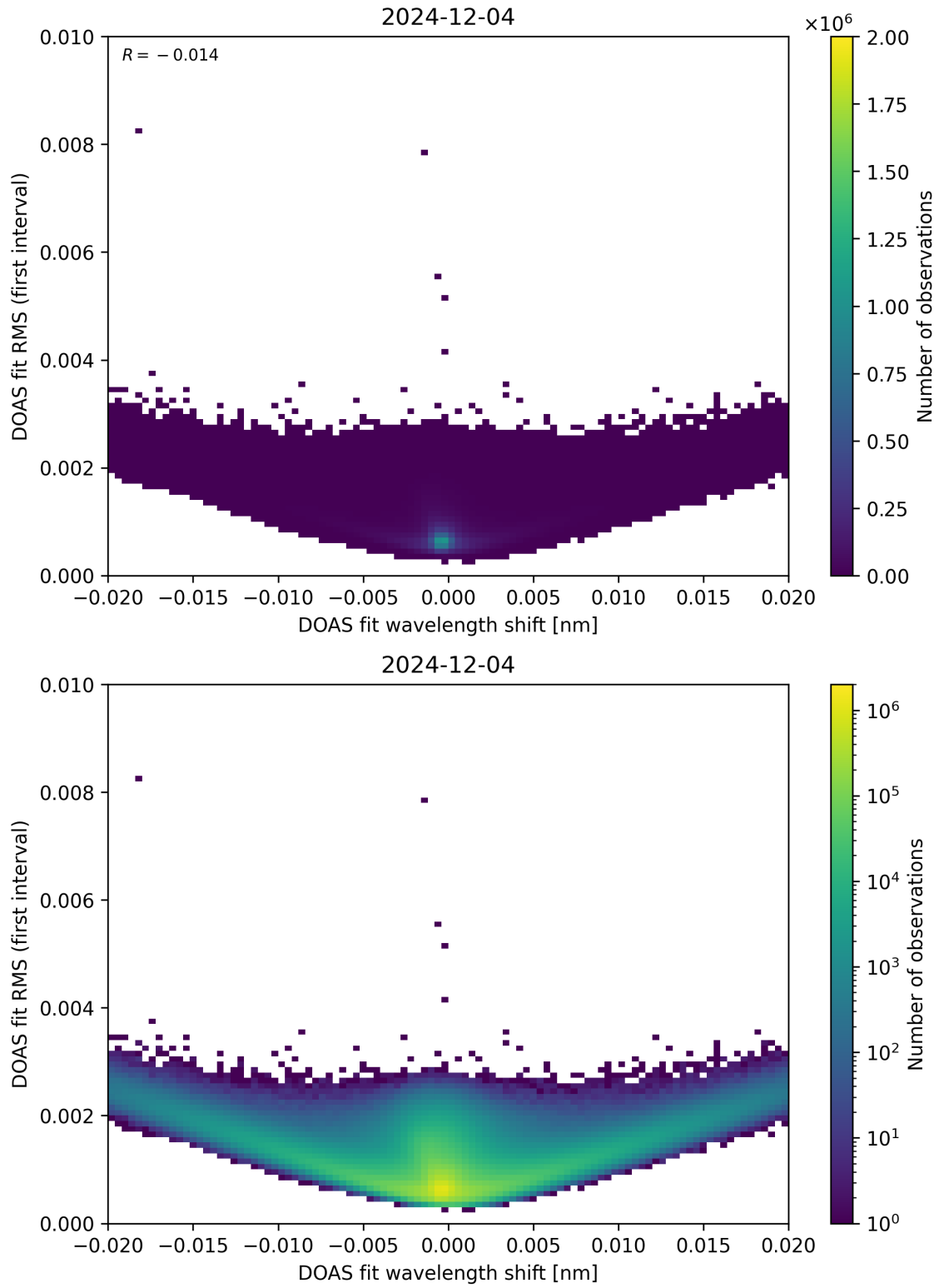
Figure 64: Scatter density plot of “DOAS fit wavelength shift” against “DOAS fit RMS (first interval)” for 2024-12-03 to 2024-12-05.
