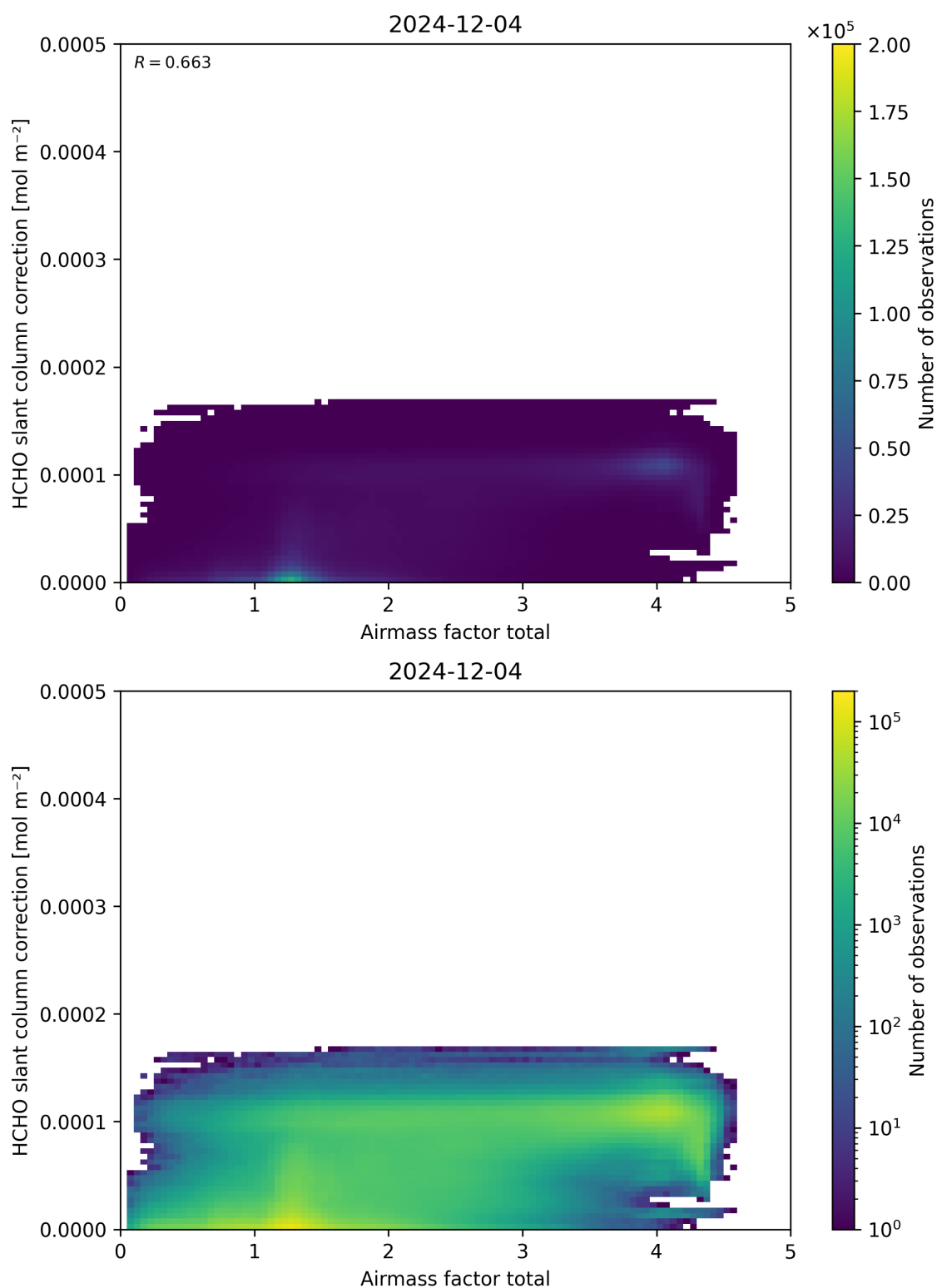
Figure 102: Scatter density plot of “Airmass factor total” against “HCHO slant column correction” for 2024-12-03 to 2024-12-05.
