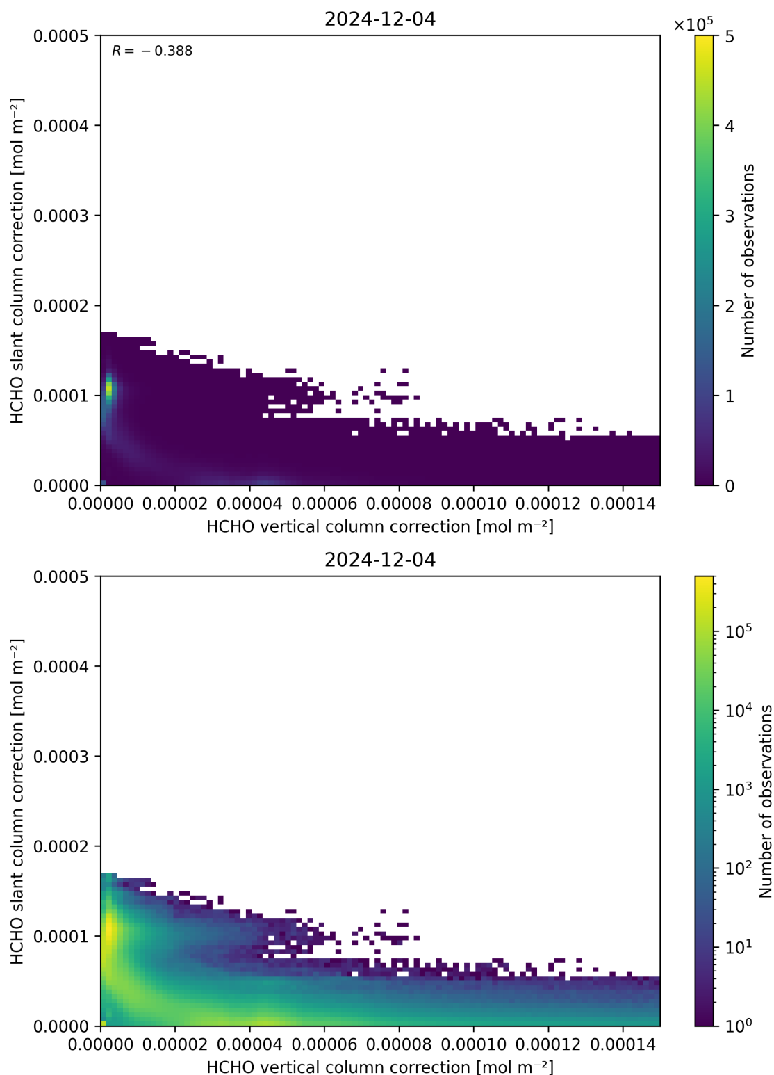
Figure 117: Scatter density plot of “HCHO vertical column correction” against “HCHO slant column correction” for 2024-12-03 to 2024-12-05.
