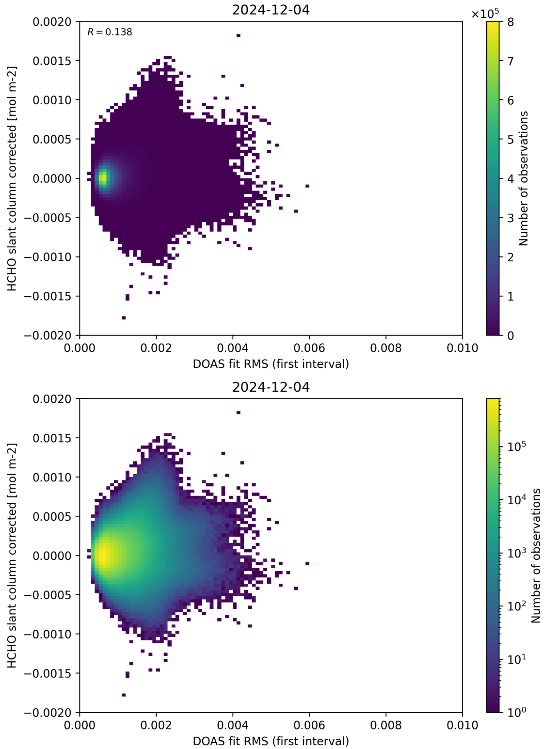
Figure 62: Scatter density plot of “DOAS fit RMS (first interval)” against “HCHO slant column corrected” for 2024-12-03 to 2024-12-05.
