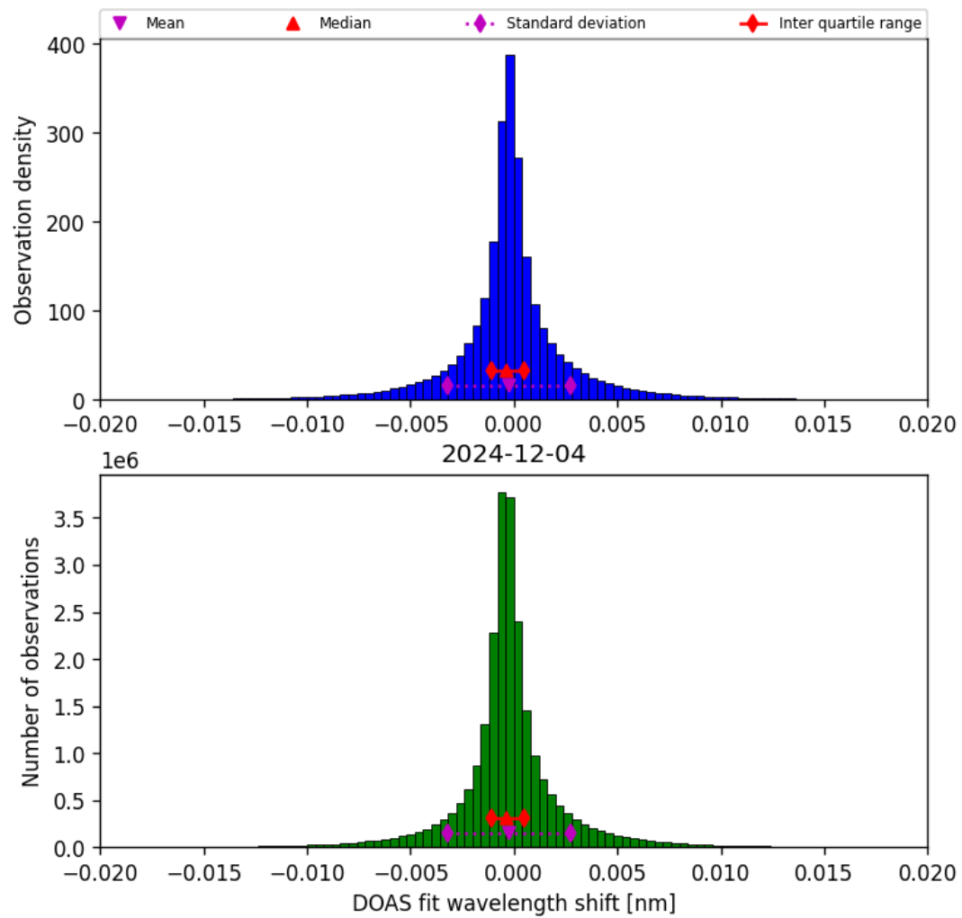
Figure 44: Histogram of “DOAS fit wavelength shift” for 2024-12-03 to 2024-12-05
