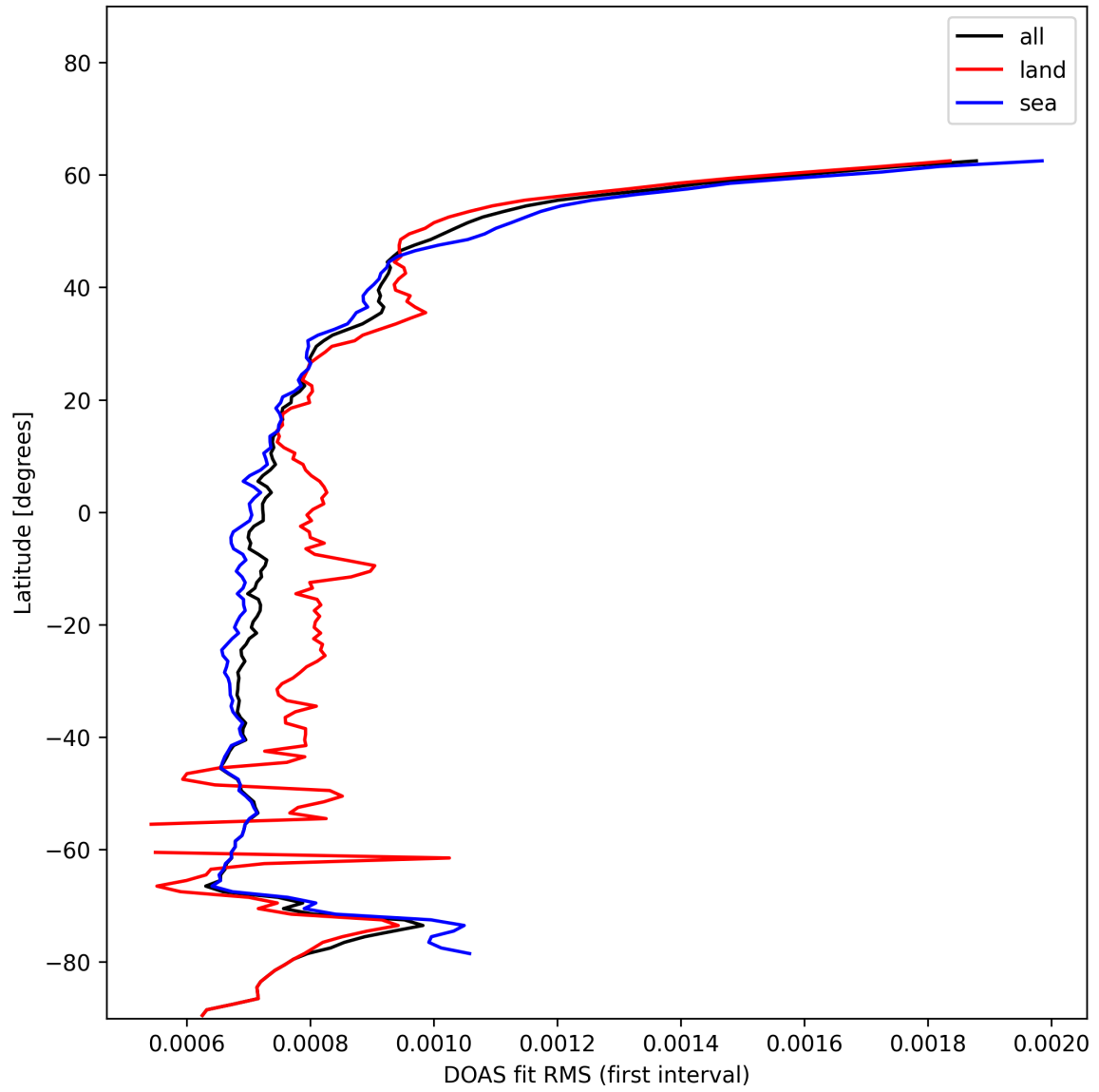
Figure 32: Zonal average of “DOAS fit RMS (first interval)” for 2024-12-03 to 2024-12-05.
