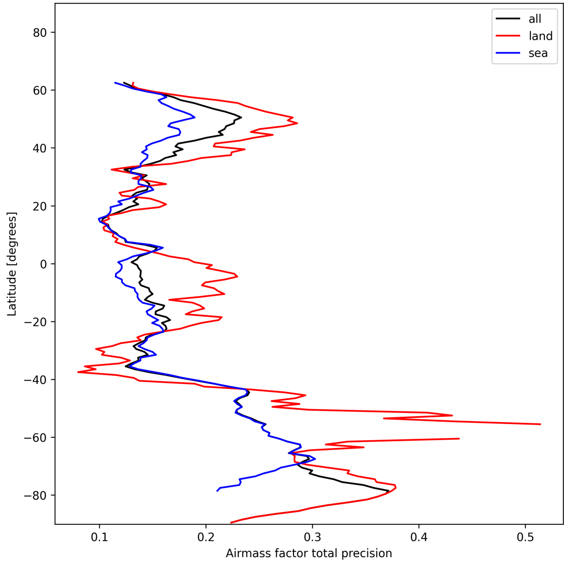
Figure 27: Zonal average of “Airmass factor total precision” for 2024-12-03 to 2024-12-05.
