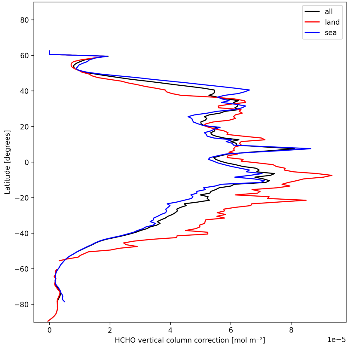
Figure 23: Zonal average of “HCHO vertical column correction” for 2024-12-03 to 2024-12-05.
