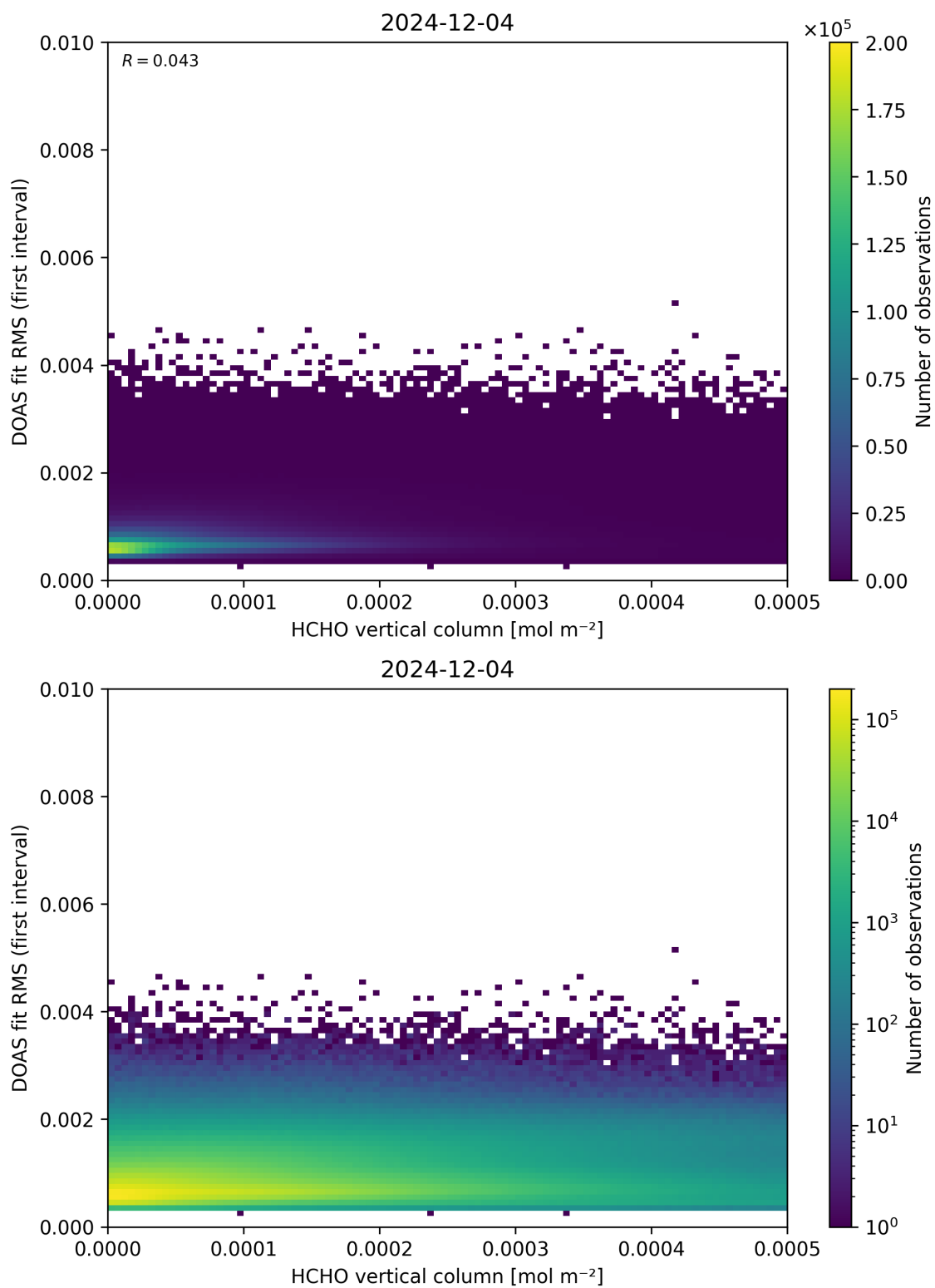
Figure 123: Scatter density plot of “HCHO vertical column” against “DOAS fit RMS (first interval)” for 2024-12-03 to 2024-12-05.
