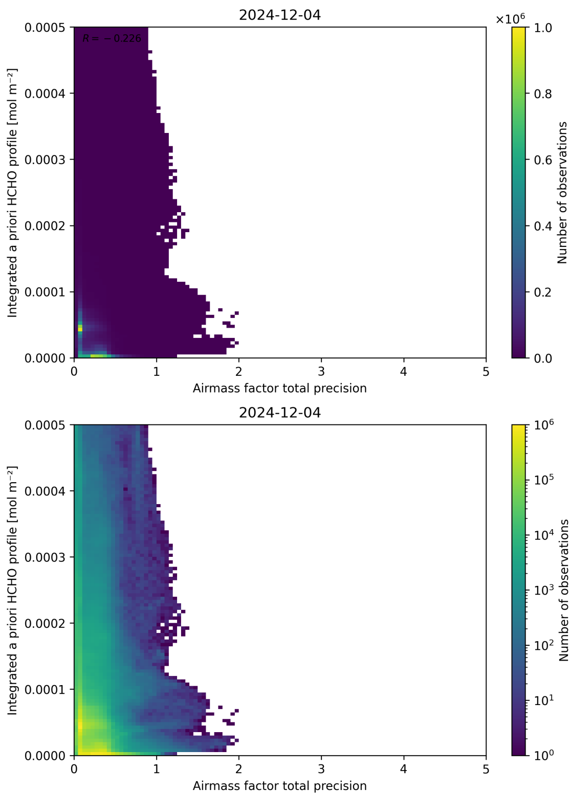
Figure 111: Scatter density plot of “Airmass factor total precision” against “Integrated a priori HCHO profile” for 2024-12-03 to 2024-12-05.
