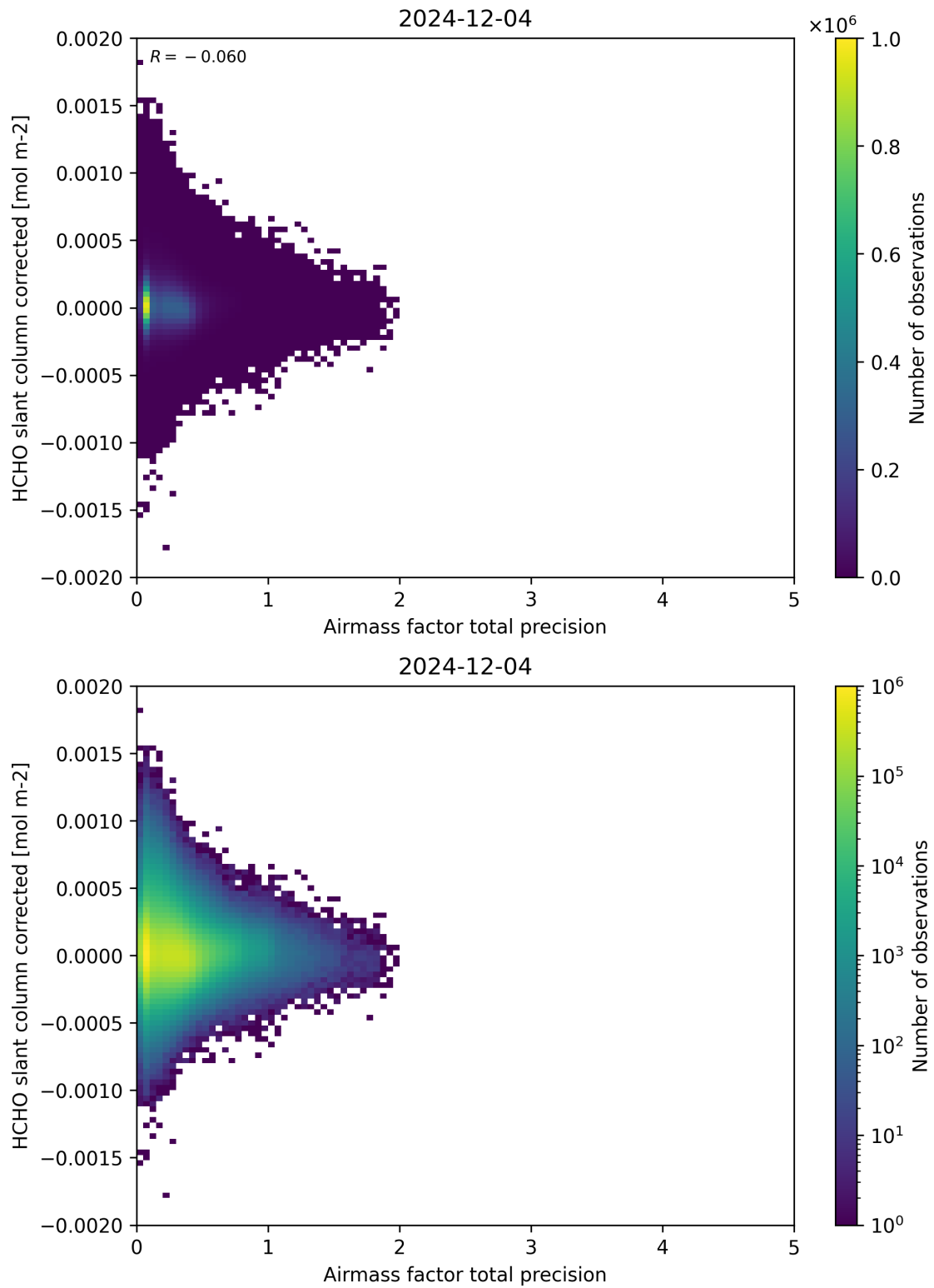
Figure 109: Scatter density plot of “Airmass factor total precision” against “HCHO slant column corrected” for 2024-12-03 to 2024-12-05.
