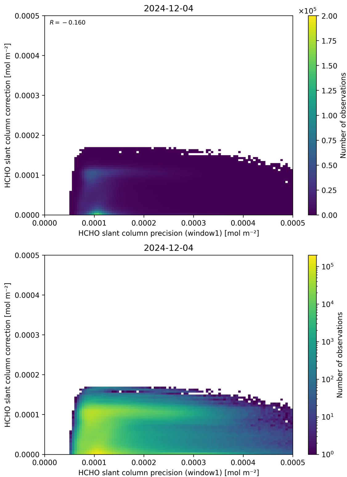
Figure 93: Scatter density plot of “HCHO slant column precision (window1)” against “HCHO slant column correction” for 2024-12-03 to 2024-12-05.
