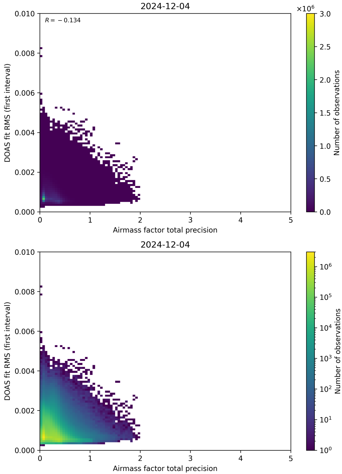
Figure 105: Scatter density plot of “Airmass factor total precision” against “DOAS fit RMS (first interval)” for 2024-12-03 to 2024-12-05.
