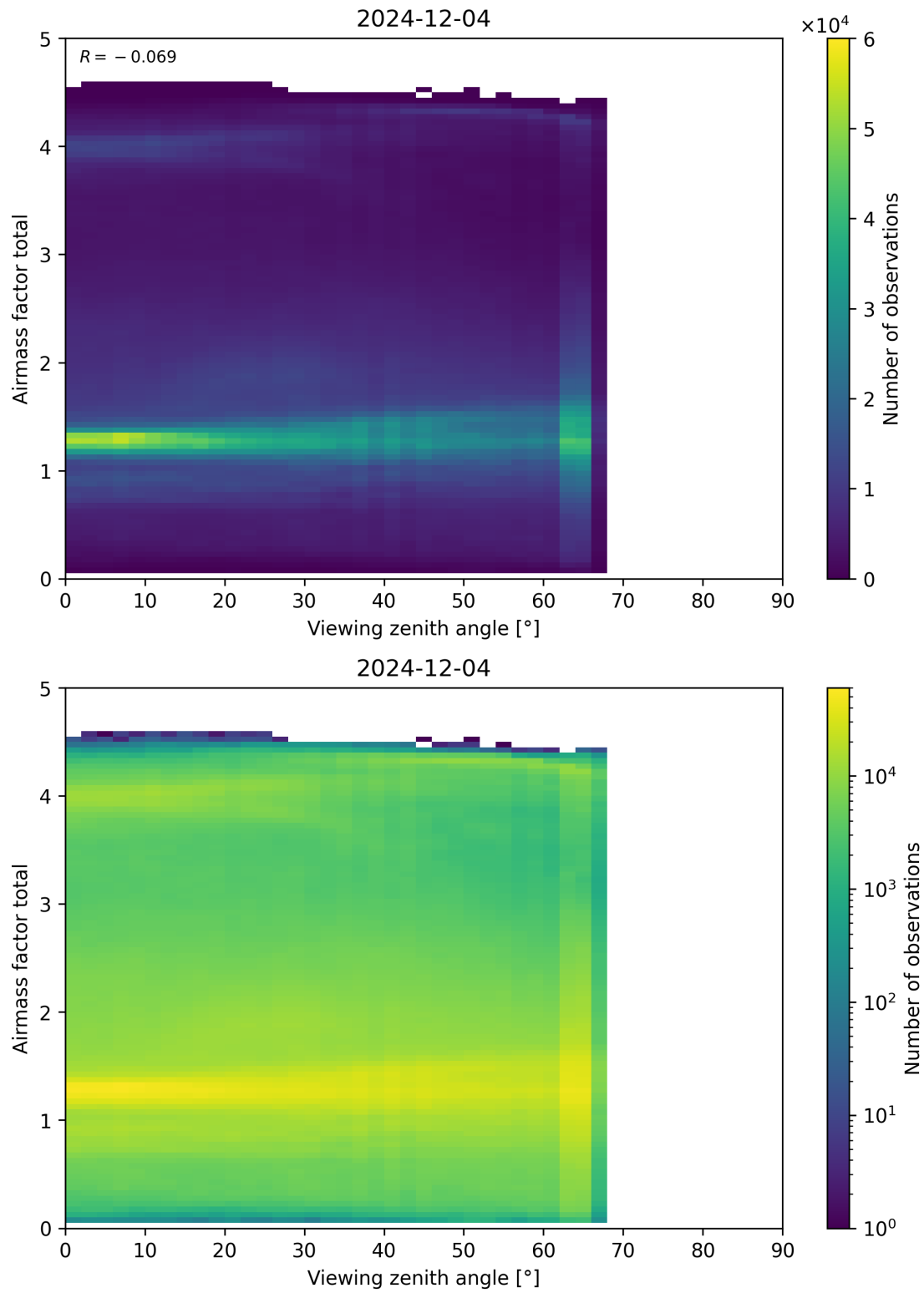
Figure 190: Scatter density plot of “Viewing zenith angle” against “Airmass factor total” for 2024-12-03 to 2024-12-05.
