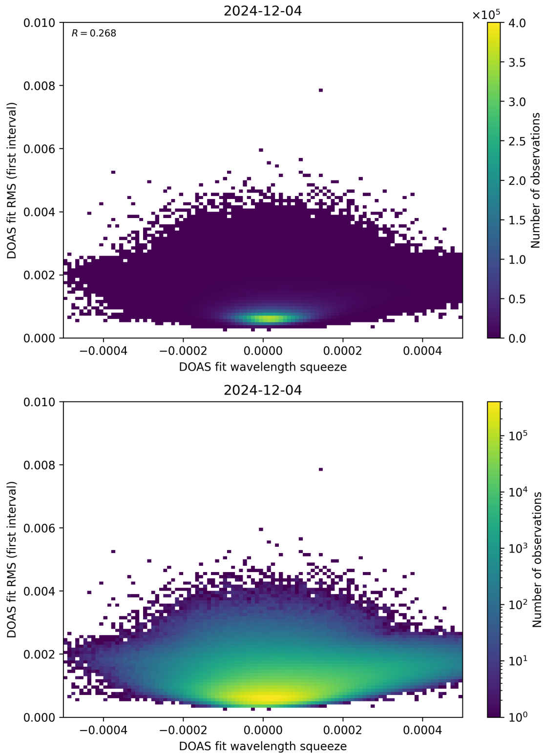
Figure 68: Scatter density plot of “DOAS fit wavelength squeeze” against “DOAS fit RMS (first interval)” for 2024-12-03 to 2024-12-05.
