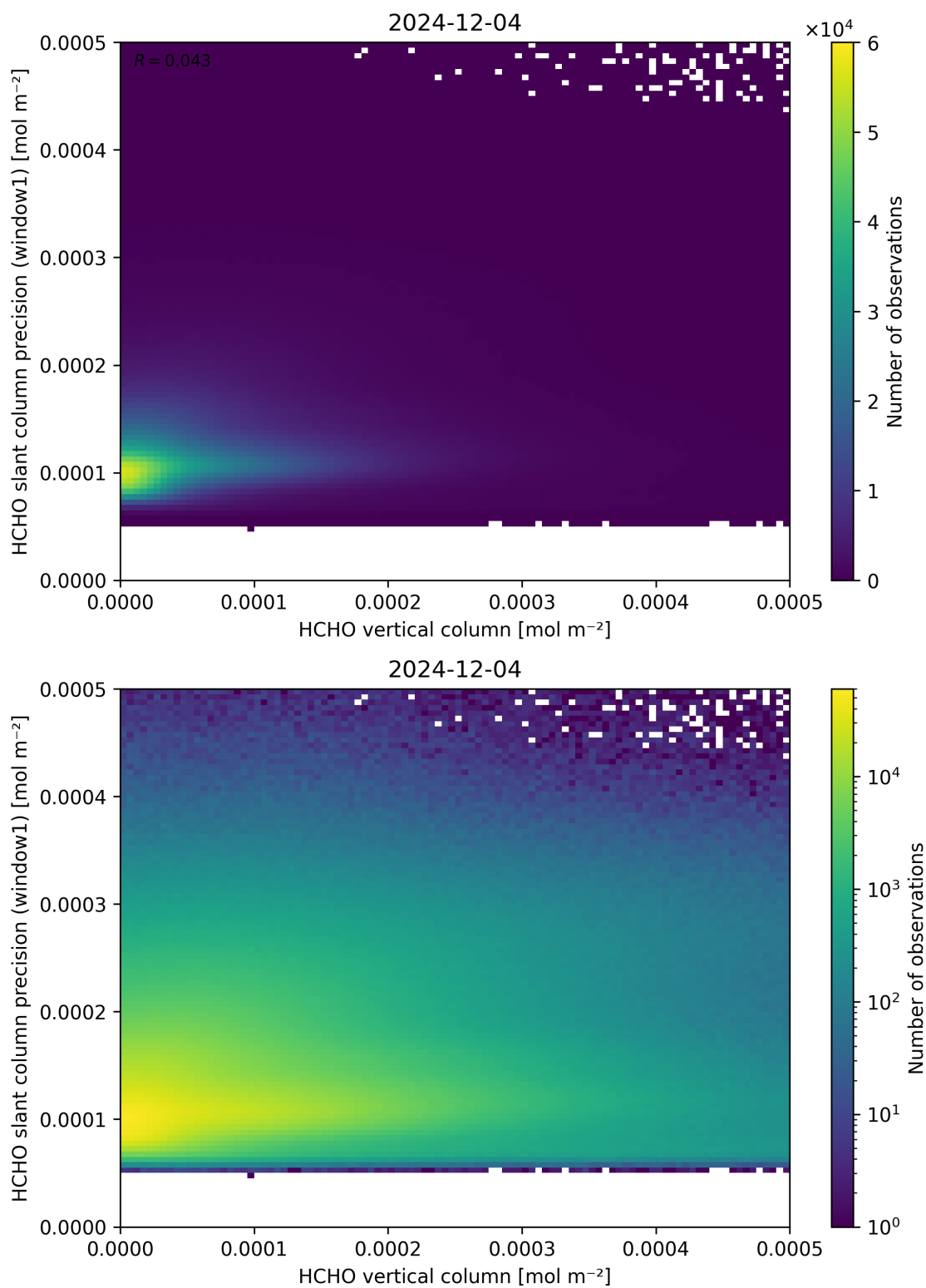
Figure 130: Scatter density plot of “HCHO vertical column” against “HCHO slant column precision (window1)” for 2024-12-03 to 2024-12-05.
