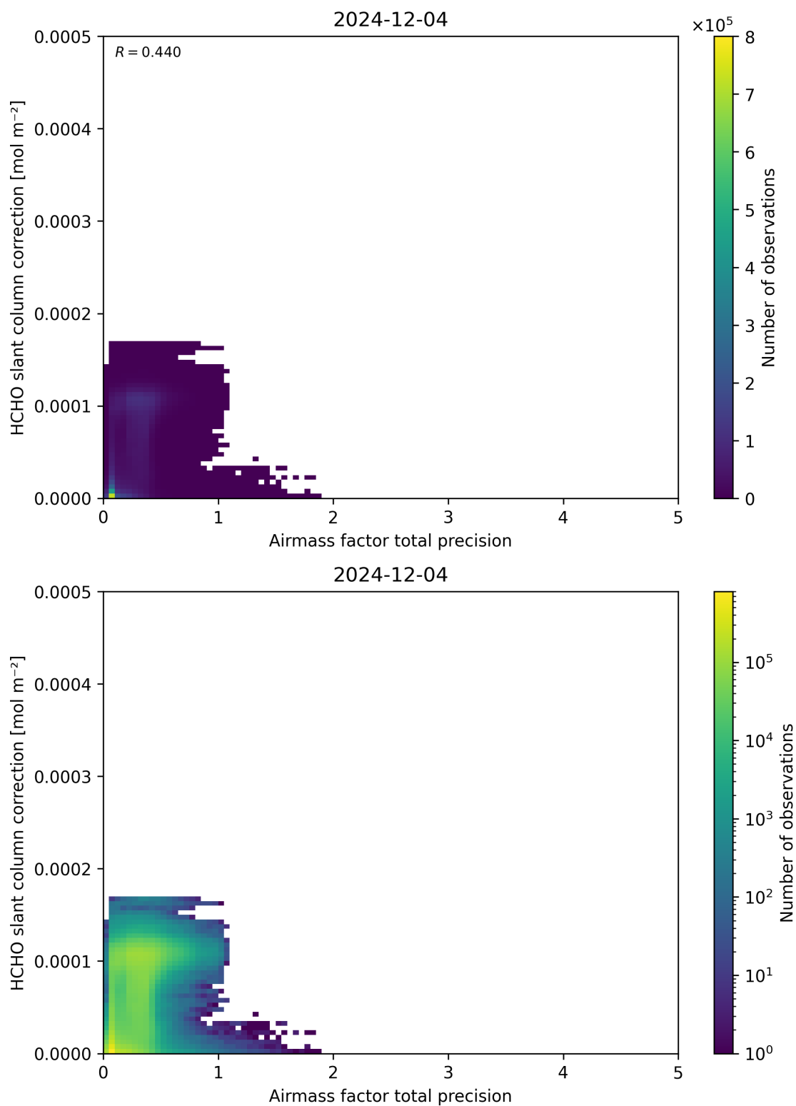
Figure 110: Scatter density plot of “Airmass factor total precision” against “HCHO slant column correction” for 2024-12-03 to 2024-12-05.
