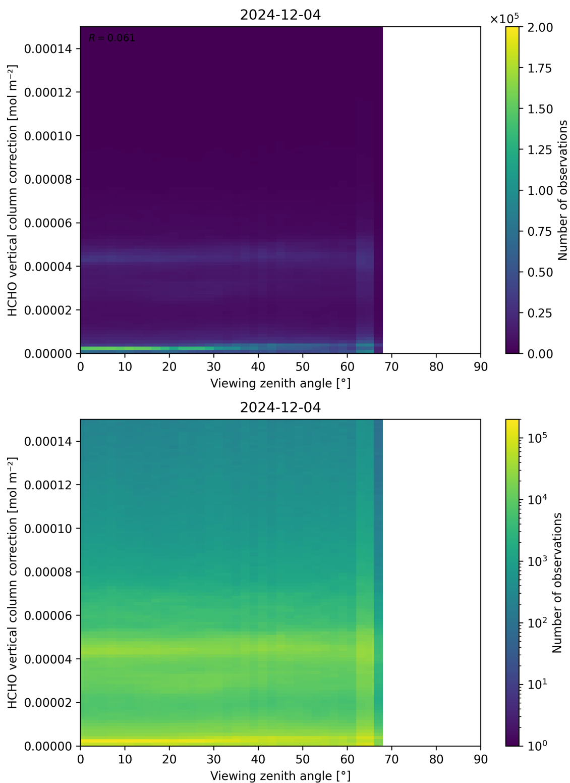
Figure 193: Scatter density plot of “Viewing zenith angle” against “HCHO vertical column correction” for 2024-12-03 to 2024-12-05.
