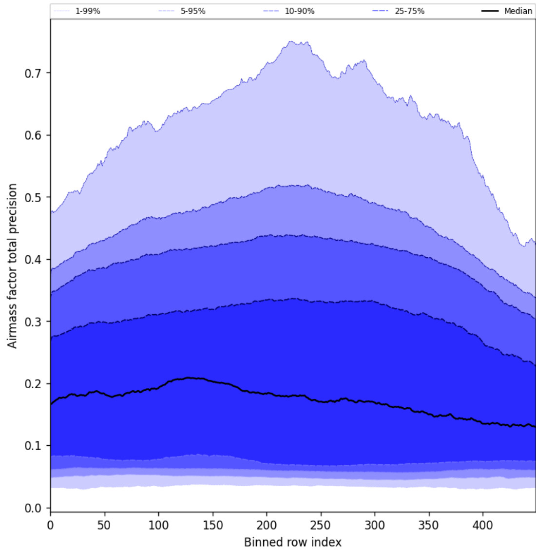
Figure 55: Along track statistics of “Airmass factor total precision” for 2024-12-03 to 2024-12-05
