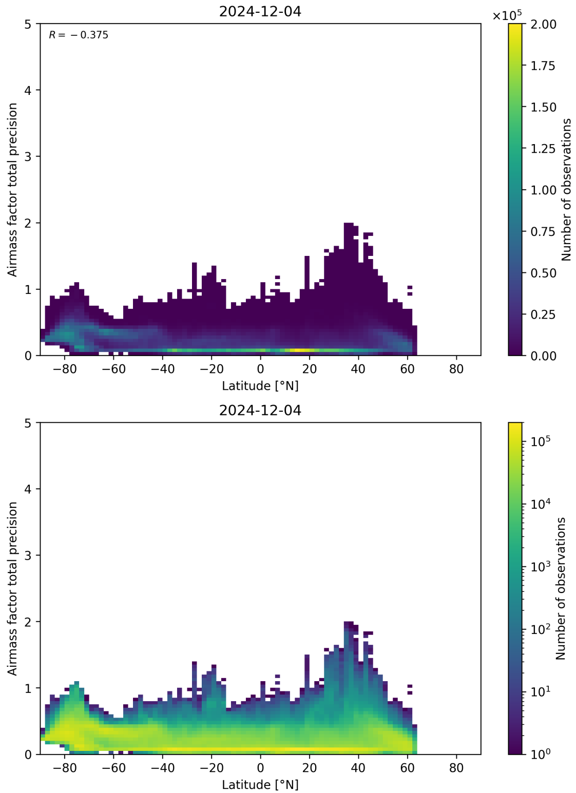
Figure 162: Scatter density plot of “Latitude” against “Airmass factor total precision” for 2024-12-03 to 2024-12-05.
