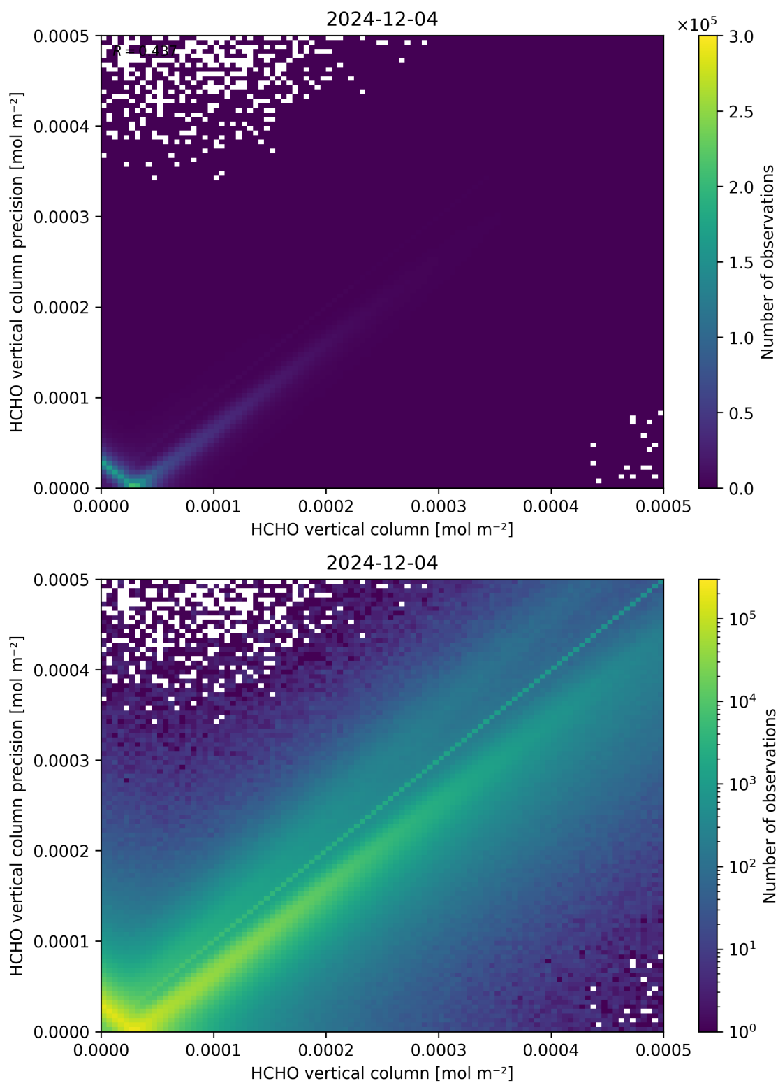
Figure 134: Scatter density plot of “HCHO vertical column” against “HCHO vertical column precision” for 2024-12-03 to 2024-12-05.
