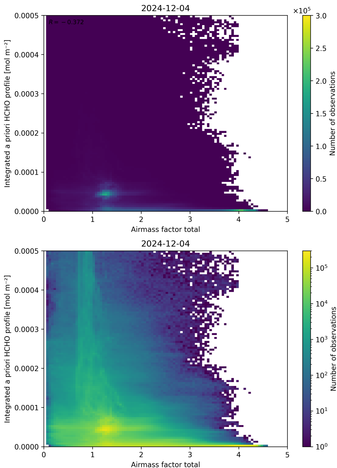
Figure 104: Scatter density plot of “Airmass factor total” against “Integrated a priori HCHO profile” for 2024-12-03 to 2024-12-05.
