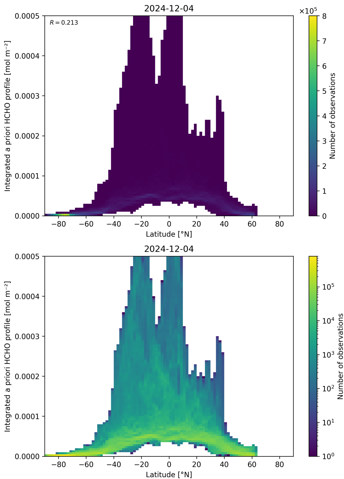
Figure 166: Scatter density plot of “Latitude” against “Integrated a priori HCHO profile” for 2024-12-03 to 2024-12-05.
