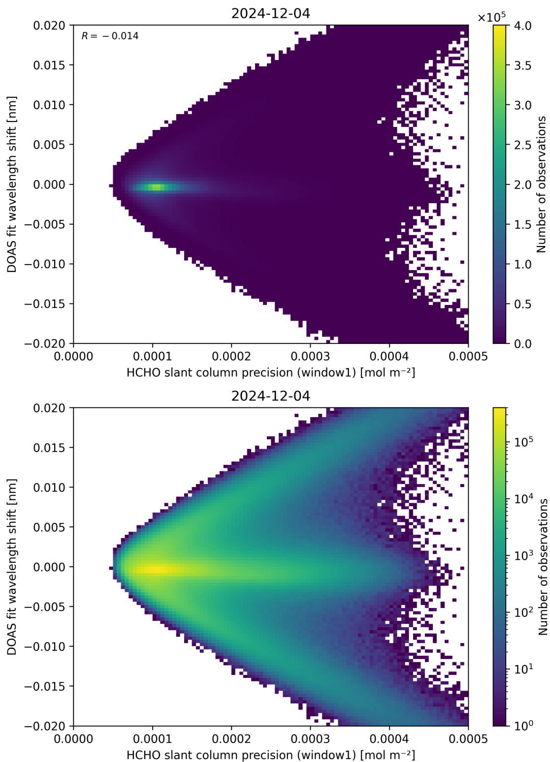
Figure 89: Scatter density plot of “HCHO slant column precision (window1)” against “DOAS fit wavelength shift” for 2024-12-03 to 2024-12-05.
