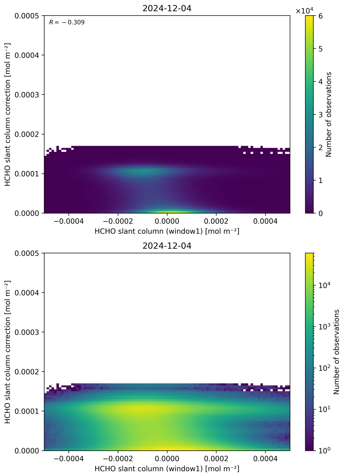
Figure 83: Scatter density plot of “HCHO slant column (window1)” against “HCHO slant column correction” for 2024-12-03 to 2024-12-05.
