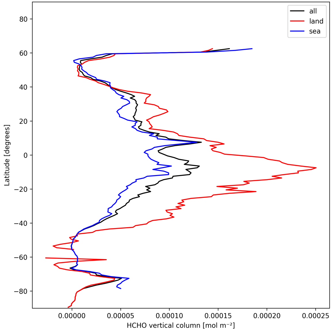
Figure 21: Zonal average of “HCHO vertical column” for 2024-12-03 to 2024-12-05.
