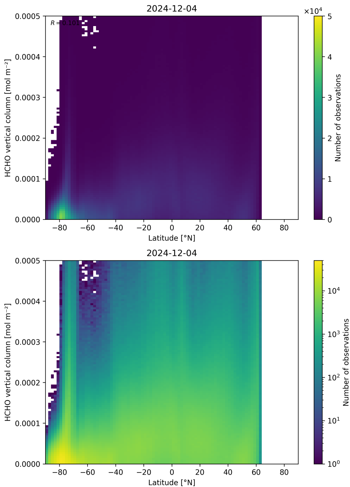
Figure 163: Scatter density plot of “Latitude” against “HCHO vertical column” for 2024-12-03 to 2024-12-05.
