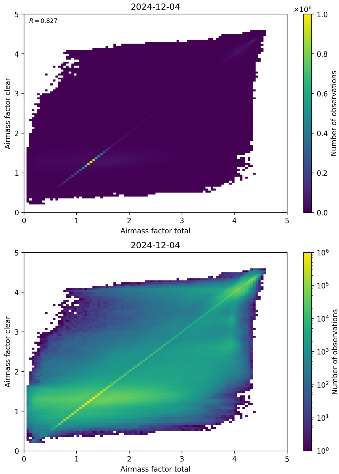
Figure 100: Scatter density plot of “Airmass factor total” against “Airmass factor clear” for 2024-12-03 to 2024-12-05.
