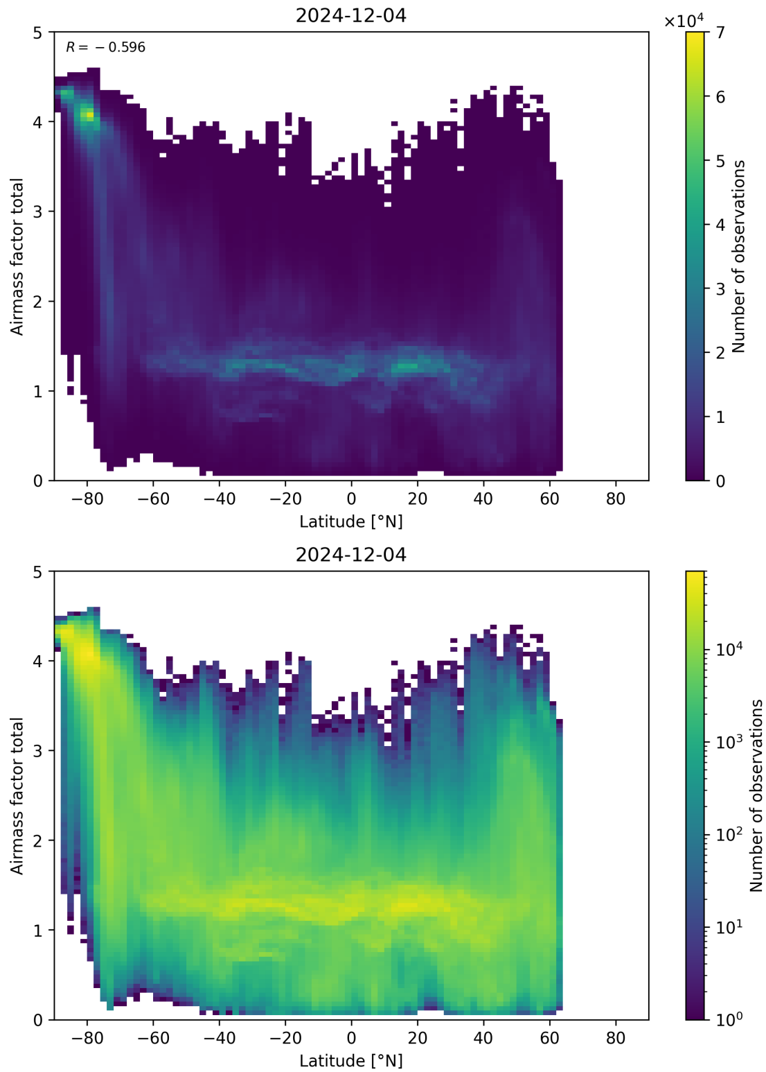
Figure 161: Scatter density plot of “Latitude” against “Airmass factor total” for 2024-12-03 to 2024-12-05.
