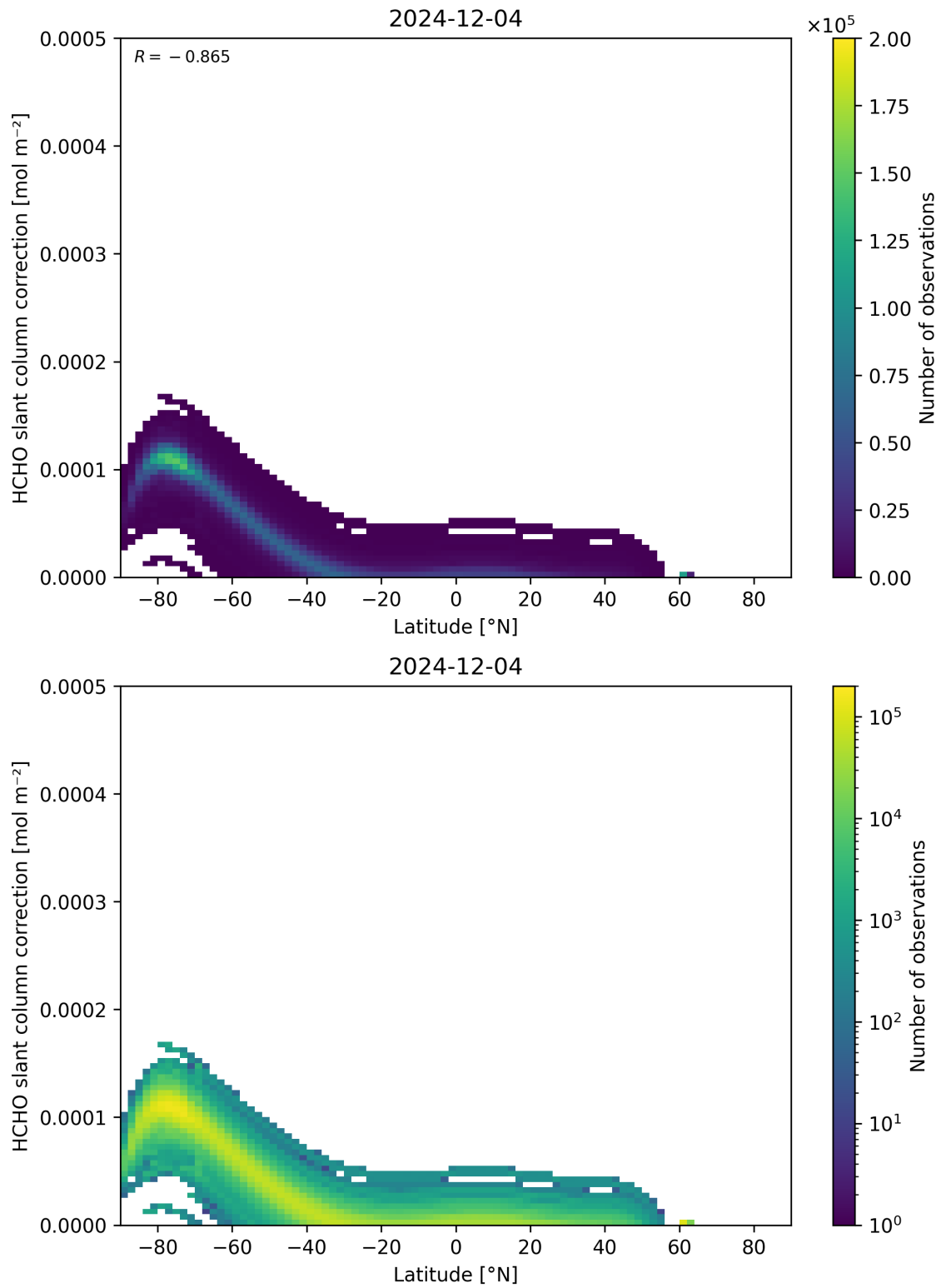
Figure 158: Scatter density plot of “Latitude” against “HCHO slant column correction” for 2024-12-03 to 2024-12-05.
