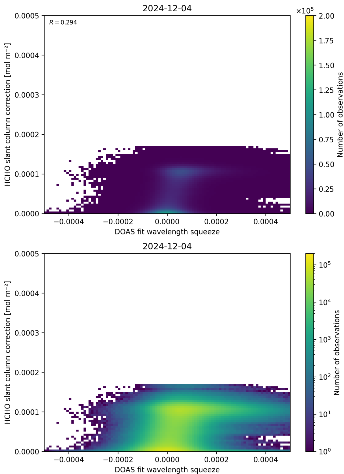
Figure 70: Scatter density plot of “DOAS fit wavelength squeeze” against “HCHO slant column correction” for 2024-12-03 to 2024-12-05.
