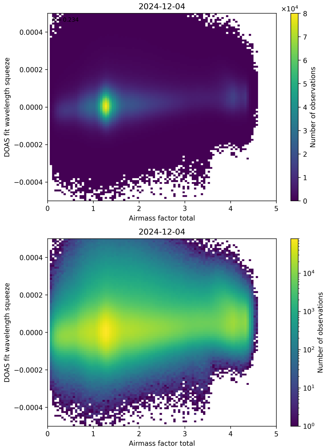
Figure 99: Scatter density plot of “Airmass factor total” against “DOAS fit wavelength squeeze” for 2024-12-03 to 2024-12-05.
