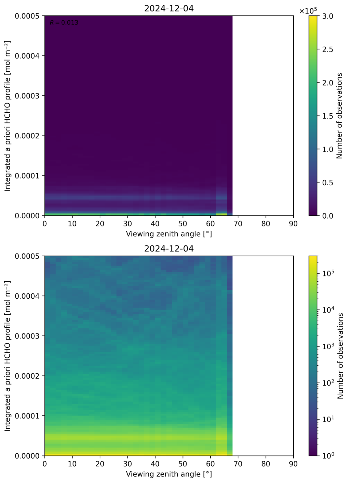
Figure 195: Scatter density plot of “Viewing zenith angle” against “Integrated a priori HCHO profile” for 2024-12-03 to 2024-12-05.
