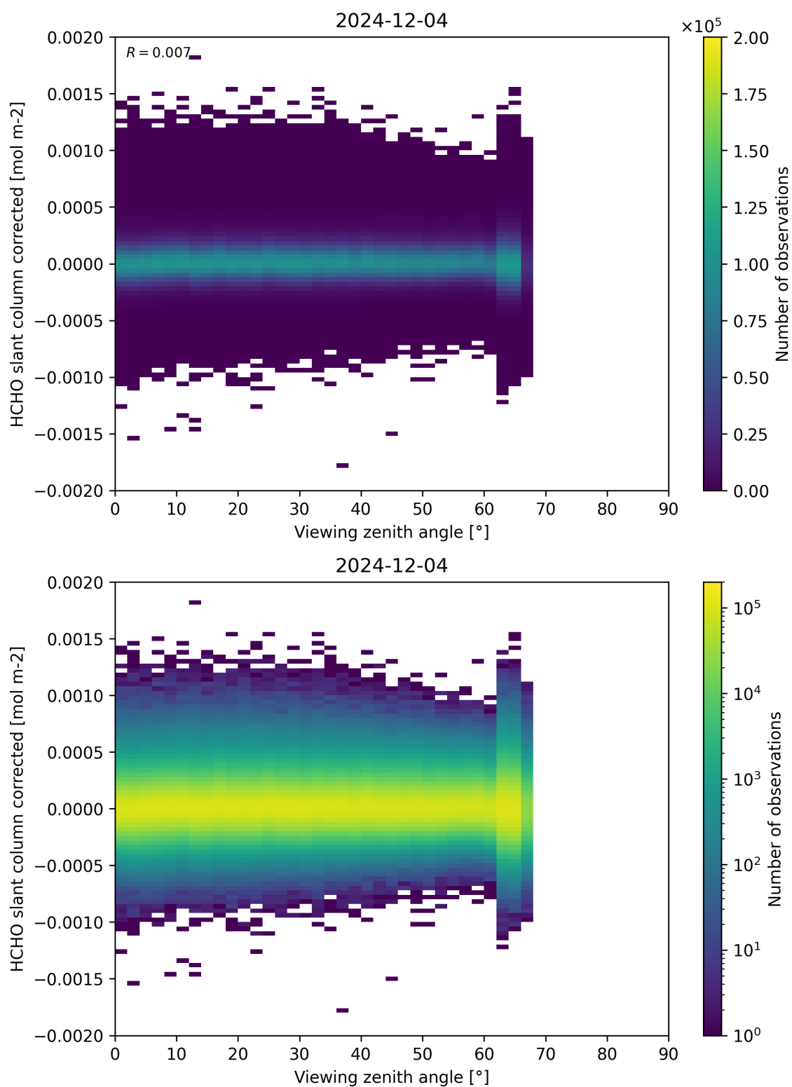
Figure 186: Scatter density plot of “Viewing zenith angle” against “HCHO slant column corrected” for 2024-12-03 to 2024-12-05.
