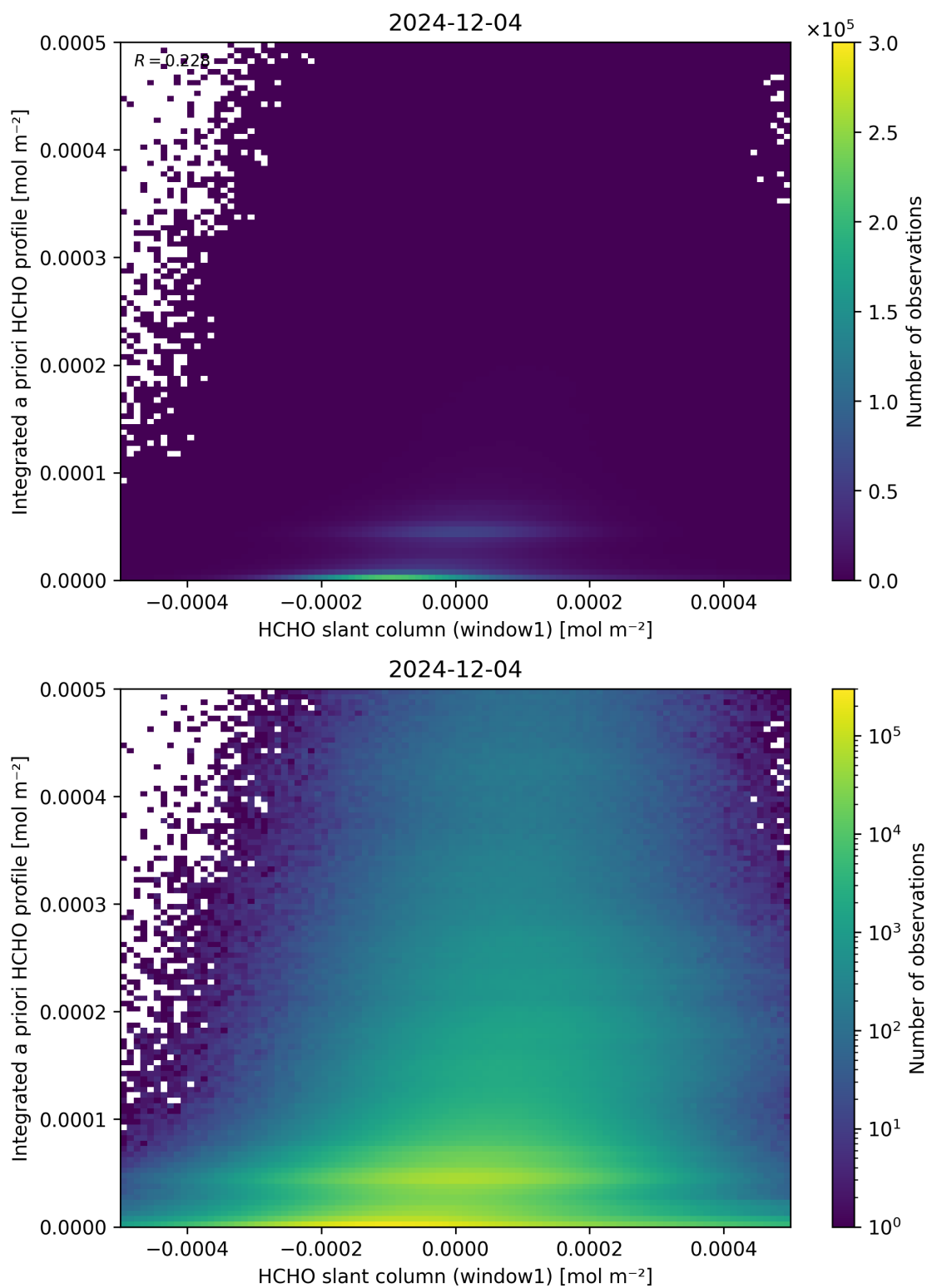
Figure 87: Scatter density plot of “HCHO slant column (window1)” against “Integrated a priori HCHO profile” for 2024-12-03 to 2024-12-05.
