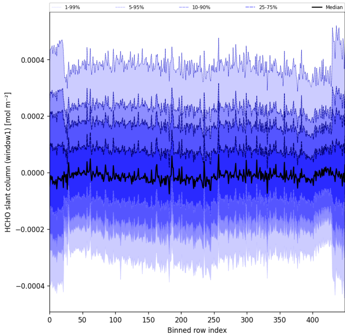
Figure 52: Along track statistics of “HCHO slant column (window1)” for 2024-12-03 to 2024-12-05
