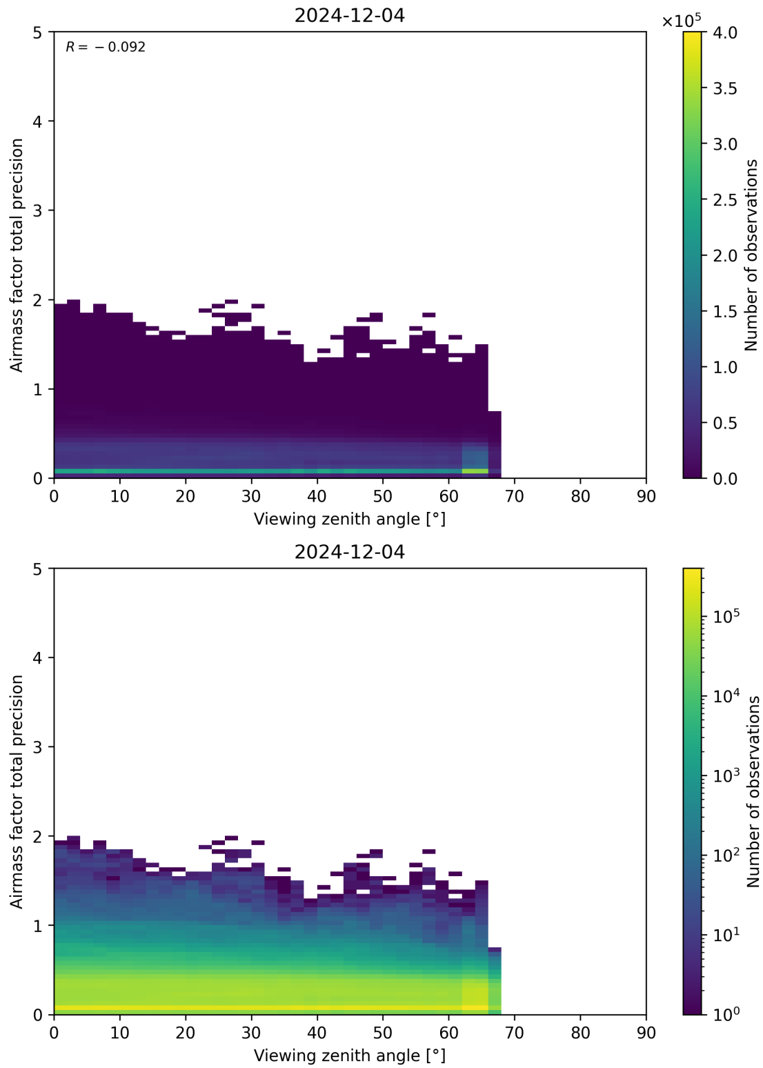
Figure 191: Scatter density plot of “Viewing zenith angle” against “Airmass factor total precision” for 2024-12-03 to 2024-12-05.
