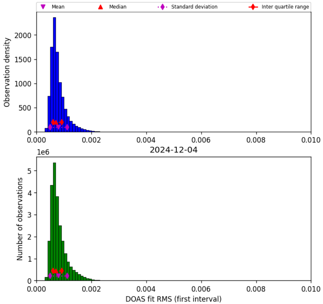
Figure 46: Histogram of “DOAS fit RMS (first interval)” for 2024-12-03 to 2024-12-05
