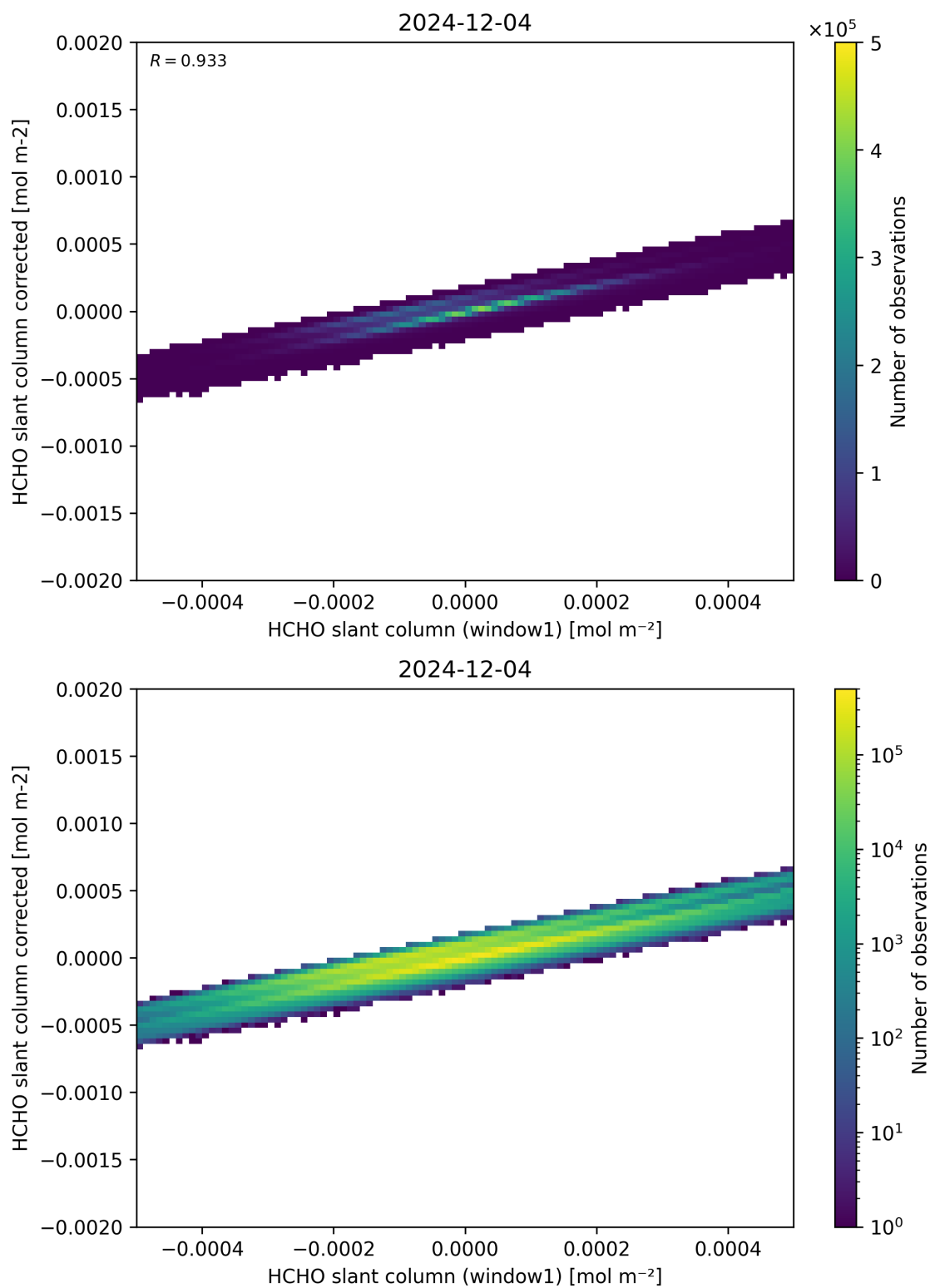
Figure 82: Scatter density plot of “HCHO slant column (window1)” against “HCHO slant column corrected” for 2024-12-03 to 2024-12-05.
