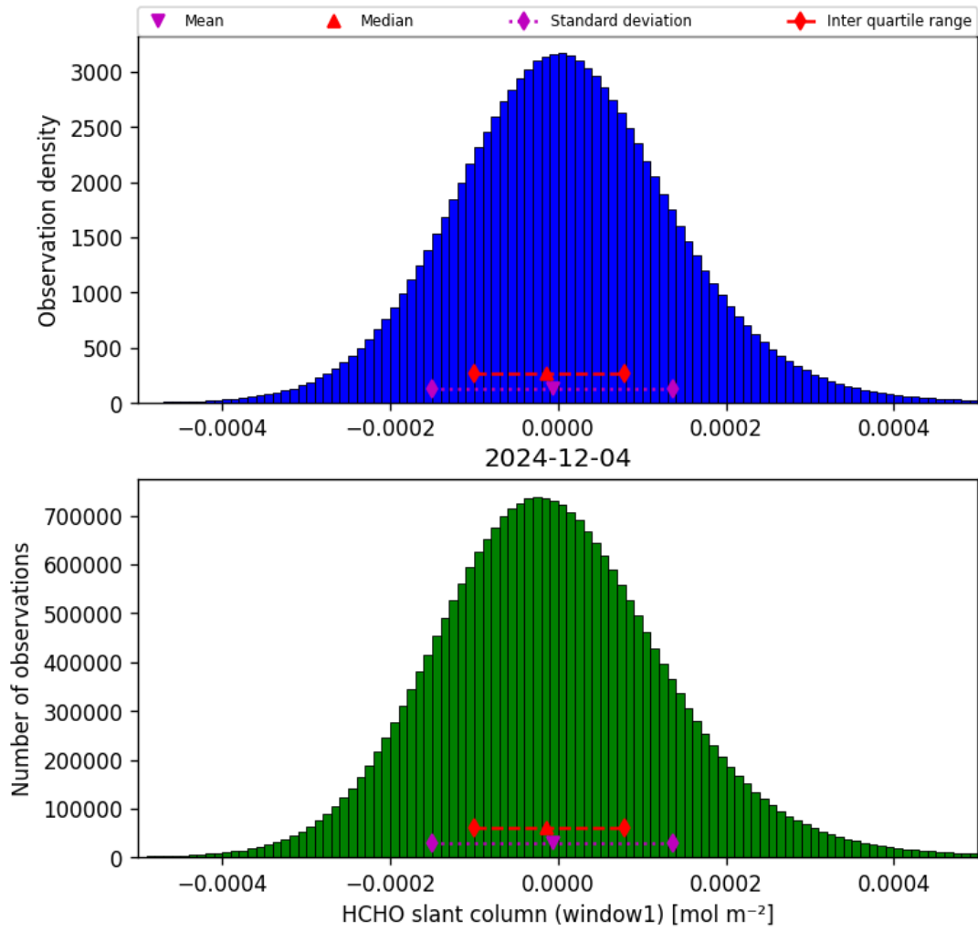
Figure 38: Histogram of “HCHO slant column (window1)” for 2024-12-03 to 2024-12-05
