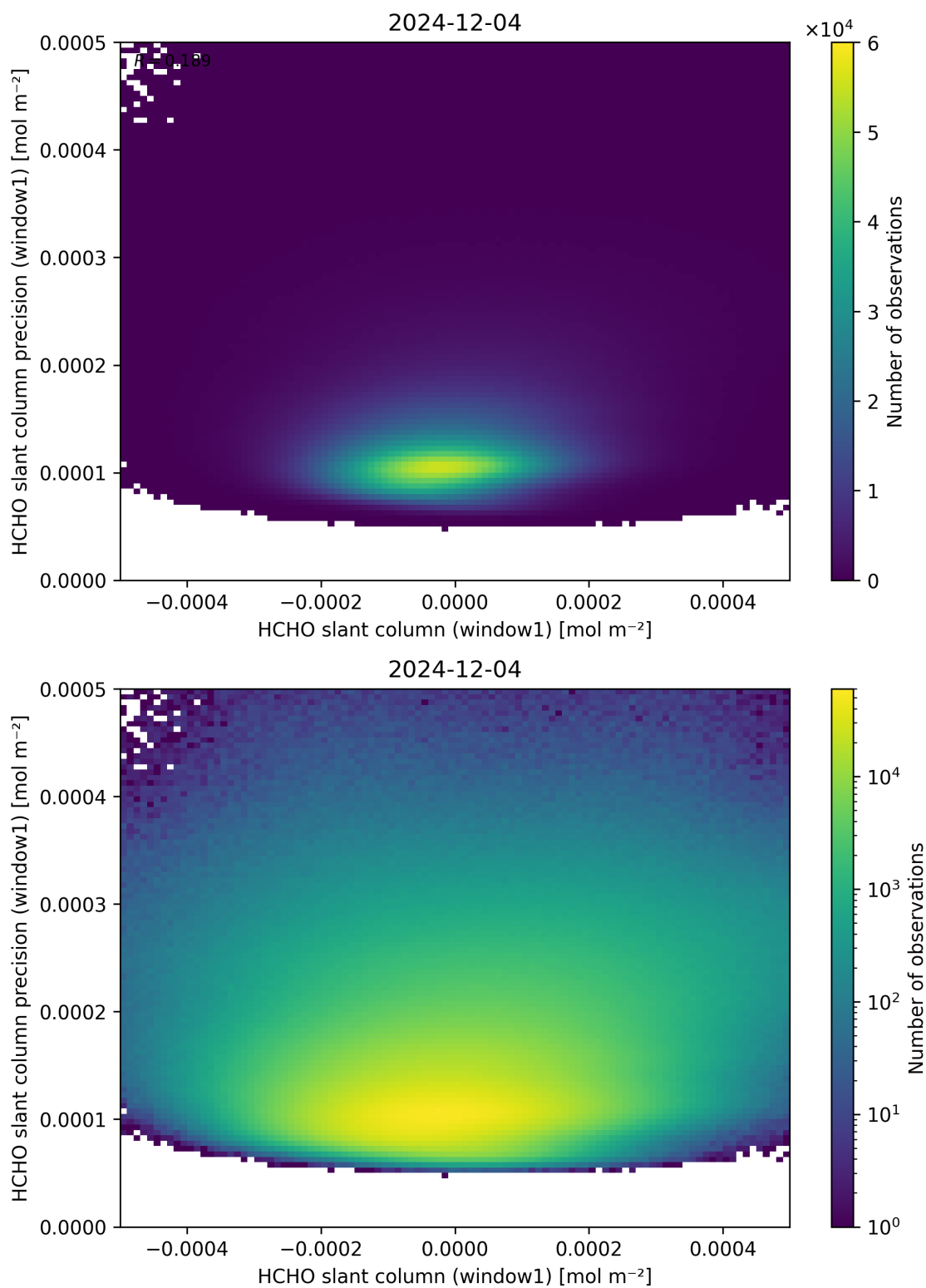
Figure 84: Scatter density plot of “HCHO slant column (window1)” against “HCHO slant column precision (window1)” for 2024-12-03 to 2024-12-05.
