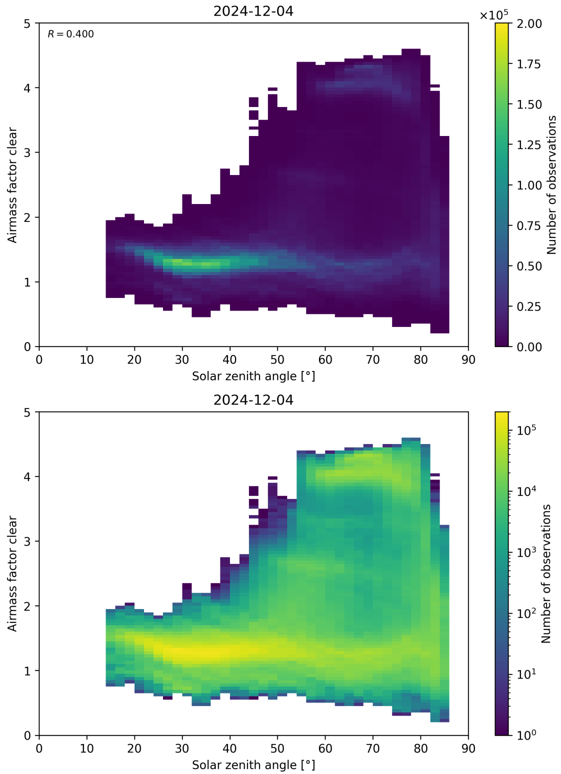
Figure 170: Scatter density plot of “Solar zenith angle” against “Airmass factor clear” for 2024-12-03 to 2024-12-05.
