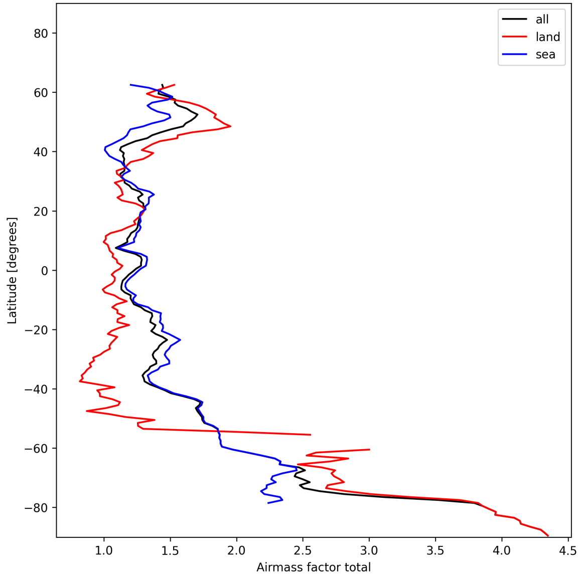
Figure 26: Zonal average of “Airmass factor total” for 2024-12-03 to 2024-12-05.
