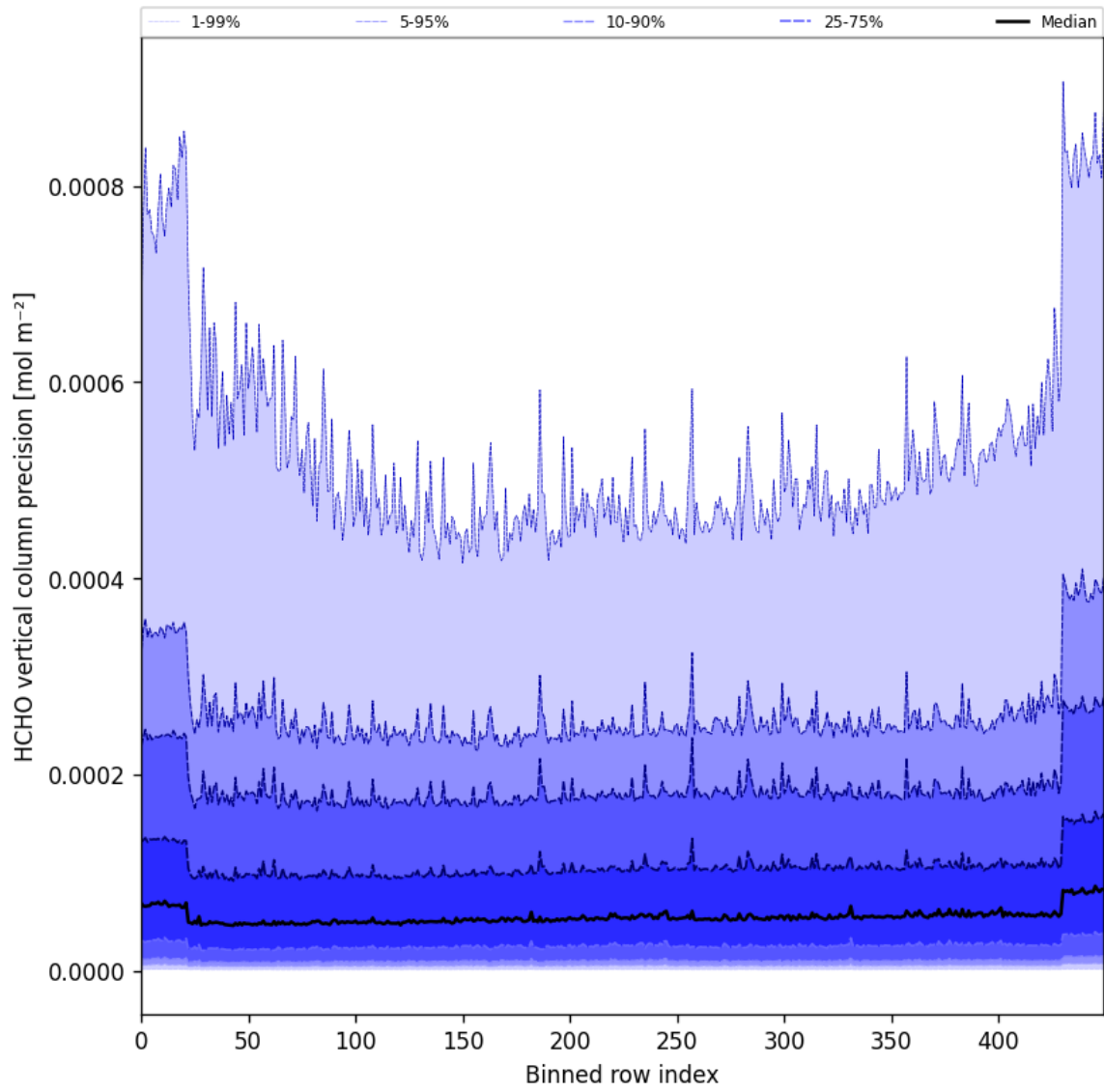
Figure 50: Along track statistics of “HCHO vertical column precision” for 2024-12-03 to 2024-12-05
