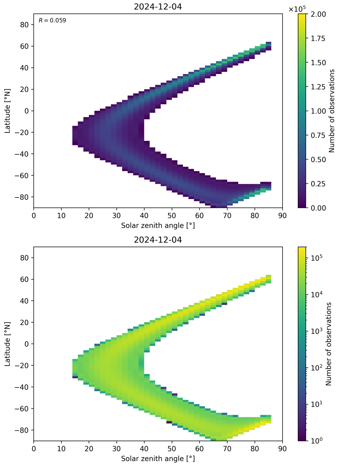
Figure 181: Scatter density plot of “Solar zenith angle” against “Latitude” for 2024-12-03 to 2024-12-05.
