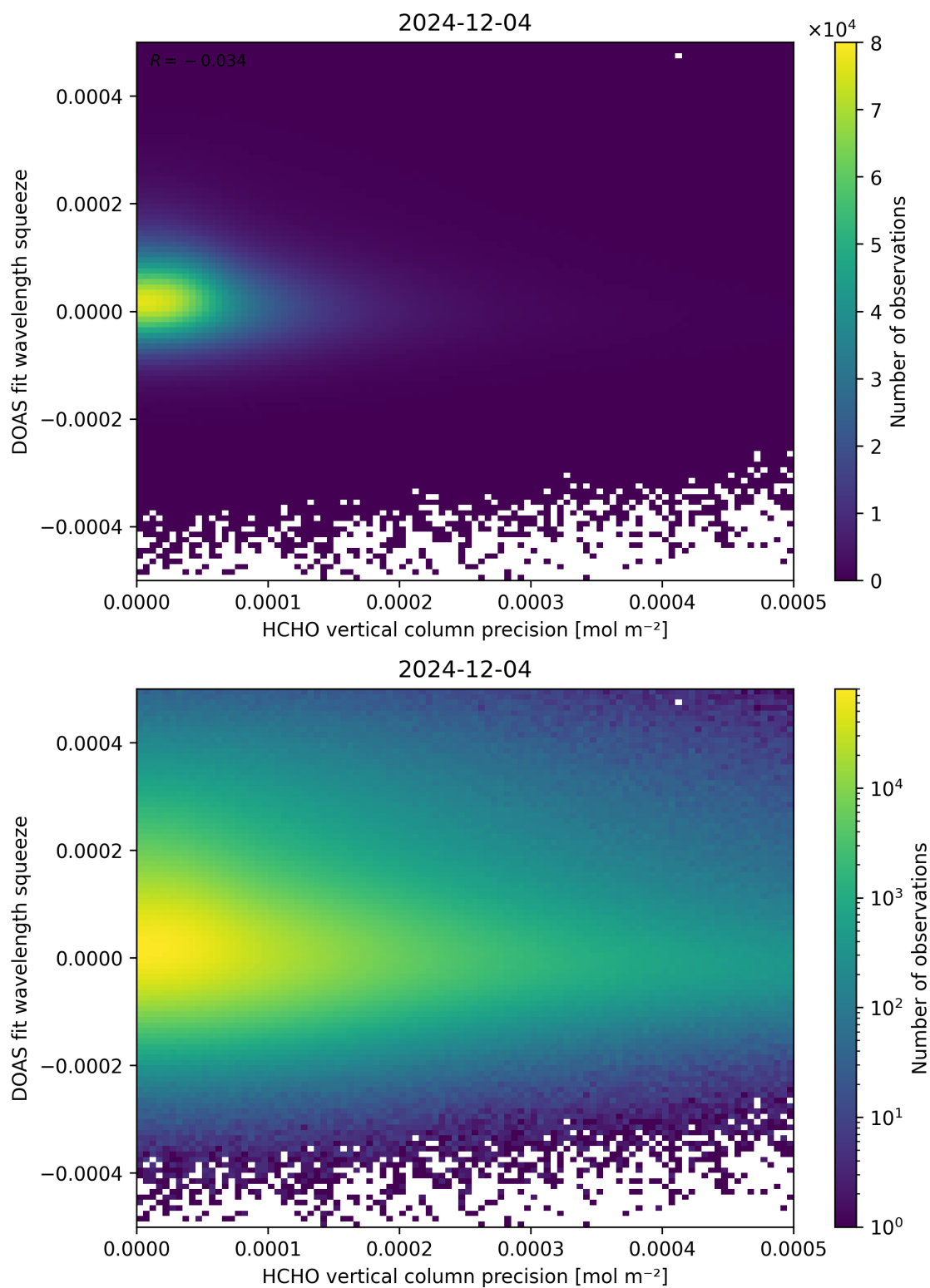
Figure 138: Scatter density plot of “HCHO vertical column precision” against “DOAS fit wavelength squeeze” for 2024-12-03 to 2024-12-05.
