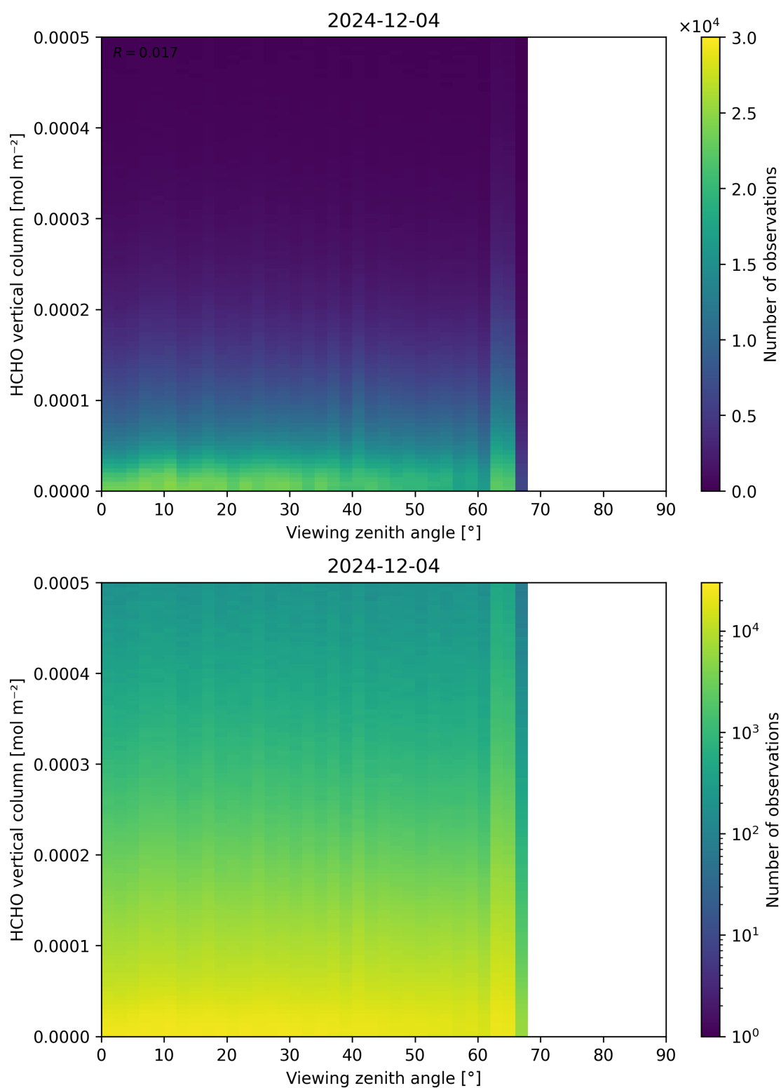
Figure 192: Scatter density plot of “Viewing zenith angle” against “HCHO vertical column” for 2024-12-03 to 2024-12-05.
