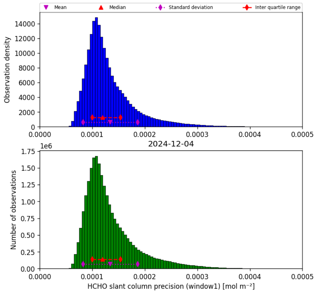
Figure 39: Histogram of “HCHO slant column precision (window1)” for 2024-12-03 to 2024-12-05
