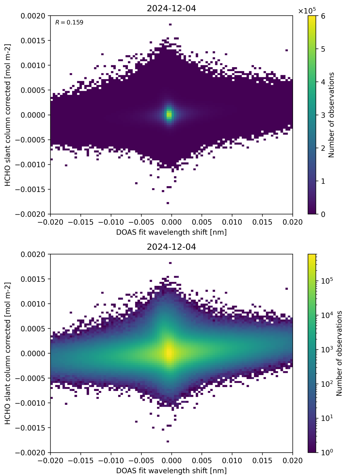
Figure 66: Scatter density plot of “DOAS fit wavelength shift” against “HCHO slant column corrected” for 2024-12-03 to 2024-12-05.
