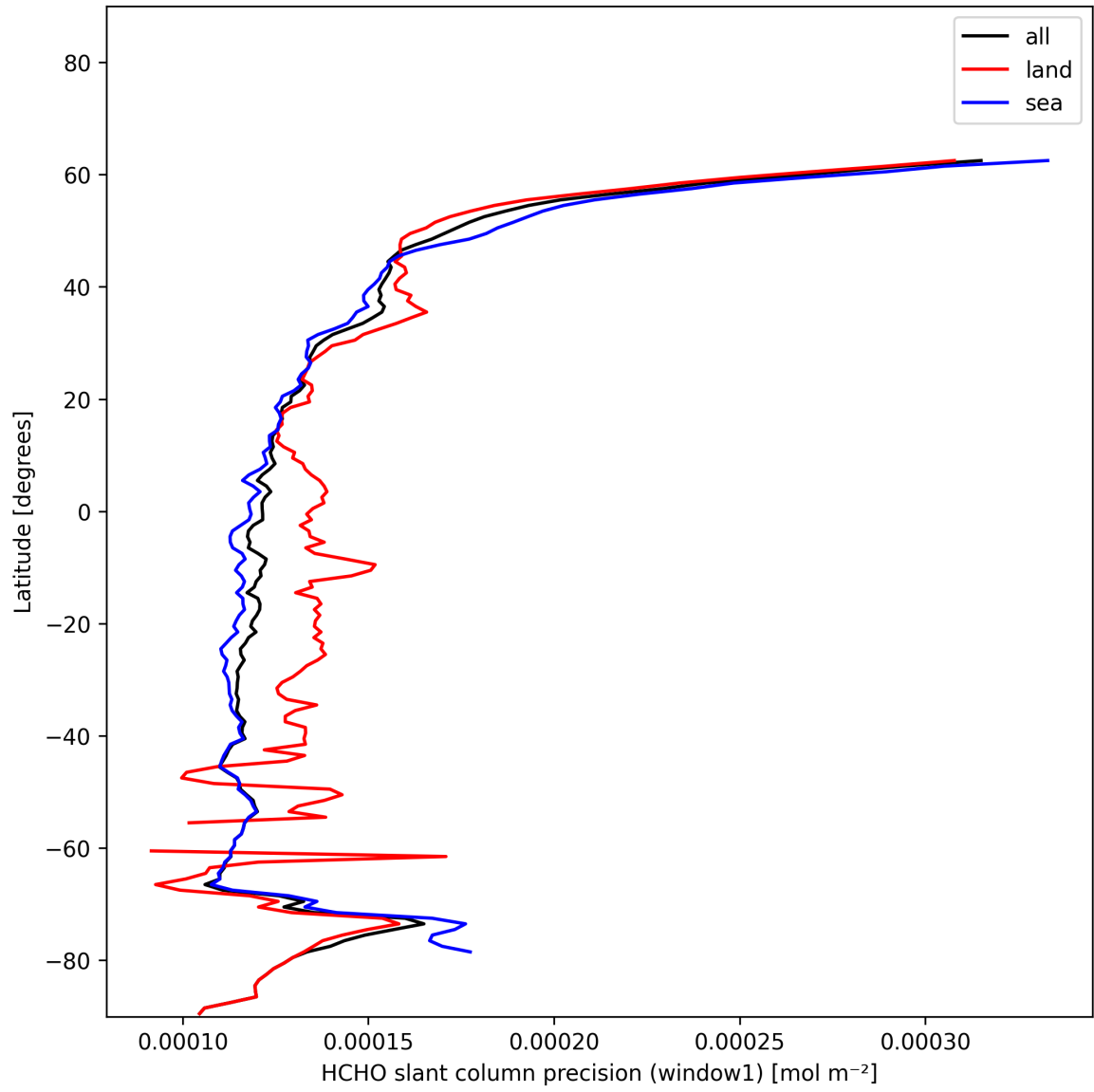
Figure 25: Zonal average of “HCHO slant column precision (window1)” for 2024-12-03 to 2024-12-05.
