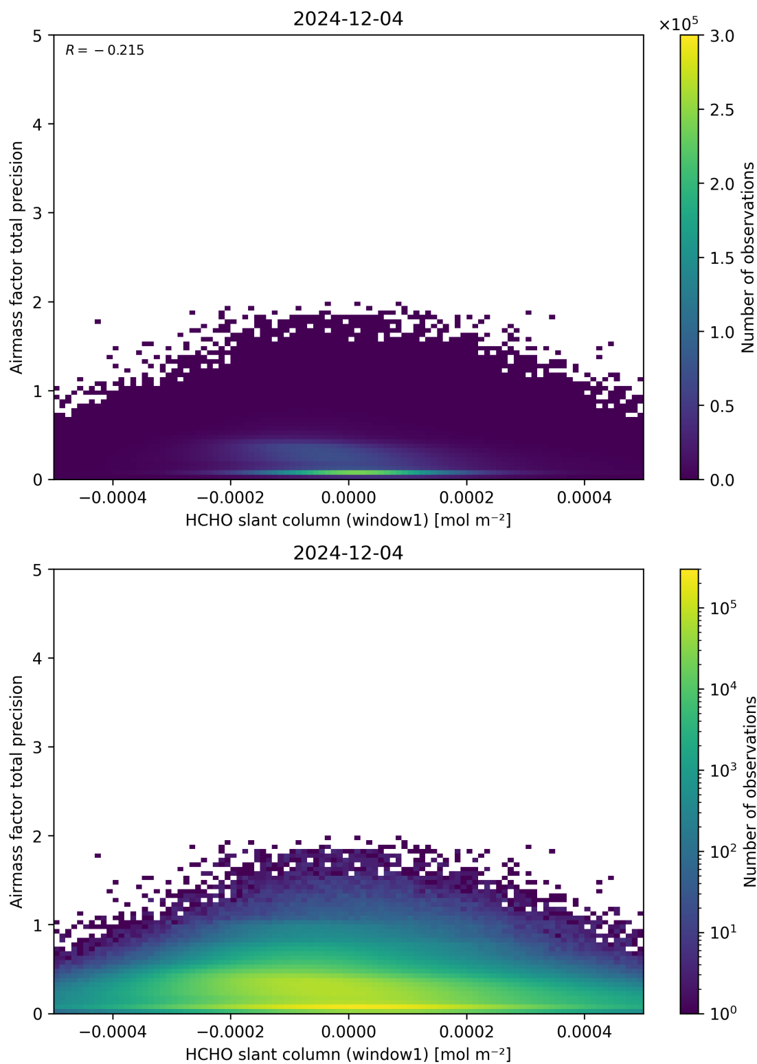
Figure 86: Scatter density plot of “HCHO slant column (window1)” against “Airmass factor total precision” for 2024-12-03 to 2024-12-05.
