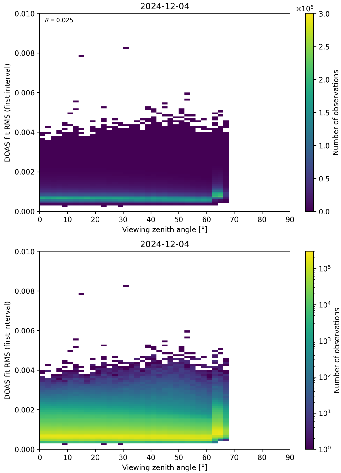
Figure 182: Scatter density plot of “Viewing zenith angle” against “DOAS fit RMS (first interval)” for 2024-12-03 to 2024-12-05.
