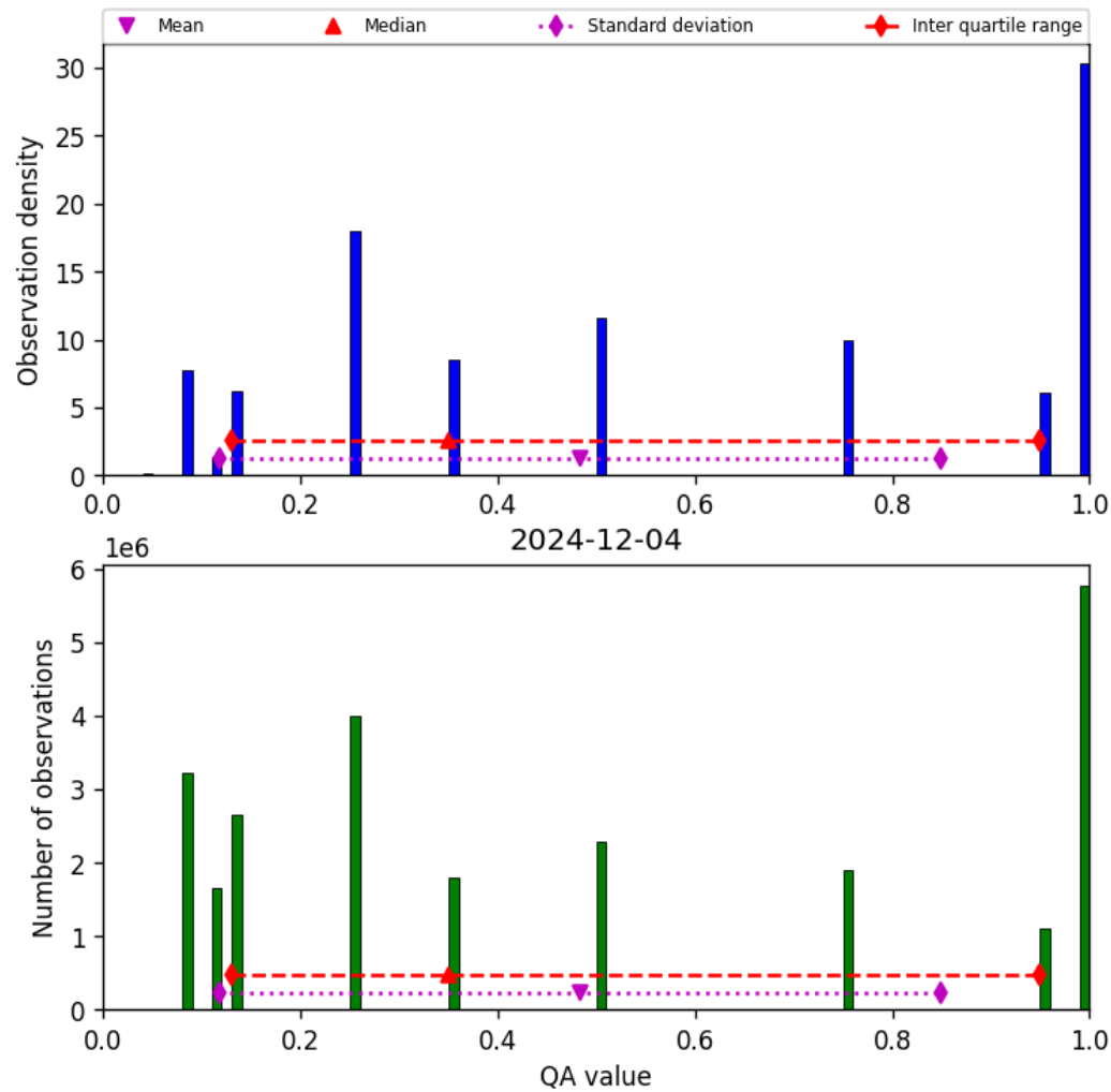
Figure 34: Histogram of “QA value” for 2024-12-03 to 2024-12-05
