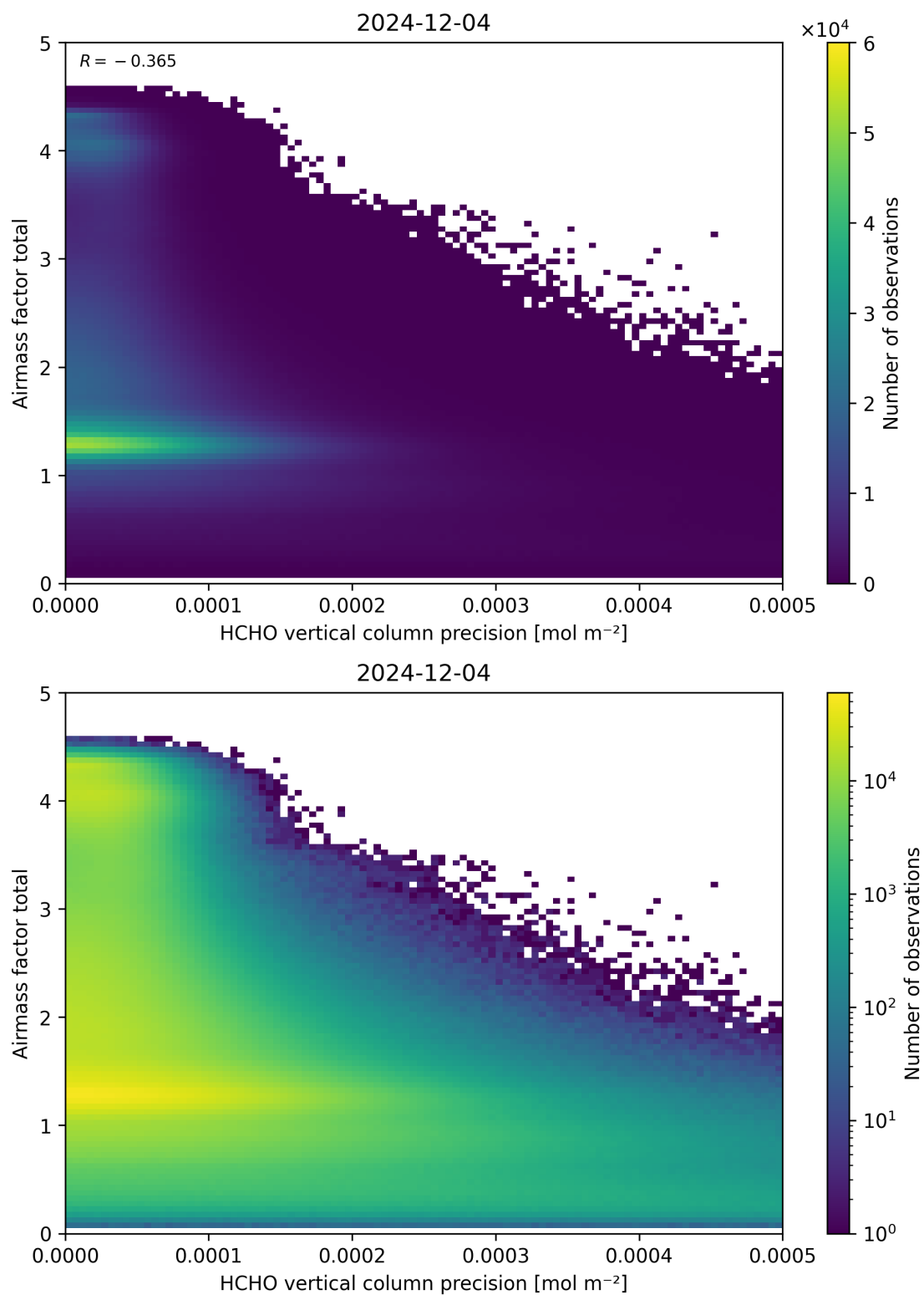
Figure 144: Scatter density plot of “HCHO vertical column precision” against “Airmass factor total” for 2024-12-03 to 2024-12-05.
