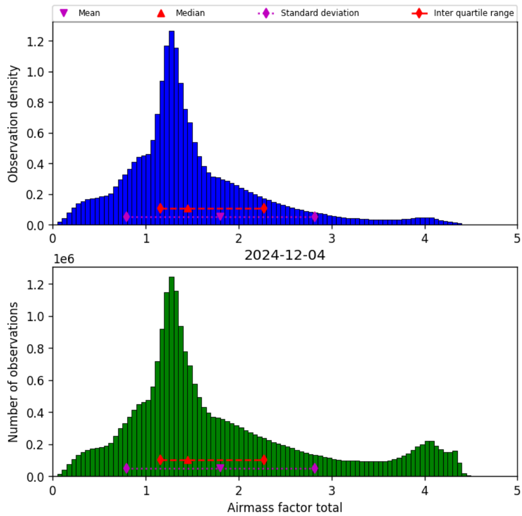
Figure 40: Histogram of “Airmass factor total” for 2024-12-03 to 2024-12-05
