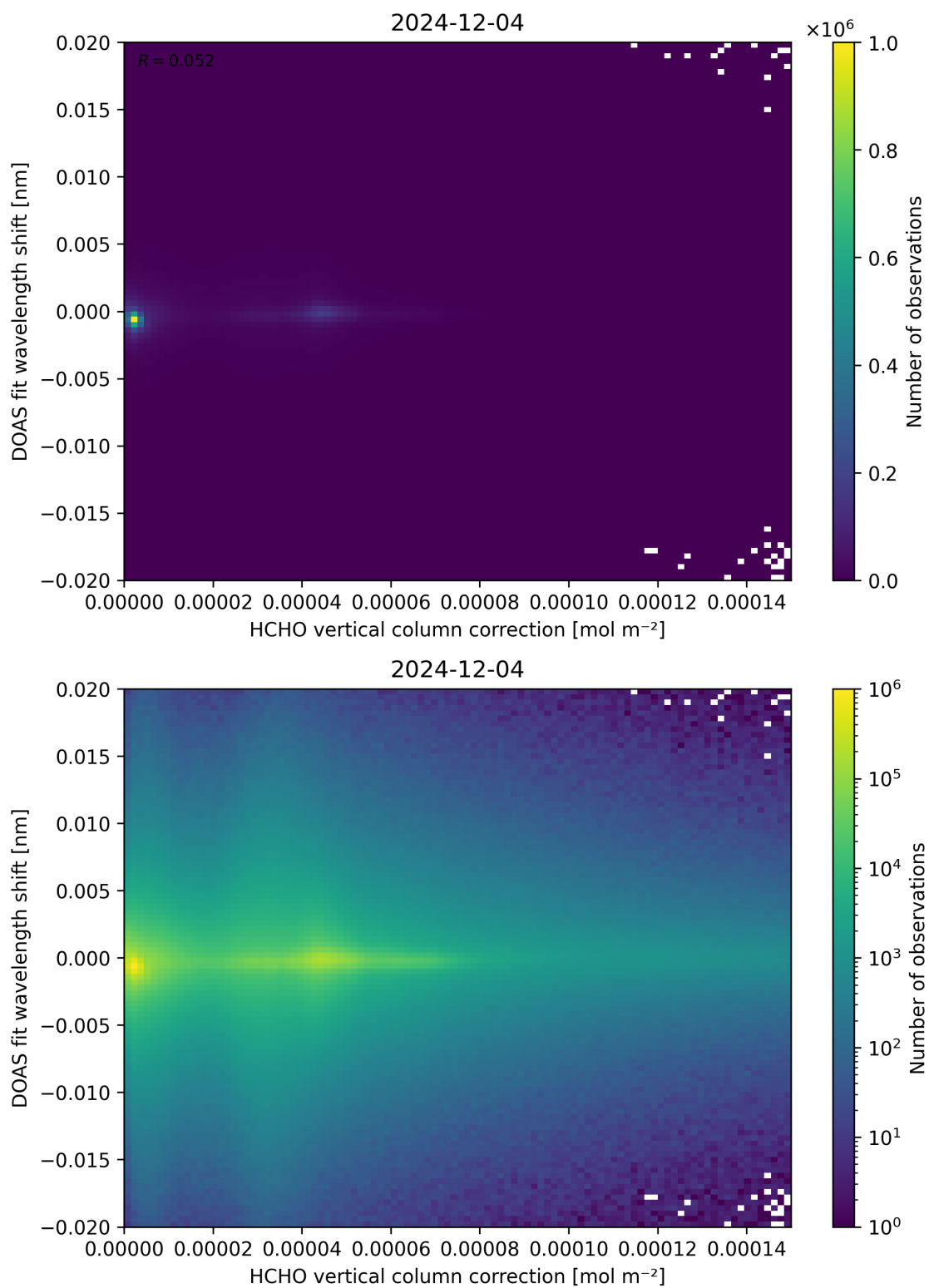
Figure 113: Scatter density plot of “HCHO vertical column correction” against “DOAS fit wavelength shift” for 2024-12-03 to 2024-12-05.
