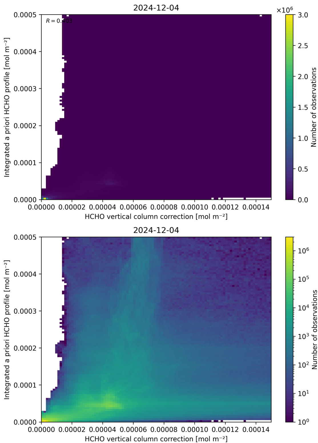
Figure 122: Scatter density plot of “HCHO vertical column correction” against “Integrated a priori HCHO profile” for 2024-12-03 to 2024-12-05.
