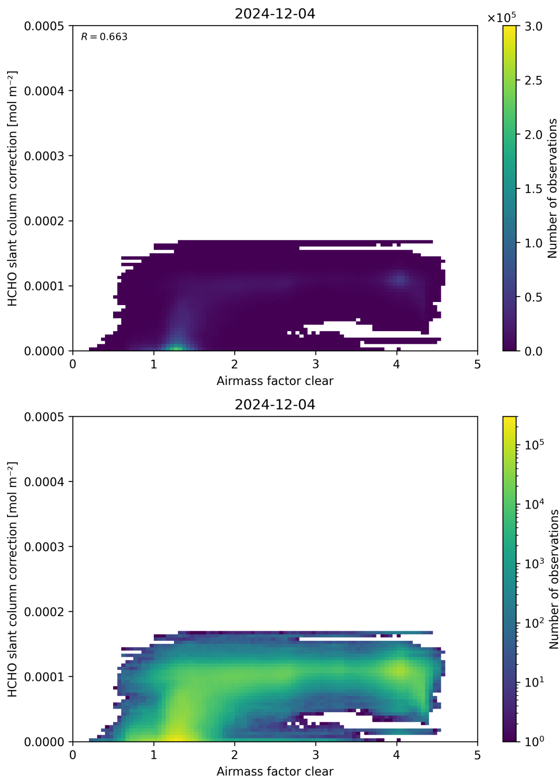
Figure 75: Scatter density plot of “Airmass factor clear” against “HCHO slant column correction” for 2024-12-03 to 2024-12-05.
