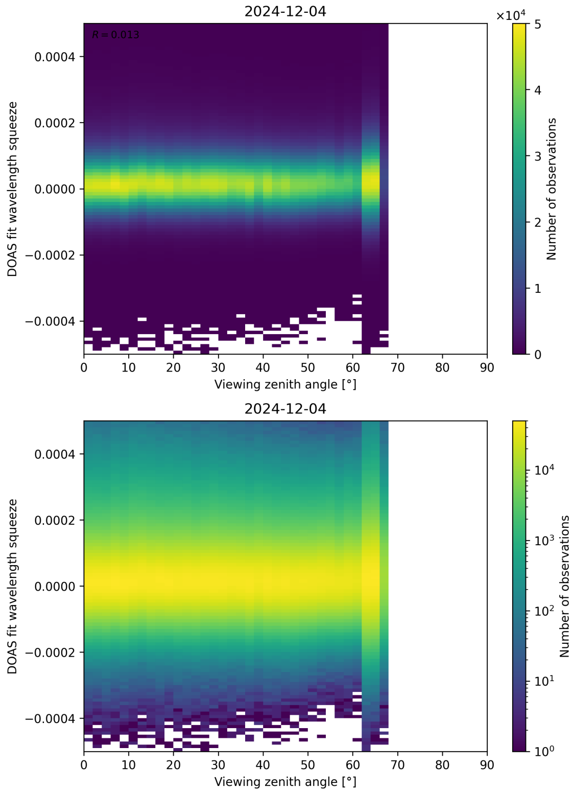
Figure 184: Scatter density plot of “Viewing zenith angle” against “DOAS fit wavelength squeeze” for 2024-12-03 to 2024-12-05.
