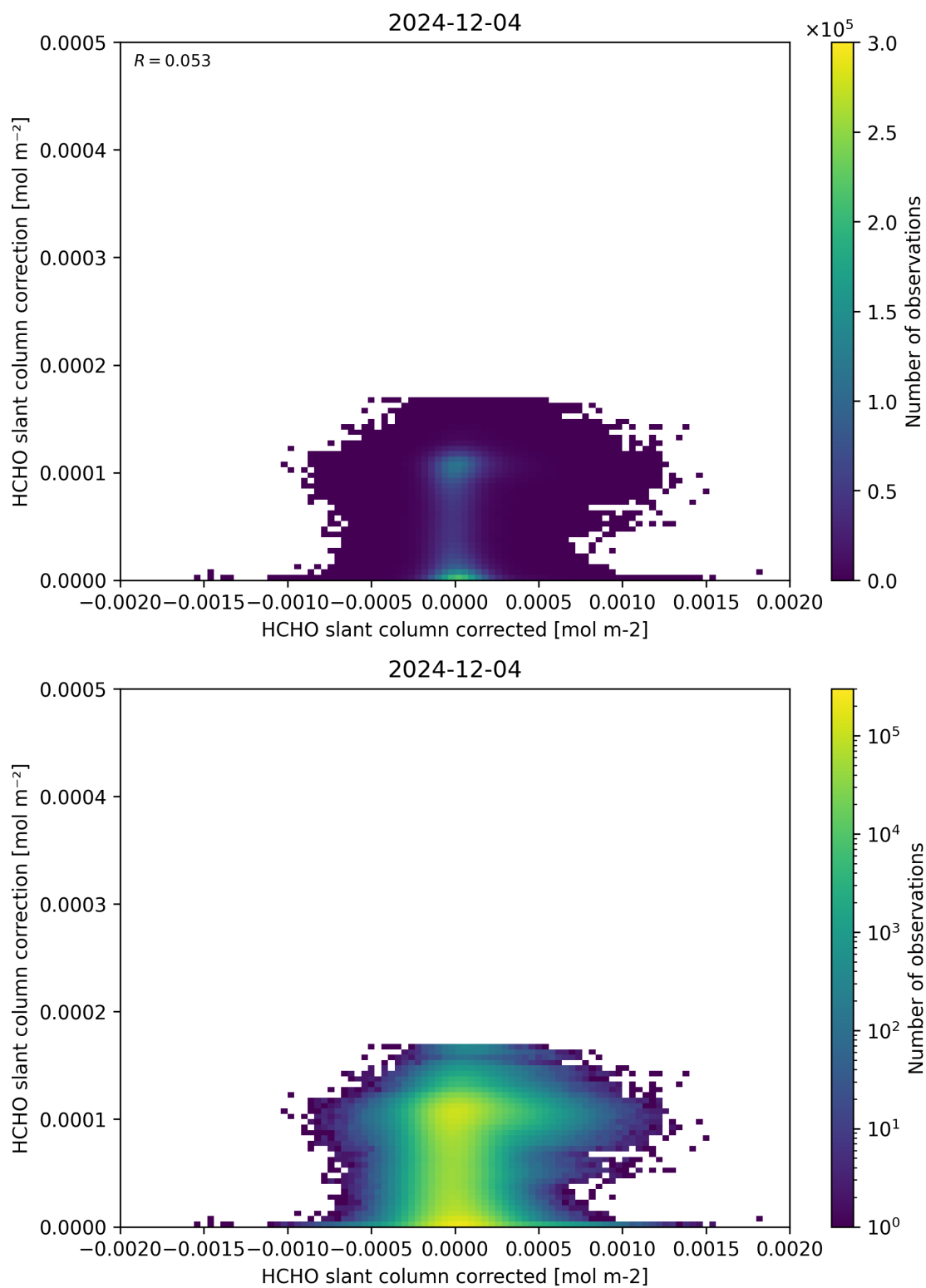
Figure 77: Scatter density plot of “HCHO slant column corrected” against “HCHO slant column correction” for 2024-12-03 to 2024-12-05.
