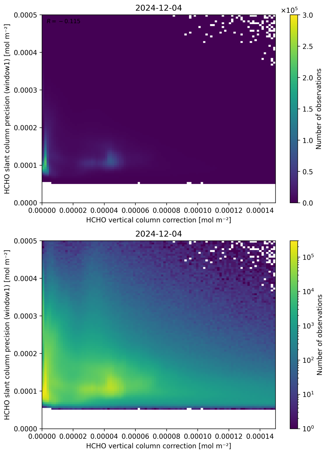
Figure 119: Scatter density plot of “HCHO vertical column correction” against “HCHO slant column precision (window1)” for 2024-12-03 to 2024-12-05.
