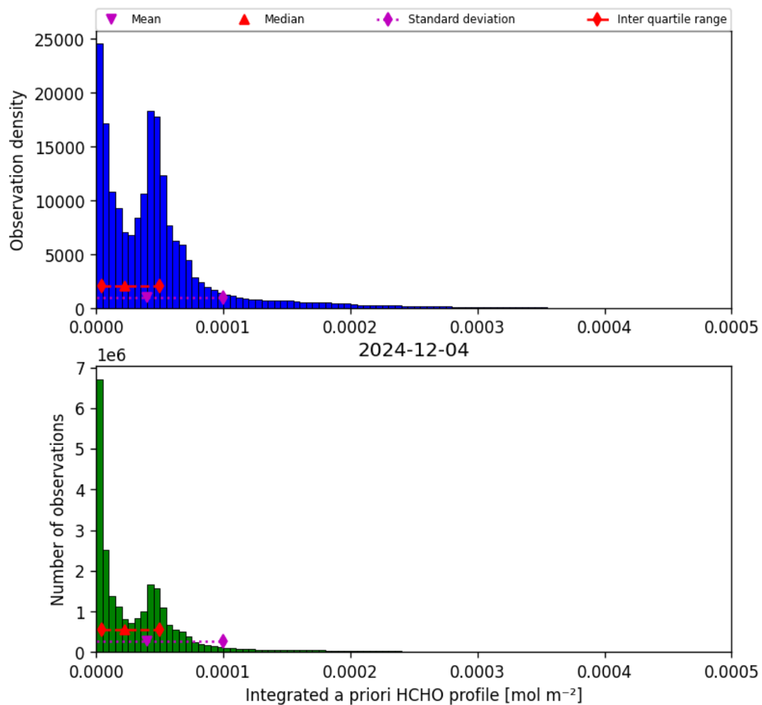
Figure 43: Histogram of “Integrated a priori HCHO profile” for 2024-12-03 to 2024-12-05
