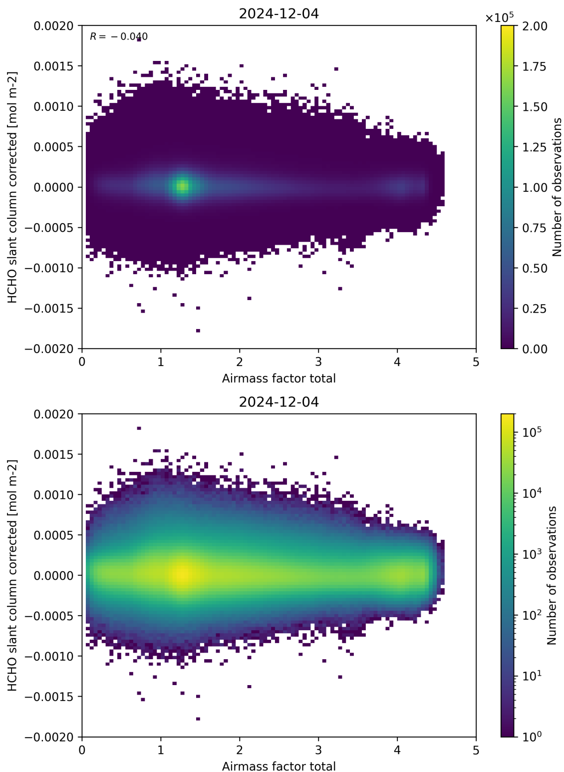
Figure 101: Scatter density plot of “Airmass factor total” against “HCHO slant column corrected” for 2024-12-03 to 2024-12-05.
