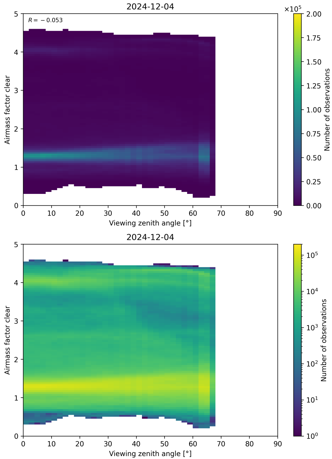
Figure 185: Scatter density plot of “Viewing zenith angle” against “Airmass factor clear” for 2024-12-03 to 2024-12-05.
