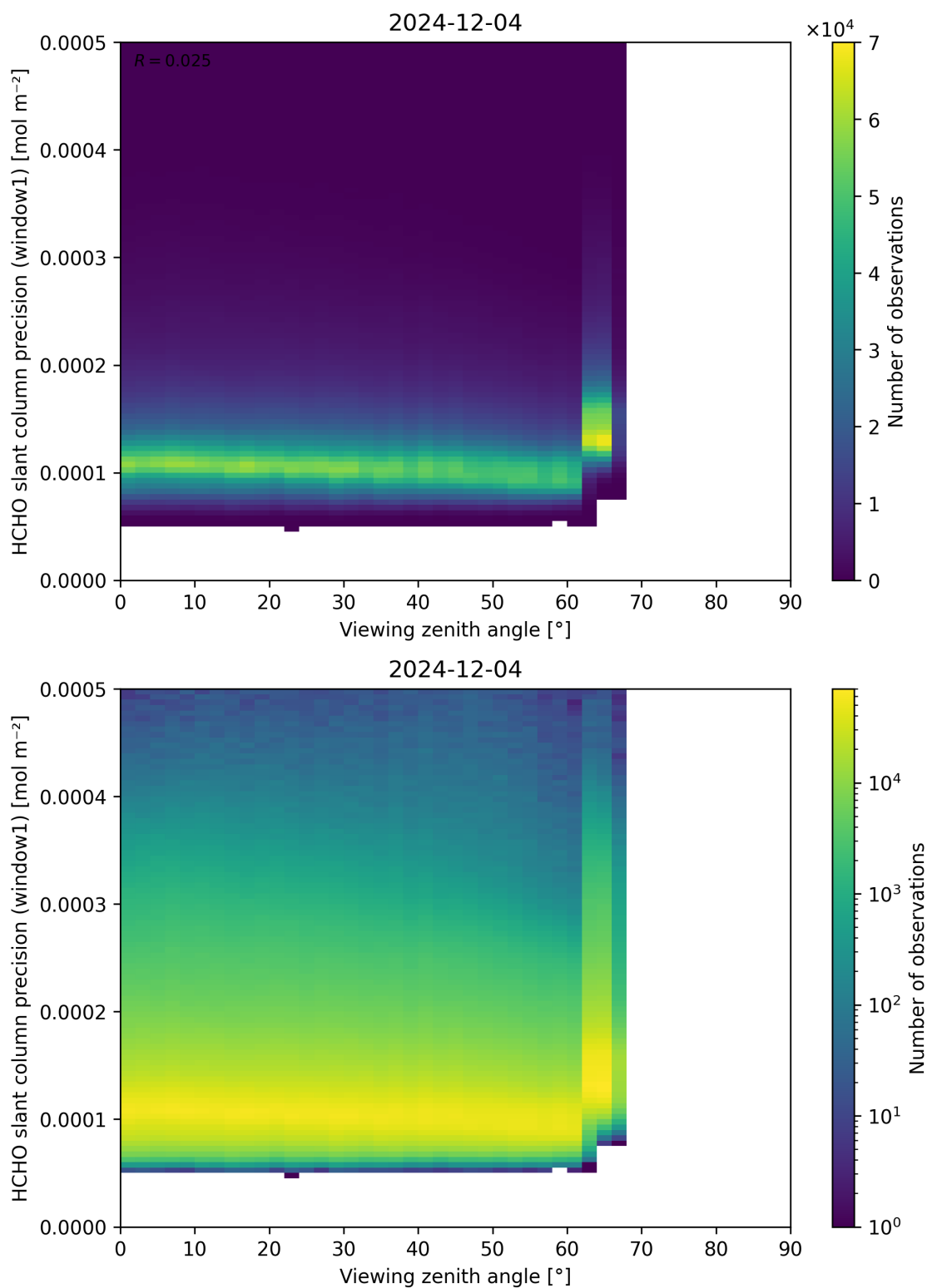
Figure 189: Scatter density plot of “Viewing zenith angle” against “HCHO slant column precision (window1)” for 2024-12-03 to 2024-12-05.
