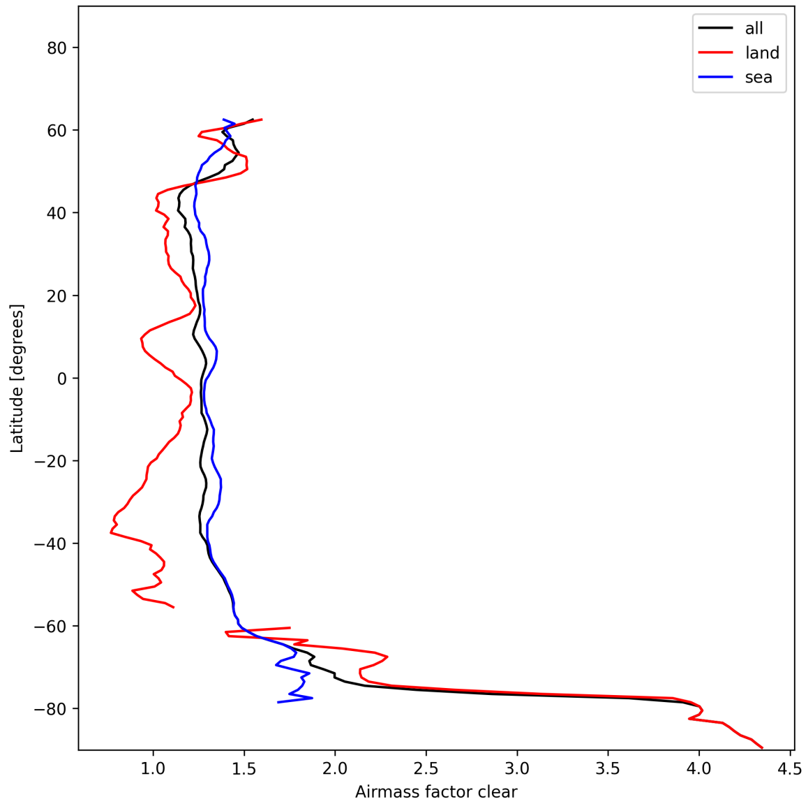
Figure 28: Zonal average of “Airmass factor clear” for 2024-12-03 to 2024-12-05.
