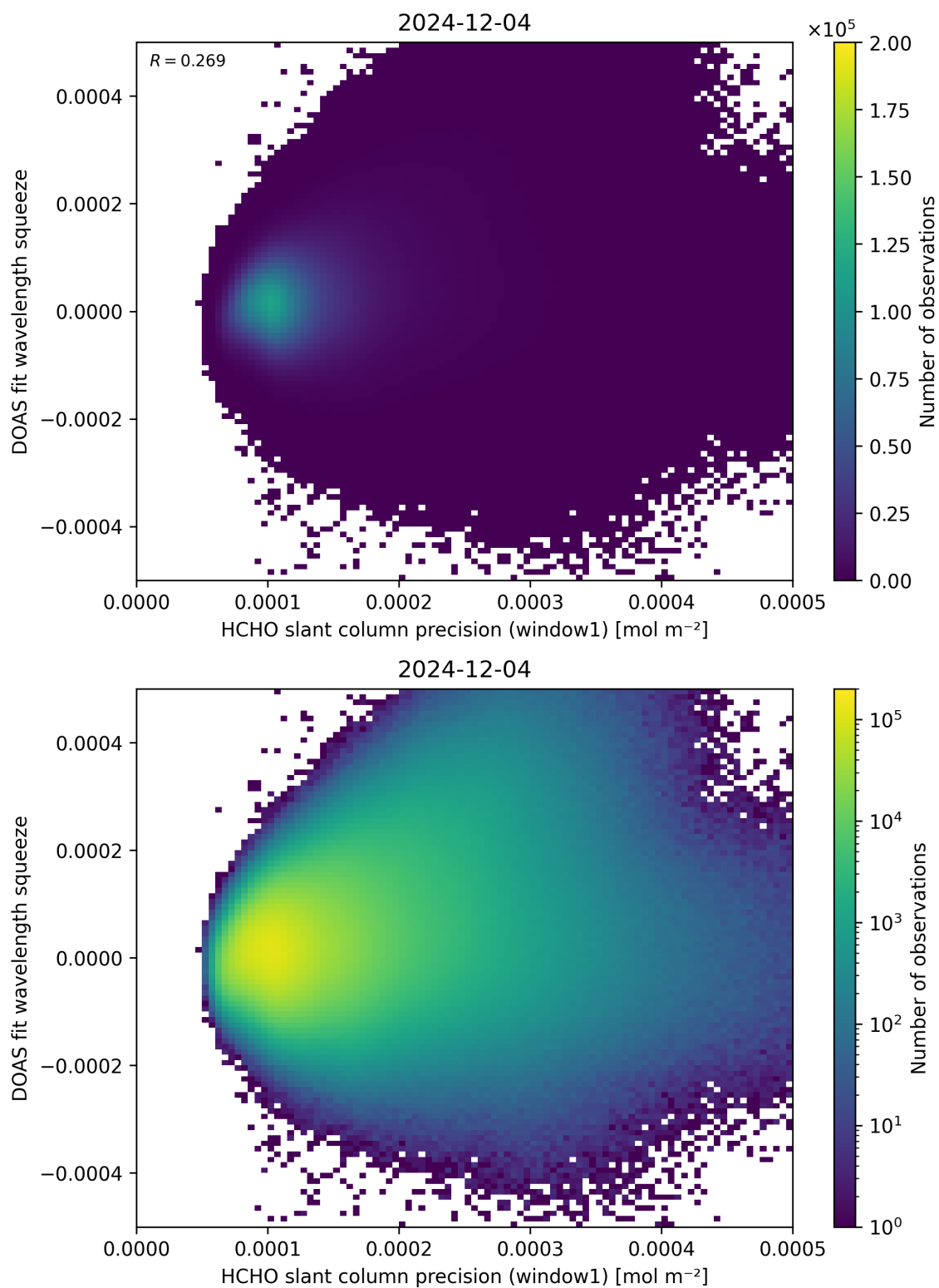
Figure 90: Scatter density plot of “HCHO slant column precision (window1)” against “DOAS fit wavelength squeeze” for 2024-12-03 to 2024-12-05.
