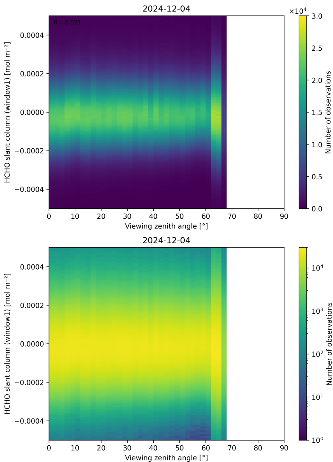
Figure 188: Scatter density plot of “Viewing zenith angle” against “HCHO slant column (window1)” for 2024-12-03 to 2024-12-05.
