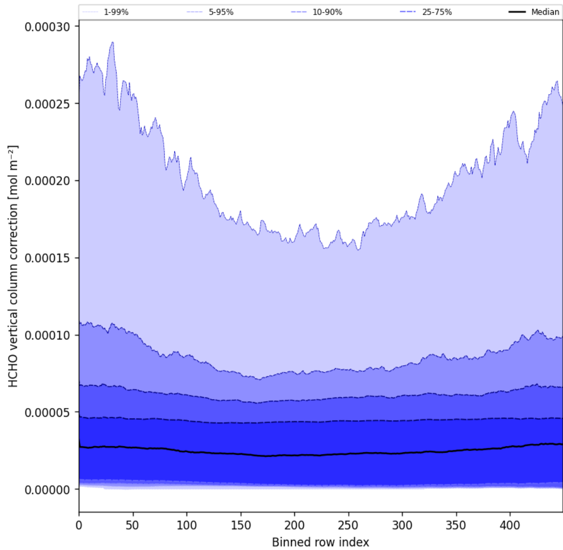
Figure 51: Along track statistics of “HCHO vertical column correction” for 2024-12-03 to 2024-12-05
