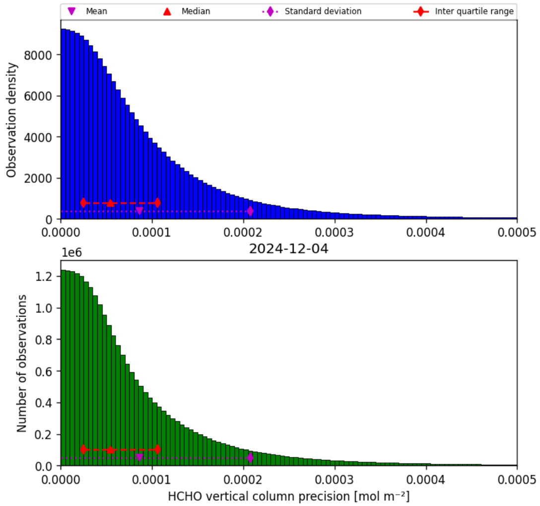
Figure 36: Histogram of “HCHO vertical column precision” for 2024-12-03 to 2024-12-05
