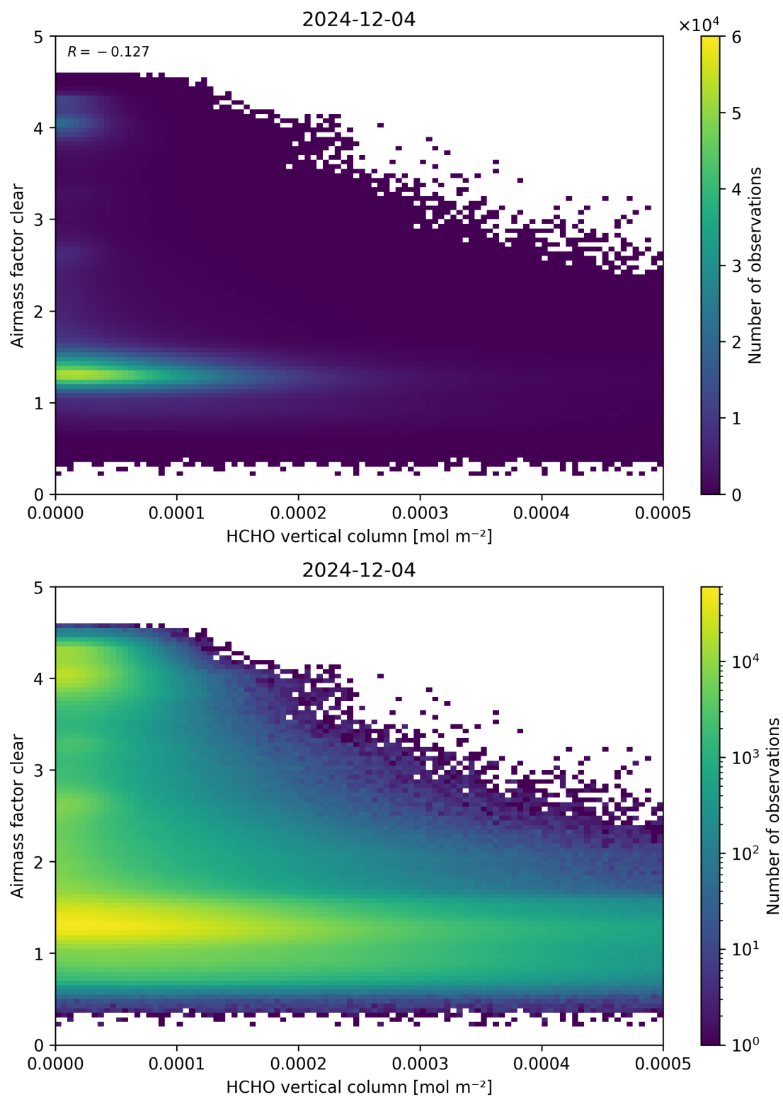
Figure 126: Scatter density plot of “HCHO vertical column” against “Airmass factor clear” for 2024-12-03 to 2024-12-05.
