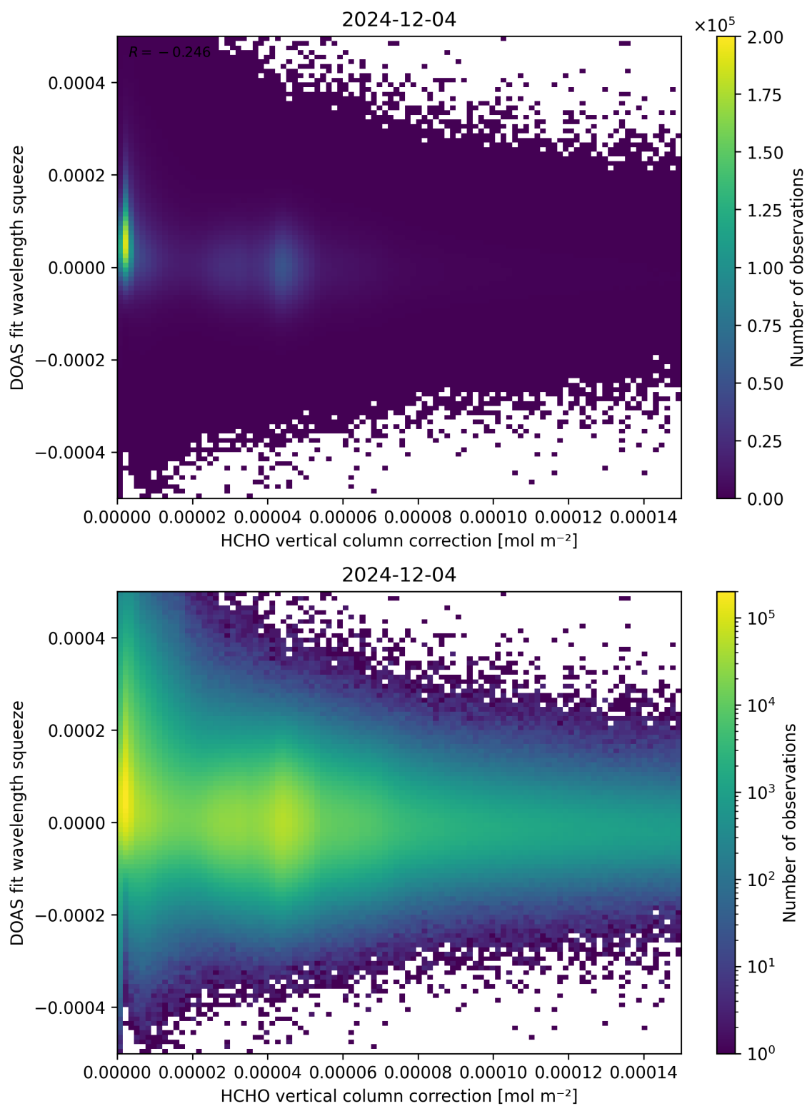
Figure 114: Scatter density plot of “HCHO vertical column correction” against “DOAS fit wavelength squeeze” for 2024-12-03 to 2024-12-05.
