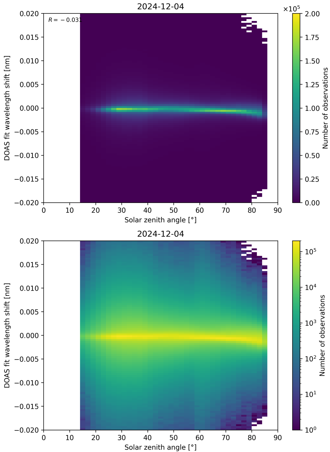
Figure 168: Scatter density plot of “Solar zenith angle” against “DOAS fit wavelength shift” for 2024-12-03 to 2024-12-05.
