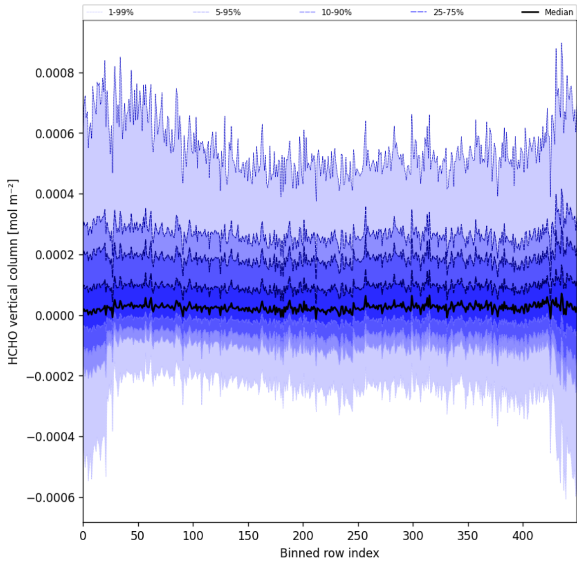
Figure 49: Along track statistics of “HCHO vertical column” for 2024-12-03 to 2024-12-05
