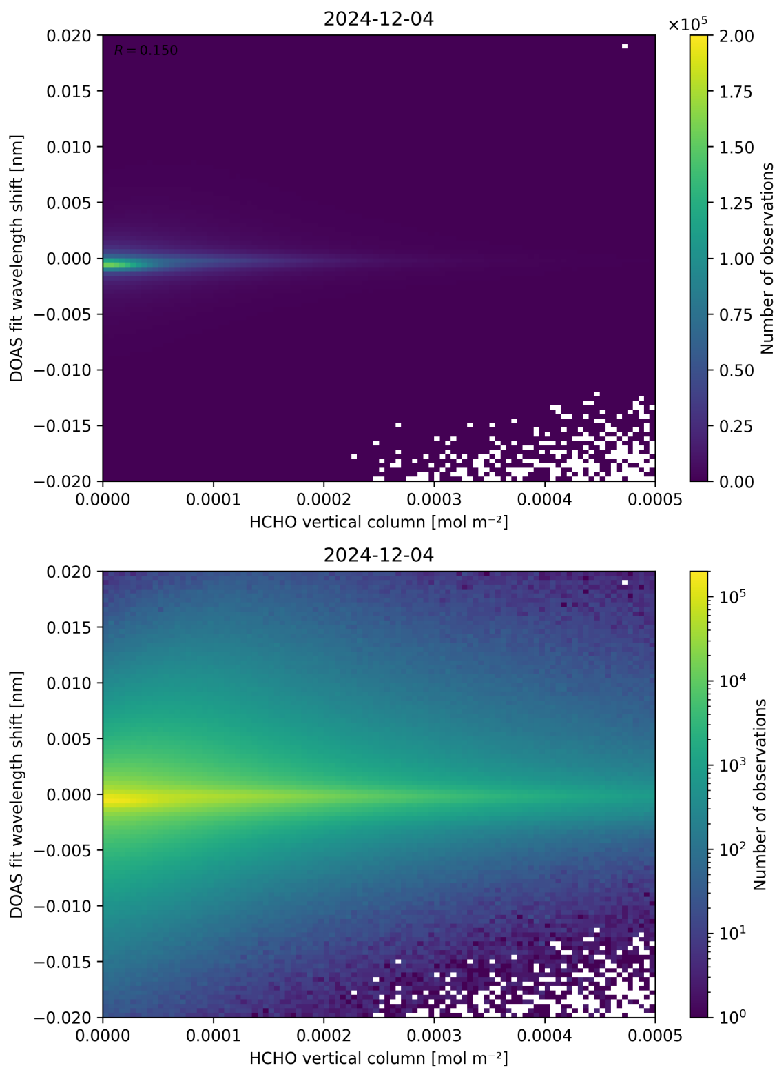
Figure 124: Scatter density plot of “HCHO vertical column” against “DOAS fit wavelength shift” for 2024-12-03 to 2024-12-05.
