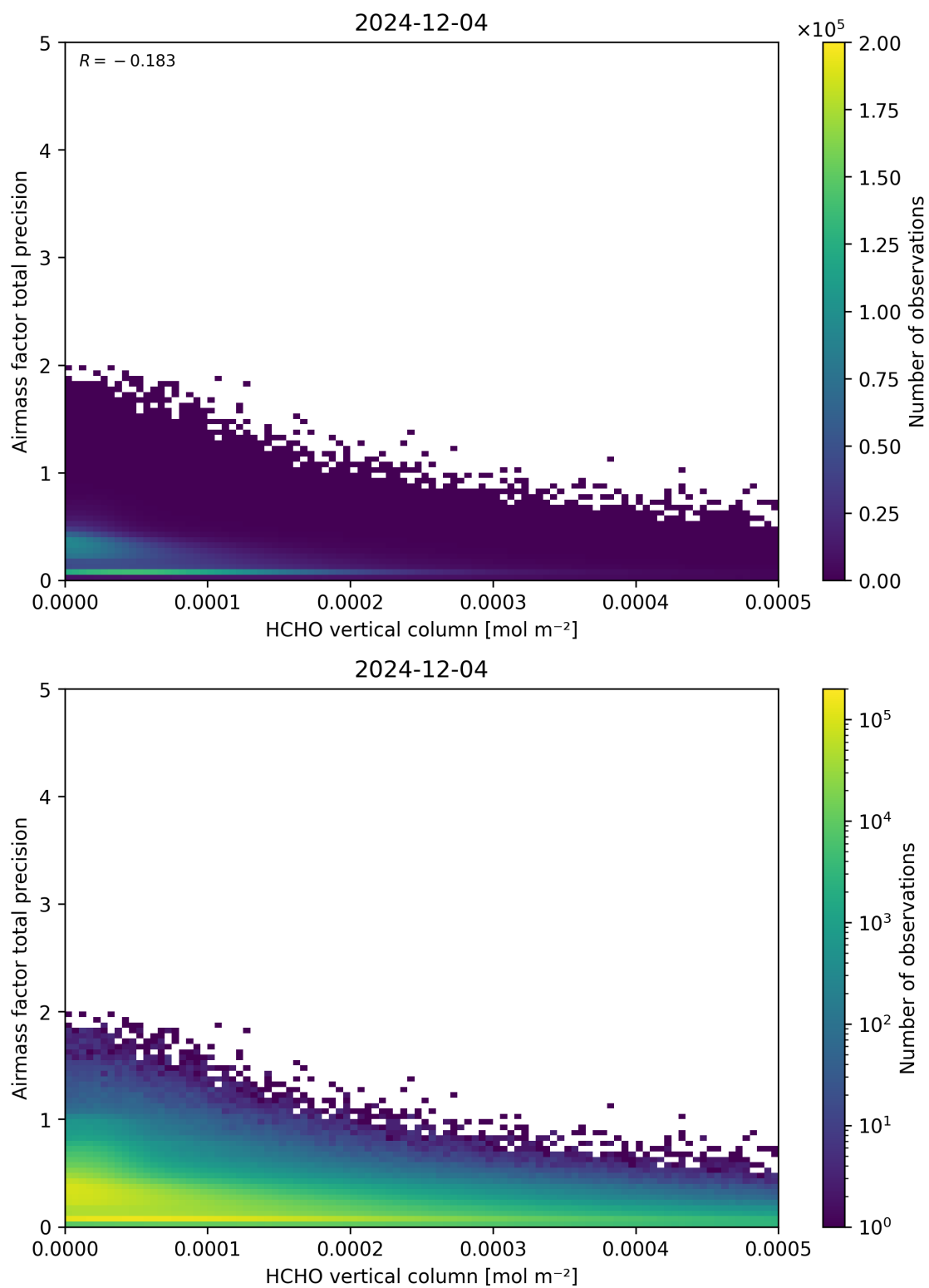
Figure 132: Scatter density plot of “HCHO vertical column” against “Airmass factor total precision” for 2024-12-03 to 2024-12-05.
