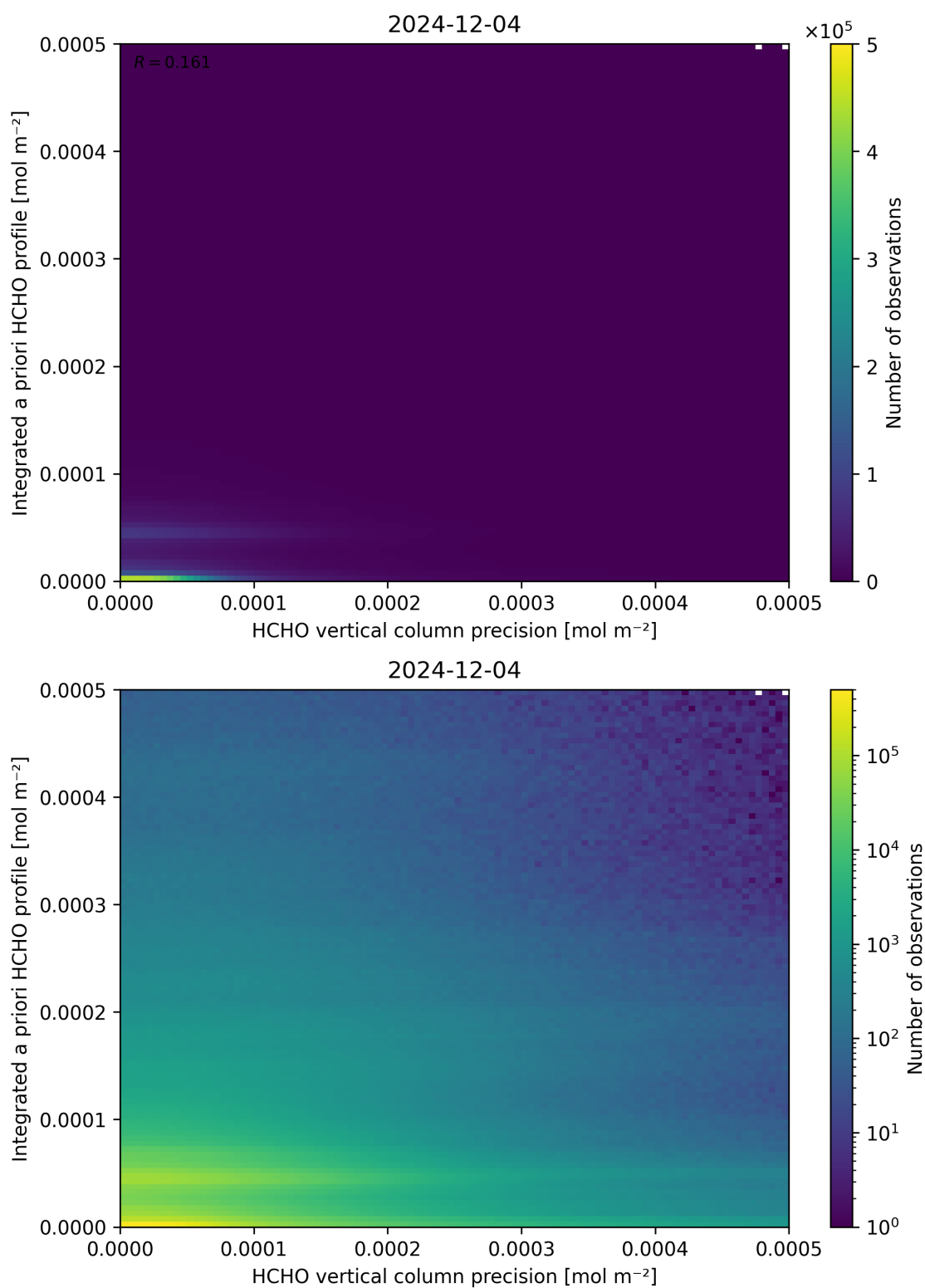
Figure 147: Scatter density plot of “HCHO vertical column precision” against “Integrated a priori HCHO profile” for 2024-12-03 to 2024-12-05.
