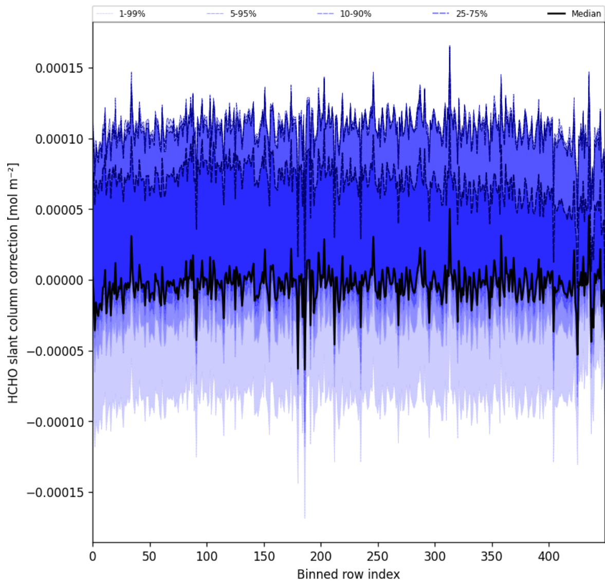
Figure 61: Along track statistics of “HCHO slant column correction” for 2024-12-03 to 2024-12-05
