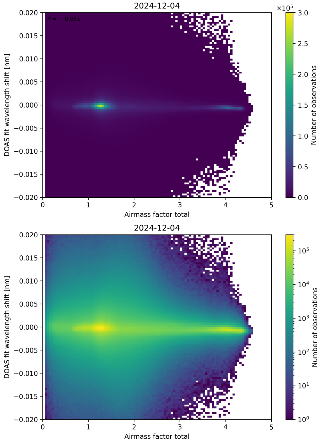
Figure 98: Scatter density plot of “Airmass factor total” against “DOAS fit wavelength shift” for 2024-12-03 to 2024-12-05.
