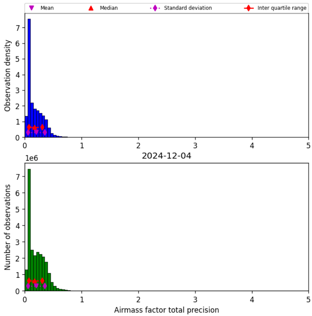
Figure 41: Histogram of “Airmass factor total precision” for 2024-12-03 to 2024-12-05
