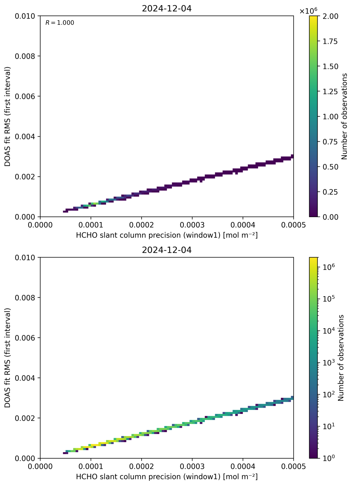
Figure 88: Scatter density plot of “HCHO slant column precision (window1)” against “DOAS fit RMS (first interval)” for 2024-12-03 to 2024-12-05.
