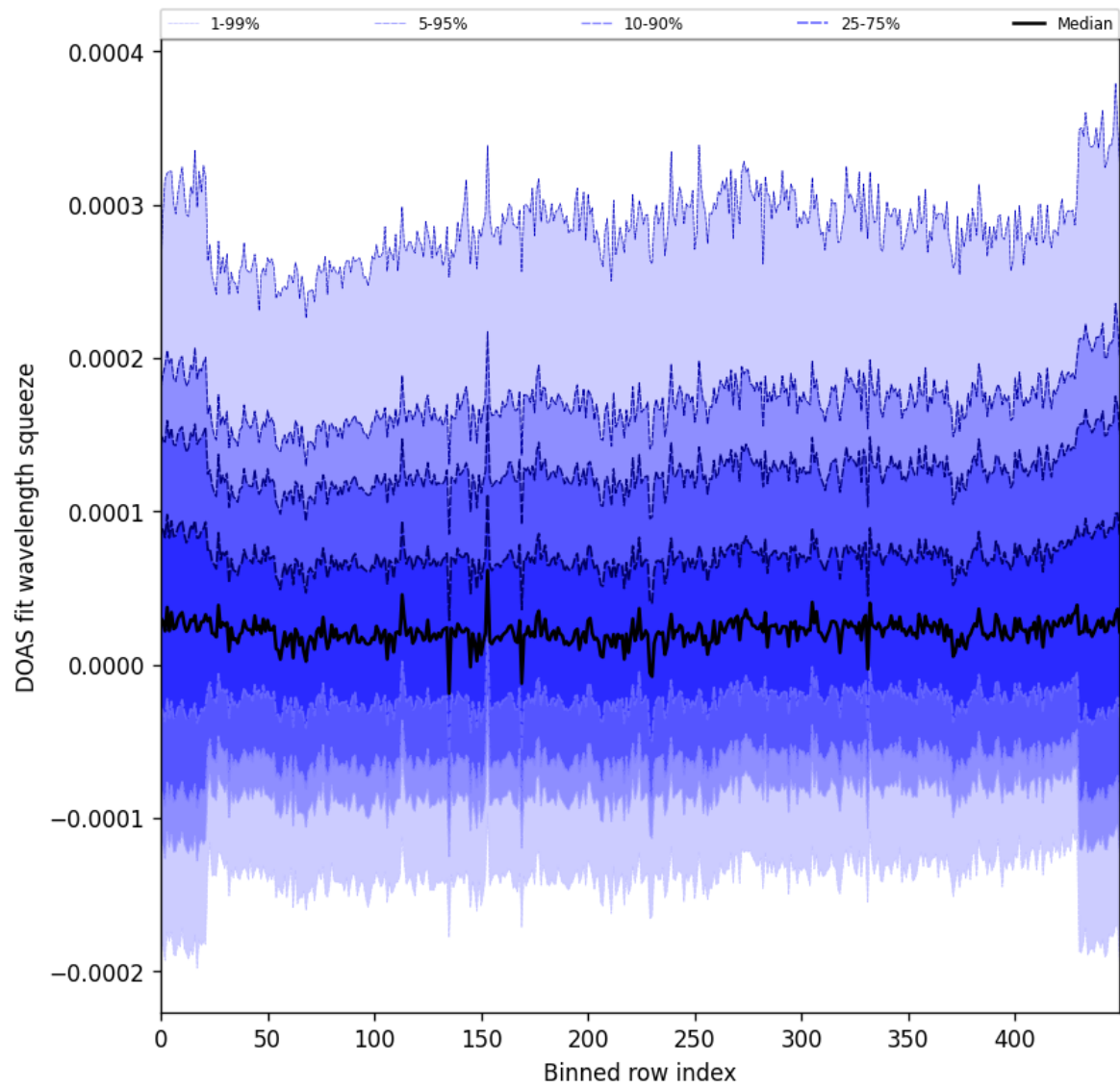
Figure 59: Along track statistics of “DOAS fit wavelength squeeze” for 2024-12-03 to 2024-12-05
