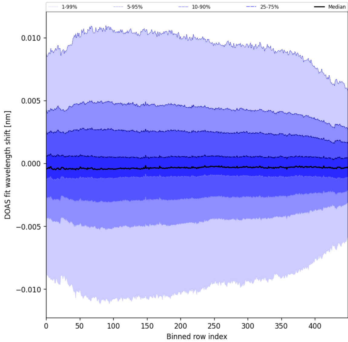
Figure 58: Along track statistics of “DOAS fit wavelength shift” for 2024-12-03 to 2024-12-05
