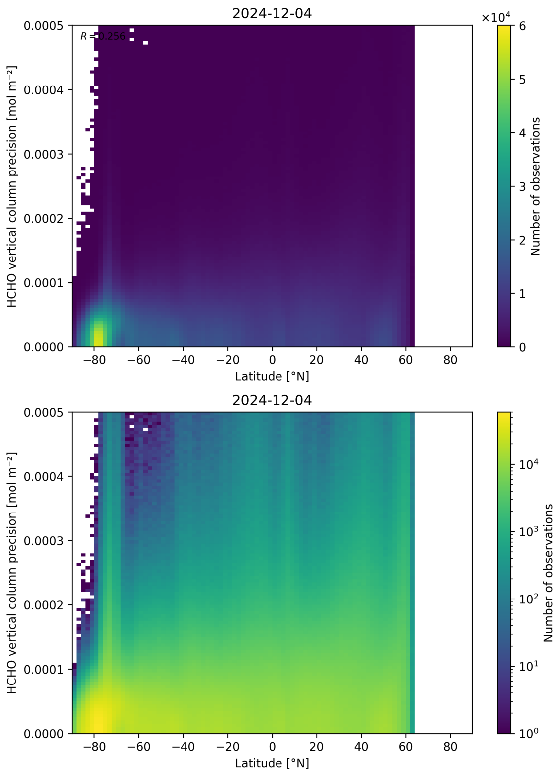
Figure 165: Scatter density plot of “Latitude” against “HCHO vertical column precision” for 2024-12-03 to 2024-12-05.
