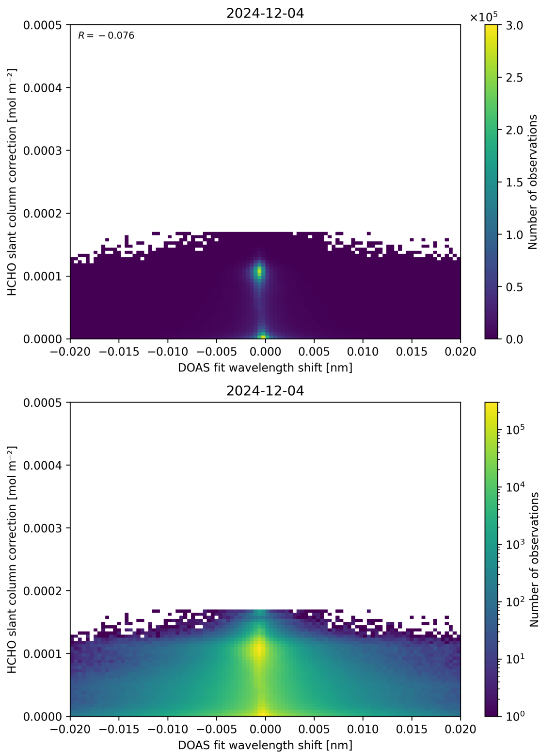
Figure 67: Scatter density plot of “DOAS fit wavelength shift” against “HCHO slant column correction” for 2024-12-03 to 2024-12-05.
