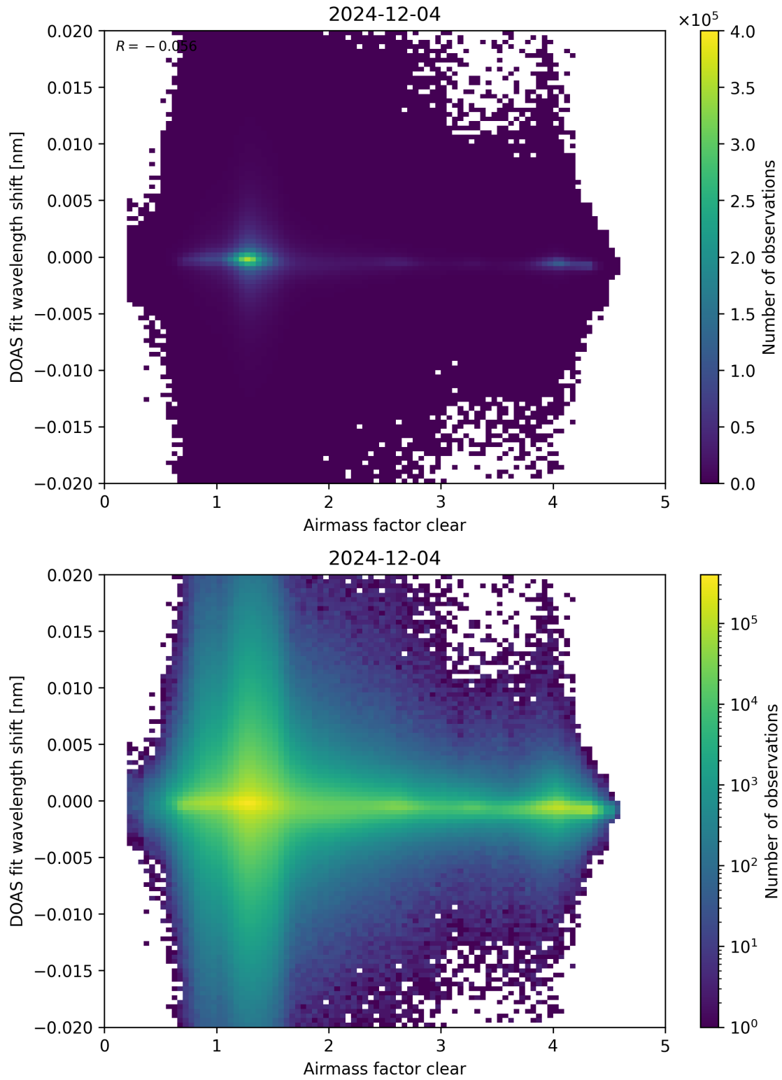
Figure 72: Scatter density plot of “Airmass factor clear” against “DOAS fit wavelength shift” for 2024-12-03 to 2024-12-05.
