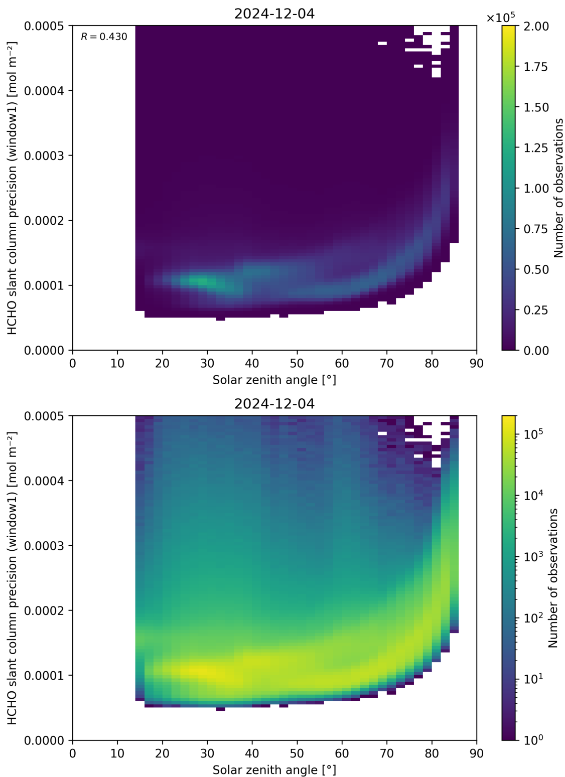
Figure 174: Scatter density plot of “Solar zenith angle” against “HCHO slant column precision (window1)” for 2024-12-03 to 2024-12-05.
