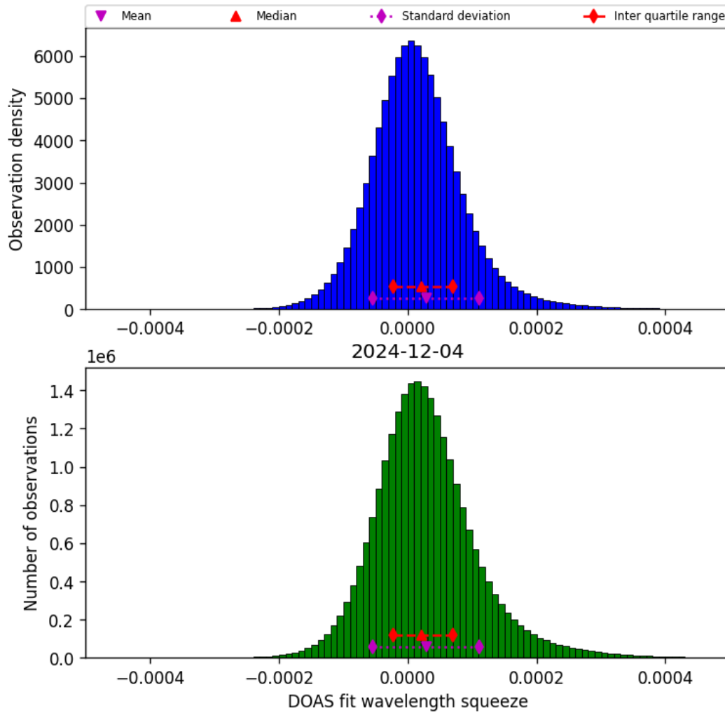
Figure 45: Histogram of “DOAS fit wavelength squeeze” for 2024-12-03 to 2024-12-05
