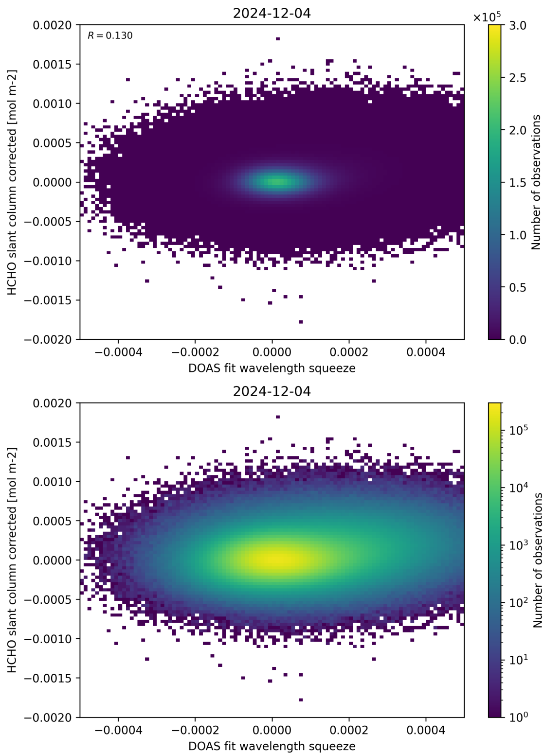
Figure 69: Scatter density plot of “DOAS fit wavelength squeeze” against “HCHO slant column corrected” for 2024-12-03 to 2024-12-05.
