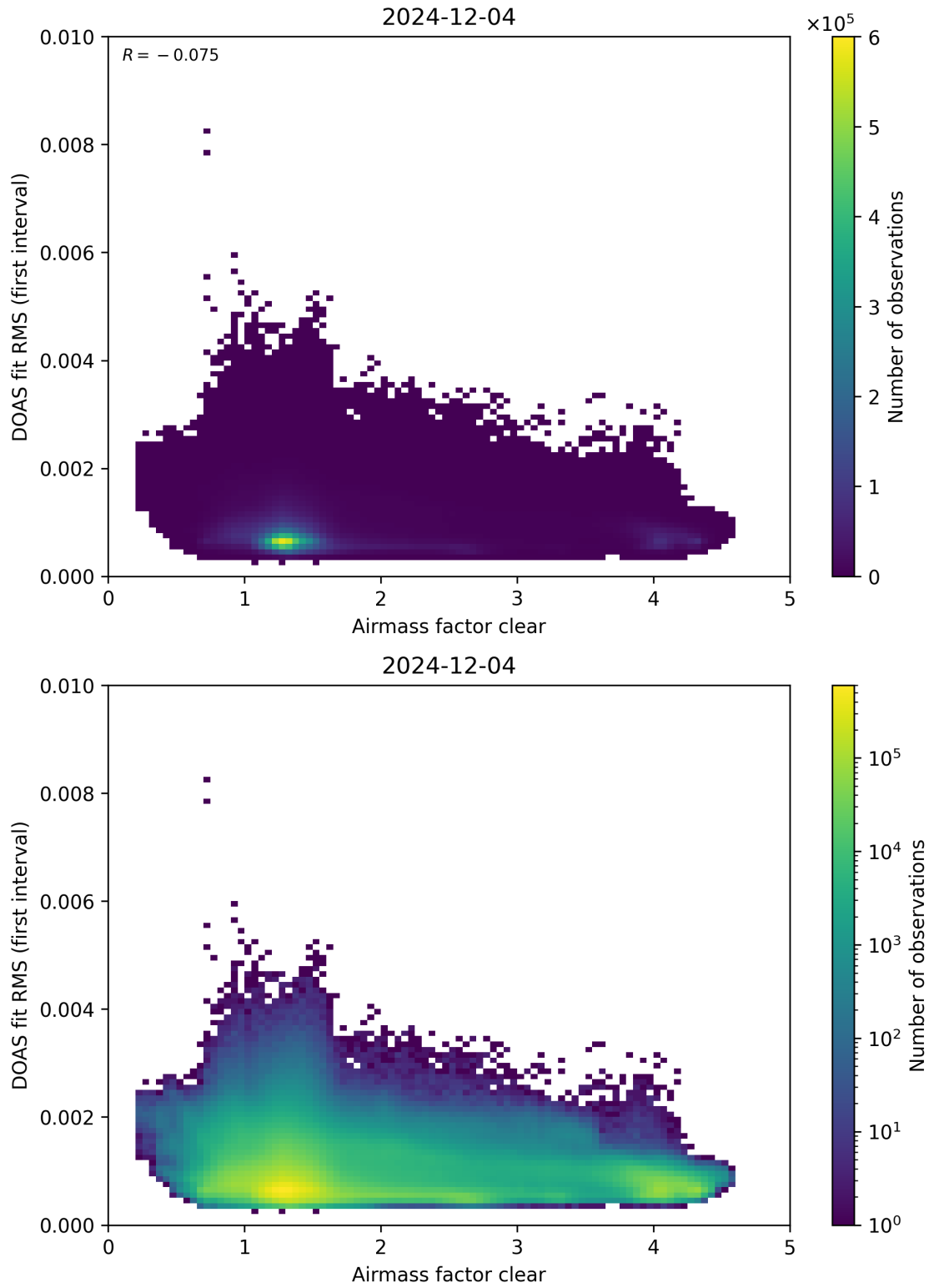
Figure 71: Scatter density plot of “Airmass factor clear” against “DOAS fit RMS (first interval)” for 2024-12-03 to 2024-12-05.
