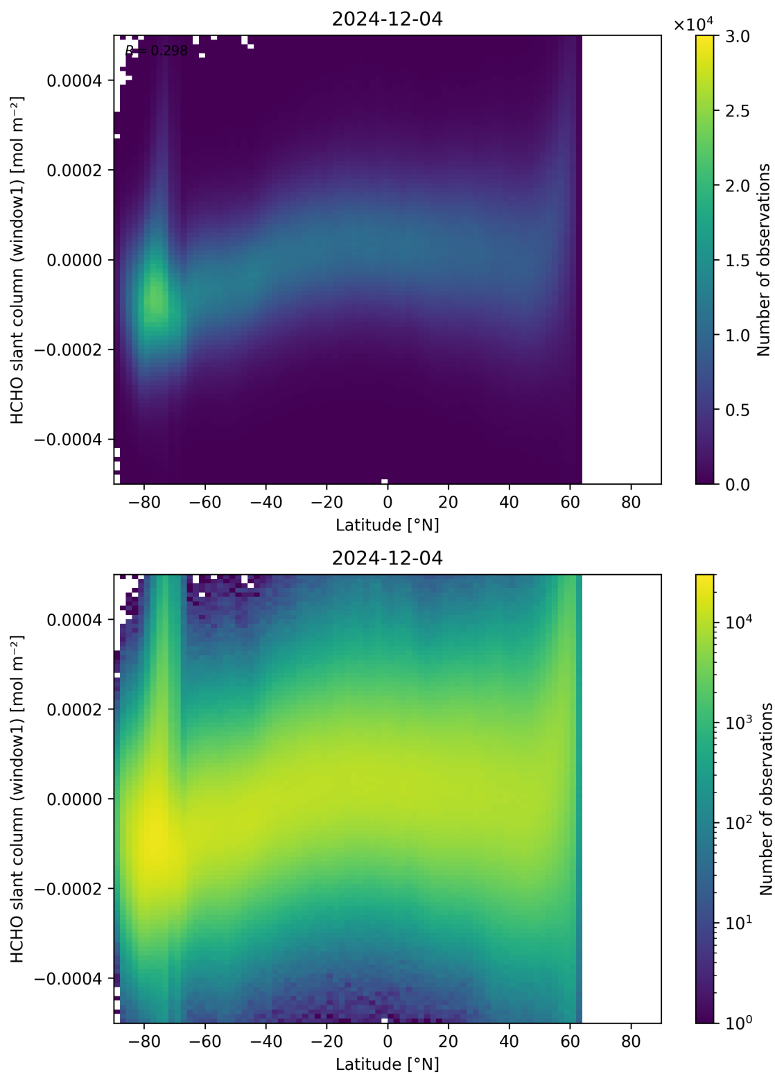
Figure 159: Scatter density plot of “Latitude” against “HCHO slant column (window1)” for 2024-12-03 to 2024-12-05.
