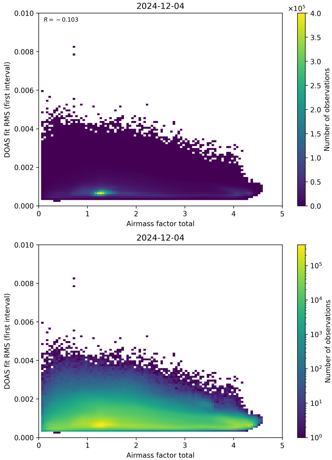
Figure 97: Scatter density plot of “Airmass factor total” against “DOAS fit RMS (first interval)” for 2024-12-03 to 2024-12-05.
