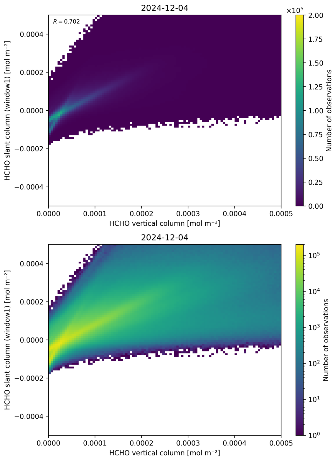
Figure 129: Scatter density plot of “HCHO vertical column” against “HCHO slant column (window1)” for 2024-12-03 to 2024-12-05.
