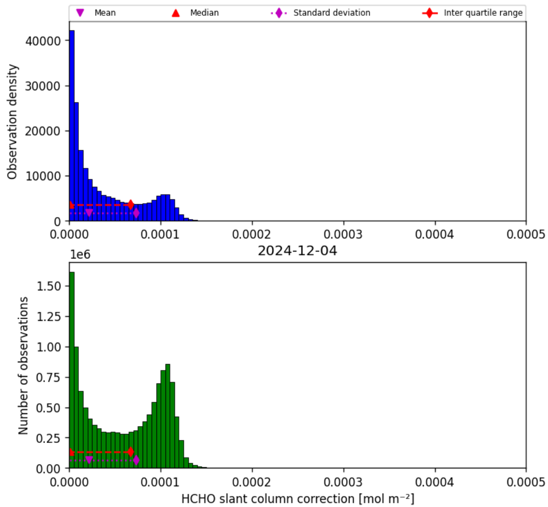
Figure 47: Histogram of “HCHO slant column correction” for 2024-12-03 to 2024-12-05
