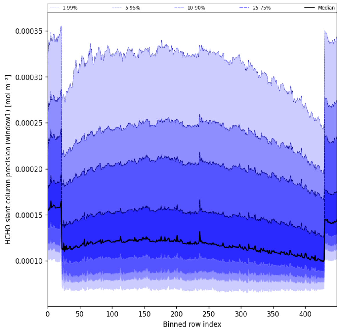
Figure 53: Along track statistics of “HCHO slant column precision (window1)” for 2024-12-03 to 2024-12-05
