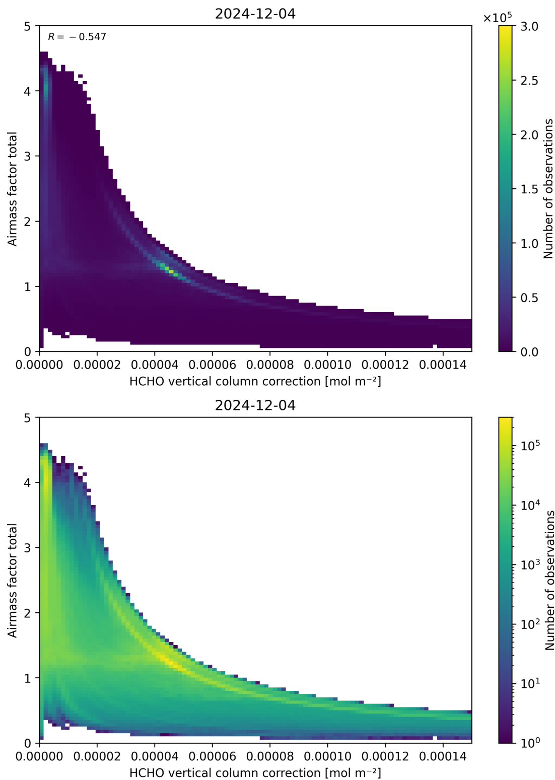
Figure 120: Scatter density plot of “HCHO vertical column correction” against “Airmass factor total” for 2024-12-03 to 2024-12-05.
