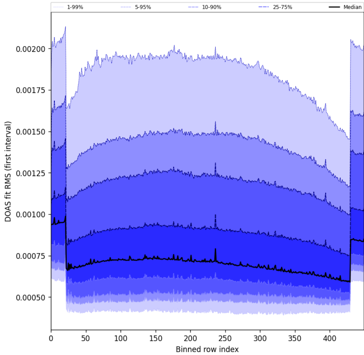
Figure 60: Along track statistics of “DOAS fit RMS (first interval)” for 2024-12-03 to 2024-12-05
