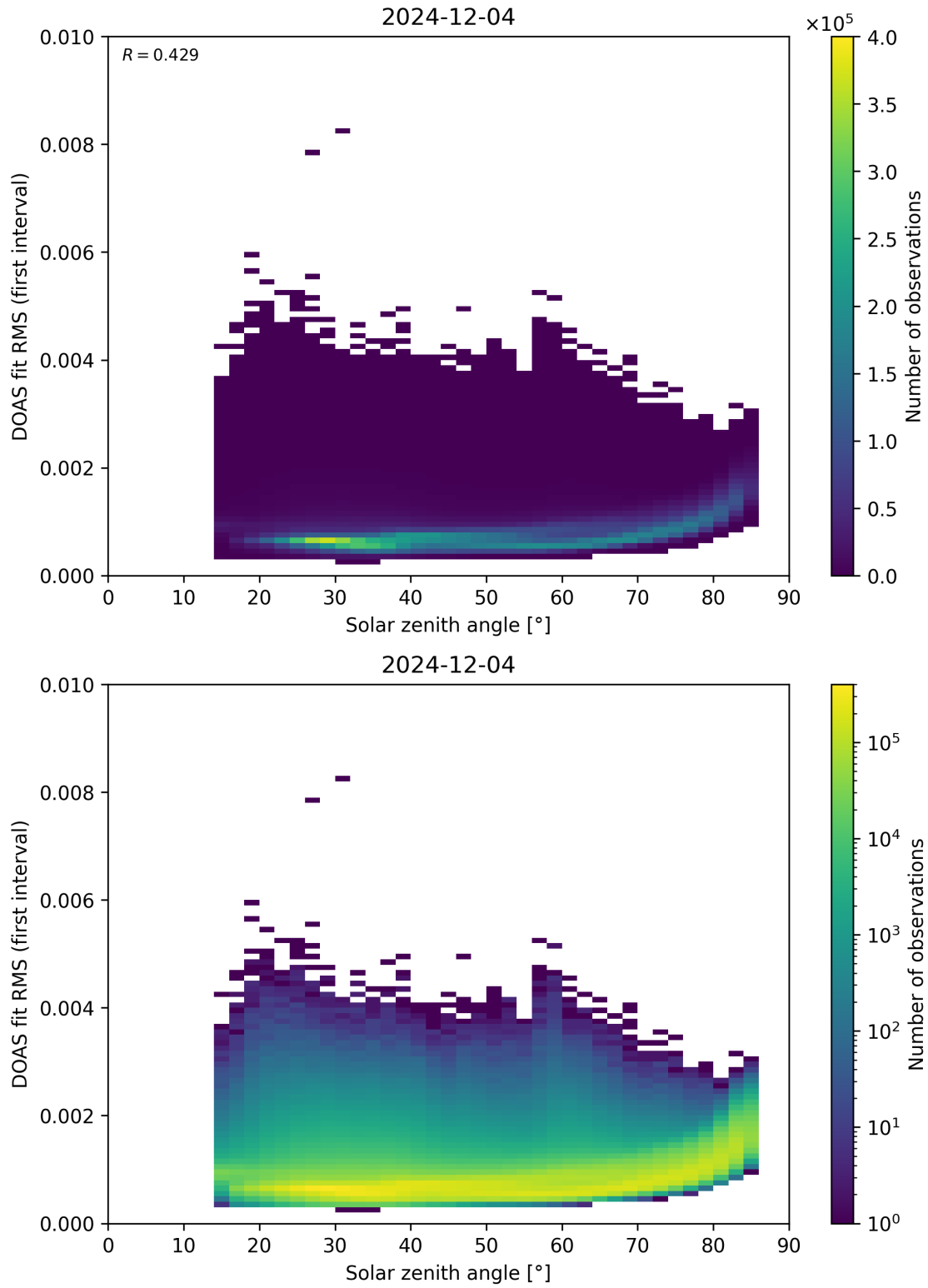
Figure 167: Scatter density plot of “Solar zenith angle” against “DOAS fit RMS (first interval)” for 2024-12-03 to 2024-12-05.
