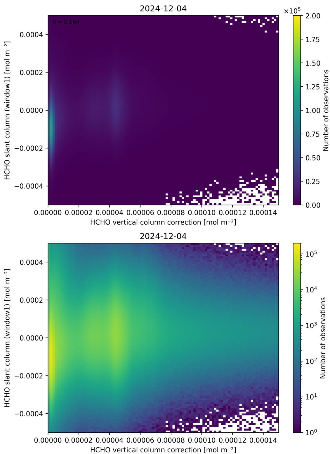
Figure 118: Scatter density plot of “HCHO vertical column correction” against “HCHO slant column (window1)” for 2024-12-03 to 2024-12-05.
