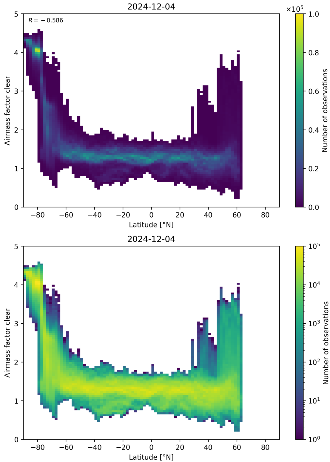
Figure 156: Scatter density plot of “Latitude” against “Airmass factor clear” for 2024-12-03 to 2024-12-05.
