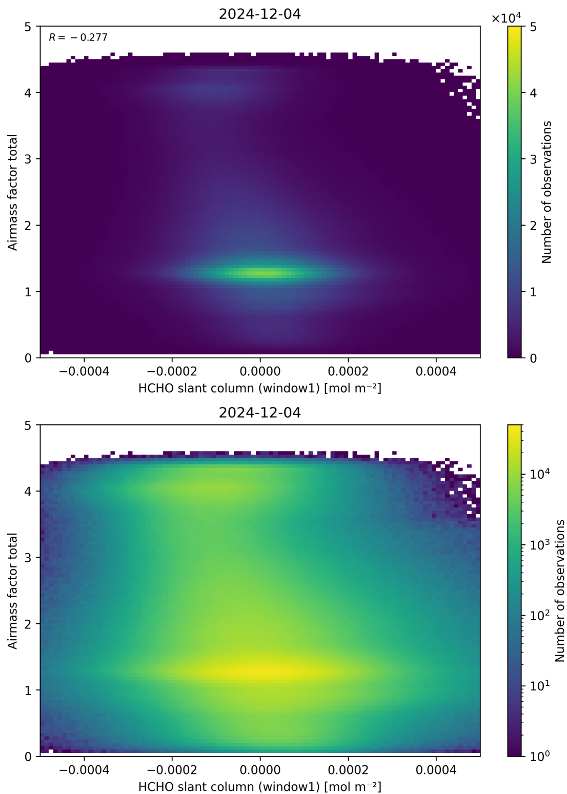
Figure 85: Scatter density plot of “HCHO slant column (window1)” against “Airmass factor total” for 2024-12-03 to 2024-12-05.
