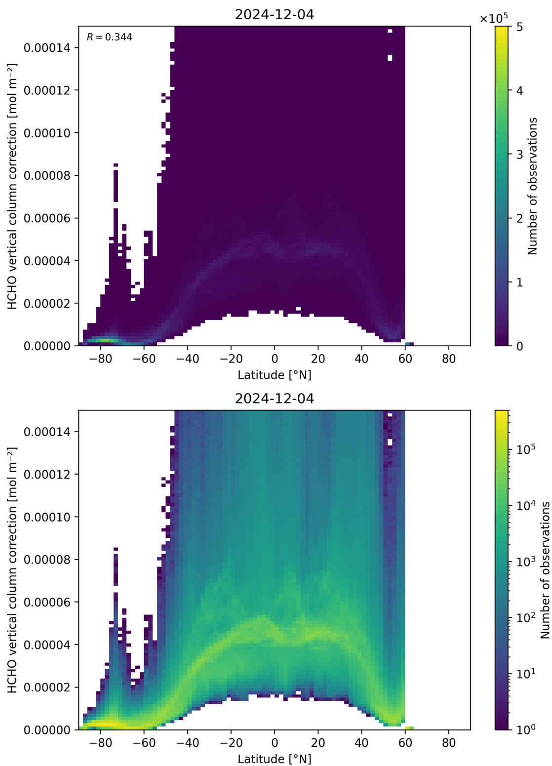
Figure 164: Scatter density plot of “Latitude” against “HCHO vertical column correction” for 2024-12-03 to 2024-12-05.
