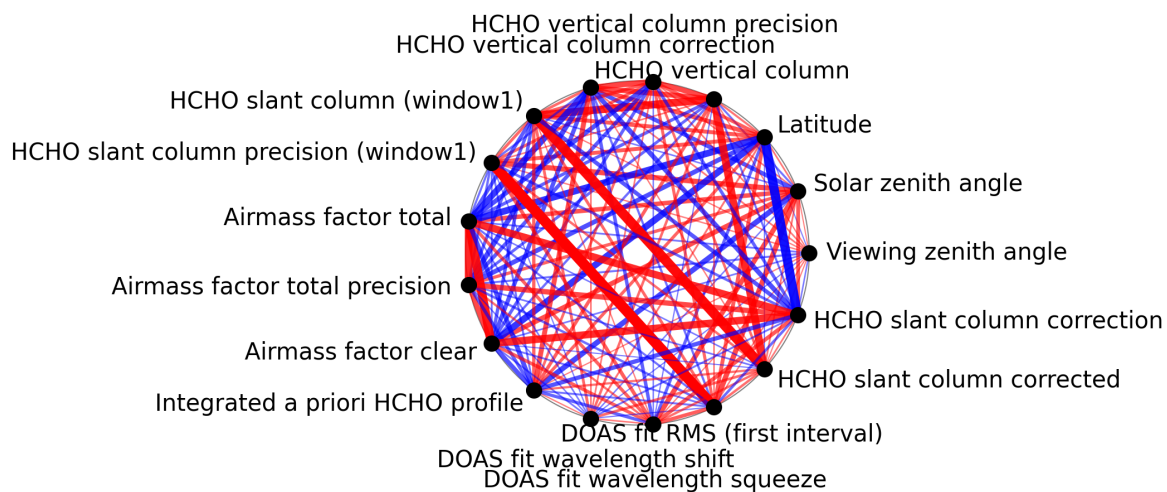
Figure 1: Map of correlation graph for 2024-12-03 to 2024-12-05.
