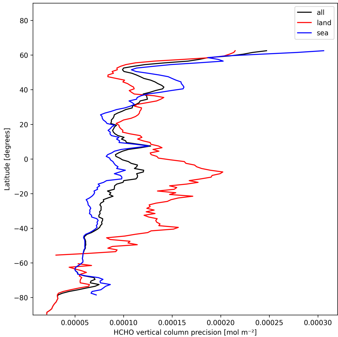
Figure 22: Zonal average of “HCHO vertical column precision” for 2024-12-03 to 2024-12-05.
