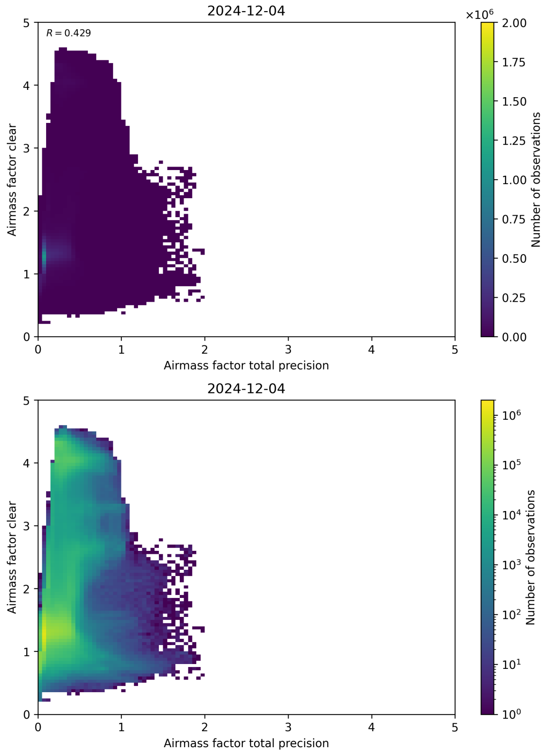
Figure 108: Scatter density plot of “Airmass factor total precision” against “Airmass factor clear” for 2024-12-03 to 2024-12-05.
