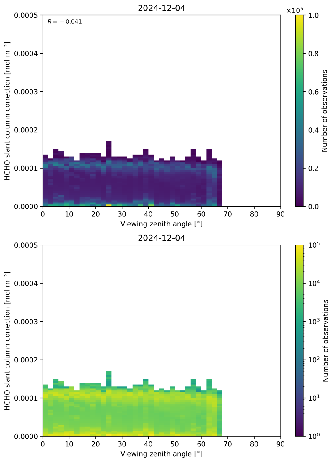
Figure 187: Scatter density plot of “Viewing zenith angle” against “HCHO slant column correction” for 2024-12-03 to 2024-12-05.
