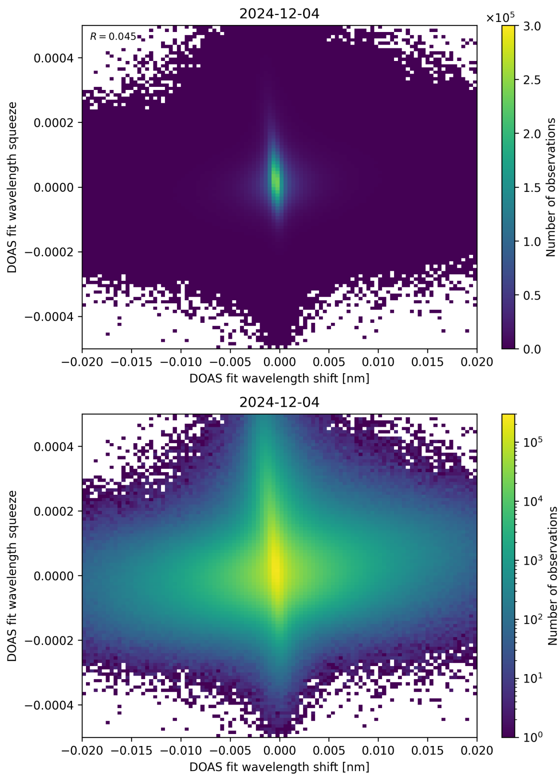
Figure 65: Scatter density plot of “DOAS fit wavelength shift” against “DOAS fit wavelength squeeze” for 2024-12-03 to 2024-12-05.
