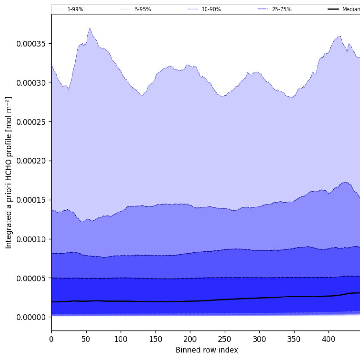
Figure 57: Along track statistics of "Integrated a priori HCHO profile" for 2024-12-03 to 2024-12-05
