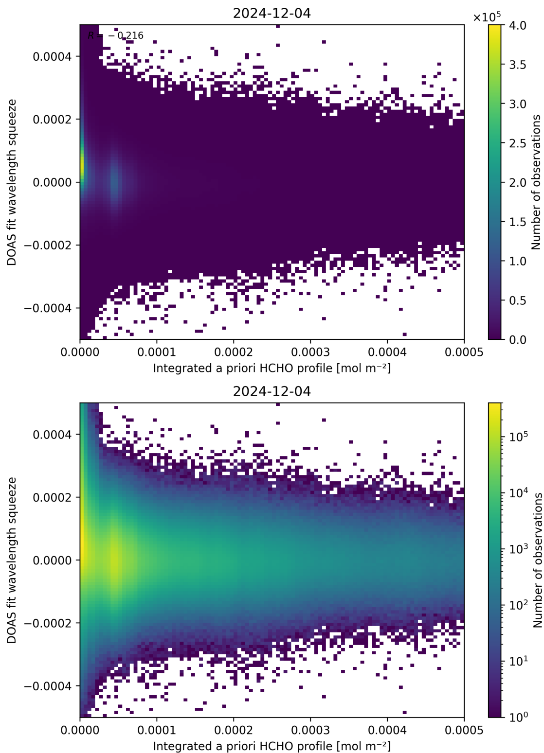
Figure 150: Scatter density plot of “Integrated a priori HCHO profile” against “DOAS fit wavelength squeeze” for 2024-12-03 to 2024-12-05.
