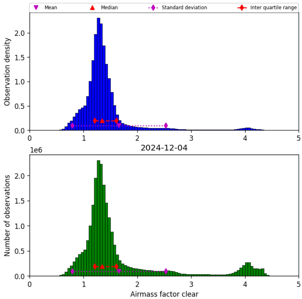
Figure 42: Histogram of “Airmass factor clear” for 2024-12-03 to 2024-12-05
