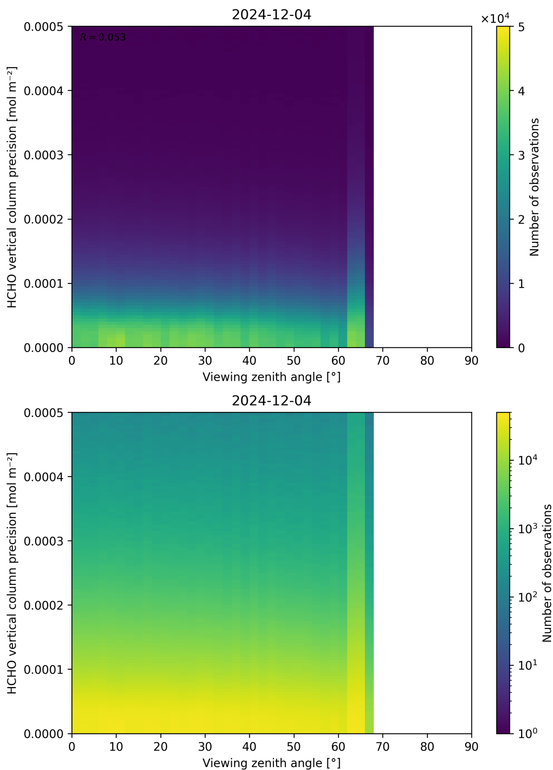
Figure 194: Scatter density plot of “Viewing zenith angle” against “HCHO vertical column precision” for 2024-12-03 to 2024-12-05.
