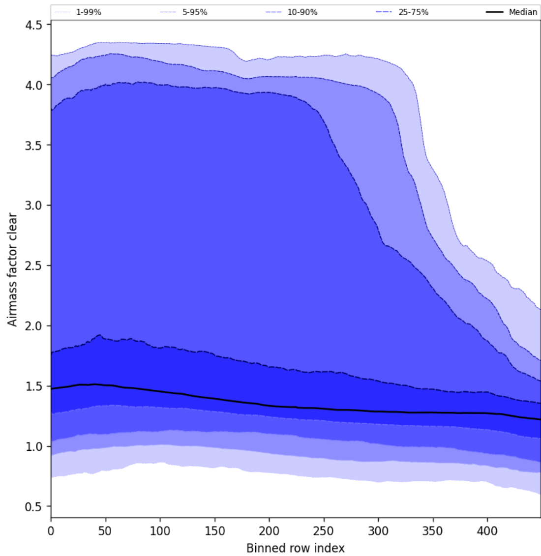
Figure 56: Along track statistics of “Airmass factor clear” for 2024-12-03 to 2024-12-05
