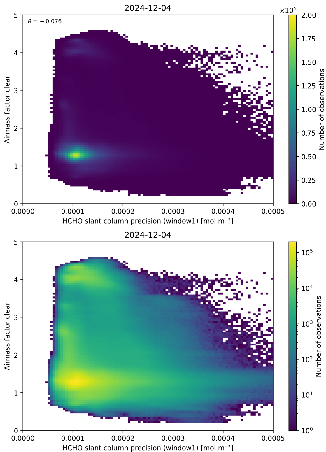
Figure 91: Scatter density plot of “HCHO slant column precision (window1)” against “Airmass factor clear” for 2024-12-03 to 2024-12-05.
