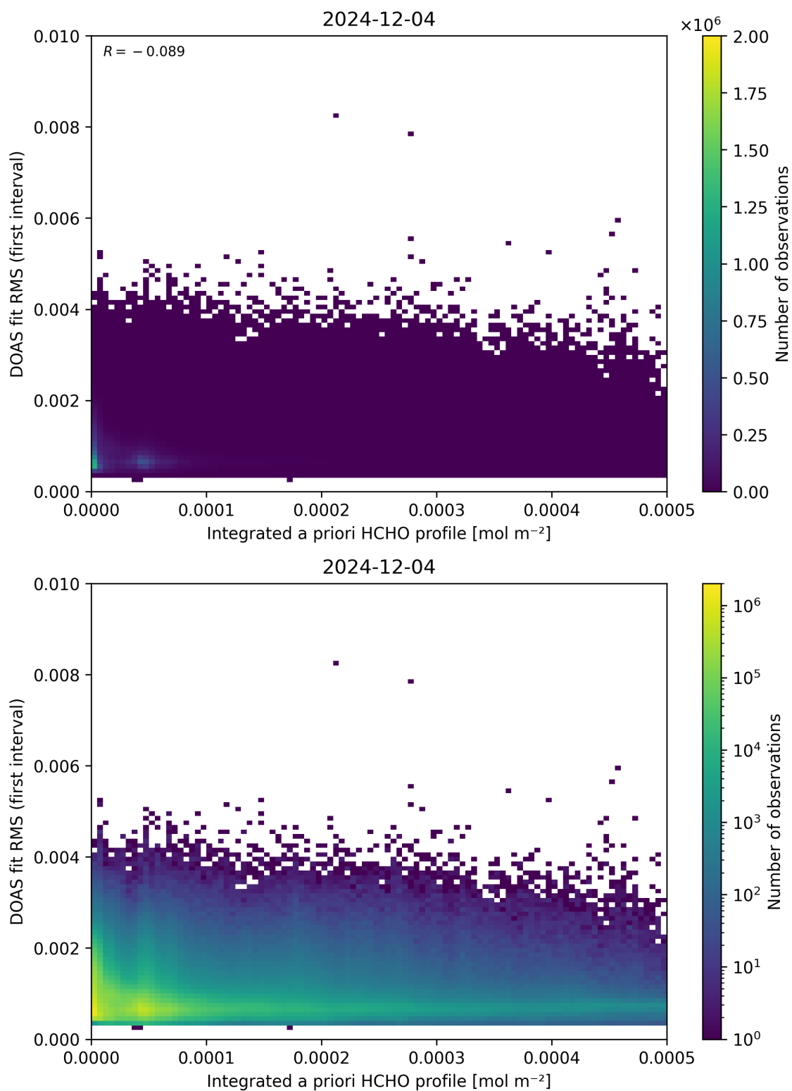
Figure 148: Scatter density plot of “Integrated a priori HCHO profile” against “DOAS fit RMS (first interval)” for 2024-12-03 to 2024-12-05.
