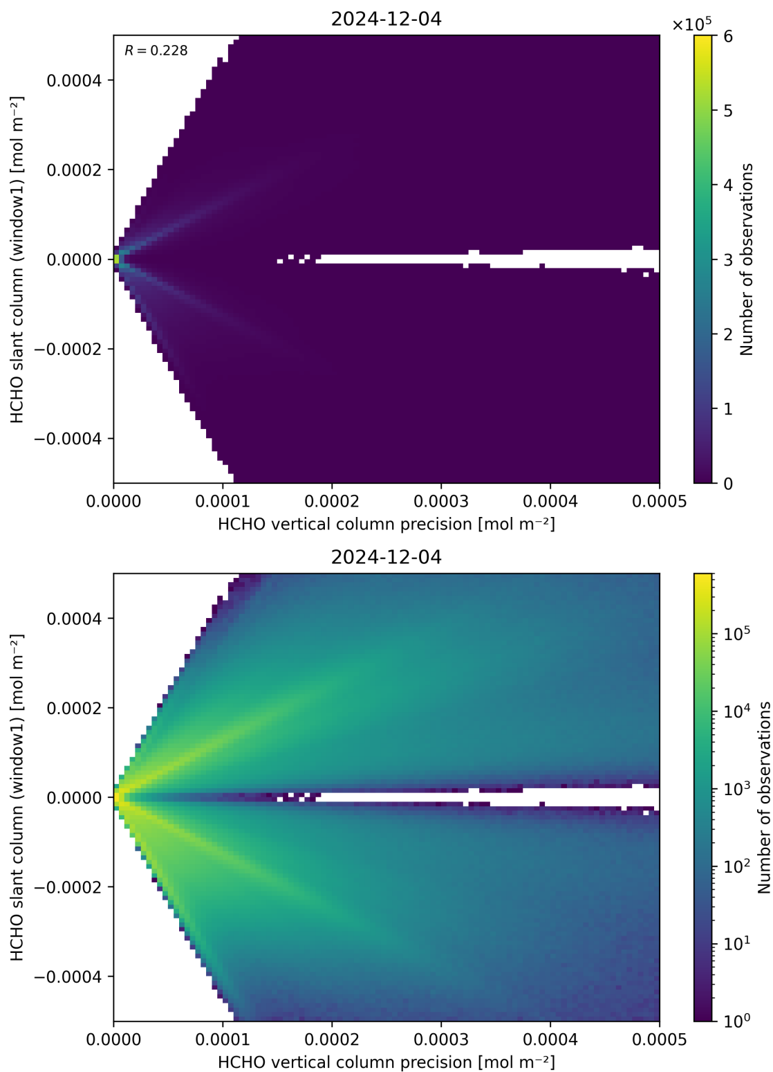
Figure 142: Scatter density plot of “HCHO vertical column precision” against “HCHO slant column (window1)” for 2024-12-03 to 2024-12-05.
