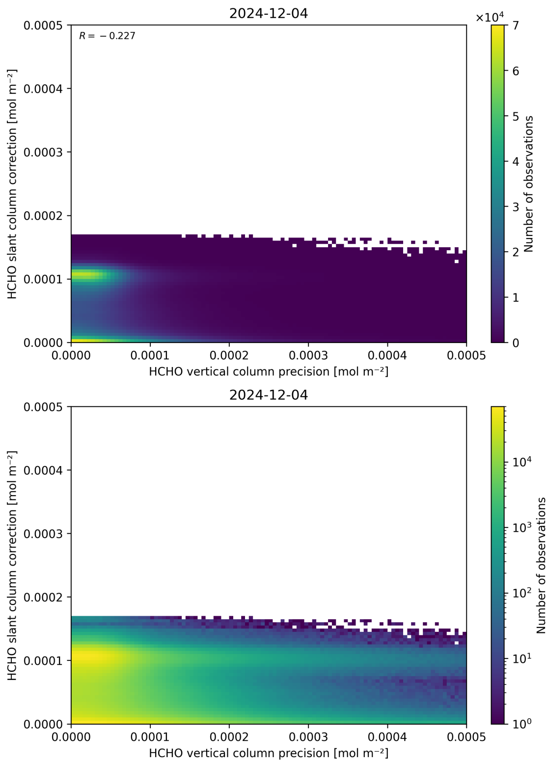
Figure 141: Scatter density plot of “HCHO vertical column precision” against “HCHO slant column correction” for 2024-12-03 to 2024-12-05.
