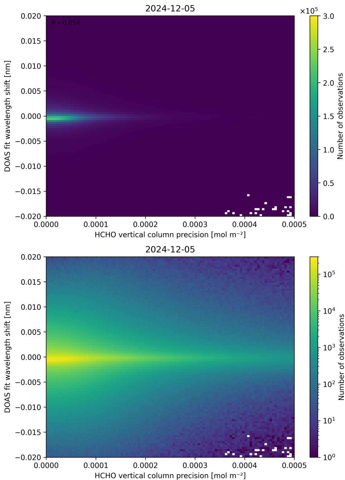
Figure 137: Scatter density plot of “HCHO vertical column precision” against “DOAS fit wavelength shift” for 2024-12-04 to 2024-12-06.
