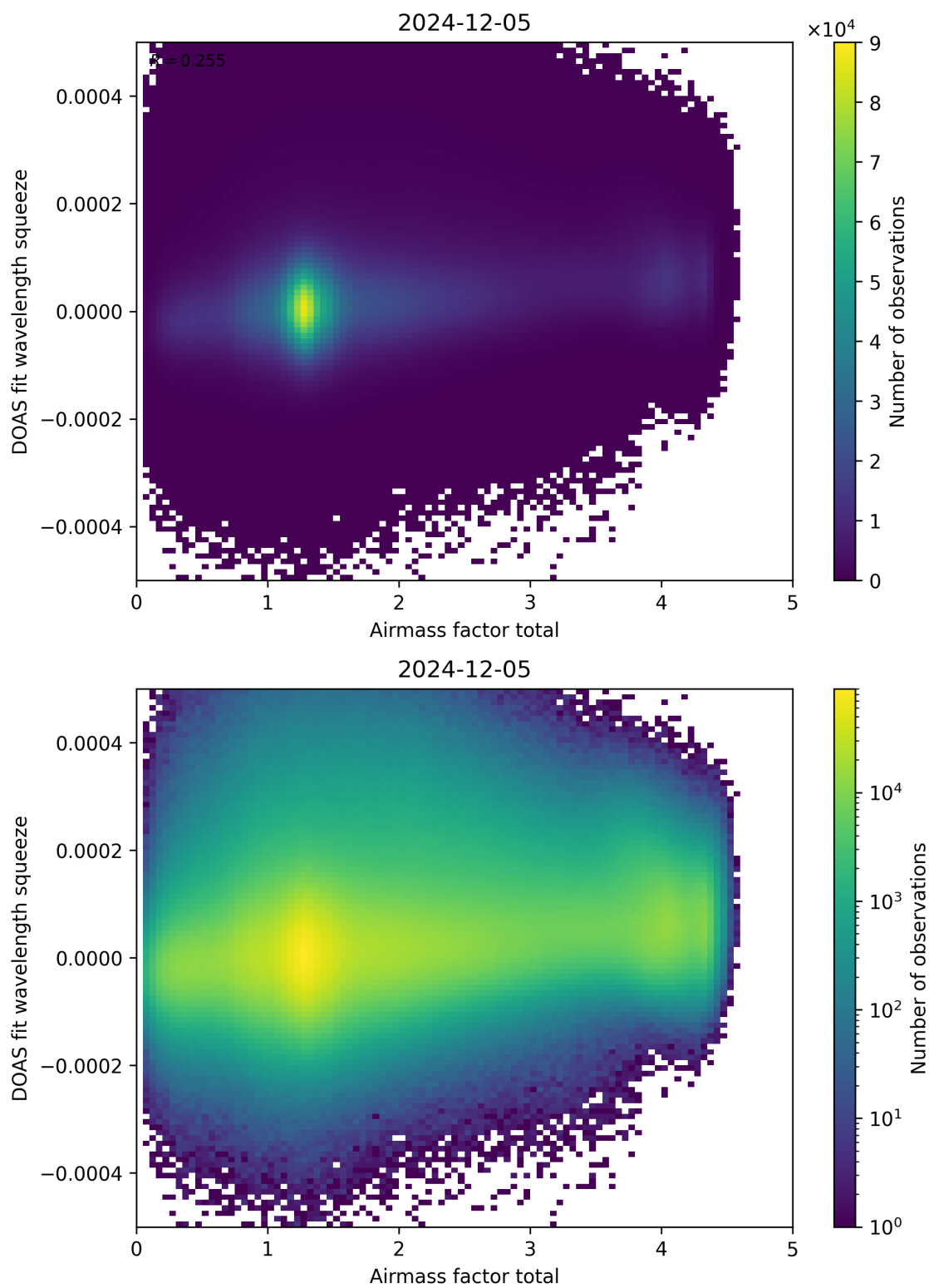
Figure 99: Scatter density plot of “Airmass factor total” against “DOAS fit wavelength squeeze” for 2024-12-04 to 2024-12-06.
