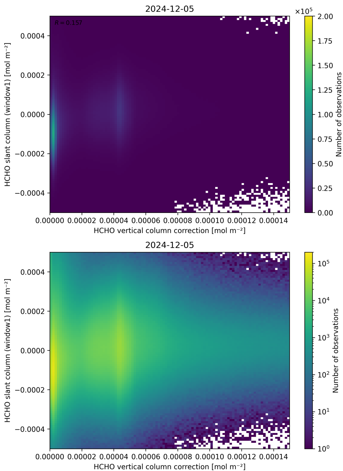
Figure 118: Scatter density plot of “HCHO vertical column correction” against “HCHO slant column (window1)” for 2024-12-04 to 2024-12-06.
