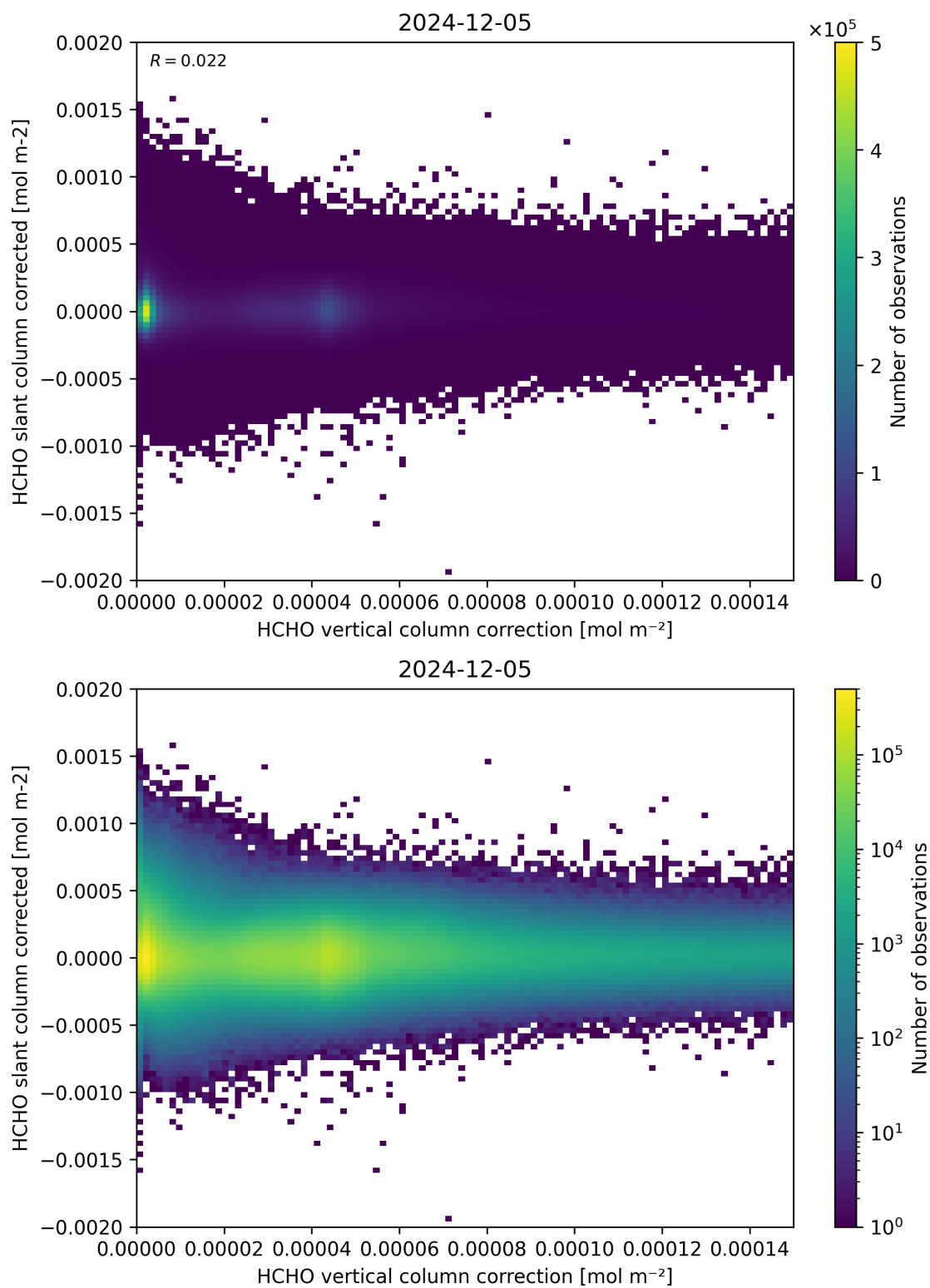
Figure 116: Scatter density plot of “HCHO vertical column correction” against “HCHO slant column corrected” for 2024-12-04 to 2024-12-06.
