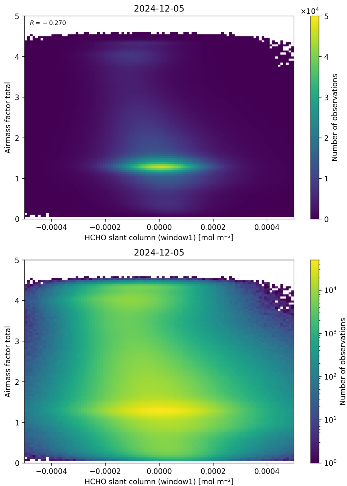
Figure 85: Scatter density plot of “HCHO slant column (window1)” against “Airmass factor total” for 2024-12-04 to 2024-12-06.
