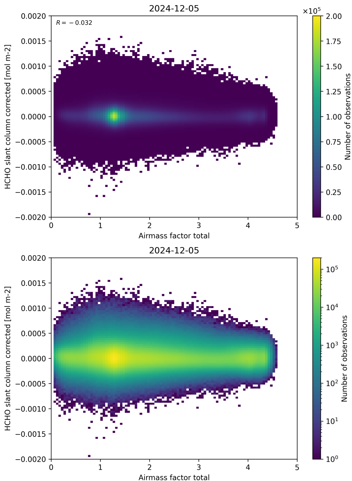
Figure 101: Scatter density plot of “Airmass factor total” against “HCHO slant column corrected” for 2024-12-04 to 2024-12-06.
