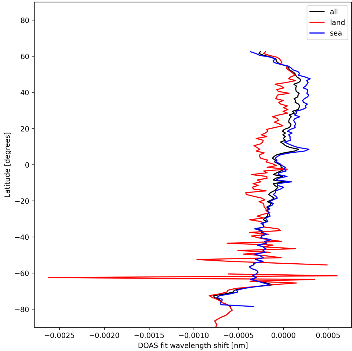
Figure 30: Zonal average of “DOAS fit wavelength shift” for 2024-12-04 to 2024-12-06.
