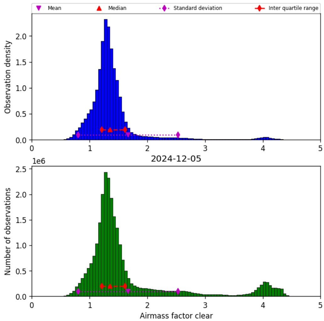
Figure 42: Histogram of “Airmass factor clear” for 2024-12-04 to 2024-12-06
