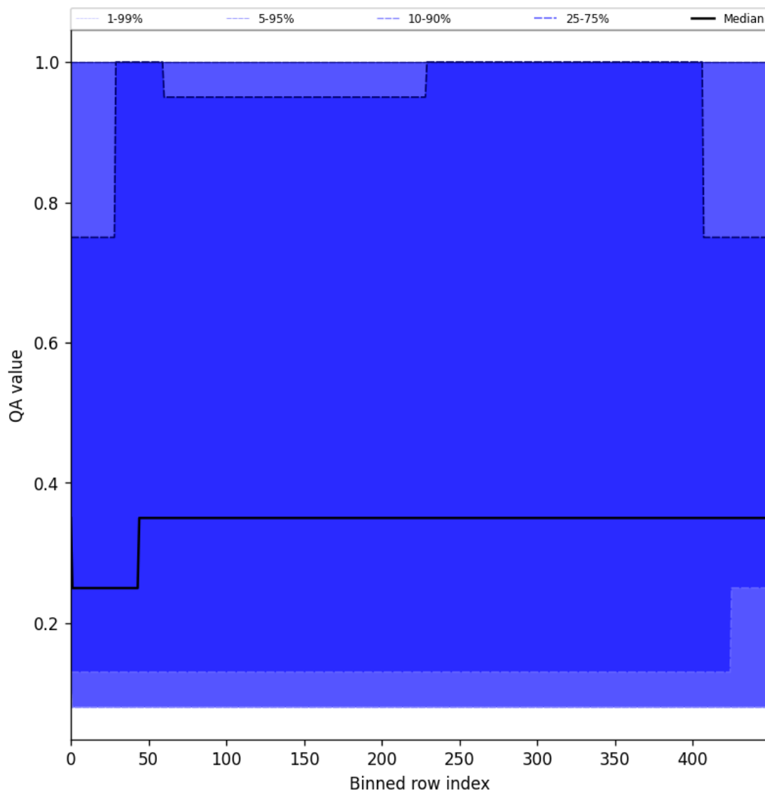
Figure 48: Along track statistics of “QA value” for 2024-12-04 to 2024-12-06
