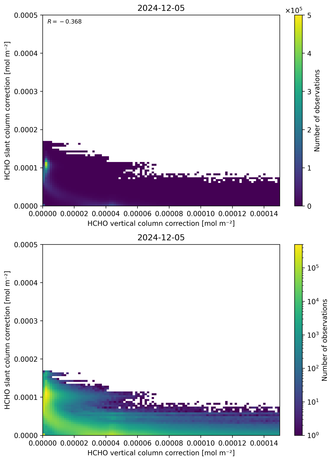
Figure 117: Scatter density plot of “HCHO vertical column correction” against “HCHO slant column correction” for 2024-12-04 to 2024-12-06.
