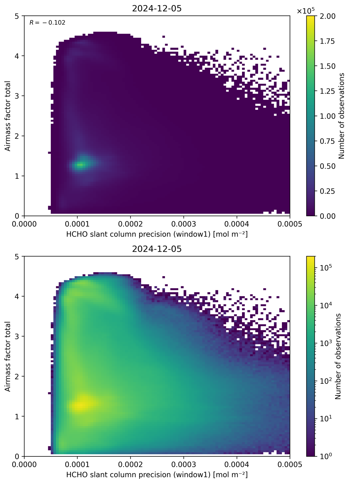
Figure 94: Scatter density plot of “HCHO slant column precision (window1)” against “Airmass factor total” for 2024-12-04 to 2024-12-06.
