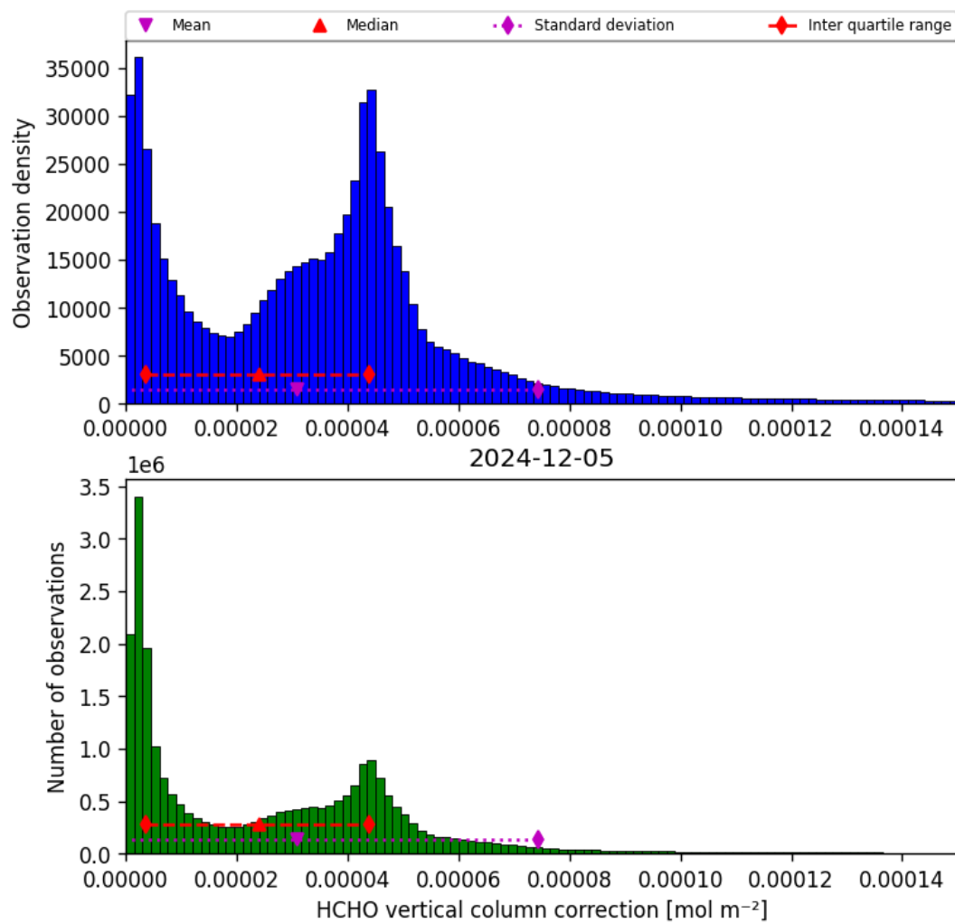
Figure 37: Histogram of “HCHO vertical column correction” for 2024-12-04 to 2024-12-06
