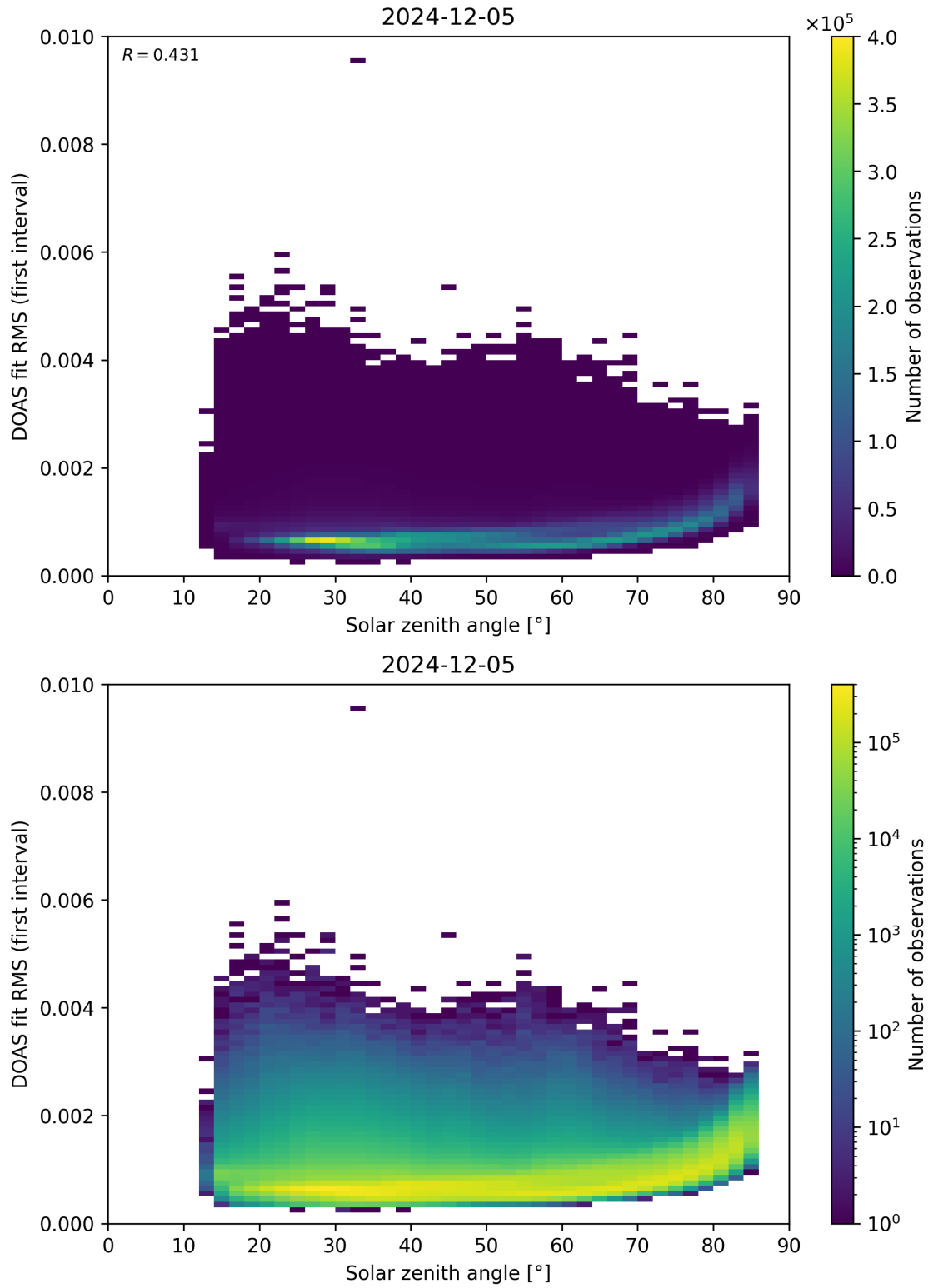
Figure 167: Scatter density plot of “Solar zenith angle” against “DOAS fit RMS (first interval)” for 2024-12-04 to 2024-12-06.
