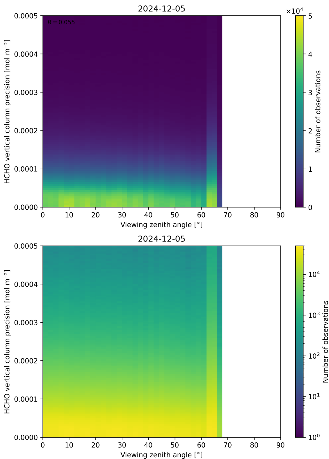
Figure 194: Scatter density plot of “Viewing zenith angle” against “HCHO vertical column precision” for 2024-12-04 to 2024-12-06.
