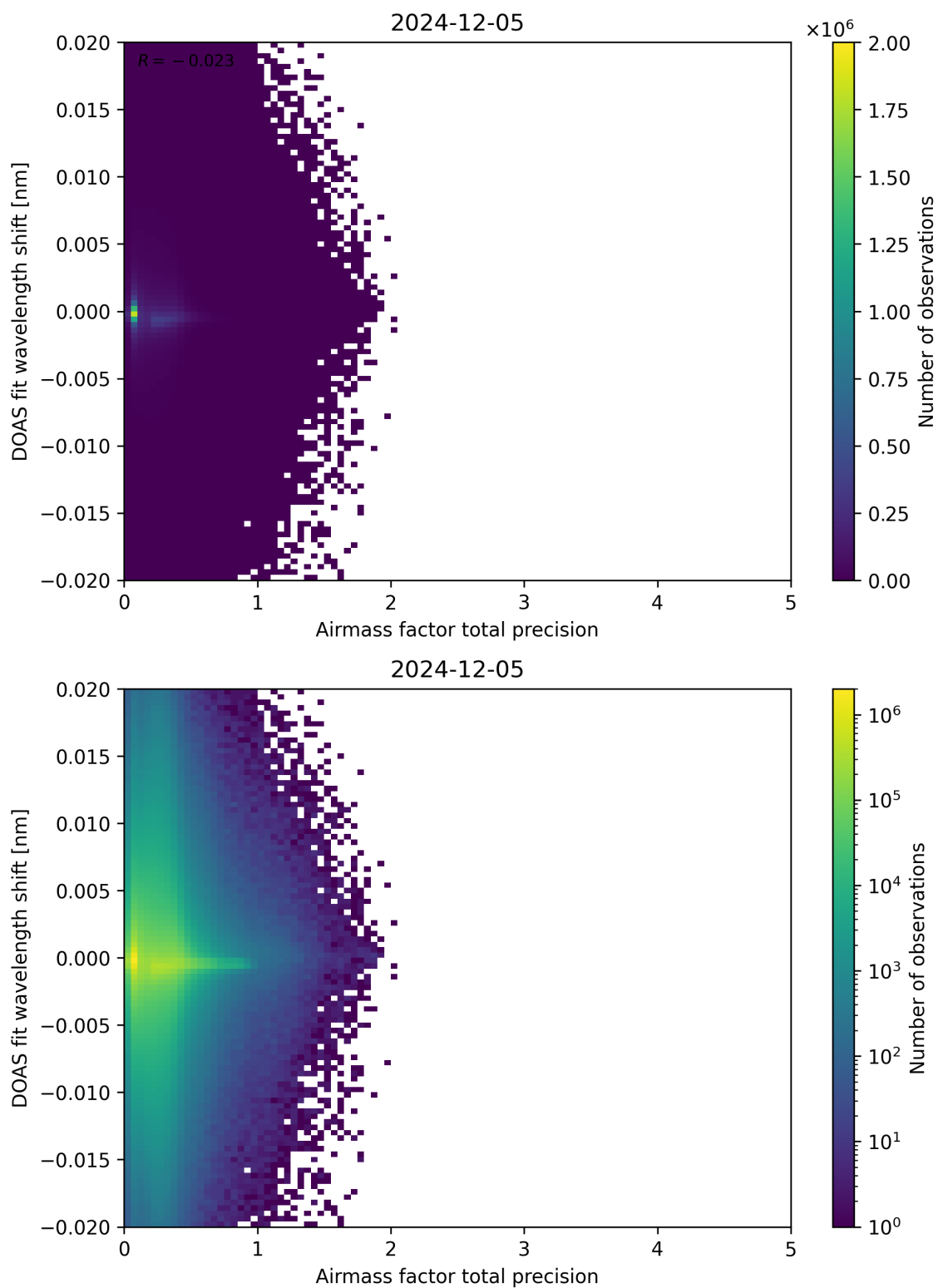
Figure 106: Scatter density plot of “Airmass factor total precision” against “DOAS fit wavelength shift” for 2024-12-04 to 2024-12-06.
