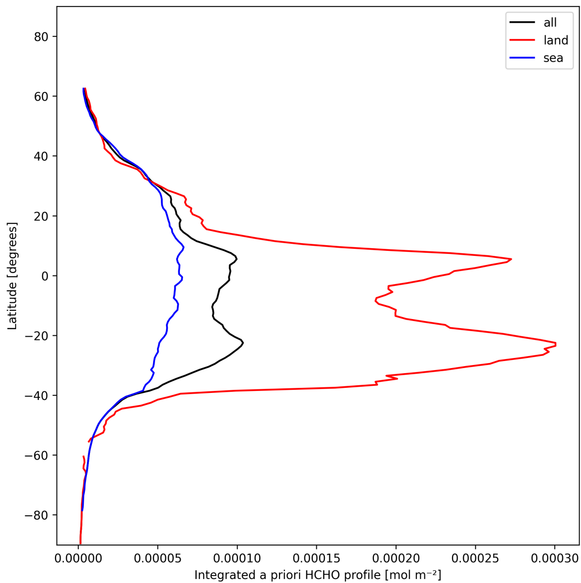
Figure 29: Zonal average of “Integrated a priori HCHO profile” for 2024-12-04 to 2024-12-06.
