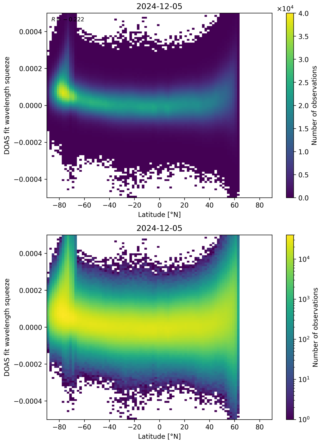
Figure 155: Scatter density plot of “Latitude” against “DOAS fit wavelength squeeze” for 2024-12-04 to 2024-12-06.
