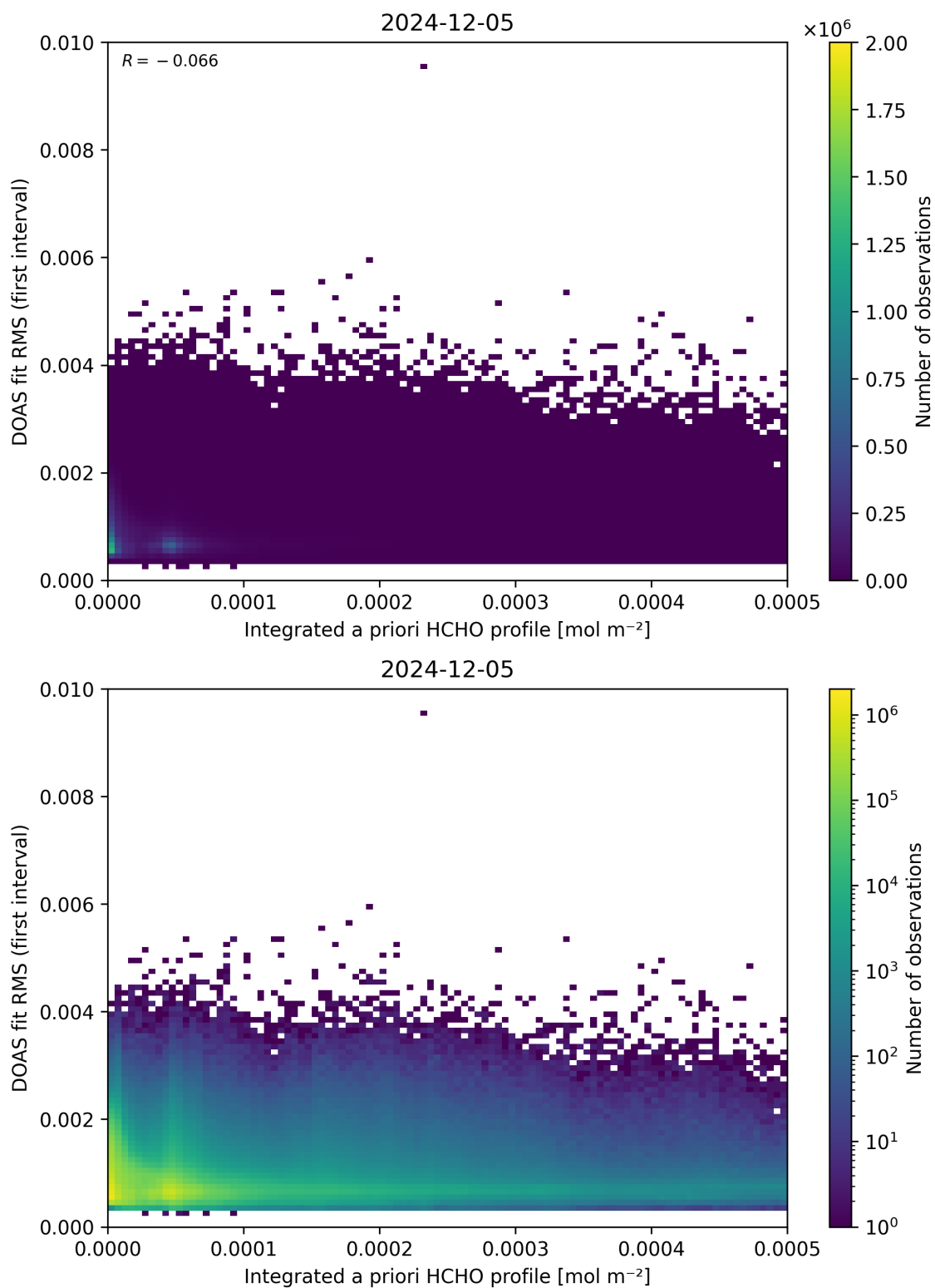
Figure 148: Scatter density plot of “Integrated a priori HCHO profile” against “DOAS fit RMS (first interval)” for 2024-12-04 to 2024-12-06.
