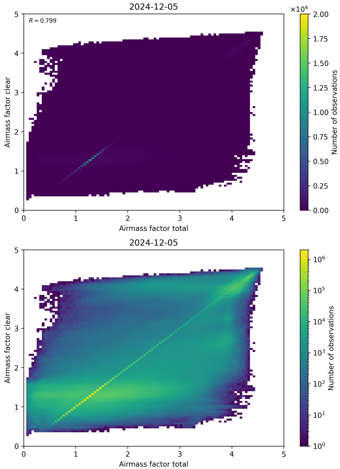
Figure 100: Scatter density plot of “Airmass factor total” against “Airmass factor clear” for 2024-12-04 to 2024-12-06.
