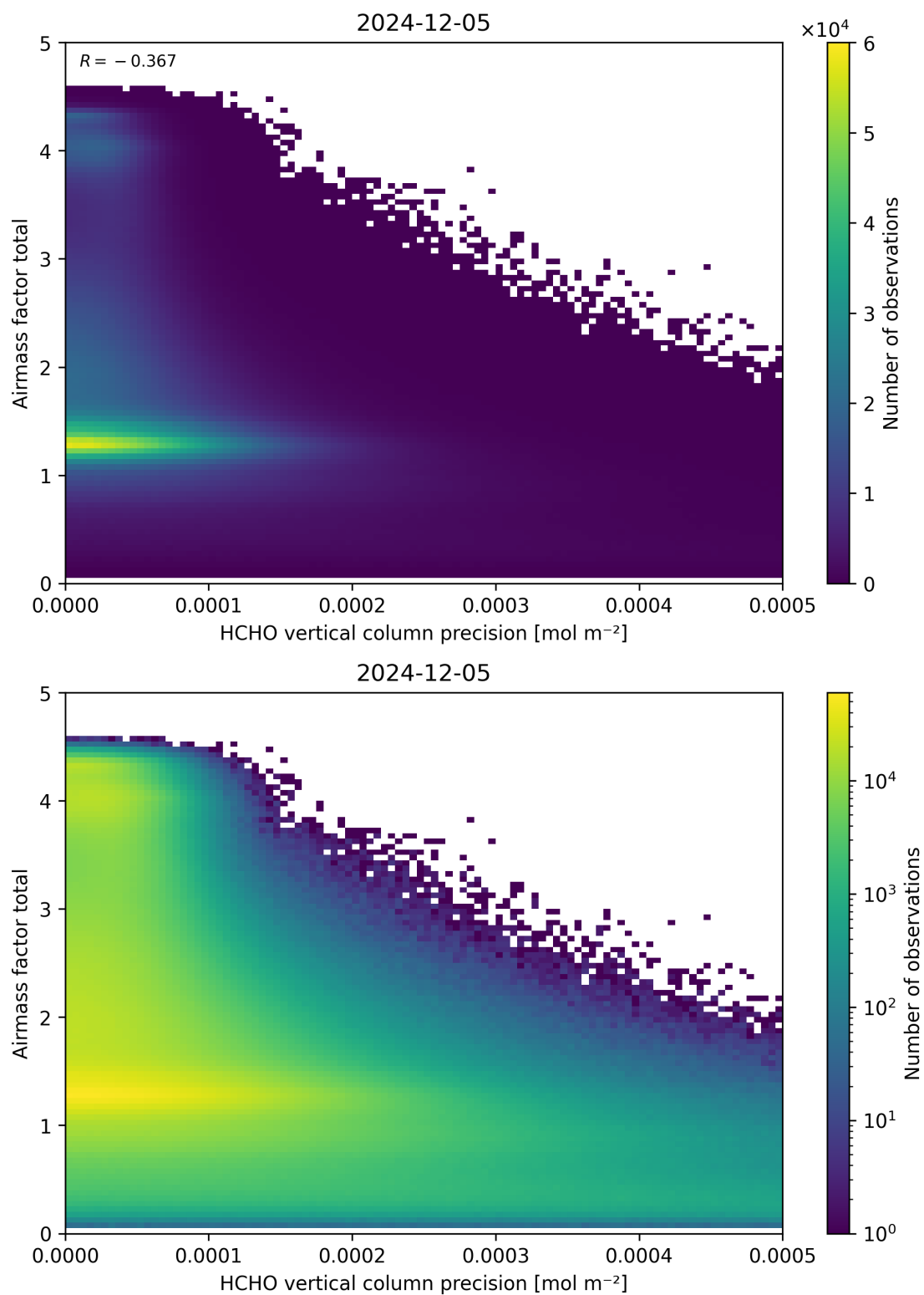
Figure 144: Scatter density plot of “HCHO vertical column precision” against “Airmass factor total” for 2024-12-04 to 2024-12-06.
