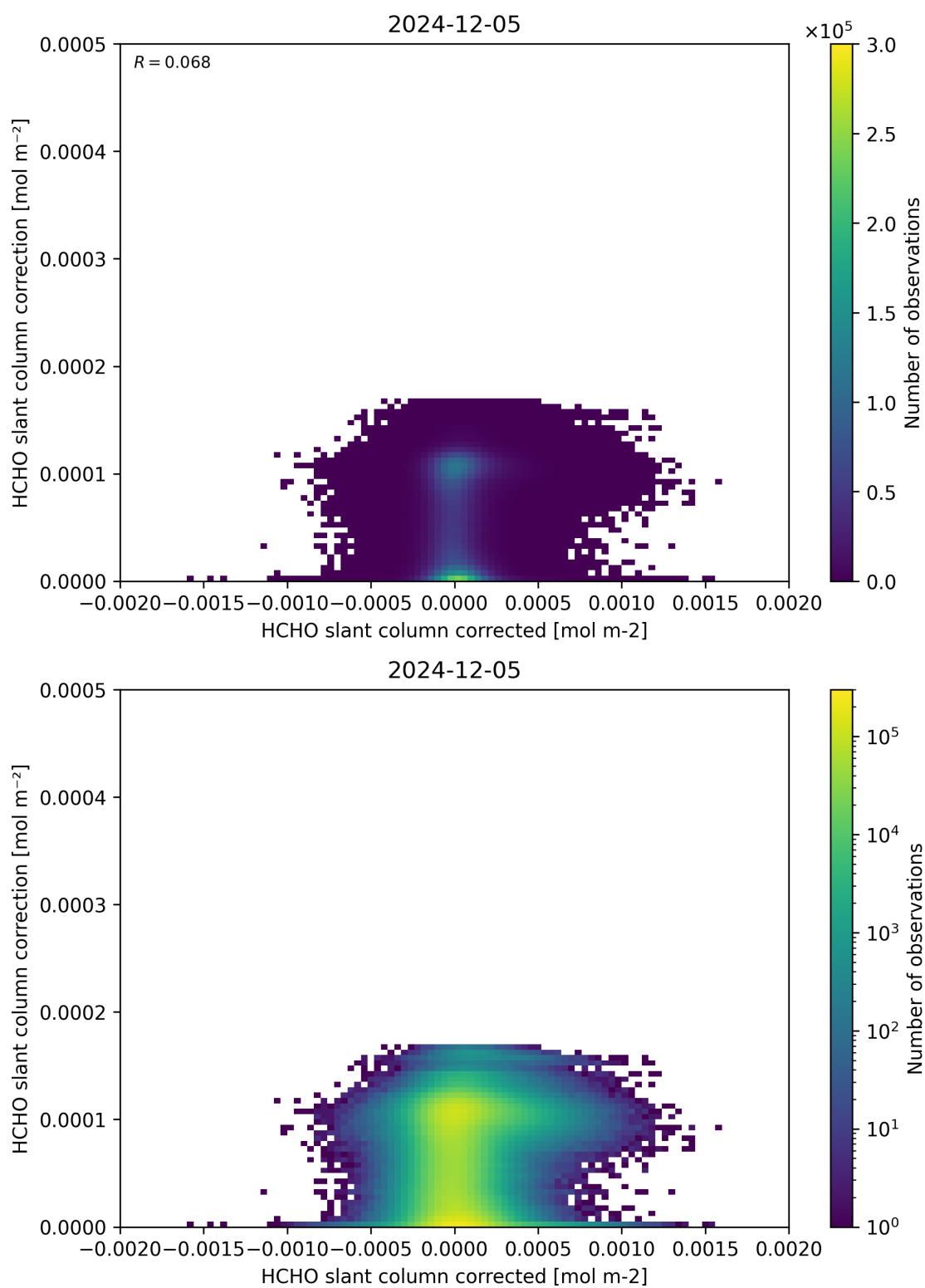
Figure 77: Scatter density plot of “HCHO slant column corrected” against “HCHO slant column correction” for 2024-12-04 to 2024-12-06.
