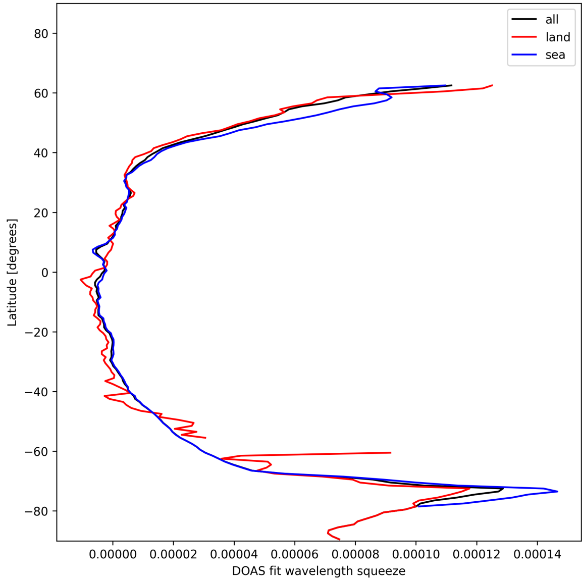
Figure 31: Zonal average of “DOAS fit wavelength squeeze” for 2024-12-04 to 2024-12-06.
