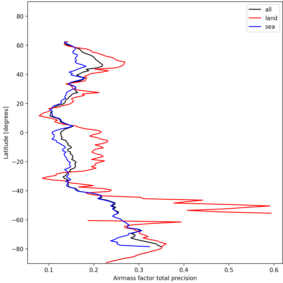
Figure 27: Zonal average of “Airmass factor total precision” for 2024-12-04 to 2024-12-06.
