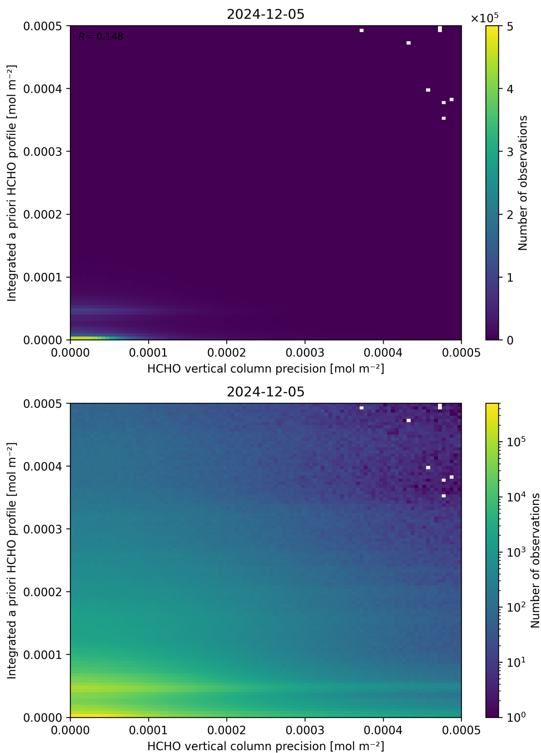
Figure 147: Scatter density plot of “HCHO vertical column precision” against “Integrated a priori HCHO profile” for 2024-12-04 to 2024-12-06.
