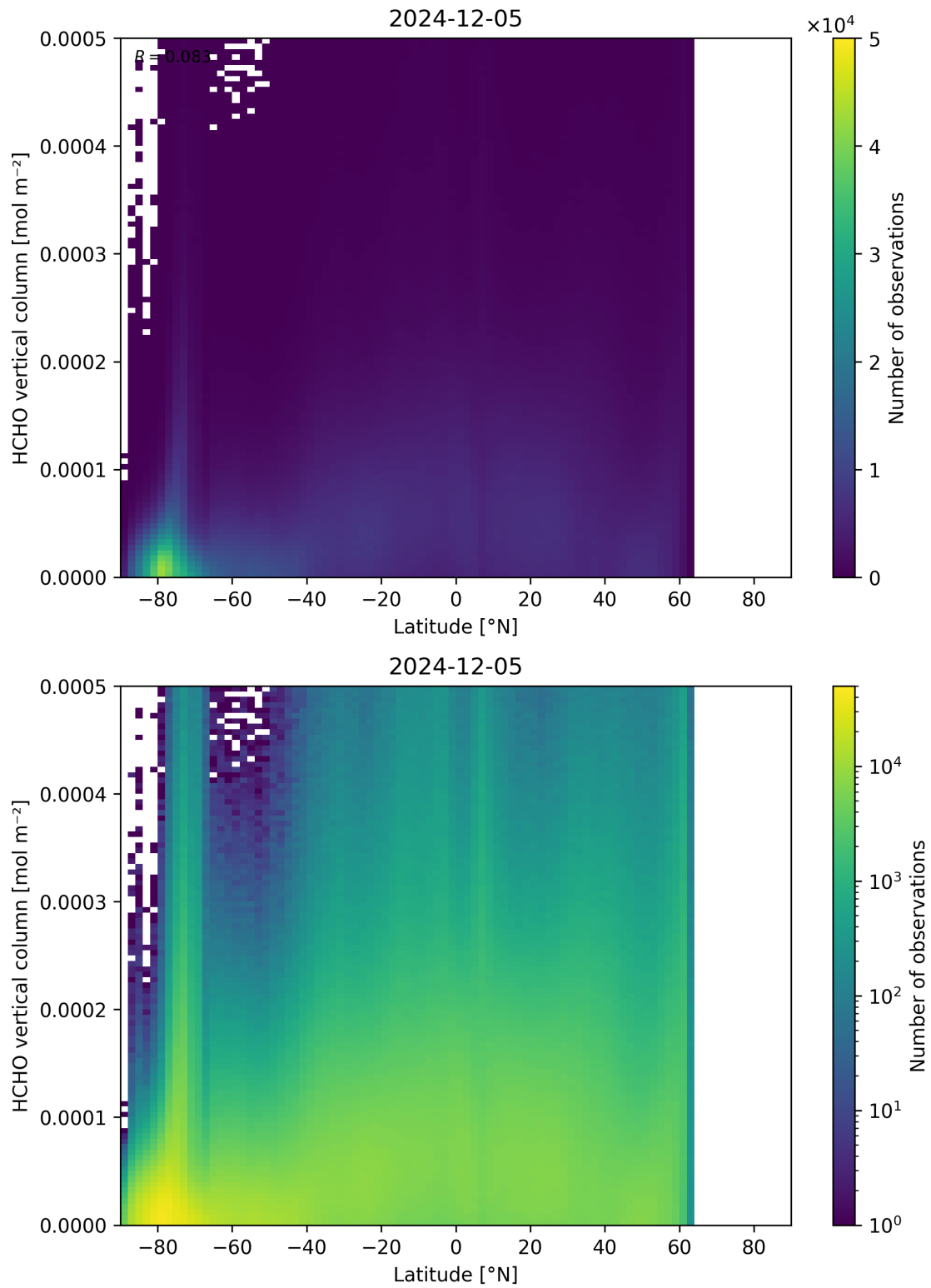
Figure 163: Scatter density plot of “Latitude” against “HCHO vertical column” for 2024-12-04 to 2024-12-06.
