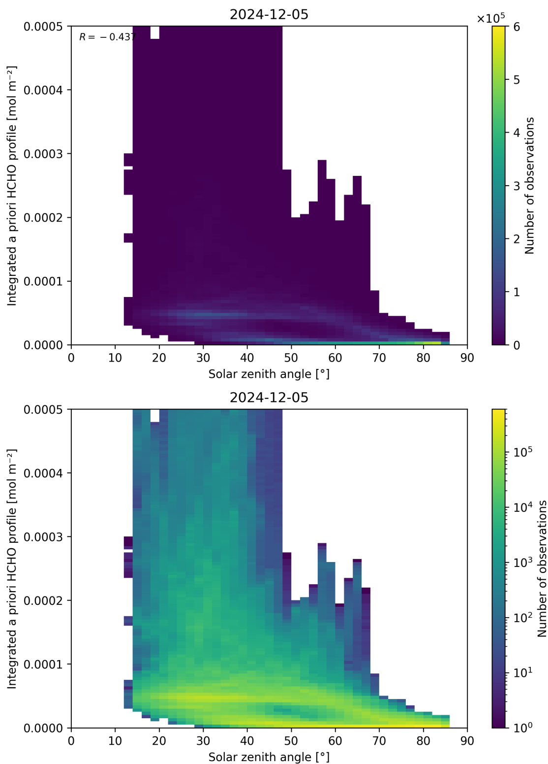
Figure 180: Scatter density plot of “Solar zenith angle” against “Integrated a priori HCHO profile” for 2024-12-04 to 2024-12-06.
