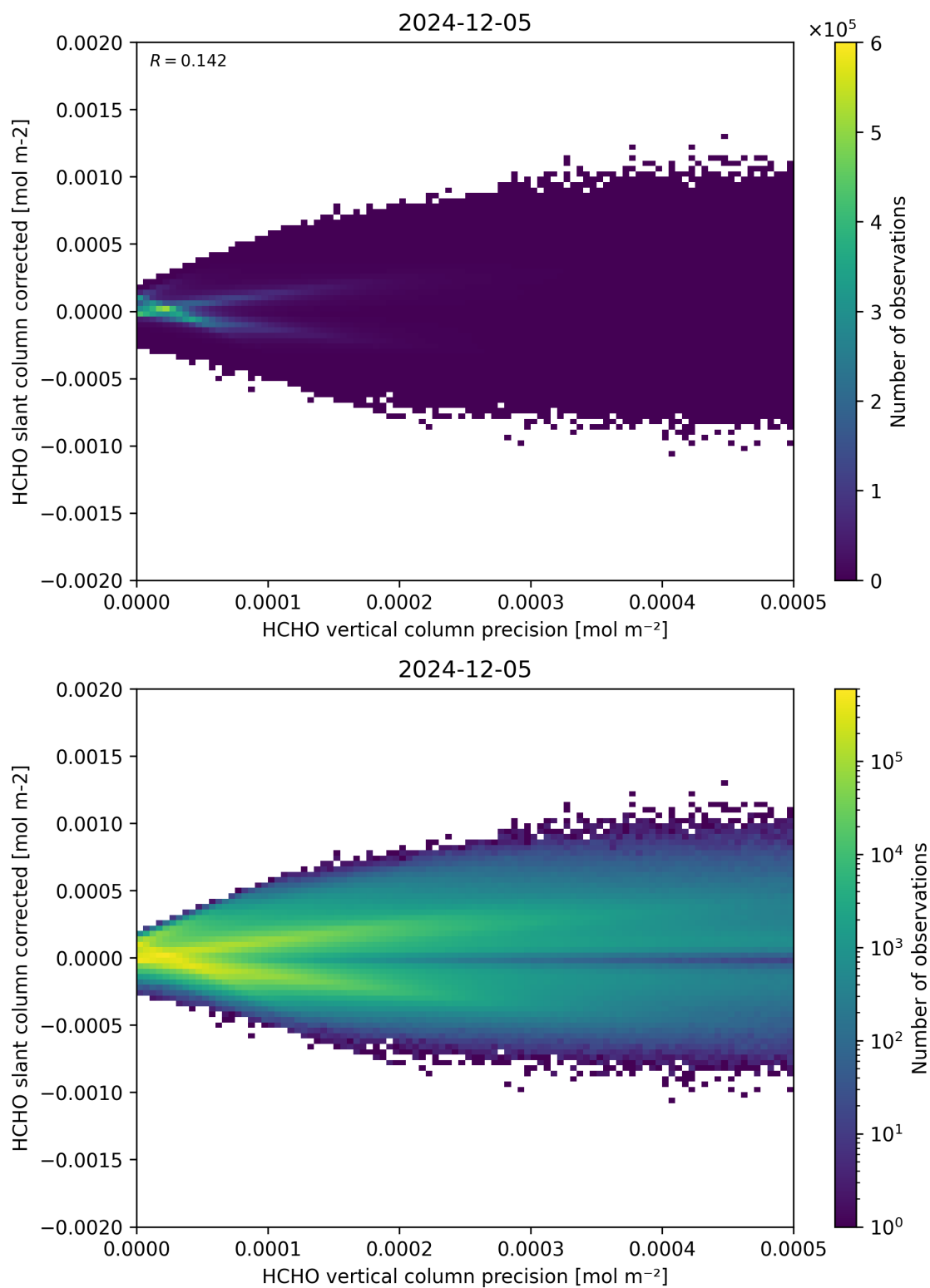
Figure 140: Scatter density plot of “HCHO vertical column precision” against “HCHO slant column corrected” for 2024-12-04 to 2024-12-06.
