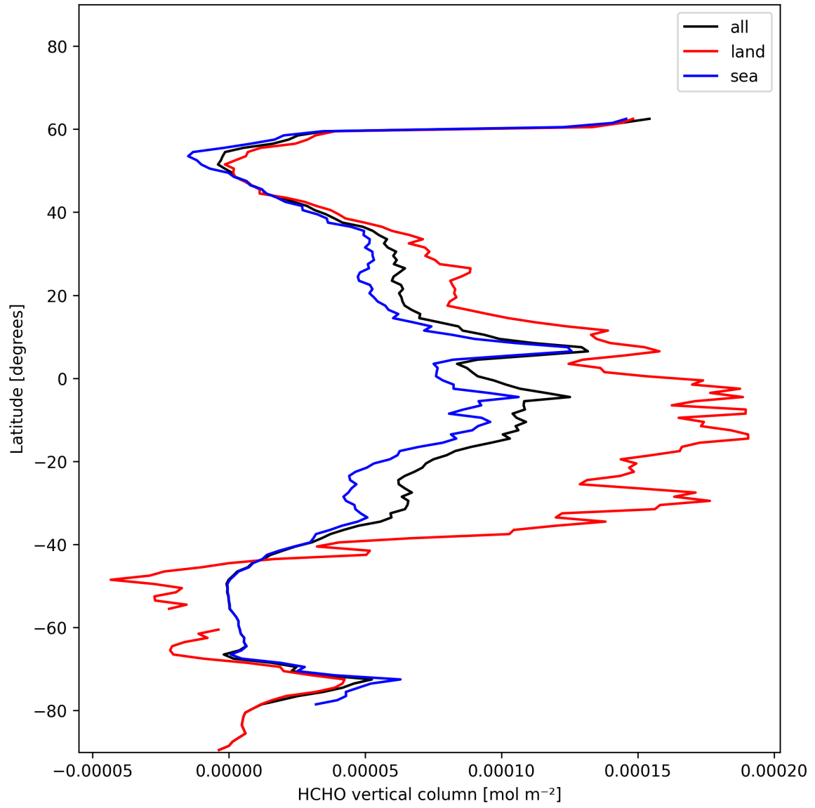
Figure 21: Zonal average of “HCHO vertical column” for 2024-12-04 to 2024-12-06.
