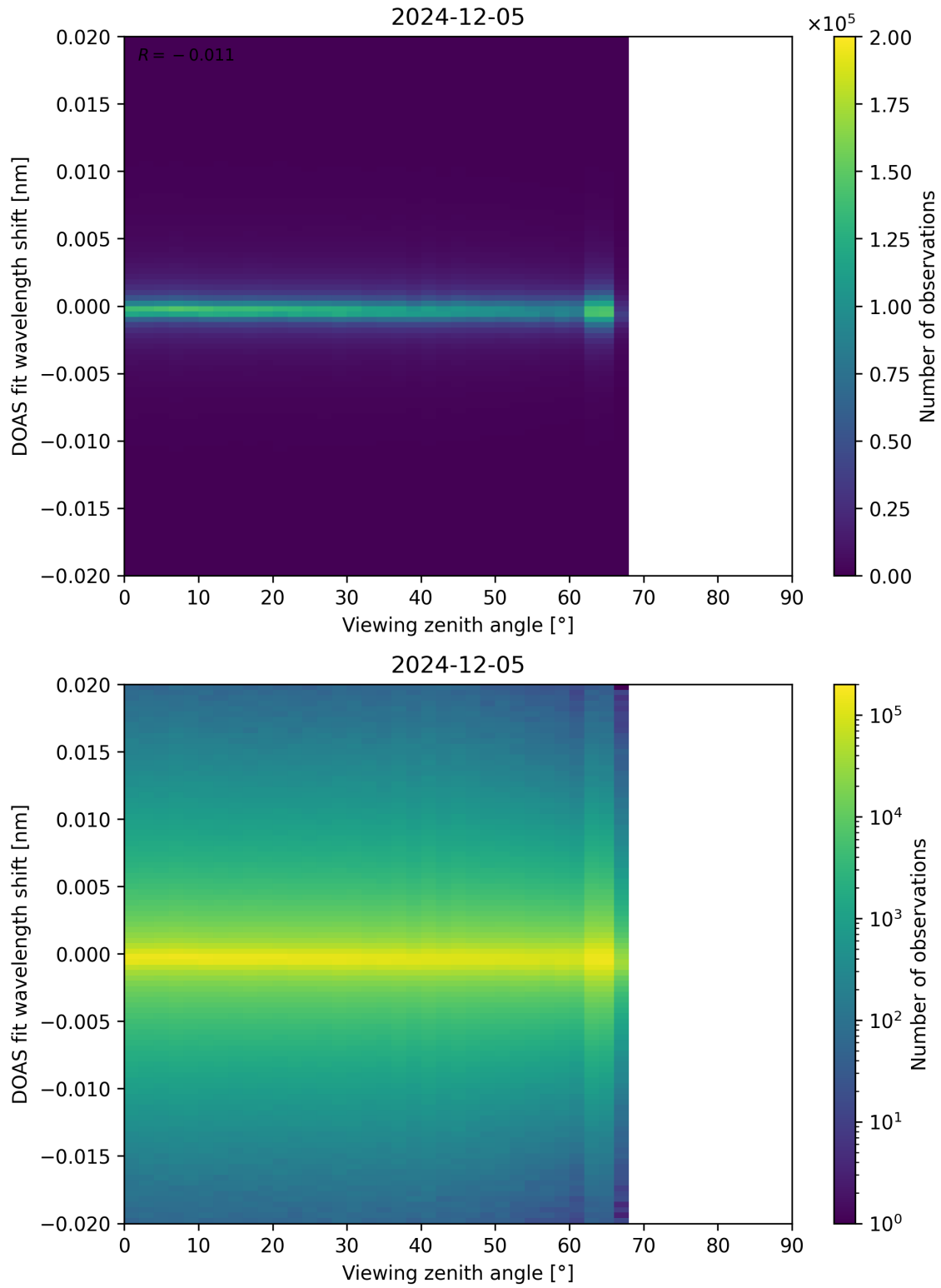
Figure 183: Scatter density plot of “Viewing zenith angle” against “DOAS fit wavelength shift” for 2024-12-04 to 2024-12-06.
