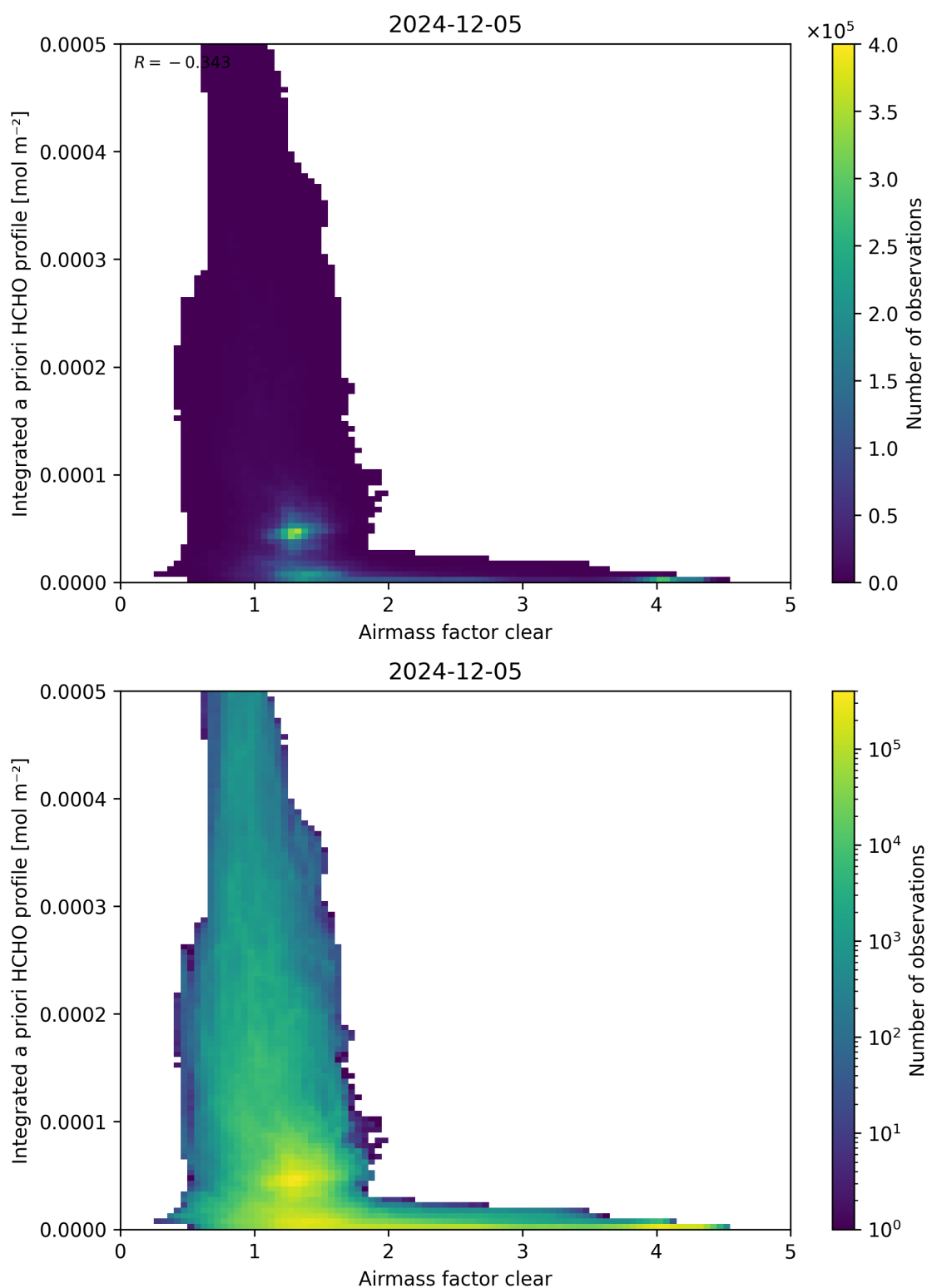
Figure 76: Scatter density plot of “Airmass factor clear” against “Integrated a priori HCHO profile” for 2024-12-04 to 2024-12-06.
