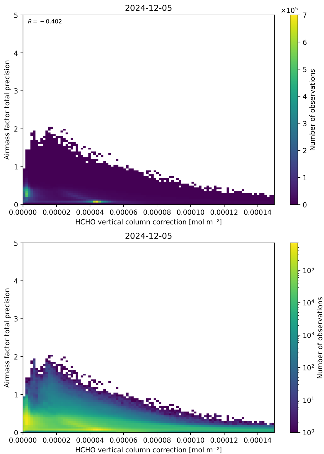
Figure 121: Scatter density plot of “HCHO vertical column correction” against “Airmass factor total precision” for 2024-12-04 to 2024-12-06.
