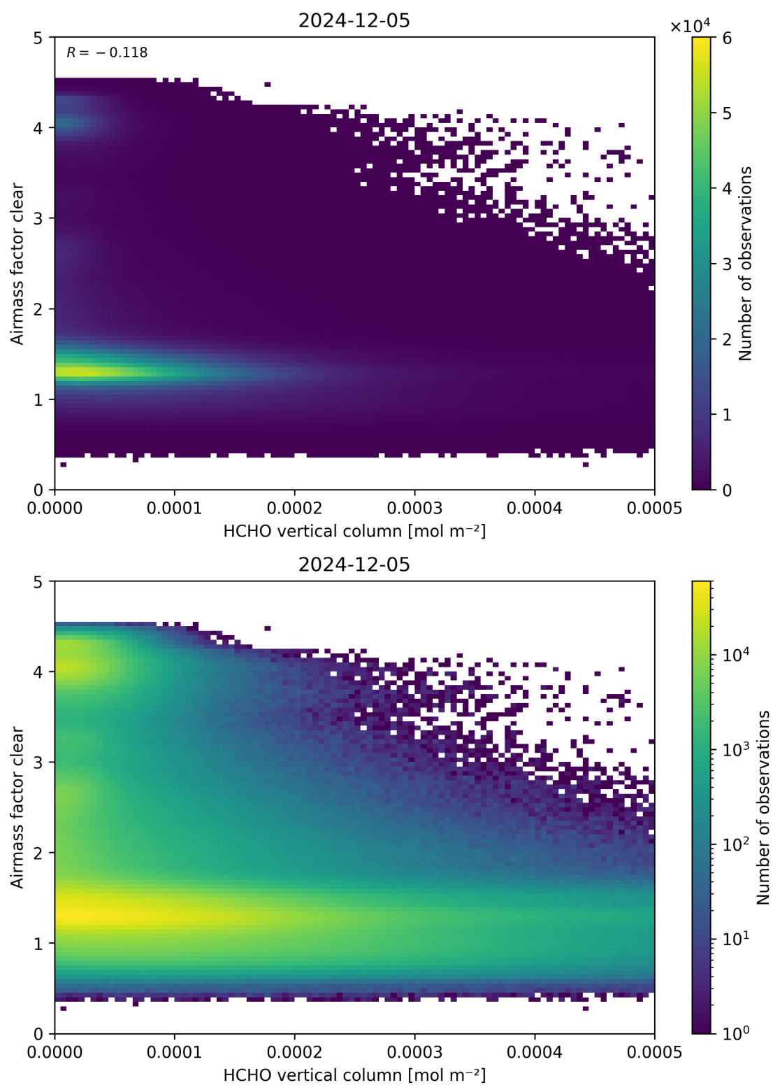
Figure 126: Scatter density plot of “HCHO vertical column” against “Airmass factor clear” for 2024-12-04 to 2024-12-06.
