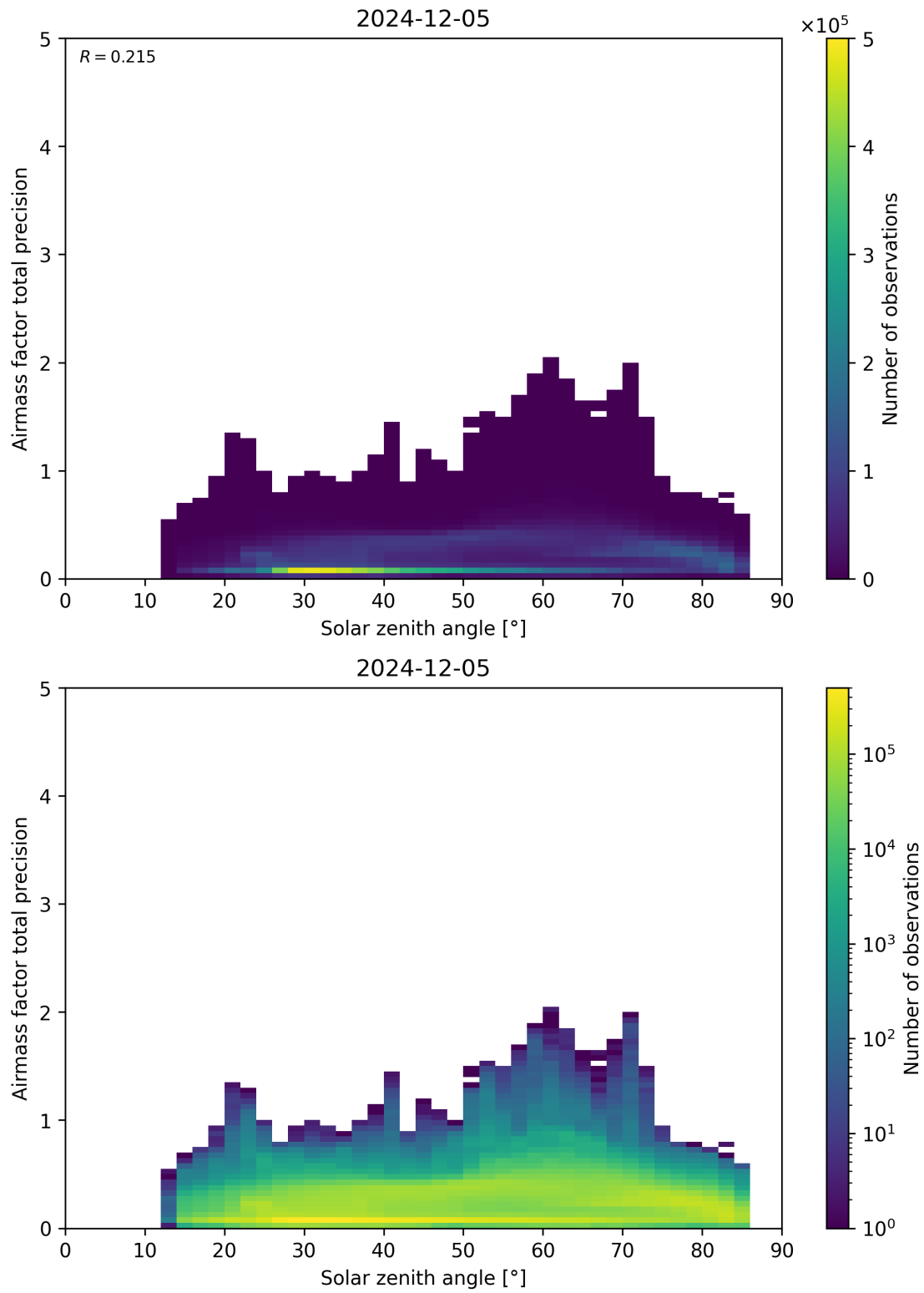
Figure 176: Scatter density plot of “Solar zenith angle” against “Airmass factor total precision” for 2024-12-04 to 2024-12-06.
