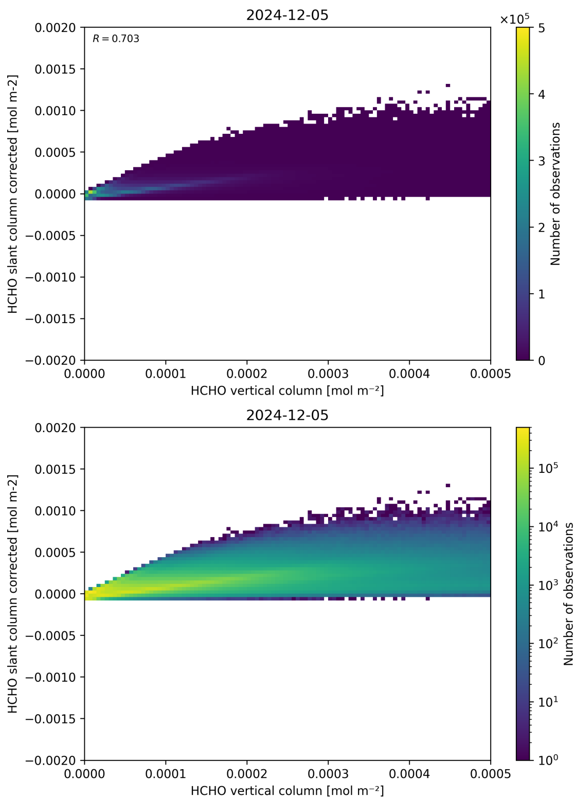
Figure 127: Scatter density plot of “HCHO vertical column” against “HCHO slant column corrected” for 2024-12-04 to 2024-12-06.
