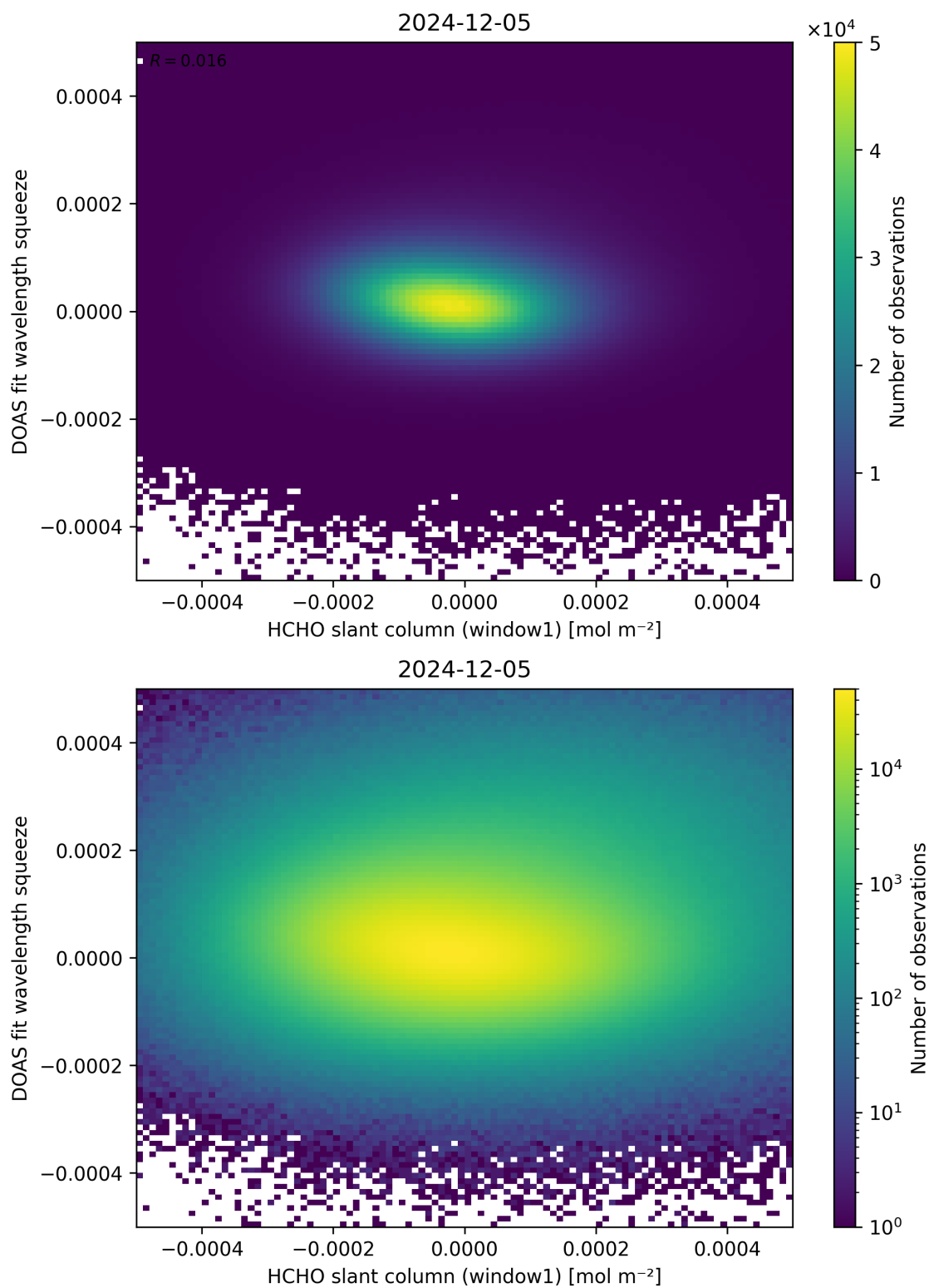
Figure 80: Scatter density plot of “HCHO slant column (window1)” against “DOAS fit wavelength squeeze” for 2024-12-04 to 2024-12-06.
