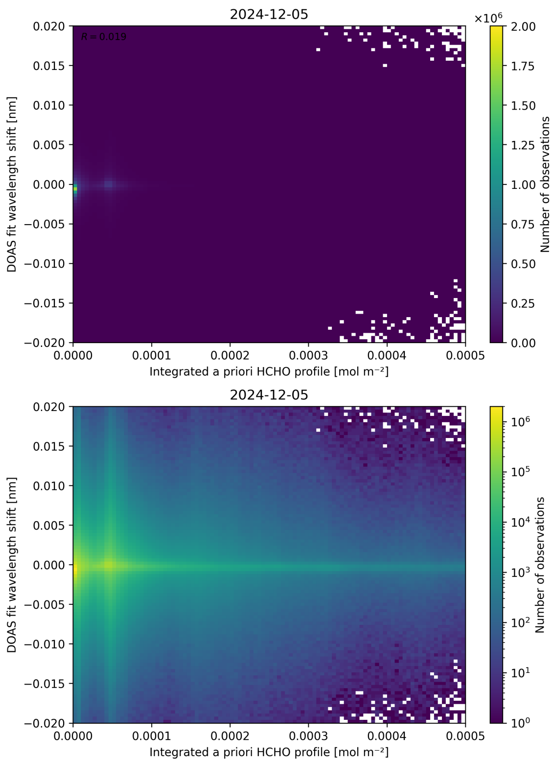
Figure 149: Scatter density plot of “Integrated a priori HCHO profile” against “DOAS fit wavelength shift” for 2024-12-04 to 2024-12-06.
