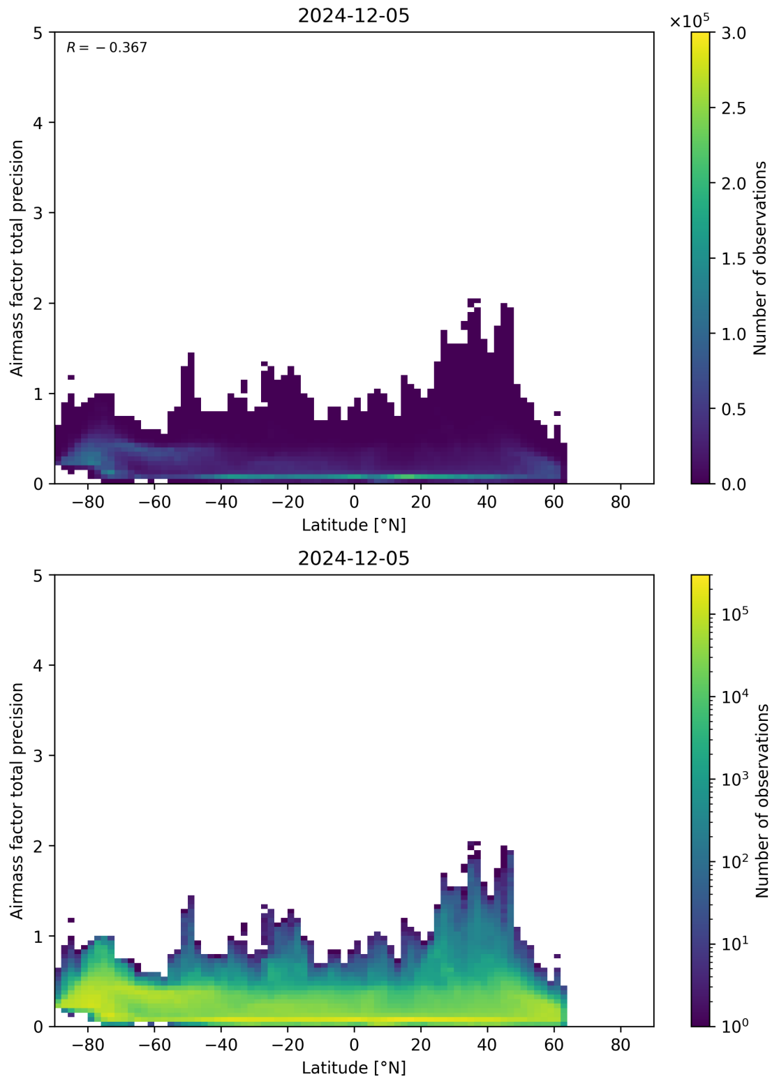
Figure 162: Scatter density plot of “Latitude” against “Airmass factor total precision” for 2024-12-04 to 2024-12-06.
