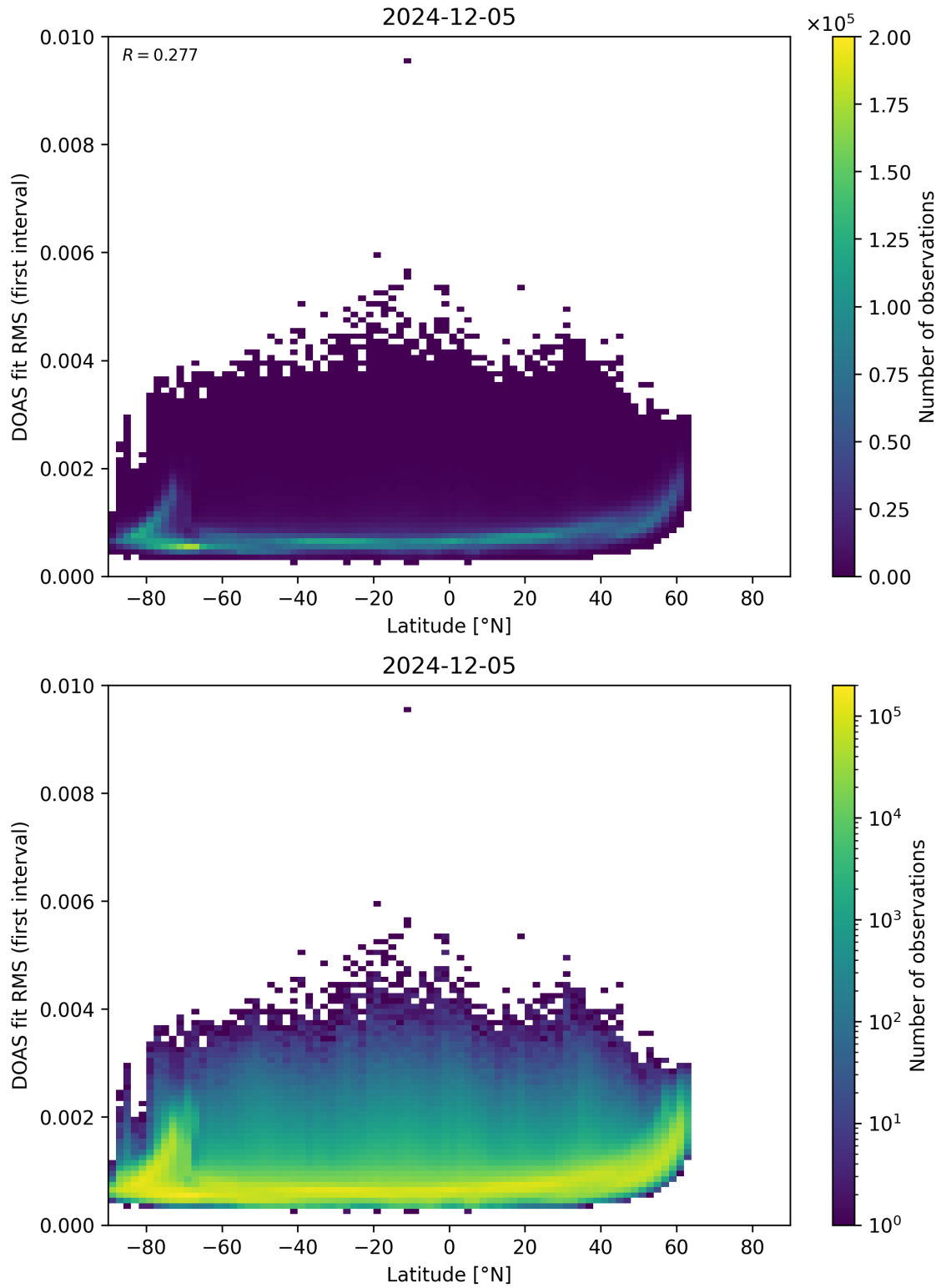
Figure 153: Scatter density plot of “Latitude” against “DOAS fit RMS (first interval)” for 2024-12-04 to 2024-12-06.
