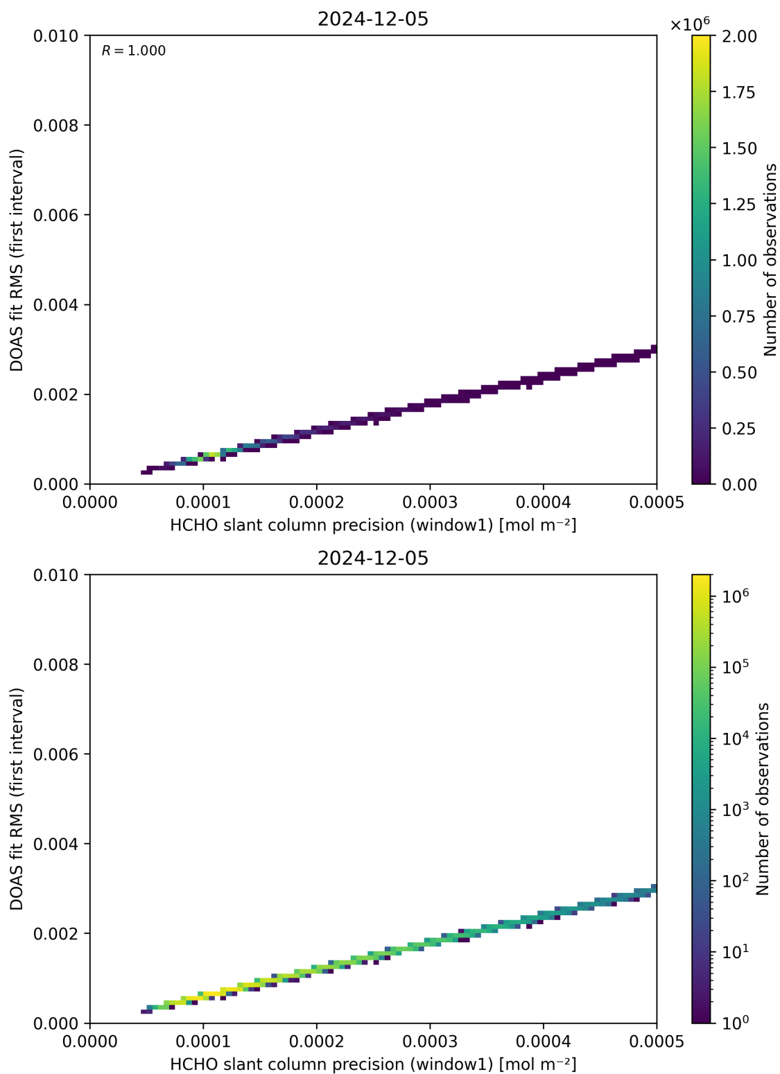
Figure 88: Scatter density plot of “HCHO slant column precision (window1)” against “DOAS fit RMS (first interval)” for 2024-12-04 to 2024-12-06.
