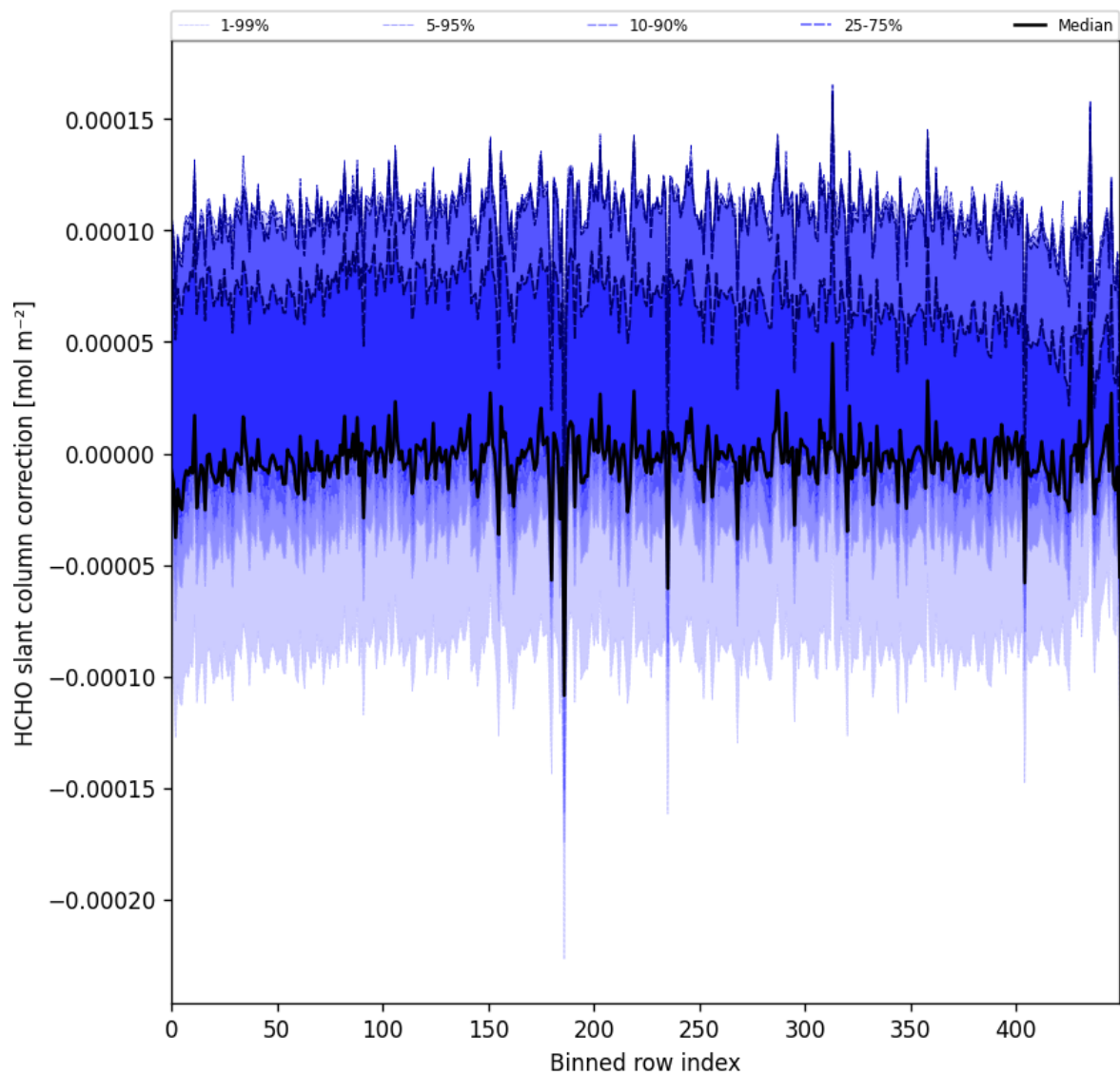
Figure 61: Along track statistics of “HCHO slant column correction” for 2024-12-04 to 2024-12-06
