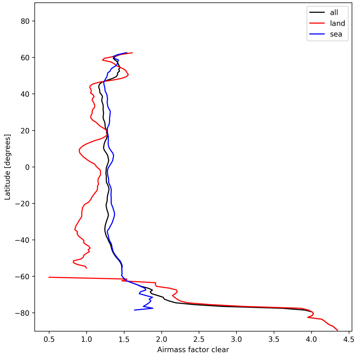
Figure 28: Zonal average of “Airmass factor clear” for 2024-12-04 to 2024-12-06.
