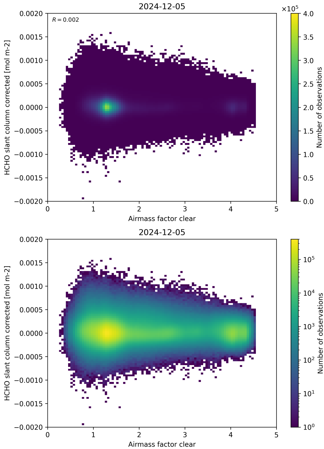
Figure 74: Scatter density plot of “Airmass factor clear” against “HCHO slant column corrected” for 2024-12-04 to 2024-12-06.
