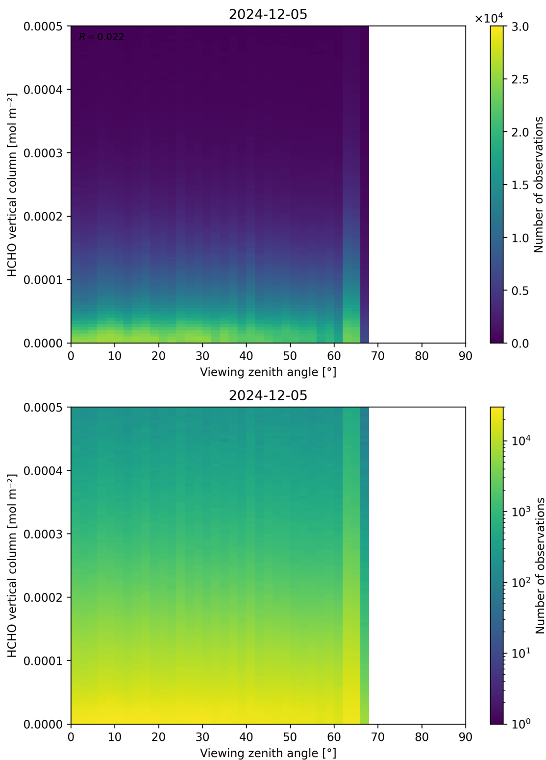
Figure 192: Scatter density plot of “Viewing zenith angle” against “HCHO vertical column” for 2024-12-04 to 2024-12-06.
