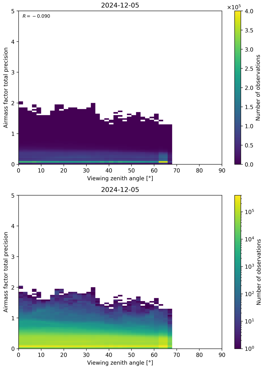
Figure 191: Scatter density plot of “Viewing zenith angle” against “Airmass factor total precision” for 2024-12-04 to 2024-12-06.
