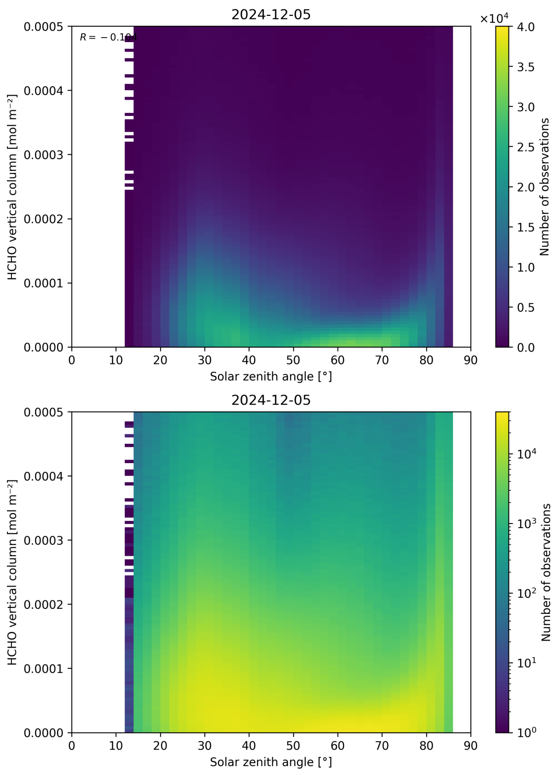
Figure 177: Scatter density plot of “Solar zenith angle” against “HCHO vertical column” for 2024-12-04 to 2024-12-06.
