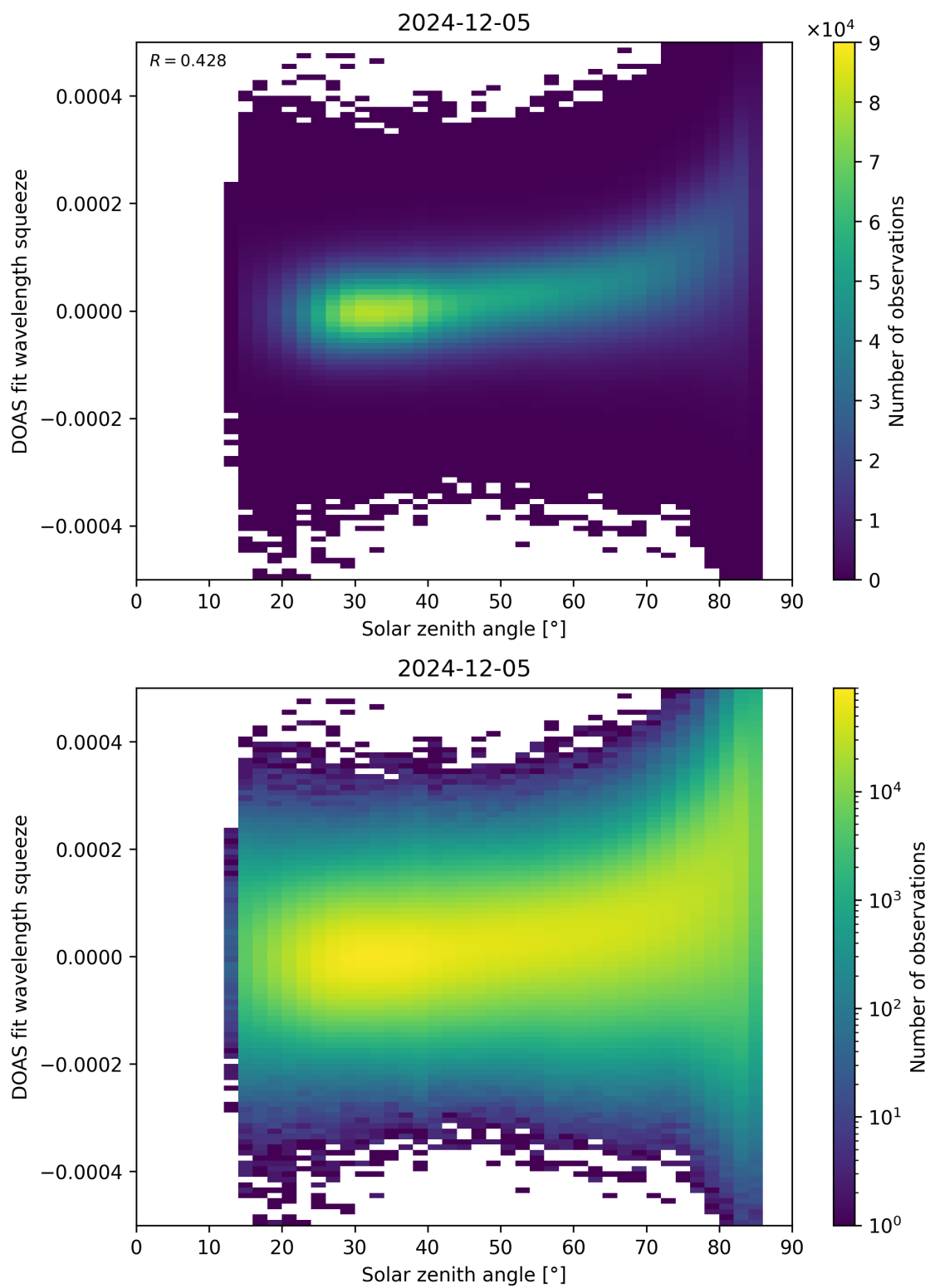
Figure 169: Scatter density plot of “Solar zenith angle” against “DOAS fit wavelength squeeze” for 2024-12-04 to 2024-12-06.
