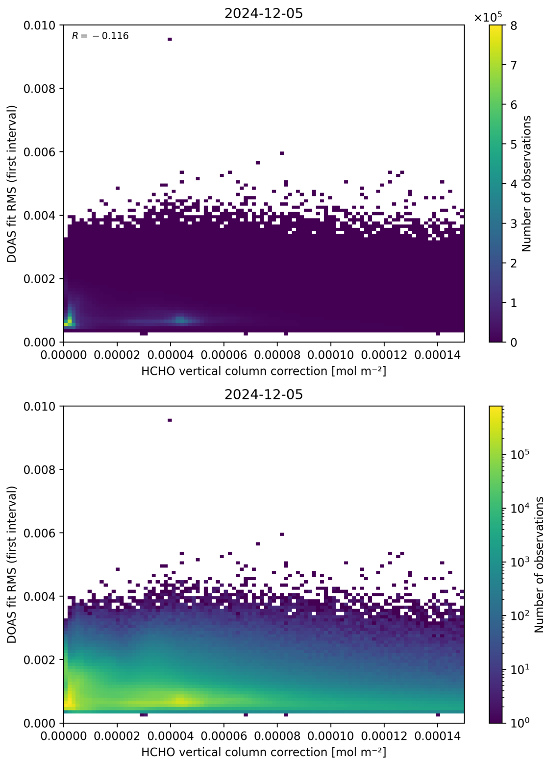
Figure 112: Scatter density plot of “HCHO vertical column correction” against “DOAS fit RMS (first interval)” for 2024-12-04 to 2024-12-06.
