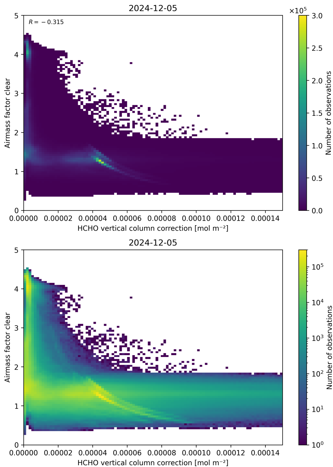
Figure 115: Scatter density plot of “HCHO vertical column correction” against “Airmass factor clear” for 2024-12-04 to 2024-12-06.
