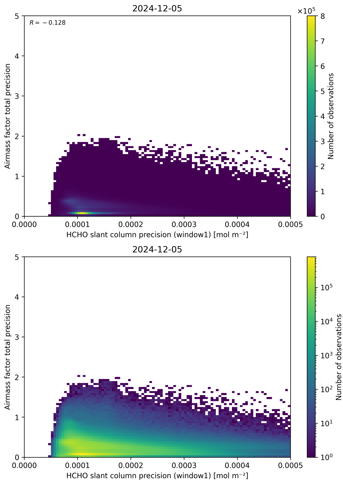
Figure 95: Scatter density plot of “HCHO slant column precision (window1)” against “Airmass factor total precision” for 2024-12-04 to 2024-12-06.
