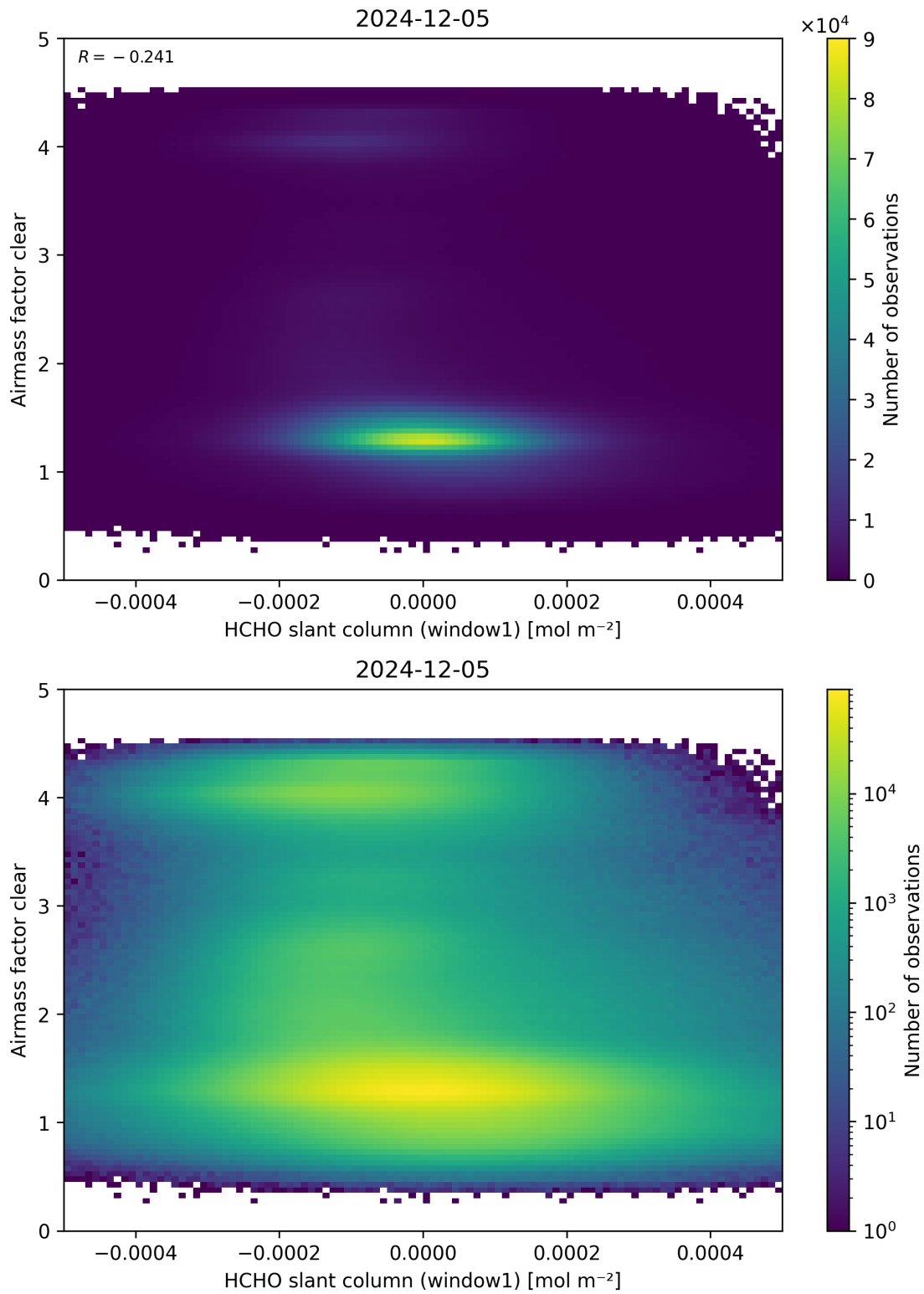
Figure 81: Scatter density plot of “HCHO slant column (window1)” against “Airmass factor clear” for 2024-12-04 to 2024-12-06.
