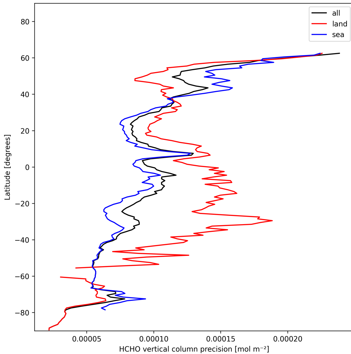
Figure 22: Zonal average of “HCHO vertical column precision” for 2024-12-04 to 2024-12-06.
