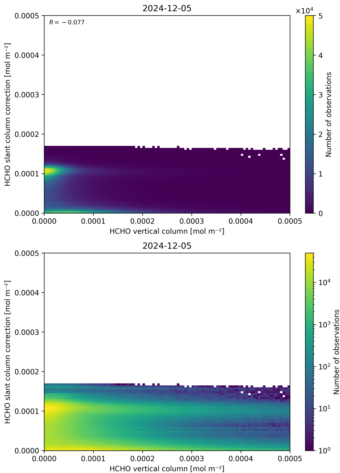
Figure 128: Scatter density plot of “HCHO vertical column” against “HCHO slant column correction” for 2024-12-04 to 2024-12-06.
