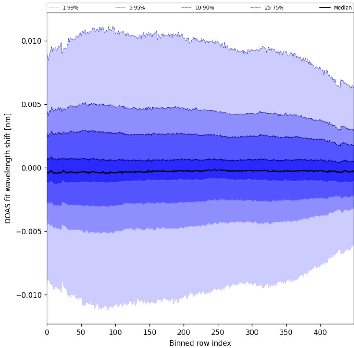
Figure 58: Along track statistics of “DOAS fit wavelength shift” for 2024-12-04 to 2024-12-06
