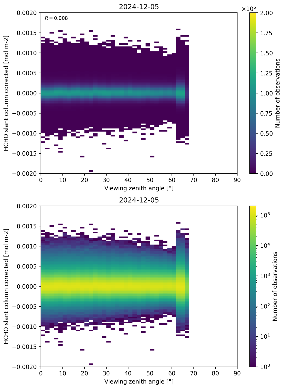
Figure 186: Scatter density plot of “Viewing zenith angle” against “HCHO slant column corrected” for 2024-12-04 to 2024-12-06.
