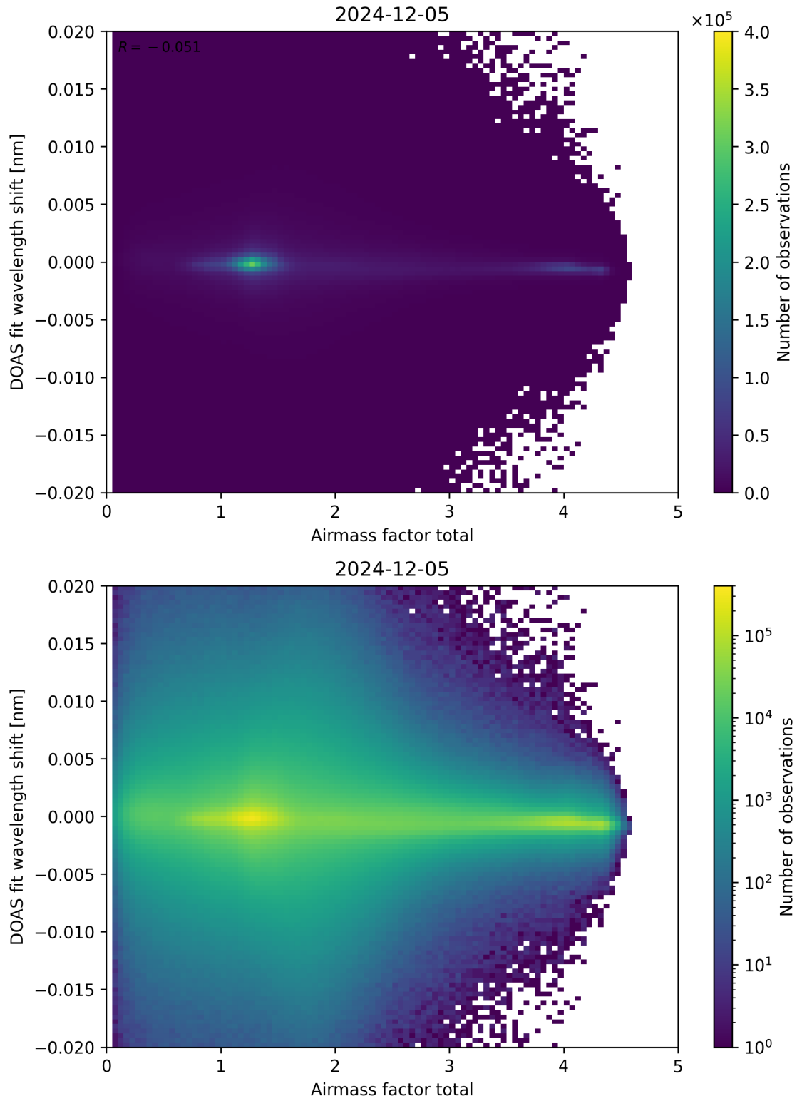
Figure 98: Scatter density plot of “Airmass factor total” against “DOAS fit wavelength shift” for 2024-12-04 to 2024-12-06.
