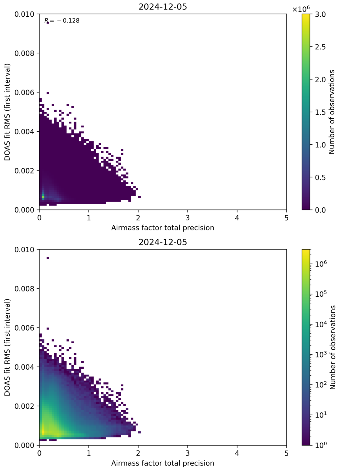
Figure 105: Scatter density plot of “Airmass factor total precision” against “DOAS fit RMS (first interval)” for 2024-12-04 to 2024-12-06.
