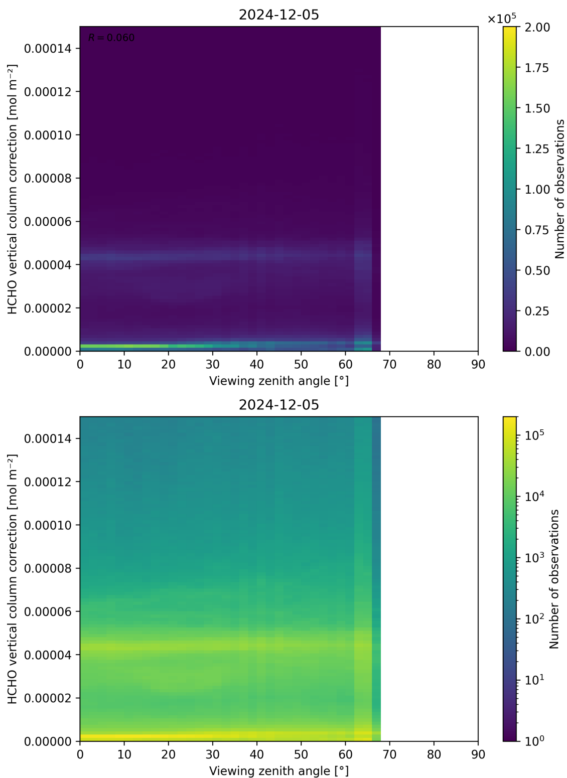
Figure 193: Scatter density plot of “Viewing zenith angle” against “HCHO vertical column correction” for 2024-12-04 to 2024-12-06.
