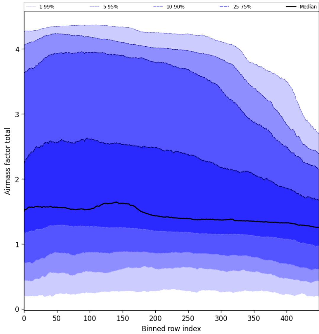
Figure 54: Along track statistics of “Airmass factor total” for 2024-12-04 to 2024-12-06
