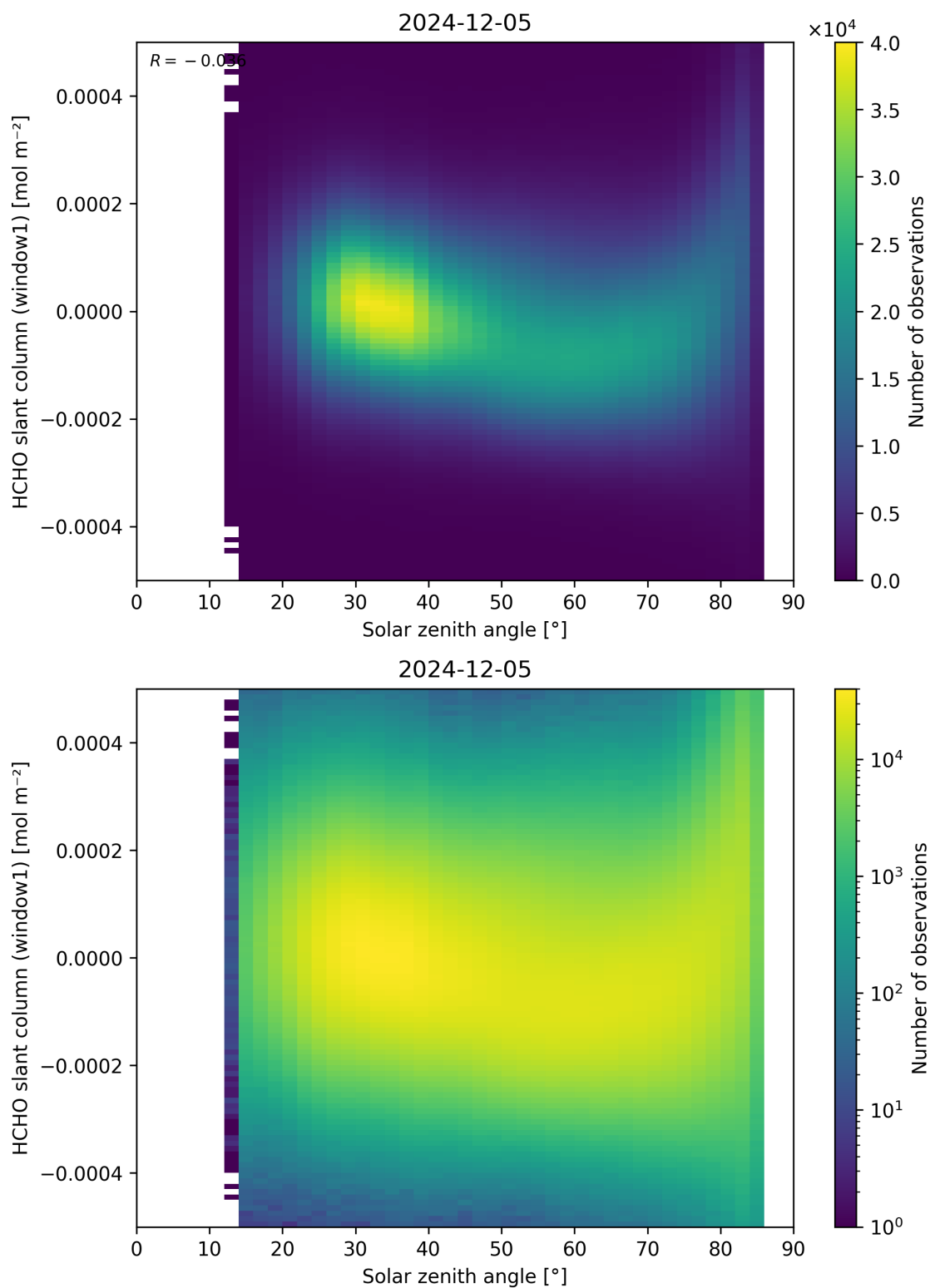
Figure 173: Scatter density plot of “Solar zenith angle” against “HCHO slant column (window1)” for 2024-12-04 to 2024-12-06.
