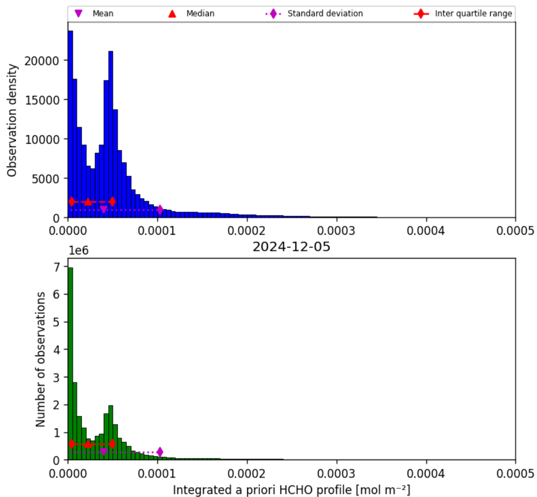
Figure 43: Histogram of “Integrated a priori HCHO profile” for 2024-12-04 to 2024-12-06
