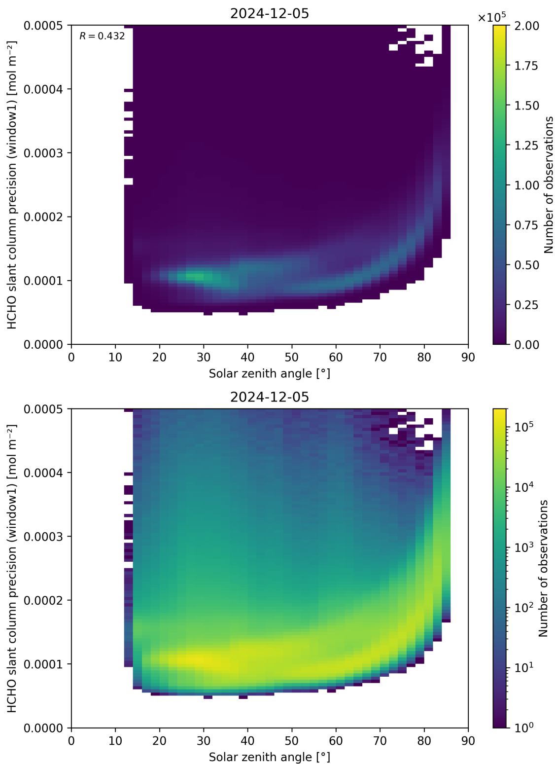
Figure 174: Scatter density plot of “Solar zenith angle” against “HCHO slant column precision (window1)” for 2024-12-04 to 2024-12-06.
