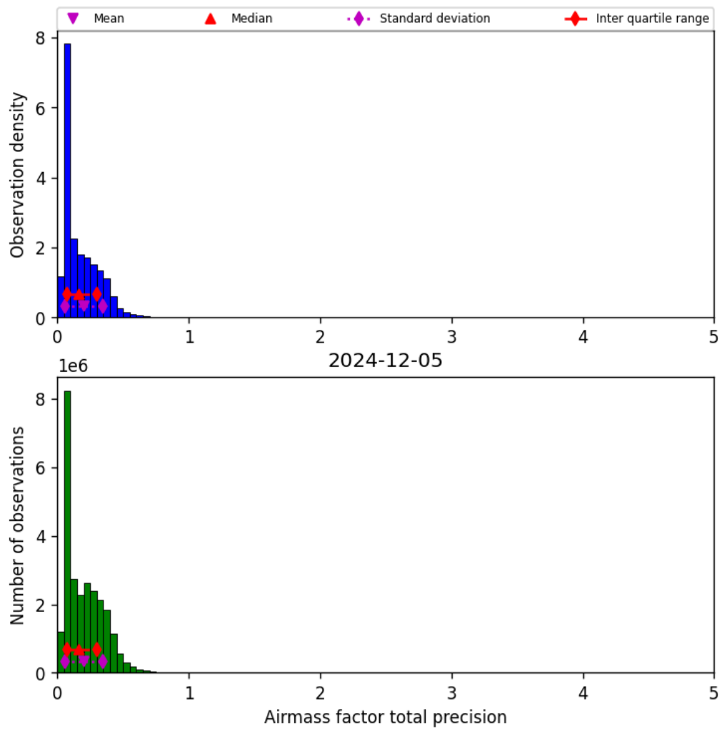
Figure 41: Histogram of “Airmass factor total precision” for 2024-12-04 to 2024-12-06
