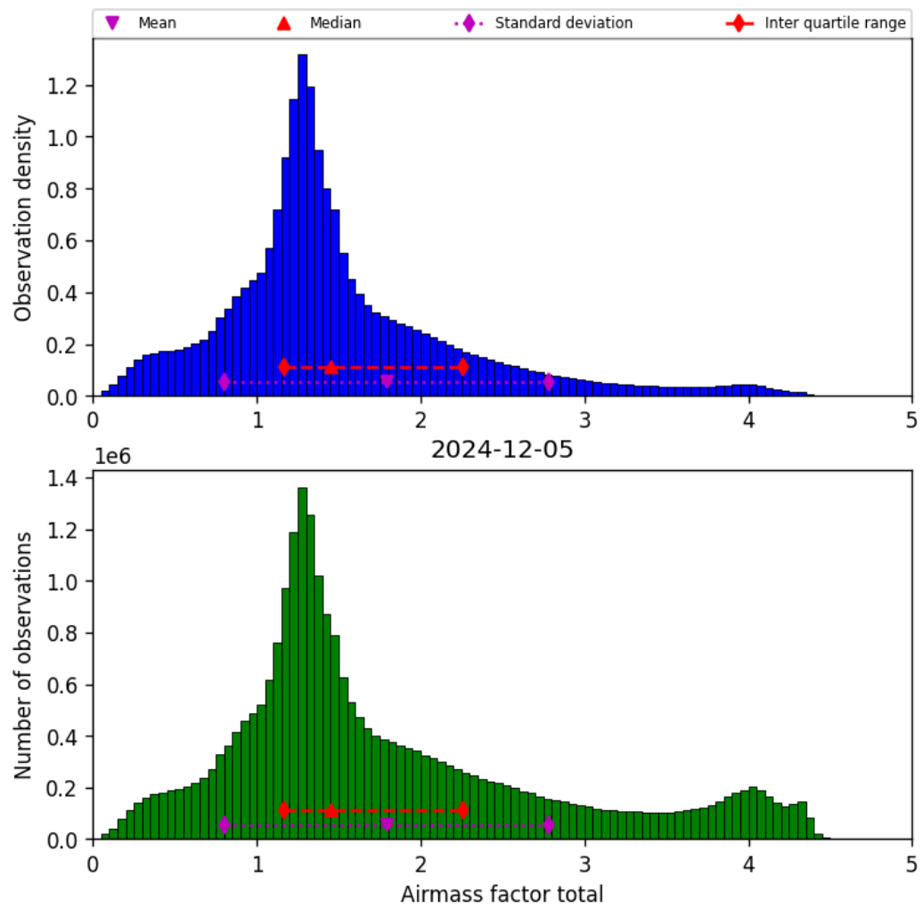
Figure 40: Histogram of “Airmass factor total” for 2024-12-04 to 2024-12-06
