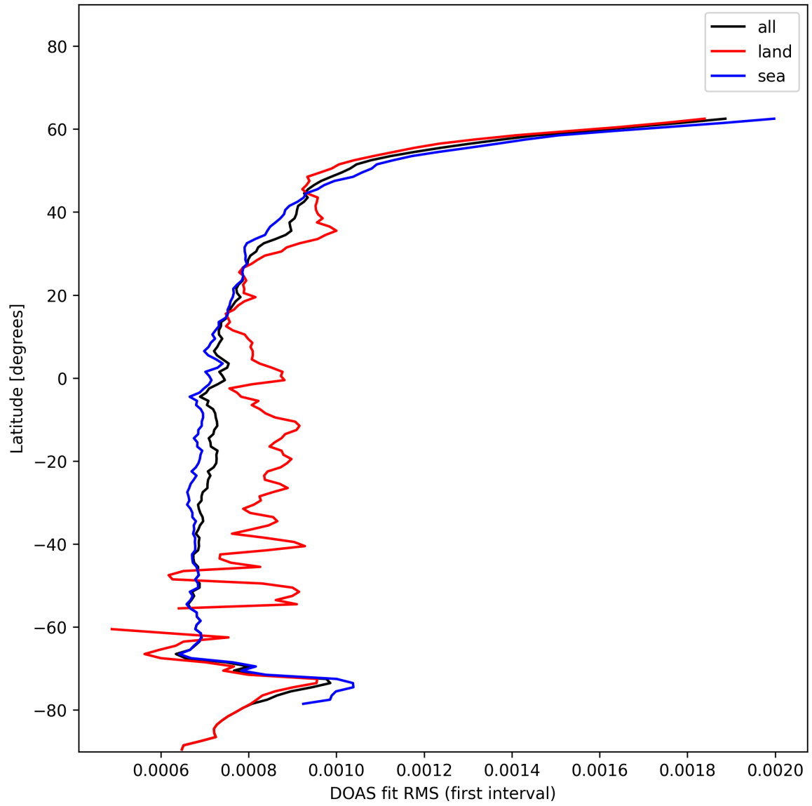
Figure 32: Zonal average of “DOAS fit RMS (first interval)” for 2024-12-04 to 2024-12-06.
