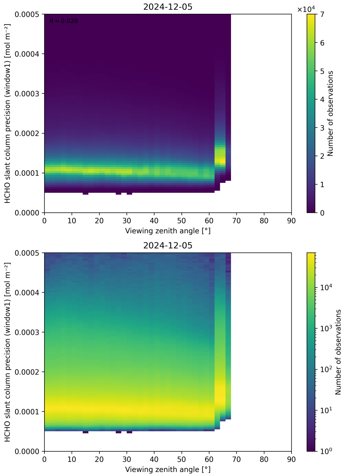
Figure 189: Scatter density plot of “Viewing zenith angle” against “HCHO slant column precision (window1)” for 2024-12-04 to 2024-12-06.
