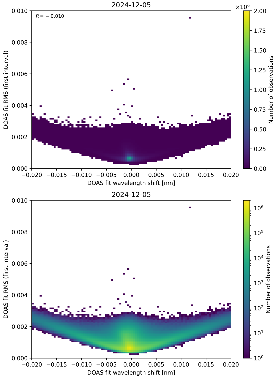
Figure 64: Scatter density plot of “DOAS fit wavelength shift” against “DOAS fit RMS (first interval)” for 2024-12-04 to 2024-12-06.
