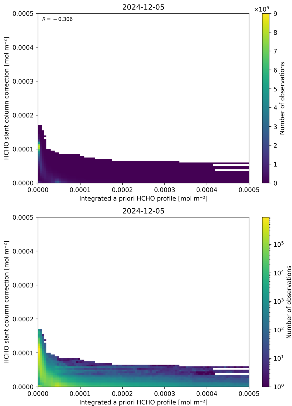
Figure 152: Scatter density plot of “Integrated a priori HCHO profile” against “HCHO slant column correction” for 2024-12-04 to 2024-12-06.
