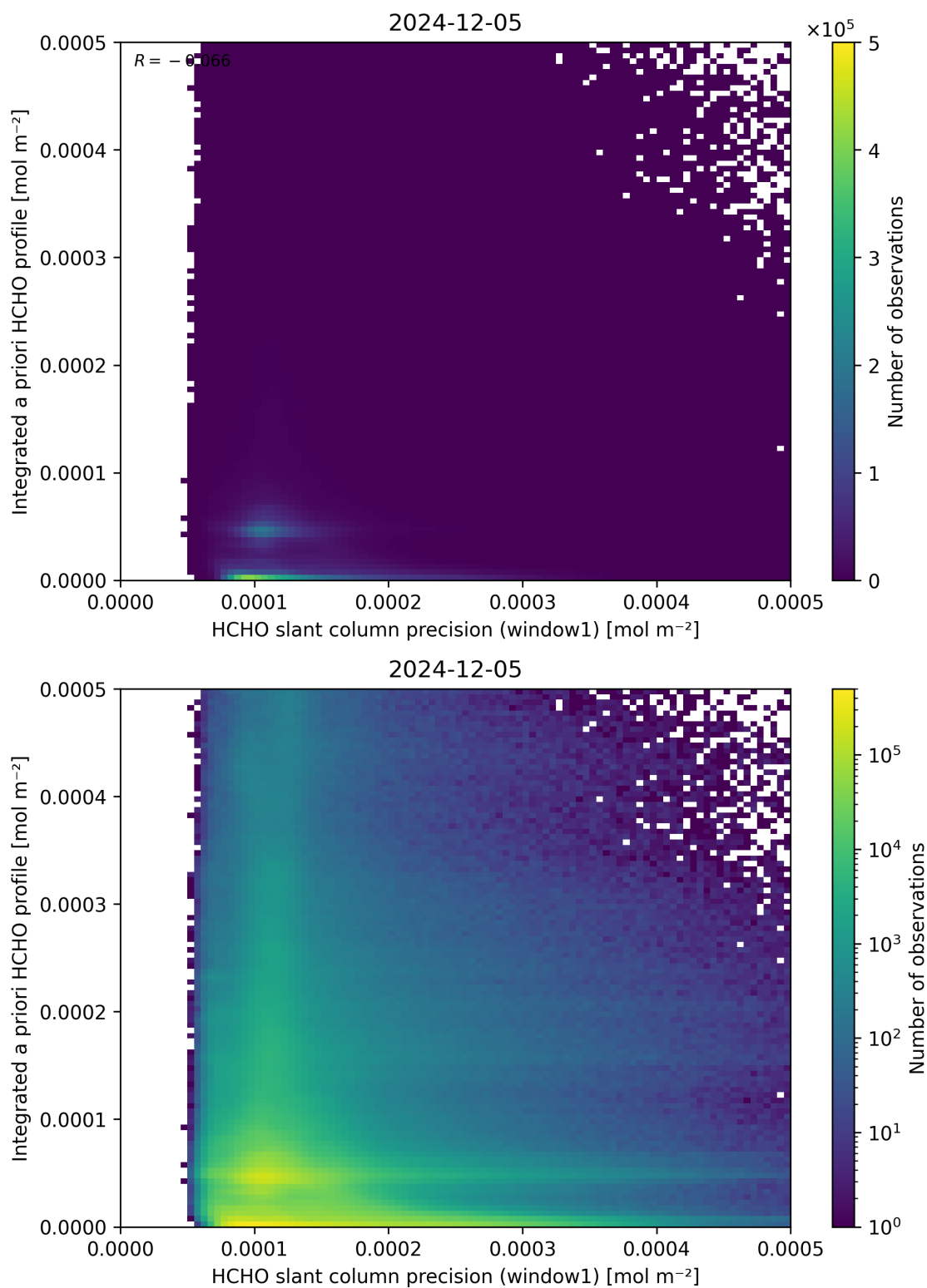
Figure 96: Scatter density plot of “HCHO slant column precision (window1)” against “Integrated a priori HCHO profile” for 2024-12-04 to 2024-12-06.
