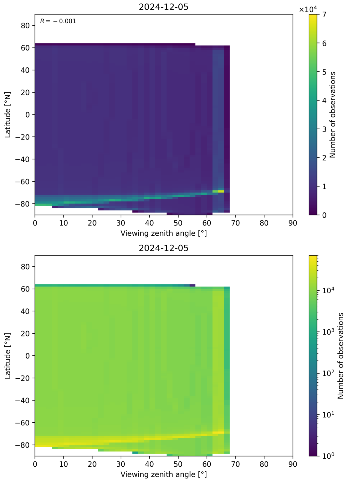
Figure 196: Scatter density plot of “Viewing zenith angle” against “Latitude” for 2024-12-04 to 2024-12-06.
