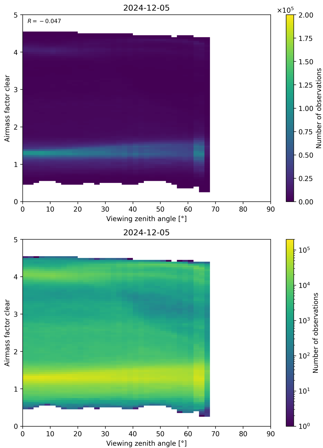
Figure 185: Scatter density plot of “Viewing zenith angle” against “Airmass factor clear” for 2024-12-04 to 2024-12-06.
