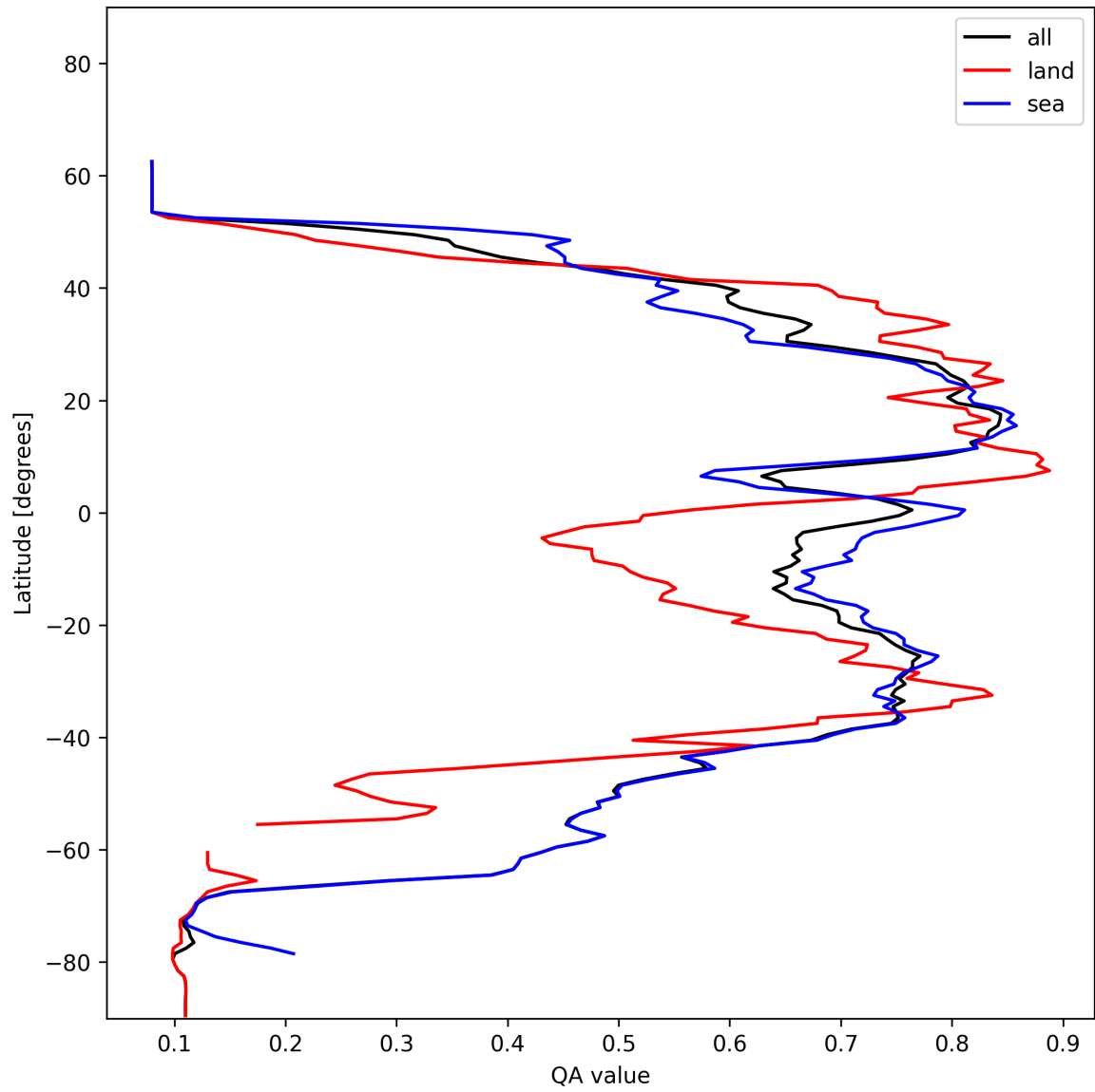
Figure 20: Zonal average of “QA value” for 2024-12-04 to 2024-12-06.
