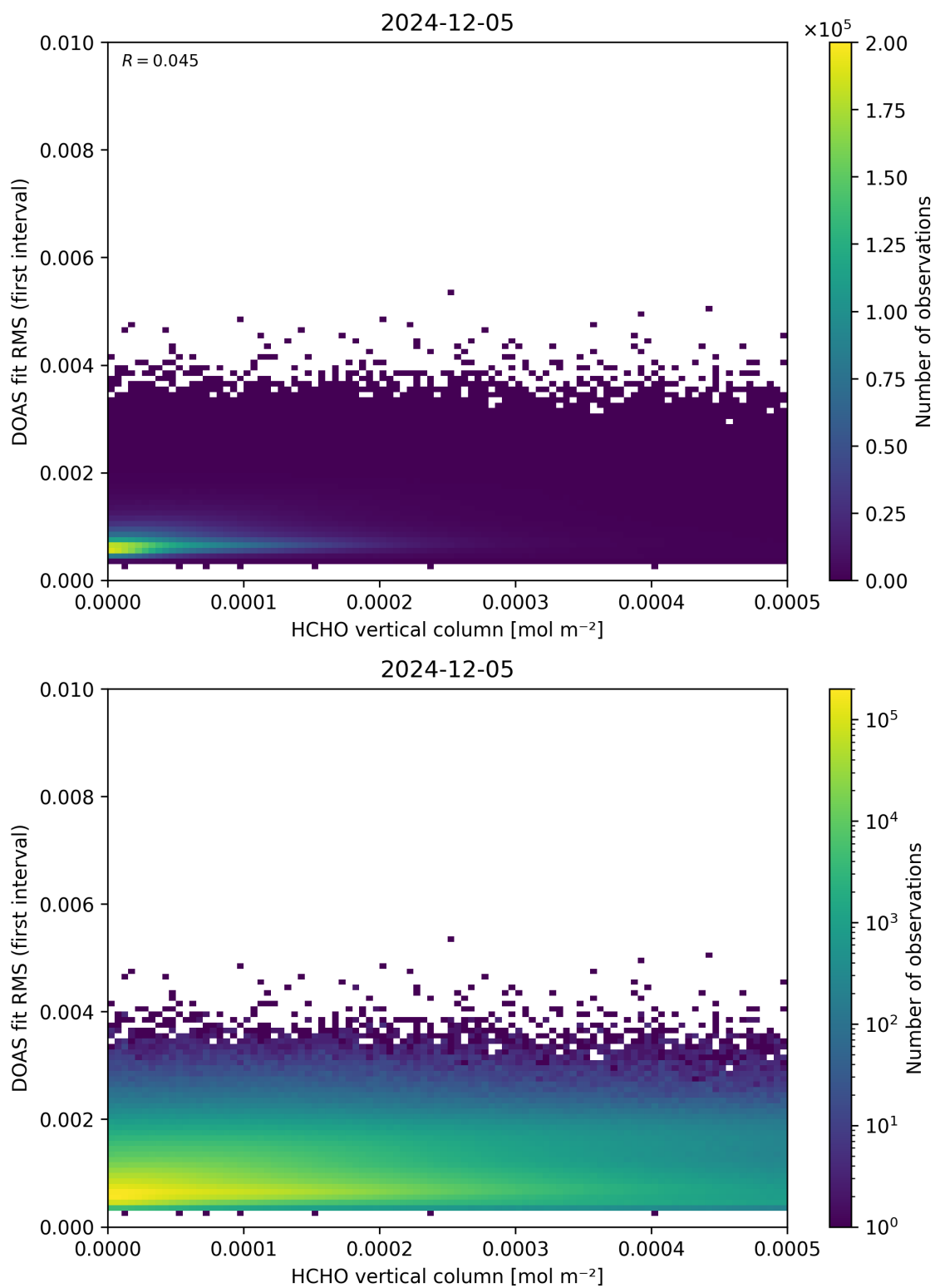
Figure 123: Scatter density plot of “HCHO vertical column” against “DOAS fit RMS (first interval)” for 2024-12-04 to 2024-12-06.
