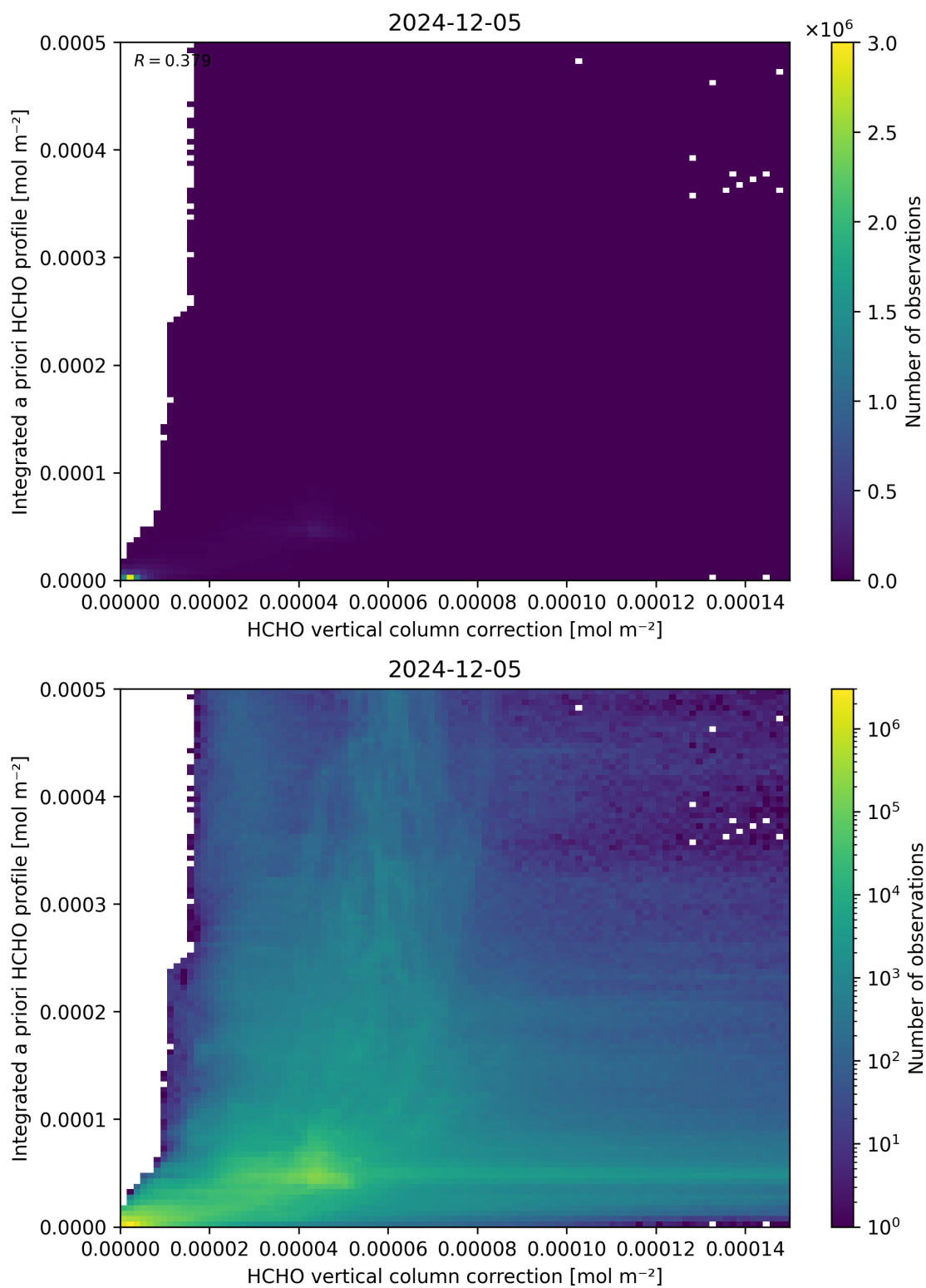
Figure 122: Scatter density plot of “HCHO vertical column correction” against “Integrated a priori HCHO profile” for 2024-12-04 to 2024-12-06.
