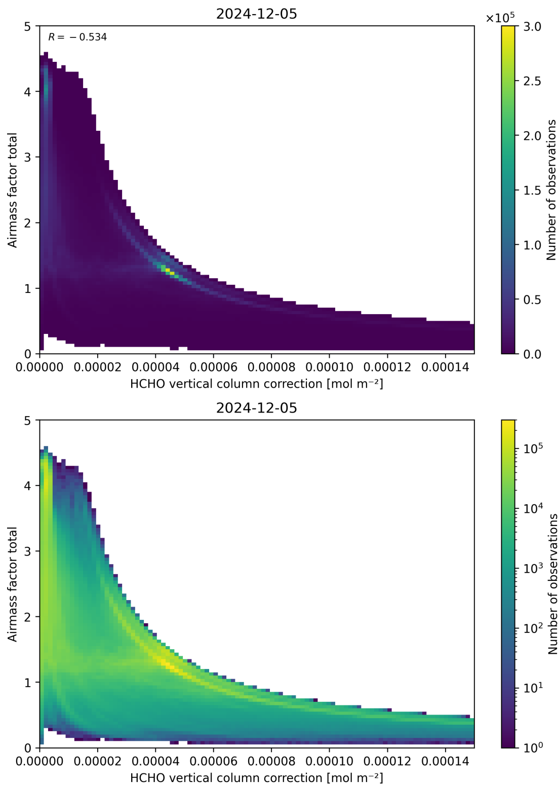
Figure 120: Scatter density plot of “HCHO vertical column correction” against “Airmass factor total” for 2024-12-04 to 2024-12-06.
