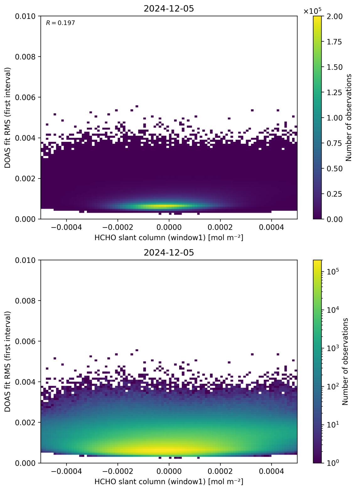
Figure 78: Scatter density plot of “HCHO slant column (window1)” against “DOAS fit RMS (first interval)” for 2024-12-04 to 2024-12-06.
