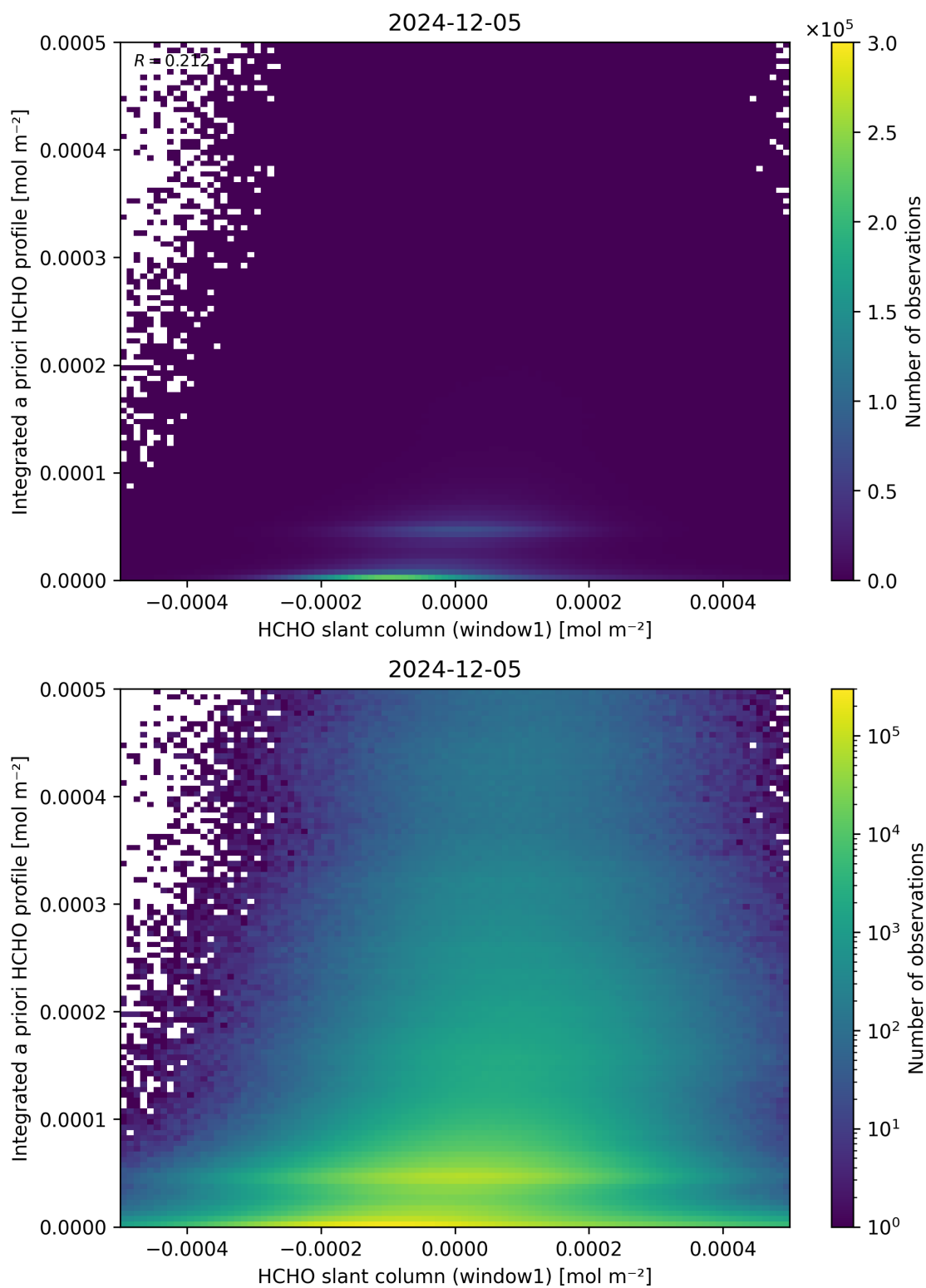
Figure 87: Scatter density plot of “HCHO slant column (window1)” against “Integrated a priori HCHO profile” for 2024-12-04 to 2024-12-06.
