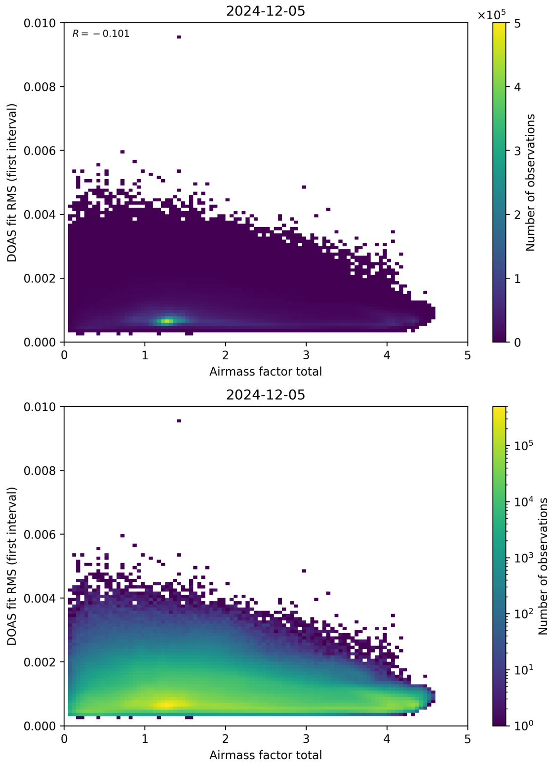
Figure 97: Scatter density plot of “Airmass factor total” against “DOAS fit RMS (first interval)” for 2024-12-04 to 2024-12-06.
