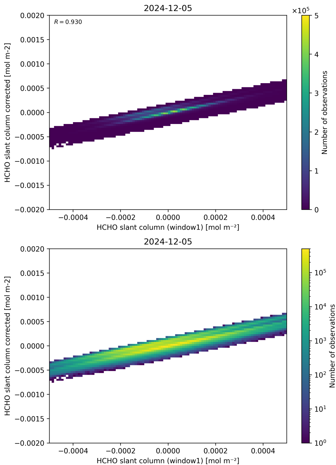
Figure 82: Scatter density plot of “HCHO slant column (window1)” against “HCHO slant column corrected” for 2024-12-04 to 2024-12-06.
