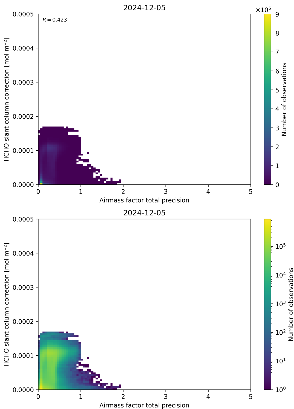
Figure 110: Scatter density plot of “Airmass factor total precision” against “HCHO slant column correction” for 2024-12-04 to 2024-12-06.
