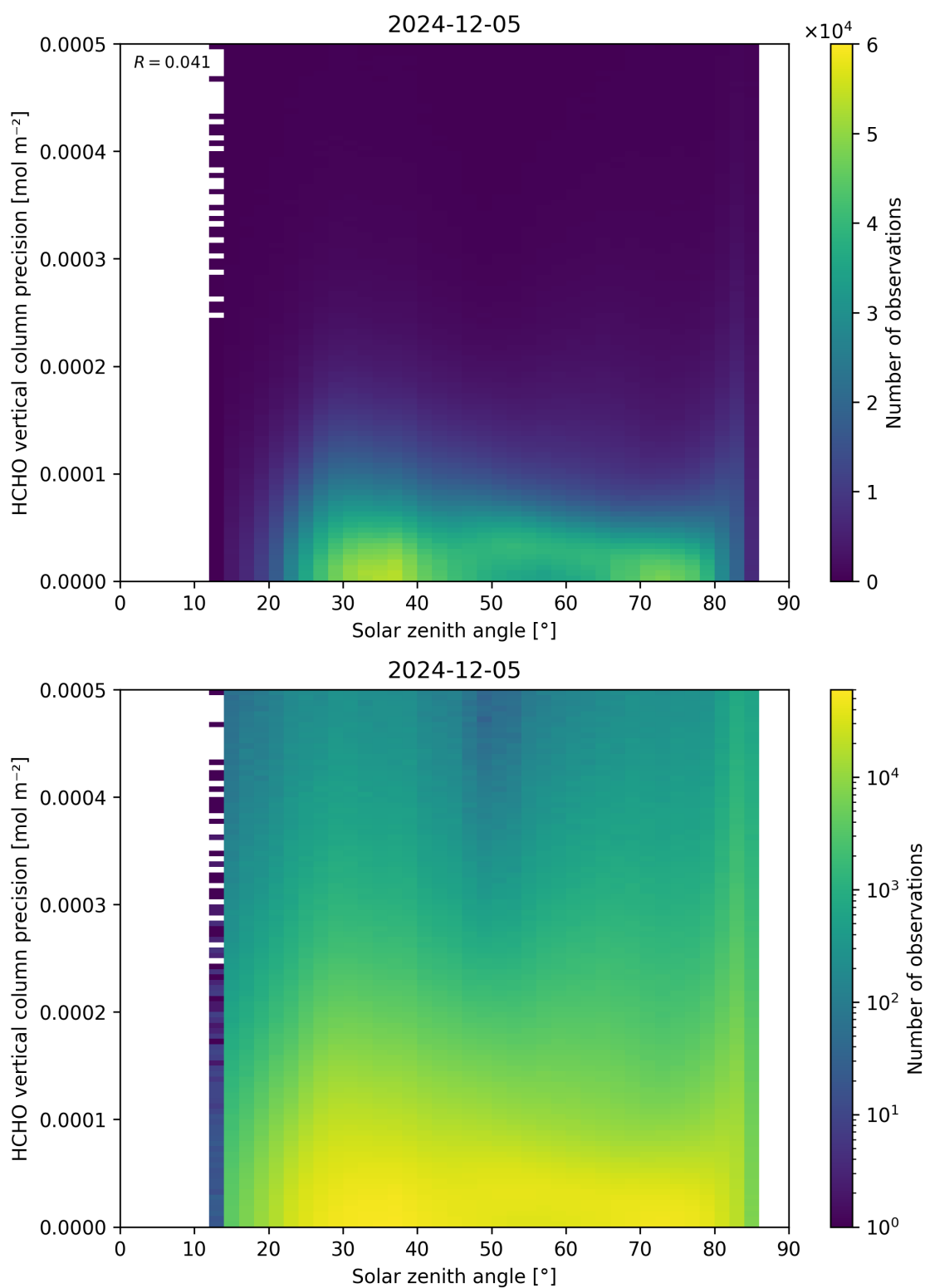
Figure 179: Scatter density plot of “Solar zenith angle” against “HCHO vertical column precision” for 2024-12-04 to 2024-12-06.
