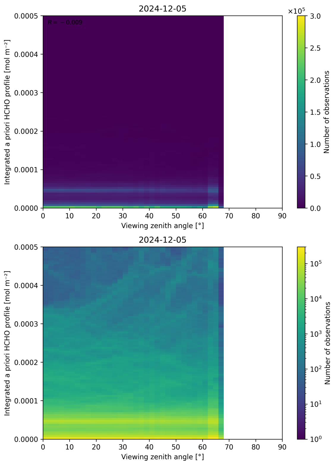
Figure 195: Scatter density plot of “Viewing zenith angle” against “Integrated a priori HCHO profile” for 2024-12-04 to 2024-12-06.
