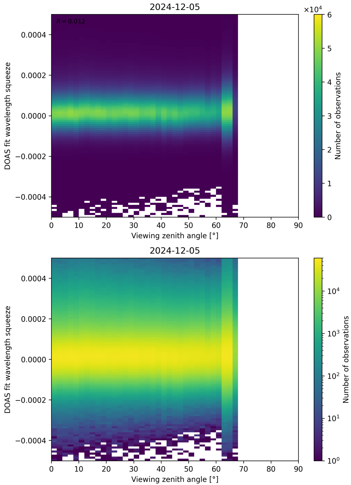
Figure 184: Scatter density plot of “Viewing zenith angle” against “DOAS fit wavelength squeeze” for 2024-12-04 to 2024-12-06.
