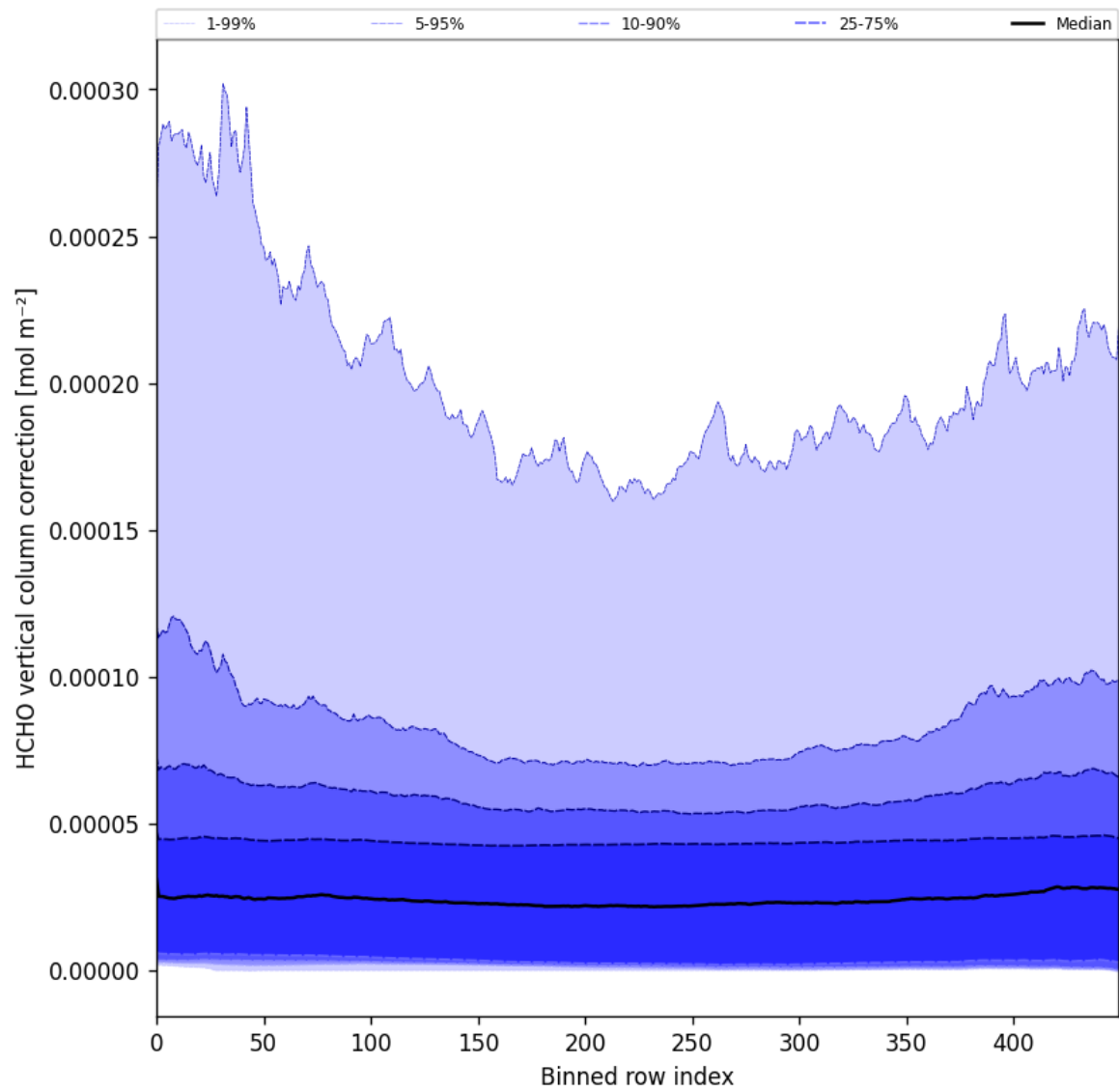
Figure 51: Along track statistics of “HCHO vertical column correction” for 2024-12-04 to 2024-12-06
