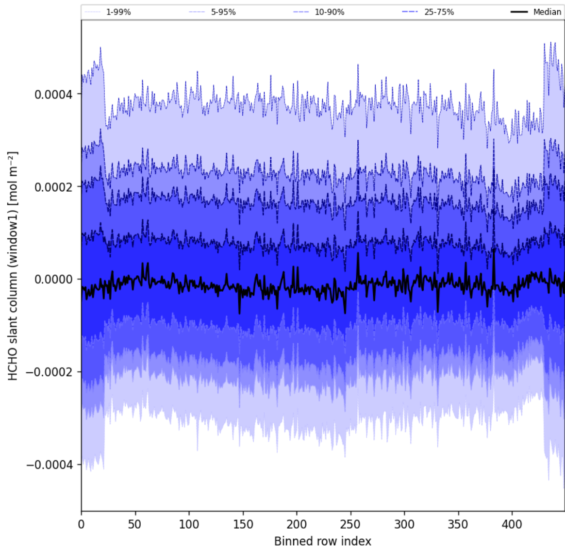
Figure 52: Along track statistics of “HCHO slant column (window1)” for 2024-12-04 to 2024-12-06
