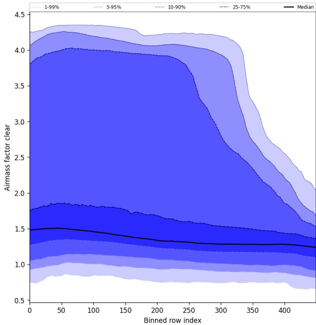
Figure 56: Along track statistics of “Airmass factor clear” for 2024-12-04 to 2024-12-06
