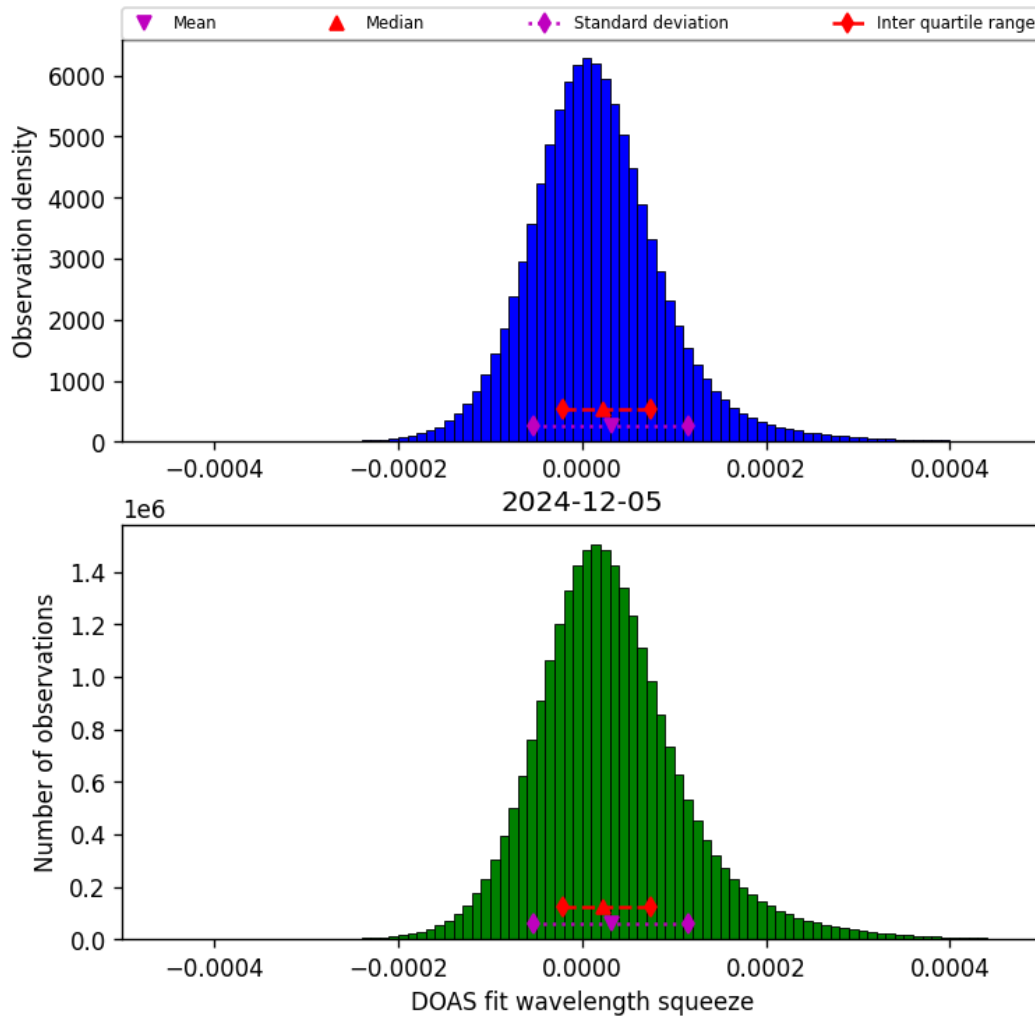
Figure 45: Histogram of “DOAS fit wavelength squeeze” for 2024-12-04 to 2024-12-06
