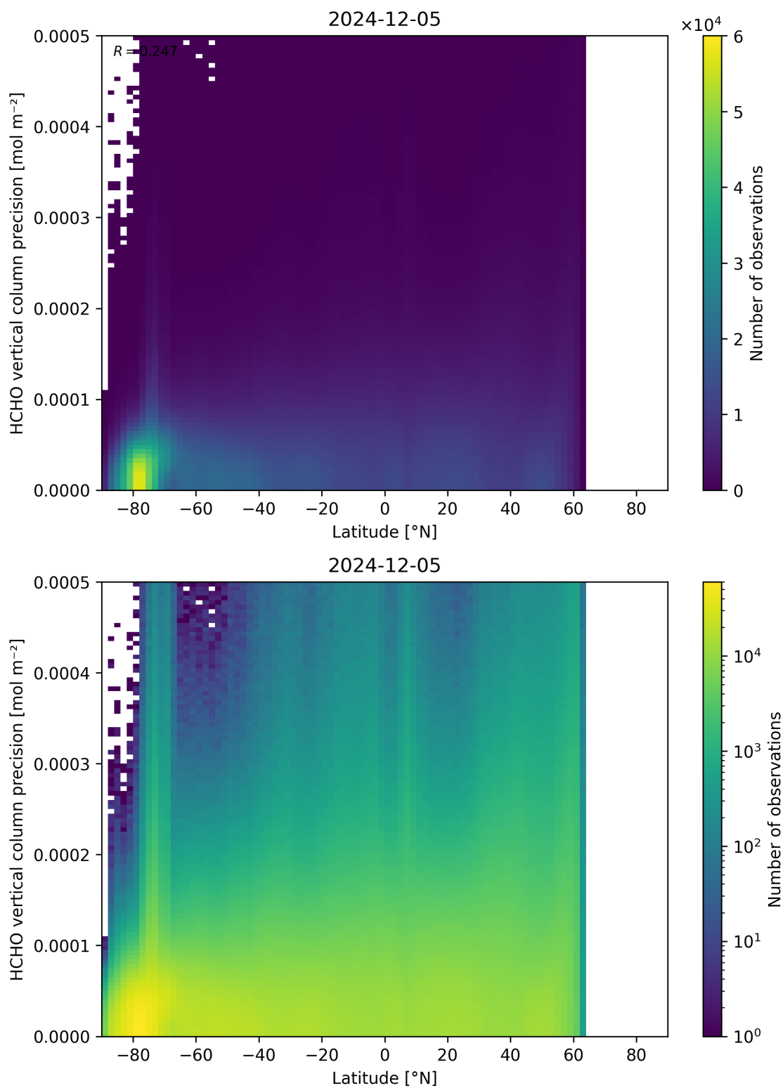
Figure 165: Scatter density plot of “Latitude” against “HCHO vertical column precision” for 2024-12-04 to 2024-12-06.
