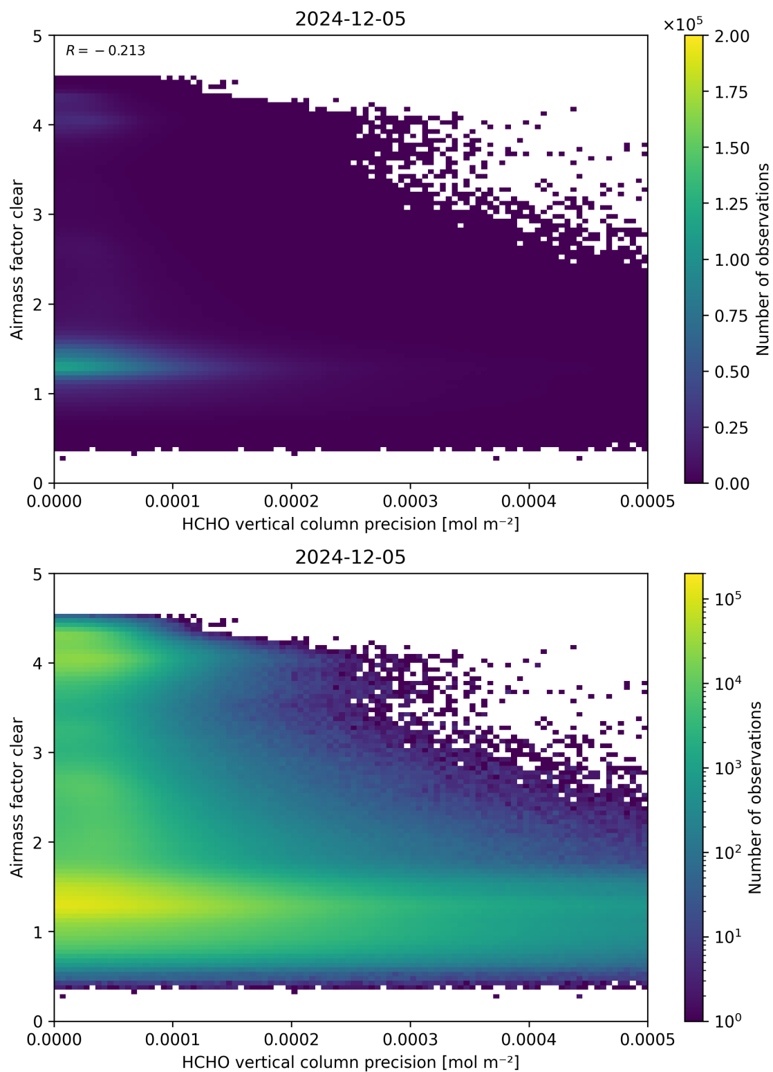
Figure 139: Scatter density plot of “HCHO vertical column precision” against “Airmass factor clear” for 2024-12-04 to 2024-12-06.
