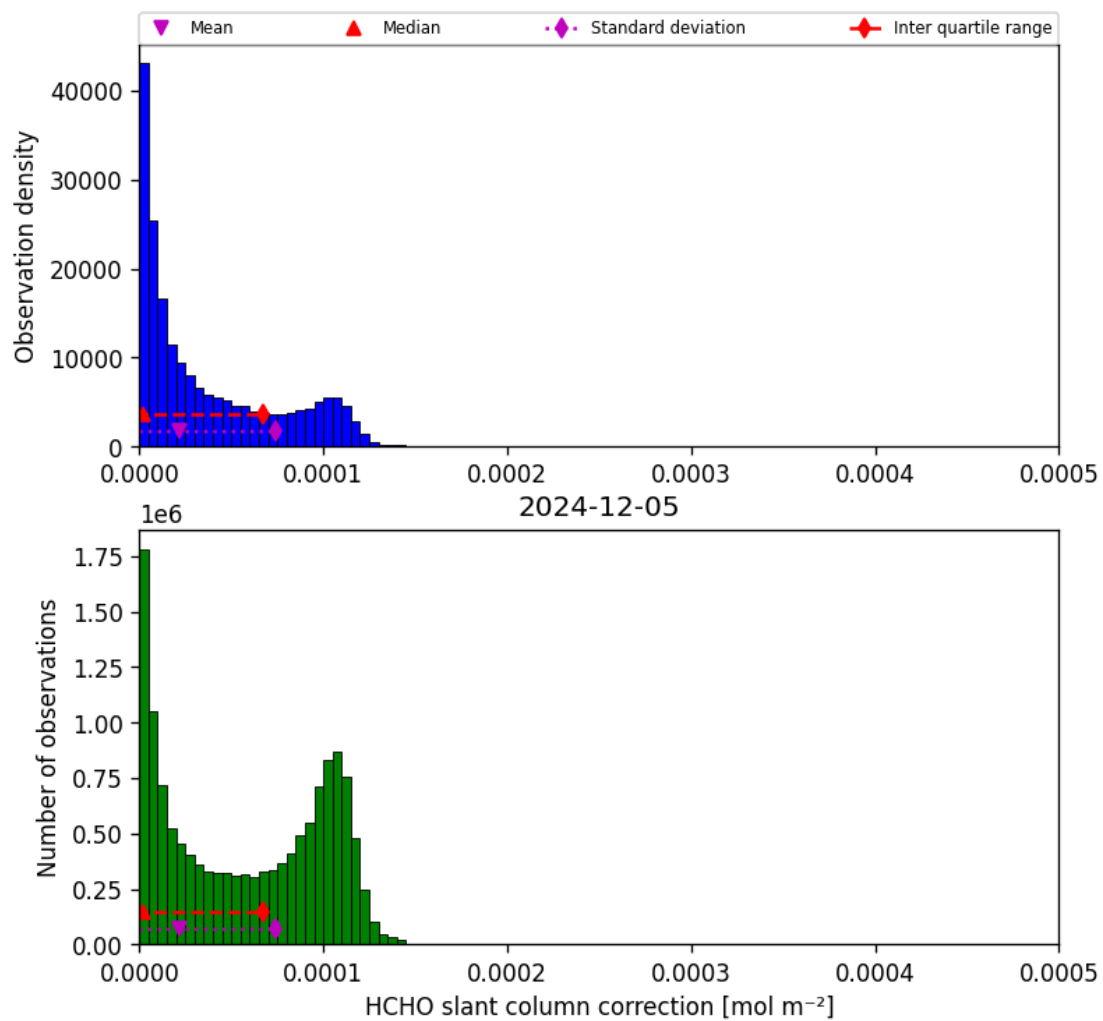
Figure 47: Histogram of “HCHO slant column correction” for 2024-12-04 to 2024-12-06
