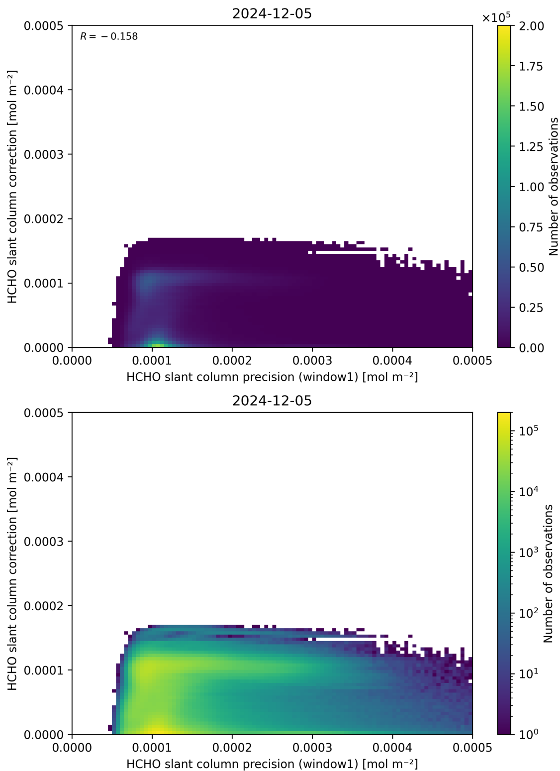
Figure 93: Scatter density plot of “HCHO slant column precision (window1)” against “HCHO slant column correction” for 2024-12-04 to 2024-12-06.
