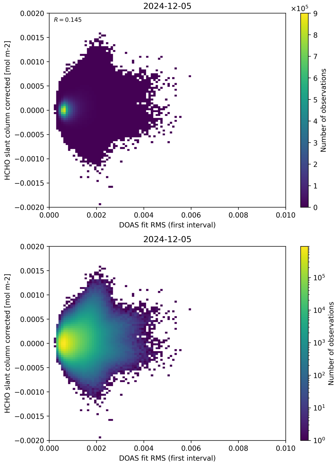
Figure 62: Scatter density plot of “DOAS fit RMS (first interval)” against “HCHO slant column corrected” for 2024-12-04 to 2024-12-06.
