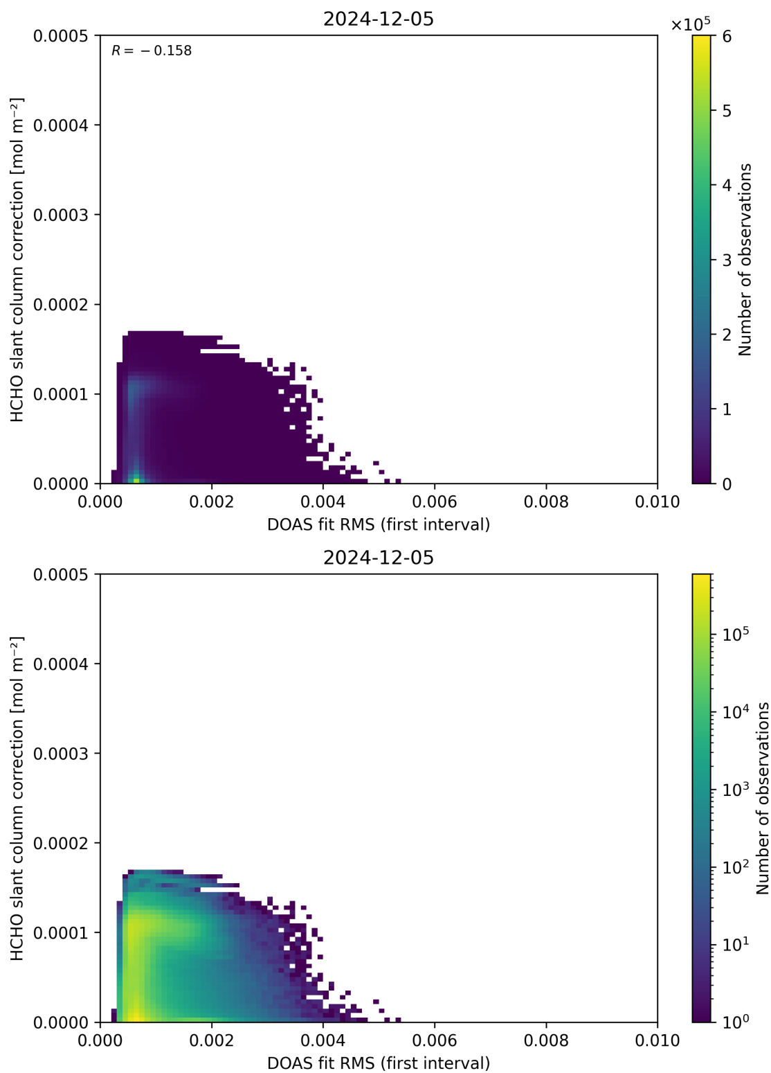
Figure 63: Scatter density plot of “DOAS fit RMS (first interval)” against “HCHO slant column correction” for 2024-12-04 to 2024-12-06.
