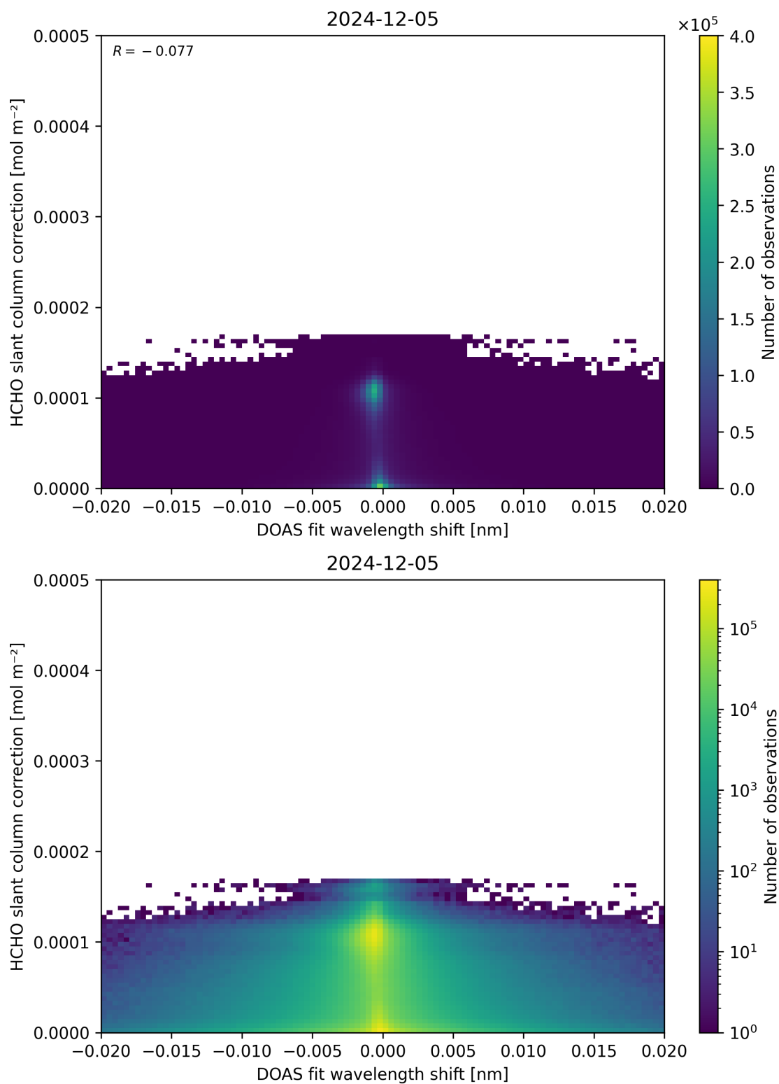
Figure 67: Scatter density plot of “DOAS fit wavelength shift” against “HCHO slant column correction” for 2024-12-04 to 2024-12-06.
