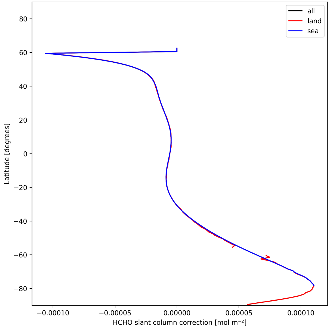
Figure 33: Zonal average of “HCHO slant column correction” for 2024-12-04 to 2024-12-06.
