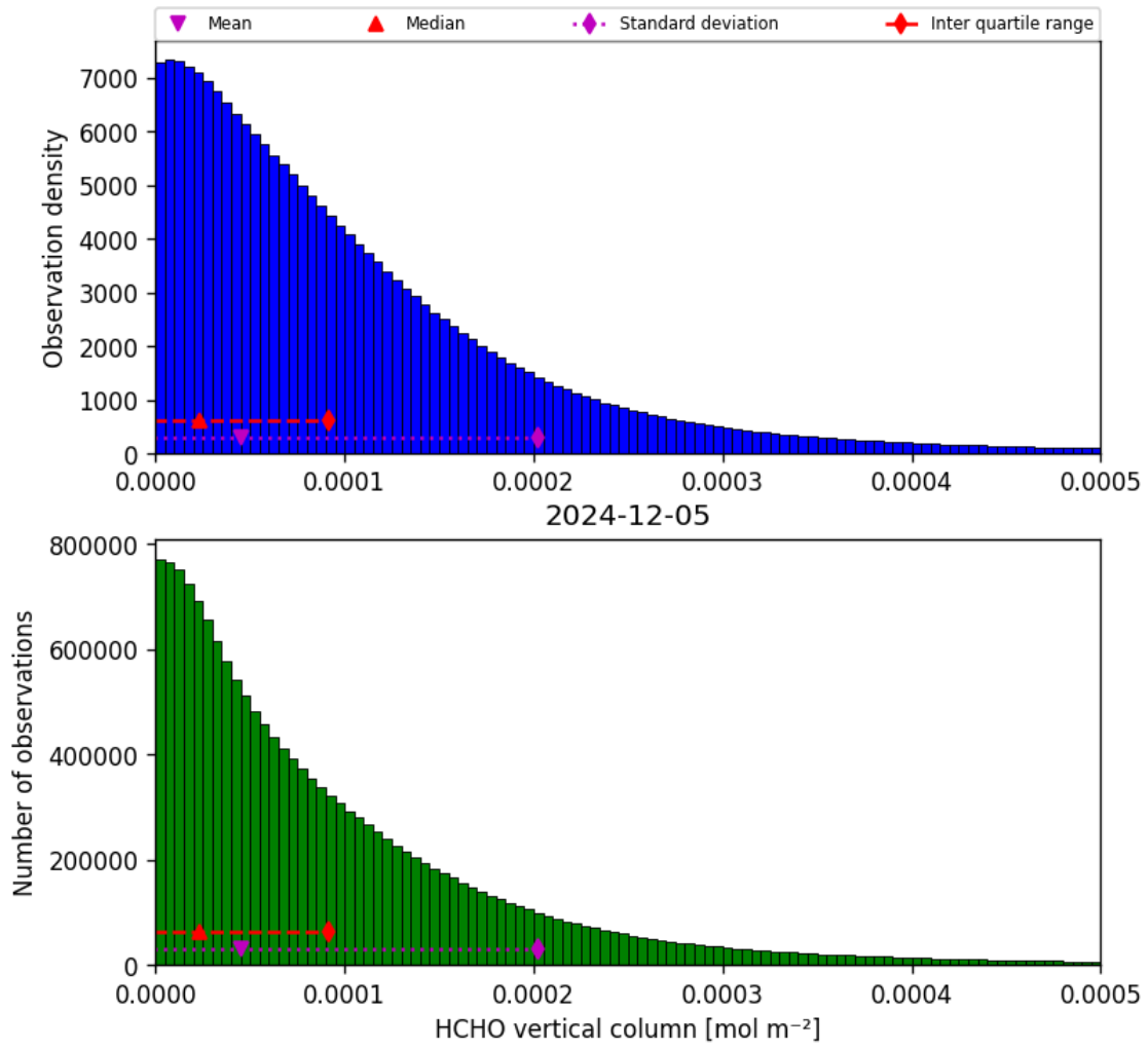
Figure 35: Histogram of “HCHO vertical column” for 2024-12-04 to 2024-12-06
