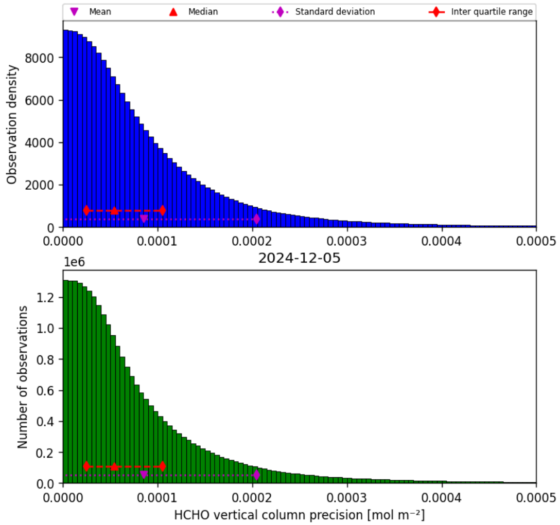
Figure 36: Histogram of “HCHO vertical column precision” for 2024-12-04 to 2024-12-06
