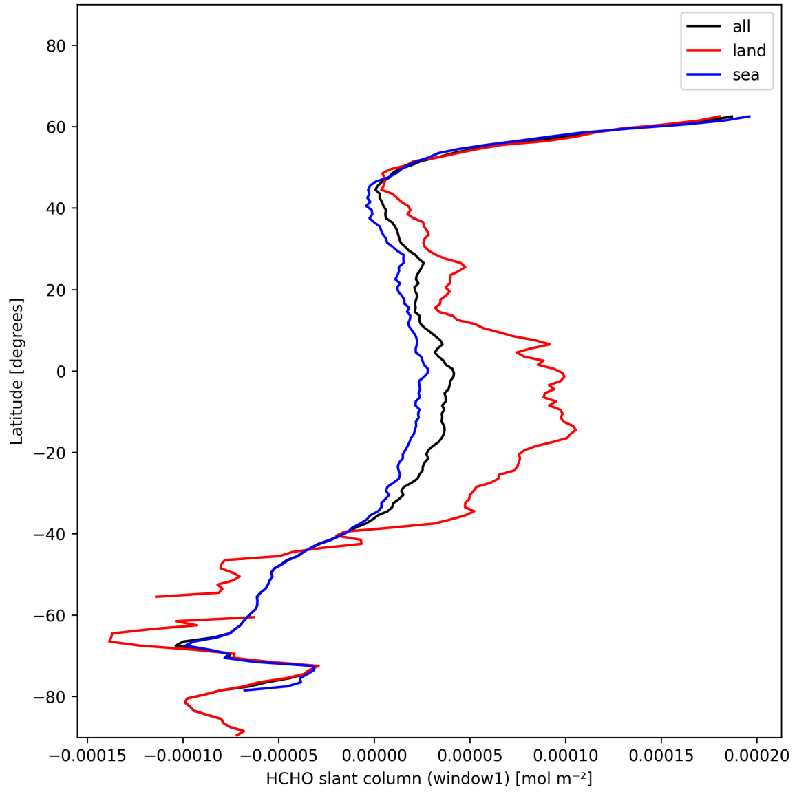
Figure 24: Zonal average of “HCHO slant column (window1)” for 2024-12-04 to 2024-12-06.
