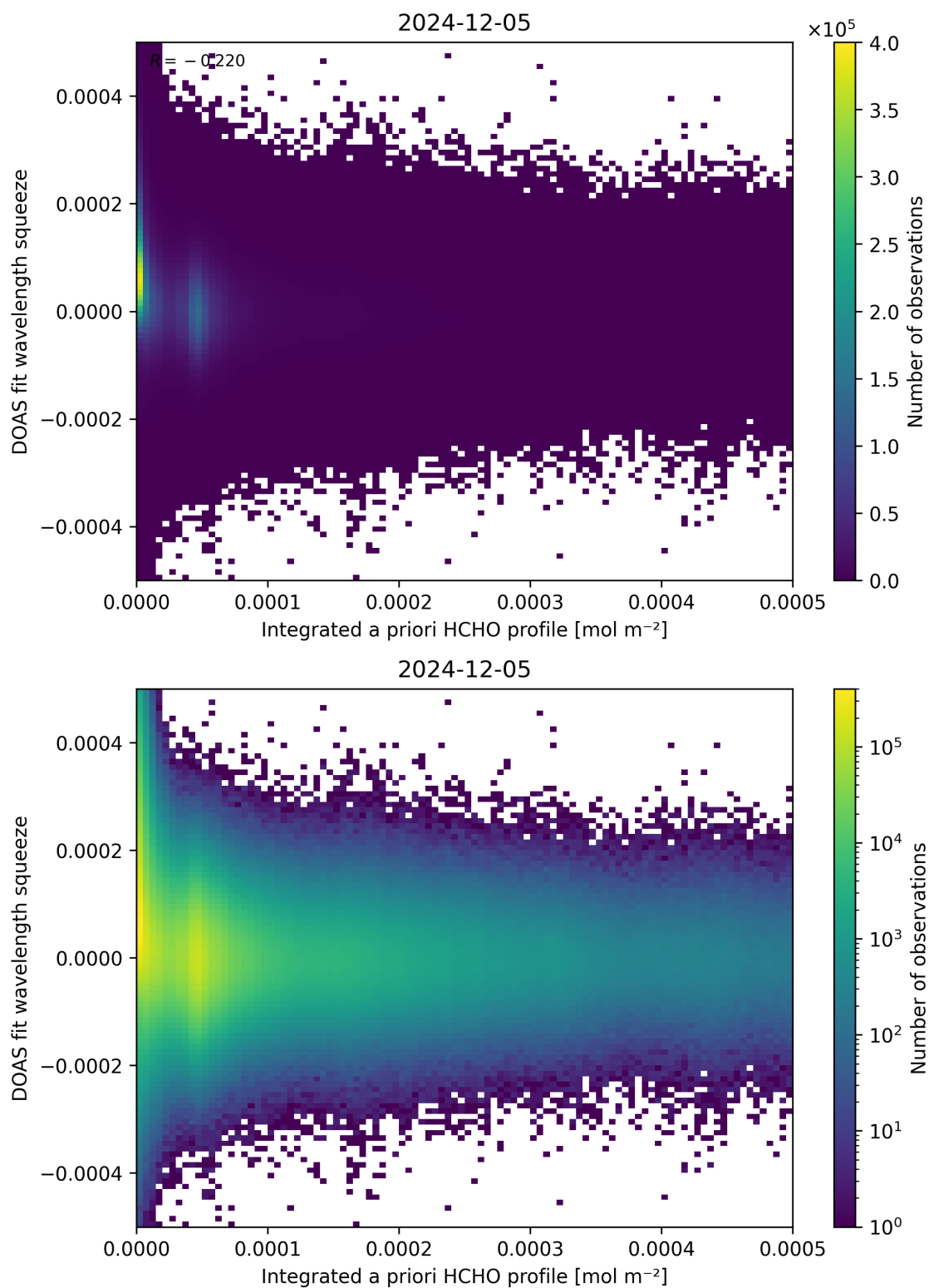
Figure 150: Scatter density plot of “Integrated a priori HCHO profile” against “DOAS fit wavelength squeeze” for 2024-12-04 to 2024-12-06.
