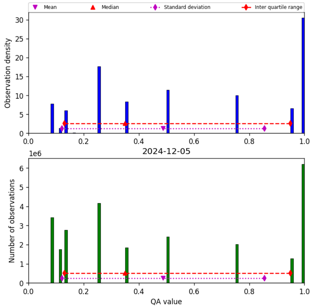
Figure 34: Histogram of “QA value” for 2024-12-04 to 2024-12-06
