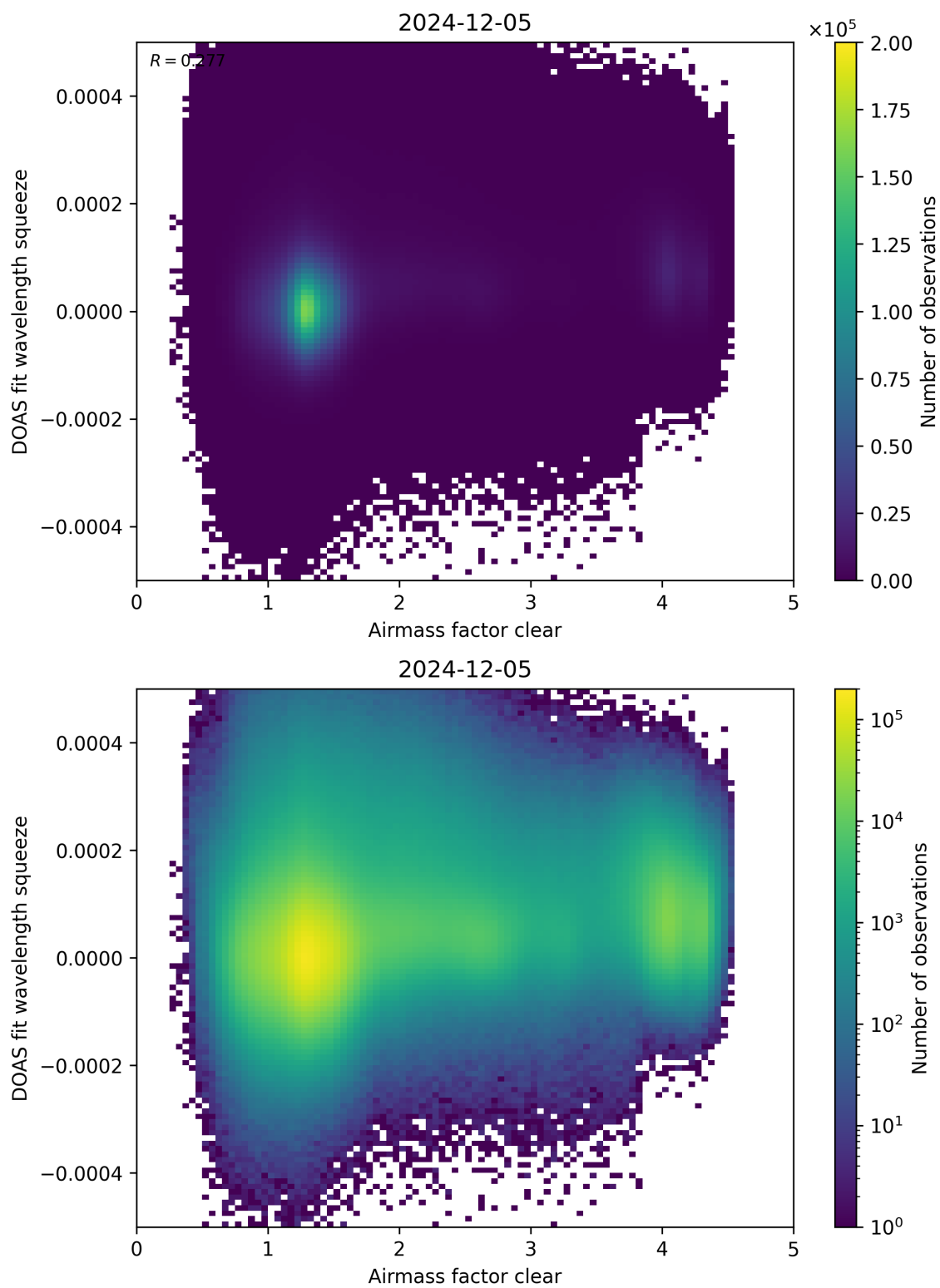
Figure 73: Scatter density plot of “Airmass factor clear” against “DOAS fit wavelength squeeze” for 2024-12-04 to 2024-12-06.
