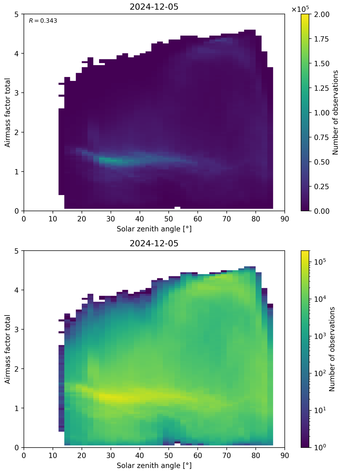
Figure 175: Scatter density plot of “Solar zenith angle” against “Airmass factor total” for 2024-12-04 to 2024-12-06.
