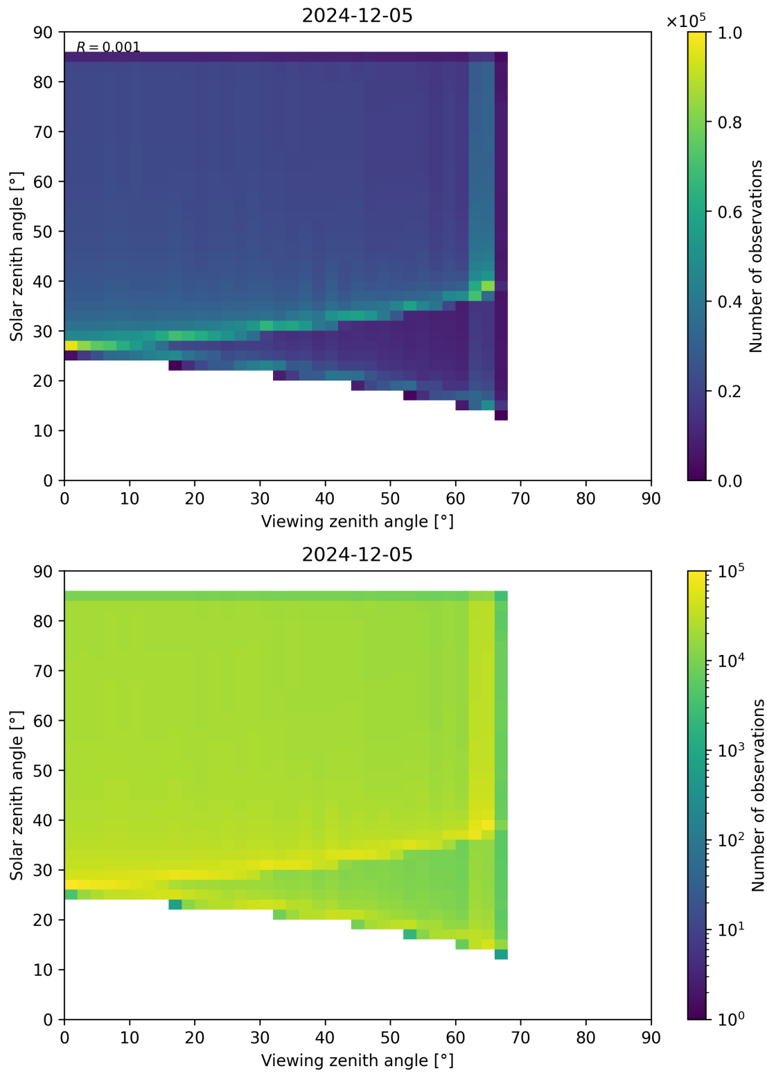
Figure 197: Scatter density plot of “Viewing zenith angle” against “Solar zenith angle” for 2024-12-04 to 2024-12-06.
