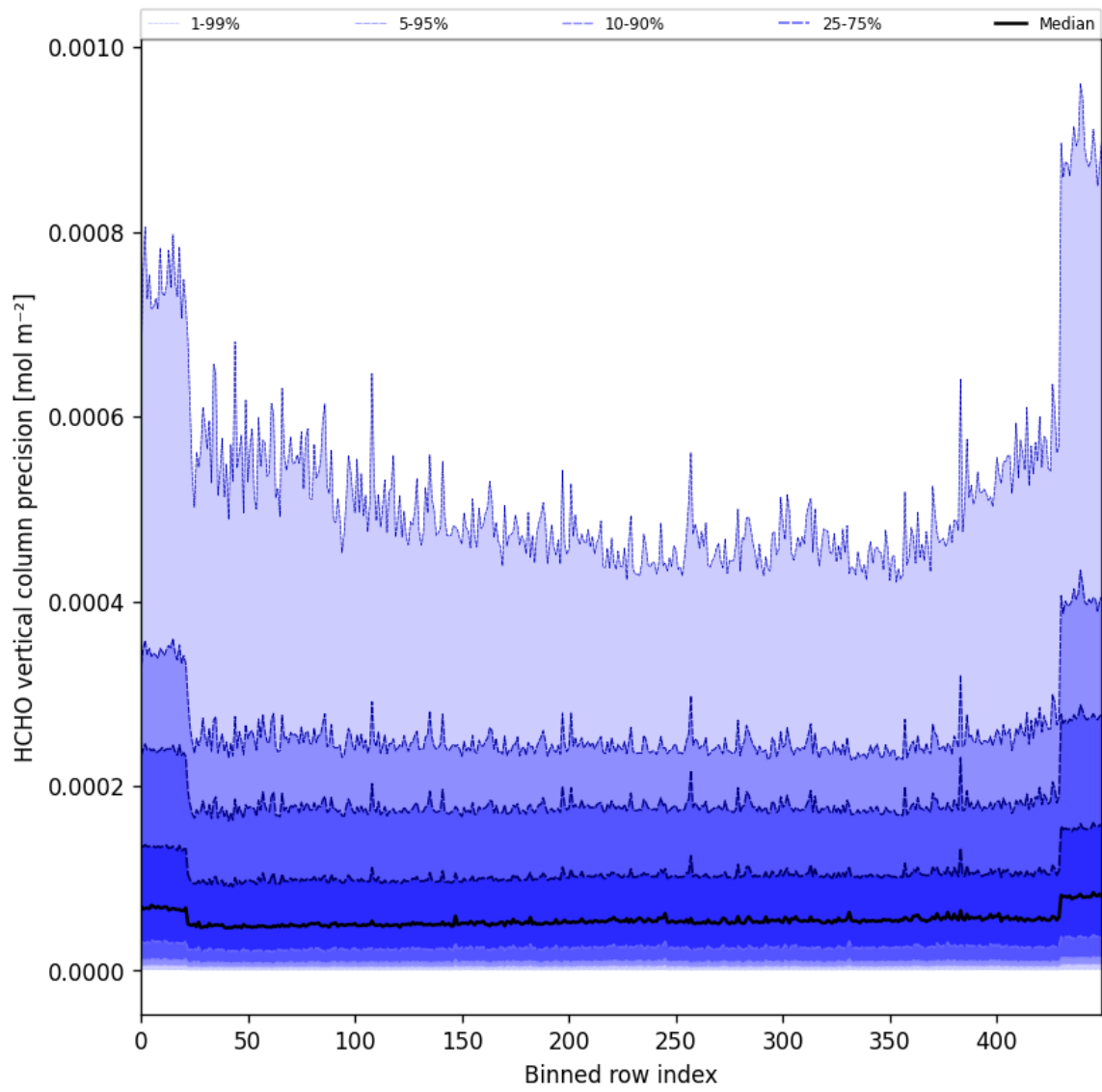
Figure 50: Along track statistics of “HCHO vertical column precision” for 2024-12-04 to 2024-12-06
