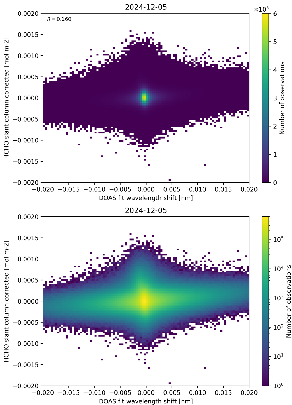
Figure 66: Scatter density plot of “DOAS fit wavelength shift” against “HCHO slant column corrected” for 2024-12-04 to 2024-12-06.
