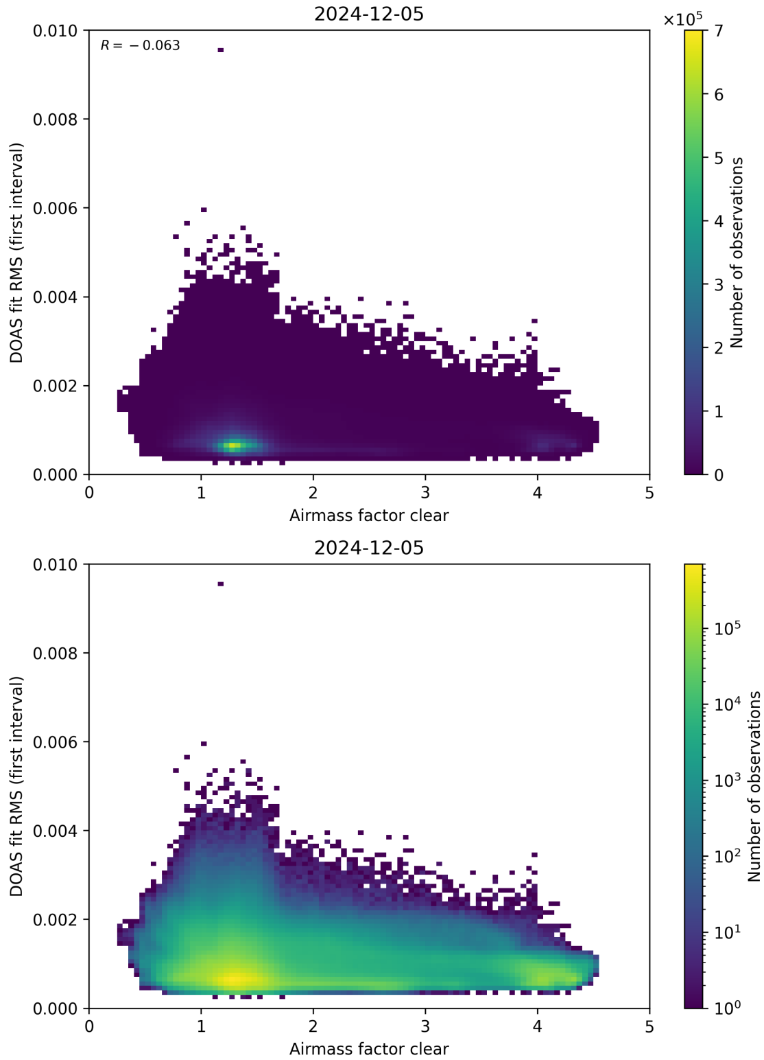
Figure 71: Scatter density plot of “Airmass factor clear” against “DOAS fit RMS (first interval)” for 2024-12-04 to 2024-12-06.
