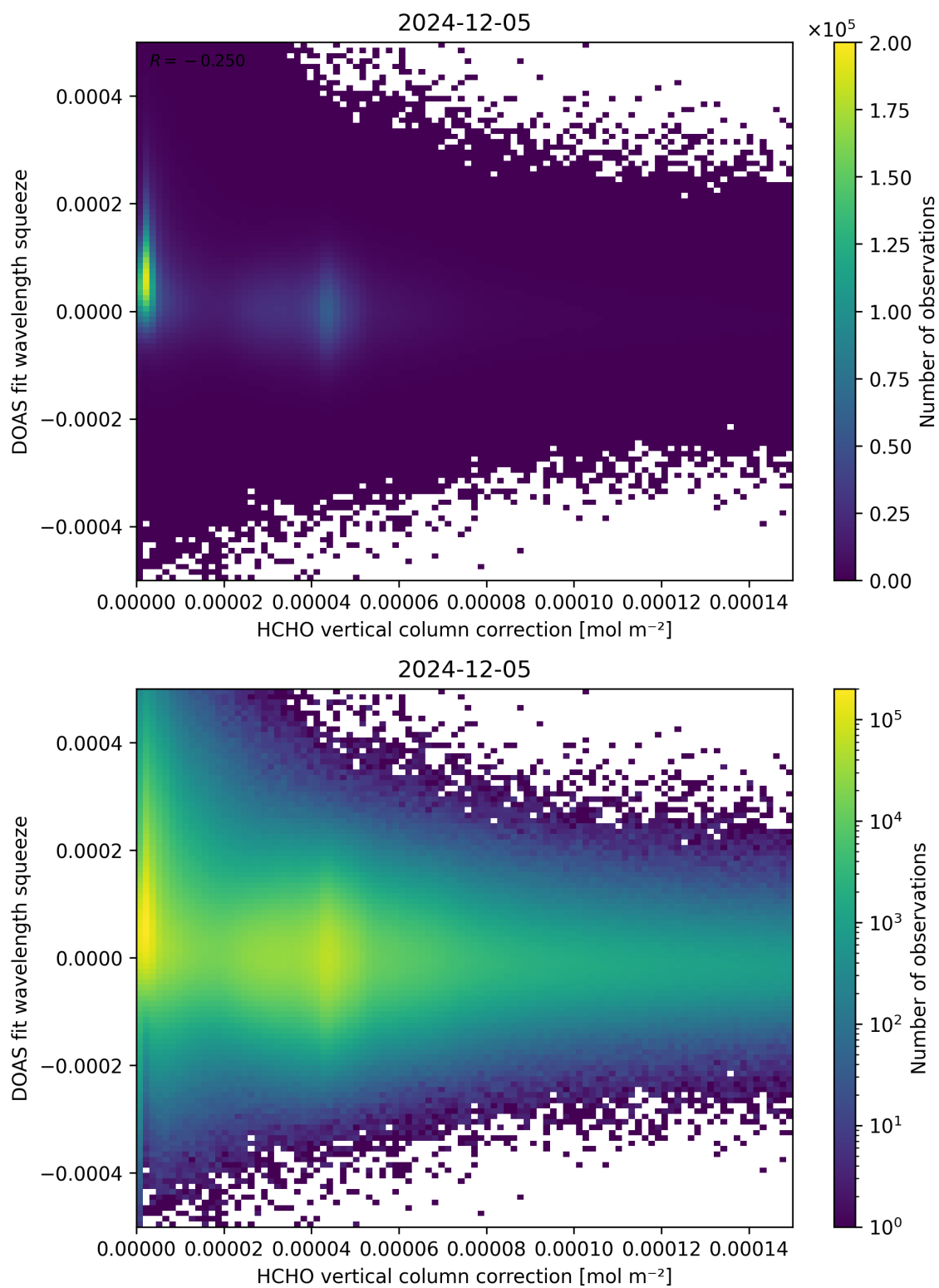
Figure 114: Scatter density plot of “HCHO vertical column correction” against “DOAS fit wavelength squeeze” for 2024-12-04 to 2024-12-06.
