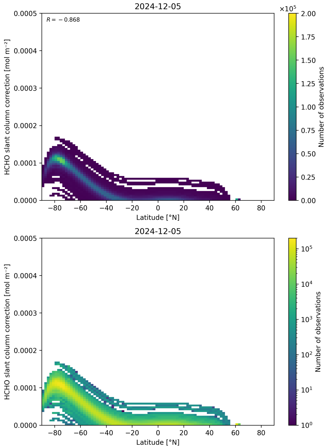
Figure 158: Scatter density plot of “Latitude” against “HCHO slant column correction” for 2024-12-04 to 2024-12-06.
