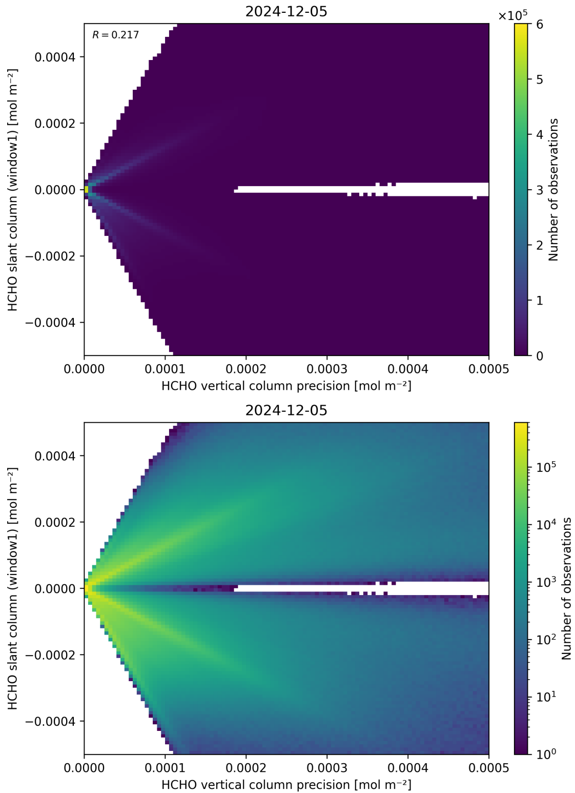
Figure 142: Scatter density plot of “HCHO vertical column precision” against “HCHO slant column (window1)” for 2024-12-04 to 2024-12-06.
