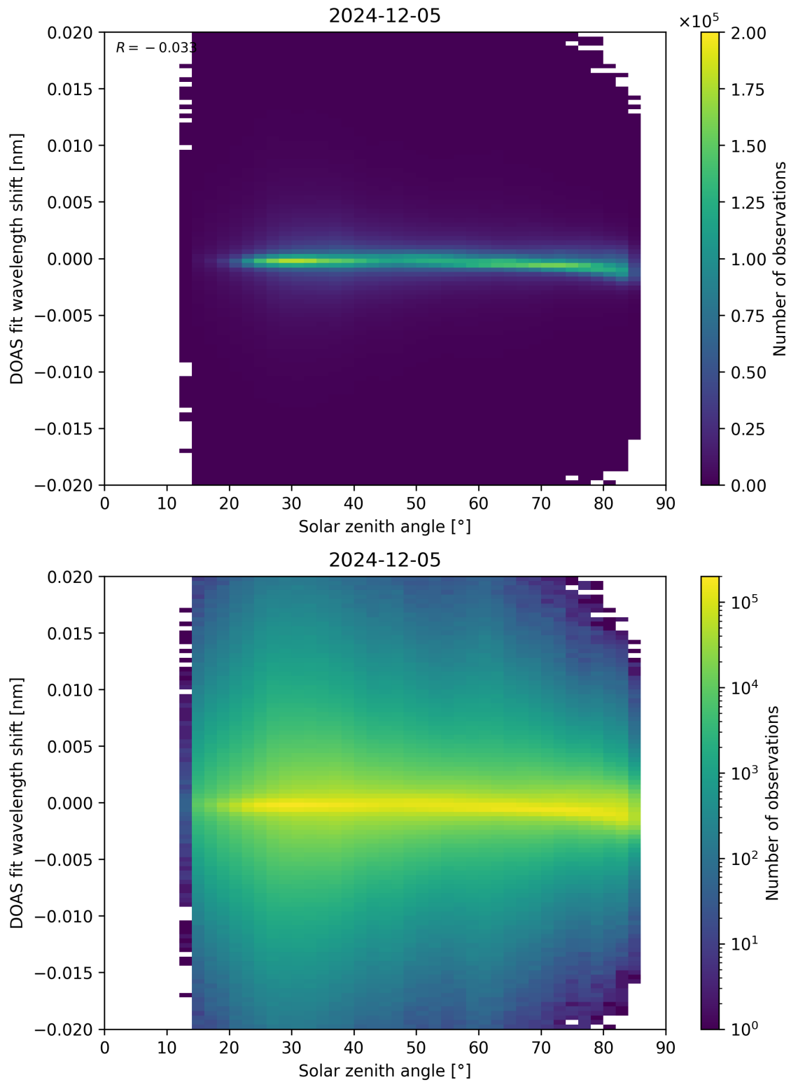
Figure 168: Scatter density plot of “Solar zenith angle” against “DOAS fit wavelength shift” for 2024-12-04 to 2024-12-06.
