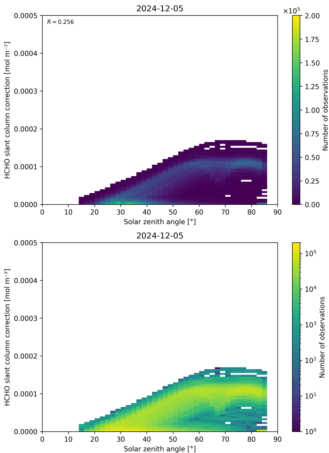
Figure 172: Scatter density plot of “Solar zenith angle” against “HCHO slant column correction” for 2024-12-04 to 2024-12-06.
