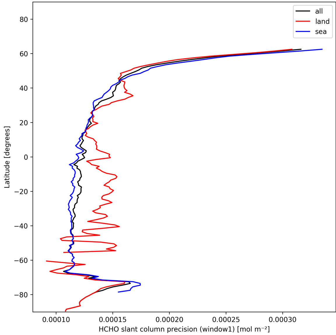
Figure 25: Zonal average of “HCHO slant column precision (window1)” for 2024-12-04 to 2024-12-06.
