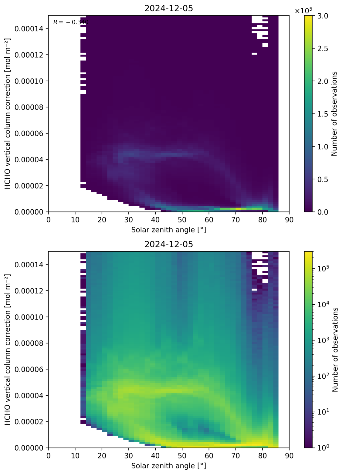
Figure 178: Scatter density plot of “Solar zenith angle” against “HCHO vertical column correction” for 2024-12-04 to 2024-12-06.
