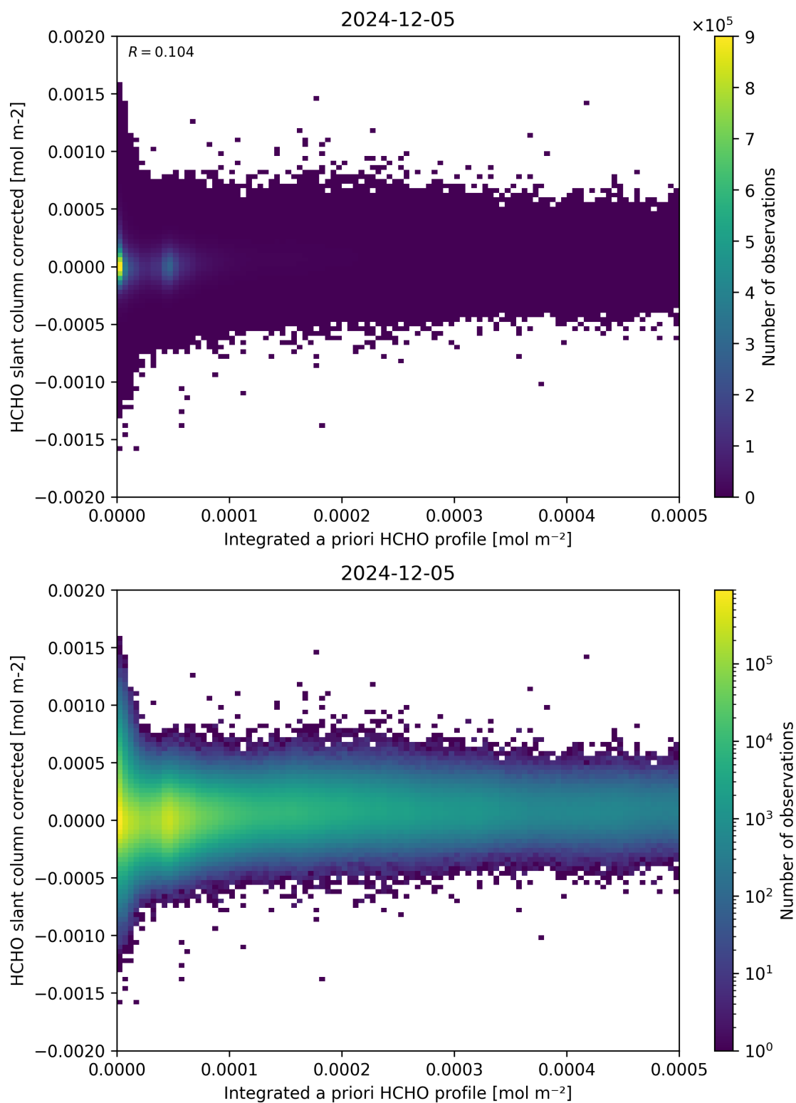
Figure 151: Scatter density plot of “Integrated a priori HCHO profile” against “HCHO slant column corrected” for 2024-12-04 to 2024-12-06.
