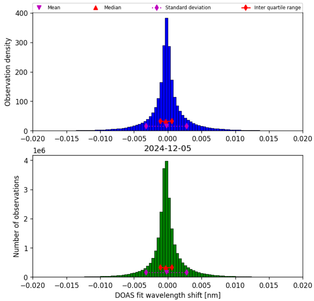
Figure 44: Histogram of “DOAS fit wavelength shift” for 2024-12-04 to 2024-12-06
