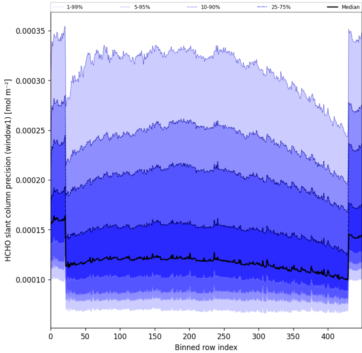
Figure 53: Along track statistics of “HCHO slant column precision (window1)” for 2024-12-04 to 2024-12-06
