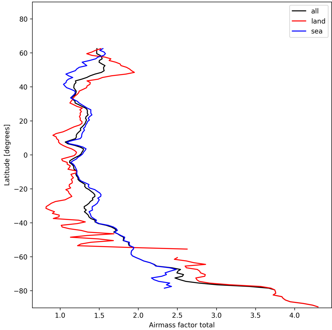
Figure 26: Zonal average of “Airmass factor total” for 2024-12-04 to 2024-12-06.
