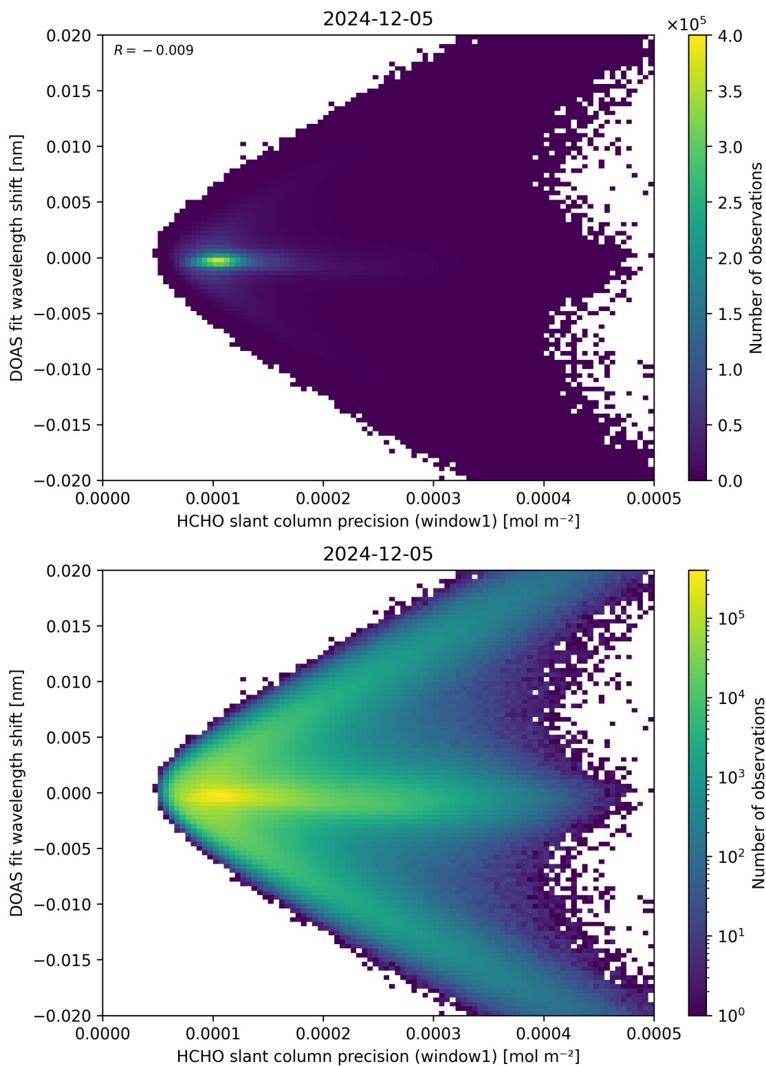
Figure 89: Scatter density plot of “HCHO slant column precision (window1)” against “DOAS fit wavelength shift” for 2024-12-04 to 2024-12-06.
