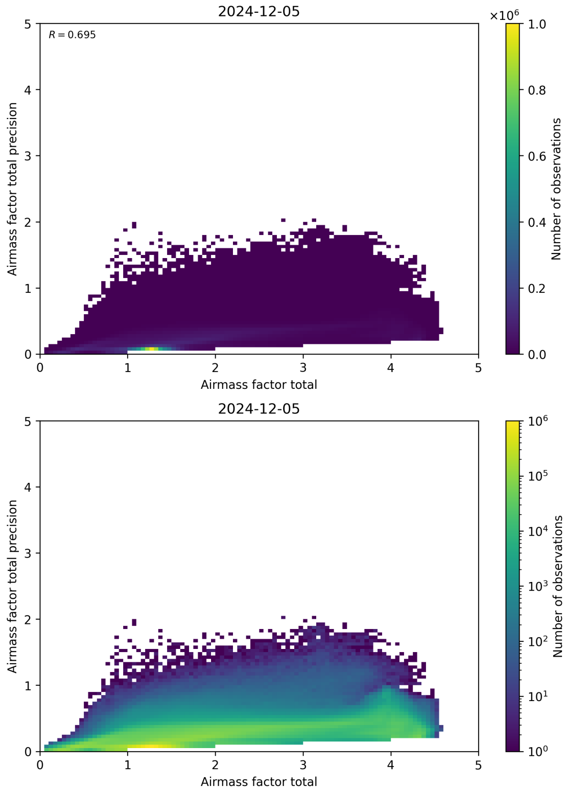
Figure 103: Scatter density plot of “Airmass factor total” against “Airmass factor total precision” for 2024-12-04 to 2024-12-06.
