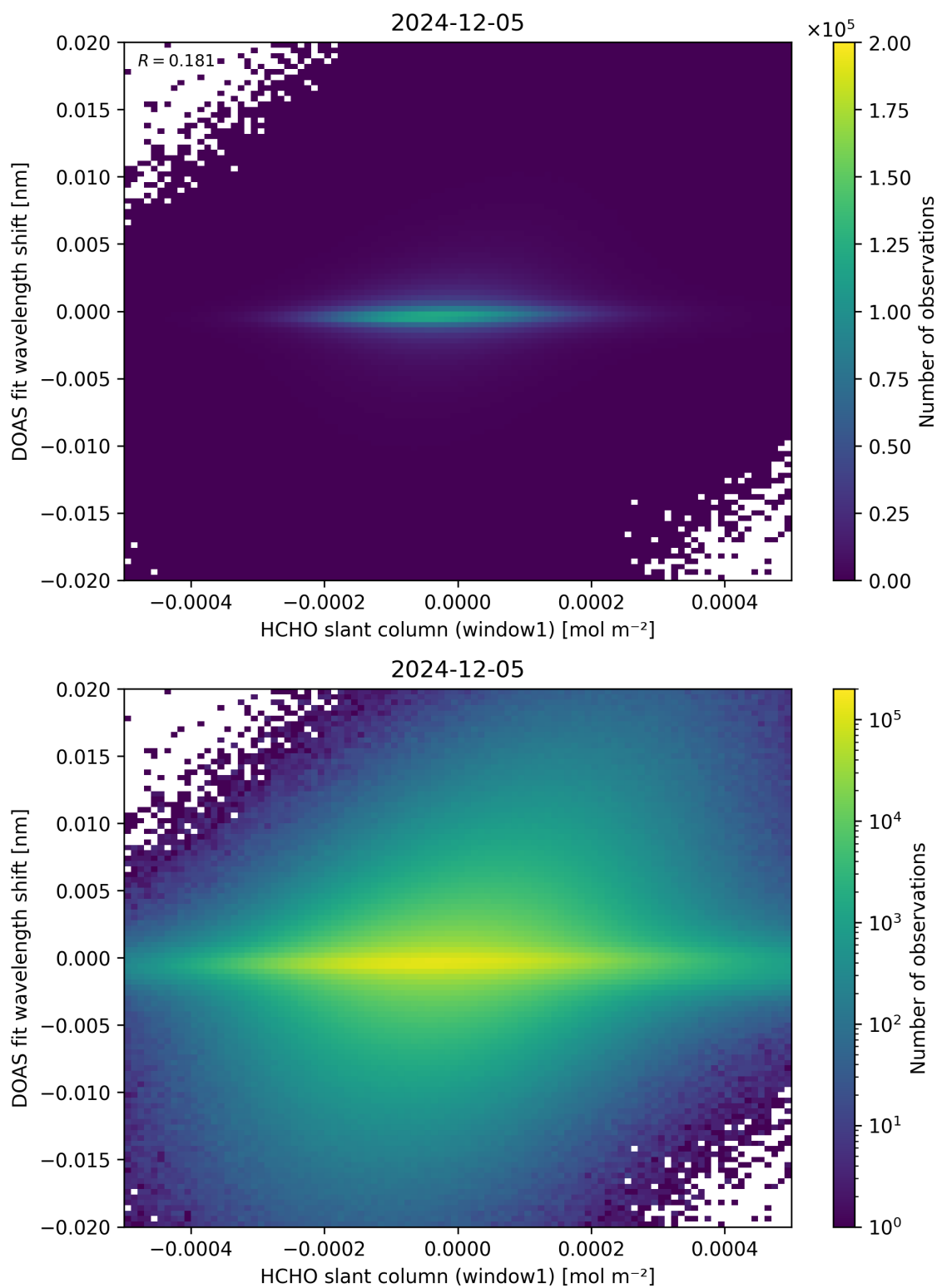
Figure 79: Scatter density plot of “HCHO slant column (window1)” against “DOAS fit wavelength shift” for 2024-12-04 to 2024-12-06.
