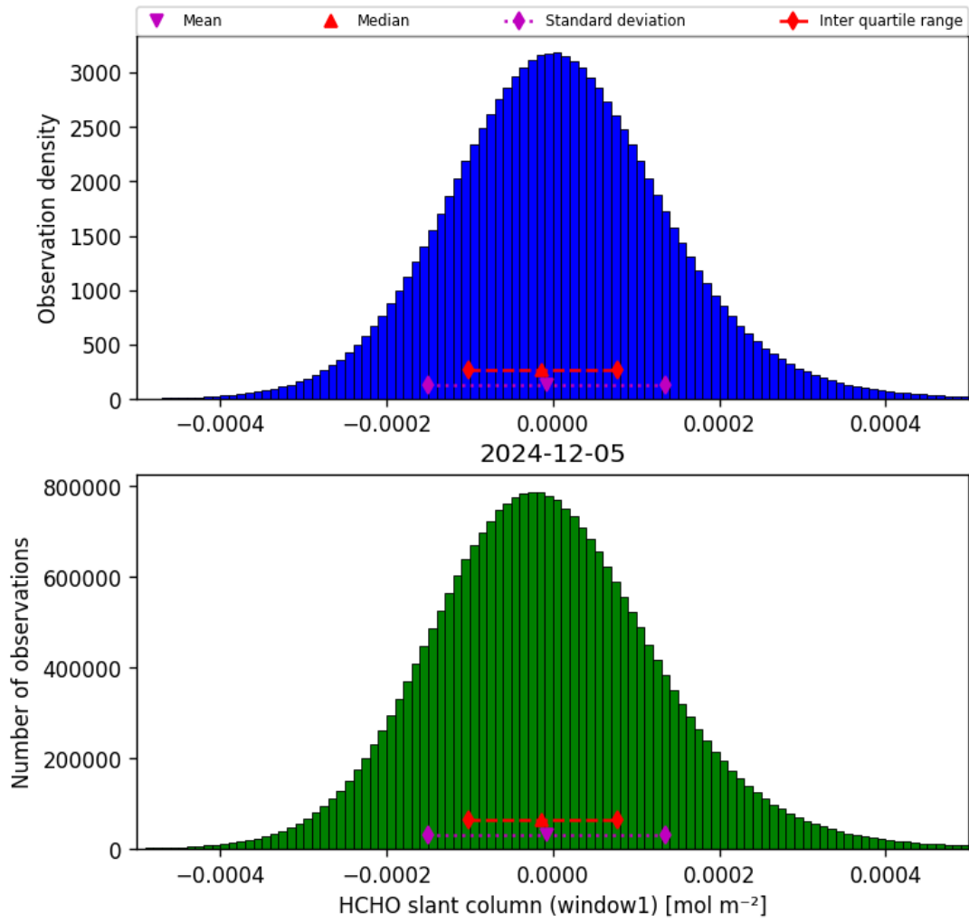
Figure 38: Histogram of “HCHO slant column (window1)” for 2024-12-04 to 2024-12-06
