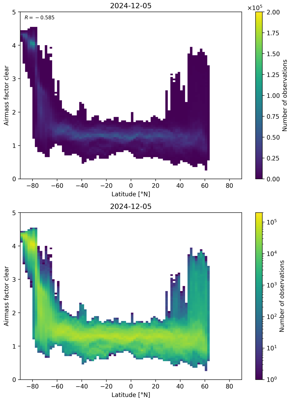
Figure 156: Scatter density plot of “Latitude” against “Airmass factor clear” for 2024-12-04 to 2024-12-06.
