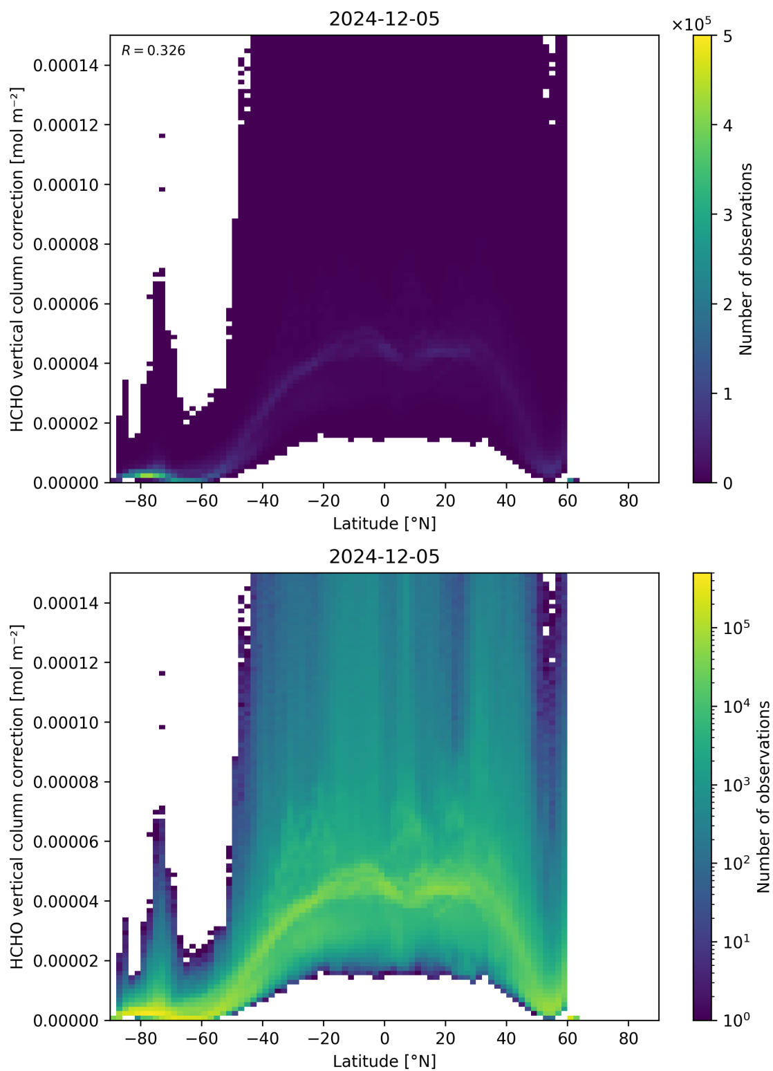
Figure 164: Scatter density plot of “Latitude” against “HCHO vertical column correction” for 2024-12-04 to 2024-12-06.
