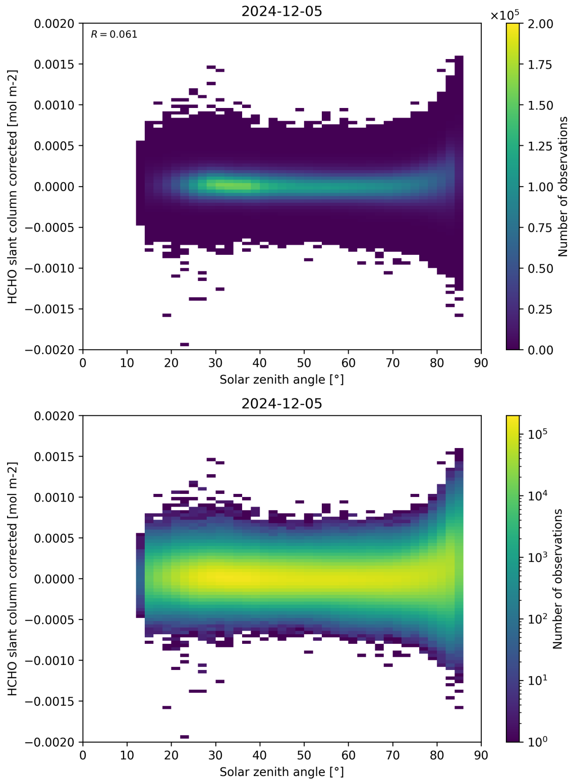
Figure 171: Scatter density plot of “Solar zenith angle” against “HCHO slant column corrected” for 2024-12-04 to 2024-12-06.
