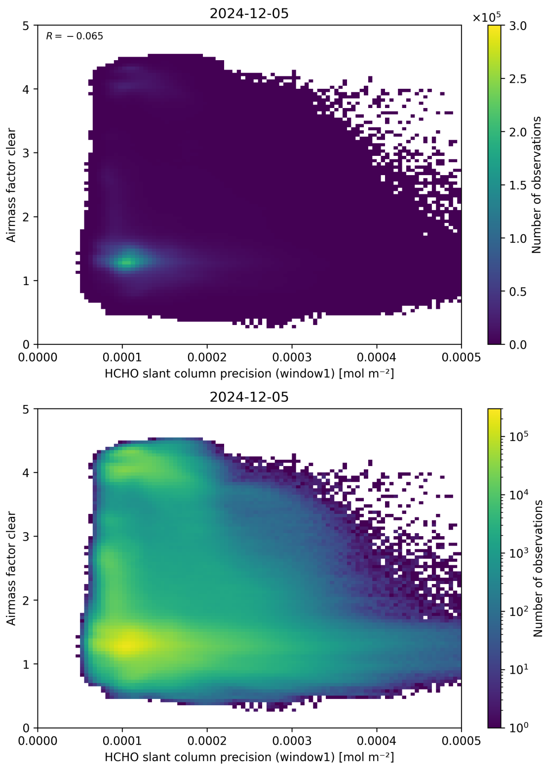
Figure 91: Scatter density plot of “HCHO slant column precision (window1)” against “Airmass factor clear” for 2024-12-04 to 2024-12-06.
