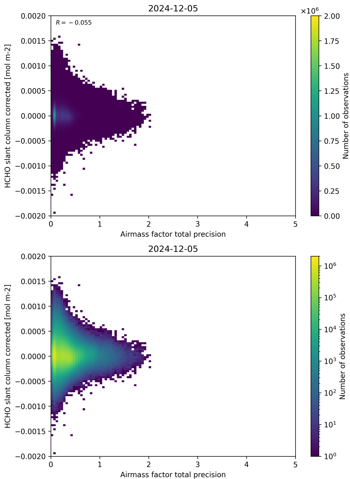
Figure 109: Scatter density plot of “Airmass factor total precision” against “HCHO slant column corrected” for 2024-12-04 to 2024-12-06.
