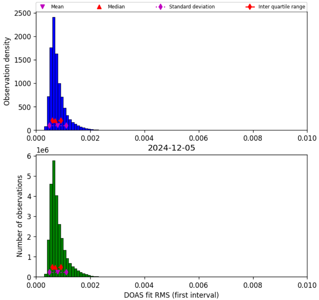
Figure 46: Histogram of “DOAS fit RMS (first interval)” for 2024-12-04 to 2024-12-06
