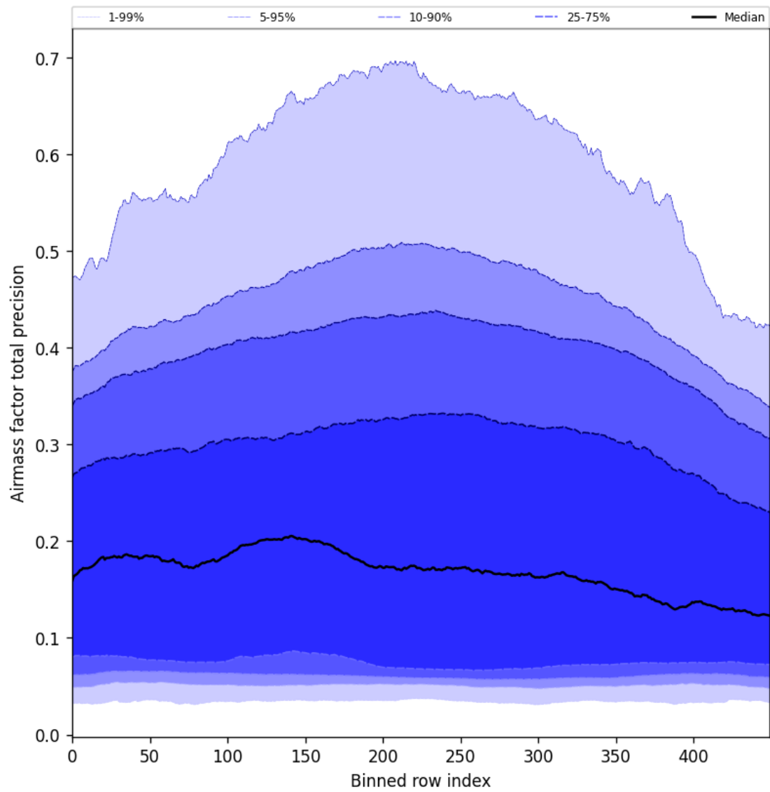
Figure 55: Along track statistics of “Airmass factor total precision” for 2024-12-04 to 2024-12-06
