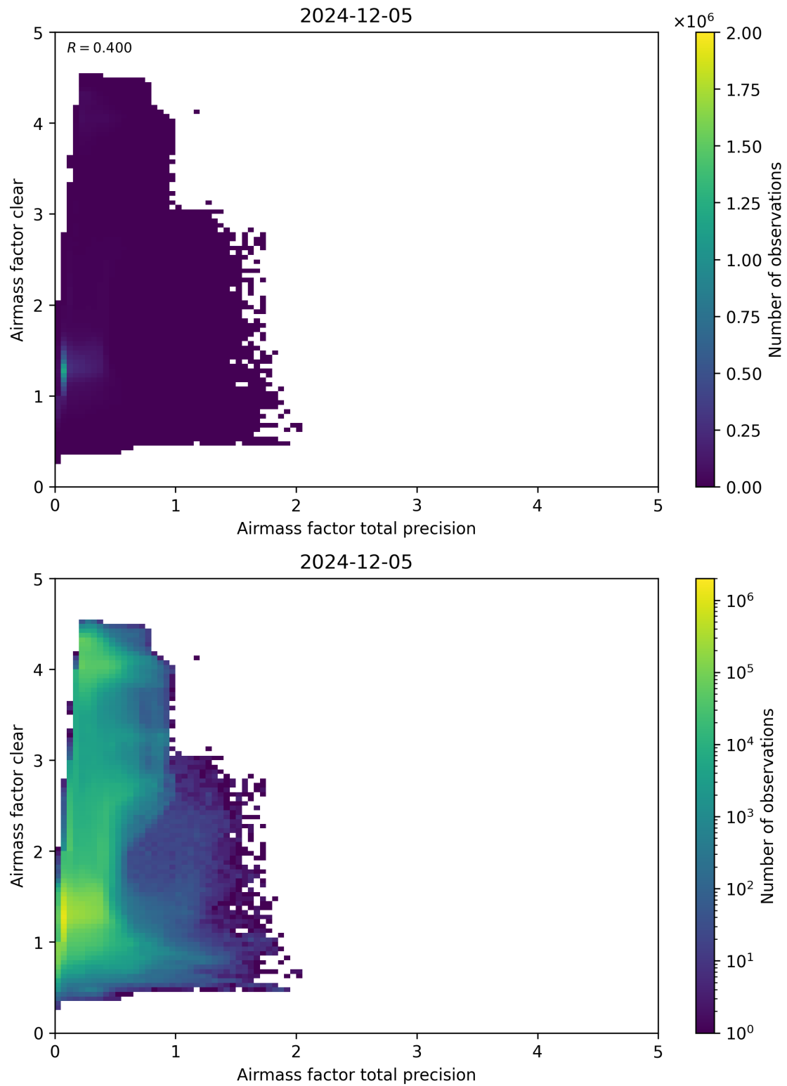
Figure 108: Scatter density plot of “Airmass factor total precision” against “Airmass factor clear” for 2024-12-04 to 2024-12-06.
