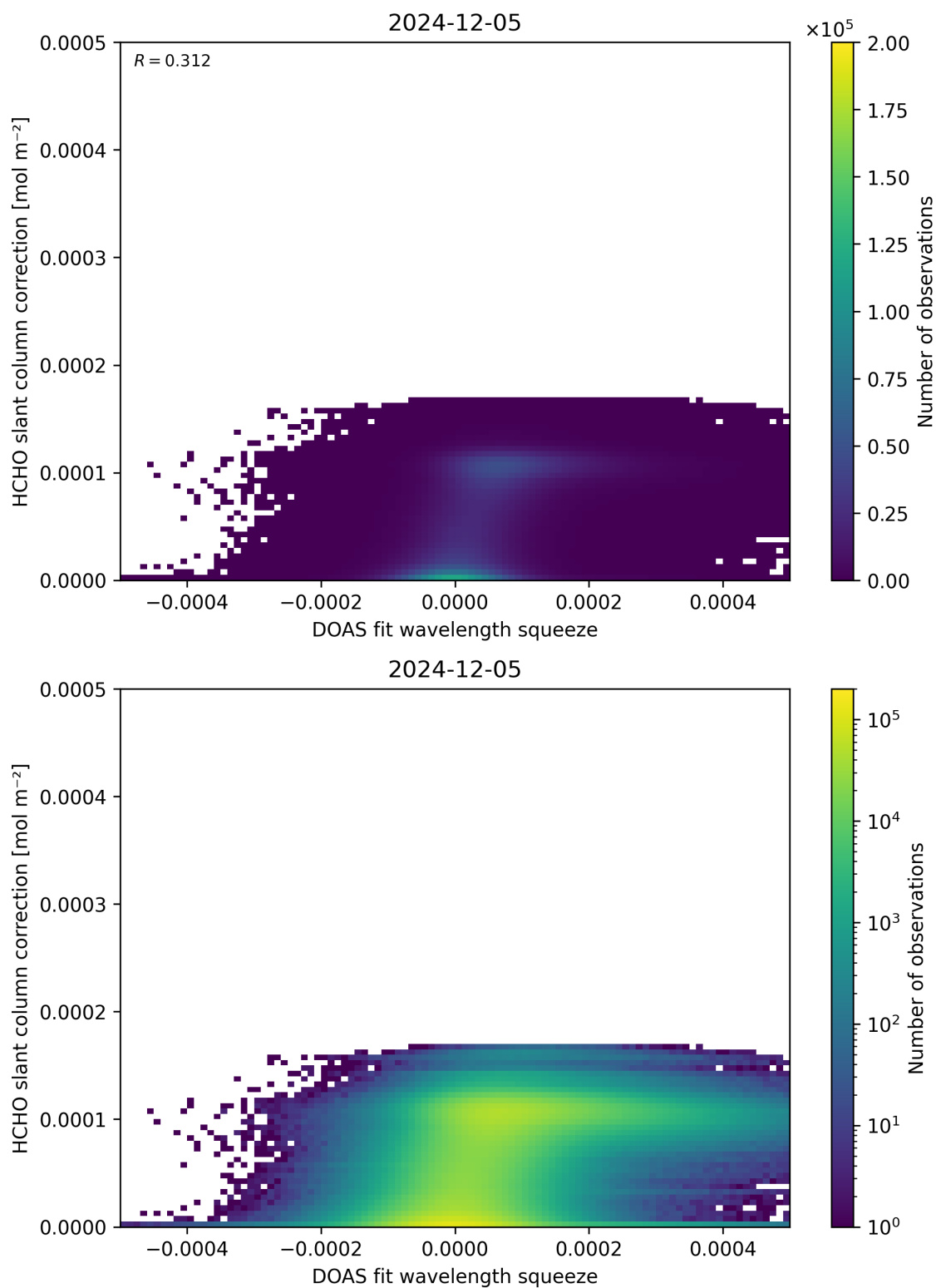
Figure 70: Scatter density plot of “DOAS fit wavelength squeeze” against “HCHO slant column correction” for 2024-12-04 to 2024-12-06.
