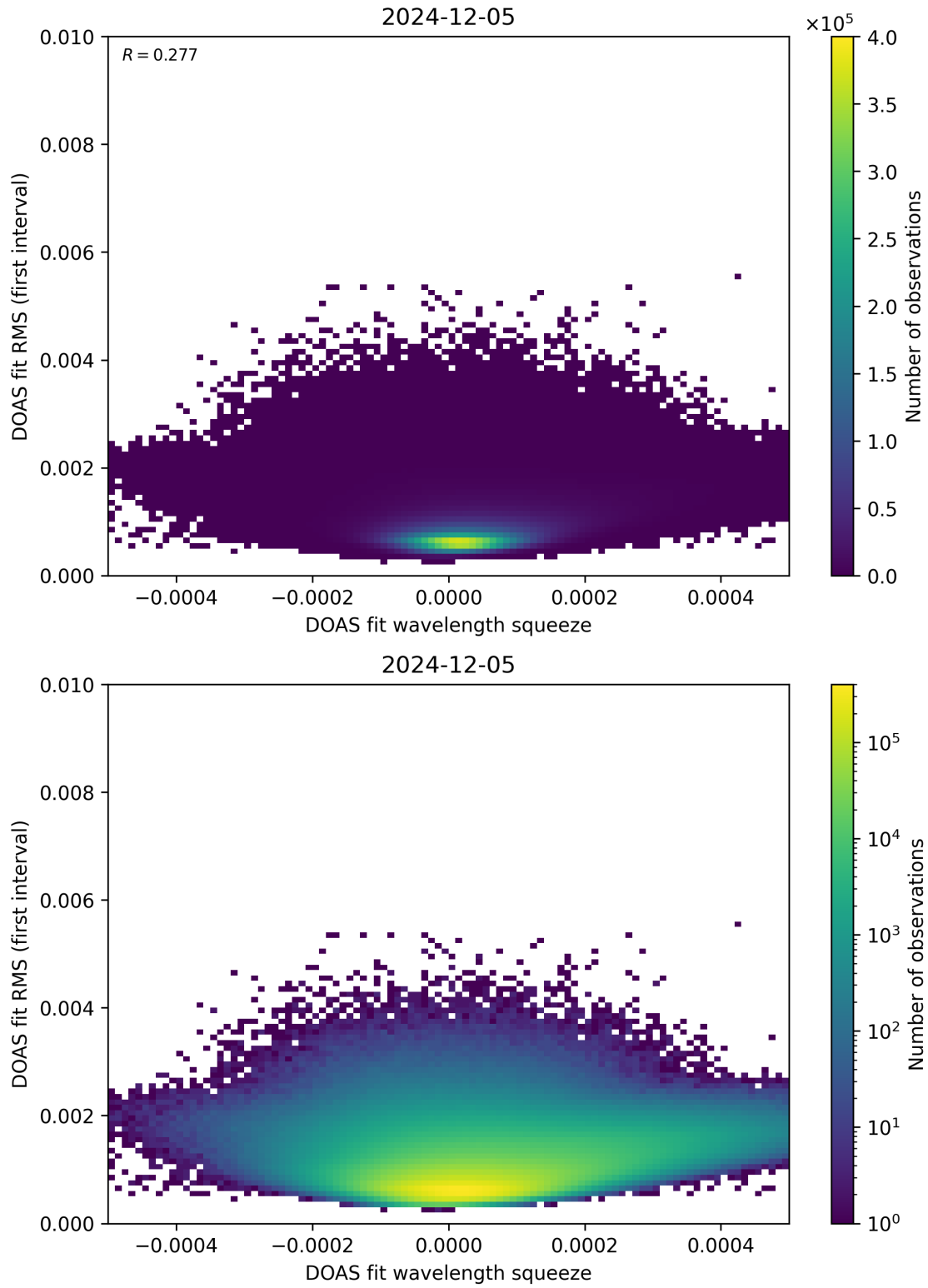
Figure 68: Scatter density plot of “DOAS fit wavelength squeeze” against “DOAS fit RMS (first interval)” for 2024-12-04 to 2024-12-06.
