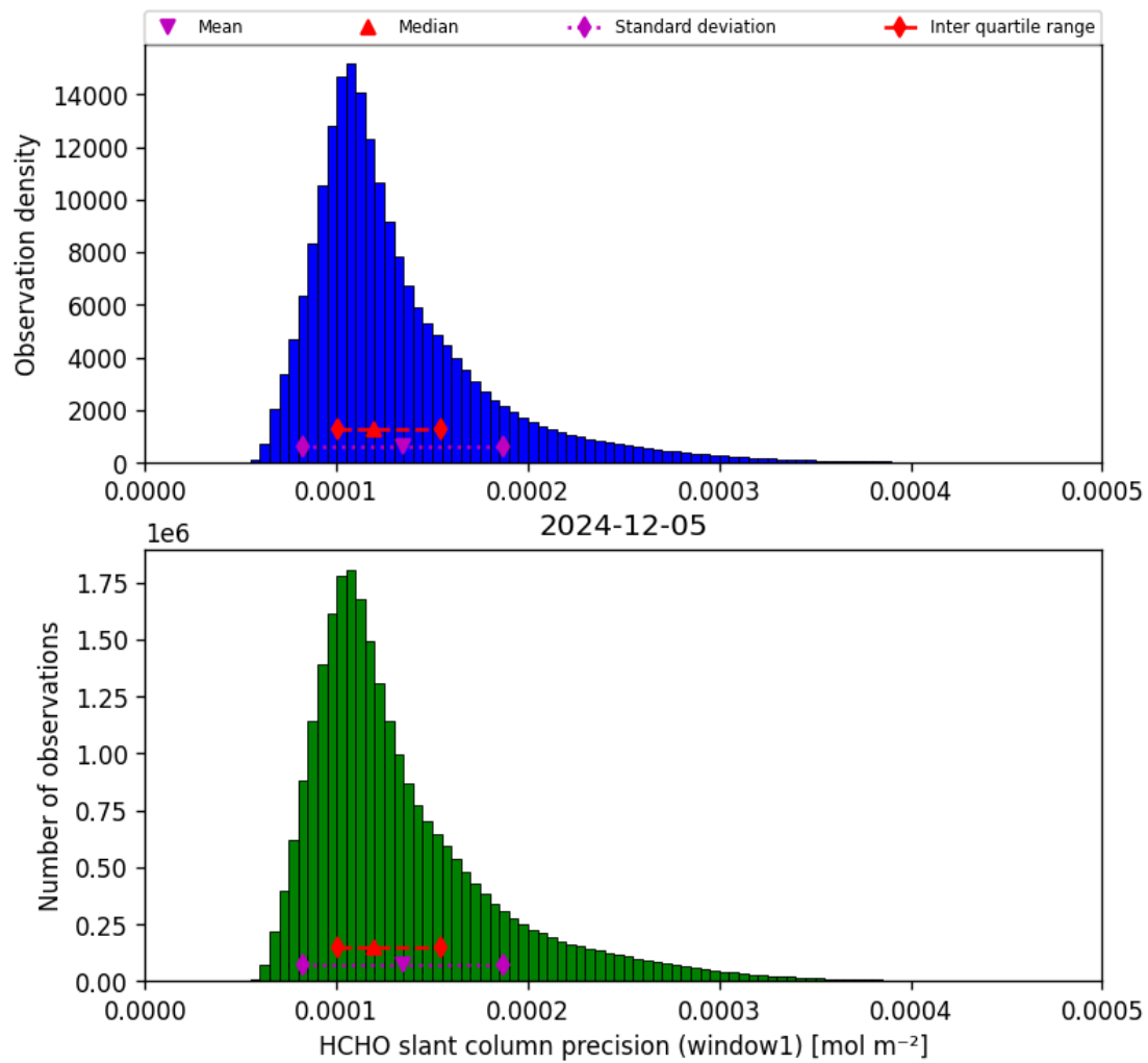
Figure 39: Histogram of “HCHO slant column precision (window1)” for 2024-12-04 to 2024-12-06
