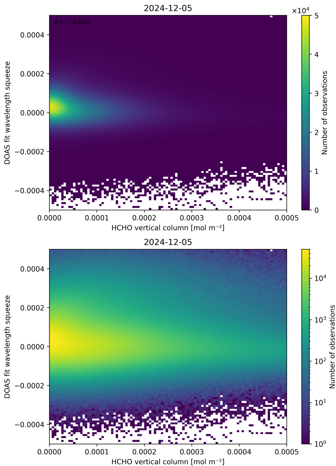
Figure 125: Scatter density plot of “HCHO vertical column” against “DOAS fit wavelength squeeze” for 2024-12-04 to 2024-12-06.
