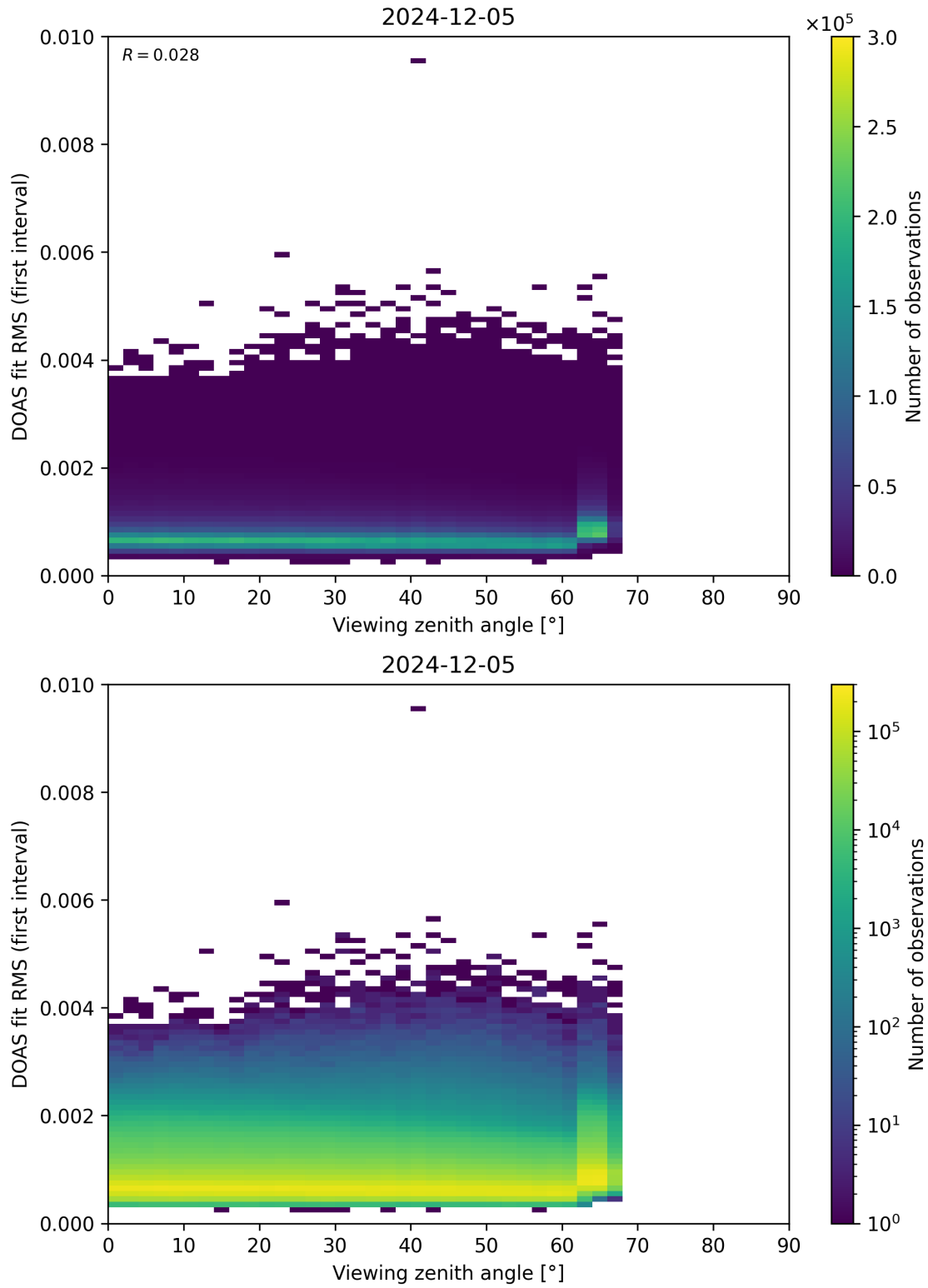
Figure 182: Scatter density plot of “Viewing zenith angle” against “DOAS fit RMS (first interval)” for 2024-12-04 to 2024-12-06.
