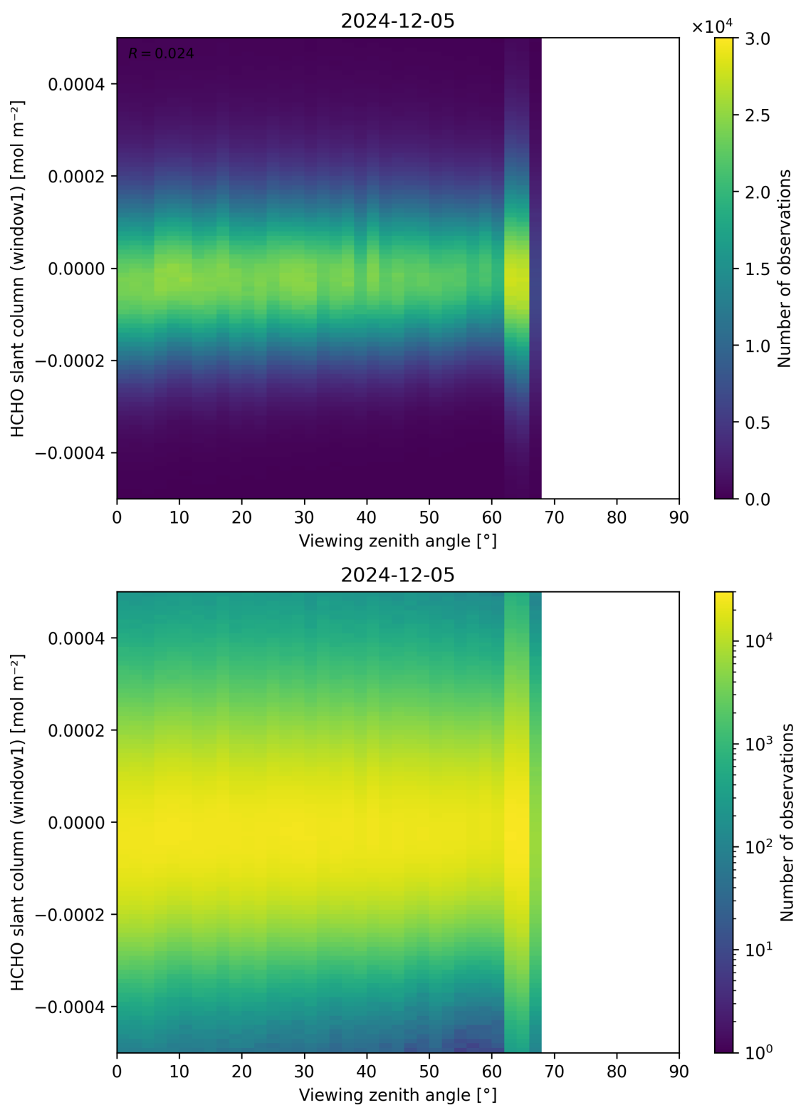
Figure 188: Scatter density plot of “Viewing zenith angle” against “HCHO slant column (window1)” for 2024-12-04 to 2024-12-06.
