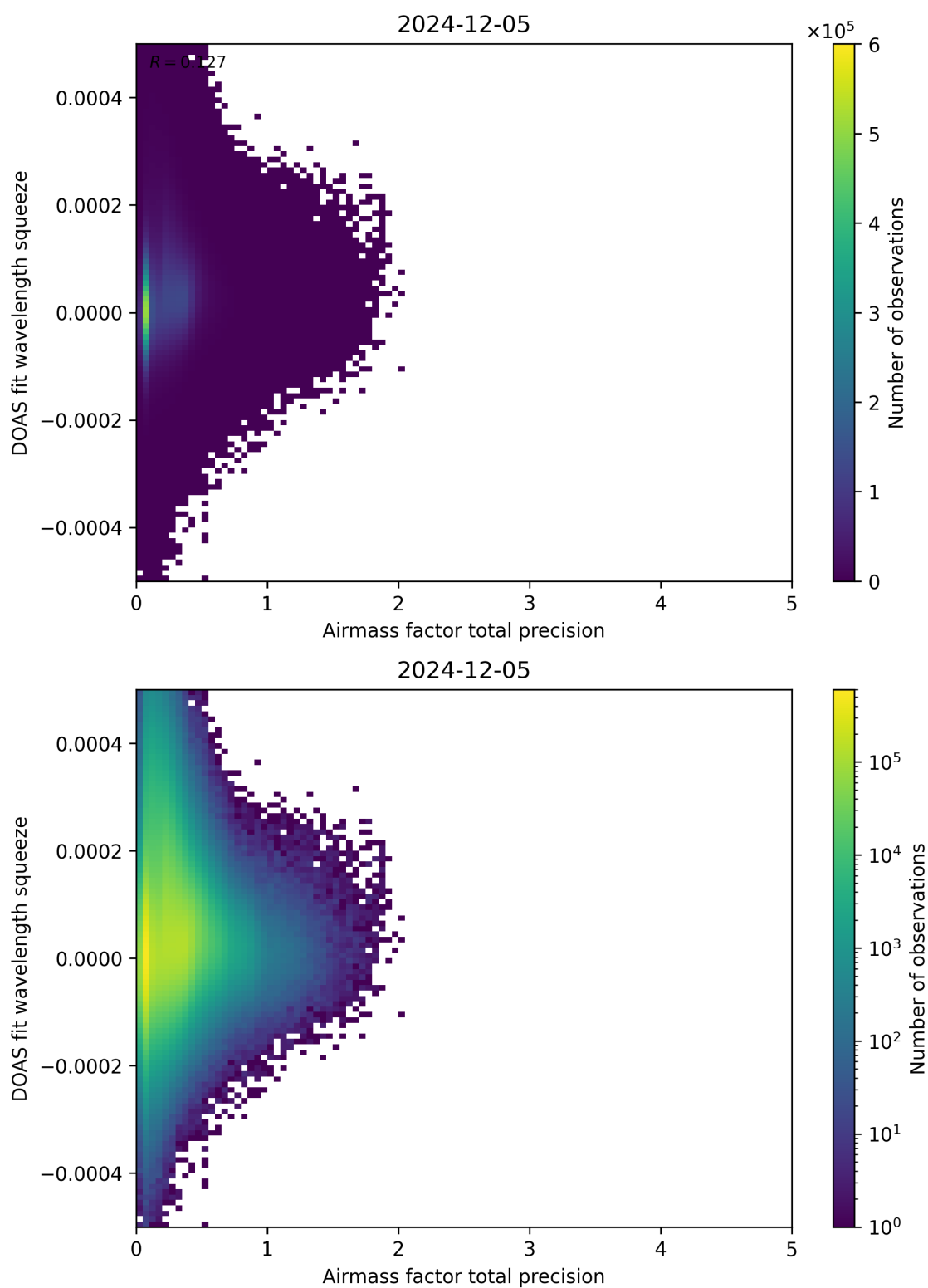
Figure 107: Scatter density plot of “Airmass factor total precision” against “DOAS fit wavelength squeeze” for 2024-12-04 to 2024-12-06.
