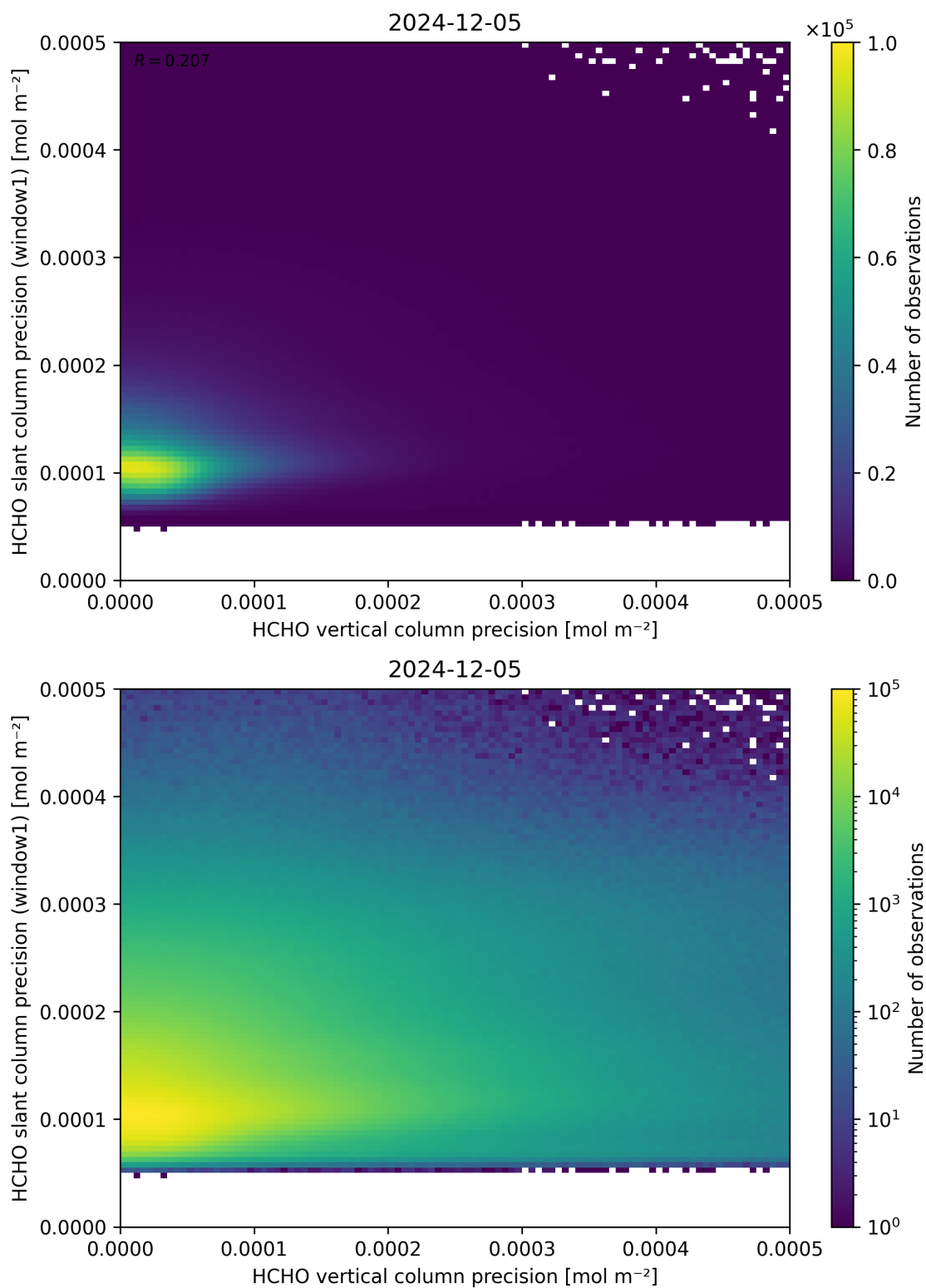
Figure 143: Scatter density plot of “HCHO vertical column precision” against “HCHO slant column precision (window1)” for 2024-12-04 to 2024-12-06.
