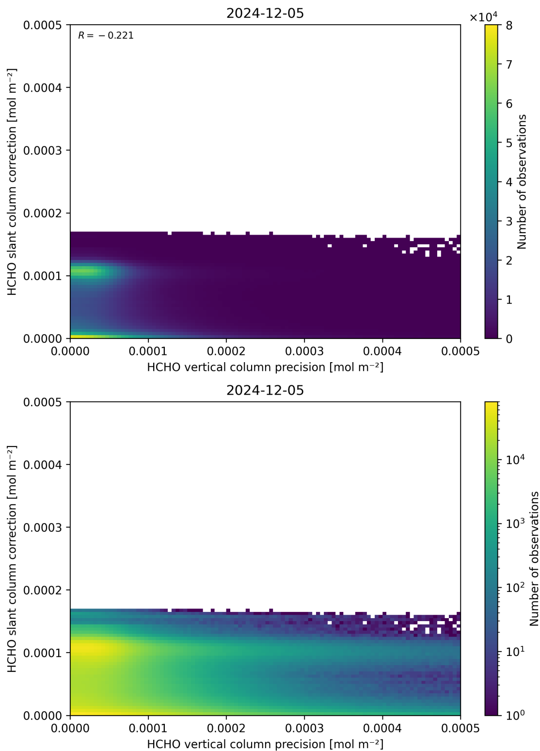
Figure 141: Scatter density plot of “HCHO vertical column precision” against “HCHO slant column correction” for 2024-12-04 to 2024-12-06.
