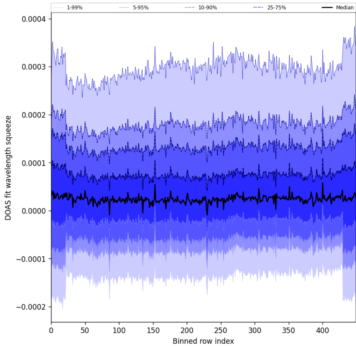
Figure 59: Along track statistics of “DOAS fit wavelength squeeze” for 2024-12-04 to 2024-12-06
