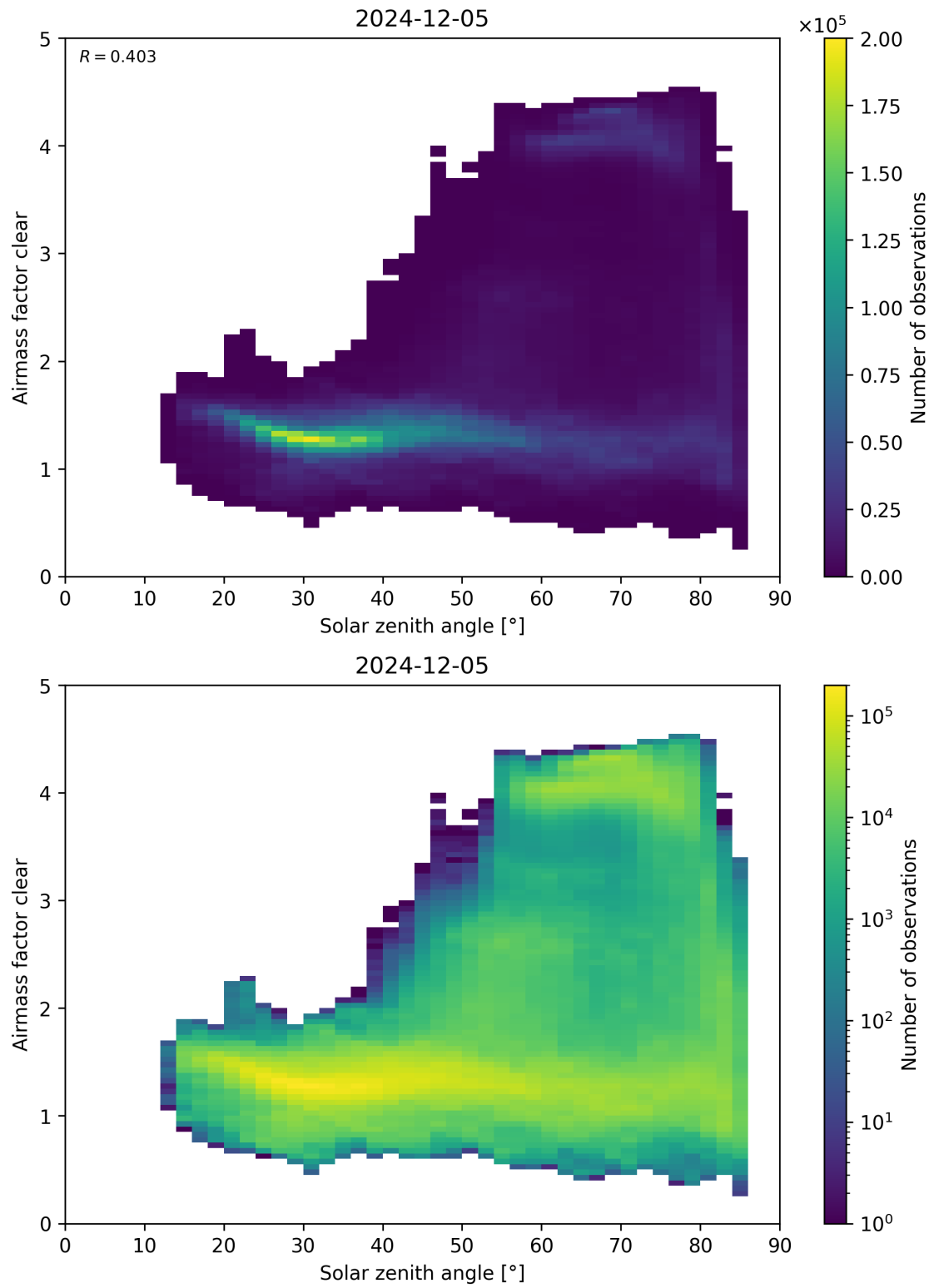
Figure 170: Scatter density plot of “Solar zenith angle” against “Airmass factor clear” for 2024-12-04 to 2024-12-06.
