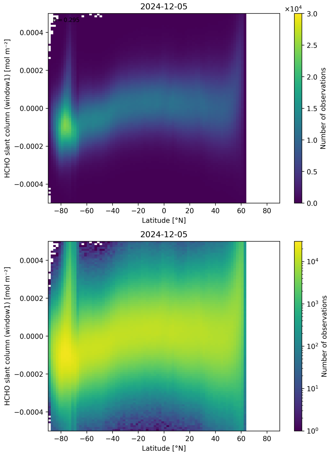
Figure 159: Scatter density plot of “Latitude” against “HCHO slant column (window1)” for 2024-12-04 to 2024-12-06.
