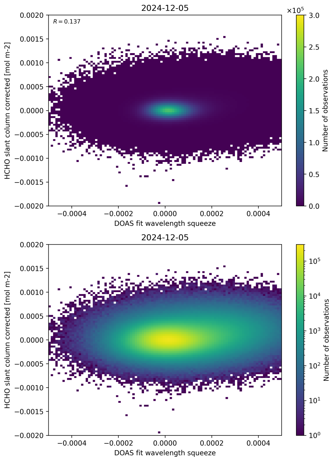
Figure 69: Scatter density plot of “DOAS fit wavelength squeeze” against “HCHO slant column corrected” for 2024-12-04 to 2024-12-06.
