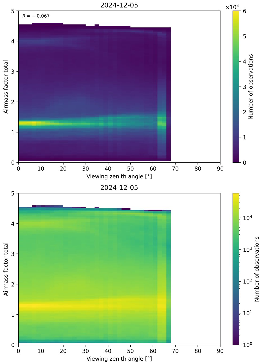
Figure 190: Scatter density plot of “Viewing zenith angle” against “Airmass factor total” for 2024-12-04 to 2024-12-06.
