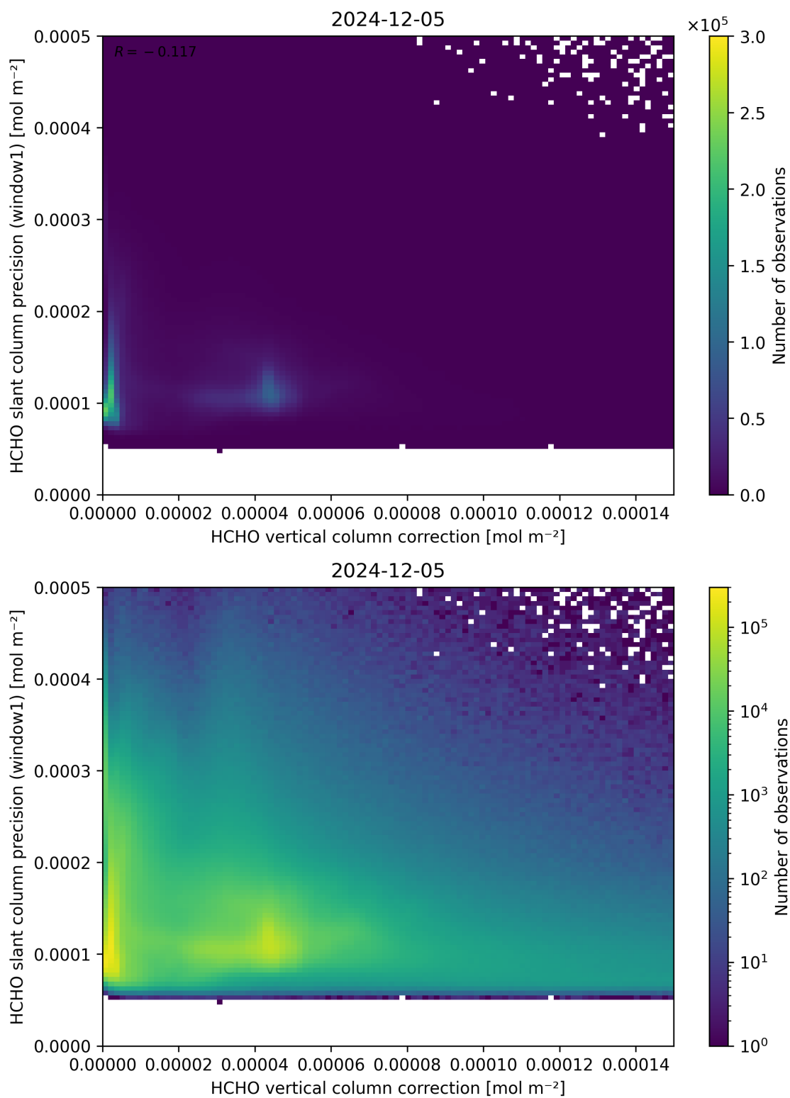
Figure 119: Scatter density plot of “HCHO vertical column correction” against “HCHO slant column precision (window1)” for 2024-12-04 to 2024-12-06.
