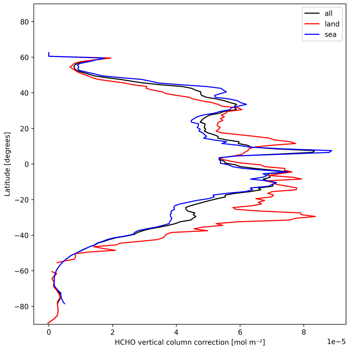
Figure 23: Zonal average of “HCHO vertical column correction” for 2024-12-04 to 2024-12-06.
