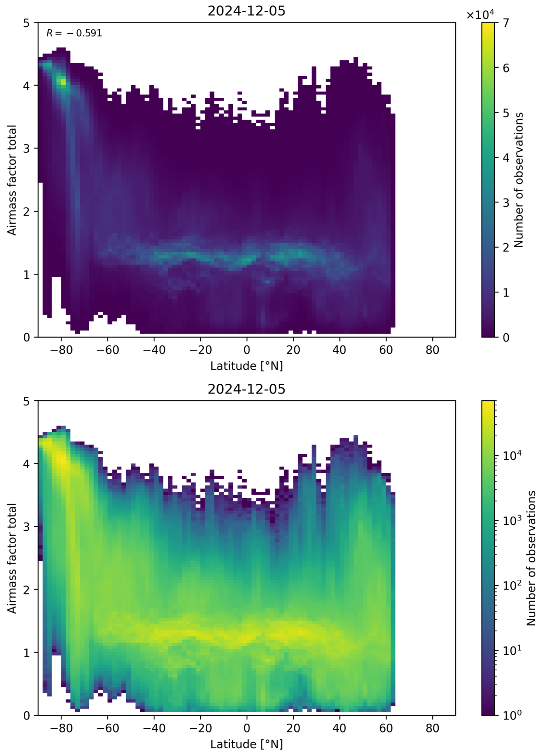
Figure 161: Scatter density plot of “Latitude” against “Airmass factor total” for 2024-12-04 to 2024-12-06.
