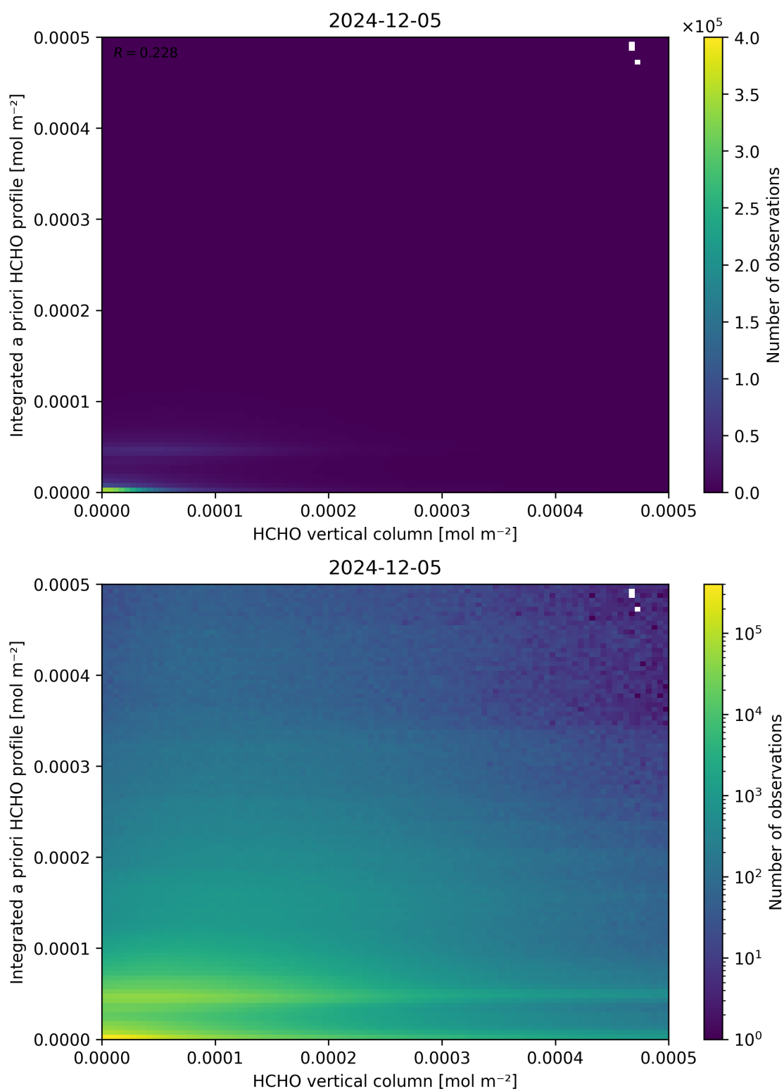
Figure 135: Scatter density plot of “HCHO vertical column” against “Integrated a priori HCHO profile” for 2024-12-04 to 2024-12-06.
