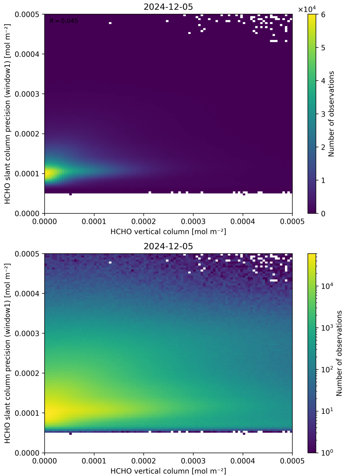
Figure 130: Scatter density plot of “HCHO vertical column” against “HCHO slant column precision (window1)” for 2024-12-04 to 2024-12-06.
