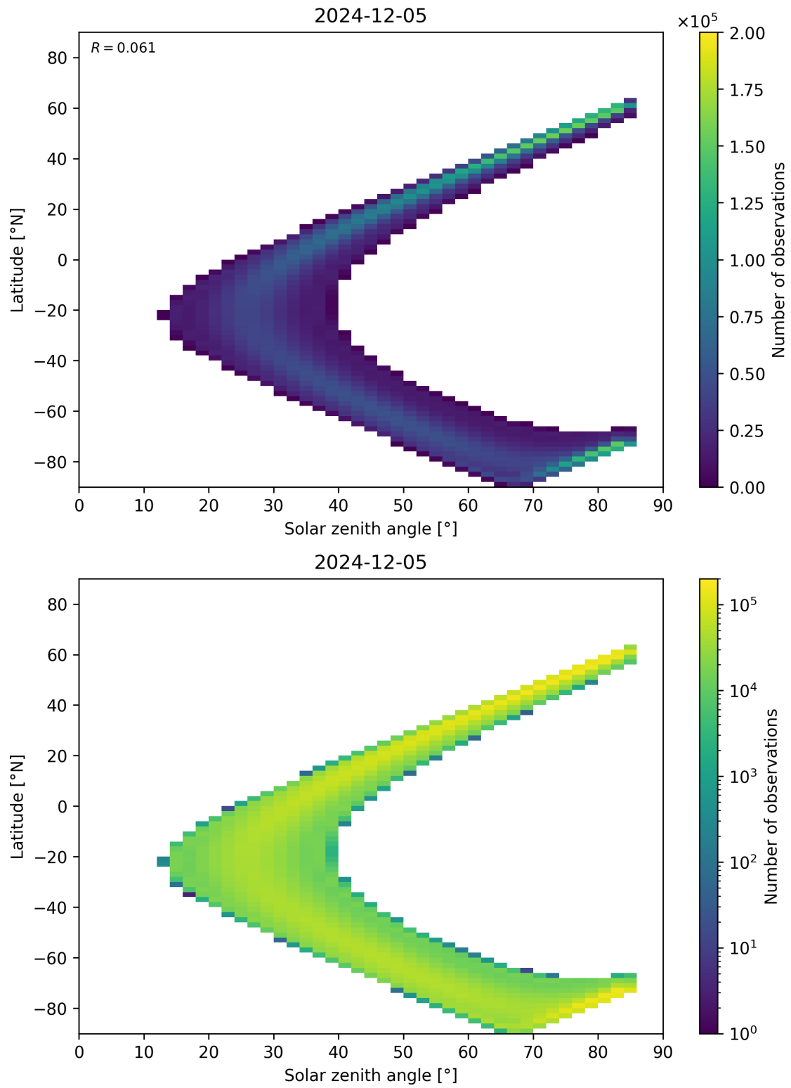
Figure 181: Scatter density plot of “Solar zenith angle” against “Latitude” for 2024-12-04 to 2024-12-06.
