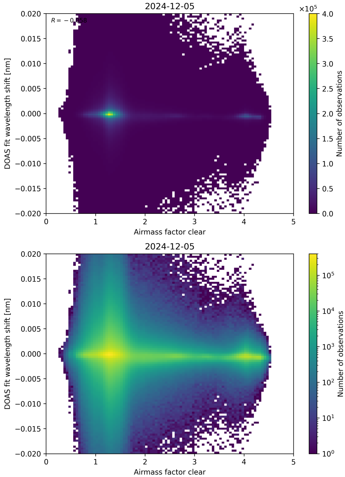
Figure 72: Scatter density plot of “Airmass factor clear” against “DOAS fit wavelength shift” for 2024-12-04 to 2024-12-06.
