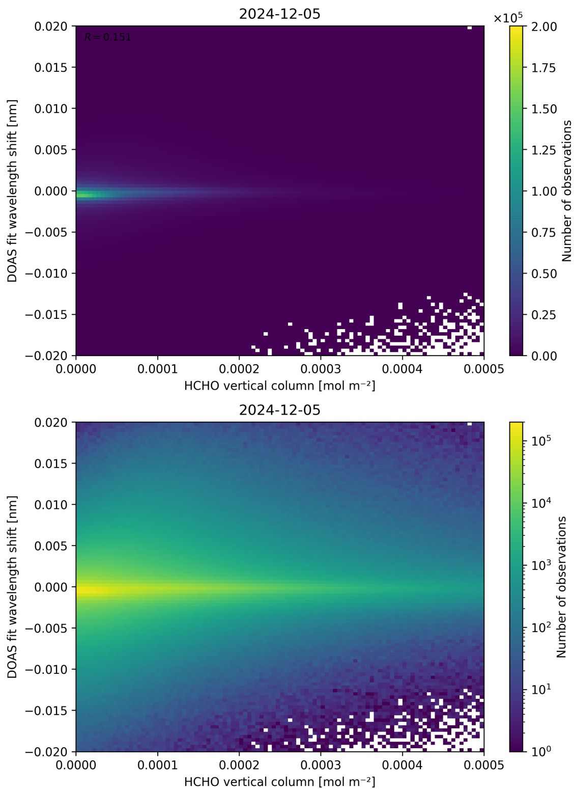
Figure 124: Scatter density plot of “HCHO vertical column” against “DOAS fit wavelength shift” for 2024-12-04 to 2024-12-06.
