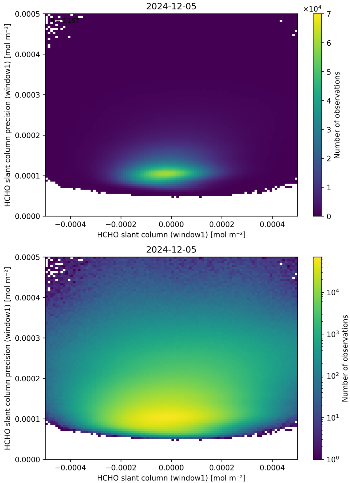
Figure 84: Scatter density plot of “HCHO slant column (window1)” against “HCHO slant column precision (window1)” for 2024-12-04 to 2024-12-06.
