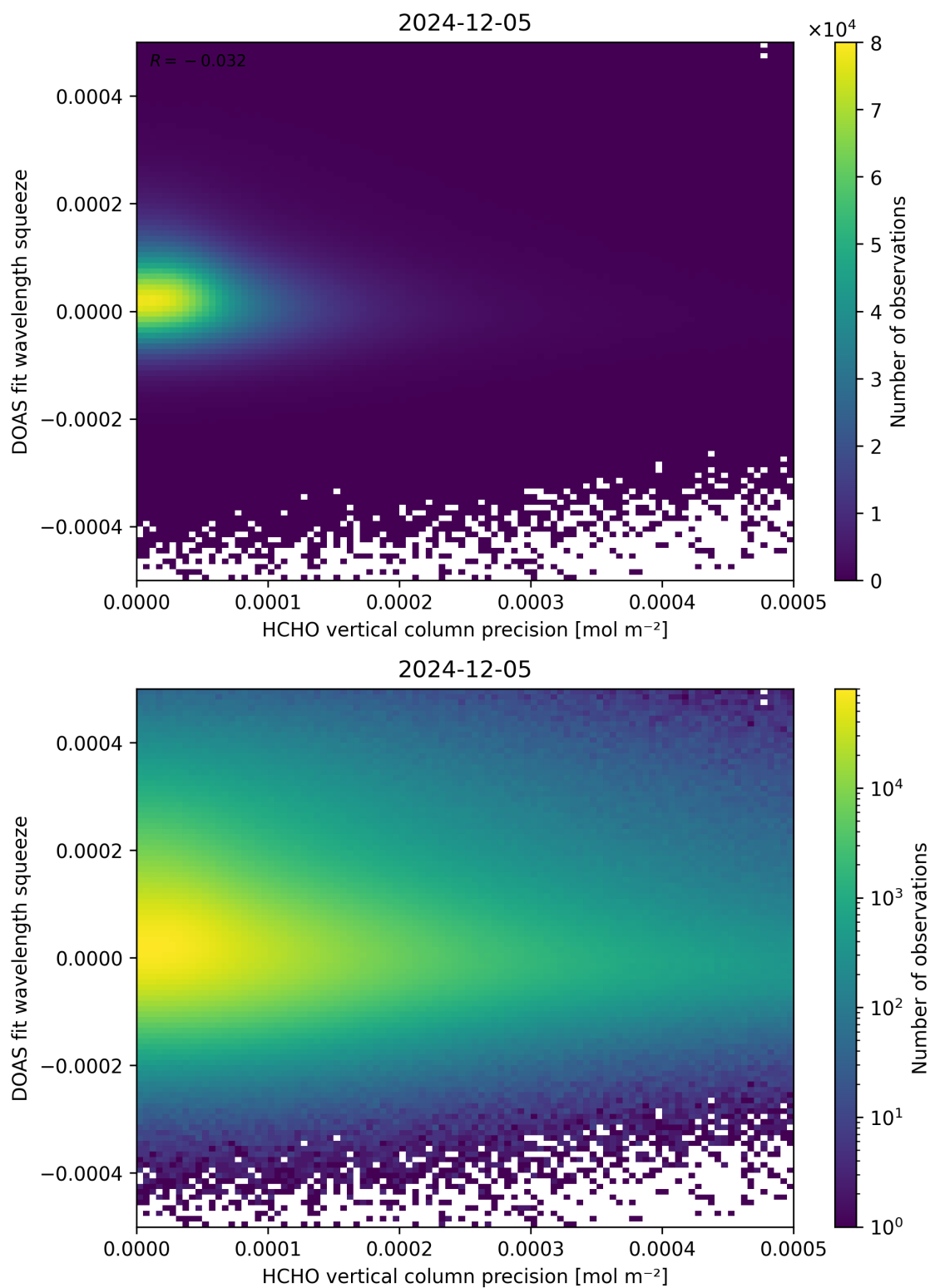
Figure 138: Scatter density plot of “HCHO vertical column precision” against “DOAS fit wavelength squeeze” for 2024-12-04 to 2024-12-06.
