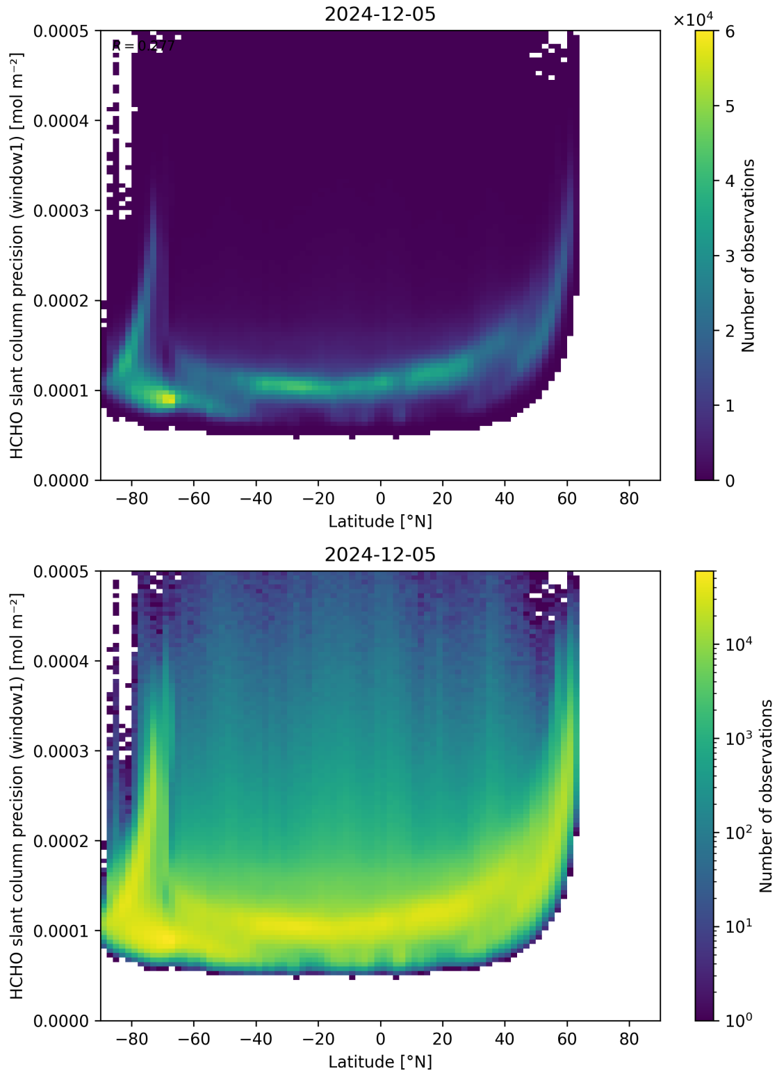
Figure 160: Scatter density plot of “Latitude” against “HCHO slant column precision (window1)” for 2024-12-04 to 2024-12-06.
