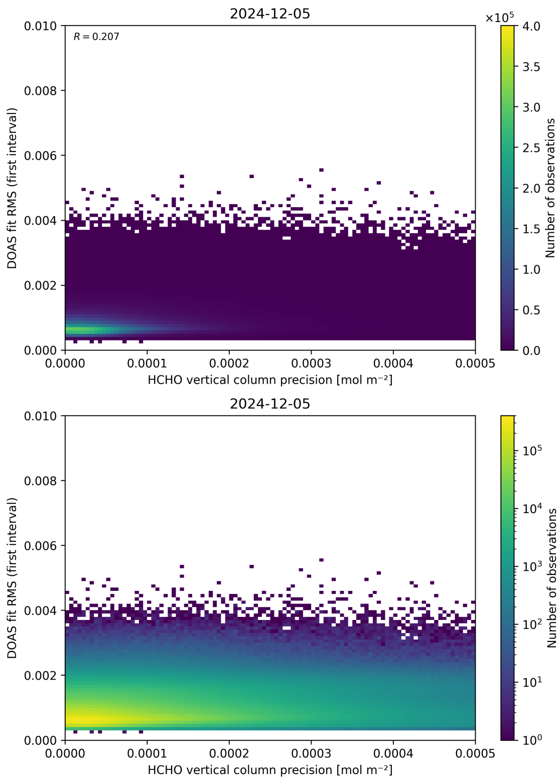
Figure 136: Scatter density plot of “HCHO vertical column precision” against “DOAS fit RMS (first interval)” for 2024-12-04 to 2024-12-06.
