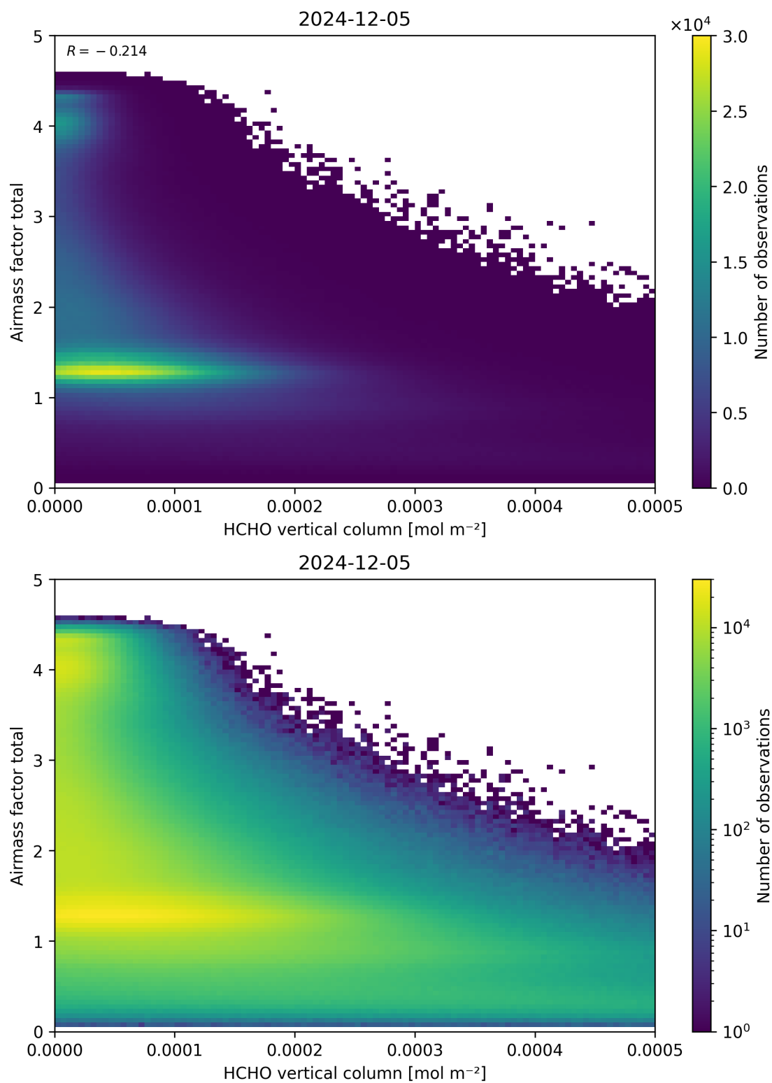
Figure 131: Scatter density plot of “HCHO vertical column” against “Airmass factor total” for 2024-12-04 to 2024-12-06.
