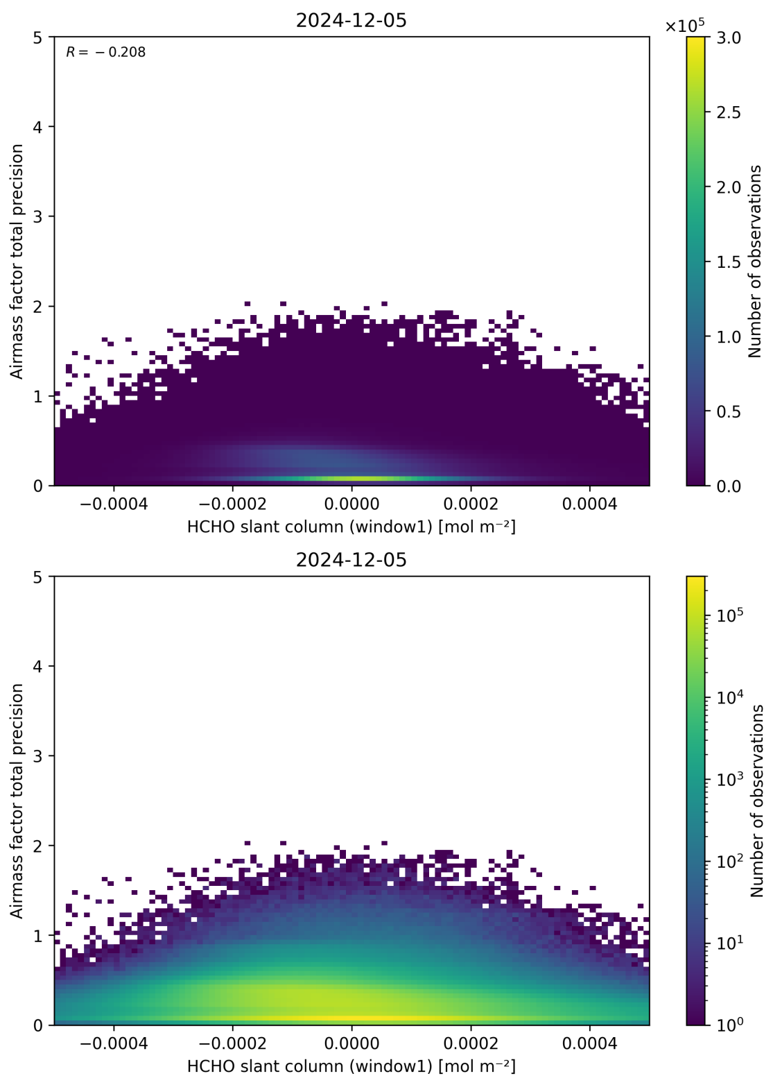
Figure 86: Scatter density plot of “HCHO slant column (window1)” against “Airmass factor total precision” for 2024-12-04 to 2024-12-06.
