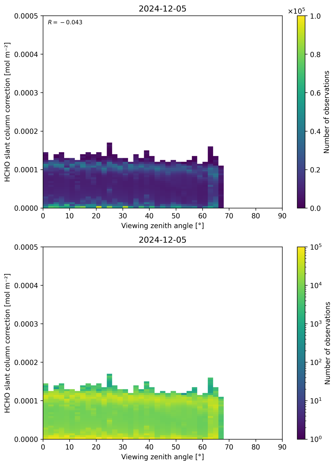
Figure 187: Scatter density plot of “Viewing zenith angle” against “HCHO slant column correction” for 2024-12-04 to 2024-12-06.
