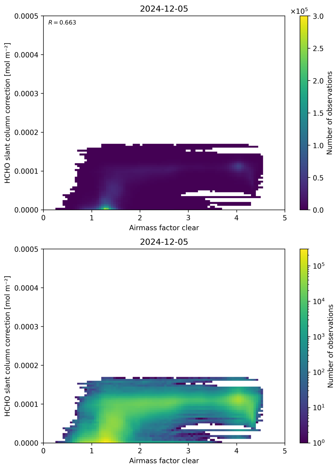
Figure 75: Scatter density plot of “Airmass factor clear” against “HCHO slant column correction” for 2024-12-04 to 2024-12-06.
