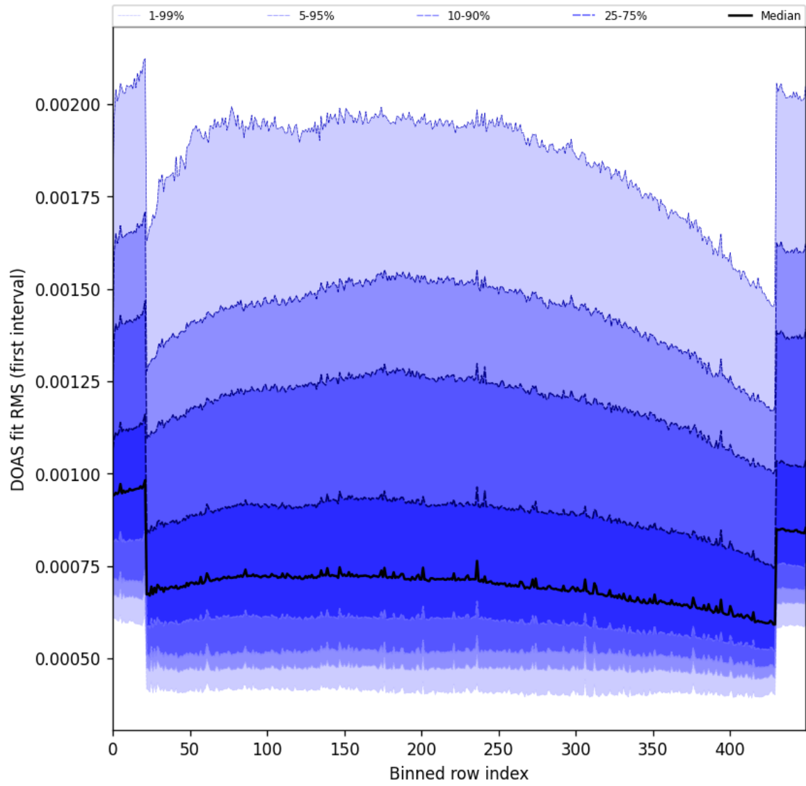
Figure 60: Along track statistics of “DOAS fit RMS (first interval)” for 2024-12-04 to 2024-12-06
