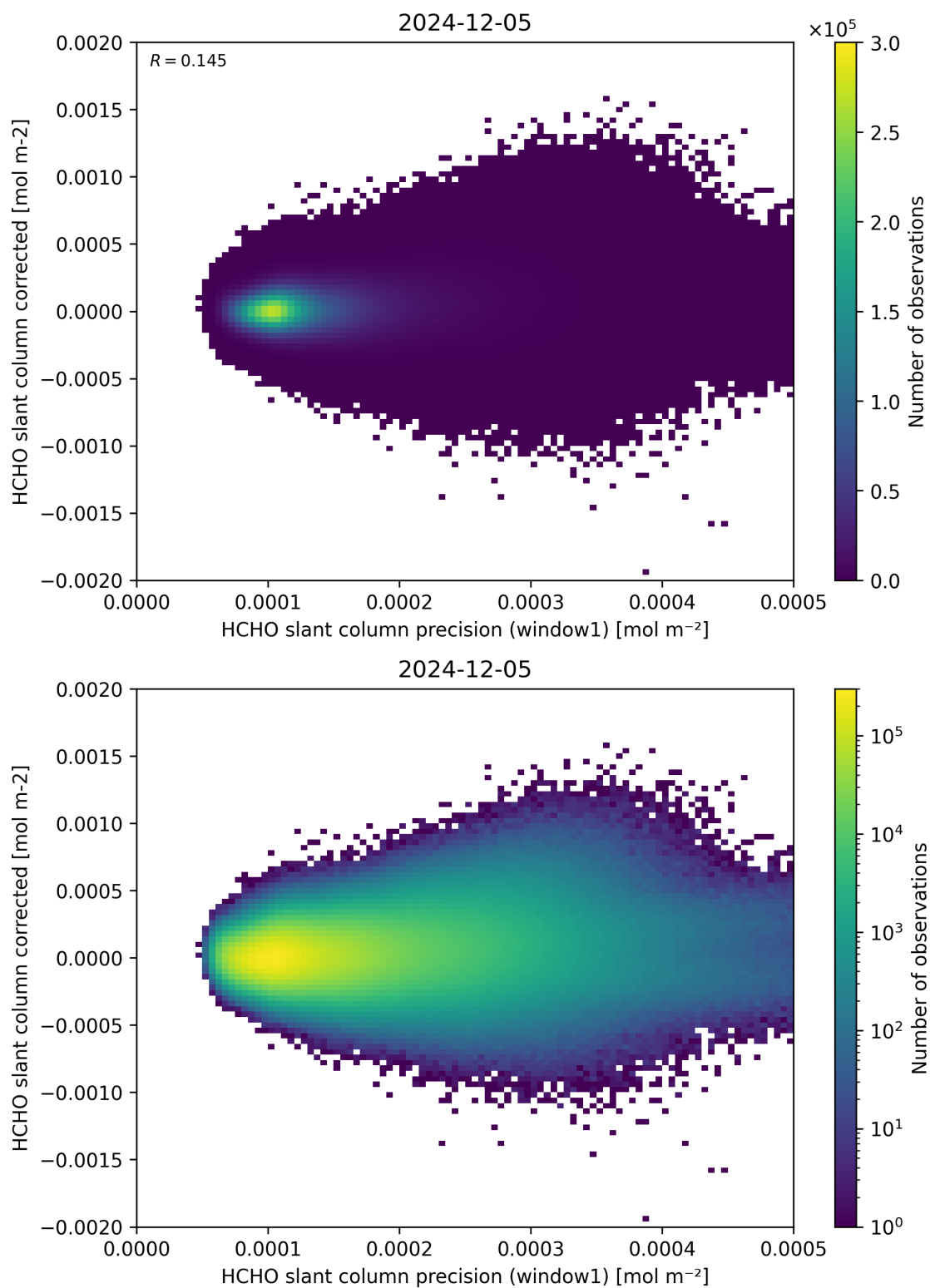
Figure 92: Scatter density plot of “HCHO slant column precision (window1)” against “HCHO slant column corrected” for 2024-12-04 to 2024-12-06.
