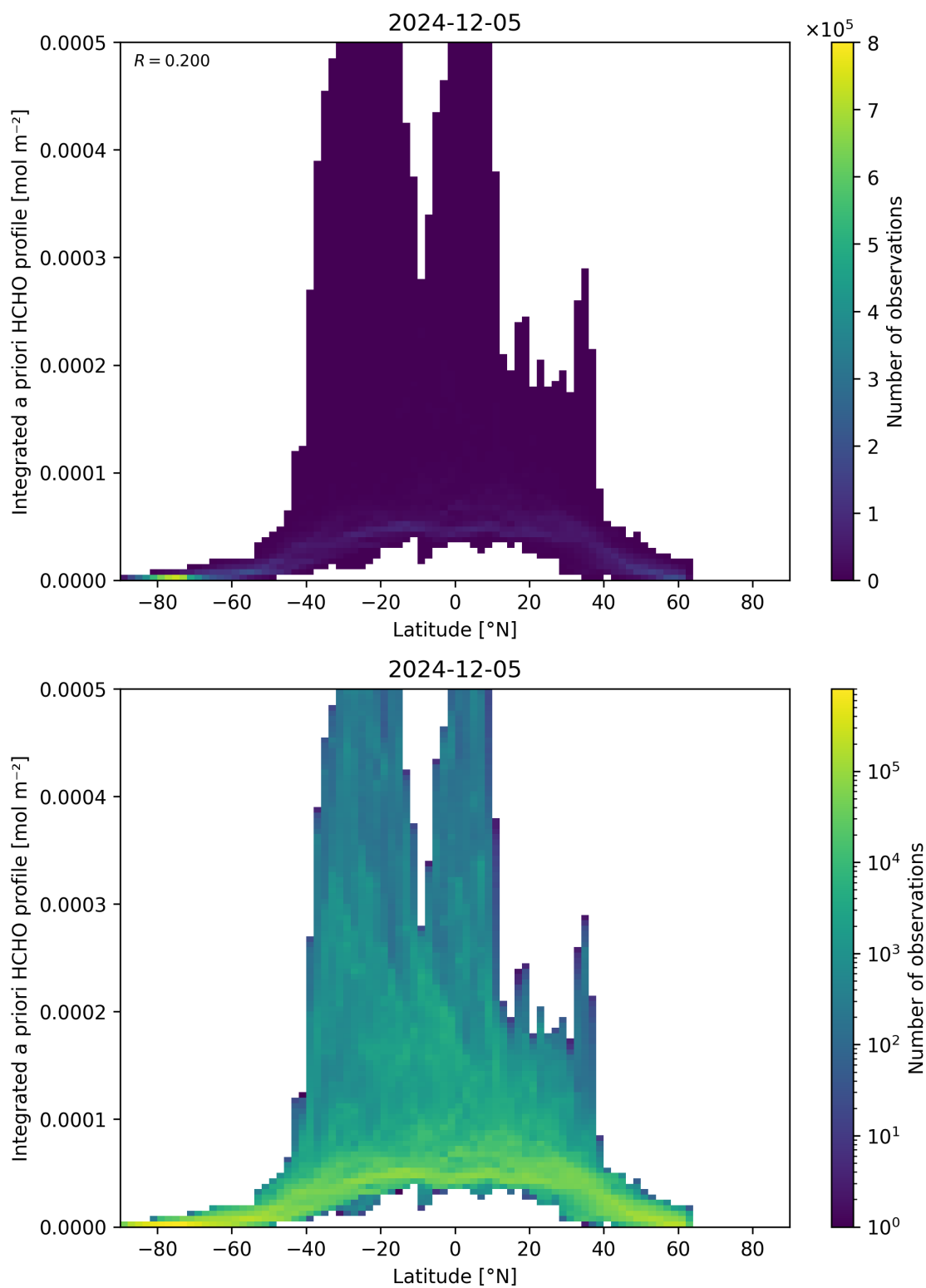
Figure 166: Scatter density plot of “Latitude” against “Integrated a priori HCHO profile” for 2024-12-04 to 2024-12-06.
