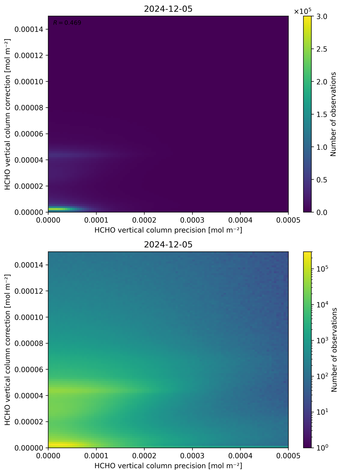
Figure 146: Scatter density plot of “HCHO vertical column precision” against “HCHO vertical column correction” for 2024-12-04 to 2024-12-06.
