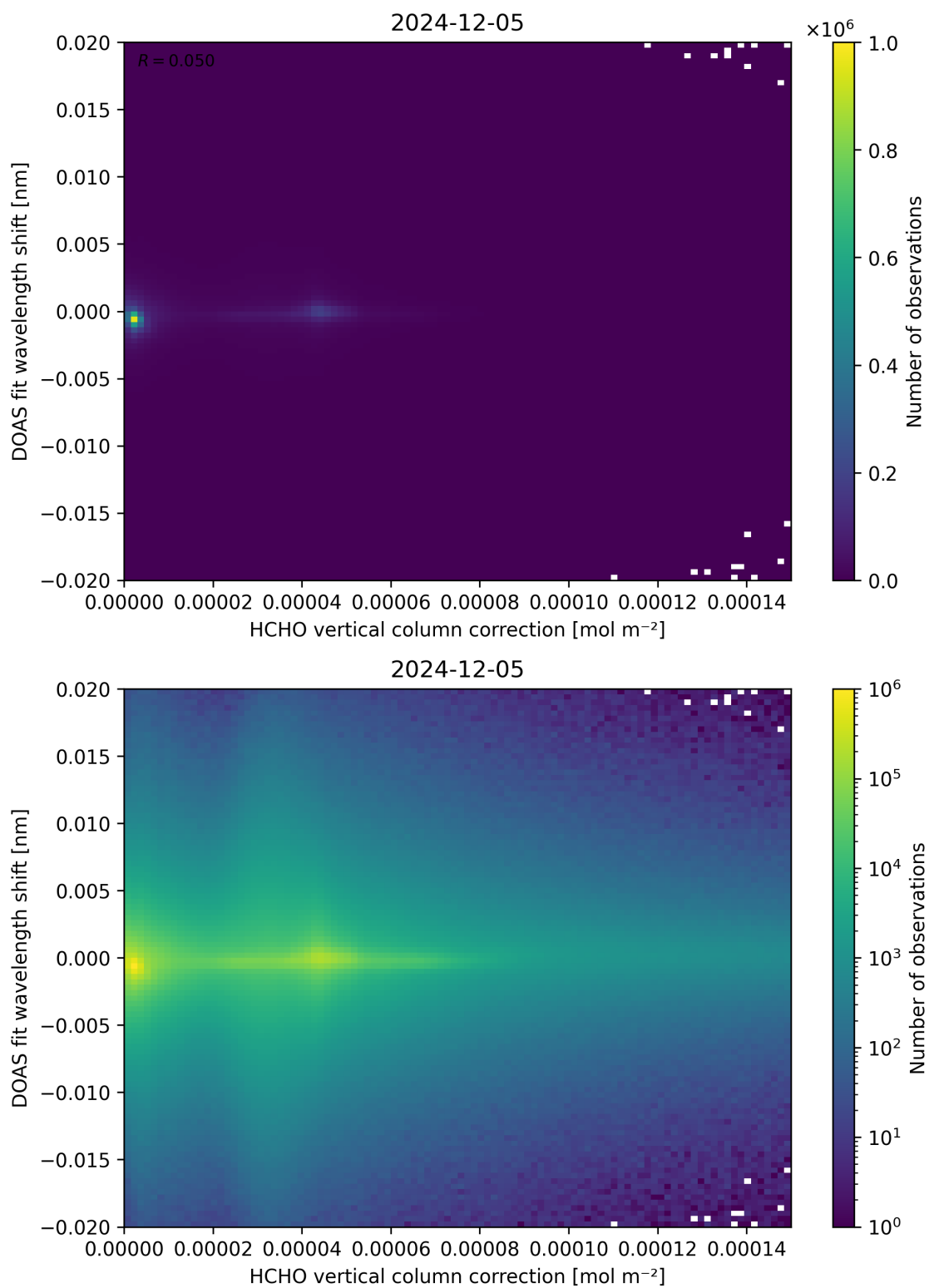
Figure 113: Scatter density plot of “HCHO vertical column correction” against “DOAS fit wavelength shift” for 2024-12-04 to 2024-12-06.
