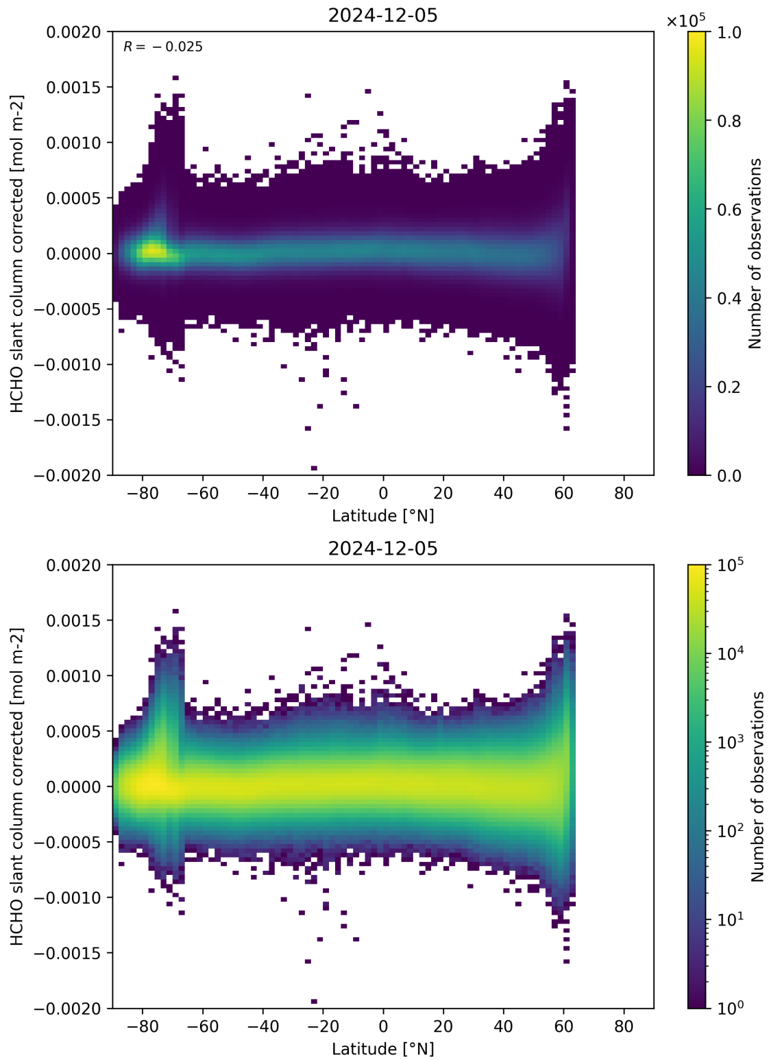
Figure 157: Scatter density plot of “Latitude” against “HCHO slant column corrected” for 2024-12-04 to 2024-12-06.
