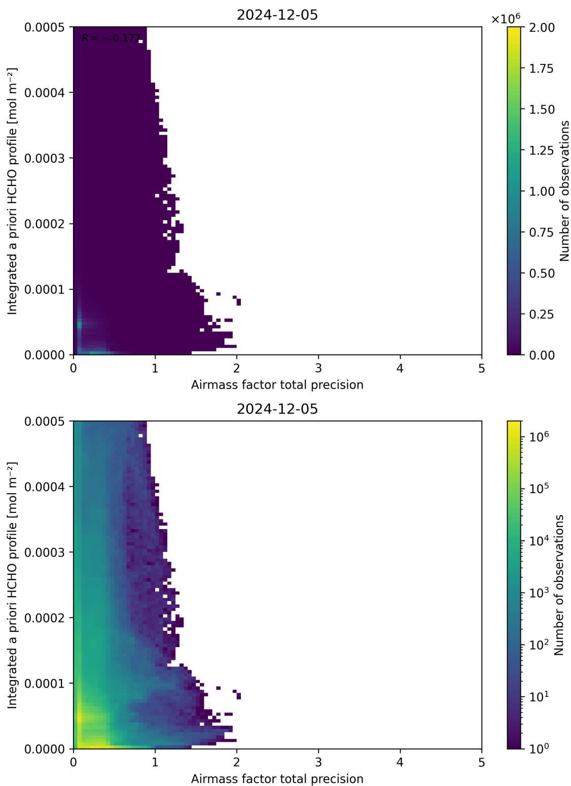
Figure 111: Scatter density plot of “Airmass factor total precision” against “Integrated a priori HCHO profile” for 2024-12-04 to 2024-12-06.
