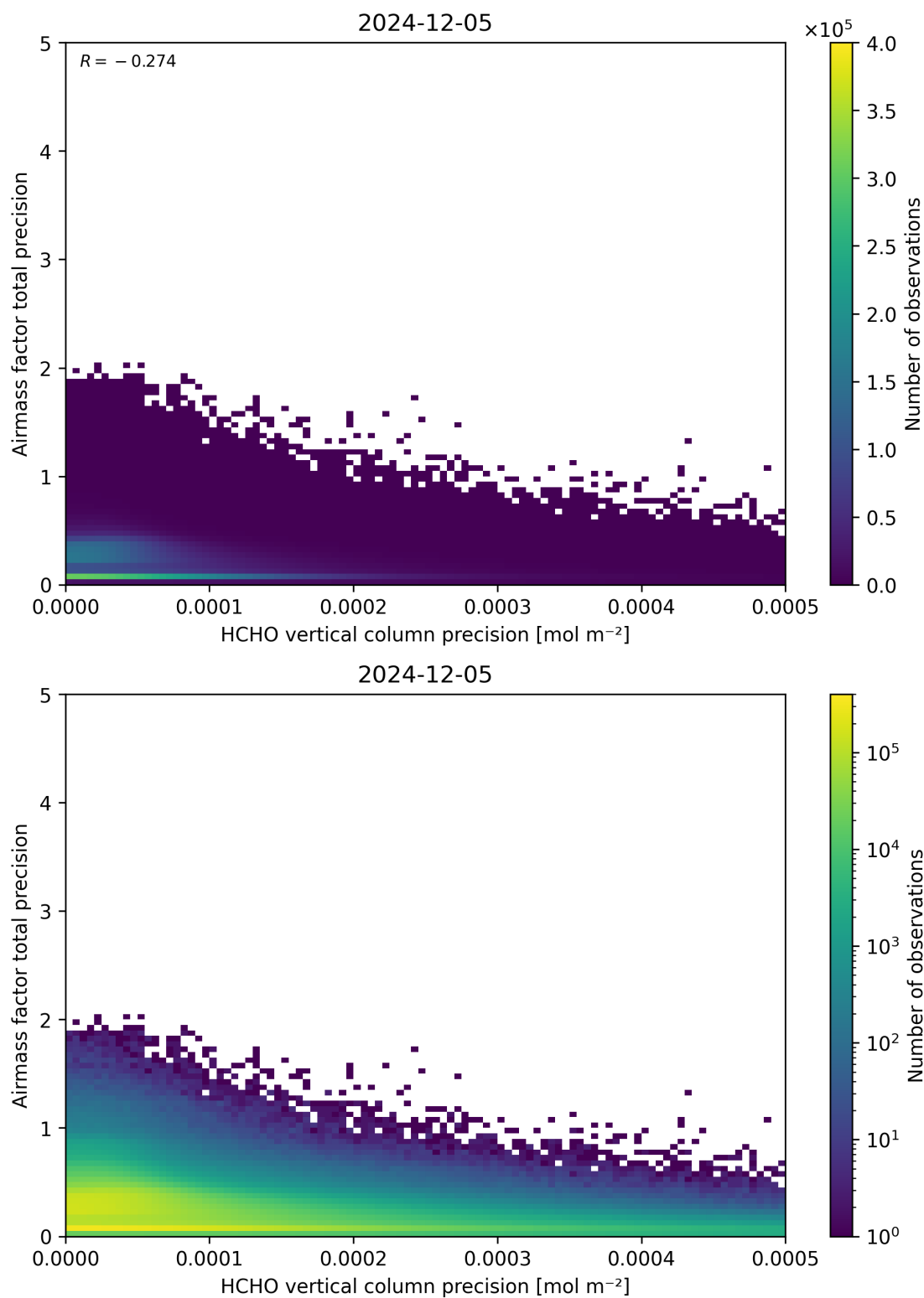
Figure 145: Scatter density plot of “HCHO vertical column precision” against “Airmass factor total precision” for 2024-12-04 to 2024-12-06.
