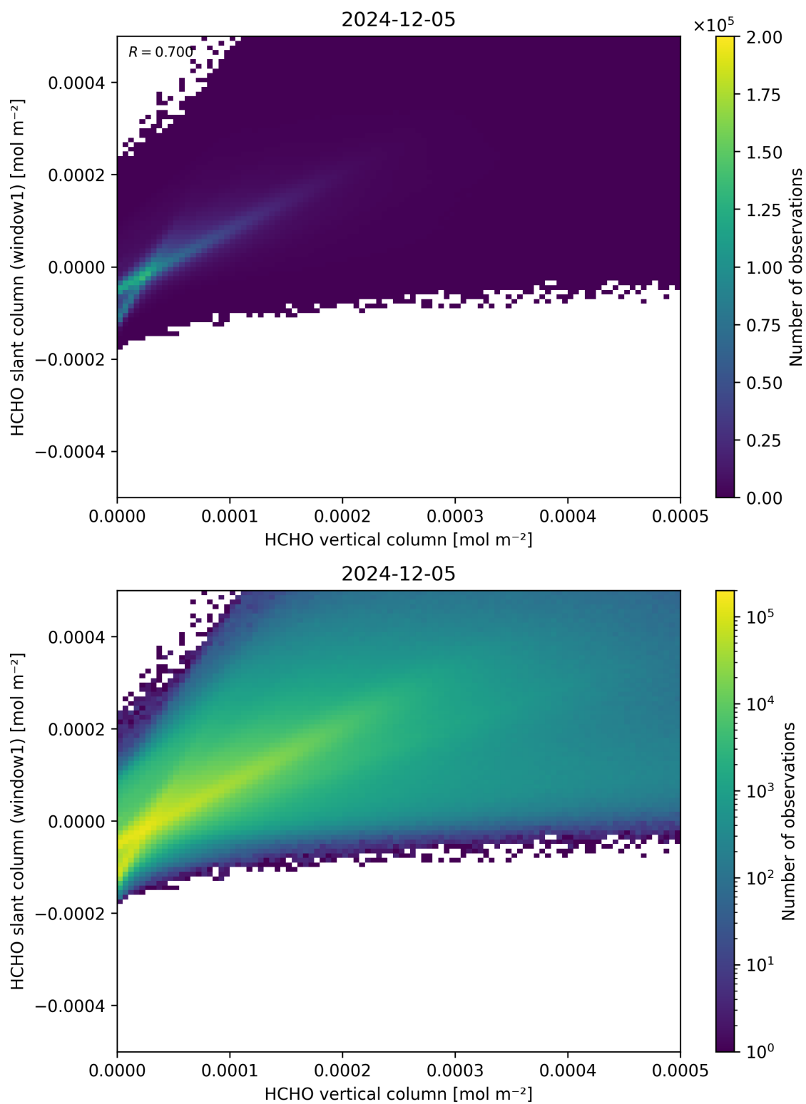
Figure 129: Scatter density plot of “HCHO vertical column” against “HCHO slant column (window1)” for 2024-12-04 to 2024-12-06.
