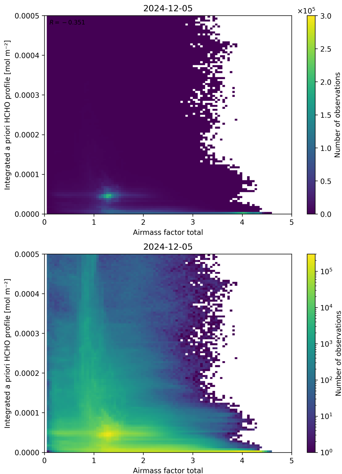
Figure 104: Scatter density plot of “Airmass factor total” against “Integrated a priori HCHO profile” for 2024-12-04 to 2024-12-06.
