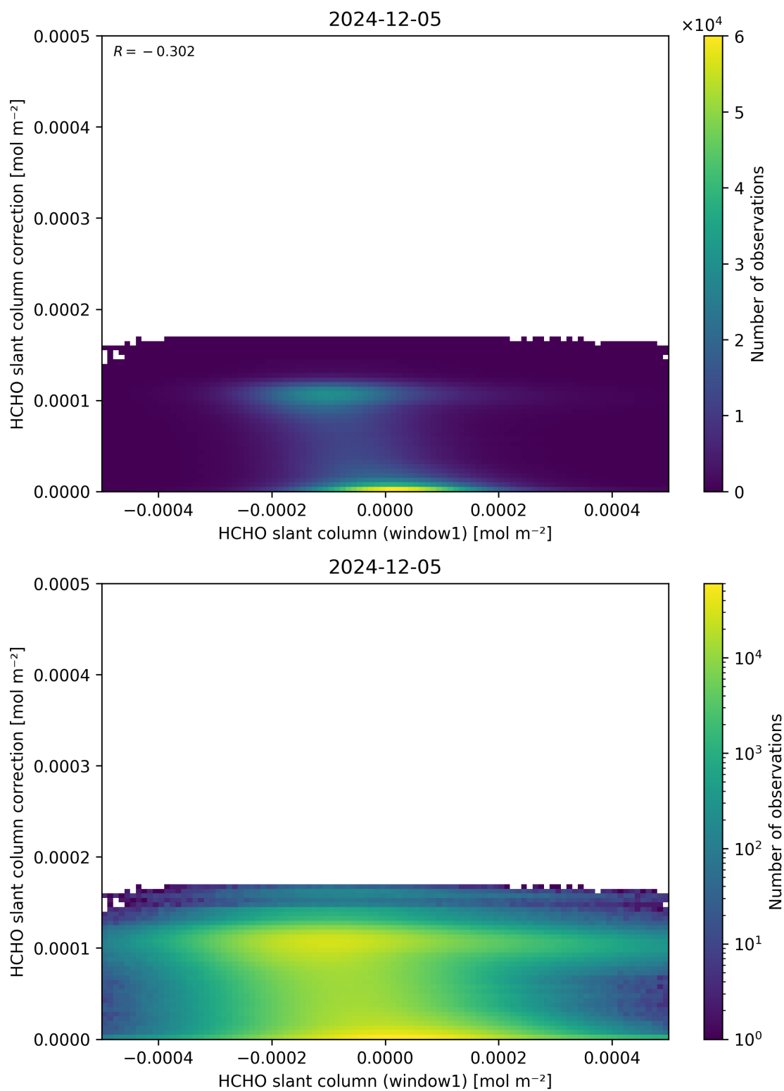
Figure 83: Scatter density plot of “HCHO slant column (window1)” against “HCHO slant column correction” for 2024-12-04 to 2024-12-06.
