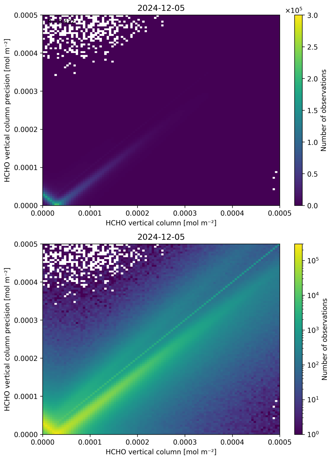
Figure 134: Scatter density plot of “HCHO vertical column” against “HCHO vertical column precision” for 2024-12-04 to 2024-12-06.
