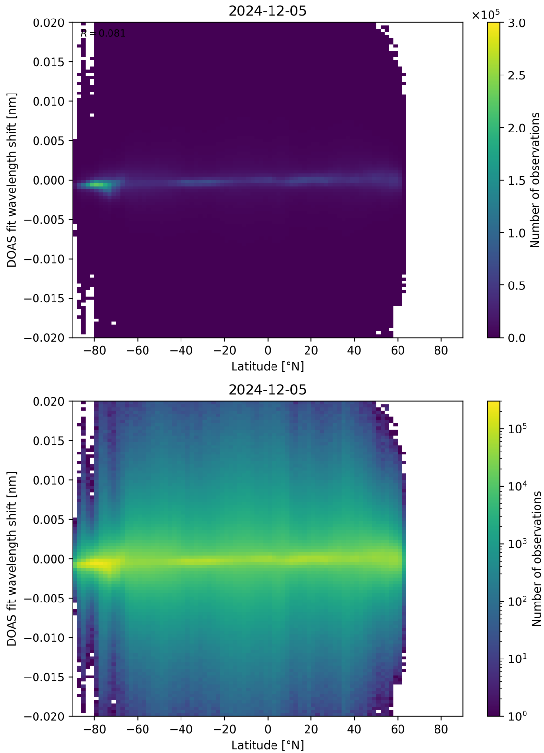
Figure 154: Scatter density plot of “Latitude” against “DOAS fit wavelength shift” for 2024-12-04 to 2024-12-06.
