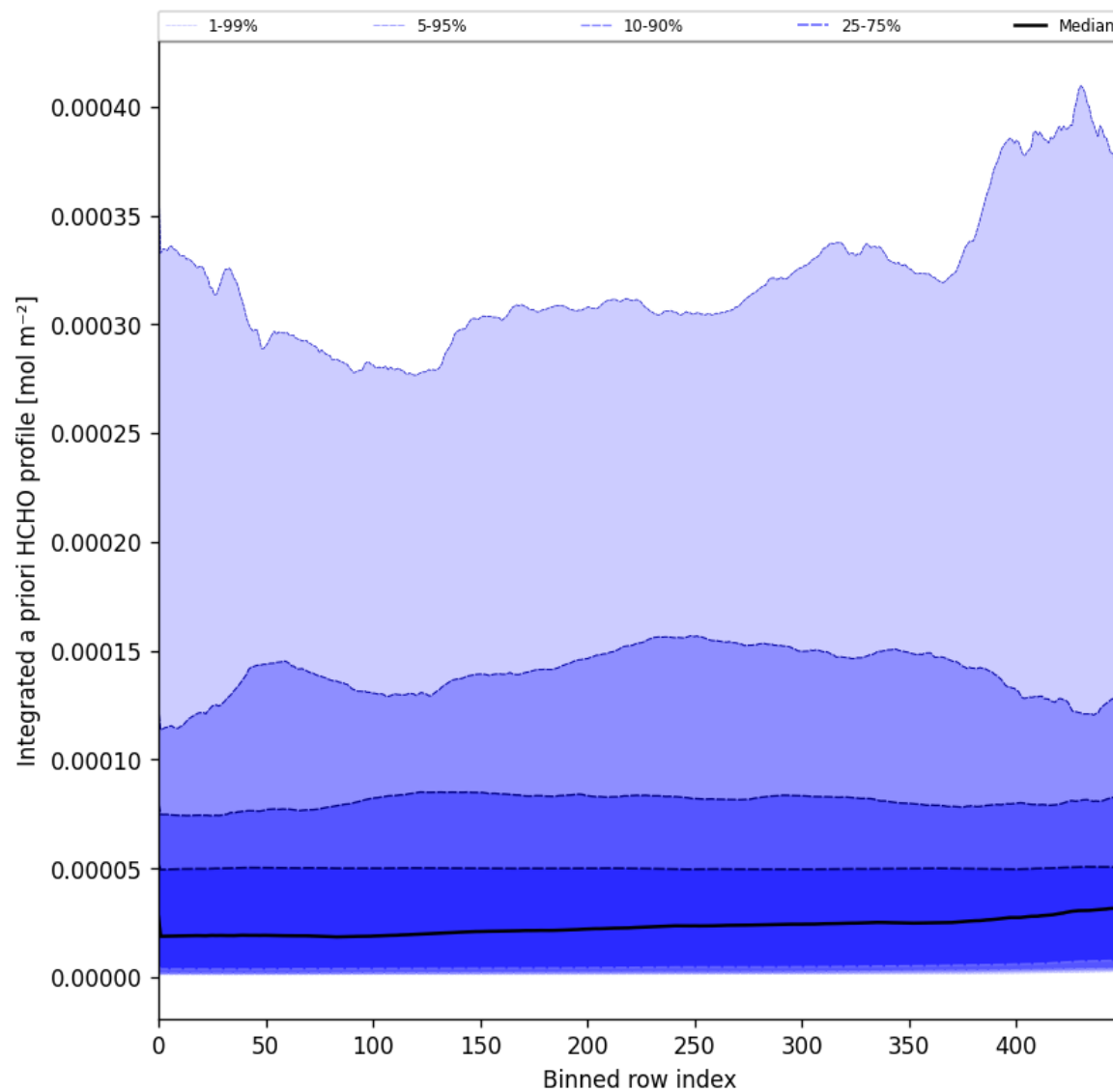
Figure 57: Along track statistics of “Integrated a priori HCHO profile” for 2024-12-04 to 2024-12-06
