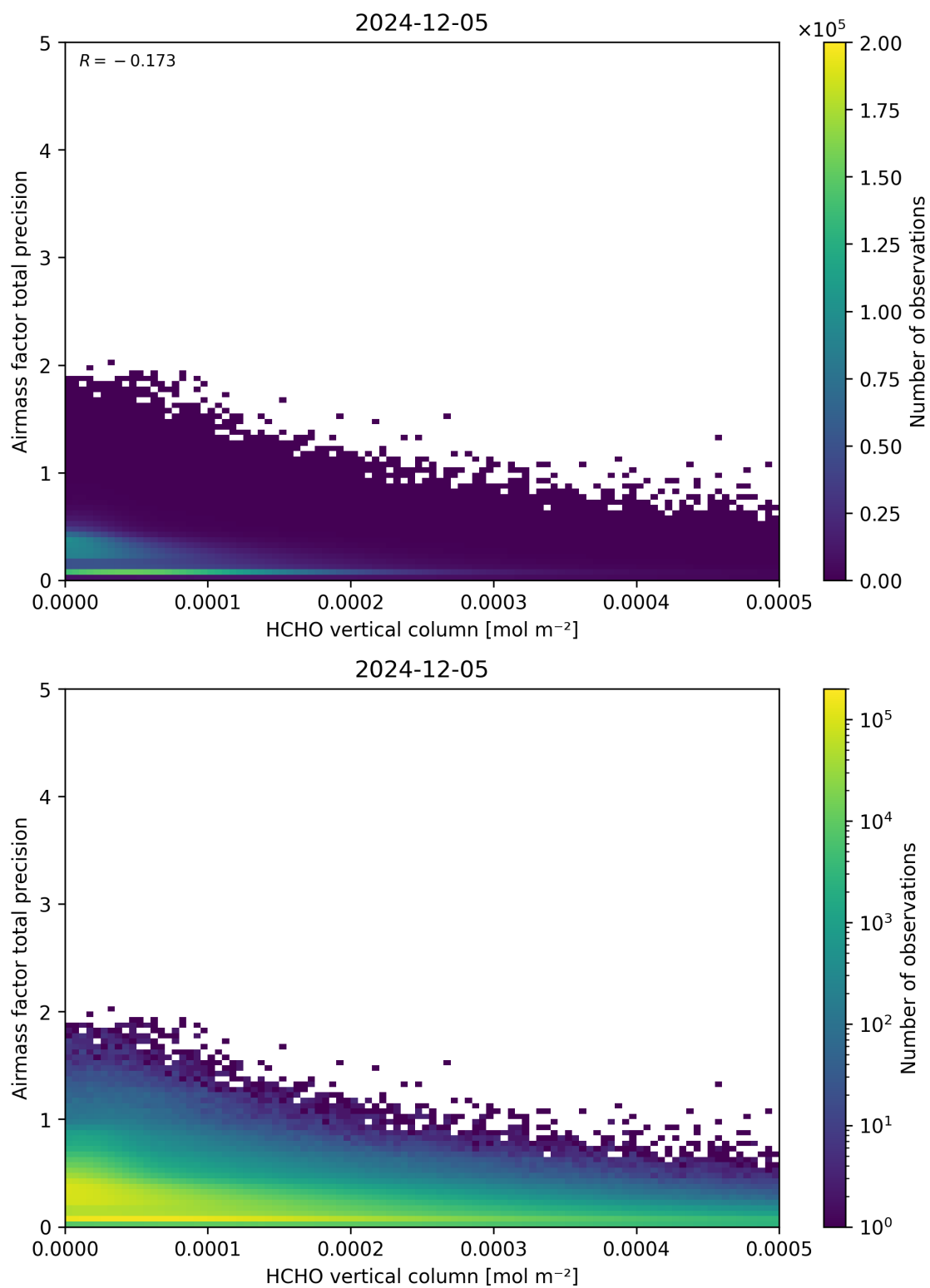
Figure 132: Scatter density plot of “HCHO vertical column” against “Airmass factor total precision” for 2024-12-04 to 2024-12-06.
