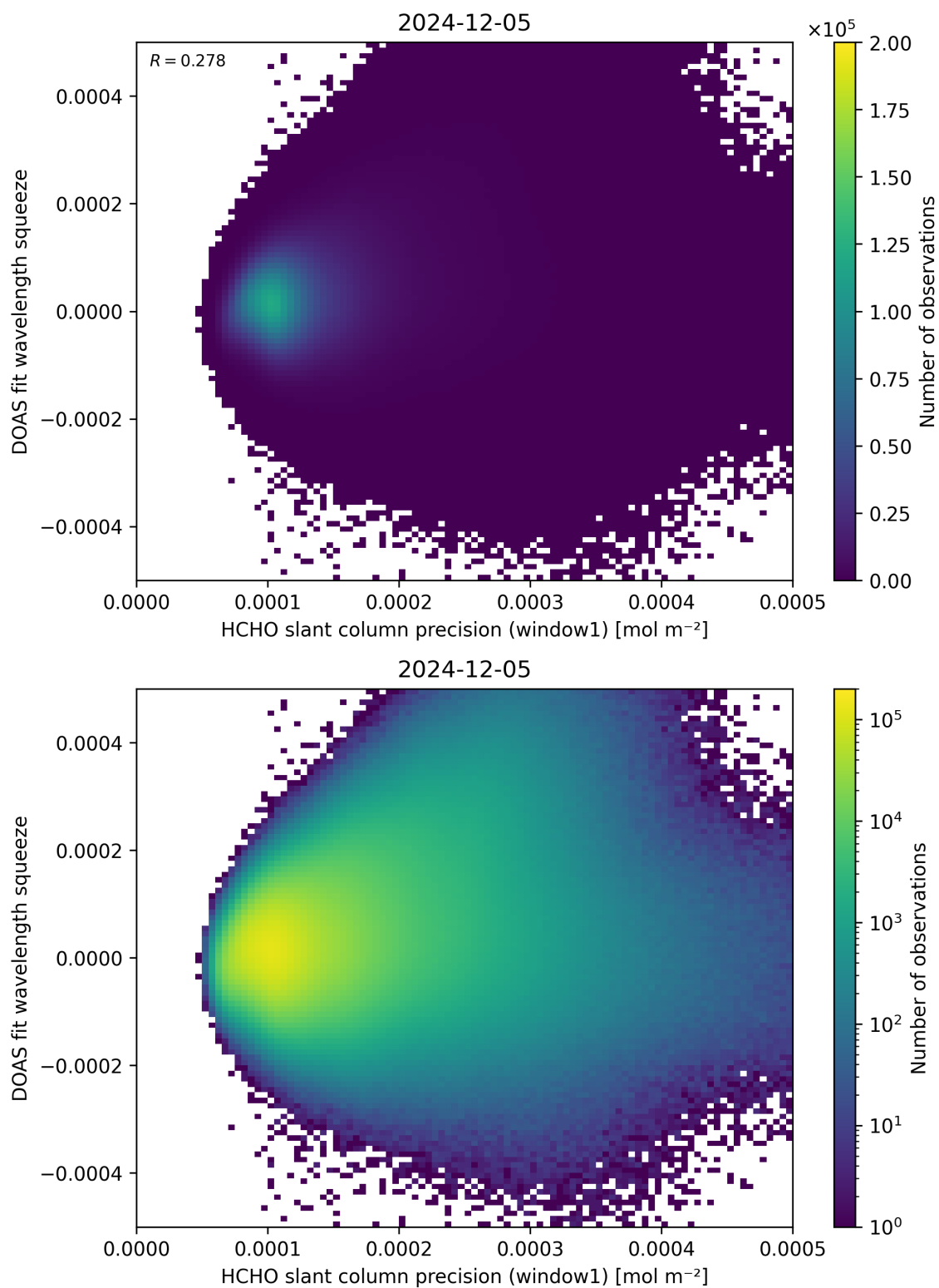
Figure 90: Scatter density plot of “HCHO slant column precision (window1)” against “DOAS fit wavelength squeeze” for 2024-12-04 to 2024-12-06.
