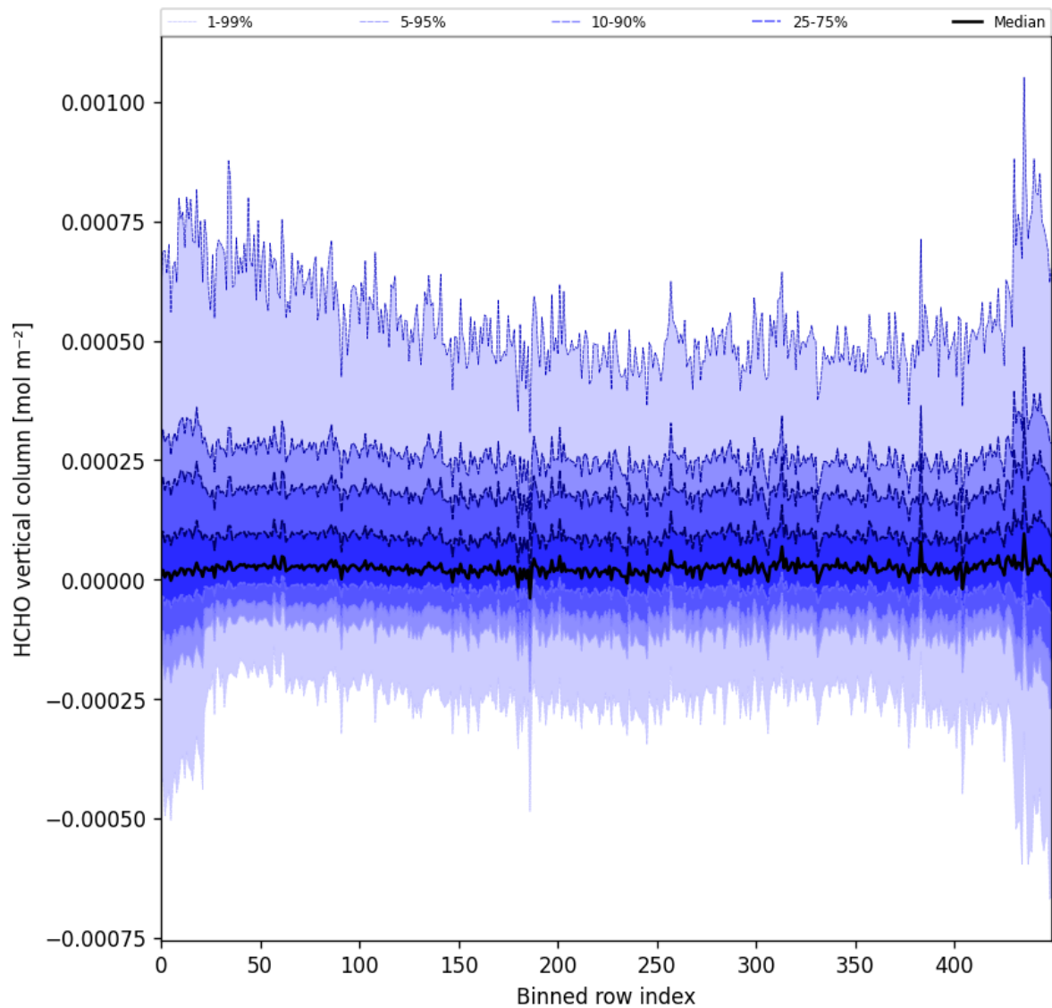
Figure 49: Along track statistics of “HCHO vertical column” for 2024-12-04 to 2024-12-06
