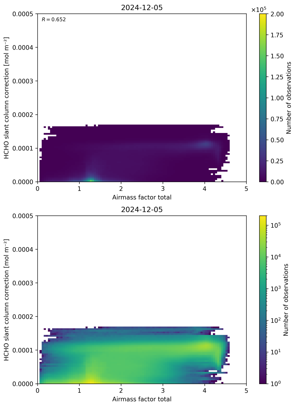
Figure 102: Scatter density plot of “Airmass factor total” against “HCHO slant column correction” for 2024-12-04 to 2024-12-06.
