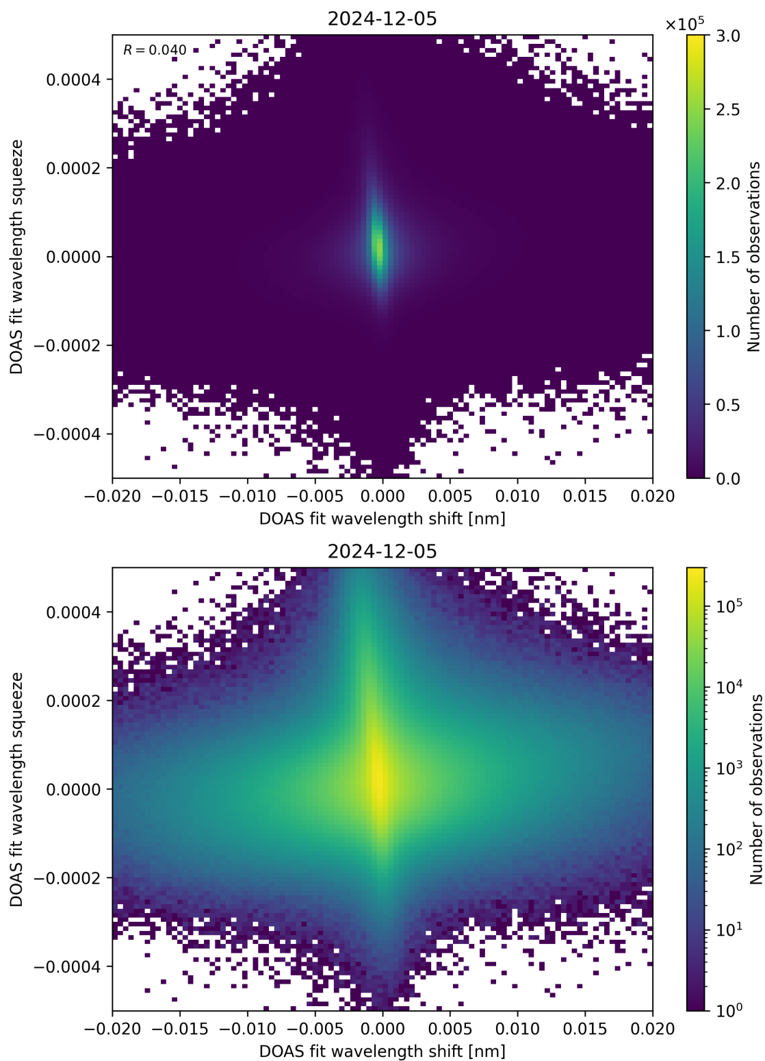
Figure 65: Scatter density plot of “DOAS fit wavelength shift” against “DOAS fit wavelength squeeze” for 2024-12-04 to 2024-12-06.
