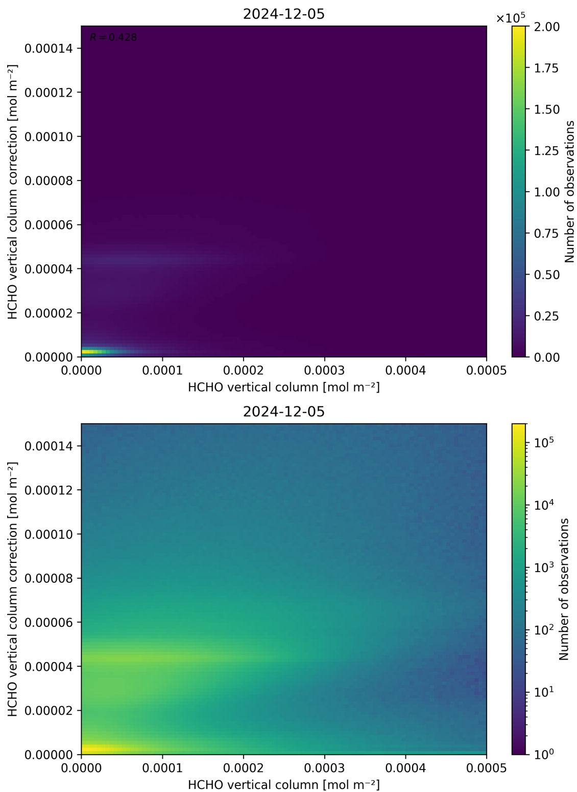
Figure 133: Scatter density plot of “HCHO vertical column” against “HCHO vertical column correction” for 2024-12-04 to 2024-12-06.
