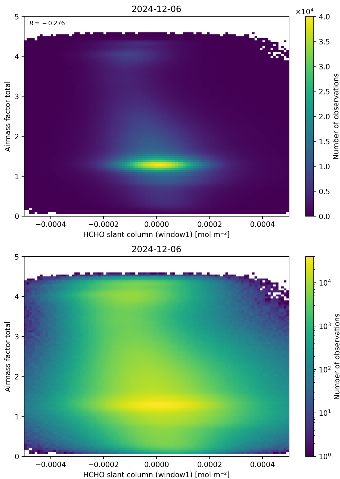
Figure 85: Scatter density plot of “HCHO slant column (window1)” against “Airmass factor total” for 2024-12-06 to 2024-12-07.
