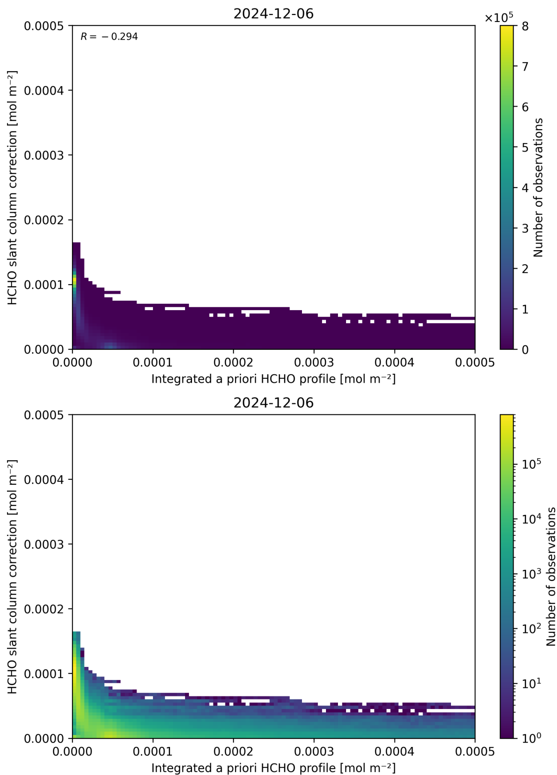
Figure 152: Scatter density plot of “Integrated a priori HCHO profile” against “HCHO slant column correction” for 2024-12-06 to 2024-12-07.
