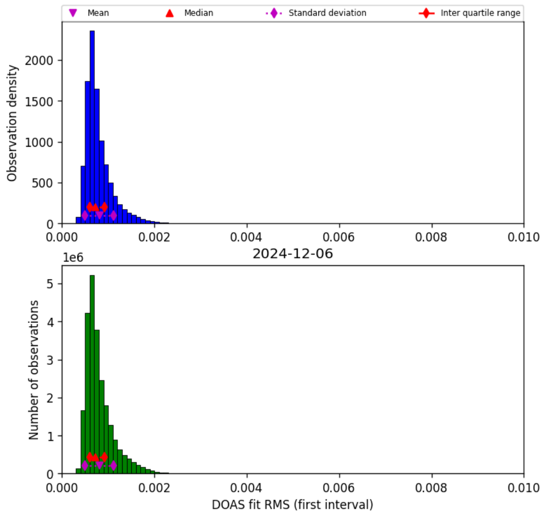
Figure 46: Histogram of “DOAS fit RMS (first interval)” for 2024-12-06 to 2024-12-07
