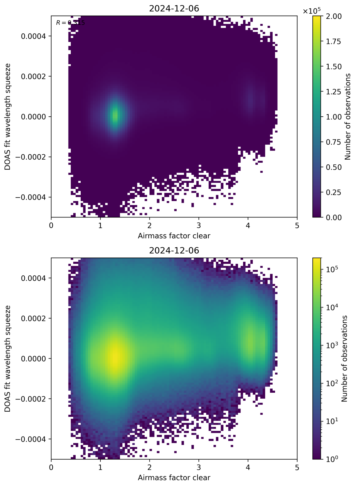
Figure 73: Scatter density plot of “Airmass factor clear” against “DOAS fit wavelength squeeze” for 2024-12-06 to 2024-12-07.
