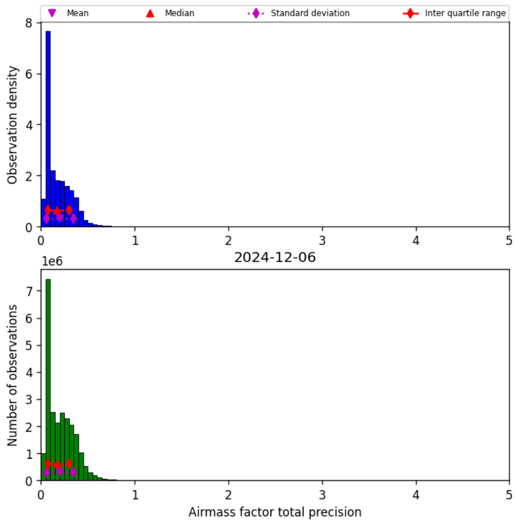
Figure 41: Histogram of “Airmass factor total precision” for 2024-12-06 to 2024-12-07
