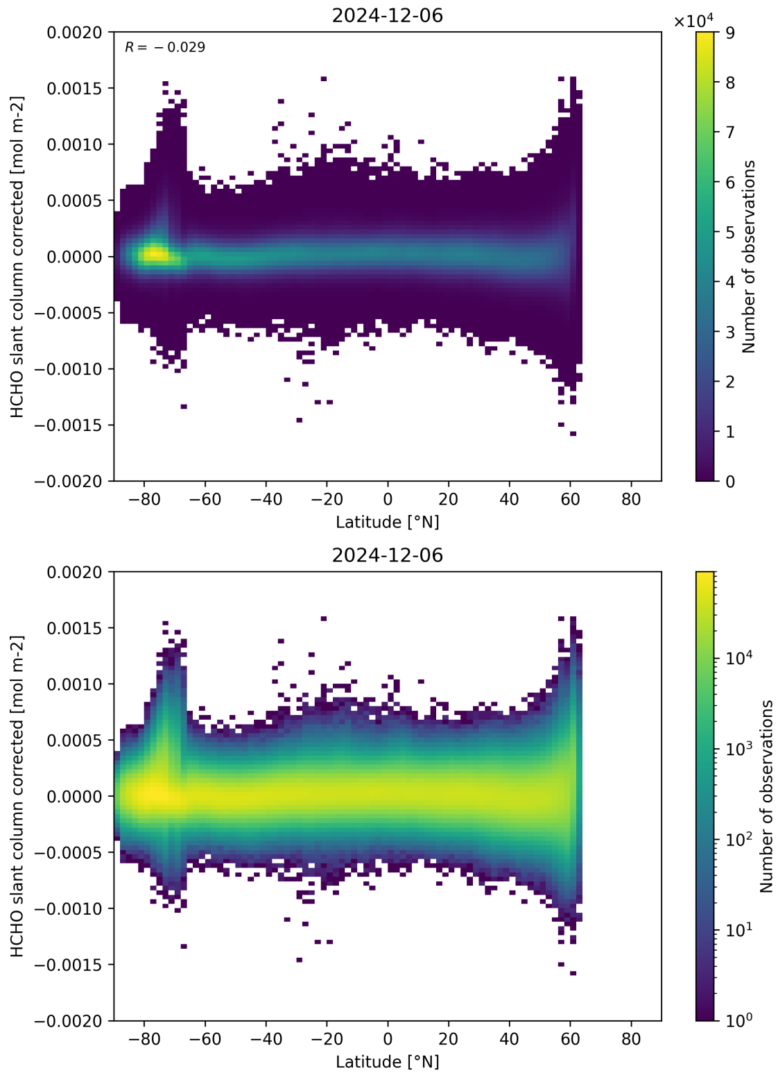
Figure 157: Scatter density plot of “Latitude” against “HCHO slant column corrected” for 2024-12-06 to 2024-12-07.
