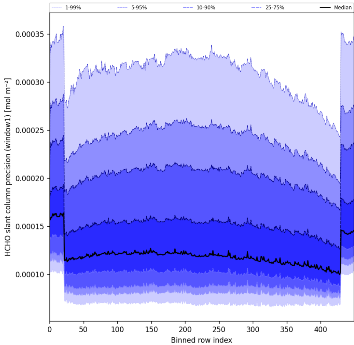
Figure 53: Along track statistics of “HCHO slant column precision (window1)” for 2024-12-06 to 2024-12-07
