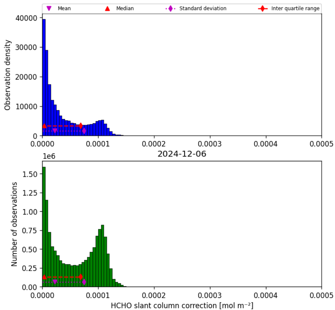
Figure 47: Histogram of “HCHO slant column correction” for 2024-12-06 to 2024-12-07
