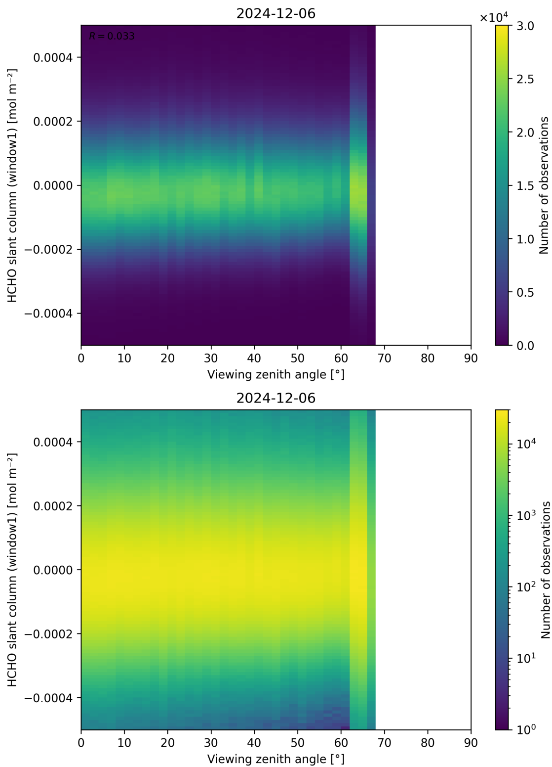
Figure 188: Scatter density plot of “Viewing zenith angle” against “HCHO slant column (window1)” for 2024-12-06 to 2024-12-07.
