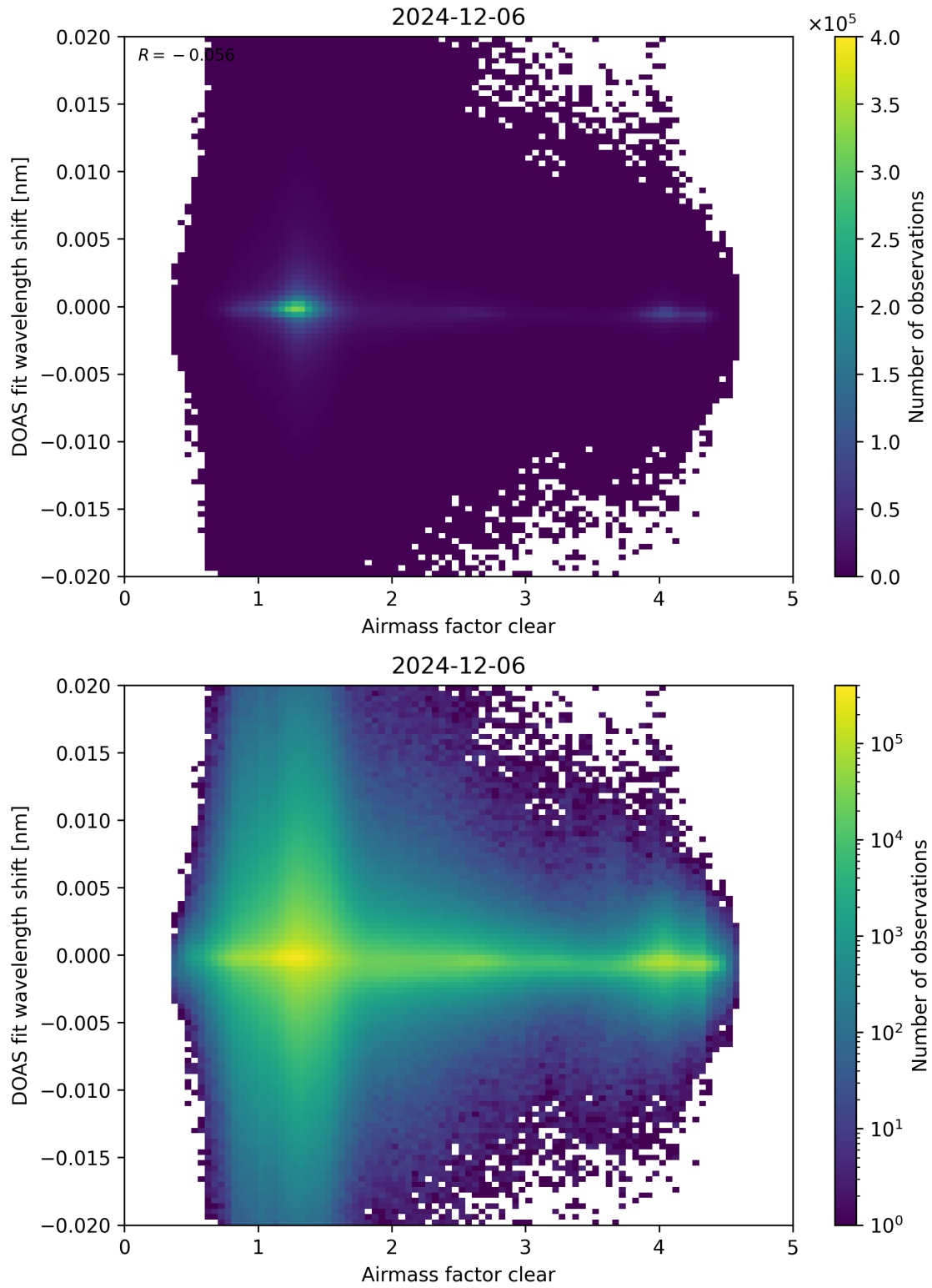
Figure 72: Scatter density plot of “Airmass factor clear” against “DOAS fit wavelength shift” for 2024-12-06 to 2024-12-07.
