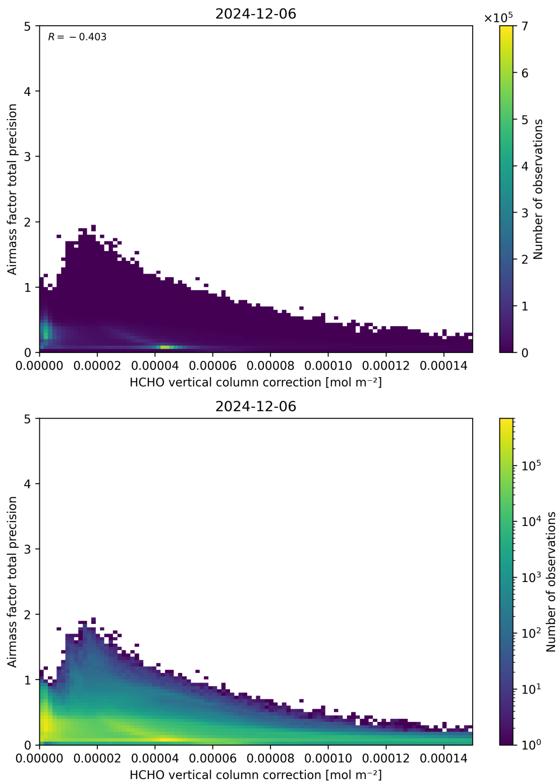
Figure 121: Scatter density plot of “HCHO vertical column correction” against “Airmass factor total precision” for 2024-12-06 to 2024-12-07.
