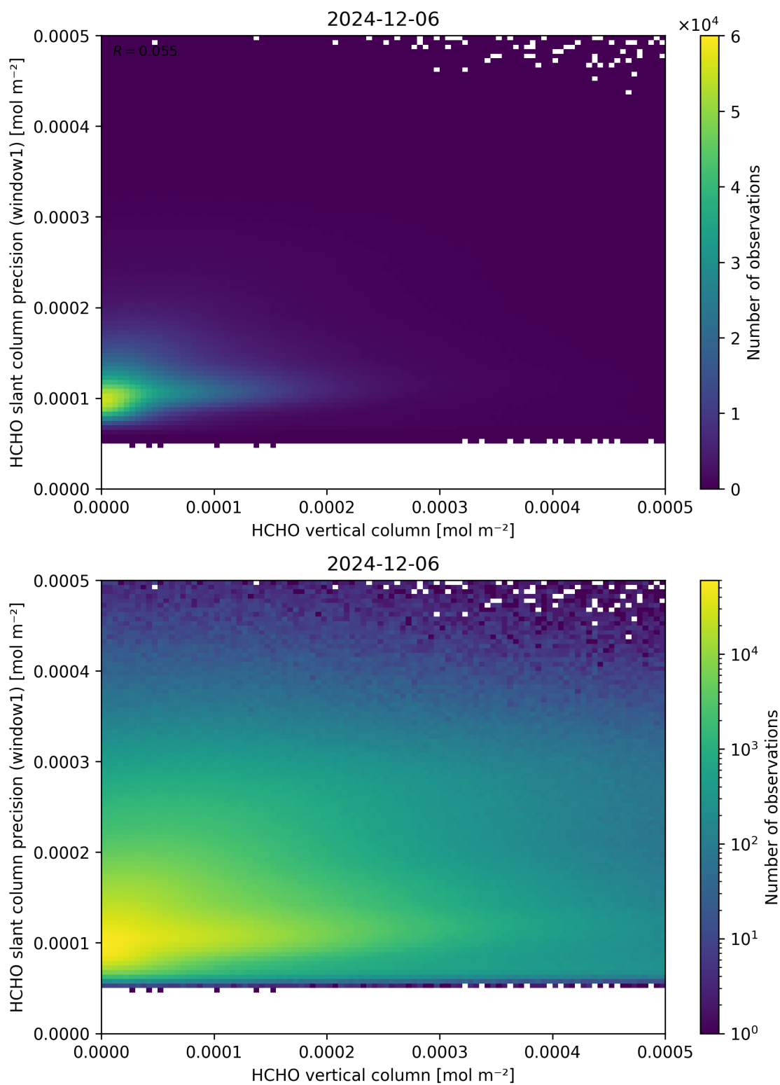
Figure 130: Scatter density plot of “HCHO vertical column” against “HCHO slant column precision (window1)” for 2024-12-06 to 2024-12-07.
