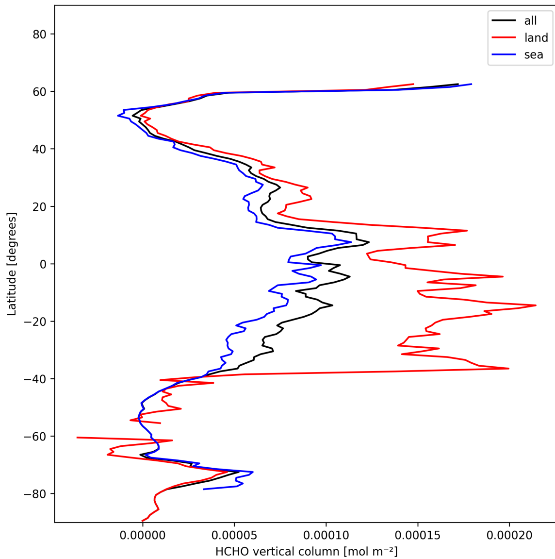
Figure 21: Zonal average of “HCHO vertical column” for 2024-12-06 to 2024-12-07.
