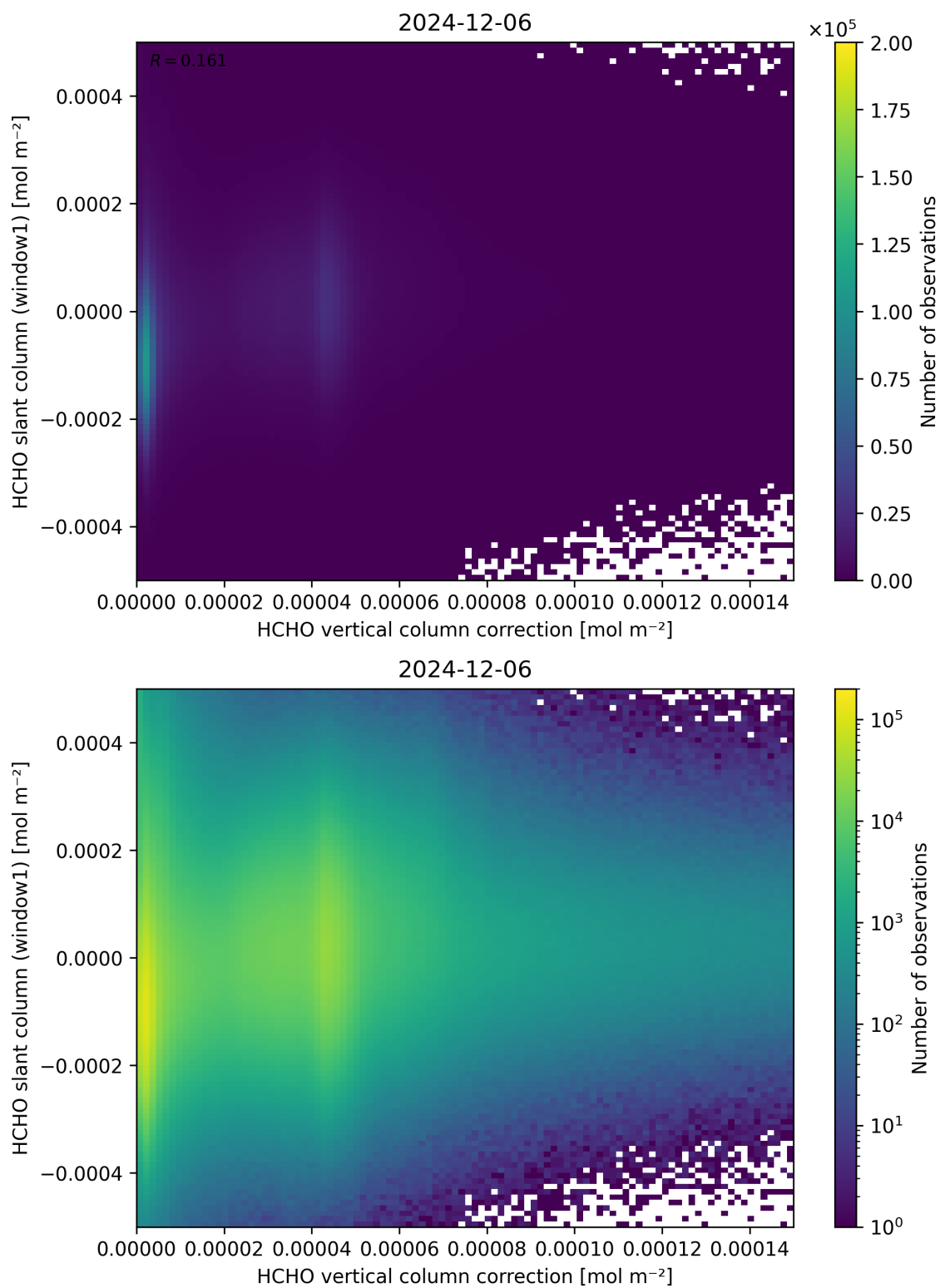
Figure 118: Scatter density plot of “HCHO vertical column correction” against “HCHO slant column (window1)” for 2024-12-06 to 2024-12-07.
