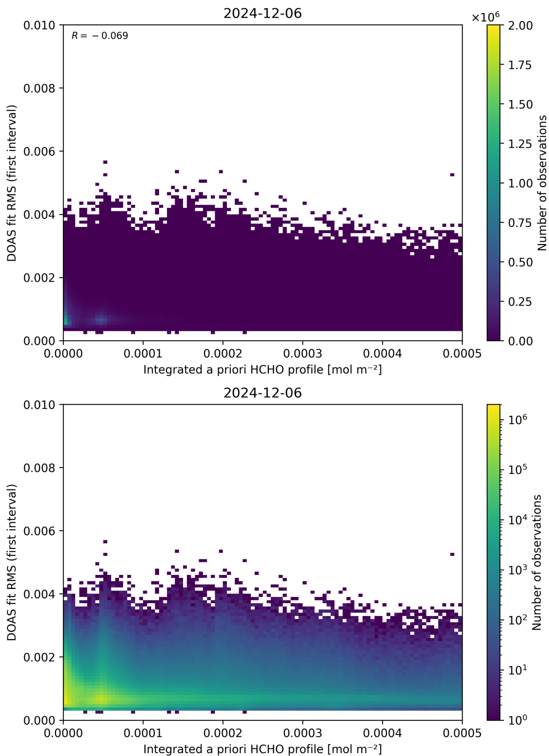
Figure 148: Scatter density plot of “Integrated a priori HCHO profile” against “DOAS fit RMS (first interval)” for 2024-12-06 to 2024-12-07.
