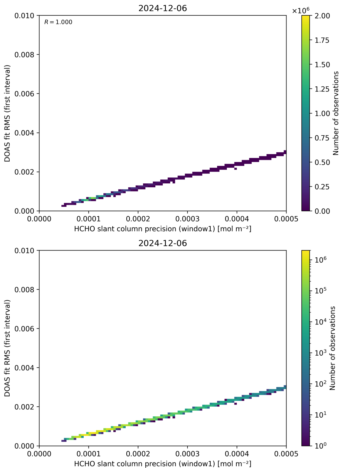
Figure 88: Scatter density plot of “HCHO slant column precision (window1)” against “DOAS fit RMS (first interval)” for 2024-12-06 to 2024-12-07.
