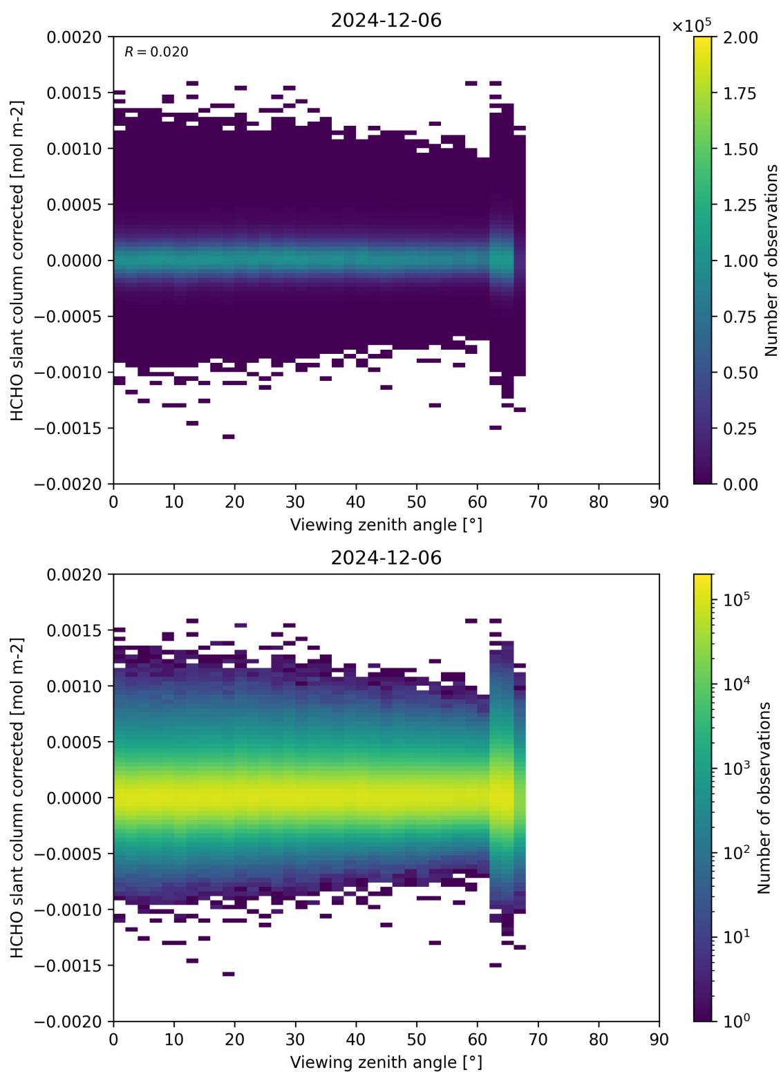
Figure 186: Scatter density plot of “Viewing zenith angle” against “HCHO slant column corrected” for 2024-12-06 to 2024-12-07.
