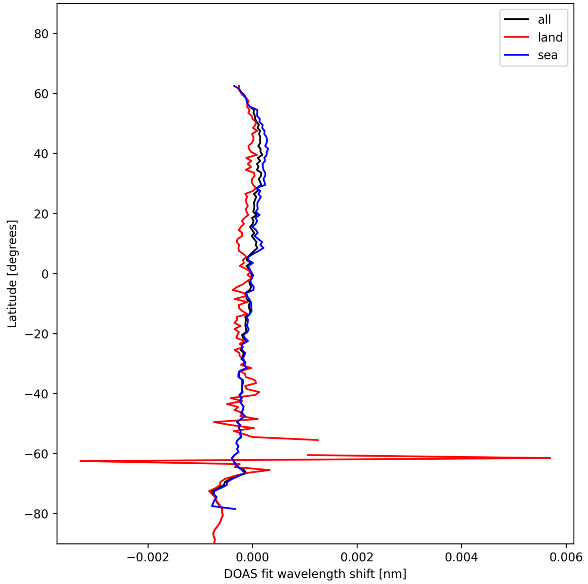
Figure 30: Zonal average of "DOAS fit wavelength shift" for 2024-12-06 to 2024-12-07.
