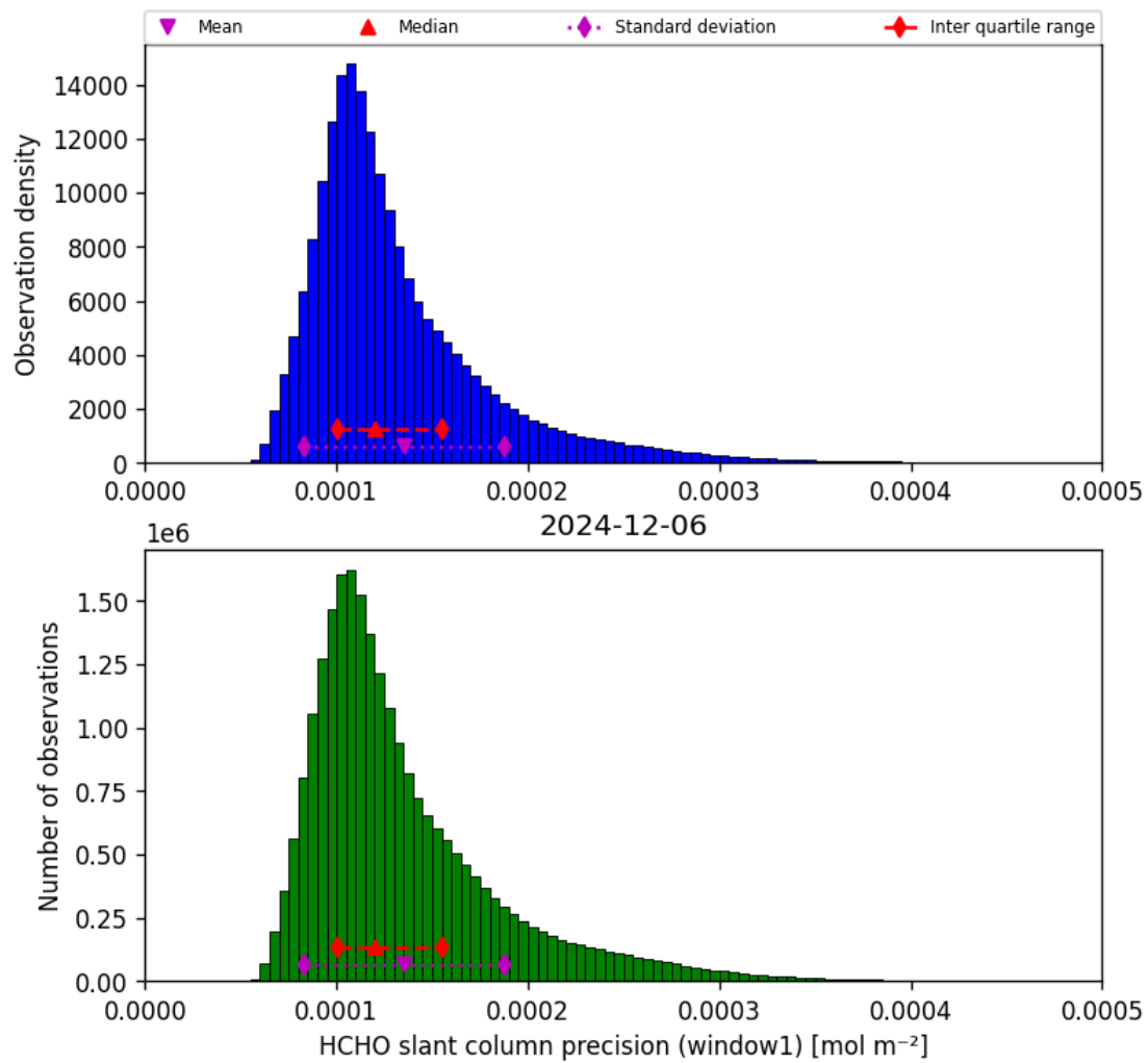
Figure 39: Histogram of “HCHO slant column precision (window1)” for 2024-12-06 to 2024-12-07
