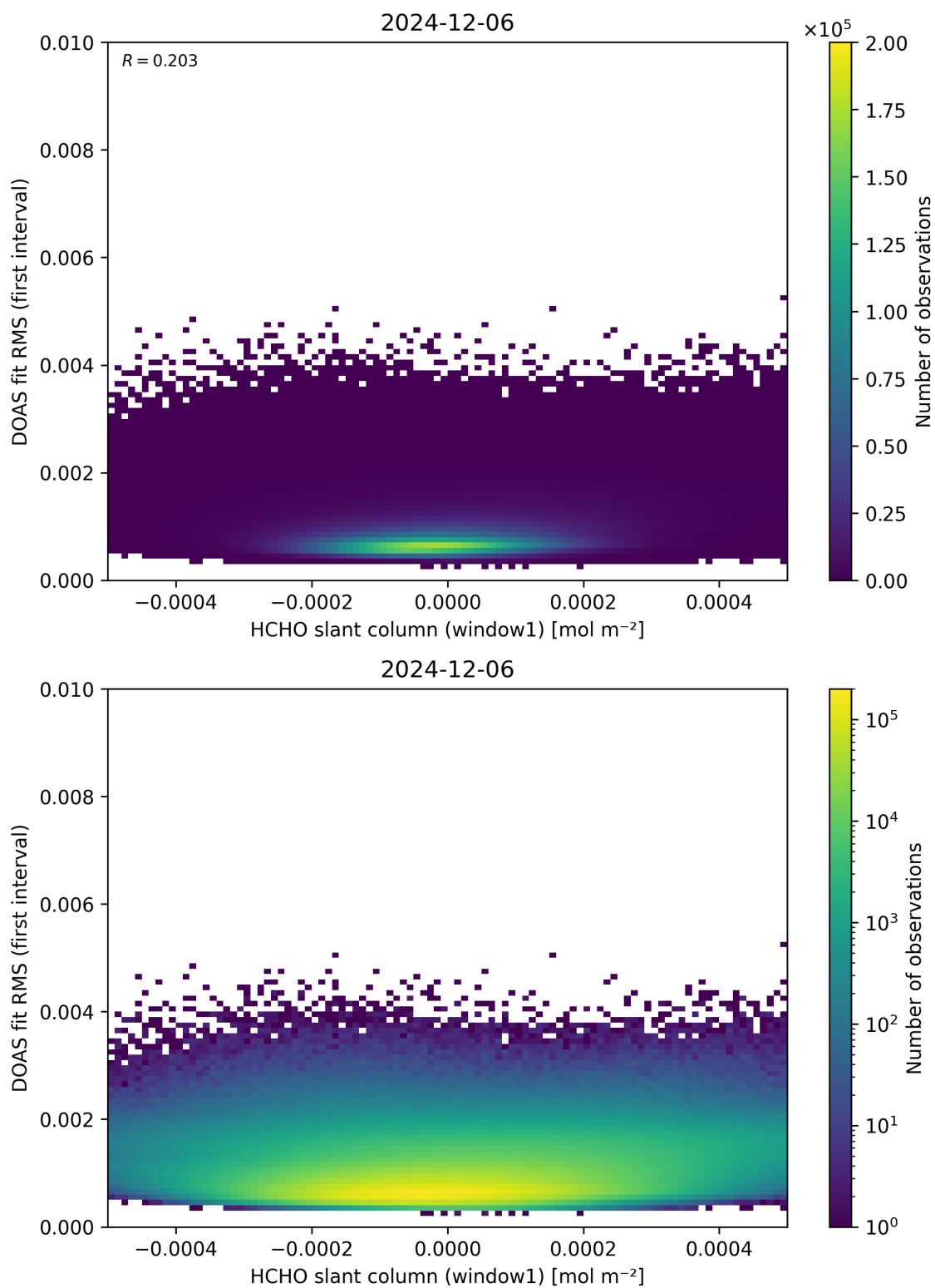
Figure 78: Scatter density plot of “HCHO slant column (window1)” against “DOAS fit RMS (first interval)” for 2024-12-06 to 2024-12-07.
