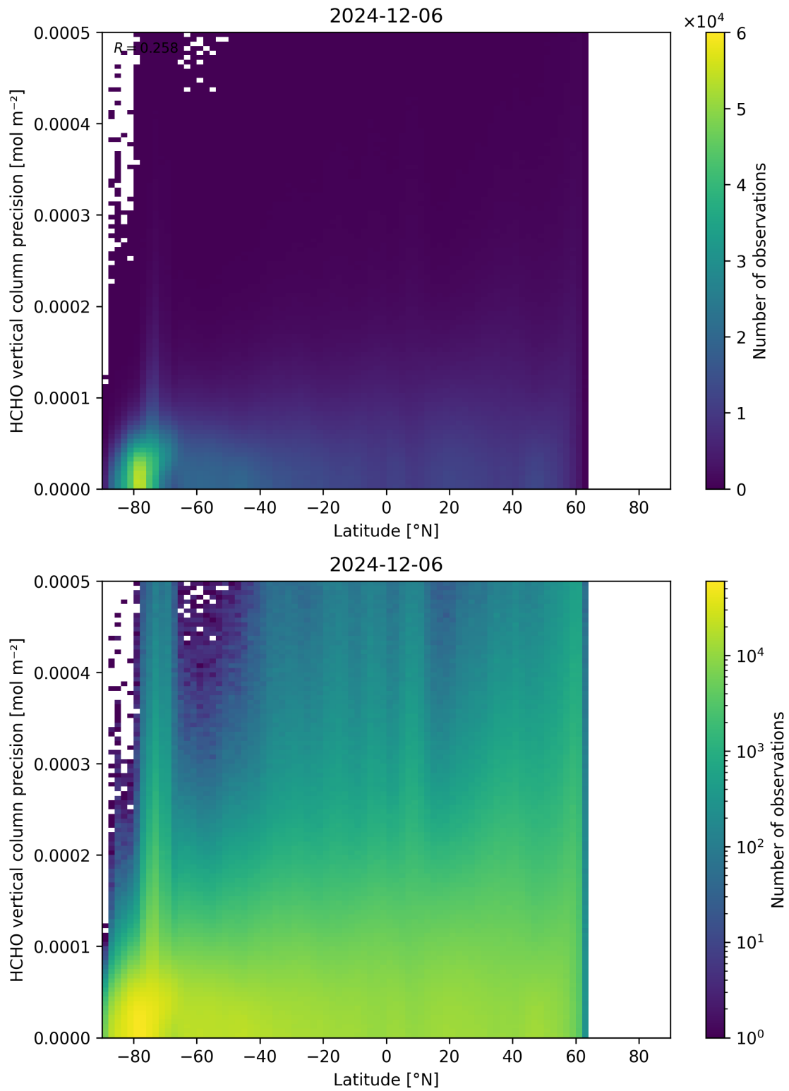
Figure 165: Scatter density plot of “Latitude” against “HCHO vertical column precision” for 2024-12-06 to 2024-12-07.
