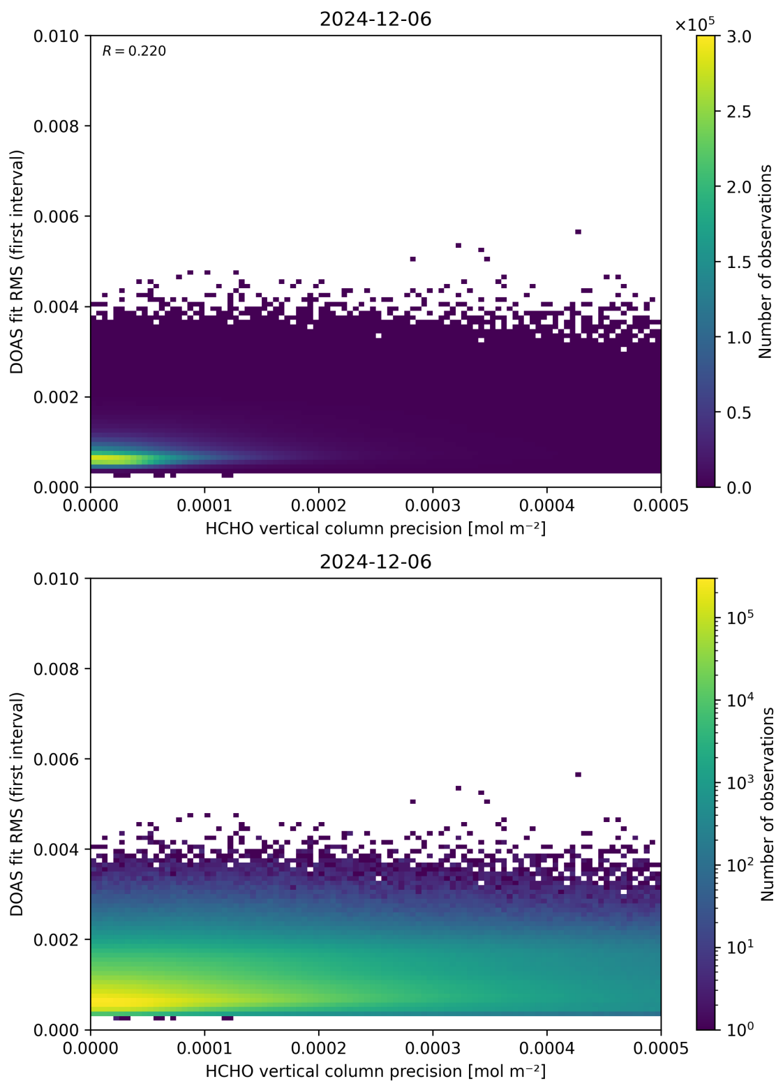
Figure 136: Scatter density plot of “HCHO vertical column precision” against “DOAS fit RMS (first interval)” for 2024-12-06 to 2024-12-07.
