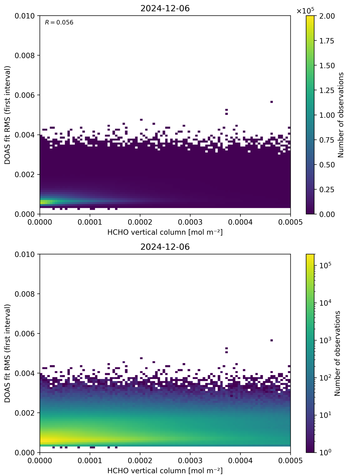
Figure 123: Scatter density plot of “HCHO vertical column” against “DOAS fit RMS (first interval)” for 2024-12-06 to 2024-12-07.
