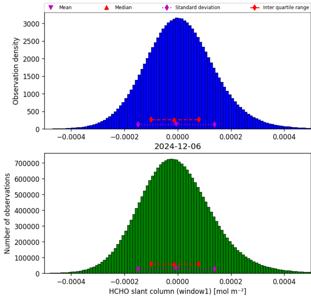
Figure 38: Histogram of “HCHO slant column (window1)” for 2024-12-06 to 2024-12-07
