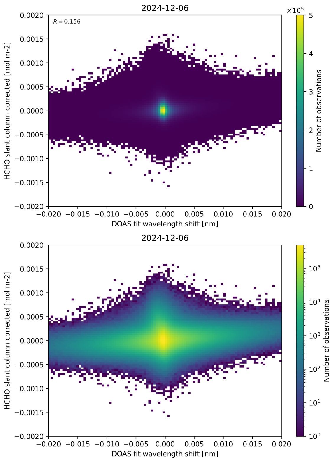
Figure 66: Scatter density plot of “DOAS fit wavelength shift” against “HCHO slant column corrected” for 2024-12-06 to 2024-12-07.
