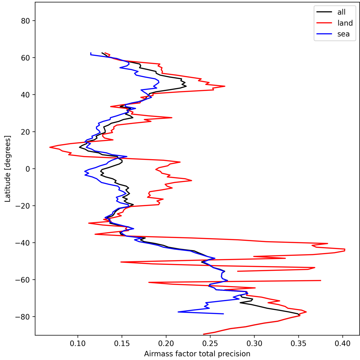
Figure 27: Zonal average of “Airmass factor total precision” for 2024-12-06 to 2024-12-07.
