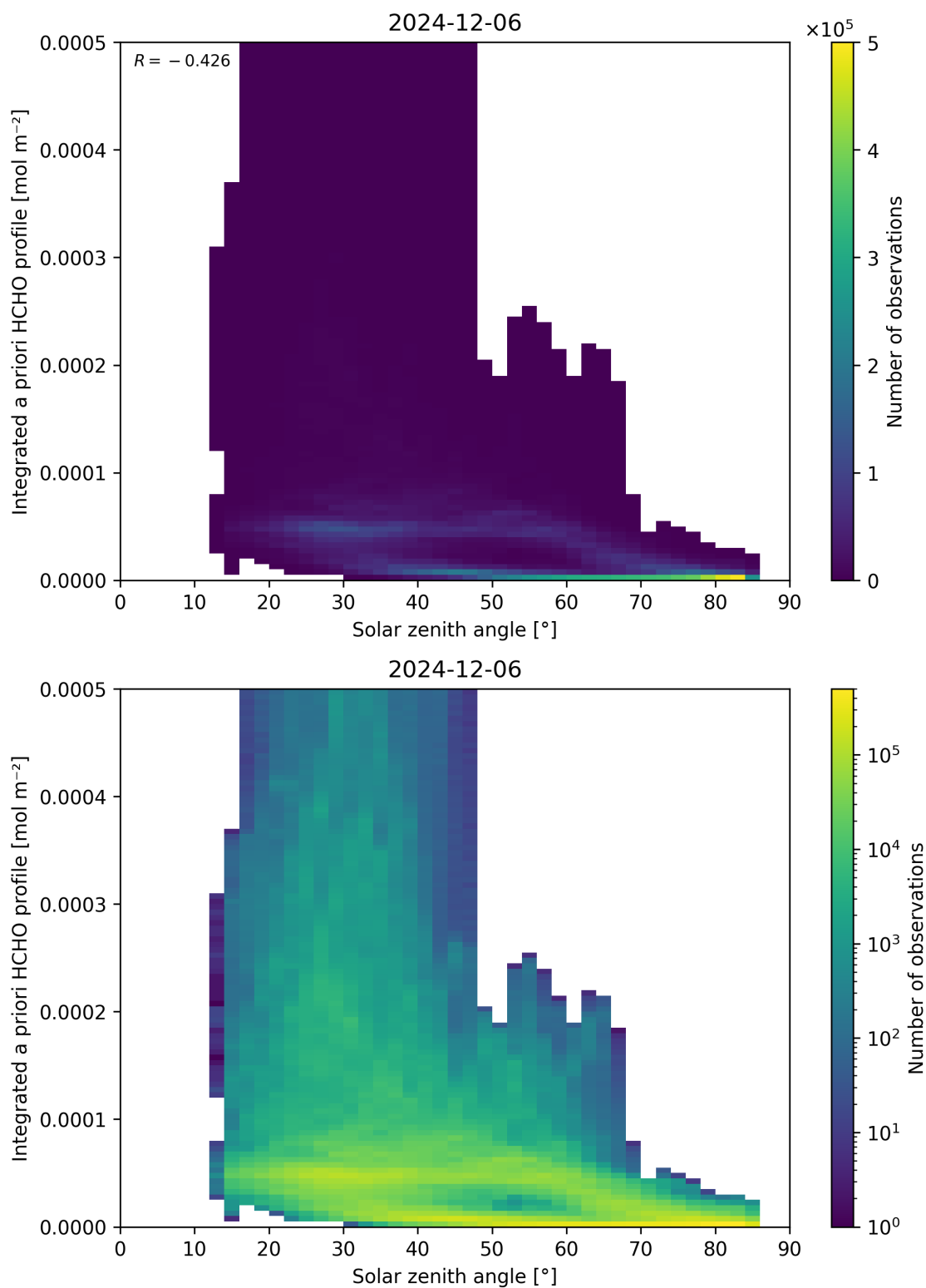
Figure 180: Scatter density plot of “Solar zenith angle” against “Integrated a priori HCHO profile” for 2024-12-06 to 2024-12-07.
