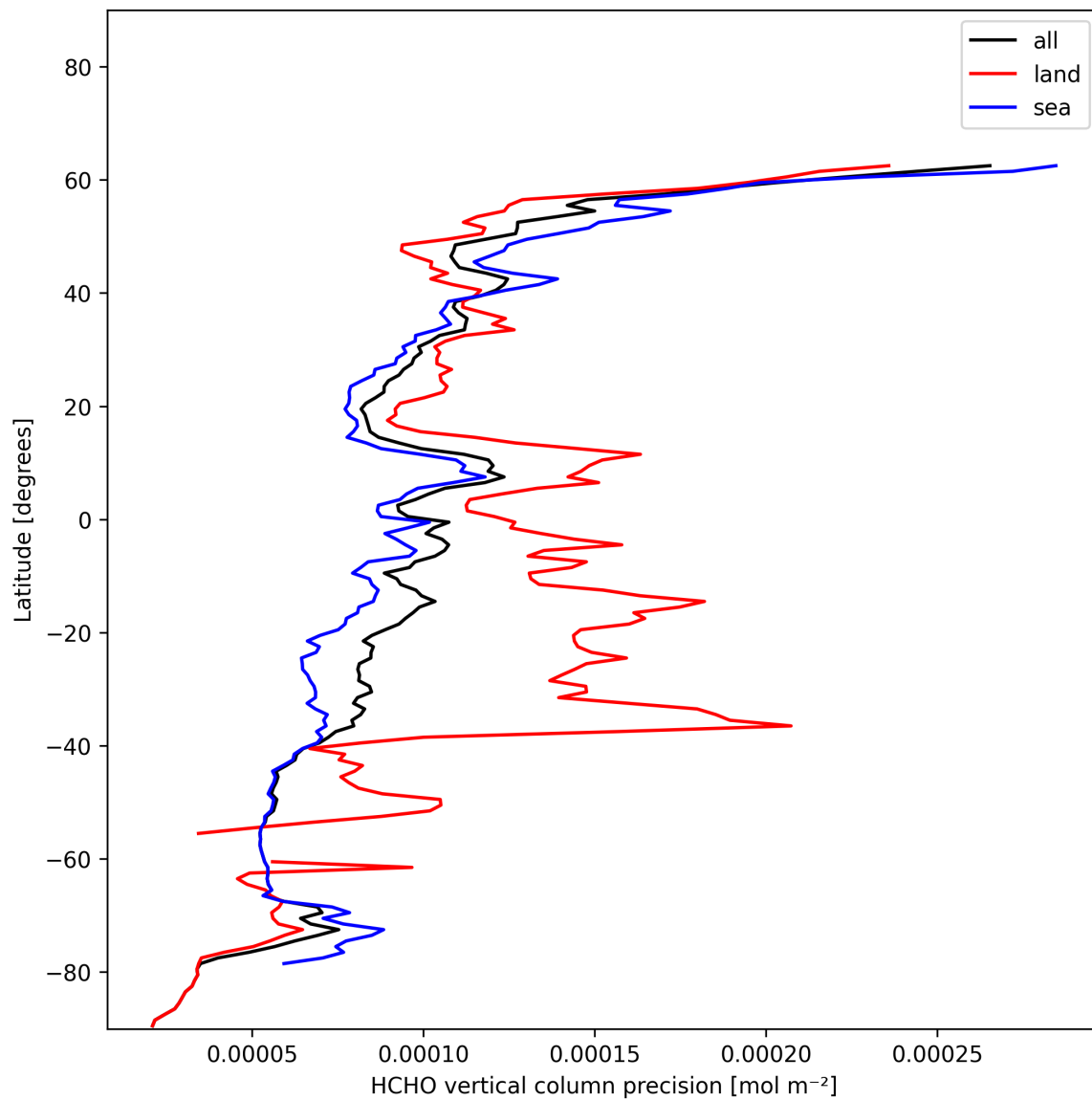
Figure 22: Zonal average of “HCHO vertical column precision” for 2024-12-06 to 2024-12-07.
