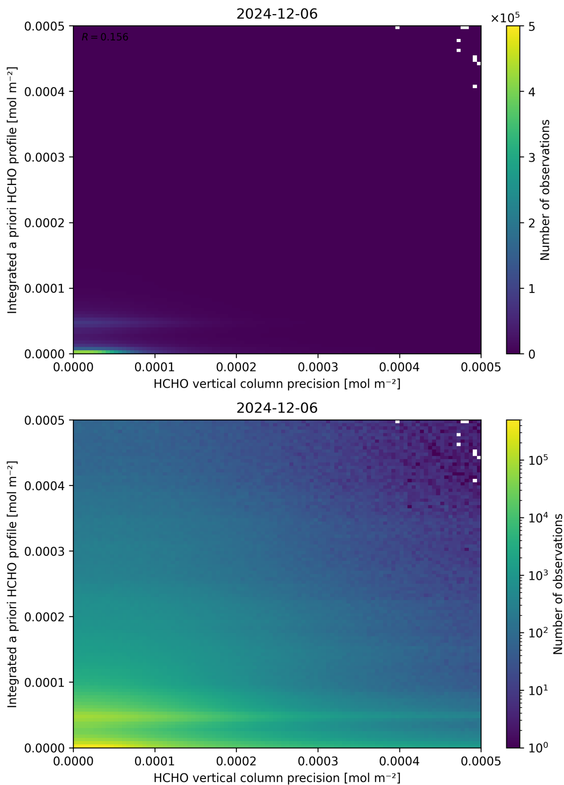
Figure 147: Scatter density plot of “HCHO vertical column precision” against “Integrated a priori HCHO profile” for 2024-12-06 to 2024-12-07.
