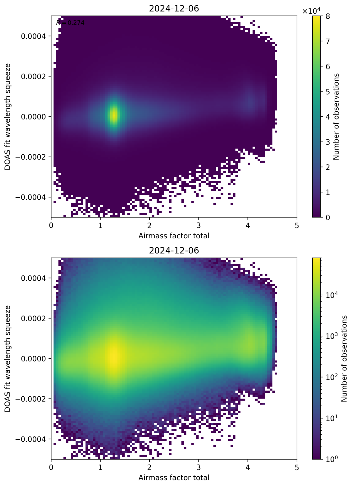
Figure 99: Scatter density plot of “Airmass factor total” against “DOAS fit wavelength squeeze” for 2024-12-06 to 2024-12-07.
