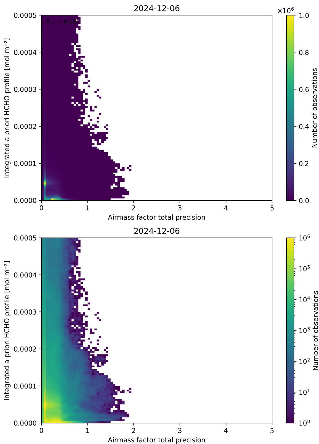
Figure 111: Scatter density plot of “Airmass factor total precision” against “Integrated a priori HCHO profile” for 2024-12-06 to 2024-12-07.
