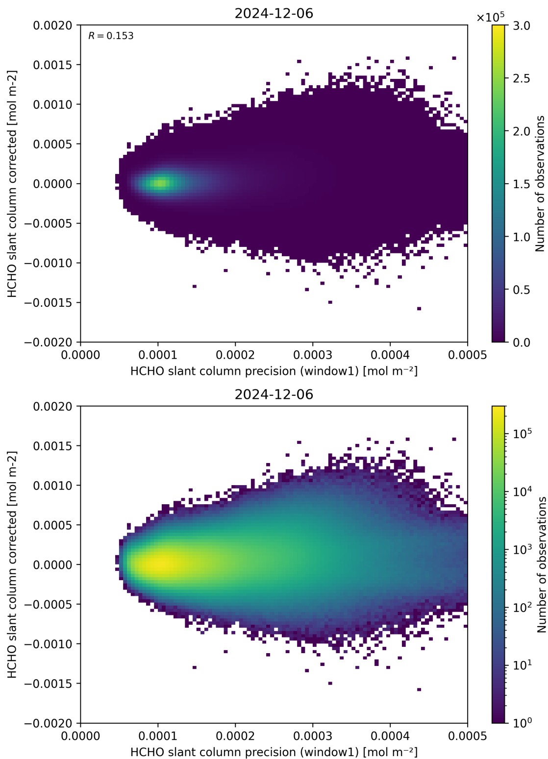
Figure 92: Scatter density plot of “HCHO slant column precision (window1)” against “HCHO slant column corrected” for 2024-12-06 to 2024-12-07.
