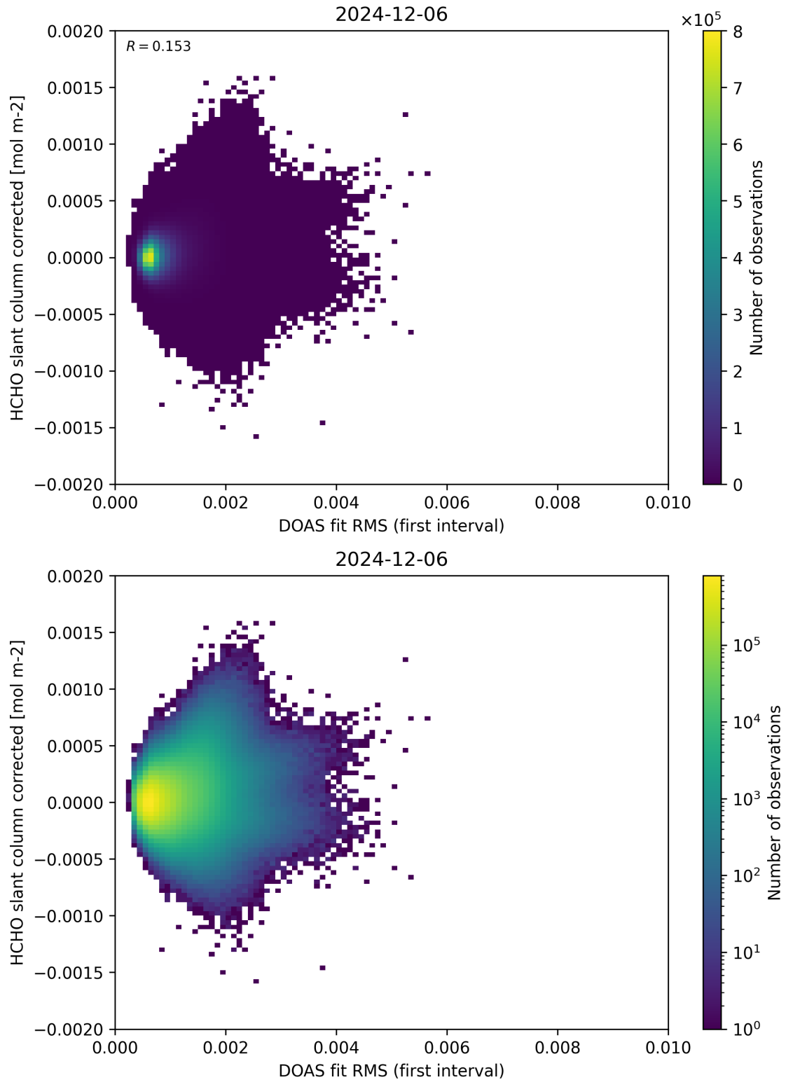
Figure 62: Scatter density plot of “DOAS fit RMS (first interval)” against “HCHO slant column corrected” for 2024-12-06 to 2024-12-07.
