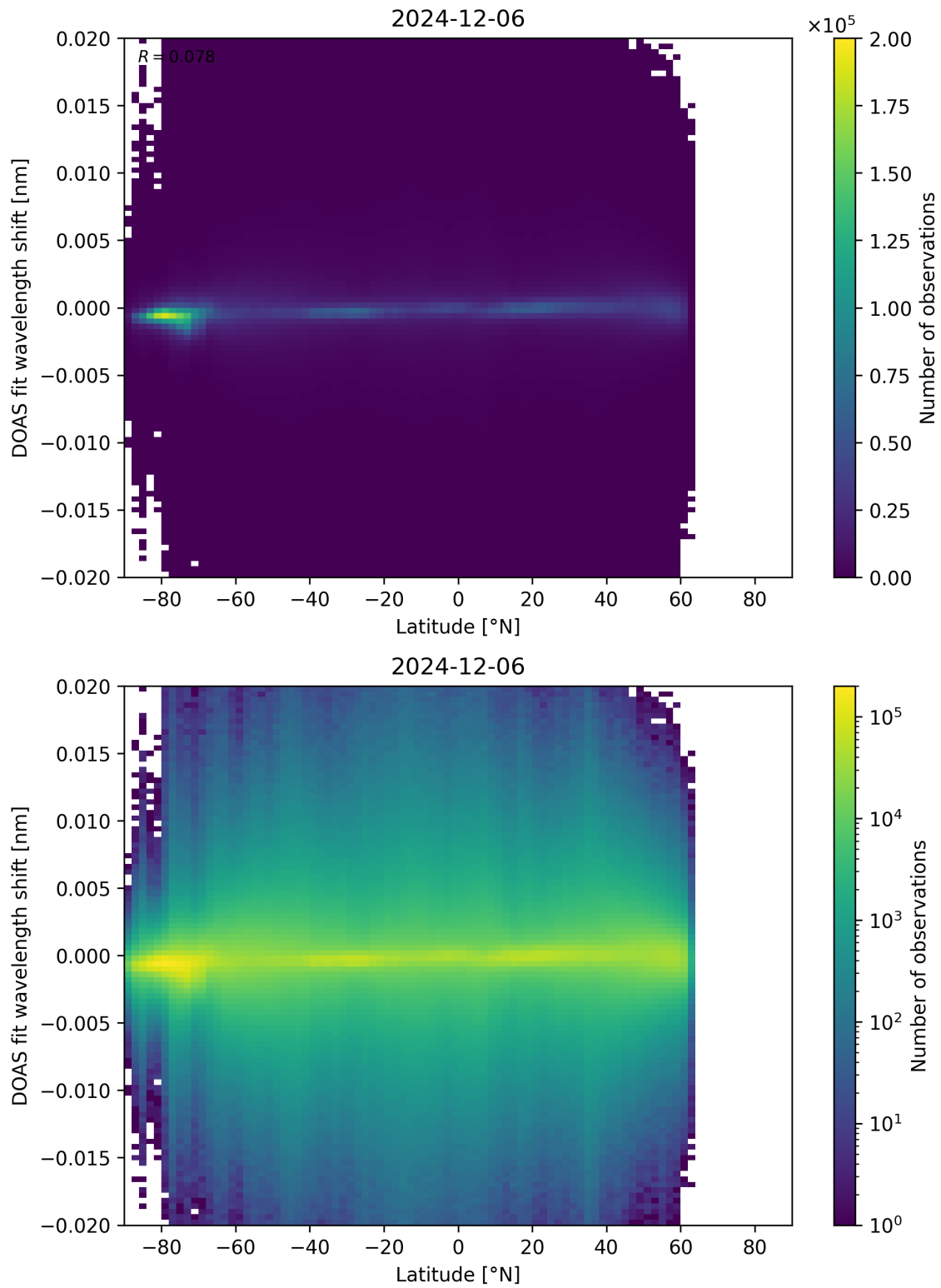
Figure 154: Scatter density plot of “Latitude” against “DOAS fit wavelength shift” for 2024-12-06 to 2024-12-07.
