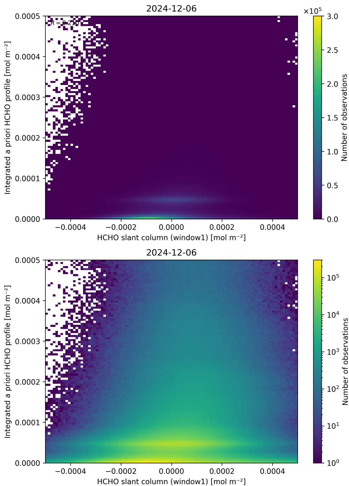
Figure 87: Scatter density plot of “HCHO slant column (window1)” against “Integrated a priori HCHO profile” for 2024-12-06 to 2024-12-07.
