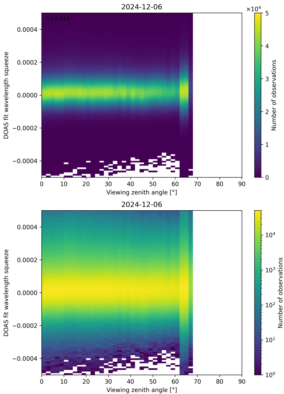
Figure 184: Scatter density plot of “Viewing zenith angle” against “DOAS fit wavelength squeeze” for 2024-12-06 to 2024-12-07.
