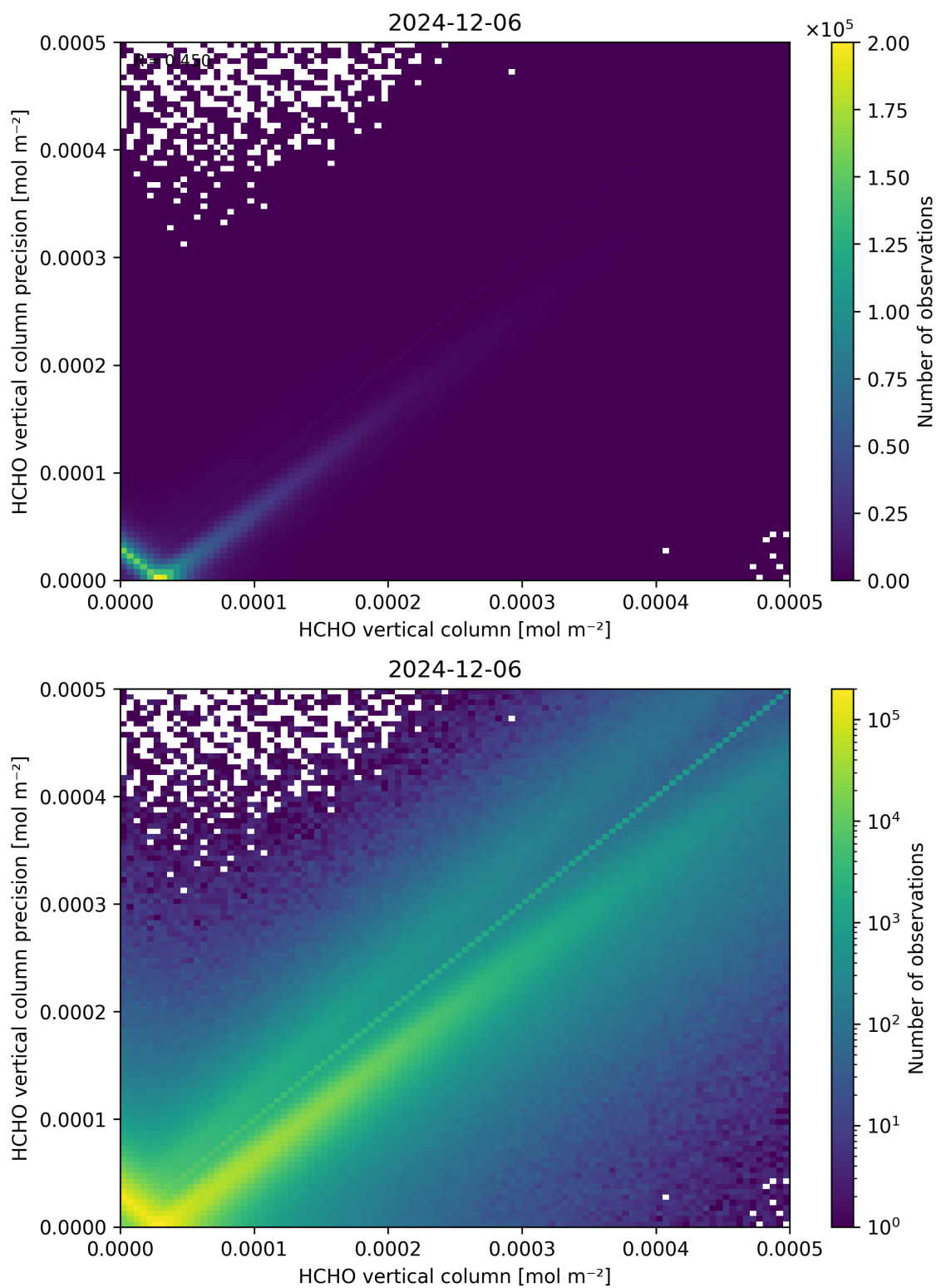
Figure 134: Scatter density plot of “HCHO vertical column” against “HCHO vertical column precision” for 2024-12-06 to 2024-12-07.
