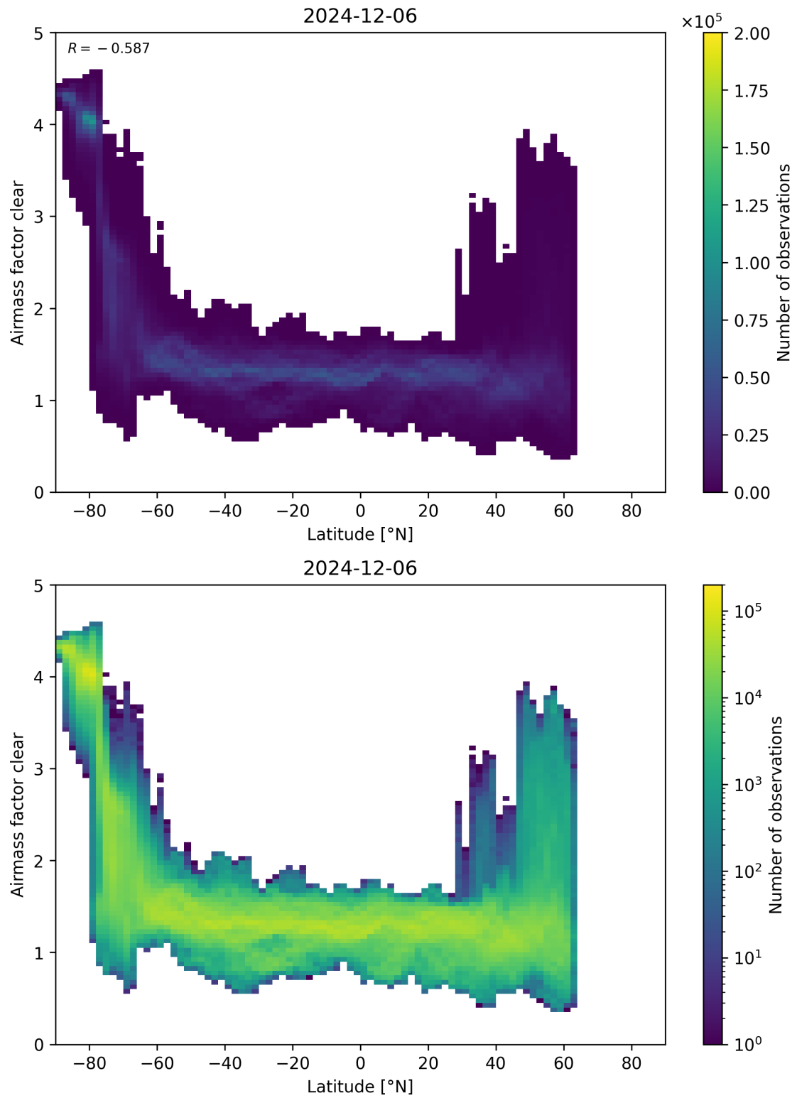
Figure 156: Scatter density plot of “Latitude” against “Airmass factor clear” for 2024-12-06 to 2024-12-07.
