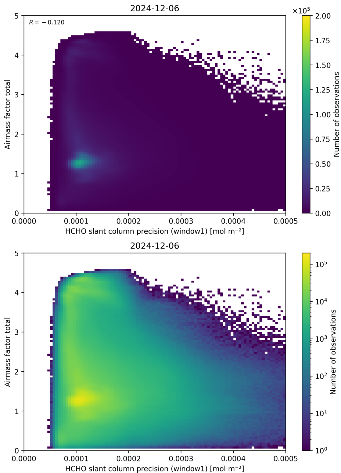
Figure 94: Scatter density plot of “HCHO slant column precision (window1)” against “Airmass factor total” for 2024-12-06 to 2024-12-07.
