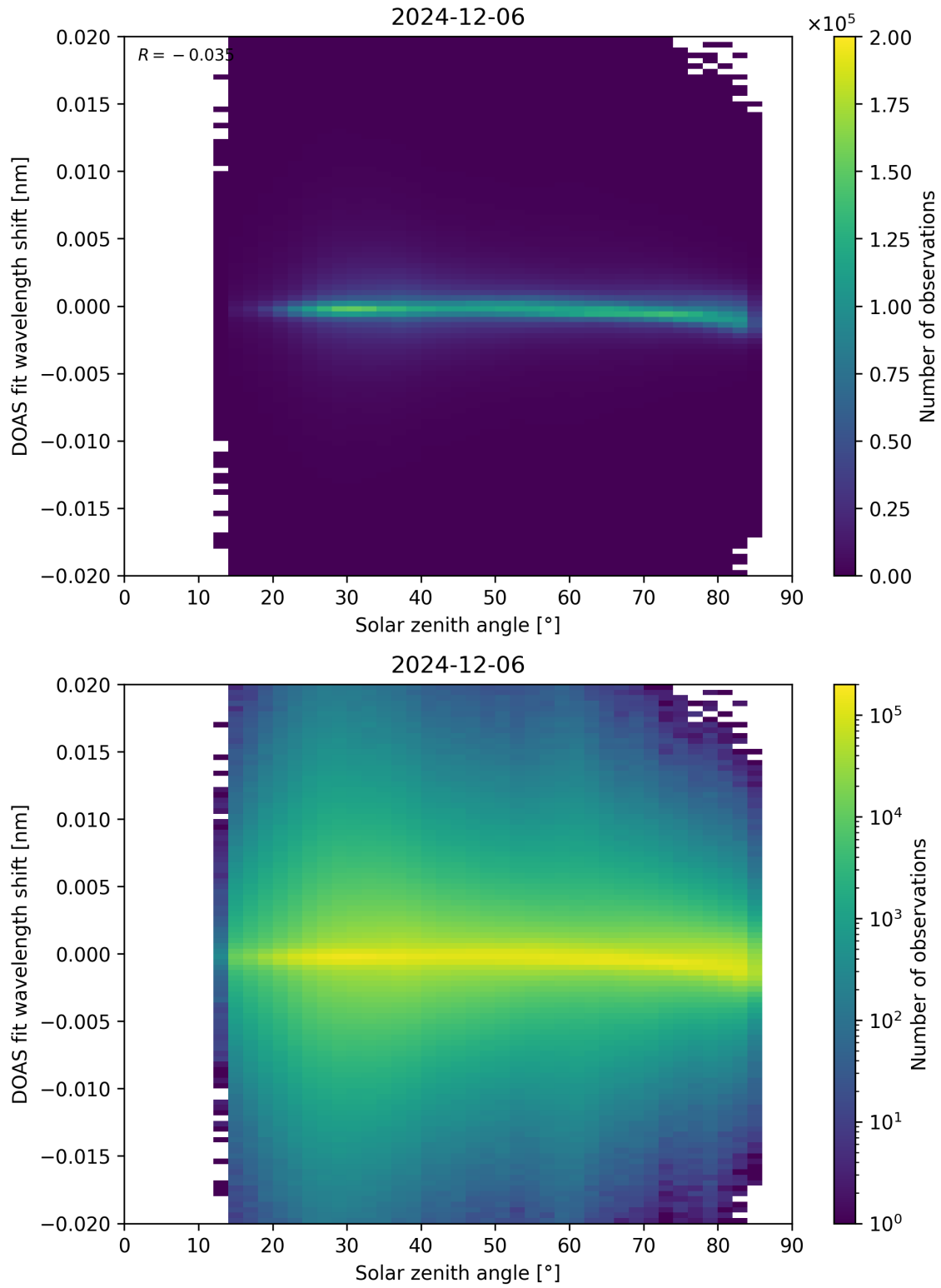
Figure 168: Scatter density plot of “Solar zenith angle” against “DOAS fit wavelength shift” for 2024-12-06 to 2024-12-07.
