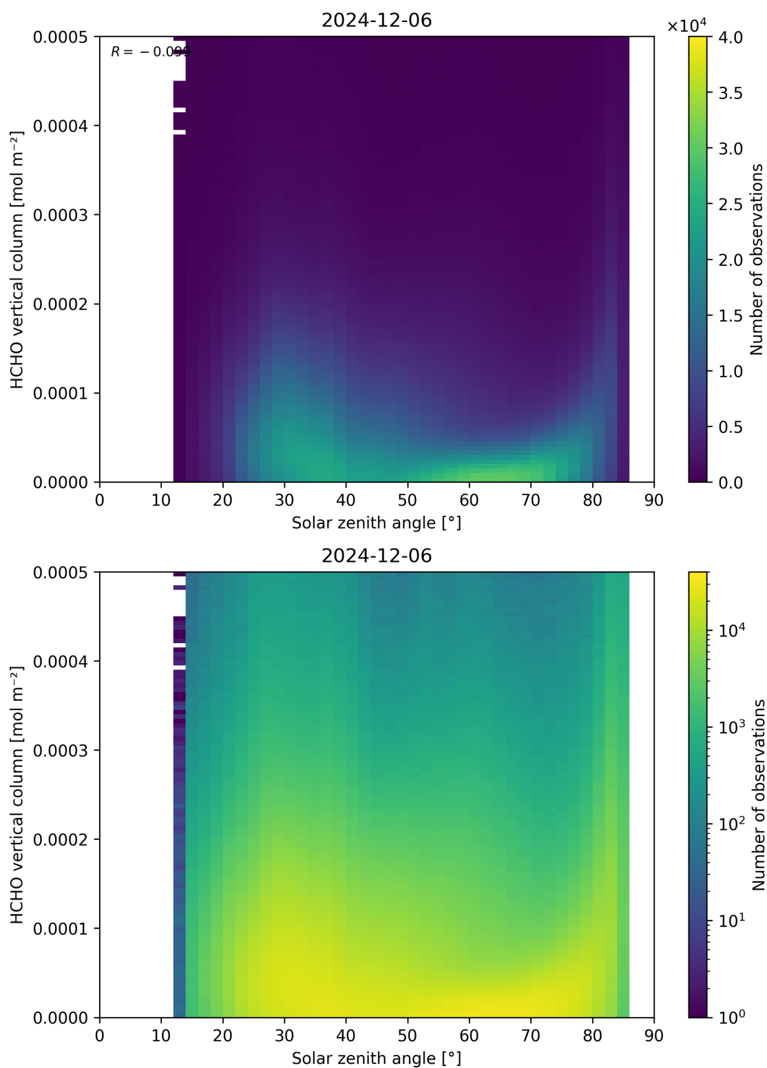
Figure 177: Scatter density plot of “Solar zenith angle” against “HCHO vertical column” for 2024-12-06 to 2024-12-07.
