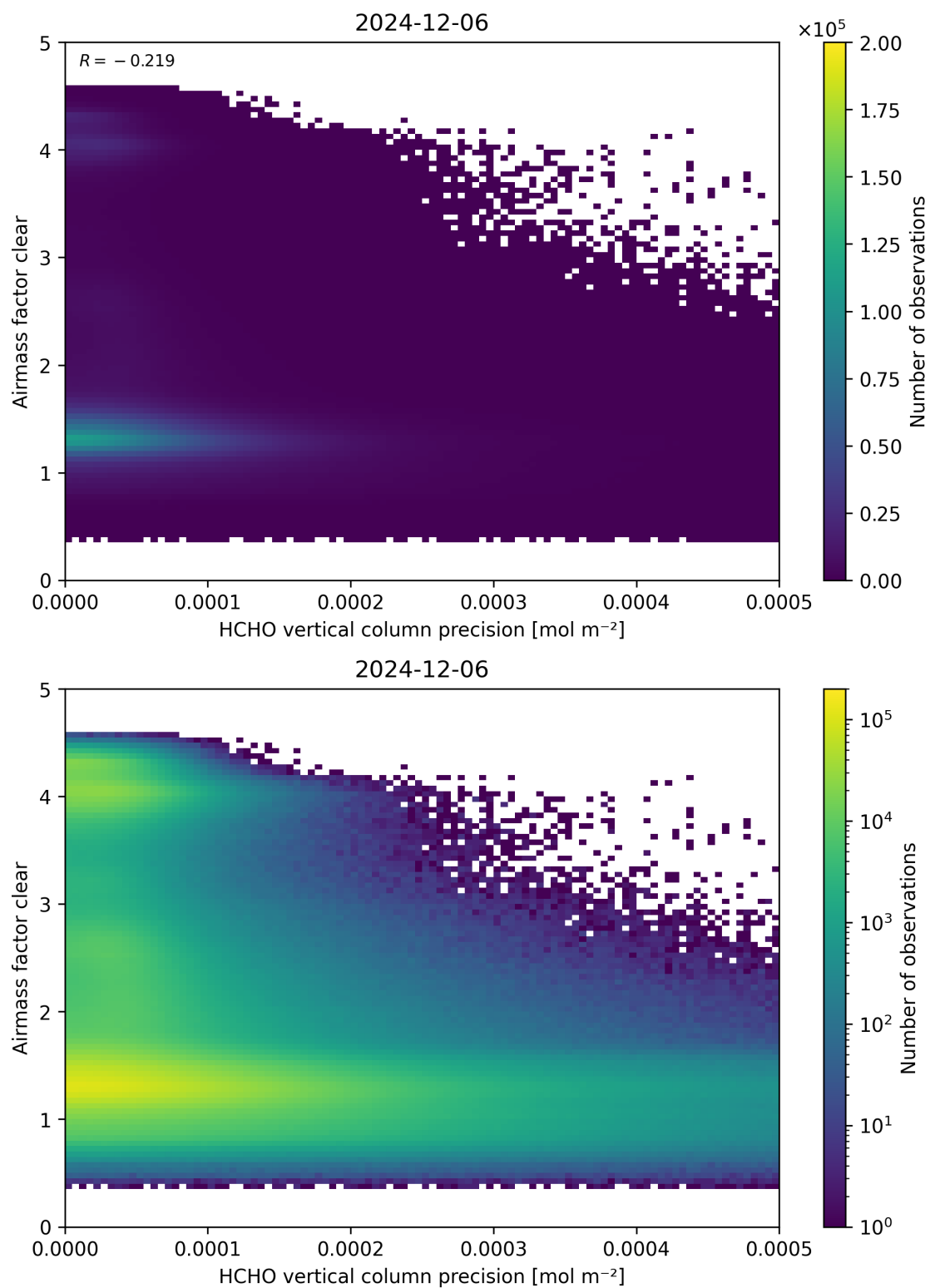
Figure 139: Scatter density plot of “HCHO vertical column precision” against “Airmass factor clear” for 2024-12-06 to 2024-12-07.
