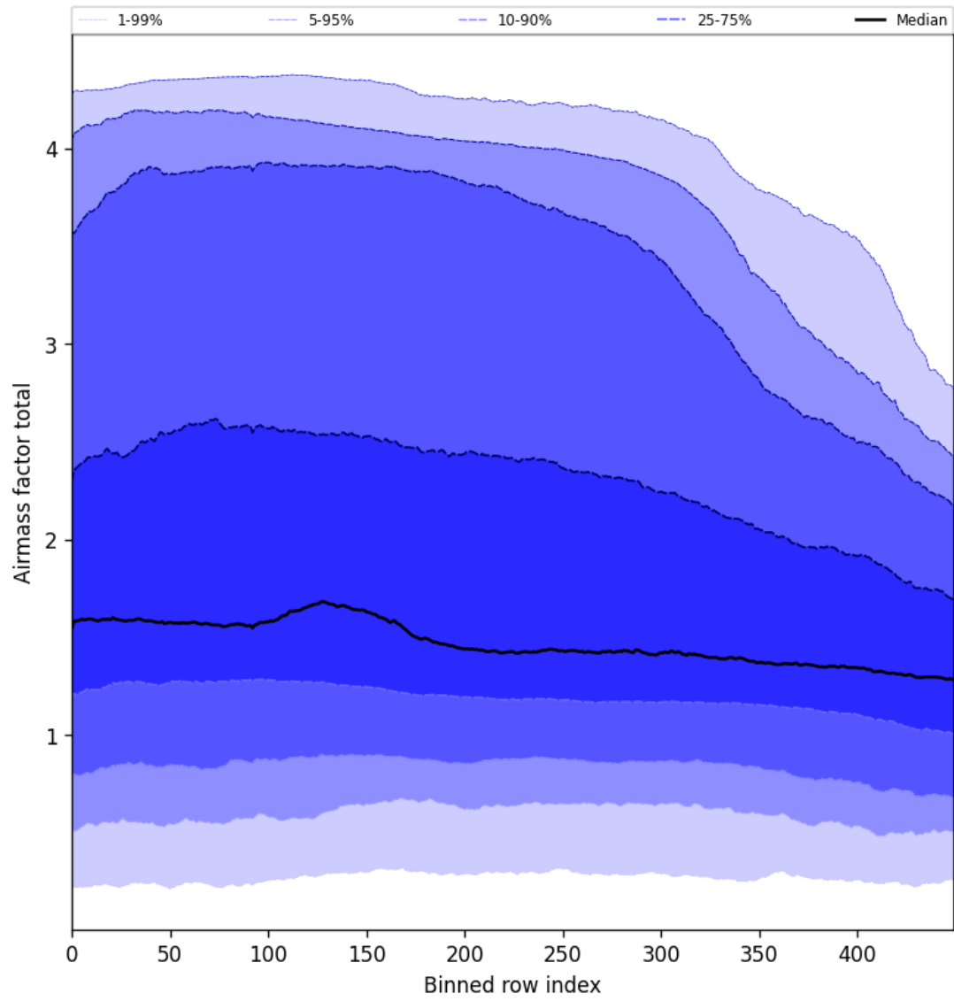
Figure 54: Along track statistics of “Airmass factor total” for 2024-12-06 to 2024-12-07
