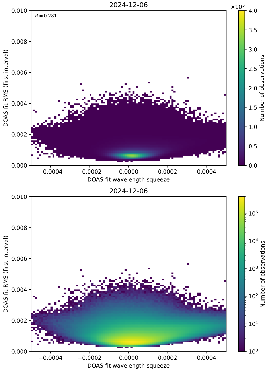
Figure 68: Scatter density plot of “DOAS fit wavelength squeeze” against “DOAS fit RMS (first interval)” for 2024-12-06 to 2024-12-07.
