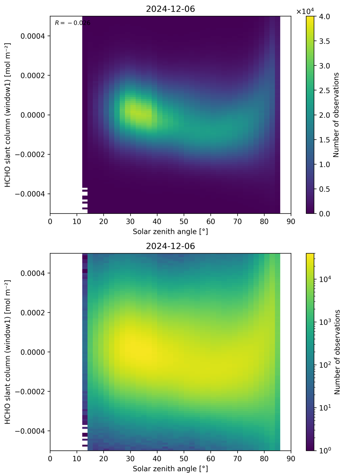
Figure 173: Scatter density plot of “Solar zenith angle” against “HCHO slant column (window1)” for 2024-12-06 to 2024-12-07.
