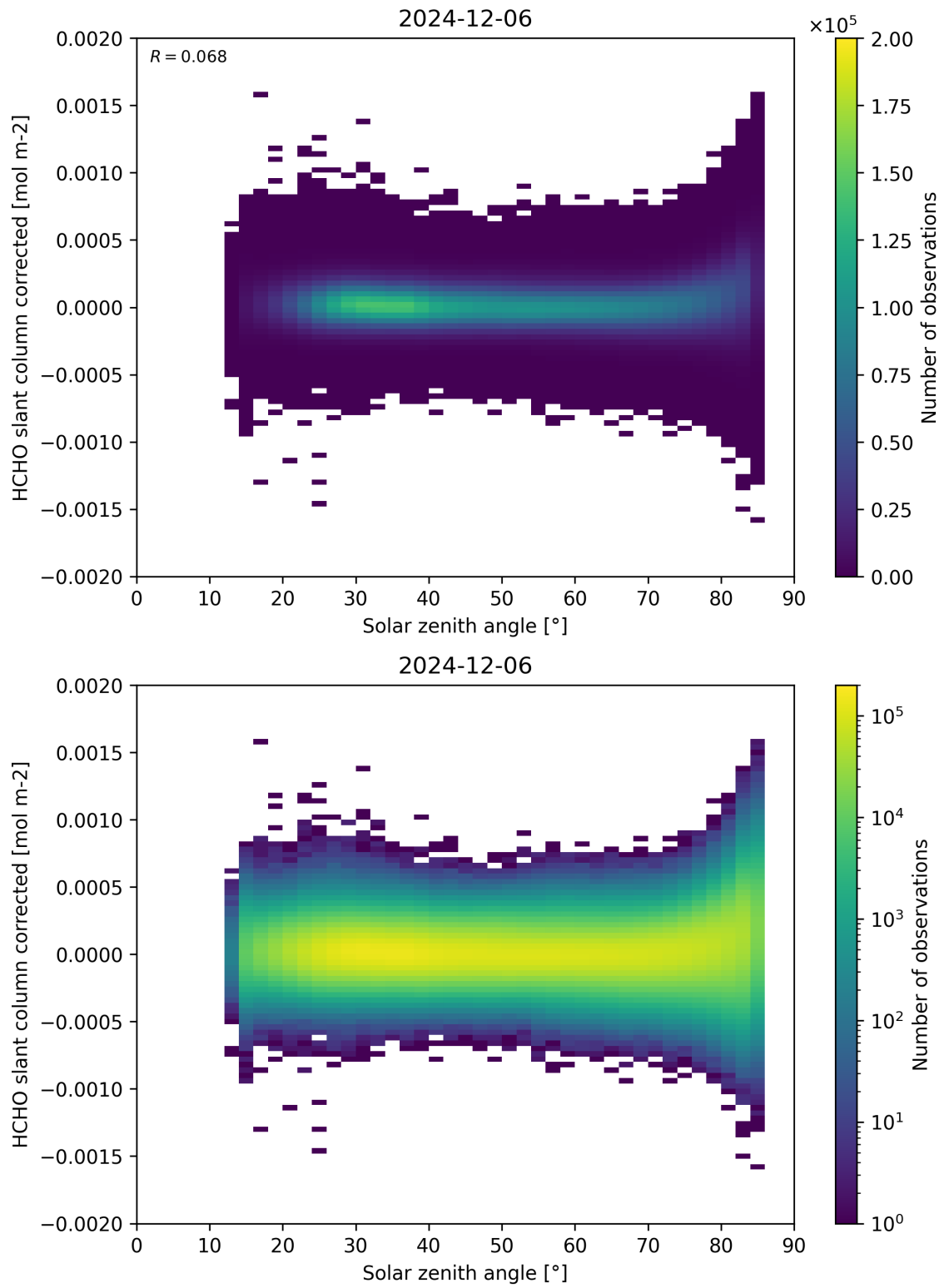
Figure 171: Scatter density plot of “Solar zenith angle” against “HCHO slant column corrected” for 2024-12-06 to 2024-12-07.
