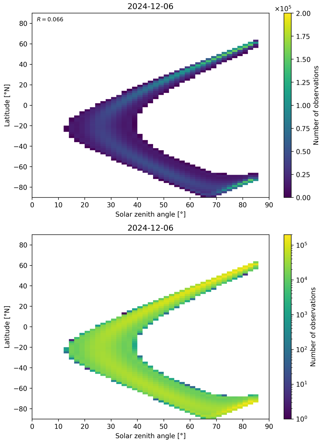
Figure 181: Scatter density plot of “Solar zenith angle” against “Latitude” for 2024-12-06 to 2024-12-07.
