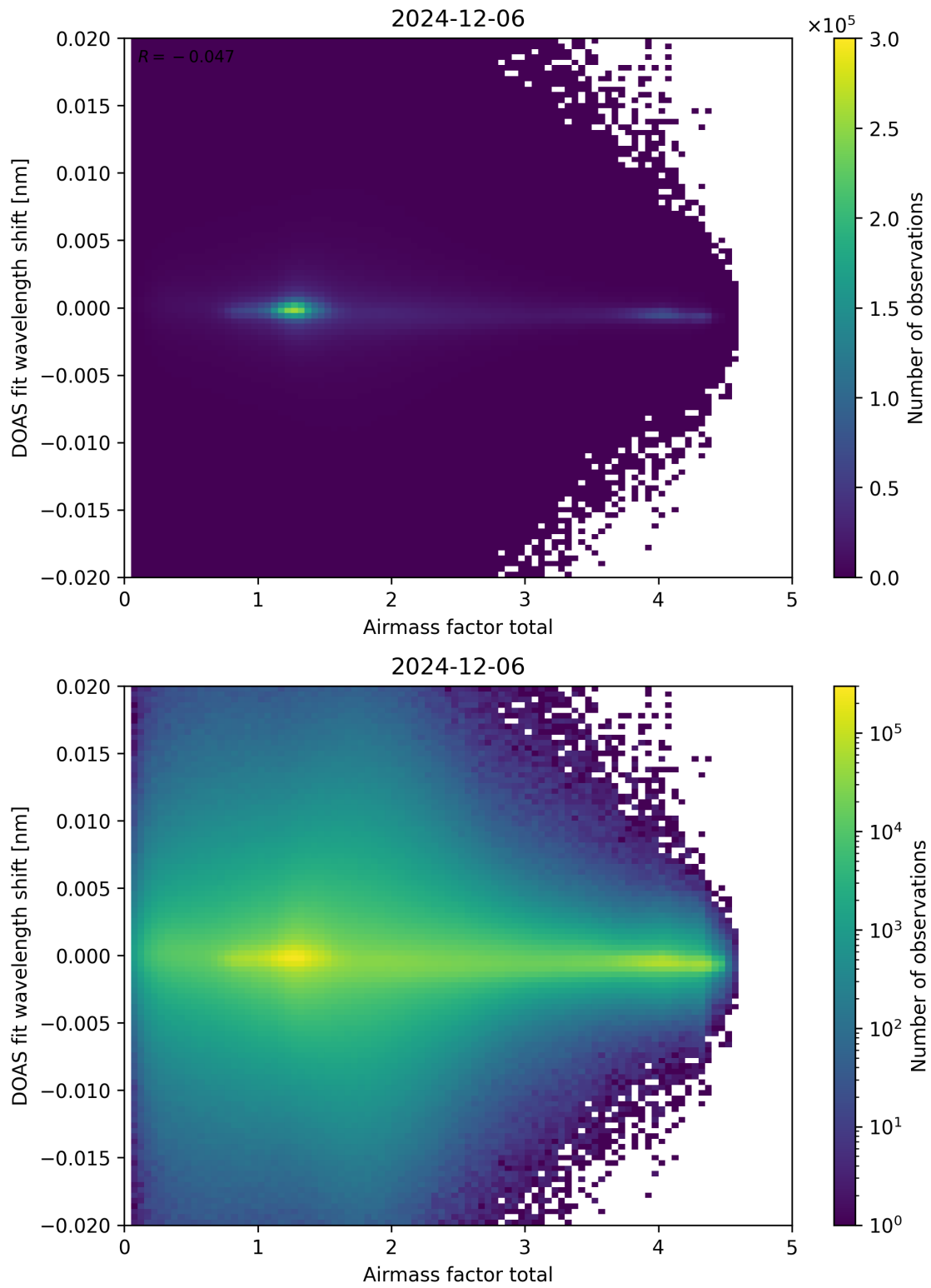
Figure 98: Scatter density plot of “Airmass factor total” against “DOAS fit wavelength shift” for 2024-12-06 to 2024-12-07.
