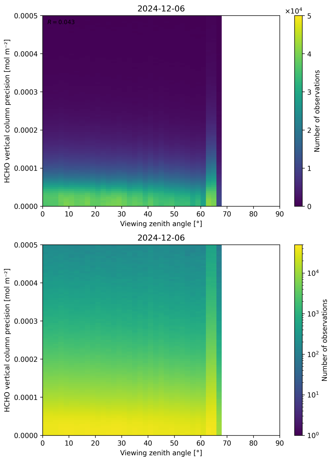
Figure 194: Scatter density plot of “Viewing zenith angle” against “HCHO vertical column precision” for 2024-12-06 to 2024-12-07.
