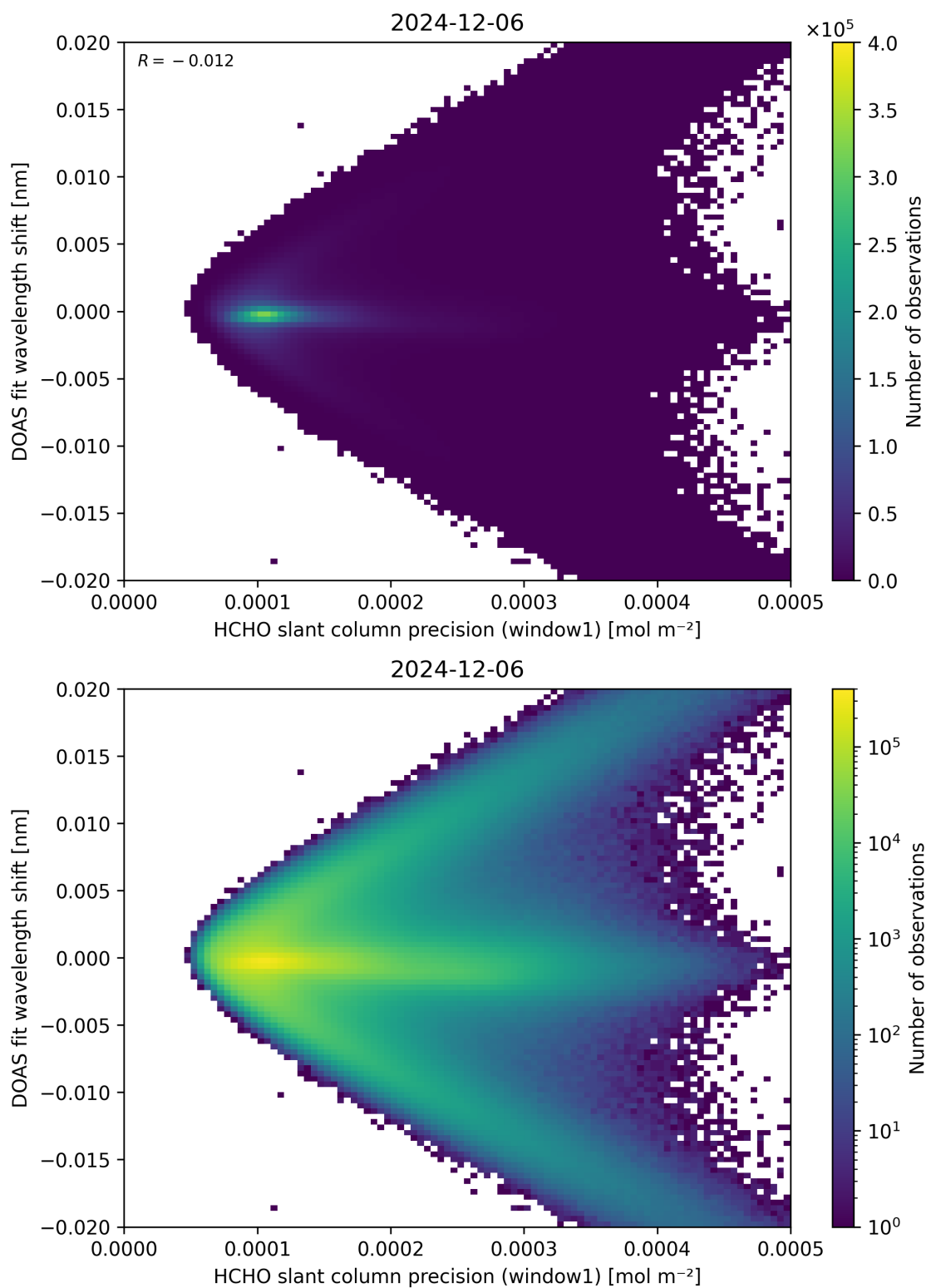
Figure 89: Scatter density plot of “HCHO slant column precision (window1)” against “DOAS fit wavelength shift” for 2024-12-06 to 2024-12-07.
