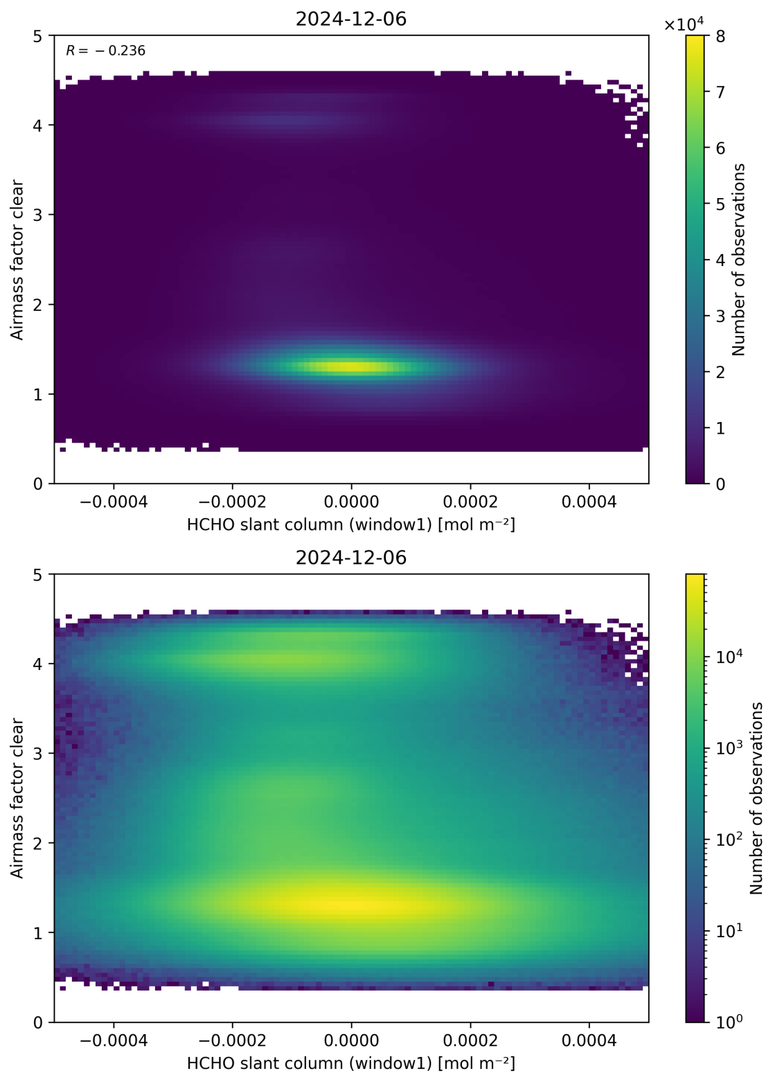
Figure 81: Scatter density plot of “HCHO slant column (window1)” against “Airmass factor clear” for 2024-12-06 to 2024-12-07.
