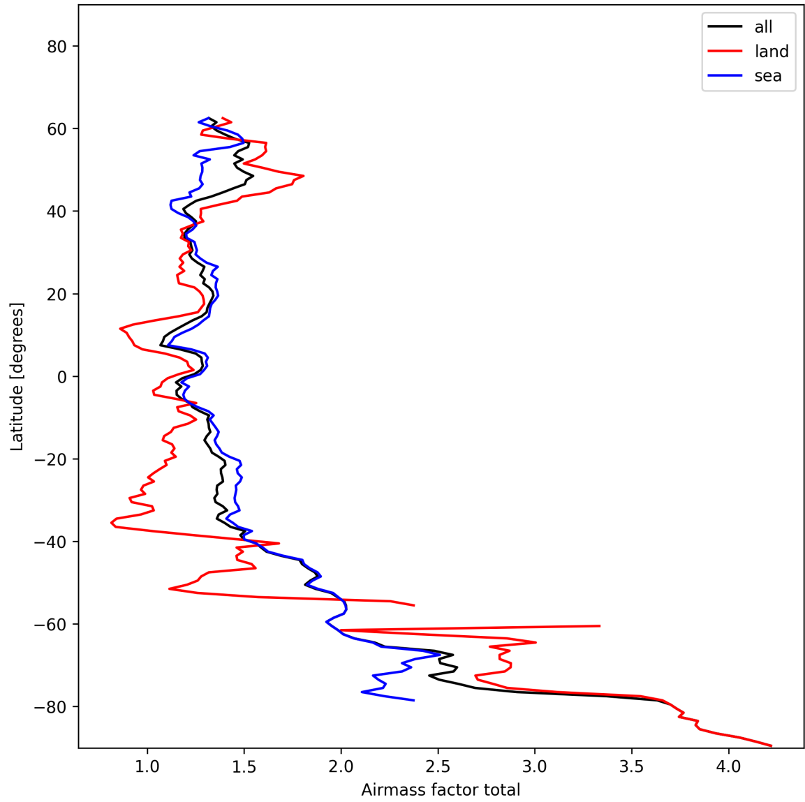
Figure 26: Zonal average of “Airmass factor total” for 2024-12-06 to 2024-12-07.
