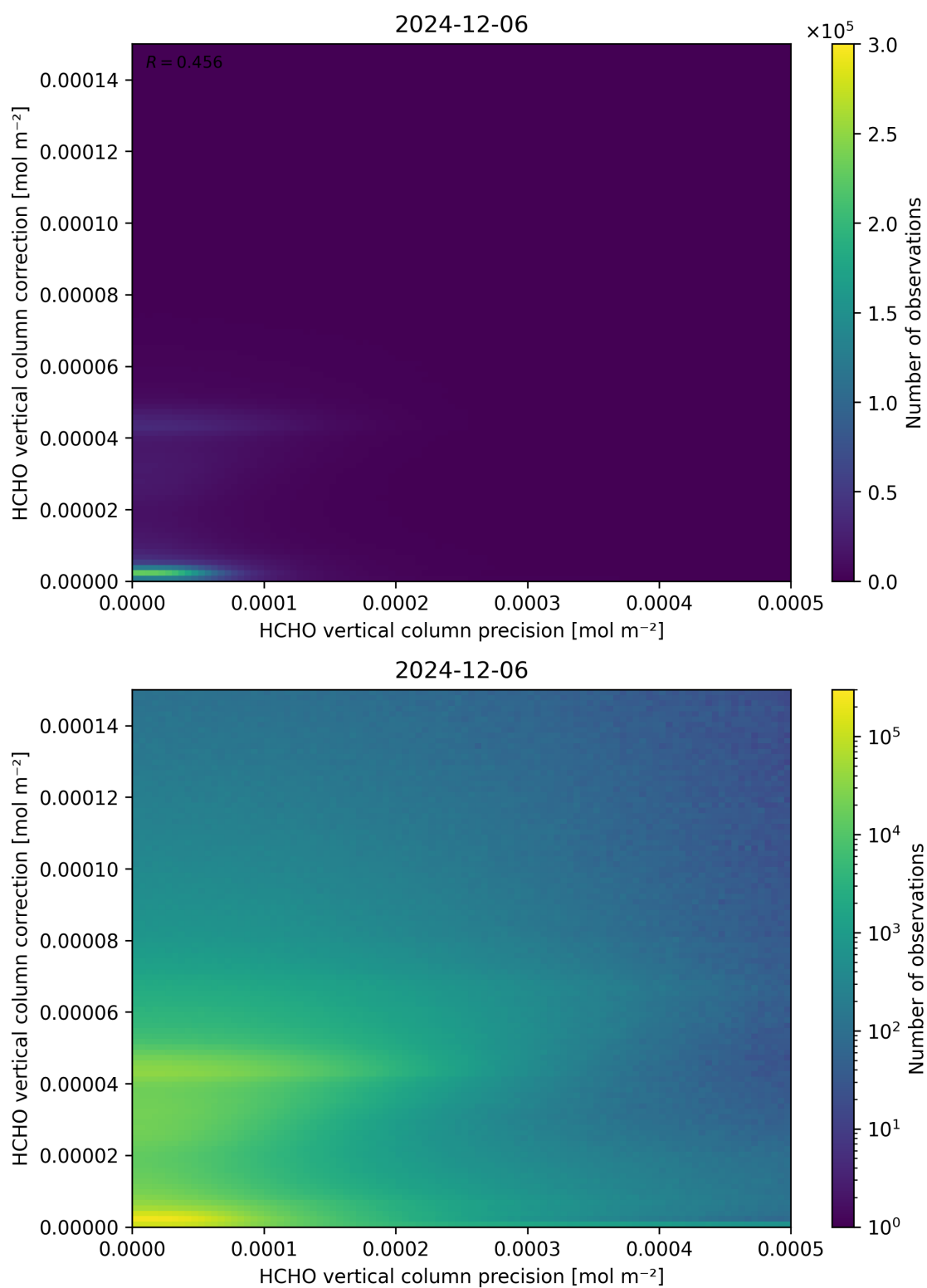
Figure 146: Scatter density plot of “HCHO vertical column precision” against “HCHO vertical column correction” for 2024-12-06 to 2024-12-07.
