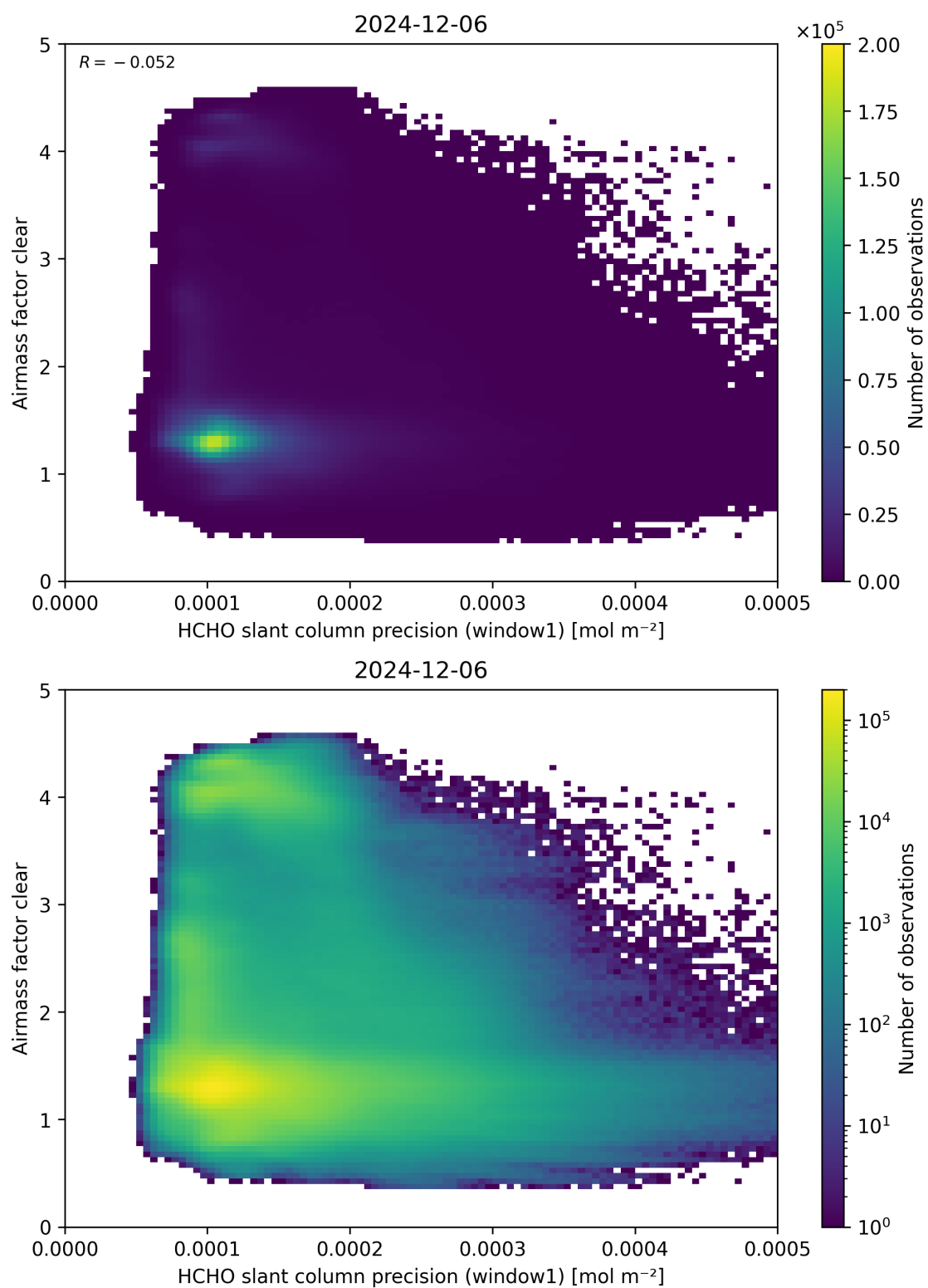
Figure 91: Scatter density plot of “HCHO slant column precision (window1)” against “Airmass factor clear” for 2024-12-06 to 2024-12-07.
