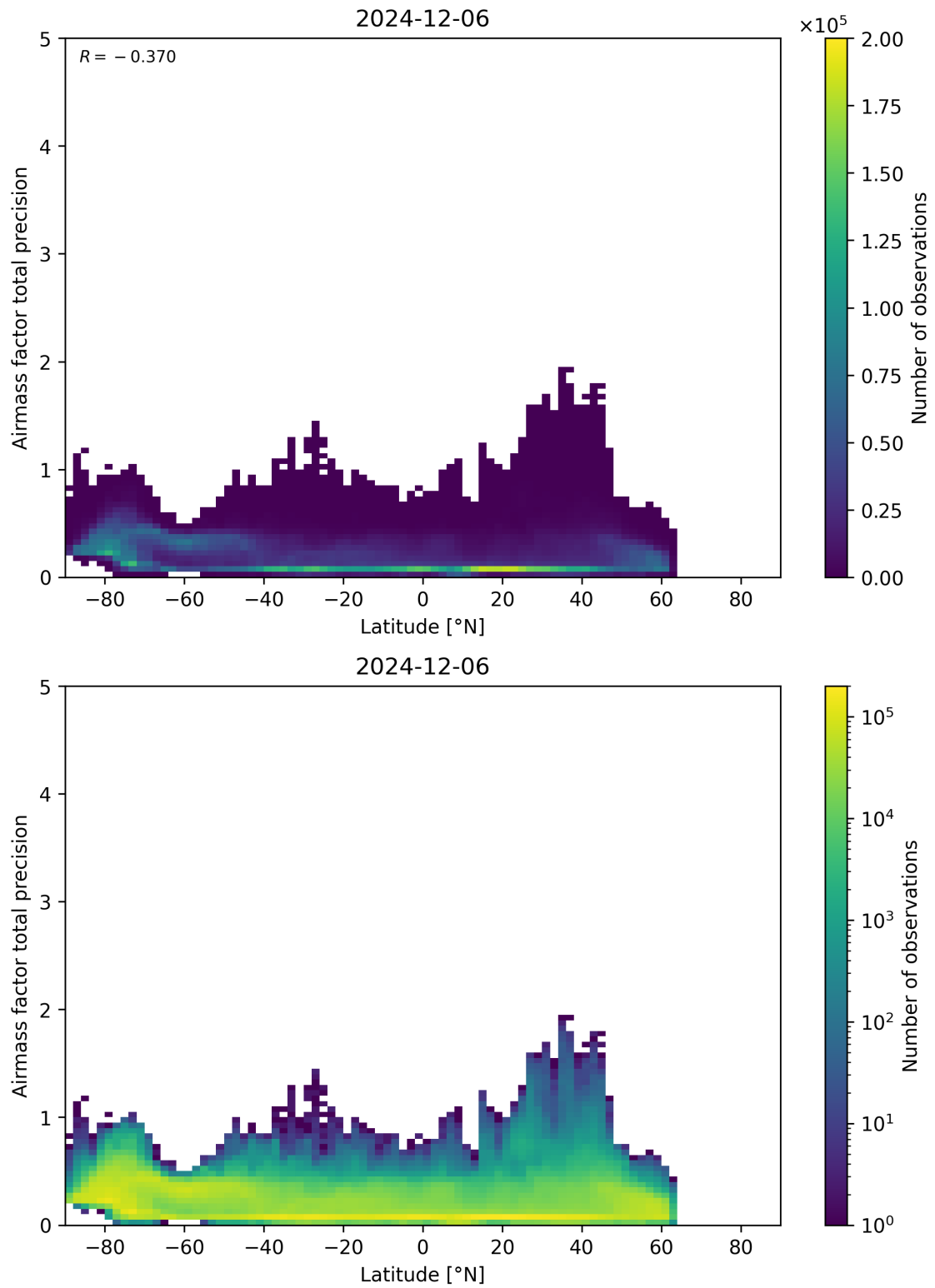
Figure 162: Scatter density plot of “Latitude” against “Airmass factor total precision” for 2024-12-06 to 2024-12-07.
