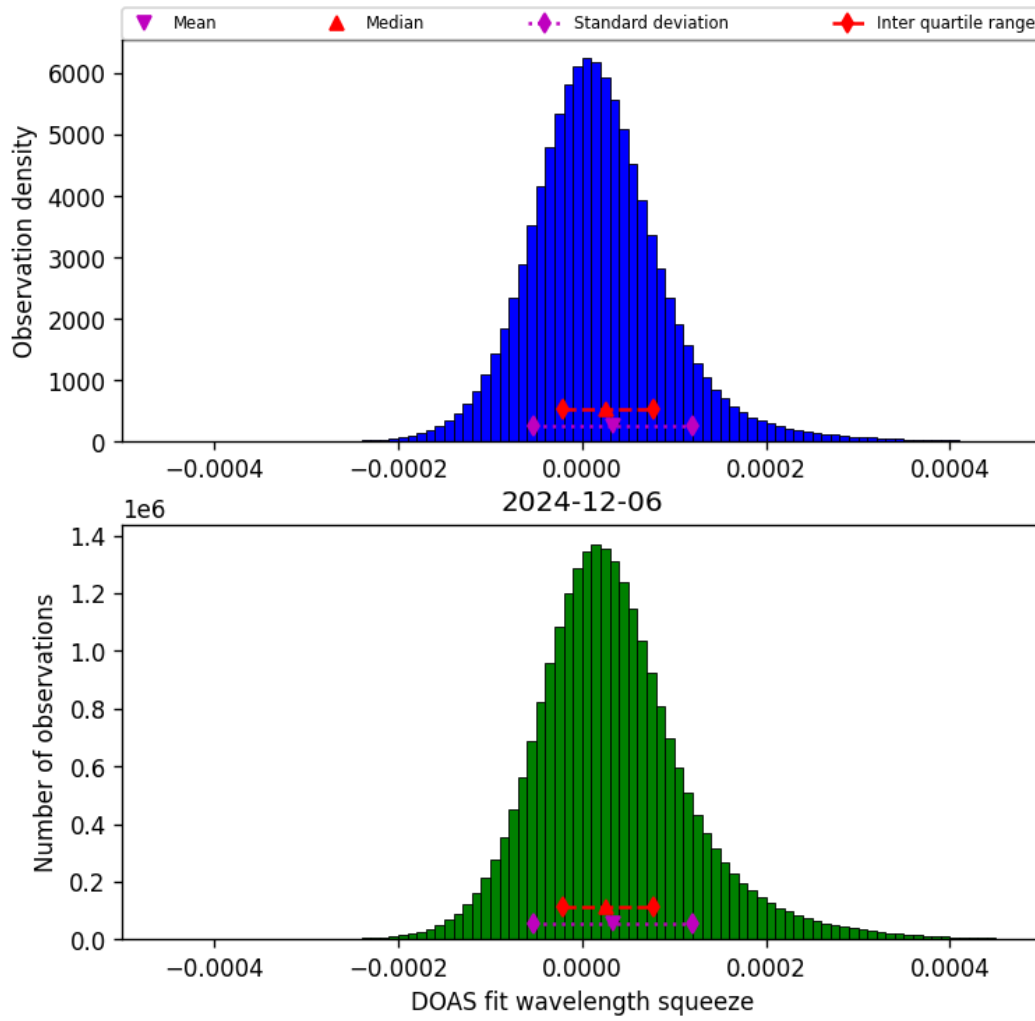
Figure 45: Histogram of “DOAS fit wavelength squeeze” for 2024-12-06 to 2024-12-07
