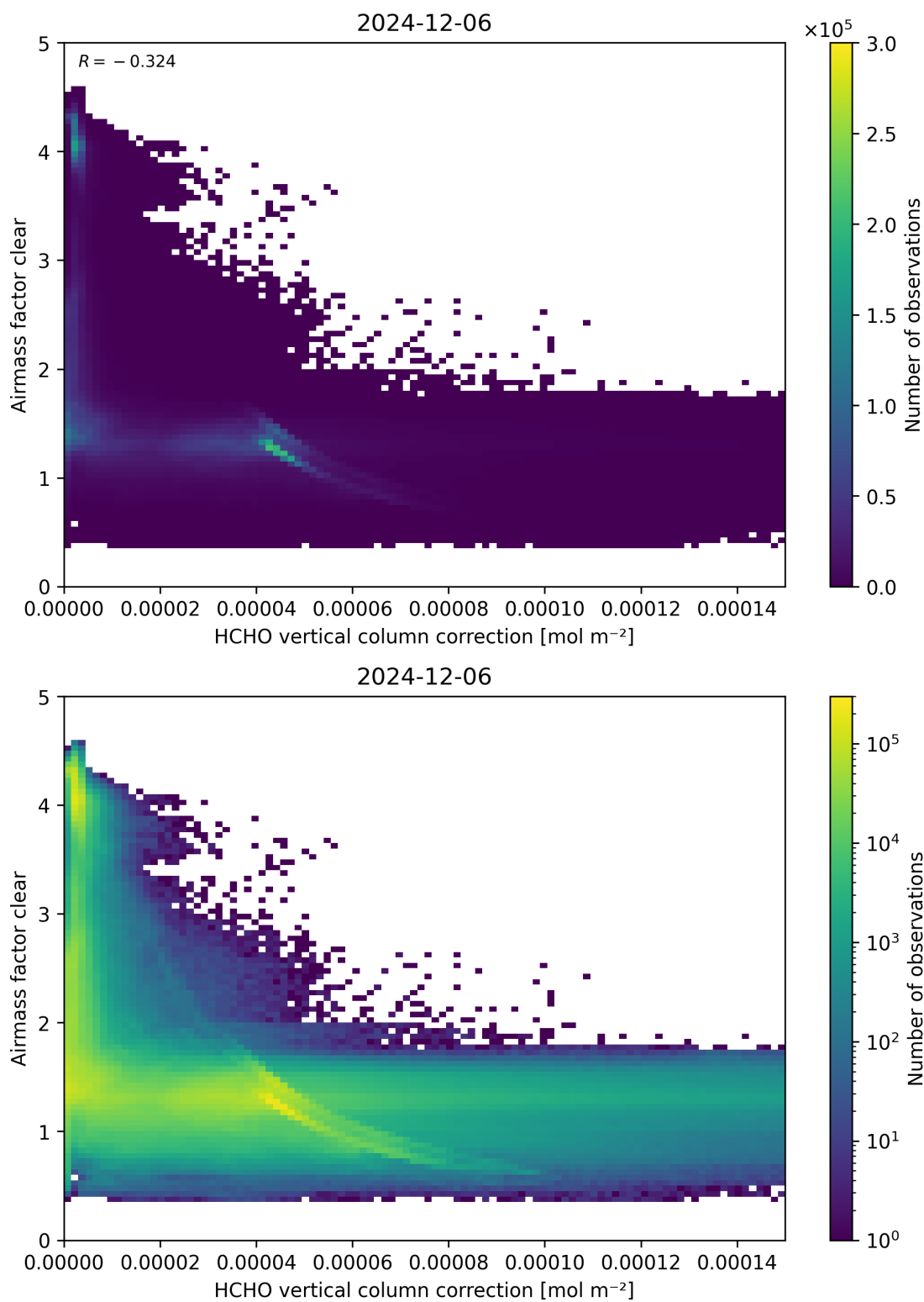
Figure 115: Scatter density plot of “HCHO vertical column correction” against “Airmass factor clear” for 2024-12-06 to 2024-12-07.
