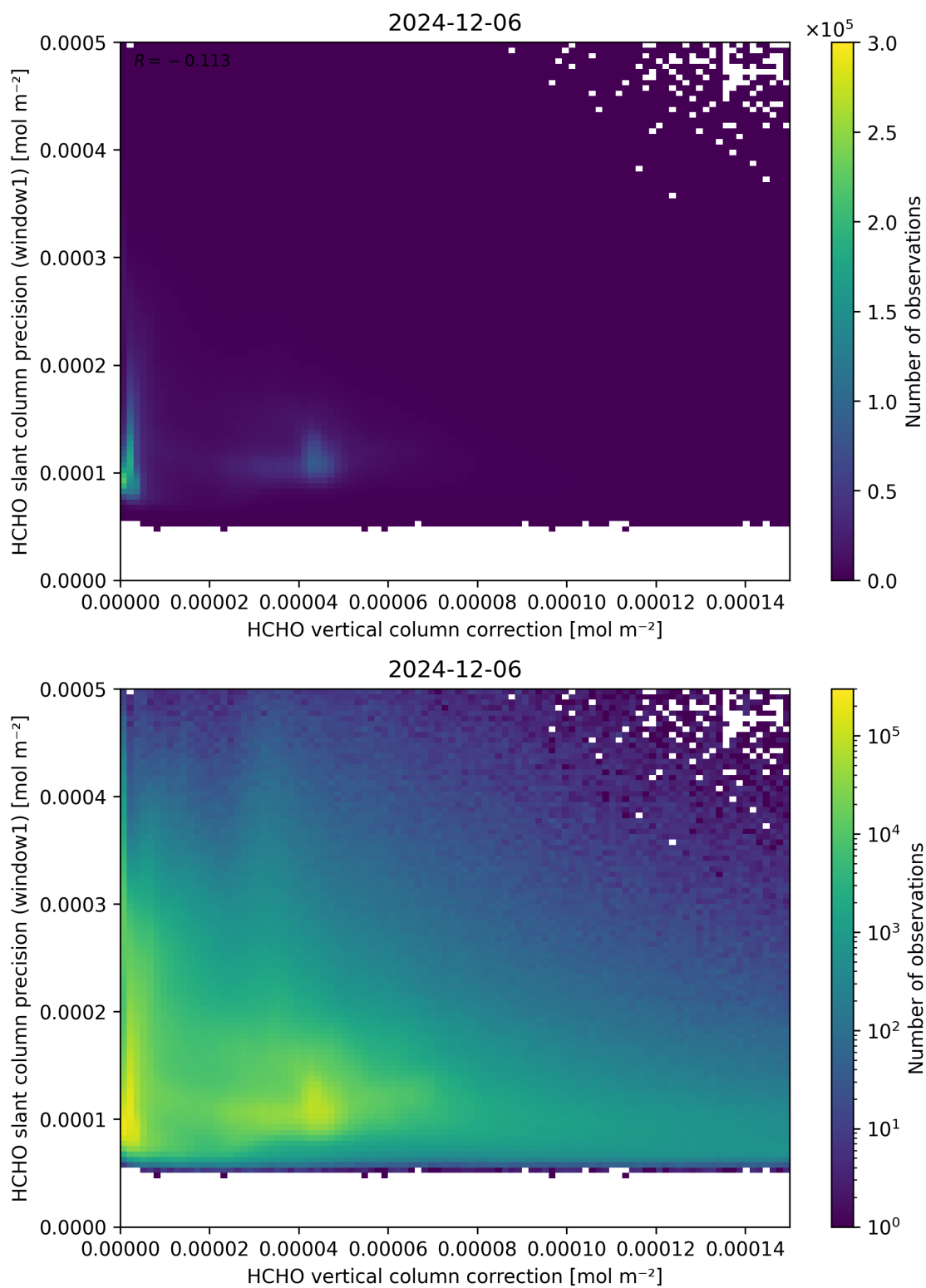
Figure 119: Scatter density plot of “HCHO vertical column correction” against “HCHO slant column precision (window1)” for 2024-12-06 to 2024-12-07.
