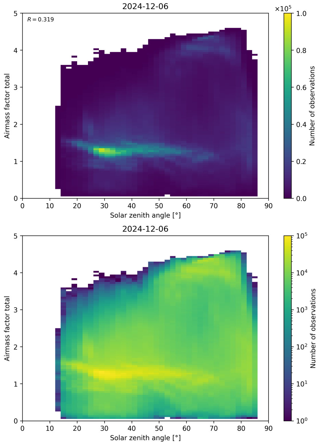
Figure 175: Scatter density plot of “Solar zenith angle” against “Airmass factor total” for 2024-12-06 to 2024-12-07.
