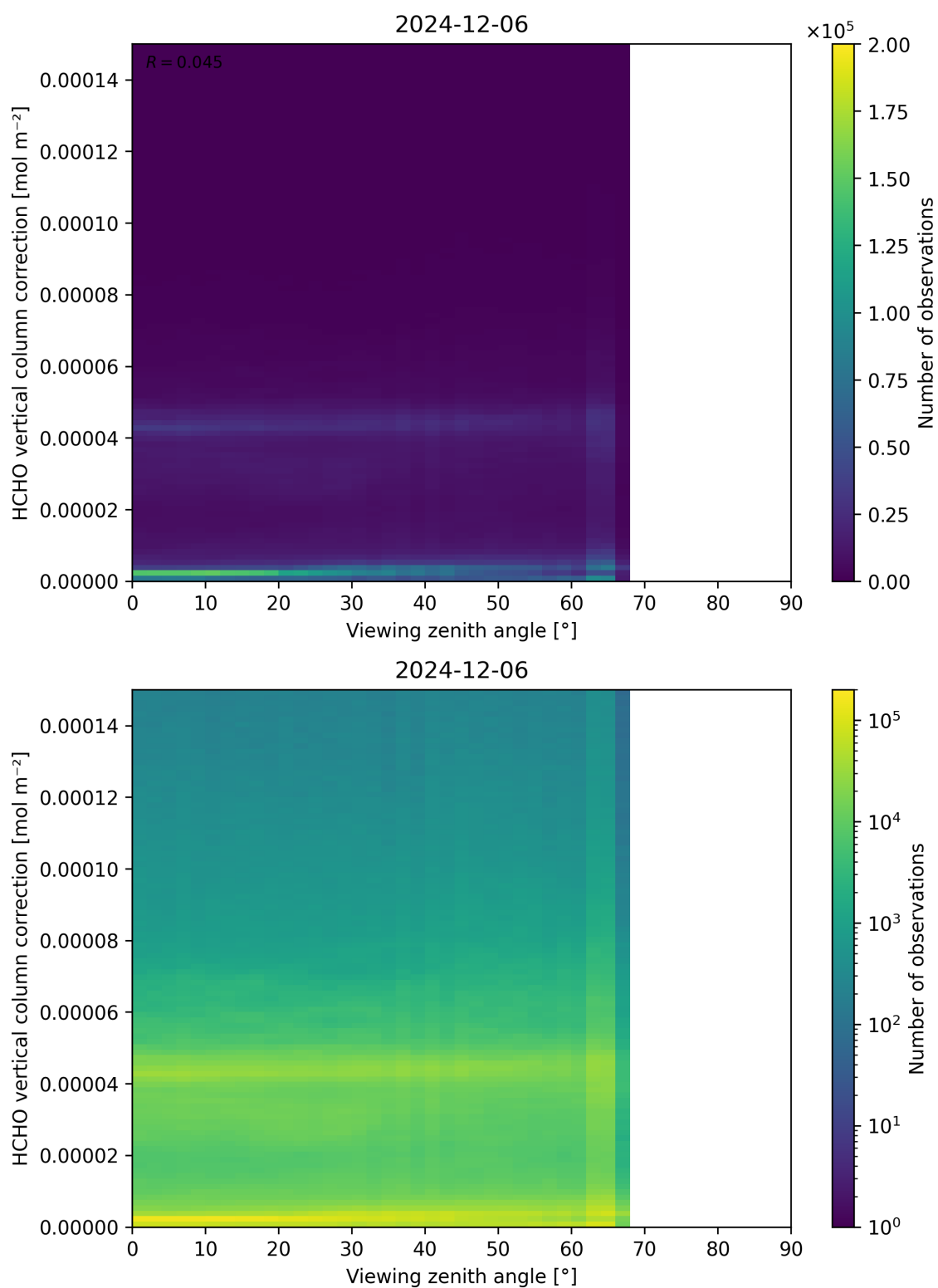
Figure 193: Scatter density plot of “Viewing zenith angle” against “HCHO vertical column correction” for 2024-12-06 to 2024-12-07.
