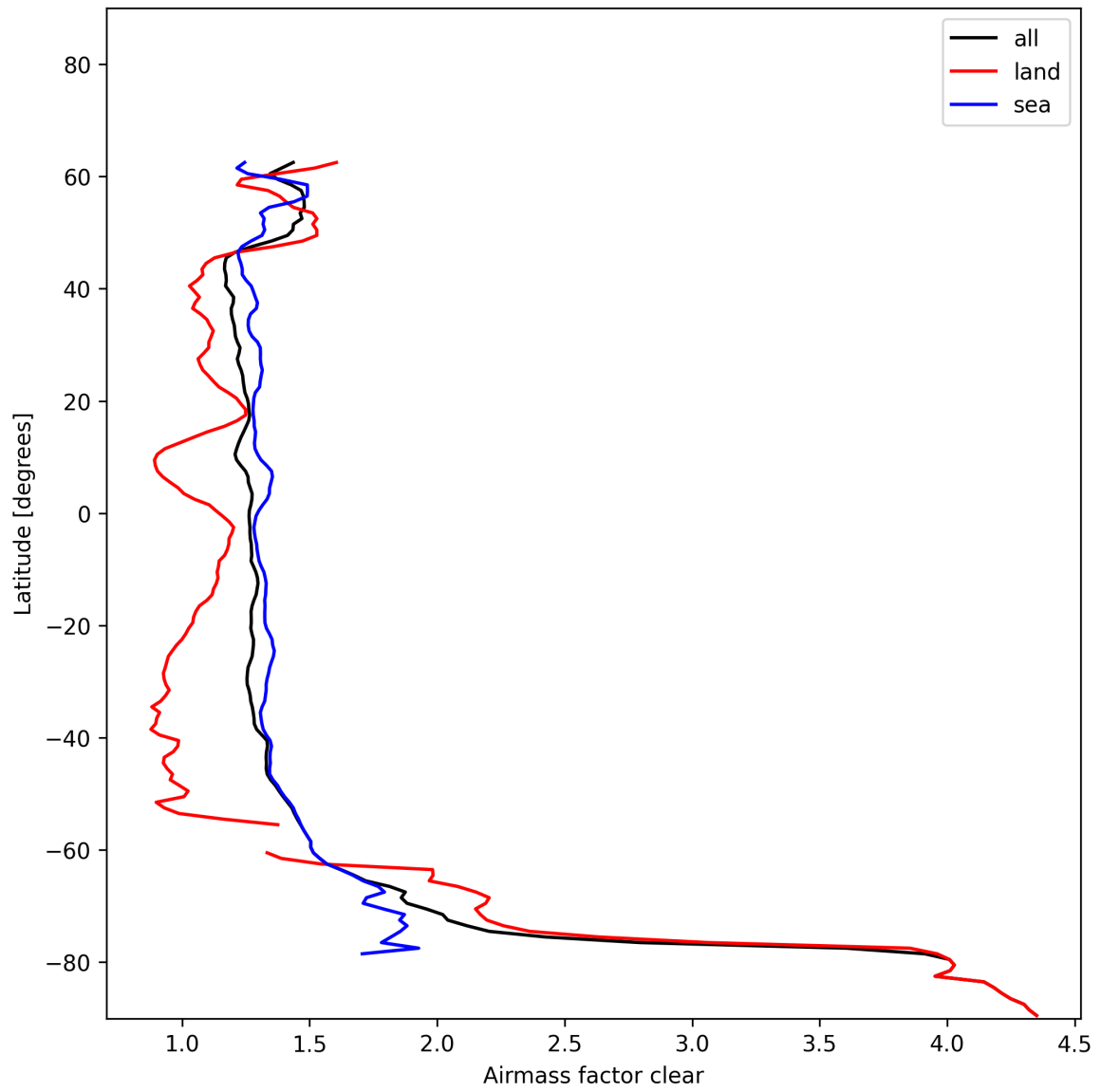
Figure 28: Zonal average of “Airmass factor clear” for 2024-12-06 to 2024-12-07.
