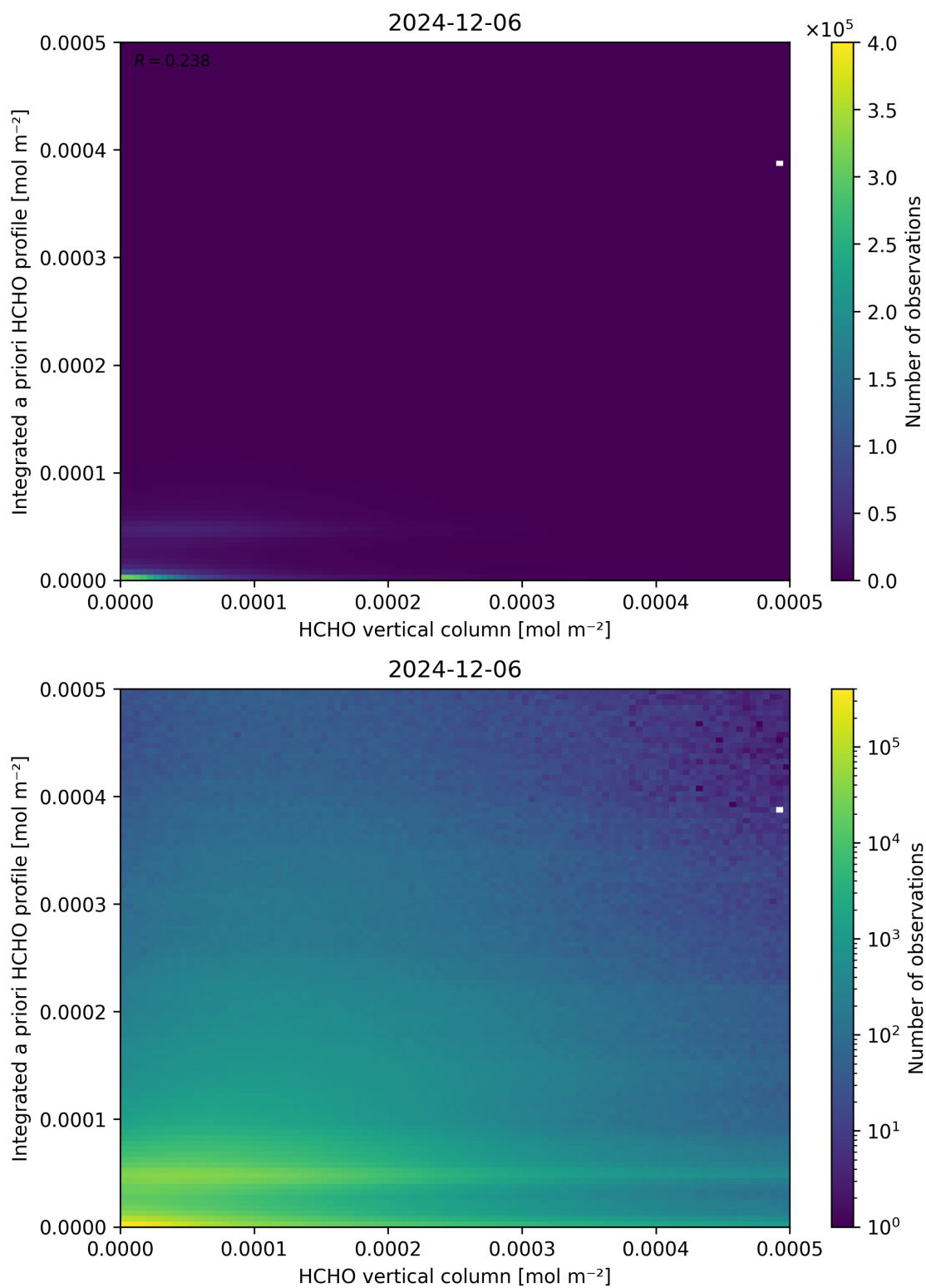
Figure 135: Scatter density plot of “HCHO vertical column” against “Integrated a priori HCHO profile” for 2024-12-06 to 2024-12-07.
