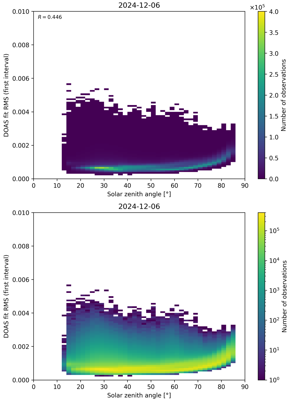
Figure 167: Scatter density plot of “Solar zenith angle” against “DOAS fit RMS (first interval)” for 2024-12-06 to 2024-12-07.
