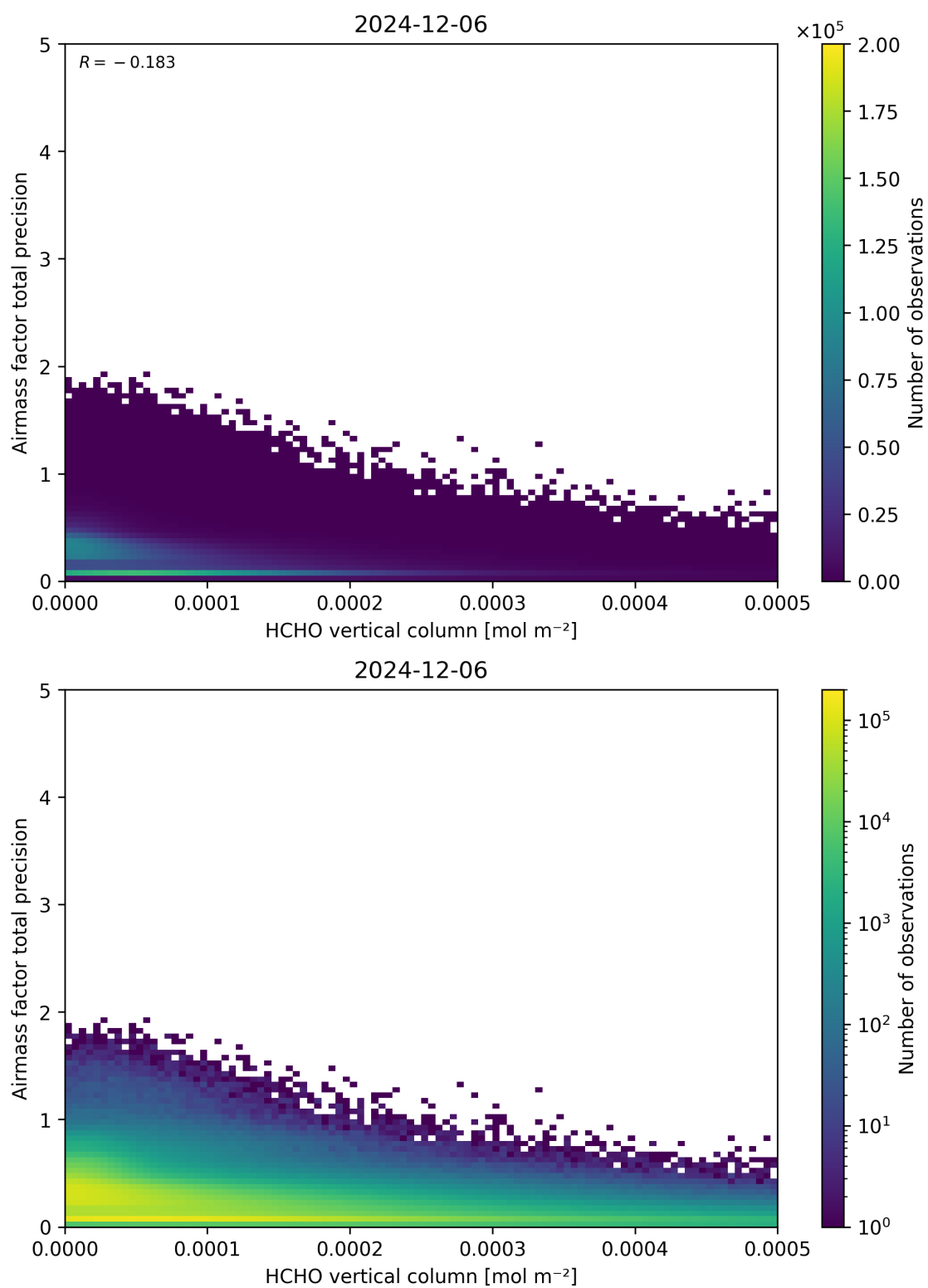
Figure 132: Scatter density plot of “HCHO vertical column” against “Airmass factor total precision” for 2024-12-06 to 2024-12-07.
