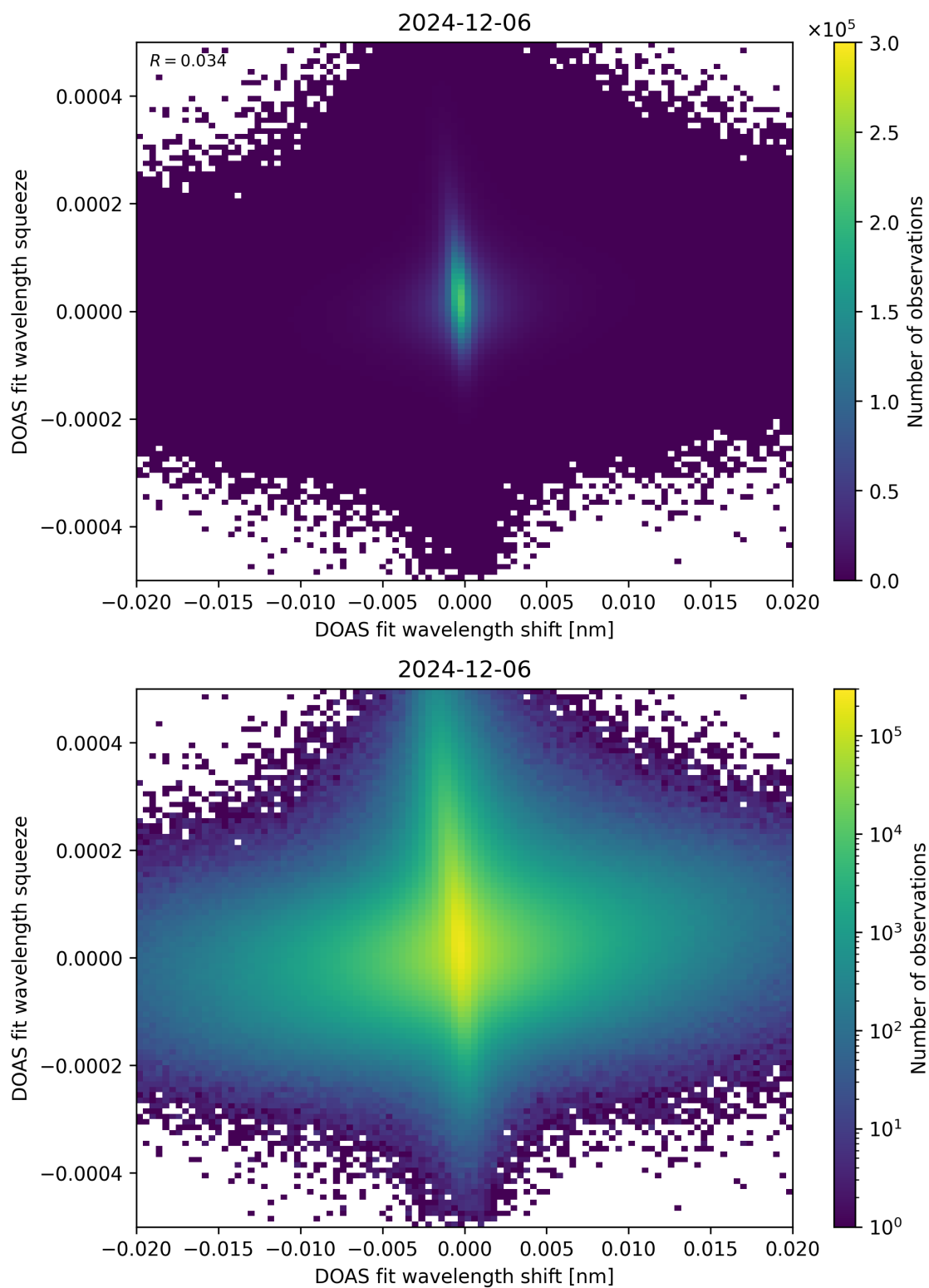
Figure 65: Scatter density plot of “DOAS fit wavelength shift” against “DOAS fit wavelength squeeze” for 2024-12-06 to 2024-12-07.
