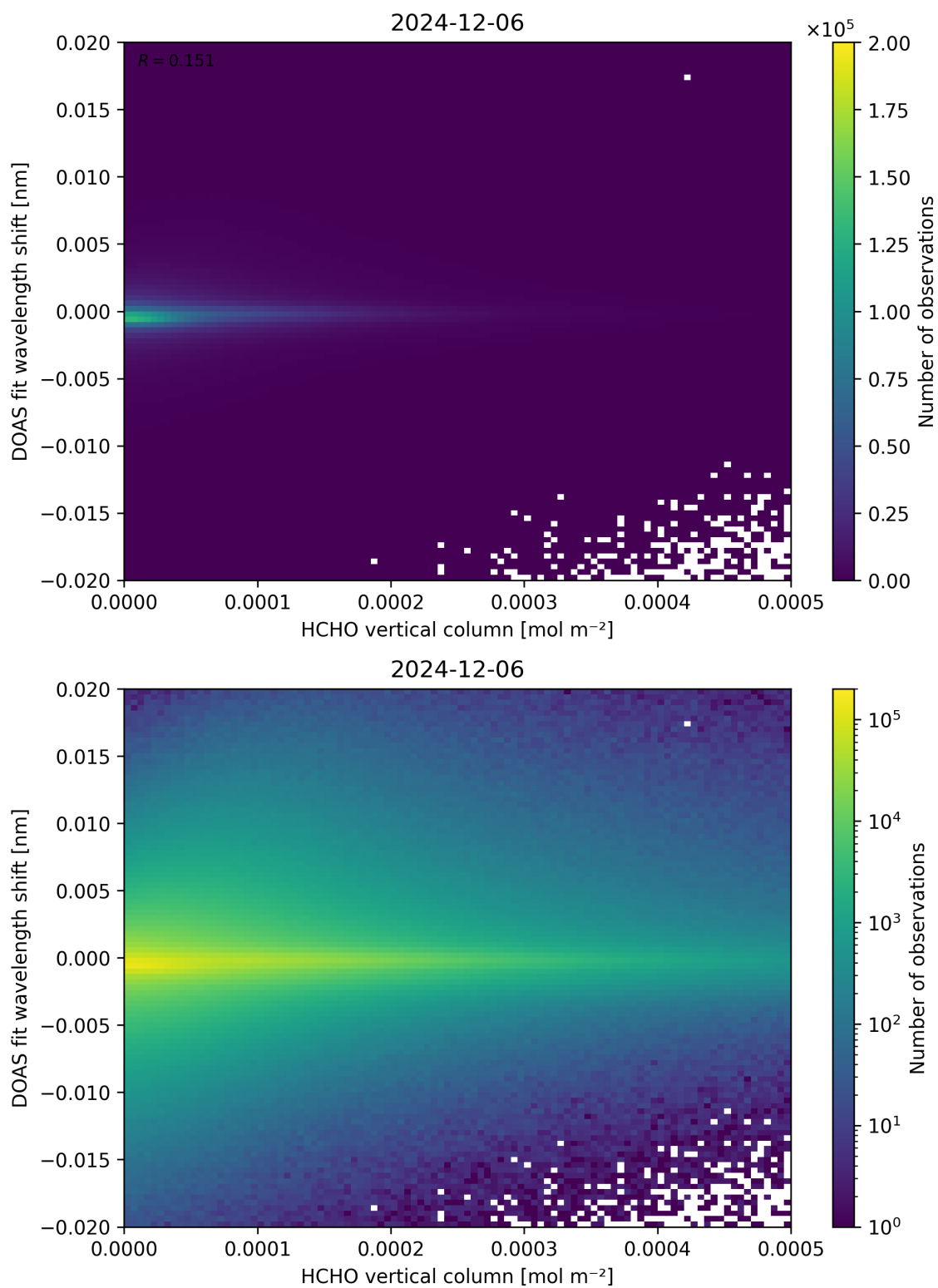
Figure 124: Scatter density plot of “HCHO vertical column” against “DOAS fit wavelength shift” for 2024-12-06 to 2024-12-07.
