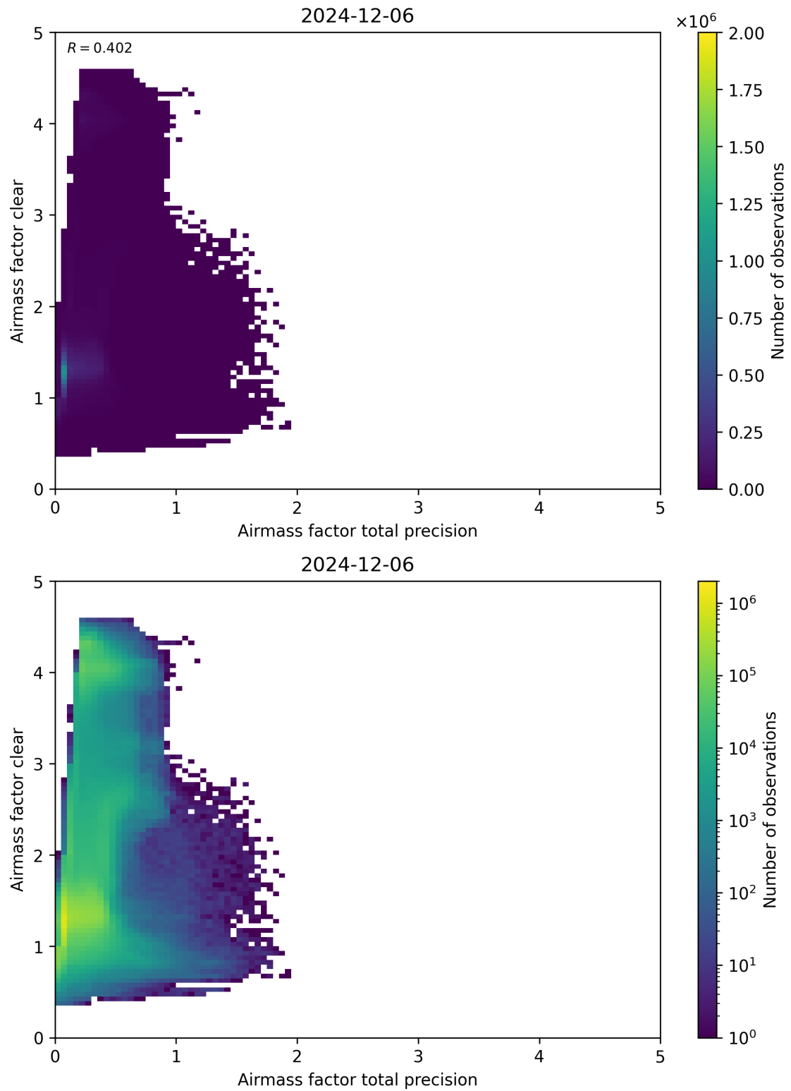
Figure 108: Scatter density plot of “Airmass factor total precision” against “Airmass factor clear” for 2024-12-06 to 2024-12-07.
