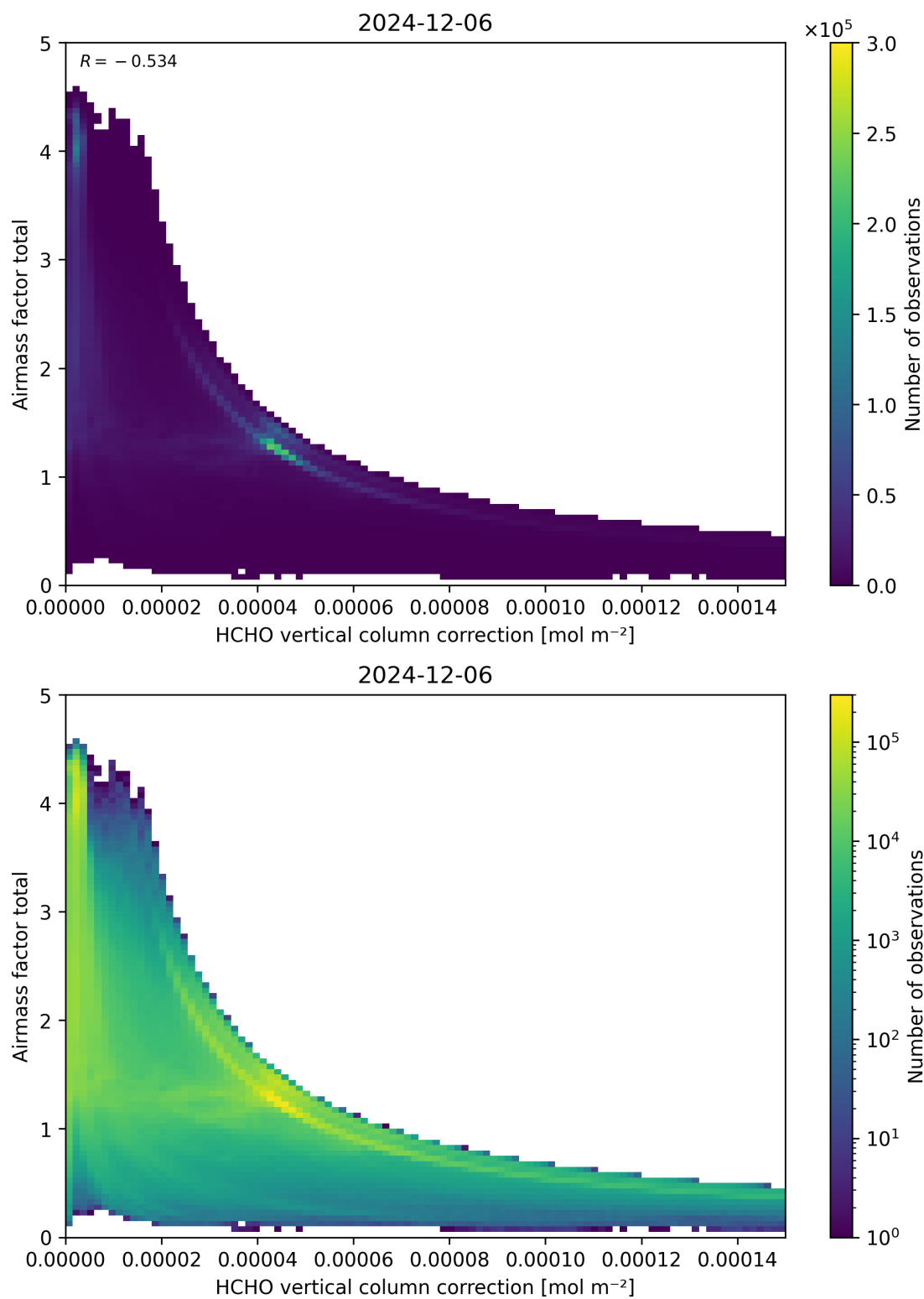
Figure 120: Scatter density plot of “HCHO vertical column correction” against “Airmass factor total” for 2024-12-06 to 2024-12-07.
