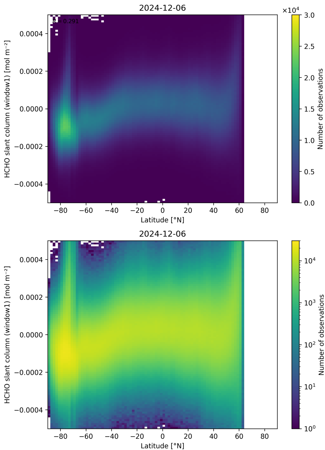
Figure 159: Scatter density plot of “Latitude” against “HCHO slant column (window1)” for 2024-12-06 to 2024-12-07.
