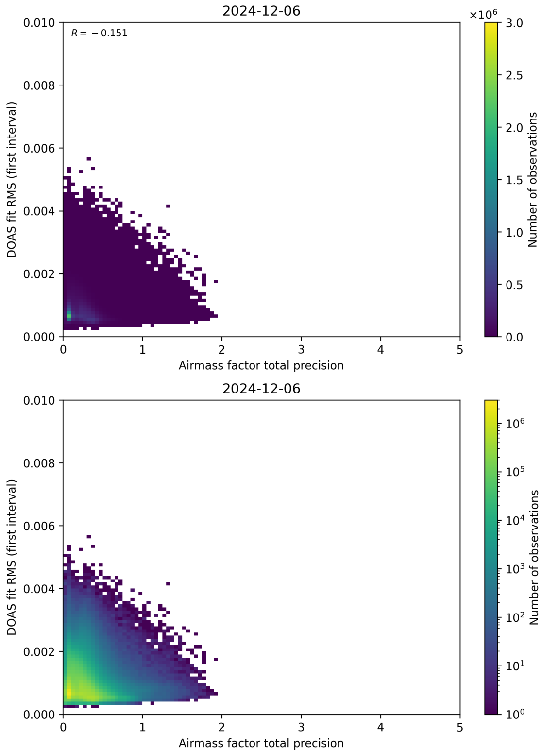
Figure 105: Scatter density plot of “Airmass factor total precision” against “DOAS fit RMS (first interval)” for 2024-12-06 to 2024-12-07.
