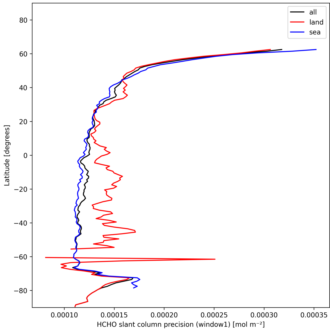
Figure 25: Zonal average of “HCHO slant column precision (window1)” for 2024-12-06 to 2024-12-07.
