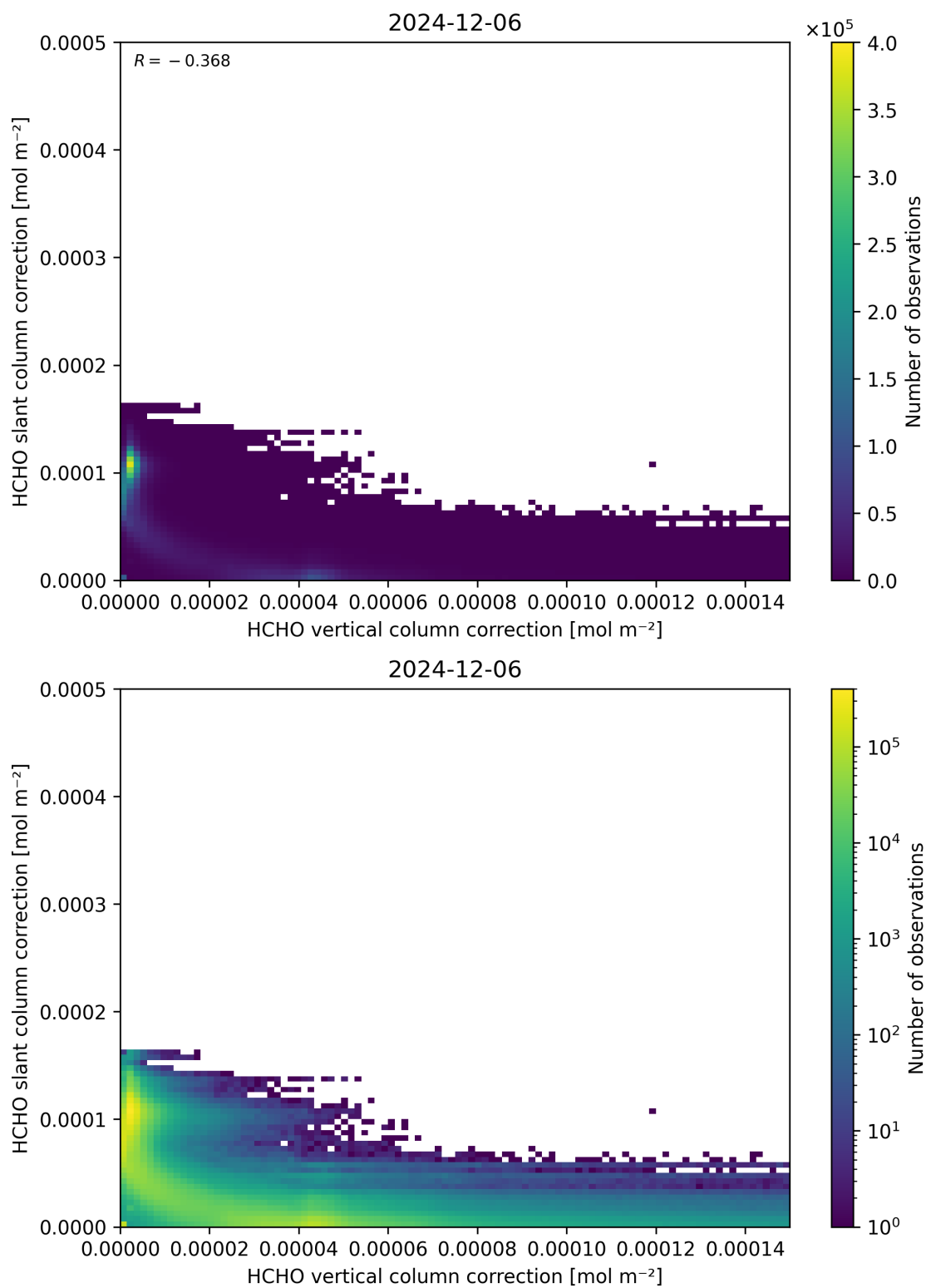
Figure 117: Scatter density plot of “HCHO vertical column correction” against “HCHO slant column correction” for 2024-12-06 to 2024-12-07.
