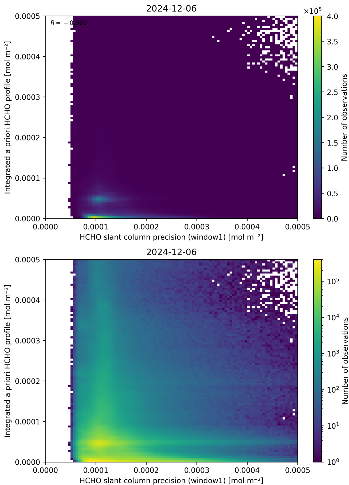
Figure 96: Scatter density plot of “HCHO slant column precision (window1)” against “Integrated a priori HCHO profile” for 2024-12-06 to 2024-12-07.
