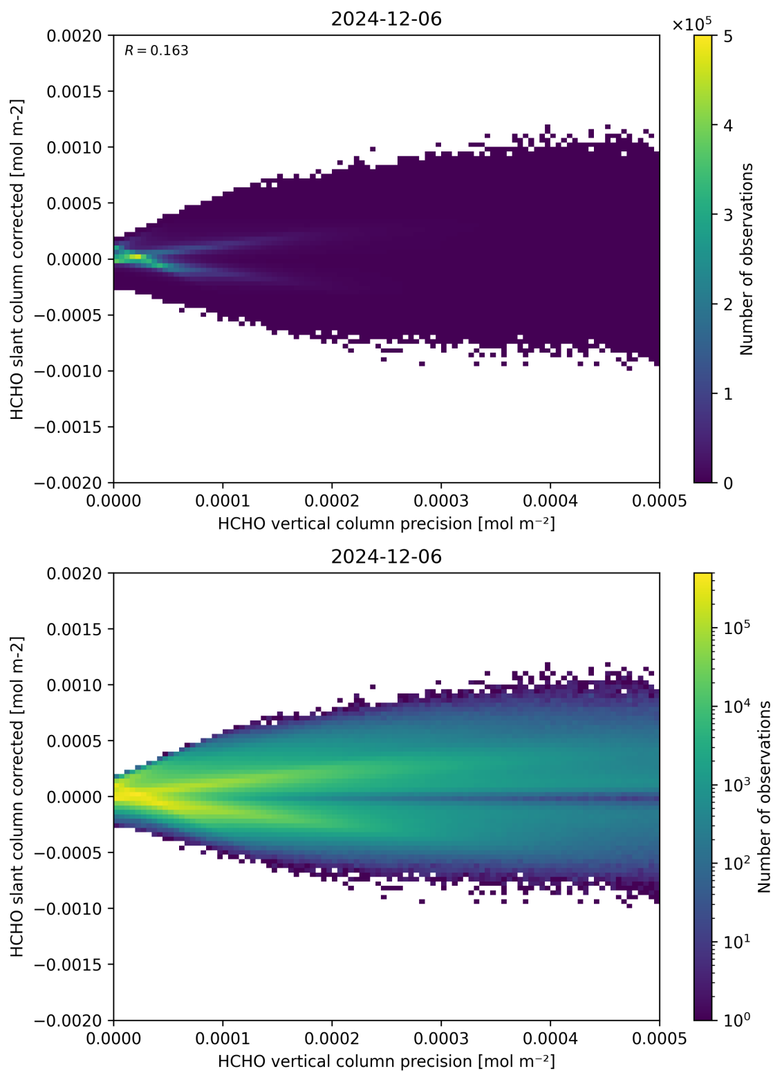
Figure 140: Scatter density plot of “HCHO vertical column precision” against “HCHO slant column corrected” for 2024-12-06 to 2024-12-07.
