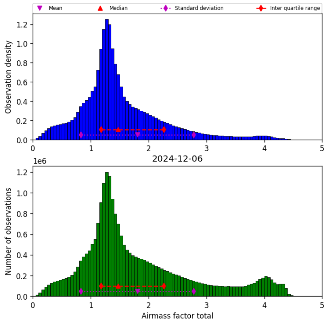
Figure 40: Histogram of “Airmass factor total” for 2024-12-06 to 2024-12-07
