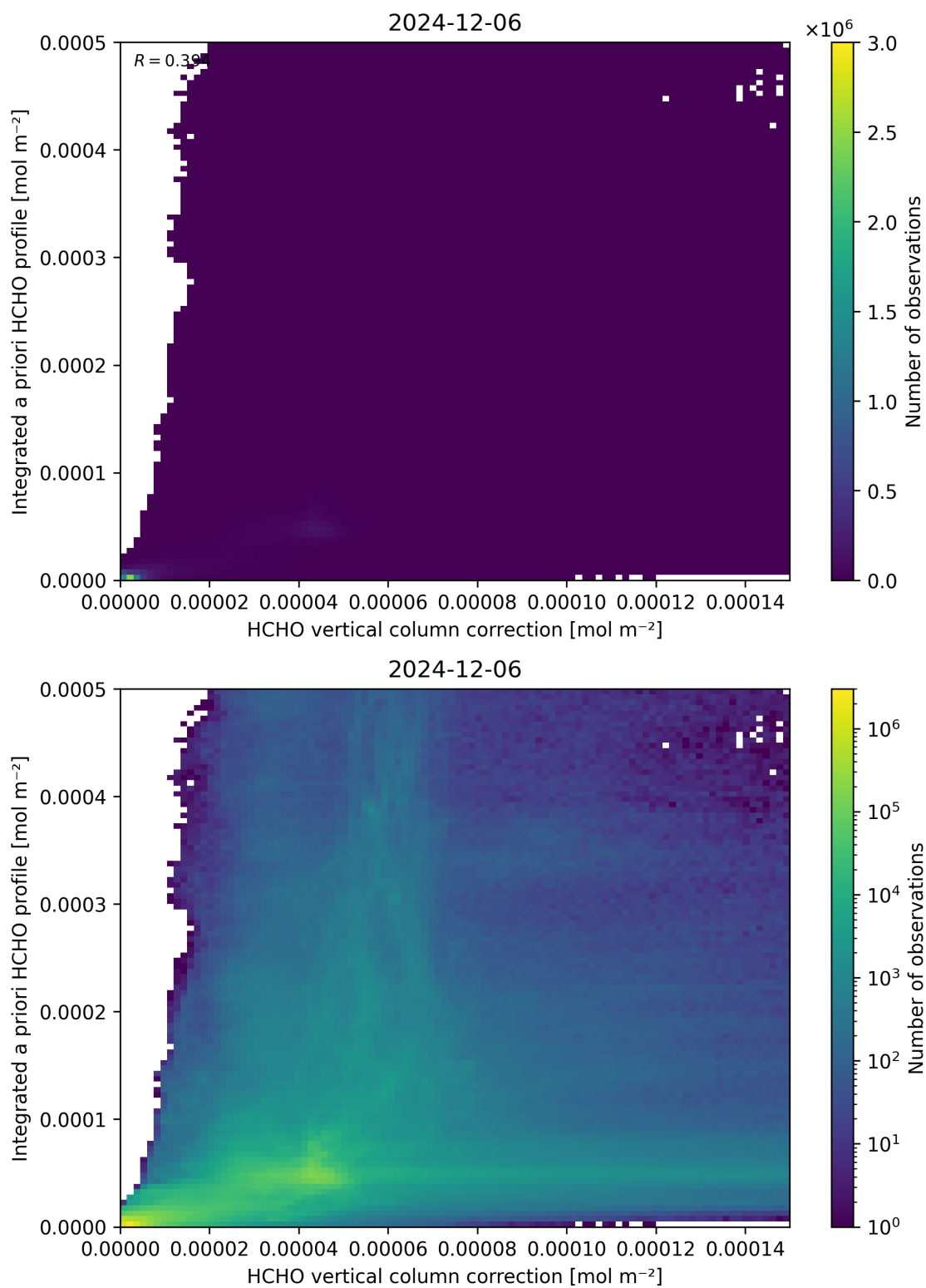
Figure 122: Scatter density plot of “HCHO vertical column correction” against “Integrated a priori HCHO profile” for 2024-12-06 to 2024-12-07.
