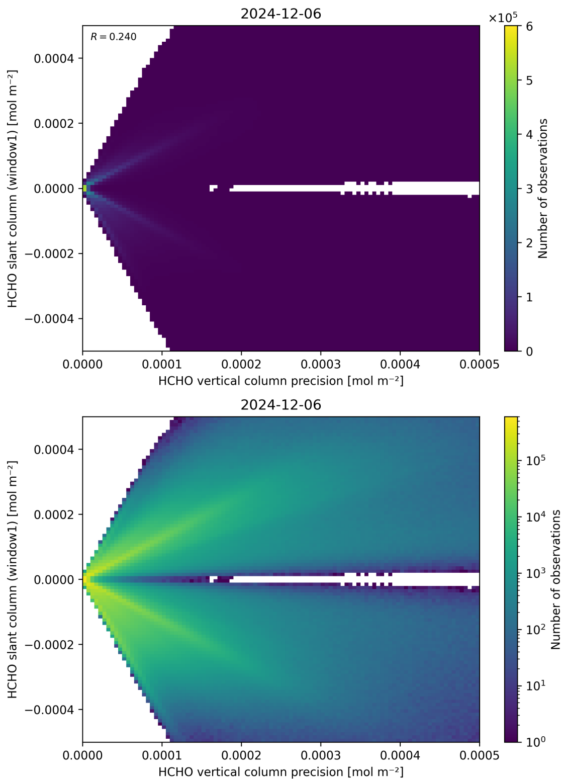
Figure 142: Scatter density plot of “HCHO vertical column precision” against “HCHO slant column (window1)” for 2024-12-06 to 2024-12-07.
