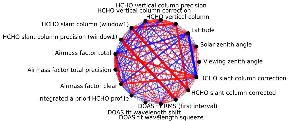
Figure 1: Map of correlation graph for 2024-12-06 to 2024-12-07.
