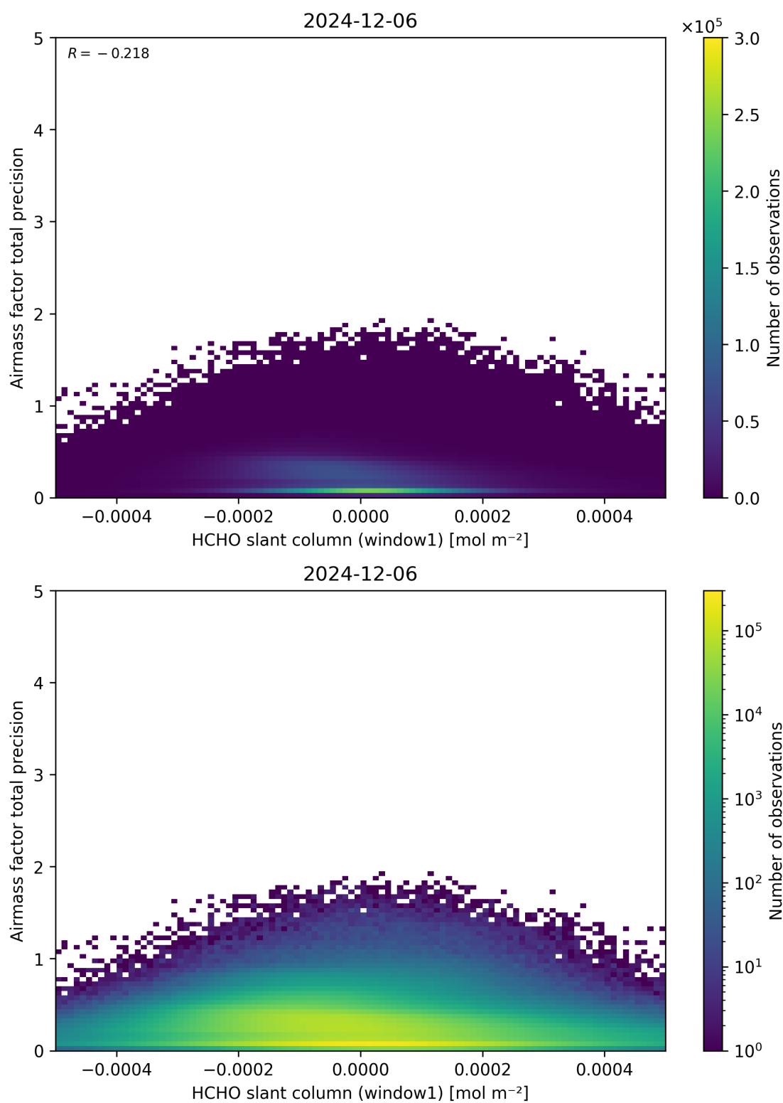
Figure 86: Scatter density plot of “HCHO slant column (window1)” against “Airmass factor total precision” for 2024-12-06 to 2024-12-07.
