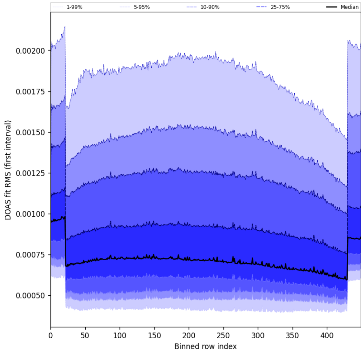
Figure 60: Along track statistics of “DOAS fit RMS (first interval)” for 2024-12-06 to 2024-12-07
