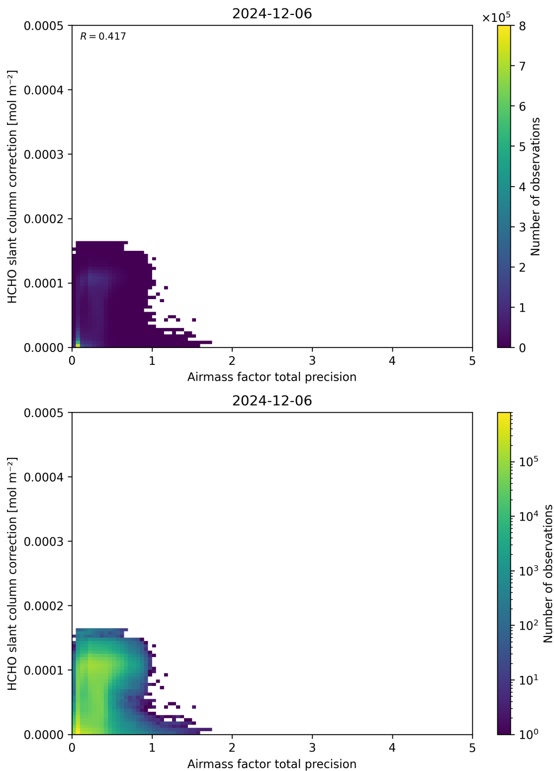
Figure 110: Scatter density plot of “Airmass factor total precision” against “HCHO slant column correction” for 2024-12-06 to 2024-12-07.
