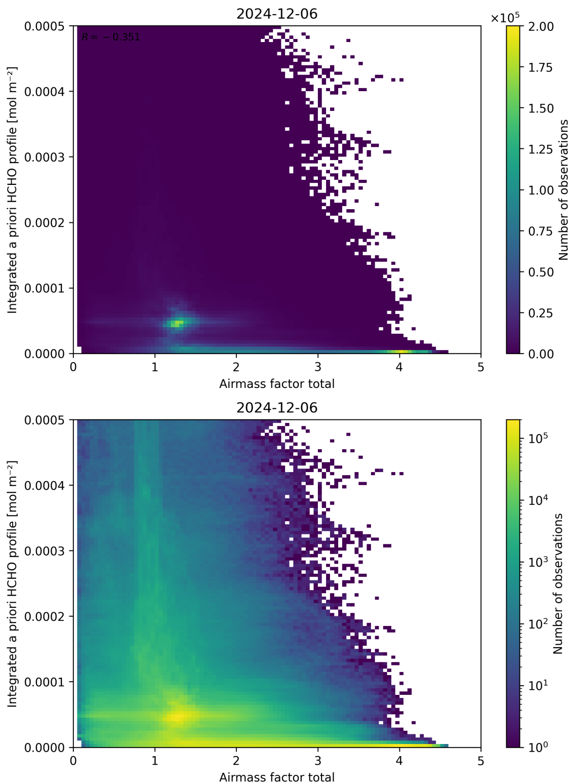
Figure 104: Scatter density plot of “Airmass factor total” against “Integrated a priori HCHO profile” for 2024-12-06 to 2024-12-07.
