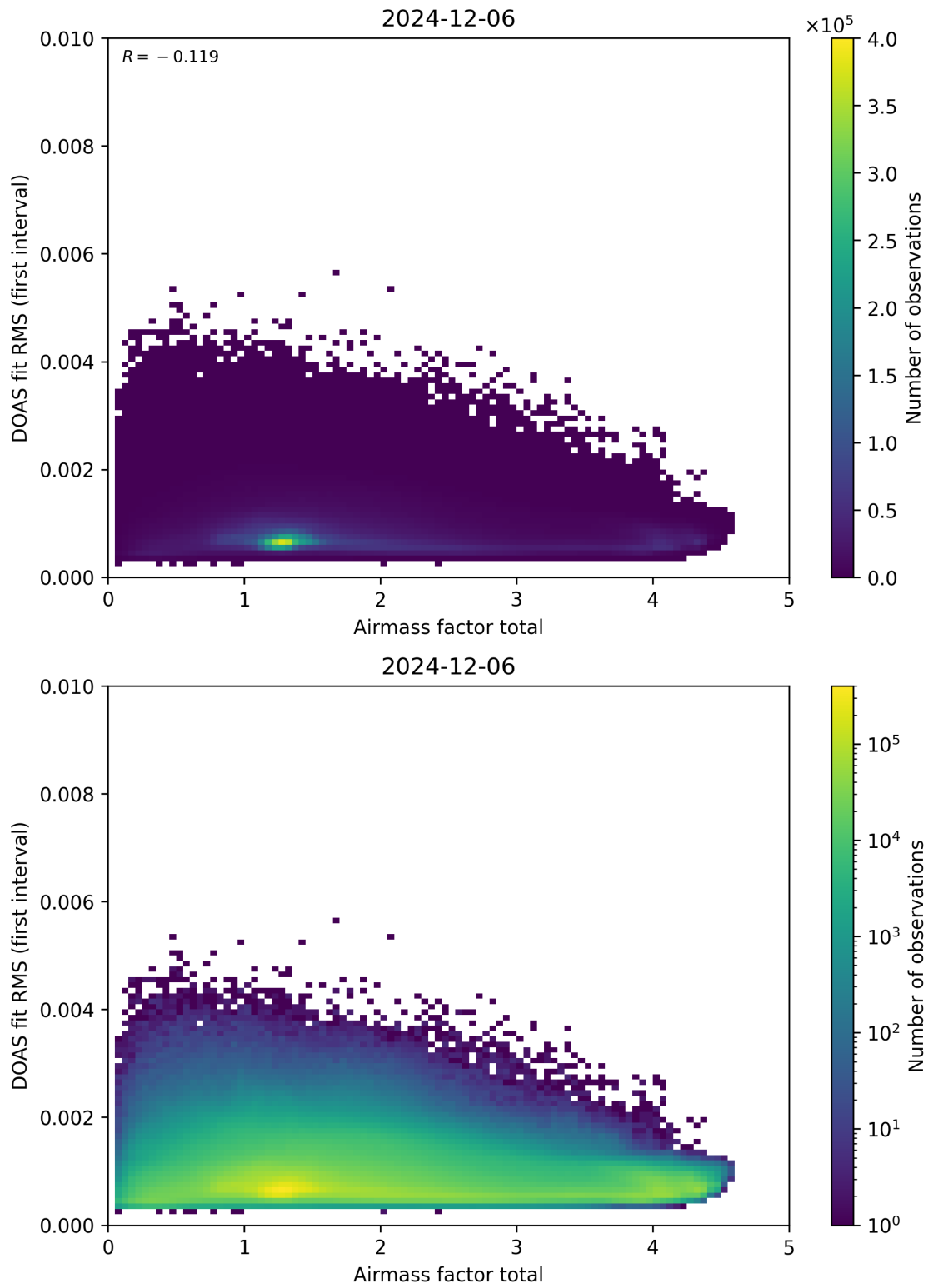
Figure 97: Scatter density plot of “Airmass factor total” against “DOAS fit RMS (first interval)” for 2024-12-06 to 2024-12-07.
