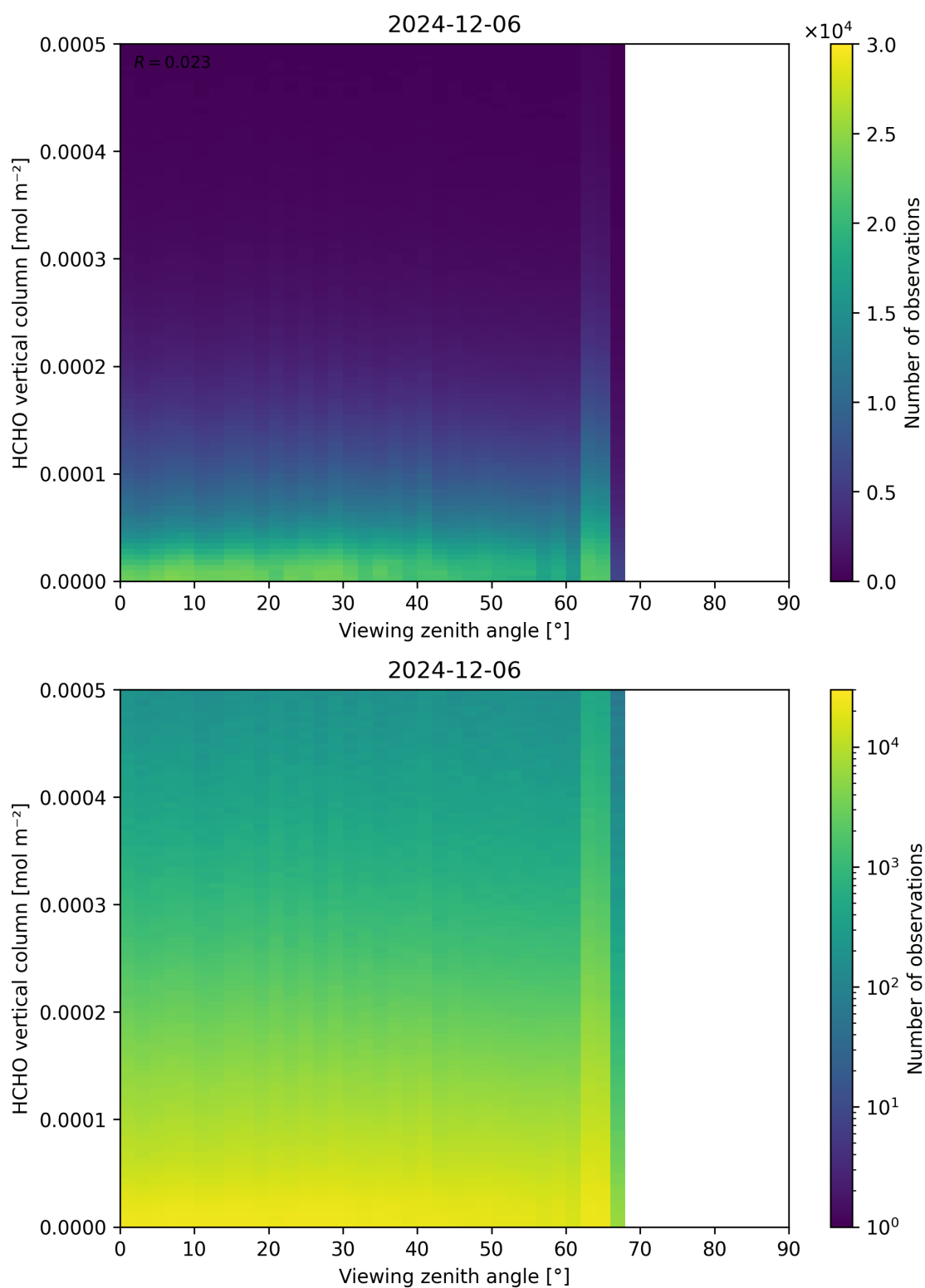
Figure 192: Scatter density plot of “Viewing zenith angle” against “HCHO vertical column” for 2024-12-06 to 2024-12-07.
