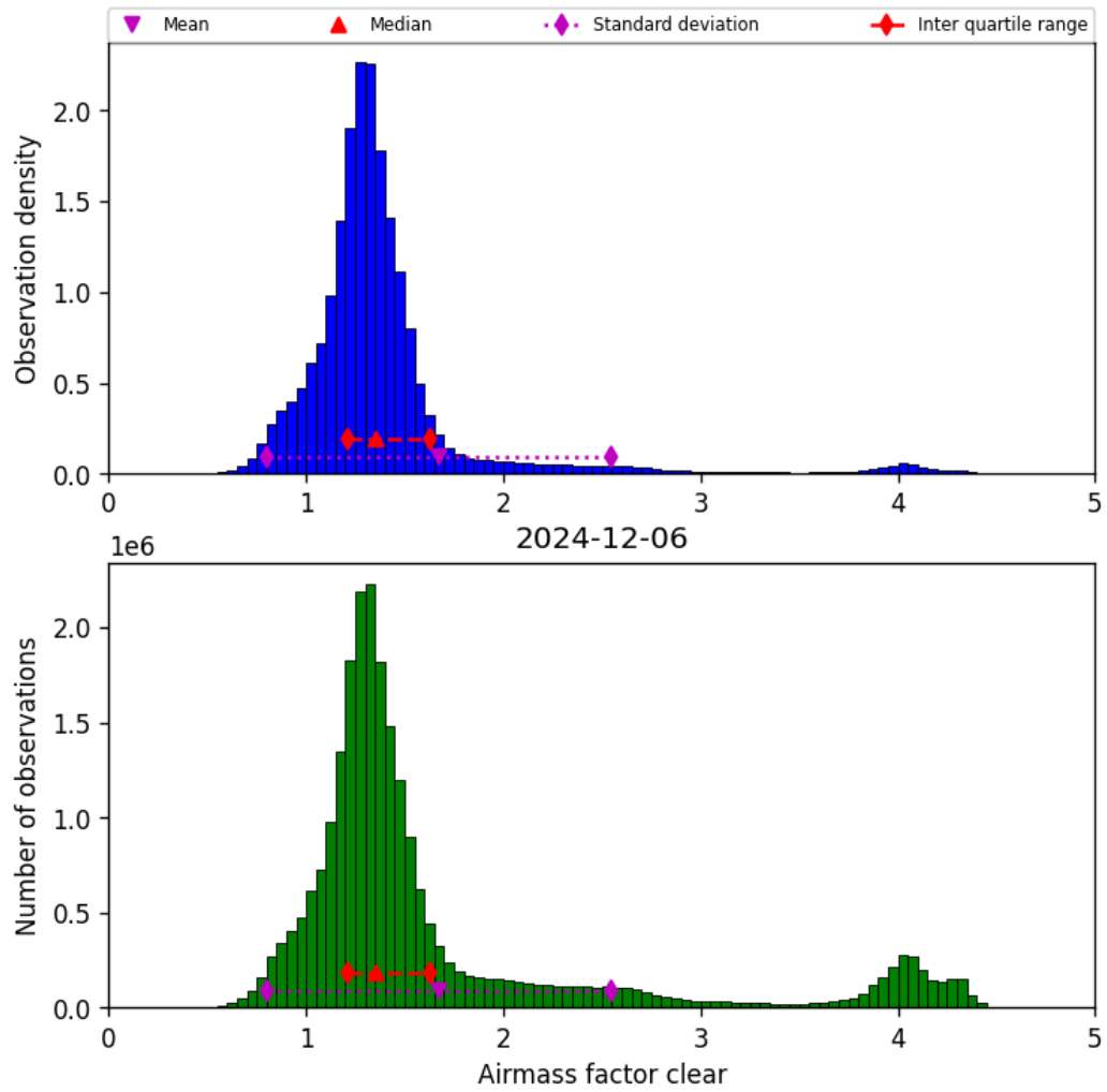
Figure 42: Histogram of “Airmass factor clear” for 2024-12-06 to 2024-12-07
