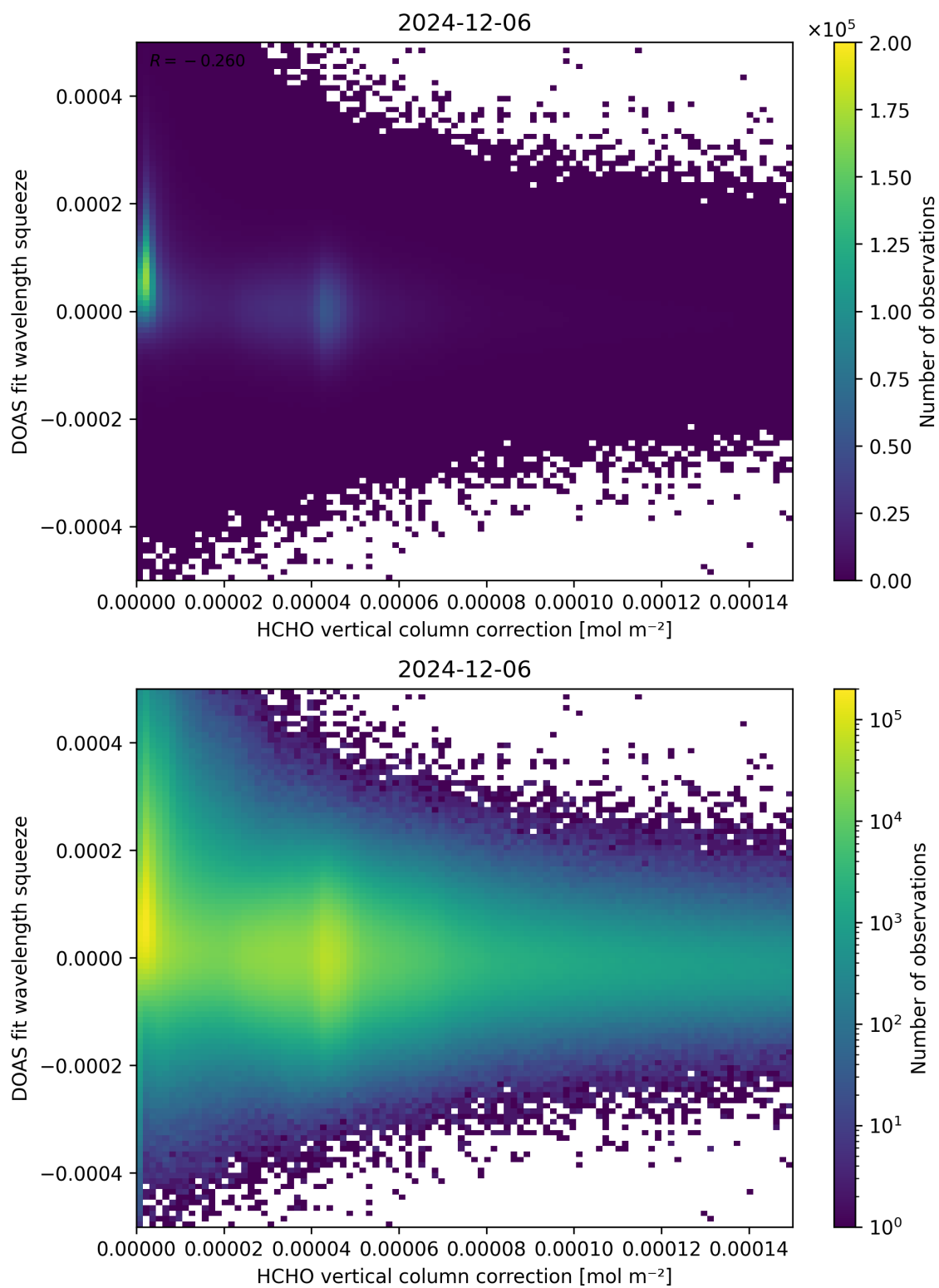
Figure 114: Scatter density plot of “HCHO vertical column correction” against “DOAS fit wavelength squeeze” for 2024-12-06 to 2024-12-07.
