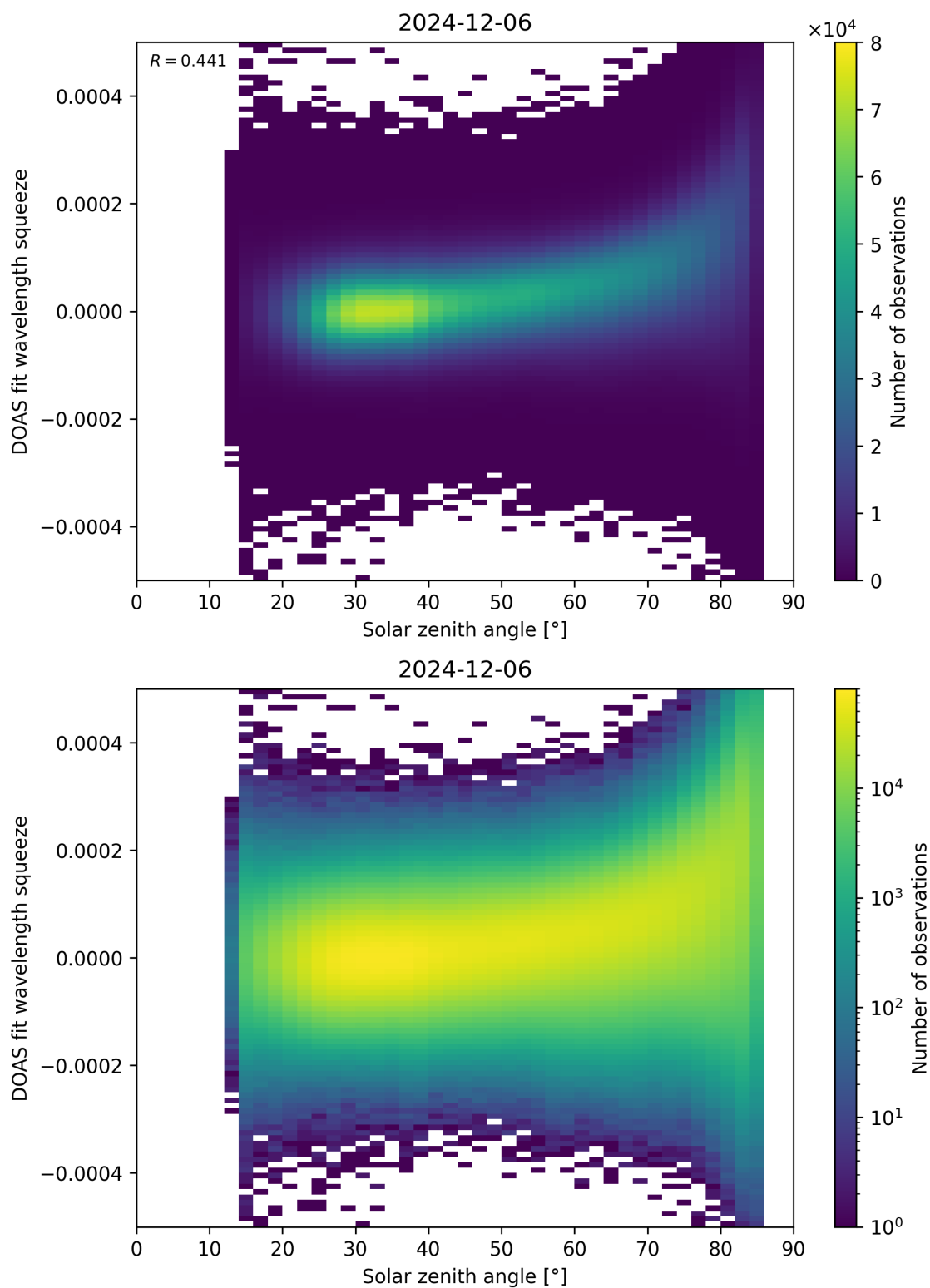
Figure 169: Scatter density plot of “Solar zenith angle” against “DOAS fit wavelength squeeze” for 2024-12-06 to 2024-12-07.
