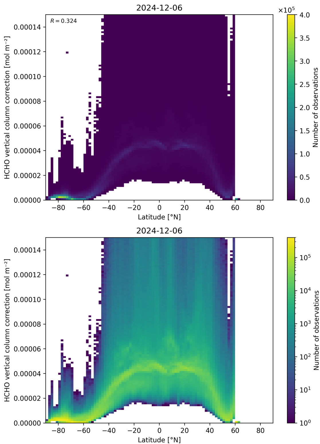
Figure 164: Scatter density plot of “Latitude” against “HCHO vertical column correction” for 2024-12-06 to 2024-12-07.
