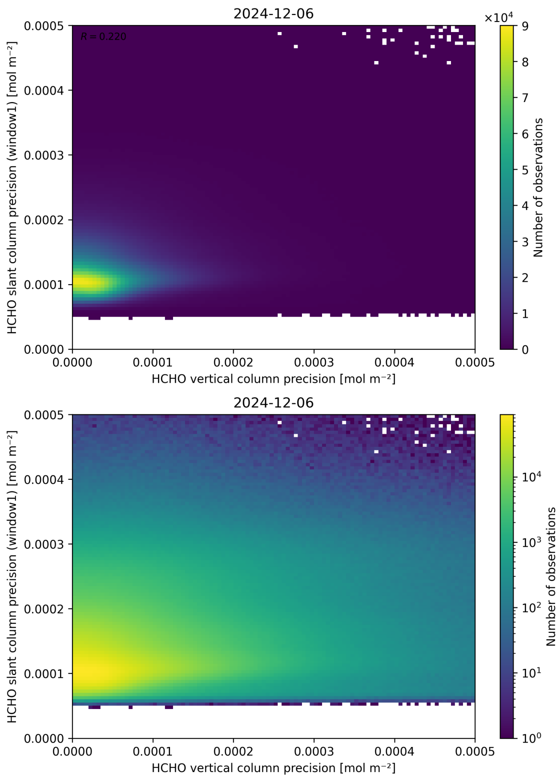
Figure 143: Scatter density plot of “HCHO vertical column precision” against “HCHO slant column precision (window1)” for 2024-12-06 to 2024-12-07.
