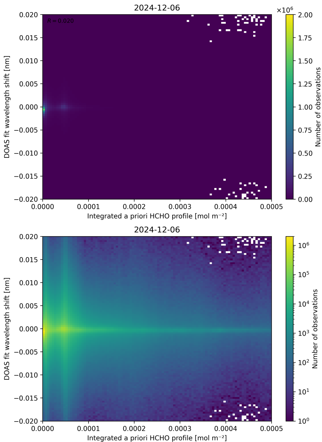
Figure 149: Scatter density plot of “Integrated a priori HCHO profile” against “DOAS fit wavelength shift” for 2024-12-06 to 2024-12-07.
