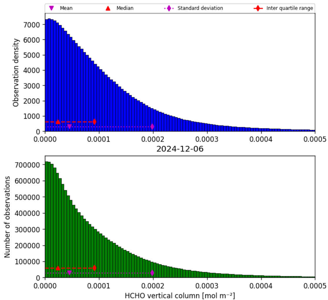
Figure 35: Histogram of “HCHO vertical column” for 2024-12-06 to 2024-12-07
