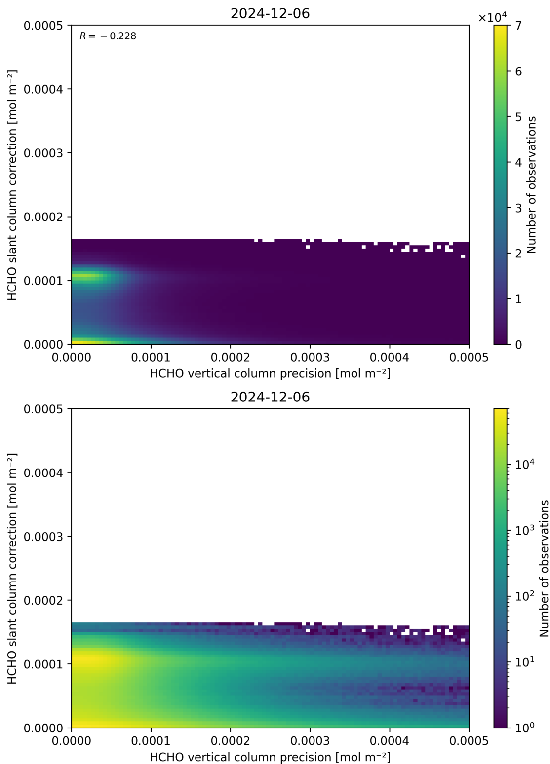
Figure 141: Scatter density plot of “HCHO vertical column precision” against “HCHO slant column correction” for 2024-12-06 to 2024-12-07.
