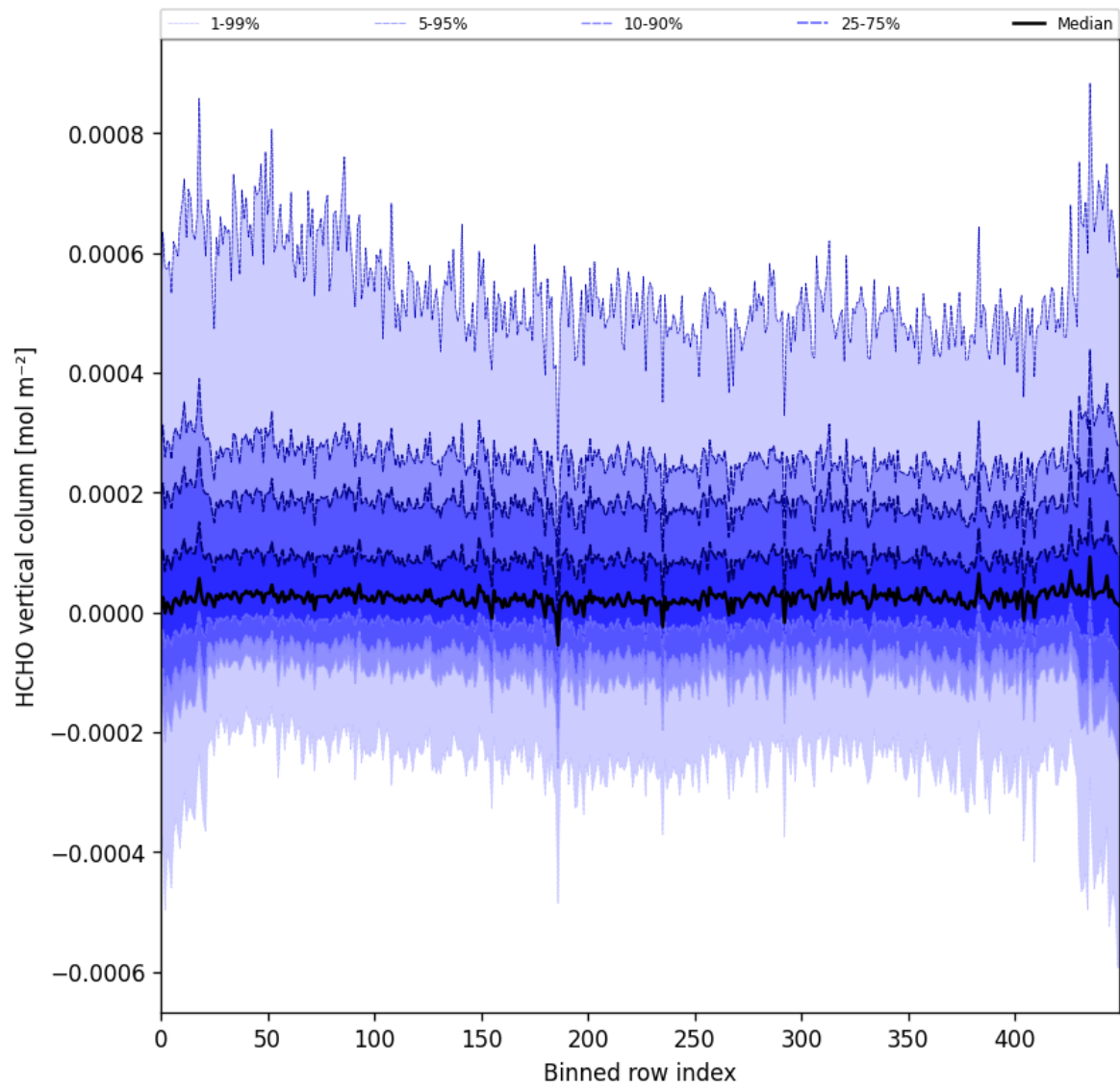
Figure 49: Along track statistics of “HCHO vertical column” for 2024-12-06 to 2024-12-07
