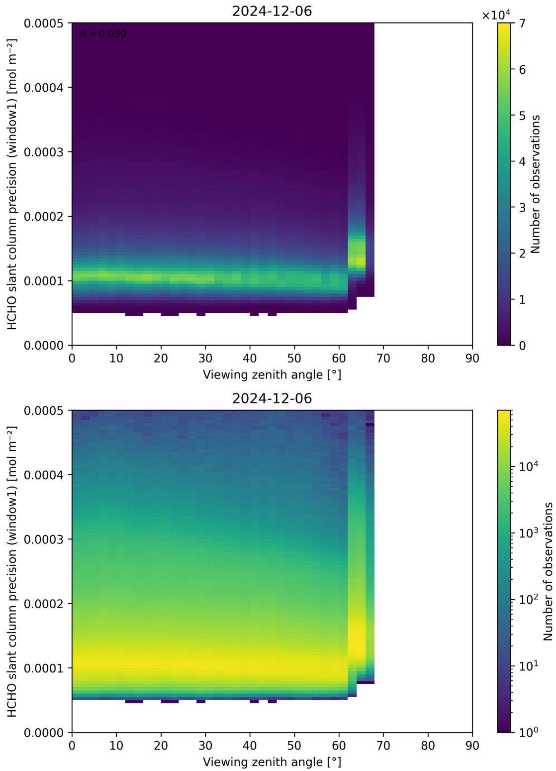
Figure 189: Scatter density plot of “Viewing zenith angle” against “HCHO slant column precision (window1)” for 2024-12-06 to 2024-12-07.
