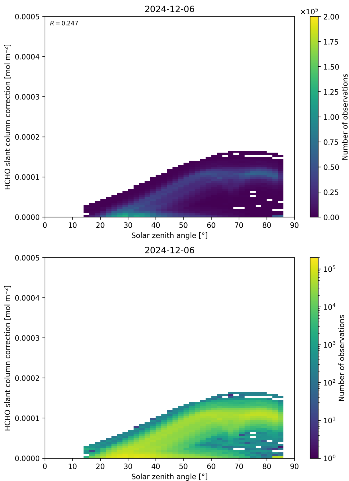
Figure 172: Scatter density plot of “Solar zenith angle” against “HCHO slant column correction” for 2024-12-06 to 2024-12-07.
