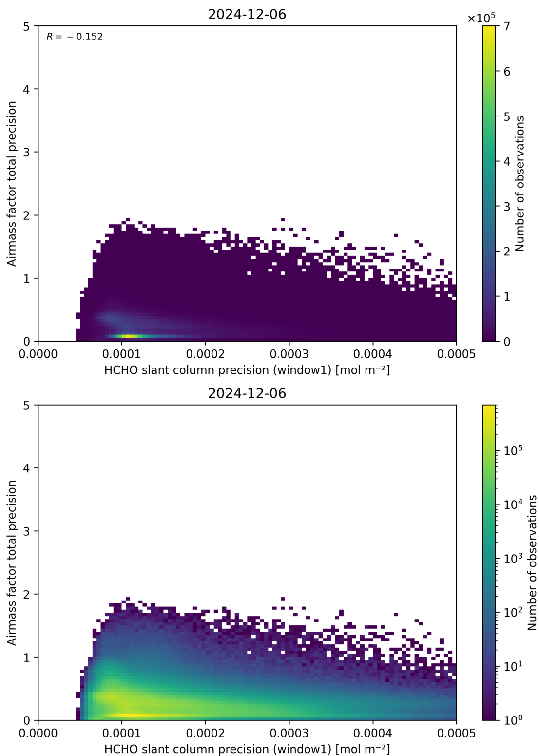
Figure 95: Scatter density plot of “HCHO slant column precision (window1)” against “Airmass factor total precision” for 2024-12-06 to 2024-12-07.
