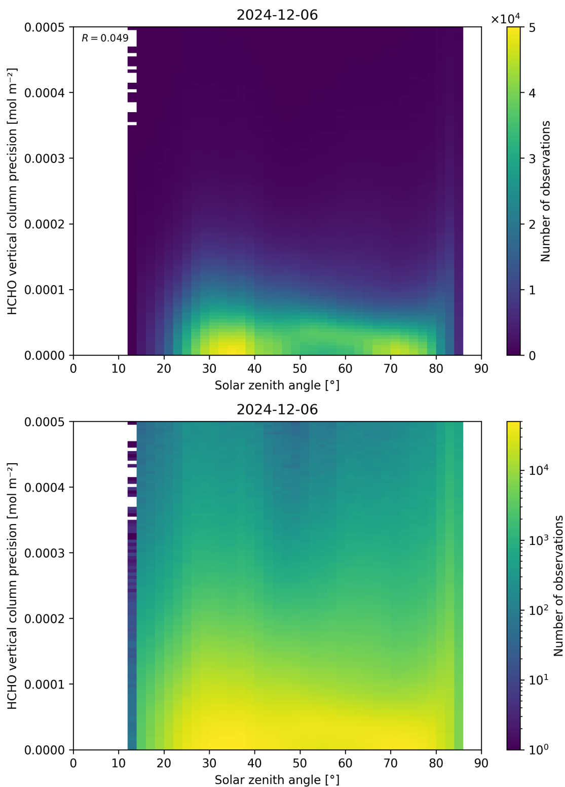
Figure 179: Scatter density plot of “Solar zenith angle” against “HCHO vertical column precision” for 2024-12-06 to 2024-12-07.
