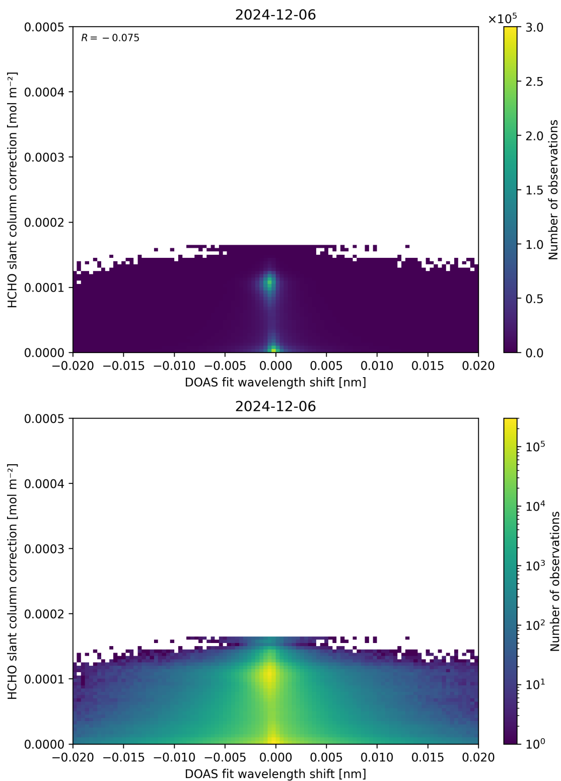
Figure 67: Scatter density plot of “DOAS fit wavelength shift” against “HCHO slant column correction” for 2024-12-06 to 2024-12-07.
