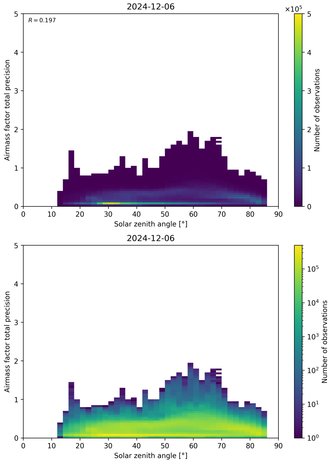
Figure 176: Scatter density plot of “Solar zenith angle” against “Airmass factor total precision” for 2024-12-06 to 2024-12-07.
