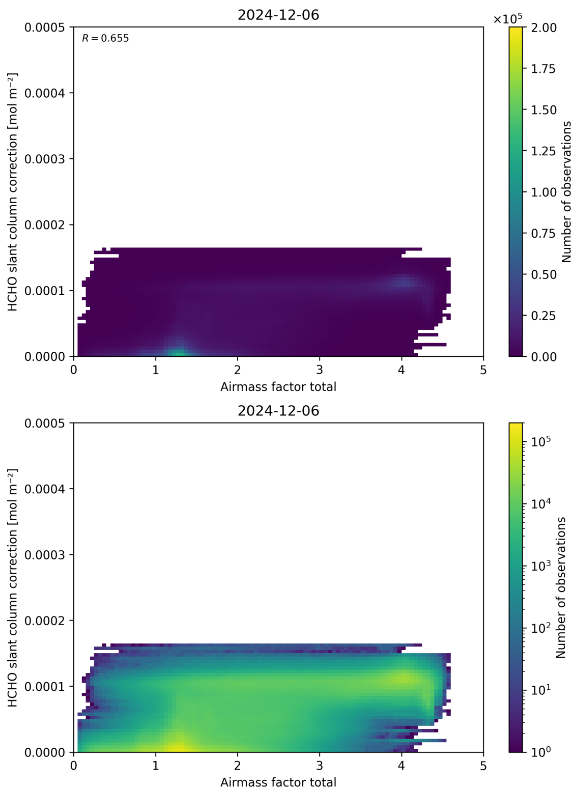
Figure 102: Scatter density plot of “Airmass factor total” against “HCHO slant column correction” for 2024-12-06 to 2024-12-07.
