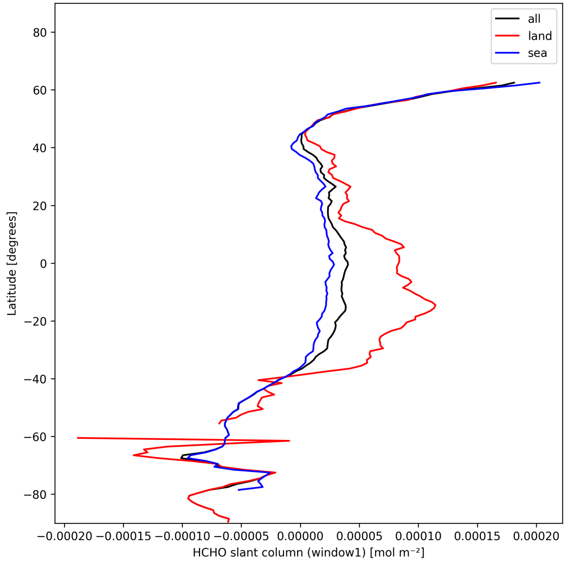
Figure 24: Zonal average of “HCHO slant column (window1)” for 2024-12-06 to 2024-12-07.
