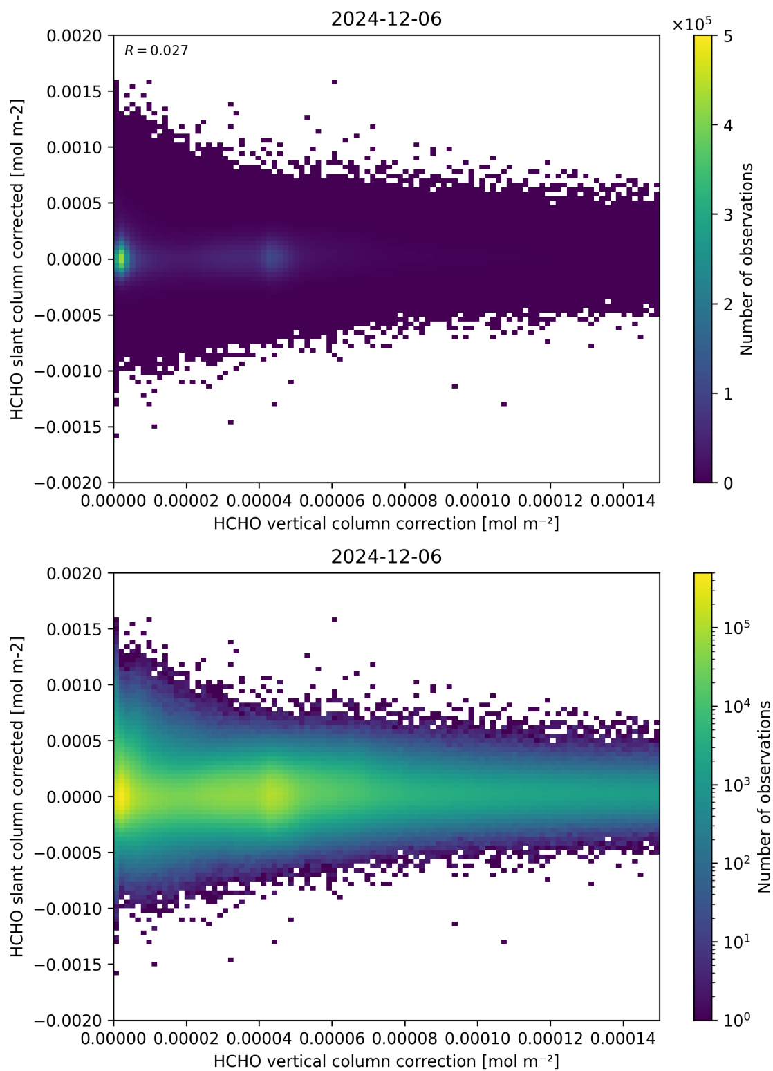
Figure 116: Scatter density plot of “HCHO vertical column correction” against “HCHO slant column corrected” for 2024-12-06 to 2024-12-07.
