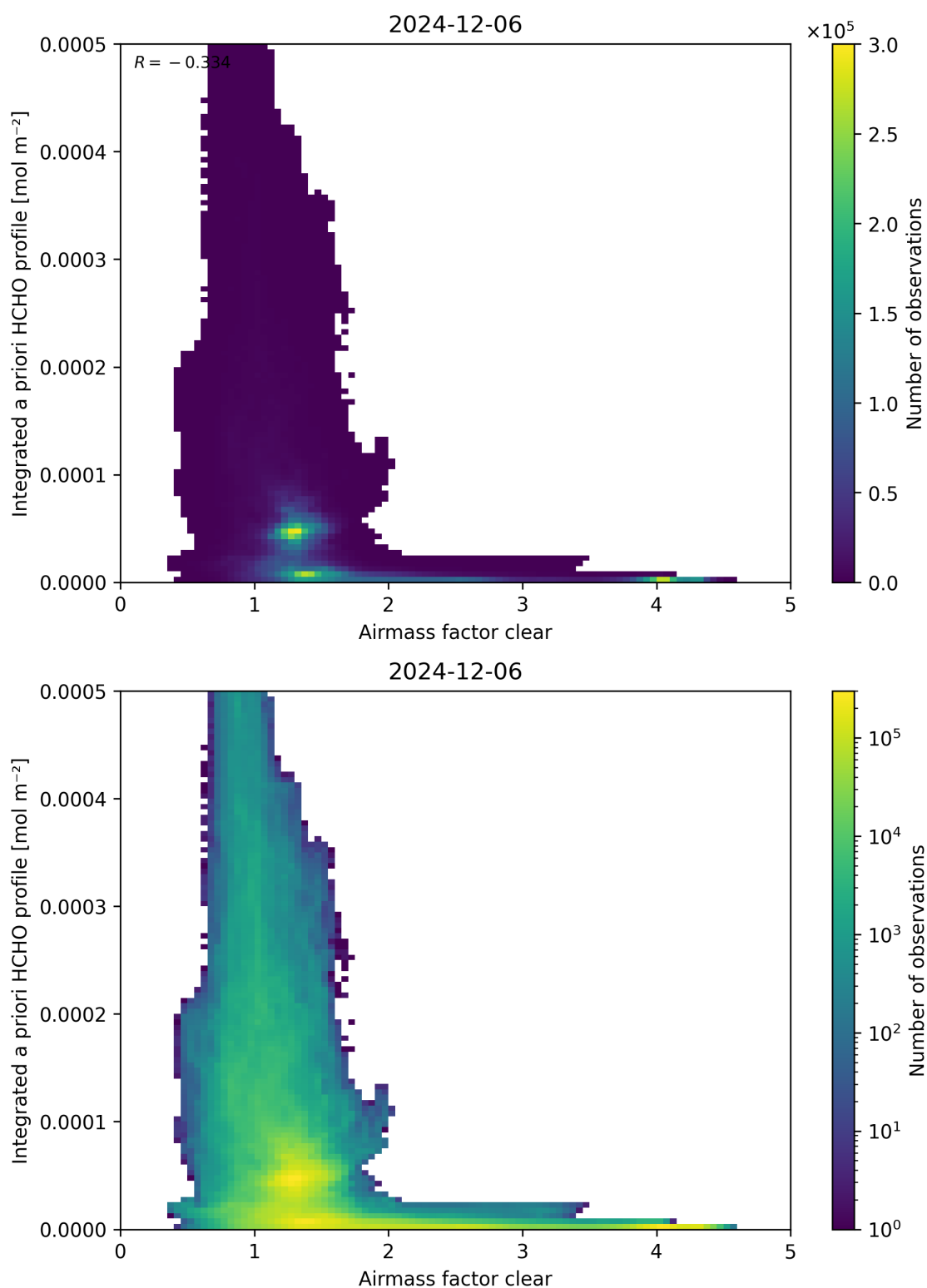
Figure 76: Scatter density plot of “Airmass factor clear” against “Integrated a priori HCHO profile” for 2024-12-06 to 2024-12-07.
