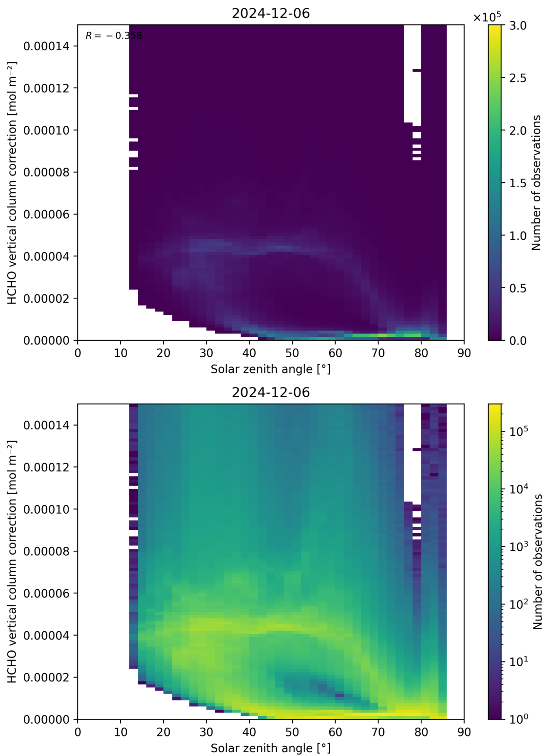
Figure 178: Scatter density plot of “Solar zenith angle” against “HCHO vertical column correction” for 2024-12-06 to 2024-12-07.
