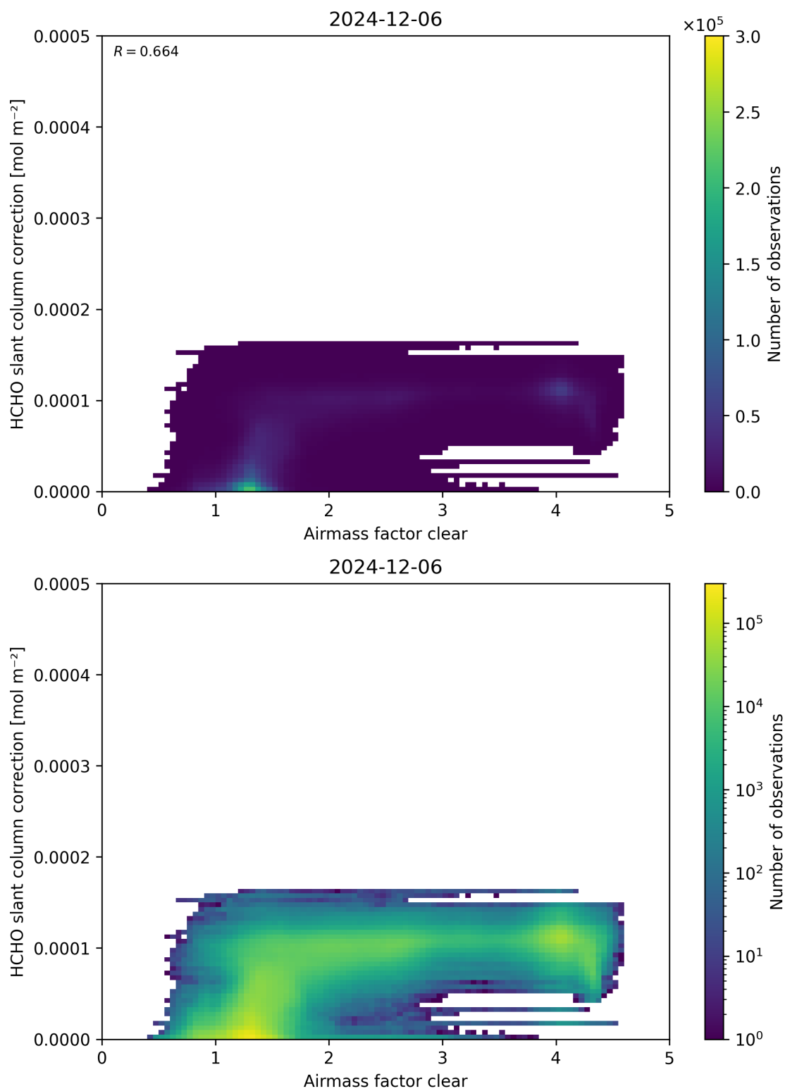
Figure 75: Scatter density plot of “Airmass factor clear” against “HCHO slant column correction” for 2024-12-06 to 2024-12-07.
