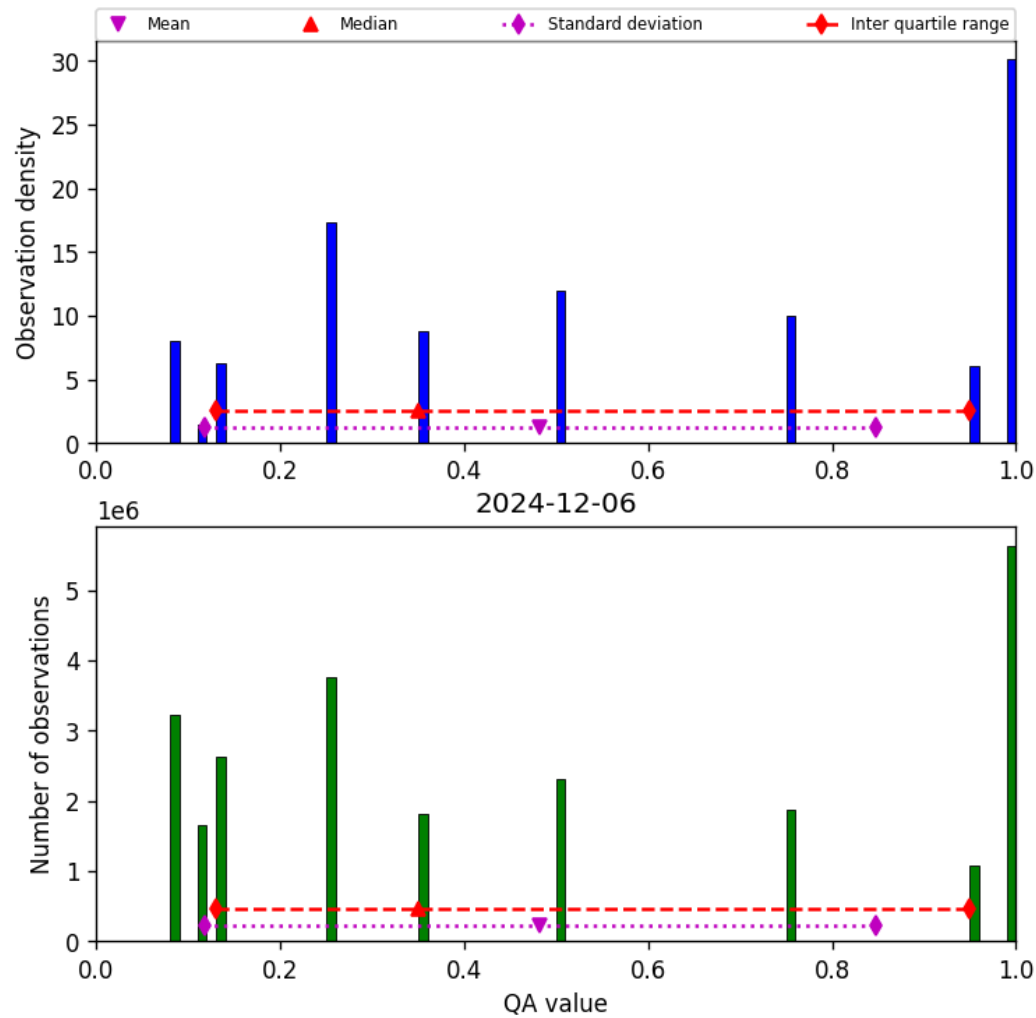
Figure 34: Histogram of “QA value” for 2024-12-06 to 2024-12-07
