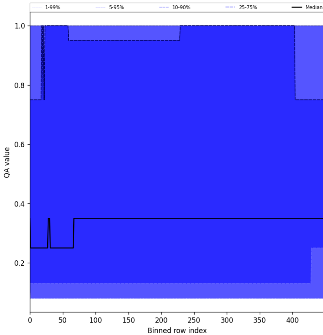
Figure 48: Along track statistics of “QA value” for 2024-12-06 to 2024-12-07
