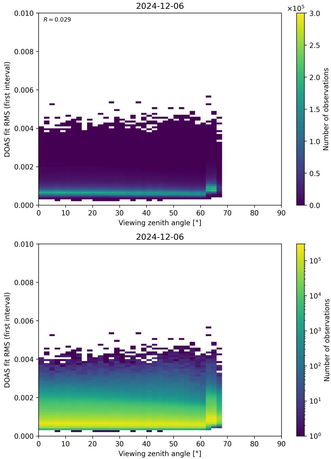
Figure 182: Scatter density plot of “Viewing zenith angle” against “DOAS fit RMS (first interval)” for 2024-12-06 to 2024-12-07.
