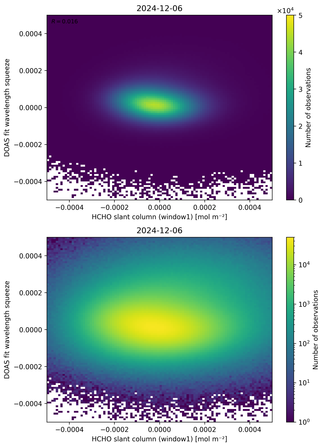
Figure 80: Scatter density plot of “HCHO slant column (window1)” against “DOAS fit wavelength squeeze” for 2024-12-06 to 2024-12-07.
