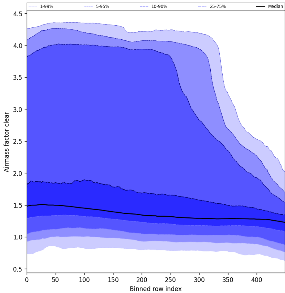
Figure 56: Along track statistics of “Air mass factor clear” for 2024-12-06 to 2024-12-07
