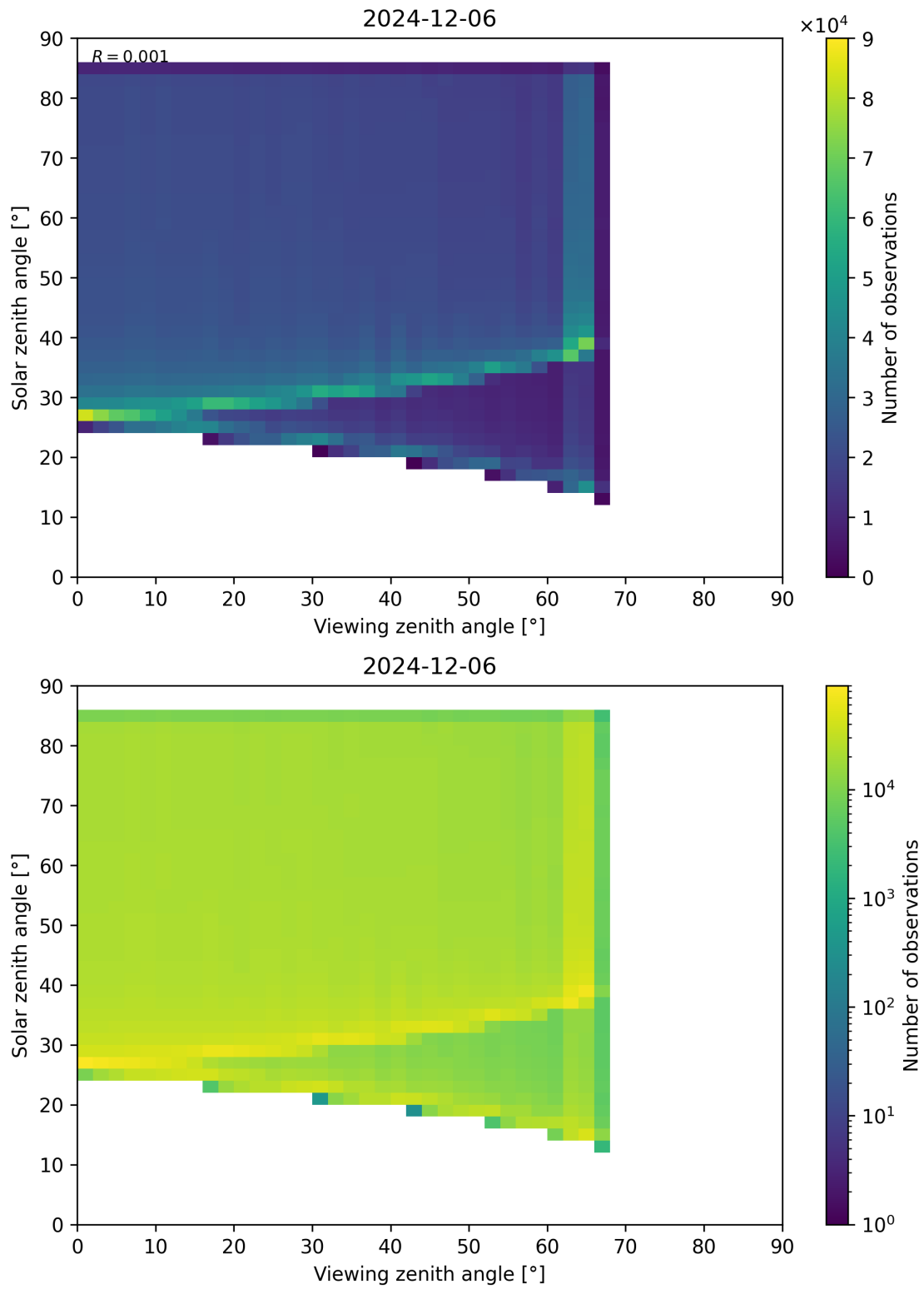
Figure 197: Scatter density plot of “Viewing zenith angle” against “Solar zenith angle” for 2024-12-06 to 2024-12-07.
