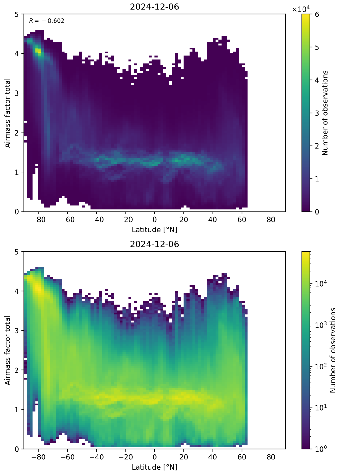
Figure 161: Scatter density plot of “Latitude” against “Airmass factor total” for 2024-12-06 to 2024-12-07.
