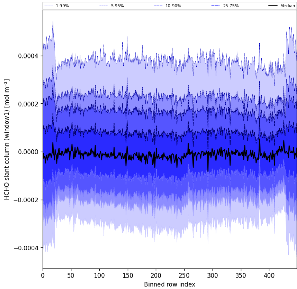
Figure 52: Along track statistics of “HCHO slant column (window1)” for 2024-12-06 to 2024-12-07
