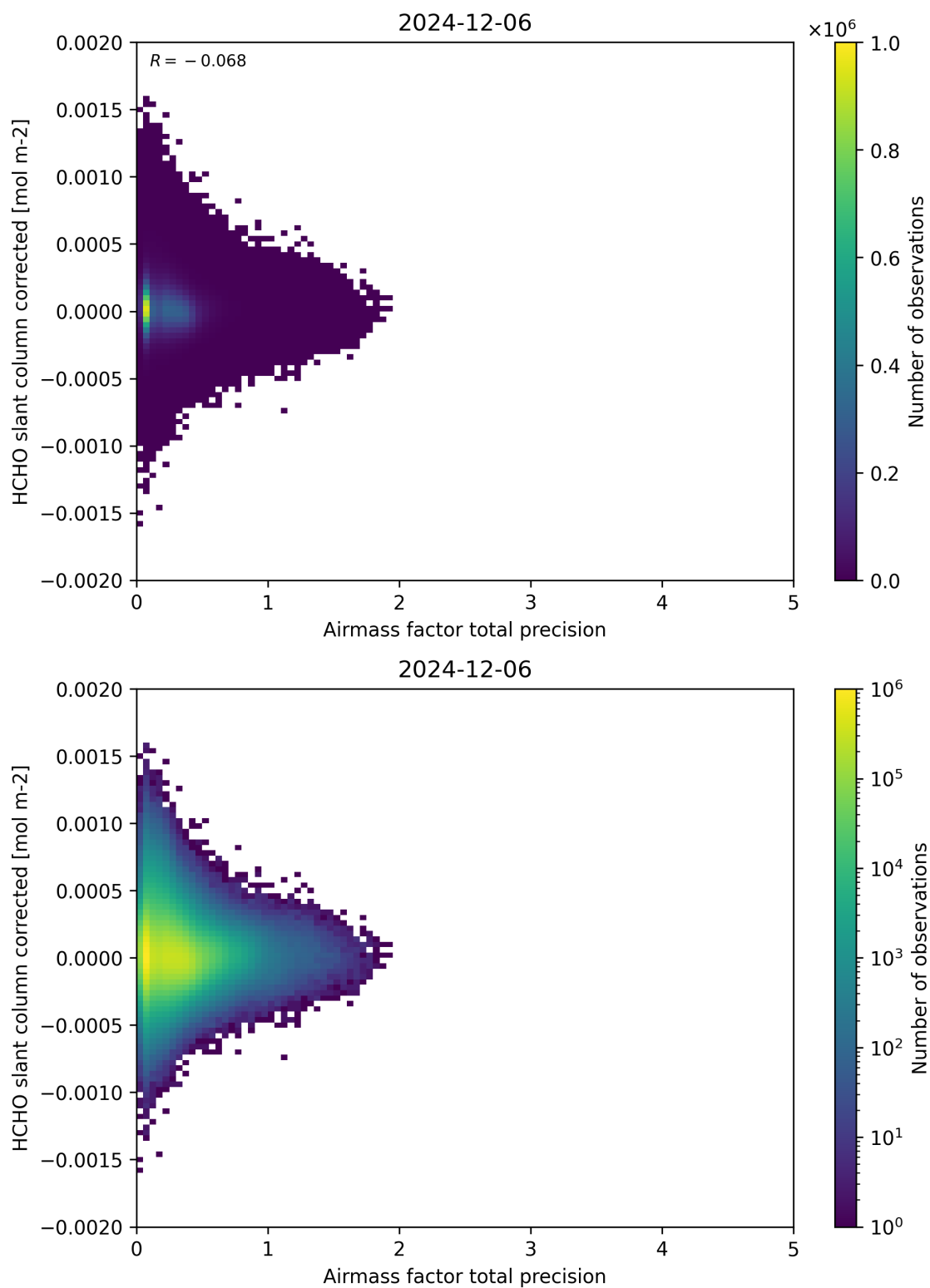
Figure 109: Scatter density plot of “Airmass factor total precision” against “HCHO slant column corrected” for 2024-12-06 to 2024-12-07.
