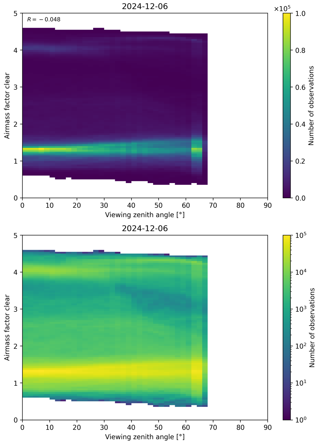
Figure 185: Scatter density plot of “Viewing zenith angle” against “Airmass factor clear” for 2024-12-06 to 2024-12-07.
