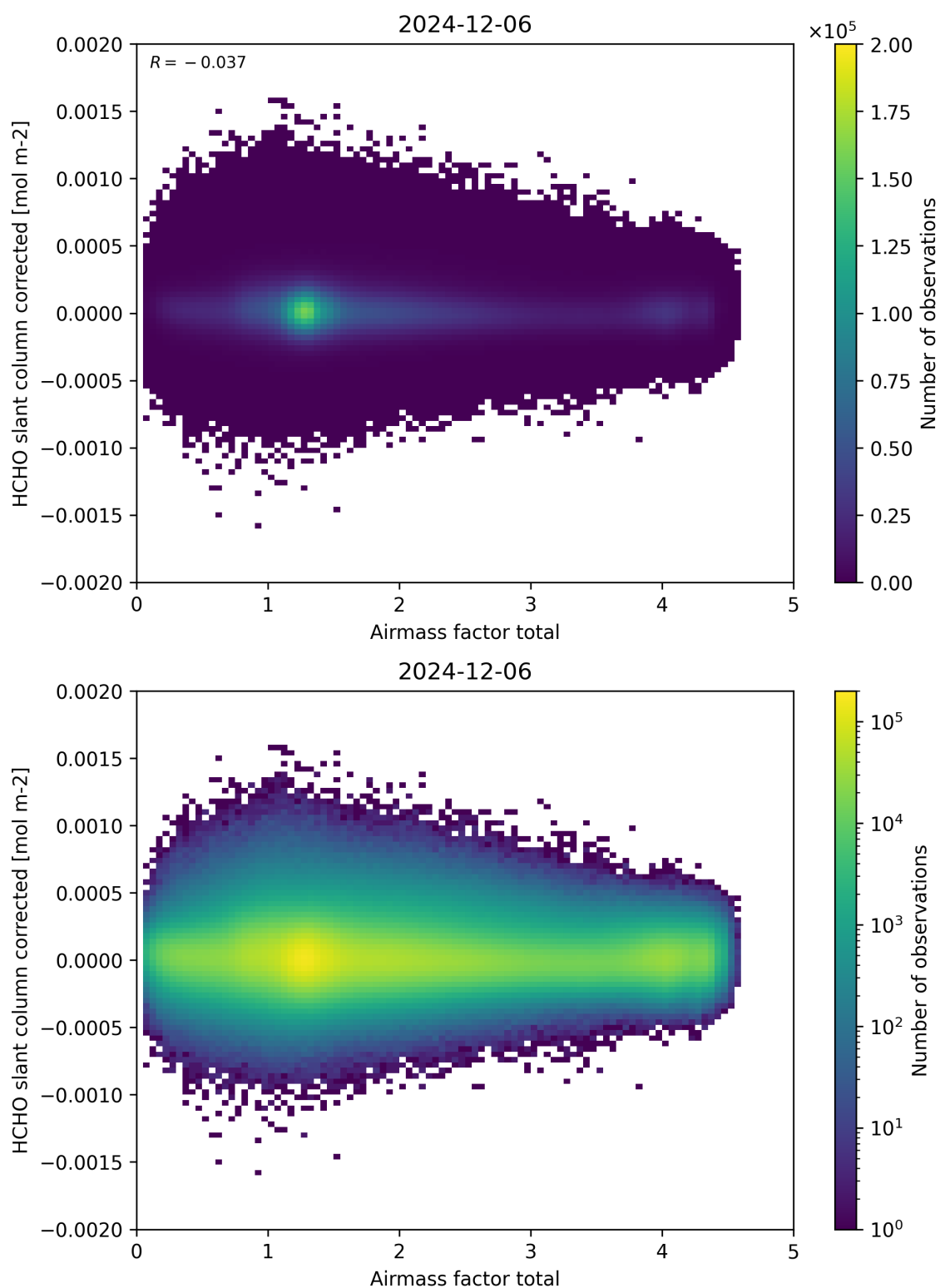
Figure 101: Scatter density plot of “Airmass factor total” against “HCHO slant column corrected” for 2024-12-06 to 2024-12-07.
