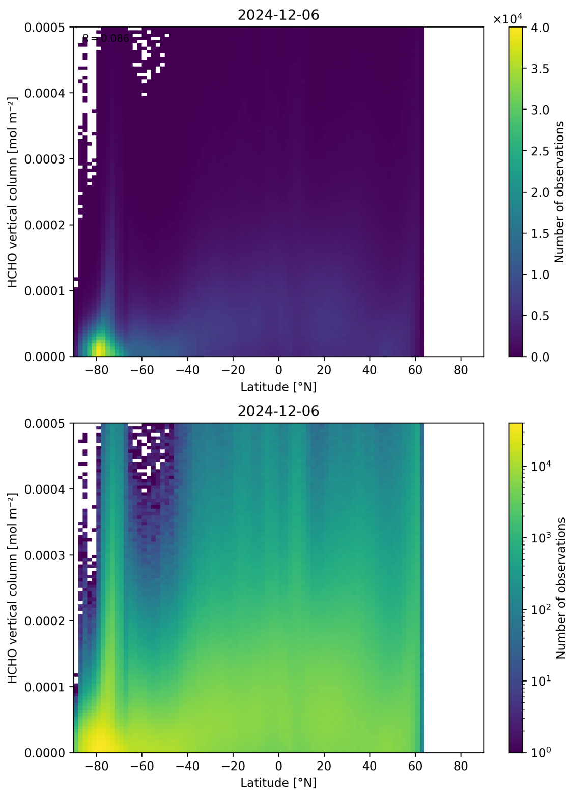
Figure 163: Scatter density plot of “Latitude” against “HCHO vertical column” for 2024-12-06 to 2024-12-07.
