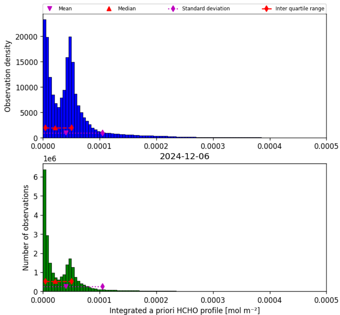
Figure 43: Histogram of “Integrated a priori HCHO profile” for 2024-12-06 to 2024-12-07
