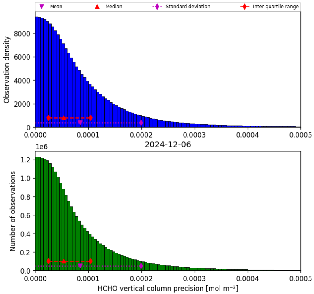
Figure 36: Histogram of “HCHO vertical column precision” for 2024-12-06 to 2024-12-07
