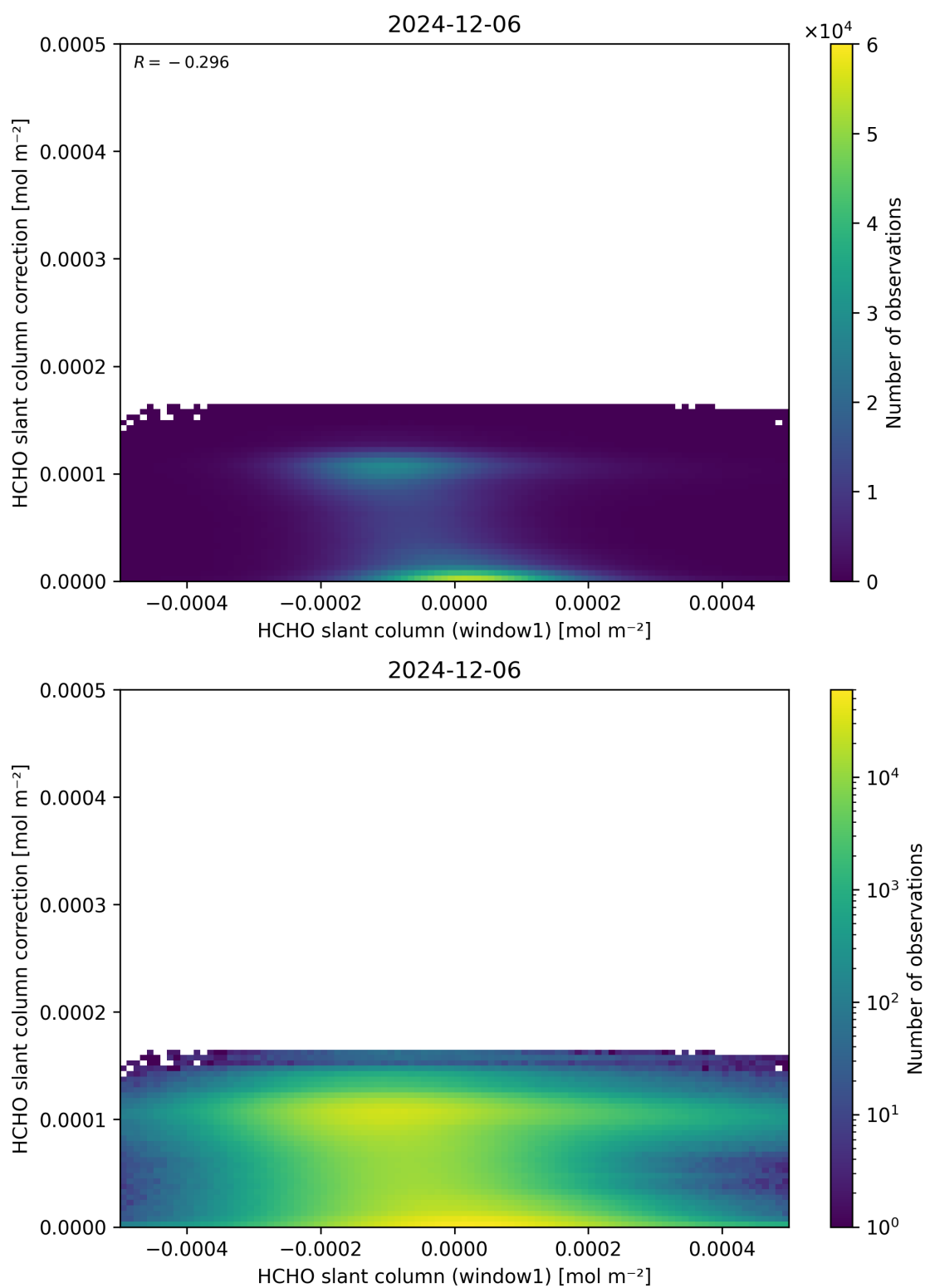
Figure 83: Scatter density plot of “HCHO slant column (window1)” against “HCHO slant column correction” for 2024-12-06 to 2024-12-07.
