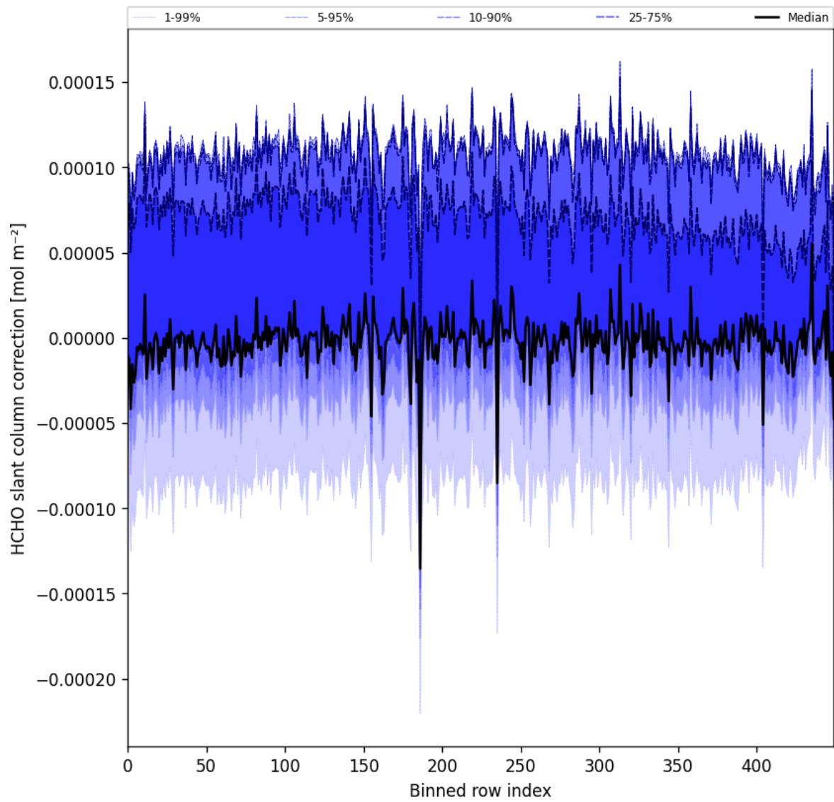
Figure 61: Along track statistics of “HCHO slant column correction” for 2024-12-06 to 2024-12-07
