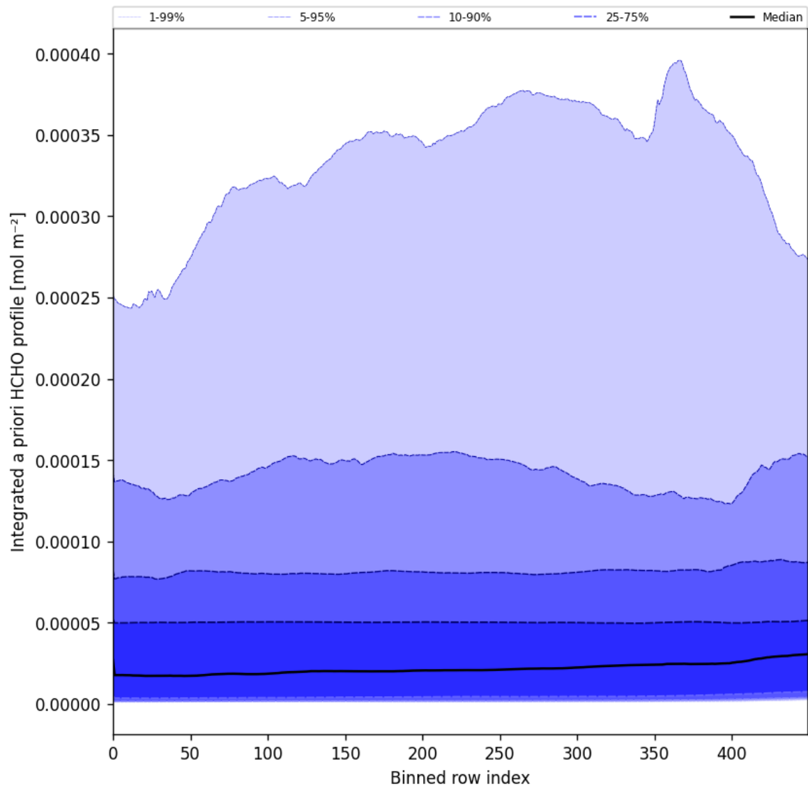
Figure 57: Along track statistics of “Integrated a priori HCHO profile” for 2024-12-06 to 2024-12-07
