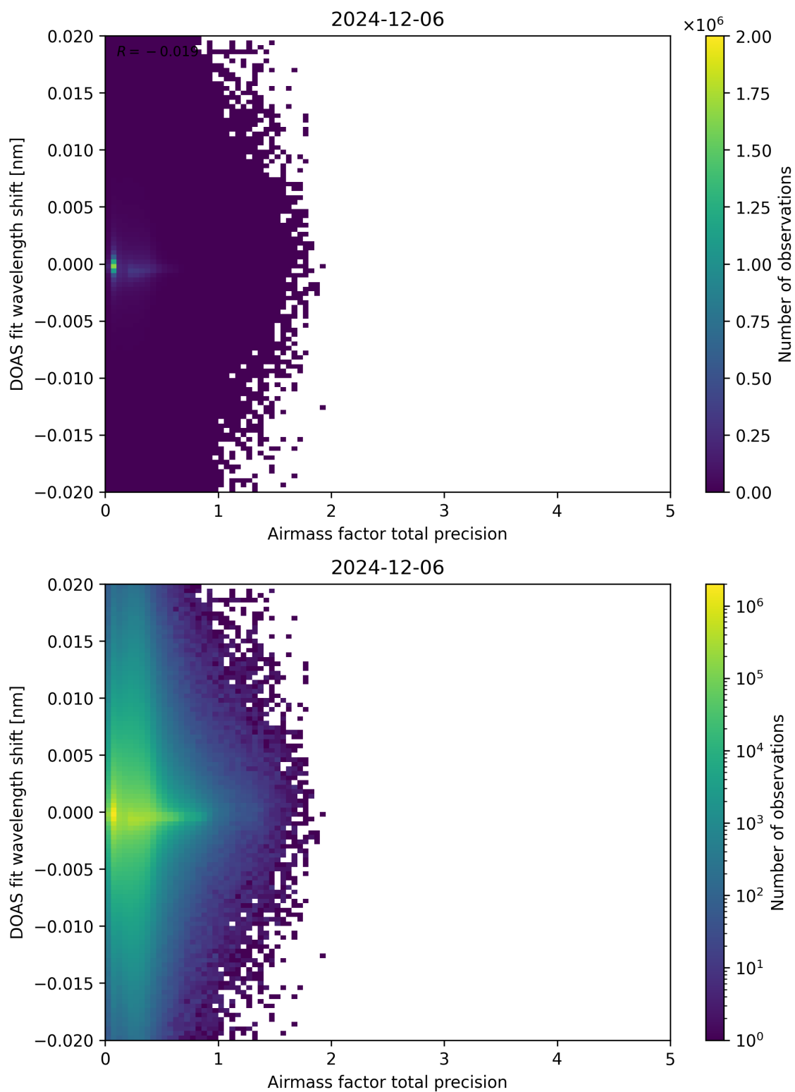
Figure 106: Scatter density plot of “Airmass factor total precision” against “DOAS fit wavelength shift” for 2024-12-06 to 2024-12-07.
