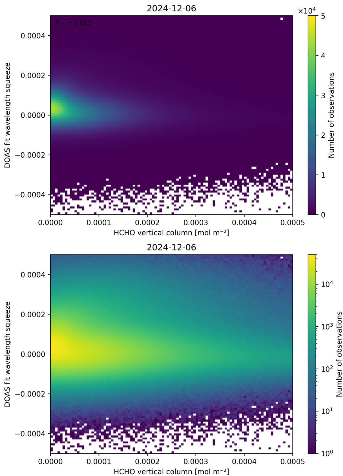
Figure 125: Scatter density plot of “HCHO vertical column” against “DOAS fit wavelength squeeze” for 2024-12-06 to 2024-12-07.
