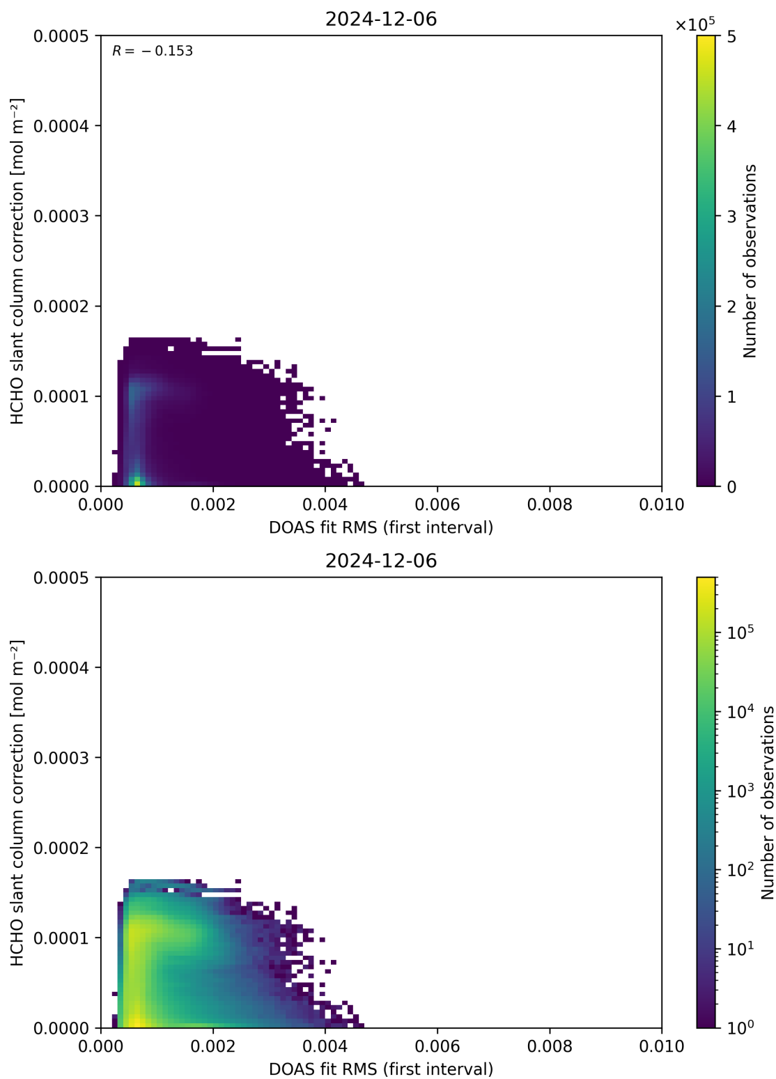
Figure 63: Scatter density plot of “DOAS fit RMS (first interval)” against “HCHO slant column correction” for 2024-12-06 to 2024-12-07.
