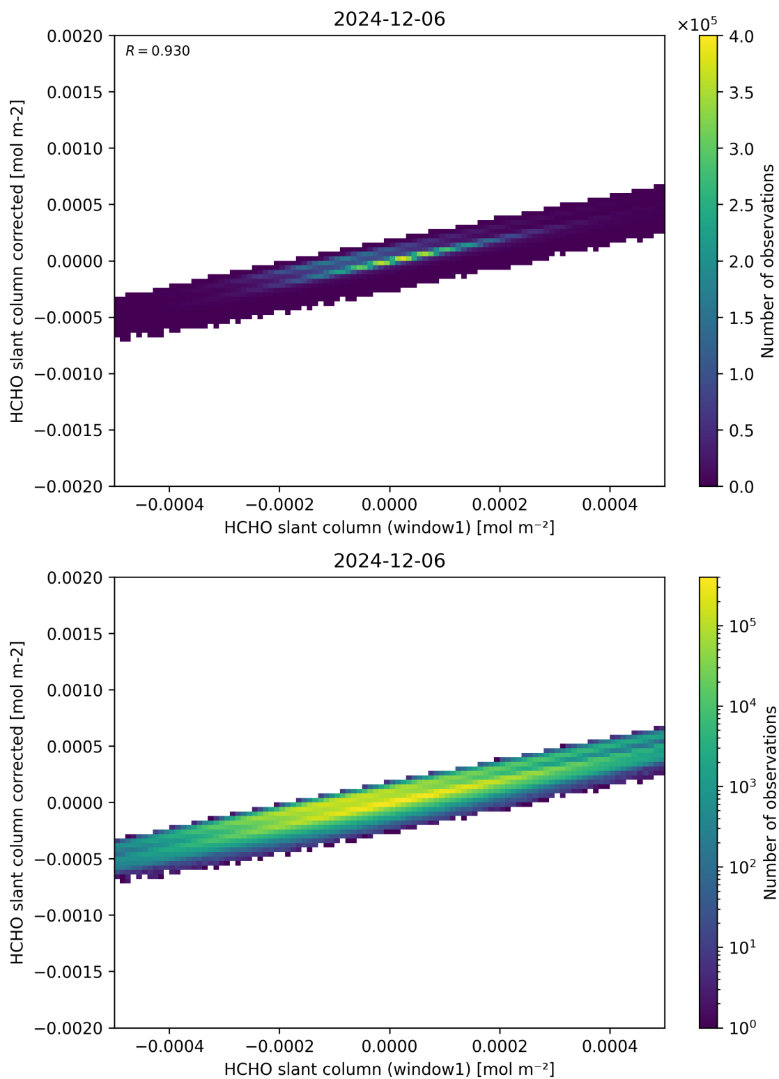
Figure 82: Scatter density plot of “HCHO slant column (window1)” against “HCHO slant column corrected” for 2024-12-06 to 2024-12-07.
