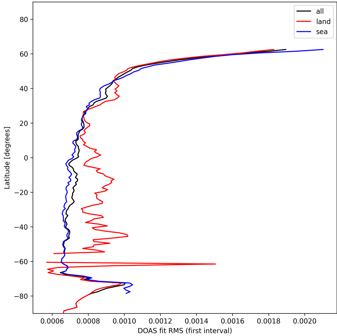
Figure 32: Zonal average of “DOAS fit RMS (first interval)” for 2024-12-06 to 2024-12-07.
