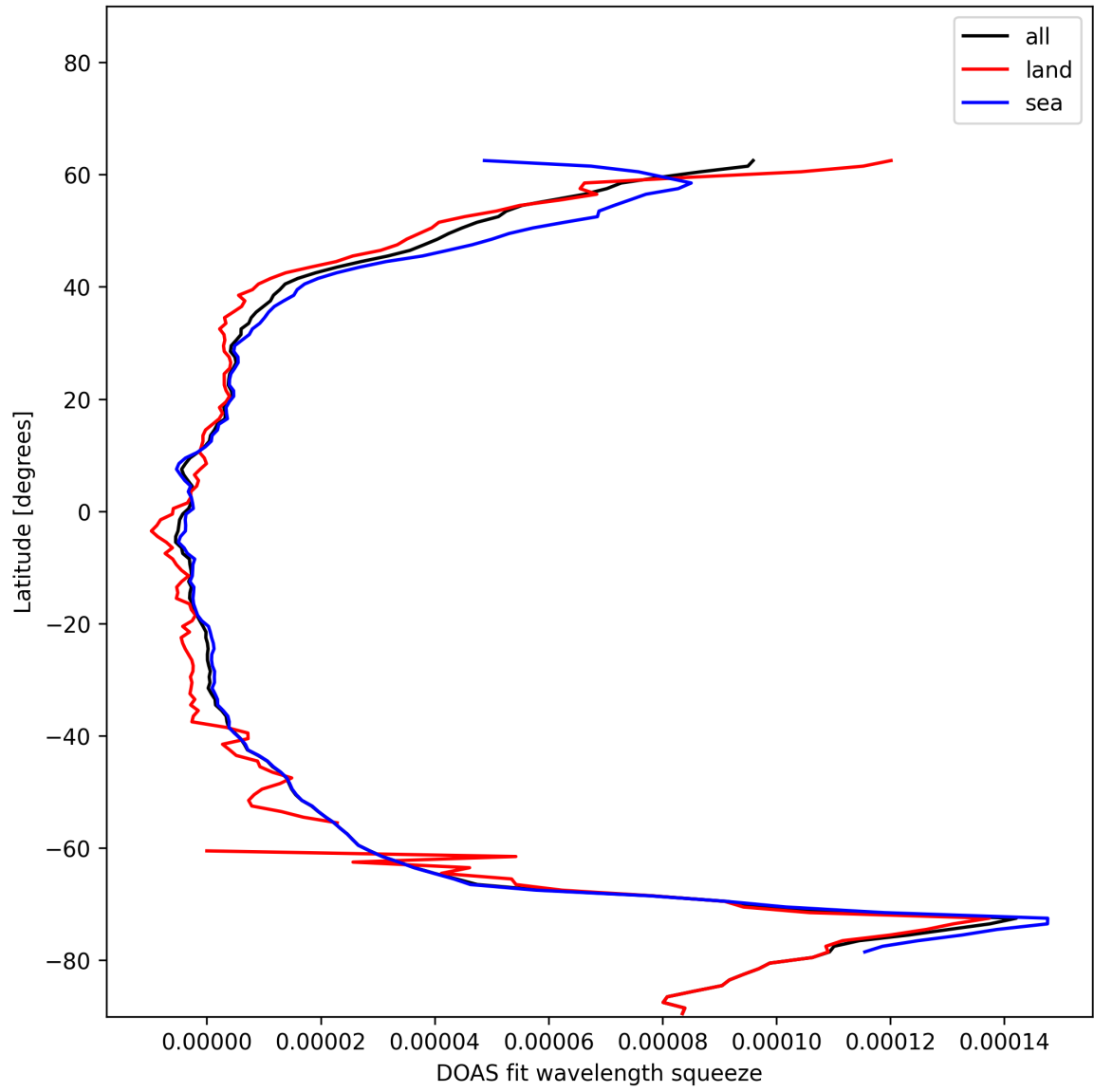
Figure 31: Zonal average of “DOAS fit wavelength squeeze” for 2024-12-06 to 2024-12-07.
