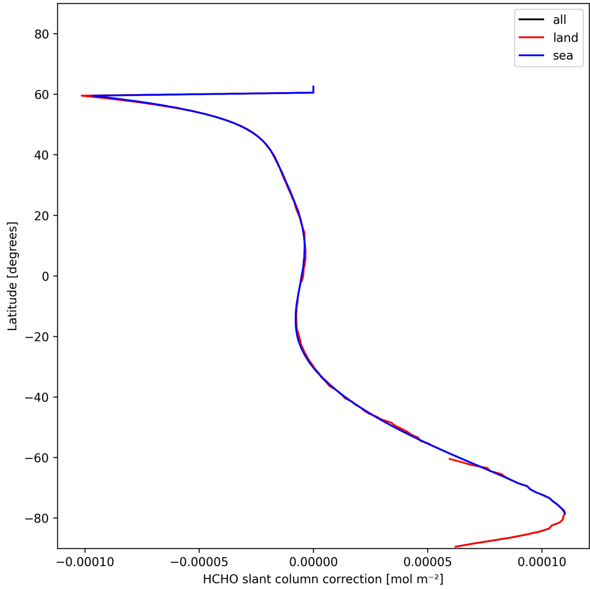
Figure 33: Zonal average of “HCHO slant column correction” for 2024-12-06 to 2024-12-07.
