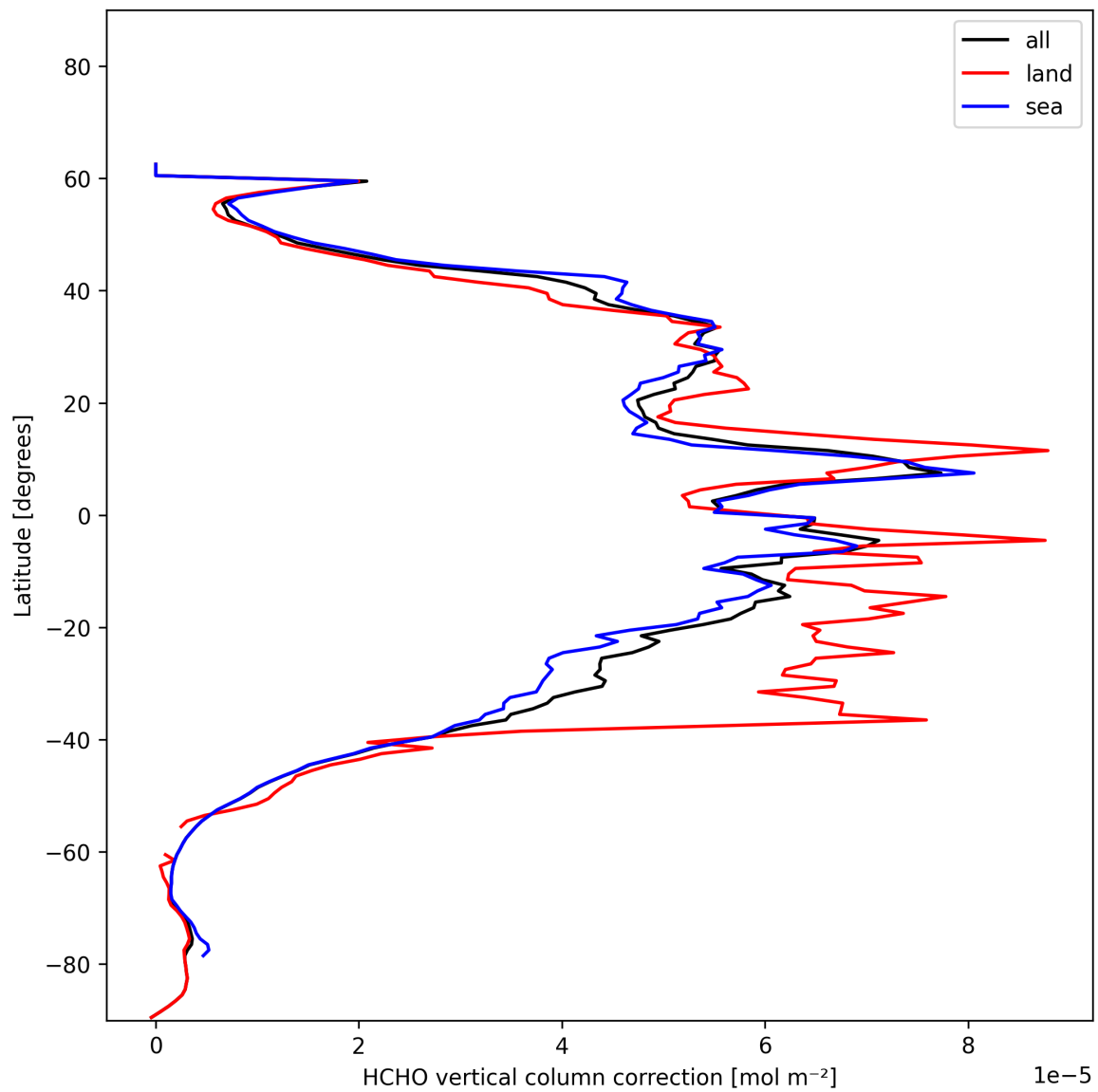
Figure 23: Zonal average of “HCHO vertical column correction” for 2024-12-06 to 2024-12-07.
