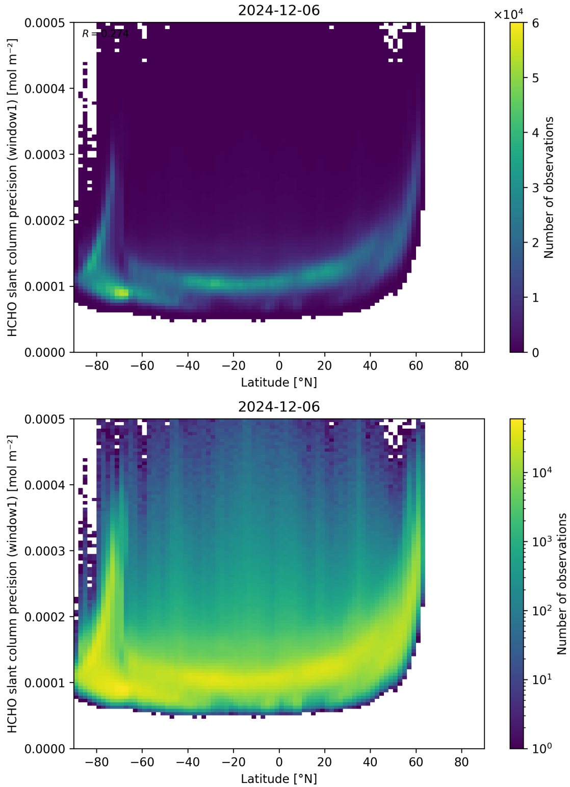
Figure 160: Scatter density plot of “Latitude” against “HCHO slant column precision (window1)” for 2024-12-06 to 2024-12-07.
