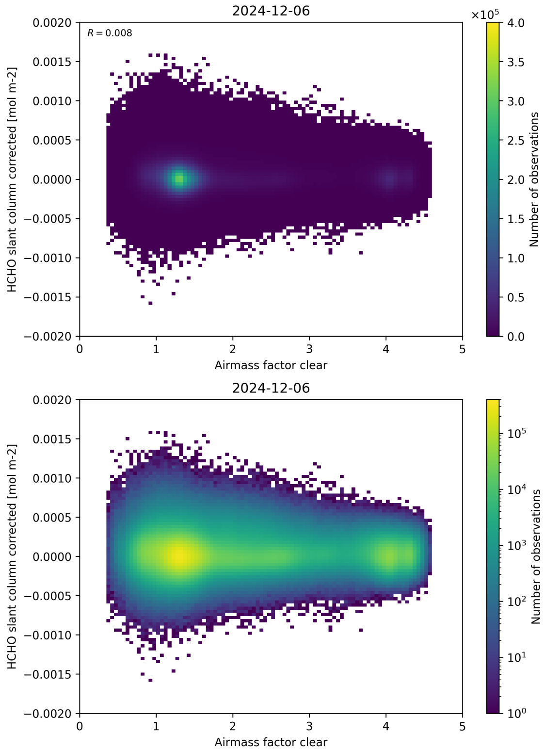
Figure 74: Scatter density plot of “Airmass factor clear” against “HCHO slant column corrected” for 2024-12-06 to 2024-12-07.
