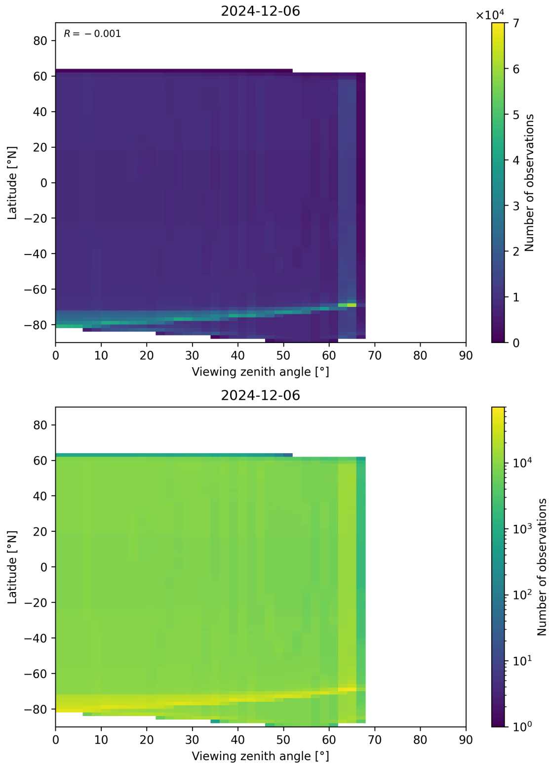
Figure 196: Scatter density plot of “Viewing zenith angle” against “Latitude” for 2024-12-06 to 2024-12-07.
