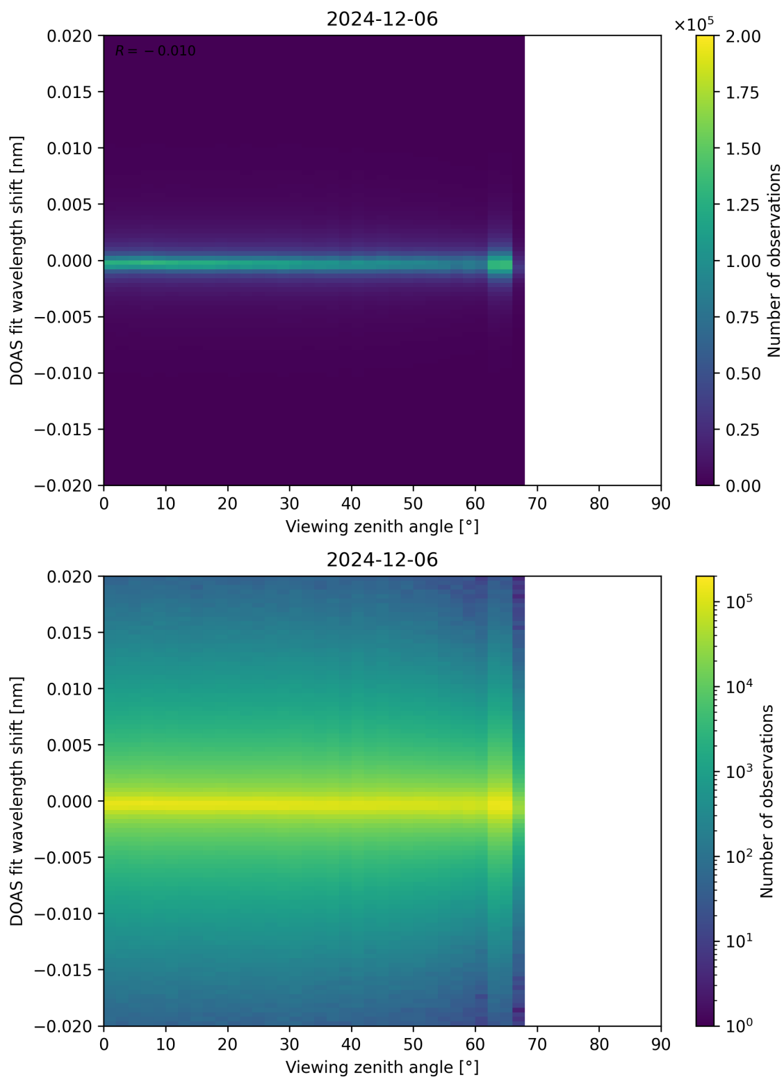
Figure 183: Scatter density plot of “Viewing zenith angle” against “DOAS fit wavelength shift” for 2024-12-06 to 2024-12-07.
