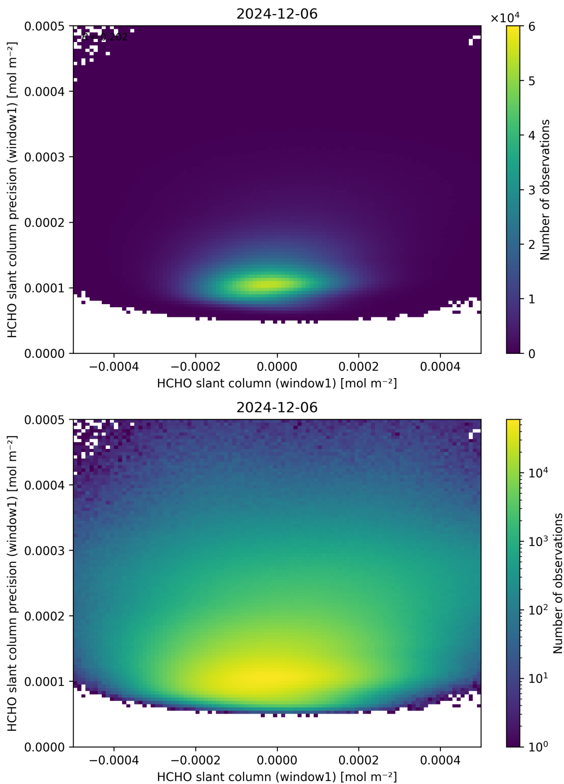
Figure 84: Scatter density plot of “HCHO slant column (window1)” against “HCHO slant column precision (window1)” for 2024-12-06 to 2024-12-07.
