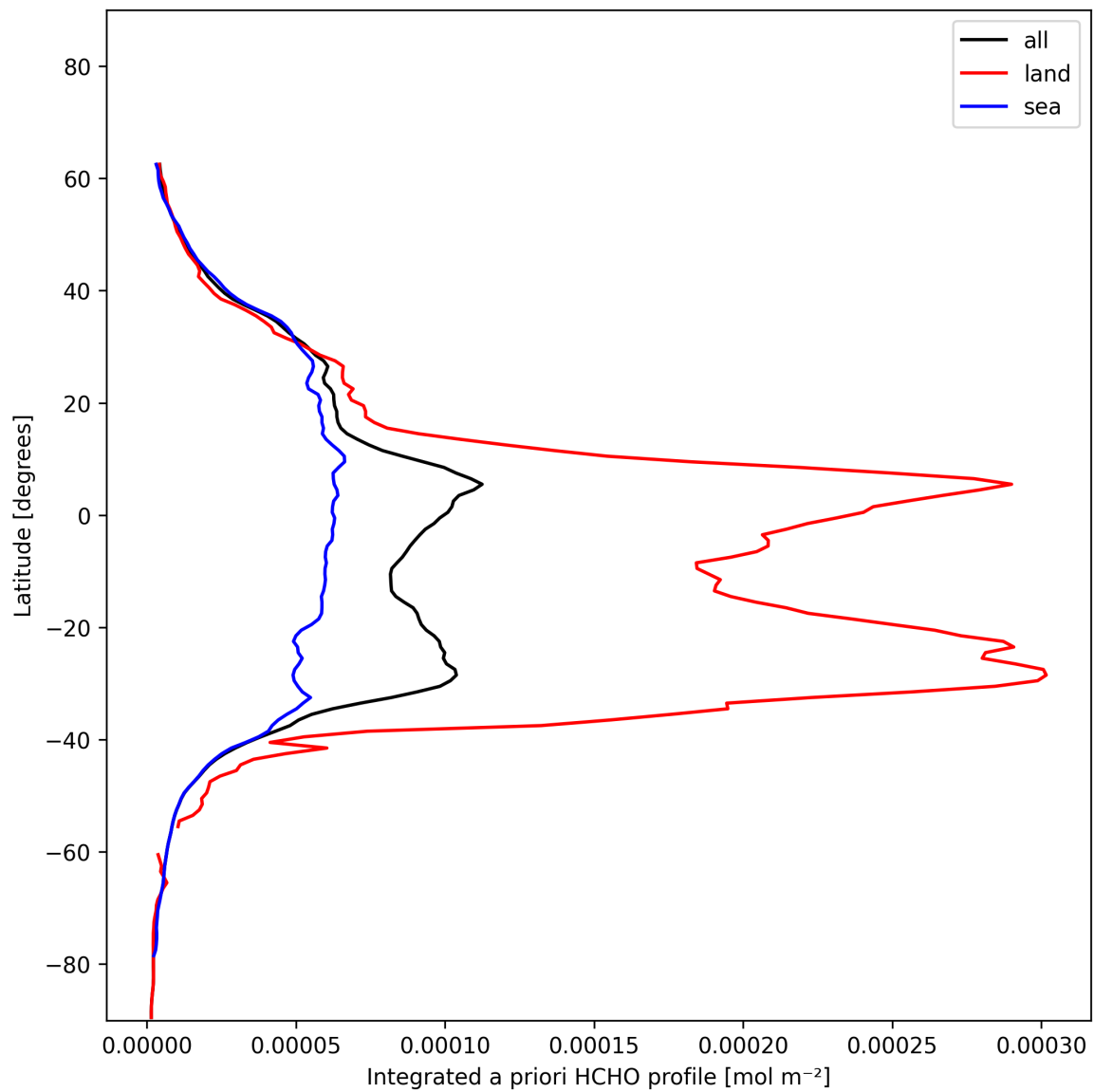
Figure 29: Zonal average of “Integrated a priori HCHO profile” for 2024-12-06 to 2024-12-07.
