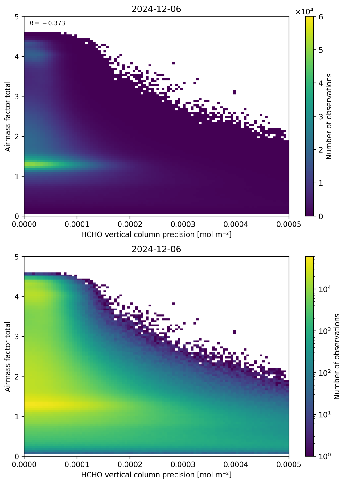
Figure 144: Scatter density plot of “HCHO vertical column precision” against “Airmass factor total” for 2024-12-06 to 2024-12-07.
