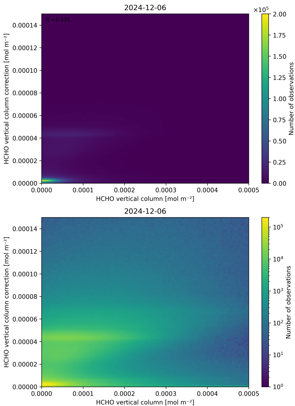
Figure 133: Scatter density plot of “HCHO vertical column” against “HCHO vertical column correction” for 2024-12-06 to 2024-12-07.
