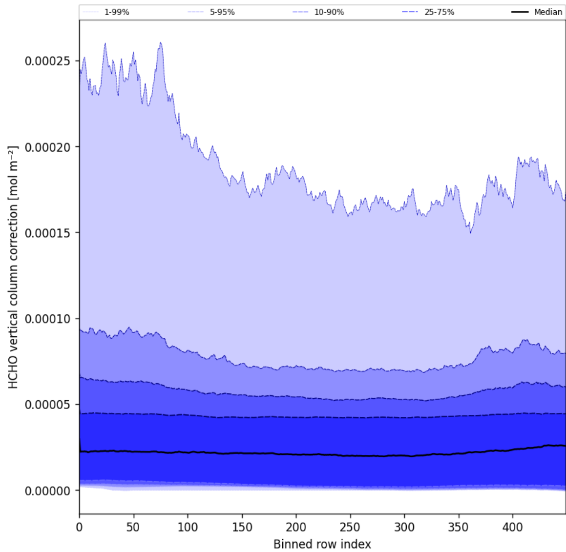
Figure 51: Along track statistics of “HCHO vertical column correction” for 2024-12-06 to 2024-12-07
