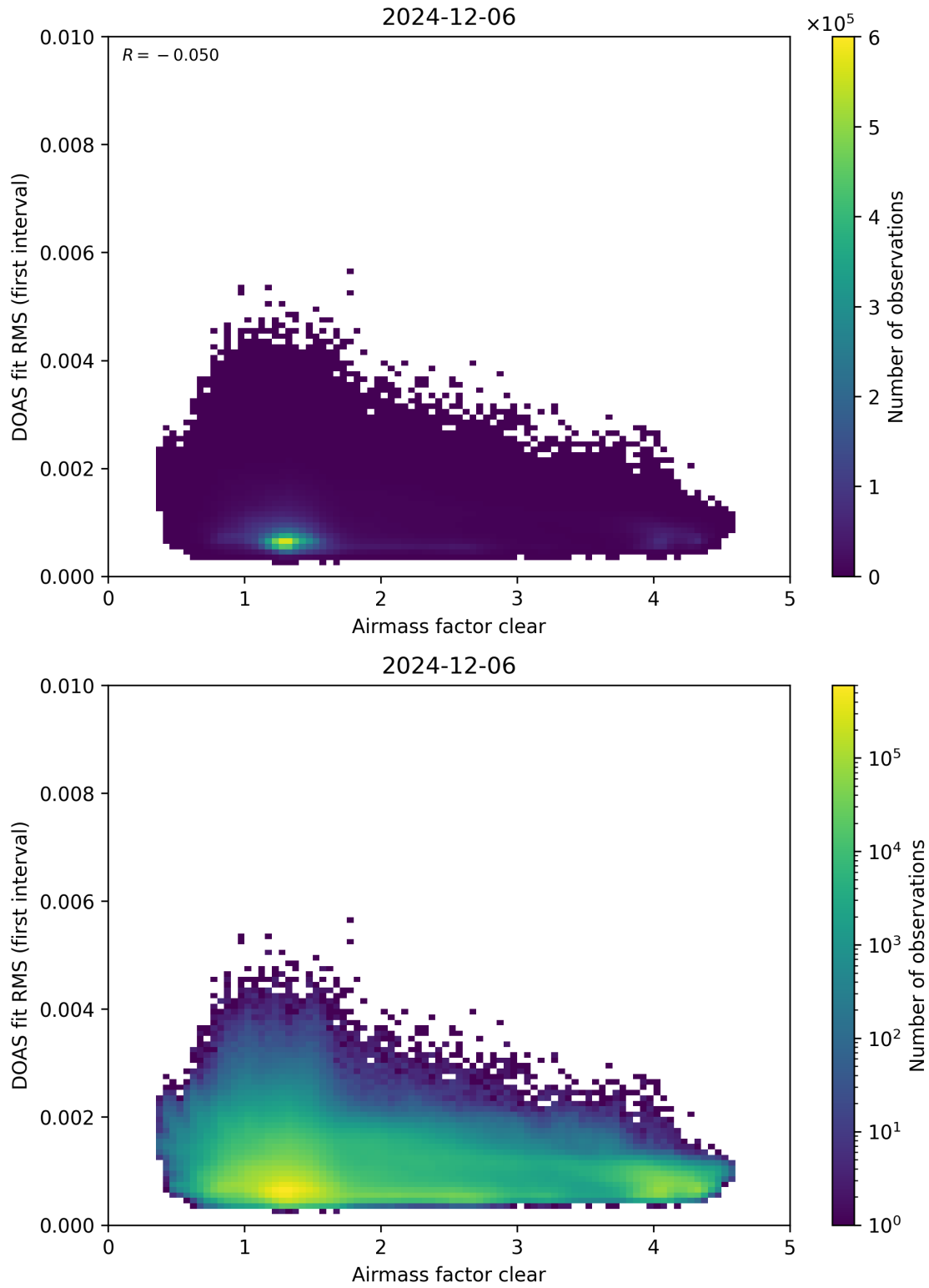
Figure 71: Scatter density plot of “Airmass factor clear” against “DOAS fit RMS (first interval)” for 2024-12-06 to 2024-12-07.
