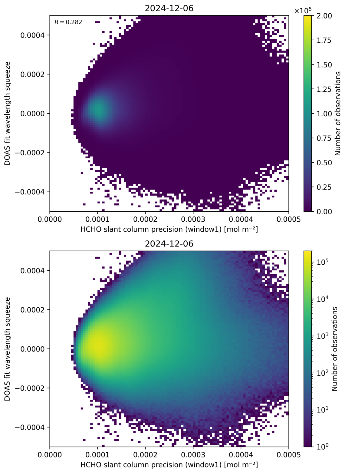
Figure 90: Scatter density plot of “HCHO slant column precision (window1)” against “DOAS fit wavelength squeeze” for 2024-12-06 to 2024-12-07.
