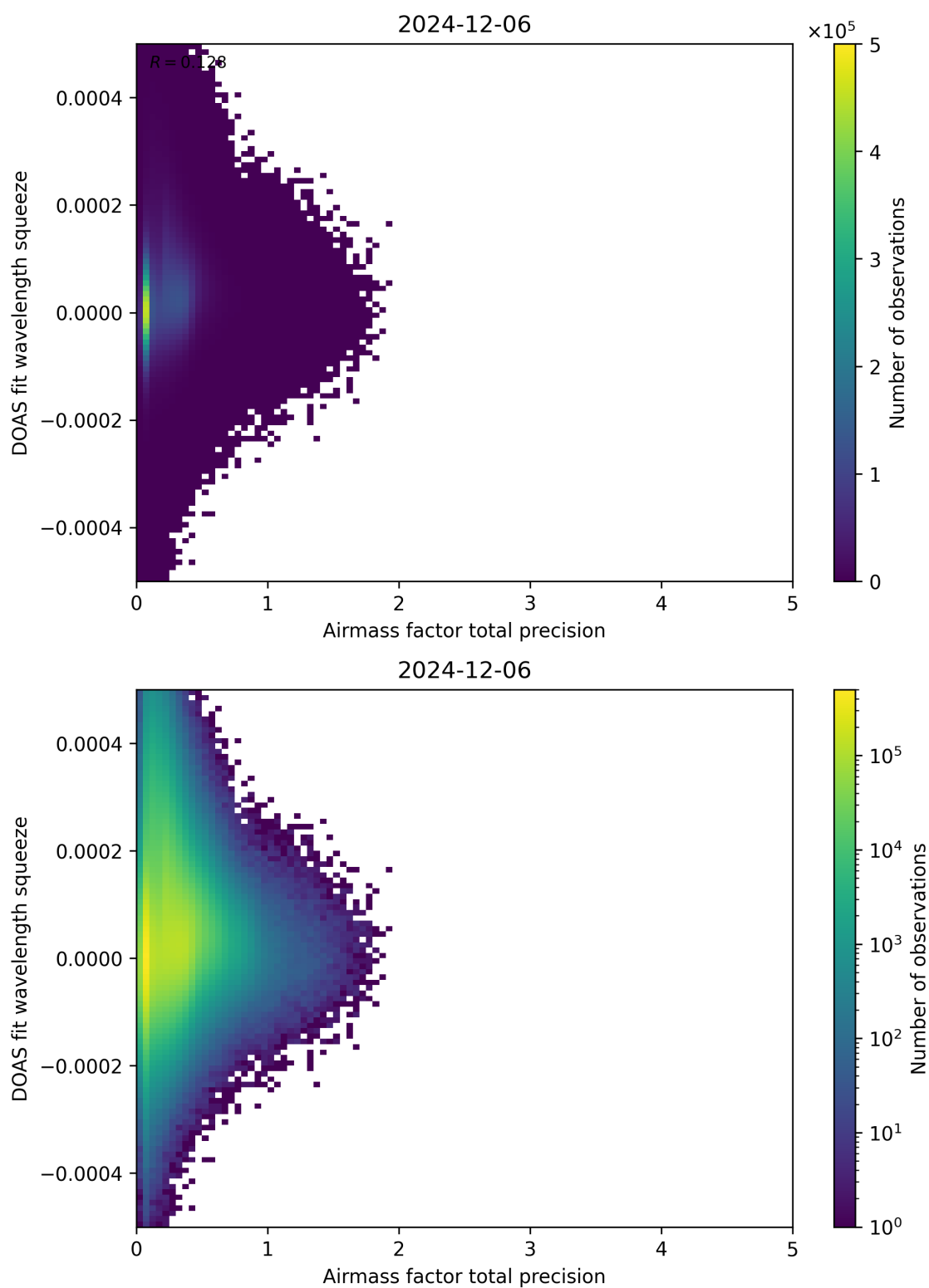
Figure 107: Scatter density plot of “Airmass factor total precision” against “DOAS fit wavelength squeeze” for 2024-12-06 to 2024-12-07.
