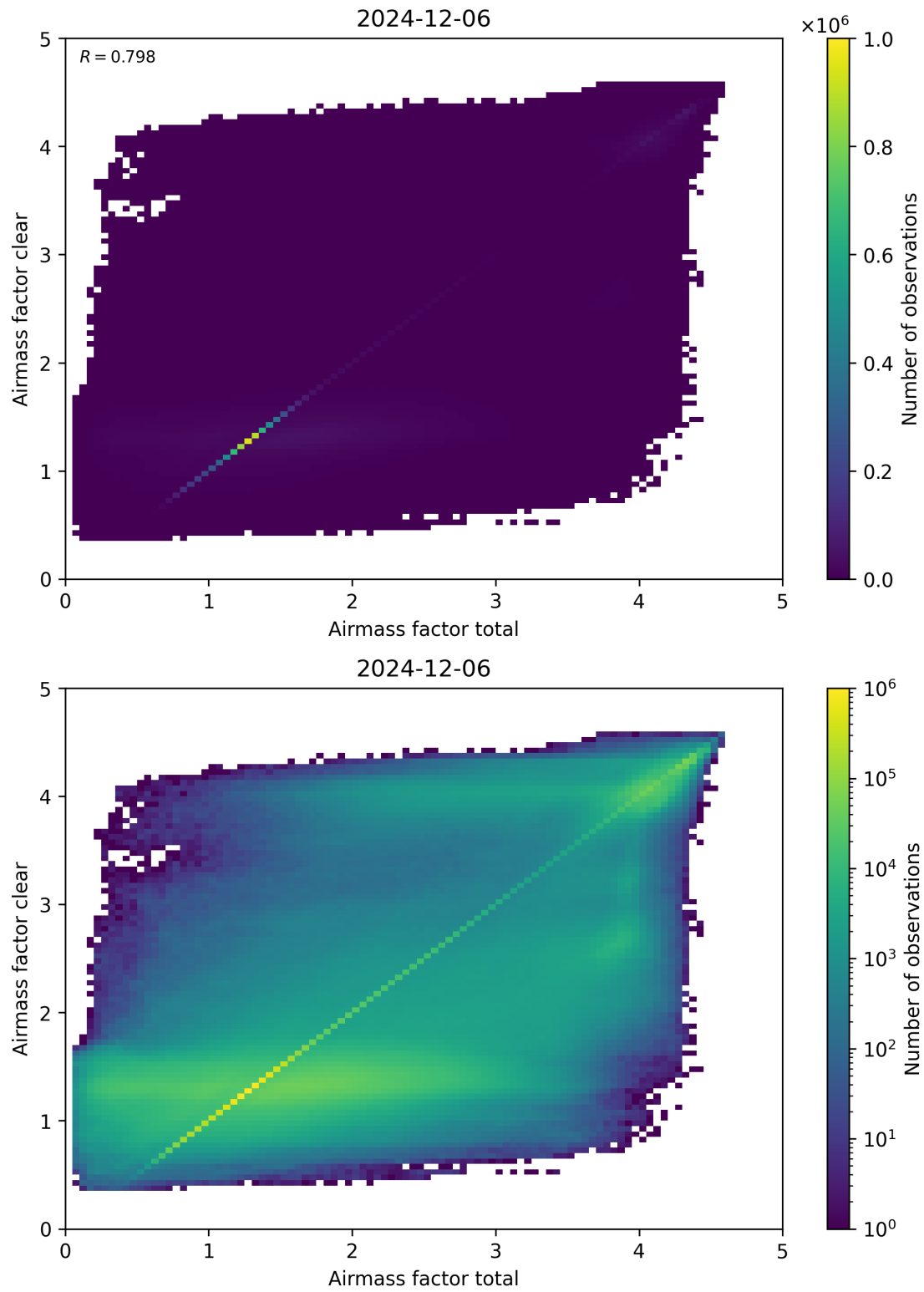
Figure 100: Scatter density plot of “Airmass factor total” against “Airmass factor clear” for 2024-12-06 to 2024-12-07.
