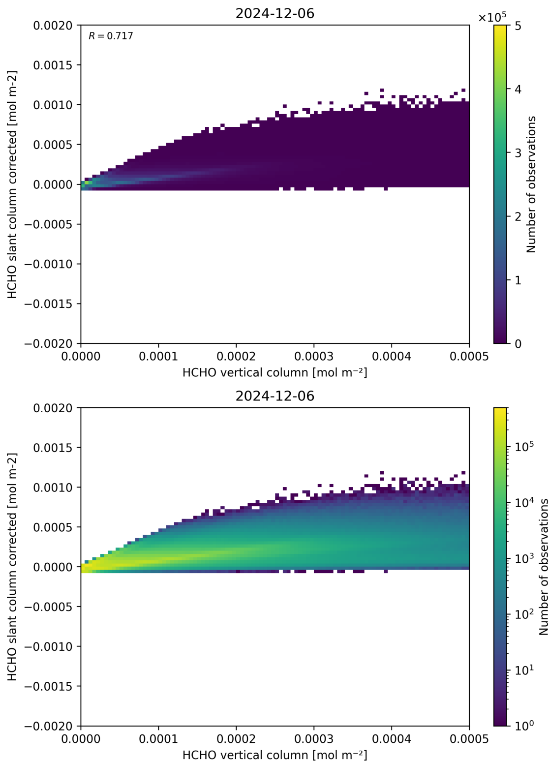
Figure 127: Scatter density plot of “HCHO vertical column” against “HCHO slant column corrected” for 2024-12-06 to 2024-12-07.
