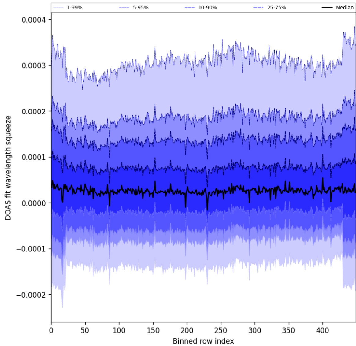
Figure 59: Along track statistics of “DOAS fit wavelength squeeze” for 2024-12-06 to 2024-12-07
