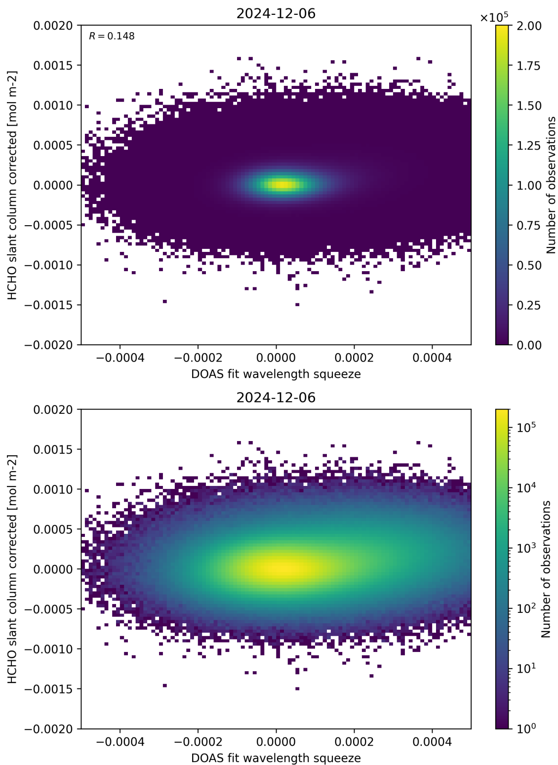
Figure 69: Scatter density plot of “DOAS fit wavelength squeeze” against “HCHO slant column corrected” for 2024-12-06 to 2024-12-07.
