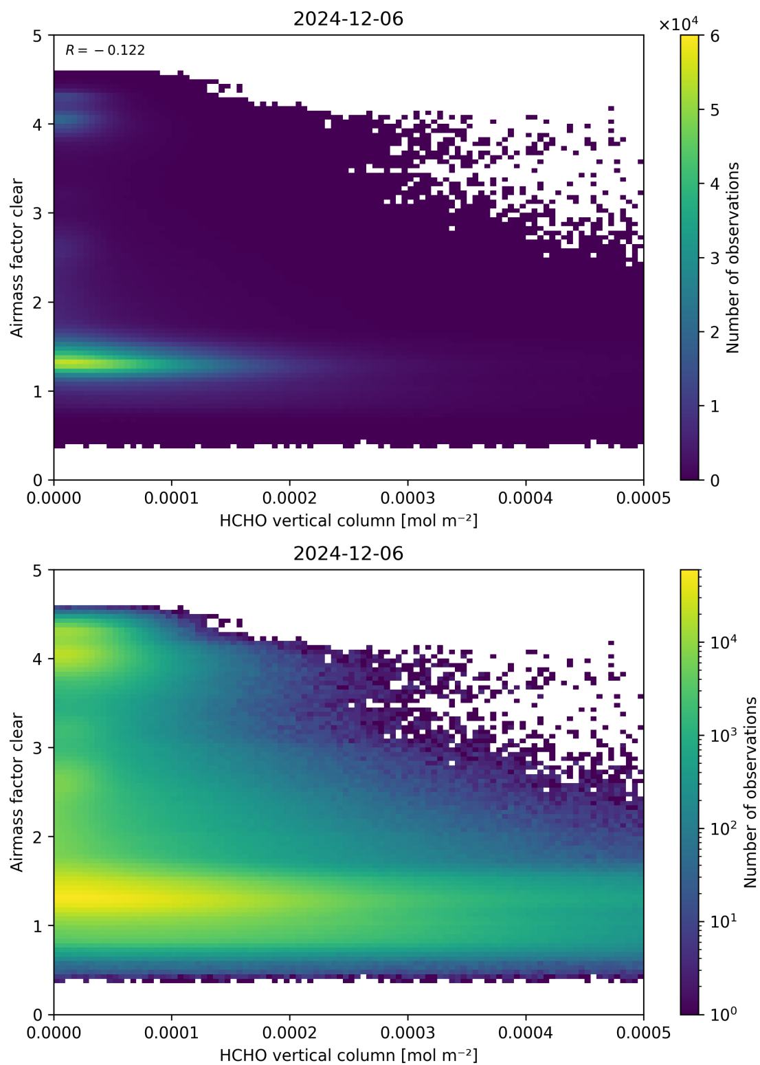
Figure 126: Scatter density plot of “HCHO vertical column” against “Airmass factor clear” for 2024-12-06 to 2024-12-07.
