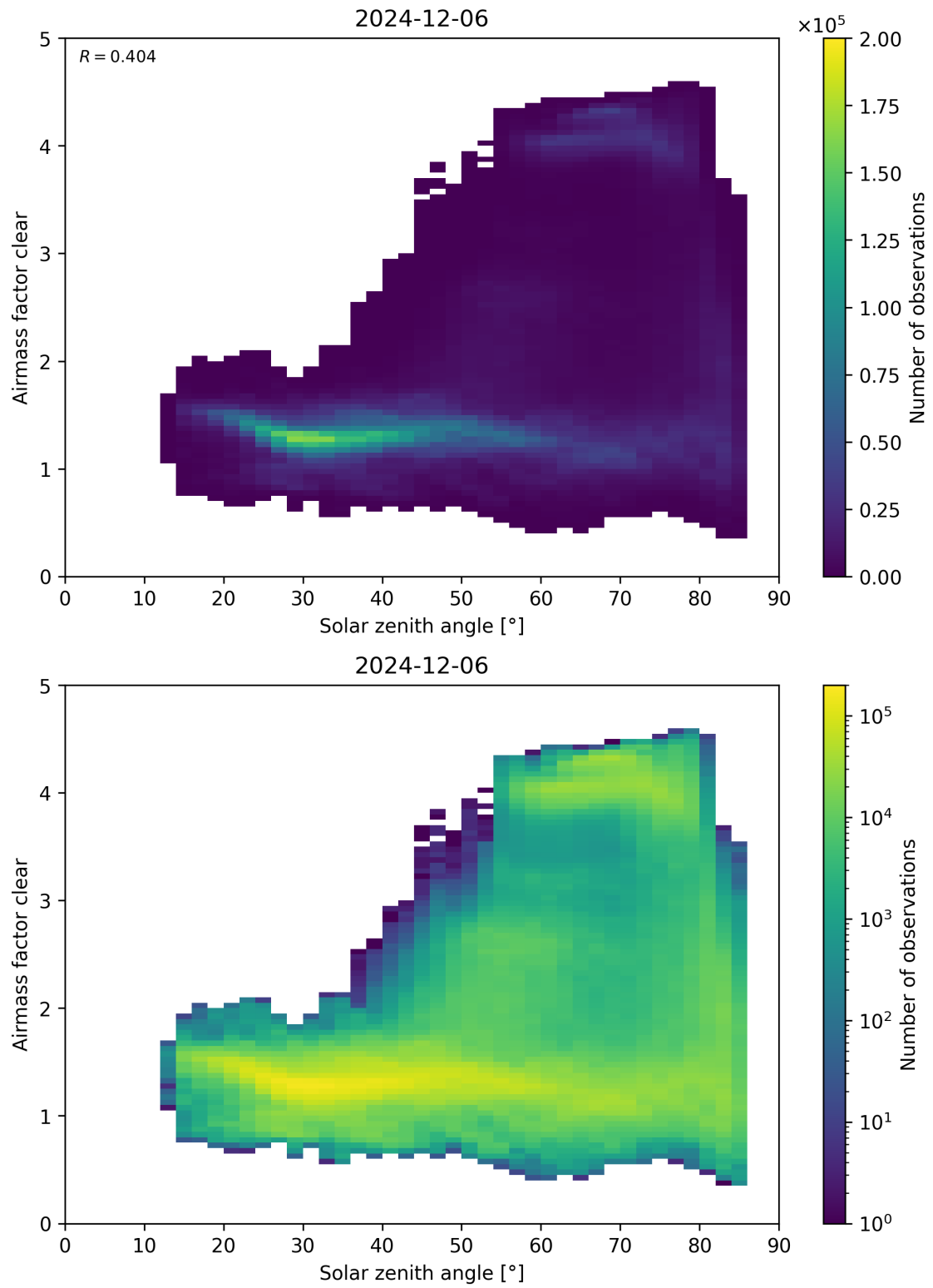
Figure 170: Scatter density plot of “Solar zenith angle” against “Airmass factor clear” for 2024-12-06 to 2024-12-07.
