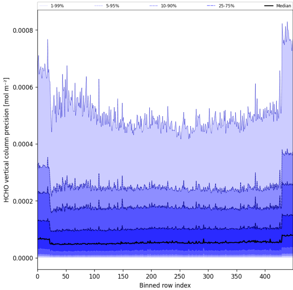
Figure 50: Along track statistics of “HCHO vertical column precision” for 2024-12-06 to 2024-12-07
