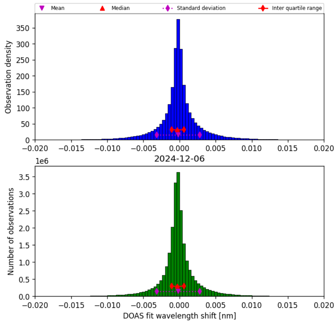
Figure 44: Histogram of “DOAS fit wavelength shift” for 2024-12-06 to 2024-12-07
