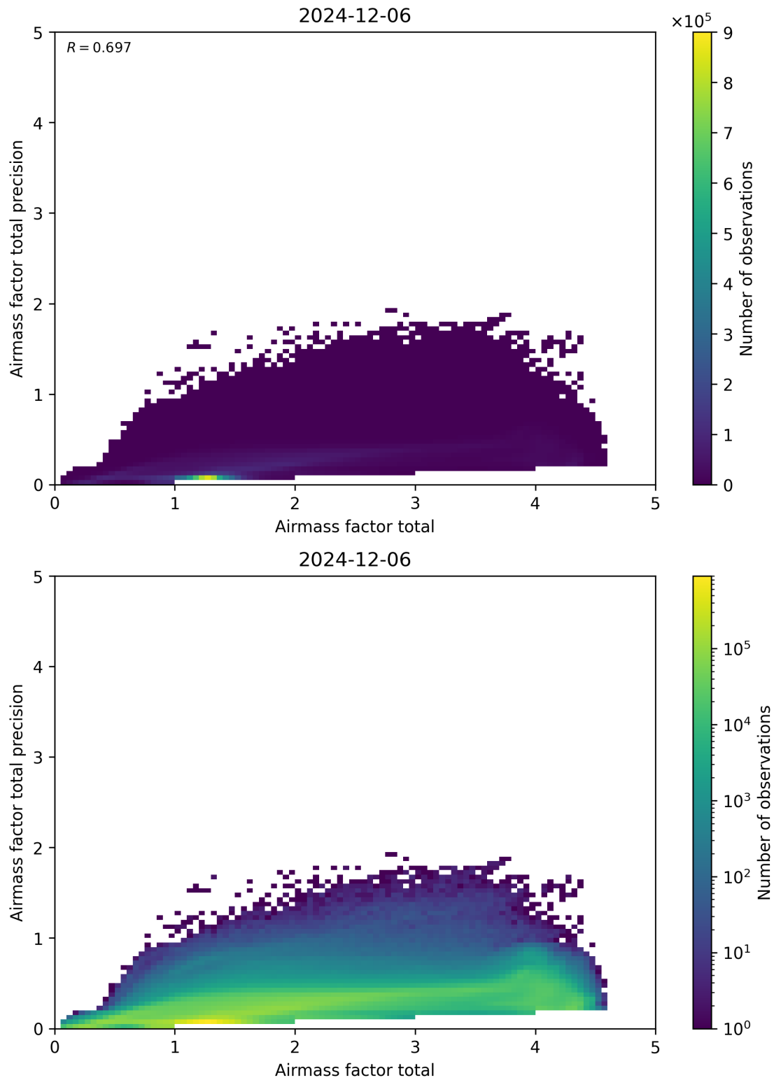
Figure 103: Scatter density plot of “Airmass factor total” against “Airmass factor total precision” for 2024-12-06 to 2024-12-07.
