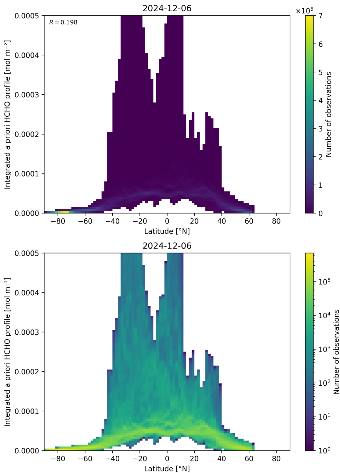
Figure 166: Scatter density plot of “Latitude” against “Integrated a priori HCHO profile” for 2024-12-06 to 2024-12-07.
