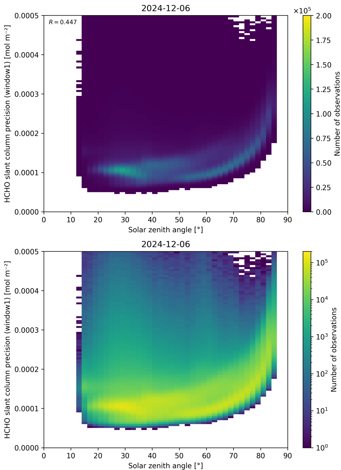
Figure 174: Scatter density plot of “Solar zenith angle” against “HCHO slant column precision (window1)” for 2024-12-06 to 2024-12-07.
