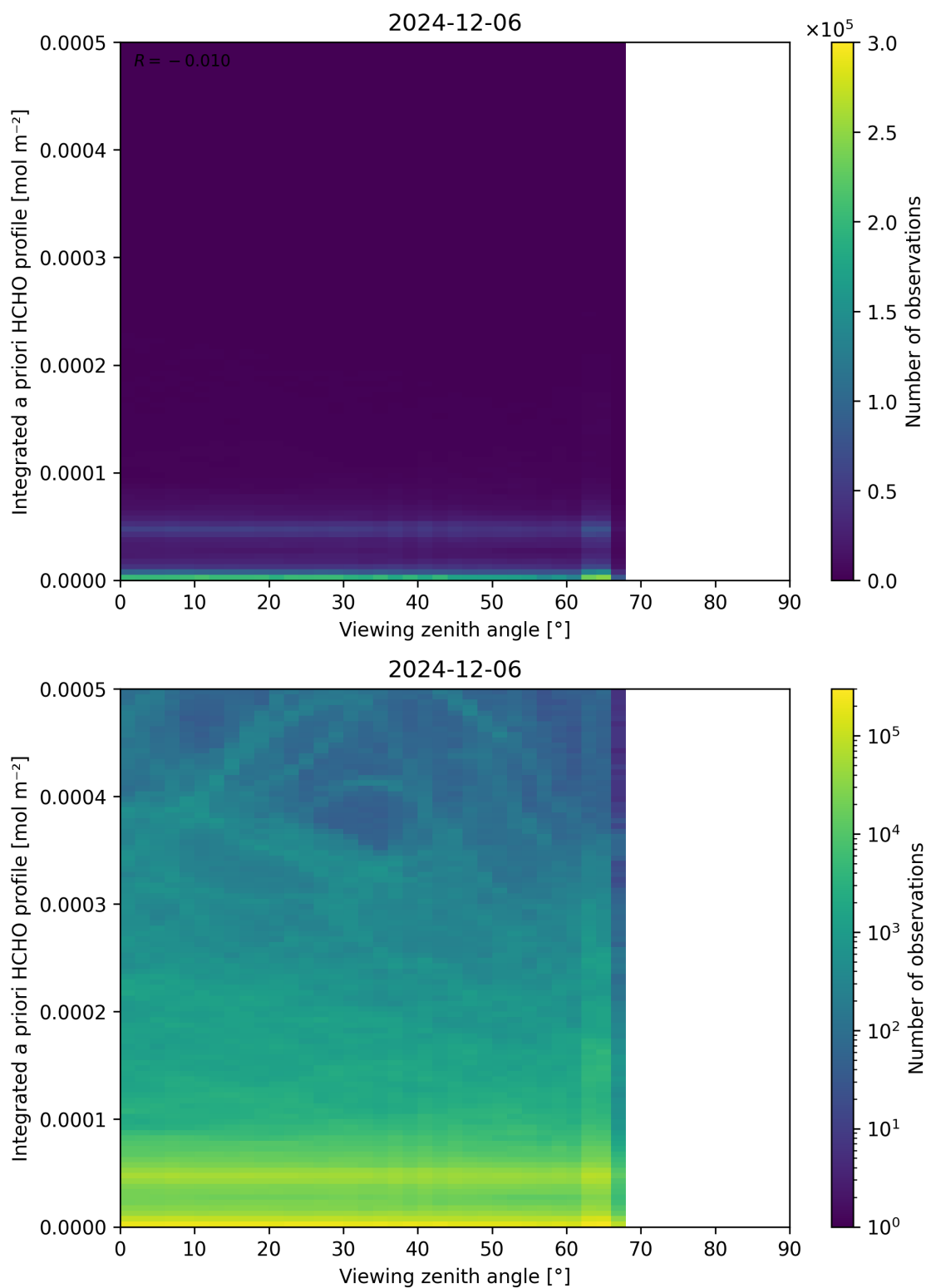
Figure 195: Scatter density plot of “Viewing zenith angle” against “Integrated a priori HCHO profile” for 2024-12-06 to 2024-12-07.
