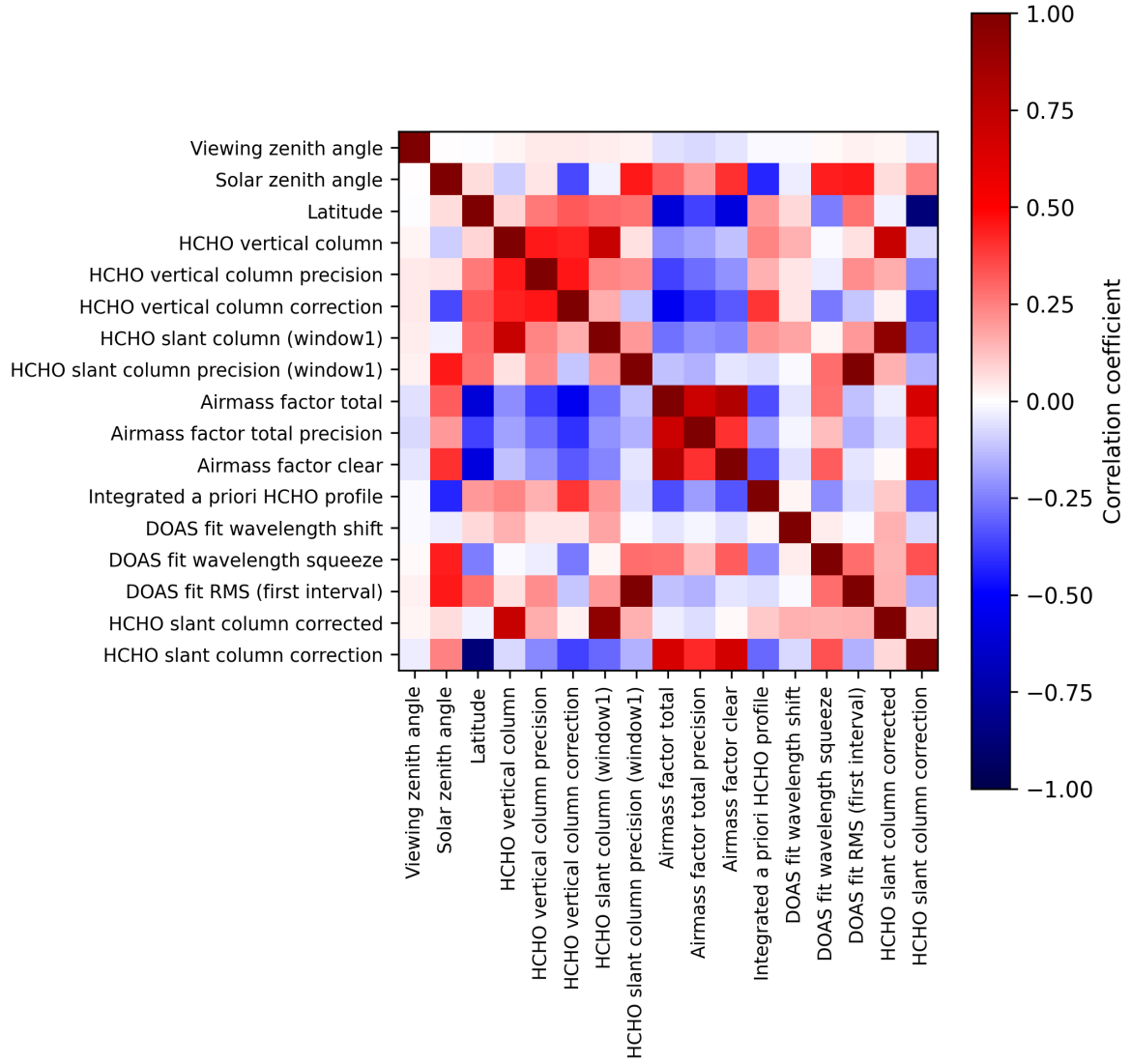
Figure 2: Map of correlation matrix for 2024-12-06 to 2024-12-07.
