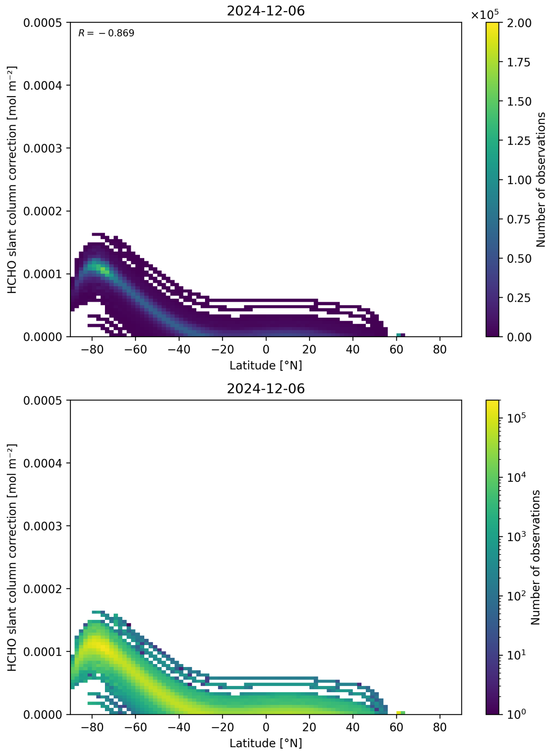
Figure 158: Scatter density plot of “Latitude” against “HCHO slant column correction” for 2024-12-06 to 2024-12-07.
