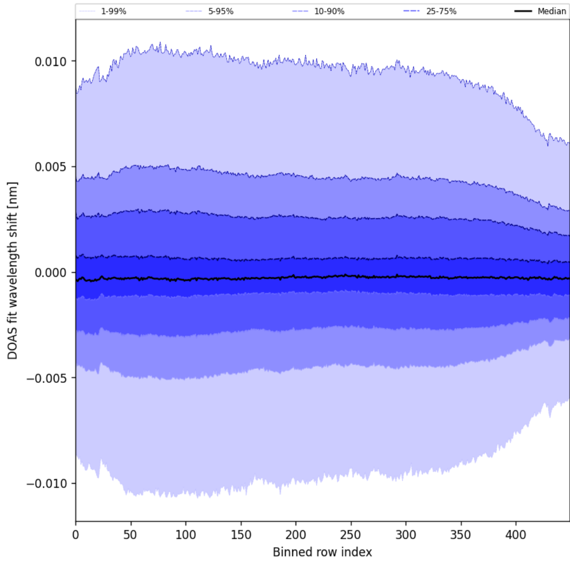
Figure 58: Along track statistics of “DOAS fit wavelength shift” for 2024-12-06 to 2024-12-07
