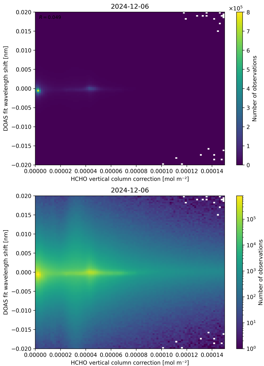
Figure 113: Scatter density plot of “HCHO vertical column correction” against “DOAS fit wavelength shift” for 2024-12-06 to 2024-12-07.
