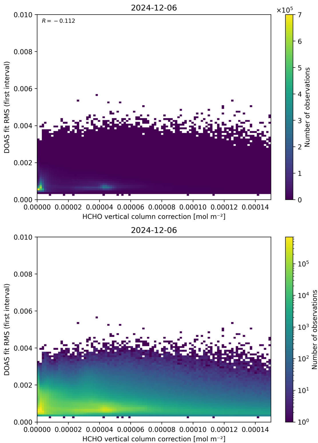
Figure 112: Scatter density plot of “HCHO vertical column correction” against “DOAS fit RMS (first interval)” for 2024-12-06 to 2024-12-07.
