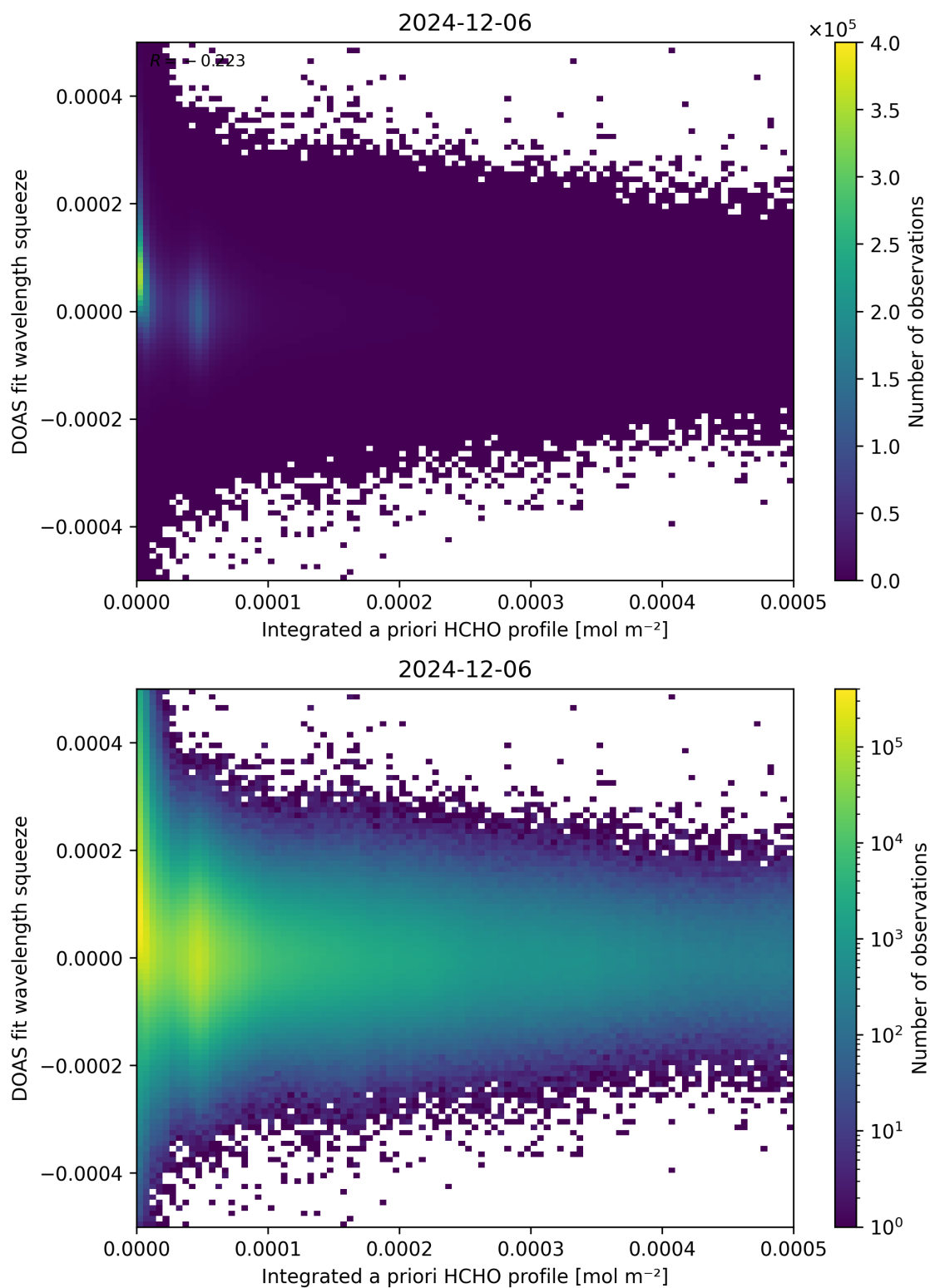
Figure 150: Scatter density plot of “Integrated a priori HCHO profile” against “DOAS fit wavelength squeeze” for 2024-12-06 to 2024-12-07.
