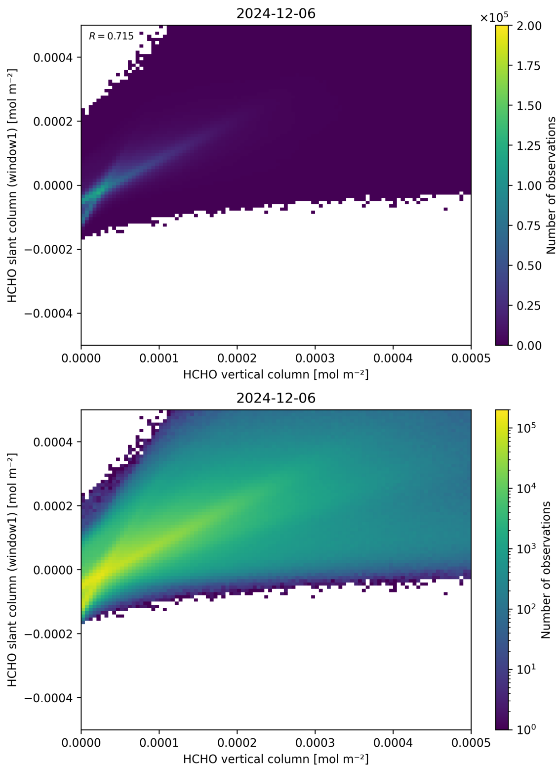
Figure 129: Scatter density plot of “HCHO vertical column” against “HCHO slant column (window1)” for 2024-12-06 to 2024-12-07.
