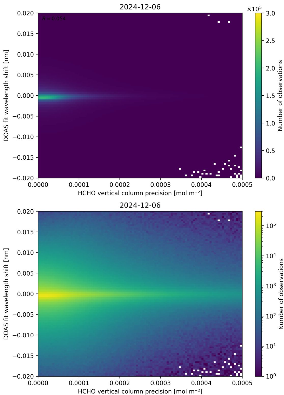
Figure 137: Scatter density plot of “HCHO vertical column precision” against “DOAS fit wavelength shift” for 2024-12-06 to 2024-12-07.
