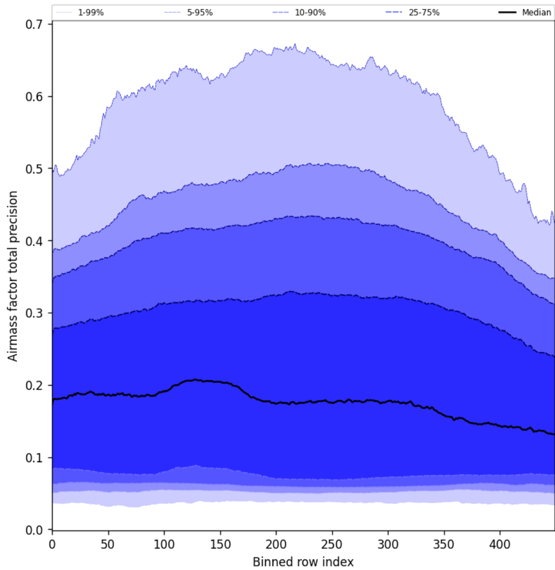
Figure 55: Along track statistics of “Airmass factor total precision” for 2024-12-06 to 2024-12-07
