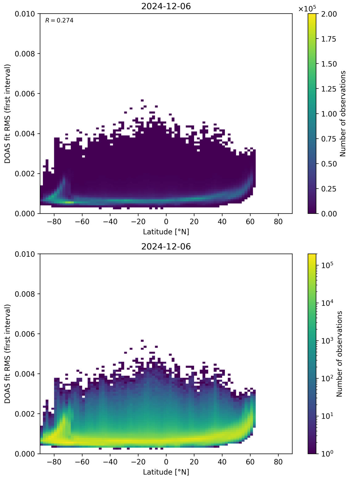
Figure 153: Scatter density plot of “Latitude” against “DOAS fit RMS (first interval)” for 2024-12-06 to 2024-12-07.
