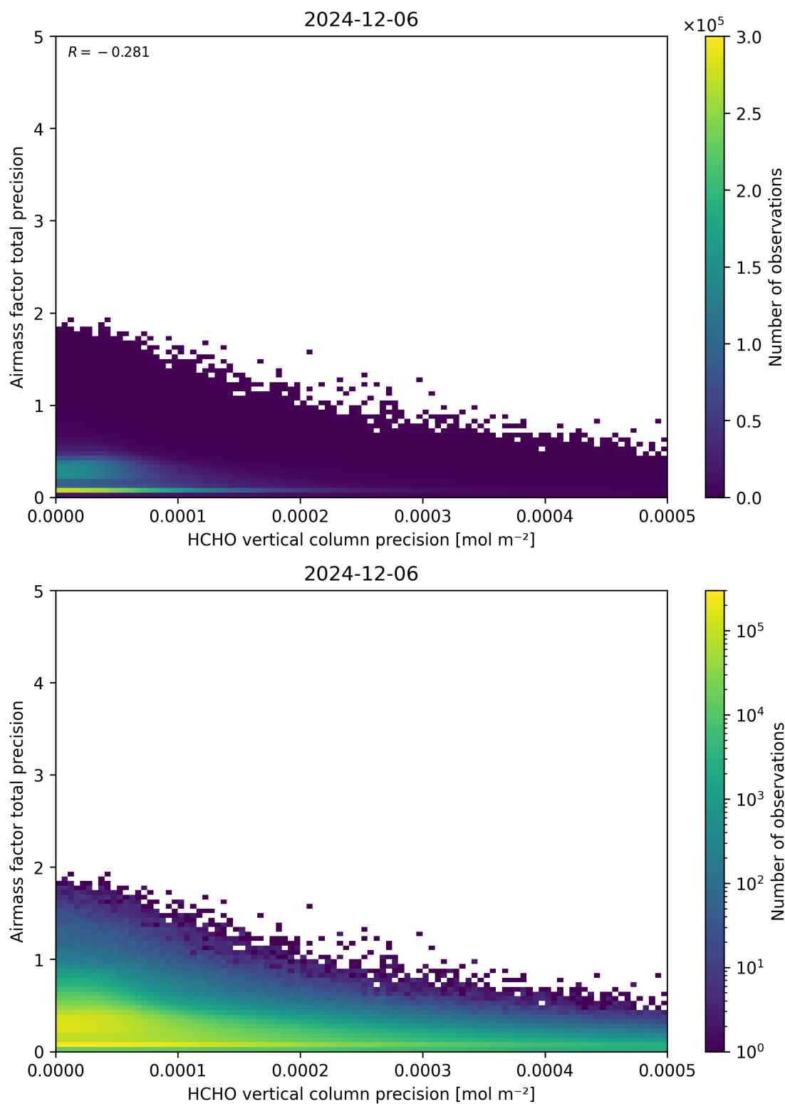
Figure 145: Scatter density plot of “HCHO vertical column precision” against “Airmass factor total precision” for 2024-12-06 to 2024-12-07.
