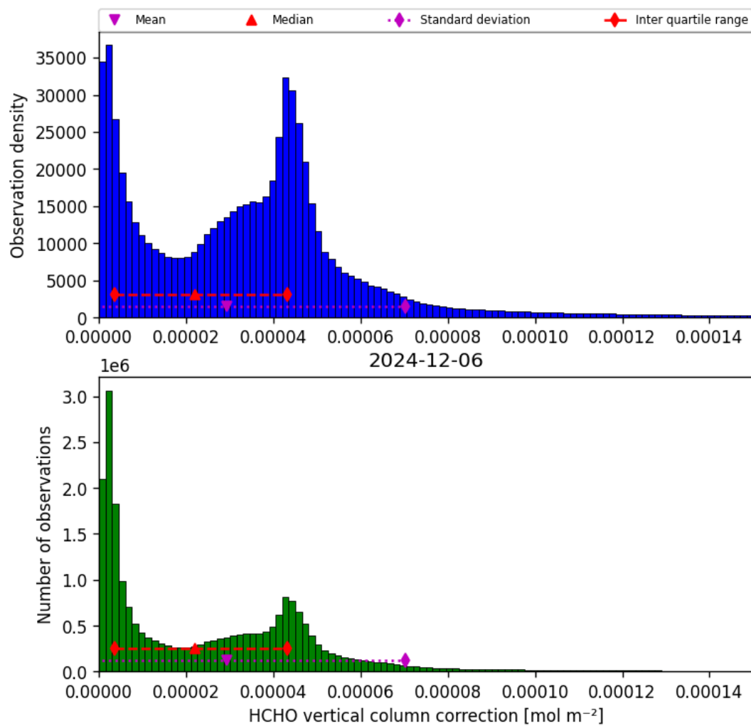
Figure 37: Histogram of “HCHO vertical column correction” for 2024-12-06 to 2024-12-07
