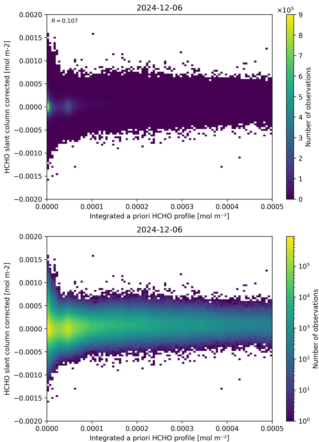
Figure 151: Scatter density plot of “Integrated a priori HCHO profile” against “HCHO slant column corrected” for 2024-12-06 to 2024-12-07.
