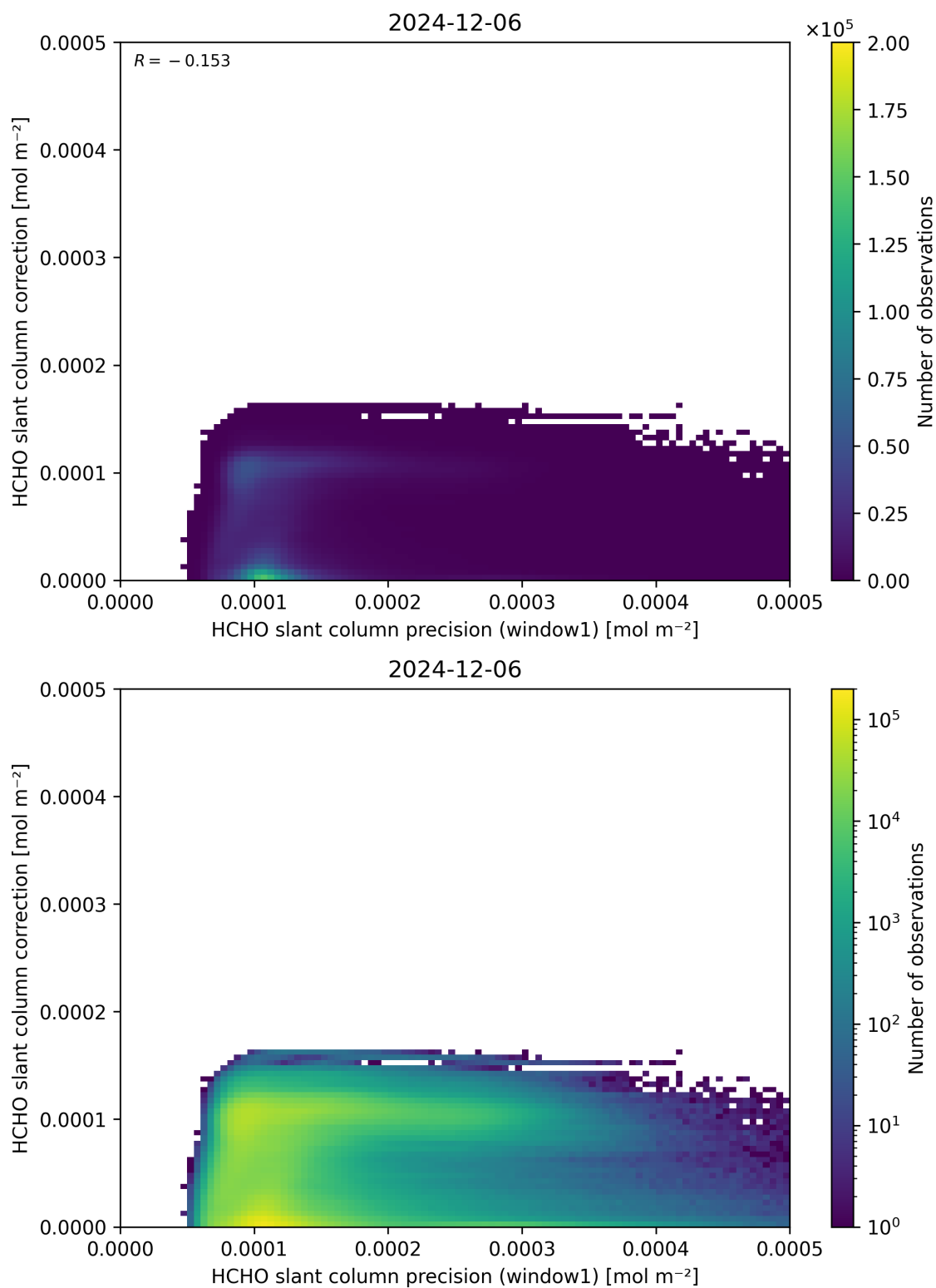
Figure 93: Scatter density plot of “HCHO slant column precision (window1)” against “HCHO slant column correction” for 2024-12-06 to 2024-12-07.
