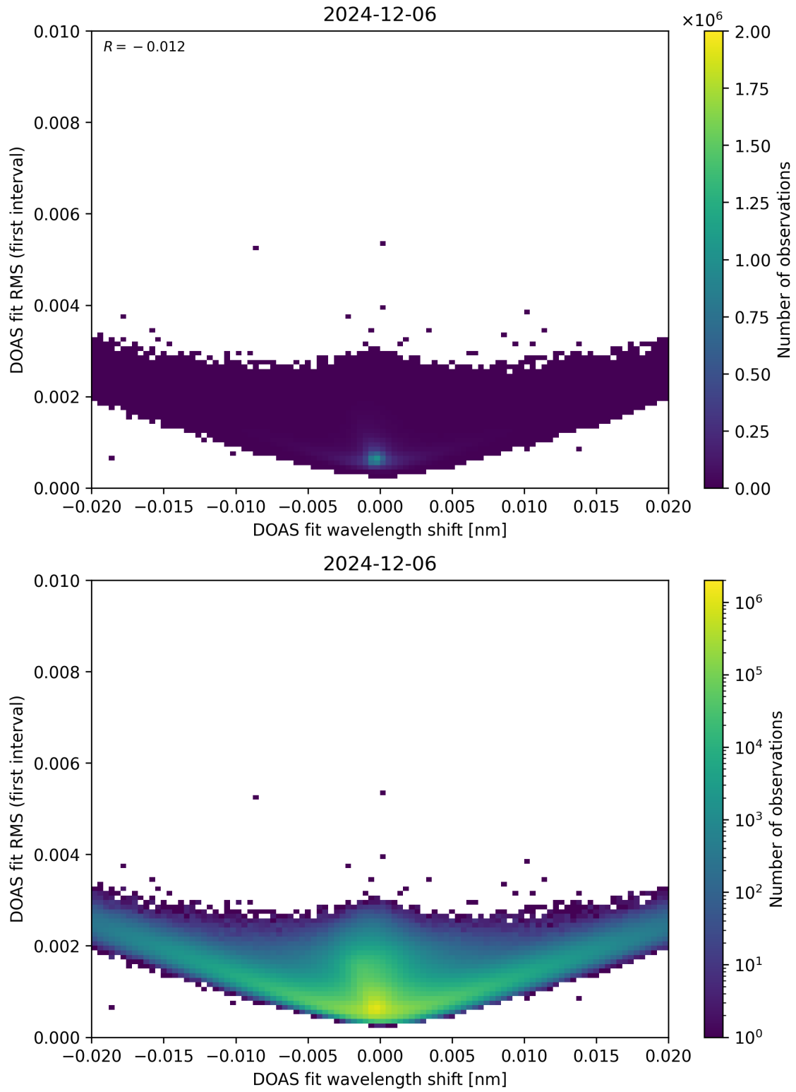
Figure 64: Scatter density plot of “DOAS fit wavelength shift” against “DOAS fit RMS (first interval)” for 2024-12-06 to 2024-12-07.
