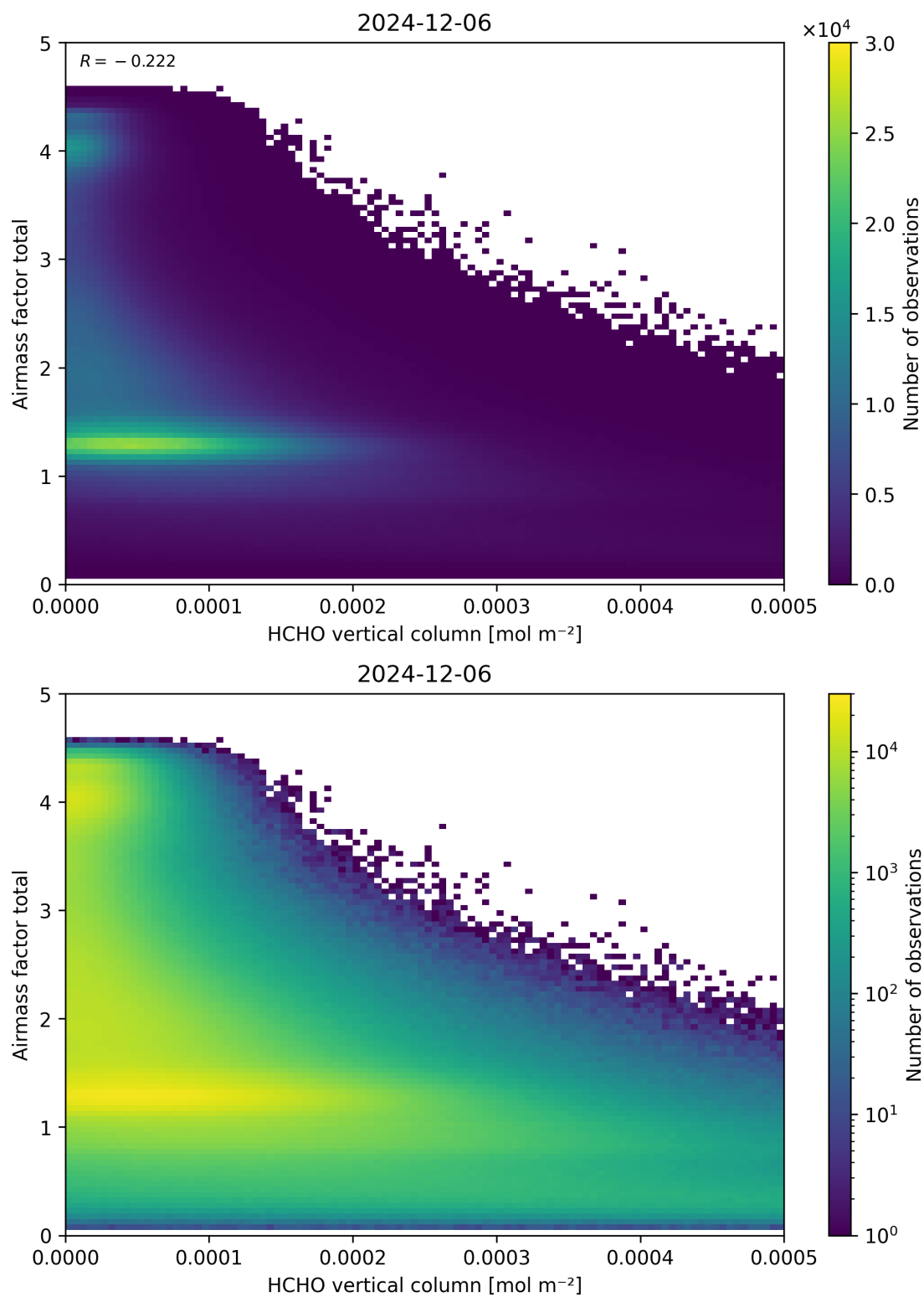
Figure 131: Scatter density plot of “HCHO vertical column” against “Airmass factor total” for 2024-12-06 to 2024-12-07.
