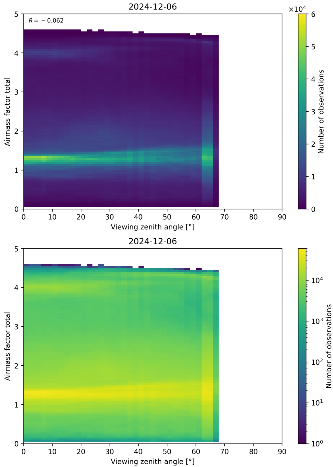
Figure 190: Scatter density plot of “Viewing zenith angle” against “Airmass factor total” for 2024-12-06 to 2024-12-07.
