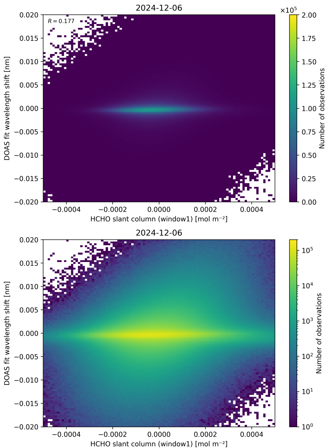
Figure 79: Scatter density plot of “HCHO slant column (window1)” against “DOAS fit wavelength shift” for 2024-12-06 to 2024-12-07.
