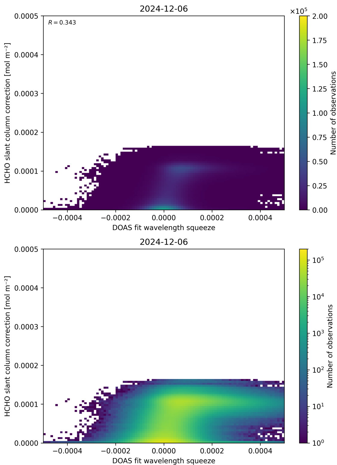
Figure 70: Scatter density plot of “DOAS fit wavelength squeeze” against “HCHO slant column correction” for 2024-12-06 to 2024-12-07.
