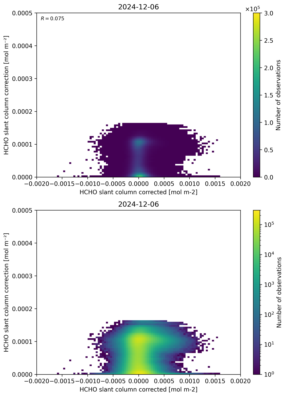
Figure 77: Scatter density plot of “HCHO slant column corrected” against “HCHO slant column correction” for 2024-12-06 to 2024-12-07.
