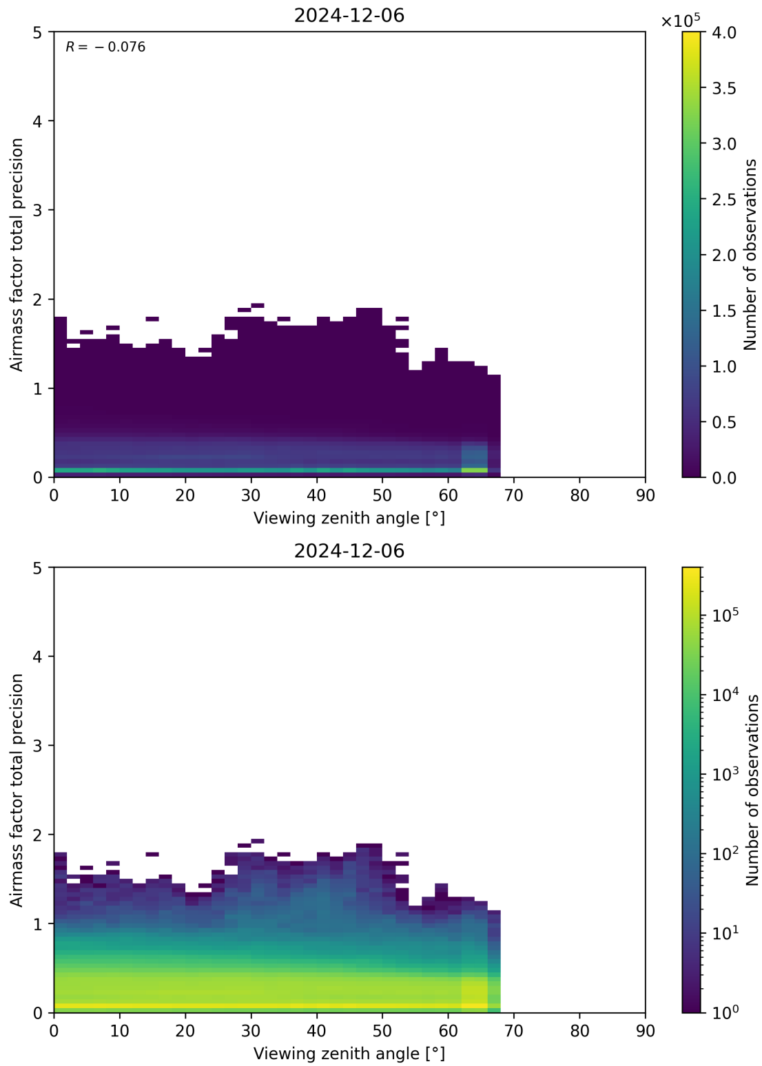
Figure 191: Scatter density plot of “Viewing zenith angle” against “Airmass factor total precision” for 2024-12-06 to 2024-12-07.
