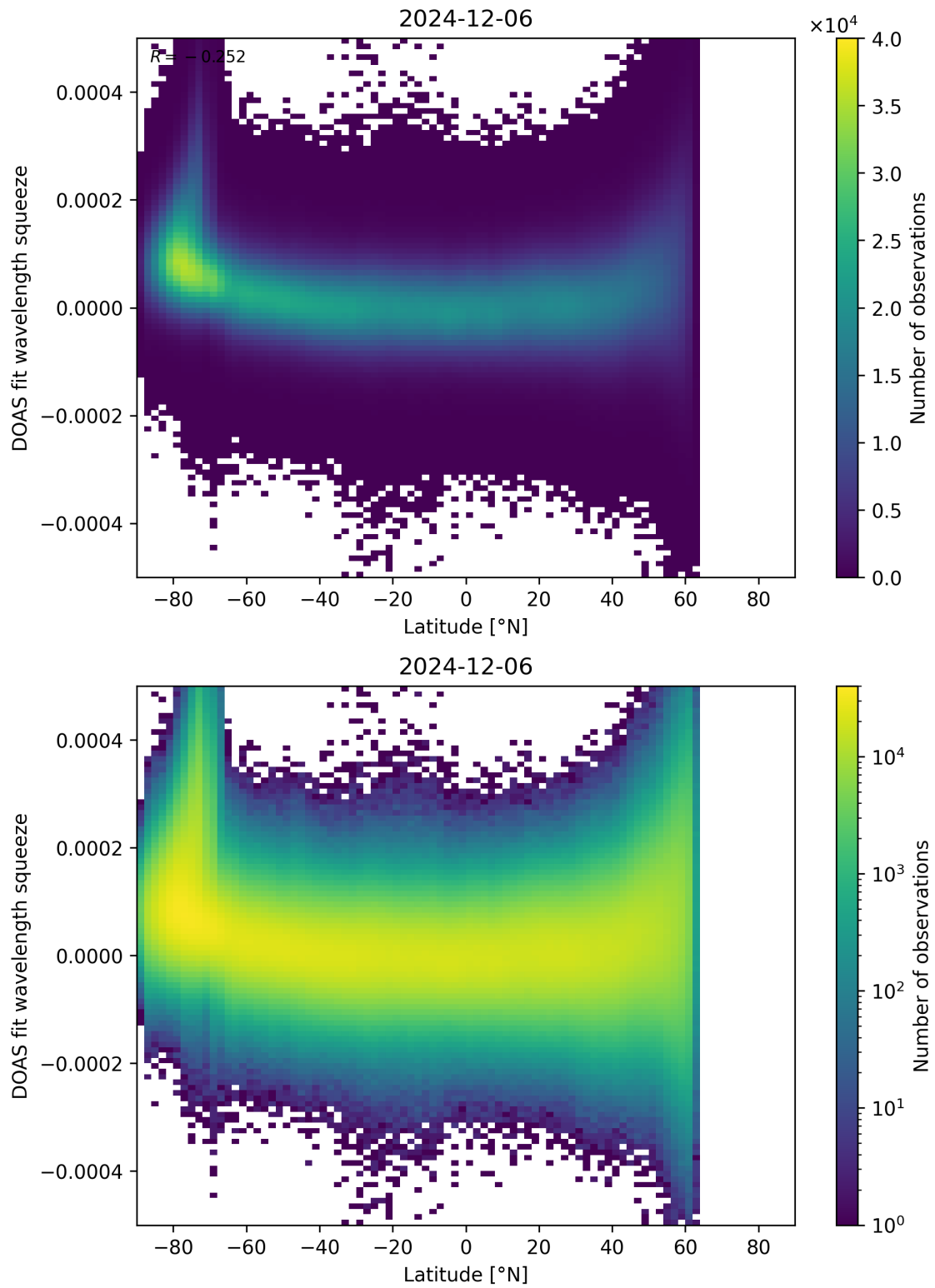
Figure 155: Scatter density plot of “Latitude” against “DOAS fit wavelength squeeze” for 2024-12-06 to 2024-12-07.
