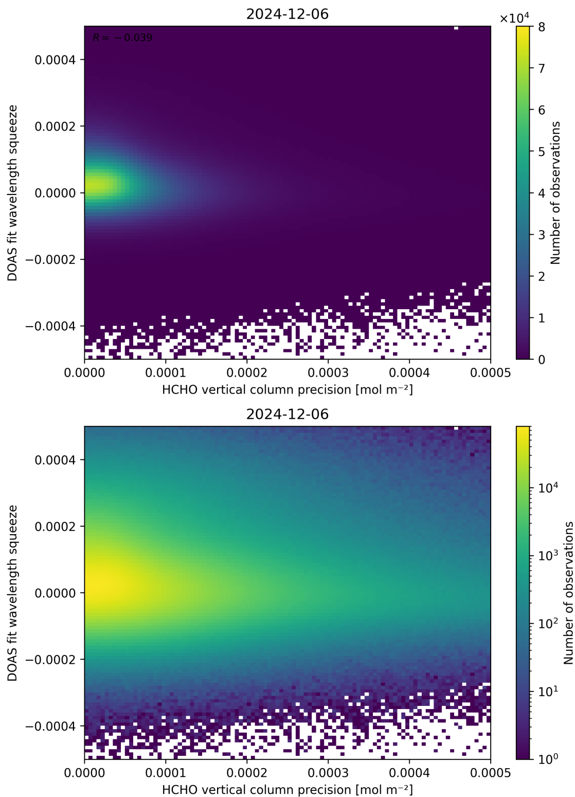
Figure 138: Scatter density plot of “HCHO vertical column precision” against “DOAS fit wavelength squeeze” for 2024-12-06 to 2024-12-07.
