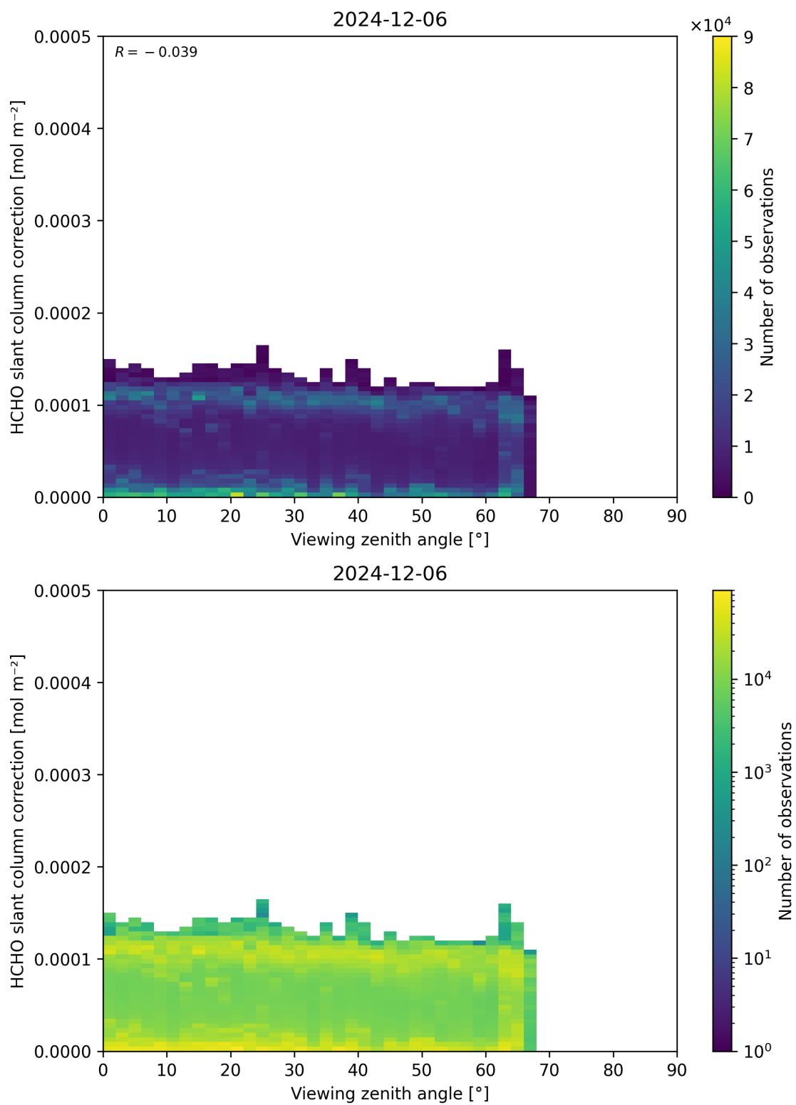
Figure 187: Scatter density plot of “Viewing zenith angle” against “HCHO slant column correction” for 2024-12-06 to 2024-12-07.
