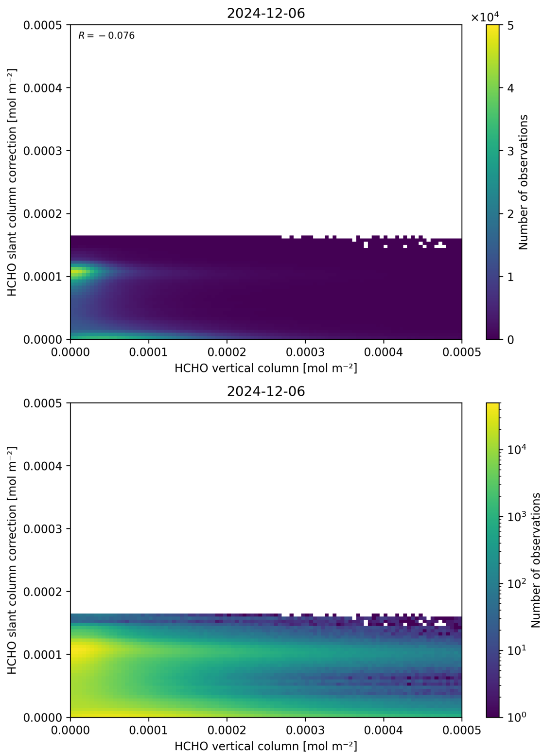
Figure 128: Scatter density plot of “HCHO vertical column” against “HCHO slant column correction” for 2024-12-06 to 2024-12-07.
