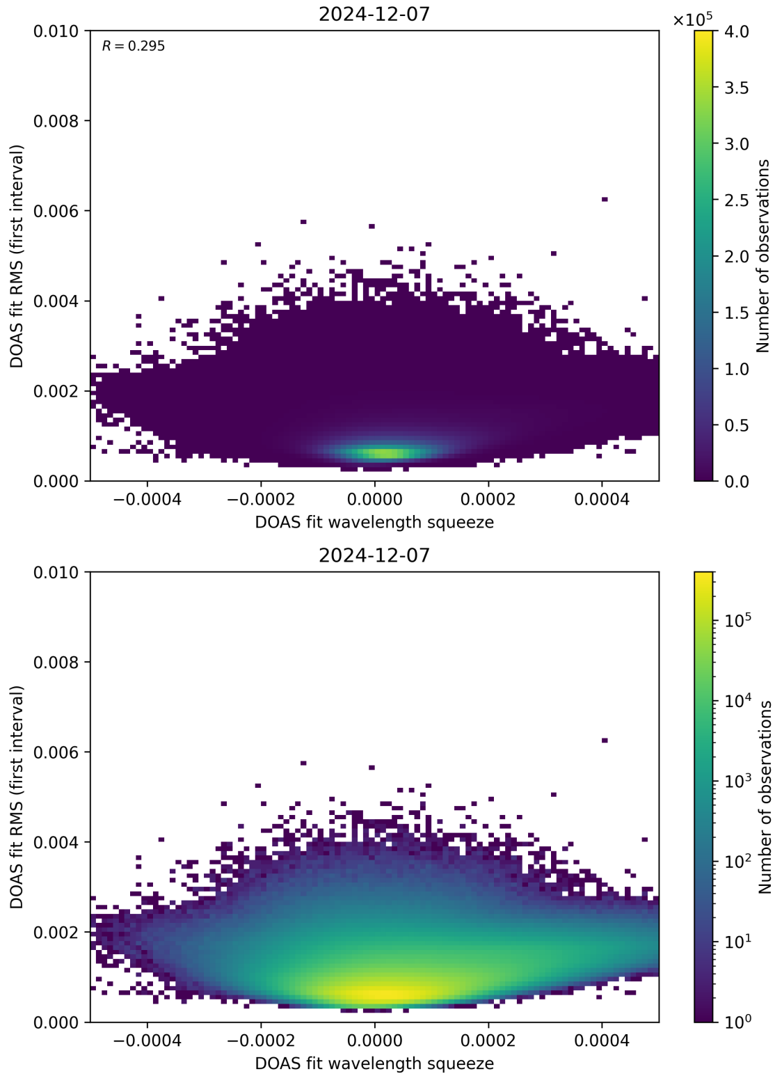
Figure 68: Scatter density plot of “DOAS fit wavelength squeeze” against “DOAS fit RMS (first interval)” for 2024-12-06 to 2024-12-08.
