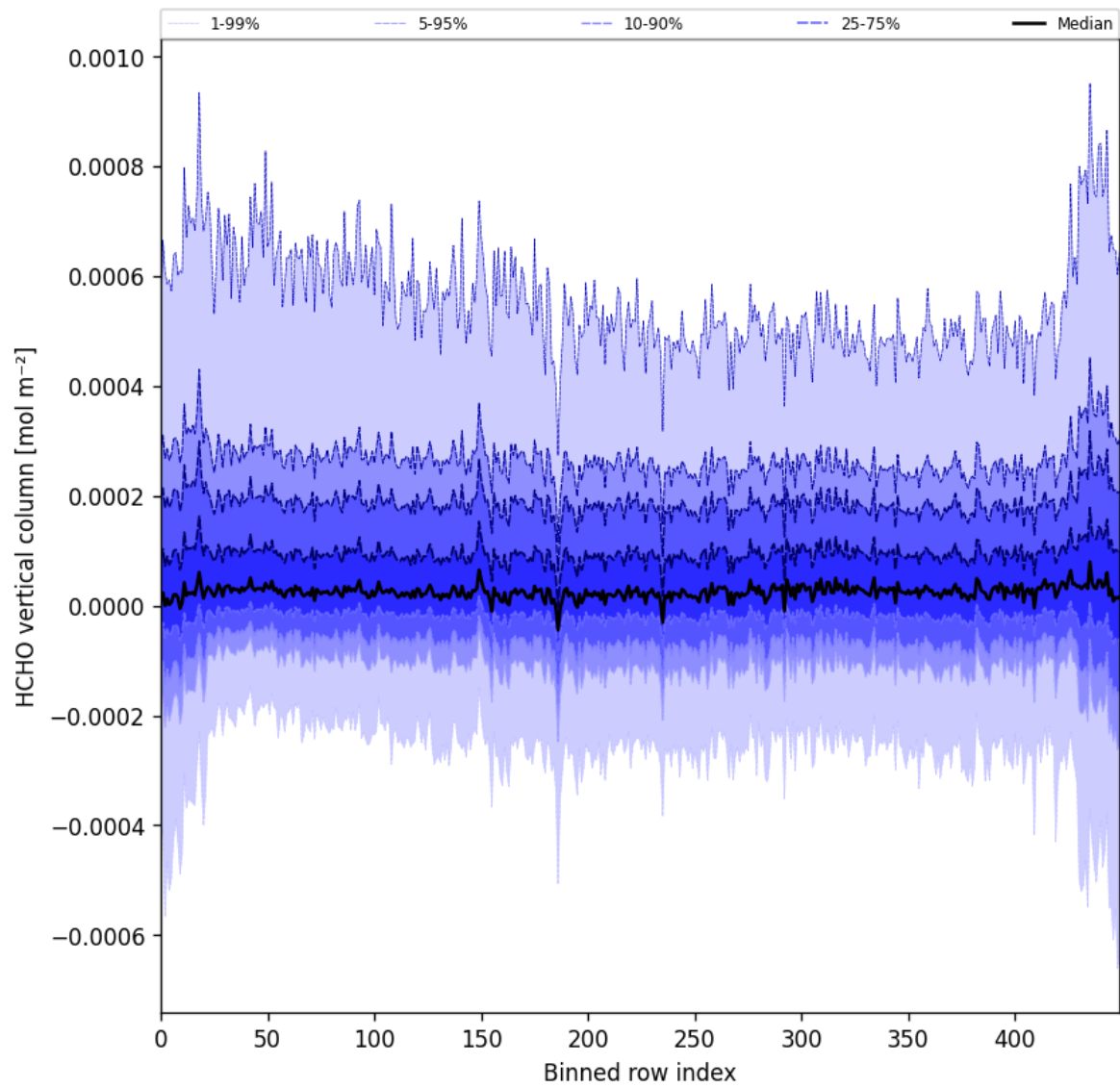
Figure 49: Along track statistics of “HCHO vertical column” for 2024-12-06 to 2024-12-08
