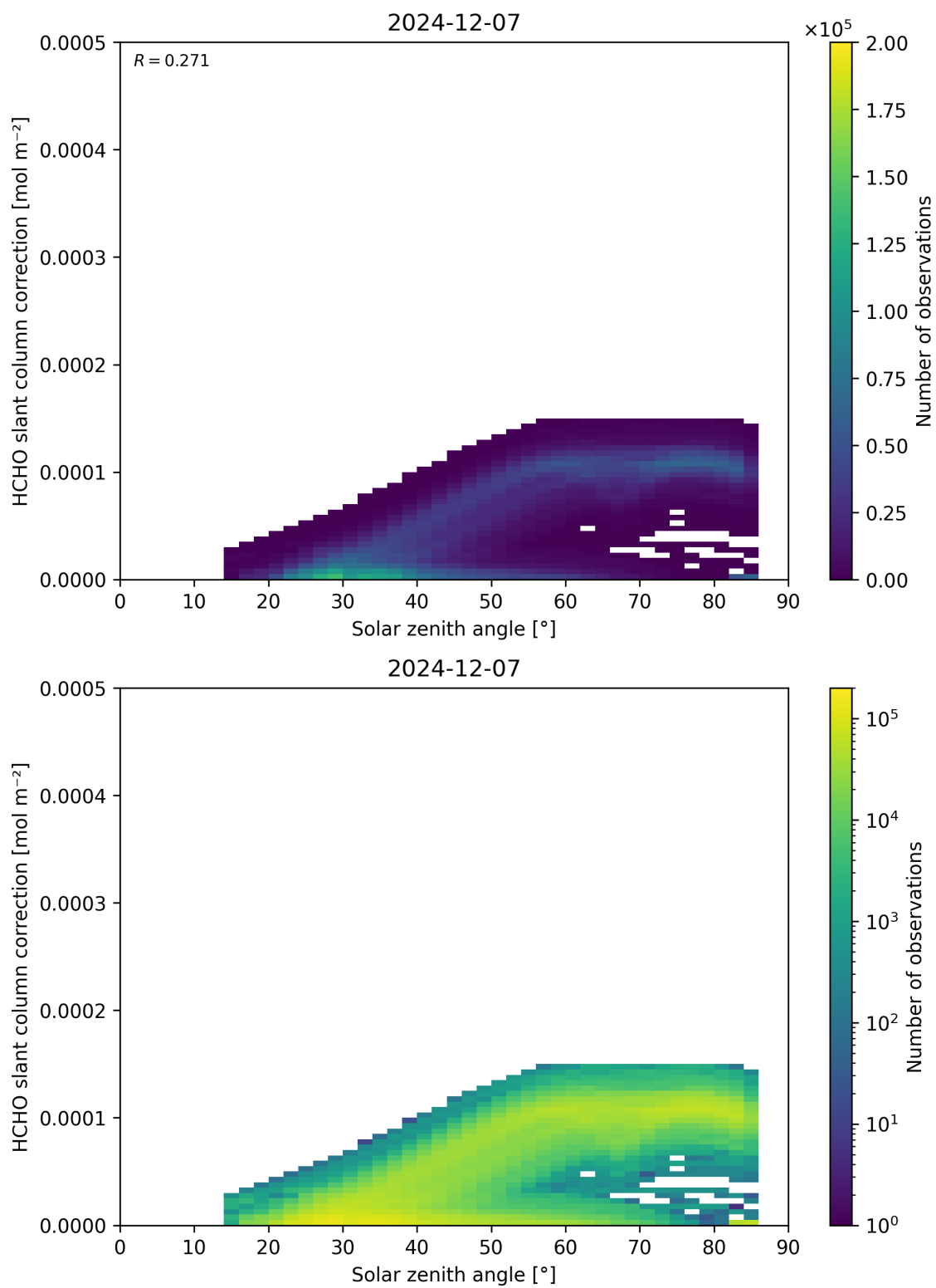
Figure 172: Scatter density plot of “Solar zenith angle” against “HCHO slant column correction” for 2024-12-06 to 2024-12-08.
