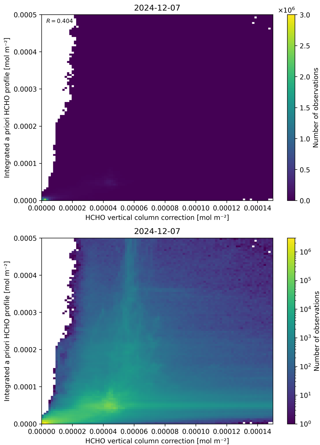
Figure 122: Scatter density plot of “HCHO vertical column correction” against “Integrated a priori HCHO profile” for 2024-12-06 to 2024-12-08.
