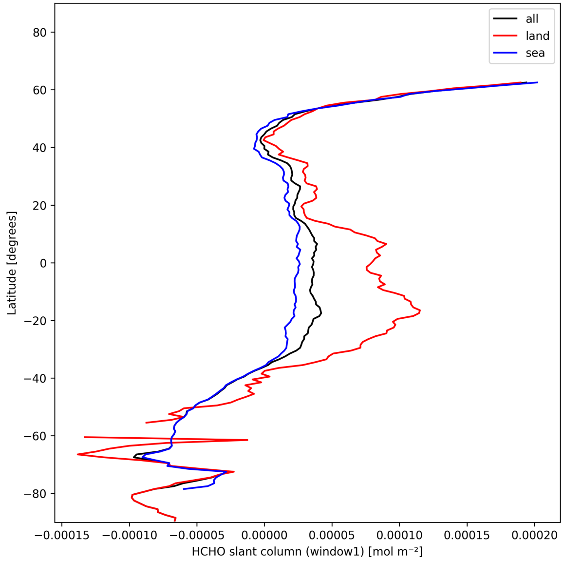
Figure 24: Zonal average of “HCHO slant column (window1)” for 2024-12-06 to 2024-12-08.
