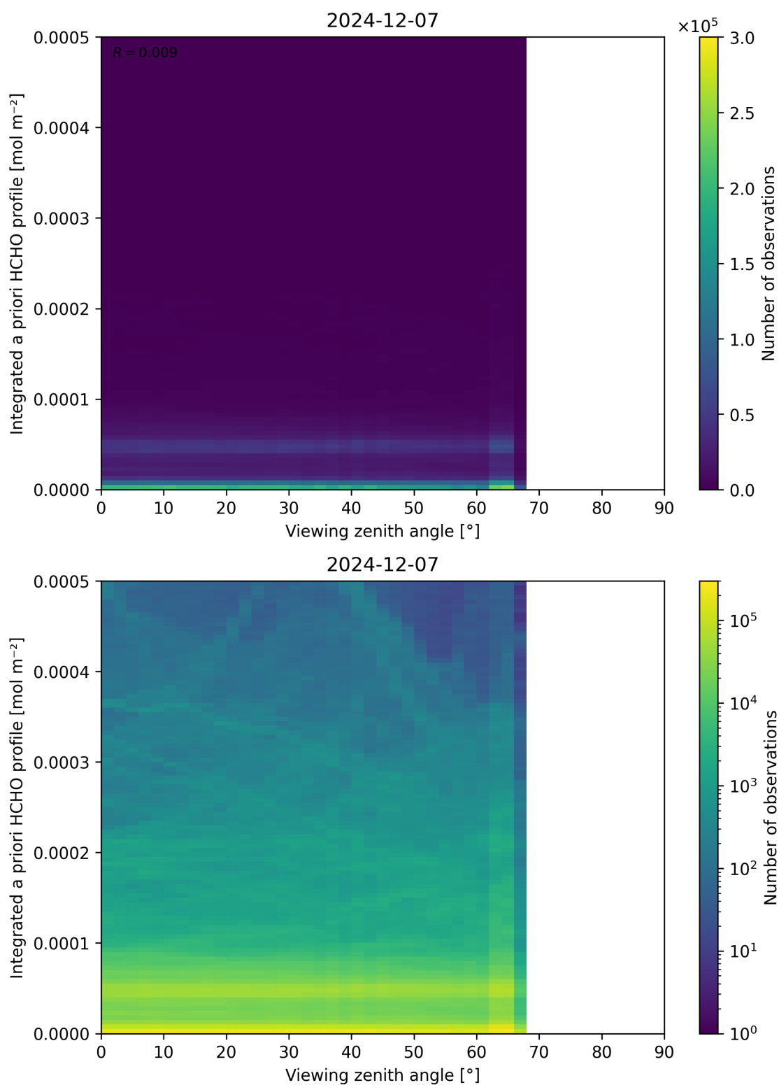
Figure 195: Scatter density plot of “Viewing zenith angle” against “Integrated a priori HCHO profile” for 2024-12-06 to 2024-12-08.
