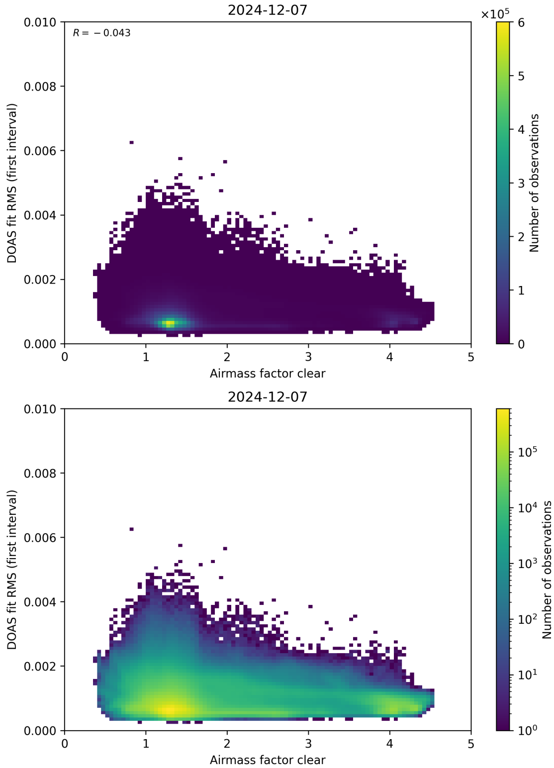
Figure 71: Scatter density plot of “Airmass factor clear” against “DOAS fit RMS (first interval)” for 2024-12-06 to 2024-12-08.
