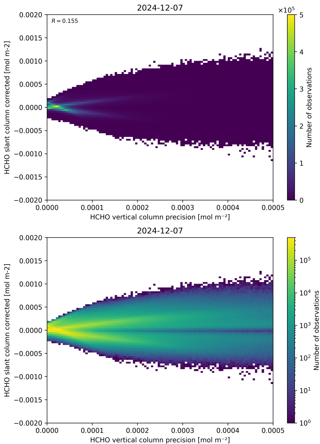
Figure 140: Scatter density plot of “HCHO vertical column precision” against “HCHO slant column corrected” for 2024-12-06 to 2024-12-08.
