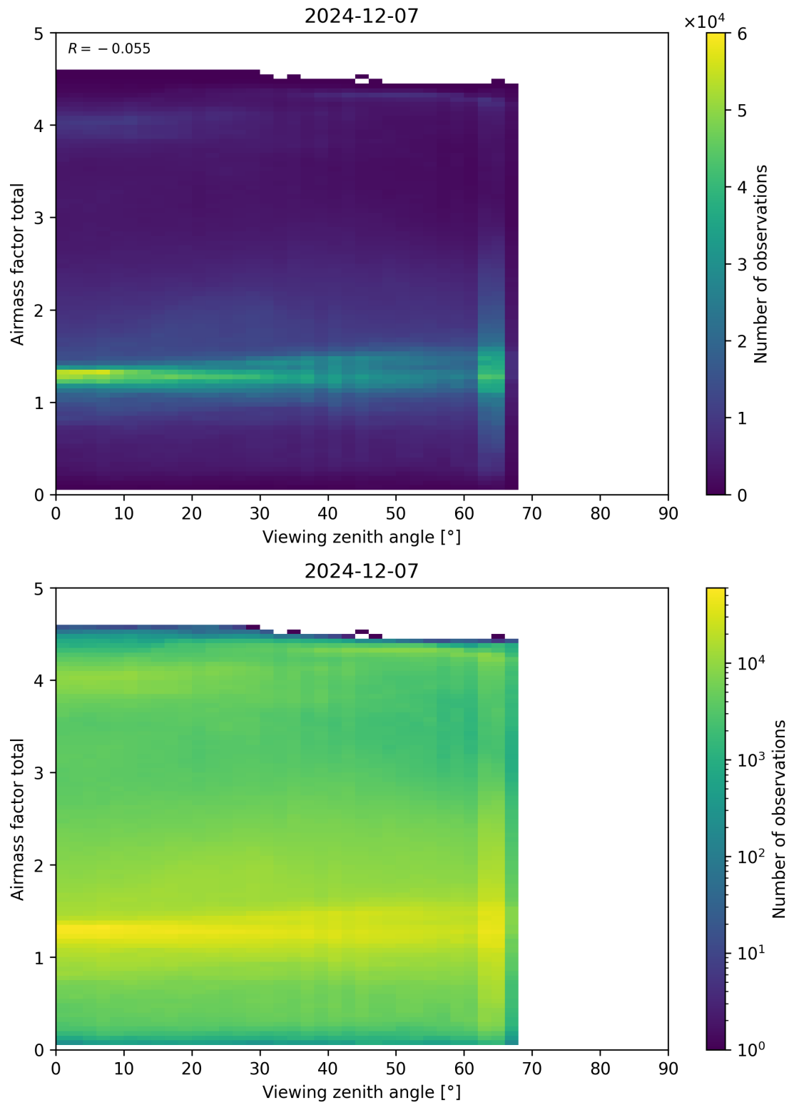
Figure 190: Scatter density plot of “Viewing zenith angle” against “Airmass factor total” for 2024-12-06 to 2024-12-08.
