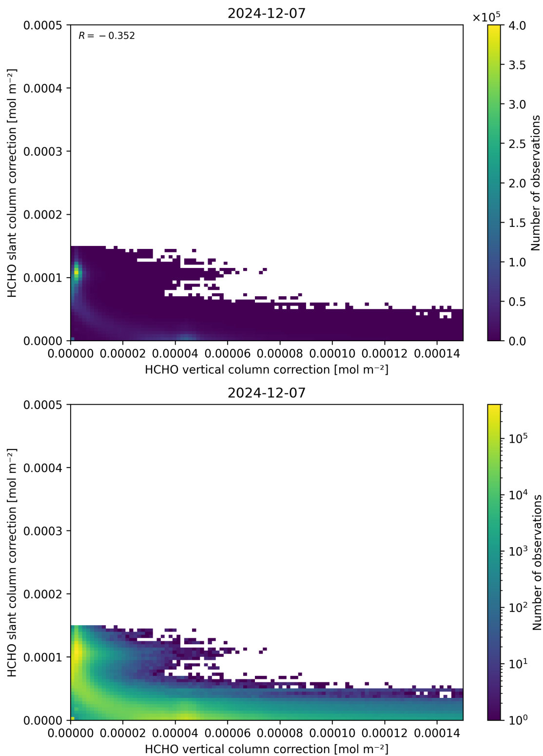
Figure 117: Scatter density plot of “HCHO vertical column correction” against “HCHO slant column correction” for 2024-12-06 to 2024-12-08.
