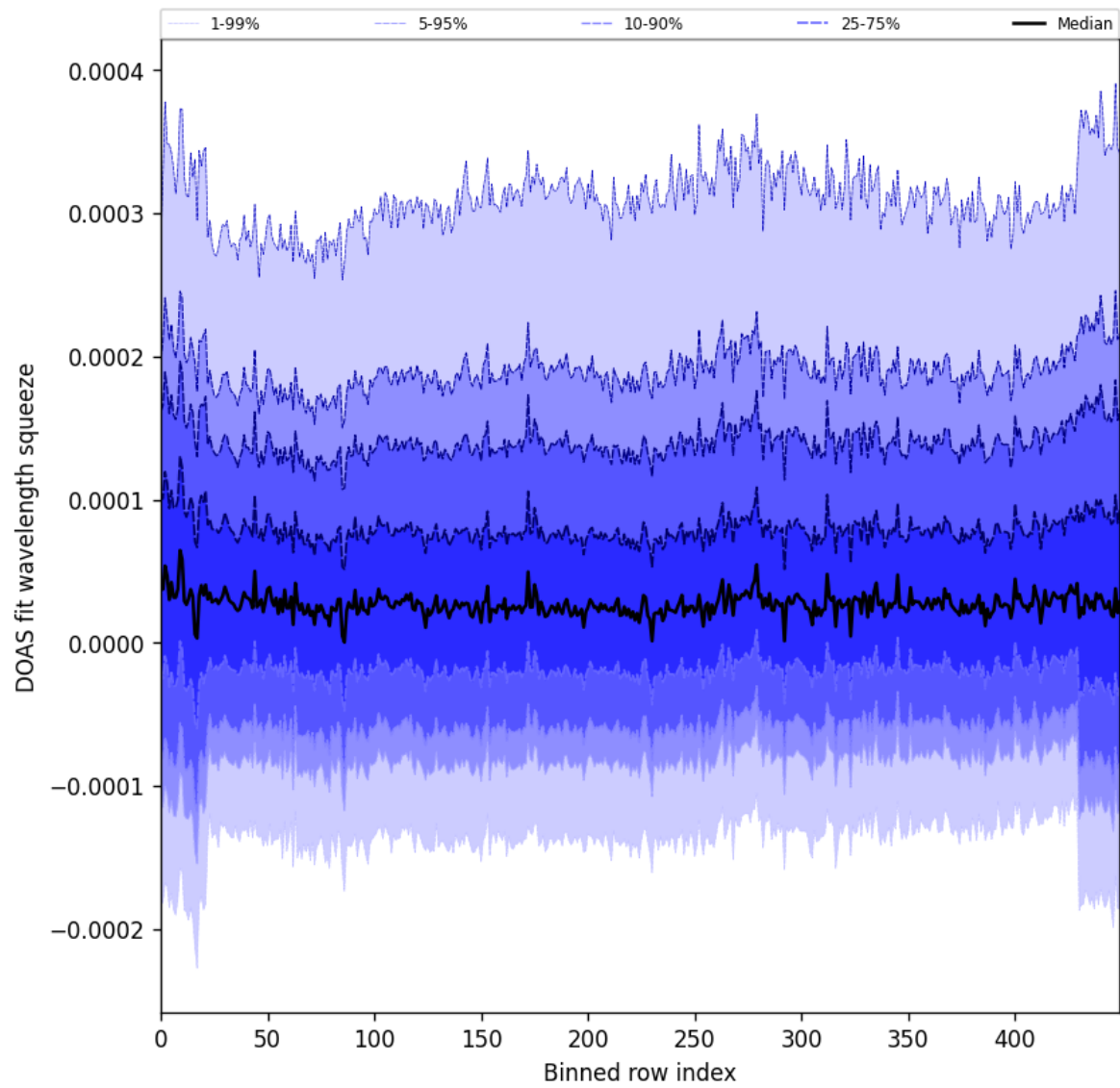
Figure 59: Along track statistics of “DOAS fit wavelength squeeze” for 2024-12-06 to 2024-12-08
