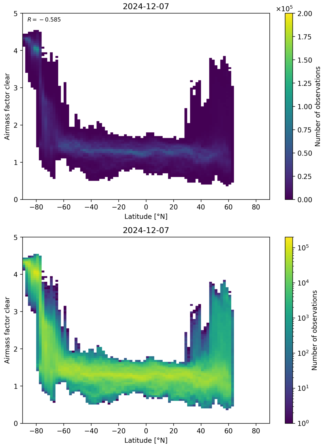
Figure 156: Scatter density plot of “Latitude” against “Airmass factor clear” for 2024-12-06 to 2024-12-08.
