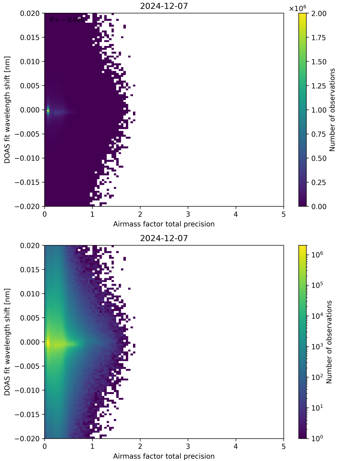
Figure 106: Scatter density plot of “Airmass factor total precision” against “DOAS fit wavelength shift” for 2024-12-06 to 2024-12-08.
