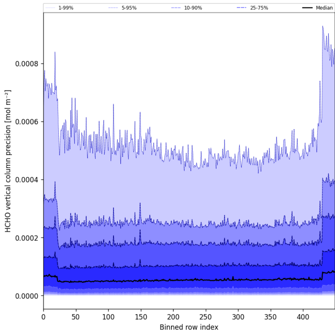
Figure 50: Along track statistics of “HCHO vertical column precision” for 2024-12-06 to 2024-12-08
