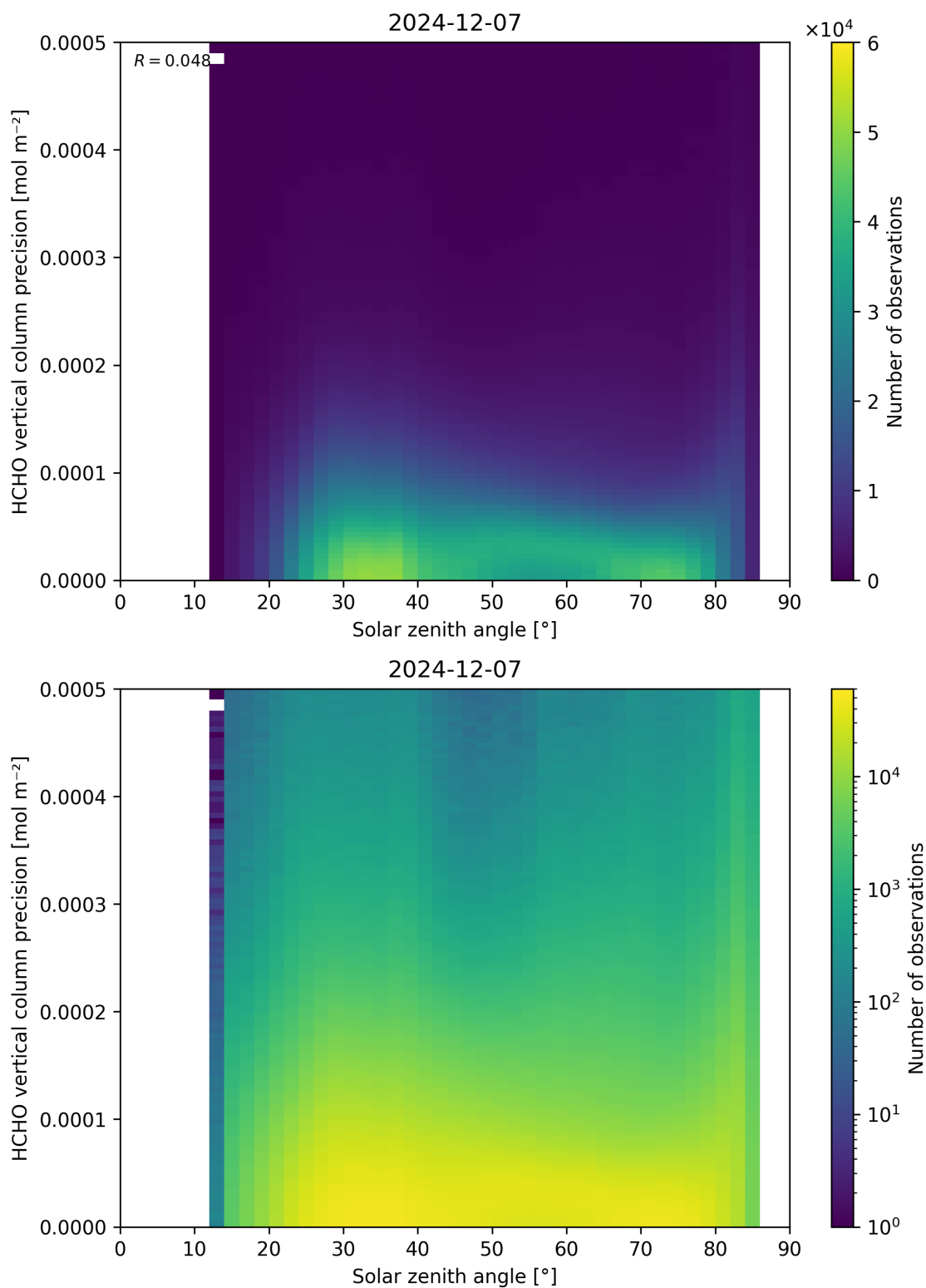
Figure 179: Scatter density plot of “Solar zenith angle” against “HCHO vertical column precision” for 2024-12-06 to 2024-12-08.
