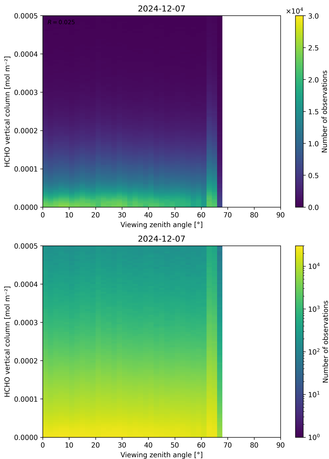
Figure 192: Scatter density plot of “Viewing zenith angle” against “HCHO vertical column” for 2024-12-06 to 2024-12-08.
