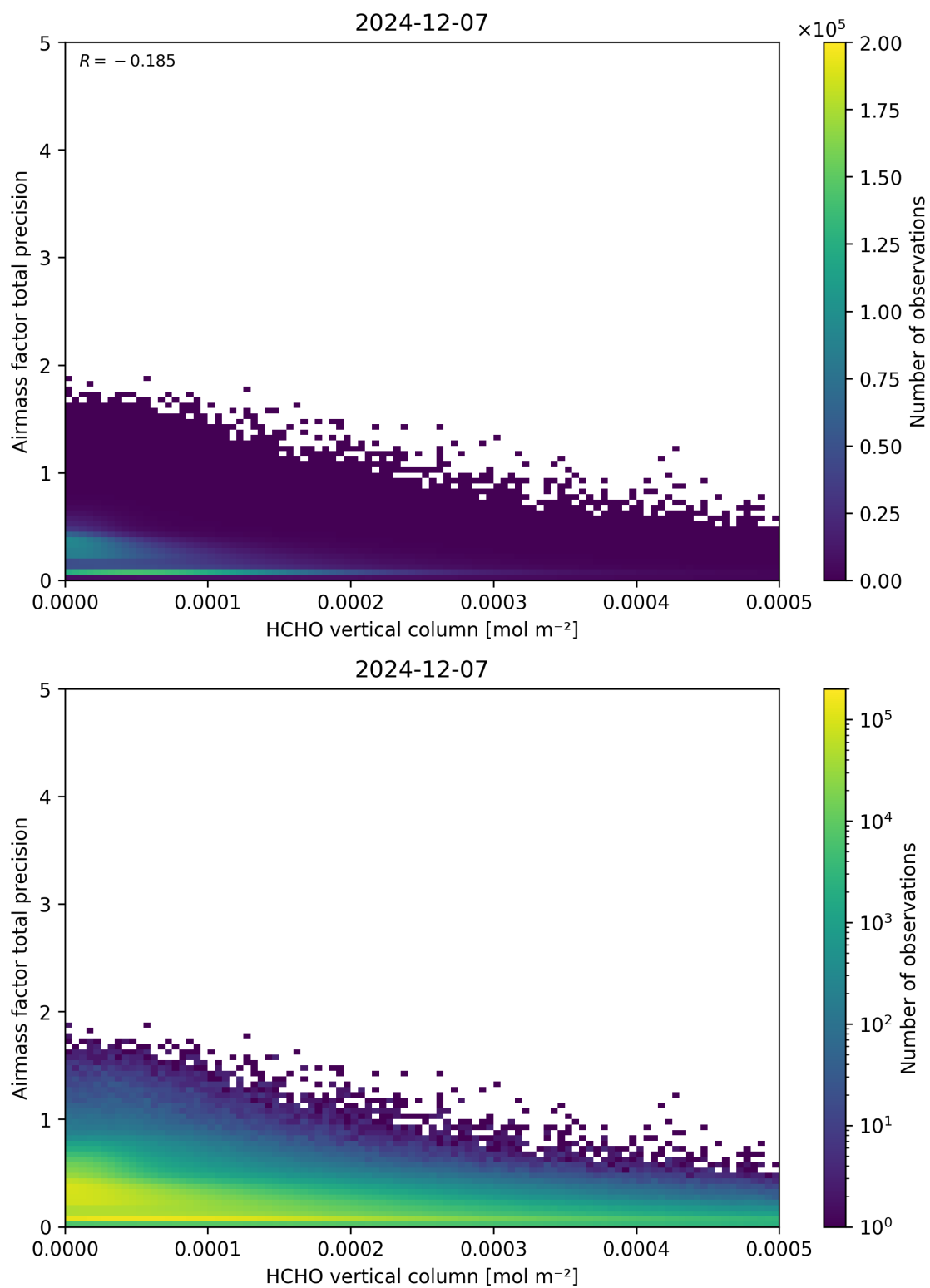
Figure 132: Scatter density plot of “HCHO vertical column” against “Airmass factor total precision” for 2024-12-06 to 2024-12-08.
