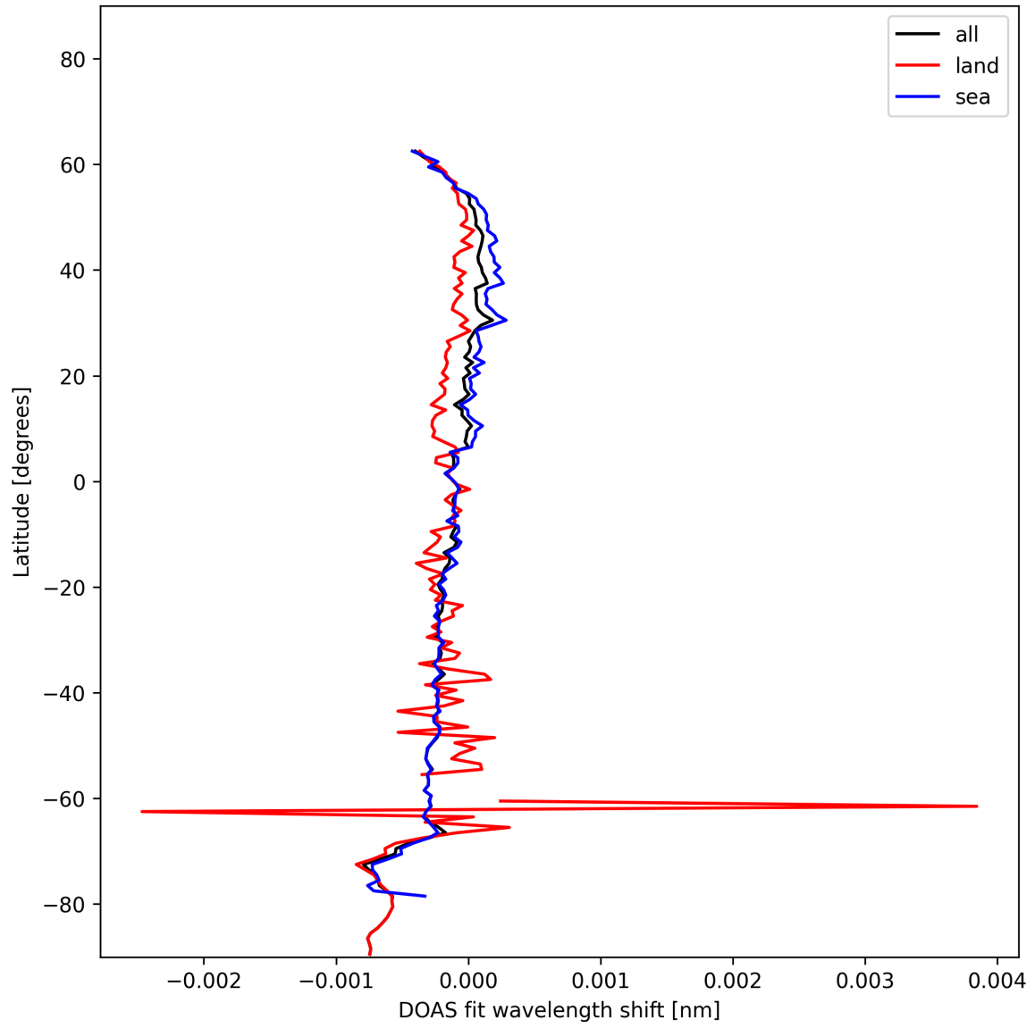
Figure 30: Zonal average of "DOAS fit wavelength shift" for 2024-12-06 to 2024-12-08.
