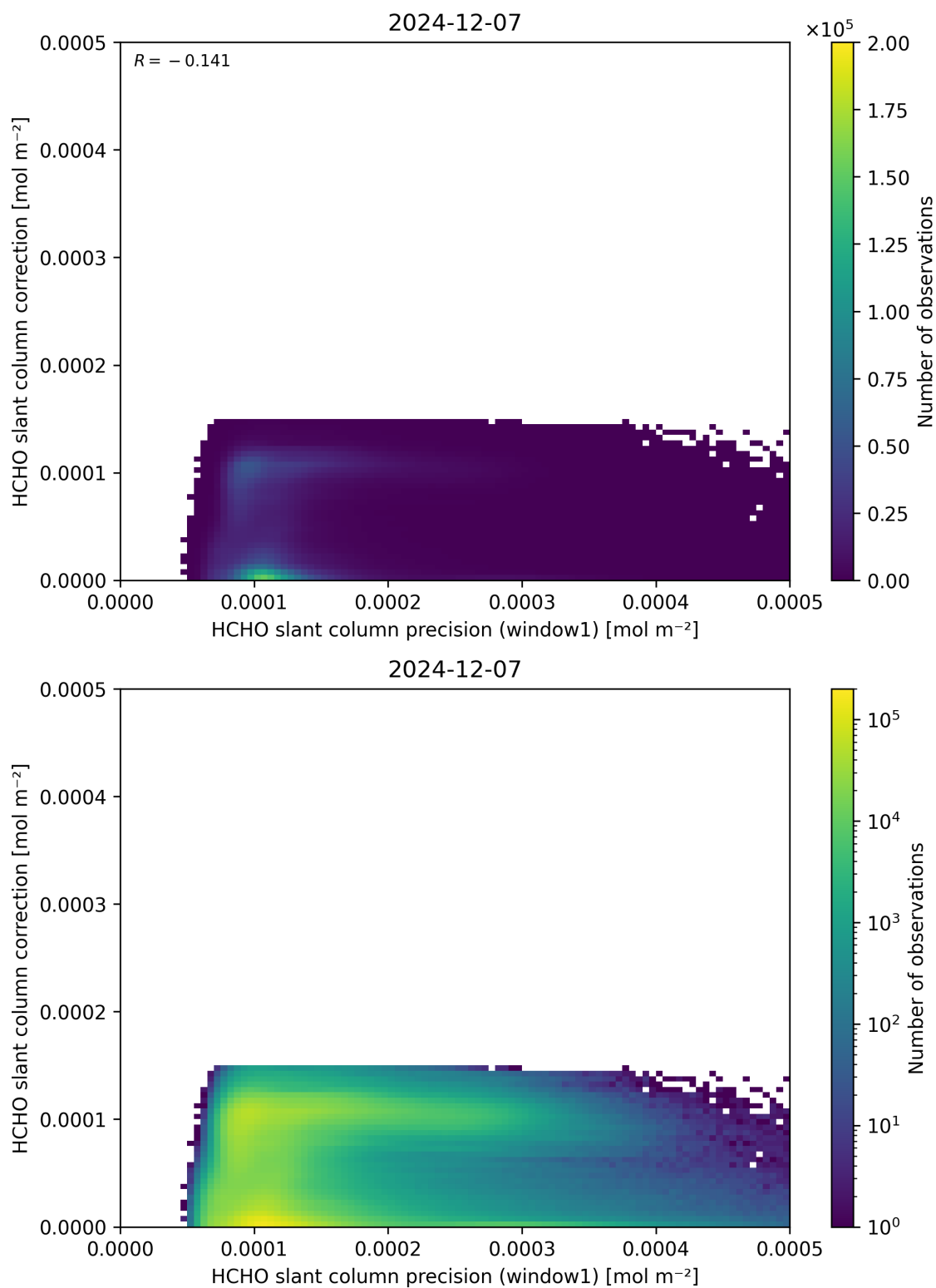
Figure 93: Scatter density plot of “HCHO slant column precision (window1)” against “HCHO slant column correction” for 2024-12-06 to 2024-12-08.
