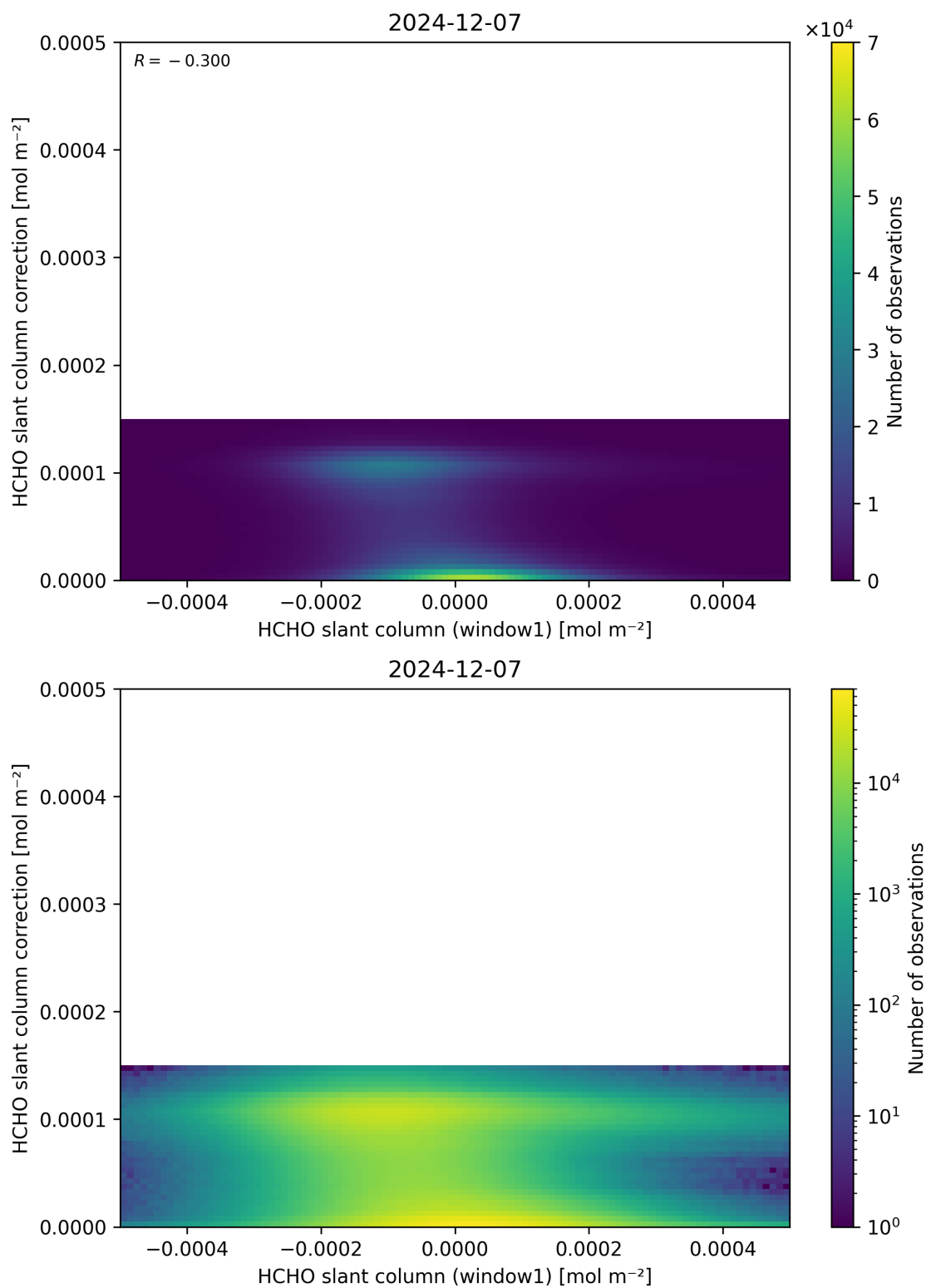
Figure 83: Scatter density plot of “HCHO slant column (window1)” against “HCHO slant column correction” for 2024-12-06 to 2024-12-08.
