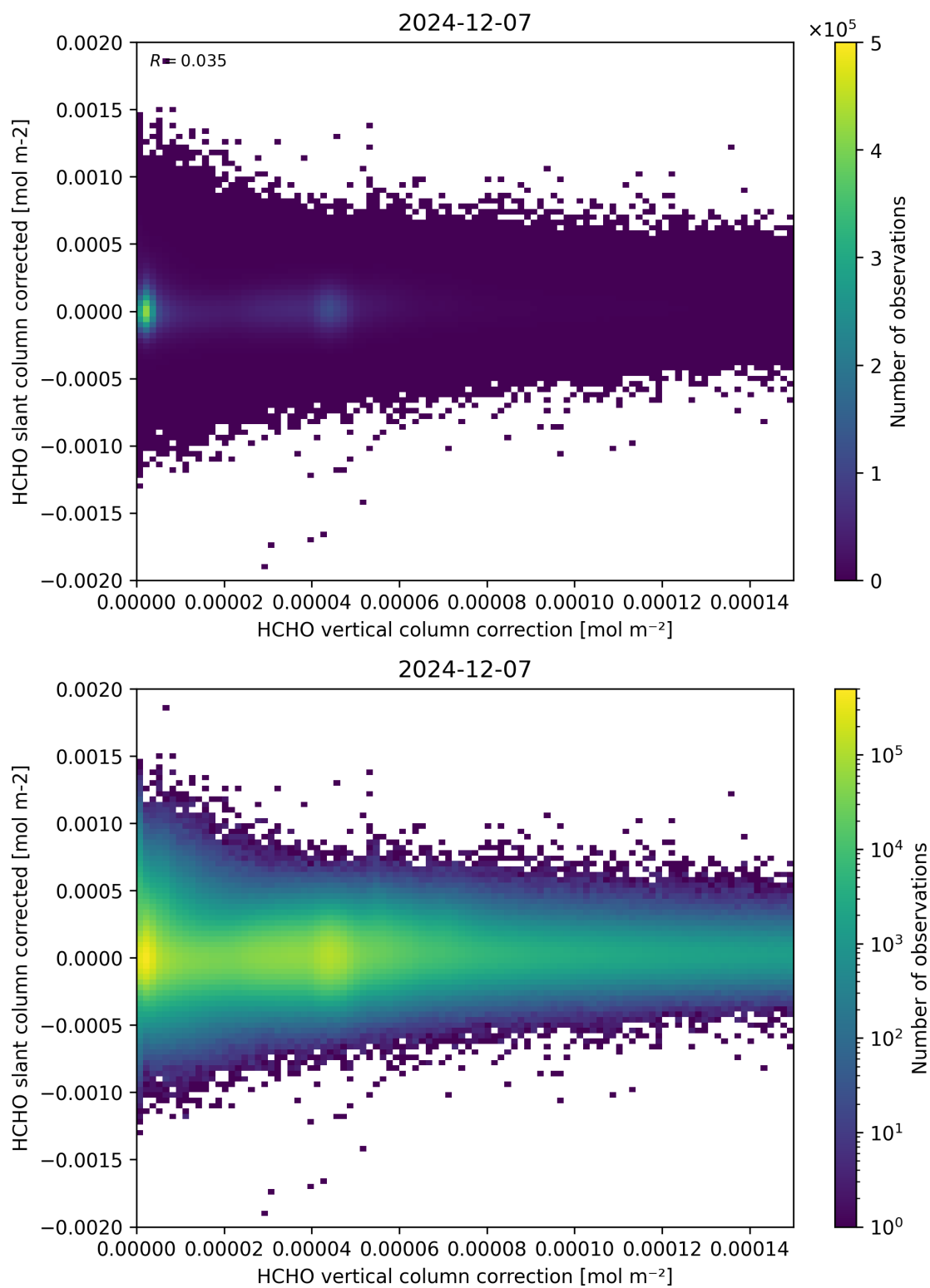
Figure 116: Scatter density plot of “HCHO vertical column correction” against “HCHO slant column corrected” for 2024-12-06 to 2024-12-08.
