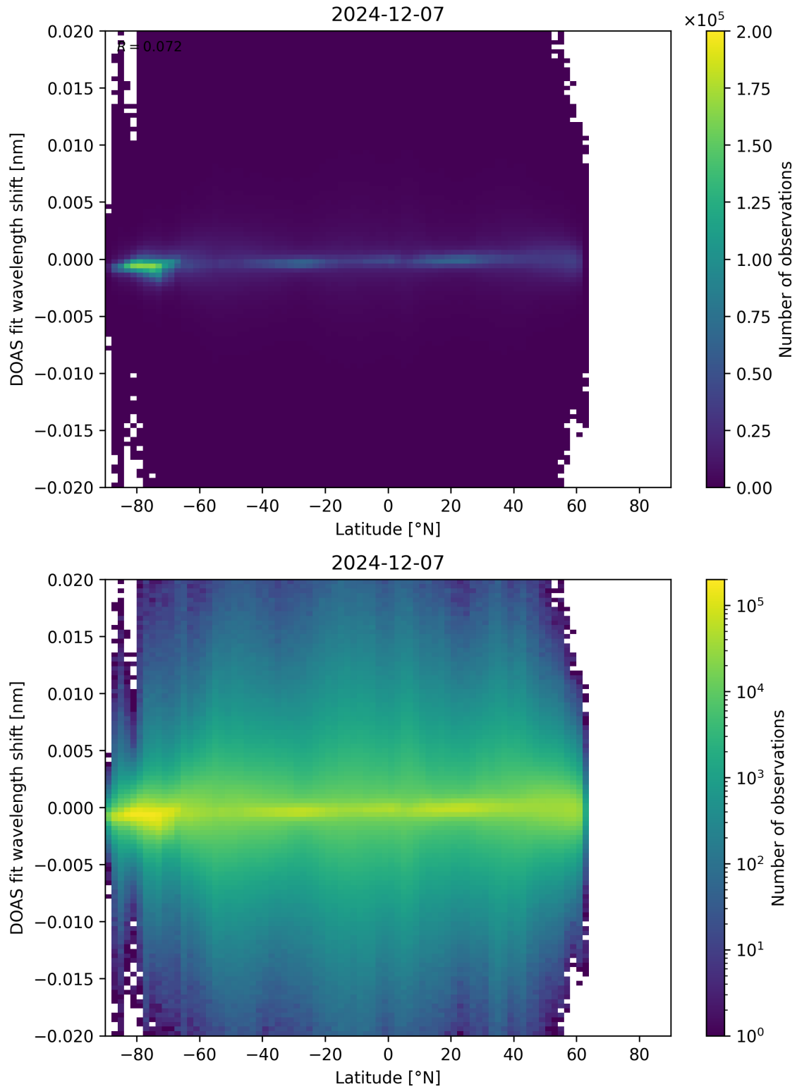
Figure 154: Scatter density plot of “Latitude” against “DOAS fit wavelength shift” for 2024-12-06 to 2024-12-08.
