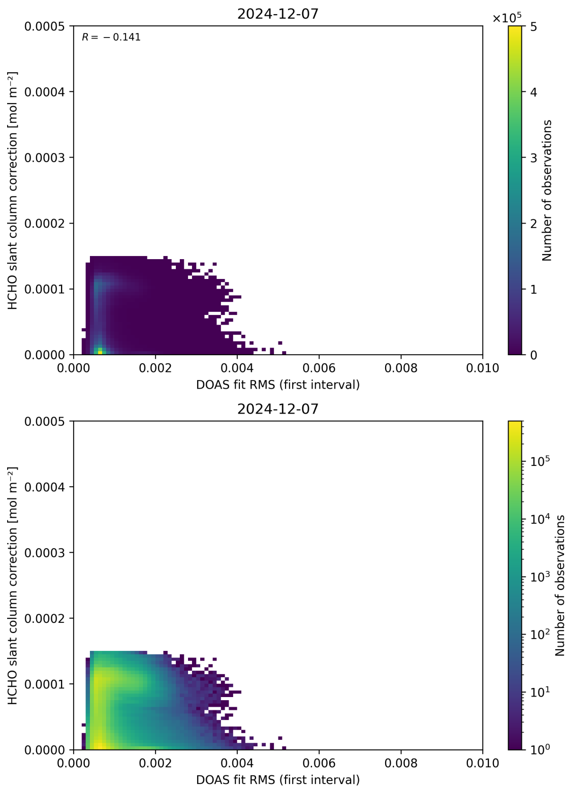
Figure 63: Scatter density plot of “DOAS fit RMS (first interval)” against “HCHO slant column correction” for 2024-12-06 to 2024-12-08.
