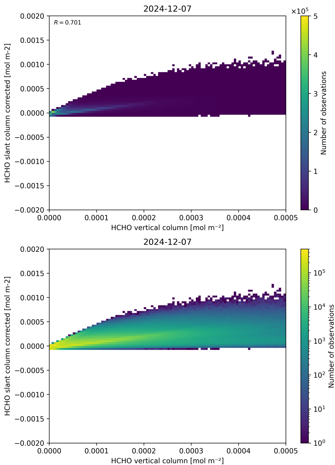
Figure 127: Scatter density plot of “HCHO vertical column” against “HCHO slant column corrected” for 2024-12-06 to 2024-12-08.
