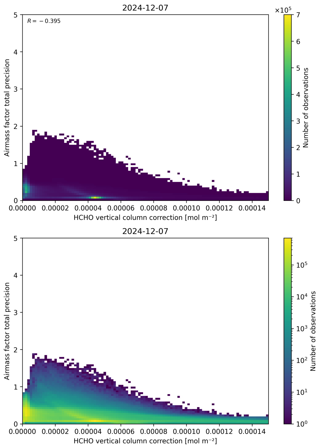
Figure 121: Scatter density plot of “HCHO vertical column correction” against “Airmass factor total precision” for 2024-12-06 to 2024-12-08.
