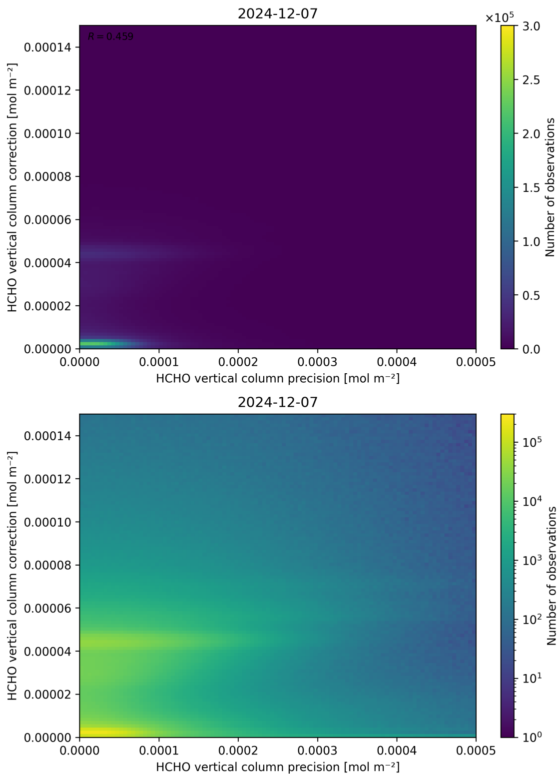
Figure 146: Scatter density plot of “HCHO vertical column precision” against “HCHO vertical column correction” for 2024-12-06 to 2024-12-08.
