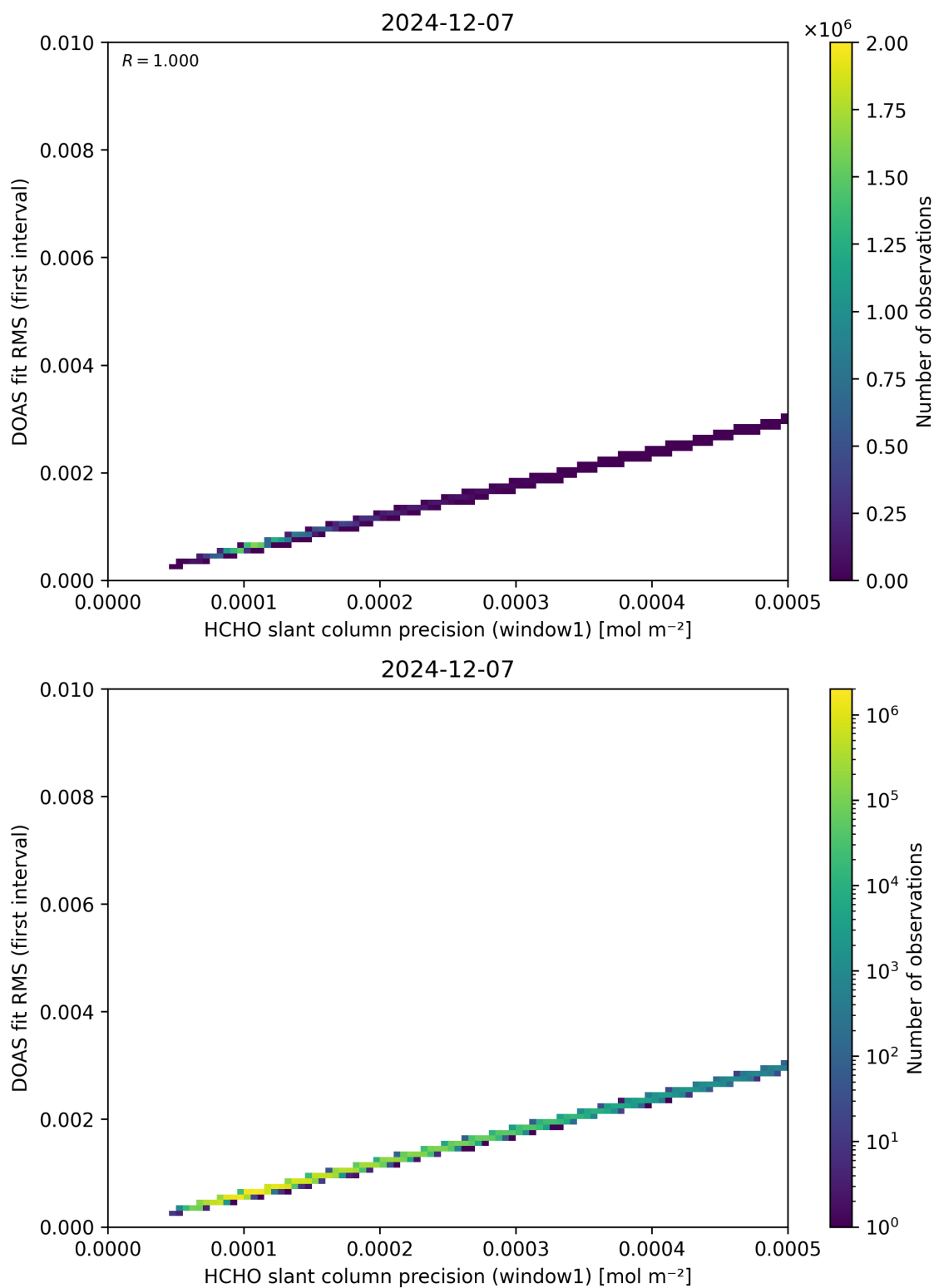
Figure 88: Scatter density plot of “HCHO slant column precision (window1)” against “DOAS fit RMS (first interval)” for 2024-12-06 to 2024-12-08.
