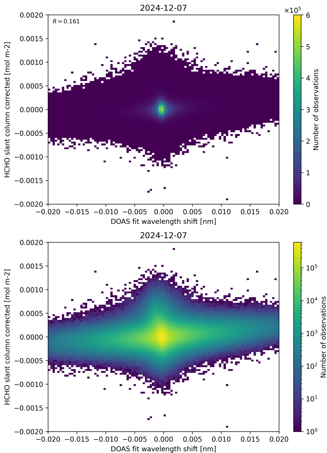
Figure 66: Scatter density plot of “DOAS fit wavelength shift” against “HCHO slant column corrected” for 2024-12-06 to 2024-12-08.
