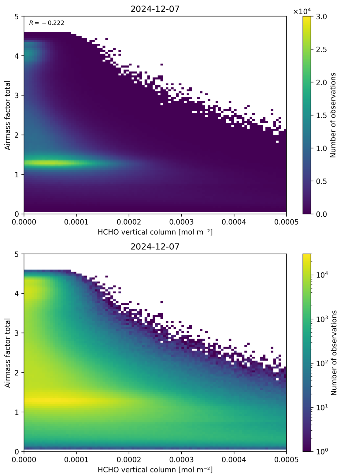
Figure 131: Scatter density plot of “HCHO vertical column” against “Airmass factor total” for 2024-12-06 to 2024-12-08.
