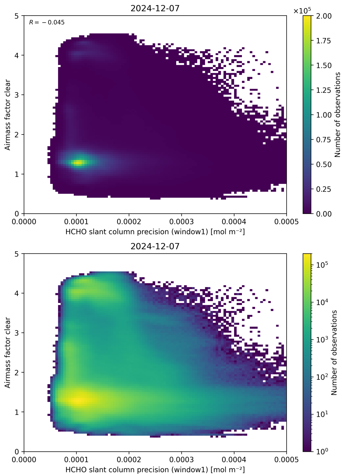
Figure 91: Scatter density plot of “HCHO slant column precision (window1)” against “Airmass factor clear” for 2024-12-06 to 2024-12-08.
