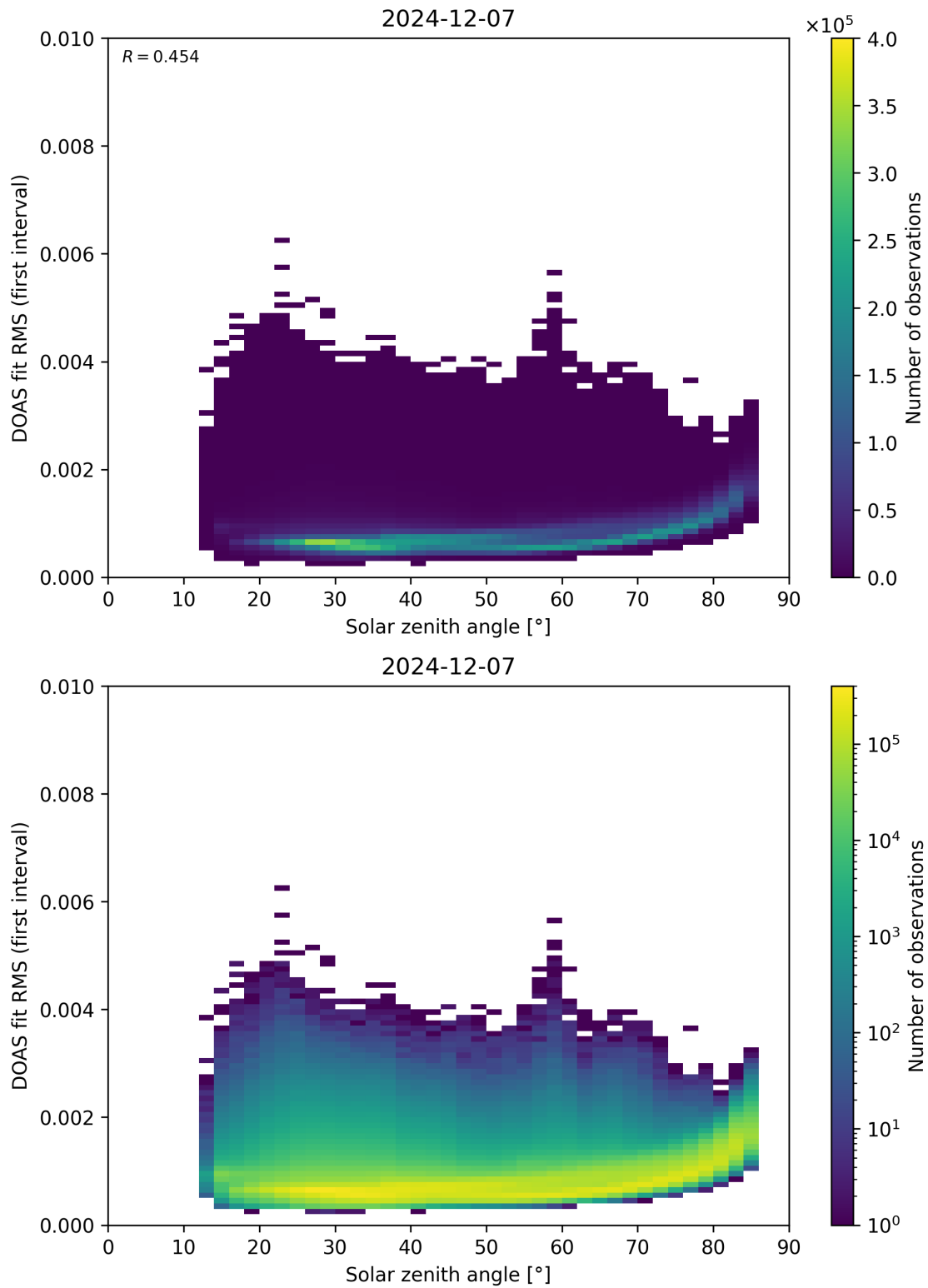
Figure 167: Scatter density plot of “Solar zenith angle” against “DOAS fit RMS (first interval)” for 2024-12-06 to 2024-12-08.
