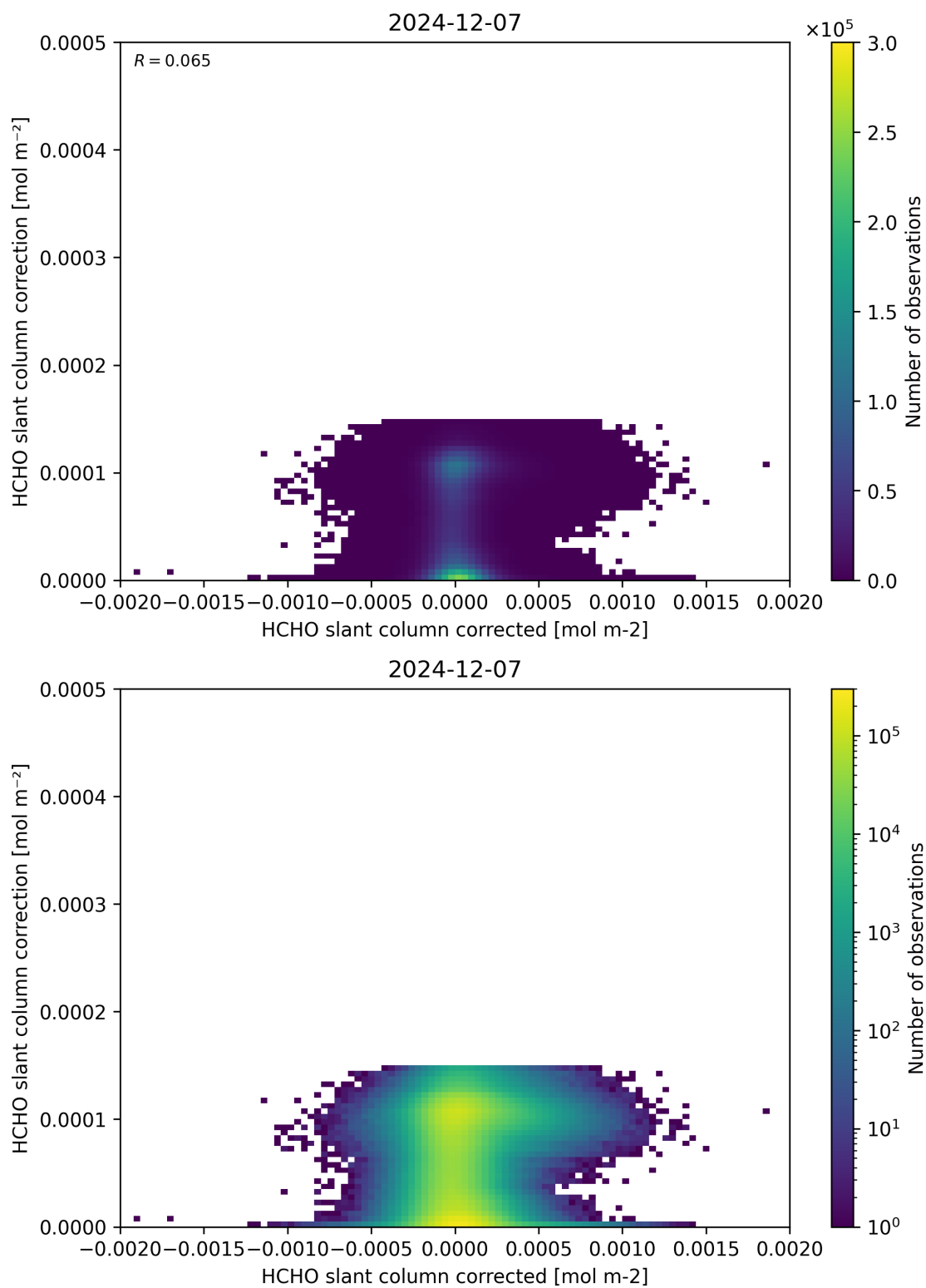
Figure 77: Scatter density plot of “HCHO slant column corrected” against “HCHO slant column correction” for 2024-12-06 to 2024-12-08.
