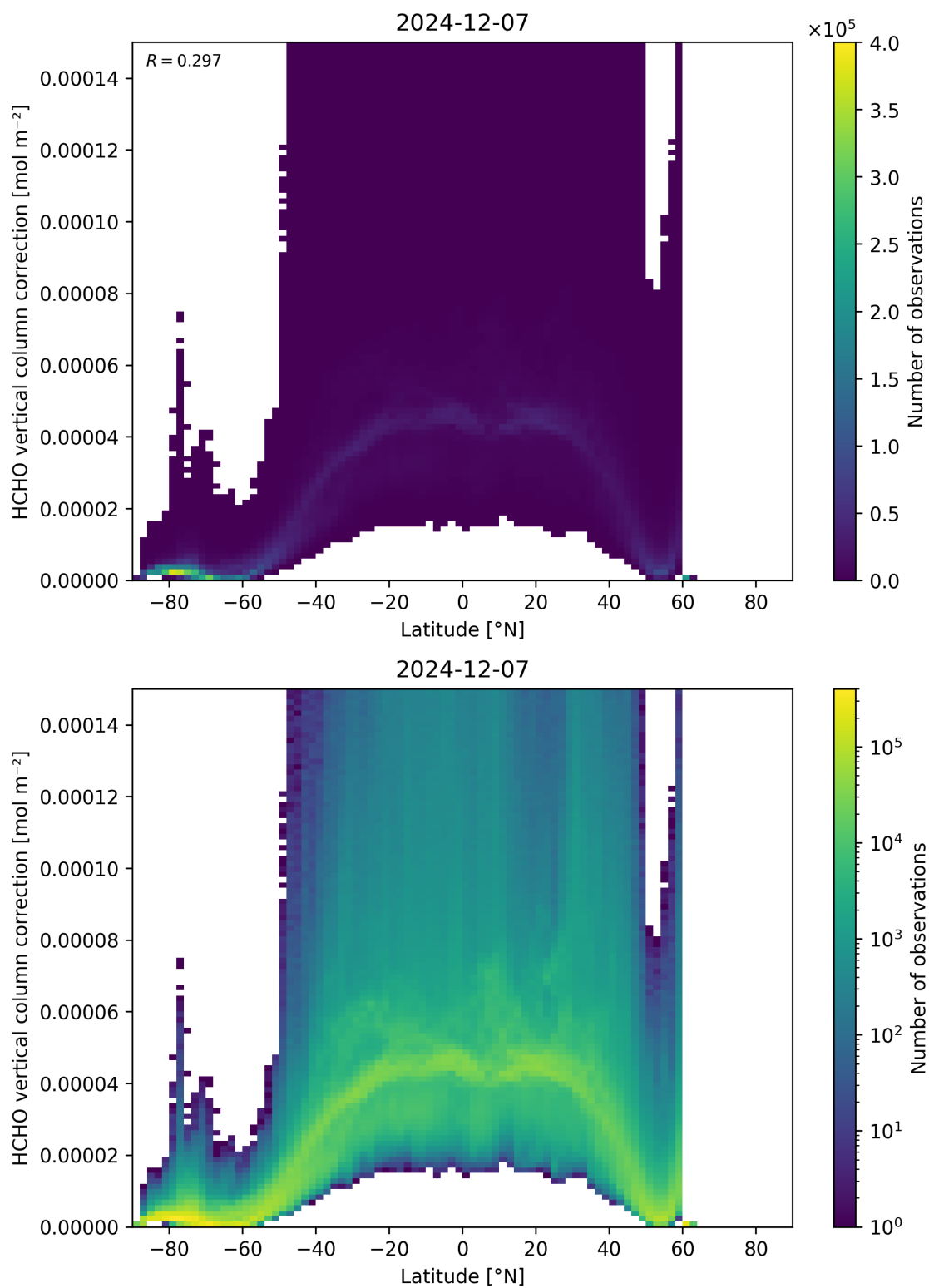
Figure 164: Scatter density plot of “Latitude” against “HCHO vertical column correction” for 2024-12-06 to 2024-12-08.
