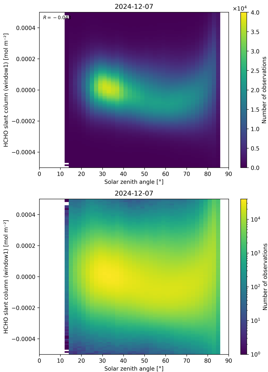
Figure 173: Scatter density plot of “Solar zenith angle” against “HCHO slant column (window1)” for 2024-12-06 to 2024-12-08.
