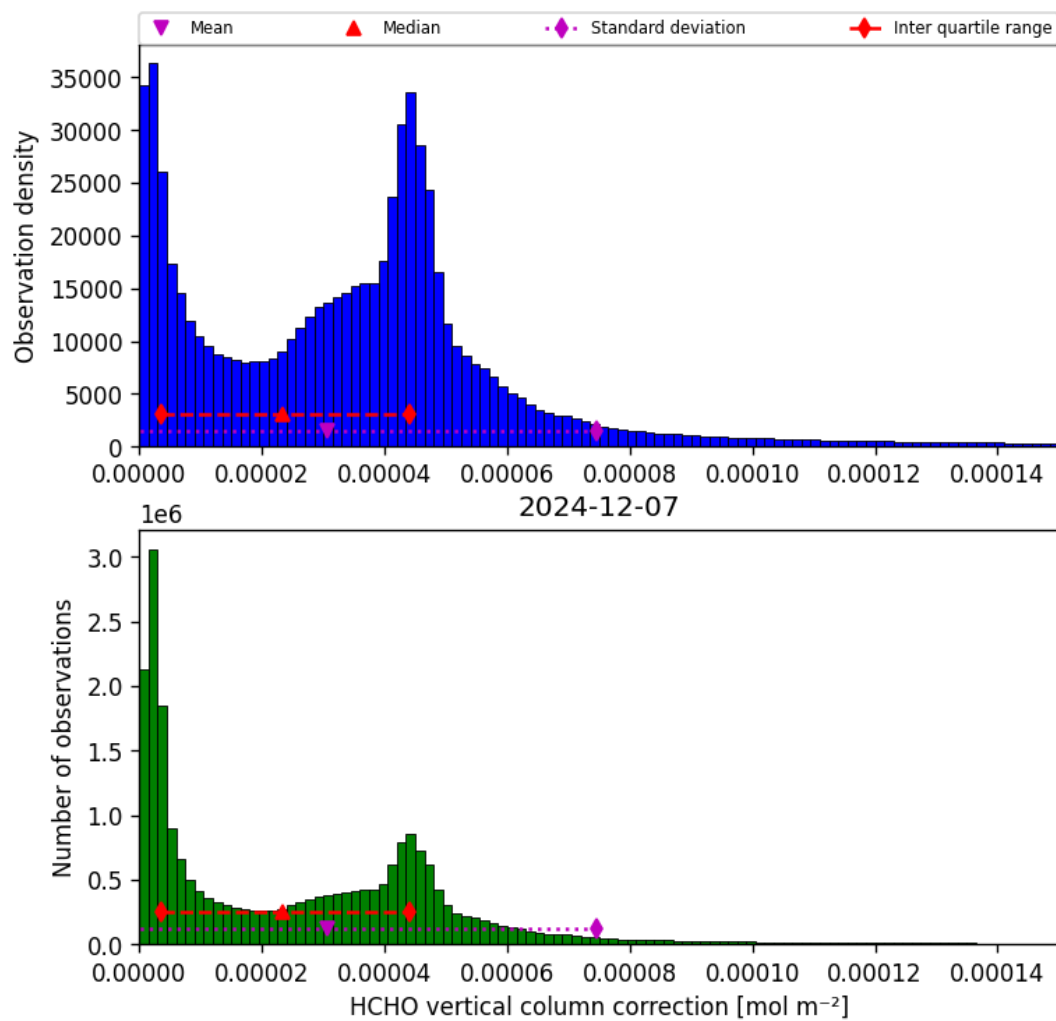
Figure 37: Histogram of “HCHO vertical column correction” for 2024-12-06 to 2024-12-08
