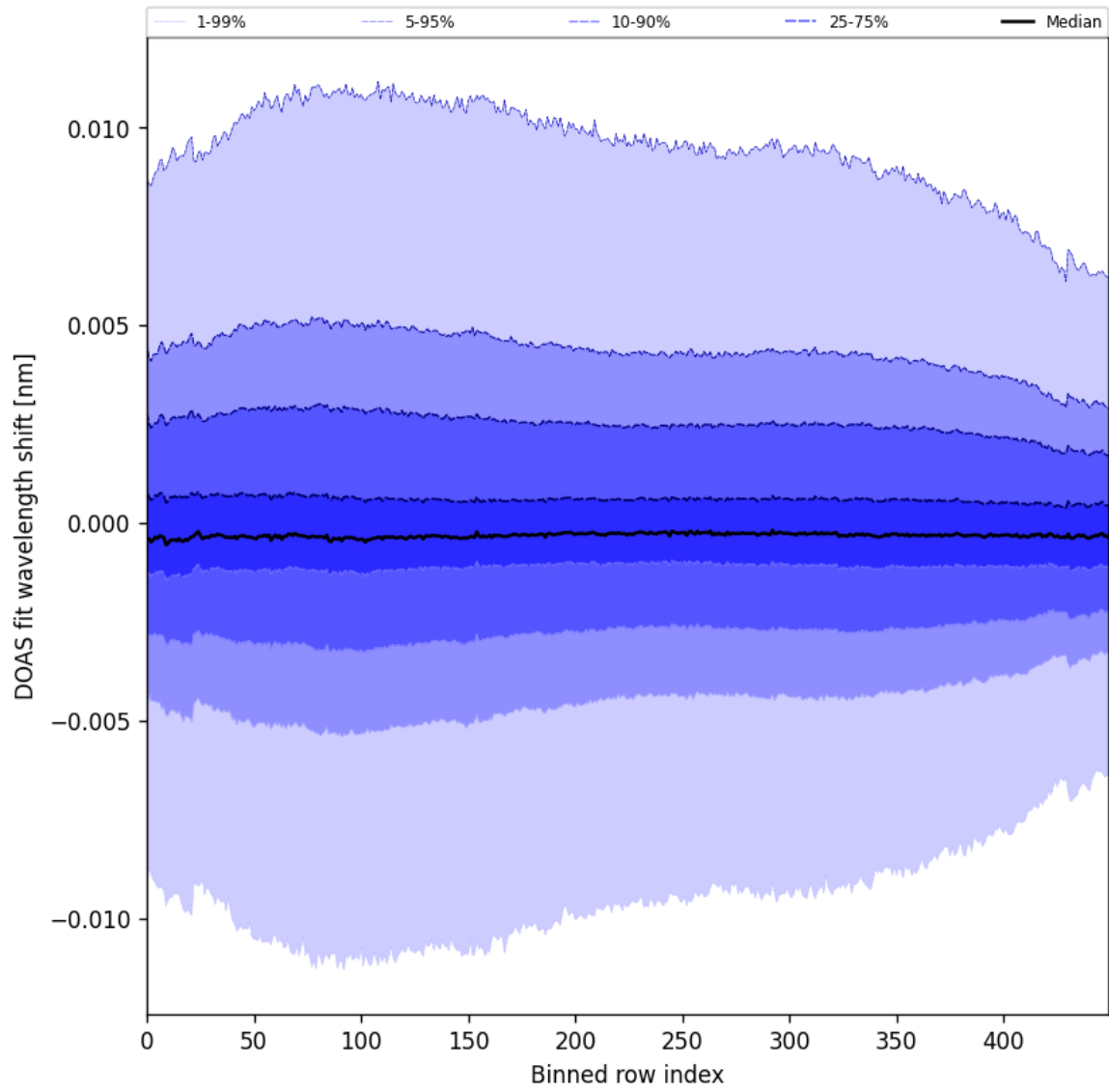
Figure 58: Along track statistics of “DOAS fit wavelength shift” for 2024-12-06 to 2024-12-08
