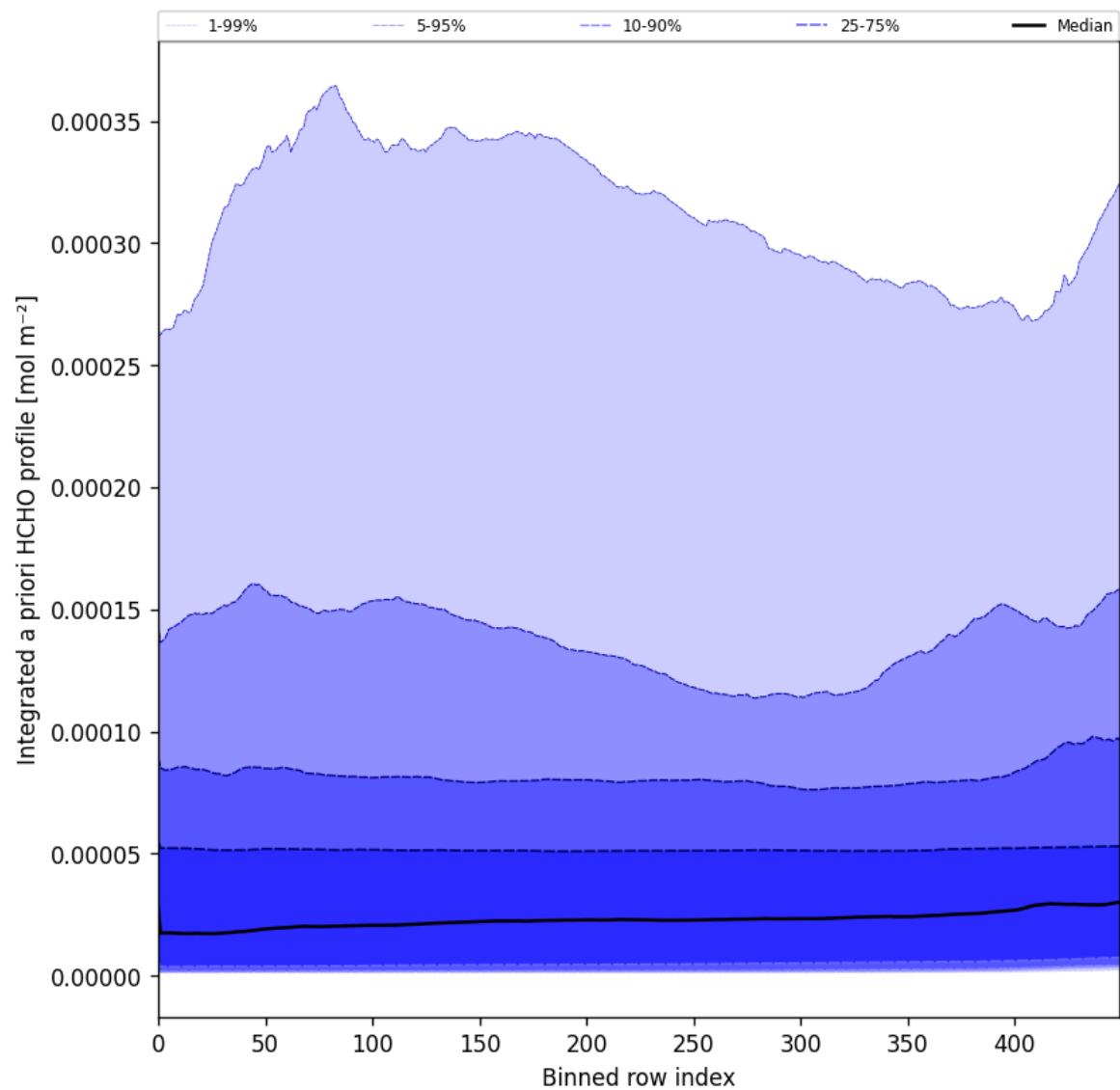
Figure 57: Along track statistics of “Integrated a priori HCHO profile” for 2024-12-06 to 2024-12-08
