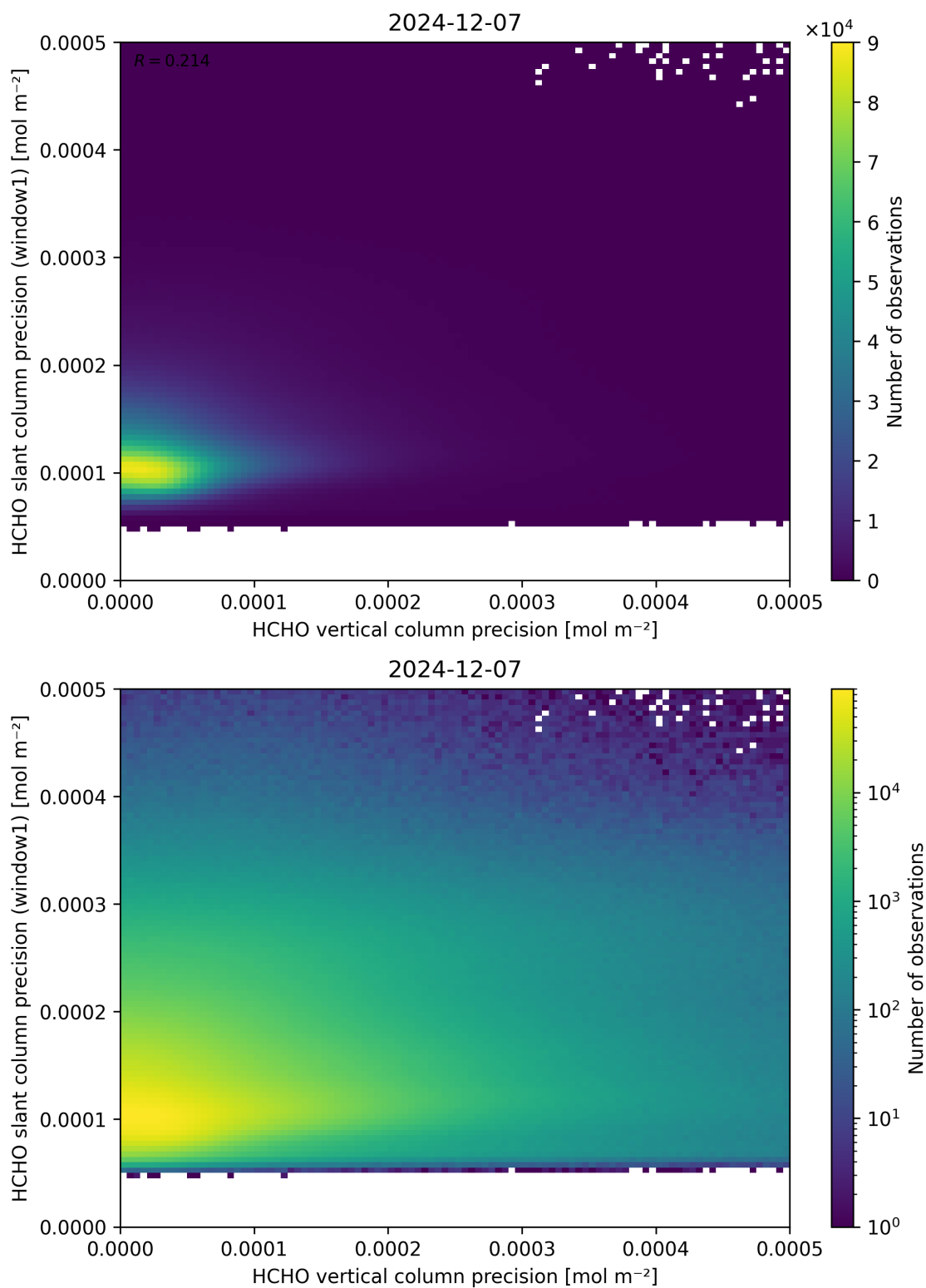
Figure 143: Scatter density plot of “HCHO vertical column precision” against “HCHO slant column precision (window1)” for 2024-12-06 to 2024-12-08.
