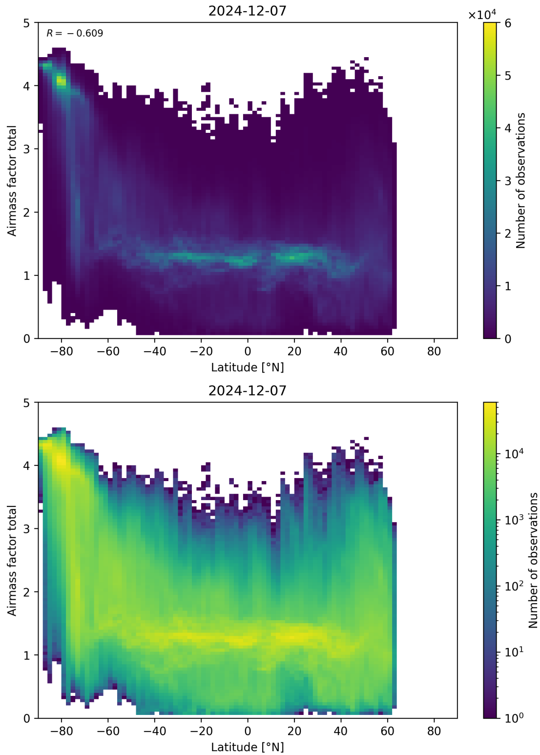
Figure 161: Scatter density plot of “Latitude” against “Airmass factor total” for 2024-12-06 to 2024-12-08.
