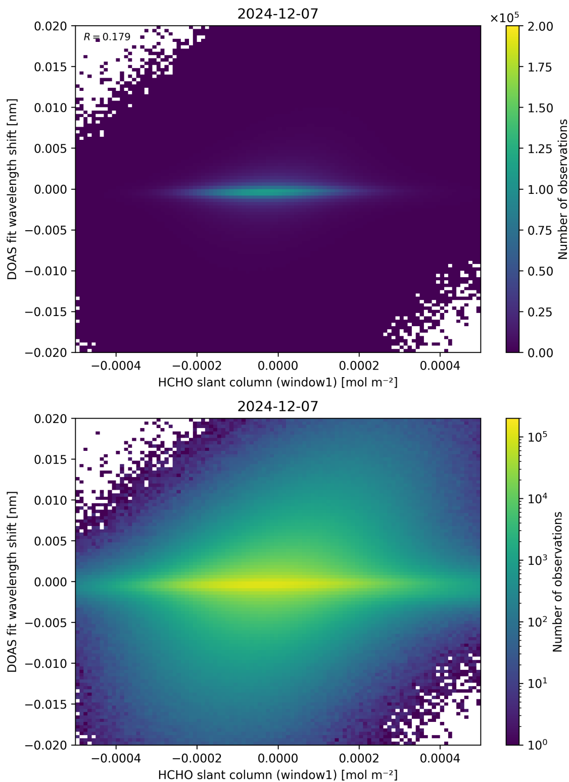
Figure 79: Scatter density plot of “HCHO slant column (window1)” against “DOAS fit wavelength shift” for 2024-12-06 to 2024-12-08.
