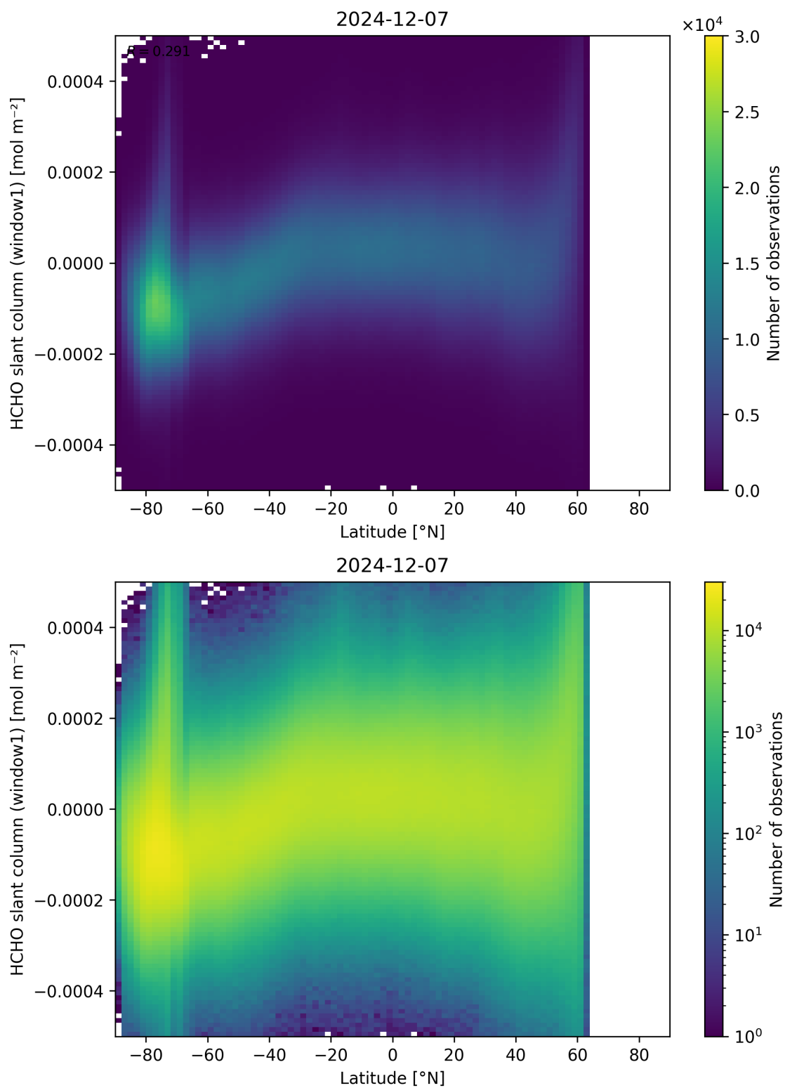
Figure 159: Scatter density plot of “Latitude” against “HCHO slant column (window1)” for 2024-12-06 to 2024-12-08.
