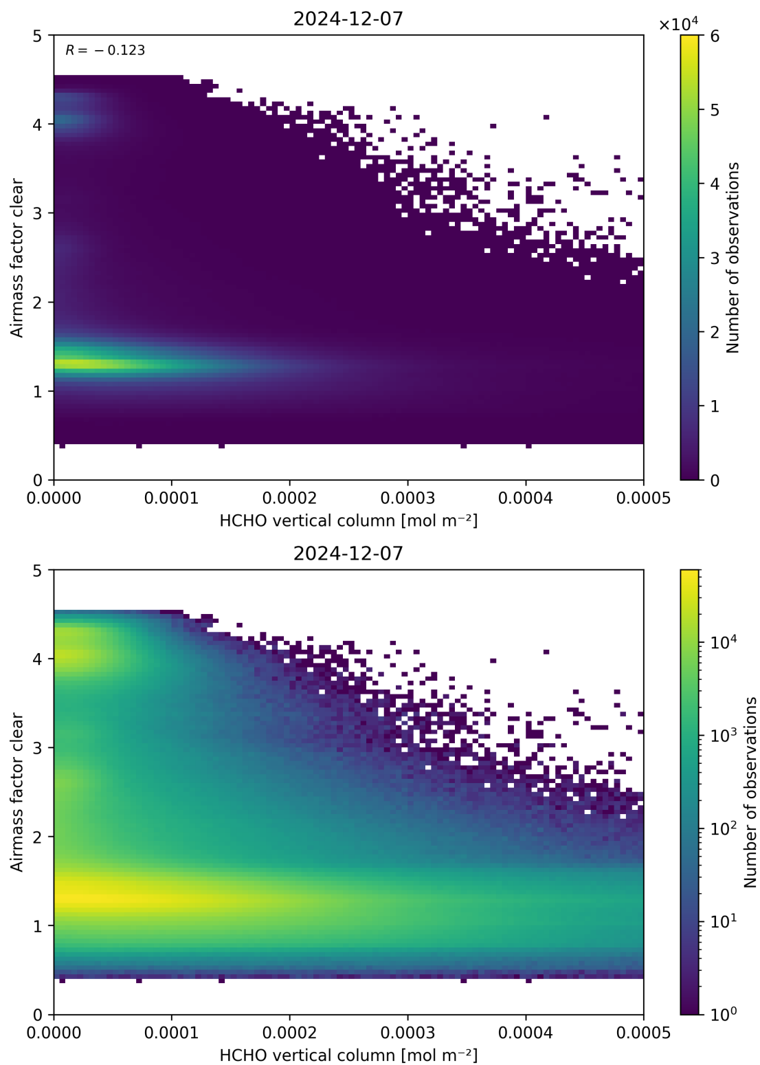
Figure 126: Scatter density plot of “HCHO vertical column” against “Airmass factor clear” for 2024-12-06 to 2024-12-08.
