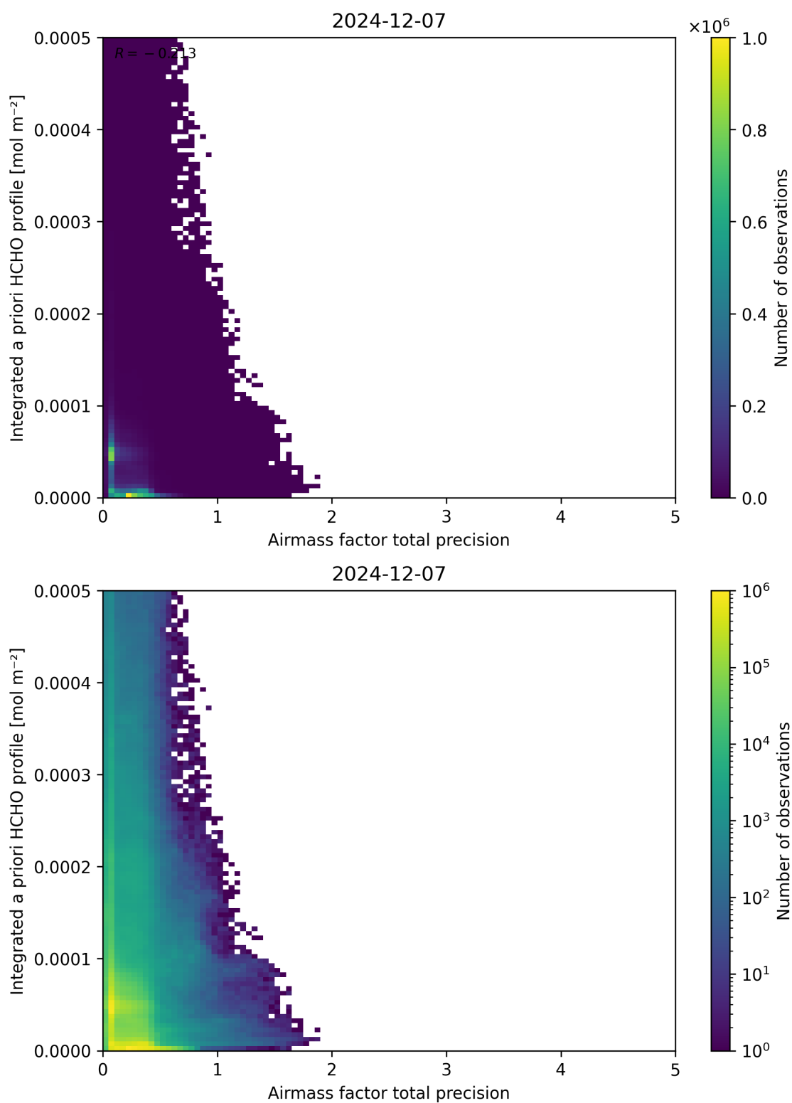
Figure 111: Scatter density plot of “Airmass factor total precision” against “Integrated a priori HCHO profile” for 2024-12-06 to 2024-12-08.
