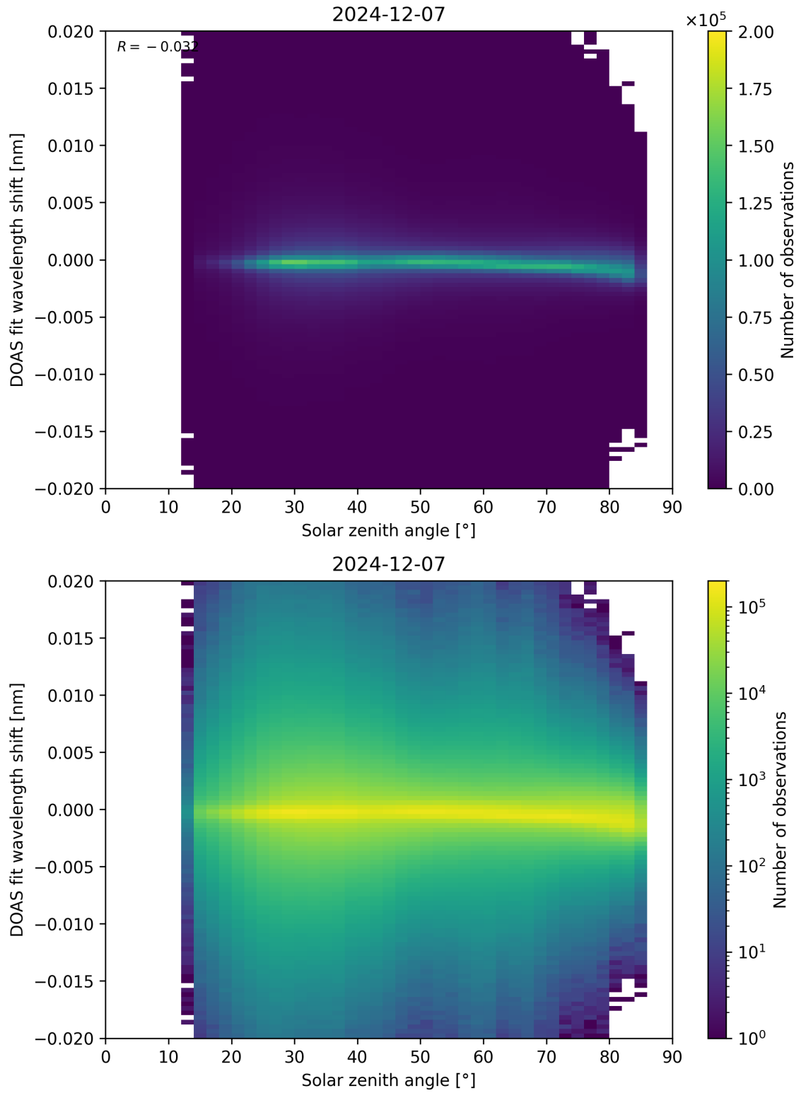
Figure 168: Scatter density plot of “Solar zenith angle” against “DOAS fit wavelength shift” for 2024-12-06 to 2024-12-08.
