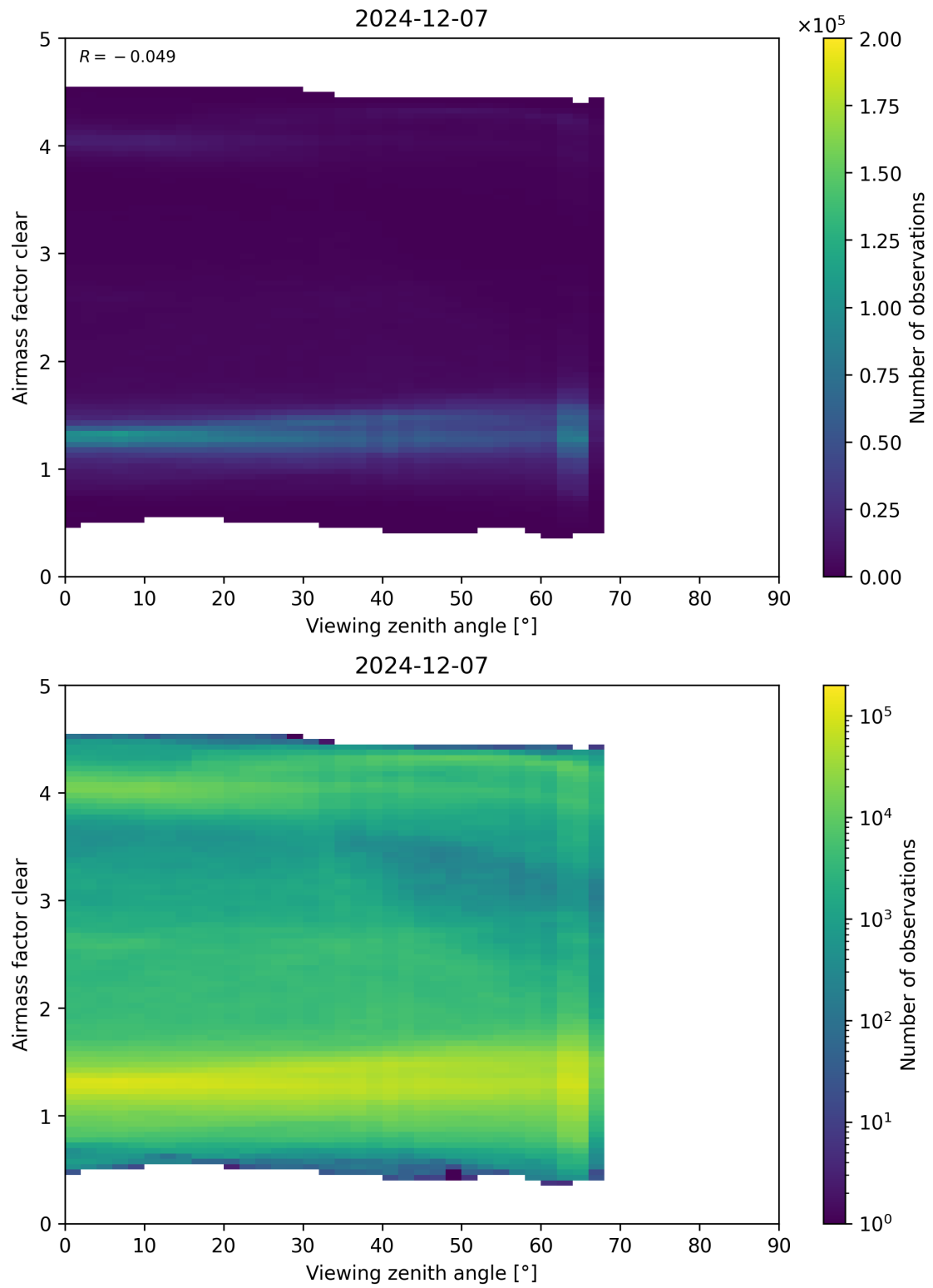
Figure 185: Scatter density plot of “Viewing zenith angle” against “Airmass factor clear” for 2024-12-06 to 2024-12-08.
