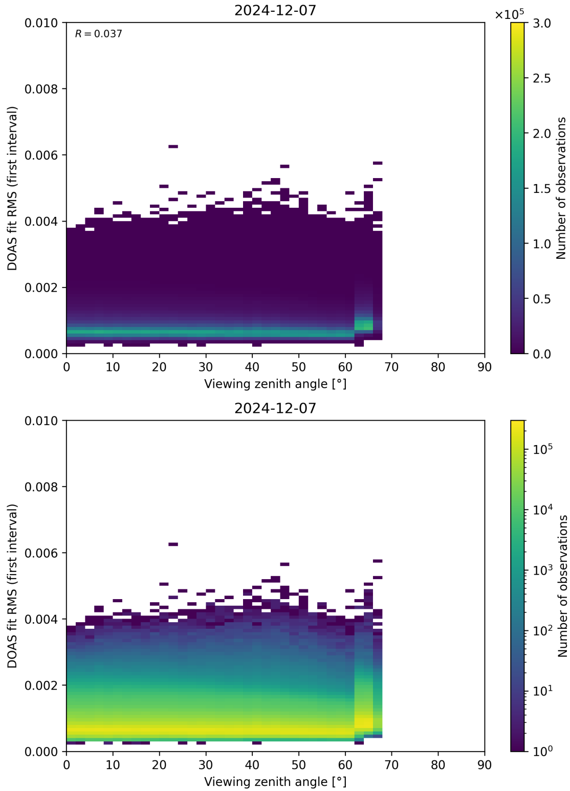
Figure 182: Scatter density plot of “Viewing zenith angle” against “DOAS fit RMS (first interval)” for 2024-12-06 to 2024-12-08.
