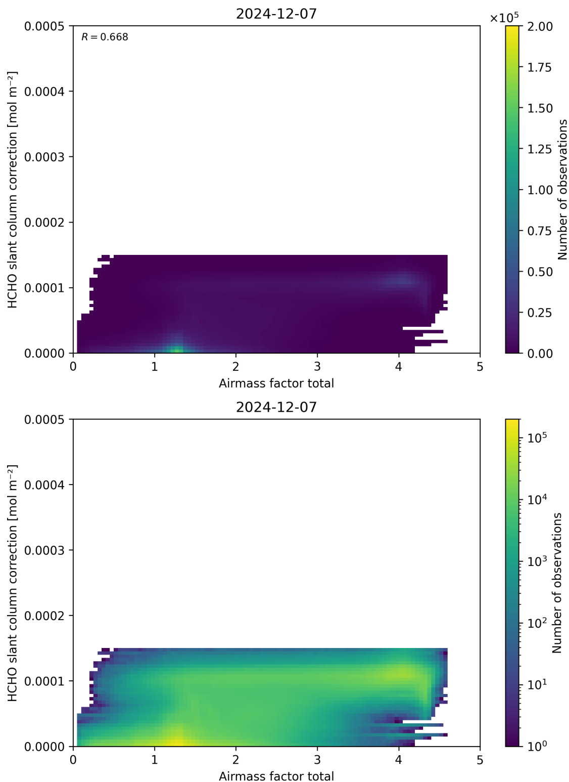
Figure 102: Scatter density plot of “Airmass factor total” against “HCHO slant column correction” for 2024-12-06 to 2024-12-08.
