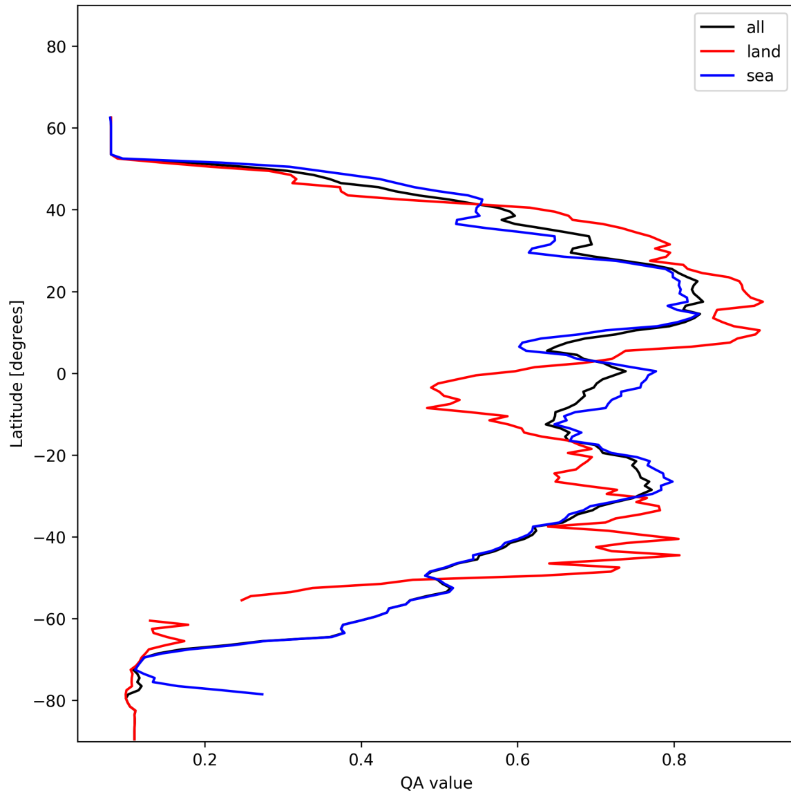
Figure 20: Zonal average of “QA value” for 2024-12-06 to 2024-12-08.
