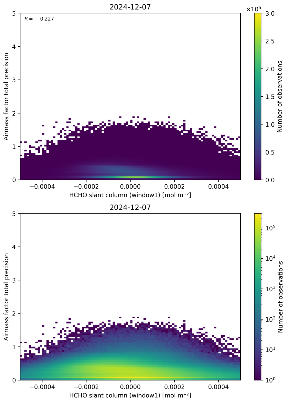
Figure 86: Scatter density plot of “HCHO slant column (window1)” against “Airmass factor total precision” for 2024-12-06 to 2024-12-08.
