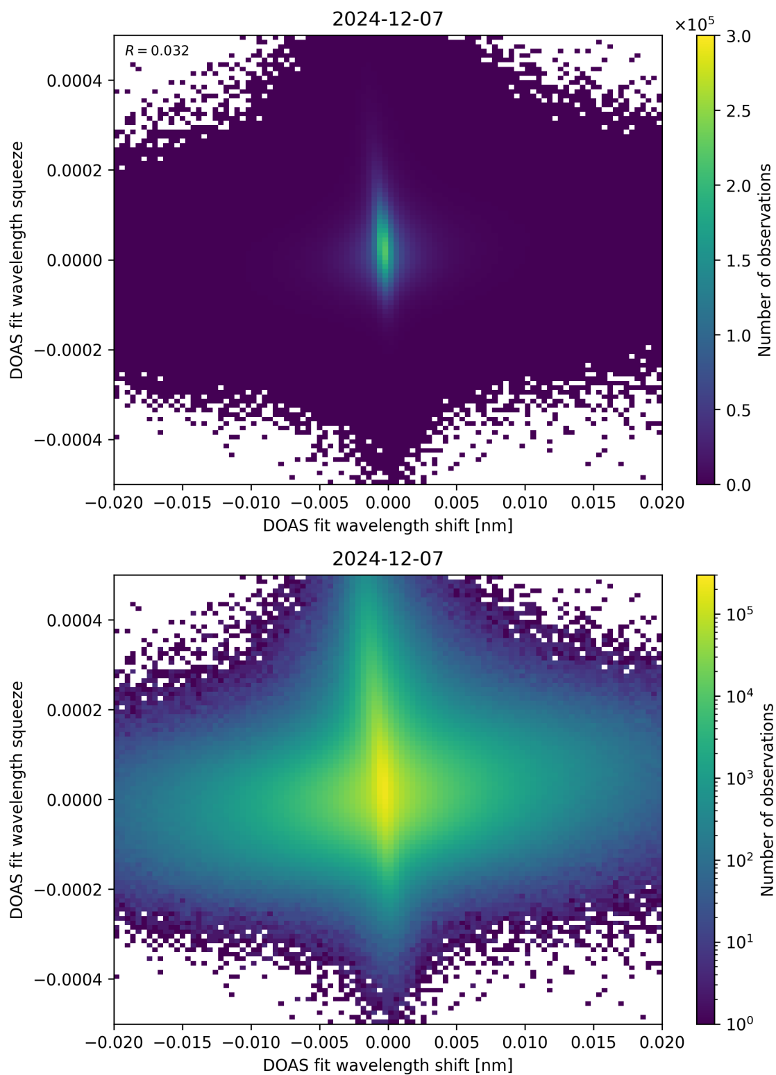
Figure 65: Scatter density plot of “DOAS fit wavelength shift” against “DOAS fit wavelength squeeze” for 2024-12-06 to 2024-12-08.
