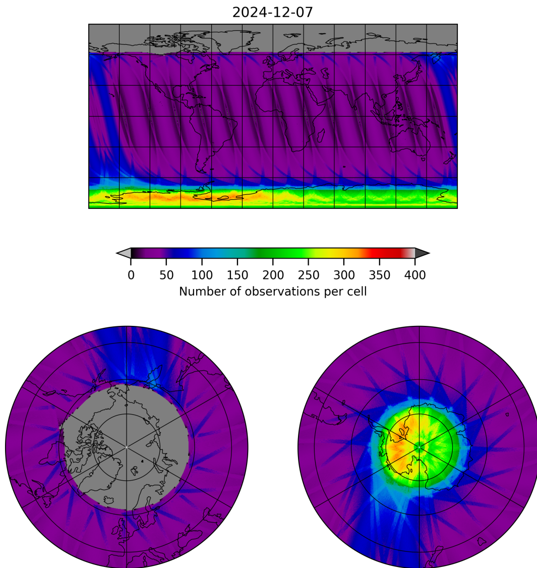
Figure 19: Map of the number of observations for 2024-12-06 to 2024-12-08
