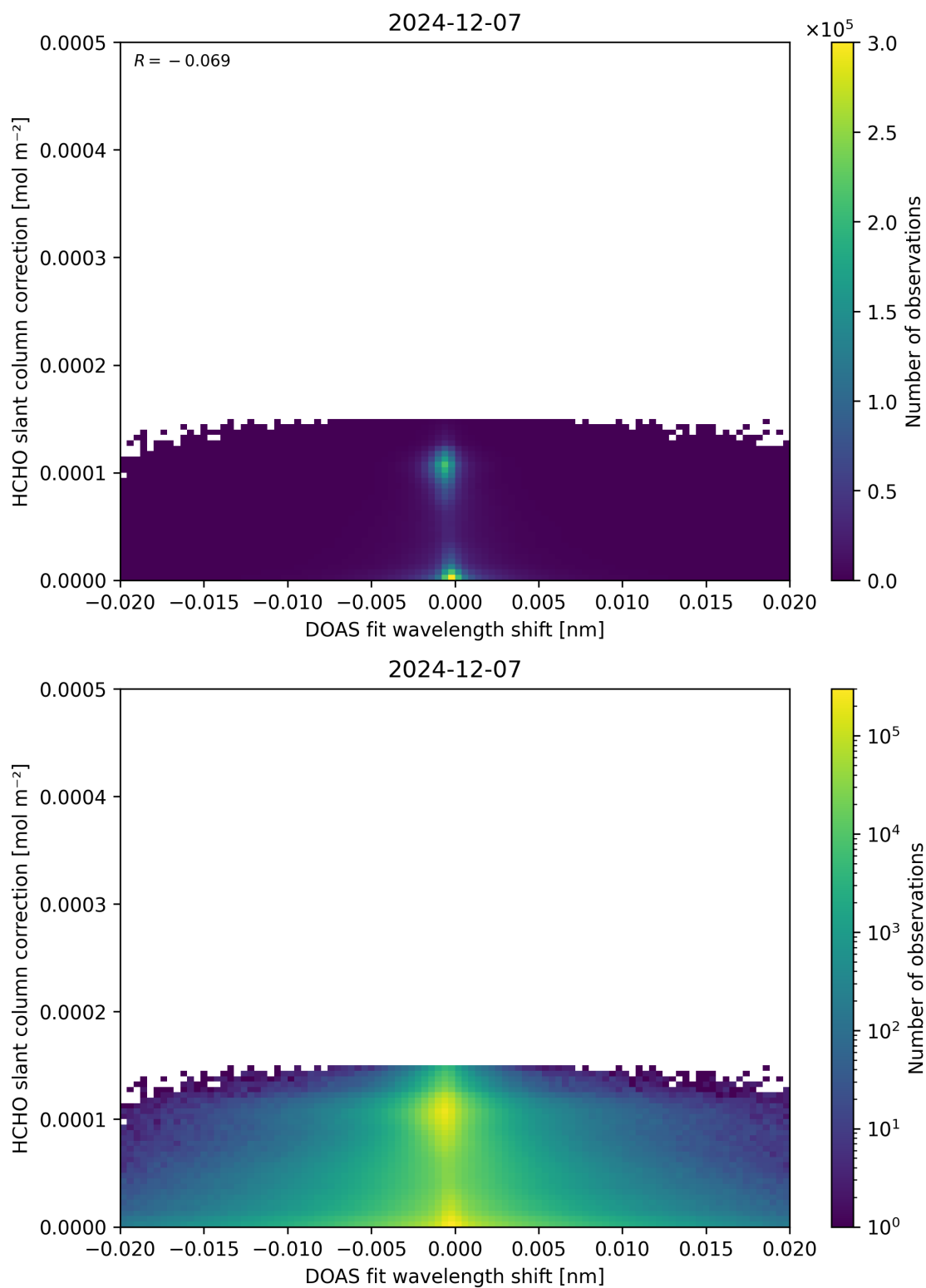
Figure 67: Scatter density plot of “DOAS fit wavelength shift” against “HCHO slant column correction” for 2024-12-06 to 2024-12-08.
