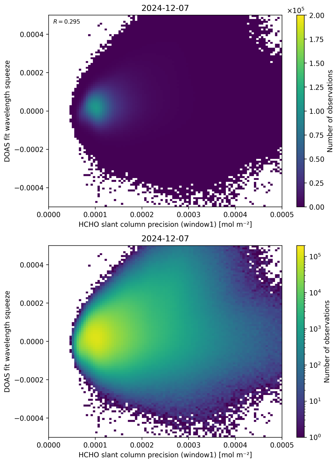
Figure 90: Scatter density plot of “HCHO slant column precision (window1)” against “DOAS fit wavelength squeeze” for 2024-12-06 to 2024-12-08.
