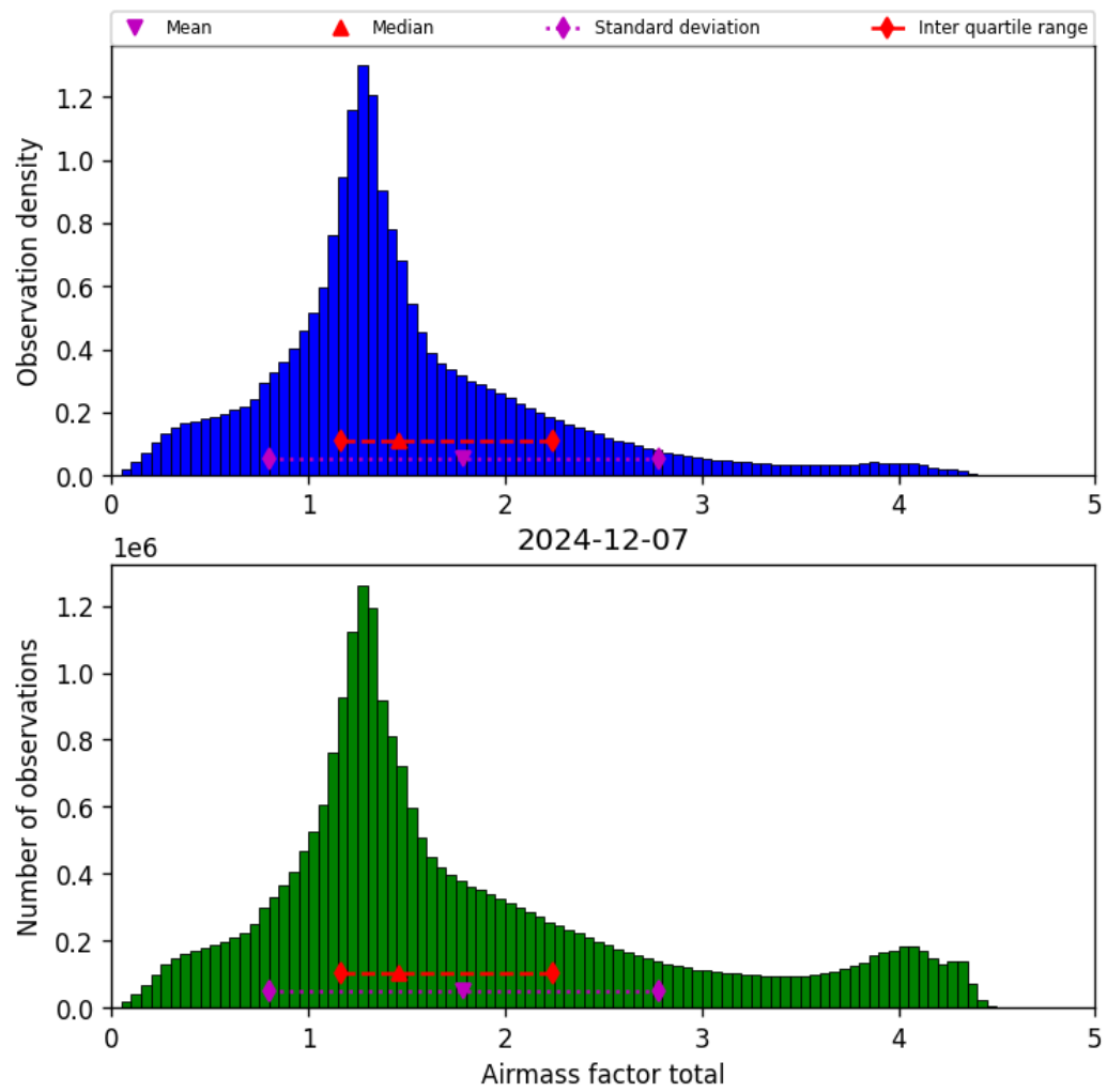
Figure 40: Histogram of “Airmass factor total” for 2024-12-06 to 2024-12-08
