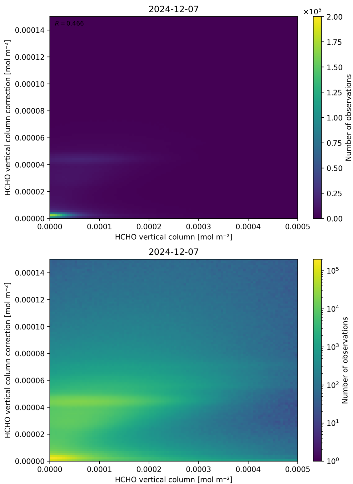
Figure 133: Scatter density plot of “HCHO vertical column” against “HCHO vertical column correction” for 2024-12-06 to 2024-12-08.
