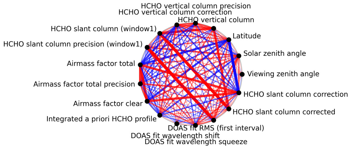
Figure 1: Map of correlation graph for 2024-12-06 to 2024-12-08.
