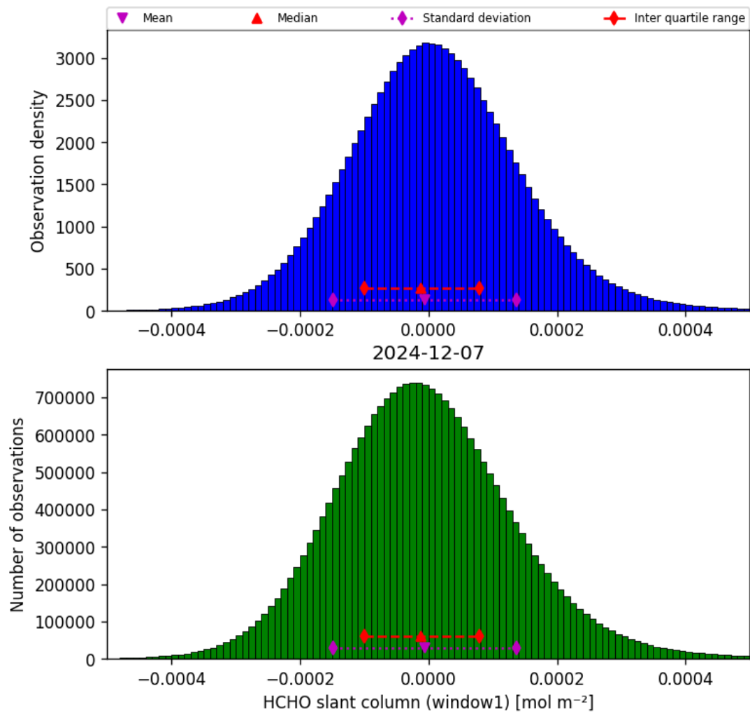
Figure 38: Histogram of “HCHO slant column (window1)” for 2024-12-06 to 2024-12-08
