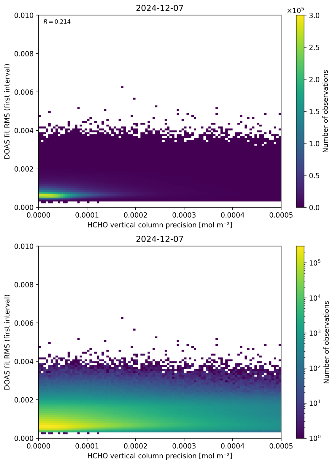
Figure 136: Scatter density plot of “HCHO vertical column precision” against “DOAS fit RMS (first interval)” for 2024-12-06 to 2024-12-08.
