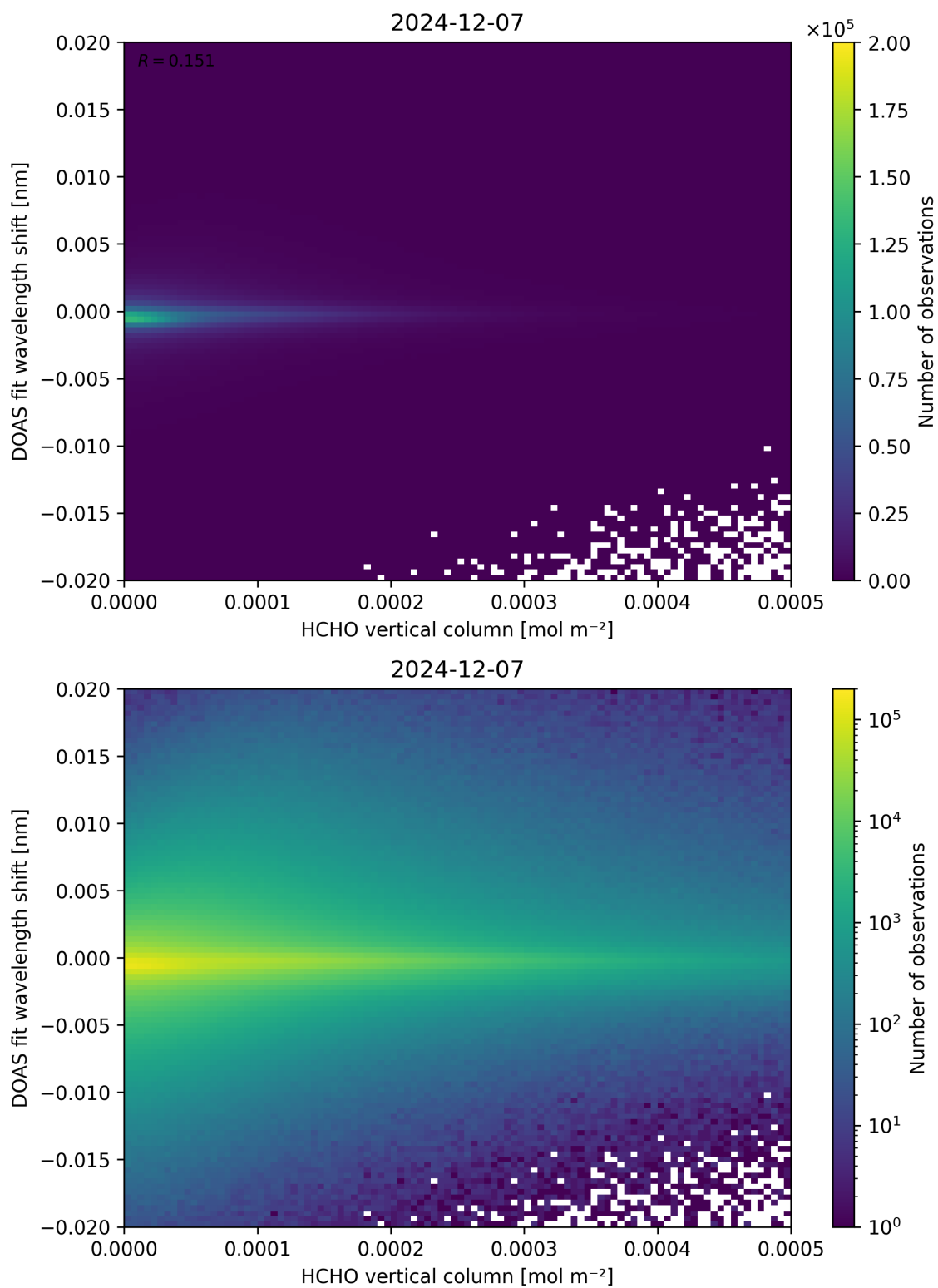
Figure 124: Scatter density plot of “HCHO vertical column” against “DOAS fit wavelength shift” for 2024-12-06 to 2024-12-08.
