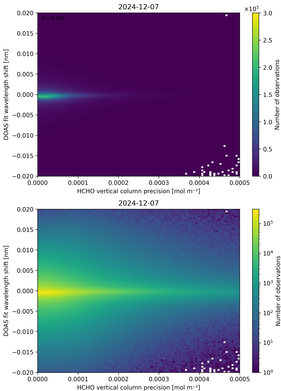
Figure 137: Scatter density plot of “HCHO vertical column precision” against “DOAS fit wavelength shift” for 2024-12-06 to 2024-12-08.
