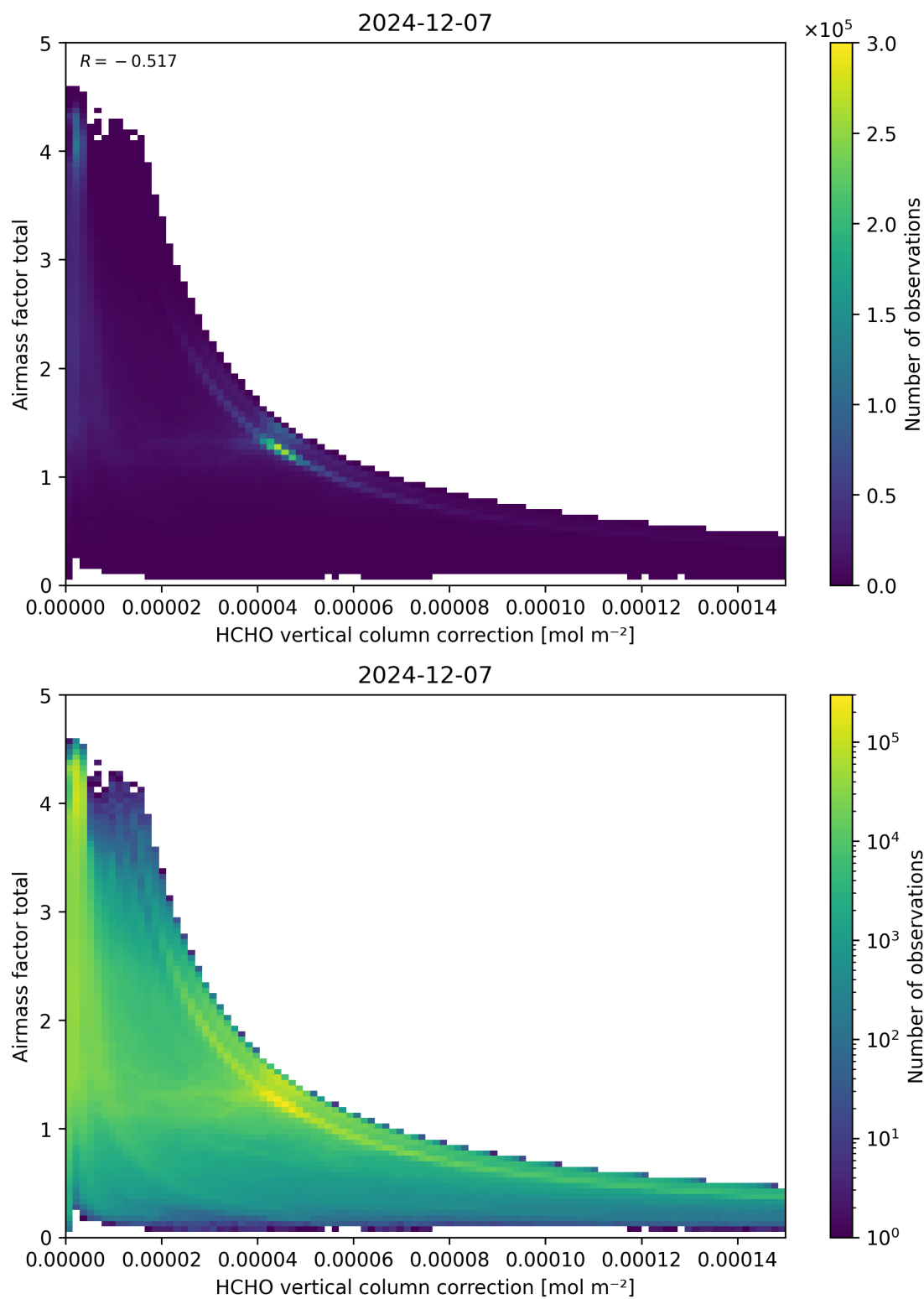
Figure 120: Scatter density plot of “HCHO vertical column correction” against “Airmass factor total” for 2024-12-06 to 2024-12-08.
