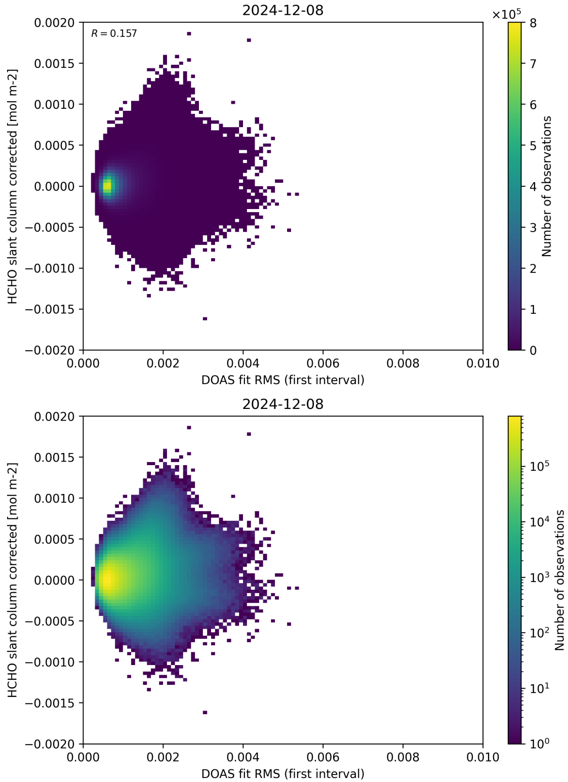
Figure 62: Scatter density plot of “DOAS fit RMS (first interval)” against “HCHO slant column corrected” for 2024-12-07 to 2024-12-09.
