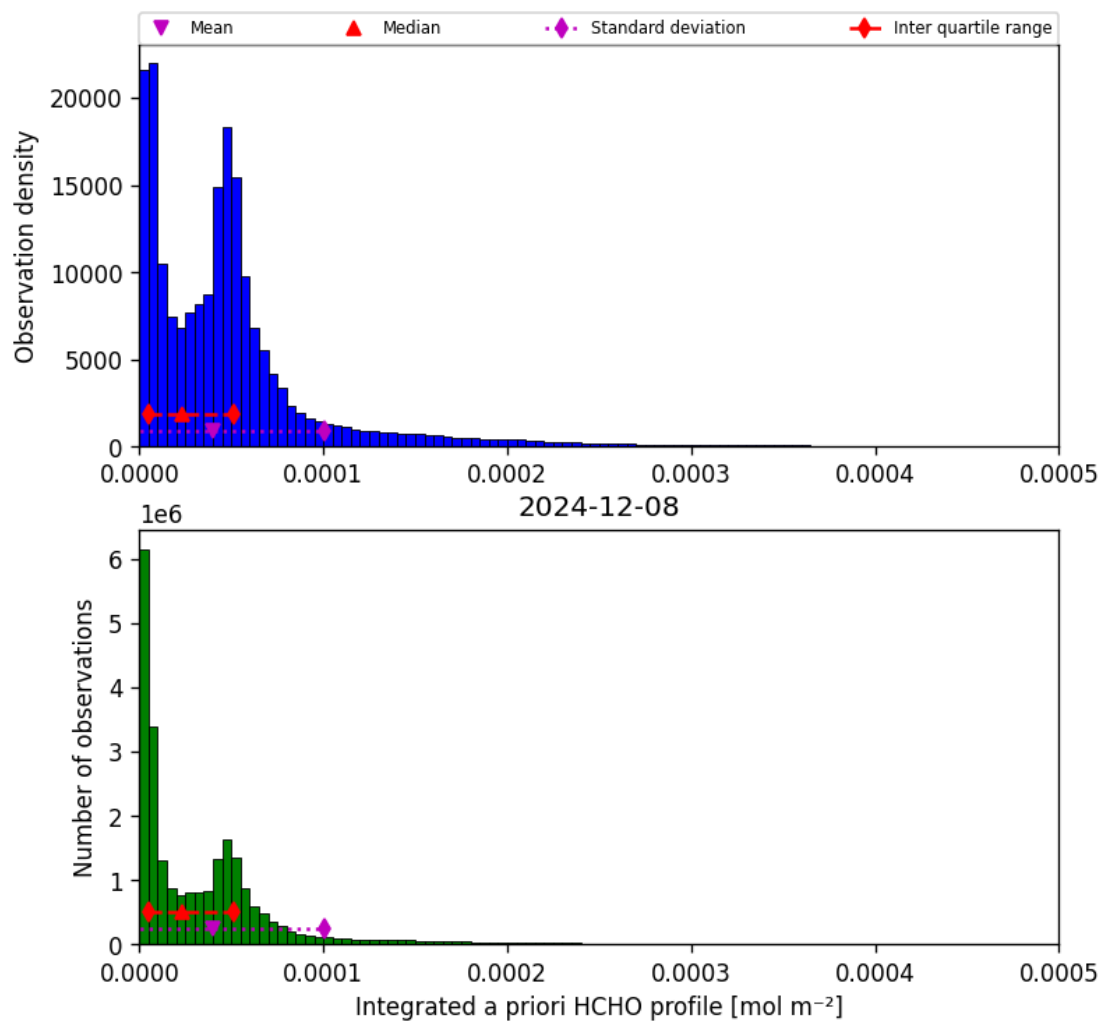
Figure 43: Histogram of “Integrated a priori HCHO profile” for 2024-12-07 to 2024-12-09
