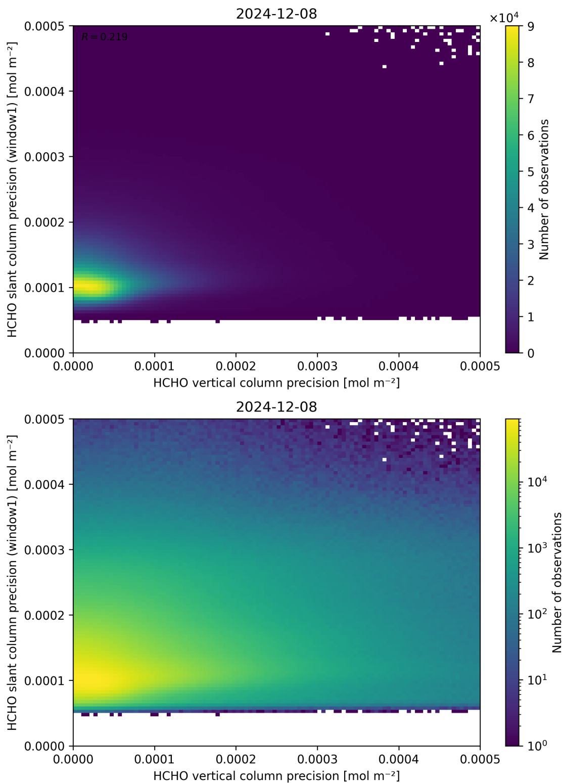
Figure 143: Scatter density plot of “HCHO vertical column precision” against “HCHO slant column precision (window1)” for 2024-12-07 to 2024-12-09.
