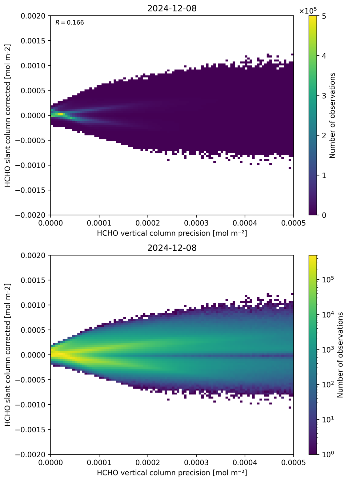
Figure 140: Scatter density plot of “HCHO vertical column precision” against “HCHO slant column corrected” for 2024-12-07 to 2024-12-09.
