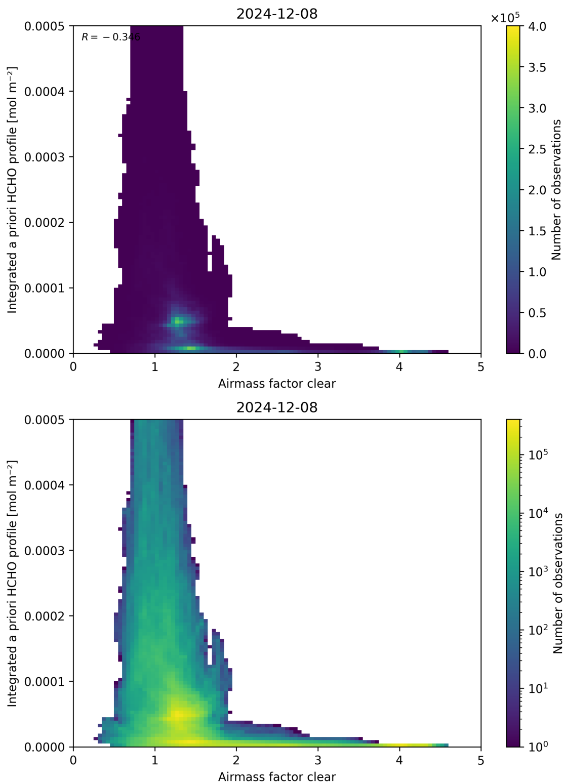
Figure 76: Scatter density plot of “Airmass factor clear” against “Integrated a priori HCHO profile” for 2024-12-07 to 2024-12-09.
