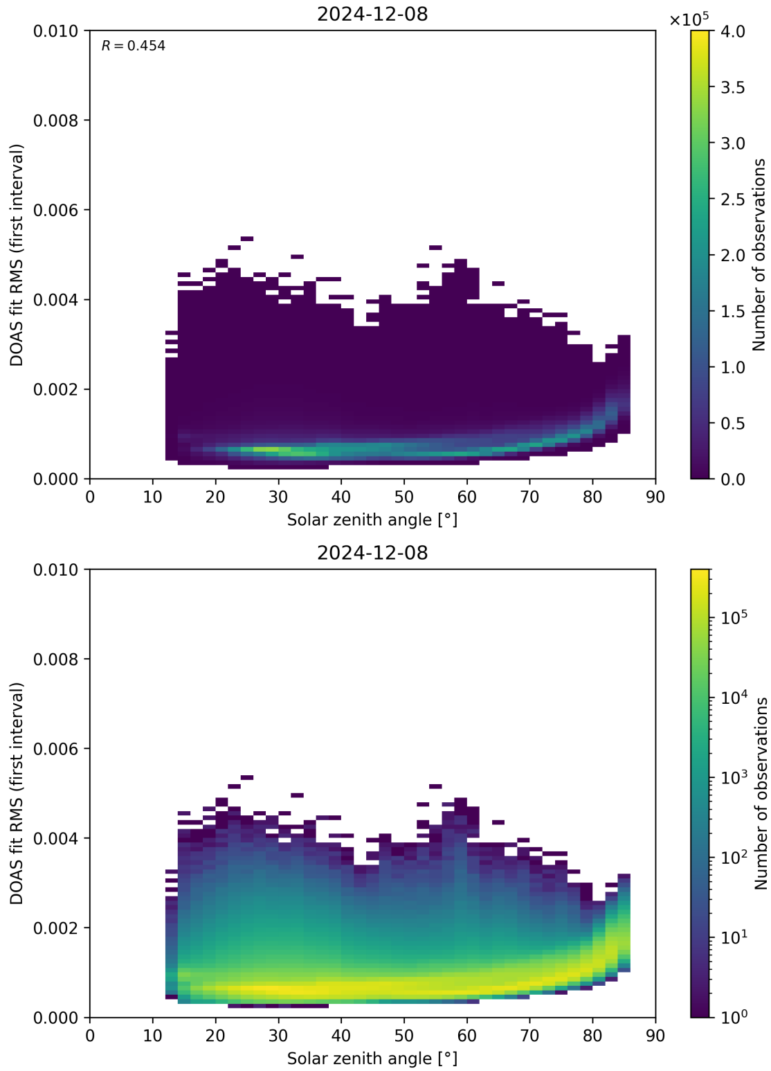
Figure 167: Scatter density plot of “Solar zenith angle” against “DOAS fit RMS (first interval)” for 2024-12-07 to 2024-12-09.
