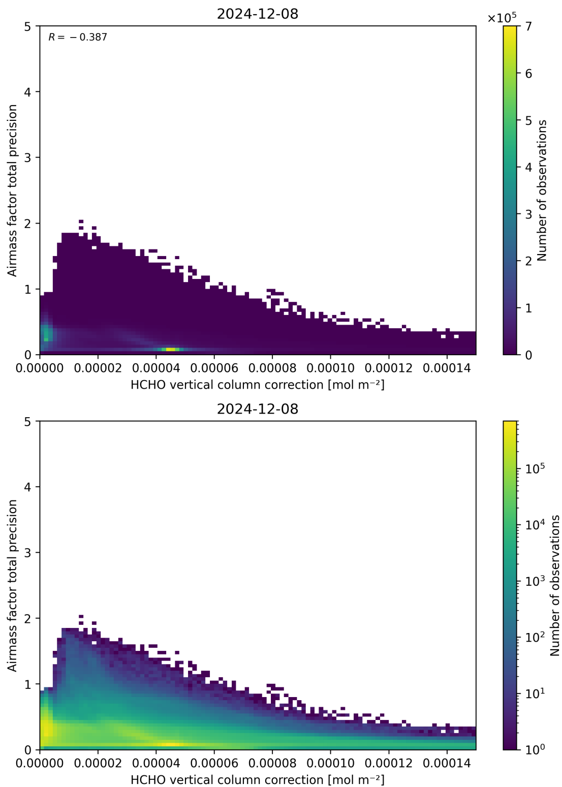
Figure 121: Scatter density plot of “HCHO vertical column correction” against “Airmass factor total precision” for 2024-12-07 to 2024-12-09.
