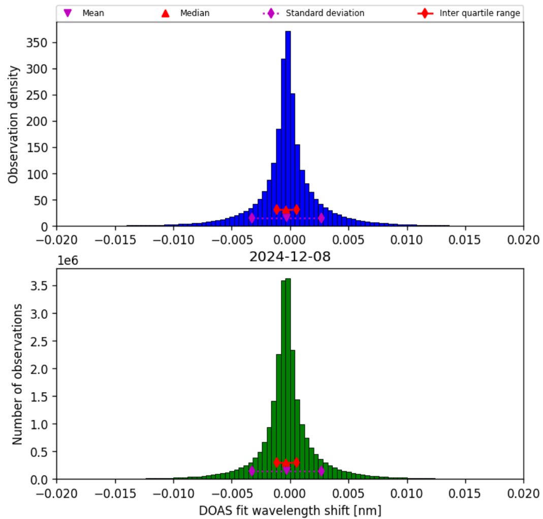
Figure 44: Histogram of “DOAS fit wavelength shift” for 2024-12-07 to 2024-12-09
