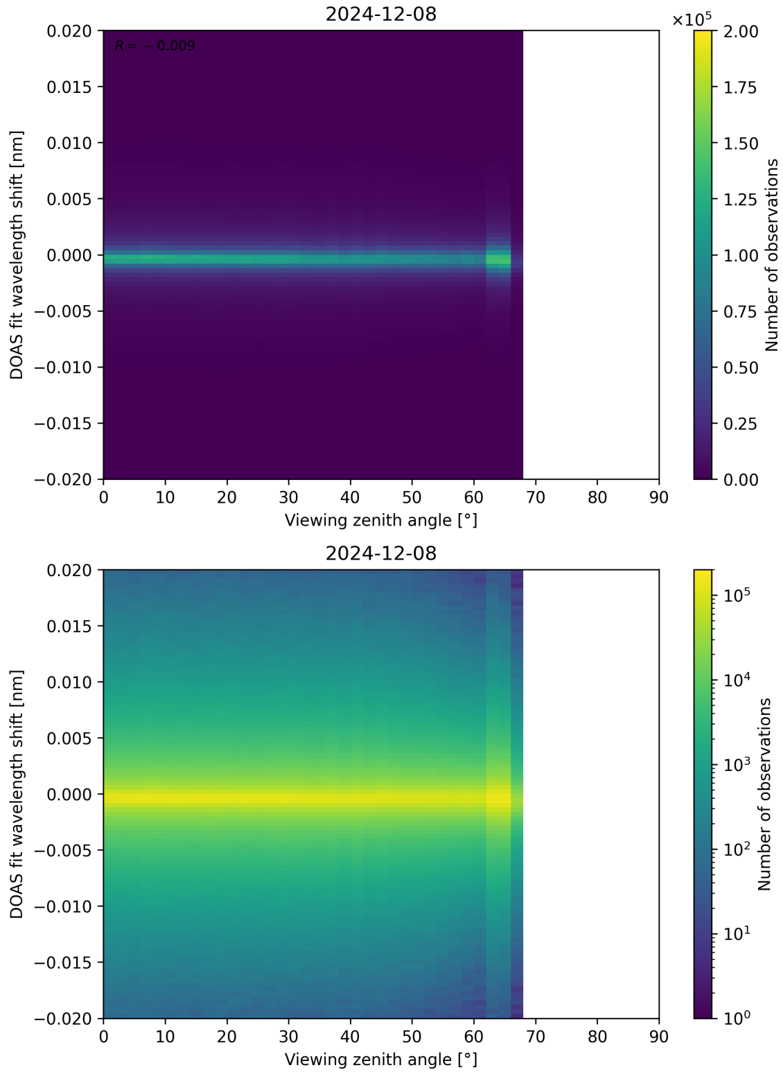
Figure 183: Scatter density plot of “Viewing zenith angle” against “DOAS fit wavelength shift” for 2024-12-07 to 2024-12-09.
