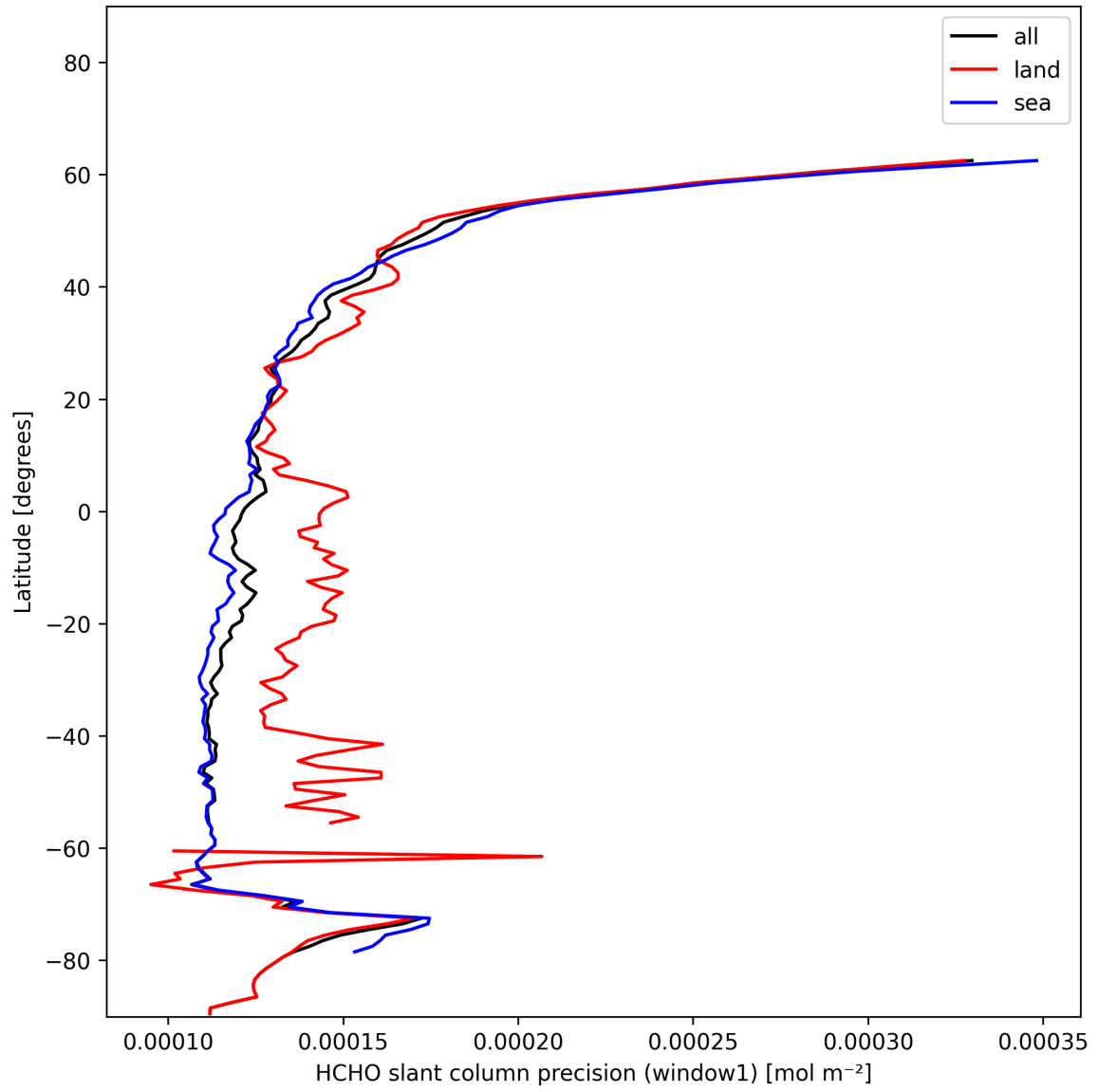
Figure 25: Zonal average of "HCHO slant column precision (window1)" for 2024-12-07 to 2024-12-09.
