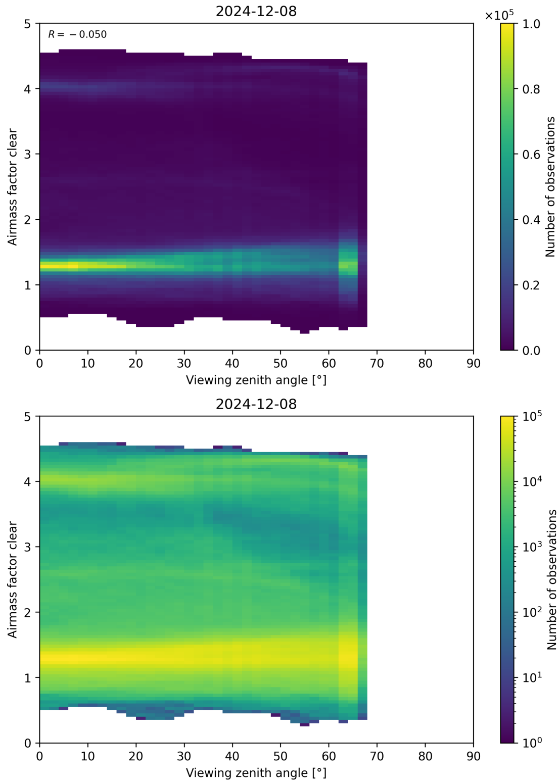
Figure 185: Scatter density plot of “Viewing zenith angle” against “Airmass factor clear” for 2024-12-07 to 2024-12-09.
