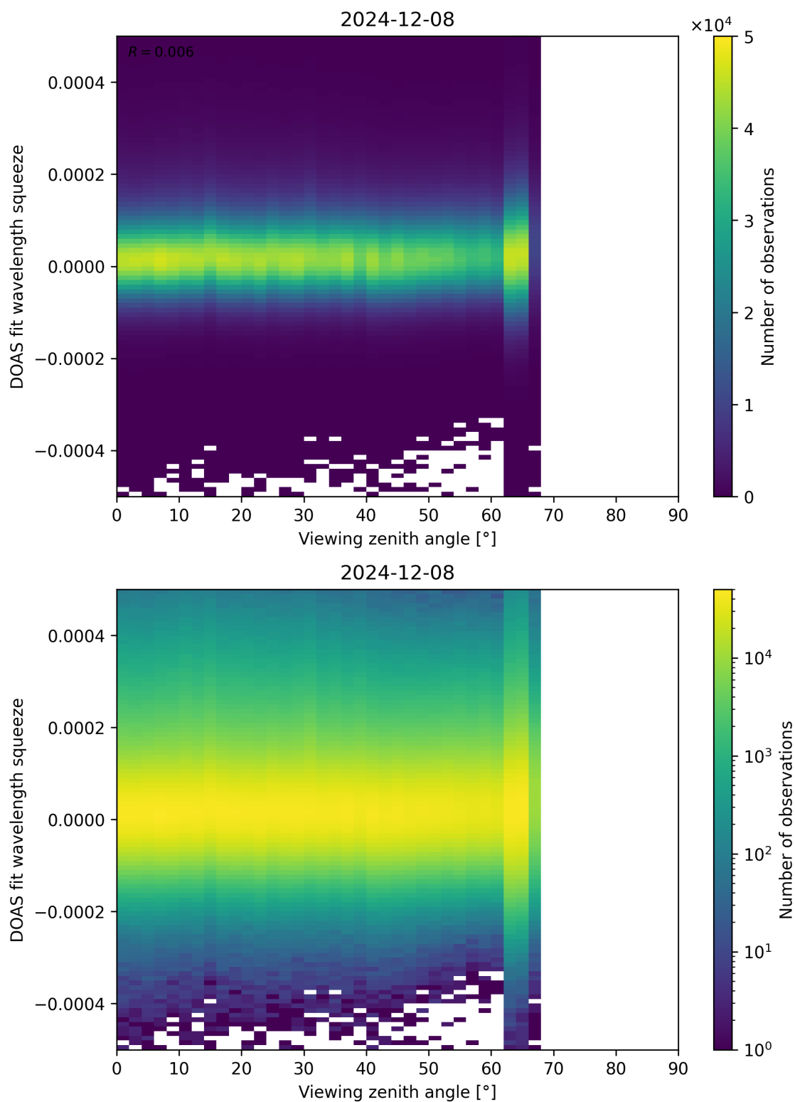
Figure 184: Scatter density plot of “Viewing zenith angle” against “DOAS fit wavelength squeeze” for 2024-12-07 to 2024-12-09.
