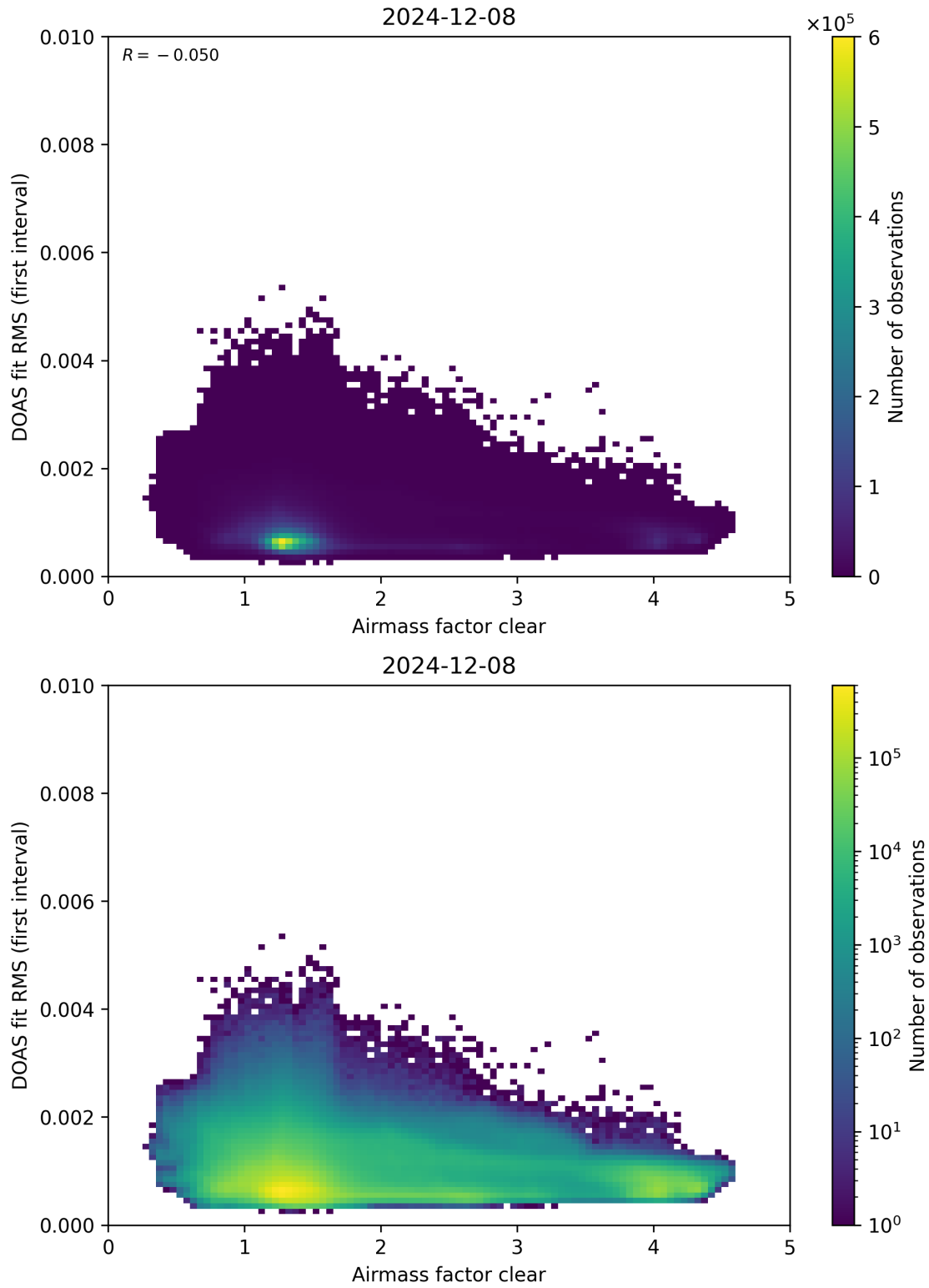
Figure 71: Scatter density plot of “Airmass factor clear” against “DOAS fit RMS (first interval)” for 2024-12-07 to 2024-12-09.
