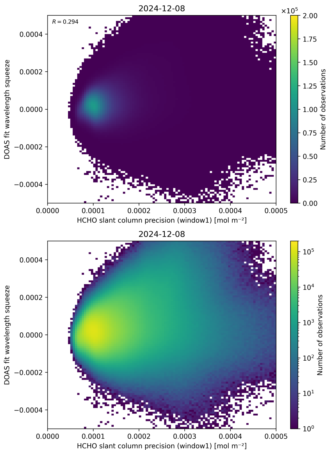
Figure 90: Scatter density plot of “HCHO slant column precision (window1)” against “DOAS fit wavelength squeeze” for 2024-12-07 to 2024-12-09.
