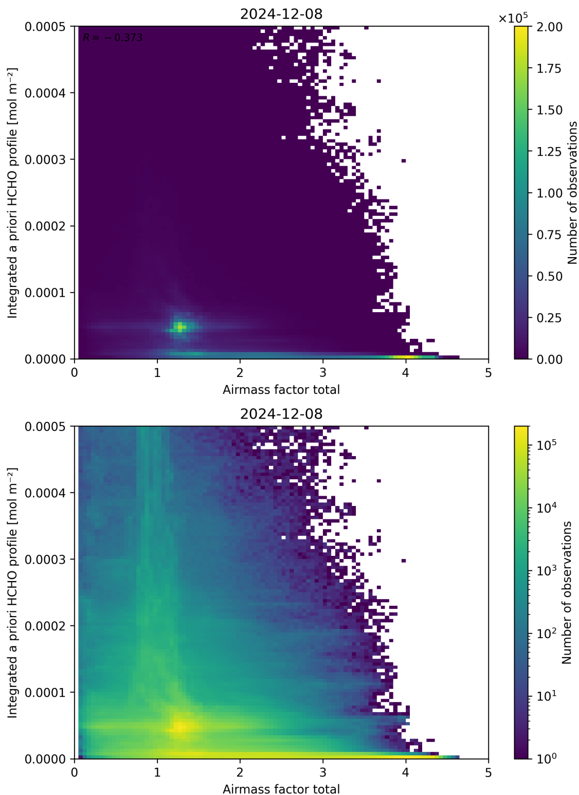
Figure 104: Scatter density plot of “Airmass factor total” against “Integrated a priori HCHO profile” for 2024-12-07 to 2024-12-09.
