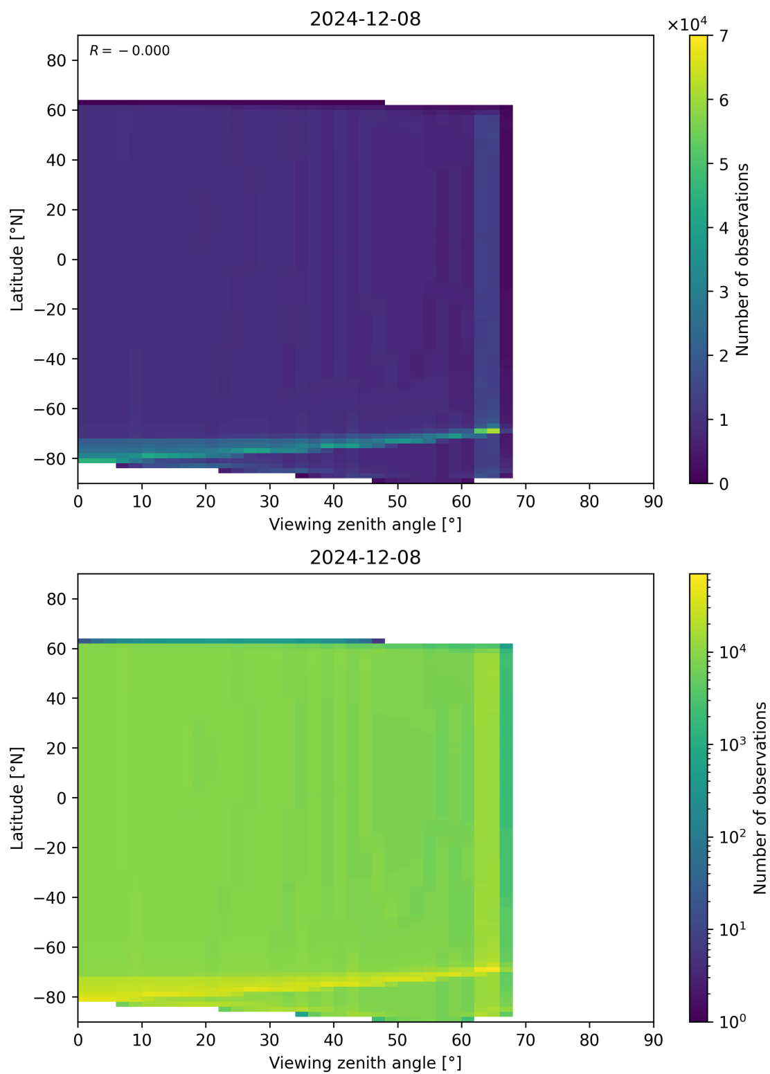
Figure 196: Scatter density plot of “Viewing zenith angle” against “Latitude” for 2024-12-07 to 2024-12-09.
