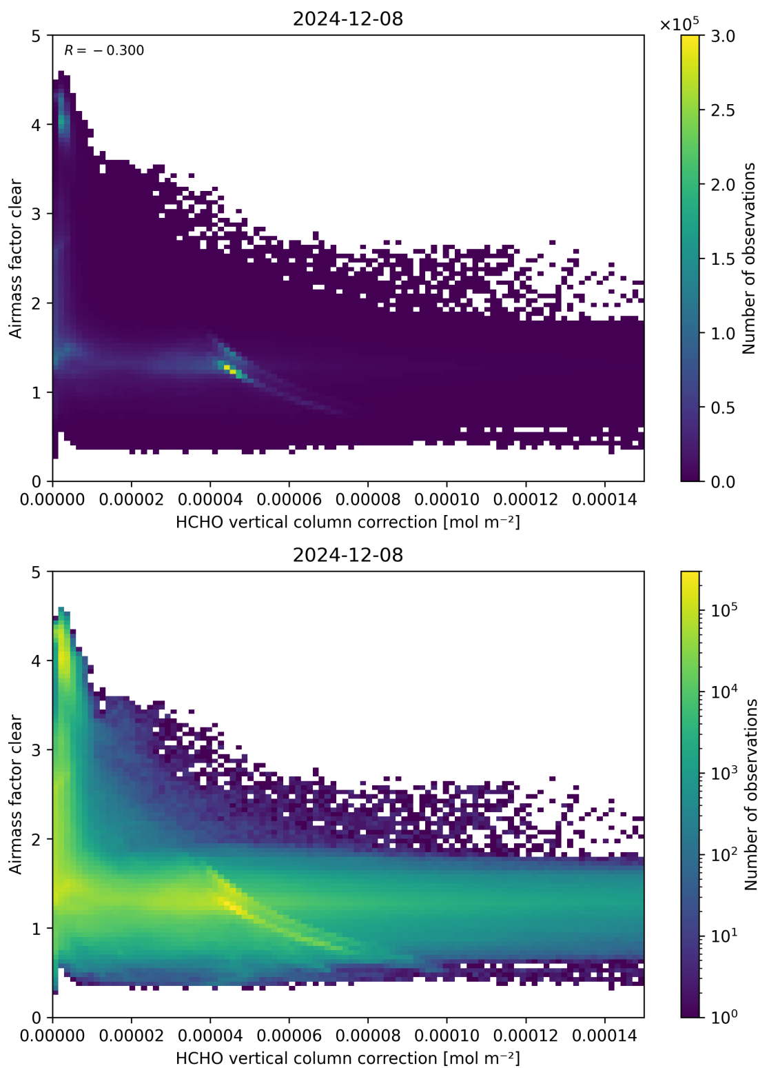
Figure 115: Scatter density plot of “HCHO vertical column correction” against “Airmass factor clear” for 2024-12-07 to 2024-12-09.
