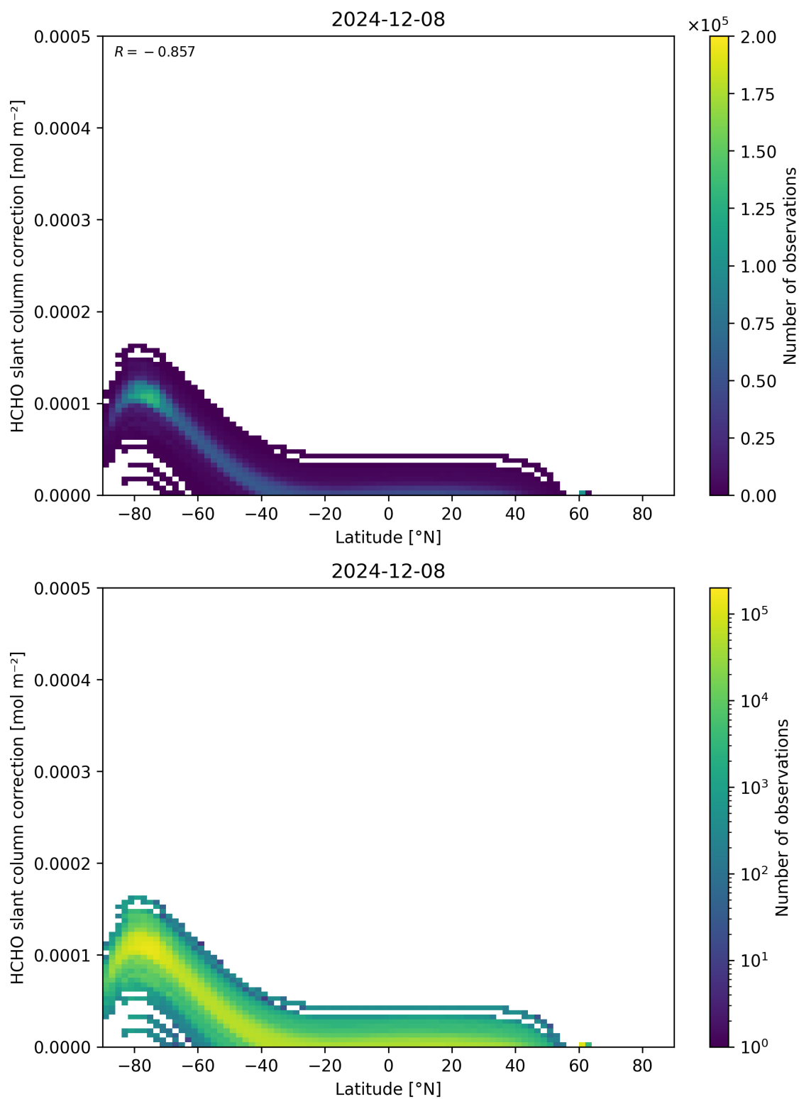
Figure 158: Scatter density plot of “Latitude” against “HCHO slant column correction” for 2024-12-07 to 2024-12-09.
