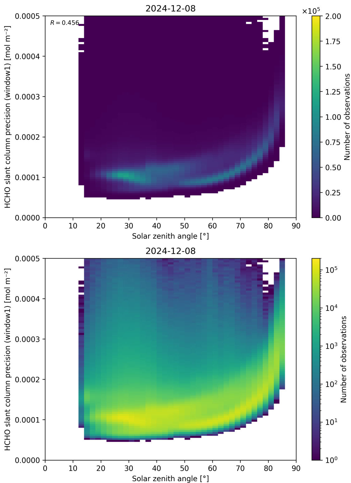
Figure 174: Scatter density plot of “Solar zenith angle” against “HCHO slant column precision (window1)” for 2024-12-07 to 2024-12-09.
