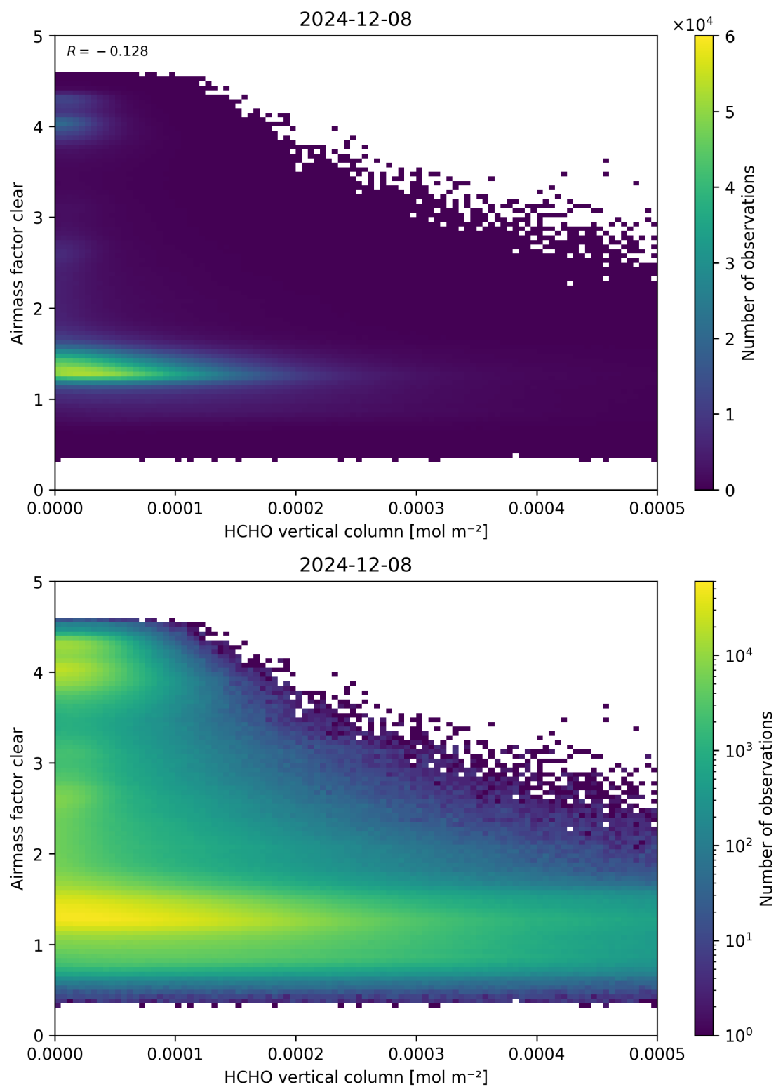
Figure 126: Scatter density plot of “HCHO vertical column” against “Airmass factor clear” for 2024-12-07 to 2024-12-09.
