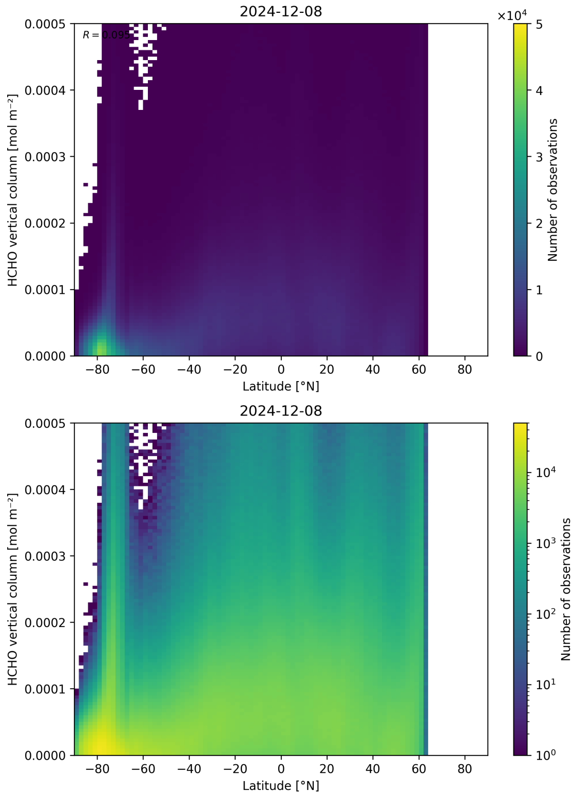
Figure 163: Scatter density plot of “Latitude” against “HCHO vertical column” for 2024-12-07 to 2024-12-09.
