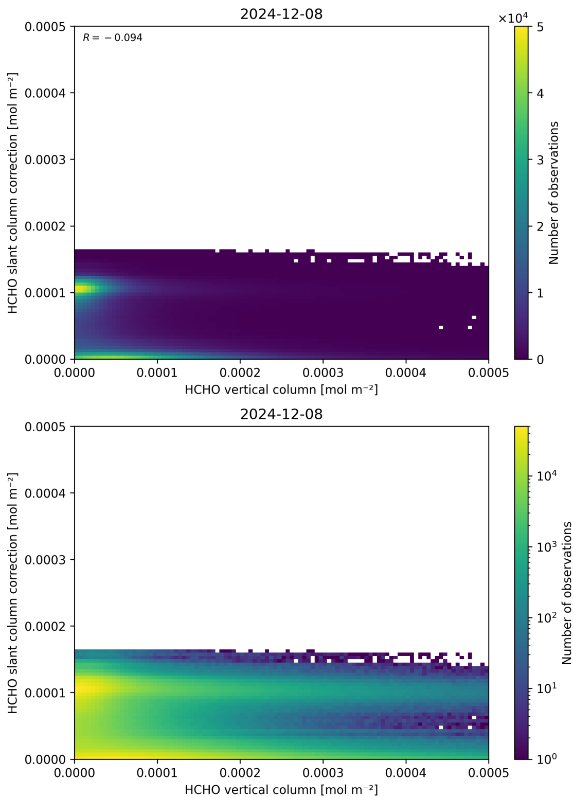
Figure 128: Scatter density plot of “HCHO vertical column” against “HCHO slant column correction” for 2024-12-07 to 2024-12-09.
