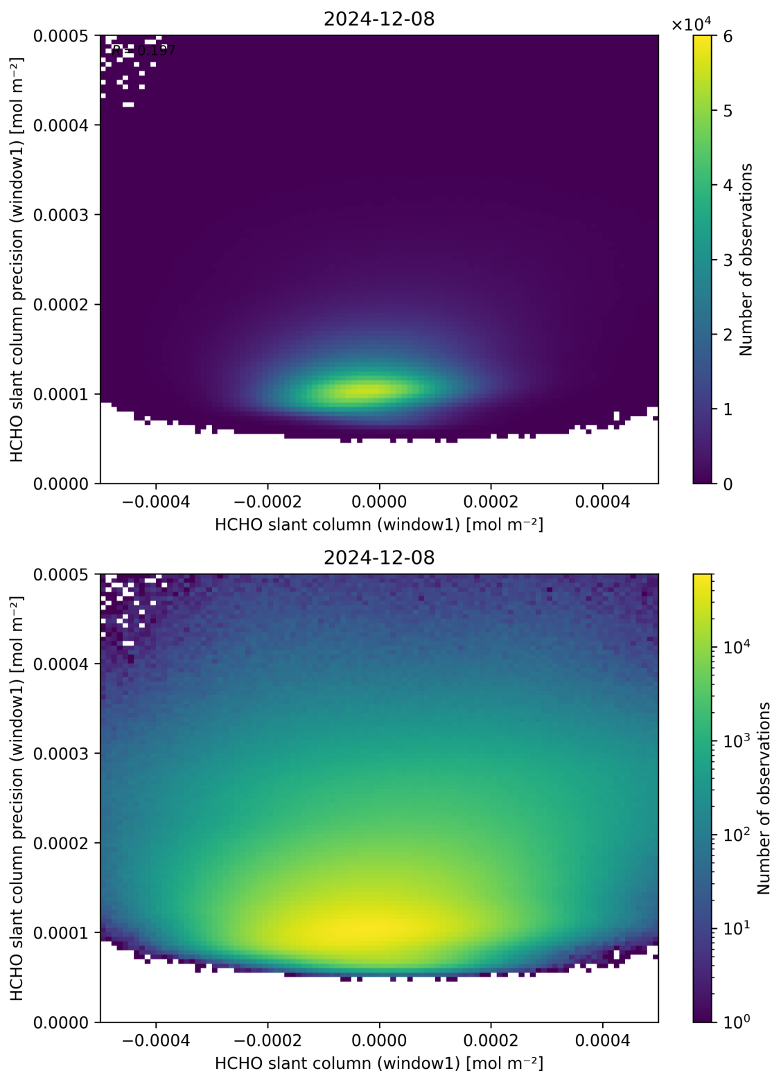
Figure 84: Scatter density plot of “HCHO slant column (window1)” against “HCHO slant column precision (window1)” for 2024-12-07 to 2024-12-09.
