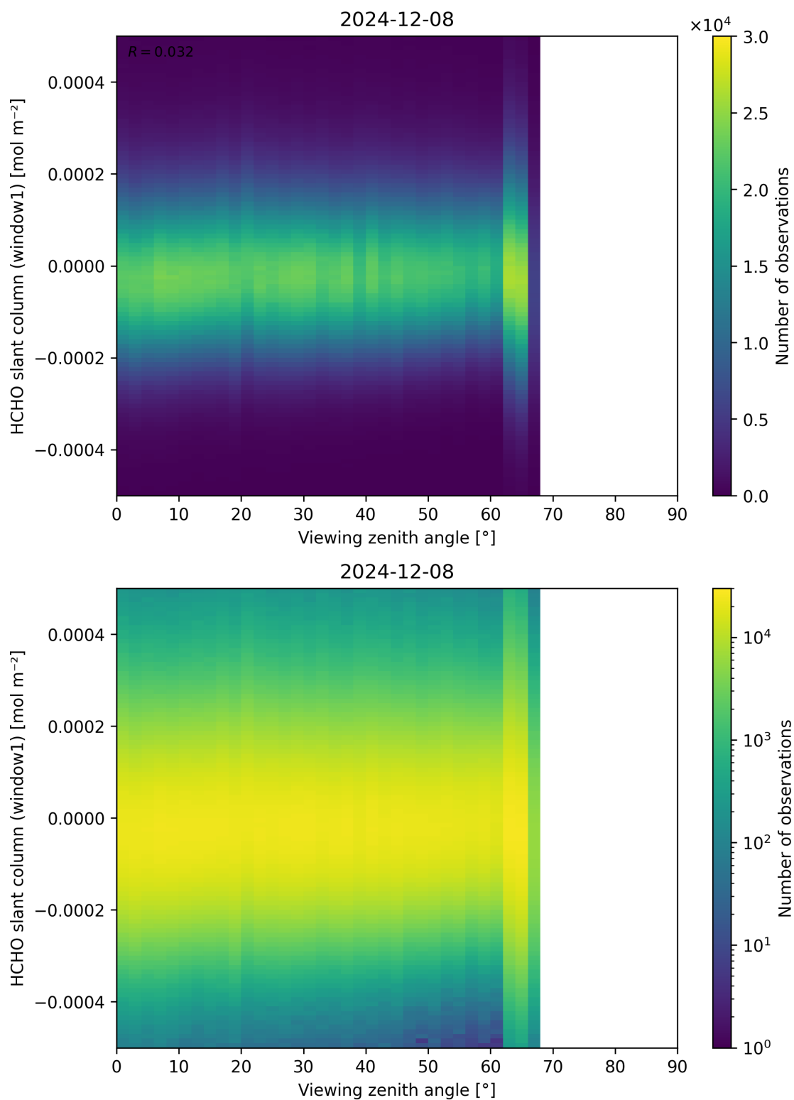
Figure 188: Scatter density plot of “Viewing zenith angle” against “HCHO slant column (window1)” for 2024-12-07 to 2024-12-09.
