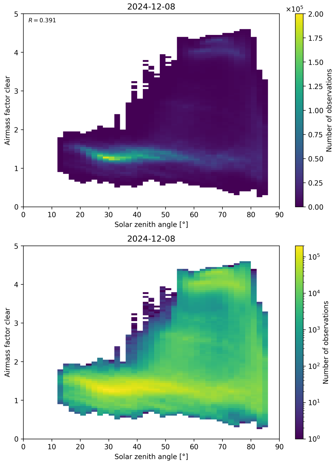
Figure 170: Scatter density plot of “Solar zenith angle” against “Airmass factor clear” for 2024-12-07 to 2024-12-09.
