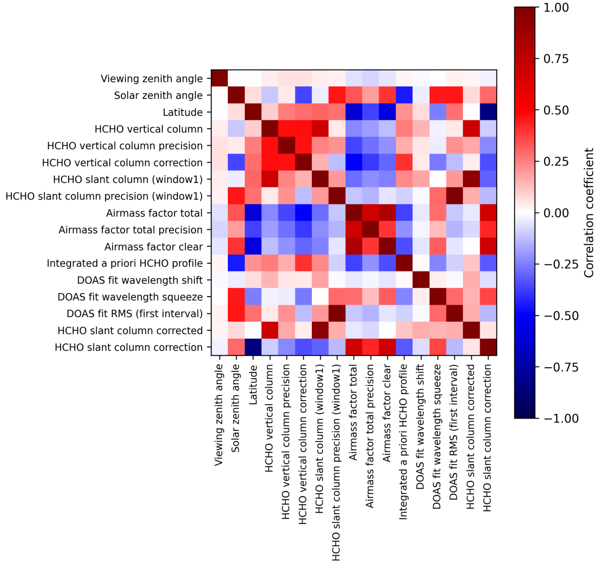
Figure 2: Map of correlation matrix for 2024-12-07 to 2024-12-09.
