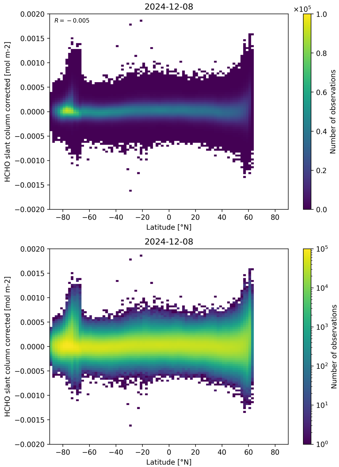
Figure 157: Scatter density plot of “Latitude” against “HCHO slant column corrected” for 2024-12-07 to 2024-12-09.
