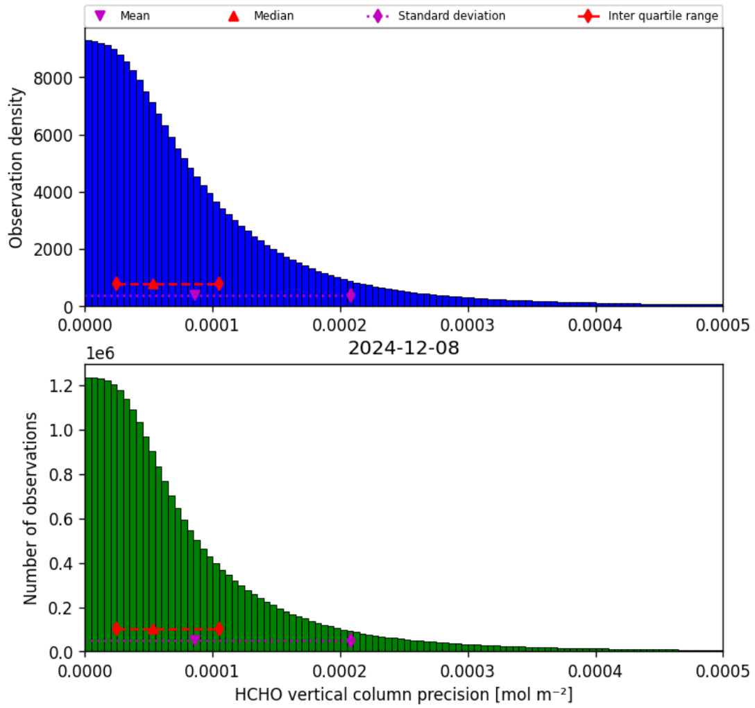
Figure 36: Histogram of “HCHO vertical column precision” for 2024-12-07 to 2024-12-09
