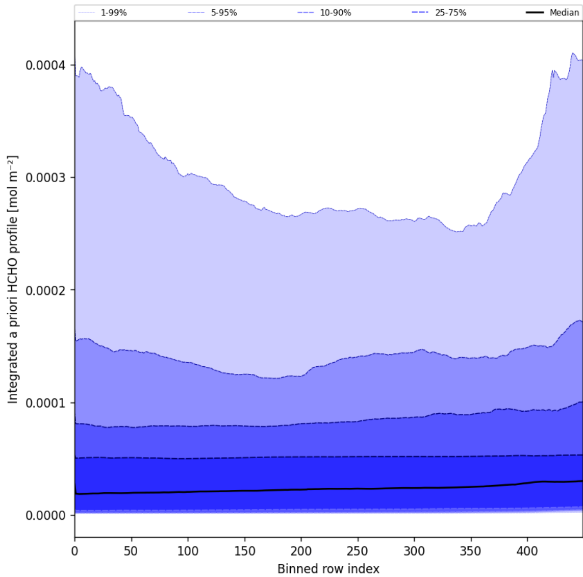
Figure 57: Along track statistics of “Integrated a priori HCHO profile” for 2024-12-07 to 2024-12-09
