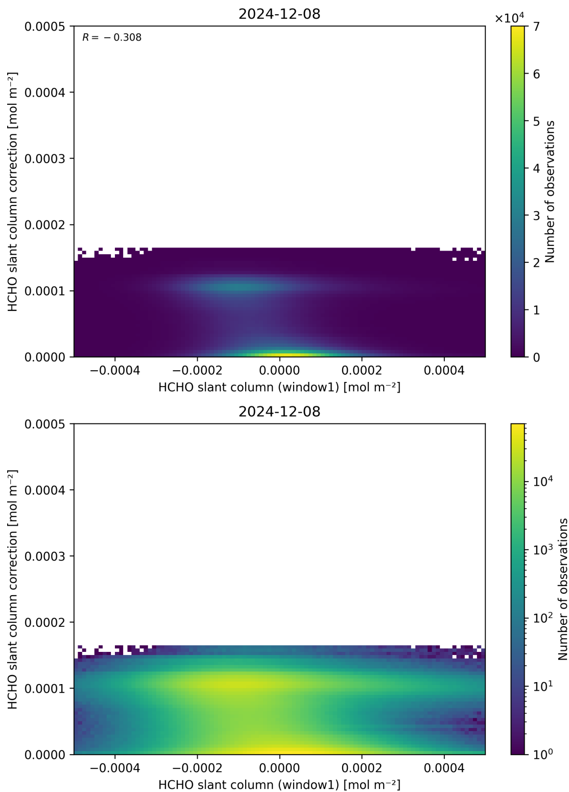
Figure 83: Scatter density plot of “HCHO slant column (window1)” against “HCHO slant column correction” for 2024-12-07 to 2024-12-09.
