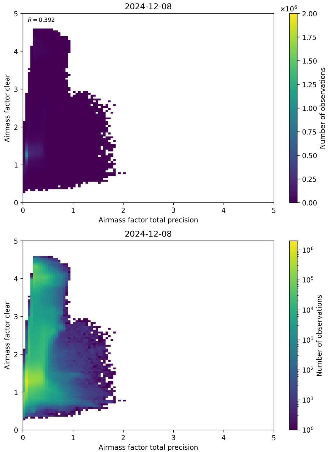
Figure 108: Scatter density plot of “Airmass factor total precision” against “Airmass factor clear” for 2024-12-07 to 2024-12-09.
