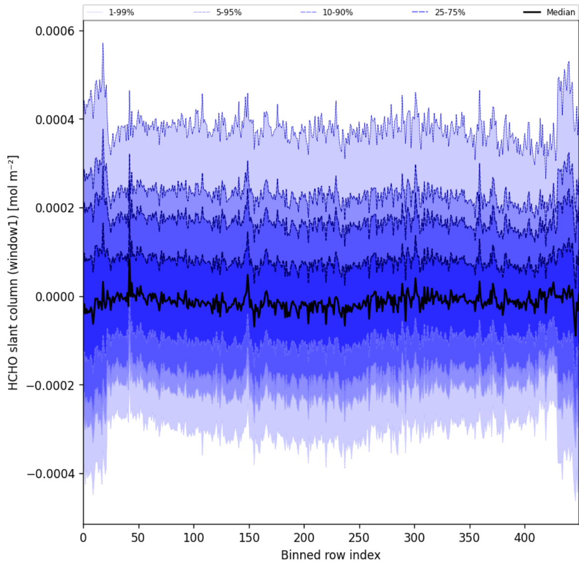
Figure 52: Along track statistics of “HCHO slant column (window1)” for 2024-12-07 to 2024-12-09
