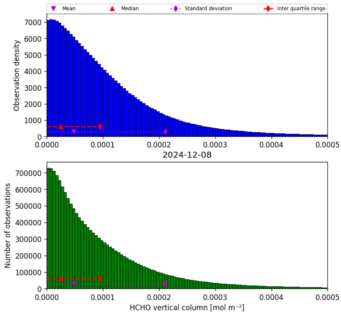
Figure 35: Histogram of “HCHO vertical column” for 2024-12-07 to 2024-12-09
