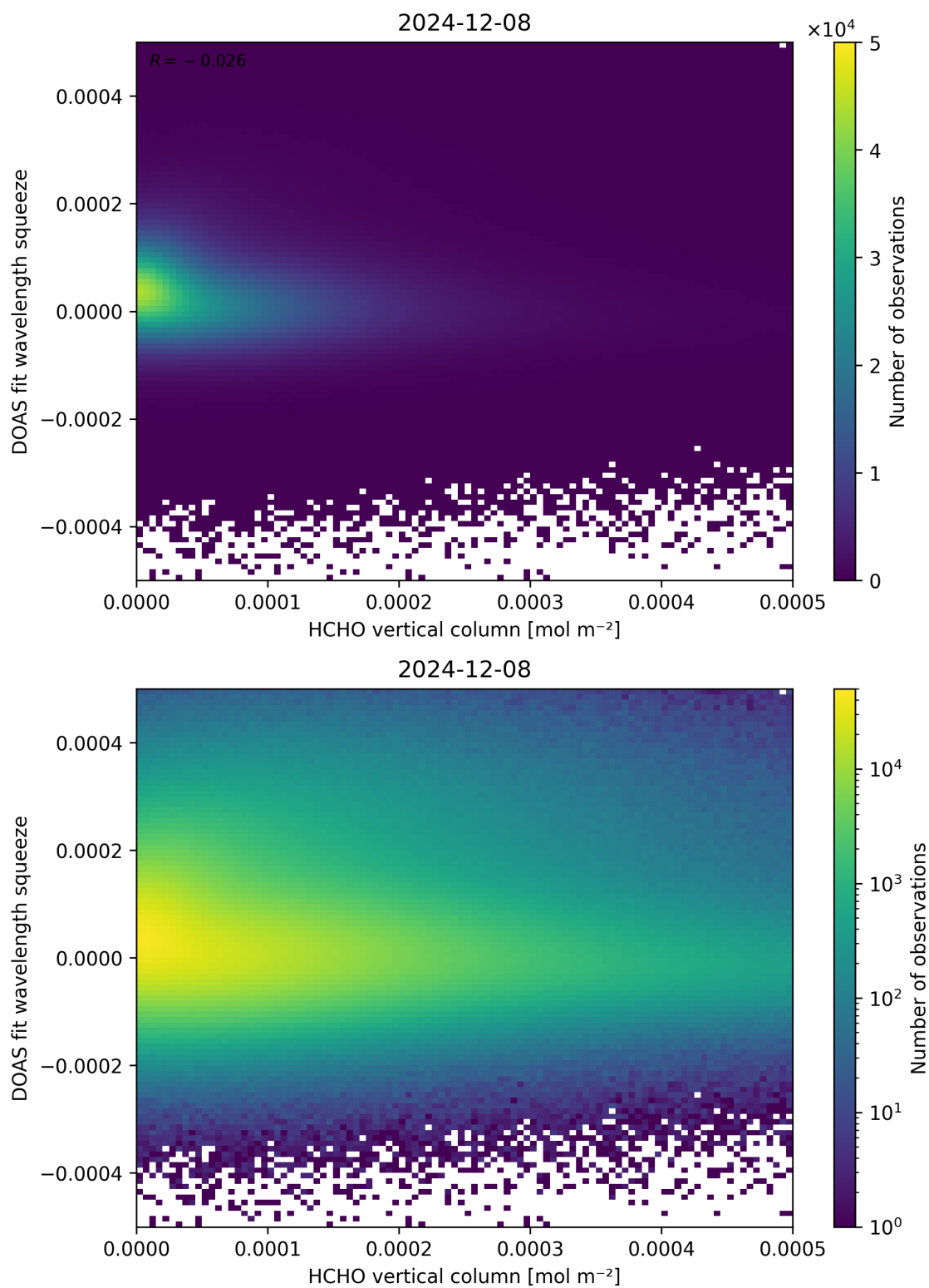
Figure 125: Scatter density plot of “HCHO vertical column” against “DOAS fit wavelength squeeze” for 2024-12-07 to 2024-12-09.
