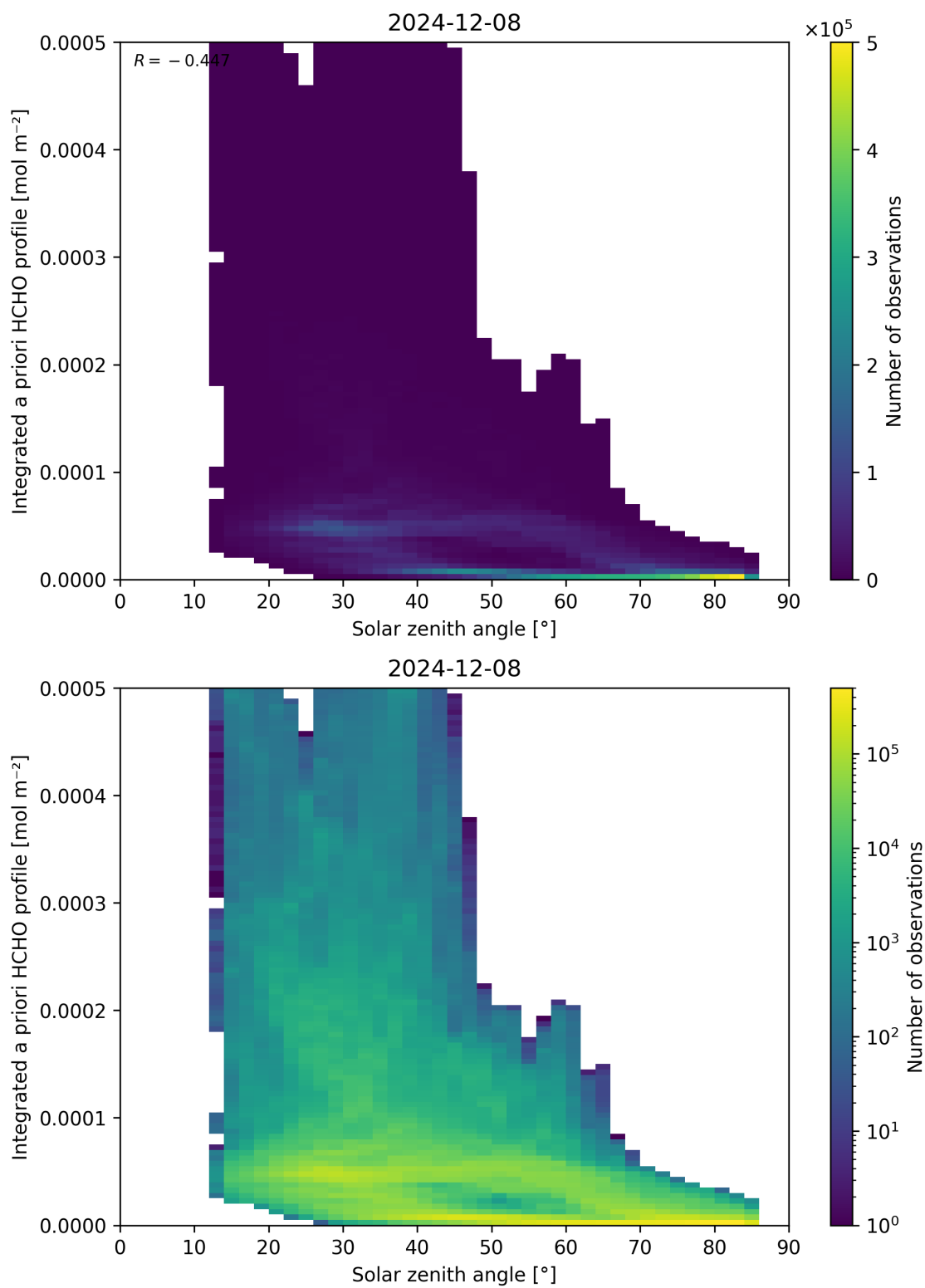
Figure 180: Scatter density plot of “Solar zenith angle” against “Integrated a priori HCHO profile” for 2024-12-07 to 2024-12-09.
