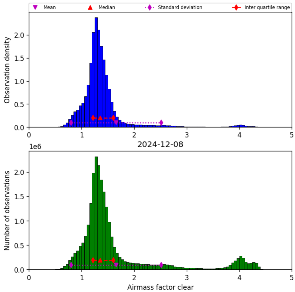
Figure 42: Histogram of “Airmass factor clear” for 2024-12-07 to 2024-12-09
