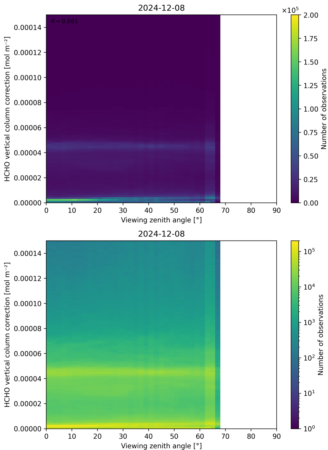
Figure 193: Scatter density plot of “Viewing zenith angle” against “HCHO vertical column correction” for 2024-12-07 to 2024-12-09.
