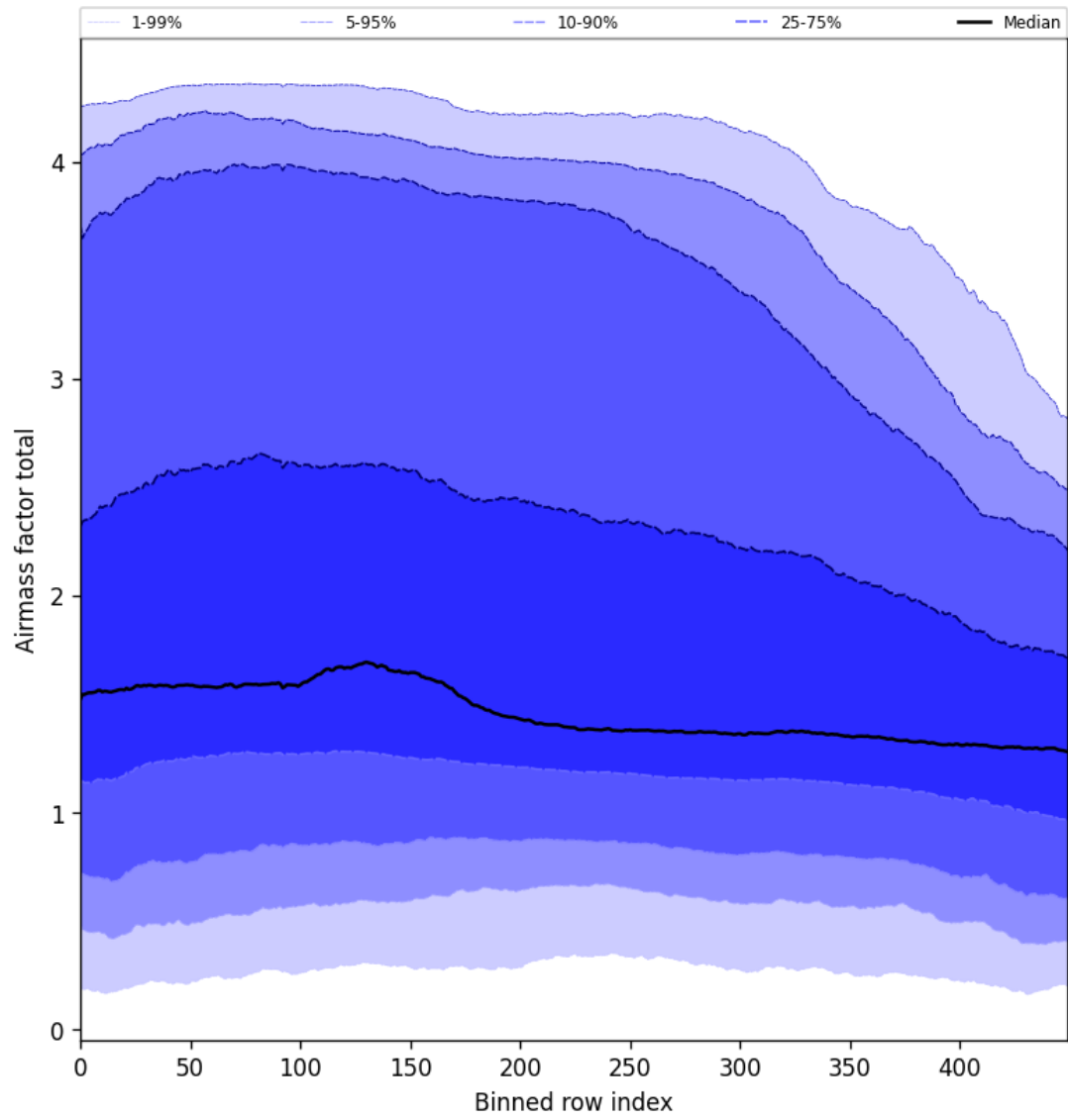
Figure 54: Along track statistics of “Airmass factor total” for 2024-12-07 to 2024-12-09
