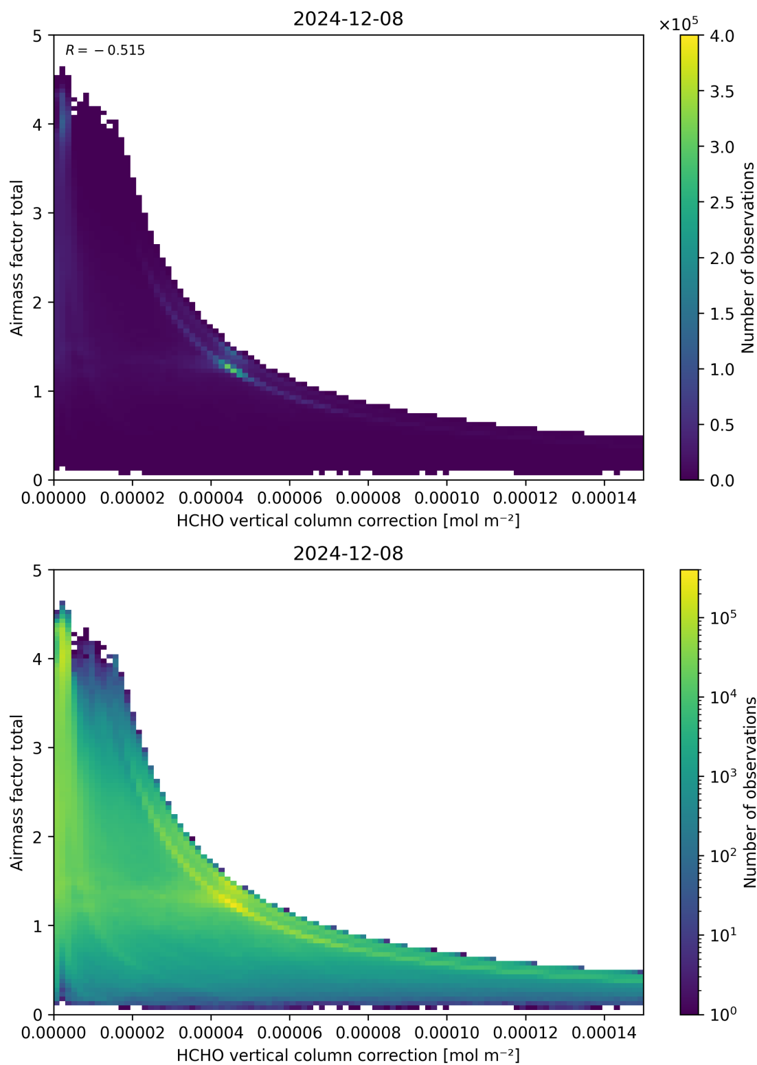
Figure 120: Scatter density plot of “HCHO vertical column correction” against “Airmass factor total” for 2024-12-07 to 2024-12-09.
