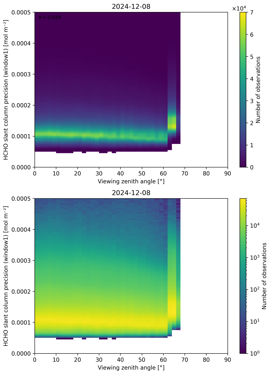
Figure 189: Scatter density plot of “Viewing zenith angle” against “HCHO slant column precision (window1)” for 2024-12-07 to 2024-12-09.
