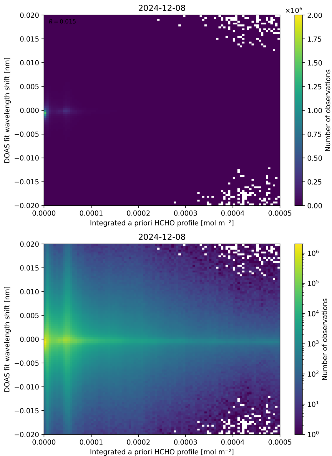
Figure 149: Scatter density plot of “Integrated a priori HCHO profile” against “DOAS fit wavelength shift” for 2024-12-07 to 2024-12-09.
