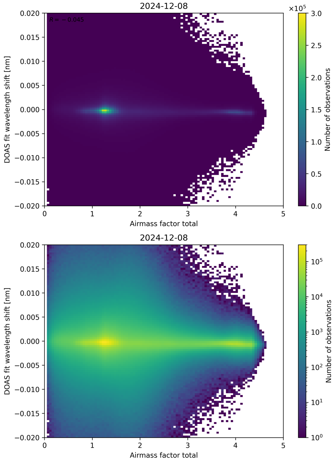
Figure 98: Scatter density plot of “Airmass factor total” against “DOAS fit wavelength shift” for 2024-12-07 to 2024-12-09.
