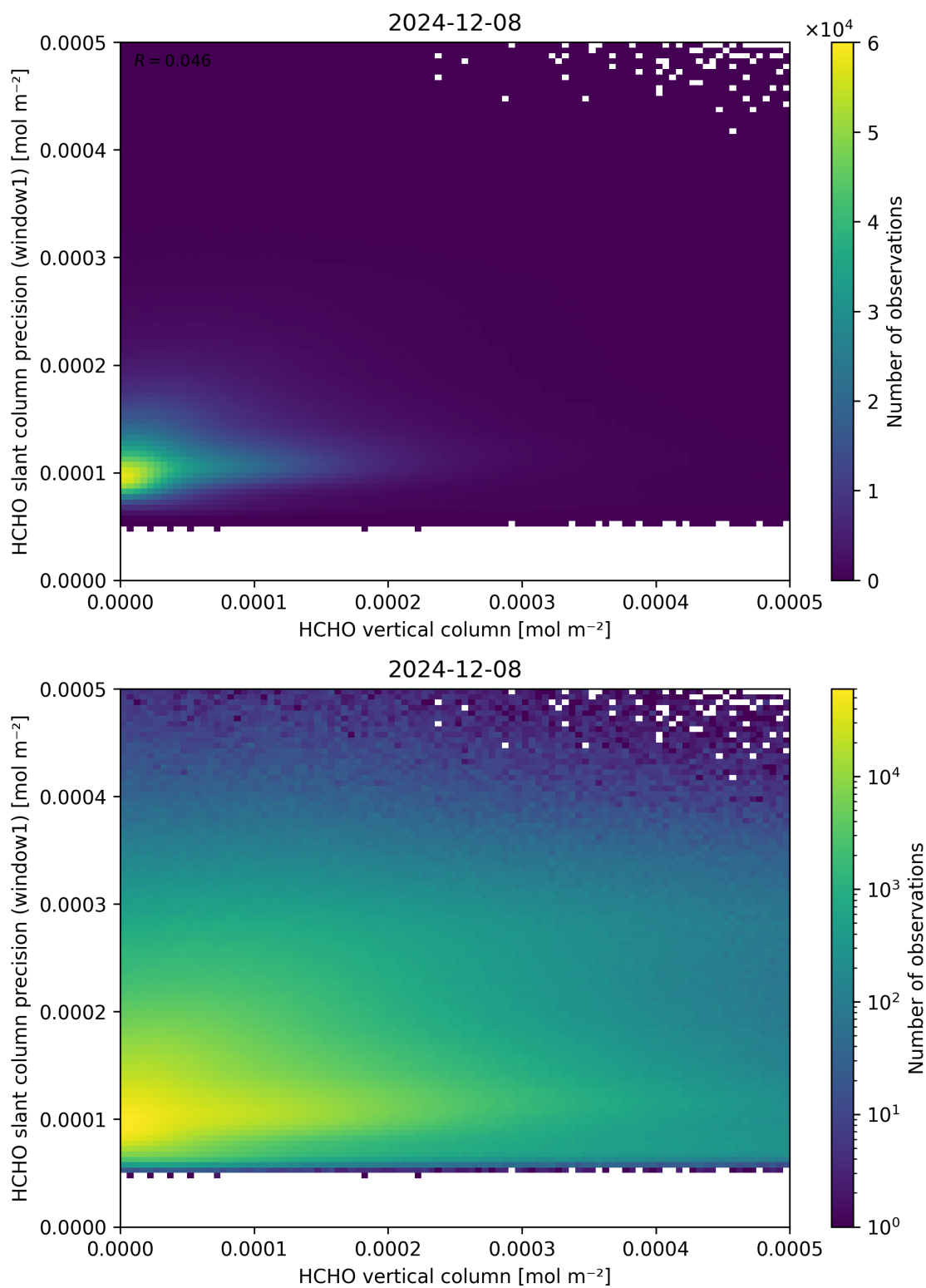
Figure 130: Scatter density plot of “HCHO vertical column” against “HCHO slant column precision (window1)” for 2024-12-07 to 2024-12-09.
