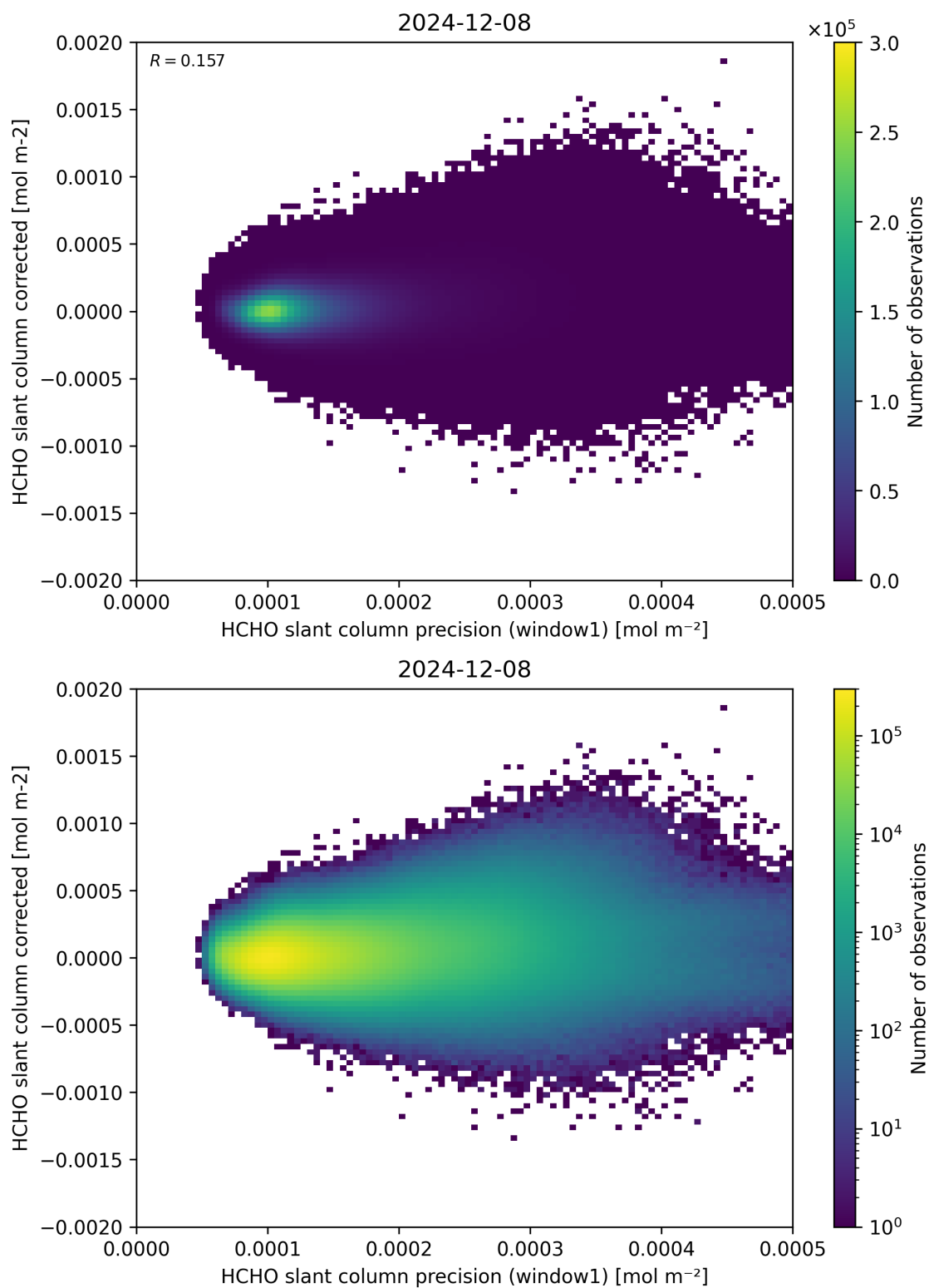
Figure 92: Scatter density plot of “HCHO slant column precision (window1)” against “HCHO slant column corrected” for 2024-12-07 to 2024-12-09.
