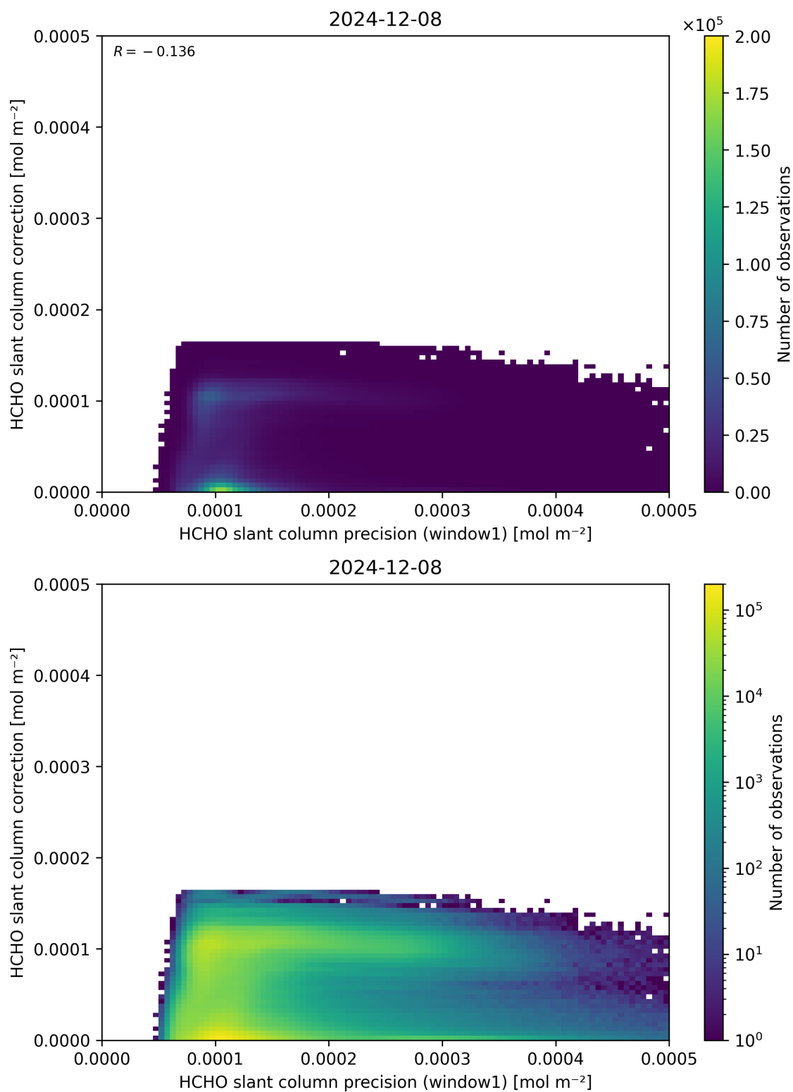
Figure 93: Scatter density plot of “HCHO slant column precision (window1)” against “HCHO slant column correction” for 2024-12-07 to 2024-12-09.
