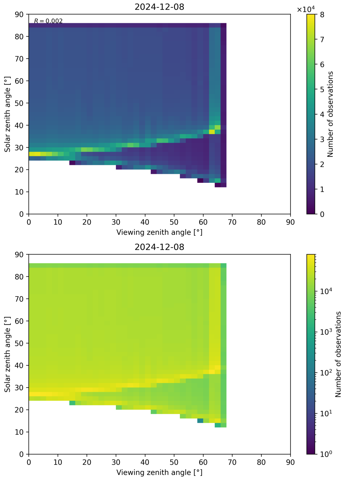
Figure 197: Scatter density plot of “Viewing zenith angle” against “Solar zenith angle” for 2024-12-07 to 2024-12-09.
