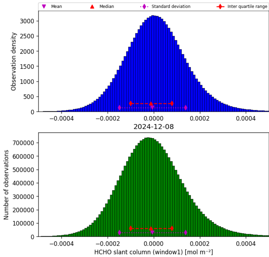
Figure 38: Histogram of “HCHO slant column (window1)” for 2024-12-07 to 2024-12-09
