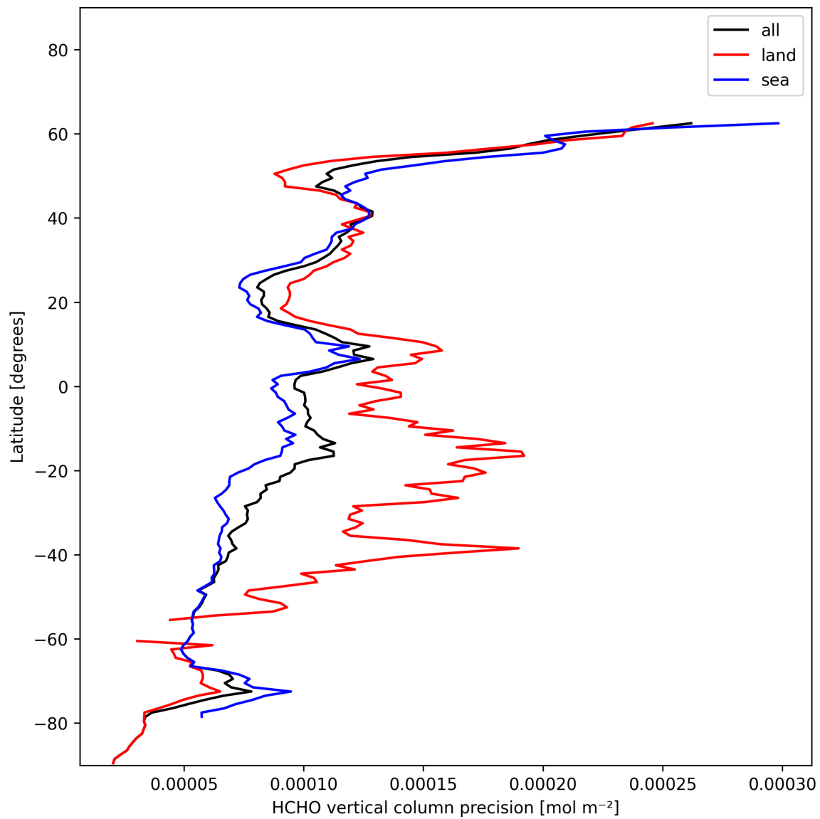
Figure 22: Zonal average of “HCHO vertical column precision” for 2024-12-07 to 2024-12-09.
