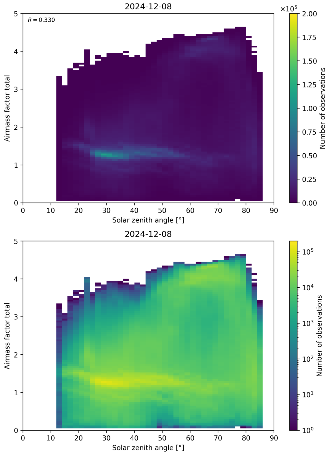
Figure 175: Scatter density plot of “Solar zenith angle” against “Airmass factor total” for 2024-12-07 to 2024-12-09.
