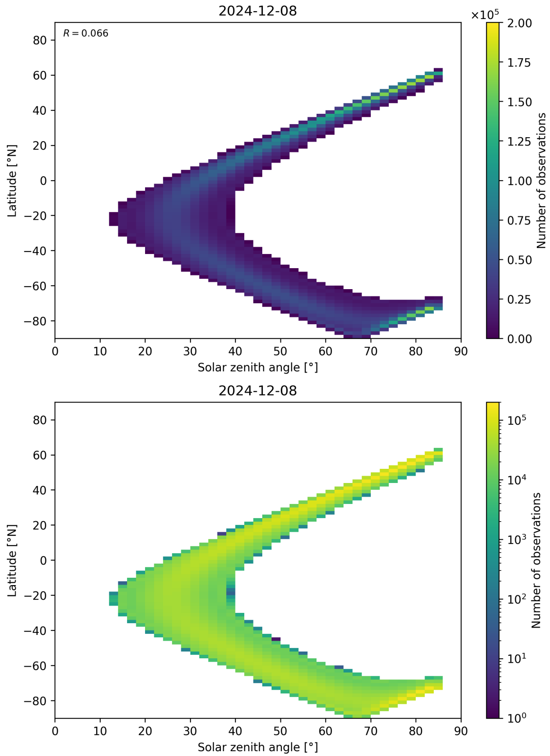
Figure 181: Scatter density plot of “Solar zenith angle” against “Latitude” for 2024-12-07 to 2024-12-09.
