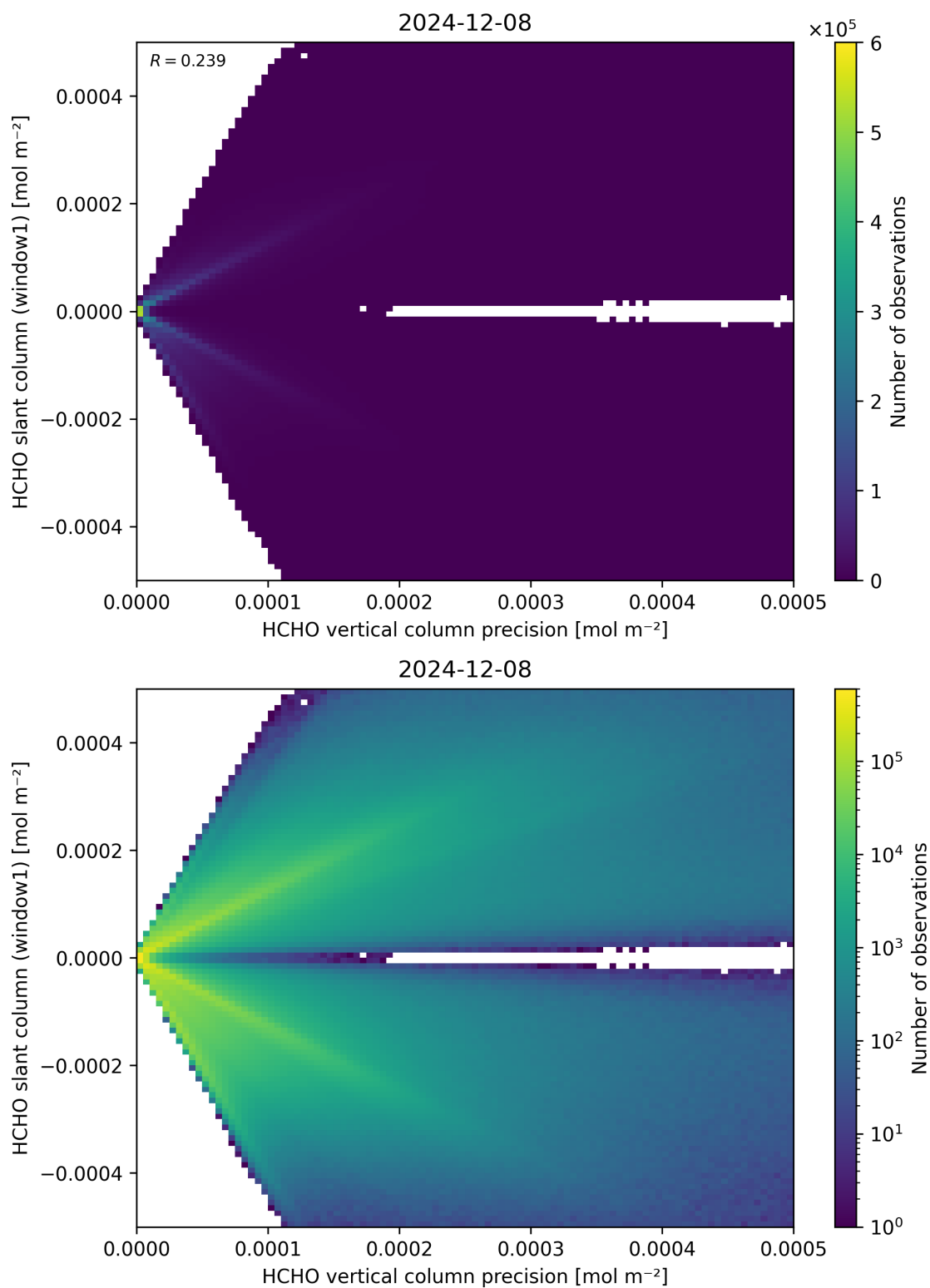
Figure 142: Scatter density plot of “HCHO vertical column precision” against “HCHO slant column (window1)” for 2024-12-07 to 2024-12-09.
