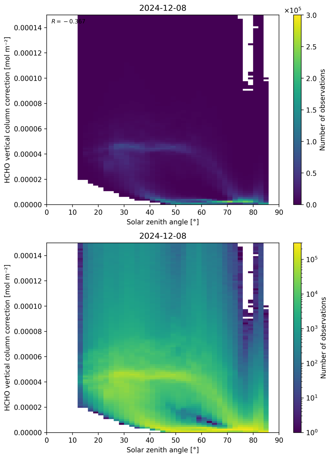
Figure 178: Scatter density plot of “Solar zenith angle” against “HCHO vertical column correction” for 2024-12-07 to 2024-12-09.
