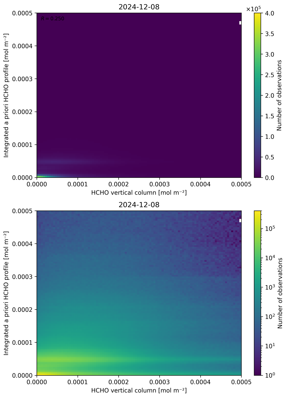
Figure 135: Scatter density plot of “HCHO vertical column” against “Integrated a priori HCHO profile” for 2024-12-07 to 2024-12-09.
