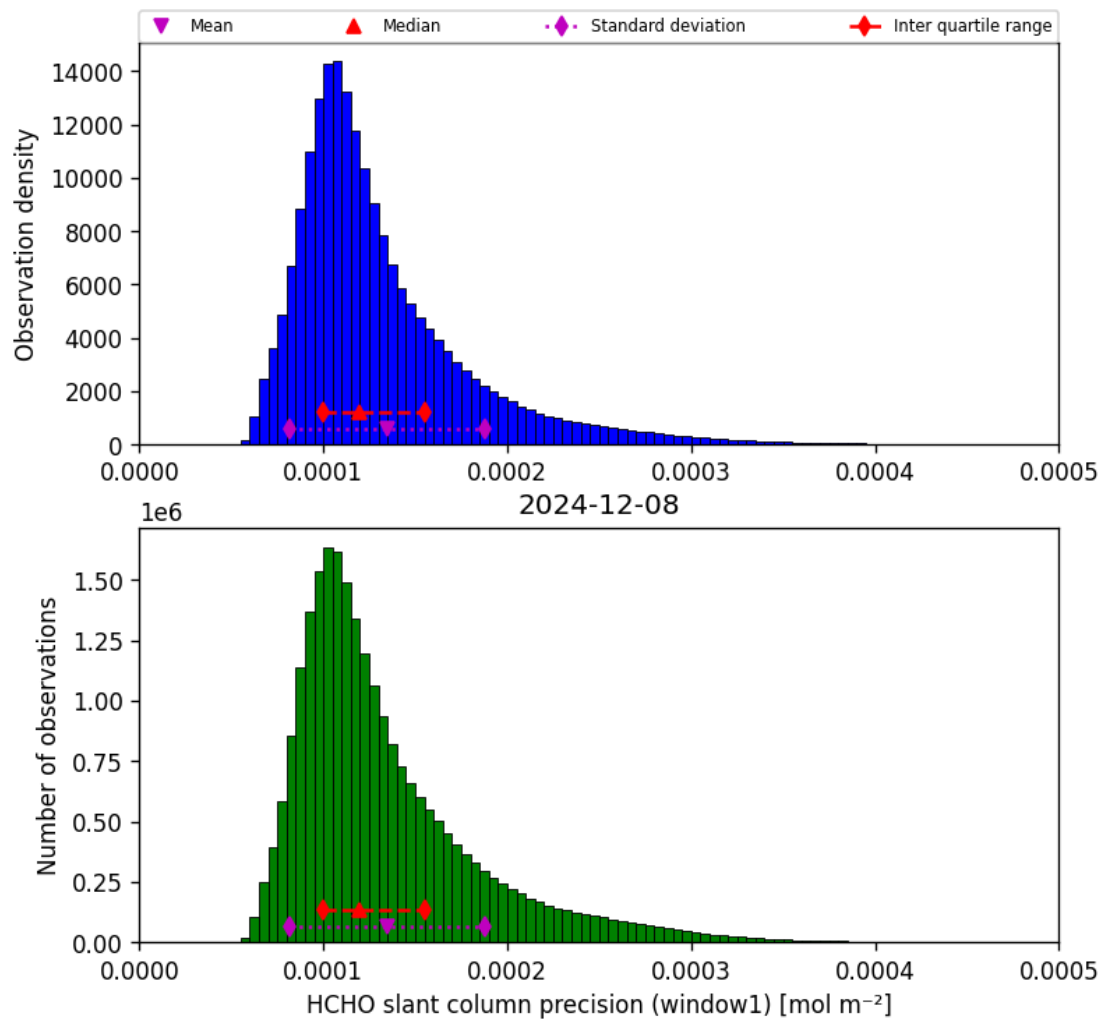
Figure 39: Histogram of “HCHO slant column precision (window1)” for 2024-12-07 to 2024-12-09
