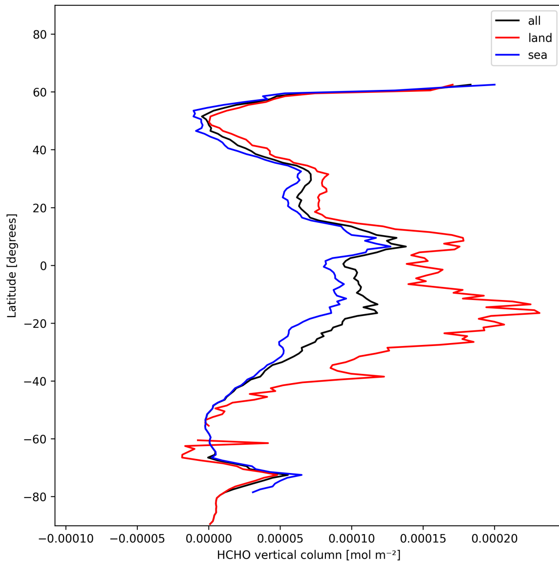
Figure 21: Zonal average of “HCHO vertical column” for 2024-12-07 to 2024-12-09.
