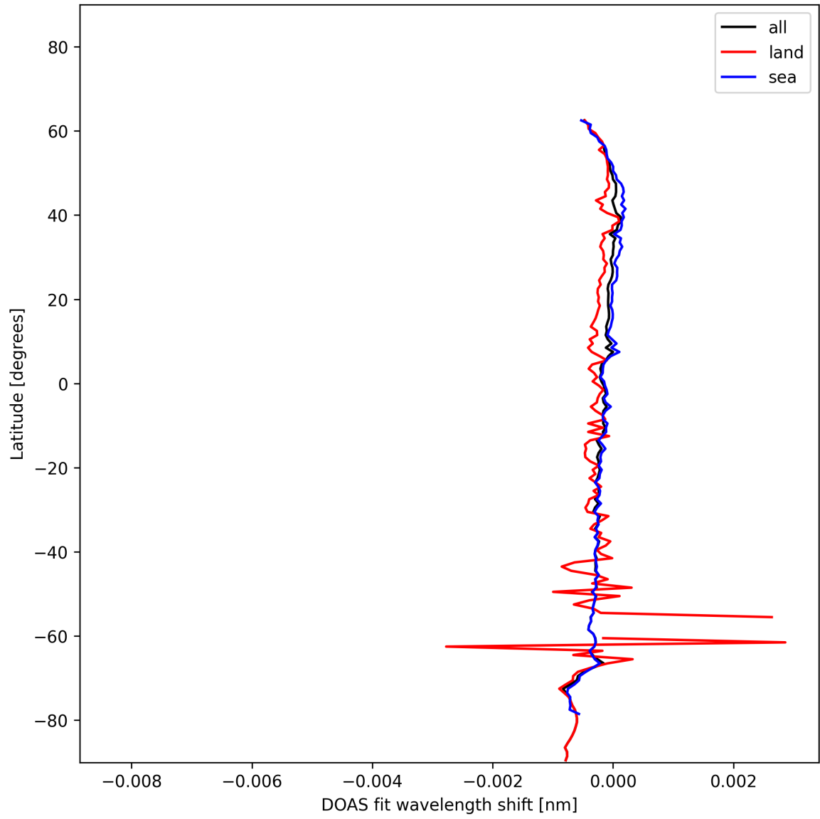
Figure 30: Zonal average of “DOAS fit wavelength shift” for 2024-12-07 to 2024-12-09.
