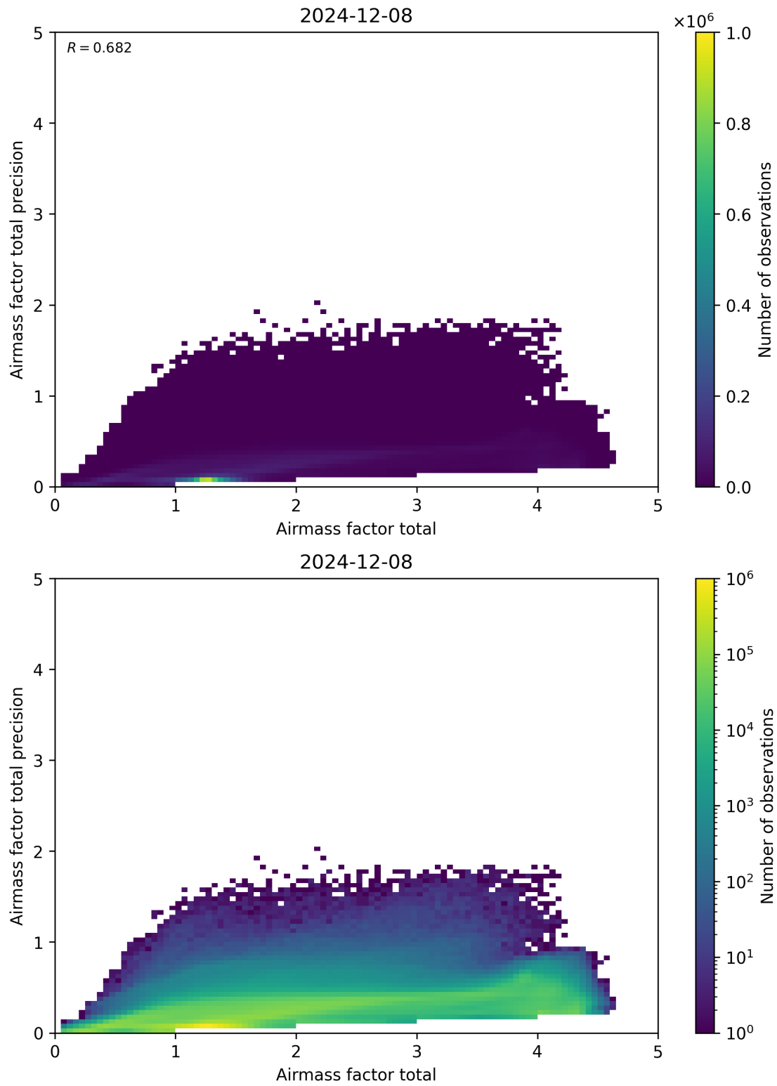
Figure 103: Scatter density plot of “Airmass factor total” against “Airmass factor total precision” for 2024-12-07 to 2024-12-09.
