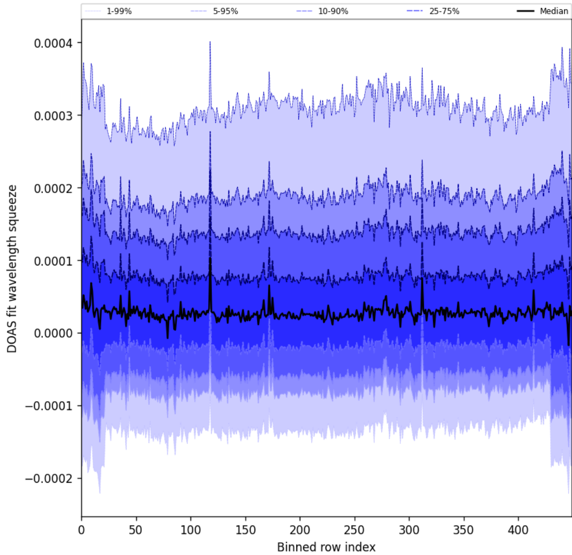
Figure 59: Along track statistics of “DOAS fit wavelength squeeze” for 2024-12-07 to 2024-12-09
