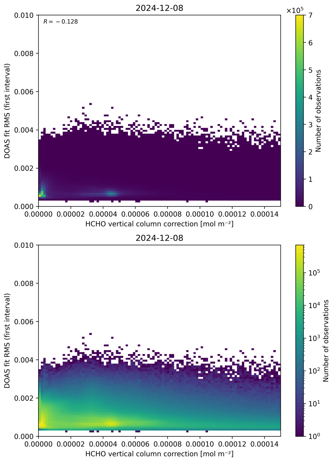
Figure 112: Scatter density plot of “HCHO vertical column correction” against “DOAS fit RMS (first interval)” for 2024-12-07 to 2024-12-09.
