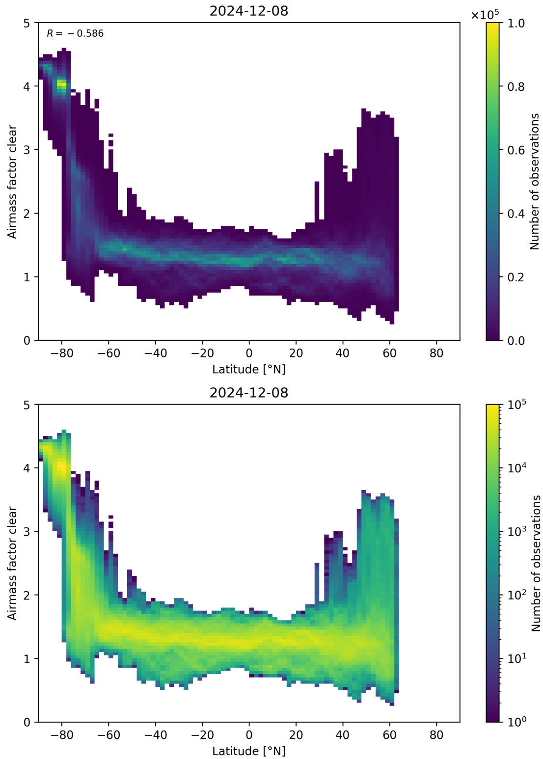
Figure 156: Scatter density plot of “Latitude” against “Airmass factor clear” for 2024-12-07 to 2024-12-09.
