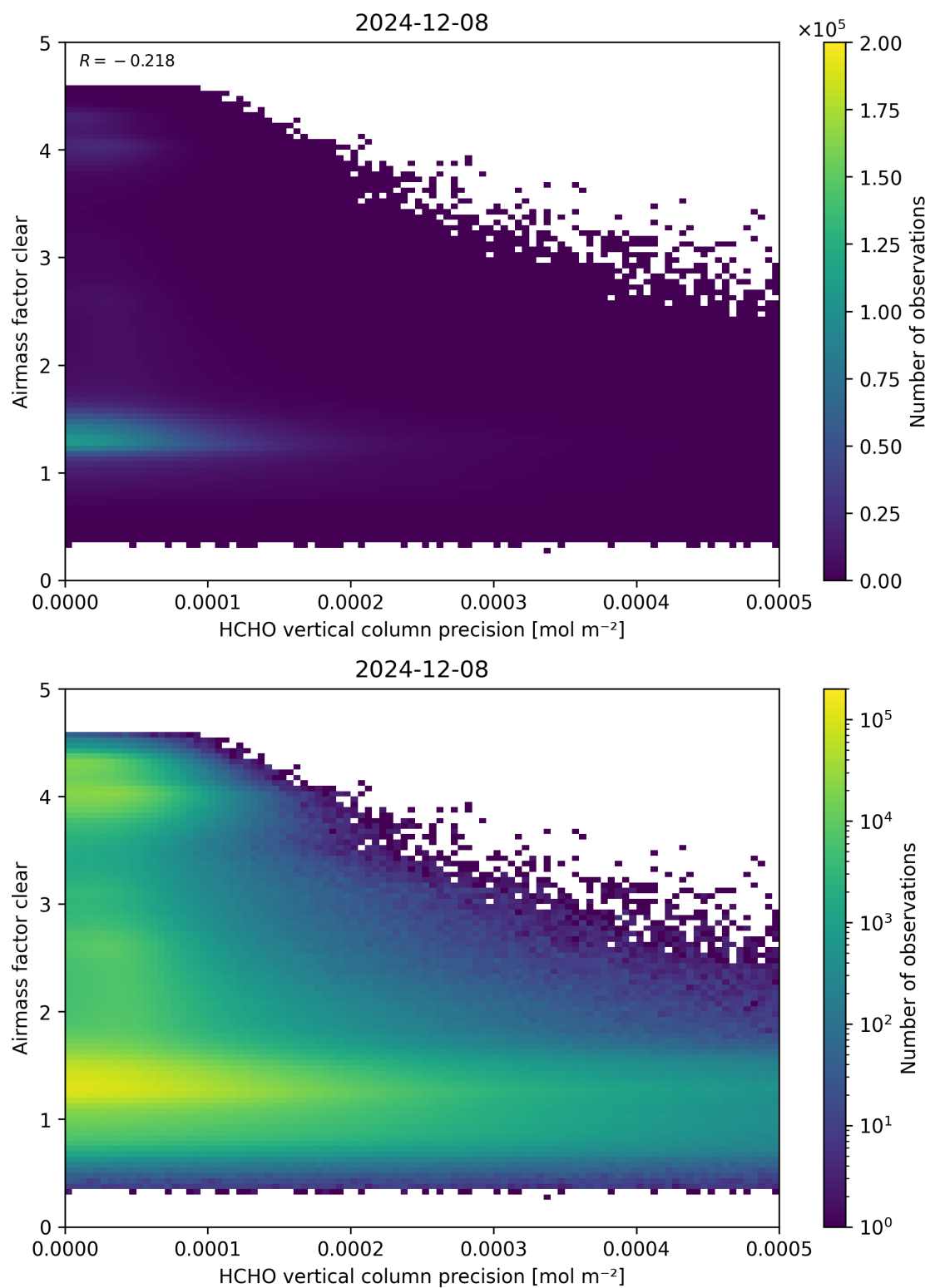
Figure 139: Scatter density plot of “HCHO vertical column precision” against “Airmass factor clear” for 2024-12-07 to 2024-12-09.
