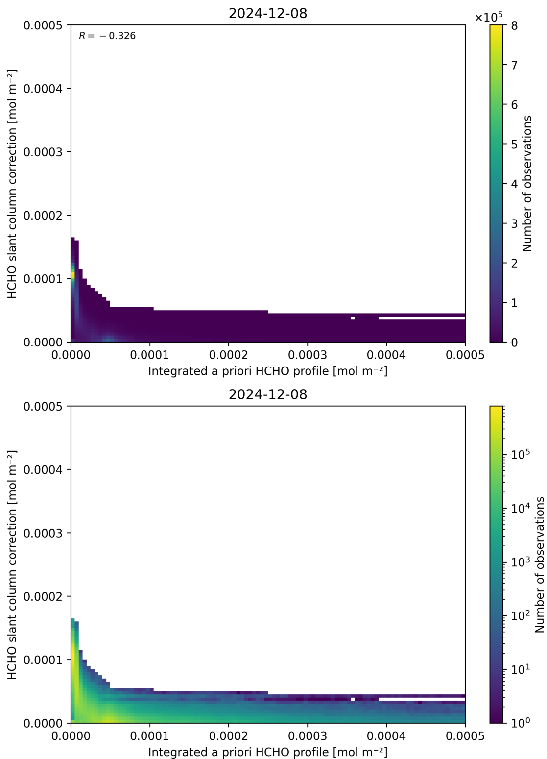
Figure 152: Scatter density plot of “Integrated a priori HCHO profile” against “HCHO slant column correction” for 2024-12-07 to 2024-12-09.
