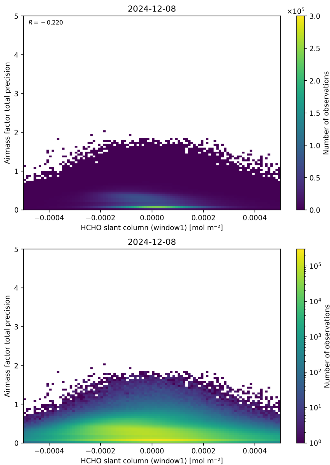
Figure 86: Scatter density plot of “HCHO slant column (window1)” against “Airmass factor total precision” for 2024-12-07 to 2024-12-09.
