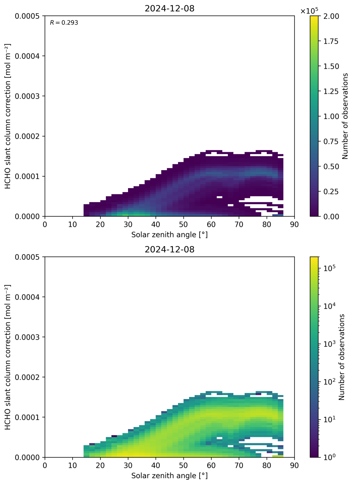
Figure 172: Scatter density plot of “Solar zenith angle” against “HCHO slant column correction” for 2024-12-07 to 2024-12-09.
