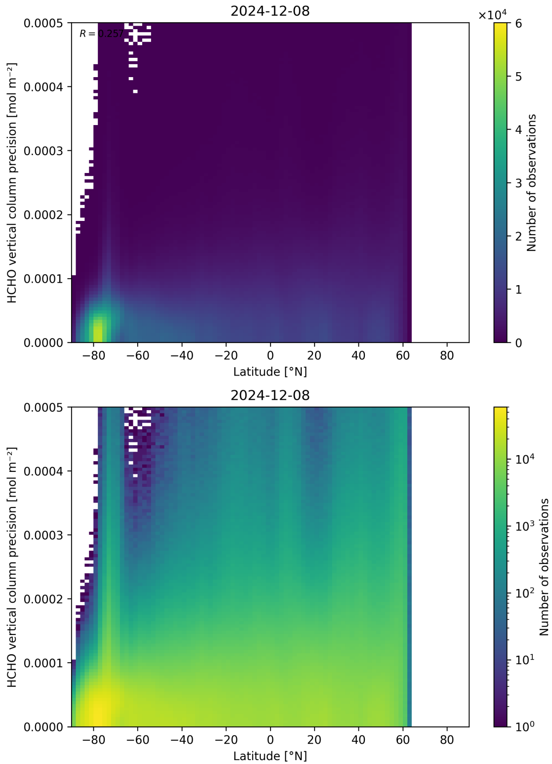
Figure 165: Scatter density plot of “Latitude” against “HCHO vertical column precision” for 2024-12-07 to 2024-12-09.
