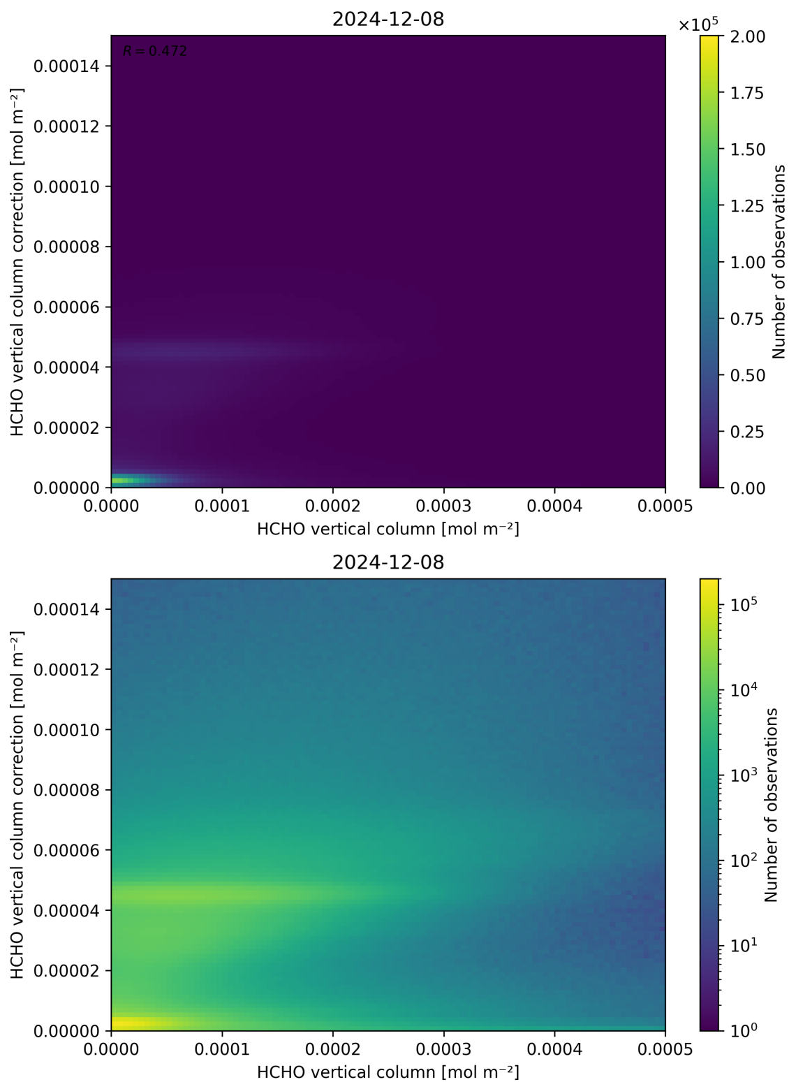
Figure 133: Scatter density plot of “HCHO vertical column” against “HCHO vertical column correction” for 2024-12-07 to 2024-12-09.
