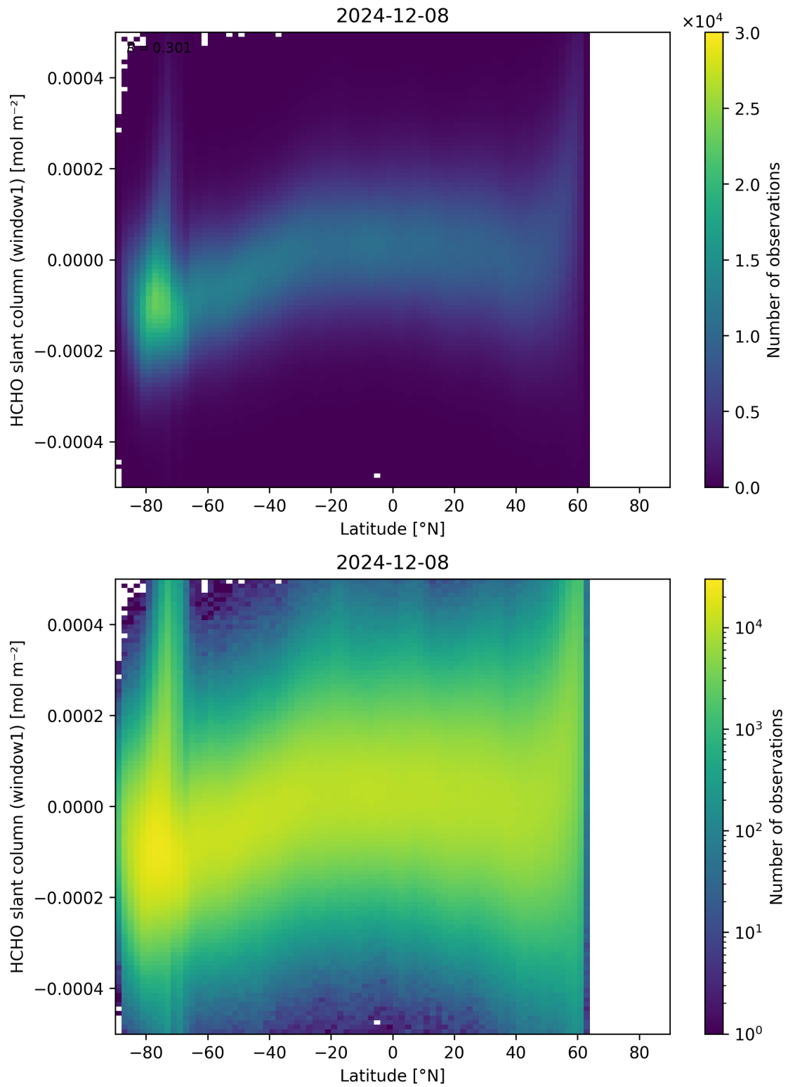
Figure 159: Scatter density plot of “Latitude” against “HCHO slant column (window1)” for 2024-12-07 to 2024-12-09.
