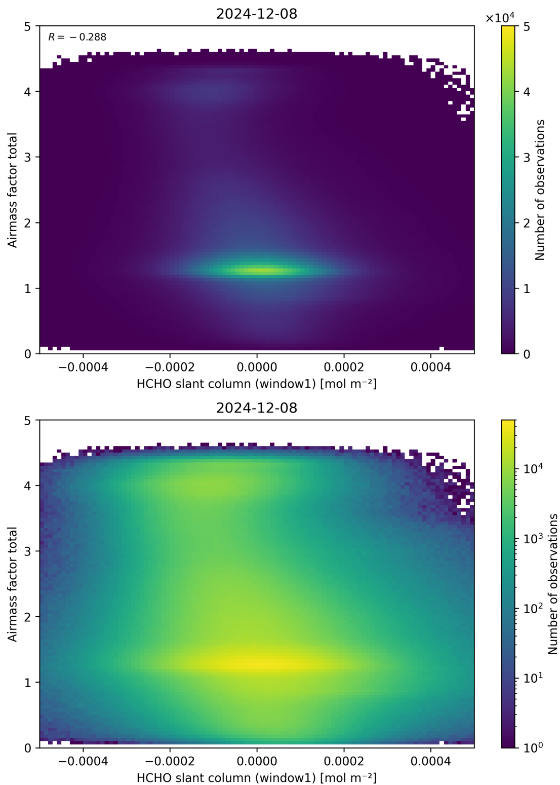
Figure 85: Scatter density plot of “HCHO slant column (window1)” against “Airmass factor total” for 2024-12-07 to 2024-12-09.
