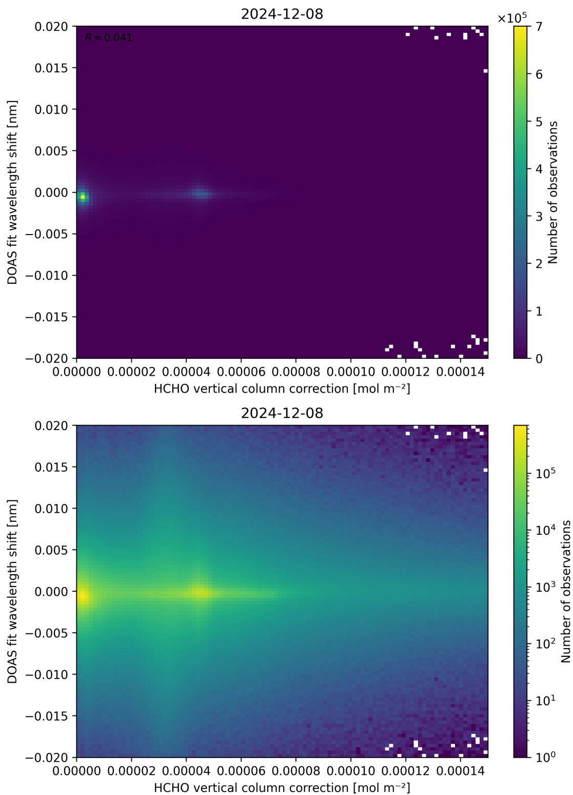
Figure 113: Scatter density plot of “HCHO vertical column correction” against “DOAS fit wavelength shift” for 2024-12-07 to 2024-12-09.
