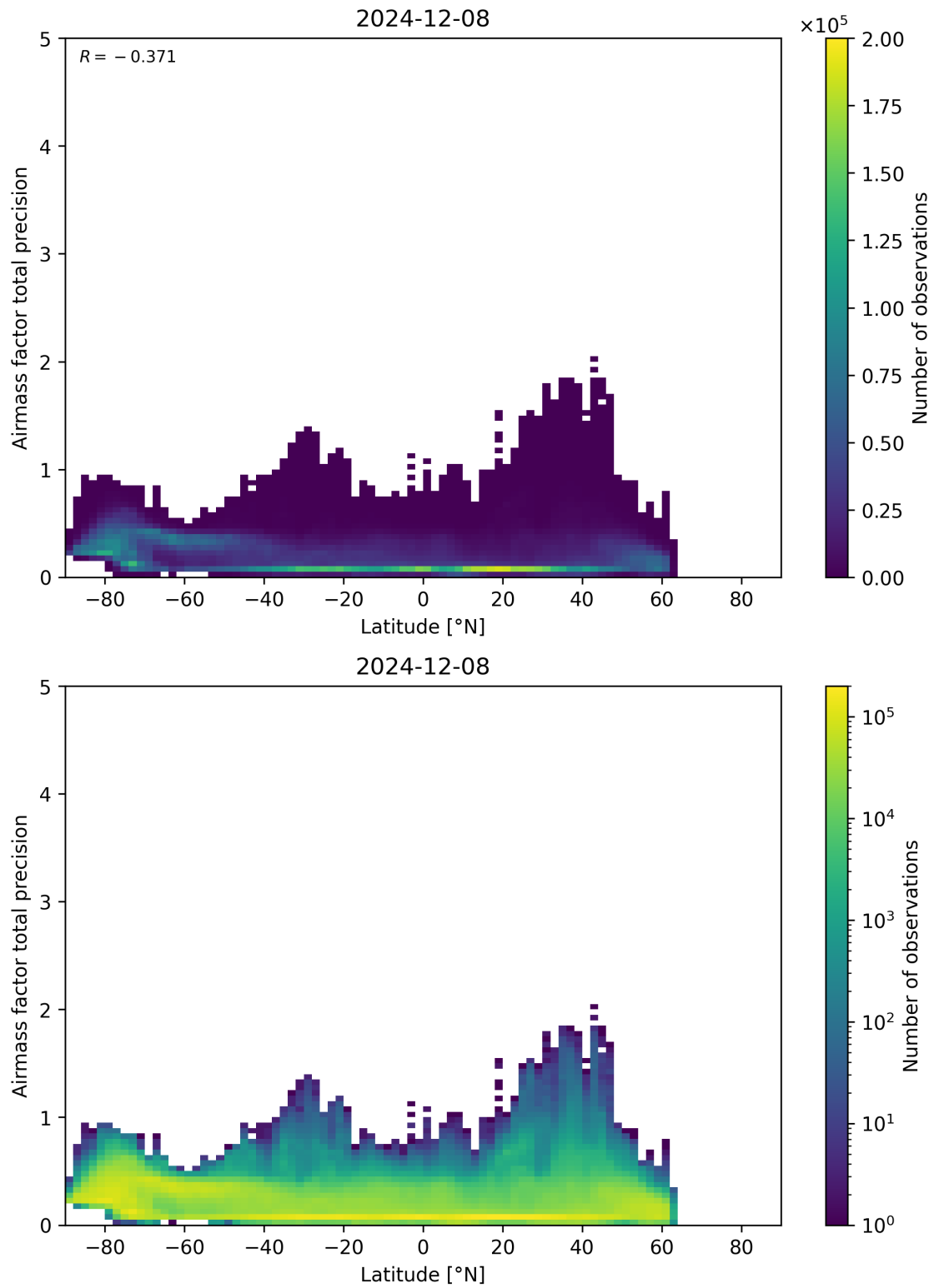
Figure 162: Scatter density plot of “Latitude” against “Airmass factor total precision” for 2024-12-07 to 2024-12-09.
