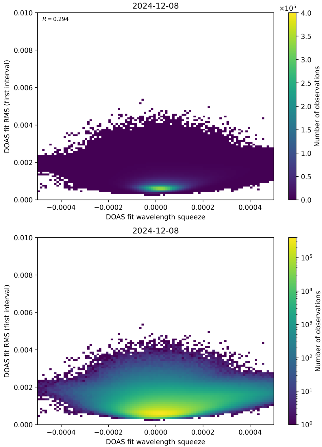
Figure 68: Scatter density plot of “DOAS fit wavelength squeeze” against “DOAS fit RMS (first interval)” for 2024-12-07 to 2024-12-09.
