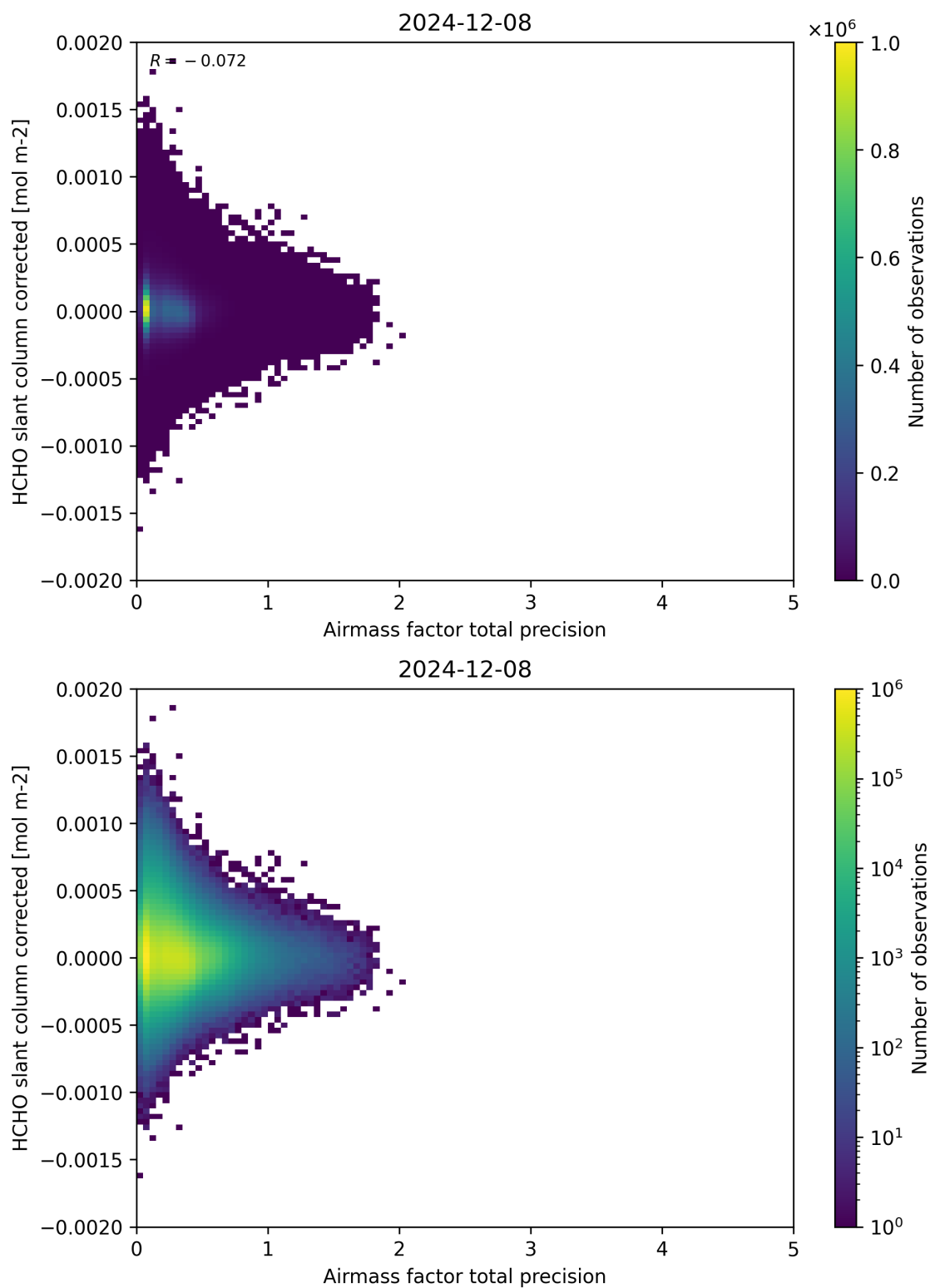
Figure 109: Scatter density plot of “Airmass factor total precision” against “HCHO slant column corrected” for 2024-12-07 to 2024-12-09.
