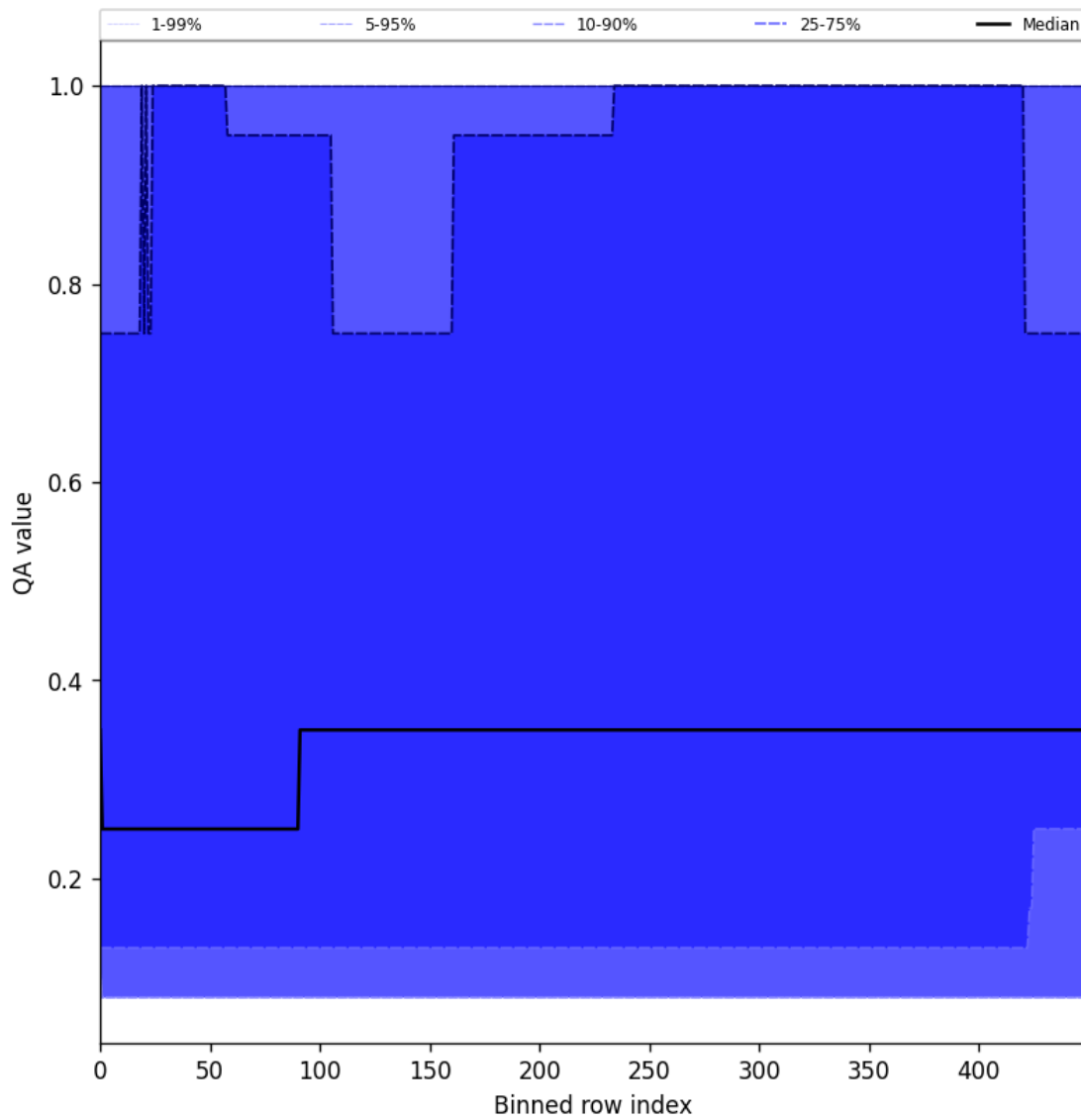
Figure 48: Along track statistics of “QA value” for 2024-12-07 to 2024-12-09
