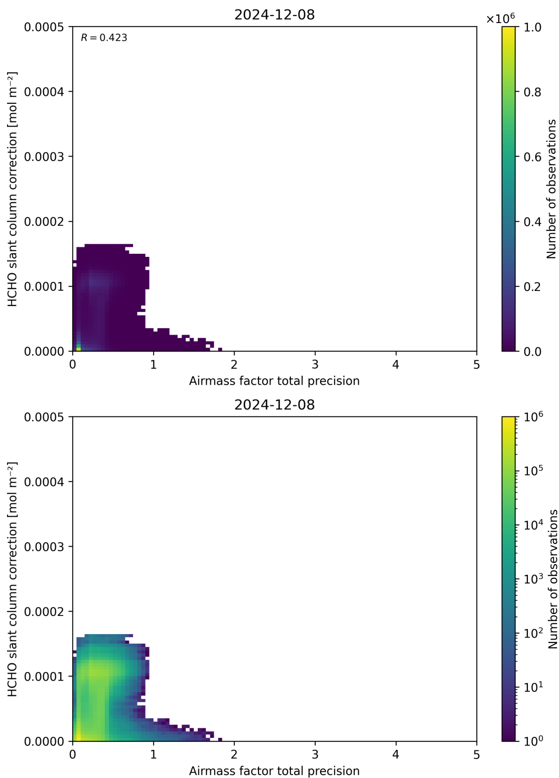
Figure 110: Scatter density plot of “Airmass factor total precision” against “HCHO slant column correction” for 2024-12-07 to 2024-12-09.
