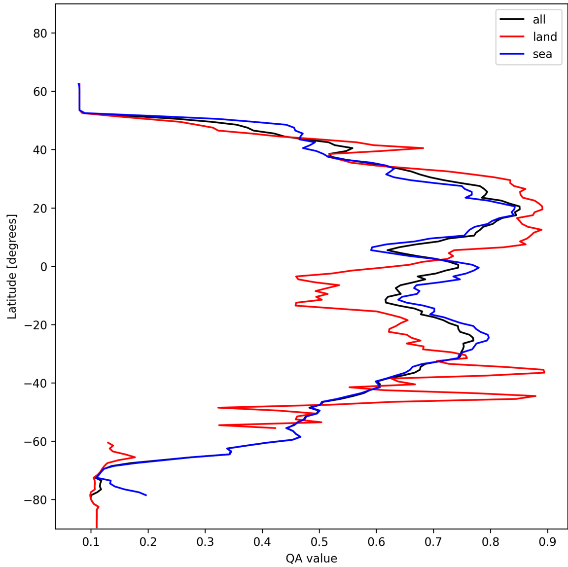
Figure 20: Zonal average of “QA value” for 2024-12-07 to 2024-12-09.
