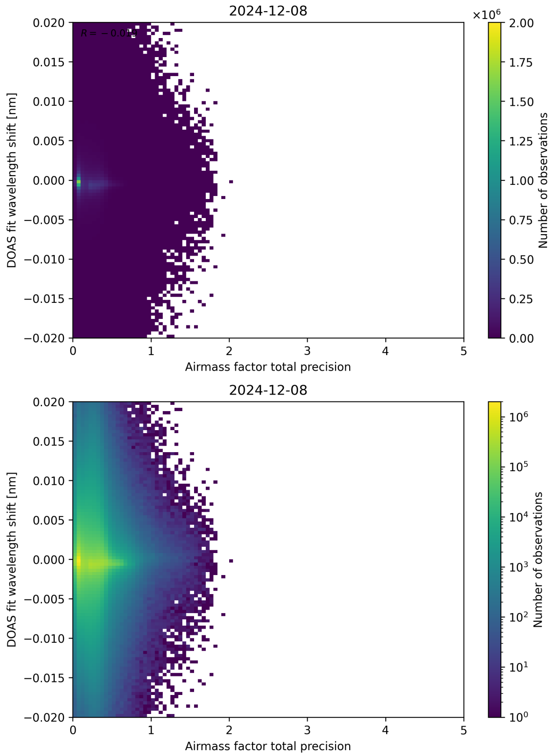
Figure 106: Scatter density plot of “Airmass factor total precision” against “DOAS fit wavelength shift” for 2024-12-07 to 2024-12-09.
