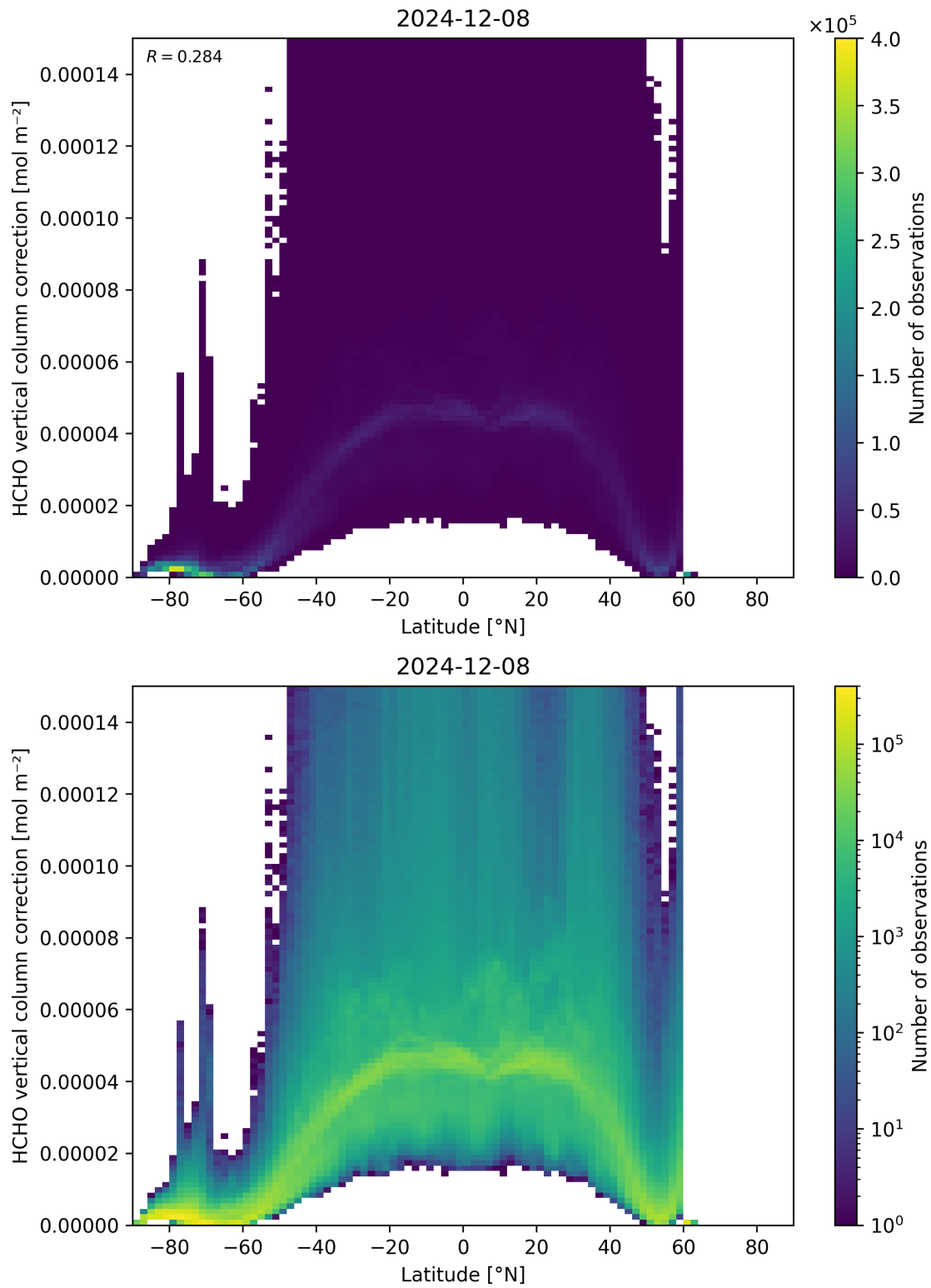
Figure 164: Scatter density plot of “Latitude” against “HCHO vertical column correction” for 2024-12-07 to 2024-12-09.
