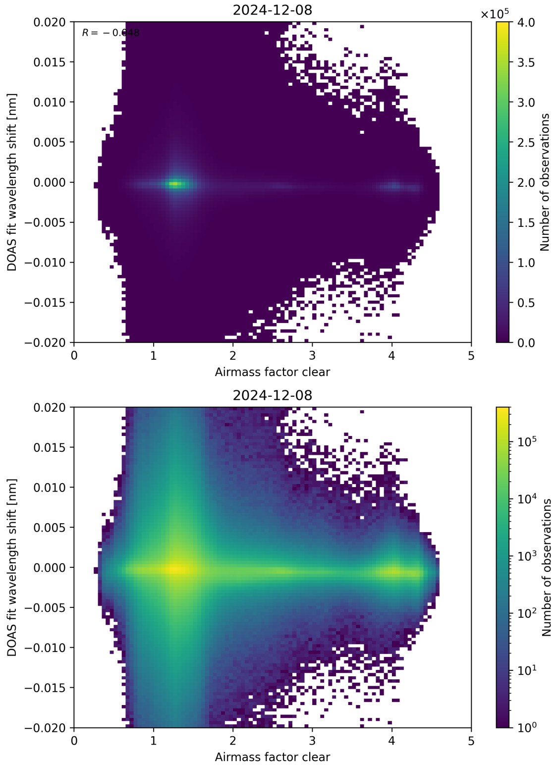
Figure 72: Scatter density plot of “Airmass factor clear” against “DOAS fit wavelength shift” for 2024-12-07 to 2024-12-09.
