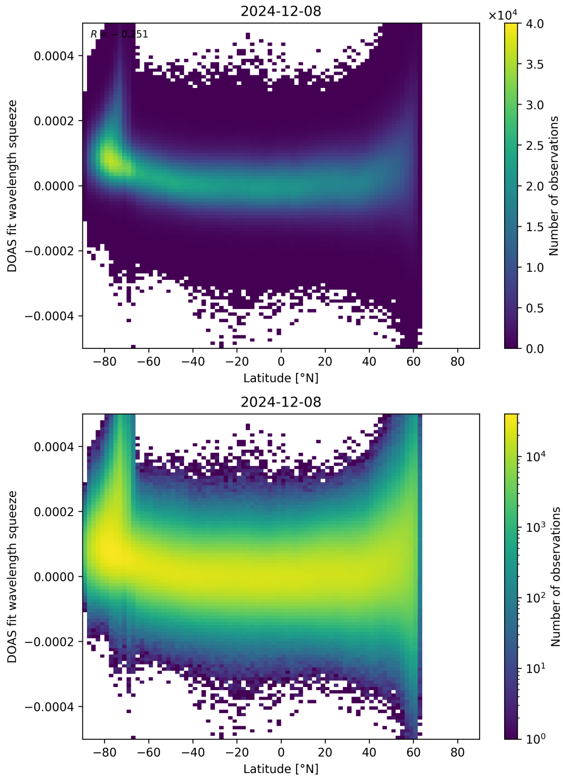
Figure 155: Scatter density plot of “Latitude” against “DOAS fit wavelength squeeze” for 2024-12-07 to 2024-12-09.
