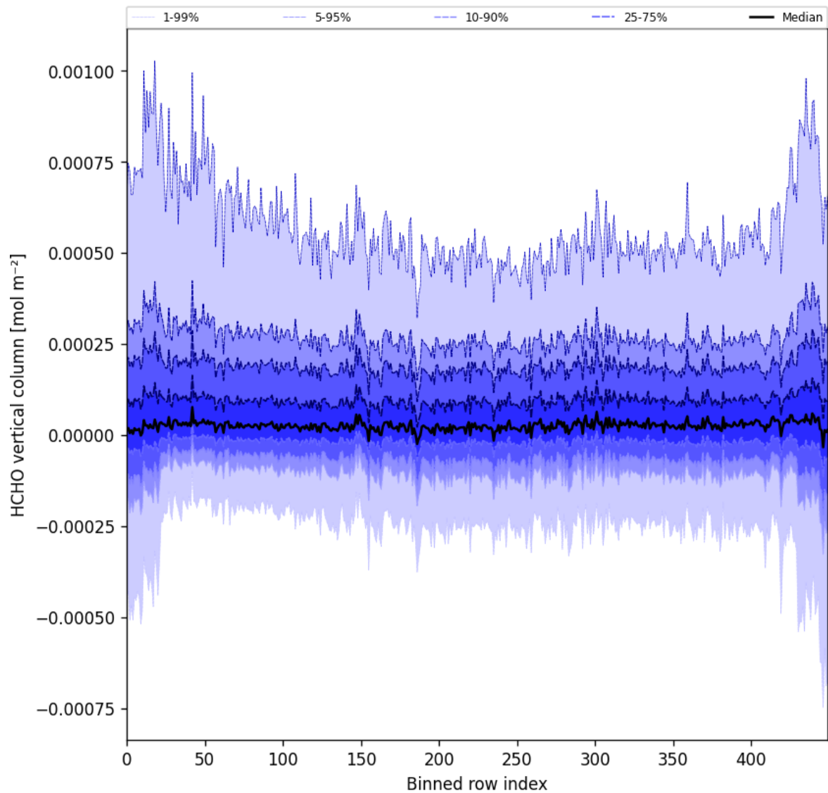
Figure 49: Along track statistics of “HCHO vertical column” for 2024-12-07 to 2024-12-09
