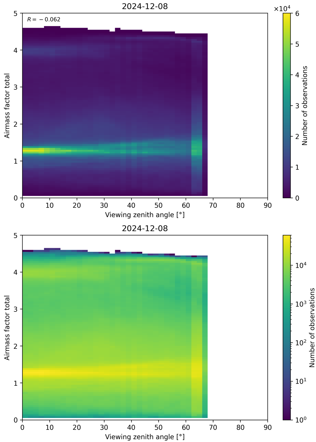
Figure 190: Scatter density plot of “Viewing zenith angle” against “Airmass factor total” for 2024-12-07 to 2024-12-09.
