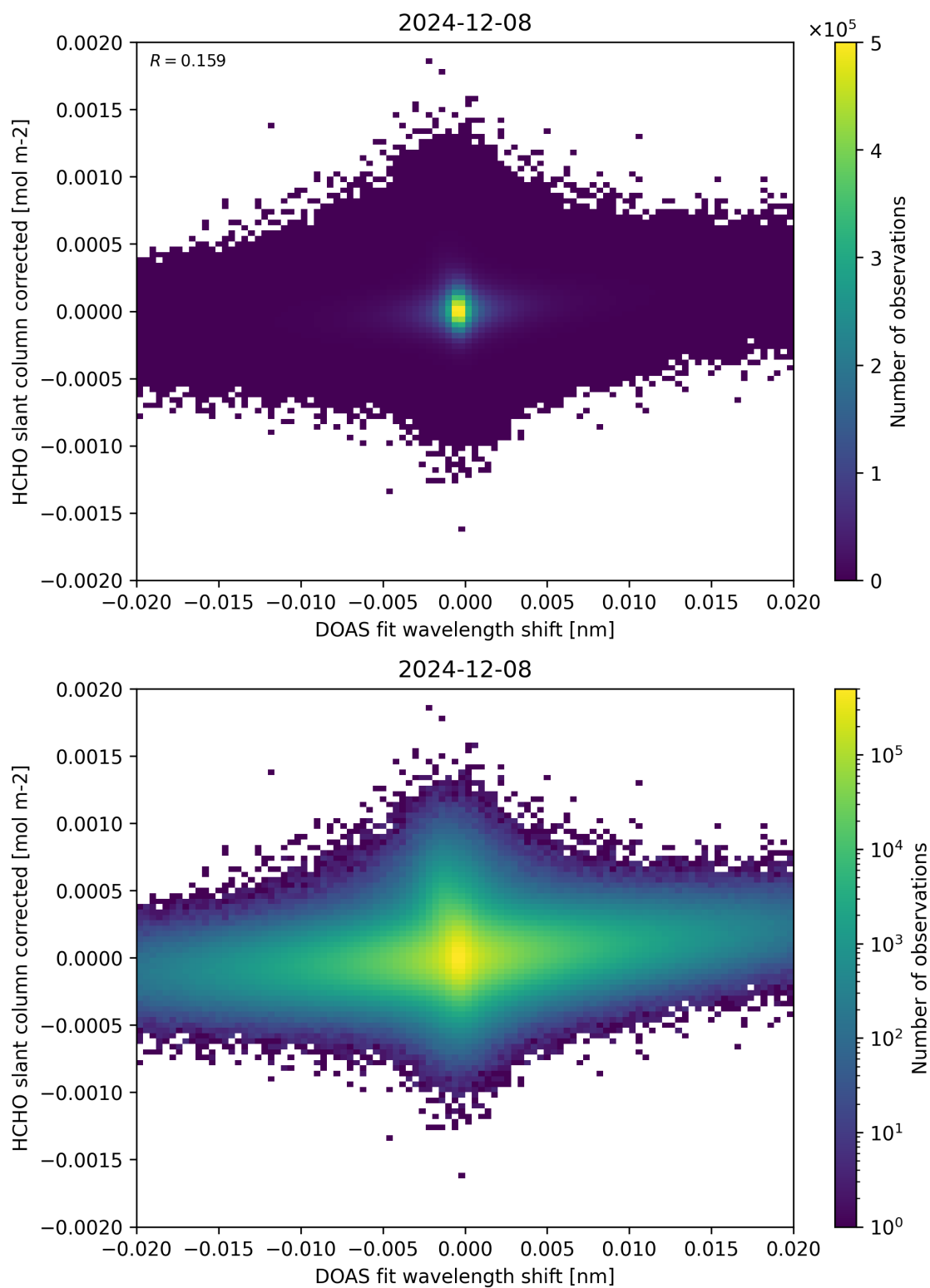
Figure 66: Scatter density plot of “DOAS fit wavelength shift” against “HCHO slant column corrected” for 2024-12-07 to 2024-12-09.
