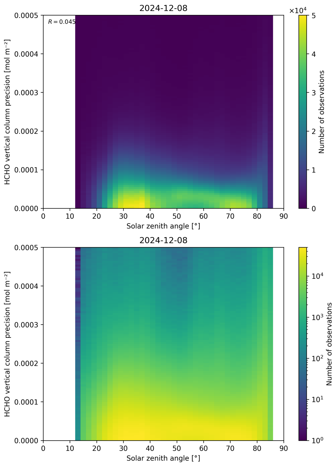
Figure 179: Scatter density plot of “Solar zenith angle” against “HCHO vertical column precision” for 2024-12-07 to 2024-12-09.
