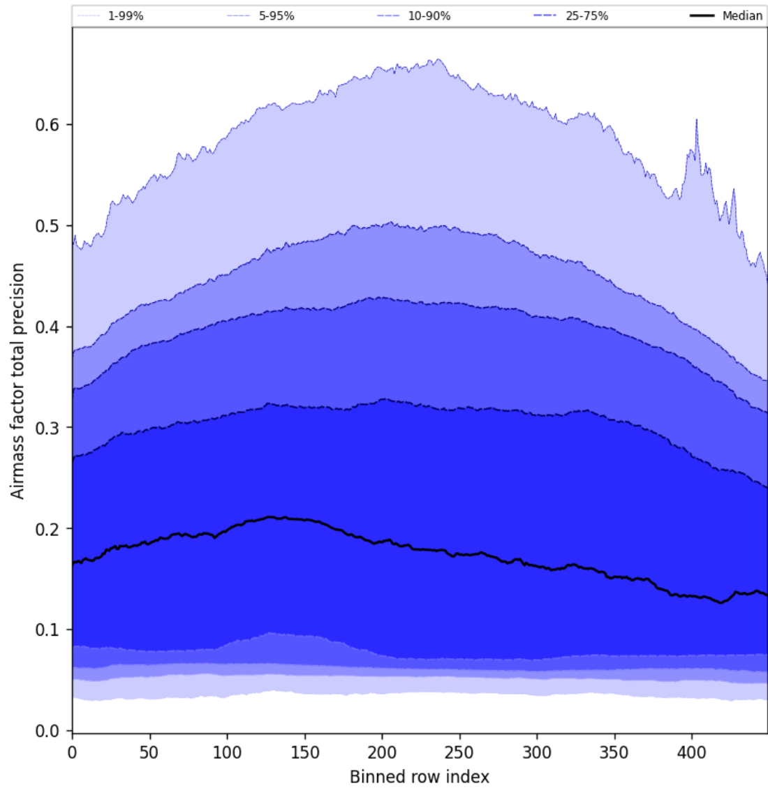
Figure 55: Along track statistics of “Airmass factor total precision” for 2024-12-07 to 2024-12-09
