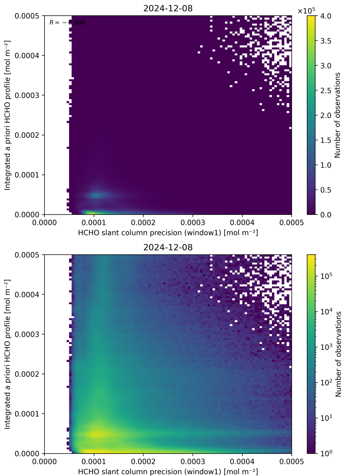
Figure 96: Scatter density plot of “HCHO slant column precision (window1)” against “Integrated a priori HCHO profile” for 2024-12-07 to 2024-12-09.
