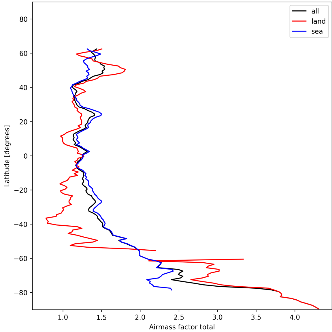
Figure 26: Zonal average of “Airmass factor total” for 2024-12-07 to 2024-12-09.
