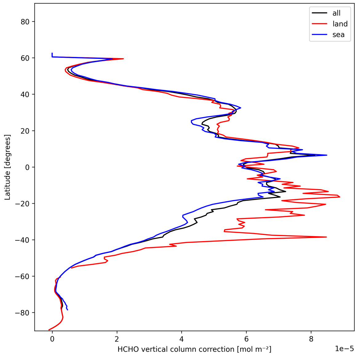
Figure 23: Zonal average of “HCHO vertical column correction” for 2024-12-07 to 2024-12-09.
