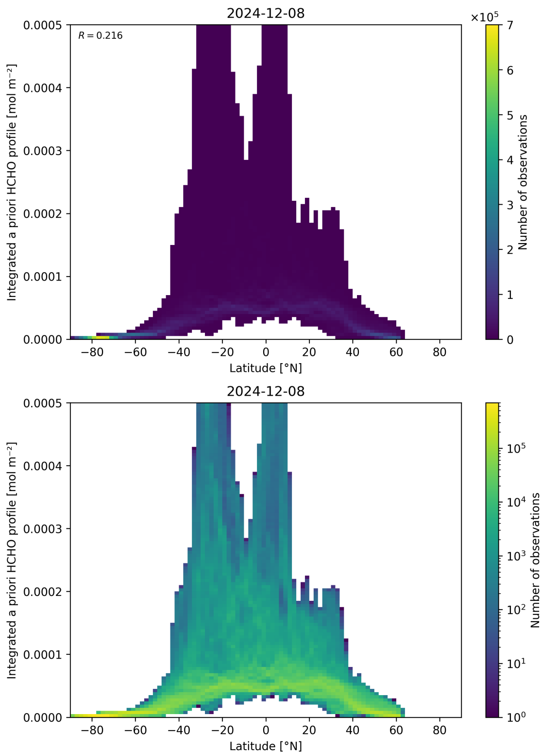
Figure 166: Scatter density plot of “Latitude” against “Integrated a priori HCHO profile” for 2024-12-07 to 2024-12-09.
