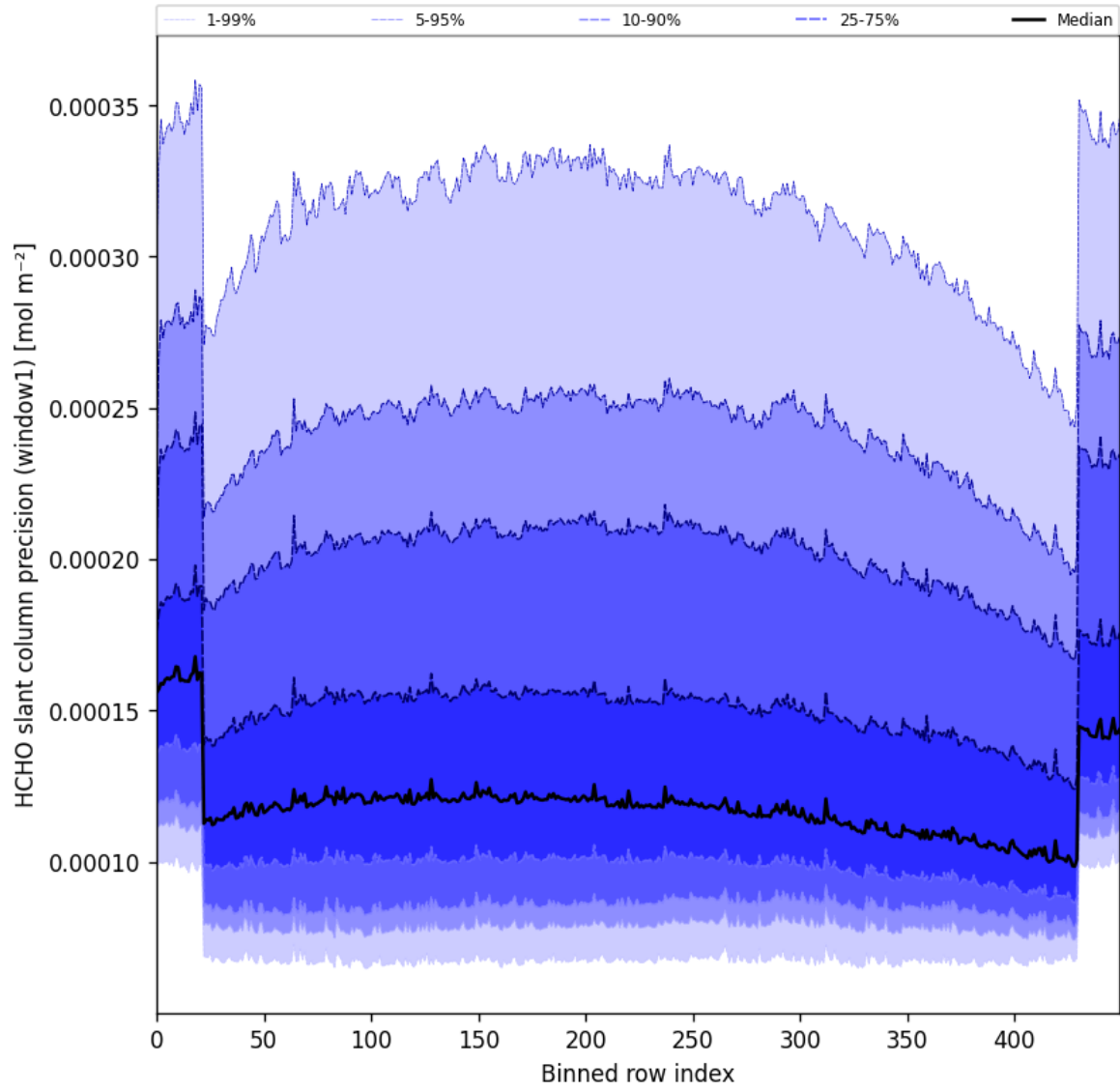
Figure 53: Along track statistics of “HCHO slant column precision (window1)” for 2024-12-07 to 2024-12-09
