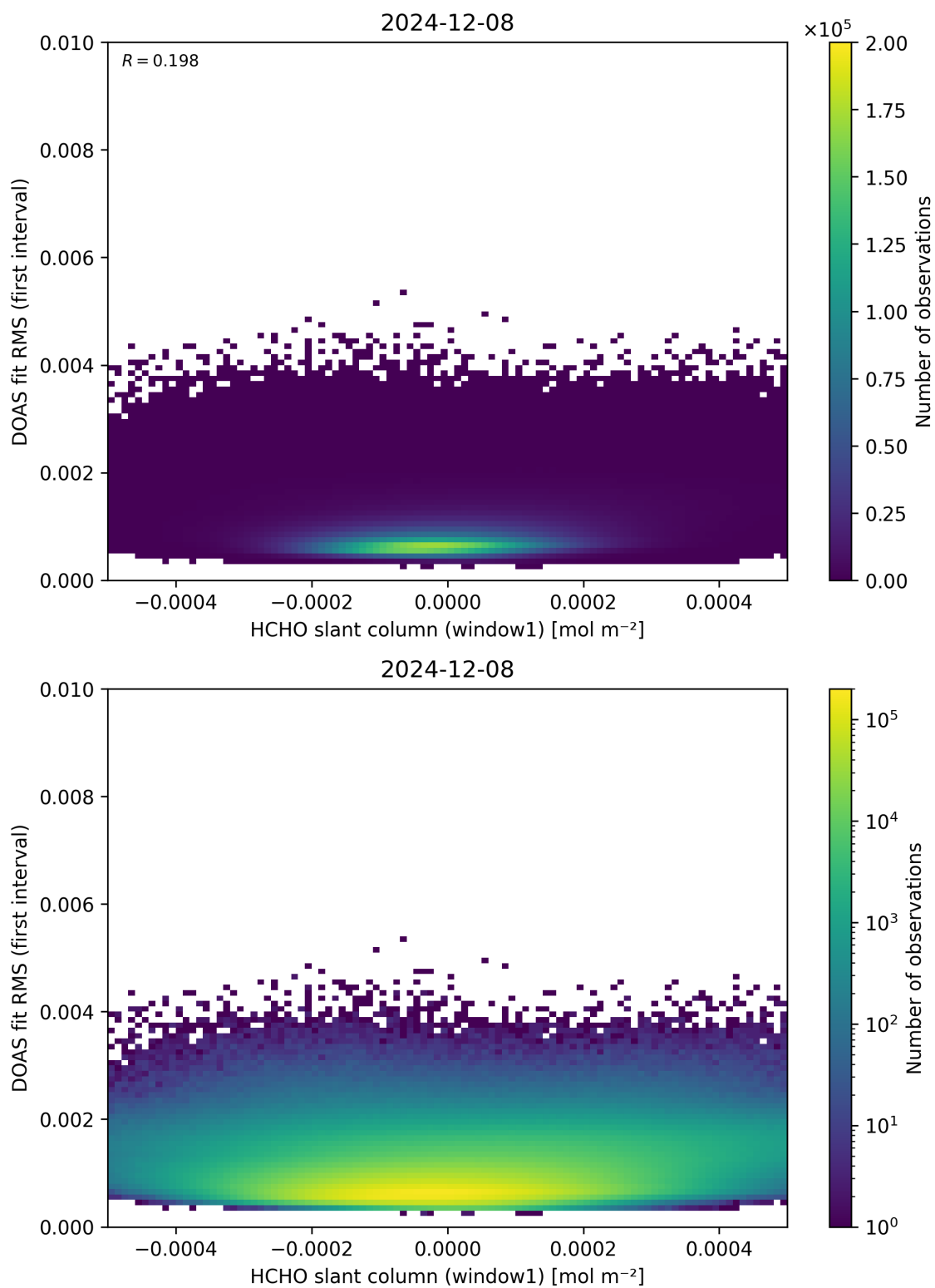
Figure 78: Scatter density plot of “HCHO slant column (window1)” against “DOAS fit RMS (first interval)” for 2024-12-07 to 2024-12-09.
