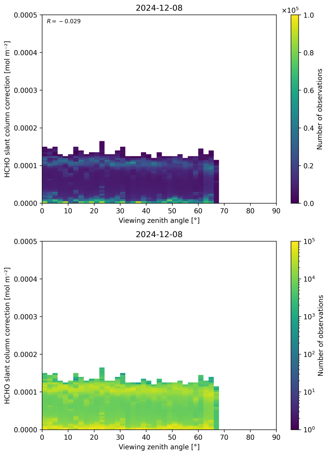
Figure 187: Scatter density plot of “Viewing zenith angle” against “HCHO slant column correction” for 2024-12-07 to 2024-12-09.
