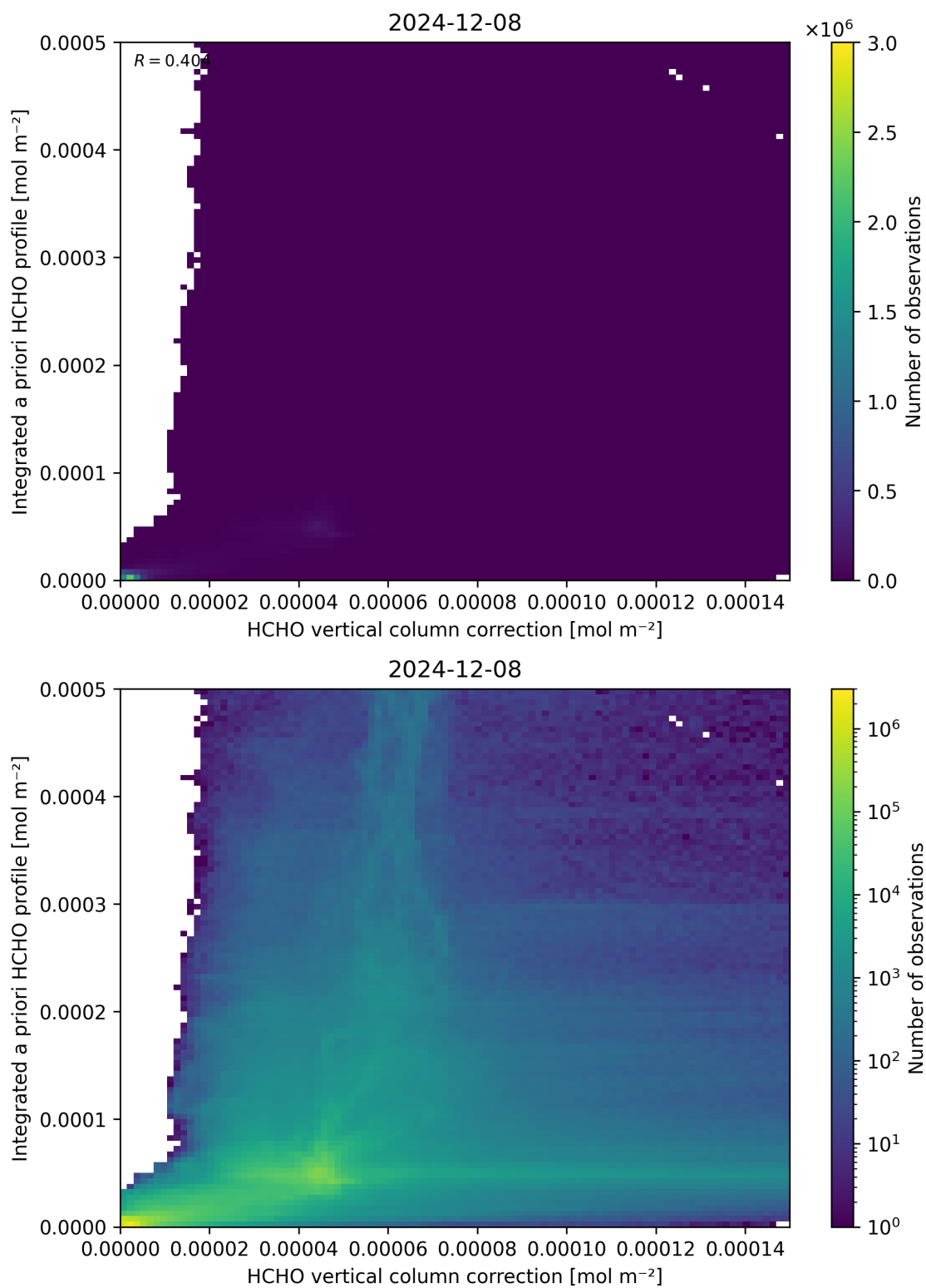
Figure 122: Scatter density plot of “HCHO vertical column correction” against “Integrated a priori HCHO profile” for 2024-12-07 to 2024-12-09.
