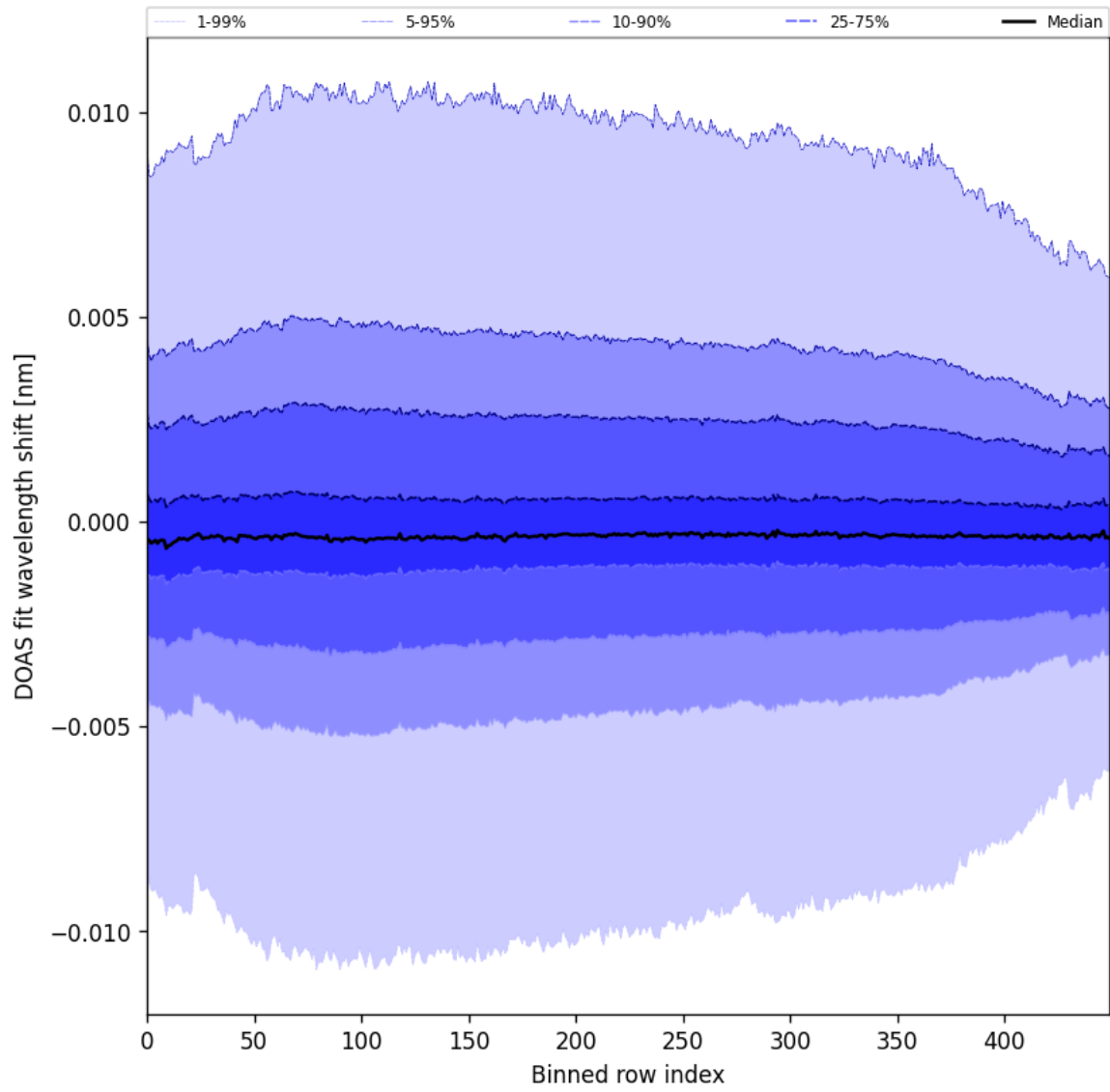
Figure 58: Along track statistics of “DOAS fit wavelength shift” for 2024-12-07 to 2024-12-09
