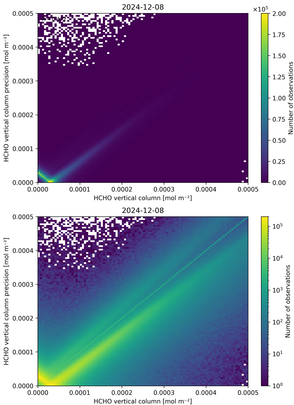
Figure 134: Scatter density plot of “HCHO vertical column” against “HCHO vertical column precision” for 2024-12-07 to 2024-12-09.
