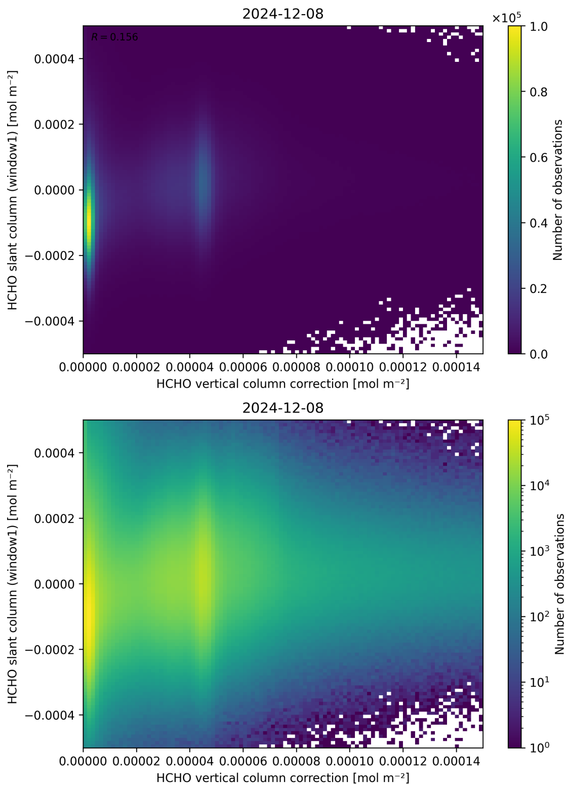
Figure 118: Scatter density plot of “HCHO vertical column correction” against “HCHO slant column (window1)” for 2024-12-07 to 2024-12-09.
