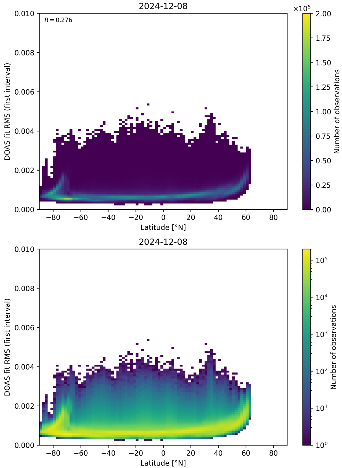
Figure 153: Scatter density plot of “Latitude” against “DOAS fit RMS (first interval)” for 2024-12-07 to 2024-12-09.
