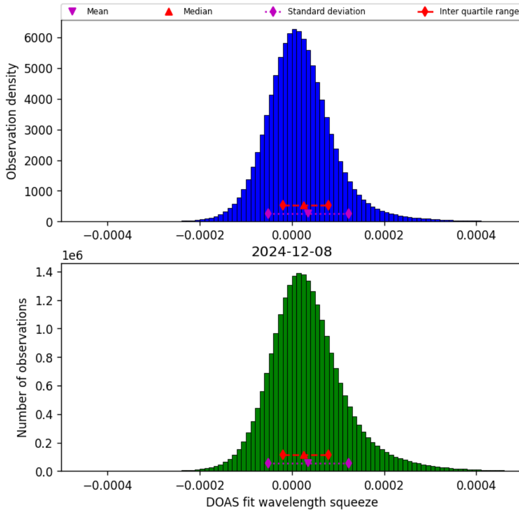
Figure 45: Histogram of “DOAS fit wavelength squeeze” for 2024-12-07 to 2024-12-09
