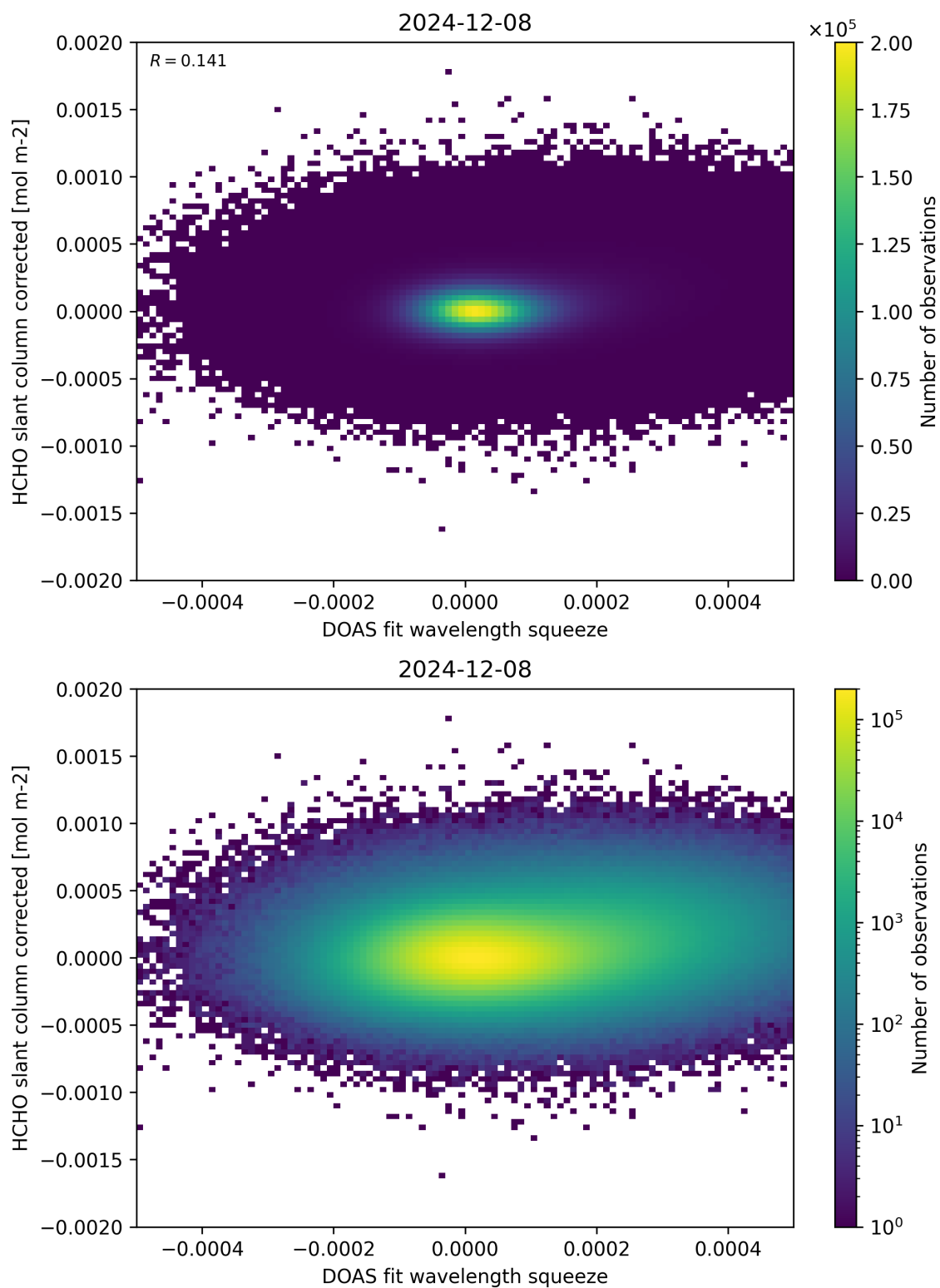
Figure 69: Scatter density plot of “DOAS fit wavelength squeeze” against “HCHO slant column corrected” for 2024-12-07 to 2024-12-09.
