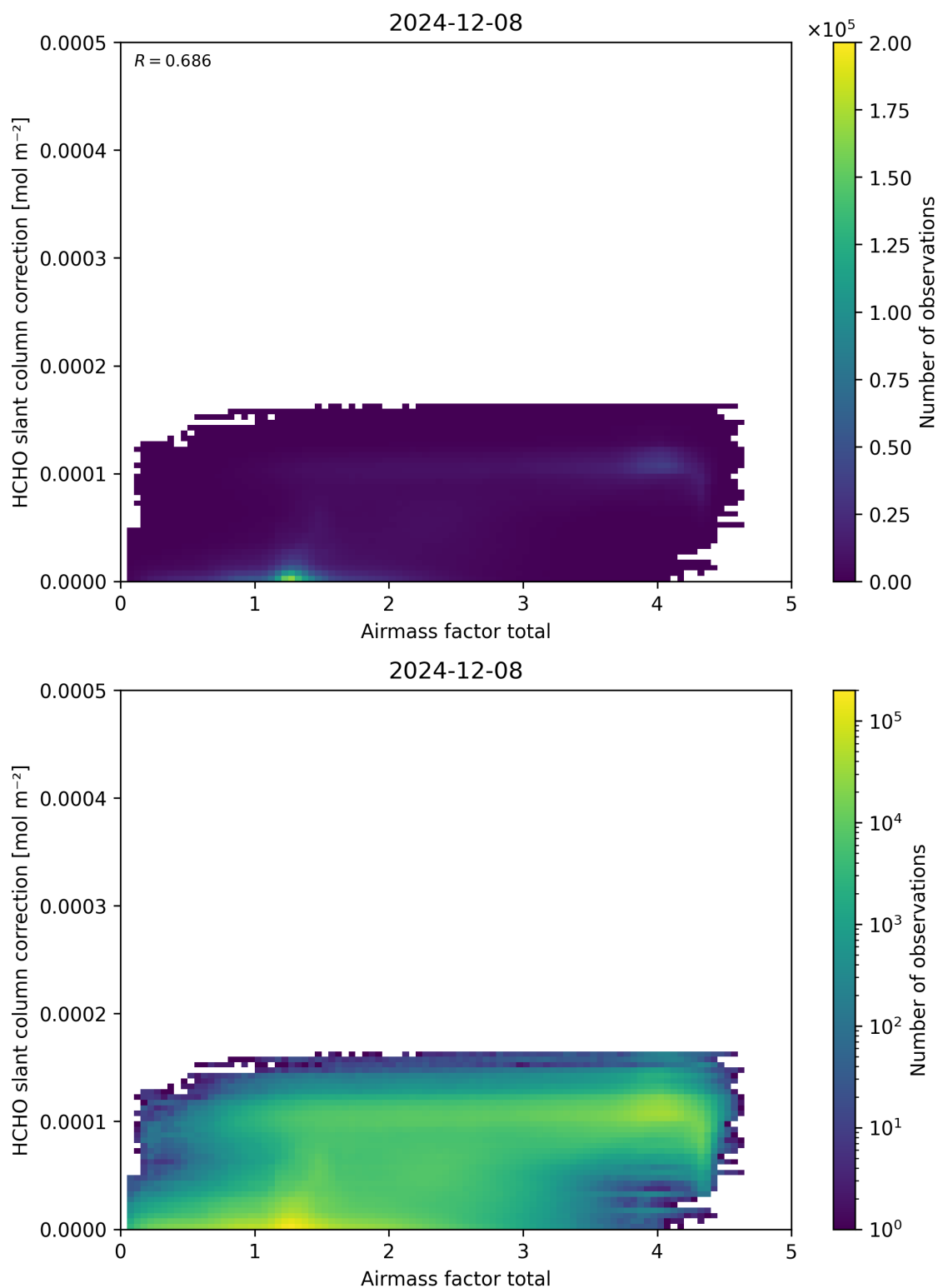
Figure 102: Scatter density plot of “Airmass factor total” against “HCHO slant column correction” for 2024-12-07 to 2024-12-09.
