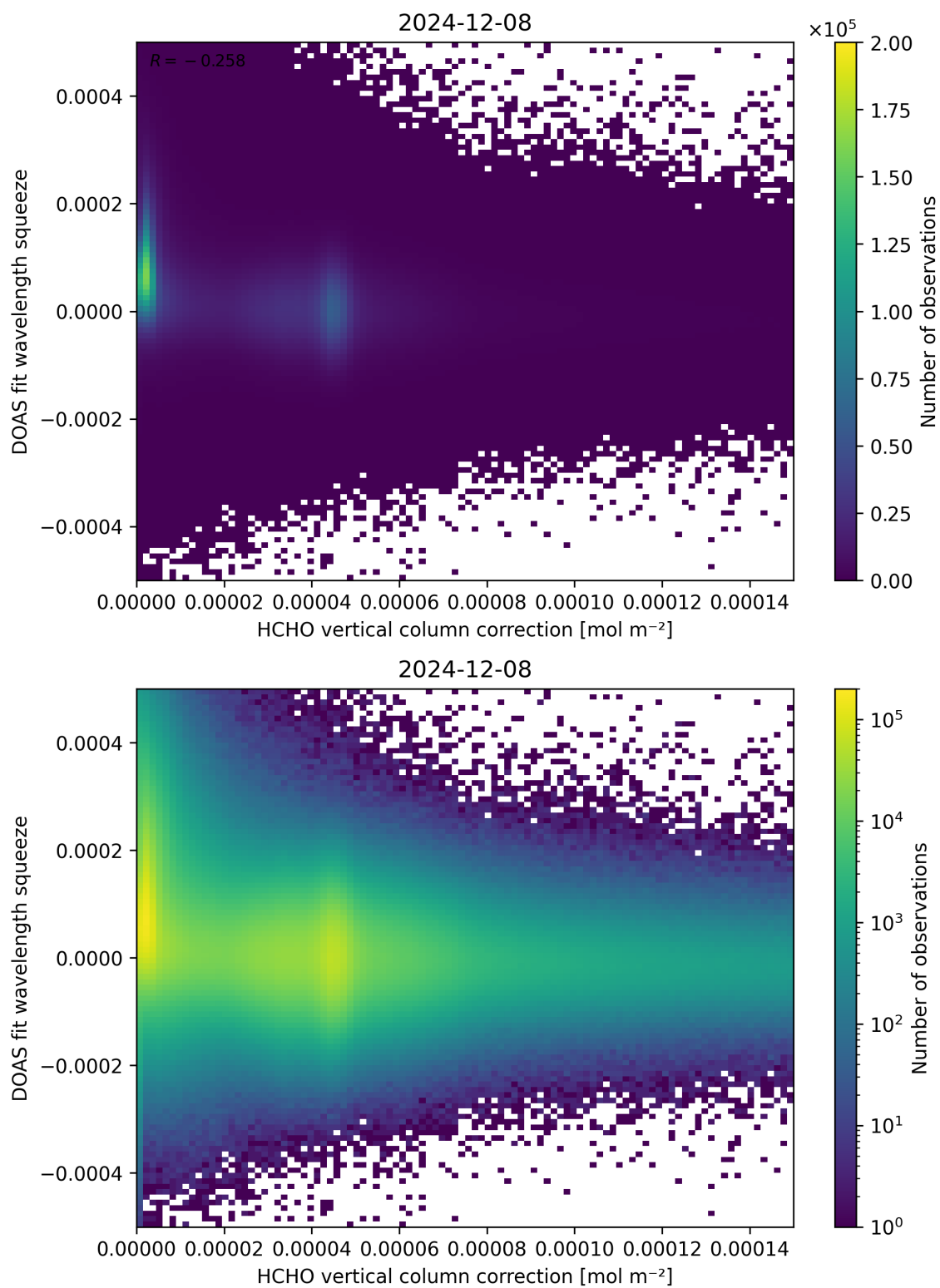
Figure 114: Scatter density plot of “HCHO vertical column correction” against “DOAS fit wavelength squeeze” for 2024-12-07 to 2024-12-09.
