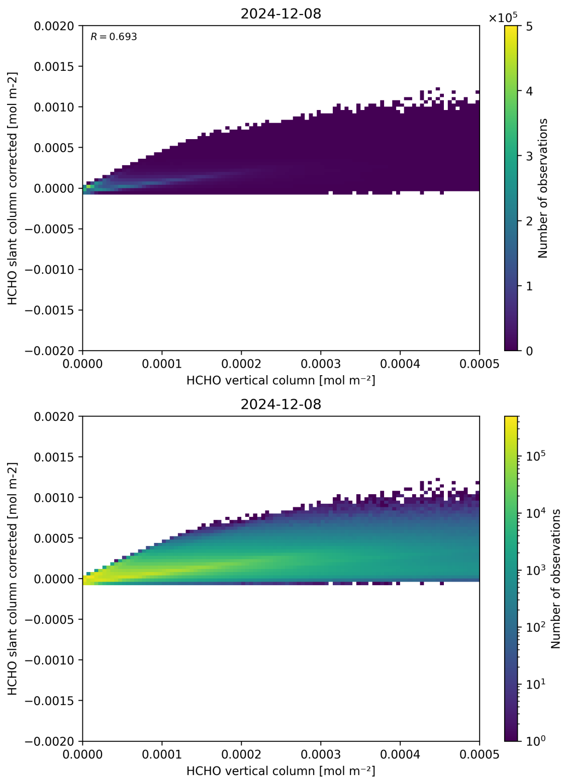
Figure 127: Scatter density plot of “HCHO vertical column” against “HCHO slant column corrected” for 2024-12-07 to 2024-12-09.
