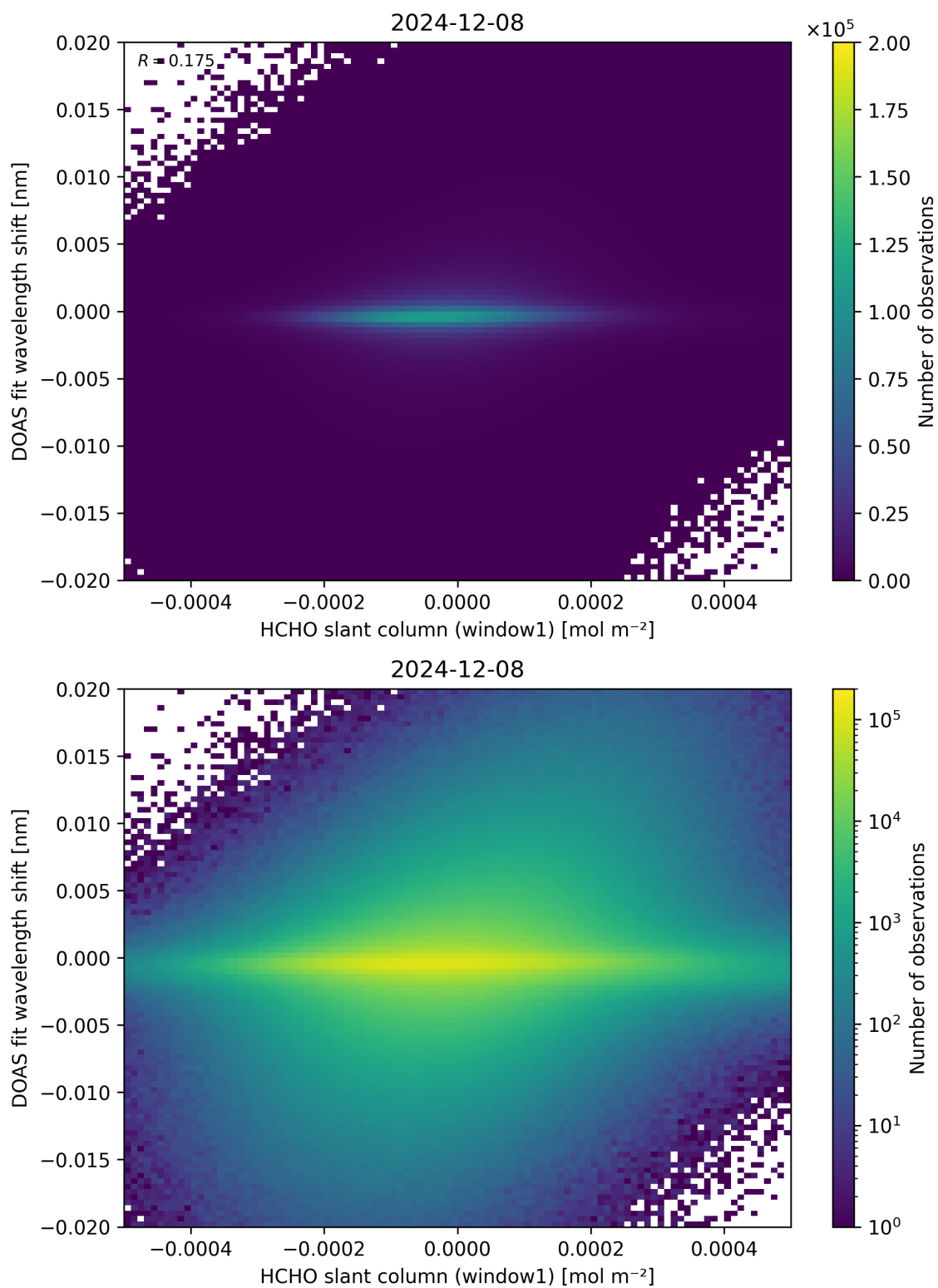
Figure 79: Scatter density plot of “HCHO slant column (window1)” against “DOAS fit wavelength shift” for 2024-12-07 to 2024-12-09.
