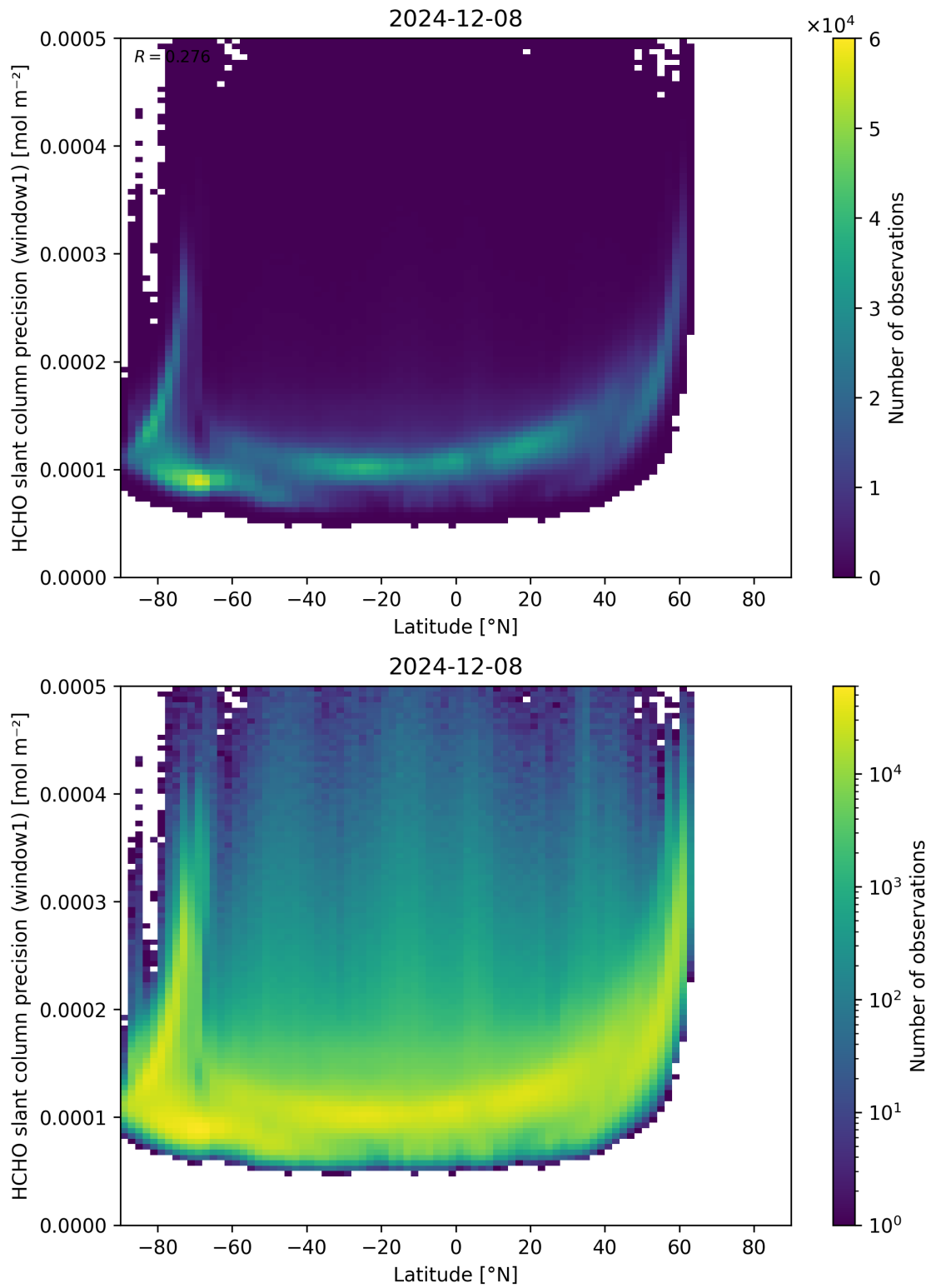
Figure 160: Scatter density plot of “Latitude” against “HCHO slant column precision (window1)” for 2024-12-07 to 2024-12-09.
