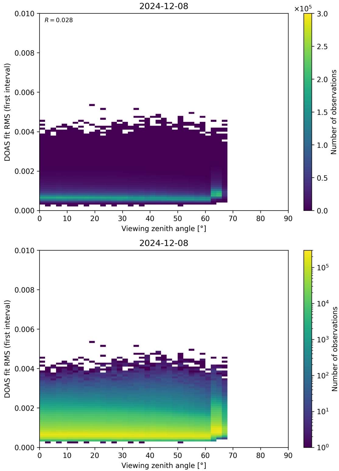
Figure 182: Scatter density plot of “Viewing zenith angle” against “DOAS fit RMS (first interval)” for 2024-12-07 to 2024-12-09.
