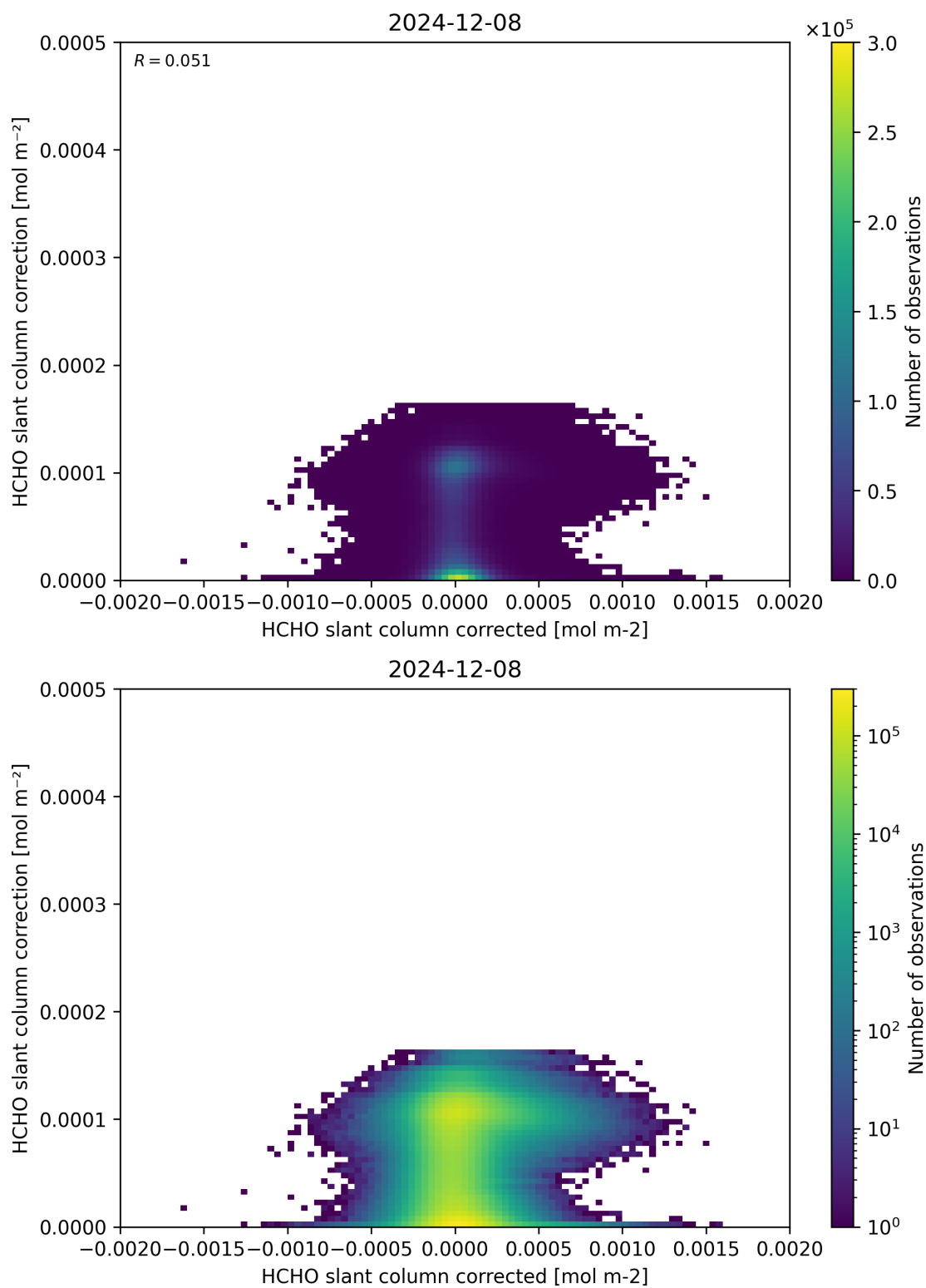
Figure 77: Scatter density plot of “HCHO slant column corrected” against “HCHO slant column correction” for 2024-12-07 to 2024-12-09.
