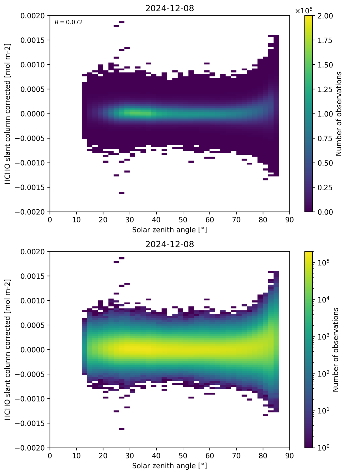
Figure 171: Scatter density plot of “Solar zenith angle” against “HCHO slant column corrected” for 2024-12-07 to 2024-12-09.
