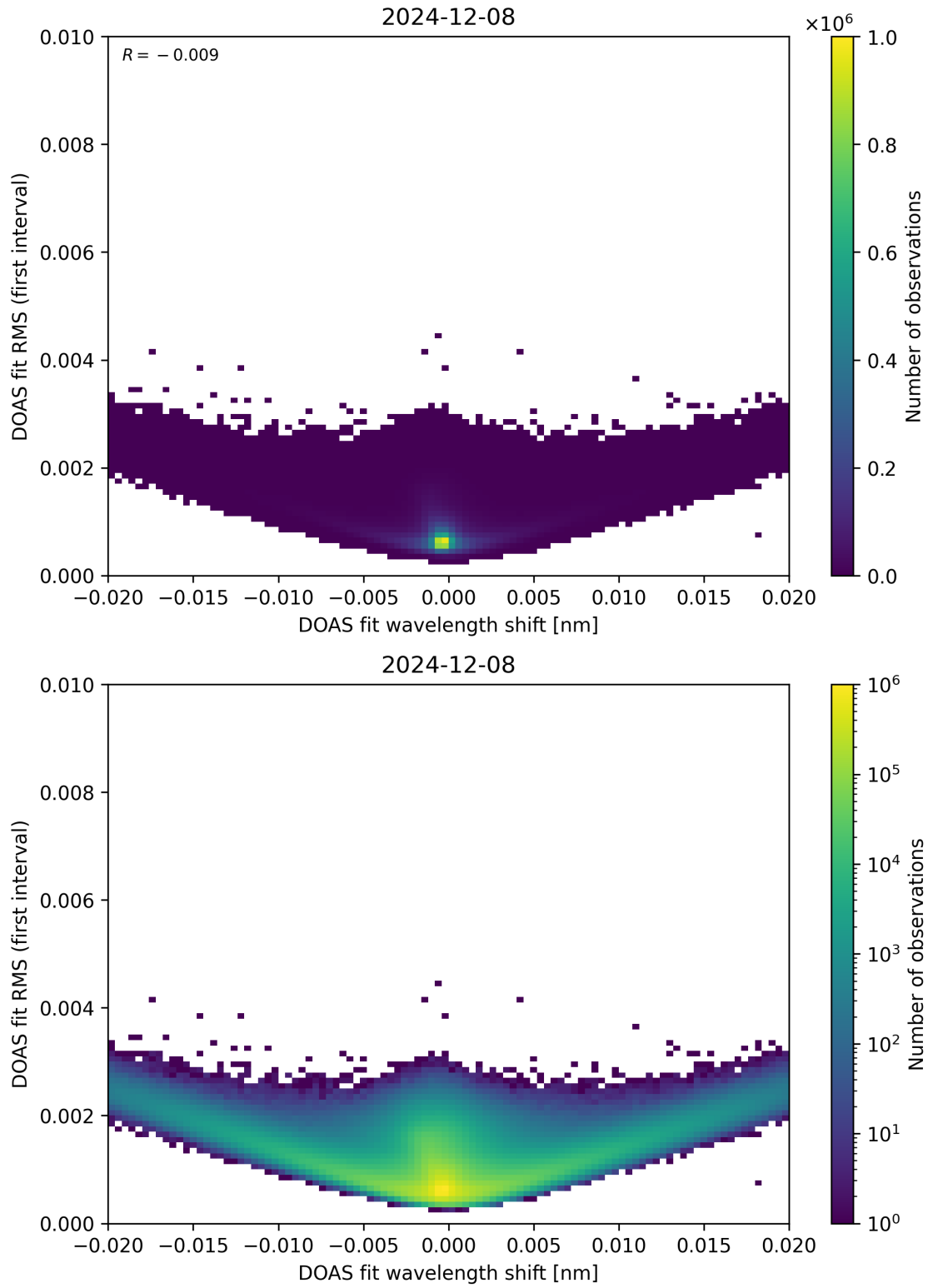
Figure 64: Scatter density plot of “DOAS fit wavelength shift” against “DOAS fit RMS (first interval)” for 2024-12-07 to 2024-12-09.
