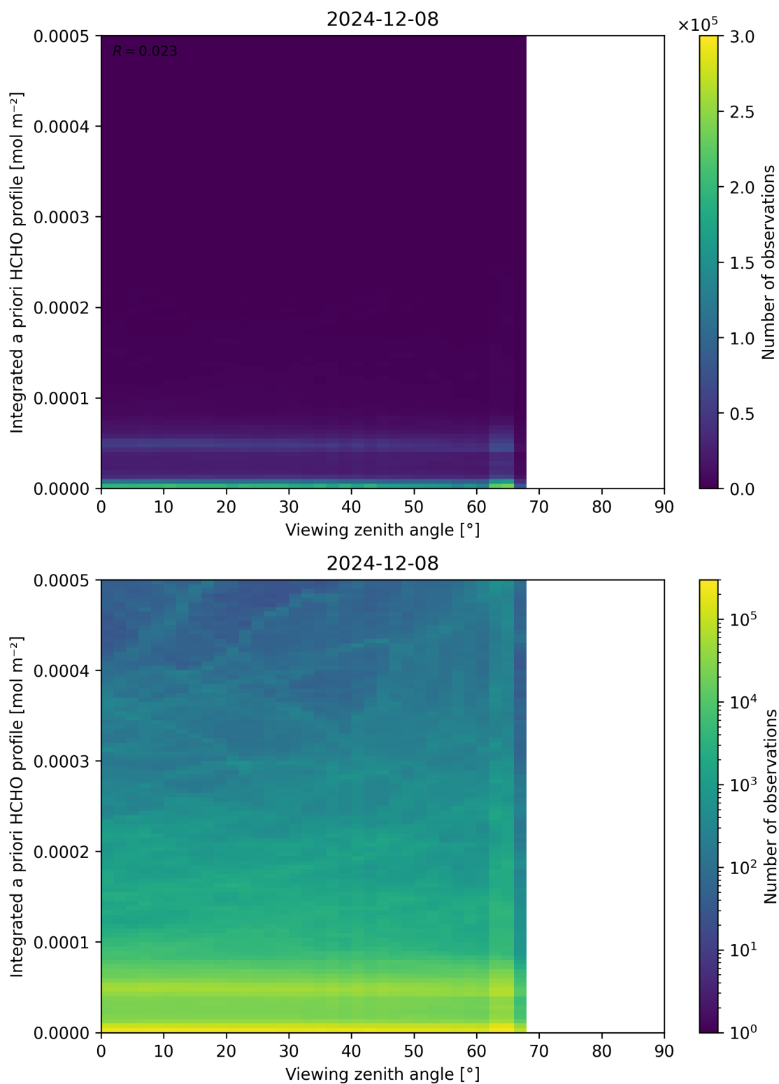
Figure 195: Scatter density plot of “Viewing zenith angle” against “Integrated a priori HCHO profile” for 2024-12-07 to 2024-12-09.
