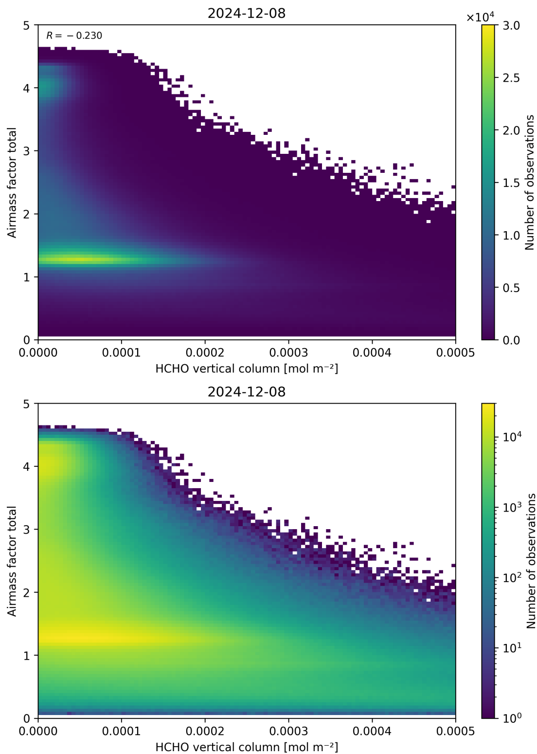
Figure 131: Scatter density plot of “HCHO vertical column” against “Airmass factor total” for 2024-12-07 to 2024-12-09.
