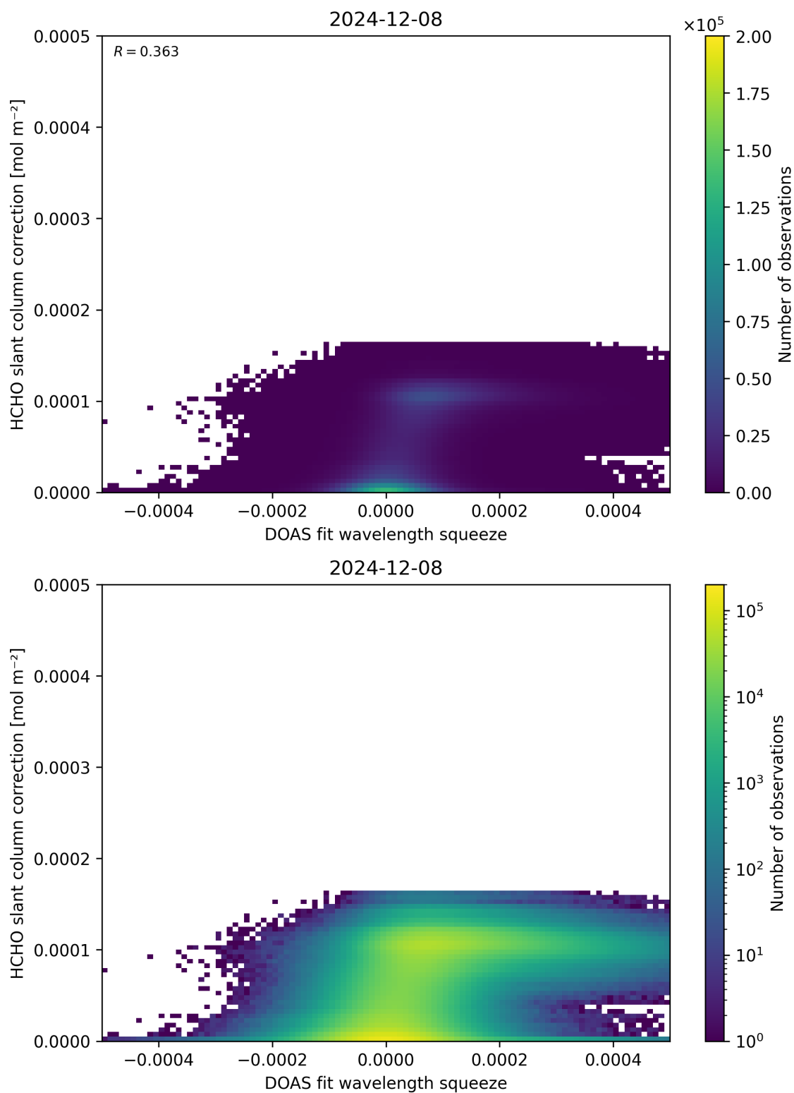
Figure 70: Scatter density plot of “DOAS fit wavelength squeeze” against “HCHO slant column correction” for 2024-12-07 to 2024-12-09.
