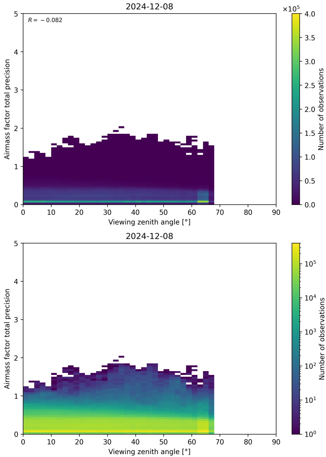
Figure 191: Scatter density plot of “Viewing zenith angle” against “Airmass factor total precision” for 2024-12-07 to 2024-12-09.
