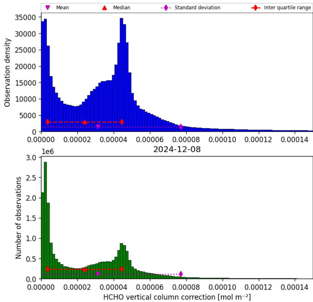
Figure 37: Histogram of “HCHO vertical column correction” for 2024-12-07 to 2024-12-09
