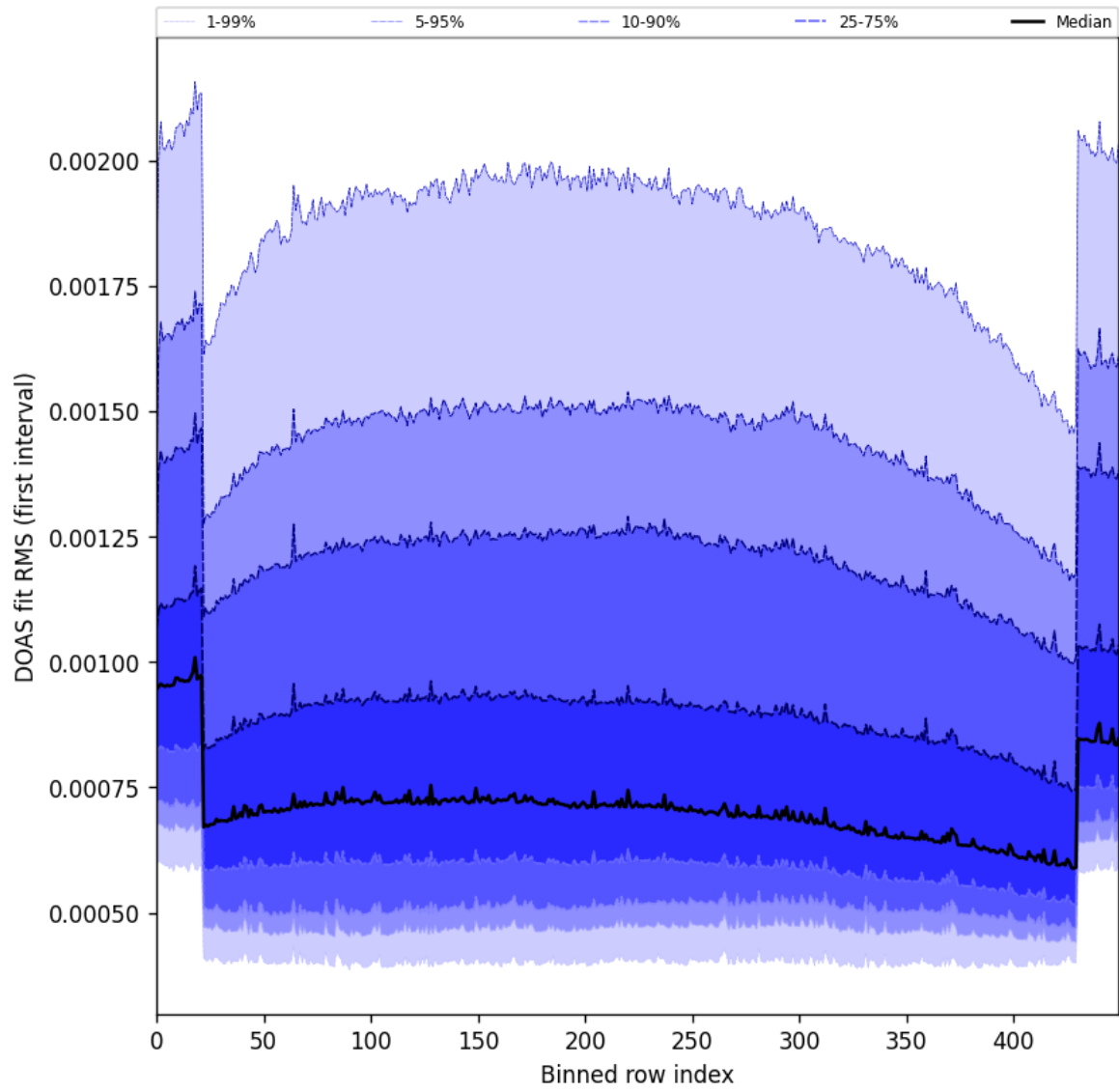
Figure 60: Along track statistics of “DOAS fit RMS (first interval)” for 2024-12-07 to 2024-12-09
