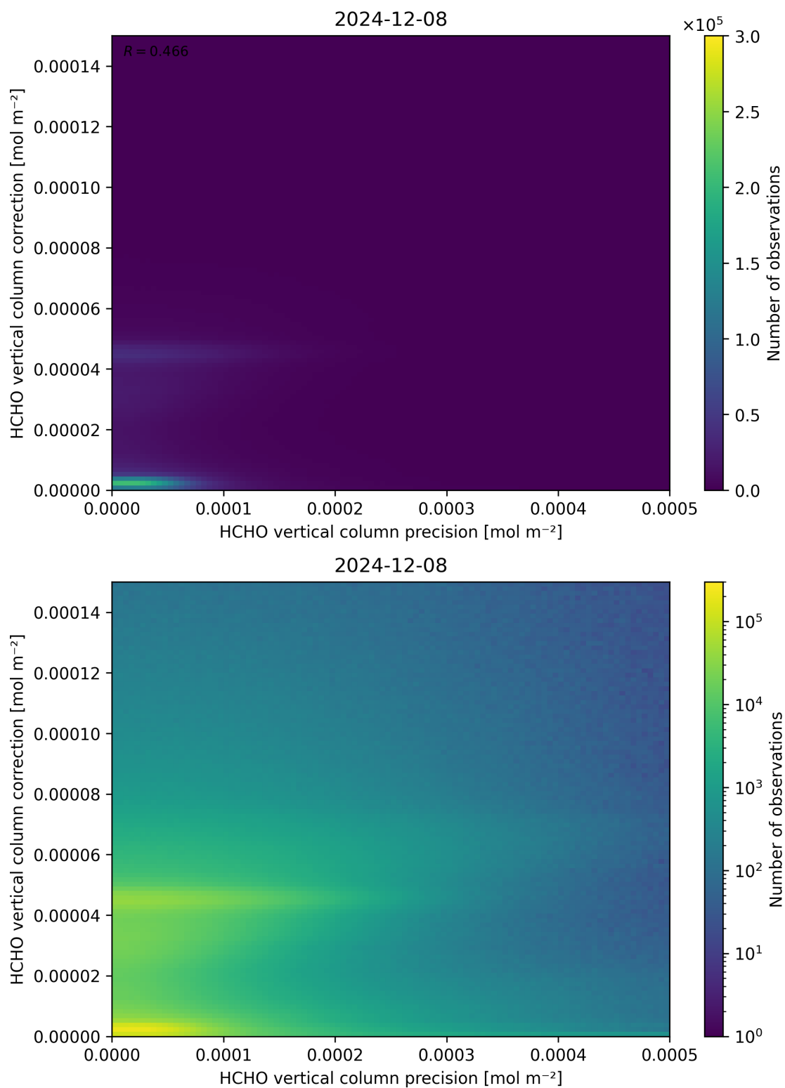
Figure 146: Scatter density plot of “HCHO vertical column precision” against “HCHO vertical column correction” for 2024-12-07 to 2024-12-09.
