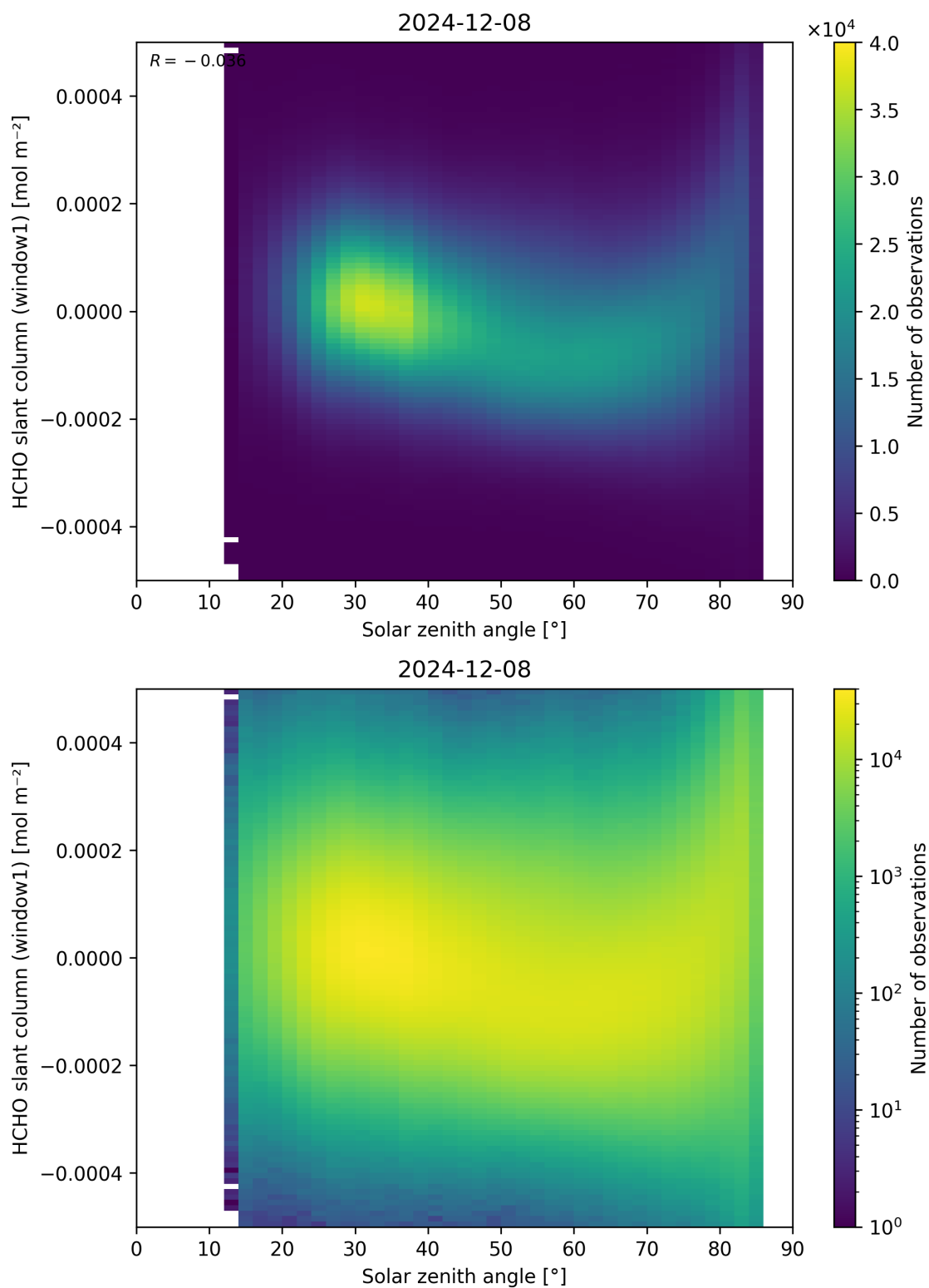
Figure 173: Scatter density plot of “Solar zenith angle” against “HCHO slant column (window1)” for 2024-12-07 to 2024-12-09.
