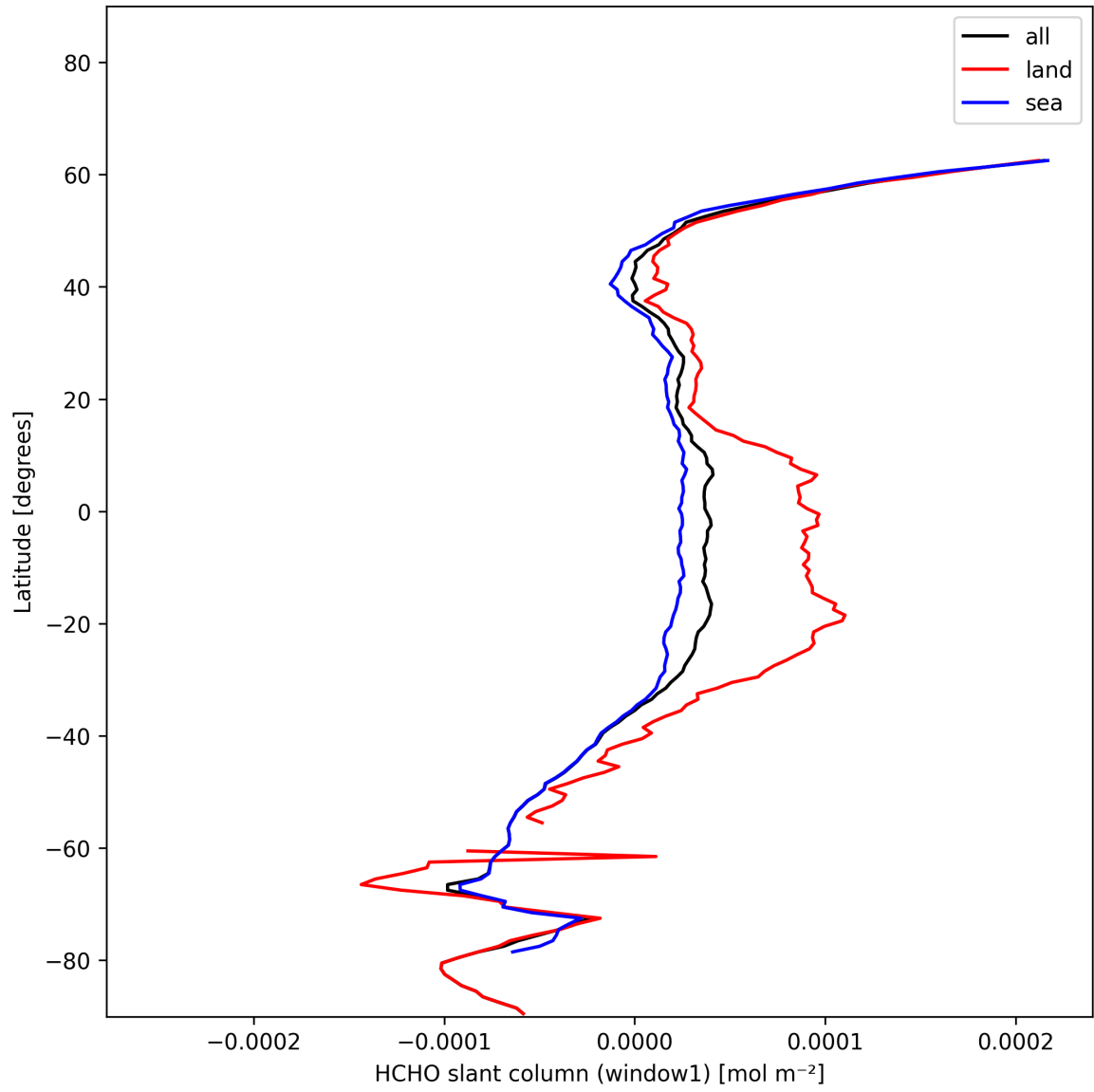
Figure 24: Zonal average of “HCHO slant column (window1)” for 2024-12-07 to 2024-12-09.
