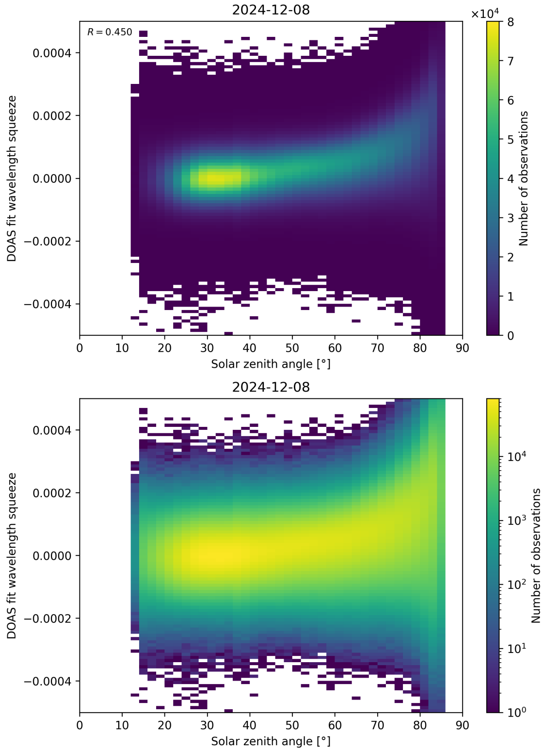
Figure 169: Scatter density plot of “Solar zenith angle” against “DOAS fit wavelength squeeze” for 2024-12-07 to 2024-12-09.
