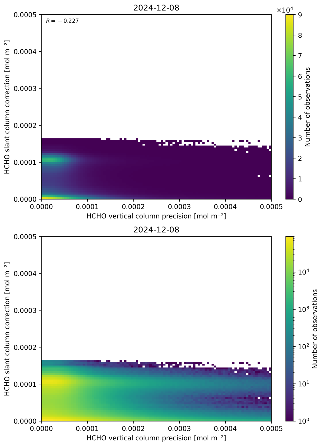
Figure 141: Scatter density plot of “HCHO vertical column precision” against “HCHO slant column correction” for 2024-12-07 to 2024-12-09.
