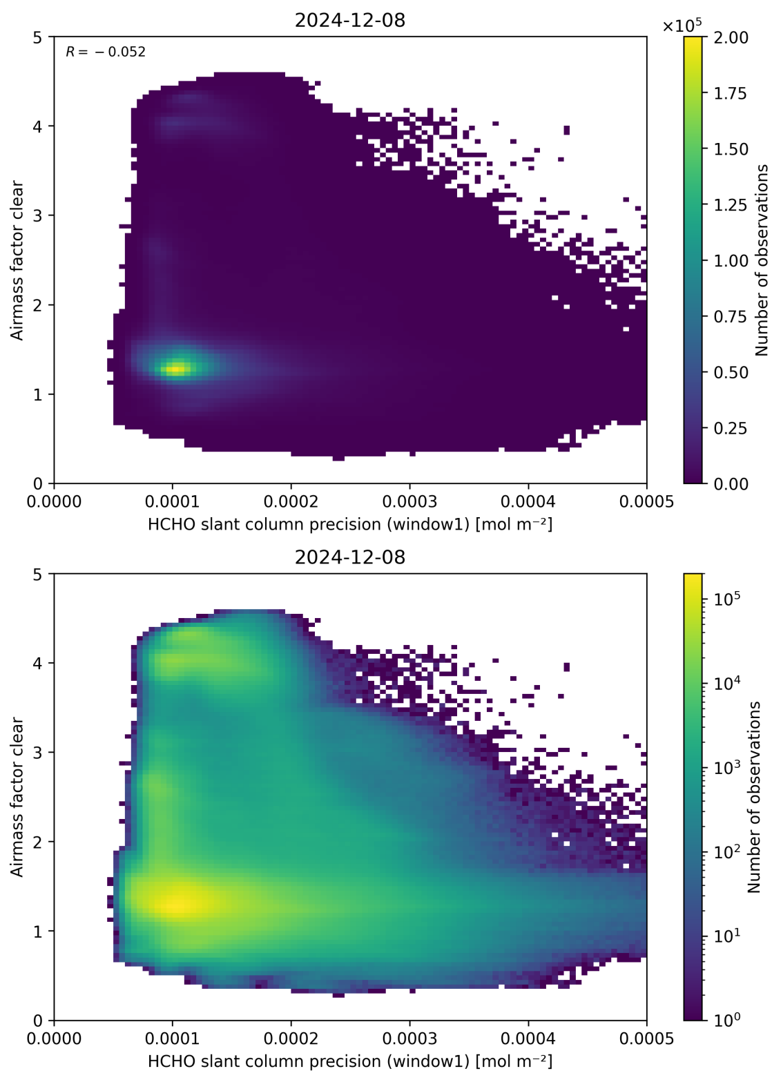
Figure 91: Scatter density plot of “HCHO slant column precision (window1)” against “Airmass factor clear” for 2024-12-07 to 2024-12-09.
