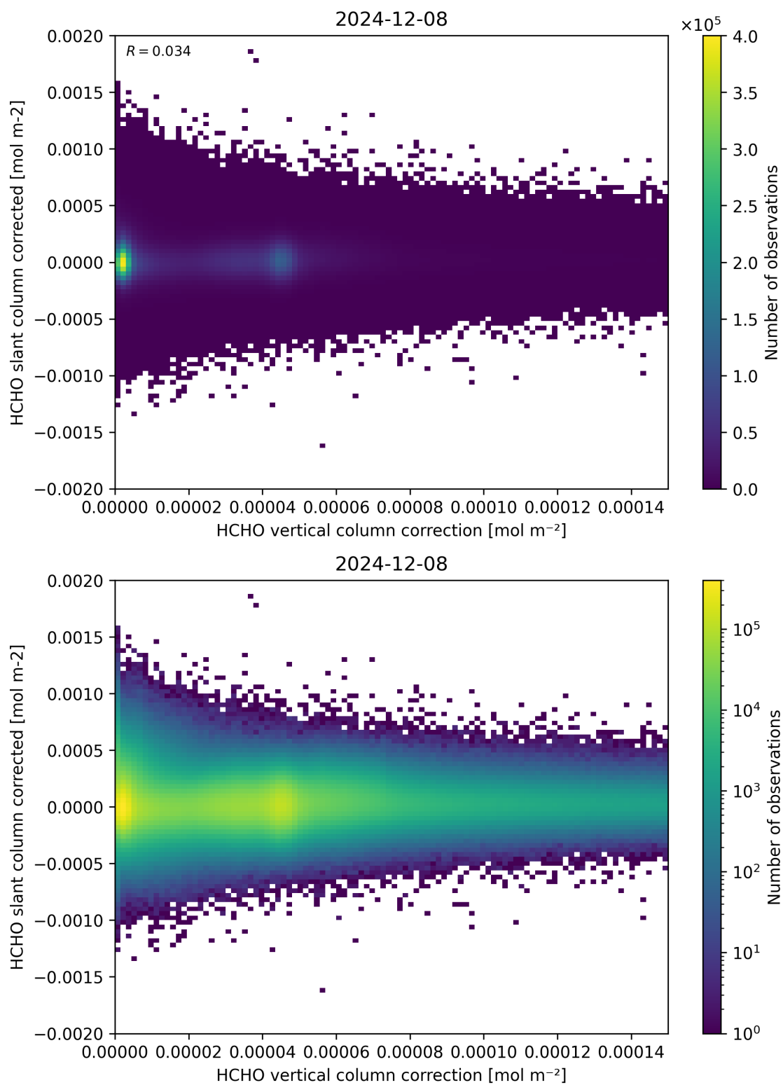
Figure 116: Scatter density plot of “HCHO vertical column correction” against “HCHO slant column corrected” for 2024-12-07 to 2024-12-09.
