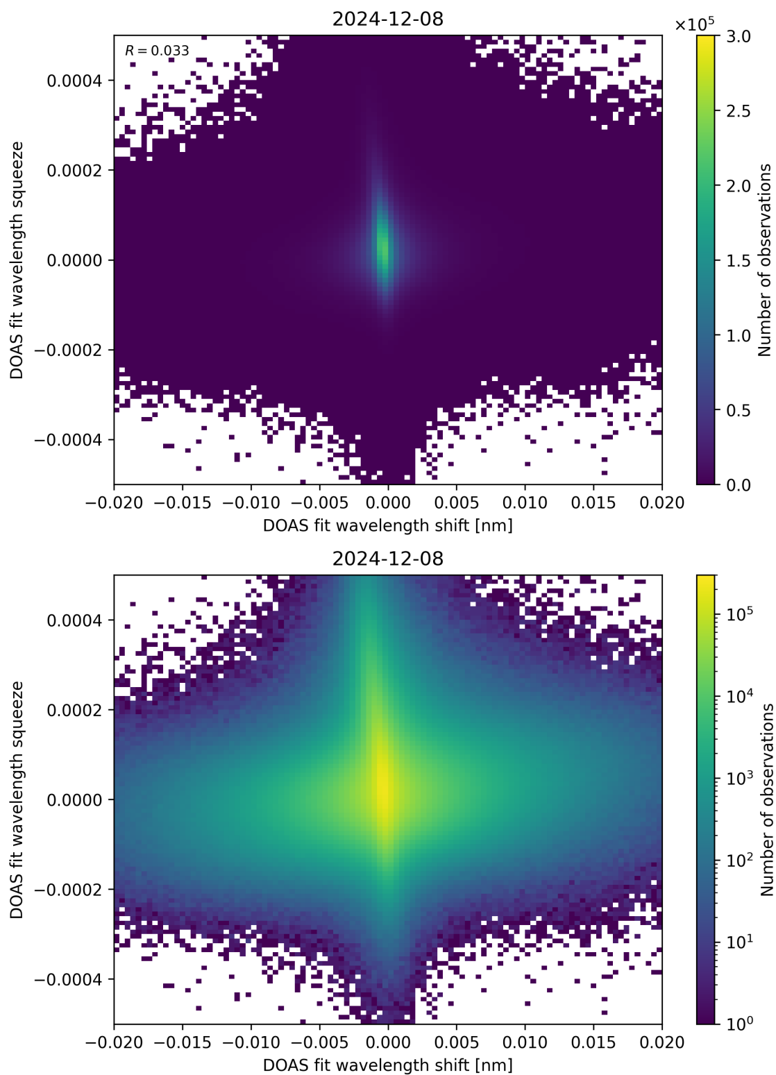
Figure 65: Scatter density plot of “DOAS fit wavelength shift” against “DOAS fit wavelength squeeze” for 2024-12-07 to 2024-12-09.
