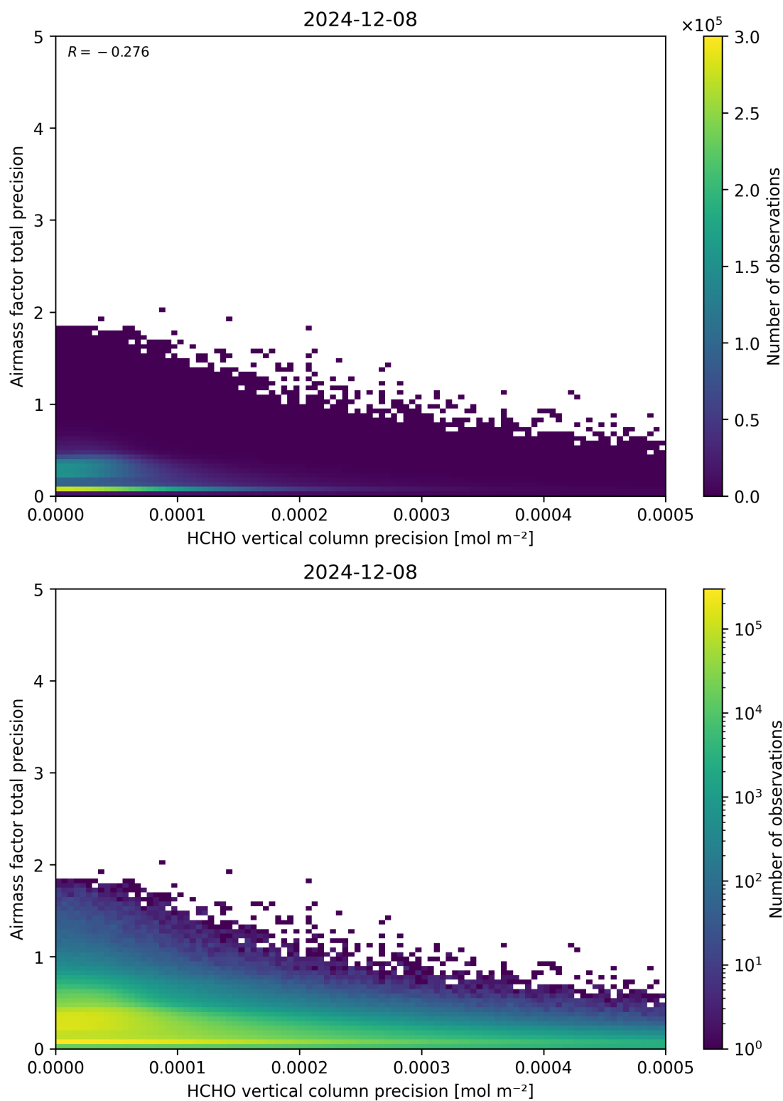
Figure 145: Scatter density plot of “HCHO vertical column precision” against “Airmass factor total precision” for 2024-12-07 to 2024-12-09.
