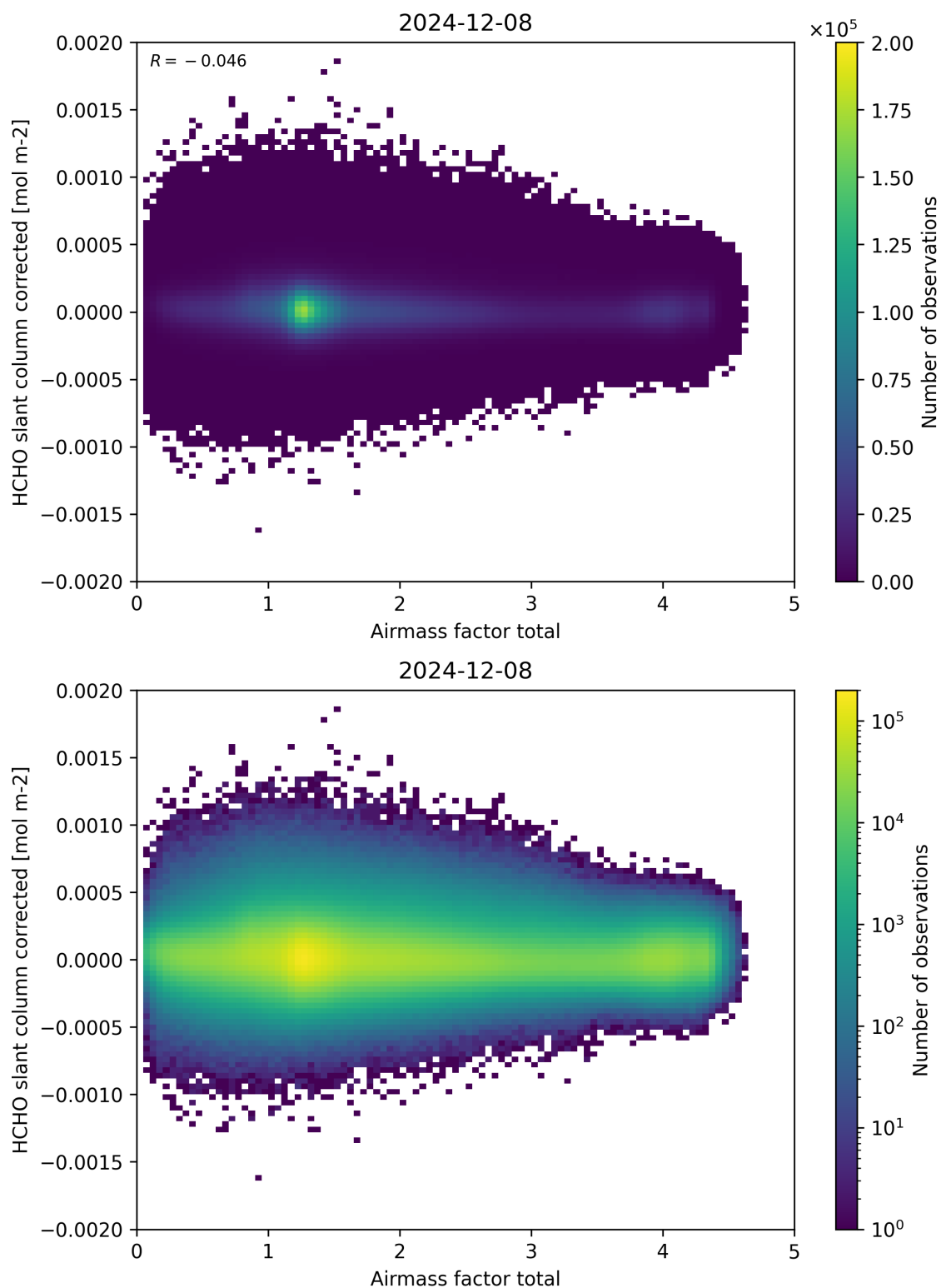
Figure 101: Scatter density plot of “Airmass factor total” against “HCHO slant column corrected” for 2024-12-07 to 2024-12-09.
