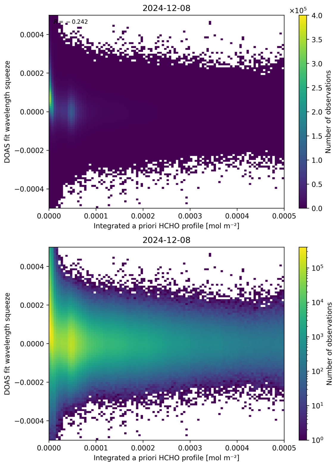
Figure 150: Scatter density plot of “Integrated a priori HCHO profile” against “DOAS fit wavelength squeeze” for 2024-12-07 to 2024-12-09.
