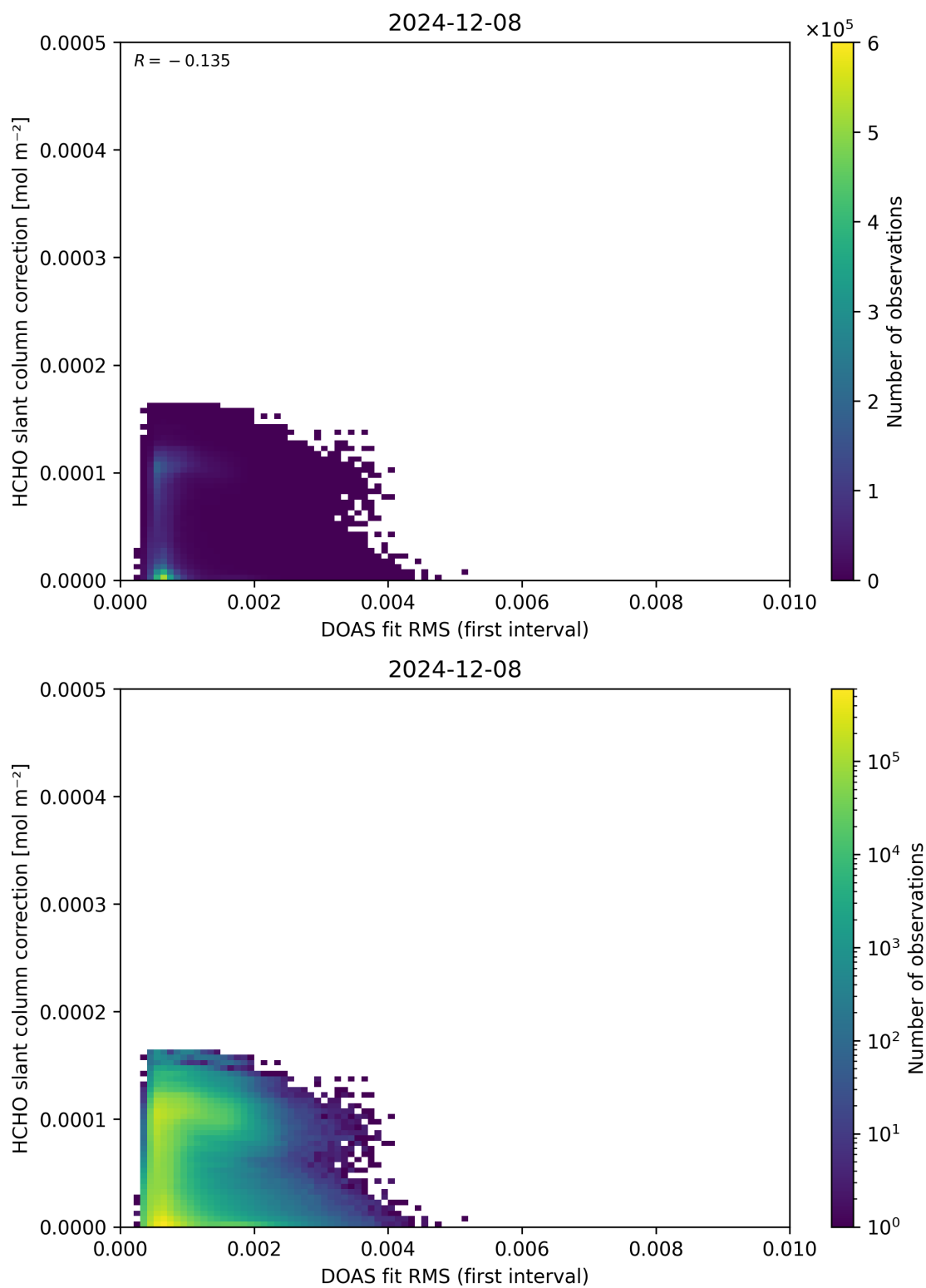
Figure 63: Scatter density plot of “DOAS fit RMS (first interval)” against “HCHO slant column correction” for 2024-12-07 to 2024-12-09.
