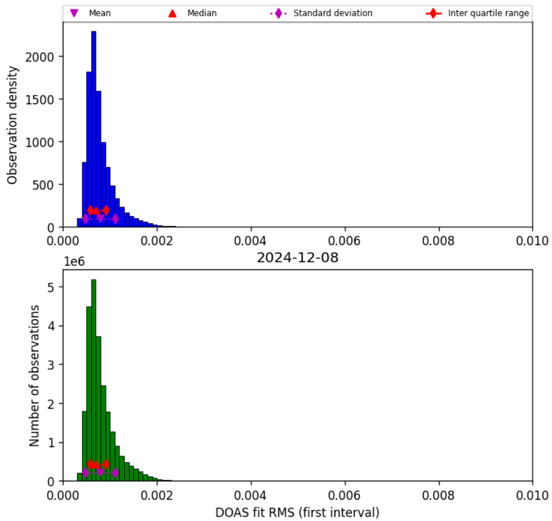
Figure 46: Histogram of “DOAS fit RMS (first interval)” for 2024-12-07 to 2024-12-09
