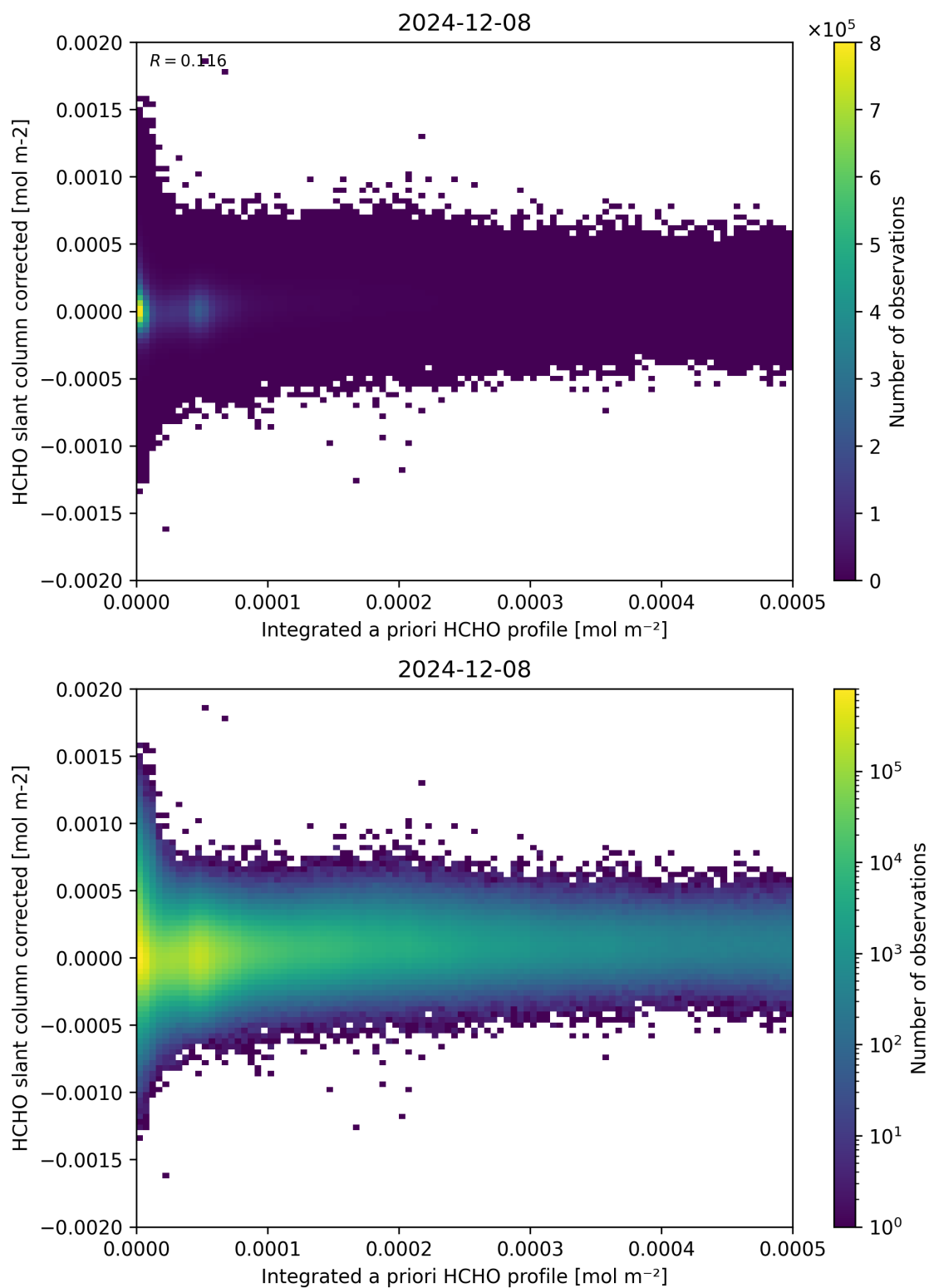
Figure 151: Scatter density plot of “Integrated a priori HCHO profile” against “HCHO slant column corrected” for 2024-12-07 to 2024-12-09.
