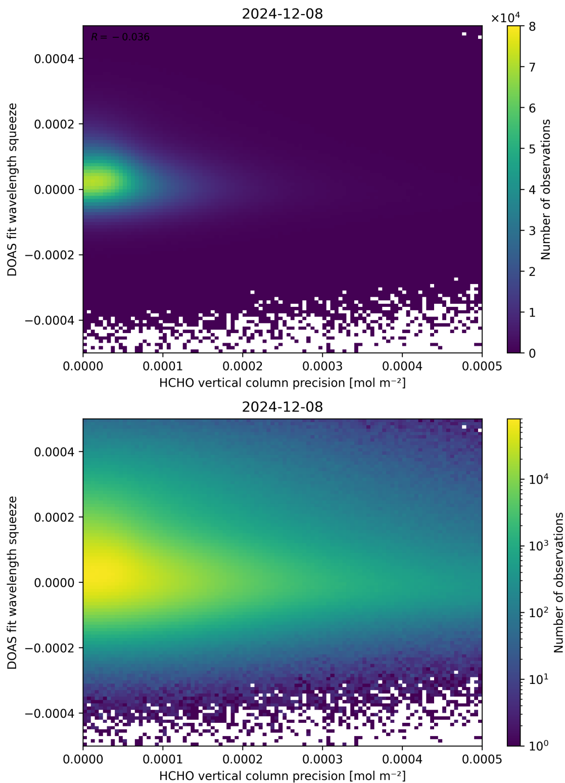
Figure 138: Scatter density plot of “HCHO vertical column precision” against “DOAS fit wavelength squeeze” for 2024-12-07 to 2024-12-09.
