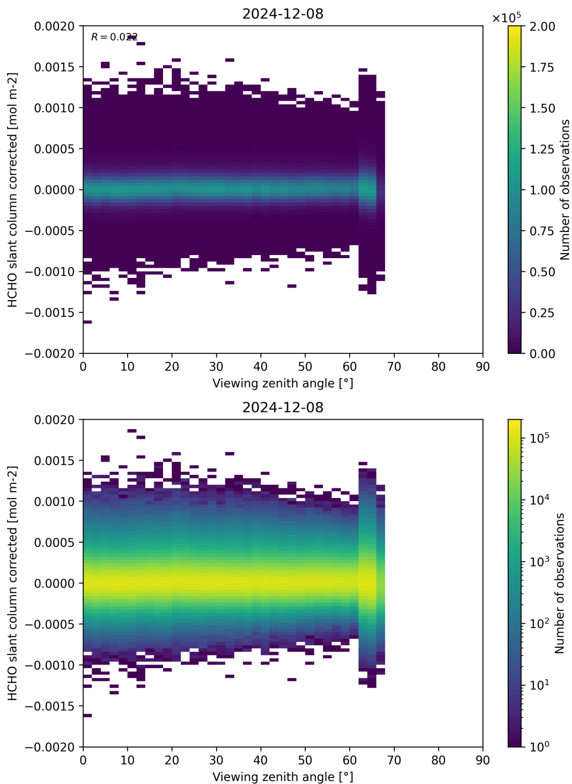
Figure 186: Scatter density plot of “Viewing zenith angle” against “HCHO slant column corrected” for 2024-12-07 to 2024-12-09.
