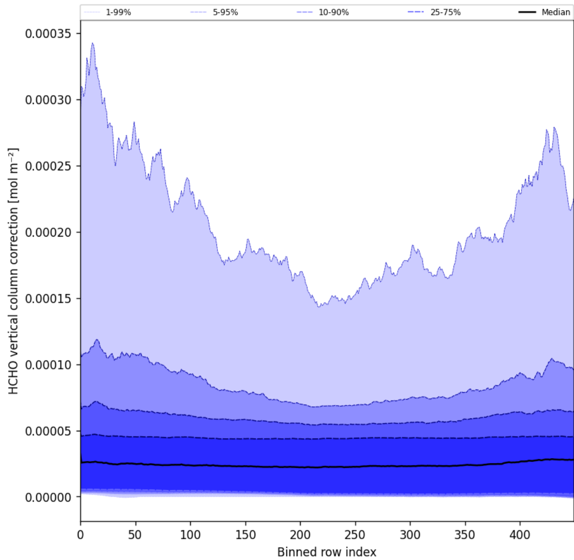
Figure 51: Along track statistics of “HCHO vertical column correction” for 2024-12-07 to 2024-12-09
