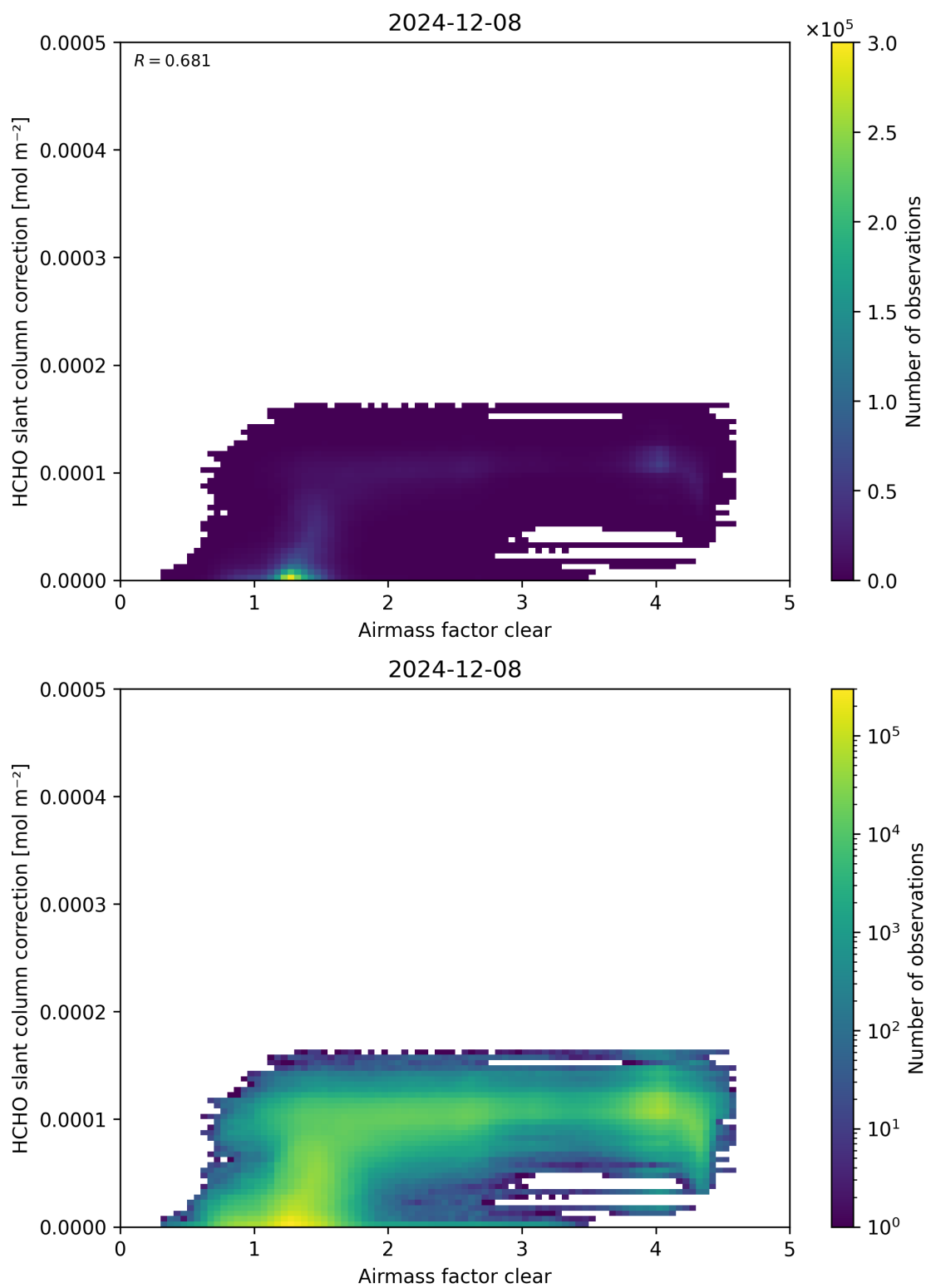
Figure 75: Scatter density plot of “Airmass factor clear” against “HCHO slant column correction” for 2024-12-07 to 2024-12-09.
