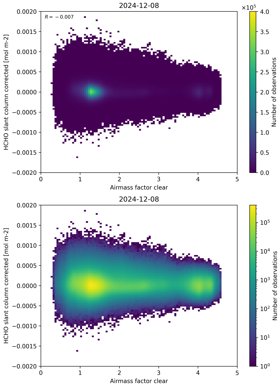
Figure 74: Scatter density plot of “Airmass factor clear” against “HCHO slant column corrected” for 2024-12-07 to 2024-12-09.
