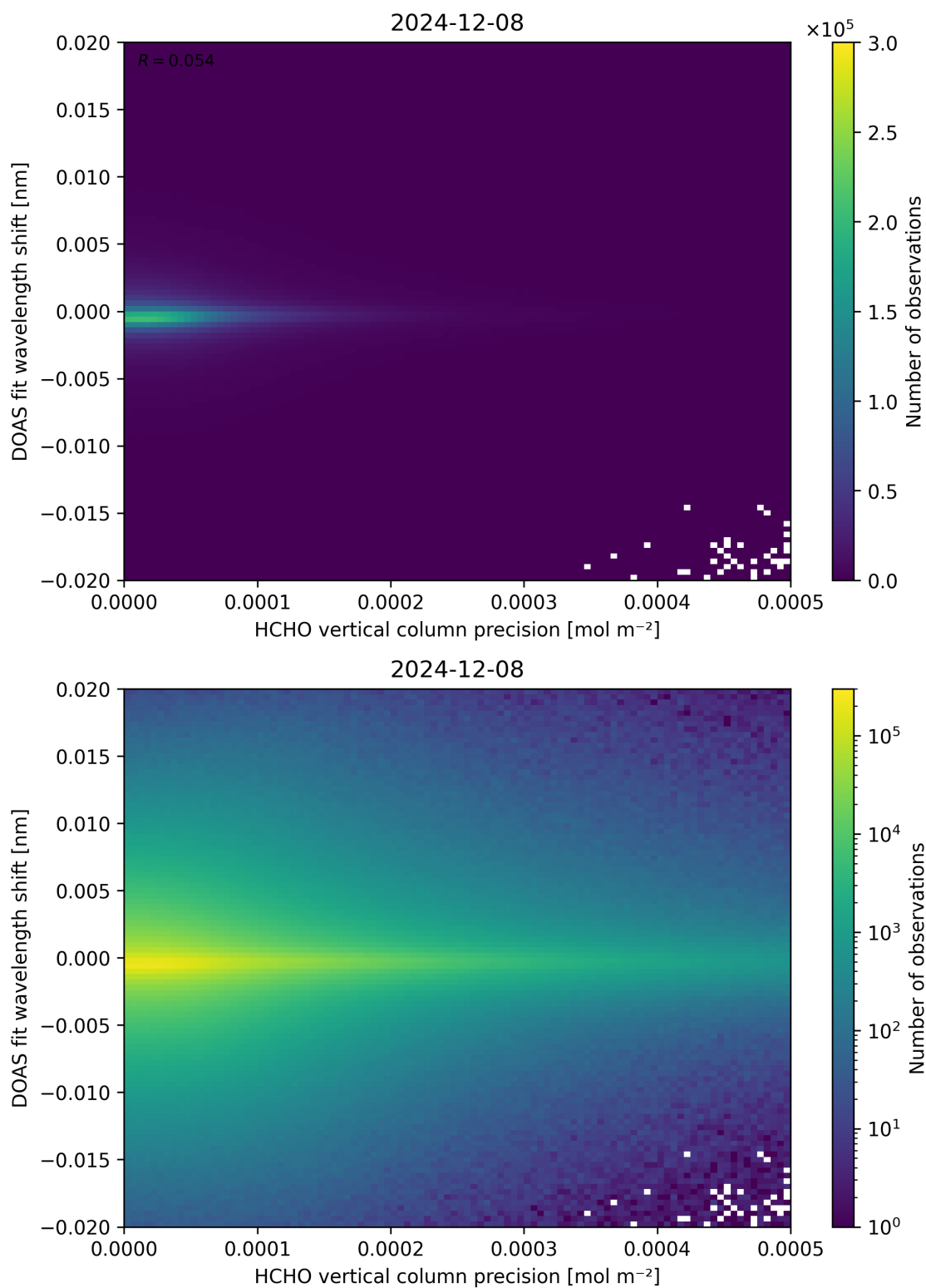
Figure 137: Scatter density plot of “HCHO vertical column precision” against “DOAS fit wavelength shift” for 2024-12-07 to 2024-12-09.
