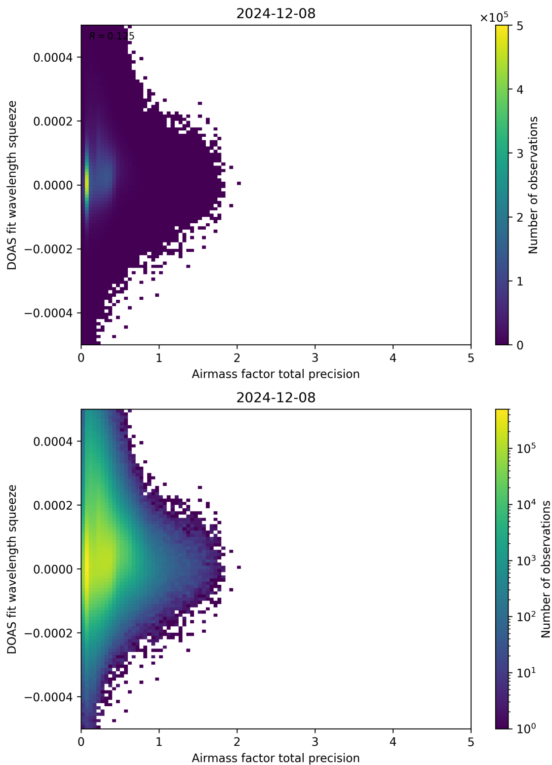
Figure 107: Scatter density plot of “Airmass factor total precision” against “DOAS fit wavelength squeeze” for 2024-12-07 to 2024-12-09.
