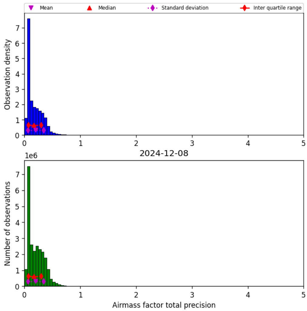
Figure 41: Histogram of “Airmass factor total precision” for 2024-12-07 to 2024-12-09
