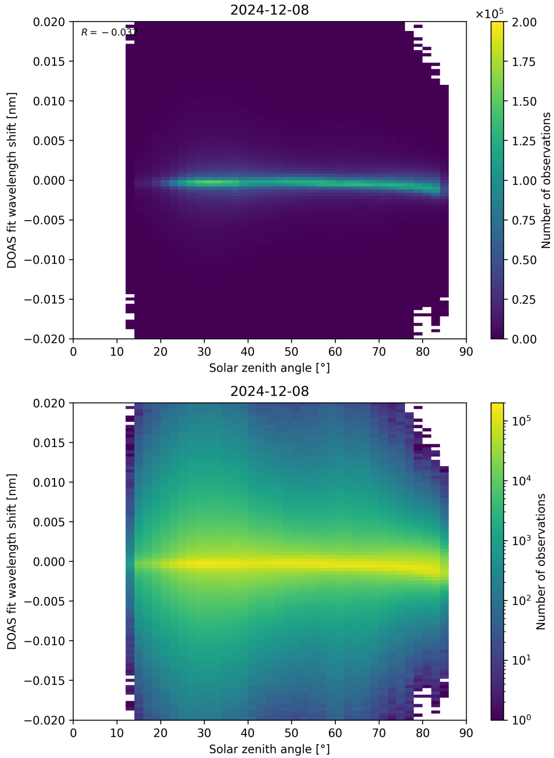
Figure 168: Scatter density plot of “Solar zenith angle” against “DOAS fit wavelength shift” for 2024-12-07 to 2024-12-09.
