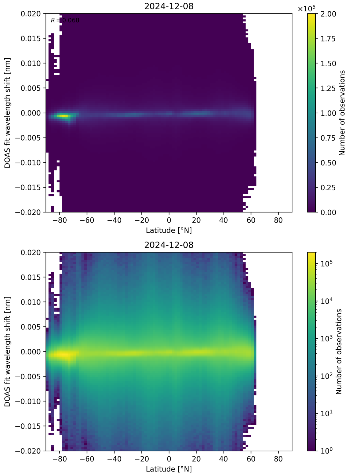
Figure 154: Scatter density plot of “Latitude” against “DOAS fit wavelength shift” for 2024-12-07 to 2024-12-09.
