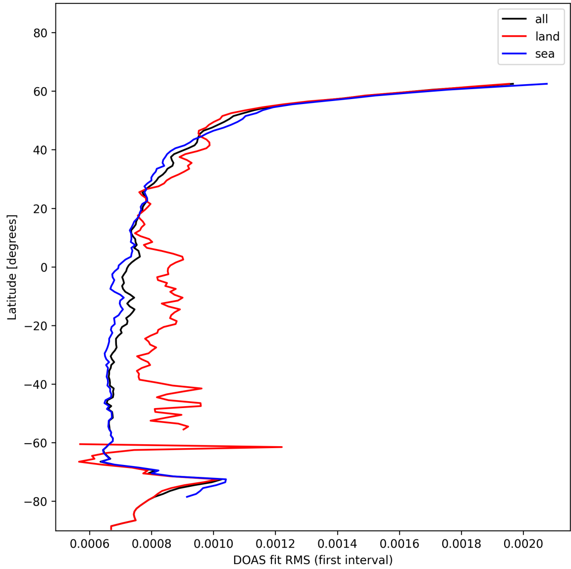
Figure 32: Zonal average of “DOAS fit RMS (first interval)” for 2024-12-07 to 2024-12-09.
