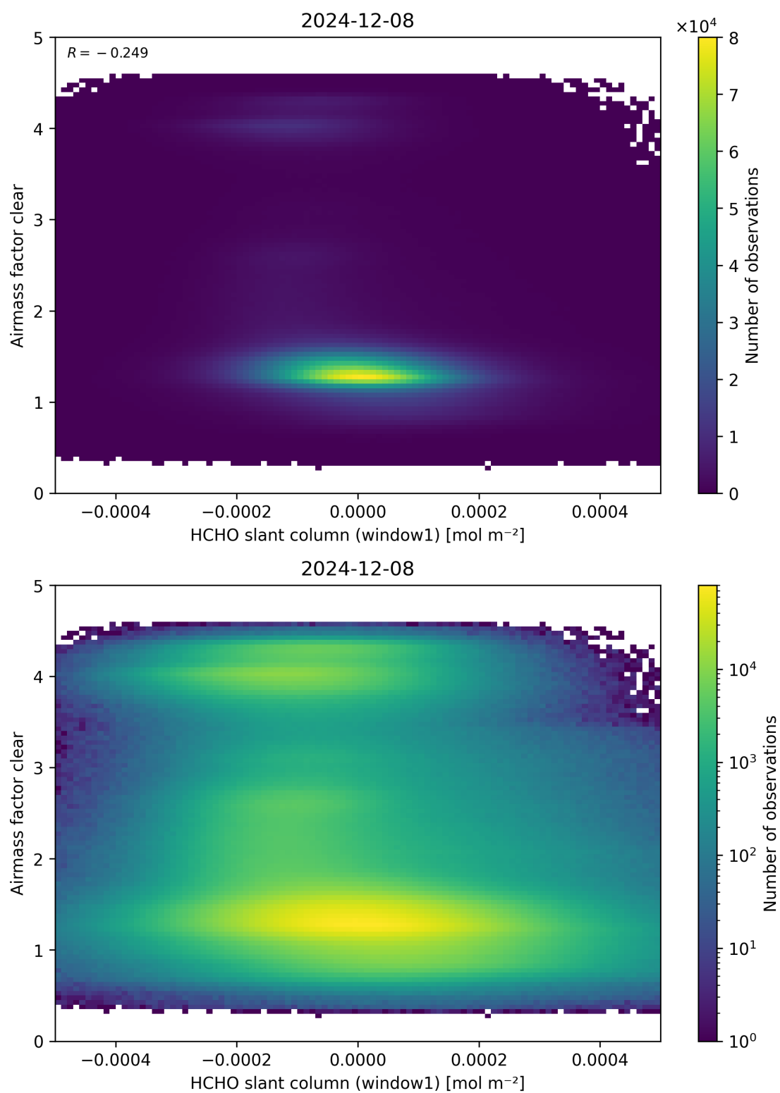
Figure 81: Scatter density plot of “HCHO slant column (window1)” against “Airmass factor clear” for 2024-12-07 to 2024-12-09.
