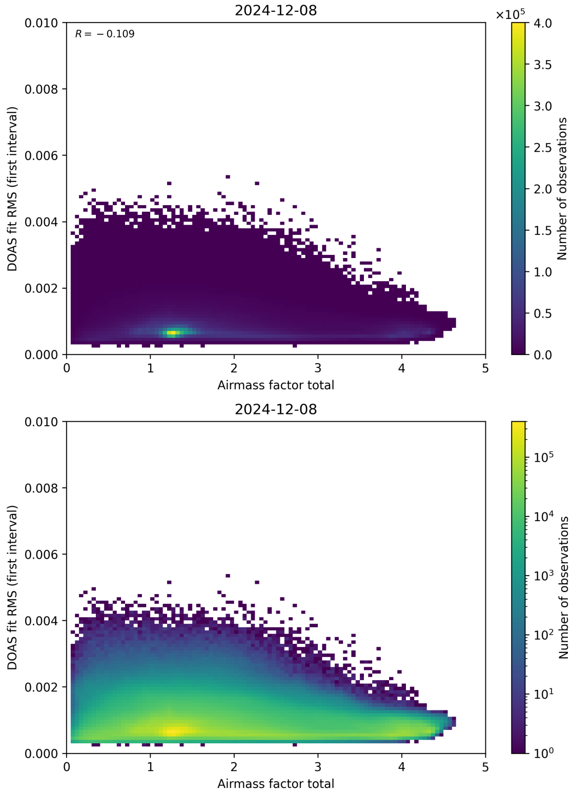
Figure 97: Scatter density plot of “Airmass factor total” against “DOAS fit RMS (first interval)” for 2024-12-07 to 2024-12-09.
