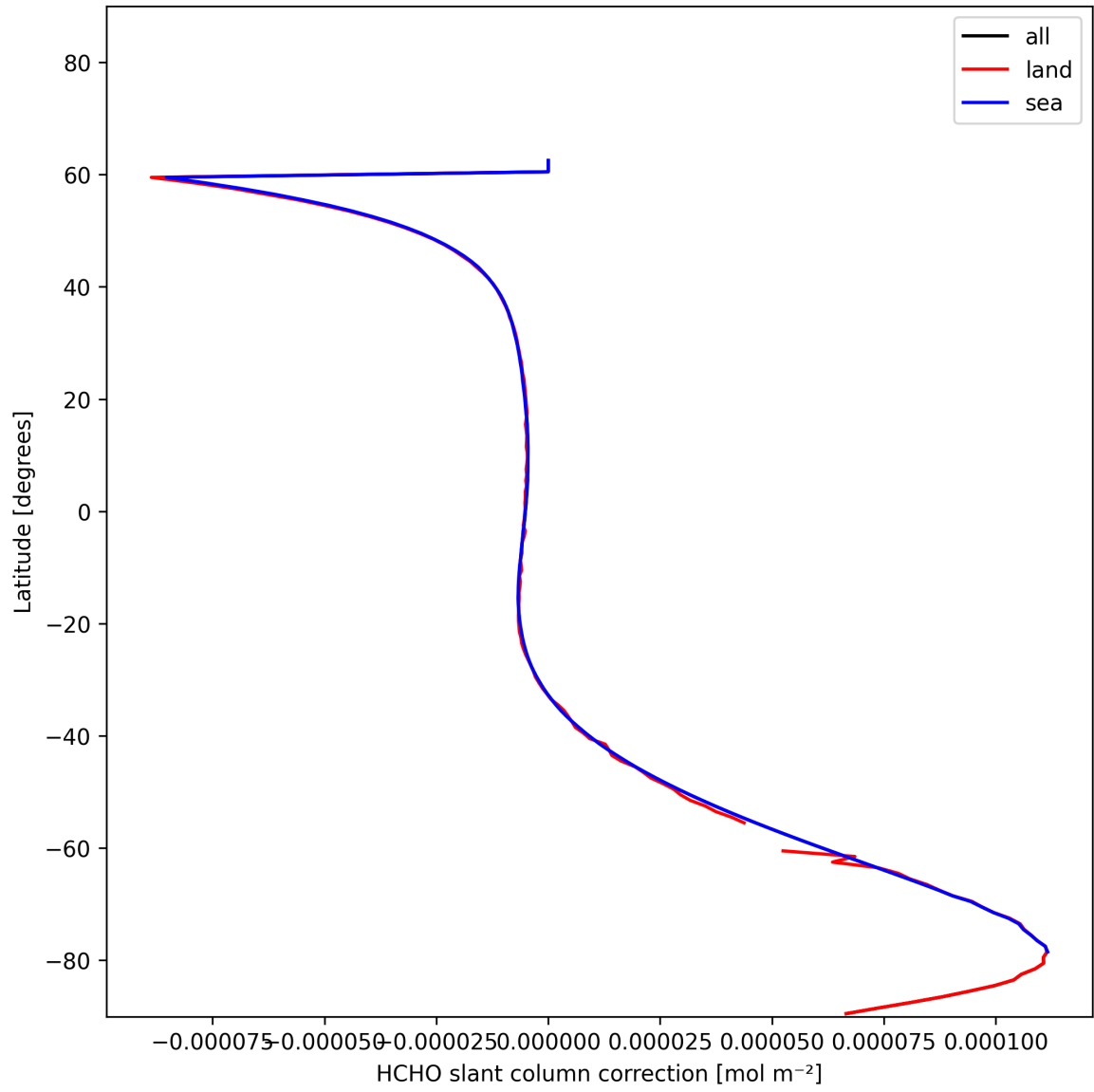
Figure 33: Zonal average of “HCHO slant column correction” for 2024-12-07 to 2024-12-09.
