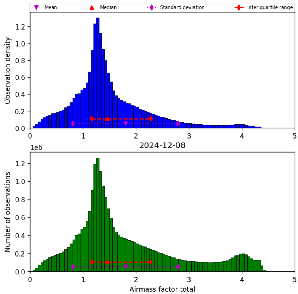
Figure 40: Histogram of “Airmass factor total” for 2024-12-07 to 2024-12-09
