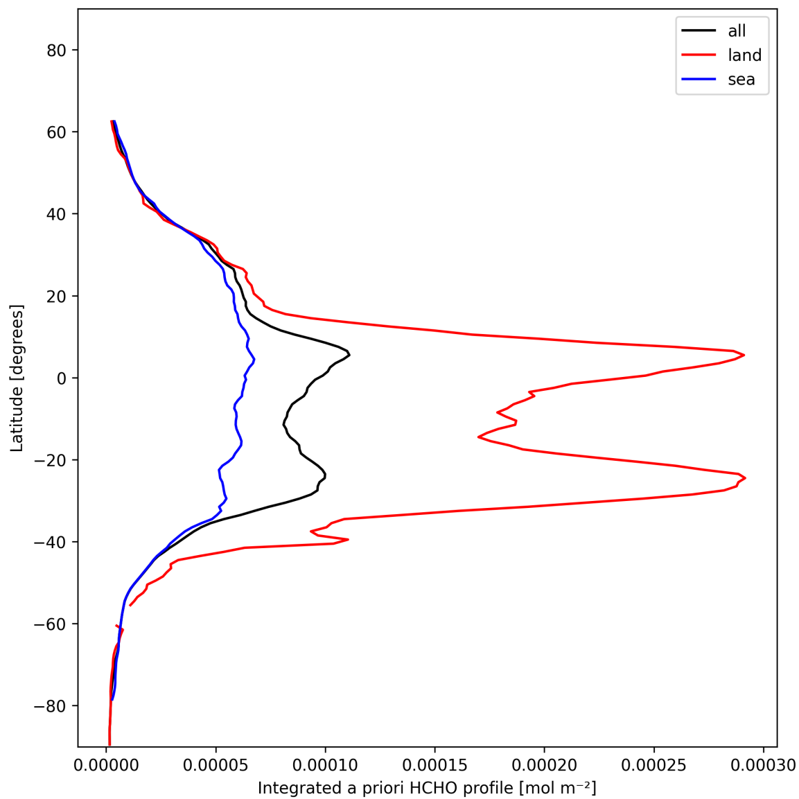
Figure 29: Zonal average of “Integrated a priori HCHO profile” for 2024-12-07 to 2024-12-09.
