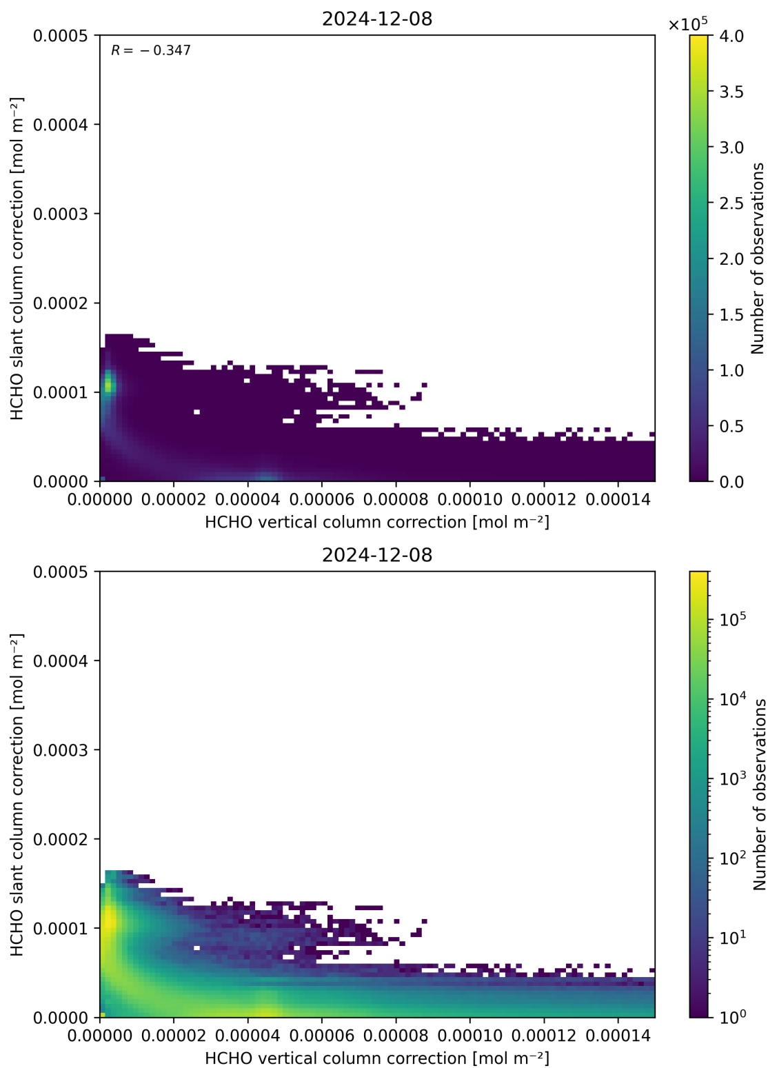
Figure 117: Scatter density plot of “HCHO vertical column correction” against “HCHO slant column correction” for 2024-12-07 to 2024-12-09.
