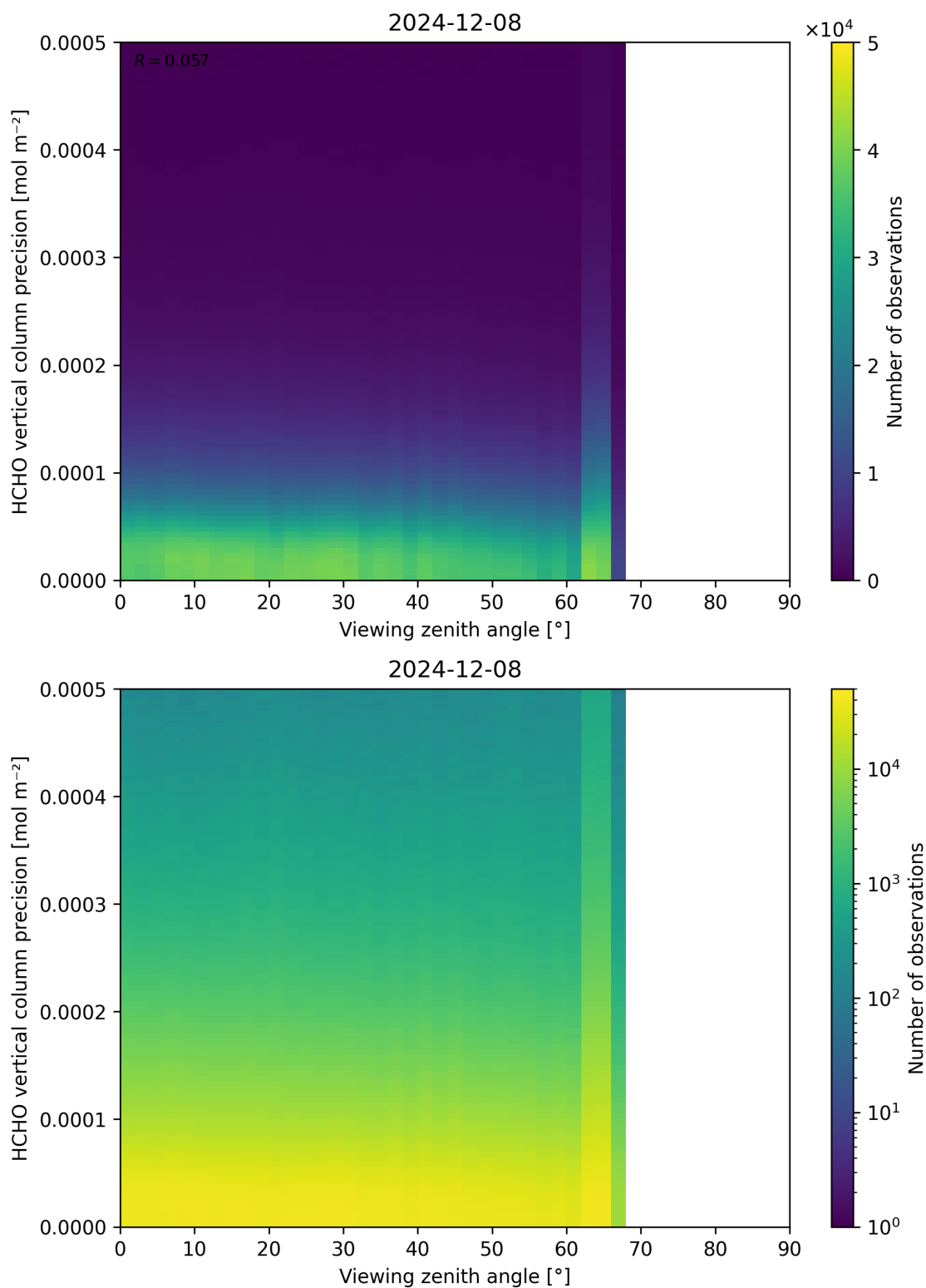
Figure 194: Scatter density plot of “Viewing zenith angle” against “HCHO vertical column precision” for 2024-12-07 to 2024-12-09.
