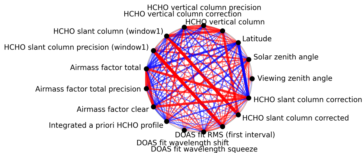
Figure 1: Map of correlation graph for 2024-12-07 to 2024-12-09.
