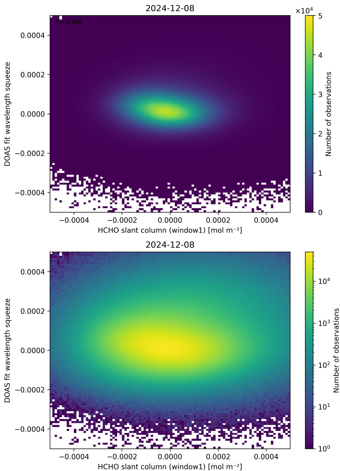
Figure 80: Scatter density plot of “HCHO slant column (window1)” against “DOAS fit wavelength squeeze” for 2024-12-07 to 2024-12-09.
