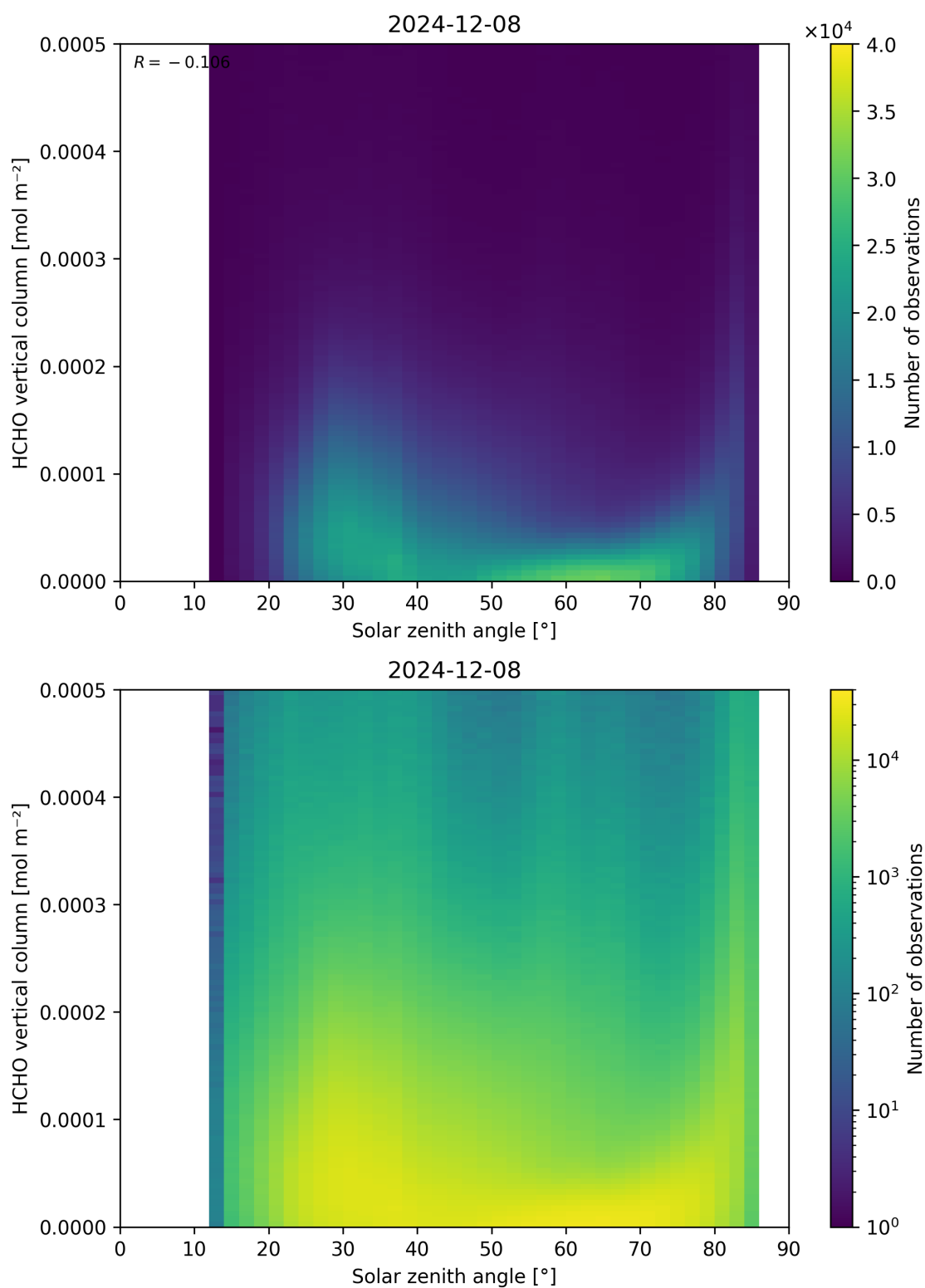
Figure 177: Scatter density plot of “Solar zenith angle” against “HCHO vertical column” for 2024-12-07 to 2024-12-09.
