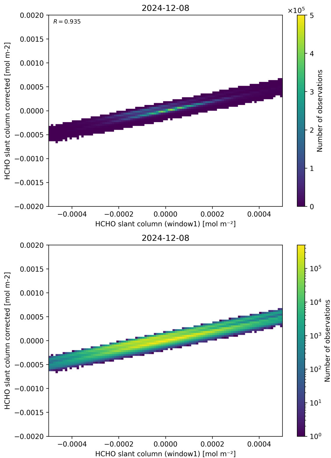
Figure 82: Scatter density plot of “HCHO slant column (window1)” against “HCHO slant column corrected” for 2024-12-07 to 2024-12-09.
