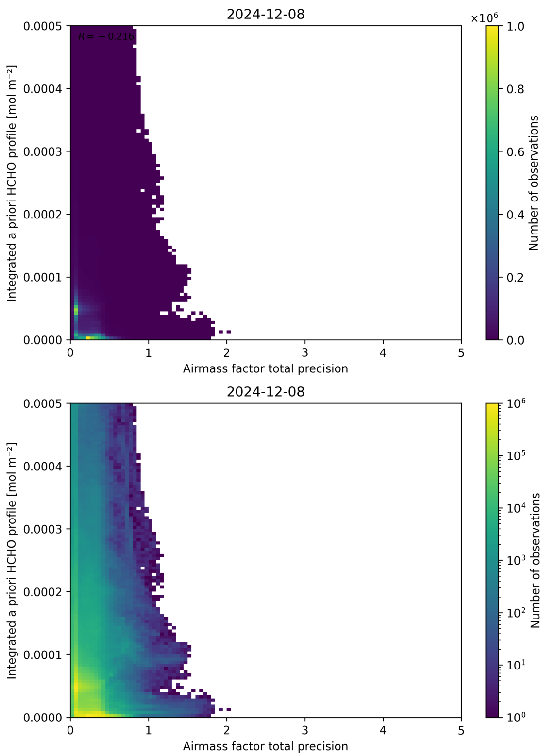
Figure 111: Scatter density plot of “Airmass factor total precision” against “Integrated a priori HCHO profile” for 2024-12-07 to 2024-12-09.
