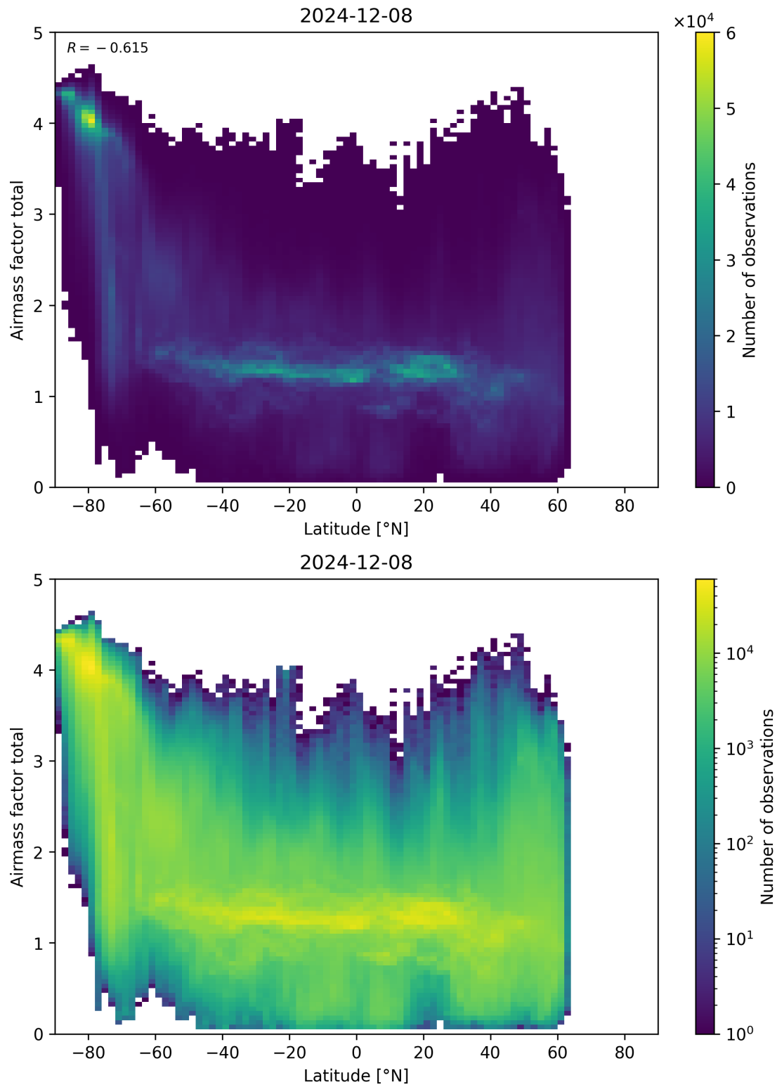
Figure 161: Scatter density plot of “Latitude” against “Airmass factor total” for 2024-12-07 to 2024-12-09.
