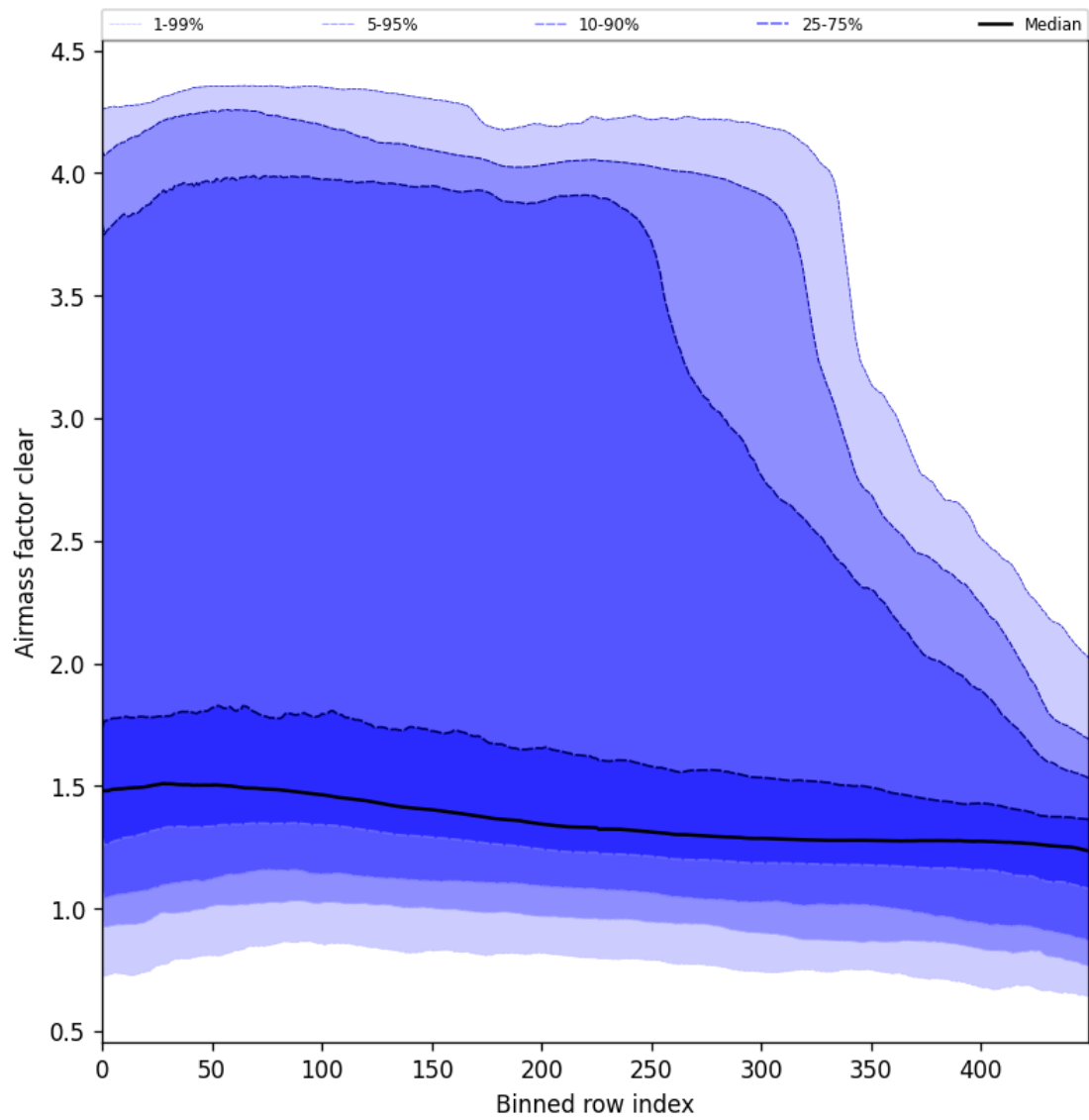
Figure 56: Along track statistics of “Air mass factor clear” for 2024-12-07 to 2024-12-09
