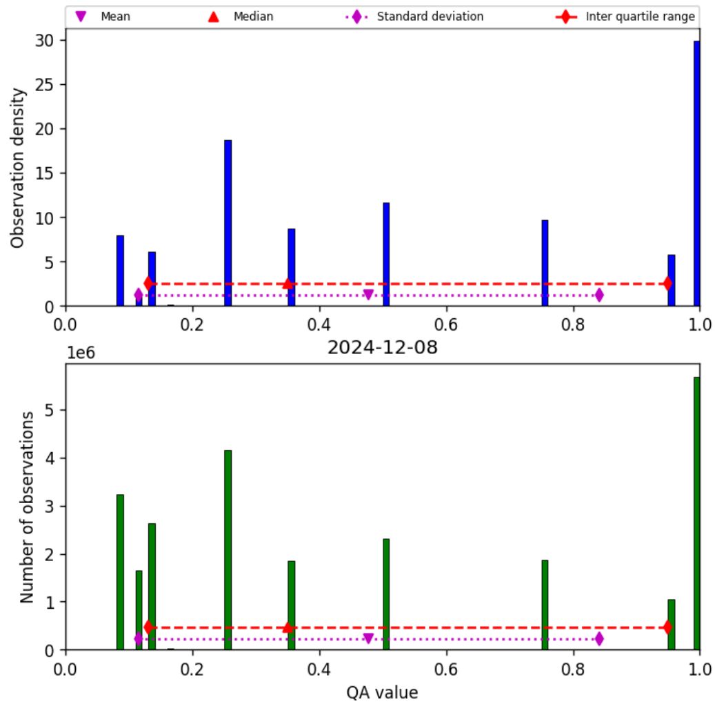
Figure 34: Histogram of “QA value” for 2024-12-07 to 2024-12-09
