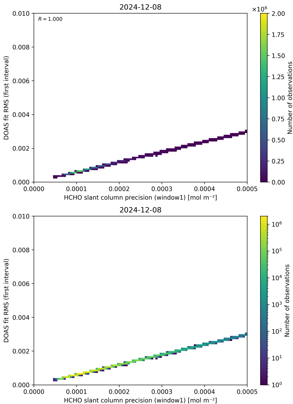
Figure 88: Scatter density plot of “HCHO slant column precision (window1)” against “DOAS fit RMS (first interval)” for 2024-12-07 to 2024-12-09.
