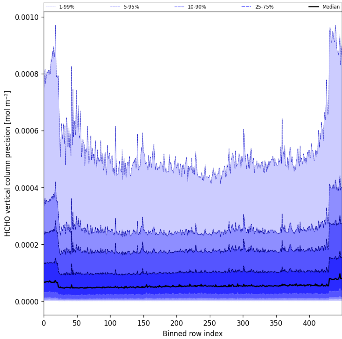
Figure 50: Along track statistics of “HCHO vertical column precision” for 2024-12-07 to 2024-12-09
