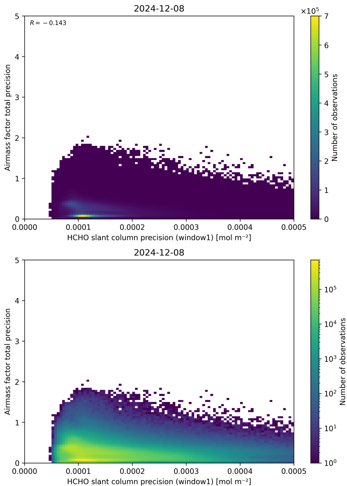
Figure 95: Scatter density plot of “HCHO slant column precision (window1)” against “Airmass factor total precision” for 2024-12-07 to 2024-12-09.
