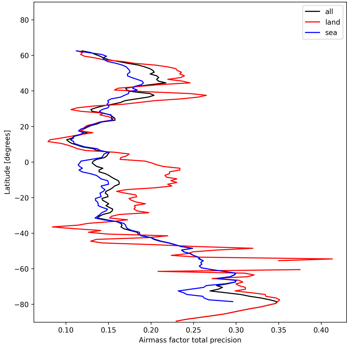
Figure 27: Zonal average of “Airmass factor total precision” for 2024-12-07 to 2024-12-09.
