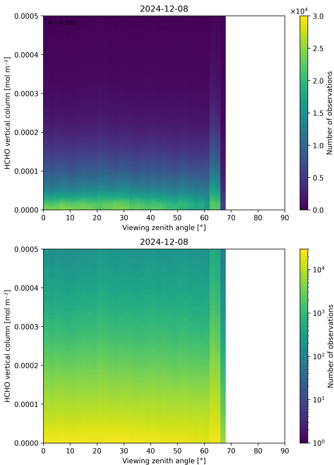
Figure 192: Scatter density plot of “Viewing zenith angle” against “HCHO vertical column” for 2024-12-07 to 2024-12-09.
