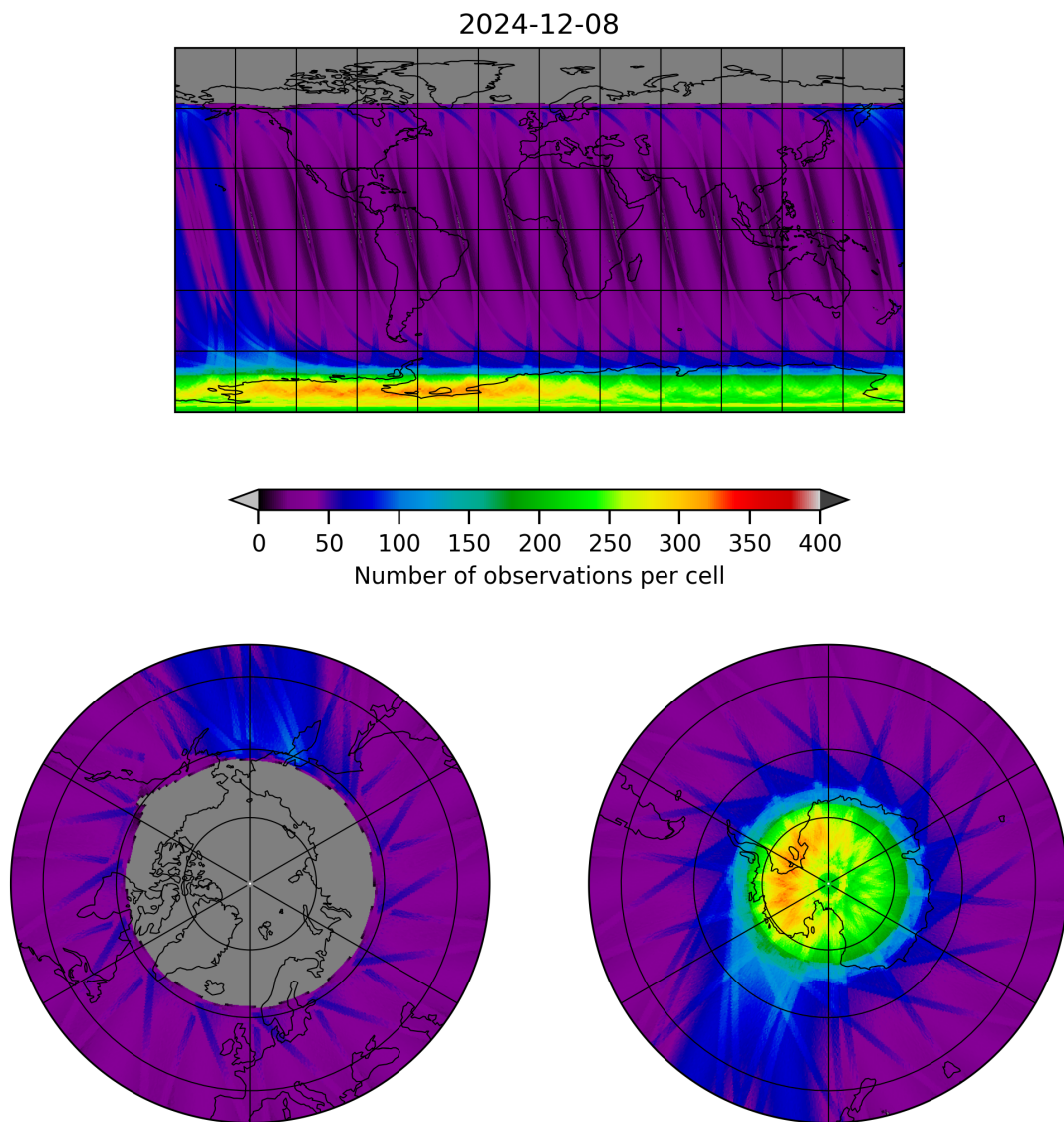
Figure 19: Map of the number of observations for 2024-12-07 to 2024-12-09
