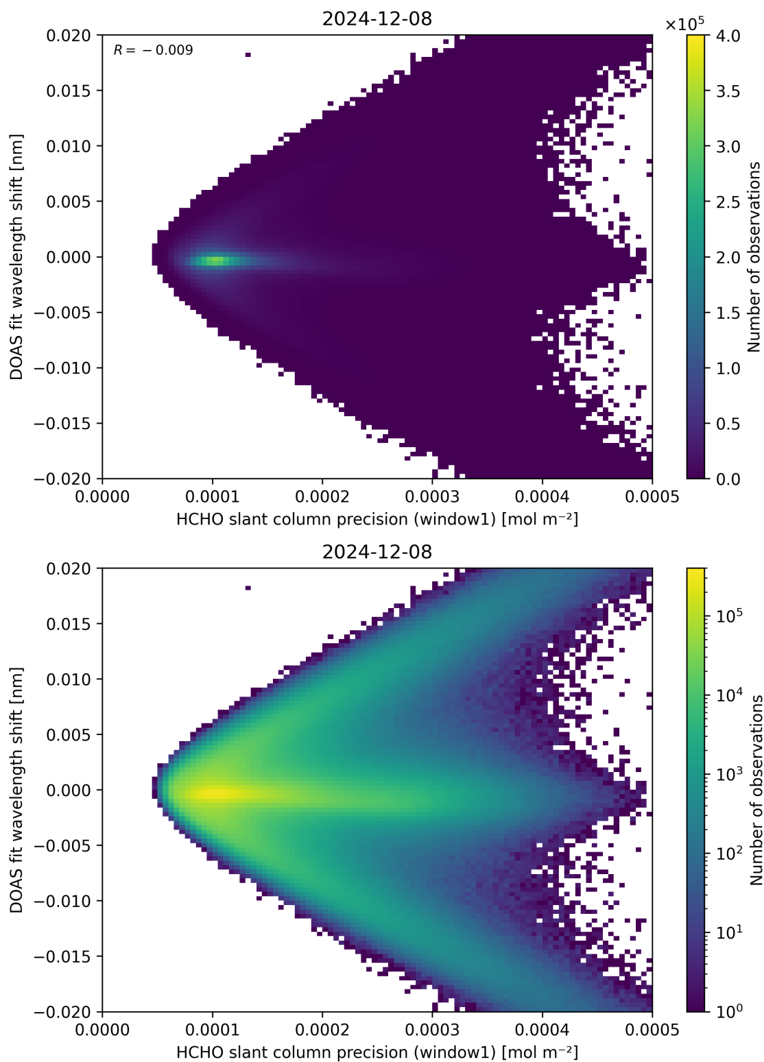
Figure 89: Scatter density plot of “HCHO slant column precision (window1)” against “DOAS fit wavelength shift” for 2024-12-07 to 2024-12-09.
