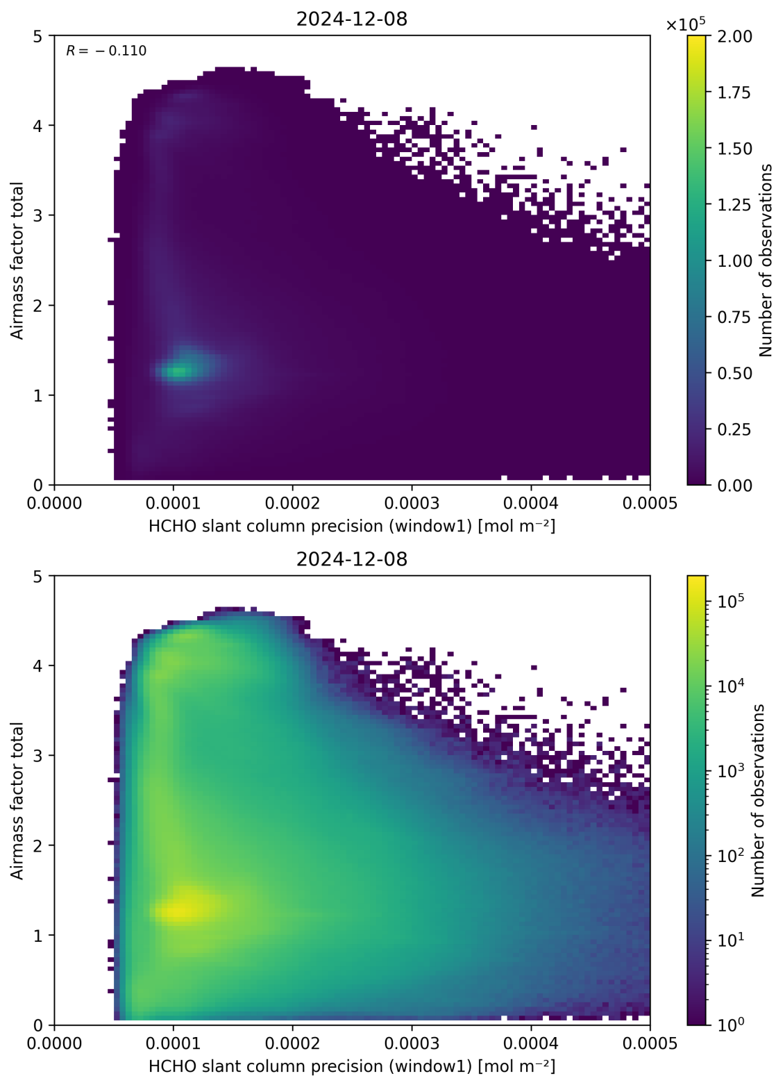
Figure 94: Scatter density plot of “HCHO slant column precision (window1)” against “Airmass factor total” for 2024-12-07 to 2024-12-09.
