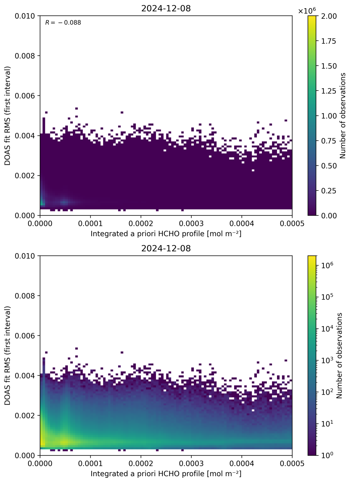
Figure 148: Scatter density plot of “Integrated a priori HCHO profile” against “DOAS fit RMS (first interval)” for 2024-12-07 to 2024-12-09.
