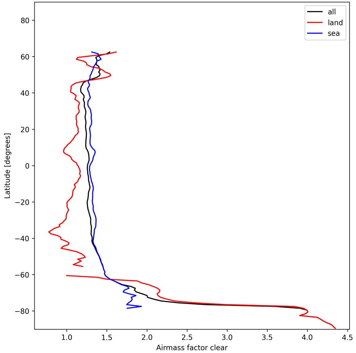
Figure 28: Zonal average of “Airmass factor clear” for 2024-12-07 to 2024-12-09.
