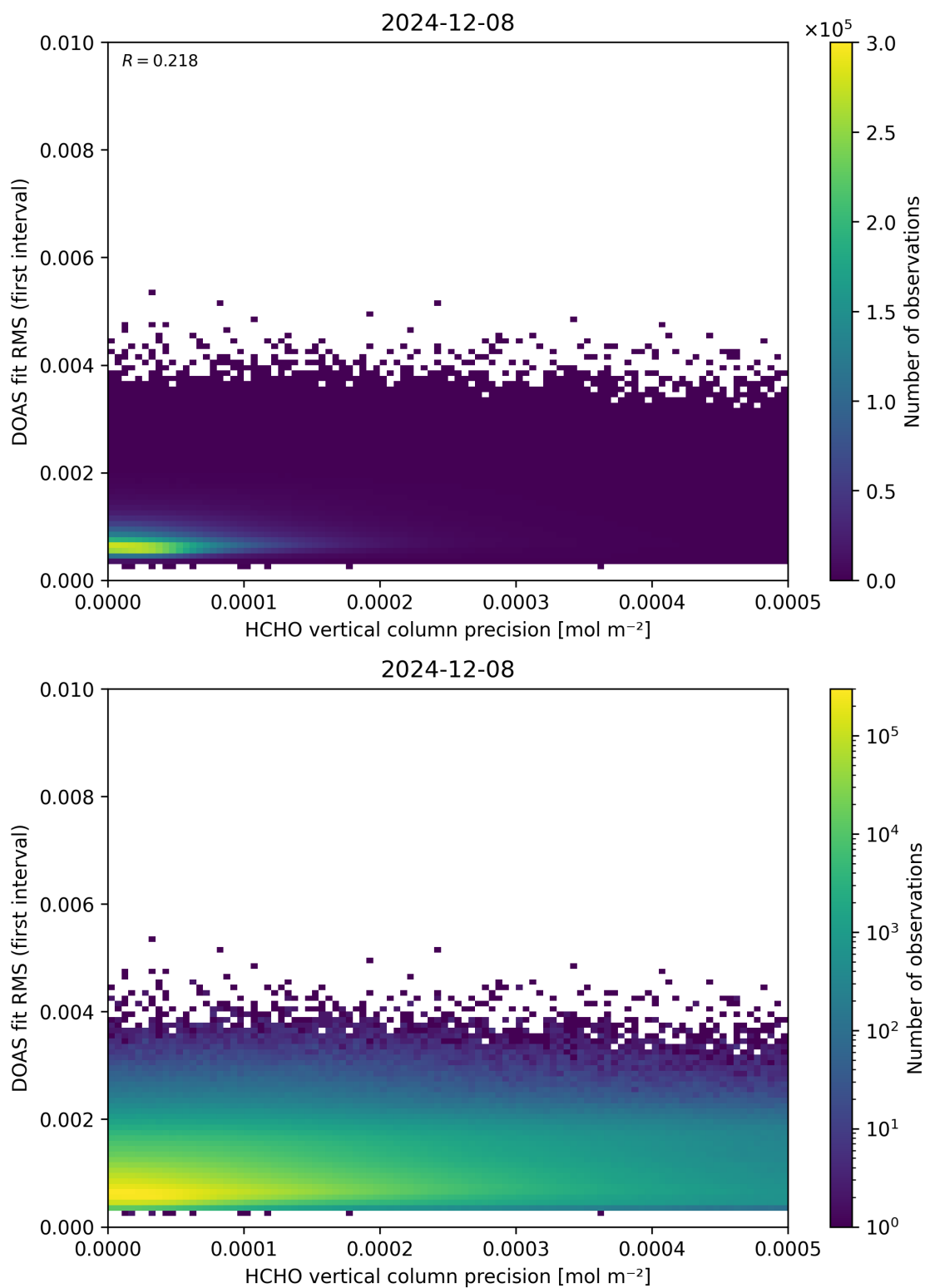
Figure 136: Scatter density plot of “HCHO vertical column precision” against “DOAS fit RMS (first interval)” for 2024-12-07 to 2024-12-09.
