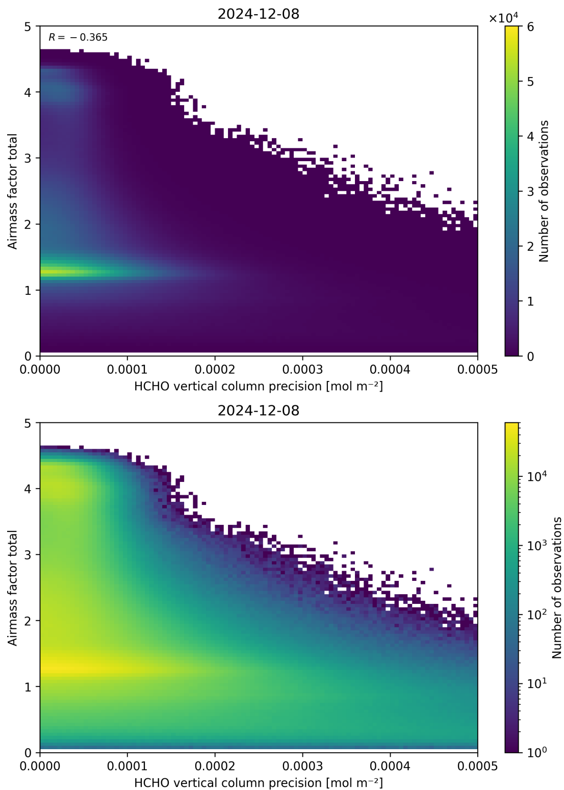
Figure 144: Scatter density plot of “HCHO vertical column precision” against “Airmass factor total” for 2024-12-07 to 2024-12-09.
