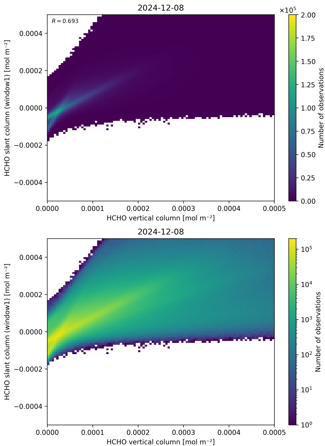
Figure 129: Scatter density plot of “HCHO vertical column” against “HCHO slant column (window1)” for 2024-12-07 to 2024-12-09.
