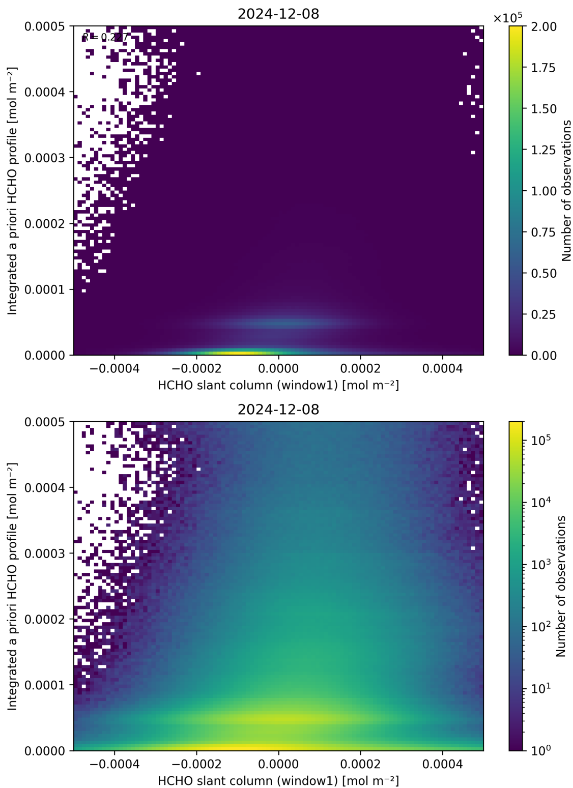
Figure 87: Scatter density plot of “HCHO slant column (window1)” against “Integrated a priori HCHO profile” for 2024-12-07 to 2024-12-09.
