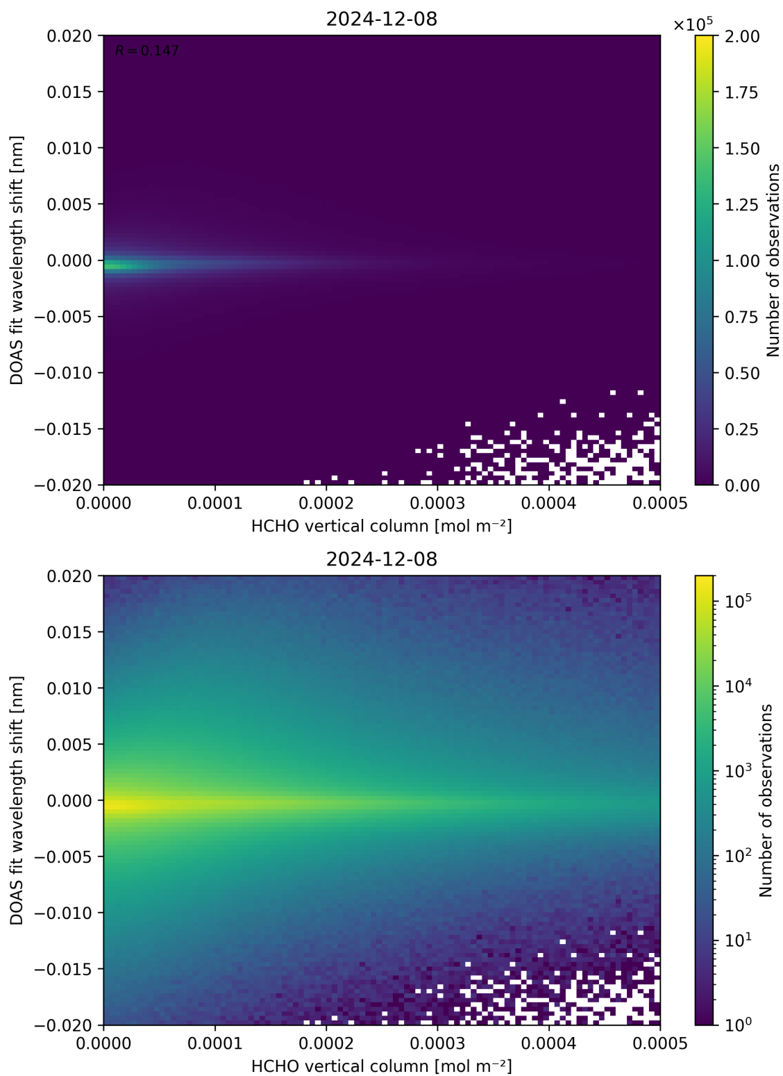
Figure 124: Scatter density plot of “HCHO vertical column” against “DOAS fit wavelength shift” for 2024-12-07 to 2024-12-09.
