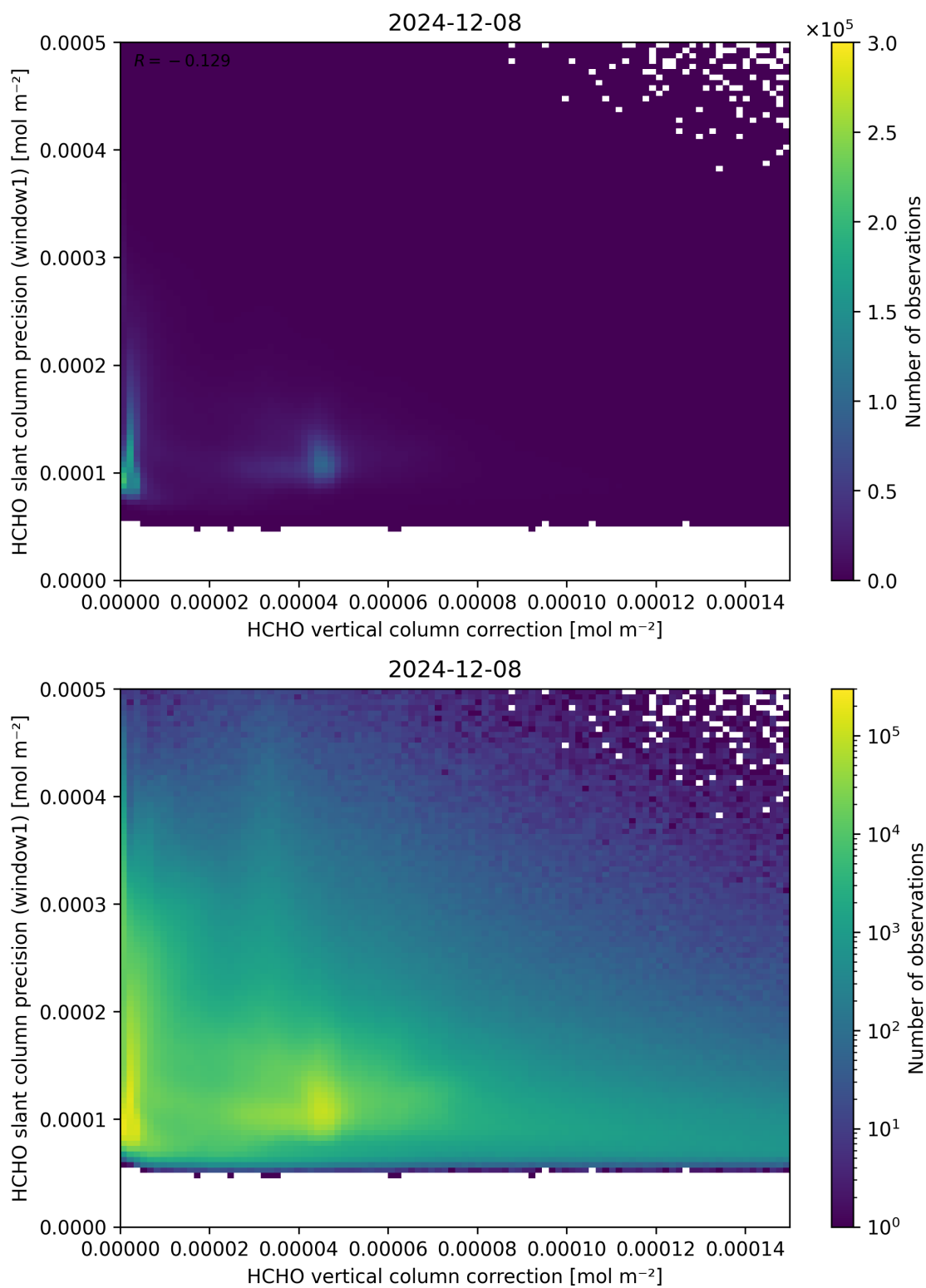
Figure 119: Scatter density plot of “HCHO vertical column correction” against “HCHO slant column precision (window1)” for 2024-12-07 to 2024-12-09.
