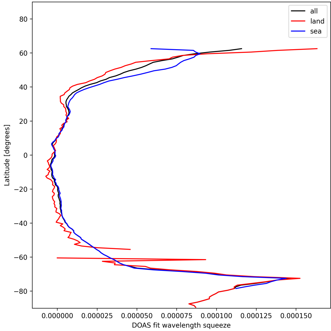
Figure 31: Zonal average of “DOAS fit wavelength squeeze” for 2024-12-07 to 2024-12-09.
