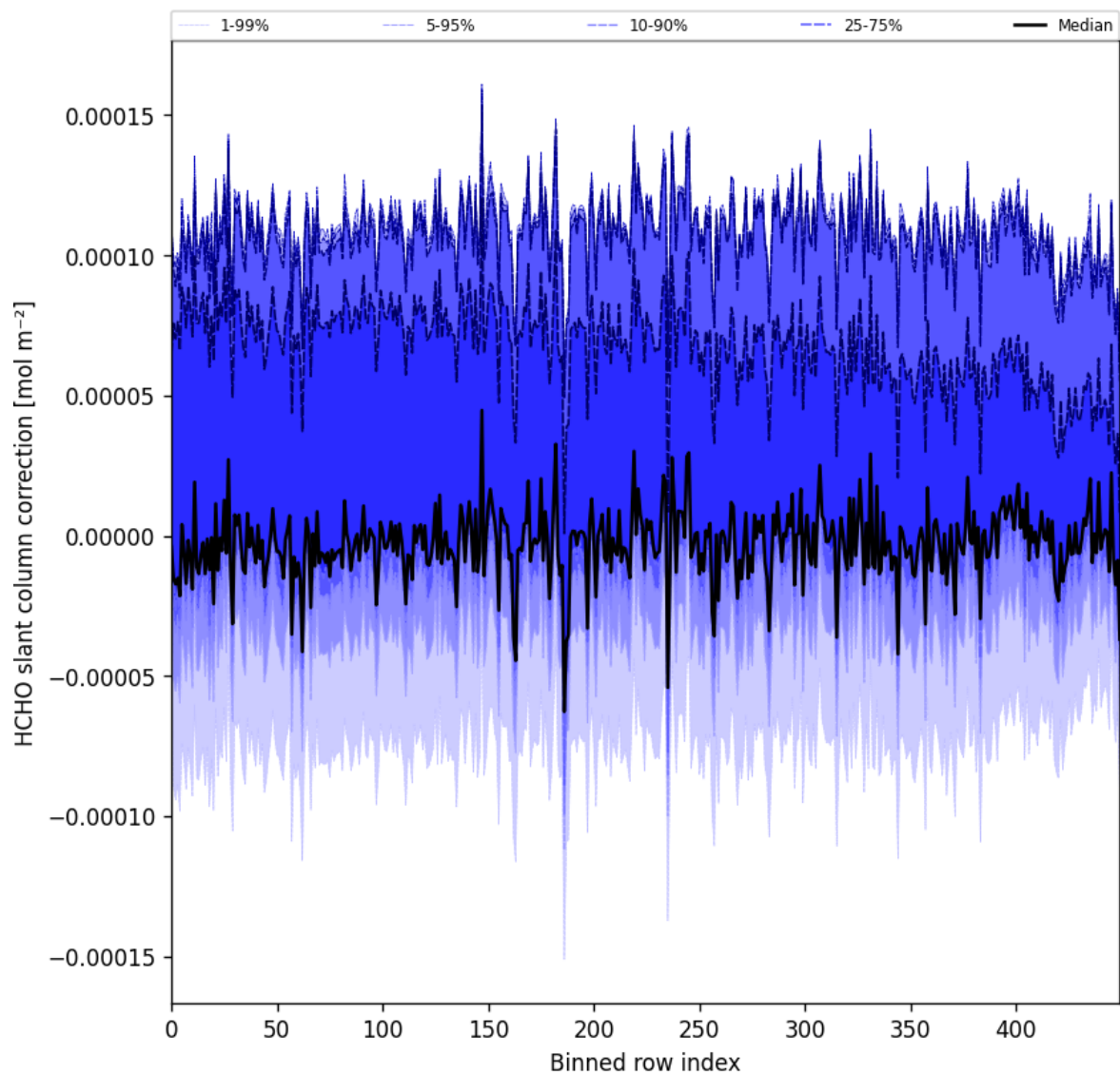
Figure 61: Along track statistics of “HCHO slant column correction” for 2024-12-07 to 2024-12-09
