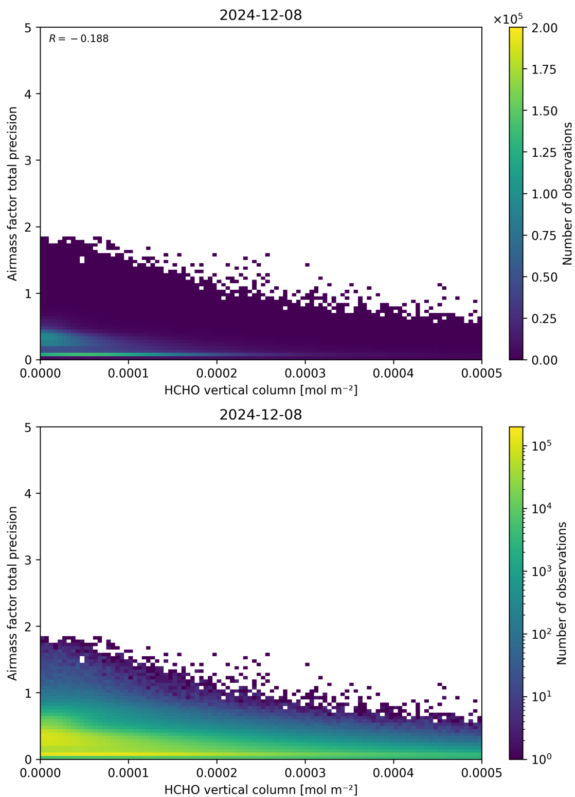
Figure 132: Scatter density plot of “HCHO vertical column” against “Airmass factor total precision” for 2024-12-07 to 2024-12-09.
