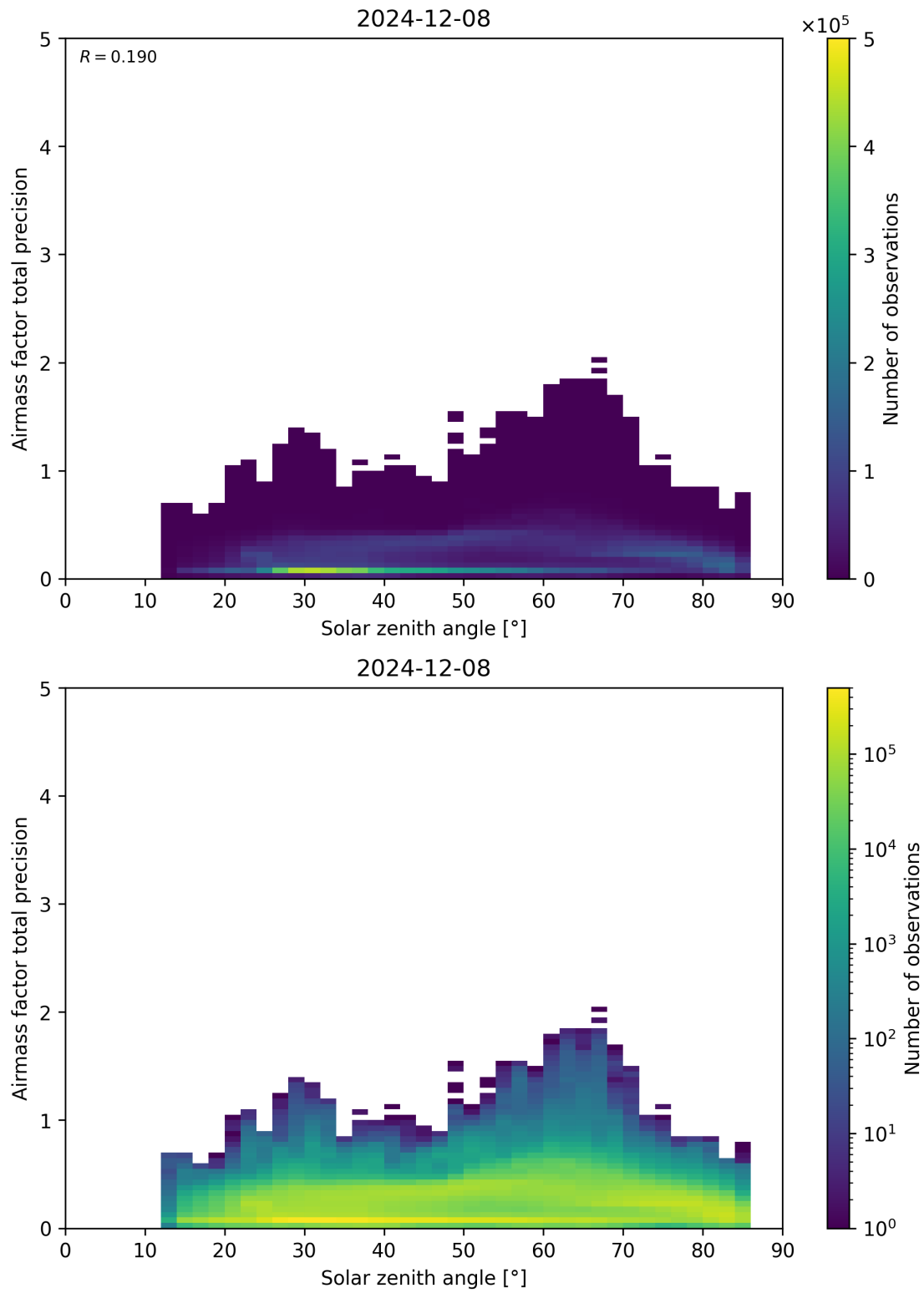
Figure 176: Scatter density plot of “Solar zenith angle” against “Airmass factor total precision” for 2024-12-07 to 2024-12-09.
