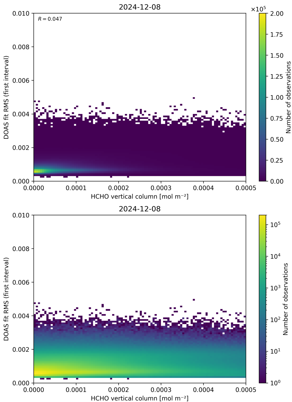
Figure 123: Scatter density plot of “HCHO vertical column” against “DOAS fit RMS (first interval)” for 2024-12-07 to 2024-12-09.
