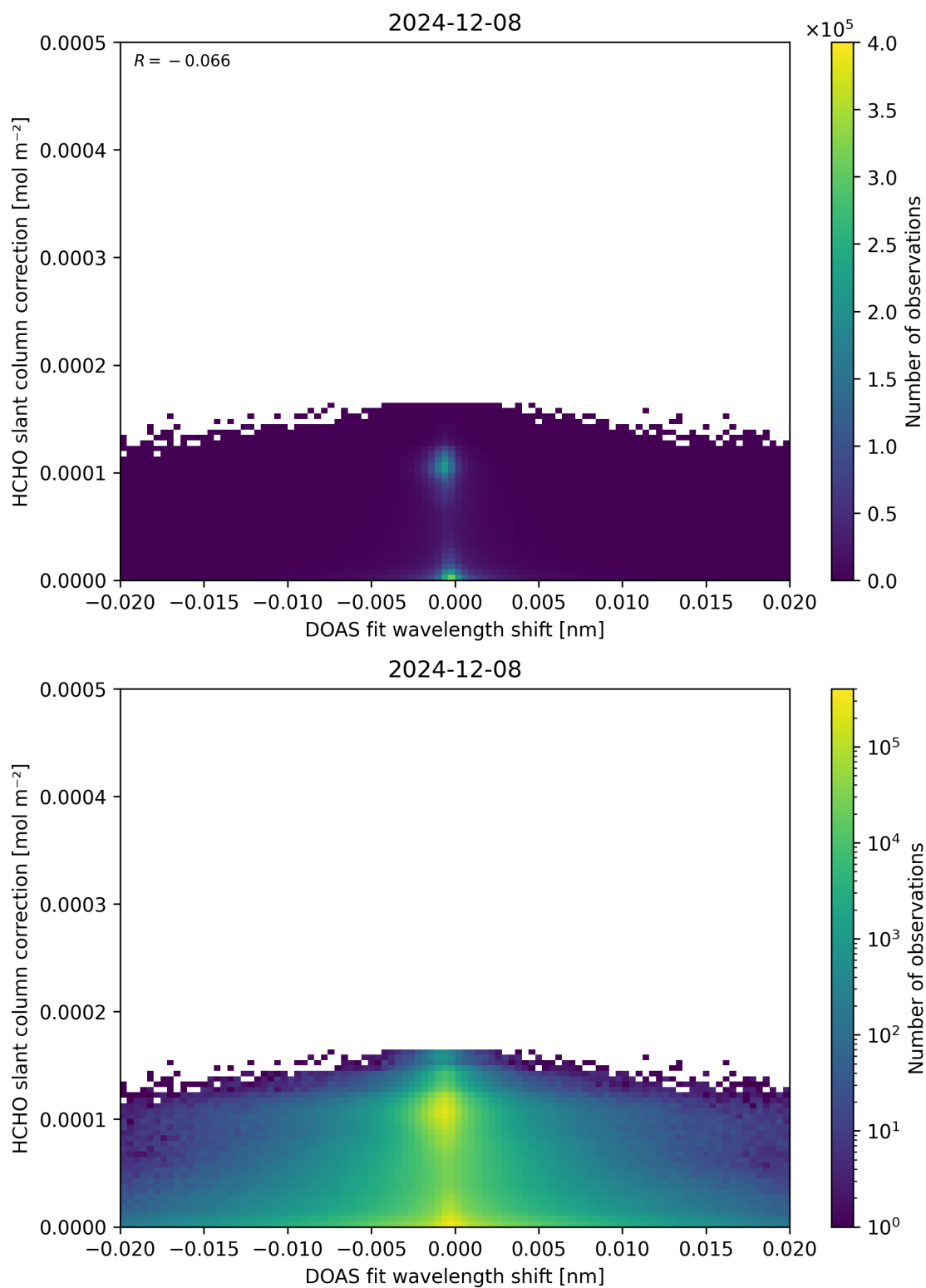
Figure 67: Scatter density plot of “DOAS fit wavelength shift” against “HCHO slant column correction” for 2024-12-07 to 2024-12-09.
