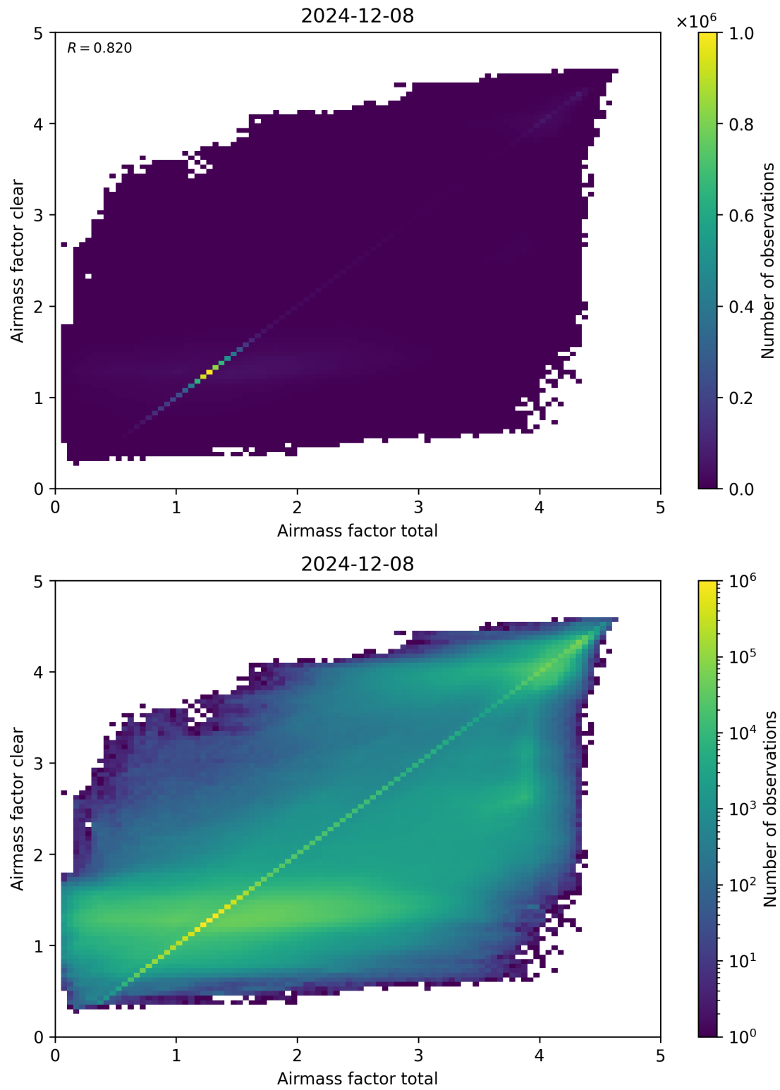
Figure 100: Scatter density plot of “Airmass factor total” against “Airmass factor clear” for 2024-12-07 to 2024-12-09.
