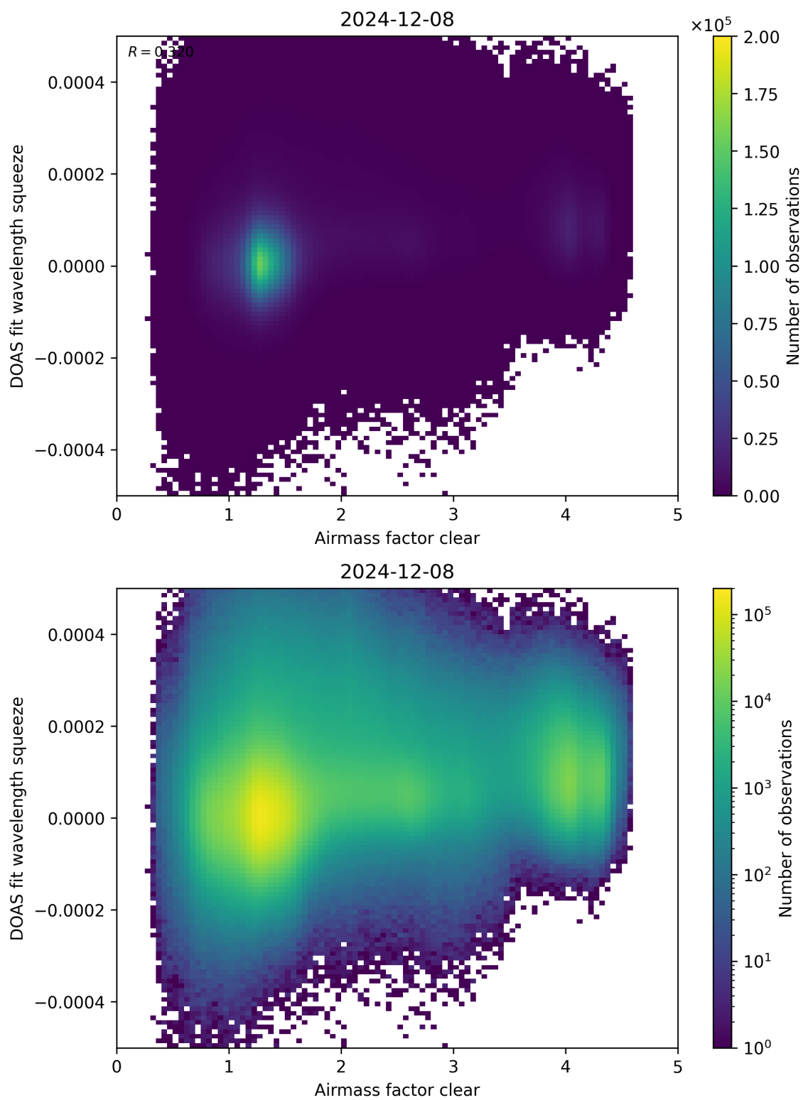
Figure 73: Scatter density plot of “Airmass factor clear” against “DOAS fit wavelength squeeze” for 2024-12-07 to 2024-12-09.
