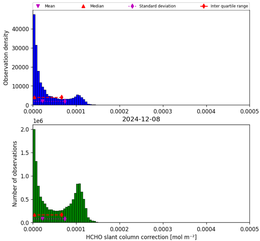
Figure 47: Histogram of “HCHO slant column correction” for 2024-12-07 to 2024-12-09
