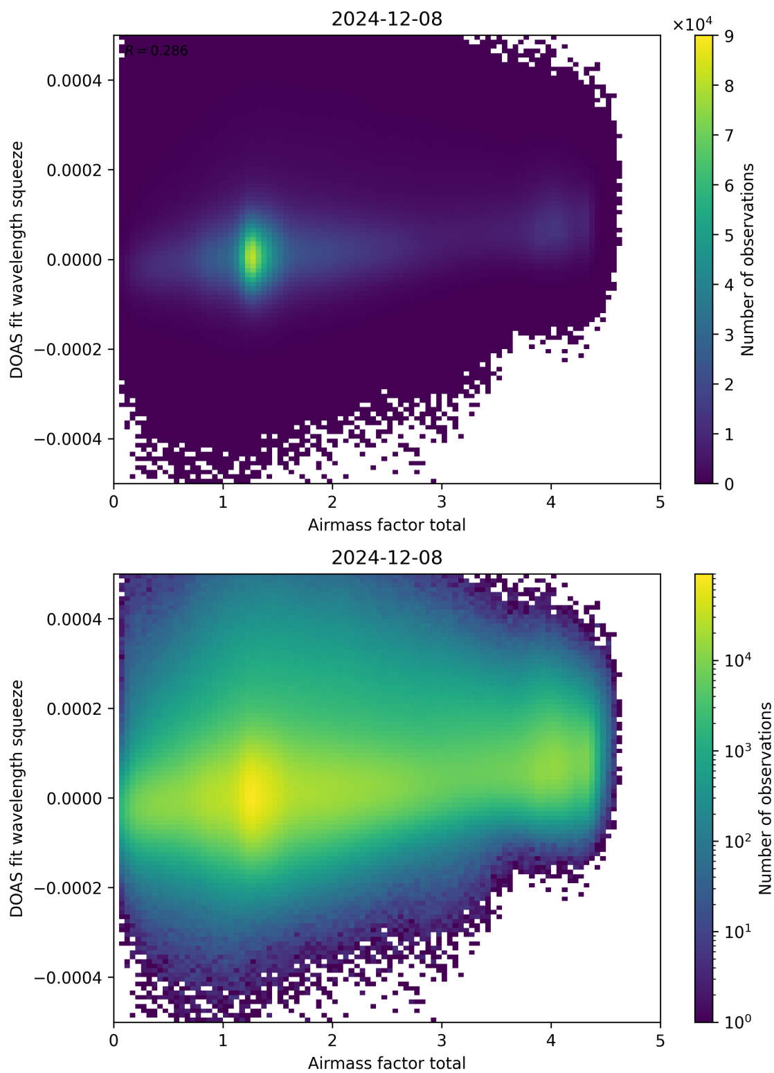
Figure 99: Scatter density plot of “Airmass factor total” against “DOAS fit wavelength squeeze” for 2024-12-07 to 2024-12-09.
