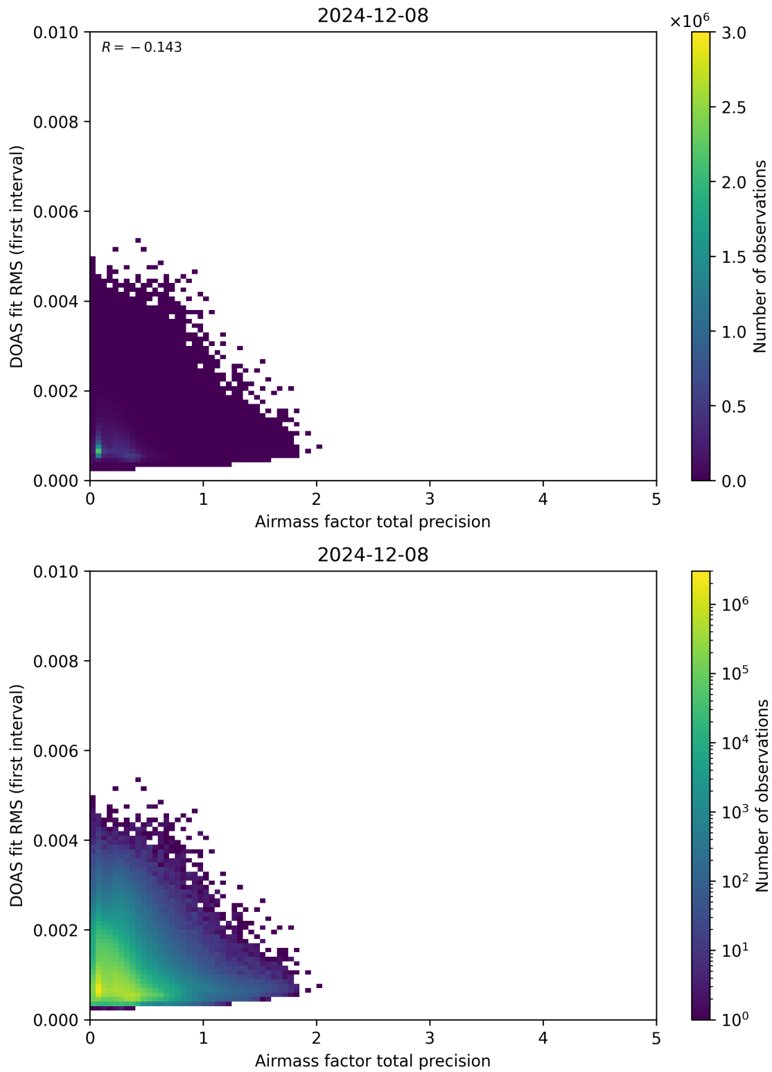
Figure 105: Scatter density plot of “Airmass factor total precision” against “DOAS fit RMS (first interval)” for 2024-12-07 to 2024-12-09.
