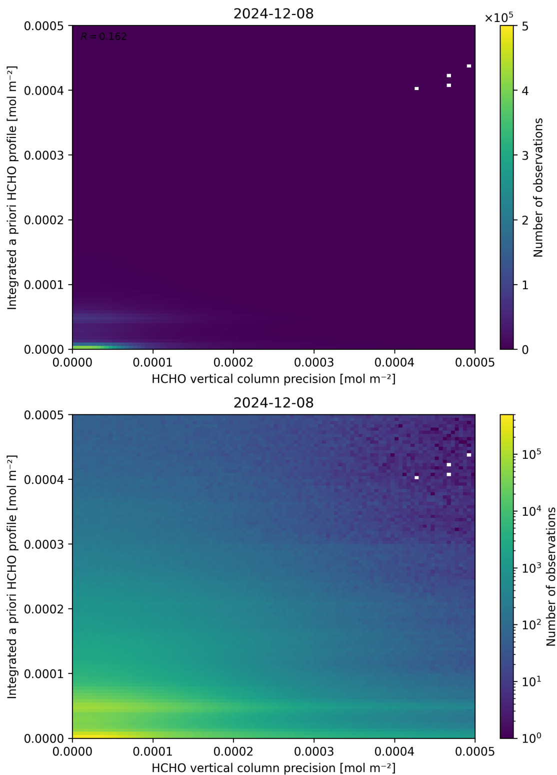
Figure 147: Scatter density plot of “HCHO vertical column precision” against “Integrated a priori HCHO profile” for 2024-12-07 to 2024-12-09.
