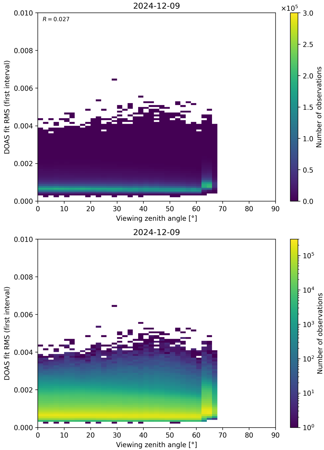
Figure 182: Scatter density plot of “Viewing zenith angle” against “DOAS fit RMS (first interval)” for 2024-12-08 to 2024-12-10.
