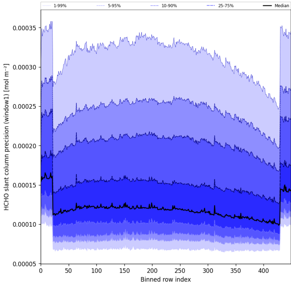
Figure 53: Along track statistics of “HCHO slant column precision (window1)” for 2024-12-08 to 2024-12-10
