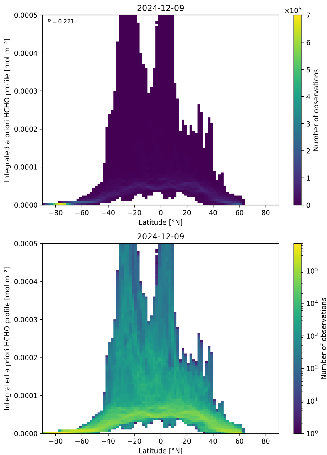
Figure 166: Scatter density plot of “Latitude” against “Integrated a priori HCHO profile” for 2024-12-08 to 2024-12-10.
