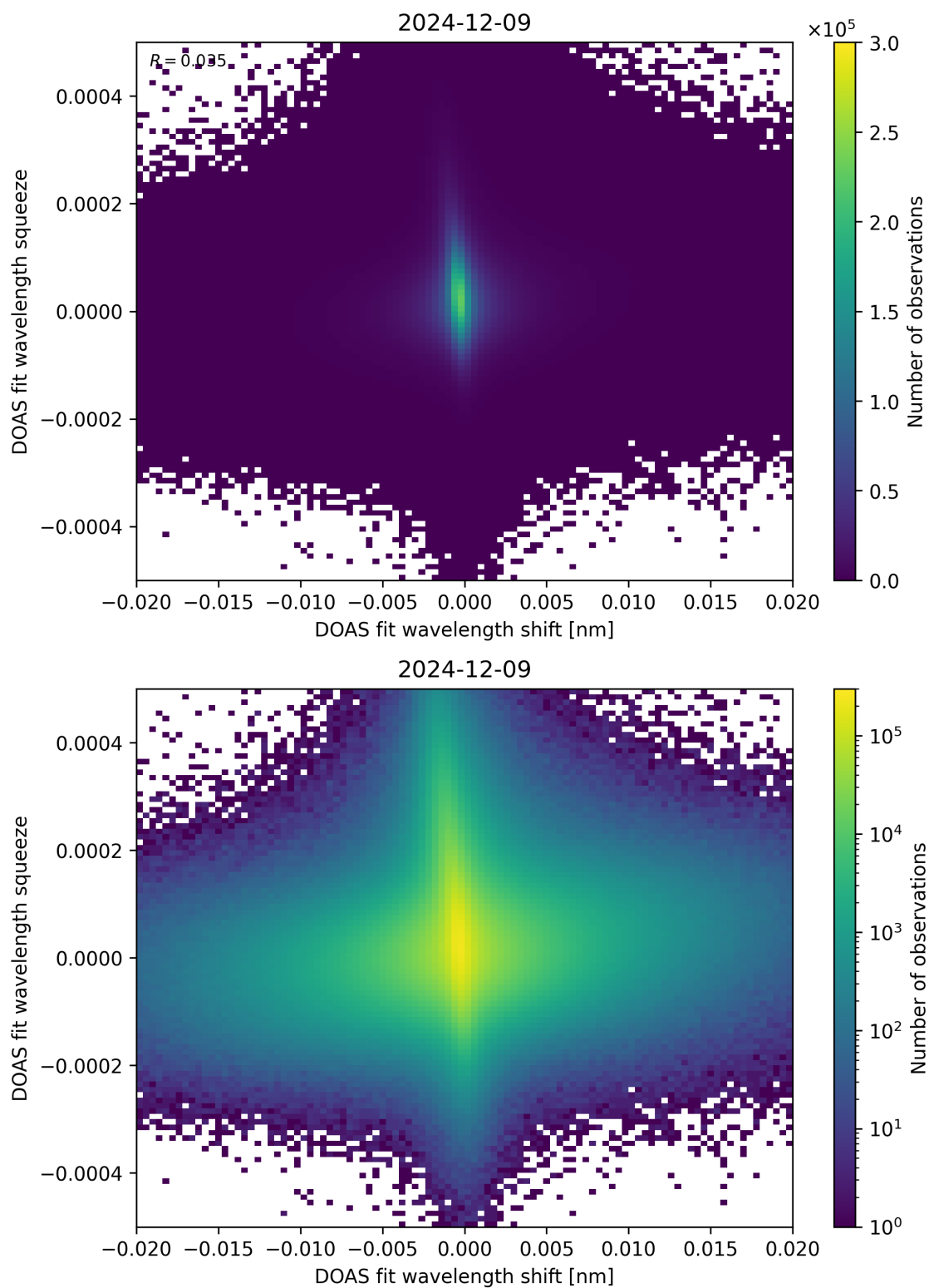
Figure 65: Scatter density plot of “DOAS fit wavelength shift” against “DOAS fit wavelength squeeze” for 2024-12-08 to 2024-12-10.
