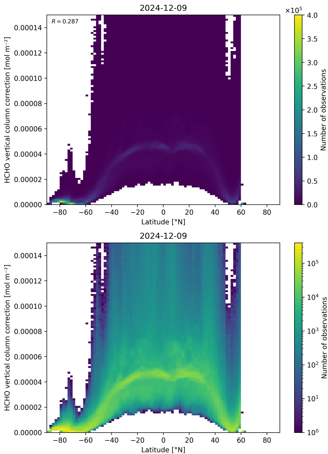
Figure 164: Scatter density plot of “Latitude” against “HCHO vertical column correction” for 2024-12-08 to 2024-12-10.
