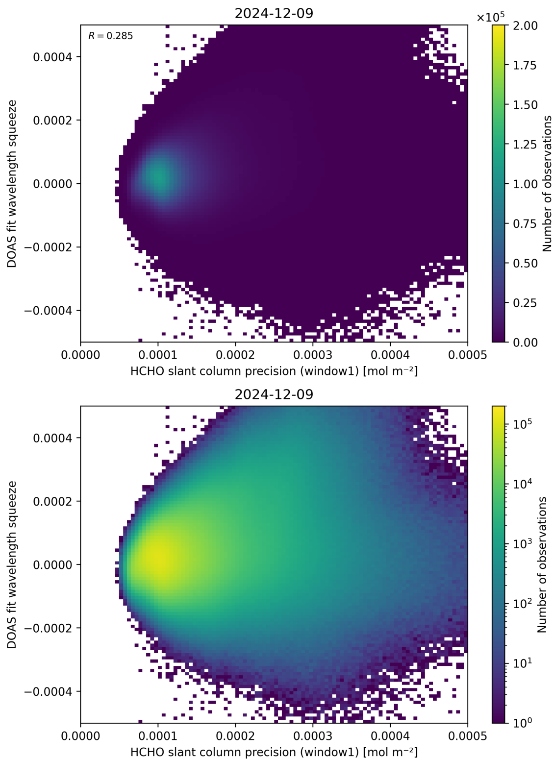
Figure 90: Scatter density plot of “HCHO slant column precision (window1)” against “DOAS fit wavelength squeeze” for 2024-12-08 to 2024-12-10.
