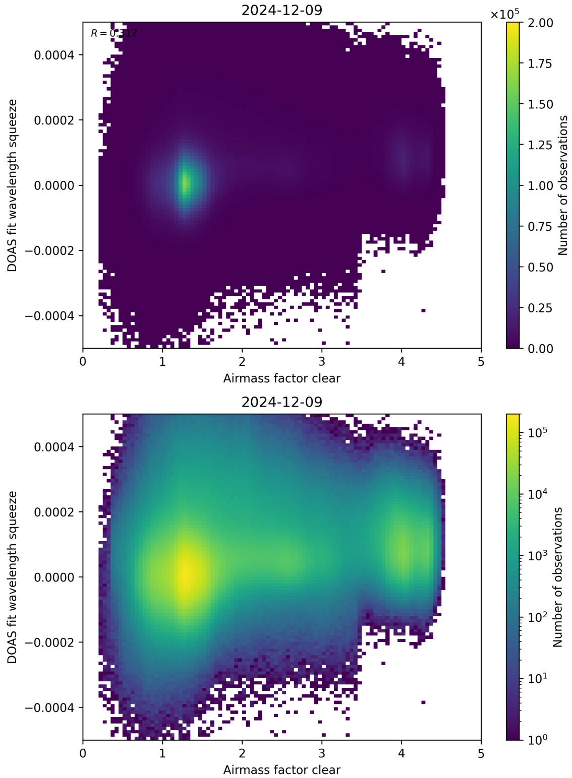
Figure 73: Scatter density plot of “Airmass factor clear” against “DOAS fit wavelength squeeze” for 2024-12-08 to 2024-12-10.
