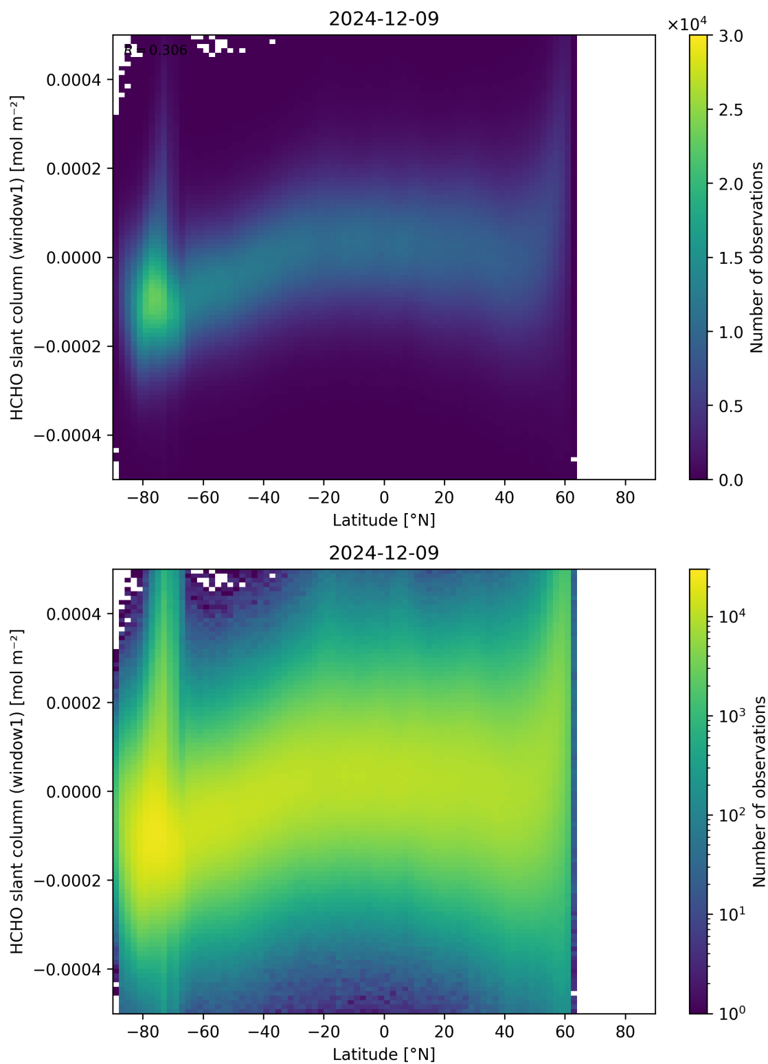
Figure 159: Scatter density plot of “Latitude” against “HCHO slant column (window1)” for 2024-12-08 to 2024-12-10.
