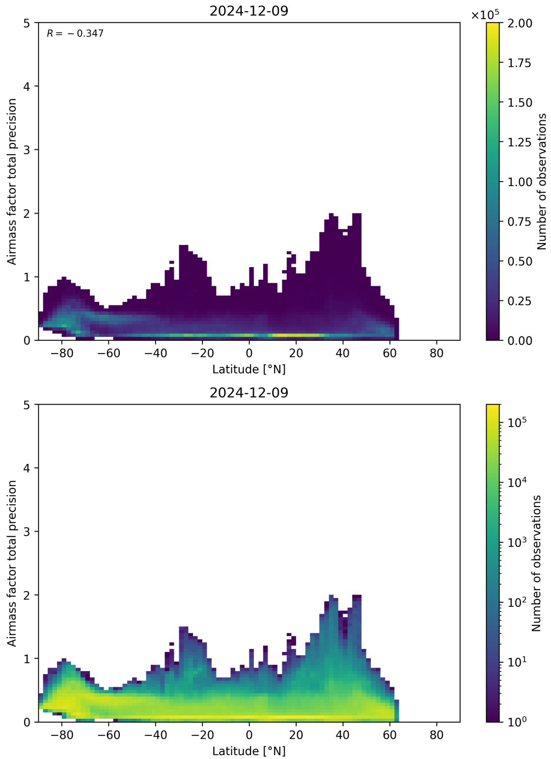
Figure 162: Scatter density plot of “Latitude” against “Airmass factor total precision” for 2024-12-08 to 2024-12-10.
