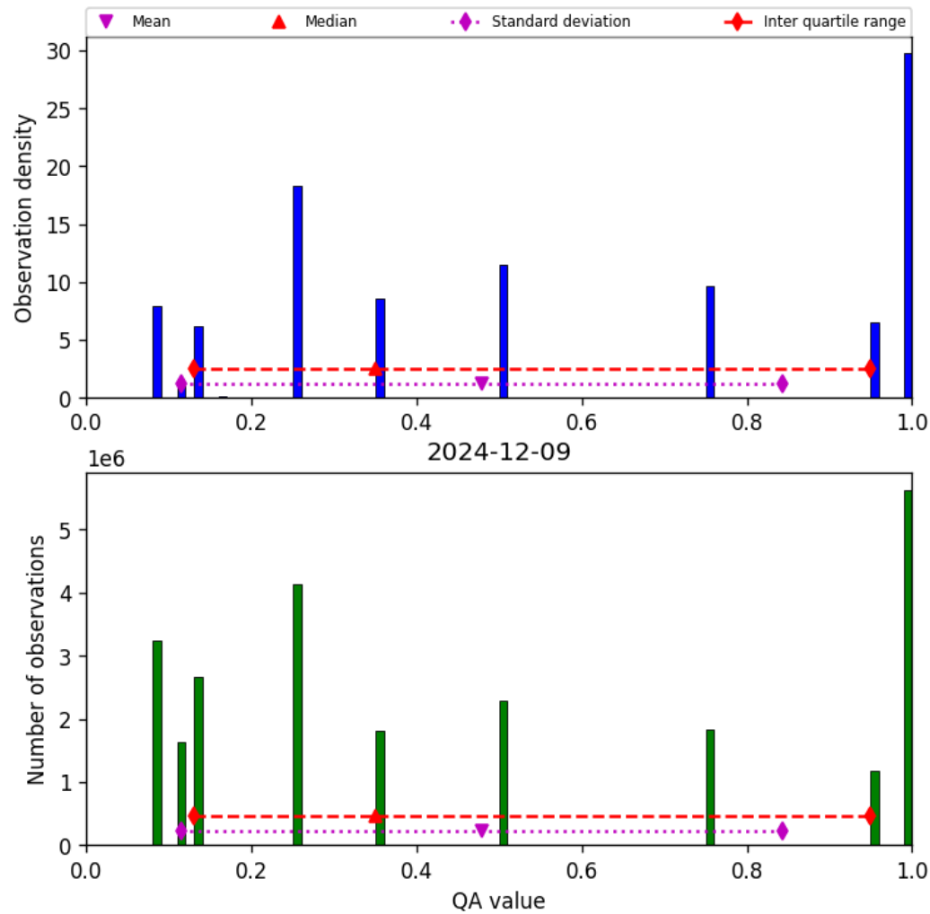
Figure 34: Histogram of “QA value” for 2024-12-08 to 2024-12-10
