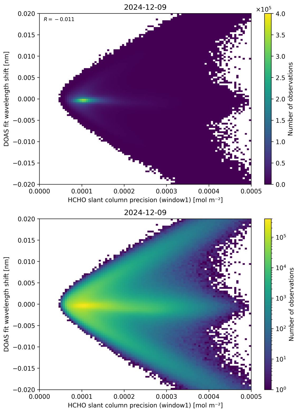
Figure 89: Scatter density plot of “HCHO slant column precision (window1)” against “DOAS fit wavelength shift” for 2024-12-08 to 2024-12-10.
