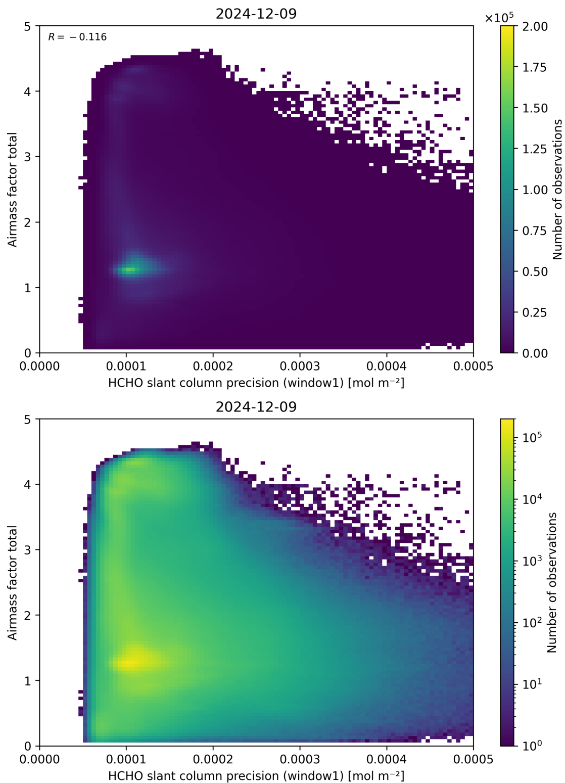
Figure 94: Scatter density plot of “HCHO slant column precision (window1)” against “Airmass factor total” for 2024-12-08 to 2024-12-10.
