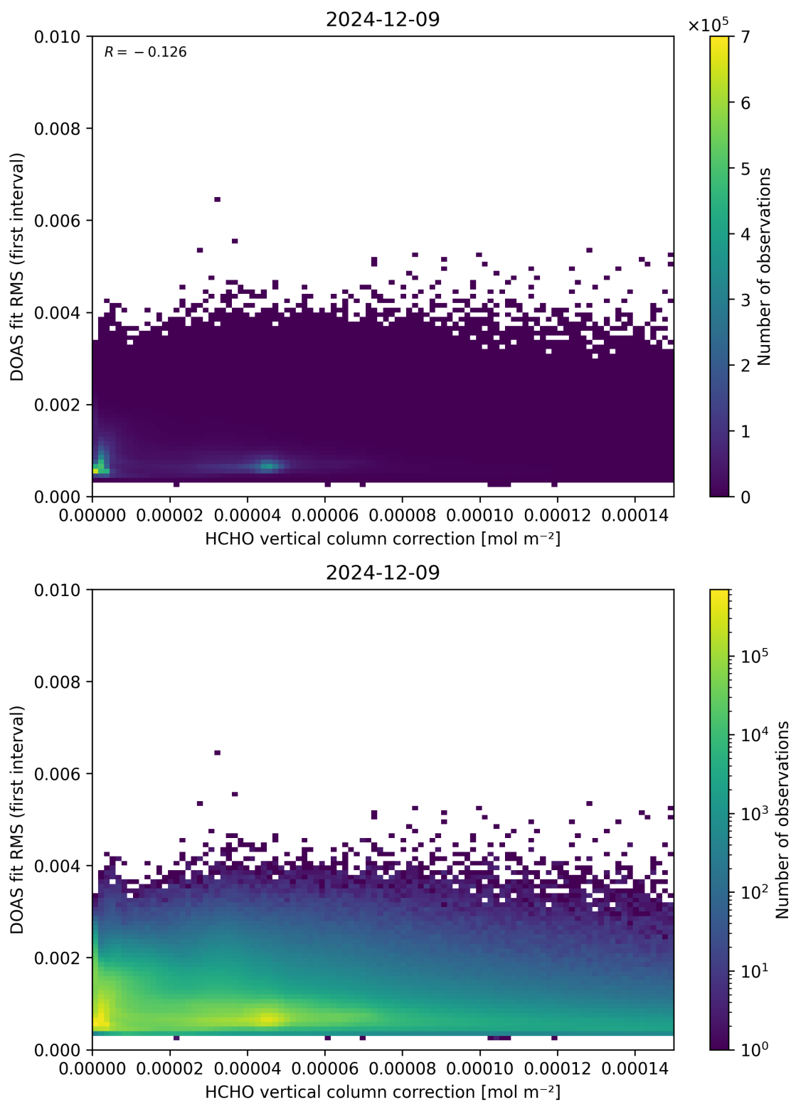
Figure 112: Scatter density plot of “HCHO vertical column correction” against “DOAS fit RMS (first interval)” for 2024-12-08 to 2024-12-10.
