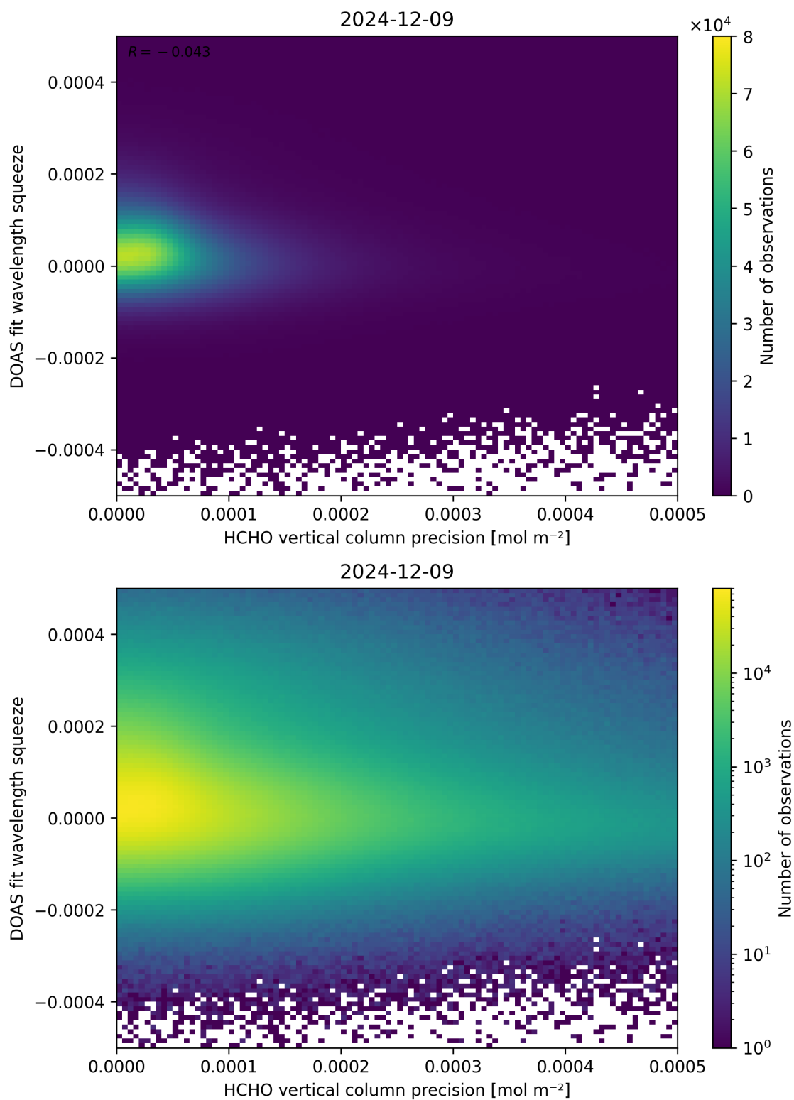
Figure 138: Scatter density plot of “HCHO vertical column precision” against “DOAS fit wavelength squeeze” for 2024-12-08 to 2024-12-10.
