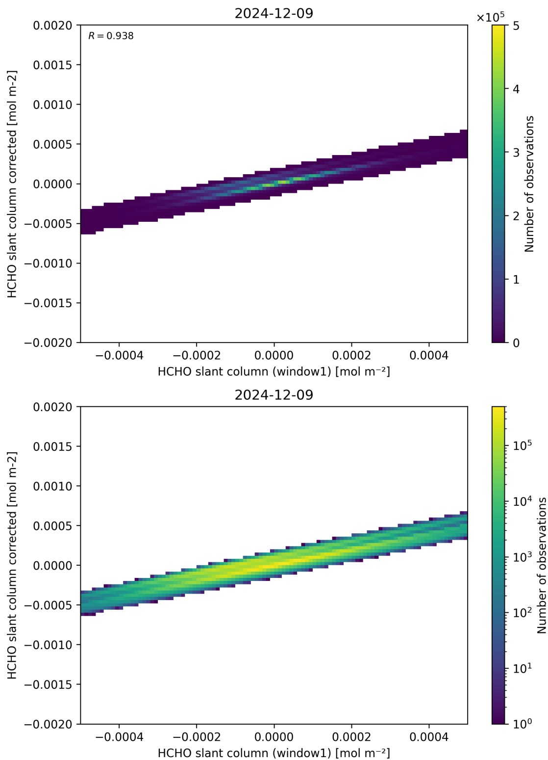
Figure 82: Scatter density plot of “HCHO slant column (window1)” against “HCHO slant column corrected” for 2024-12-08 to 2024-12-10.
