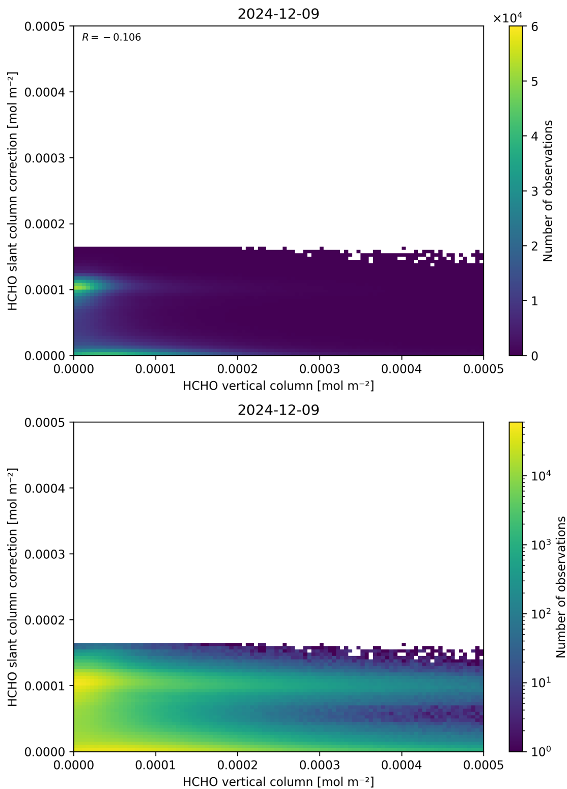
Figure 128: Scatter density plot of “HCHO vertical column” against “HCHO slant column correction” for 2024-12-08 to 2024-12-10.
