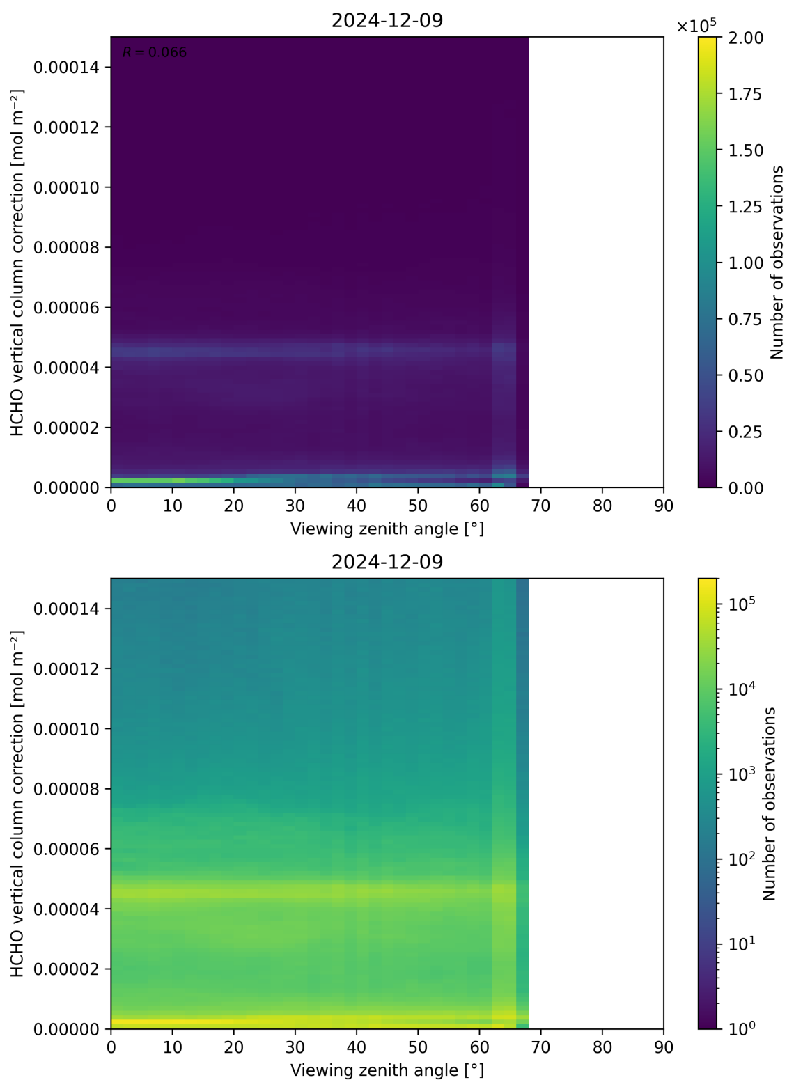
Figure 193: Scatter density plot of “Viewing zenith angle” against “HCHO vertical column correction” for 2024-12-08 to 2024-12-10.
