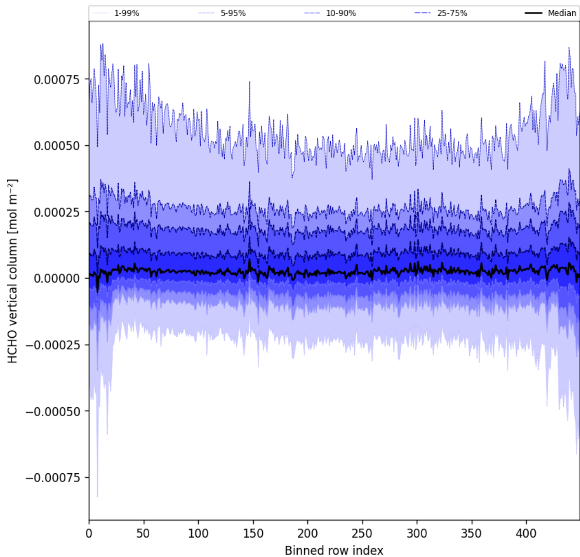
Figure 49: Along track statistics of “HCHO vertical column” for 2024-12-08 to 2024-12-10
