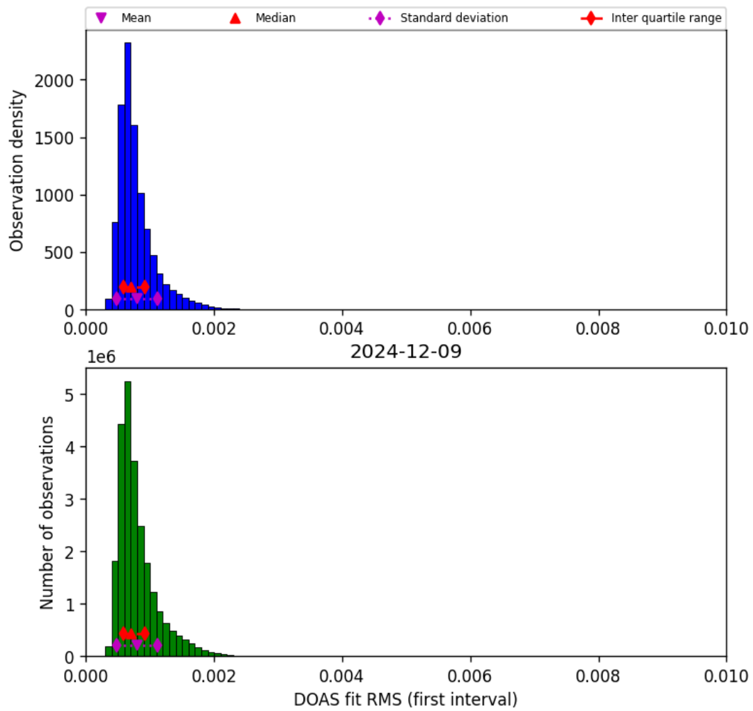
Figure 46: Histogram of “DOAS fit RMS (first interval)” for 2024-12-08 to 2024-12-10
