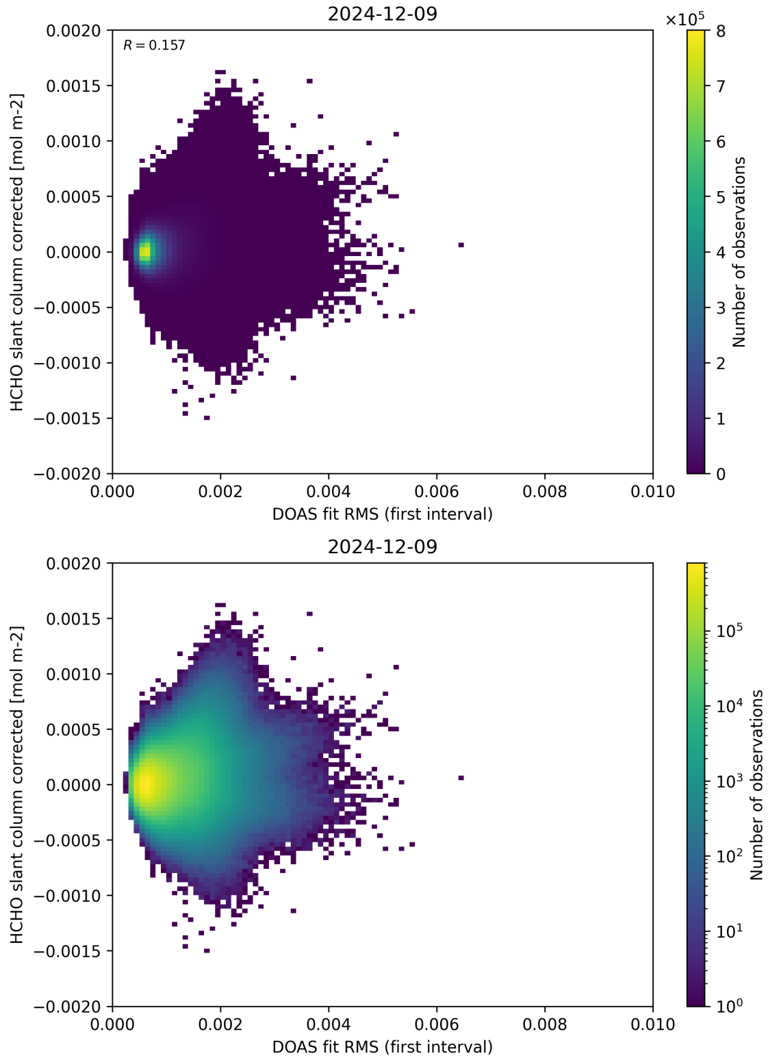
Figure 62: Scatter density plot of “DOAS fit RMS (first interval)” against “HCHO slant column corrected” for 2024-12-08 to 2024-12-10.
