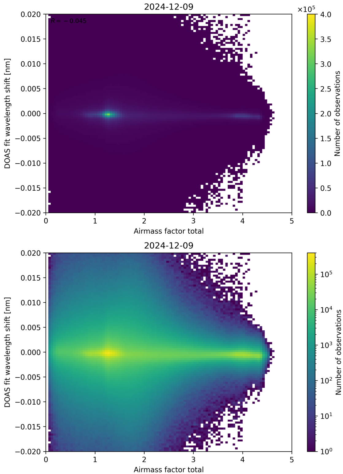
Figure 98: Scatter density plot of “Airmass factor total” against “DOAS fit wavelength shift” for 2024-12-08 to 2024-12-10.
