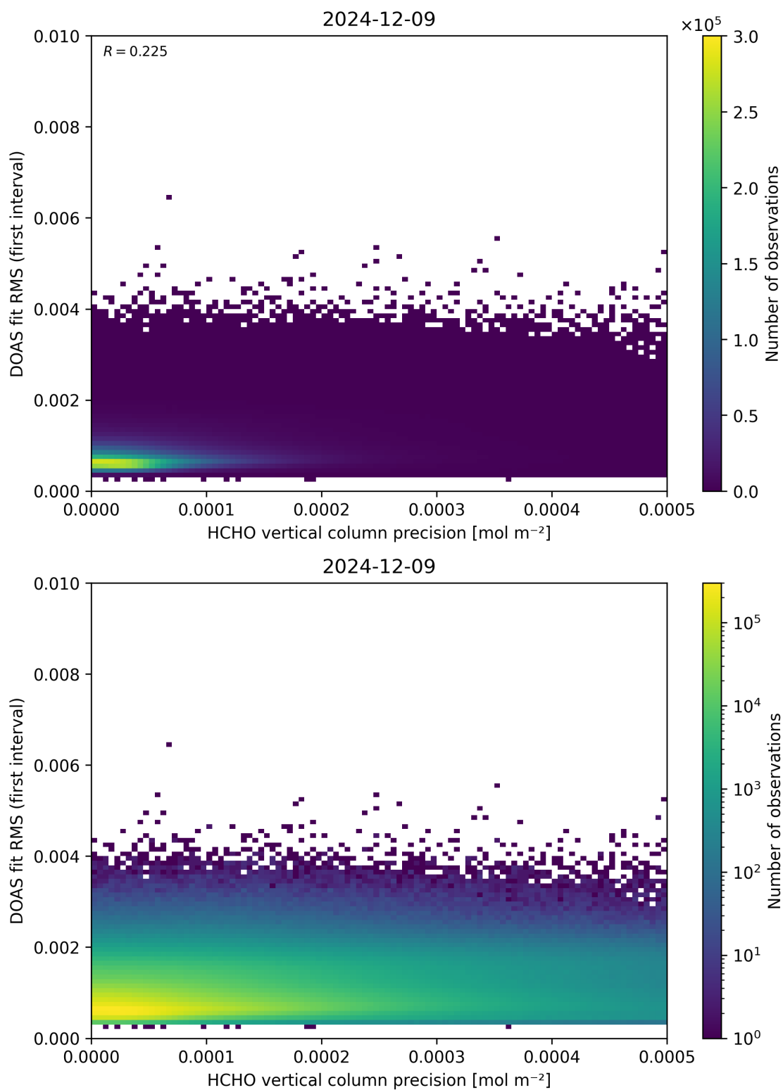
Figure 136: Scatter density plot of “HCHO vertical column precision” against “DOAS fit RMS (first interval)” for 2024-12-08 to 2024-12-10.
