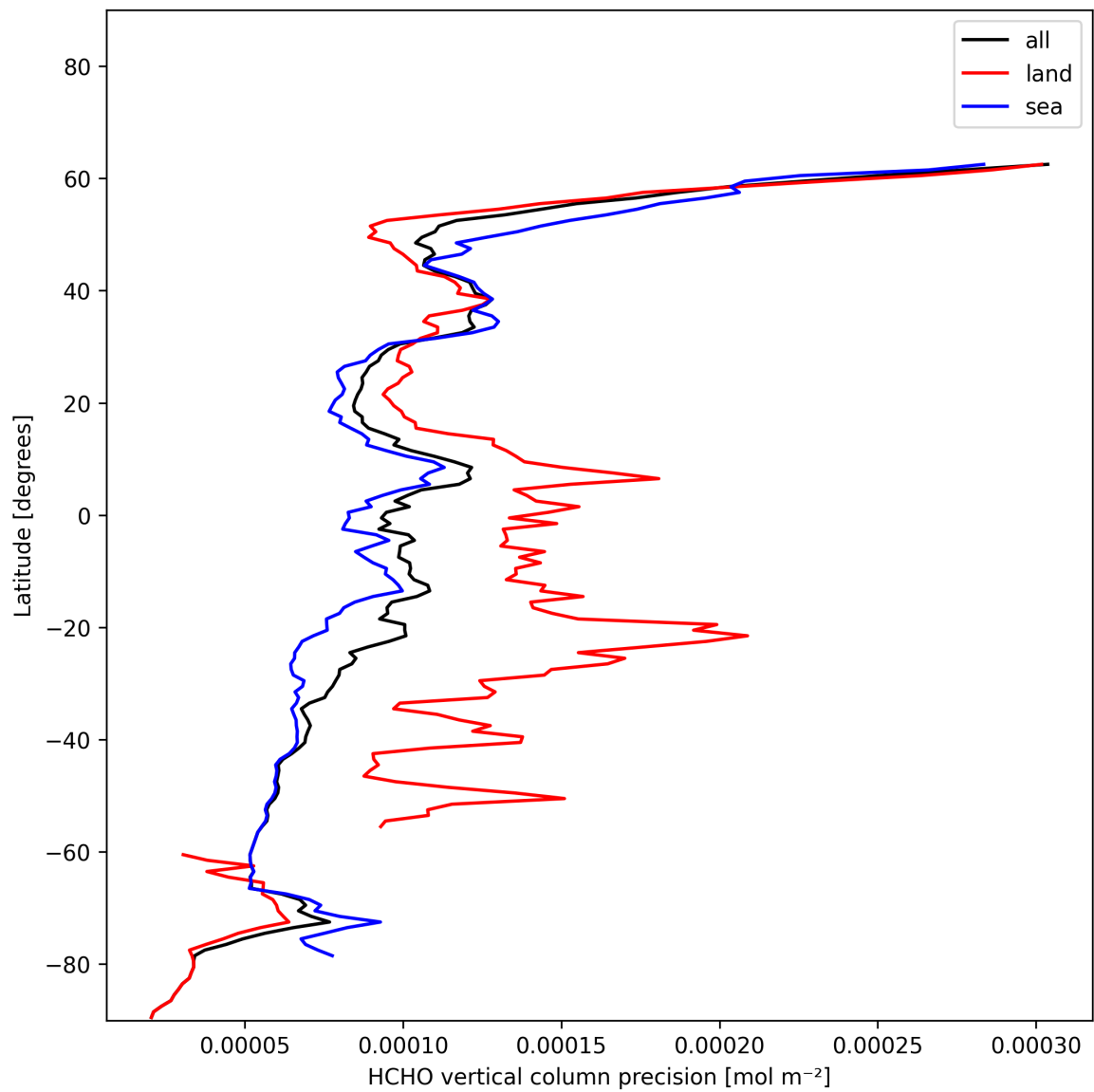
Figure 22: Zonal average of “HCHO vertical column precision” for 2024-12-08 to 2024-12-10.
