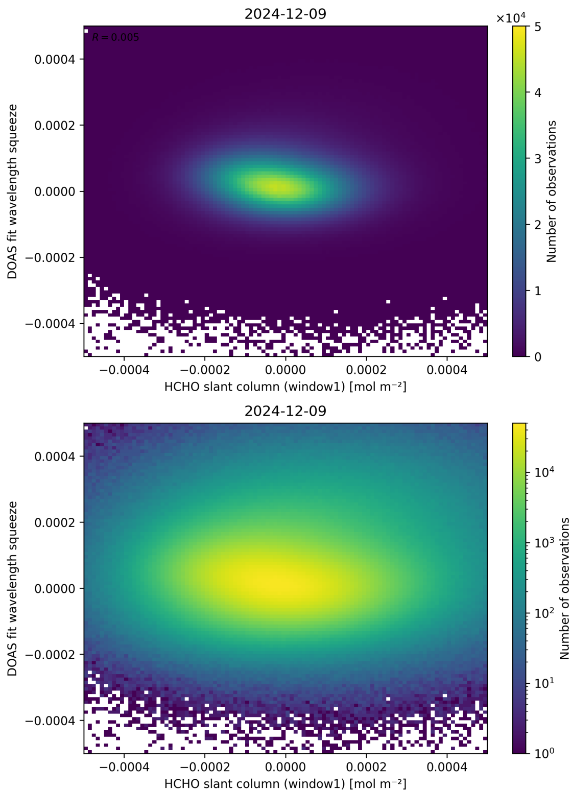
Figure 80: Scatter density plot of “HCHO slant column (window1)” against “DOAS fit wavelength squeeze” for 2024-12-08 to 2024-12-10.
