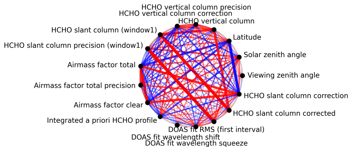
Figure 1: Map of correlation graph for 2024-12-08 to 2024-12-10.
