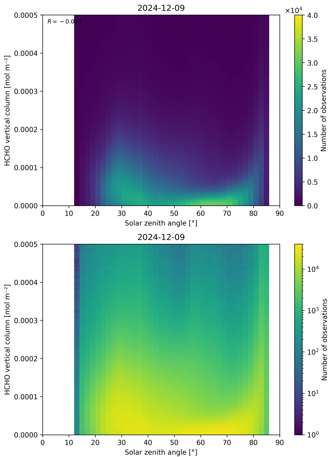
Figure 177: Scatter density plot of “Solar zenith angle” against “HCHO vertical column” for 2024-12-08 to 2024-12-10.
