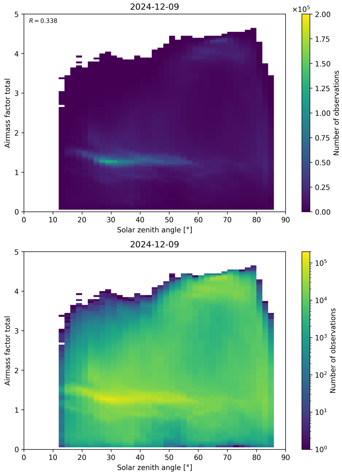
Figure 175: Scatter density plot of “Solar zenith angle” against “Airmass factor total” for 2024-12-08 to 2024-12-10.
