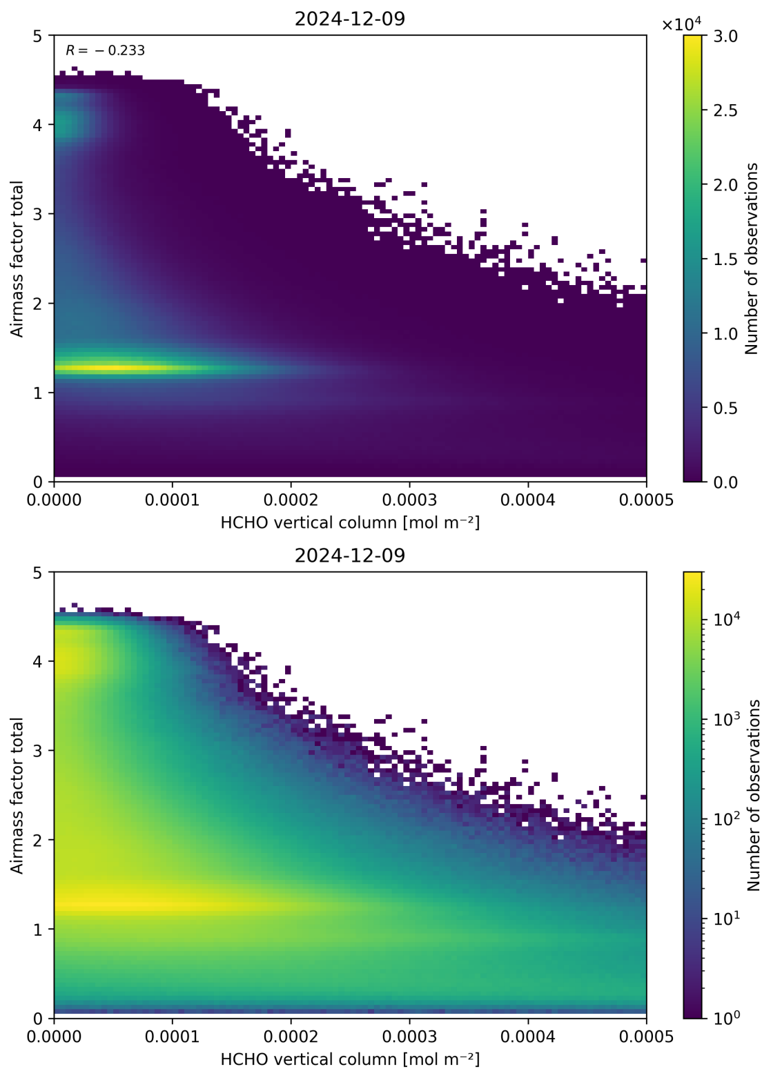
Figure 131: Scatter density plot of “HCHO vertical column” against “Airmass factor total” for 2024-12-08 to 2024-12-10.
