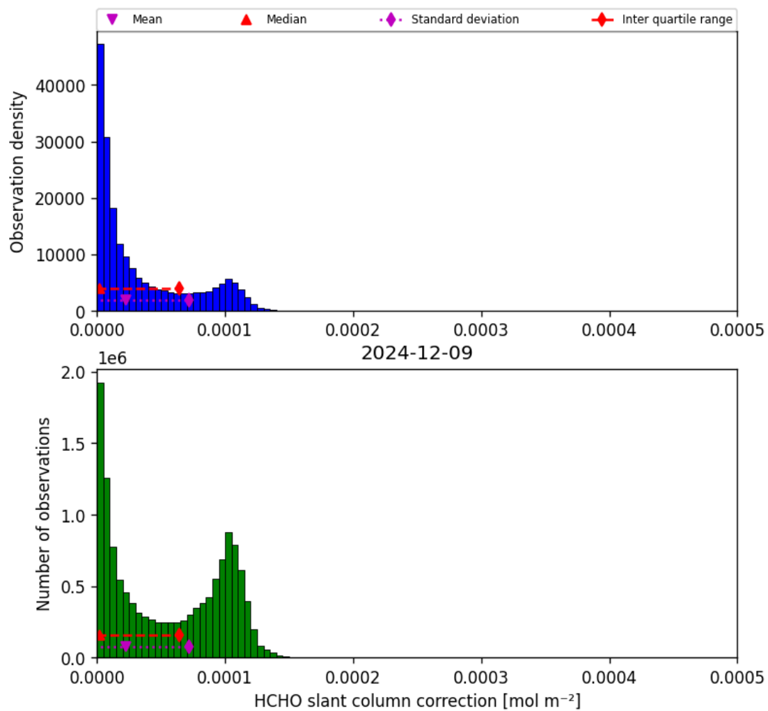
Figure 47: Histogram of “HCHO slant column correction” for 2024-12-08 to 2024-12-10
