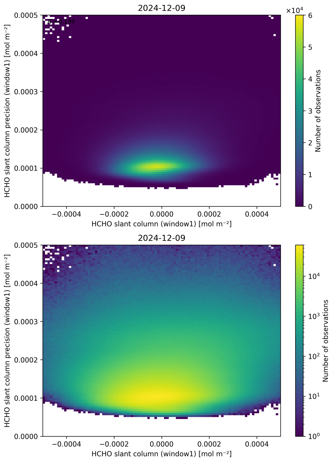
Figure 84: Scatter density plot of “HCHO slant column (window1)” against “HCHO slant column precision (window1)” for 2024-12-08 to 2024-12-10.
