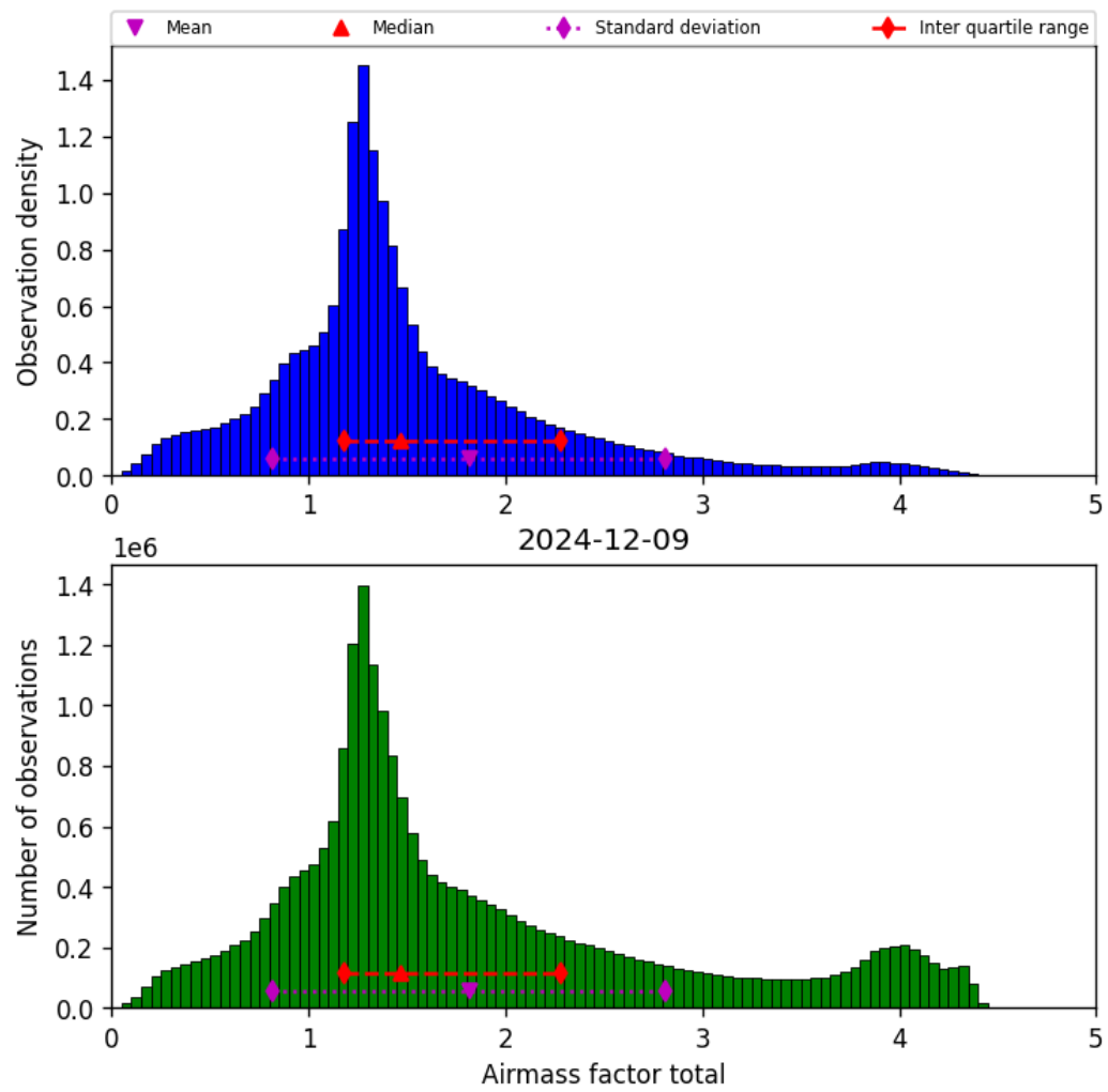
Figure 40: Histogram of “Airmass factor total” for 2024-12-08 to 2024-12-10
