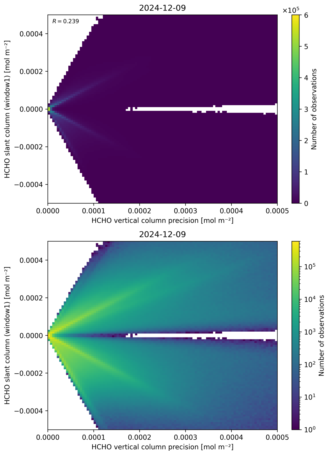
Figure 142: Scatter density plot of “HCHO vertical column precision” against “HCHO slant column (window1)” for 2024-12-08 to 2024-12-10.
