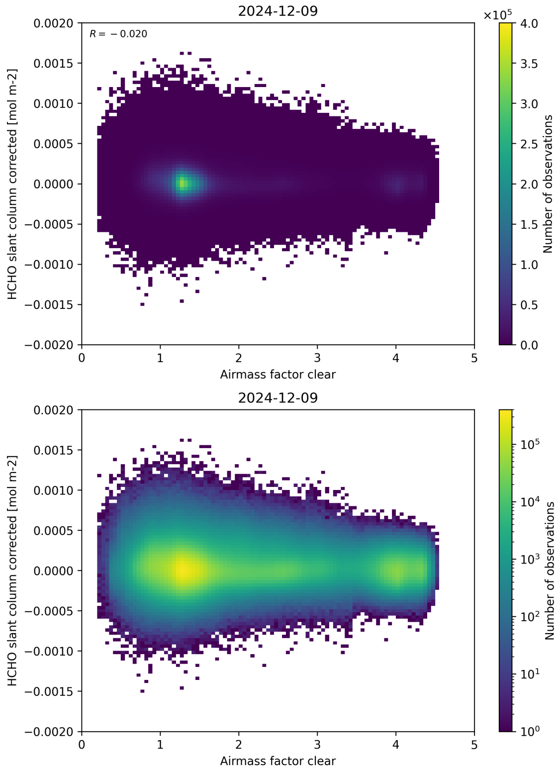
Figure 74: Scatter density plot of “Airmass factor clear” against “HCHO slant column corrected” for 2024-12-08 to 2024-12-10.
