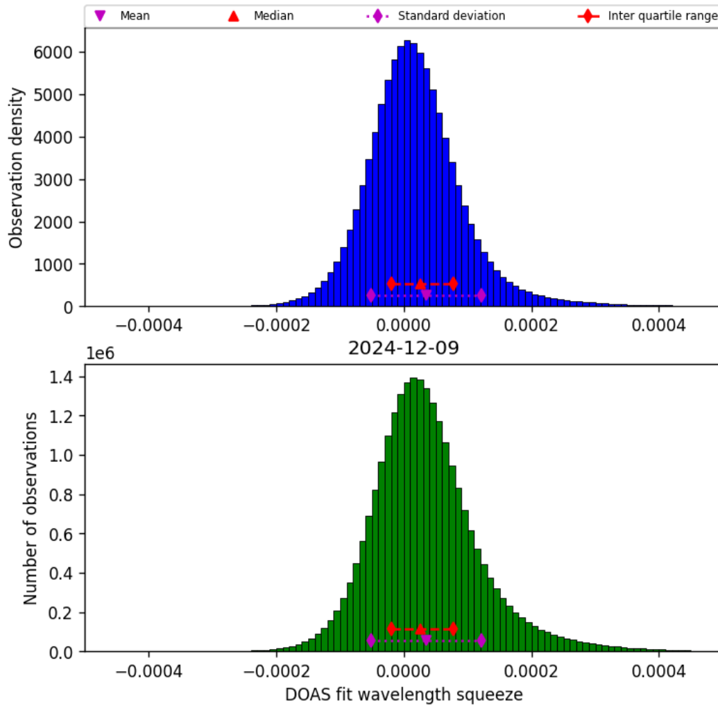
Figure 45: Histogram of “DOAS fit wavelength squeeze” for 2024-12-08 to 2024-12-10
