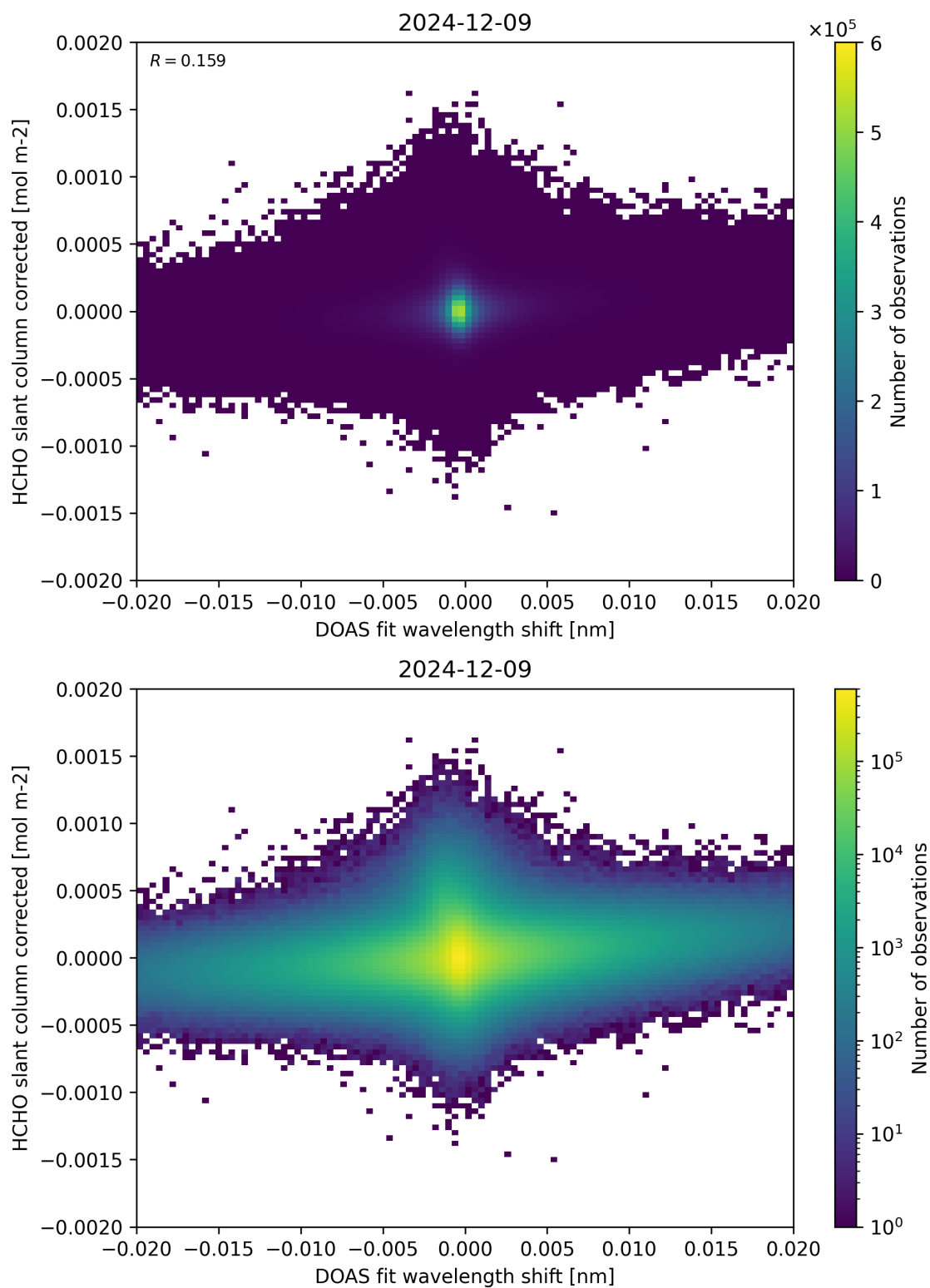
Figure 66: Scatter density plot of “DOAS fit wavelength shift” against “HCHO slant column corrected” for 2024-12-08 to 2024-12-10.
