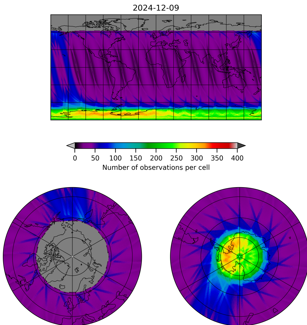
Figure 19: Map of the number of observations for 2024-12-08 to 2024-12-10
