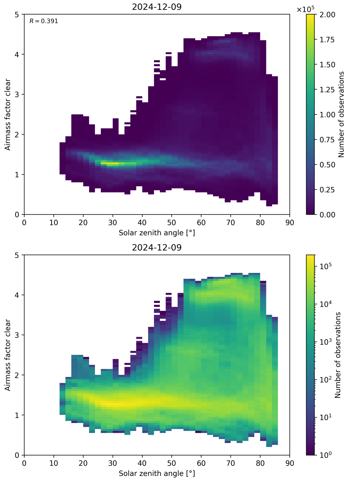
Figure 170: Scatter density plot of “Solar zenith angle” against “Airmass factor clear” for 2024-12-08 to 2024-12-10.
