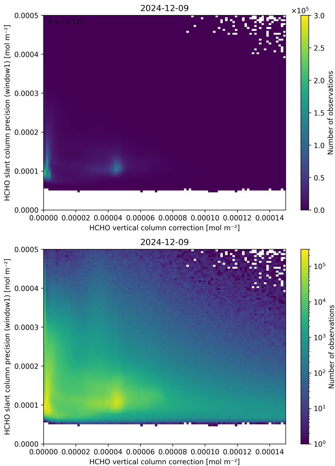
Figure 119: Scatter density plot of “HCHO vertical column correction” against “HCHO slant column precision (window1)” for 2024-12-08 to 2024-12-10.
