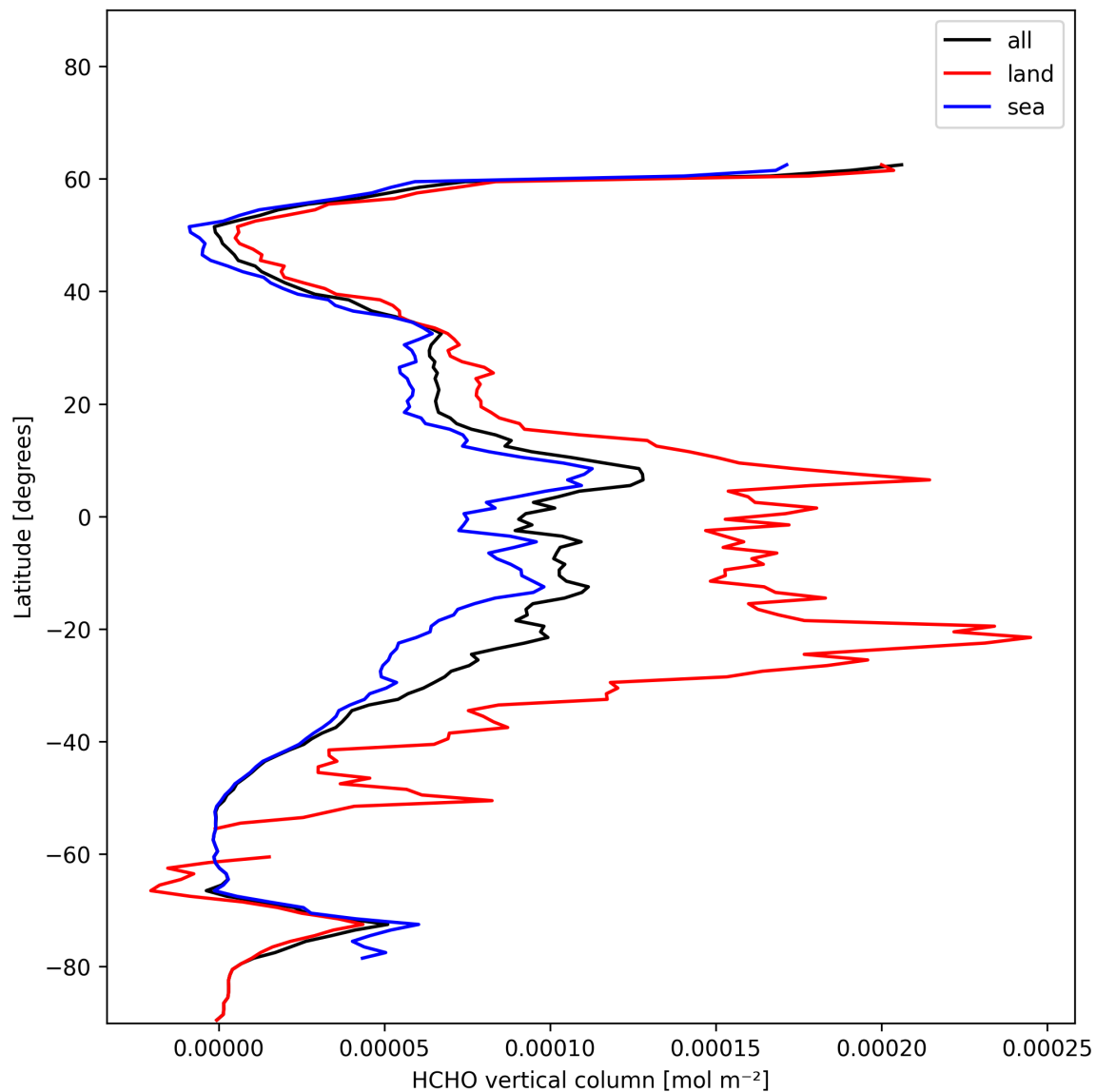
Figure 21: Zonal average of “HCHO vertical column” for 2024-12-08 to 2024-12-10.
