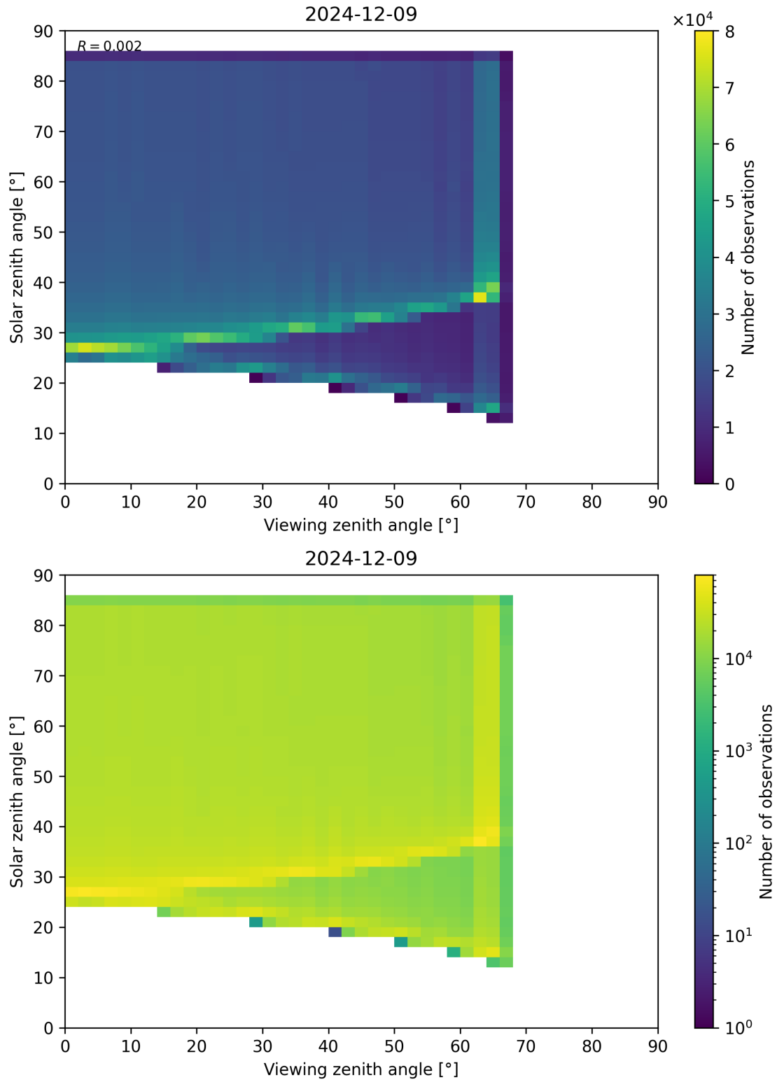
Figure 197: Scatter density plot of “Viewing zenith angle” against “Solar zenith angle” for 2024-12-08 to 2024-12-10.
