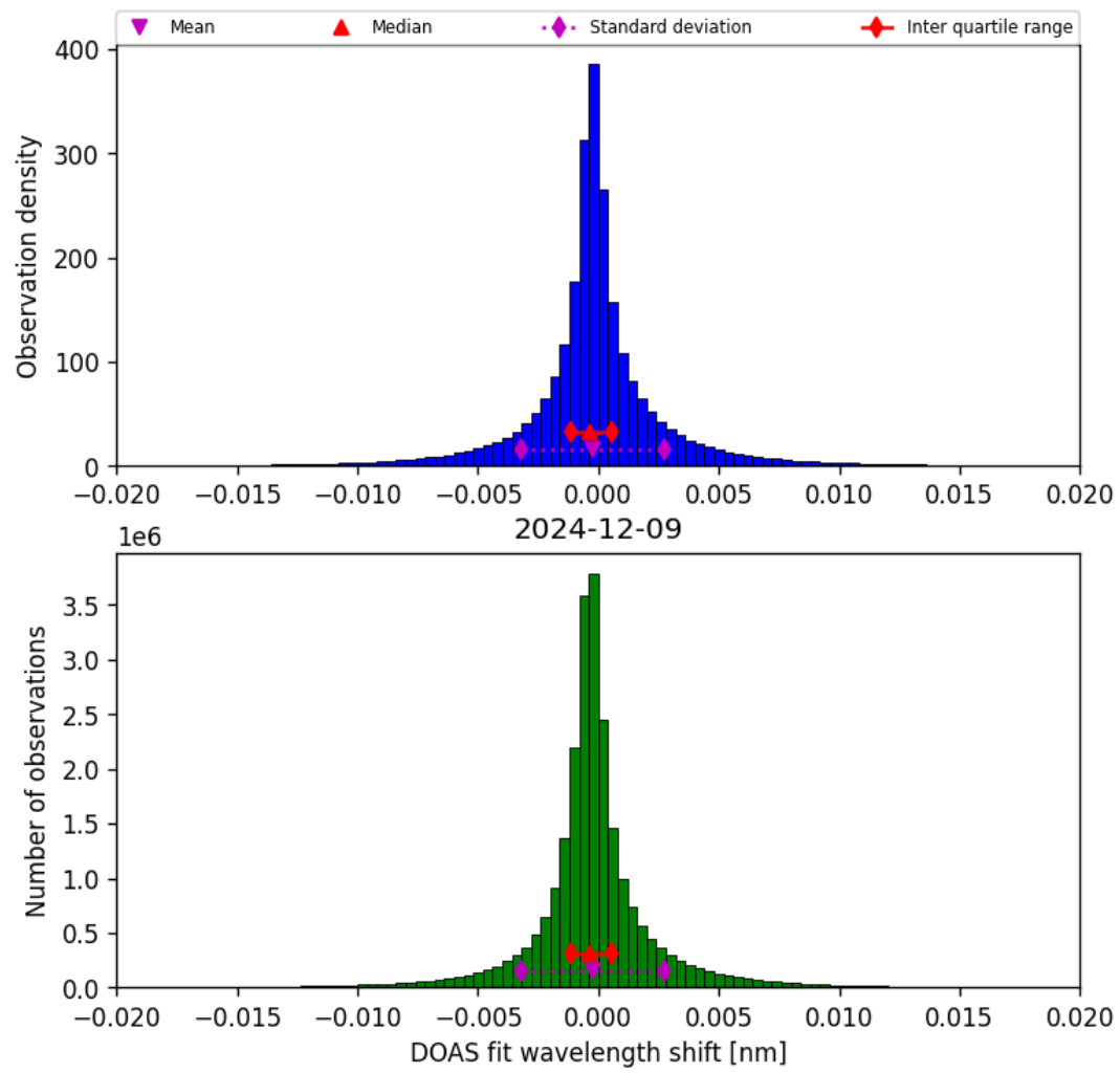
Figure 44: Histogram of “DOAS fit wavelength shift” for 2024-12-08 to 2024-12-10
