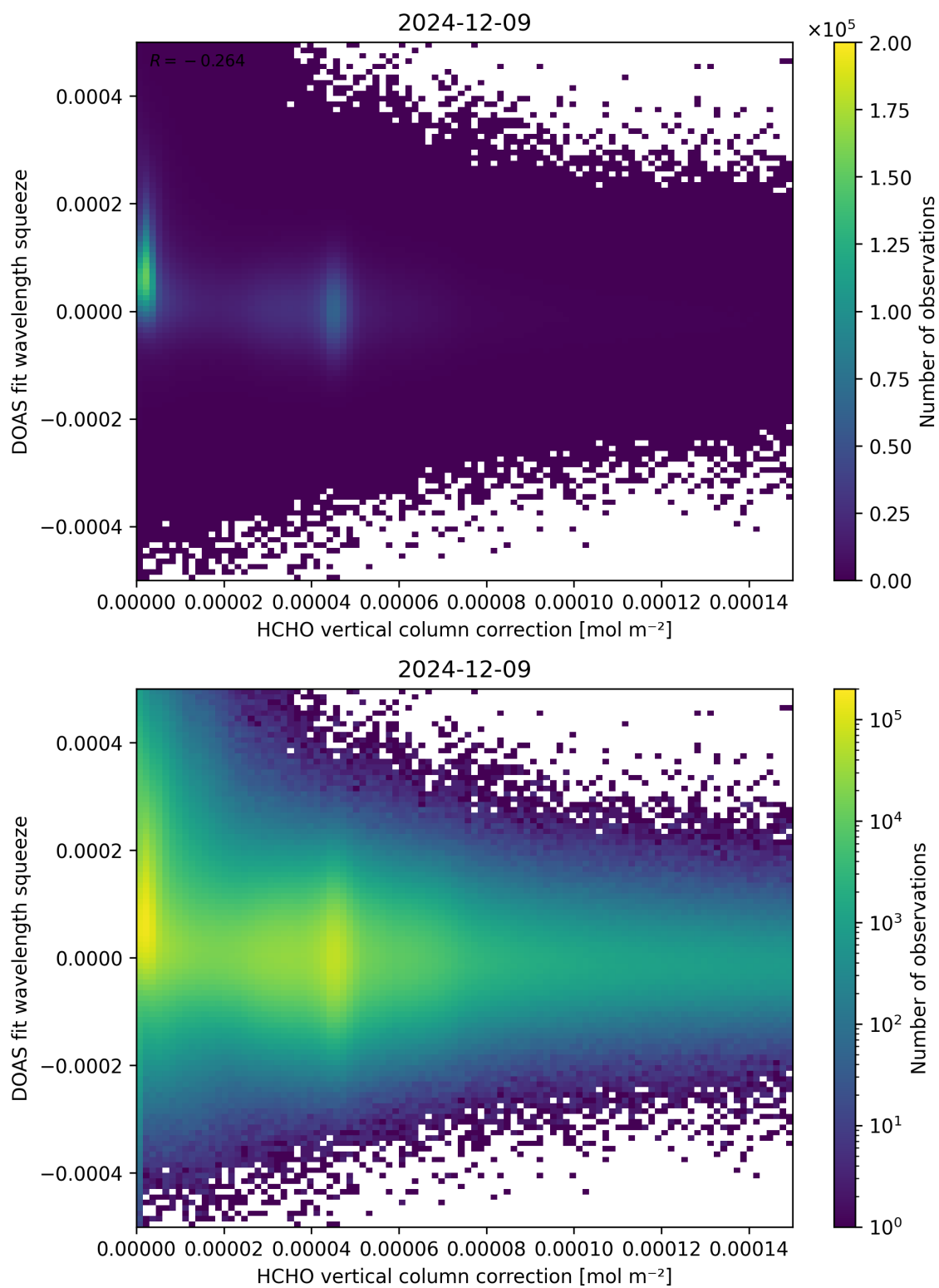
Figure 114: Scatter density plot of “HCHO vertical column correction” against “DOAS fit wavelength squeeze” for 2024-12-08 to 2024-12-10.
