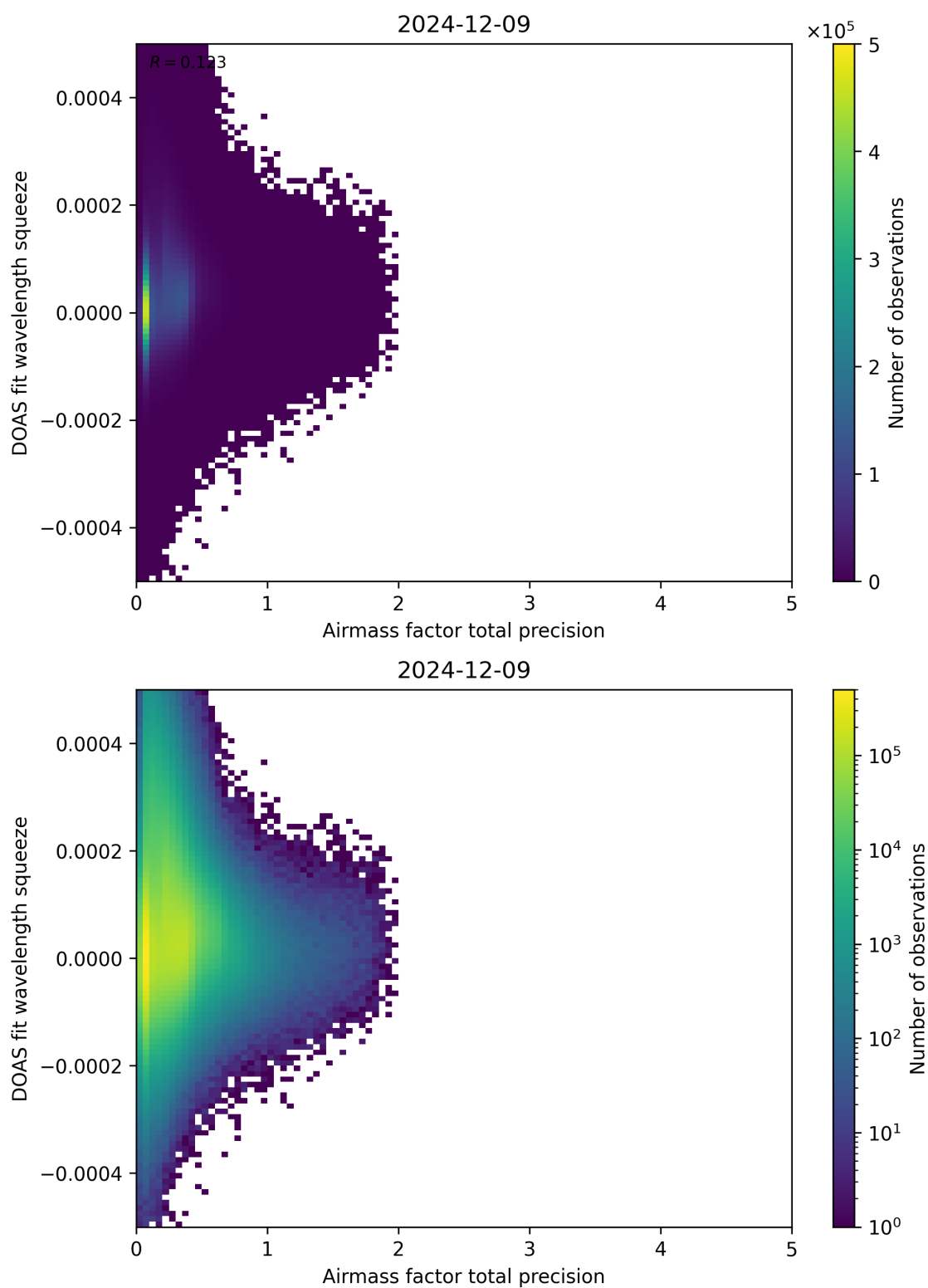
Figure 107: Scatter density plot of “Airmass factor total precision” against “DOAS fit wavelength squeeze” for 2024-12-08 to 2024-12-10.
