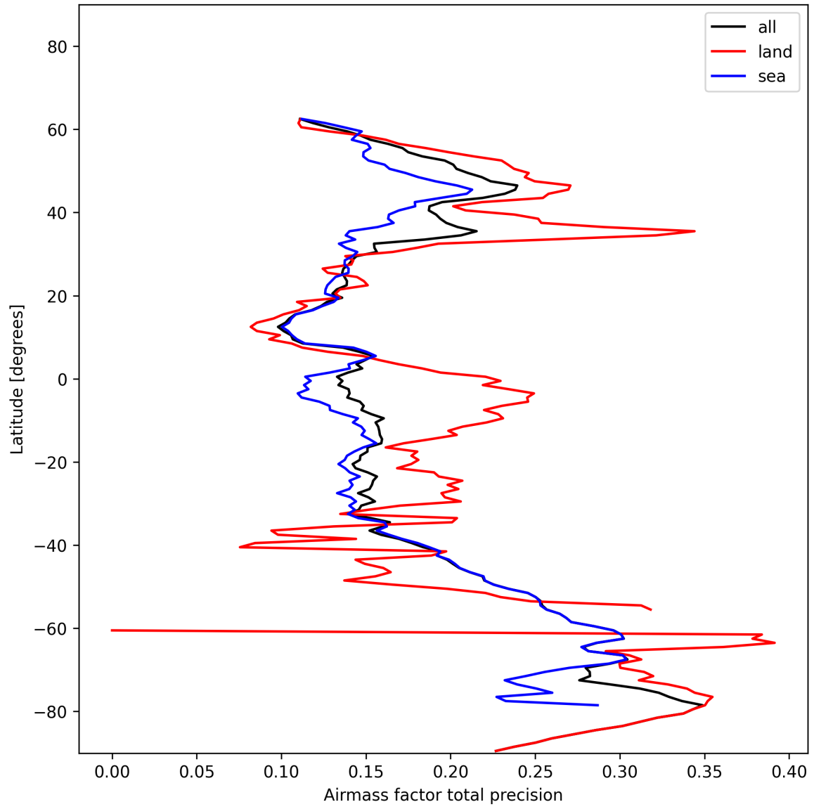
Figure 27: Zonal average of “Airmass factor total precision” for 2024-12-08 to 2024-12-10.
