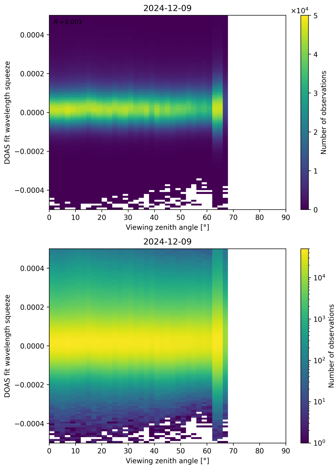
Figure 184: Scatter density plot of “Viewing zenith angle” against “DOAS fit wavelength squeeze” for 2024-12-08 to 2024-12-10.
