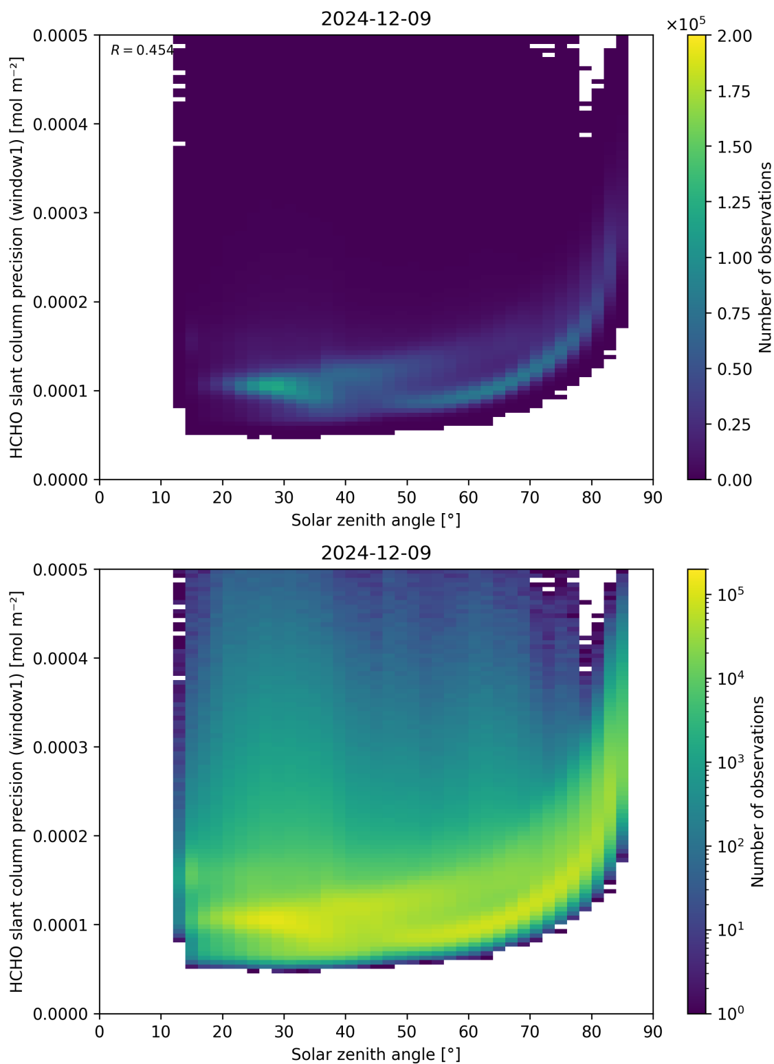
Figure 174: Scatter density plot of “Solar zenith angle” against “HCHO slant column precision (window1)” for 2024-12-08 to 2024-12-10.
