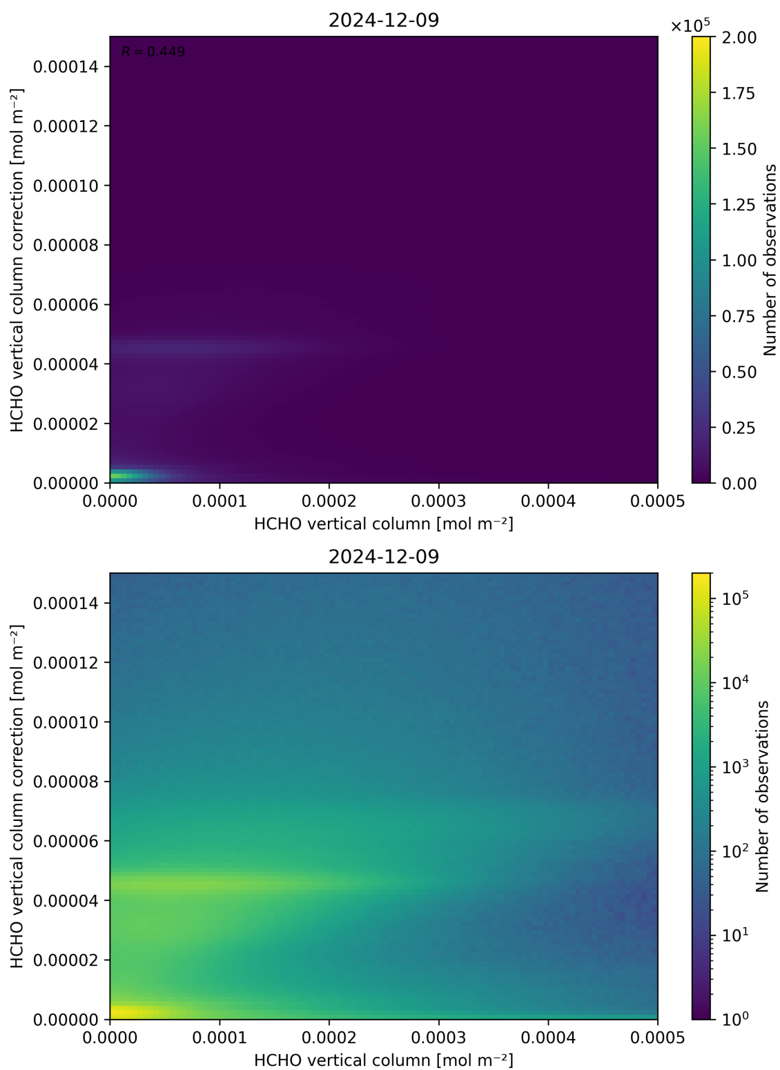
Figure 133: Scatter density plot of “HCHO vertical column” against “HCHO vertical column correction” for 2024-12-08 to 2024-12-10.
