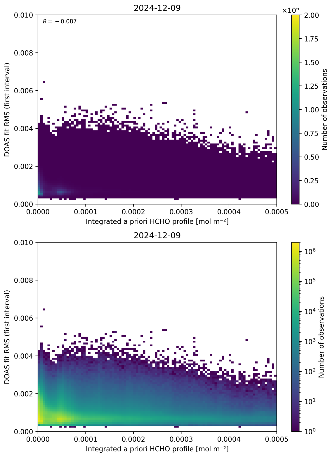
Figure 148: Scatter density plot of “Integrated a priori HCHO profile” against “DOAS fit RMS (first interval)” for 2024-12-08 to 2024-12-10.
