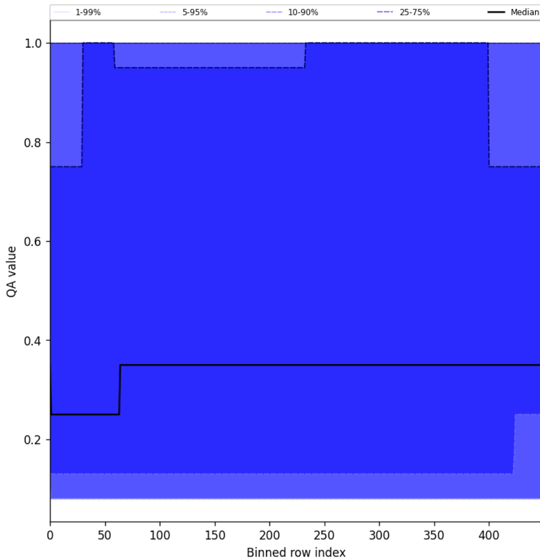
Figure 48: Along track statistics of “QA value” for 2024-12-08 to 2024-12-10
