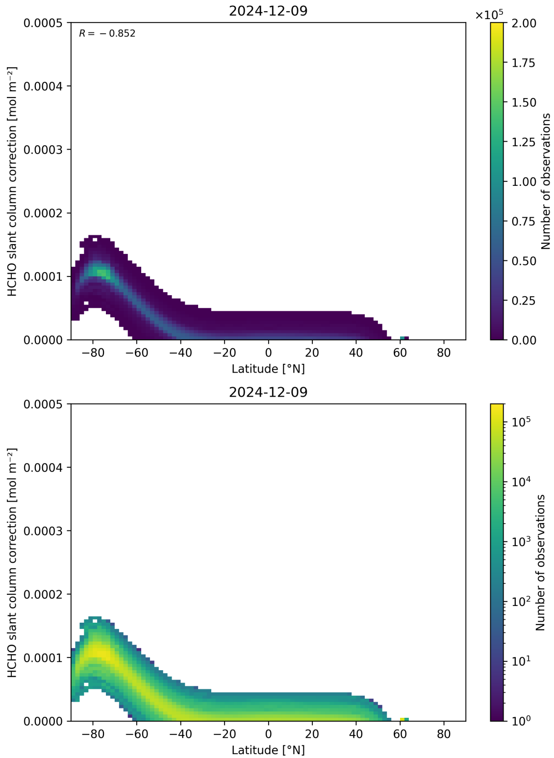
Figure 158: Scatter density plot of “Latitude” against “HCHO slant column correction” for 2024-12-08 to 2024-12-10.
