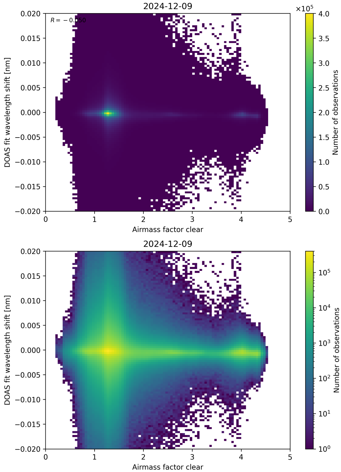
Figure 72: Scatter density plot of “Airmass factor clear” against “DOAS fit wavelength shift” for 2024-12-08 to 2024-12-10.
