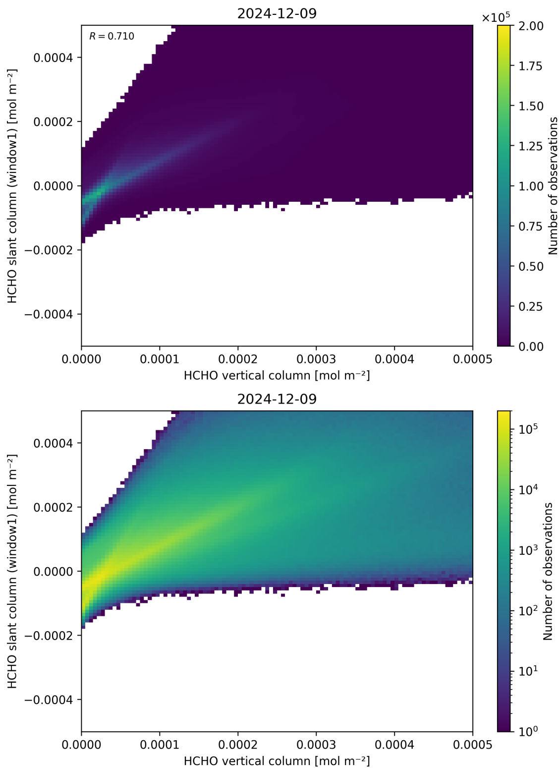
Figure 129: Scatter density plot of “HCHO vertical column” against “HCHO slant column (window1)” for 2024-12-08 to 2024-12-10.
