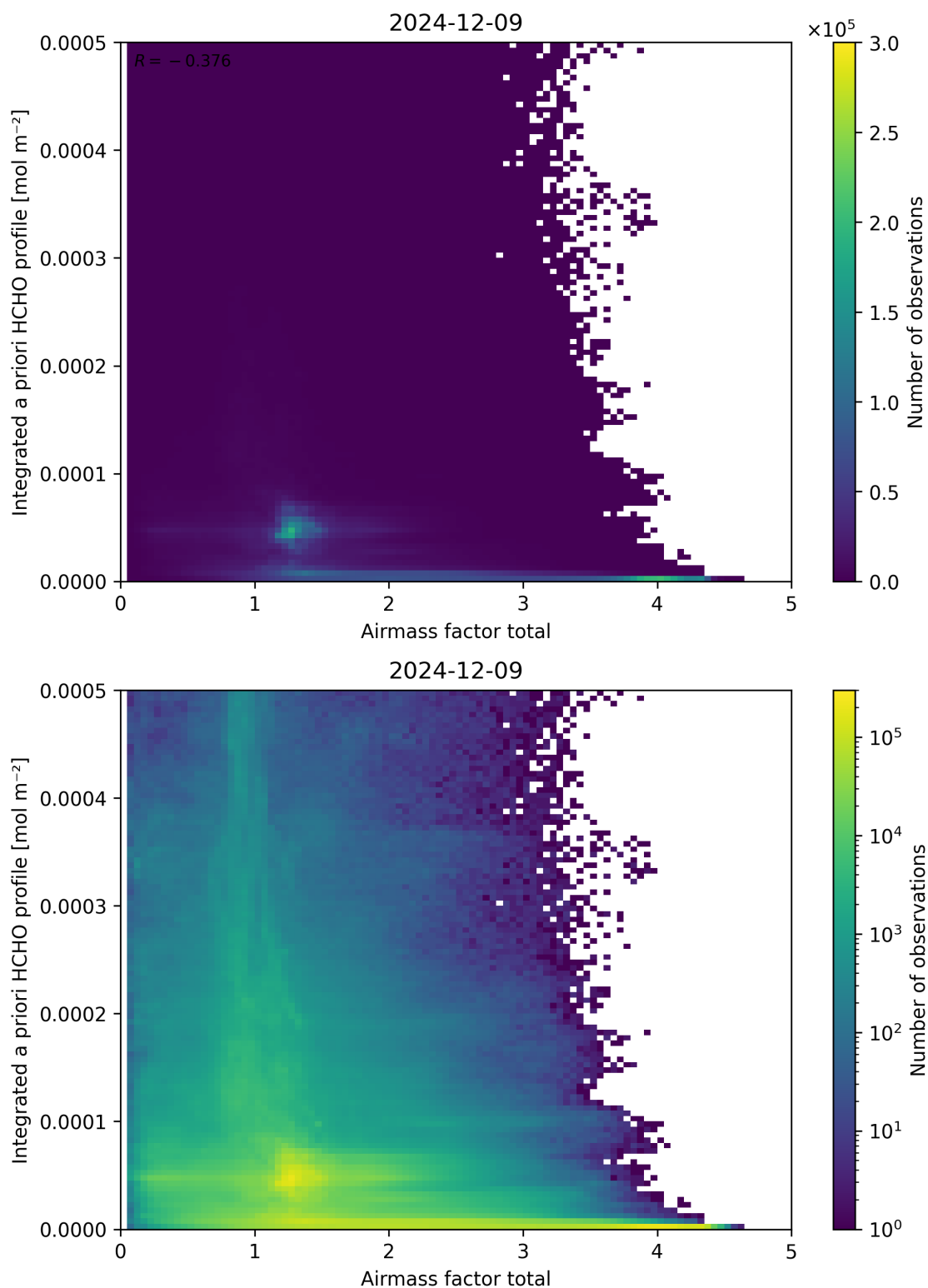
Figure 104: Scatter density plot of “Airmass factor total” against “Integrated a priori HCHO profile” for 2024-12-08 to 2024-12-10.
