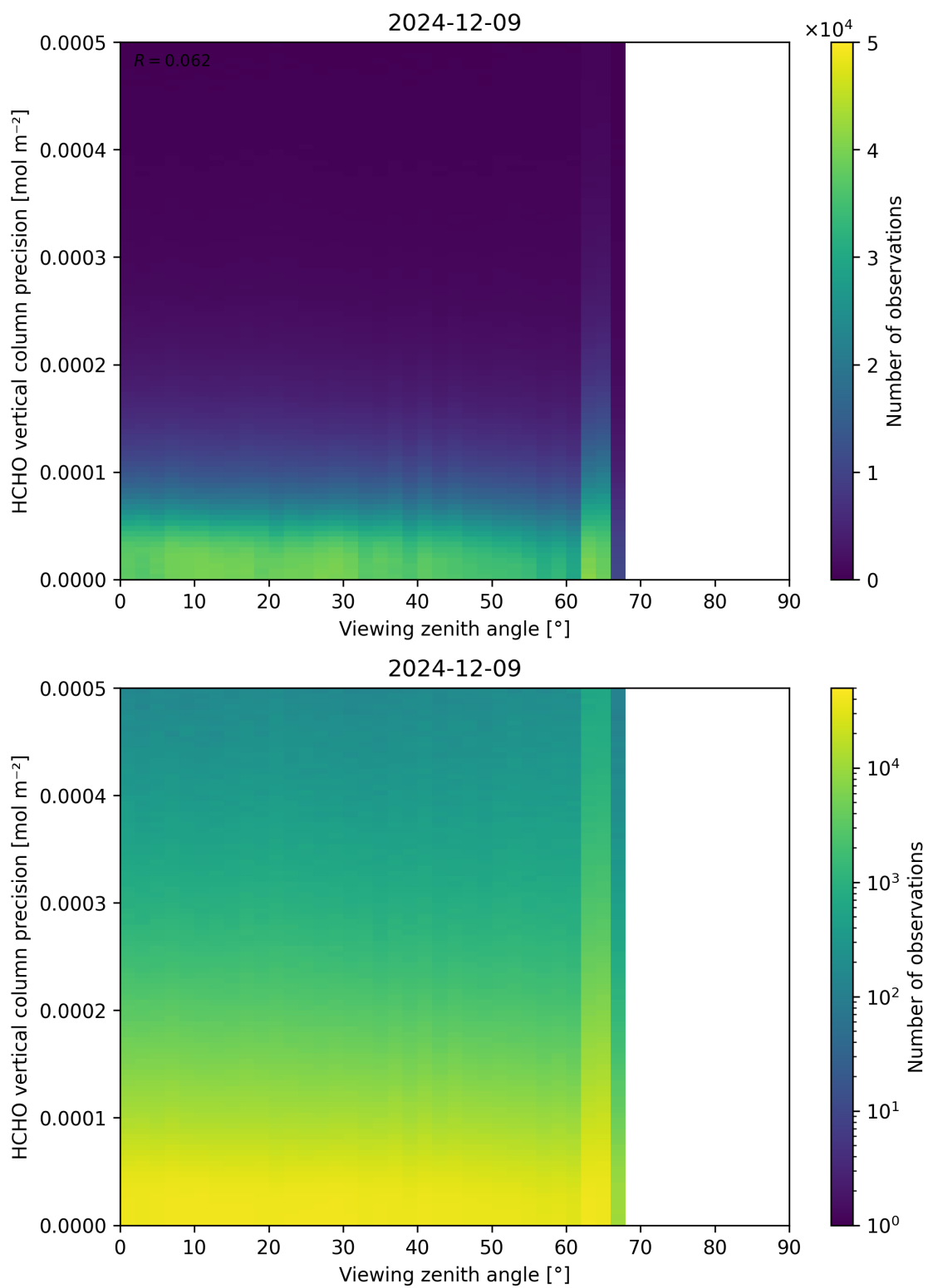
Figure 194: Scatter density plot of “Viewing zenith angle” against “HCHO vertical column precision” for 2024-12-08 to 2024-12-10.
