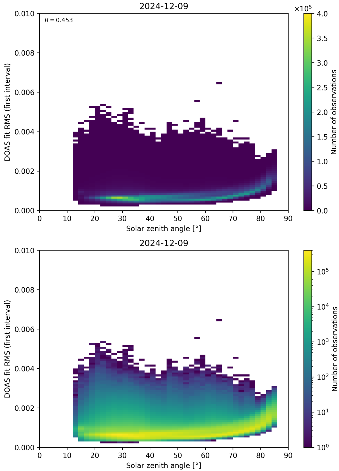
Figure 167: Scatter density plot of “Solar zenith angle” against “DOAS fit RMS (first interval)” for 2024-12-08 to 2024-12-10.
