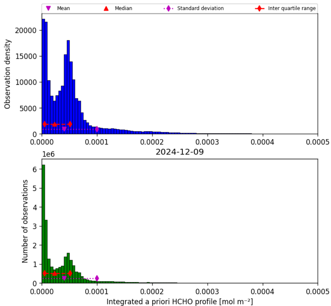
Figure 43: Histogram of “Integrated a priori HCHO profile” for 2024-12-08 to 2024-12-10
