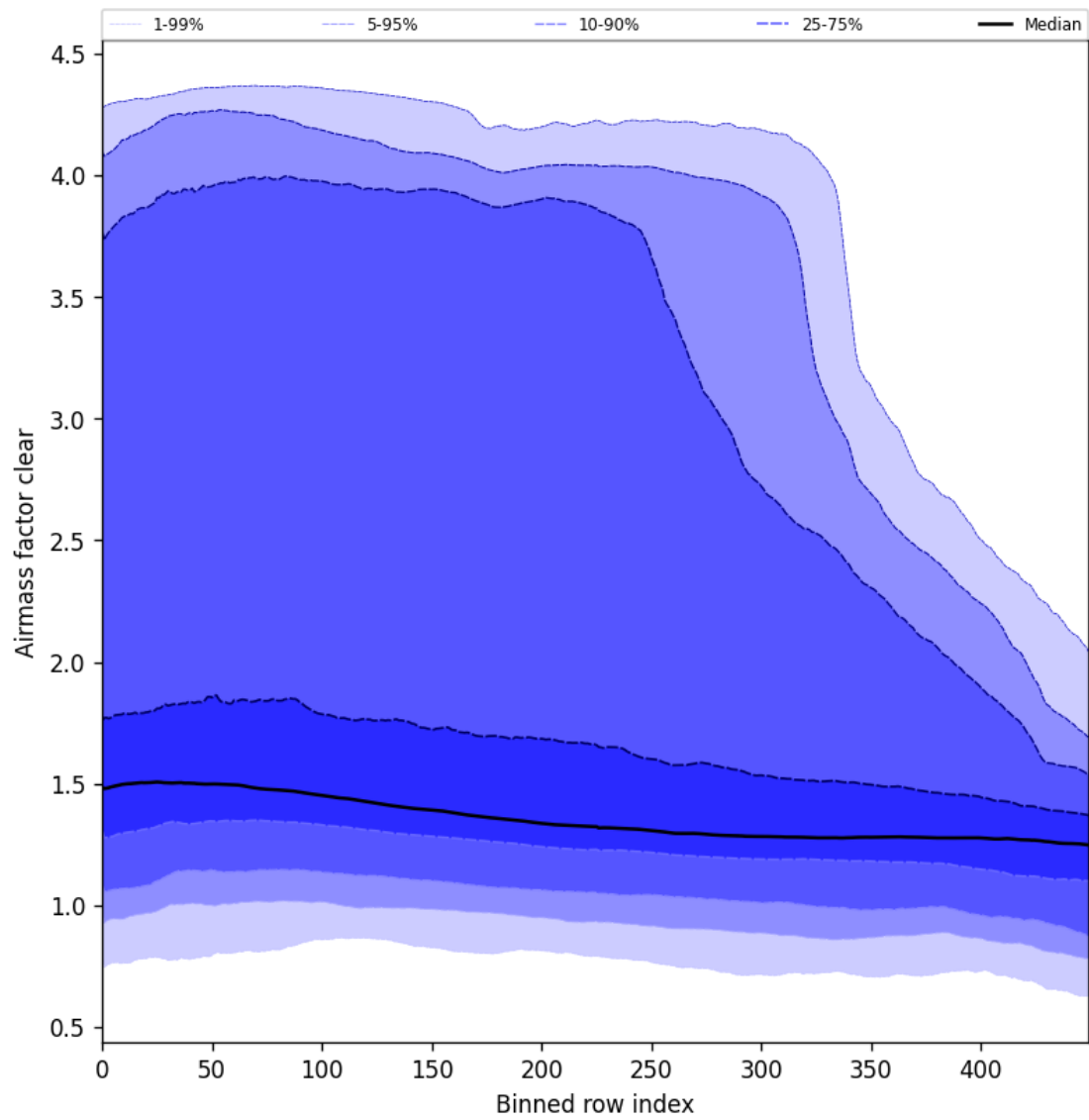
Figure 56: Along track statistics of “Air mass factor clear” for 2024-12-08 to 2024-12-10
