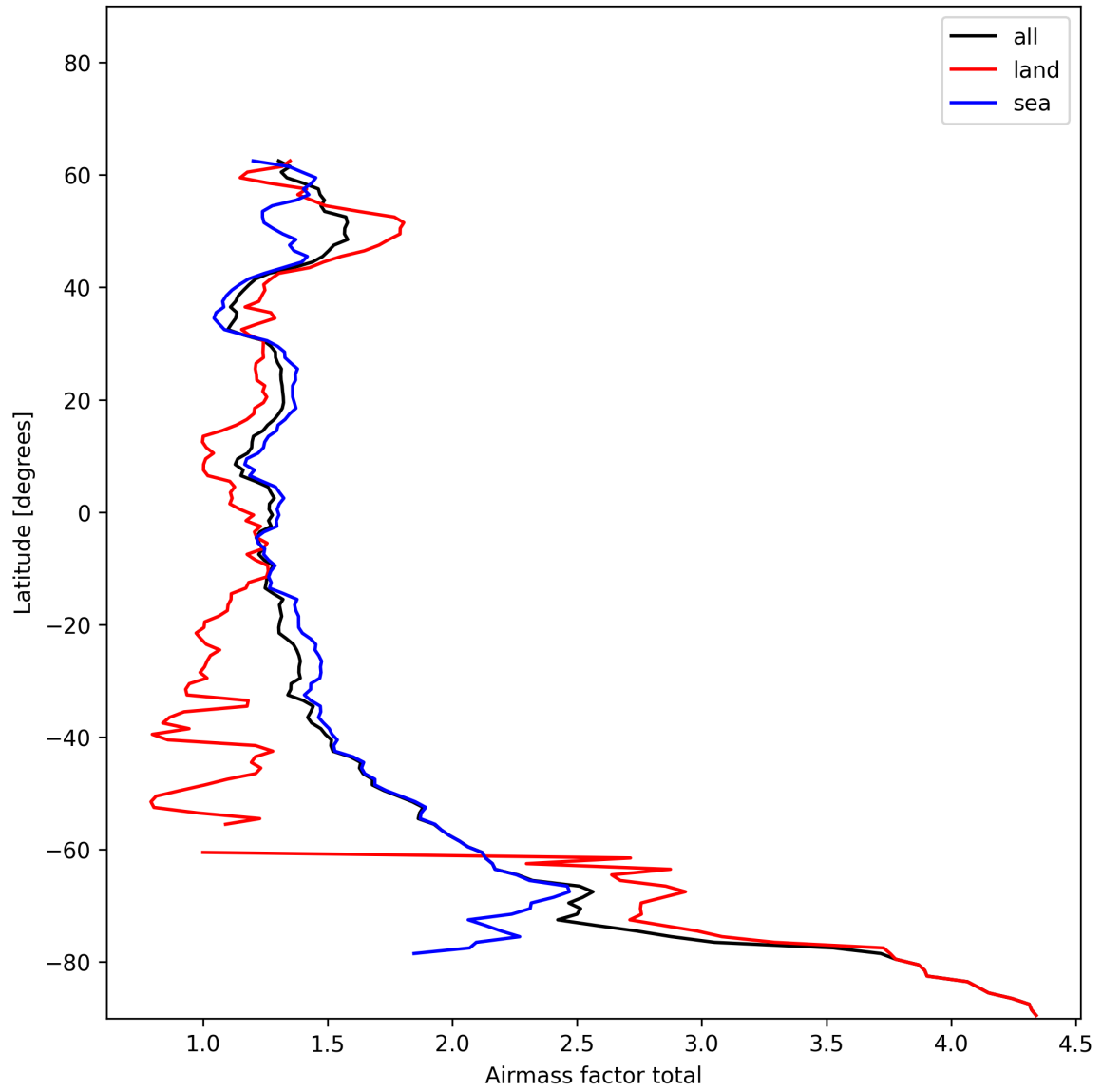
Figure 26: Zonal average of “Airmass factor total” for 2024-12-08 to 2024-12-10.
