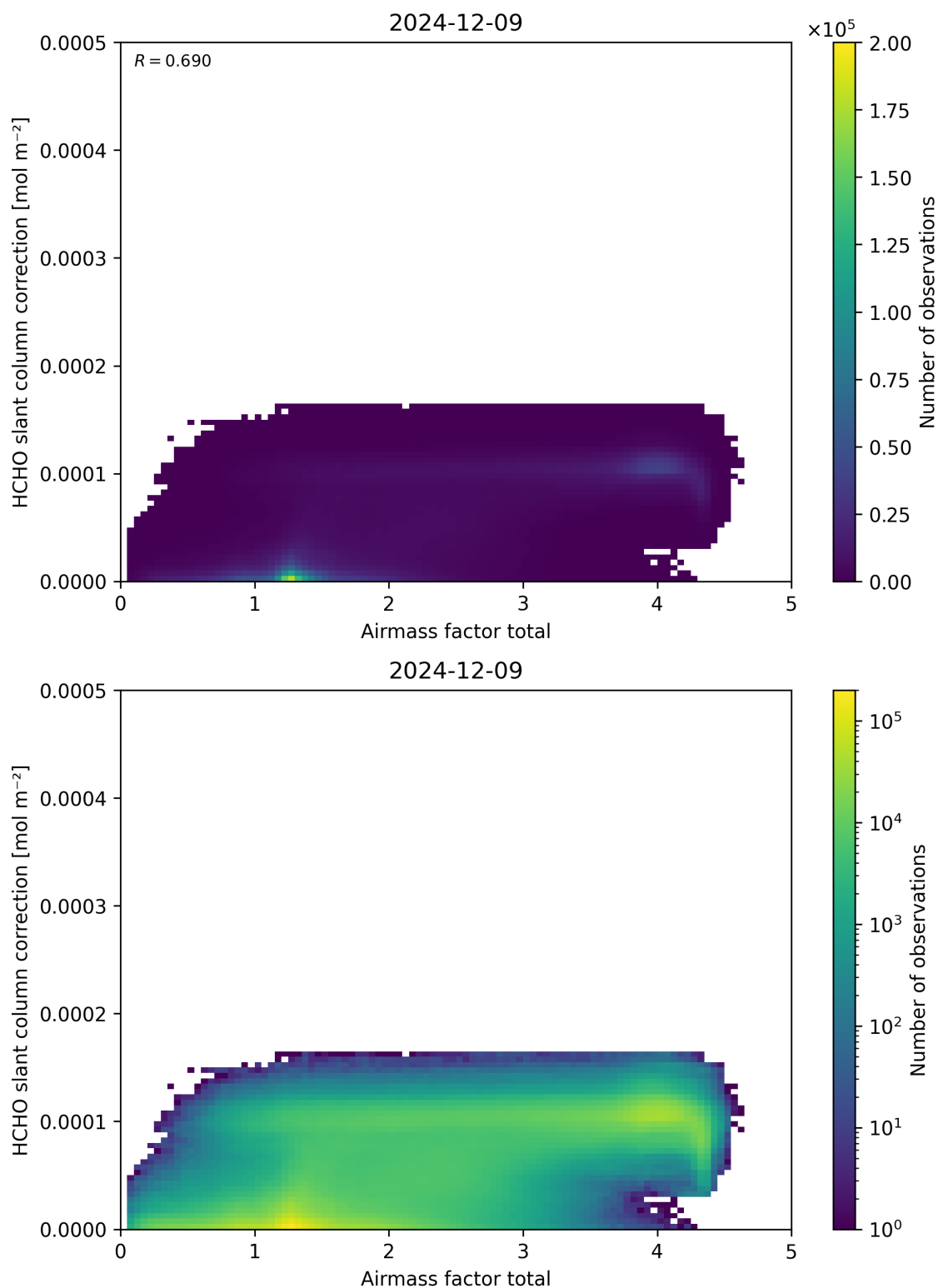
Figure 102: Scatter density plot of “Airmass factor total” against “HCHO slant column correction” for 2024-12-08 to 2024-12-10.
