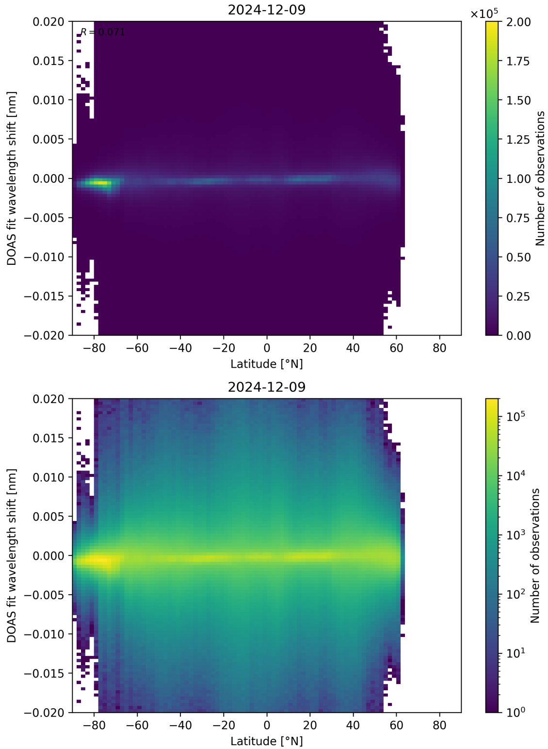
Figure 154: Scatter density plot of “Latitude” against “DOAS fit wavelength shift” for 2024-12-08 to 2024-12-10.
