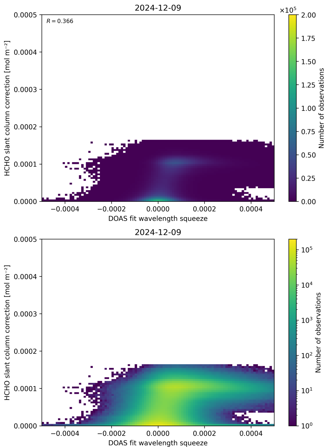
Figure 70: Scatter density plot of “DOAS fit wavelength squeeze” against “HCHO slant column correction” for 2024-12-08 to 2024-12-10.
