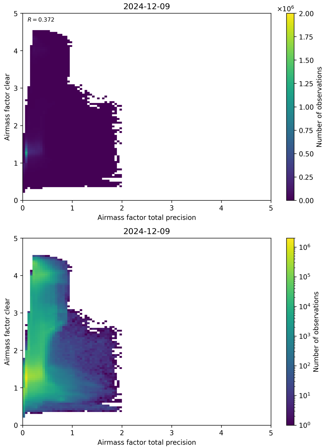
Figure 108: Scatter density plot of “Airmass factor total precision” against “Airmass factor clear” for 2024-12-08 to 2024-12-10.
