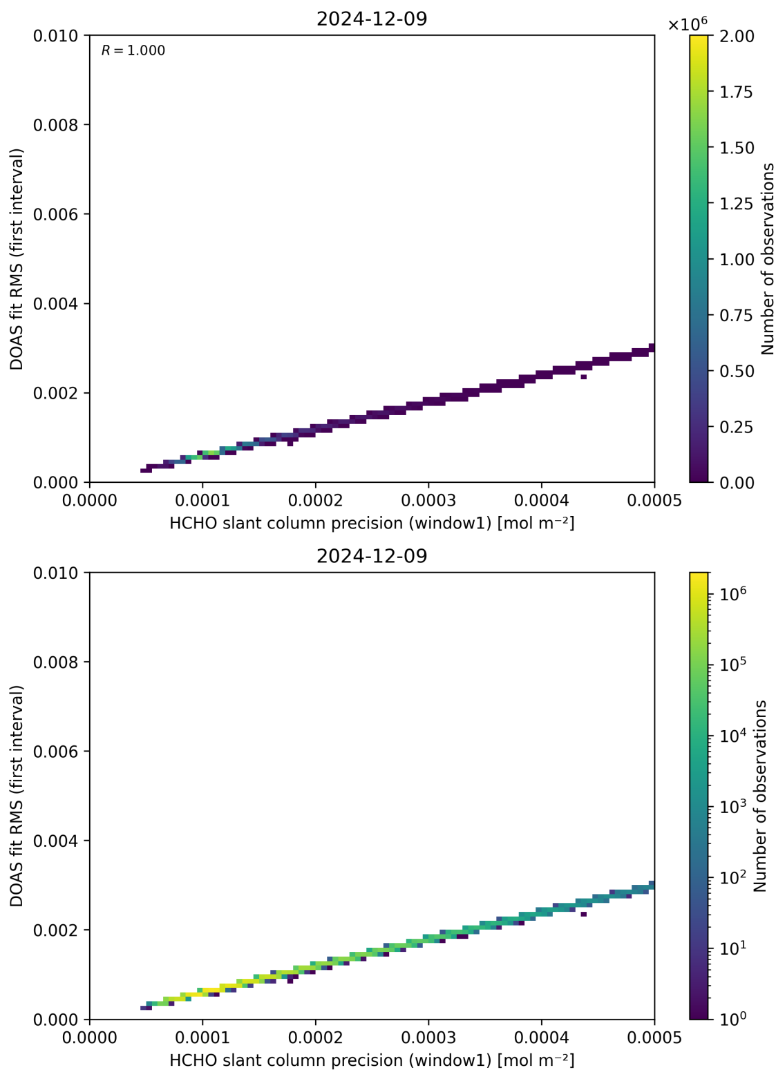
Figure 88: Scatter density plot of “HCHO slant column precision (window1)” against “DOAS fit RMS (first interval)” for 2024-12-08 to 2024-12-10.
