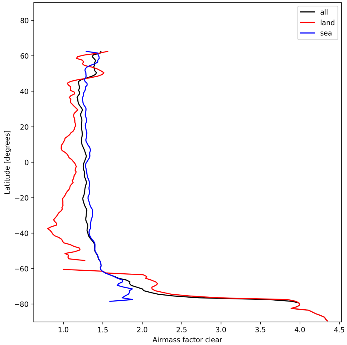
Figure 28: Zonal average of “Airmass factor clear” for 2024-12-08 to 2024-12-10.
