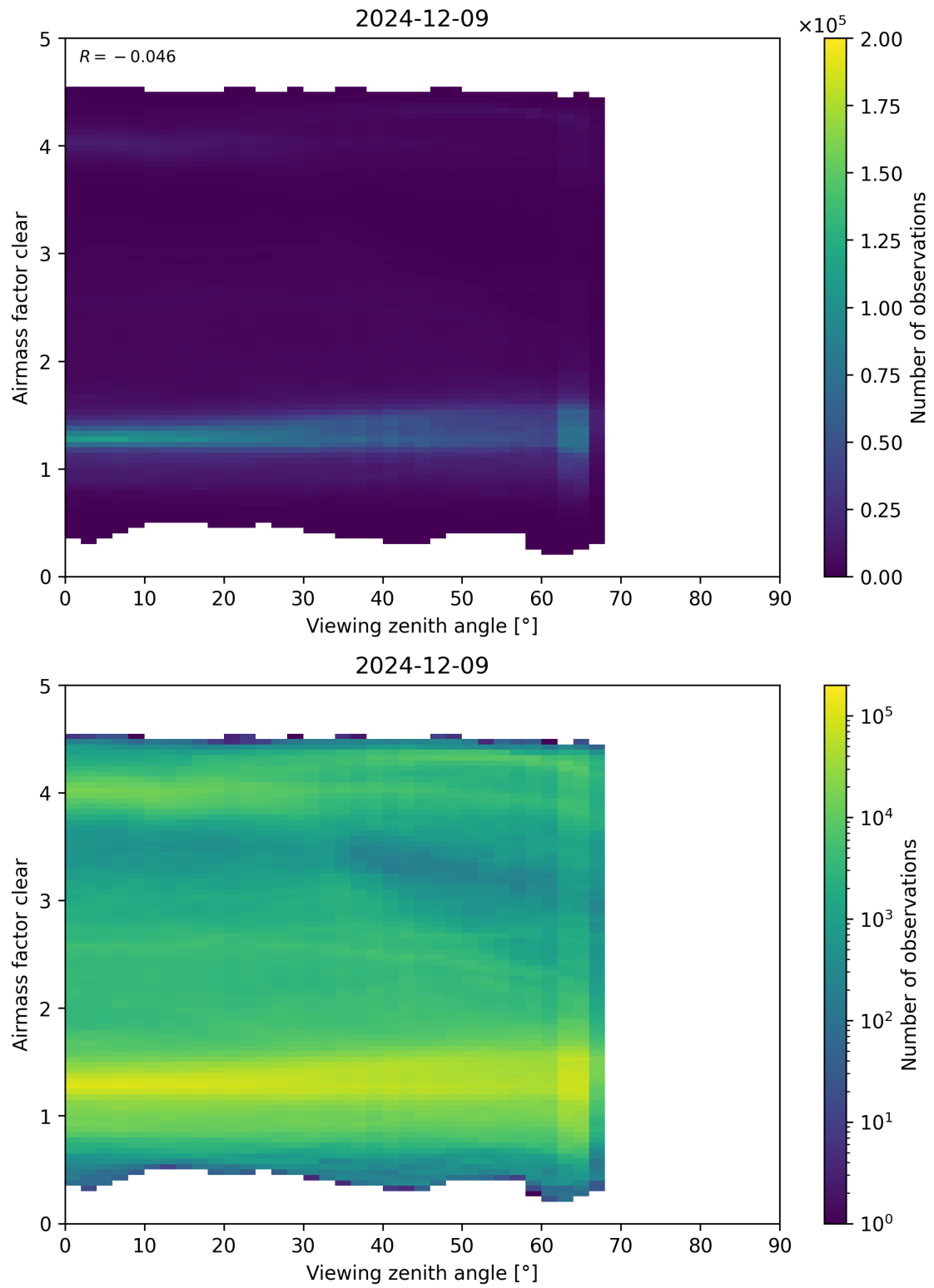
Figure 185: Scatter density plot of “Viewing zenith angle” against “Airmass factor clear” for 2024-12-08 to 2024-12-10.
