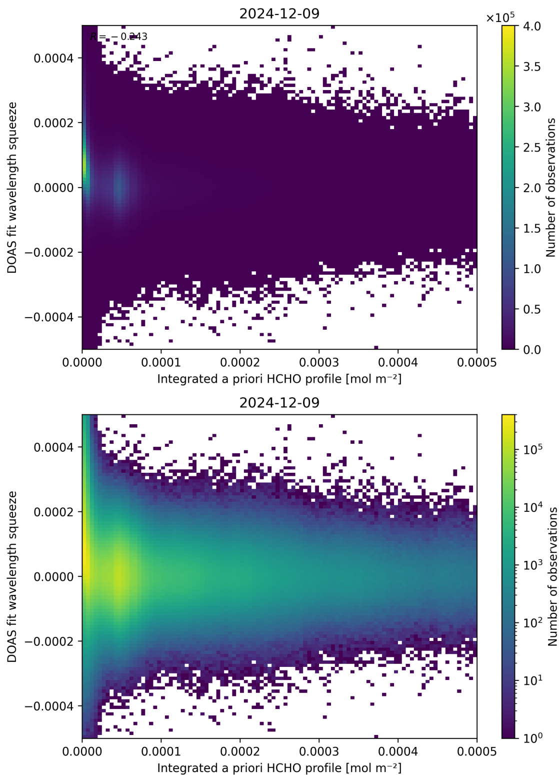
Figure 150: Scatter density plot of “Integrated a priori HCHO profile” against “DOAS fit wavelength squeeze” for 2024-12-08 to 2024-12-10.
