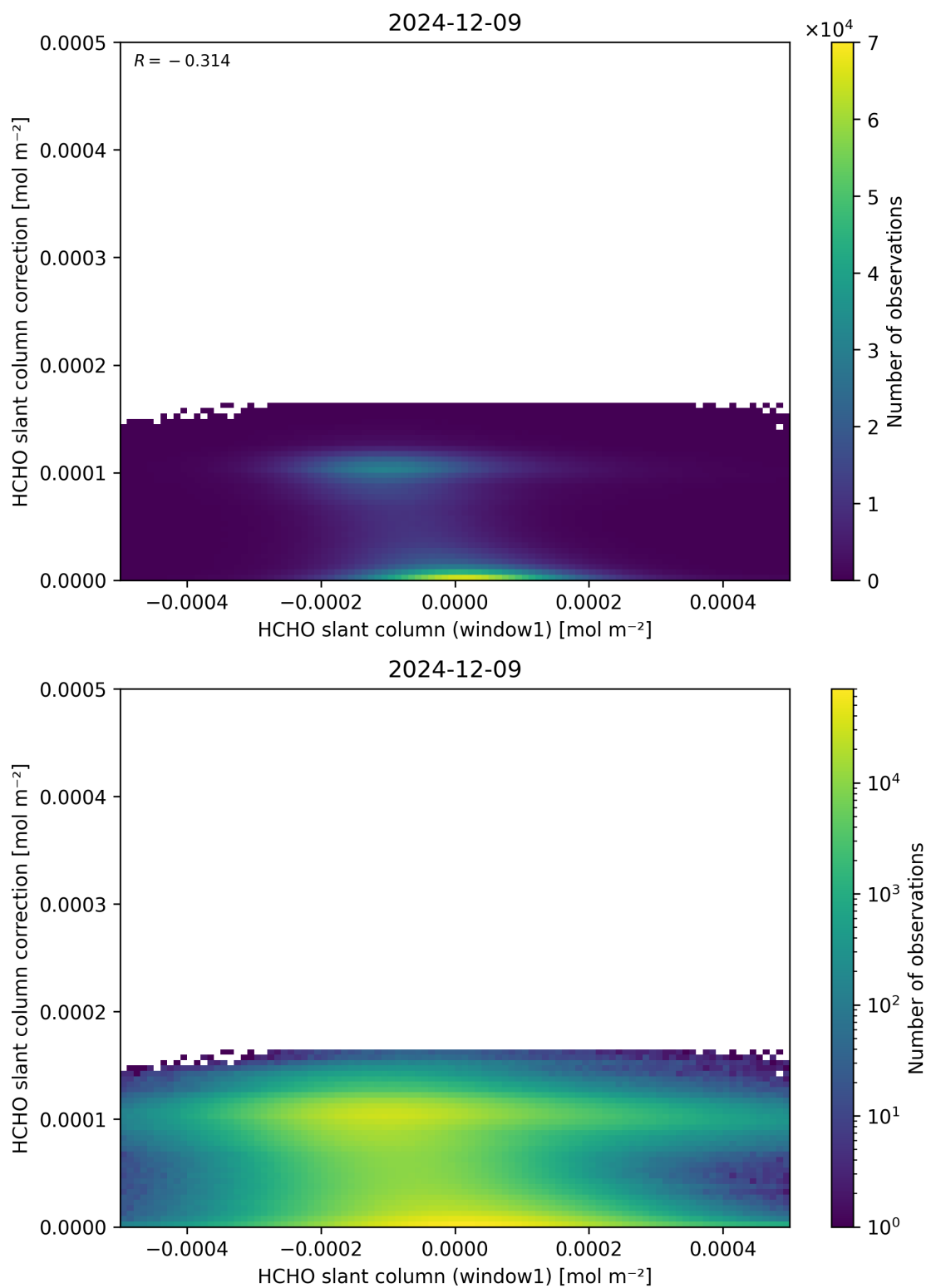
Figure 83: Scatter density plot of “HCHO slant column (window1)” against “HCHO slant column correction” for 2024-12-08 to 2024-12-10.
