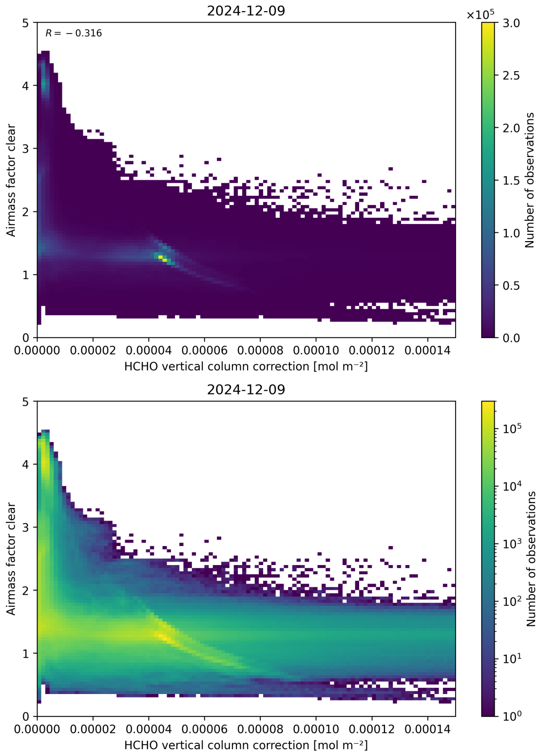
Figure 115: Scatter density plot of “HCHO vertical column correction” against “Airmass factor clear” for 2024-12-08 to 2024-12-10.
