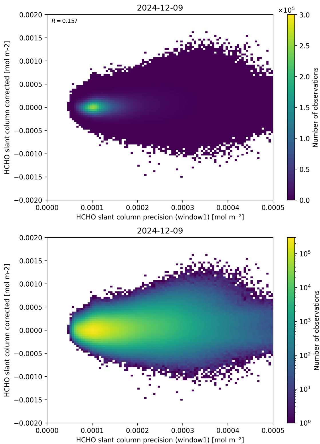
Figure 92: Scatter density plot of “HCHO slant column precision (window1)” against “HCHO slant column corrected” for 2024-12-08 to 2024-12-10.
