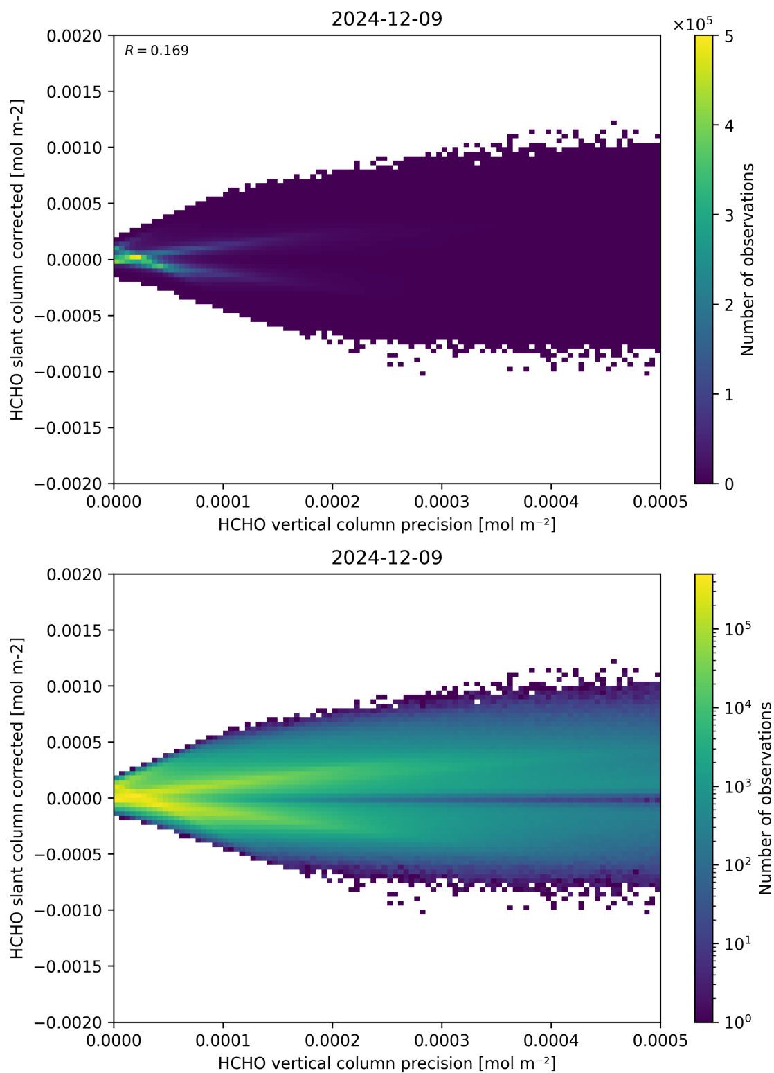
Figure 140: Scatter density plot of “HCHO vertical column precision” against “HCHO slant column corrected” for 2024-12-08 to 2024-12-10.
