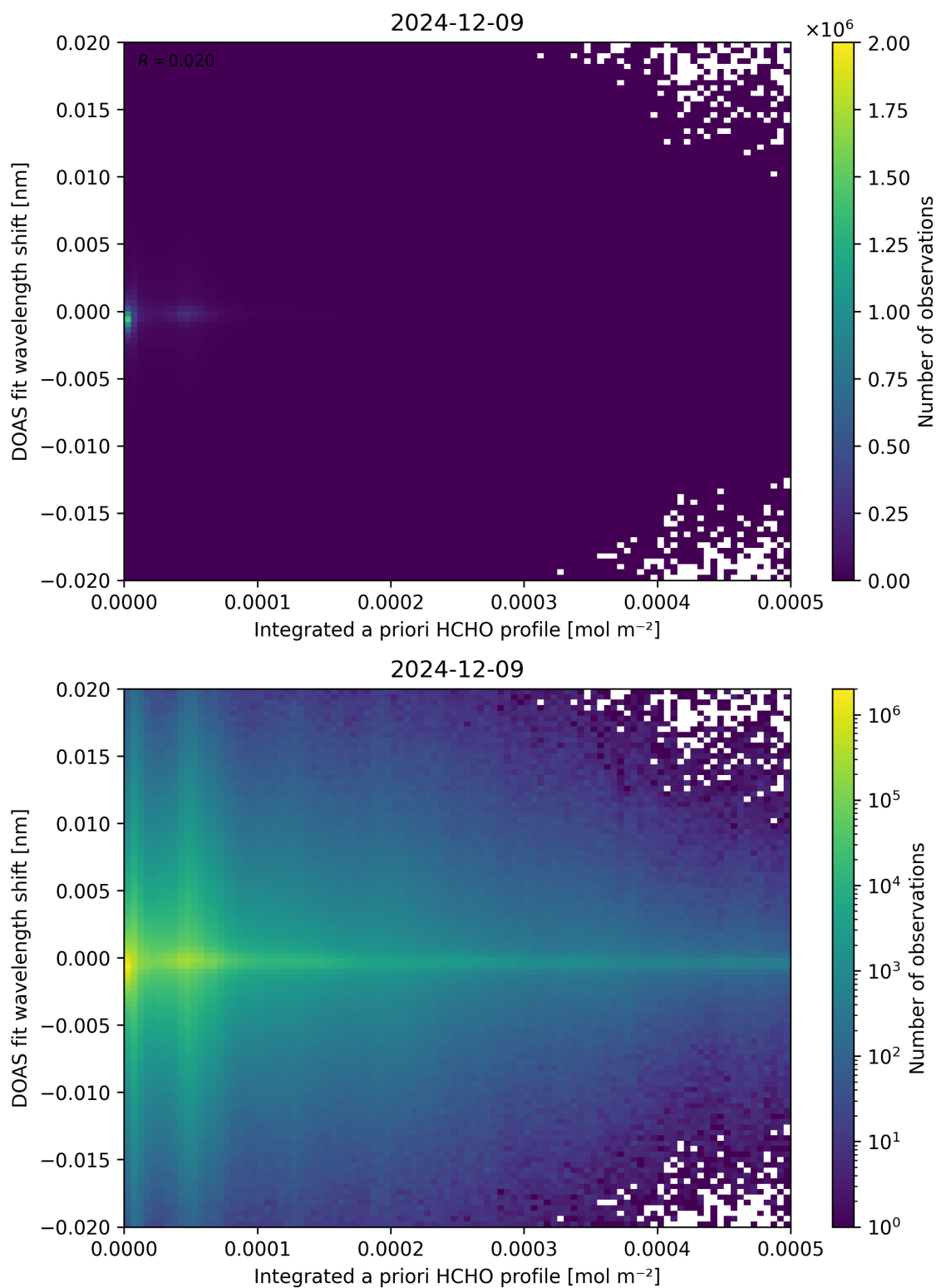
Figure 149: Scatter density plot of “Integrated a priori HCHO profile” against “DOAS fit wavelength shift” for 2024-12-08 to 2024-12-10.
