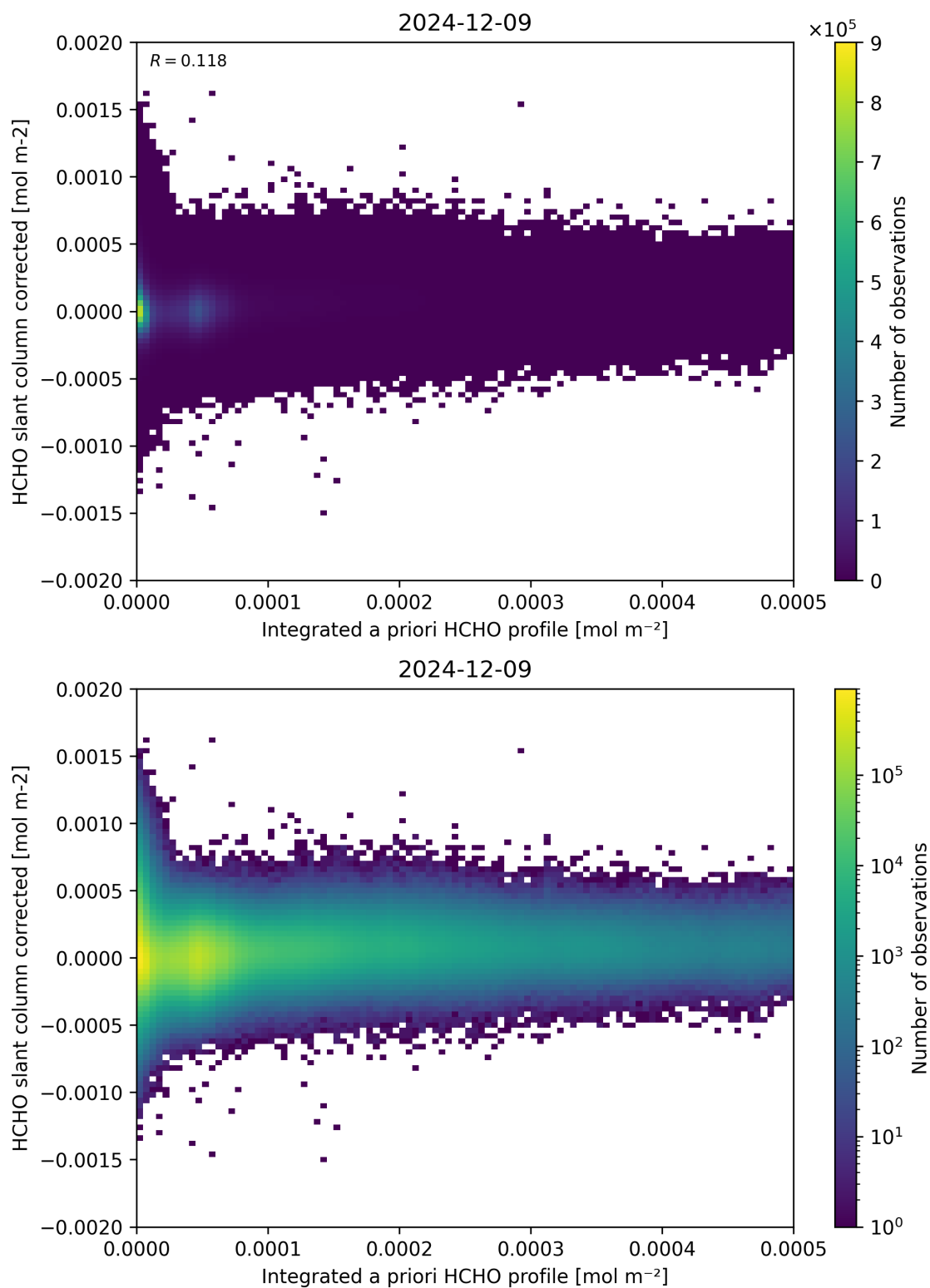
Figure 151: Scatter density plot of “Integrated a priori HCHO profile” against “HCHO slant column corrected” for 2024-12-08 to 2024-12-10.
