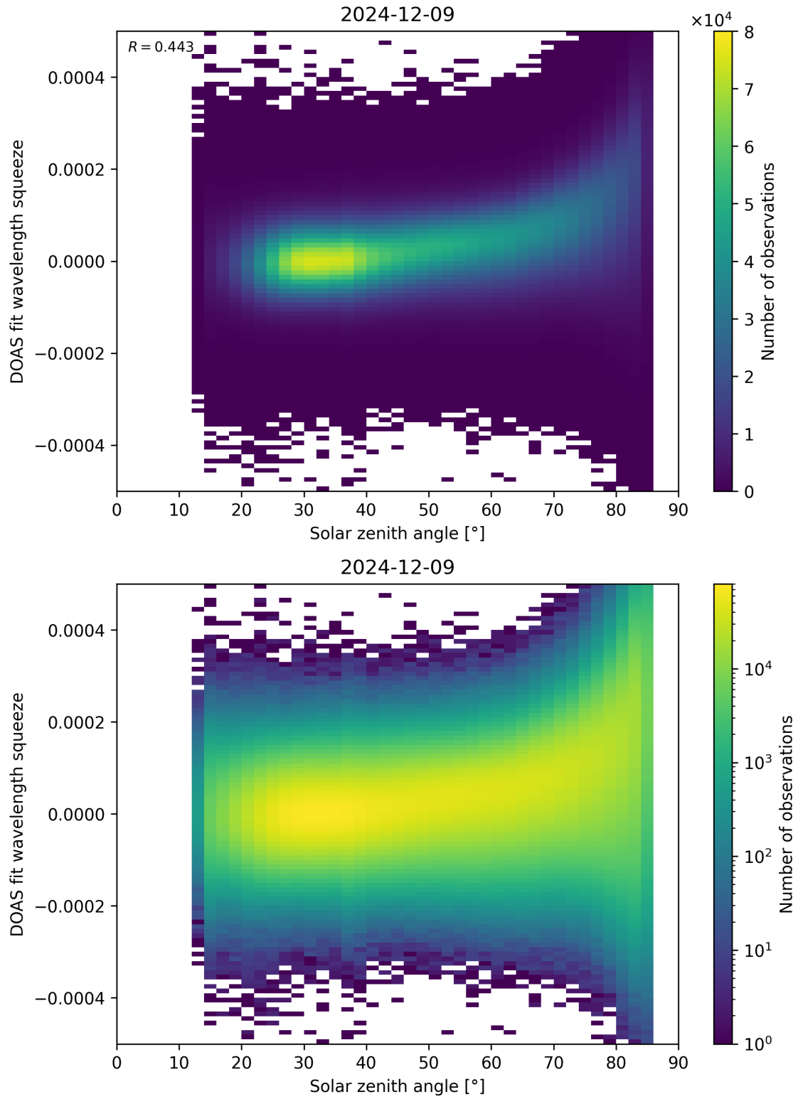
Figure 169: Scatter density plot of “Solar zenith angle” against “DOAS fit wavelength squeeze” for 2024-12-08 to 2024-12-10.
