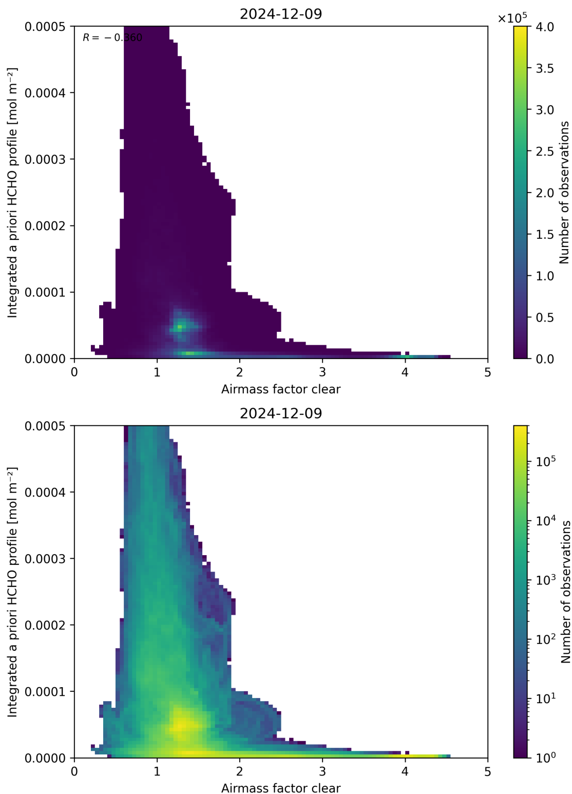
Figure 76: Scatter density plot of “Airmass factor clear” against “Integrated a priori HCHO profile” for 2024-12-08 to 2024-12-10.
