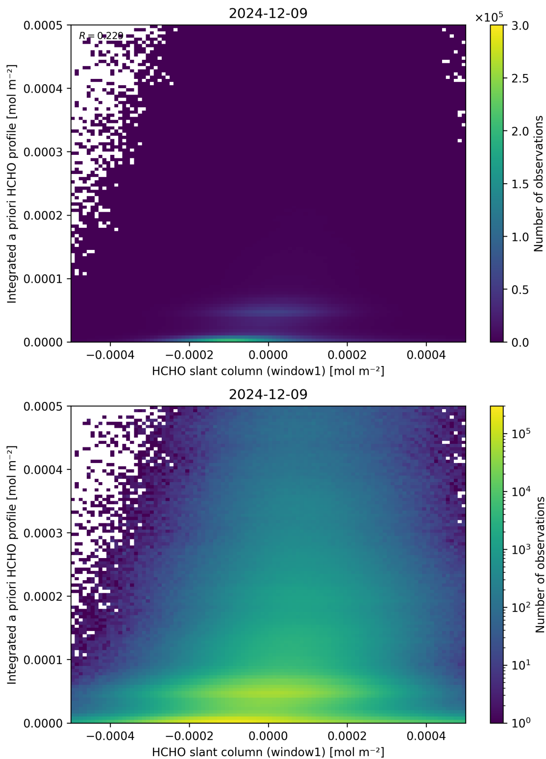
Figure 87: Scatter density plot of “HCHO slant column (window1)” against “Integrated a priori HCHO profile” for 2024-12-08 to 2024-12-10.
