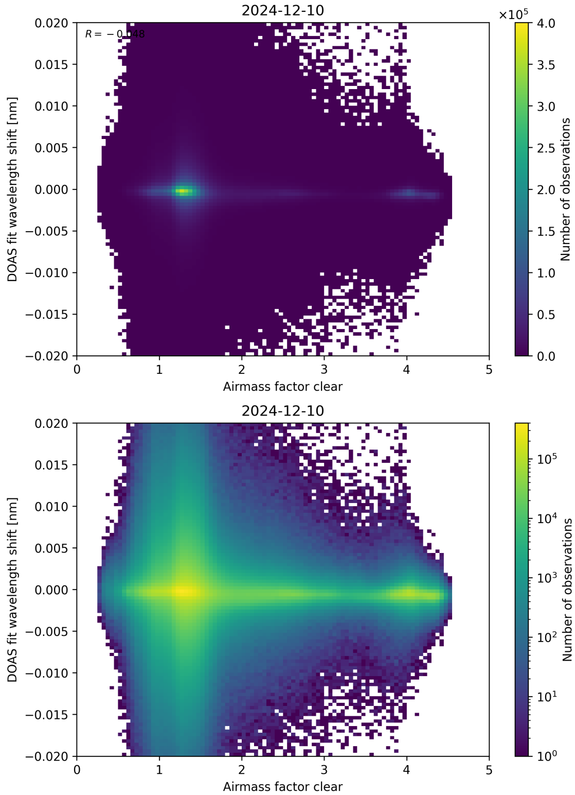
Figure 72: Scatter density plot of “Airmass factor clear” against “DOAS fit wavelength shift” for 2024-12-09 to 2024-12-11.
