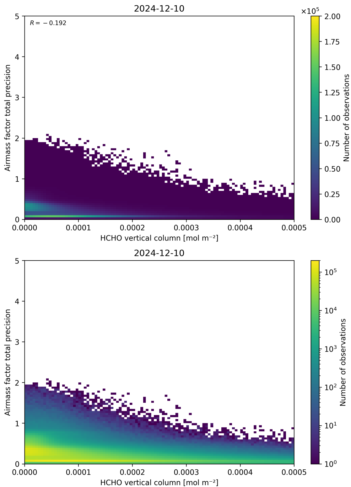
Figure 132: Scatter density plot of “HCHO vertical column” against “Airmass factor total precision” for 2024-12-09 to 2024-12-11.
