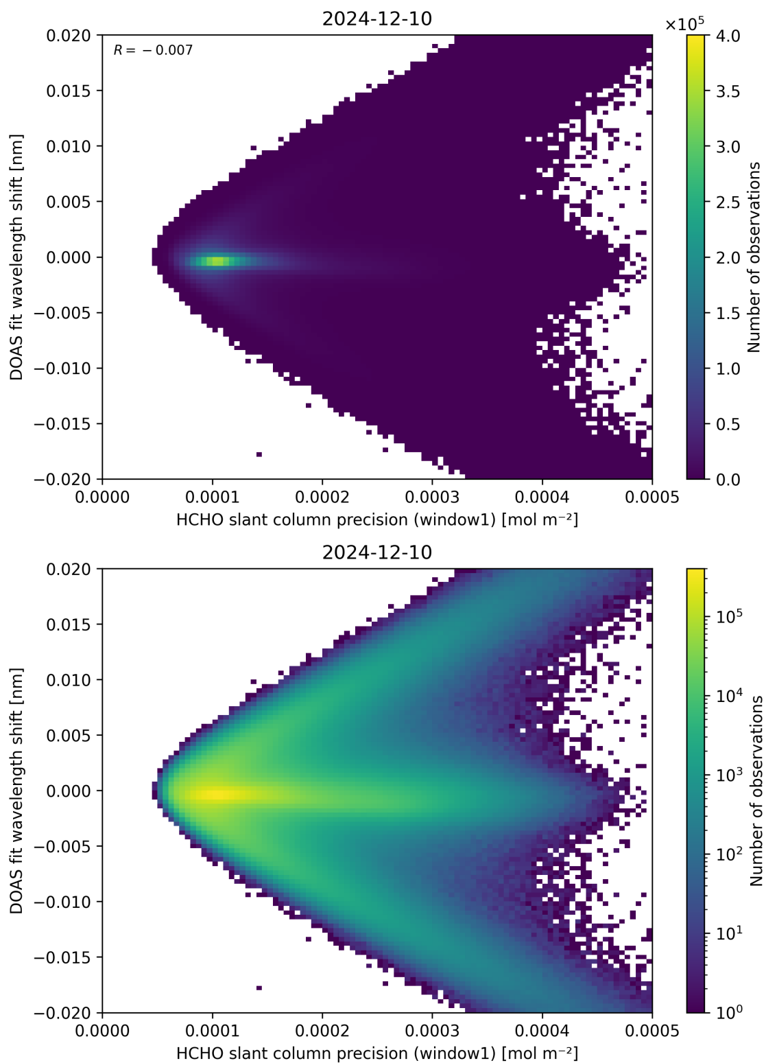
Figure 89: Scatter density plot of “HCHO slant column precision (window1)” against “DOAS fit wavelength shift” for 2024-12-09 to 2024-12-11.
