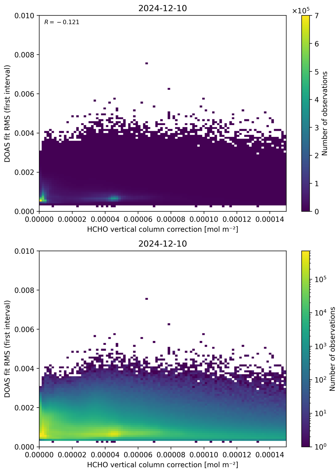
Figure 112: Scatter density plot of “HCHO vertical column correction” against “DOAS fit RMS (first interval)” for 2024-12-09 to 2024-12-11.
