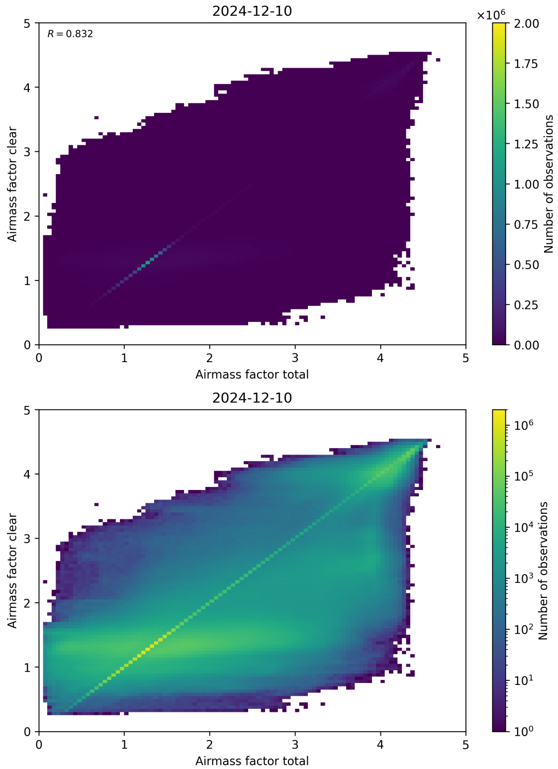
Figure 100: Scatter density plot of “Airmass factor total” against “Airmass factor clear” for 2024-12-09 to 2024-12-11.
