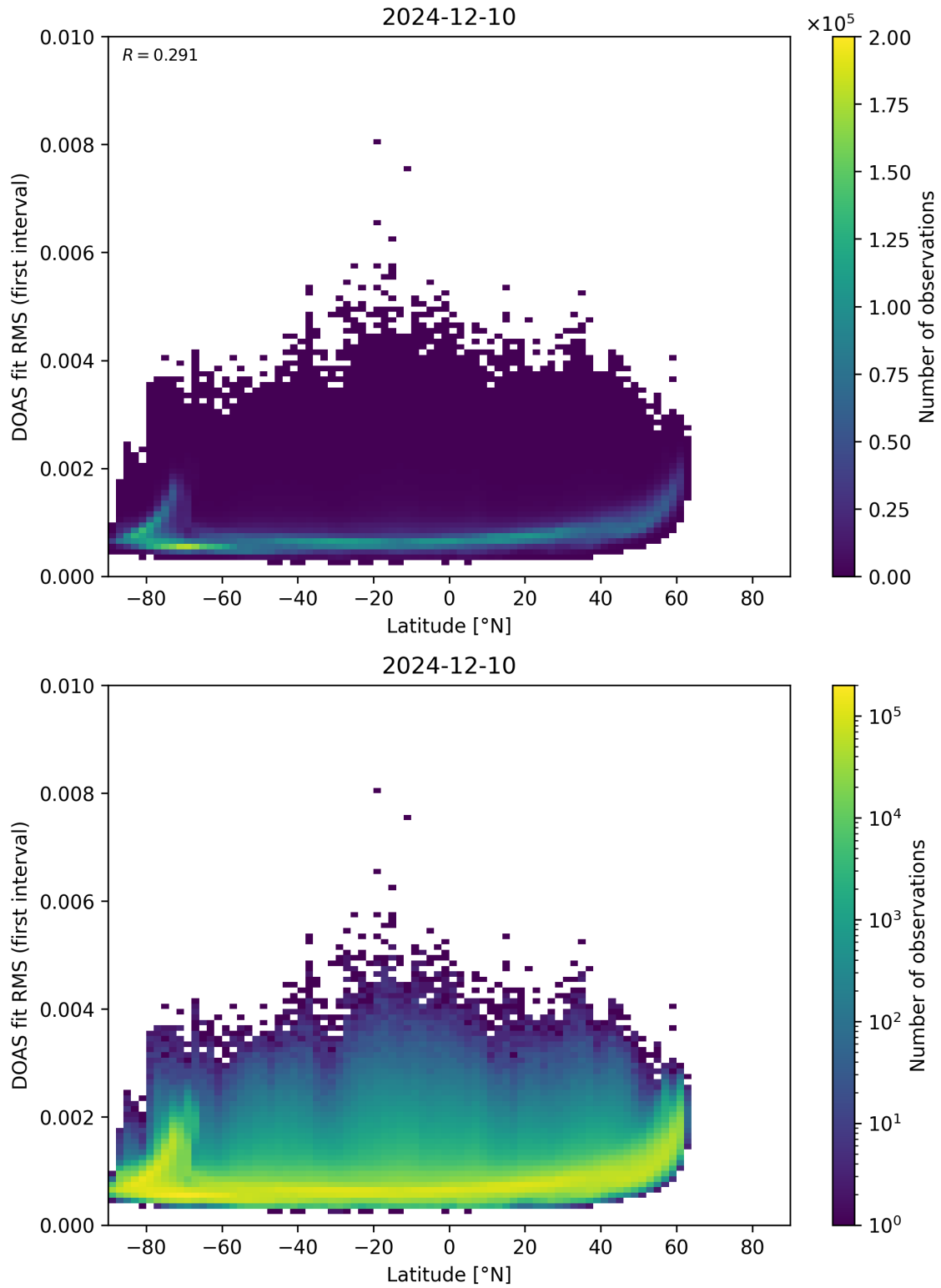
Figure 153: Scatter density plot of “Latitude” against “DOAS fit RMS (first interval)” for 2024-12-09 to 2024-12-11.
