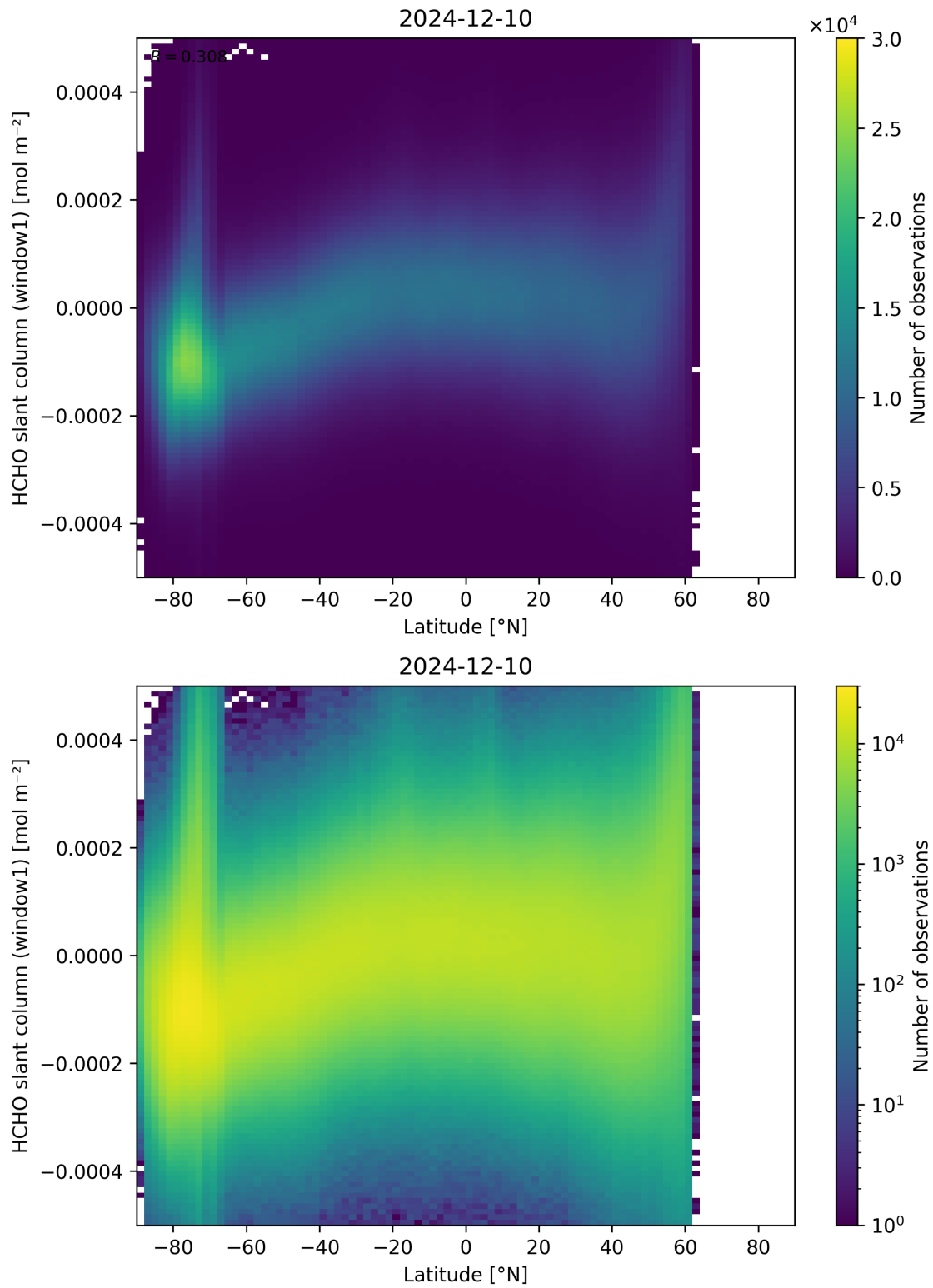
Figure 159: Scatter density plot of “Latitude” against “HCHO slant column (window1)” for 2024-12-09 to 2024-12-11.
