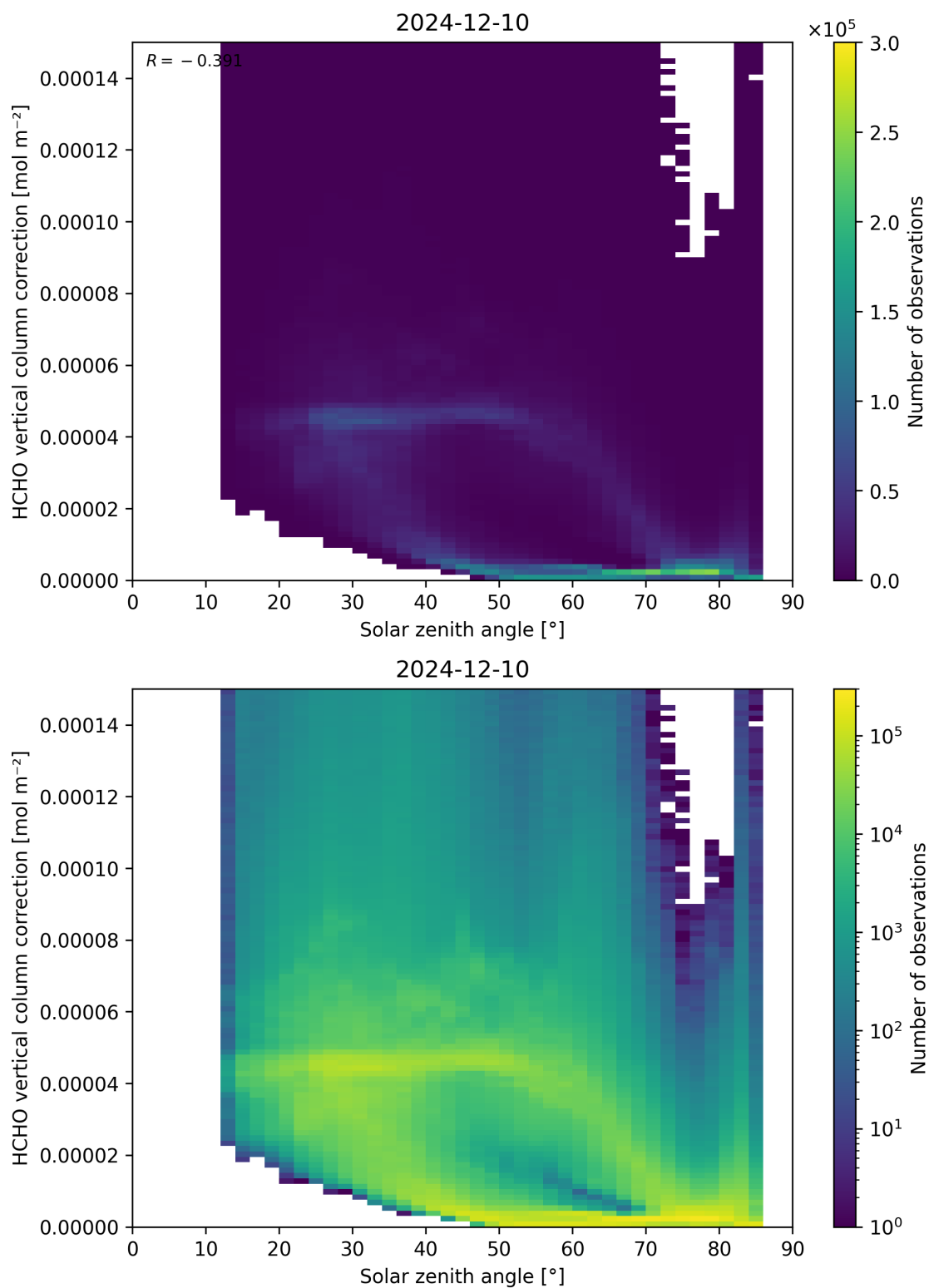
Figure 178: Scatter density plot of “Solar zenith angle” against “HCHO vertical column correction” for 2024-12-09 to 2024-12-11.
