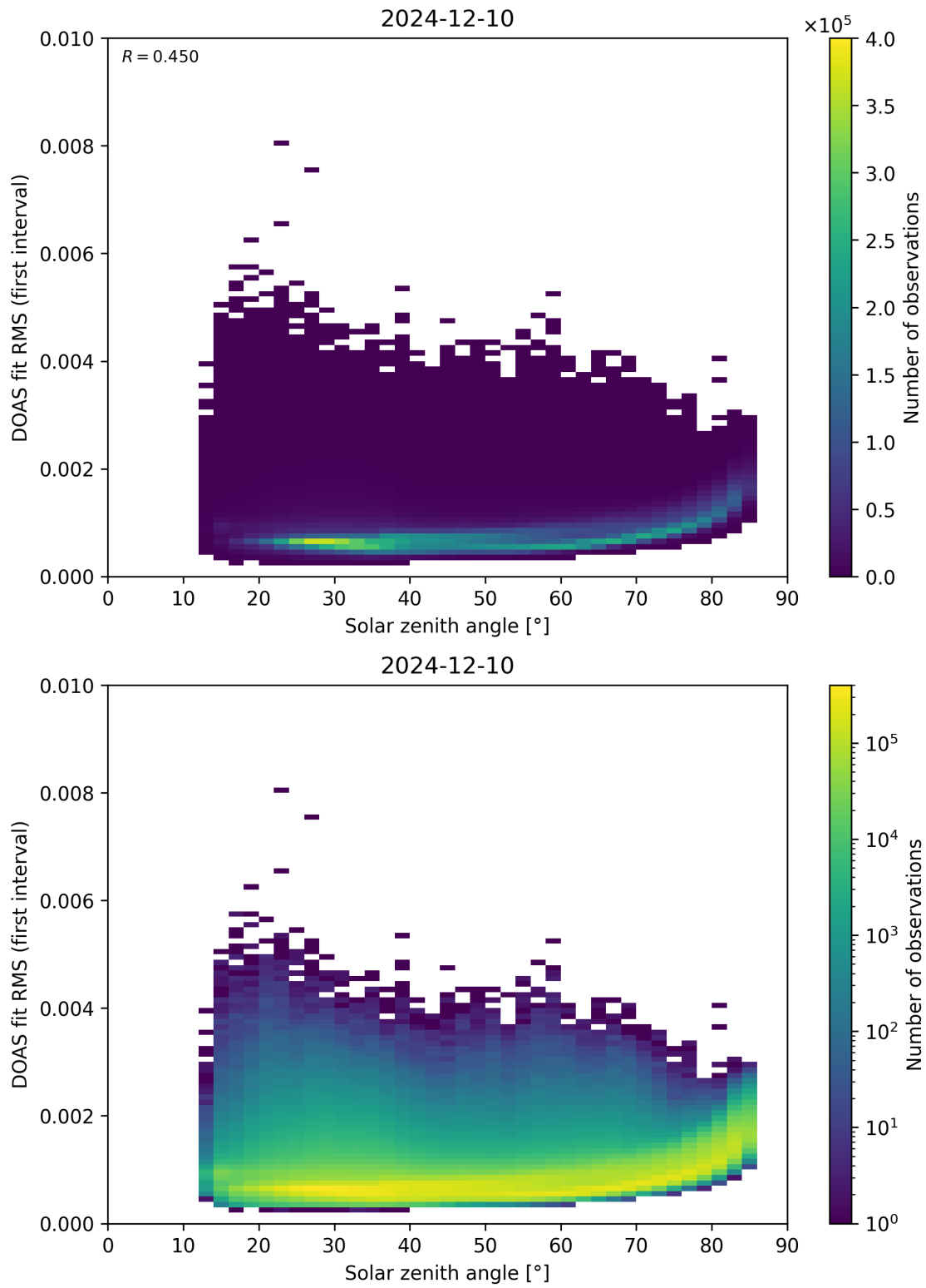
Figure 167: Scatter density plot of “Solar zenith angle” against “DOAS fit RMS (first interval)” for 2024-12-09 to 2024-12-11.
