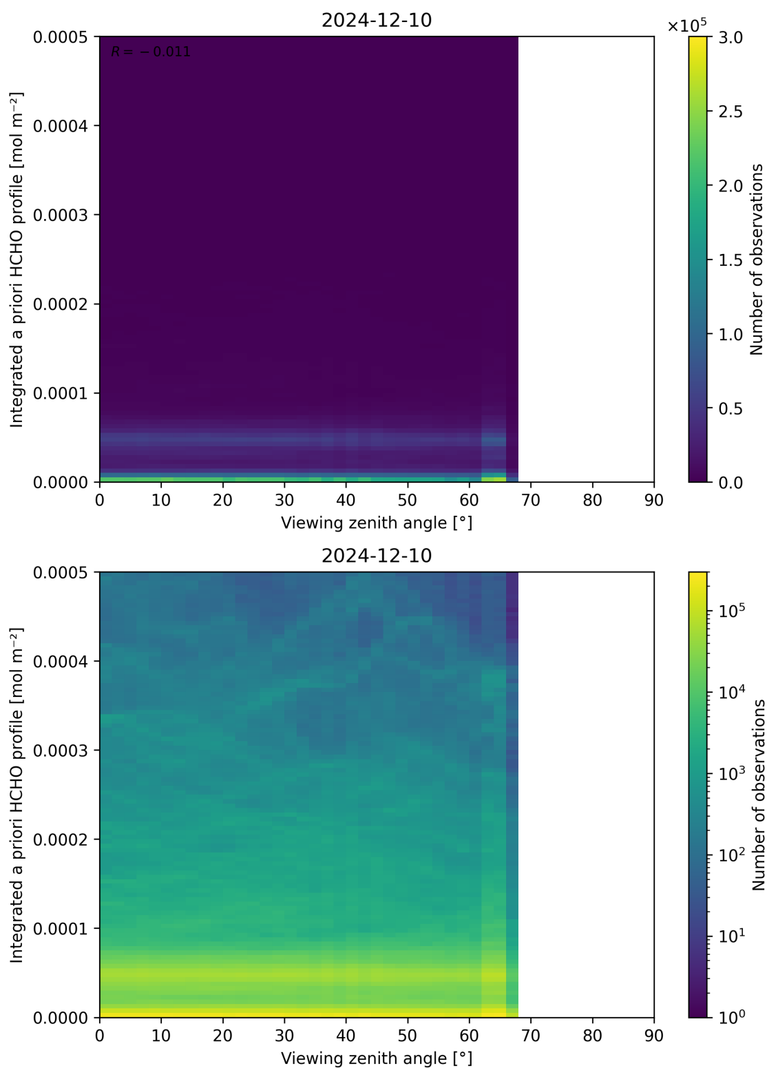
Figure 195: Scatter density plot of “Viewing zenith angle” against “Integrated a priori HCHO profile” for 2024-12-09 to 2024-12-11.
