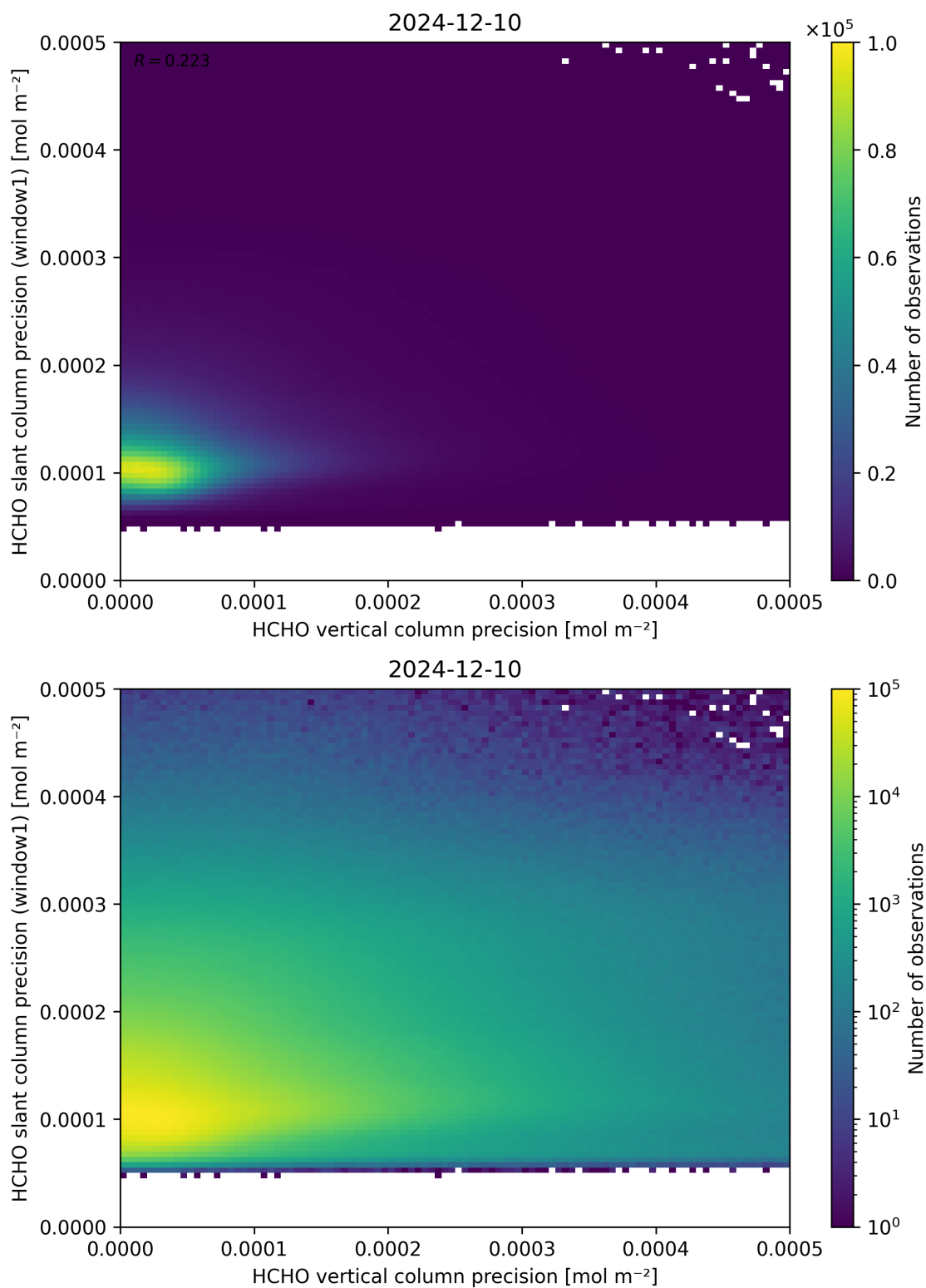
Figure 143: Scatter density plot of “HCHO vertical column precision” against “HCHO slant column precision (window1)” for 2024-12-09 to 2024-12-11.
