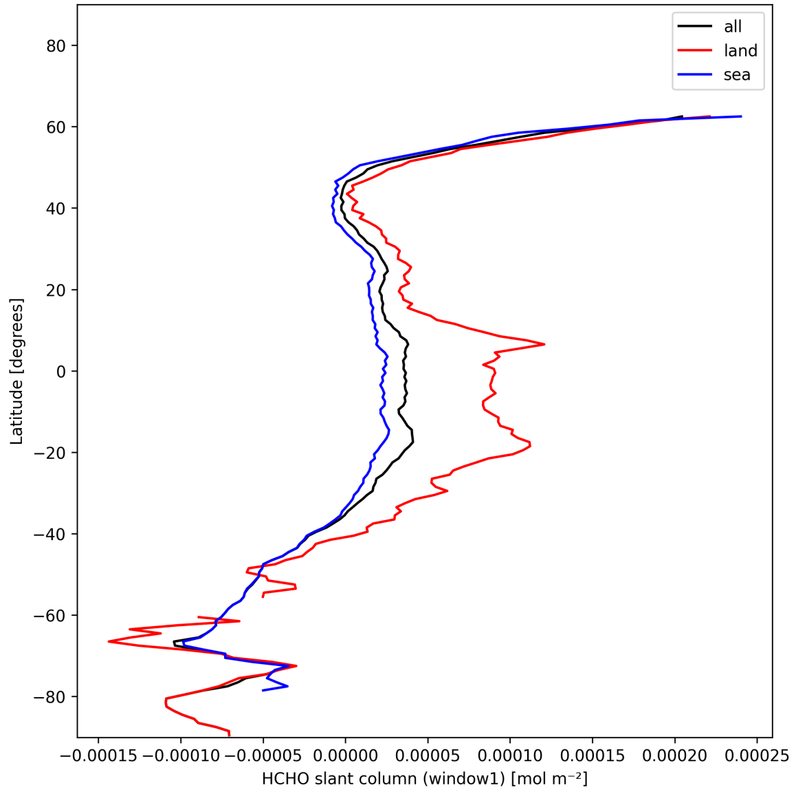
Figure 24: Zonal average of “HCHO slant column (window1)” for 2024-12-09 to 2024-12-11.
