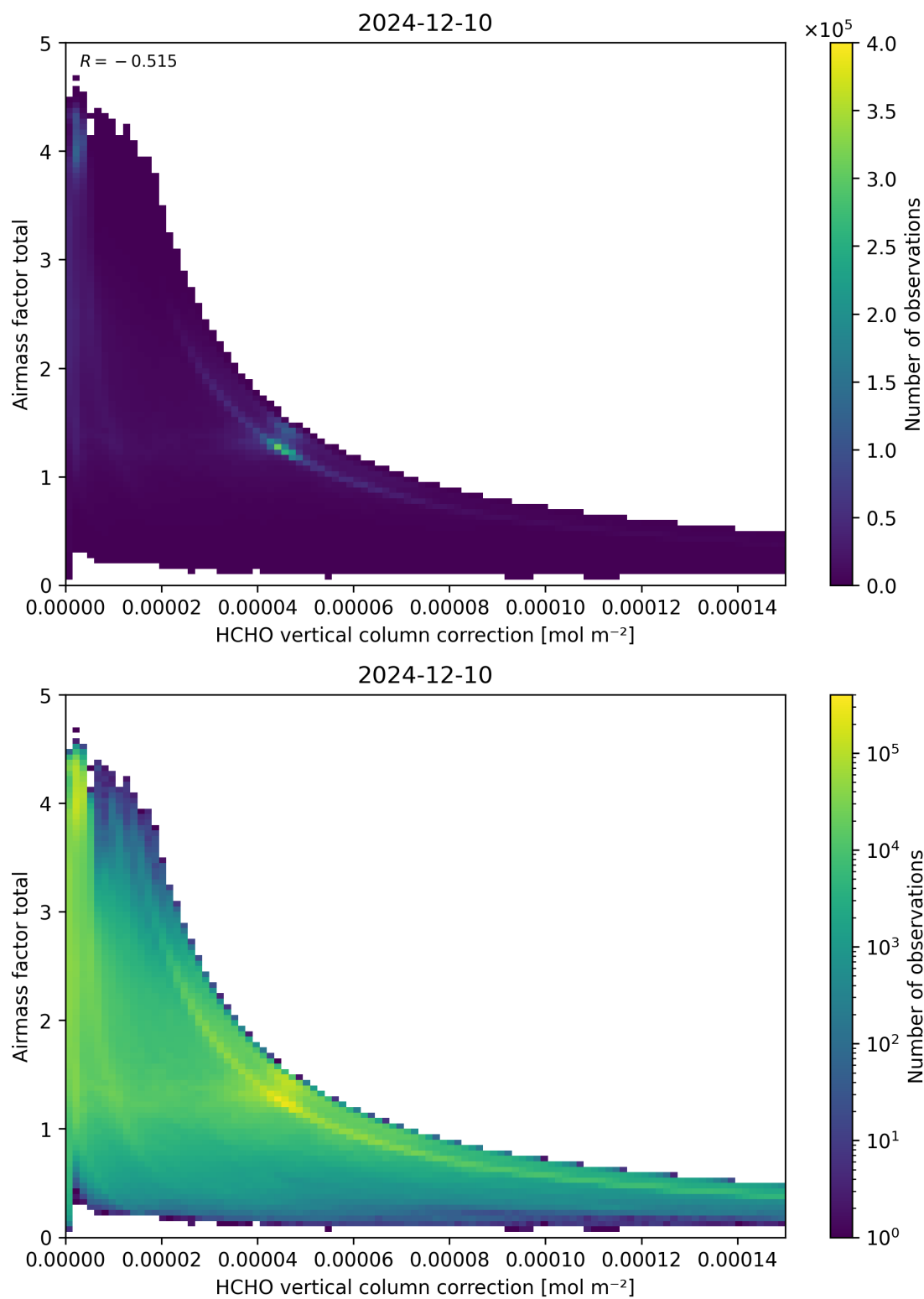
Figure 120: Scatter density plot of “HCHO vertical column correction” against “Airmass factor total” for 2024-12-09 to 2024-12-11.
