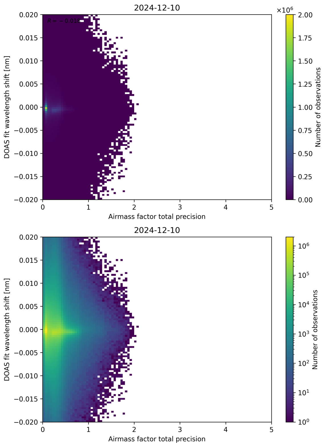
Figure 106: Scatter density plot of “Airmass factor total precision” against “DOAS fit wavelength shift” for 2024-12-09 to 2024-12-11.
