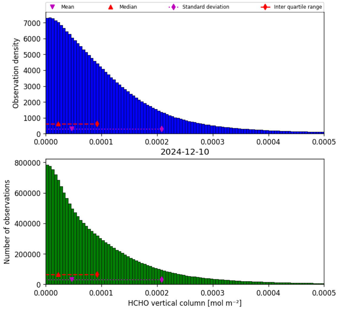
Figure 35: Histogram of “HCHO vertical column” for 2024-12-09 to 2024-12-11
