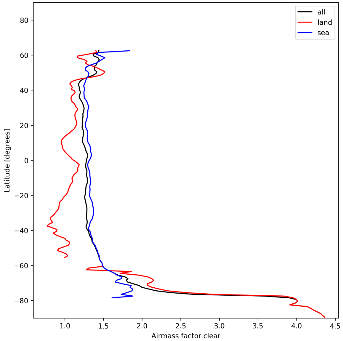
Figure 28: Zonal average of “Airmass factor clear” for 2024-12-09 to 2024-12-11.
