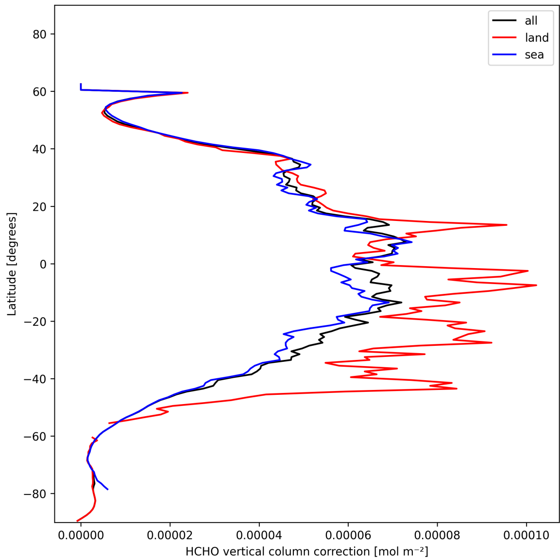
Figure 23: Zonal average of “HCHO vertical column correction” for 2024-12-09 to 2024-12-11.
