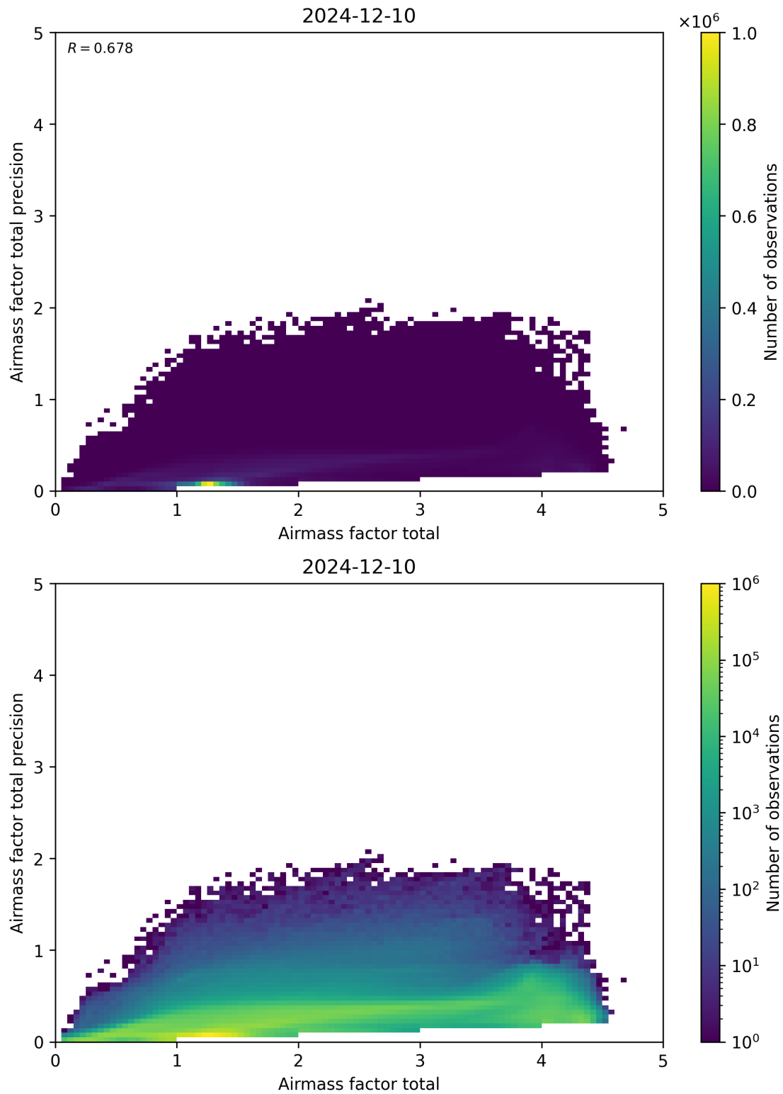
Figure 103: Scatter density plot of “Airmass factor total” against “Airmass factor total precision” for 2024-12-09 to 2024-12-11.
