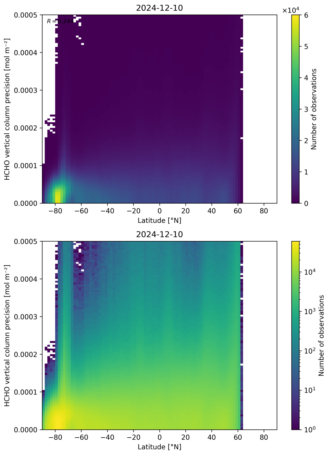
Figure 165: Scatter density plot of “Latitude” against “HCHO vertical column precision” for 2024-12-09 to 2024-12-11.
