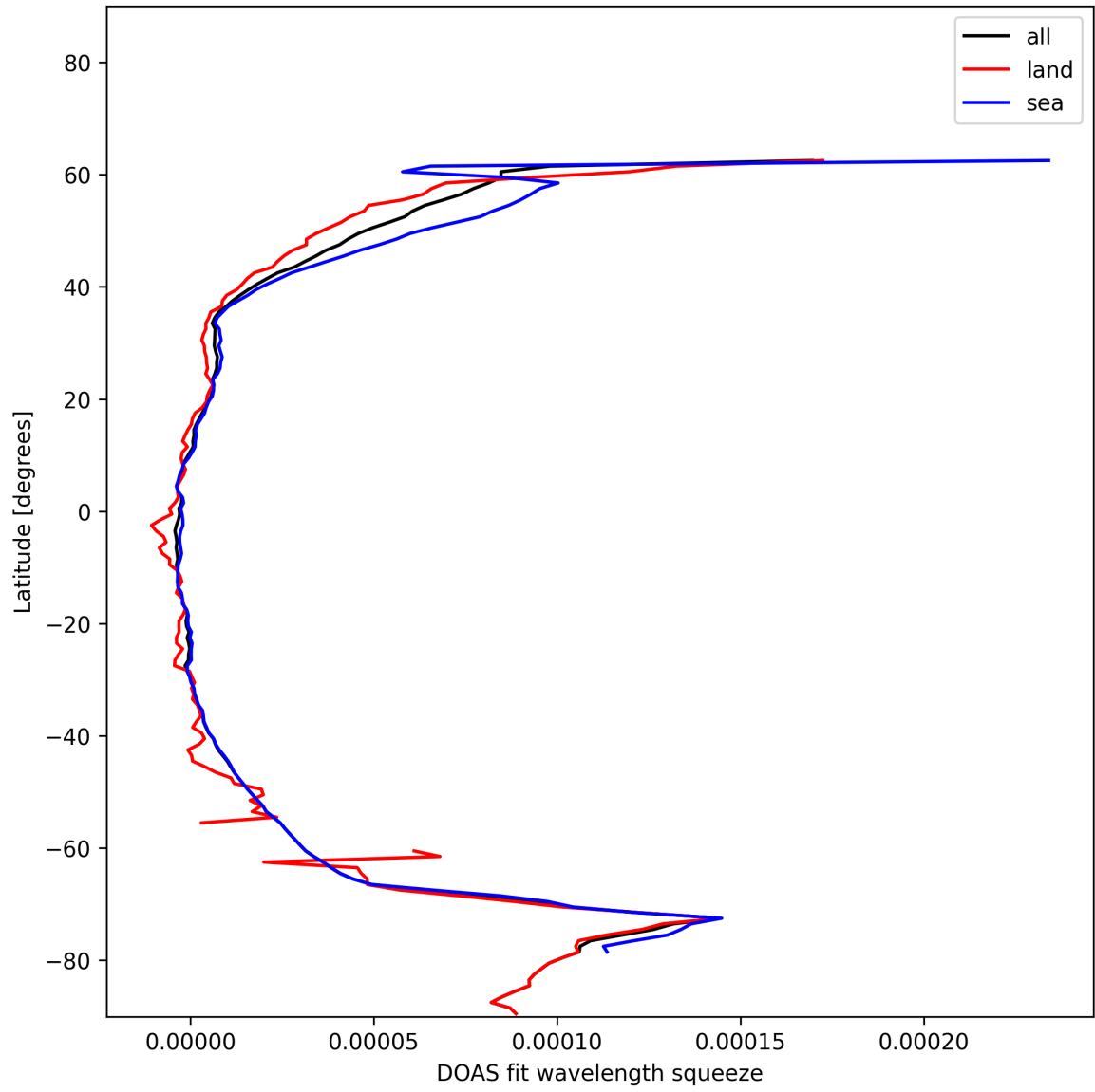
Figure 31: Zonal average of “DOAS fit wavelength squeeze” for 2024-12-09 to 2024-12-11.
