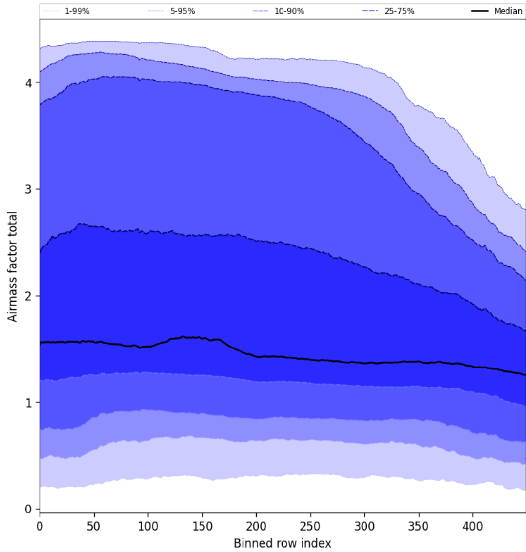
Figure 54: Along track statistics of “Airmass factor total” for 2024-12-09 to 2024-12-11
