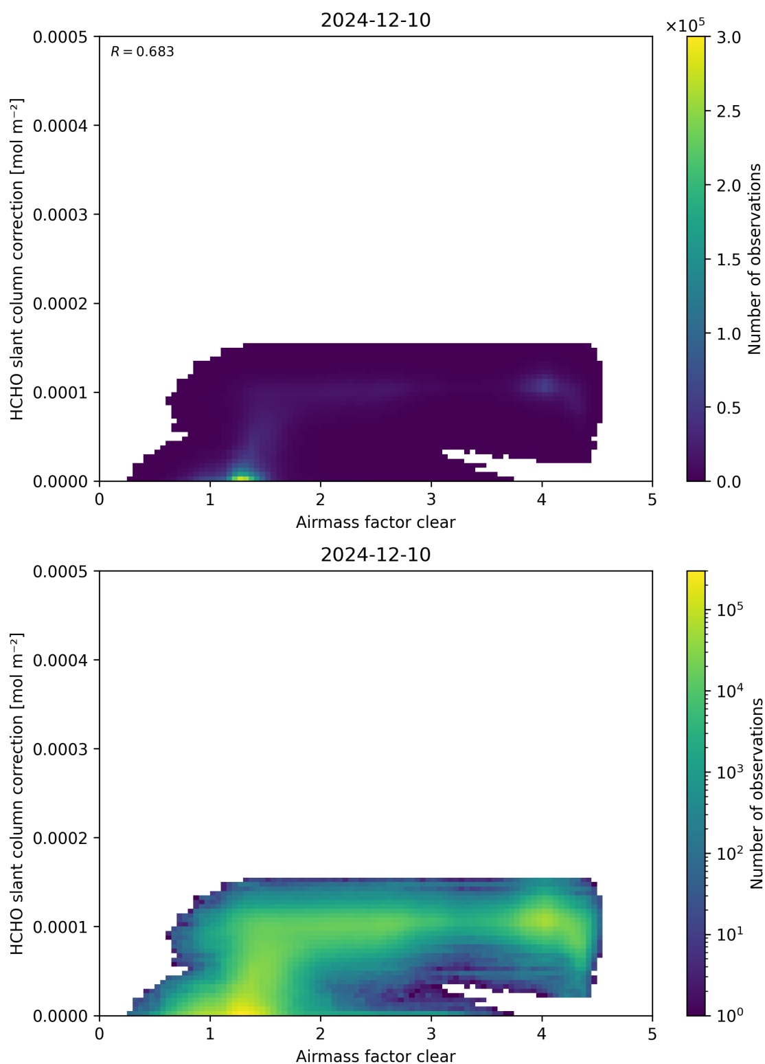
Figure 75: Scatter density plot of “Airmass factor clear” against “HCHO slant column correction” for 2024-12-09 to 2024-12-11.
