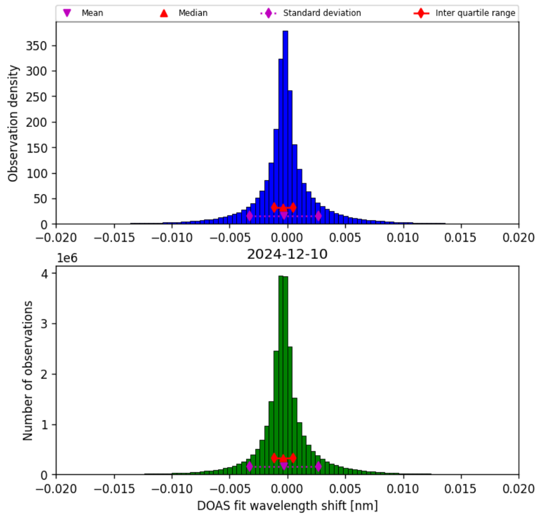
Figure 44: Histogram of “DOAS fit wavelength shift” for 2024-12-09 to 2024-12-11
