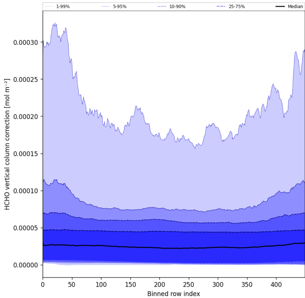
Figure 51: Along track statistics of “HCHO vertical column correction” for 2024-12-09 to 2024-12-11
