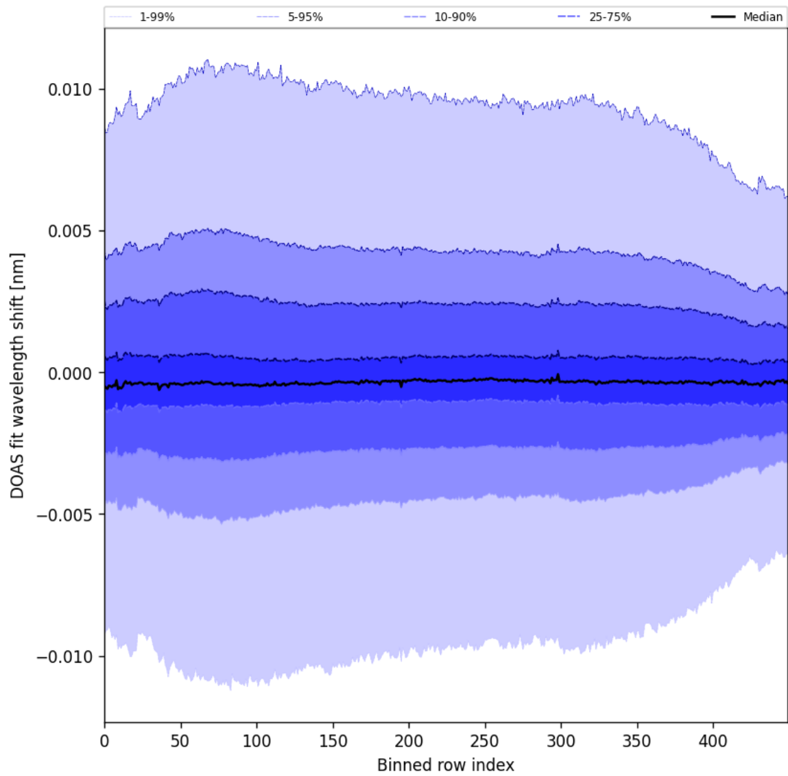
Figure 58: Along track statistics of “DOAS fit wavelength shift” for 2024-12-09 to 2024-12-11
