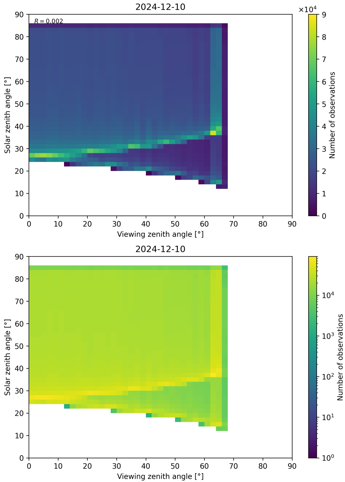
Figure 197: Scatter density plot of “Viewing zenith angle” against “Solar zenith angle” for 2024-12-09 to 2024-12-11.
