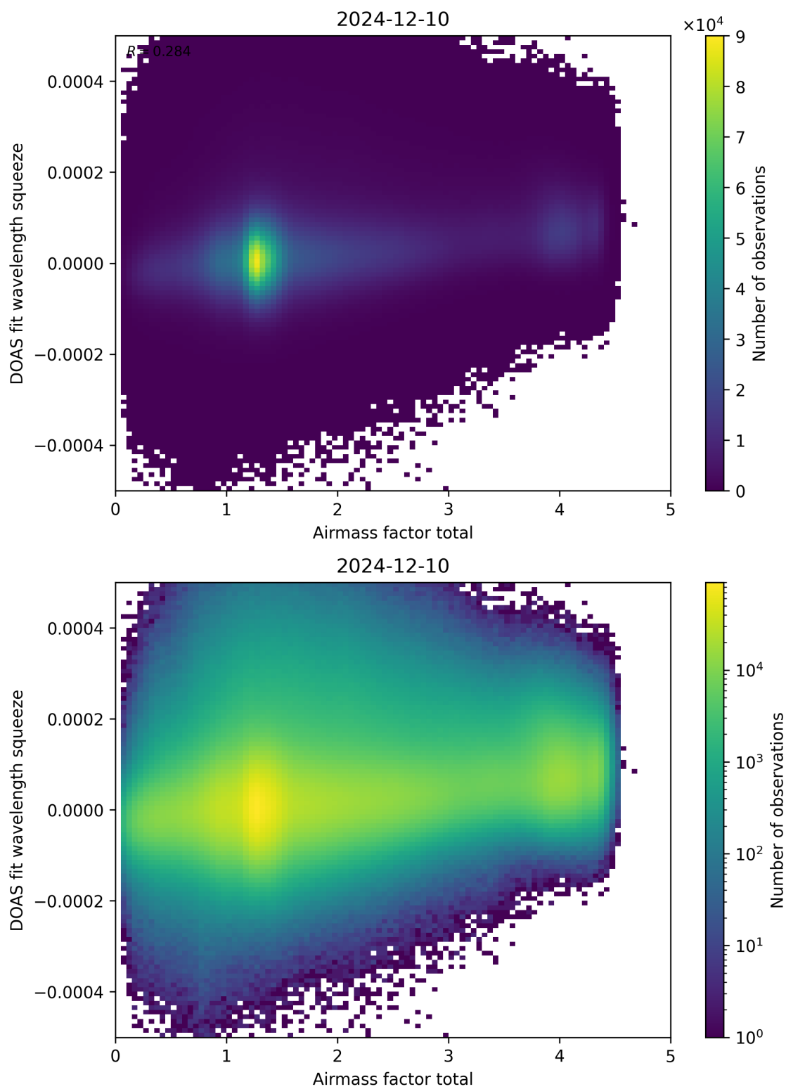
Figure 99: Scatter density plot of “Airmass factor total” against “DOAS fit wavelength squeeze” for 2024-12-09 to 2024-12-11.
