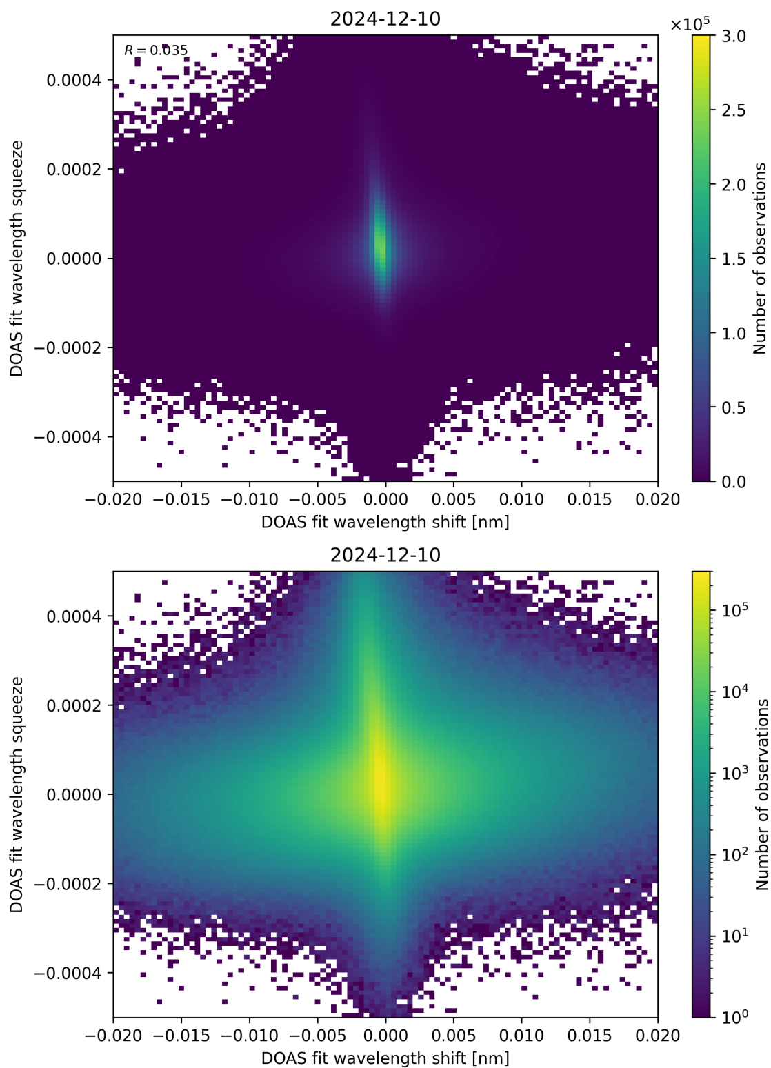
Figure 65: Scatter density plot of “DOAS fit wavelength shift” against “DOAS fit wavelength squeeze” for 2024-12-09 to 2024-12-11.
