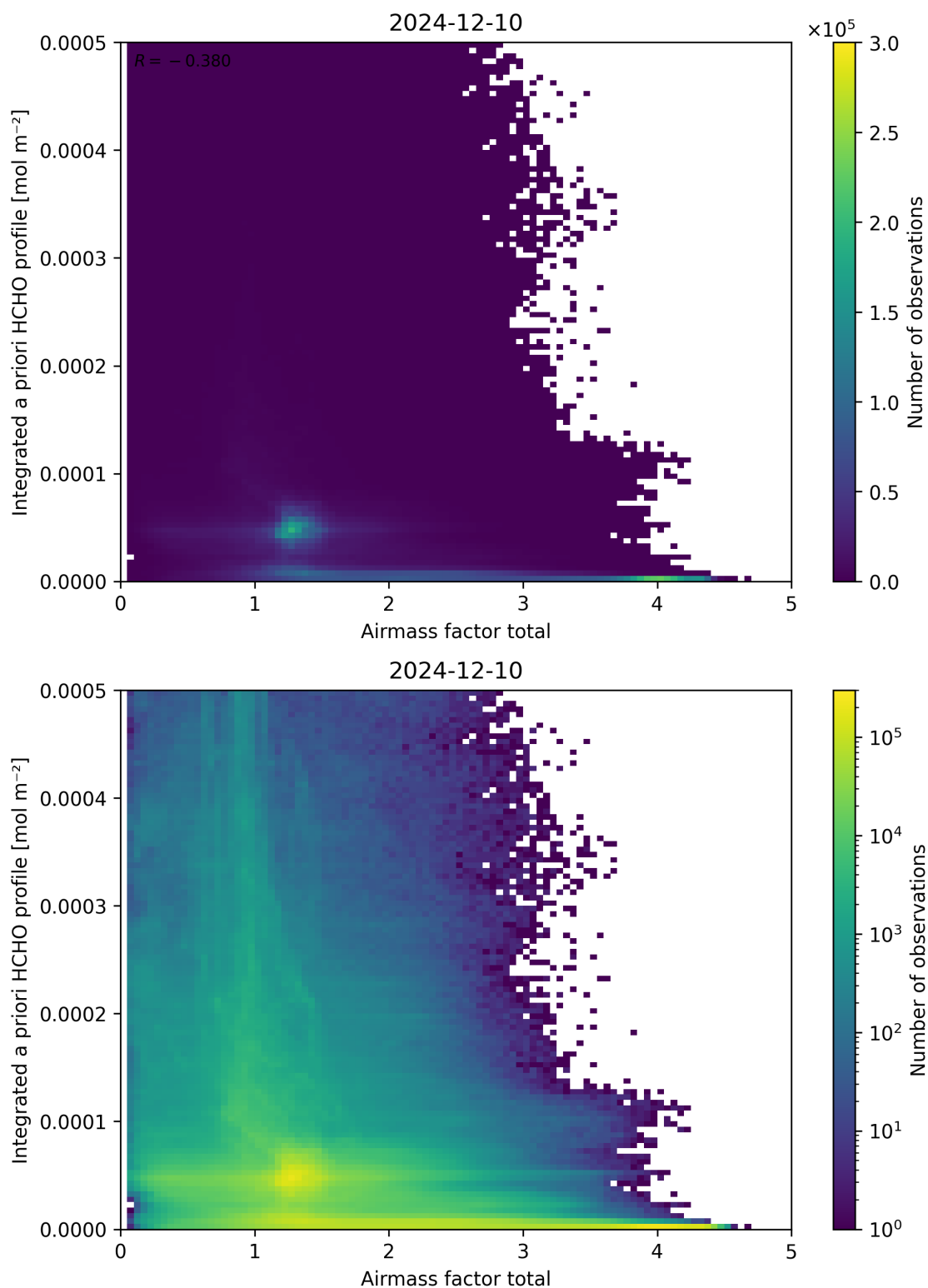
Figure 104: Scatter density plot of “Airmass factor total” against “Integrated a priori HCHO profile” for 2024-12-09 to 2024-12-11.
