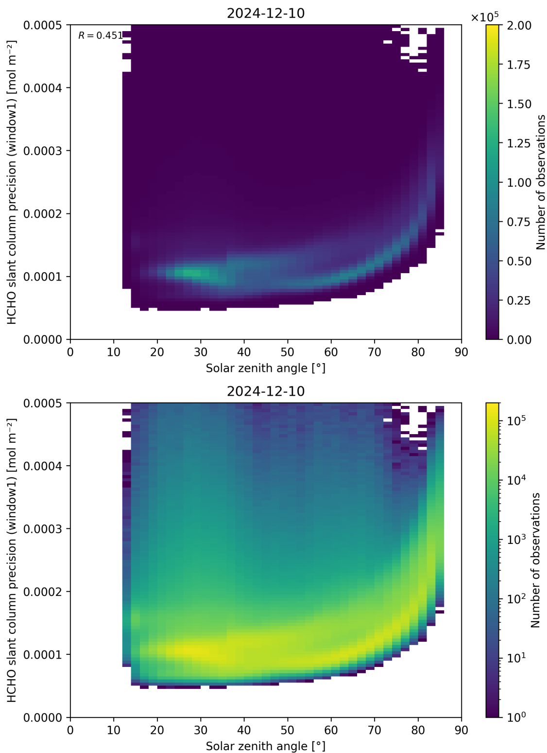
Figure 174: Scatter density plot of “Solar zenith angle” against “HCHO slant column precision (window1)” for 2024-12-09 to 2024-12-11.
