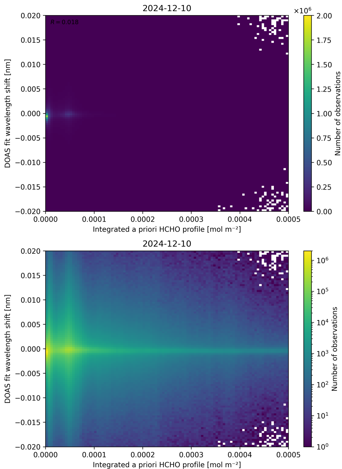
Figure 149: Scatter density plot of “Integrated a priori HCHO profile” against “DOAS fit wavelength shift” for 2024-12-09 to 2024-12-11.
