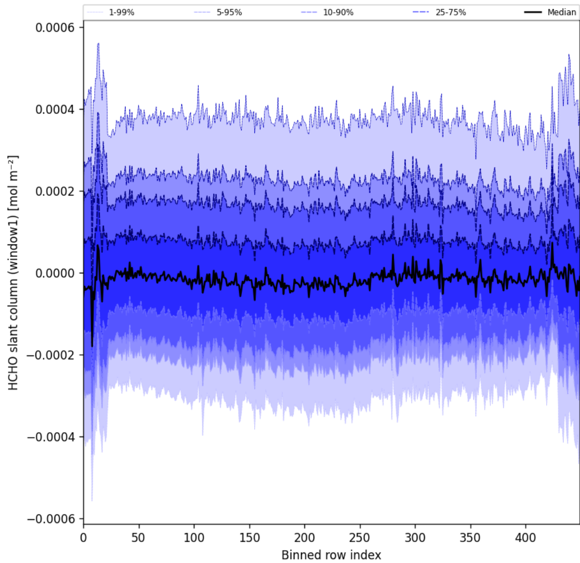
Figure 52: Along track statistics of “HCHO slant column (window1)” for 2024-12-09 to 2024-12-11
