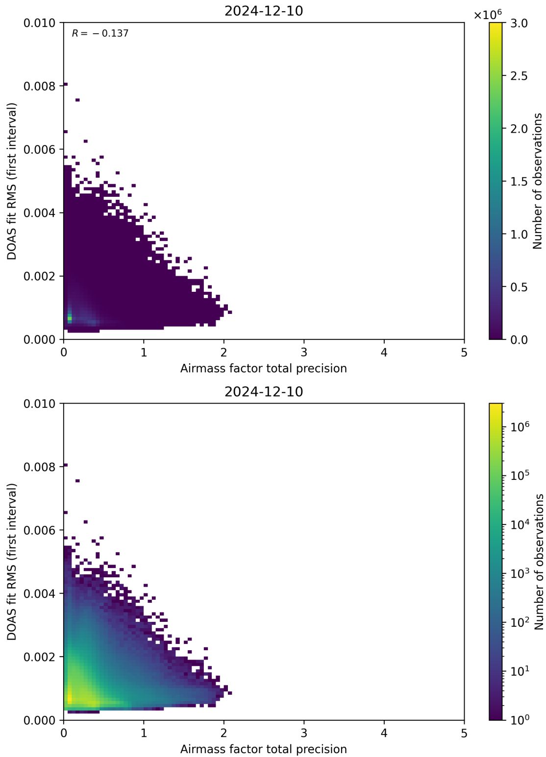
Figure 105: Scatter density plot of “Airmass factor total precision” against “DOAS fit RMS (first interval)” for 2024-12-09 to 2024-12-11.
