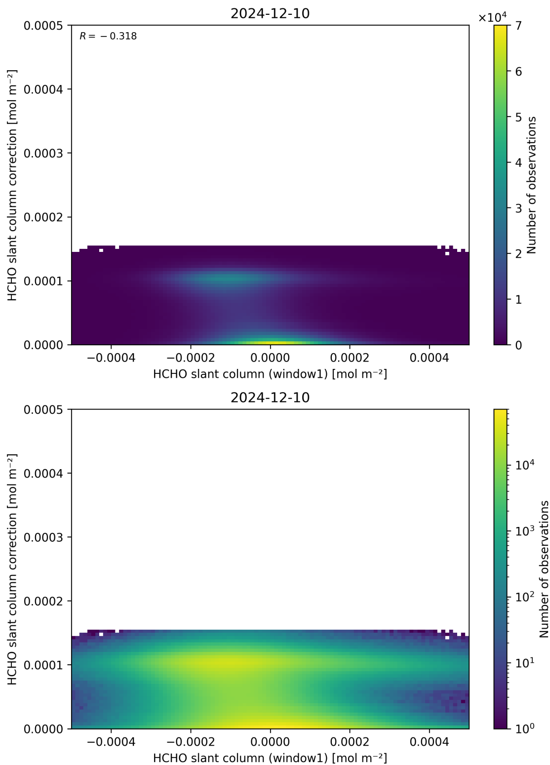
Figure 83: Scatter density plot of “HCHO slant column (window1)” against “HCHO slant column correction” for 2024-12-09 to 2024-12-11.
