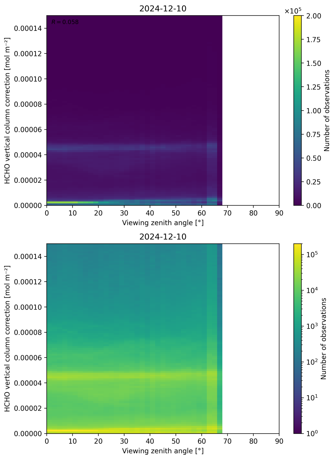
Figure 193: Scatter density plot of “Viewing zenith angle” against “HCHO vertical column correction” for 2024-12-09 to 2024-12-11.
