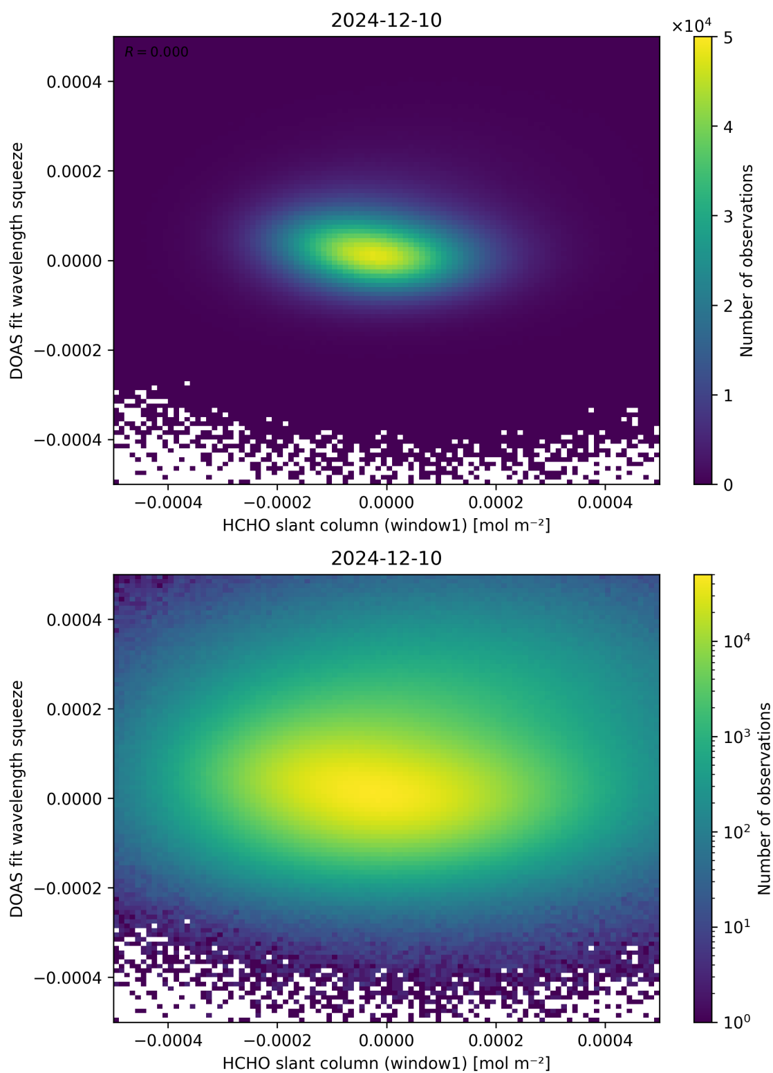
Figure 80: Scatter density plot of “HCHO slant column (window1)” against “DOAS fit wavelength squeeze” for 2024-12-09 to 2024-12-11.
