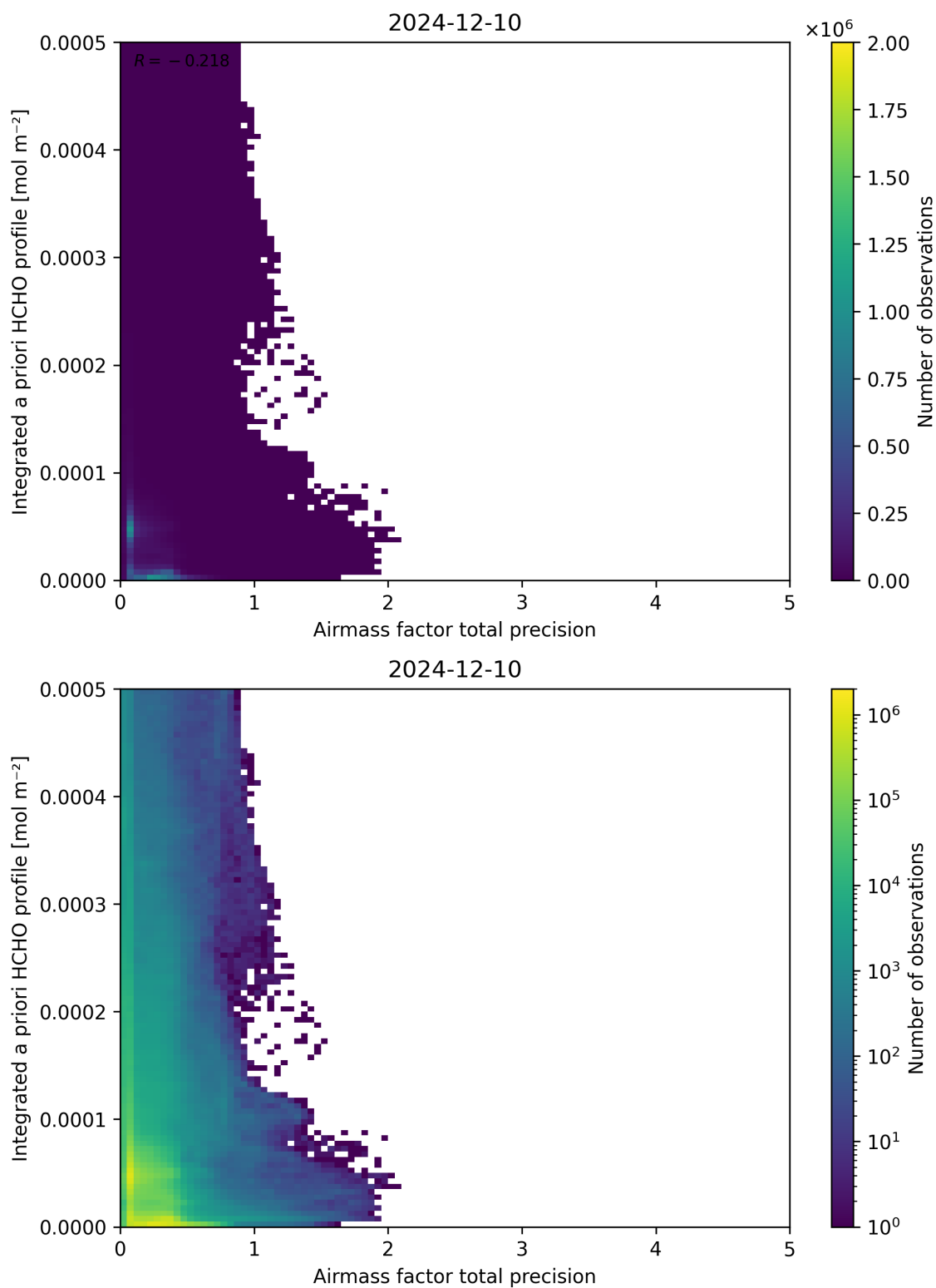
Figure 111: Scatter density plot of “Airmass factor total precision” against “Integrated a priori HCHO profile” for 2024-12-09 to 2024-12-11.
