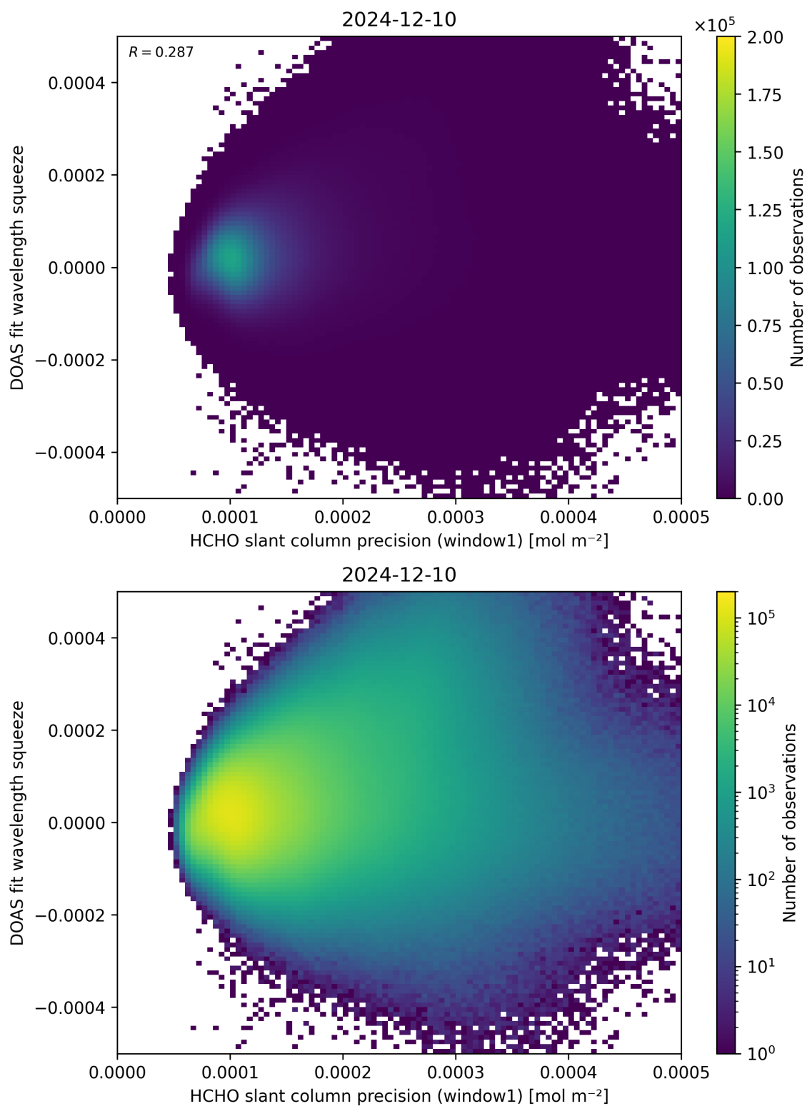
Figure 90: Scatter density plot of “HCHO slant column precision (window1)” against “DOAS fit wavelength squeeze” for 2024-12-09 to 2024-12-11.
