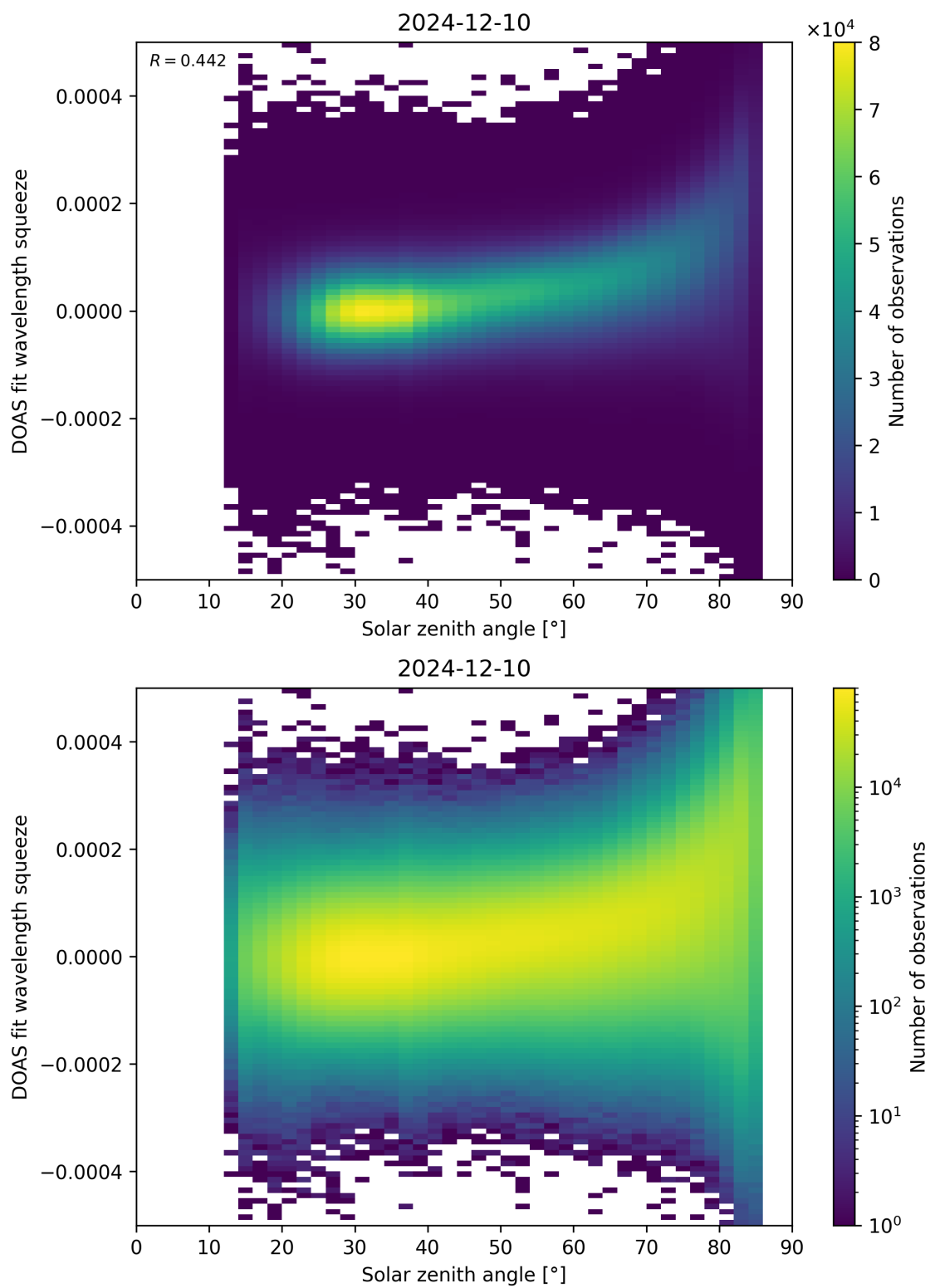
Figure 169: Scatter density plot of “Solar zenith angle” against “DOAS fit wavelength squeeze” for 2024-12-09 to 2024-12-11.
