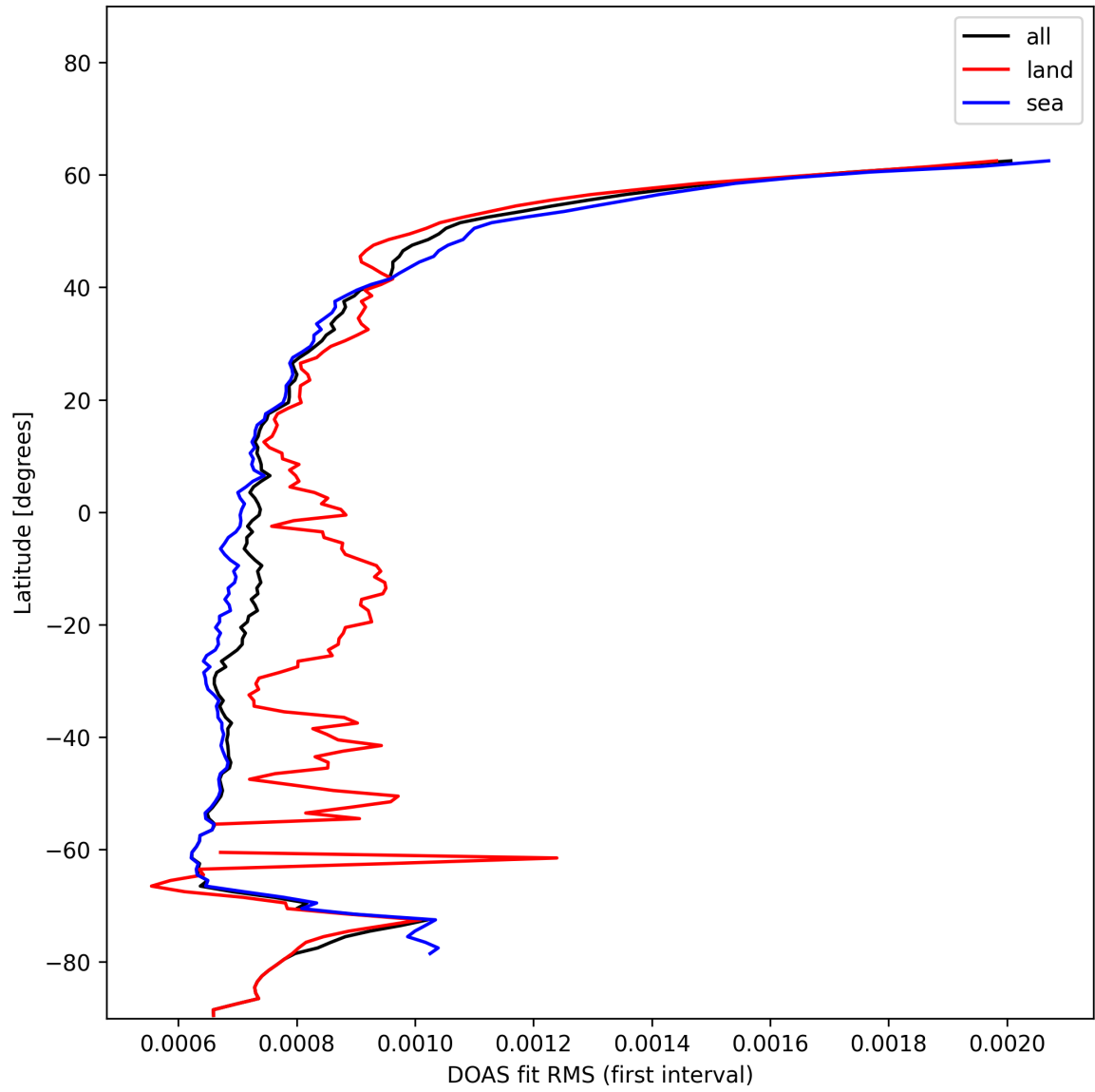
Figure 32: Zonal average of "DOAS fit RMS (first interval)" for 2024-12-09 to 2024-12-11.
