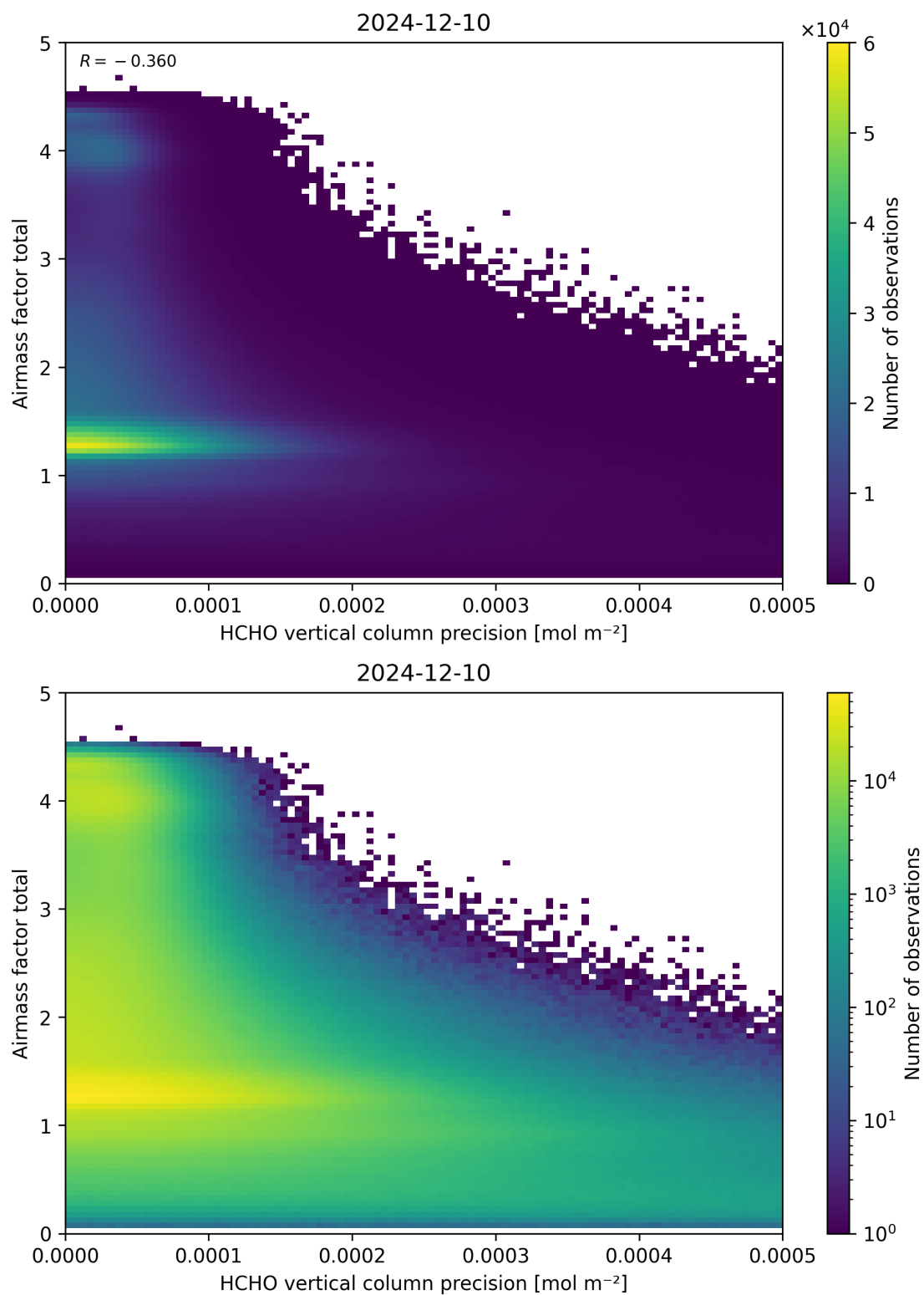
Figure 144: Scatter density plot of “HCHO vertical column precision” against “Airmass factor total” for 2024-12-09 to 2024-12-11.
