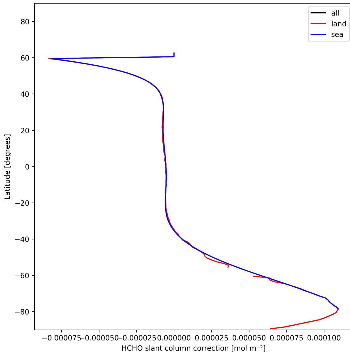
Figure 33: Zonal average of “HCHO slant column correction” for 2024-12-09 to 2024-12-11.
