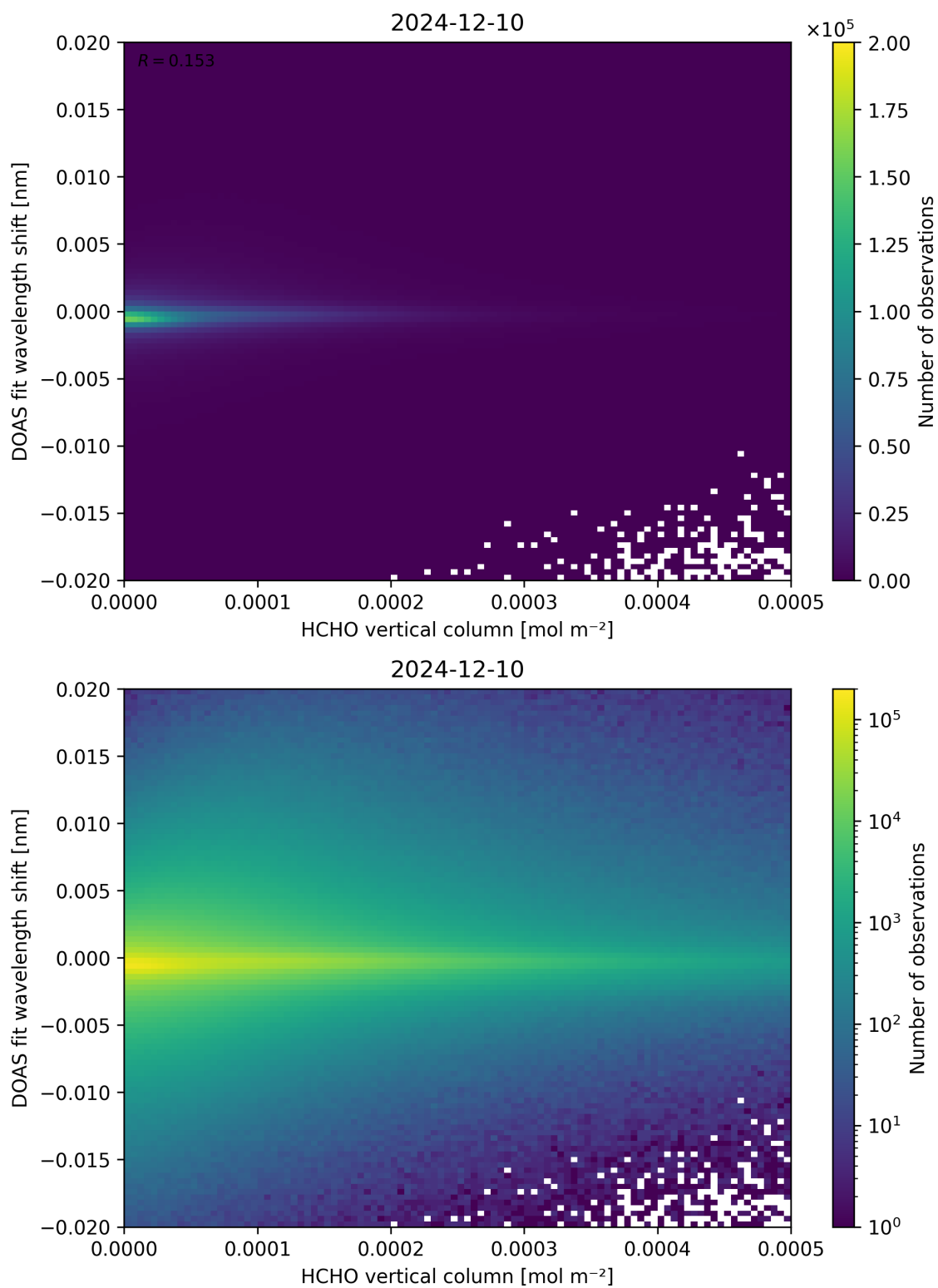
Figure 124: Scatter density plot of “HCHO vertical column” against “DOAS fit wavelength shift” for 2024-12-09 to 2024-12-11.
