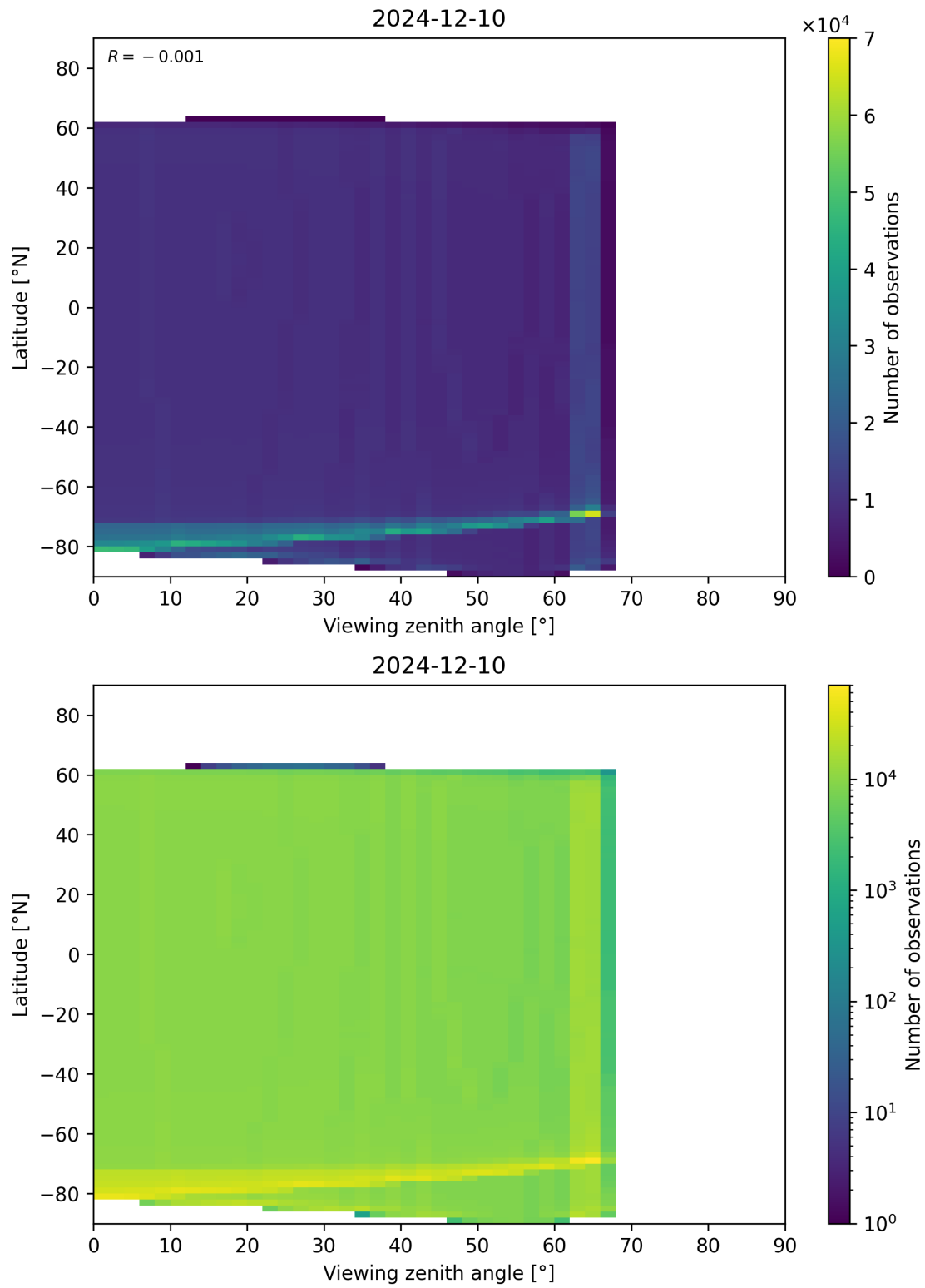
Figure 196: Scatter density plot of “Viewing zenith angle” against “Latitude” for 2024-12-09 to 2024-12-11.
