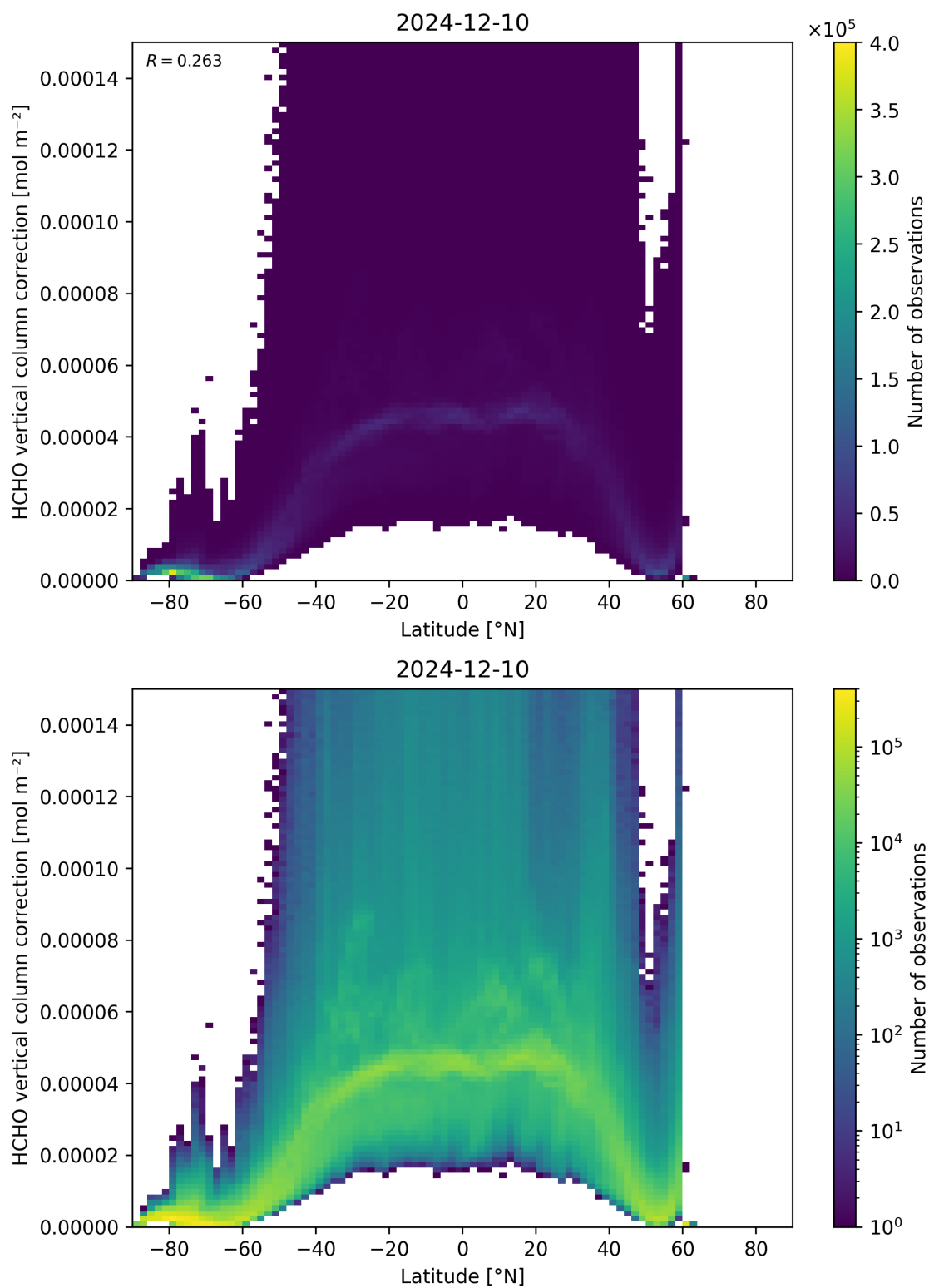
Figure 164: Scatter density plot of “Latitude” against “HCHO vertical column correction” for 2024-12-09 to 2024-12-11.
