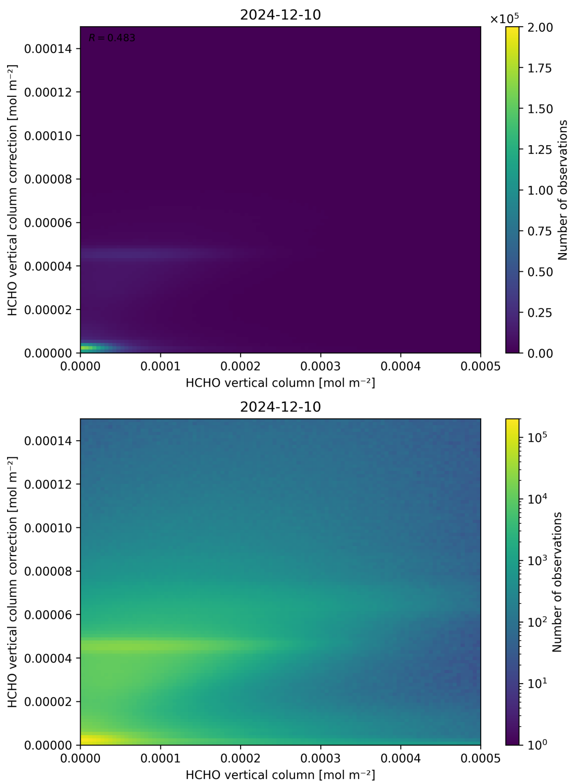
Figure 133: Scatter density plot of “HCHO vertical column” against “HCHO vertical column correction” for 2024-12-09 to 2024-12-11.
