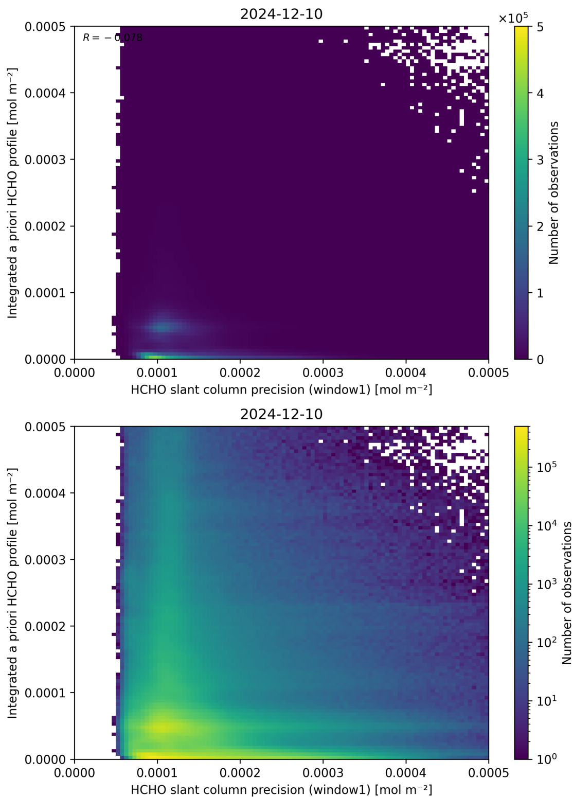
Figure 96: Scatter density plot of “HCHO slant column precision (window1)” against “Integrated a priori HCHO profile” for 2024-12-09 to 2024-12-11.
