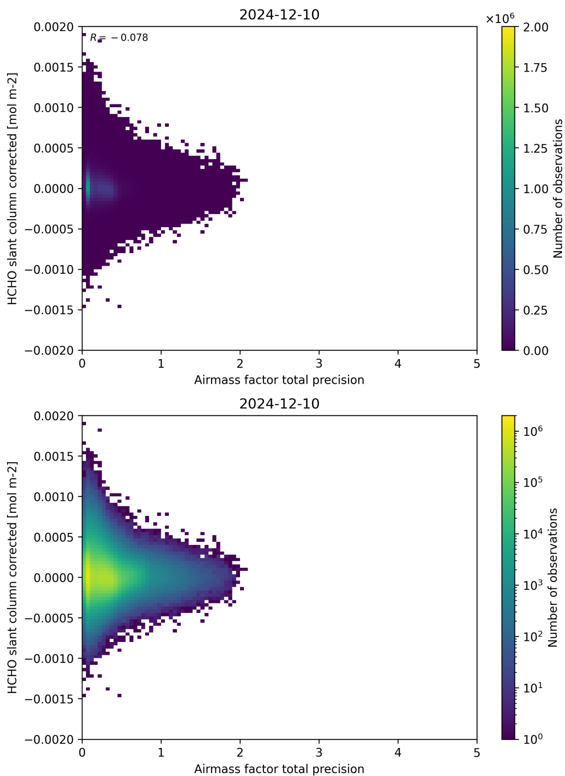
Figure 109: Scatter density plot of “Airmass factor total precision” against “HCHO slant column corrected” for 2024-12-09 to 2024-12-11.
