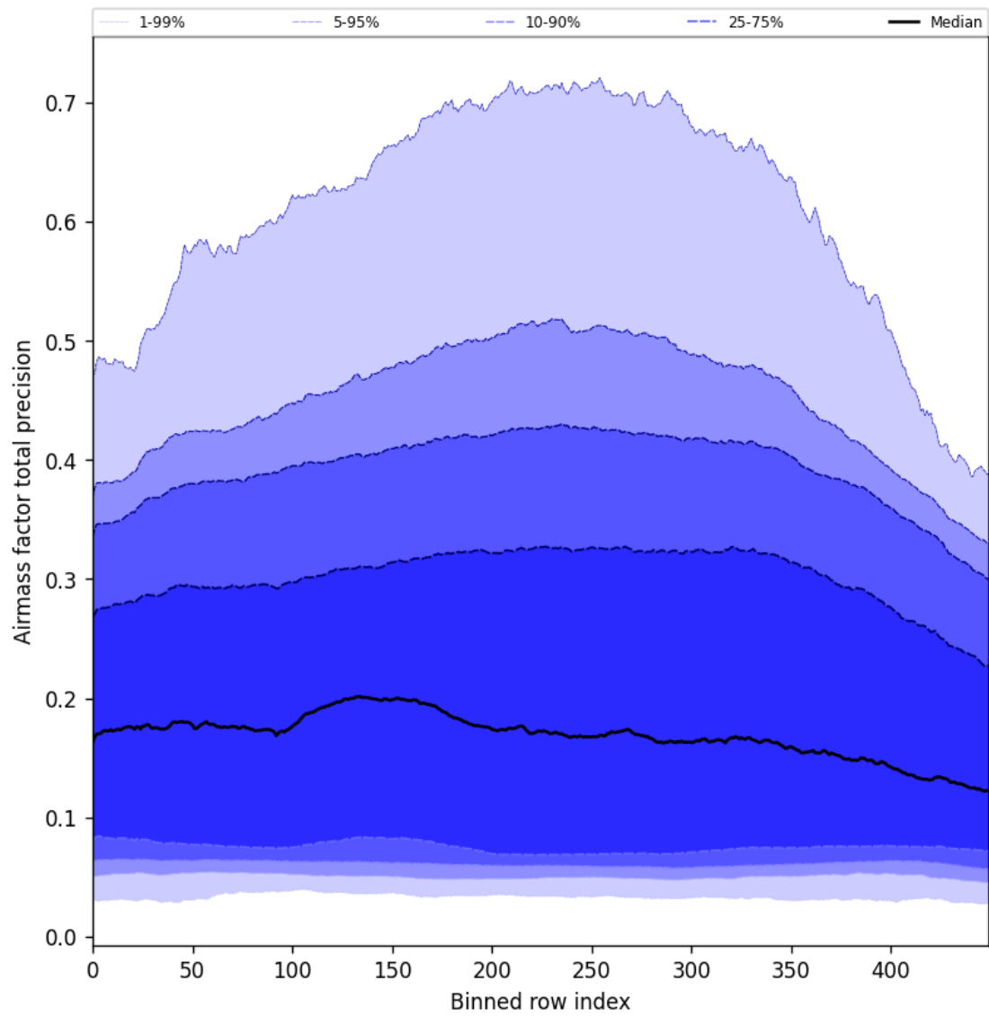
Figure 55: Along track statistics of “Airmass factor total precision” for 2024-12-09 to 2024-12-11
