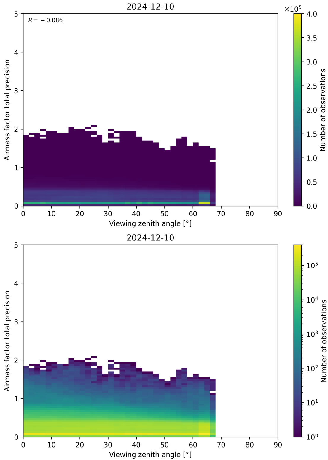
Figure 191: Scatter density plot of “Viewing zenith angle” against “Airmass factor total precision” for 2024-12-09 to 2024-12-11.
