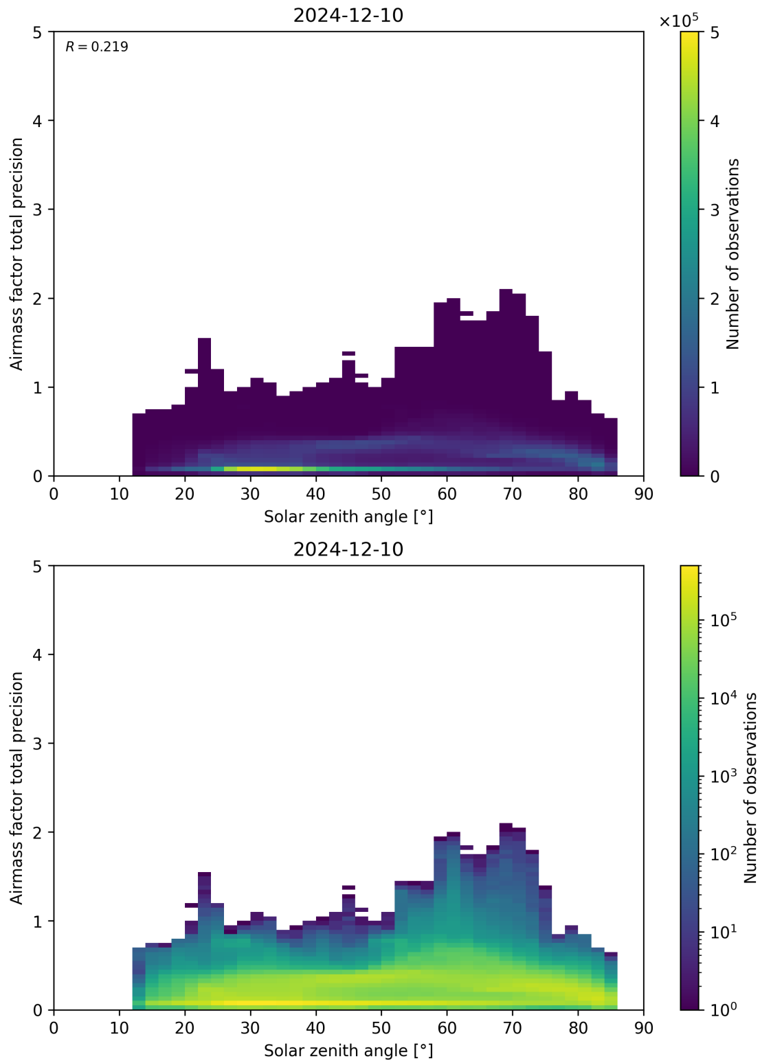
Figure 176: Scatter density plot of “Solar zenith angle” against “Airmass factor total precision” for 2024-12-09 to 2024-12-11.
