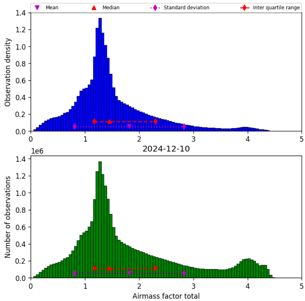
Figure 40: Histogram of “Airmass factor total” for 2024-12-09 to 2024-12-11
