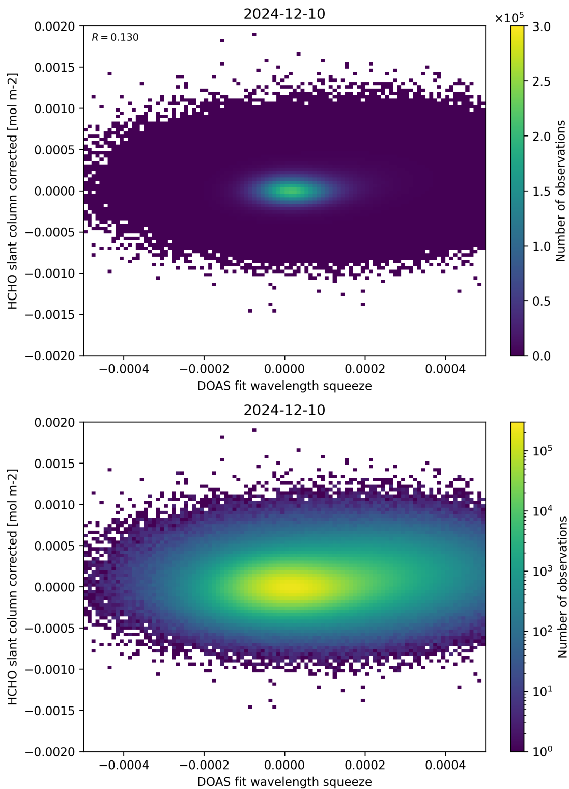
Figure 69: Scatter density plot of “DOAS fit wavelength squeeze” against “HCHO slant column corrected” for 2024-12-09 to 2024-12-11.
