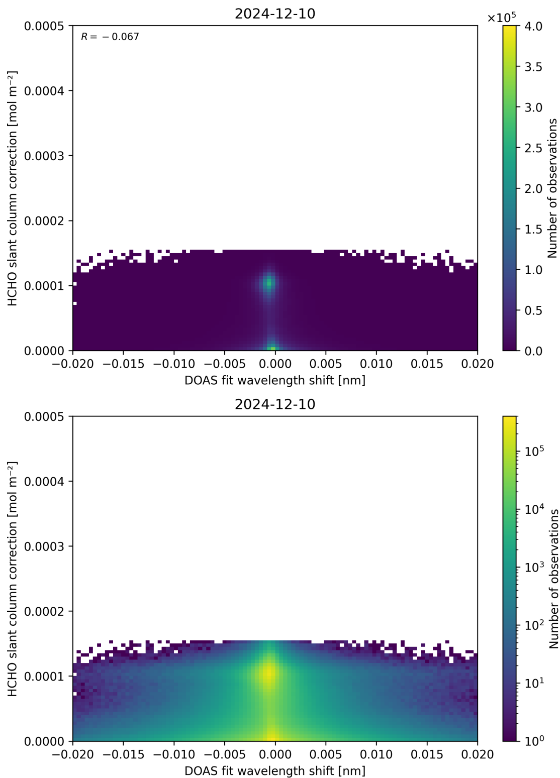
Figure 67: Scatter density plot of “DOAS fit wavelength shift” against “HCHO slant column correction” for 2024-12-09 to 2024-12-11.
