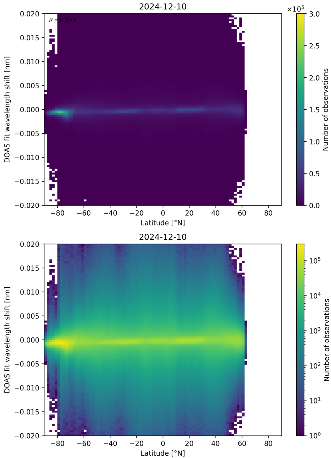
Figure 154: Scatter density plot of “Latitude” against “DOAS fit wavelength shift” for 2024-12-09 to 2024-12-11.
