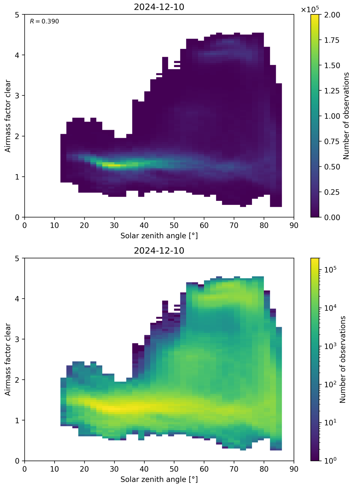
Figure 170: Scatter density plot of “Solar zenith angle” against “Airmass factor clear” for 2024-12-09 to 2024-12-11.
