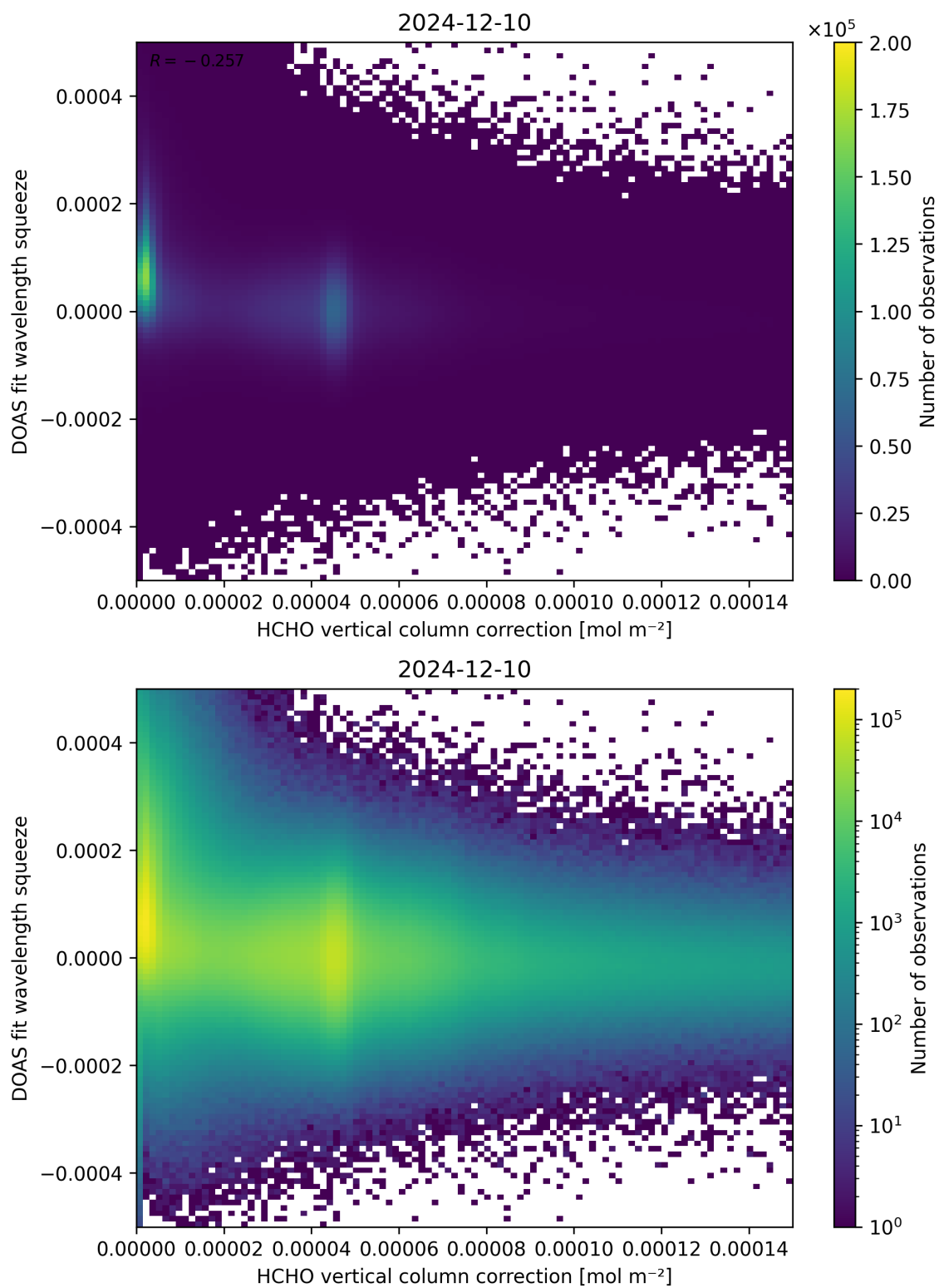
Figure 114: Scatter density plot of “HCHO vertical column correction” against “DOAS fit wavelength squeeze” for 2024-12-09 to 2024-12-11.
