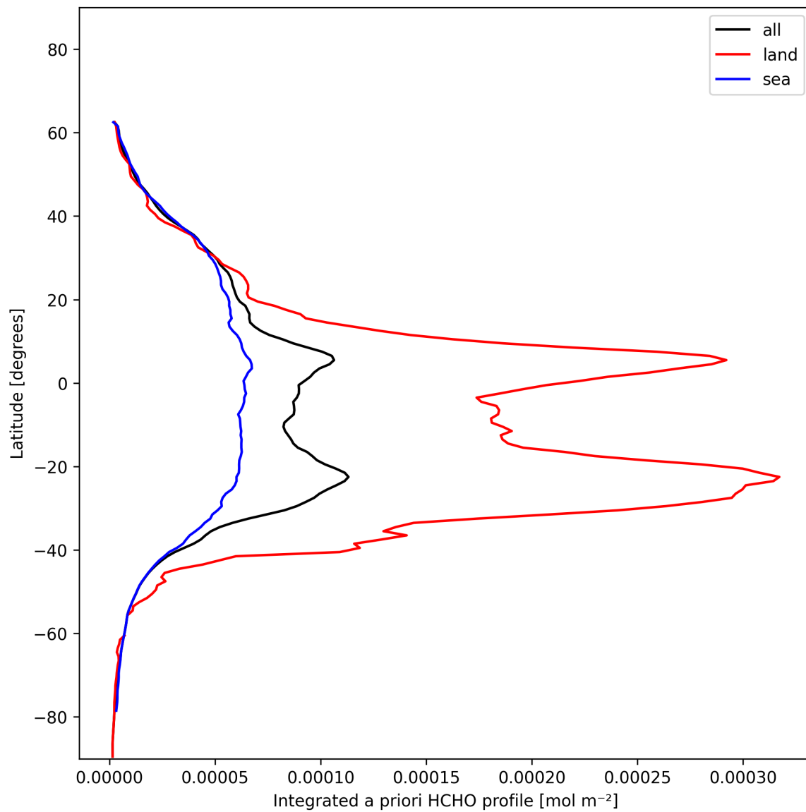
Figure 29: Zonal average of “Integrated a priori HCHO profile” for 2024-12-09 to 2024-12-11.
