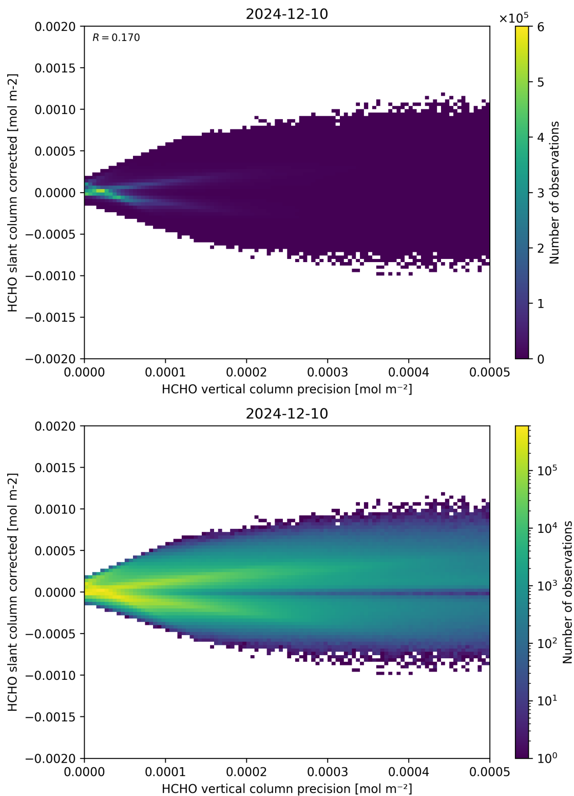
Figure 140: Scatter density plot of “HCHO vertical column precision” against “HCHO slant column corrected” for 2024-12-09 to 2024-12-11.
