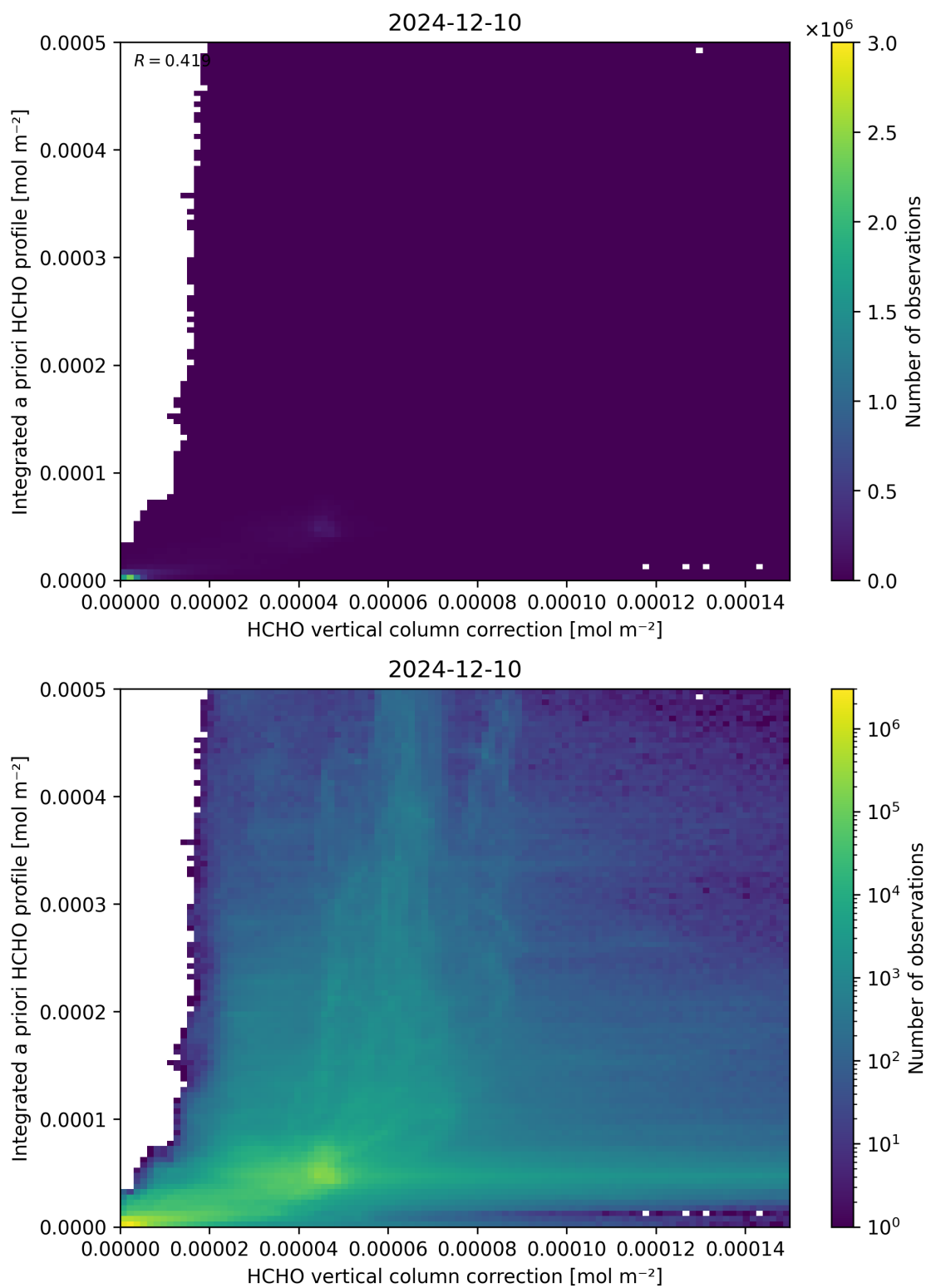
Figure 122: Scatter density plot of “HCHO vertical column correction” against “Integrated a priori HCHO profile” for 2024-12-09 to 2024-12-11.
