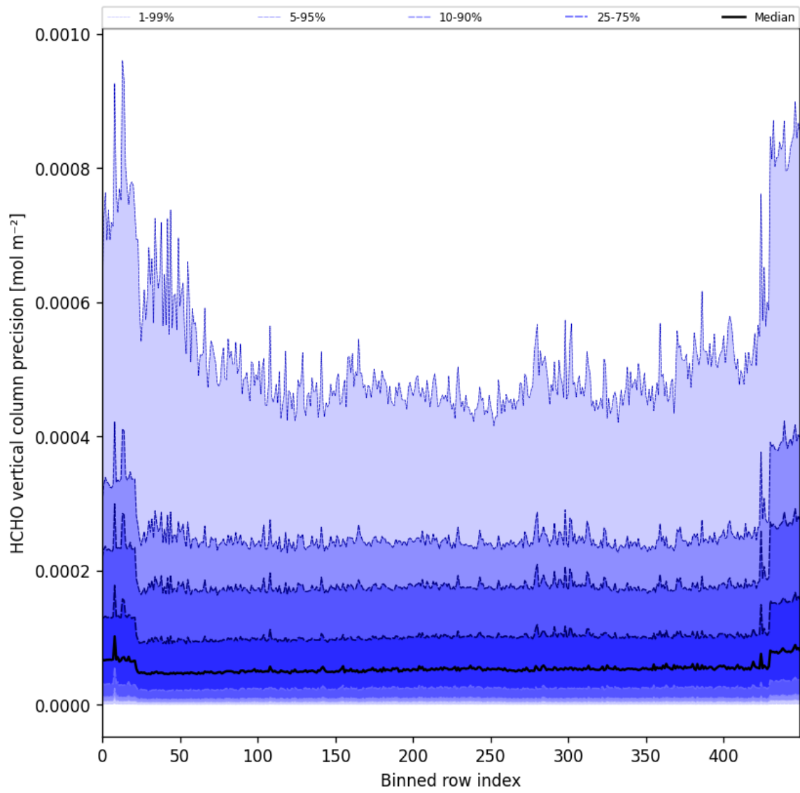
Figure 50: Along track statistics of “HCHO vertical column precision” for 2024-12-09 to 2024-12-11
