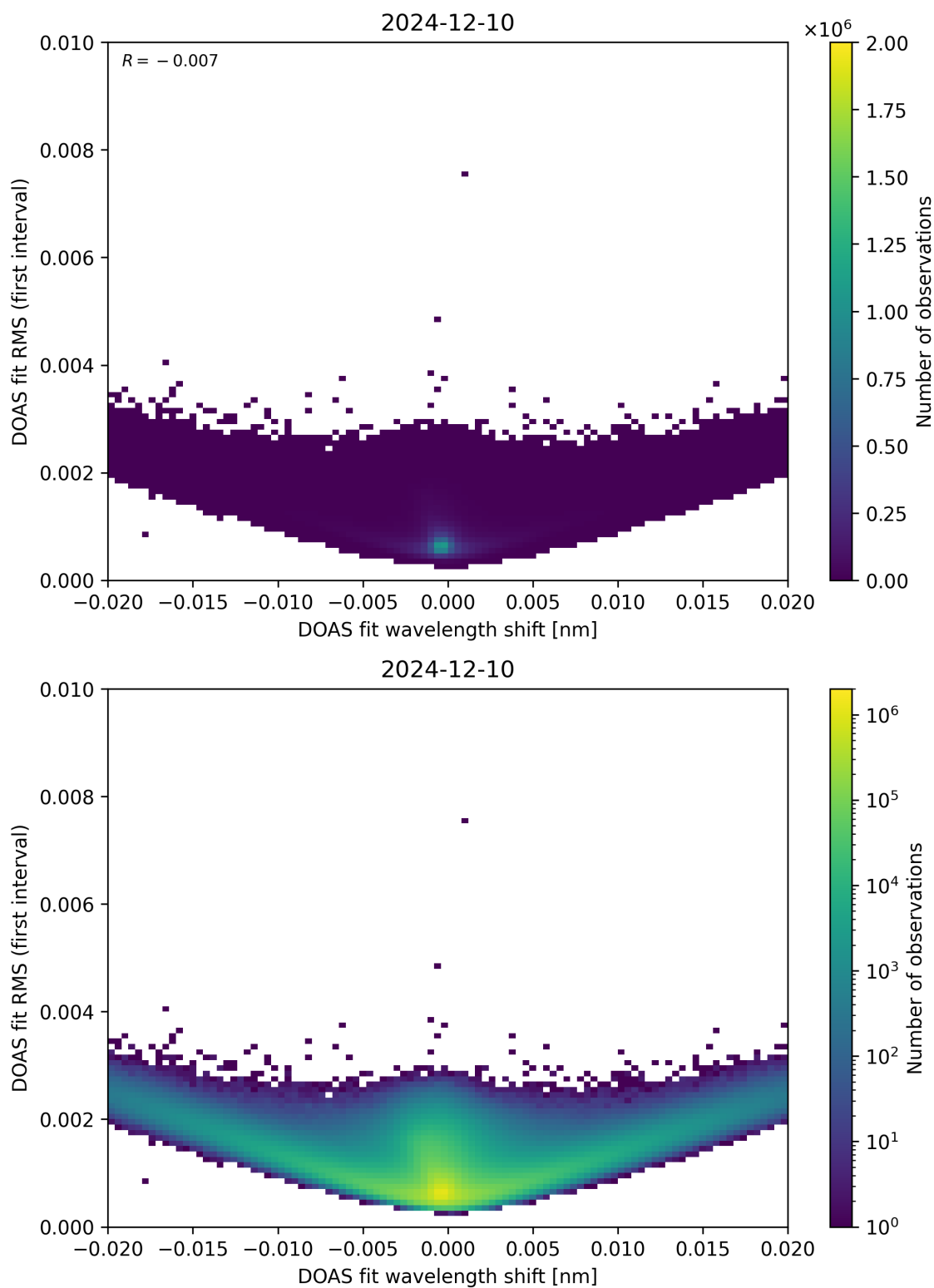
Figure 64: Scatter density plot of “DOAS fit wavelength shift” against “DOAS fit RMS (first interval)” for 2024-12-09 to 2024-12-11.
