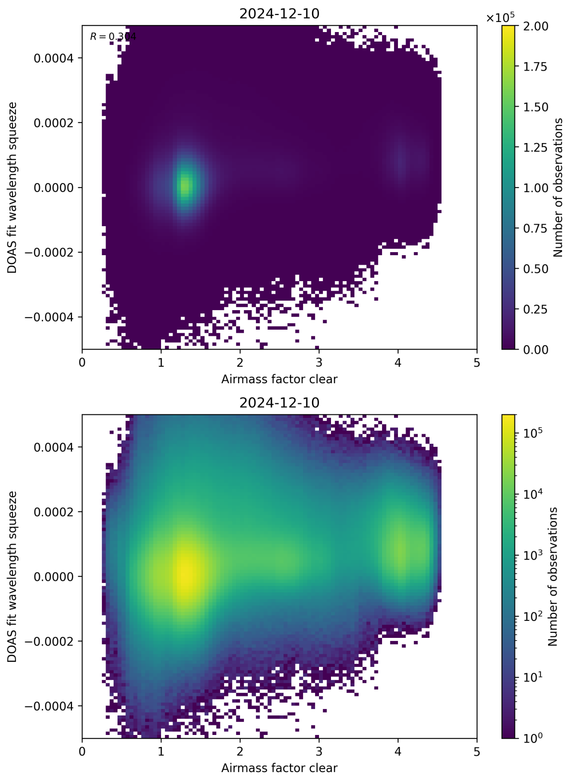
Figure 73: Scatter density plot of “Airmass factor clear” against “DOAS fit wavelength squeeze” for 2024-12-09 to 2024-12-11.
