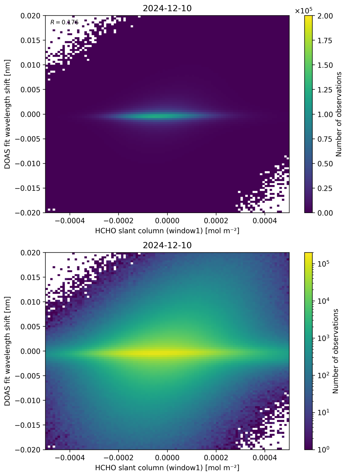
Figure 79: Scatter density plot of “HCHO slant column (window1)” against “DOAS fit wavelength shift” for 2024-12-09 to 2024-12-11.
