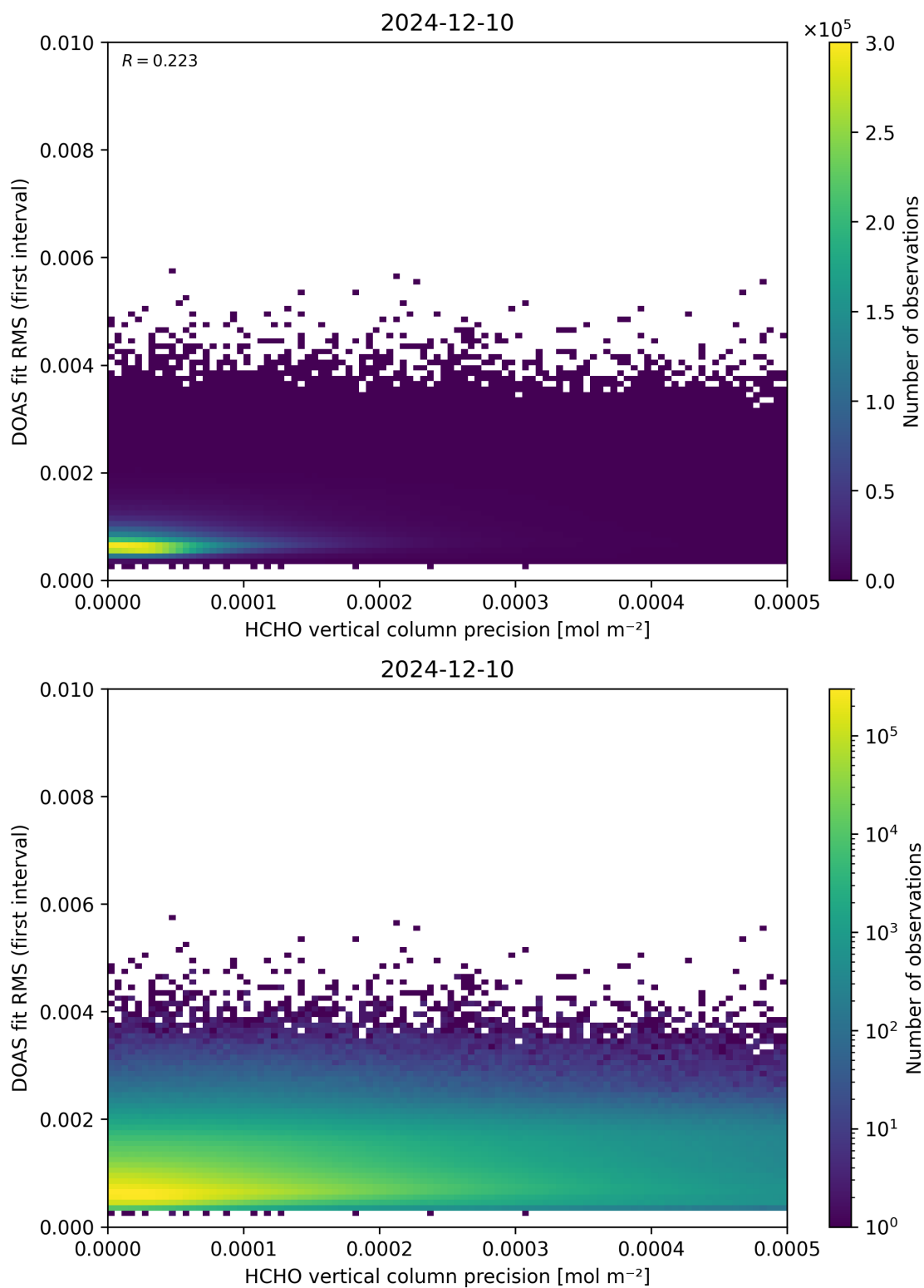
Figure 136: Scatter density plot of “HCHO vertical column precision” against “DOAS fit RMS (first interval)” for 2024-12-09 to 2024-12-11.
