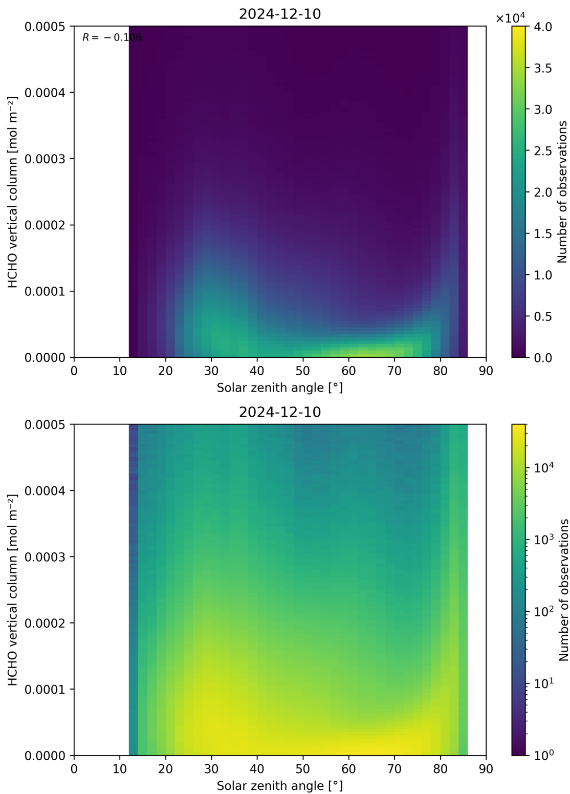
Figure 177: Scatter density plot of “Solar zenith angle” against “HCHO vertical column” for 2024-12-09 to 2024-12-11.
