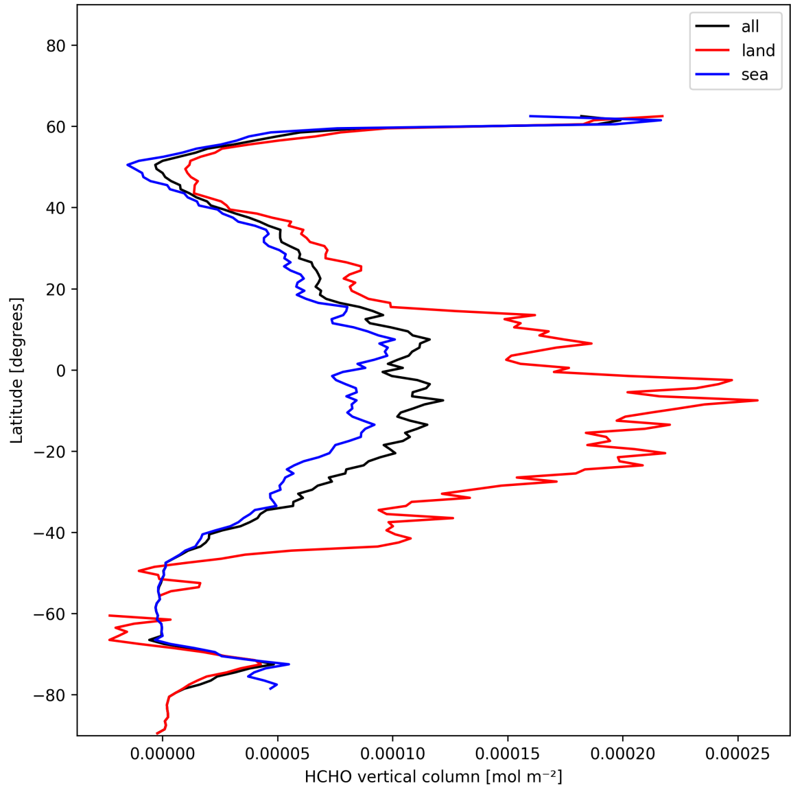
Figure 21: Zonal average of “HCHO vertical column” for 2024-12-09 to 2024-12-11.
