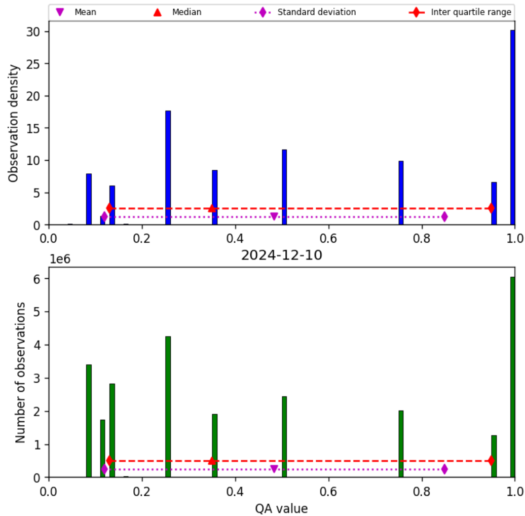
Figure 34: Histogram of “QA value” for 2024-12-09 to 2024-12-11
