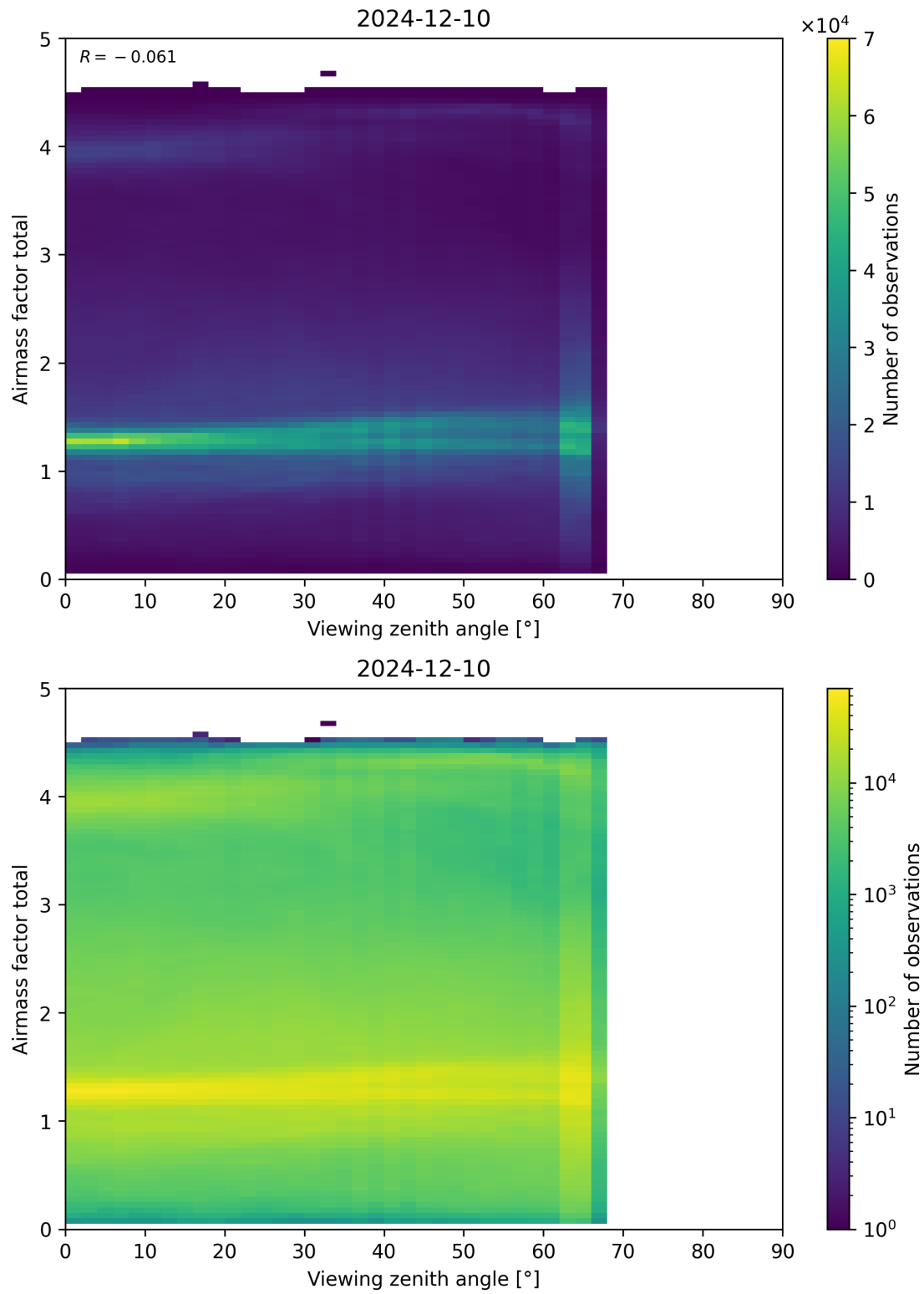
Figure 190: Scatter density plot of “Viewing zenith angle” against “Airmass factor total” for 2024-12-09 to 2024-12-11.
