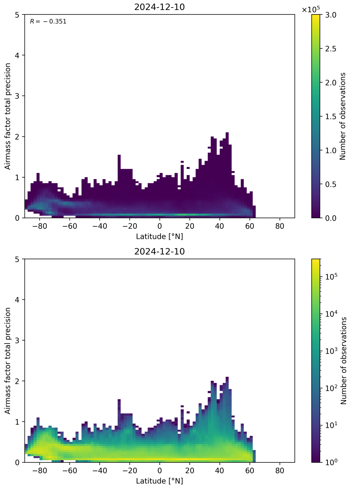
Figure 162: Scatter density plot of “Latitude” against “Airmass factor total precision” for 2024-12-09 to 2024-12-11.
