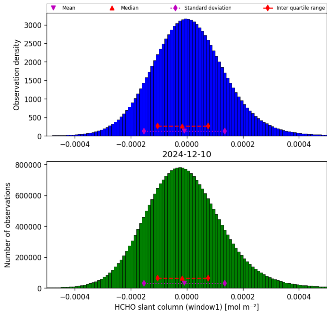
Figure 38: Histogram of “HCHO slant column (window1)” for 2024-12-09 to 2024-12-11
