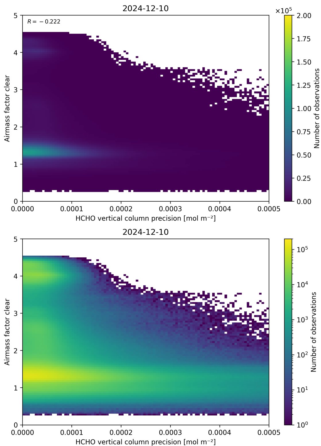
Figure 139: Scatter density plot of “HCHO vertical column precision” against “Airmass factor clear” for 2024-12-09 to 2024-12-11.
