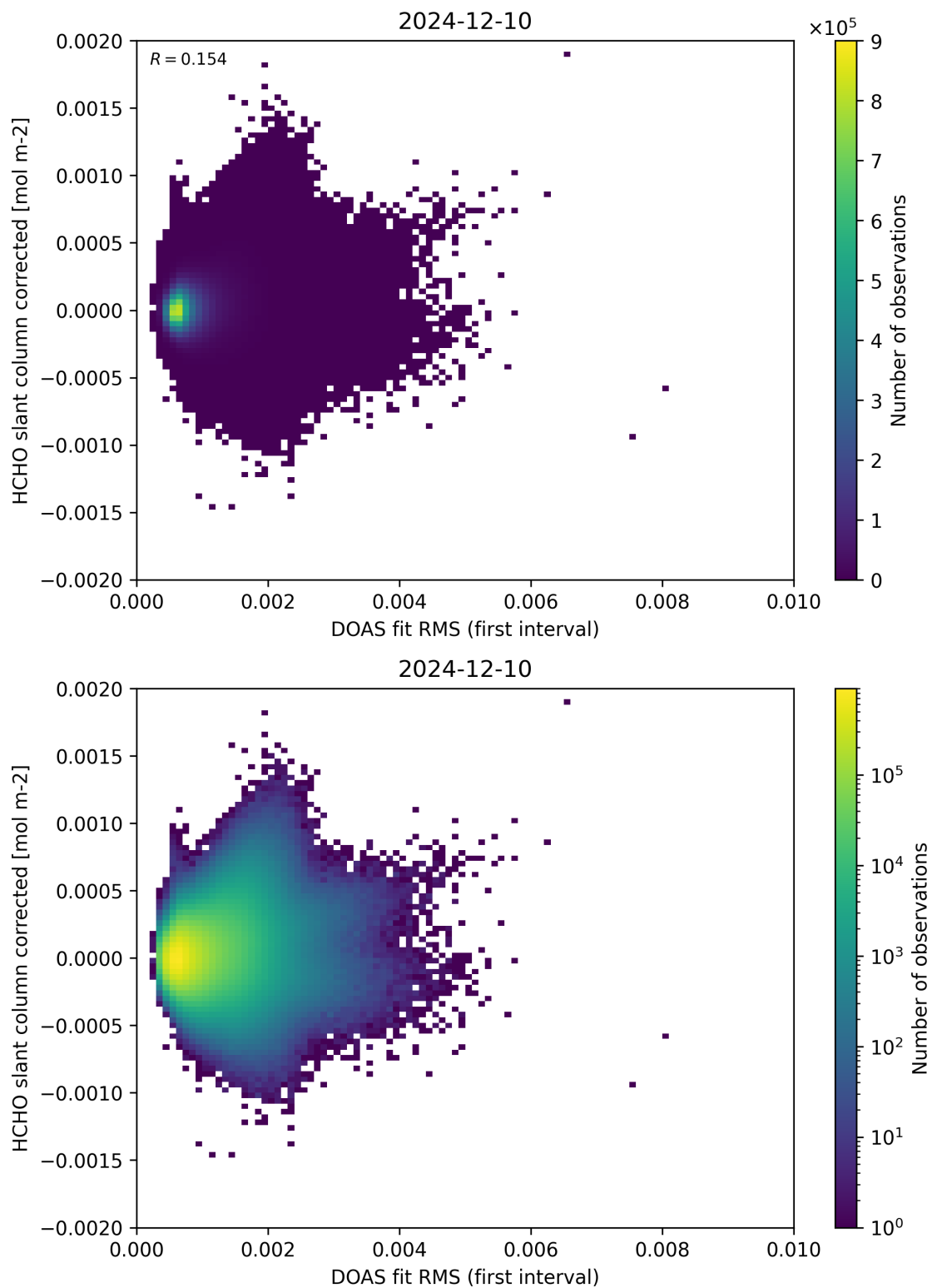
Figure 62: Scatter density plot of “DOAS fit RMS (first interval)” against “HCHO slant column corrected” for 2024-12-09 to 2024-12-11.
