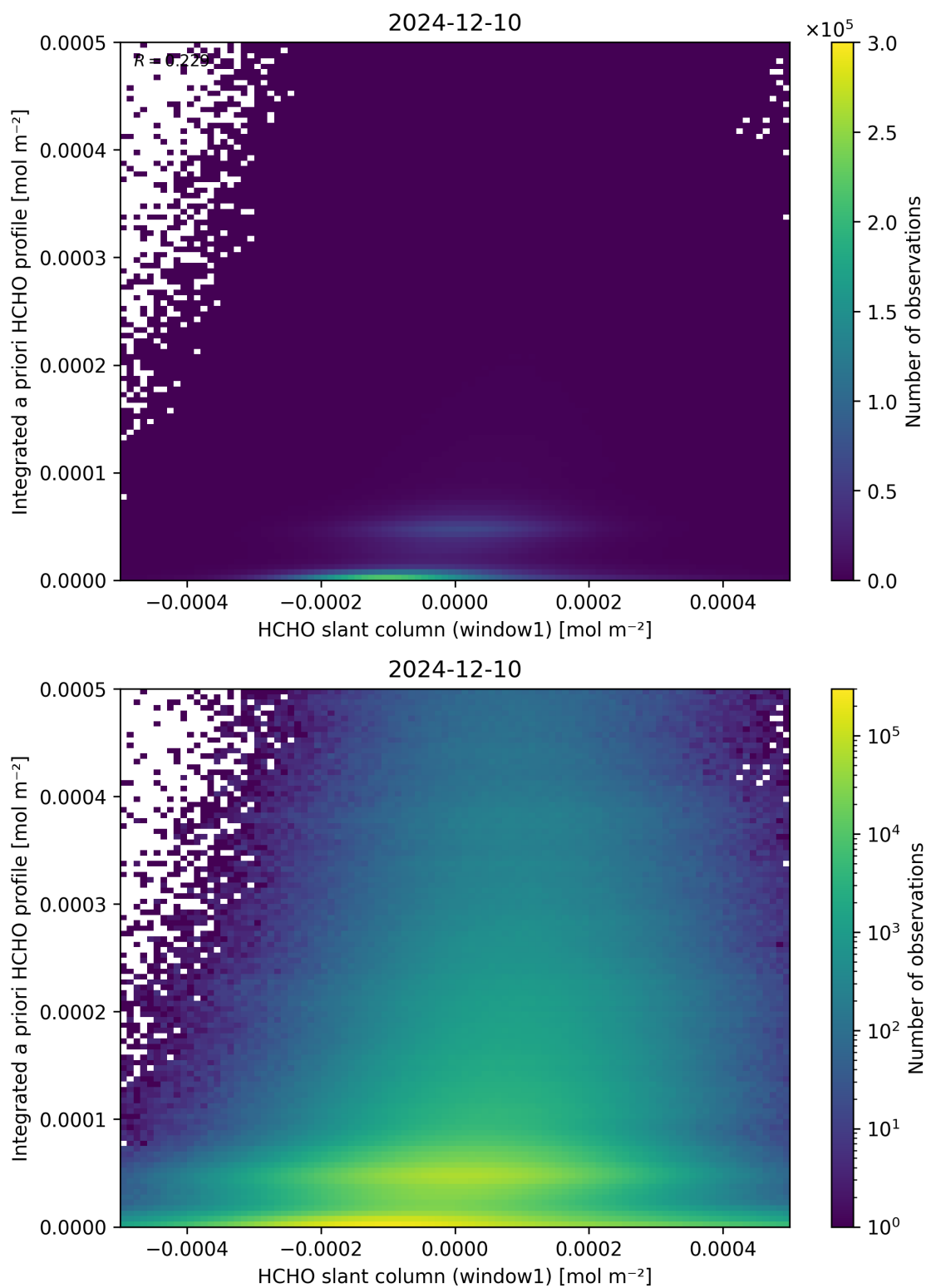
Figure 87: Scatter density plot of “HCHO slant column (window1)” against “Integrated a priori HCHO profile” for 2024-12-09 to 2024-12-11.
