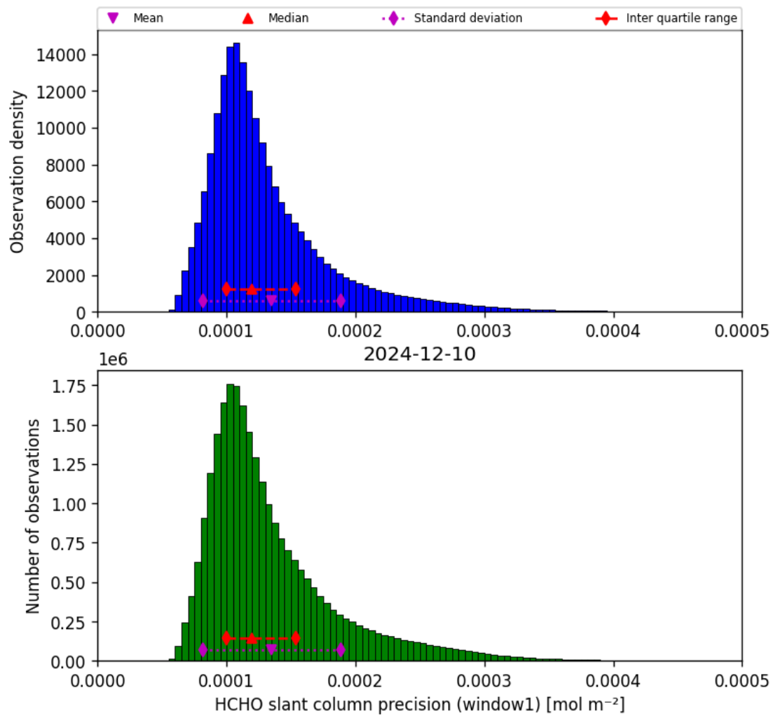
Figure 39: Histogram of “HCHO slant column precision (window1)” for 2024-12-09 to 2024-12-11
