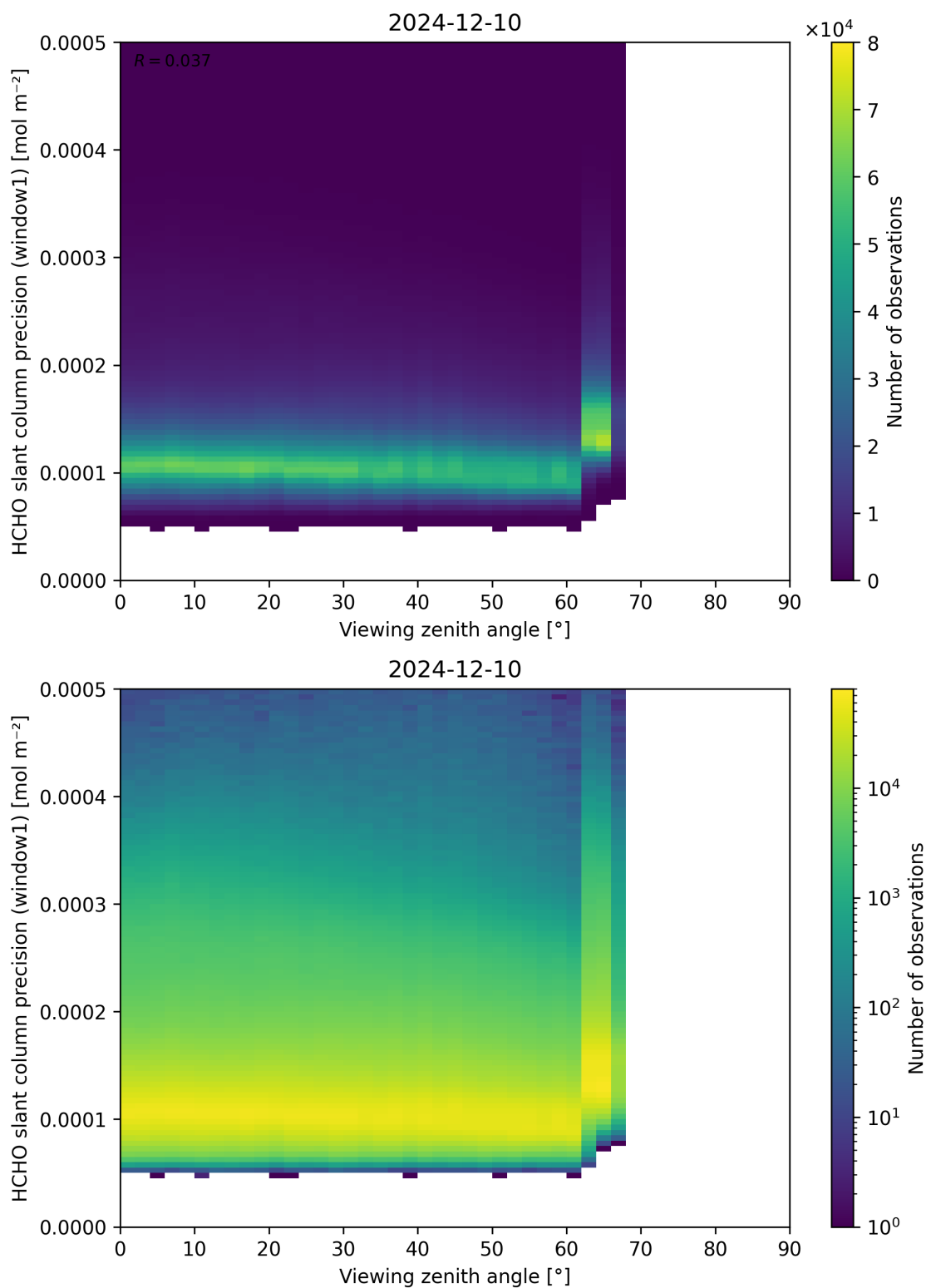
Figure 189: Scatter density plot of “Viewing zenith angle” against “HCHO slant column precision (window1)” for 2024-12-09 to 2024-12-11.
