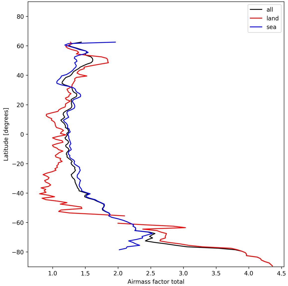
Figure 26: Zonal average of “Airmass factor total” for 2024-12-09 to 2024-12-11.
