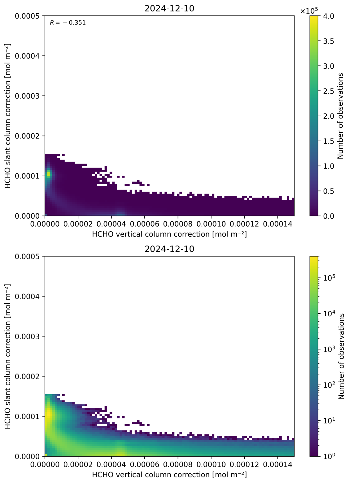
Figure 117: Scatter density plot of “HCHO vertical column correction” against “HCHO slant column correction” for 2024-12-09 to 2024-12-11.
