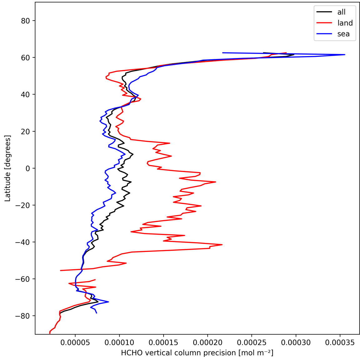
Figure 22: Zonal average of “HCHO vertical column precision” for 2024-12-09 to 2024-12-11.
