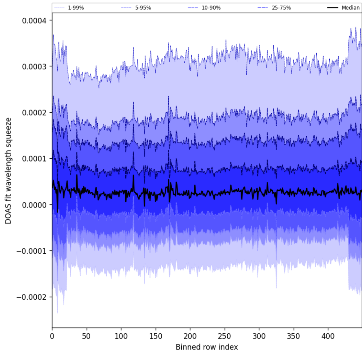
Figure 59: Along track statistics of “DOAS fit wavelength squeeze” for 2024-12-09 to 2024-12-11
