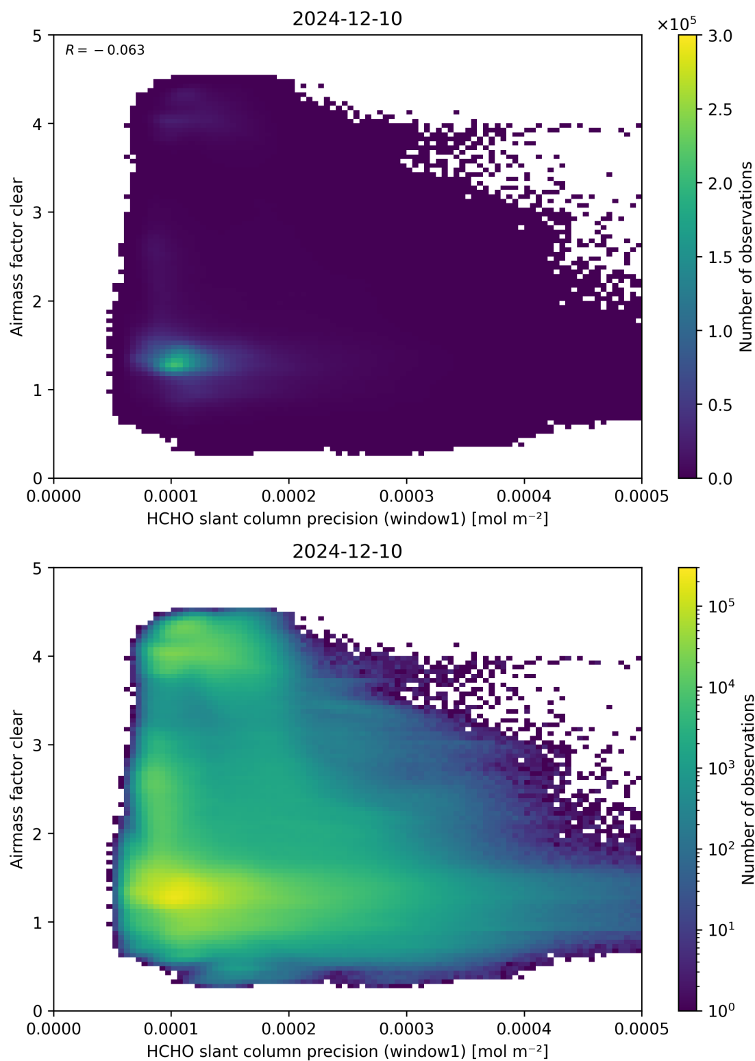
Figure 91: Scatter density plot of “HCHO slant column precision (window1)” against “Airmass factor clear” for 2024-12-09 to 2024-12-11.
