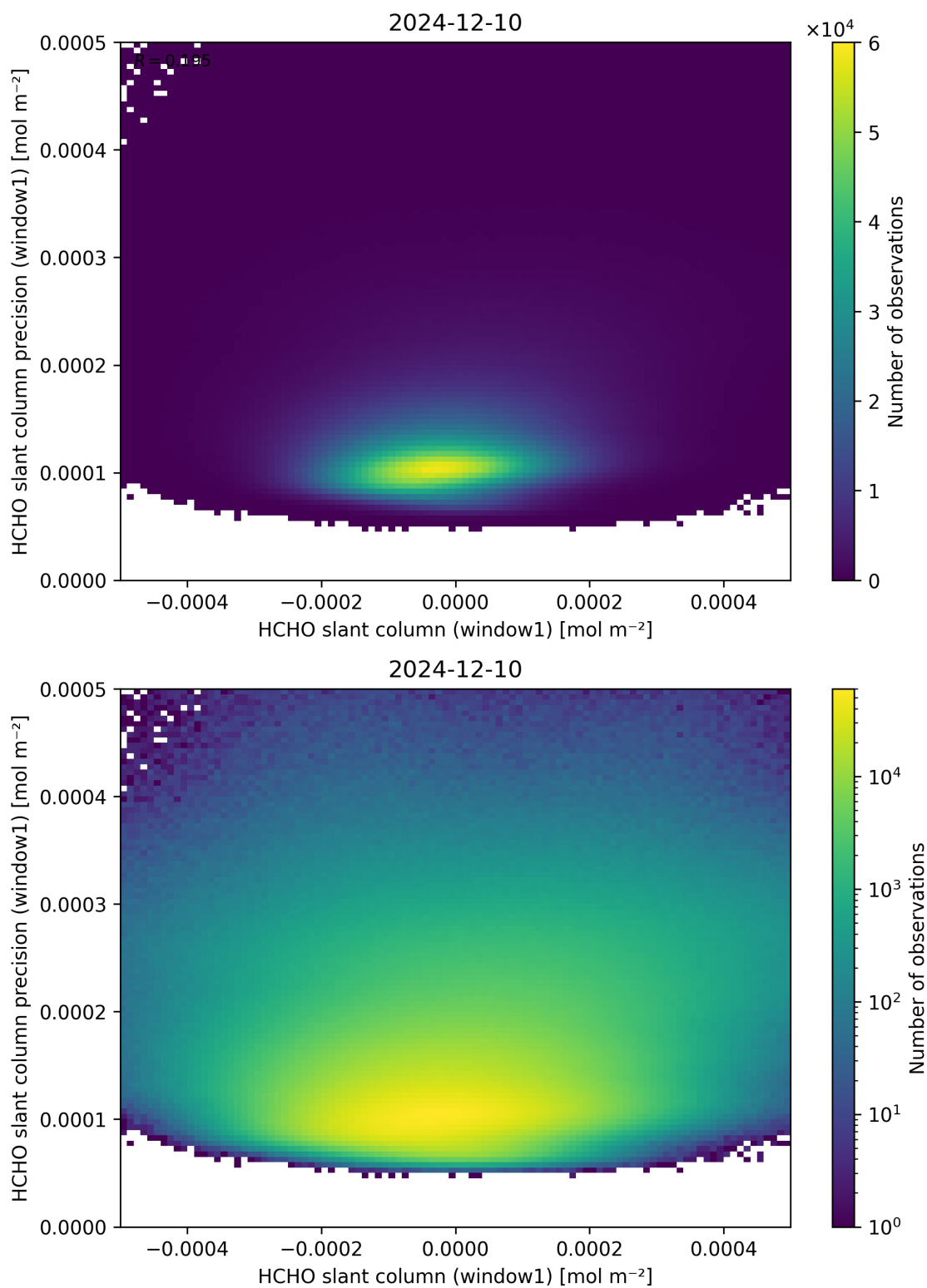
Figure 84: Scatter density plot of “HCHO slant column (window1)” against “HCHO slant column precision (window1)” for 2024-12-09 to 2024-12-11.
