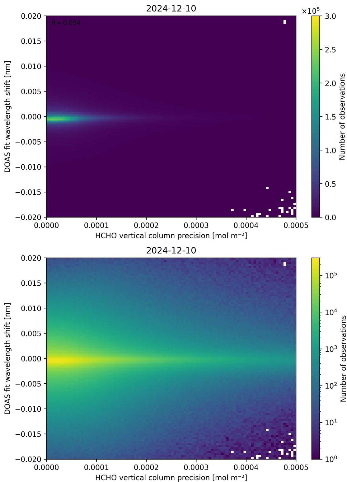
Figure 137: Scatter density plot of “HCHO vertical column precision” against “DOAS fit wavelength shift” for 2024-12-09 to 2024-12-11.
