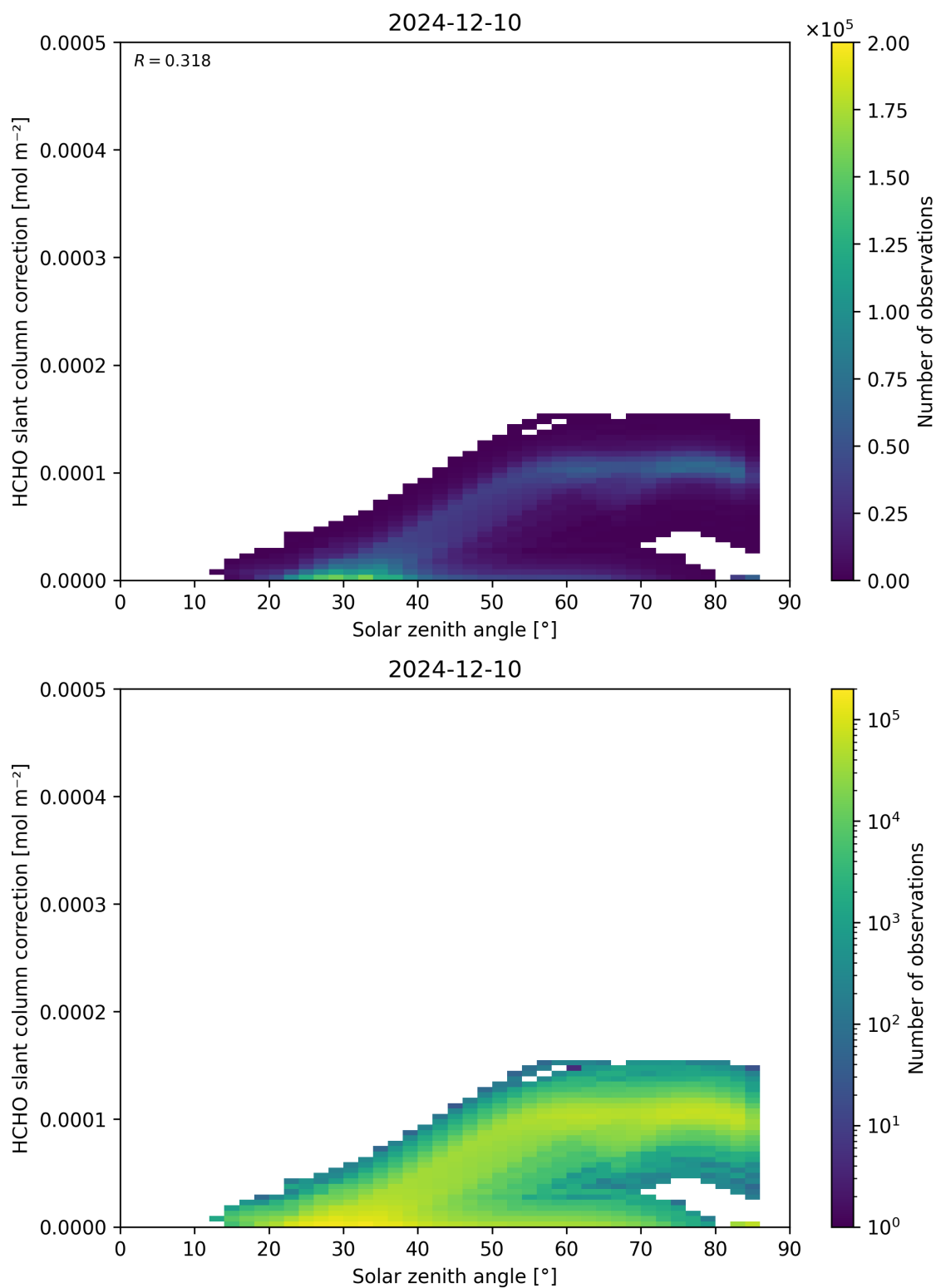
Figure 172: Scatter density plot of “Solar zenith angle” against “HCHO slant column correction” for 2024-12-09 to 2024-12-11.
