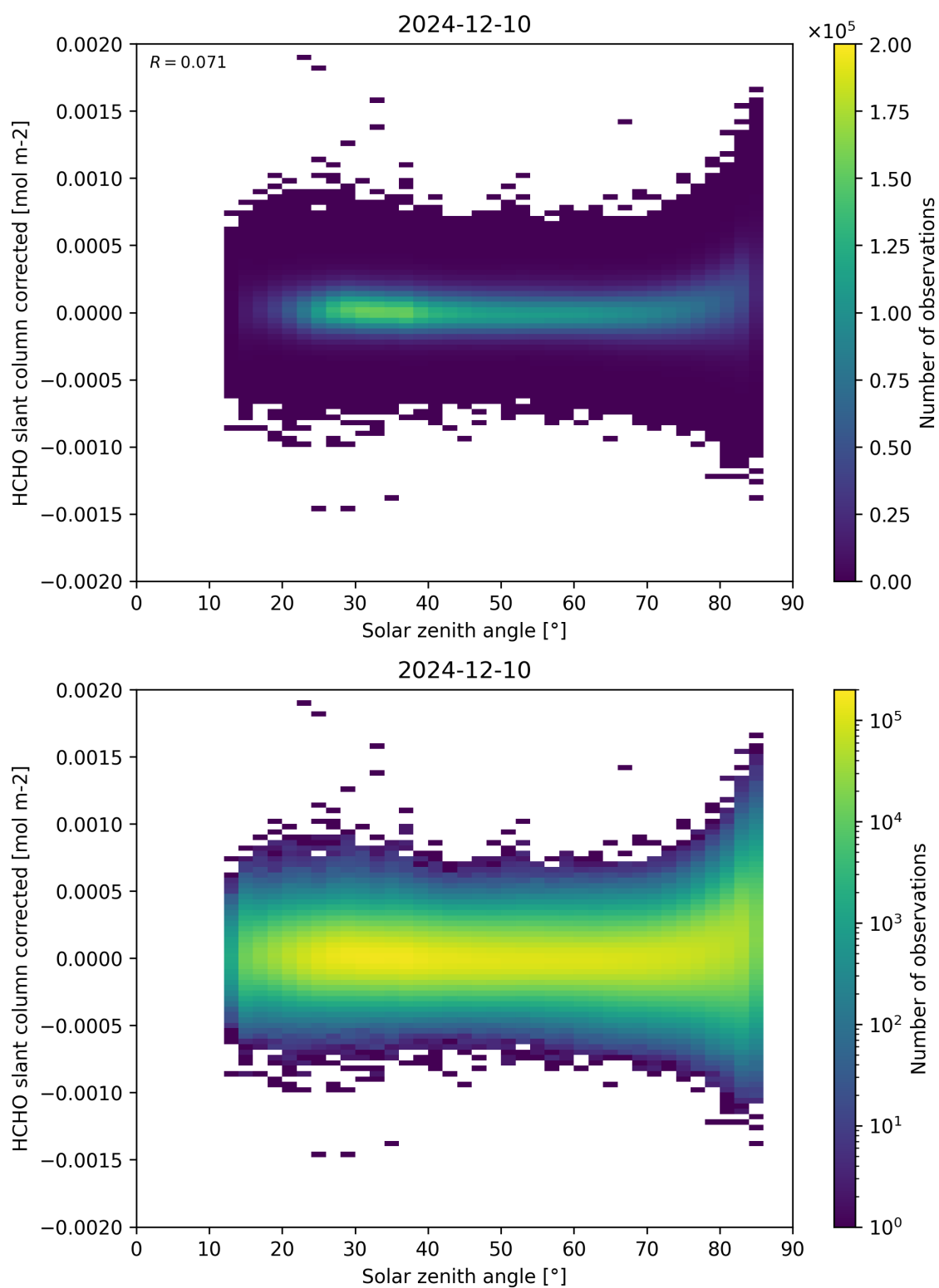
Figure 171: Scatter density plot of “Solar zenith angle” against “HCHO slant column corrected” for 2024-12-09 to 2024-12-11.
