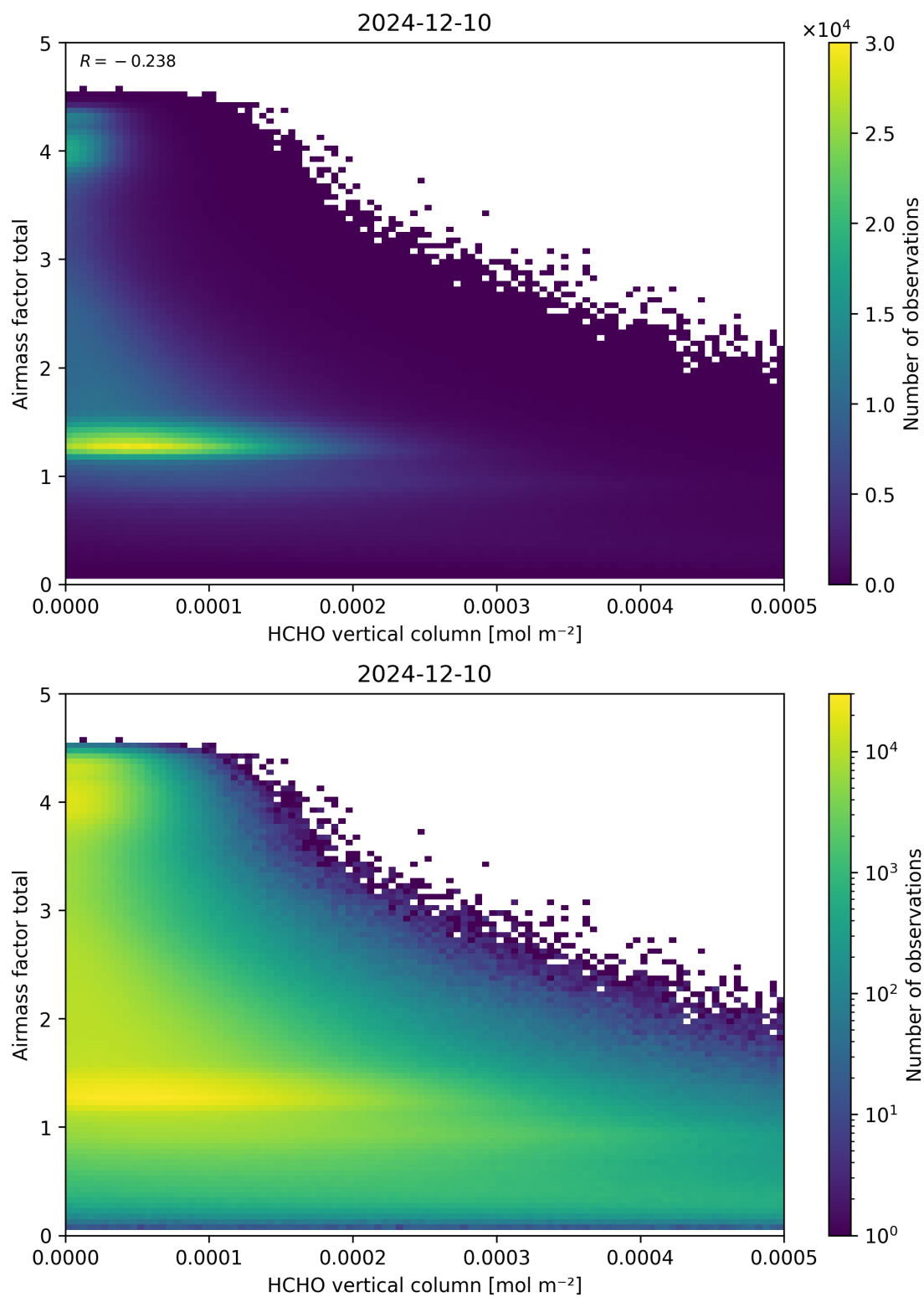
Figure 131: Scatter density plot of “HCHO vertical column” against “Airmass factor total” for 2024-12-09 to 2024-12-11.
