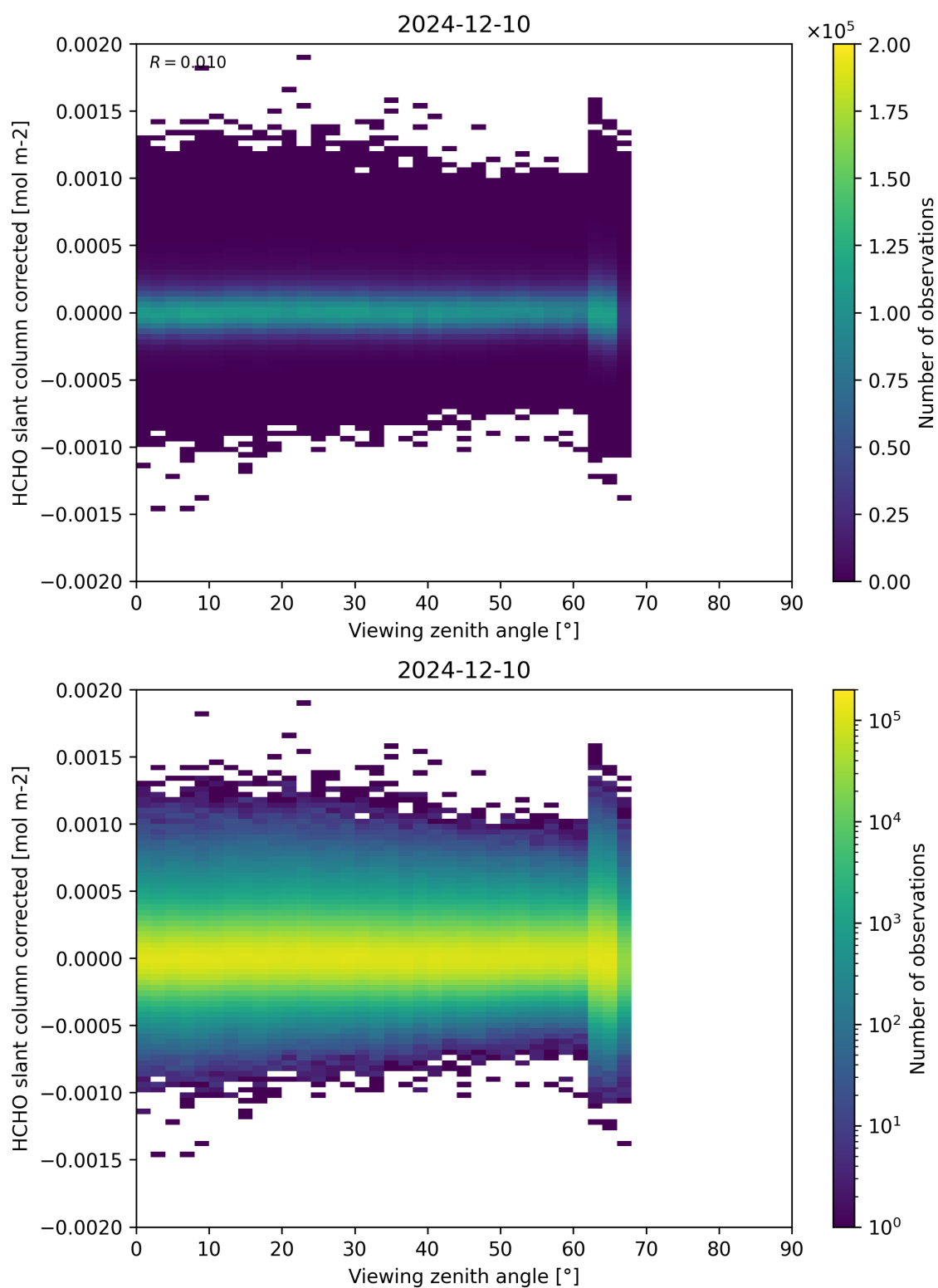
Figure 186: Scatter density plot of “Viewing zenith angle” against “HCHO slant column corrected” for 2024-12-09 to 2024-12-11.
