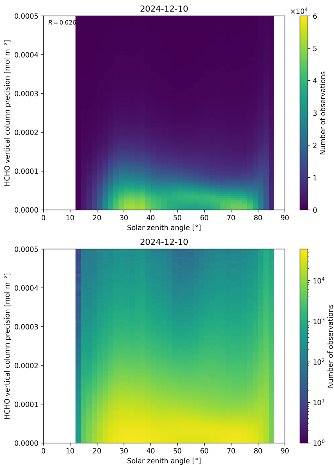
Figure 179: Scatter density plot of “Solar zenith angle” against “HCHO vertical column precision” for 2024-12-09 to 2024-12-11.
