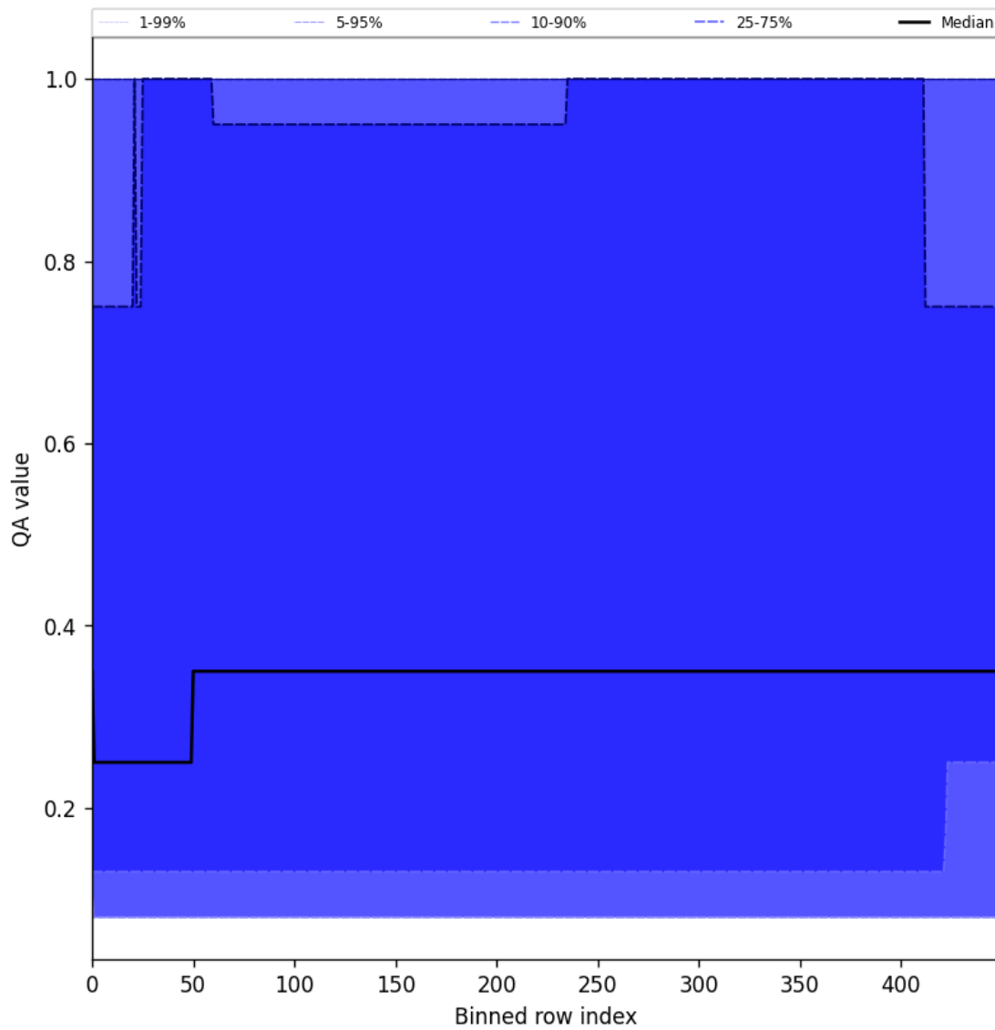
Figure 48: Along track statistics of “QA value” for 2024-12-09 to 2024-12-11
