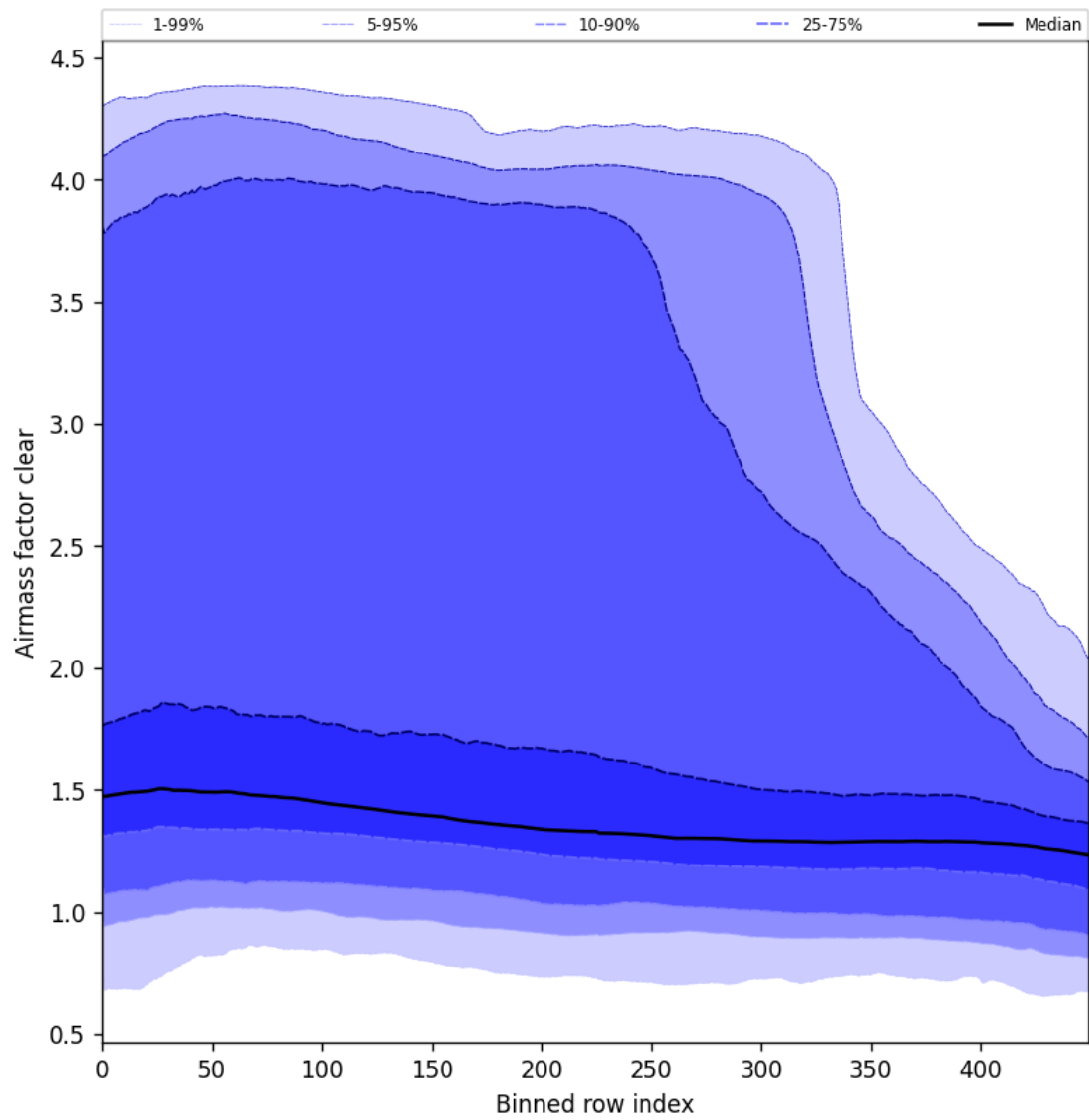
Figure 56: Along track statistics of “Airmass factor clear” for 2024-12-09 to 2024-12-11
