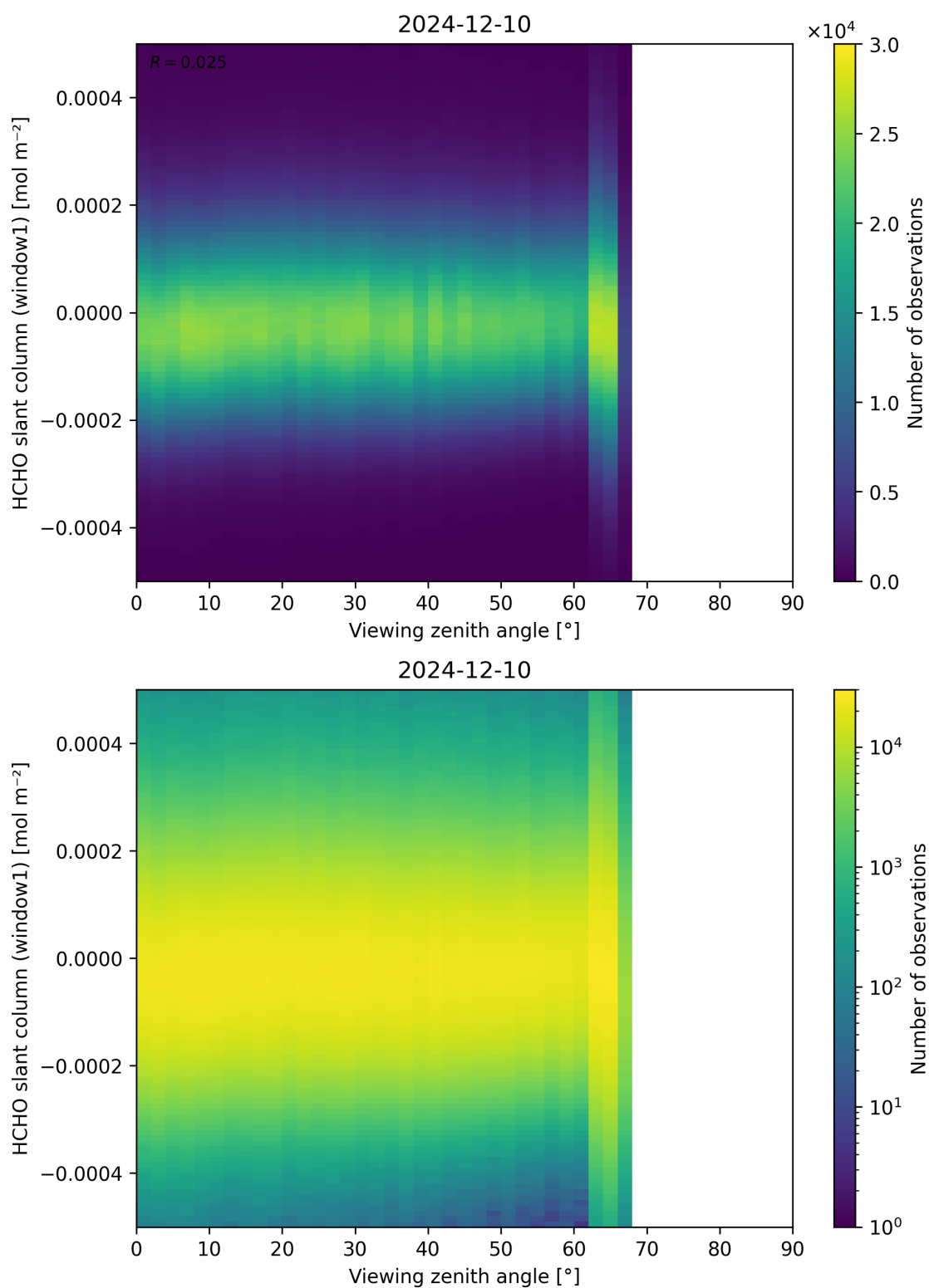
Figure 188: Scatter density plot of “Viewing zenith angle” against “HCHO slant column (window1)” for 2024-12-09 to 2024-12-11.
