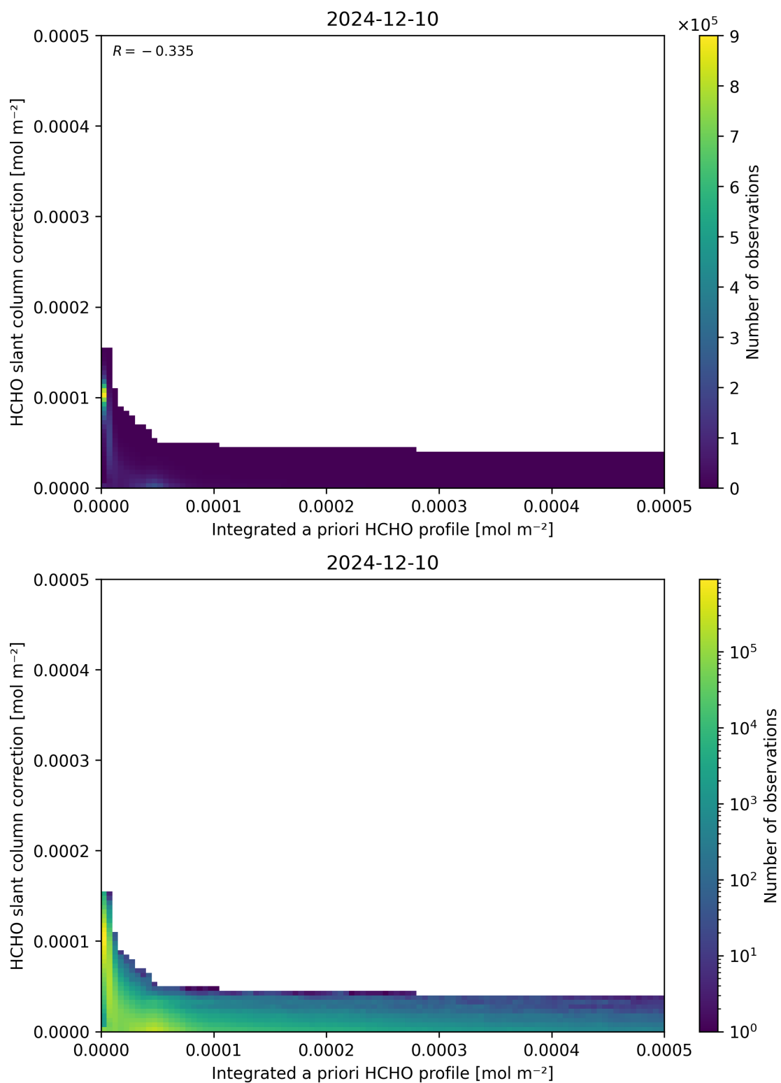
Figure 152: Scatter density plot of “Integrated a priori HCHO profile” against “HCHO slant column correction” for 2024-12-09 to 2024-12-11.
