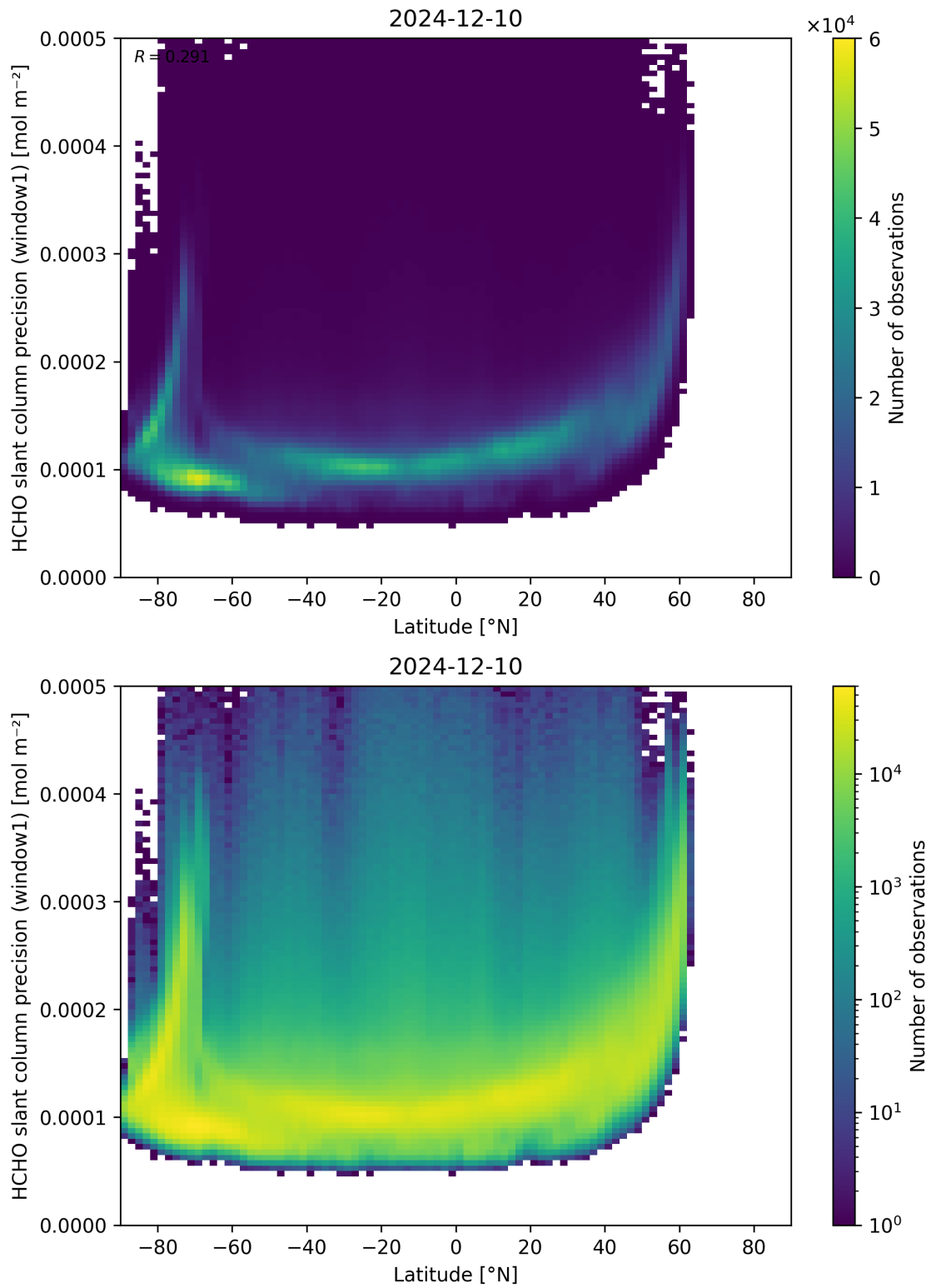
Figure 160: Scatter density plot of “Latitude” against “HCHO slant column precision (window1)” for 2024-12-09 to 2024-12-11.
