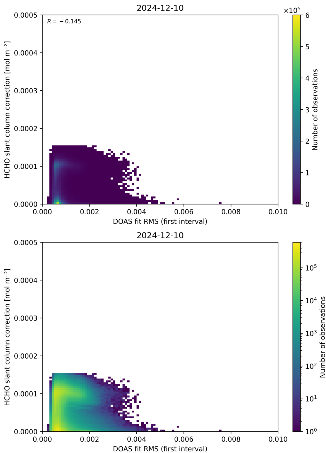
Figure 63: Scatter density plot of “DOAS fit RMS (first interval)” against “HCHO slant column correction” for 2024-12-09 to 2024-12-11.
