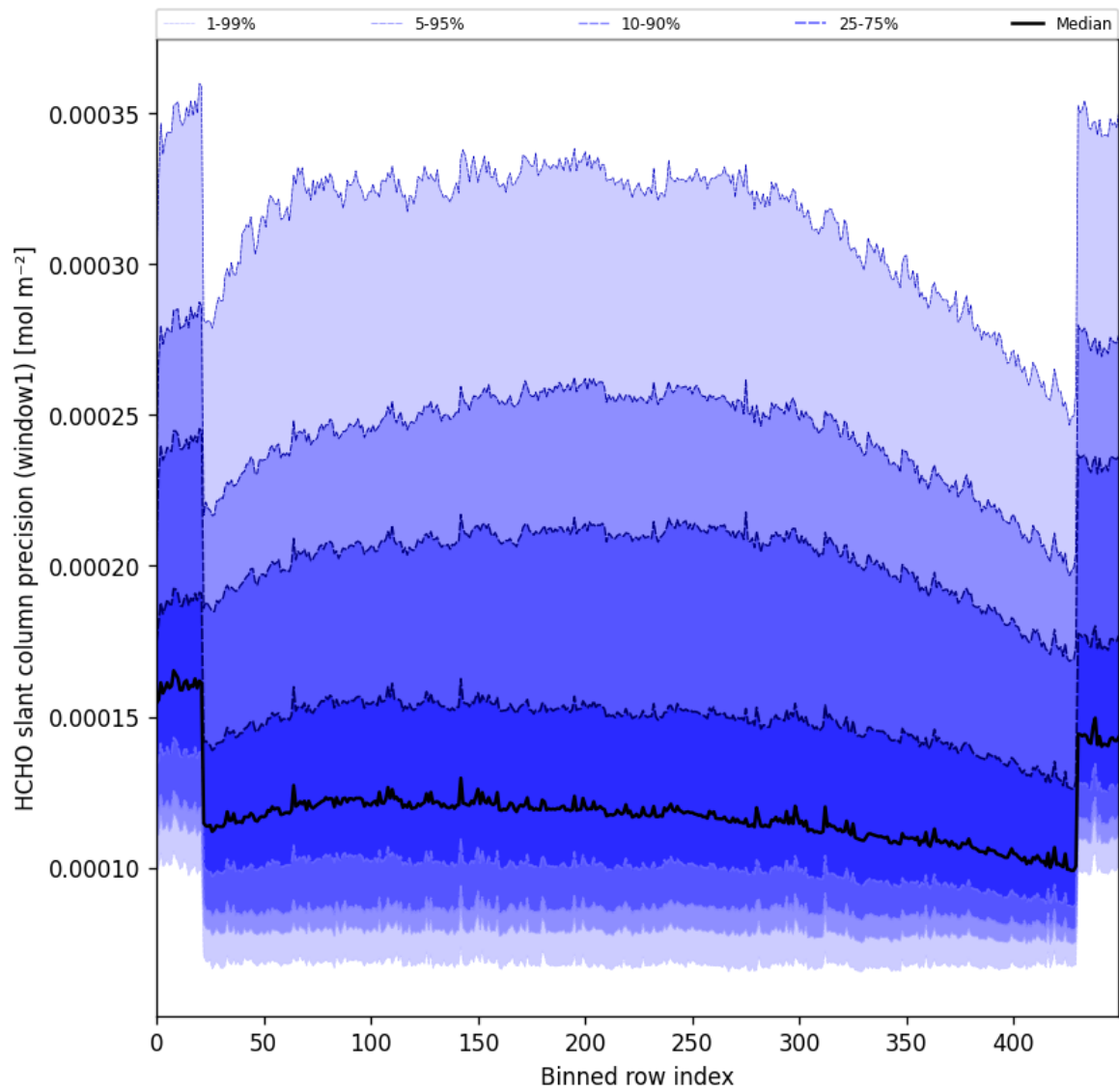
Figure 53: Along track statistics of “HCHO slant column precision (window1)” for 2024-12-09 to 2024-12-11
