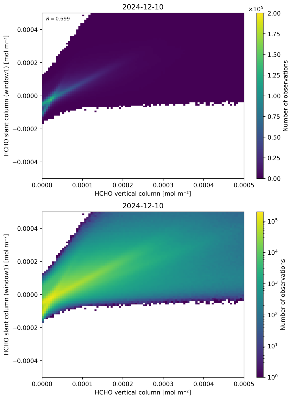
Figure 129: Scatter density plot of “HCHO vertical column” against “HCHO slant column (window1)” for 2024-12-09 to 2024-12-11.
