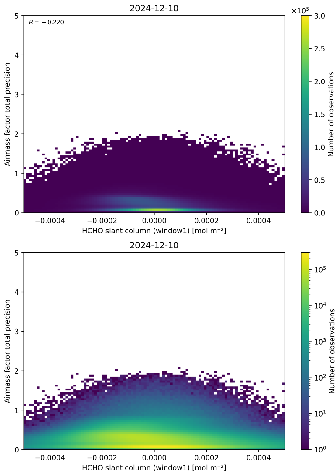
Figure 86: Scatter density plot of “HCHO slant column (window1)” against “Airmass factor total precision” for 2024-12-09 to 2024-12-11.
