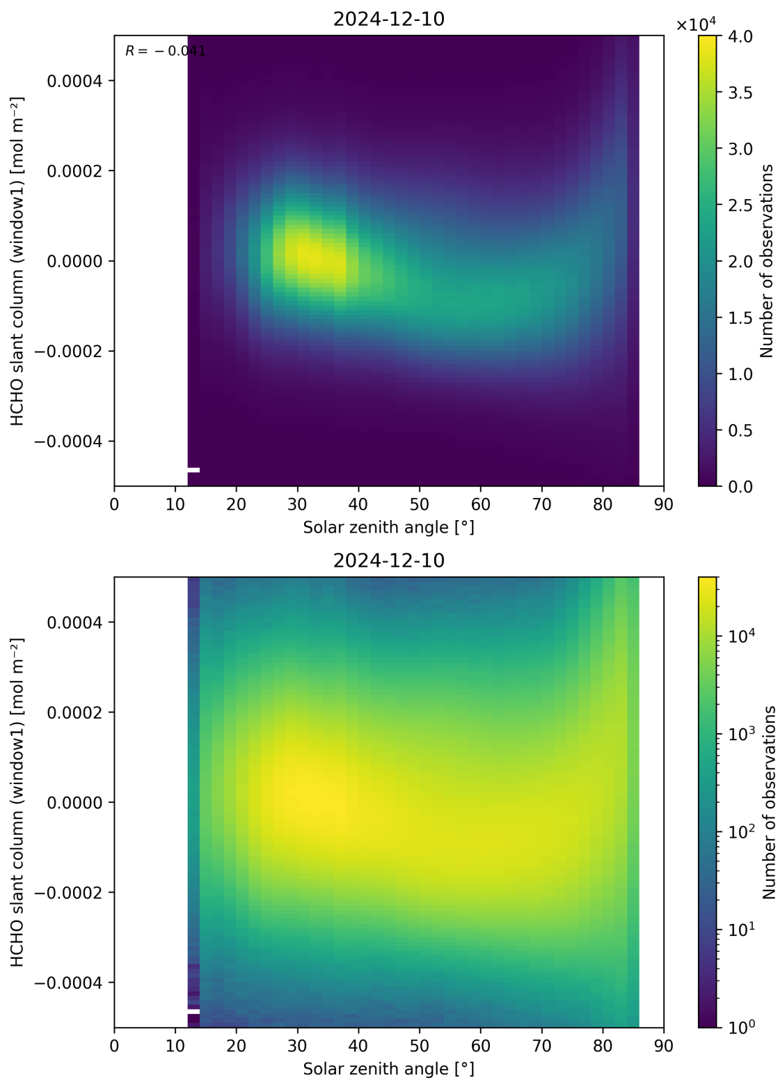
Figure 173: Scatter density plot of “Solar zenith angle” against “HCHO slant column (window1)” for 2024-12-09 to 2024-12-11.
