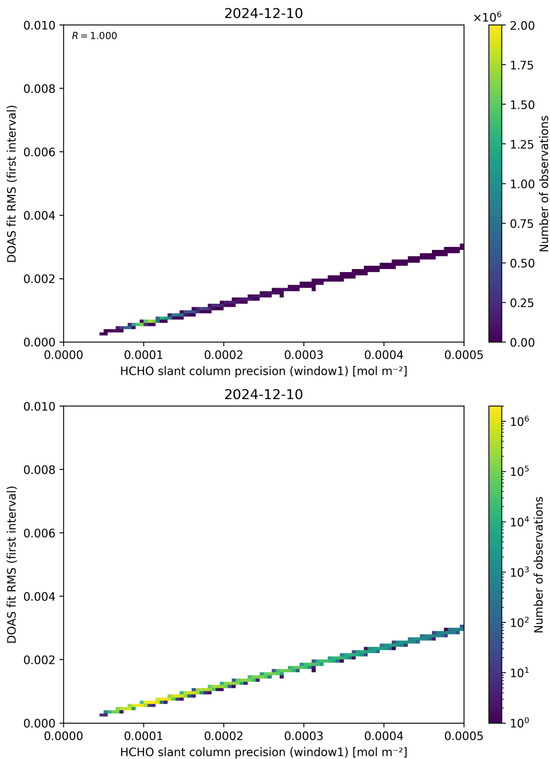
Figure 88: Scatter density plot of “HCHO slant column precision (window1)” against “DOAS fit RMS (first interval)” for 2024-12-09 to 2024-12-11.
