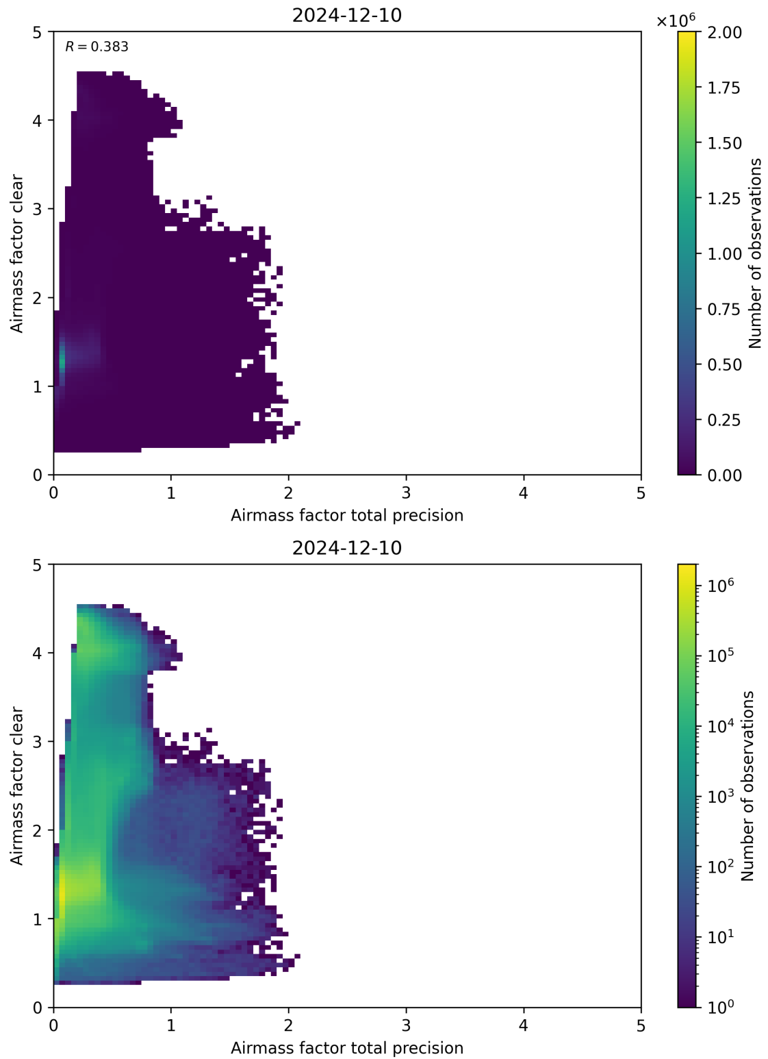
Figure 108: Scatter density plot of “Airmass factor total precision” against “Airmass factor clear” for 2024-12-09 to 2024-12-11.
