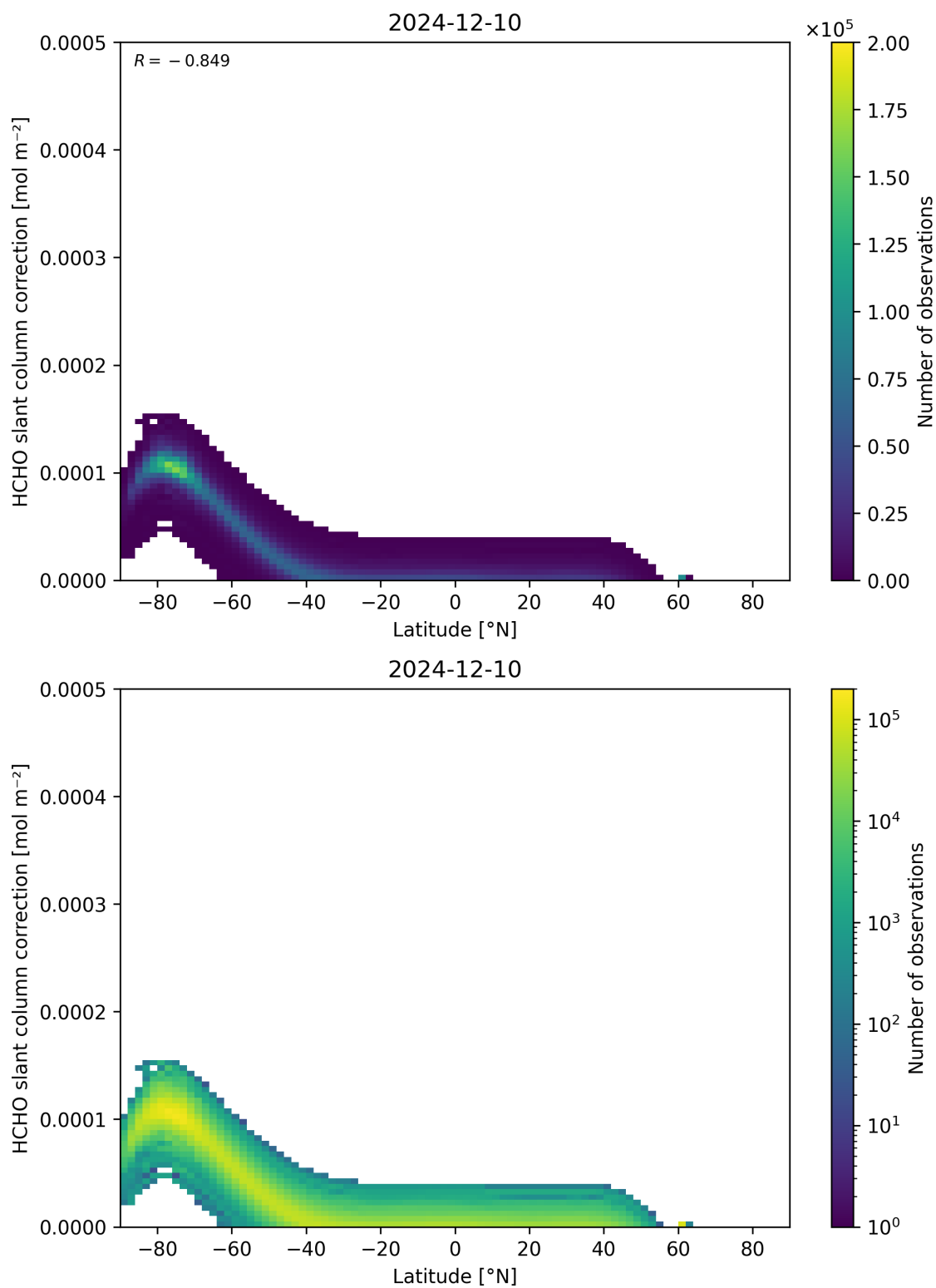
Figure 158: Scatter density plot of “Latitude” against “HCHO slant column correction” for 2024-12-09 to 2024-12-11.
