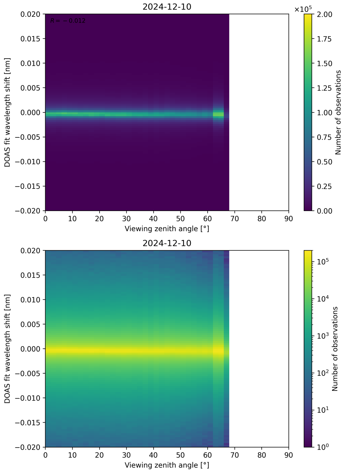
Figure 183: Scatter density plot of “Viewing zenith angle” against “DOAS fit wavelength shift” for 2024-12-09 to 2024-12-11.
