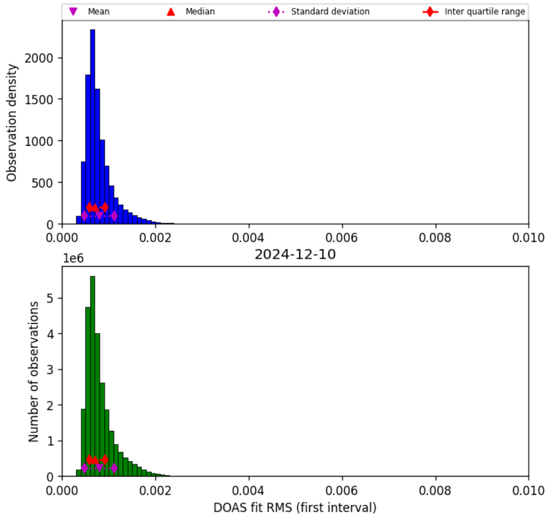
Figure 46: Histogram of “DOAS fit RMS (first interval)” for 2024-12-09 to 2024-12-11
