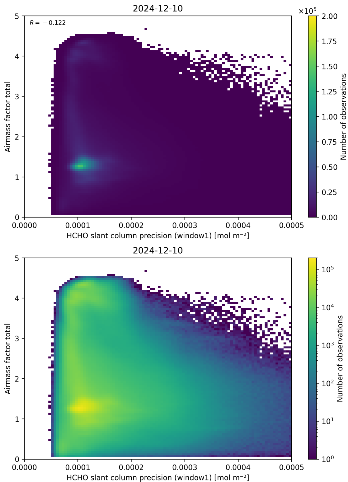
Figure 94: Scatter density plot of “HCHO slant column precision (window1)” against “Airmass factor total” for 2024-12-09 to 2024-12-11.
