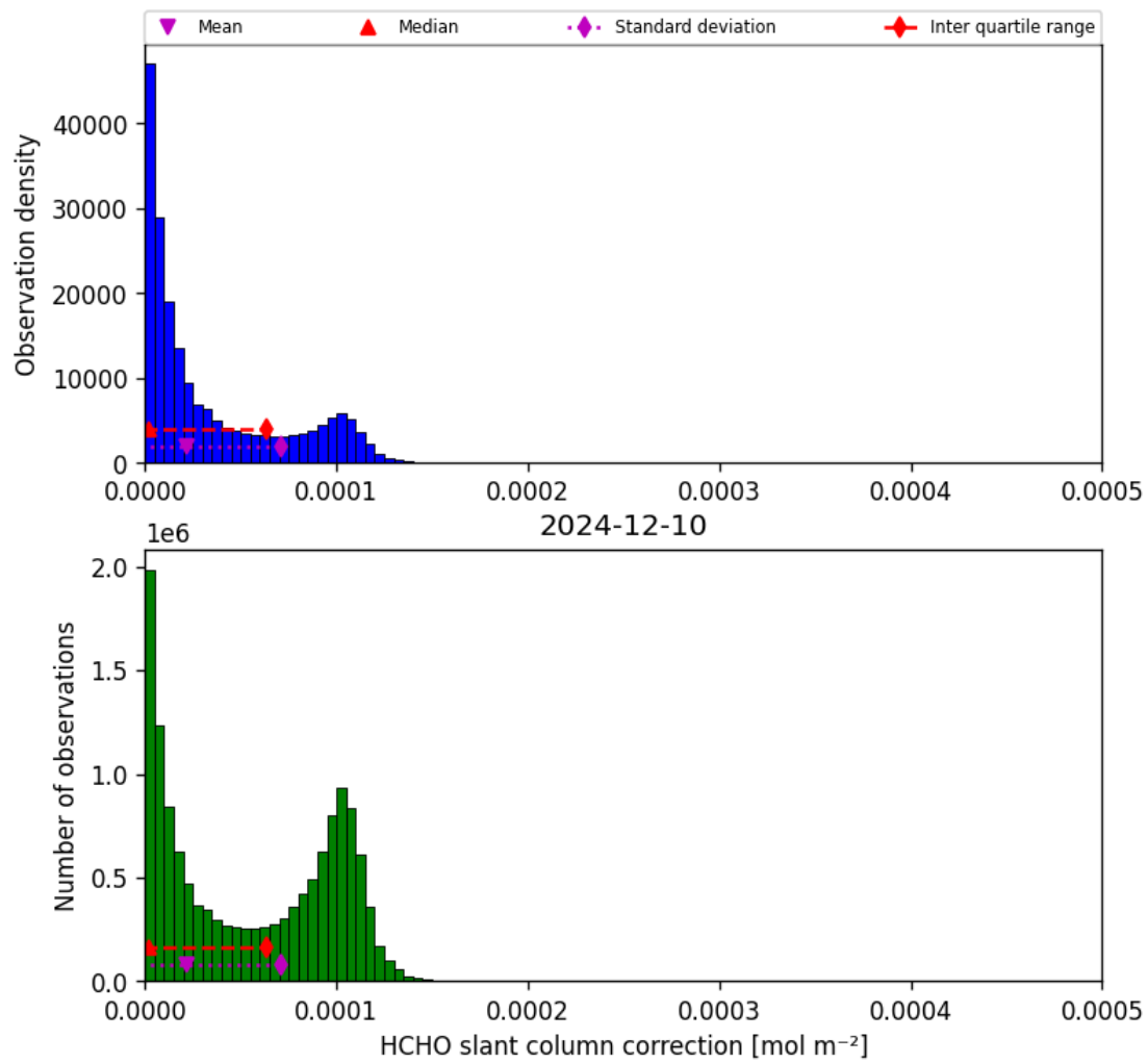
Figure 47: Histogram of “HCHO slant column correction” for 2024-12-09 to 2024-12-11
