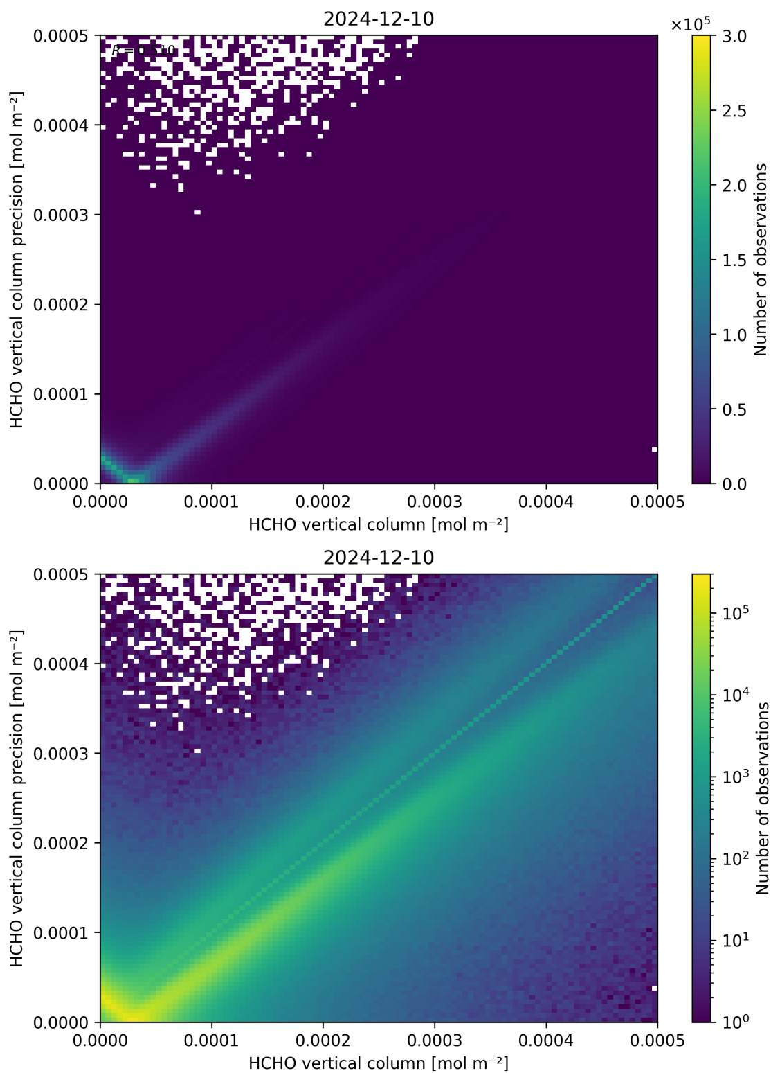
Figure 134: Scatter density plot of “HCHO vertical column” against “HCHO vertical column precision” for 2024-12-09 to 2024-12-11.
