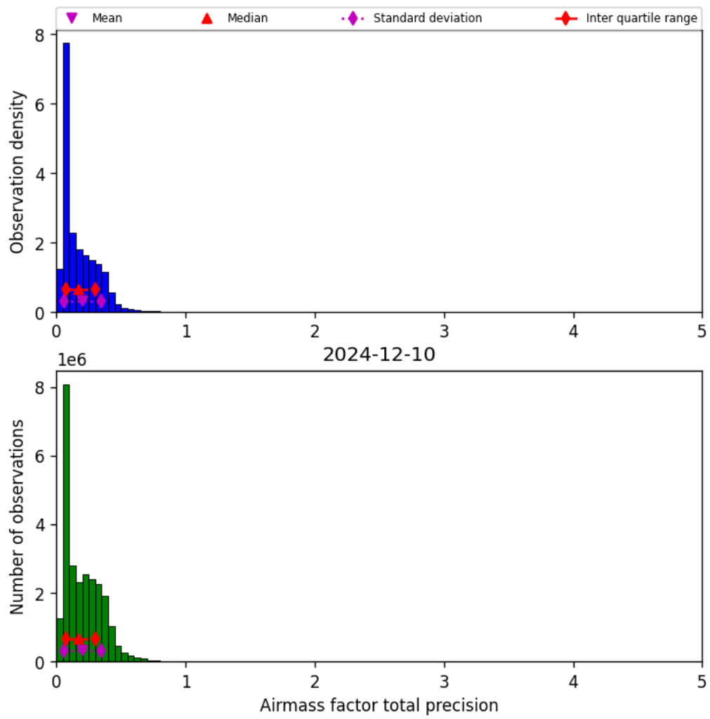
Figure 41: Histogram of “Airmass factor total precision” for 2024-12-09 to 2024-12-11
