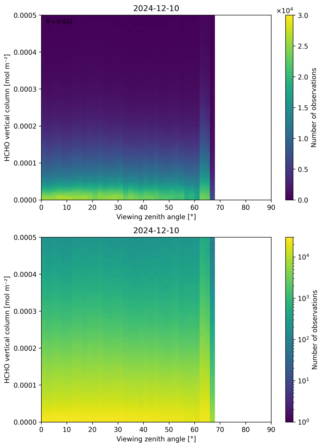
Figure 192: Scatter density plot of “Viewing zenith angle” against “HCHO vertical column” for 2024-12-09 to 2024-12-11.
