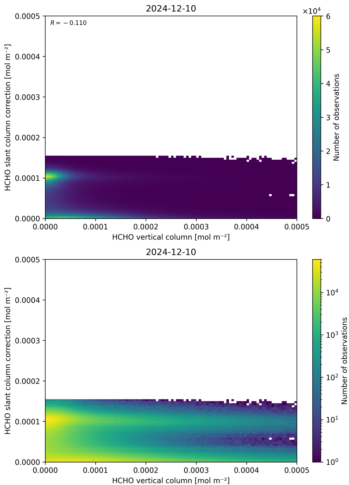
Figure 128: Scatter density plot of “HCHO vertical column” against “HCHO slant column correction” for 2024-12-09 to 2024-12-11.
