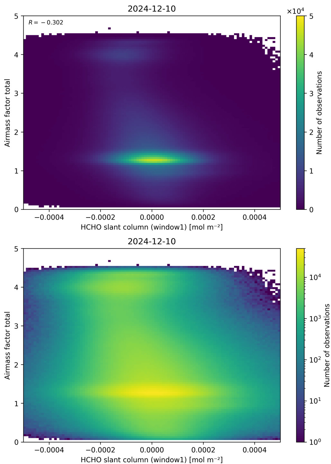
Figure 85: Scatter density plot of “HCHO slant column (window1)” against “Airmass factor total” for 2024-12-09 to 2024-12-11.
