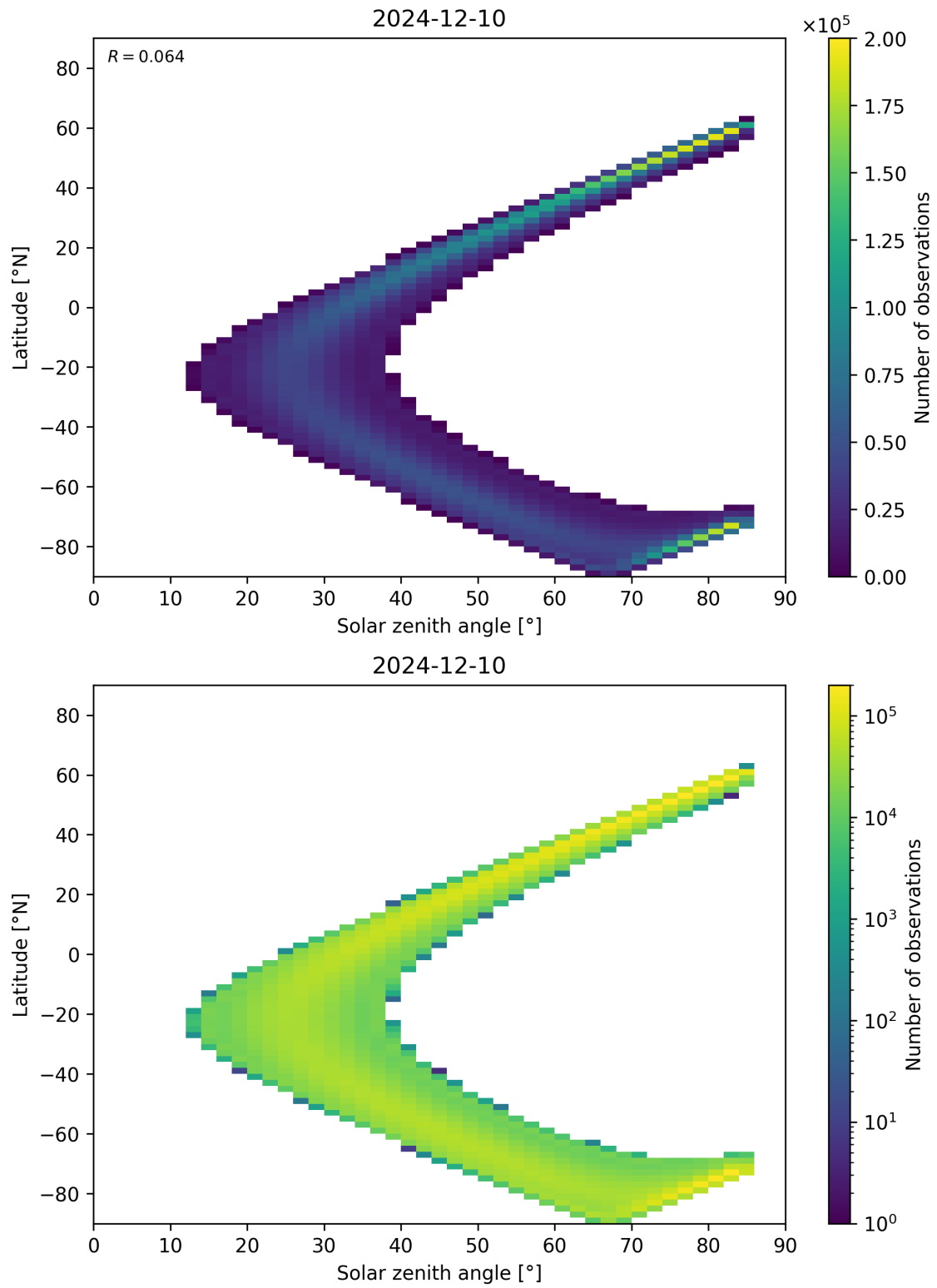
Figure 181: Scatter density plot of “Solar zenith angle” against “Latitude” for 2024-12-09 to 2024-12-11.
