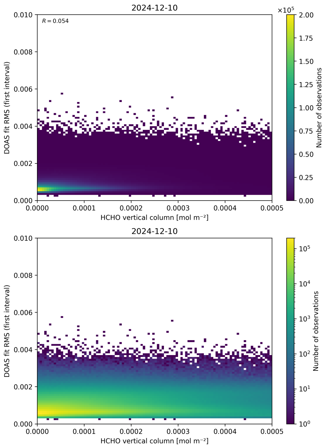
Figure 123: Scatter density plot of “HCHO vertical column” against “DOAS fit RMS (first interval)” for 2024-12-09 to 2024-12-11.
