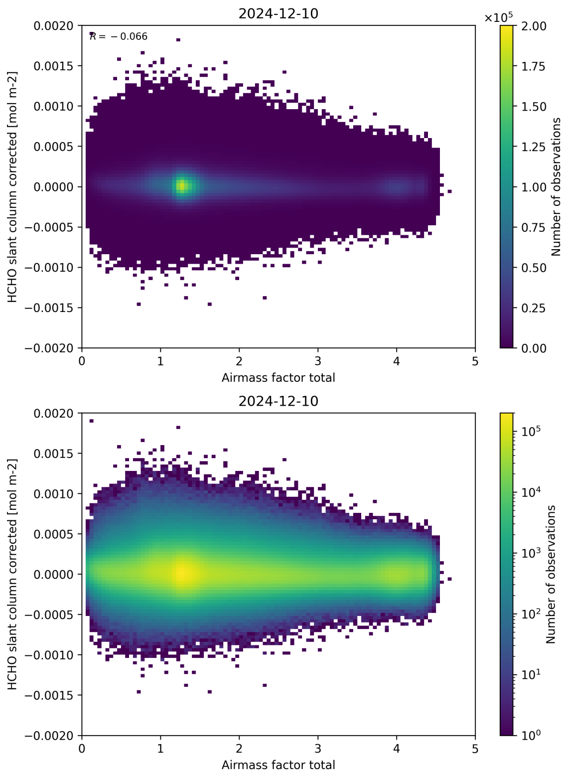
Figure 101: Scatter density plot of “Airmass factor total” against “HCHO slant column corrected” for 2024-12-09 to 2024-12-11.
