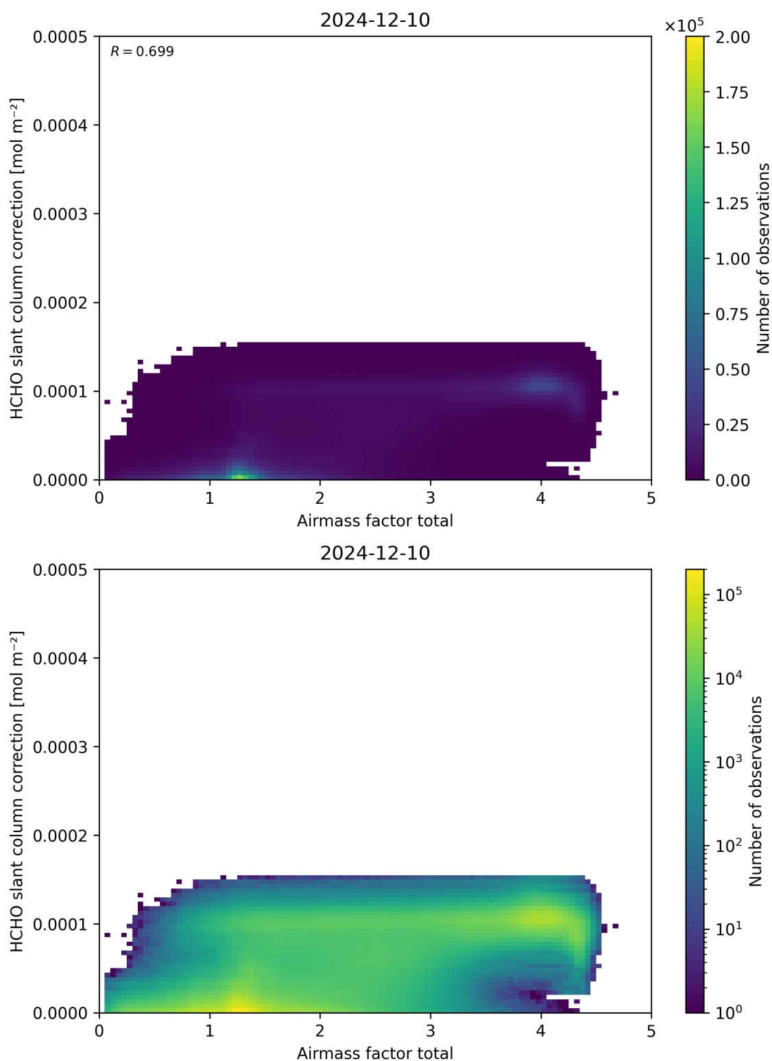
Figure 102: Scatter density plot of “Airmass factor total” against “HCHO slant column correction” for 2024-12-09 to 2024-12-11.
