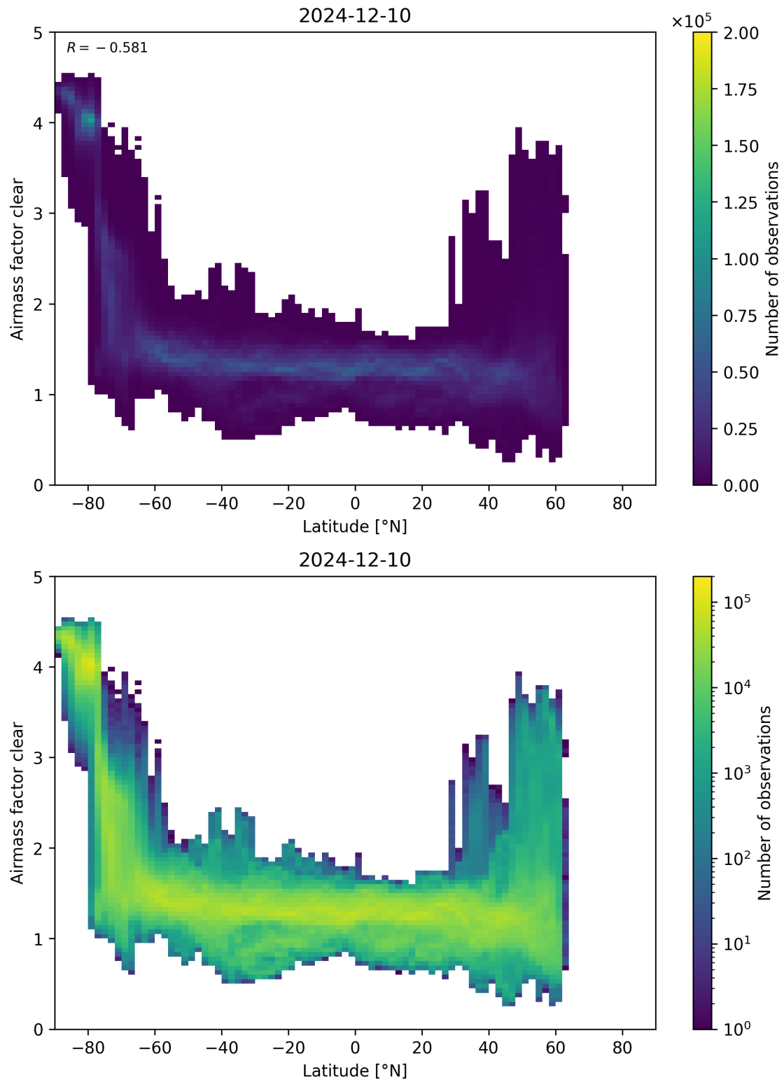
Figure 156: Scatter density plot of “Latitude” against “Airmass factor clear” for 2024-12-09 to 2024-12-11.
