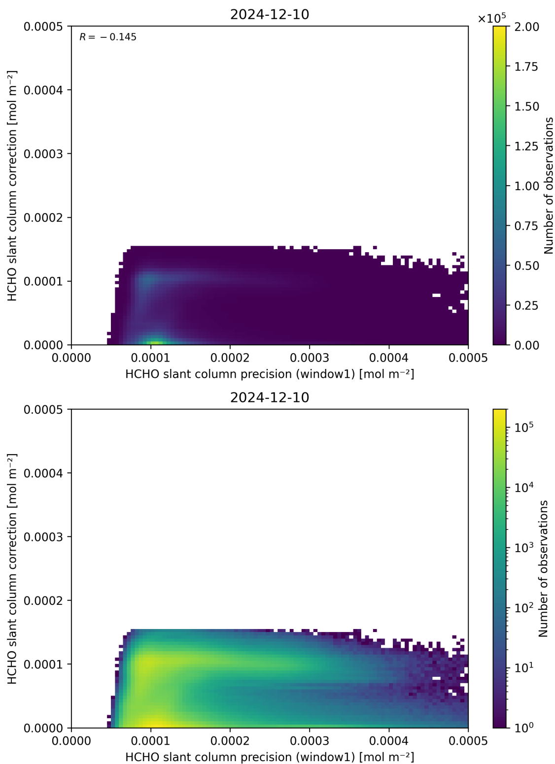
Figure 93: Scatter density plot of “HCHO slant column precision (window1)” against “HCHO slant column correction” for 2024-12-09 to 2024-12-11.
