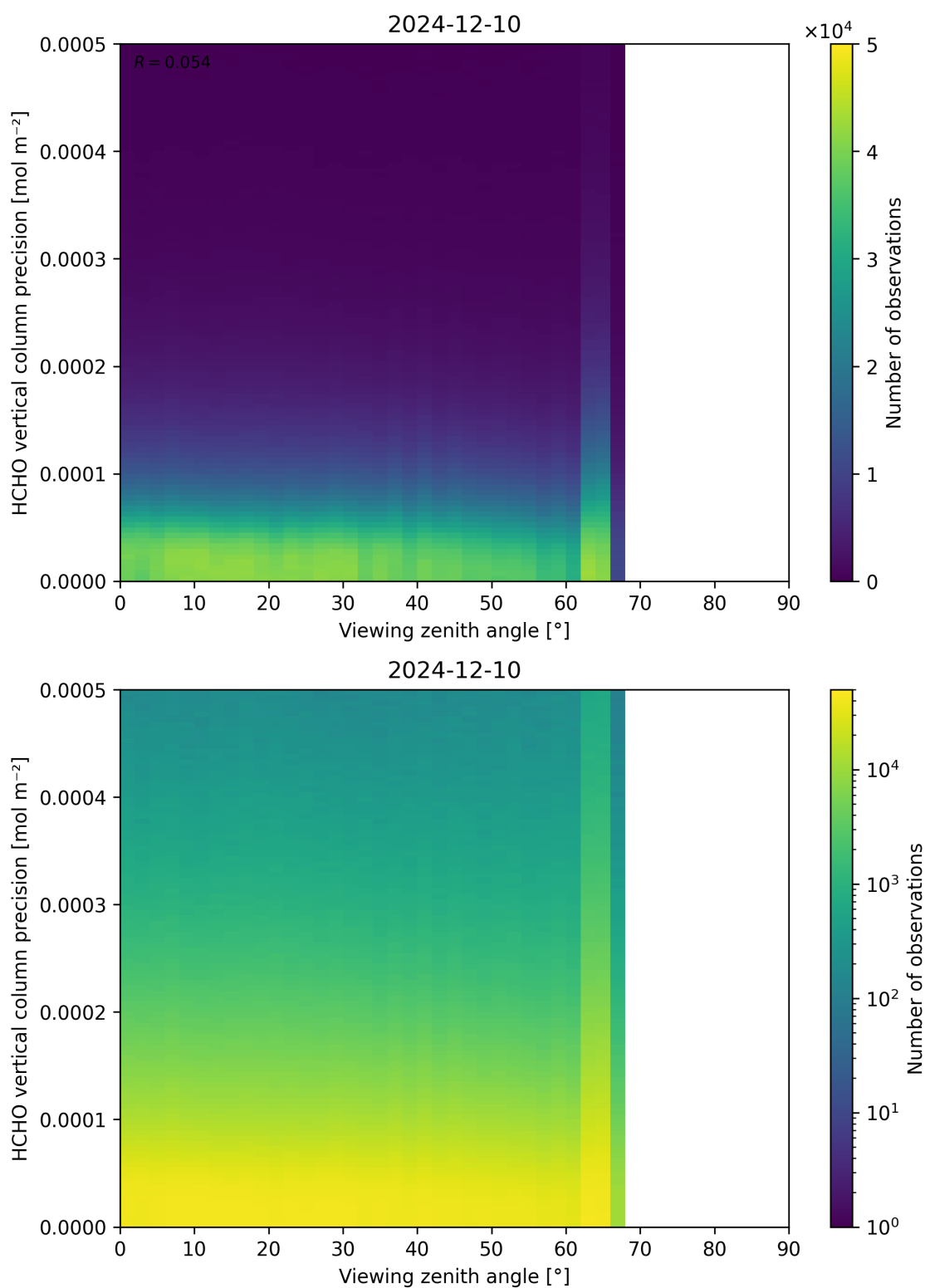
Figure 194: Scatter density plot of “Viewing zenith angle” against “HCHO vertical column precision” for 2024-12-09 to 2024-12-11.
