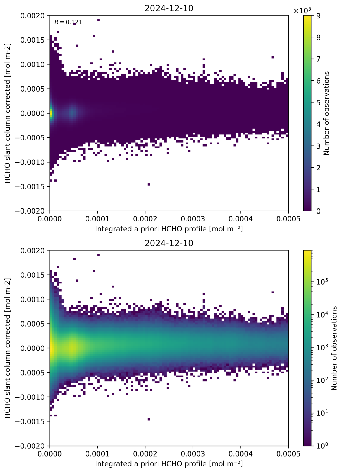
Figure 151: Scatter density plot of “Integrated a priori HCHO profile” against “HCHO slant column corrected” for 2024-12-09 to 2024-12-11.
