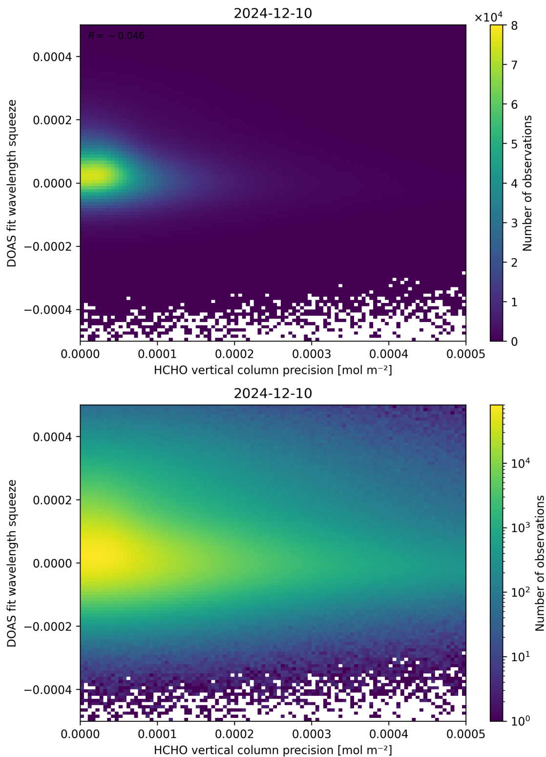
Figure 138: Scatter density plot of “HCHO vertical column precision” against “DOAS fit wavelength squeeze” for 2024-12-09 to 2024-12-11.
