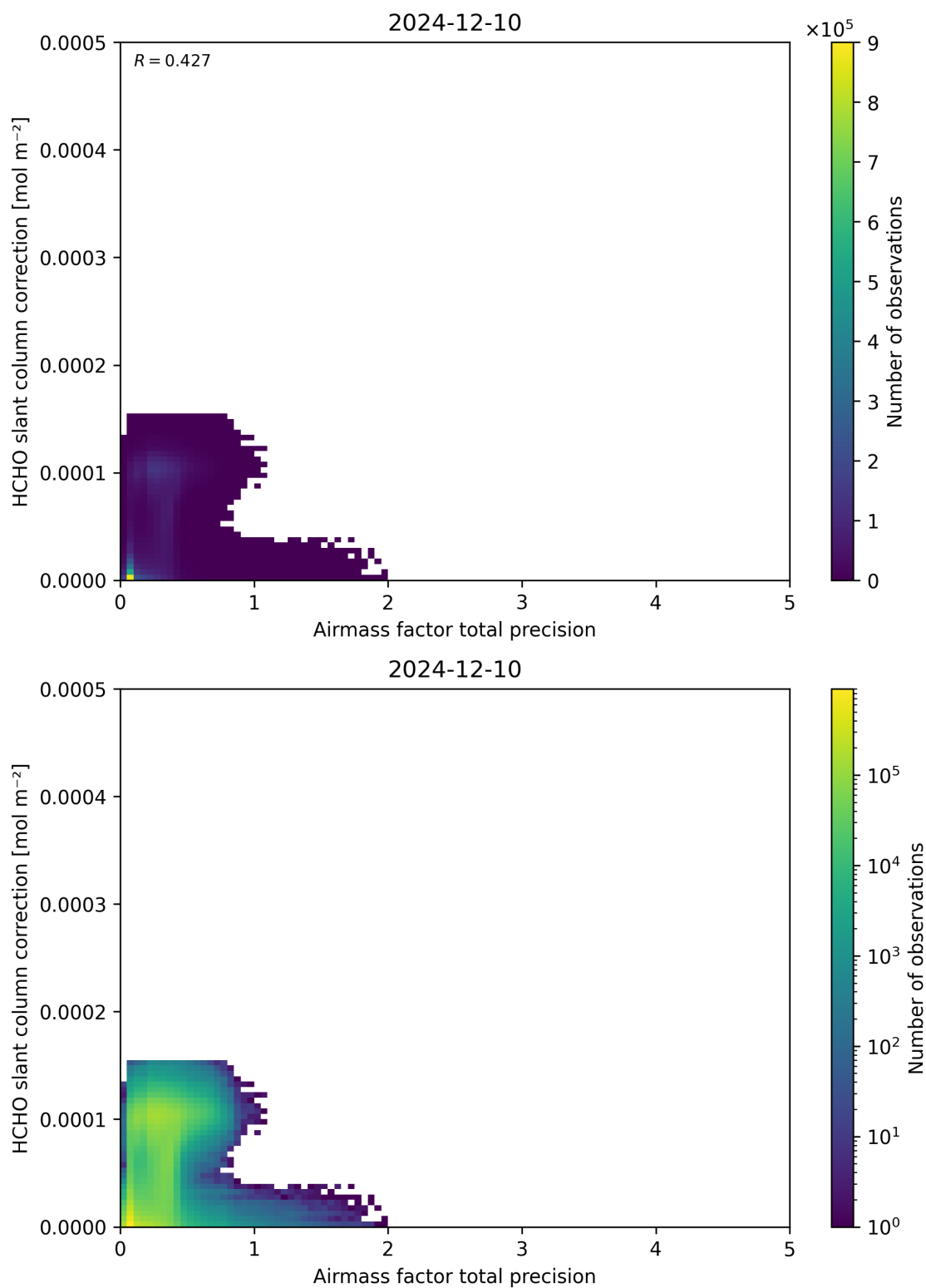
Figure 110: Scatter density plot of “Airmass factor total precision” against “HCHO slant column correction” for 2024-12-09 to 2024-12-11.
