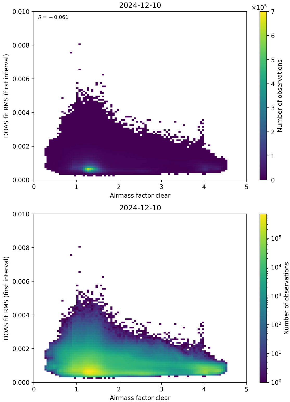
Figure 71: Scatter density plot of “Airmass factor clear” against “DOAS fit RMS (first interval)” for 2024-12-09 to 2024-12-11.
