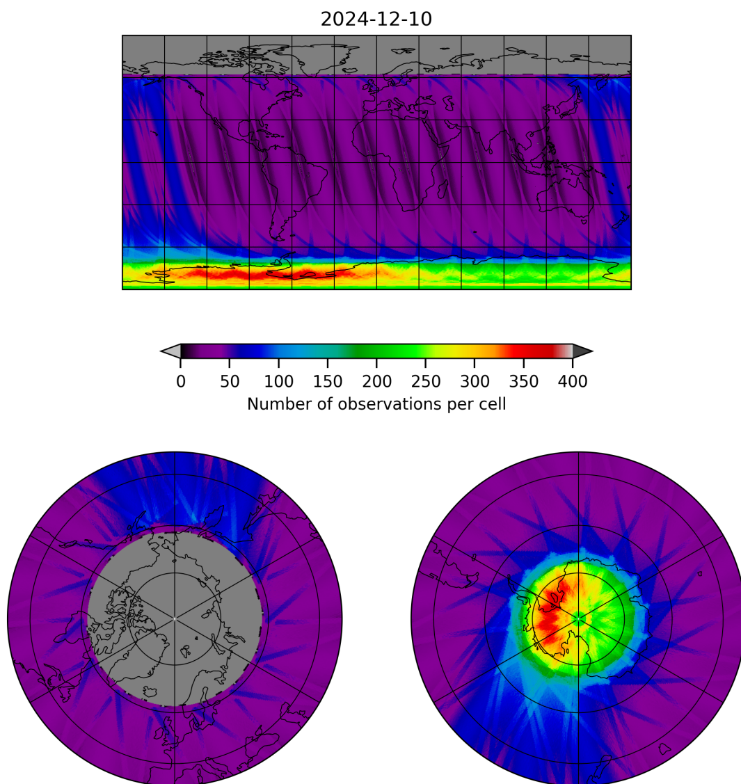
Figure 19: Map of the number of observations for 2024-12-09 to 2024-12-11
