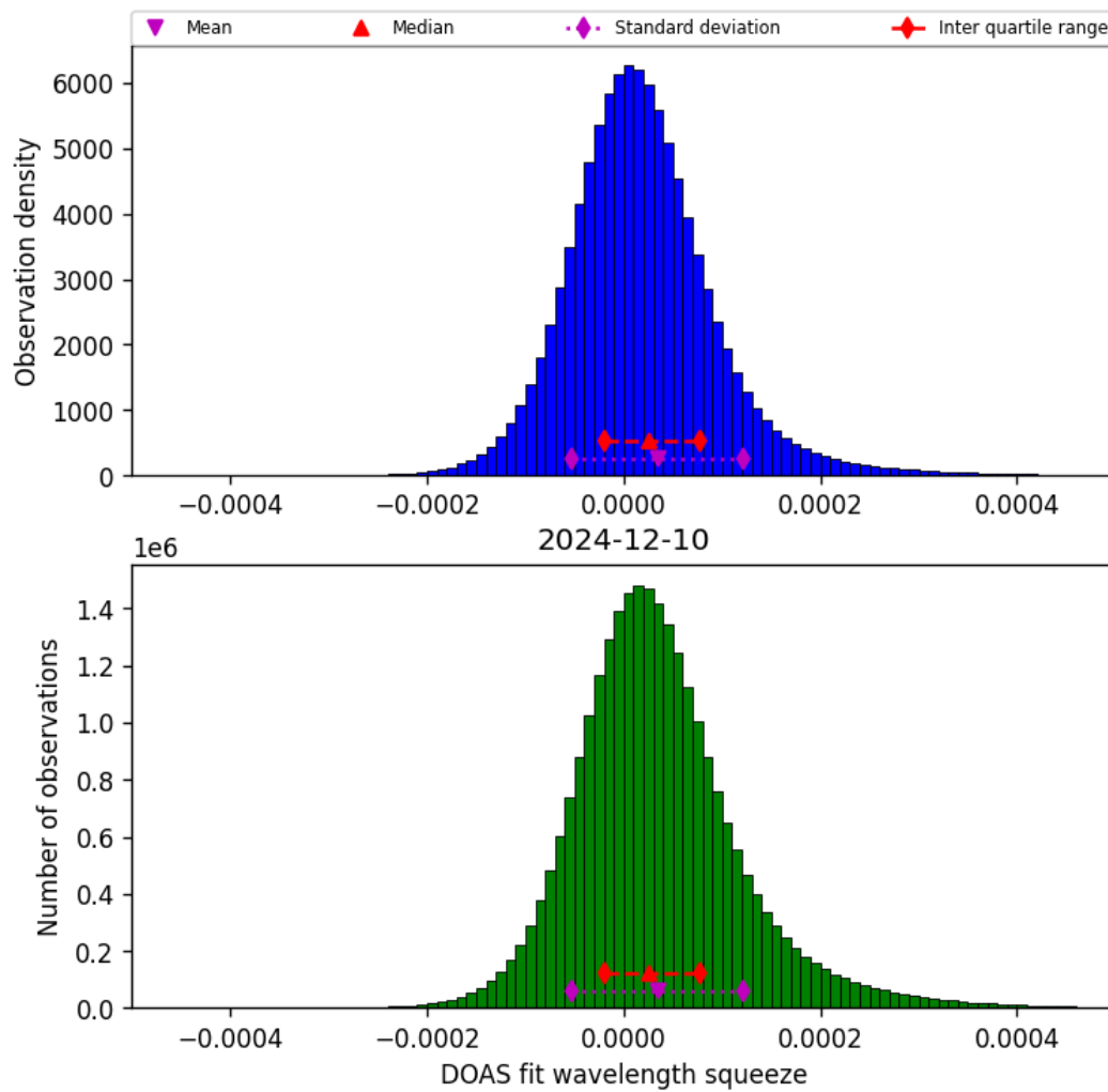
Figure 45: Histogram of “DOAS fit wavelength squeeze” for 2024-12-09 to 2024-12-11
