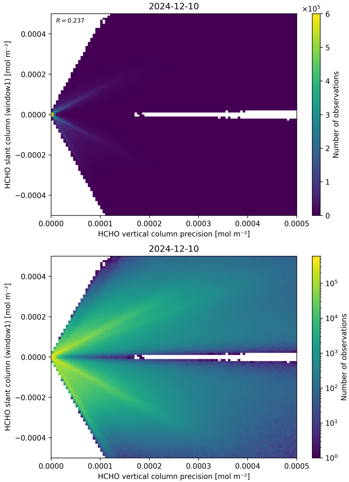
Figure 142: Scatter density plot of “HCHO vertical column precision” against “HCHO slant column (window1)” for 2024-12-09 to 2024-12-11.
