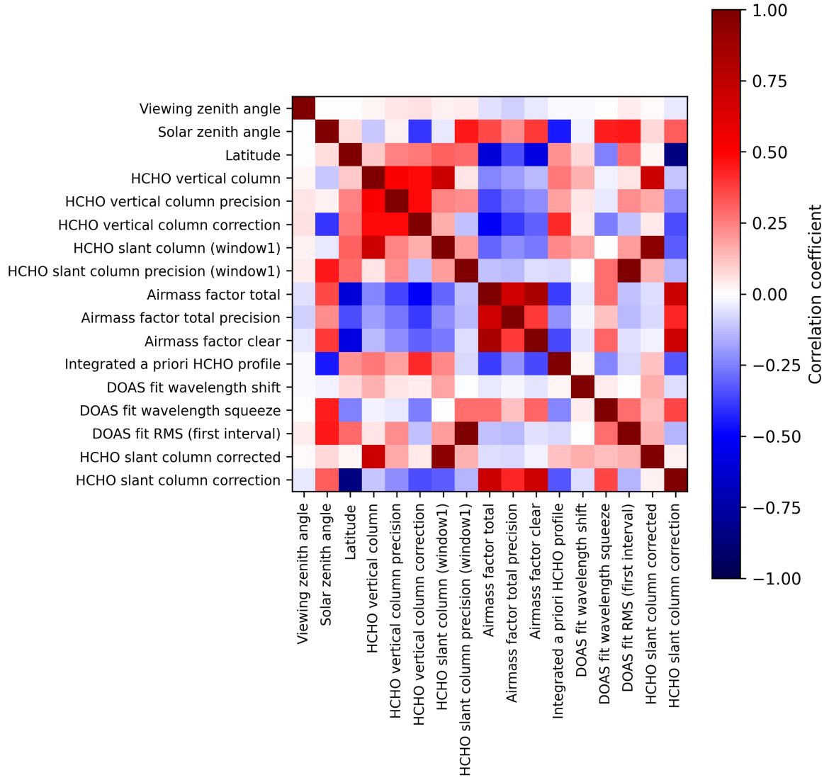
Figure 2: Map of correlation matrix for 2024-12-09 to 2024-12-11.
