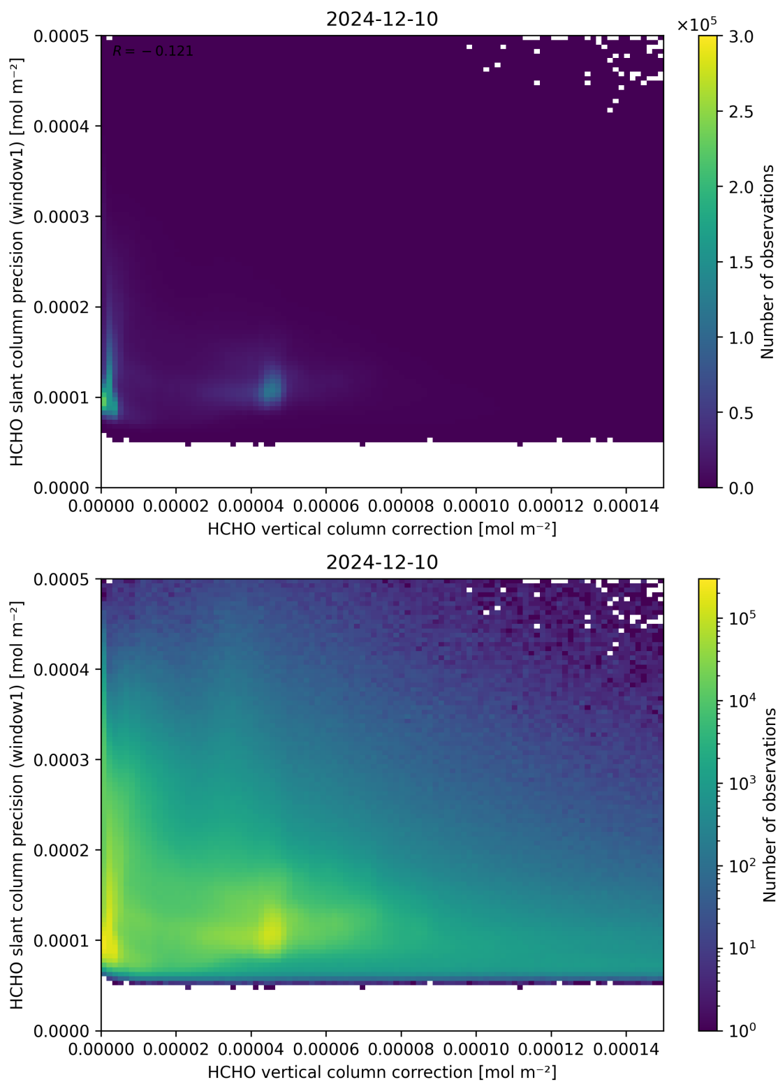
Figure 119: Scatter density plot of “HCHO vertical column correction” against “HCHO slant column precision (window1)” for 2024-12-09 to 2024-12-11.
