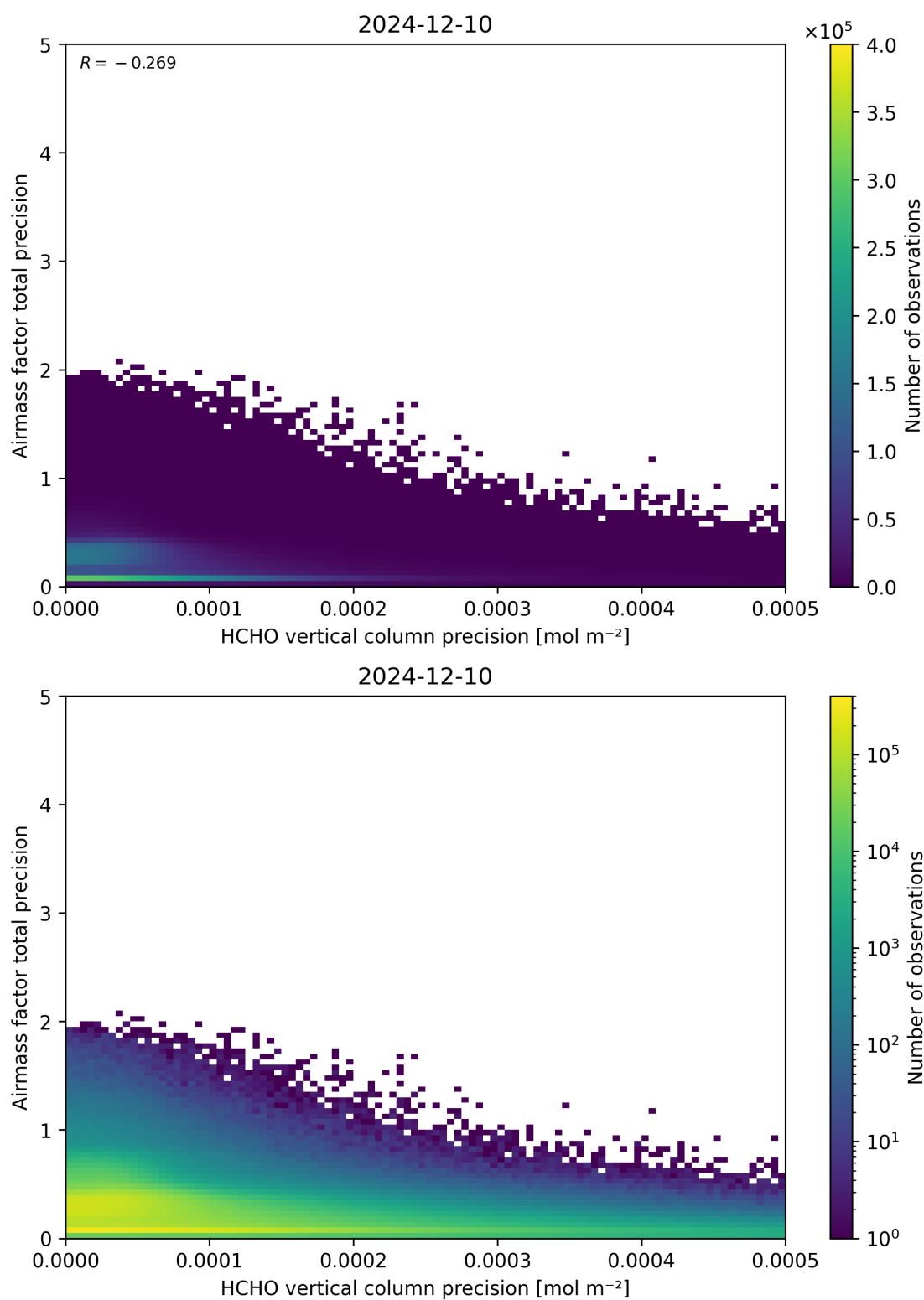
Figure 145: Scatter density plot of “HCHO vertical column precision” against “Airmass factor total precision” for 2024-12-09 to 2024-12-11.
