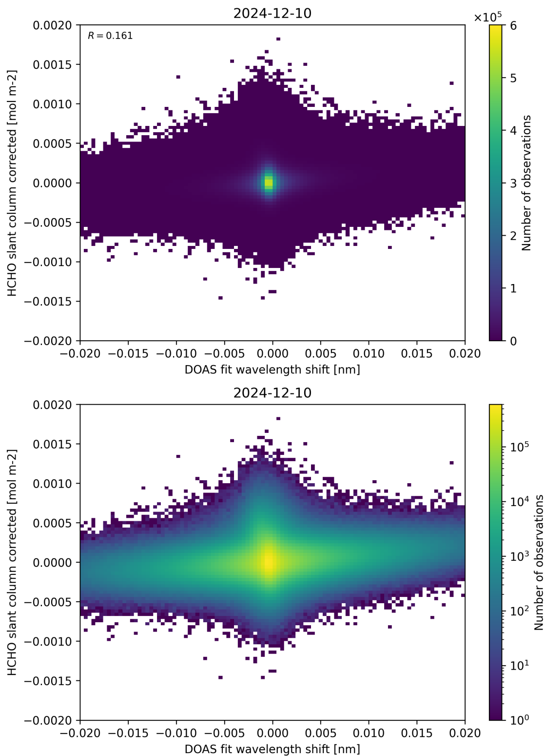
Figure 66: Scatter density plot of “DOAS fit wavelength shift” against “HCHO slant column corrected” for 2024-12-09 to 2024-12-11.
