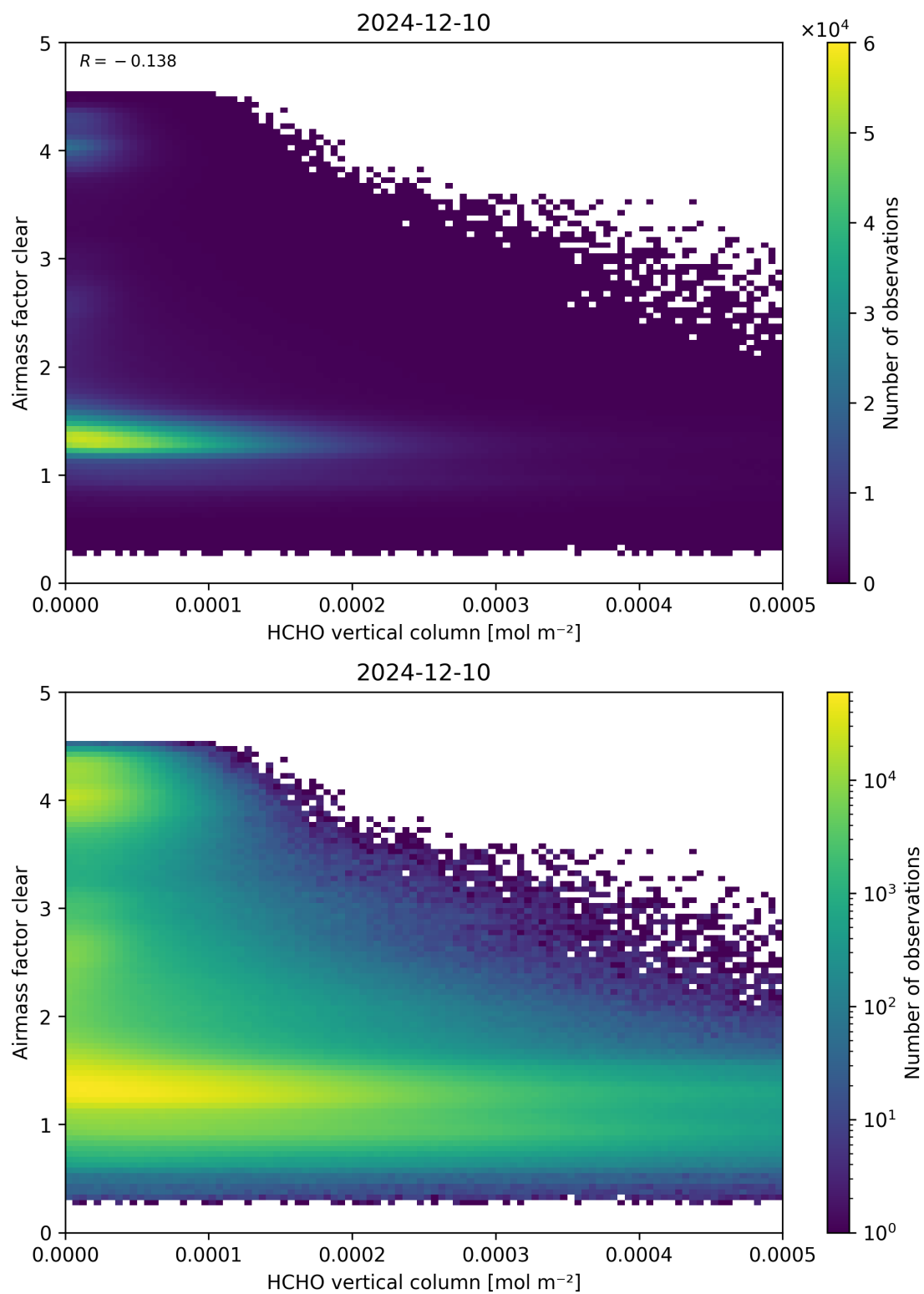
Figure 126: Scatter density plot of “HCHO vertical column” against “Airmass factor clear” for 2024-12-09 to 2024-12-11.
