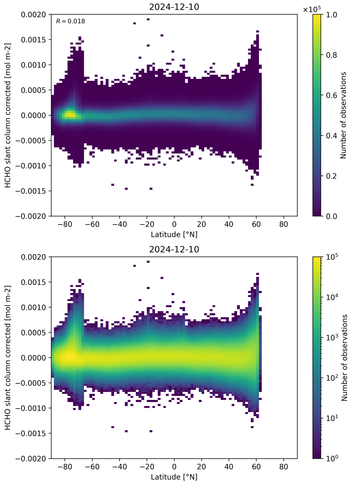
Figure 157: Scatter density plot of “Latitude” against “HCHO slant column corrected” for 2024-12-09 to 2024-12-11.
