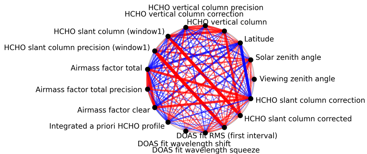
Figure 1: Map of correlation graph for 2024-12-09 to 2024-12-11.
