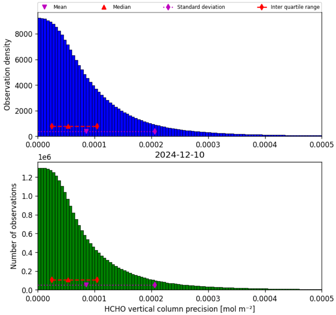
Figure 36: Histogram of “HCHO vertical column precision” for 2024-12-09 to 2024-12-11
