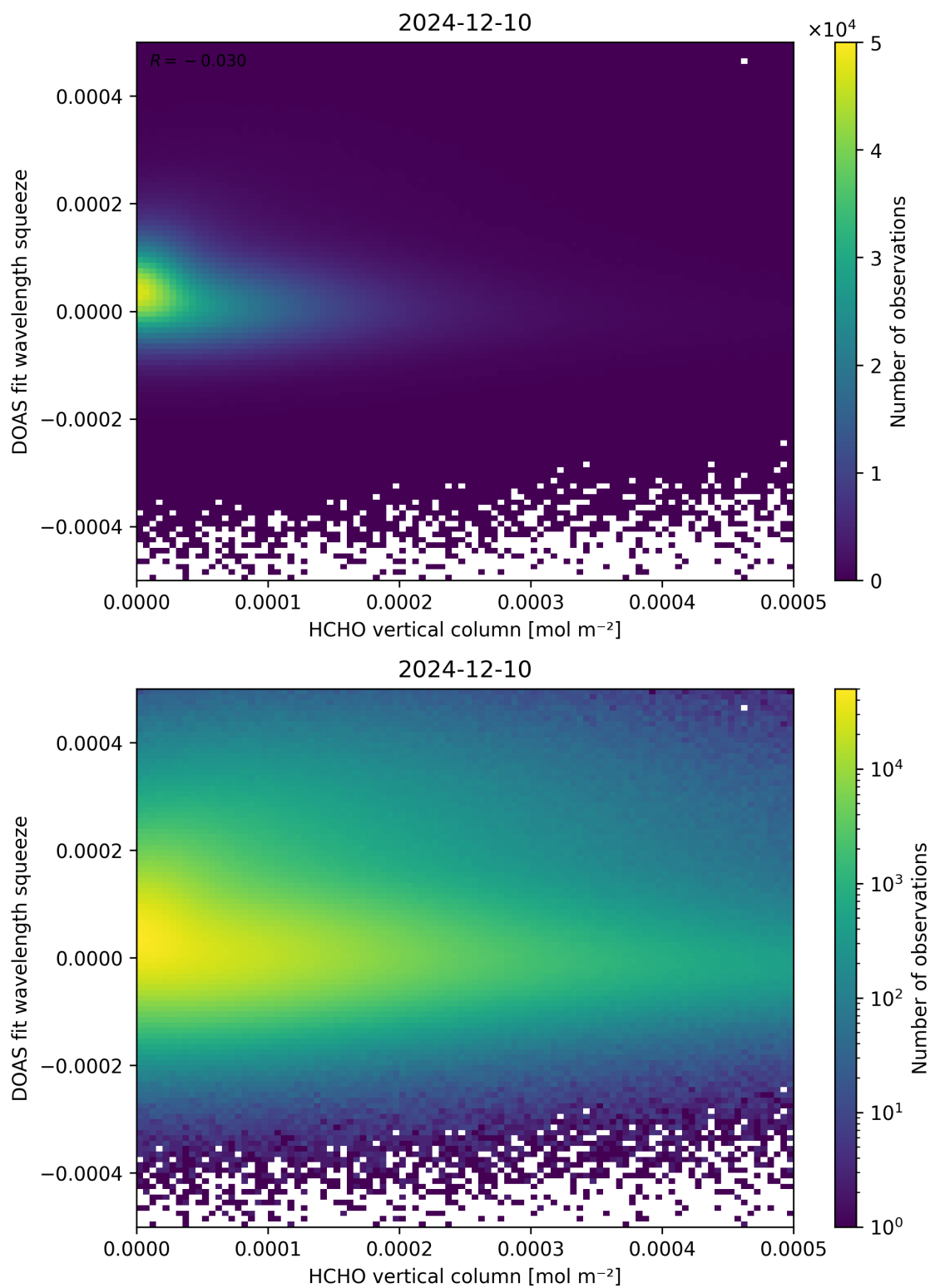
Figure 125: Scatter density plot of “HCHO vertical column” against “DOAS fit wavelength squeeze” for 2024-12-09 to 2024-12-11.
