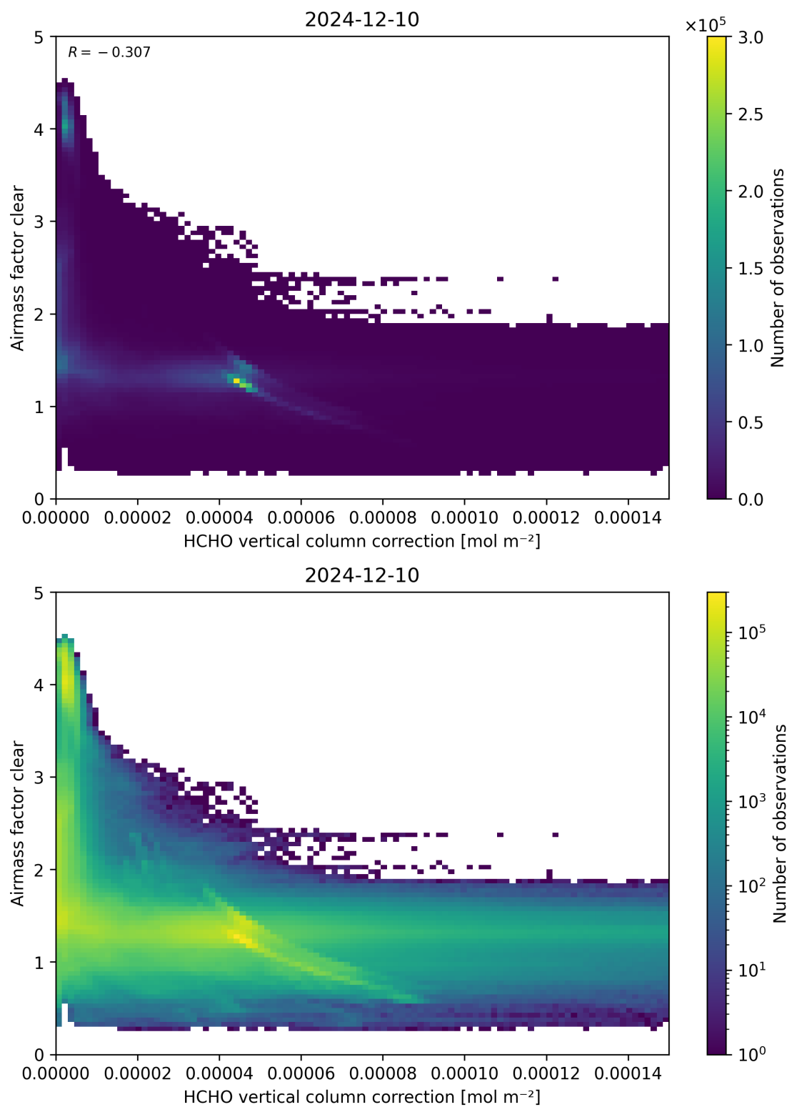
Figure 115: Scatter density plot of “HCHO vertical column correction” against “Airmass factor clear” for 2024-12-09 to 2024-12-11.
