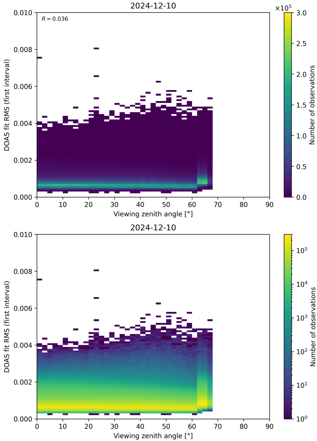
Figure 182: Scatter density plot of “Viewing zenith angle” against “DOAS fit RMS (first interval)” for 2024-12-09 to 2024-12-11.
