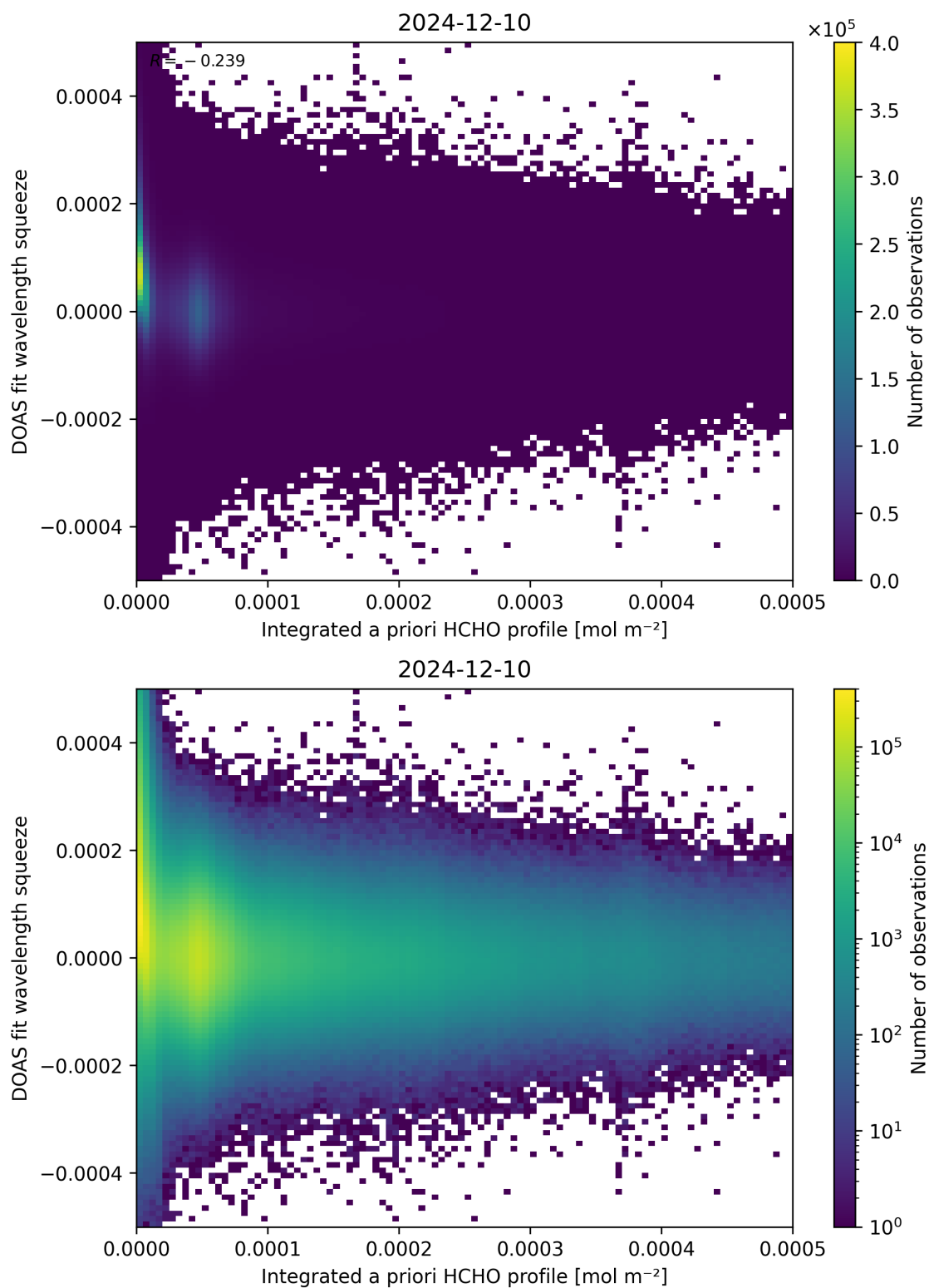
Figure 150: Scatter density plot of “Integrated a priori HCHO profile” against “DOAS fit wavelength squeeze” for 2024-12-09 to 2024-12-11.
