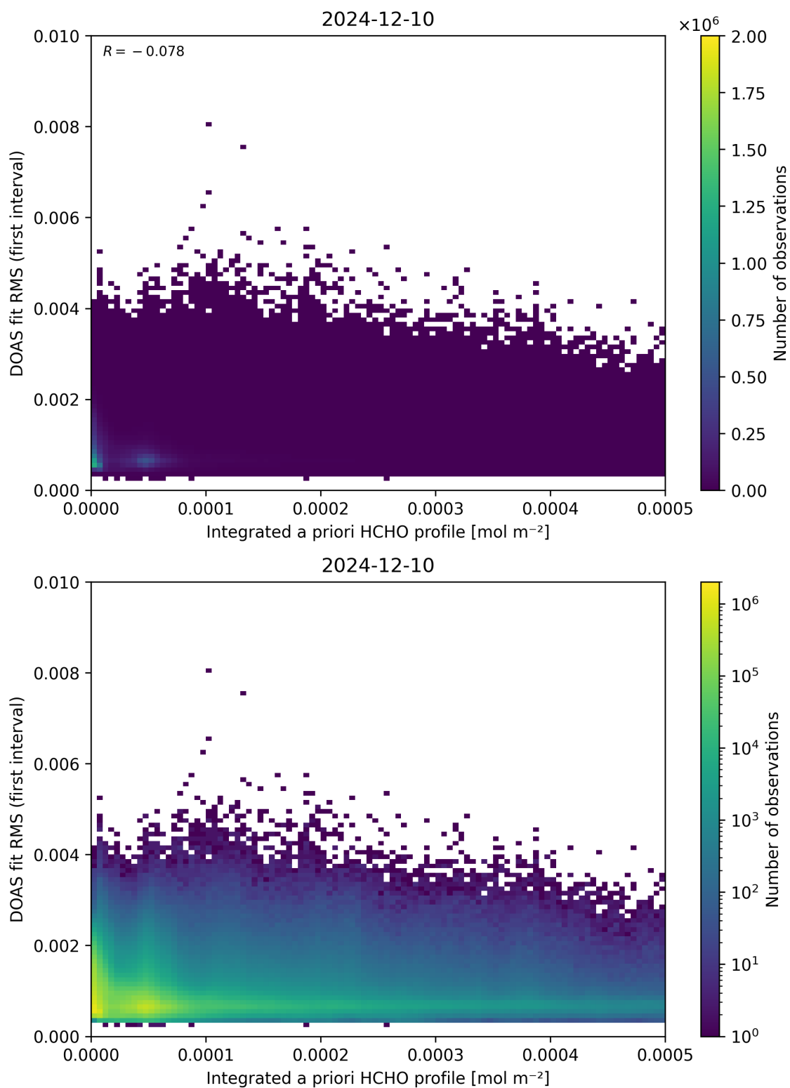
Figure 148: Scatter density plot of “Integrated a priori HCHO profile” against “DOAS fit RMS (first interval)” for 2024-12-09 to 2024-12-11.
