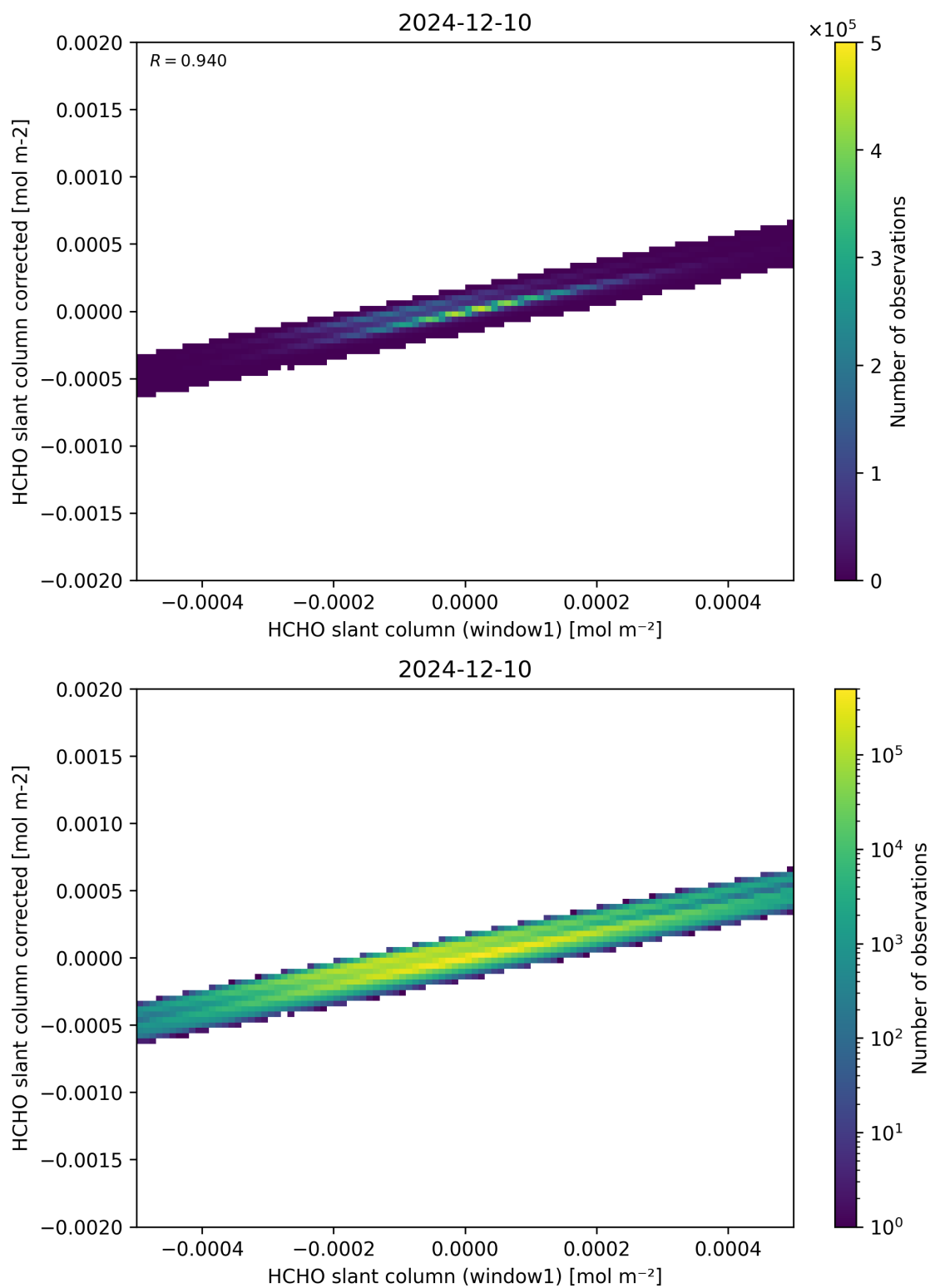
Figure 82: Scatter density plot of “HCHO slant column (window1)” against “HCHO slant column corrected” for 2024-12-09 to 2024-12-11.
