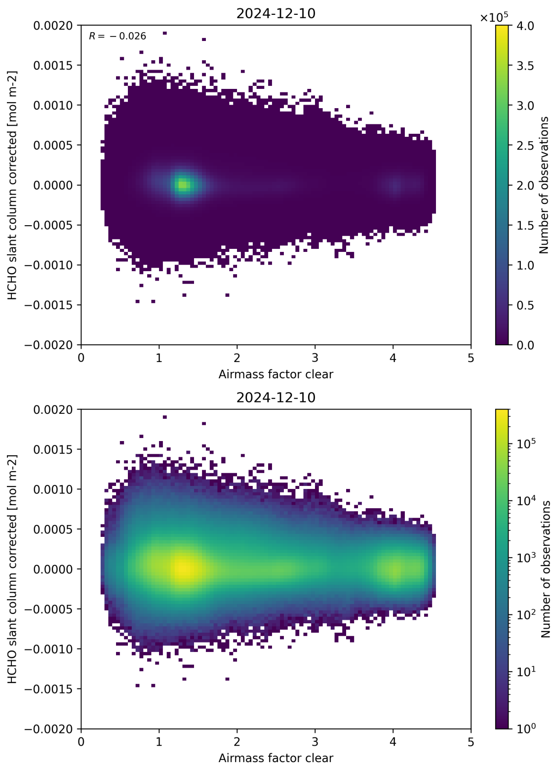
Figure 74: Scatter density plot of “Airmass factor clear” against “HCHO slant column corrected” for 2024-12-09 to 2024-12-11.
