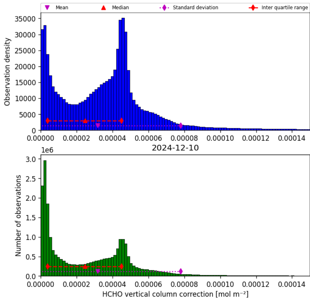
Figure 37: Histogram of “HCHO vertical column correction” for 2024-12-09 to 2024-12-11
