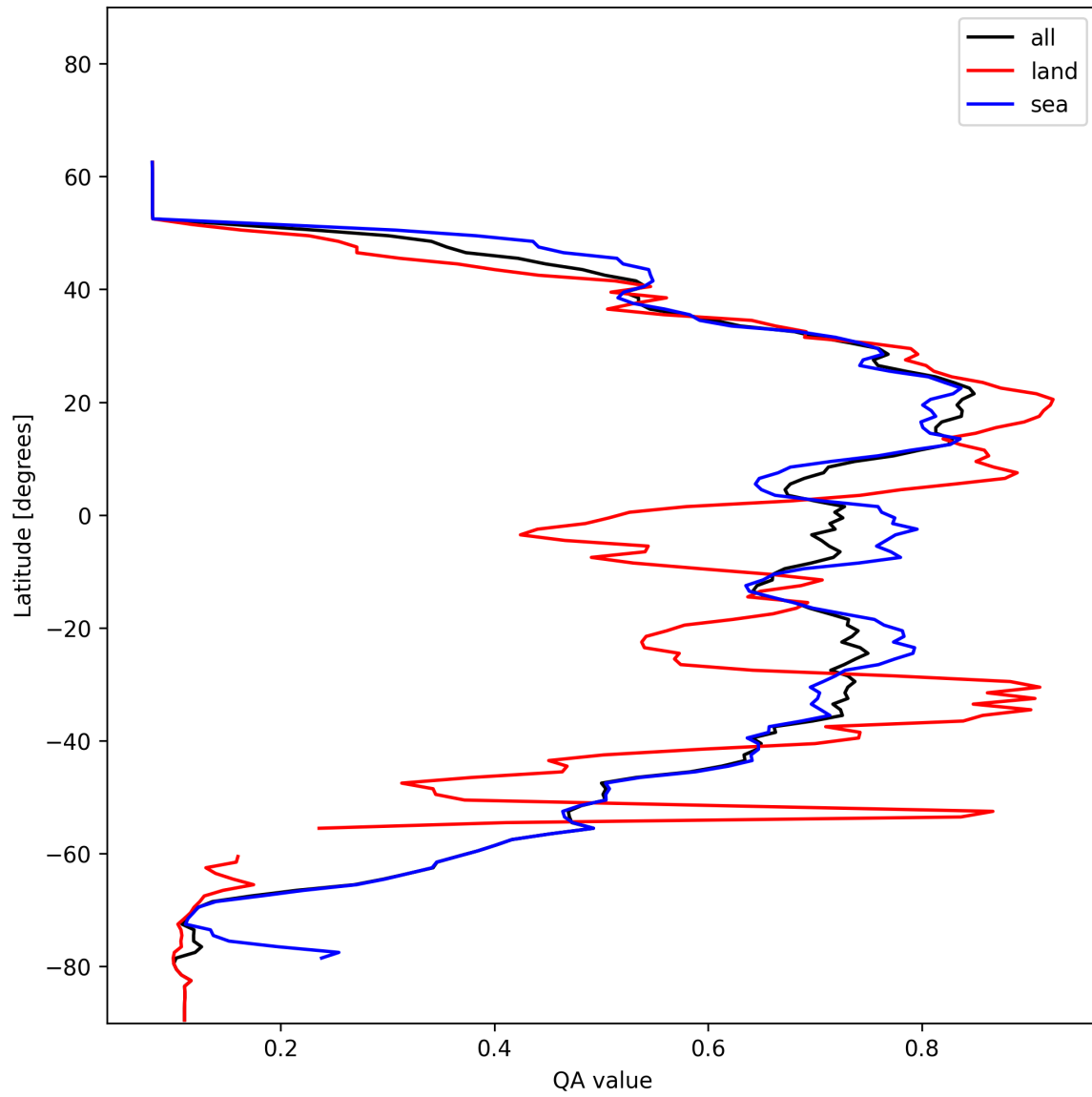
Figure 20: Zonal average of “QA value” for 2024-12-09 to 2024-12-11.
