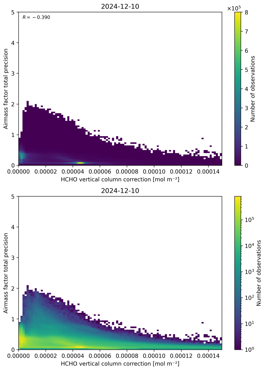
Figure 121: Scatter density plot of “HCHO vertical column correction” against “Airmass factor total precision” for 2024-12-09 to 2024-12-11.
