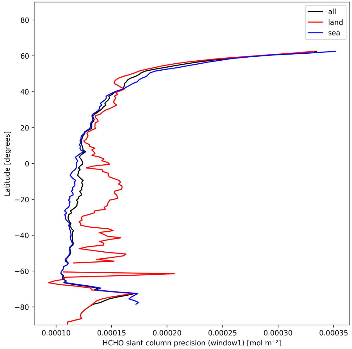
Figure 25: Zonal average of “HCHO slant column precision (window1)” for 2024-12-09 to 2024-12-11.
