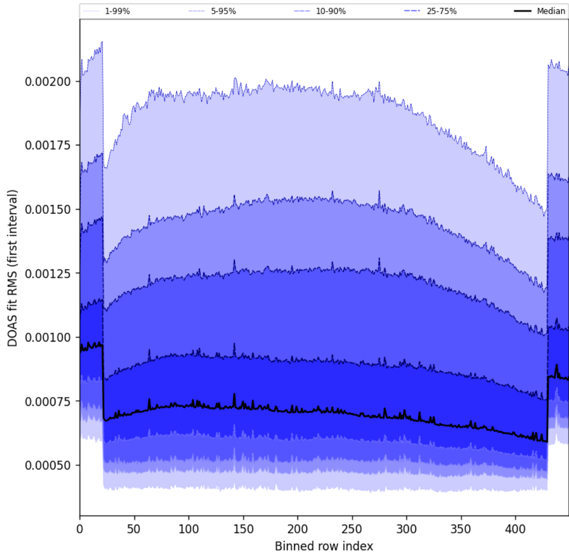
Figure 60: Along track statistics of “DOAS fit RMS (first interval)” for 2024-12-09 to 2024-12-11
