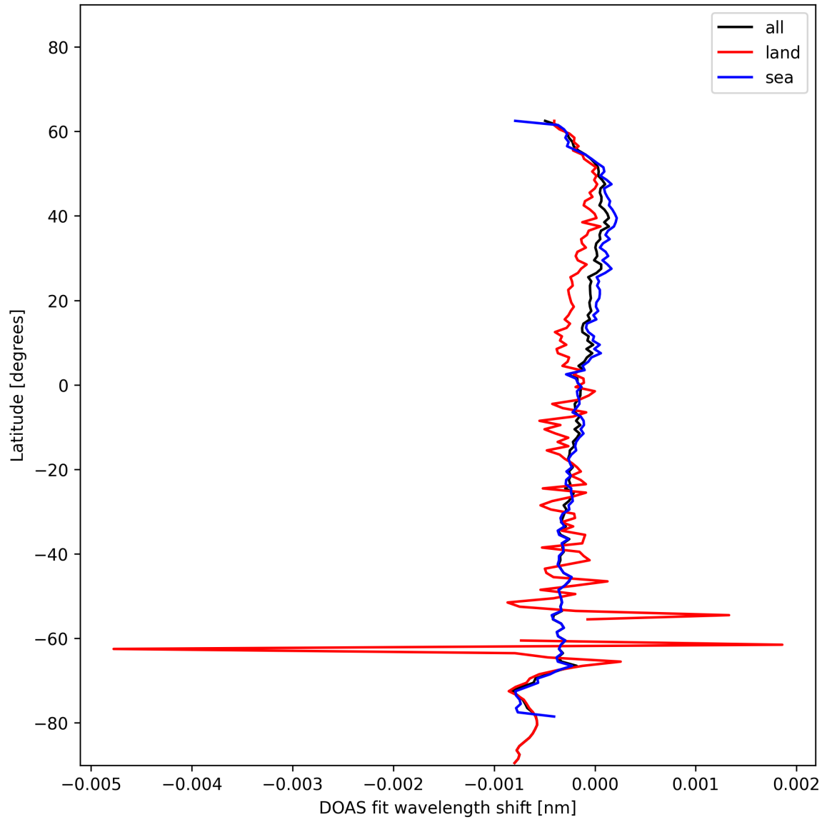
Figure 30: Zonal average of “DOAS fit wavelength shift” for 2024-12-09 to 2024-12-11.
