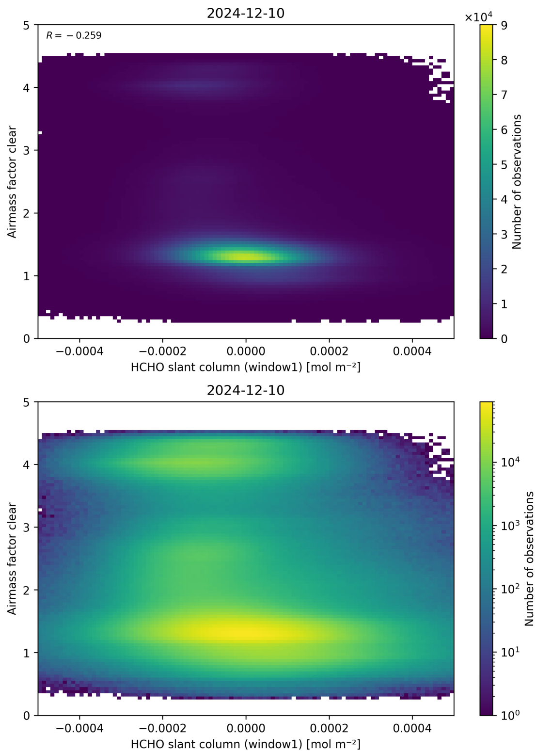
Figure 81: Scatter density plot of “HCHO slant column (window1)” against “Airmass factor clear” for 2024-12-09 to 2024-12-11.
