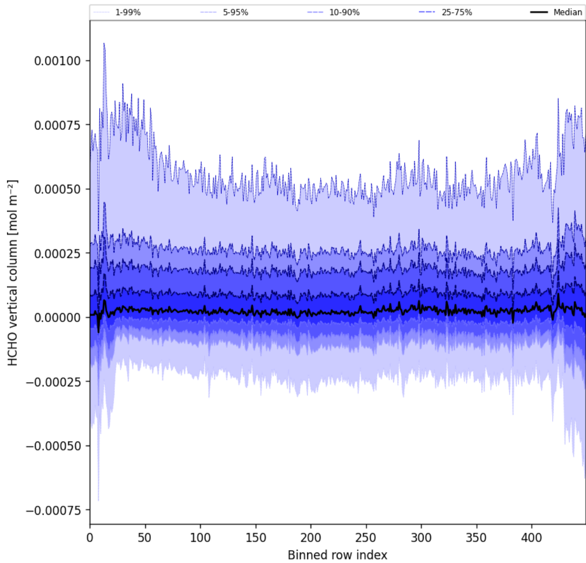
Figure 49: Along track statistics of “HCHO vertical column” for 2024-12-09 to 2024-12-11
