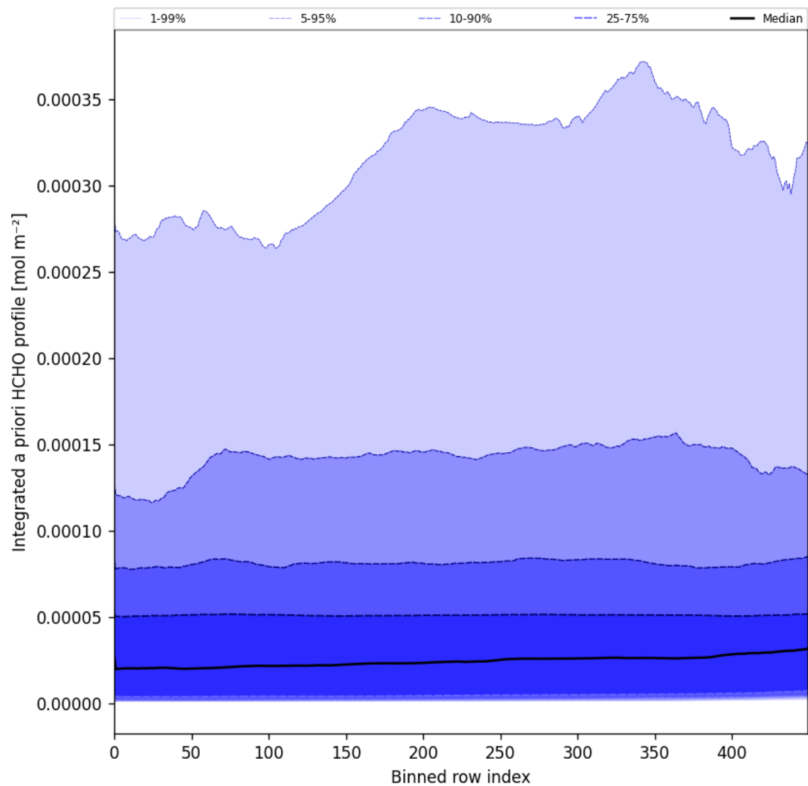
Figure 57: Along track statistics of "Integrated a priori HCHO profile" for 2024-12-09 to 2024-12-11
