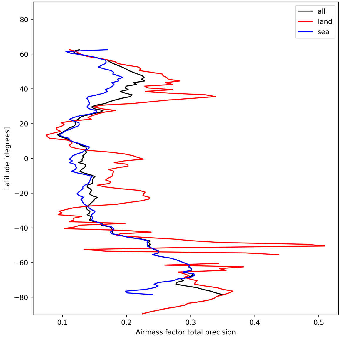
Figure 27: Zonal average of “Airmass factor total precision” for 2024-12-09 to 2024-12-11.
