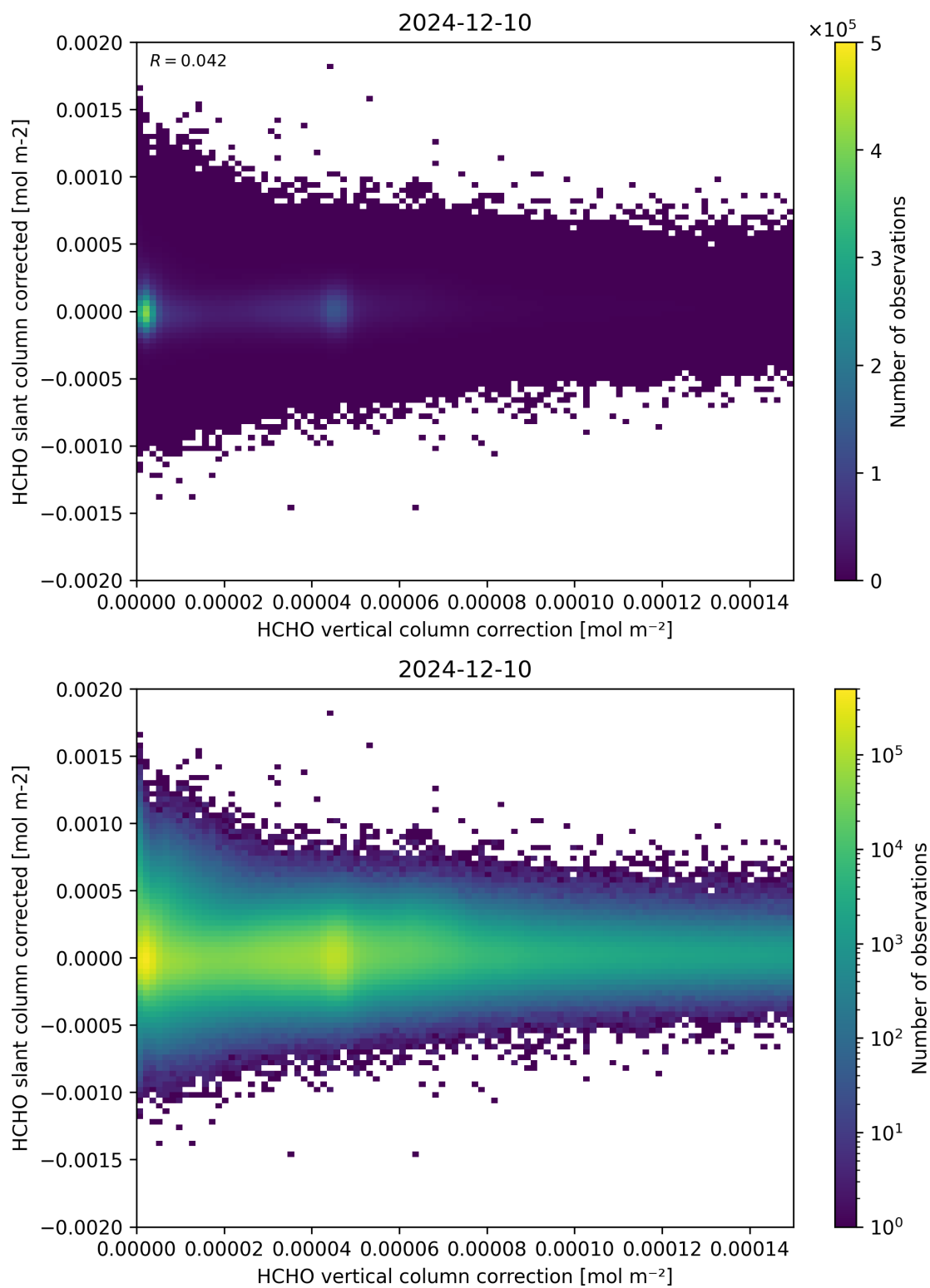
Figure 116: Scatter density plot of “HCHO vertical column correction” against “HCHO slant column corrected” for 2024-12-09 to 2024-12-11.
