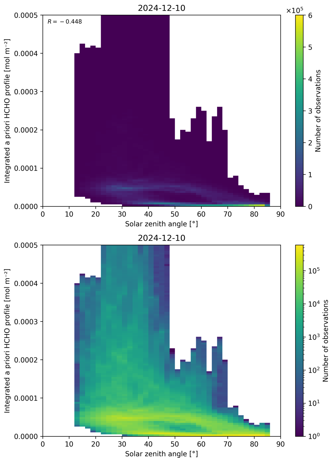
Figure 180: Scatter density plot of “Solar zenith angle” against “Integrated a priori HCHO profile” for 2024-12-09 to 2024-12-11.
