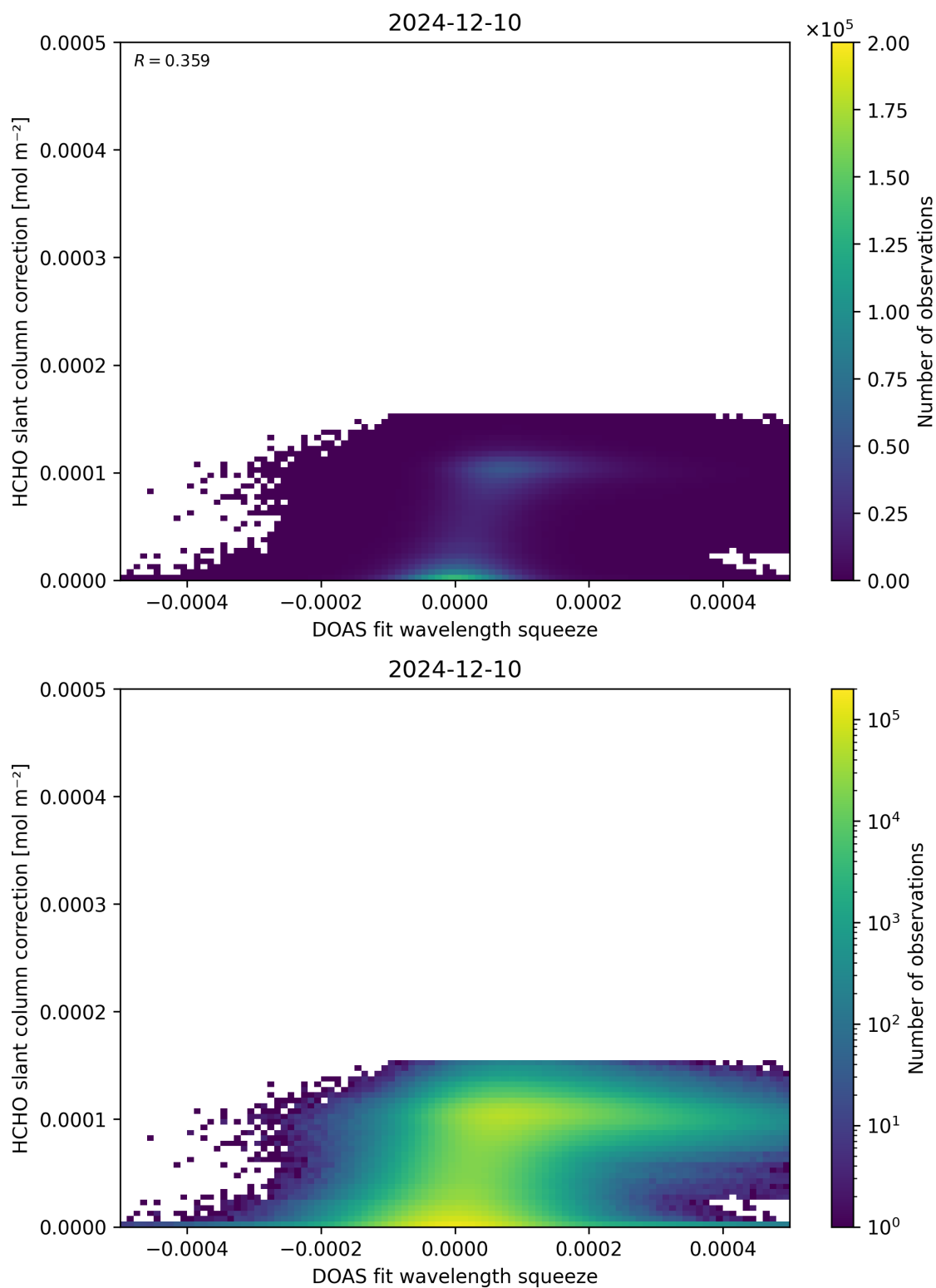
Figure 70: Scatter density plot of “DOAS fit wavelength squeeze” against “HCHO slant column correction” for 2024-12-09 to 2024-12-11.
