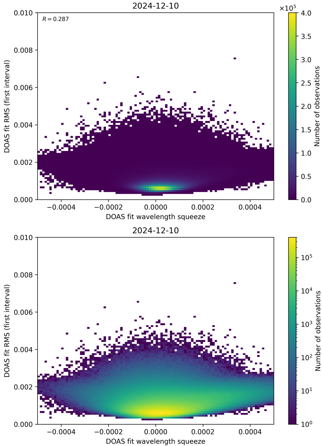
Figure 68: Scatter density plot of “DOAS fit wavelength squeeze” against “DOAS fit RMS (first interval)” for 2024-12-09 to 2024-12-11.
