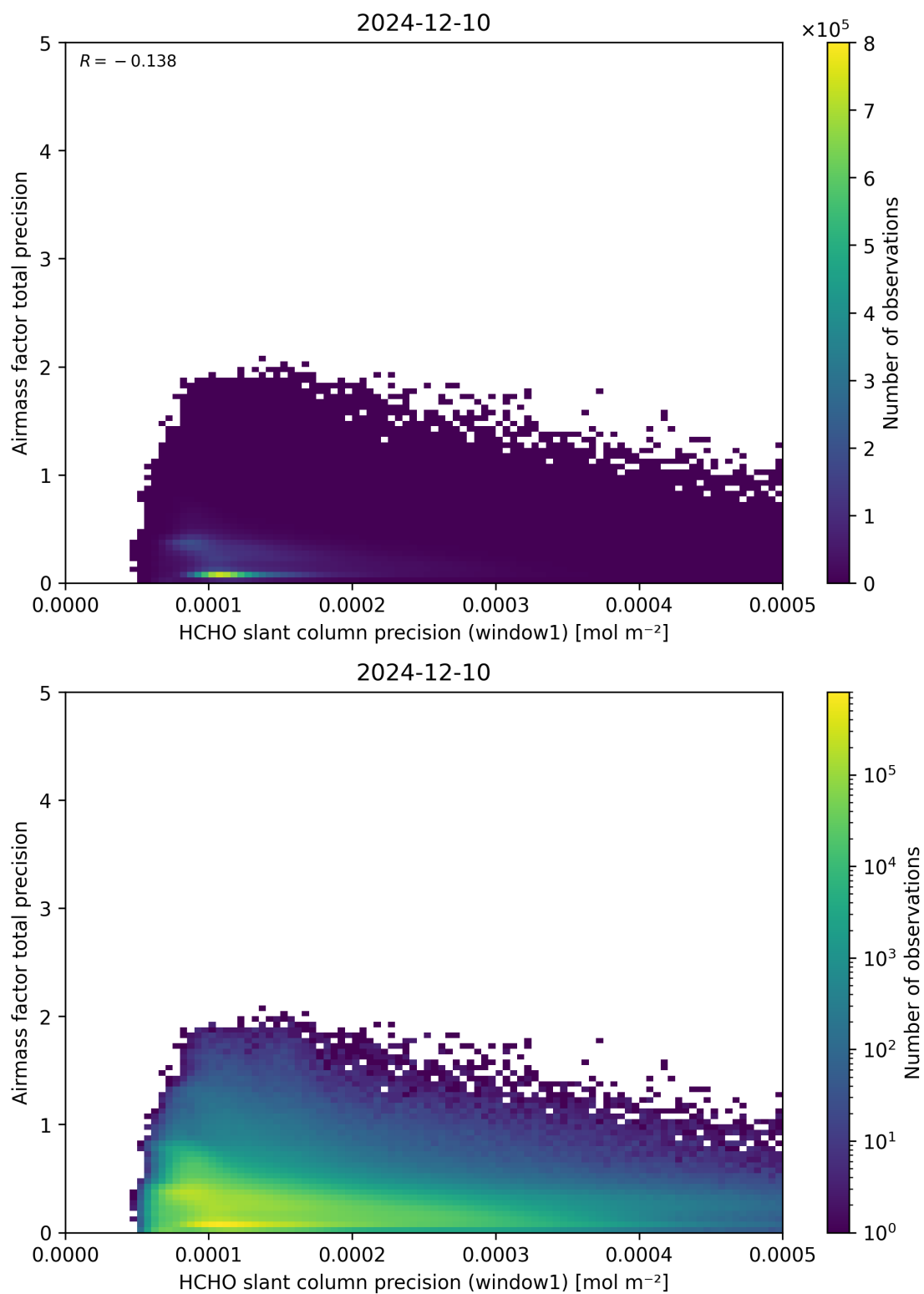
Figure 95: Scatter density plot of “HCHO slant column precision (window1)” against “Airmass factor total precision” for 2024-12-09 to 2024-12-11.
