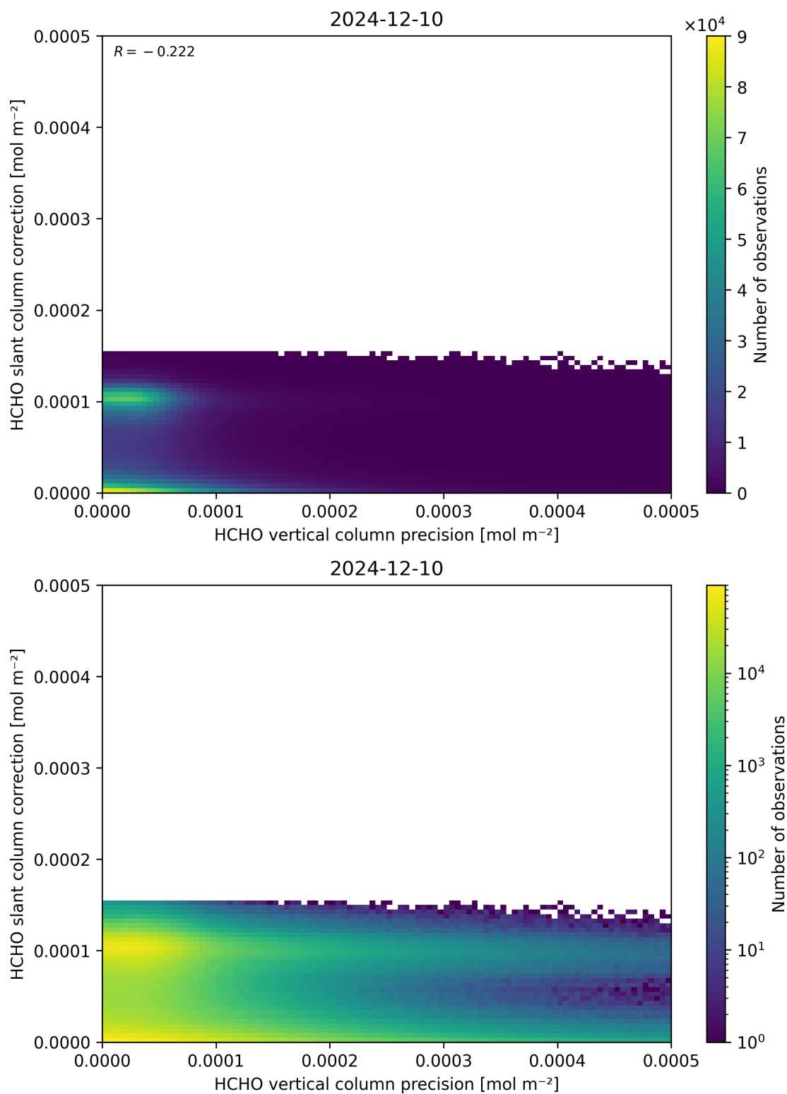
Figure 141: Scatter density plot of “HCHO vertical column precision” against “HCHO slant column correction” for 2024-12-09 to 2024-12-11.
