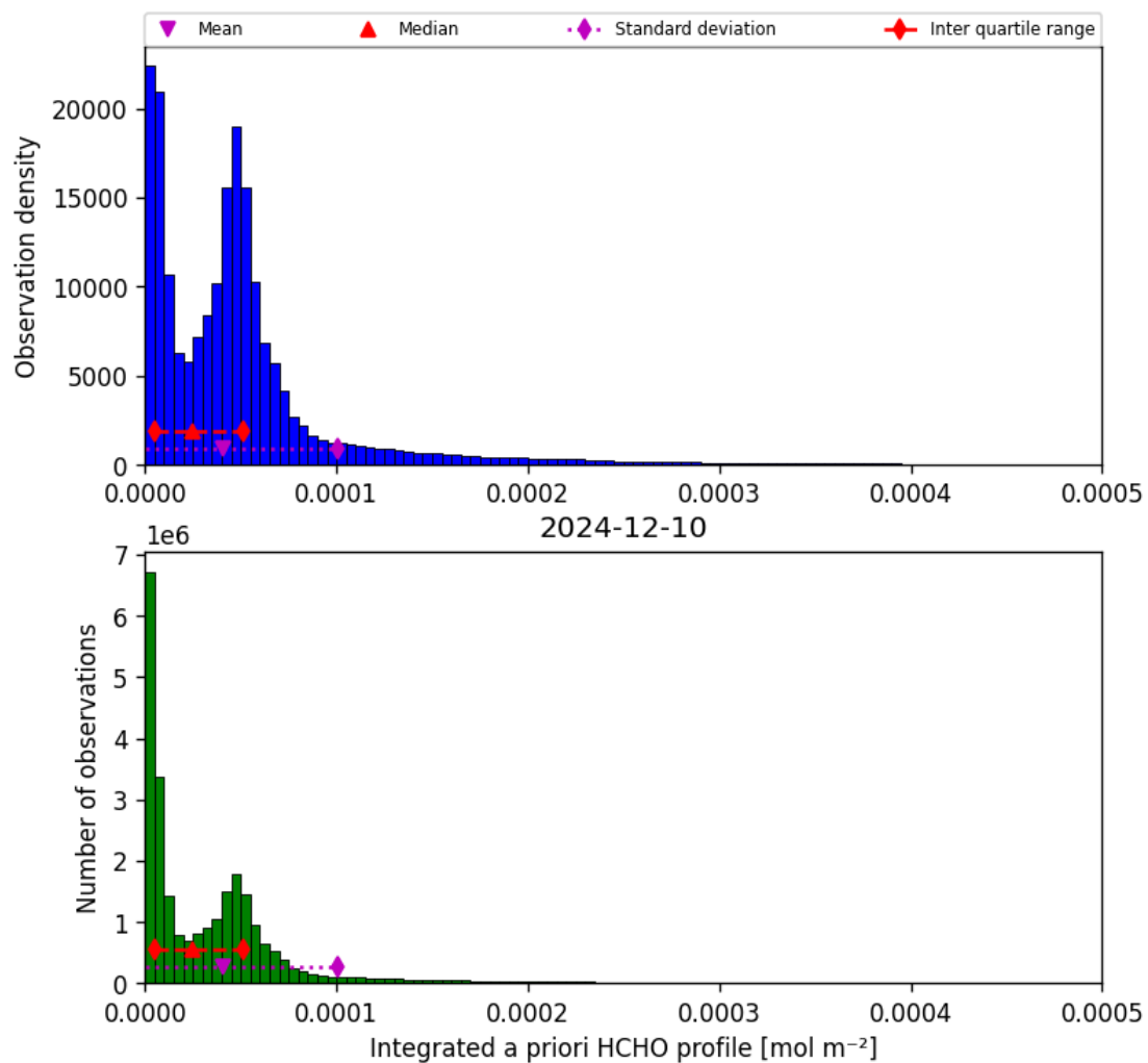
Figure 43: Histogram of “Integrated a priori HCHO profile” for 2024-12-09 to 2024-12-11
