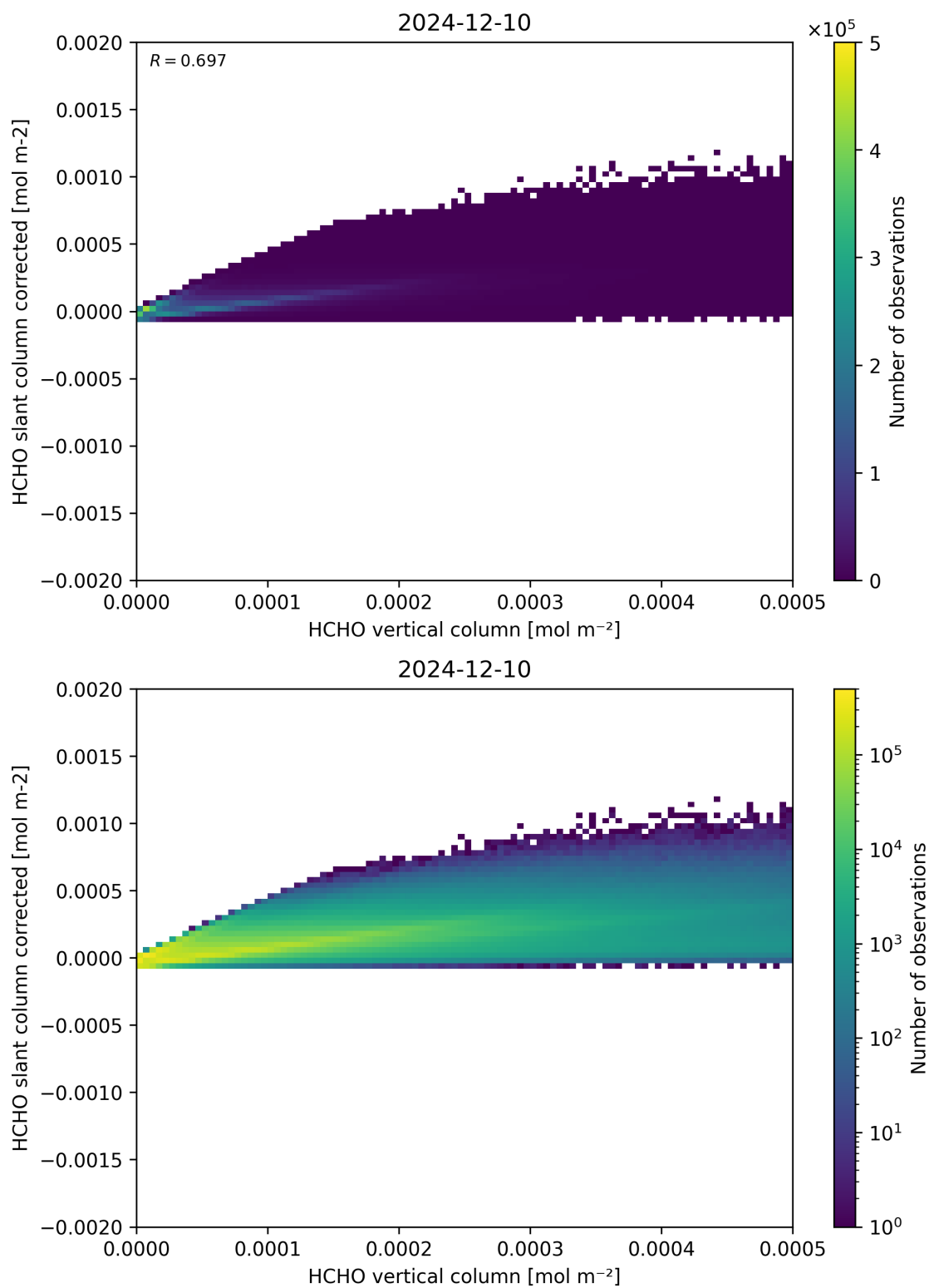
Figure 127: Scatter density plot of “HCHO vertical column” against “HCHO slant column corrected” for 2024-12-09 to 2024-12-11.
