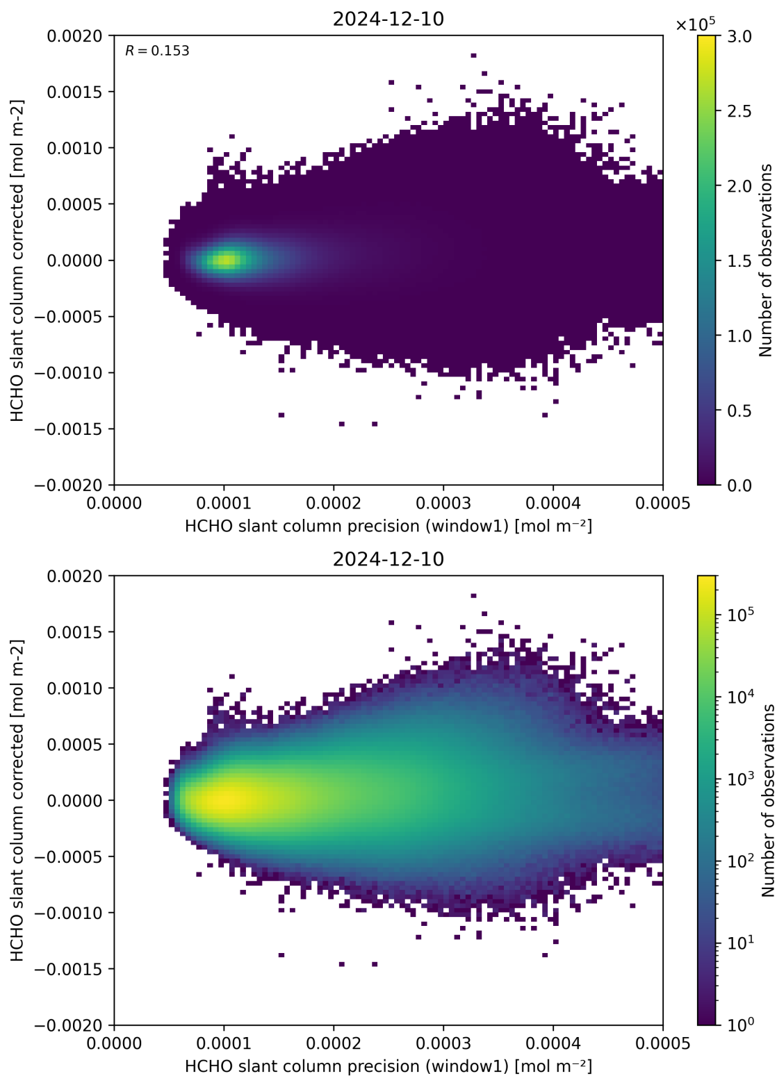
Figure 92: Scatter density plot of “HCHO slant column precision (window1)” against “HCHO slant column corrected” for 2024-12-09 to 2024-12-11.
