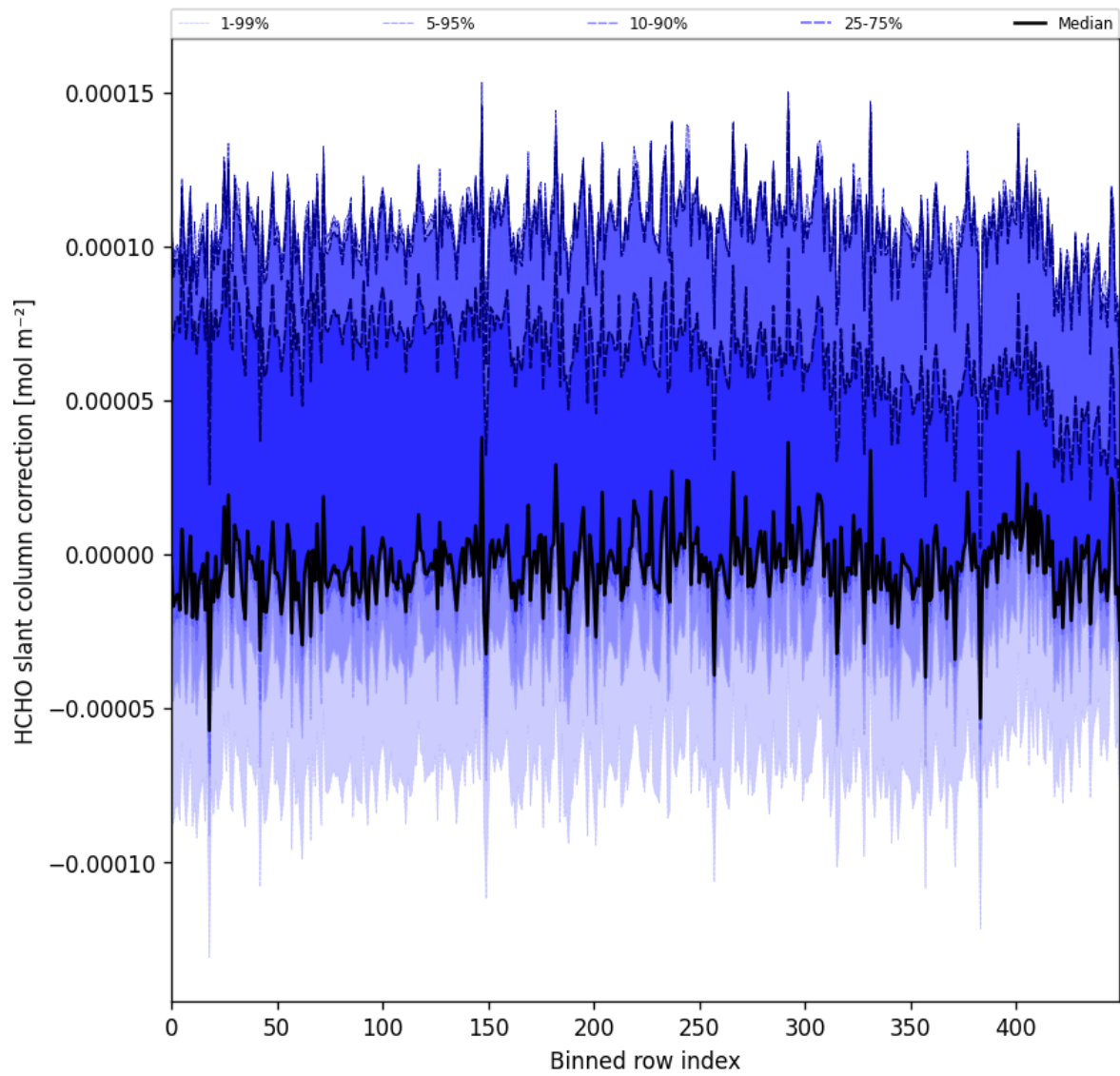
Figure 61: Along track statistics of “HCHO slant column correction” for 2024-12-09 to 2024-12-11
