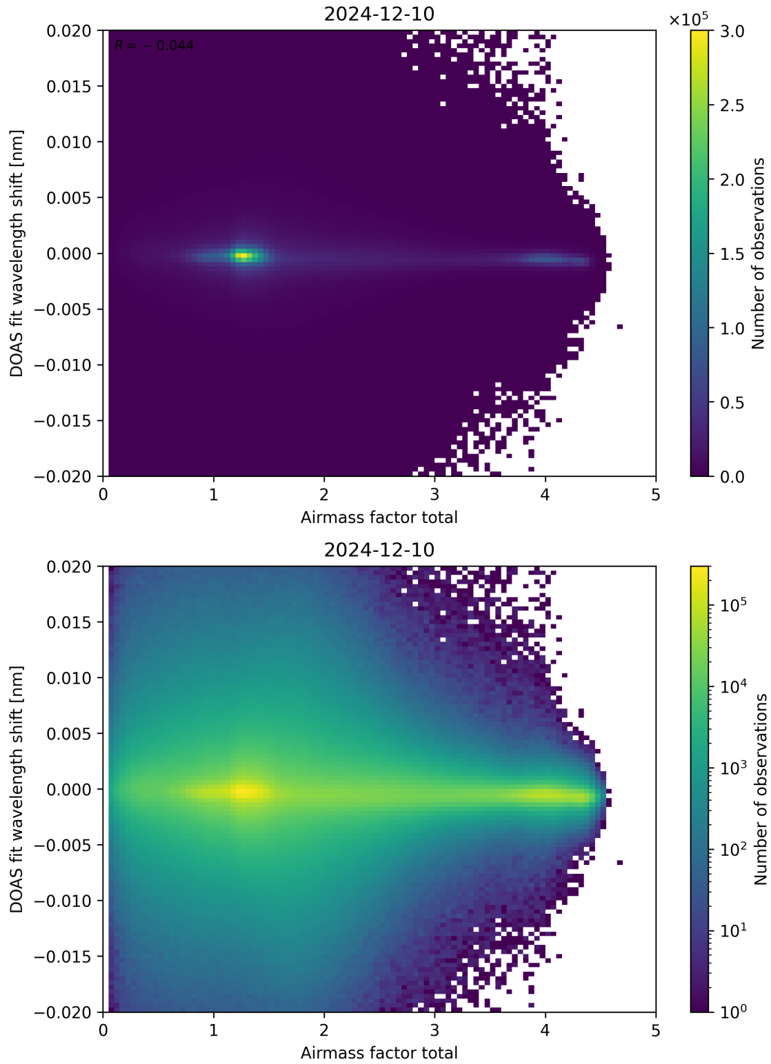
Figure 98: Scatter density plot of “Airmass factor total” against “DOAS fit wavelength shift” for 2024-12-09 to 2024-12-11.
