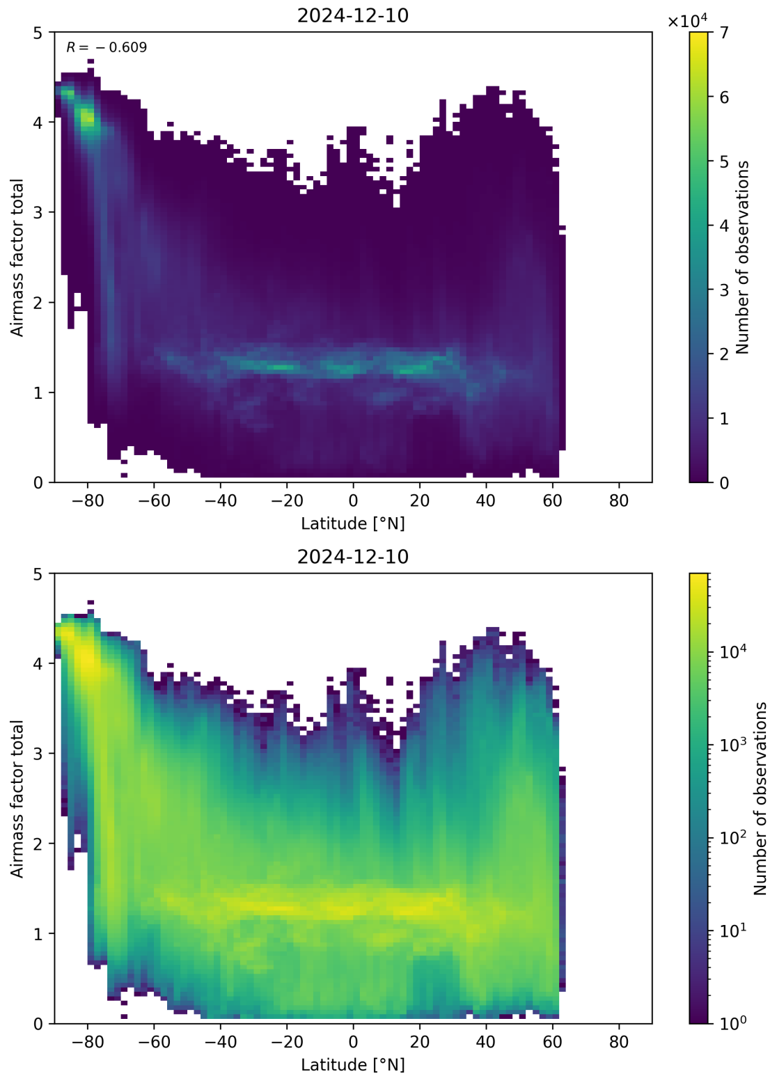
Figure 161: Scatter density plot of “Latitude” against “Airmass factor total” for 2024-12-09 to 2024-12-11.
