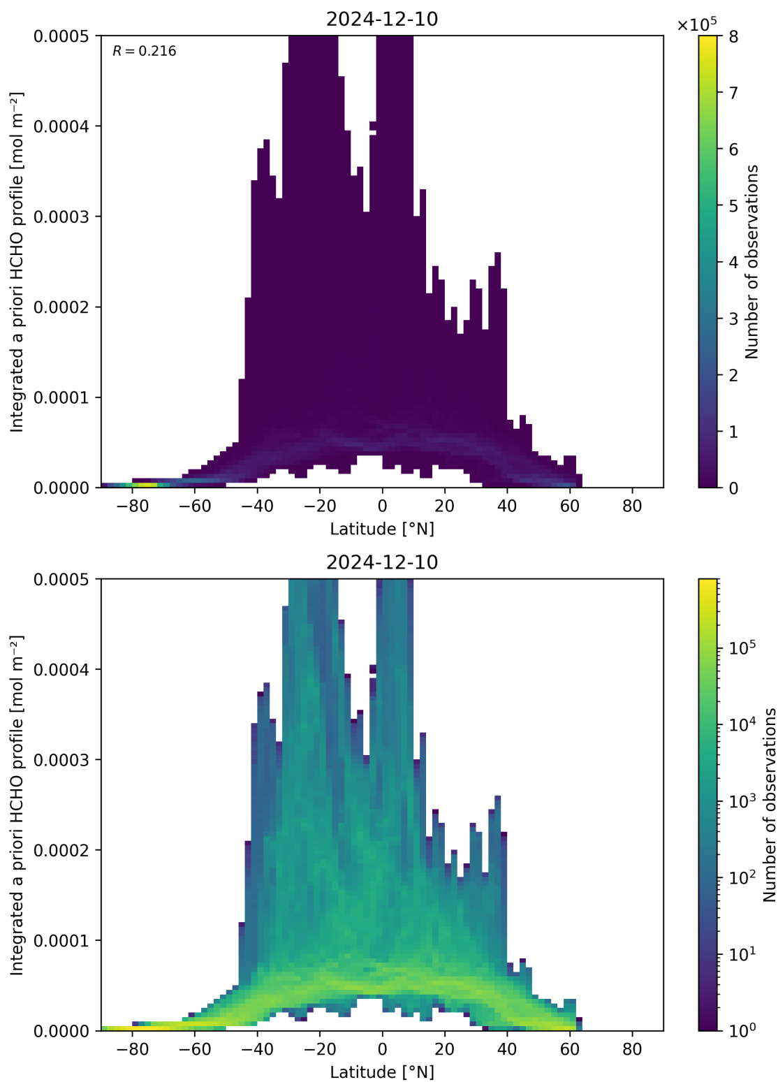
Figure 166: Scatter density plot of “Latitude” against “Integrated a priori HCHO profile” for 2024-12-09 to 2024-12-11.
