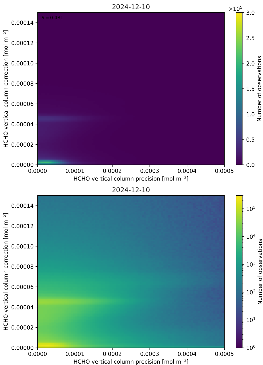
Figure 146: Scatter density plot of “HCHO vertical column precision” against “HCHO vertical column correction” for 2024-12-09 to 2024-12-11.
