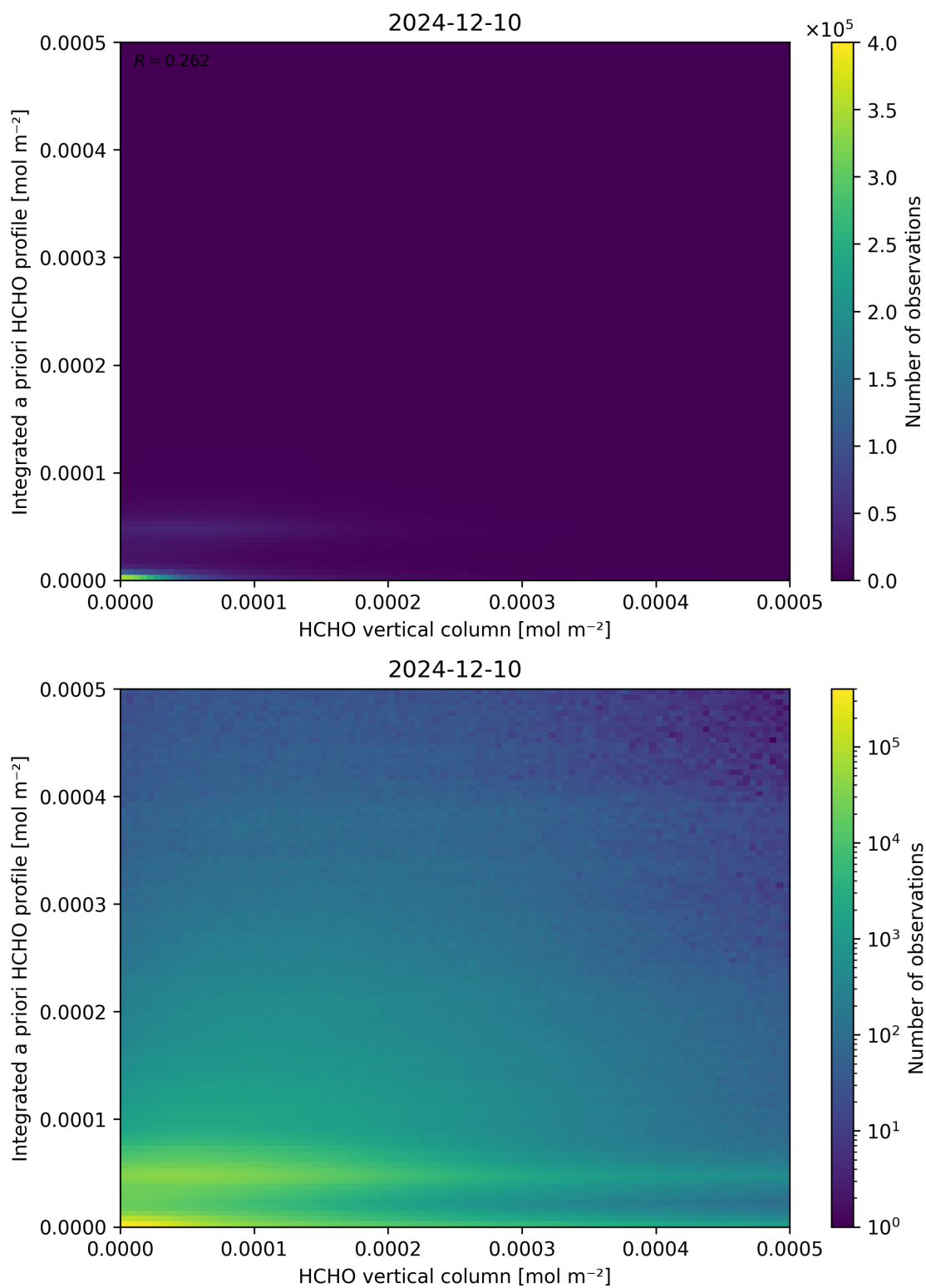
Figure 135: Scatter density plot of “HCHO vertical column” against “Integrated a priori HCHO profile” for 2024-12-09 to 2024-12-11.
