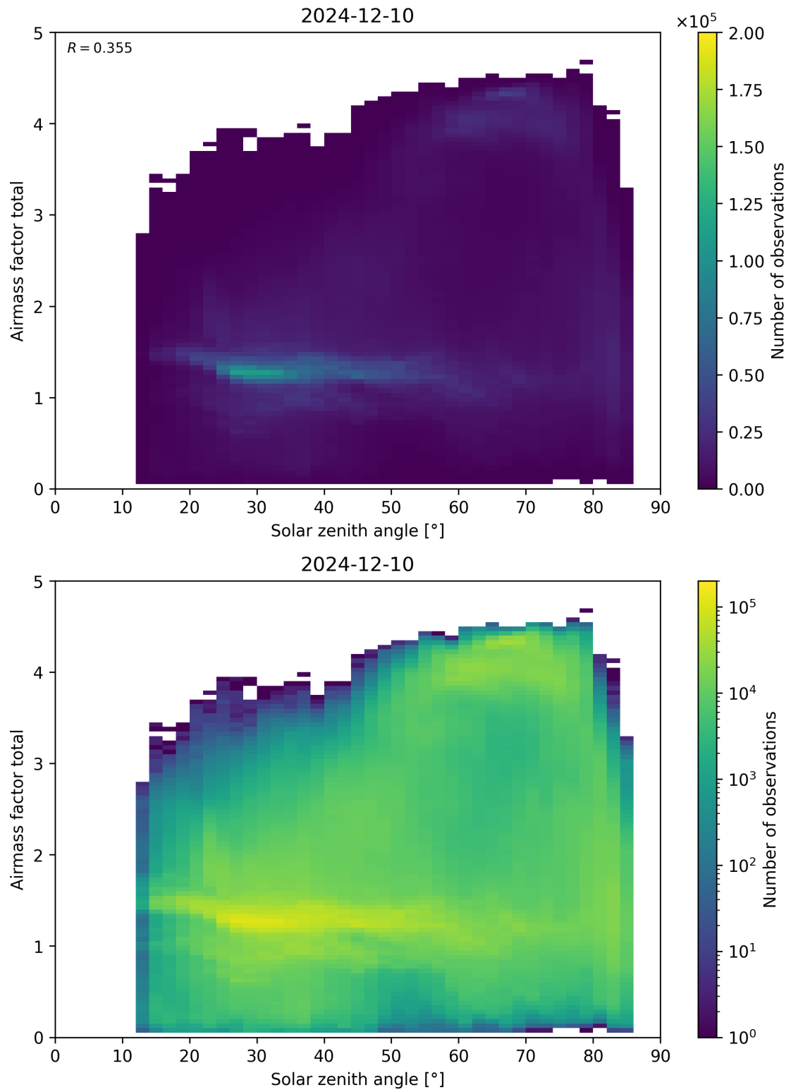
Figure 175: Scatter density plot of “Solar zenith angle” against “Airmass factor total” for 2024-12-09 to 2024-12-11.
