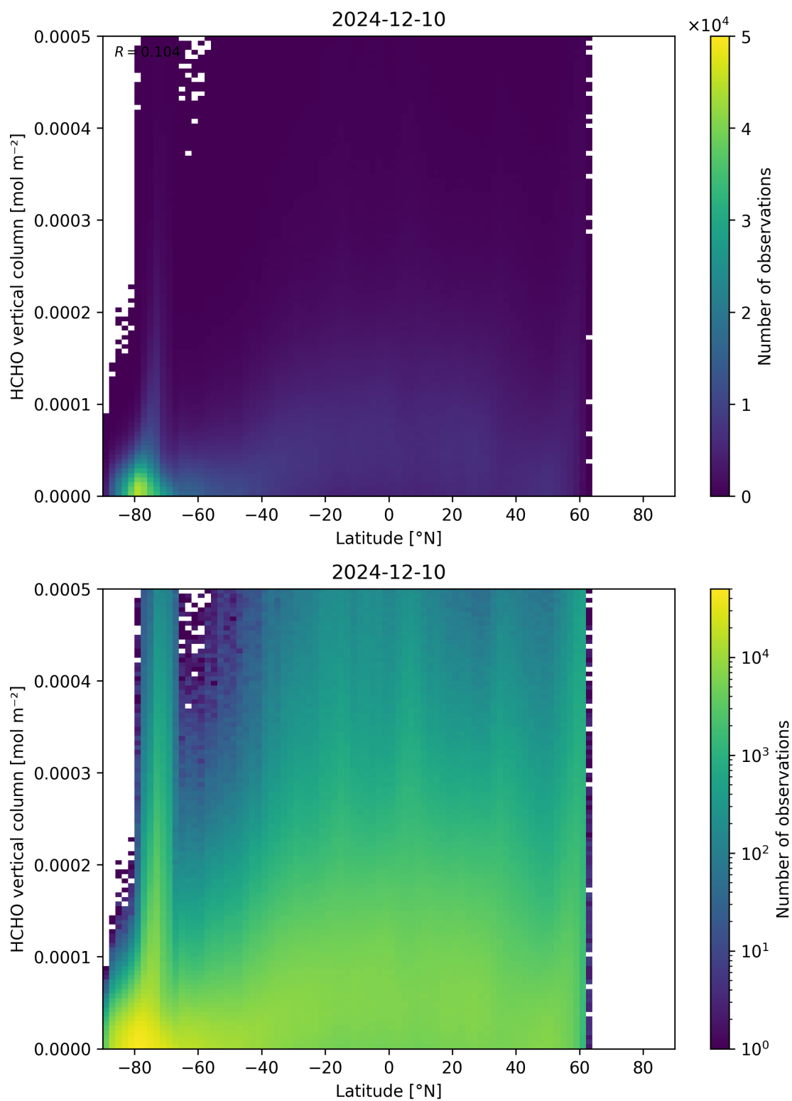
Figure 163: Scatter density plot of “Latitude” against “HCHO vertical column” for 2024-12-09 to 2024-12-11.
