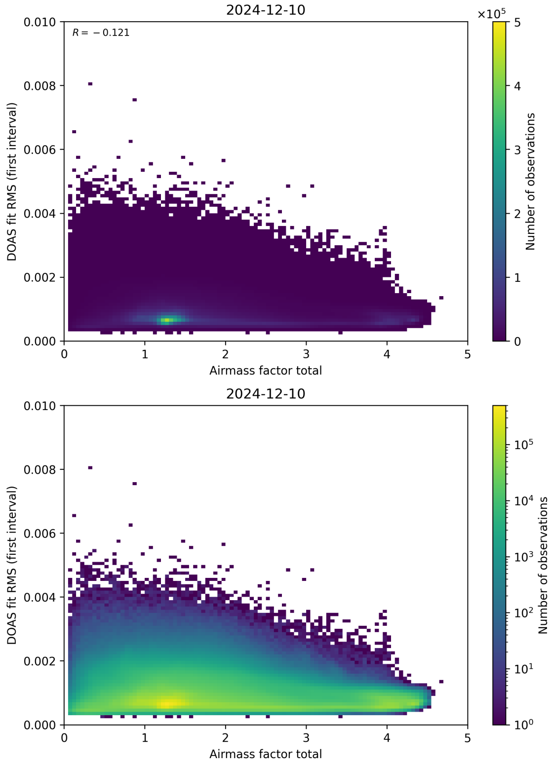
Figure 97: Scatter density plot of “Airmass factor total” against “DOAS fit RMS (first interval)” for 2024-12-09 to 2024-12-11.
