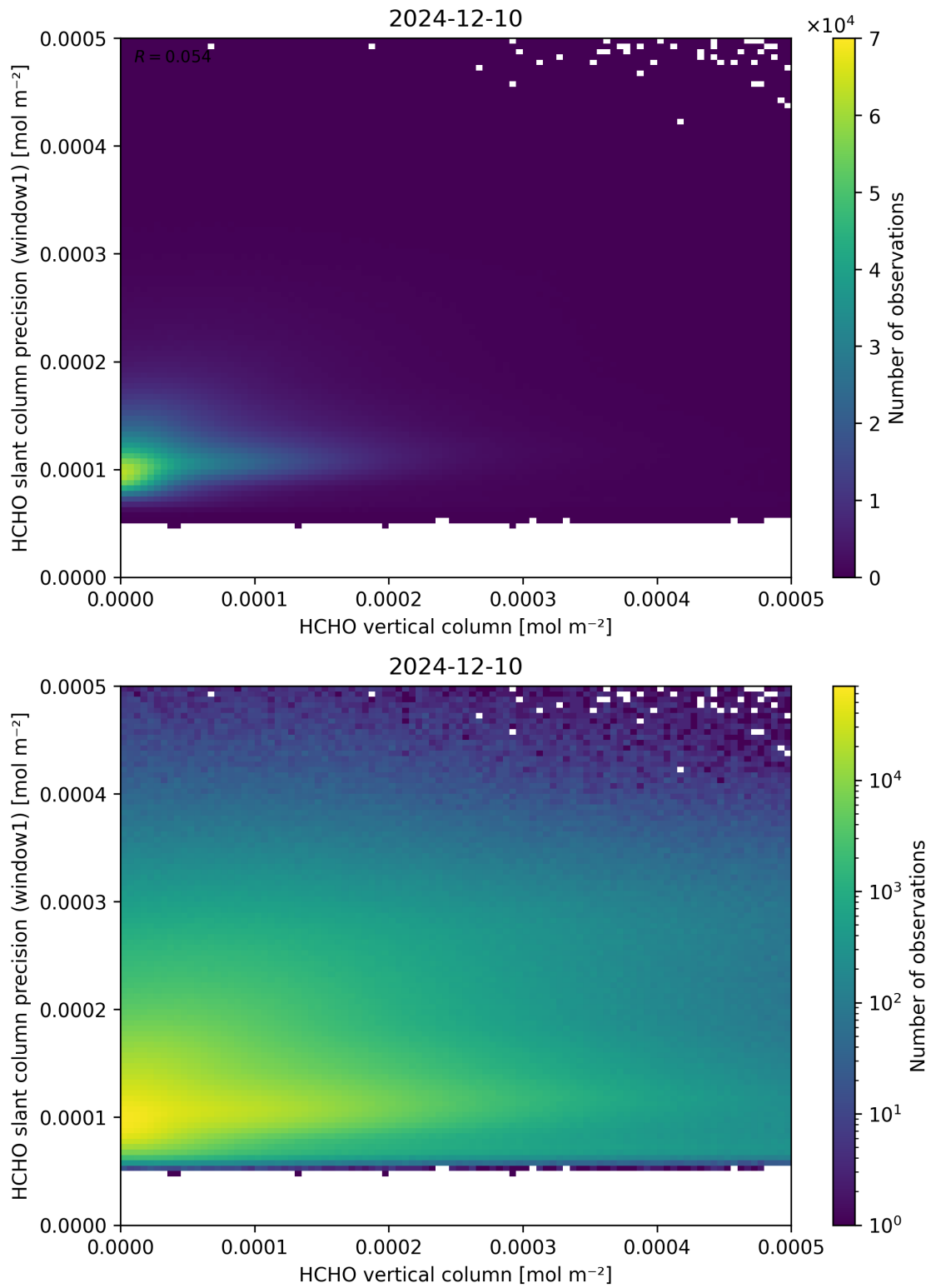
Figure 130: Scatter density plot of “HCHO vertical column” against “HCHO slant column precision (window1)” for 2024-12-09 to 2024-12-11.
