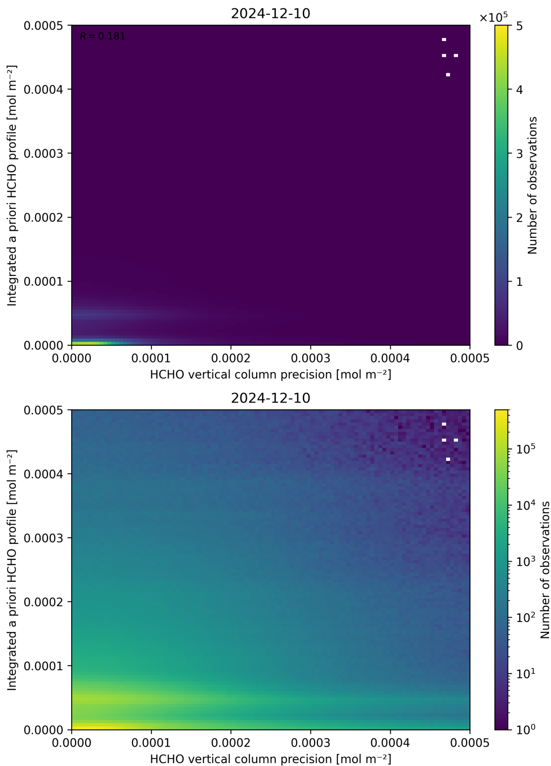
Figure 147: Scatter density plot of “HCHO vertical column precision” against “Integrated a priori HCHO profile” for 2024-12-09 to 2024-12-11.
