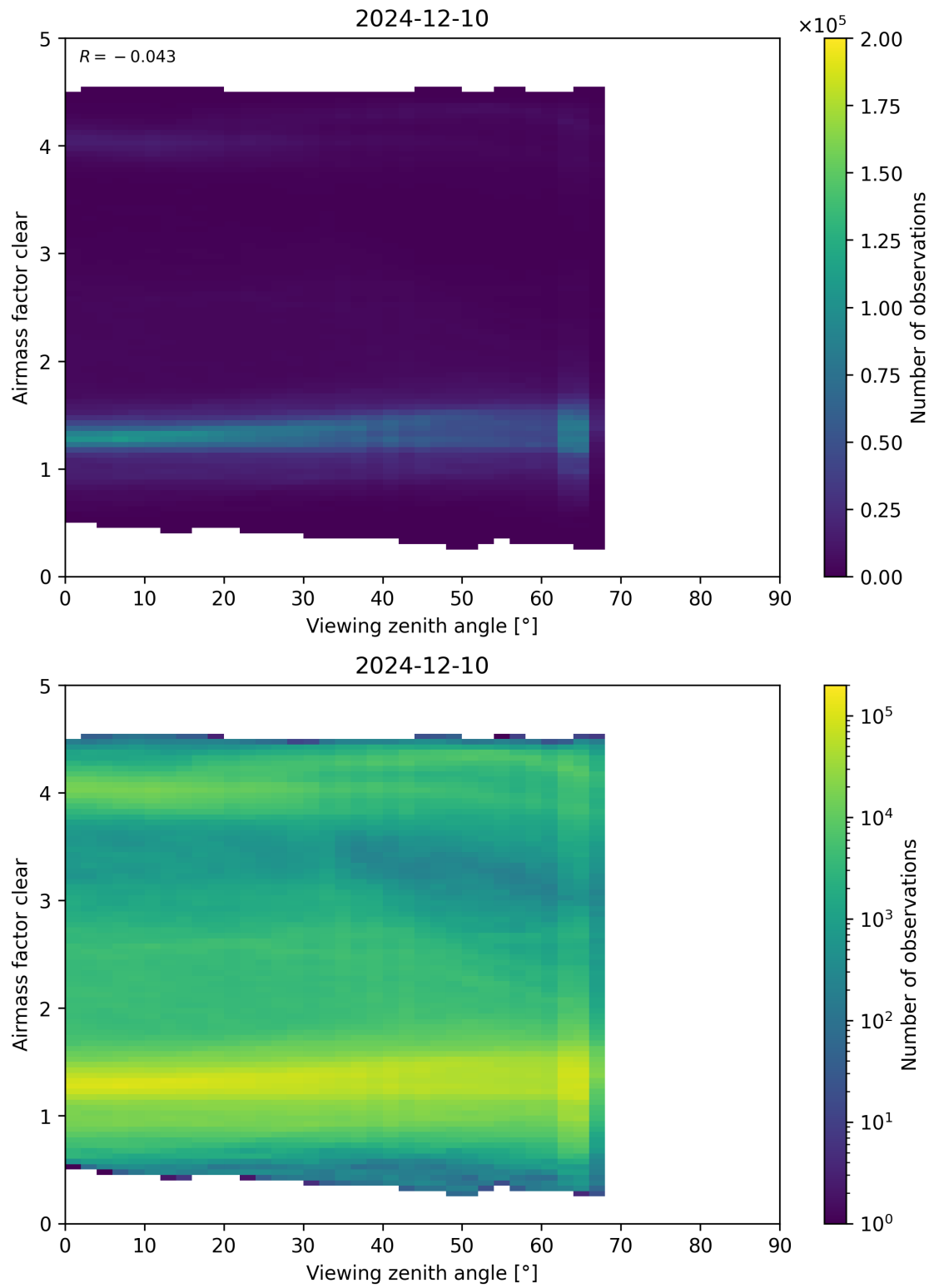
Figure 185: Scatter density plot of “Viewing zenith angle” against “Airmass factor clear” for 2024-12-09 to 2024-12-11.
