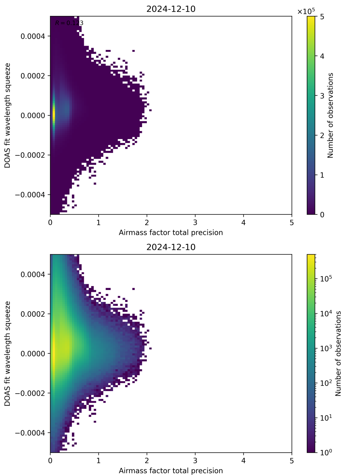
Figure 107: Scatter density plot of “Airmass factor total precision” against “DOAS fit wavelength squeeze” for 2024-12-09 to 2024-12-11.
