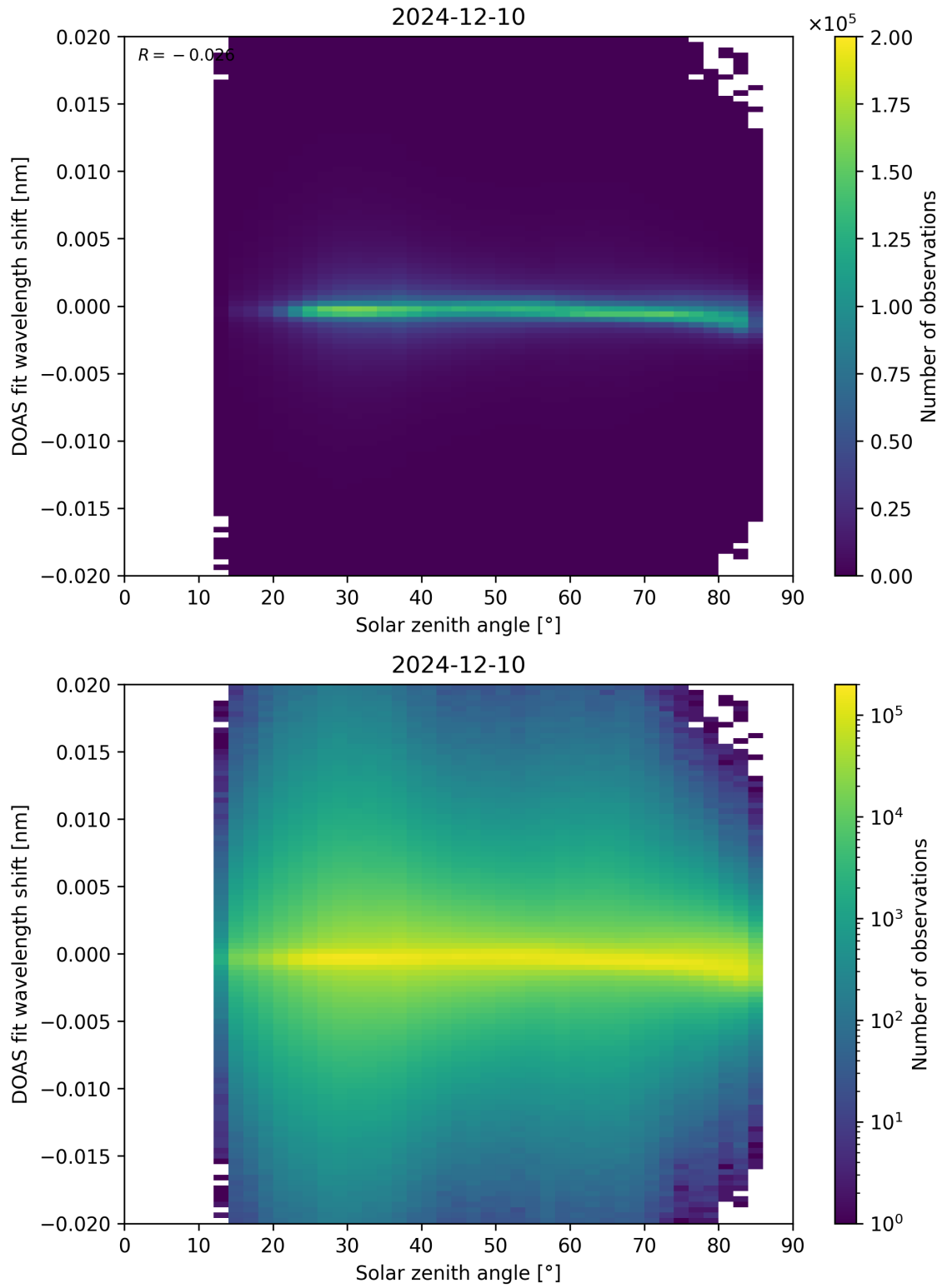
Figure 168: Scatter density plot of “Solar zenith angle” against “DOAS fit wavelength shift” for 2024-12-09 to 2024-12-11.
