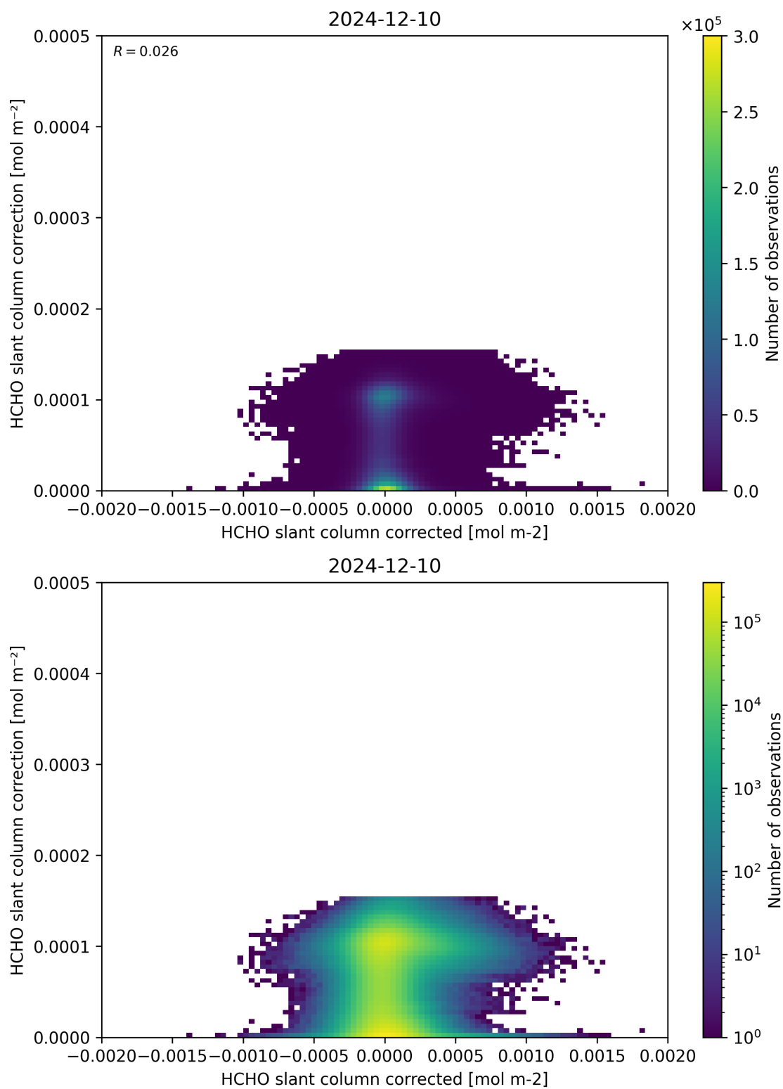
Figure 77: Scatter density plot of “HCHO slant column corrected” against “HCHO slant column correction” for 2024-12-09 to 2024-12-11.
