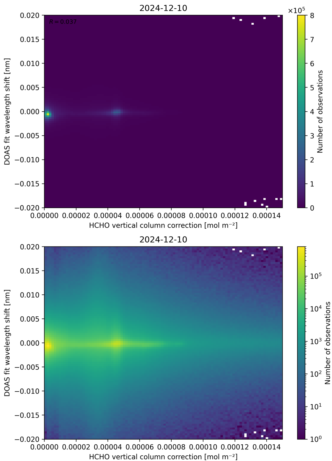
Figure 113: Scatter density plot of “HCHO vertical column correction” against “DOAS fit wavelength shift” for 2024-12-09 to 2024-12-11.
