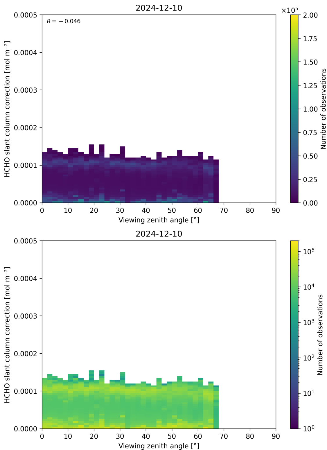
Figure 187: Scatter density plot of “Viewing zenith angle” against “HCHO slant column correction” for 2024-12-09 to 2024-12-11.
