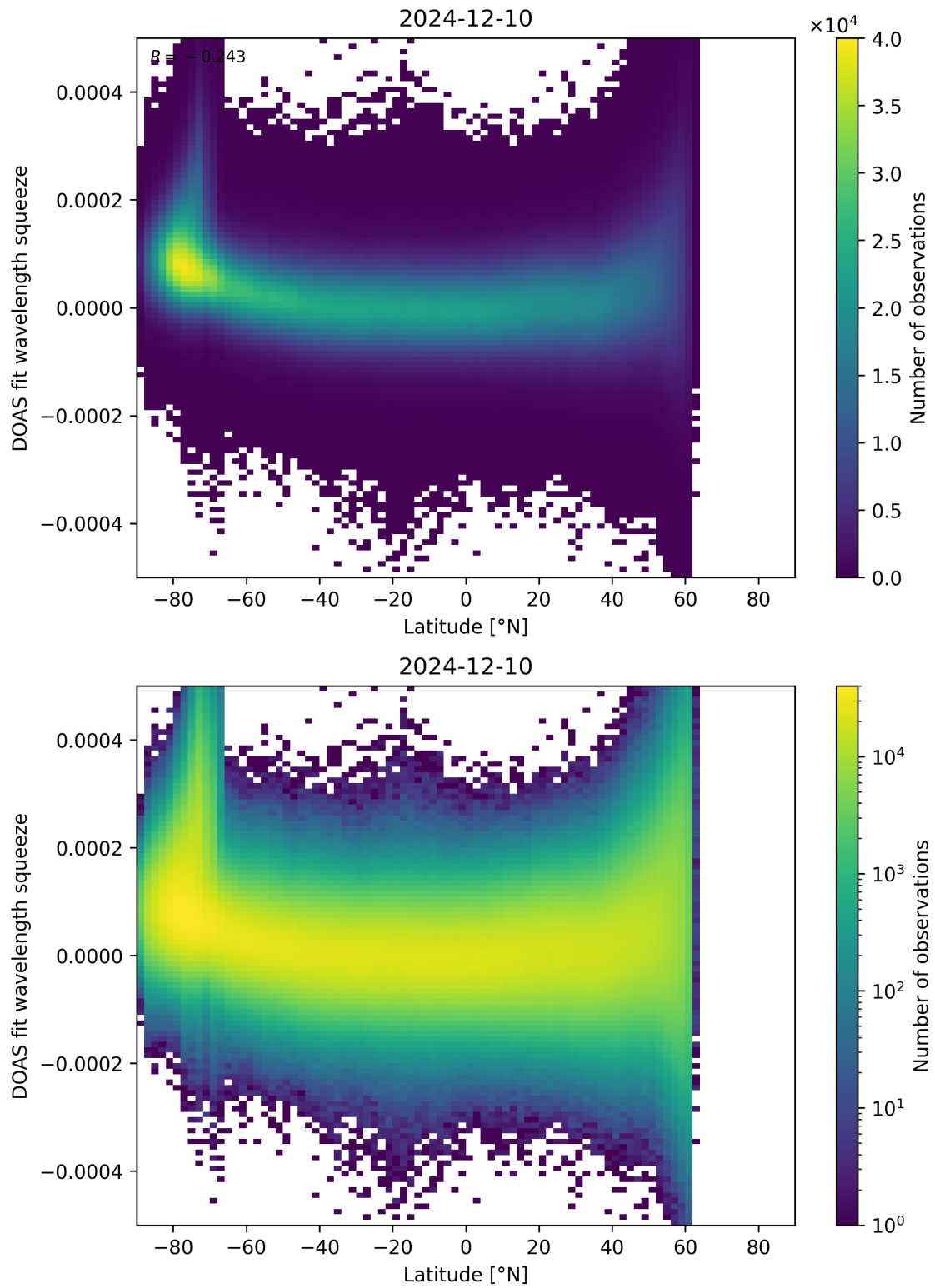
Figure 155: Scatter density plot of “Latitude” against “DOAS fit wavelength squeeze” for 2024-12-09 to 2024-12-11.
