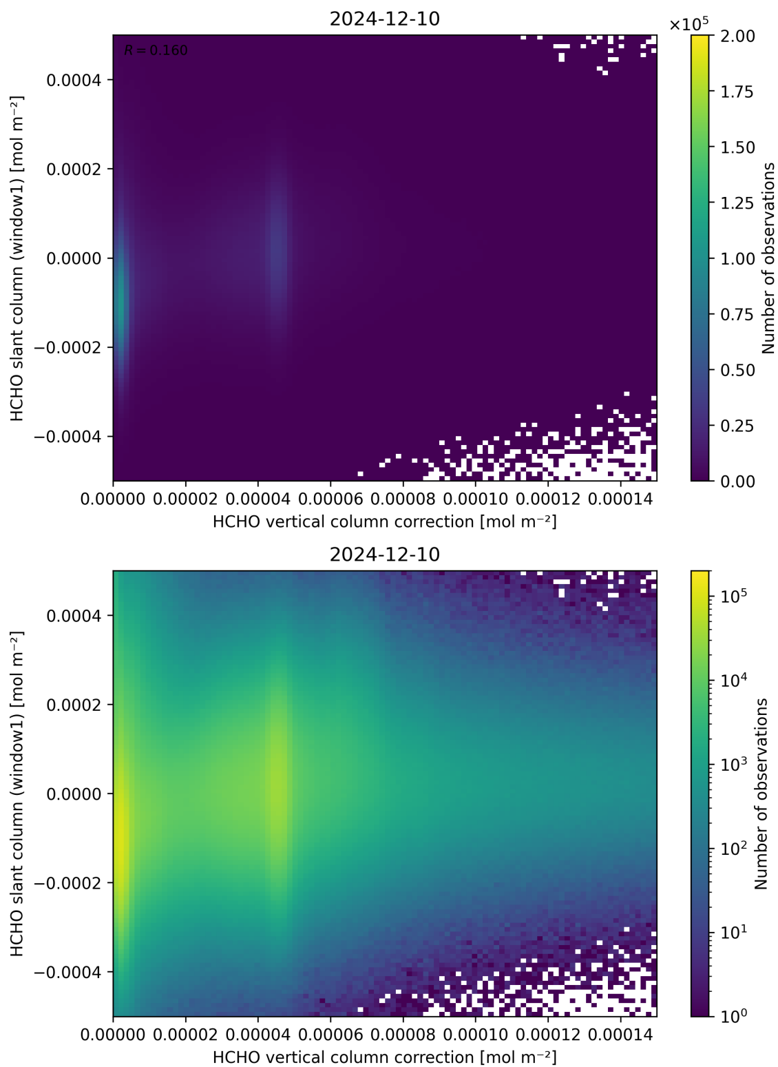
Figure 118: Scatter density plot of “HCHO vertical column correction” against “HCHO slant column (window1)” for 2024-12-09 to 2024-12-11.
