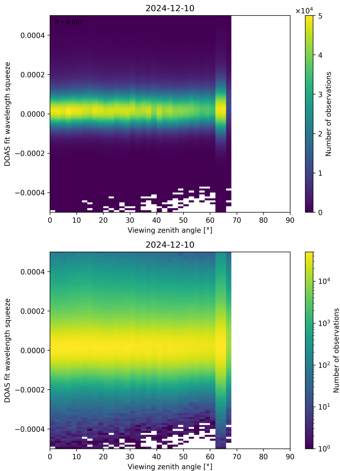
Figure 184: Scatter density plot of “Viewing zenith angle” against “DOAS fit wavelength squeeze” for 2024-12-09 to 2024-12-11.
