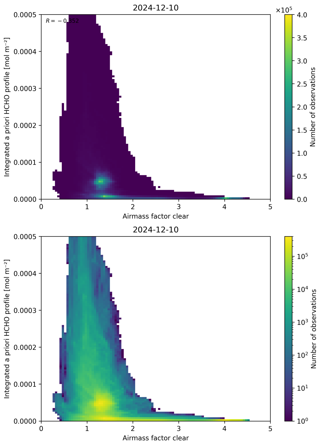
Figure 76: Scatter density plot of “Airmass factor clear” against “Integrated a priori HCHO profile” for 2024-12-09 to 2024-12-11.
