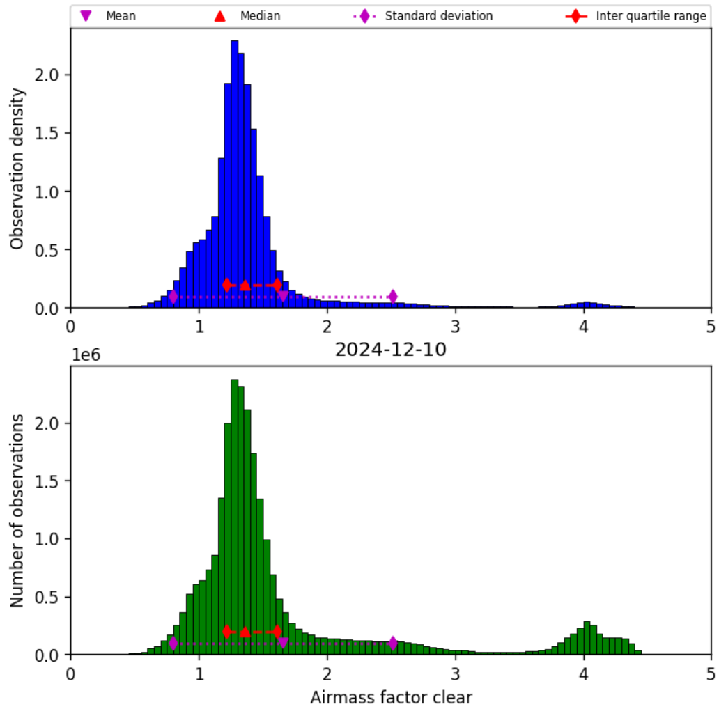
Figure 42: Histogram of “Airmass factor clear” for 2024-12-09 to 2024-12-11
