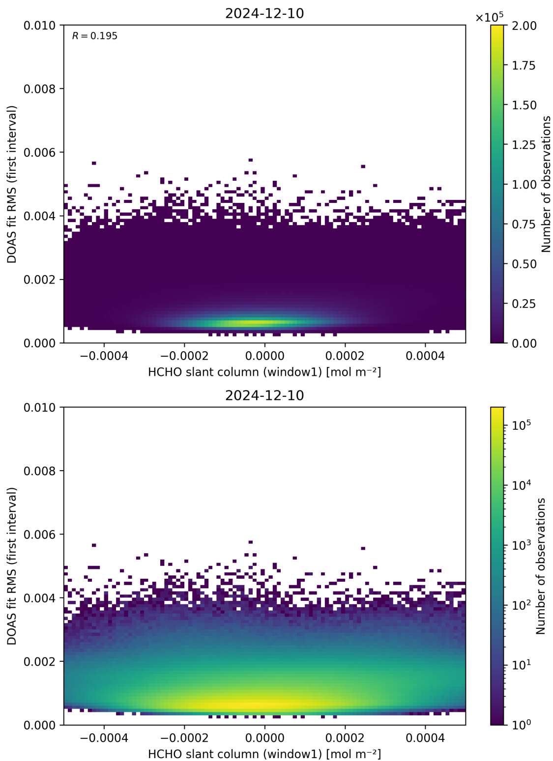
Figure 78: Scatter density plot of “HCHO slant column (window1)” against “DOAS fit RMS (first interval)” for 2024-12-09 to 2024-12-11.
