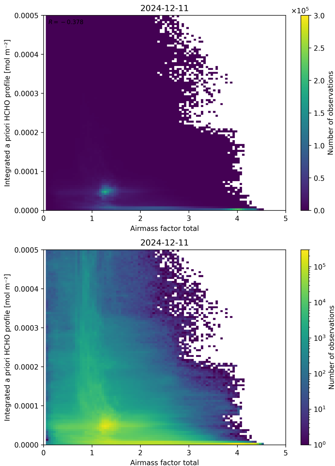
Figure 104: Scatter density plot of “Airmass factor total” against “Integrated a priori HCHO profile” for 2024-12-11 to 2024-12-12.
