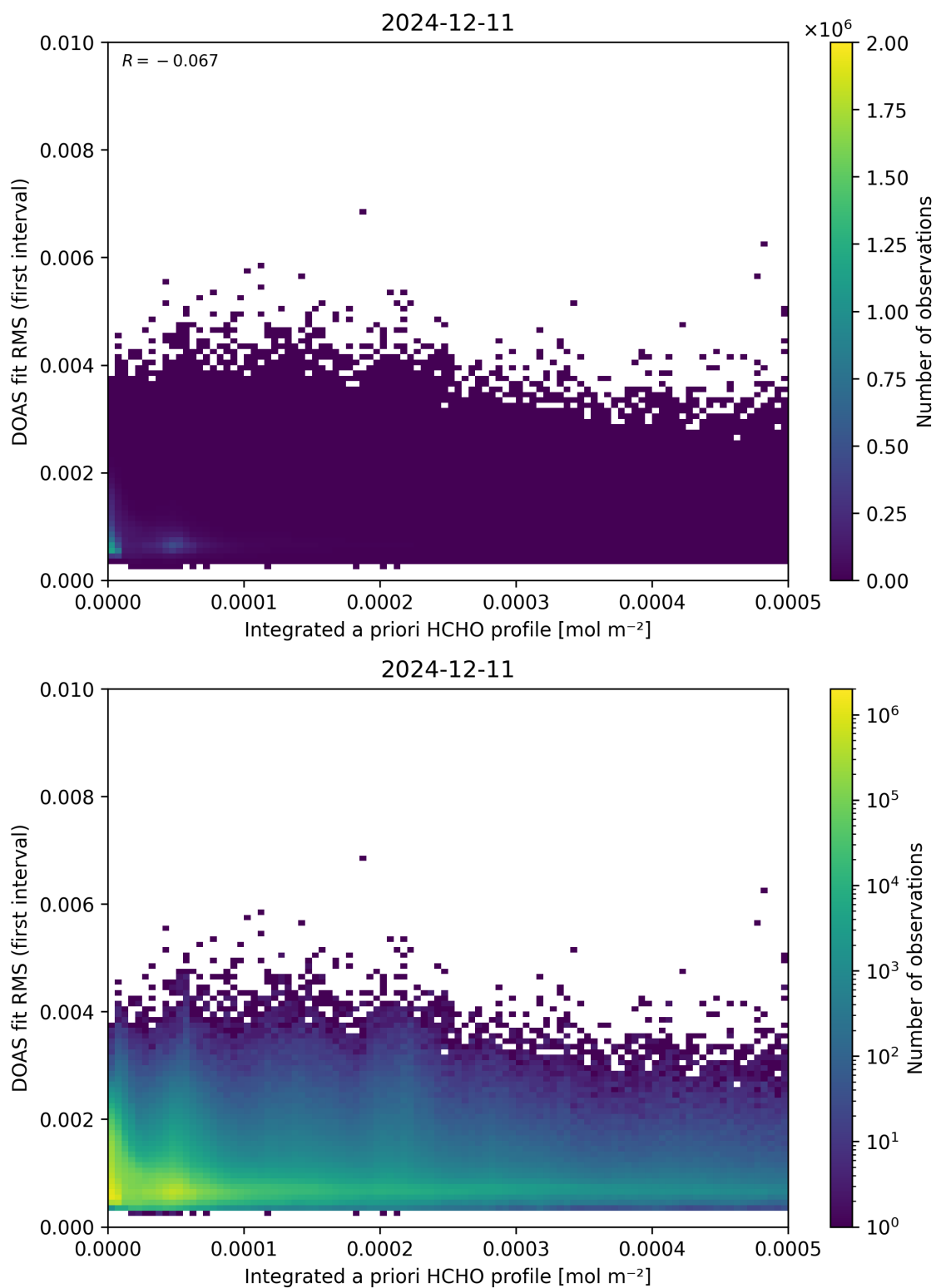
Figure 148: Scatter density plot of “Integrated a priori HCHO profile” against “DOAS fit RMS (first interval)” for 2024-12-11 to 2024-12-12.
