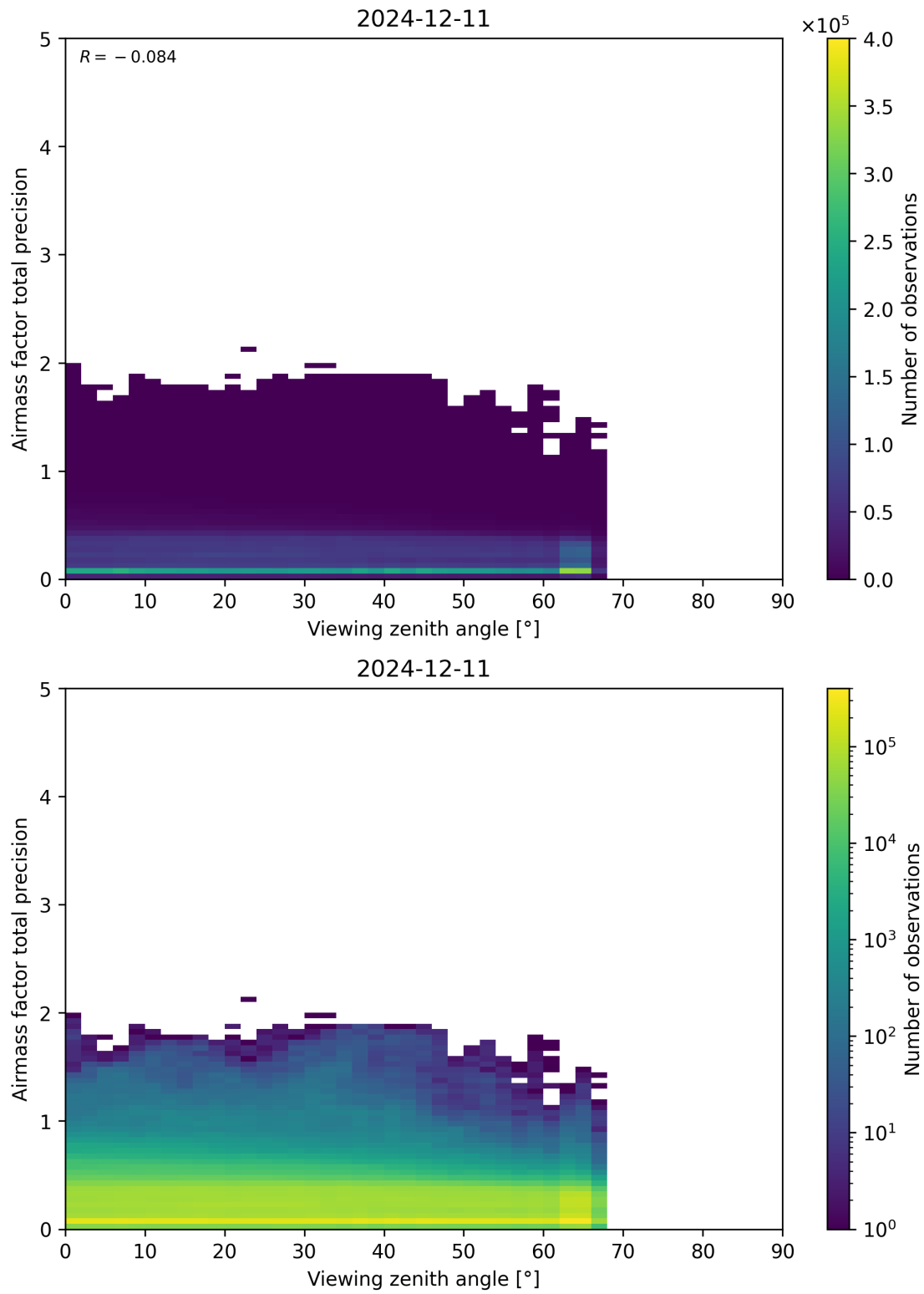
Figure 191: Scatter density plot of “Viewing zenith angle” against “Airmass factor total precision” for 2024-12-11 to 2024-12-12.
