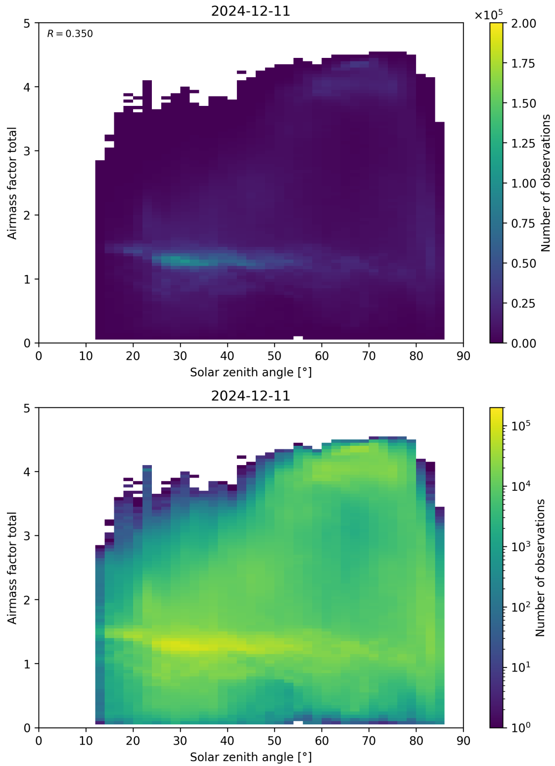
Figure 175: Scatter density plot of “Solar zenith angle” against “Airmass factor total” for 2024-12-11 to 2024-12-12.
