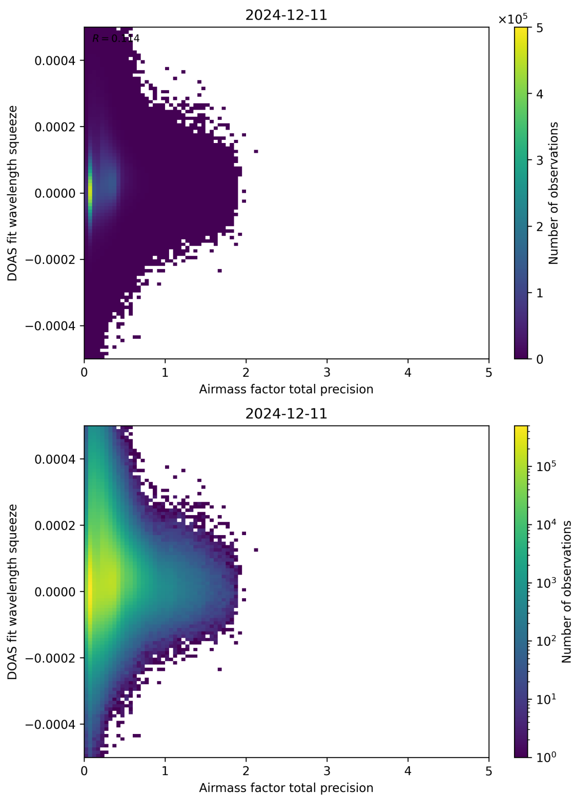
Figure 107: Scatter density plot of “Airmass factor total precision” against “DOAS fit wavelength squeeze” for 2024-12-11 to 2024-12-12.
