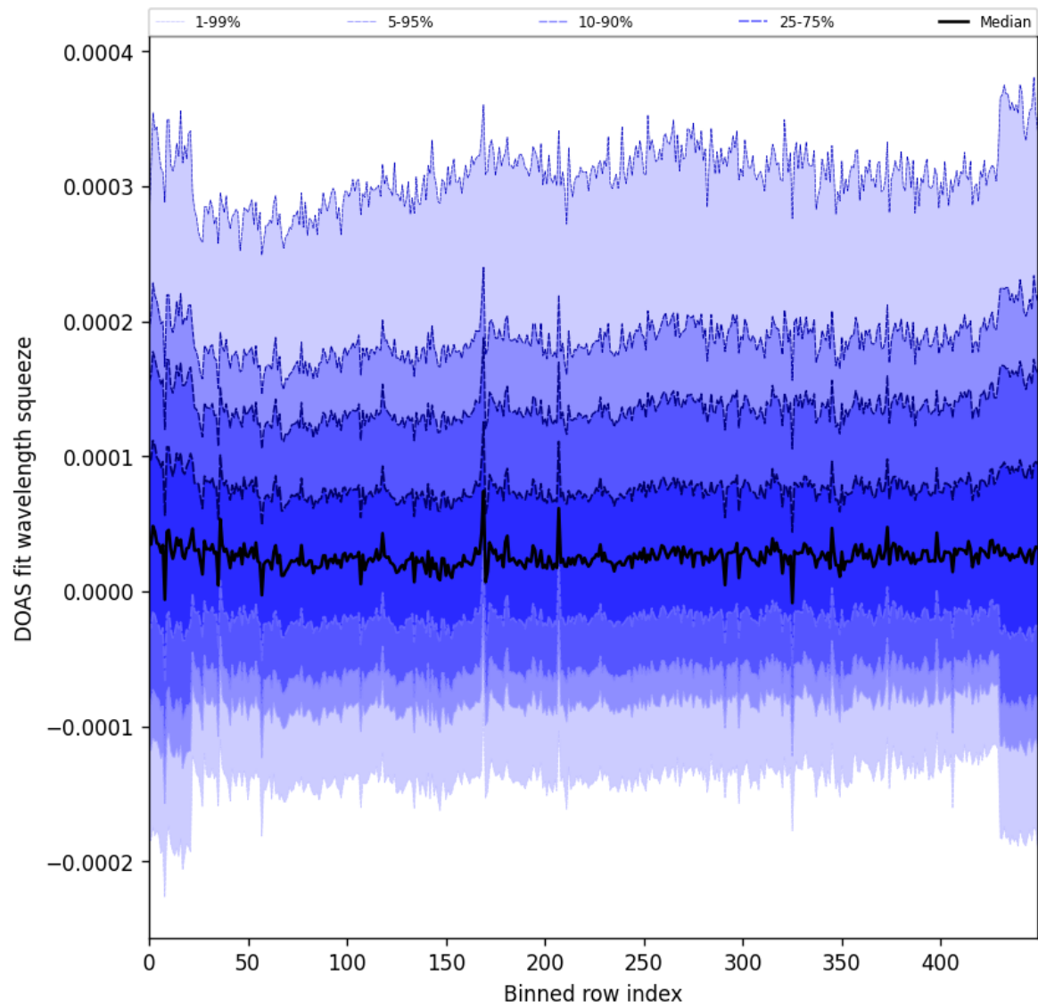
Figure 59: Along track statistics of “DOAS fit wavelength squeeze” for 2024-12-11 to 2024-12-12
