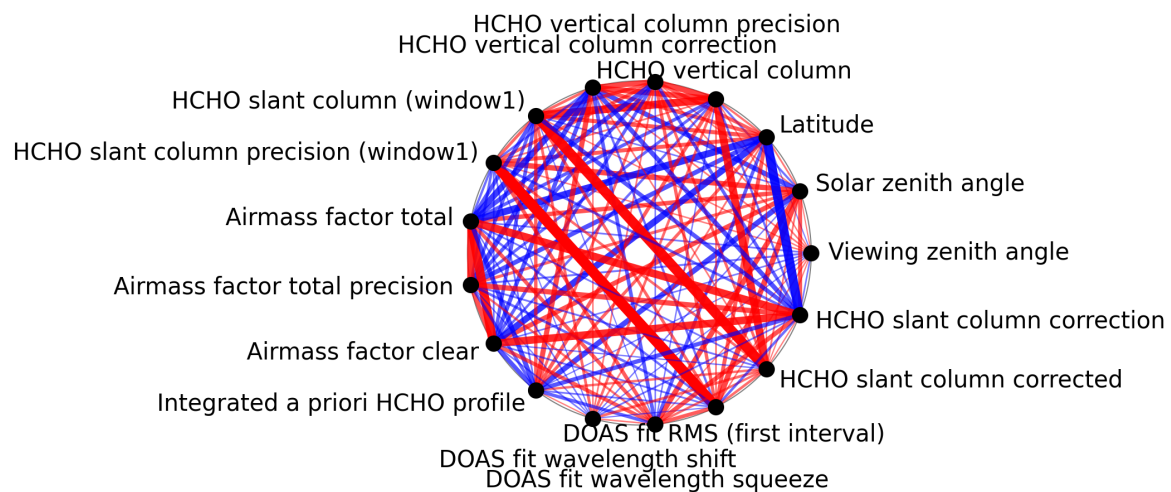
Figure 1: Map of correlation graph for 2024-12-11 to 2024-12-12.
