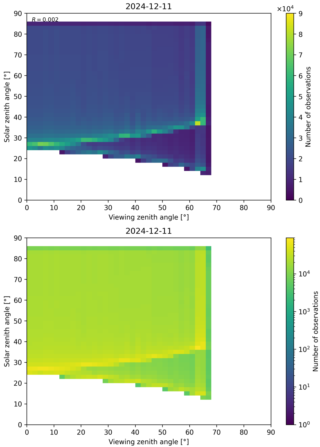
Figure 197: Scatter density plot of “Viewing zenith angle” against “Solar zenith angle” for 2024-12-11 to 2024-12-12.
