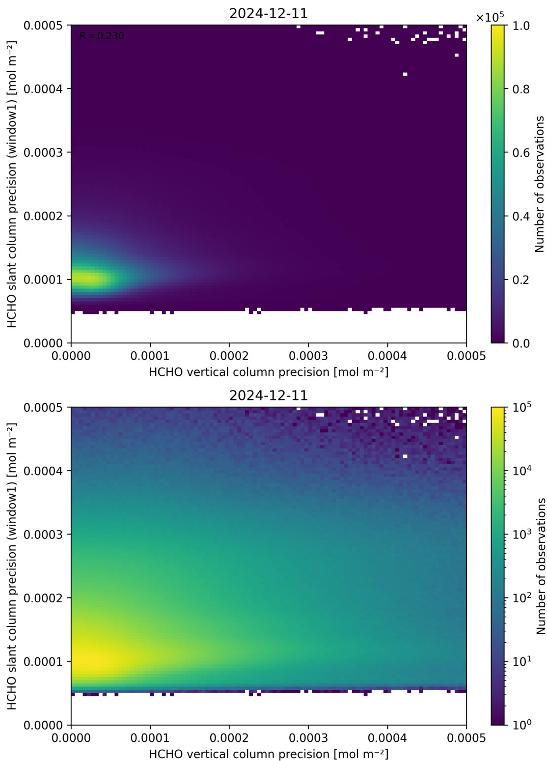
Figure 143: Scatter density plot of “HCHO vertical column precision” against “HCHO slant column precision (window1)” for 2024-12-11 to 2024-12-12.
