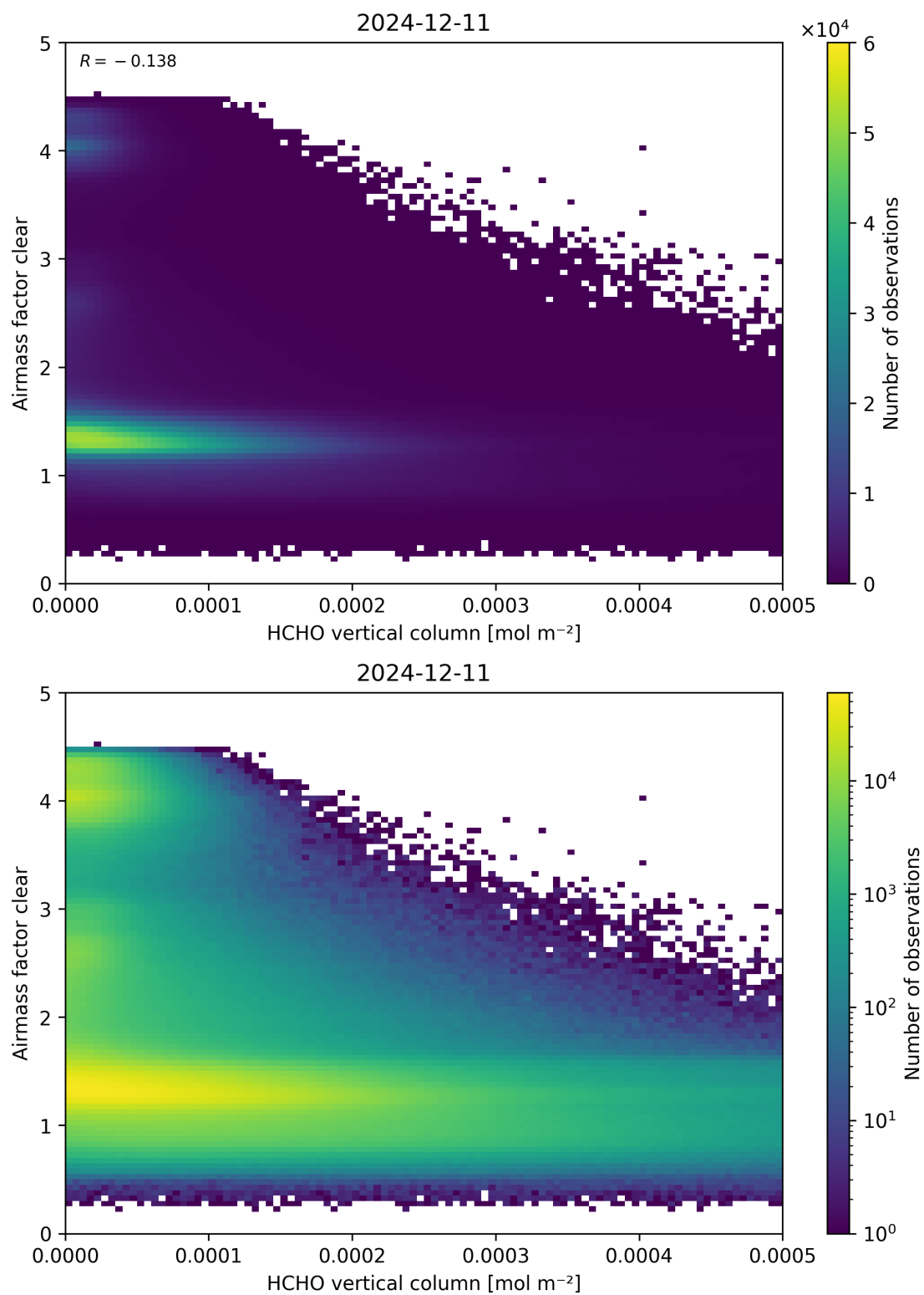
Figure 126: Scatter density plot of “HCHO vertical column” against “Airmass factor clear” for 2024-12-11 to 2024-12-12.
