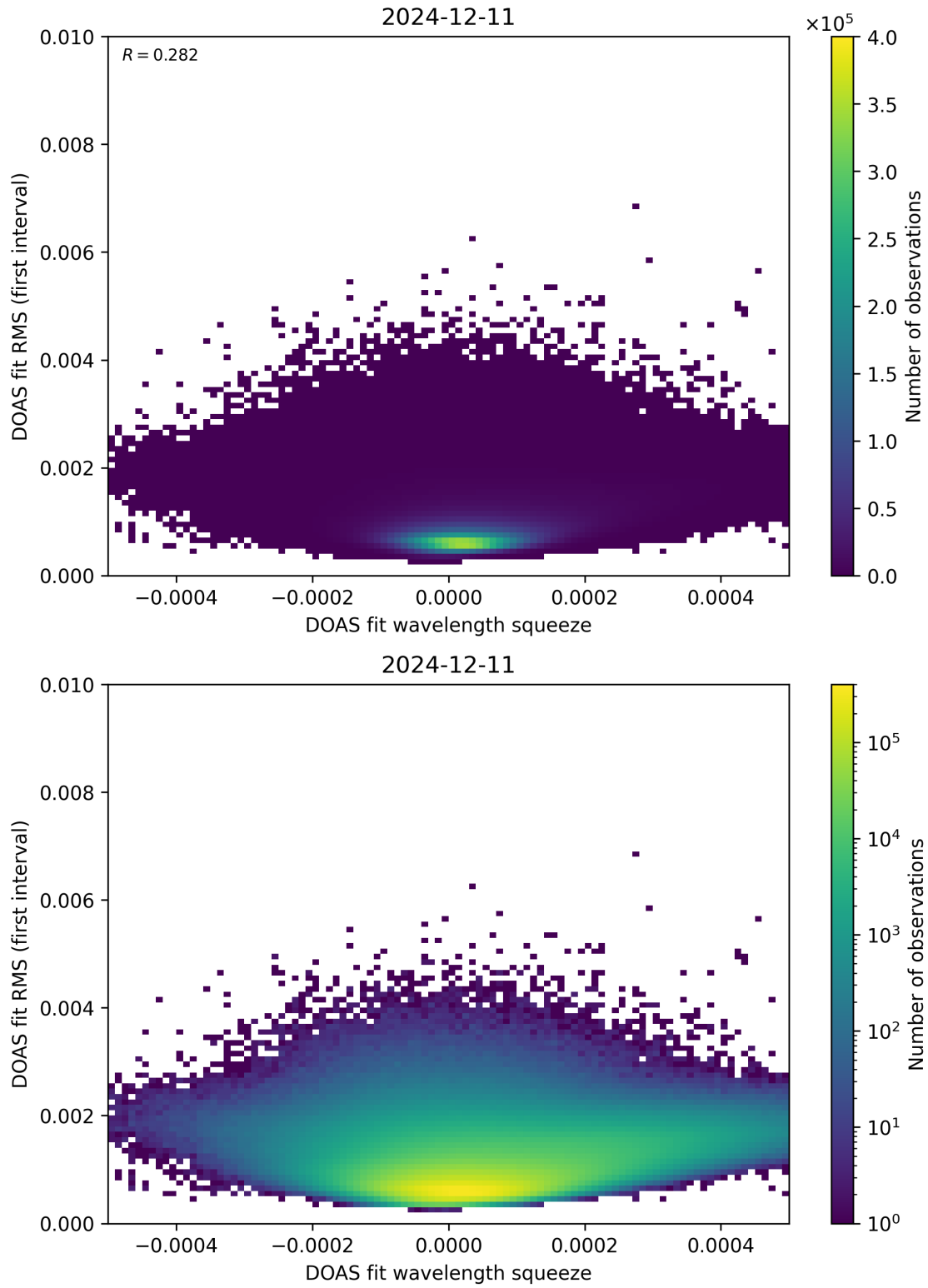
Figure 68: Scatter density plot of “DOAS fit wavelength squeeze” against “DOAS fit RMS (first interval)” for 2024-12-11 to 2024-12-12.
