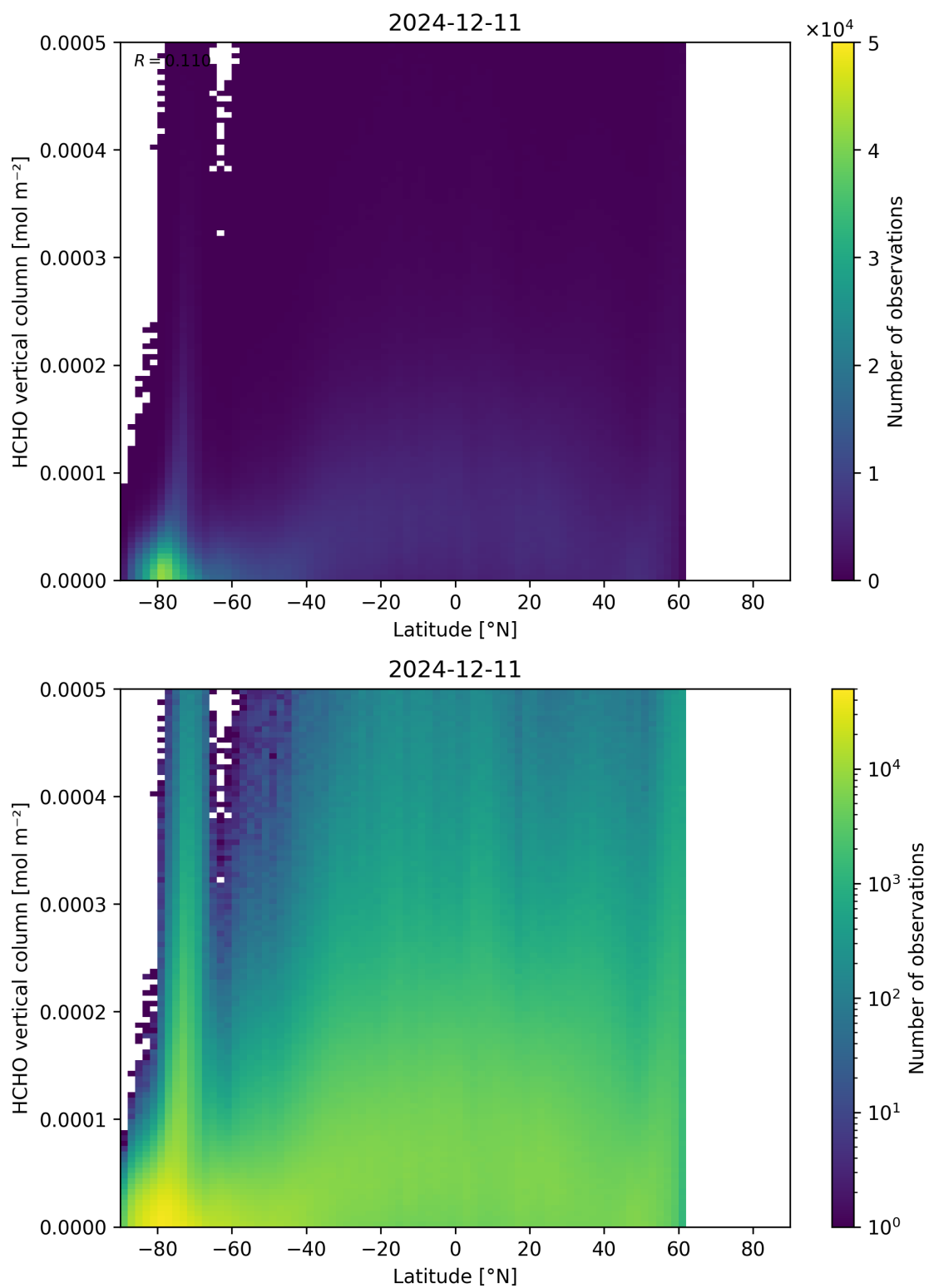
Figure 163: Scatter density plot of “Latitude” against “HCHO vertical column” for 2024-12-11 to 2024-12-12.
