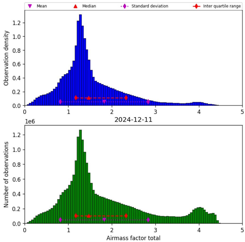
Figure 40: Histogram of “Airmass factor total” for 2024-12-11 to 2024-12-12
