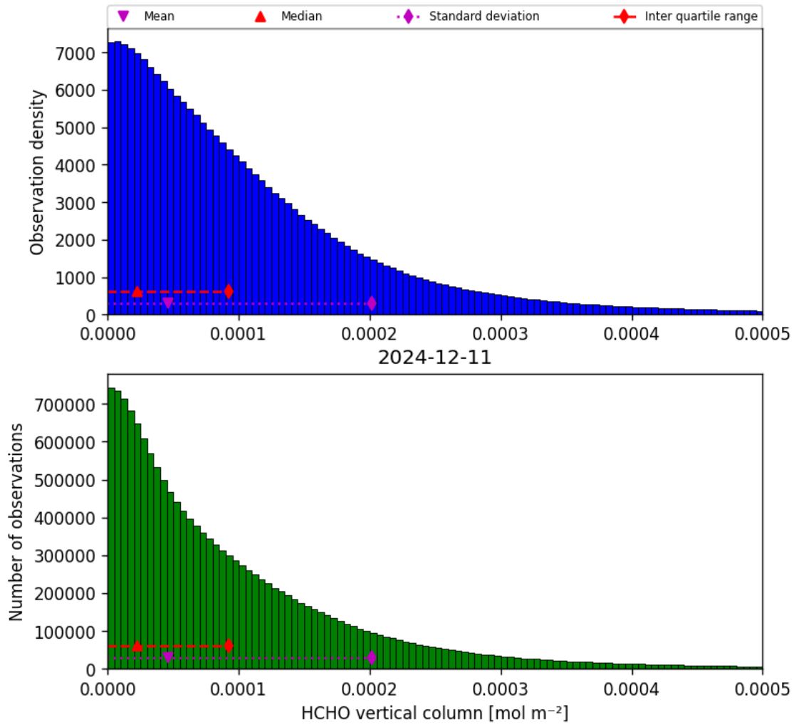
Figure 35: Histogram of “HCHO vertical column” for 2024-12-11 to 2024-12-12
