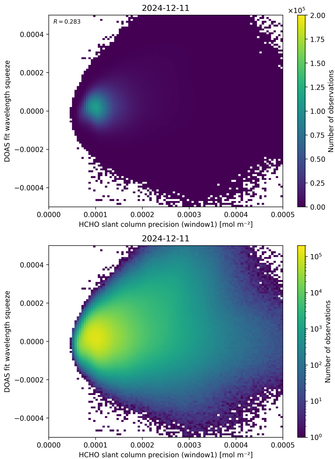
Figure 90: Scatter density plot of “HCHO slant column precision (window1)” against “DOAS fit wavelength squeeze” for 2024-12-11 to 2024-12-12.
