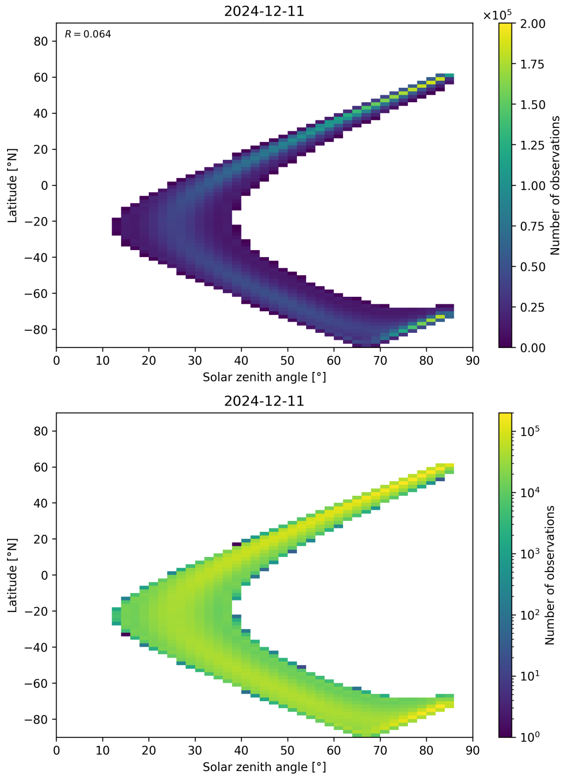
Figure 181: Scatter density plot of “Solar zenith angle” against “Latitude” for 2024-12-11 to 2024-12-12.
