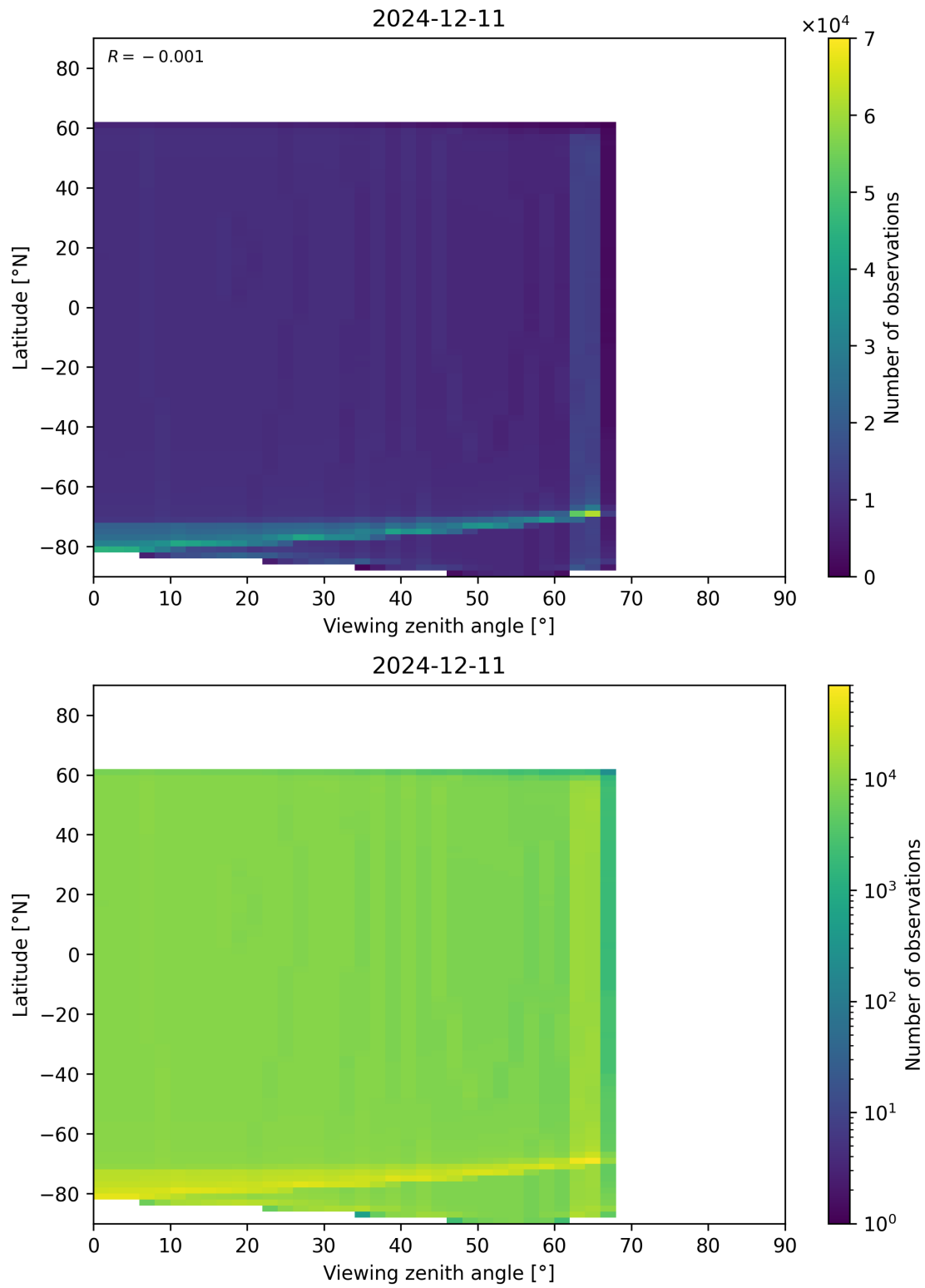
Figure 196: Scatter density plot of “Viewing zenith angle” against “Latitude” for 2024-12-11 to 2024-12-12.
