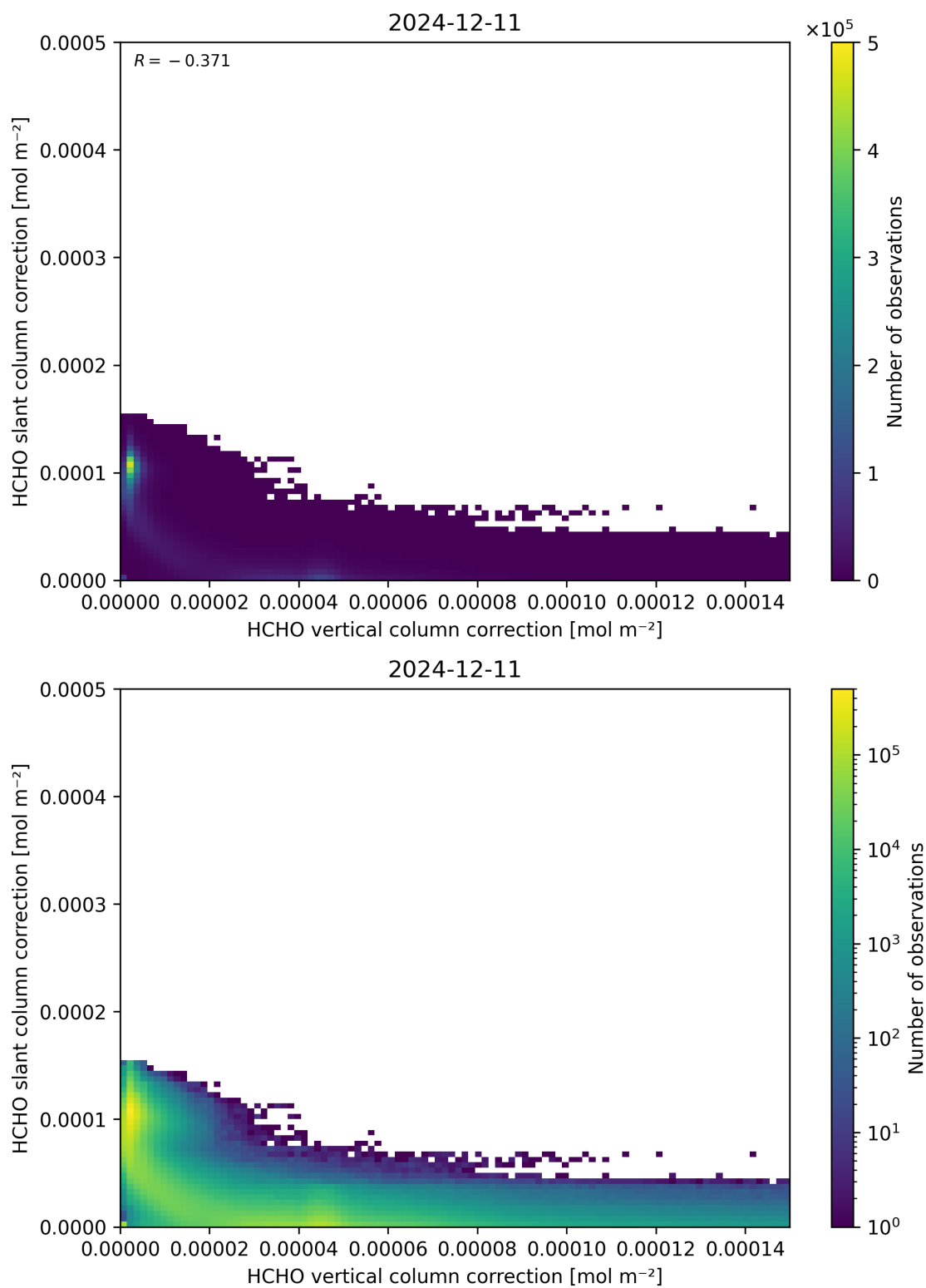
Figure 117: Scatter density plot of “HCHO vertical column correction” against “HCHO slant column correction” for 2024-12-11 to 2024-12-12.
