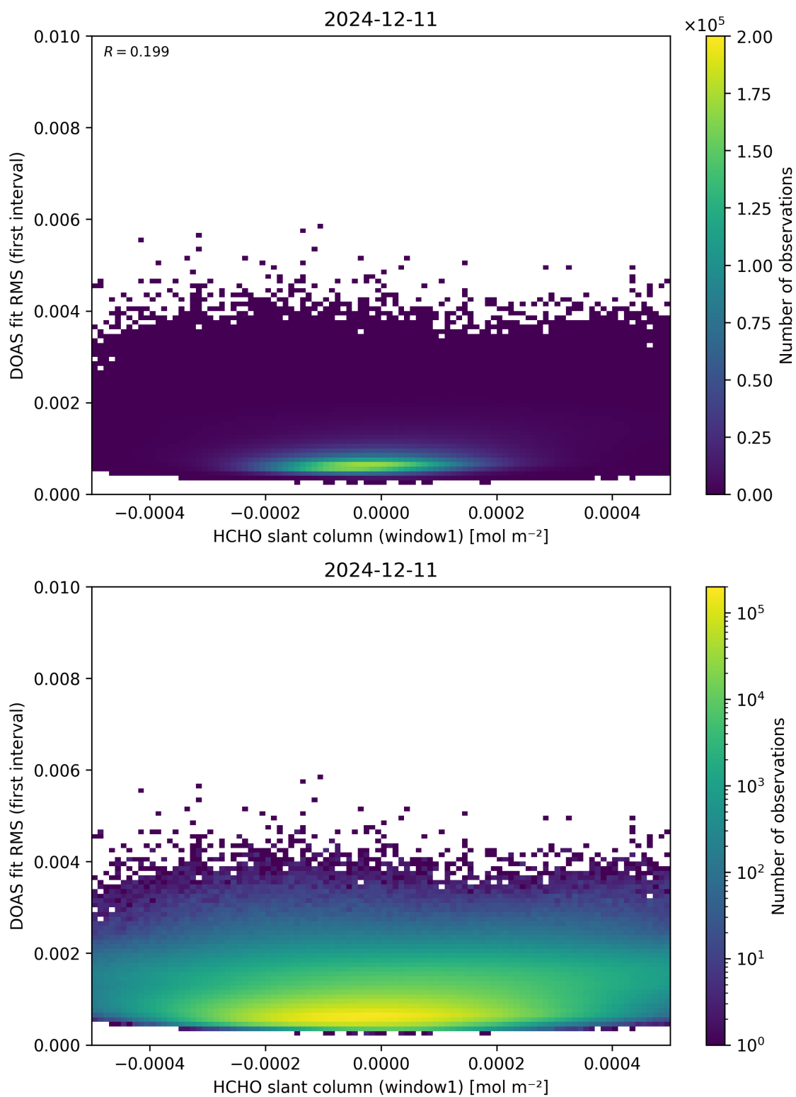
Figure 78: Scatter density plot of “HCHO slant column (window1)” against “DOAS fit RMS (first interval)” for 2024-12-11 to 2024-12-12.
