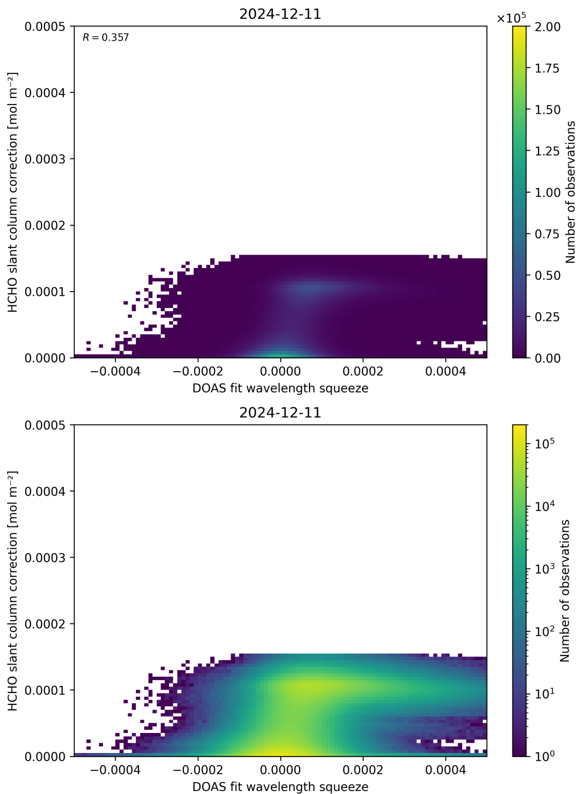
Figure 70: Scatter density plot of “DOAS fit wavelength squeeze” against “HCHO slant column correction” for 2024-12-11 to 2024-12-12.
