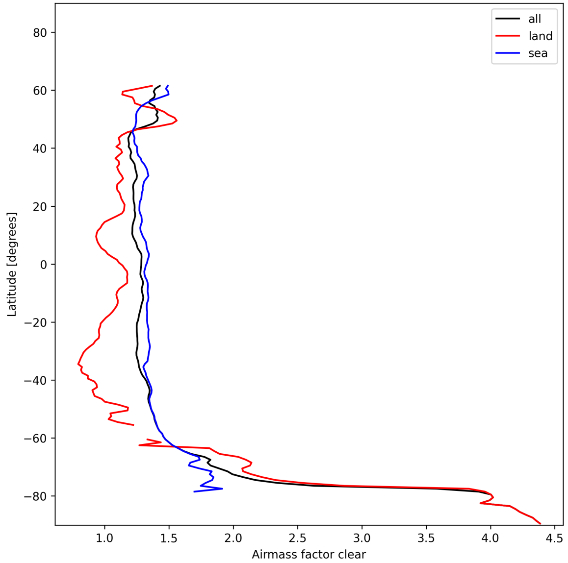
Figure 28: Zonal average of “Airmass factor clear” for 2024-12-11 to 2024-12-12.
