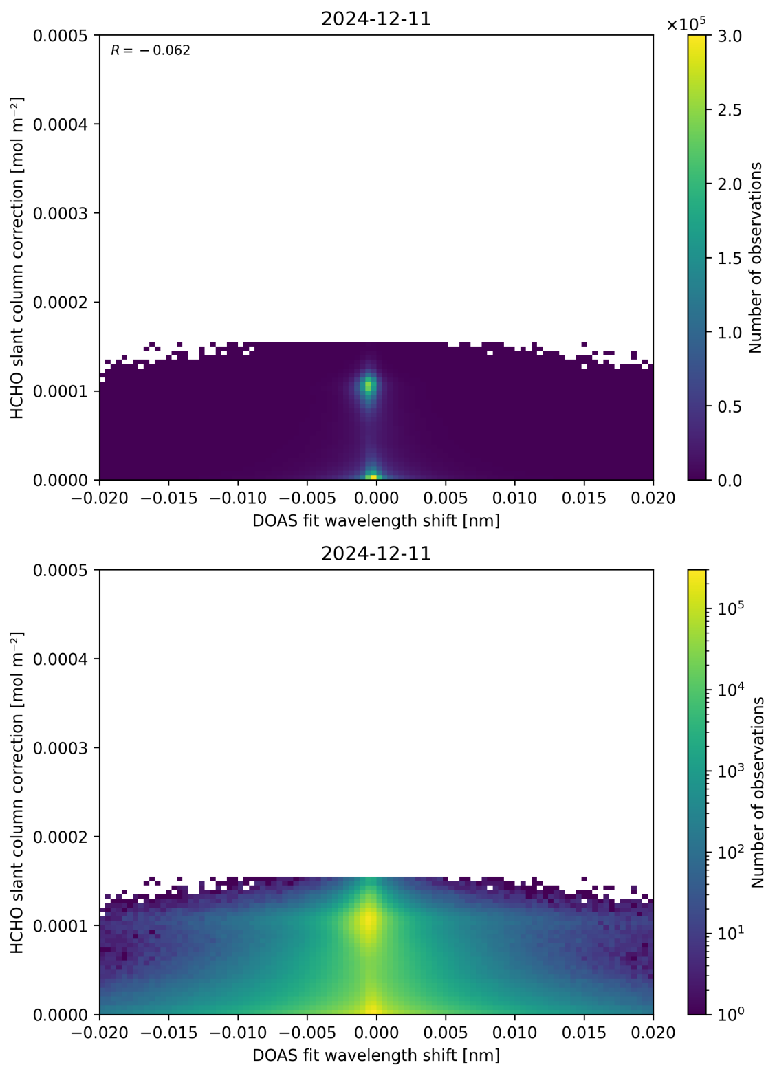
Figure 67: Scatter density plot of “DOAS fit wavelength shift” against “HCHO slant column correction” for 2024-12-11 to 2024-12-12.
