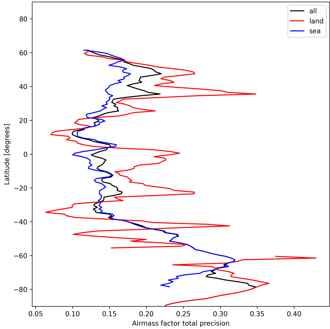
Figure 27: Zonal average of “Airmass factor total precision” for 2024-12-11 to 2024-12-12.
