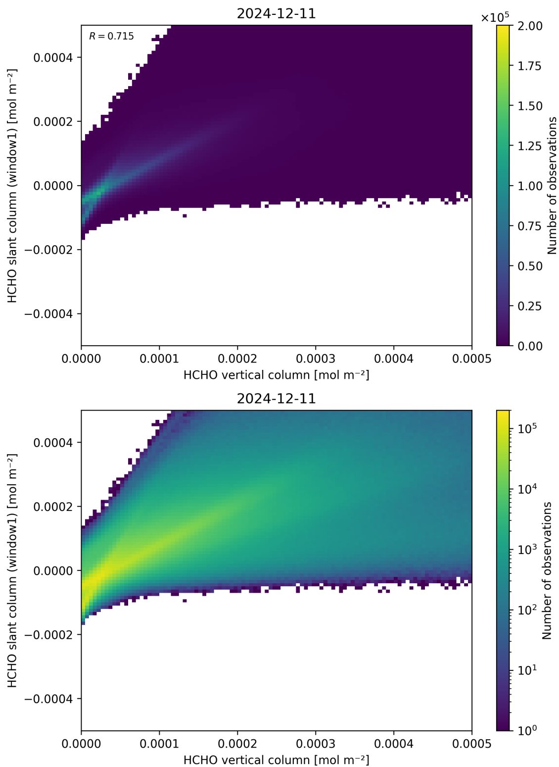
Figure 129: Scatter density plot of “HCHO vertical column” against “HCHO slant column (window1)” for 2024-12-11 to 2024-12-12.
