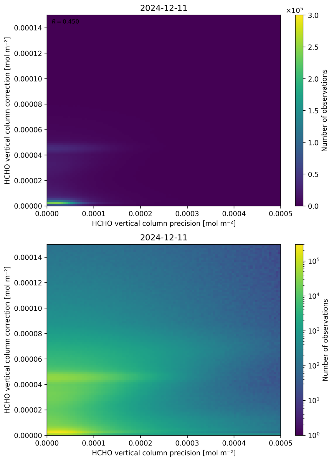
Figure 146: Scatter density plot of “HCHO vertical column precision” against “HCHO vertical column correction” for 2024-12-11 to 2024-12-12.
