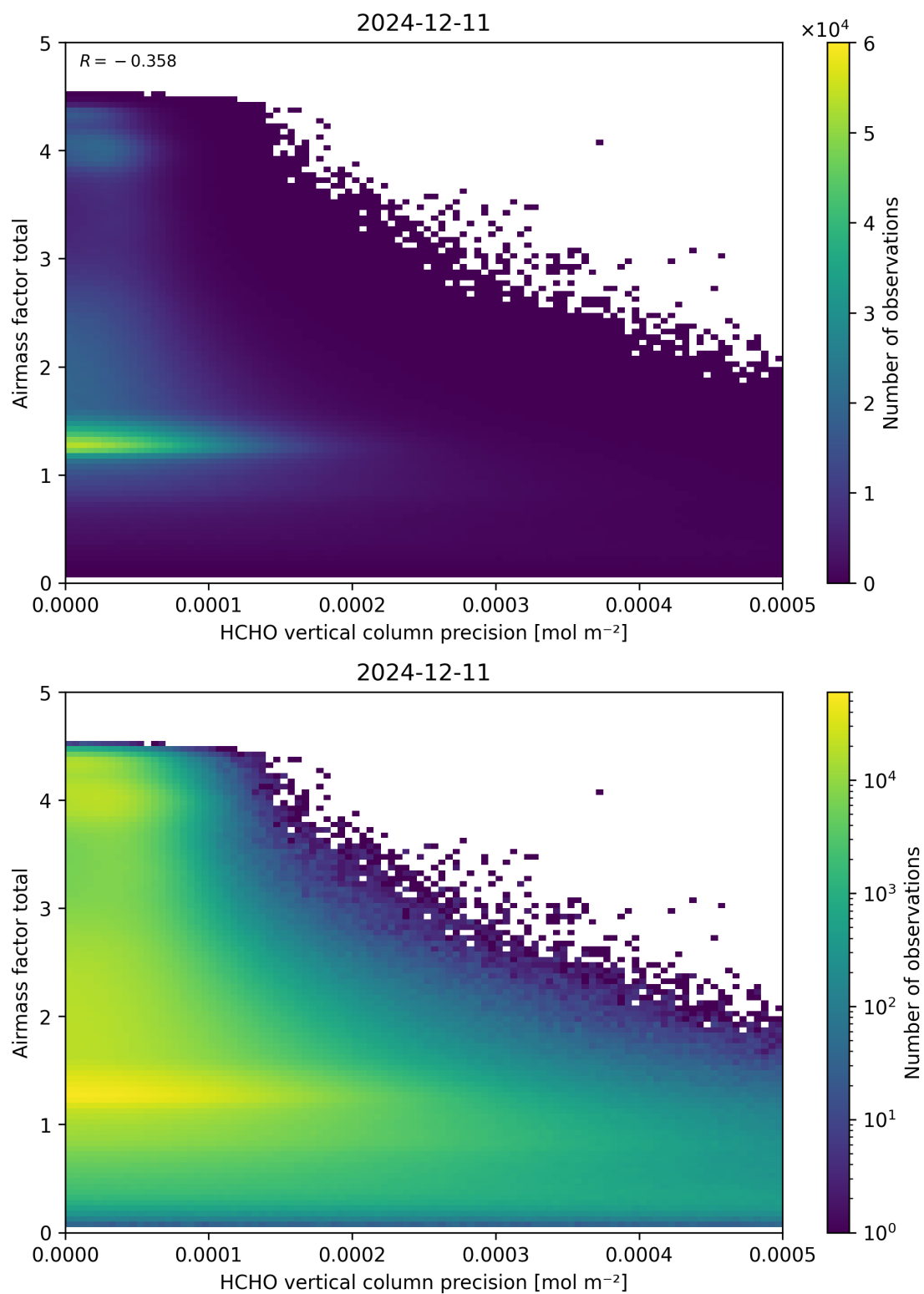
Figure 144: Scatter density plot of “HCHO vertical column precision” against “Airmass factor total” for 2024-12-11 to 2024-12-12.
