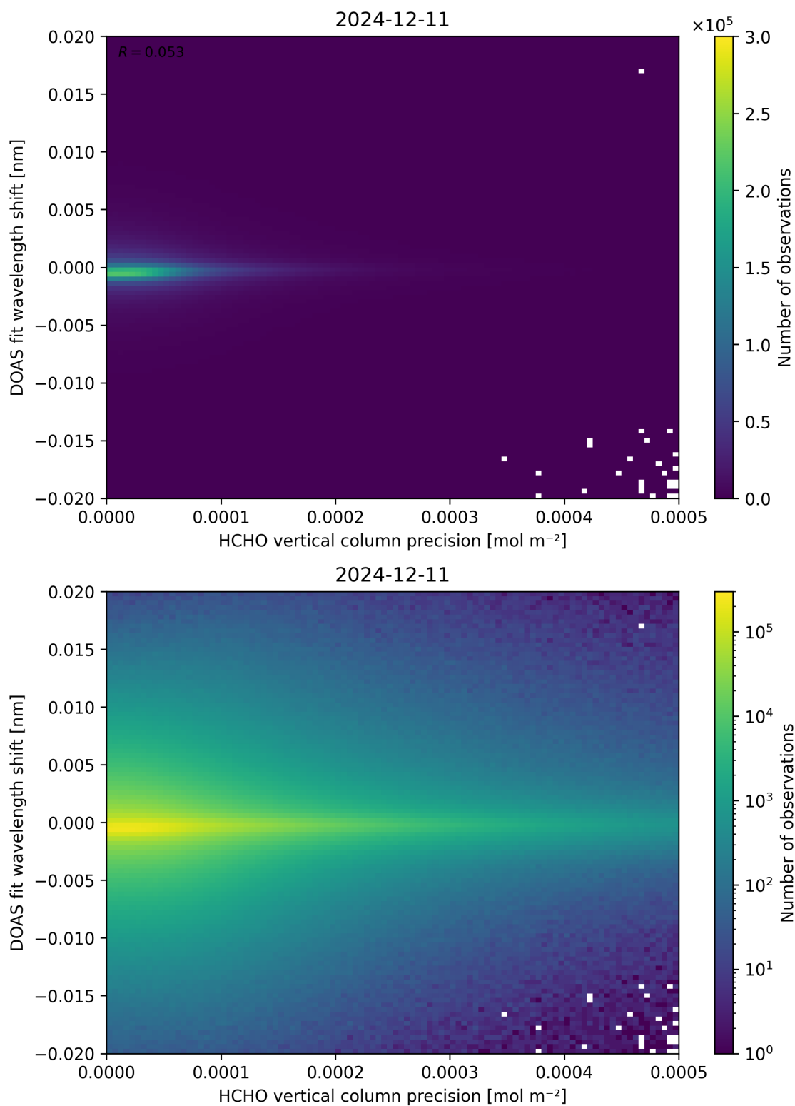
Figure 137: Scatter density plot of “HCHO vertical column precision” against “DOAS fit wavelength shift” for 2024-12-11 to 2024-12-12.
