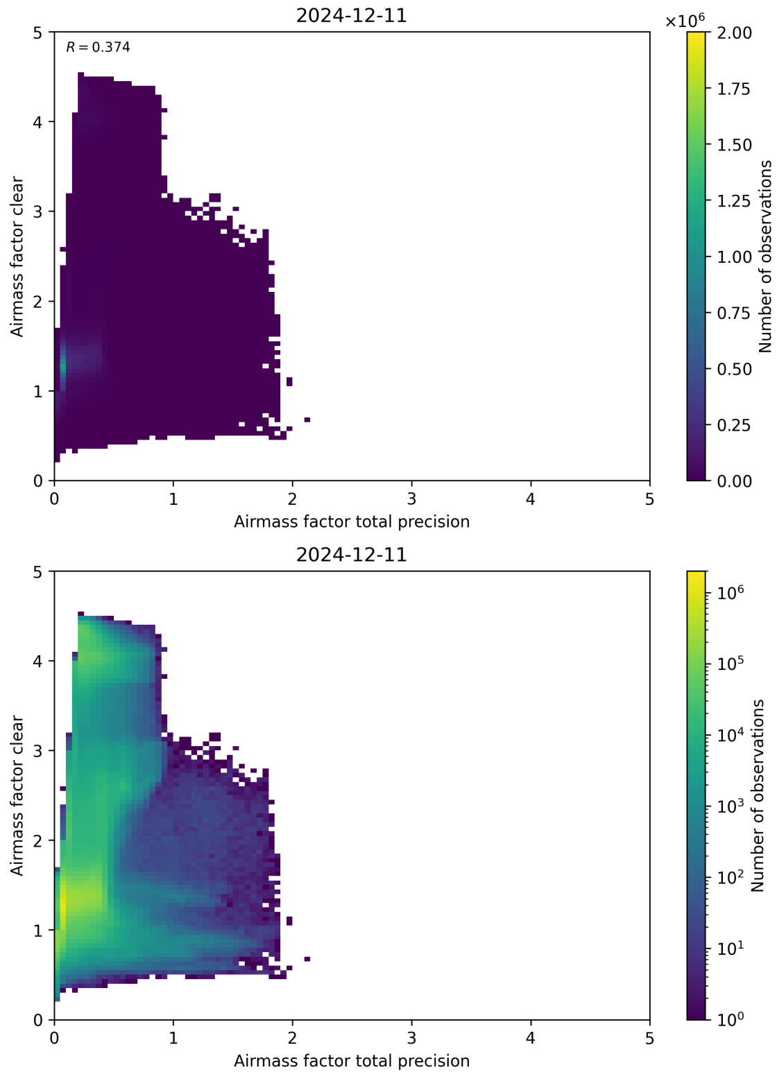
Figure 108: Scatter density plot of “Airmass factor total precision” against “Airmass factor clear” for 2024-12-11 to 2024-12-12.
