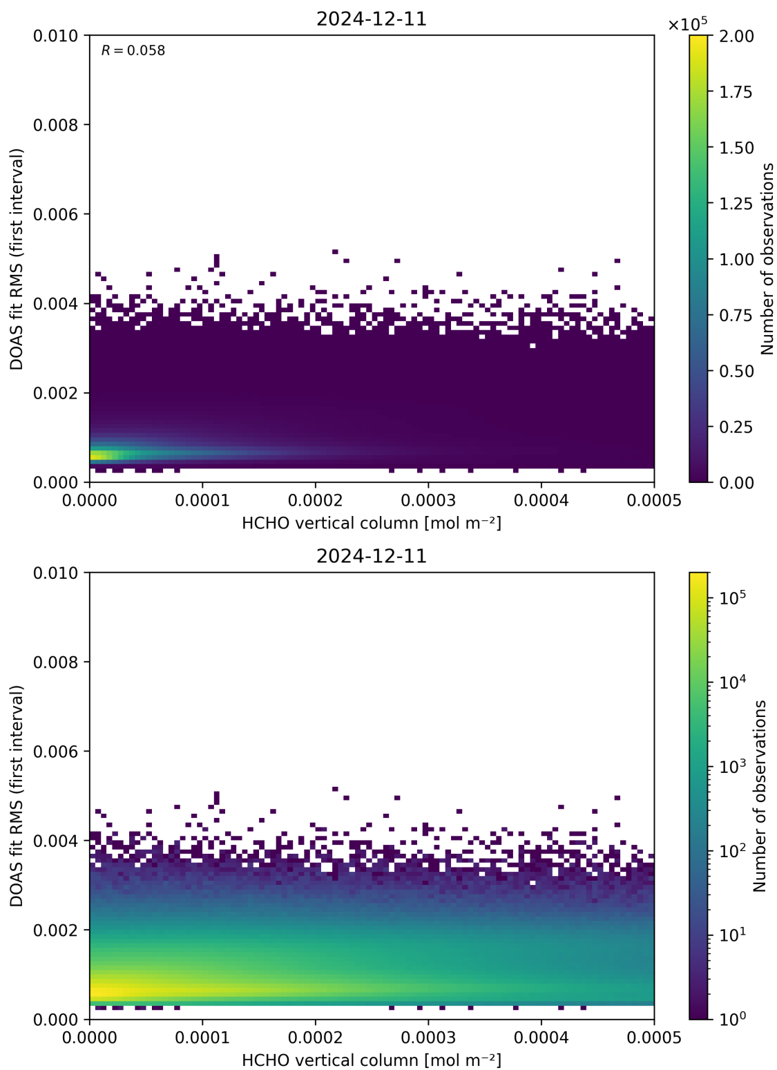
Figure 123: Scatter density plot of “HCHO vertical column” against “DOAS fit RMS (first interval)” for 2024-12-11 to 2024-12-12.
