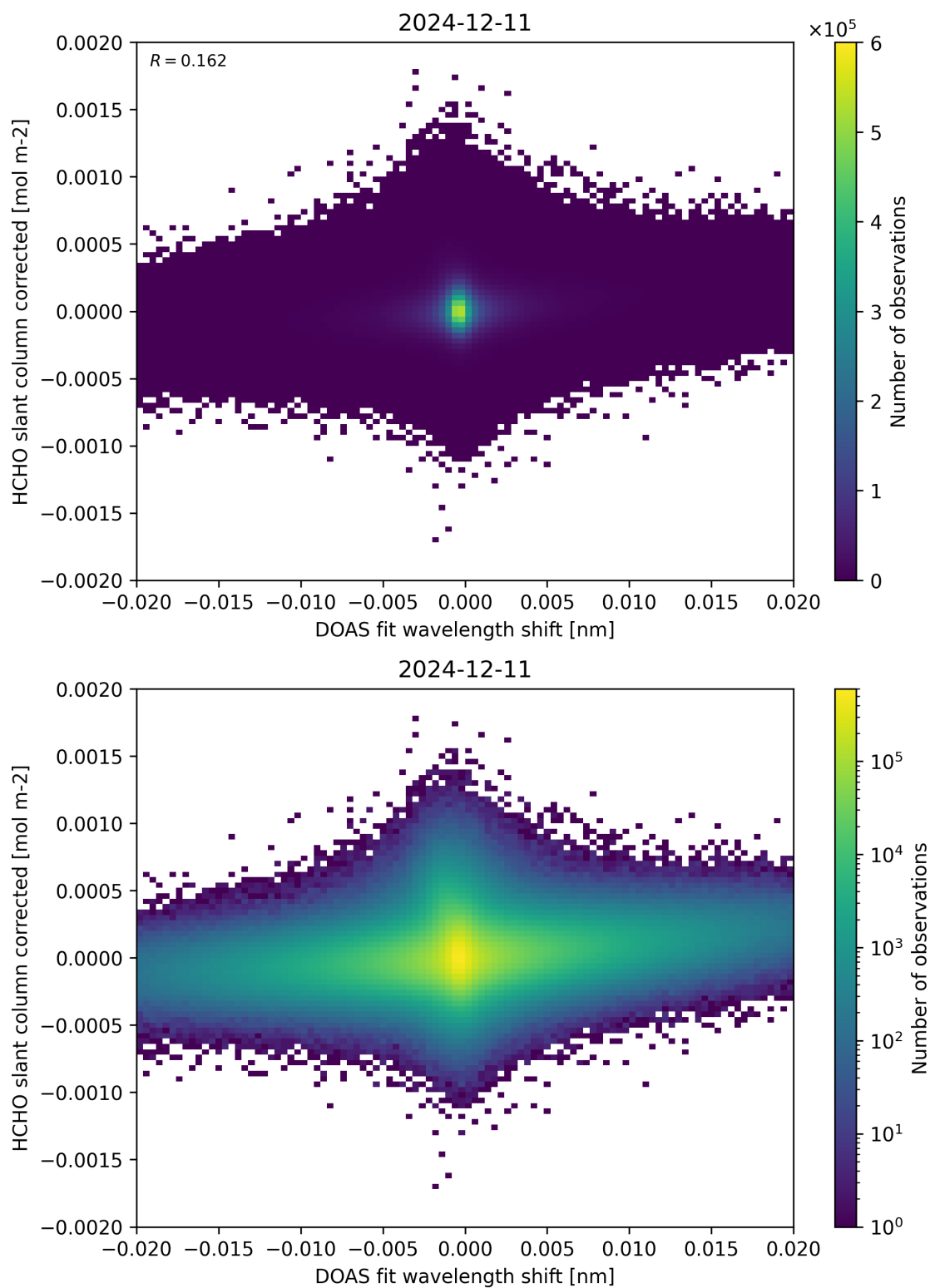
Figure 66: Scatter density plot of “DOAS fit wavelength shift” against “HCHO slant column corrected” for 2024-12-11 to 2024-12-12.
