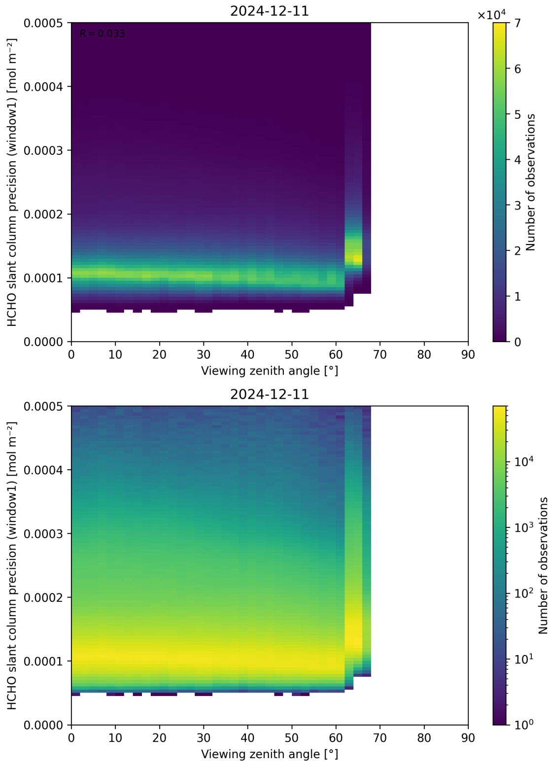
Figure 189: Scatter density plot of “Viewing zenith angle” against “HCHO slant column precision (window1)” for 2024-12-11 to 2024-12-12.
