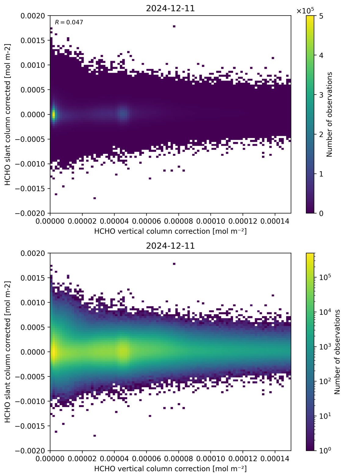
Figure 116: Scatter density plot of “HCHO vertical column correction” against “HCHO slant column corrected” for 2024-12-11 to 2024-12-12.
