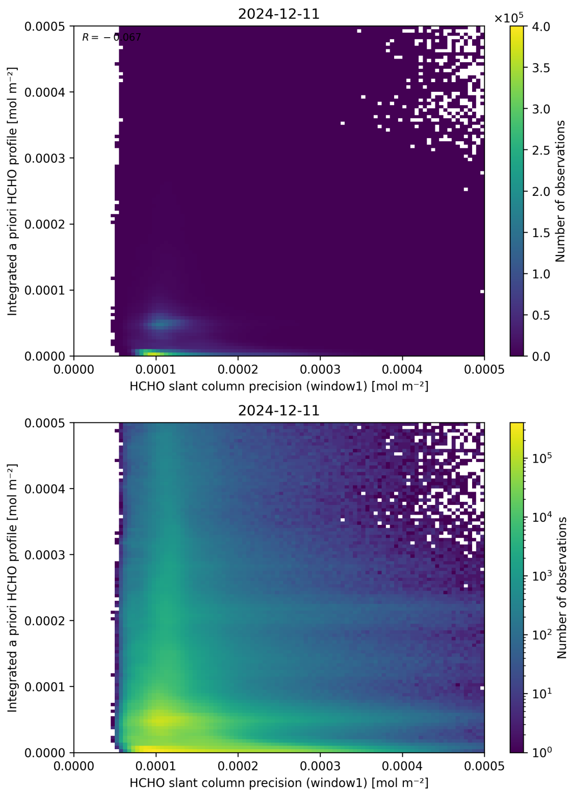
Figure 96: Scatter density plot of “HCHO slant column precision (window1)” against “Integrated a priori HCHO profile” for 2024-12-11 to 2024-12-12.
