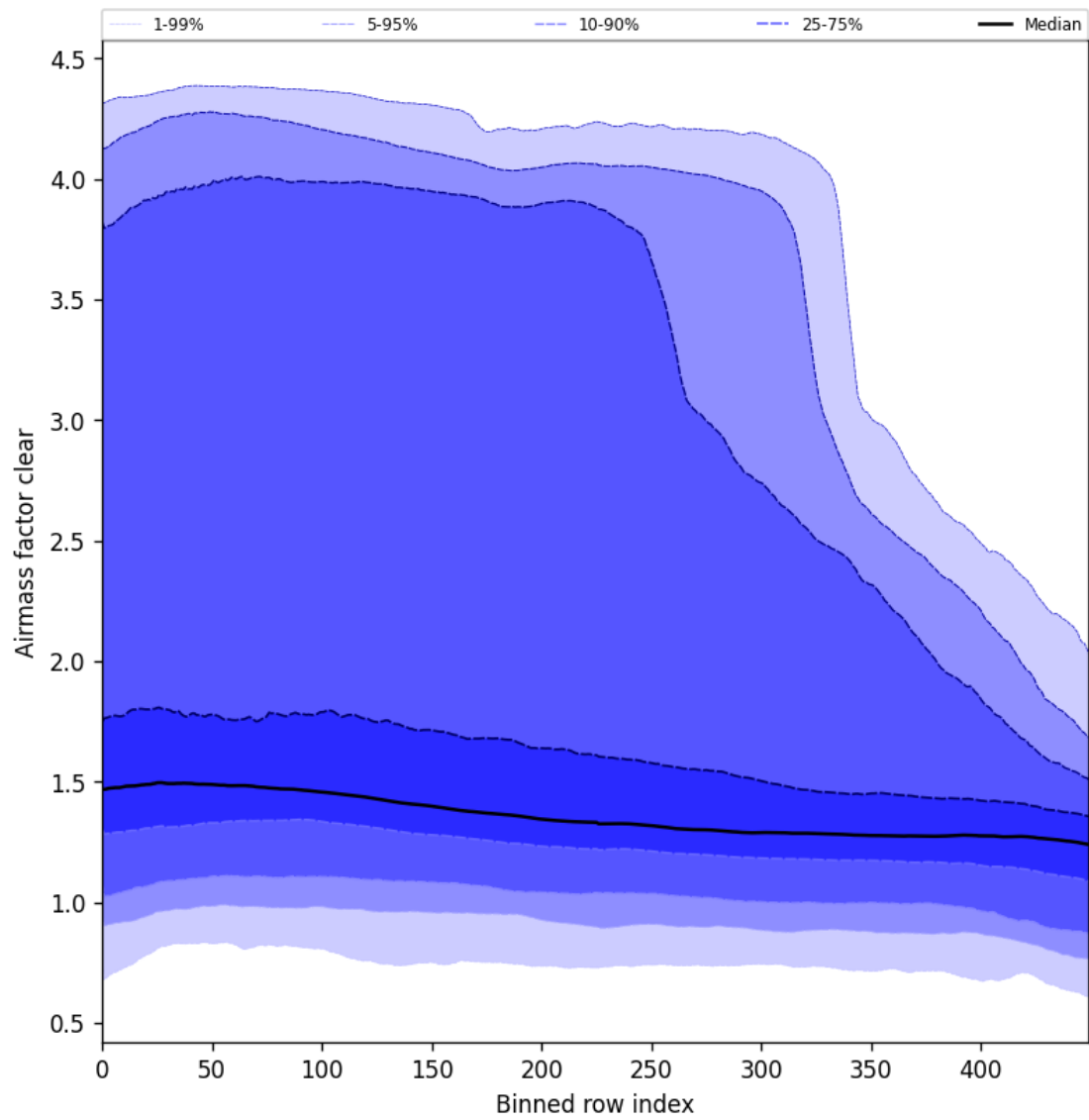
Figure 56: Along track statistics of “Air mass factor clear” for 2024-12-11 to 2024-12-12
