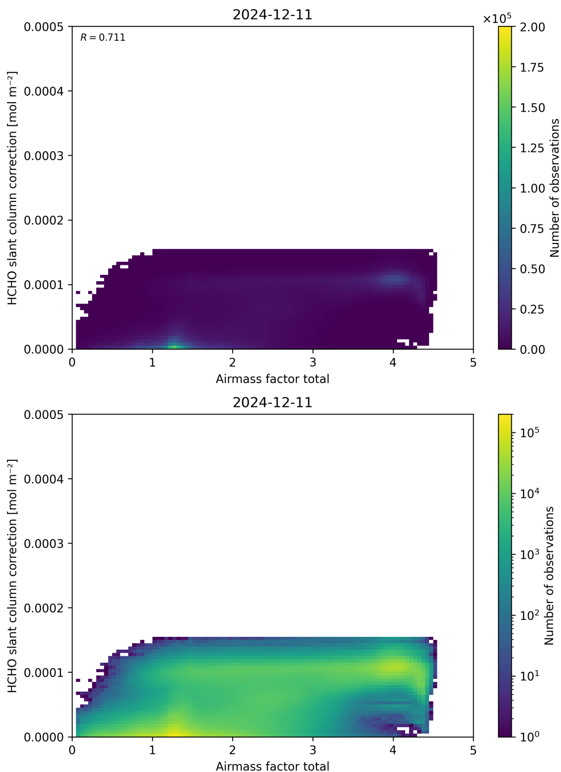
Figure 102: Scatter density plot of “Airmass factor total” against “HCHO slant column correction” for 2024-12-11 to 2024-12-12.
