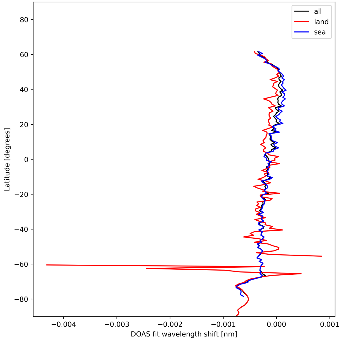
Figure 30: Zonal average of “DOAS fit wavelength shift” for 2024-12-11 to 2024-12-12.
