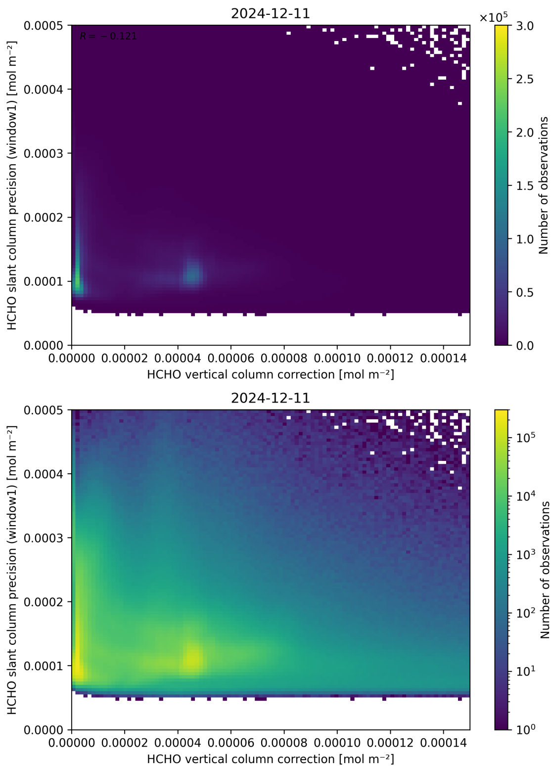
Figure 119: Scatter density plot of “HCHO vertical column correction” against “HCHO slant column precision (window1)” for 2024-12-11 to 2024-12-12.
