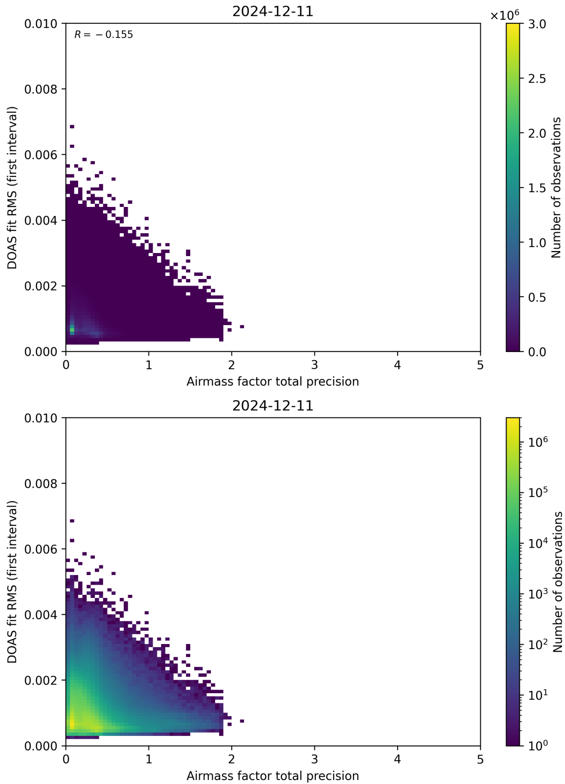
Figure 105: Scatter density plot of “Airmass factor total precision” against “DOAS fit RMS (first interval)” for 2024-12-11 to 2024-12-12.
