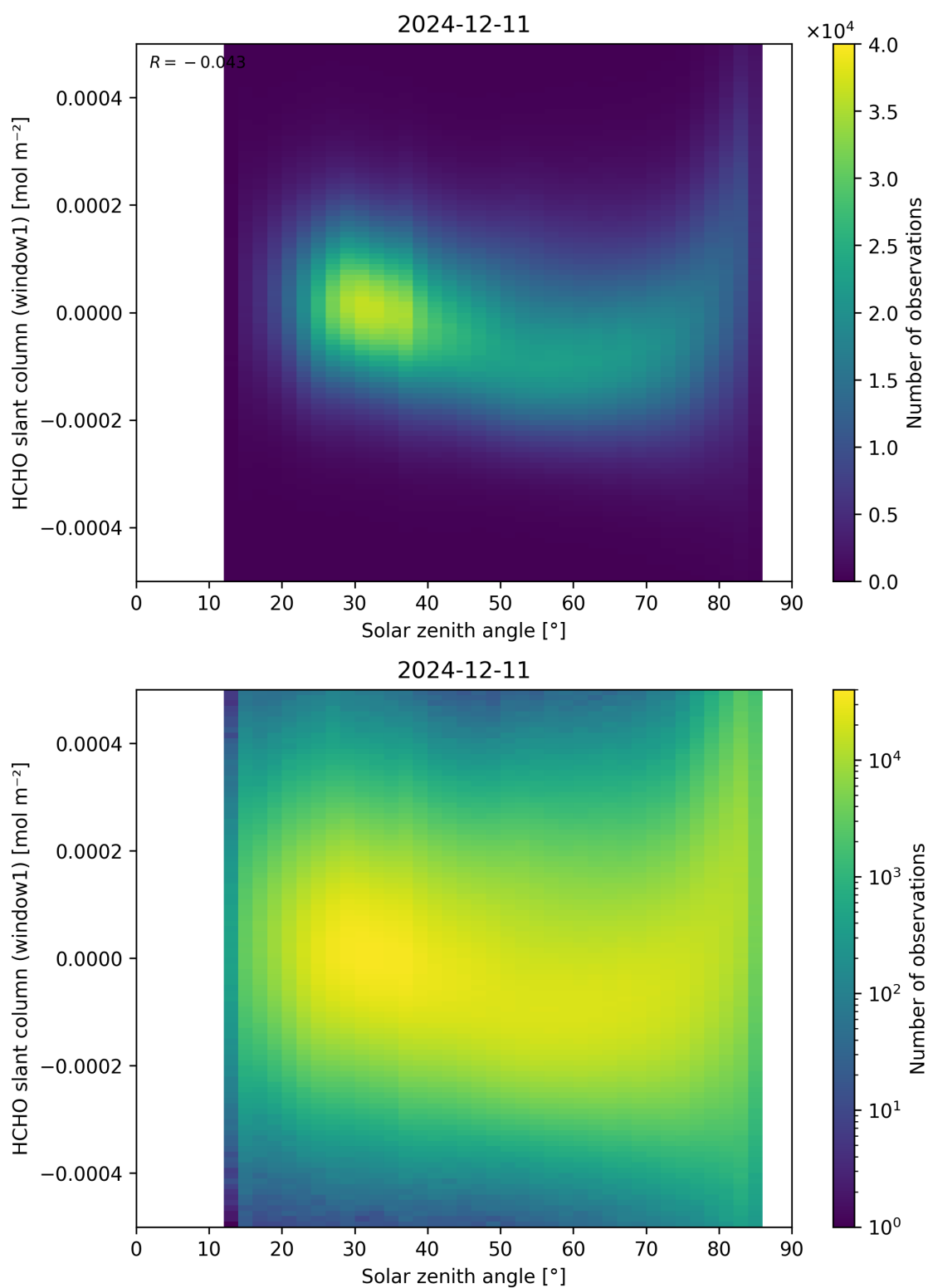
Figure 173: Scatter density plot of “Solar zenith angle” against “HCHO slant column (window1)” for 2024-12-11 to 2024-12-12.
