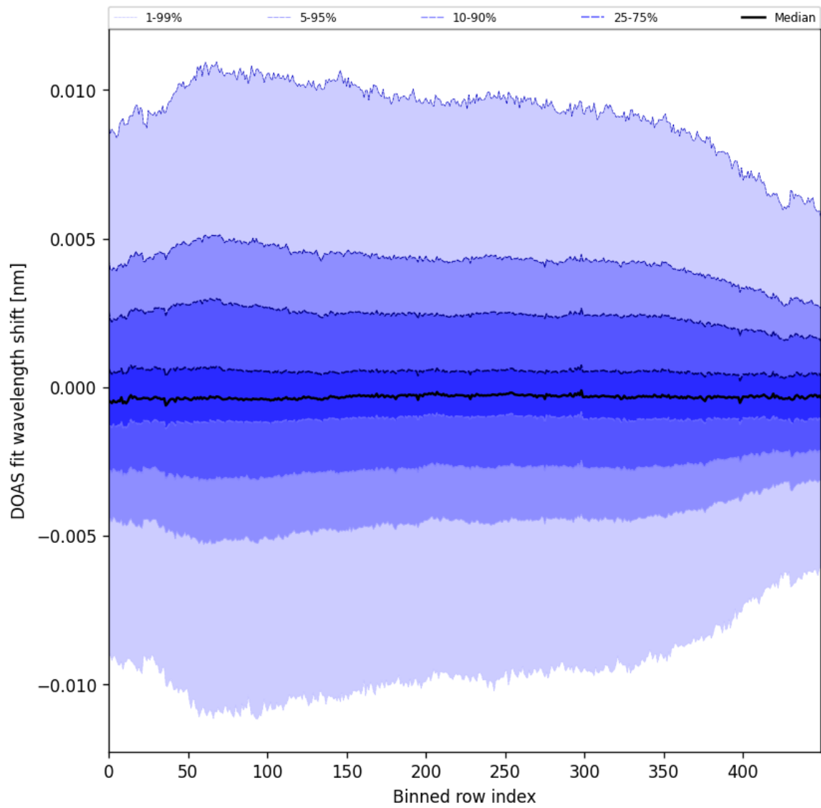
Figure 58: Along track statistics of “DOAS fit wavelength shift” for 2024-12-11 to 2024-12-12
