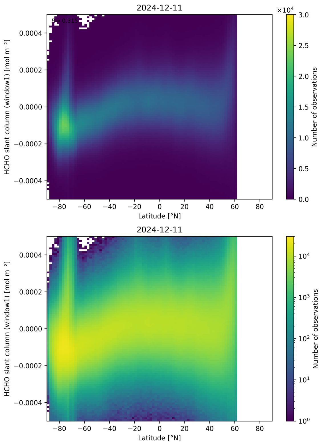
Figure 159: Scatter density plot of “Latitude” against “HCHO slant column (window1)” for 2024-12-11 to 2024-12-12.
