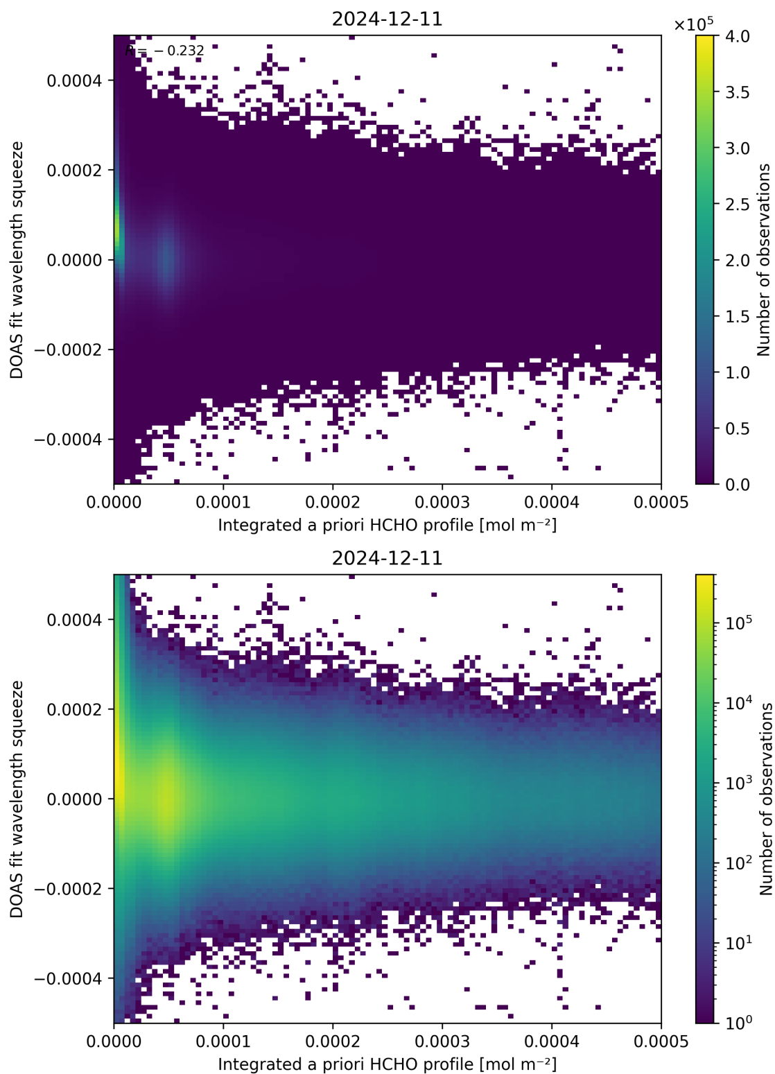
Figure 150: Scatter density plot of “Integrated a priori HCHO profile” against “DOAS fit wavelength squeeze” for 2024-12-11 to 2024-12-12.
