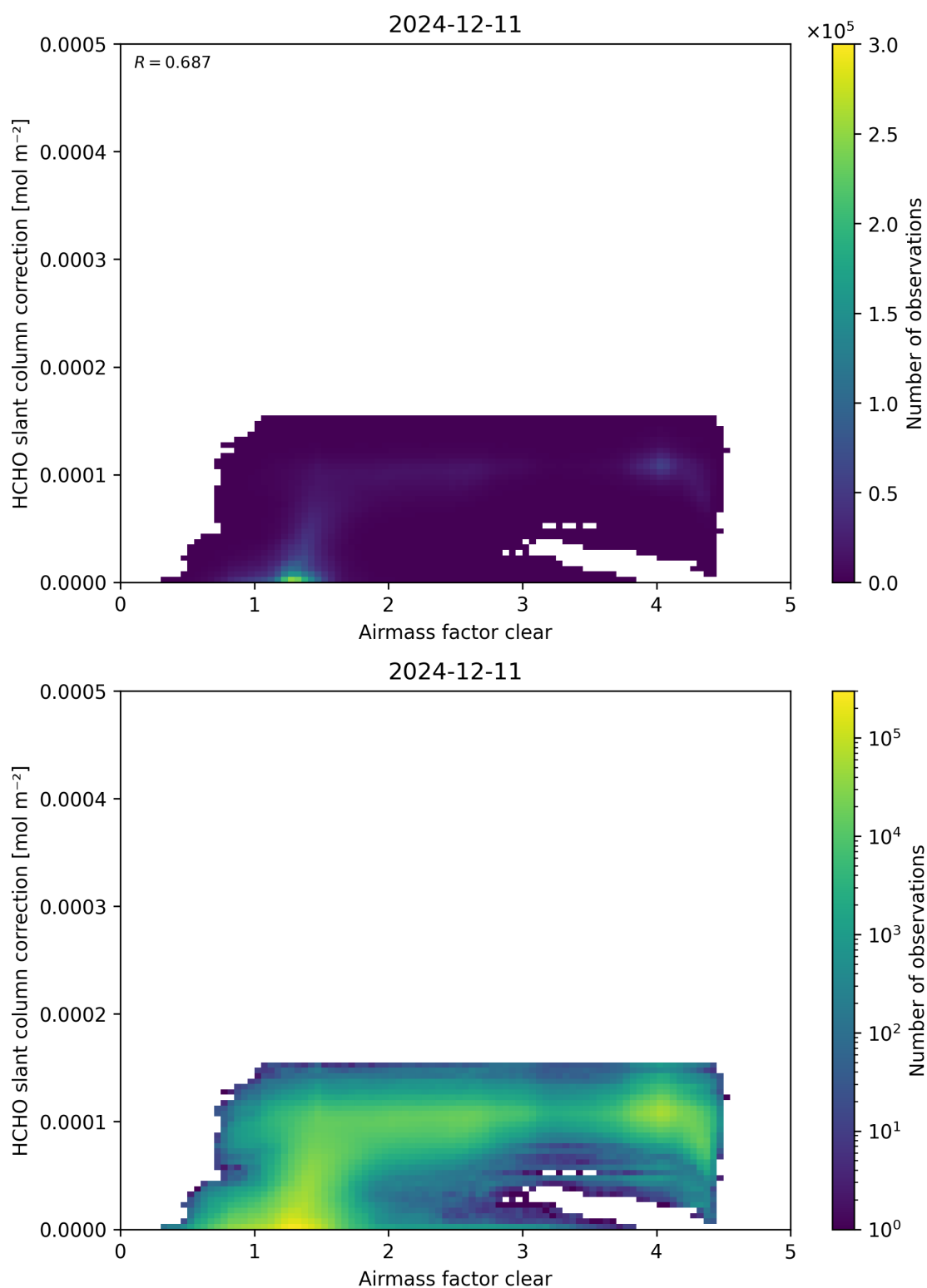
Figure 75: Scatter density plot of “Airmass factor clear” against “HCHO slant column correction” for 2024-12-11 to 2024-12-12.
