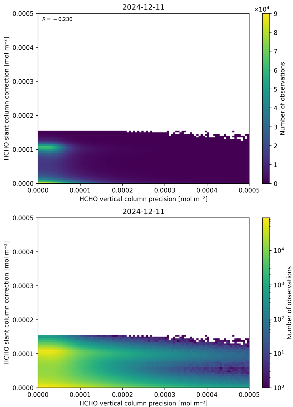
Figure 141: Scatter density plot of “HCHO vertical column precision” against “HCHO slant column correction” for 2024-12-11 to 2024-12-12.
