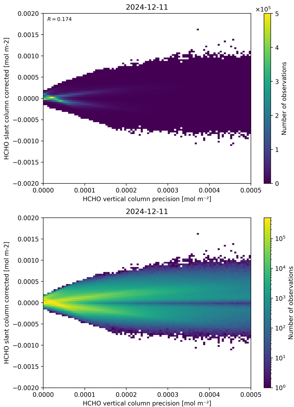
Figure 140: Scatter density plot of “HCHO vertical column precision” against “HCHO slant column corrected” for 2024-12-11 to 2024-12-12.
