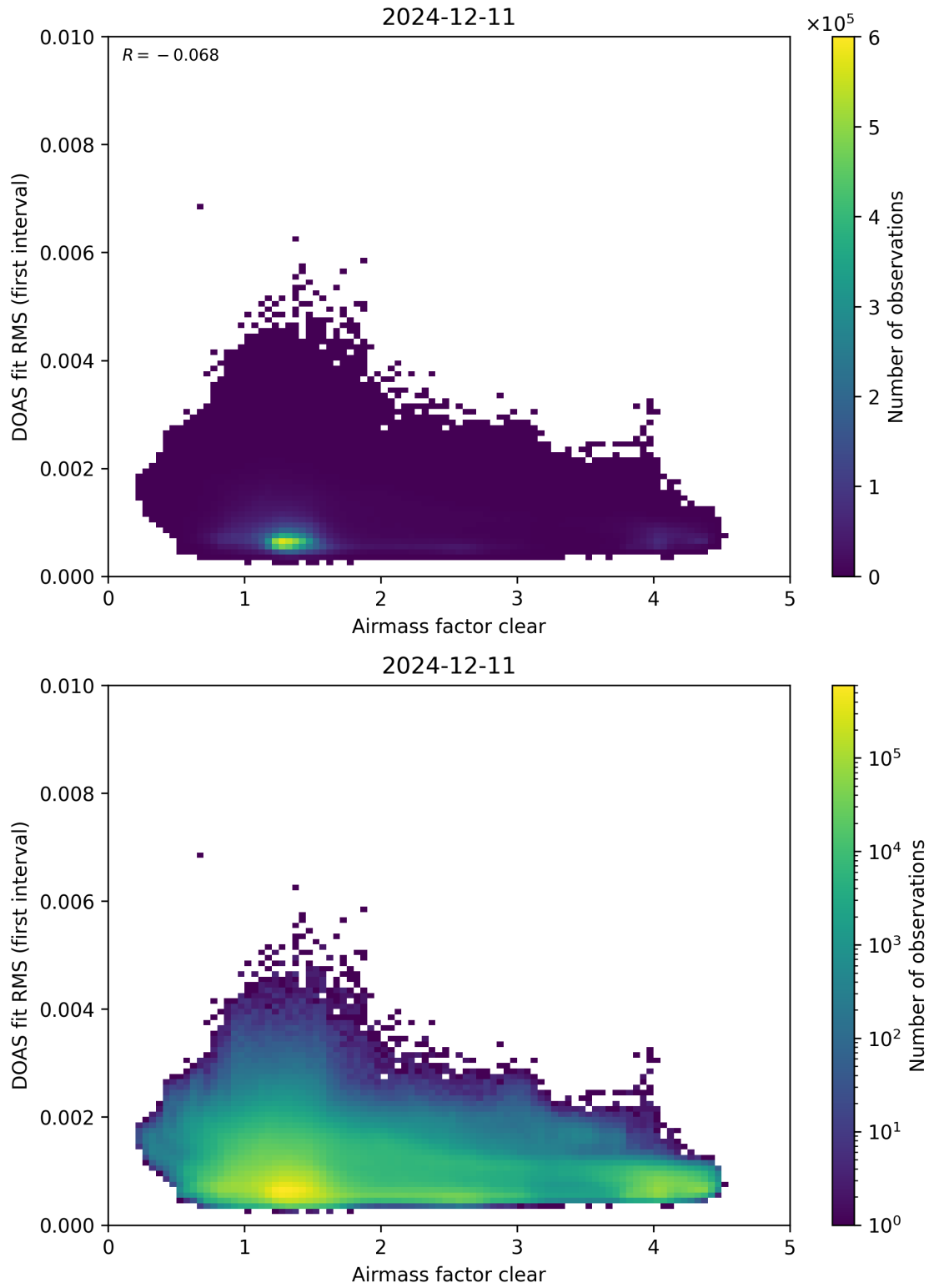
Figure 71: Scatter density plot of “Airmass factor clear” against “DOAS fit RMS (first interval)” for 2024-12-11 to 2024-12-12.
