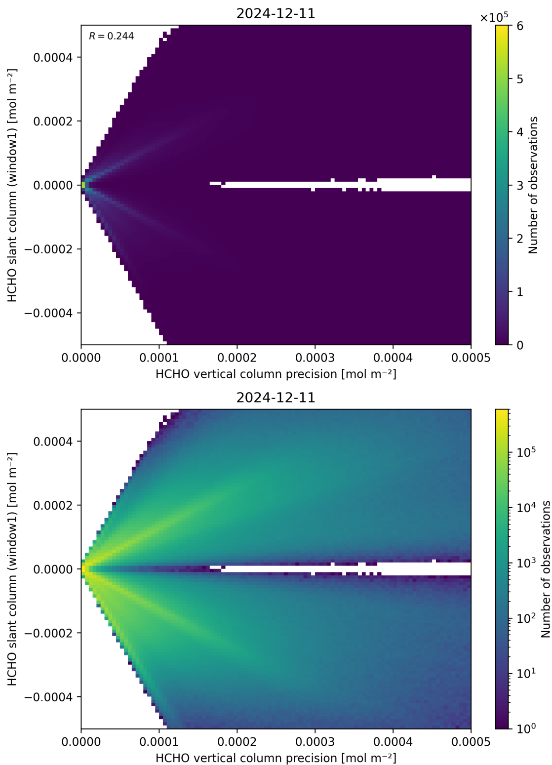
Figure 142: Scatter density plot of “HCHO vertical column precision” against “HCHO slant column (window1)” for 2024-12-11 to 2024-12-12.
