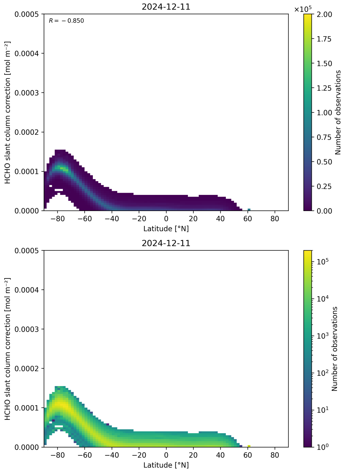
Figure 158: Scatter density plot of “Latitude” against “HCHO slant column correction” for 2024-12-11 to 2024-12-12.
