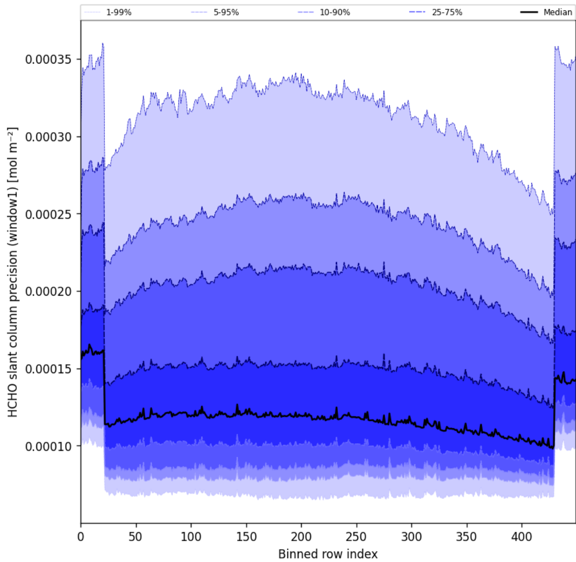
Figure 53: Along track statistics of “HCHO slant column precision (window1)” for 2024-12-11 to 2024-12-12
