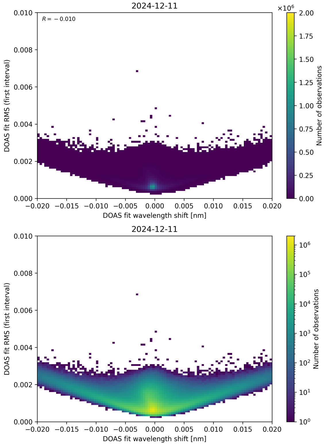
Figure 64: Scatter density plot of “DOAS fit wavelength shift” against “DOAS fit RMS (first interval)” for 2024-12-11 to 2024-12-12.
