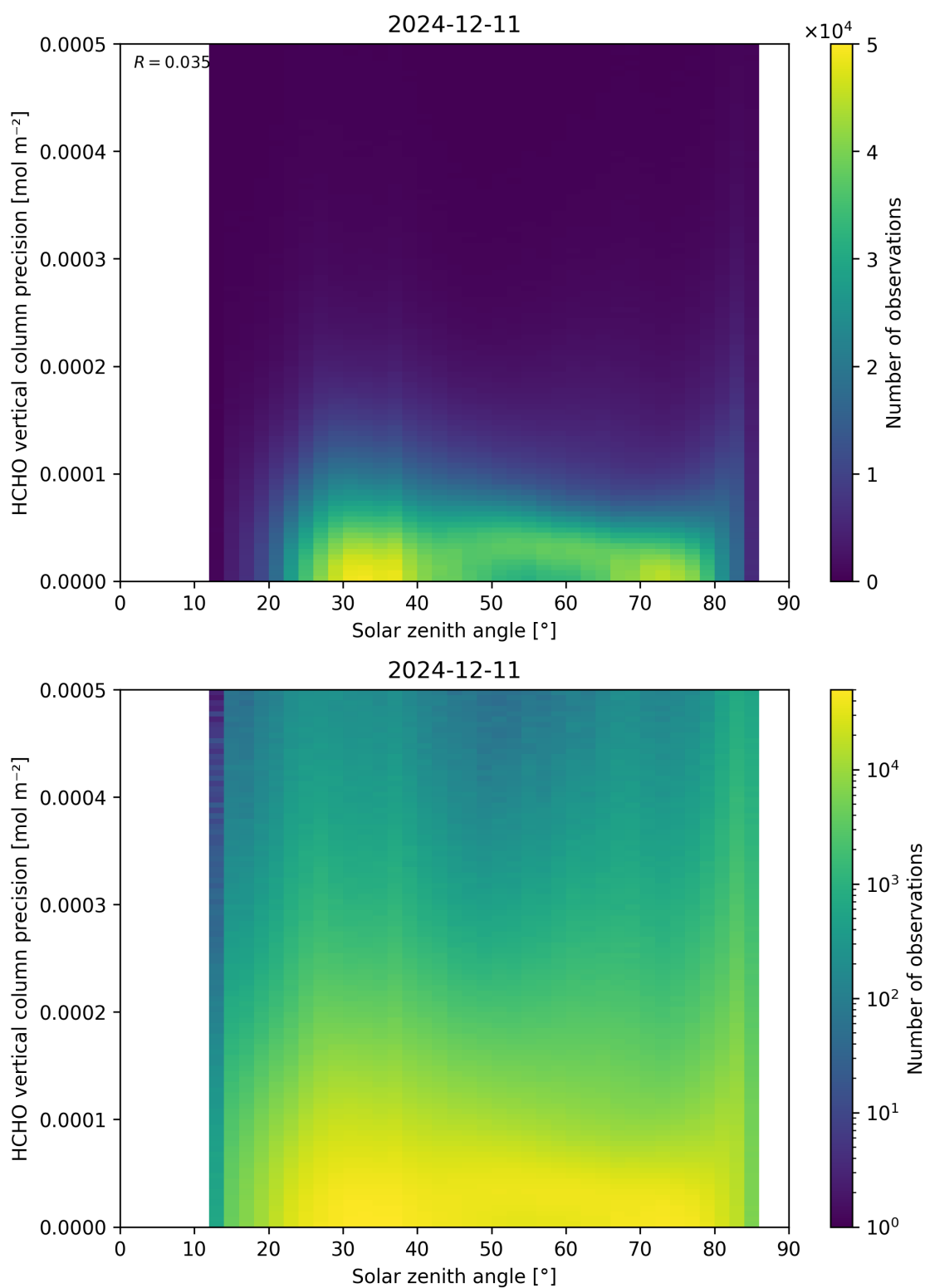
Figure 179: Scatter density plot of “Solar zenith angle” against “HCHO vertical column precision” for 2024-12-11 to 2024-12-12.
