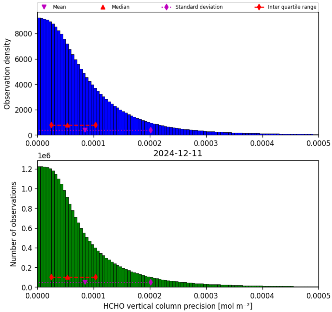
Figure 36: Histogram of “HCHO vertical column precision” for 2024-12-11 to 2024-12-12
