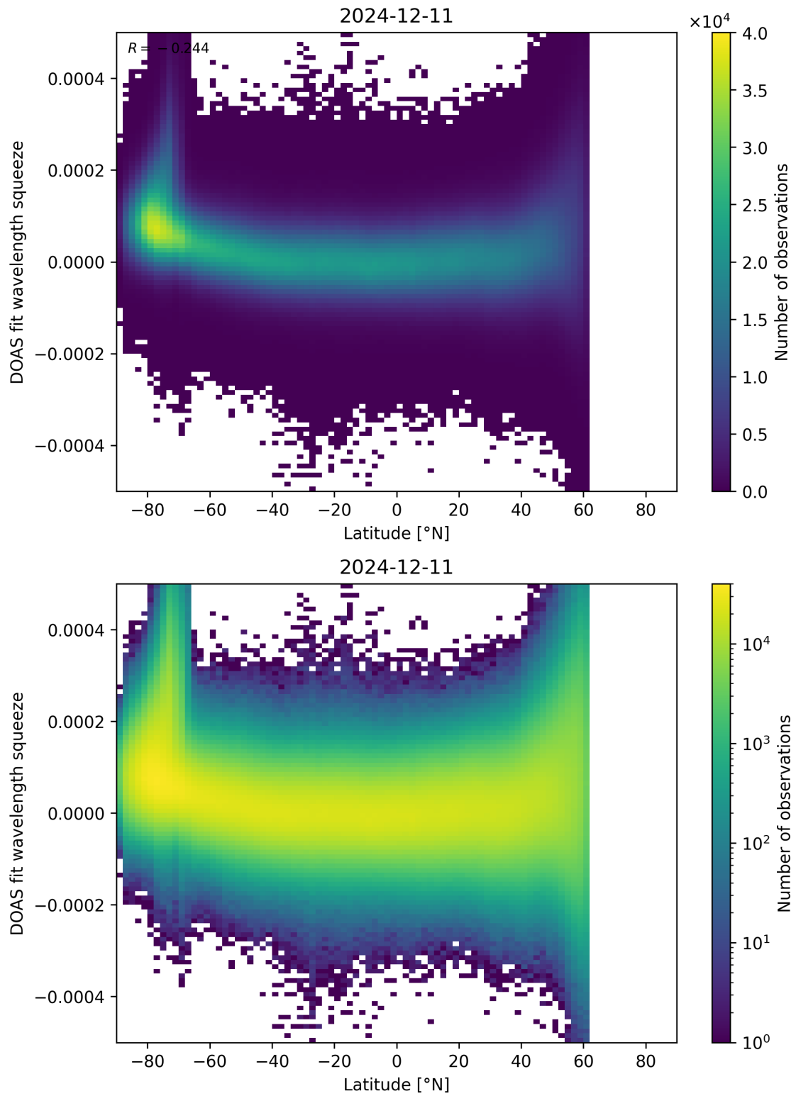
Figure 155: Scatter density plot of “Latitude” against “DOAS fit wavelength squeeze” for 2024-12-11 to 2024-12-12.
