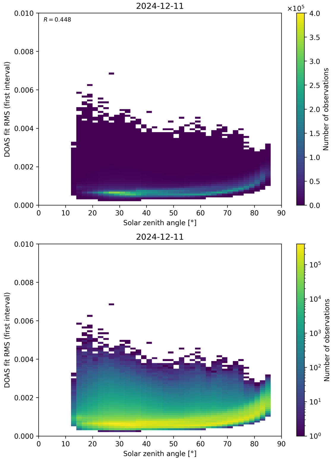
Figure 167: Scatter density plot of “Solar zenith angle” against “DOAS fit RMS (first interval)” for 2024-12-11 to 2024-12-12.
