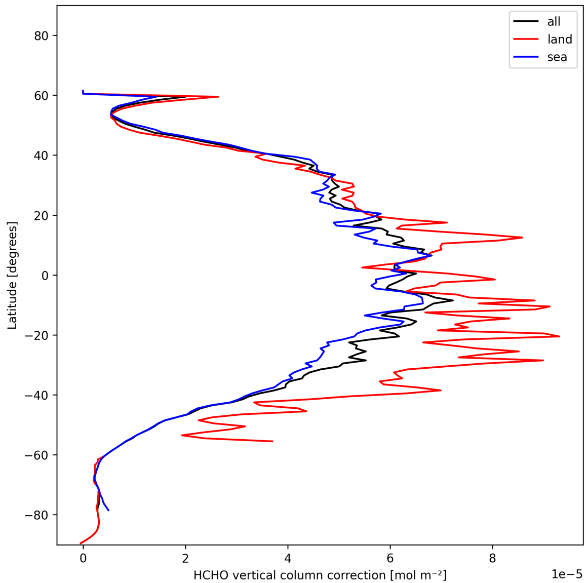
Figure 23: Zonal average of “HCHO vertical column correction” for 2024-12-11 to 2024-12-12.
