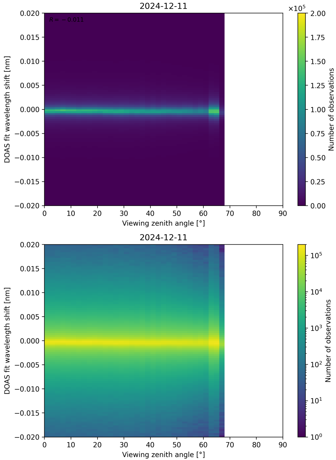
Figure 183: Scatter density plot of “Viewing zenith angle” against “DOAS fit wavelength shift” for 2024-12-11 to 2024-12-12.
