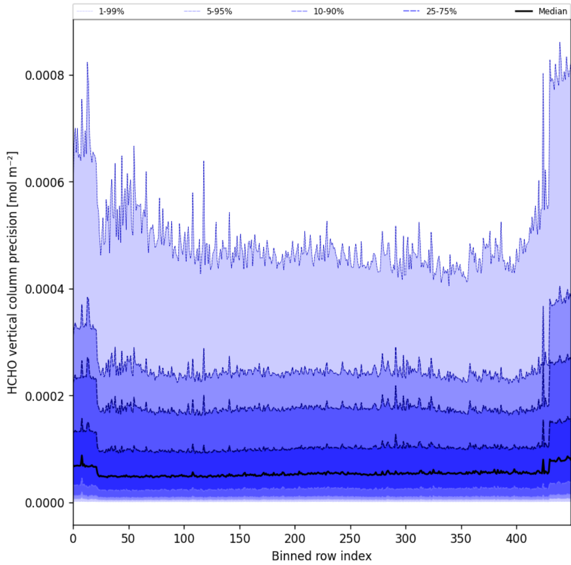
Figure 50: Along track statistics of “HCHO vertical column precision” for 2024-12-11 to 2024-12-12
