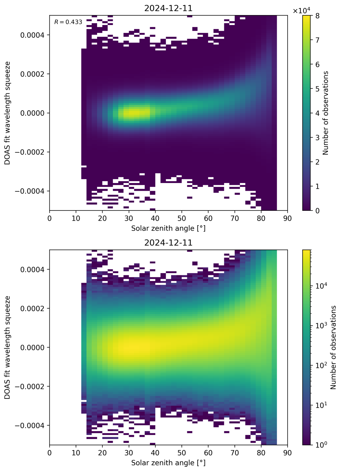
Figure 169: Scatter density plot of “Solar zenith angle” against “DOAS fit wavelength squeeze” for 2024-12-11 to 2024-12-12.
