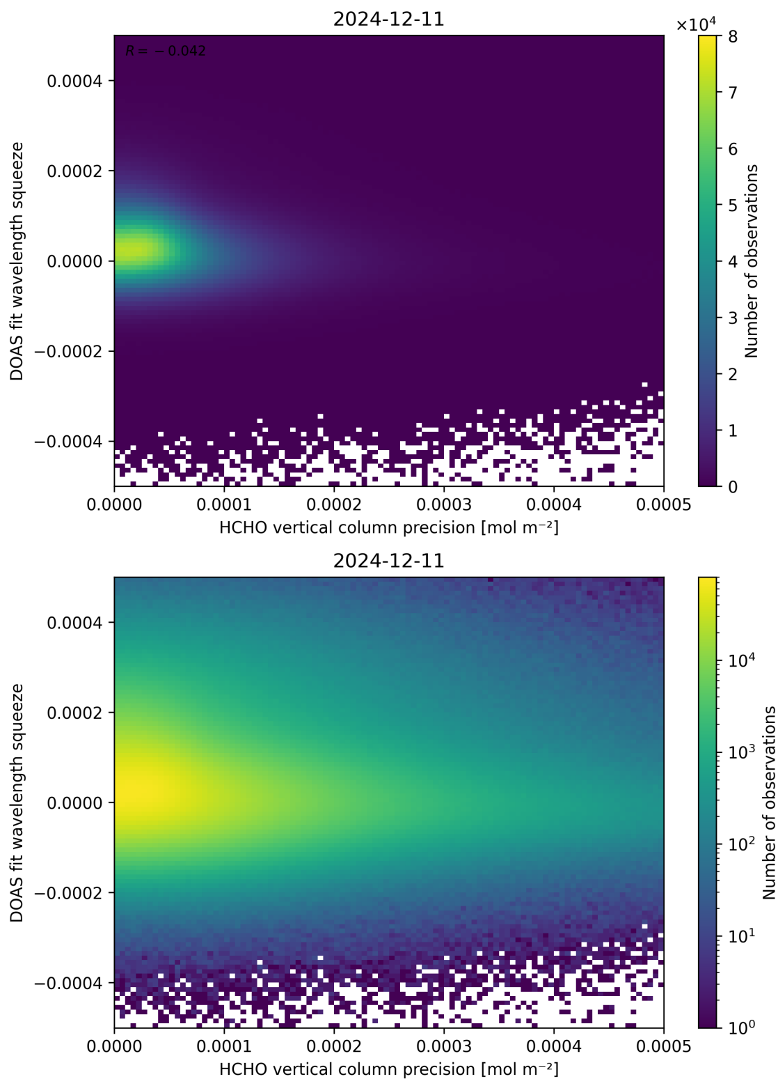
Figure 138: Scatter density plot of “HCHO vertical column precision” against “DOAS fit wavelength squeeze” for 2024-12-11 to 2024-12-12.
