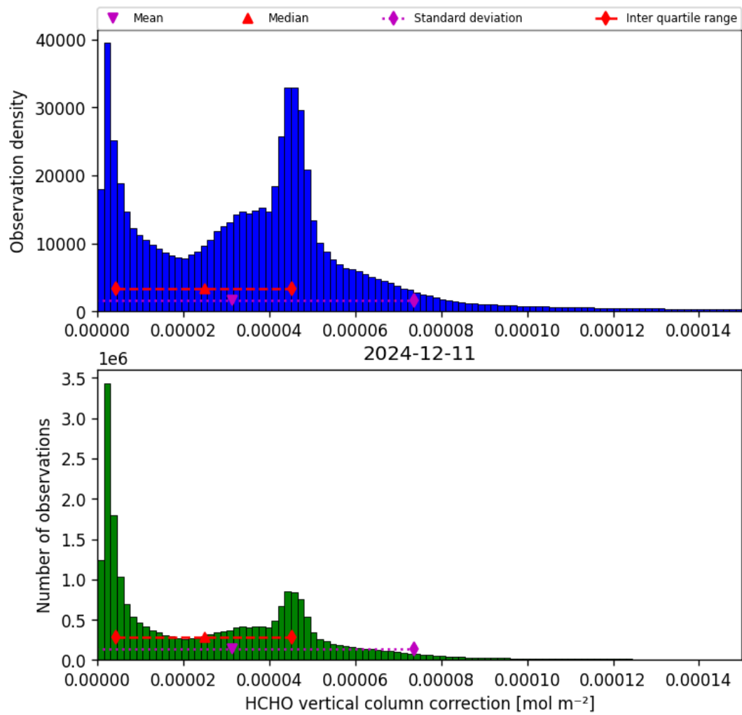
Figure 37: Histogram of “HCHO vertical column correction” for 2024-12-11 to 2024-12-12
