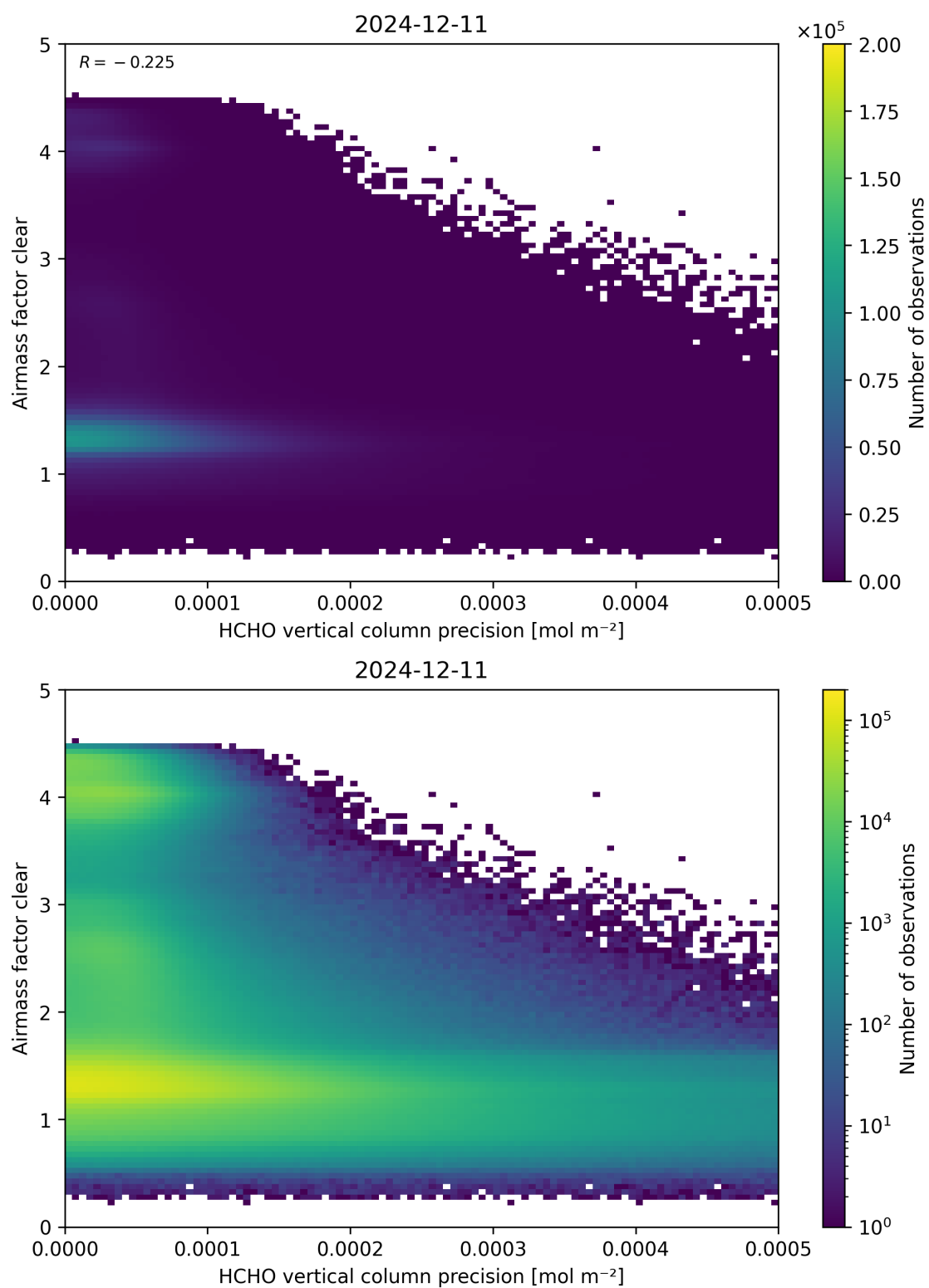
Figure 139: Scatter density plot of “HCHO vertical column precision” against “Airmass factor clear” for 2024-12-11 to 2024-12-12.
