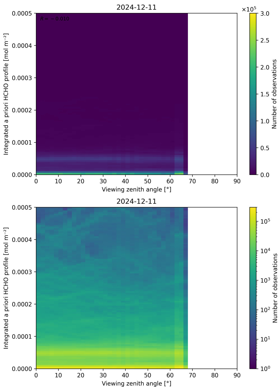
Figure 195: Scatter density plot of “Viewing zenith angle” against “Integrated a priori HCHO profile” for 2024-12-11 to 2024-12-12.
