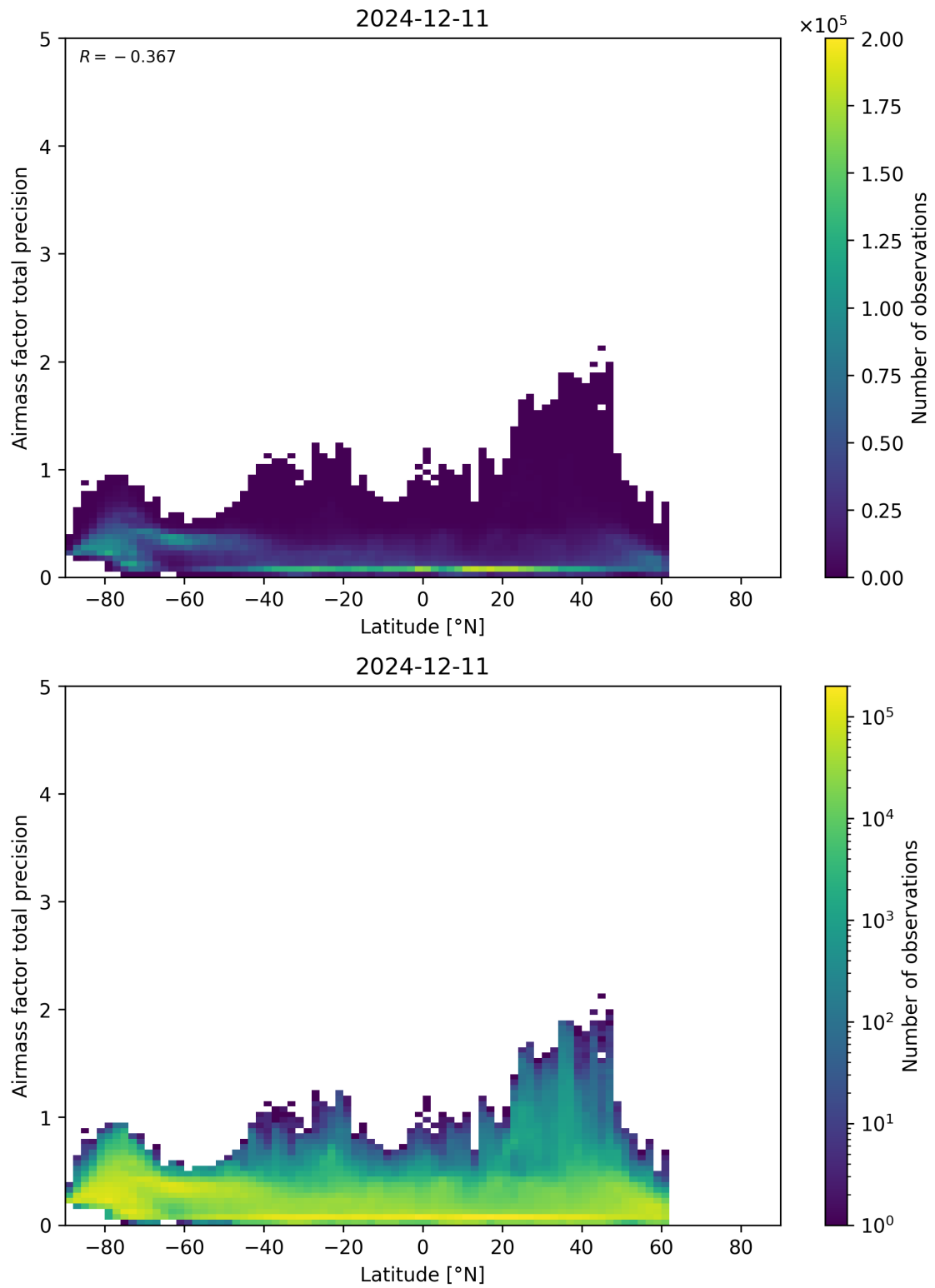
Figure 162: Scatter density plot of “Latitude” against “Airmass factor total precision” for 2024-12-11 to 2024-12-12.
