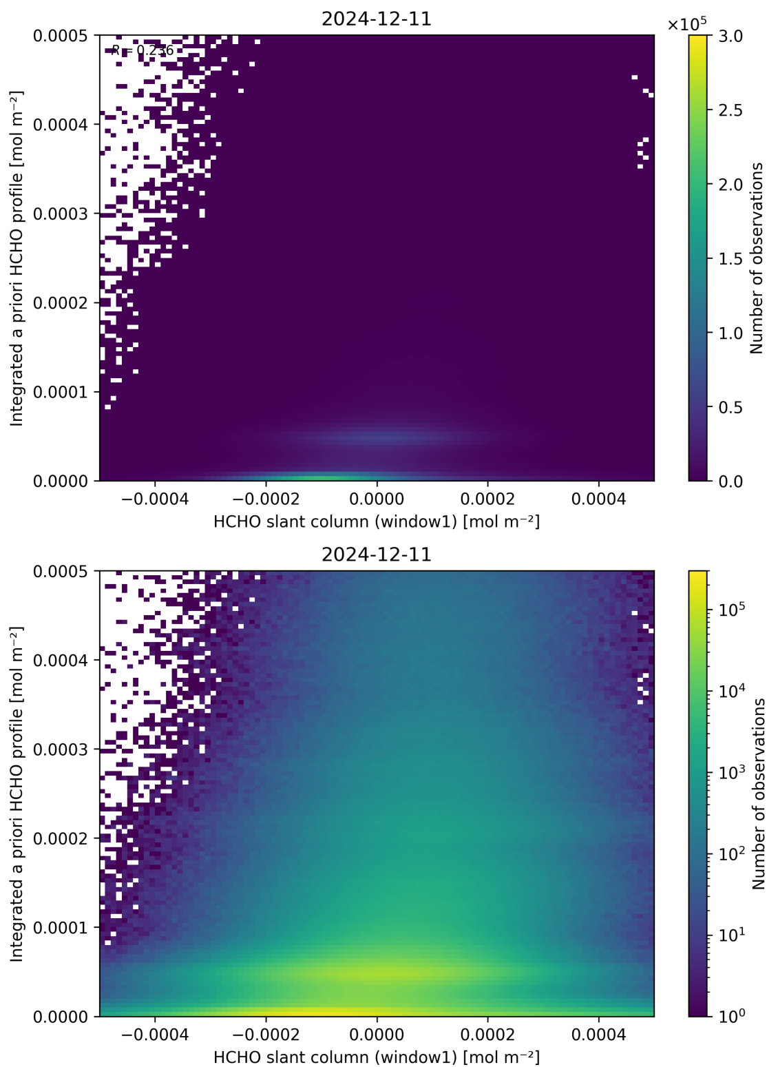
Figure 87: Scatter density plot of “HCHO slant column (window1)” against “Integrated a priori HCHO profile” for 2024-12-11 to 2024-12-12.
