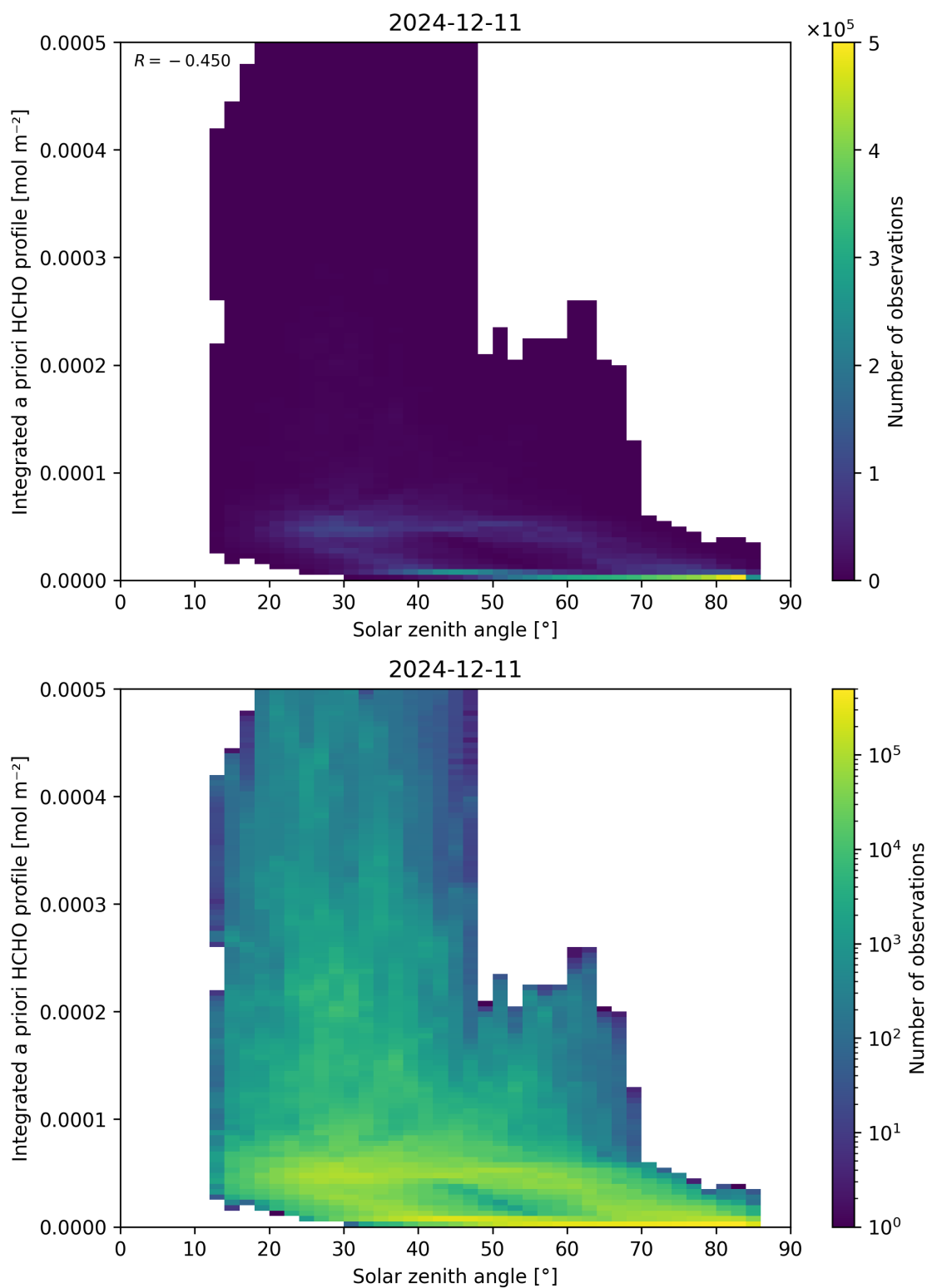
Figure 180: Scatter density plot of “Solar zenith angle” against “Integrated a priori HCHO profile” for 2024-12-11 to 2024-12-12.
