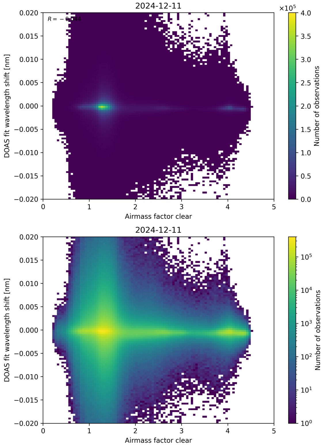
Figure 72: Scatter density plot of “Airmass factor clear” against “DOAS fit wavelength shift” for 2024-12-11 to 2024-12-12.
