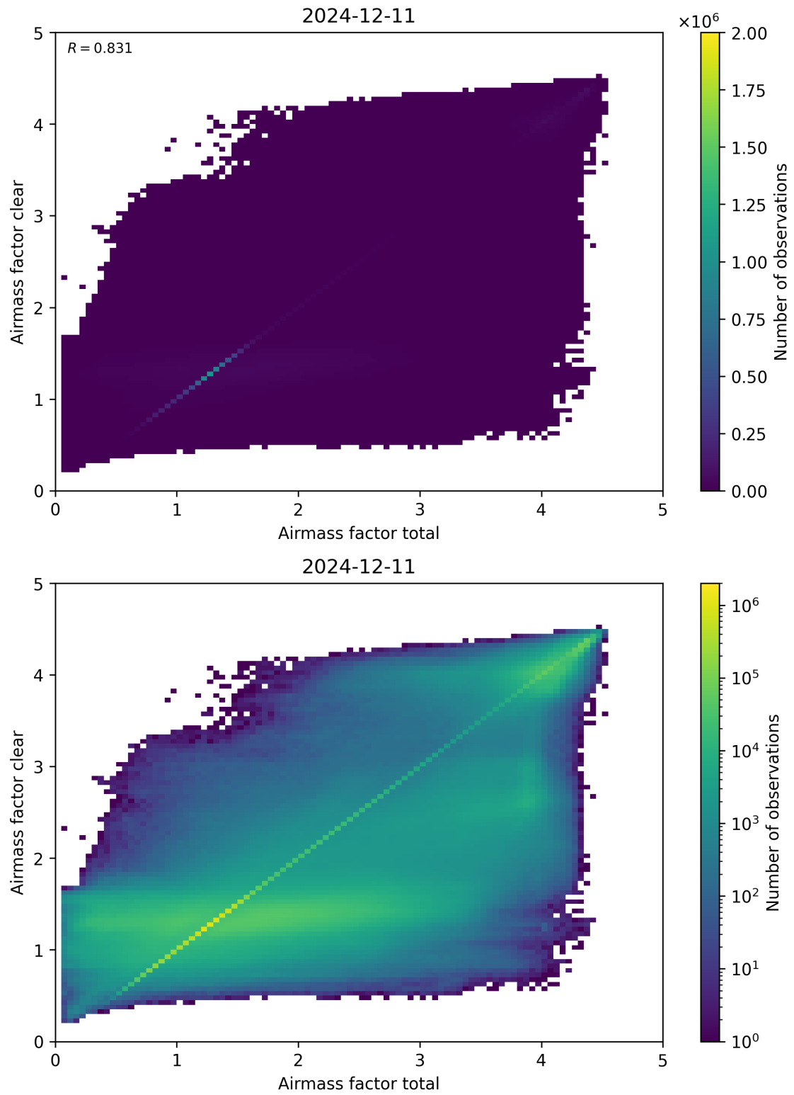
Figure 100: Scatter density plot of “Airmass factor total” against “Airmass factor clear” for 2024-12-11 to 2024-12-12.
