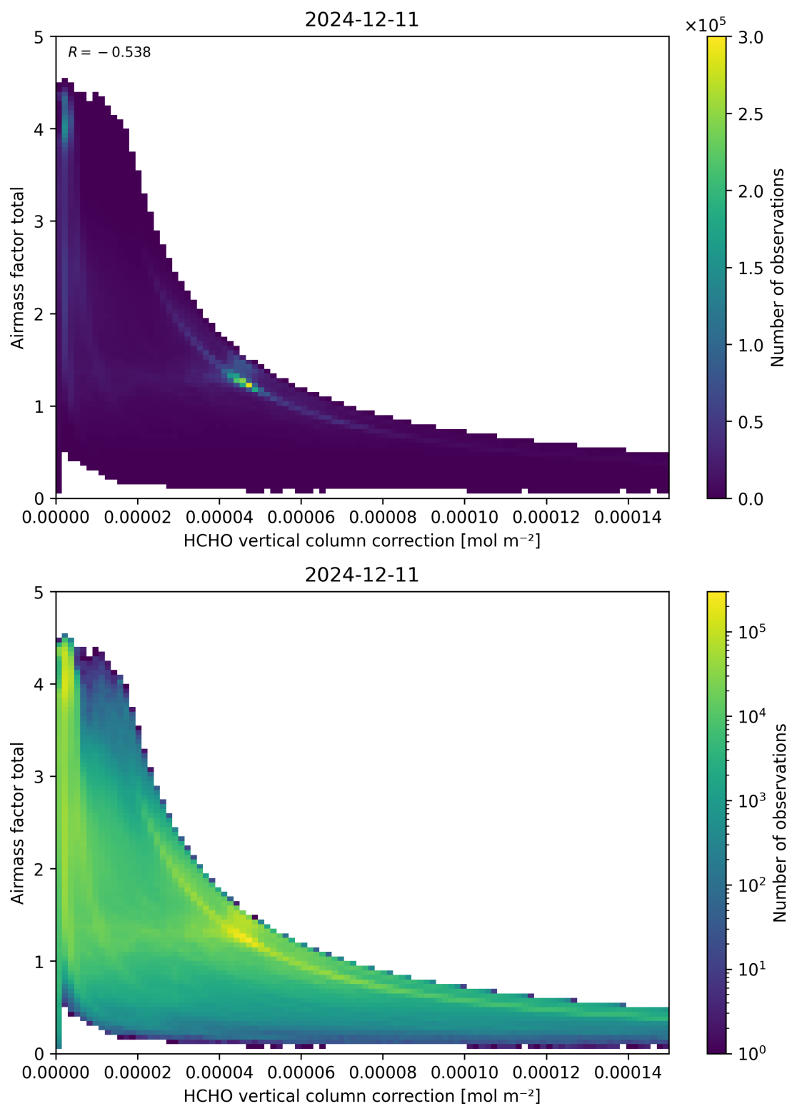
Figure 120: Scatter density plot of “HCHO vertical column correction” against “Airmass factor total” for 2024-12-11 to 2024-12-12.
