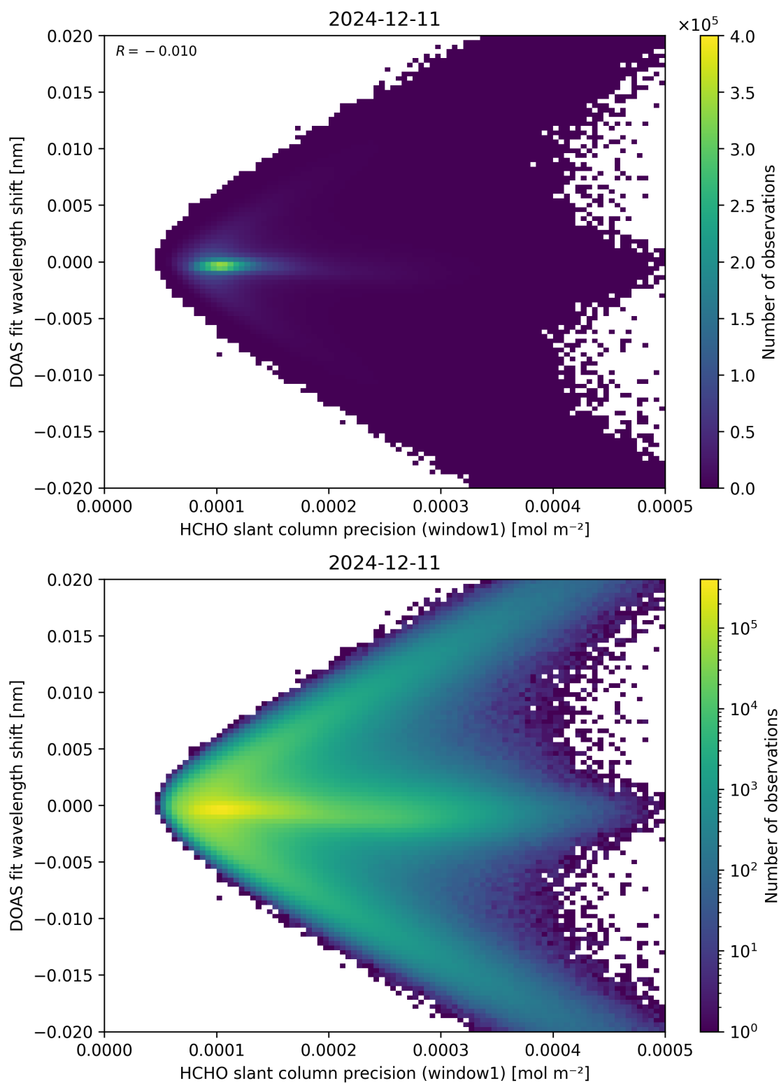
Figure 89: Scatter density plot of “HCHO slant column precision (window1)” against “DOAS fit wavelength shift” for 2024-12-11 to 2024-12-12.
