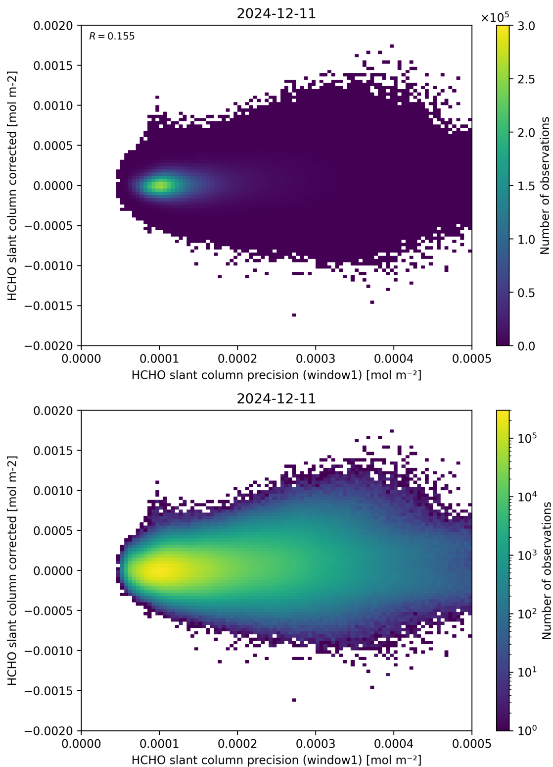
Figure 92: Scatter density plot of “HCHO slant column precision (window1)” against “HCHO slant column corrected” for 2024-12-11 to 2024-12-12.
