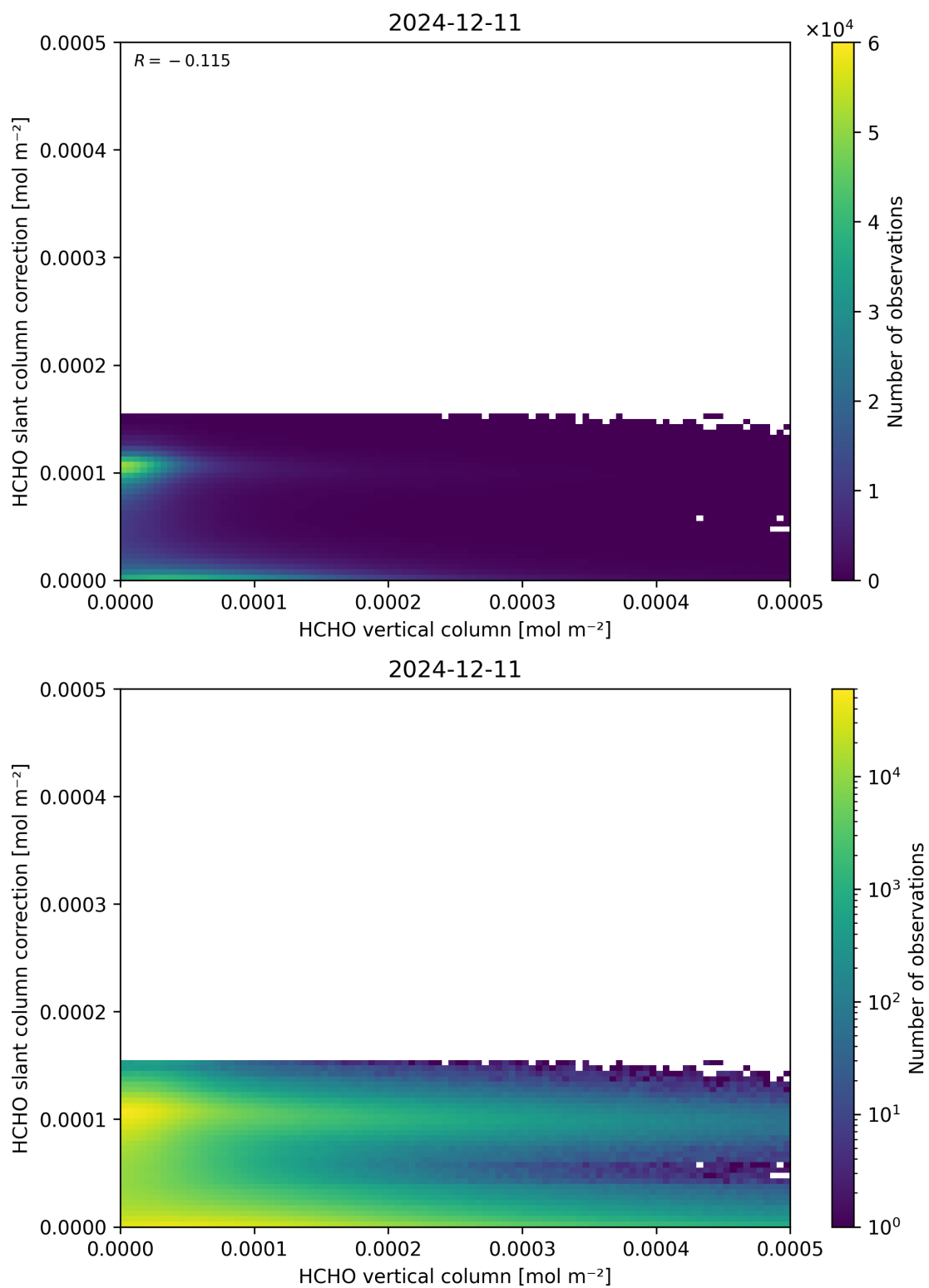
Figure 128: Scatter density plot of “HCHO vertical column” against “HCHO slant column correction” for 2024-12-11 to 2024-12-12.
