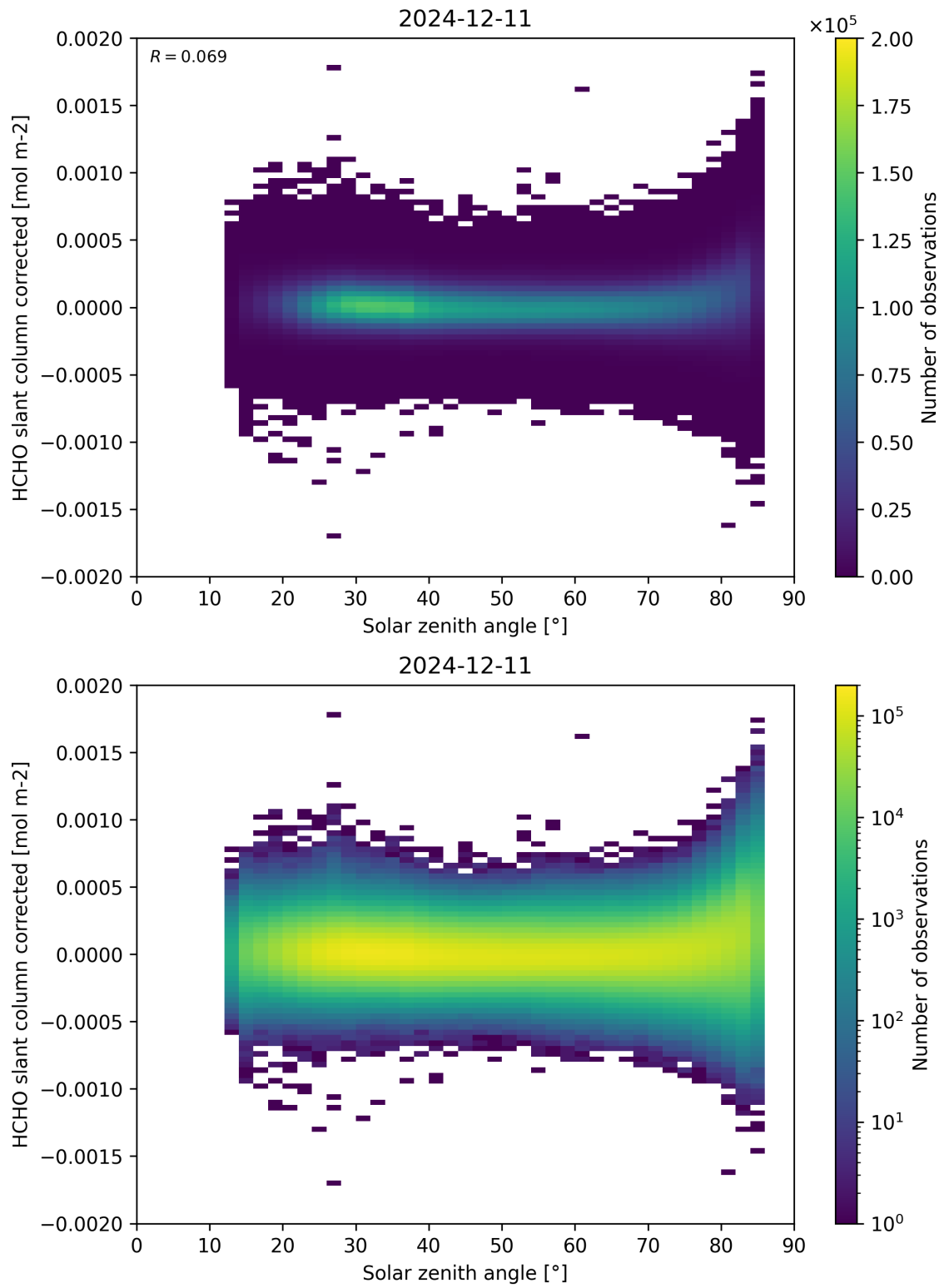
Figure 171: Scatter density plot of “Solar zenith angle” against “HCHO slant column corrected” for 2024-12-11 to 2024-12-12.
