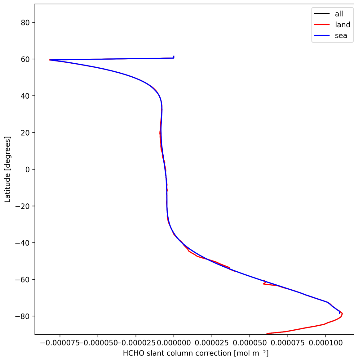
Figure 33: Zonal average of “HCHO slant column correction” for 2024-12-11 to 2024-12-12.
