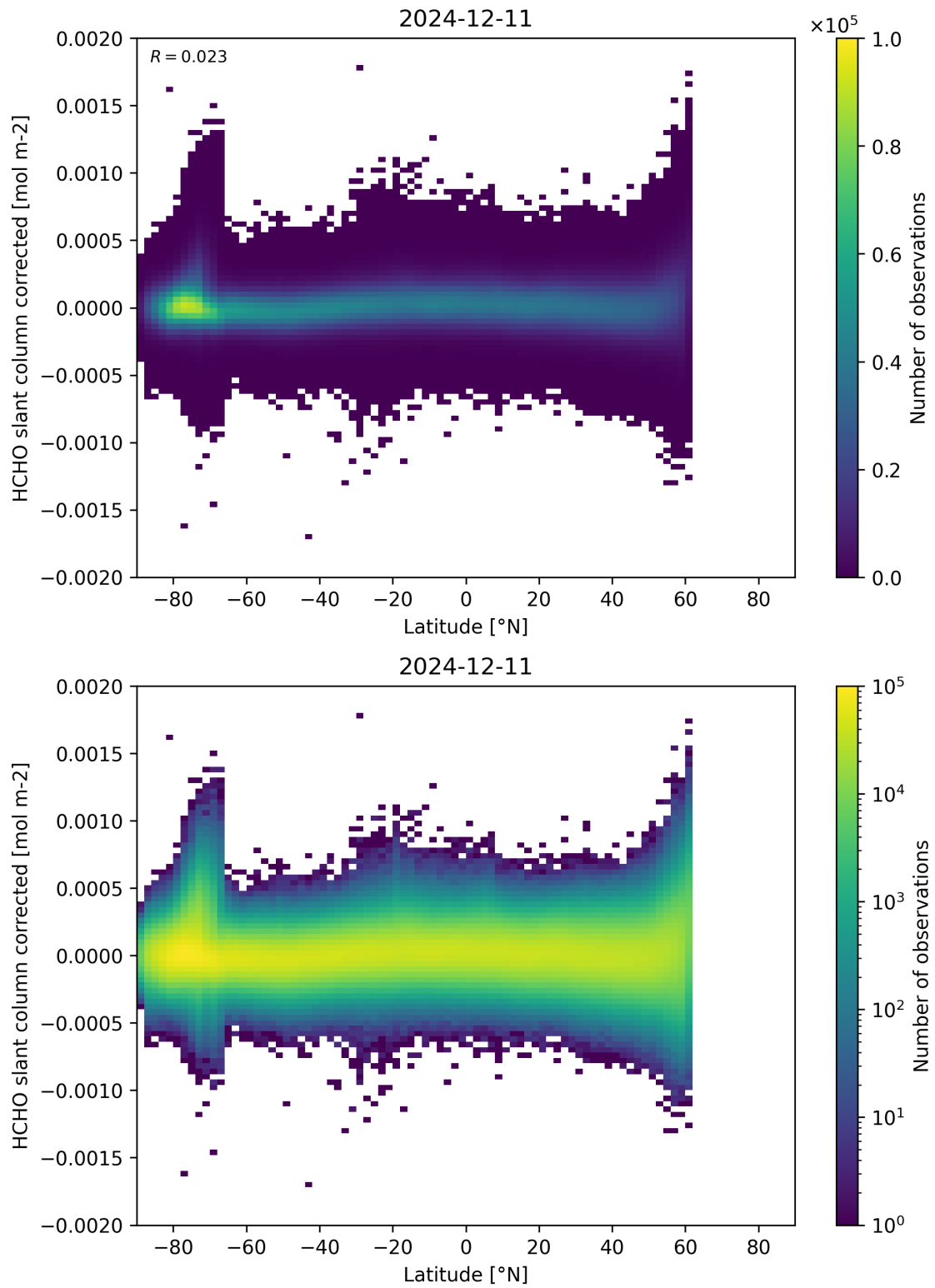
Figure 157: Scatter density plot of “Latitude” against “HCHO slant column corrected” for 2024-12-11 to 2024-12-12.
