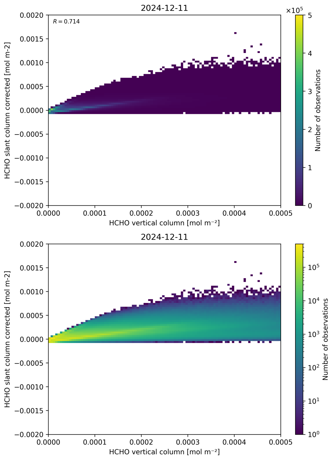
Figure 127: Scatter density plot of “HCHO vertical column” against “HCHO slant column corrected” for 2024-12-11 to 2024-12-12.
