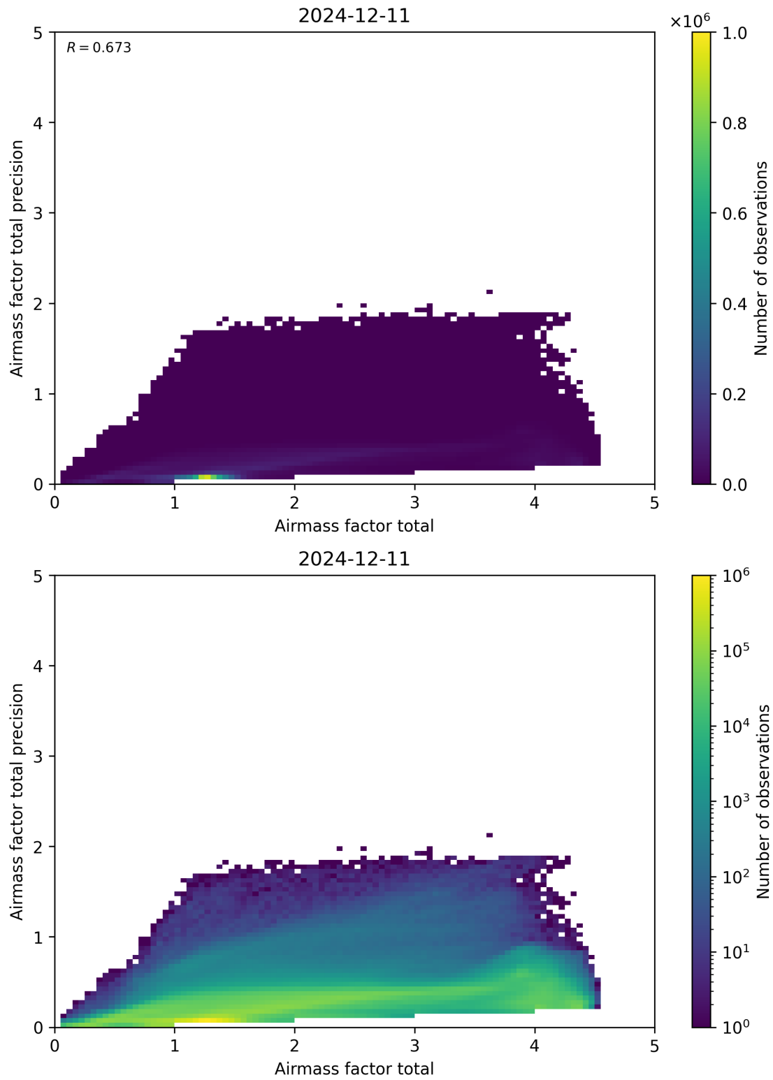
Figure 103: Scatter density plot of “Airmass factor total” against “Airmass factor total precision” for 2024-12-11 to 2024-12-12.
