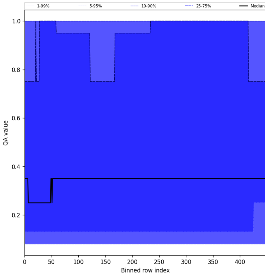
Figure 48: Along track statistics of “QA value” for 2024-12-11 to 2024-12-12
