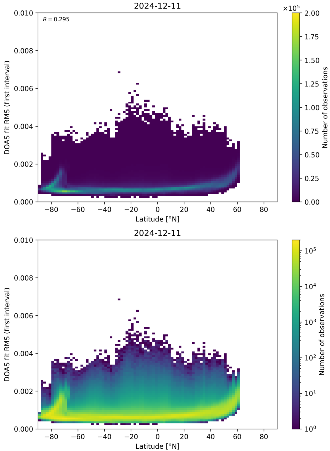
Figure 153: Scatter density plot of “Latitude” against “DOAS fit RMS (first interval)” for 2024-12-11 to 2024-12-12.
