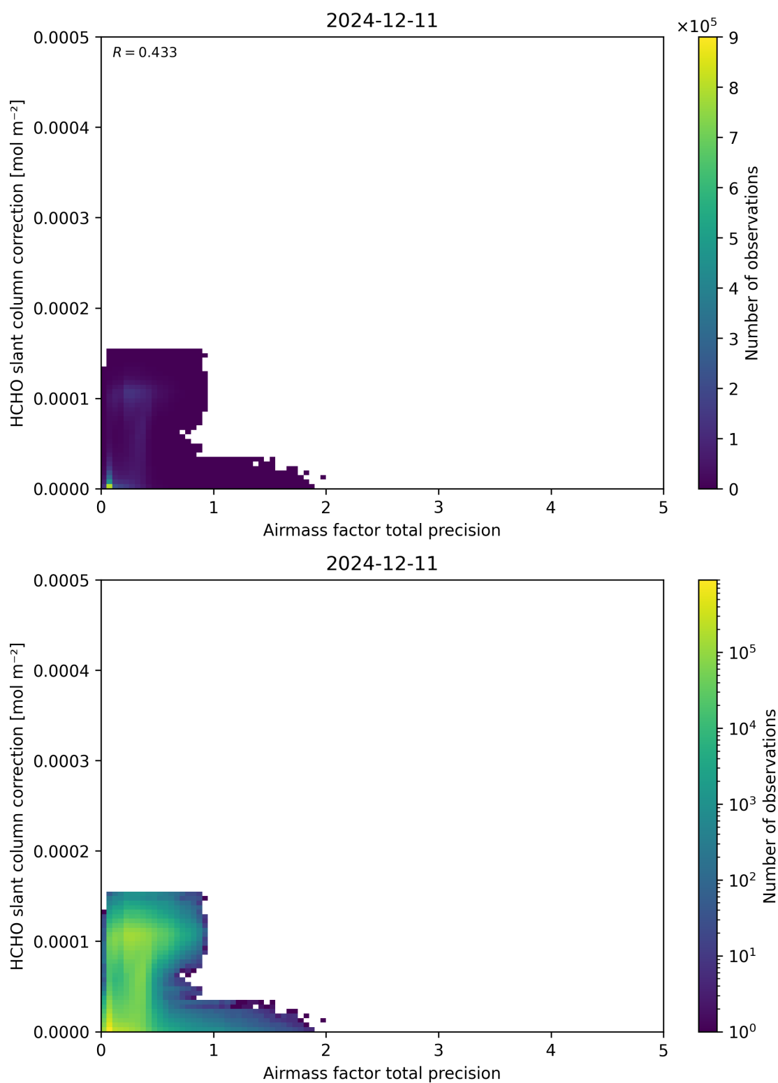
Figure 110: Scatter density plot of “Airmass factor total precision” against “HCHO slant column correction” for 2024-12-11 to 2024-12-12.
