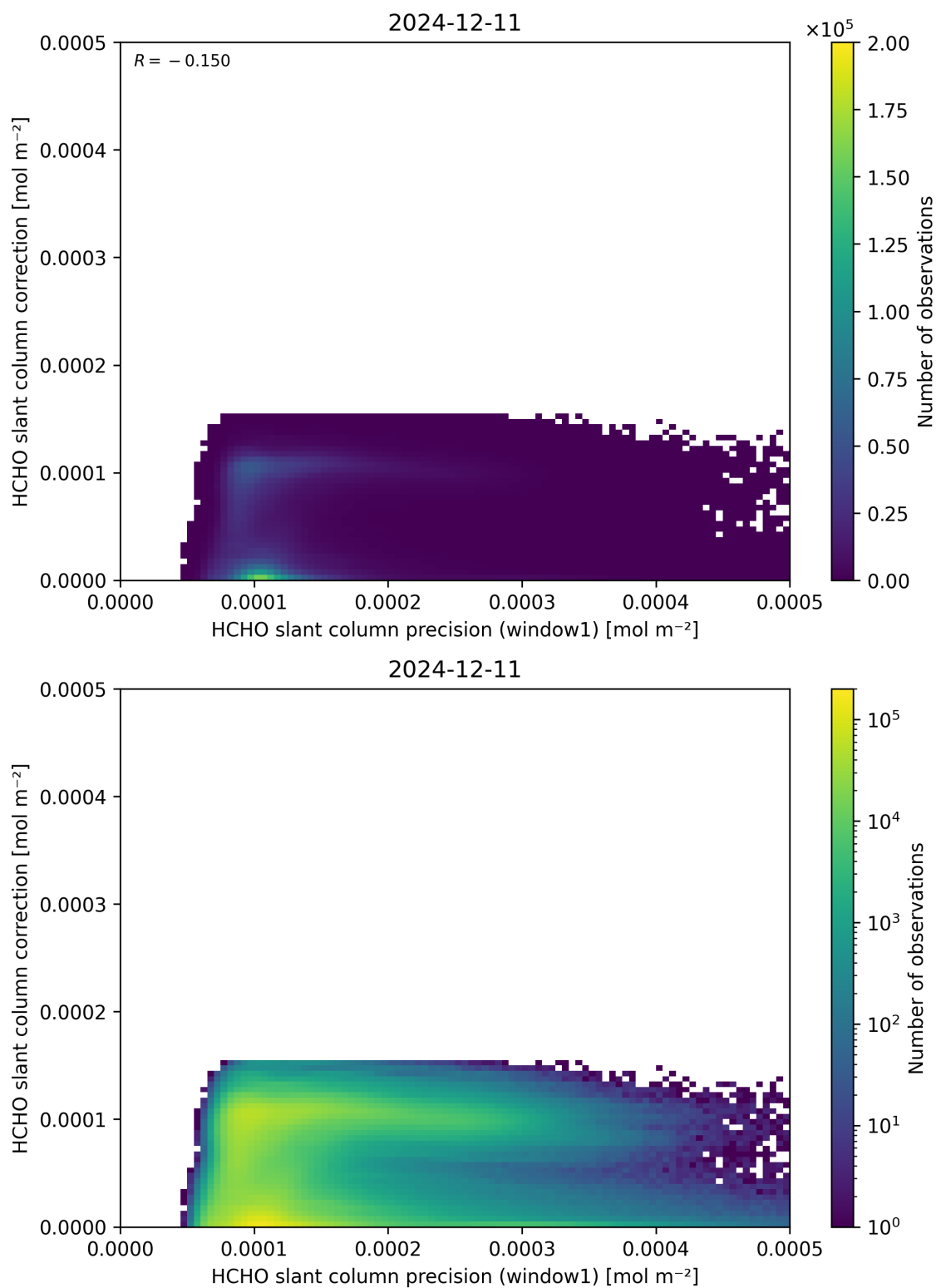
Figure 93: Scatter density plot of “HCHO slant column precision (window1)” against “HCHO slant column correction” for 2024-12-11 to 2024-12-12.
