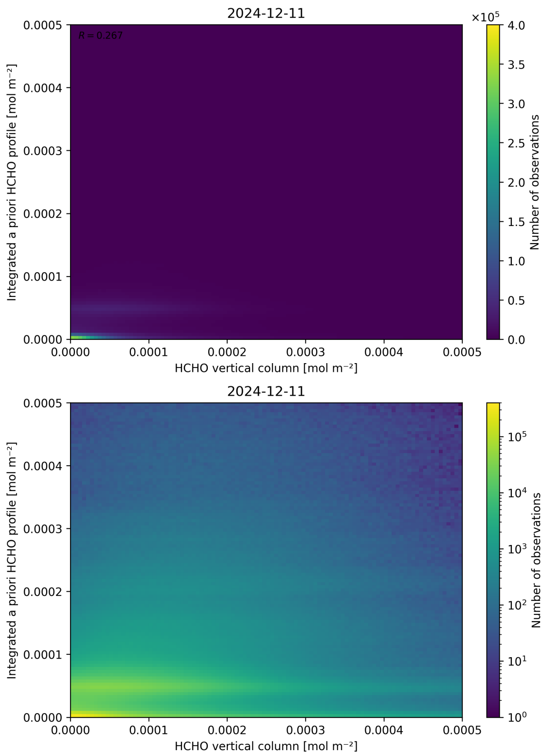
Figure 135: Scatter density plot of “HCHO vertical column” against “Integrated a priori HCHO profile” for 2024-12-11 to 2024-12-12.
