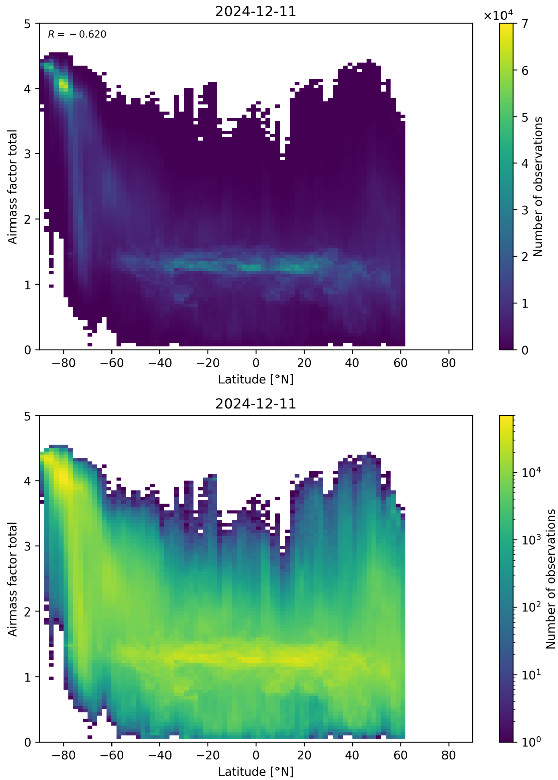
Figure 161: Scatter density plot of “Latitude” against “Airmass factor total” for 2024-12-11 to 2024-12-12.
