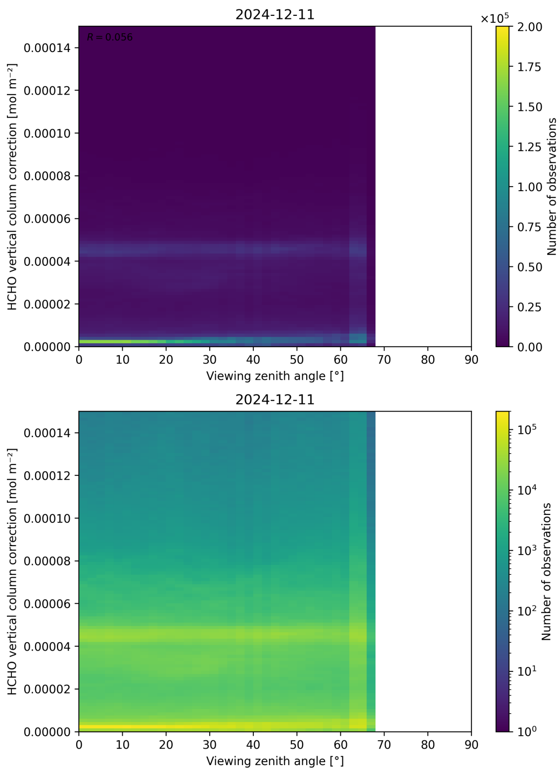
Figure 193: Scatter density plot of “Viewing zenith angle” against “HCHO vertical column correction” for 2024-12-11 to 2024-12-12.
