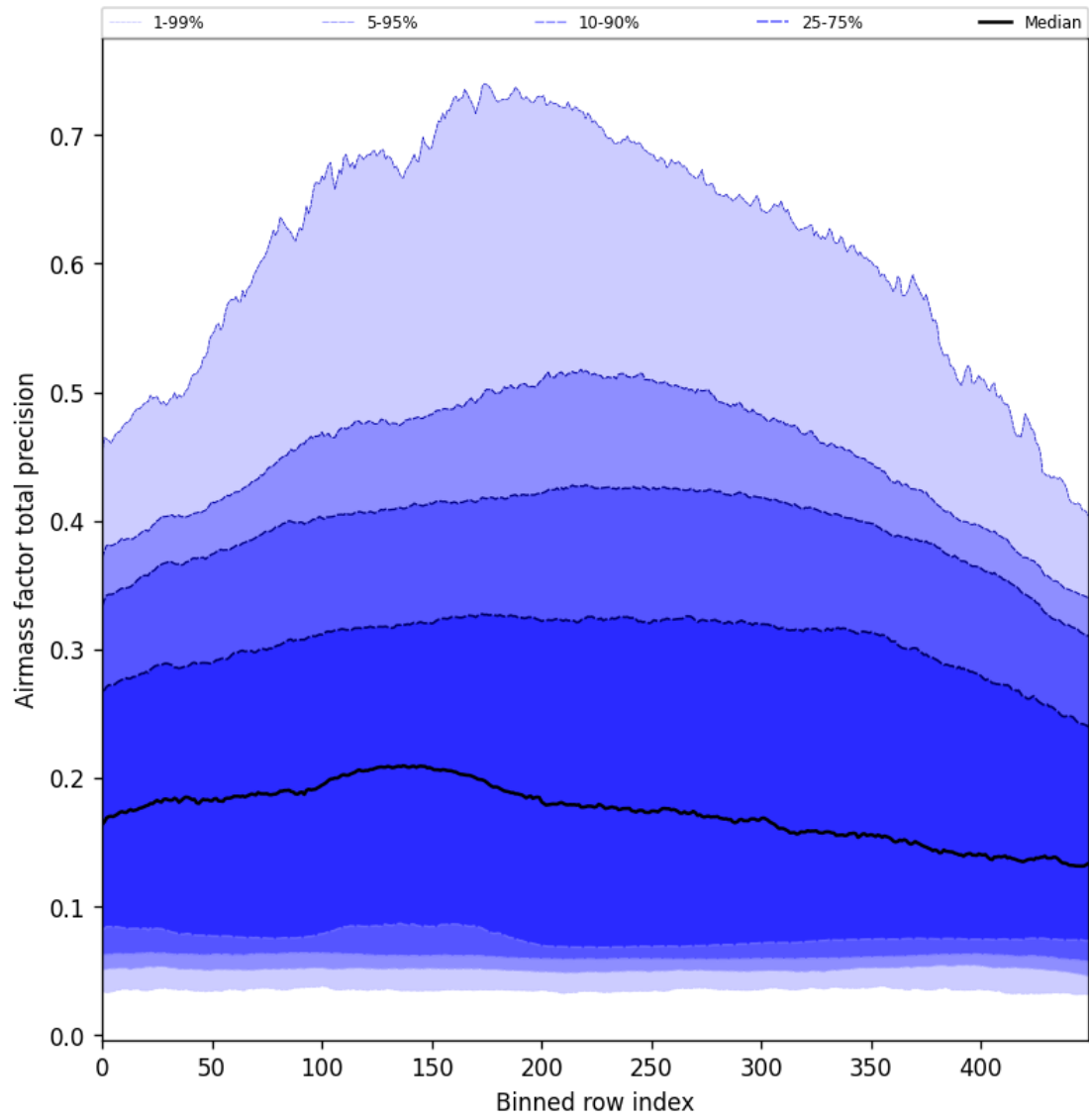
Figure 55: Along track statistics of “Airmass factor total precision” for 2024-12-11 to 2024-12-12
