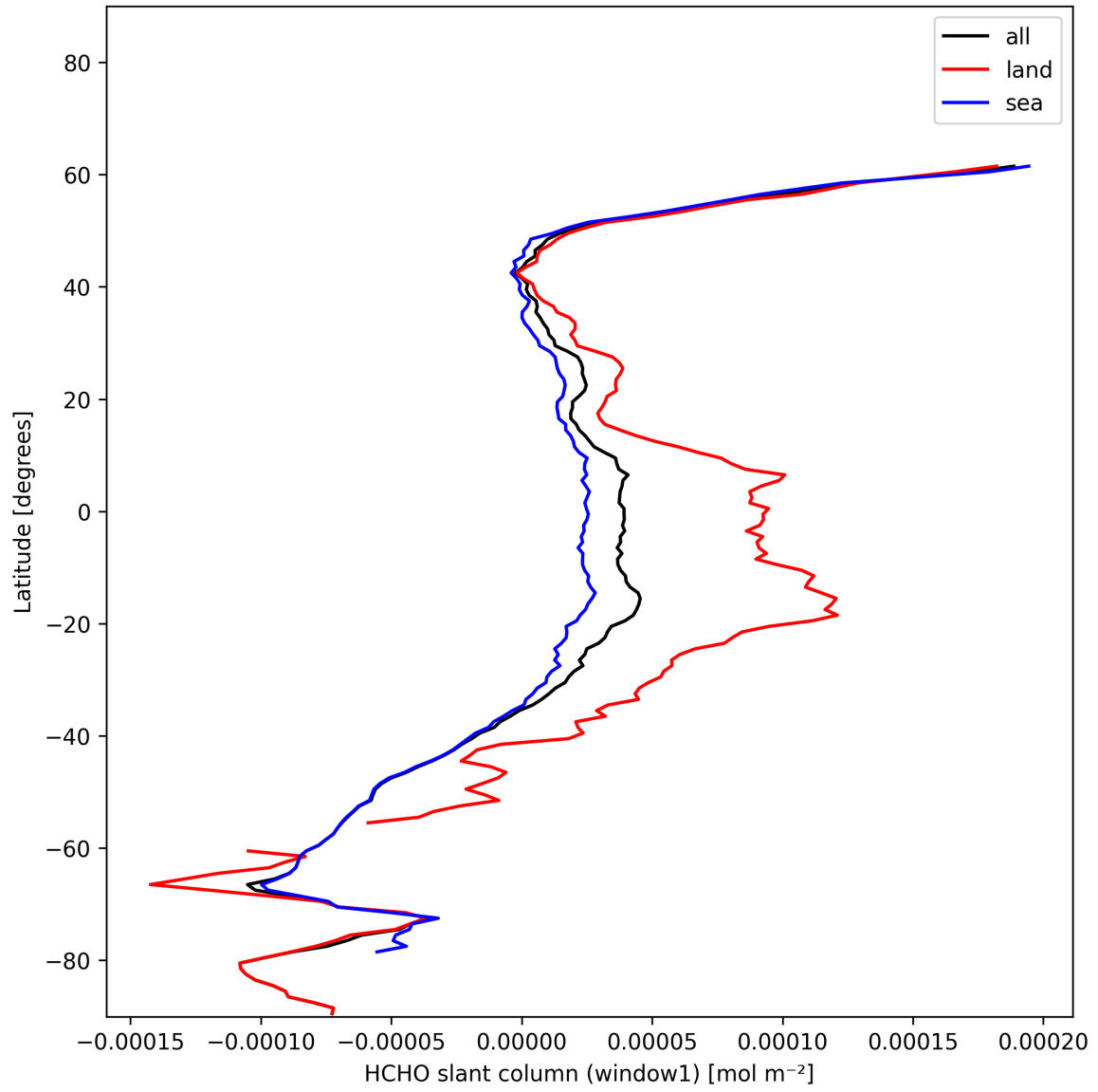
Figure 24: Zonal average of “HCHO slant column (window1)” for 2024-12-11 to 2024-12-12.
