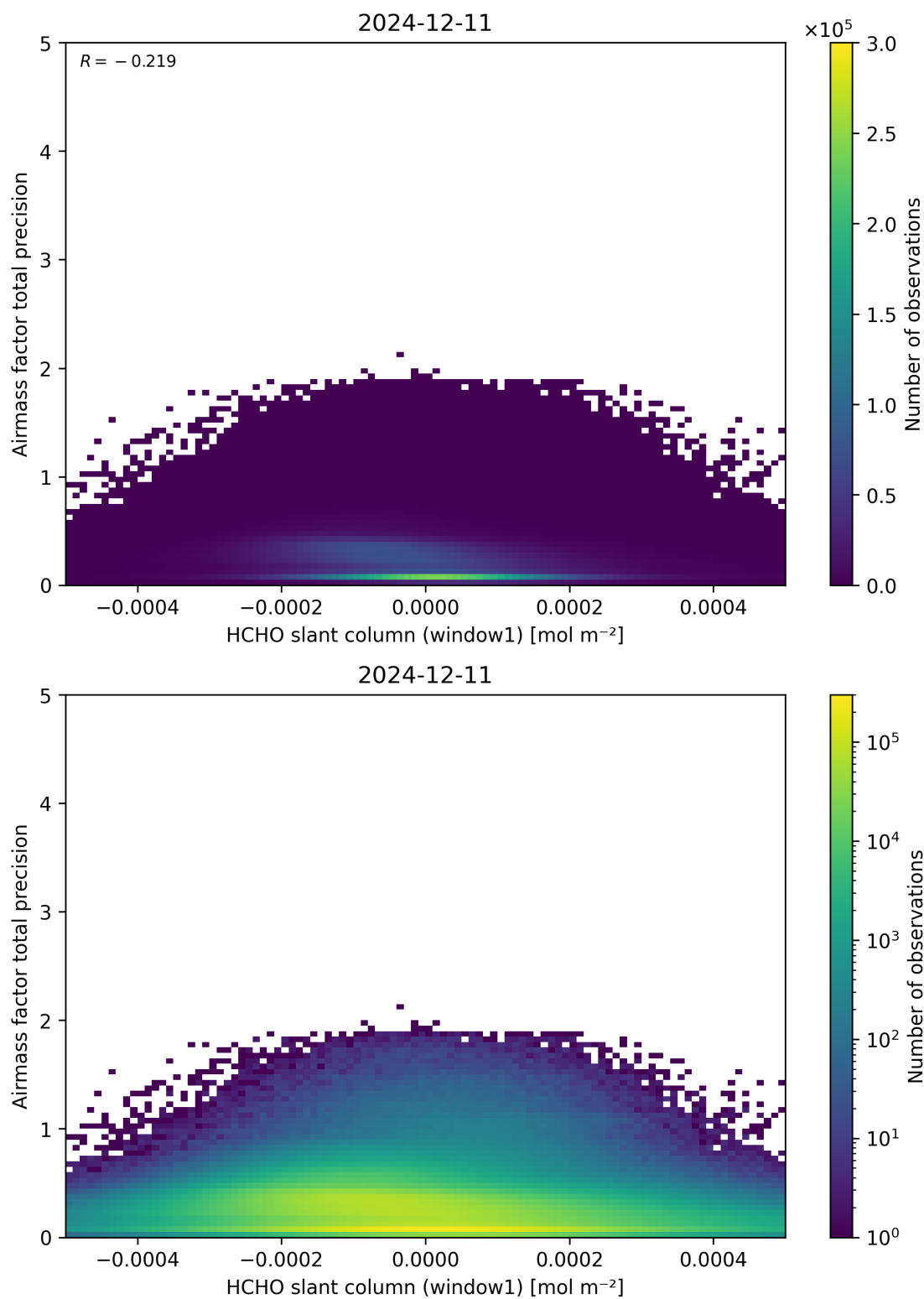
Figure 86: Scatter density plot of “HCHO slant column (window1)” against “Airmass factor total precision” for 2024-12-11 to 2024-12-12.
