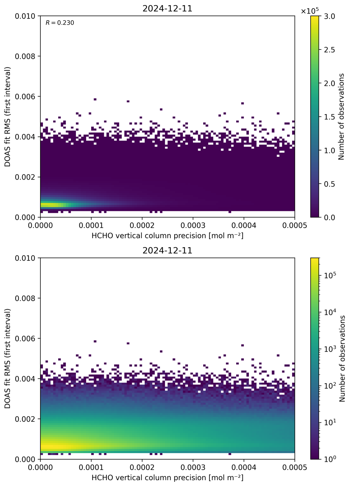
Figure 136: Scatter density plot of “HCHO vertical column precision” against “DOAS fit RMS (first interval)” for 2024-12-11 to 2024-12-12.
