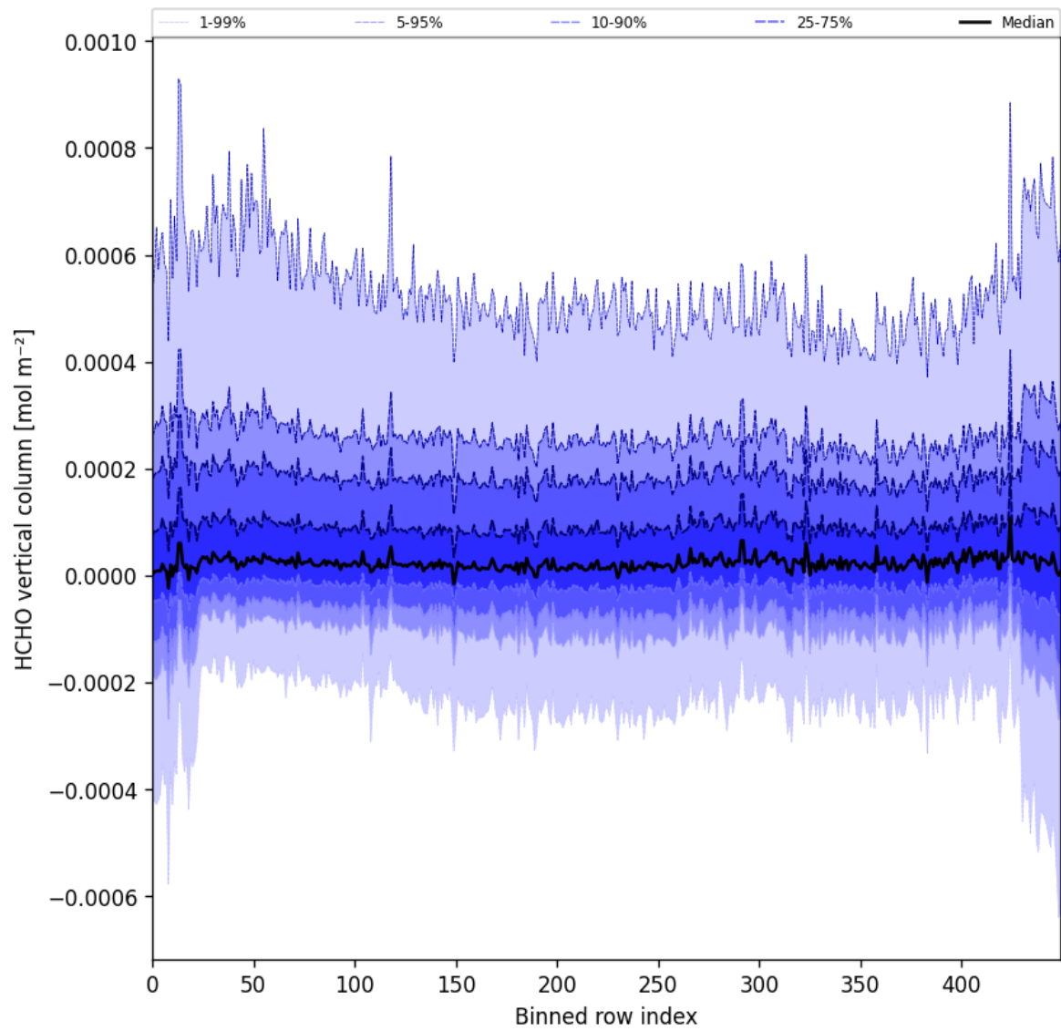
Figure 49: Along track statistics of “HCHO vertical column” for 2024-12-11 to 2024-12-12
