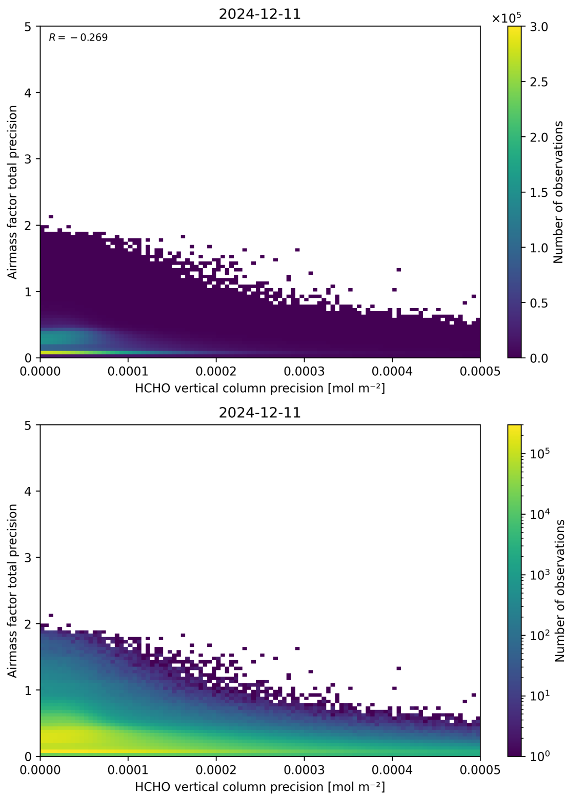
Figure 145: Scatter density plot of “HCHO vertical column precision” against “Airmass factor total precision” for 2024-12-11 to 2024-12-12.
