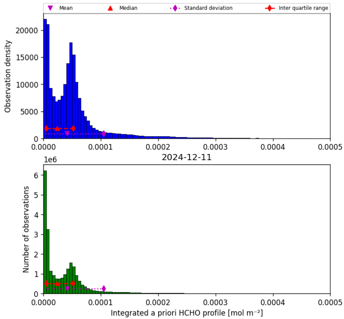
Figure 43: Histogram of “Integrated a priori HCHO profile” for 2024-12-11 to 2024-12-12
