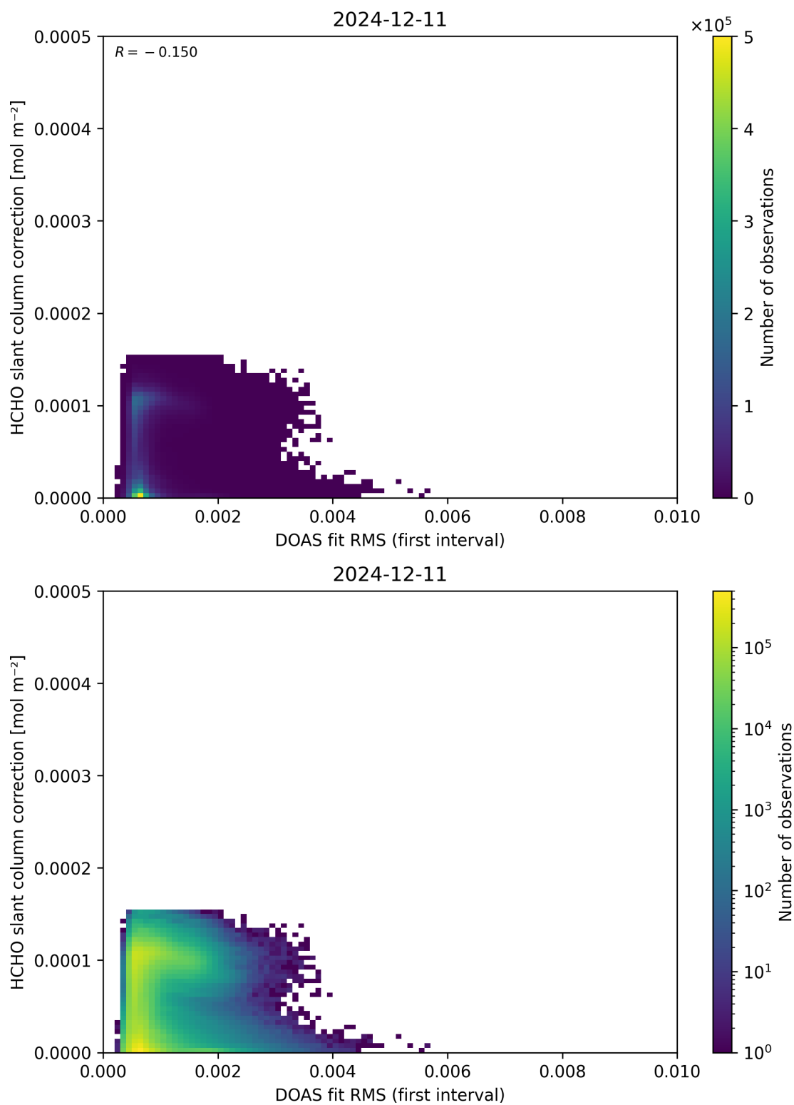
Figure 63: Scatter density plot of “DOAS fit RMS (first interval)” against “HCHO slant column correction” for 2024-12-11 to 2024-12-12.
