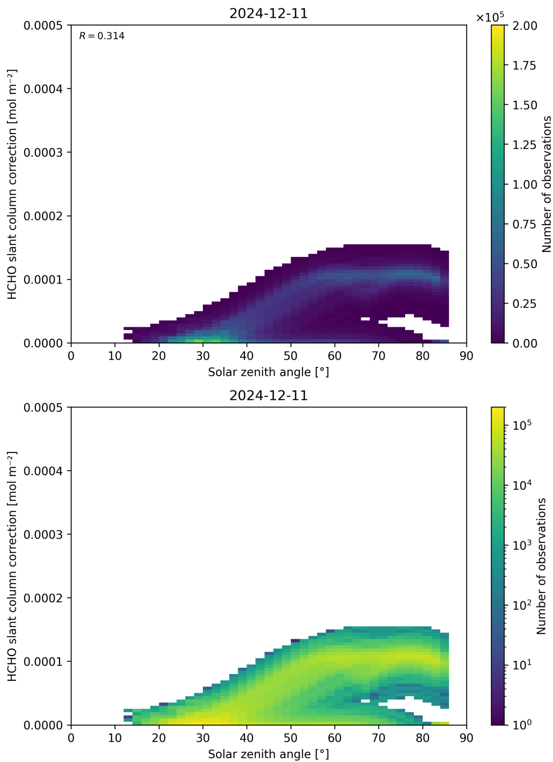
Figure 172: Scatter density plot of “Solar zenith angle” against “HCHO slant column correction” for 2024-12-11 to 2024-12-12.
