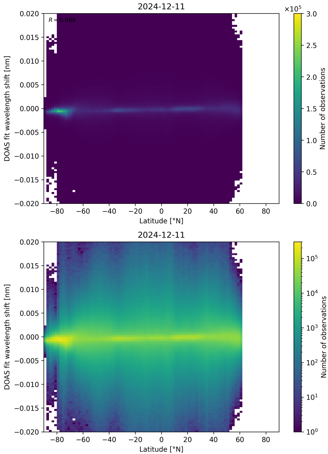
Figure 154: Scatter density plot of “Latitude” against “DOAS fit wavelength shift” for 2024-12-11 to 2024-12-12.
