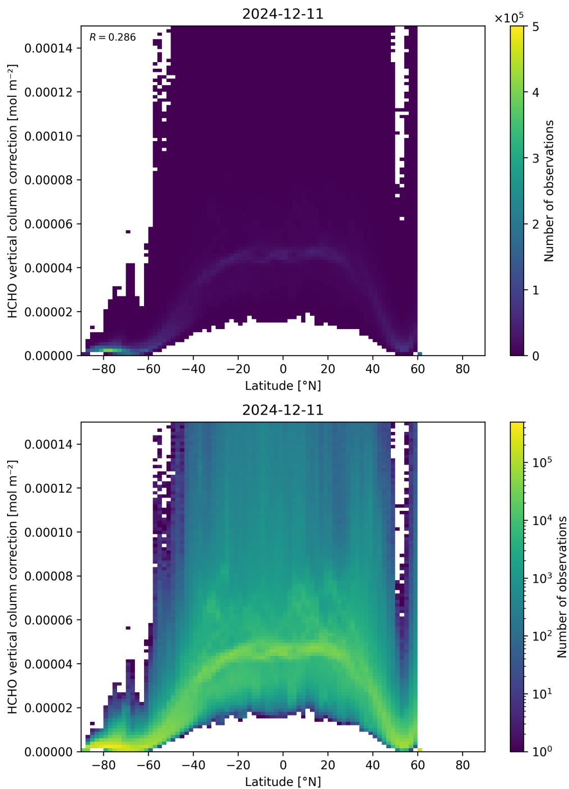
Figure 164: Scatter density plot of “Latitude” against “HCHO vertical column correction” for 2024-12-11 to 2024-12-12.
