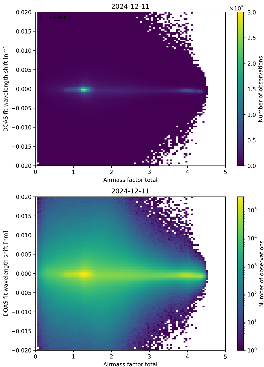
Figure 98: Scatter density plot of “Airmass factor total” against “DOAS fit wavelength shift” for 2024-12-11 to 2024-12-12.
