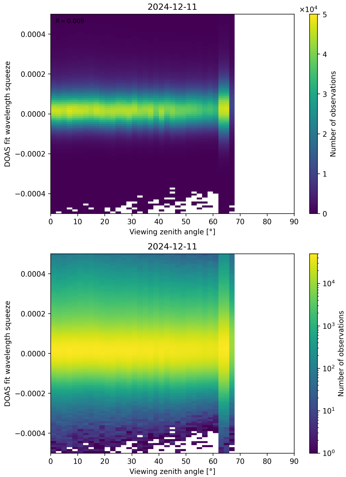
Figure 184: Scatter density plot of “Viewing zenith angle” against “DOAS fit wavelength squeeze” for 2024-12-11 to 2024-12-12.
