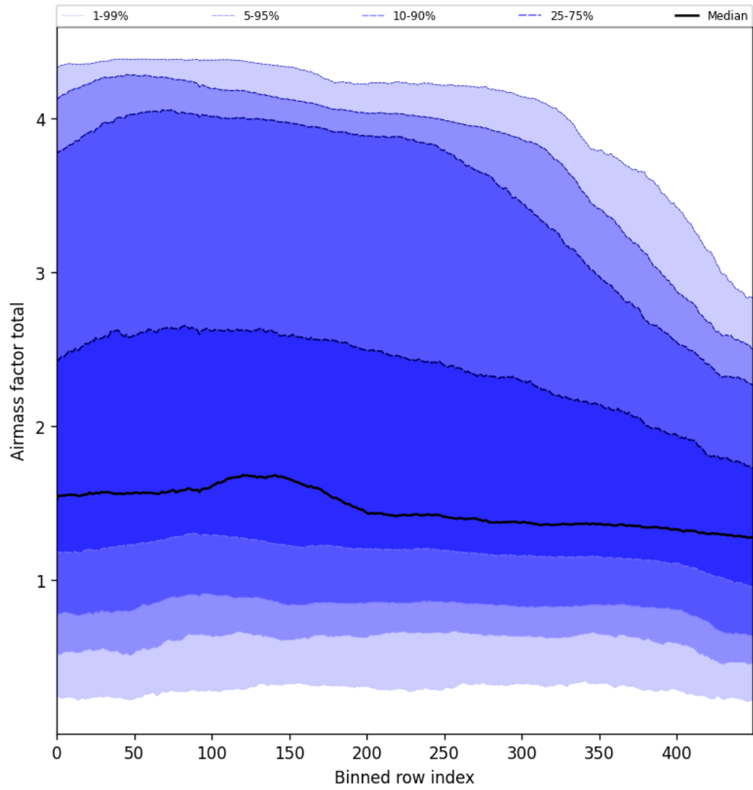
Figure 54: Along track statistics of “Airmass factor total” for 2024-12-11 to 2024-12-12
