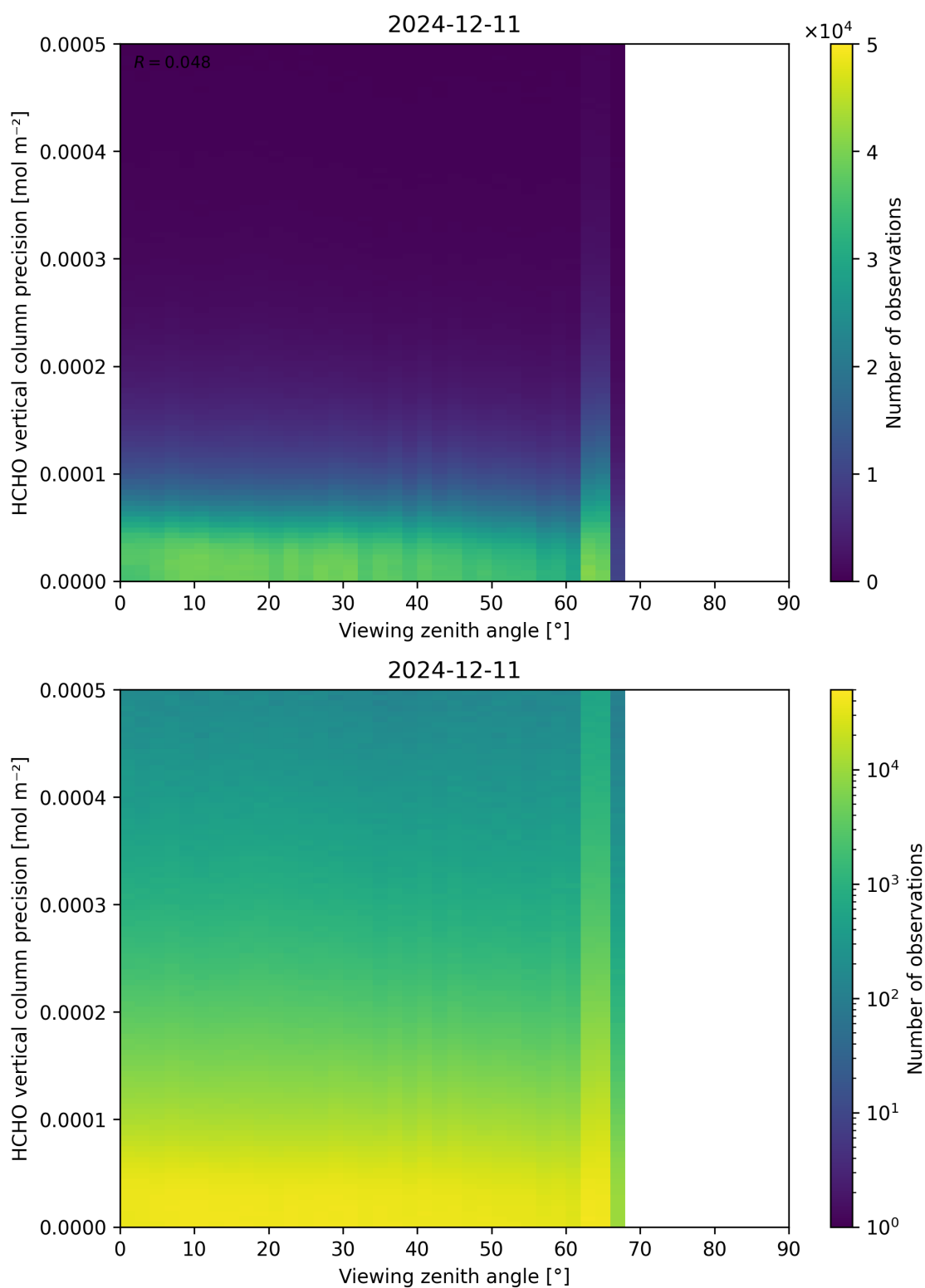
Figure 194: Scatter density plot of “Viewing zenith angle” against “HCHO vertical column precision” for 2024-12-11 to 2024-12-12.
