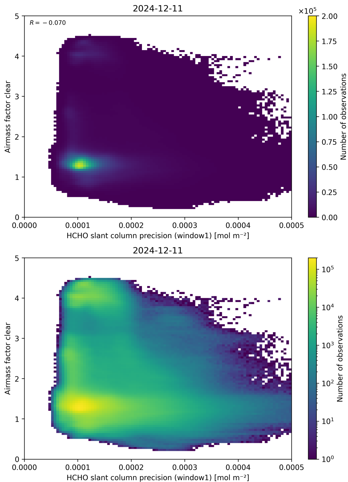
Figure 91: Scatter density plot of “HCHO slant column precision (window1)” against “Airmass factor clear” for 2024-12-11 to 2024-12-12.
