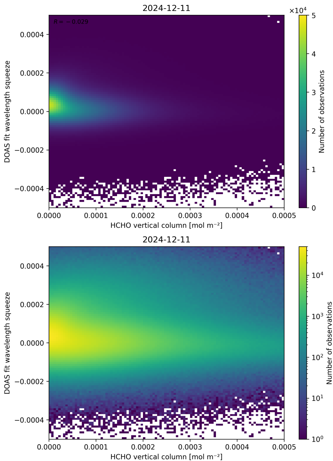
Figure 125: Scatter density plot of “HCHO vertical column” against “DOAS fit wavelength squeeze” for 2024-12-11 to 2024-12-12.
