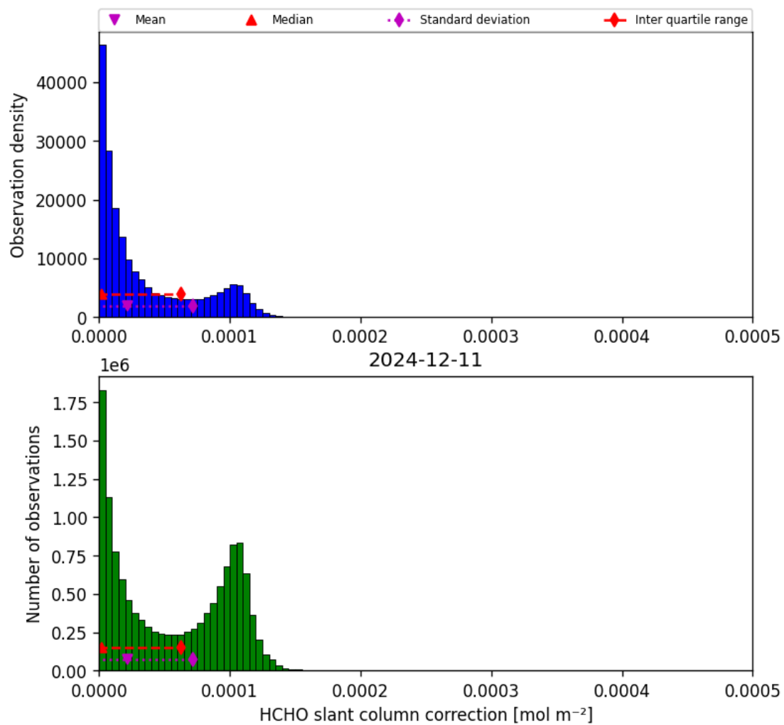
Figure 47: Histogram of “HCHO slant column correction” for 2024-12-11 to 2024-12-12
