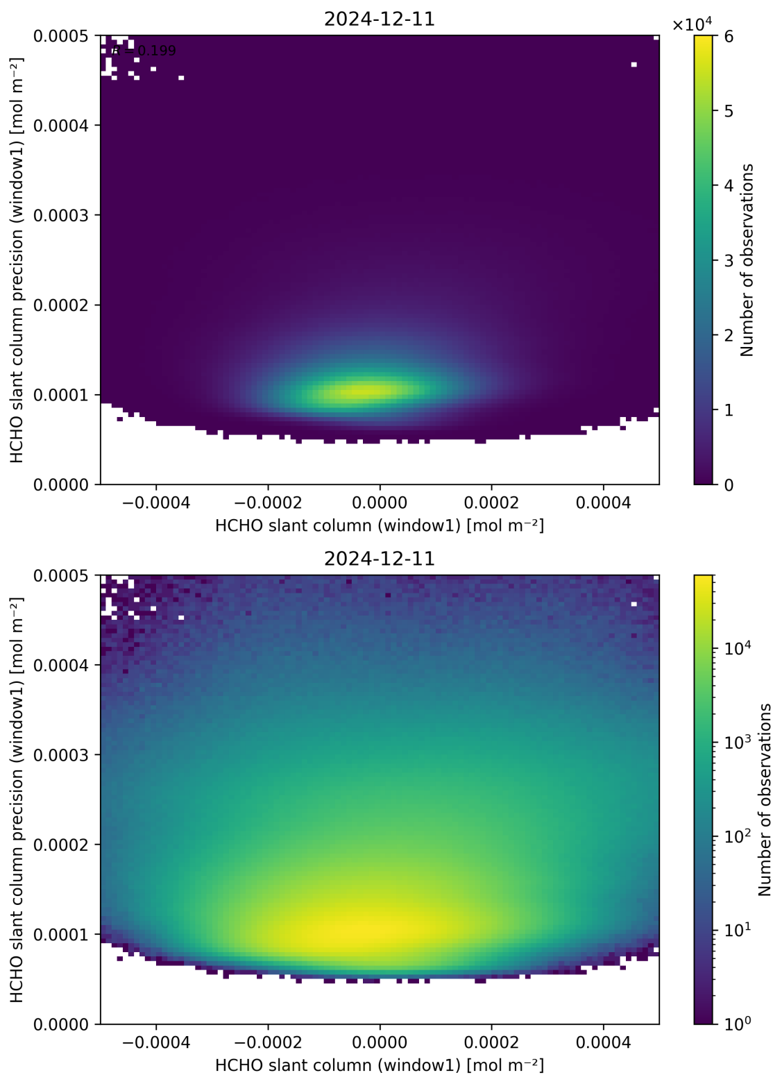
Figure 84: Scatter density plot of “HCHO slant column (window1)” against “HCHO slant column precision (window1)” for 2024-12-11 to 2024-12-12.
