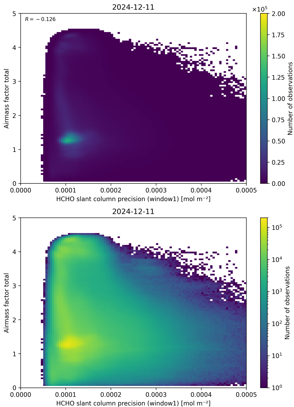
Figure 94: Scatter density plot of “HCHO slant column precision (window1)” against “Airmass factor total” for 2024-12-11 to 2024-12-12.
