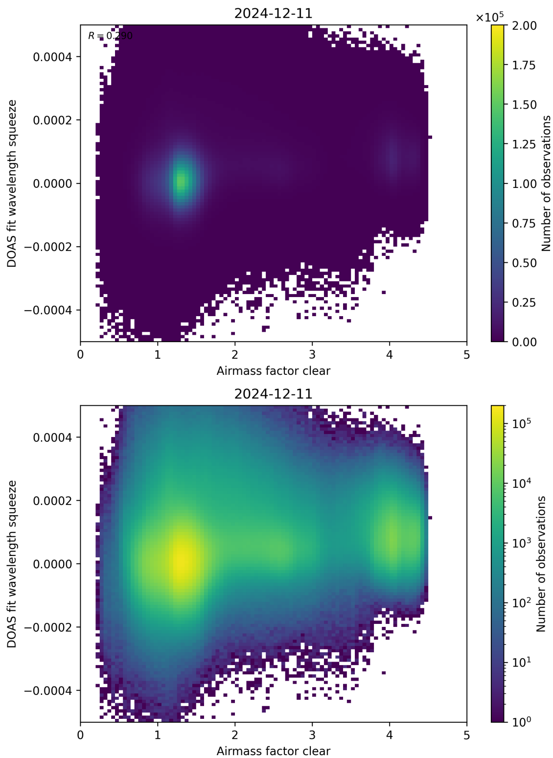
Figure 73: Scatter density plot of “Airmass factor clear” against “DOAS fit wavelength squeeze” for 2024-12-11 to 2024-12-12.
