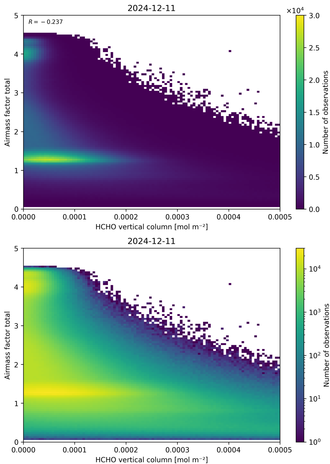
Figure 131: Scatter density plot of “HCHO vertical column” against “Airmass factor total” for 2024-12-11 to 2024-12-12.
