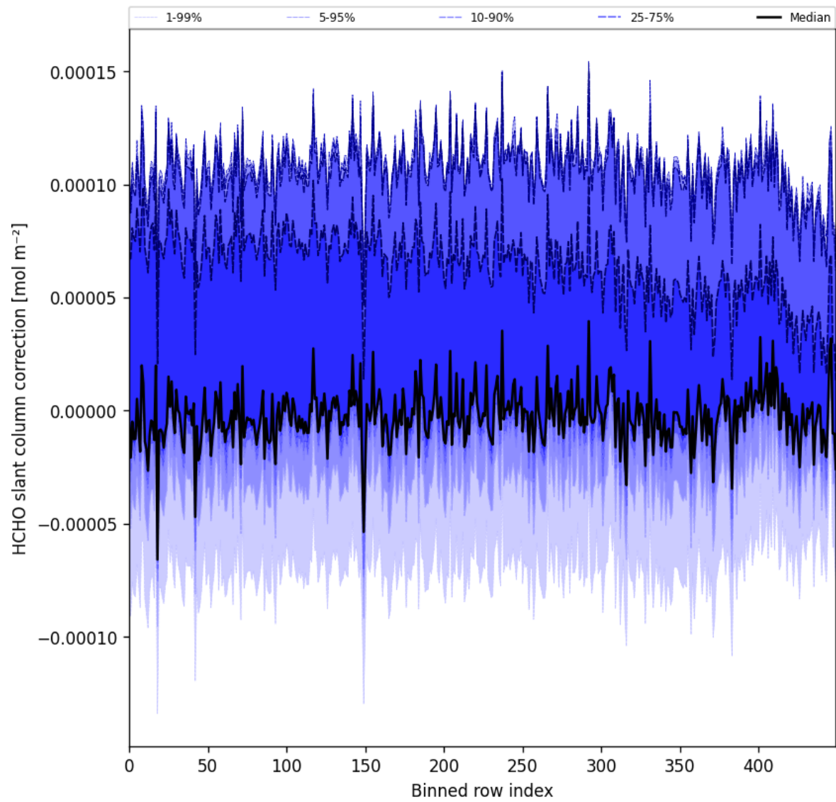
Figure 61: Along track statistics of "HCHO slant column correction" for 2024-12-11 to 2024-12-12
