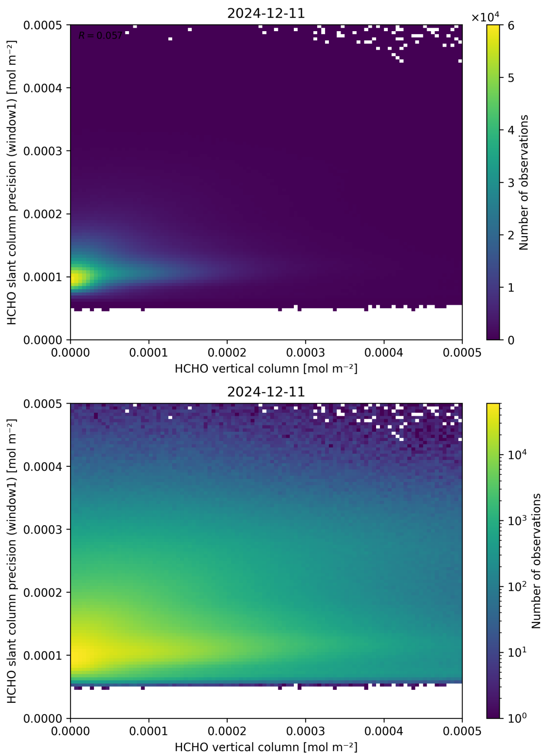
Figure 130: Scatter density plot of “HCHO vertical column” against “HCHO slant column precision (window1)” for 2024-12-11 to 2024-12-12.
