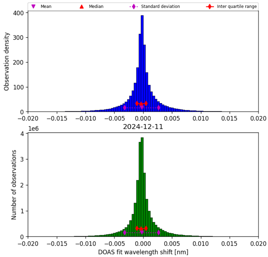
Figure 44: Histogram of “DOAS fit wavelength shift” for 2024-12-11 to 2024-12-12
