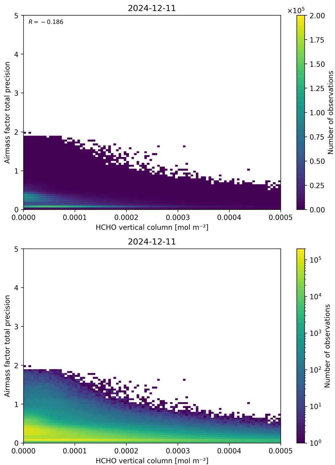
Figure 132: Scatter density plot of “HCHO vertical column” against “Airmass factor total precision” for 2024-12-11 to 2024-12-12.
