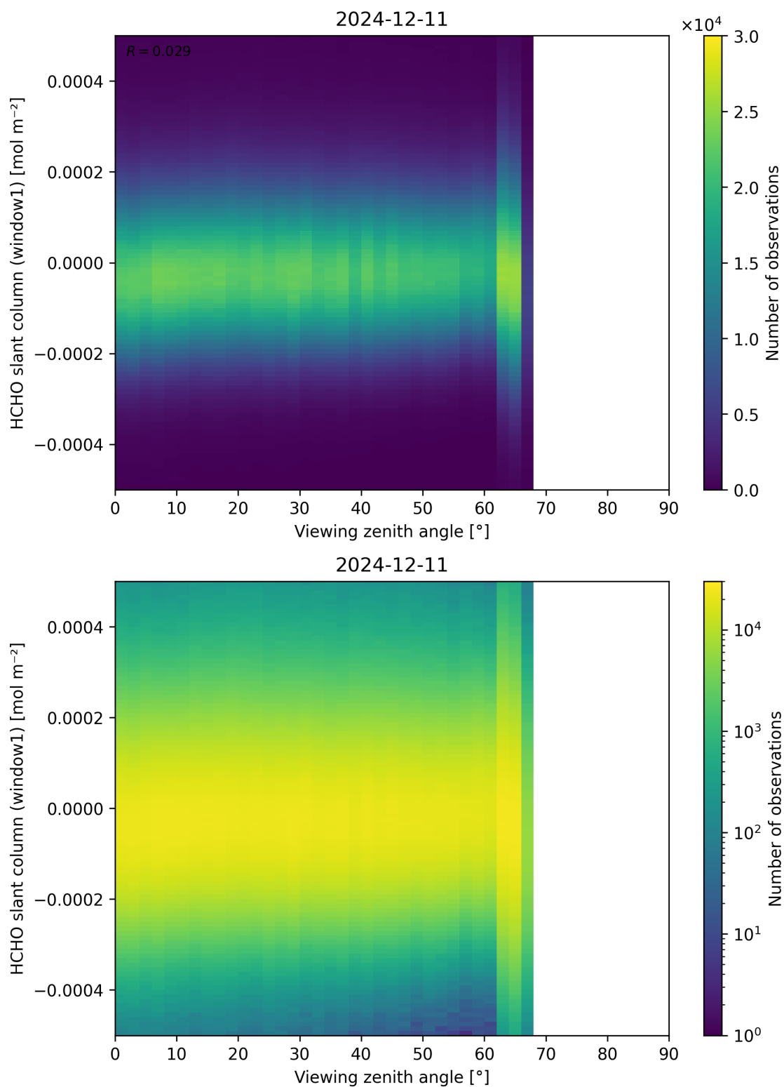
Figure 188: Scatter density plot of “Viewing zenith angle” against “HCHO slant column (window1)” for 2024-12-11 to 2024-12-12.
