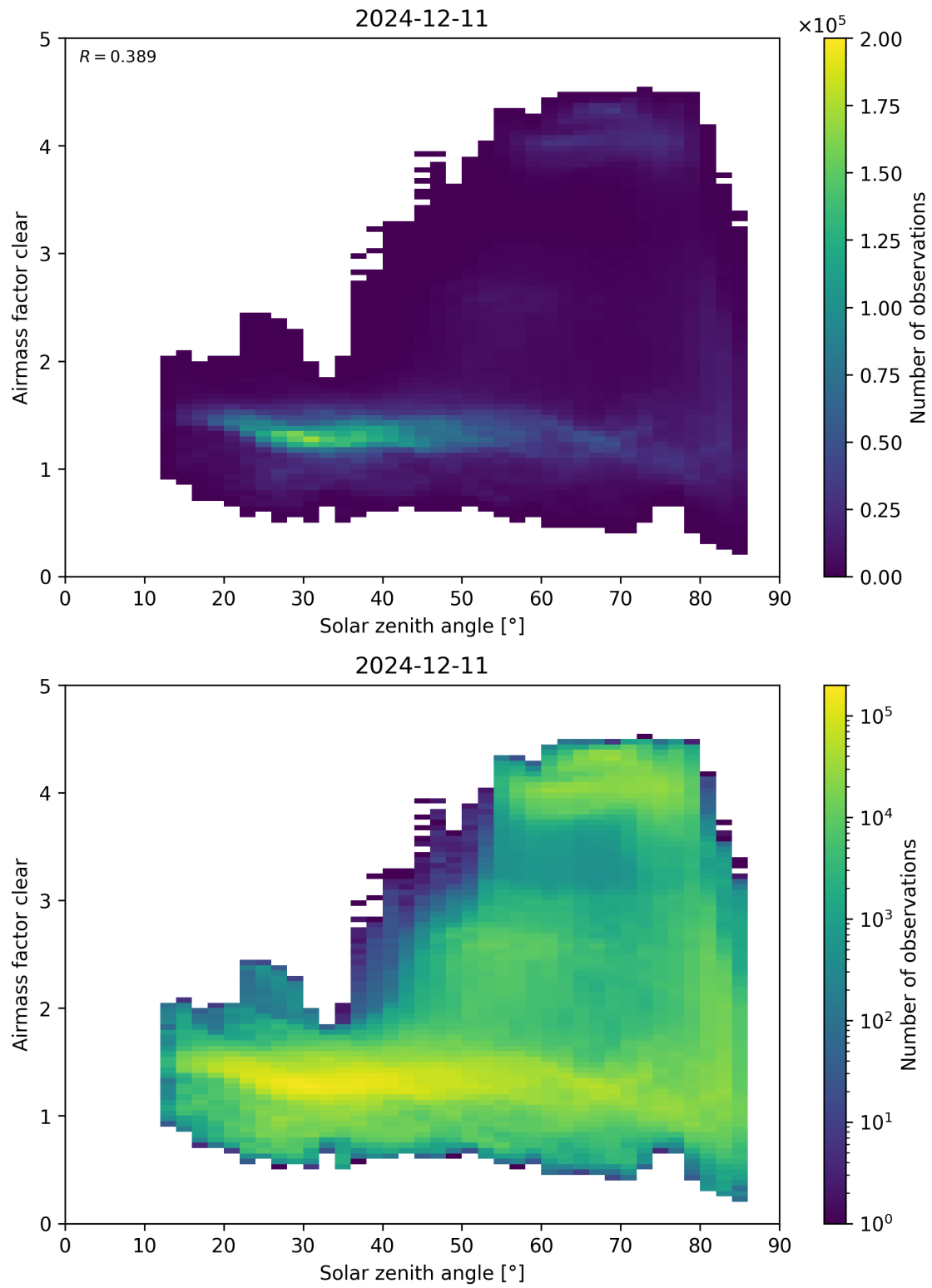
Figure 170: Scatter density plot of “Solar zenith angle” against “Airmass factor clear” for 2024-12-11 to 2024-12-12.
