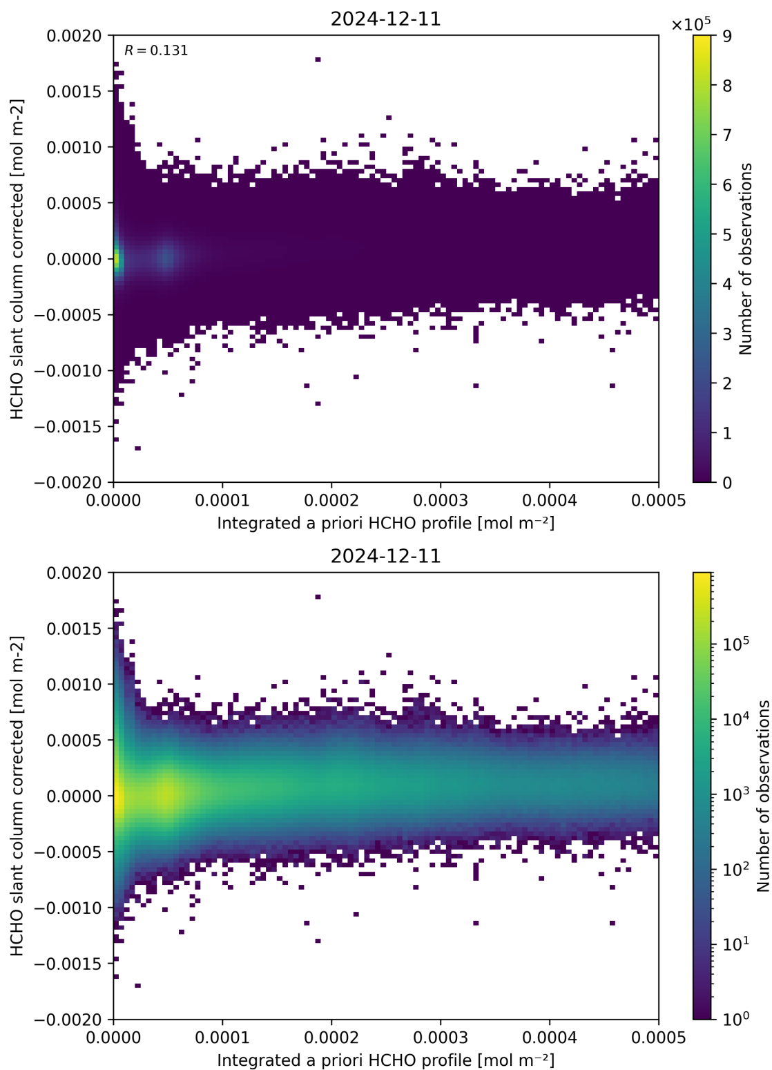
Figure 151: Scatter density plot of “Integrated a priori HCHO profile” against “HCHO slant column corrected” for 2024-12-11 to 2024-12-12.
