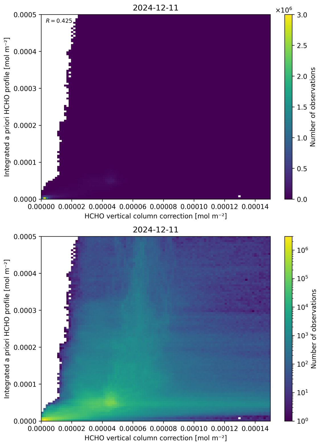
Figure 122: Scatter density plot of “HCHO vertical column correction” against “Integrated a priori HCHO profile” for 2024-12-11 to 2024-12-12.
