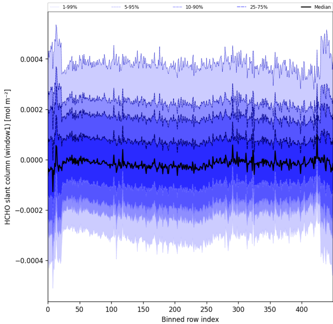
Figure 52: Along track statistics of “HCHO slant column (window1)” for 2024-12-11 to 2024-12-12
