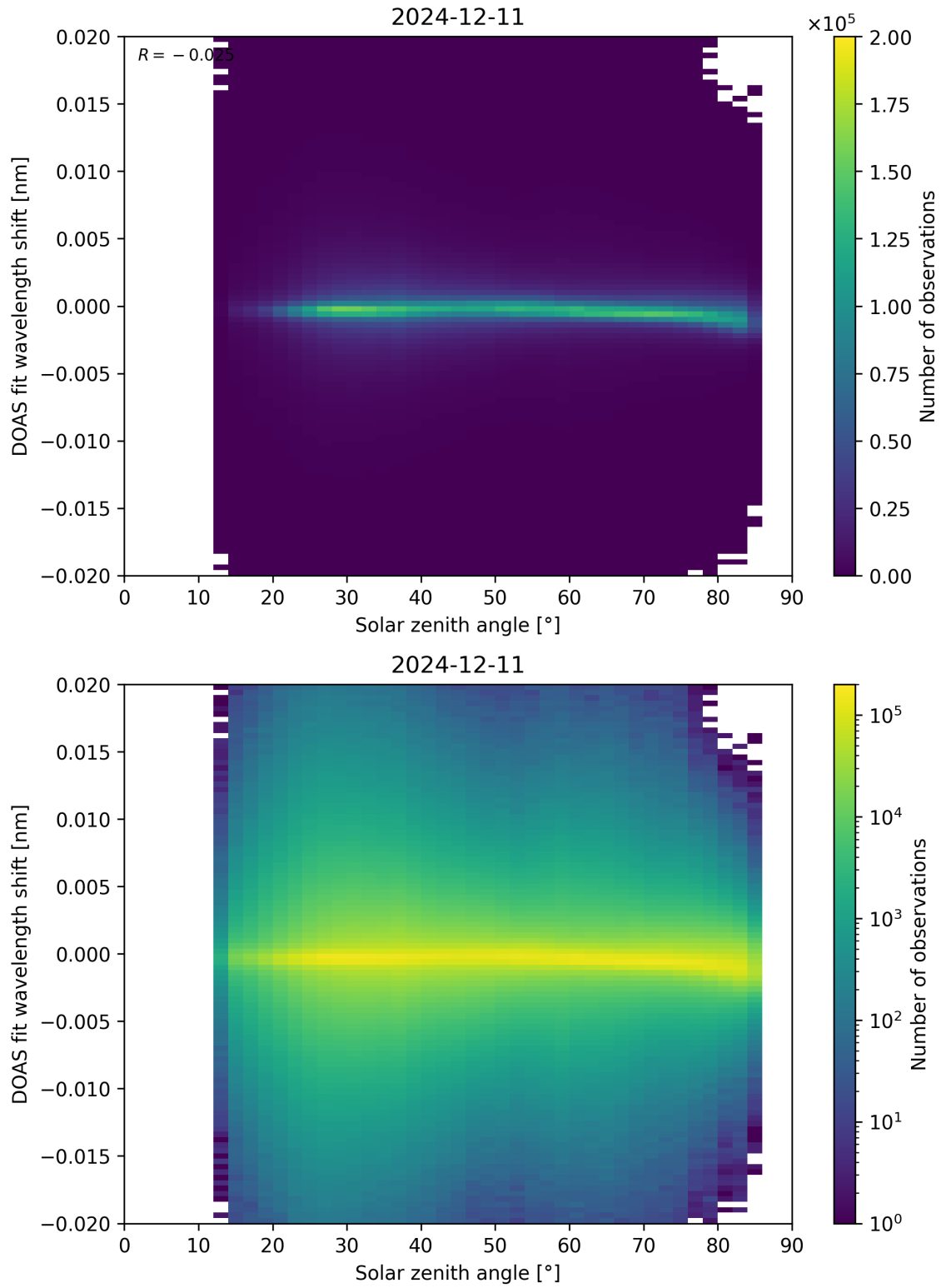
Figure 168: Scatter density plot of “Solar zenith angle” against “DOAS fit wavelength shift” for 2024-12-11 to 2024-12-12.
