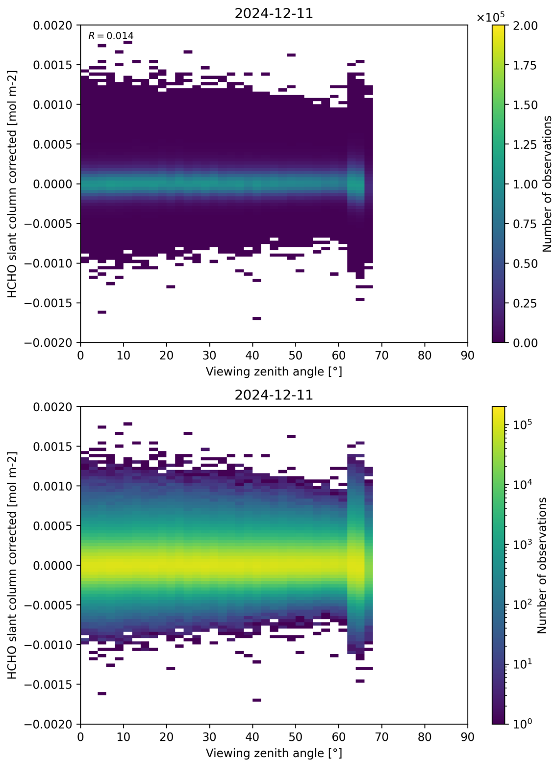
Figure 186: Scatter density plot of “Viewing zenith angle” against “HCHO slant column corrected” for 2024-12-11 to 2024-12-12.
