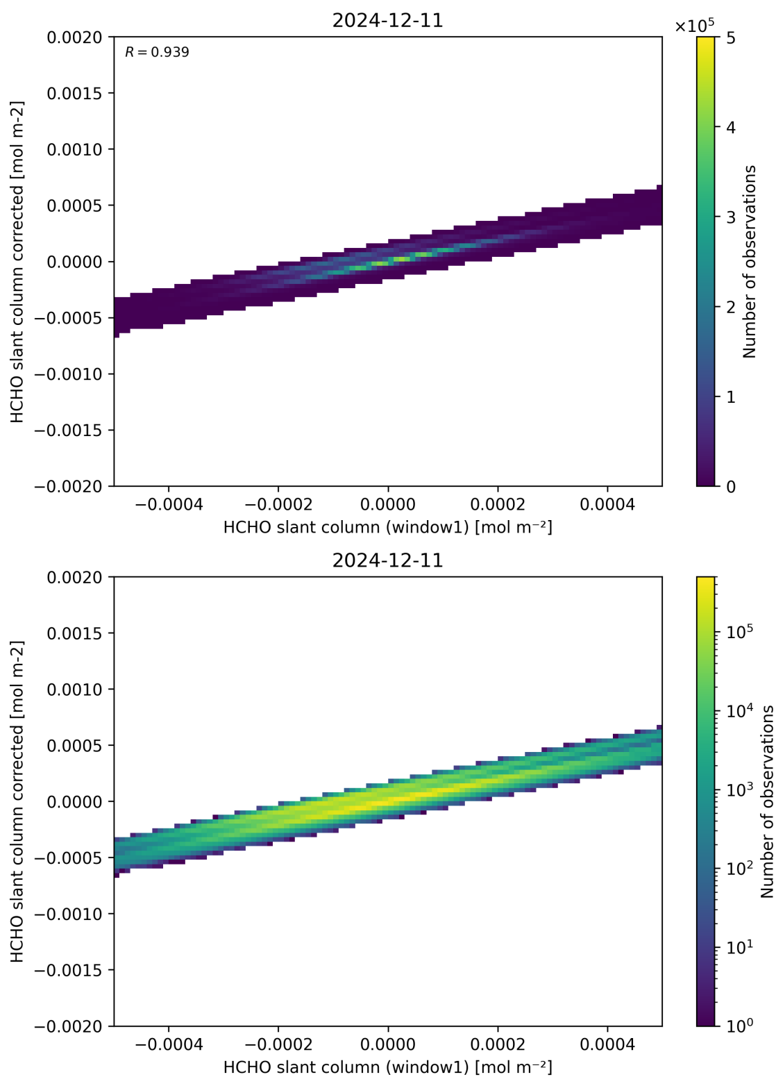
Figure 82: Scatter density plot of “HCHO slant column (window1)” against “HCHO slant column corrected” for 2024-12-11 to 2024-12-12.
