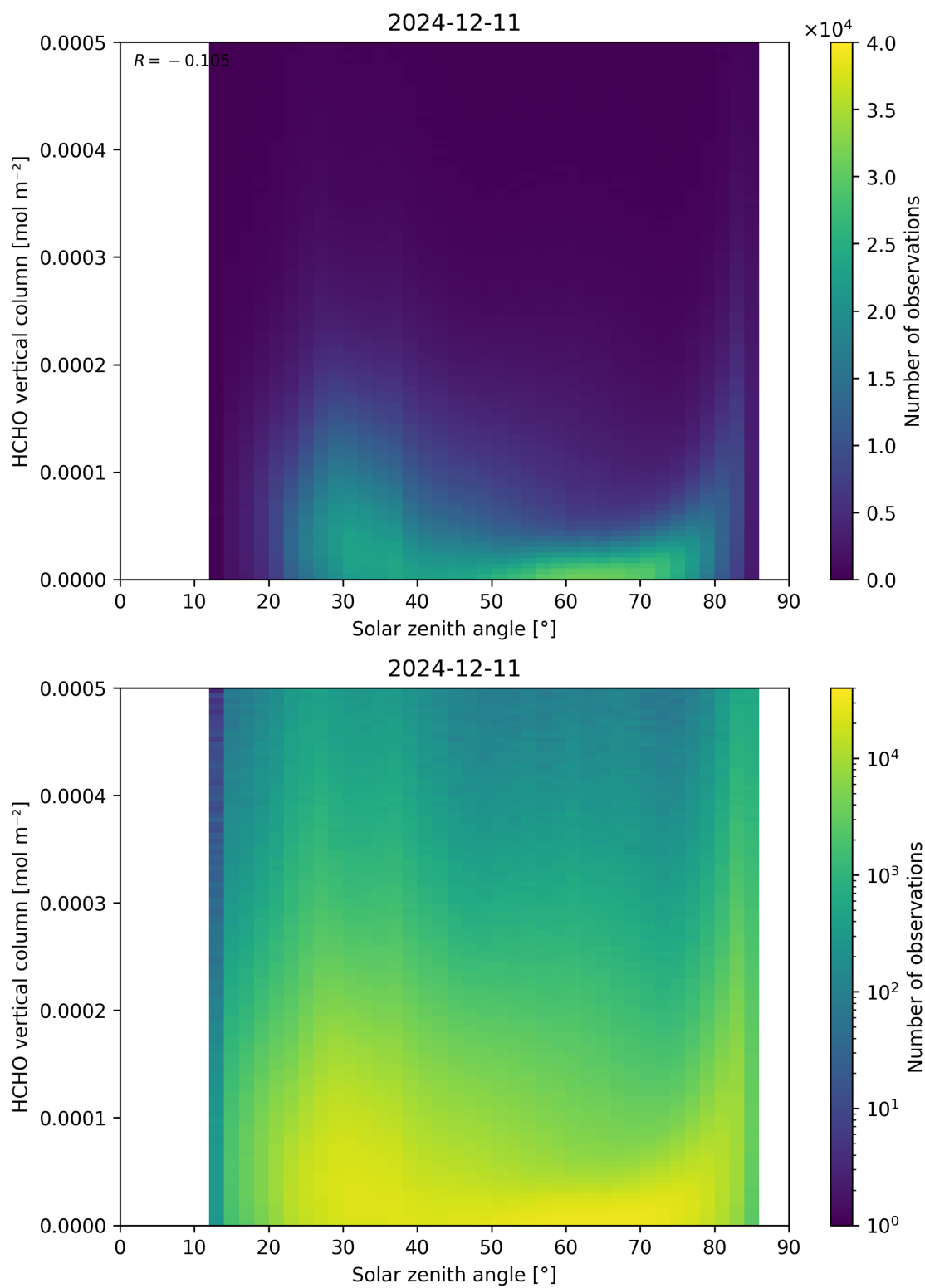
Figure 177: Scatter density plot of “Solar zenith angle” against “HCHO vertical column” for 2024-12-11 to 2024-12-12.
