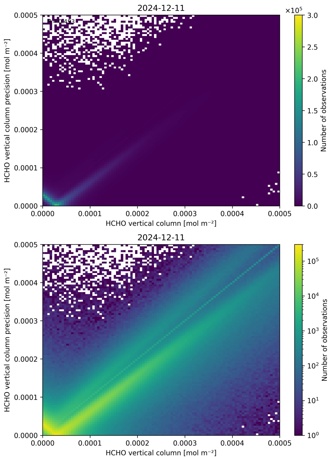
Figure 134: Scatter density plot of “HCHO vertical column” against “HCHO vertical column precision” for 2024-12-11 to 2024-12-12.
