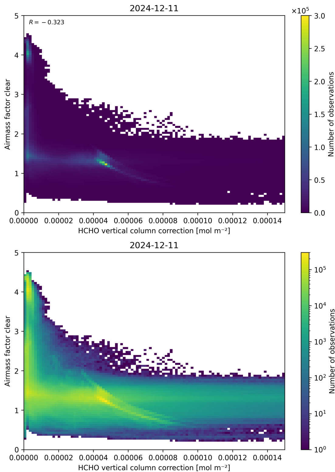
Figure 115: Scatter density plot of “HCHO vertical column correction” against “Airmass factor clear” for 2024-12-11 to 2024-12-12.
