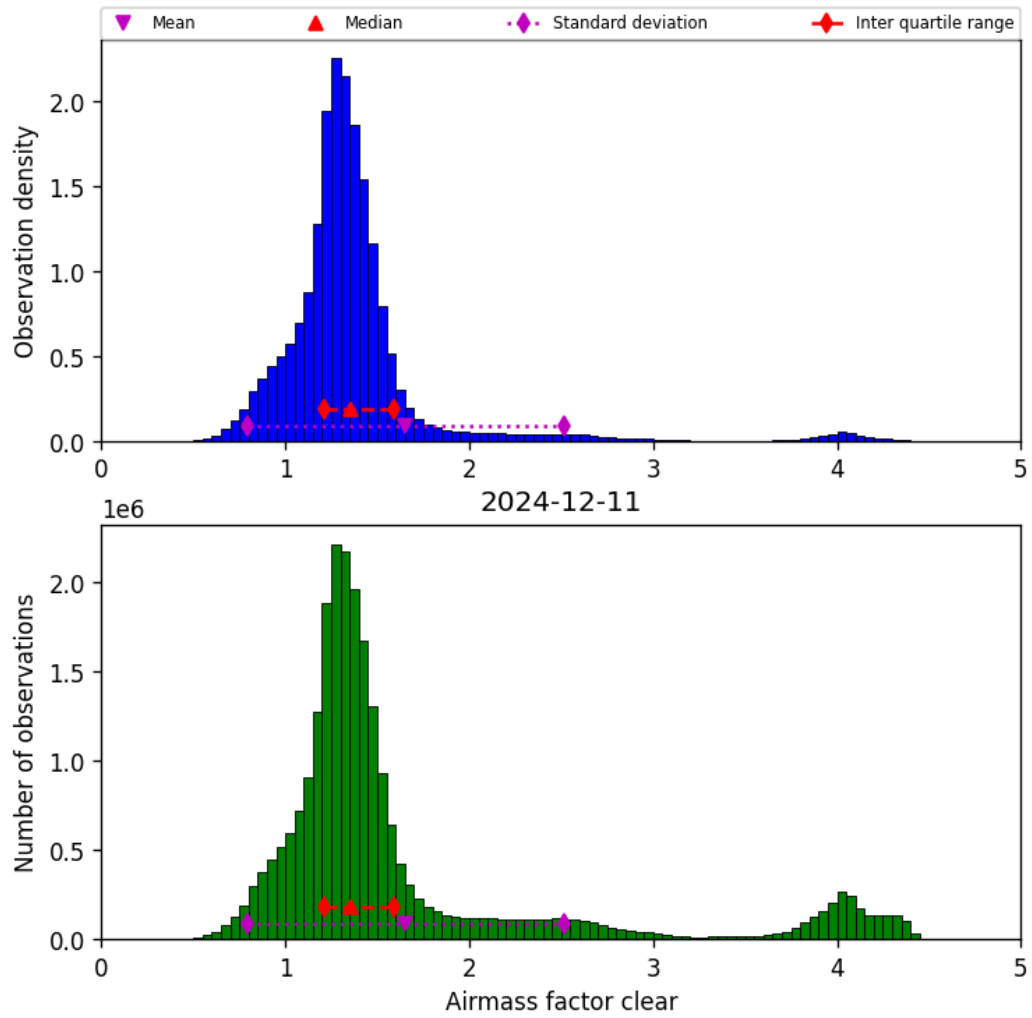
Figure 42: Histogram of “Airmass factor clear” for 2024-12-11 to 2024-12-12
