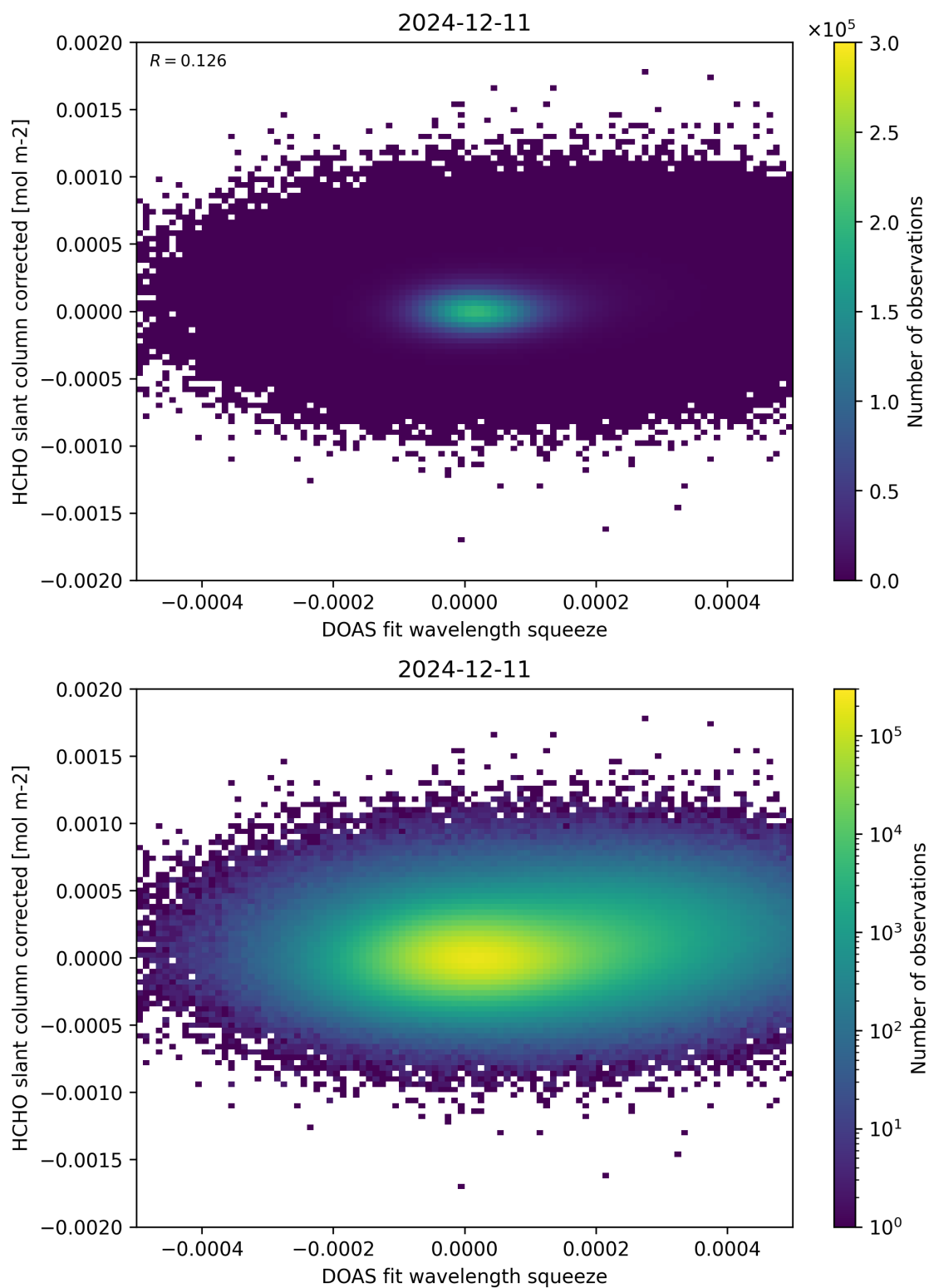
Figure 69: Scatter density plot of “DOAS fit wavelength squeeze” against “HCHO slant column corrected” for 2024-12-11 to 2024-12-12.
