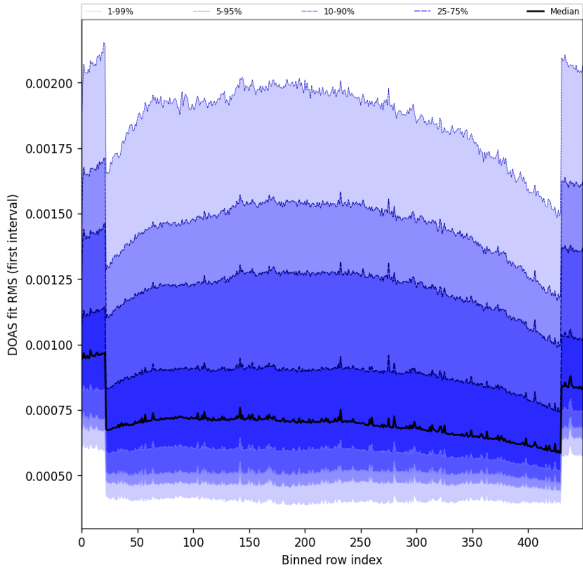
Figure 60: Along track statistics of “DOAS fit RMS (first interval)” for 2024-12-11 to 2024-12-12
