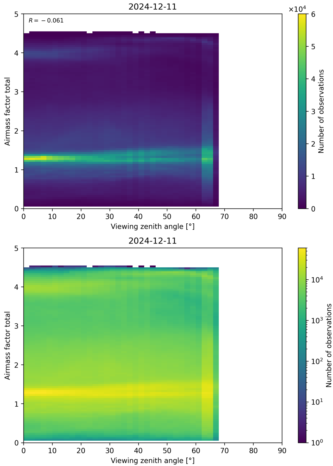
Figure 190: Scatter density plot of “Viewing zenith angle” against “Airmass factor total” for 2024-12-11 to 2024-12-12.
