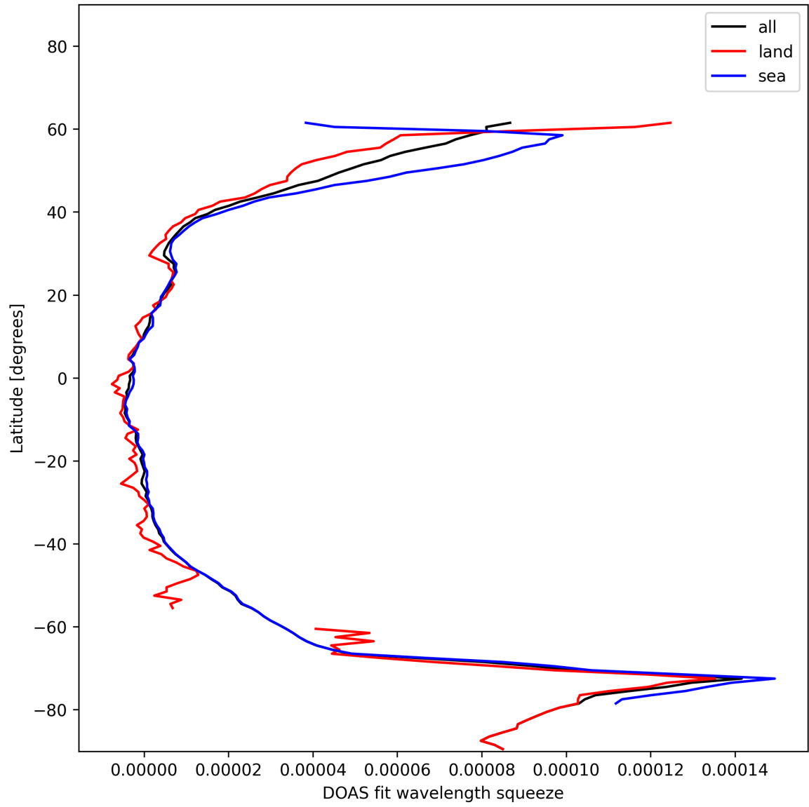
Figure 31: Zonal average of “DOAS fit wavelength squeeze” for 2024-12-11 to 2024-12-12.
