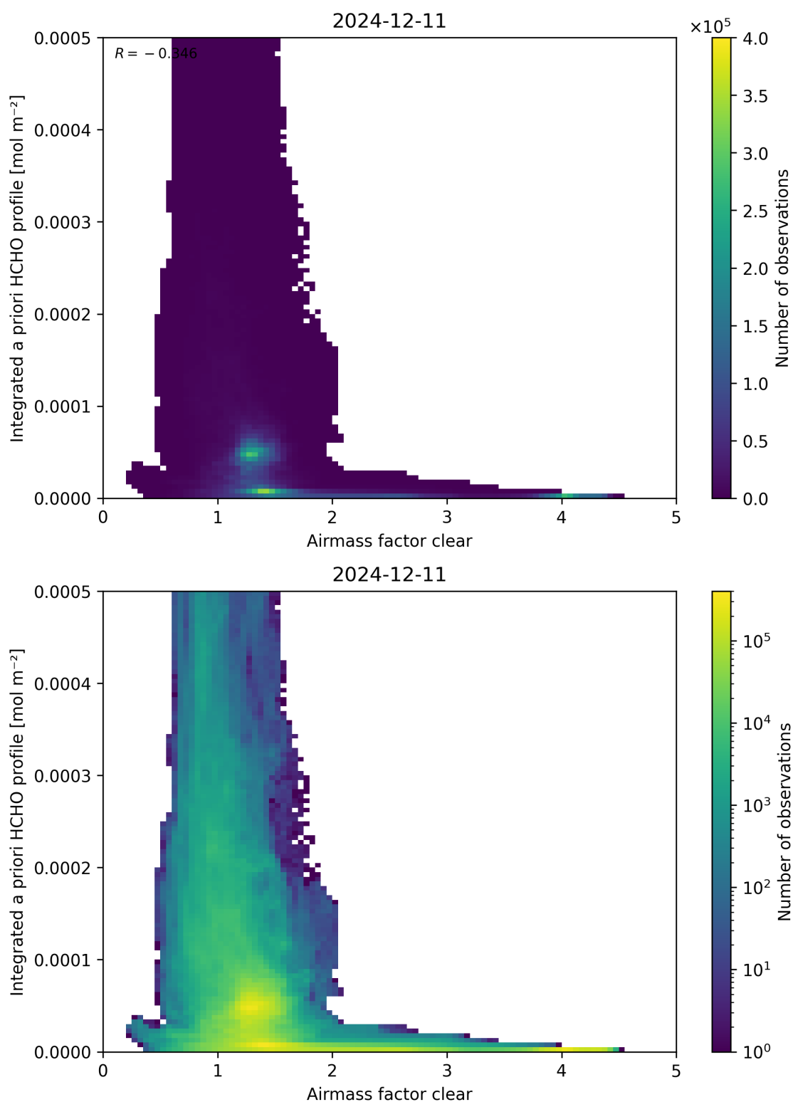
Figure 76: Scatter density plot of “Airmass factor clear” against “Integrated a priori HCHO profile” for 2024-12-11 to 2024-12-12.
