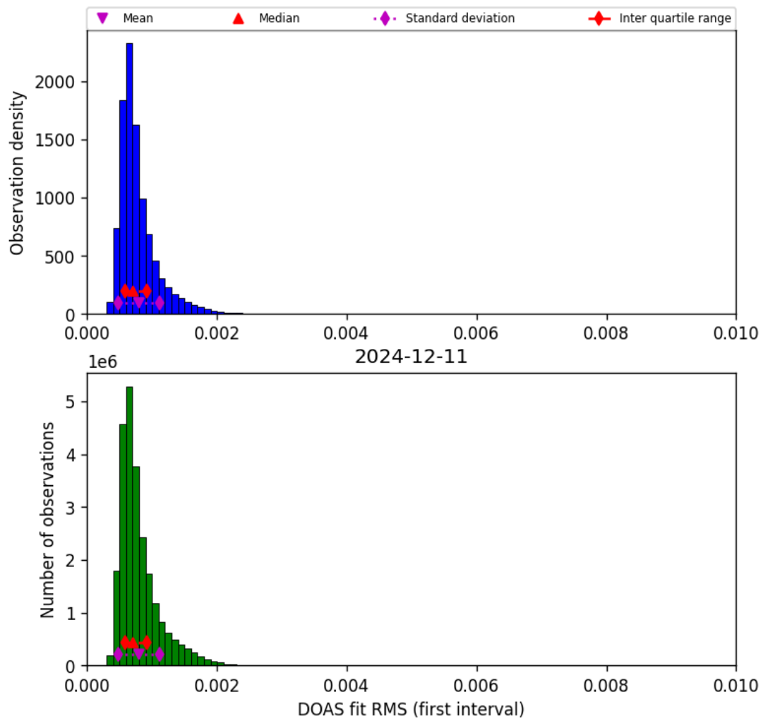
Figure 46: Histogram of “DOAS fit RMS (first interval)” for 2024-12-11 to 2024-12-12
