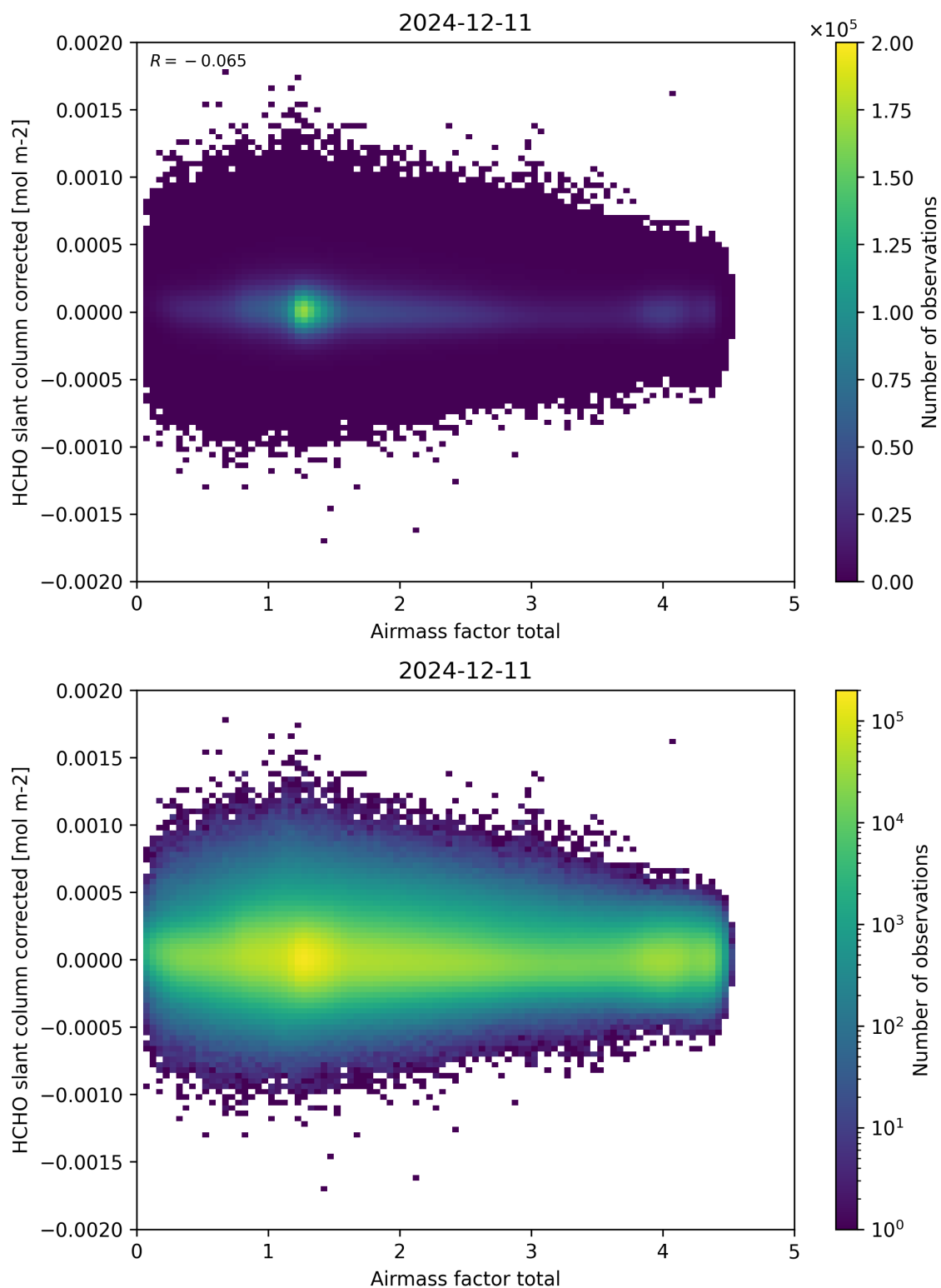
Figure 101: Scatter density plot of “Airmass factor total” against “HCHO slant column corrected” for 2024-12-11 to 2024-12-12.
