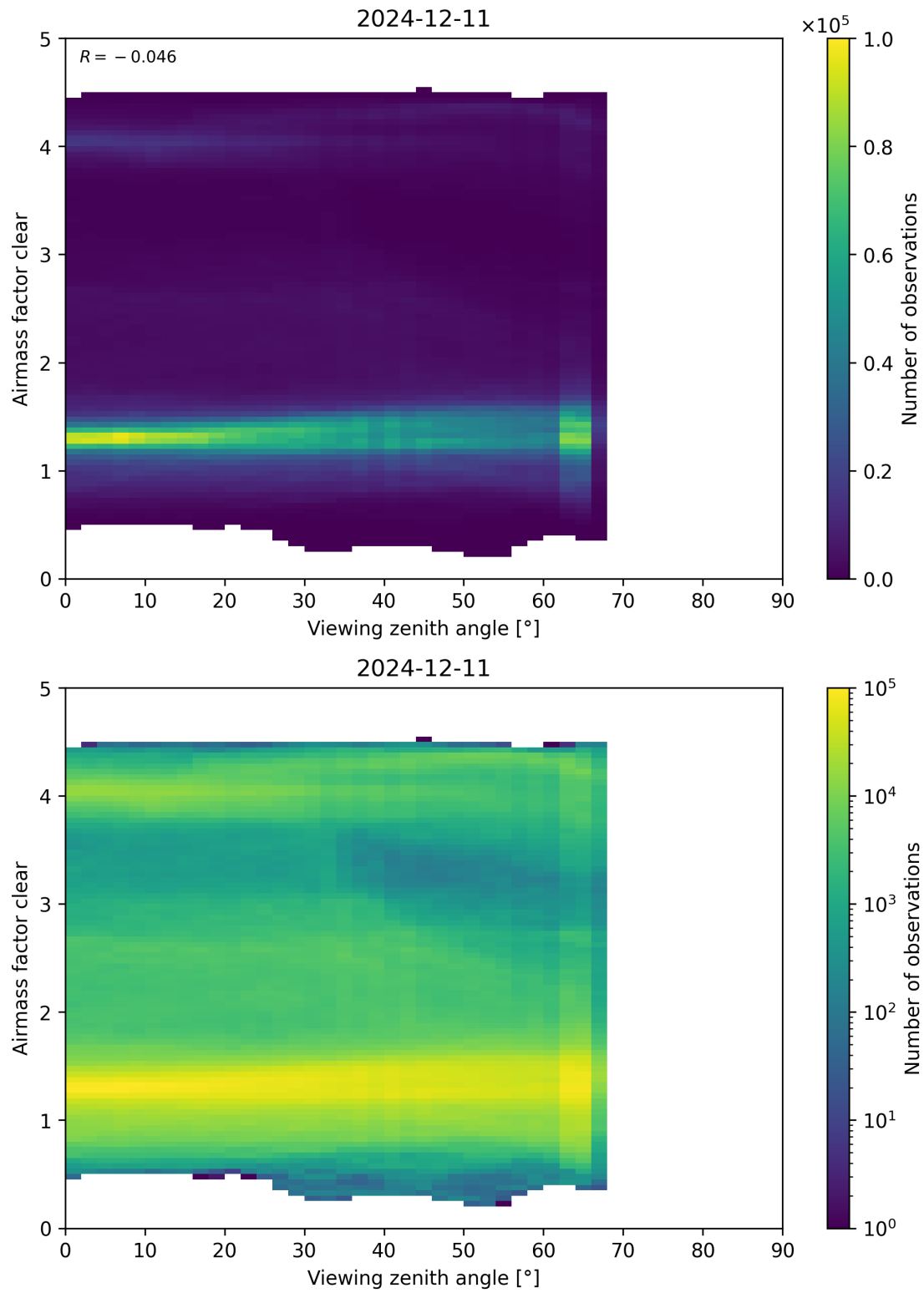
Figure 185: Scatter density plot of “Viewing zenith angle” against “Airmass factor clear” for 2024-12-11 to 2024-12-12.
