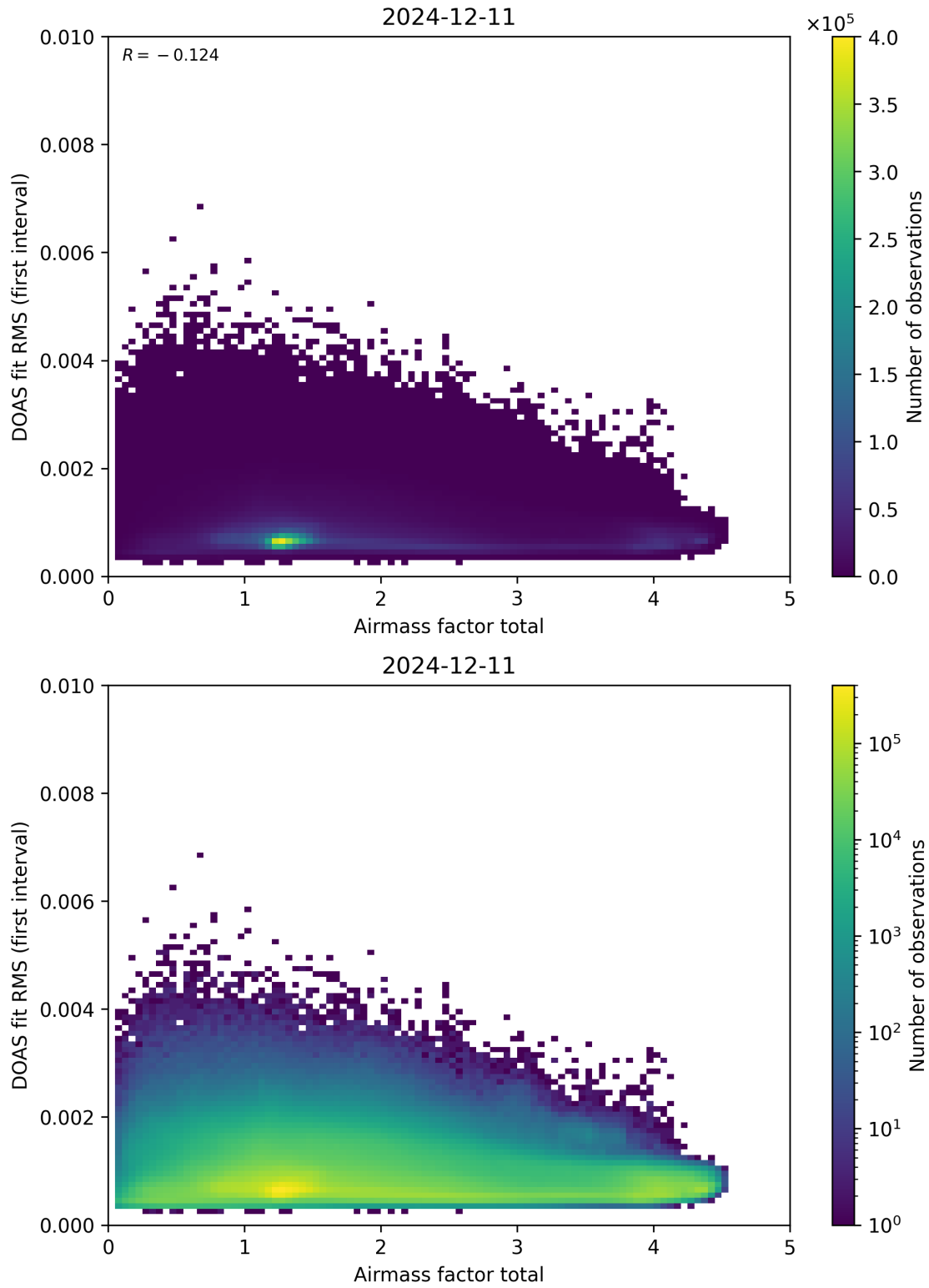
Figure 97: Scatter density plot of “Airmass factor total” against “DOAS fit RMS (first interval)” for 2024-12-11 to 2024-12-12.
