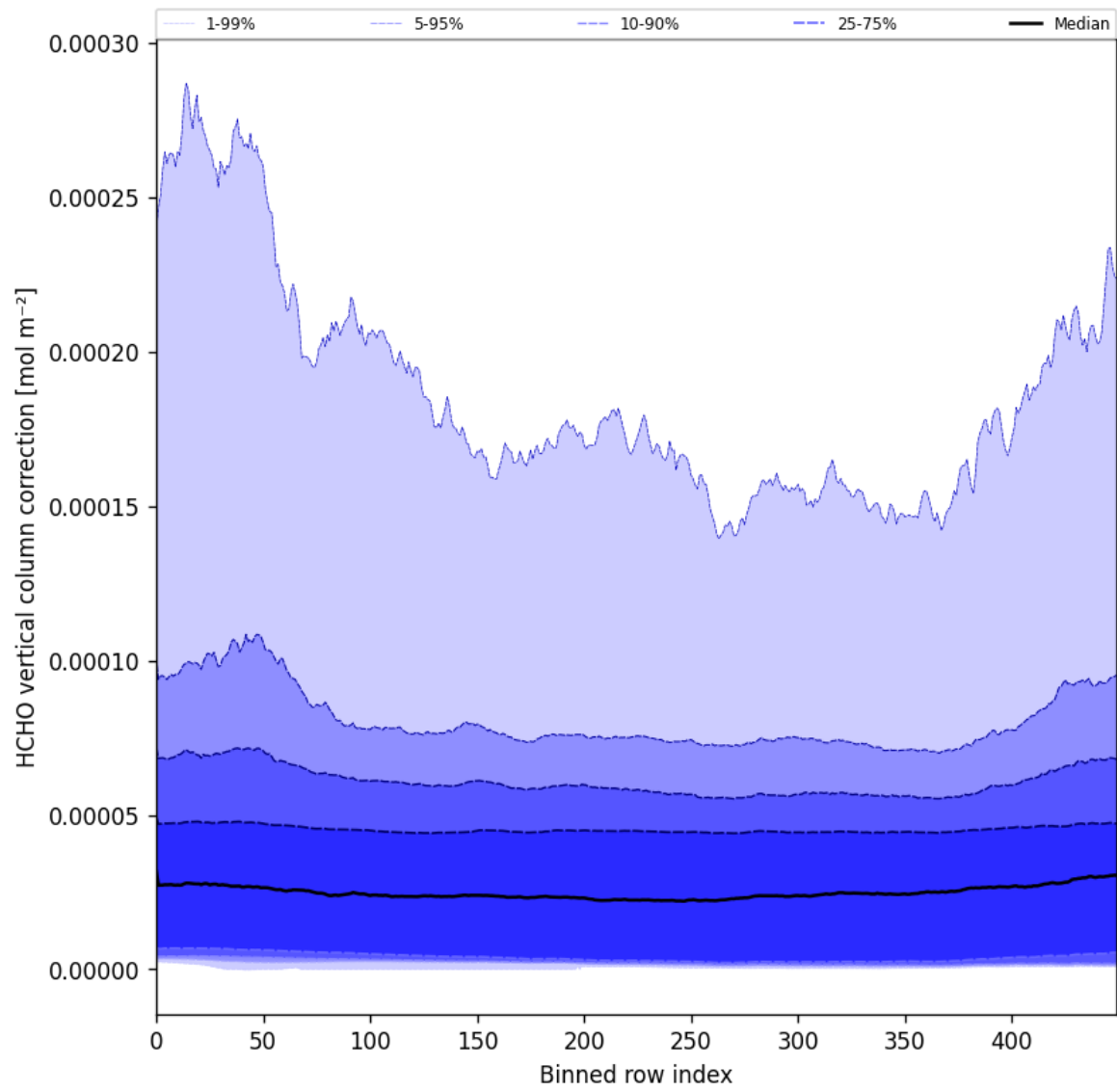
Figure 51: Along track statistics of “HCHO vertical column correction” for 2024-12-11 to 2024-12-12
