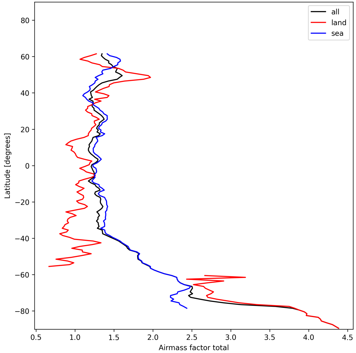
Figure 26: Zonal average of “Airmass factor total” for 2024-12-11 to 2024-12-12.
