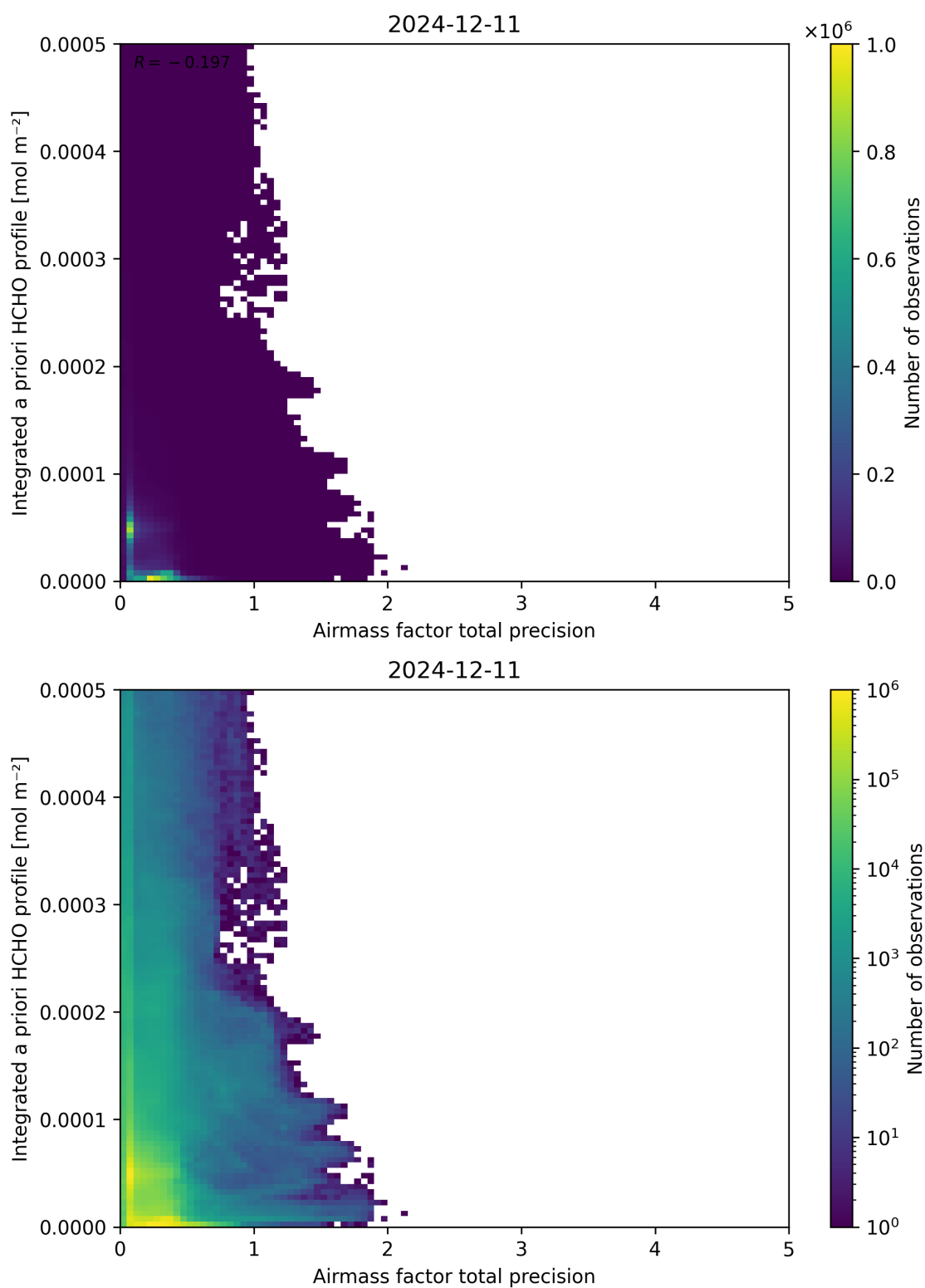
Figure 111: Scatter density plot of “Airmass factor total precision” against “Integrated a priori HCHO profile” for 2024-12-11 to 2024-12-12.
