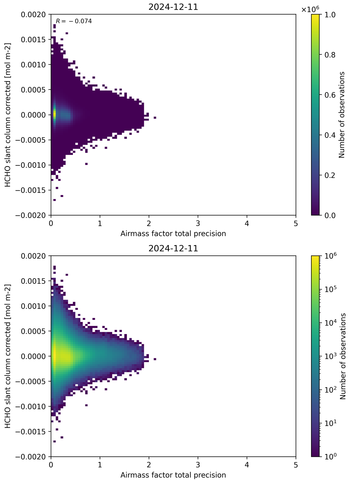
Figure 109: Scatter density plot of “Airmass factor total precision” against “HCHO slant column corrected” for 2024-12-11 to 2024-12-12.
