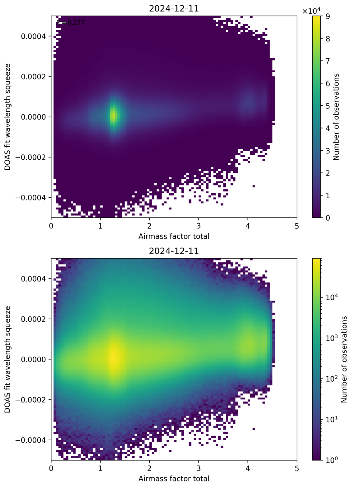
Figure 99: Scatter density plot of “Airmass factor total” against “DOAS fit wavelength squeeze” for 2024-12-11 to 2024-12-12.
