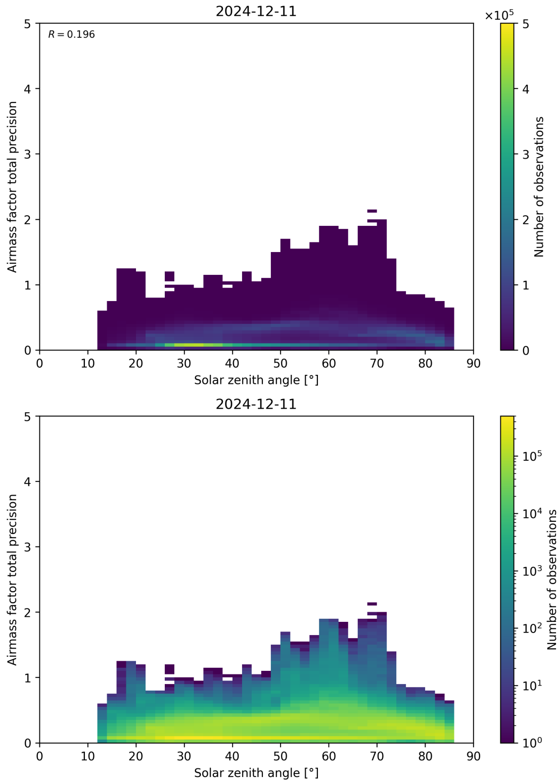
Figure 176: Scatter density plot of “Solar zenith angle” against “Airmass factor total precision” for 2024-12-11 to 2024-12-12.
