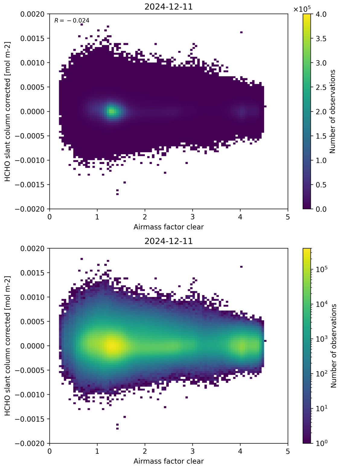
Figure 74: Scatter density plot of “Airmass factor clear” against “HCHO slant column corrected” for 2024-12-11 to 2024-12-12.
