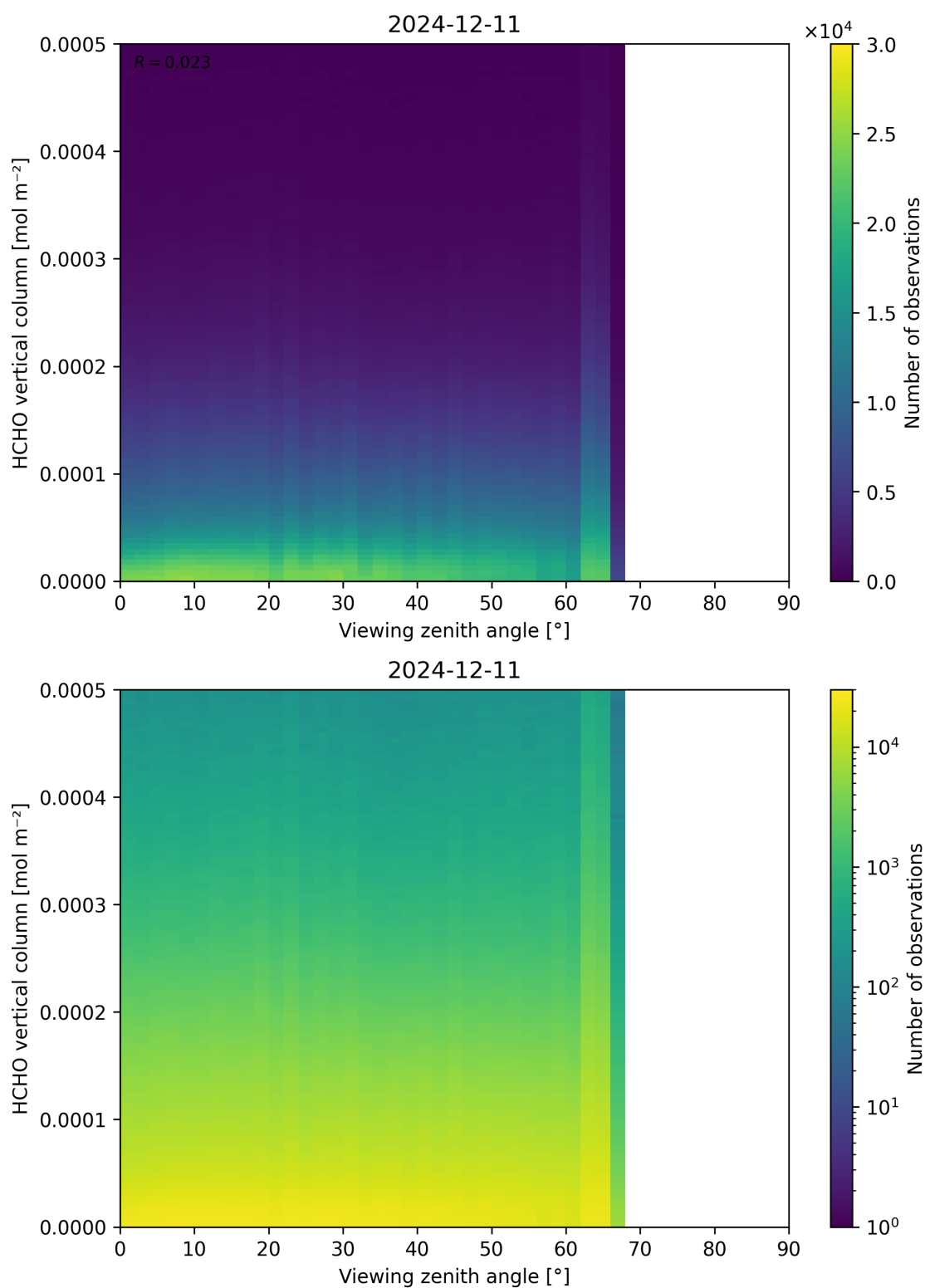
Figure 192: Scatter density plot of “Viewing zenith angle” against “HCHO vertical column” for 2024-12-11 to 2024-12-12.
