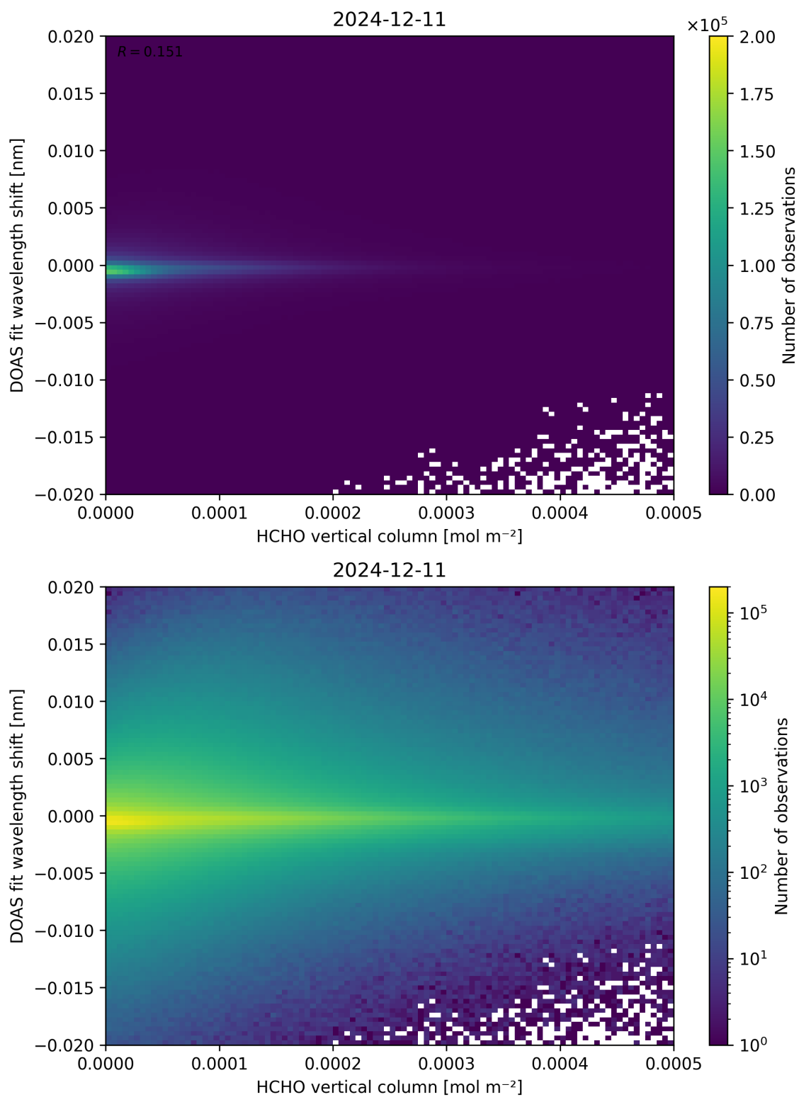
Figure 124: Scatter density plot of “HCHO vertical column” against “DOAS fit wavelength shift” for 2024-12-11 to 2024-12-12.
