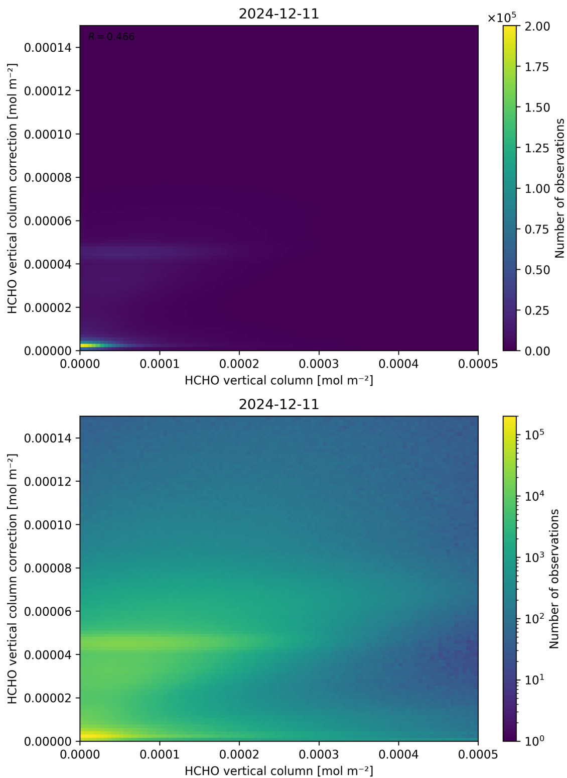
Figure 133: Scatter density plot of “HCHO vertical column” against “HCHO vertical column correction” for 2024-12-11 to 2024-12-12.
