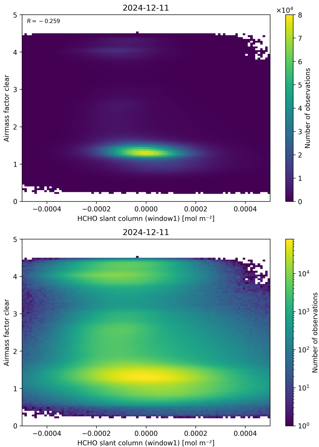
Figure 81: Scatter density plot of “HCHO slant column (window1)” against “Airmass factor clear” for 2024-12-11 to 2024-12-12.
