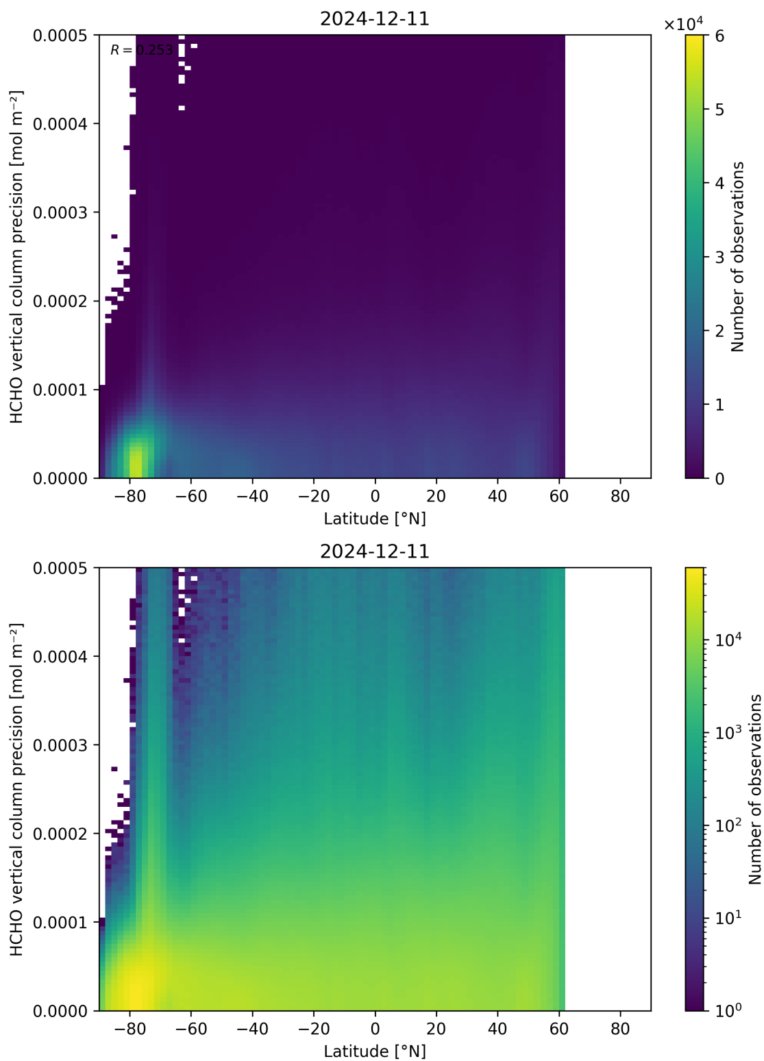
Figure 165: Scatter density plot of “Latitude” against “HCHO vertical column precision” for 2024-12-11 to 2024-12-12.
