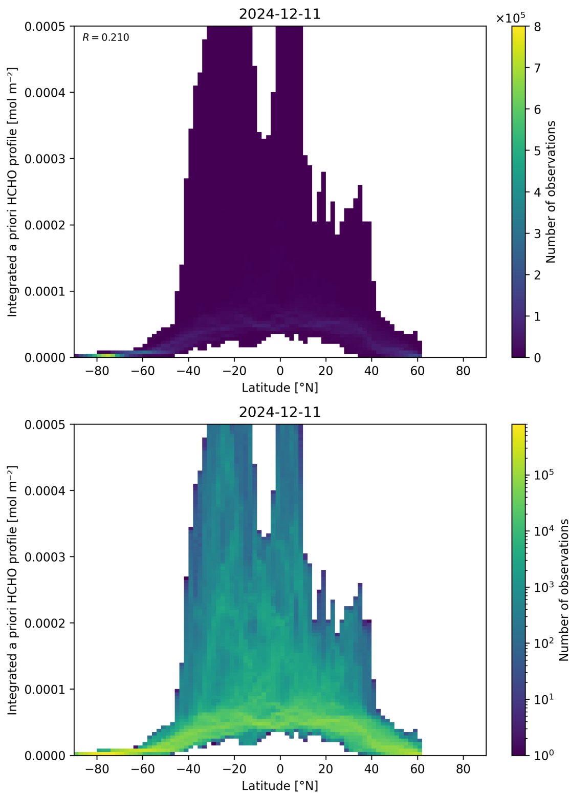
Figure 166: Scatter density plot of “Latitude” against “Integrated a priori HCHO profile” for 2024-12-11 to 2024-12-12.
