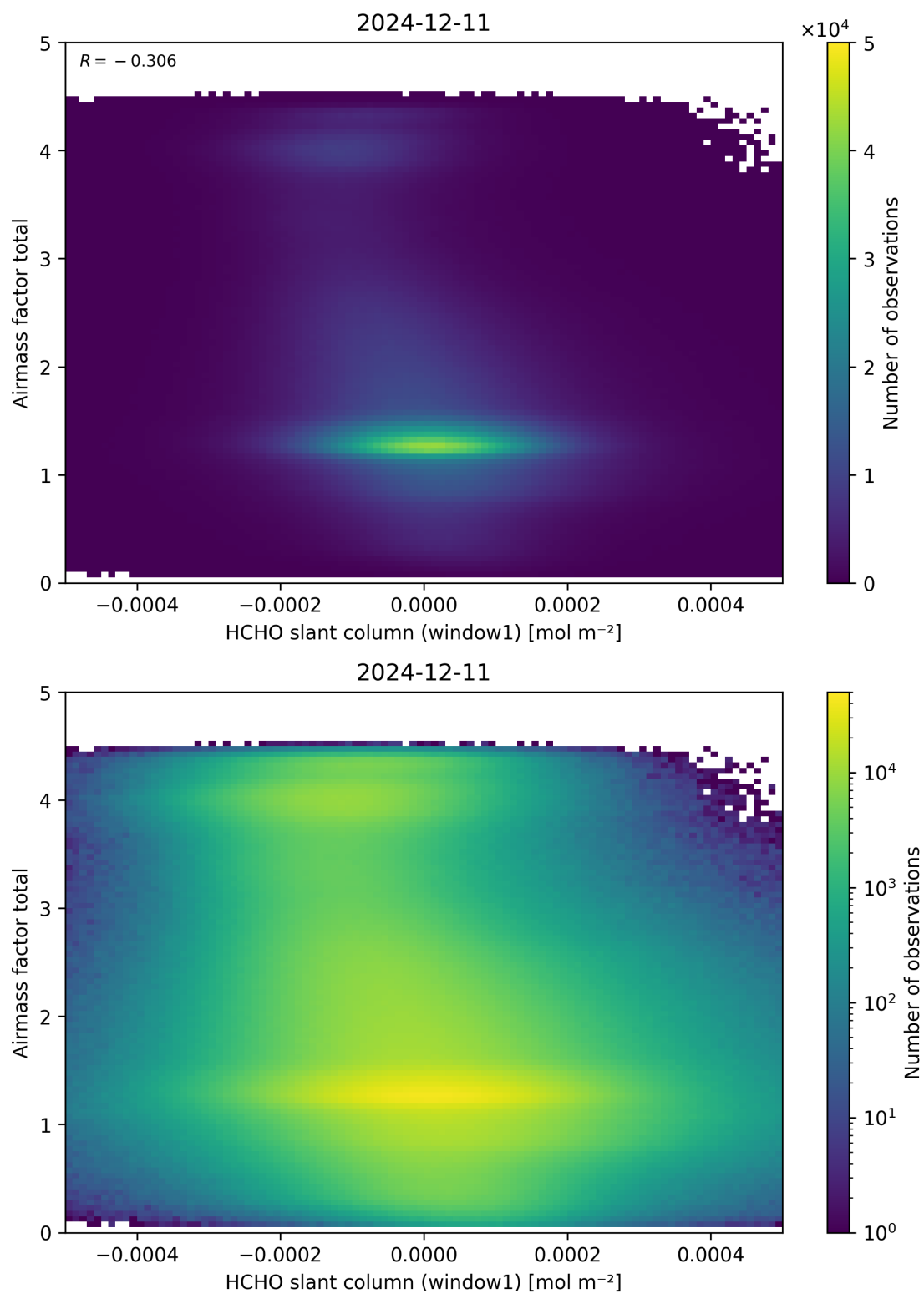
Figure 85: Scatter density plot of “HCHO slant column (window1)” against “Airmass factor total” for 2024-12-11 to 2024-12-12.
