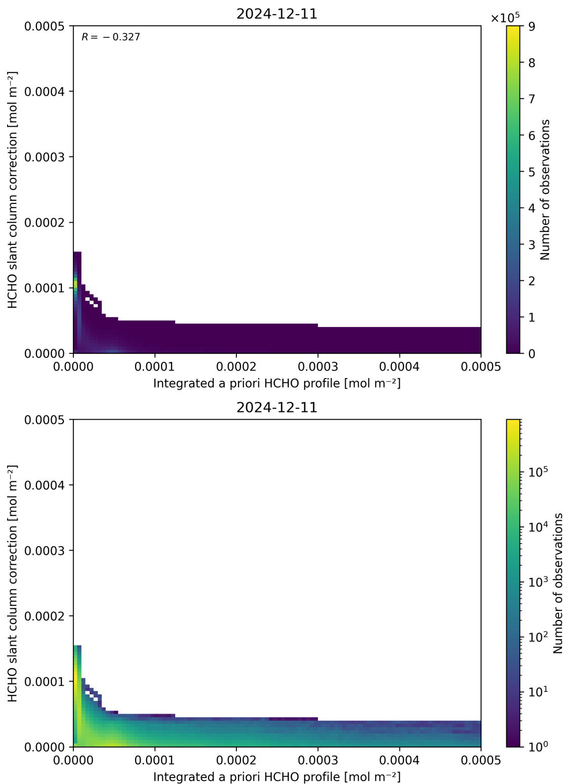
Figure 152: Scatter density plot of “Integrated a priori HCHO profile” against “HCHO slant column correction” for 2024-12-11 to 2024-12-12.
