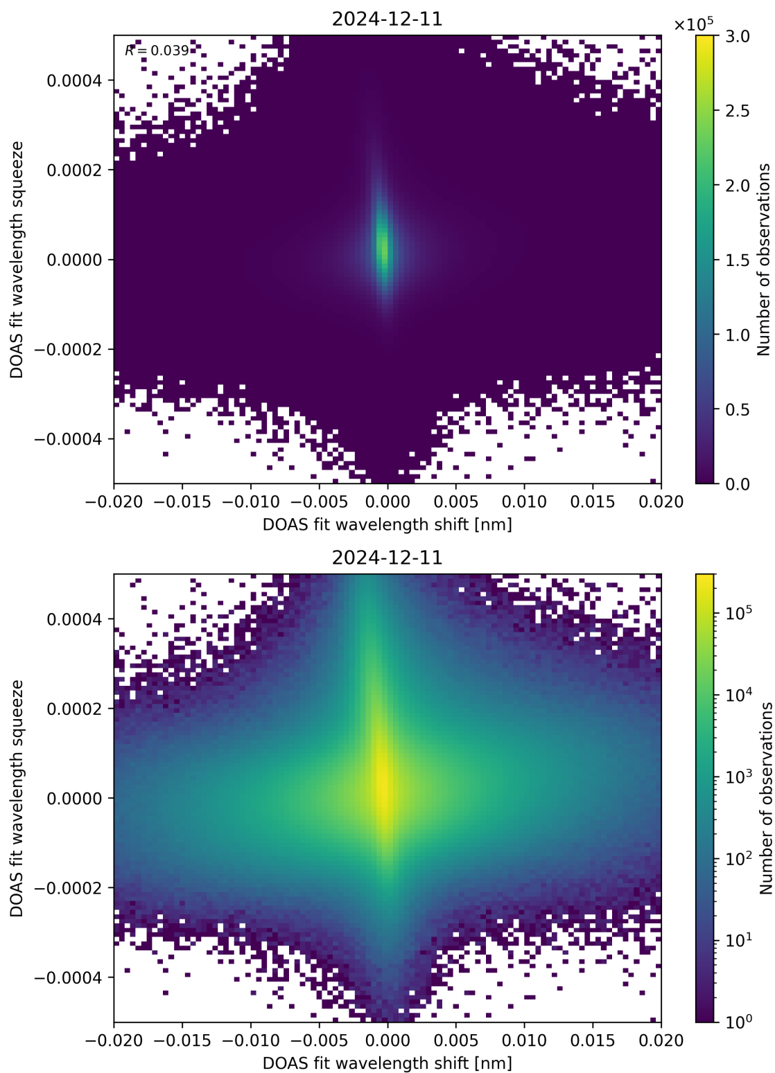
Figure 65: Scatter density plot of “DOAS fit wavelength shift” against “DOAS fit wavelength squeeze” for 2024-12-11 to 2024-12-12.
