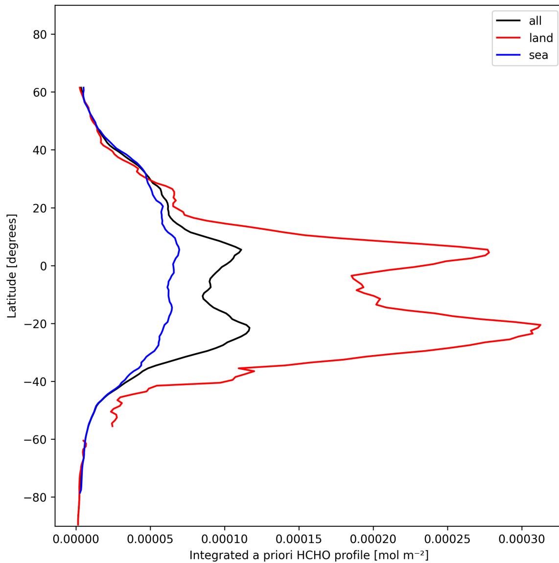
Figure 29: Zonal average of “Integrated a priori HCHO profile” for 2024-12-11 to 2024-12-12.
