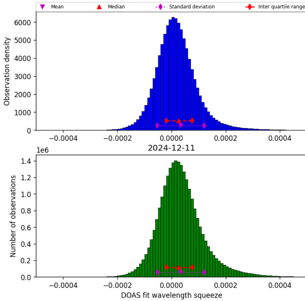
Figure 45: Histogram of “DOAS fit wavelength squeeze” for 2024-12-11 to 2024-12-12
