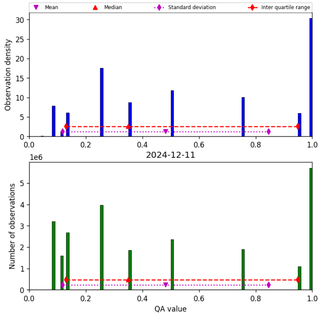
Figure 34: Histogram of “QA value” for 2024-12-11 to 2024-12-12
