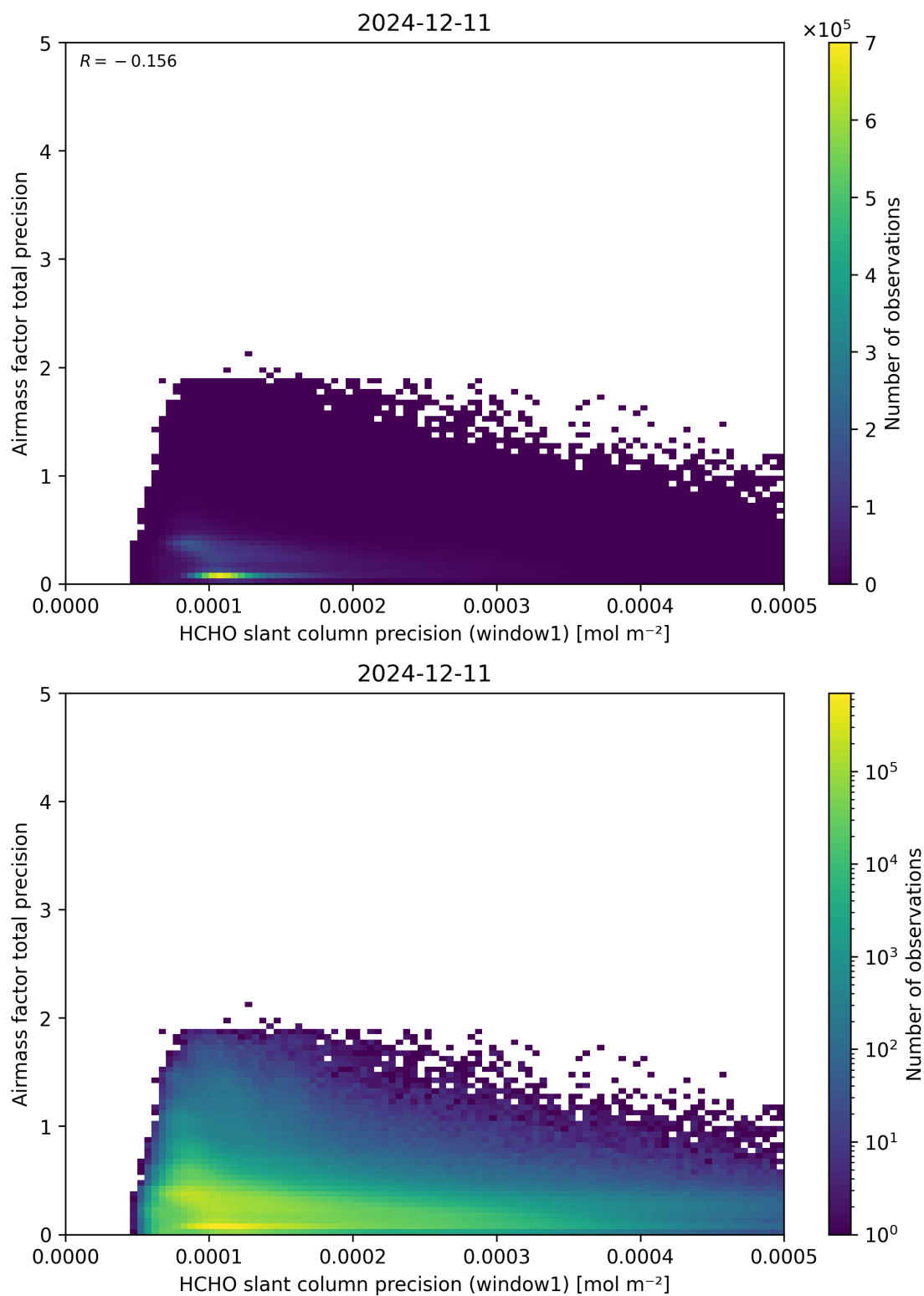
Figure 95: Scatter density plot of “HCHO slant column precision (window1)” against “Airmass factor total precision” for 2024-12-11 to 2024-12-12.
