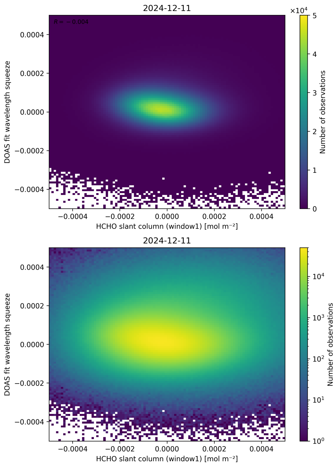
Figure 80: Scatter density plot of “HCHO slant column (window1)” against “DOAS fit wavelength squeeze” for 2024-12-11 to 2024-12-12.
