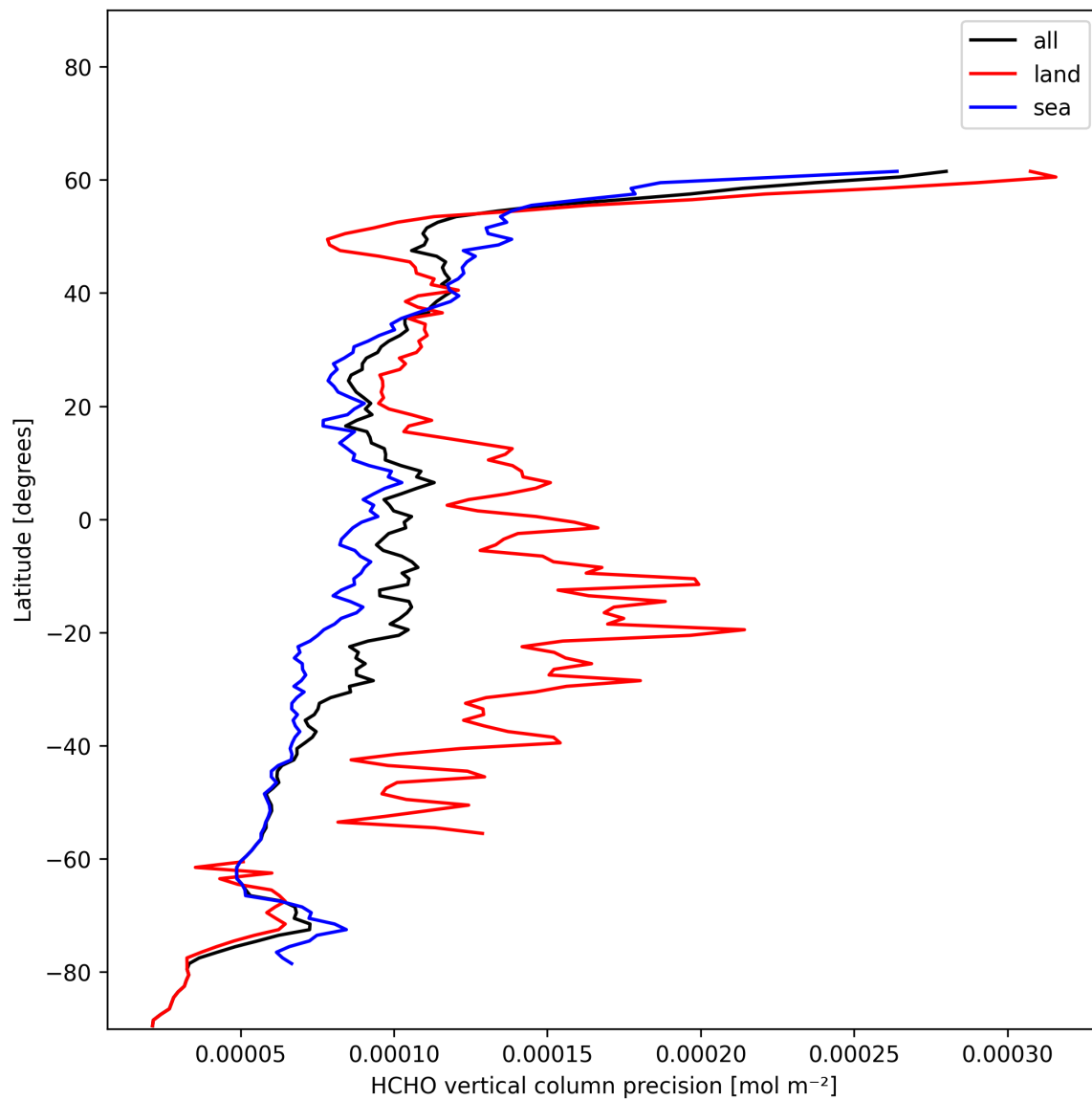
Figure 22: Zonal average of "HCHO vertical column precision" for 2024-12-11 to 2024-12-12.
