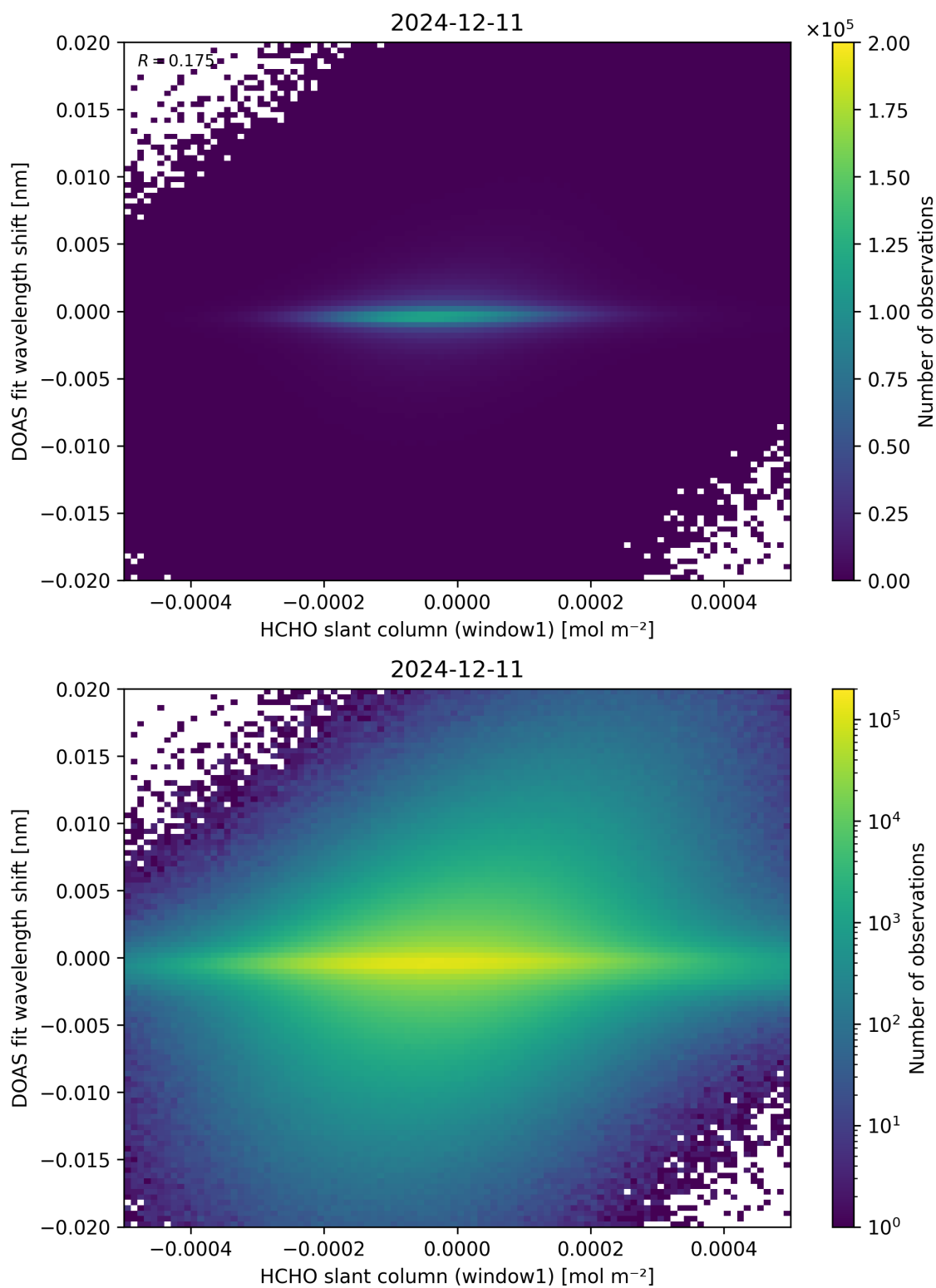
Figure 79: Scatter density plot of “HCHO slant column (window1)” against “DOAS fit wavelength shift” for 2024-12-11 to 2024-12-12.
