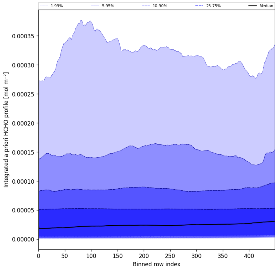
Figure 57: Along track statistics of "Integrated a priori HCHO profile" for 2024-12-11 to 2024-12-12
