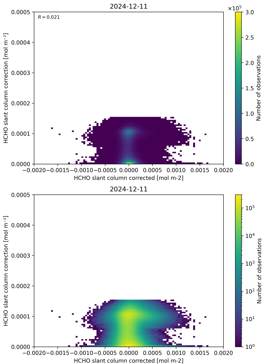
Figure 77: Scatter density plot of “HCHO slant column corrected” against “HCHO slant column correction” for 2024-12-11 to 2024-12-12.
