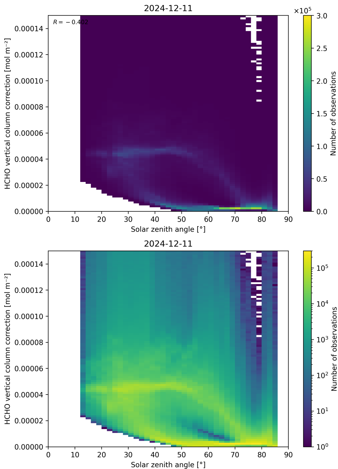
Figure 178: Scatter density plot of “Solar zenith angle” against “HCHO vertical column correction” for 2024-12-11 to 2024-12-12.
