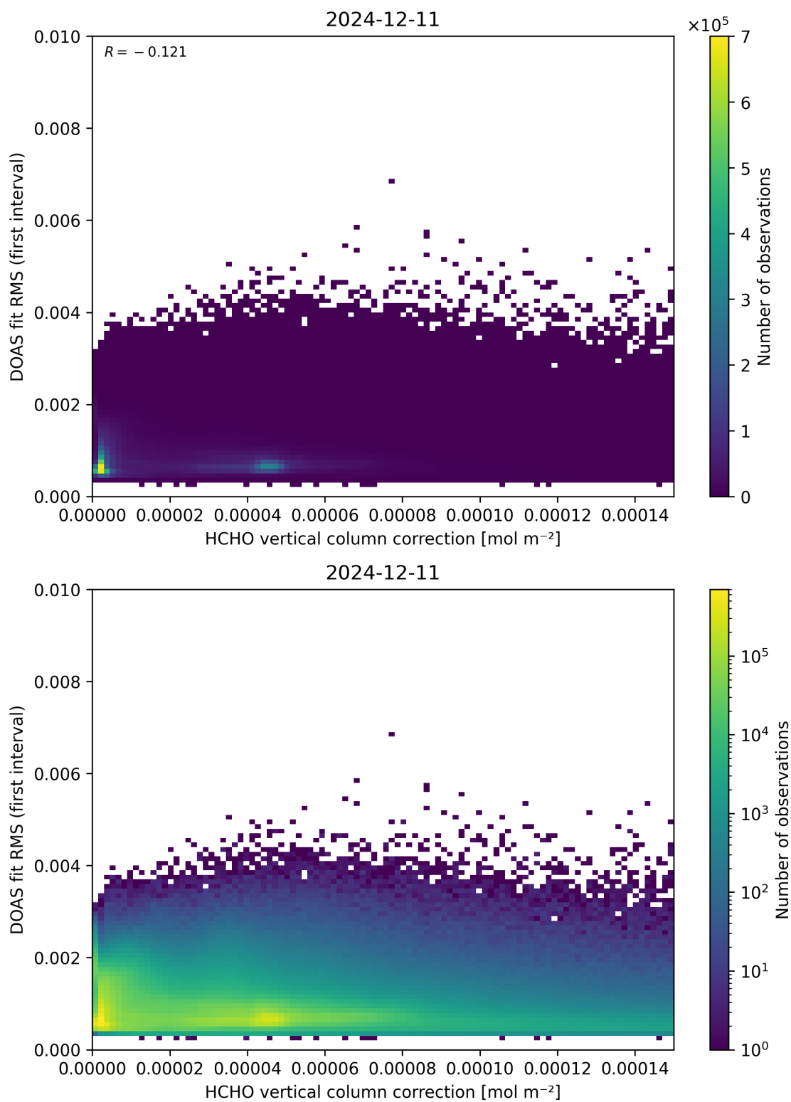
Figure 112: Scatter density plot of “HCHO vertical column correction” against “DOAS fit RMS (first interval)” for 2024-12-11 to 2024-12-12.
