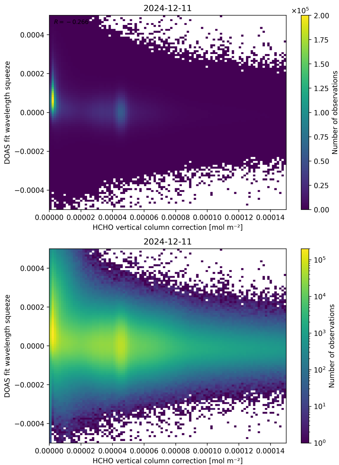
Figure 114: Scatter density plot of “HCHO vertical column correction” against “DOAS fit wavelength squeeze” for 2024-12-11 to 2024-12-12.
