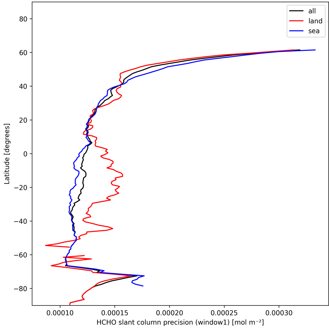
Figure 25: Zonal average of “HCHO slant column precision (window1)” for 2024-12-11 to 2024-12-12.
