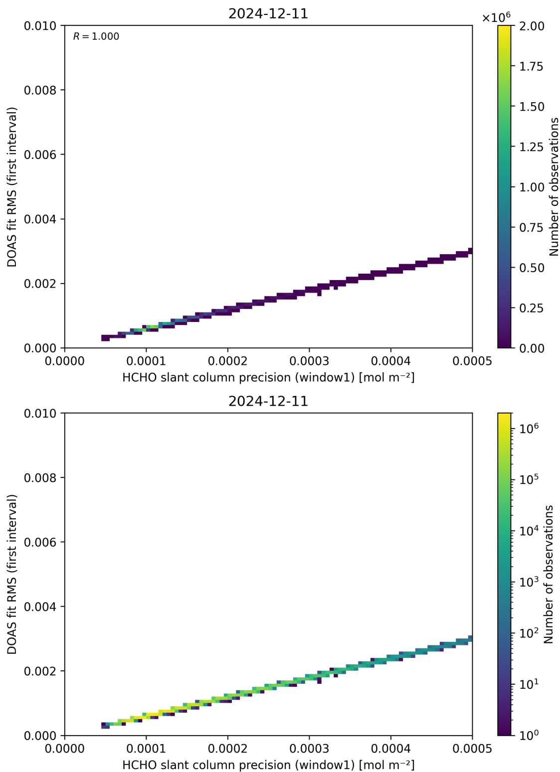
Figure 88: Scatter density plot of “HCHO slant column precision (window1)” against “DOAS fit RMS (first interval)” for 2024-12-11 to 2024-12-12.
