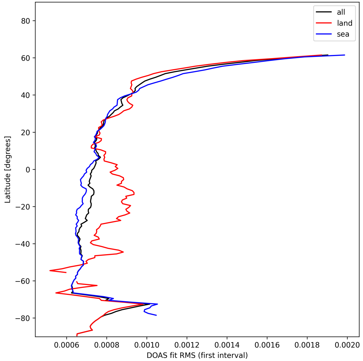
Figure 32: Zonal average of “DOAS fit RMS (first interval)” for 2024-12-11 to 2024-12-12.
