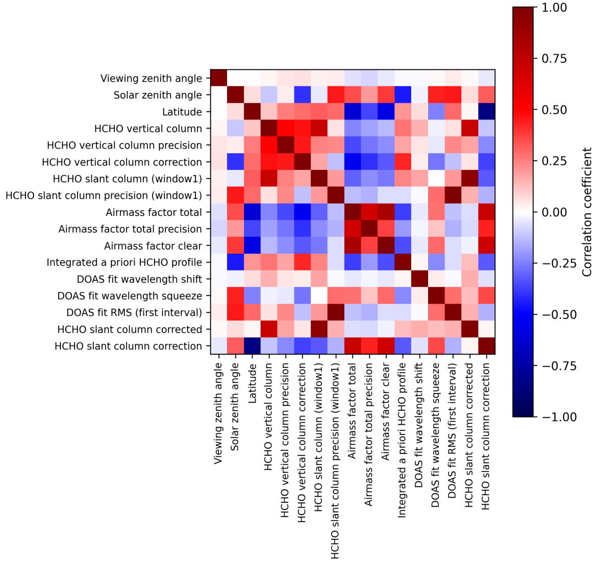
Figure 2: Map of correlation matrix for 2024-12-11 to 2024-12-12.
