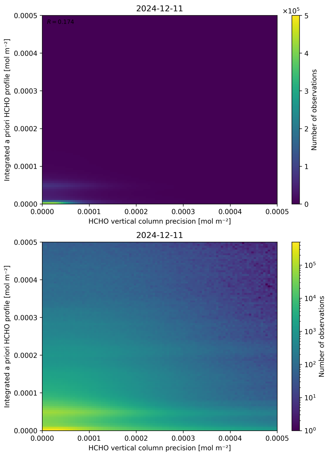
Figure 147: Scatter density plot of “HCHO vertical column precision” against “Integrated a priori HCHO profile” for 2024-12-11 to 2024-12-12.
