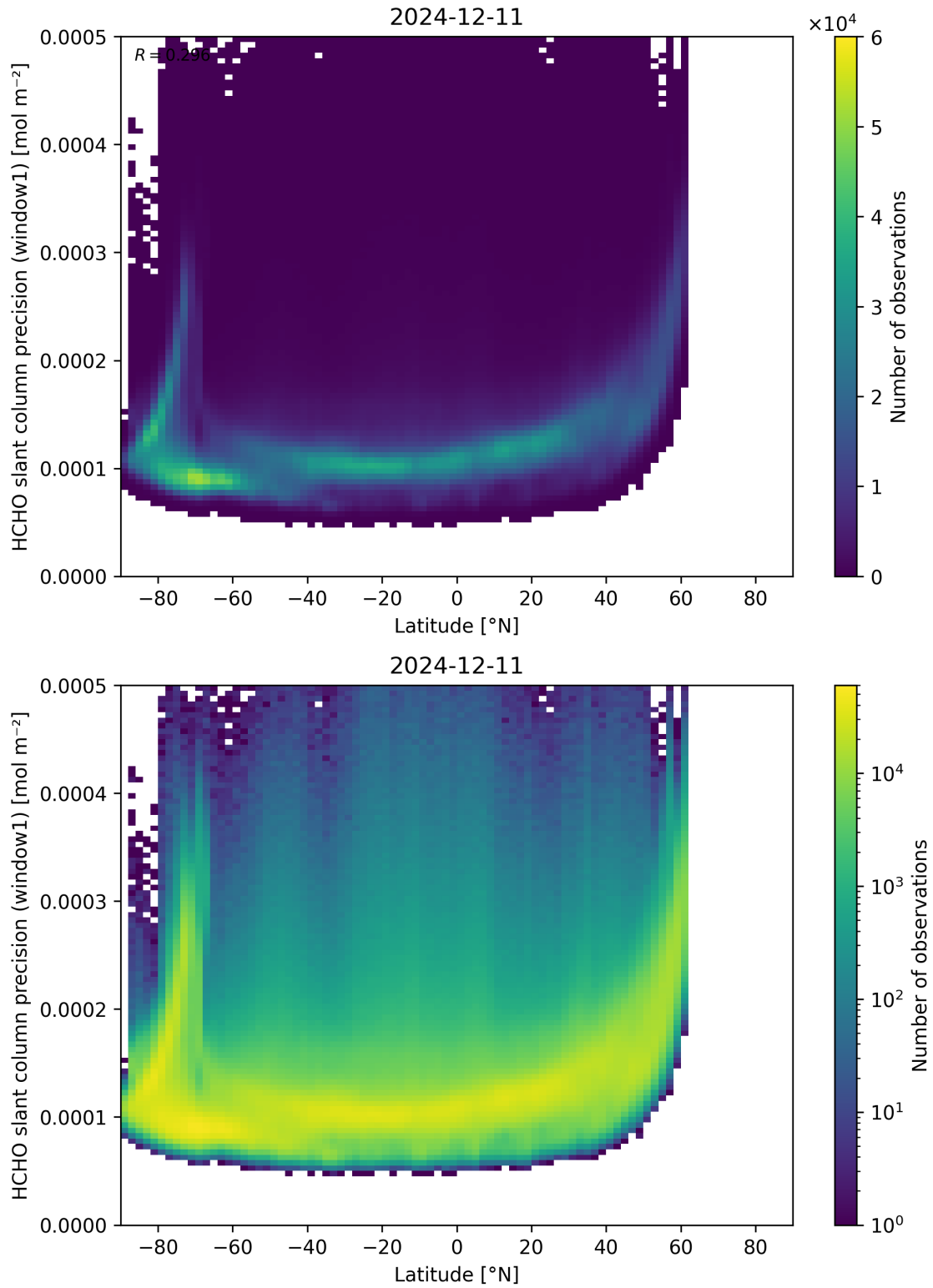
Figure 160: Scatter density plot of “Latitude” against “HCHO slant column precision (window1)” for 2024-12-11 to 2024-12-12.
