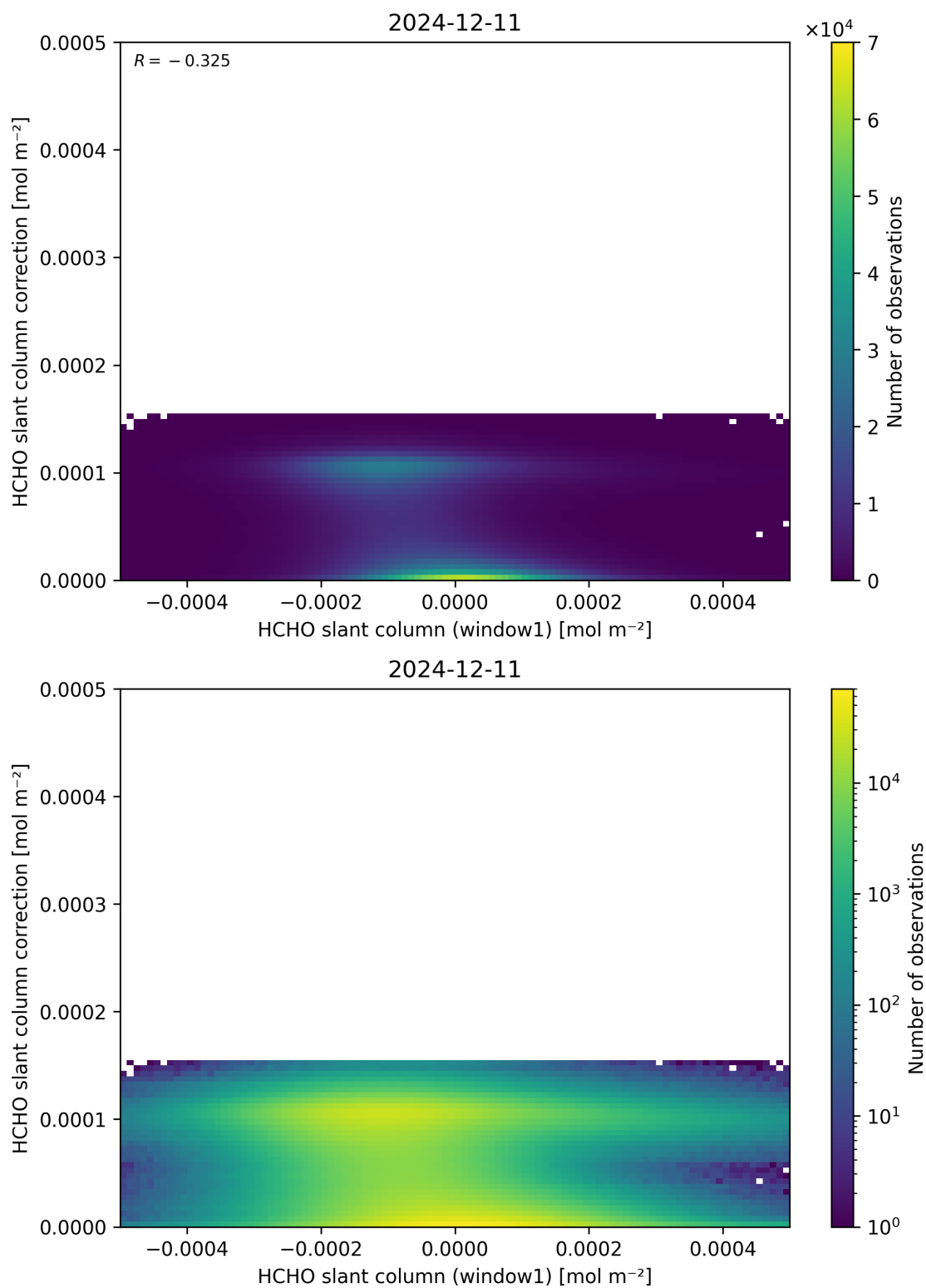
Figure 83: Scatter density plot of “HCHO slant column (window1)” against “HCHO slant column correction” for 2024-12-11 to 2024-12-12.
