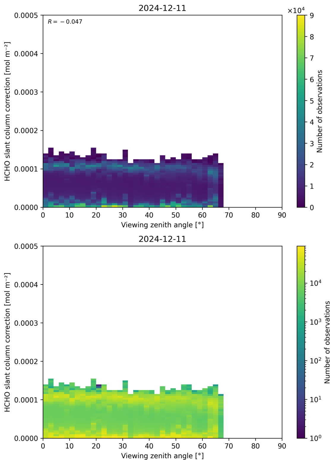
Figure 187: Scatter density plot of “Viewing zenith angle” against “HCHO slant column correction” for 2024-12-11 to 2024-12-12.
