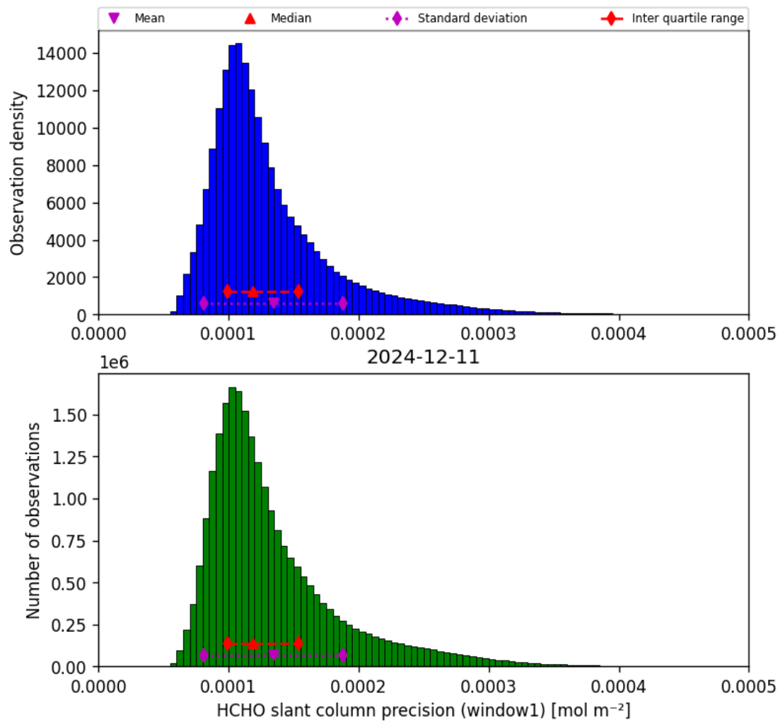
Figure 39: Histogram of “HCHO slant column precision (window1)” for 2024-12-11 to 2024-12-12
