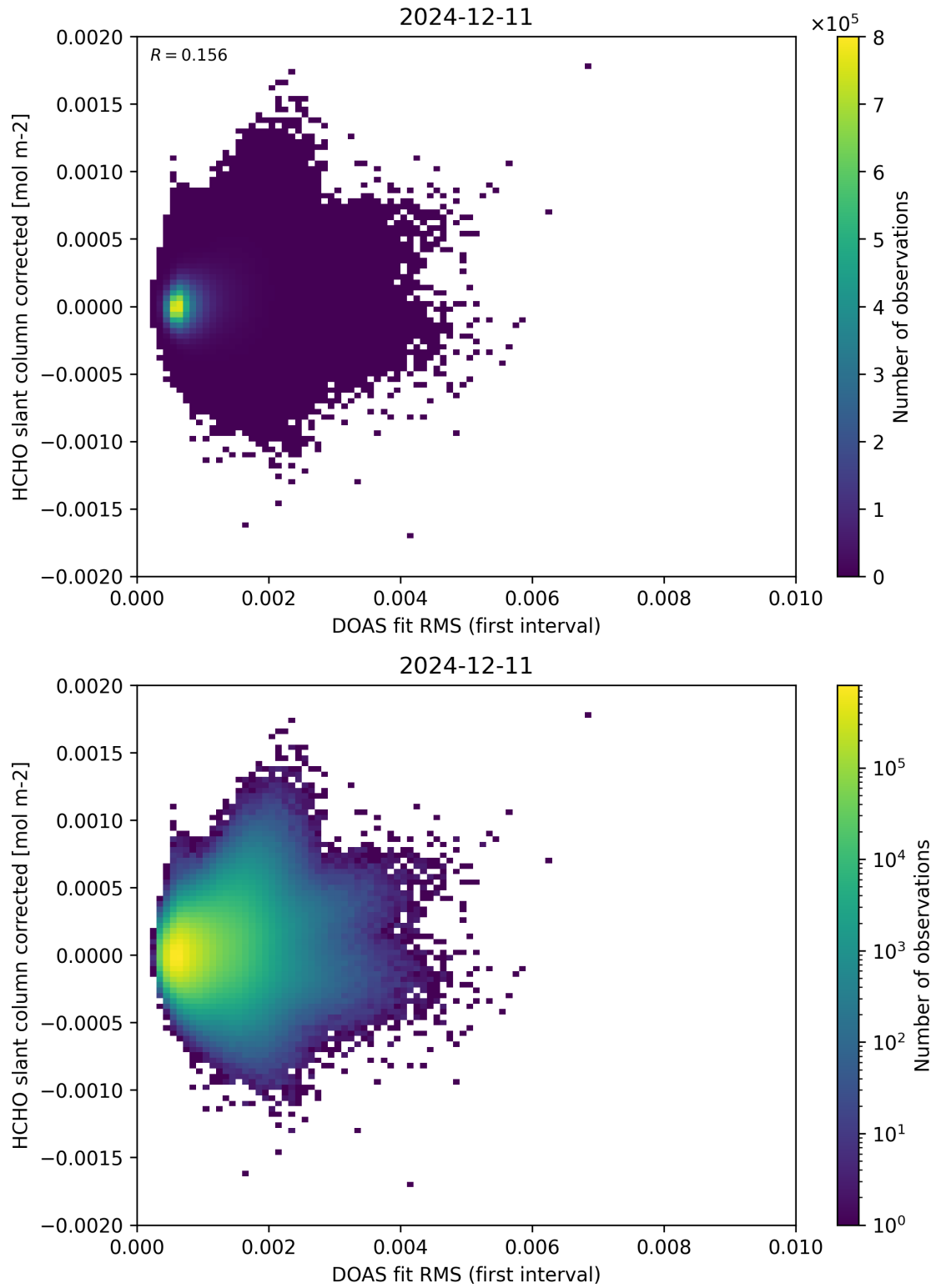
Figure 62: Scatter density plot of “DOAS fit RMS (first interval)” against “HCHO slant column corrected” for 2024-12-11 to 2024-12-12.
