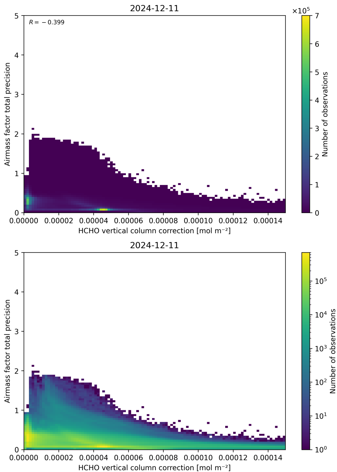
Figure 121: Scatter density plot of “HCHO vertical column correction” against “Airmass factor total precision” for 2024-12-11 to 2024-12-12.
