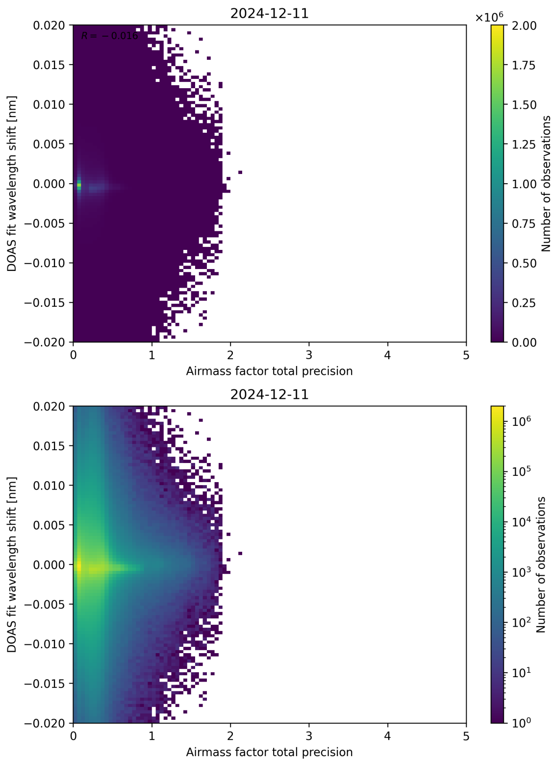
Figure 106: Scatter density plot of “Airmass factor total precision” against “DOAS fit wavelength shift” for 2024-12-11 to 2024-12-12.
