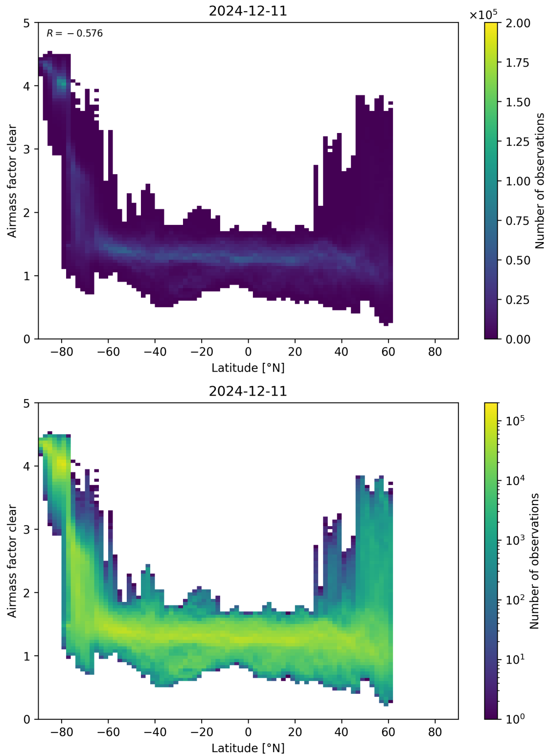
Figure 156: Scatter density plot of “Latitude” against “Airmass factor clear” for 2024-12-11 to 2024-12-12.
