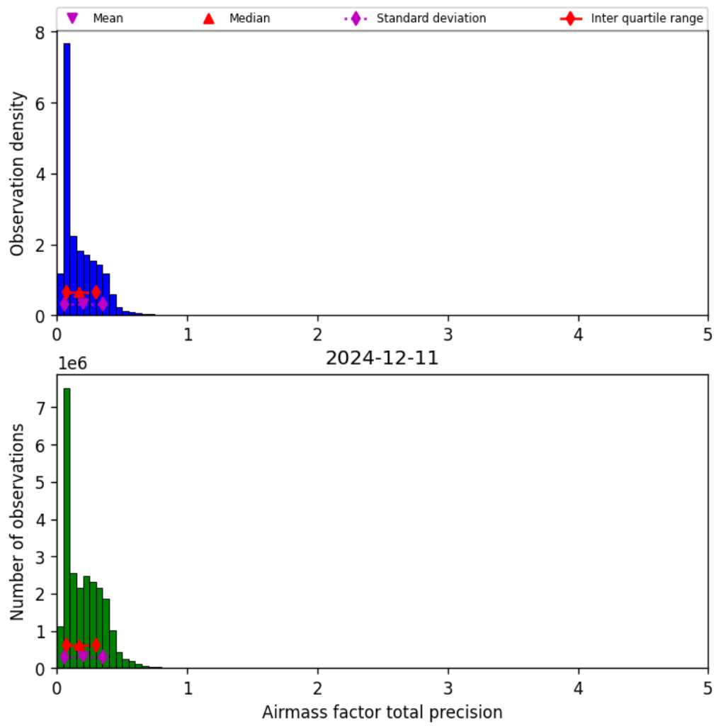
Figure 41: Histogram of “Airmass factor total precision” for 2024-12-11 to 2024-12-12
