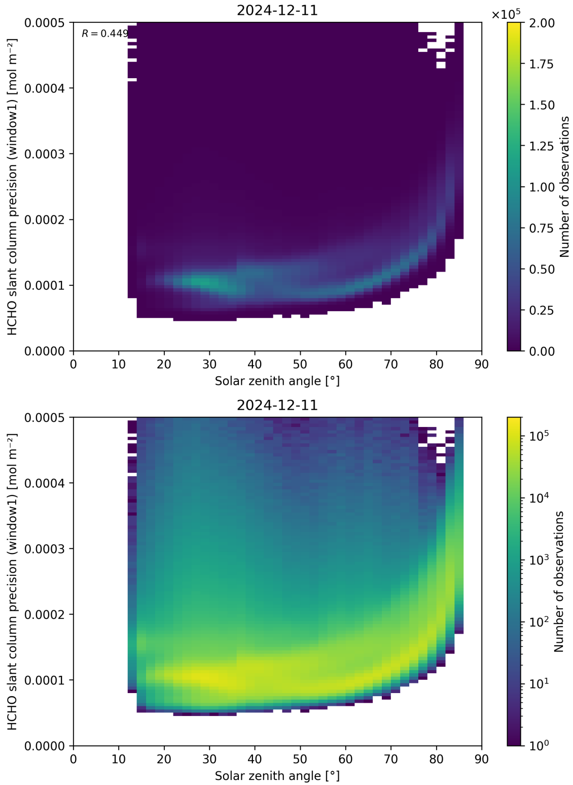
Figure 174: Scatter density plot of “Solar zenith angle” against “HCHO slant column precision (window1)” for 2024-12-11 to 2024-12-12.
