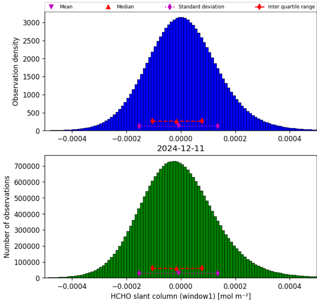
Figure 38: Histogram of “HCHO slant column (window1)” for 2024-12-11 to 2024-12-12
