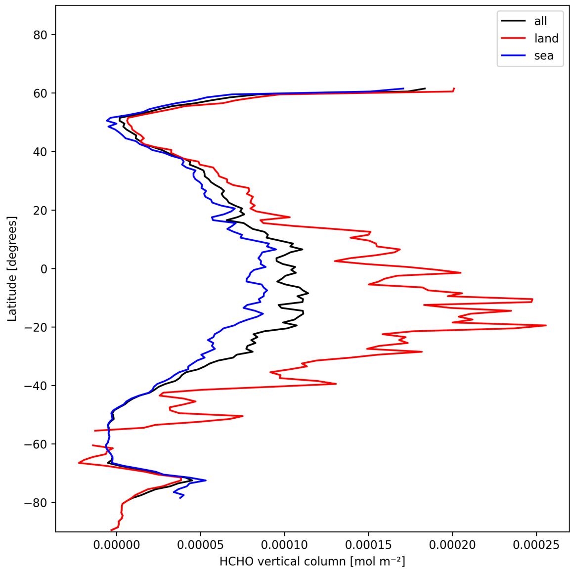
Figure 21: Zonal average of “HCHO vertical column” for 2024-12-11 to 2024-12-12.
