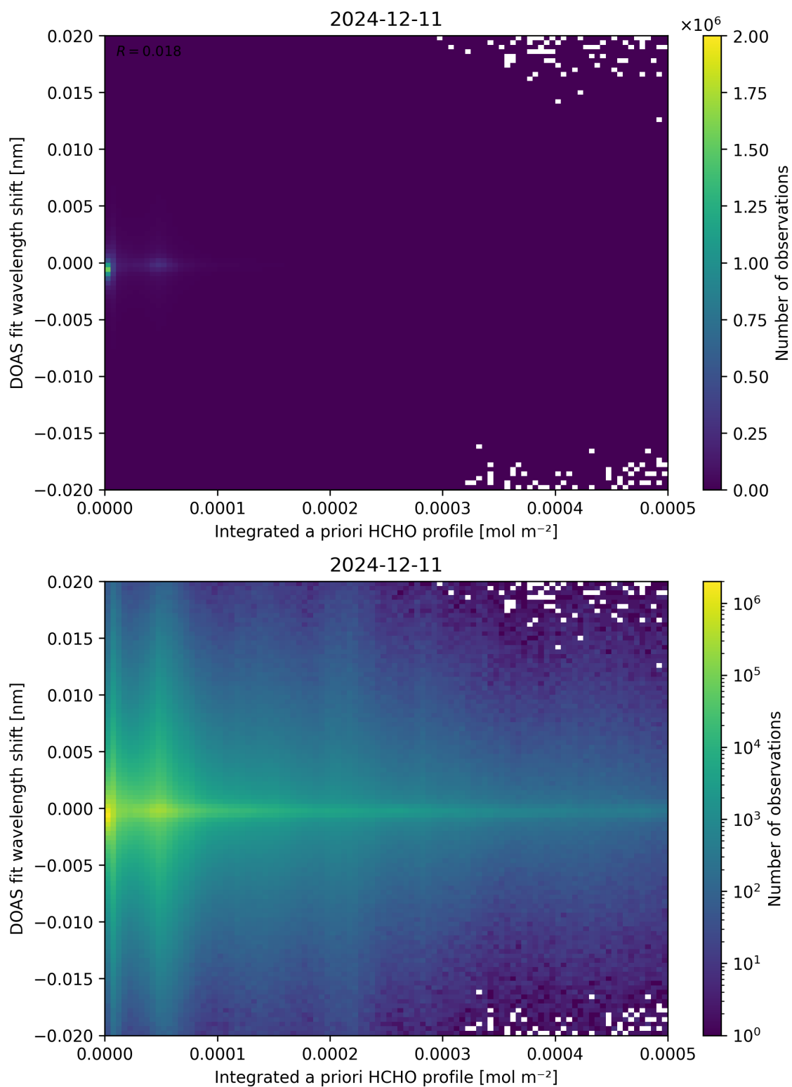
Figure 149: Scatter density plot of “Integrated a priori HCHO profile” against “DOAS fit wavelength shift” for 2024-12-11 to 2024-12-12.
