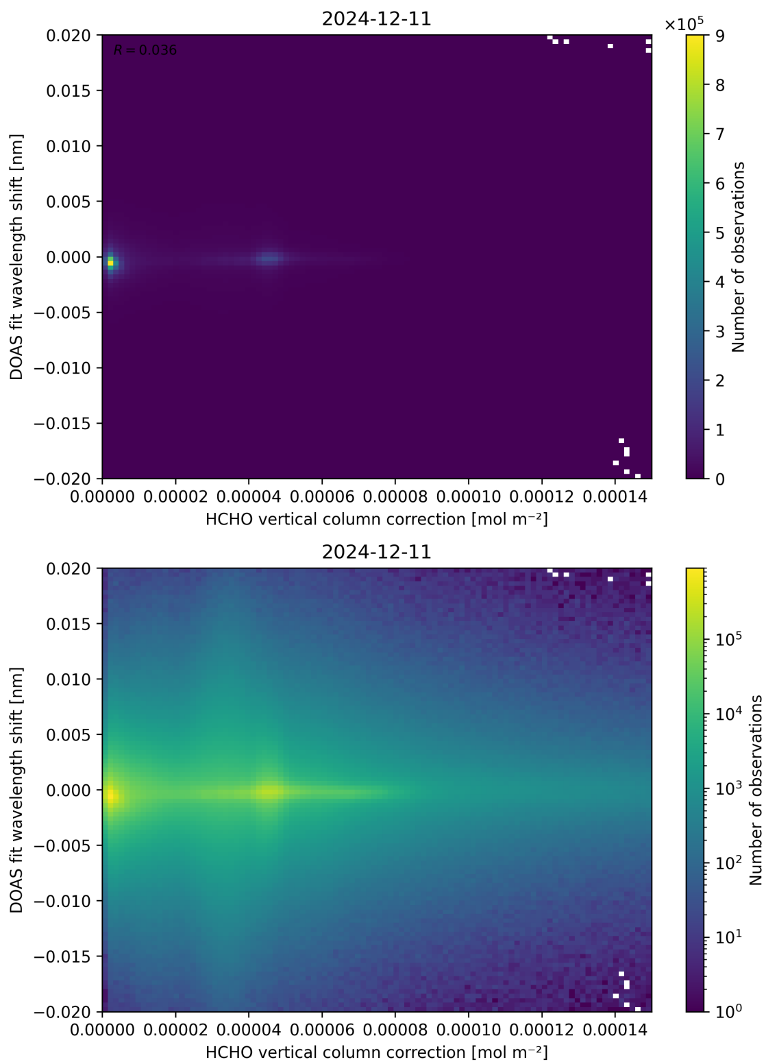
Figure 113: Scatter density plot of “HCHO vertical column correction” against “DOAS fit wavelength shift” for 2024-12-11 to 2024-12-12.
