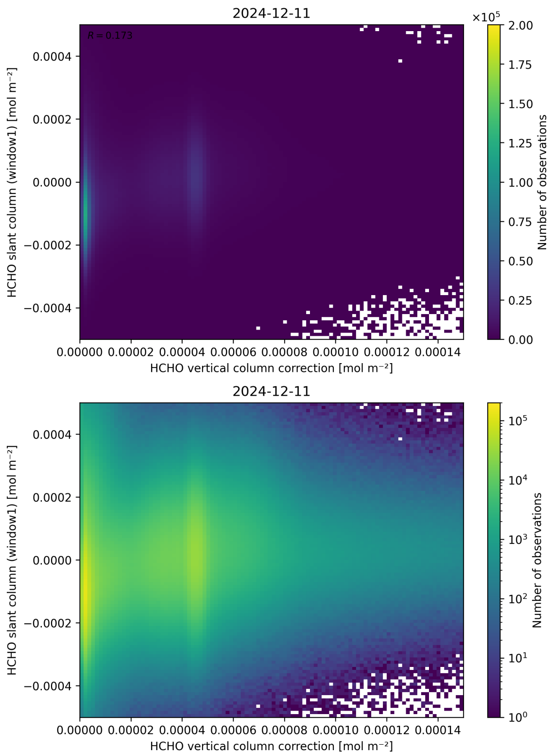
Figure 118: Scatter density plot of “HCHO vertical column correction” against “HCHO slant column (window1)” for 2024-12-11 to 2024-12-12.
