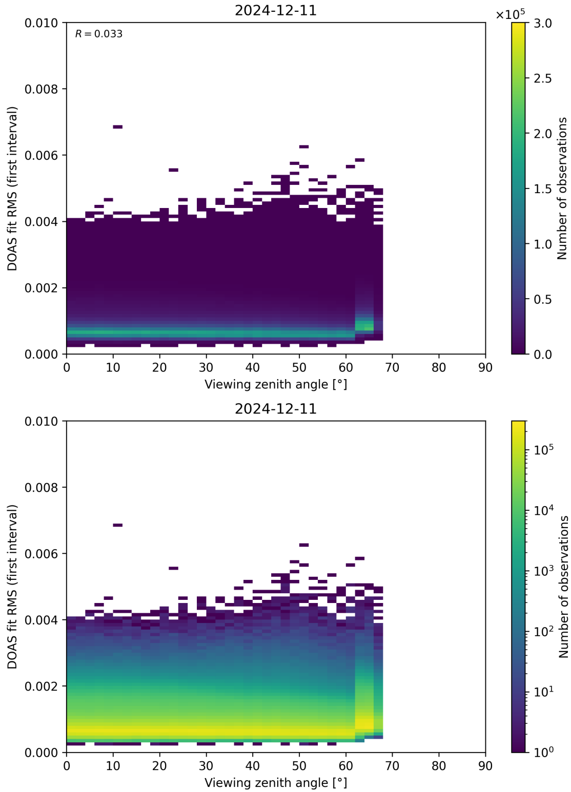
Figure 182: Scatter density plot of “Viewing zenith angle” against “DOAS fit RMS (first interval)” for 2024-12-11 to 2024-12-12.
