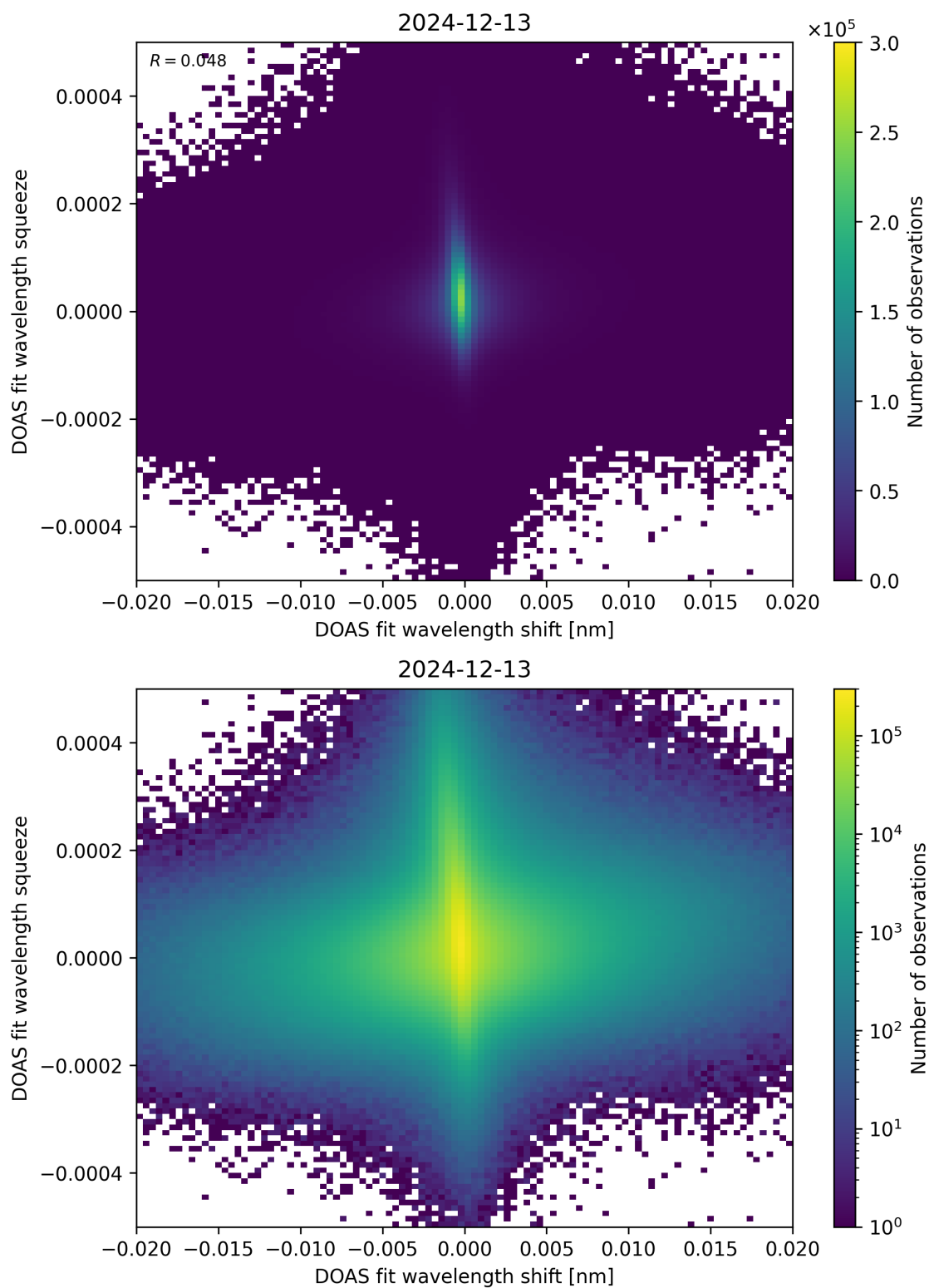
Figure 65: Scatter density plot of “DOAS fit wavelength shift” against “DOAS fit wavelength squeeze” for 2024-12-12 to 2024-12-14.
