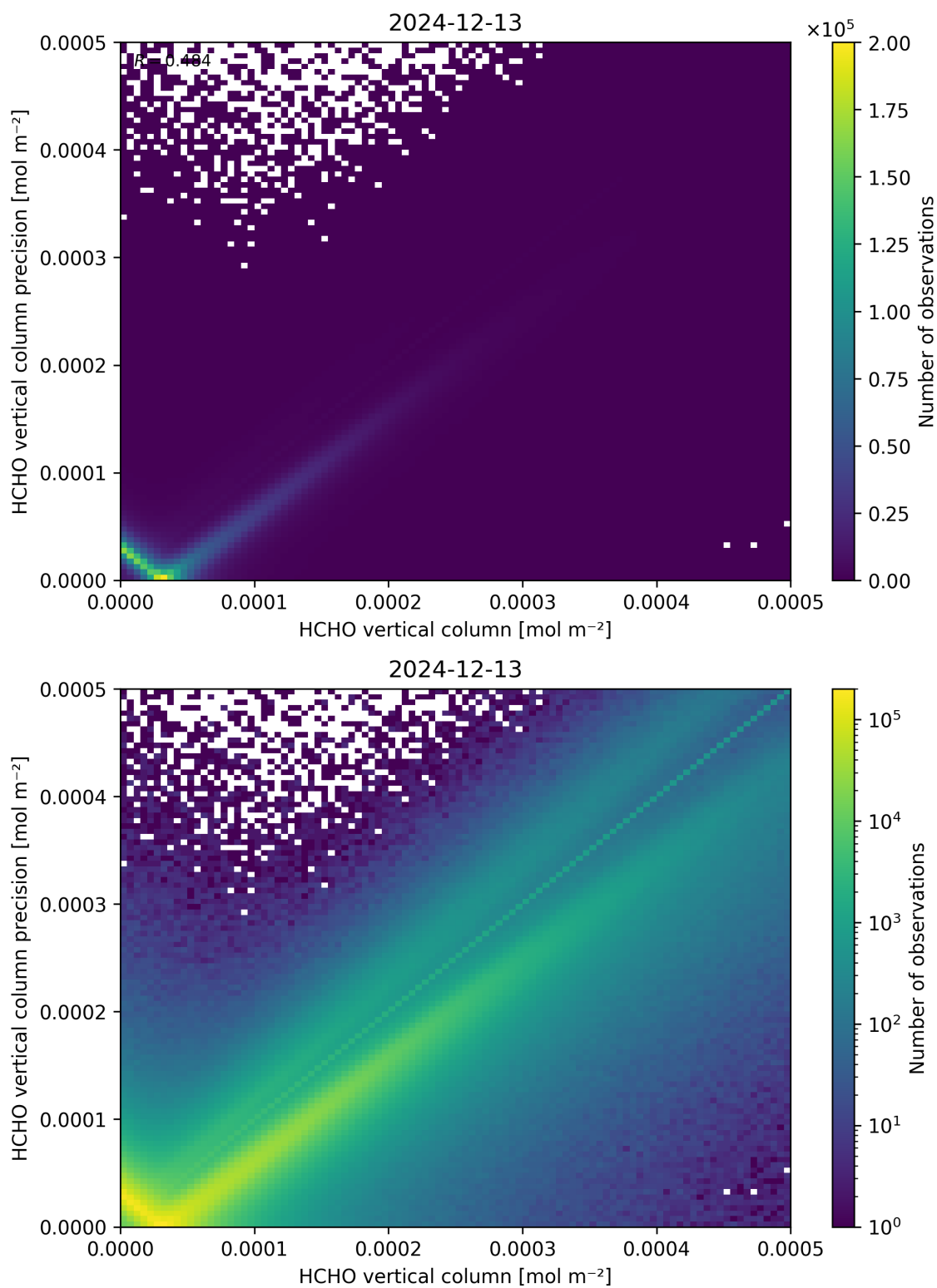
Figure 134: Scatter density plot of “HCHO vertical column” against “HCHO vertical column precision” for 2024-12-12 to 2024-12-14.
