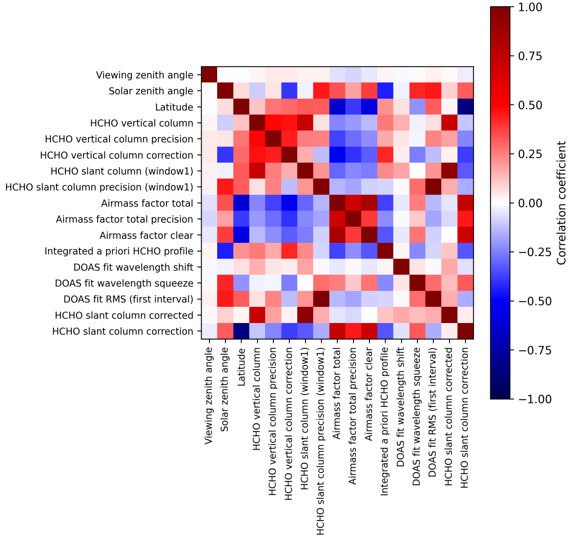
Figure 2: Map of correlation matrix for 2024-12-12 to 2024-12-14.
