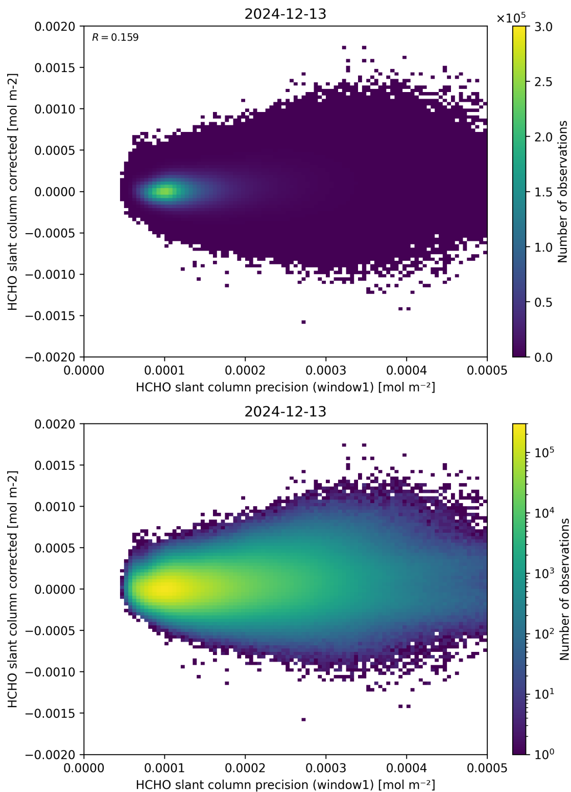
Figure 92: Scatter density plot of “HCHO slant column precision (window1)” against “HCHO slant column corrected” for 2024-12-12 to 2024-12-14.
