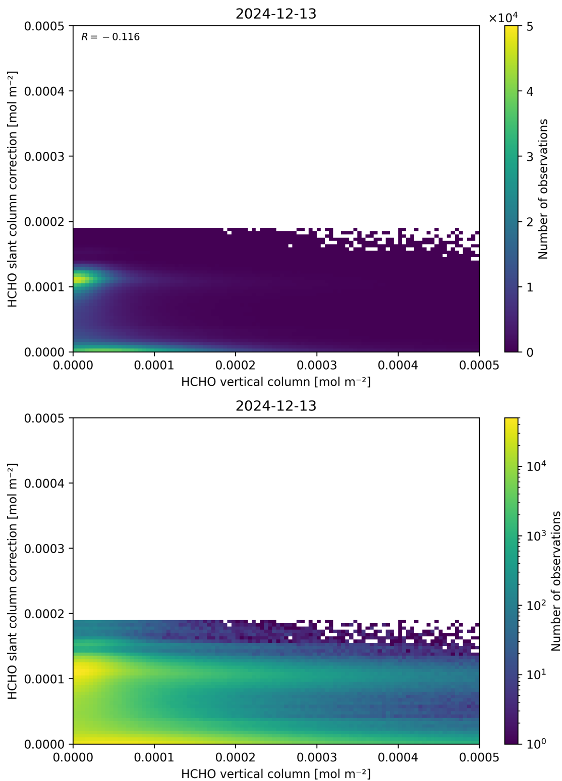
Figure 128: Scatter density plot of “HCHO vertical column” against “HCHO slant column correction” for 2024-12-12 to 2024-12-14.
