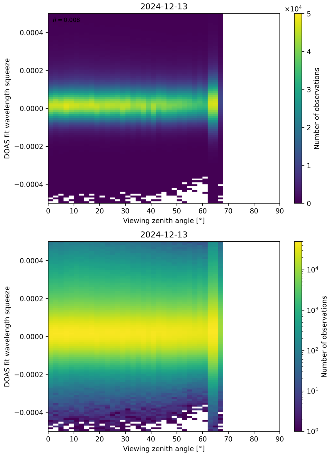
Figure 184: Scatter density plot of “Viewing zenith angle” against “DOAS fit wavelength squeeze” for 2024-12-12 to 2024-12-14.
