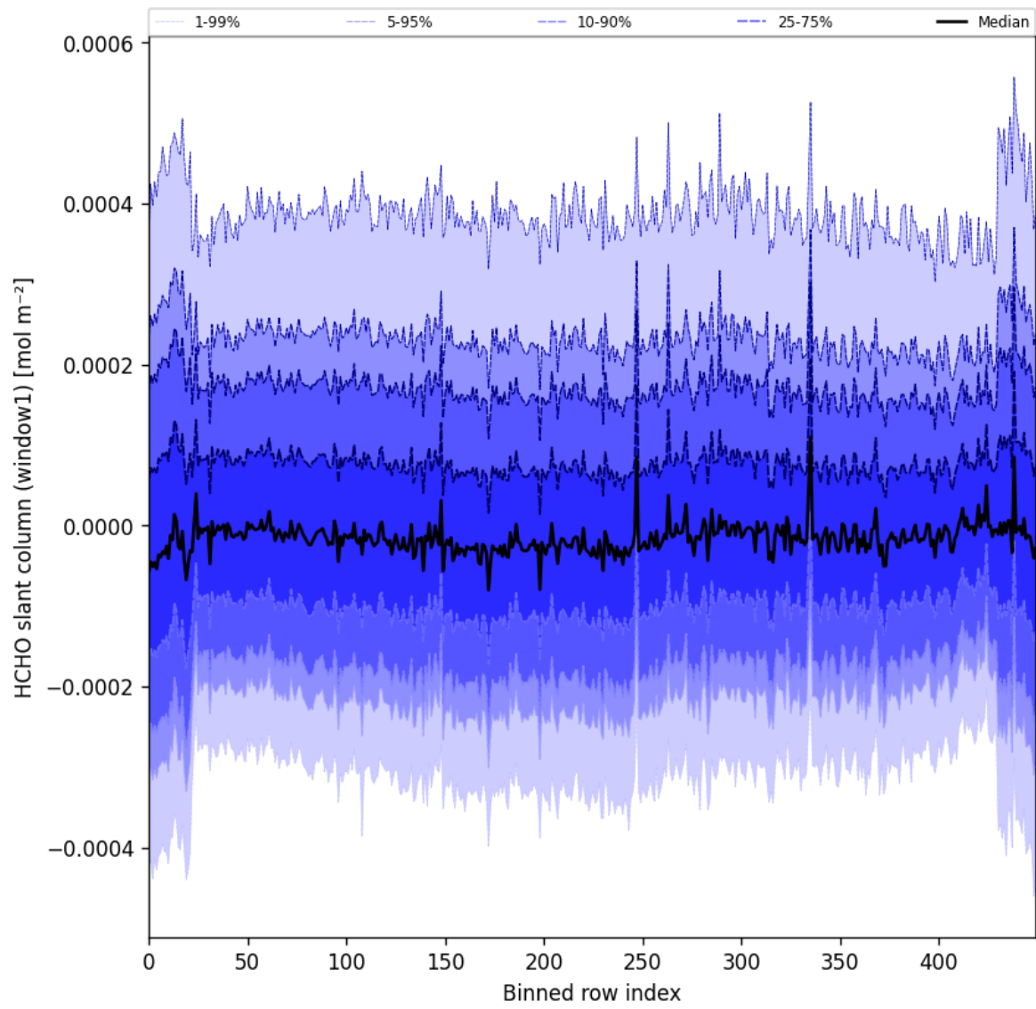
Figure 52: Along track statistics of “HCHO slant column (window1)” for 2024-12-12 to 2024-12-14
