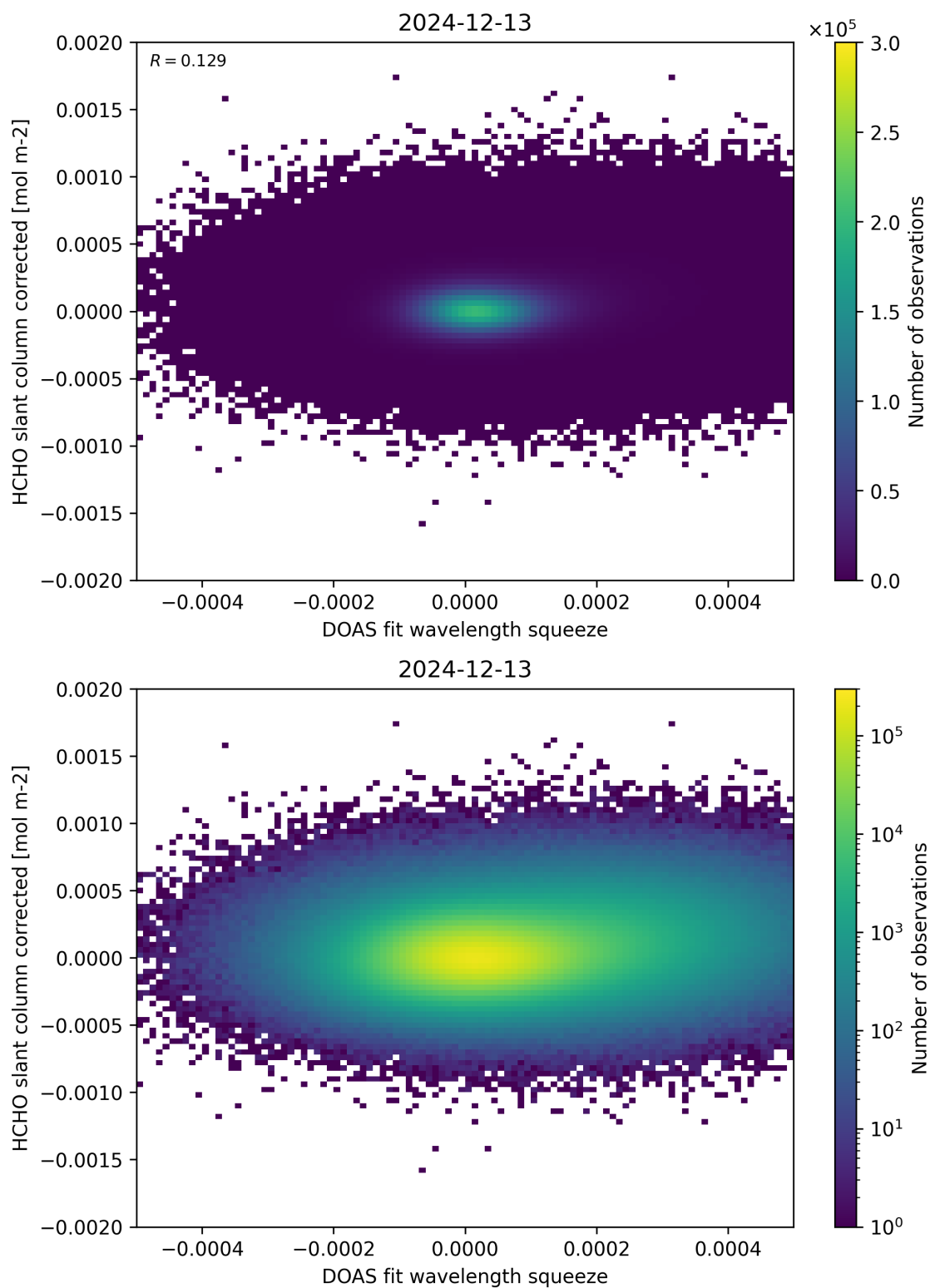
Figure 69: Scatter density plot of “DOAS fit wavelength squeeze” against “HCHO slant column corrected” for 2024-12-12 to 2024-12-14.
