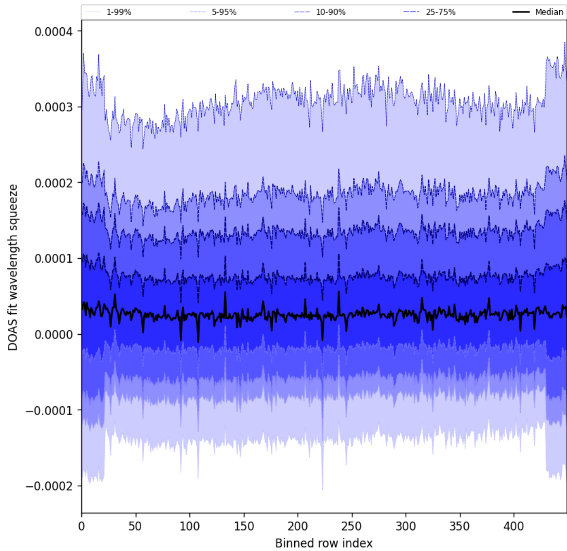
Figure 59: Along track statistics of “DOAS fit wavelength squeeze” for 2024-12-12 to 2024-12-14
