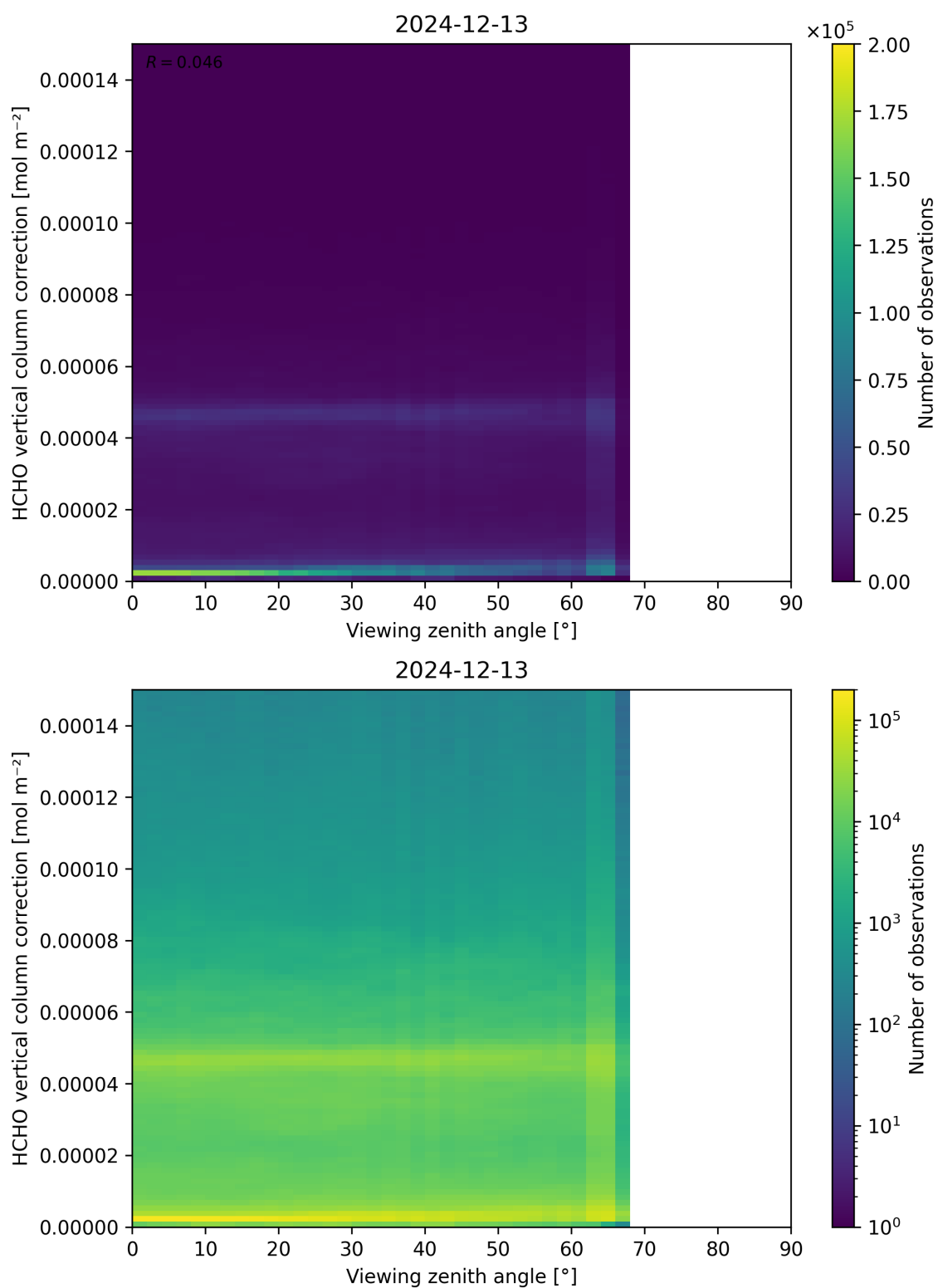
Figure 193: Scatter density plot of “Viewing zenith angle” against “HCHO vertical column correction” for 2024-12-12 to 2024-12-14.
