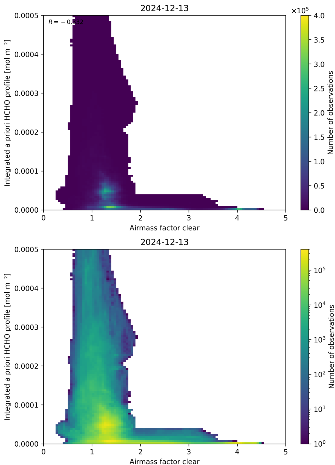
Figure 76: Scatter density plot of “Airmass factor clear” against “Integrated a priori HCHO profile” for 2024-12-12 to 2024-12-14.
