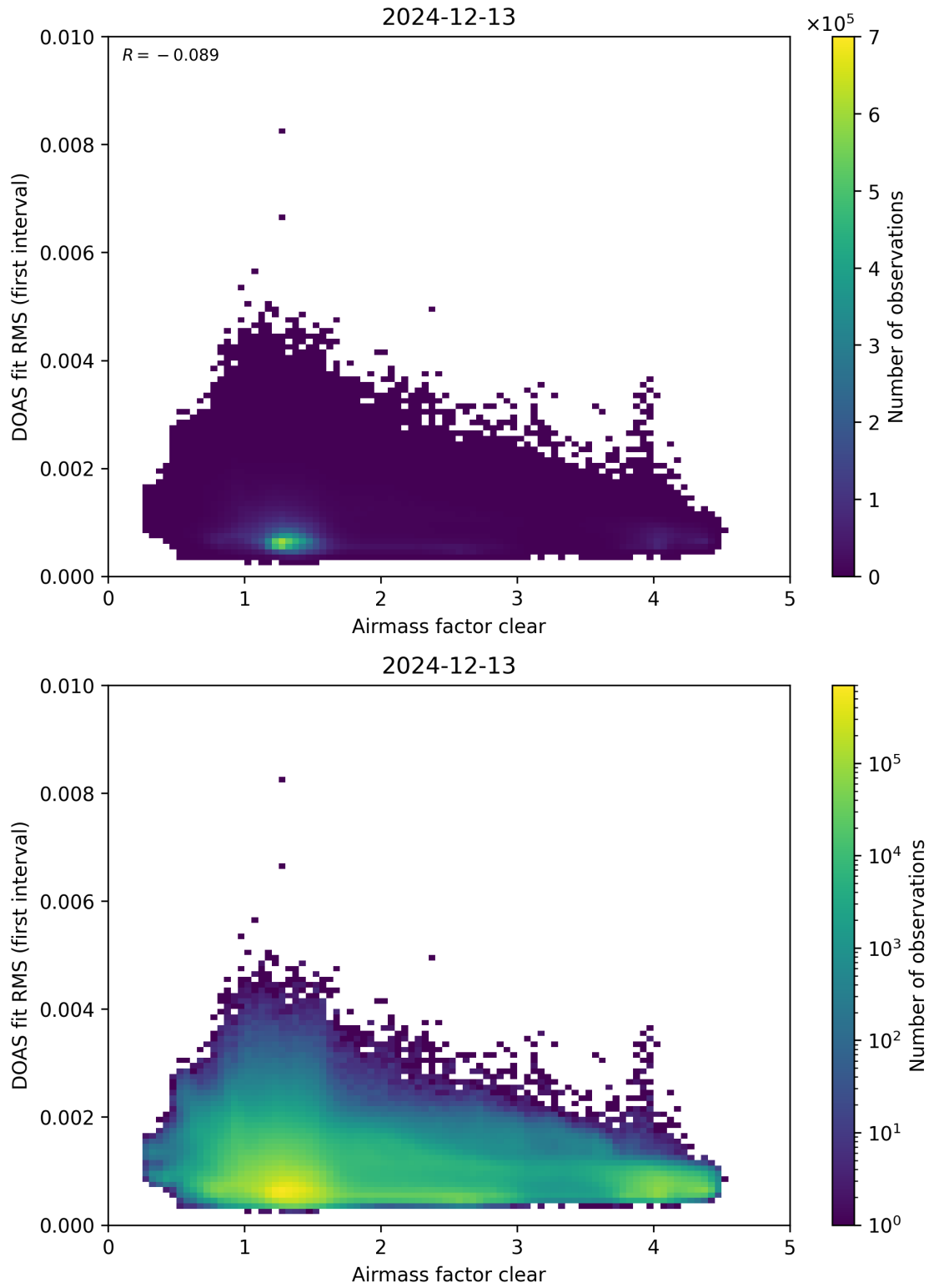
Figure 71: Scatter density plot of “Airmass factor clear” against “DOAS fit RMS (first interval)” for 2024-12-12 to 2024-12-14.
