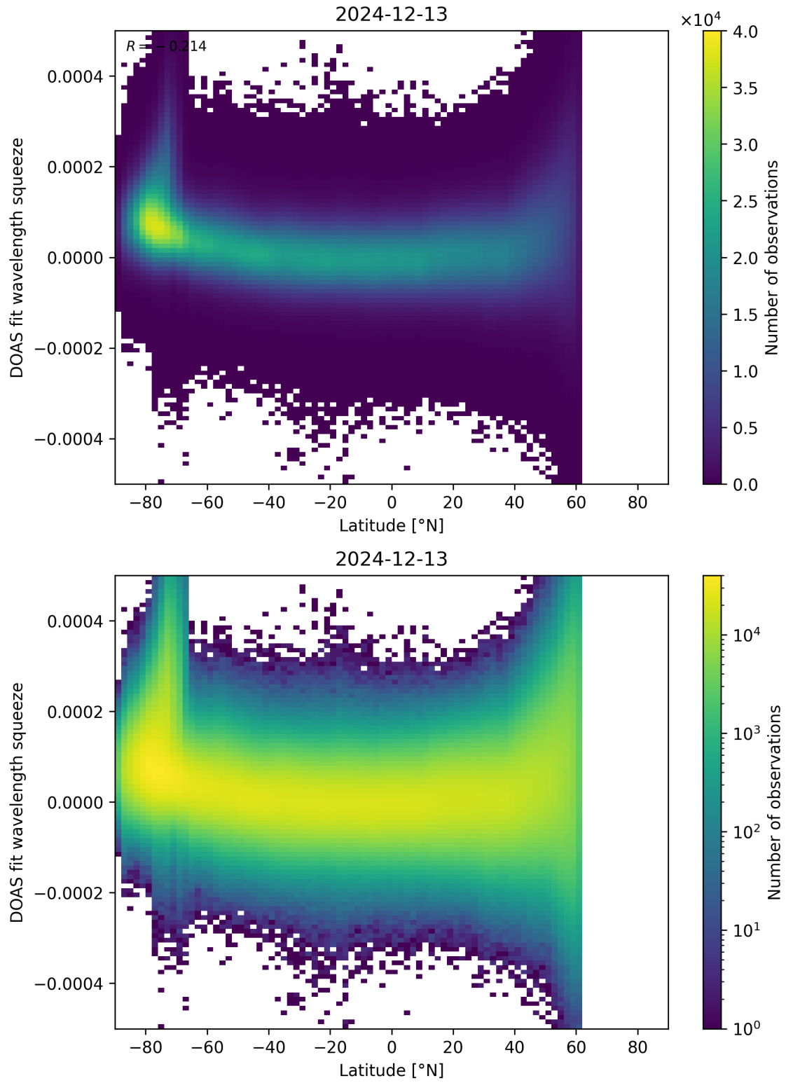
Figure 155: Scatter density plot of “Latitude” against “DOAS fit wavelength squeeze” for 2024-12-12 to 2024-12-14.
