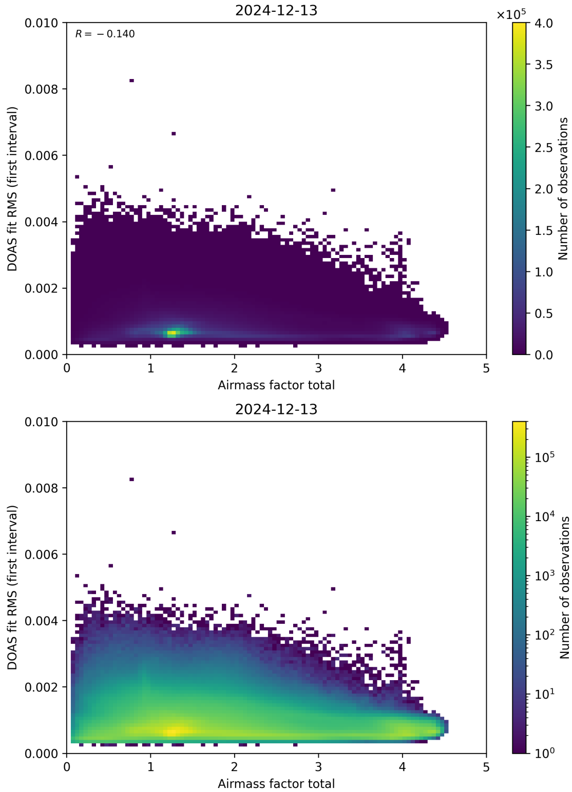
Figure 97: Scatter density plot of “Airmass factor total” against “DOAS fit RMS (first interval)” for 2024-12-12 to 2024-12-14.
