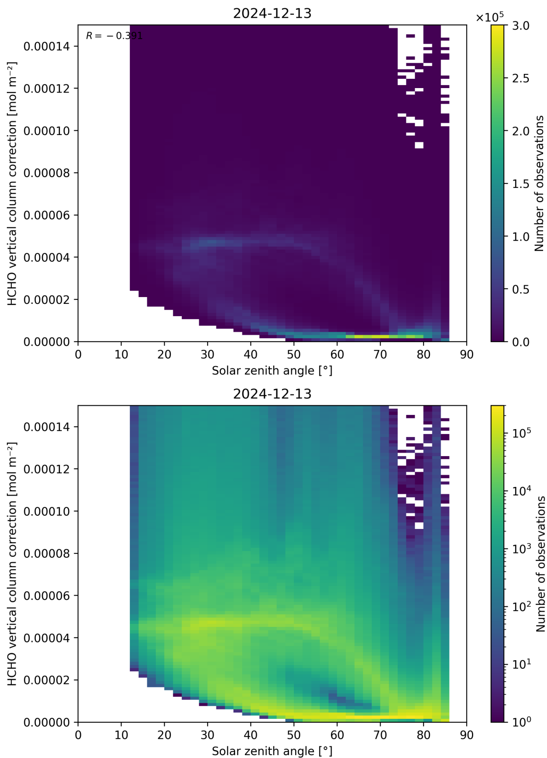
Figure 178: Scatter density plot of “Solar zenith angle” against “HCHO vertical column correction” for 2024-12-12 to 2024-12-14.
