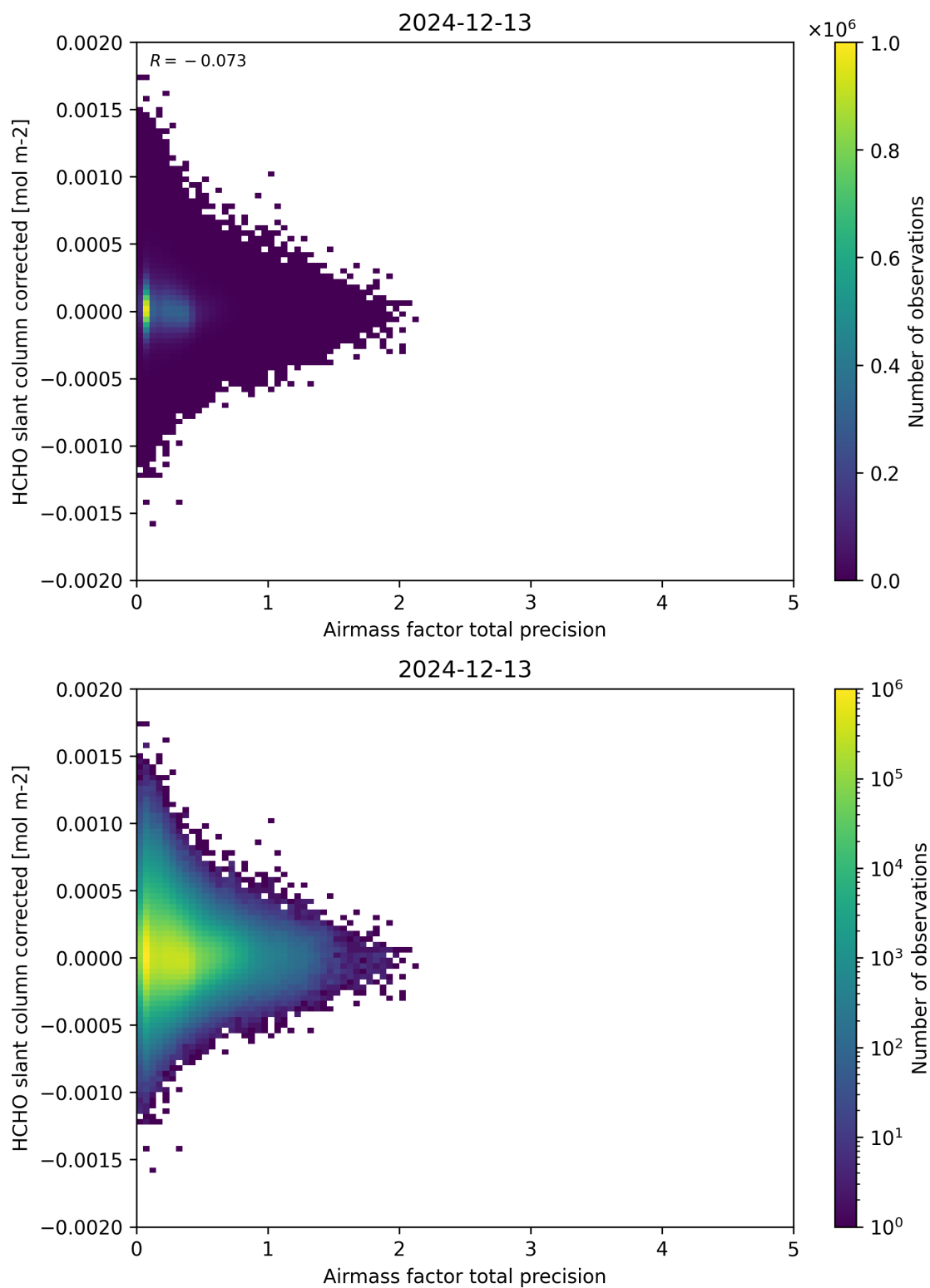
Figure 109: Scatter density plot of “Airmass factor total precision” against “HCHO slant column corrected” for 2024-12-12 to 2024-12-14.
