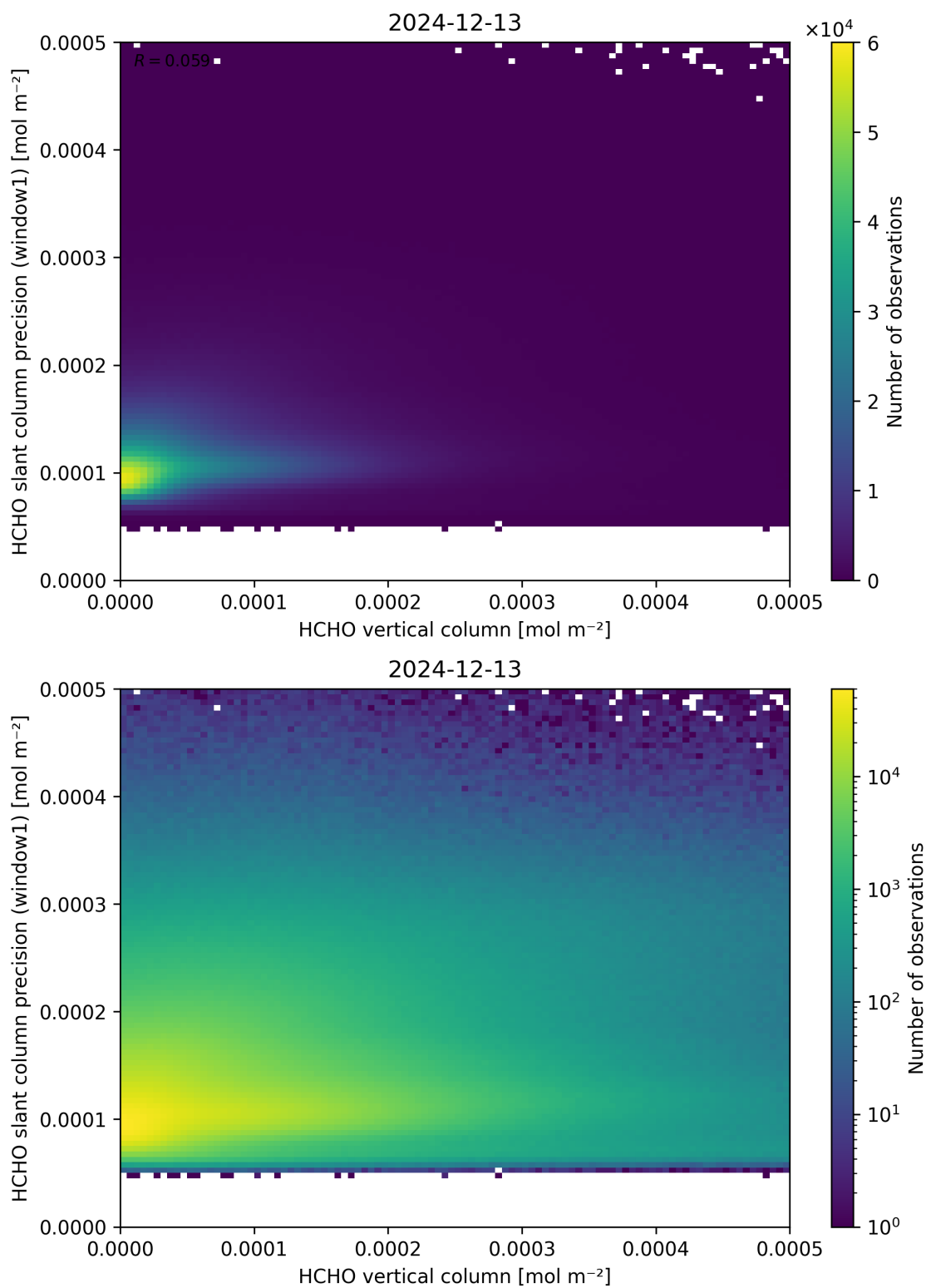
Figure 130: Scatter density plot of “HCHO vertical column” against “HCHO slant column precision (window1)” for 2024-12-12 to 2024-12-14.
