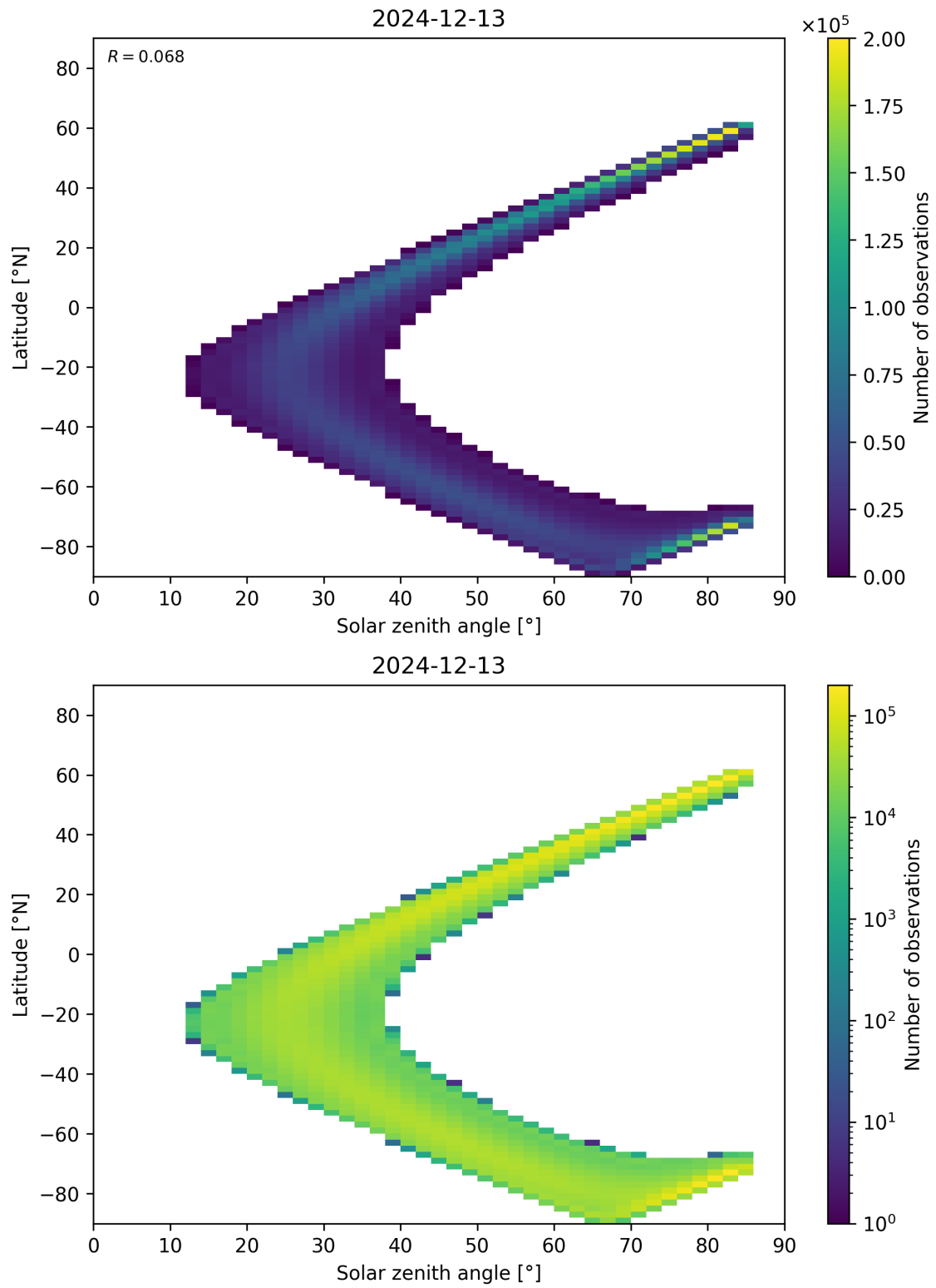
Figure 181: Scatter density plot of “Solar zenith angle” against “Latitude” for 2024-12-12 to 2024-12-14.
