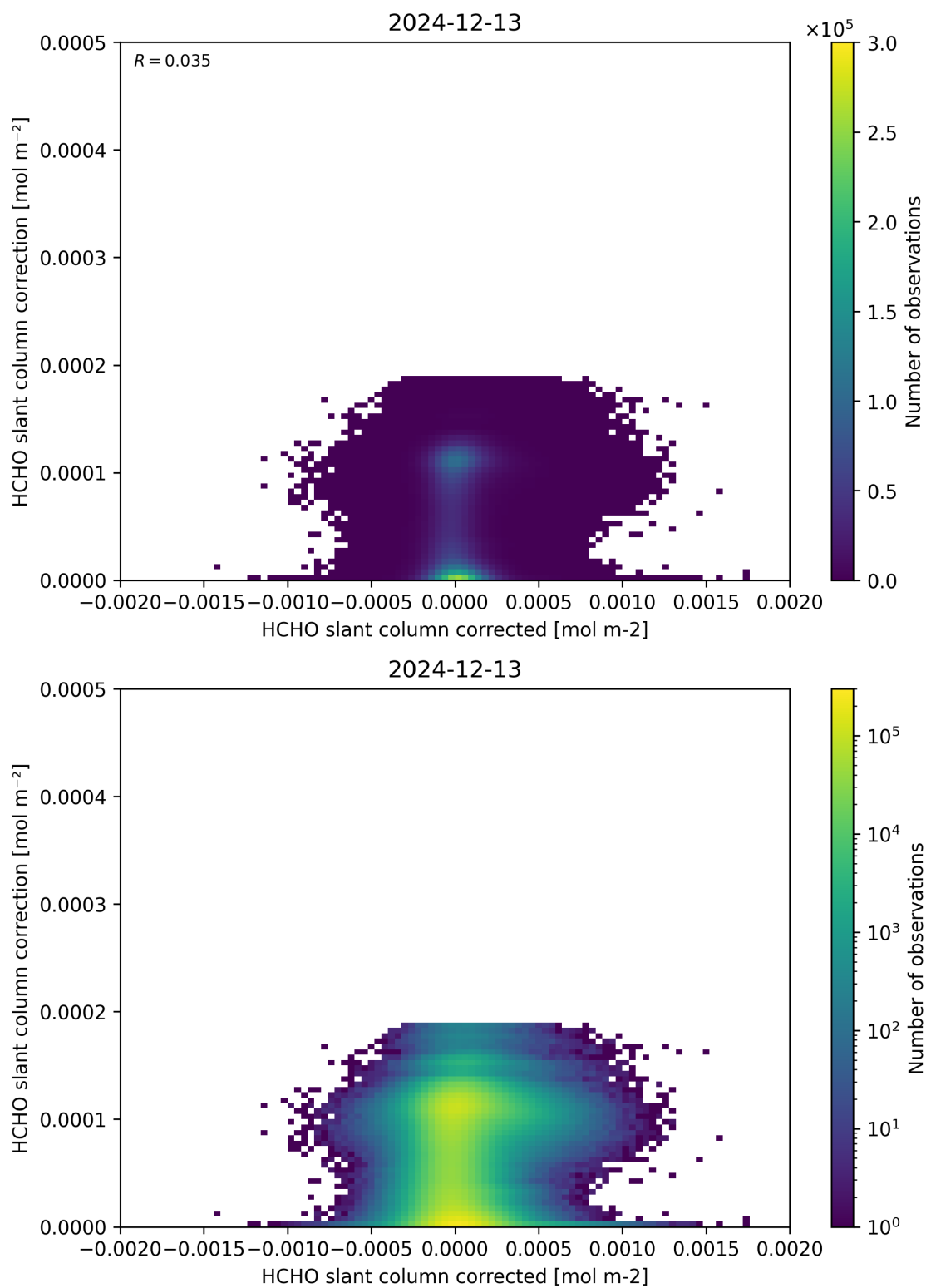
Figure 77: Scatter density plot of “HCHO slant column corrected” against “HCHO slant column correction” for 2024-12-12 to 2024-12-14.
