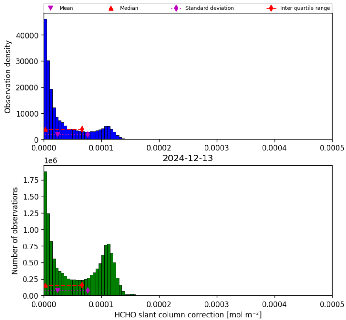
Figure 47: Histogram of “HCHO slant column correction” for 2024-12-12 to 2024-12-14
