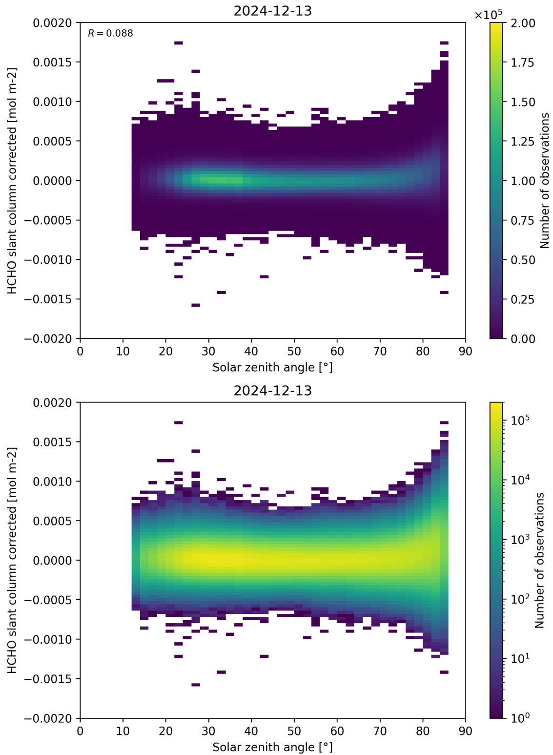
Figure 171: Scatter density plot of “Solar zenith angle” against “HCHO slant column corrected” for 2024-12-12 to 2024-12-14.
