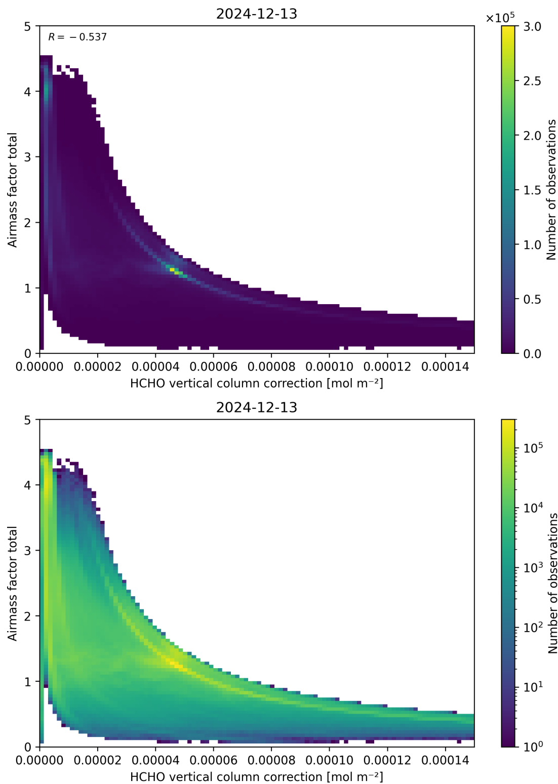
Figure 120: Scatter density plot of “HCHO vertical column correction” against “Airmass factor total” for 2024-12-12 to 2024-12-14.
