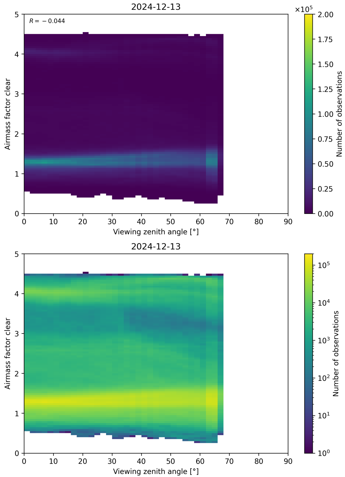
Figure 185: Scatter density plot of “Viewing zenith angle” against “Airmass factor clear” for 2024-12-12 to 2024-12-14.
