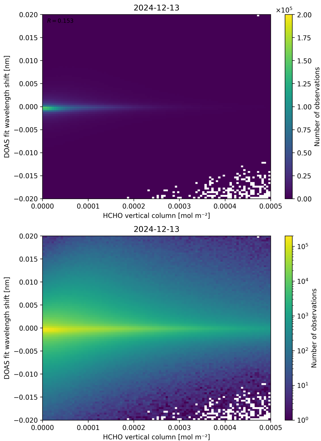
Figure 124: Scatter density plot of “HCHO vertical column” against “DOAS fit wavelength shift” for 2024-12-12 to 2024-12-14.
