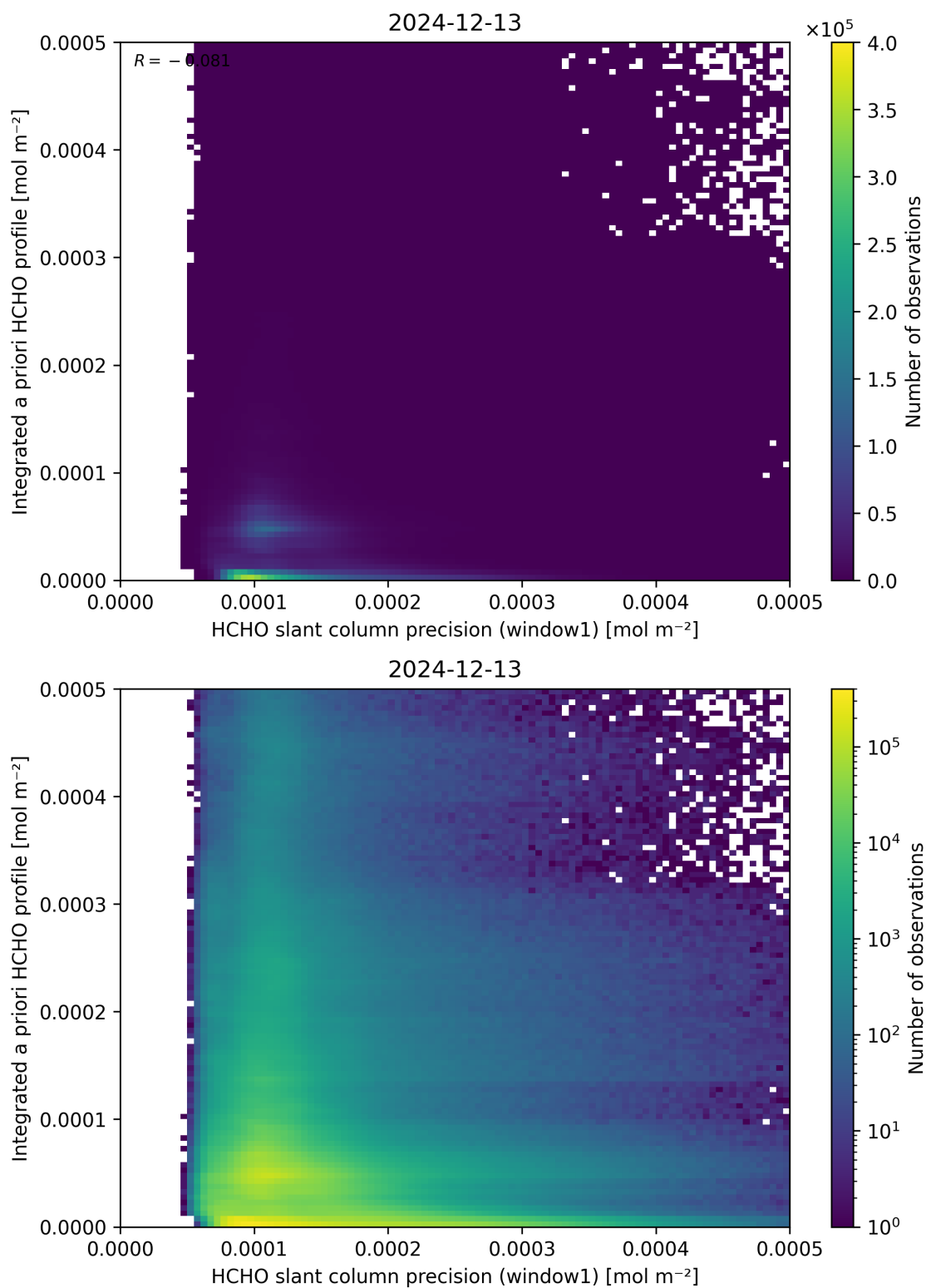
Figure 96: Scatter density plot of “HCHO slant column precision (window1)” against “Integrated a priori HCHO profile” for 2024-12-12 to 2024-12-14.
