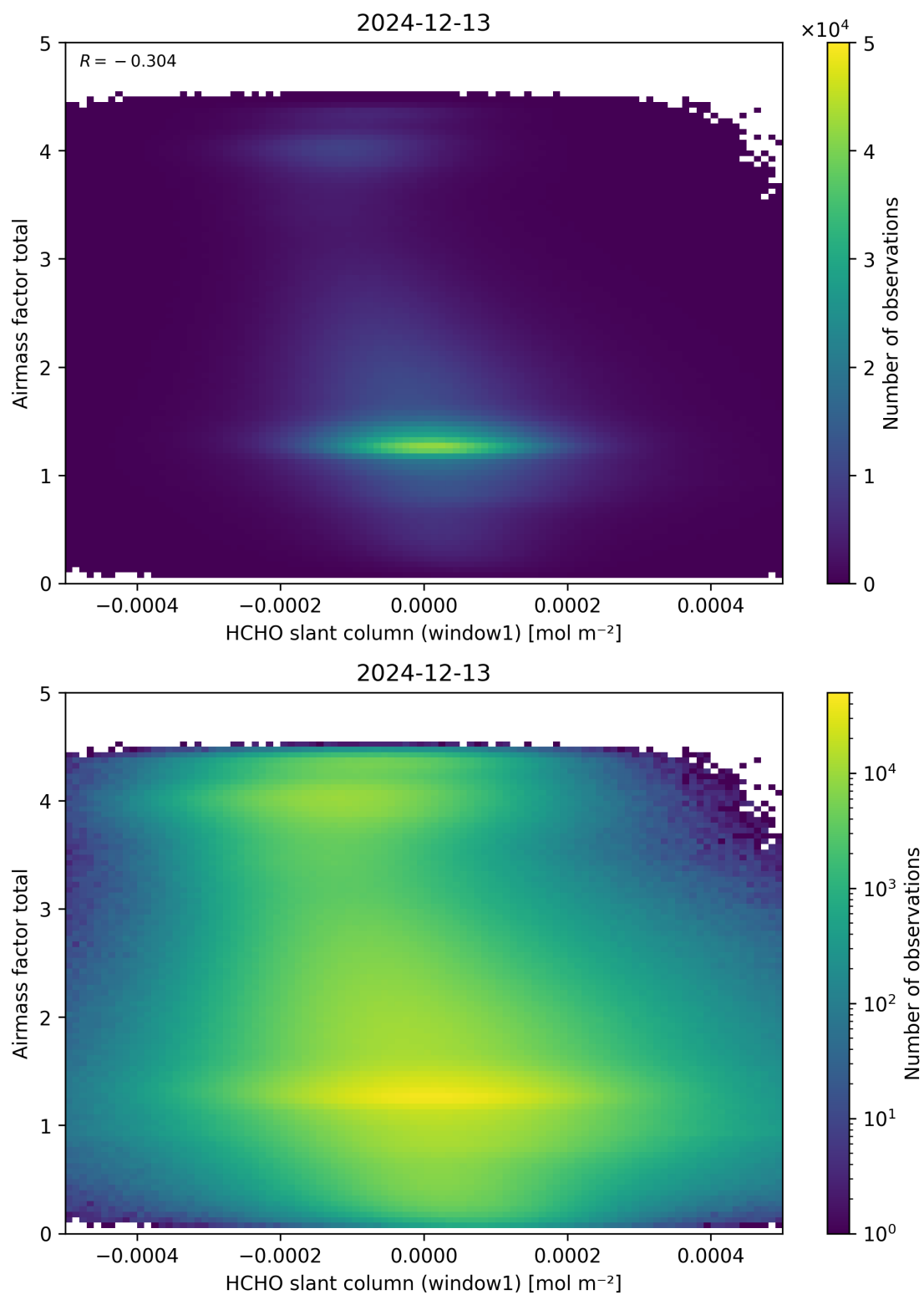
Figure 85: Scatter density plot of “HCHO slant column (window1)” against “Airmass factor total” for 2024-12-12 to 2024-12-14.
