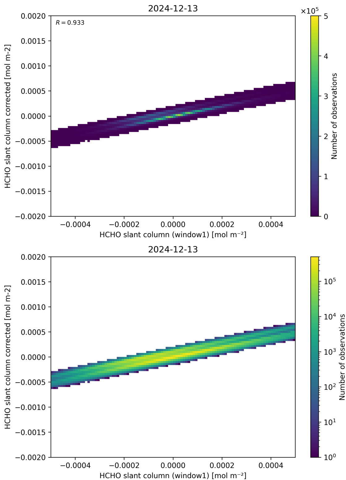
Figure 82: Scatter density plot of “HCHO slant column (window1)” against “HCHO slant column corrected” for 2024-12-12 to 2024-12-14.
