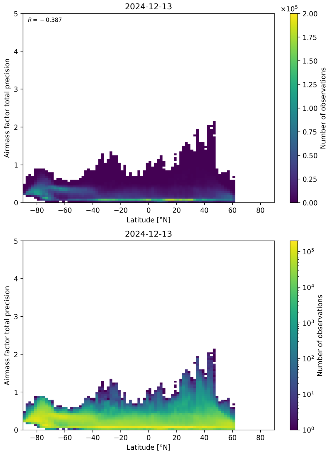
Figure 162: Scatter density plot of “Latitude” against “Airmass factor total precision” for 2024-12-12 to 2024-12-14.
