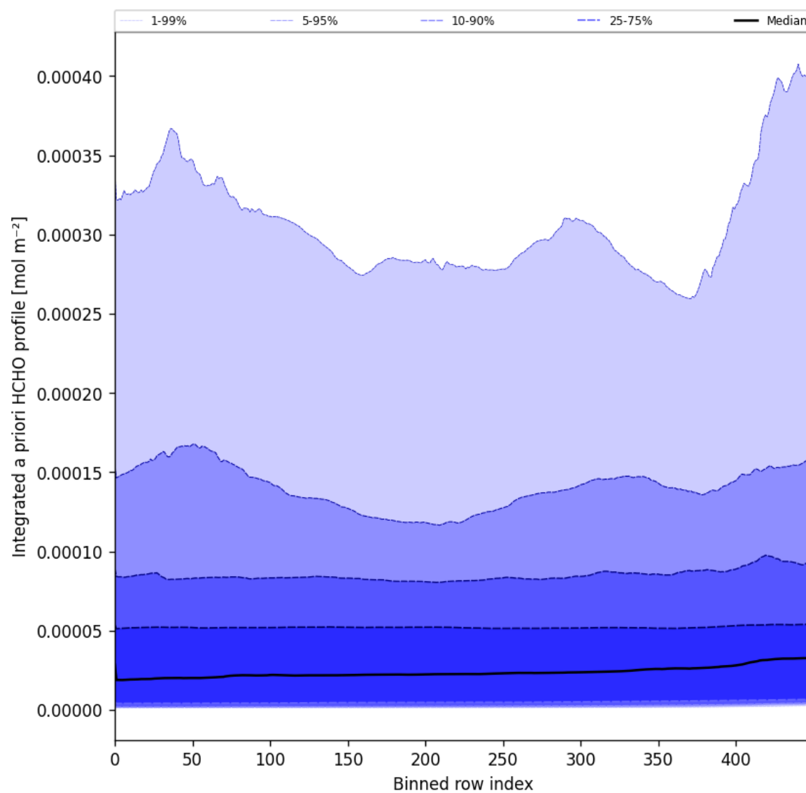
Figure 57: Along track statistics of “Integrated a priori HCHO profile” for 2024-12-12 to 2024-12-14
