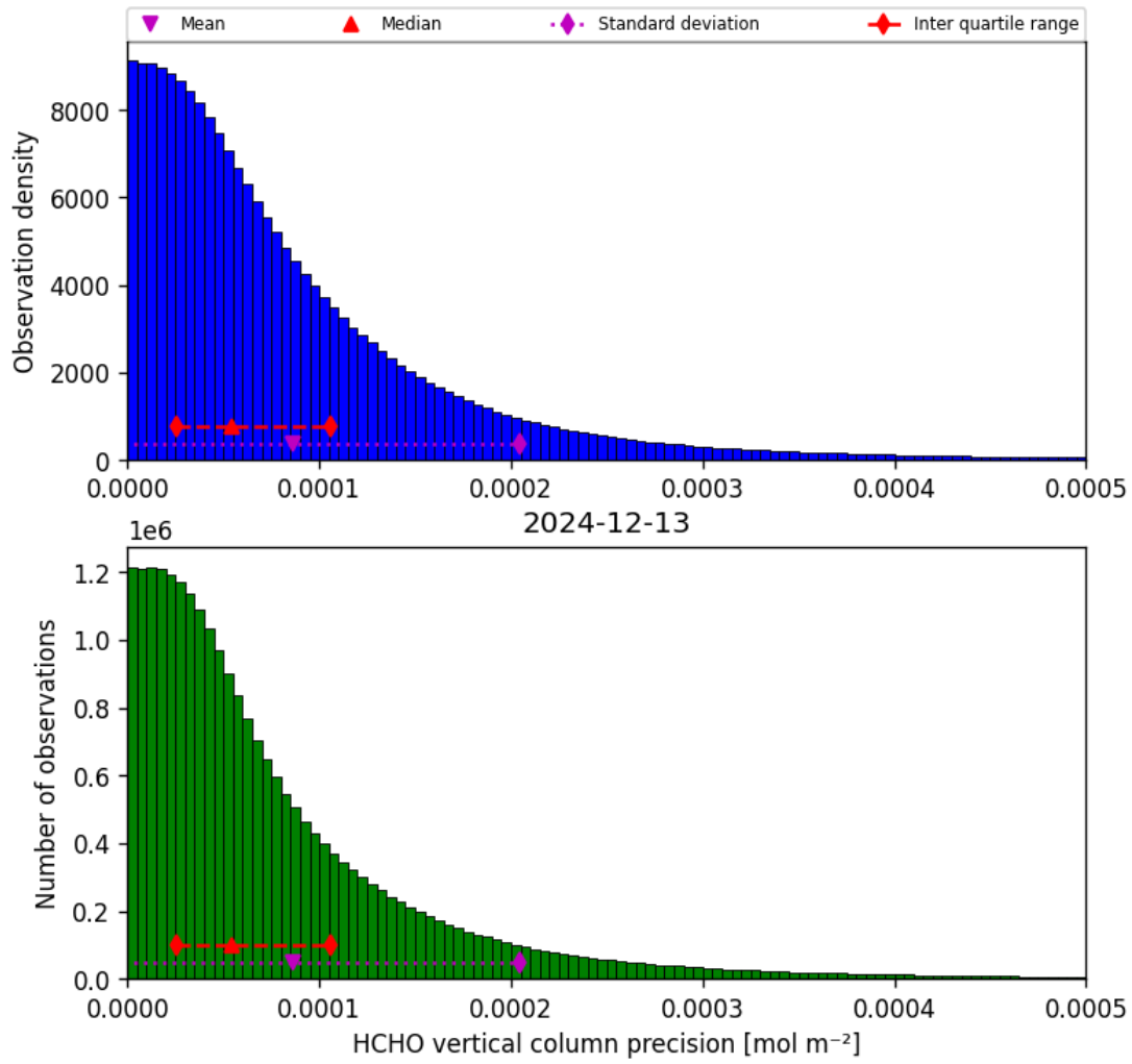
Figure 36: Histogram of “HCHO vertical column precision” for 2024-12-12 to 2024-12-14
