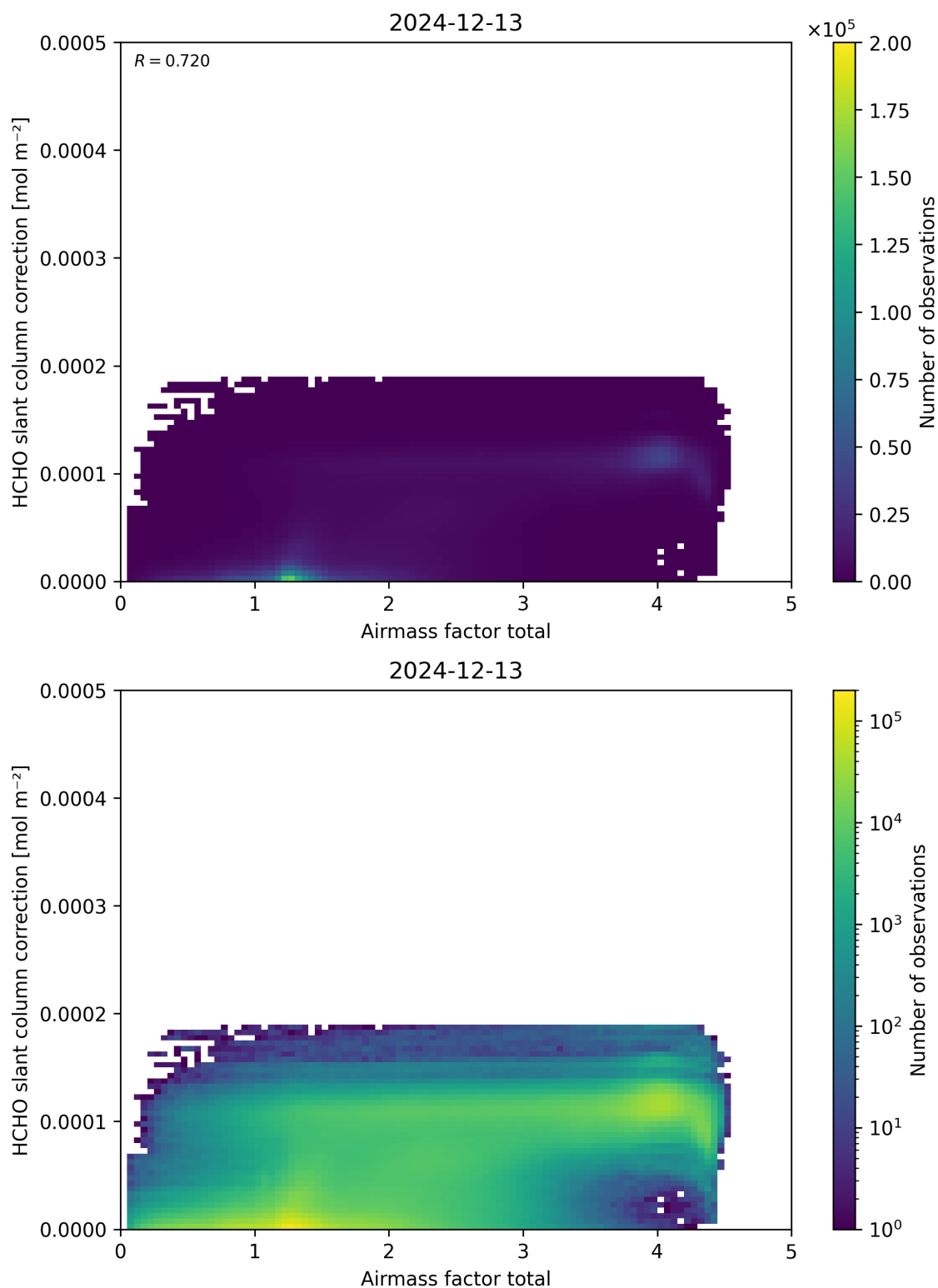
Figure 102: Scatter density plot of “Airmass factor total” against “HCHO slant column correction” for 2024-12-12 to 2024-12-14.
