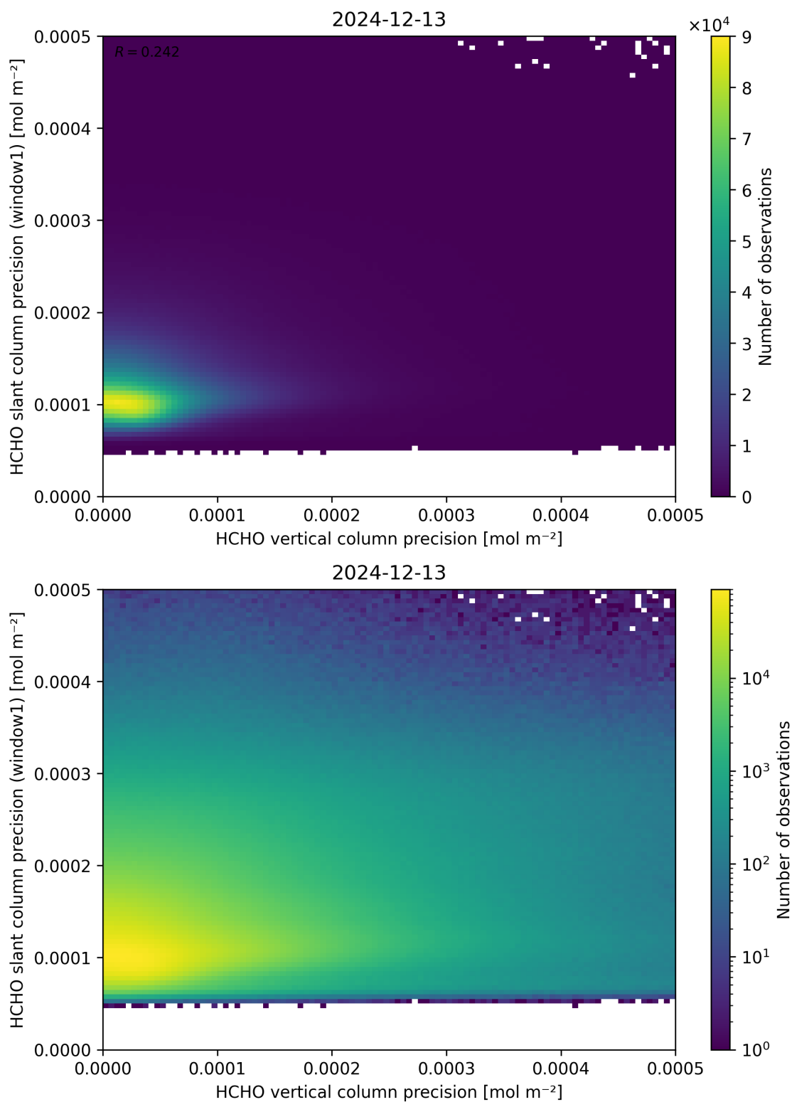
Figure 143: Scatter density plot of “HCHO vertical column precision” against “HCHO slant column precision (window1)” for 2024-12-12 to 2024-12-14.
