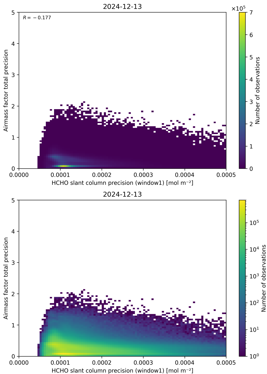
Figure 95: Scatter density plot of “HCHO slant column precision (window1)” against “Airmass factor total precision” for 2024-12-12 to 2024-12-14.
