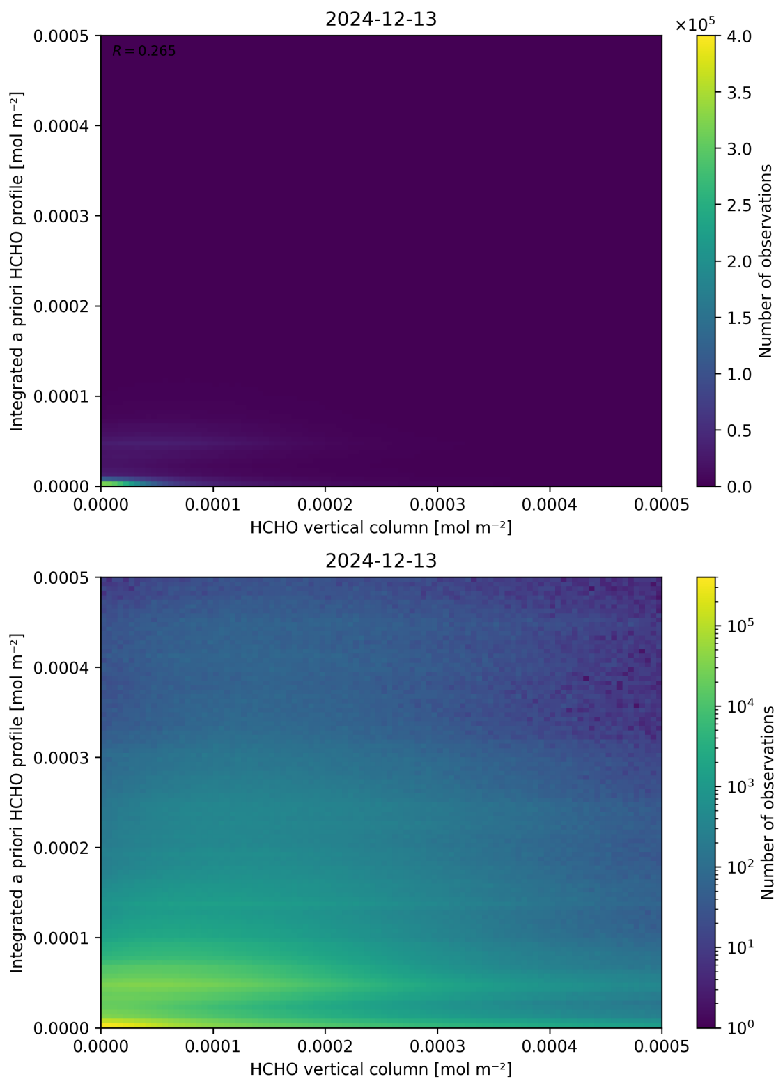
Figure 135: Scatter density plot of “HCHO vertical column” against “Integrated a priori HCHO profile” for 2024-12-12 to 2024-12-14.
