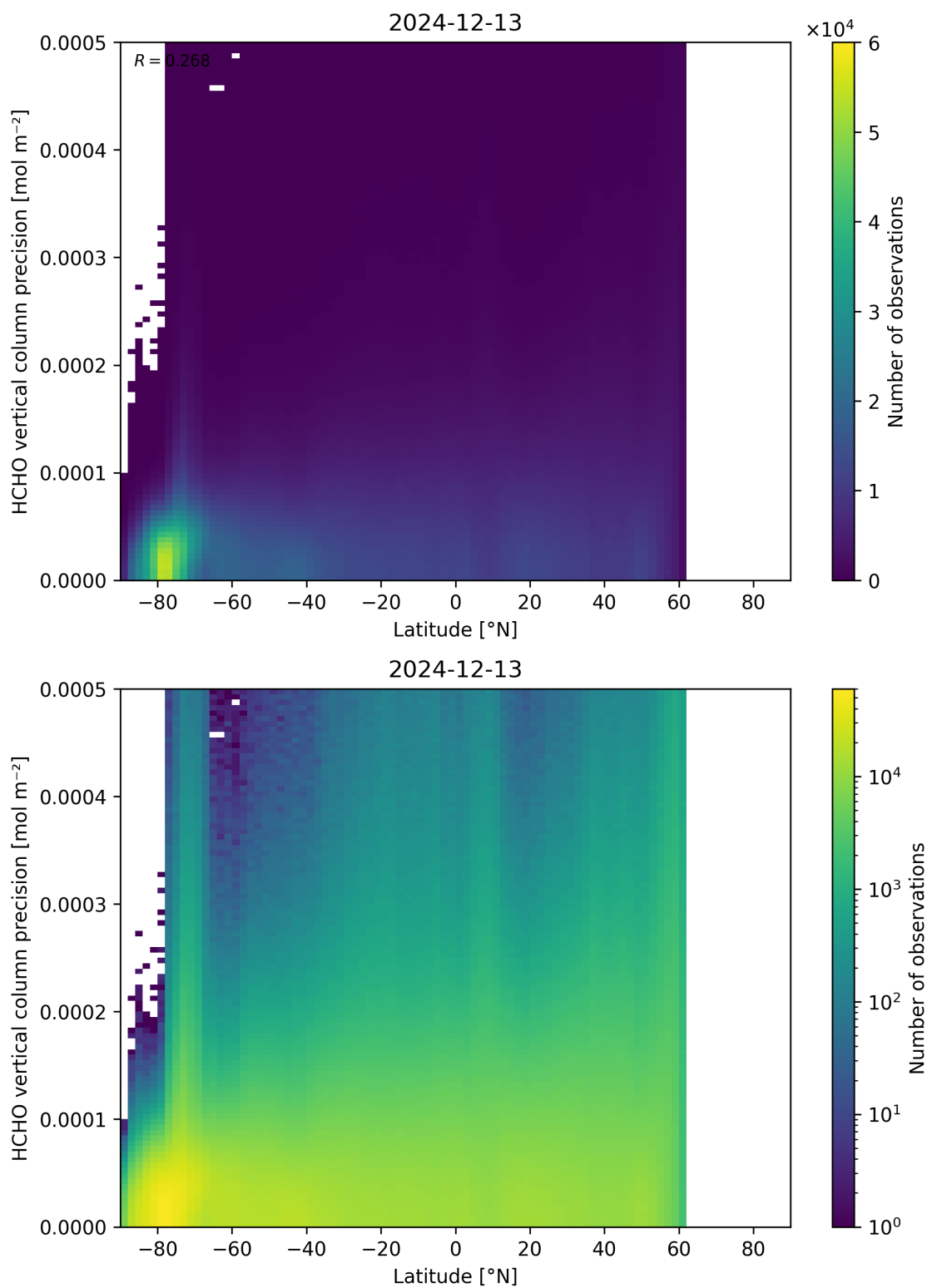
Figure 165: Scatter density plot of “Latitude” against “HCHO vertical column precision” for 2024-12-12 to 2024-12-14.
