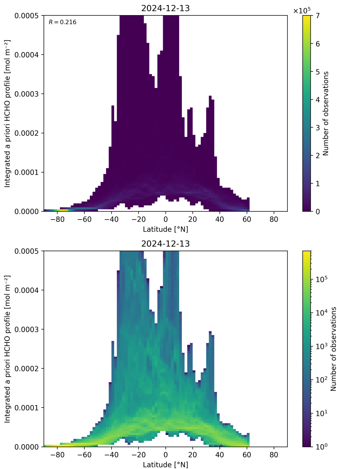
Figure 166: Scatter density plot of “Latitude” against “Integrated a priori HCHO profile” for 2024-12-12 to 2024-12-14.
