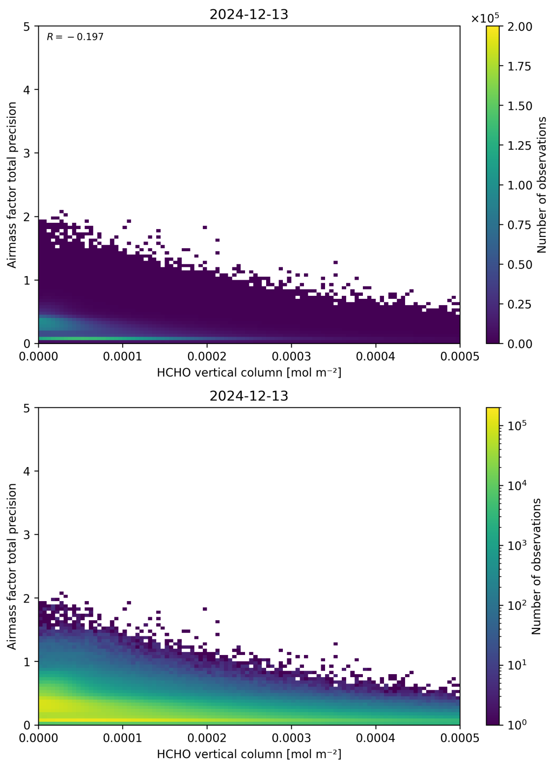
Figure 132: Scatter density plot of “HCHO vertical column” against “Airmass factor total precision” for 2024-12-12 to 2024-12-14.
