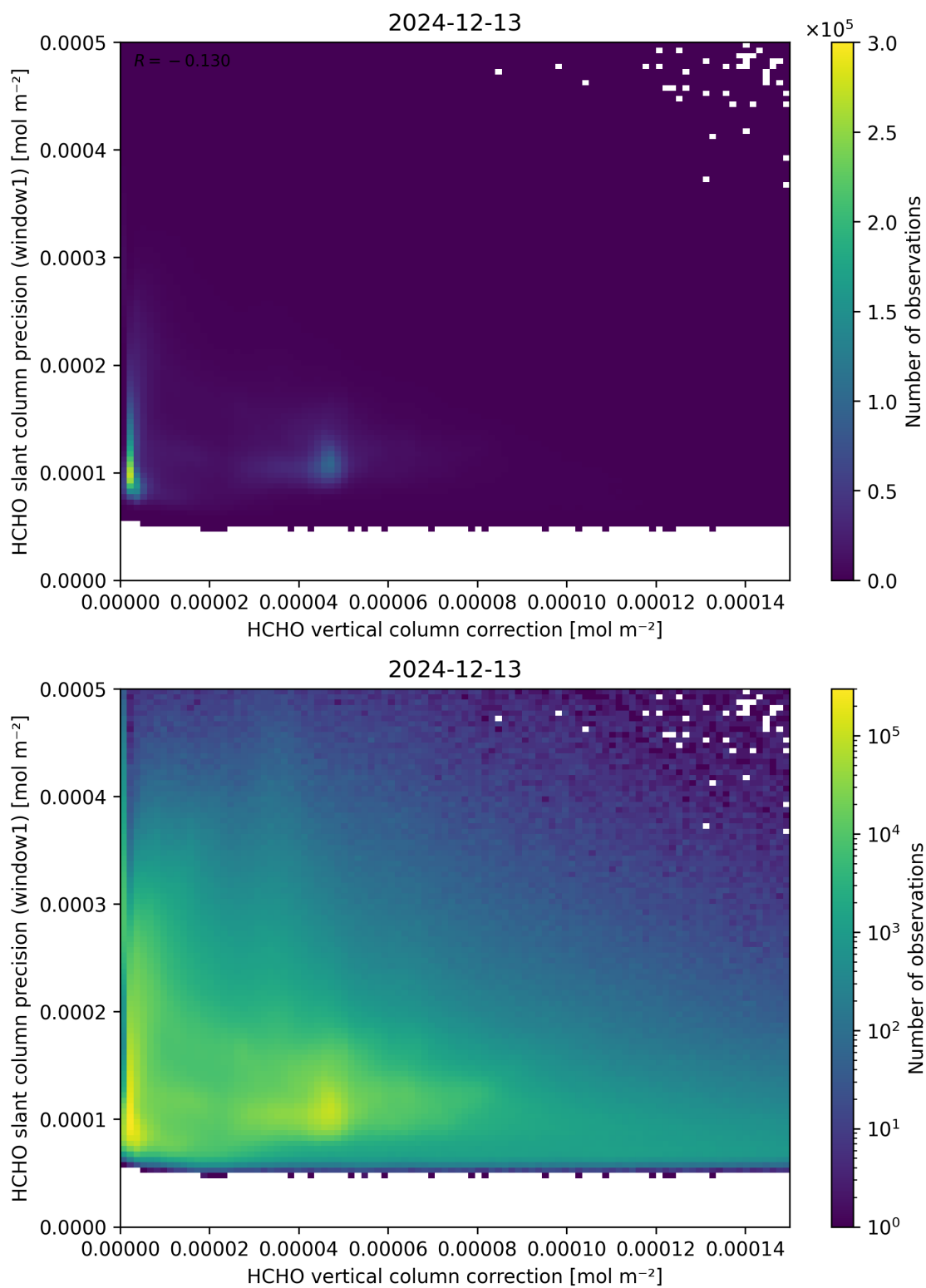
Figure 119: Scatter density plot of “HCHO vertical column correction” against “HCHO slant column precision (window1)” for 2024-12-12 to 2024-12-14.
