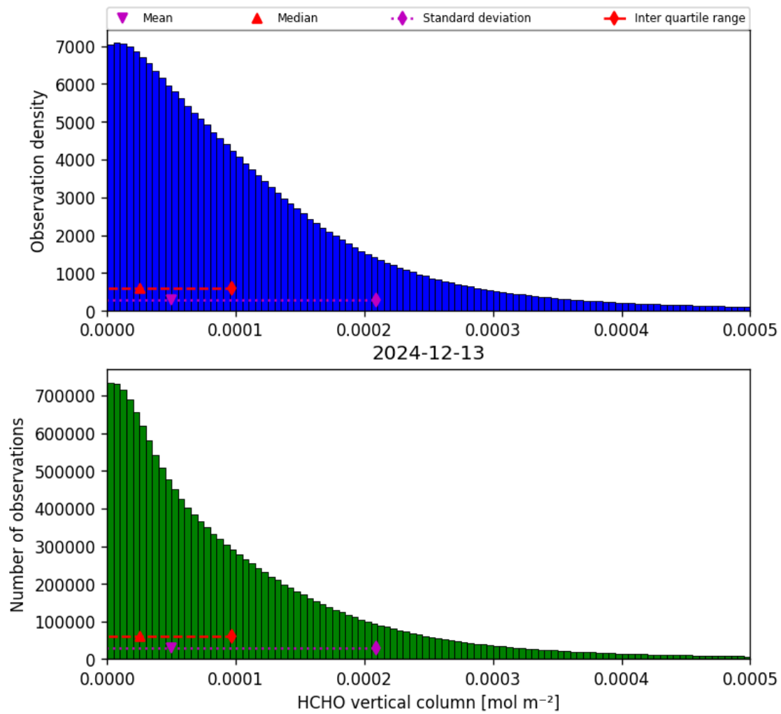
Figure 35: Histogram of “HCHO vertical column” for 2024-12-12 to 2024-12-14
