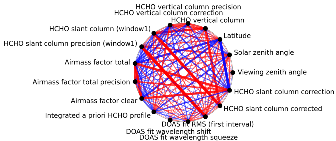
Figure 1: Map of correlation graph for 2024-12-12 to 2024-12-14.
