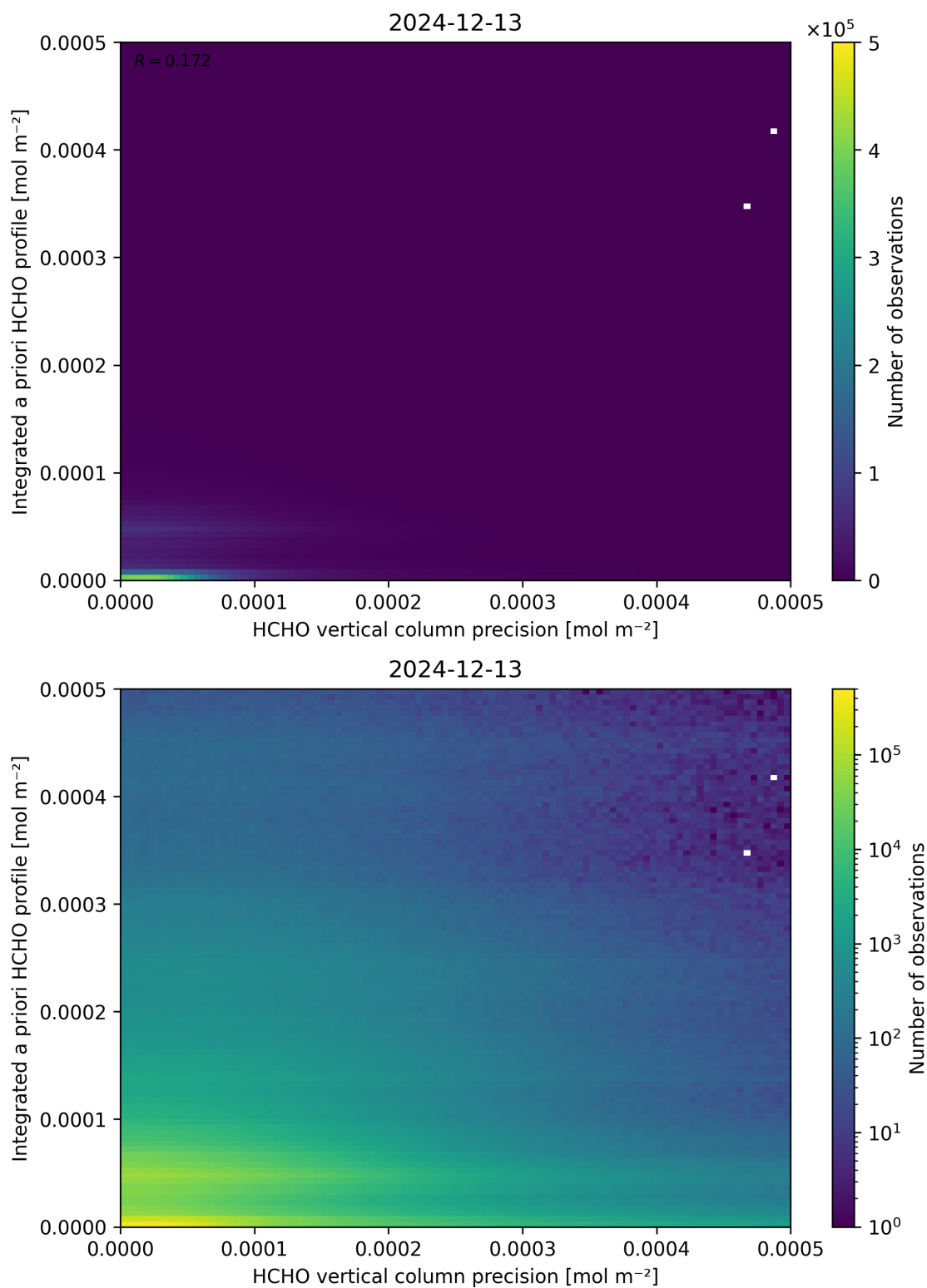
Figure 147: Scatter density plot of “HCHO vertical column precision” against “Integrated a priori HCHO profile” for 2024-12-12 to 2024-12-14.
