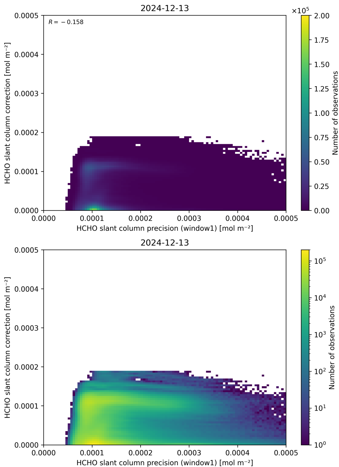
Figure 93: Scatter density plot of “HCHO slant column precision (window1)” against “HCHO slant column correction” for 2024-12-12 to 2024-12-14.
