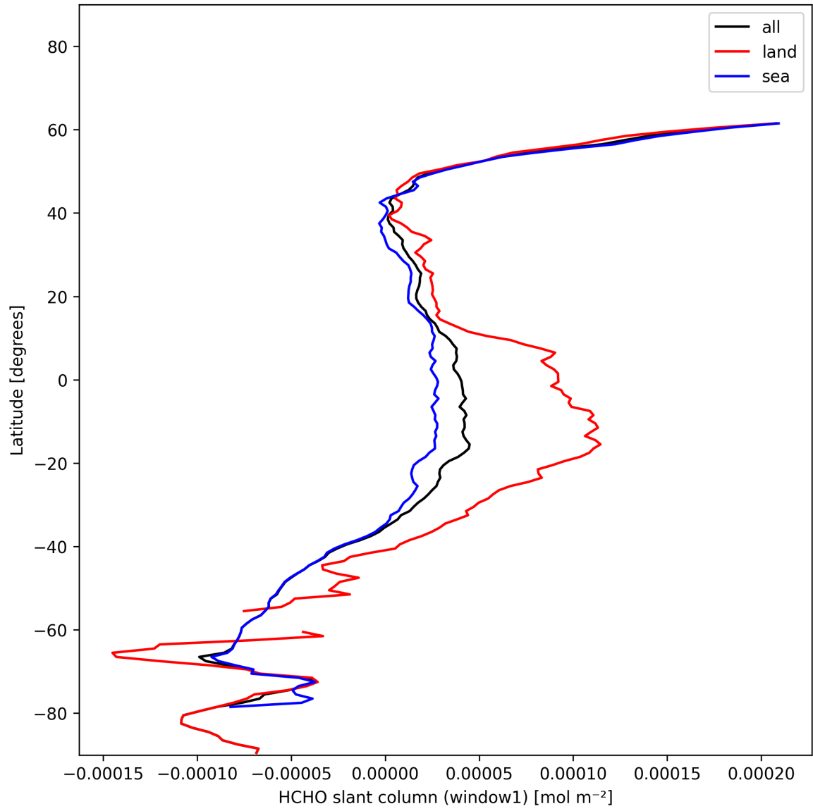
Figure 24: Zonal average of “HCHO slant column (window1)” for 2024-12-12 to 2024-12-14.
