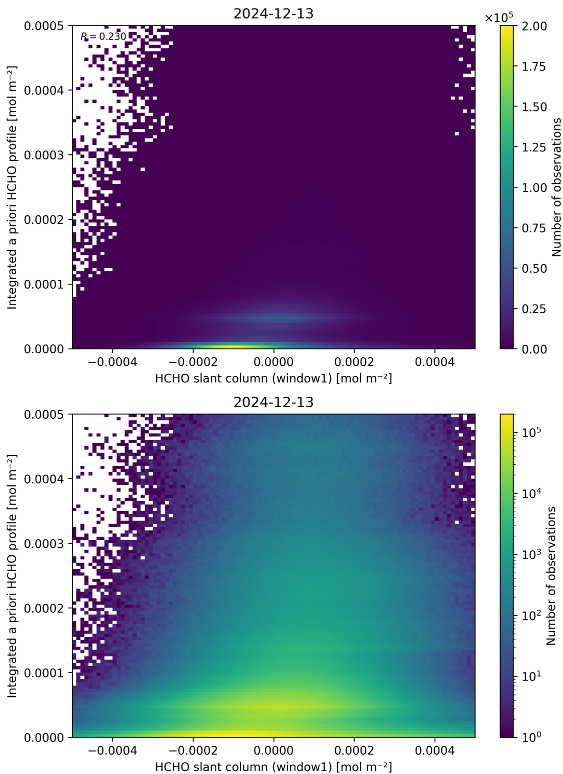
Figure 87: Scatter density plot of “HCHO slant column (window1)” against “Integrated a priori HCHO profile” for 2024-12-12 to 2024-12-14.
