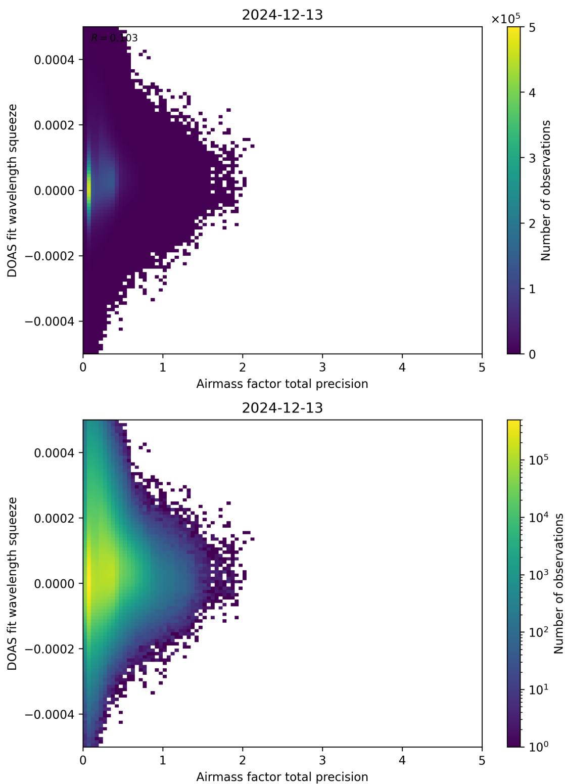
Figure 107: Scatter density plot of “Airmass factor total precision” against “DOAS fit wavelength squeeze” for 2024-12-12 to 2024-12-14.
