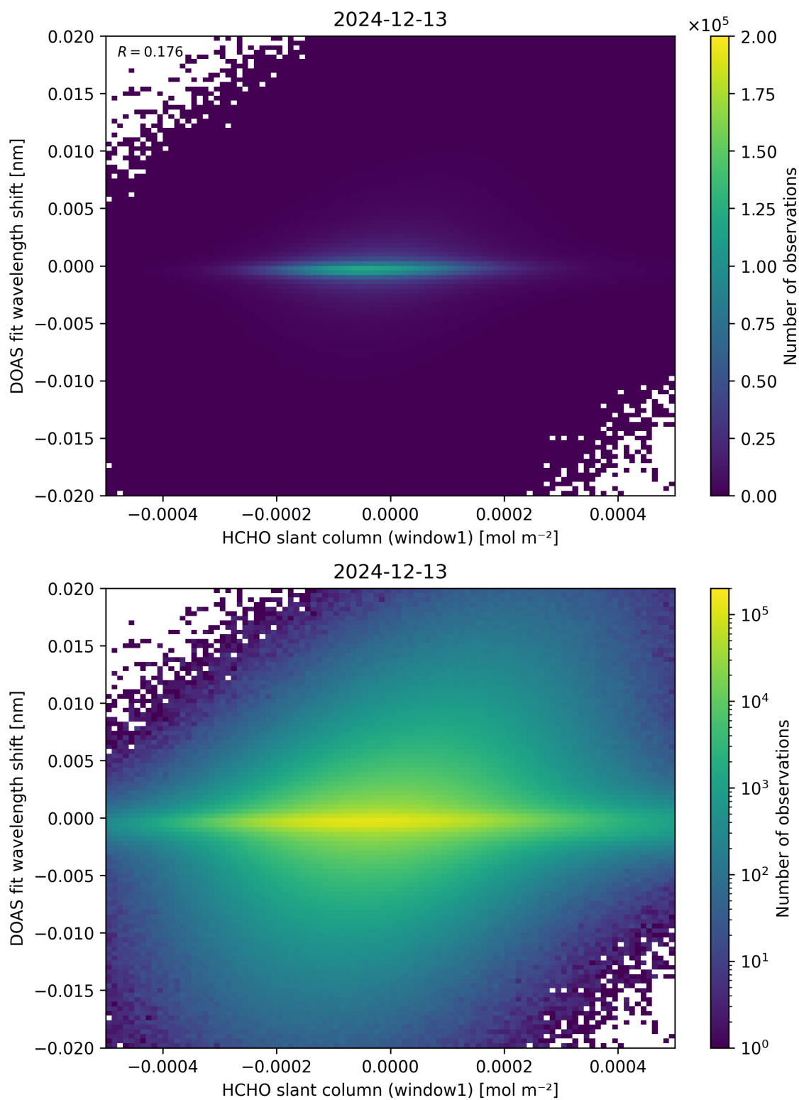
Figure 79: Scatter density plot of “HCHO slant column (window1)” against “DOAS fit wavelength shift” for 2024-12-12 to 2024-12-14.
