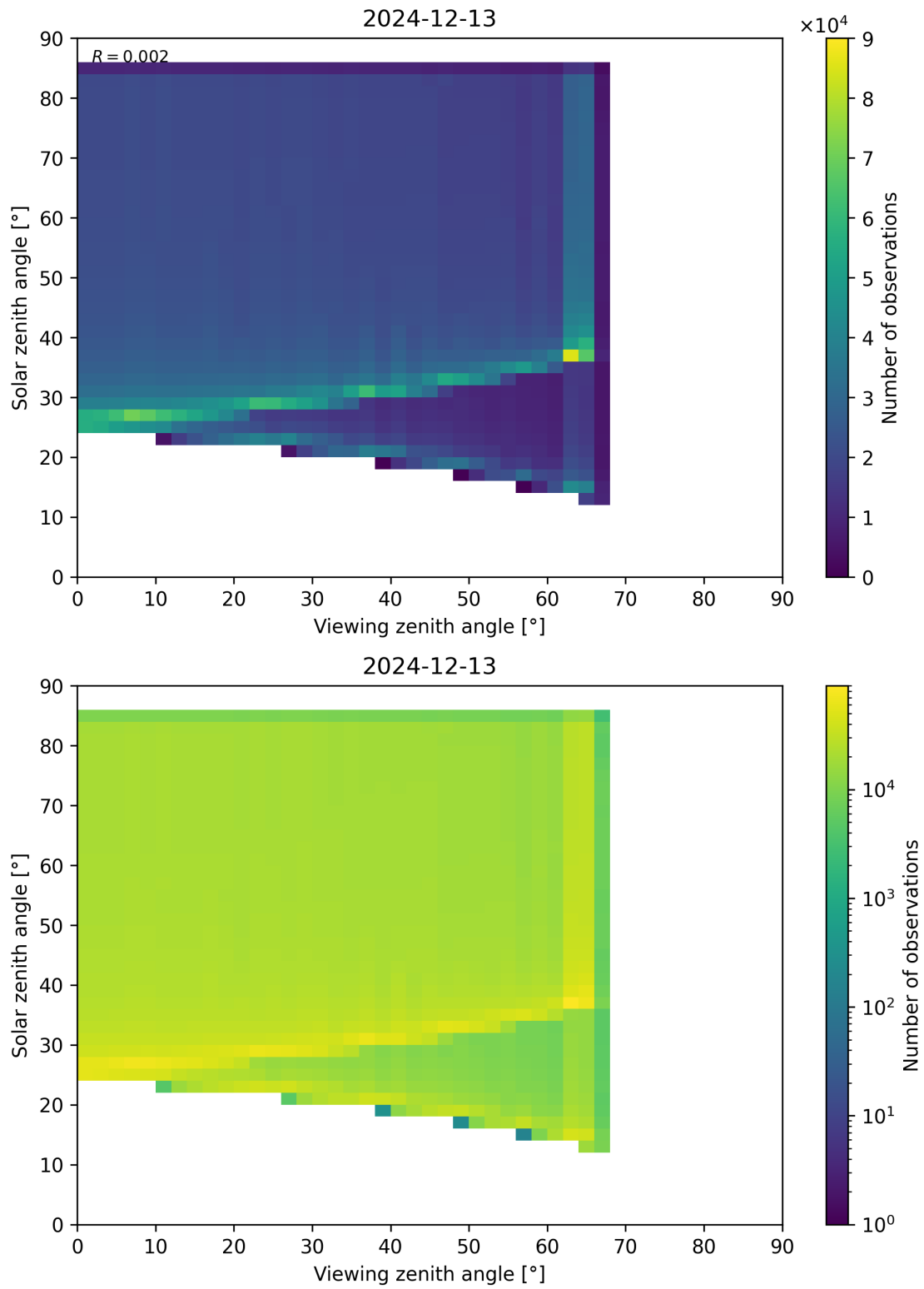
Figure 197: Scatter density plot of “Viewing zenith angle” against “Solar zenith angle” for 2024-12-12 to 2024-12-14.
