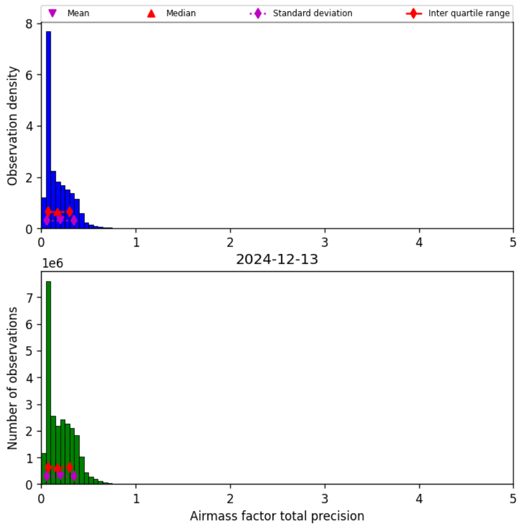
Figure 41: Histogram of “Airmass factor total precision” for 2024-12-12 to 2024-12-14
