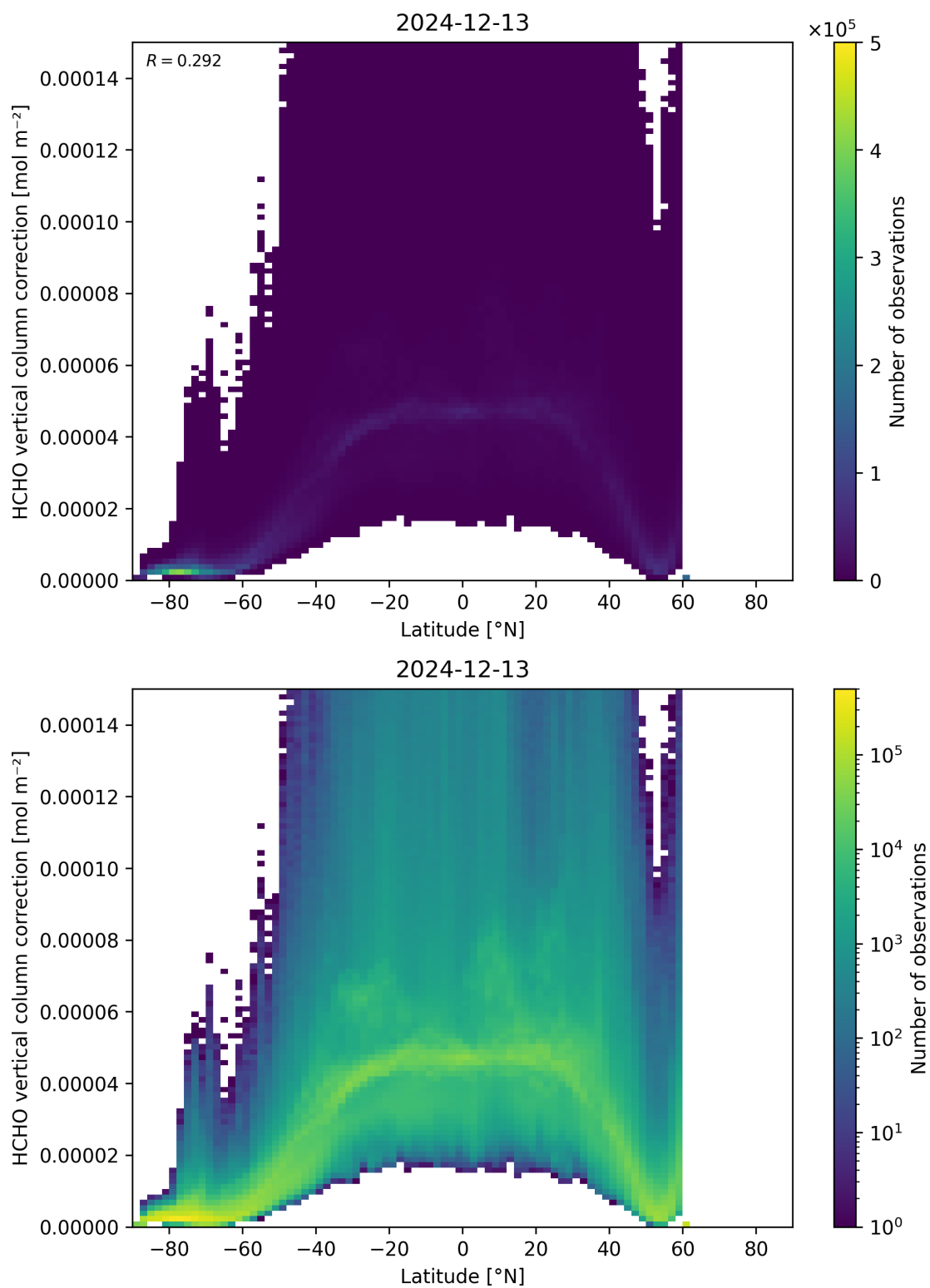
Figure 164: Scatter density plot of “Latitude” against “HCHO vertical column correction” for 2024-12-12 to 2024-12-14.
