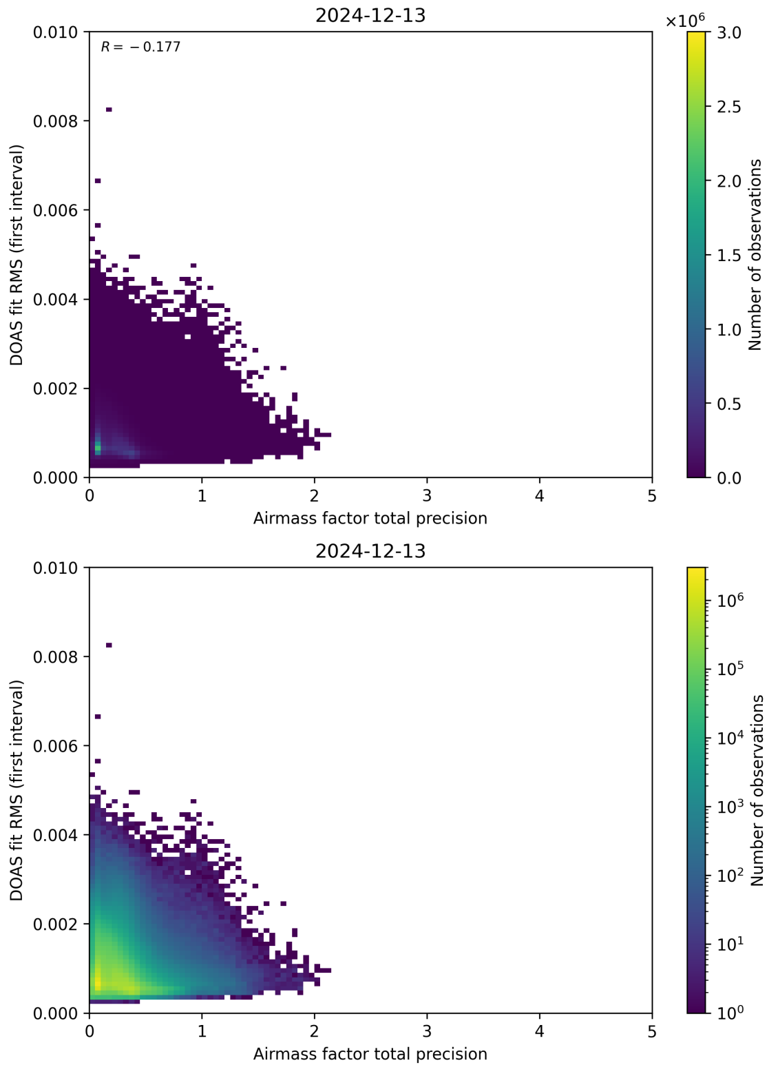
Figure 105: Scatter density plot of “Airmass factor total precision” against “DOAS fit RMS (first interval)” for 2024-12-12 to 2024-12-14.
