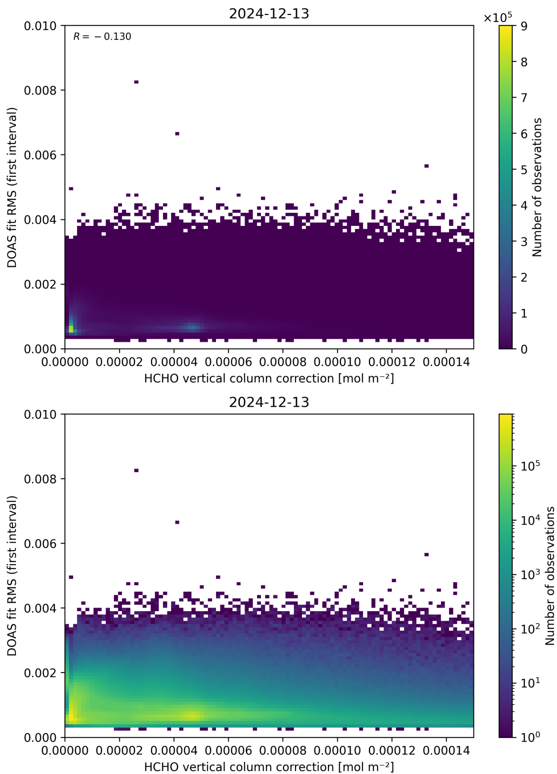
Figure 112: Scatter density plot of “HCHO vertical column correction” against “DOAS fit RMS (first interval)” for 2024-12-12 to 2024-12-14.
