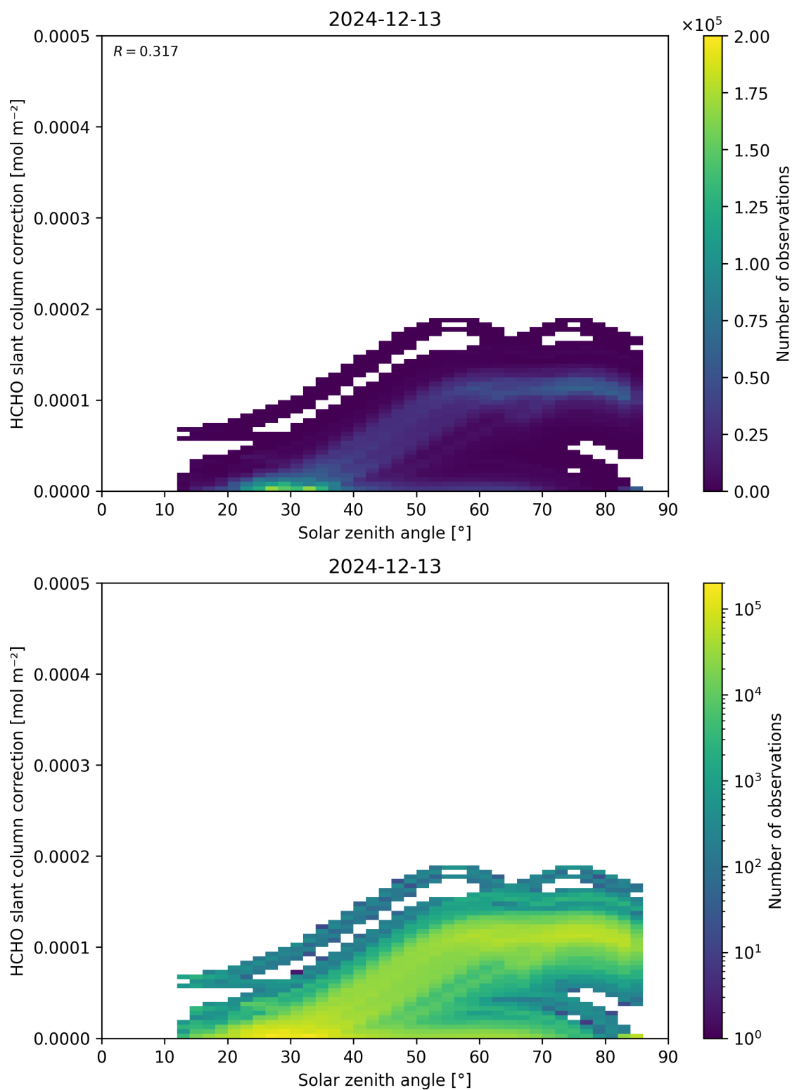
Figure 172: Scatter density plot of “Solar zenith angle” against “HCHO slant column correction” for 2024-12-12 to 2024-12-14.
