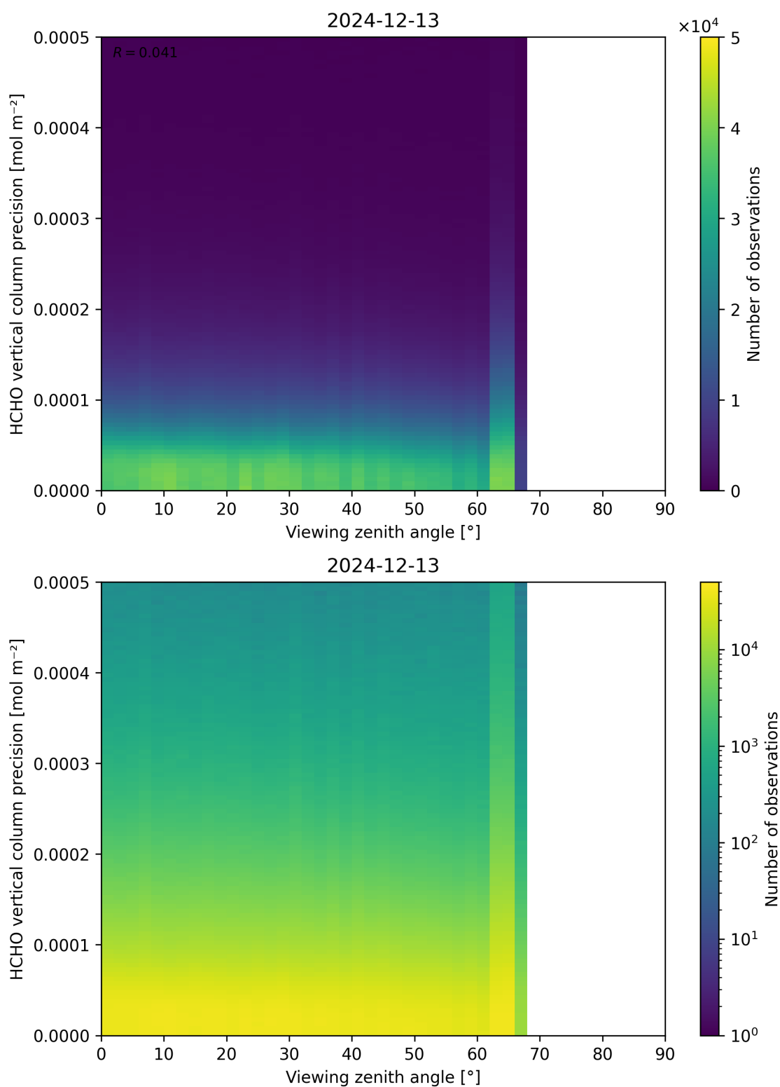
Figure 194: Scatter density plot of “Viewing zenith angle” against “HCHO vertical column precision” for 2024-12-12 to 2024-12-14.
