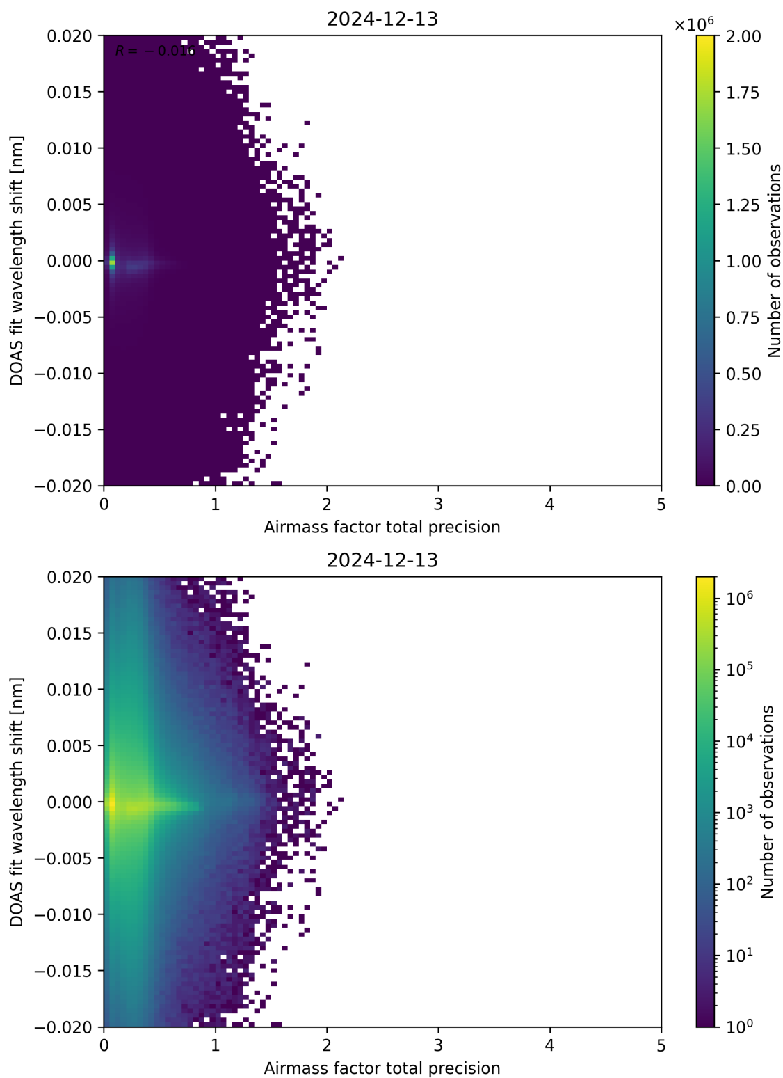
Figure 106: Scatter density plot of “Airmass factor total precision” against “DOAS fit wavelength shift” for 2024-12-12 to 2024-12-14.
