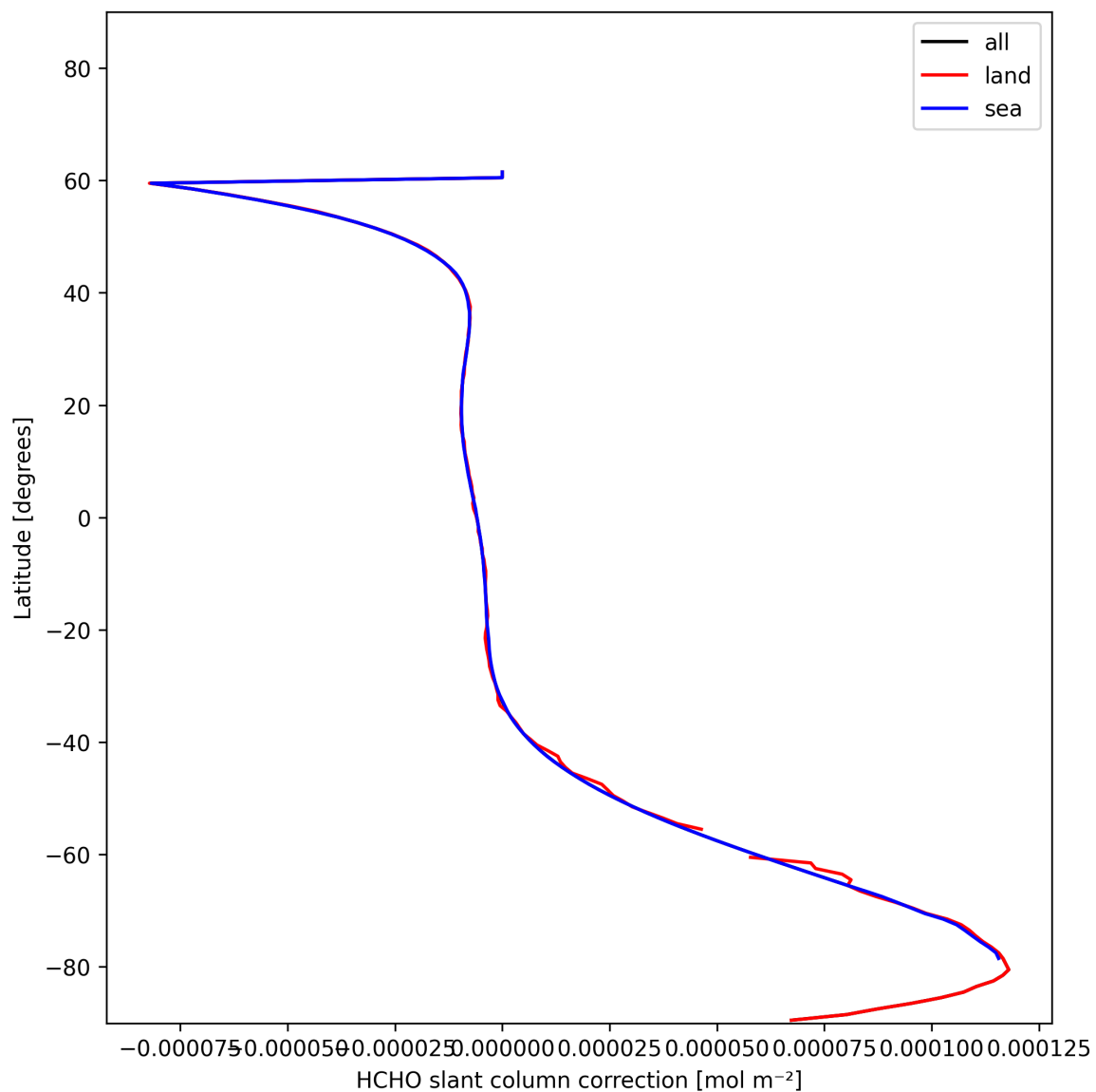
Figure 33: Zonal average of “HCHO slant column correction” for 2024-12-12 to 2024-12-14.
