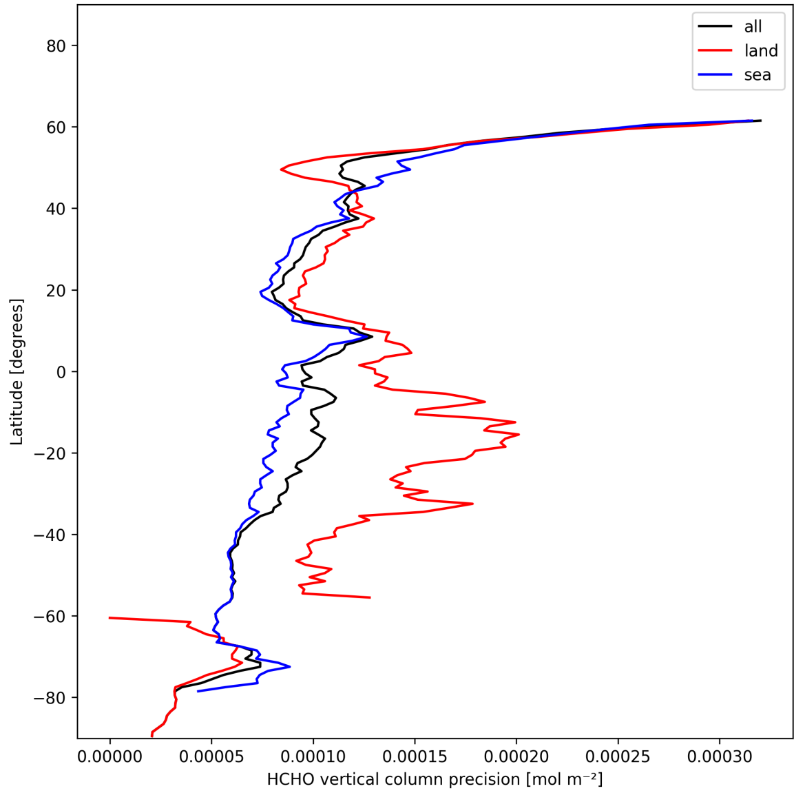
Figure 22: Zonal average of "HCHO vertical column precision" for 2024-12-12 to 2024-12-14.
