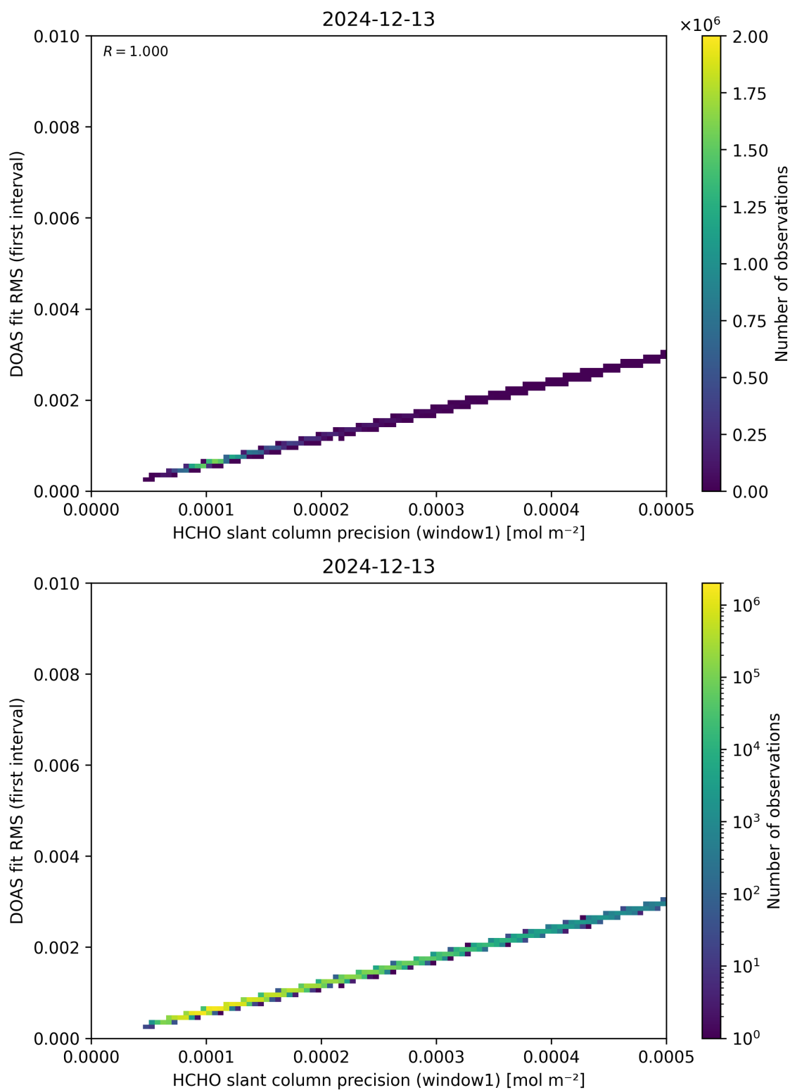
Figure 88: Scatter density plot of “HCHO slant column precision (window1)” against “DOAS fit RMS (first interval)” for 2024-12-12 to 2024-12-14.
