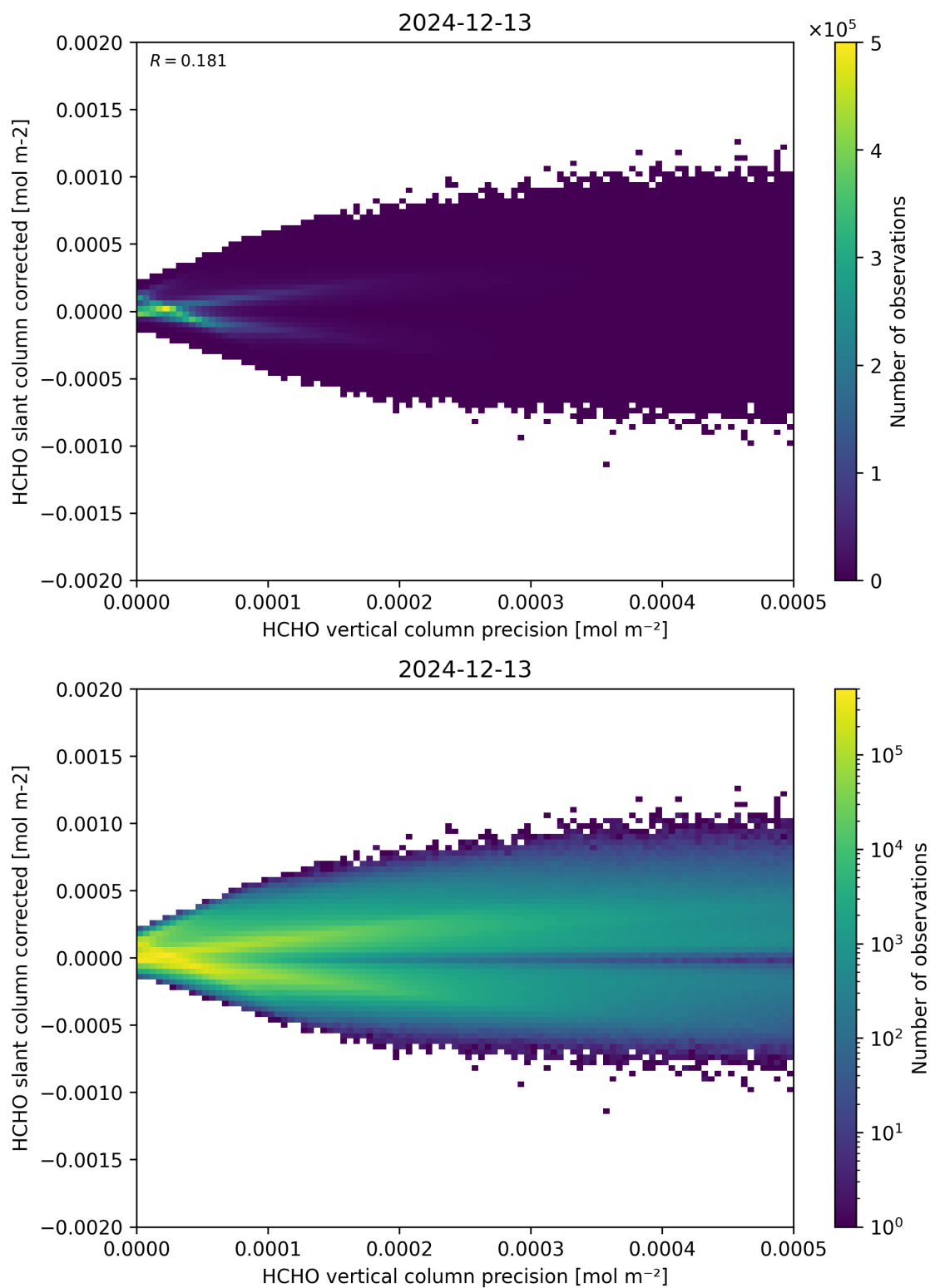
Figure 140: Scatter density plot of “HCHO vertical column precision” against “HCHO slant column corrected” for 2024-12-12 to 2024-12-14.
