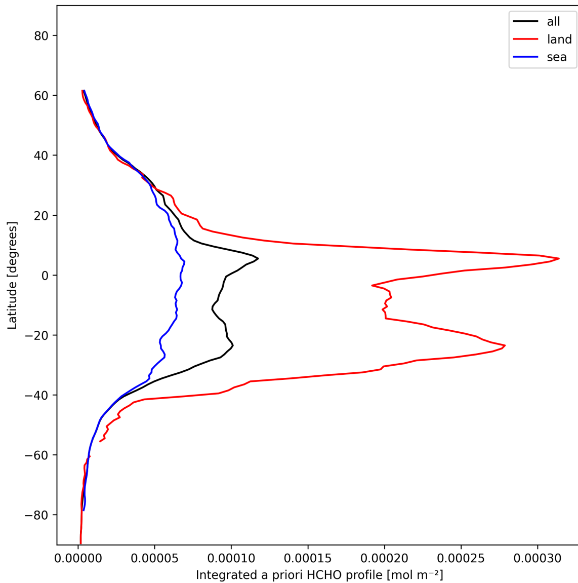
Figure 29: Zonal average of “Integrated a priori HCHO profile” for 2024-12-12 to 2024-12-14.
