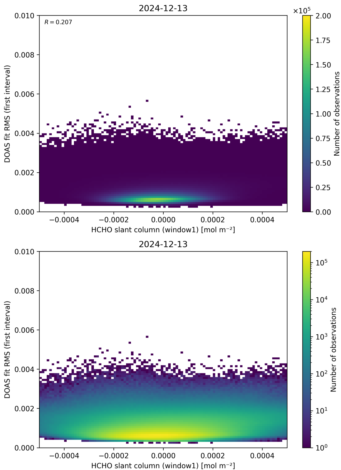
Figure 78: Scatter density plot of “HCHO slant column (window1)” against “DOAS fit RMS (first interval)” for 2024-12-12 to 2024-12-14.
