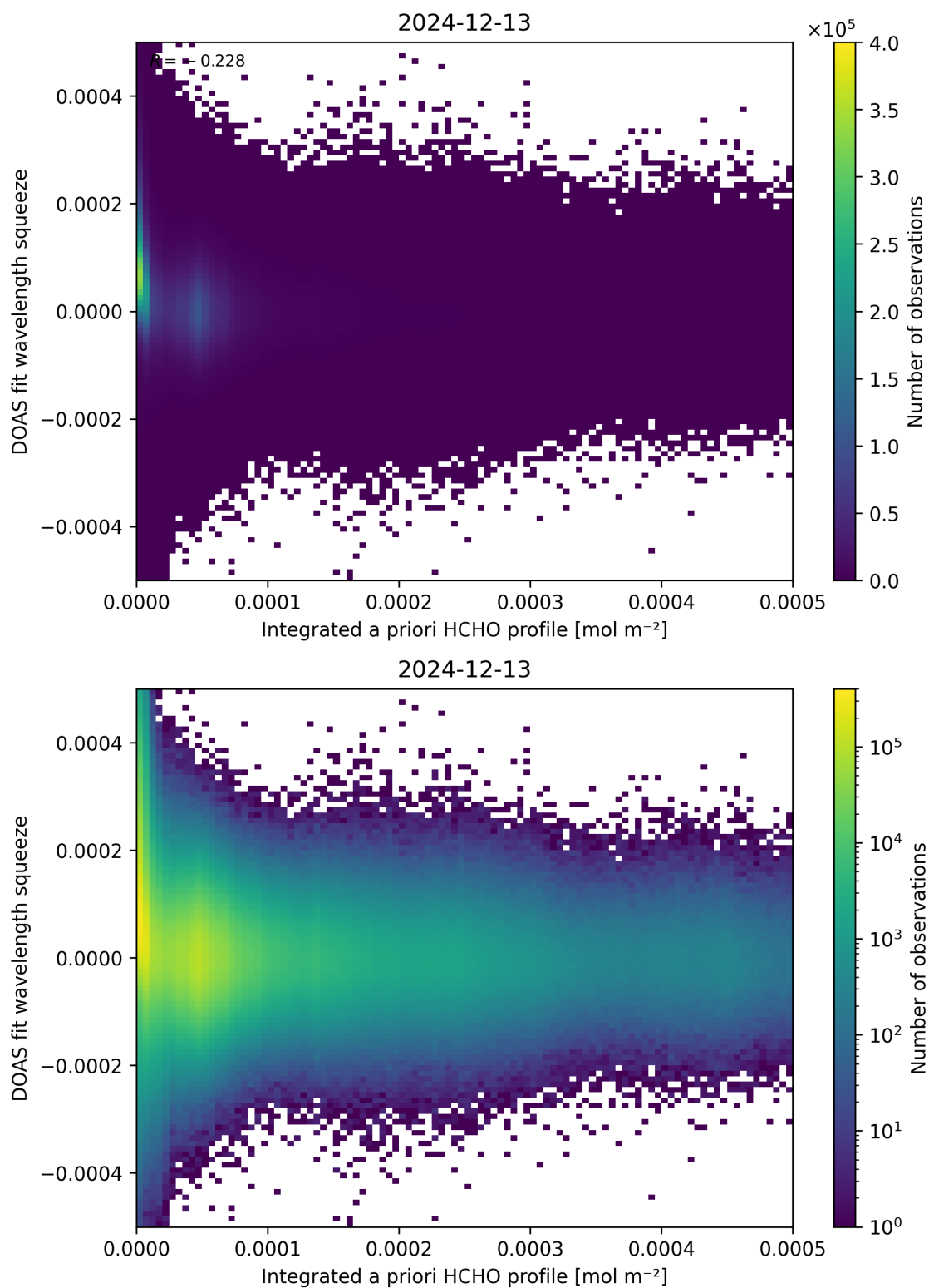
Figure 150: Scatter density plot of “Integrated a priori HCHO profile” against “DOAS fit wavelength squeeze” for 2024-12-12 to 2024-12-14.
