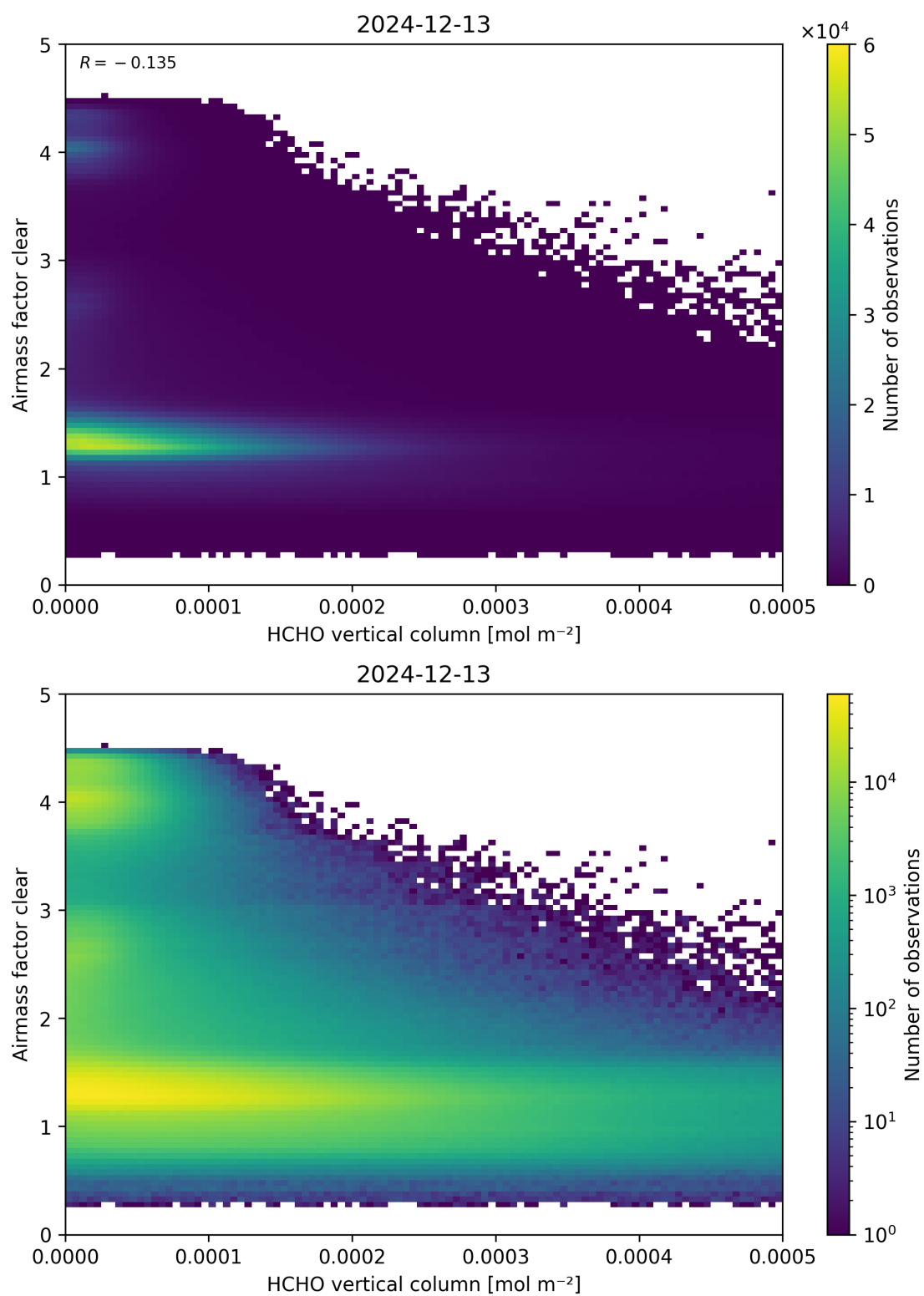
Figure 126: Scatter density plot of “HCHO vertical column” against “Airmass factor clear” for 2024-12-12 to 2024-12-14.
