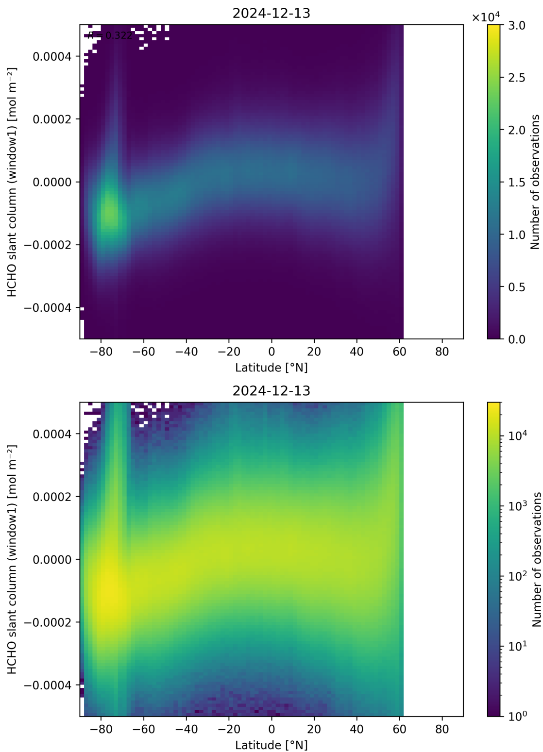
Figure 159: Scatter density plot of “Latitude” against “HCHO slant column (window1)” for 2024-12-12 to 2024-12-14.
