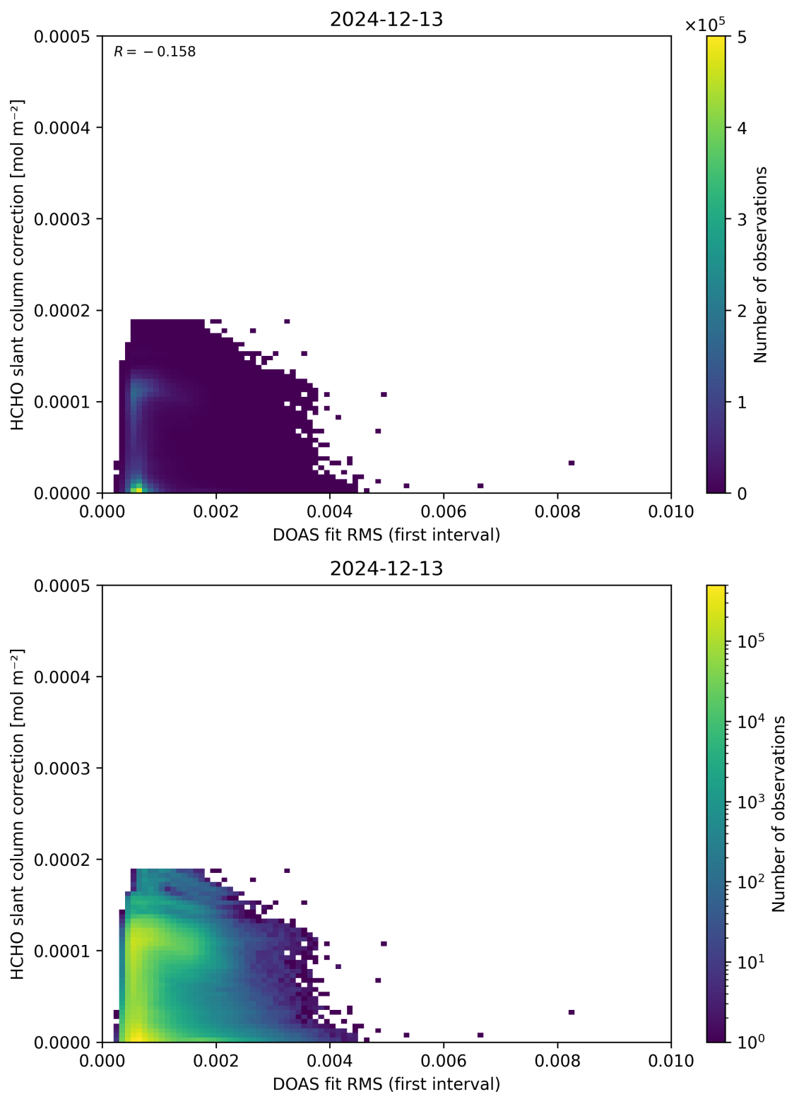
Figure 63: Scatter density plot of “DOAS fit RMS (first interval)” against “HCHO slant column correction” for 2024-12-12 to 2024-12-14.
