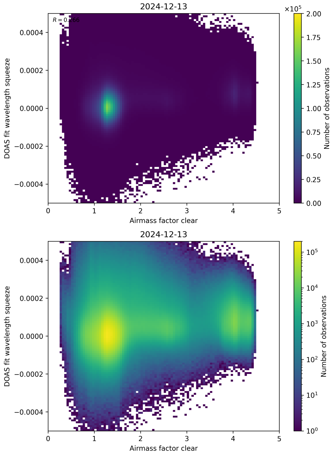
Figure 73: Scatter density plot of “Airmass factor clear” against “DOAS fit wavelength squeeze” for 2024-12-12 to 2024-12-14.
