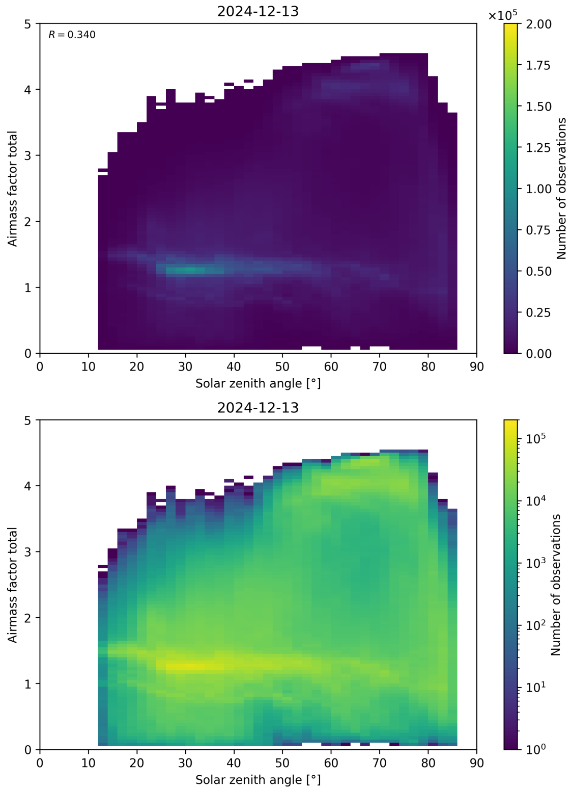
Figure 175: Scatter density plot of “Solar zenith angle” against “Airmass factor total” for 2024-12-12 to 2024-12-14.
