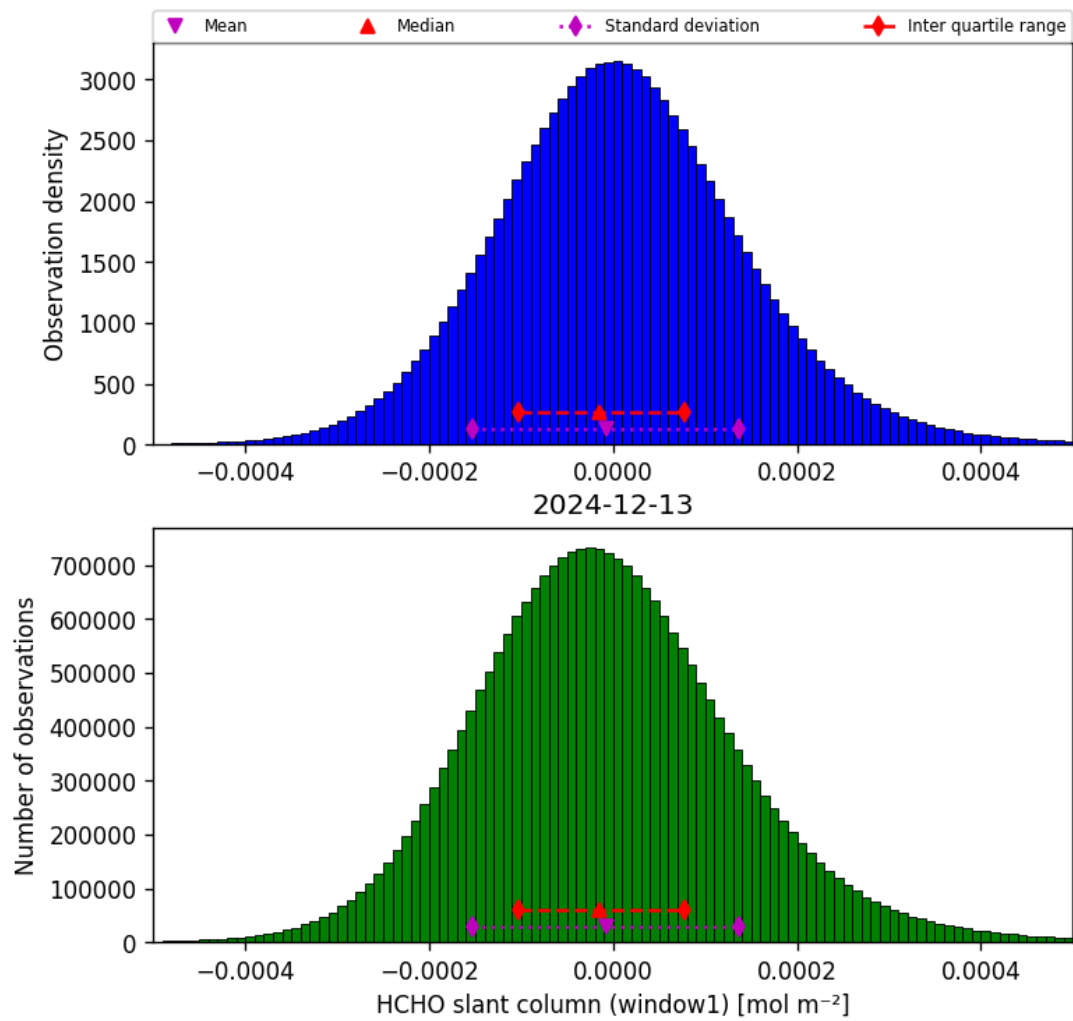
Figure 38: Histogram of “HCHO slant column (window1)” for 2024-12-12 to 2024-12-14
