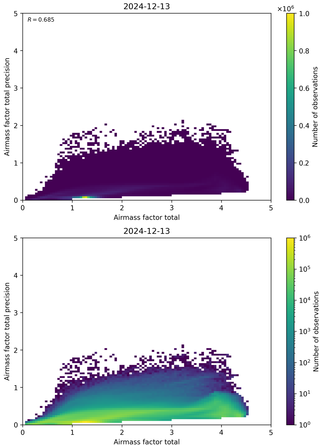
Figure 103: Scatter density plot of “Airmass factor total” against “Airmass factor total precision” for 2024-12-12 to 2024-12-14.
