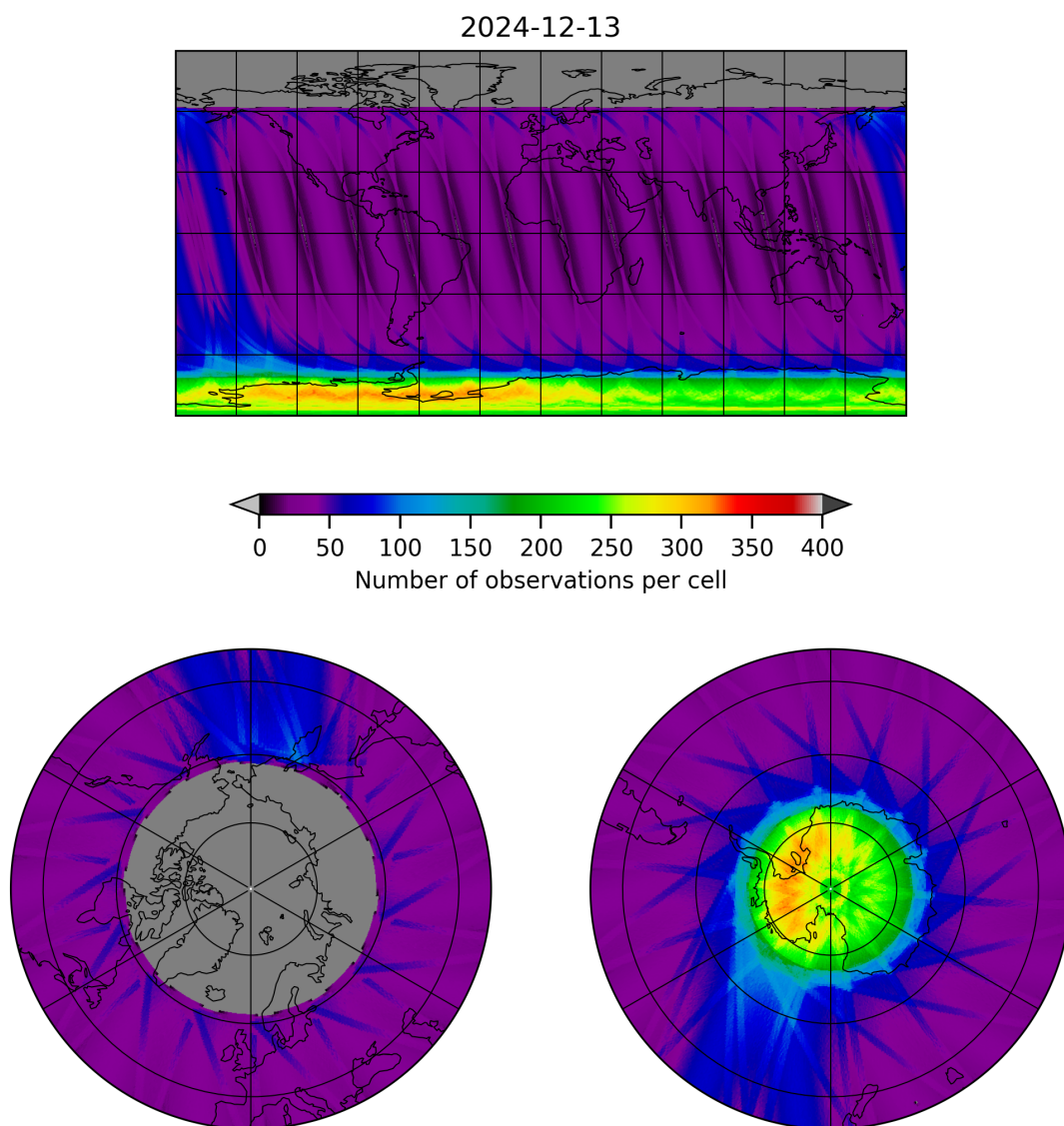
Figure 19: Map of the number of observations for 2024-12-12 to 2024-12-14
