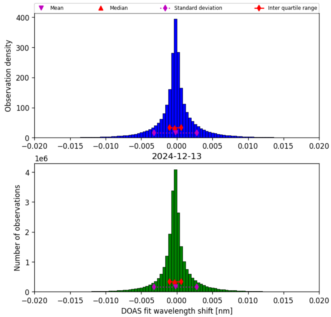
Figure 44: Histogram of “DOAS fit wavelength shift” for 2024-12-12 to 2024-12-14
