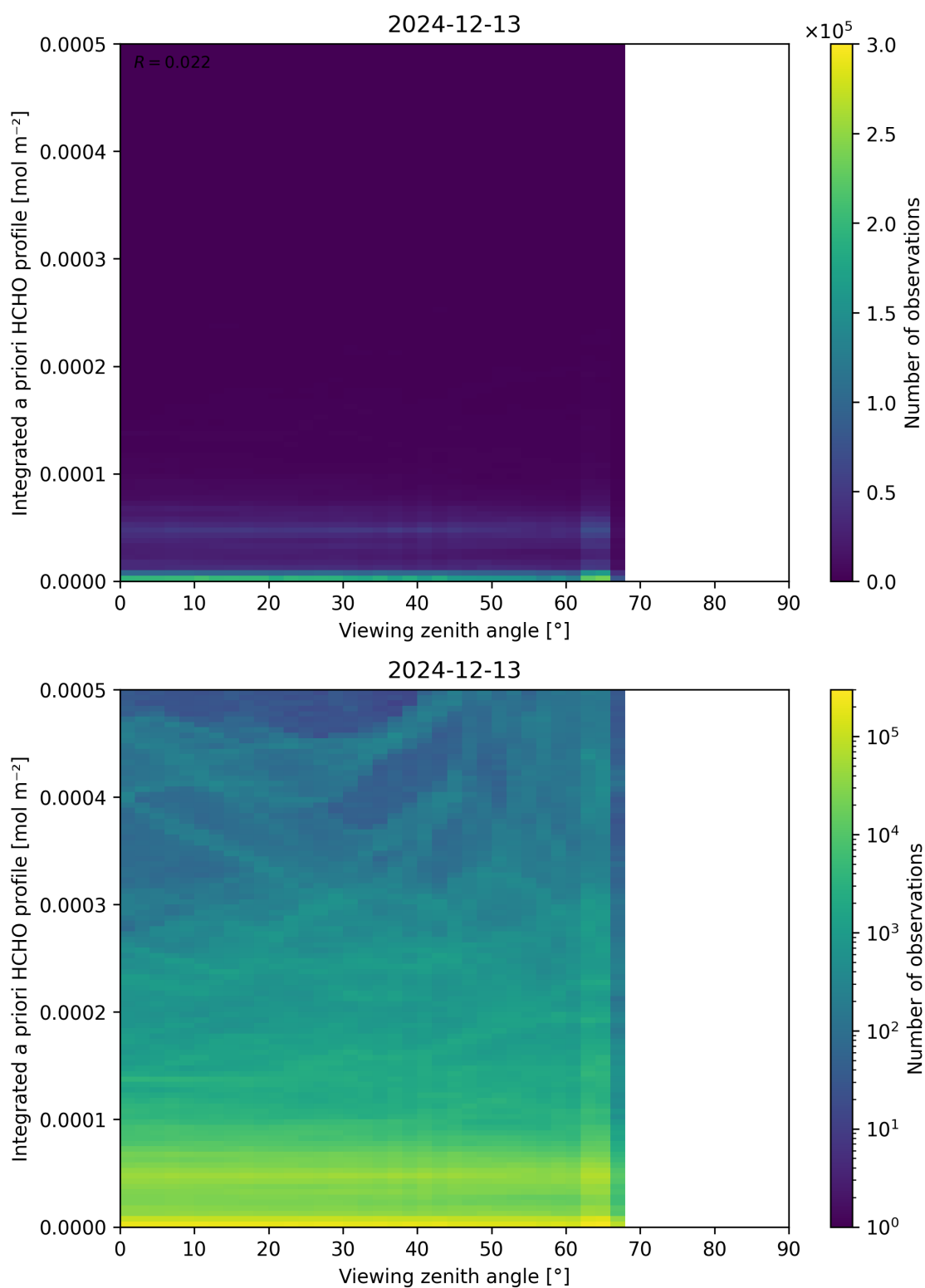
Figure 195: Scatter density plot of “Viewing zenith angle” against “Integrated a priori HCHO profile” for 2024-12-12 to 2024-12-14.
