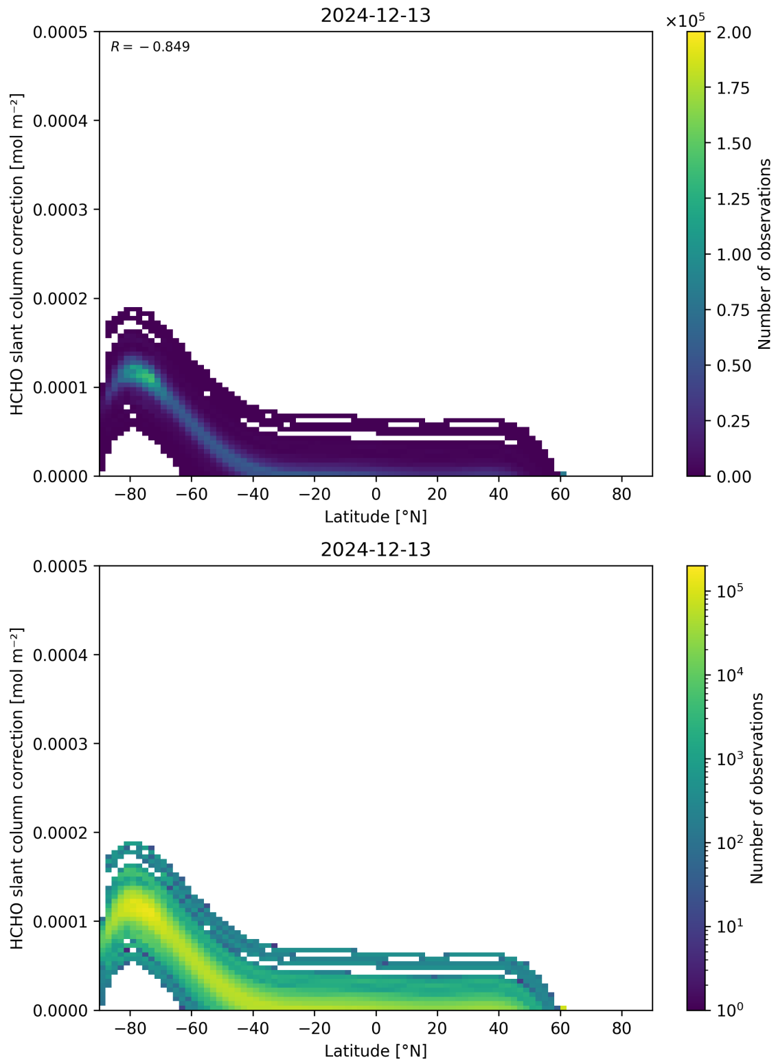
Figure 158: Scatter density plot of “Latitude” against “HCHO slant column correction” for 2024-12-12 to 2024-12-14.
