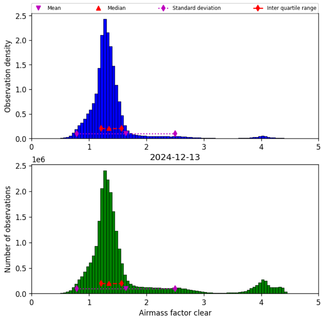
Figure 42: Histogram of “Airmass factor clear” for 2024-12-12 to 2024-12-14
