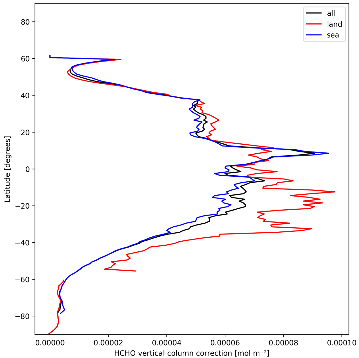
Figure 23: Zonal average of “HCHO vertical column correction” for 2024-12-12 to 2024-12-14.
