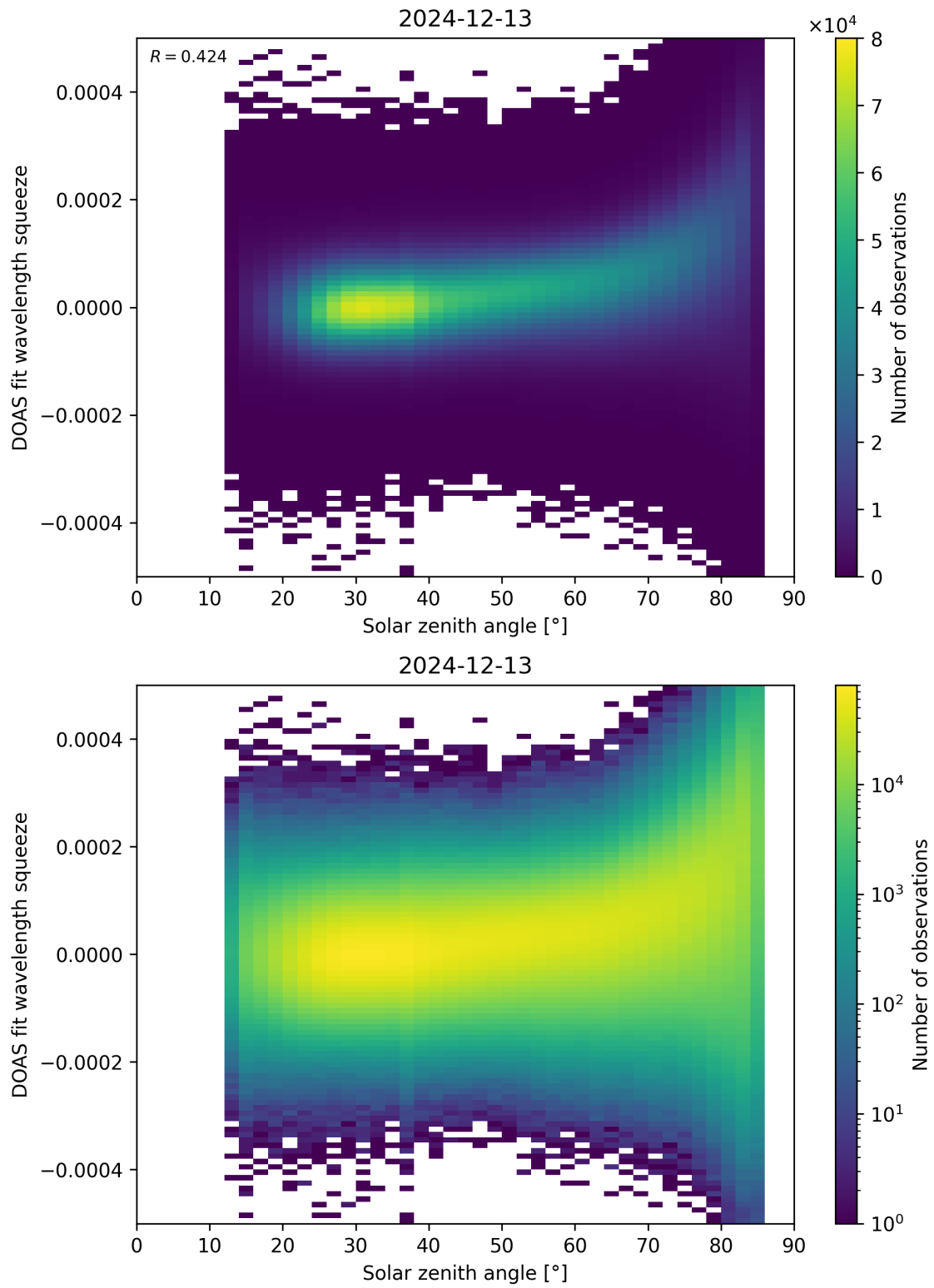
Figure 169: Scatter density plot of “Solar zenith angle” against “DOAS fit wavelength squeeze” for 2024-12-12 to 2024-12-14.
