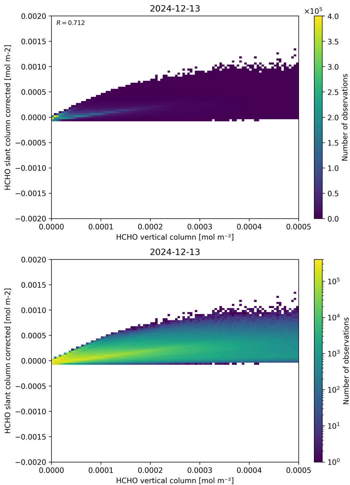
Figure 127: Scatter density plot of “HCHO vertical column” against “HCHO slant column corrected” for 2024-12-12 to 2024-12-14.
