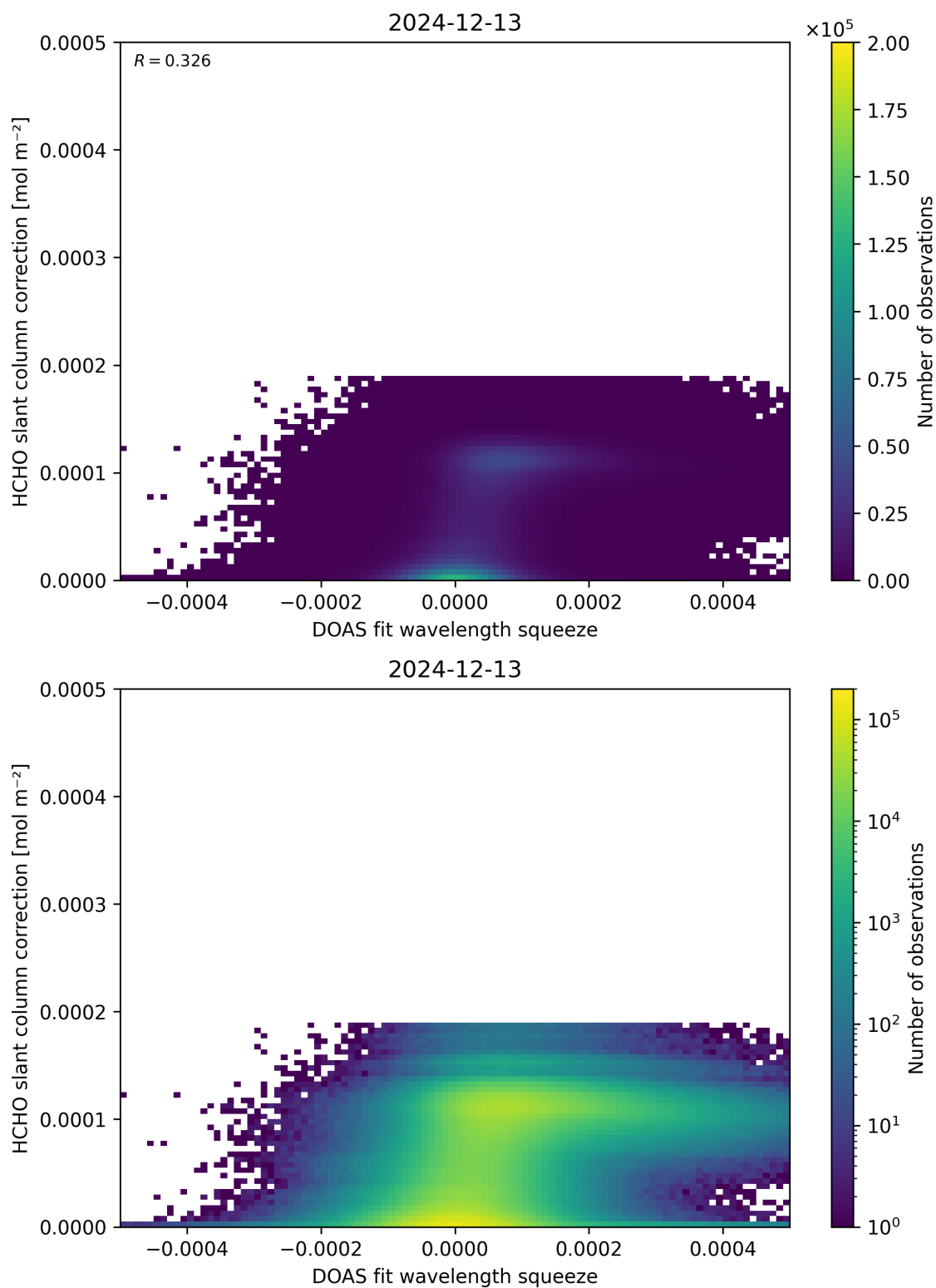
Figure 70: Scatter density plot of “DOAS fit wavelength squeeze” against “HCHO slant column correction” for 2024-12-12 to 2024-12-14.
