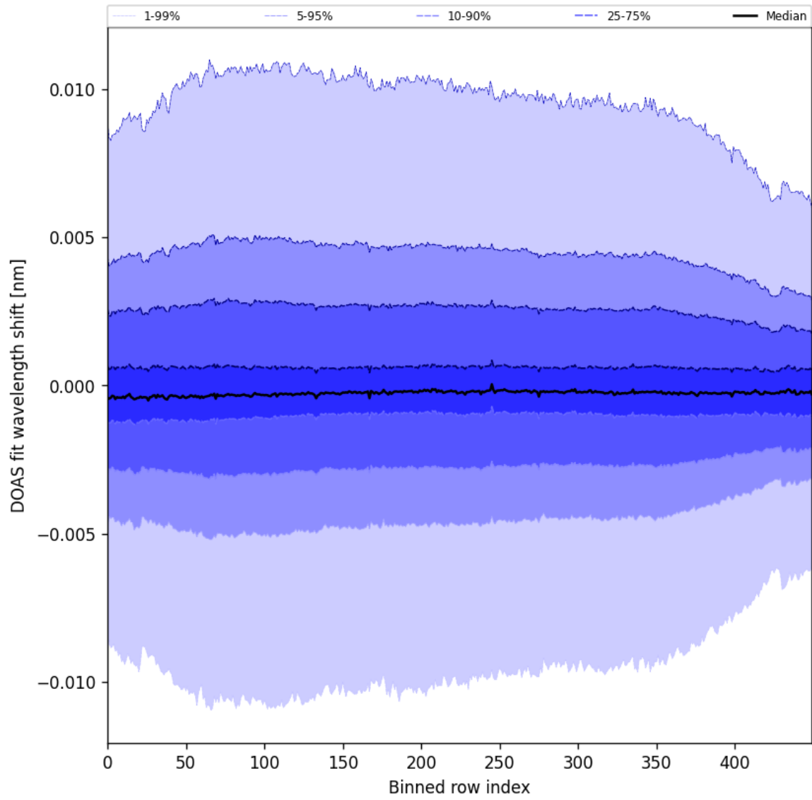
Figure 58: Along track statistics of “DOAS fit wavelength shift” for 2024-12-12 to 2024-12-14
