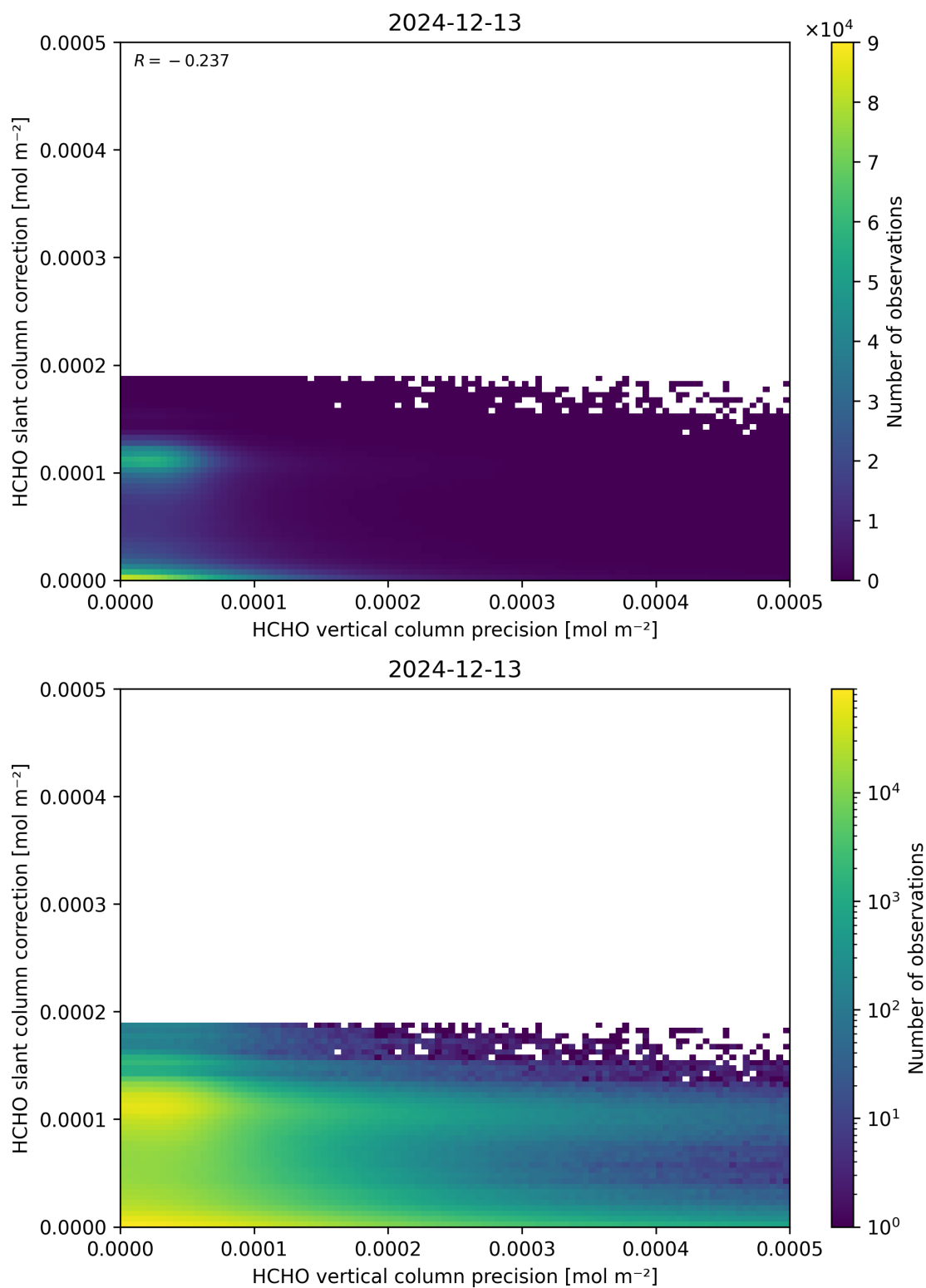
Figure 141: Scatter density plot of “HCHO vertical column precision” against “HCHO slant column correction” for 2024-12-12 to 2024-12-14.
