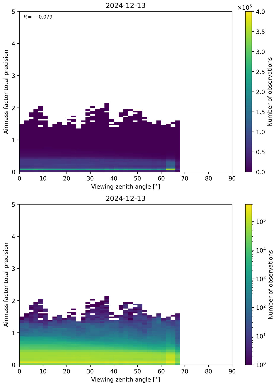
Figure 191: Scatter density plot of “Viewing zenith angle” against “Airmass factor total precision” for 2024-12-12 to 2024-12-14.
