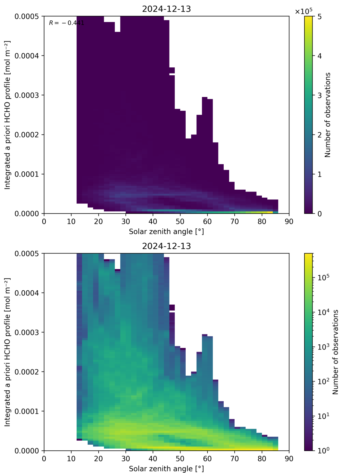
Figure 180: Scatter density plot of “Solar zenith angle” against “Integrated a priori HCHO profile” for 2024-12-12 to 2024-12-14.
