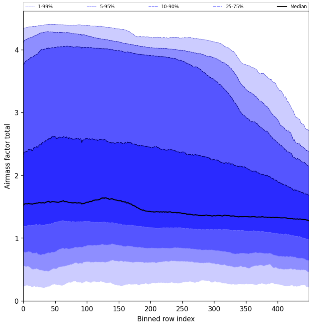
Figure 54: Along track statistics of “Airmass factor total” for 2024-12-12 to 2024-12-14
