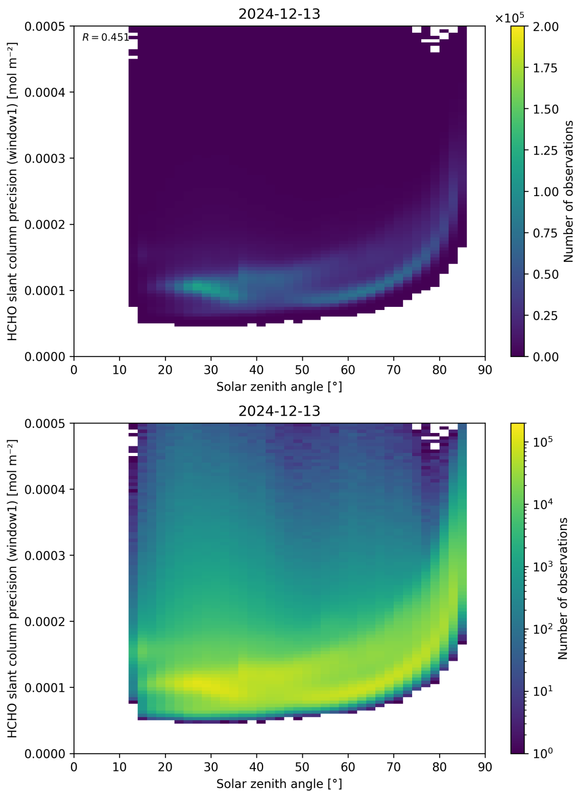
Figure 174: Scatter density plot of “Solar zenith angle” against “HCHO slant column precision (window1)” for 2024-12-12 to 2024-12-14.
