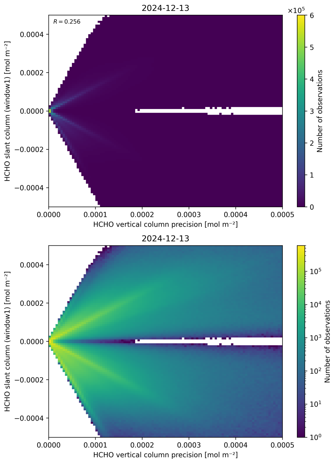
Figure 142: Scatter density plot of “HCHO vertical column precision” against “HCHO slant column (window1)” for 2024-12-12 to 2024-12-14.
