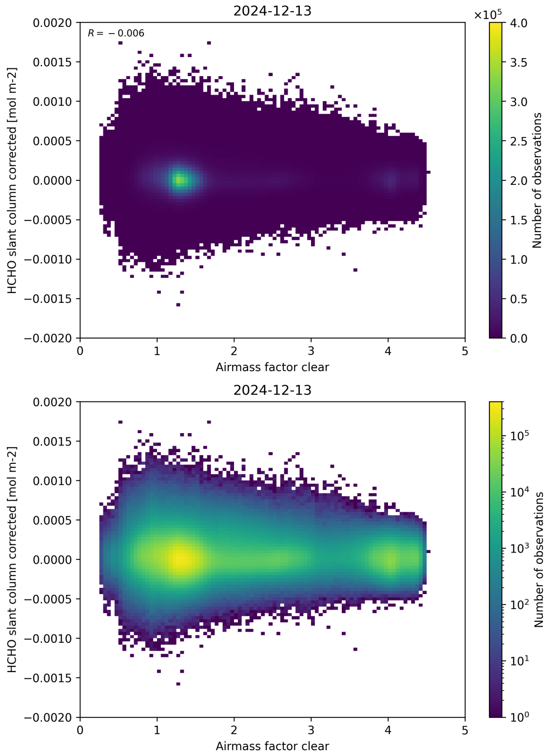
Figure 74: Scatter density plot of “Airmass factor clear” against “HCHO slant column corrected” for 2024-12-12 to 2024-12-14.
