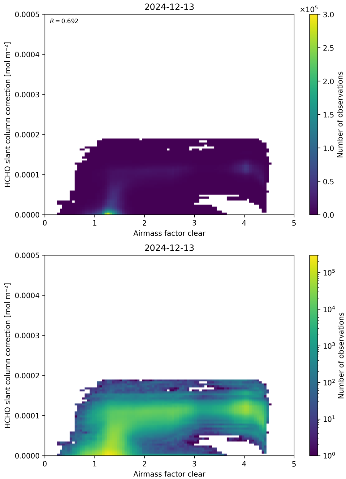
Figure 75: Scatter density plot of “Airmass factor clear” against “HCHO slant column correction” for 2024-12-12 to 2024-12-14.
