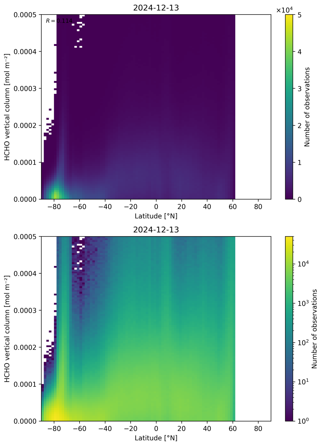
Figure 163: Scatter density plot of “Latitude” against “HCHO vertical column” for 2024-12-12 to 2024-12-14.
