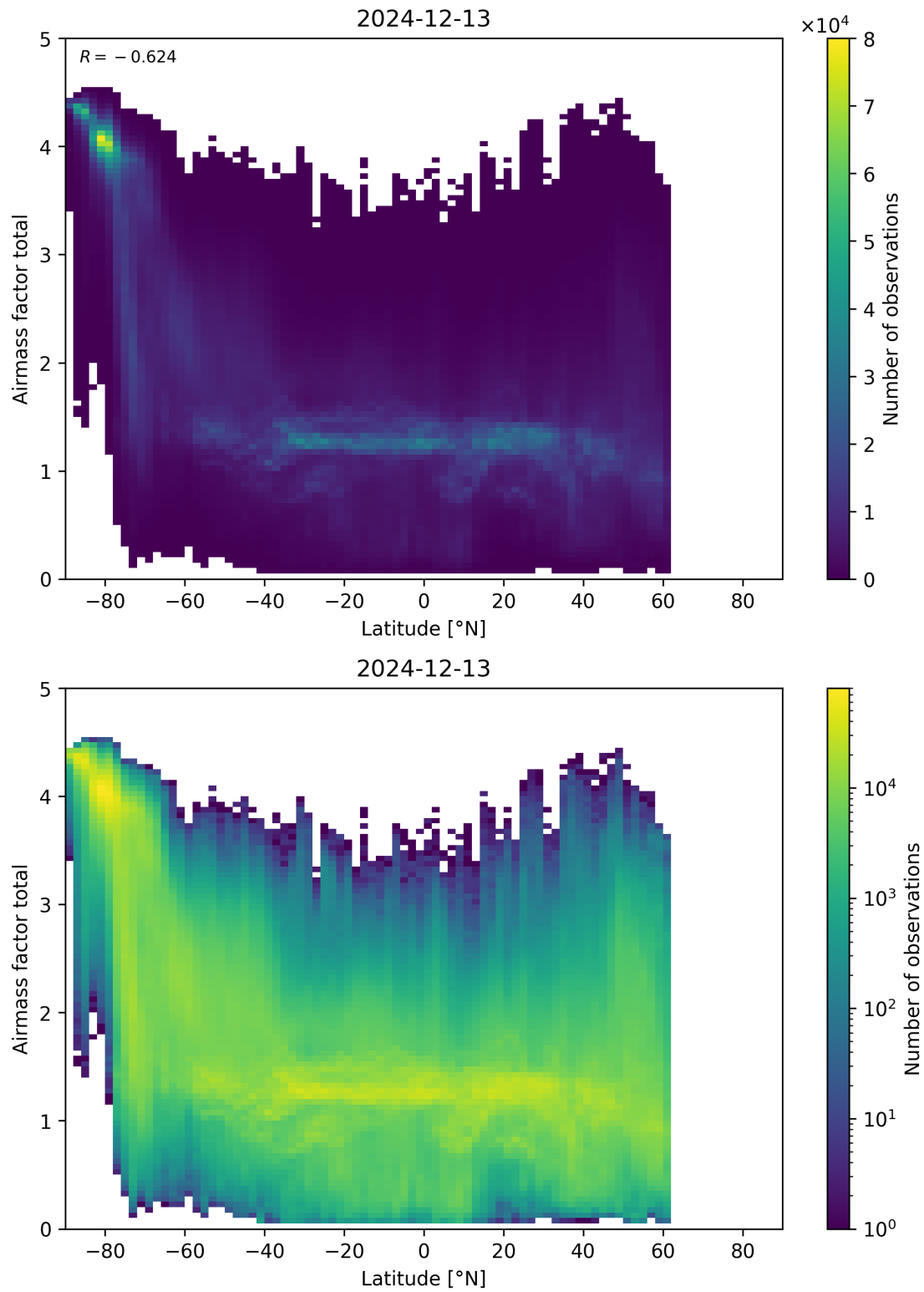
Figure 161: Scatter density plot of “Latitude” against “Airmass factor total” for 2024-12-12 to 2024-12-14.
