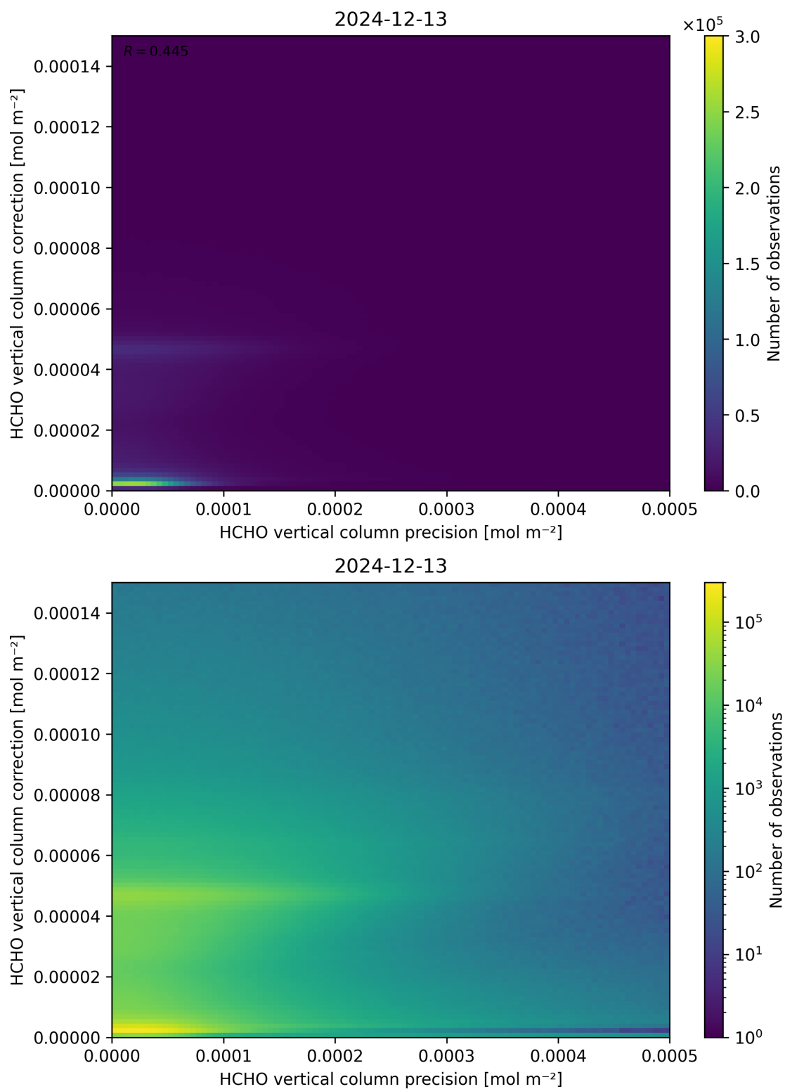
Figure 146: Scatter density plot of “HCHO vertical column precision” against “HCHO vertical column correction” for 2024-12-12 to 2024-12-14.
