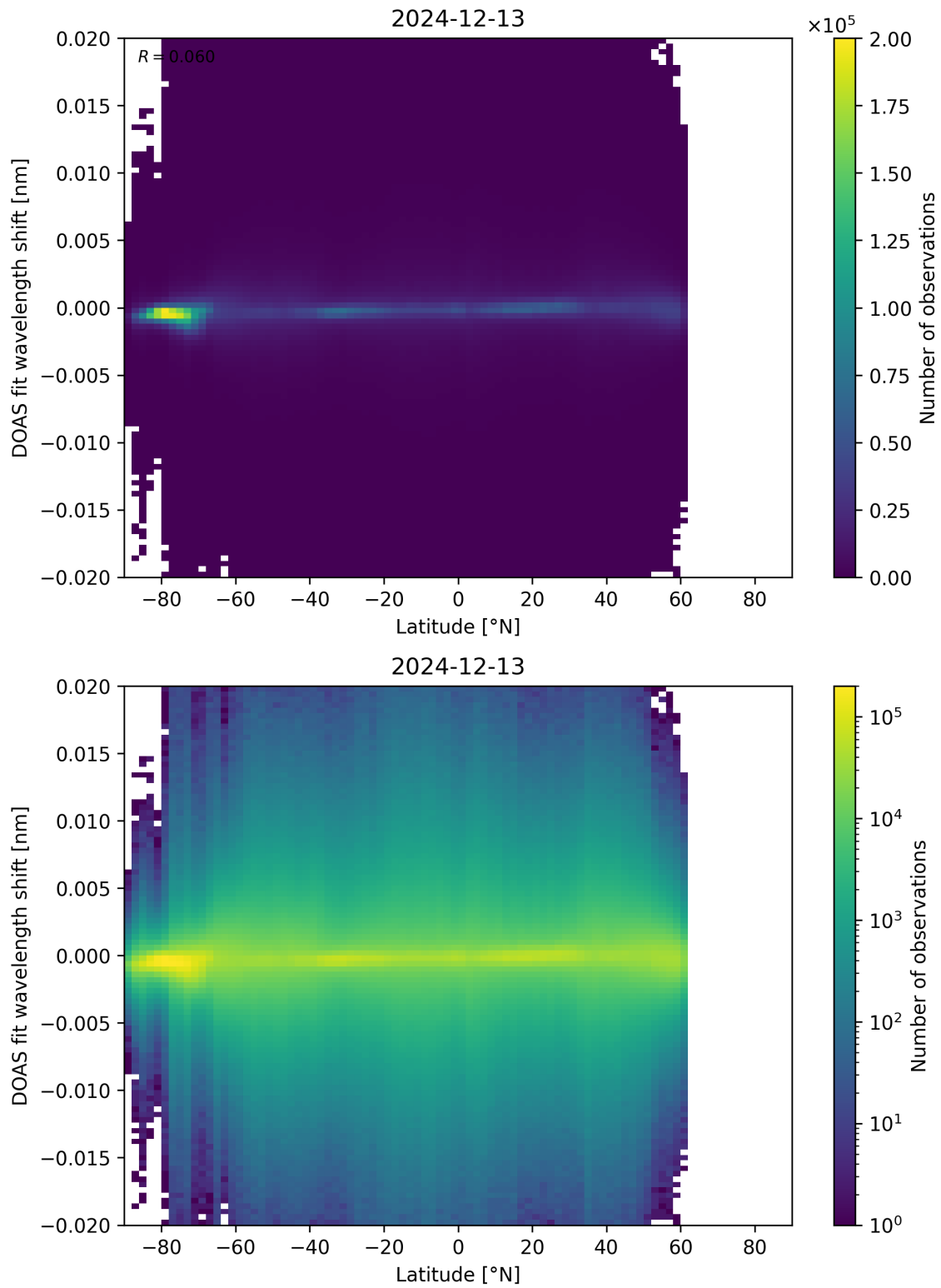
Figure 154: Scatter density plot of “Latitude” against “DOAS fit wavelength shift” for 2024-12-12 to 2024-12-14.
