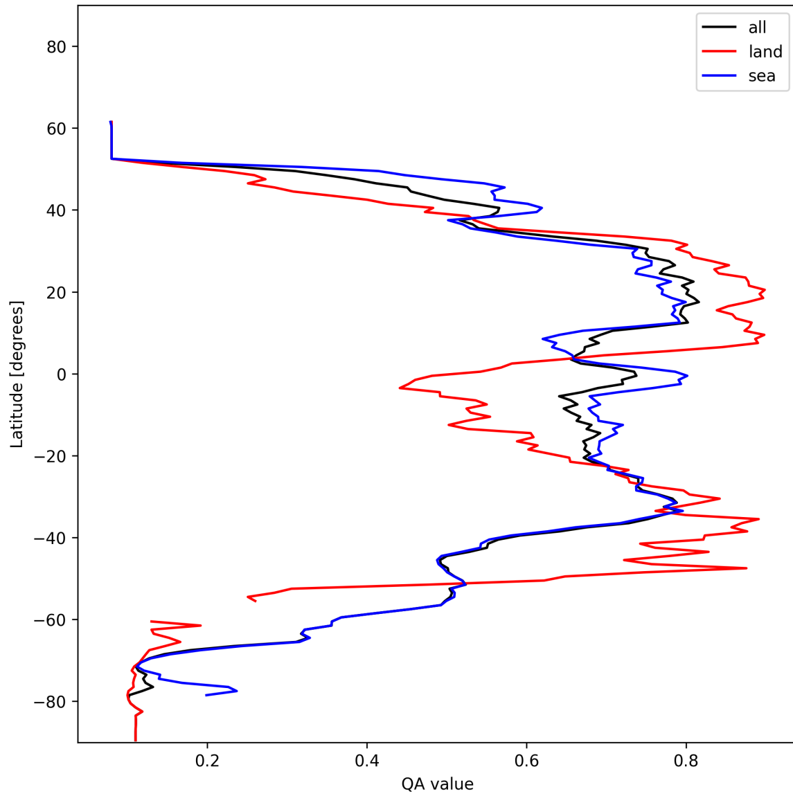
Figure 20: Zonal average of “QA value” for 2024-12-12 to 2024-12-14.
