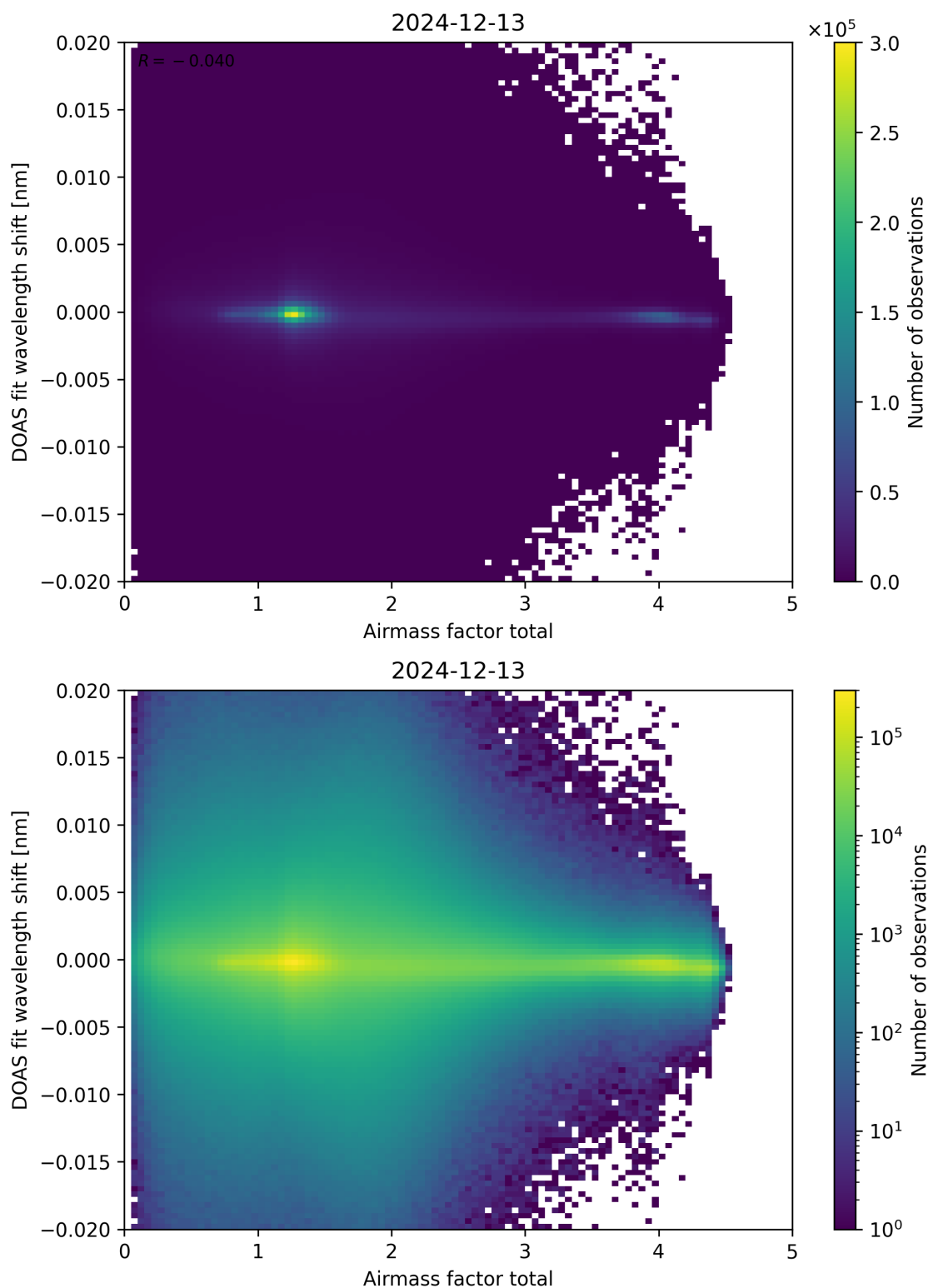
Figure 98: Scatter density plot of “Airmass factor total” against “DOAS fit wavelength shift” for 2024-12-12 to 2024-12-14.
