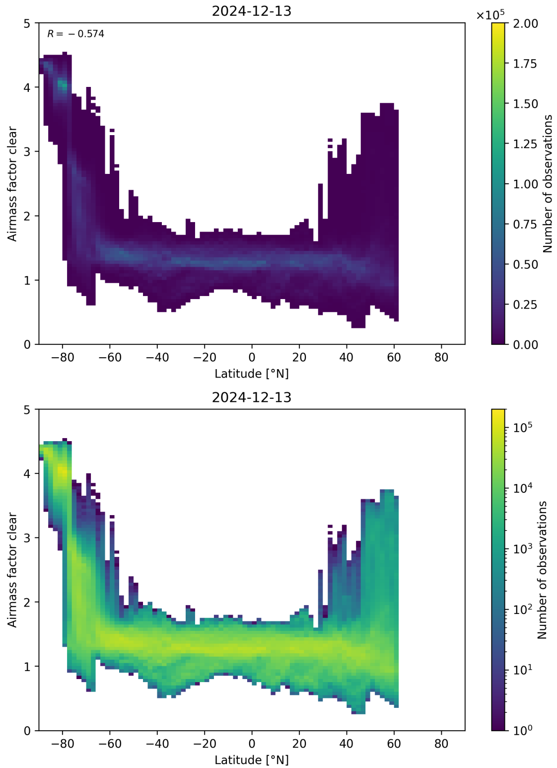
Figure 156: Scatter density plot of “Latitude” against “Airmass factor clear” for 2024-12-12 to 2024-12-14.
