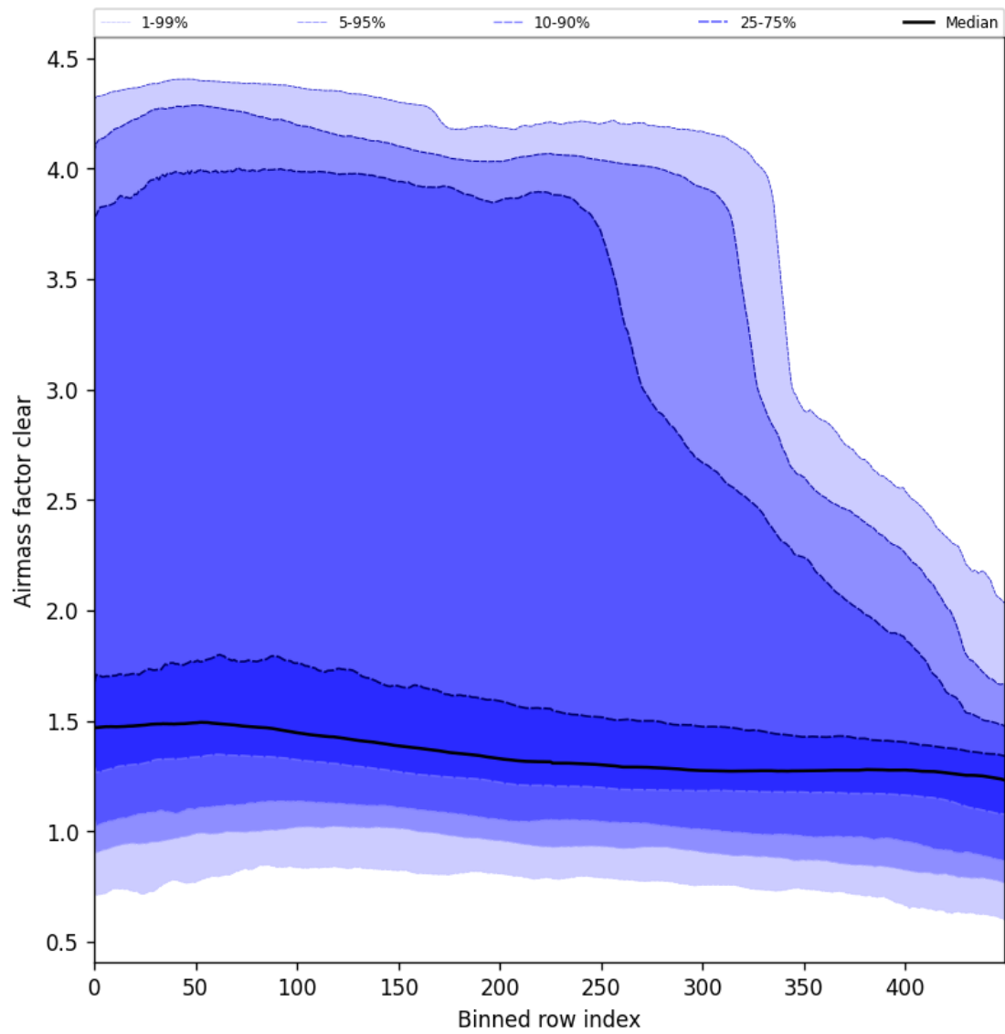
Figure 56: Along track statistics of “Airmass factor clear” for 2024-12-12 to 2024-12-14
