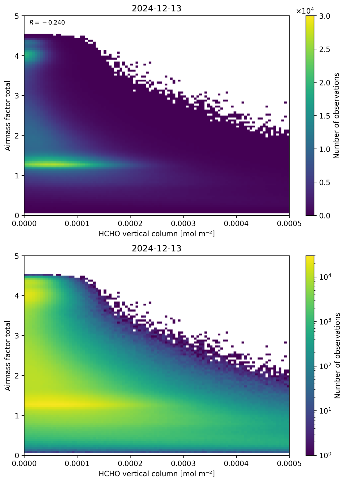
Figure 131: Scatter density plot of “HCHO vertical column” against “Airmass factor total” for 2024-12-12 to 2024-12-14.
