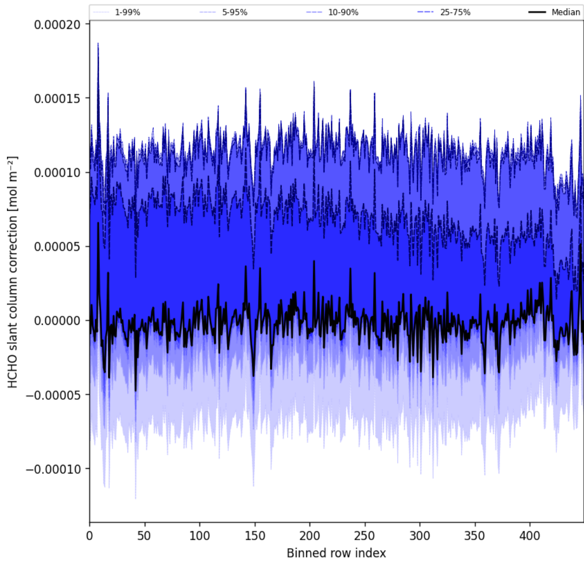
Figure 61: Along track statistics of “HCHO slant column correction” for 2024-12-12 to 2024-12-14
