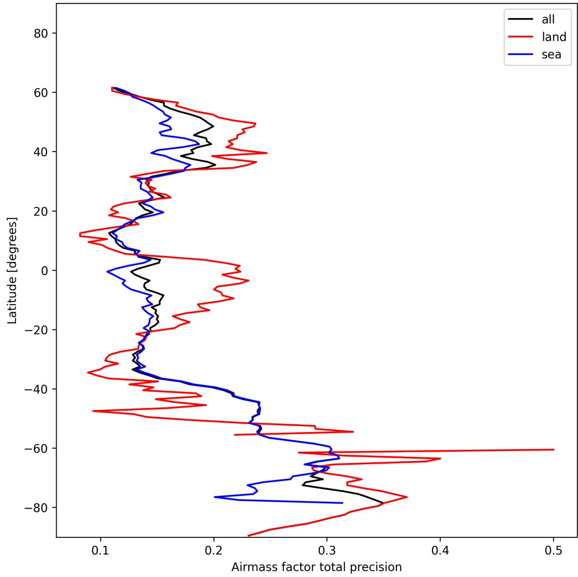
Figure 27: Zonal average of “Airmass factor total precision” for 2024-12-12 to 2024-12-14.
