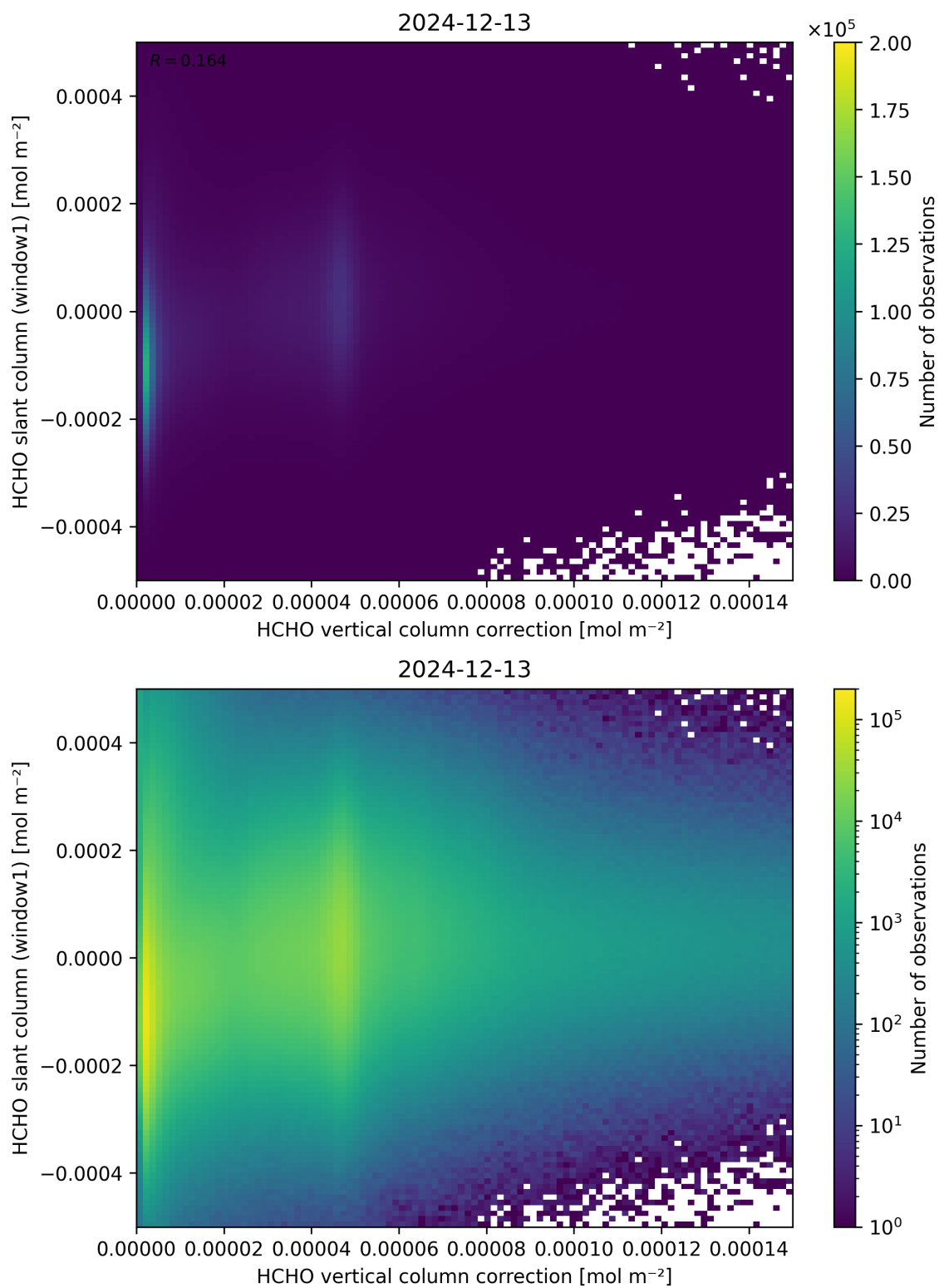
Figure 118: Scatter density plot of “HCHO vertical column correction” against “HCHO slant column (window1)” for 2024-12-12 to 2024-12-14.
