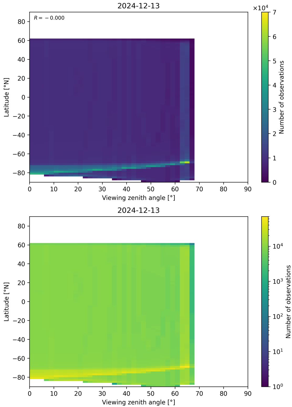
Figure 196: Scatter density plot of “Viewing zenith angle” against “Latitude” for 2024-12-12 to 2024-12-14.
