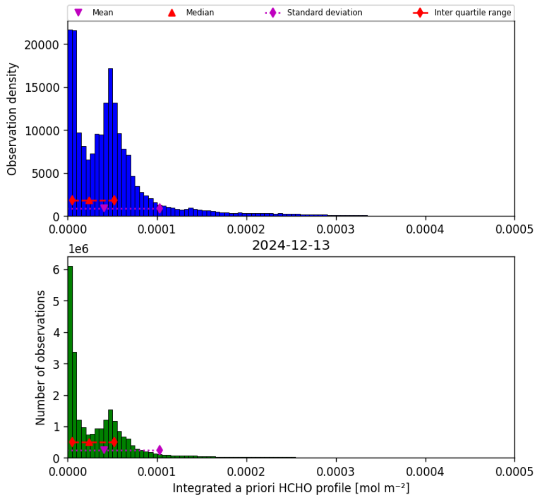
Figure 43: Histogram of “Integrated a priori HCHO profile” for 2024-12-12 to 2024-12-14
