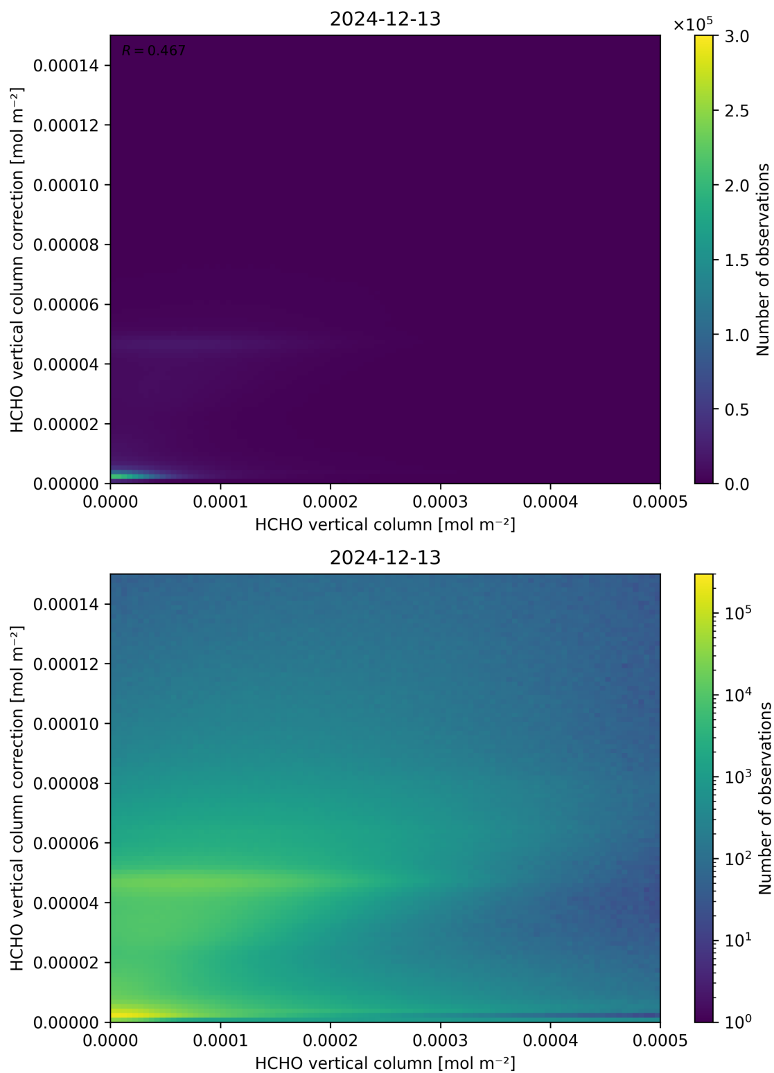
Figure 133: Scatter density plot of “HCHO vertical column” against “HCHO vertical column correction” for 2024-12-12 to 2024-12-14.
