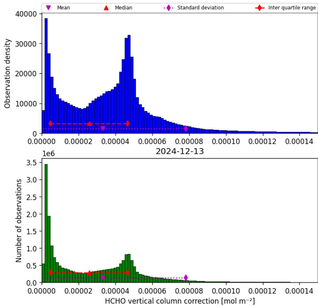
Figure 37: Histogram of “HCHO vertical column correction” for 2024-12-12 to 2024-12-14
