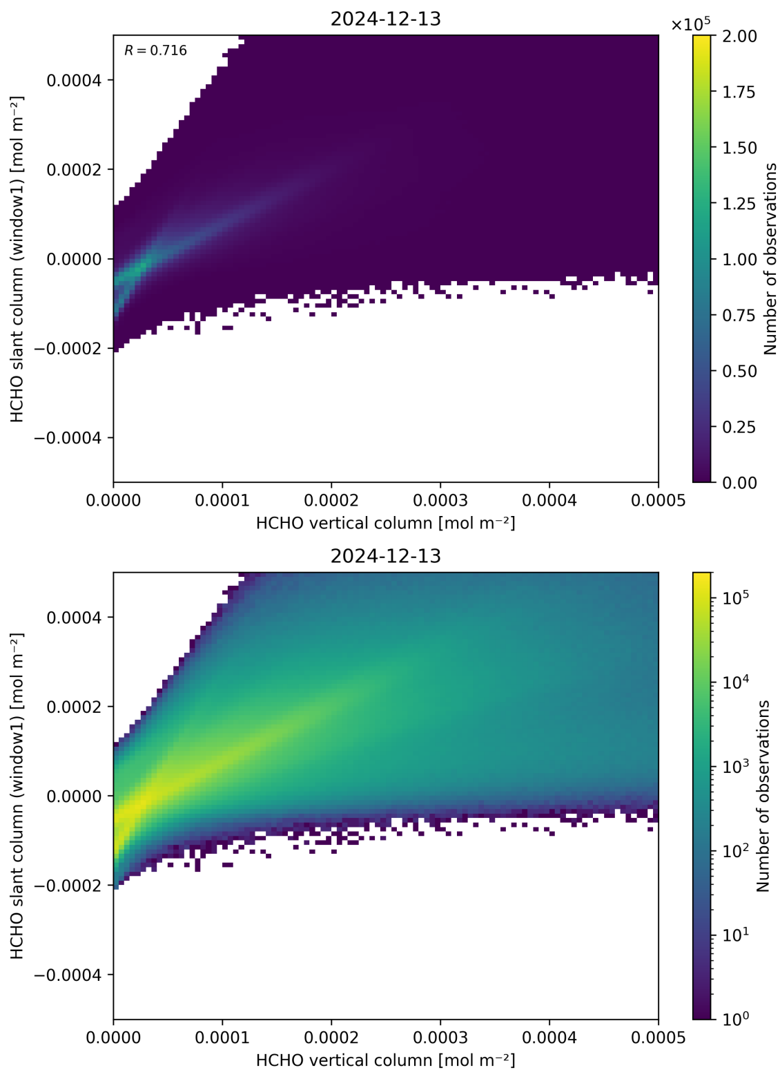
Figure 129: Scatter density plot of “HCHO vertical column” against “HCHO slant column (window1)” for 2024-12-12 to 2024-12-14.
