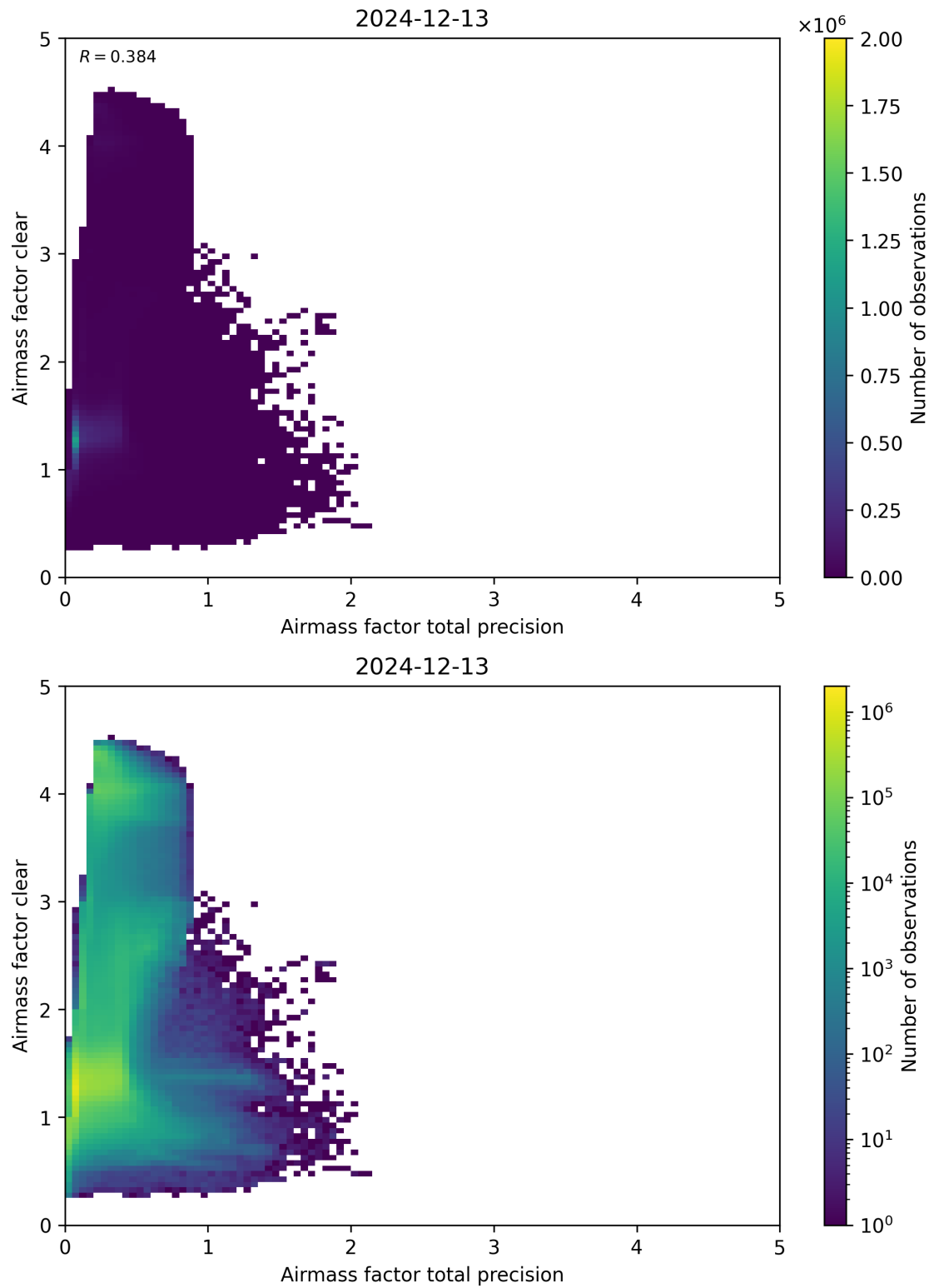
Figure 108: Scatter density plot of “Airmass factor total precision” against “Airmass factor clear” for 2024-12-12 to 2024-12-14.
