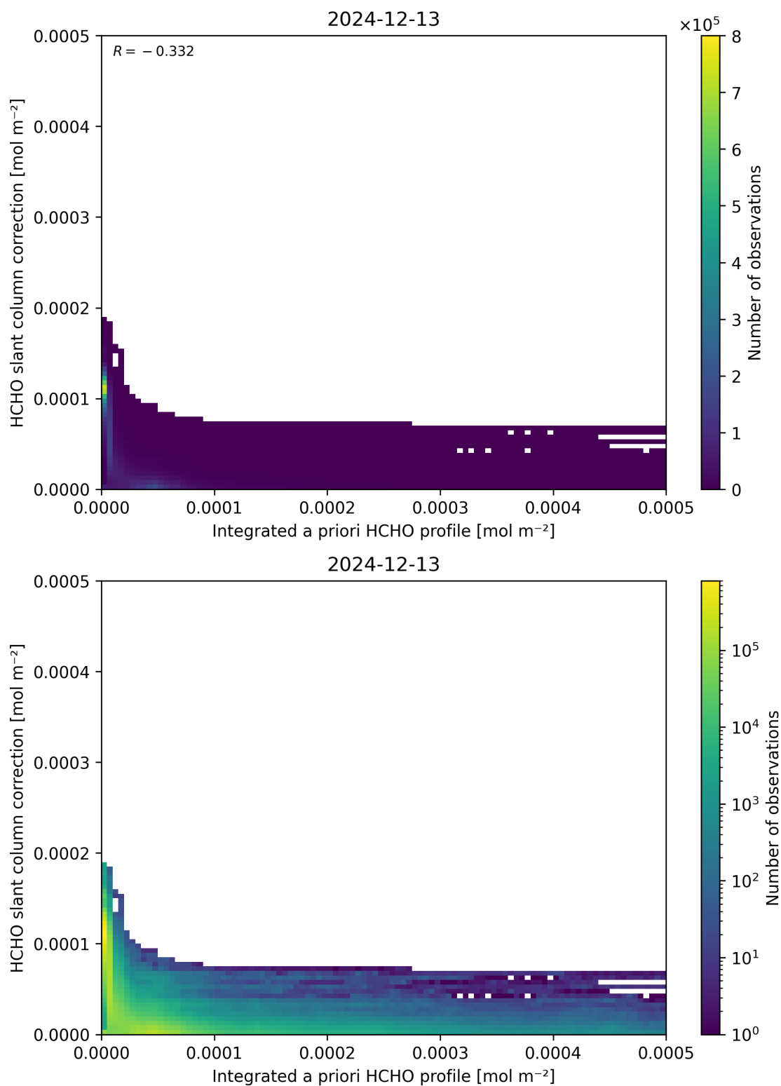
Figure 152: Scatter density plot of “Integrated a priori HCHO profile” against “HCHO slant column correction” for 2024-12-12 to 2024-12-14.
