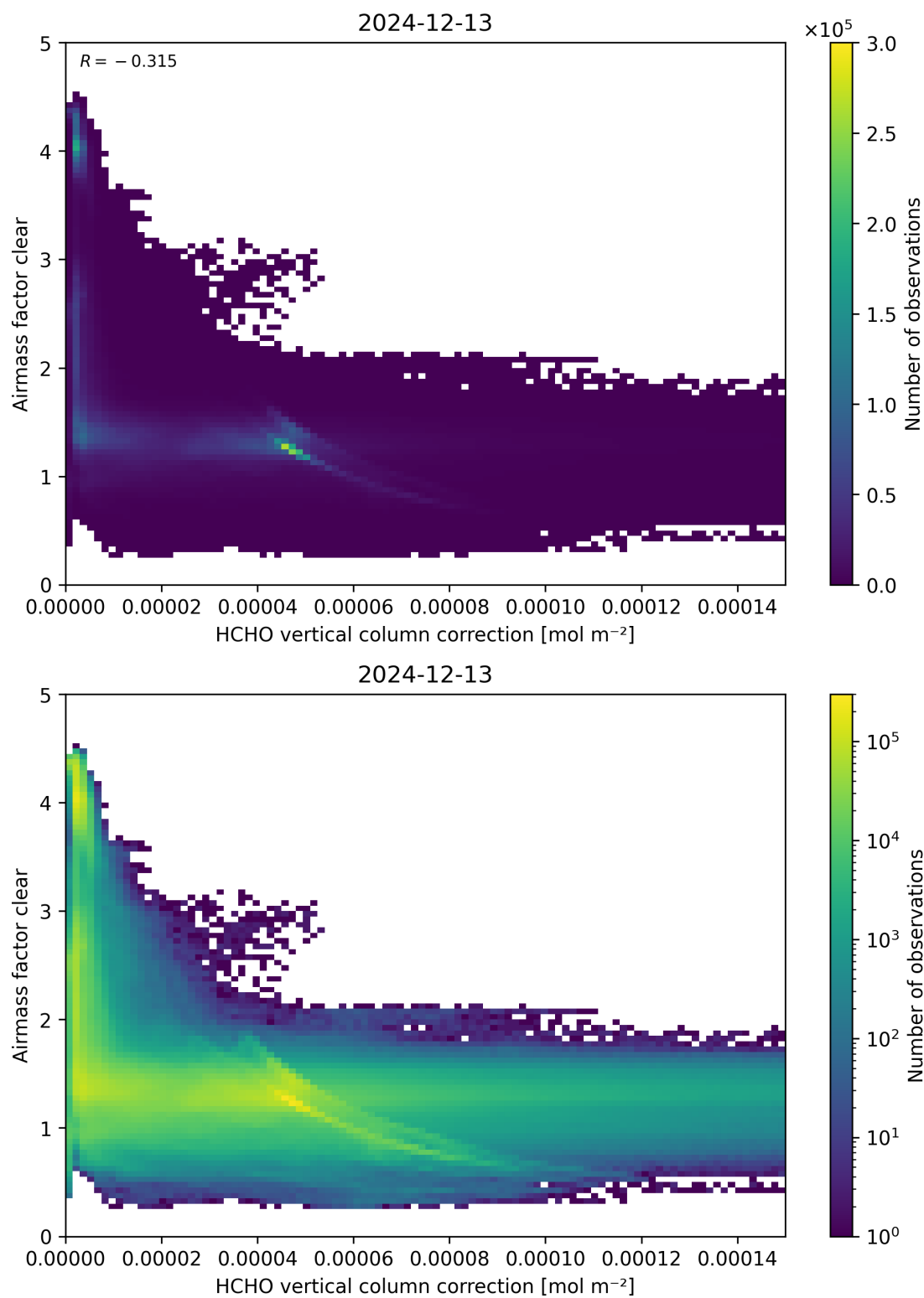
Figure 115: Scatter density plot of “HCHO vertical column correction” against “Airmass factor clear” for 2024-12-12 to 2024-12-14.
