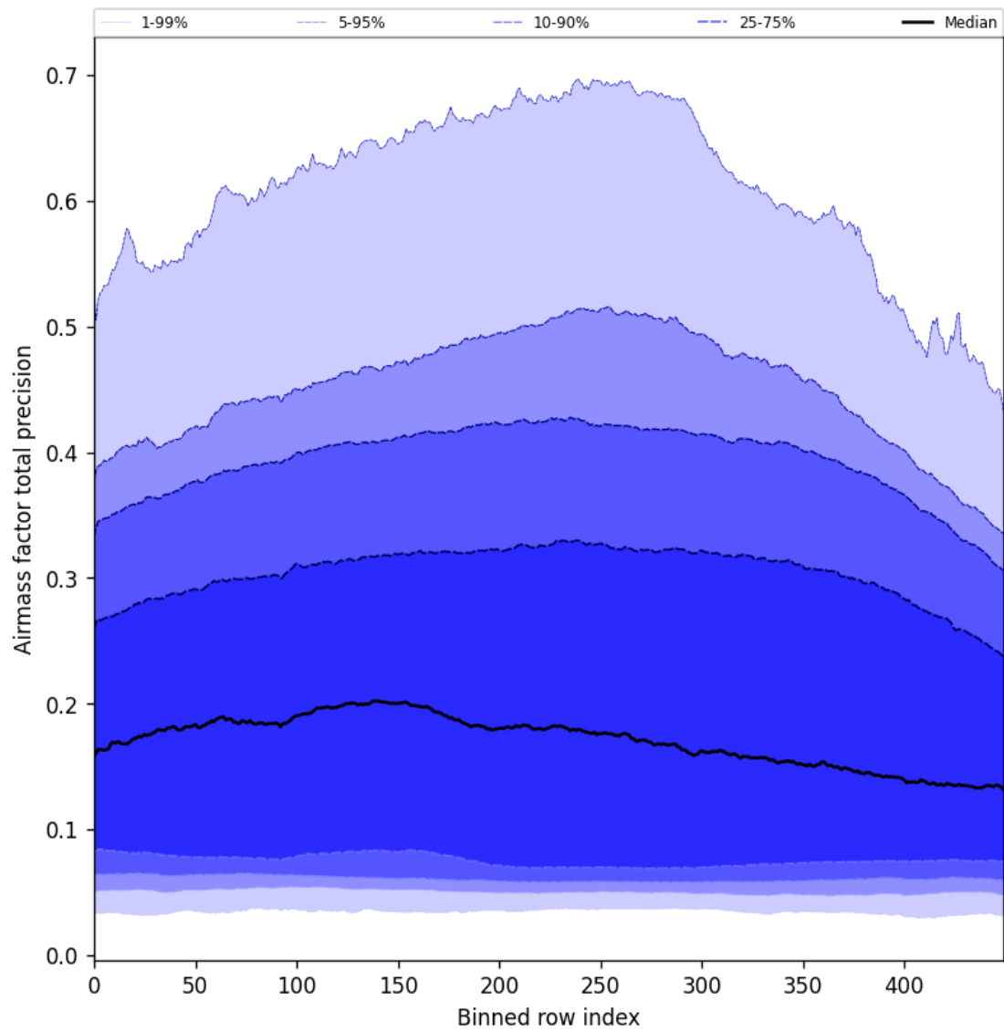
Figure 55: Along track statistics of “Airmass factor total precision” for 2024-12-12 to 2024-12-14
