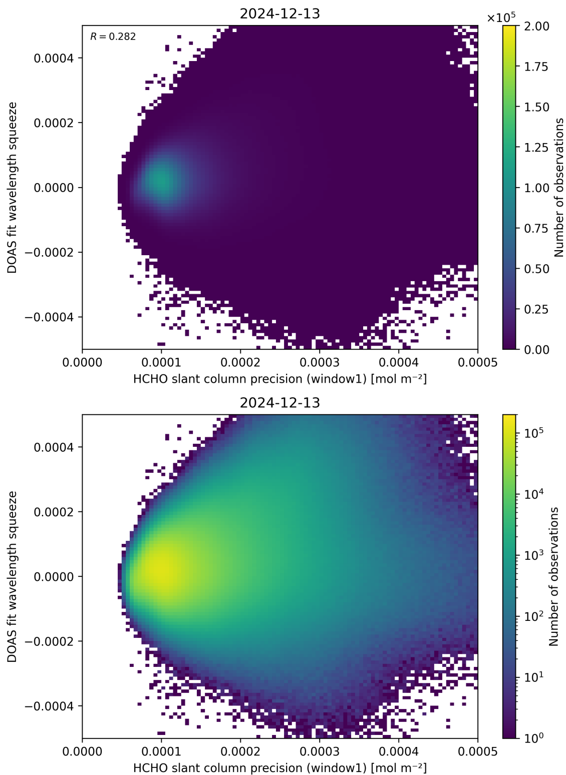
Figure 90: Scatter density plot of “HCHO slant column precision (window1)” against “DOAS fit wavelength squeeze” for 2024-12-12 to 2024-12-14.
