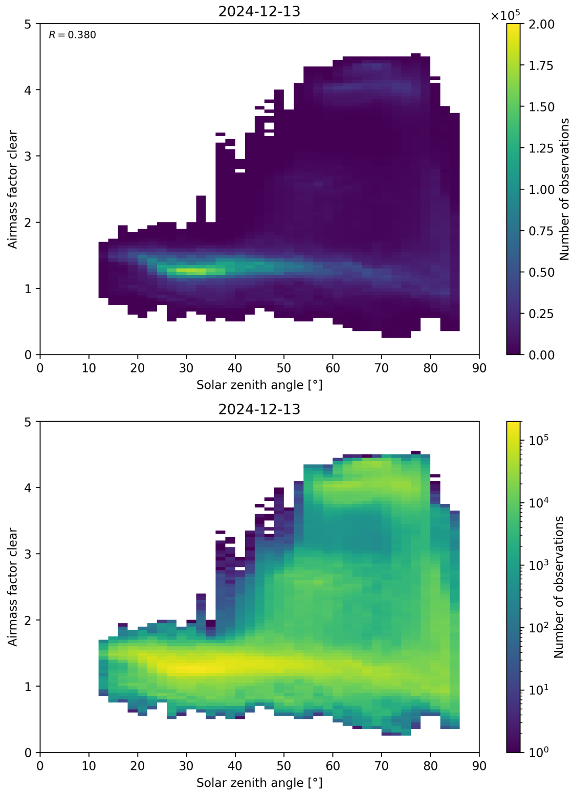
Figure 170: Scatter density plot of “Solar zenith angle” against “Airmass factor clear” for 2024-12-12 to 2024-12-14.
