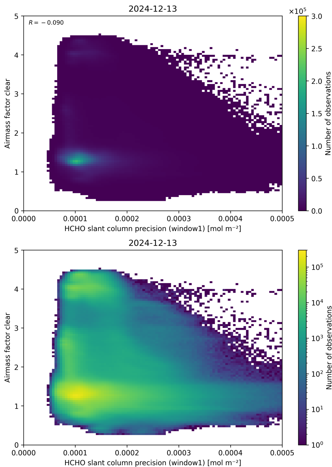
Figure 91: Scatter density plot of “HCHO slant column precision (window1)” against “Airmass factor clear” for 2024-12-12 to 2024-12-14.
