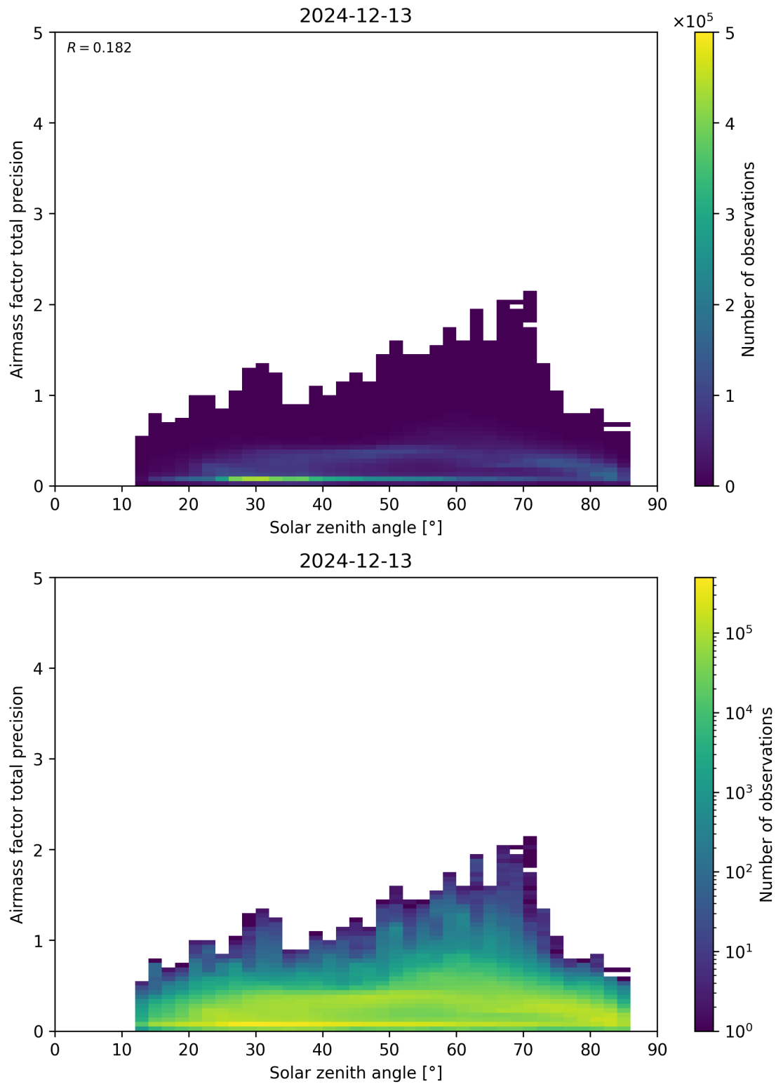
Figure 176: Scatter density plot of “Solar zenith angle” against “Airmass factor total precision” for 2024-12-12 to 2024-12-14.
