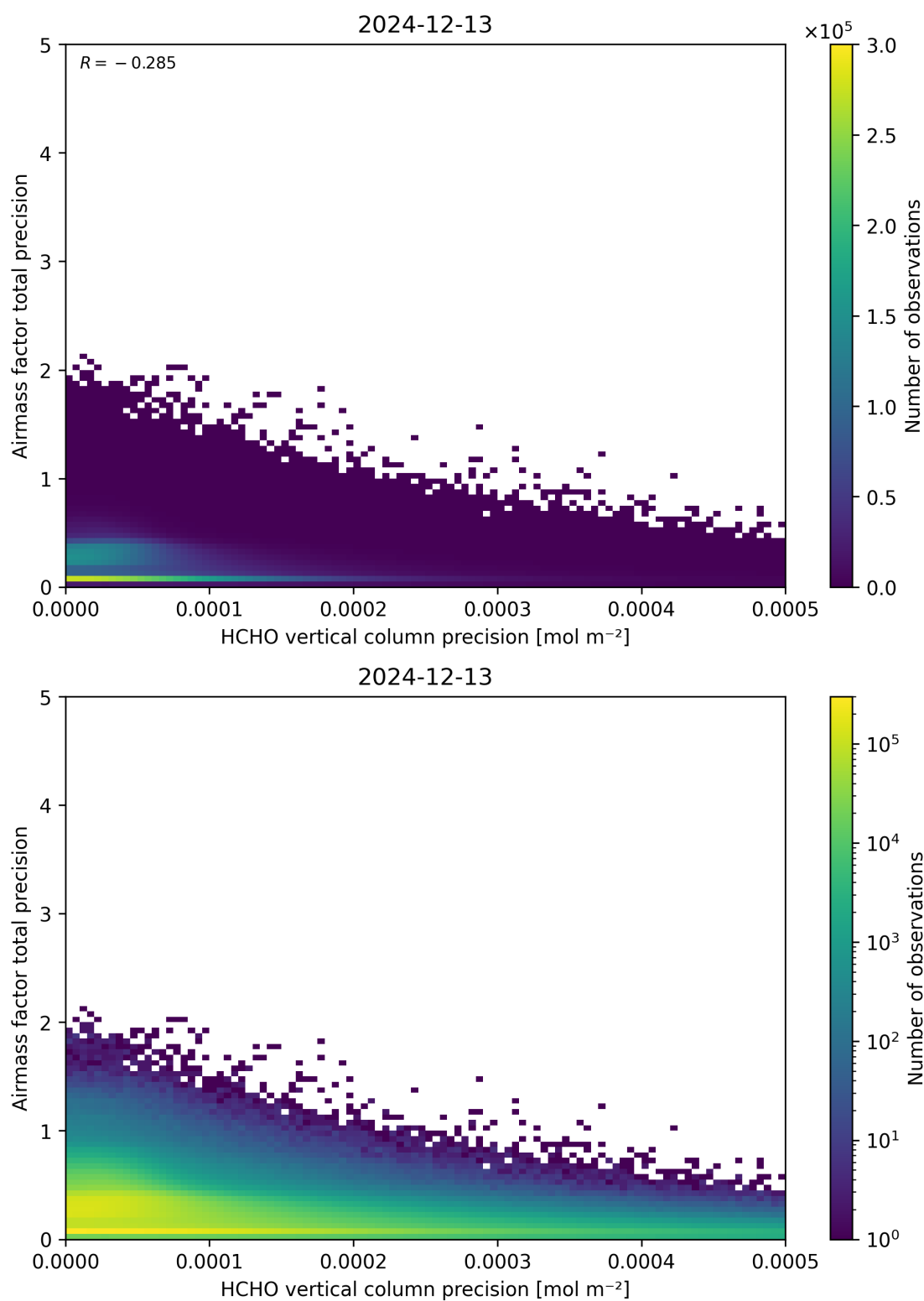
Figure 145: Scatter density plot of “HCHO vertical column precision” against “Airmass factor total precision” for 2024-12-12 to 2024-12-14.
