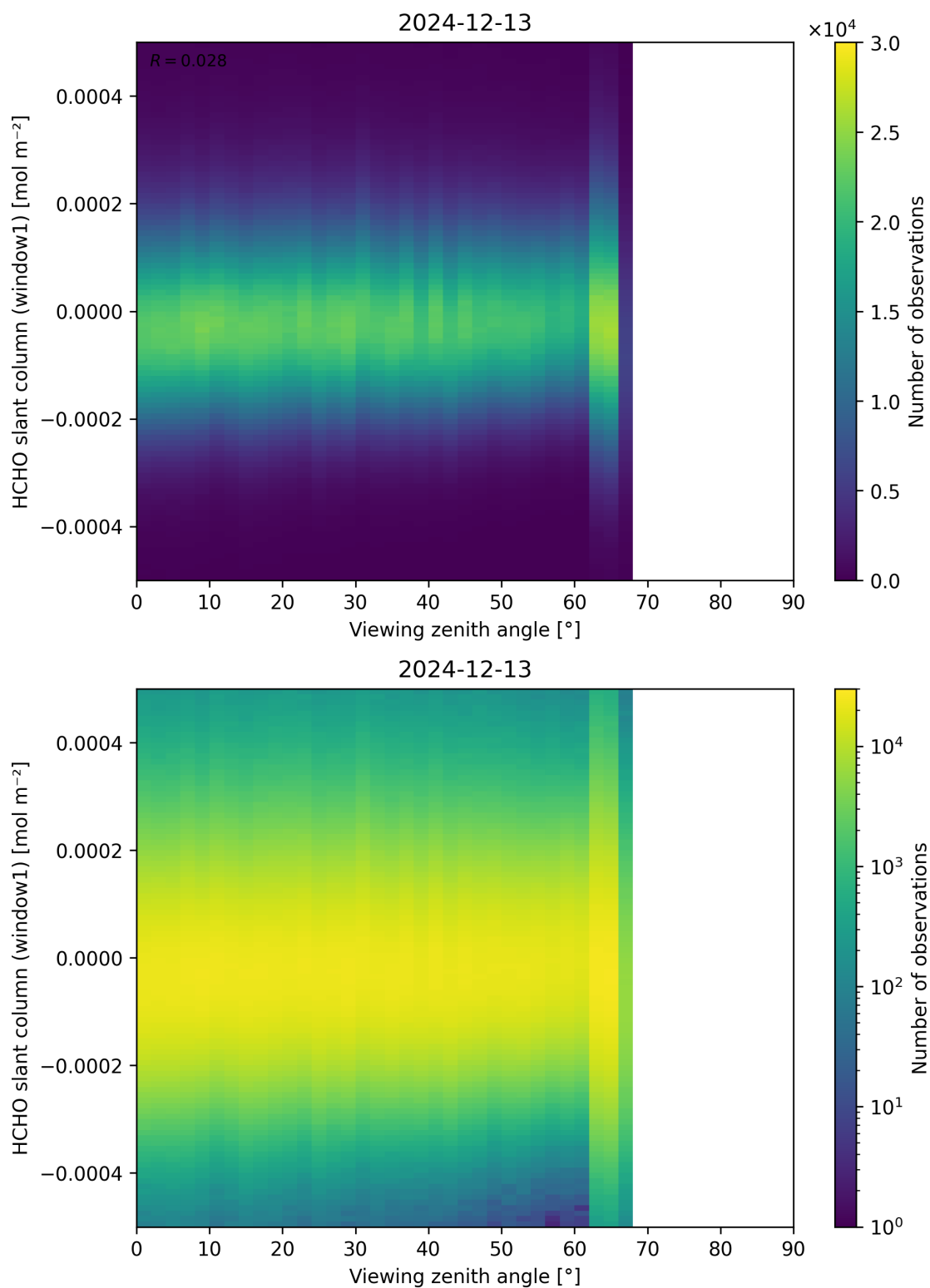
Figure 188: Scatter density plot of “Viewing zenith angle” against “HCHO slant column (window1)” for 2024-12-12 to 2024-12-14.
