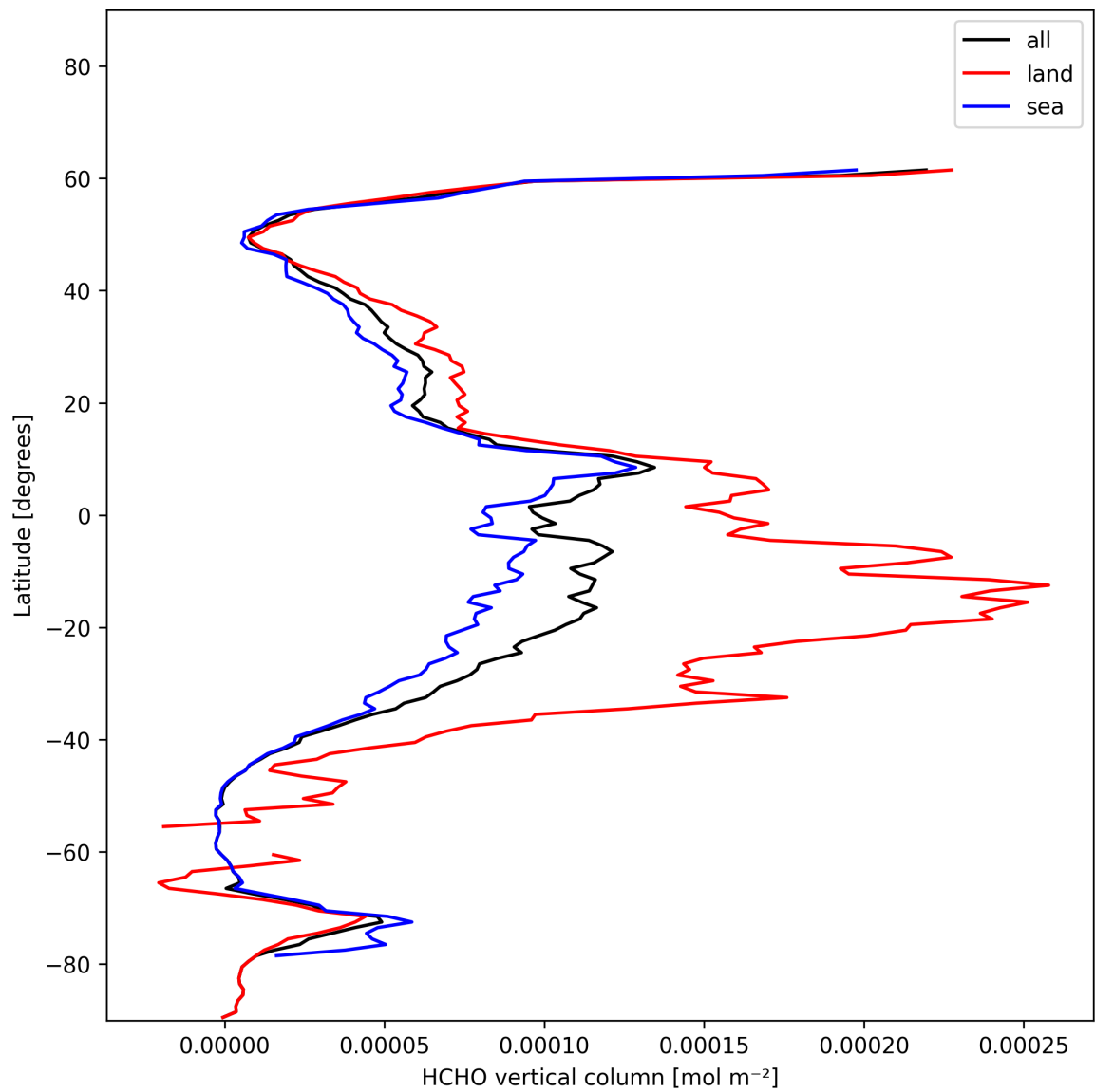
Figure 21: Zonal average of “HCHO vertical column” for 2024-12-12 to 2024-12-14.
