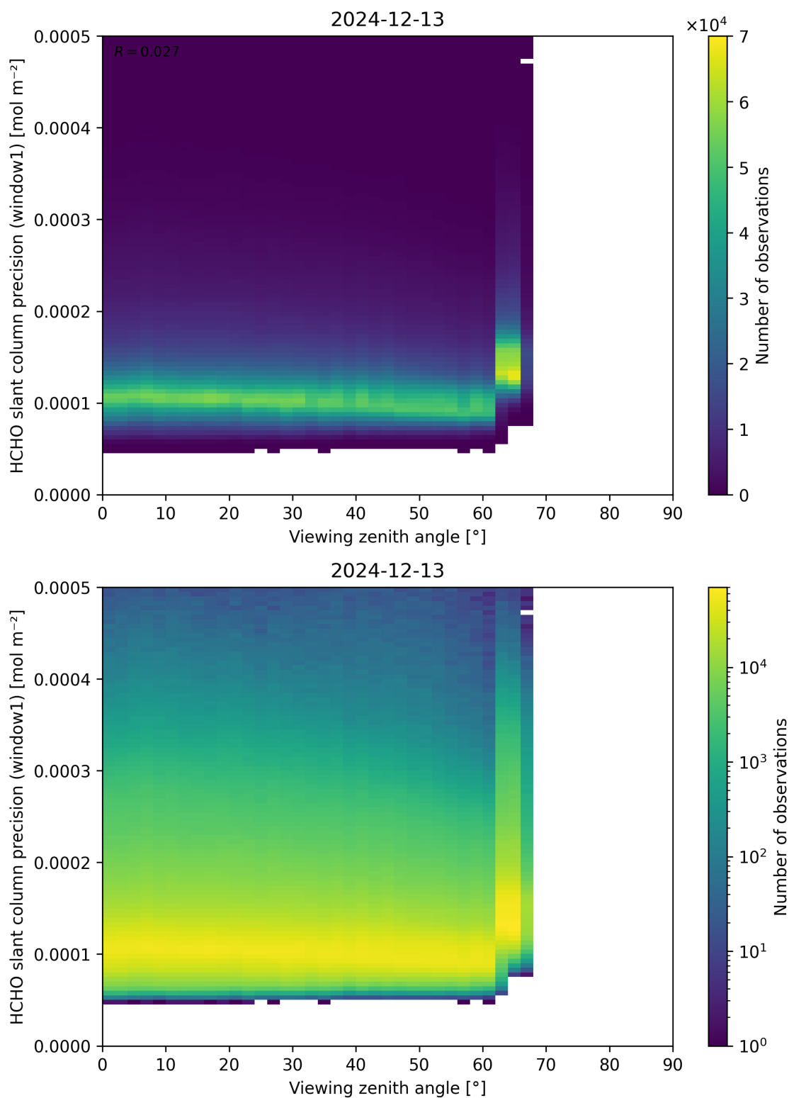
Figure 189: Scatter density plot of “Viewing zenith angle” against “HCHO slant column precision (window1)” for 2024-12-12 to 2024-12-14.
