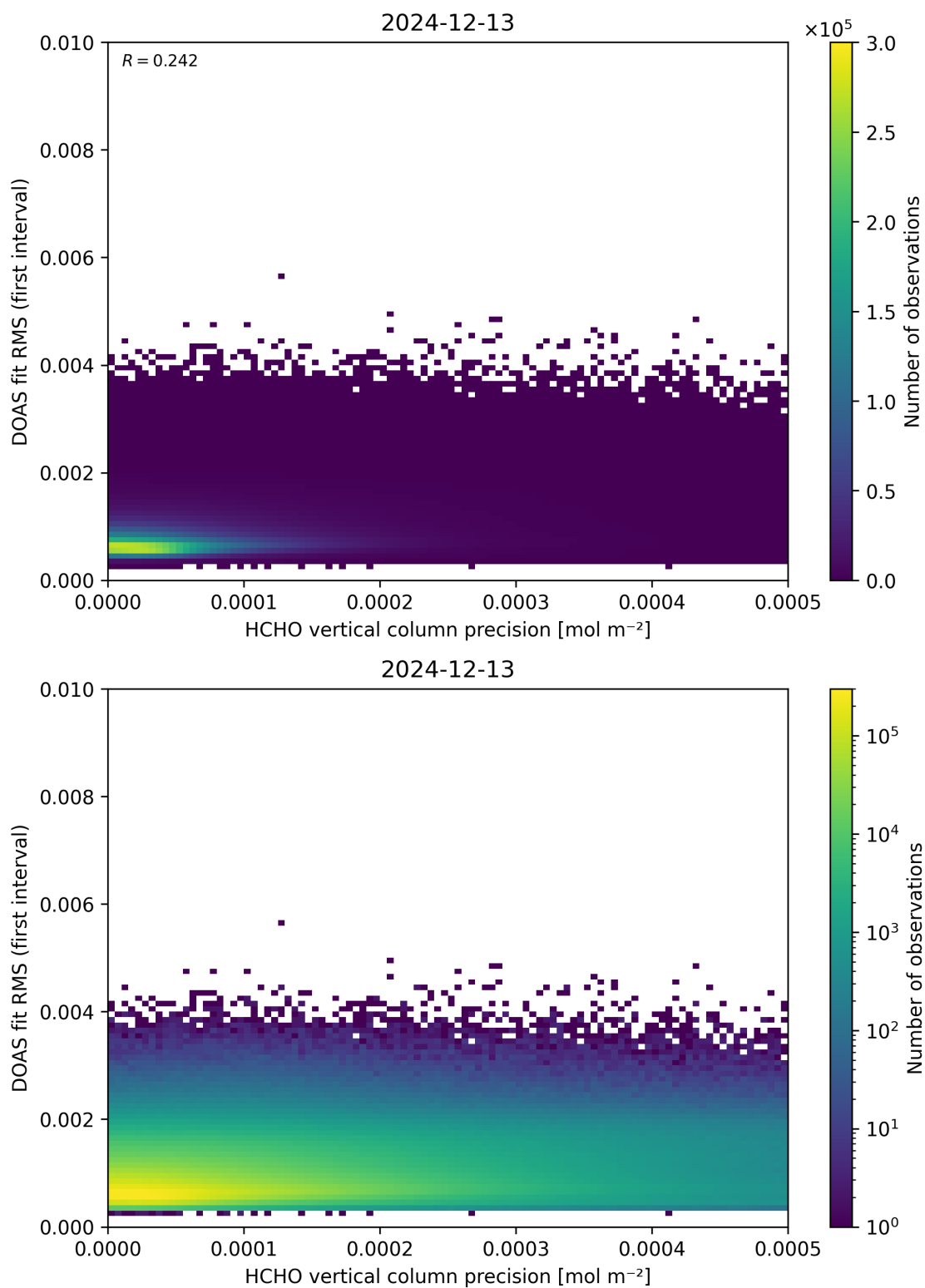
Figure 136: Scatter density plot of “HCHO vertical column precision” against “DOAS fit RMS (first interval)” for 2024-12-12 to 2024-12-14.
