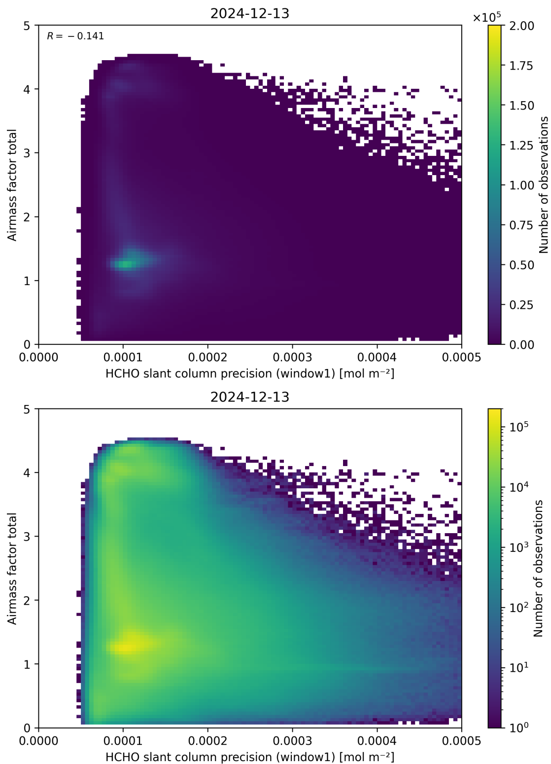
Figure 94: Scatter density plot of “HCHO slant column precision (window1)” against “Airmass factor total” for 2024-12-12 to 2024-12-14.
