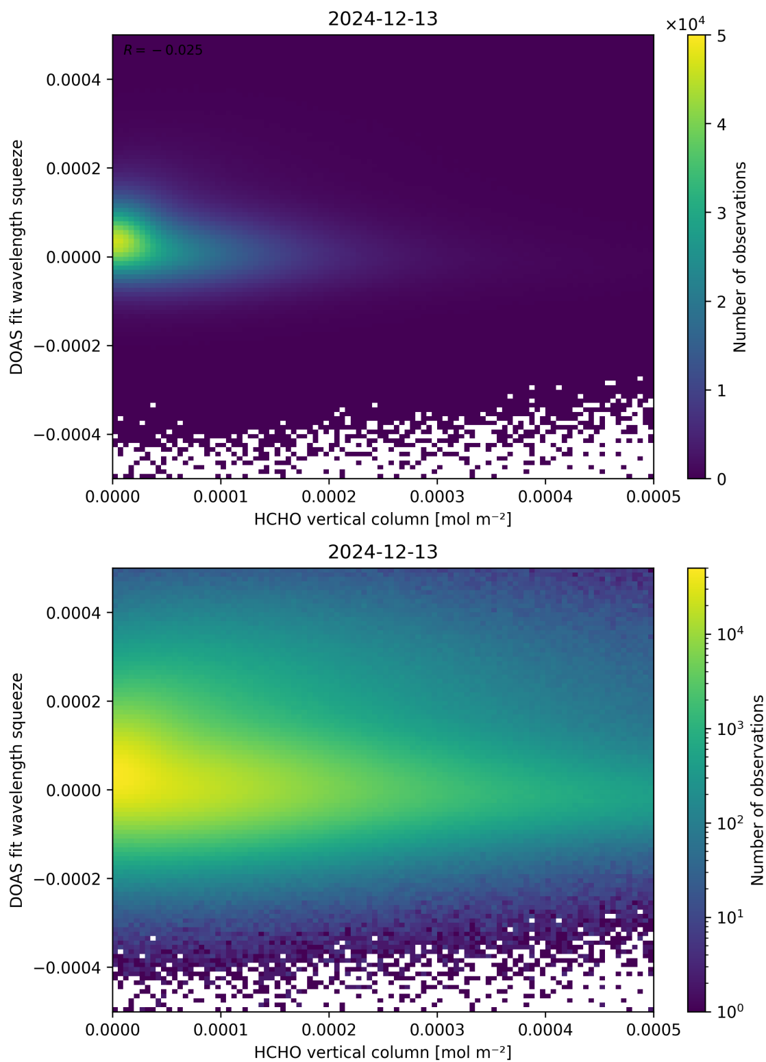
Figure 125: Scatter density plot of “HCHO vertical column” against “DOAS fit wavelength squeeze” for 2024-12-12 to 2024-12-14.
