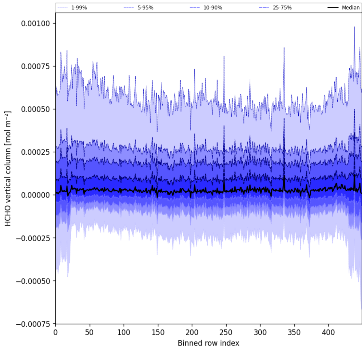
Figure 49: Along track statistics of “HCHO vertical column” for 2024-12-12 to 2024-12-14
