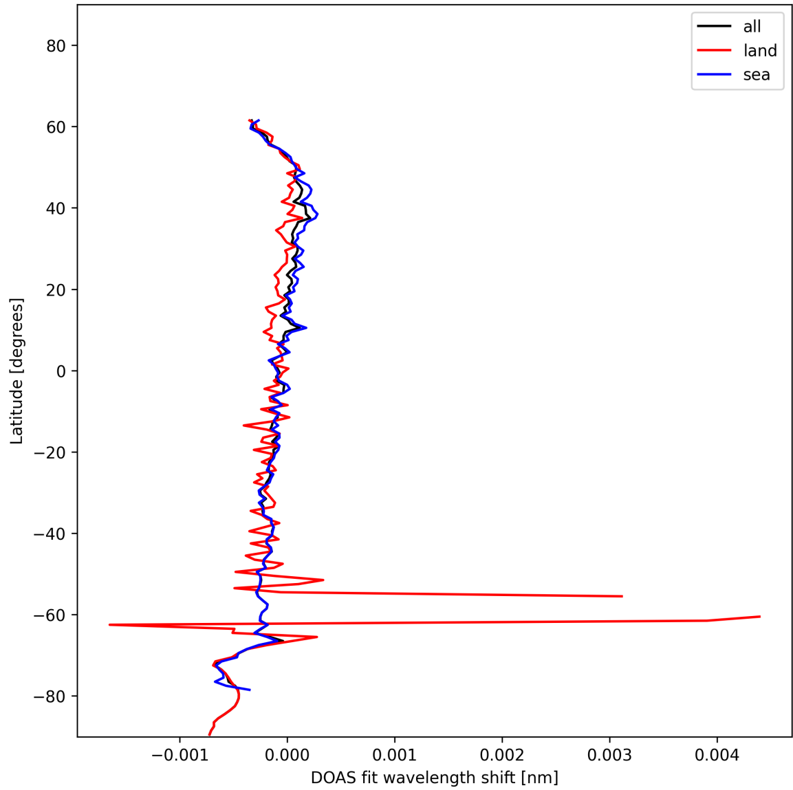
Figure 30: Zonal average of "DOAS fit wavelength shift" for 2024-12-12 to 2024-12-14.
