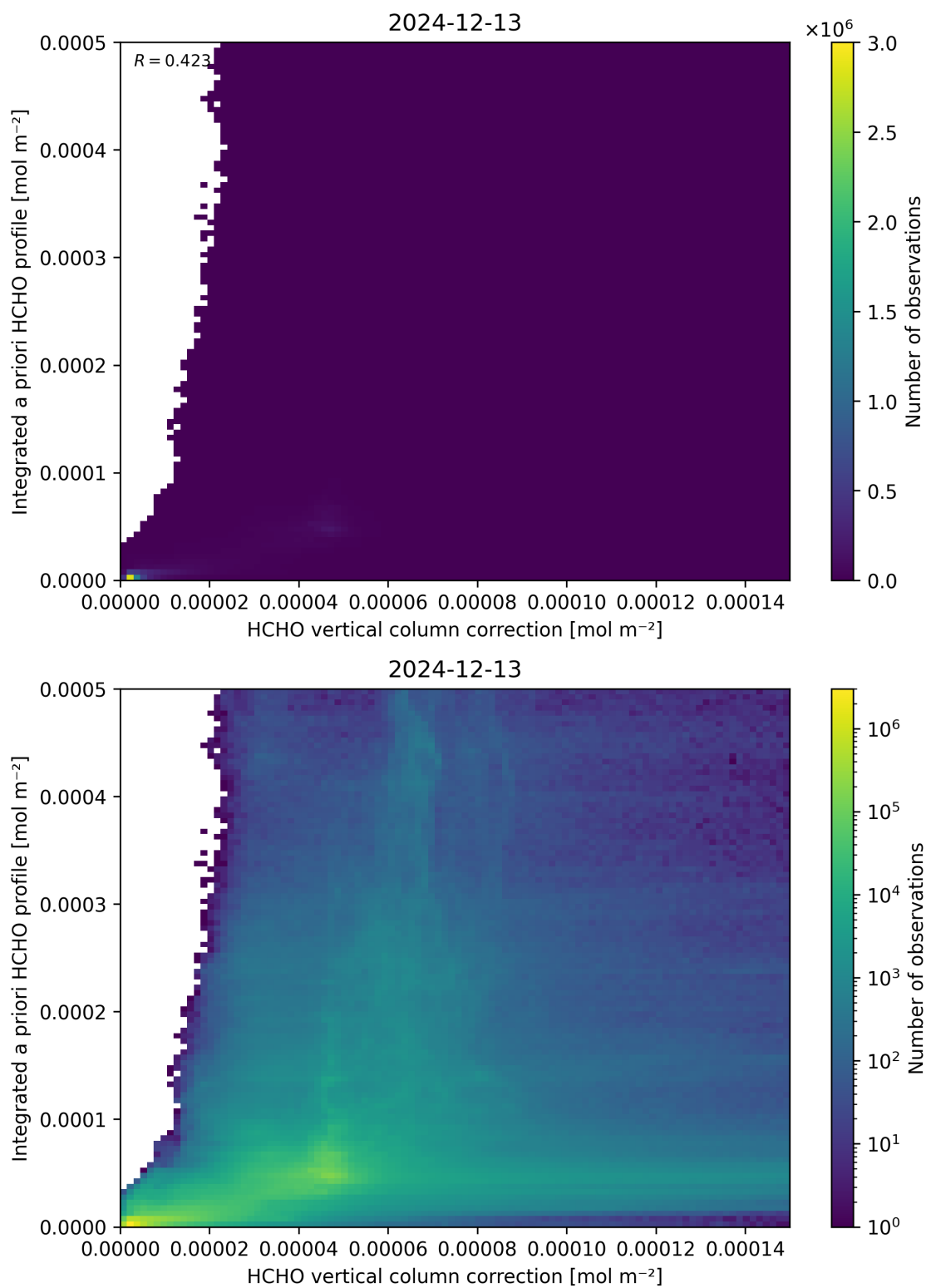
Figure 122: Scatter density plot of “HCHO vertical column correction” against “Integrated a priori HCHO profile” for 2024-12-12 to 2024-12-14.
