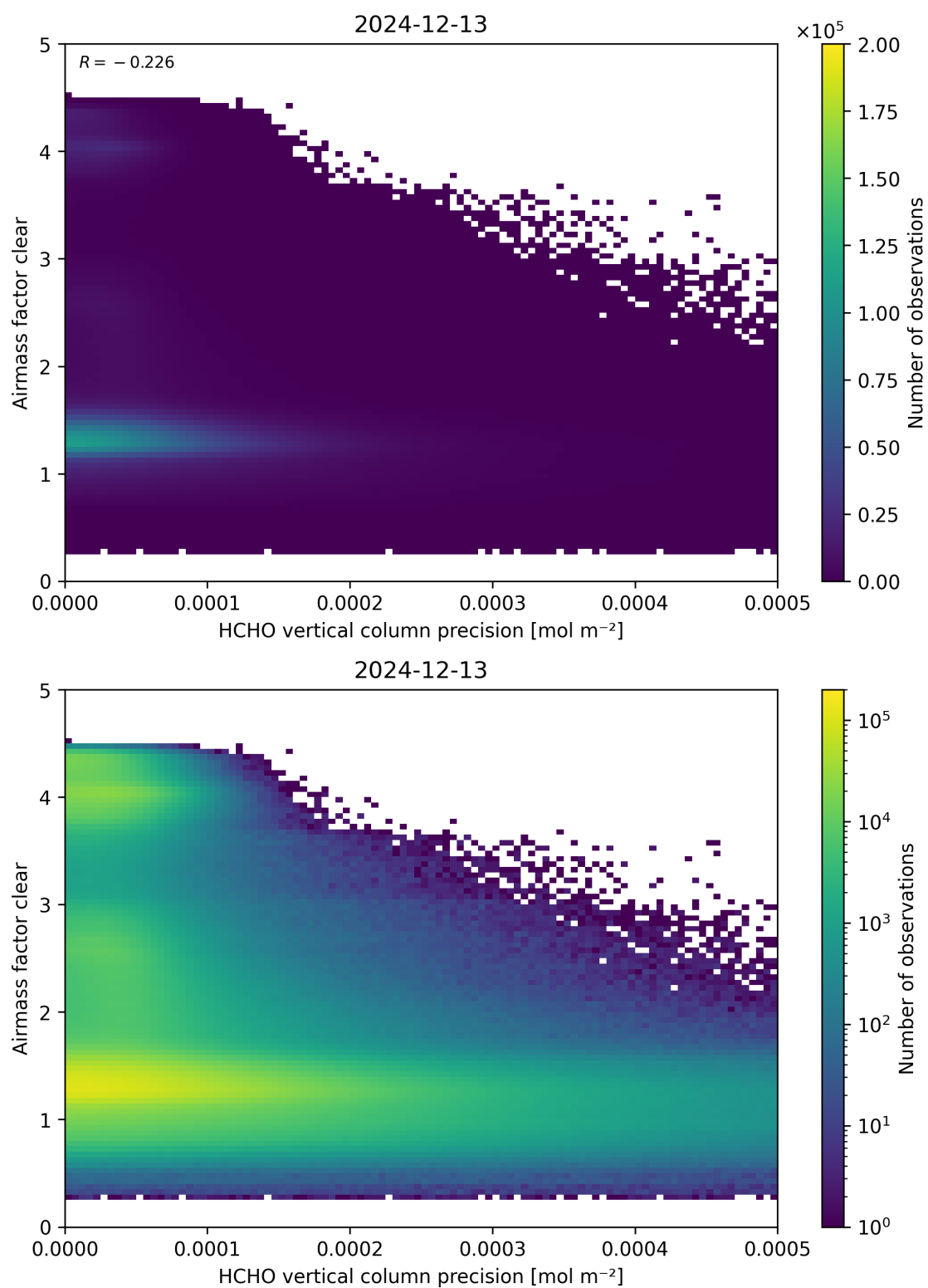
Figure 139: Scatter density plot of “HCHO vertical column precision” against “Airmass factor clear” for 2024-12-12 to 2024-12-14.
