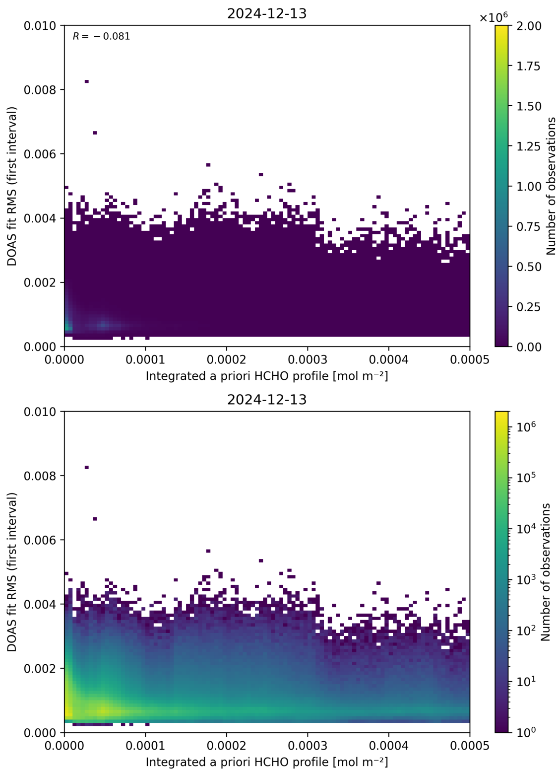
Figure 148: Scatter density plot of “Integrated a priori HCHO profile” against “DOAS fit RMS (first interval)” for 2024-12-12 to 2024-12-14.
