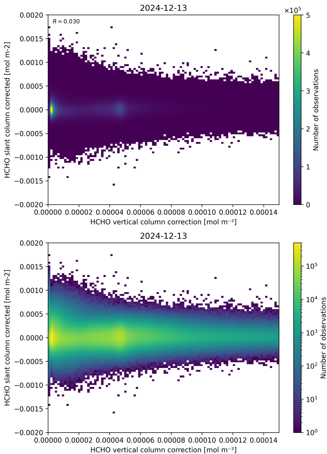
Figure 116: Scatter density plot of “HCHO vertical column correction” against “HCHO slant column corrected” for 2024-12-12 to 2024-12-14.
