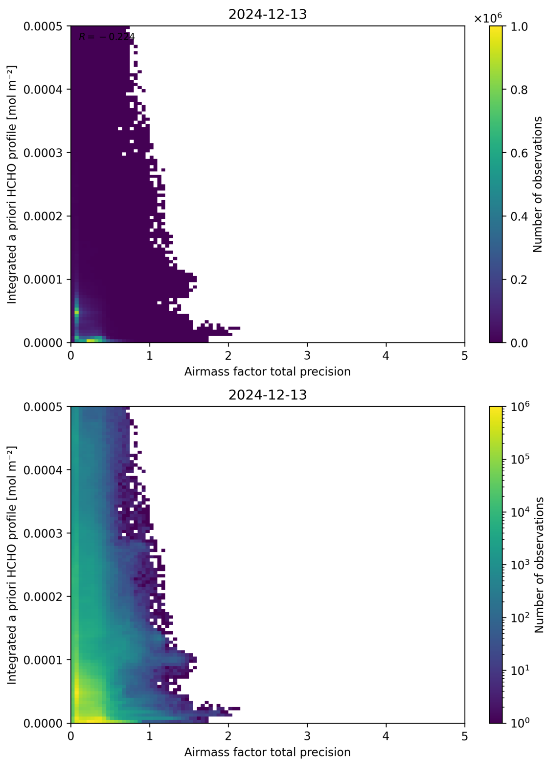
Figure 111: Scatter density plot of “Airmass factor total precision” against “Integrated a priori HCHO profile” for 2024-12-12 to 2024-12-14.
