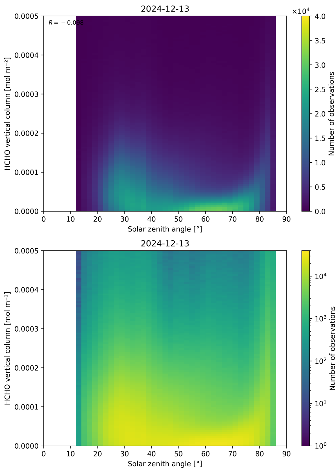
Figure 177: Scatter density plot of “Solar zenith angle” against “HCHO vertical column” for 2024-12-12 to 2024-12-14.
