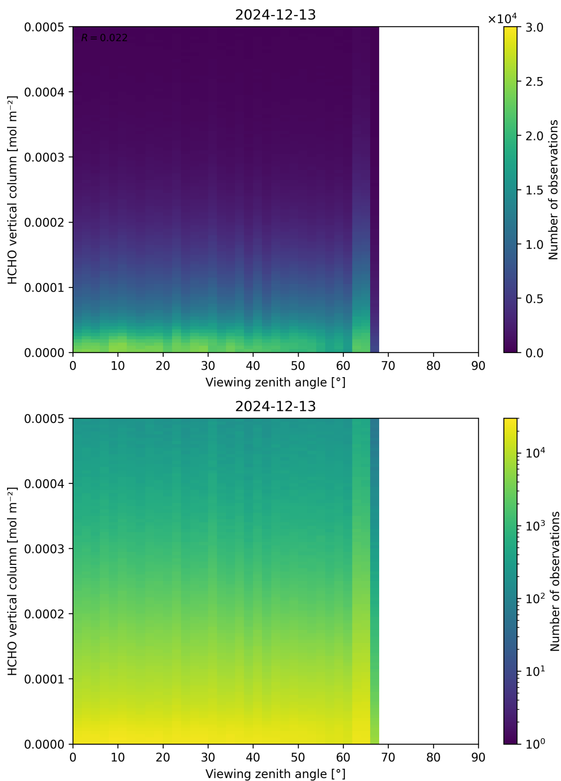
Figure 192: Scatter density plot of “Viewing zenith angle” against “HCHO vertical column” for 2024-12-12 to 2024-12-14.
