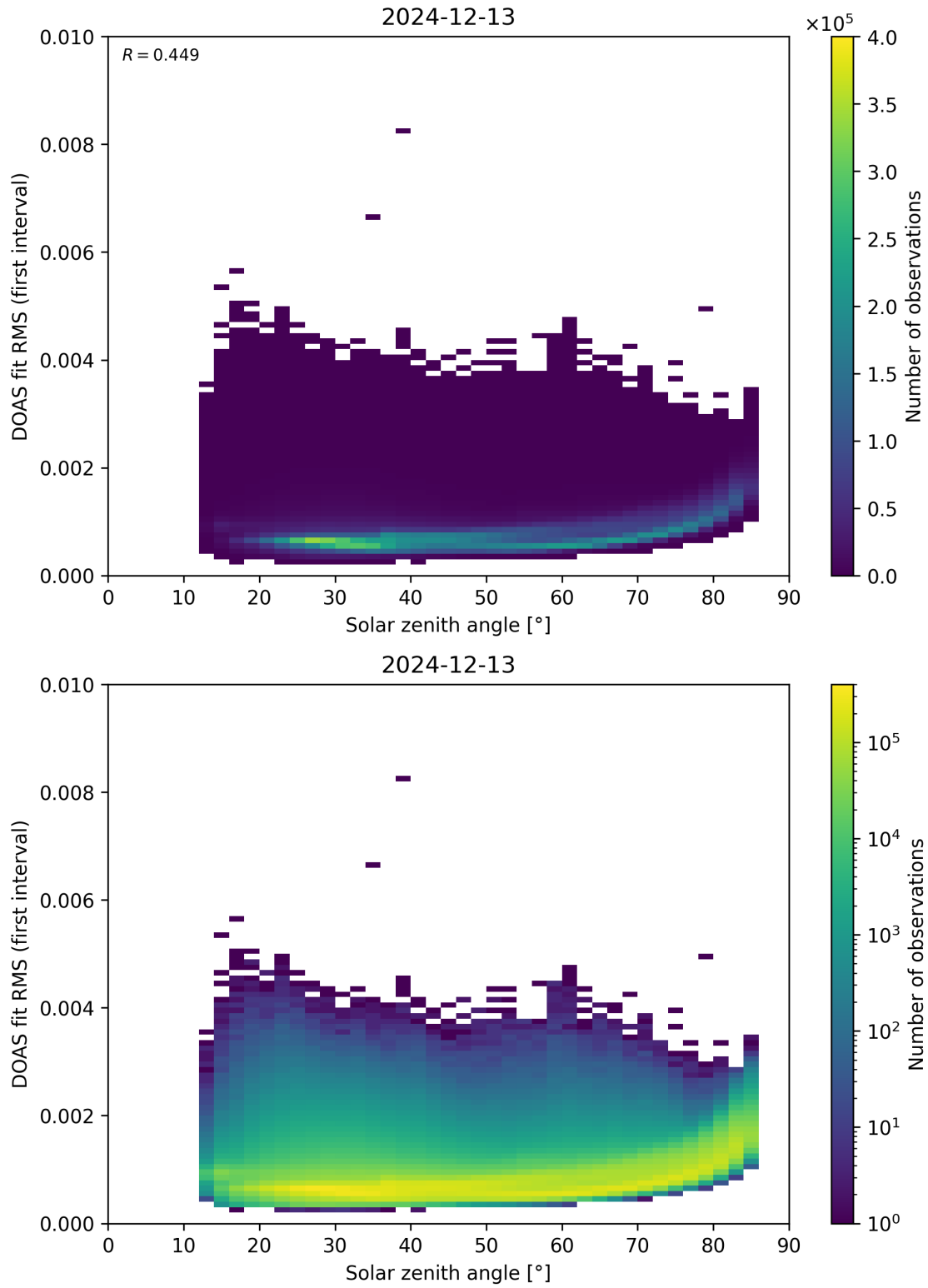
Figure 167: Scatter density plot of “Solar zenith angle” against “DOAS fit RMS (first interval)” for 2024-12-12 to 2024-12-14.
