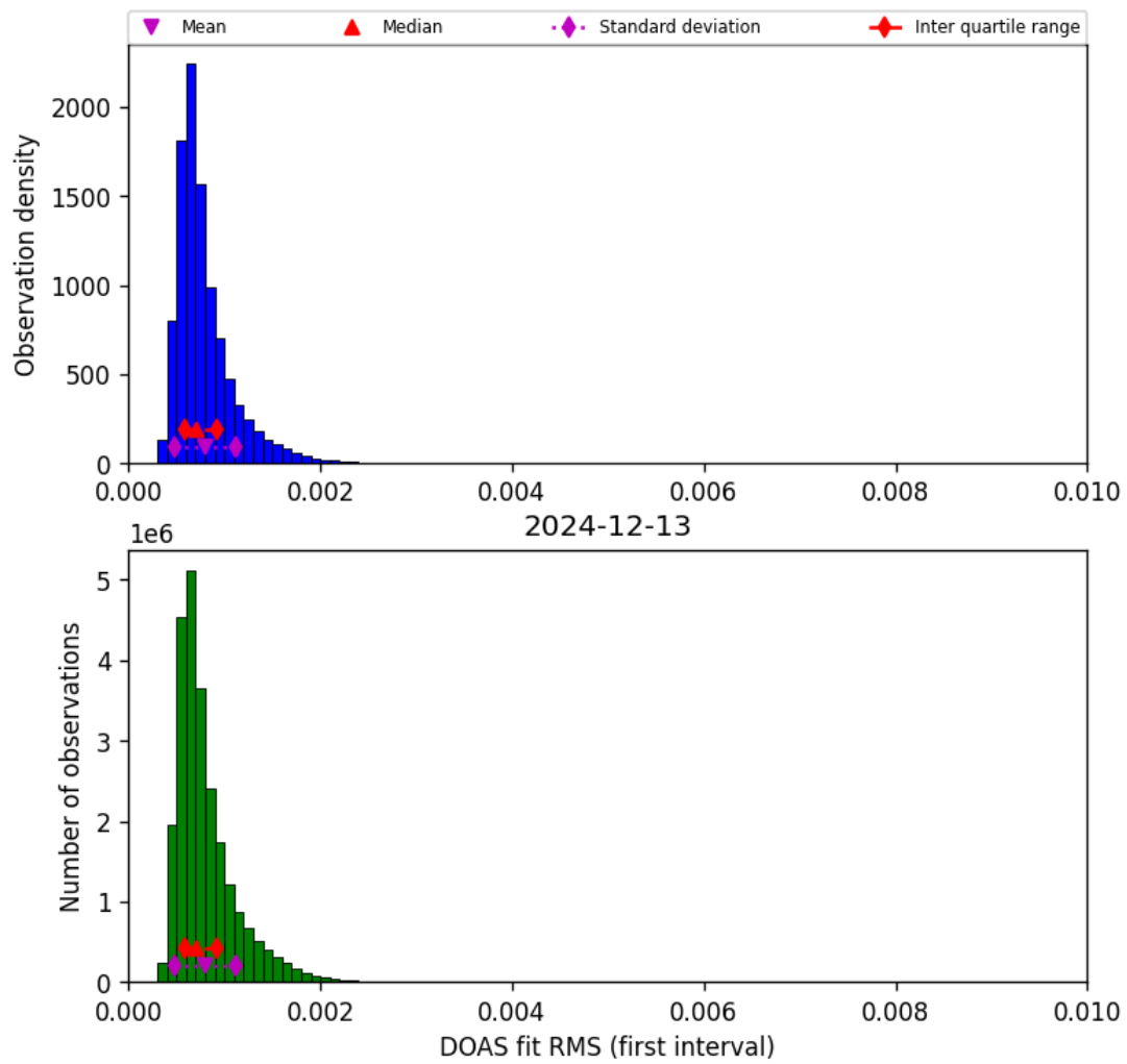
Figure 46: Histogram of “DOAS fit RMS (first interval)” for 2024-12-12 to 2024-12-14
