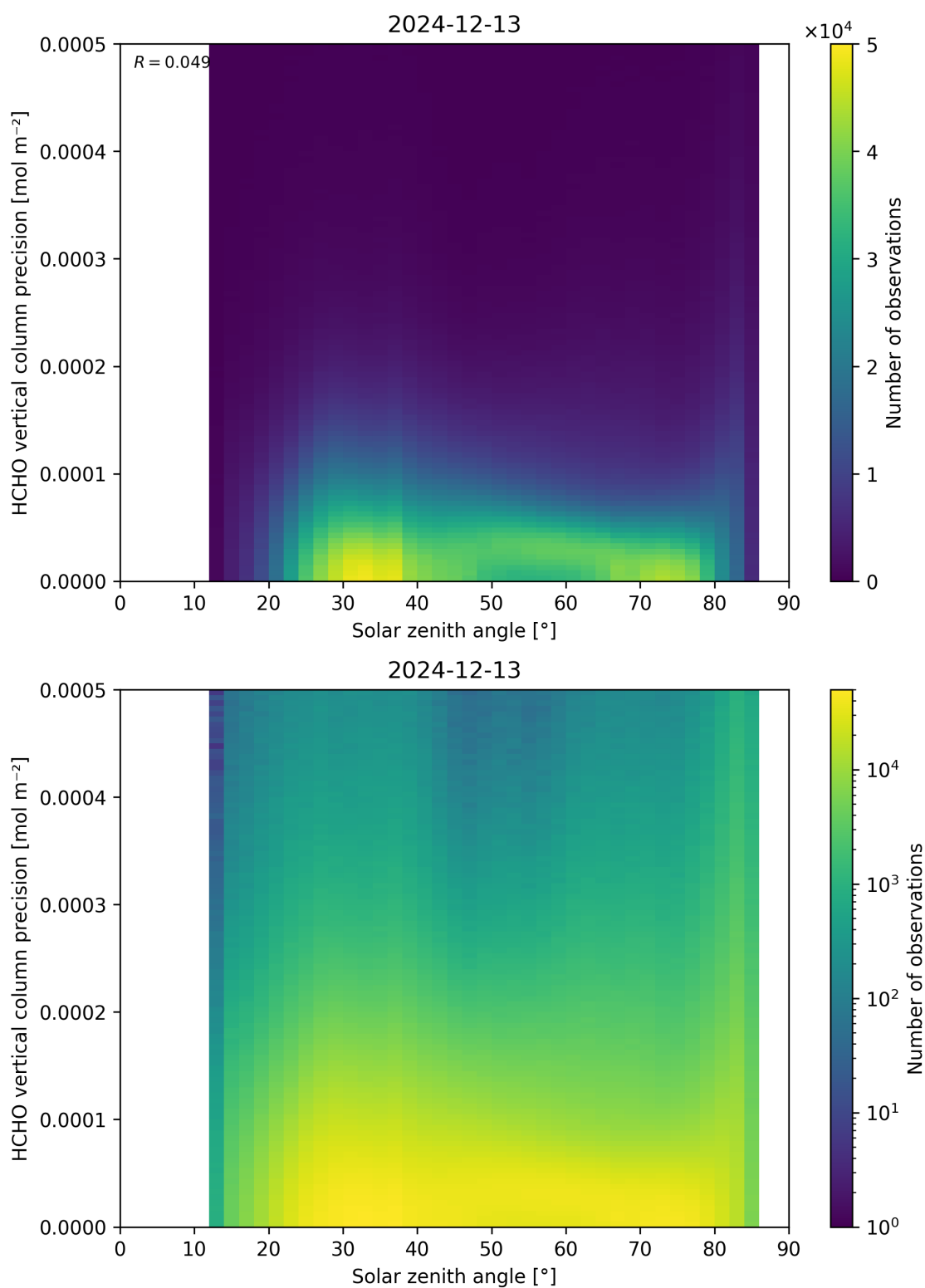
Figure 179: Scatter density plot of “Solar zenith angle” against “HCHO vertical column precision” for 2024-12-12 to 2024-12-14.
