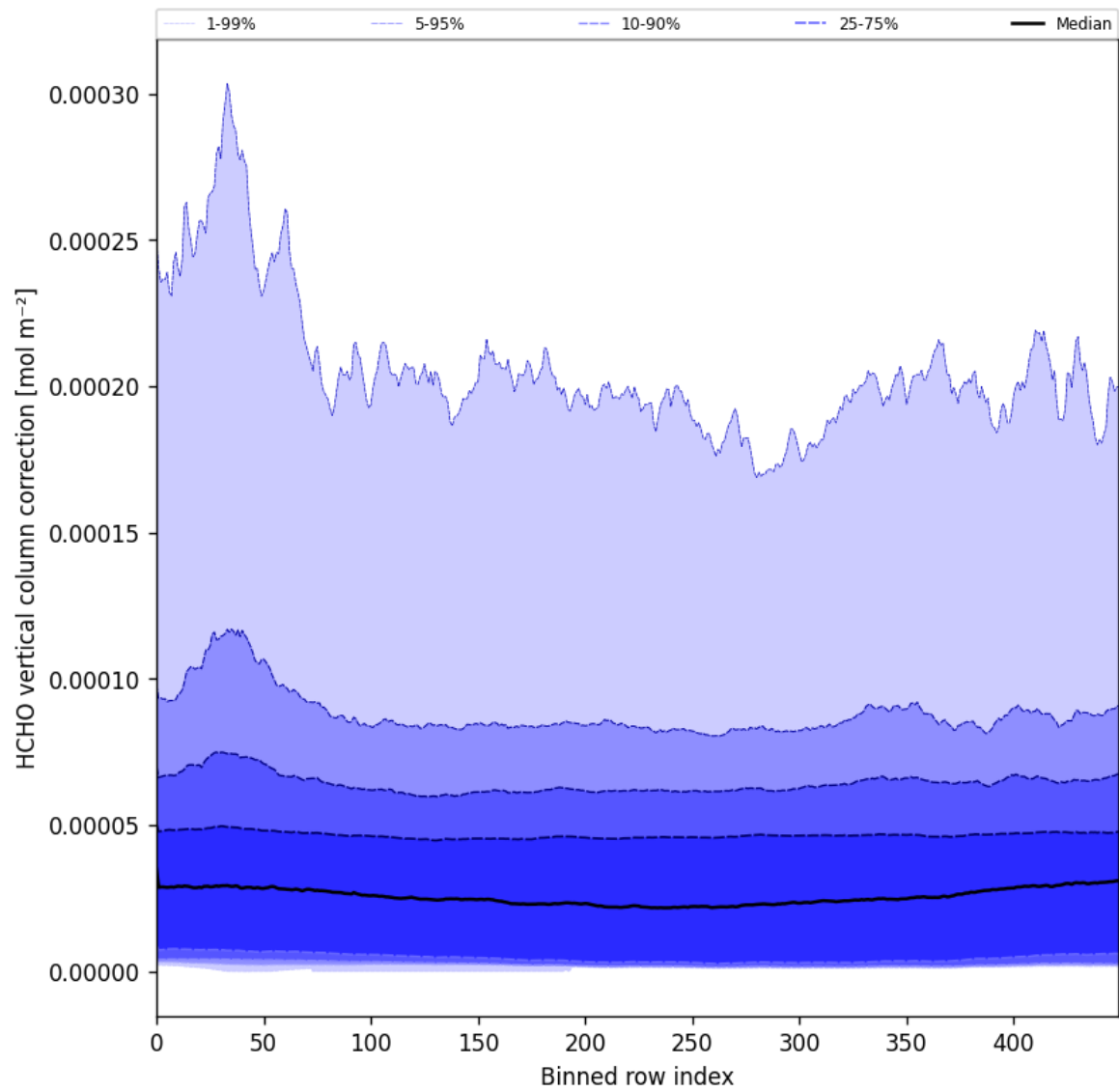
Figure 51: Along track statistics of “HCHO vertical column correction” for 2024-12-12 to 2024-12-14
