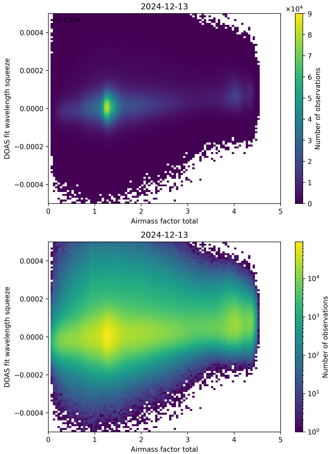
Figure 99: Scatter density plot of “Airmass factor total” against “DOAS fit wavelength squeeze” for 2024-12-12 to 2024-12-14.
