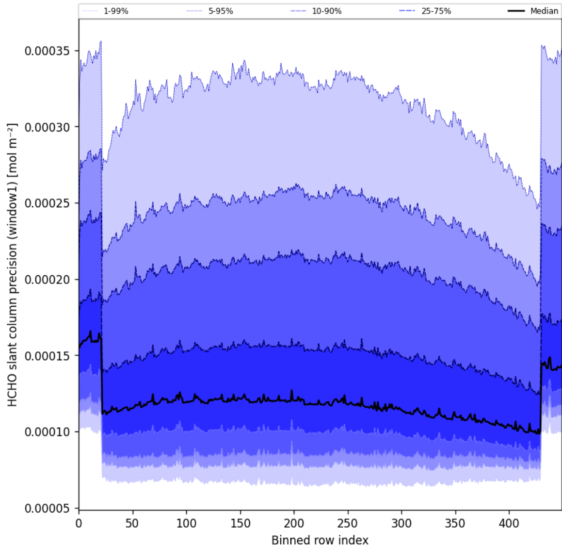
Figure 53: Along track statistics of “HCHO slant column precision (window1)” for 2024-12-12 to 2024-12-14
