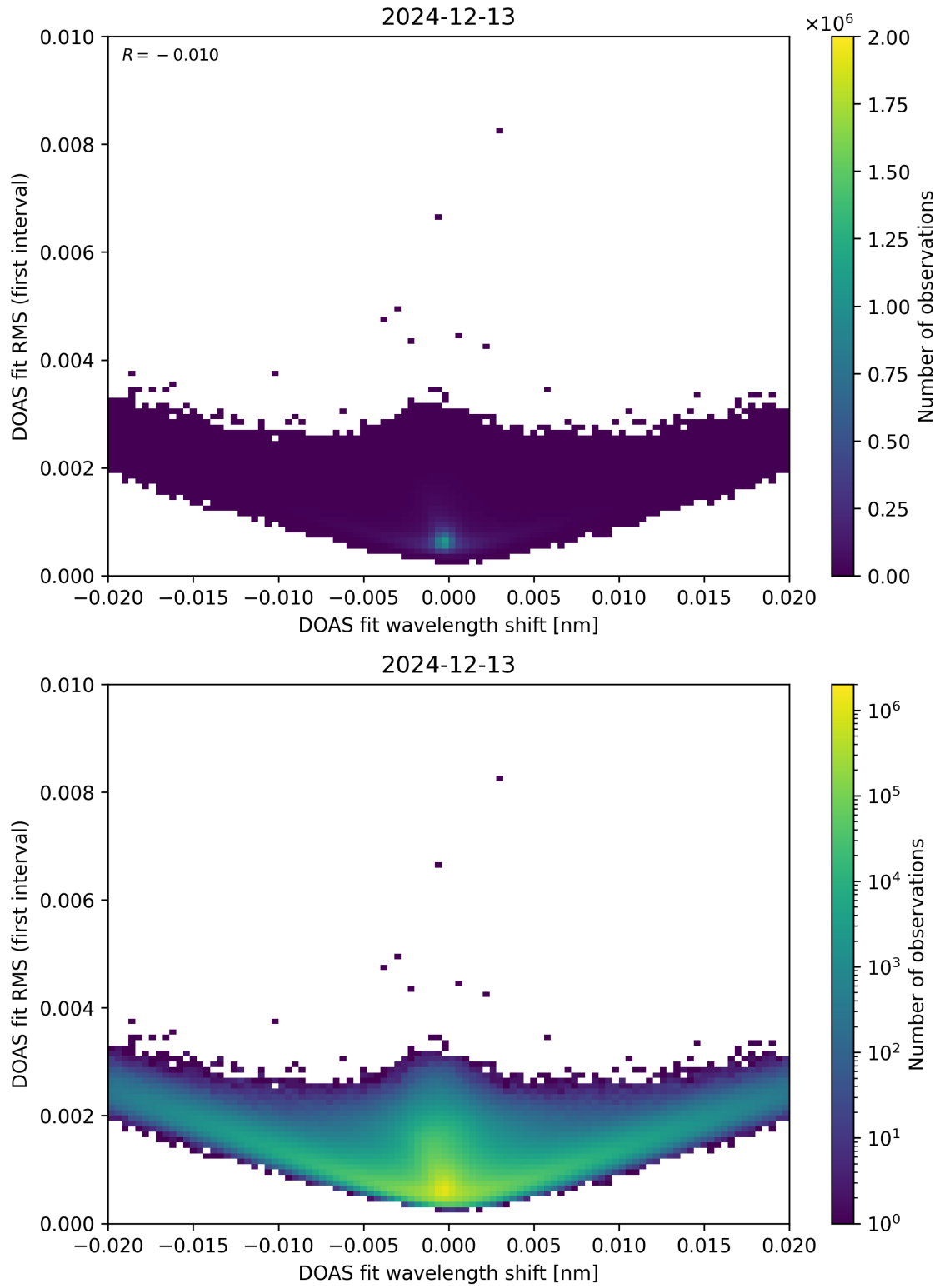
Figure 64: Scatter density plot of “DOAS fit wavelength shift” against “DOAS fit RMS (first interval)” for 2024-12-12 to 2024-12-14.
