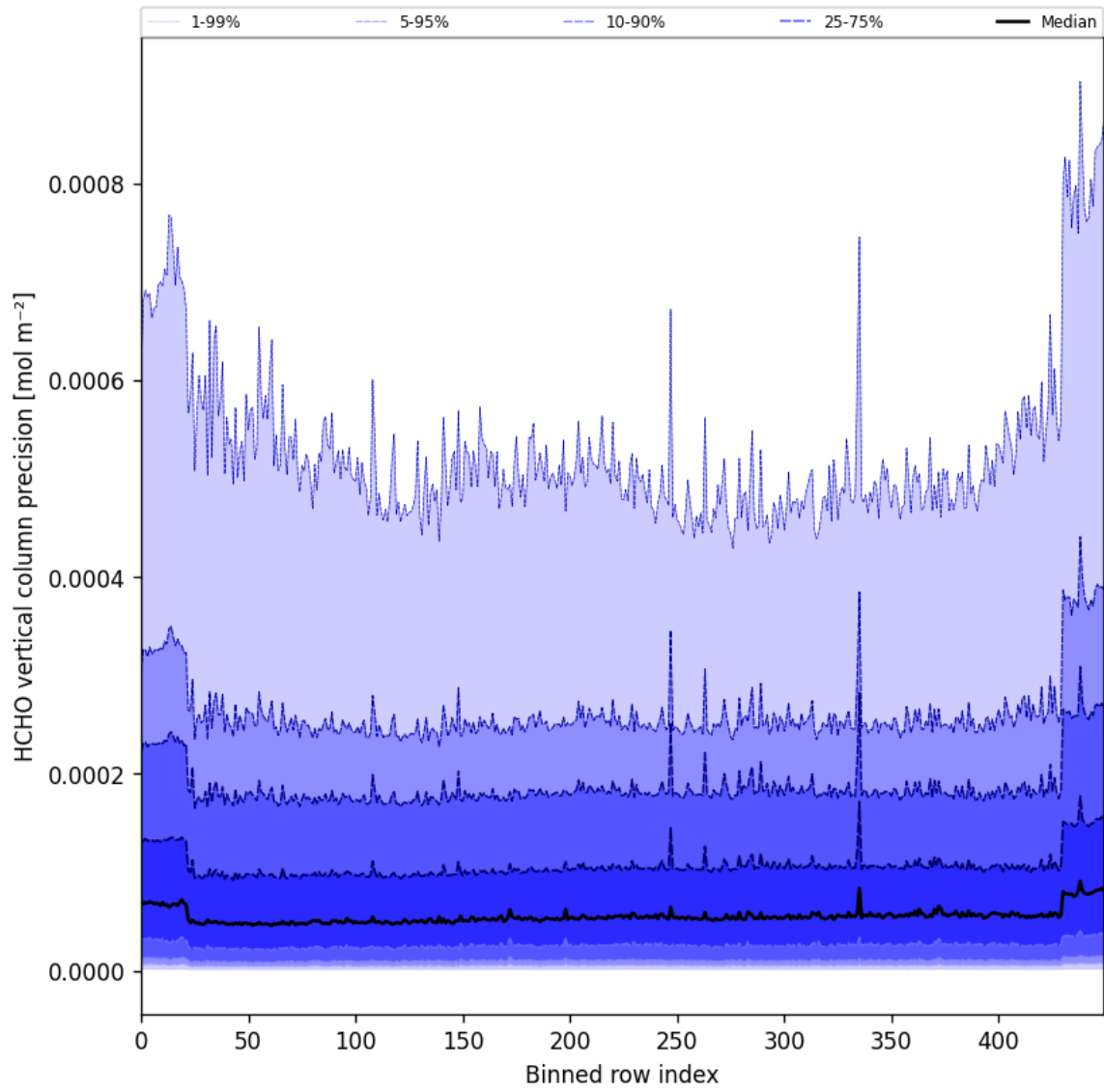
Figure 50: Along track statistics of “HCHO vertical column precision” for 2024-12-12 to 2024-12-14
