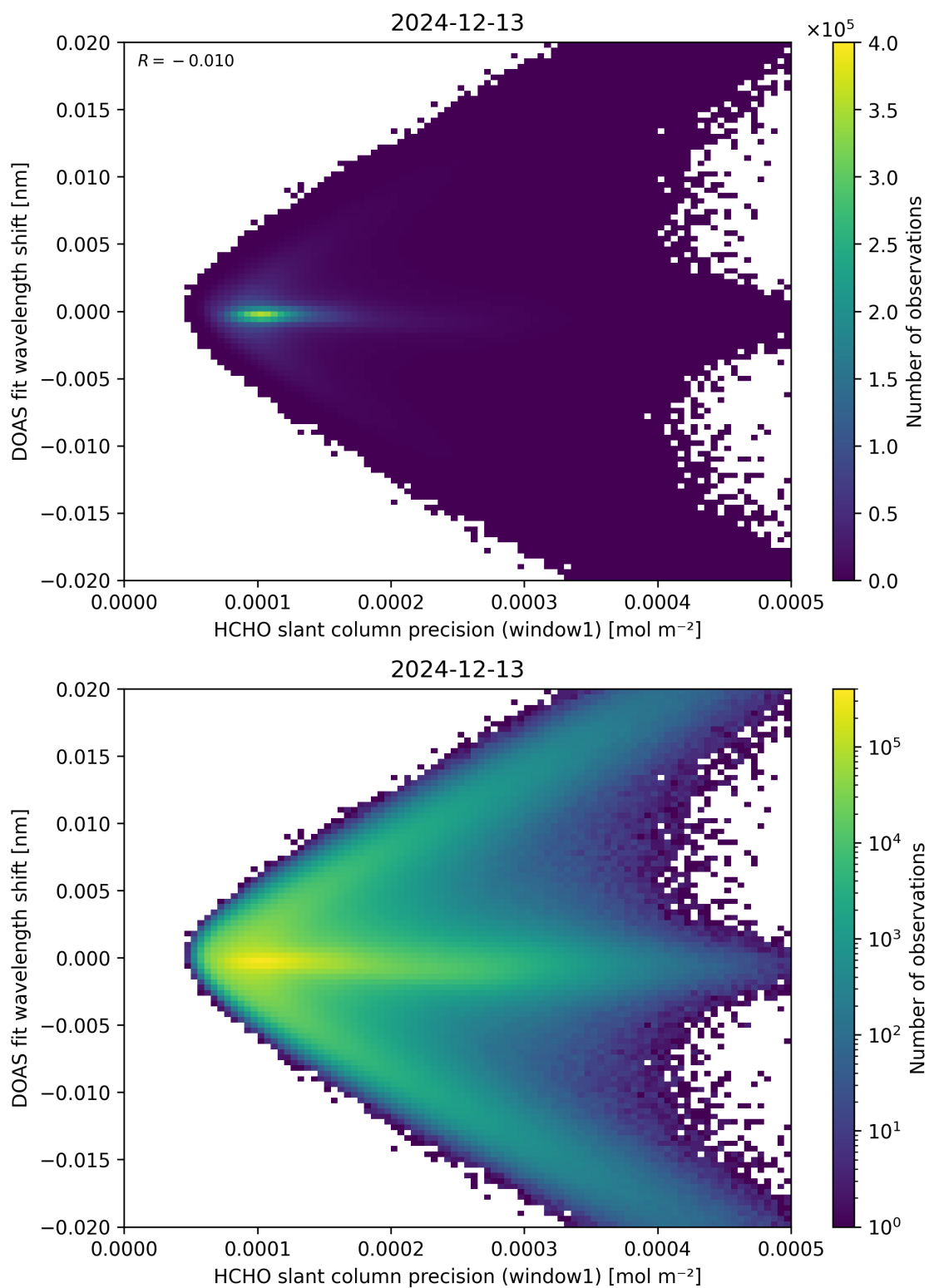
Figure 89: Scatter density plot of “HCHO slant column precision (window1)” against “DOAS fit wavelength shift” for 2024-12-12 to 2024-12-14.
