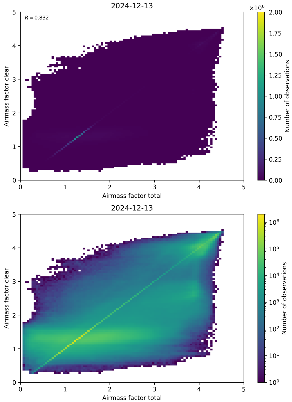
Figure 100: Scatter density plot of “Airmass factor total” against “Airmass factor clear” for 2024-12-12 to 2024-12-14.
