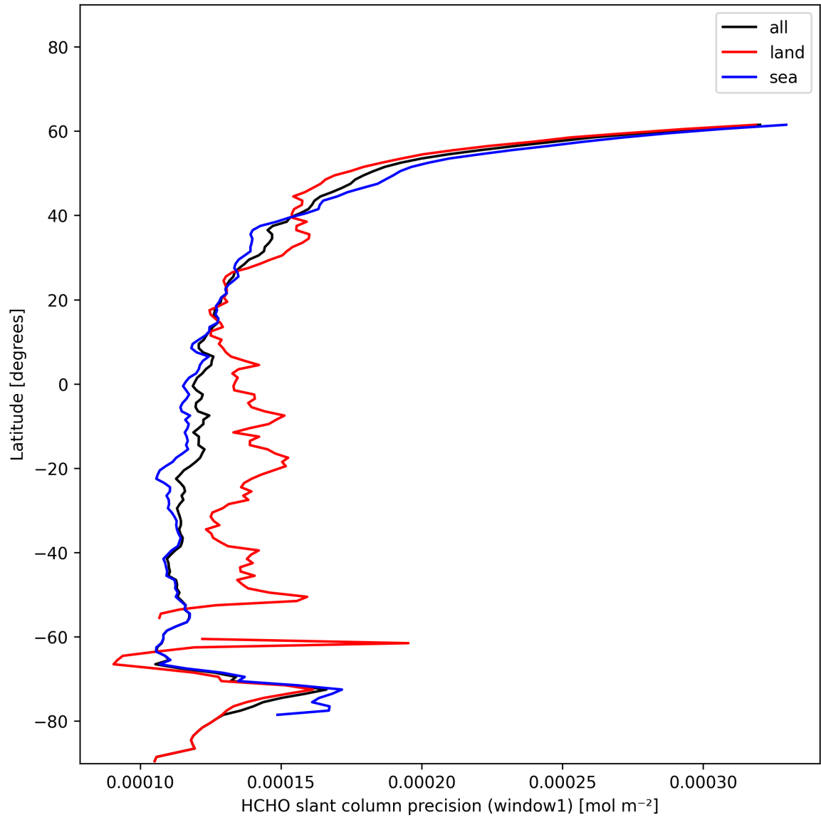
Figure 25: Zonal average of “HCHO slant column precision (window1)” for 2024-12-12 to 2024-12-14.
