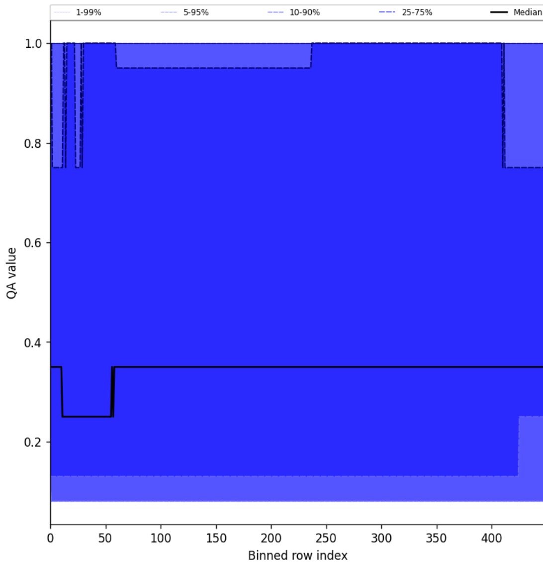
Figure 48: Along track statistics of “QA value” for 2024-12-12 to 2024-12-14
