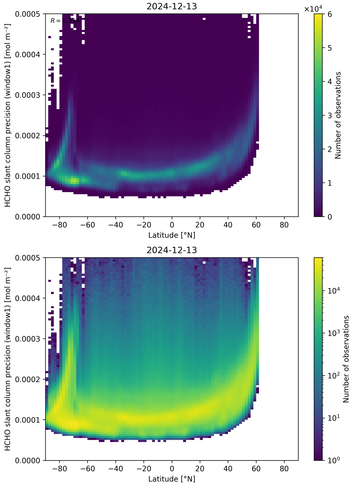
Figure 160: Scatter density plot of “Latitude” against “HCHO slant column precision (window1)” for 2024-12-12 to 2024-12-14.
