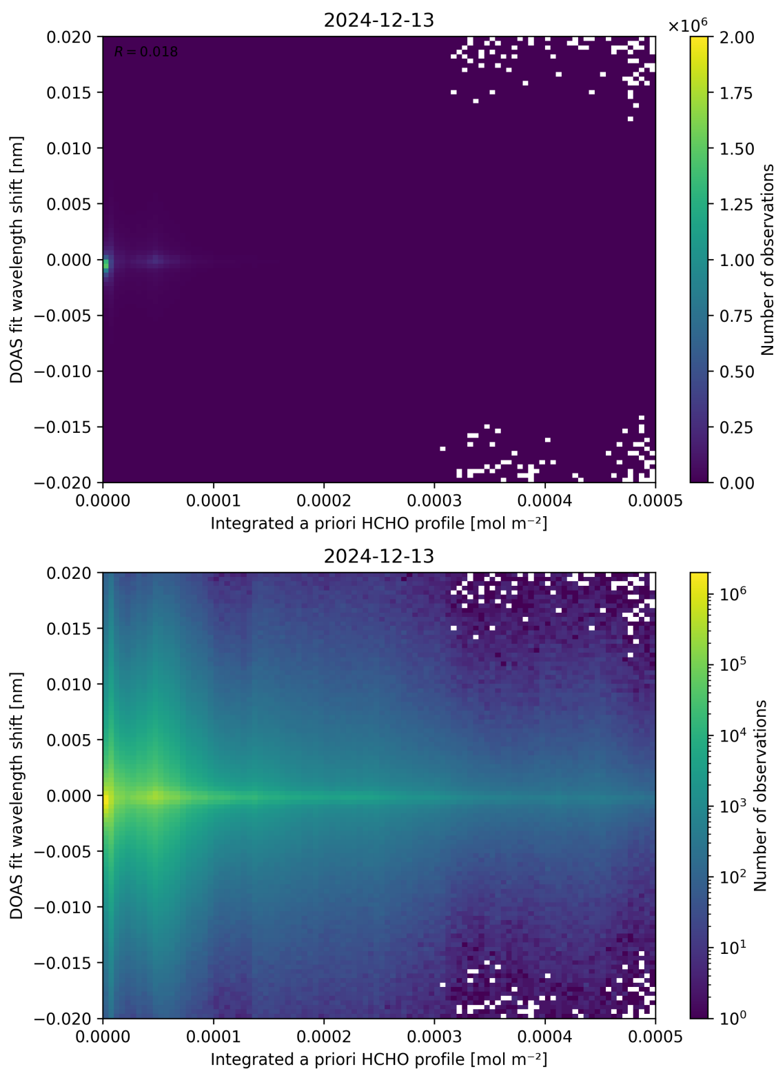
Figure 149: Scatter density plot of “Integrated a priori HCHO profile” against “DOAS fit wavelength shift” for 2024-12-12 to 2024-12-14.
