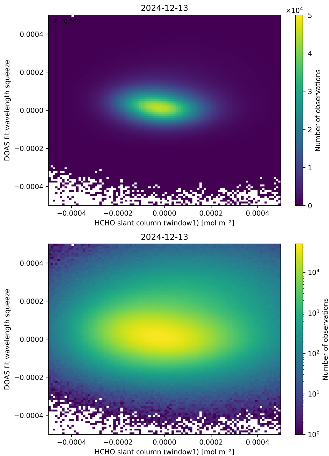
Figure 80: Scatter density plot of “HCHO slant column (window1)” against “DOAS fit wavelength squeeze” for 2024-12-12 to 2024-12-14.
