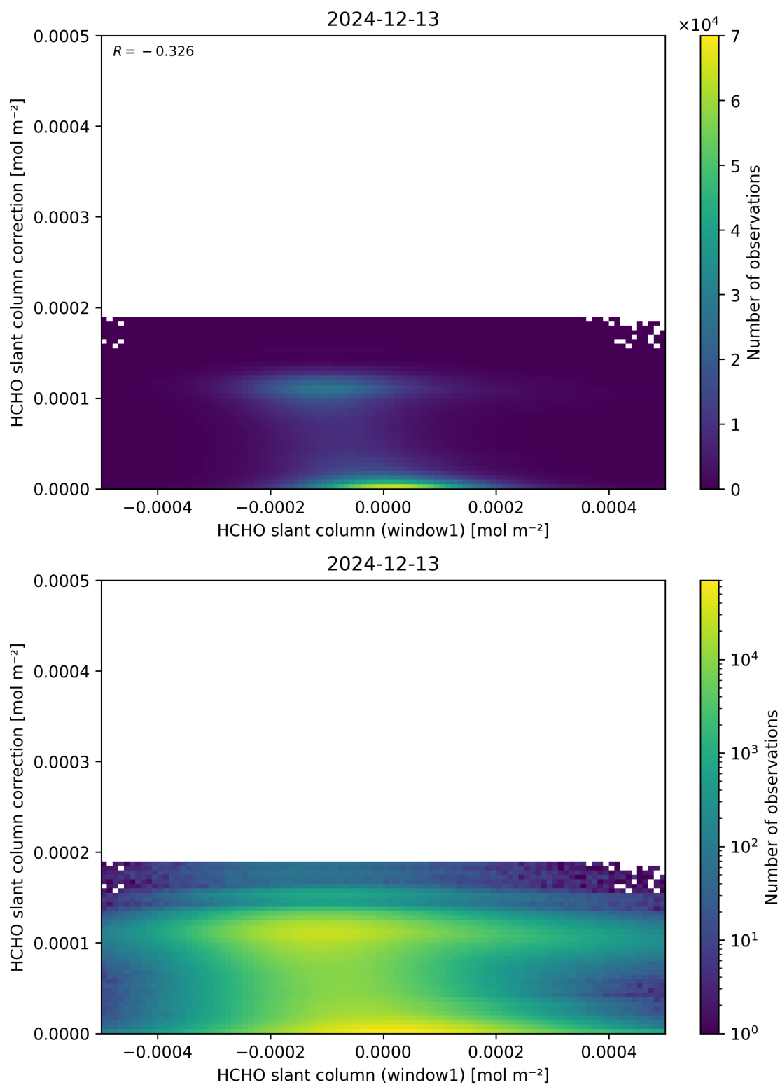
Figure 83: Scatter density plot of “HCHO slant column (window1)” against “HCHO slant column correction” for 2024-12-12 to 2024-12-14.
