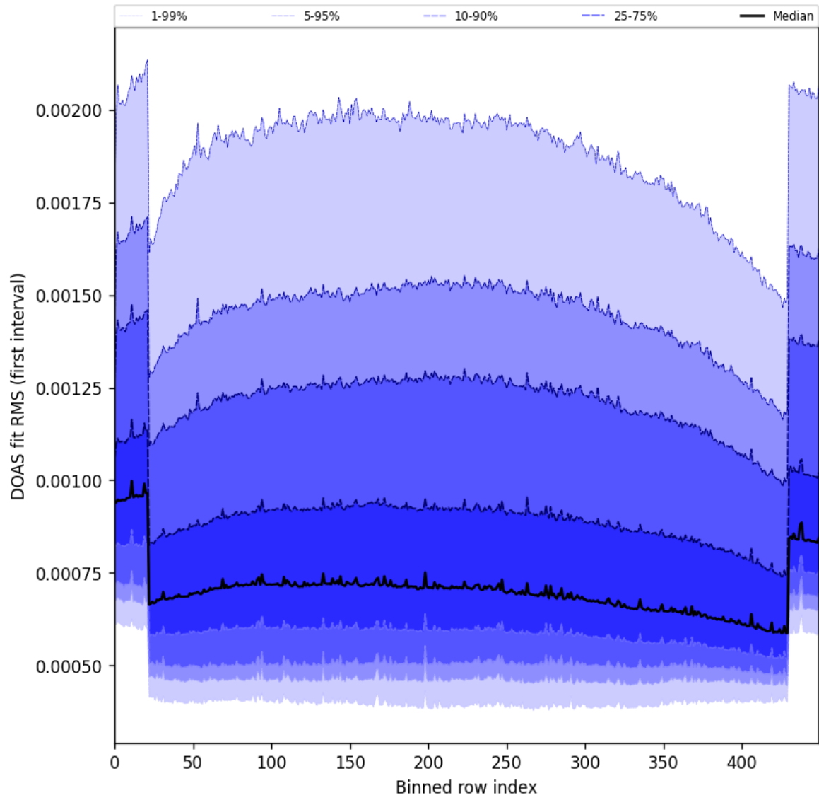
Figure 60: Along track statistics of “DOAS fit RMS (first interval)” for 2024-12-12 to 2024-12-14
