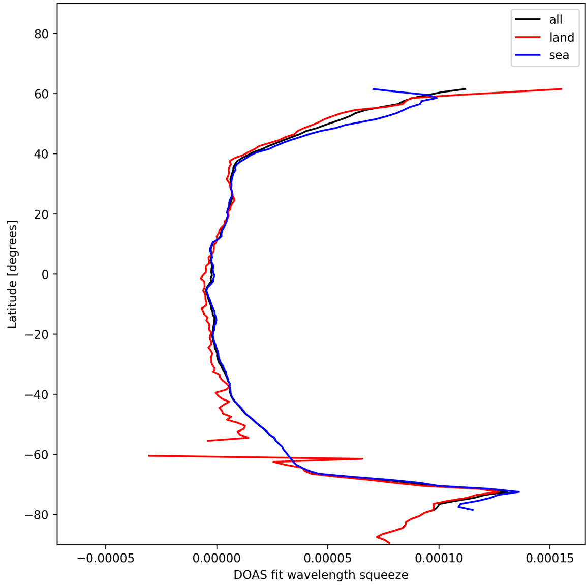
Figure 31: Zonal average of “DOAS fit wavelength squeeze” for 2024-12-12 to 2024-12-14.
