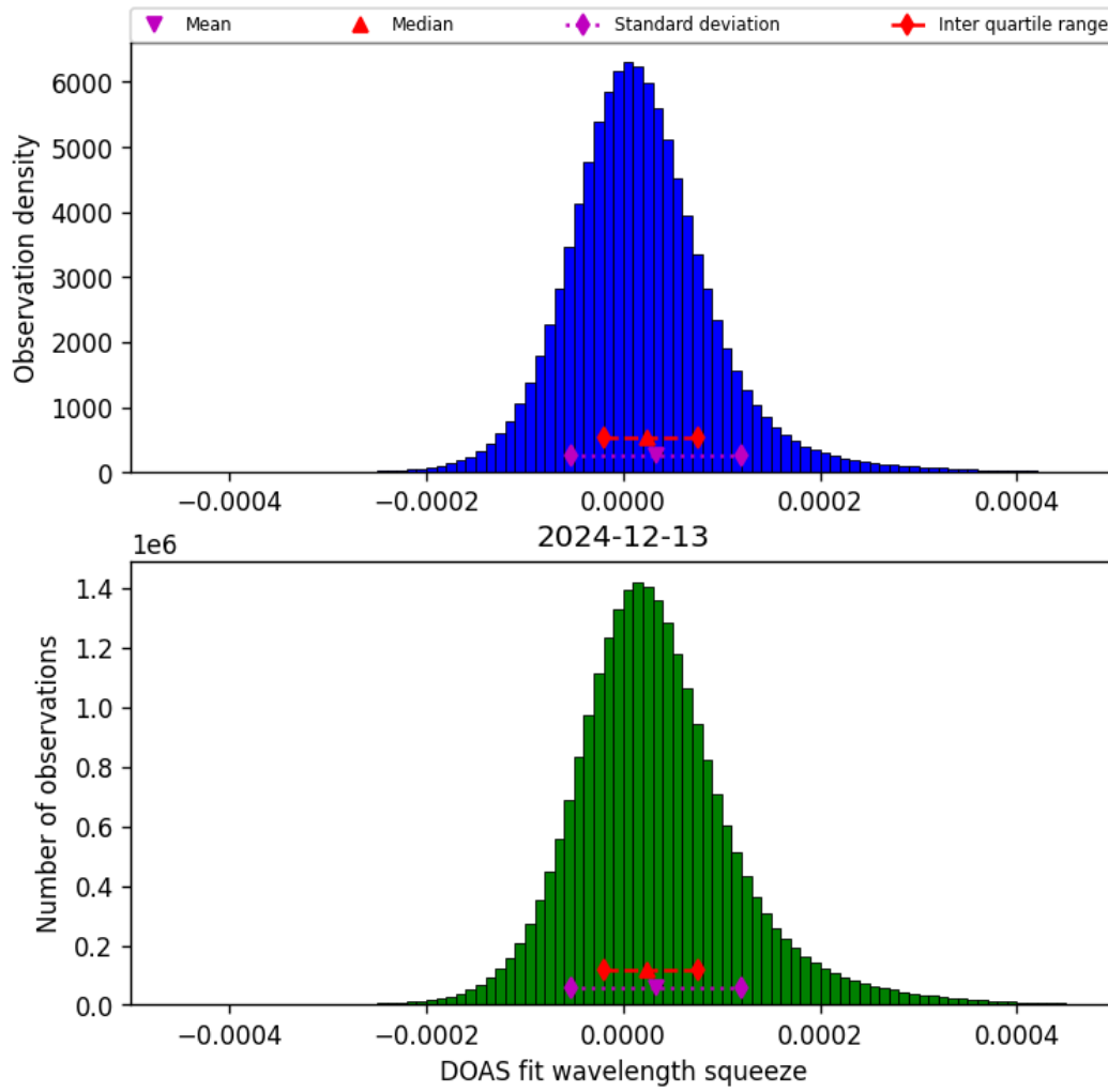
Figure 45: Histogram of “DOAS fit wavelength squeeze” for 2024-12-12 to 2024-12-14
