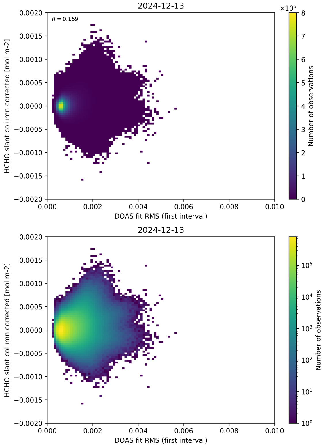
Figure 62: Scatter density plot of “DOAS fit RMS (first interval)” against “HCHO slant column corrected” for 2024-12-12 to 2024-12-14.
