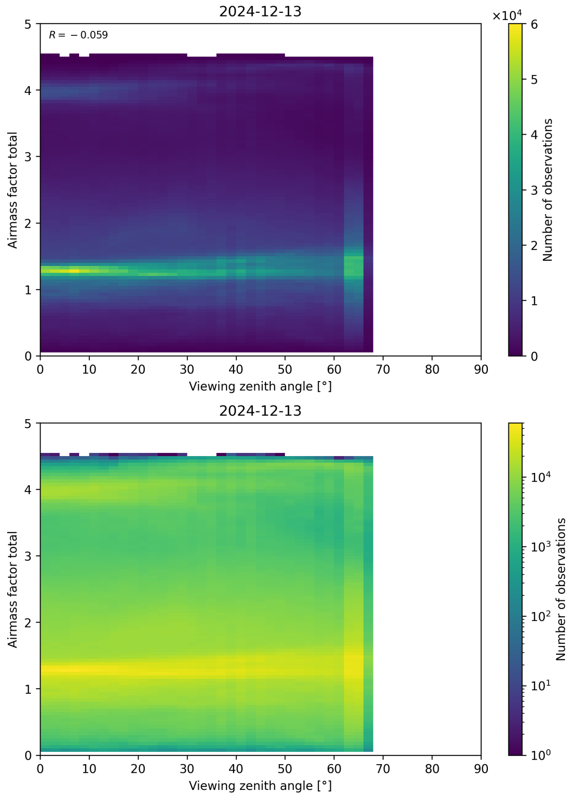
Figure 190: Scatter density plot of “Viewing zenith angle” against “Airmass factor total” for 2024-12-12 to 2024-12-14.
