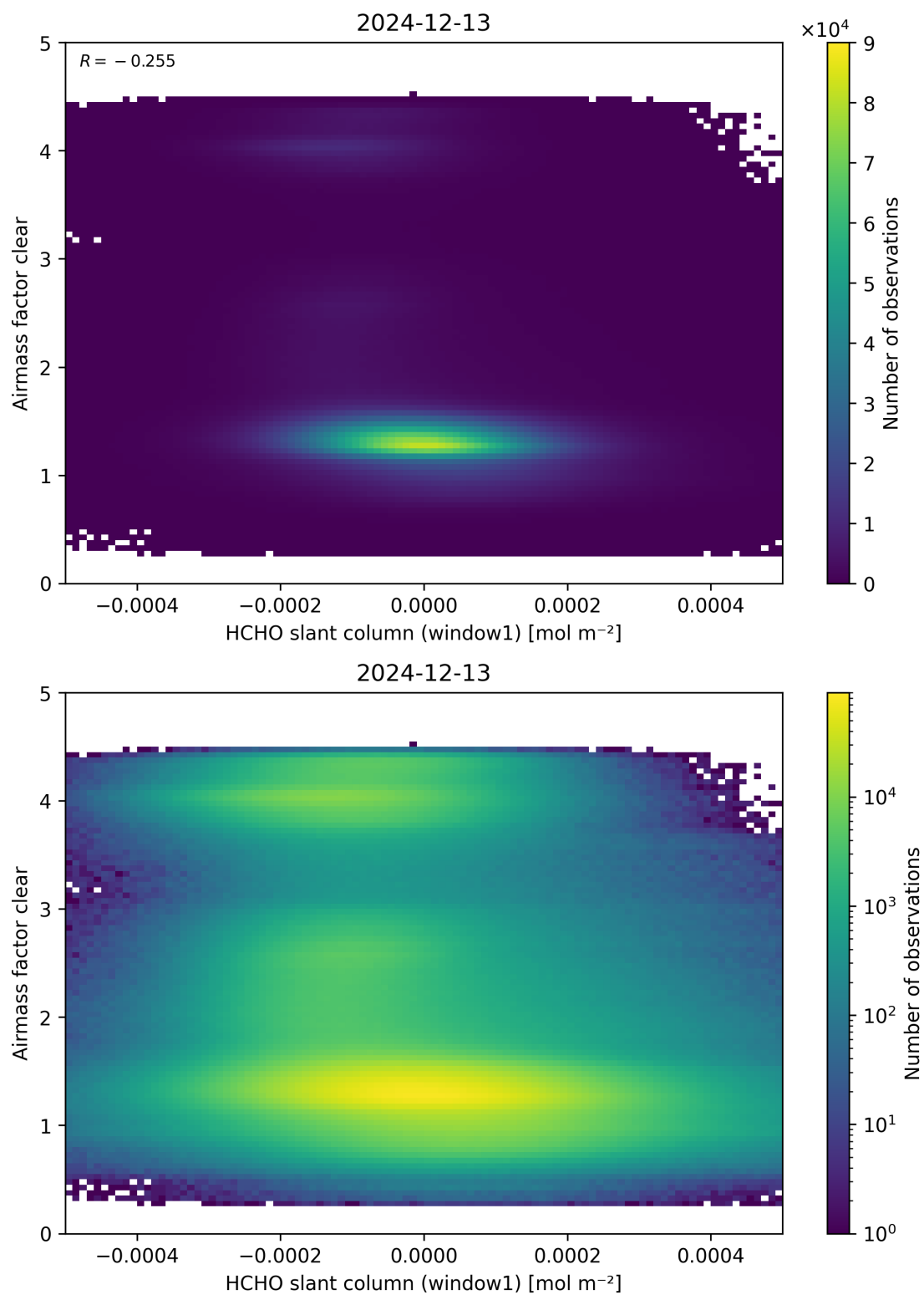
Figure 81: Scatter density plot of “HCHO slant column (window1)” against “Airmass factor clear” for 2024-12-12 to 2024-12-14.
