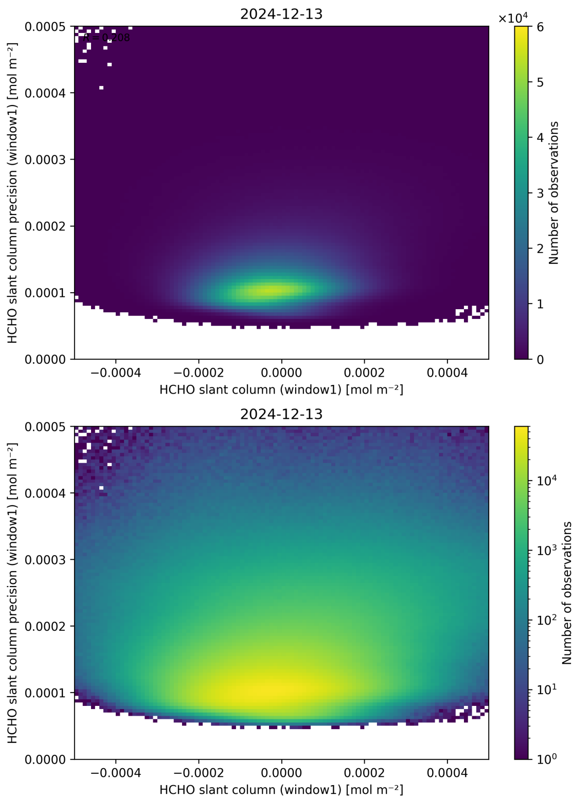
Figure 84: Scatter density plot of “HCHO slant column (window1)” against “HCHO slant column precision (window1)” for 2024-12-12 to 2024-12-14.
