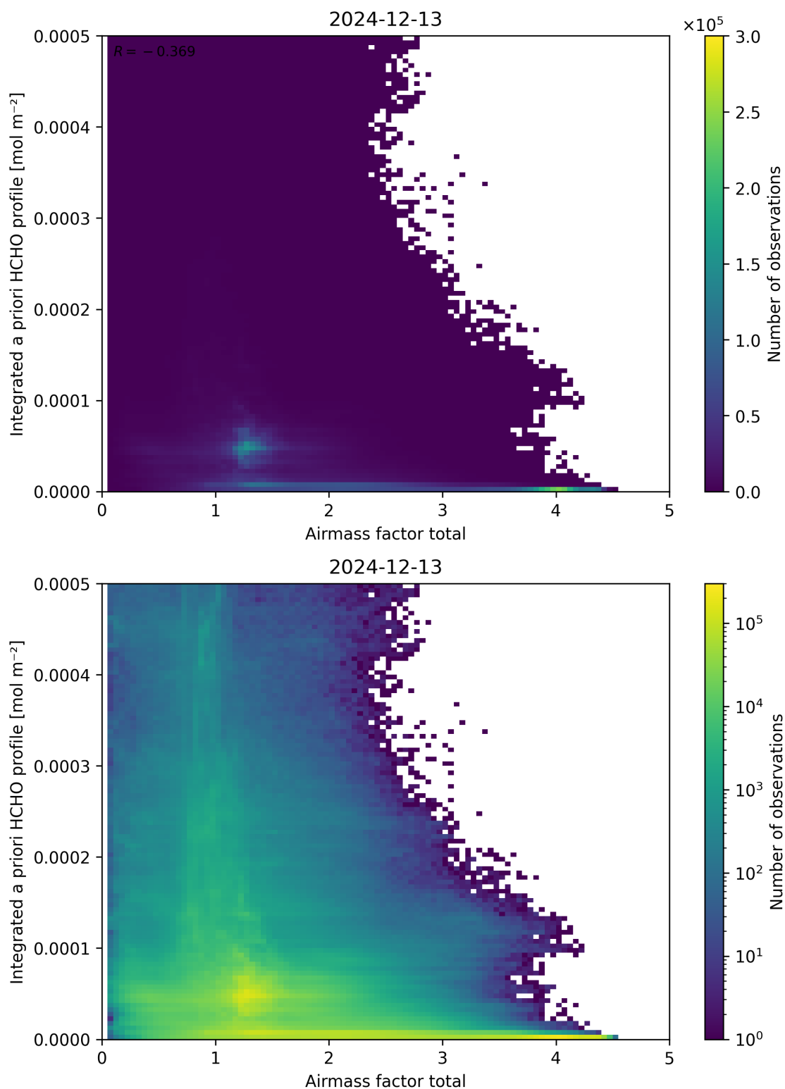
Figure 104: Scatter density plot of “Airmass factor total” against “Integrated a priori HCHO profile” for 2024-12-12 to 2024-12-14.
