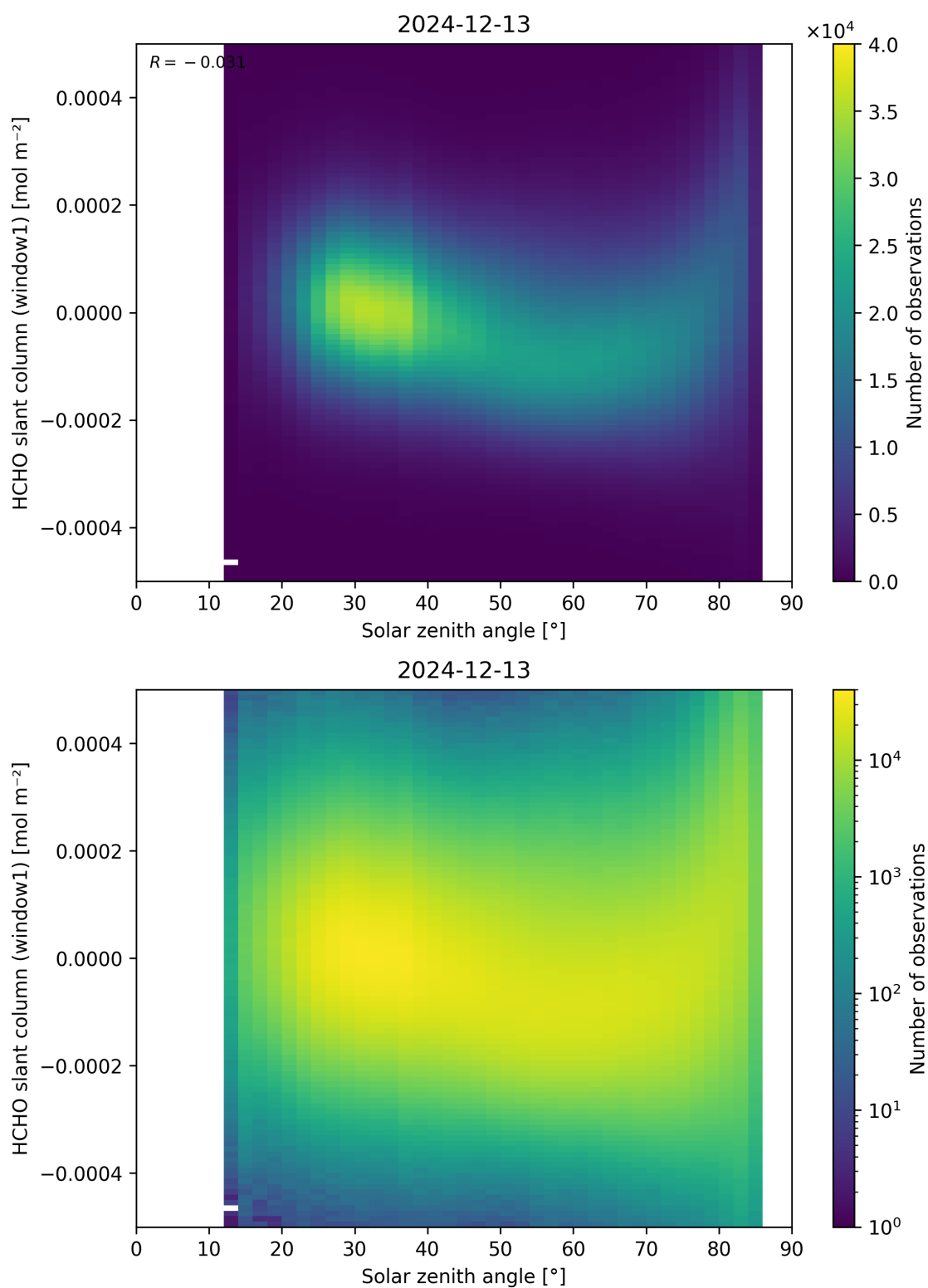
Figure 173: Scatter density plot of “Solar zenith angle” against “HCHO slant column (window1)” for 2024-12-12 to 2024-12-14.
