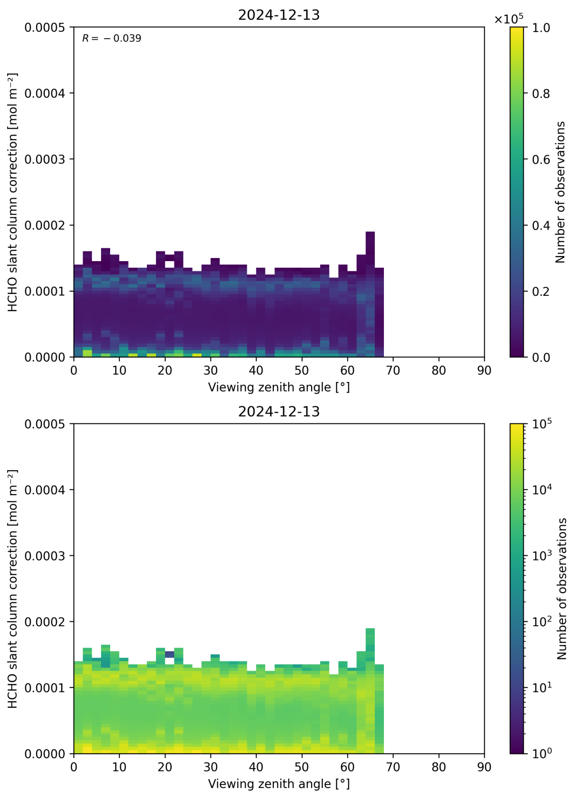
Figure 187: Scatter density plot of “Viewing zenith angle” against “HCHO slant column correction” for 2024-12-12 to 2024-12-14.
