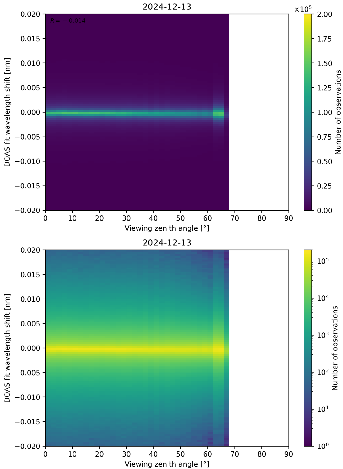
Figure 183: Scatter density plot of “Viewing zenith angle” against “DOAS fit wavelength shift” for 2024-12-12 to 2024-12-14.
