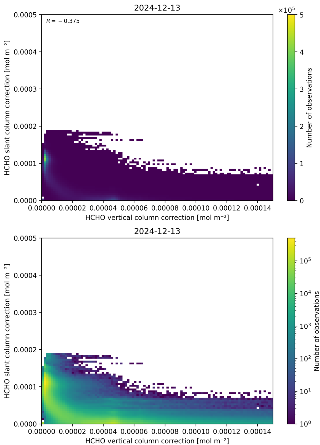
Figure 117: Scatter density plot of “HCHO vertical column correction” against “HCHO slant column correction” for 2024-12-12 to 2024-12-14.
