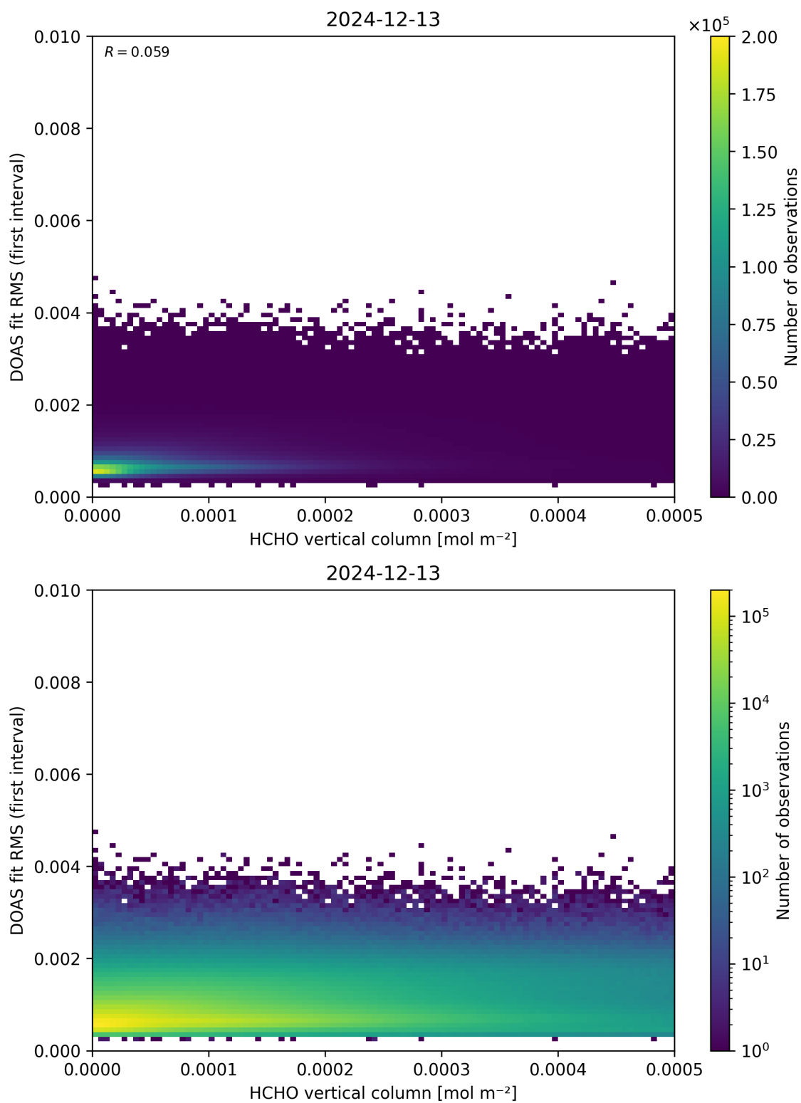
Figure 123: Scatter density plot of “HCHO vertical column” against “DOAS fit RMS (first interval)” for 2024-12-12 to 2024-12-14.
