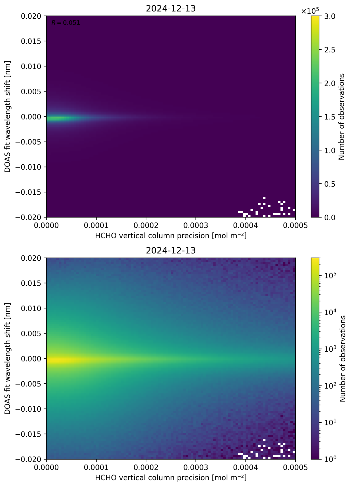
Figure 137: Scatter density plot of “HCHO vertical column precision” against “DOAS fit wavelength shift” for 2024-12-12 to 2024-12-14.
