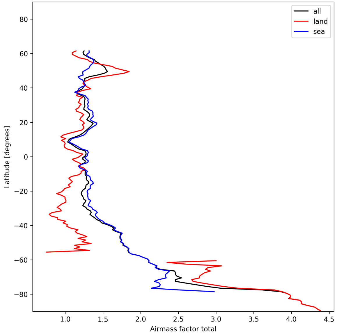
Figure 26: Zonal average of “Airmass factor total” for 2024-12-12 to 2024-12-14.
