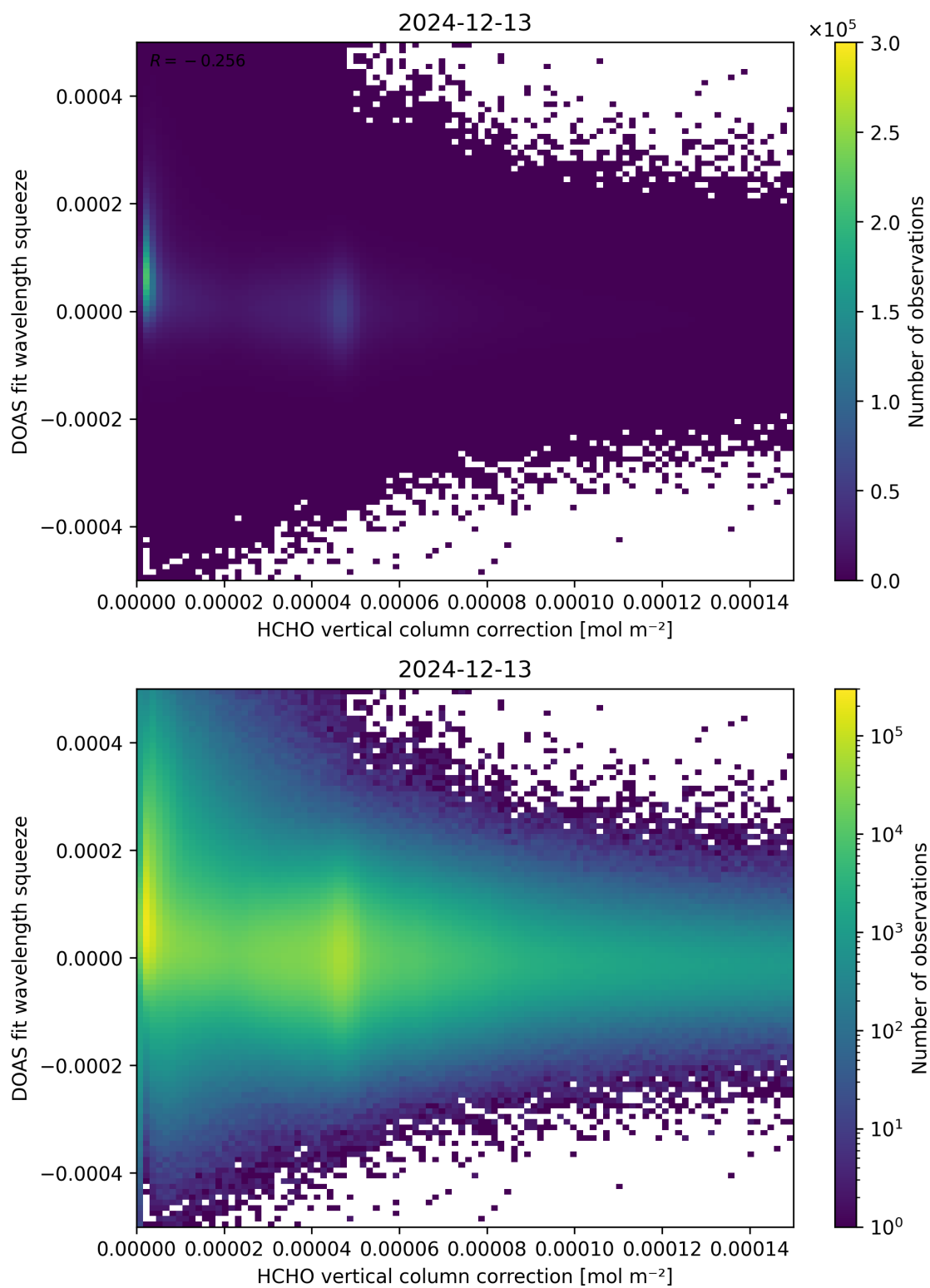
Figure 114: Scatter density plot of “HCHO vertical column correction” against “DOAS fit wavelength squeeze” for 2024-12-12 to 2024-12-14.
