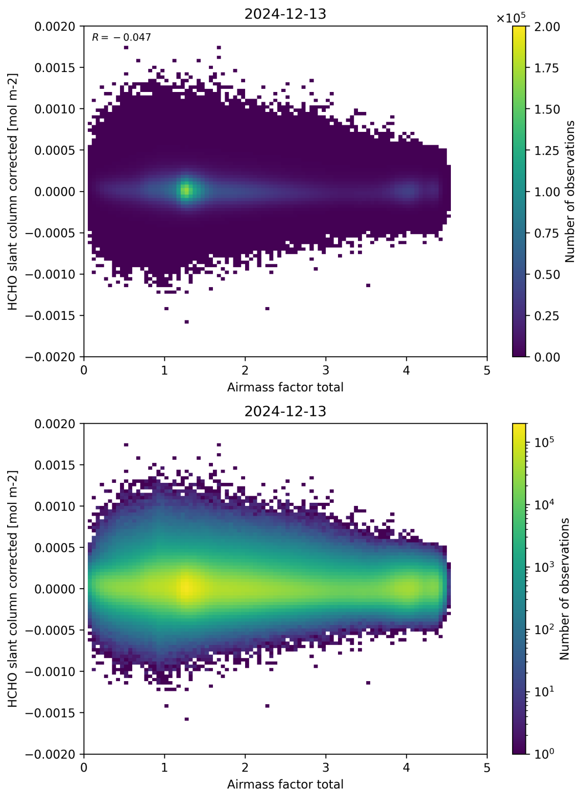
Figure 101: Scatter density plot of “Airmass factor total” against “HCHO slant column corrected” for 2024-12-12 to 2024-12-14.
