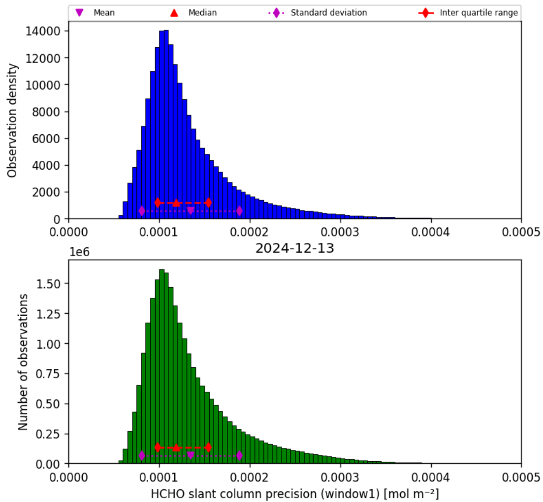
Figure 39: Histogram of “HCHO slant column precision (window1)” for 2024-12-12 to 2024-12-14
