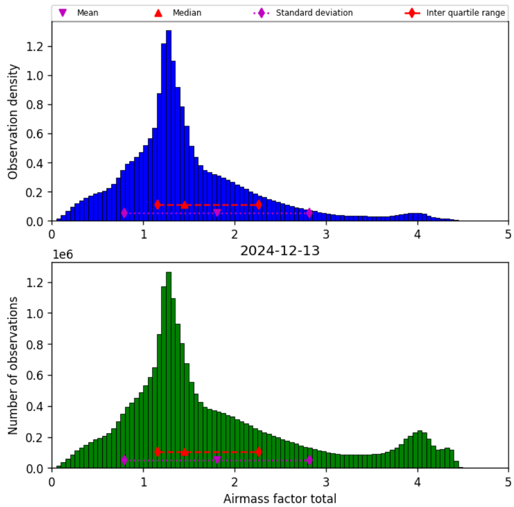
Figure 40: Histogram of “Airmass factor total” for 2024-12-12 to 2024-12-14
