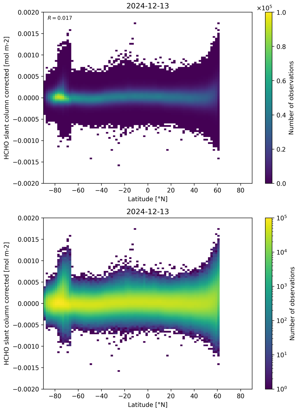
Figure 157: Scatter density plot of “Latitude” against “HCHO slant column corrected” for 2024-12-12 to 2024-12-14.
