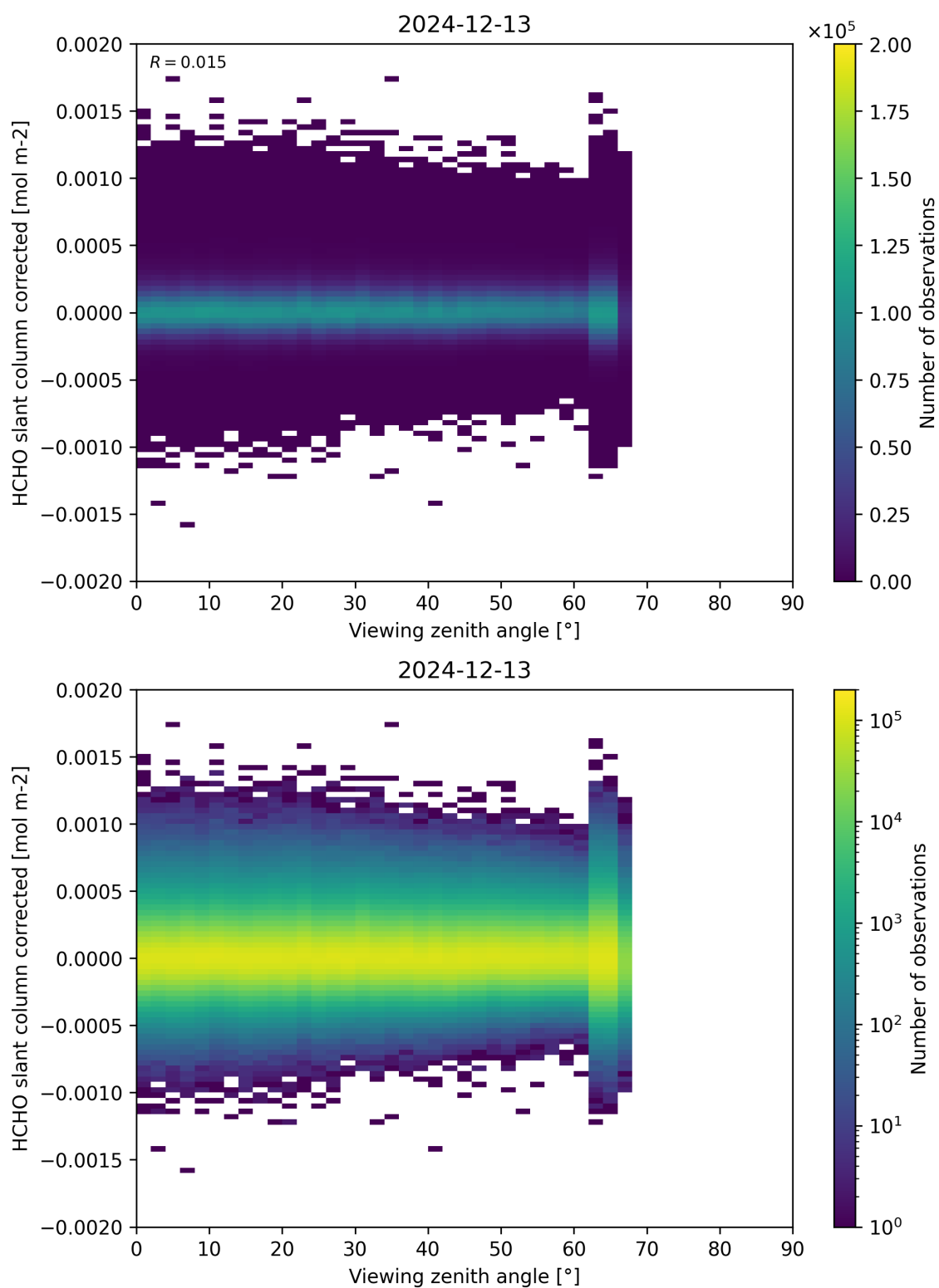
Figure 186: Scatter density plot of “Viewing zenith angle” against “HCHO slant column corrected” for 2024-12-12 to 2024-12-14.
