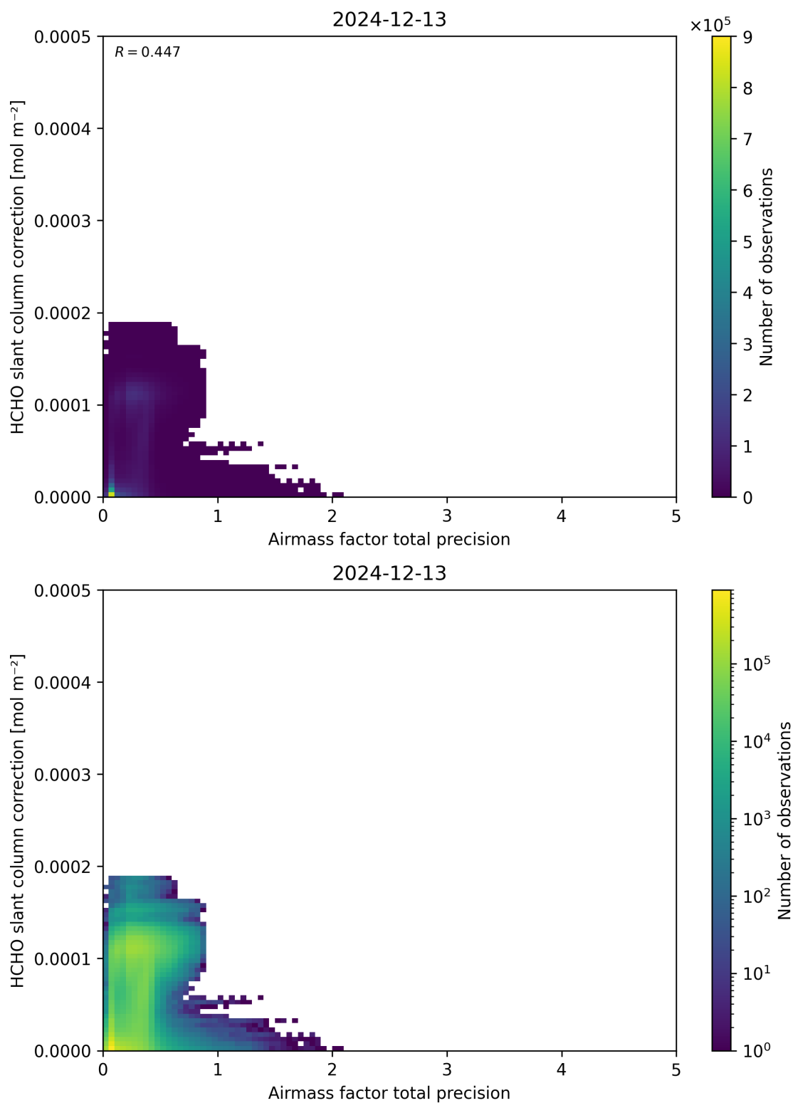
Figure 110: Scatter density plot of “Airmass factor total precision” against “HCHO slant column correction” for 2024-12-12 to 2024-12-14.
