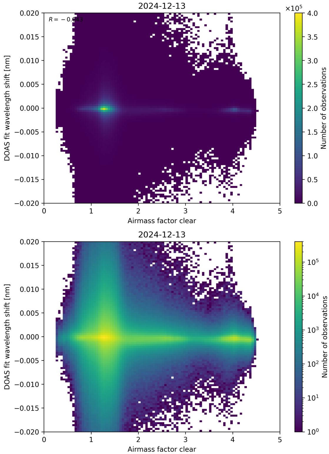
Figure 72: Scatter density plot of “Airmass factor clear” against “DOAS fit wavelength shift” for 2024-12-12 to 2024-12-14.
