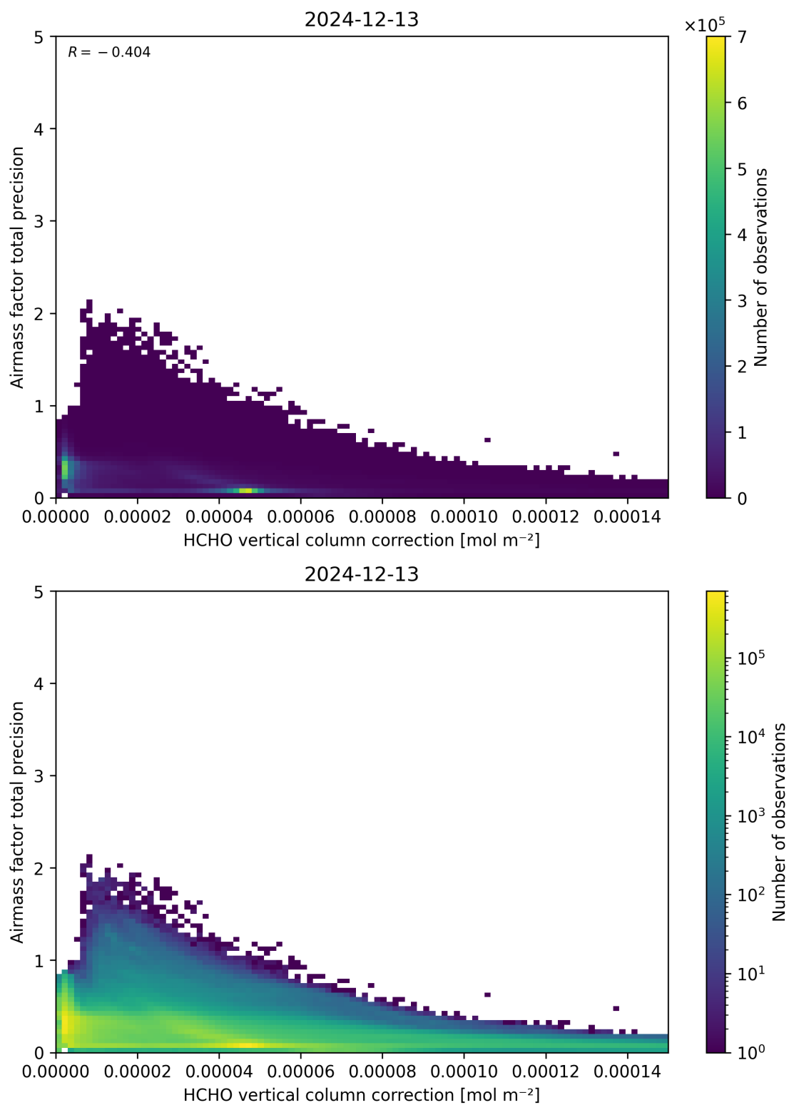
Figure 121: Scatter density plot of “HCHO vertical column correction” against “Airmass factor total precision” for 2024-12-12 to 2024-12-14.
