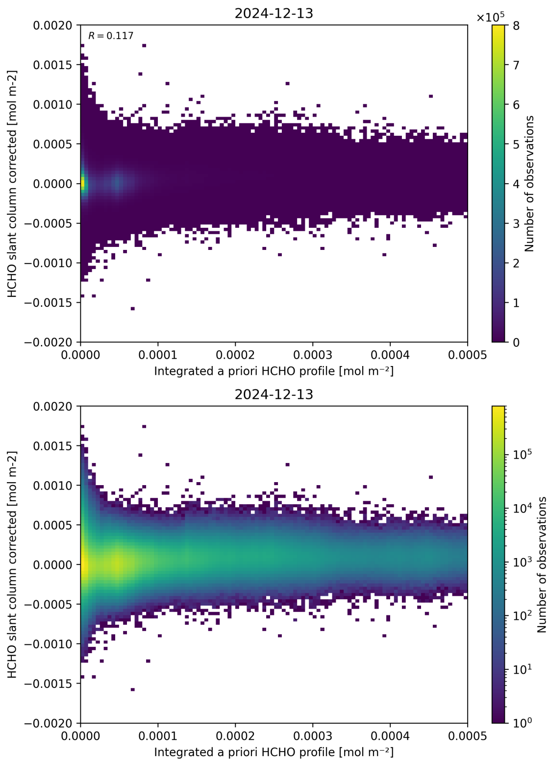
Figure 151: Scatter density plot of “Integrated a priori HCHO profile” against “HCHO slant column corrected” for 2024-12-12 to 2024-12-14.
