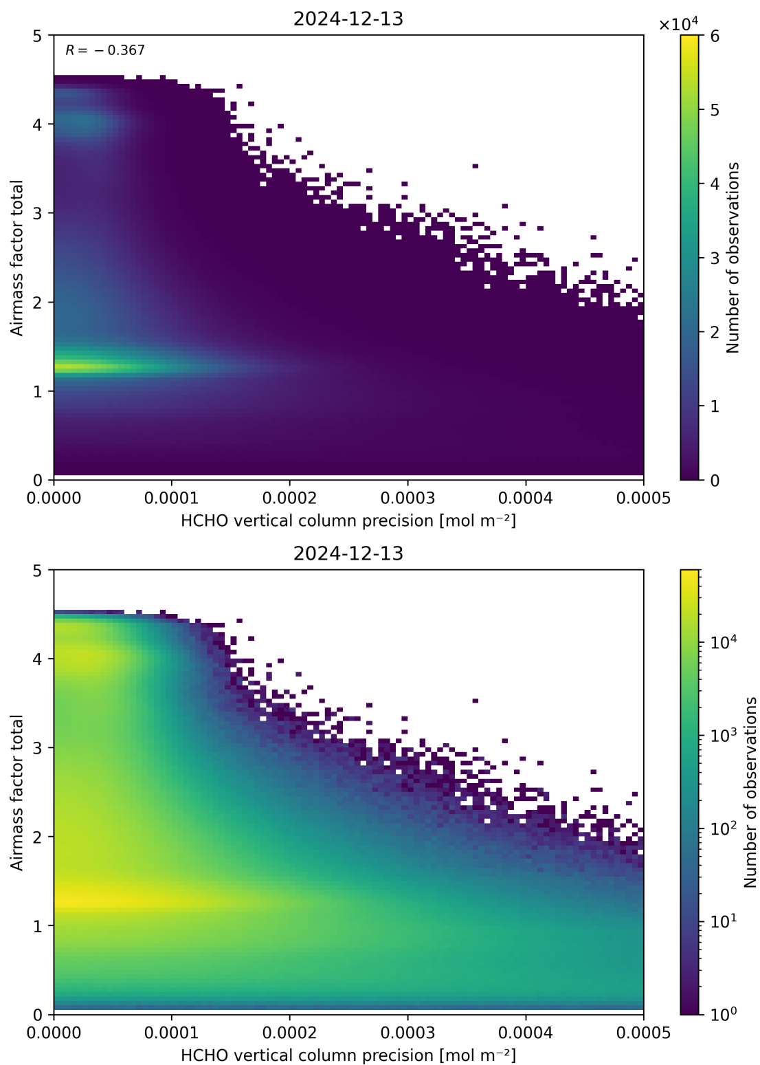
Figure 144: Scatter density plot of “HCHO vertical column precision” against “Airmass factor total” for 2024-12-12 to 2024-12-14.
