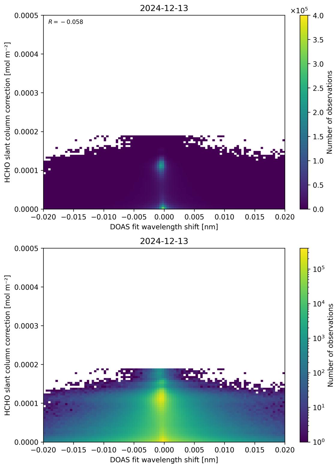
Figure 67: Scatter density plot of “DOAS fit wavelength shift” against “HCHO slant column correction” for 2024-12-12 to 2024-12-14.
