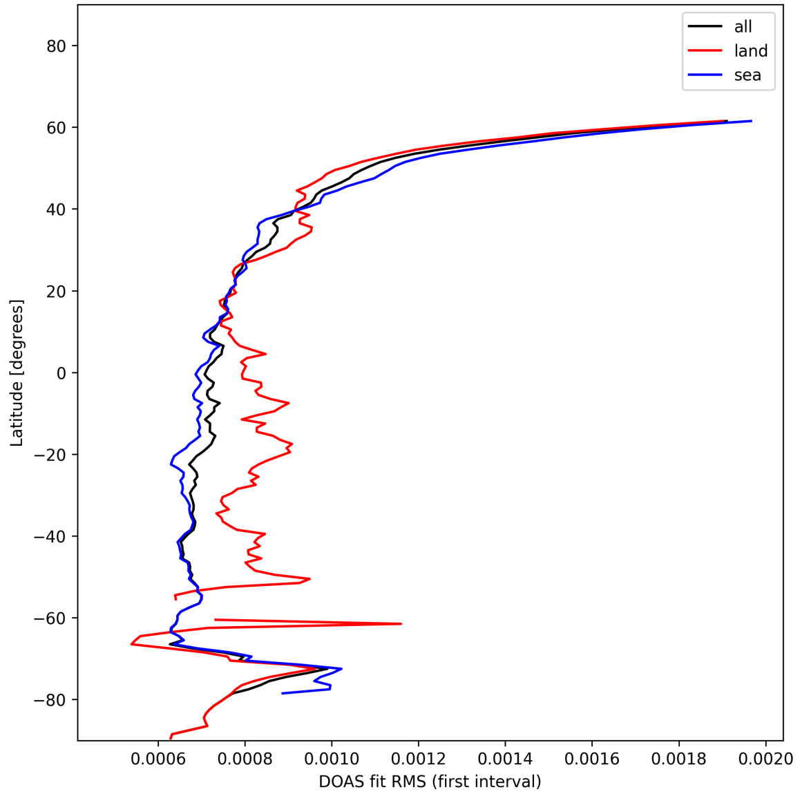
Figure 32: Zonal average of “DOAS fit RMS (first interval)” for 2024-12-12 to 2024-12-14.
