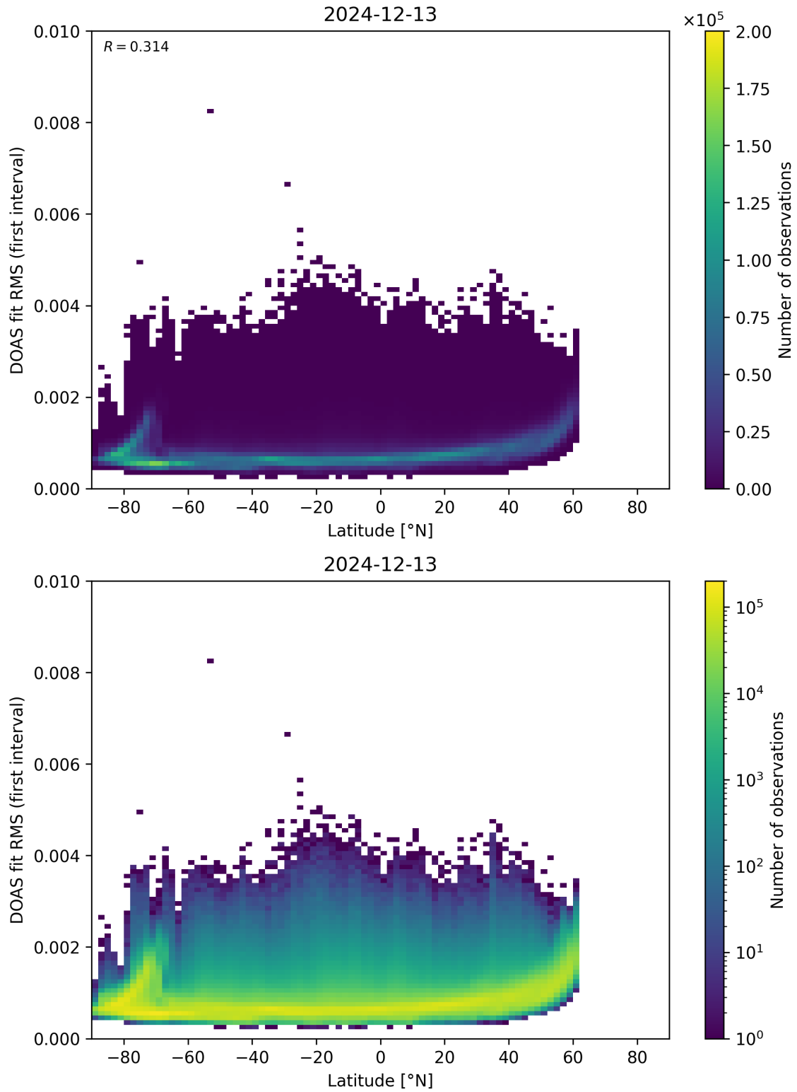
Figure 153: Scatter density plot of “Latitude” against “DOAS fit RMS (first interval)” for 2024-12-12 to 2024-12-14.
