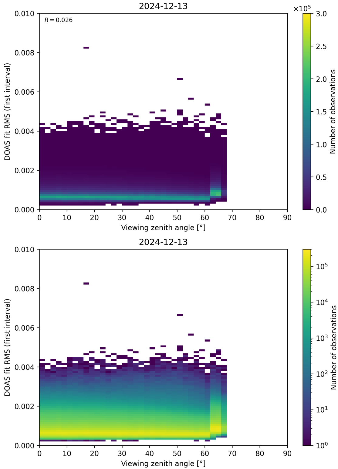
Figure 182: Scatter density plot of “Viewing zenith angle” against “DOAS fit RMS (first interval)” for 2024-12-12 to 2024-12-14.
