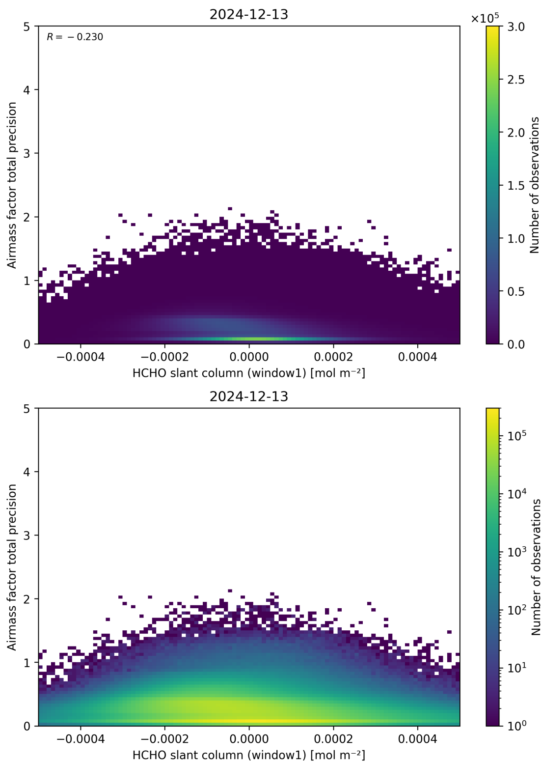
Figure 86: Scatter density plot of “HCHO slant column (window1)” against “Airmass factor total precision” for 2024-12-12 to 2024-12-14.
