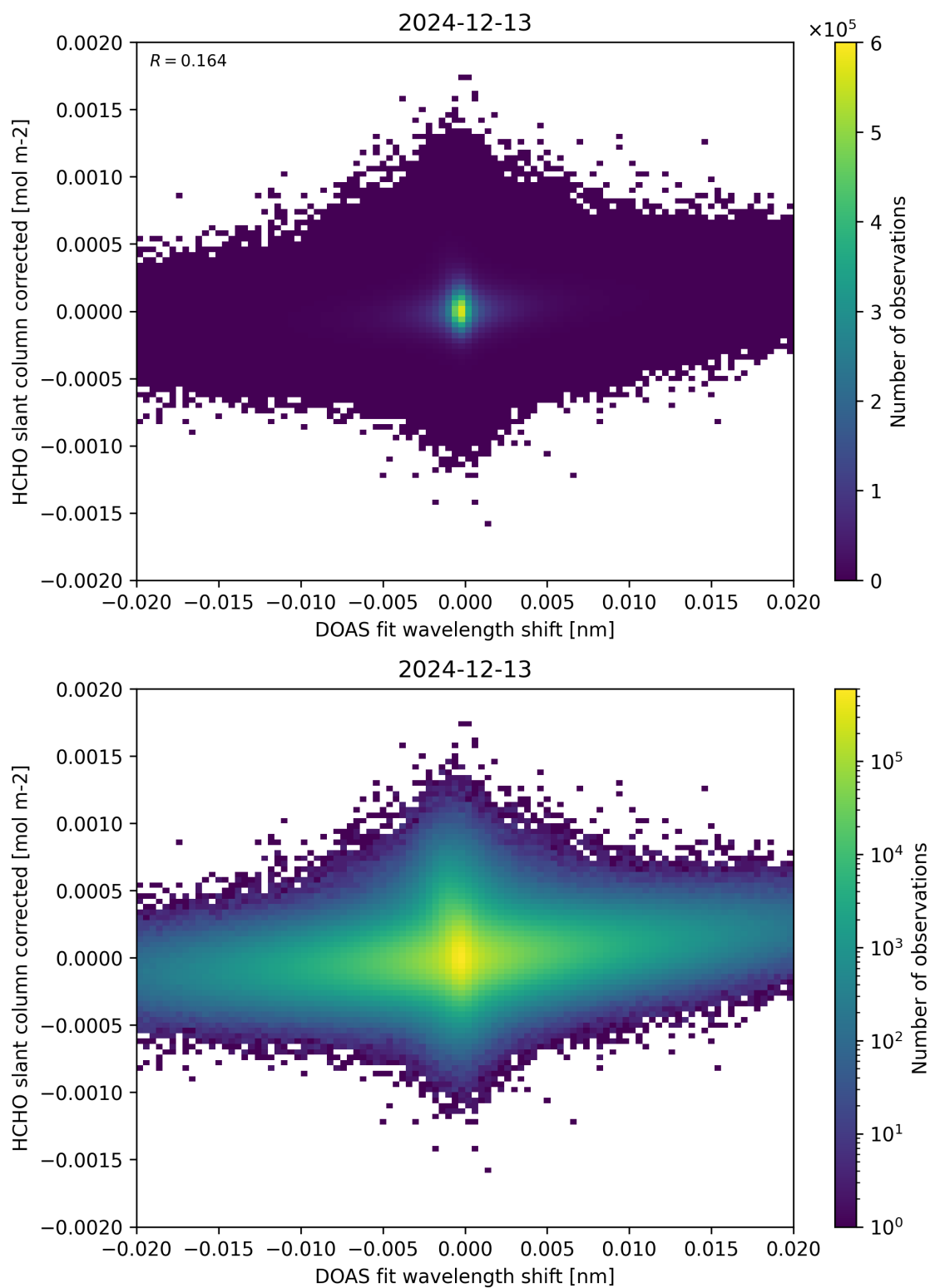
Figure 66: Scatter density plot of “DOAS fit wavelength shift” against “HCHO slant column corrected” for 2024-12-12 to 2024-12-14.
