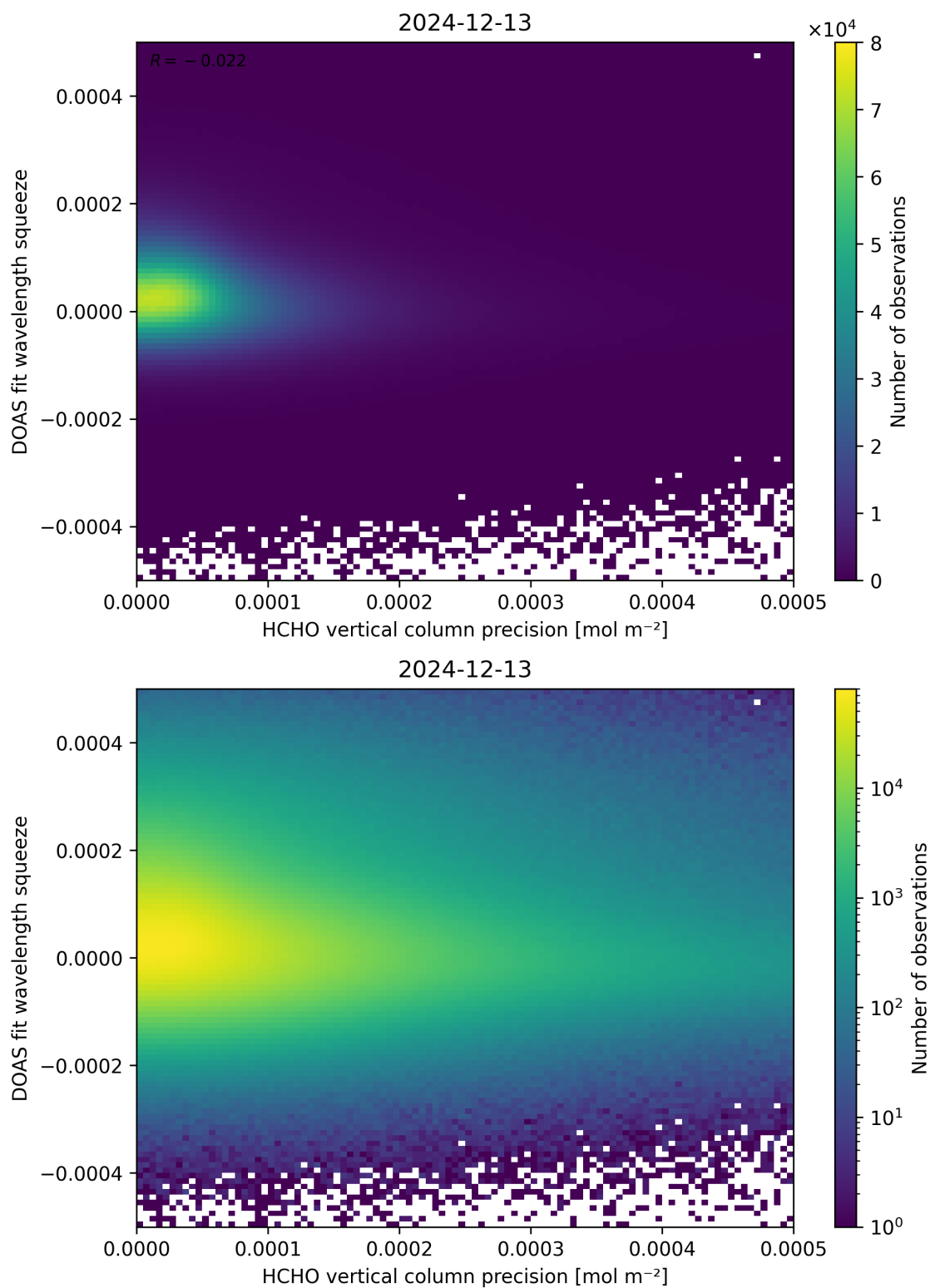
Figure 138: Scatter density plot of “HCHO vertical column precision” against “DOAS fit wavelength squeeze” for 2024-12-12 to 2024-12-14.
