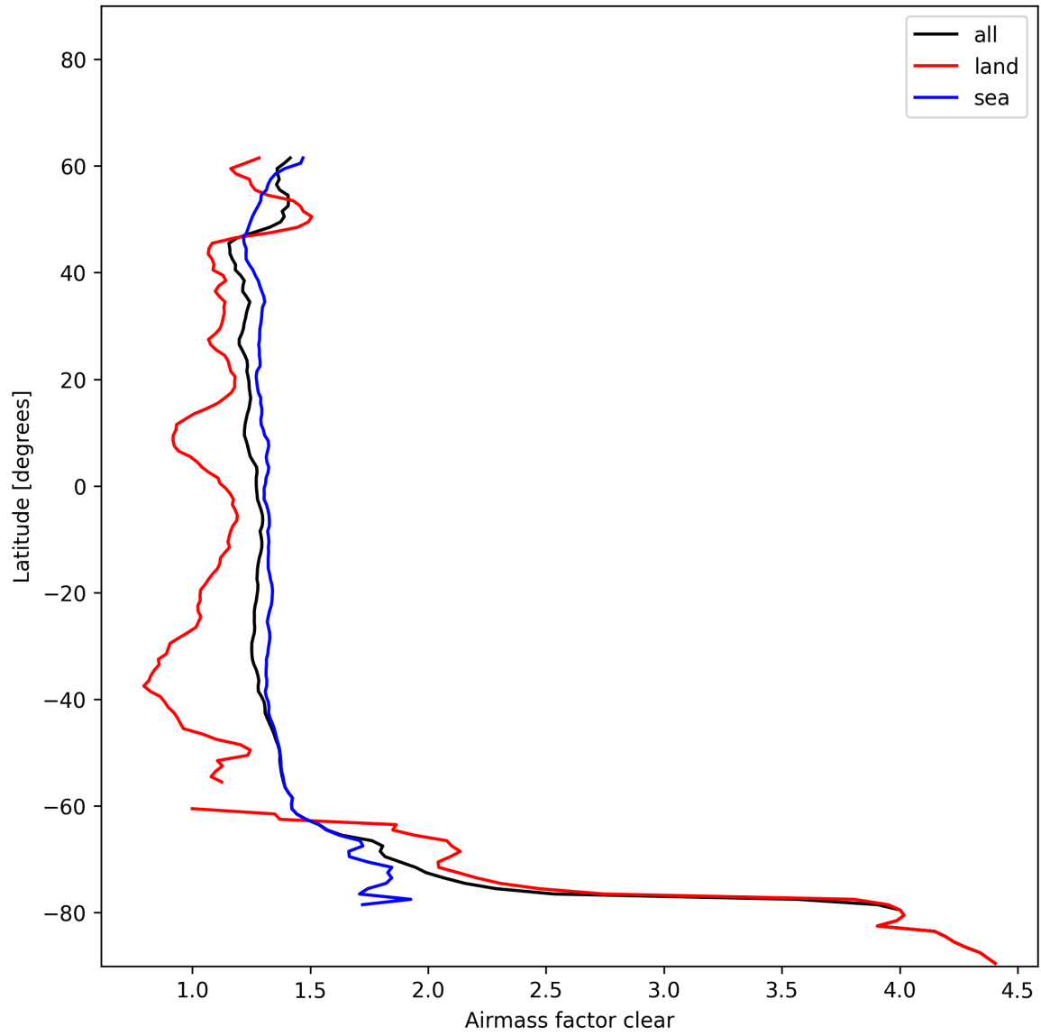
Figure 28: Zonal average of “Airmass factor clear” for 2024-12-12 to 2024-12-14.
