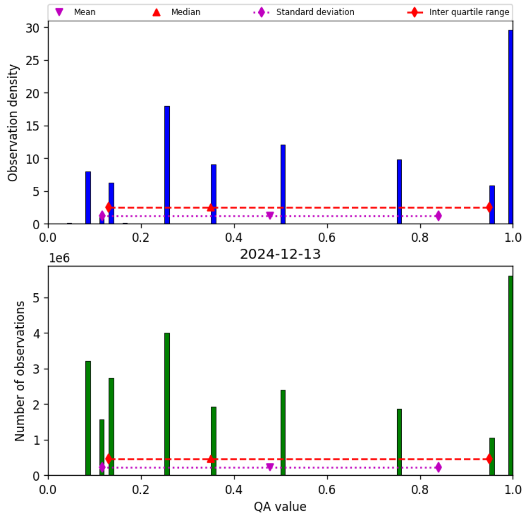
Figure 34: Histogram of “QA value” for 2024-12-12 to 2024-12-14
