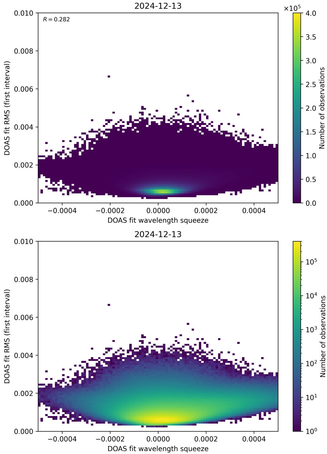
Figure 68: Scatter density plot of “DOAS fit wavelength squeeze” against “DOAS fit RMS (first interval)” for 2024-12-12 to 2024-12-14.
