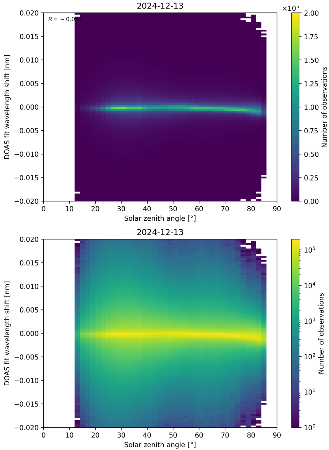
Figure 168: Scatter density plot of “Solar zenith angle” against “DOAS fit wavelength shift” for 2024-12-12 to 2024-12-14.
