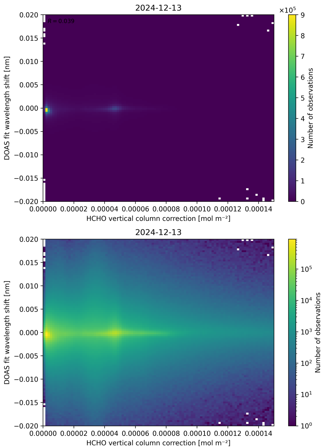
Figure 113: Scatter density plot of “HCHO vertical column correction” against “DOAS fit wavelength shift” for 2024-12-12 to 2024-12-14.
