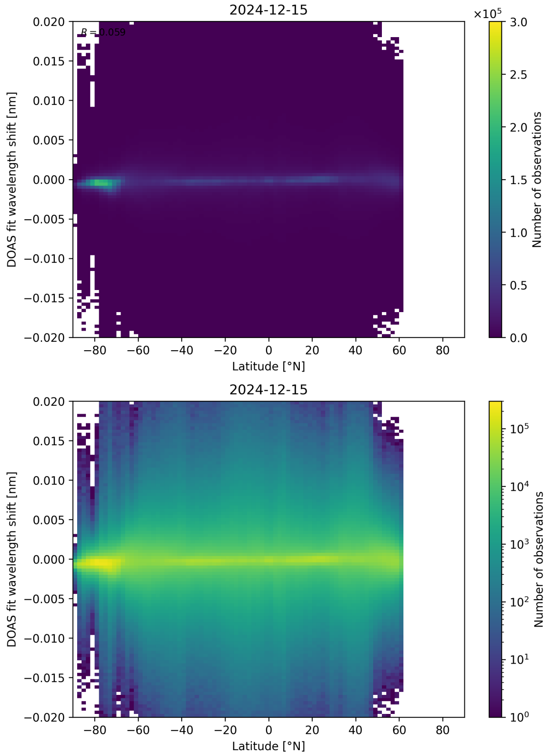
Figure 154: Scatter density plot of “Latitude” against “DOAS fit wavelength shift” for 2024-12-14 to 2024-12-16.
