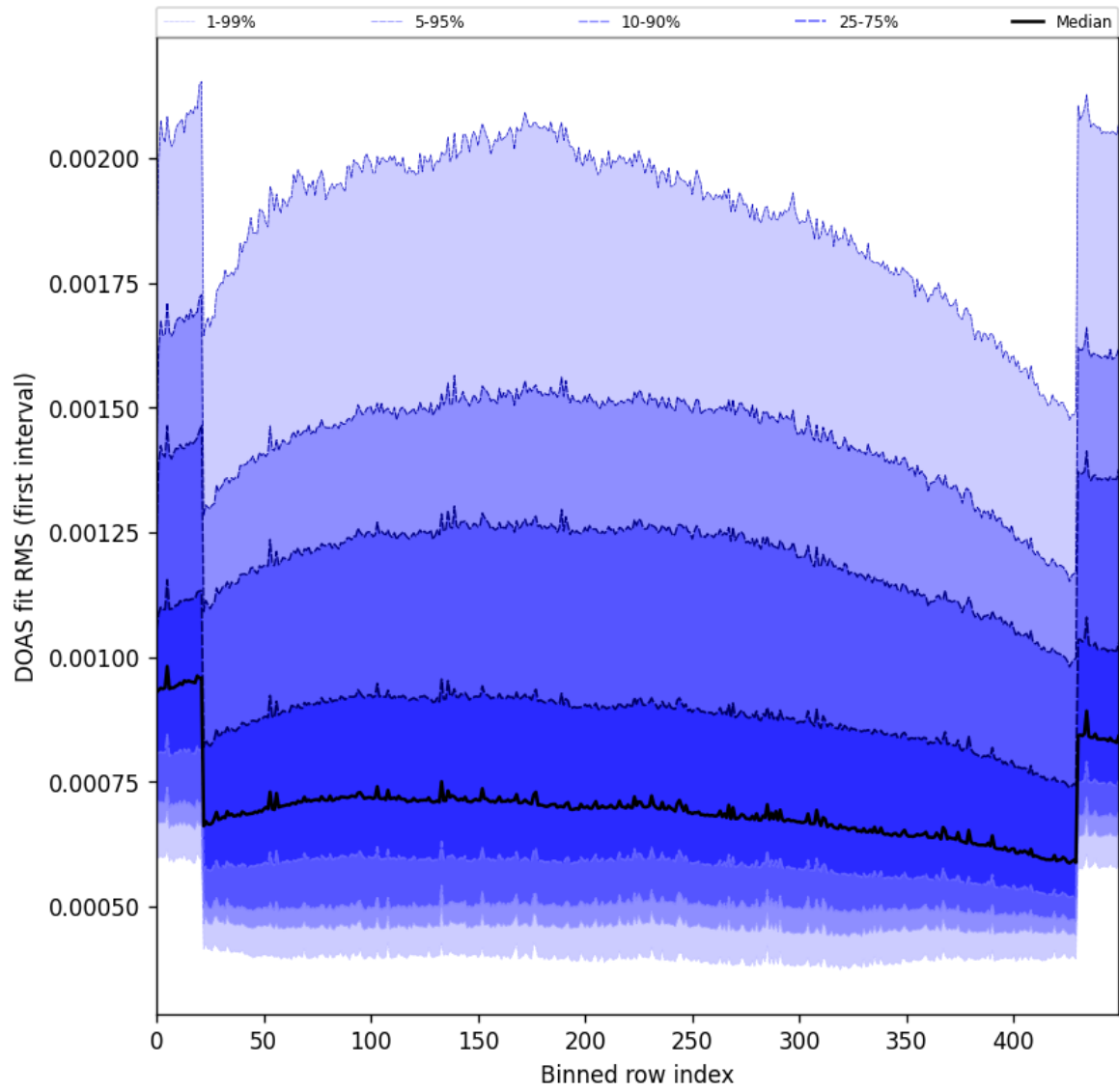
Figure 60: Along track statistics of “DOAS fit RMS (first interval)” for 2024-12-14 to 2024-12-16
