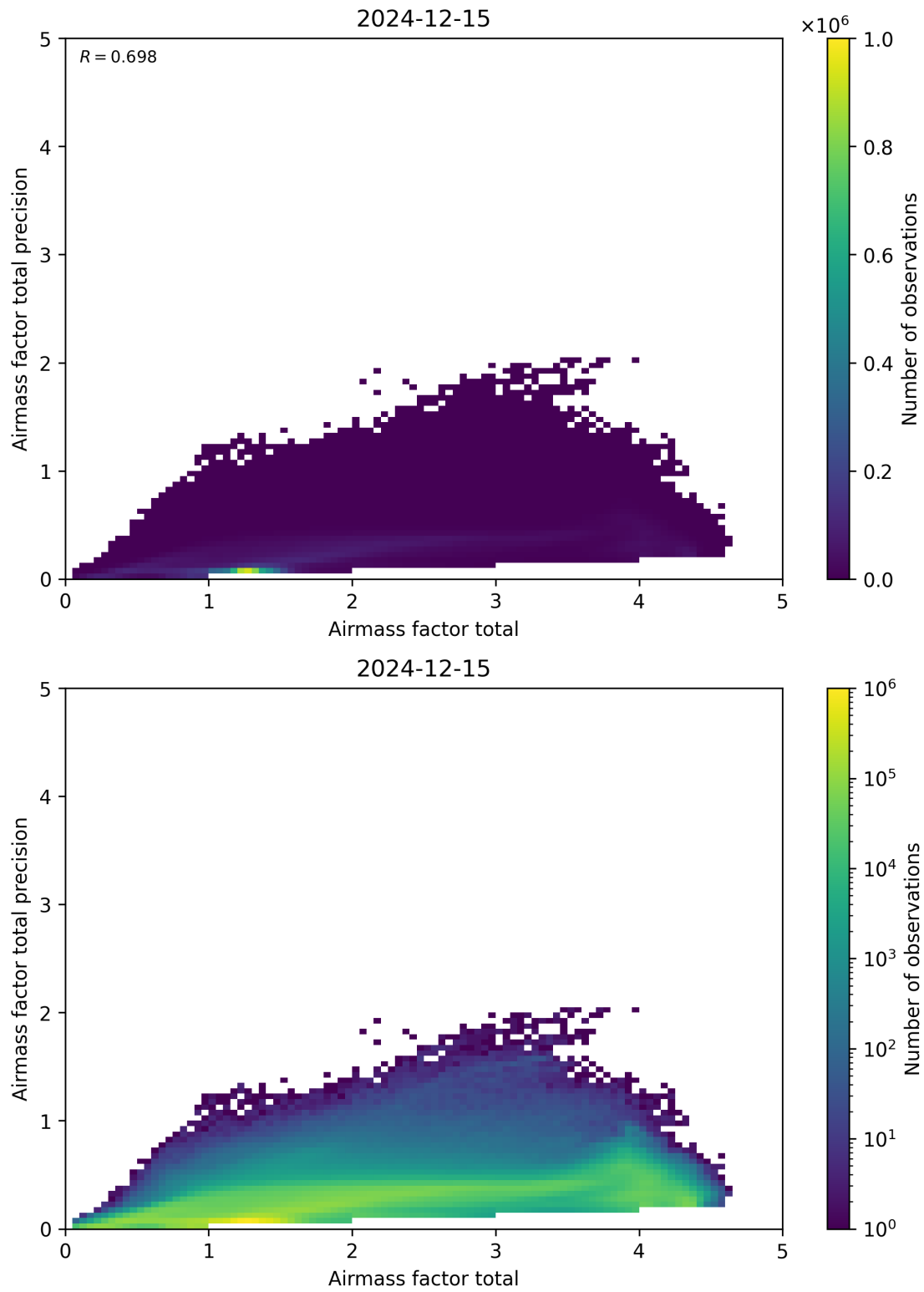
Figure 103: Scatter density plot of “Airmass factor total” against “Airmass factor total precision” for 2024-12-14 to 2024-12-16.
