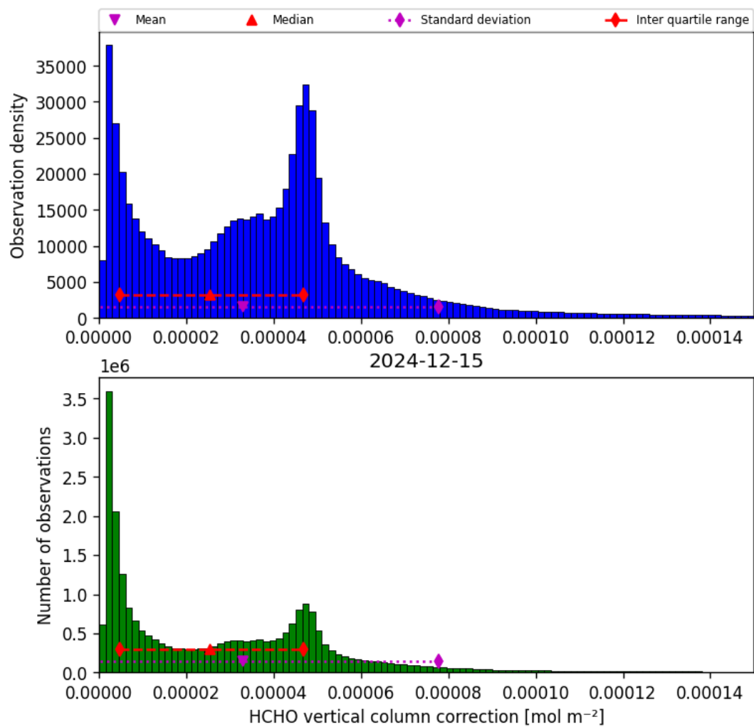
Figure 37: Histogram of “HCHO vertical column correction” for 2024-12-14 to 2024-12-16
