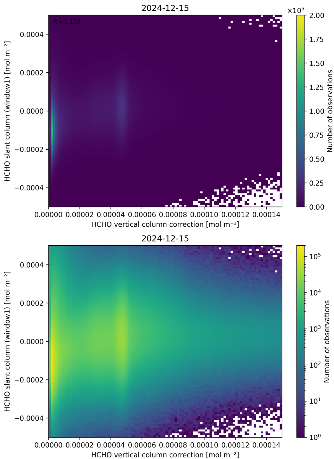
Figure 118: Scatter density plot of “HCHO vertical column correction” against “HCHO slant column (window1)” for 2024-12-14 to 2024-12-16.
