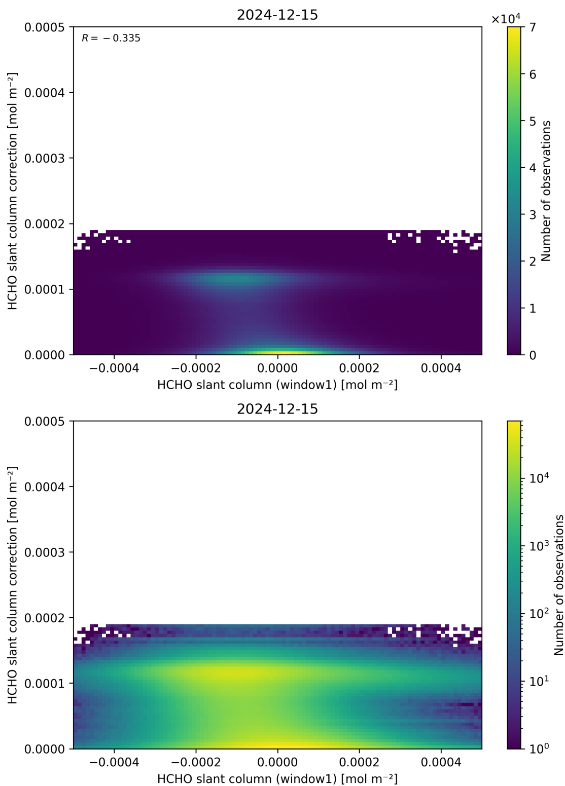
Figure 83: Scatter density plot of “HCHO slant column (window1)” against “HCHO slant column correction” for 2024-12-14 to 2024-12-16.
