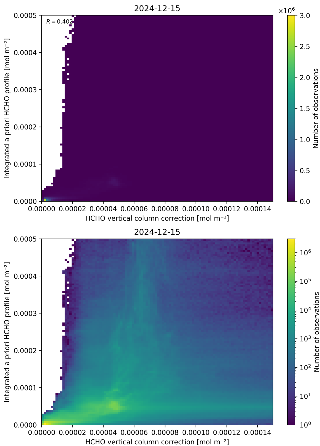
Figure 122: Scatter density plot of “HCHO vertical column correction” against “Integrated a priori HCHO profile” for 2024-12-14 to 2024-12-16.
