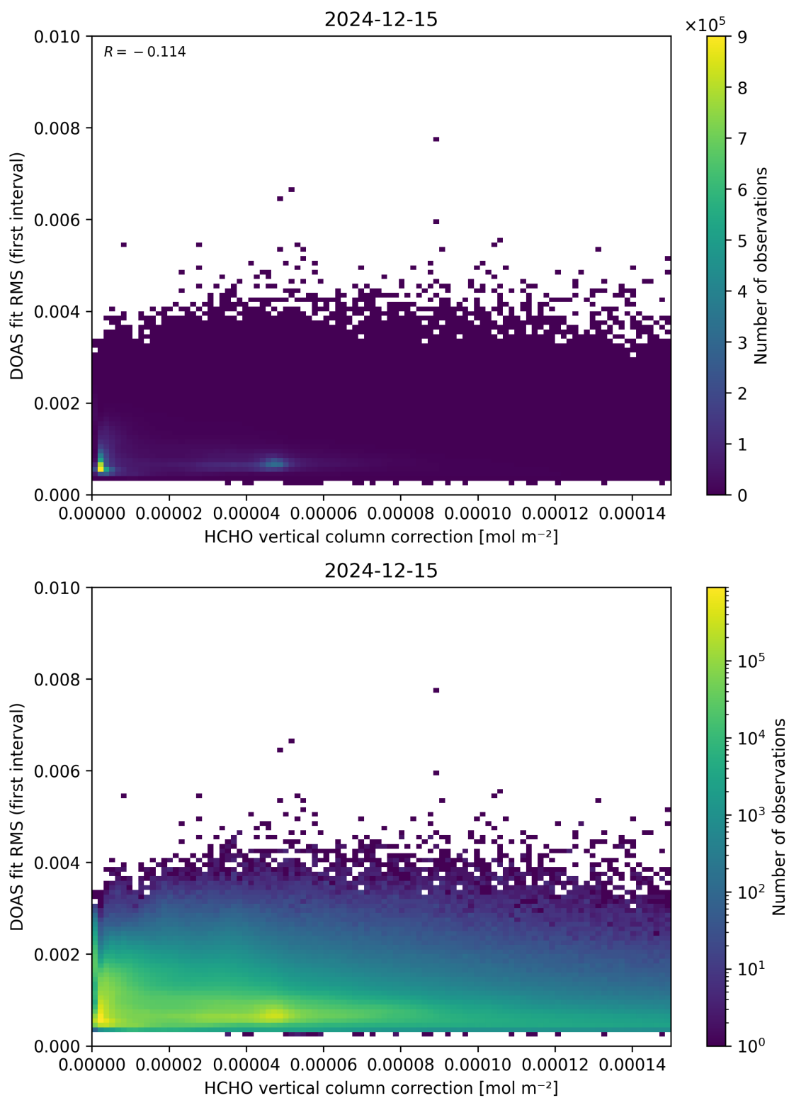
Figure 112: Scatter density plot of “HCHO vertical column correction” against “DOAS fit RMS (first interval)” for 2024-12-14 to 2024-12-16.
