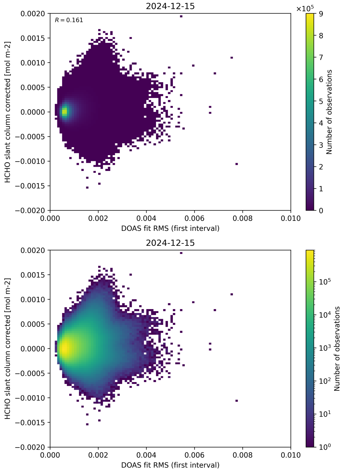
Figure 62: Scatter density plot of “DOAS fit RMS (first interval)” against “HCHO slant column corrected” for 2024-12-14 to 2024-12-16.
