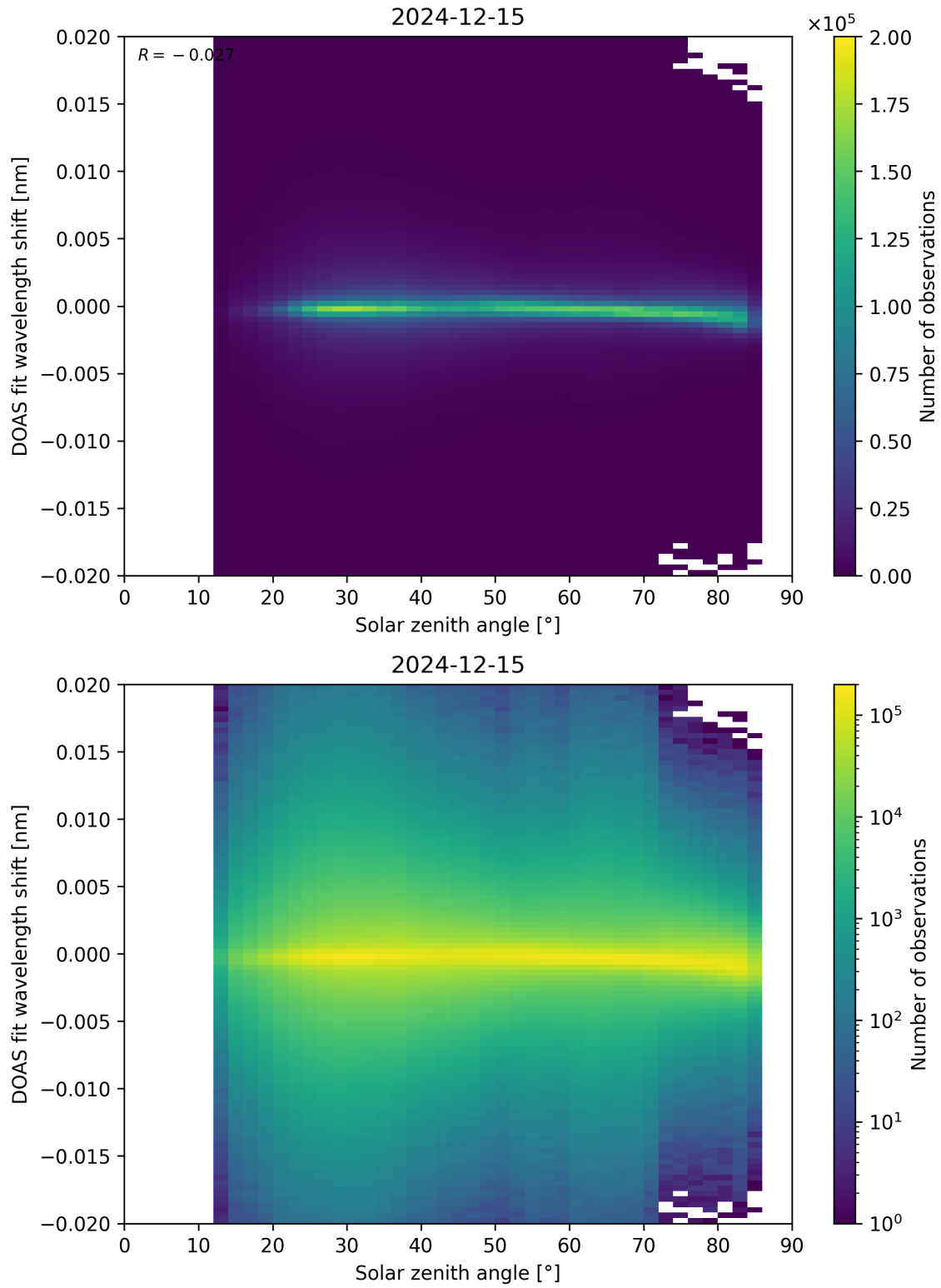
Figure 168: Scatter density plot of “Solar zenith angle” against “DOAS fit wavelength shift” for 2024-12-14 to 2024-12-16.
