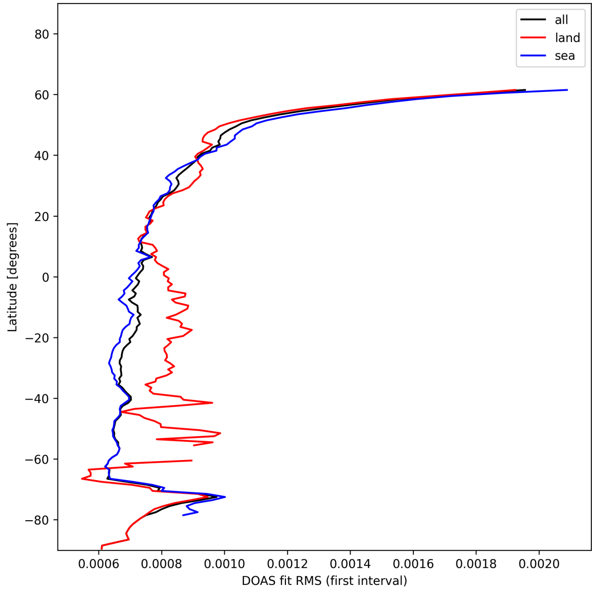
Figure 32: Zonal average of “DOAS fit RMS (first interval)” for 2024-12-14 to 2024-12-16.
