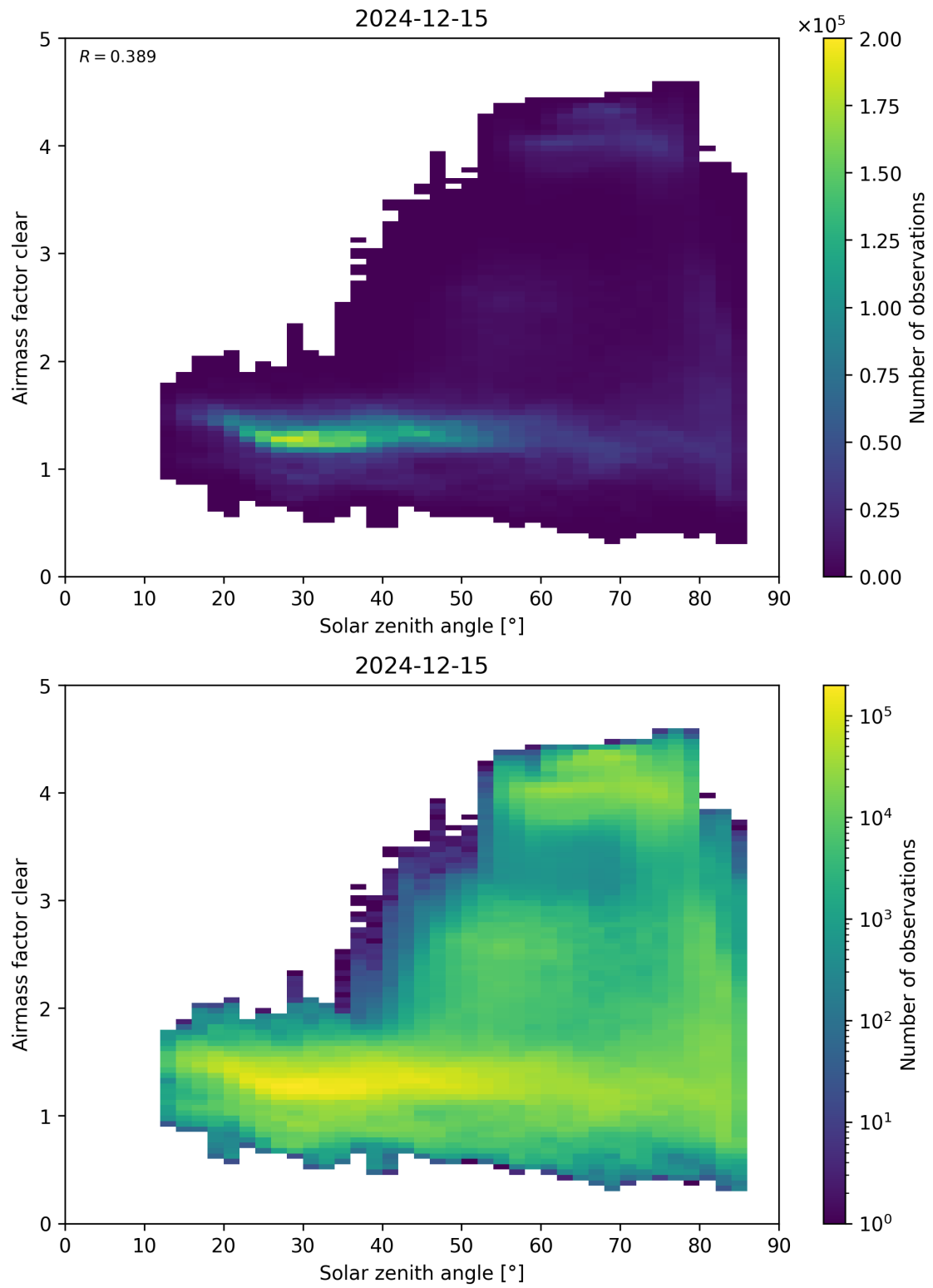
Figure 170: Scatter density plot of “Solar zenith angle” against “Airmass factor clear” for 2024-12-14 to 2024-12-16.
