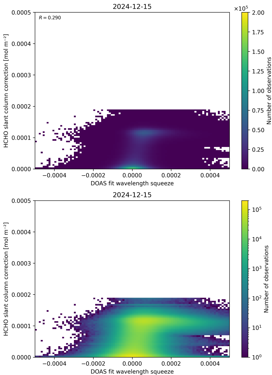
Figure 70: Scatter density plot of “DOAS fit wavelength squeeze” against “HCHO slant column correction” for 2024-12-14 to 2024-12-16.
