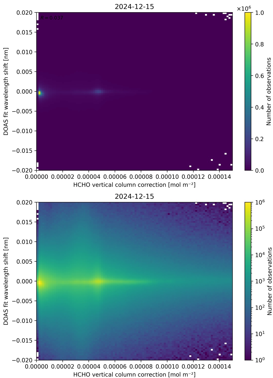
Figure 113: Scatter density plot of “HCHO vertical column correction” against “DOAS fit wavelength shift” for 2024-12-14 to 2024-12-16.
