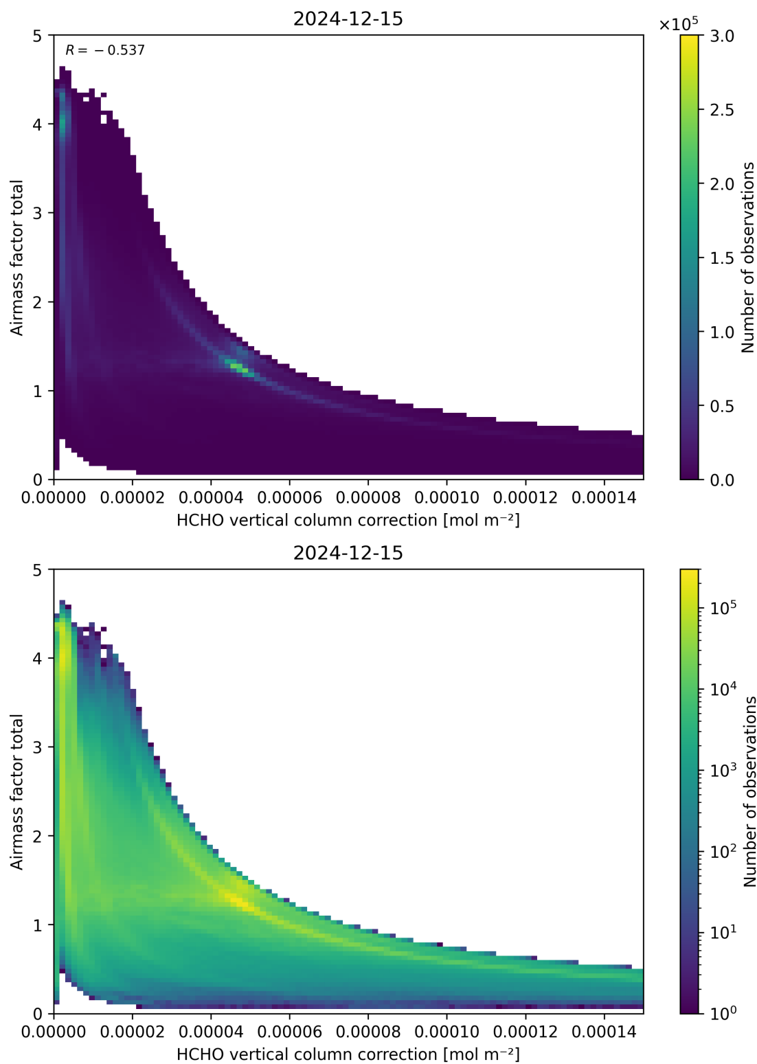
Figure 120: Scatter density plot of “HCHO vertical column correction” against “Airmass factor total” for 2024-12-14 to 2024-12-16.
