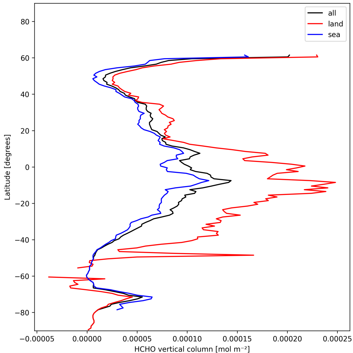
Figure 21: Zonal average of “HCHO vertical column” for 2024-12-14 to 2024-12-16.
