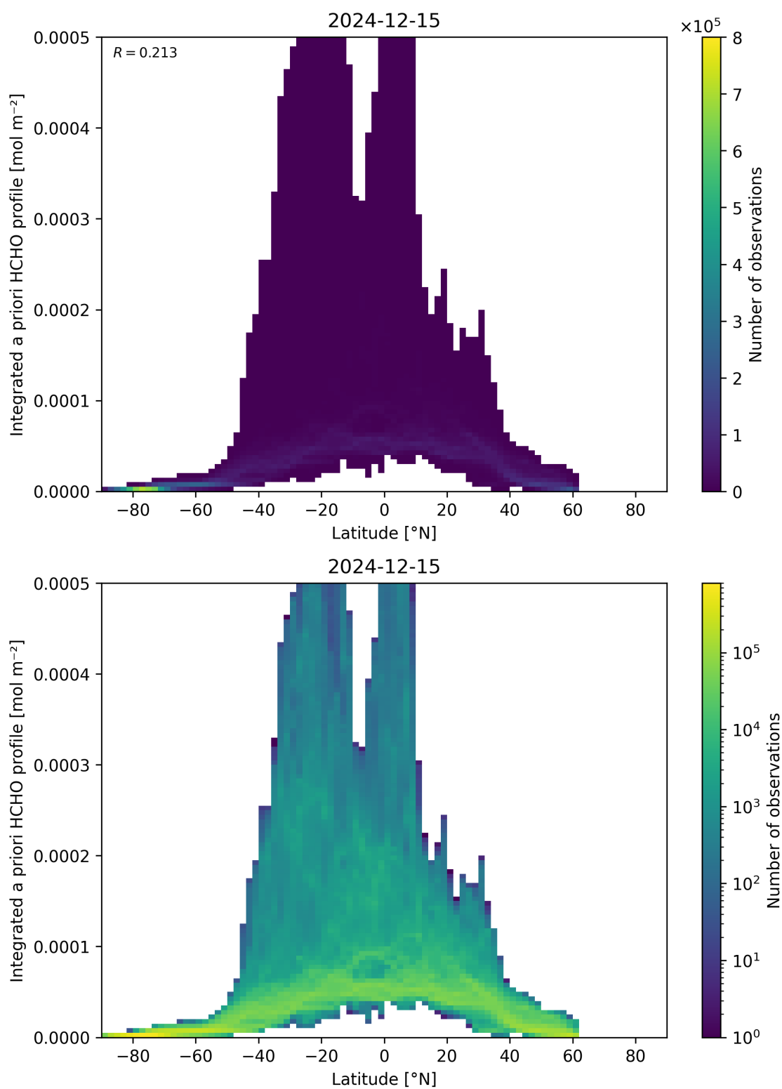
Figure 166: Scatter density plot of “Latitude” against “Integrated a priori HCHO profile” for 2024-12-14 to 2024-12-16.
