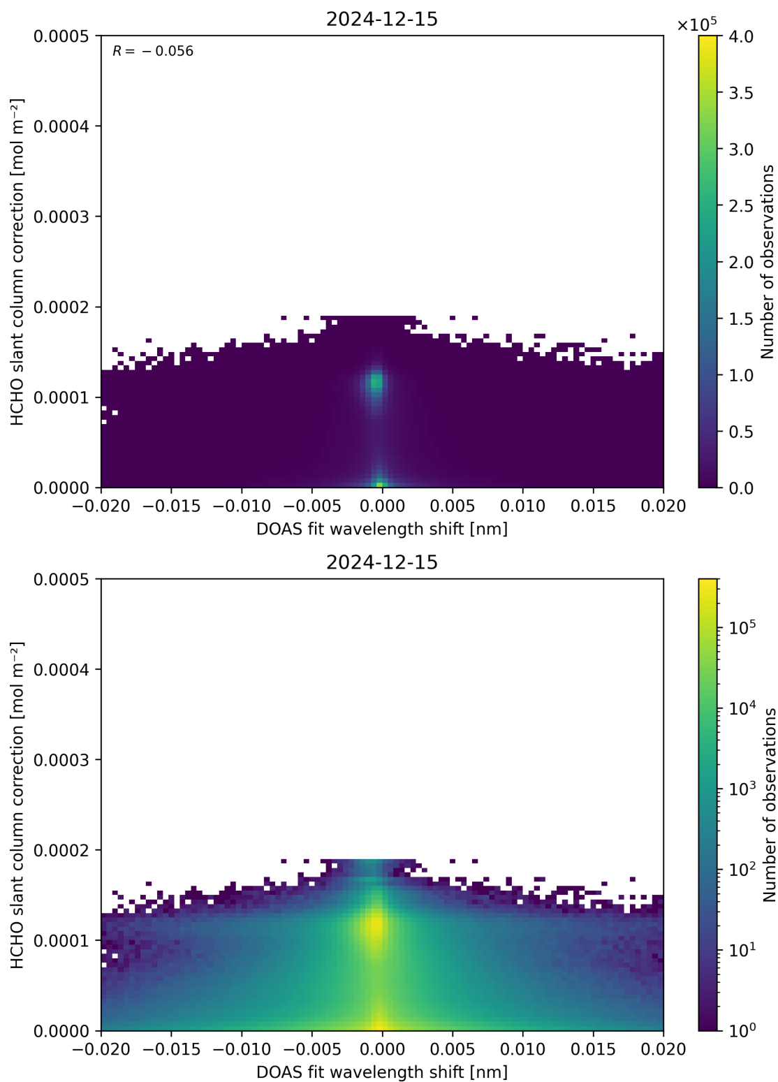
Figure 67: Scatter density plot of “DOAS fit wavelength shift” against “HCHO slant column correction” for 2024-12-14 to 2024-12-16.
