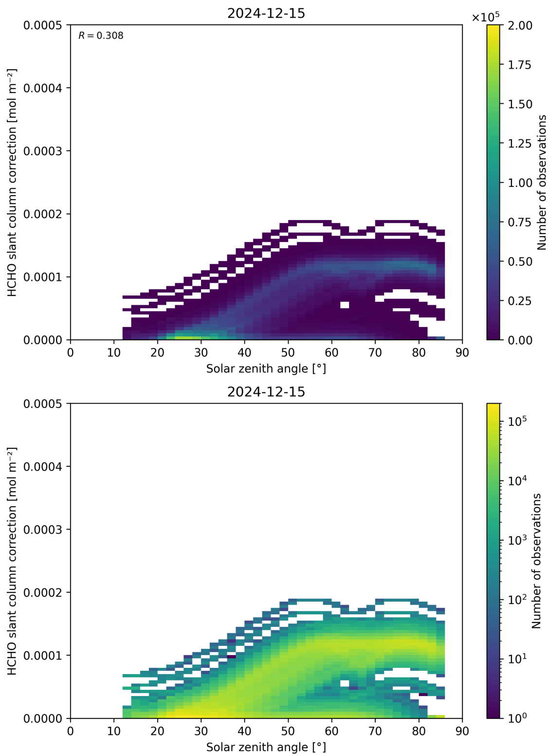
Figure 172: Scatter density plot of “Solar zenith angle” against “HCHO slant column correction” for 2024-12-14 to 2024-12-16.
