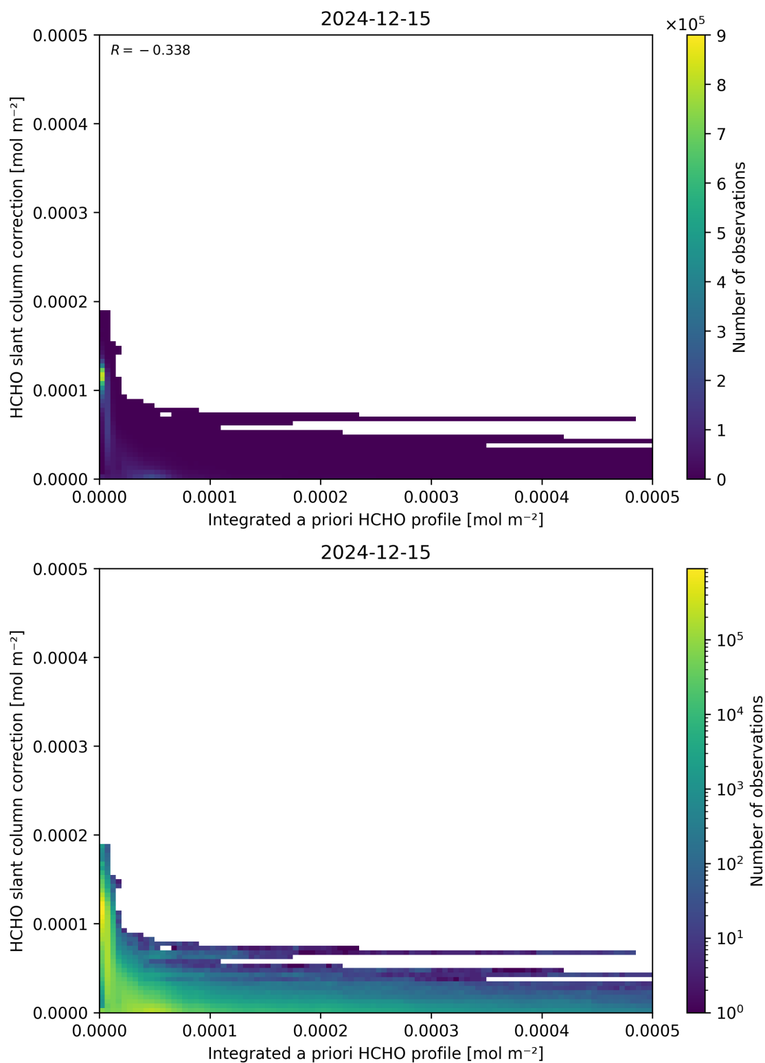
Figure 152: Scatter density plot of “Integrated a priori HCHO profile” against “HCHO slant column correction” for 2024-12-14 to 2024-12-16.
