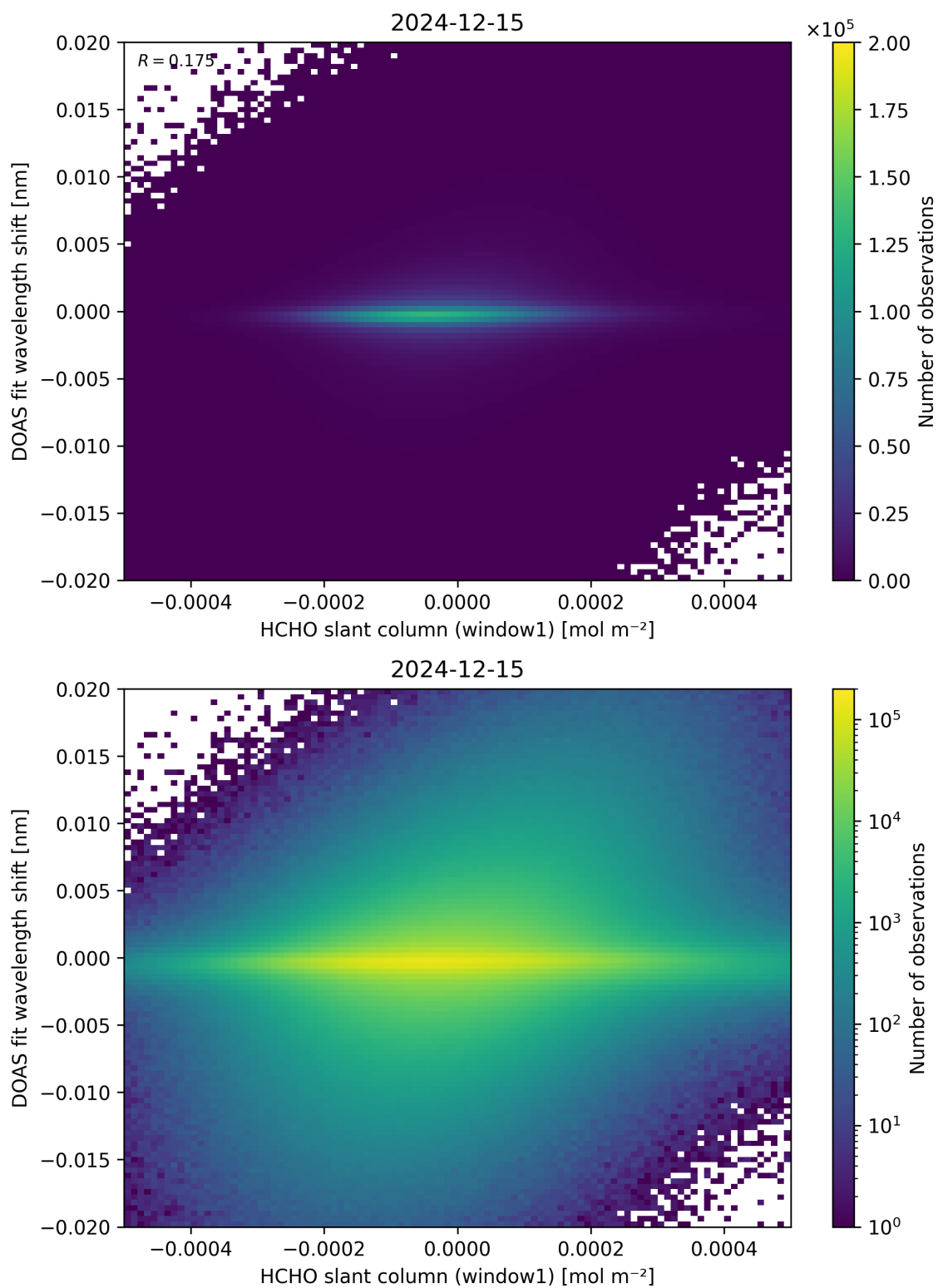
Figure 79: Scatter density plot of “HCHO slant column (window1)” against “DOAS fit wavelength shift” for 2024-12-14 to 2024-12-16.
