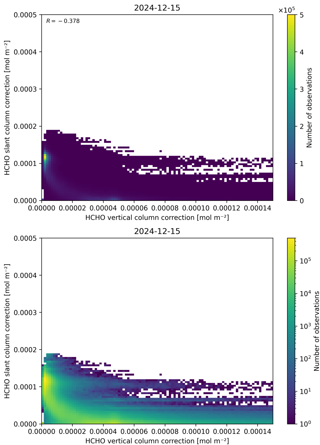
Figure 117: Scatter density plot of “HCHO vertical column correction” against “HCHO slant column correction” for 2024-12-14 to 2024-12-16.
