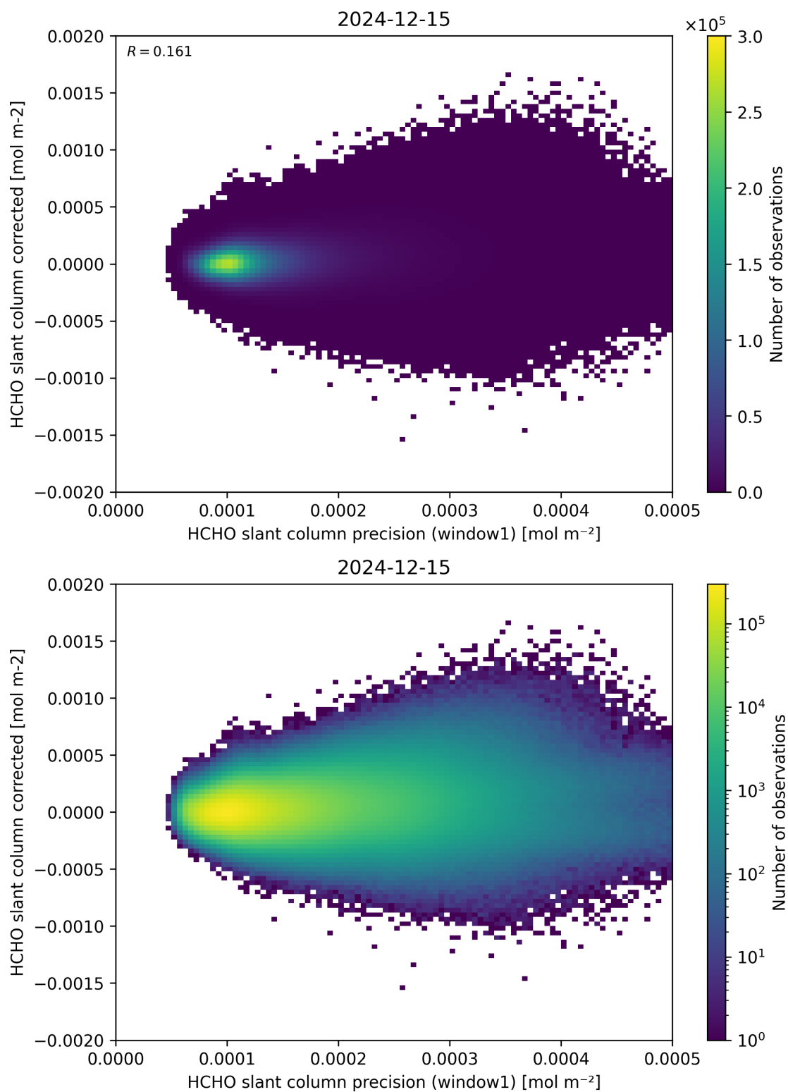
Figure 92: Scatter density plot of “HCHO slant column precision (window1)” against “HCHO slant column corrected” for 2024-12-14 to 2024-12-16.
