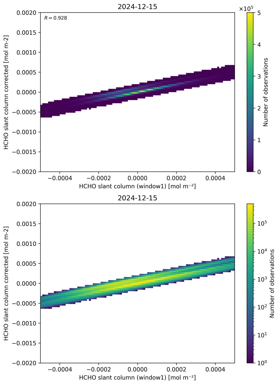
Figure 82: Scatter density plot of “HCHO slant column (window1)” against “HCHO slant column corrected” for 2024-12-14 to 2024-12-16.
