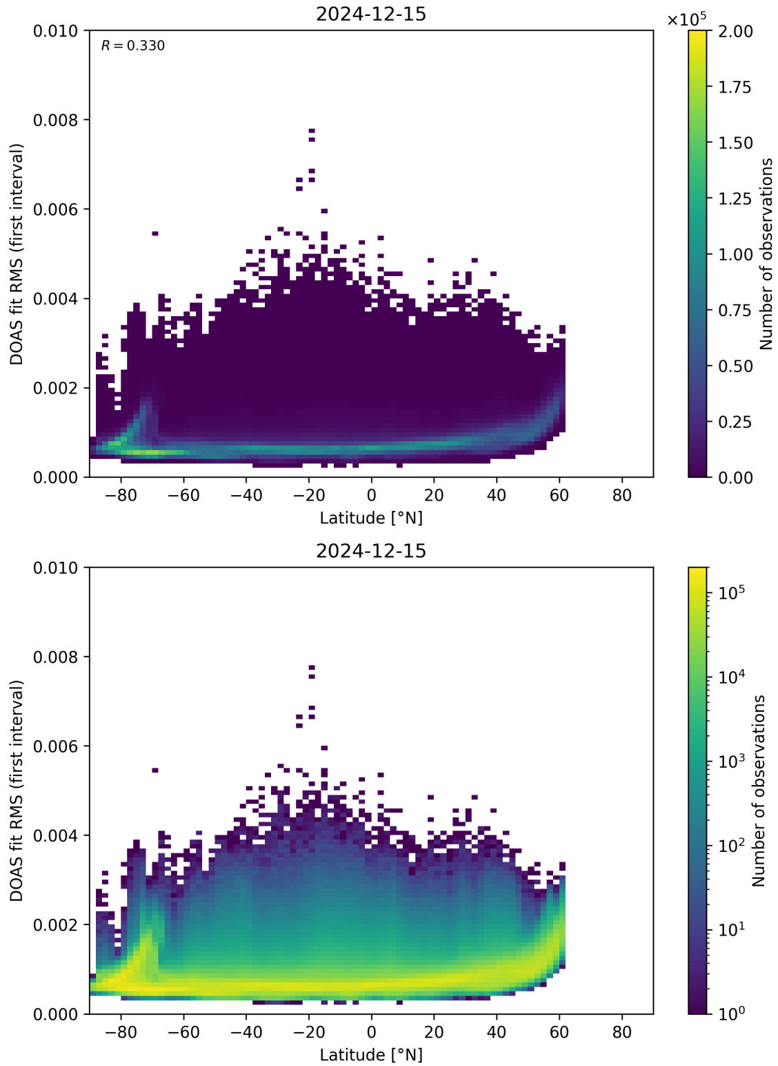
Figure 153: Scatter density plot of “Latitude” against “DOAS fit RMS (first interval)” for 2024-12-14 to 2024-12-16.
