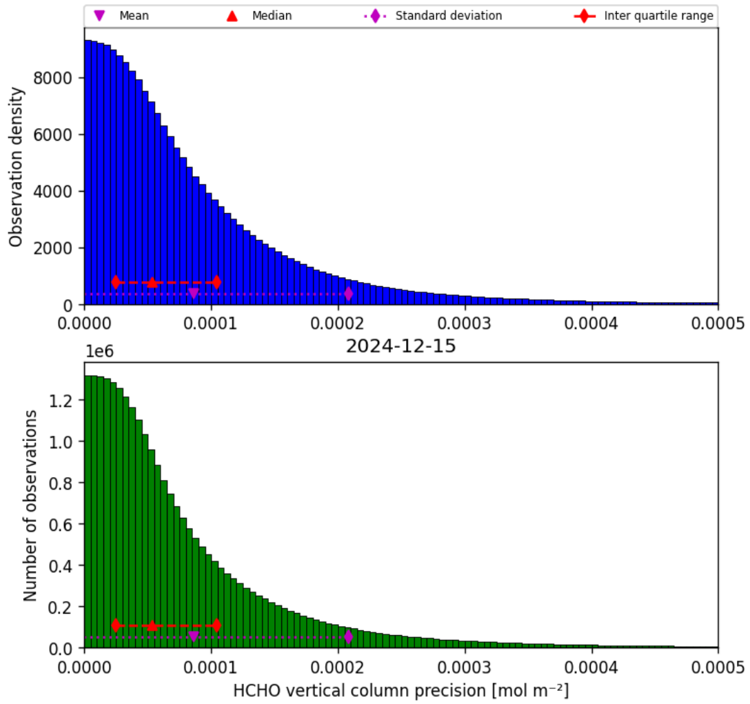
Figure 36: Histogram of “HCHO vertical column precision” for 2024-12-14 to 2024-12-16
