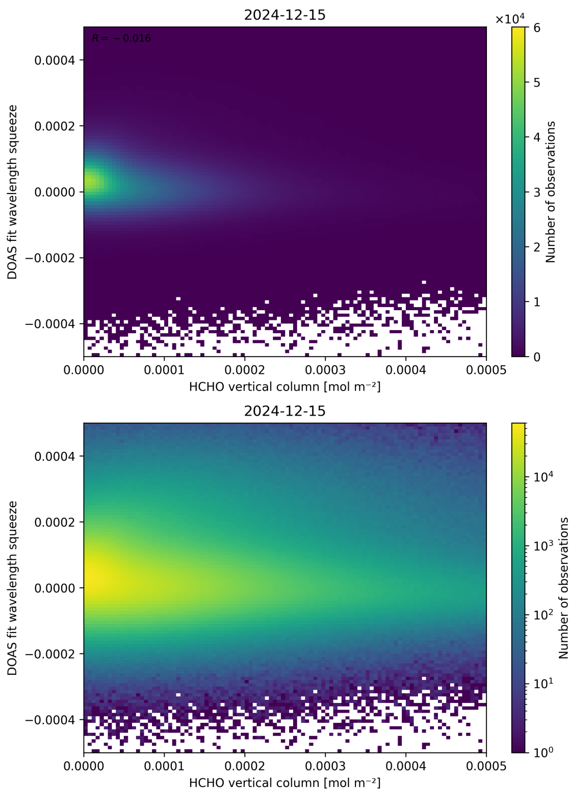
Figure 125: Scatter density plot of “HCHO vertical column” against “DOAS fit wavelength squeeze” for 2024-12-14 to 2024-12-16.
