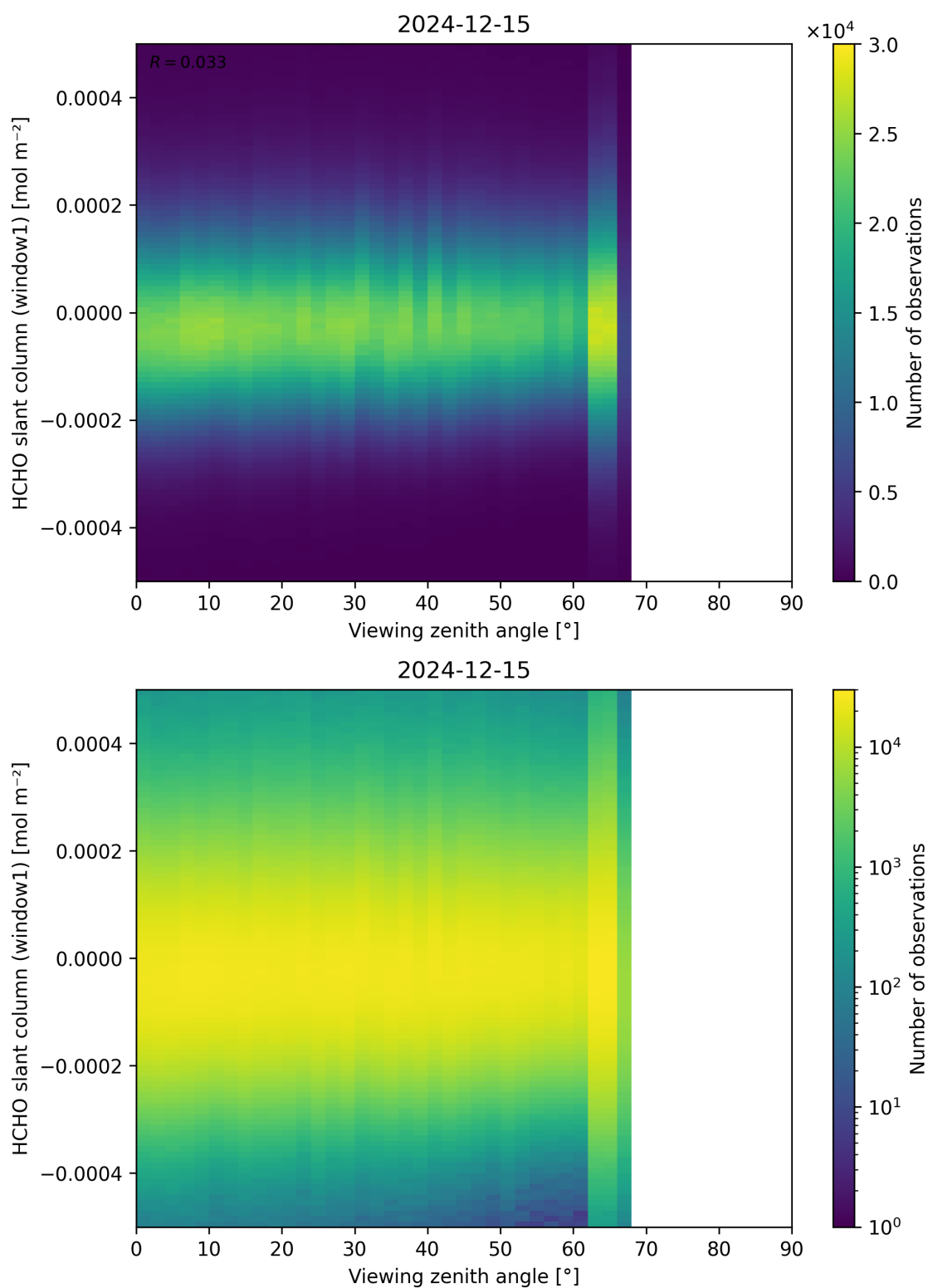
Figure 188: Scatter density plot of “Viewing zenith angle” against “HCHO slant column (window1)” for 2024-12-14 to 2024-12-16.
