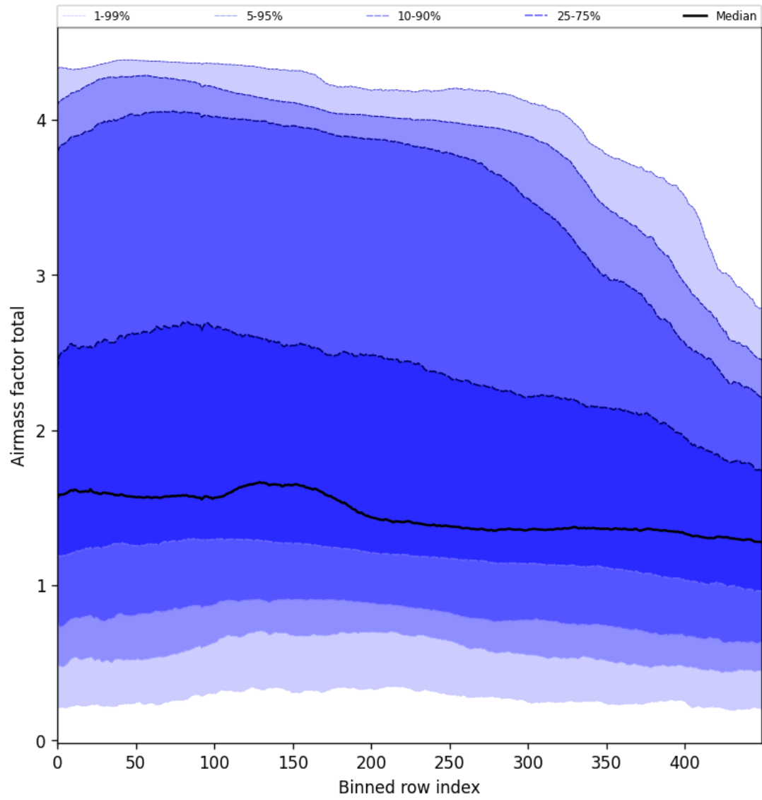
Figure 54: Along track statistics of “Airmass factor total” for 2024-12-14 to 2024-12-16
