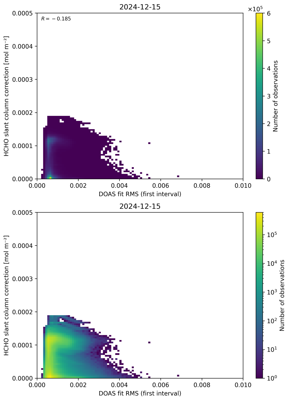
Figure 63: Scatter density plot of “DOAS fit RMS (first interval)” against “HCHO slant column correction” for 2024-12-14 to 2024-12-16.
