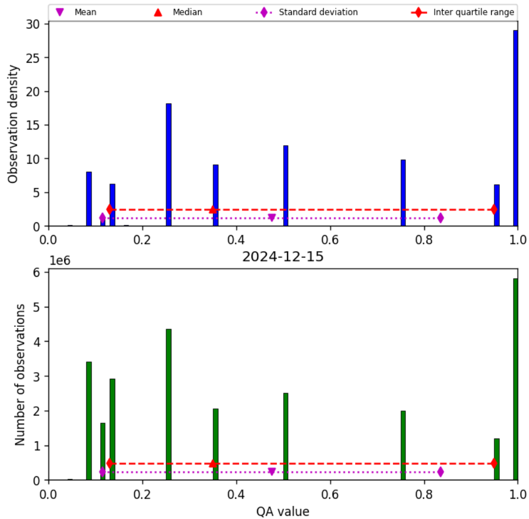
Figure 34: Histogram of “QA value” for 2024-12-14 to 2024-12-16
