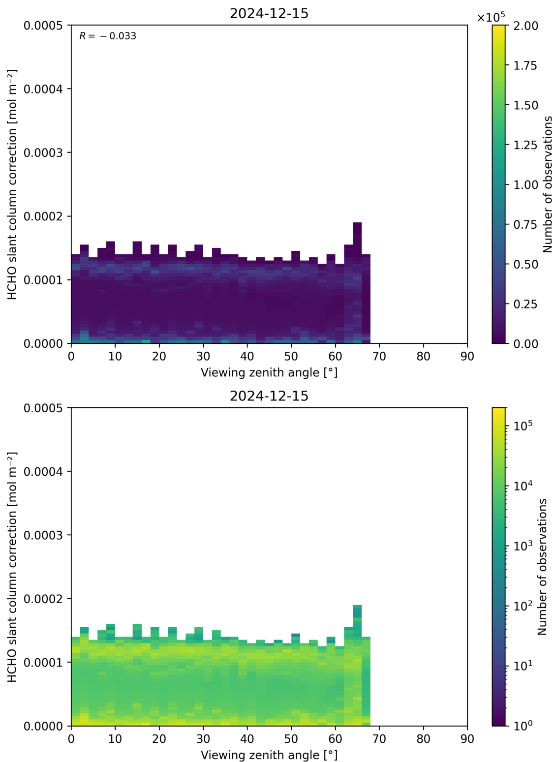
Figure 187: Scatter density plot of “Viewing zenith angle” against “HCHO slant column correction” for 2024-12-14 to 2024-12-16.
