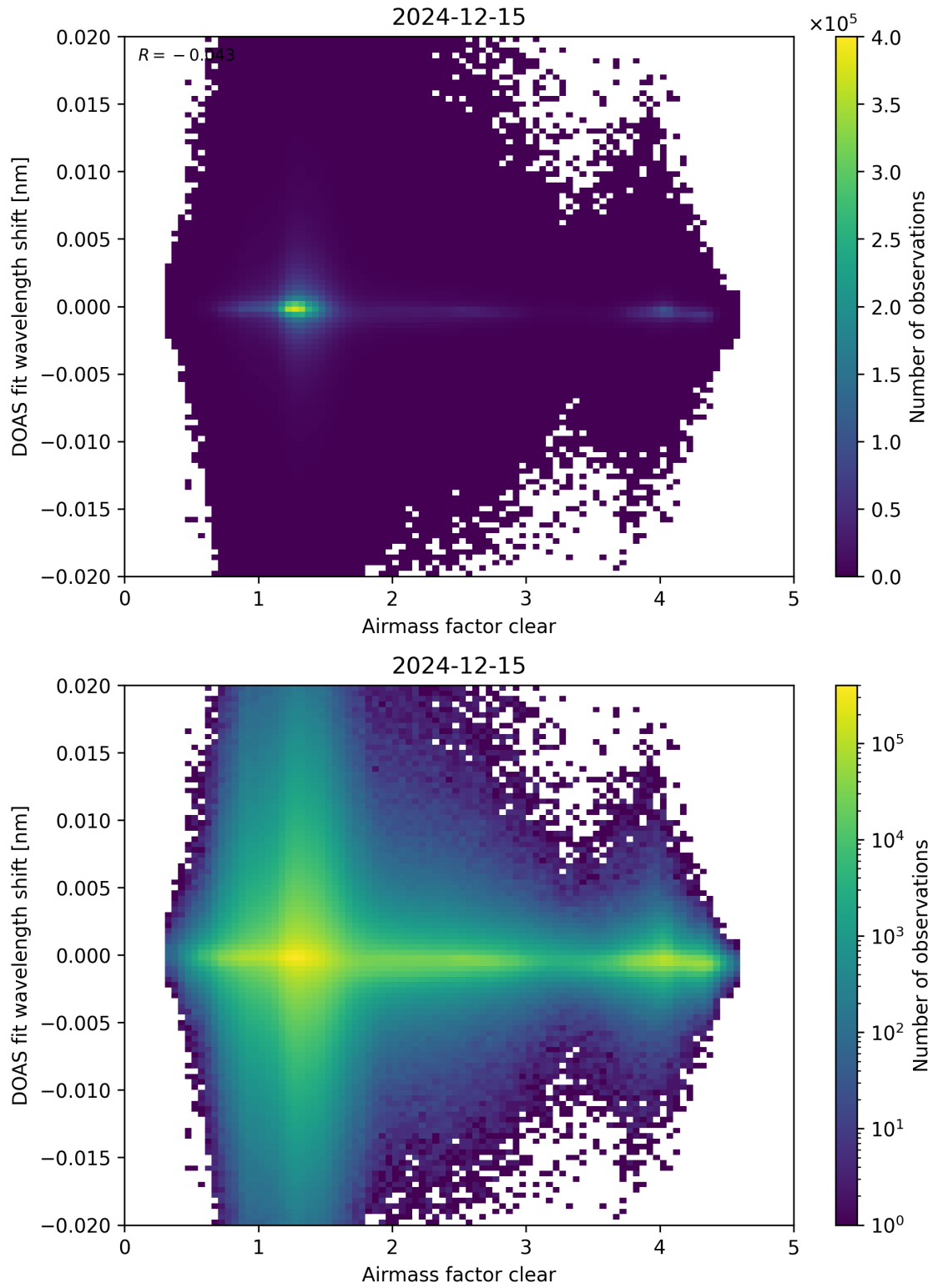
Figure 72: Scatter density plot of “Airmass factor clear” against “DOAS fit wavelength shift” for 2024-12-14 to 2024-12-16.
