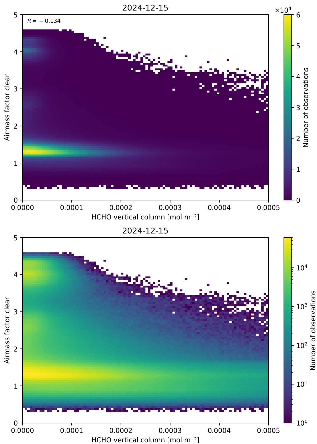
Figure 126: Scatter density plot of “HCHO vertical column” against “Airmass factor clear” for 2024-12-14 to 2024-12-16.
