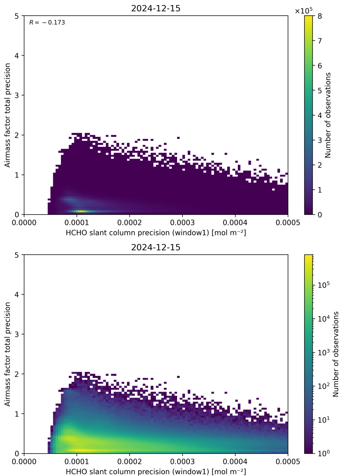
Figure 95: Scatter density plot of “HCHO slant column precision (window1)” against “Airmass factor total precision” for 2024-12-14 to 2024-12-16.
