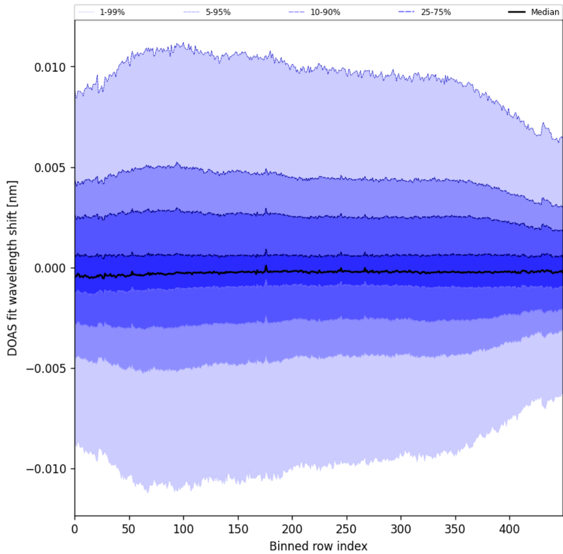
Figure 58: Along track statistics of “DOAS fit wavelength shift” for 2024-12-14 to 2024-12-16
