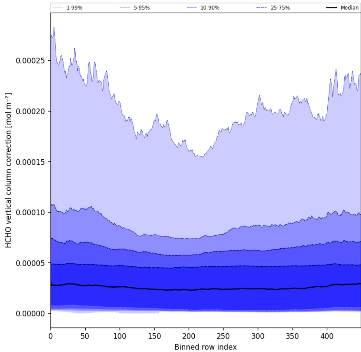
Figure 51: Along track statistics of “HCHO vertical column correction” for 2024-12-14 to 2024-12-16
