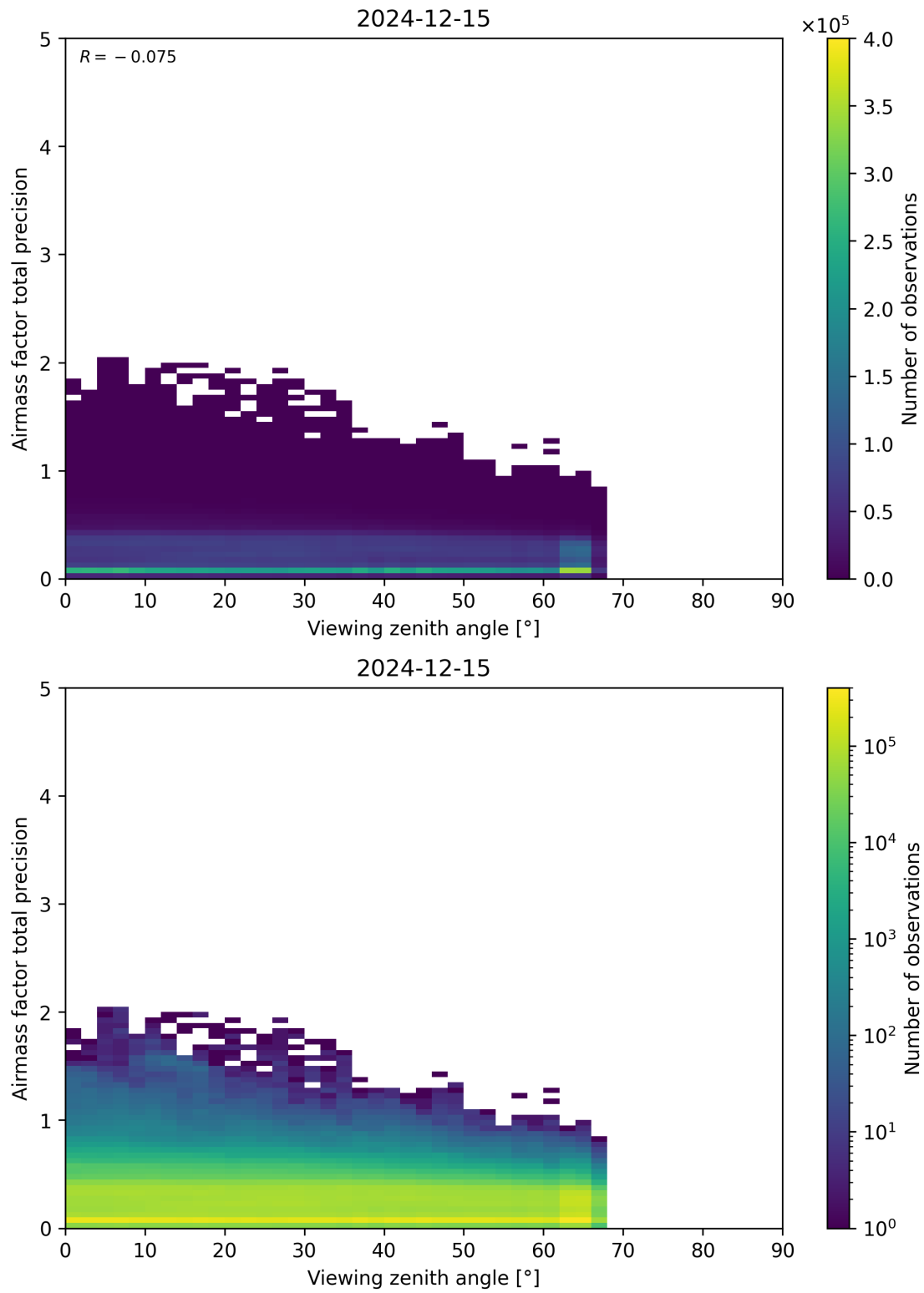
Figure 191: Scatter density plot of “Viewing zenith angle” against “Airmass factor total precision” for 2024-12-14 to 2024-12-16.
