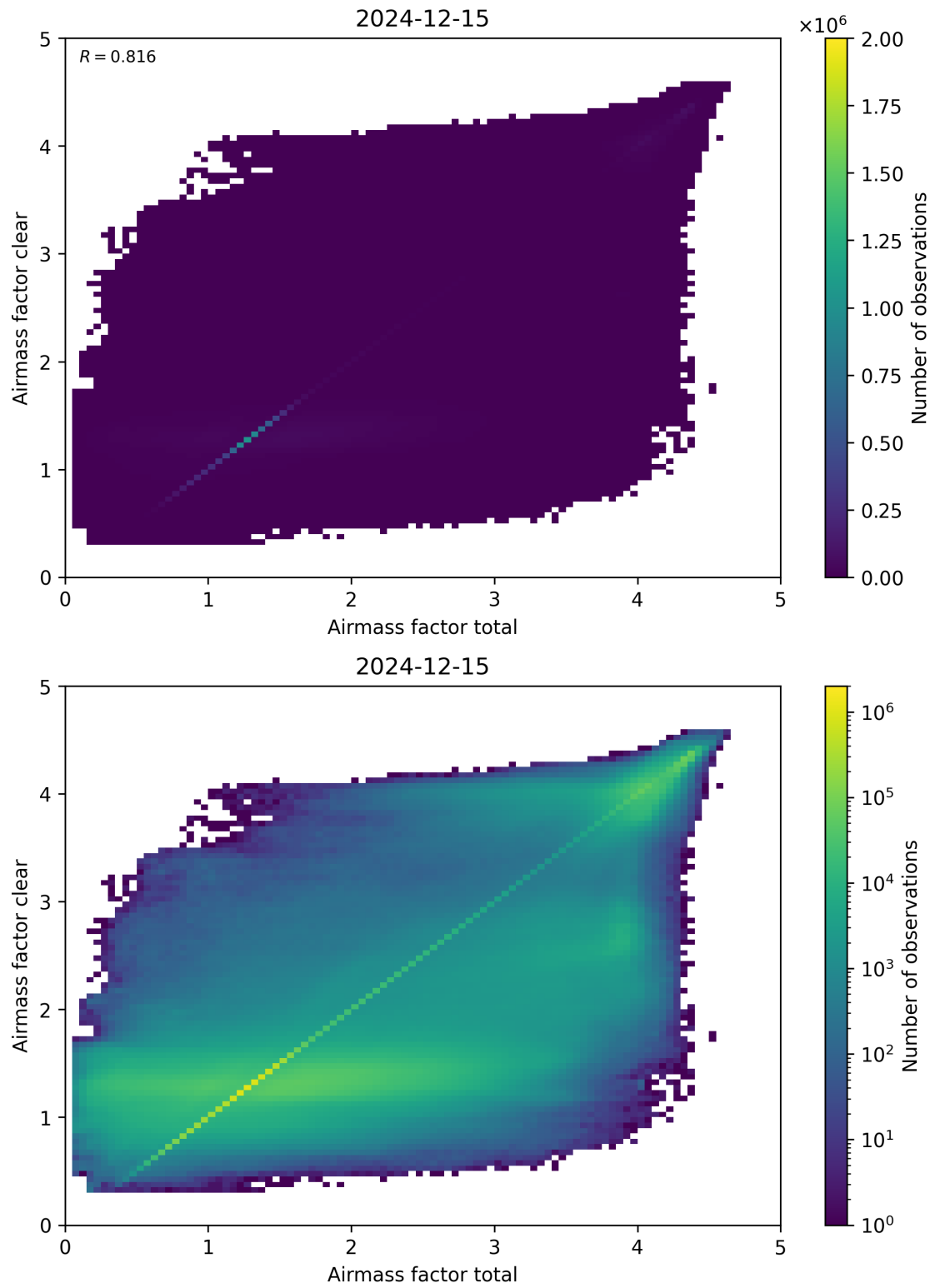
Figure 100: Scatter density plot of “Airmass factor total” against “Airmass factor clear” for 2024-12-14 to 2024-12-16.
