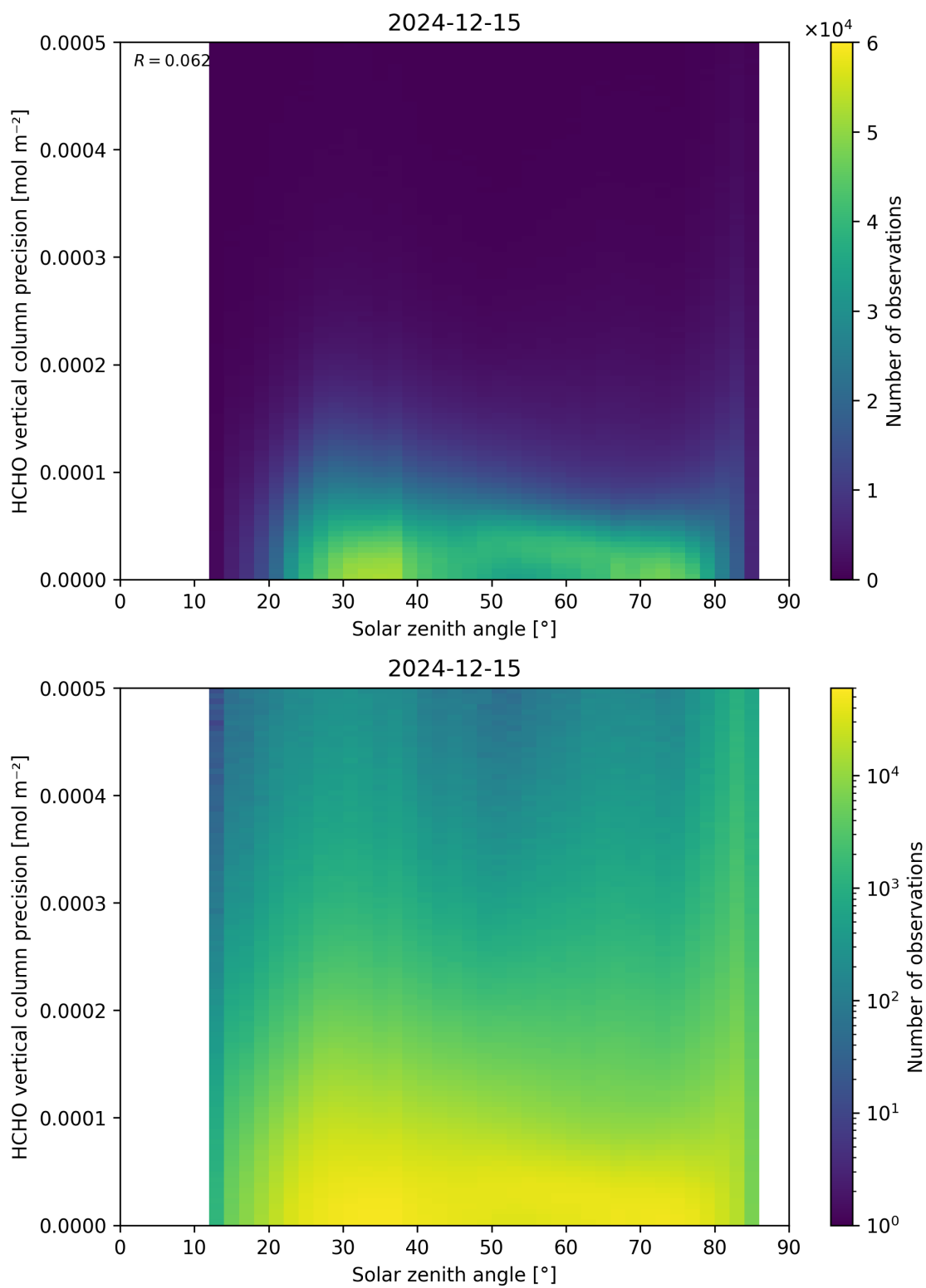
Figure 179: Scatter density plot of “Solar zenith angle” against “HCHO vertical column precision” for 2024-12-14 to 2024-12-16.
