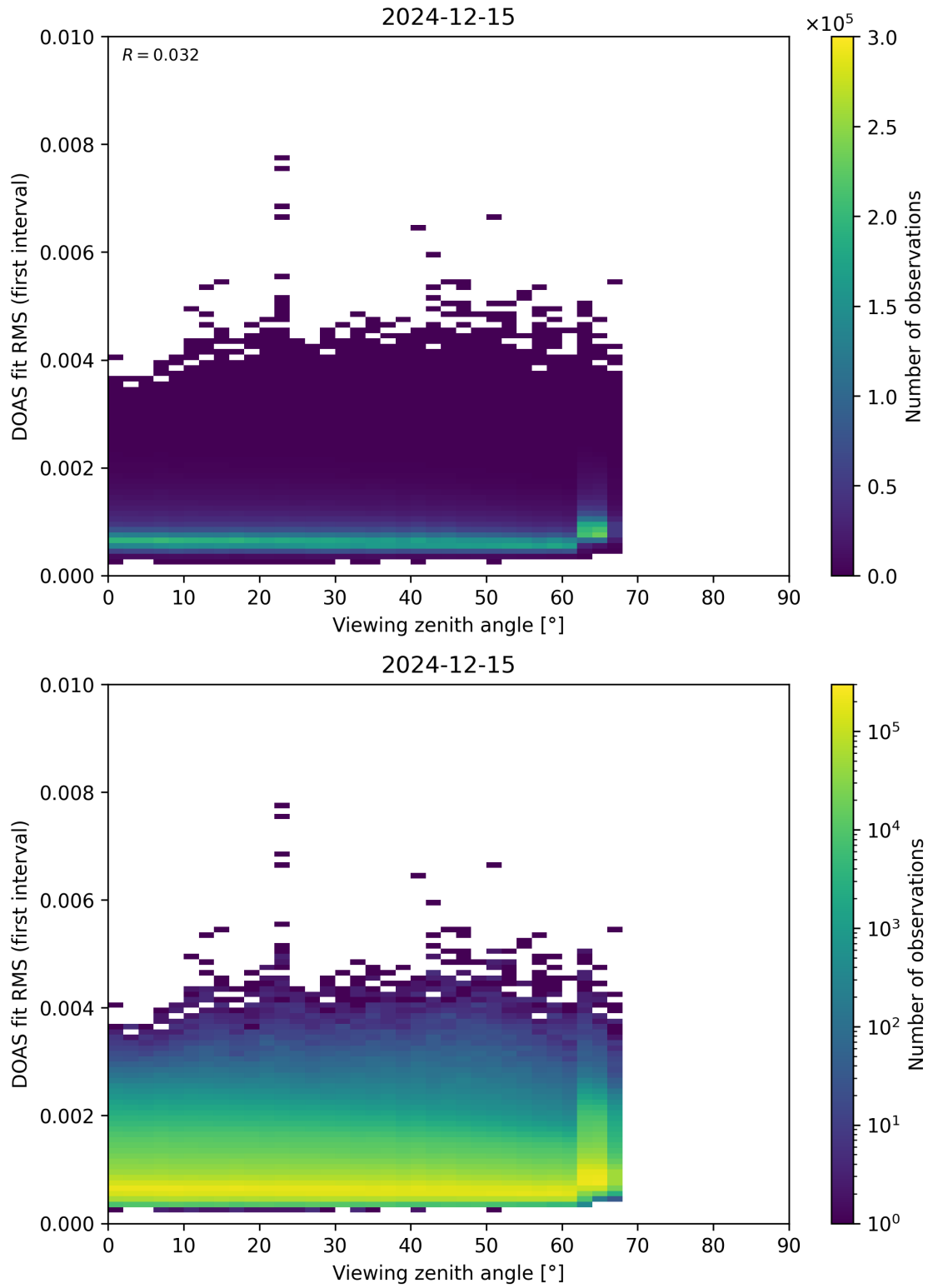
Figure 182: Scatter density plot of “Viewing zenith angle” against “DOAS fit RMS (first interval)” for 2024-12-14 to 2024-12-16.
