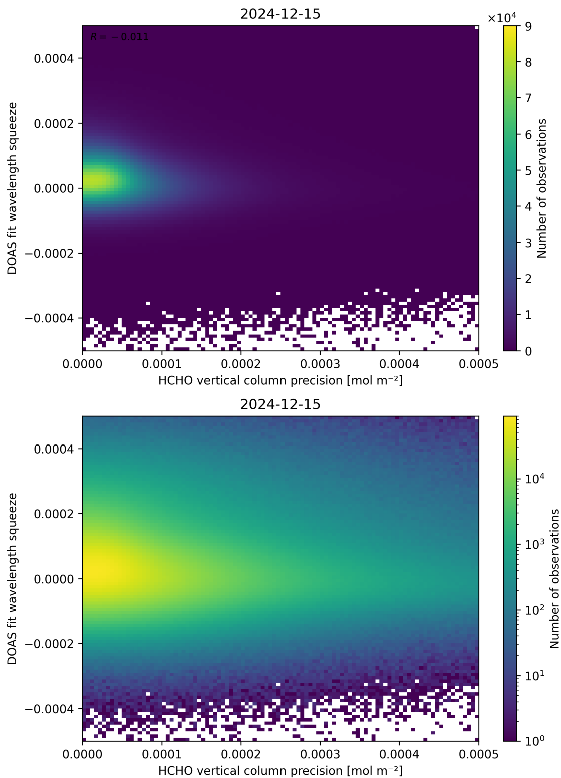
Figure 138: Scatter density plot of “HCHO vertical column precision” against “DOAS fit wavelength squeeze” for 2024-12-14 to 2024-12-16.
