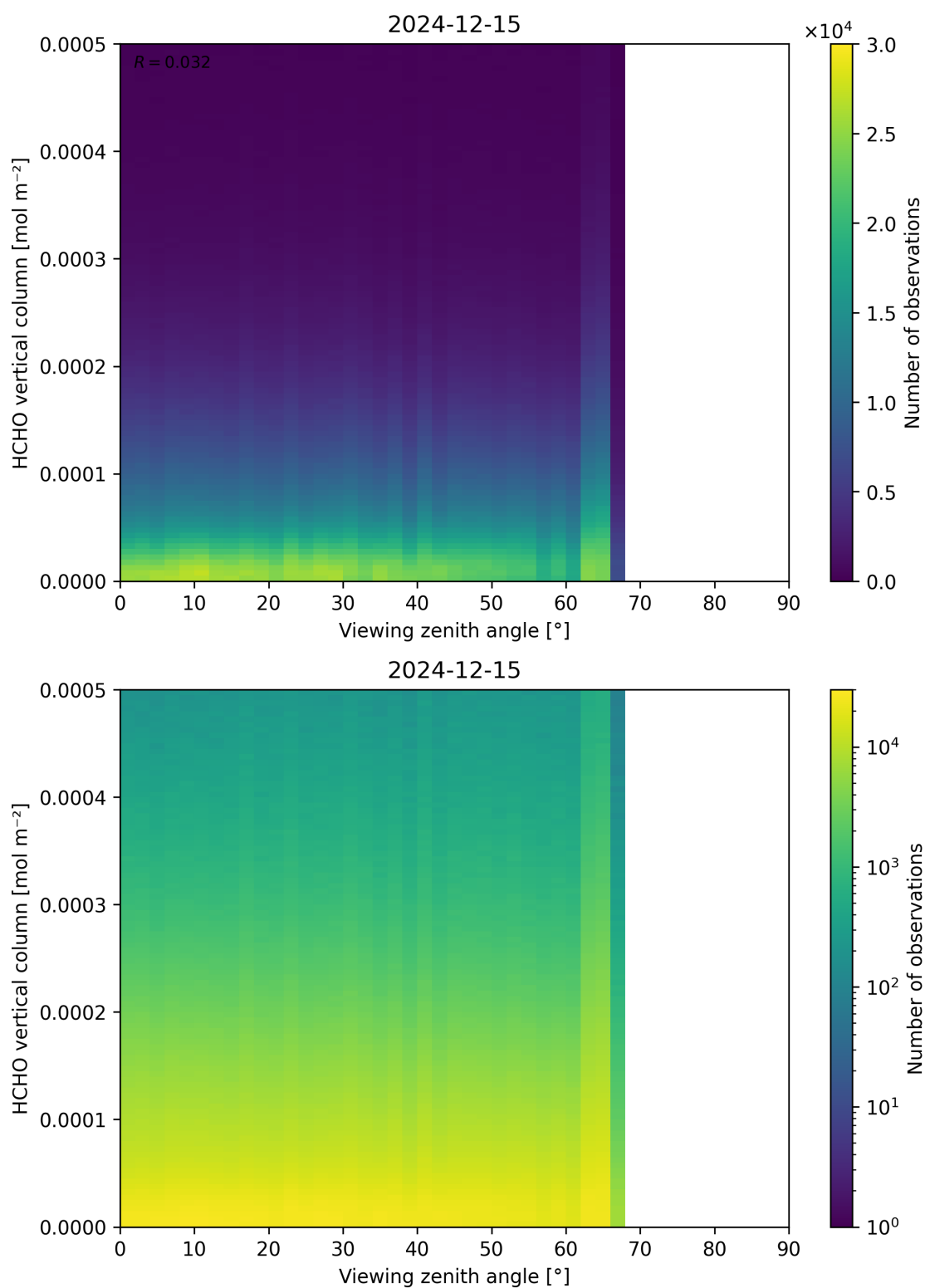
Figure 192: Scatter density plot of “Viewing zenith angle” against “HCHO vertical column” for 2024-12-14 to 2024-12-16.
