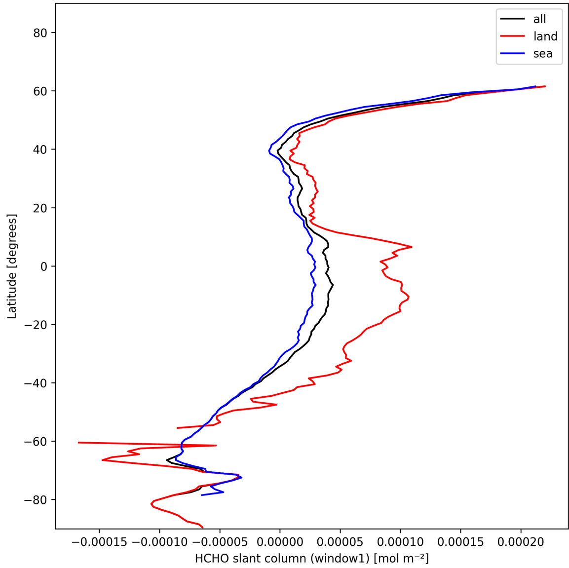
Figure 24: Zonal average of “HCHO slant column (window1)” for 2024-12-14 to 2024-12-16.
