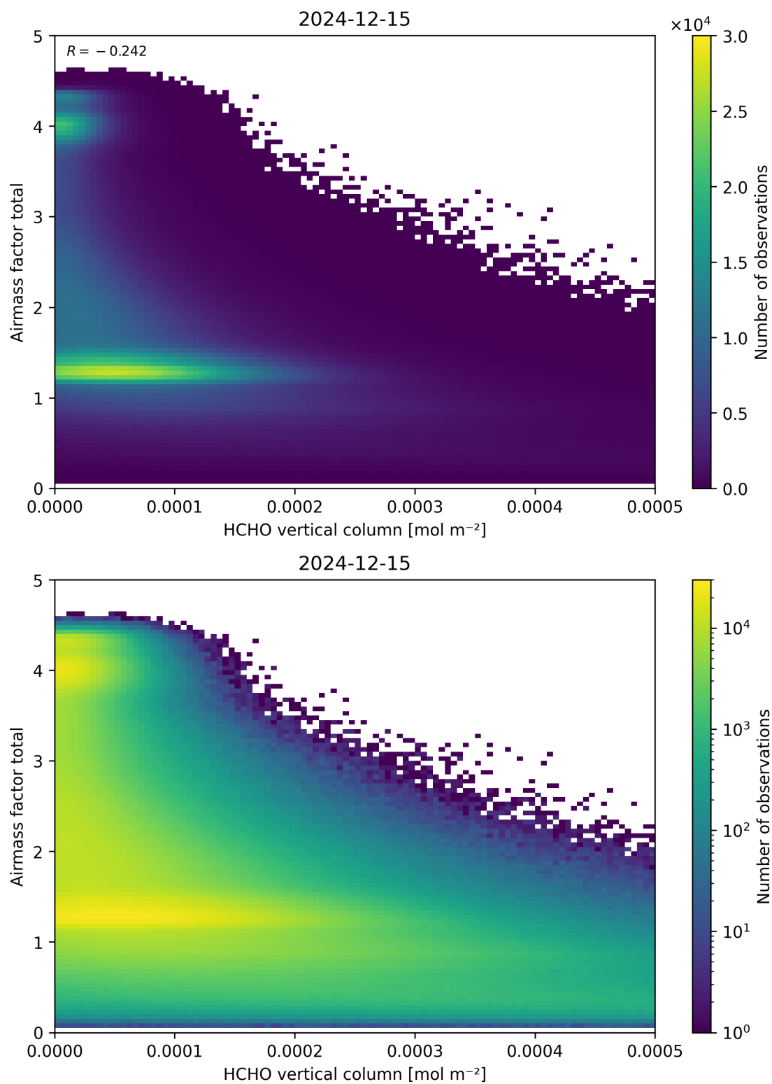
Figure 131: Scatter density plot of “HCHO vertical column” against “Airmass factor total” for 2024-12-14 to 2024-12-16.
