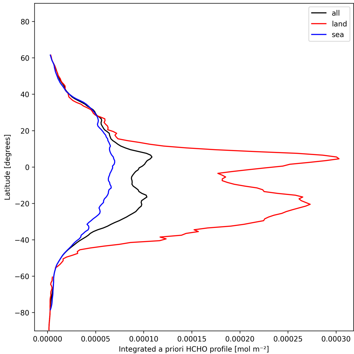
Figure 29: Zonal average of “Integrated a priori HCHO profile” for 2024-12-14 to 2024-12-16.
