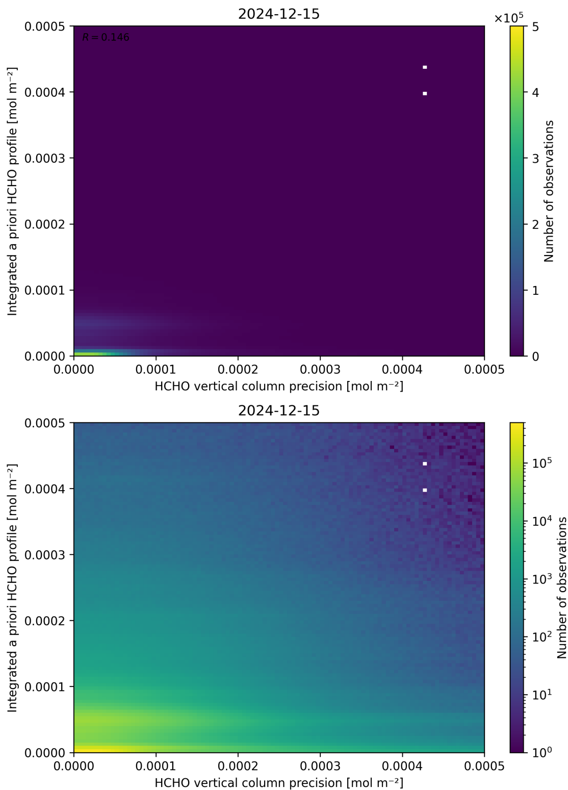
Figure 147: Scatter density plot of “HCHO vertical column precision” against “Integrated a priori HCHO profile” for 2024-12-14 to 2024-12-16.
