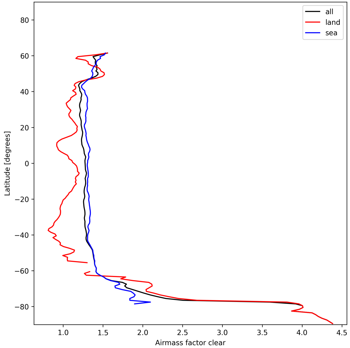
Figure 28: Zonal average of “Airmass factor clear” for 2024-12-14 to 2024-12-16.
