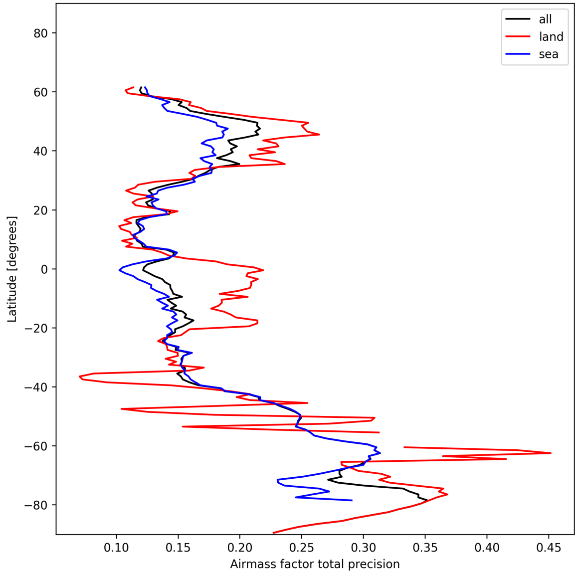
Figure 27: Zonal average of “Airmass factor total precision” for 2024-12-14 to 2024-12-16.
