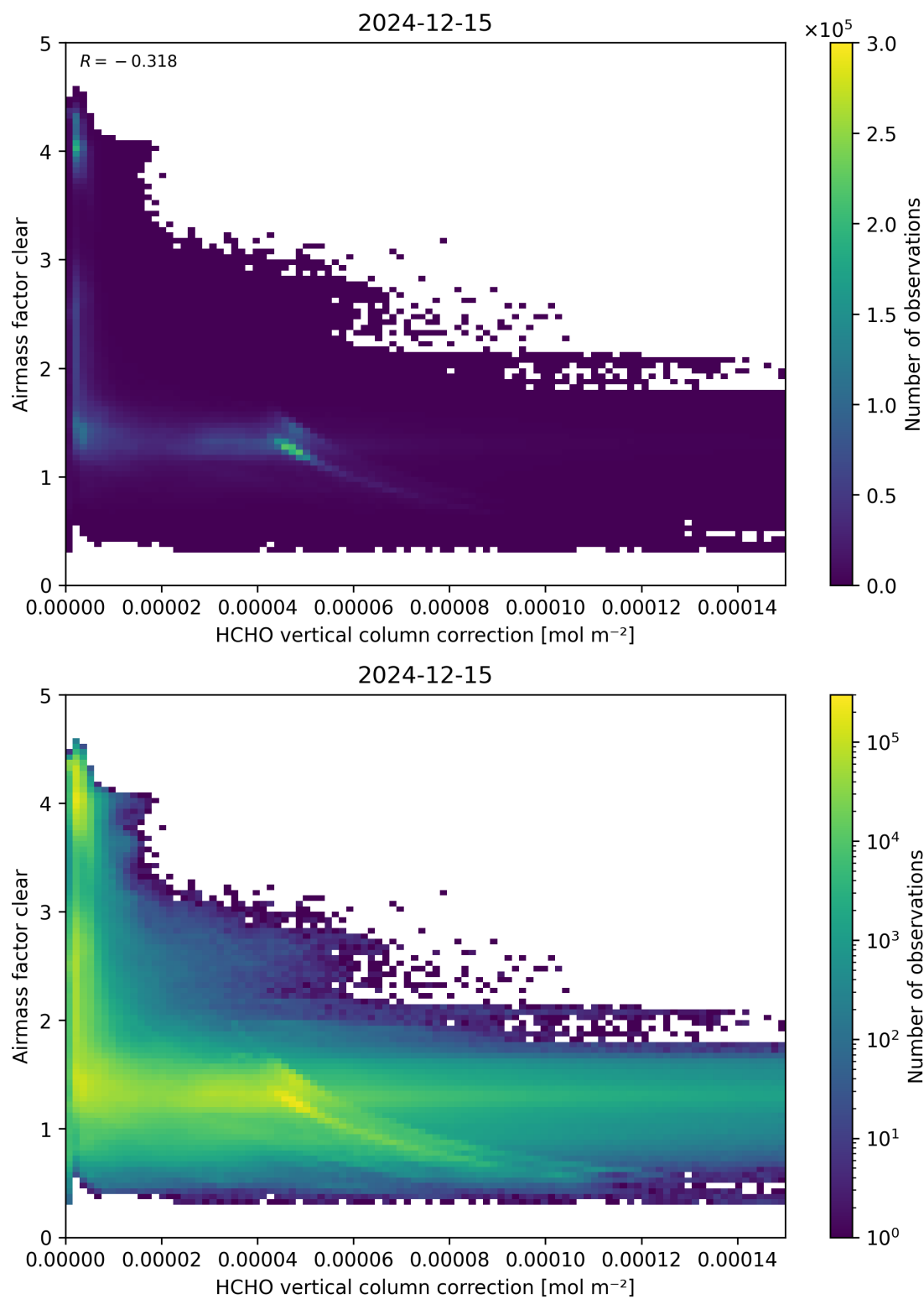
Figure 115: Scatter density plot of “HCHO vertical column correction” against “Airmass factor clear” for 2024-12-14 to 2024-12-16.
