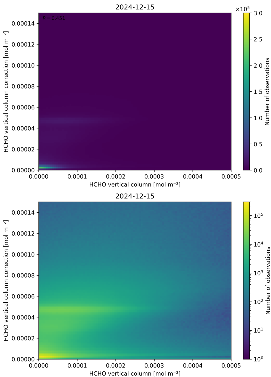
Figure 133: Scatter density plot of “HCHO vertical column” against “HCHO vertical column correction” for 2024-12-14 to 2024-12-16.
