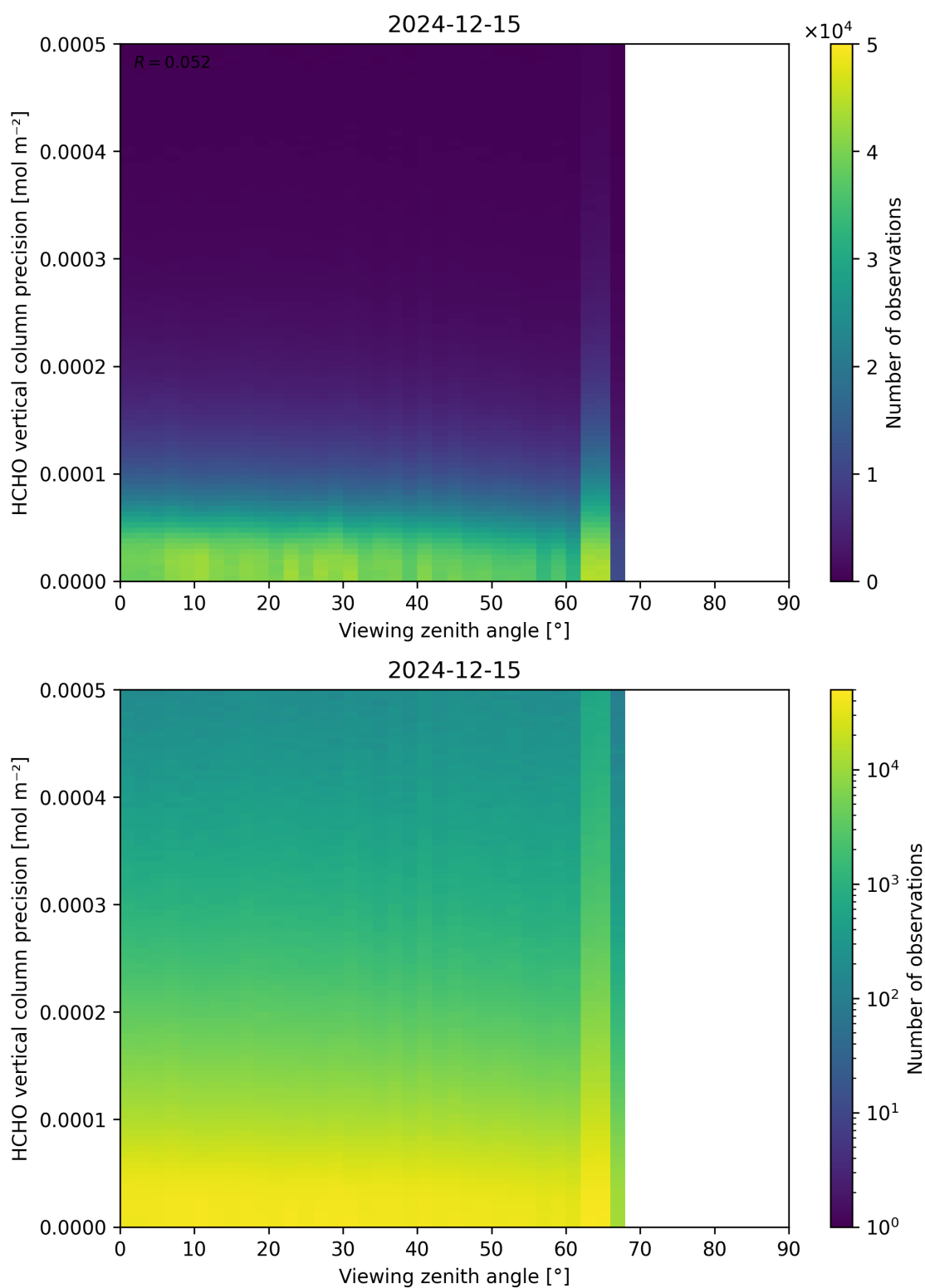
Figure 194: Scatter density plot of “Viewing zenith angle” against “HCHO vertical column precision” for 2024-12-14 to 2024-12-16.
