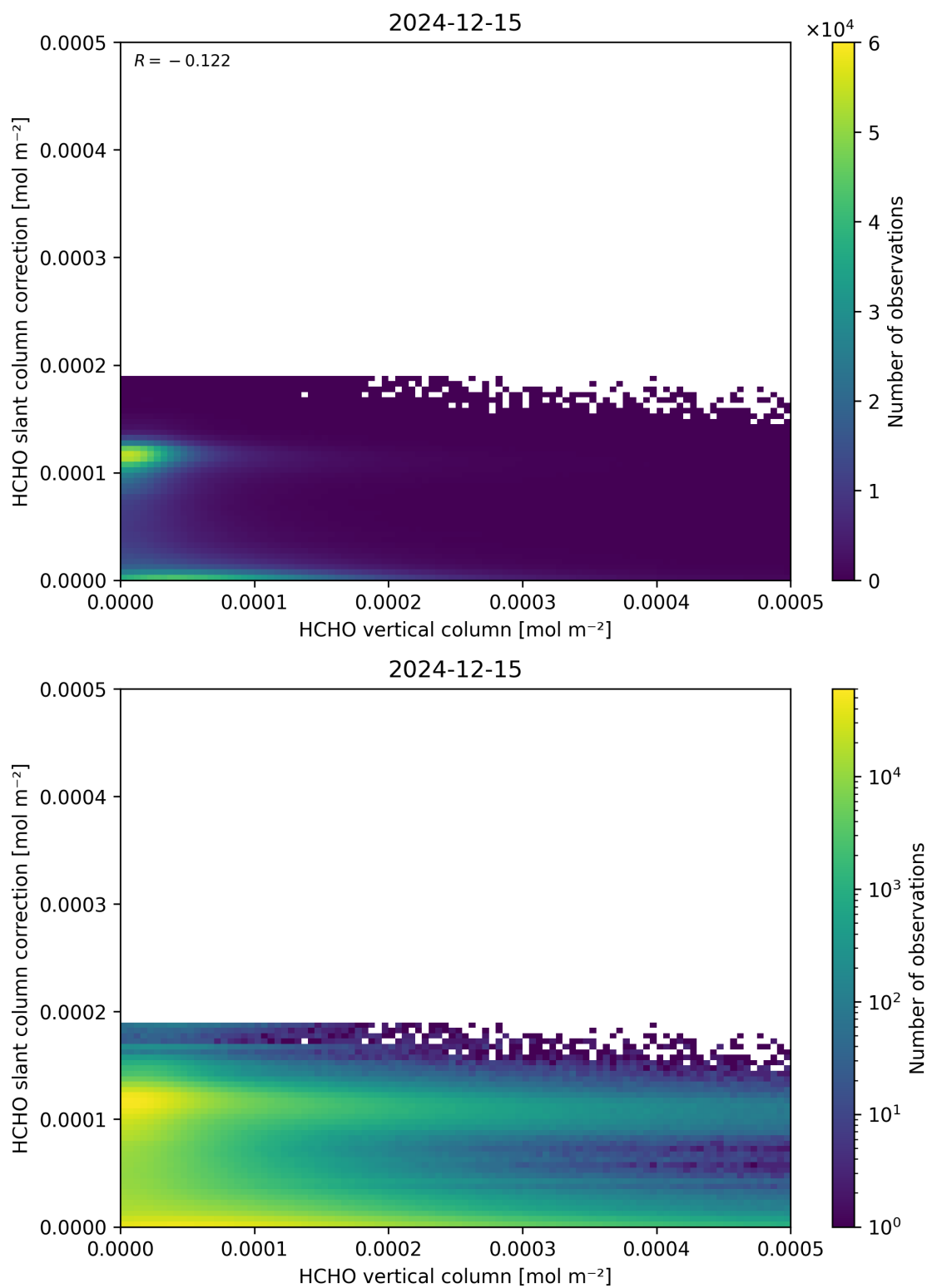
Figure 128: Scatter density plot of “HCHO vertical column” against “HCHO slant column correction” for 2024-12-14 to 2024-12-16.
