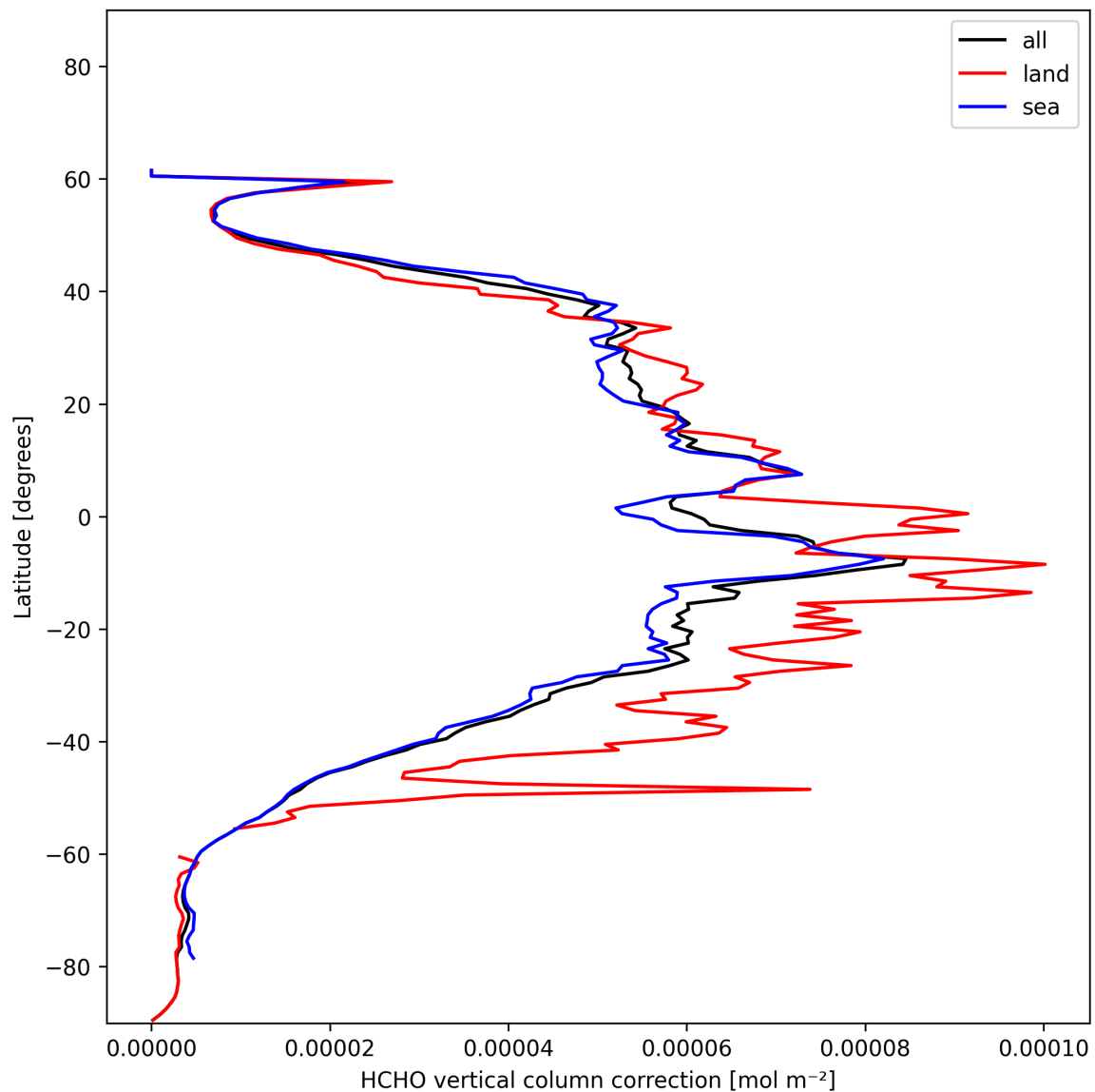
Figure 23: Zonal average of “HCHO vertical column correction” for 2024-12-14 to 2024-12-16.
