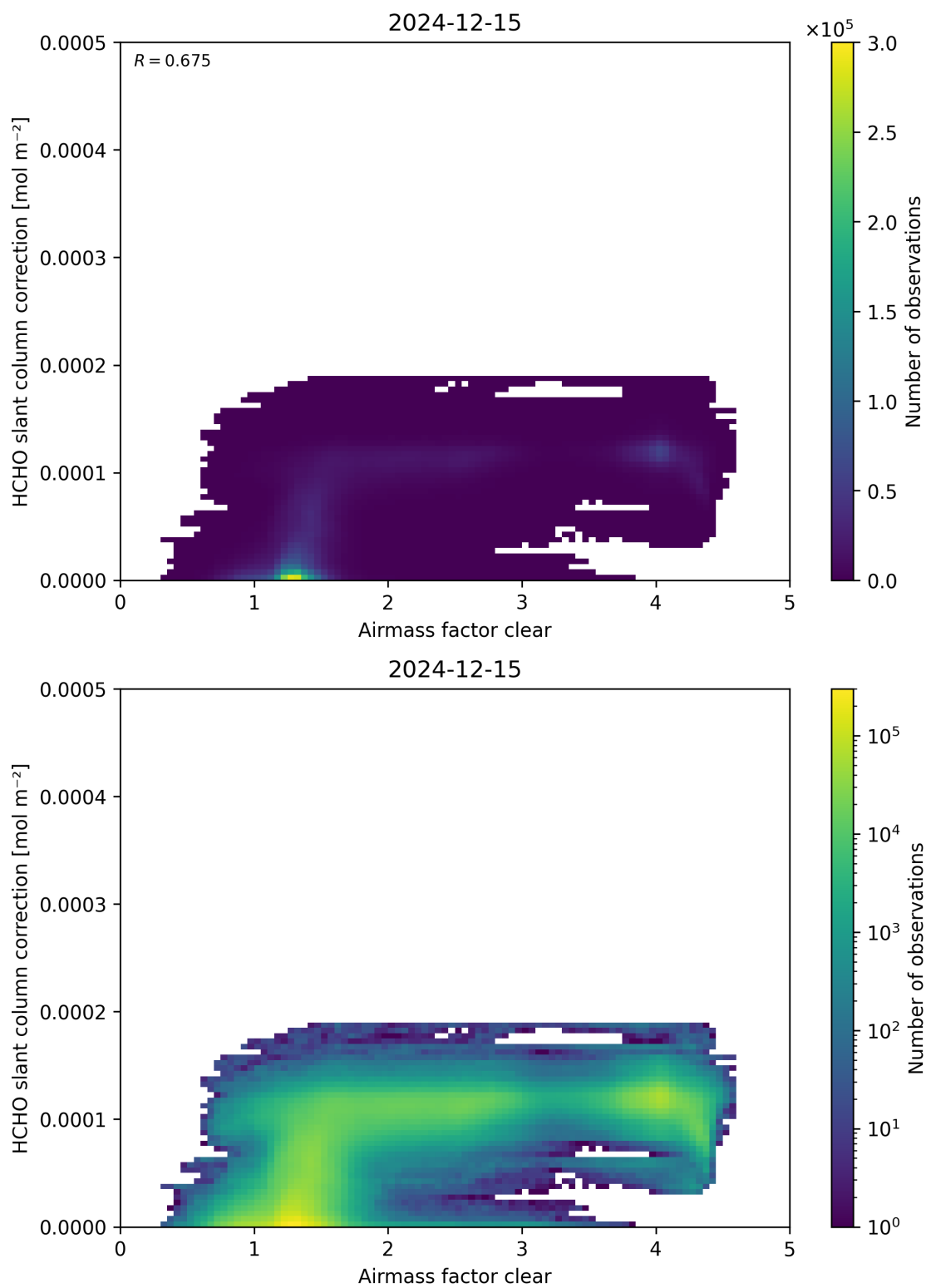
Figure 75: Scatter density plot of “Airmass factor clear” against “HCHO slant column correction” for 2024-12-14 to 2024-12-16.
