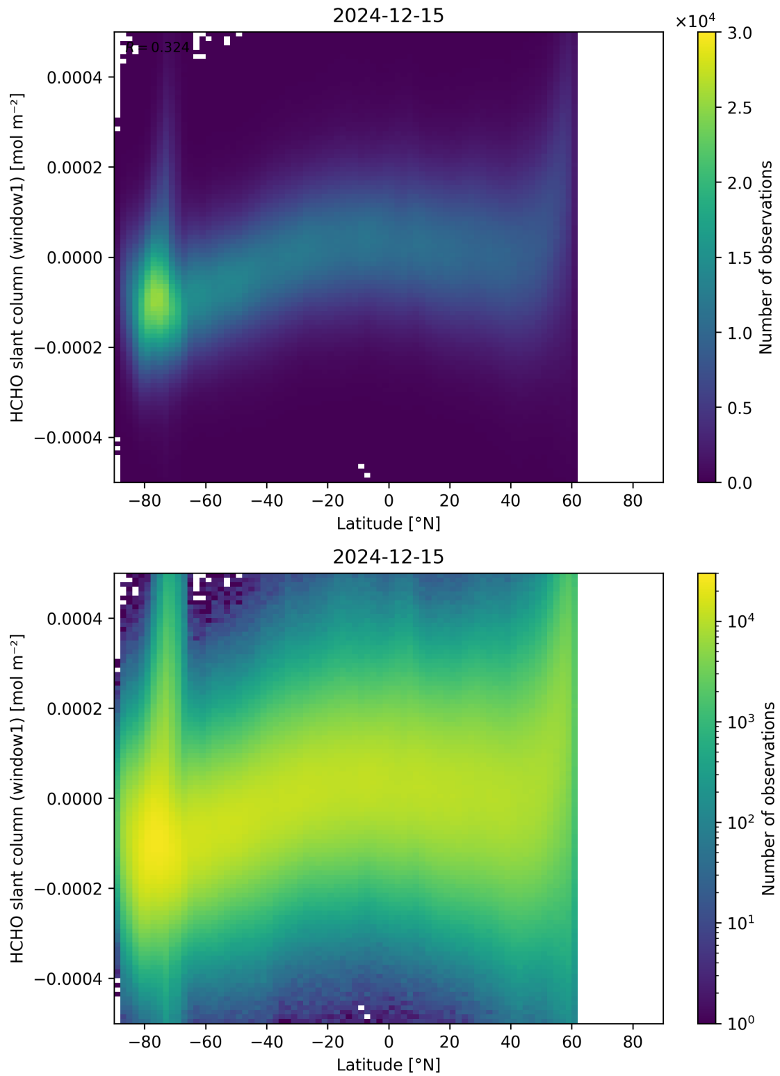
Figure 159: Scatter density plot of “Latitude” against “HCHO slant column (window1)” for 2024-12-14 to 2024-12-16.
