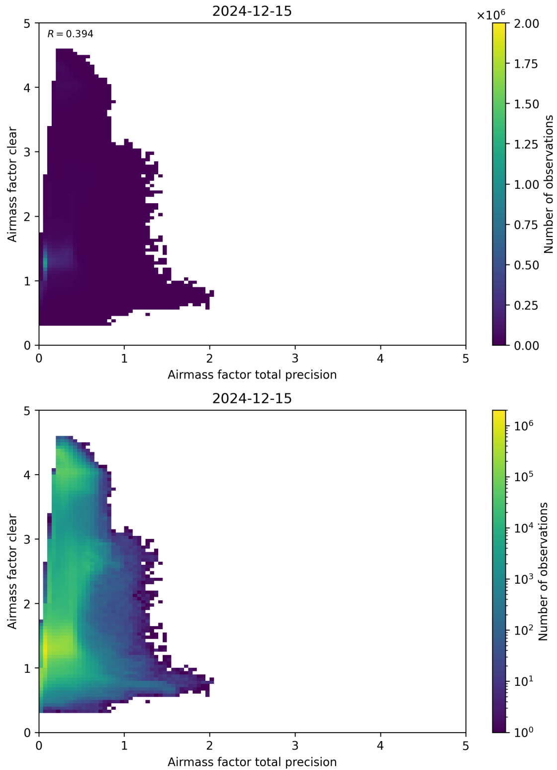
Figure 108: Scatter density plot of “Airmass factor total precision” against “Airmass factor clear” for 2024-12-14 to 2024-12-16.
