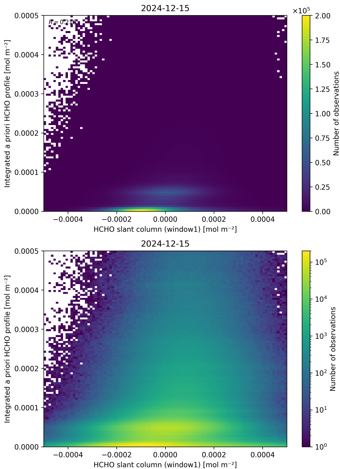
Figure 87: Scatter density plot of “HCHO slant column (window1)” against “Integrated a priori HCHO profile” for 2024-12-14 to 2024-12-16.
