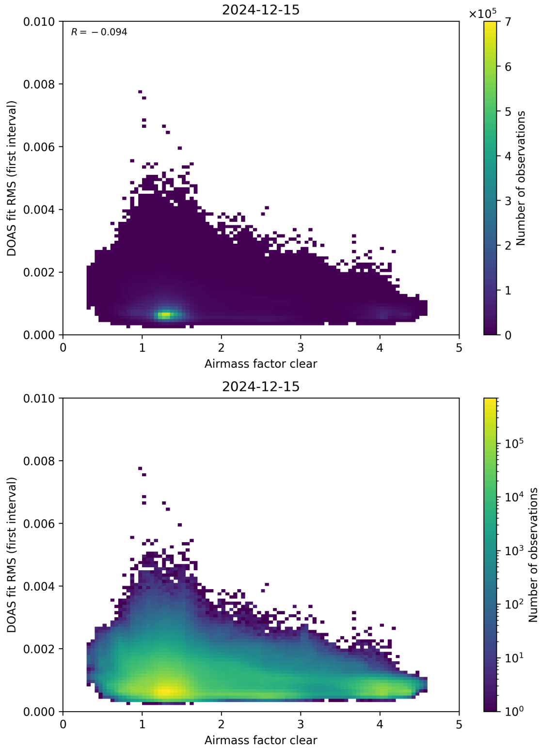
Figure 71: Scatter density plot of “Airmass factor clear” against “DOAS fit RMS (first interval)” for 2024-12-14 to 2024-12-16.
