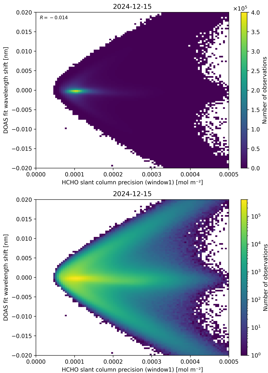
Figure 89: Scatter density plot of “HCHO slant column precision (window1)” against “DOAS fit wavelength shift” for 2024-12-14 to 2024-12-16.
