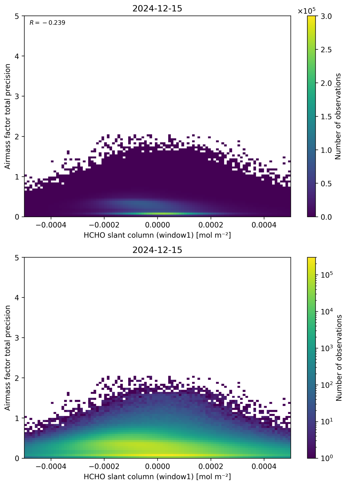
Figure 86: Scatter density plot of “HCHO slant column (window1)” against “Airmass factor total precision” for 2024-12-14 to 2024-12-16.
