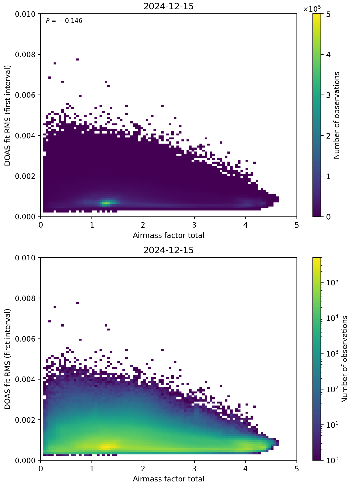
Figure 97: Scatter density plot of “Airmass factor total” against “DOAS fit RMS (first interval)” for 2024-12-14 to 2024-12-16.
