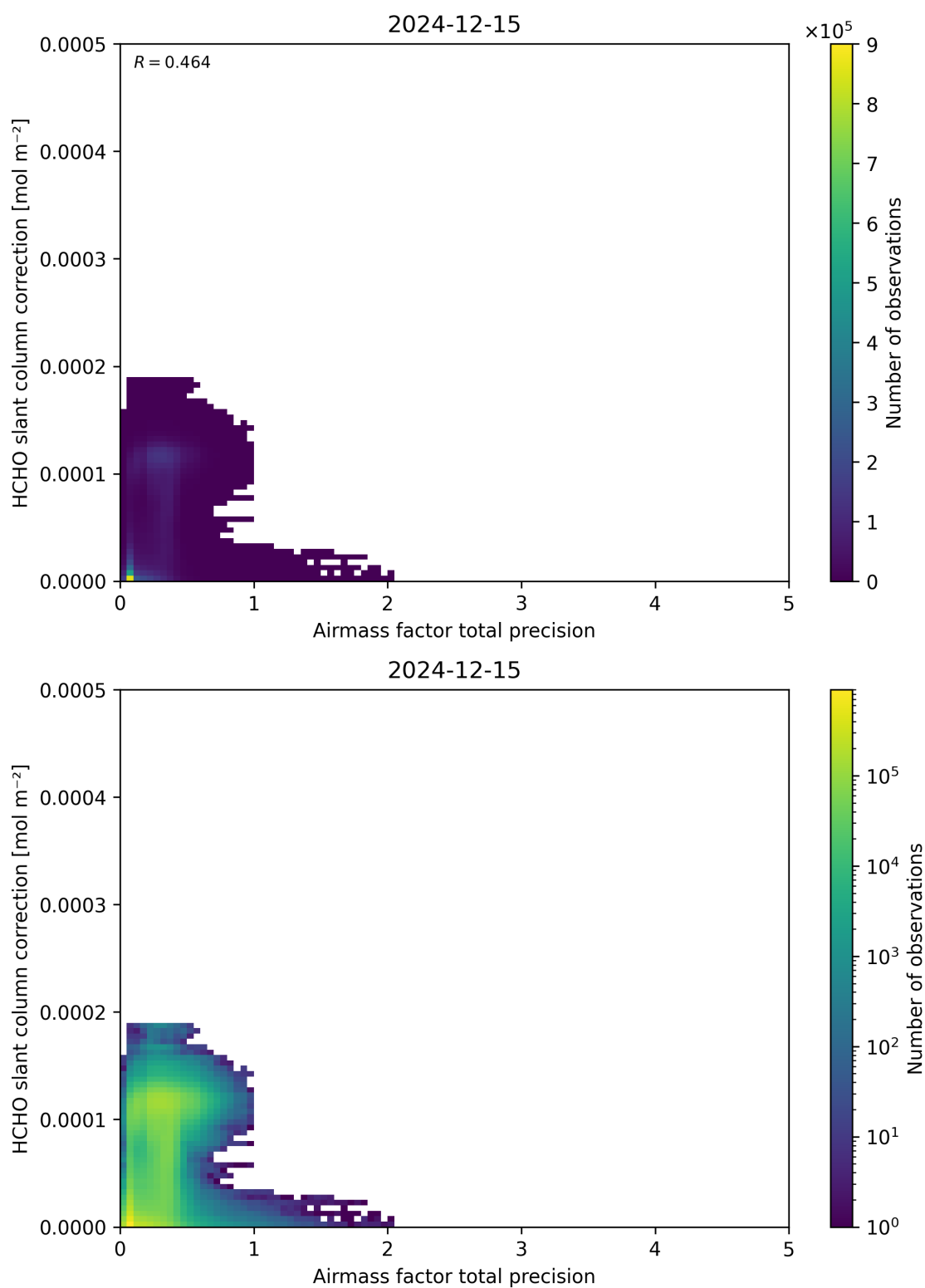
Figure 110: Scatter density plot of “Airmass factor total precision” against “HCHO slant column correction” for 2024-12-14 to 2024-12-16.
