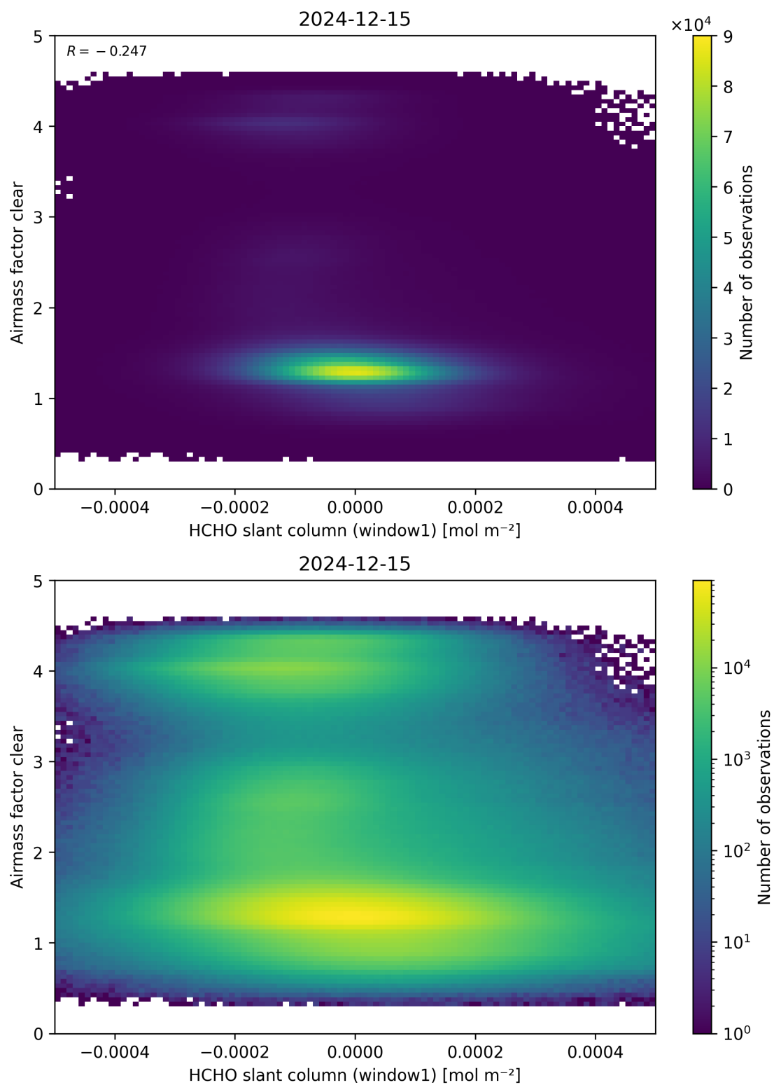
Figure 81: Scatter density plot of “HCHO slant column (window1)” against “Airmass factor clear” for 2024-12-14 to 2024-12-16.
