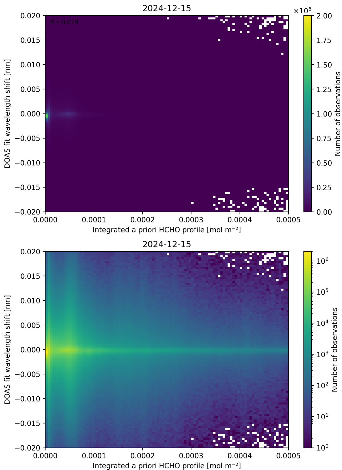
Figure 149: Scatter density plot of “Integrated a priori HCHO profile” against “DOAS fit wavelength shift” for 2024-12-14 to 2024-12-16.
