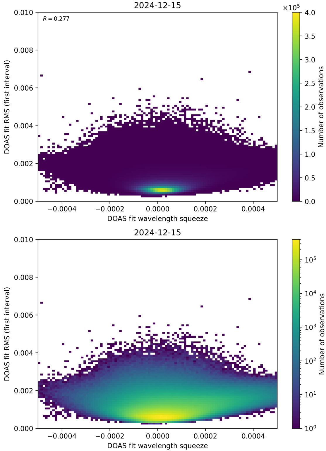
Figure 68: Scatter density plot of “DOAS fit wavelength squeeze” against “DOAS fit RMS (first interval)” for 2024-12-14 to 2024-12-16.
