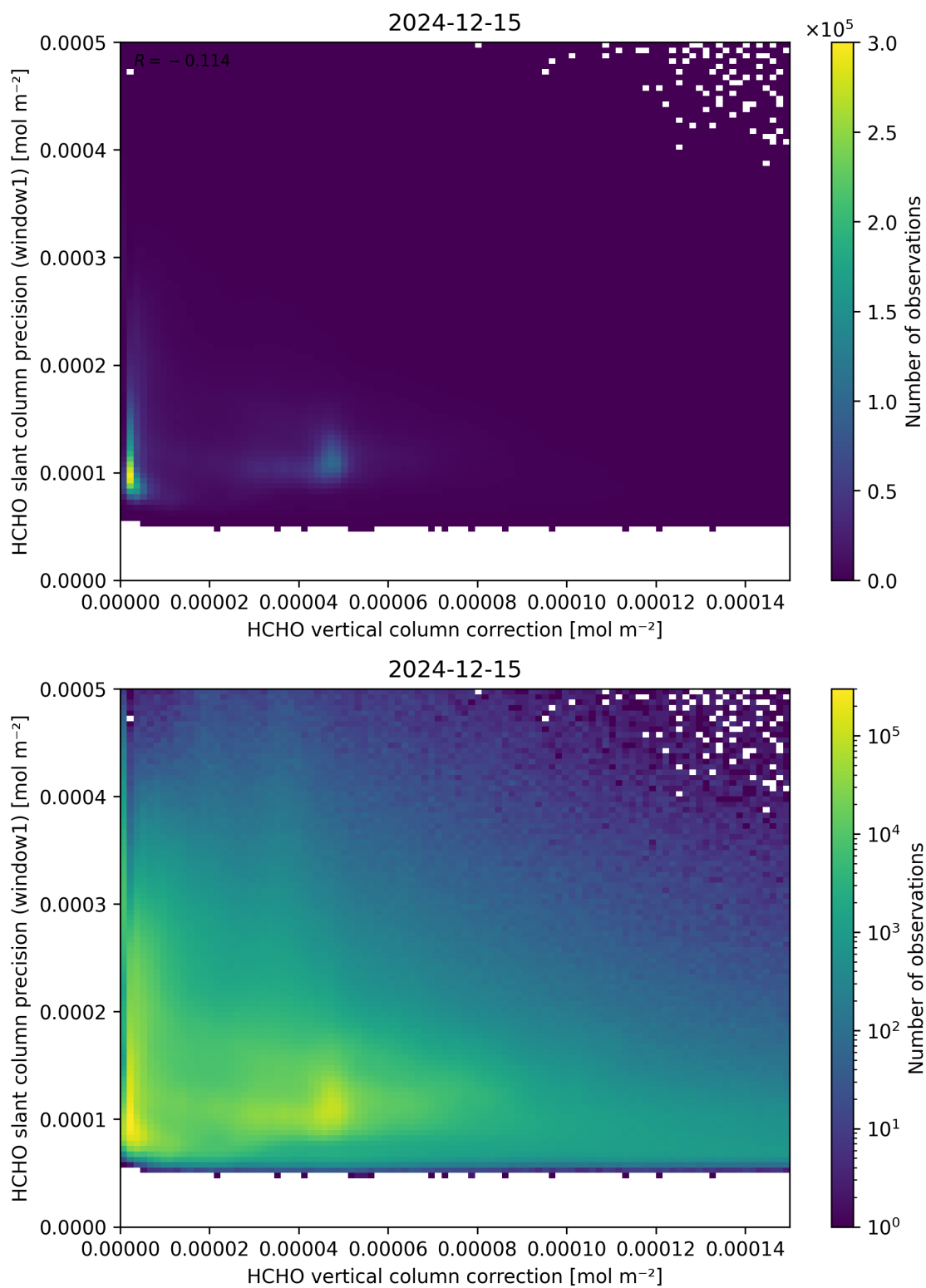
Figure 119: Scatter density plot of “HCHO vertical column correction” against “HCHO slant column precision (window1)” for 2024-12-14 to 2024-12-16.
