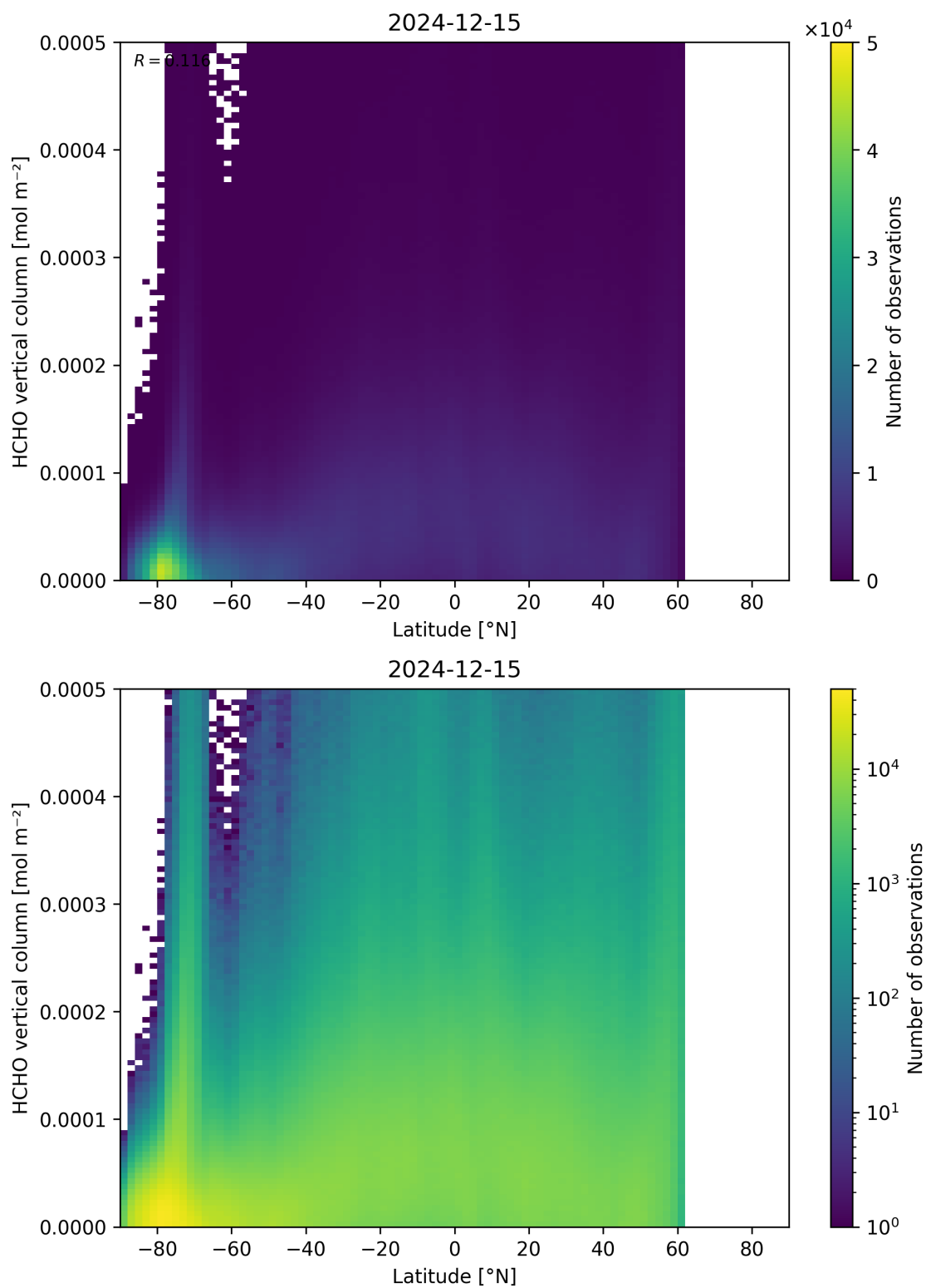
Figure 163: Scatter density plot of “Latitude” against “HCHO vertical column” for 2024-12-14 to 2024-12-16.
