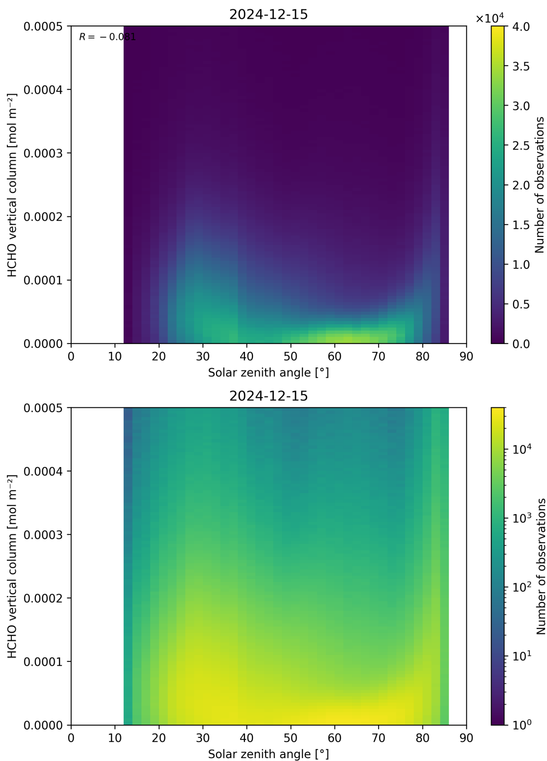
Figure 177: Scatter density plot of “Solar zenith angle” against “HCHO vertical column” for 2024-12-14 to 2024-12-16.
