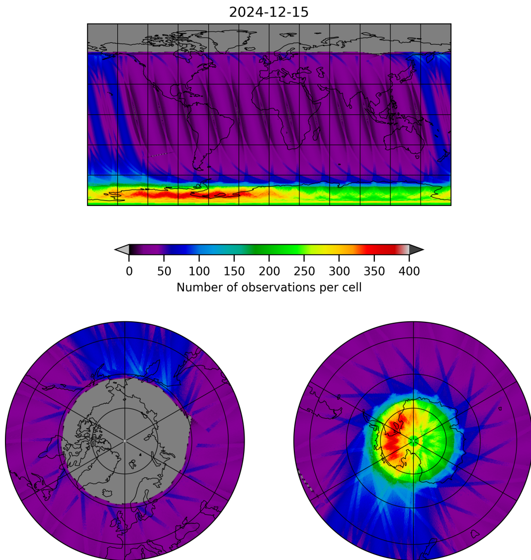
Figure 19: Map of the number of observations for 2024-12-14 to 2024-12-16
