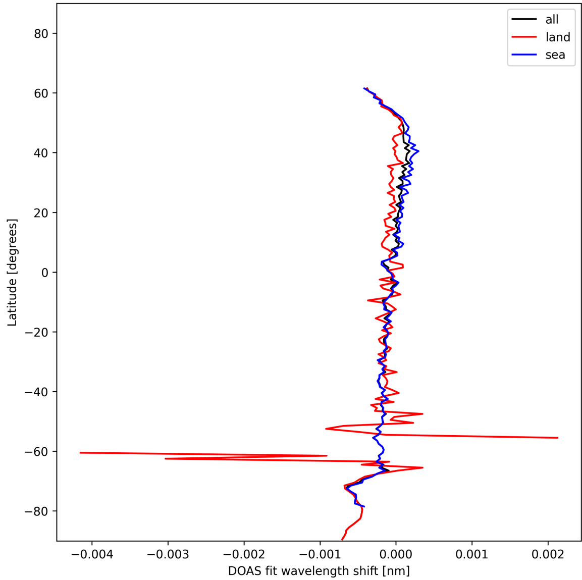
Figure 30: Zonal average of “DOAS fit wavelength shift” for 2024-12-14 to 2024-12-16.
