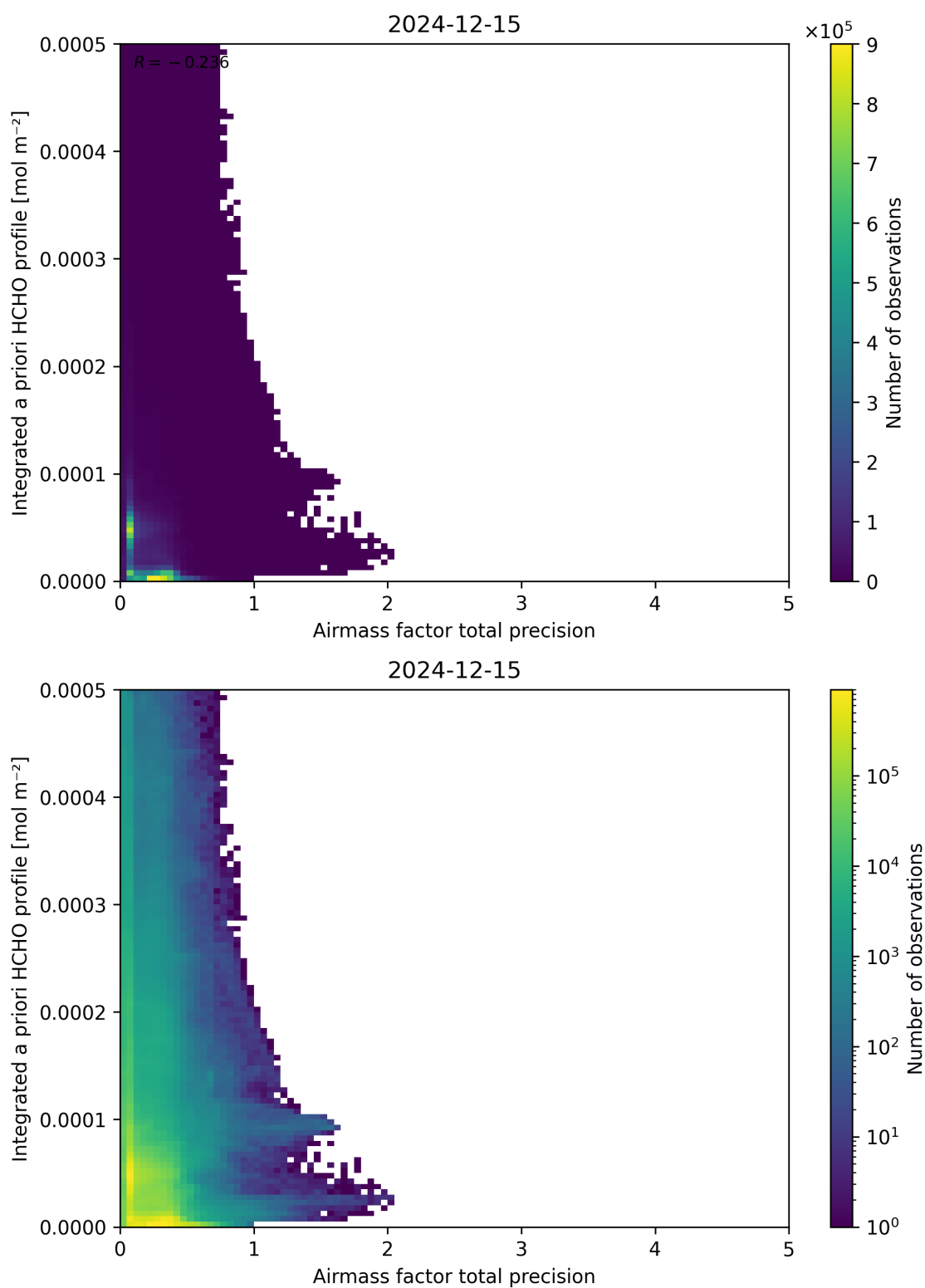
Figure 111: Scatter density plot of “Airmass factor total precision” against “Integrated a priori HCHO profile” for 2024-12-14 to 2024-12-16.
