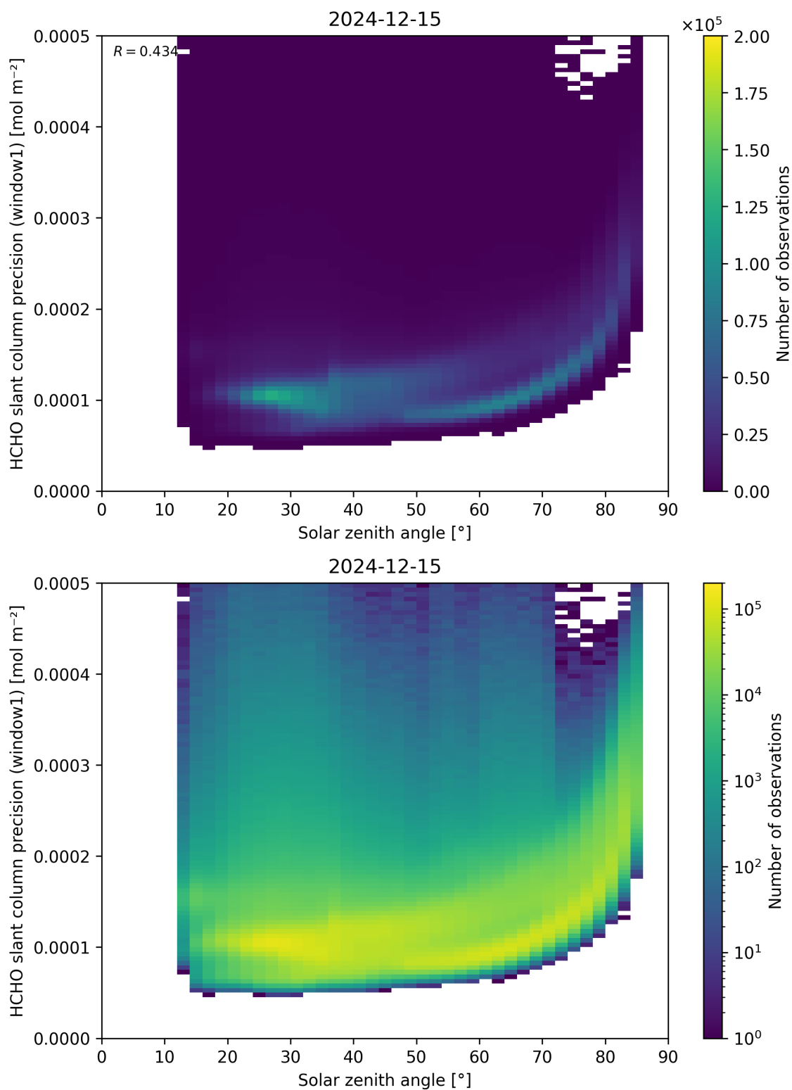
Figure 174: Scatter density plot of “Solar zenith angle” against “HCHO slant column precision (window1)” for 2024-12-14 to 2024-12-16.
