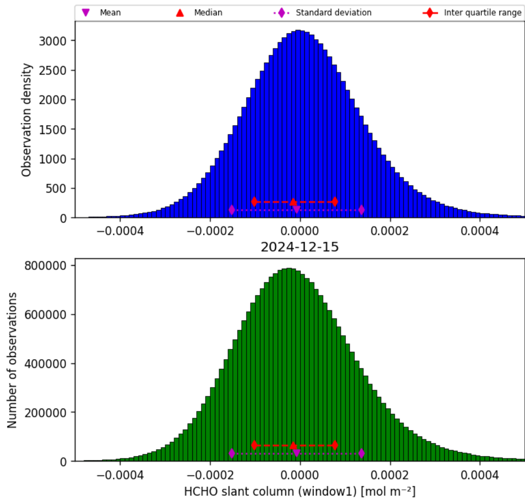
Figure 38: Histogram of “HCHO slant column (window1)” for 2024-12-14 to 2024-12-16
