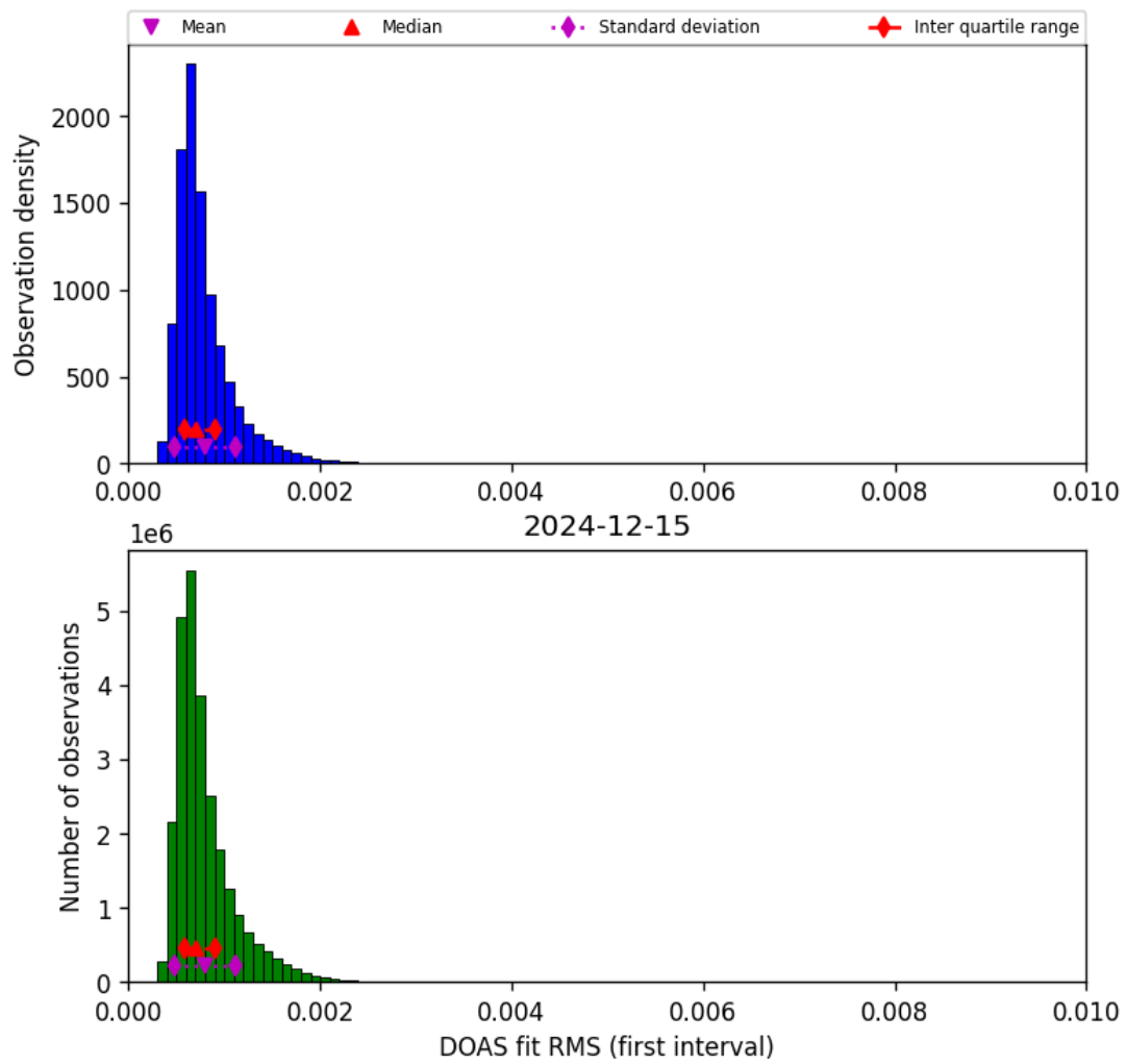
Figure 46: Histogram of “DOAS fit RMS (first interval)” for 2024-12-14 to 2024-12-16
