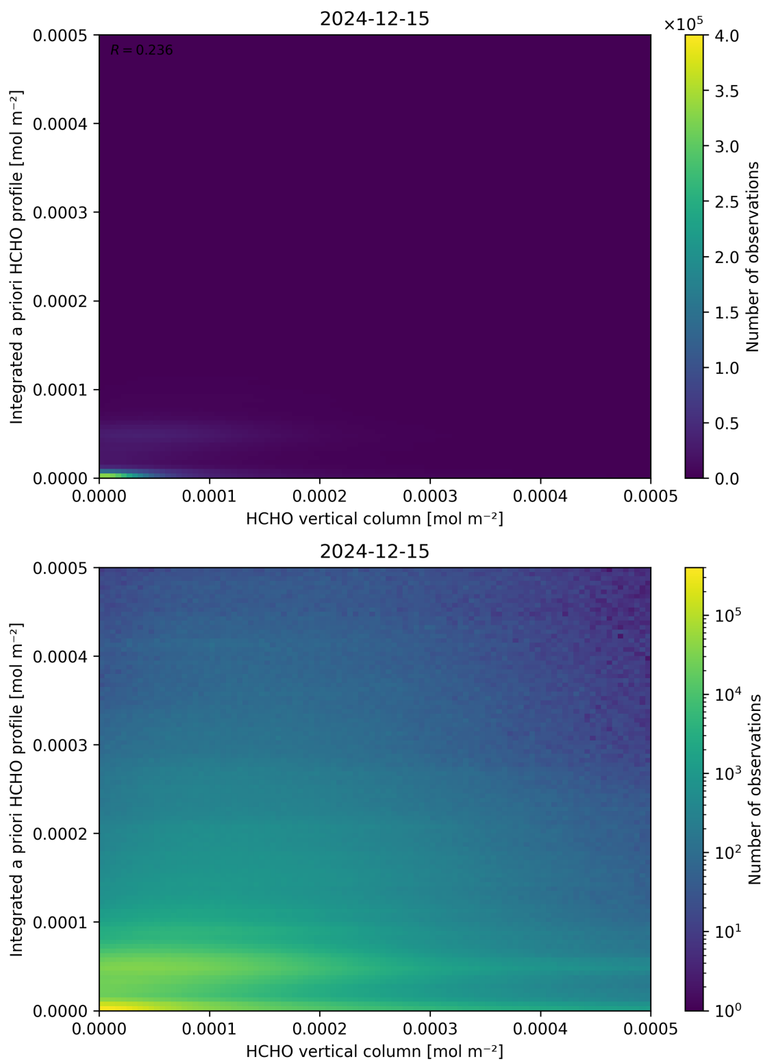
Figure 135: Scatter density plot of “HCHO vertical column” against “Integrated a priori HCHO profile” for 2024-12-14 to 2024-12-16.
