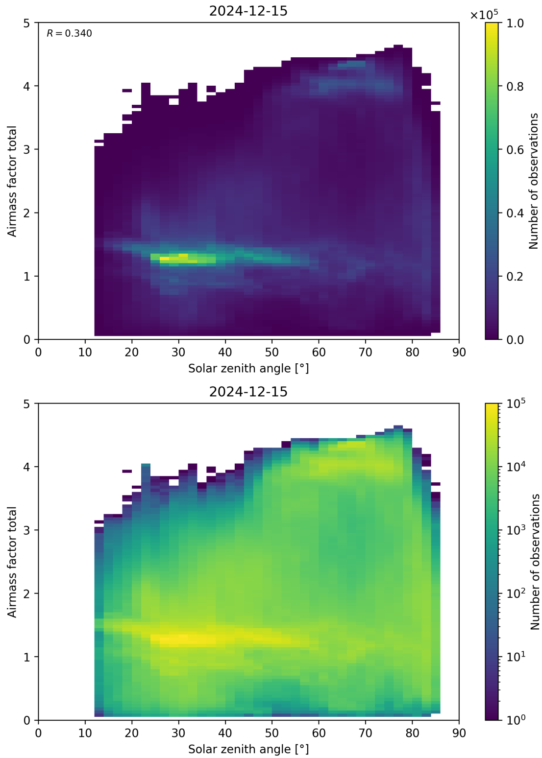
Figure 175: Scatter density plot of “Solar zenith angle” against “Airmass factor total” for 2024-12-14 to 2024-12-16.
