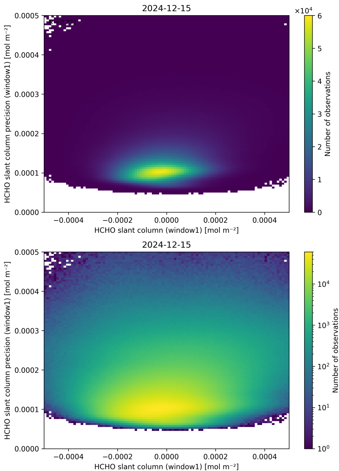
Figure 84: Scatter density plot of “HCHO slant column (window1)” against “HCHO slant column precision (window1)” for 2024-12-14 to 2024-12-16.
