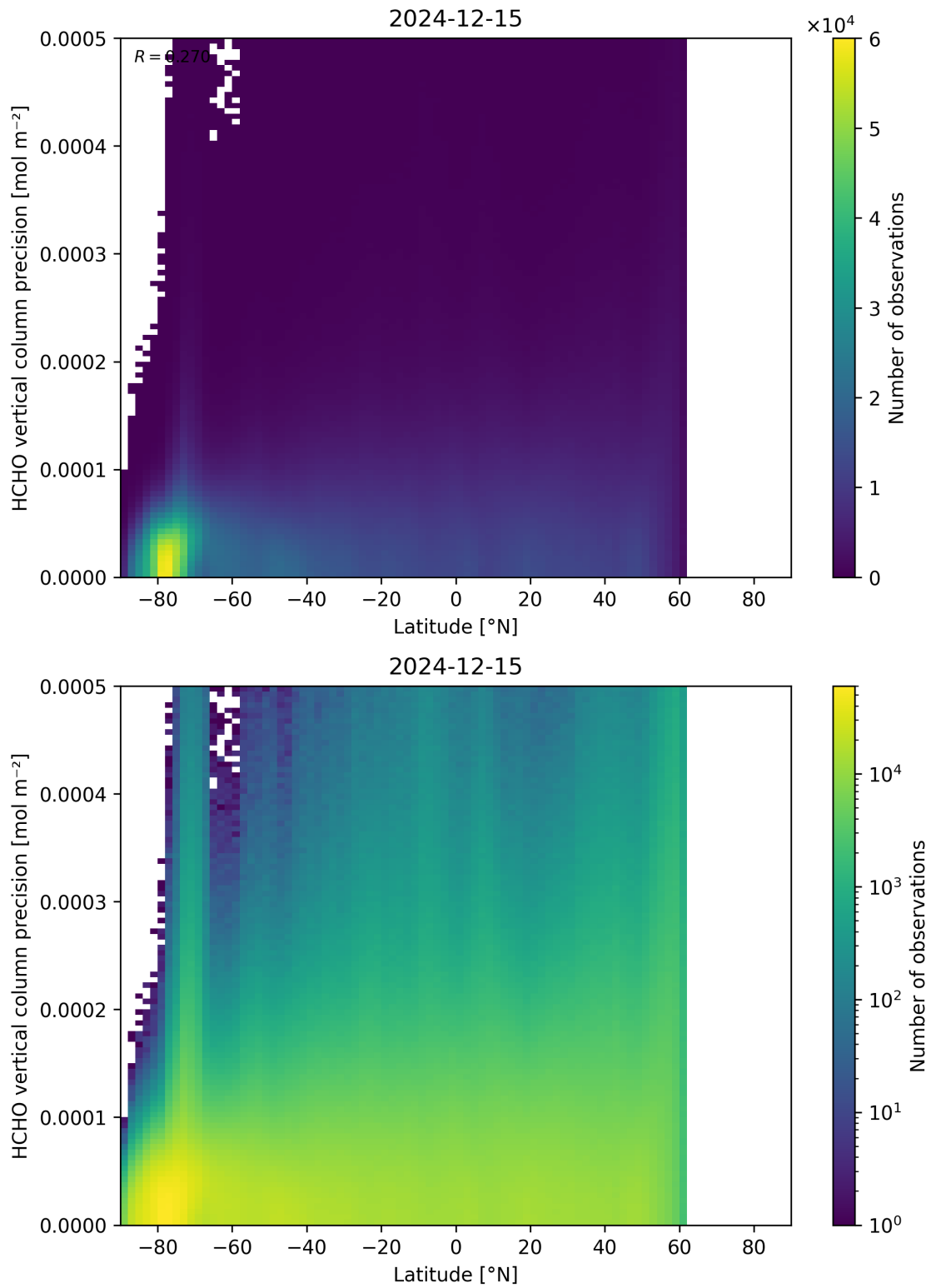
Figure 165: Scatter density plot of “Latitude” against “HCHO vertical column precision” for 2024-12-14 to 2024-12-16.
