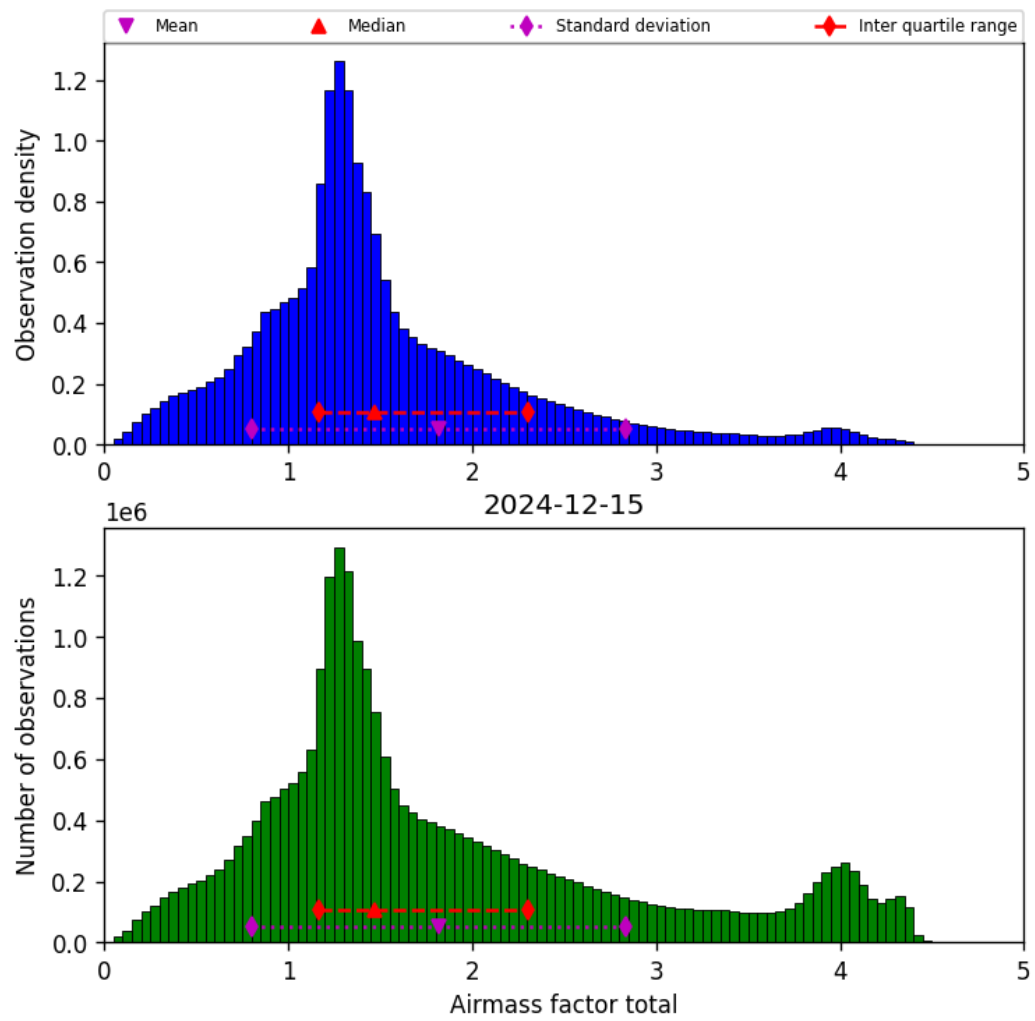
Figure 40: Histogram of “Airmass factor total” for 2024-12-14 to 2024-12-16
