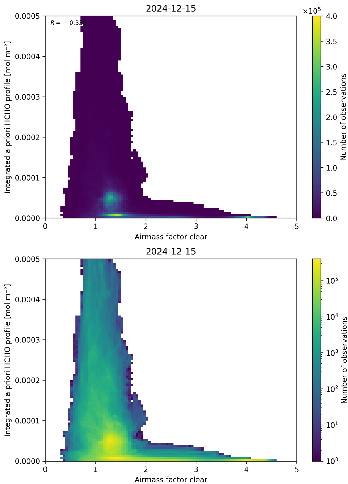
Figure 76: Scatter density plot of “Airmass factor clear” against “Integrated a priori HCHO profile” for 2024-12-14 to 2024-12-16.
