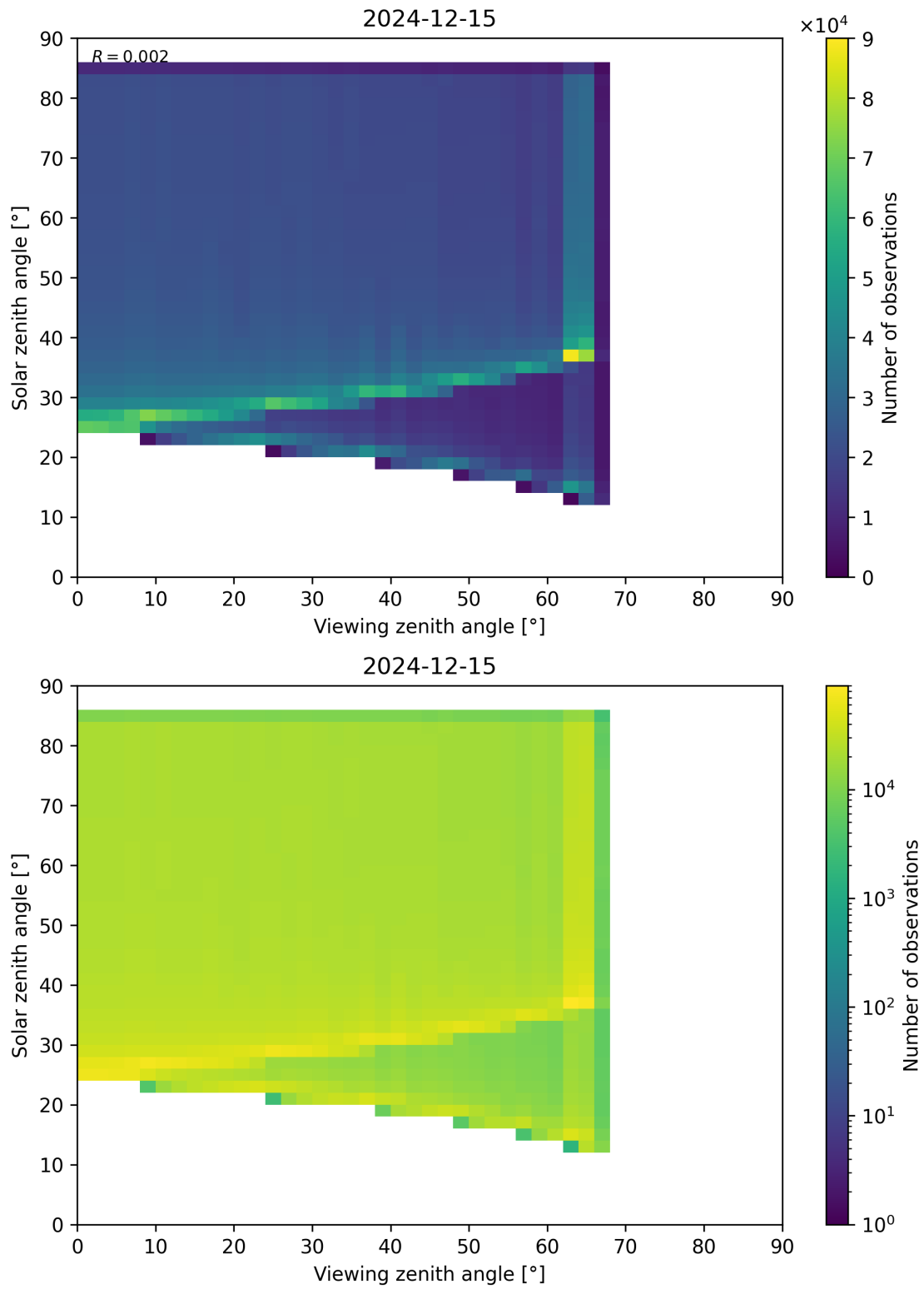
Figure 197: Scatter density plot of “Viewing zenith angle” against “Solar zenith angle” for 2024-12-14 to 2024-12-16.
