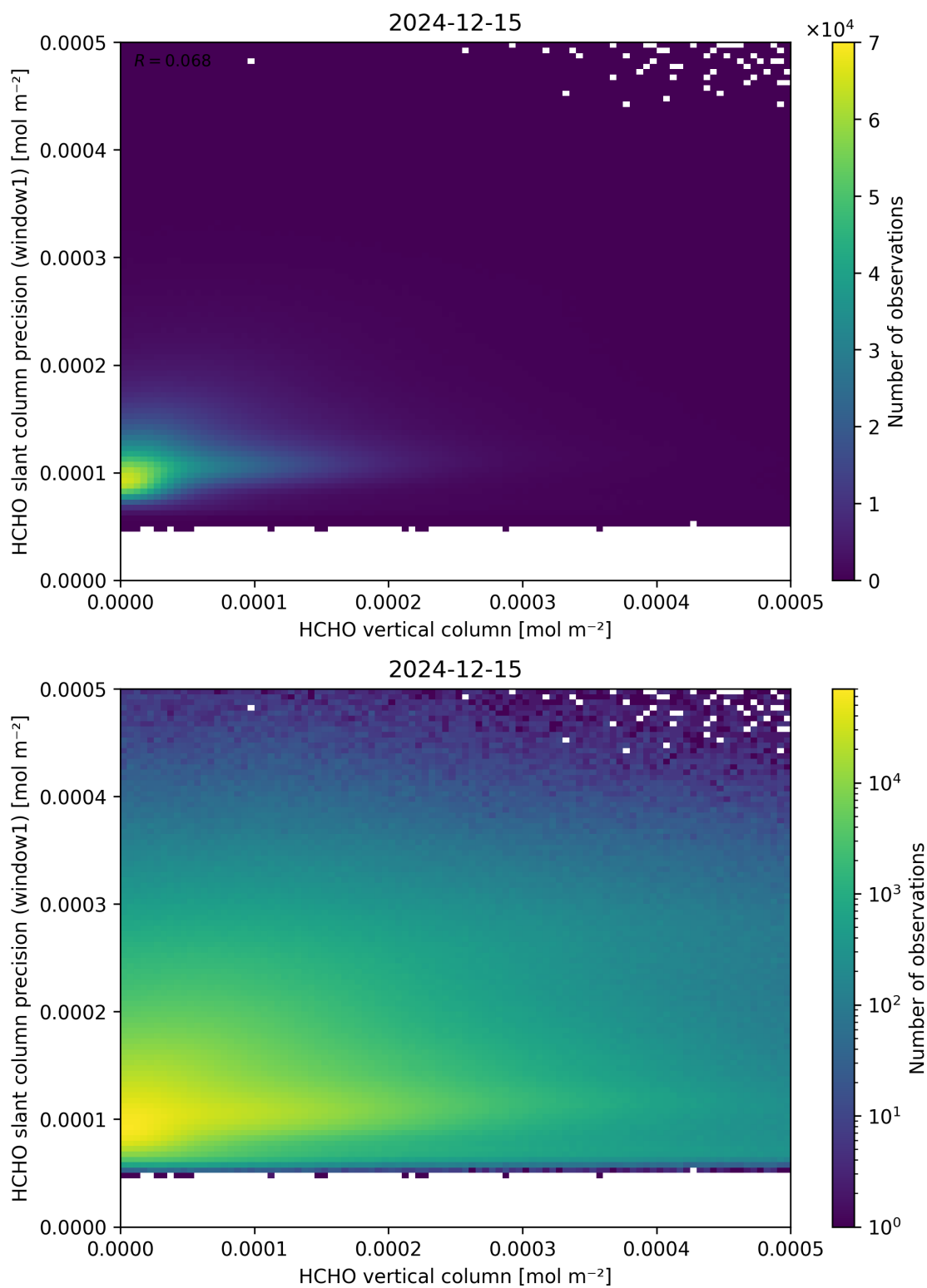
Figure 130: Scatter density plot of “HCHO vertical column” against “HCHO slant column precision (window1)” for 2024-12-14 to 2024-12-16.
