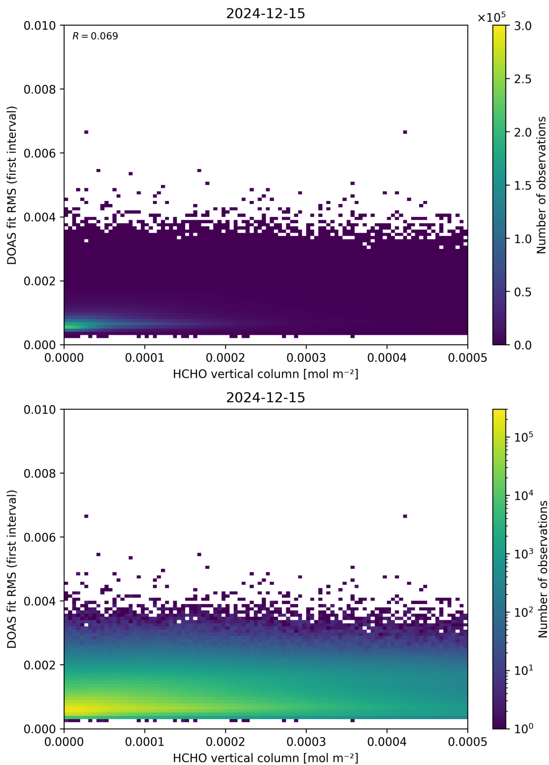
Figure 123: Scatter density plot of “HCHO vertical column” against “DOAS fit RMS (first interval)” for 2024-12-14 to 2024-12-16.
