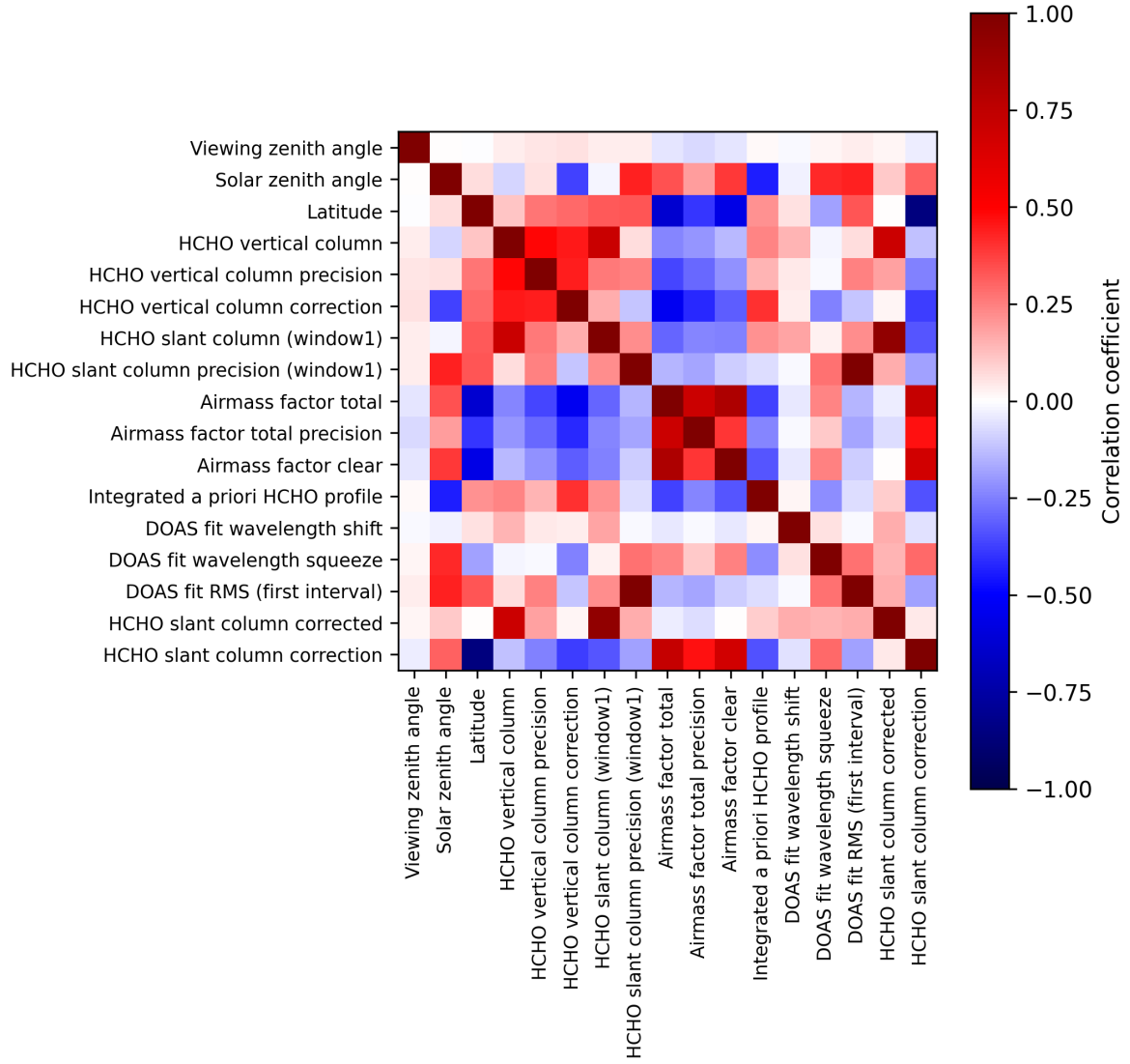
Figure 2: Map of correlation matrix for 2024-12-14 to 2024-12-16.
