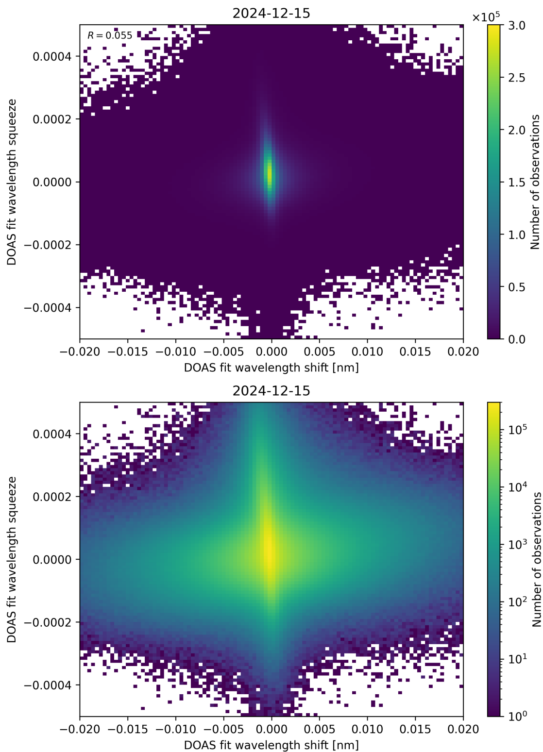
Figure 65: Scatter density plot of “DOAS fit wavelength shift” against “DOAS fit wavelength squeeze” for 2024-12-14 to 2024-12-16.
