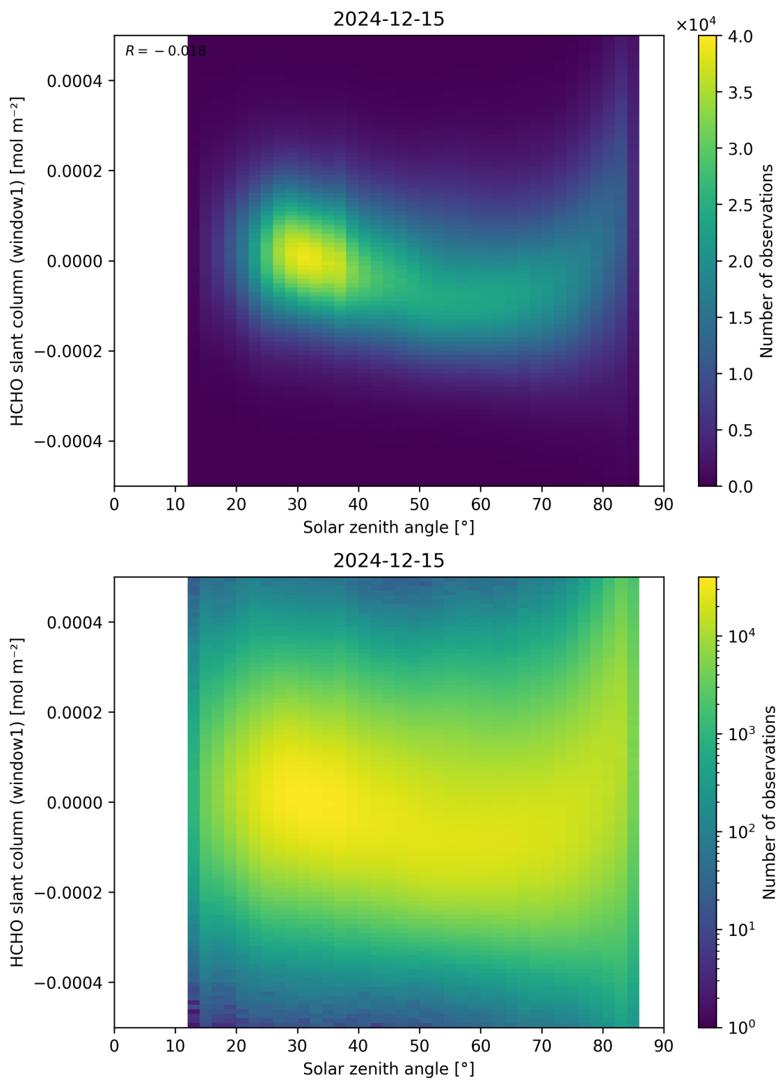
Figure 173: Scatter density plot of “Solar zenith angle” against “HCHO slant column (window1)” for 2024-12-14 to 2024-12-16.
