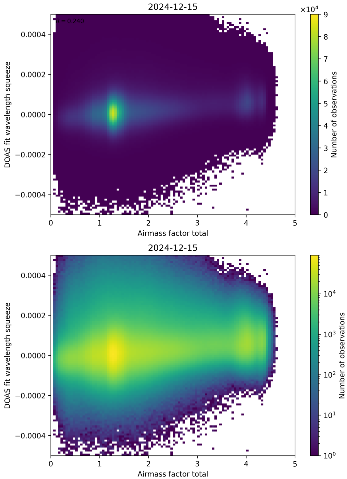
Figure 99: Scatter density plot of “Airmass factor total” against “DOAS fit wavelength squeeze” for 2024-12-14 to 2024-12-16.
