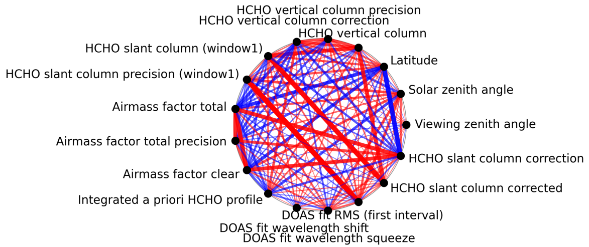
Figure 1: Map of correlation graph for 2024-12-14 to 2024-12-16.
