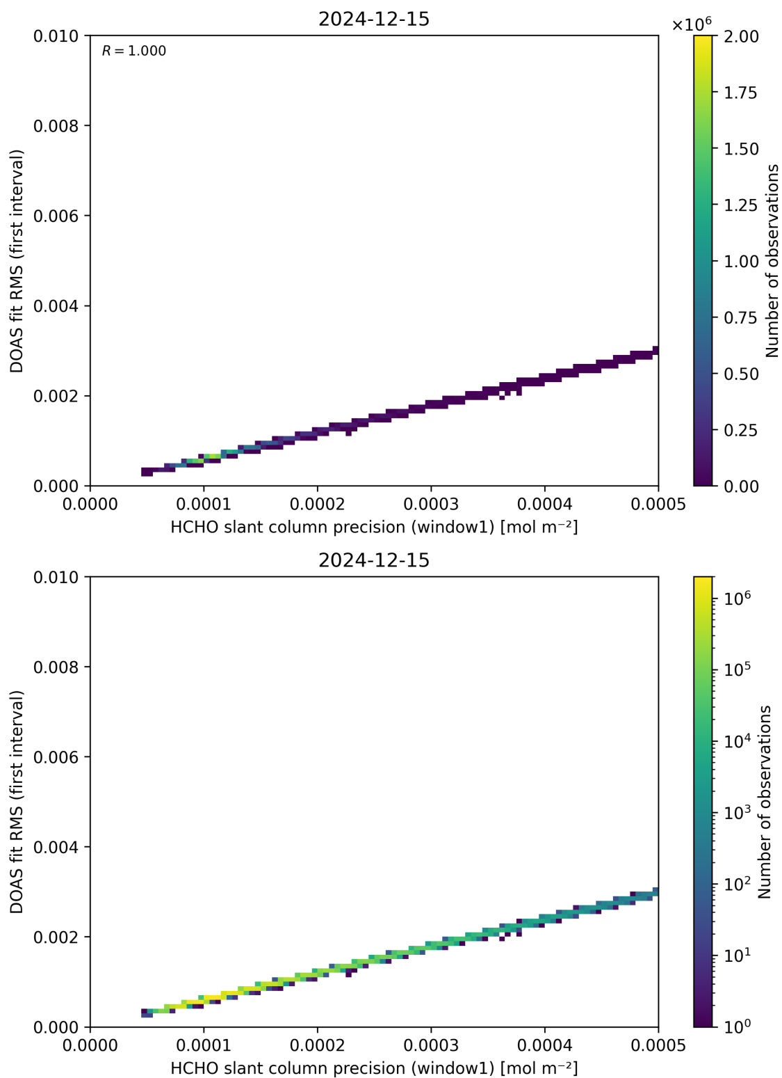
Figure 88: Scatter density plot of “HCHO slant column precision (window1)” against “DOAS fit RMS (first interval)” for 2024-12-14 to 2024-12-16.
