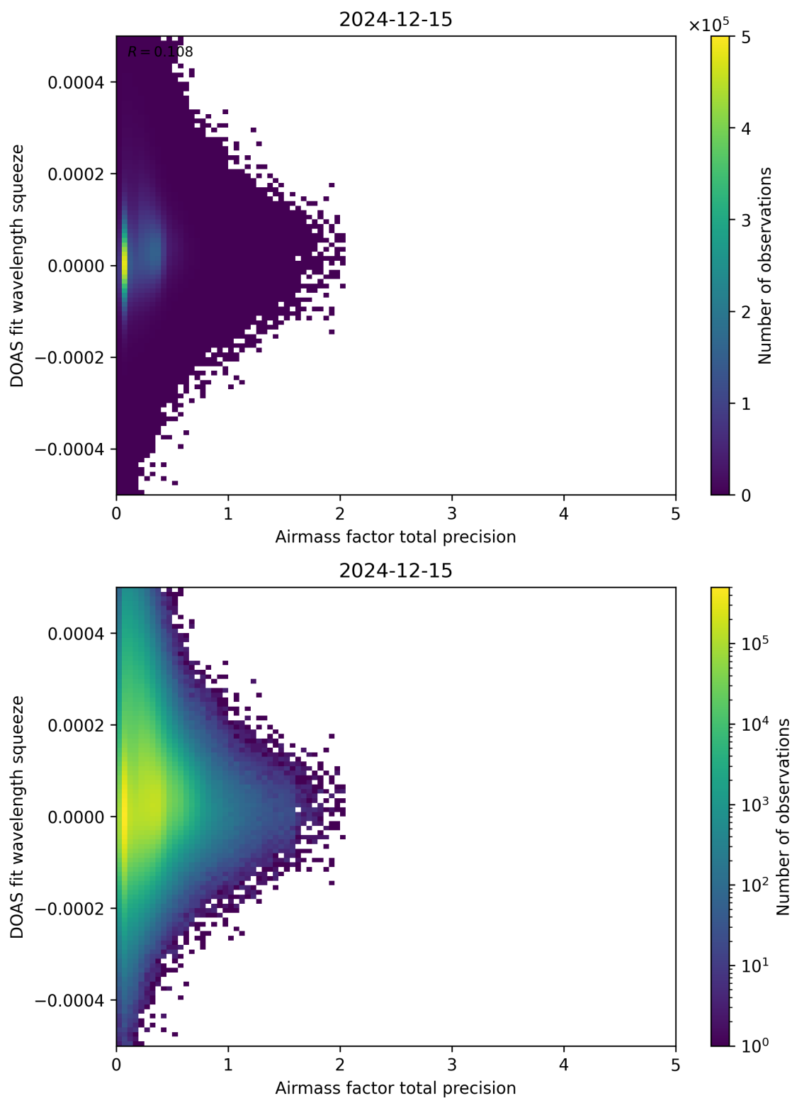
Figure 107: Scatter density plot of “Airmass factor total precision” against “DOAS fit wavelength squeeze” for 2024-12-14 to 2024-12-16.
