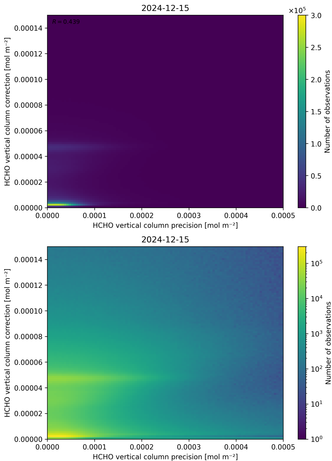
Figure 146: Scatter density plot of “HCHO vertical column precision” against “HCHO vertical column correction” for 2024-12-14 to 2024-12-16.
