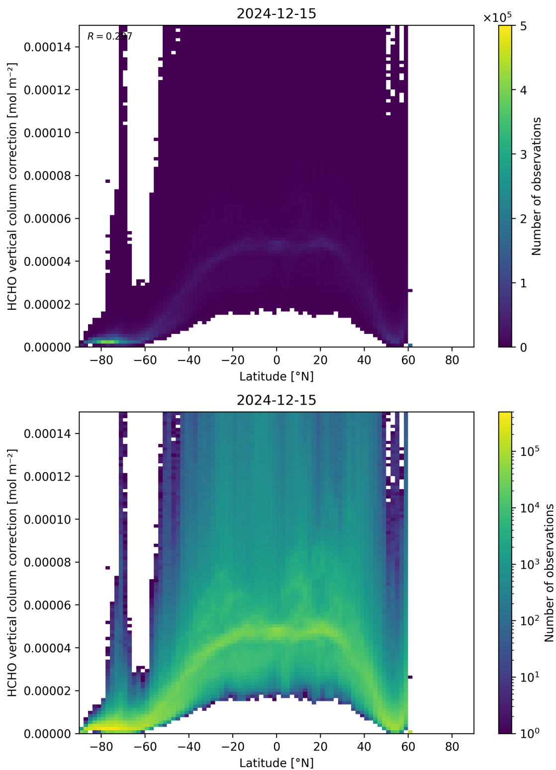
Figure 164: Scatter density plot of “Latitude” against “HCHO vertical column correction” for 2024-12-14 to 2024-12-16.
