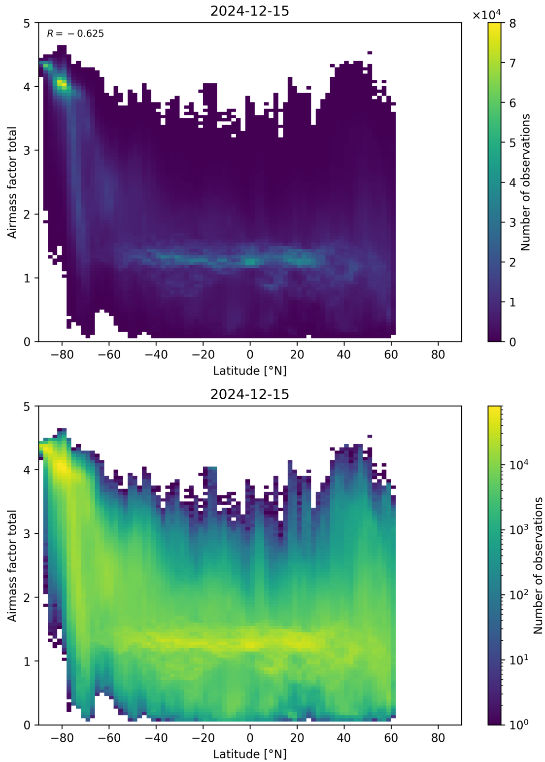
Figure 161: Scatter density plot of “Latitude” against “Airmass factor total” for 2024-12-14 to 2024-12-16.
