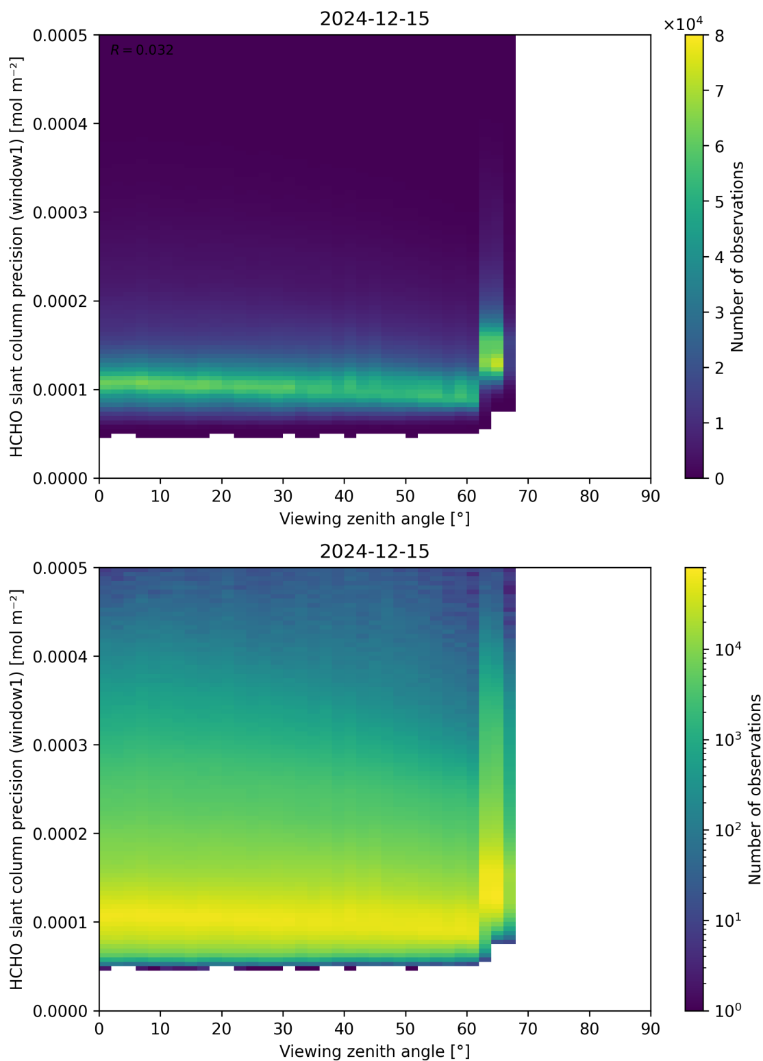
Figure 189: Scatter density plot of “Viewing zenith angle” against “HCHO slant column precision (window1)” for 2024-12-14 to 2024-12-16.
