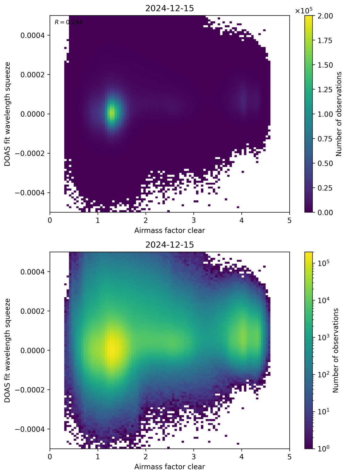
Figure 73: Scatter density plot of “Airmass factor clear” against “DOAS fit wavelength squeeze” for 2024-12-14 to 2024-12-16.
