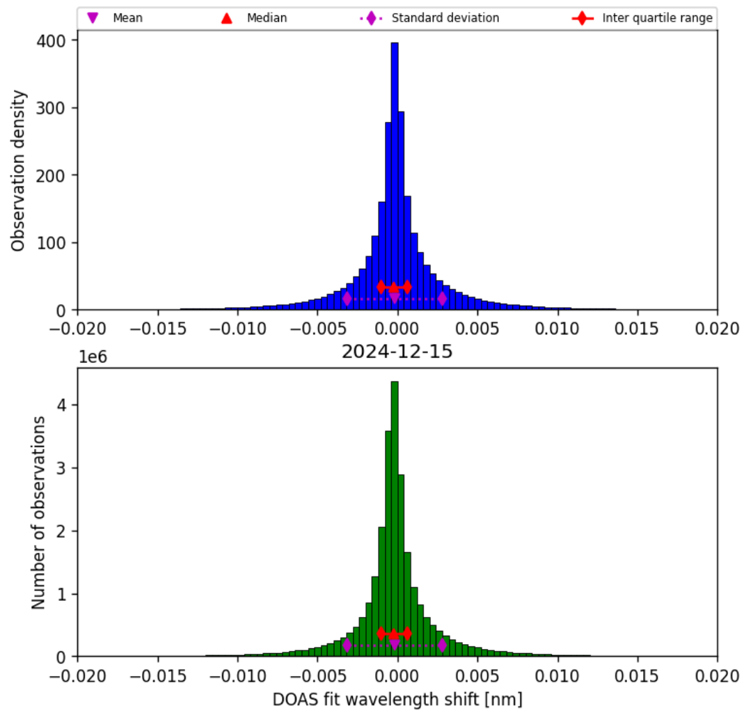
Figure 44: Histogram of “DOAS fit wavelength shift” for 2024-12-14 to 2024-12-16
