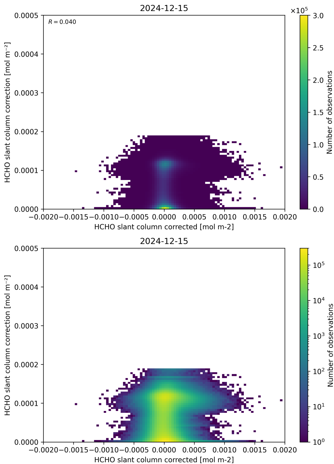
Figure 77: Scatter density plot of “HCHO slant column corrected” against “HCHO slant column correction” for 2024-12-14 to 2024-12-16.
