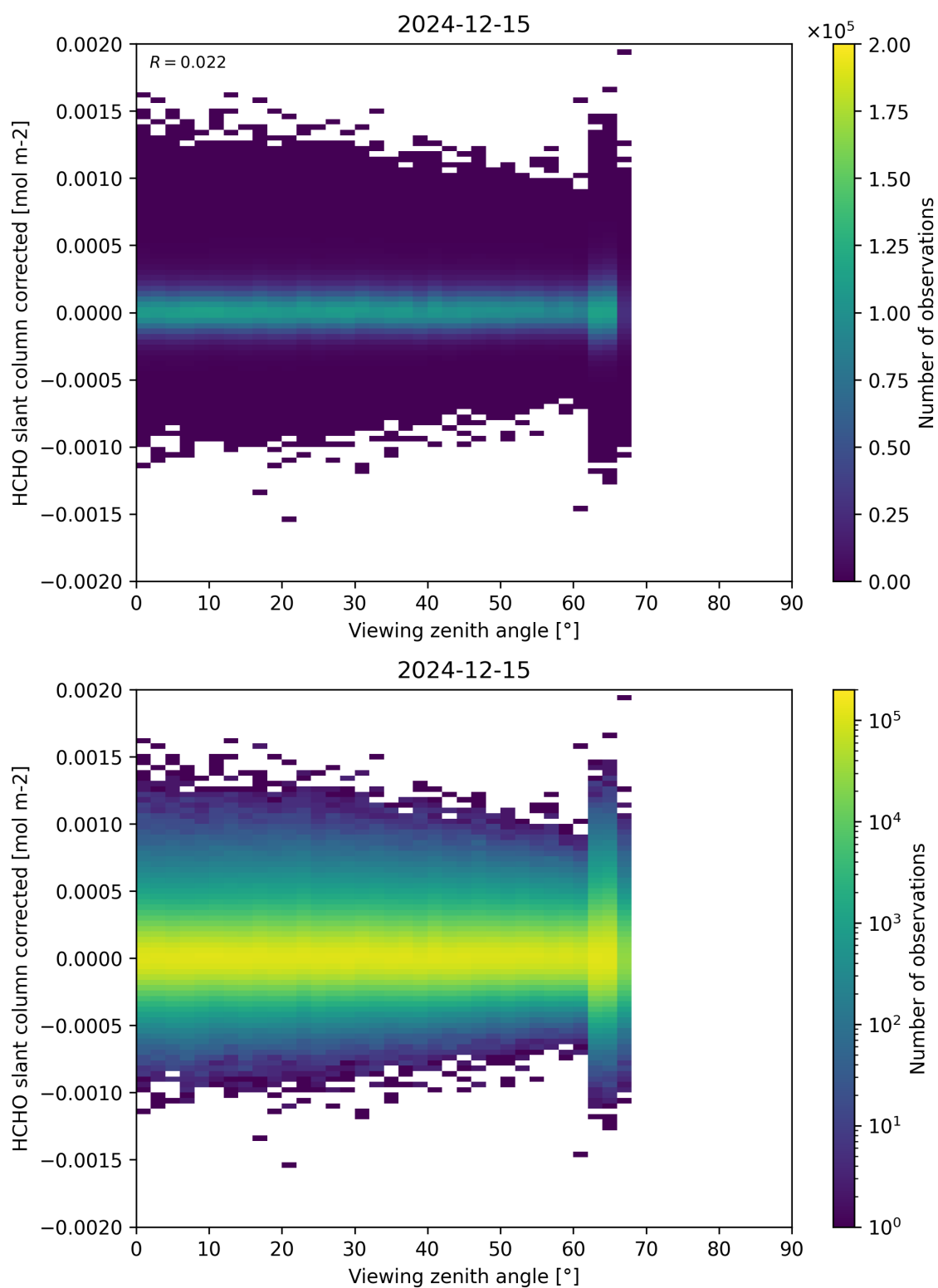
Figure 186: Scatter density plot of “Viewing zenith angle” against “HCHO slant column corrected” for 2024-12-14 to 2024-12-16.
