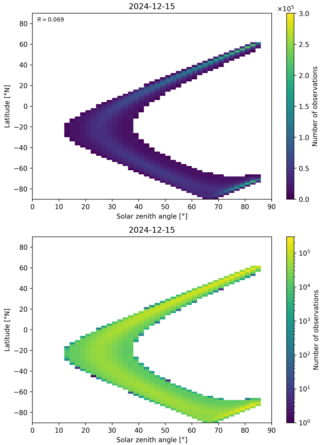
Figure 181: Scatter density plot of “Solar zenith angle” against “Latitude” for 2024-12-14 to 2024-12-16.
