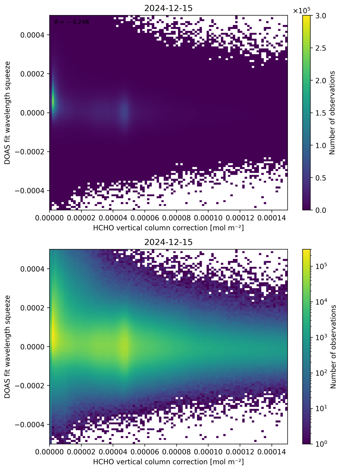
Figure 114: Scatter density plot of “HCHO vertical column correction” against “DOAS fit wavelength squeeze” for 2024-12-14 to 2024-12-16.
