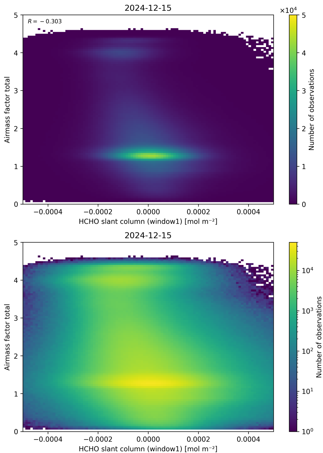
Figure 85: Scatter density plot of “HCHO slant column (window1)” against “Airmass factor total” for 2024-12-14 to 2024-12-16.
