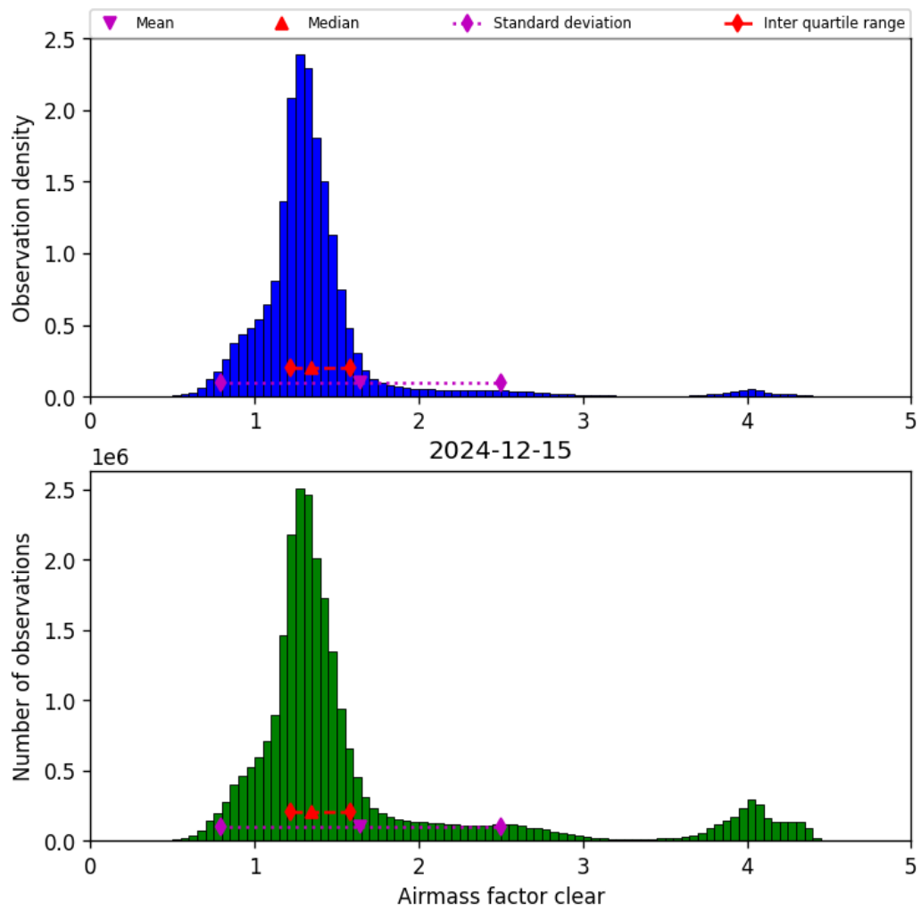
Figure 42: Histogram of “Airmass factor clear” for 2024-12-14 to 2024-12-16
