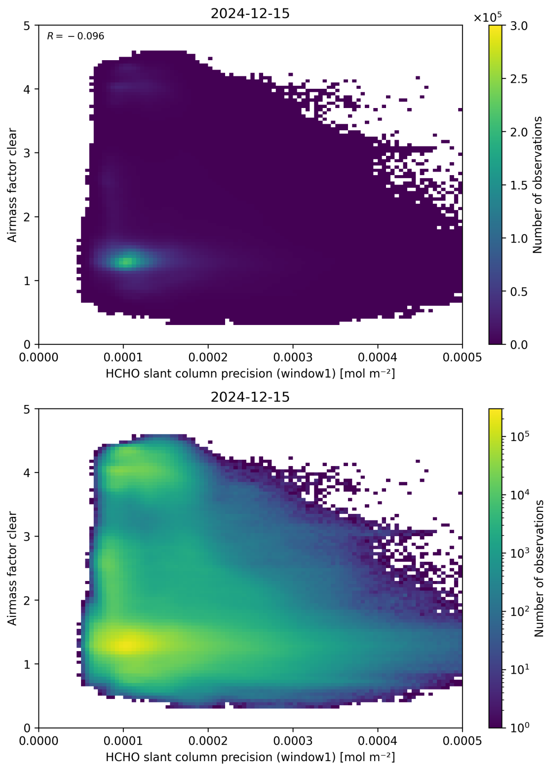
Figure 91: Scatter density plot of “HCHO slant column precision (window1)” against “Airmass factor clear” for 2024-12-14 to 2024-12-16.
