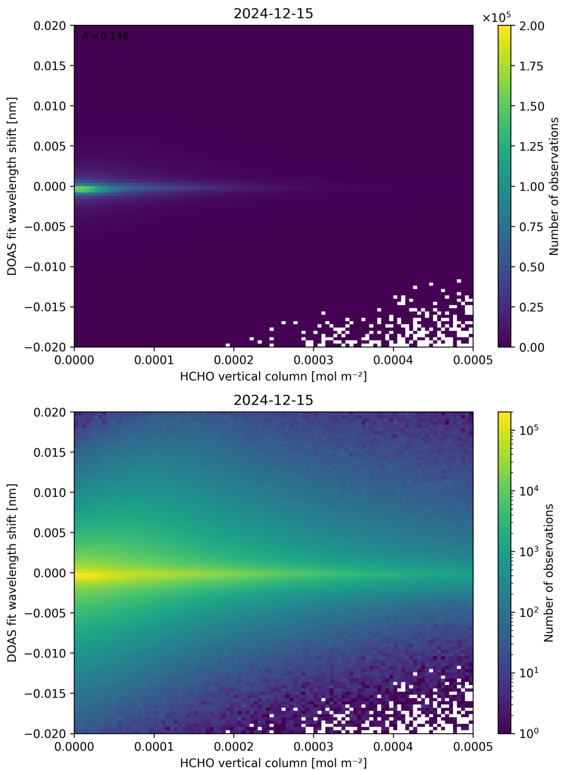
Figure 124: Scatter density plot of “HCHO vertical column” against “DOAS fit wavelength shift” for 2024-12-14 to 2024-12-16.
