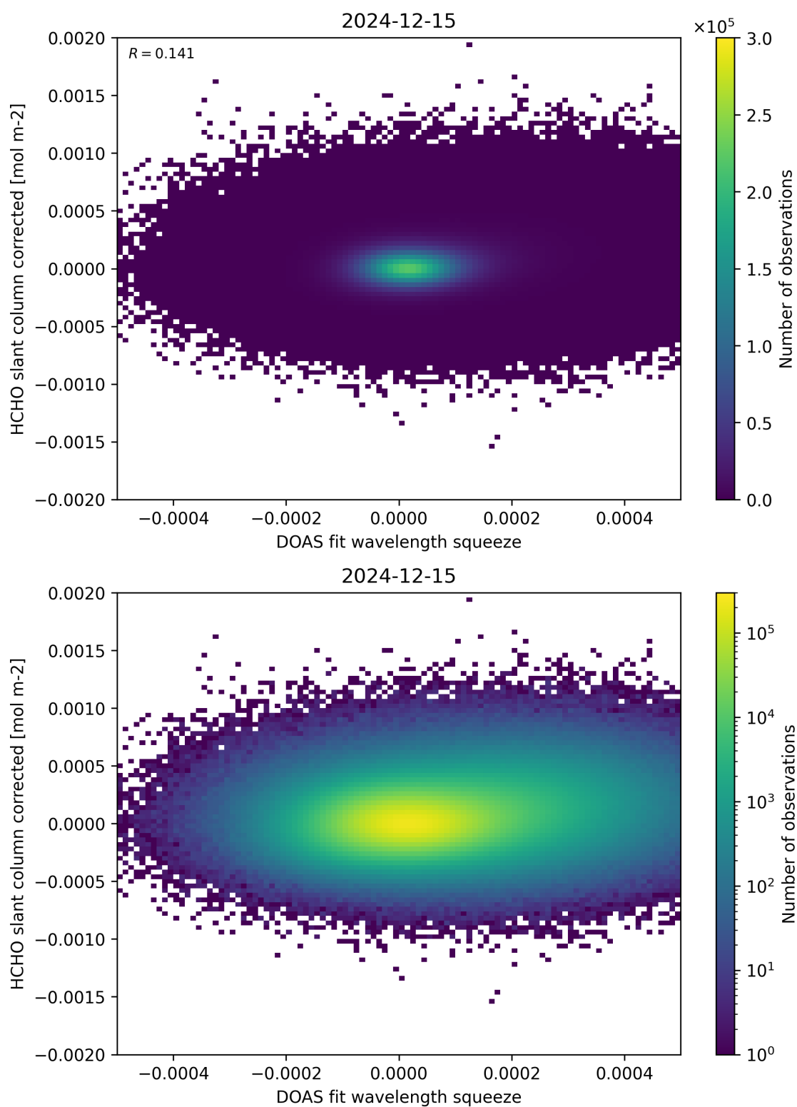
Figure 69: Scatter density plot of “DOAS fit wavelength squeeze” against “HCHO slant column corrected” for 2024-12-14 to 2024-12-16.
