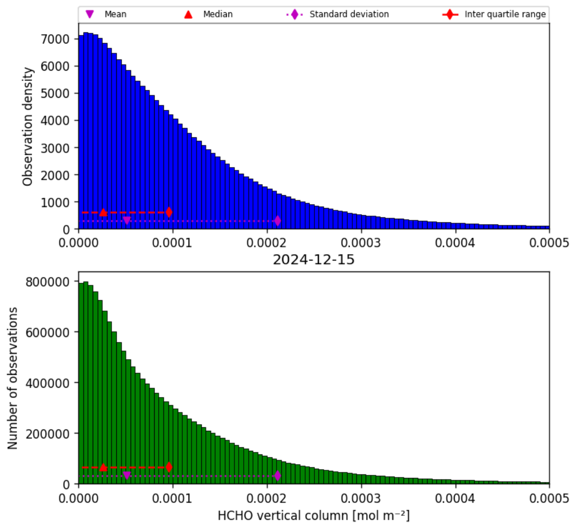
Figure 35: Histogram of “HCHO vertical column” for 2024-12-14 to 2024-12-16
