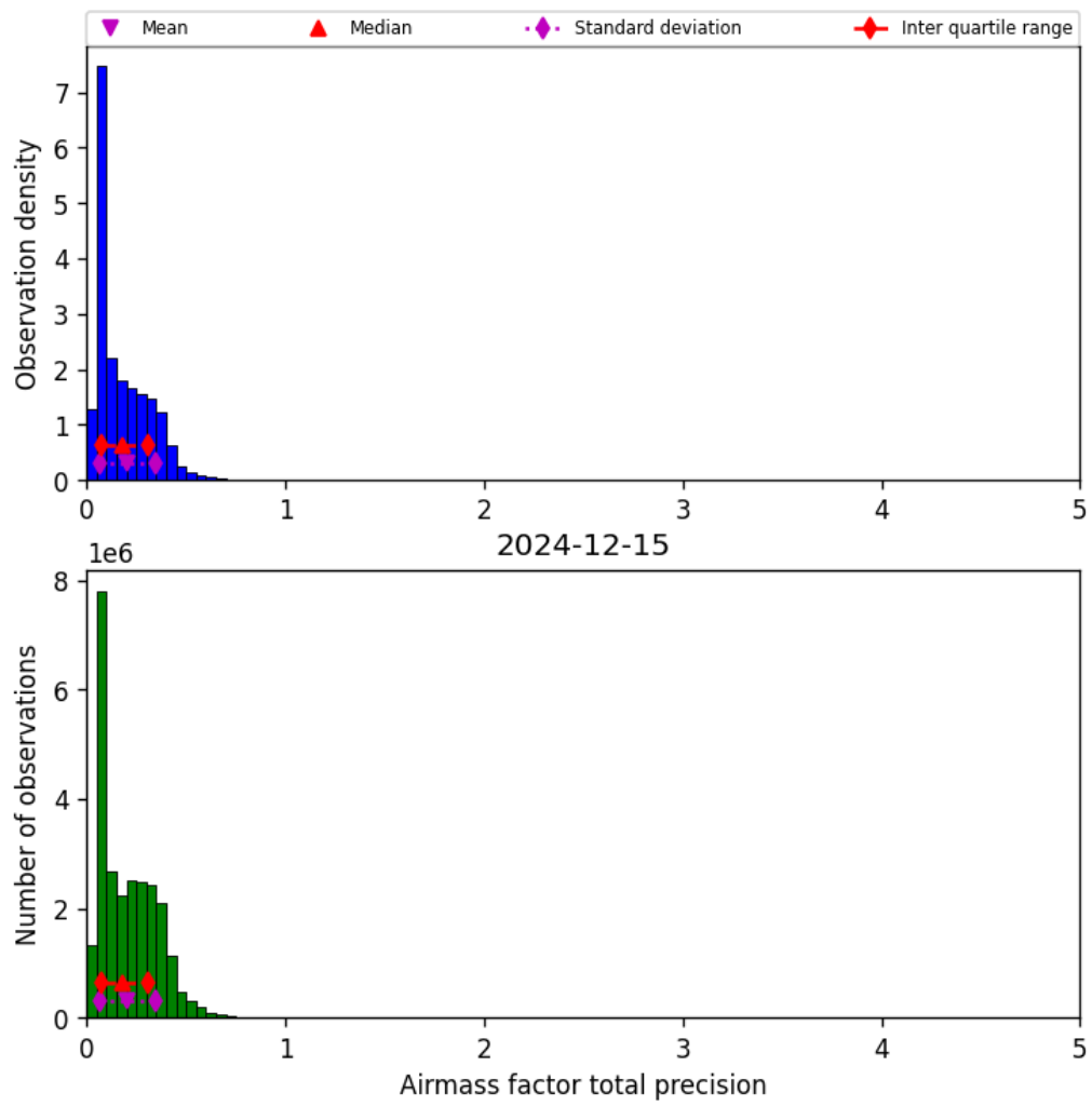
Figure 41: Histogram of "Airmass factor total precision" for 2024-12-14 to 2024-12-16
