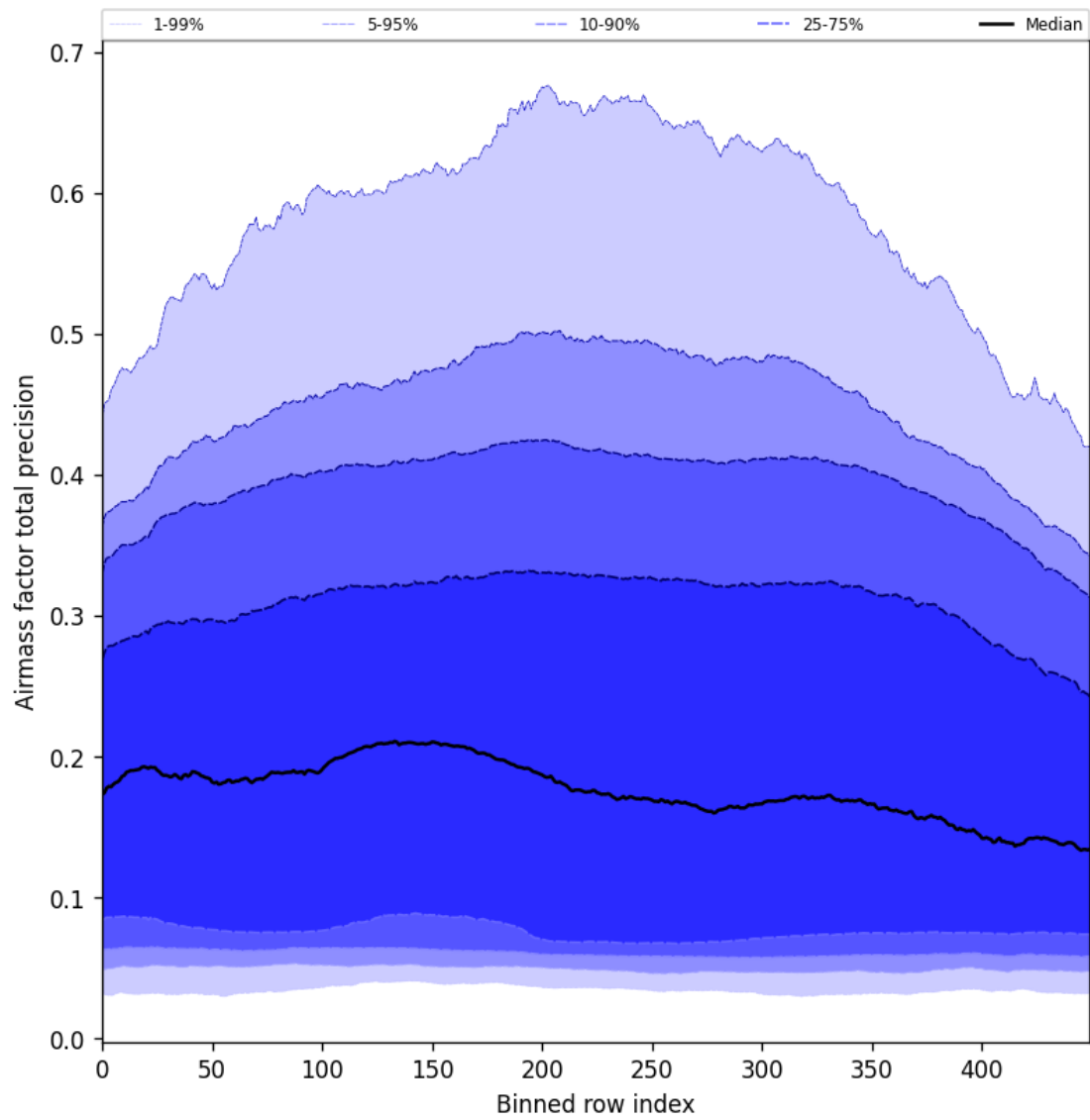
Figure 55: Along track statistics of “Airmass factor total precision” for 2024-12-14 to 2024-12-16
