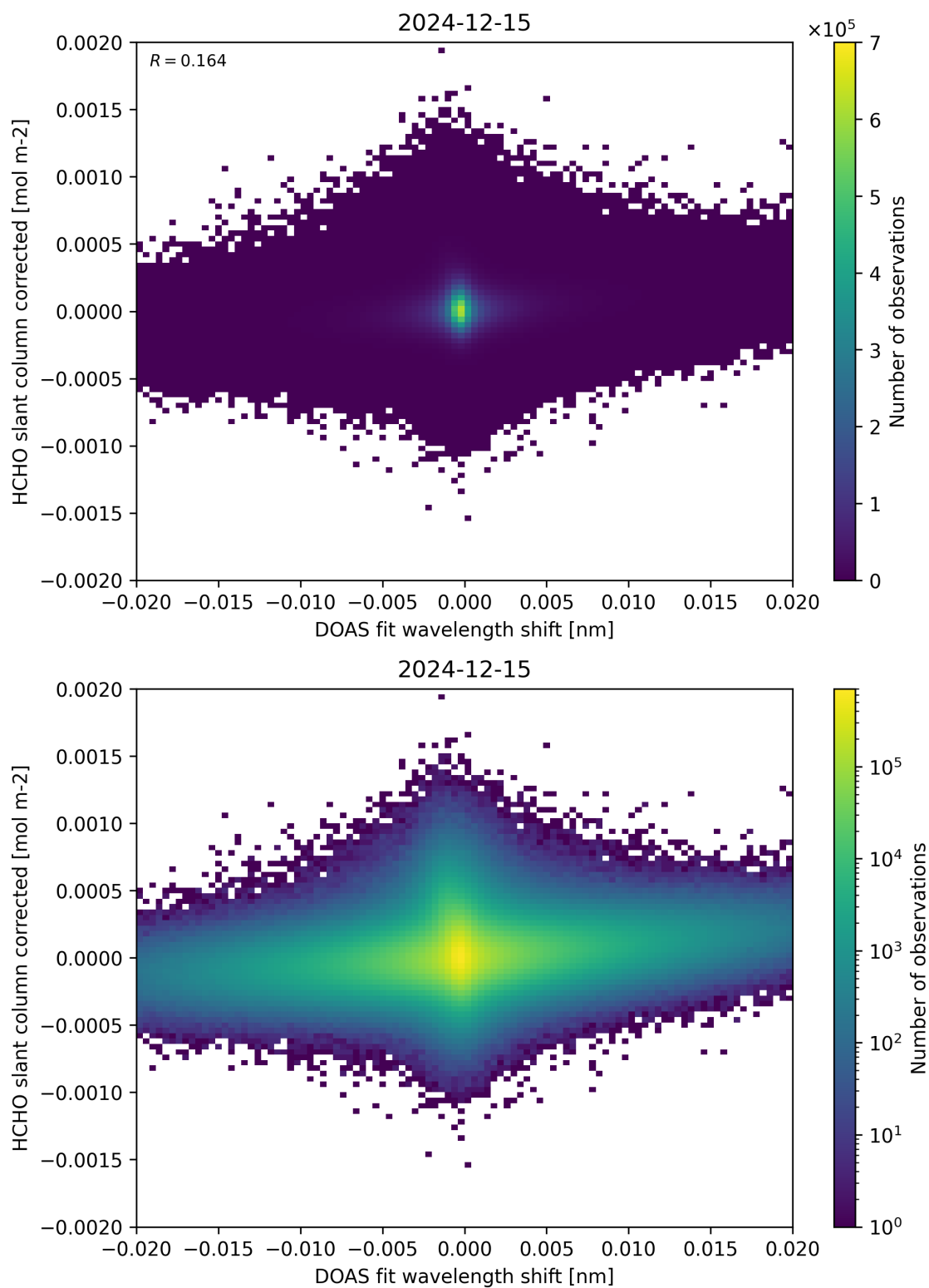
Figure 66: Scatter density plot of “DOAS fit wavelength shift” against “HCHO slant column corrected” for 2024-12-14 to 2024-12-16.
