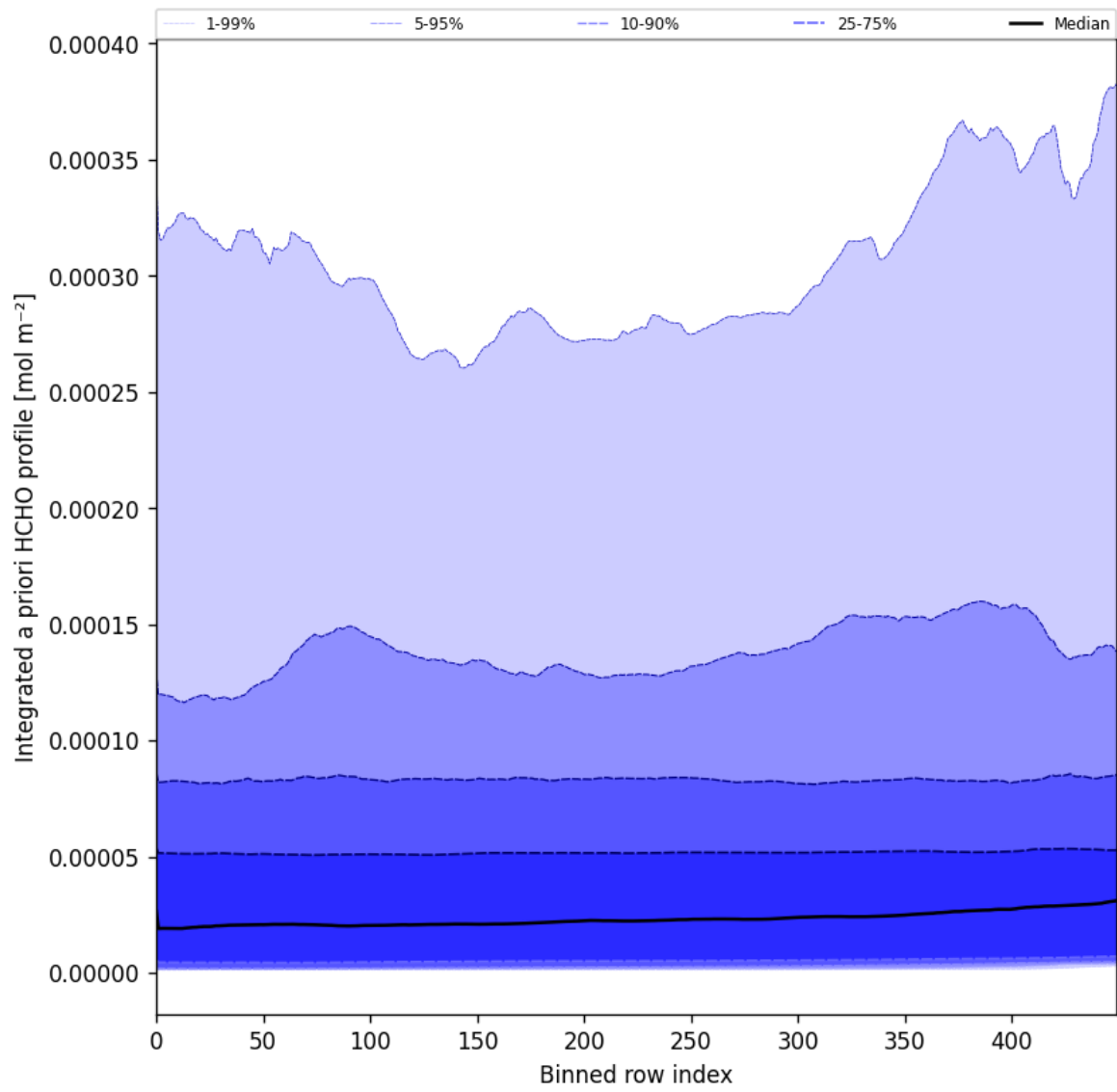
Figure 57: Along track statistics of “Integrated a priori HCHO profile” for 2024-12-14 to 2024-12-16
