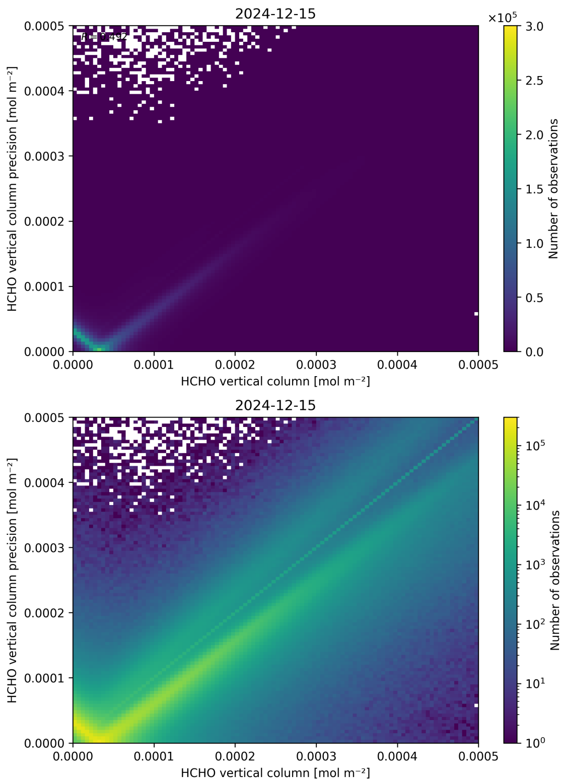
Figure 134: Scatter density plot of “HCHO vertical column” against “HCHO vertical column precision” for 2024-12-14 to 2024-12-16.
