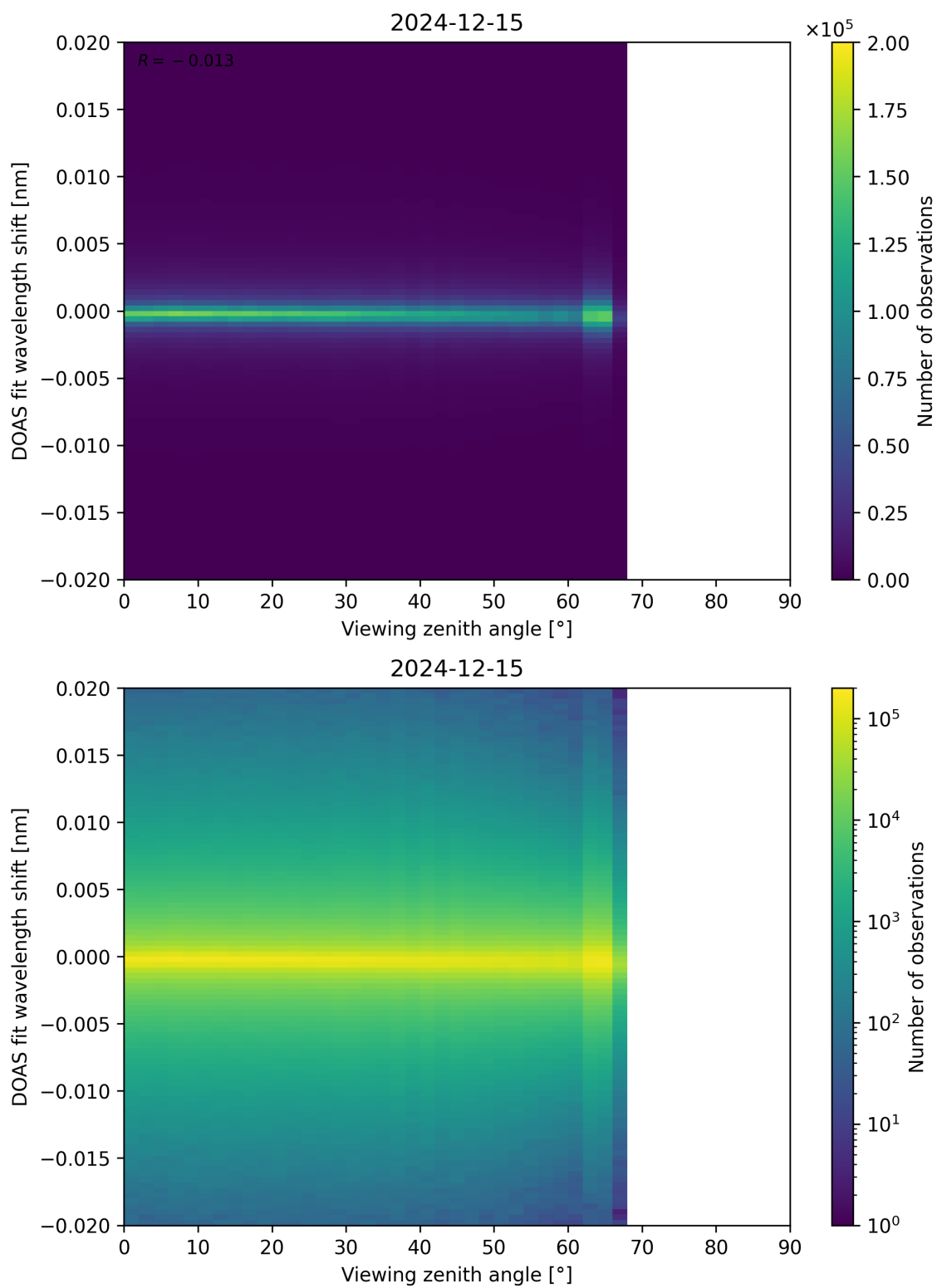
Figure 183: Scatter density plot of “Viewing zenith angle” against “DOAS fit wavelength shift” for 2024-12-14 to 2024-12-16.
