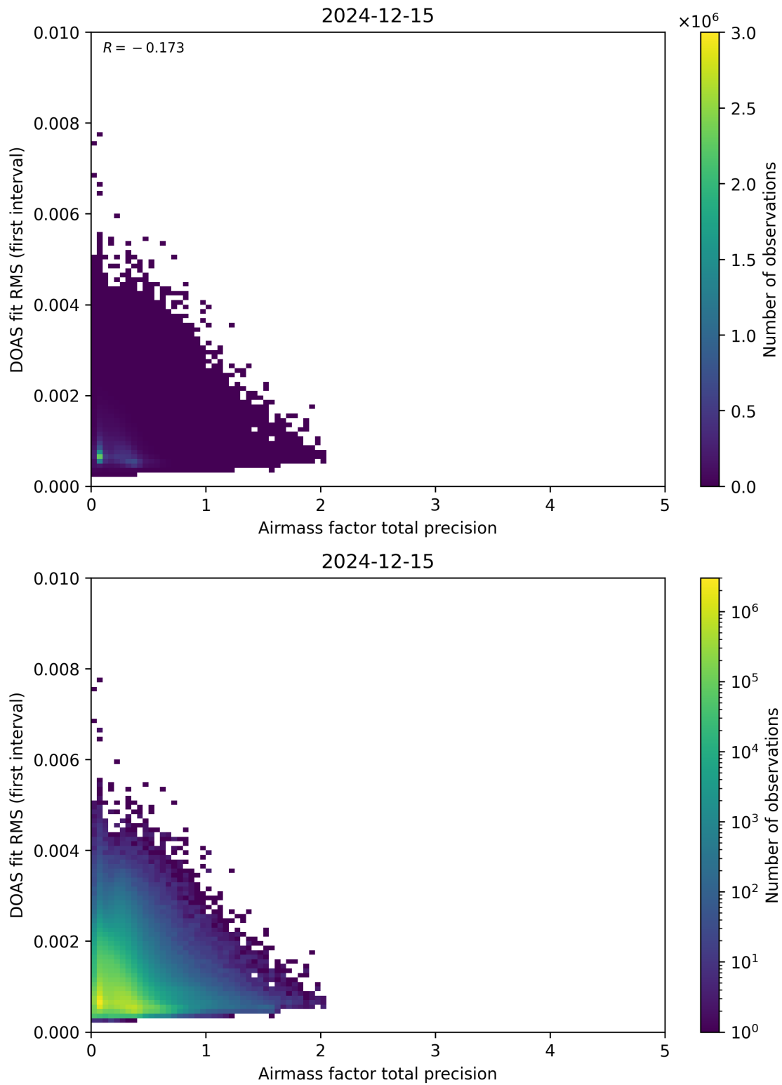
Figure 105: Scatter density plot of “Airmass factor total precision” against “DOAS fit RMS (first interval)” for 2024-12-14 to 2024-12-16.
