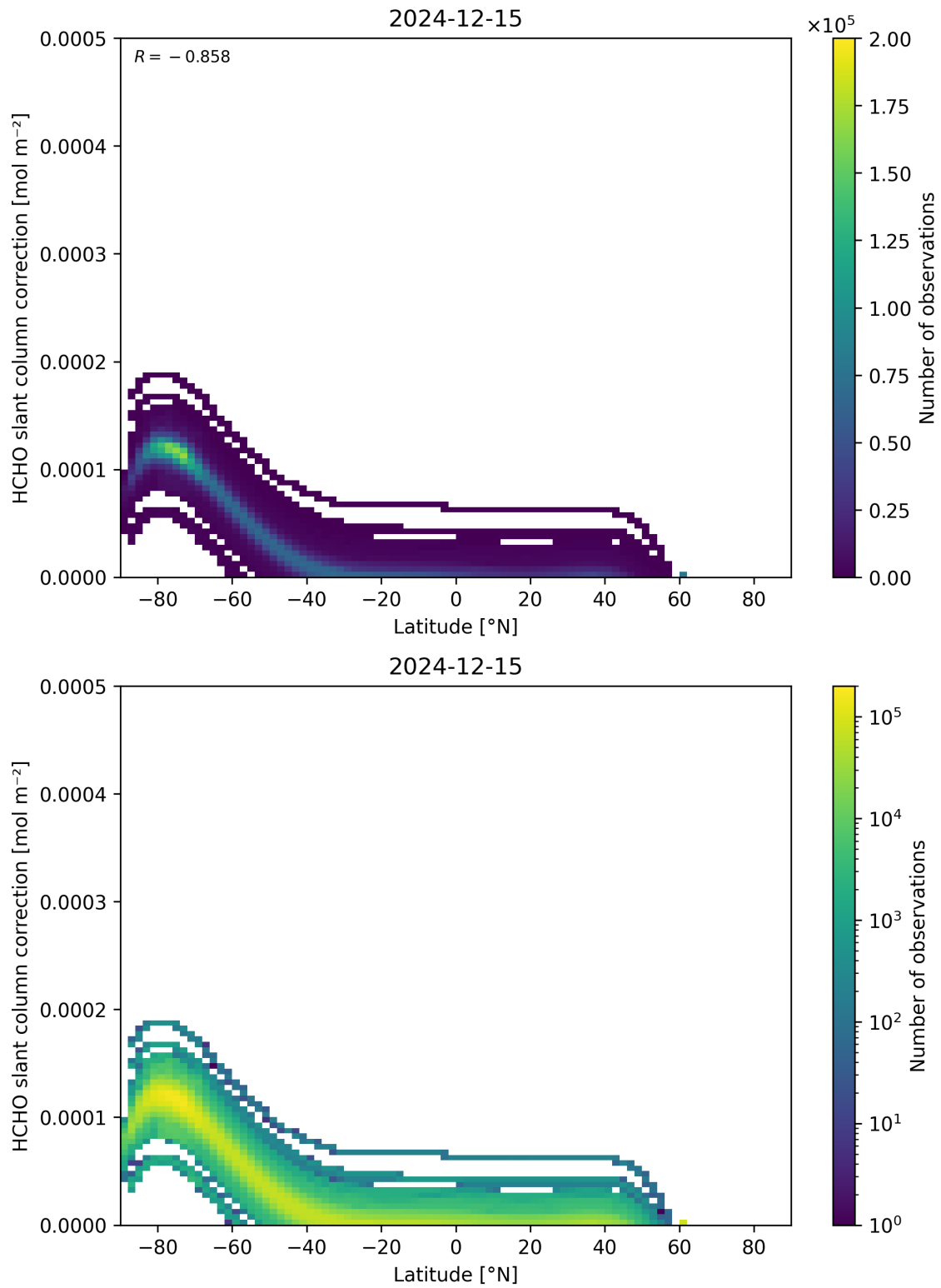
Figure 158: Scatter density plot of “Latitude” against “HCHO slant column correction” for 2024-12-14 to 2024-12-16.
