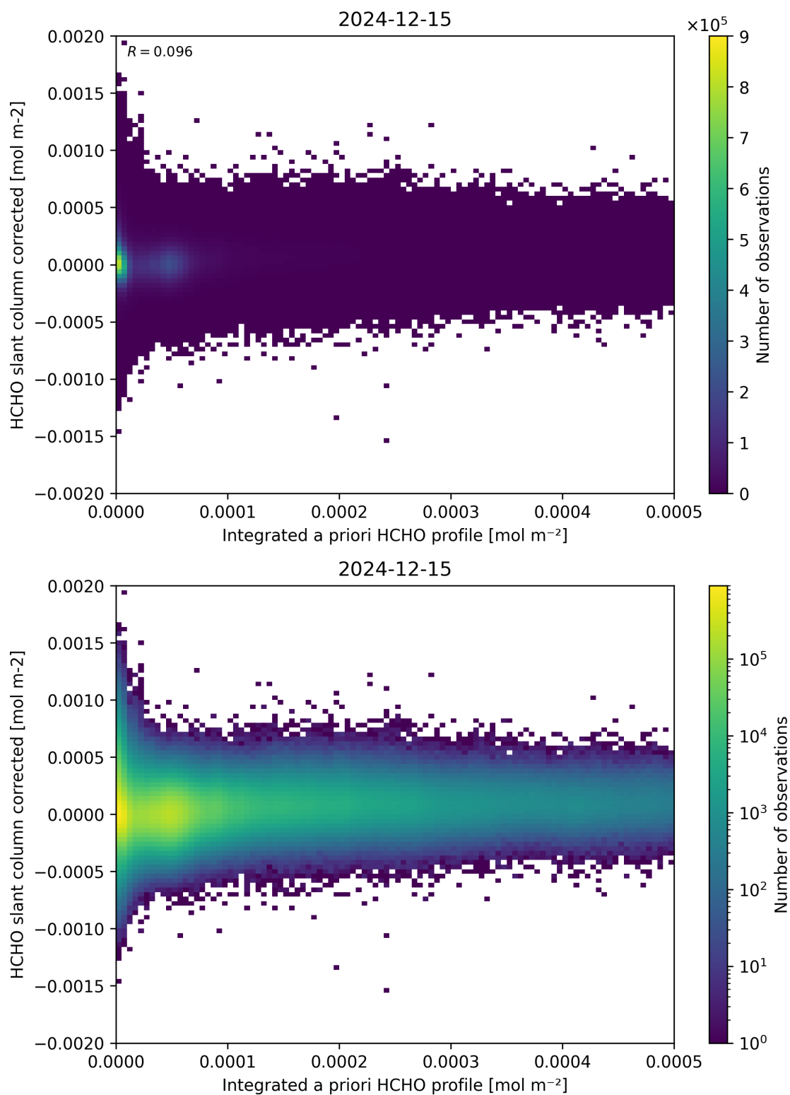
Figure 151: Scatter density plot of “Integrated a priori HCHO profile” against “HCHO slant column corrected” for 2024-12-14 to 2024-12-16.
