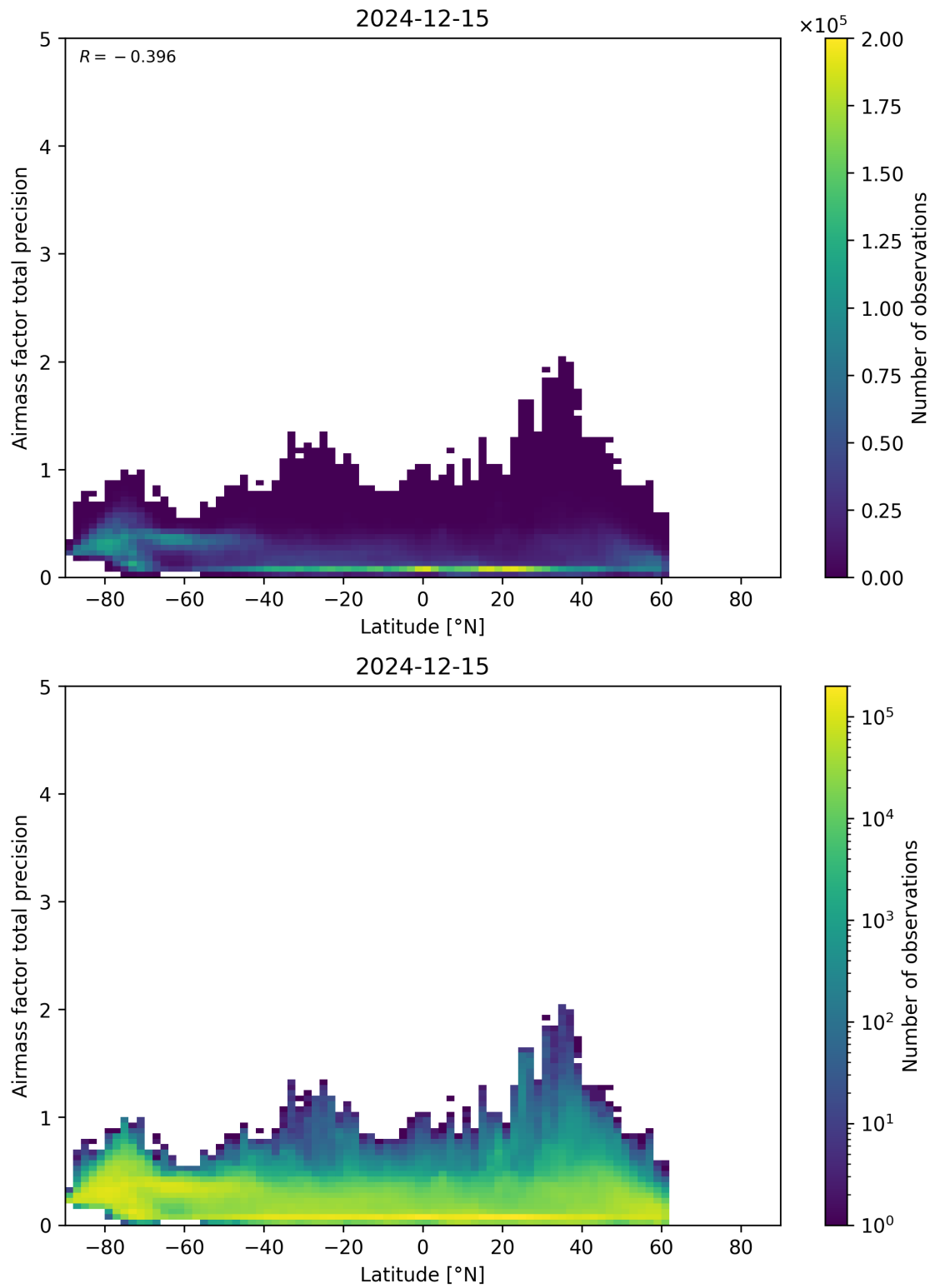
Figure 162: Scatter density plot of “Latitude” against “Airmass factor total precision” for 2024-12-14 to 2024-12-16.
