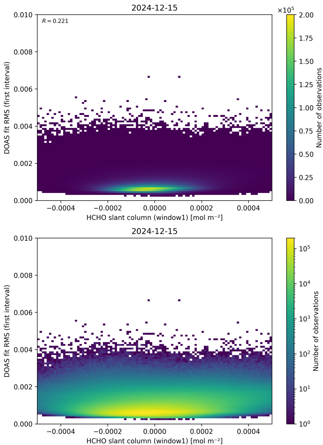
Figure 78: Scatter density plot of “HCHO slant column (window1)” against “DOAS fit RMS (first interval)” for 2024-12-14 to 2024-12-16.
