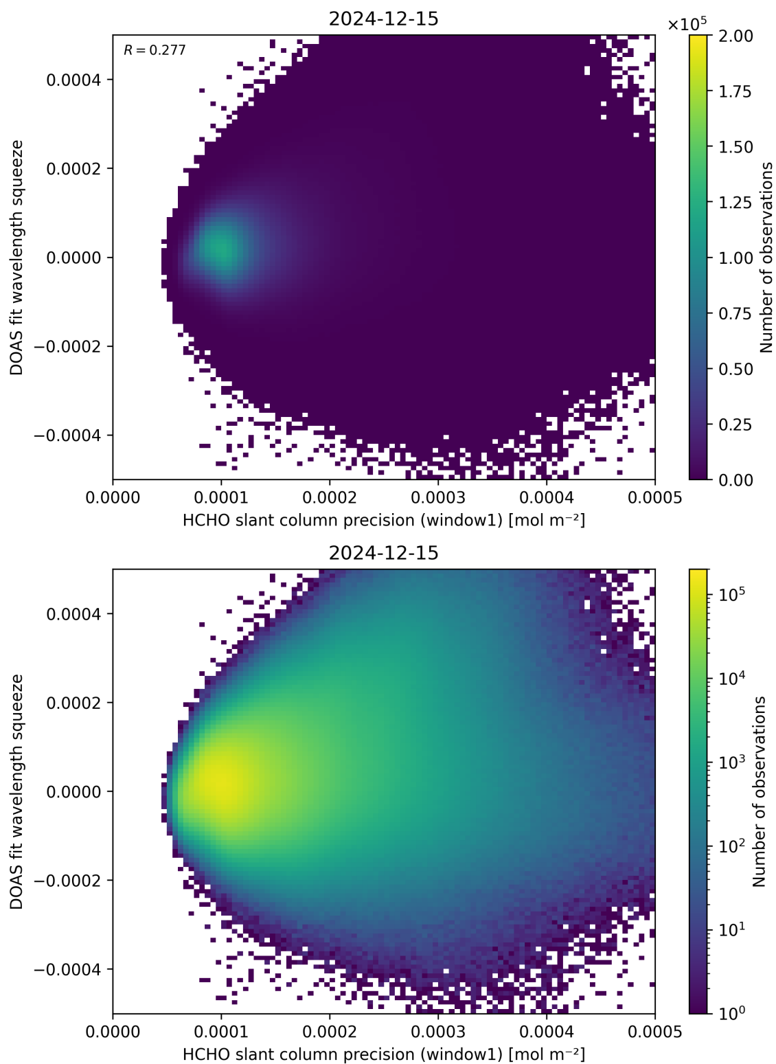
Figure 90: Scatter density plot of “HCHO slant column precision (window1)” against “DOAS fit wavelength squeeze” for 2024-12-14 to 2024-12-16.
