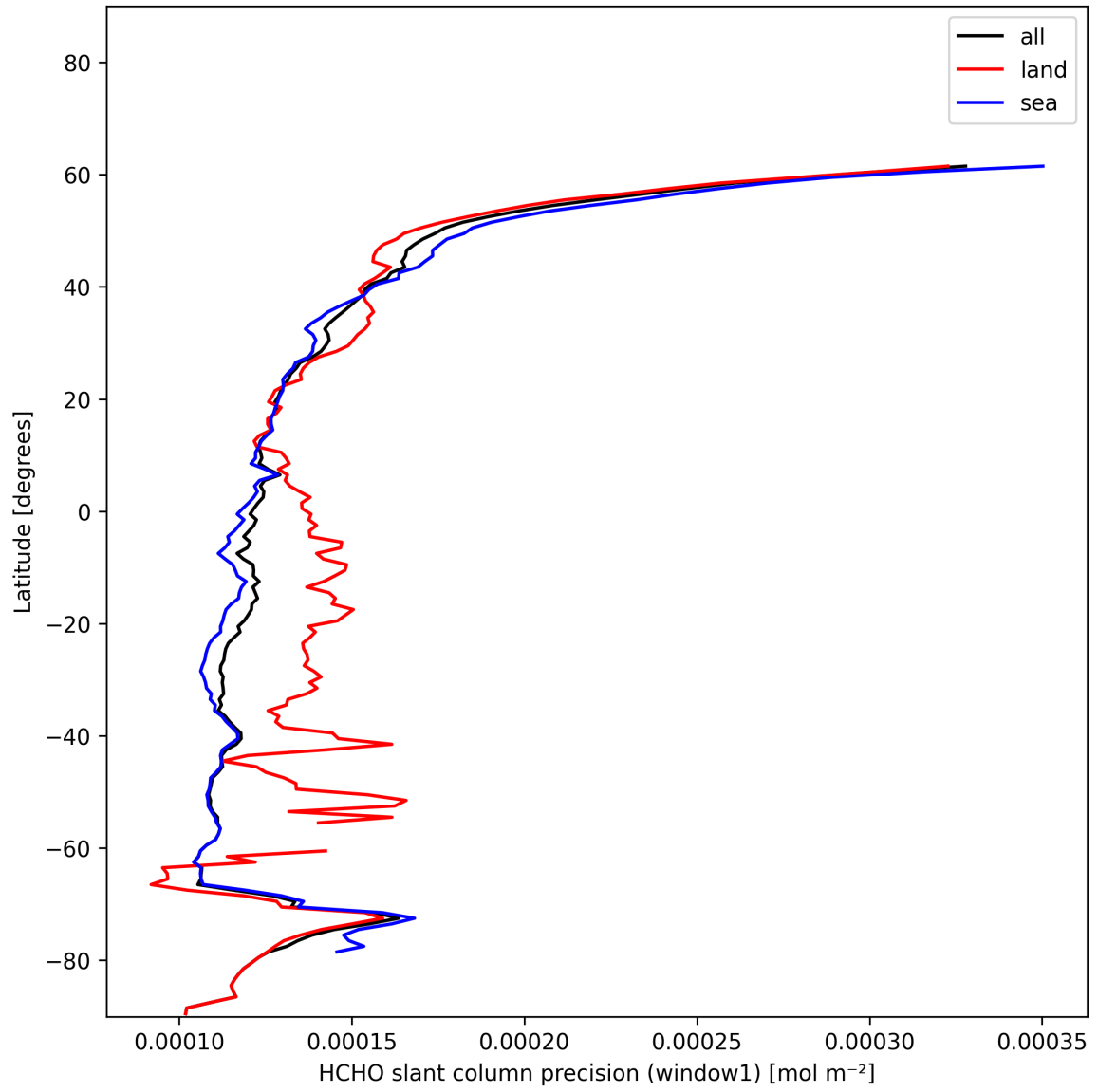
Figure 25: Zonal average of “HCHO slant column precision (window1)” for 2024-12-14 to 2024-12-16.
