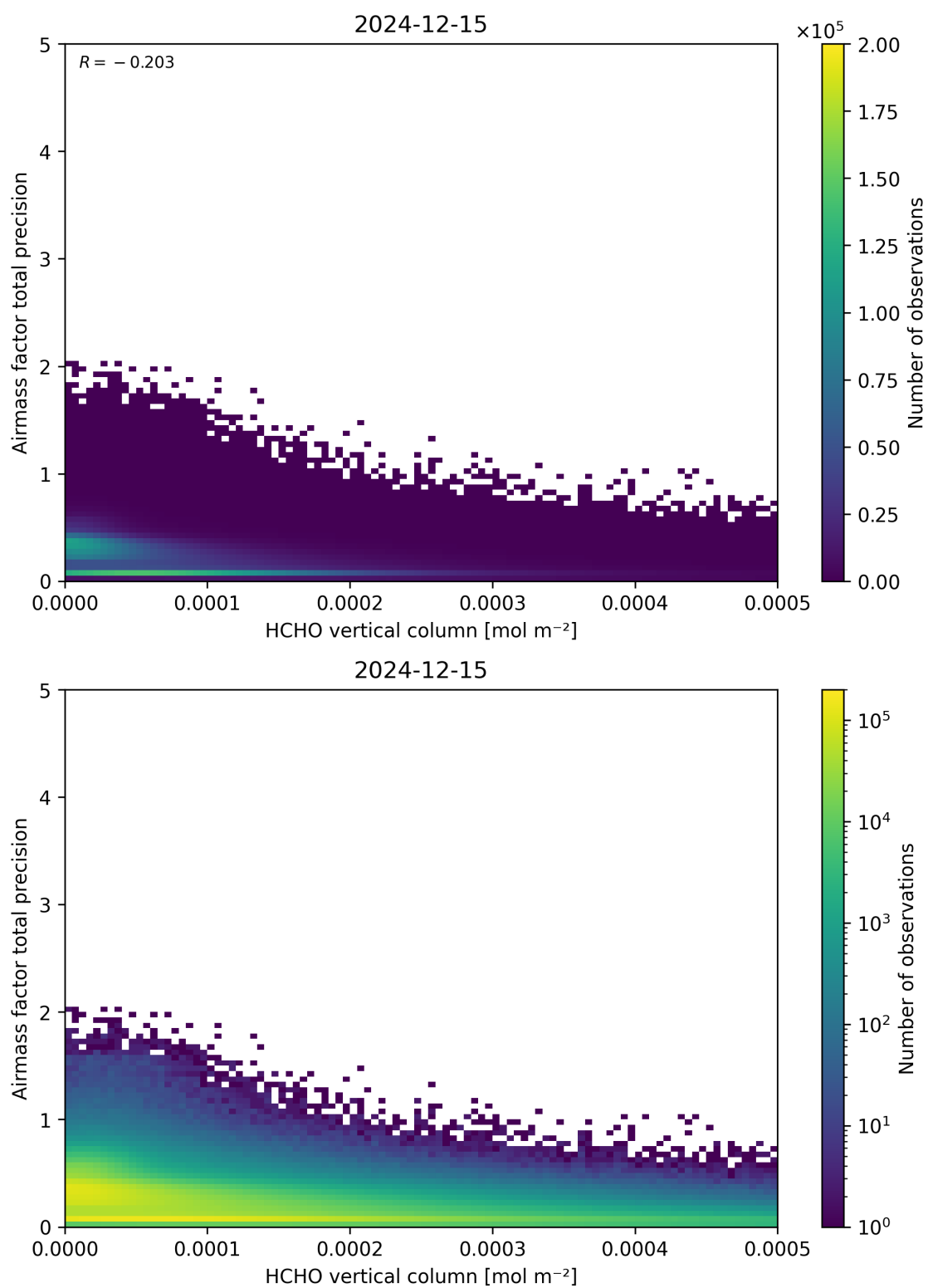
Figure 132: Scatter density plot of “HCHO vertical column” against “Airmass factor total precision” for 2024-12-14 to 2024-12-16.
