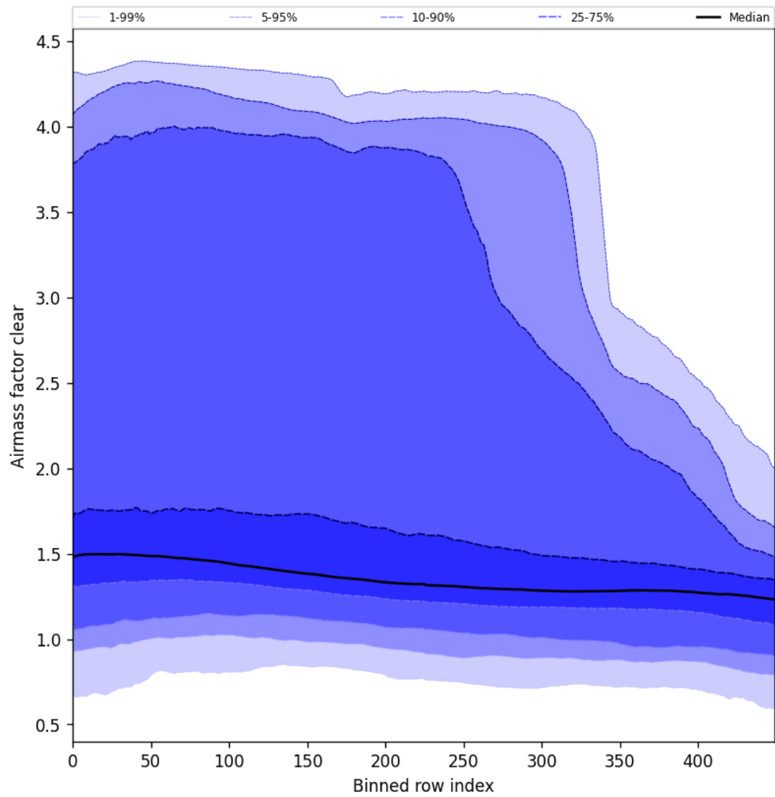
Figure 56: Along track statistics of “Air mass factor clear” for 2024-12-14 to 2024-12-16
