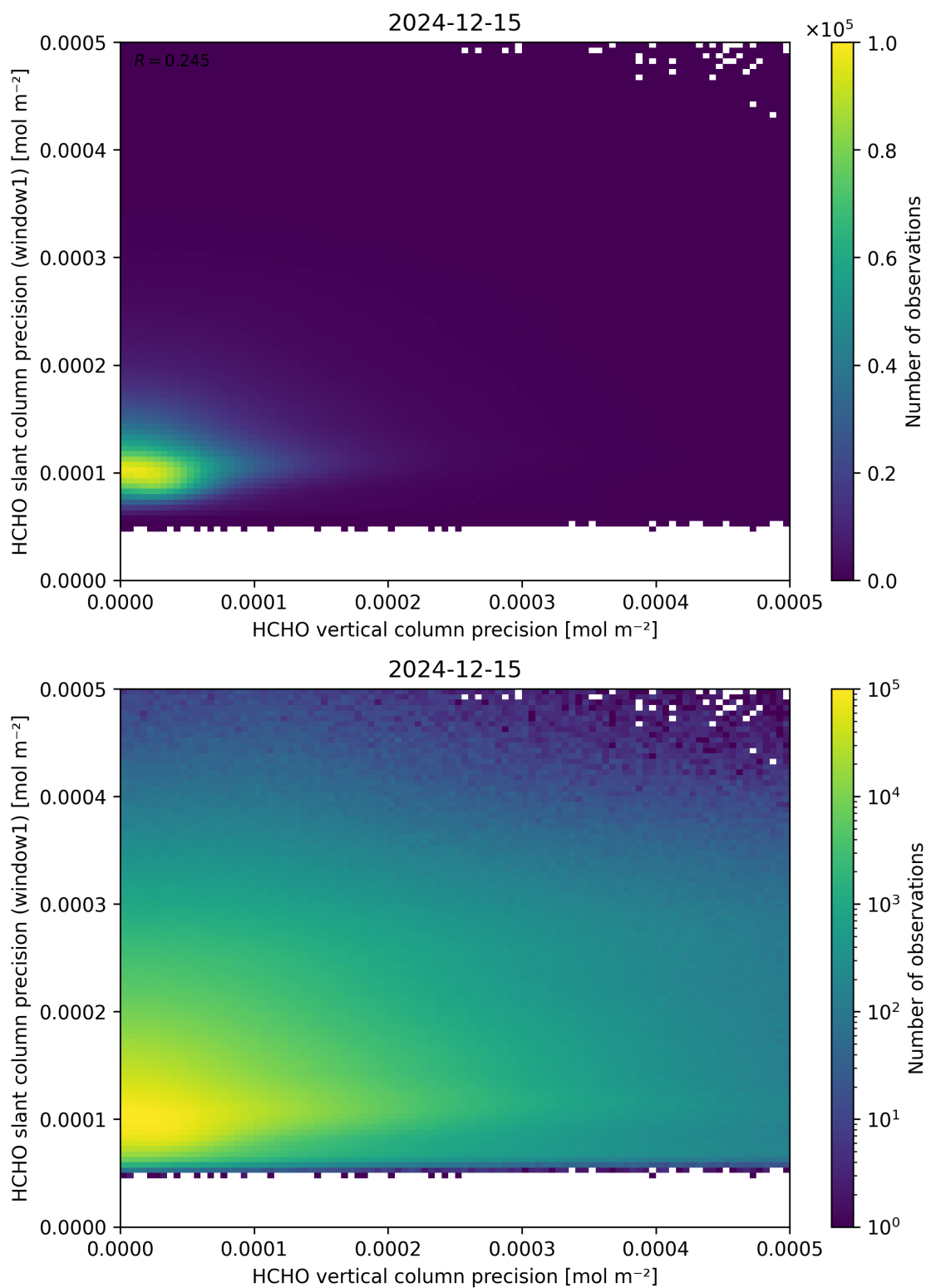
Figure 143: Scatter density plot of “HCHO vertical column precision” against “HCHO slant column precision (window1)” for 2024-12-14 to 2024-12-16.
