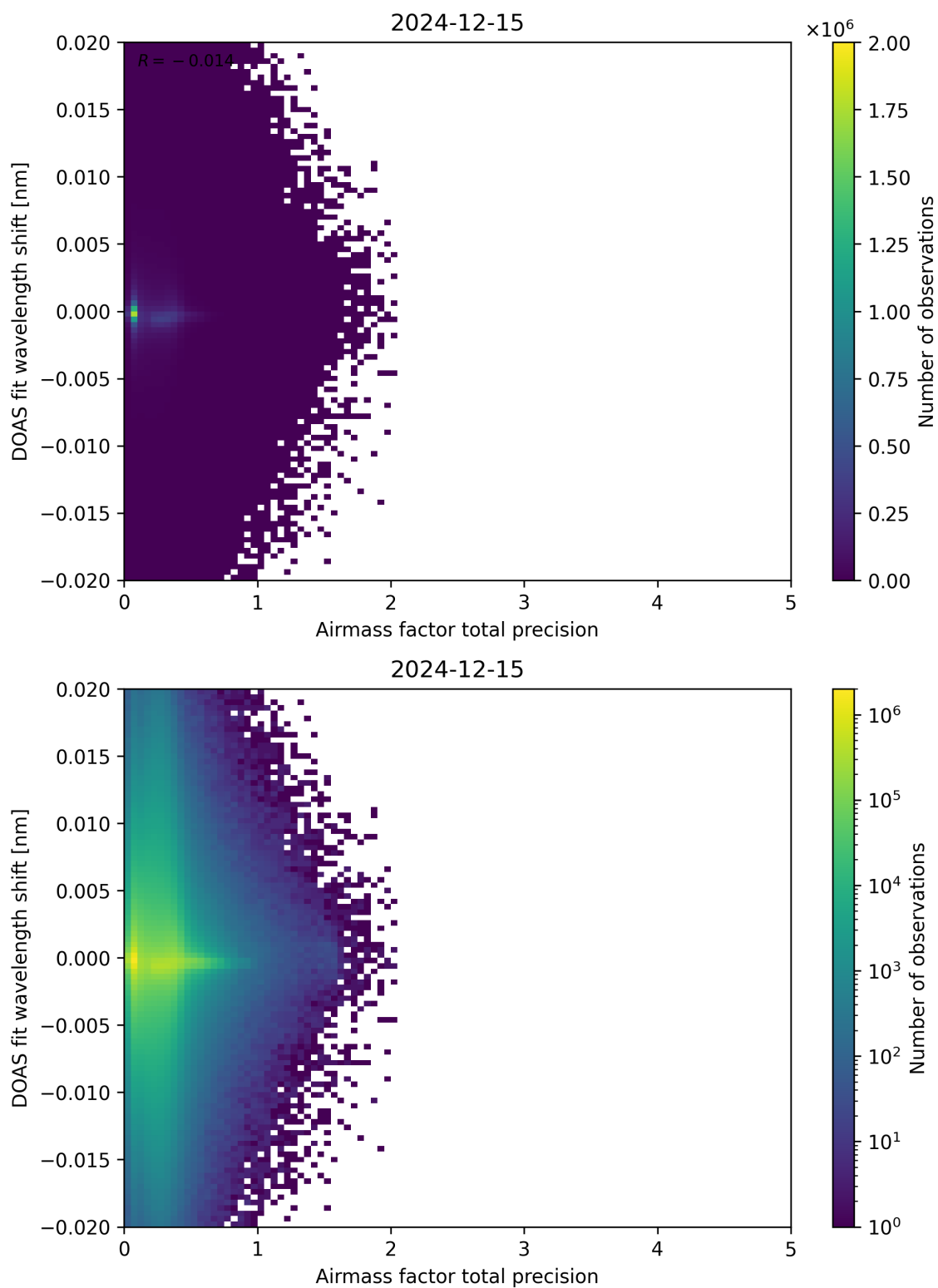
Figure 106: Scatter density plot of “Airmass factor total precision” against “DOAS fit wavelength shift” for 2024-12-14 to 2024-12-16.
