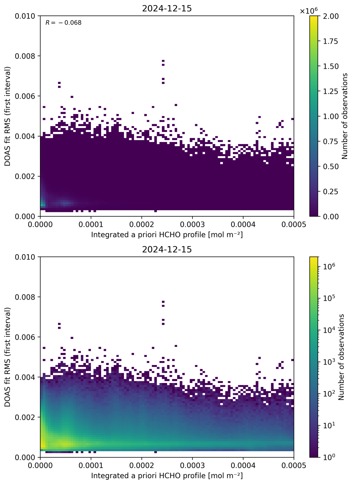
Figure 148: Scatter density plot of “Integrated a priori HCHO profile” against “DOAS fit RMS (first interval)” for 2024-12-14 to 2024-12-16.
