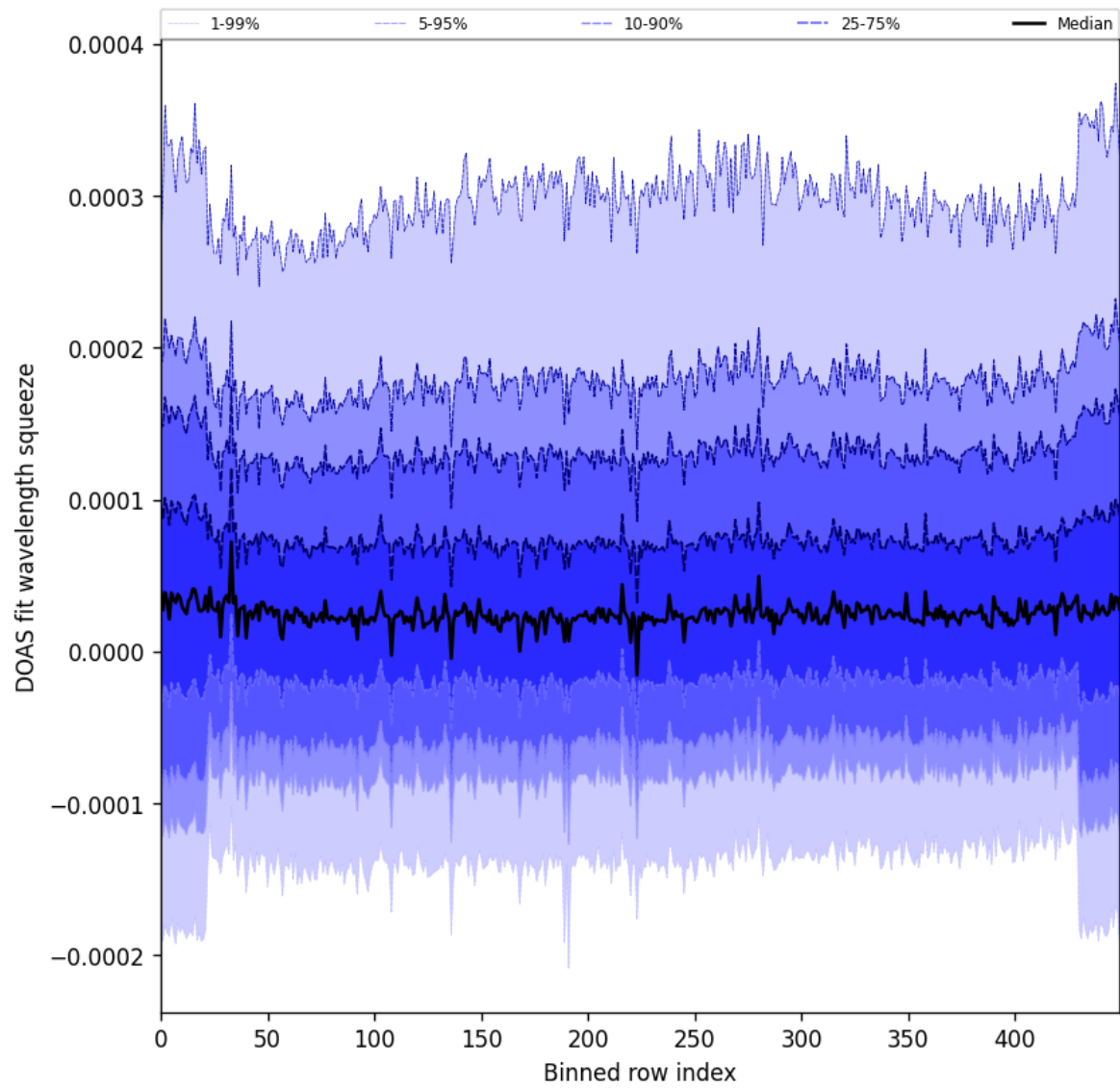
Figure 59: Along track statistics of “DOAS fit wavelength squeeze” for 2024-12-14 to 2024-12-16
