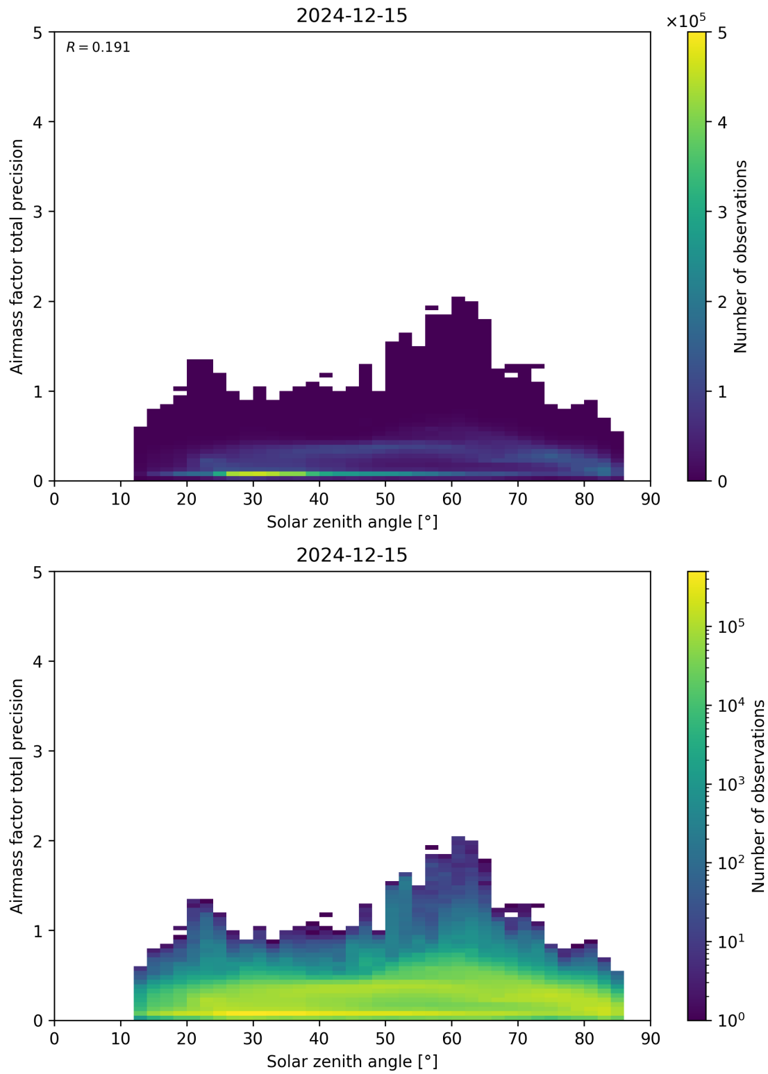
Figure 176: Scatter density plot of “Solar zenith angle” against “Airmass factor total precision” for 2024-12-14 to 2024-12-16.
