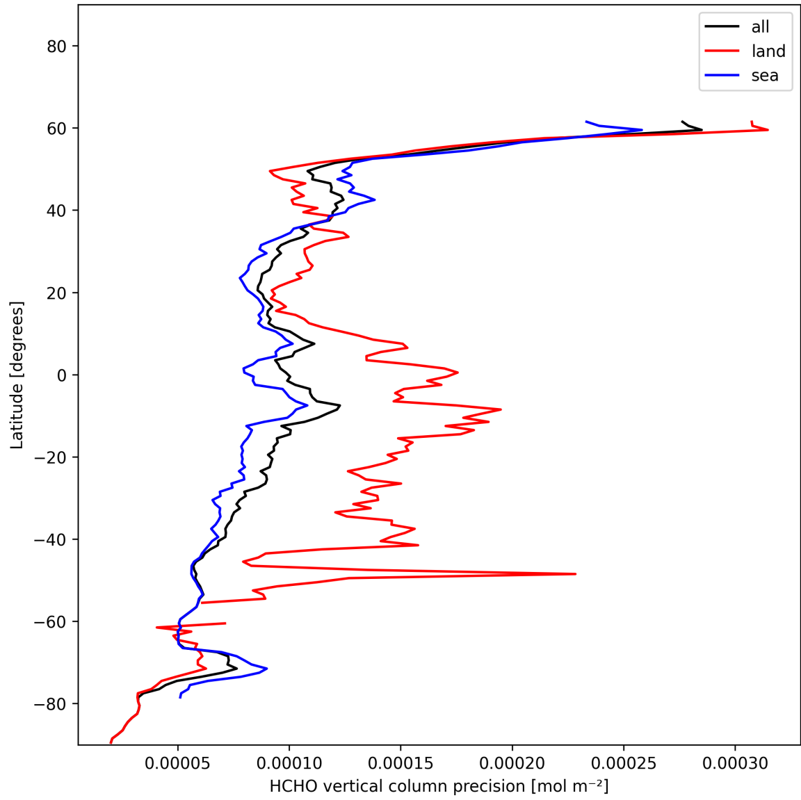
Figure 22: Zonal average of “HCHO vertical column precision” for 2024-12-14 to 2024-12-16.
