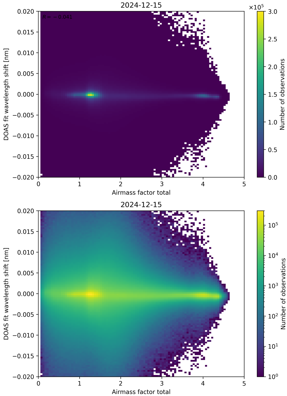
Figure 98: Scatter density plot of “Airmass factor total” against “DOAS fit wavelength shift” for 2024-12-14 to 2024-12-16.
