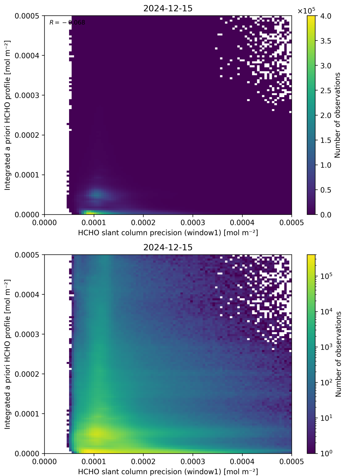
Figure 96: Scatter density plot of “HCHO slant column precision (window1)” against “Integrated a priori HCHO profile” for 2024-12-14 to 2024-12-16.
