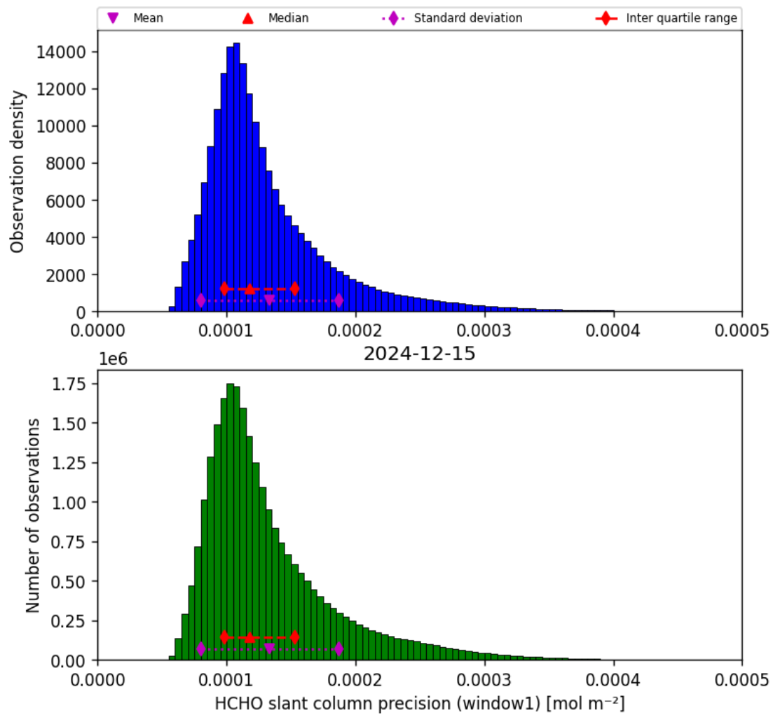
Figure 39: Histogram of “HCHO slant column precision (window1)” for 2024-12-14 to 2024-12-16
