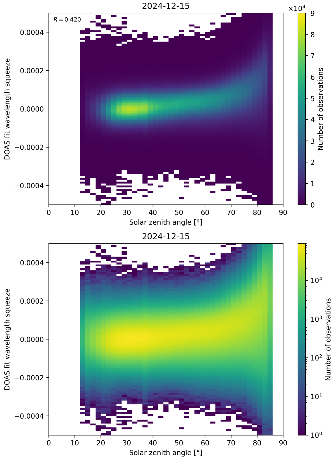
Figure 169: Scatter density plot of “Solar zenith angle” against “DOAS fit wavelength squeeze” for 2024-12-14 to 2024-12-16.
