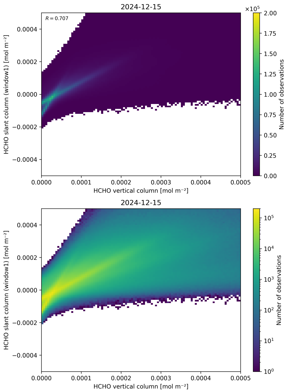
Figure 129: Scatter density plot of “HCHO vertical column” against “HCHO slant column (window1)” for 2024-12-14 to 2024-12-16.
