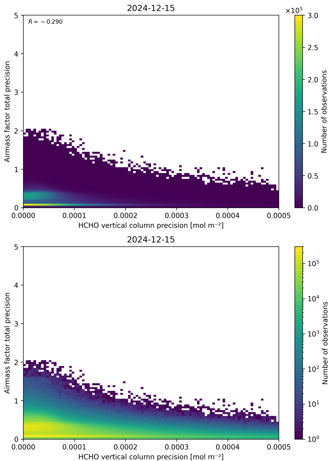
Figure 145: Scatter density plot of “HCHO vertical column precision” against “Airmass factor total precision” for 2024-12-14 to 2024-12-16.
