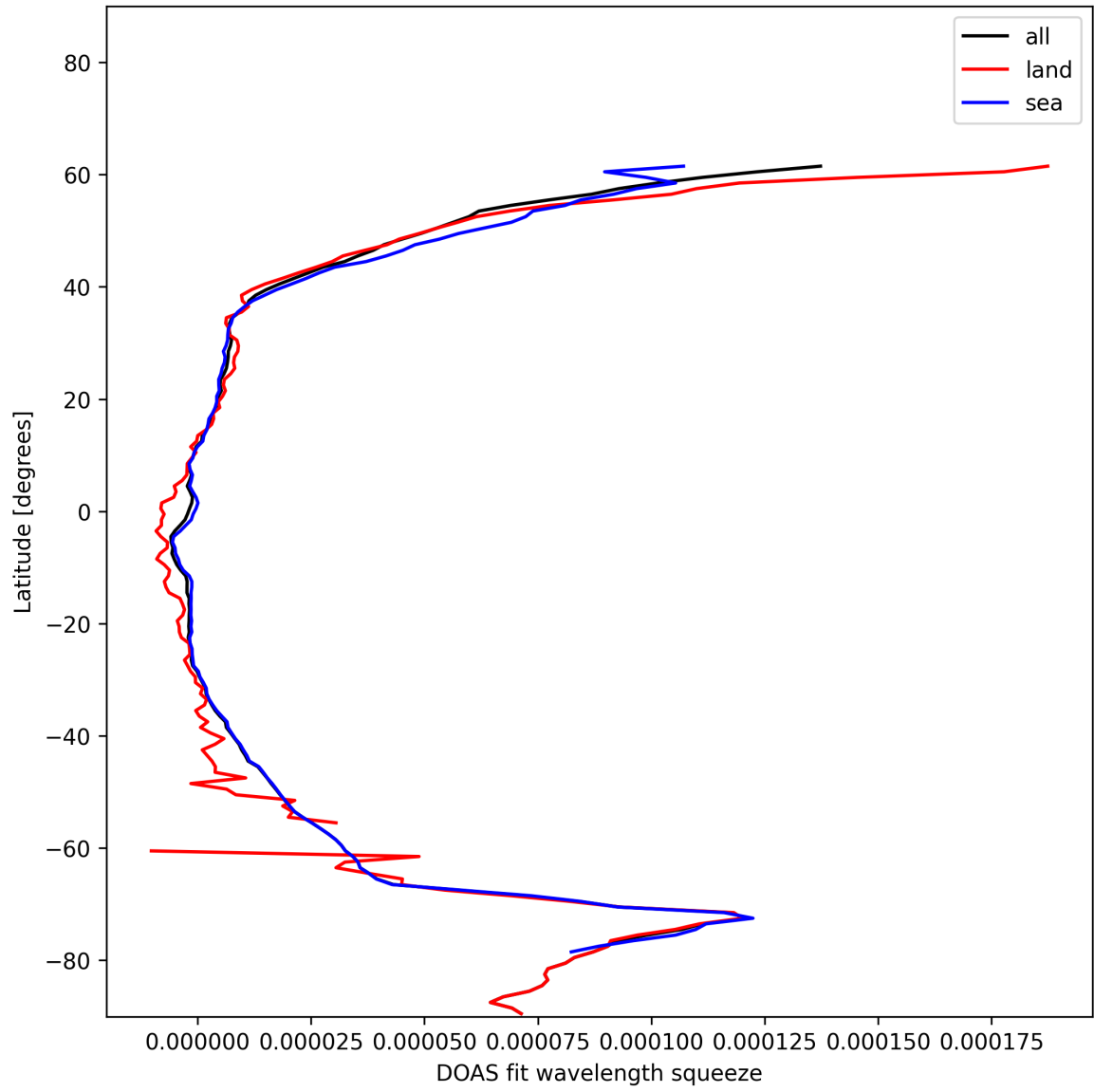
Figure 31: Zonal average of “DOAS fit wavelength squeeze” for 2024-12-14 to 2024-12-16.
