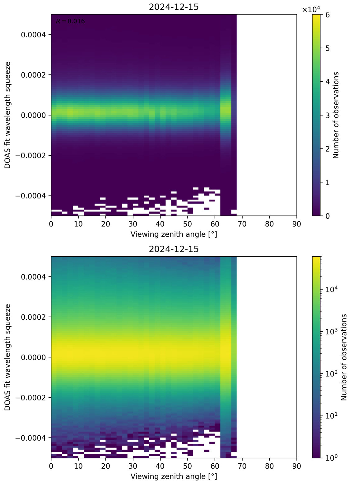
Figure 184: Scatter density plot of “Viewing zenith angle” against “DOAS fit wavelength squeeze” for 2024-12-14 to 2024-12-16.
