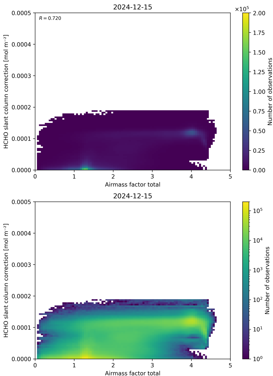
Figure 102: Scatter density plot of “Airmass factor total” against “HCHO slant column correction” for 2024-12-14 to 2024-12-16.
