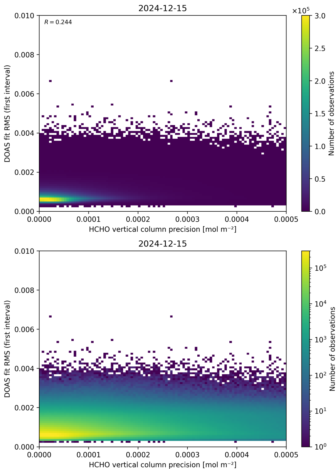
Figure 136: Scatter density plot of “HCHO vertical column precision” against “DOAS fit RMS (first interval)” for 2024-12-14 to 2024-12-16.
