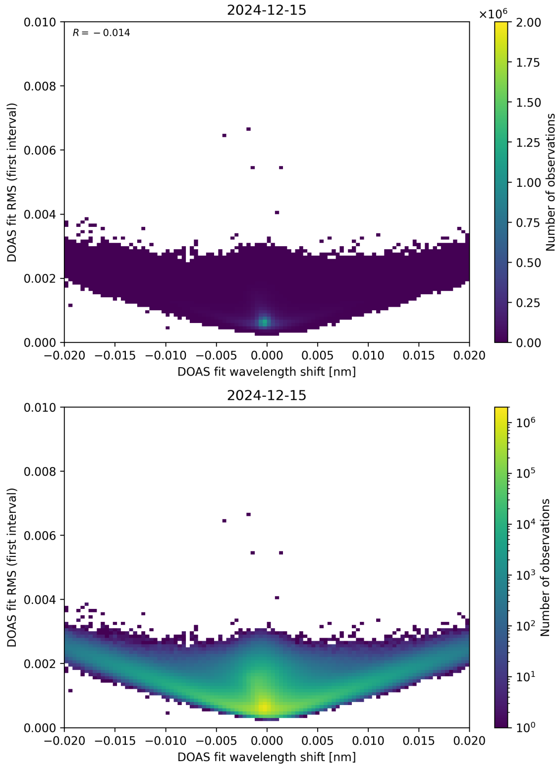
Figure 64: Scatter density plot of “DOAS fit wavelength shift” against “DOAS fit RMS (first interval)” for 2024-12-14 to 2024-12-16.
