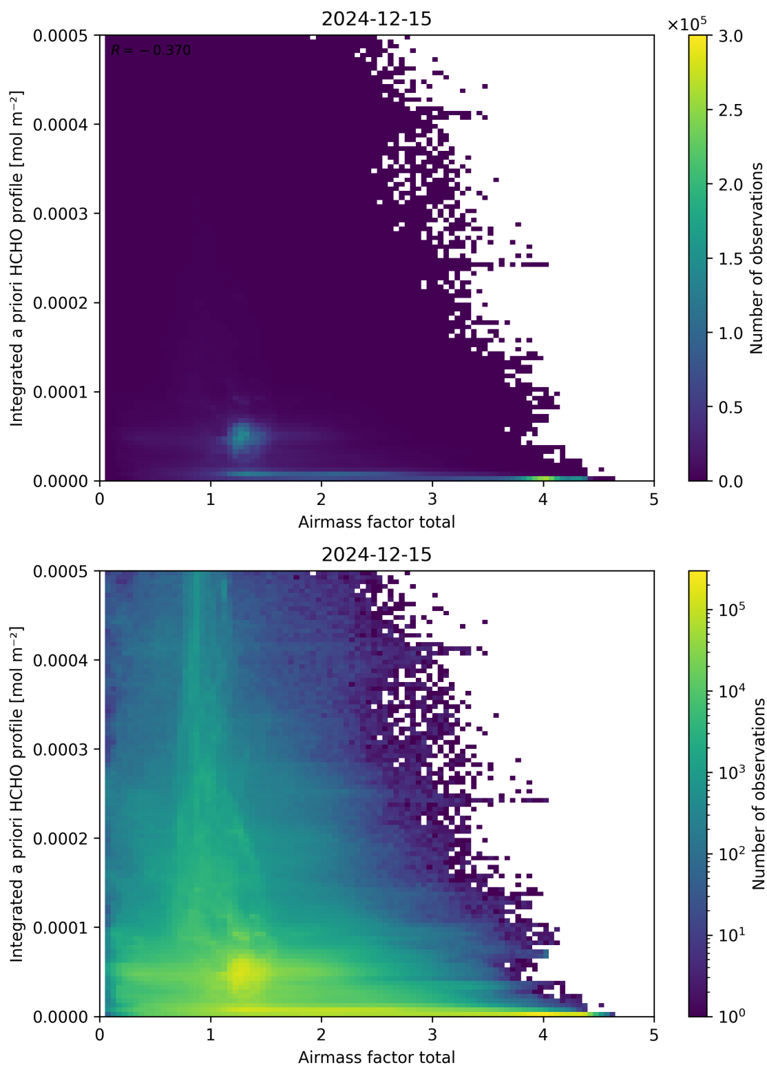
Figure 104: Scatter density plot of “Airmass factor total” against “Integrated a priori HCHO profile” for 2024-12-14 to 2024-12-16.
