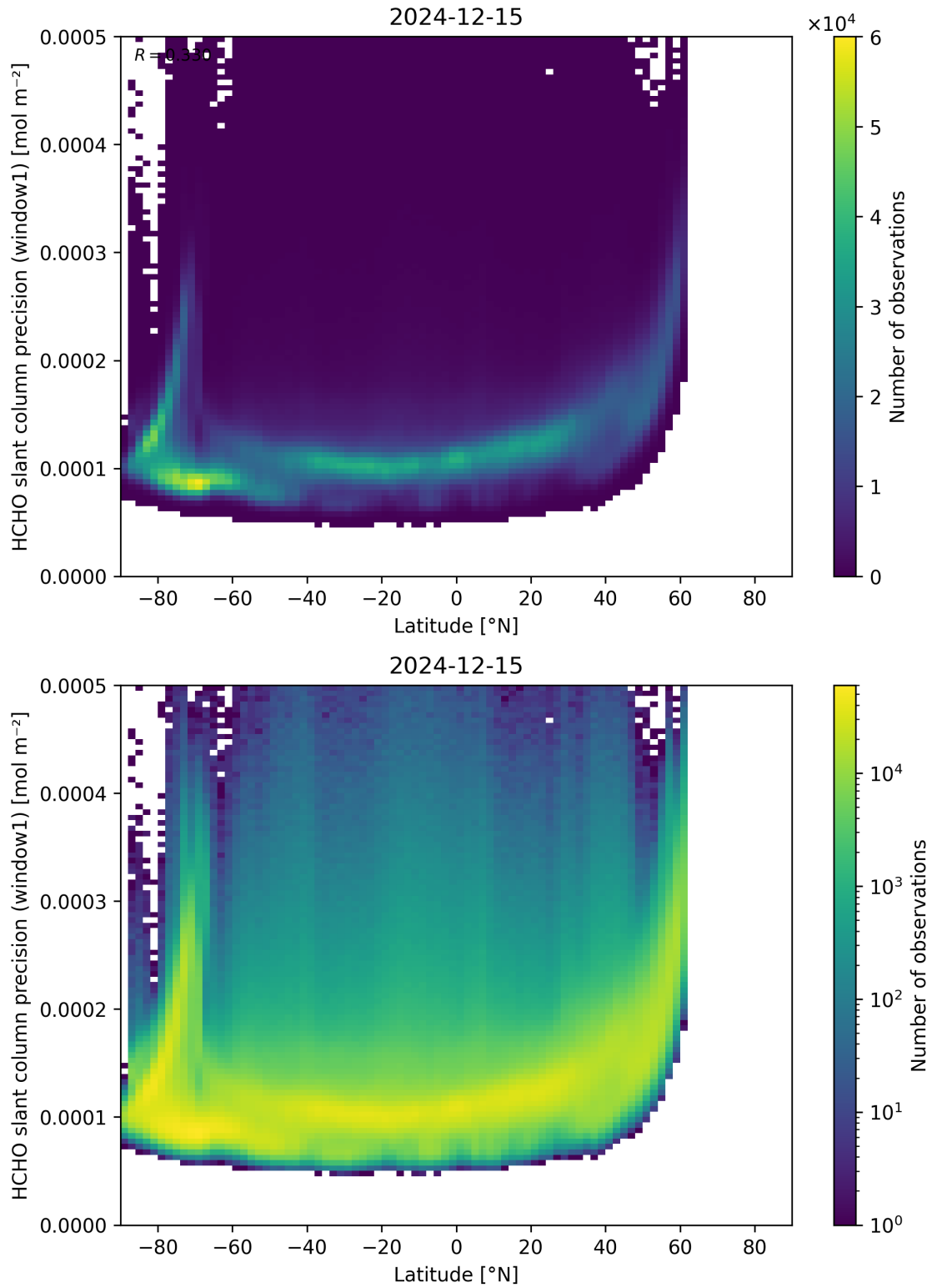
Figure 160: Scatter density plot of “Latitude” against “HCHO slant column precision (window1)” for 2024-12-14 to 2024-12-16.
