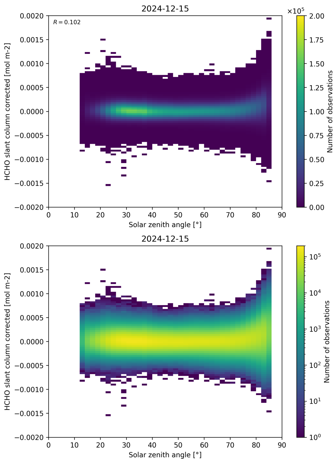
Figure 171: Scatter density plot of “Solar zenith angle” against “HCHO slant column corrected” for 2024-12-14 to 2024-12-16.
