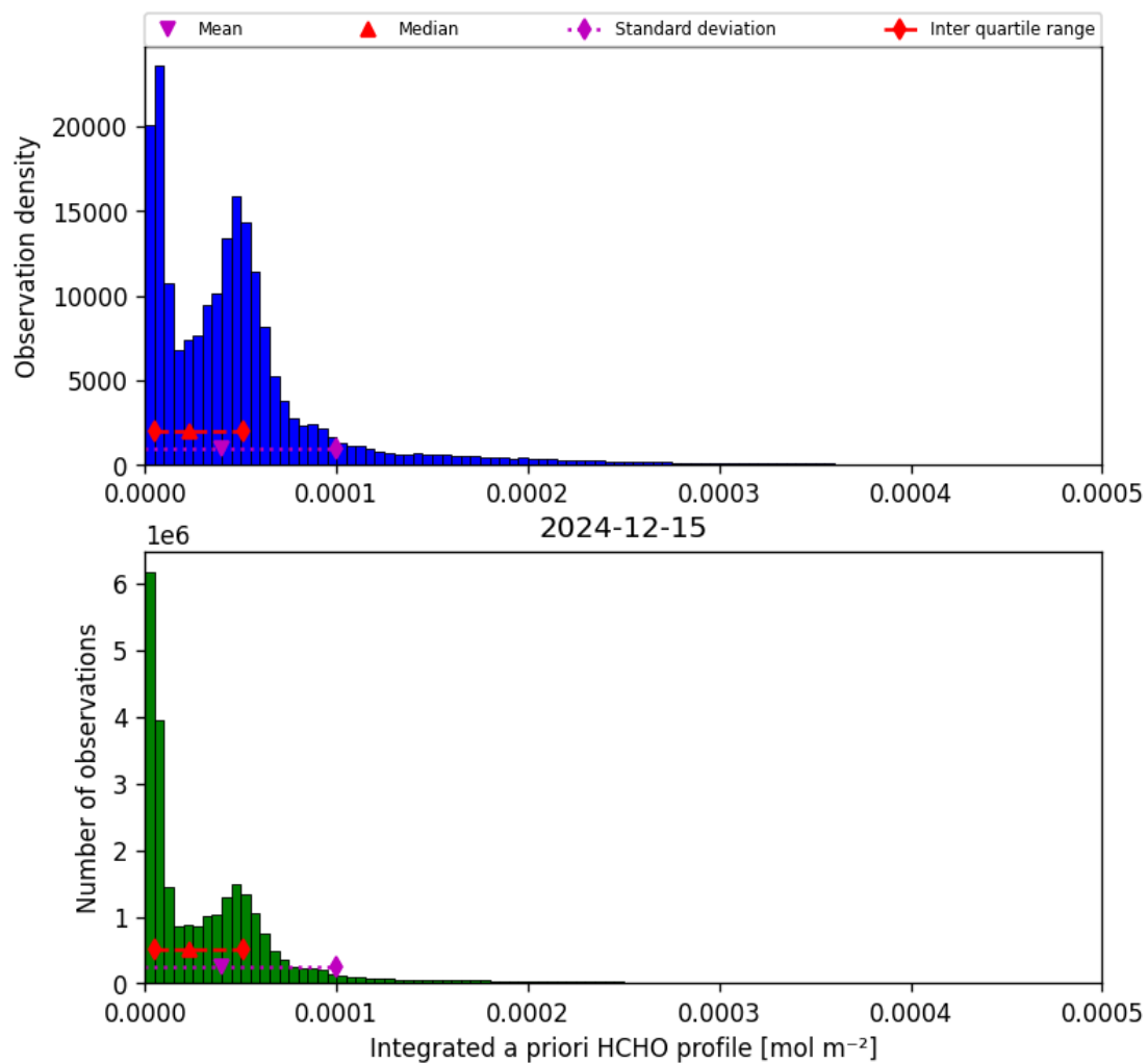
Figure 43: Histogram of “Integrated a priori HCHO profile” for 2024-12-14 to 2024-12-16
