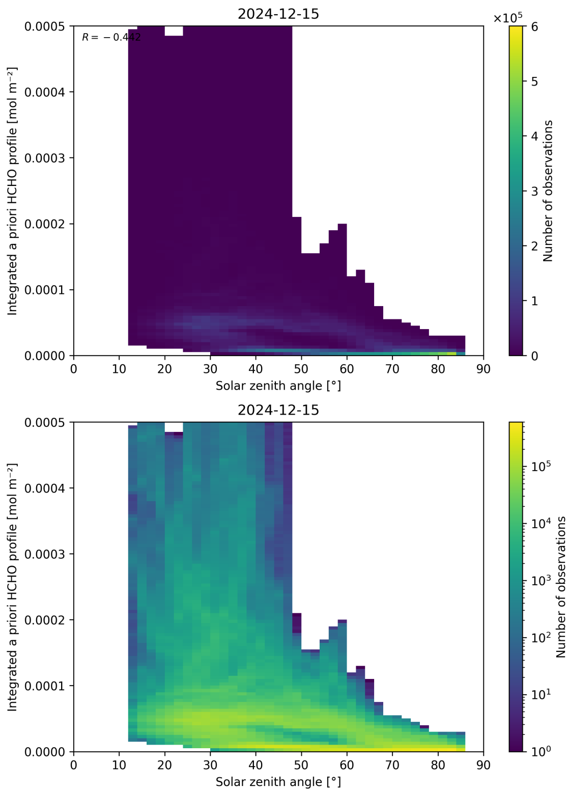
Figure 180: Scatter density plot of “Solar zenith angle” against “Integrated a priori HCHO profile” for 2024-12-14 to 2024-12-16.
