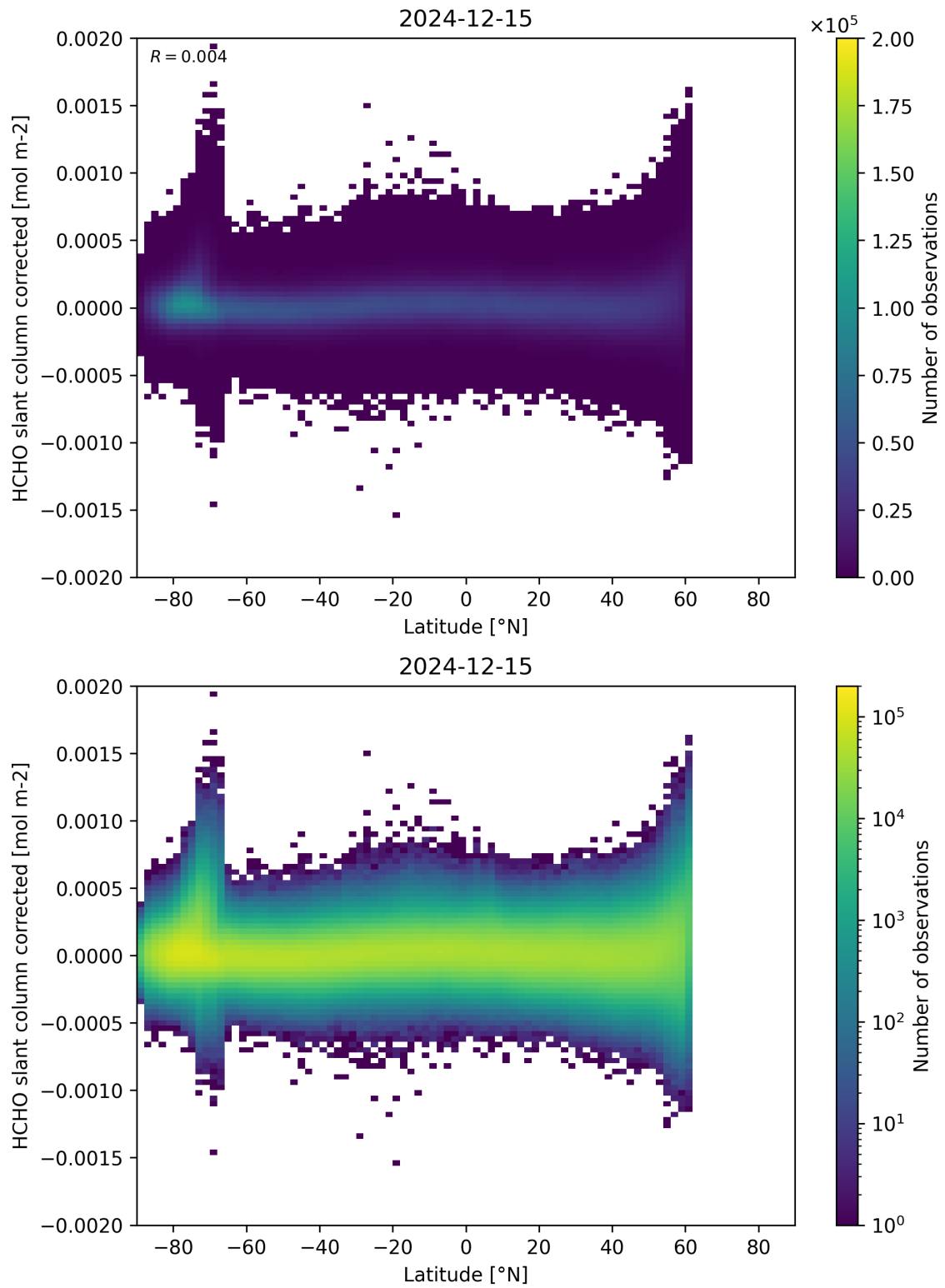
Figure 157: Scatter density plot of “Latitude” against “HCHO slant column corrected” for 2024-12-14 to 2024-12-16.
