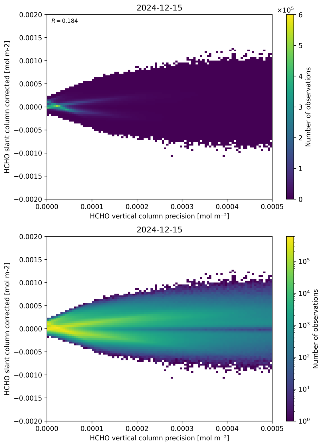
Figure 140: Scatter density plot of “HCHO vertical column precision” against “HCHO slant column corrected” for 2024-12-14 to 2024-12-16.
