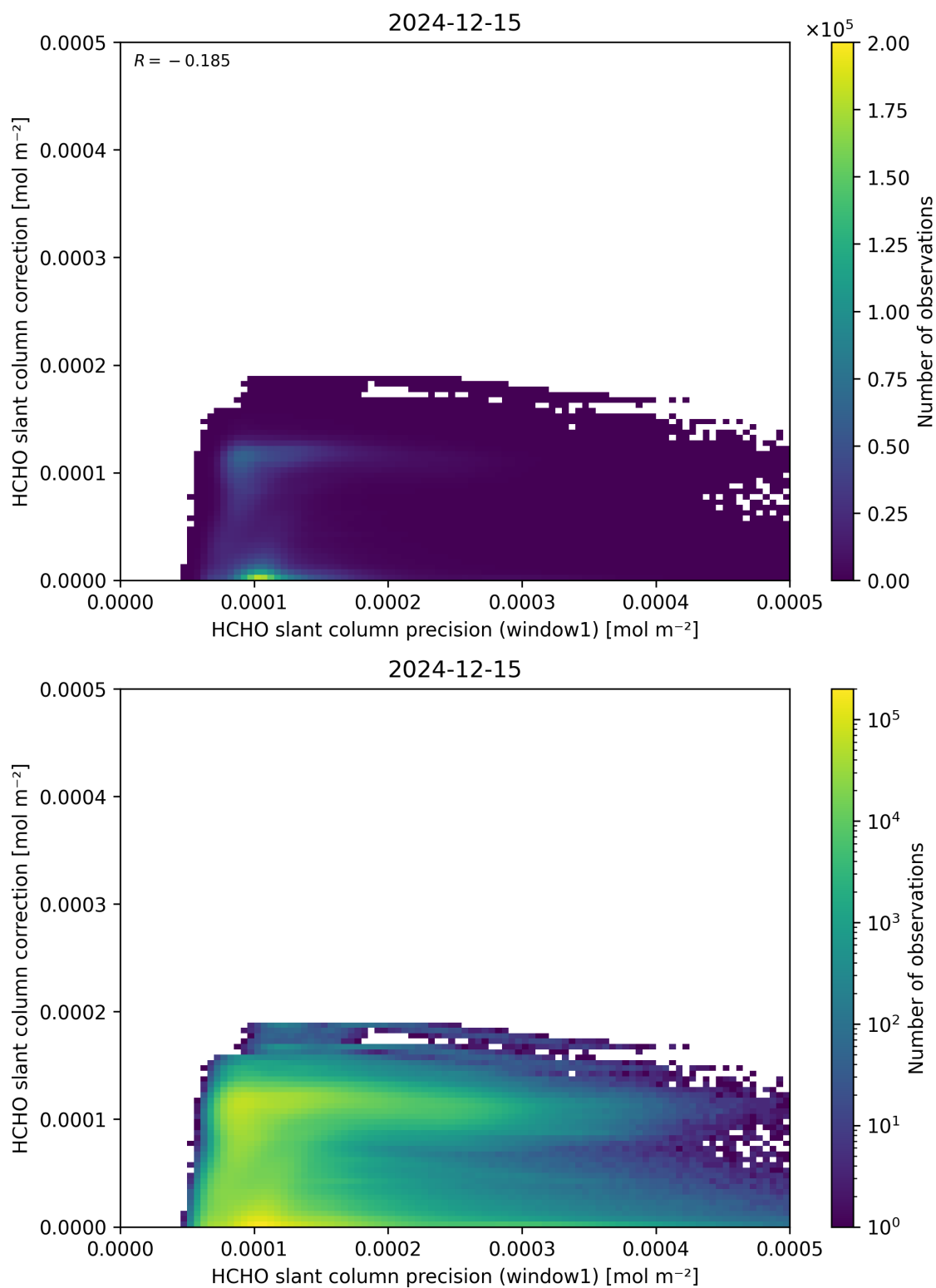
Figure 93: Scatter density plot of “HCHO slant column precision (window1)” against “HCHO slant column correction” for 2024-12-14 to 2024-12-16.
