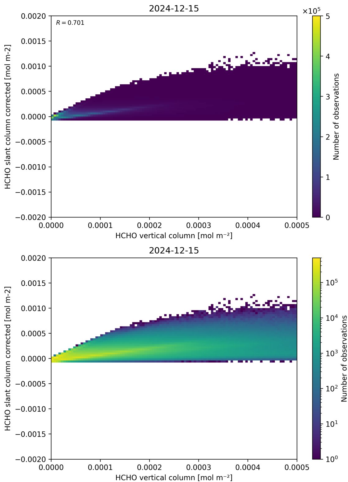
Figure 127: Scatter density plot of “HCHO vertical column” against “HCHO slant column corrected” for 2024-12-14 to 2024-12-16.
