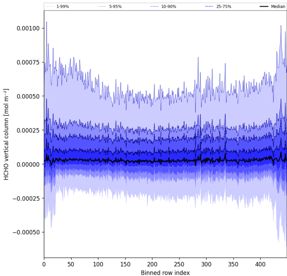
Figure 49: Along track statistics of “HCHO vertical column” for 2024-12-14 to 2024-12-16
