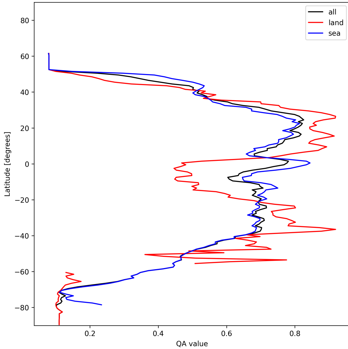
Figure 20: Zonal average of “QA value” for 2024-12-14 to 2024-12-16.
