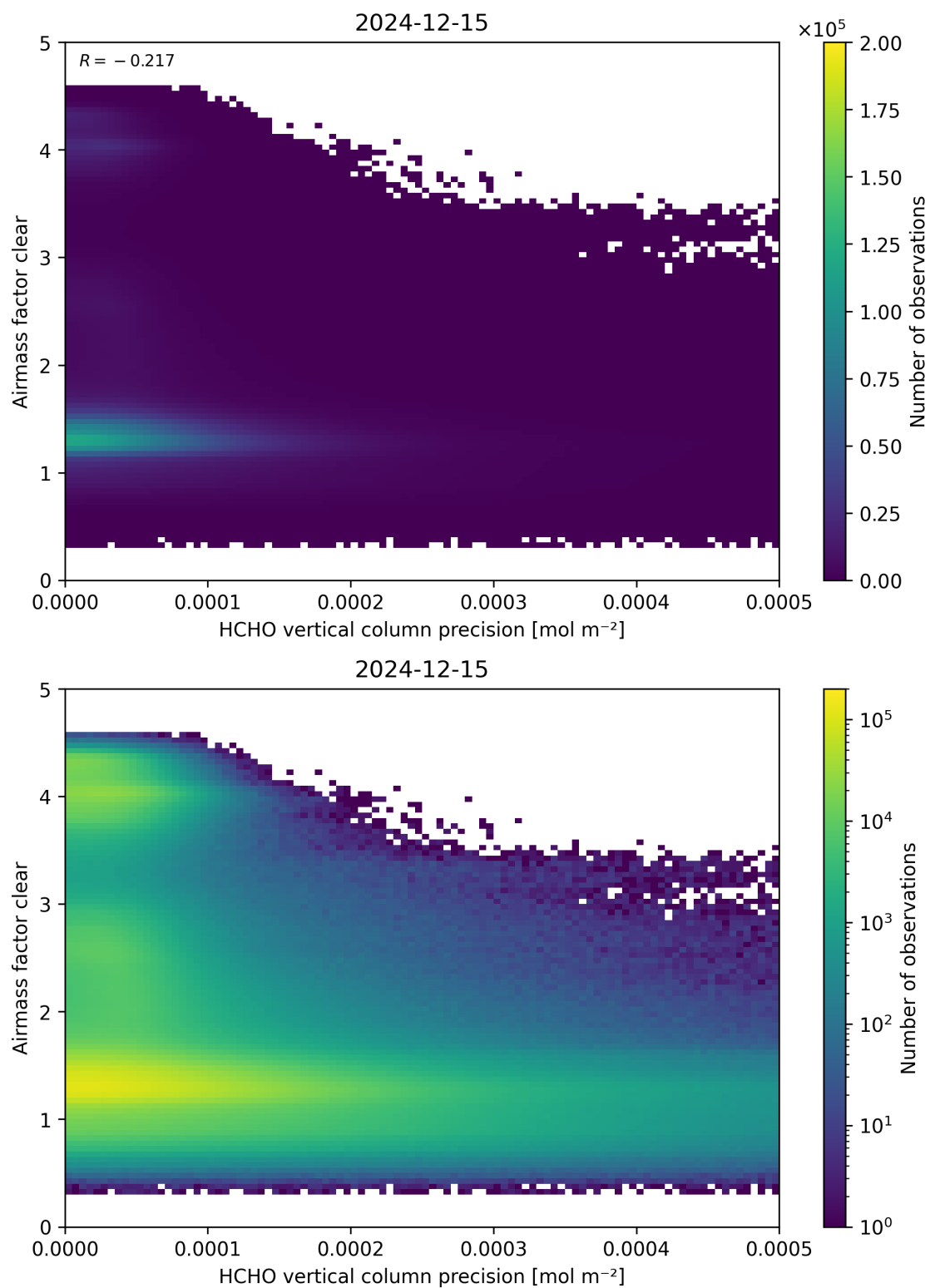
Figure 139: Scatter density plot of “HCHO vertical column precision” against “Airmass factor clear” for 2024-12-14 to 2024-12-16.
