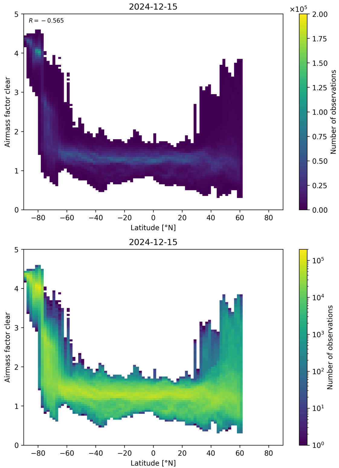
Figure 156: Scatter density plot of “Latitude” against “Airmass factor clear” for 2024-12-14 to 2024-12-16.
