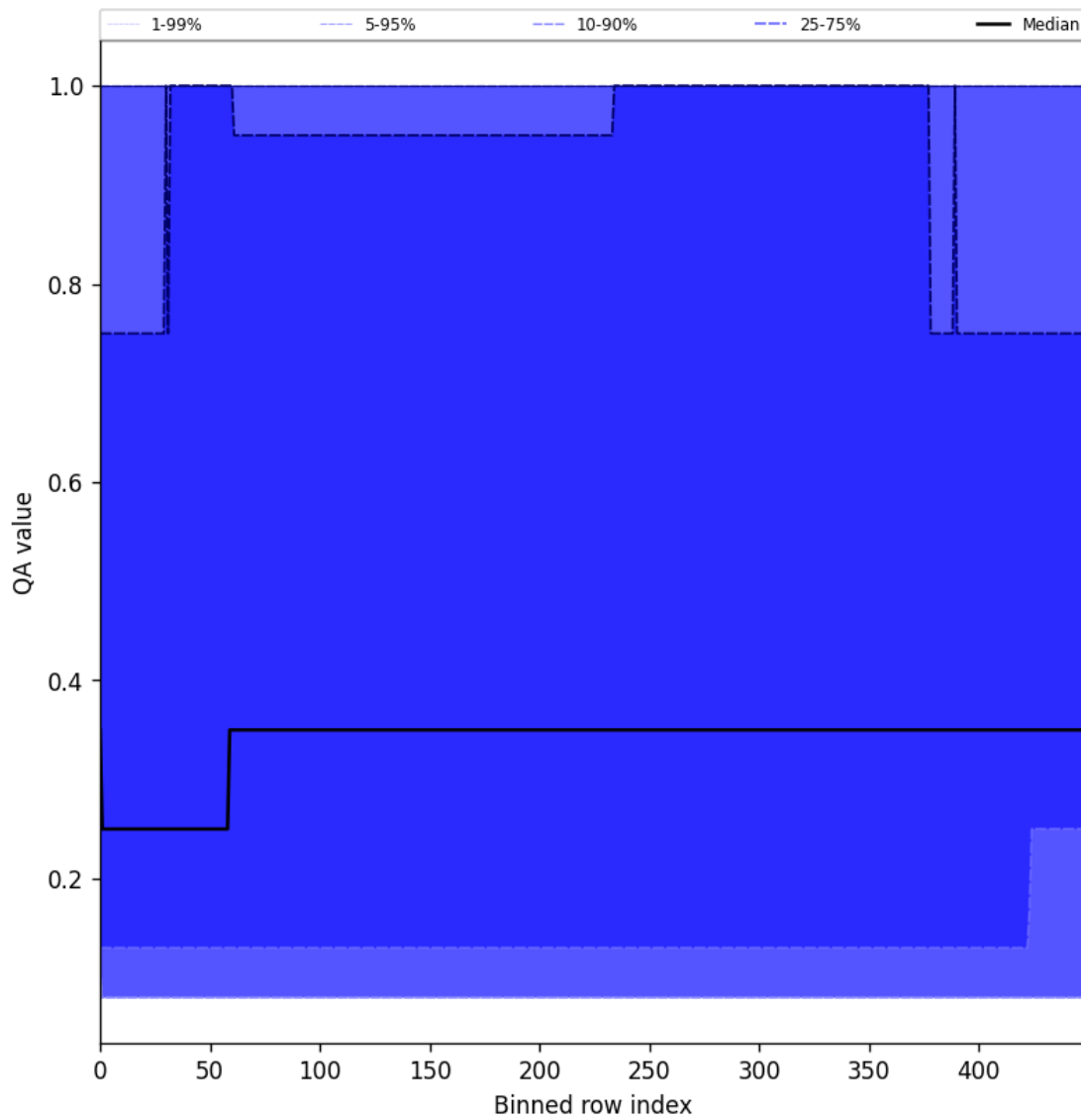
Figure 48: Along track statistics of “QA value” for 2024-12-14 to 2024-12-16
