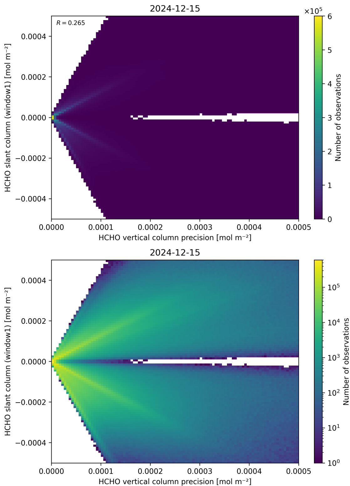
Figure 142: Scatter density plot of “HCHO vertical column precision” against “HCHO slant column (window1)” for 2024-12-14 to 2024-12-16.
