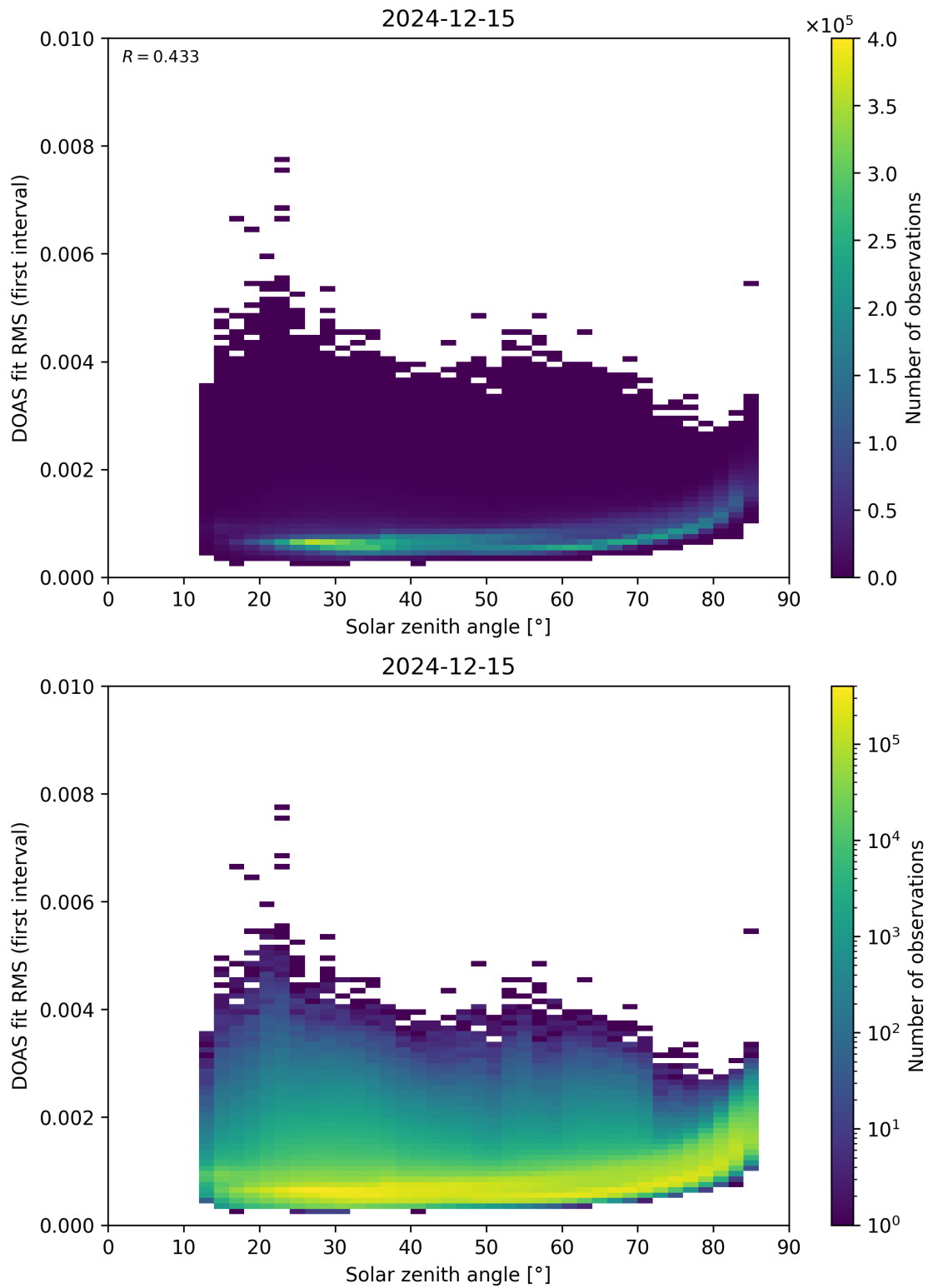
Figure 167: Scatter density plot of “Solar zenith angle” against “DOAS fit RMS (first interval)” for 2024-12-14 to 2024-12-16.
