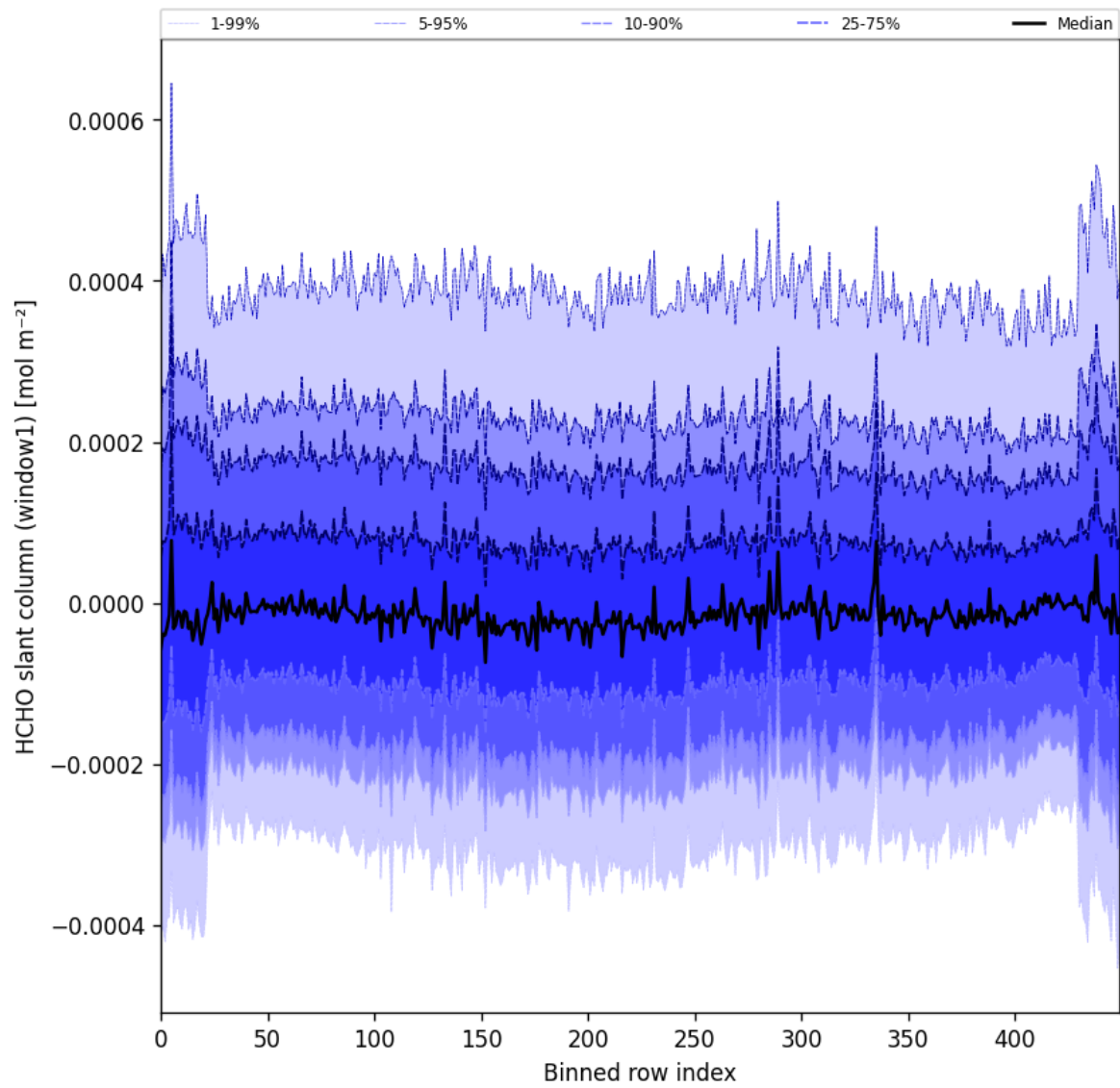
Figure 52: Along track statistics of “HCHO slant column (window1)” for 2024-12-14 to 2024-12-16
