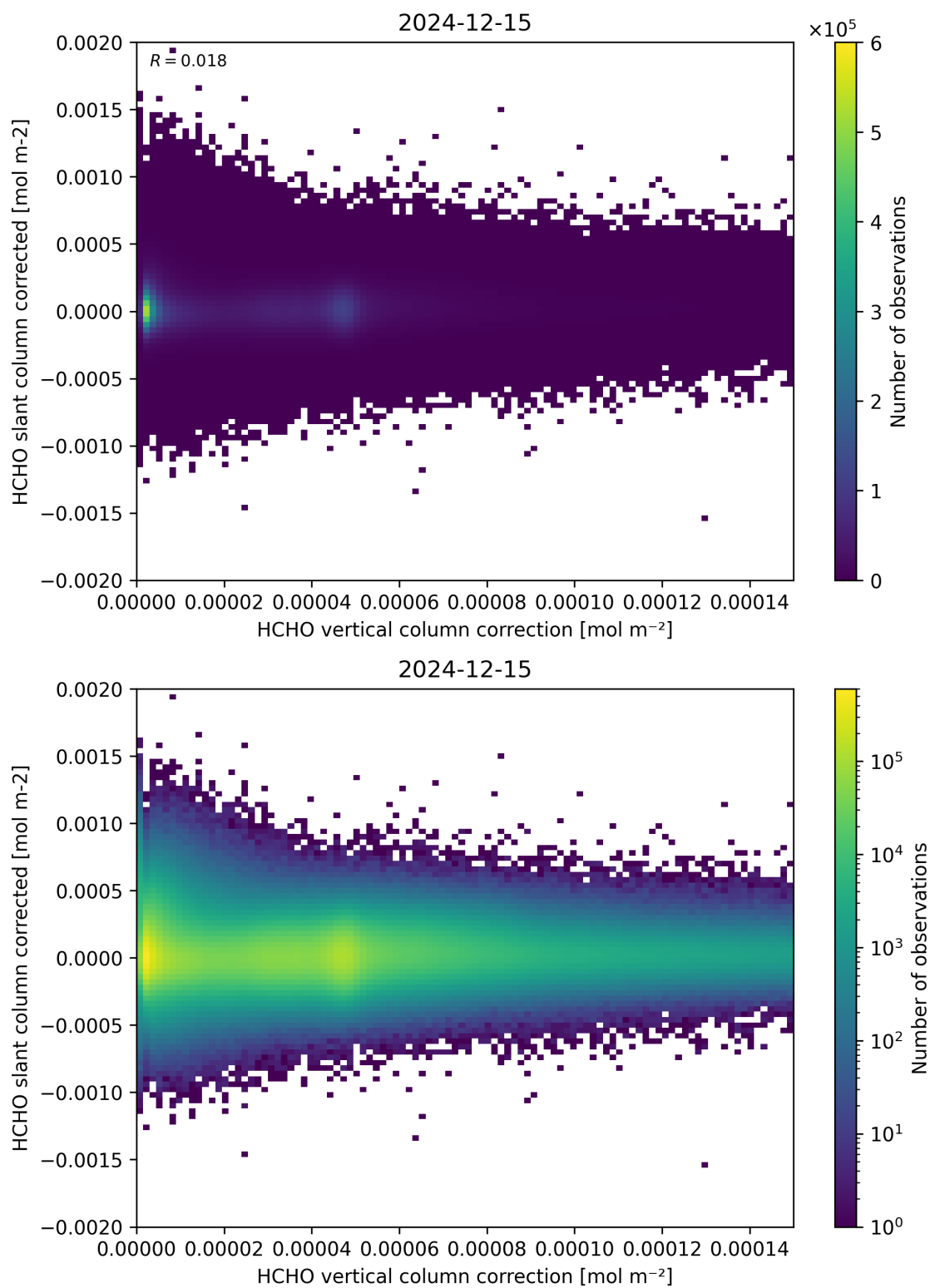
Figure 116: Scatter density plot of “HCHO vertical column correction” against “HCHO slant column corrected” for 2024-12-14 to 2024-12-16.
