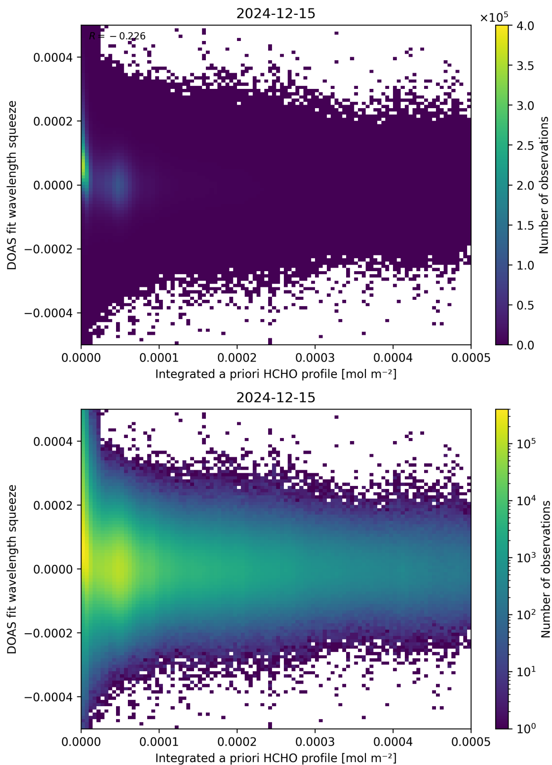
Figure 150: Scatter density plot of “Integrated a priori HCHO profile” against “DOAS fit wavelength squeeze” for 2024-12-14 to 2024-12-16.
