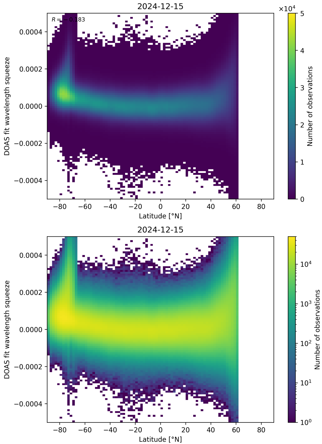
Figure 155: Scatter density plot of “Latitude” against “DOAS fit wavelength squeeze” for 2024-12-14 to 2024-12-16.
