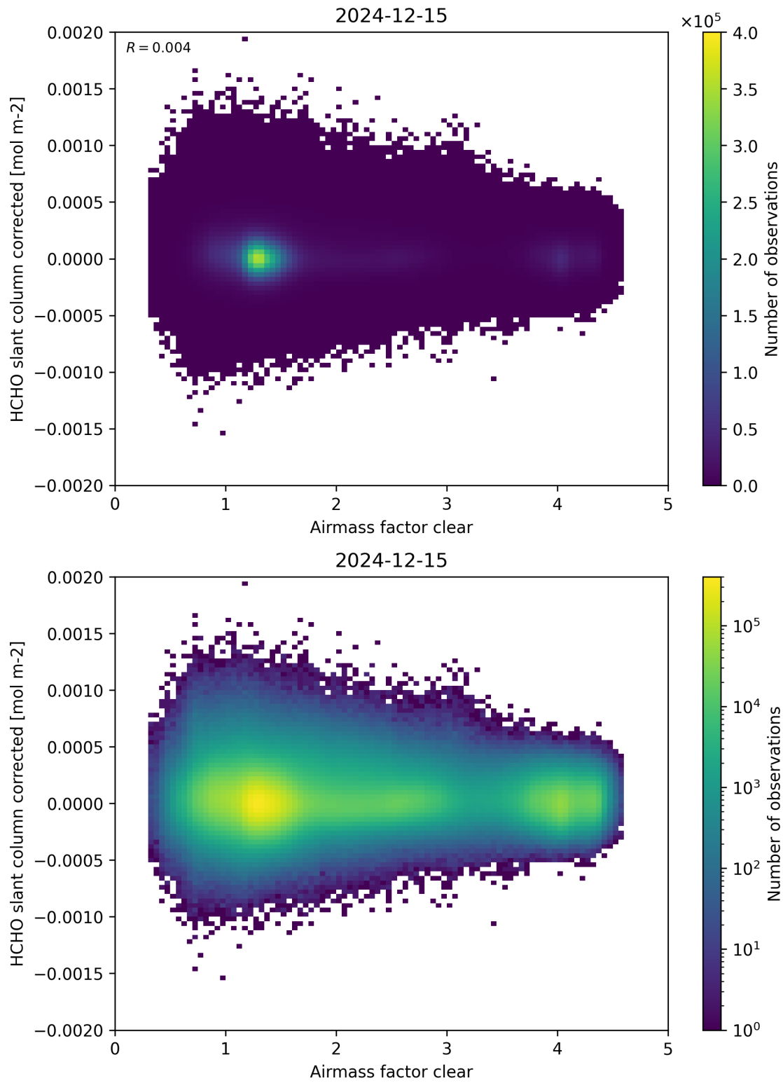
Figure 74: Scatter density plot of “Airmass factor clear” against “HCHO slant column corrected” for 2024-12-14 to 2024-12-16.
