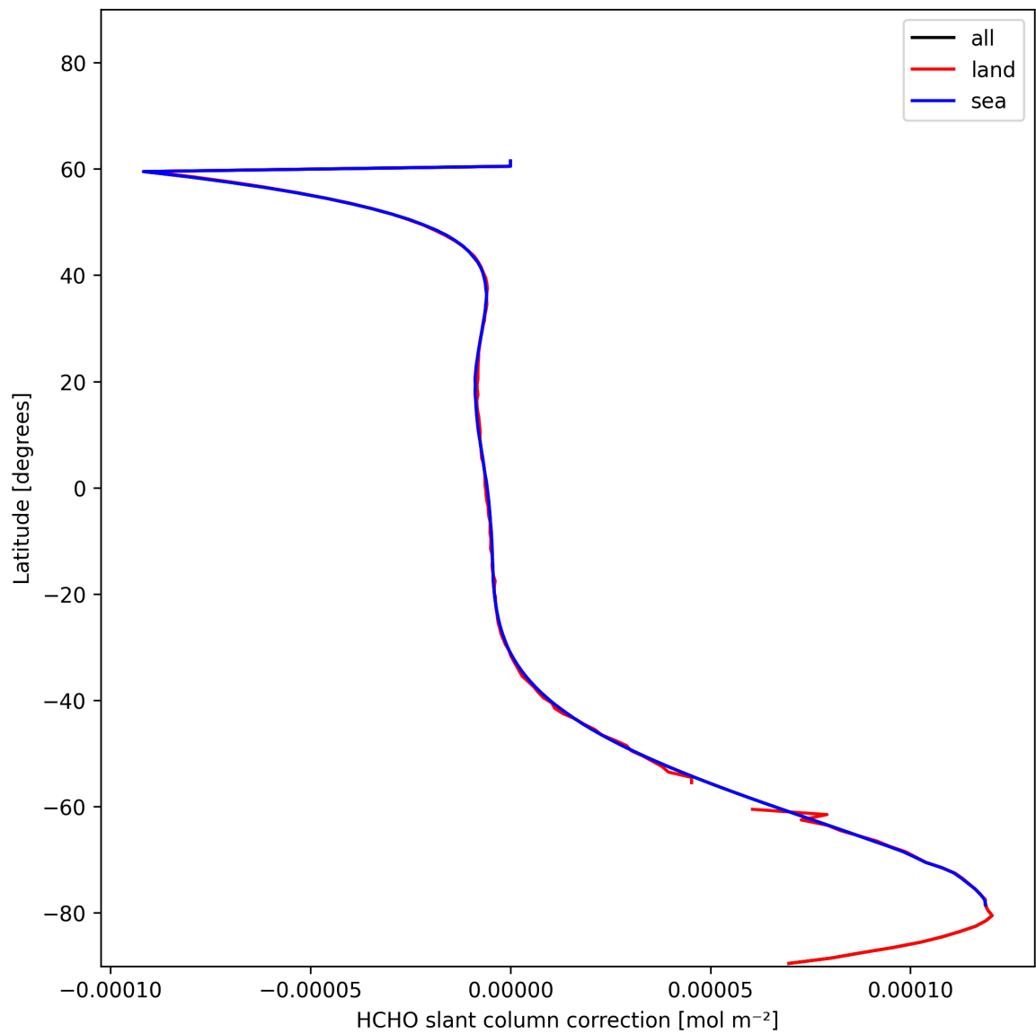
Figure 33: Zonal average of “HCHO slant column correction” for 2024-12-14 to 2024-12-16.
