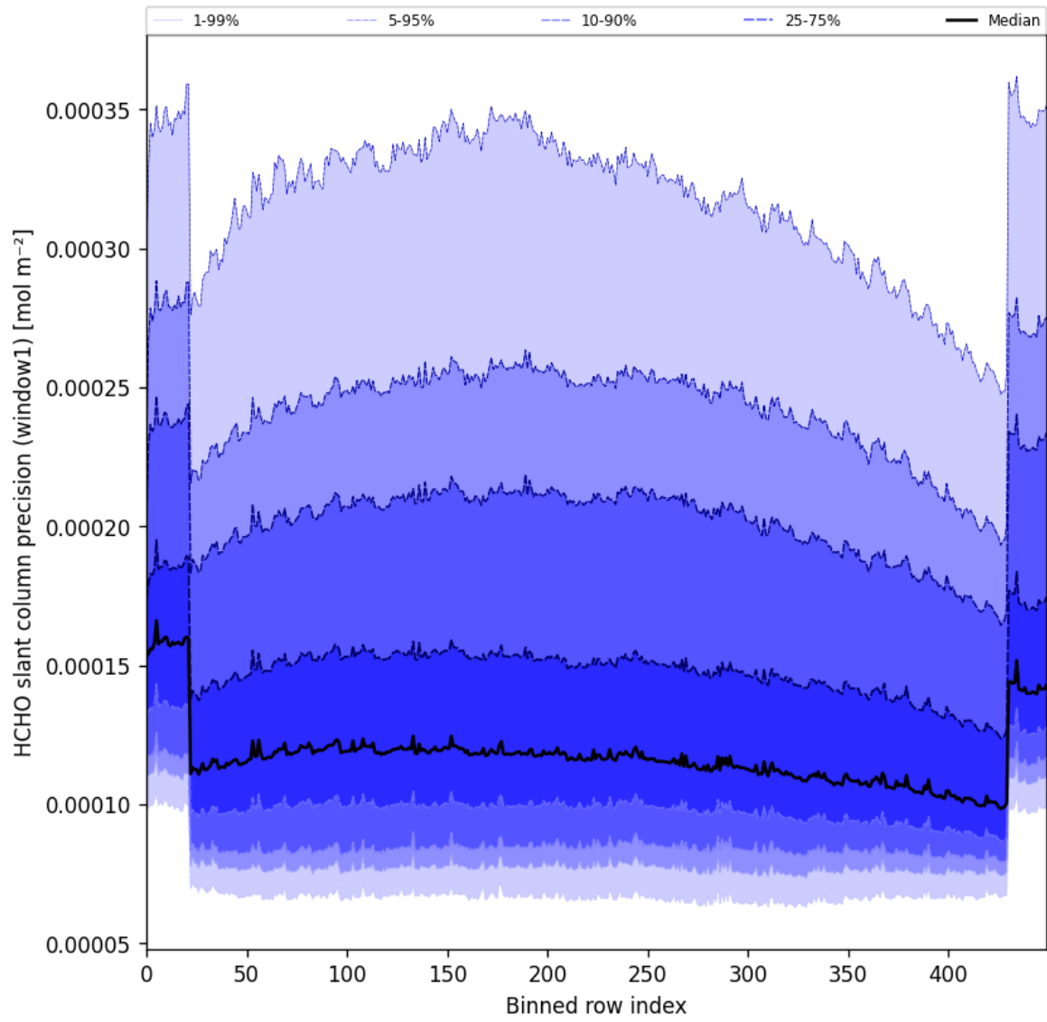
Figure 53: Along track statistics of “HCHO slant column precision (window1)” for 2024-12-14 to 2024-12-16
