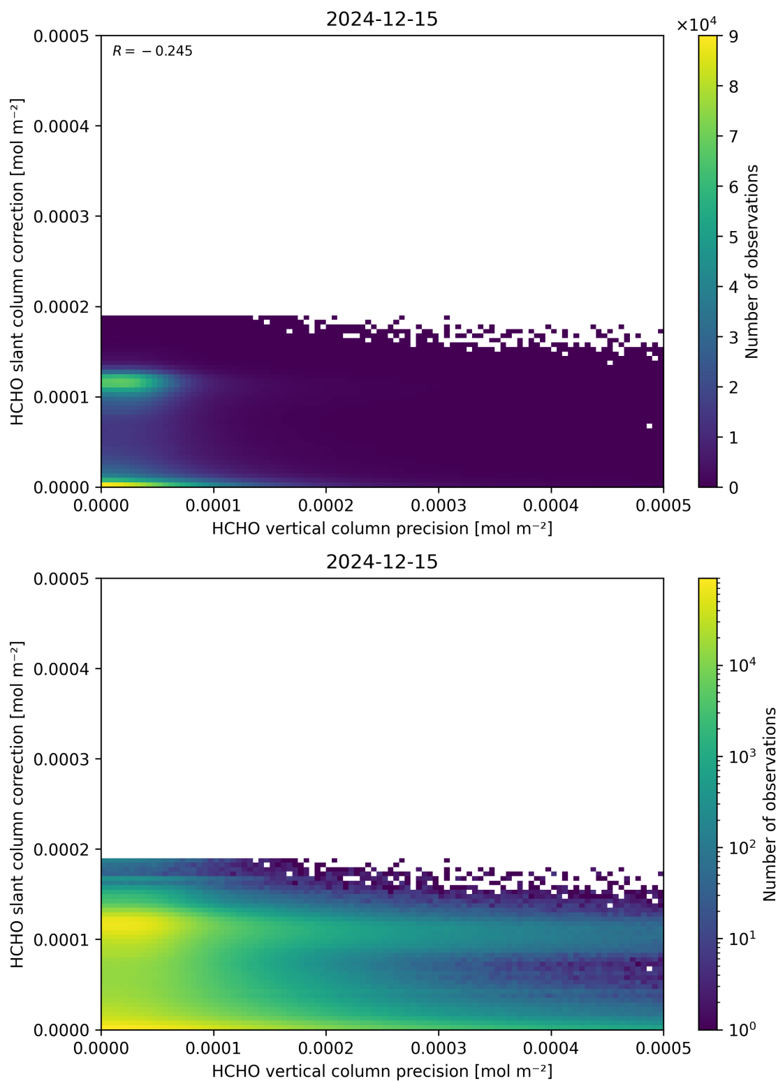
Figure 141: Scatter density plot of “HCHO vertical column precision” against “HCHO slant column correction” for 2024-12-14 to 2024-12-16.
