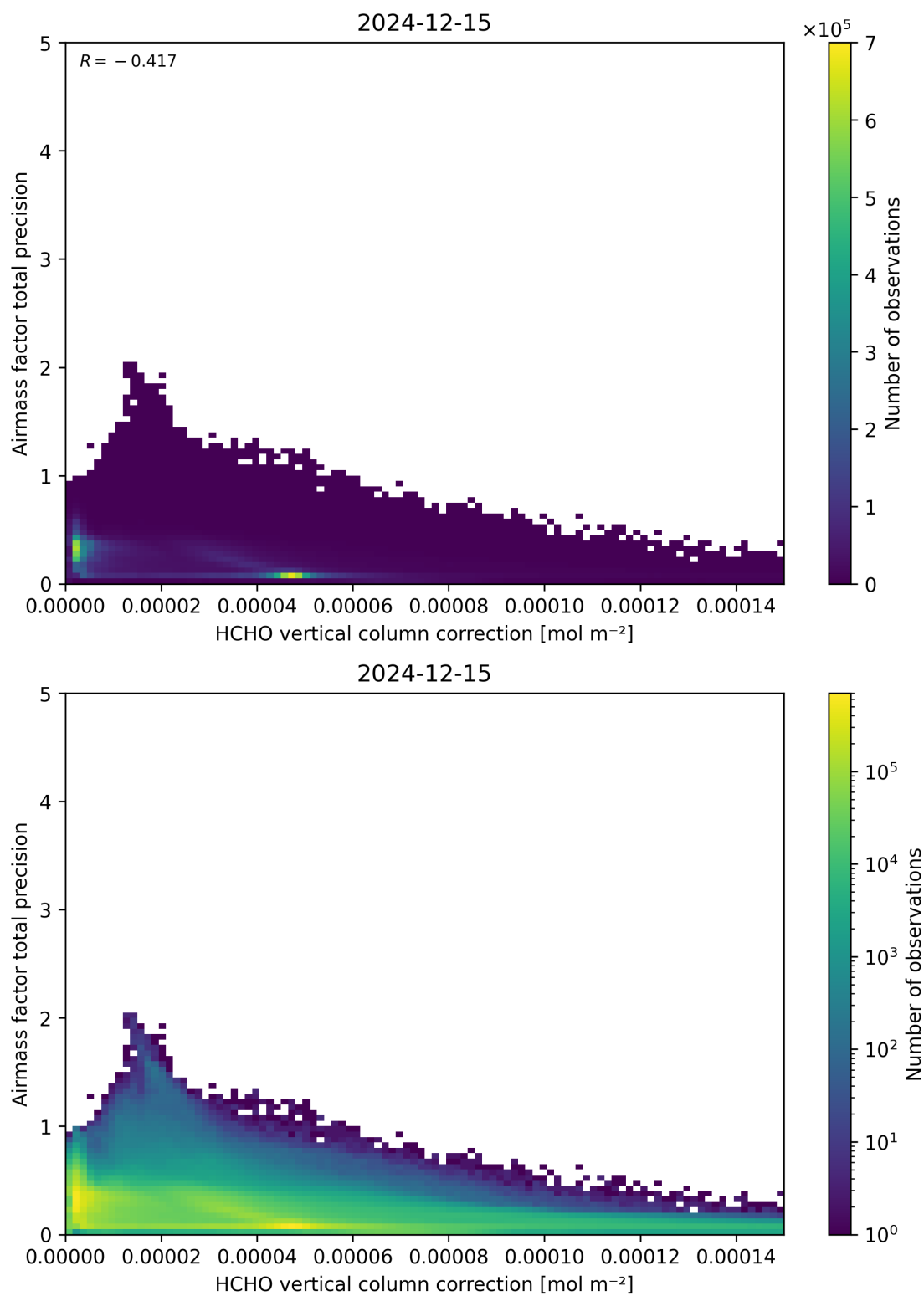
Figure 121: Scatter density plot of “HCHO vertical column correction” against “Airmass factor total precision” for 2024-12-14 to 2024-12-16.
