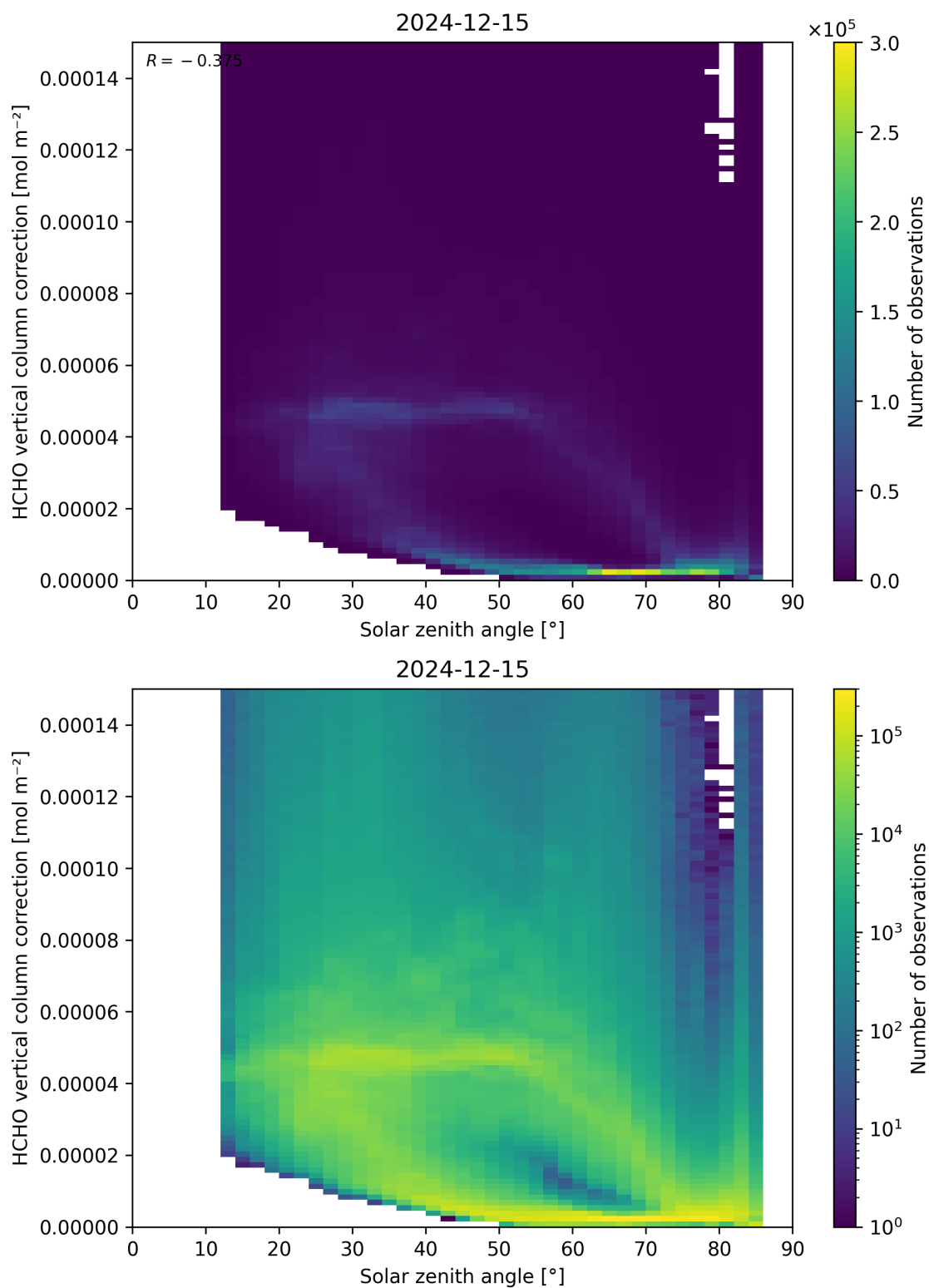
Figure 178: Scatter density plot of “Solar zenith angle” against “HCHO vertical column correction” for 2024-12-14 to 2024-12-16.
