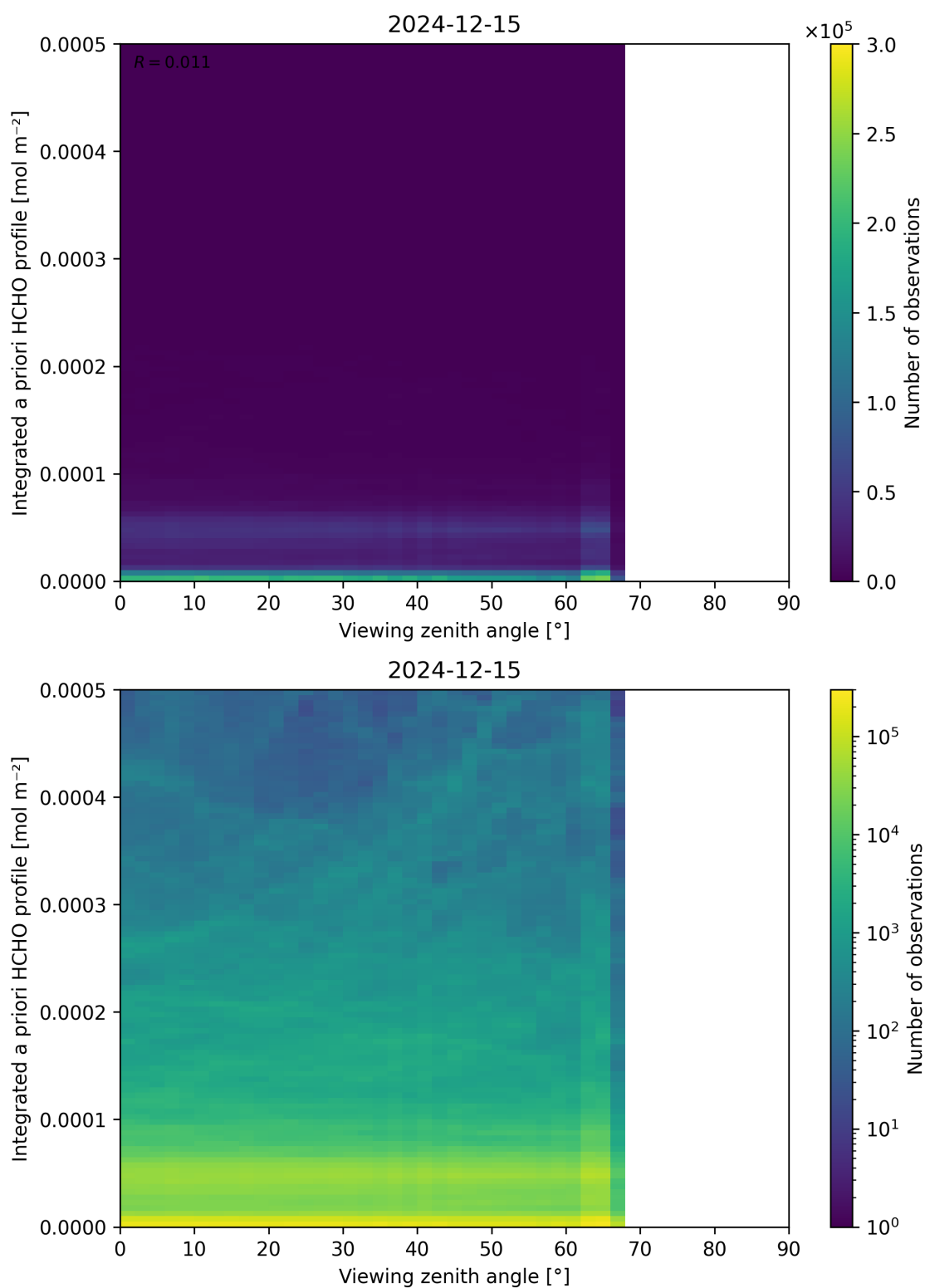
Figure 195: Scatter density plot of “Viewing zenith angle” against “Integrated a priori HCHO profile” for 2024-12-14 to 2024-12-16.
