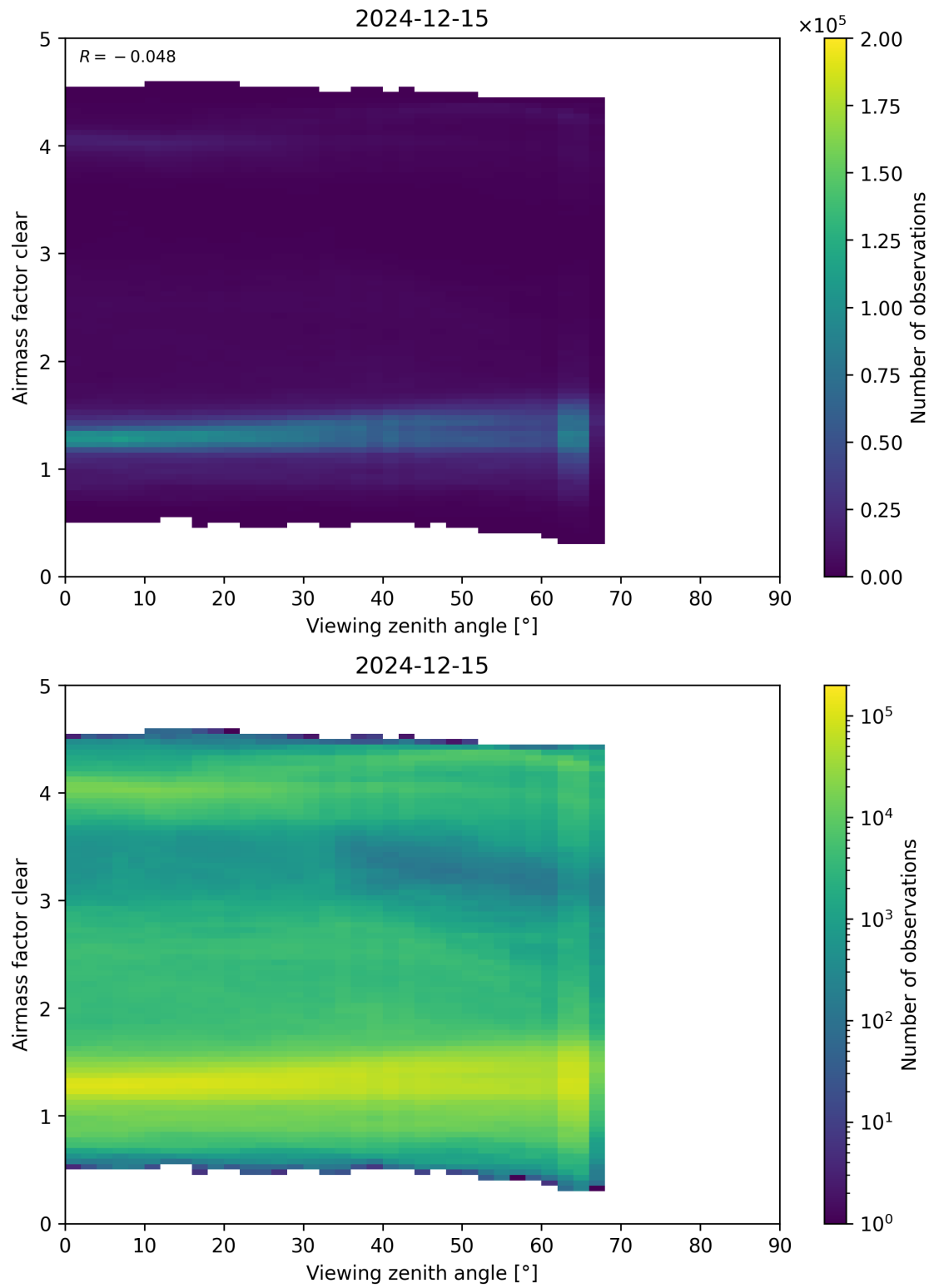
Figure 185: Scatter density plot of “Viewing zenith angle” against “Airmass factor clear” for 2024-12-14 to 2024-12-16.
