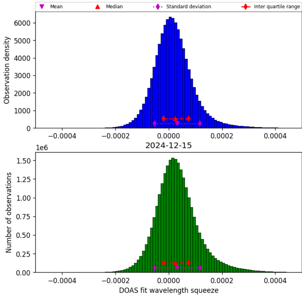
Figure 45: Histogram of “DOAS fit wavelength squeeze” for 2024-12-14 to 2024-12-16
