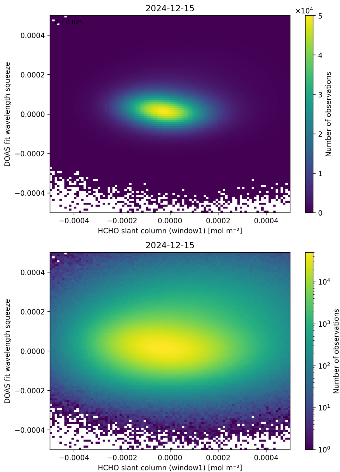
Figure 80: Scatter density plot of “HCHO slant column (window1)” against “DOAS fit wavelength squeeze” for 2024-12-14 to 2024-12-16.
