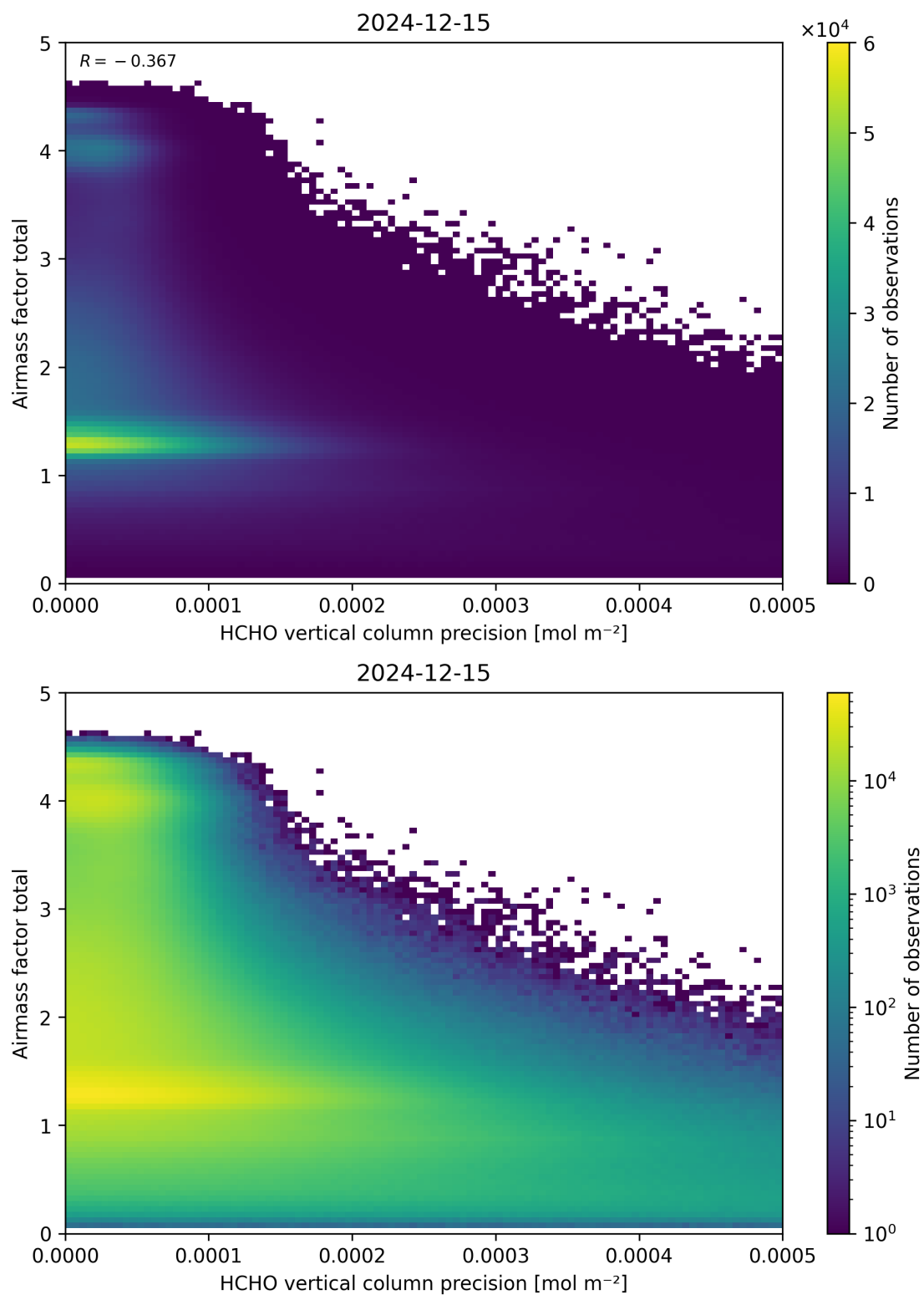
Figure 144: Scatter density plot of “HCHO vertical column precision” against “Airmass factor total” for 2024-12-14 to 2024-12-16.
