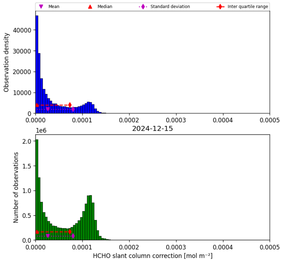
Figure 47: Histogram of “HCHO slant column correction” for 2024-12-14 to 2024-12-16
