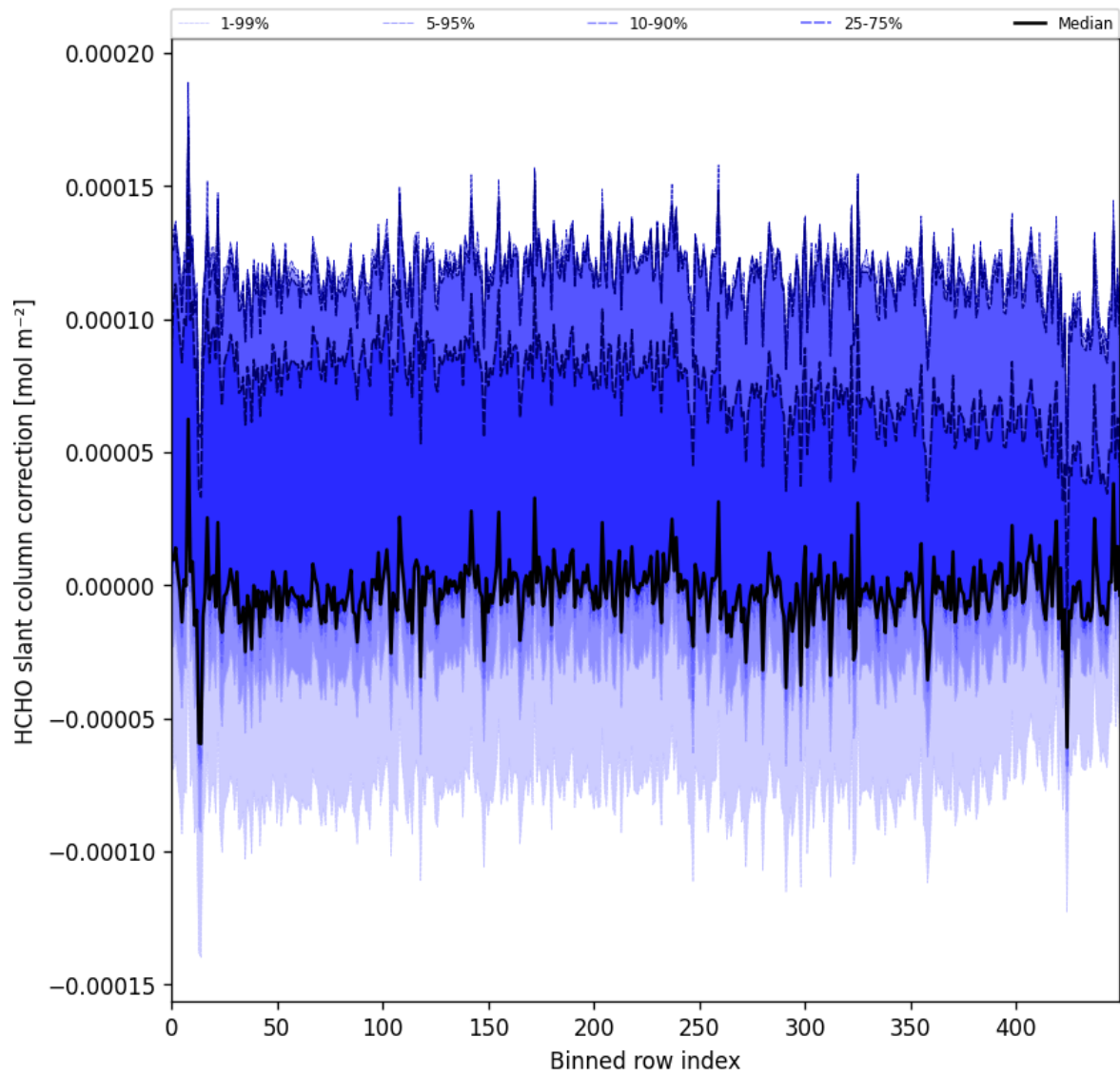
Figure 61: Along track statistics of “HCHO slant column correction” for 2024-12-14 to 2024-12-16
