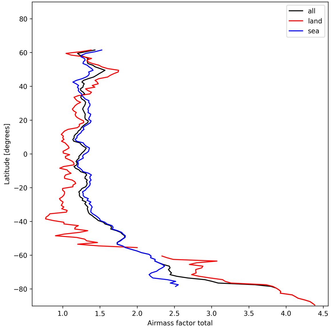
Figure 26: Zonal average of “Airmass factor total” for 2024-12-14 to 2024-12-16.
