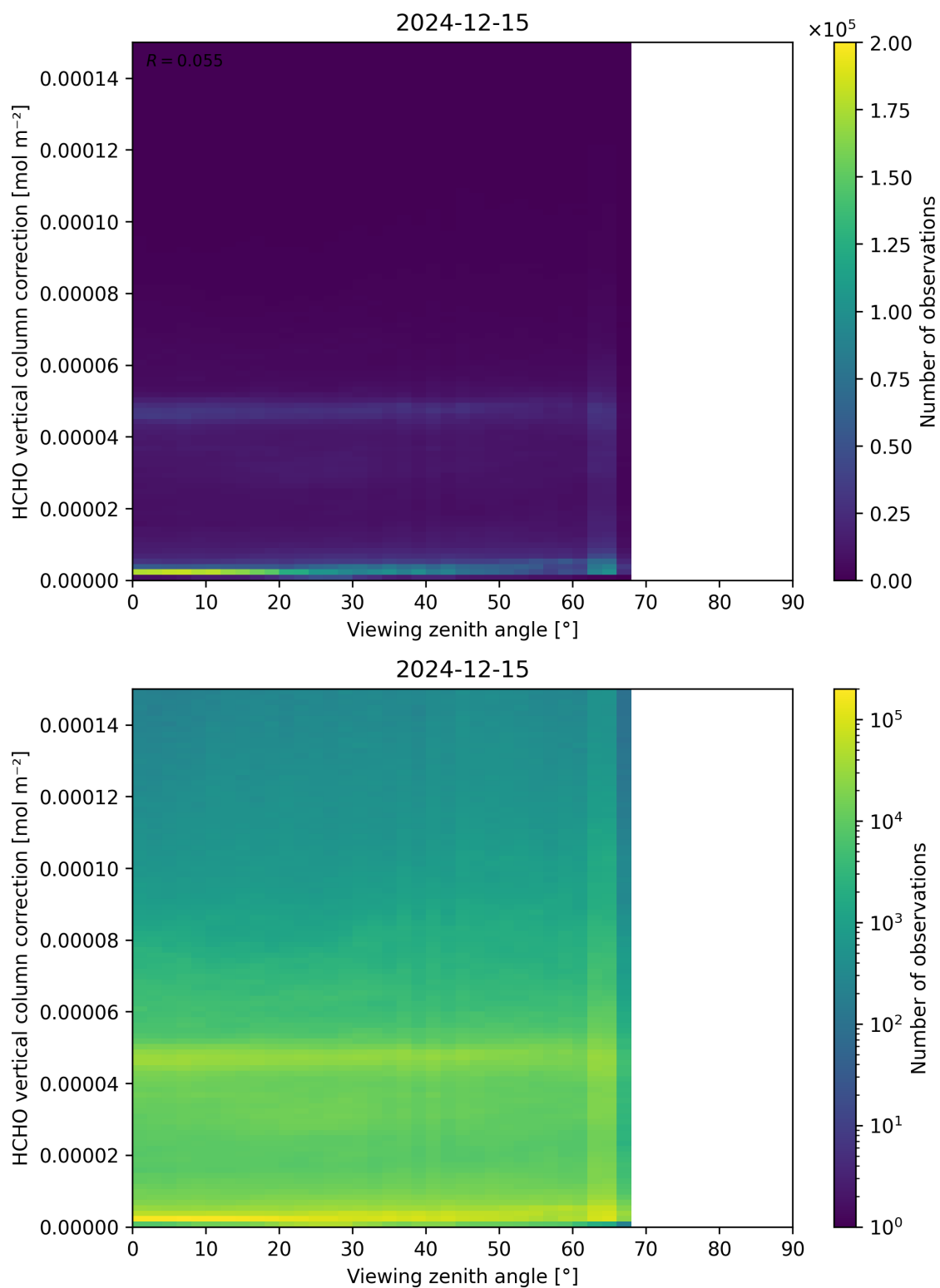
Figure 193: Scatter density plot of “Viewing zenith angle” against “HCHO vertical column correction” for 2024-12-14 to 2024-12-16.
