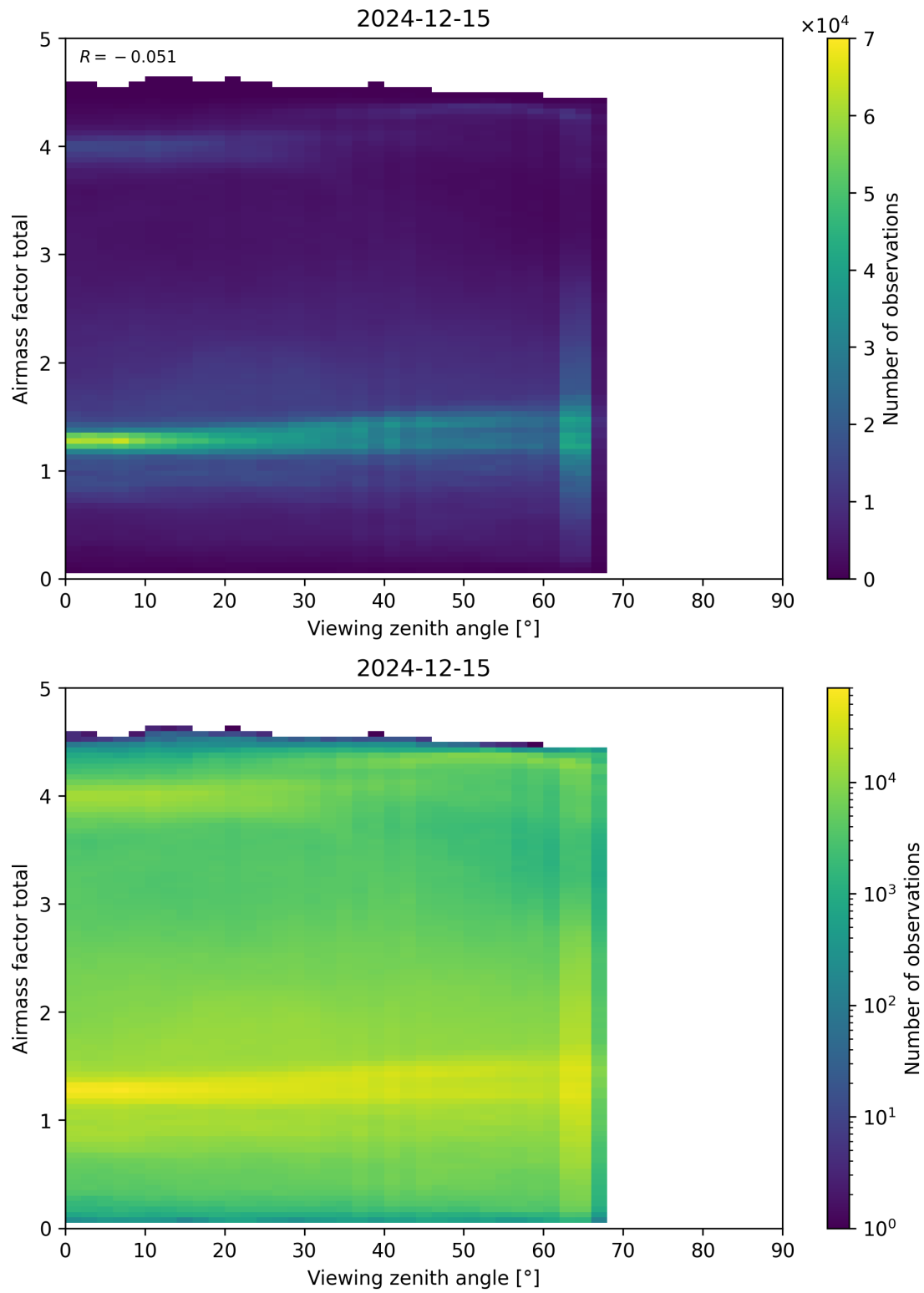
Figure 190: Scatter density plot of “Viewing zenith angle” against “Airmass factor total” for 2024-12-14 to 2024-12-16.
