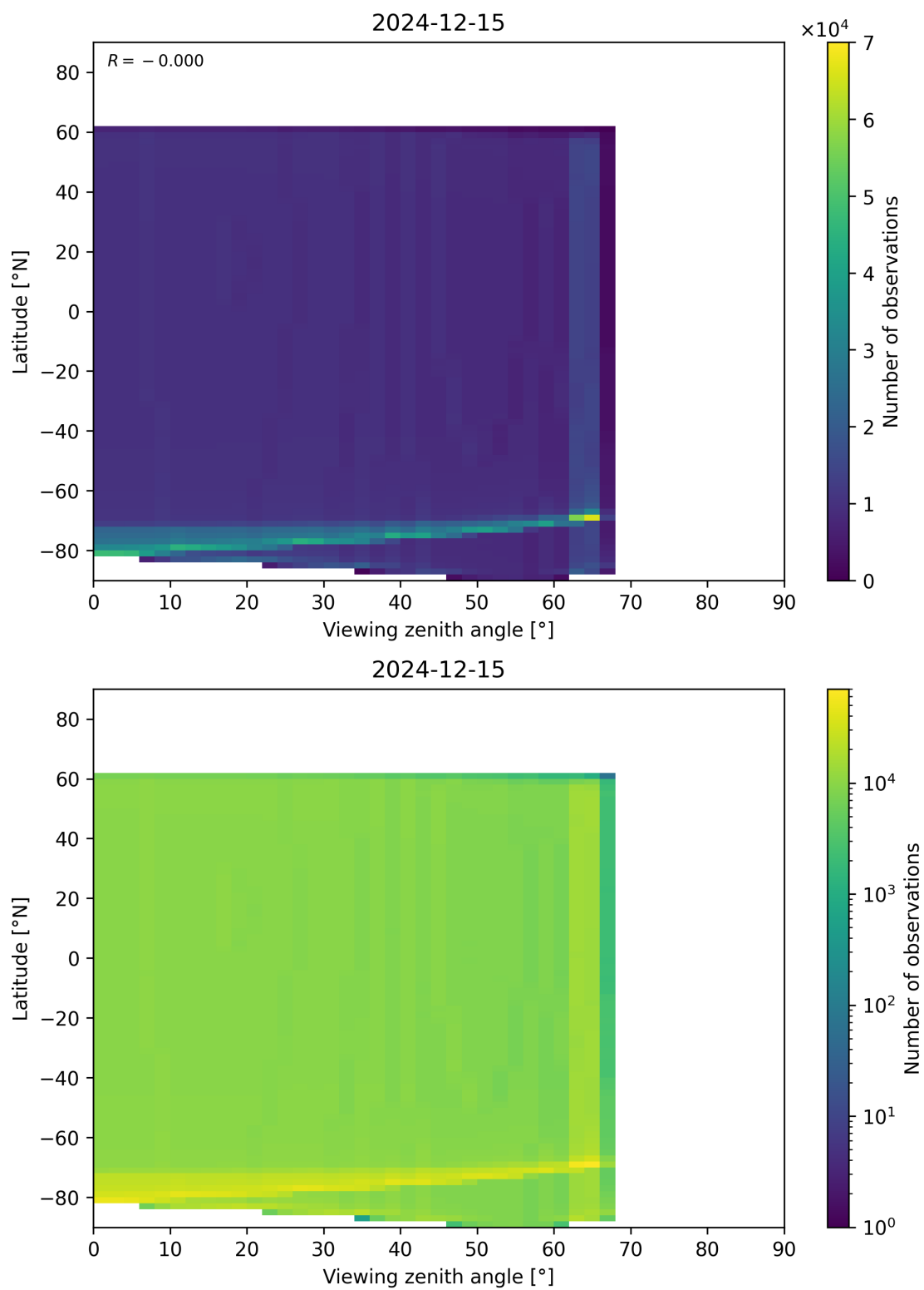
Figure 196: Scatter density plot of “Viewing zenith angle” against “Latitude” for 2024-12-14 to 2024-12-16.
