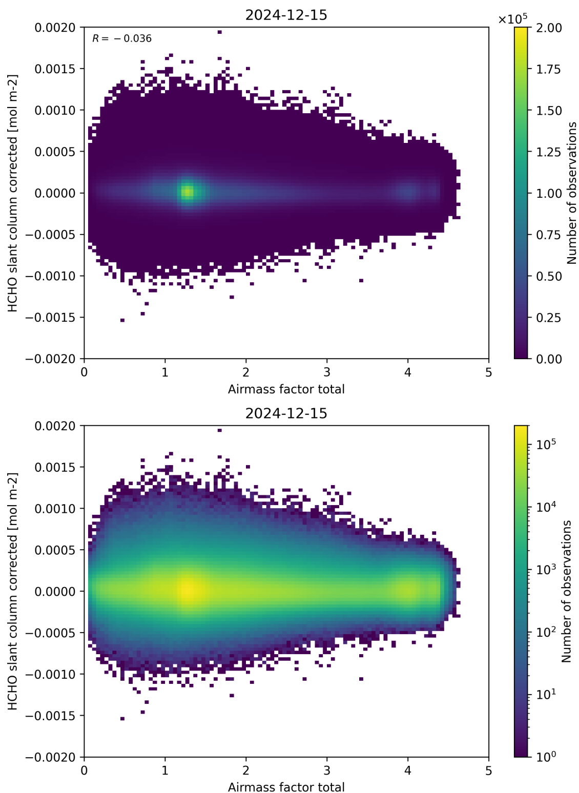
Figure 101: Scatter density plot of “Airmass factor total” against “HCHO slant column corrected” for 2024-12-14 to 2024-12-16.
