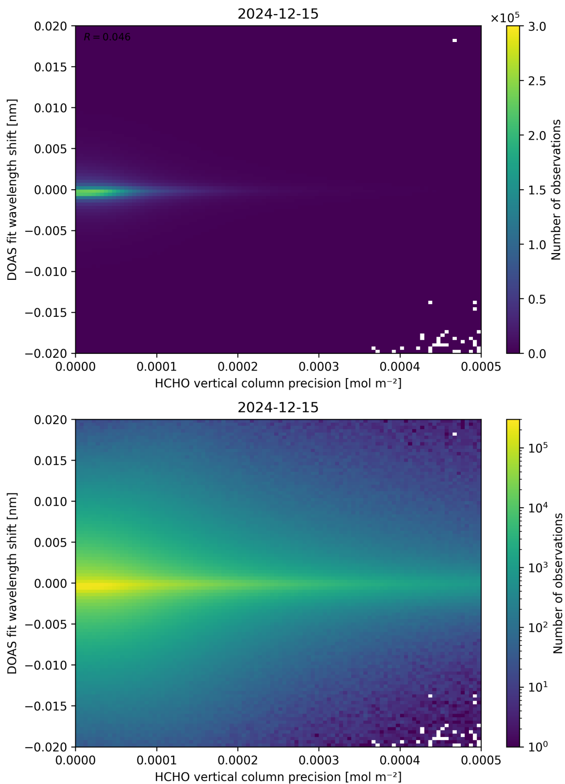
Figure 137: Scatter density plot of “HCHO vertical column precision” against “DOAS fit wavelength shift” for 2024-12-14 to 2024-12-16.
