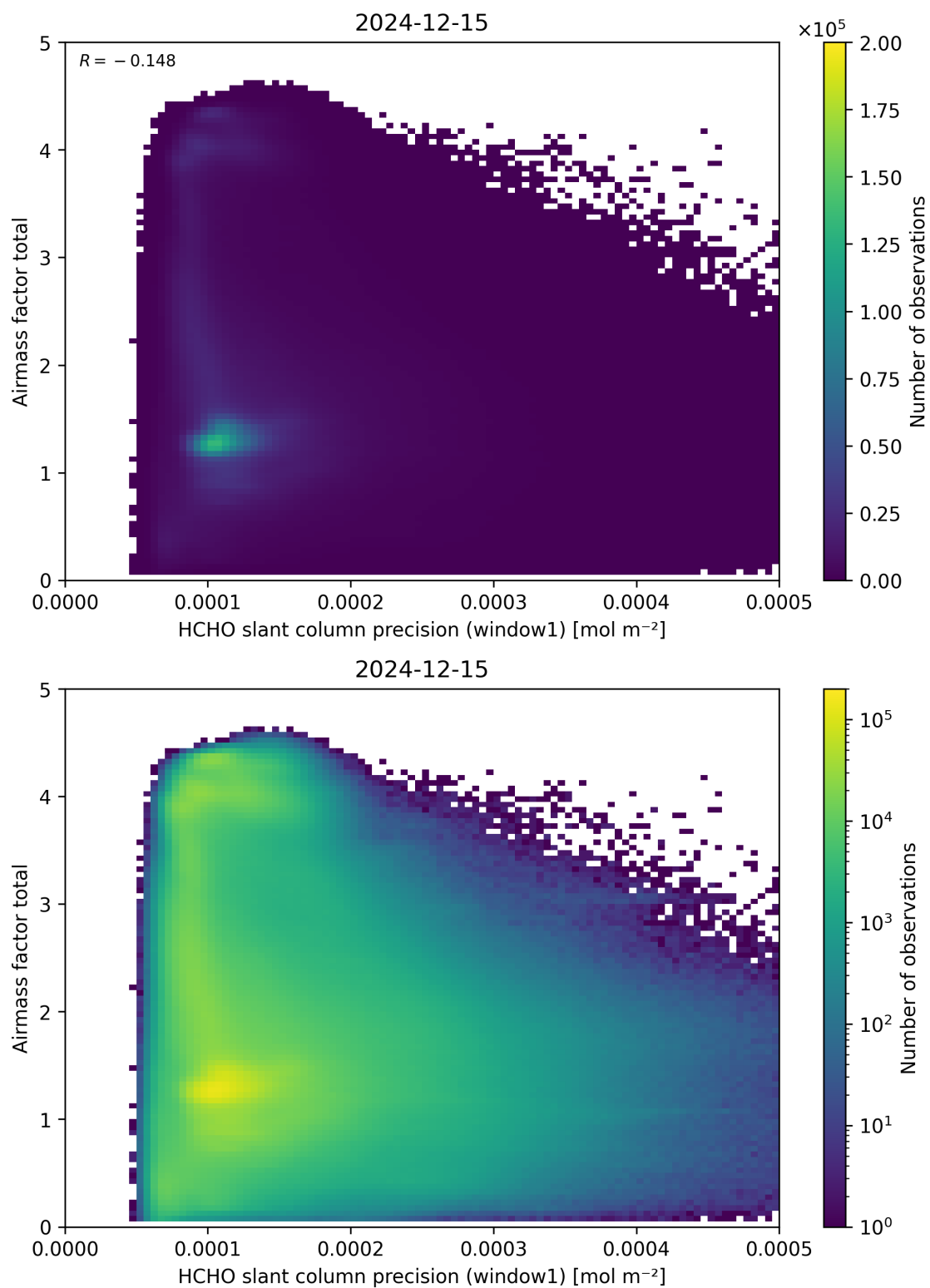
Figure 94: Scatter density plot of “HCHO slant column precision (window1)” against “Airmass factor total” for 2024-12-14 to 2024-12-16.
