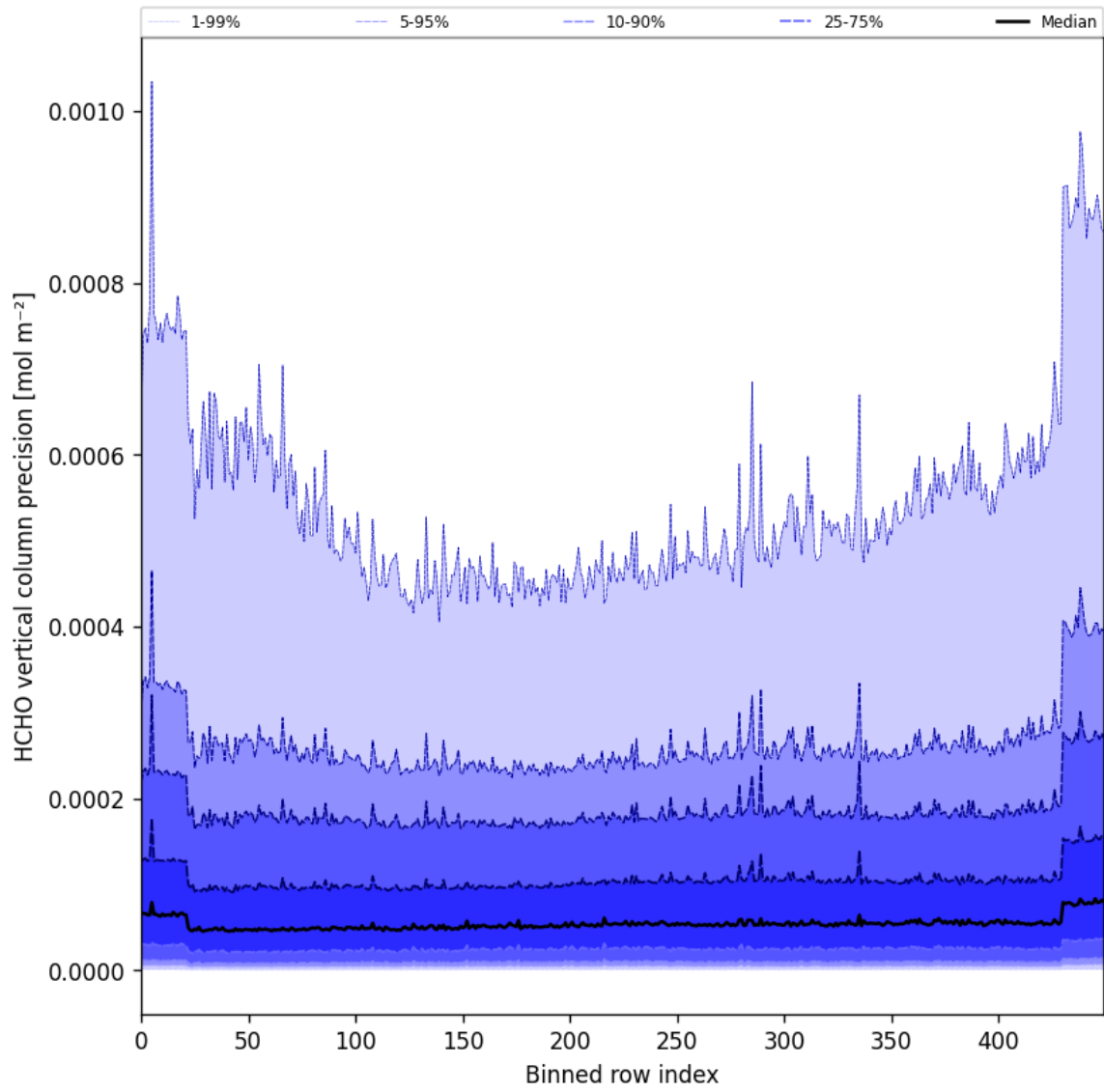
Figure 50: Along track statistics of “HCHO vertical column precision” for 2024-12-14 to 2024-12-16
