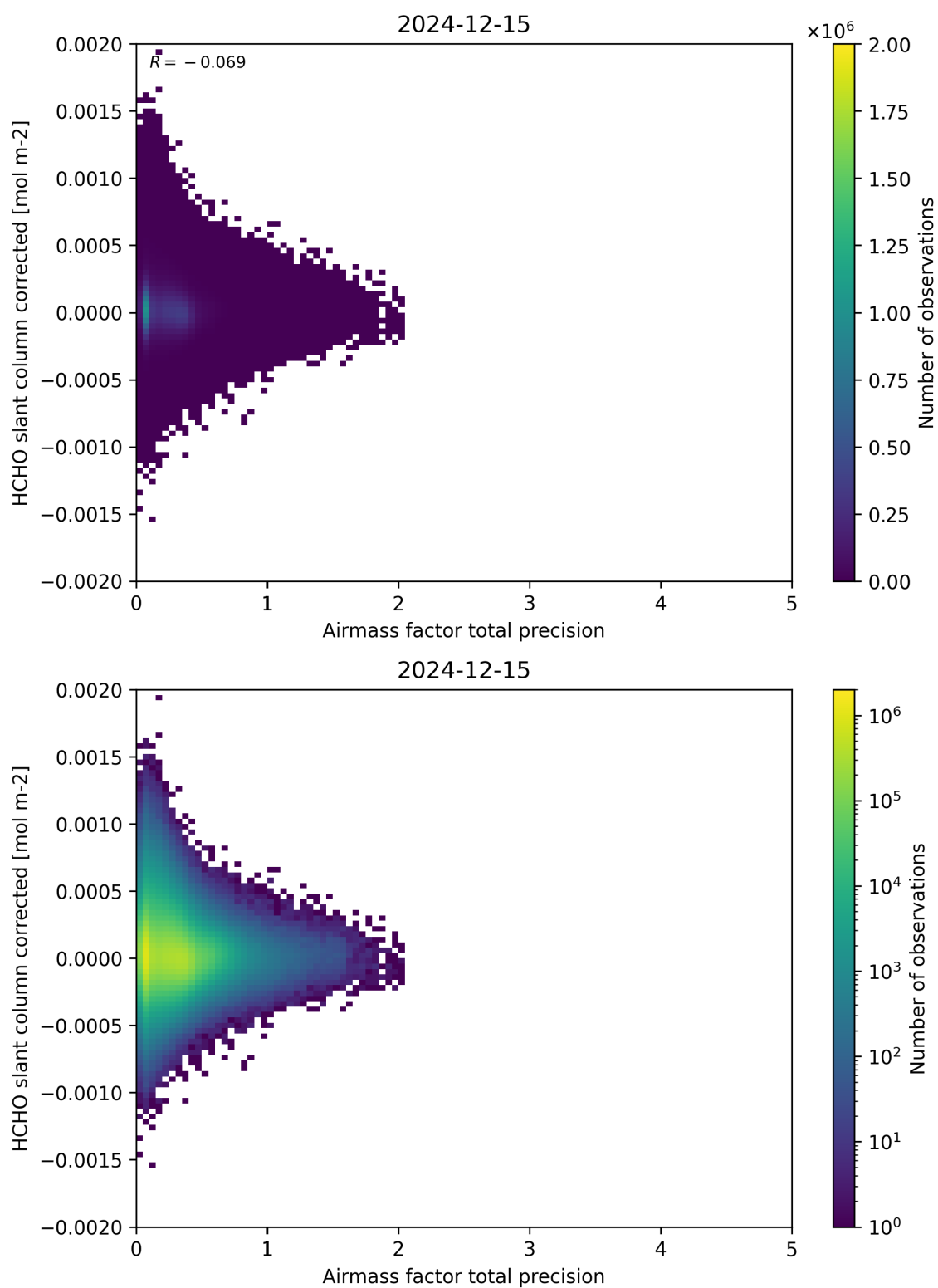
Figure 109: Scatter density plot of “Airmass factor total precision” against “HCHO slant column corrected” for 2024-12-14 to 2024-12-16.
