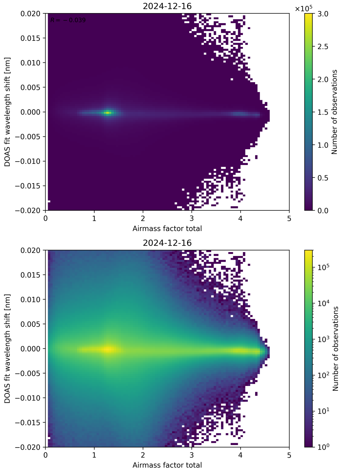
Figure 98: Scatter density plot of “Airmass factor total” against “DOAS fit wavelength shift” for 2024-12-16 to 2024-12-17.
