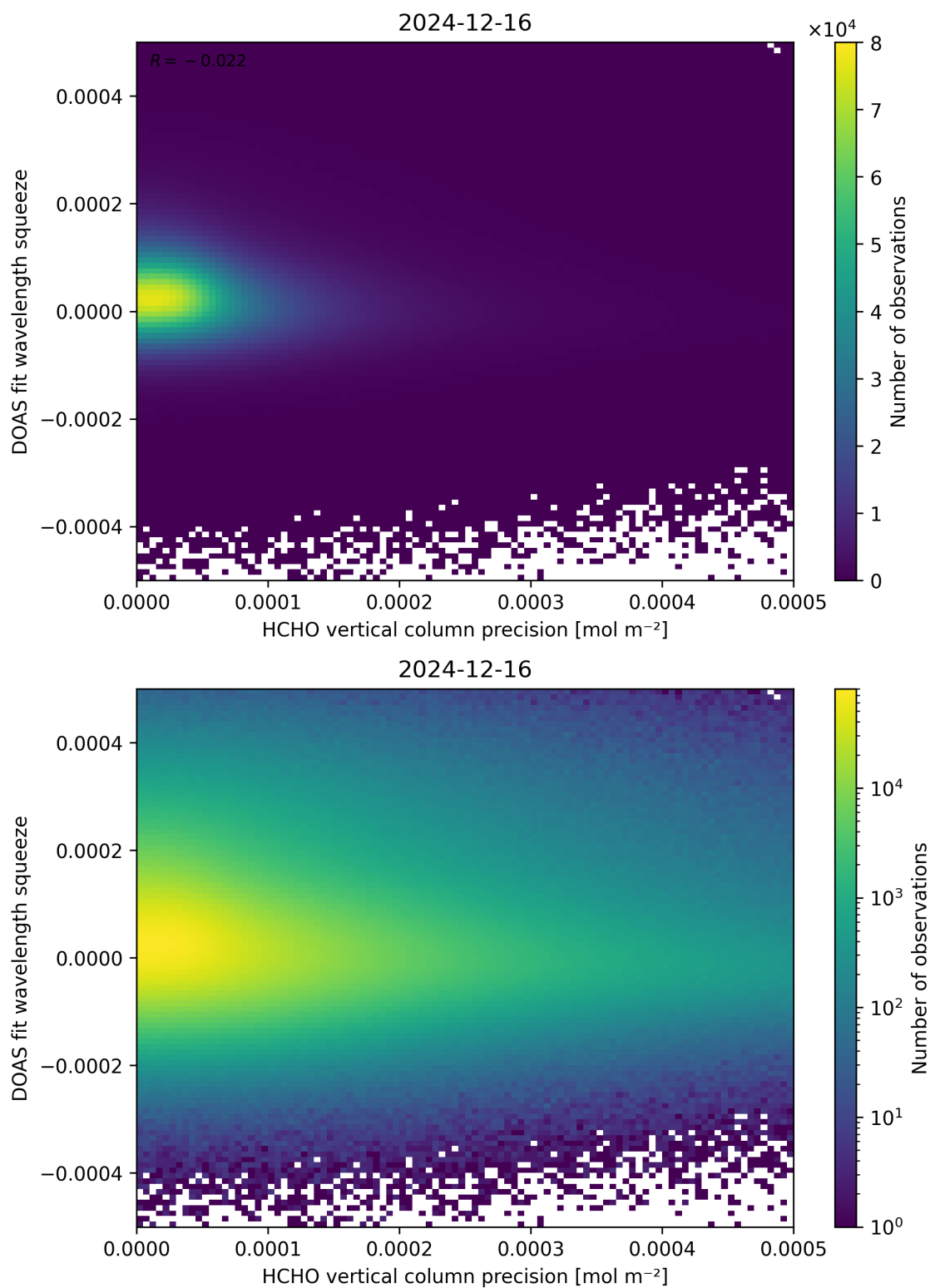
Figure 138: Scatter density plot of “HCHO vertical column precision” against “DOAS fit wavelength squeeze” for 2024-12-16 to 2024-12-17.
