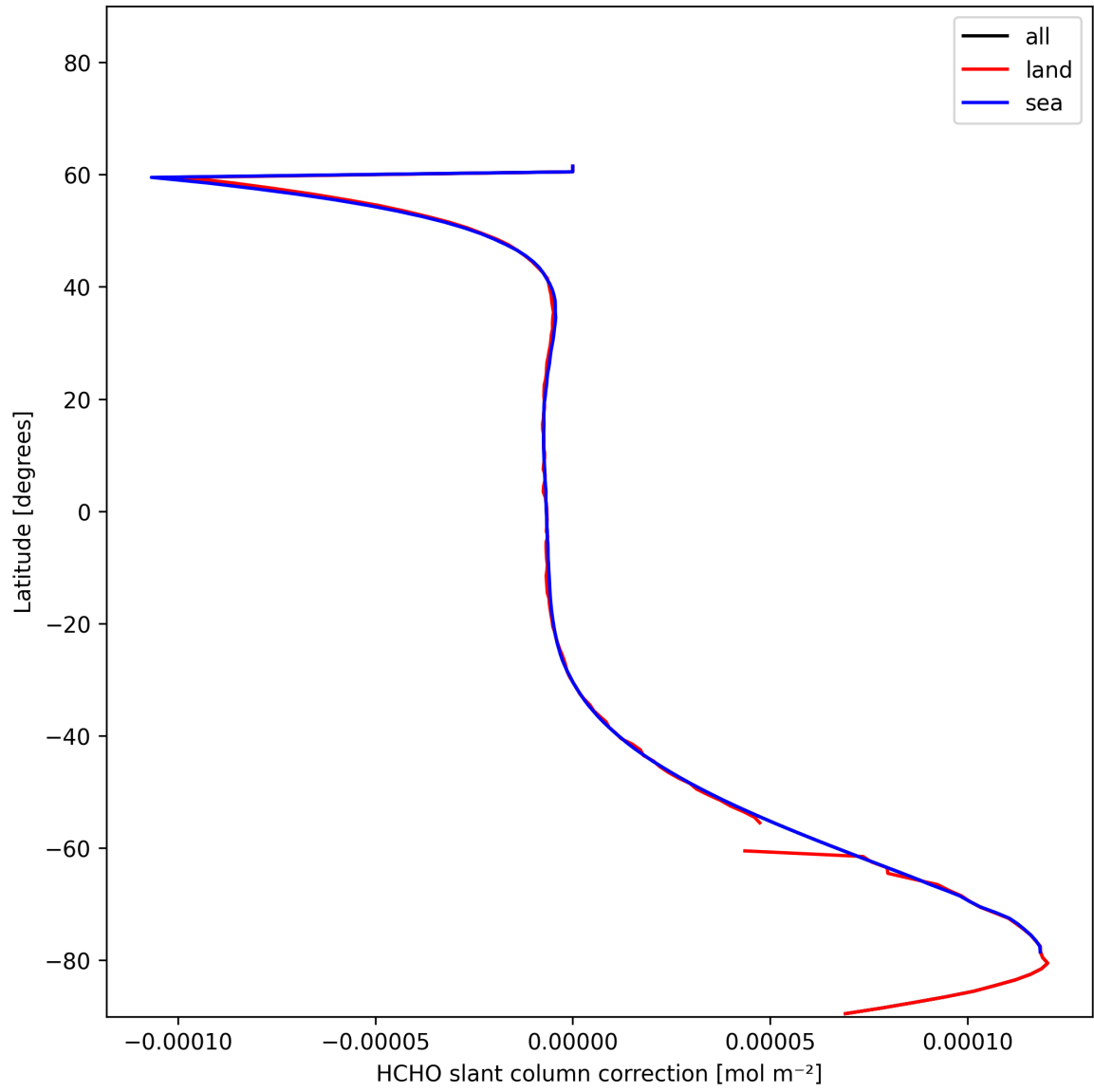
Figure 33: Zonal average of "HCHO slant column correction" for 2024-12-16 to 2024-12-17.
