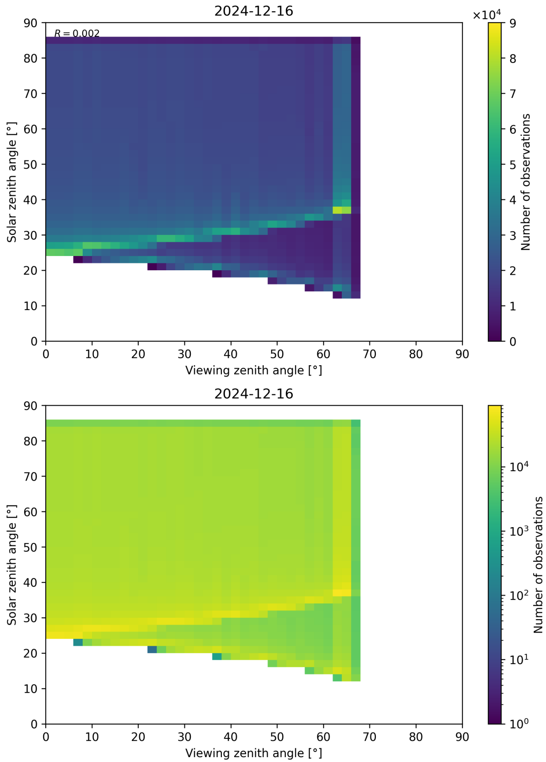
Figure 197: Scatter density plot of “Viewing zenith angle” against “Solar zenith angle” for 2024-12-16 to 2024-12-17.
