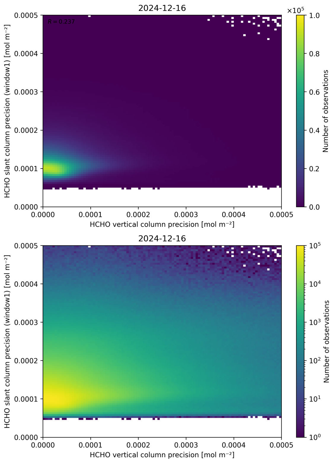
Figure 143: Scatter density plot of “HCHO vertical column precision” against “HCHO slant column precision (window1)” for 2024-12-16 to 2024-12-17.
