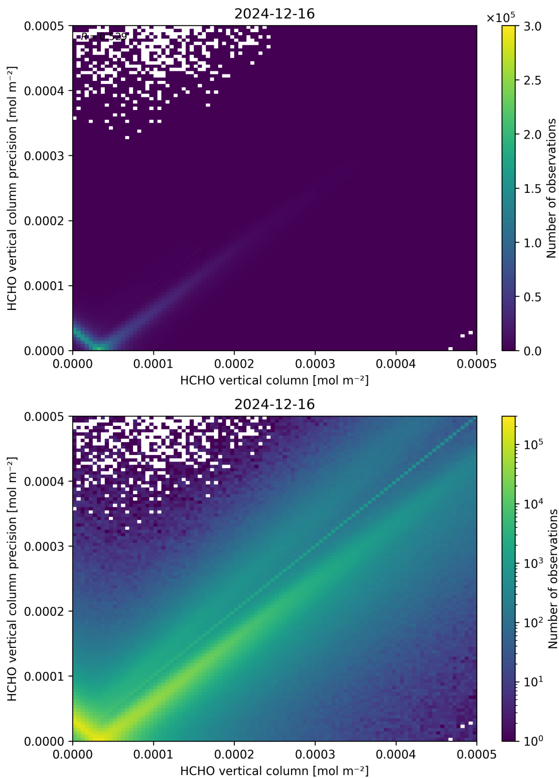
Figure 134: Scatter density plot of “HCHO vertical column” against “HCHO vertical column precision” for 2024-12-16 to 2024-12-17.
