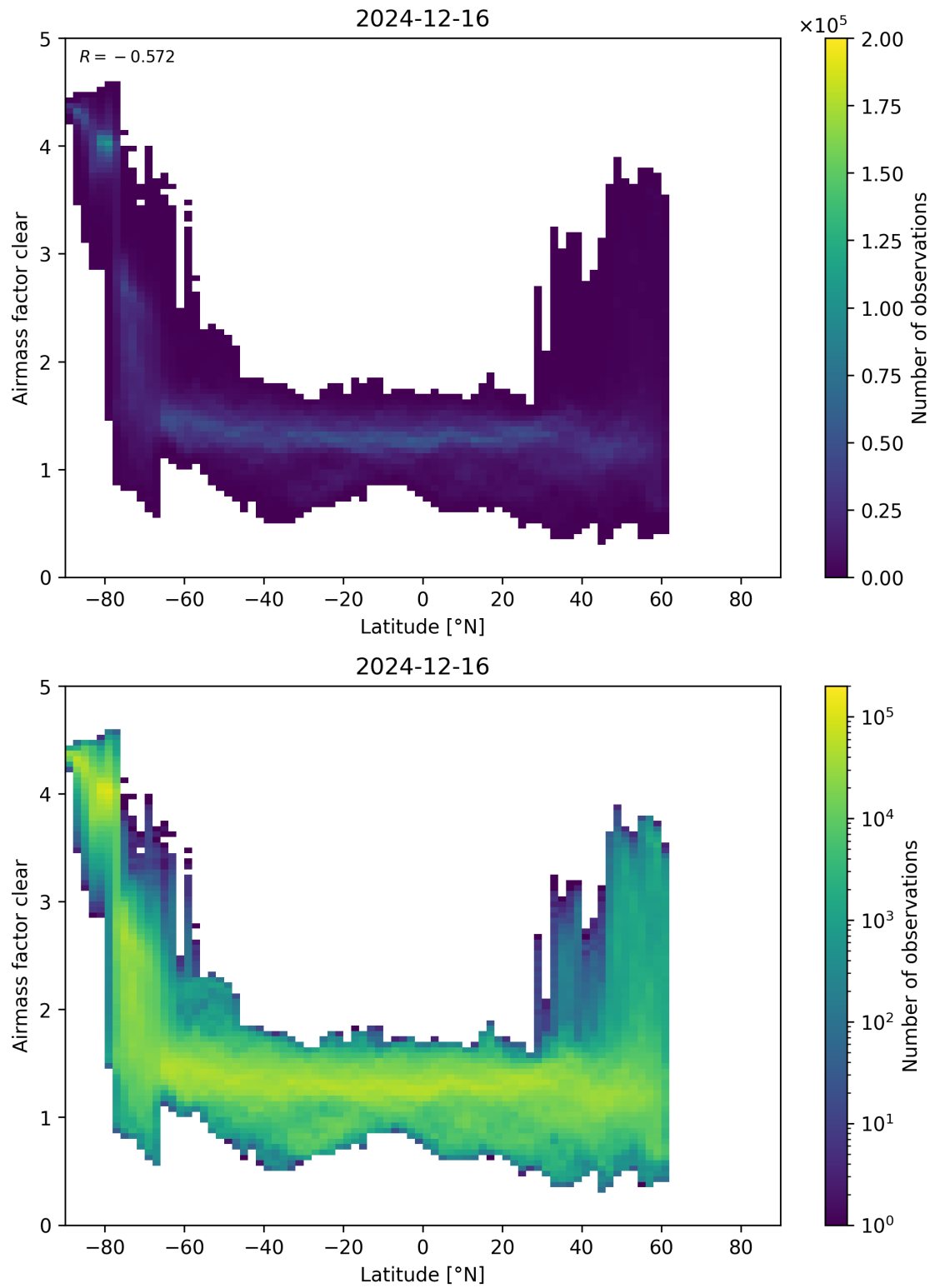
Figure 156: Scatter density plot of “Latitude” against “Airmass factor clear” for 2024-12-16 to 2024-12-17.
