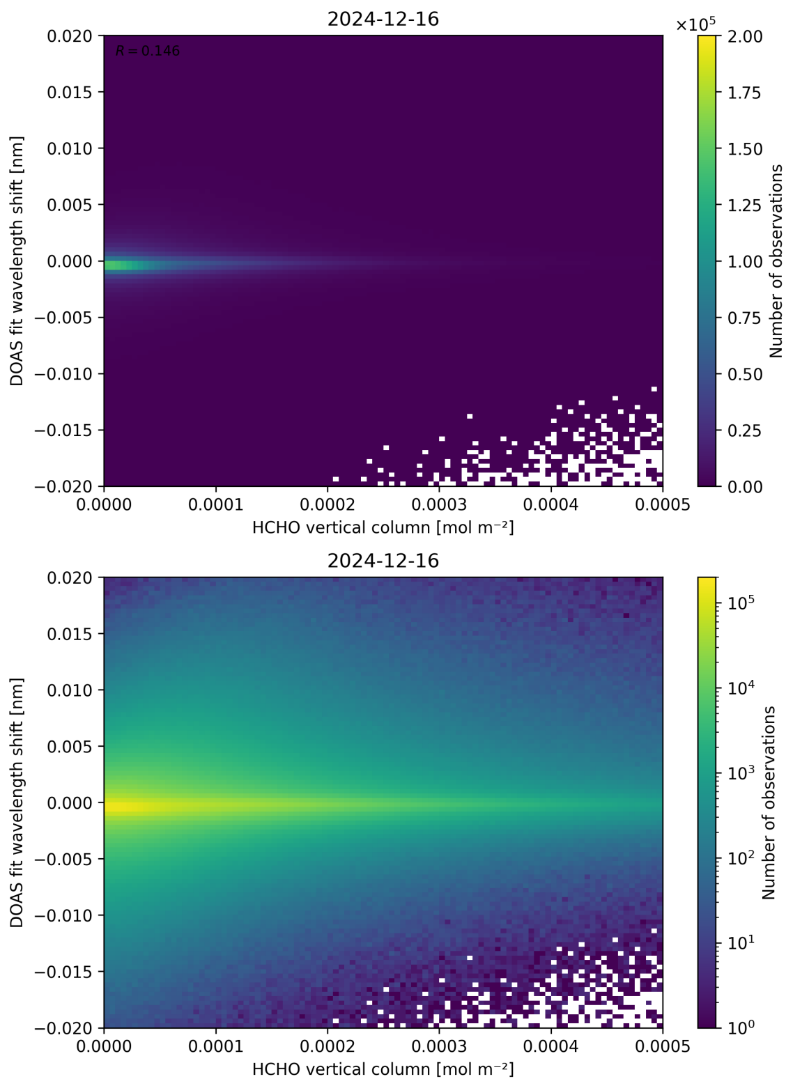
Figure 124: Scatter density plot of “HCHO vertical column” against “DOAS fit wavelength shift” for 2024-12-16 to 2024-12-17.
