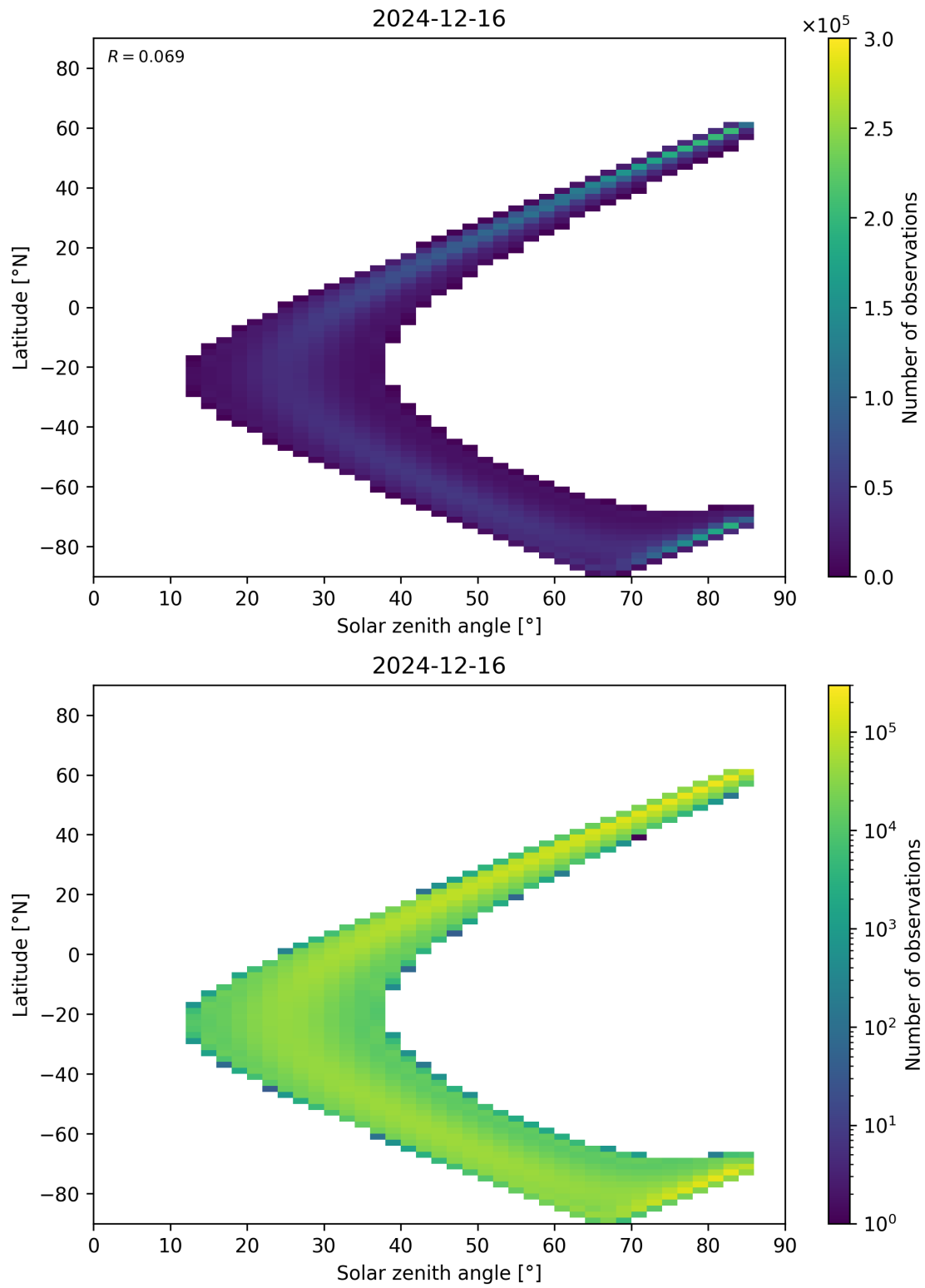
Figure 181: Scatter density plot of “Solar zenith angle” against “Latitude” for 2024-12-16 to 2024-12-17.
