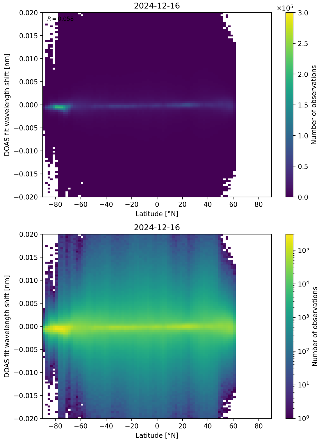
Figure 154: Scatter density plot of “Latitude” against “DOAS fit wavelength shift” for 2024-12-16 to 2024-12-17.
