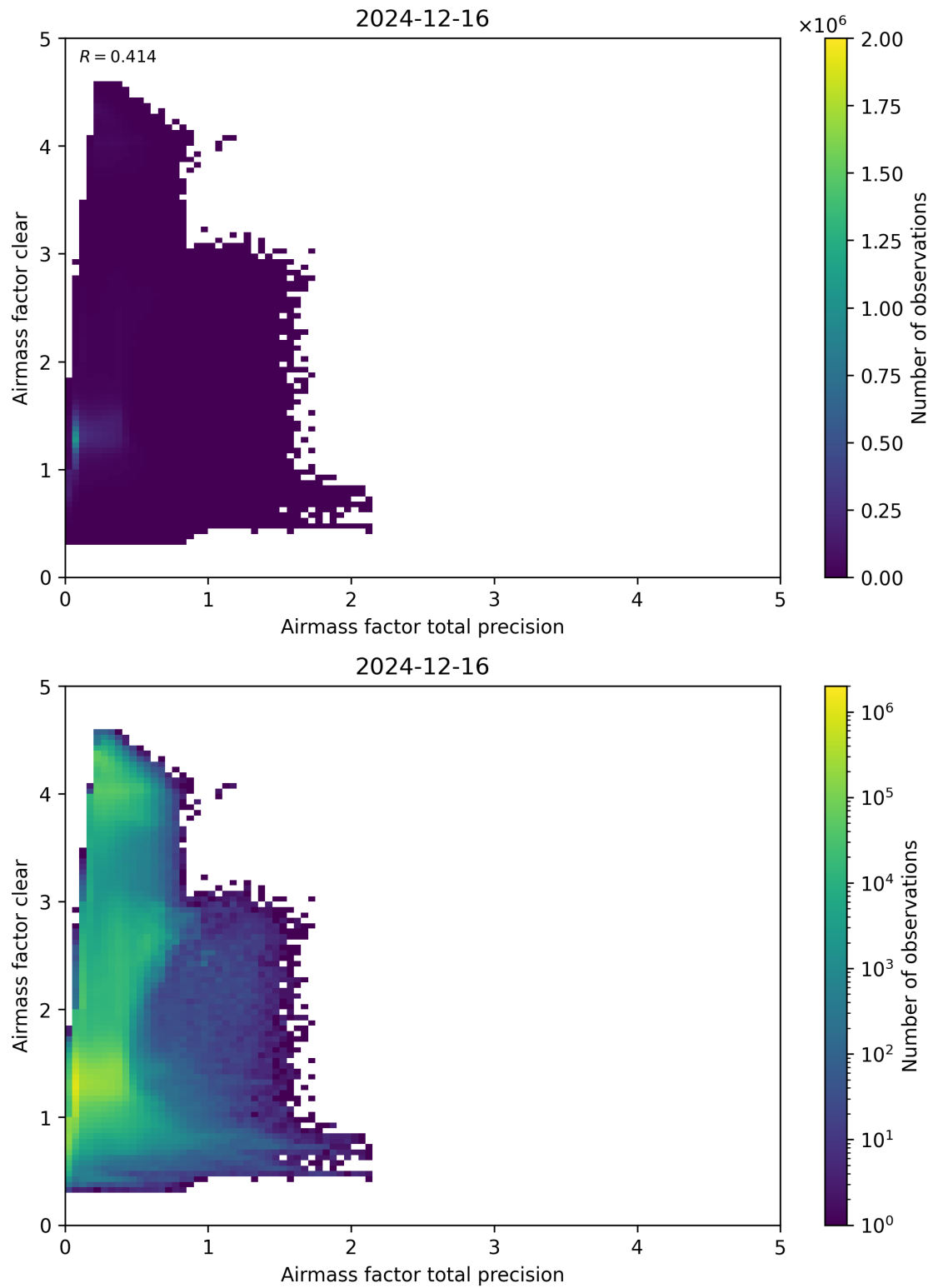
Figure 108: Scatter density plot of “Airmass factor total precision” against “Airmass factor clear” for 2024-12-16 to 2024-12-17.
