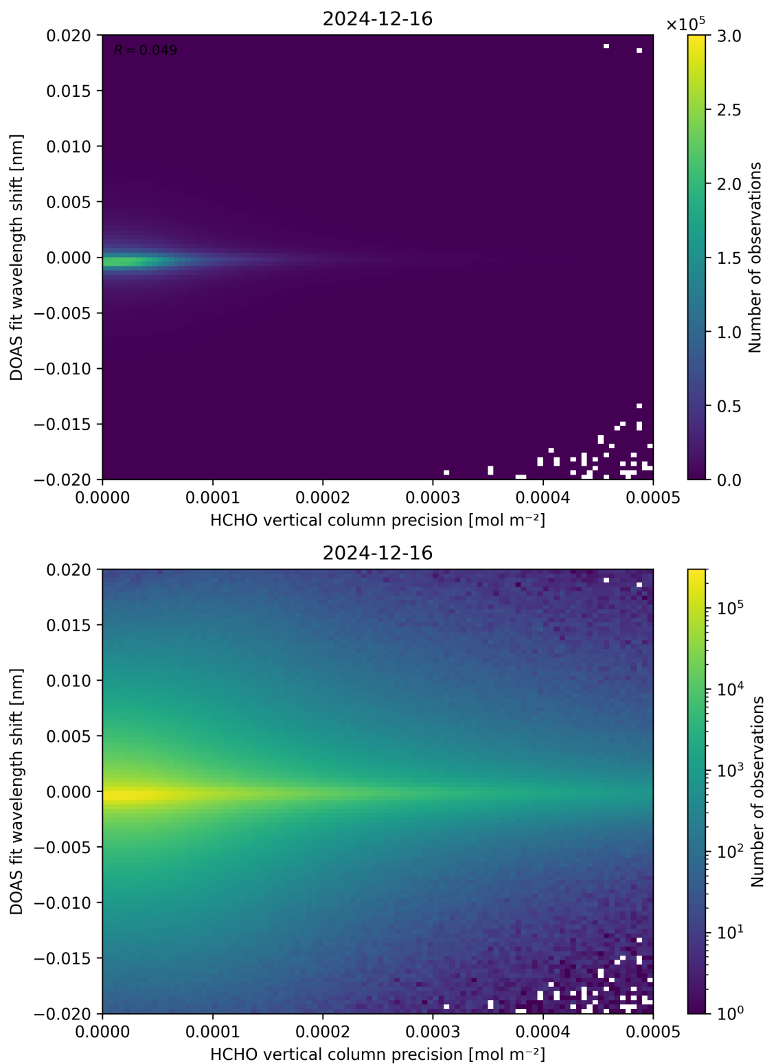
Figure 137: Scatter density plot of “HCHO vertical column precision” against “DOAS fit wavelength shift” for 2024-12-16 to 2024-12-17.
