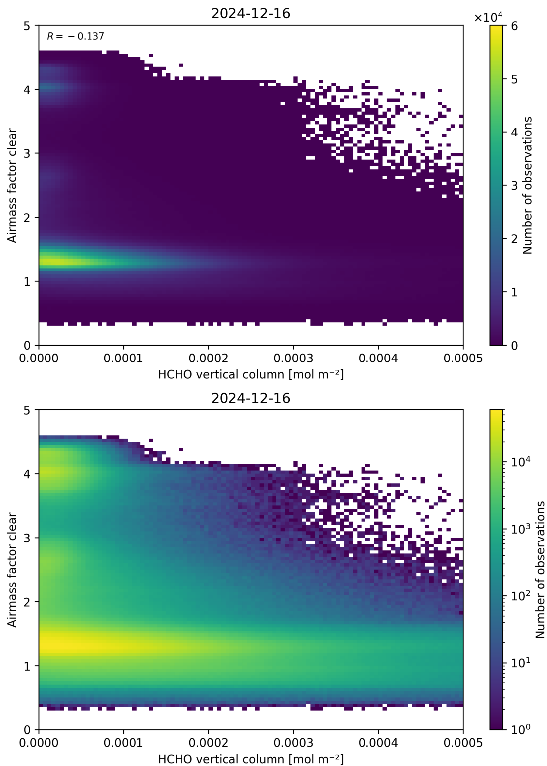
Figure 126: Scatter density plot of “HCHO vertical column” against “Airmass factor clear” for 2024-12-16 to 2024-12-17.
