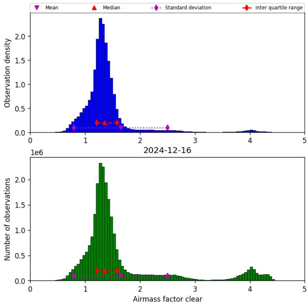
Figure 42: Histogram of “Airmass factor clear” for 2024-12-16 to 2024-12-17
