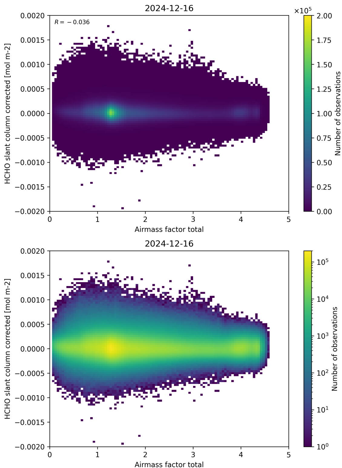
Figure 101: Scatter density plot of “Airmass factor total” against “HCHO slant column corrected” for 2024-12-16 to 2024-12-17.
