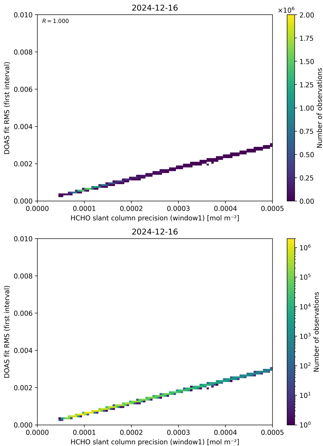
Figure 88: Scatter density plot of “HCHO slant column precision (window1)” against “DOAS fit RMS (first interval)” for 2024-12-16 to 2024-12-17.
