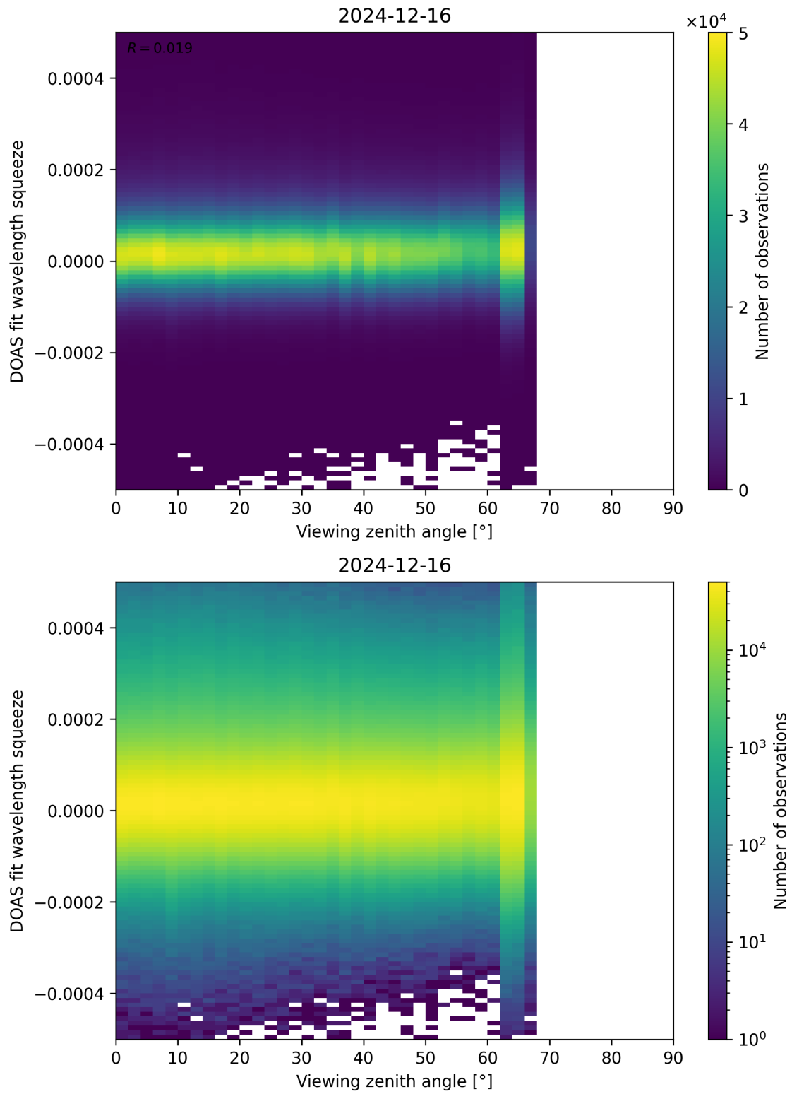
Figure 184: Scatter density plot of “Viewing zenith angle” against “DOAS fit wavelength squeeze” for 2024-12-16 to 2024-12-17.
