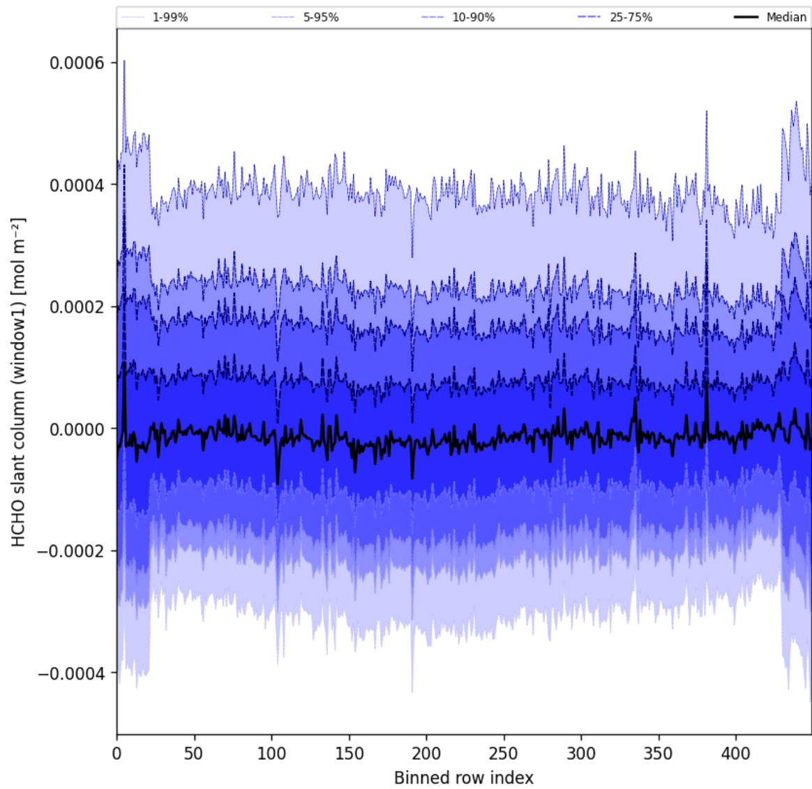
Figure 52: Along track statistics of “HCHO slant column (window1)” for 2024-12-16 to 2024-12-17
