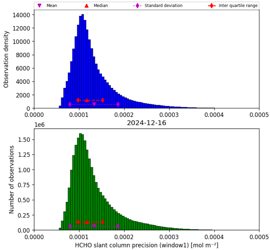
Figure 39: Histogram of “HCHO slant column precision (window1)” for 2024-12-16 to 2024-12-17
