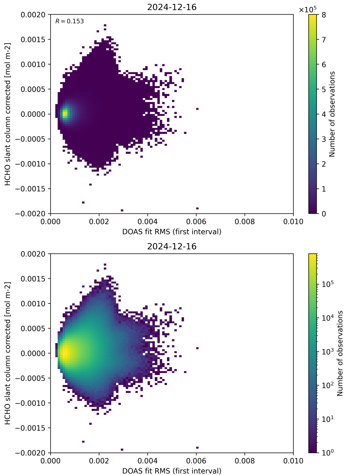
Figure 62: Scatter density plot of “DOAS fit RMS (first interval)” against “HCHO slant column corrected” for 2024-12-16 to 2024-12-17.
