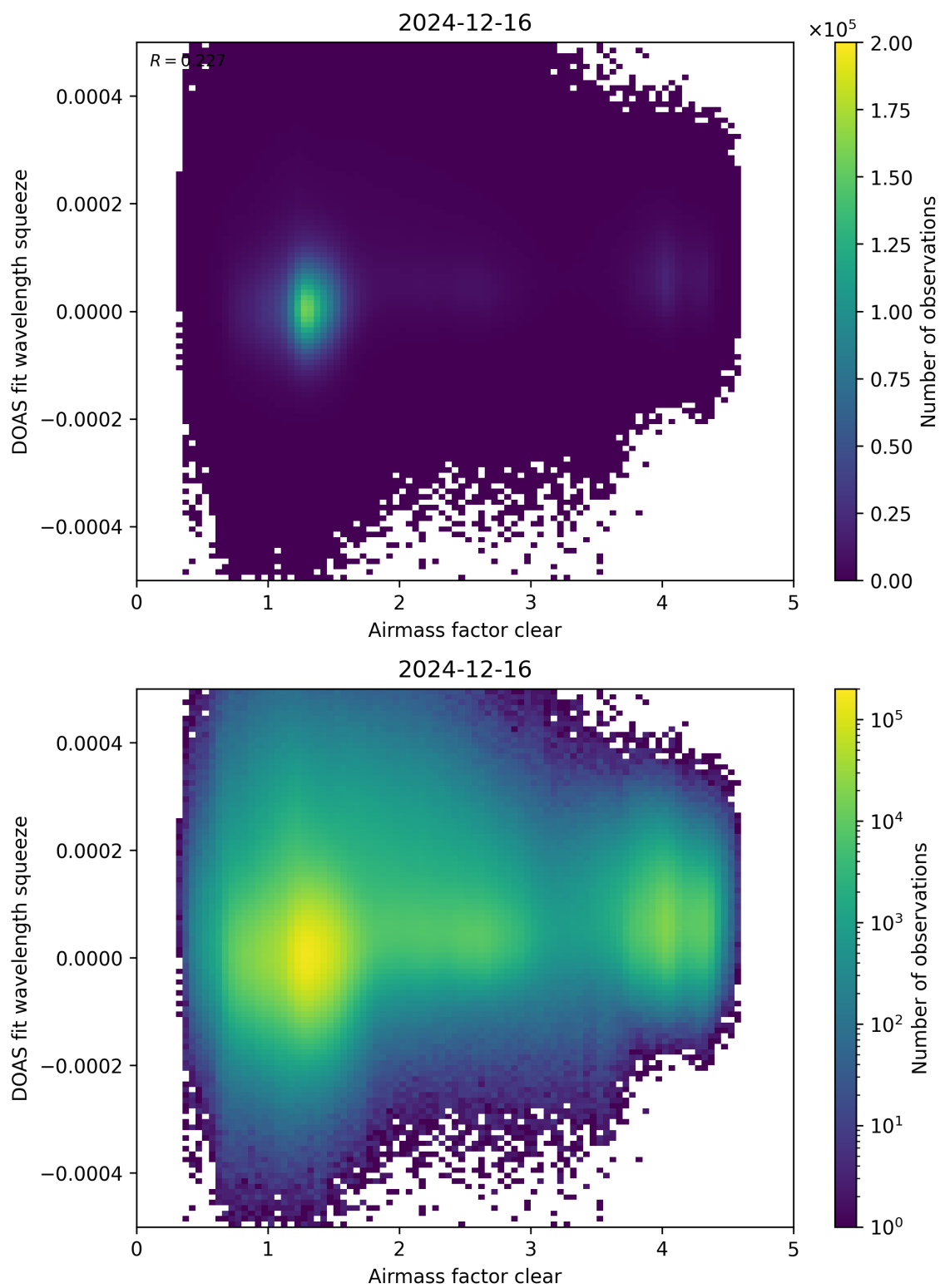
Figure 73: Scatter density plot of “Airmass factor clear” against “DOAS fit wavelength squeeze” for 2024-12-16 to 2024-12-17.
