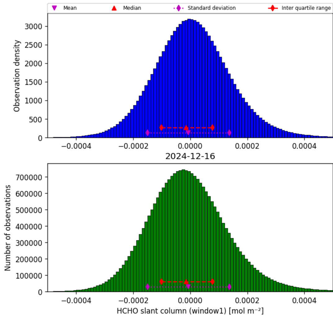
Figure 38: Histogram of “HCHO slant column (window1)” for 2024-12-16 to 2024-12-17
