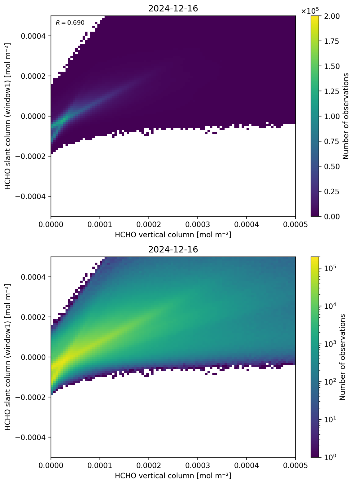
Figure 129: Scatter density plot of “HCHO vertical column” against “HCHO slant column (window1)” for 2024-12-16 to 2024-12-17.
