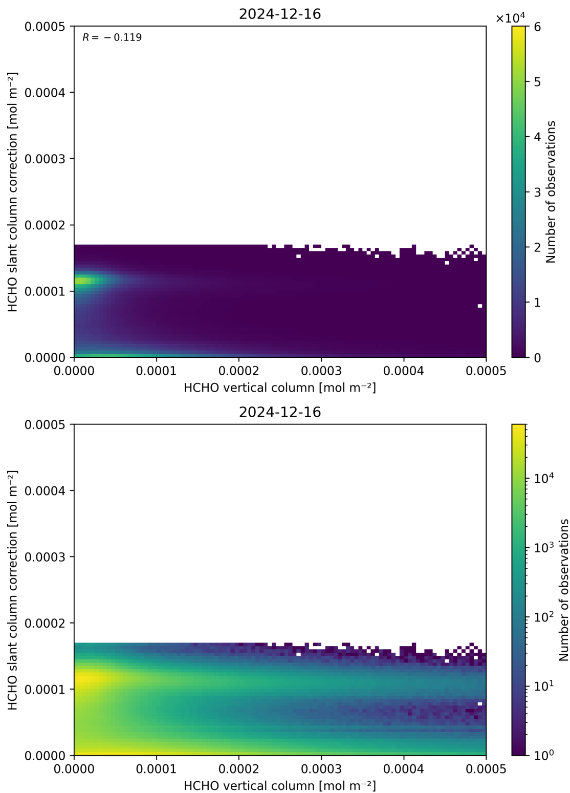
Figure 128: Scatter density plot of “HCHO vertical column” against “HCHO slant column correction” for 2024-12-16 to 2024-12-17.
