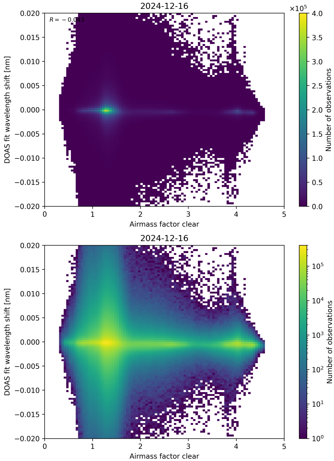
Figure 72: Scatter density plot of “Airmass factor clear” against “DOAS fit wavelength shift” for 2024-12-16 to 2024-12-17.
