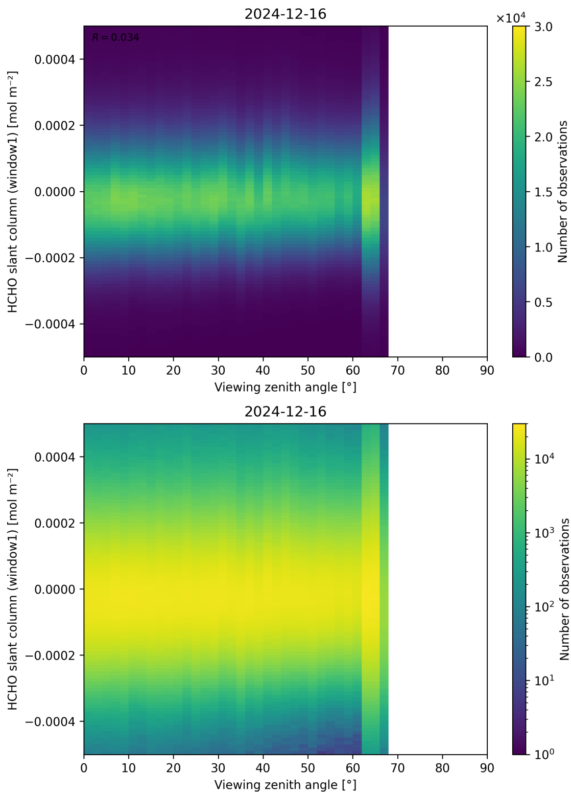
Figure 188: Scatter density plot of “Viewing zenith angle” against “HCHO slant column (window1)” for 2024-12-16 to 2024-12-17.
