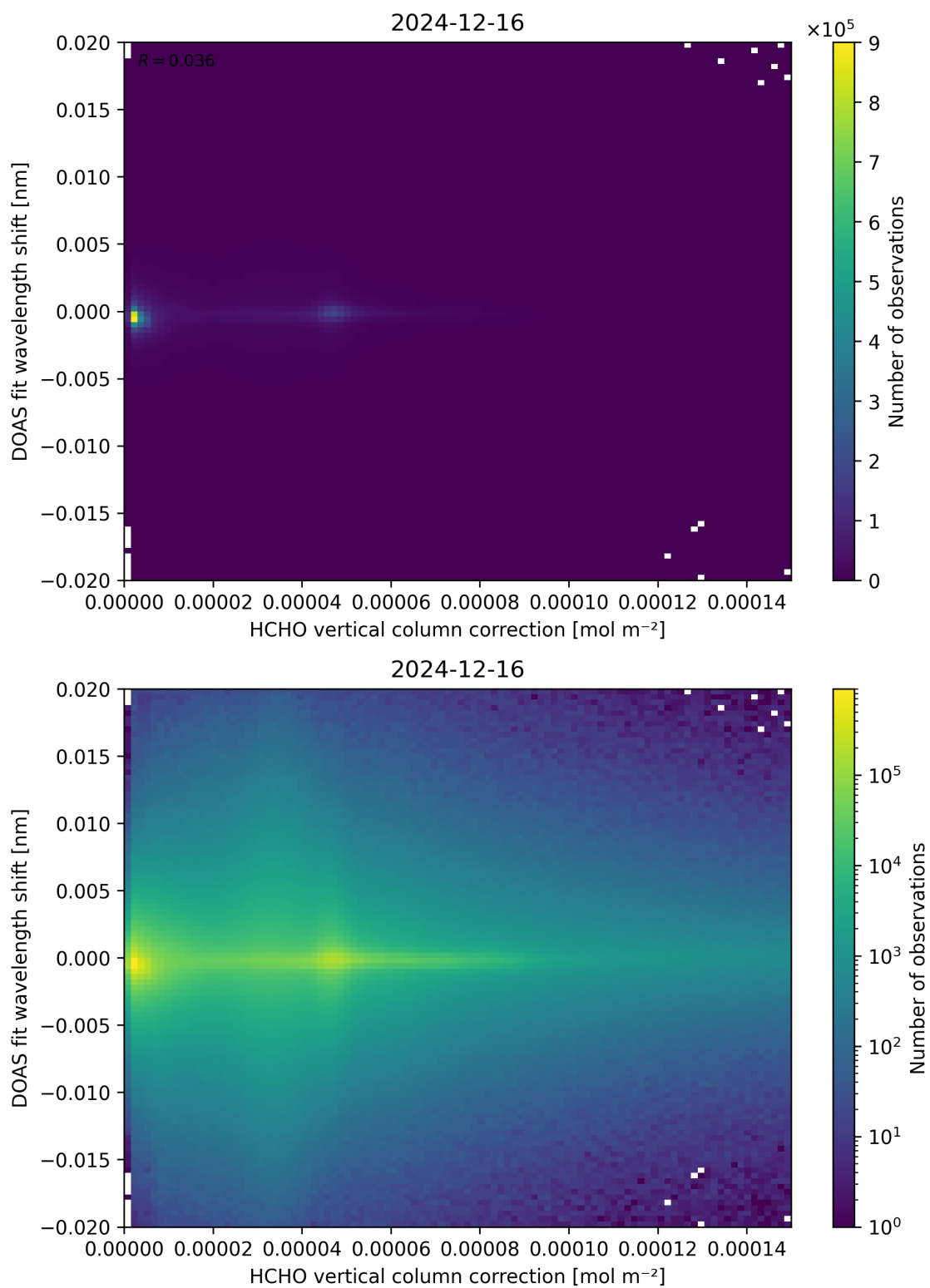
Figure 113: Scatter density plot of “HCHO vertical column correction” against “DOAS fit wavelength shift” for 2024-12-16 to 2024-12-17.
