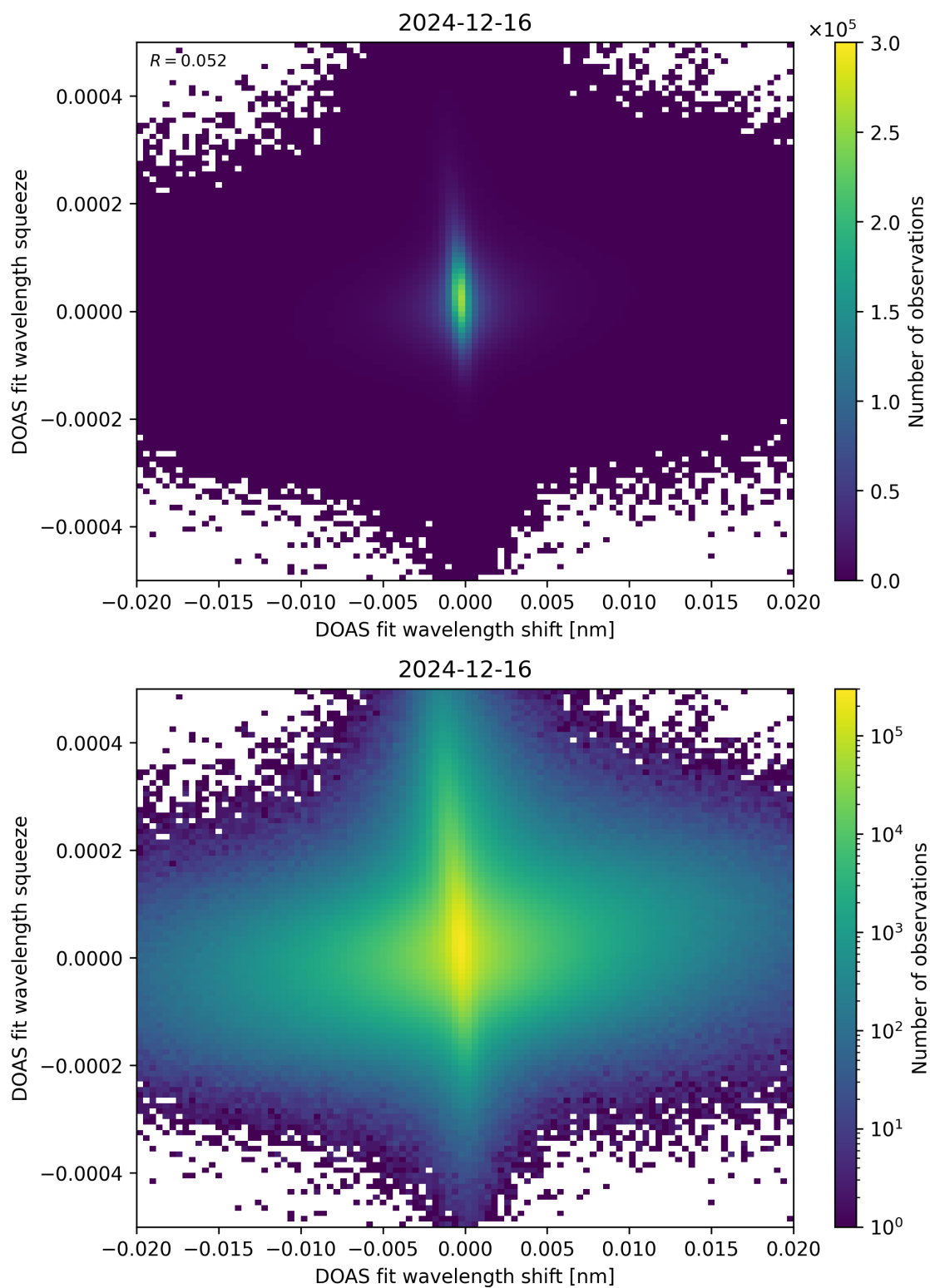
Figure 65: Scatter density plot of “DOAS fit wavelength shift” against “DOAS fit wavelength squeeze” for 2024-12-16 to 2024-12-17.
