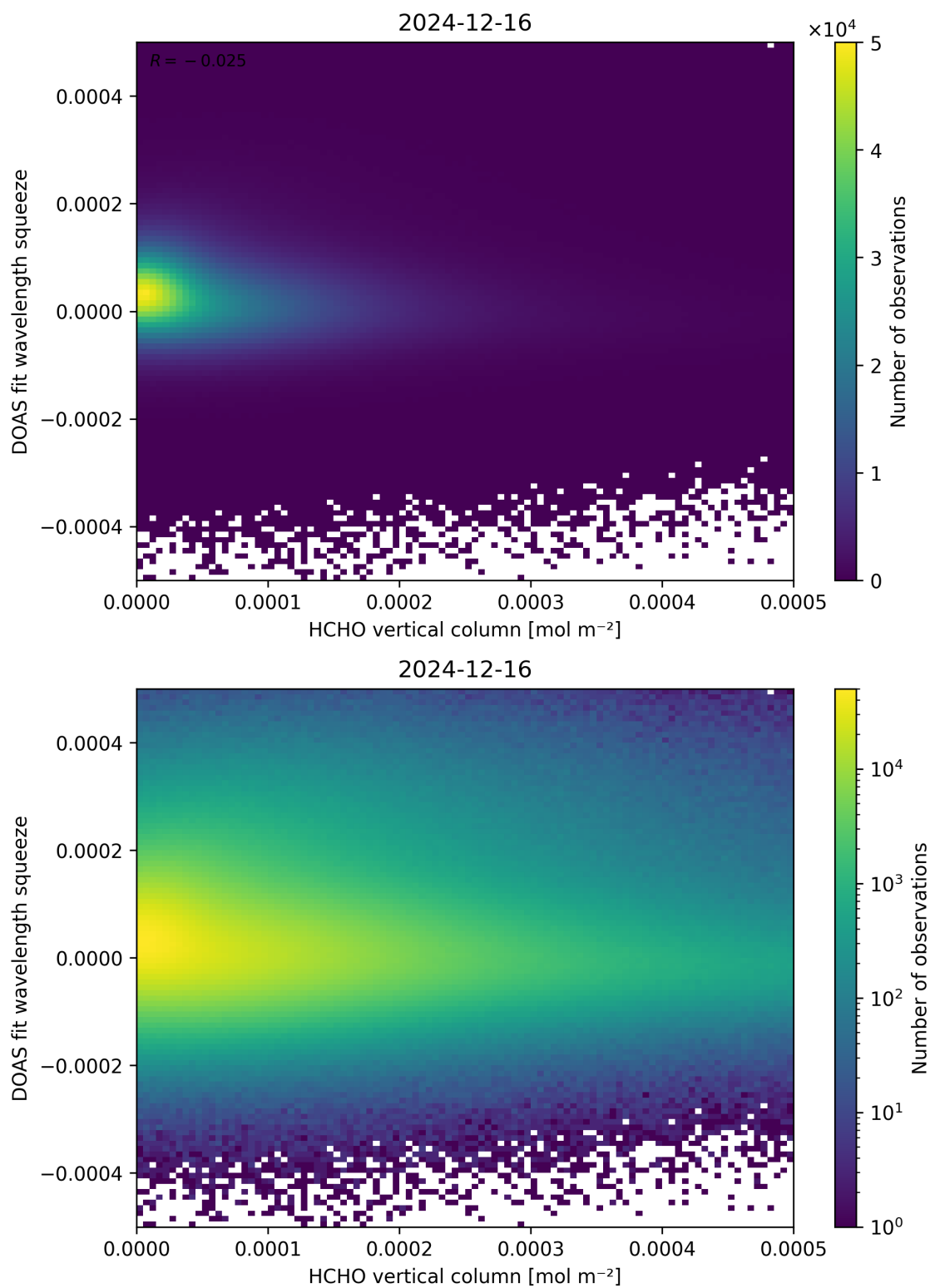
Figure 125: Scatter density plot of “HCHO vertical column” against “DOAS fit wavelength squeeze” for 2024-12-16 to 2024-12-17.
