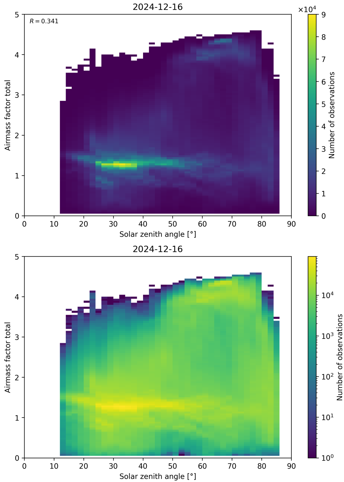
Figure 175: Scatter density plot of “Solar zenith angle” against “Airmass factor total” for 2024-12-16 to 2024-12-17.
