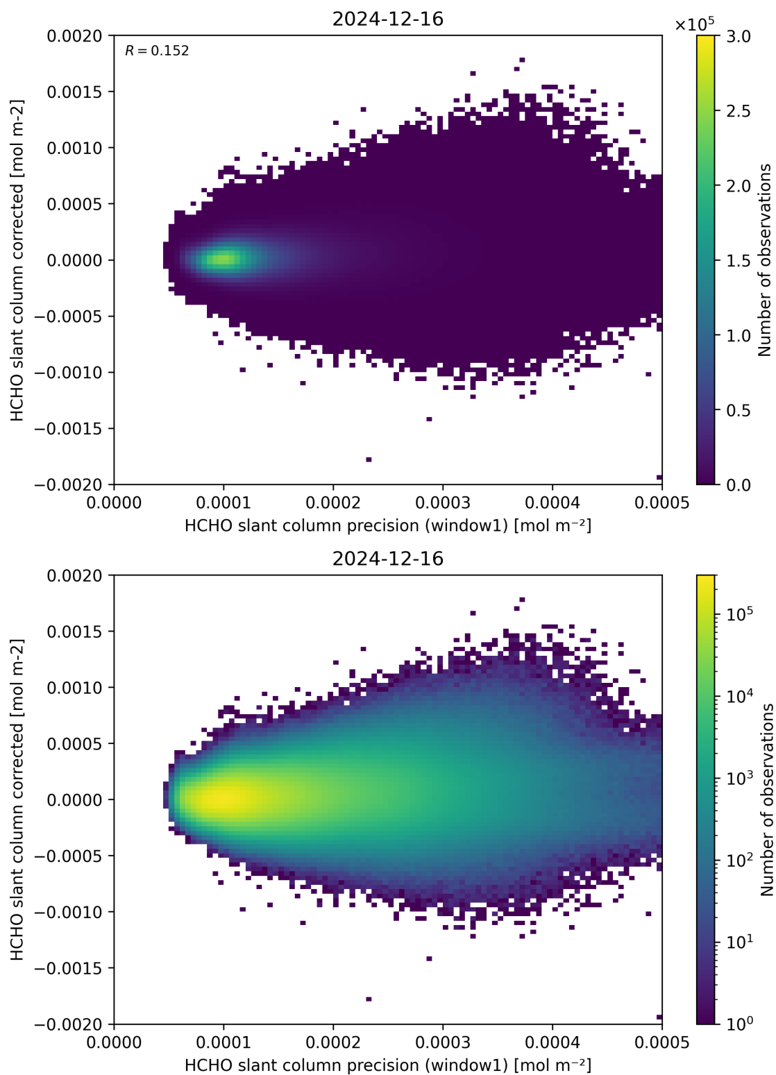
Figure 92: Scatter density plot of “HCHO slant column precision (window1)” against “HCHO slant column corrected” for 2024-12-16 to 2024-12-17.
