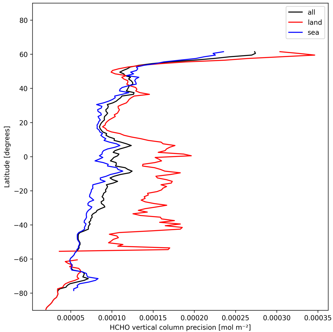
Figure 22: Zonal average of “HCHO vertical column precision” for 2024-12-16 to 2024-12-17.
