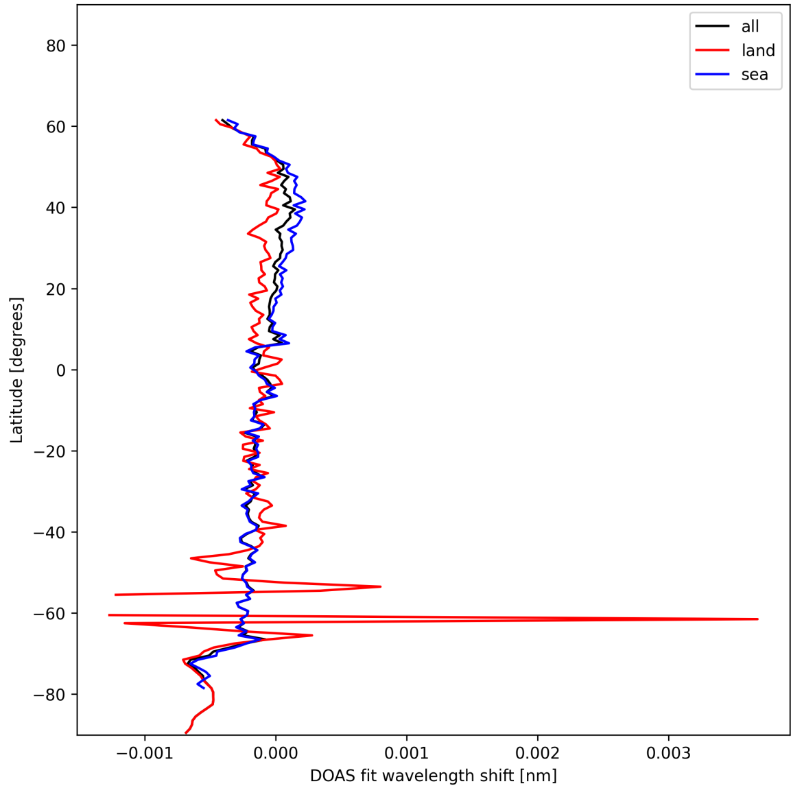
Figure 30: Zonal average of “DOAS fit wavelength shift” for 2024-12-16 to 2024-12-17.
