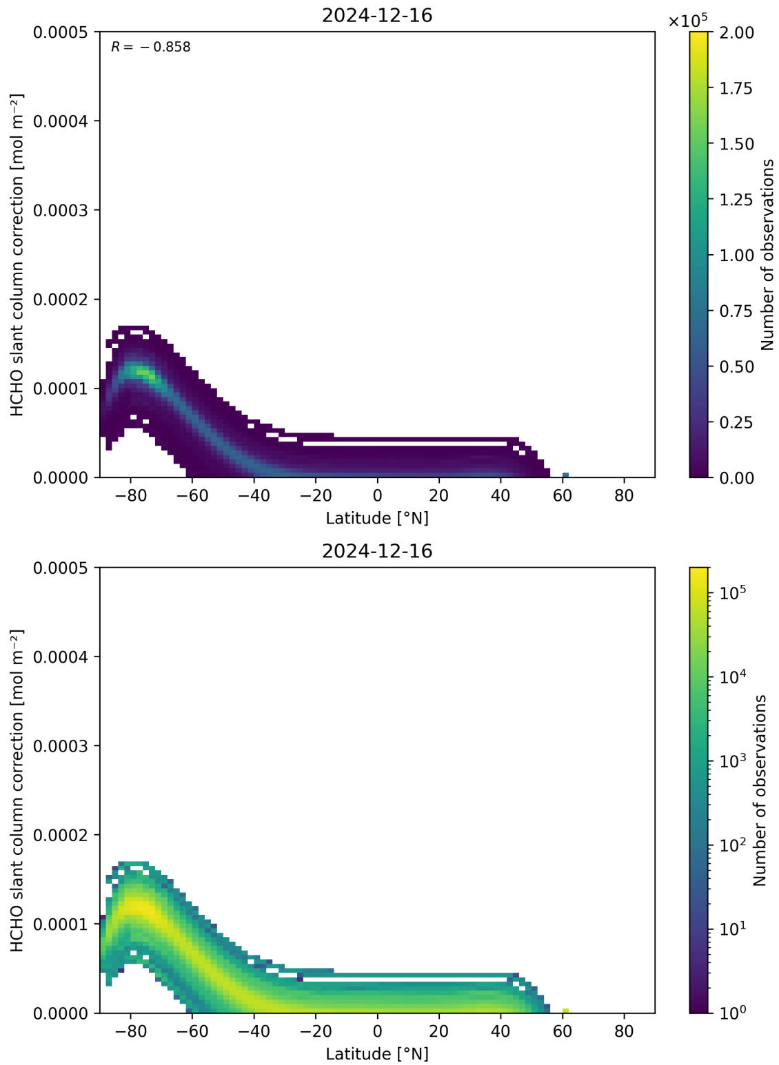
Figure 158: Scatter density plot of “Latitude” against “HCHO slant column correction” for 2024-12-16 to 2024-12-17.
