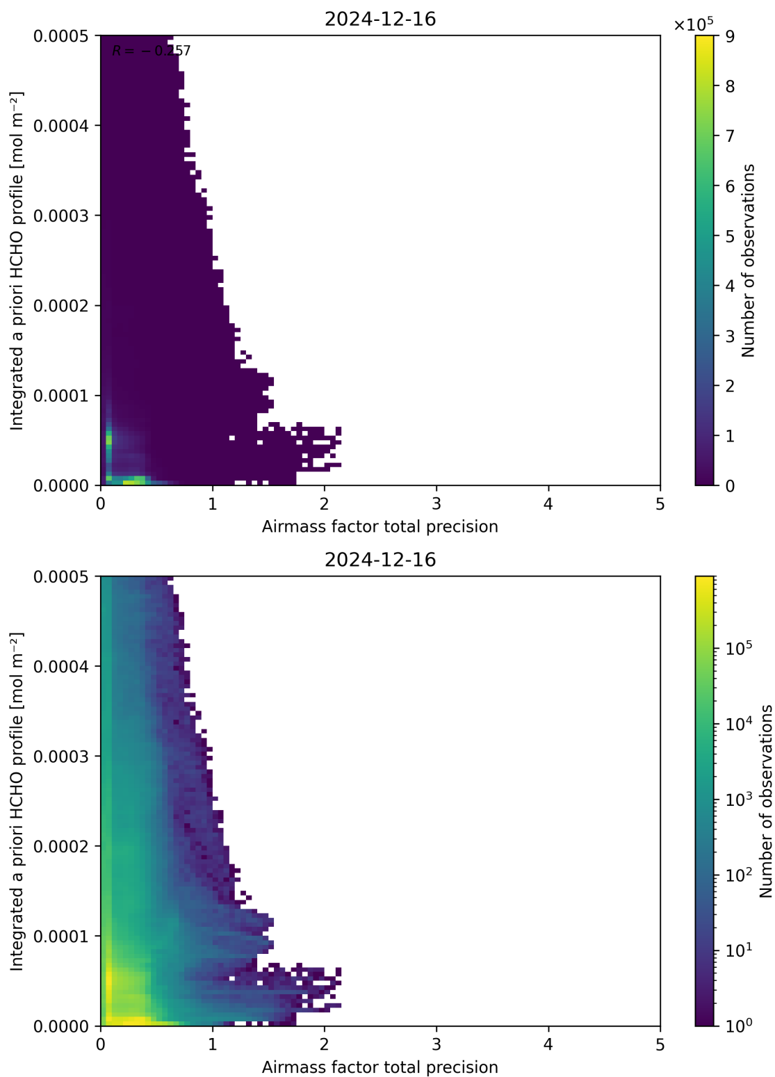
Figure 111: Scatter density plot of “Airmass factor total precision” against “Integrated a priori HCHO profile” for 2024-12-16 to 2024-12-17.
