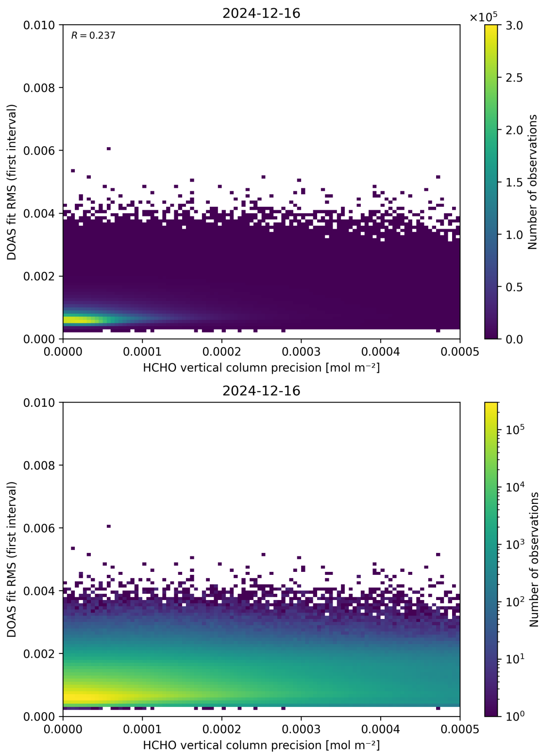
Figure 136: Scatter density plot of “HCHO vertical column precision” against “DOAS fit RMS (first interval)” for 2024-12-16 to 2024-12-17.
