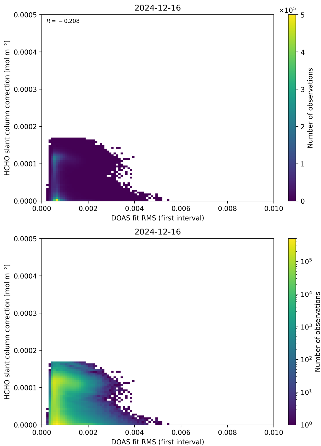
Figure 63: Scatter density plot of “DOAS fit RMS (first interval)” against “HCHO slant column correction” for 2024-12-16 to 2024-12-17.
