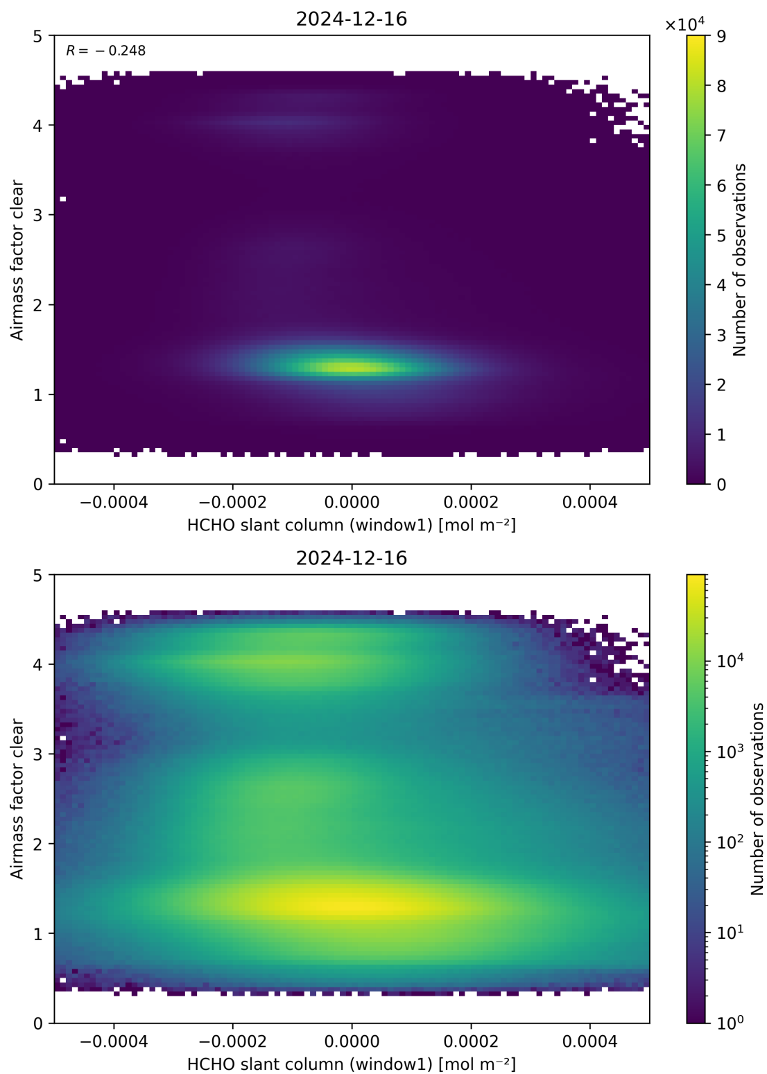
Figure 81: Scatter density plot of “HCHO slant column (window1)” against “Airmass factor clear” for 2024-12-16 to 2024-12-17.
