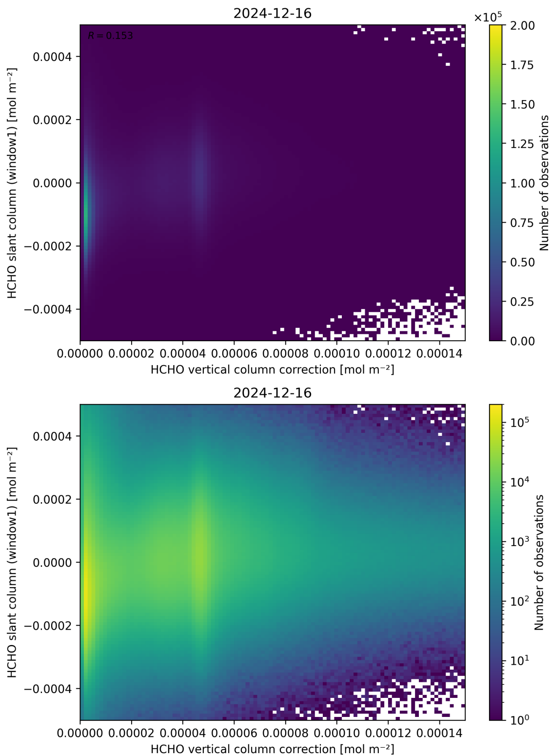
Figure 118: Scatter density plot of “HCHO vertical column correction” against “HCHO slant column (window1)” for 2024-12-16 to 2024-12-17.
