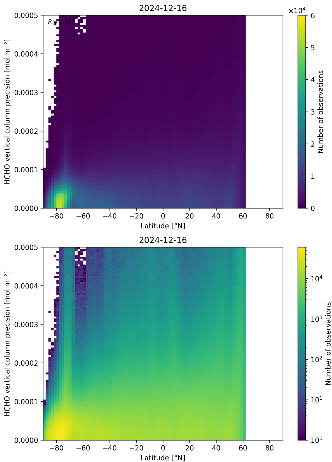
Figure 165: Scatter density plot of “Latitude” against “HCHO vertical column precision” for 2024-12-16 to 2024-12-17.
