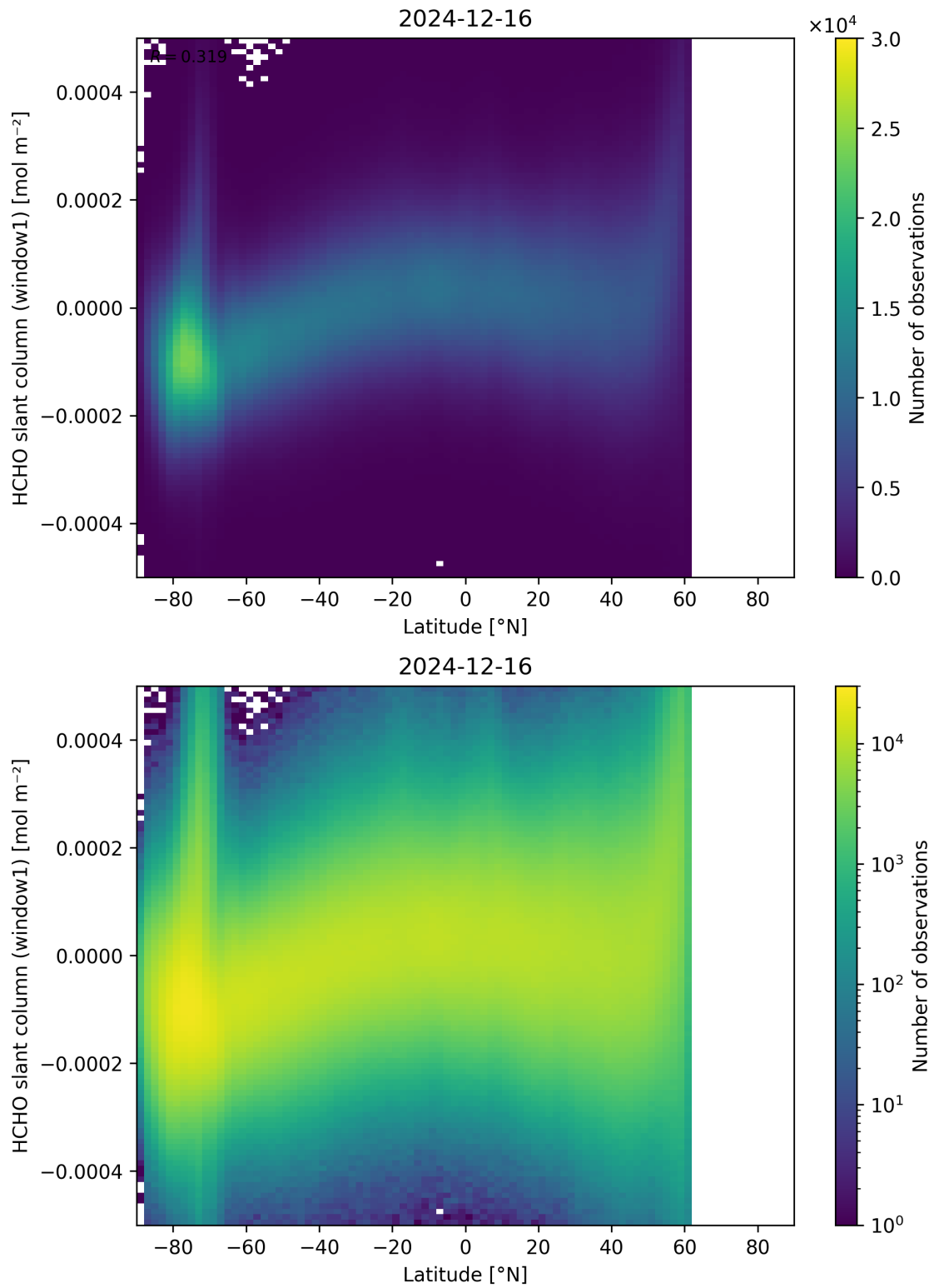
Figure 159: Scatter density plot of “Latitude” against “HCHO slant column (window1)” for 2024-12-16 to 2024-12-17.
