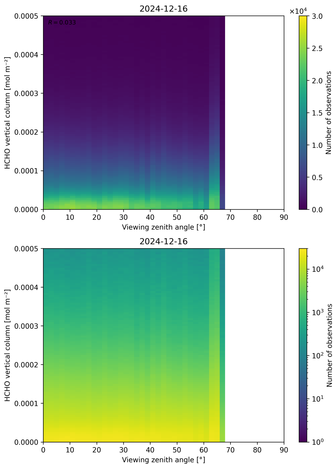
Figure 192: Scatter density plot of “Viewing zenith angle” against “HCHO vertical column” for 2024-12-16 to 2024-12-17.
