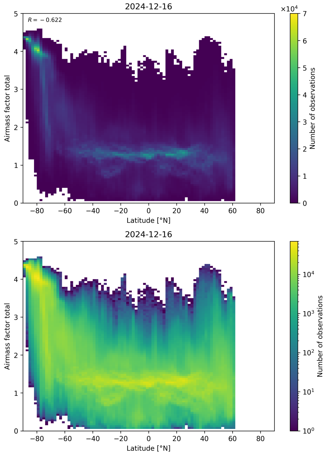
Figure 161: Scatter density plot of “Latitude” against “Airmass factor total” for 2024-12-16 to 2024-12-17.
