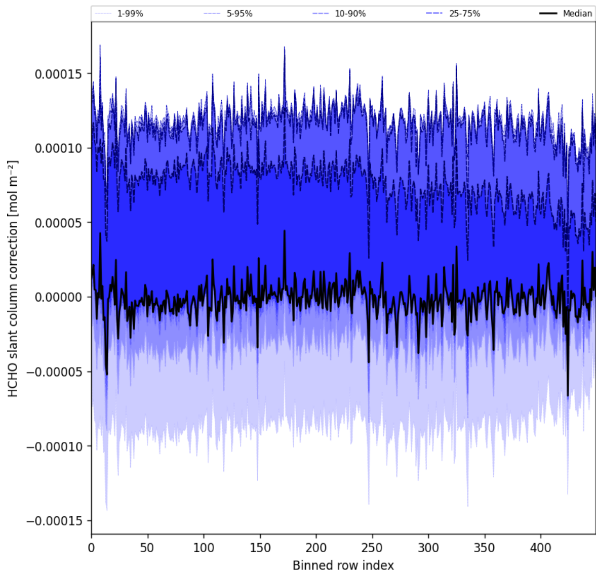
Figure 61: Along track statistics of “HCHO slant column correction” for 2024-12-16 to 2024-12-17
