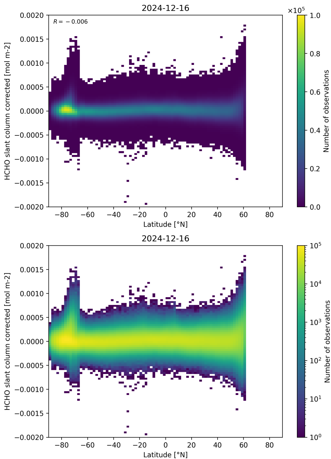
Figure 157: Scatter density plot of “Latitude” against “HCHO slant column corrected” for 2024-12-16 to 2024-12-17.
