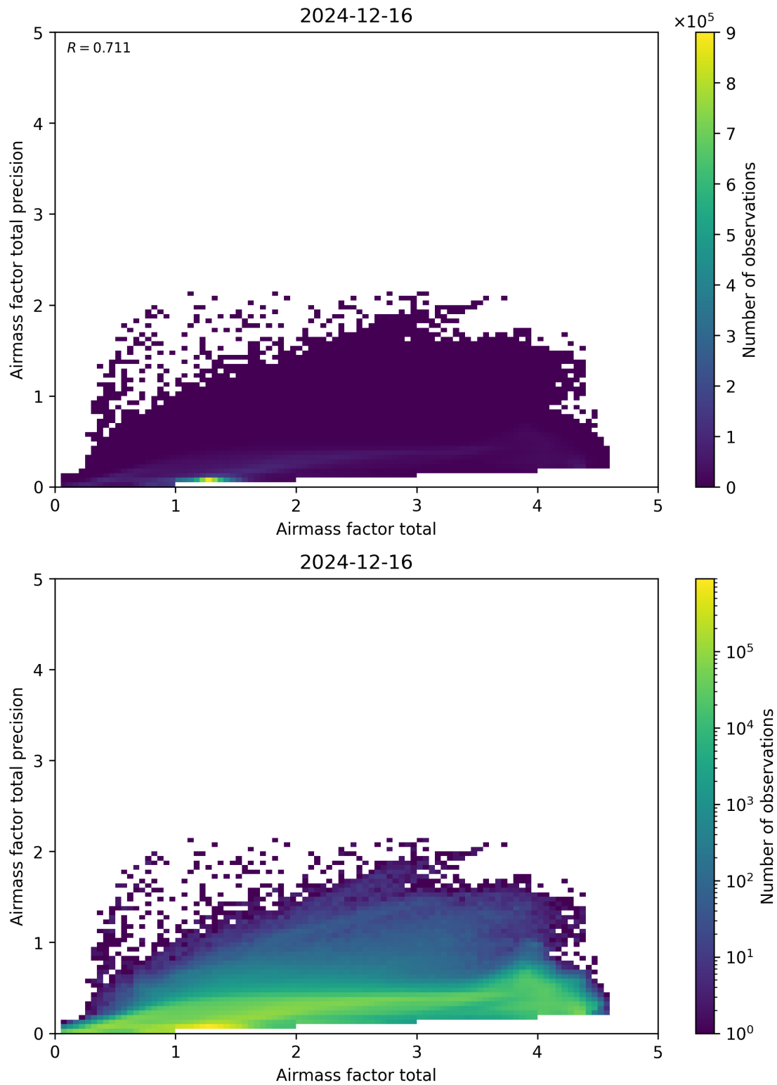
Figure 103: Scatter density plot of “Airmass factor total” against “Airmass factor total precision” for 2024-12-16 to 2024-12-17.
