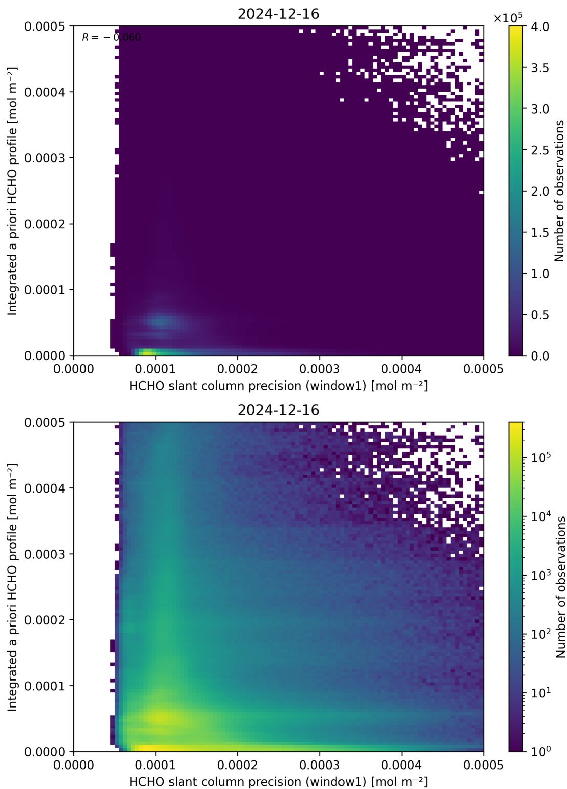
Figure 96: Scatter density plot of “HCHO slant column precision (window1)” against “Integrated a priori HCHO profile” for 2024-12-16 to 2024-12-17.
