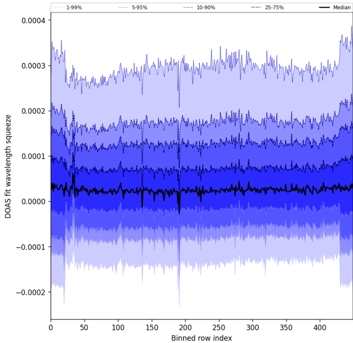
Figure 59: Along track statistics of “DOAS fit wavelength squeeze” for 2024-12-16 to 2024-12-17
