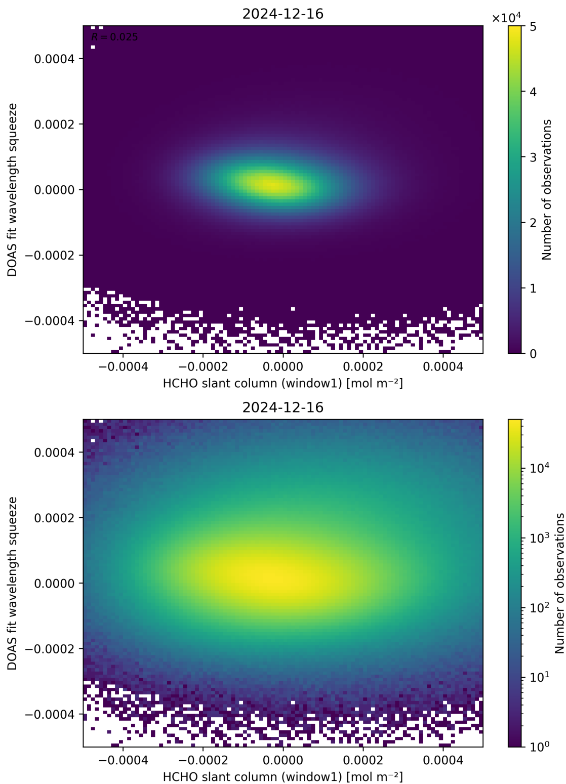
Figure 80: Scatter density plot of “HCHO slant column (window1)” against “DOAS fit wavelength squeeze” for 2024-12-16 to 2024-12-17.
