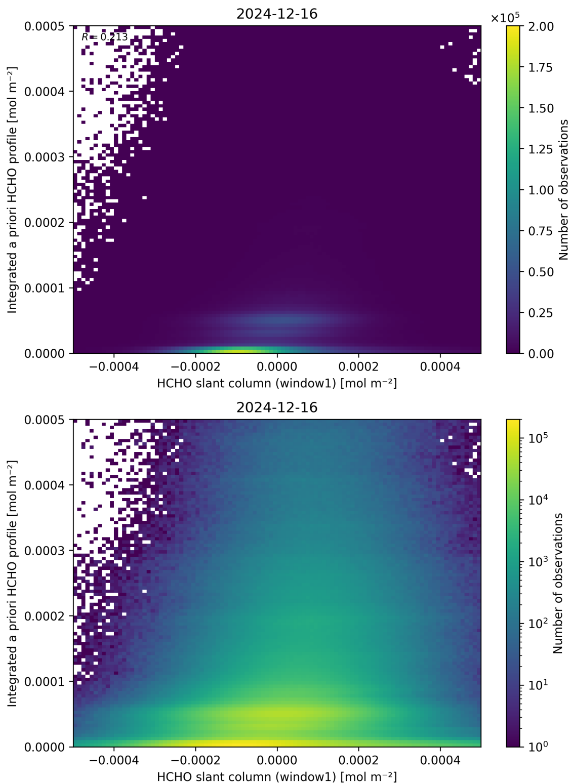
Figure 87: Scatter density plot of “HCHO slant column (window1)” against “Integrated a priori HCHO profile” for 2024-12-16 to 2024-12-17.
