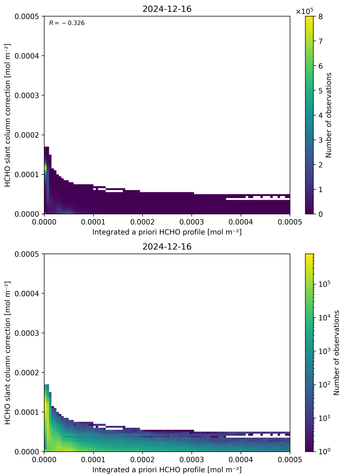
Figure 152: Scatter density plot of “Integrated a priori HCHO profile” against “HCHO slant column correction” for 2024-12-16 to 2024-12-17.
