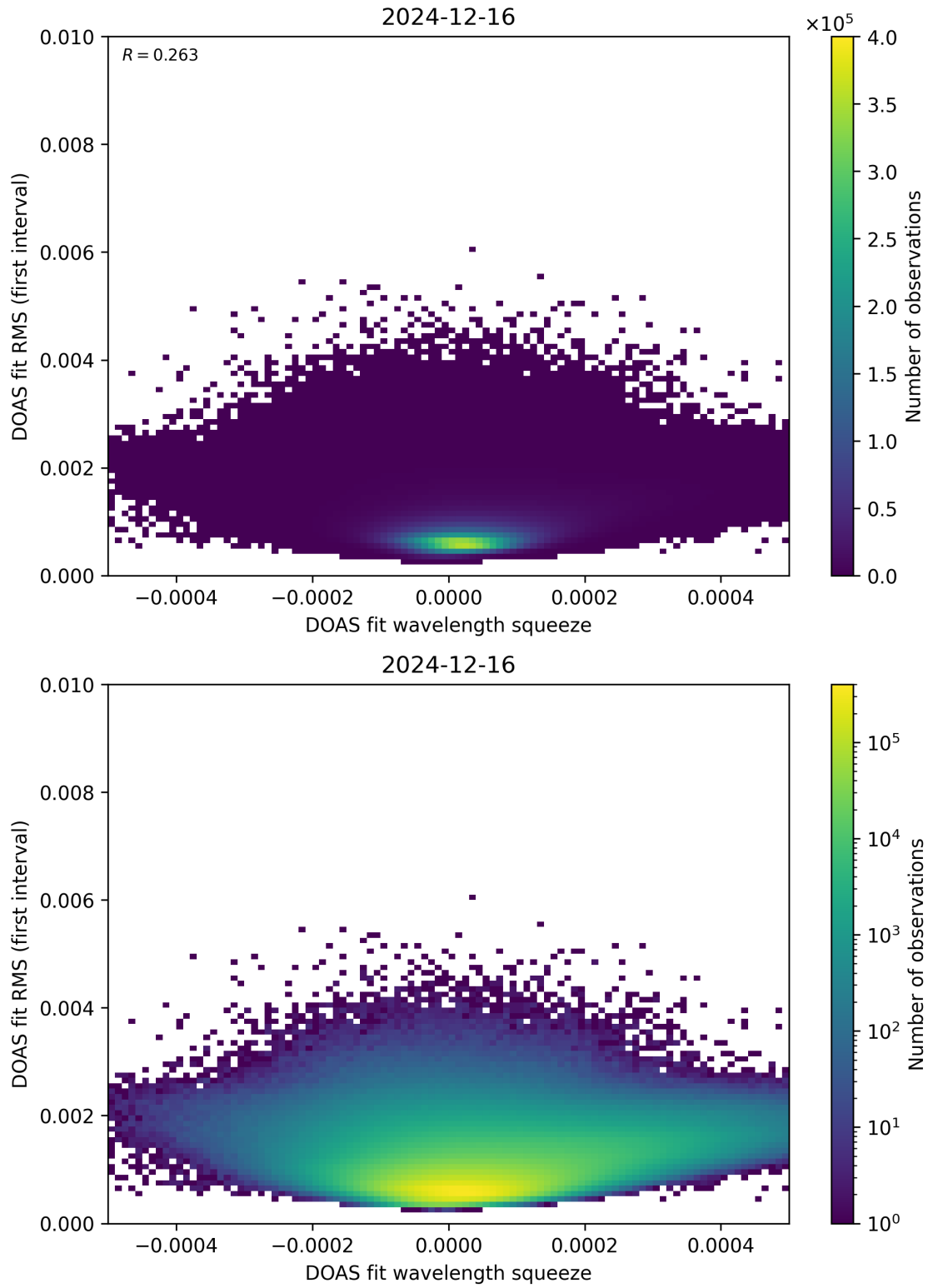
Figure 68: Scatter density plot of “DOAS fit wavelength squeeze” against “DOAS fit RMS (first interval)” for 2024-12-16 to 2024-12-17.
