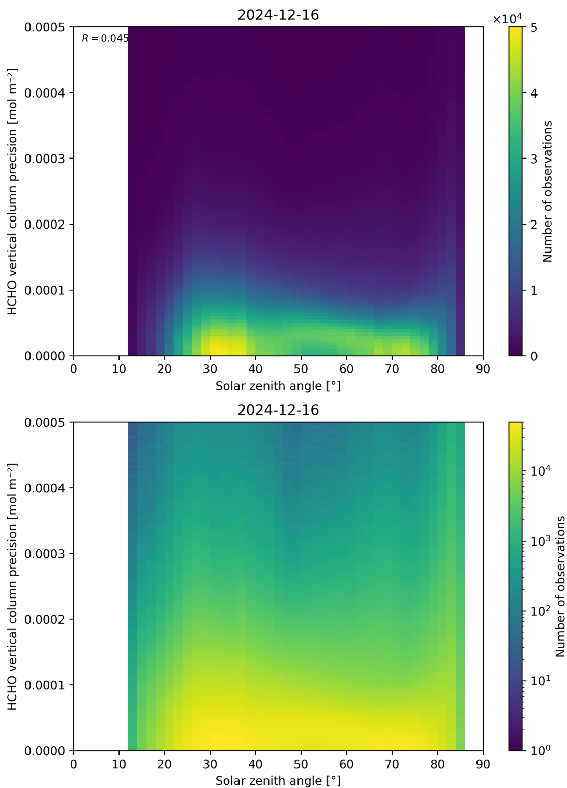
Figure 179: Scatter density plot of “Solar zenith angle” against “HCHO vertical column precision” for 2024-12-16 to 2024-12-17.
