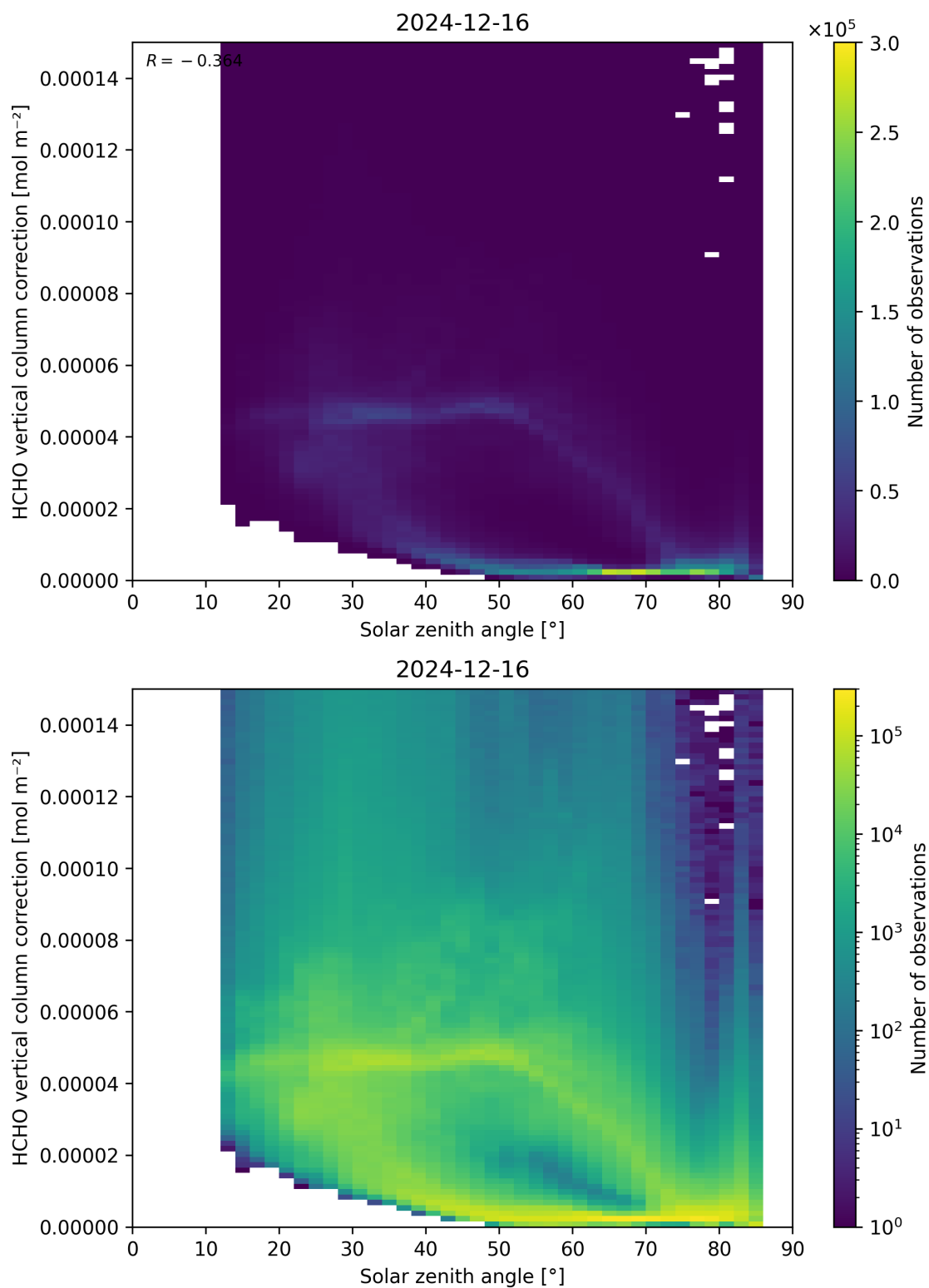
Figure 178: Scatter density plot of “Solar zenith angle” against “HCHO vertical column correction” for 2024-12-16 to 2024-12-17.
