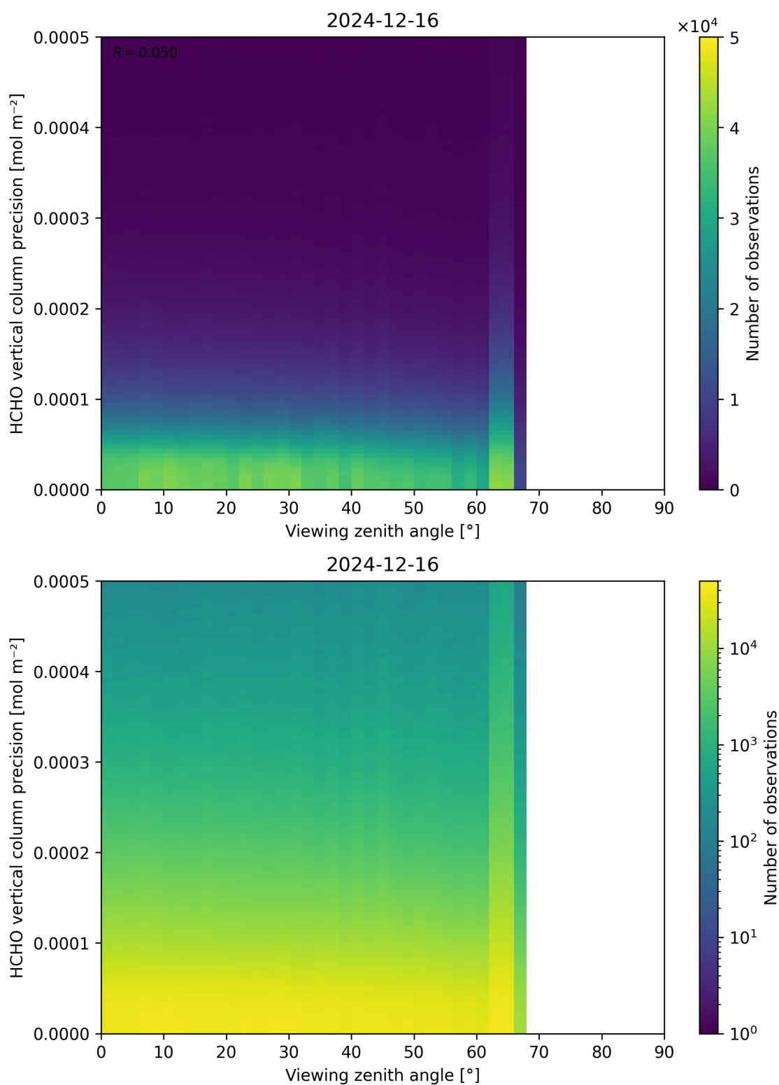
Figure 194: Scatter density plot of “Viewing zenith angle” against “HCHO vertical column precision” for 2024-12-16 to 2024-12-17.
