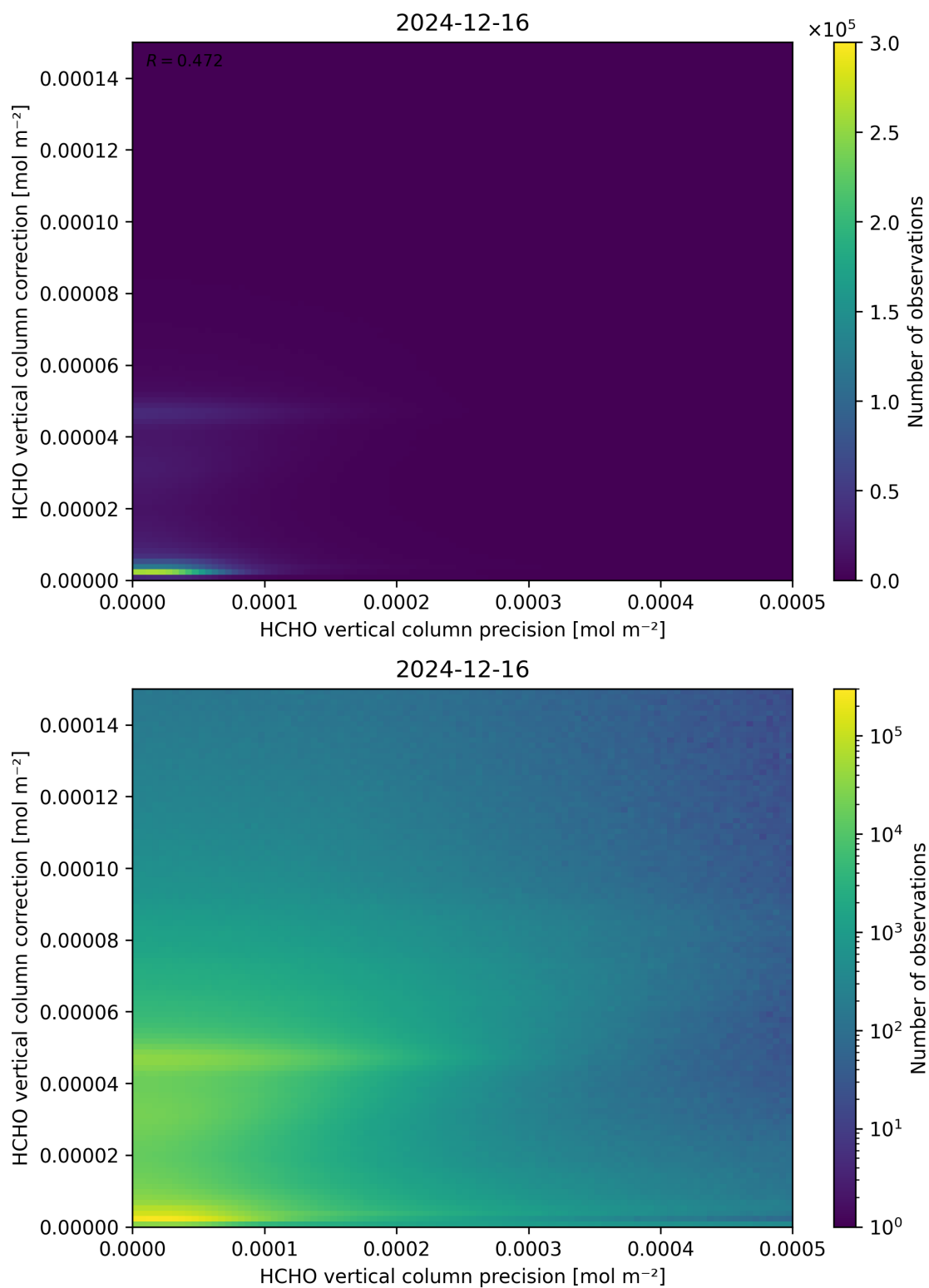
Figure 146: Scatter density plot of “HCHO vertical column precision” against “HCHO vertical column correction” for 2024-12-16 to 2024-12-17.
