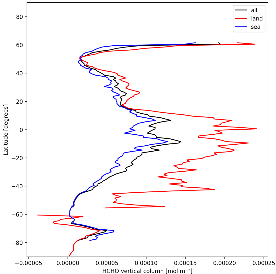
Figure 21: Zonal average of “HCHO vertical column” for 2024-12-16 to 2024-12-17.
