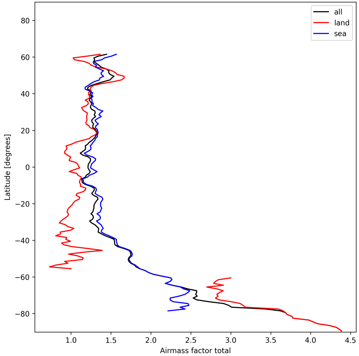
Figure 26: Zonal average of “Airmass factor total” for 2024-12-16 to 2024-12-17.
