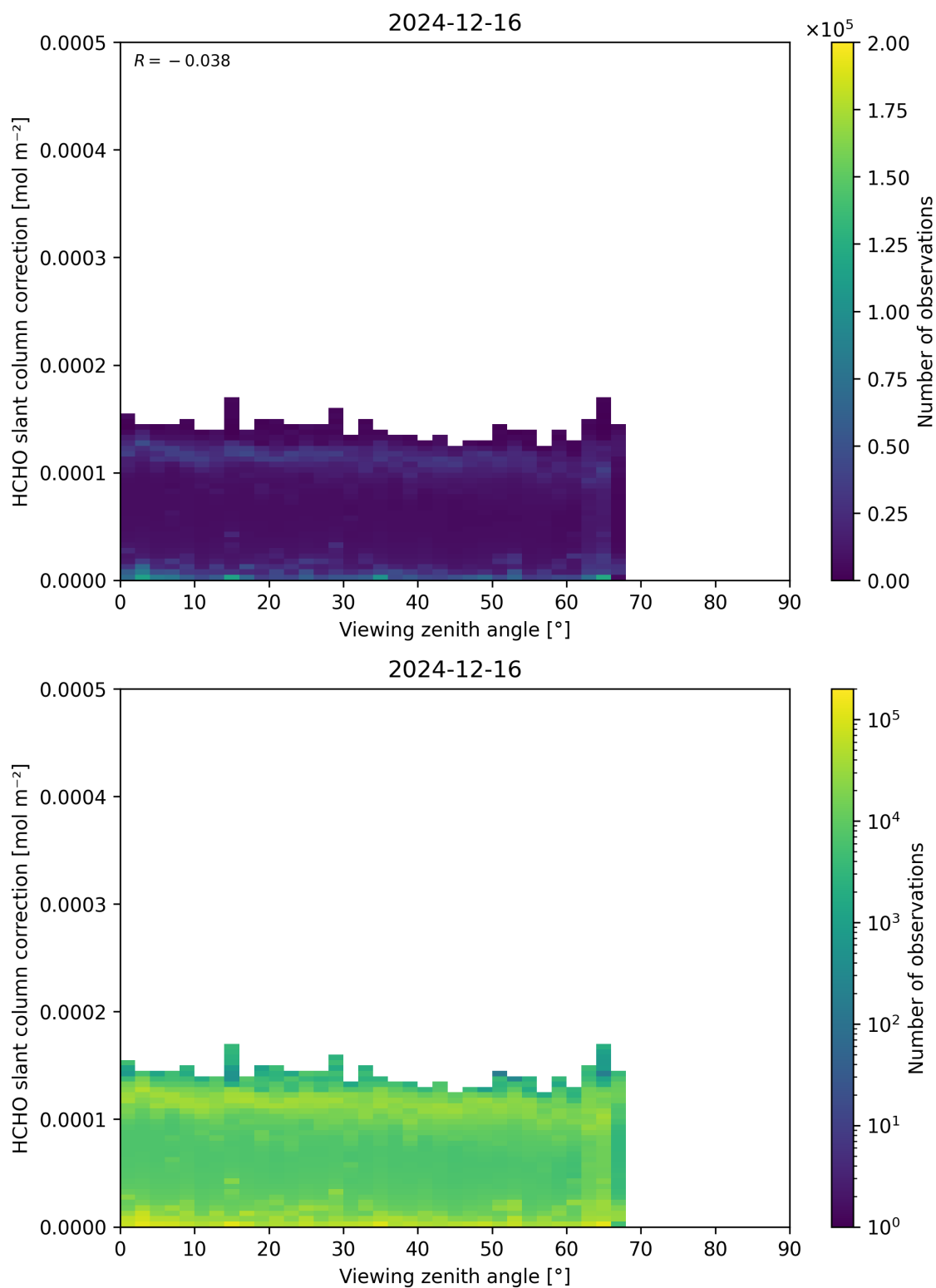
Figure 187: Scatter density plot of “Viewing zenith angle” against “HCHO slant column correction” for 2024-12-16 to 2024-12-17.
