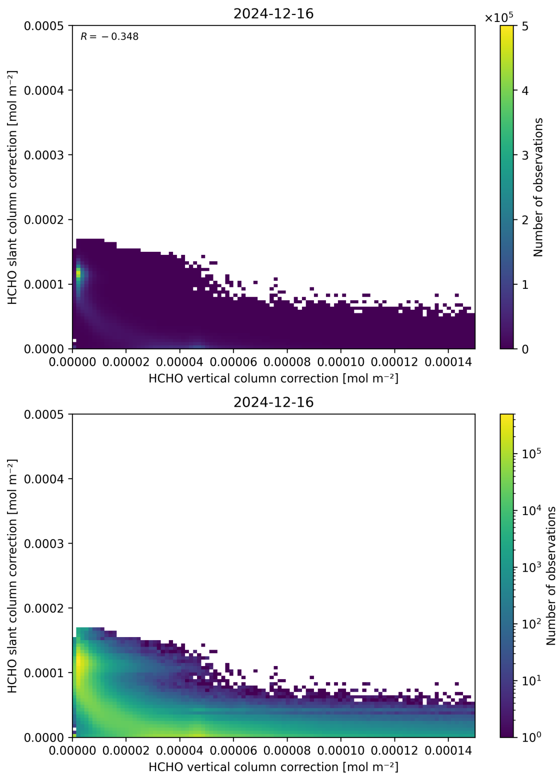
Figure 117: Scatter density plot of “HCHO vertical column correction” against “HCHO slant column correction” for 2024-12-16 to 2024-12-17.
