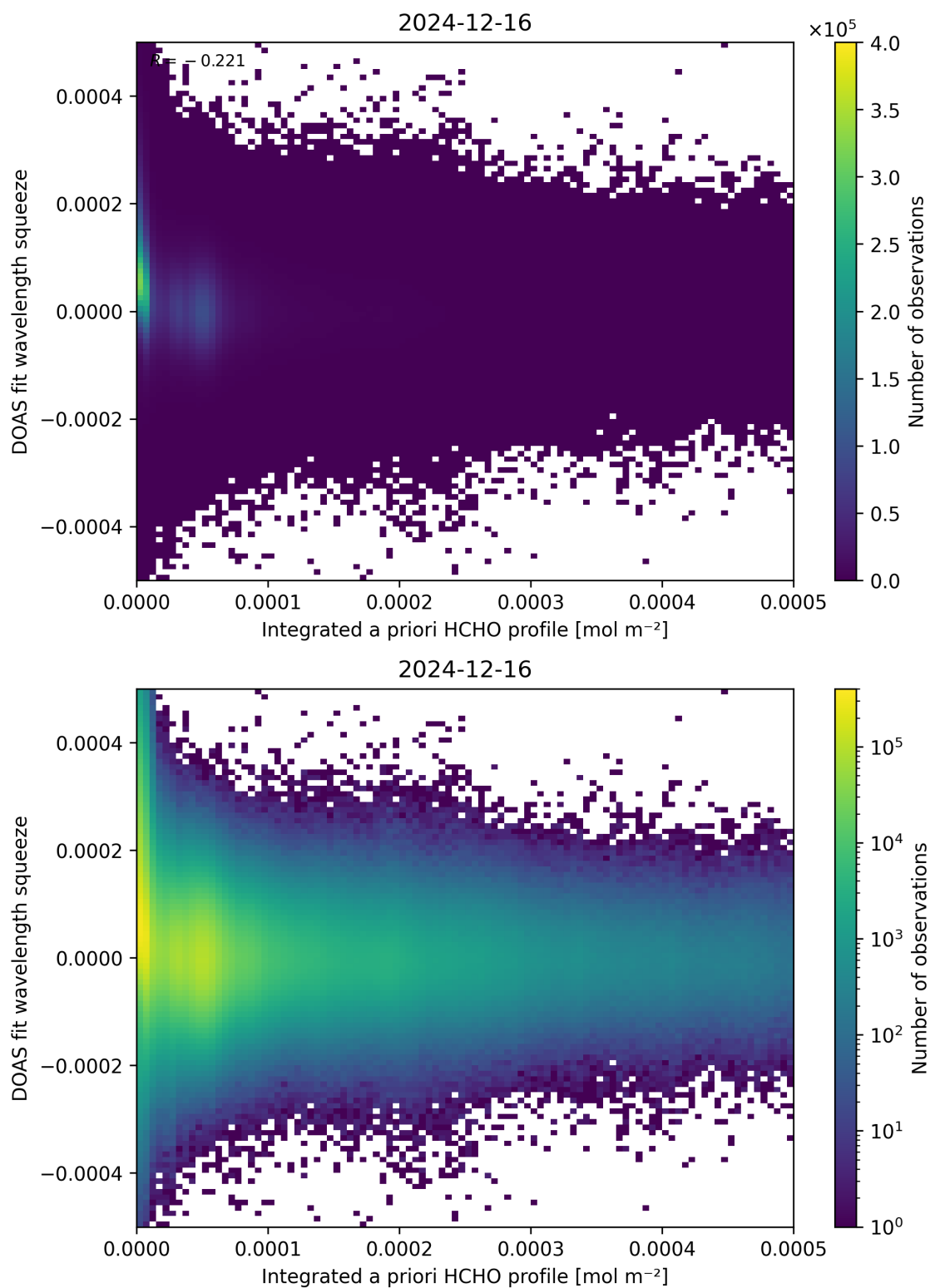
Figure 150: Scatter density plot of “Integrated a priori HCHO profile” against “DOAS fit wavelength squeeze” for 2024-12-16 to 2024-12-17.
