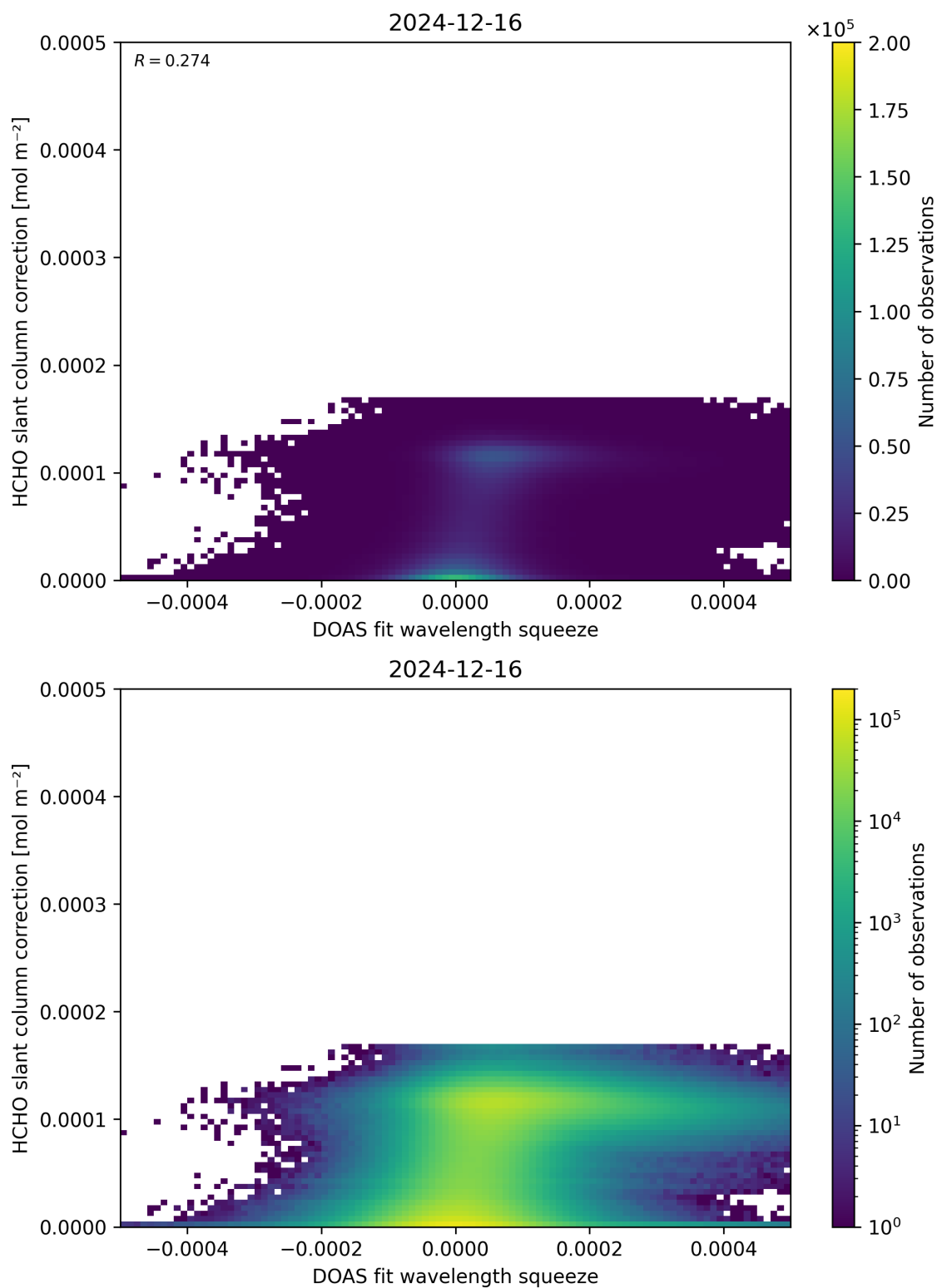
Figure 70: Scatter density plot of “DOAS fit wavelength squeeze” against “HCHO slant column correction” for 2024-12-16 to 2024-12-17.
