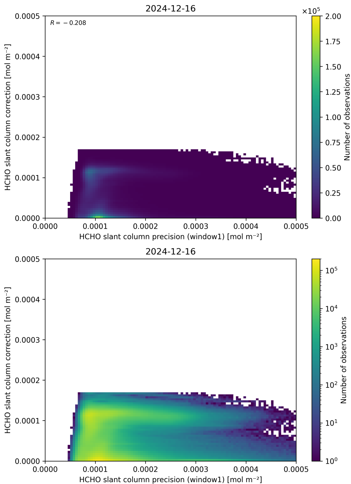
Figure 93: Scatter density plot of “HCHO slant column precision (window1)” against “HCHO slant column correction” for 2024-12-16 to 2024-12-17.
