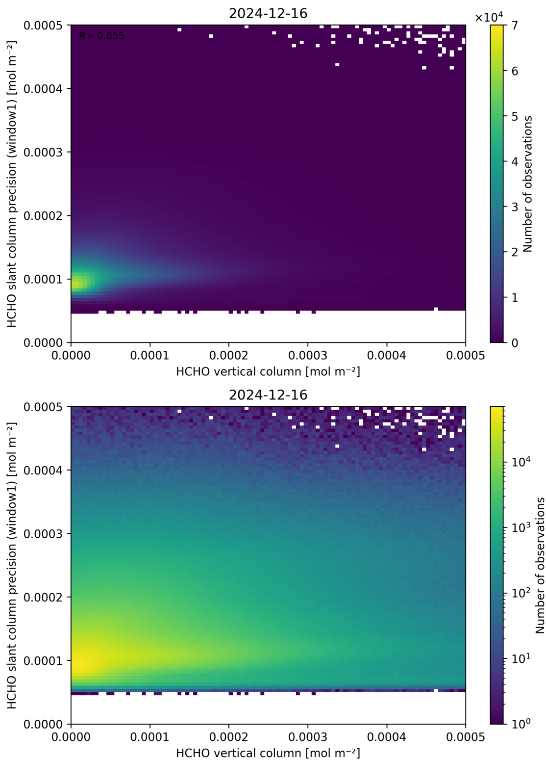
Figure 130: Scatter density plot of “HCHO vertical column” against “HCHO slant column precision (window1)” for 2024-12-16 to 2024-12-17.
