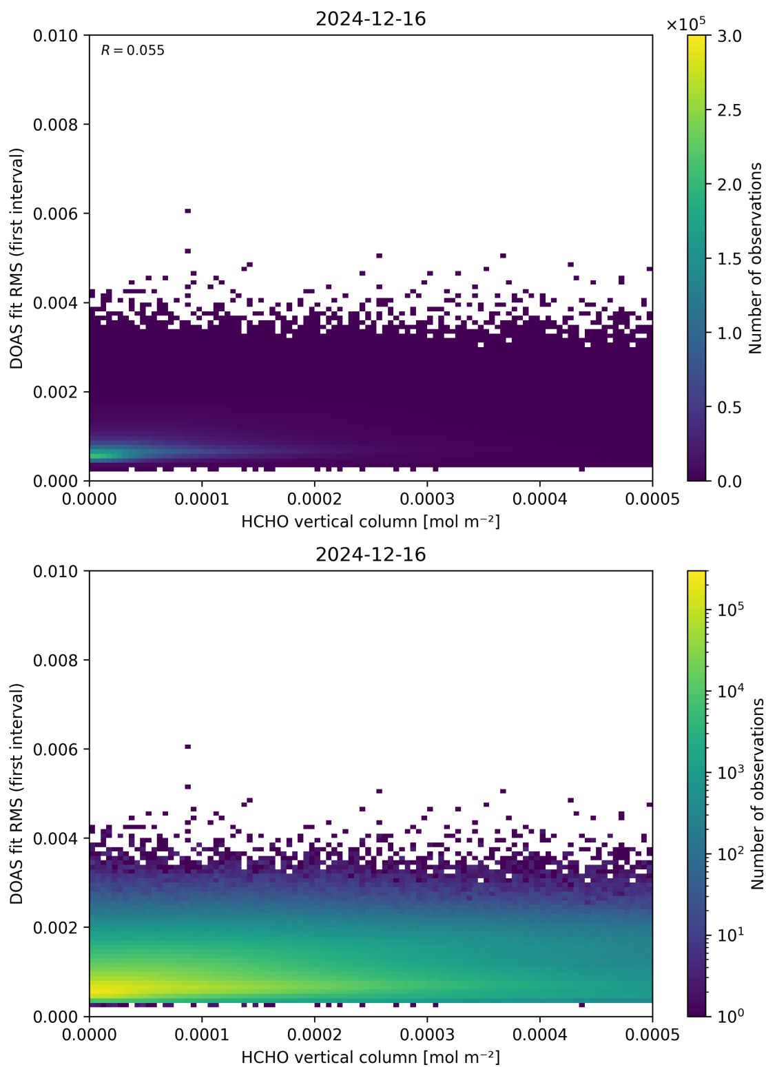
Figure 123: Scatter density plot of “HCHO vertical column” against “DOAS fit RMS (first interval)” for 2024-12-16 to 2024-12-17.
