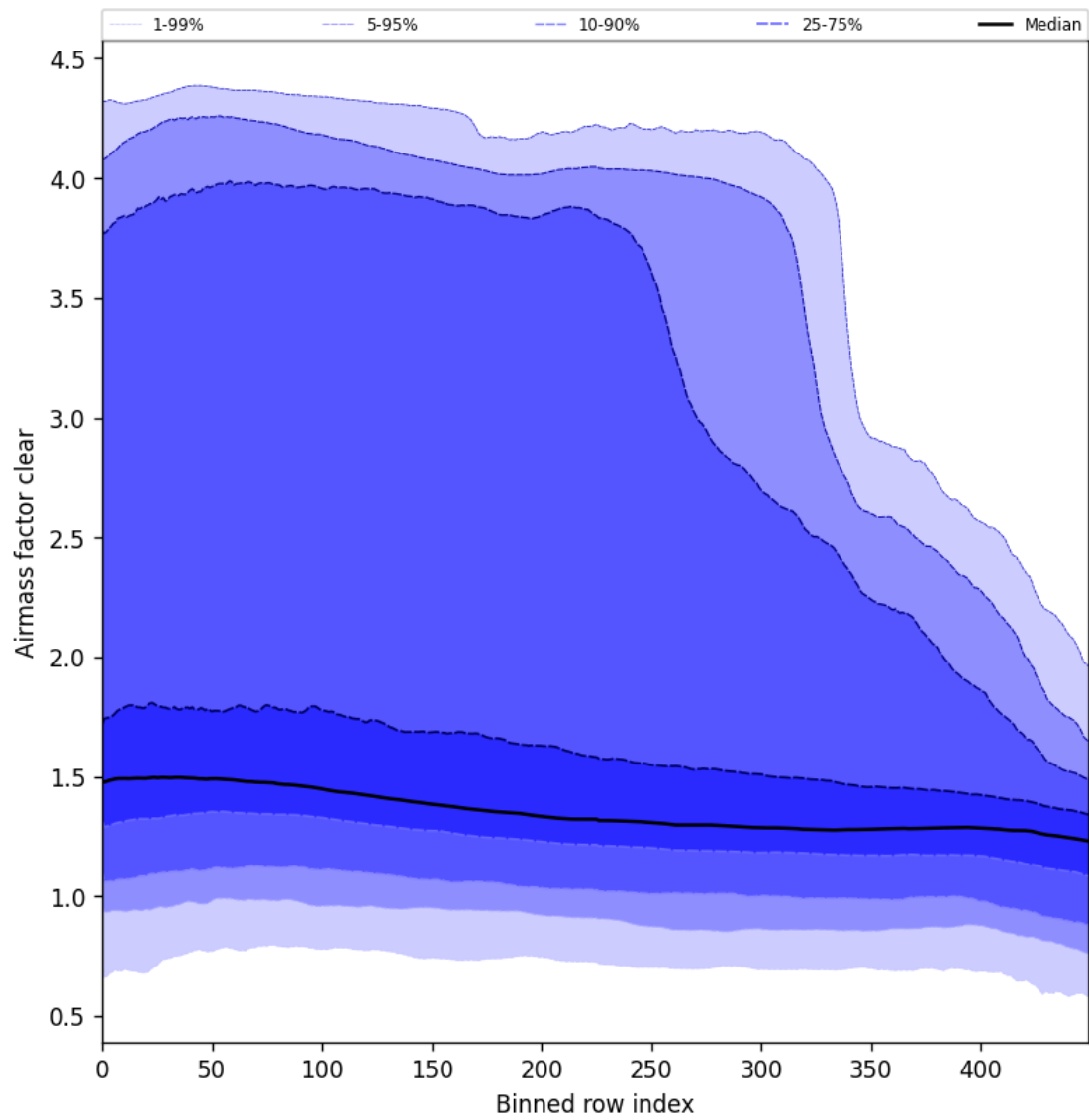
Figure 56: Along track statistics of “Airmass factor clear” for 2024-12-16 to 2024-12-17
