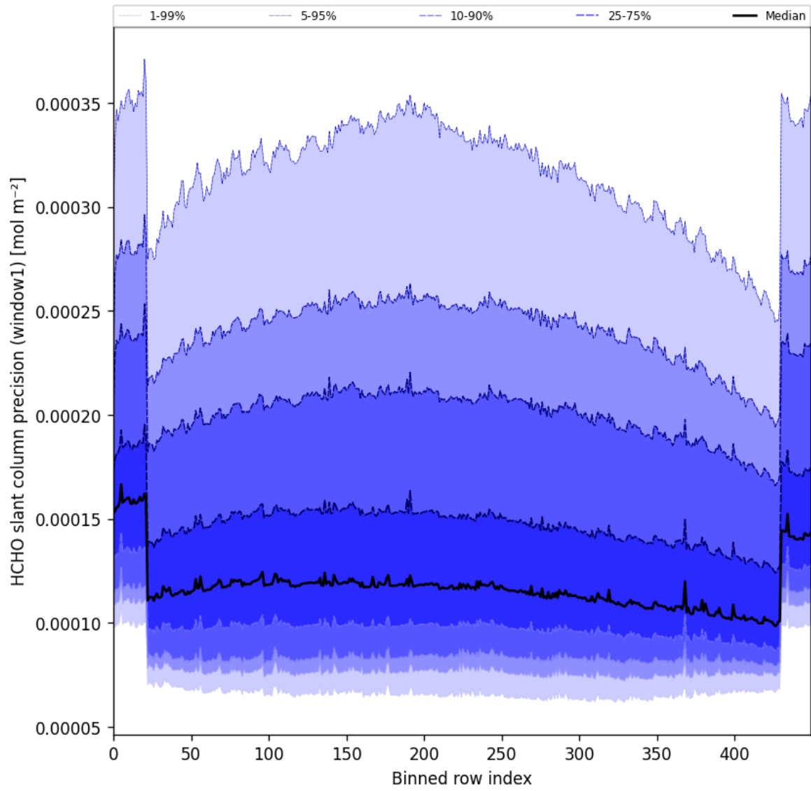
Figure 53: Along track statistics of “HCHO slant column precision (window1)” for 2024-12-16 to 2024-12-17
