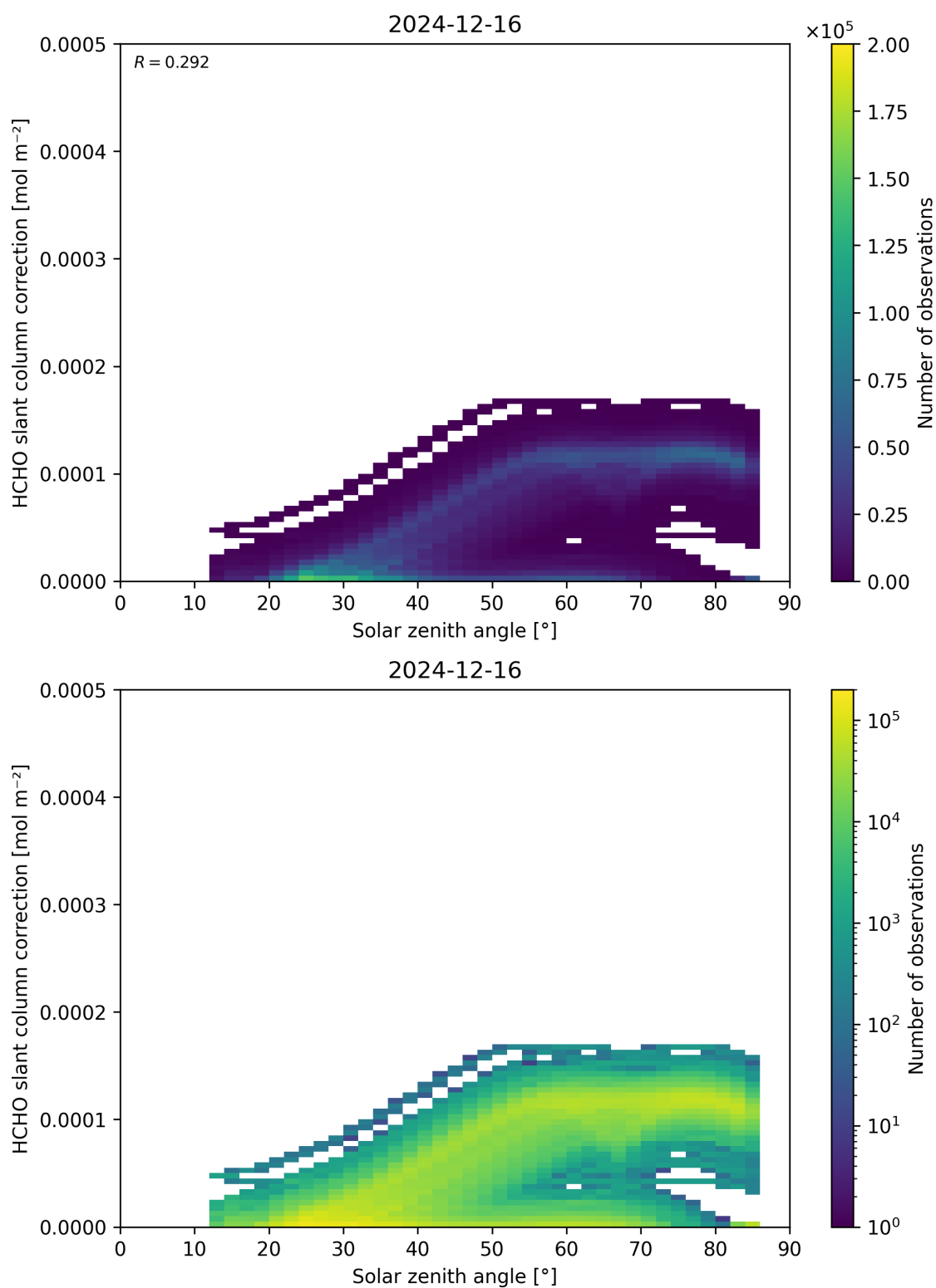
Figure 172: Scatter density plot of “Solar zenith angle” against “HCHO slant column correction” for 2024-12-16 to 2024-12-17.
