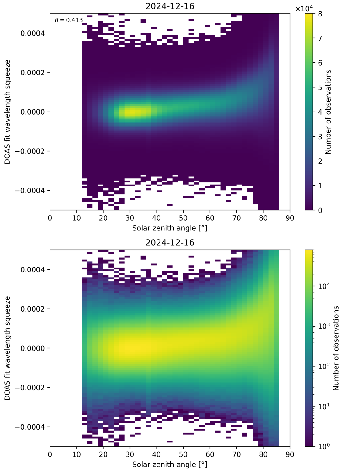
Figure 169: Scatter density plot of “Solar zenith angle” against “DOAS fit wavelength squeeze” for 2024-12-16 to 2024-12-17.
