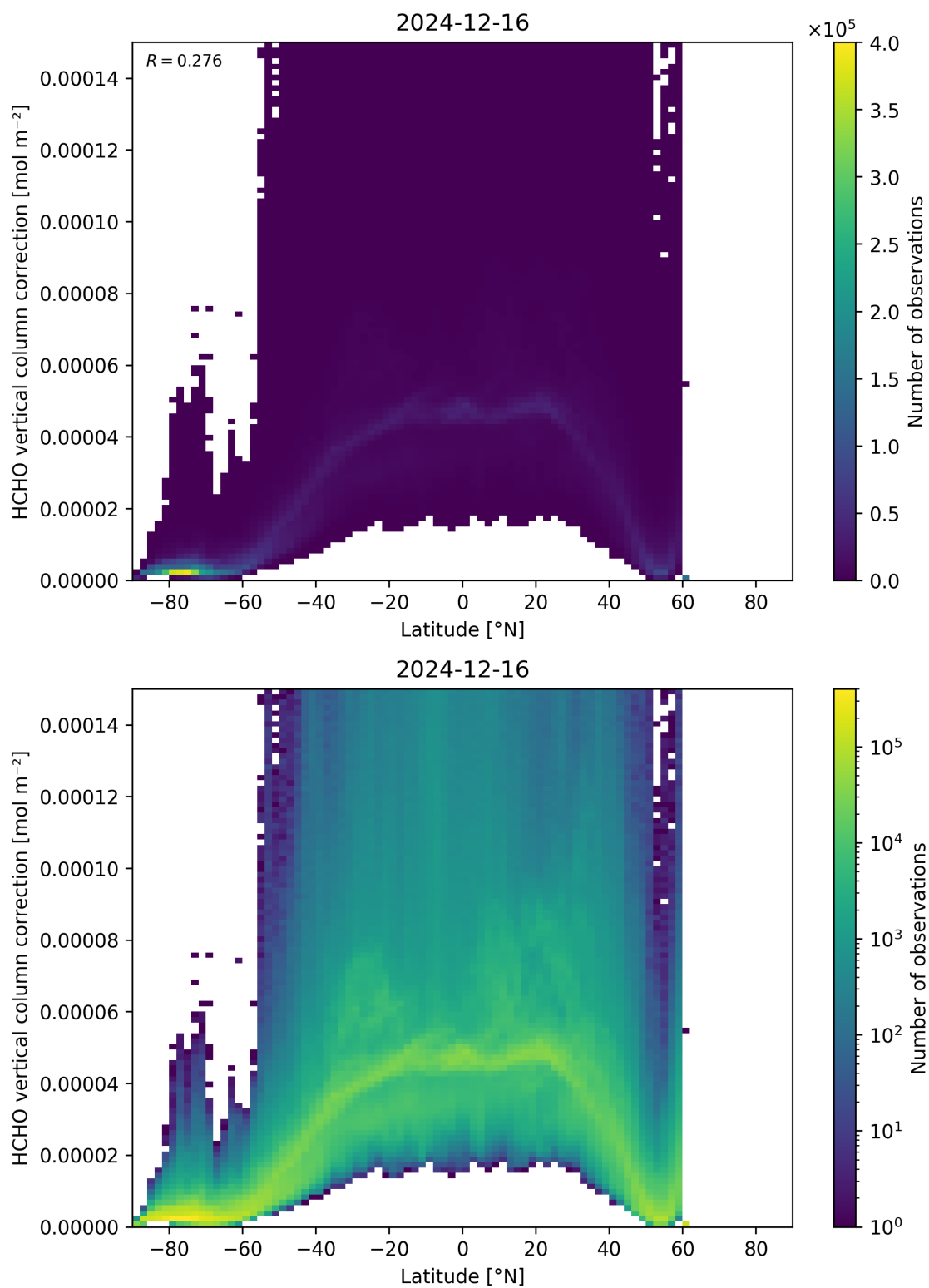
Figure 164: Scatter density plot of “Latitude” against “HCHO vertical column correction” for 2024-12-16 to 2024-12-17.
