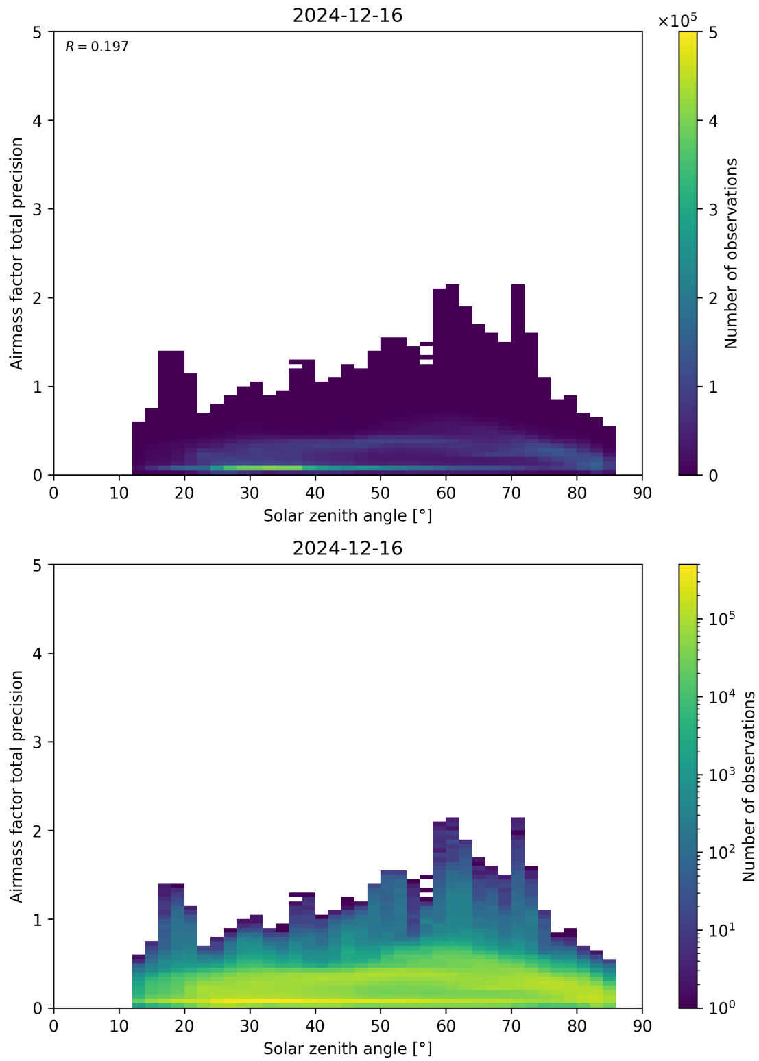
Figure 176: Scatter density plot of “Solar zenith angle” against “Airmass factor total precision” for 2024-12-16 to 2024-12-17.
