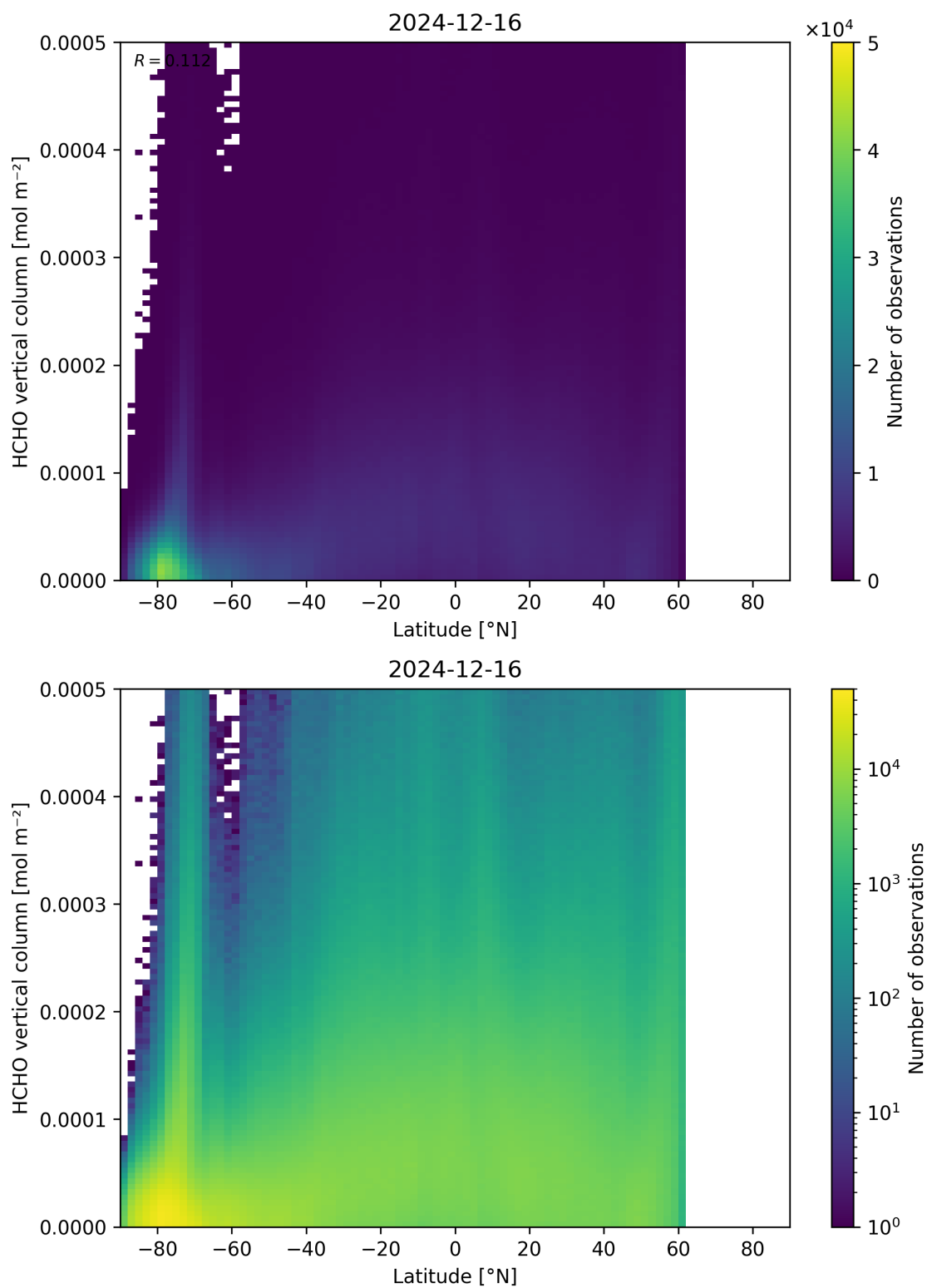
Figure 163: Scatter density plot of “Latitude” against “HCHO vertical column” for 2024-12-16 to 2024-12-17.
