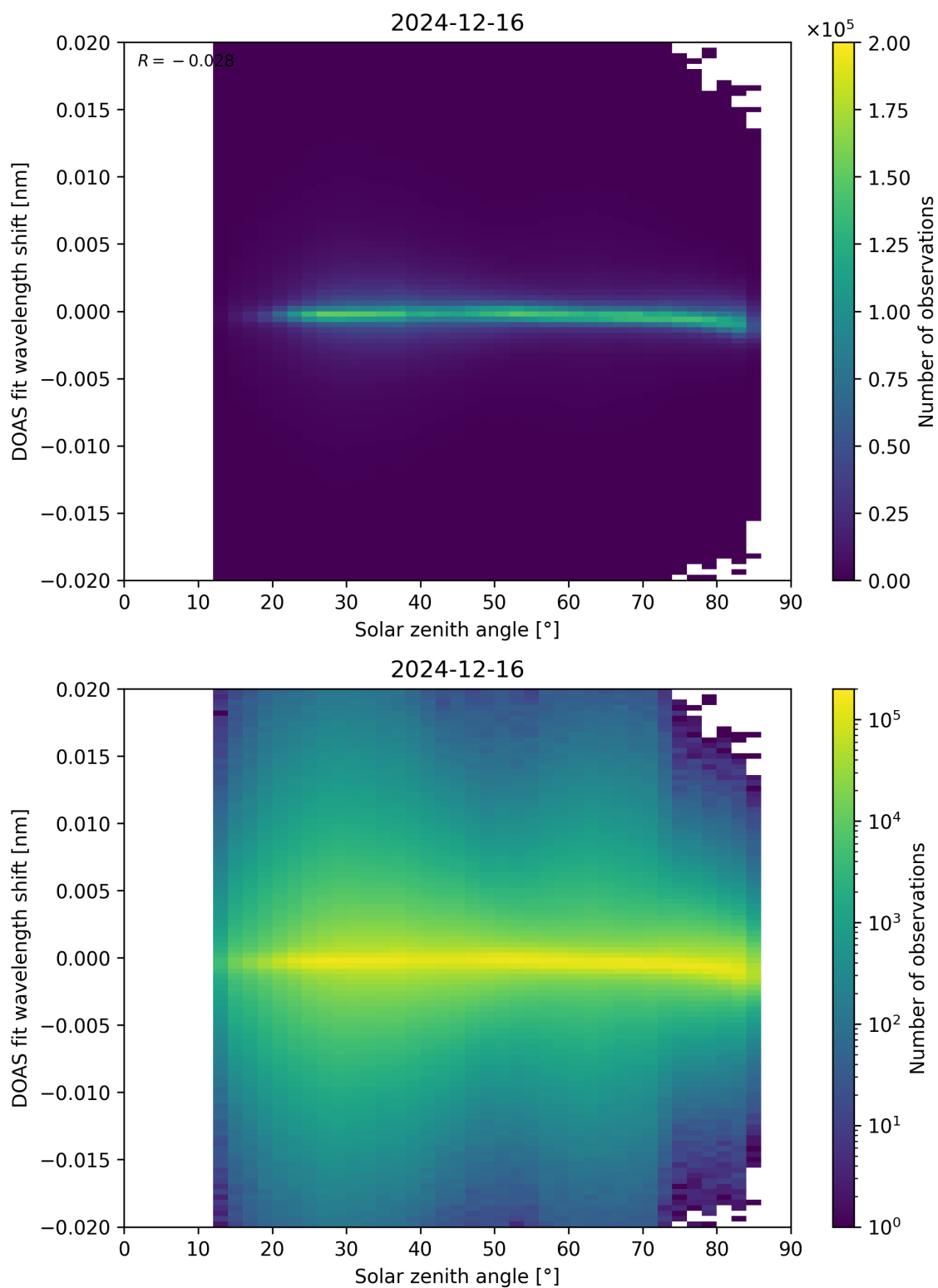
Figure 168: Scatter density plot of “Solar zenith angle” against “DOAS fit wavelength shift” for 2024-12-16 to 2024-12-17.
