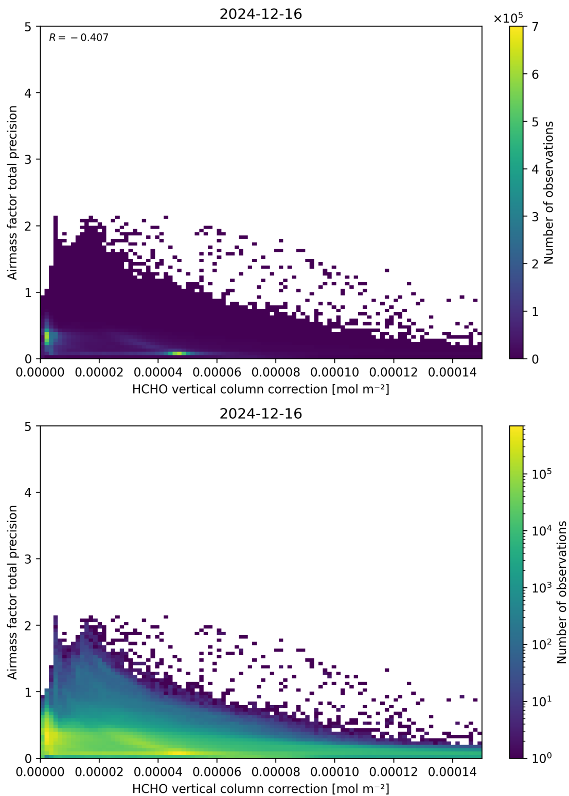
Figure 121: Scatter density plot of “HCHO vertical column correction” against “Airmass factor total precision” for 2024-12-16 to 2024-12-17.
