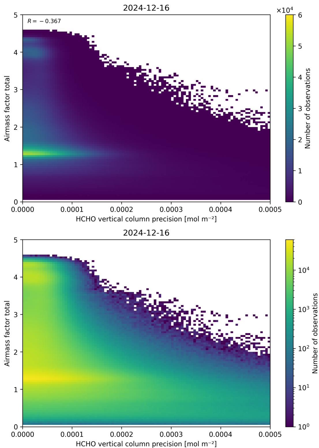
Figure 144: Scatter density plot of “HCHO vertical column precision” against “Airmass factor total” for 2024-12-16 to 2024-12-17.
