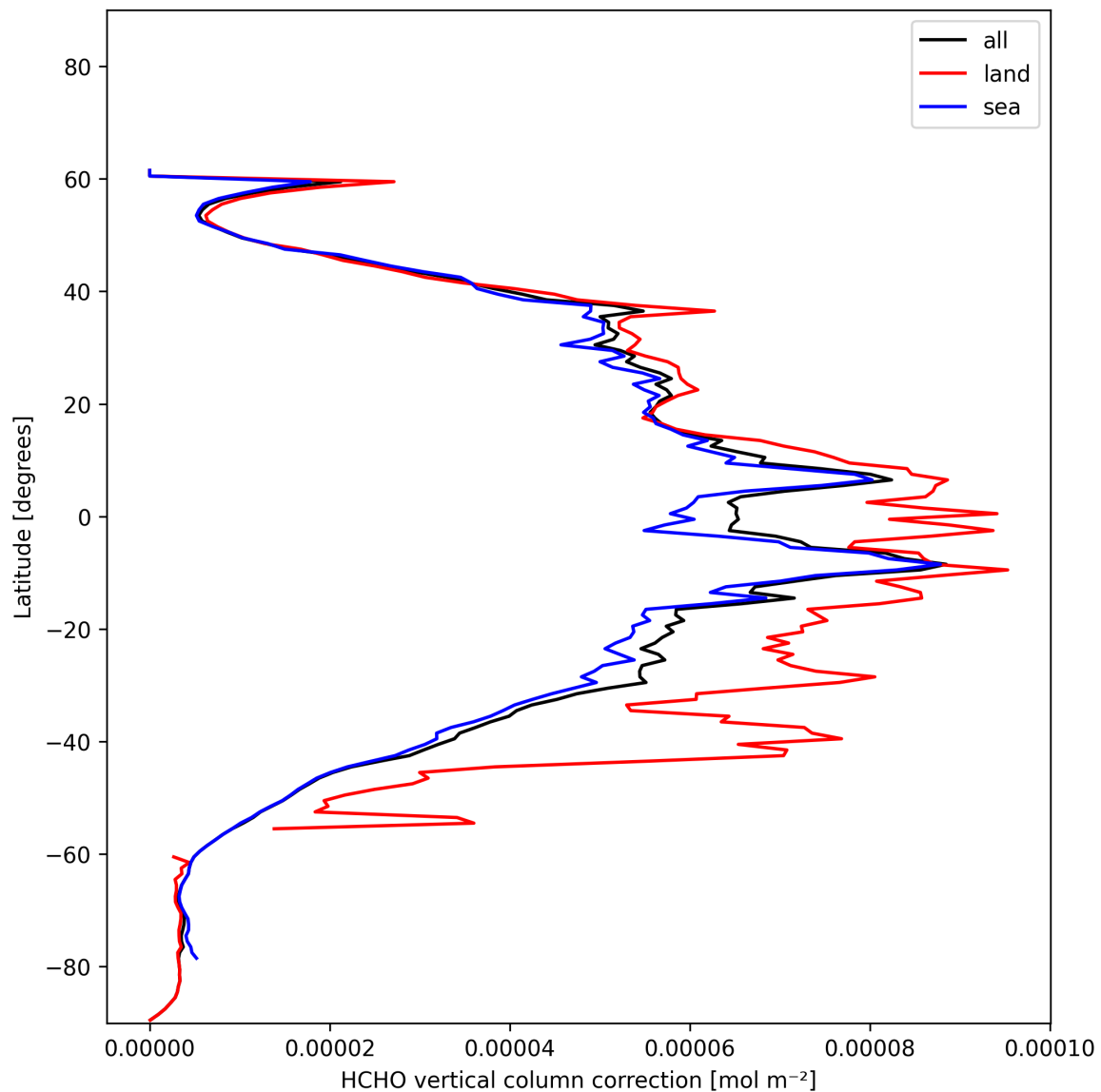
Figure 23: Zonal average of “HCHO vertical column correction” for 2024-12-16 to 2024-12-17.
