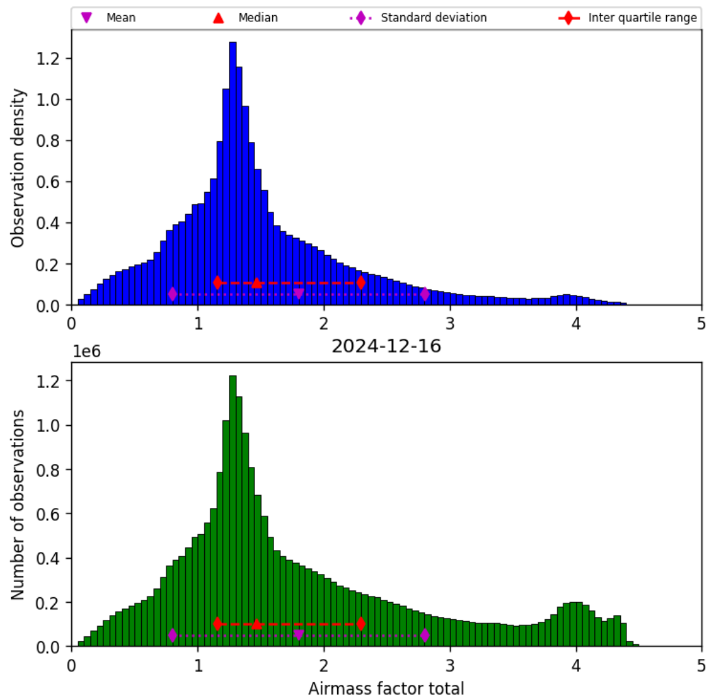
Figure 40: Histogram of “Airmass factor total” for 2024-12-16 to 2024-12-17
