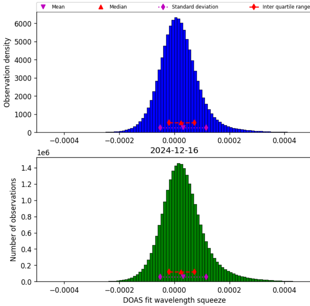
Figure 45: Histogram of “DOAS fit wavelength squeeze” for 2024-12-16 to 2024-12-17
