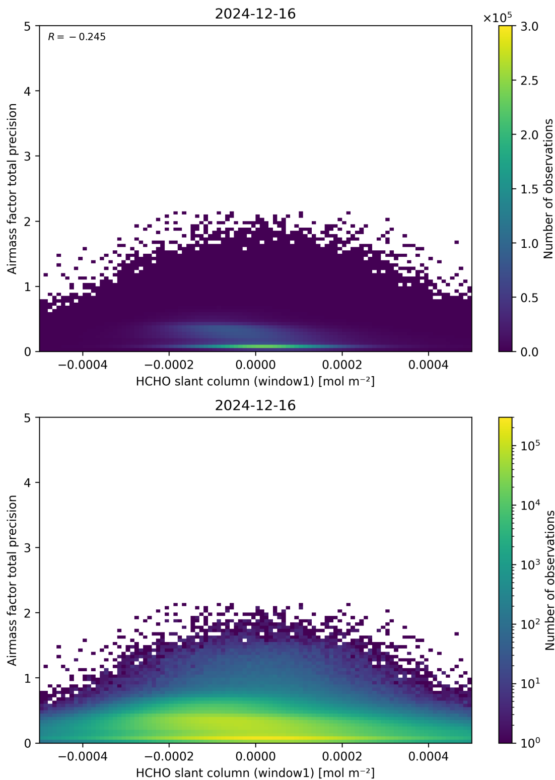
Figure 86: Scatter density plot of “HCHO slant column (window1)” against “Airmass factor total precision” for 2024-12-16 to 2024-12-17.
