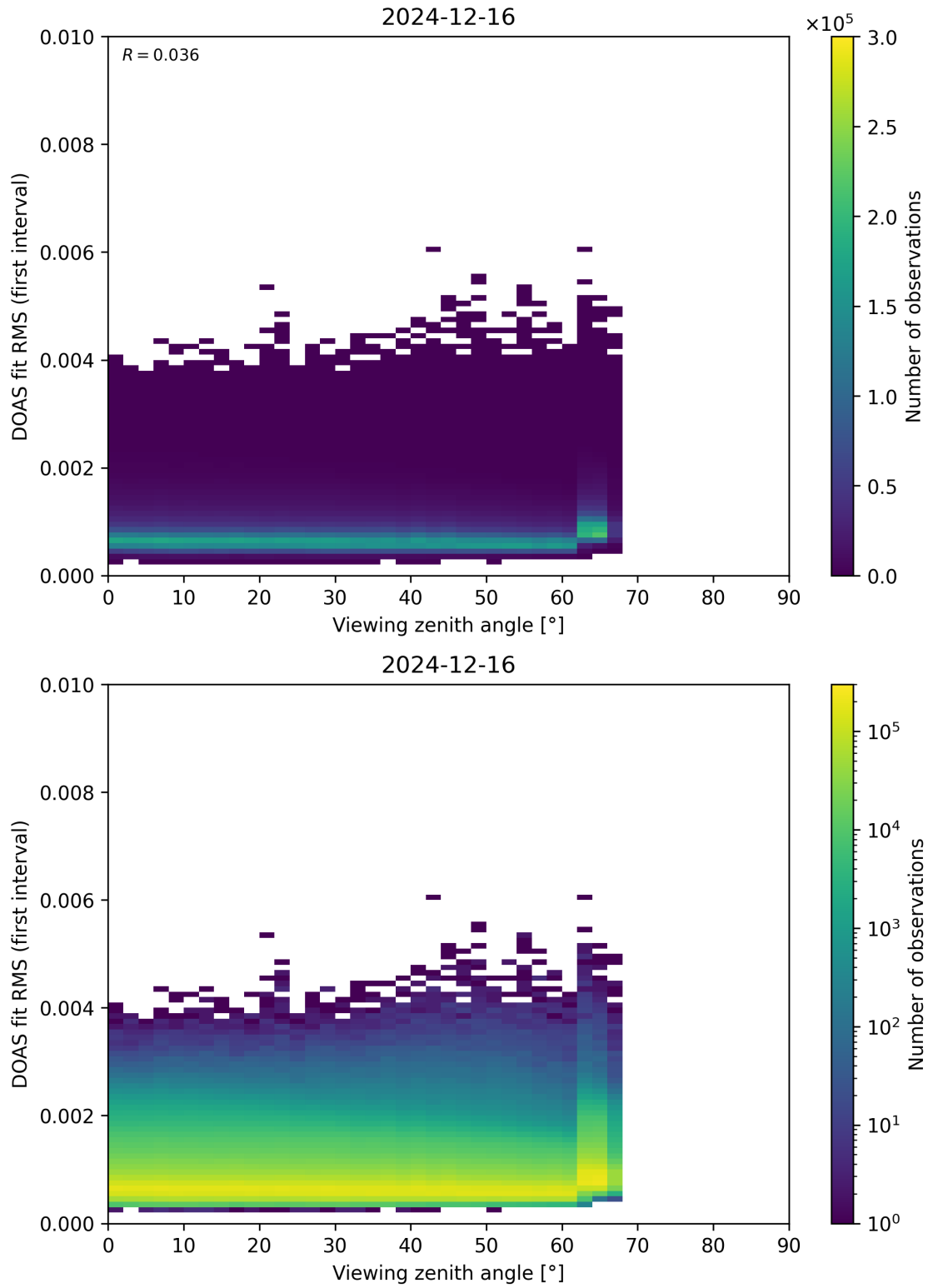
Figure 182: Scatter density plot of “Viewing zenith angle” against “DOAS fit RMS (first interval)” for 2024-12-16 to 2024-12-17.
