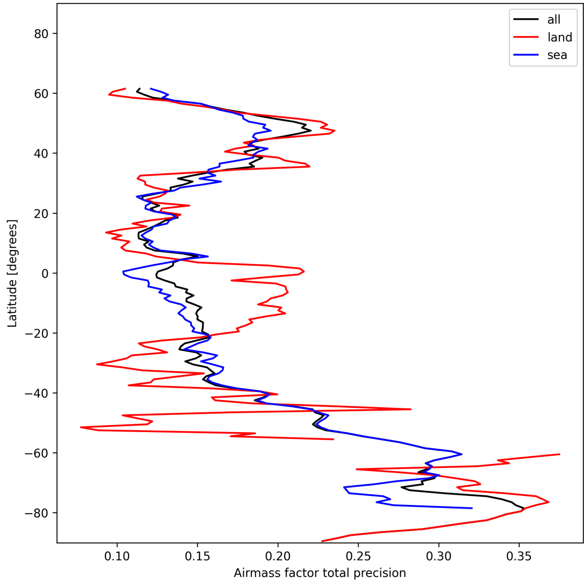
Figure 27: Zonal average of “Airmass factor total precision” for 2024-12-16 to 2024-12-17.
