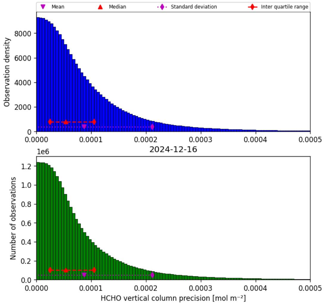
Figure 36: Histogram of “HCHO vertical column precision” for 2024-12-16 to 2024-12-17
