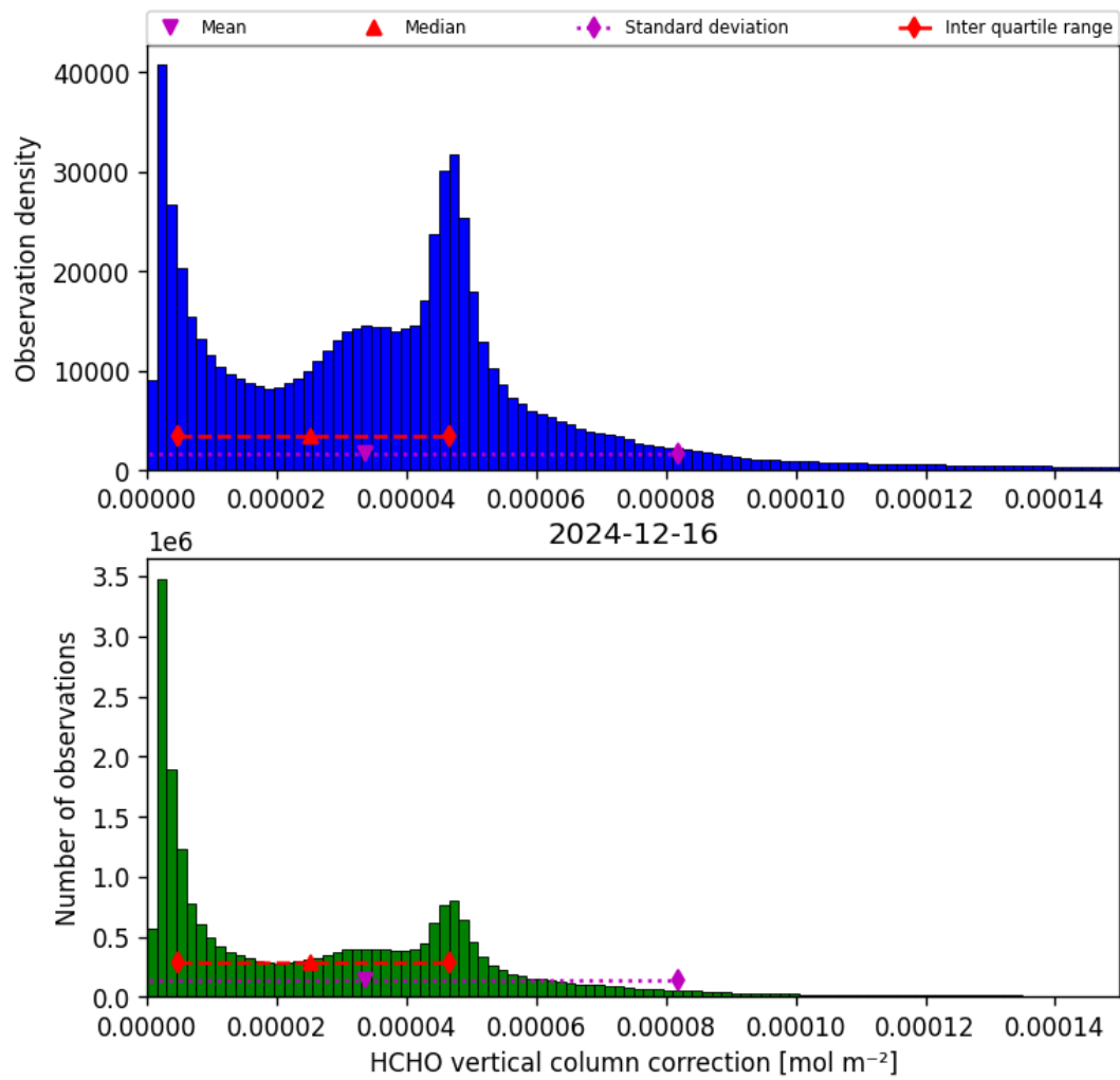
Figure 37: Histogram of “HCHO vertical column correction” for 2024-12-16 to 2024-12-17
