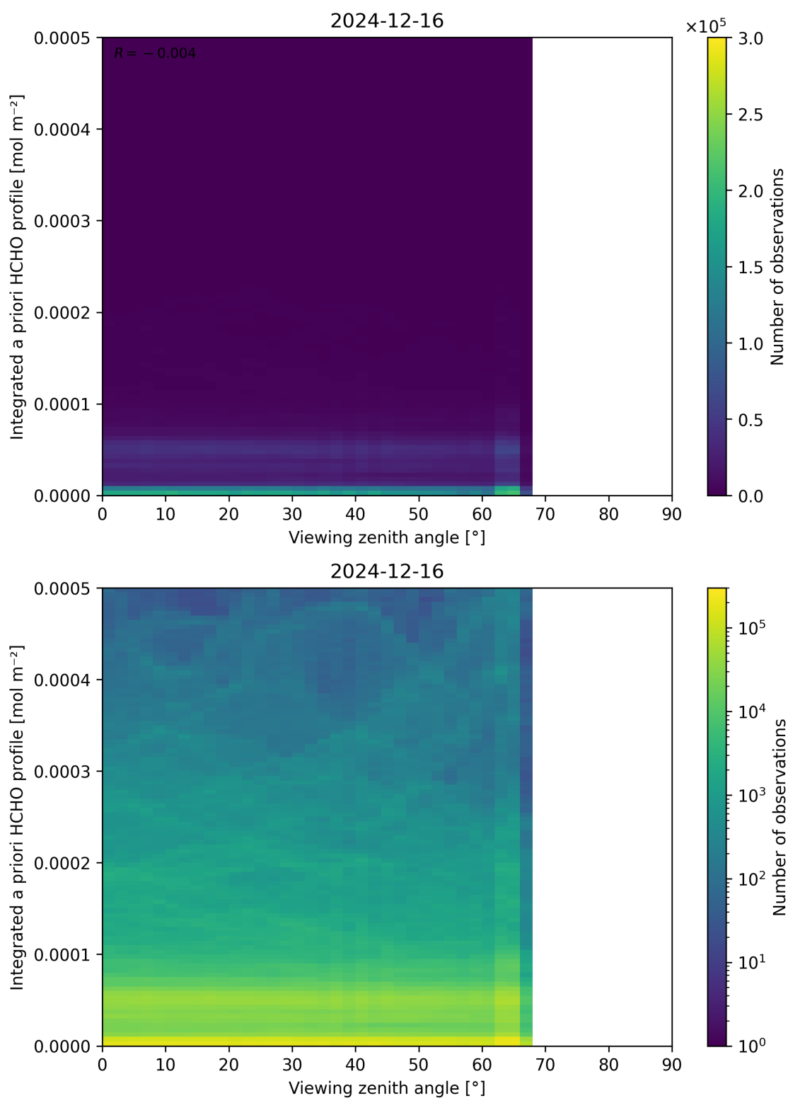
Figure 195: Scatter density plot of “Viewing zenith angle” against “Integrated a priori HCHO profile” for 2024-12-16 to 2024-12-17.
