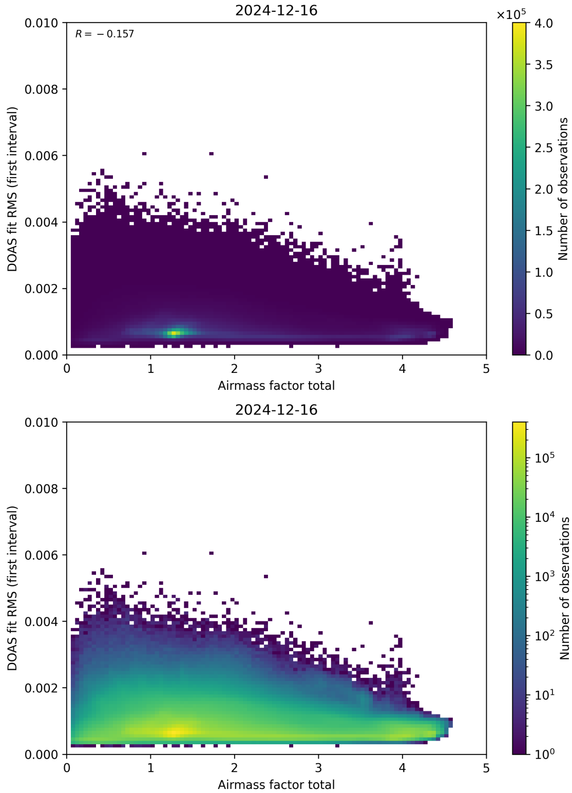
Figure 97: Scatter density plot of “Airmass factor total” against “DOAS fit RMS (first interval)” for 2024-12-16 to 2024-12-17.
