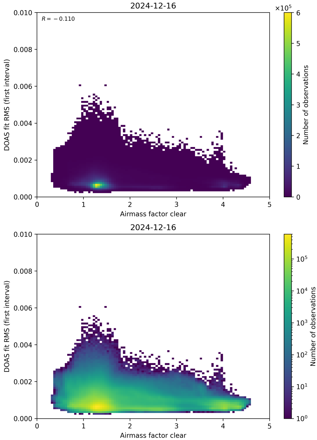
Figure 71: Scatter density plot of “Airmass factor clear” against “DOAS fit RMS (first interval)” for 2024-12-16 to 2024-12-17.
