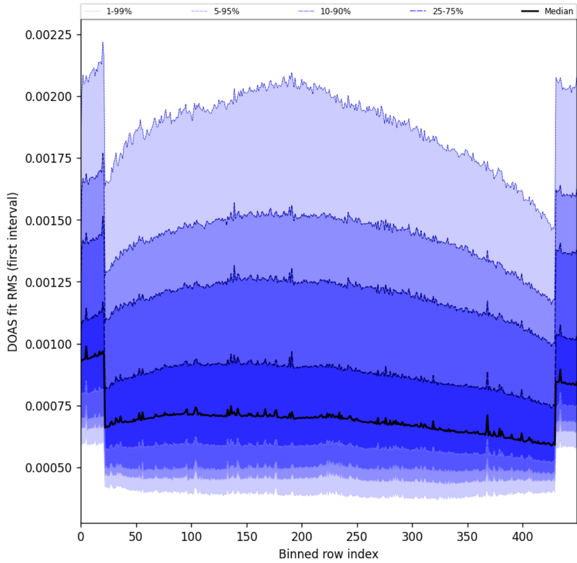
Figure 60: Along track statistics of “DOAS fit RMS (first interval)” for 2024-12-16 to 2024-12-17
