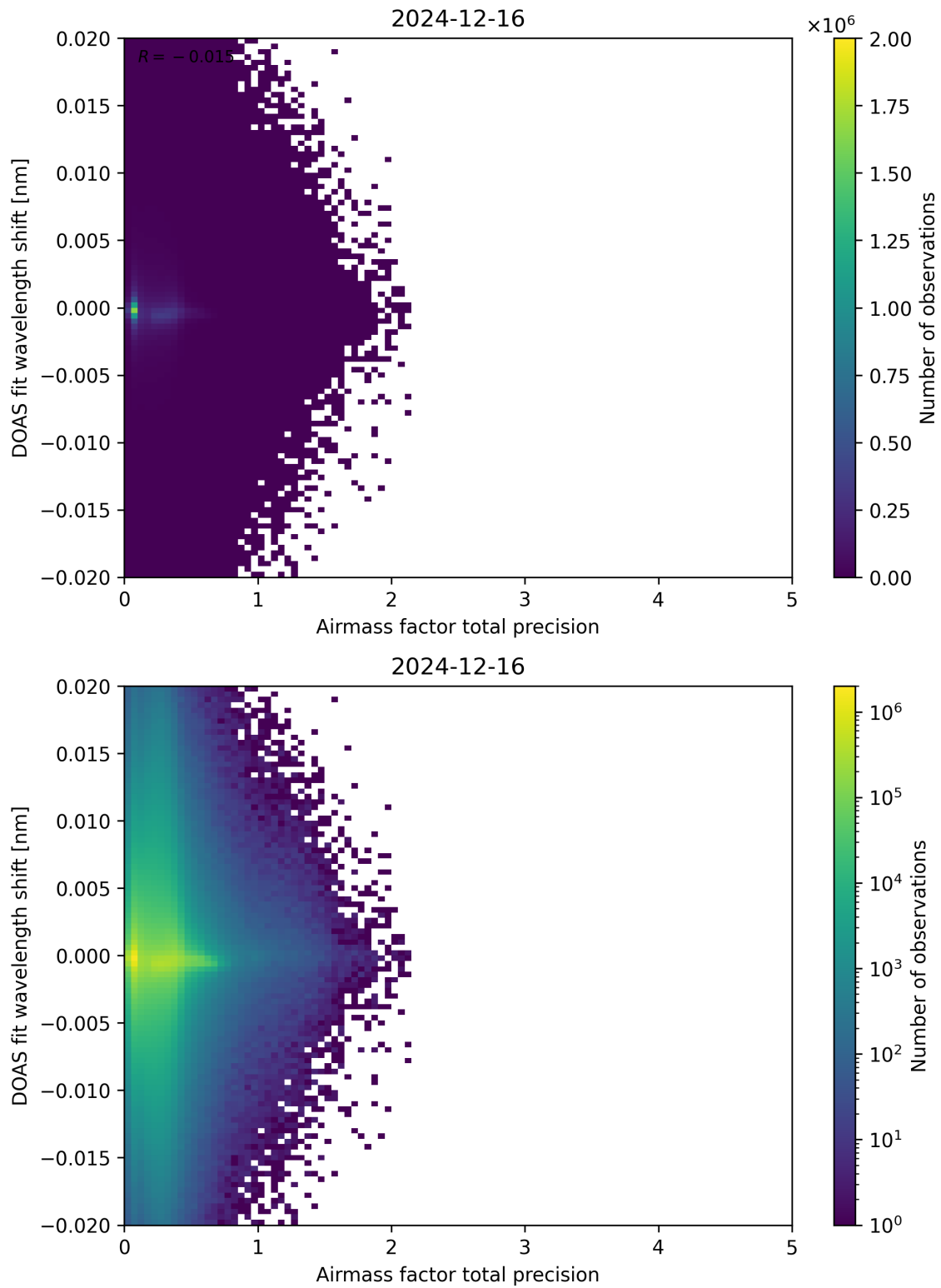
Figure 106: Scatter density plot of “Airmass factor total precision” against “DOAS fit wavelength shift” for 2024-12-16 to 2024-12-17.
