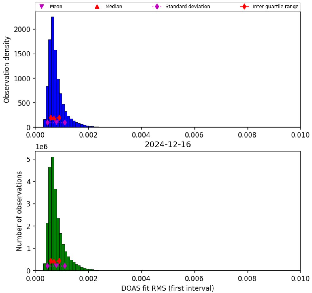
Figure 46: Histogram of “DOAS fit RMS (first interval)” for 2024-12-16 to 2024-12-17
