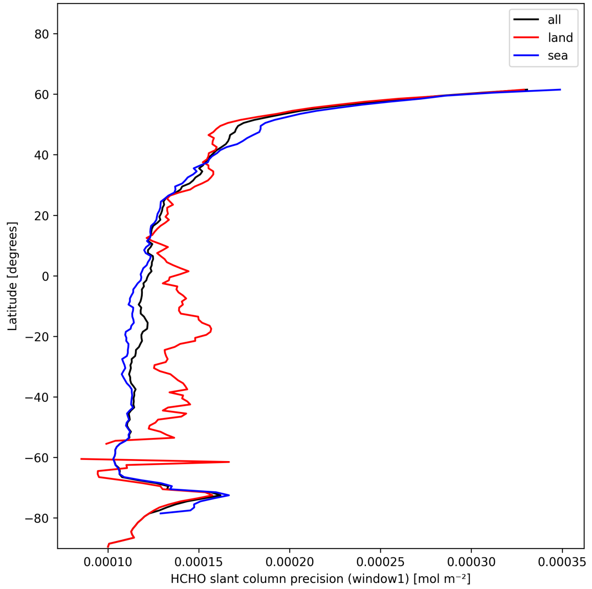
Figure 25: Zonal average of "HCHO slant column precision (window1)" for 2024-12-16 to 2024-12-17.
