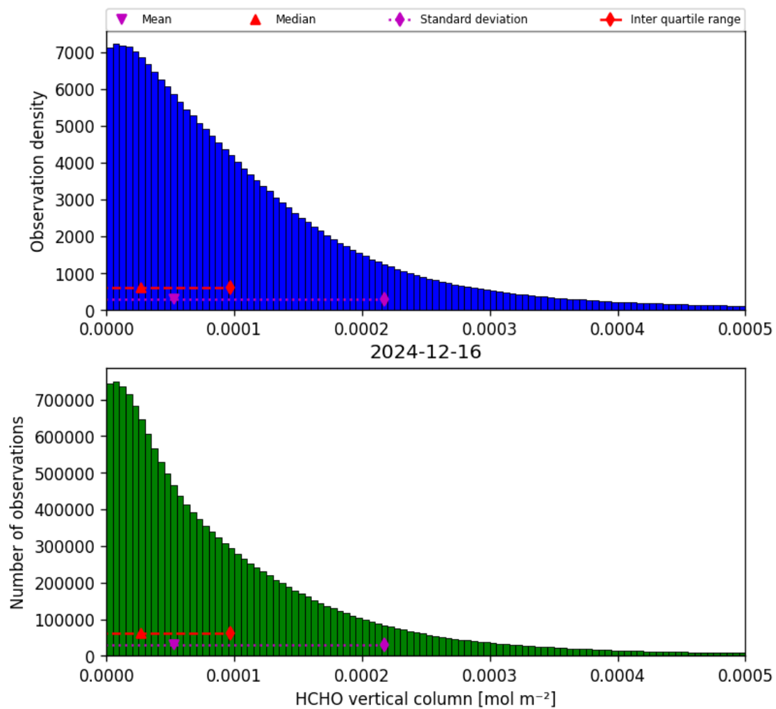
Figure 35: Histogram of “HCHO vertical column” for 2024-12-16 to 2024-12-17
