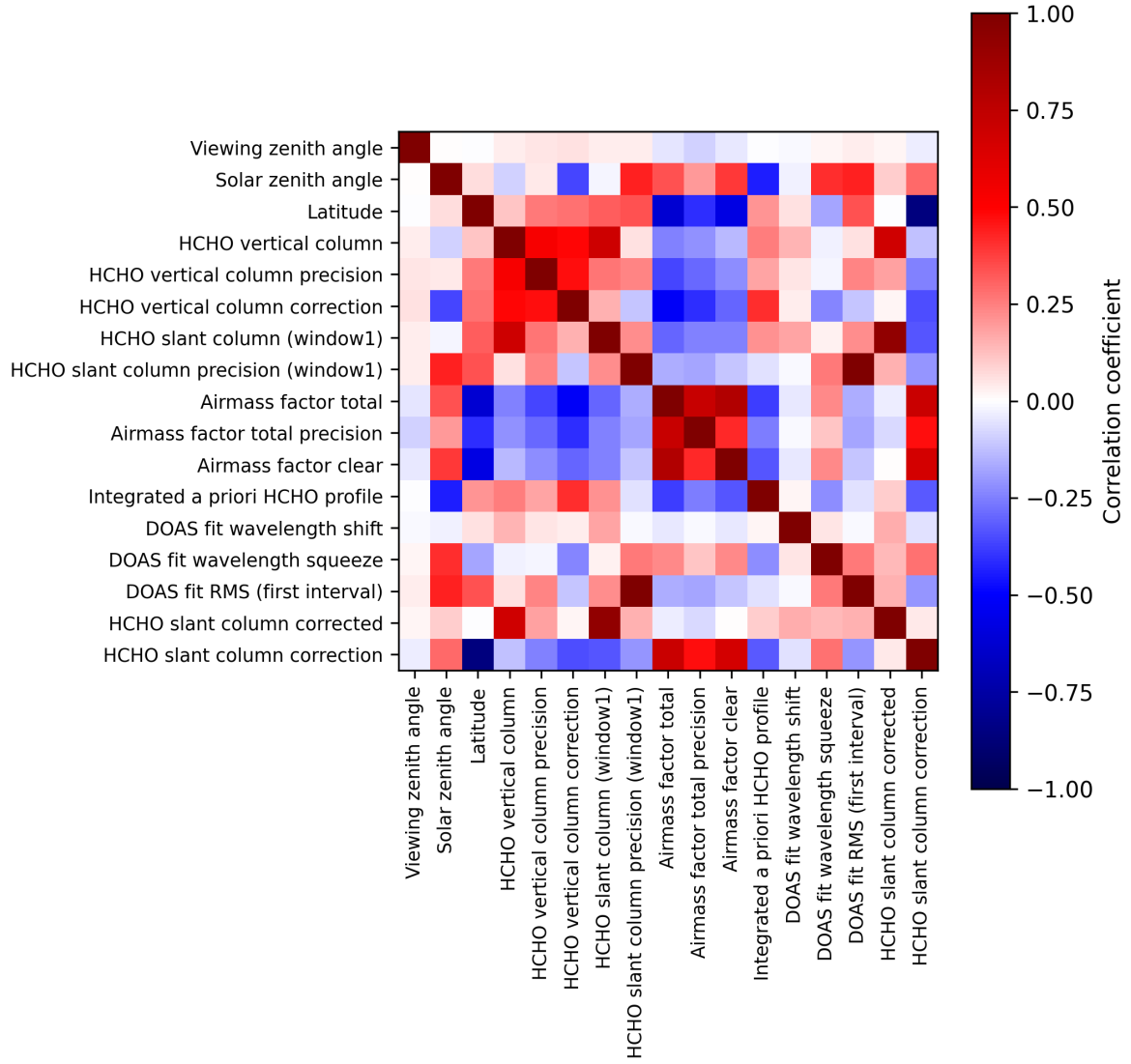
Figure 2: Map of correlation matrix for 2024-12-16 to 2024-12-17.
