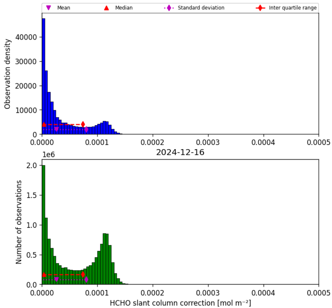
Figure 47: Histogram of “HCHO slant column correction” for 2024-12-16 to 2024-12-17
