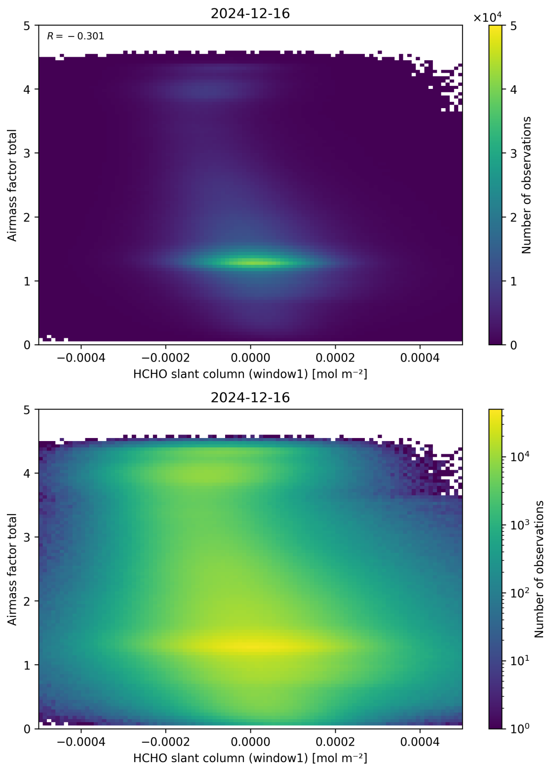
Figure 85: Scatter density plot of “HCHO slant column (window1)” against “Airmass factor total” for 2024-12-16 to 2024-12-17.
