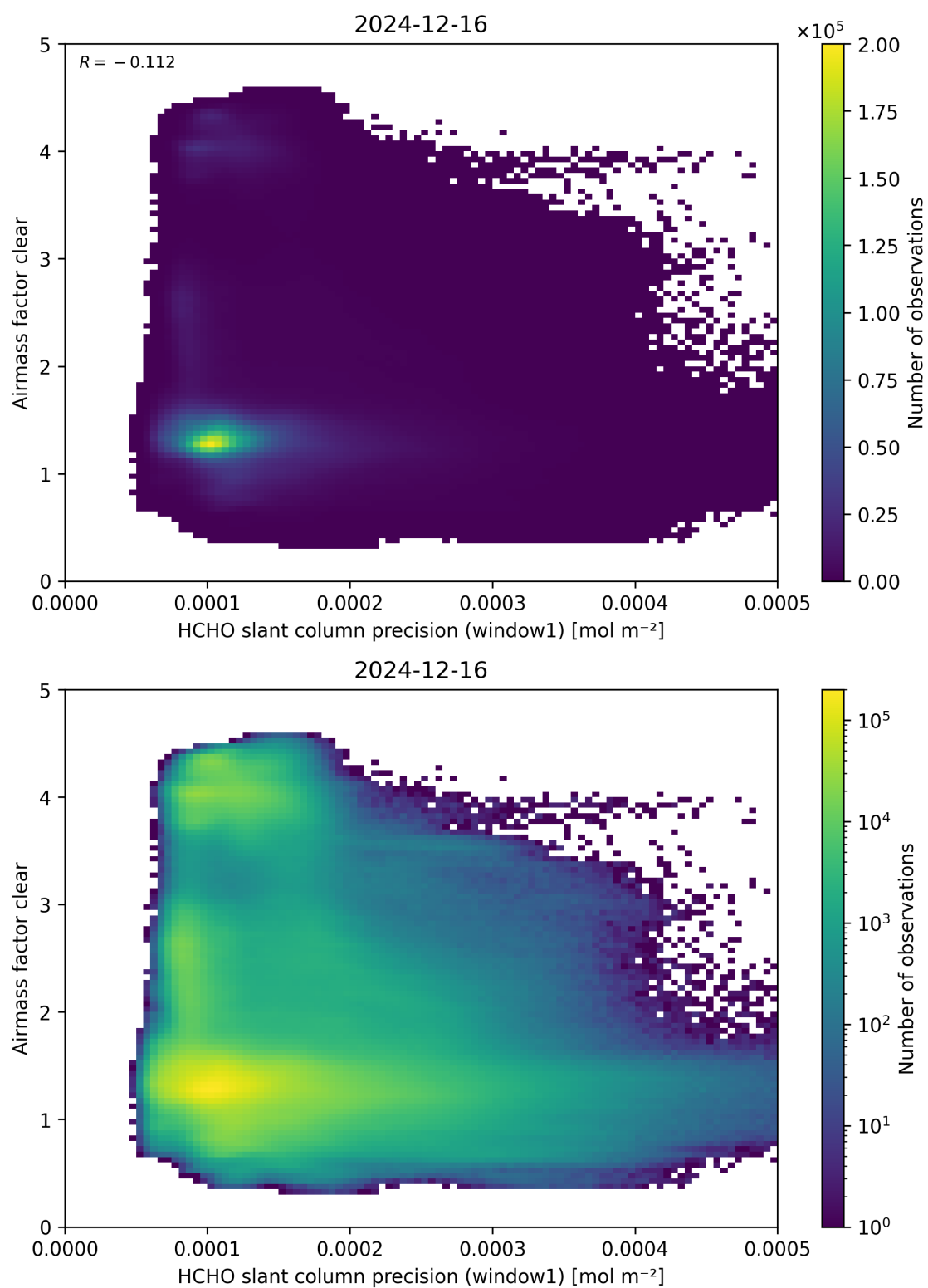
Figure 91: Scatter density plot of “HCHO slant column precision (window1)” against “Airmass factor clear” for 2024-12-16 to 2024-12-17.
