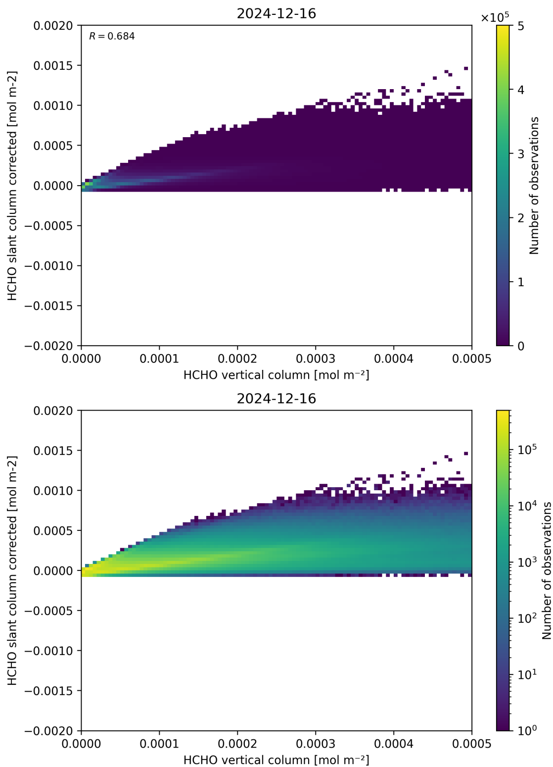
Figure 127: Scatter density plot of “HCHO vertical column” against “HCHO slant column corrected” for 2024-12-16 to 2024-12-17.
