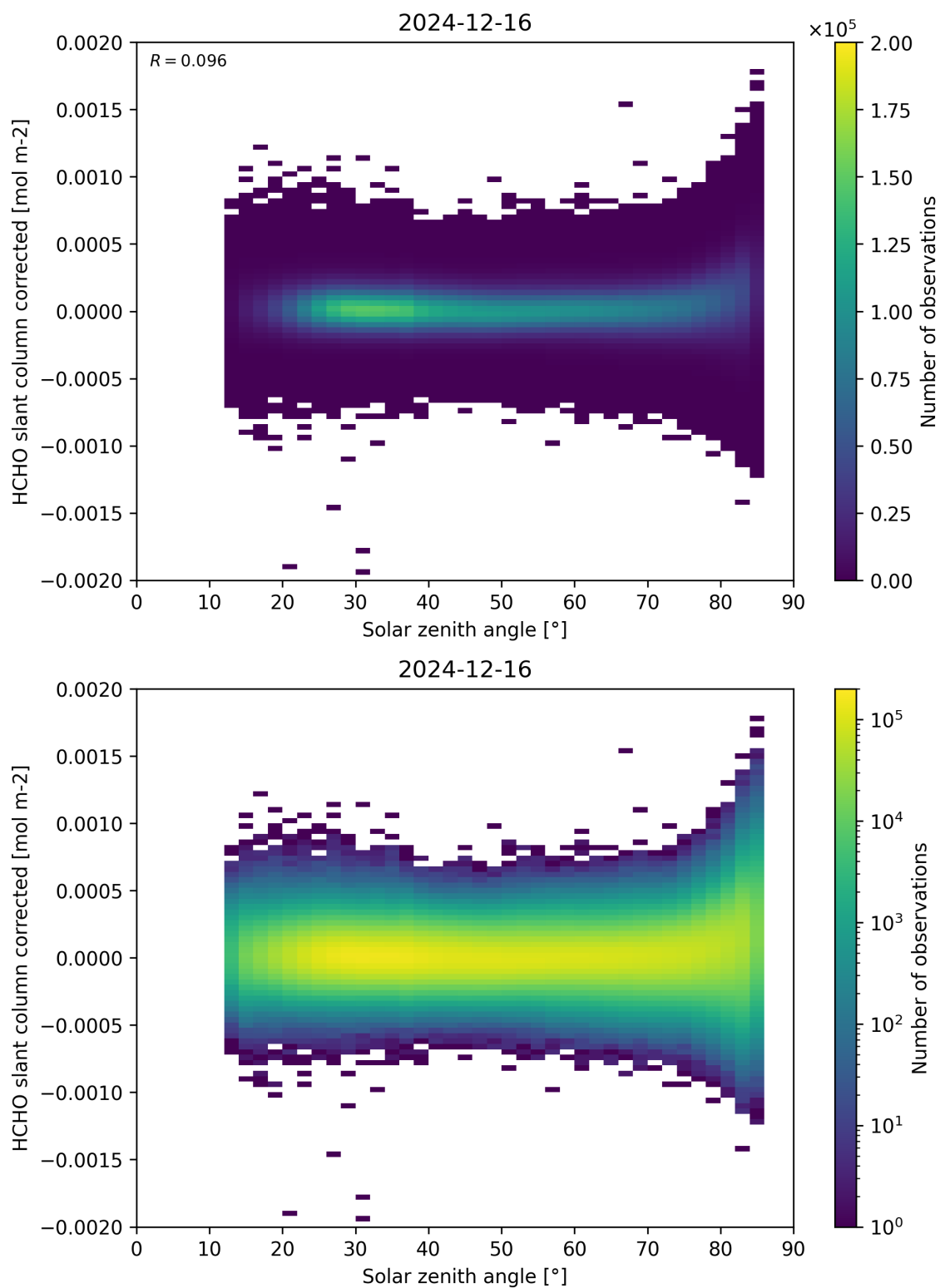
Figure 171: Scatter density plot of “Solar zenith angle” against “HCHO slant column corrected” for 2024-12-16 to 2024-12-17.
