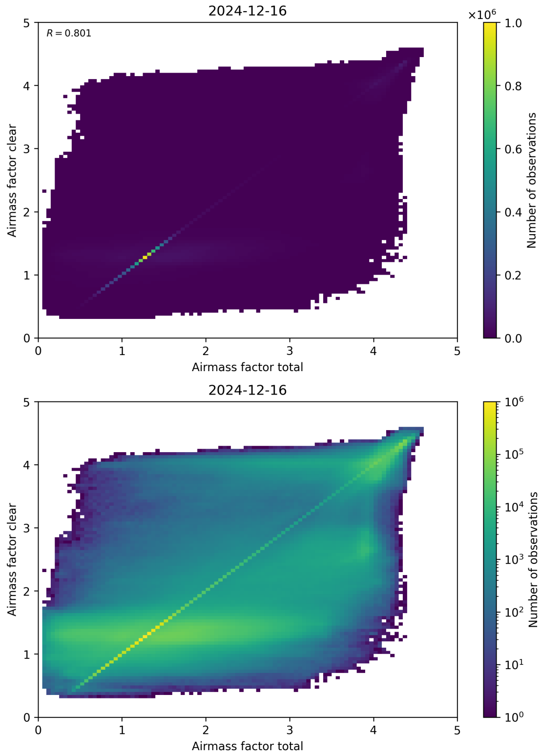
Figure 100: Scatter density plot of “Airmass factor total” against “Airmass factor clear” for 2024-12-16 to 2024-12-17.
