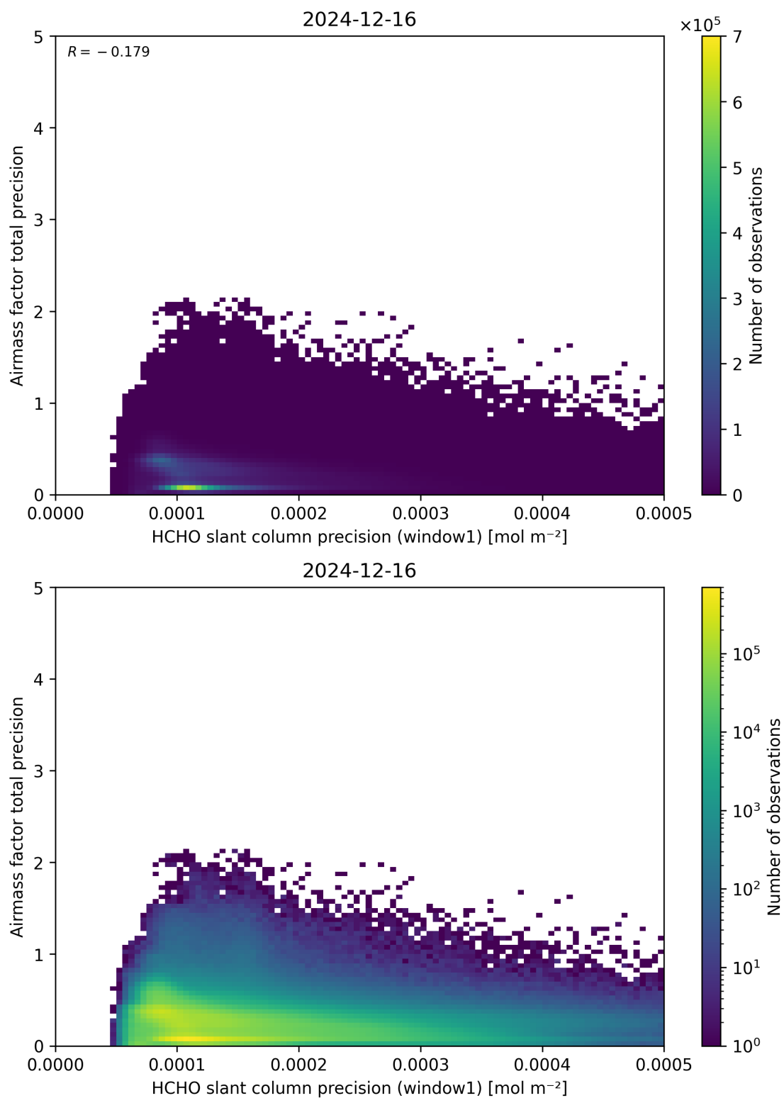
Figure 95: Scatter density plot of “HCHO slant column precision (window1)” against “Airmass factor total precision” for 2024-12-16 to 2024-12-17.
