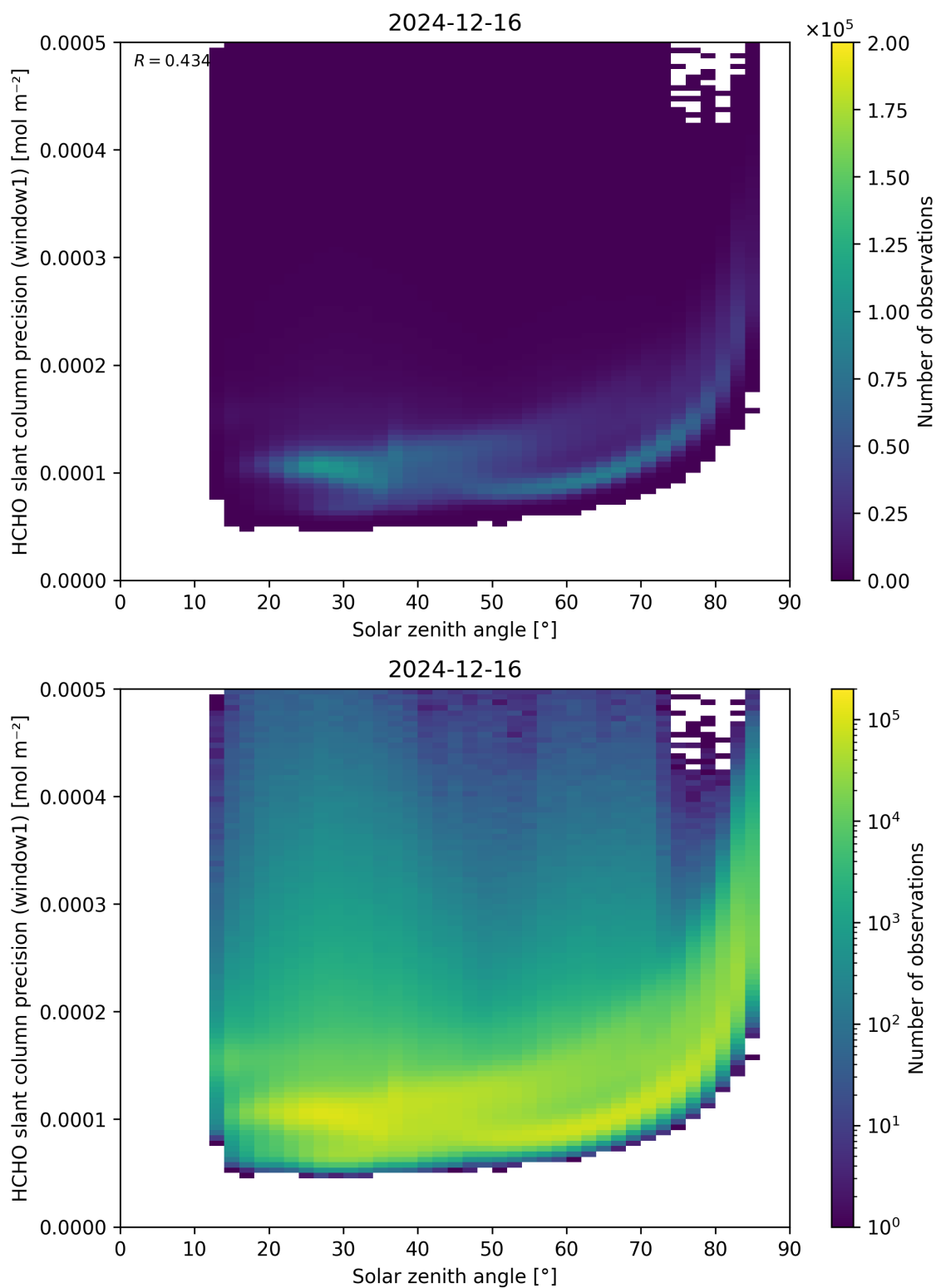
Figure 174: Scatter density plot of “Solar zenith angle” against “HCHO slant column precision (window1)” for 2024-12-16 to 2024-12-17.
