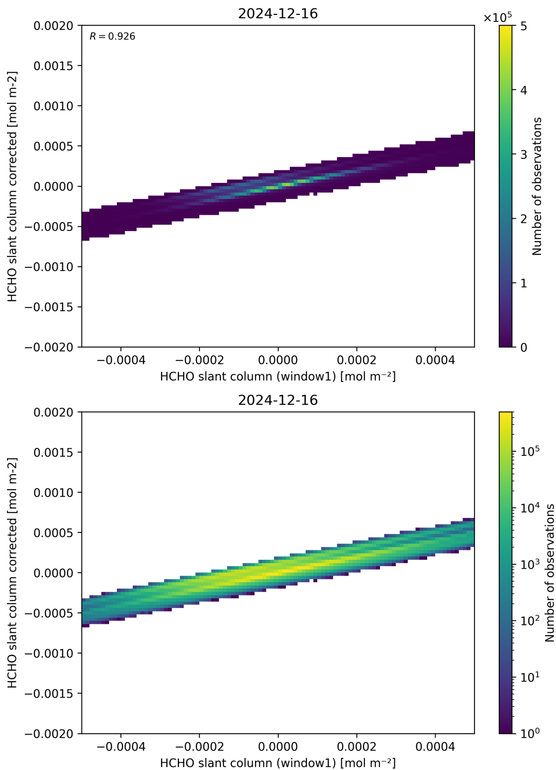
Figure 82: Scatter density plot of “HCHO slant column (window1)” against “HCHO slant column corrected” for 2024-12-16 to 2024-12-17.
