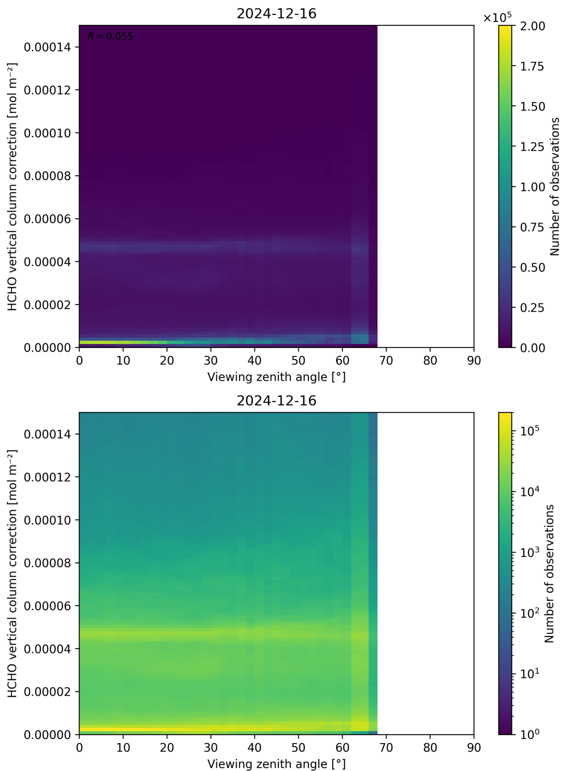
Figure 193: Scatter density plot of “Viewing zenith angle” against “HCHO vertical column correction” for 2024-12-16 to 2024-12-17.
