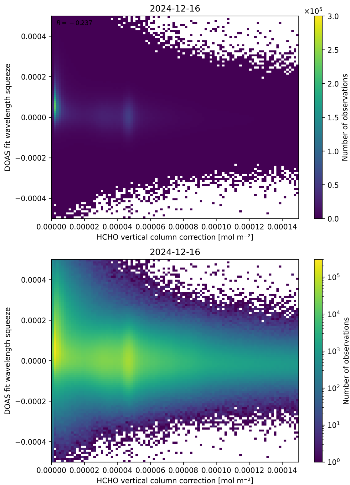
Figure 114: Scatter density plot of “HCHO vertical column correction” against “DOAS fit wavelength squeeze” for 2024-12-16 to 2024-12-17.
