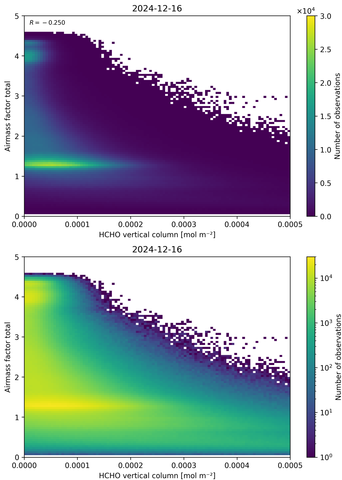
Figure 131: Scatter density plot of “HCHO vertical column” against “Airmass factor total” for 2024-12-16 to 2024-12-17.
