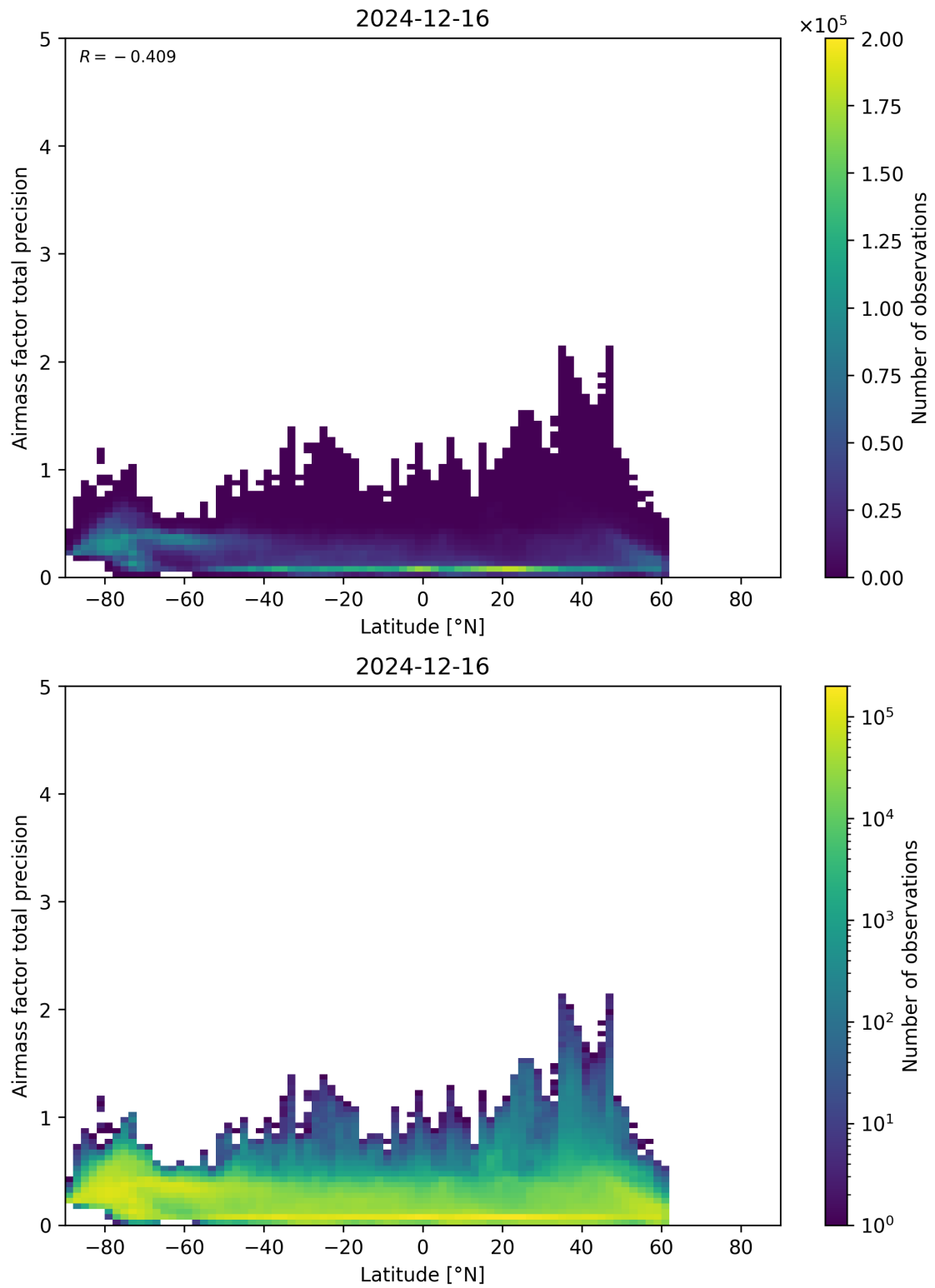
Figure 162: Scatter density plot of “Latitude” against “Airmass factor total precision” for 2024-12-16 to 2024-12-17.
