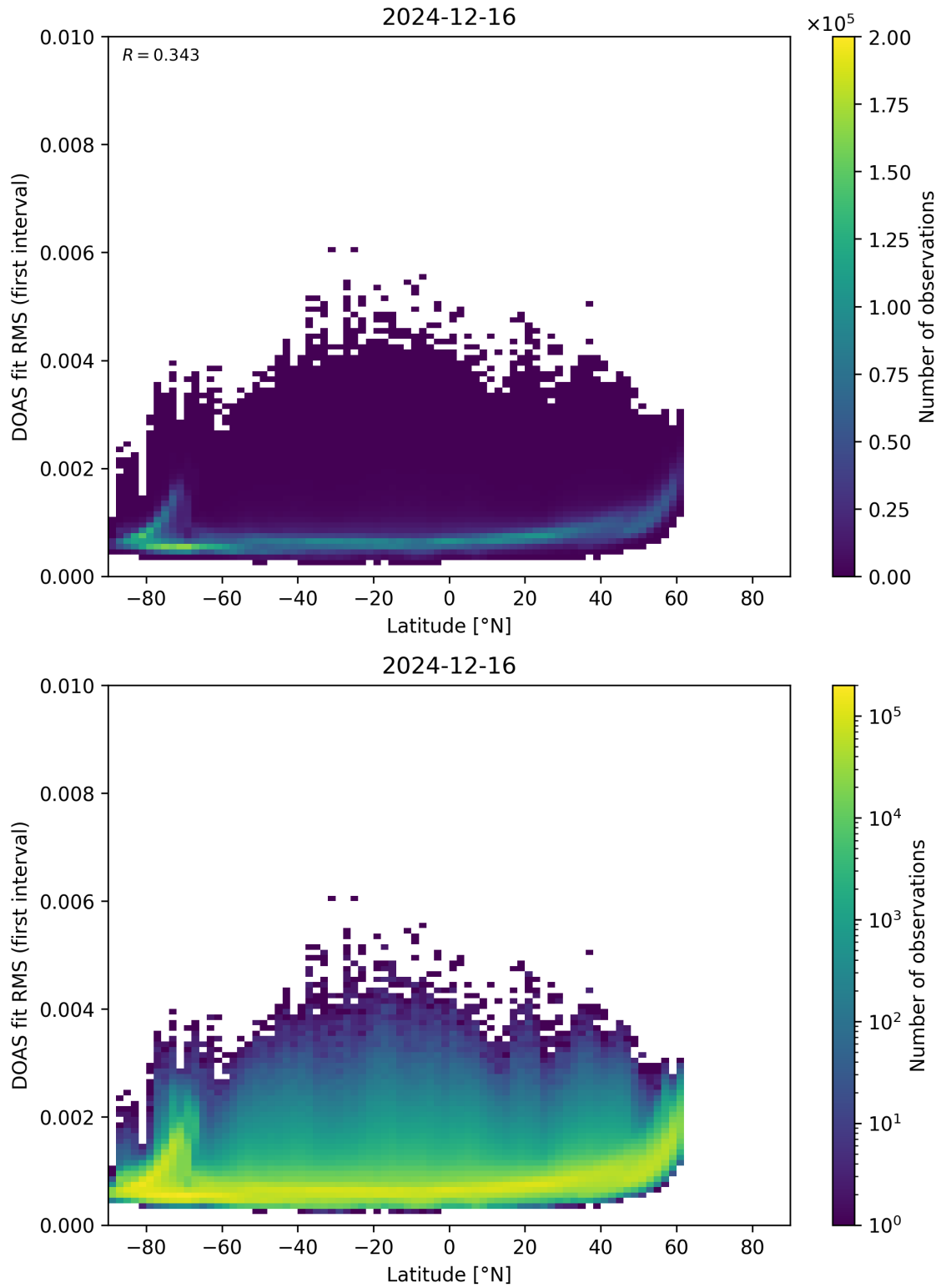
Figure 153: Scatter density plot of “Latitude” against “DOAS fit RMS (first interval)” for 2024-12-16 to 2024-12-17.
