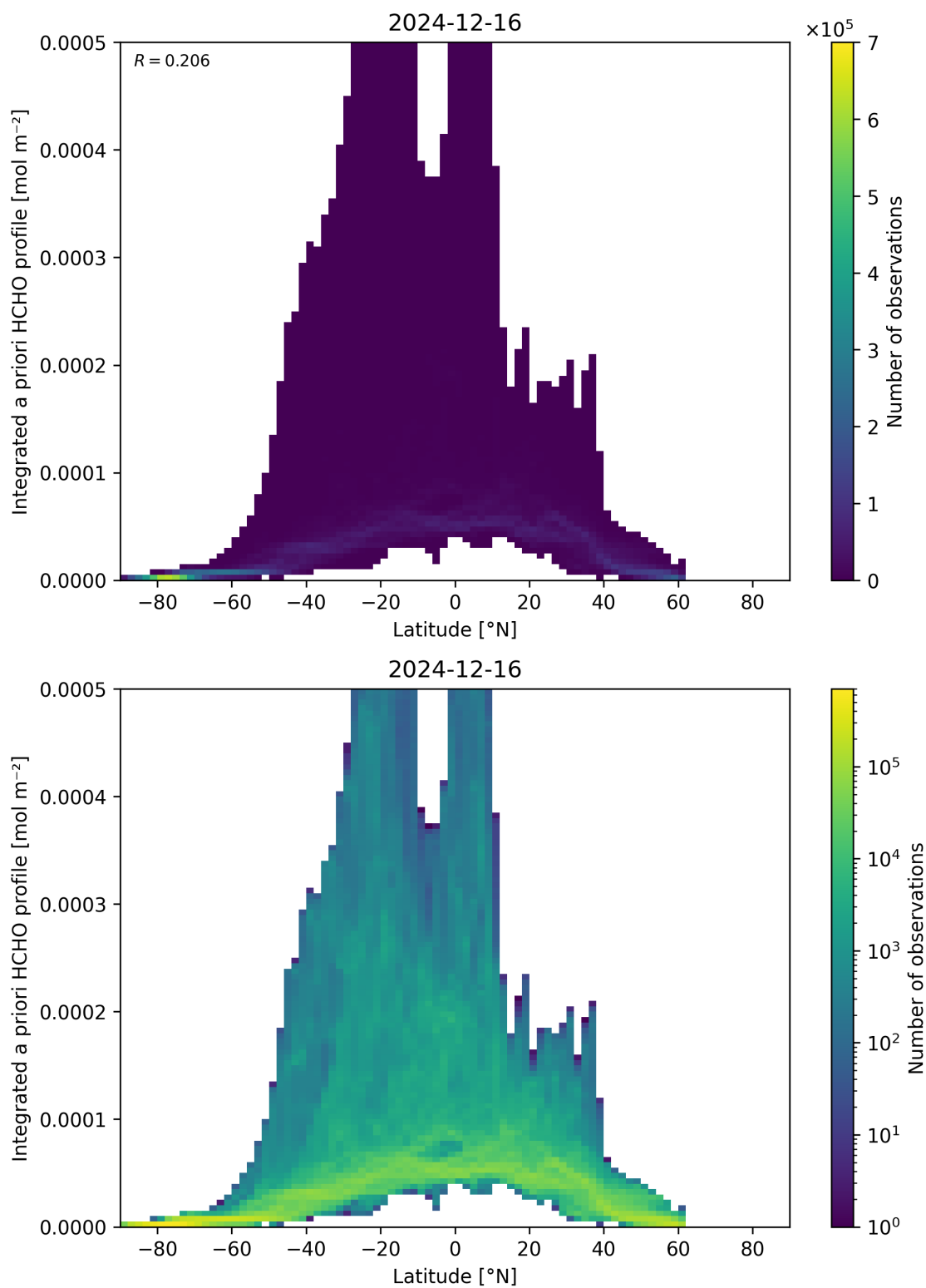
Figure 166: Scatter density plot of “Latitude” against “Integrated a priori HCHO profile” for 2024-12-16 to 2024-12-17.
