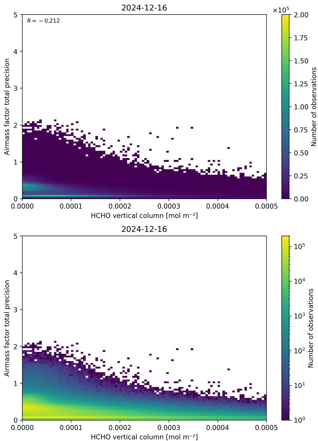
Figure 132: Scatter density plot of “HCHO vertical column” against “Airmass factor total precision” for 2024-12-16 to 2024-12-17.
