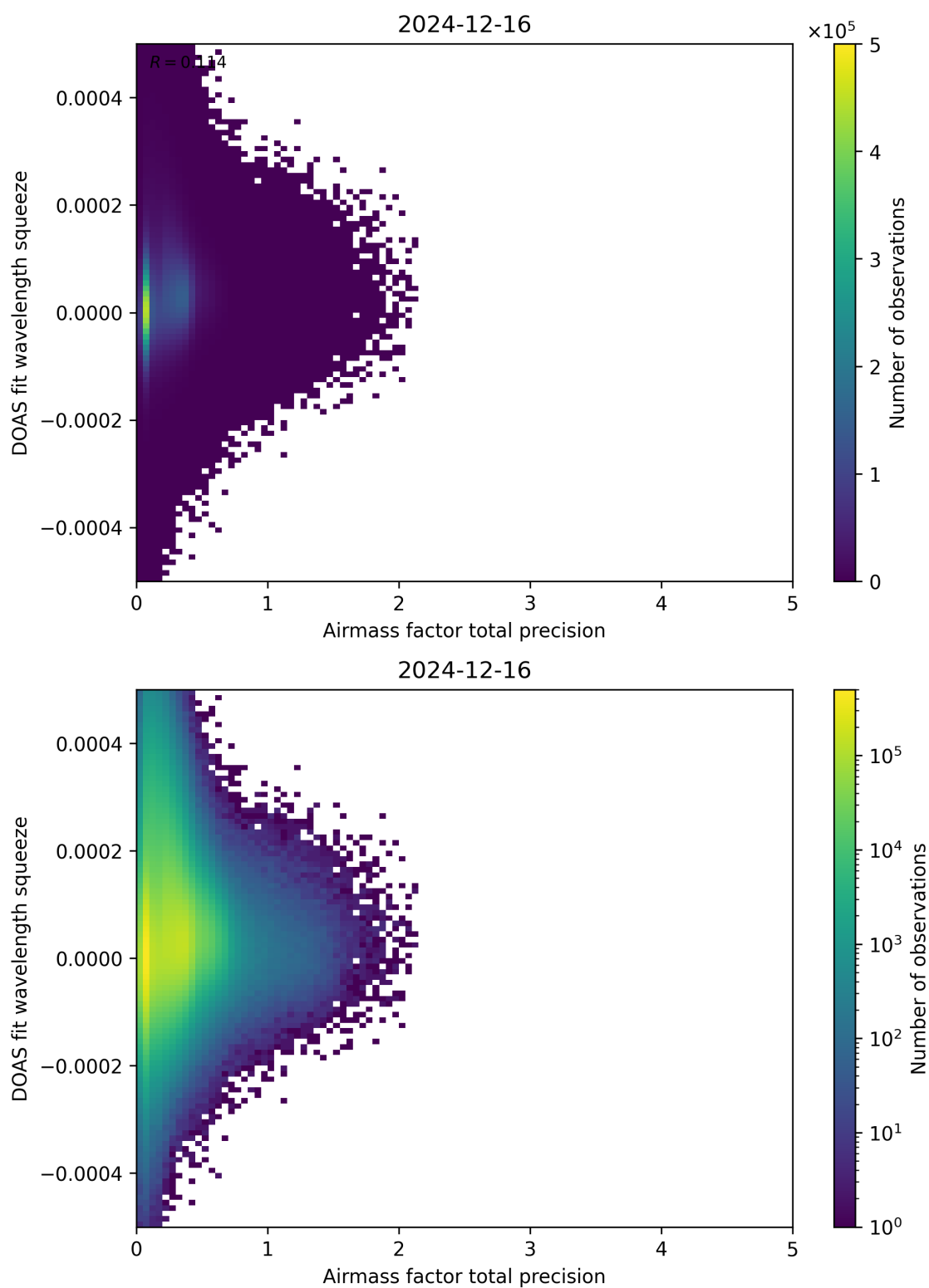
Figure 107: Scatter density plot of “Airmass factor total precision” against “DOAS fit wavelength squeeze” for 2024-12-16 to 2024-12-17.
