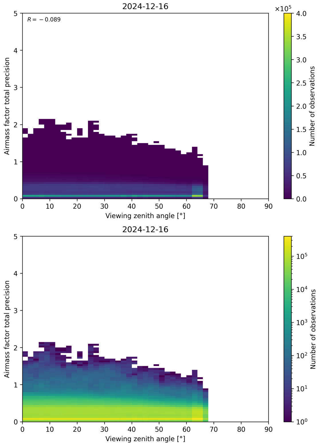
Figure 191: Scatter density plot of “Viewing zenith angle” against “Airmass factor total precision” for 2024-12-16 to 2024-12-17.
