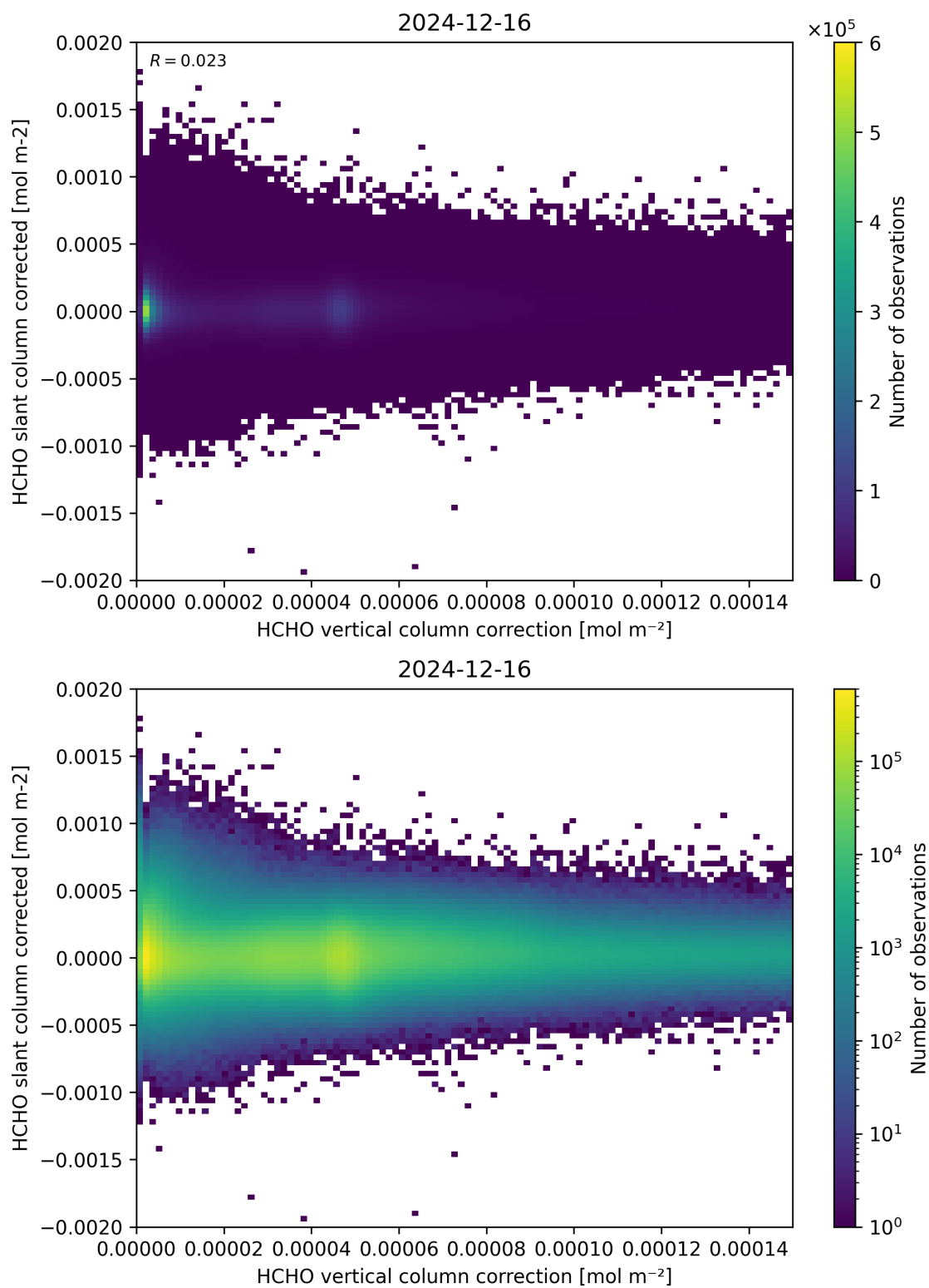
Figure 116: Scatter density plot of “HCHO vertical column correction” against “HCHO slant column corrected” for 2024-12-16 to 2024-12-17.
