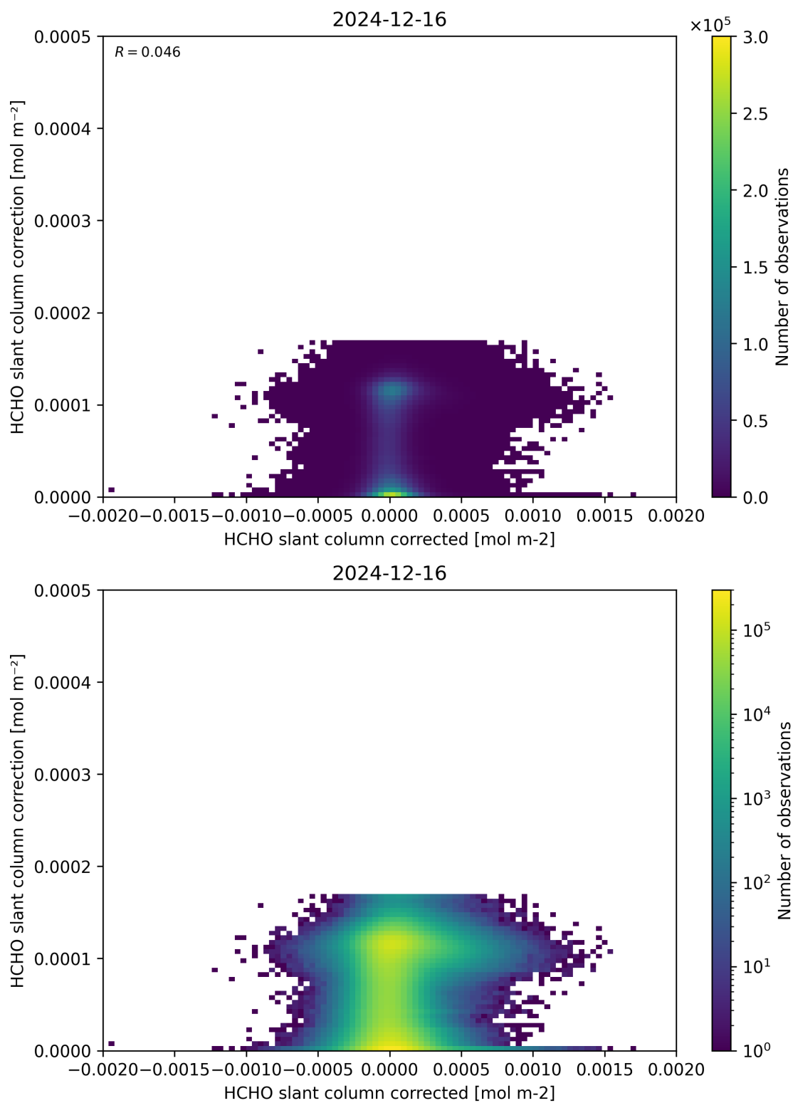
Figure 77: Scatter density plot of “HCHO slant column corrected” against “HCHO slant column correction” for 2024-12-16 to 2024-12-17.
