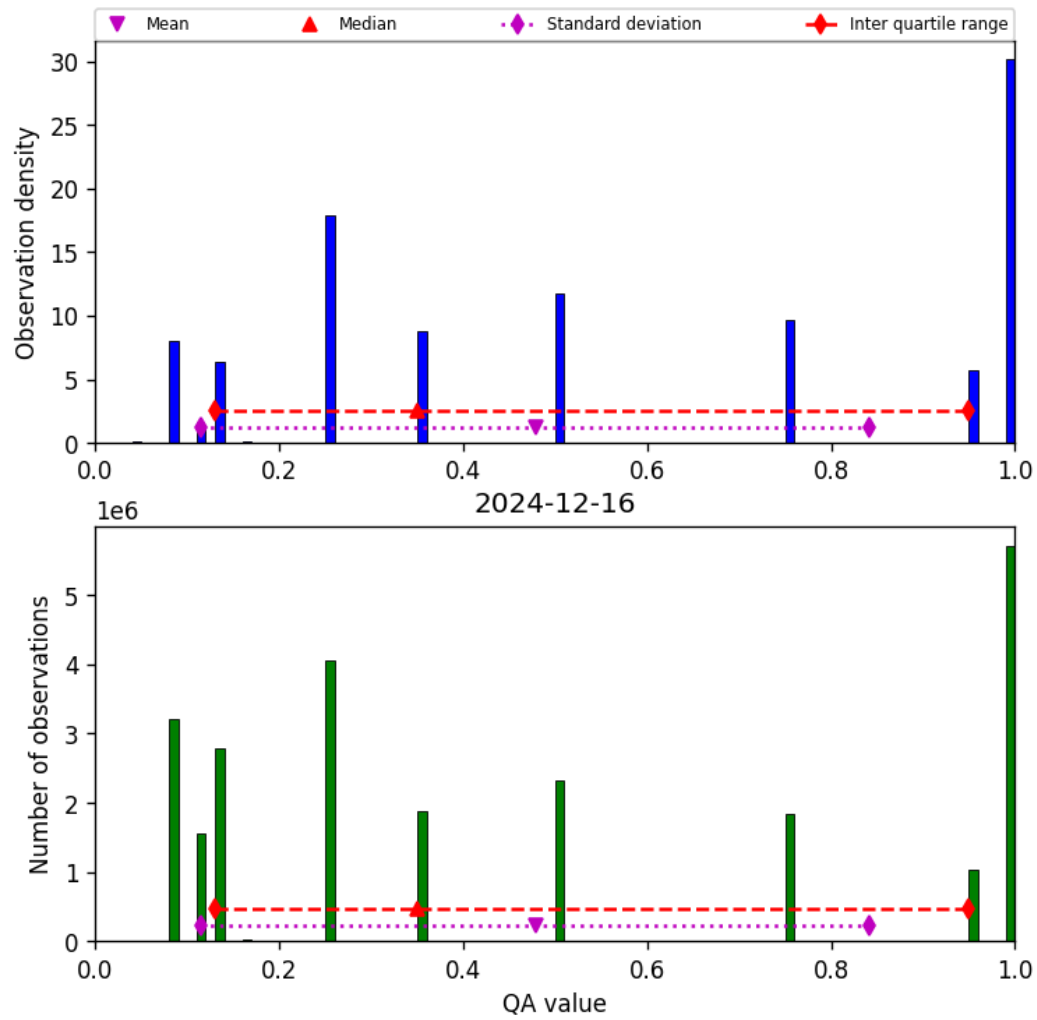
Figure 34: Histogram of “QA value” for 2024-12-16 to 2024-12-17
