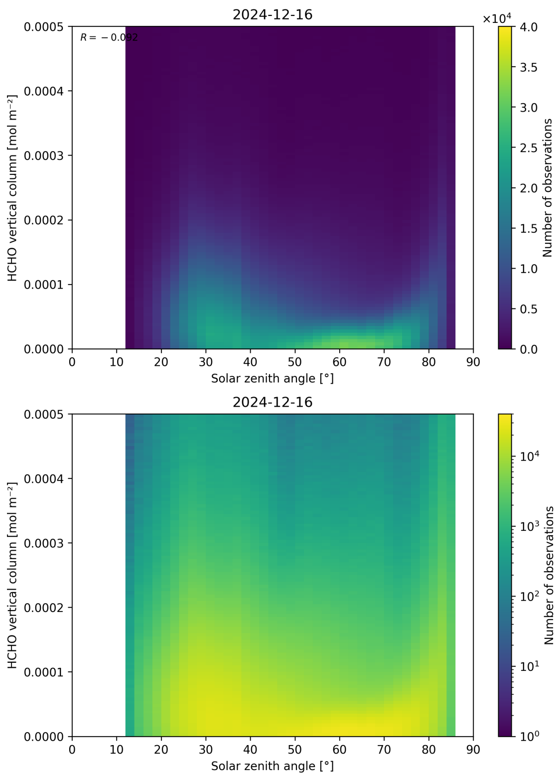
Figure 177: Scatter density plot of “Solar zenith angle” against “HCHO vertical column” for 2024-12-16 to 2024-12-17.
