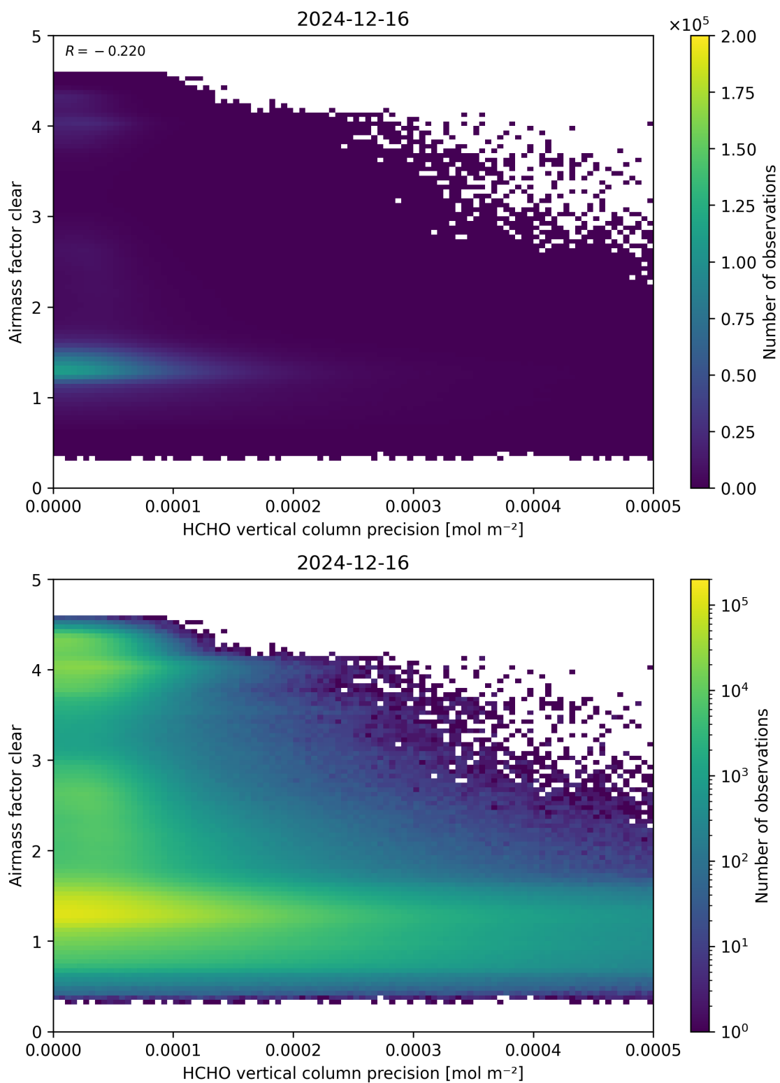
Figure 139: Scatter density plot of “HCHO vertical column precision” against “Airmass factor clear” for 2024-12-16 to 2024-12-17.
