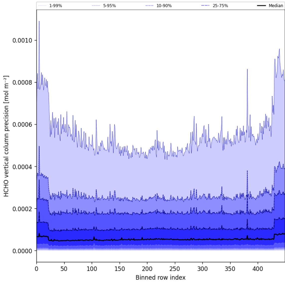
Figure 50: Along track statistics of “HCHO vertical column precision” for 2024-12-16 to 2024-12-17
