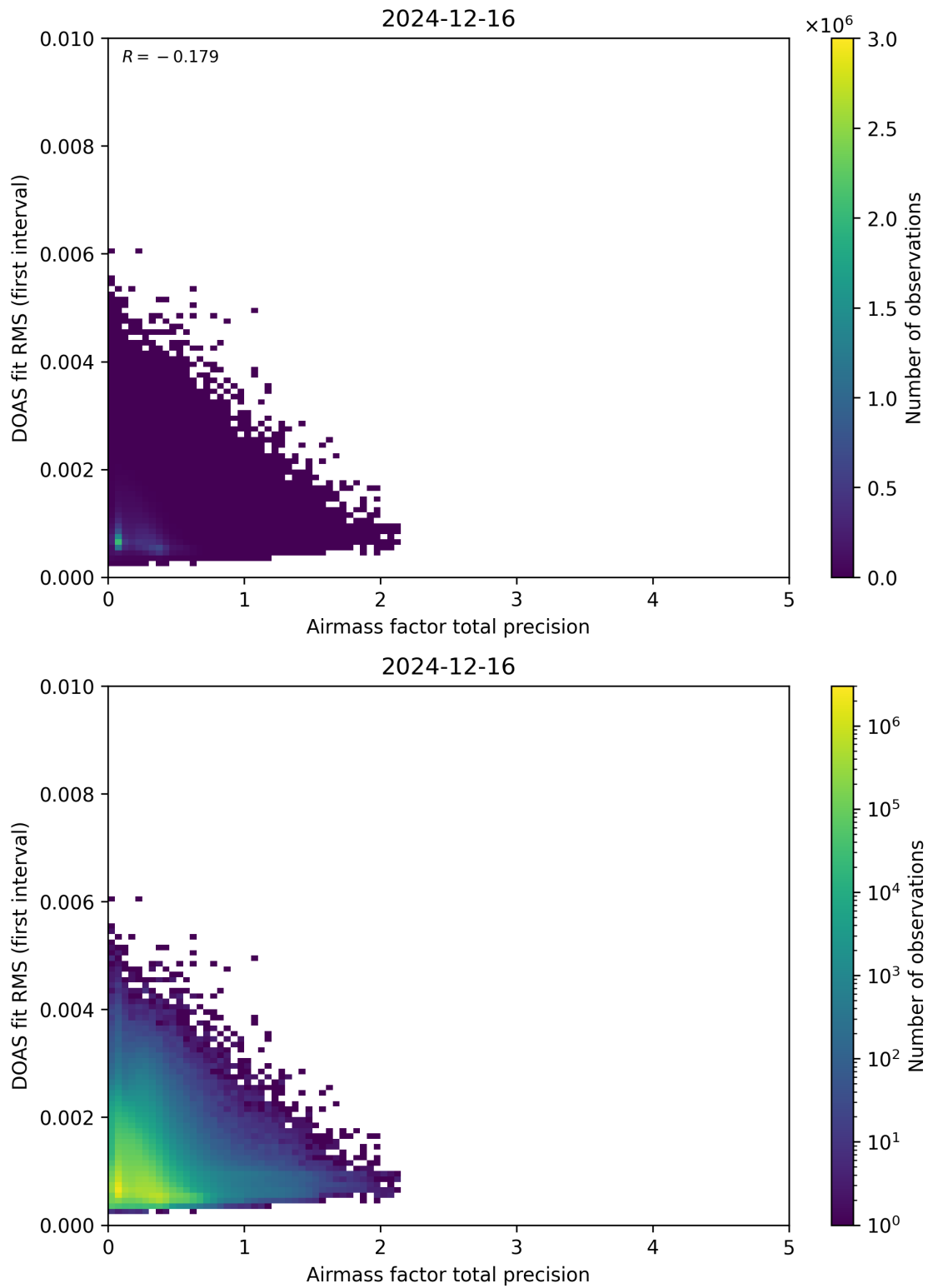
Figure 105: Scatter density plot of “Airmass factor total precision” against “DOAS fit RMS (first interval)” for 2024-12-16 to 2024-12-17.
