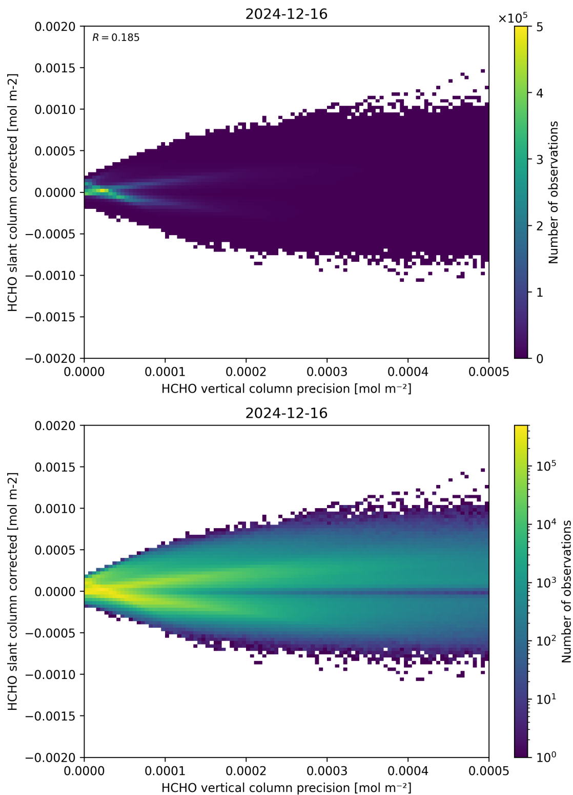
Figure 140: Scatter density plot of “HCHO vertical column precision” against “HCHO slant column corrected” for 2024-12-16 to 2024-12-17.
