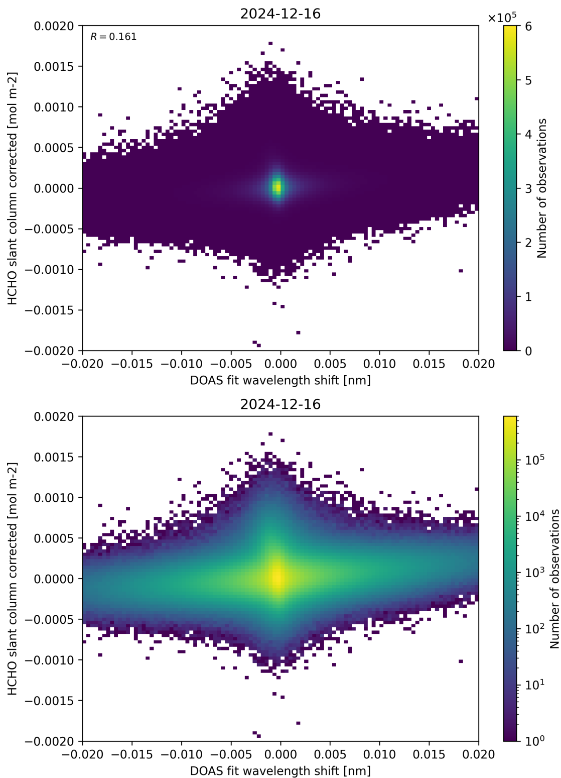
Figure 66: Scatter density plot of “DOAS fit wavelength shift” against “HCHO slant column corrected” for 2024-12-16 to 2024-12-17.
