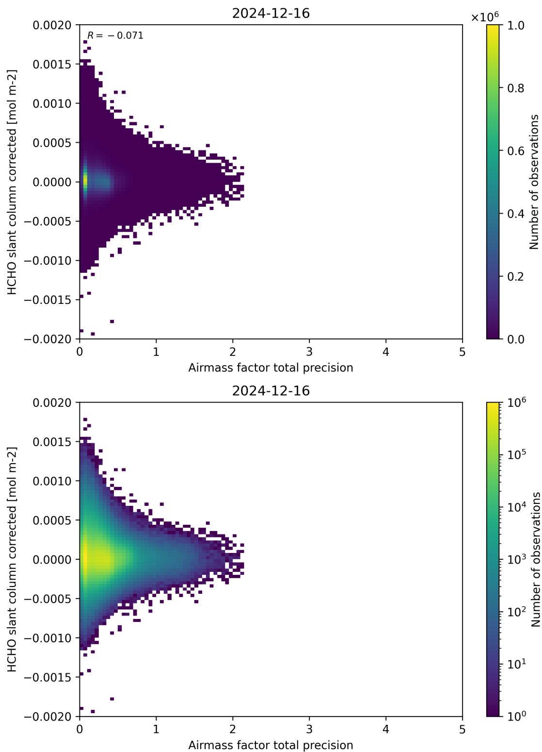
Figure 109: Scatter density plot of “Airmass factor total precision” against “HCHO slant column corrected” for 2024-12-16 to 2024-12-17.
