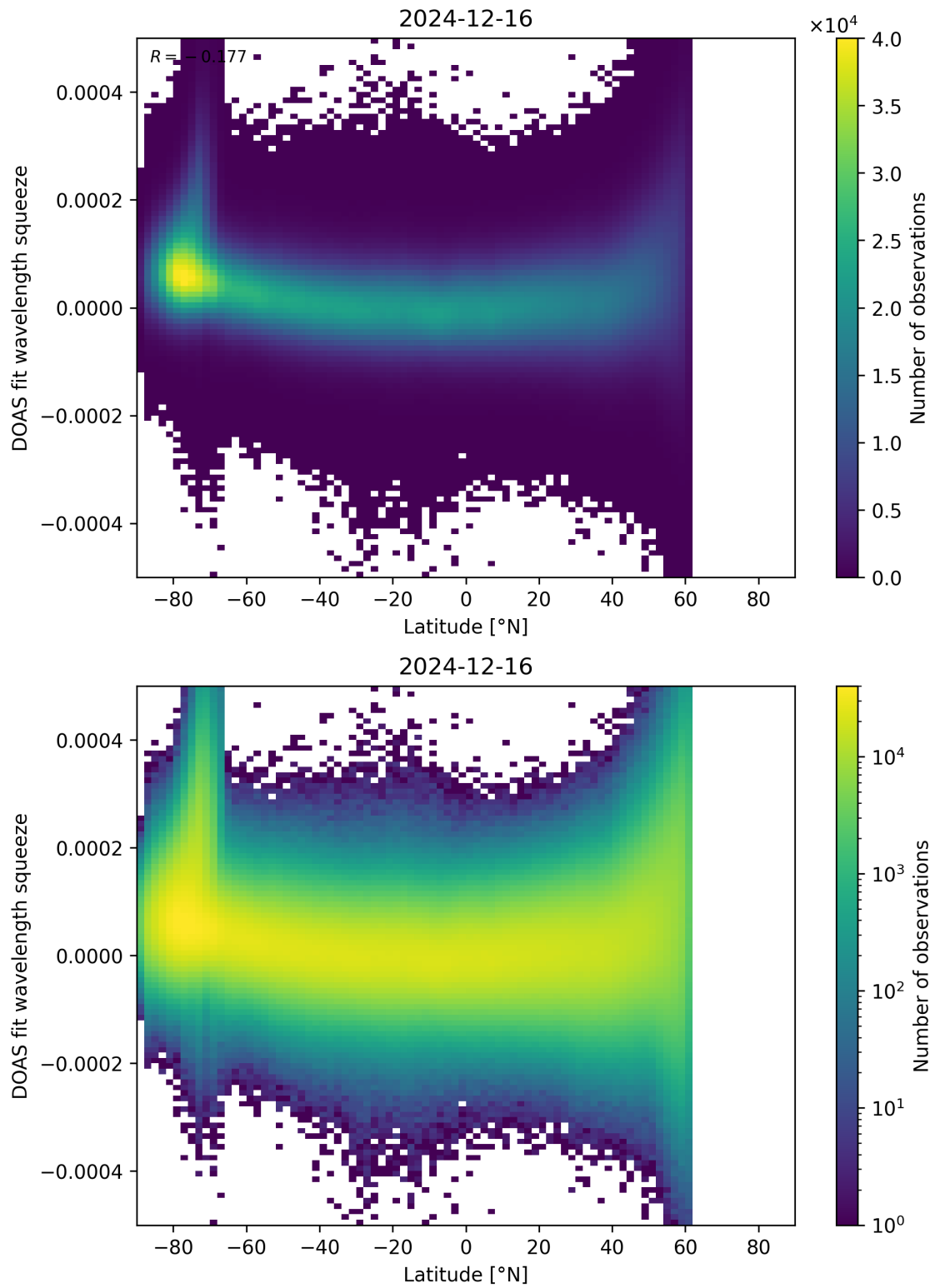
Figure 155: Scatter density plot of “Latitude” against “DOAS fit wavelength squeeze” for 2024-12-16 to 2024-12-17.
