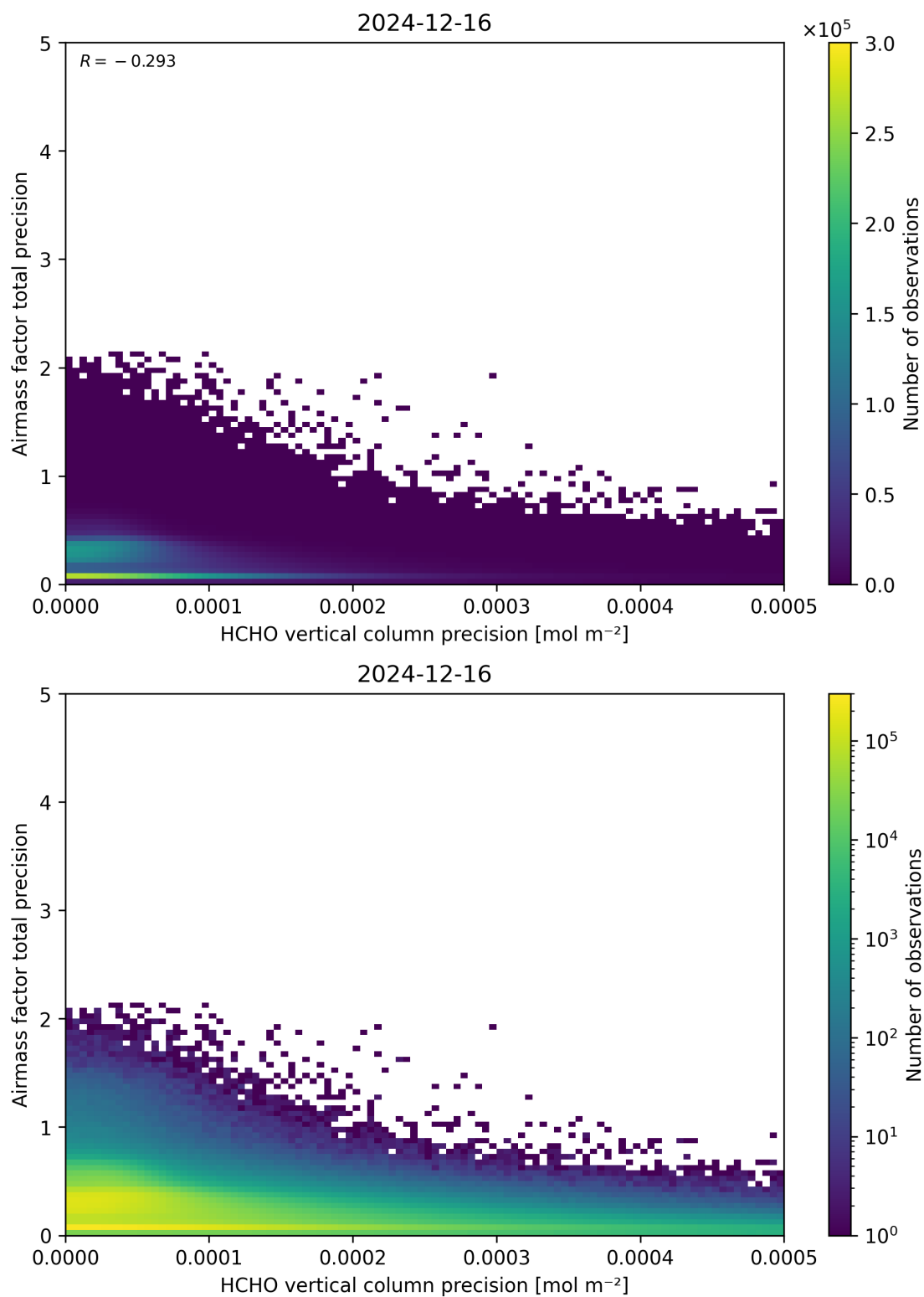
Figure 145: Scatter density plot of “HCHO vertical column precision” against “Airmass factor total precision” for 2024-12-16 to 2024-12-17.
