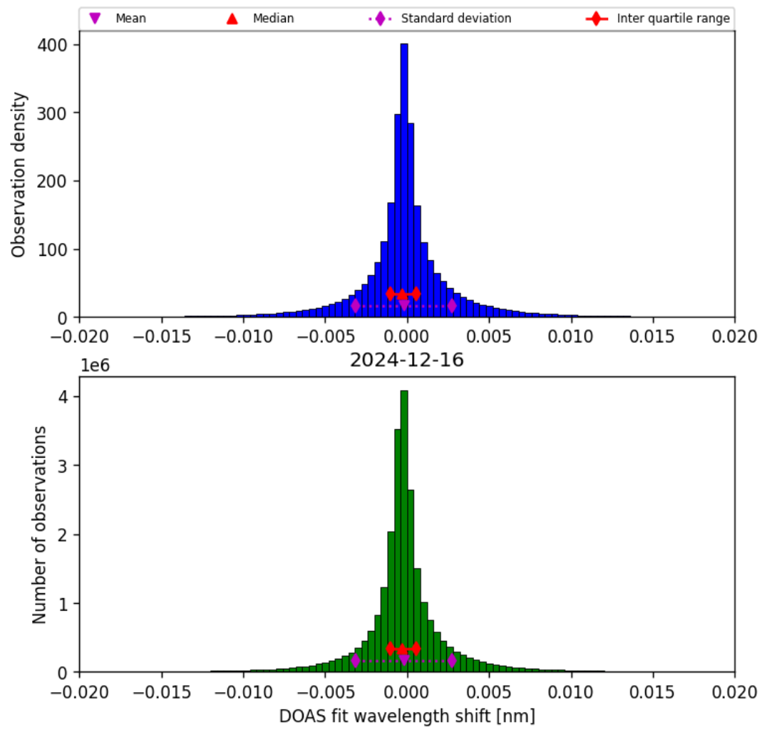
Figure 44: Histogram of “DOAS fit wavelength shift” for 2024-12-16 to 2024-12-17
