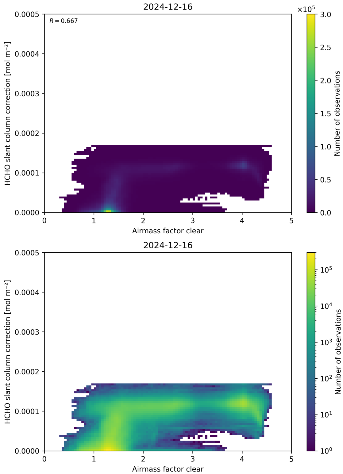
Figure 75: Scatter density plot of “Airmass factor clear” against “HCHO slant column correction” for 2024-12-16 to 2024-12-17.
