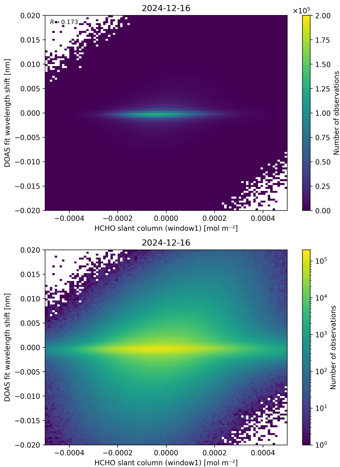
Figure 79: Scatter density plot of “HCHO slant column (window1)” against “DOAS fit wavelength shift” for 2024-12-16 to 2024-12-17.
