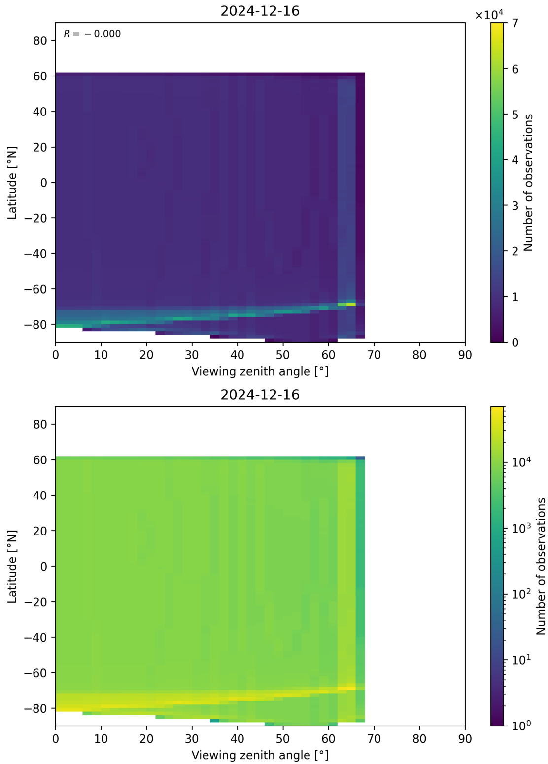
Figure 196: Scatter density plot of “Viewing zenith angle” against “Latitude” for 2024-12-16 to 2024-12-17.
