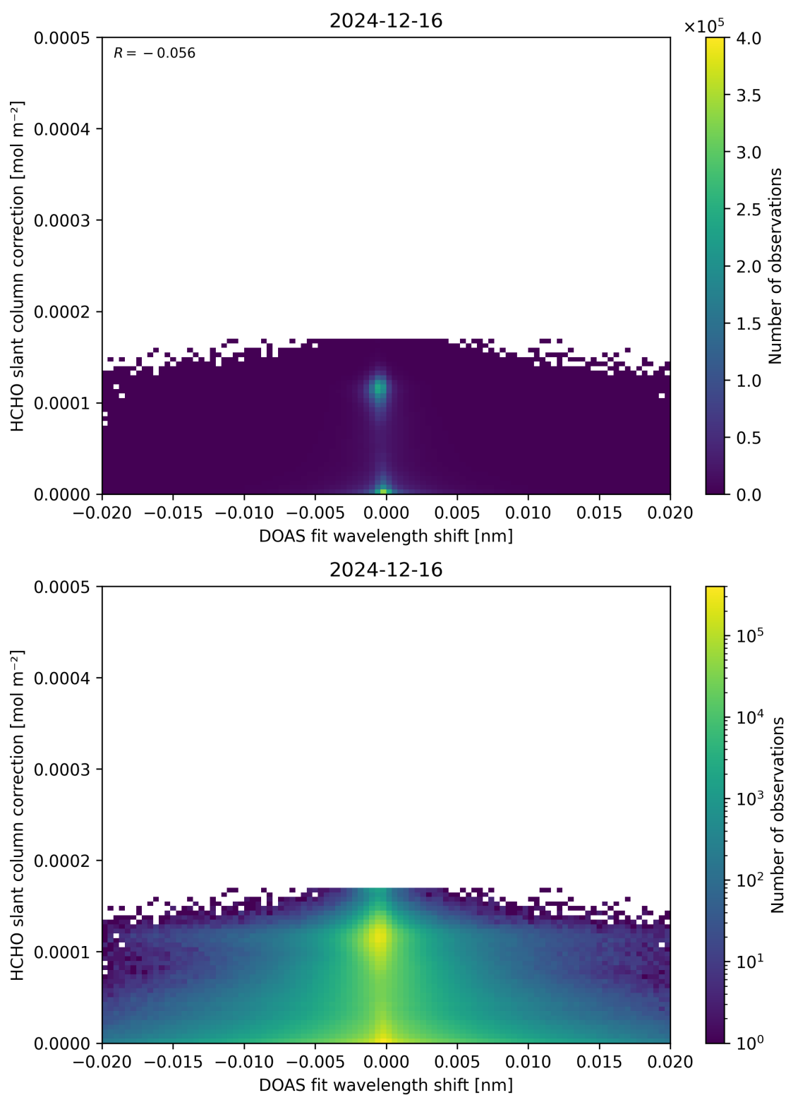
Figure 67: Scatter density plot of “DOAS fit wavelength shift” against “HCHO slant column correction” for 2024-12-16 to 2024-12-17.
