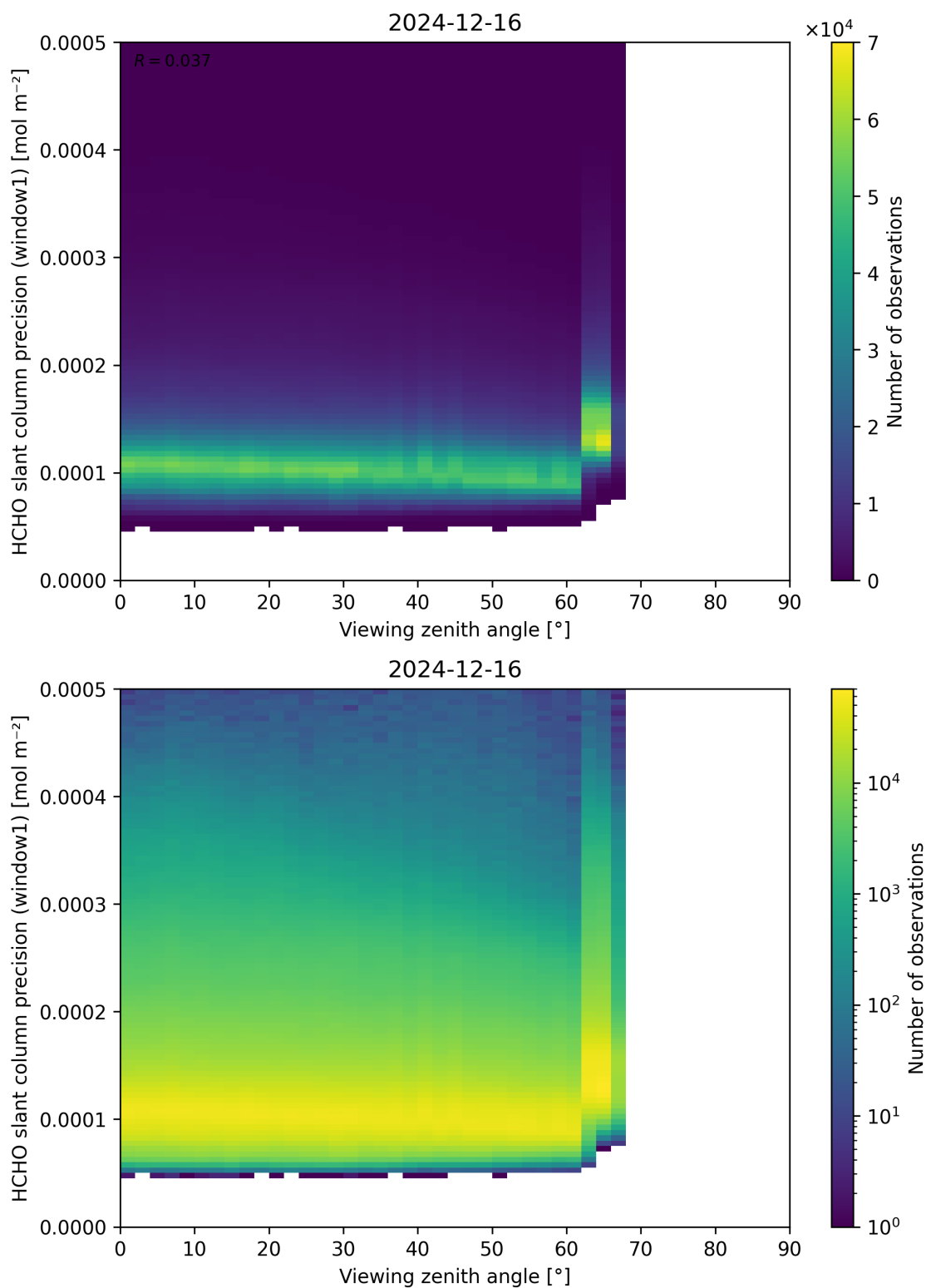
Figure 189: Scatter density plot of “Viewing zenith angle” against “HCHO slant column precision (window1)” for 2024-12-16 to 2024-12-17.
