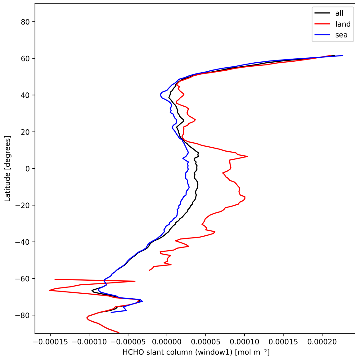
Figure 24: Zonal average of “HCHO slant column (window1)” for 2024-12-16 to 2024-12-17.
