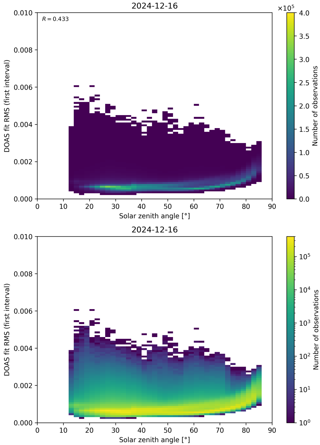
Figure 167: Scatter density plot of “Solar zenith angle” against “DOAS fit RMS (first interval)” for 2024-12-16 to 2024-12-17.
