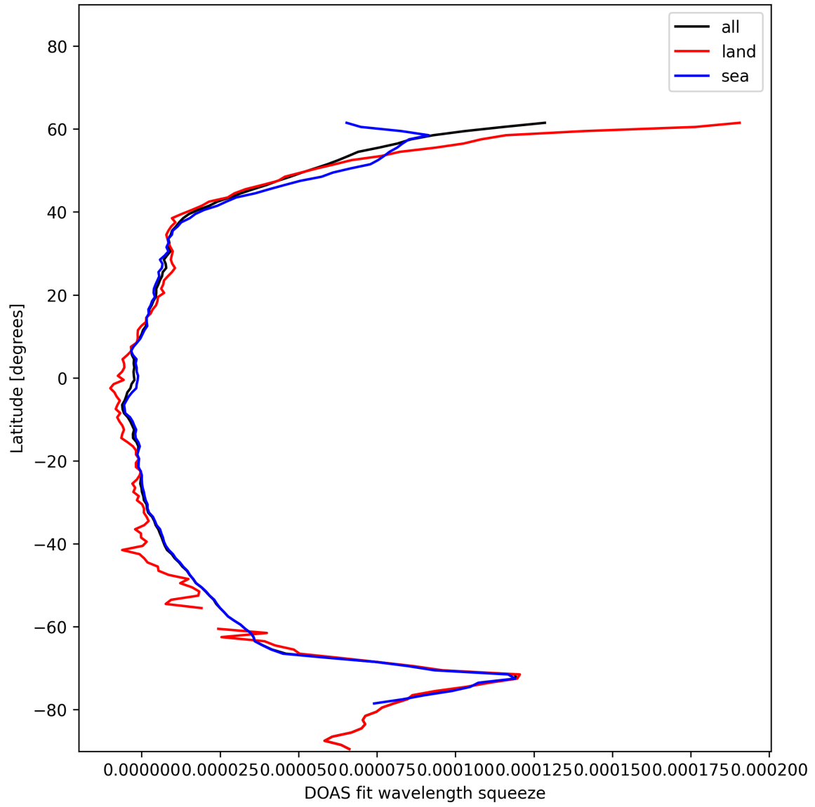
Figure 31: Zonal average of “DOAS fit wavelength squeeze” for 2024-12-16 to 2024-12-17.
