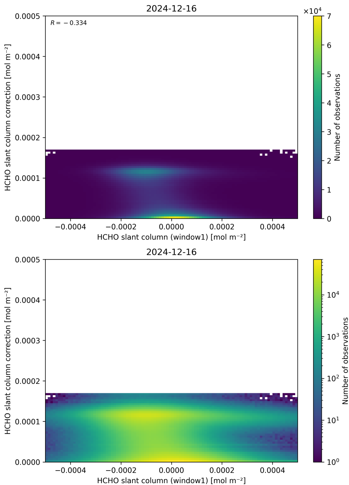
Figure 83: Scatter density plot of “HCHO slant column (window1)” against “HCHO slant column correction” for 2024-12-16 to 2024-12-17.
