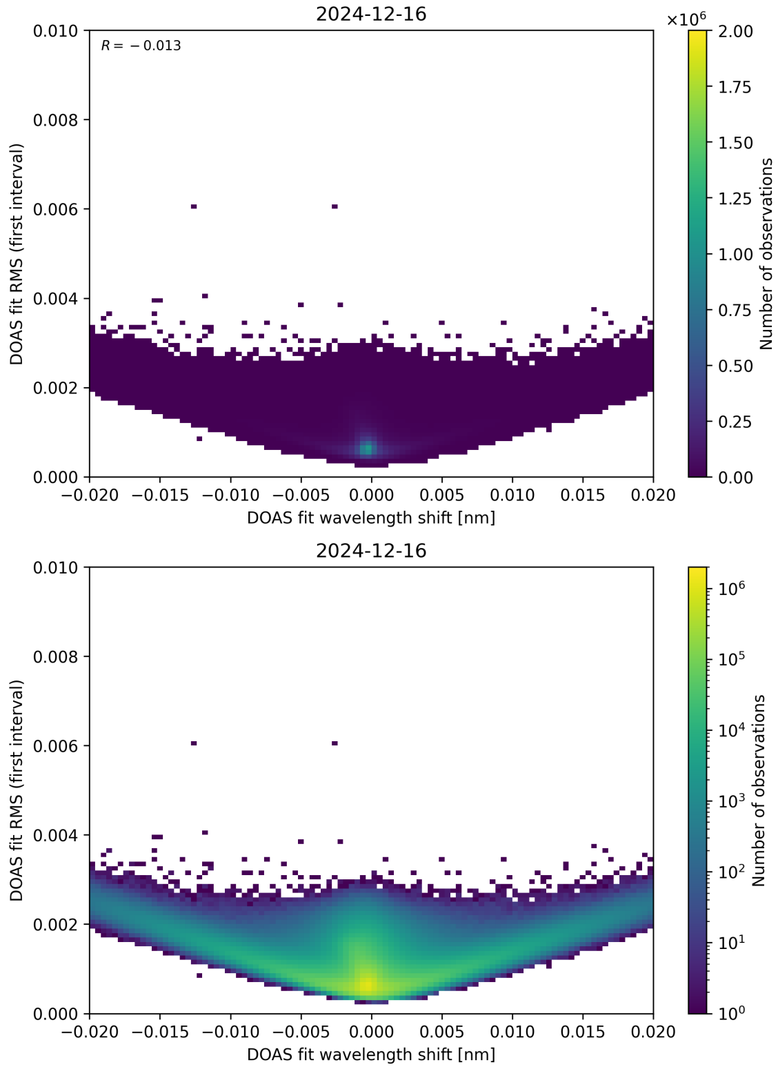
Figure 64: Scatter density plot of “DOAS fit wavelength shift” against “DOAS fit RMS (first interval)” for 2024-12-16 to 2024-12-17.
