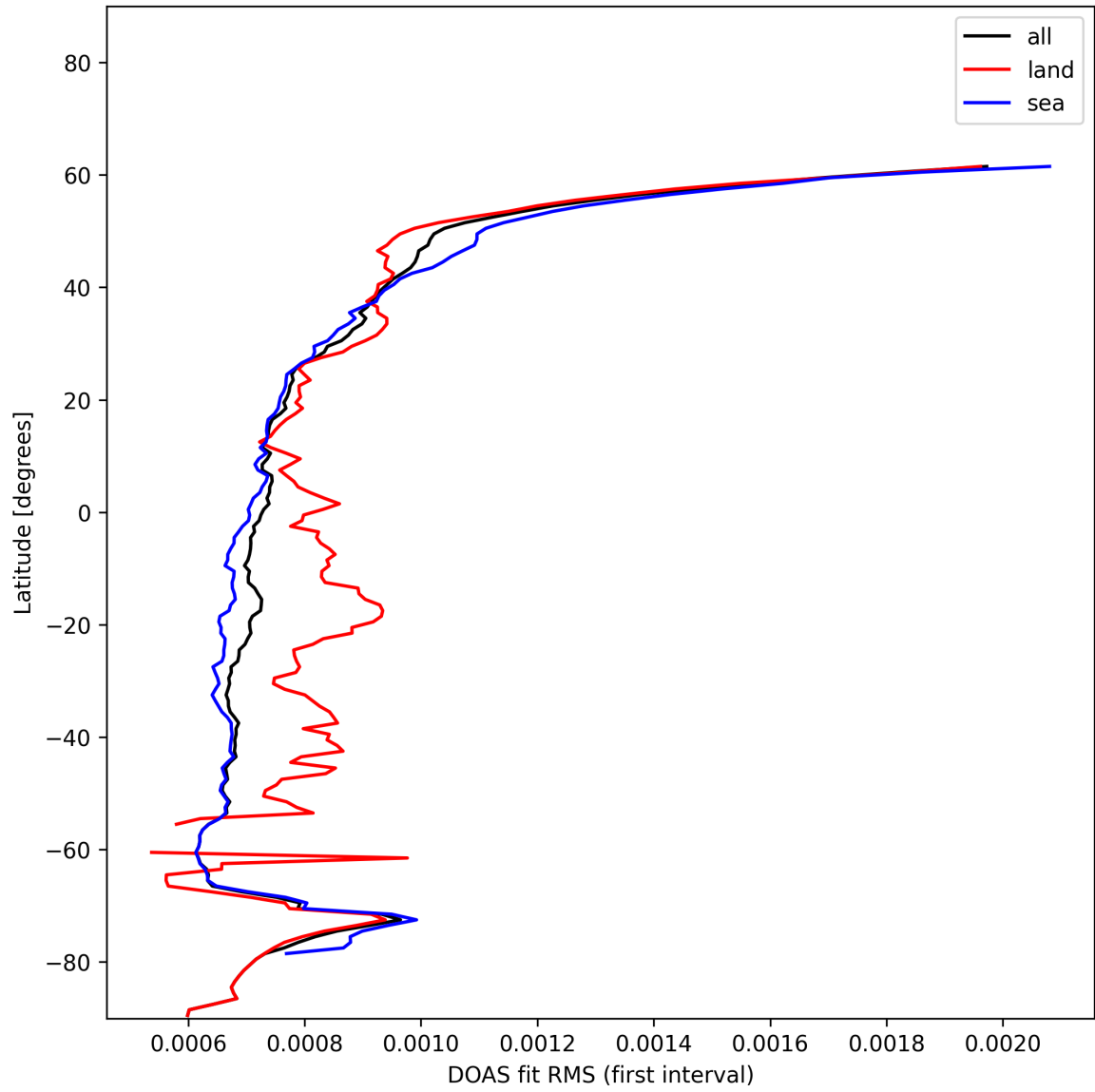
Figure 32: Zonal average of “DOAS fit RMS (first interval)” for 2024-12-16 to 2024-12-17.
