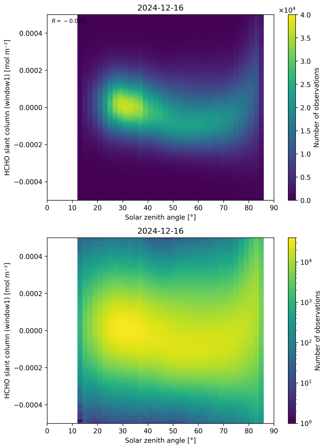
Figure 173: Scatter density plot of “Solar zenith angle” against “HCHO slant column (window1)” for 2024-12-16 to 2024-12-17.
