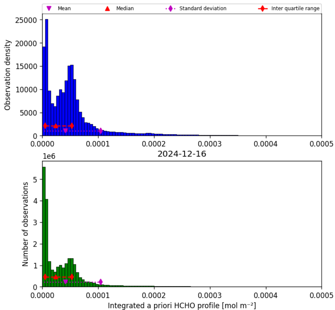
Figure 43: Histogram of “Integrated a priori HCHO profile” for 2024-12-16 to 2024-12-17
