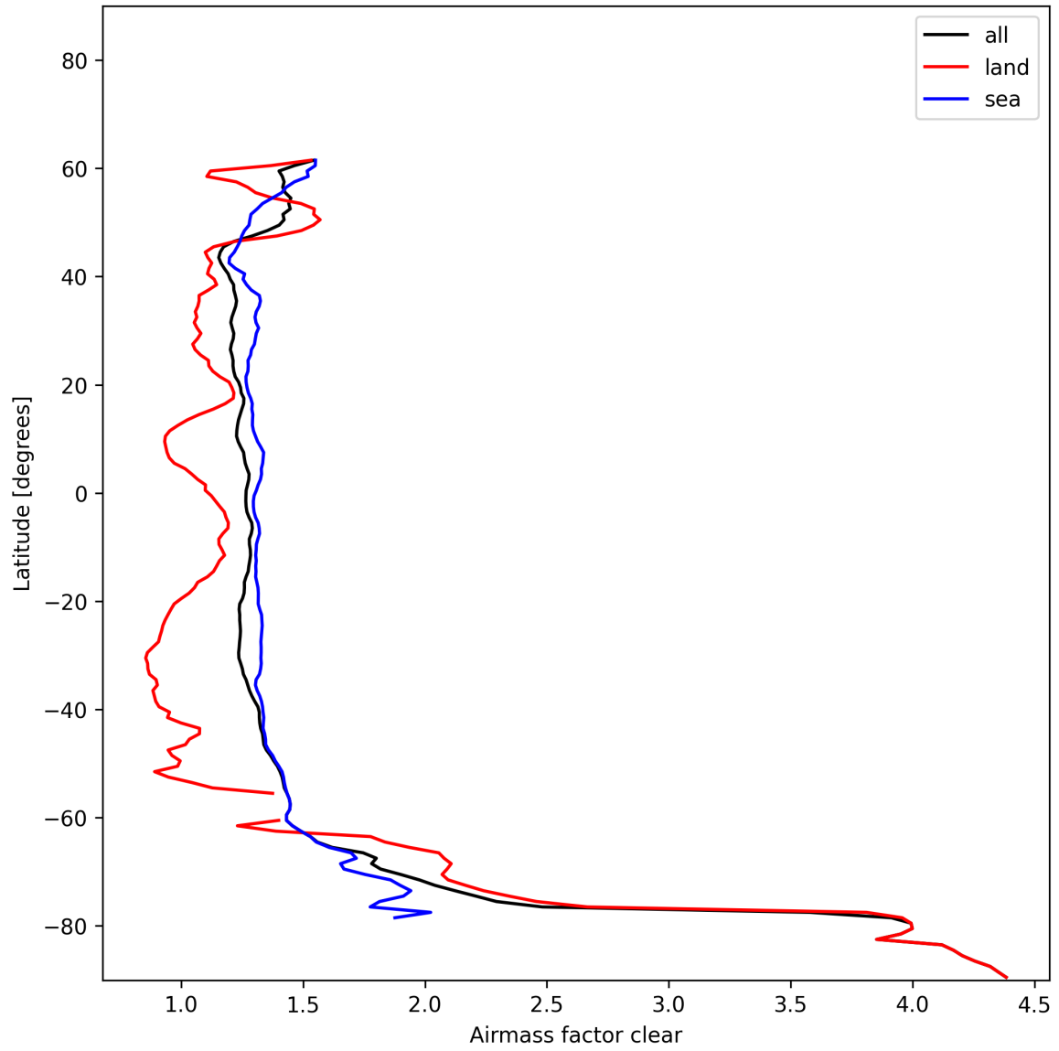
Figure 28: Zonal average of “Airmass factor clear” for 2024-12-16 to 2024-12-17.
