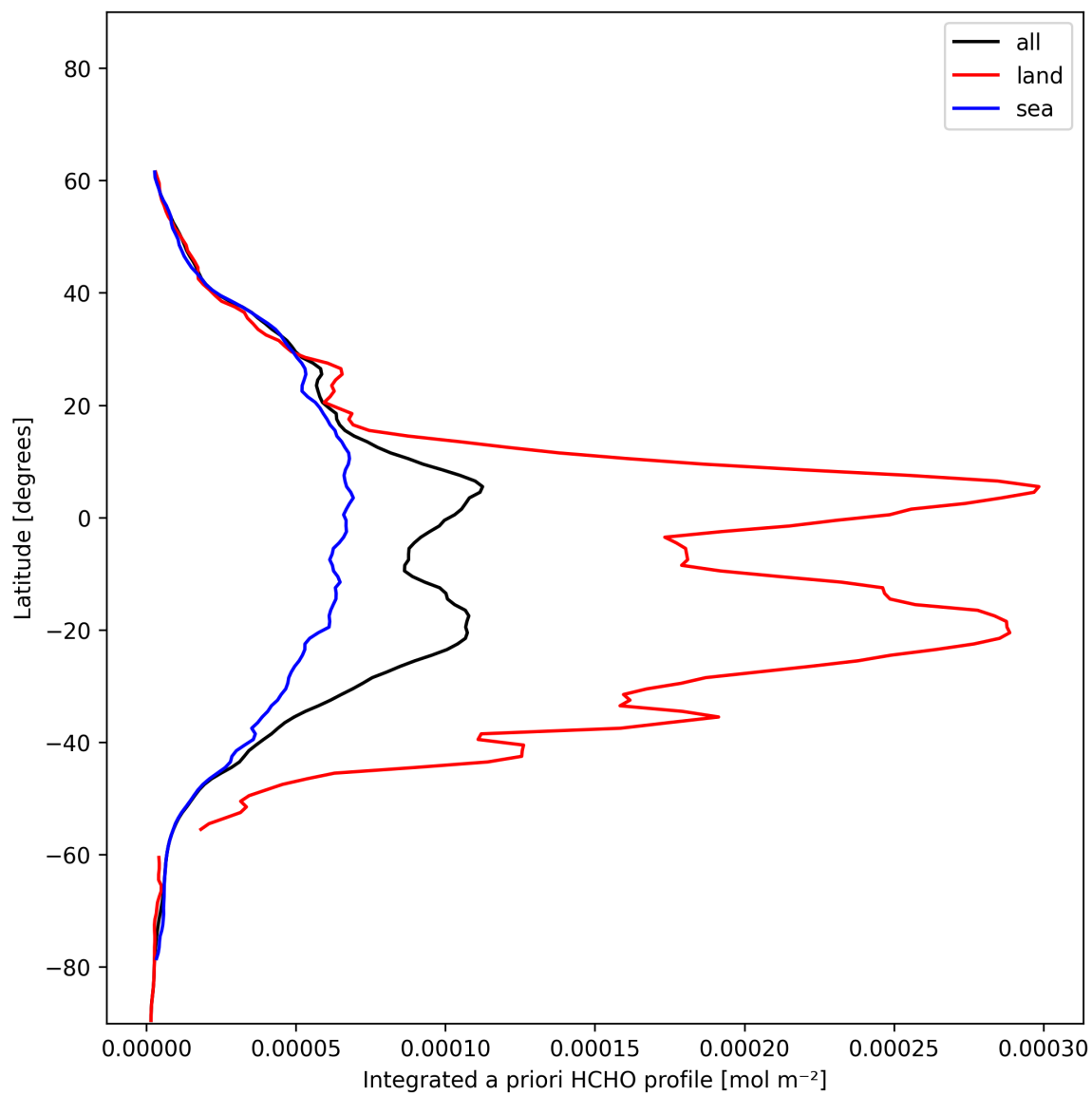
Figure 29: Zonal average of “Integrated a priori HCHO profile” for 2024-12-16 to 2024-12-17.
