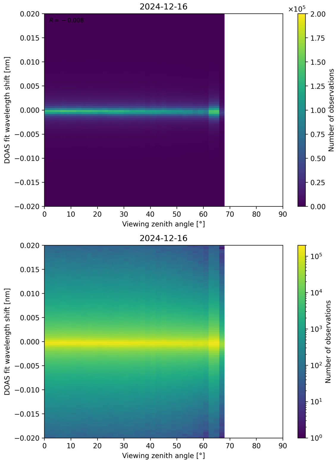
Figure 183: Scatter density plot of “Viewing zenith angle” against “DOAS fit wavelength shift” for 2024-12-16 to 2024-12-17.
