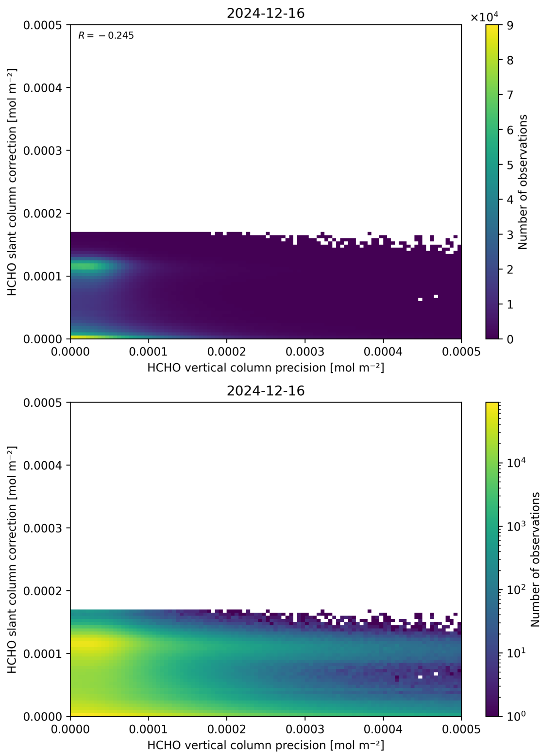
Figure 141: Scatter density plot of “HCHO vertical column precision” against “HCHO slant column correction” for 2024-12-16 to 2024-12-17.
