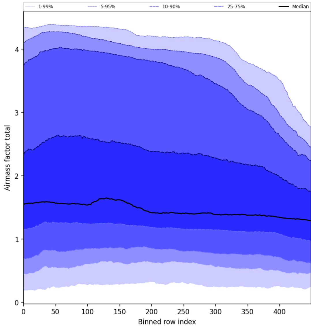
Figure 54: Along track statistics of “Airmass factor total” for 2024-12-16 to 2024-12-17
