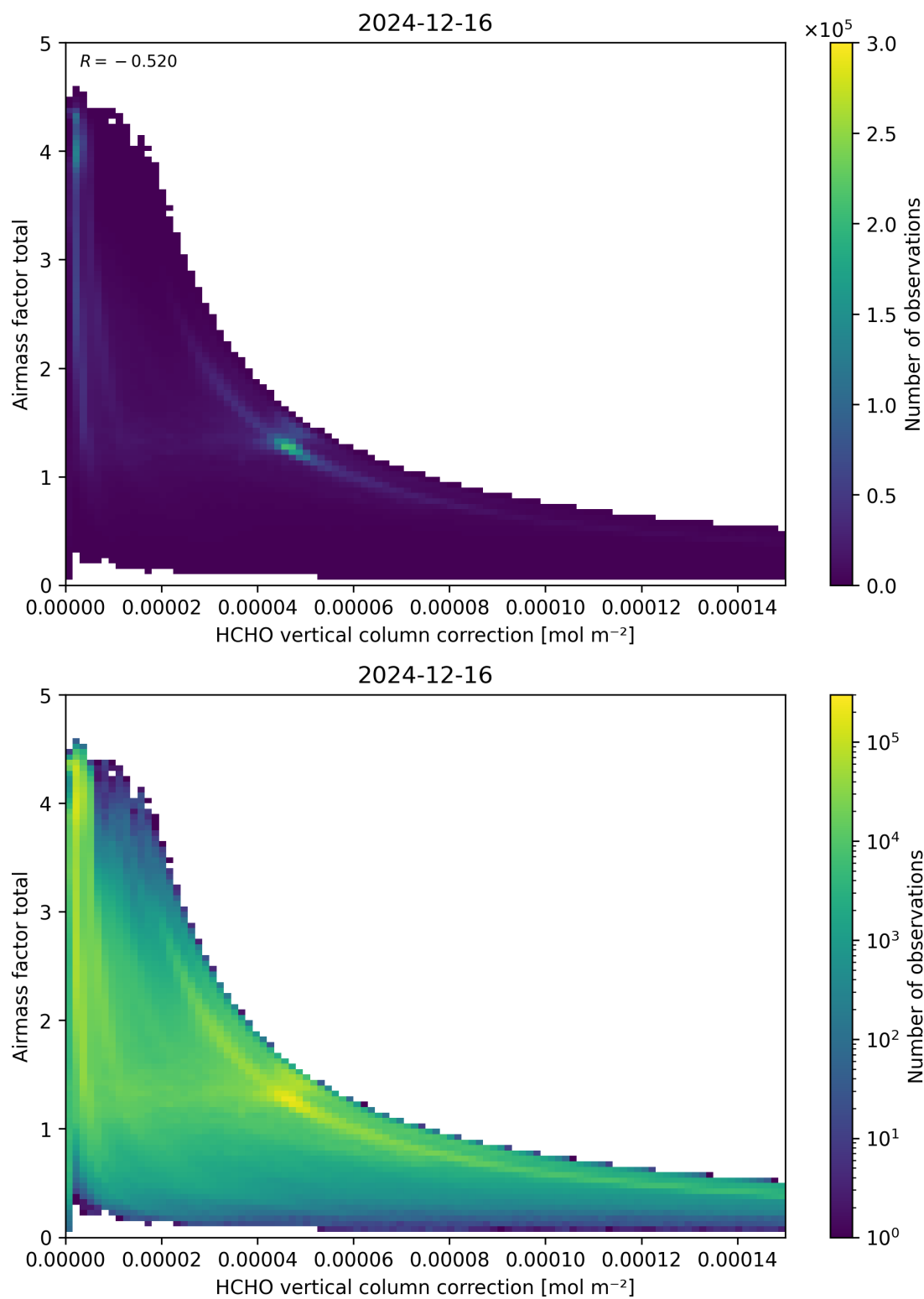
Figure 120: Scatter density plot of “HCHO vertical column correction” against “Airmass factor total” for 2024-12-16 to 2024-12-17.
