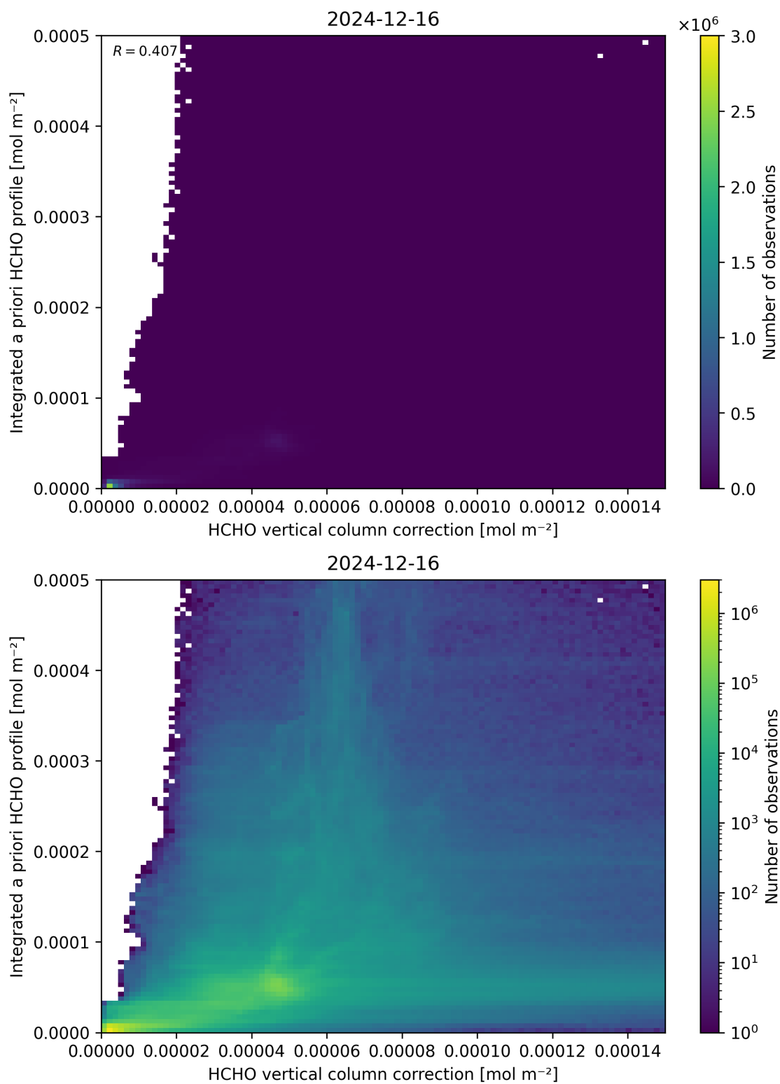
Figure 122: Scatter density plot of “HCHO vertical column correction” against “Integrated a priori HCHO profile” for 2024-12-16 to 2024-12-17.
