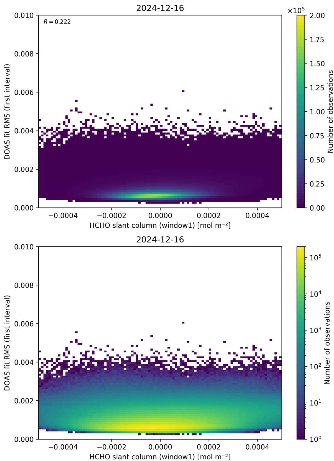
Figure 78: Scatter density plot of “HCHO slant column (window1)” against “DOAS fit RMS (first interval)” for 2024-12-16 to 2024-12-17.
