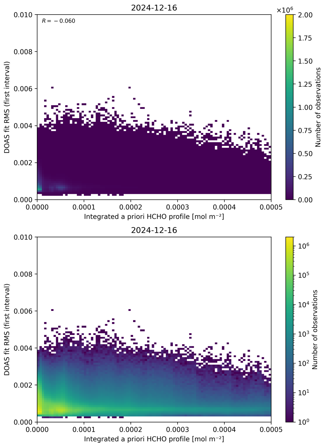
Figure 148: Scatter density plot of “Integrated a priori HCHO profile” against “DOAS fit RMS (first interval)” for 2024-12-16 to 2024-12-17.
