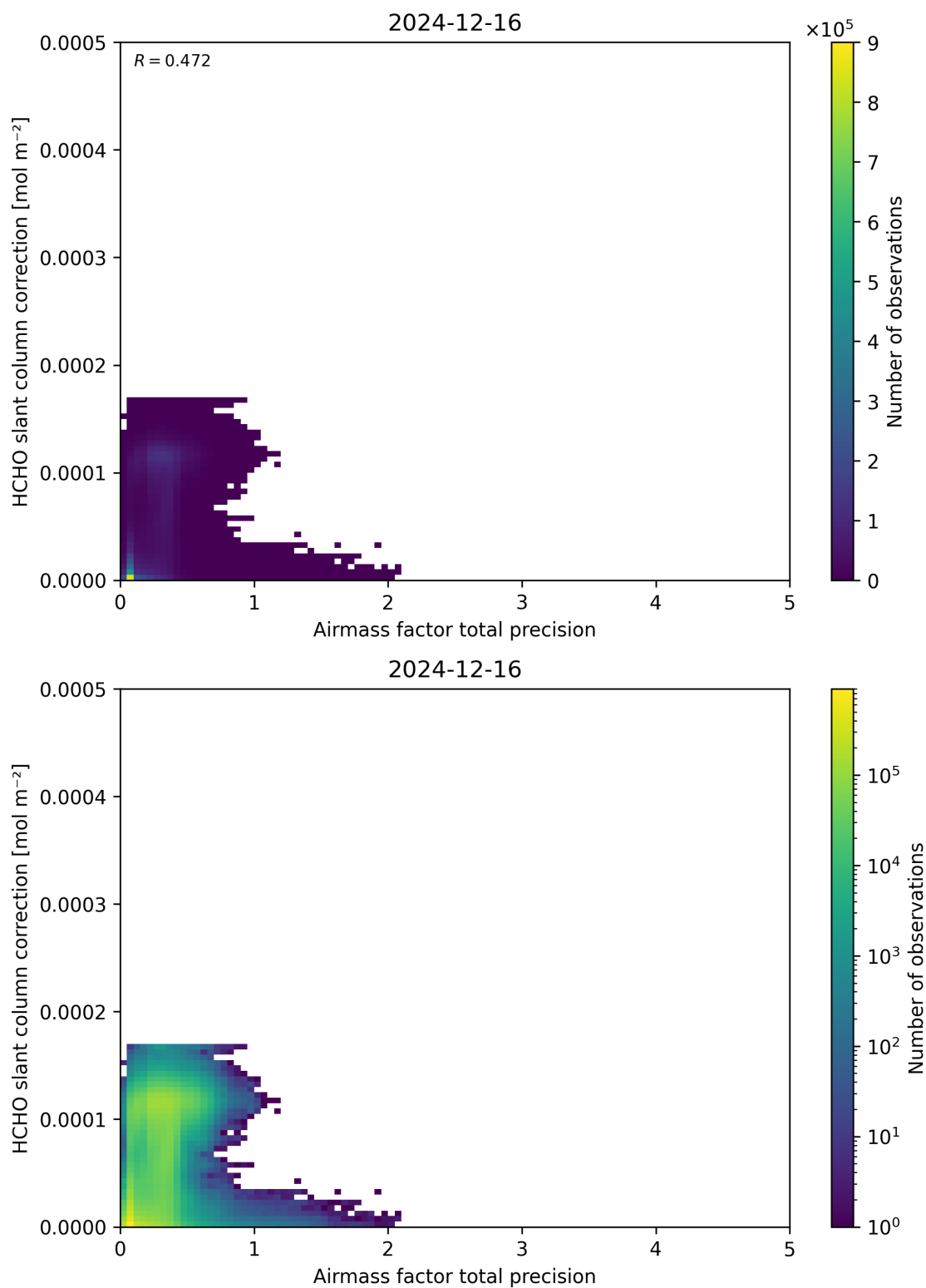
Figure 110: Scatter density plot of “Airmass factor total precision” against “HCHO slant column correction” for 2024-12-16 to 2024-12-17.
