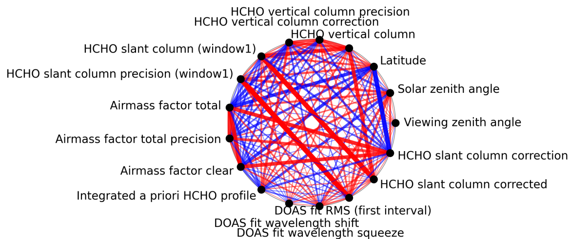
Figure 1: Map of correlation graph for 2024-12-16 to 2024-12-17.
