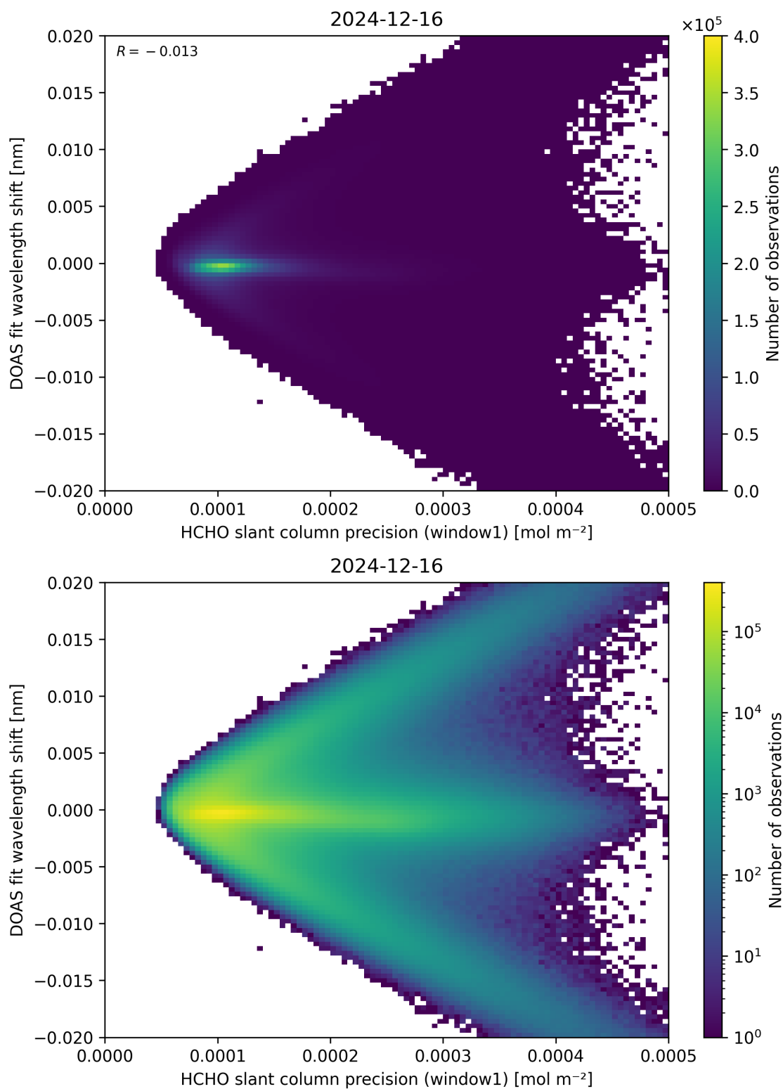
Figure 89: Scatter density plot of “HCHO slant column precision (window1)” against “DOAS fit wavelength shift” for 2024-12-16 to 2024-12-17.
