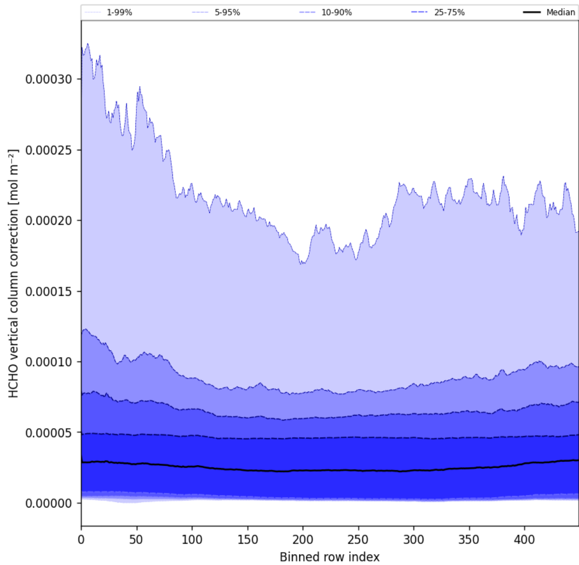
Figure 51: Along track statistics of “HCHO vertical column correction” for 2024-12-16 to 2024-12-17
