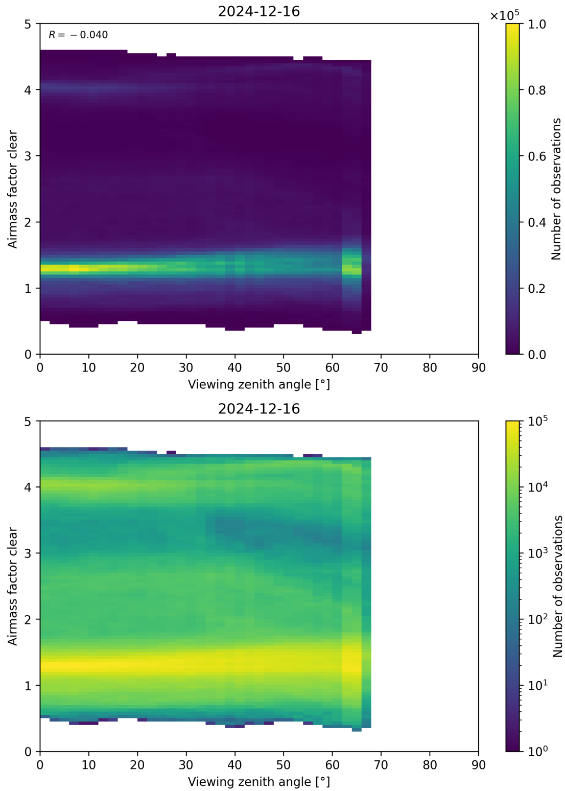
Figure 185: Scatter density plot of “Viewing zenith angle” against “Airmass factor clear” for 2024-12-16 to 2024-12-17.
