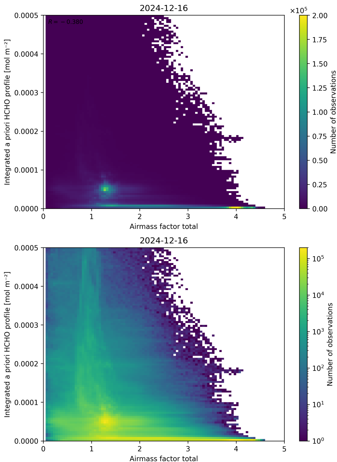
Figure 104: Scatter density plot of “Airmass factor total” against “Integrated a priori HCHO profile” for 2024-12-16 to 2024-12-17.
