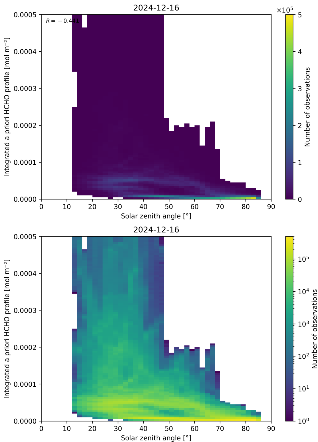
Figure 180: Scatter density plot of “Solar zenith angle” against “Integrated a priori HCHO profile” for 2024-12-16 to 2024-12-17.
