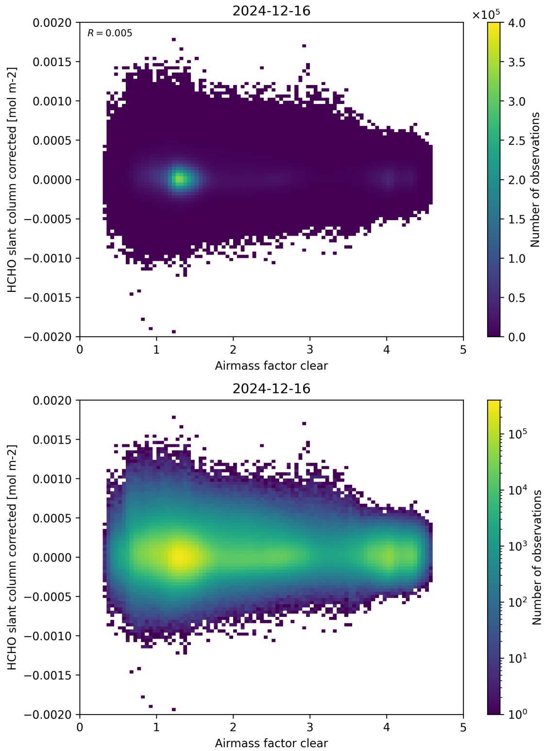
Figure 74: Scatter density plot of “Airmass factor clear” against “HCHO slant column corrected” for 2024-12-16 to 2024-12-17.
