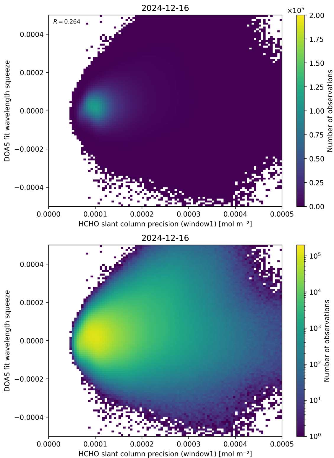
Figure 90: Scatter density plot of “HCHO slant column precision (window1)” against “DOAS fit wavelength squeeze” for 2024-12-16 to 2024-12-17.
