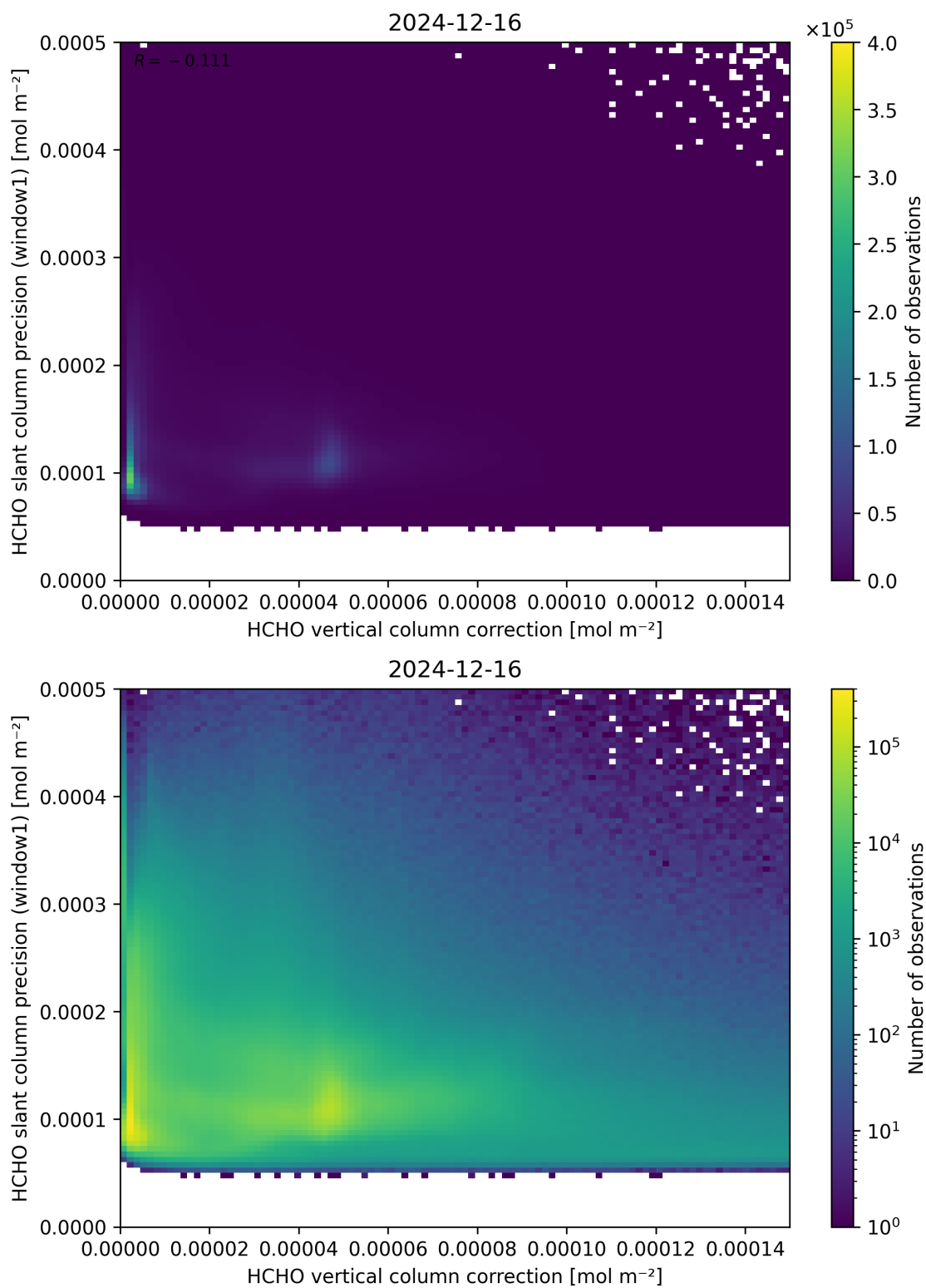
Figure 119: Scatter density plot of “HCHO vertical column correction” against “HCHO slant column precision (window1)” for 2024-12-16 to 2024-12-17.
