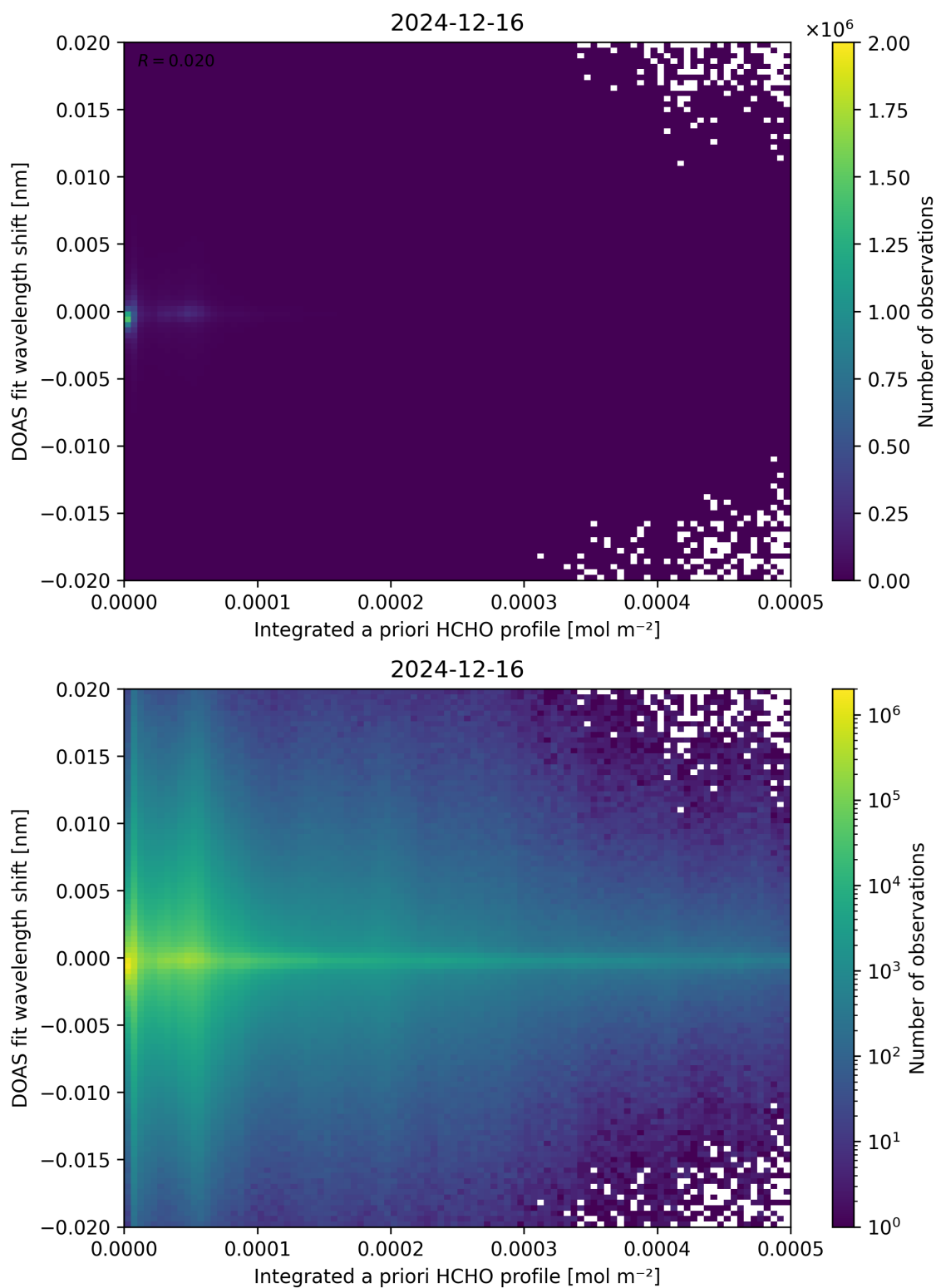
Figure 149: Scatter density plot of “Integrated a priori HCHO profile” against “DOAS fit wavelength shift” for 2024-12-16 to 2024-12-17.
