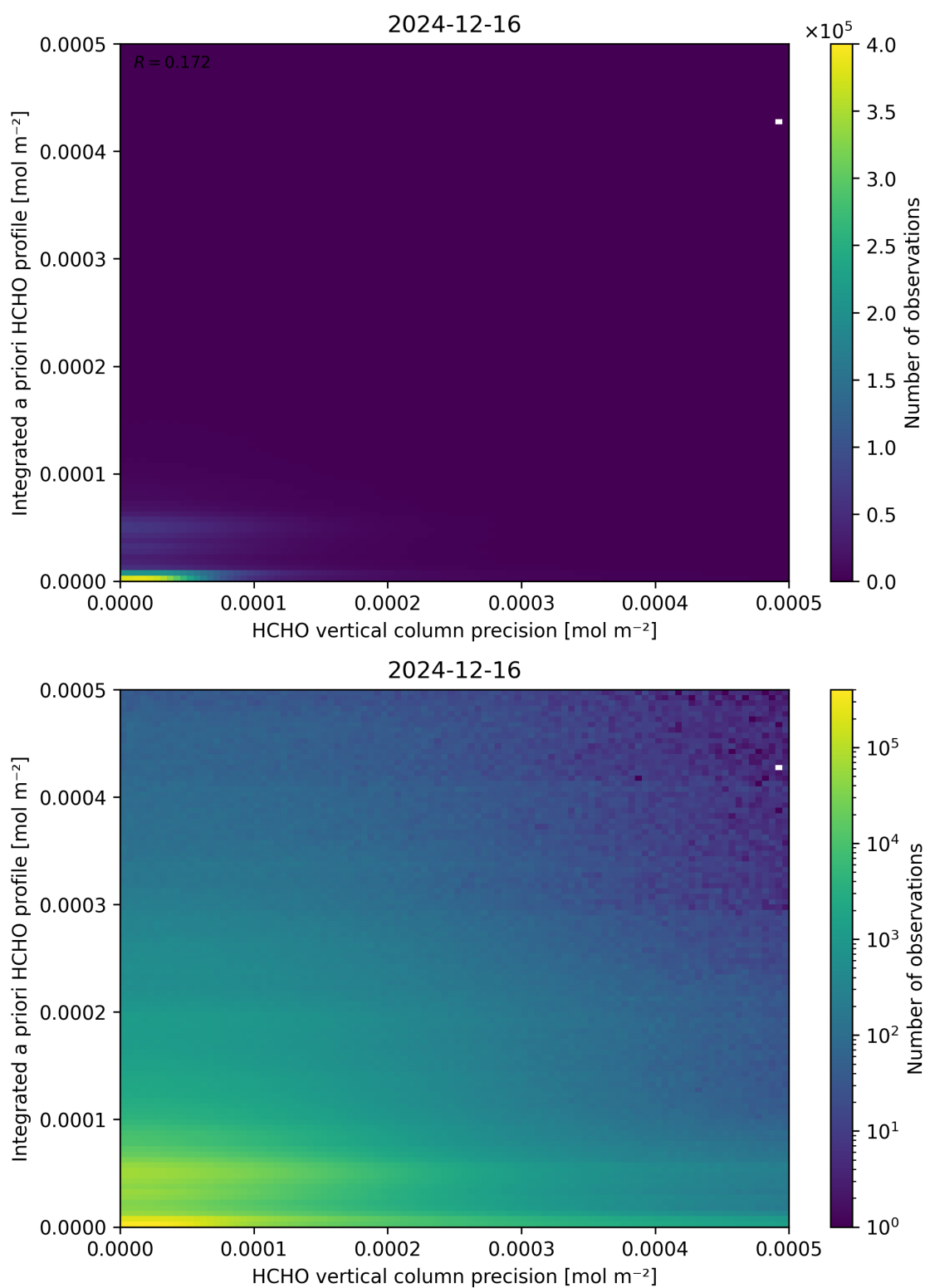
Figure 147: Scatter density plot of “HCHO vertical column precision” against “Integrated a priori HCHO profile” for 2024-12-16 to 2024-12-17.
