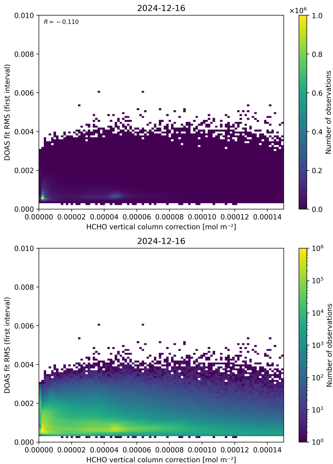
Figure 112: Scatter density plot of “HCHO vertical column correction” against “DOAS fit RMS (first interval)” for 2024-12-16 to 2024-12-17.
