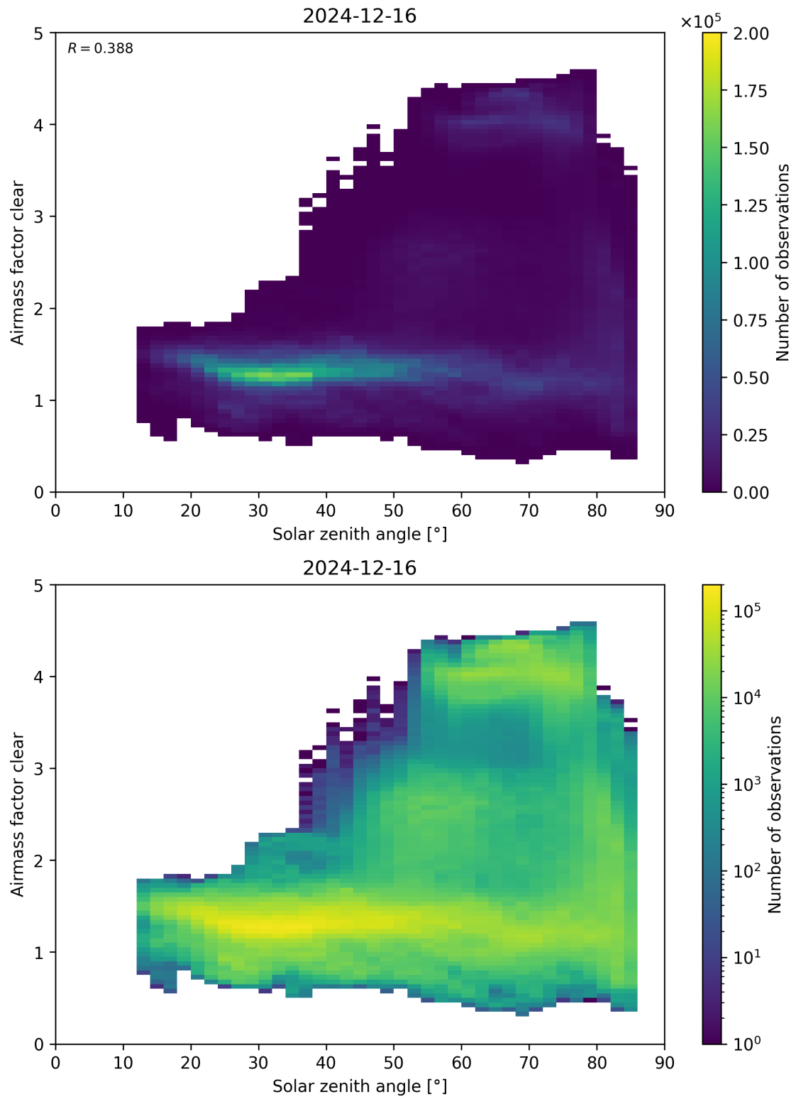
Figure 170: Scatter density plot of “Solar zenith angle” against “Airmass factor clear” for 2024-12-16 to 2024-12-17.
