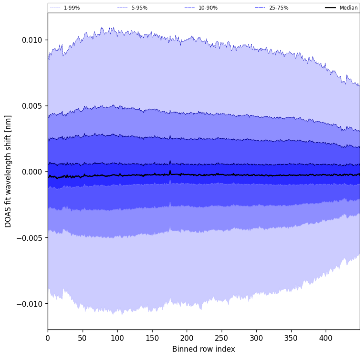
Figure 58: Along track statistics of “DOAS fit wavelength shift” for 2024-12-16 to 2024-12-17
