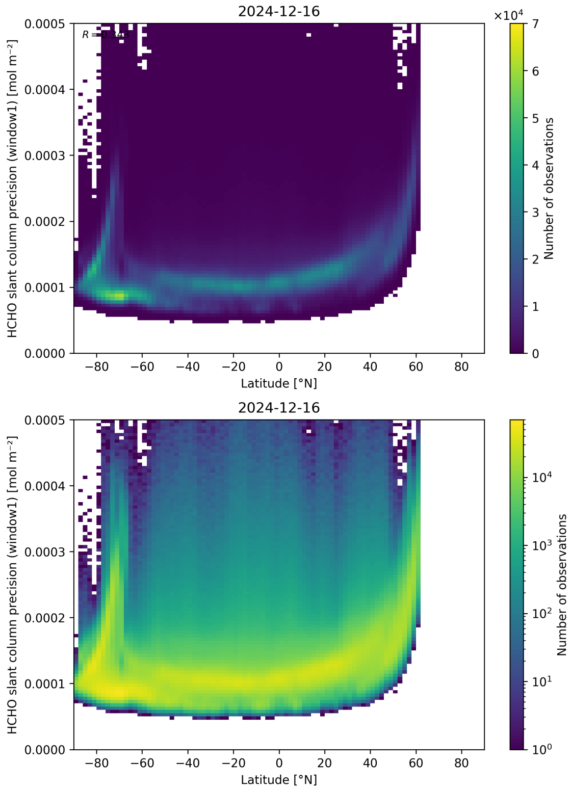
Figure 160: Scatter density plot of “Latitude” against “HCHO slant column precision (window1)” for 2024-12-16 to 2024-12-17.
