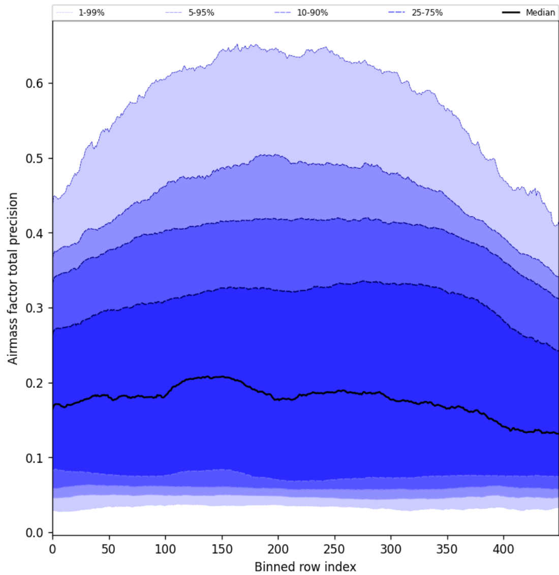
Figure 55: Along track statistics of “Airmass factor total precision” for 2024-12-16 to 2024-12-17
