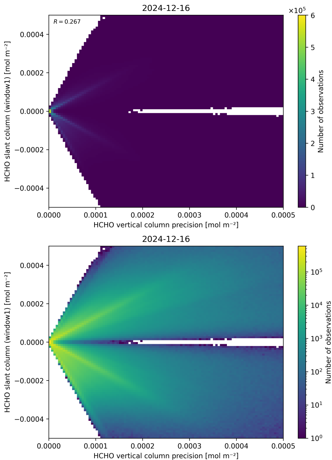
Figure 142: Scatter density plot of “HCHO vertical column precision” against “HCHO slant column (window1)” for 2024-12-16 to 2024-12-17.
