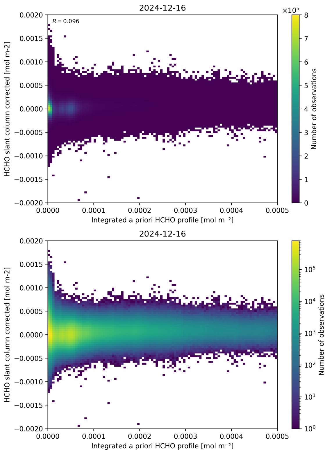
Figure 151: Scatter density plot of “Integrated a priori HCHO profile” against “HCHO slant column corrected” for 2024-12-16 to 2024-12-17.
