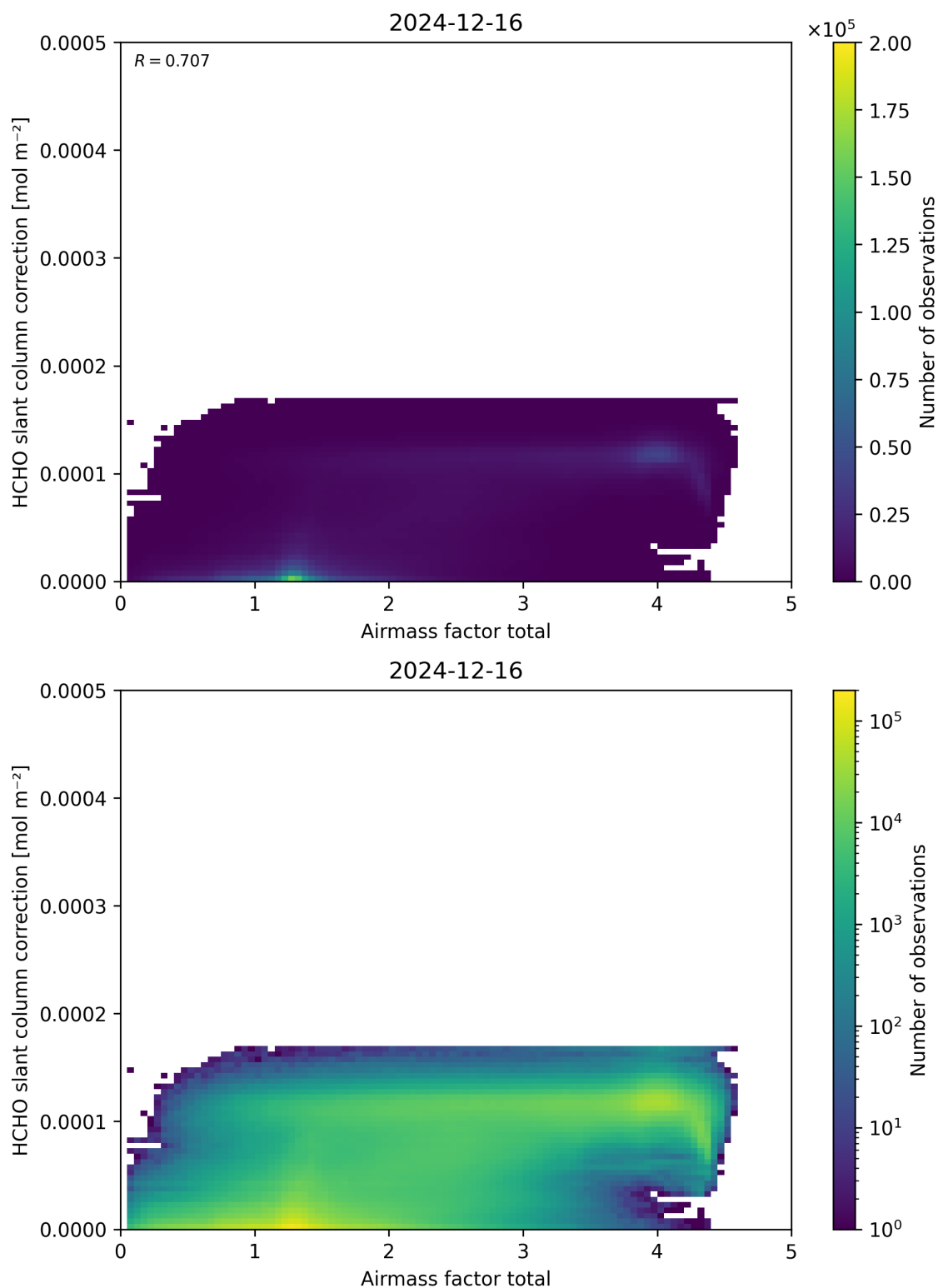
Figure 102: Scatter density plot of “Airmass factor total” against “HCHO slant column correction” for 2024-12-16 to 2024-12-17.
