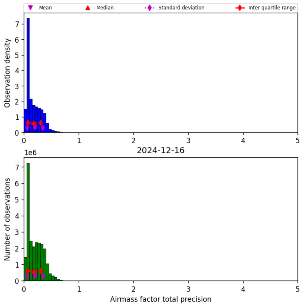
Figure 41: Histogram of “Airmass factor total precision” for 2024-12-16 to 2024-12-17
