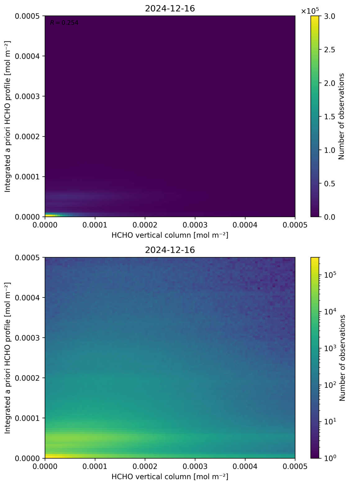
Figure 135: Scatter density plot of “HCHO vertical column” against “Integrated a priori HCHO profile” for 2024-12-16 to 2024-12-17.
