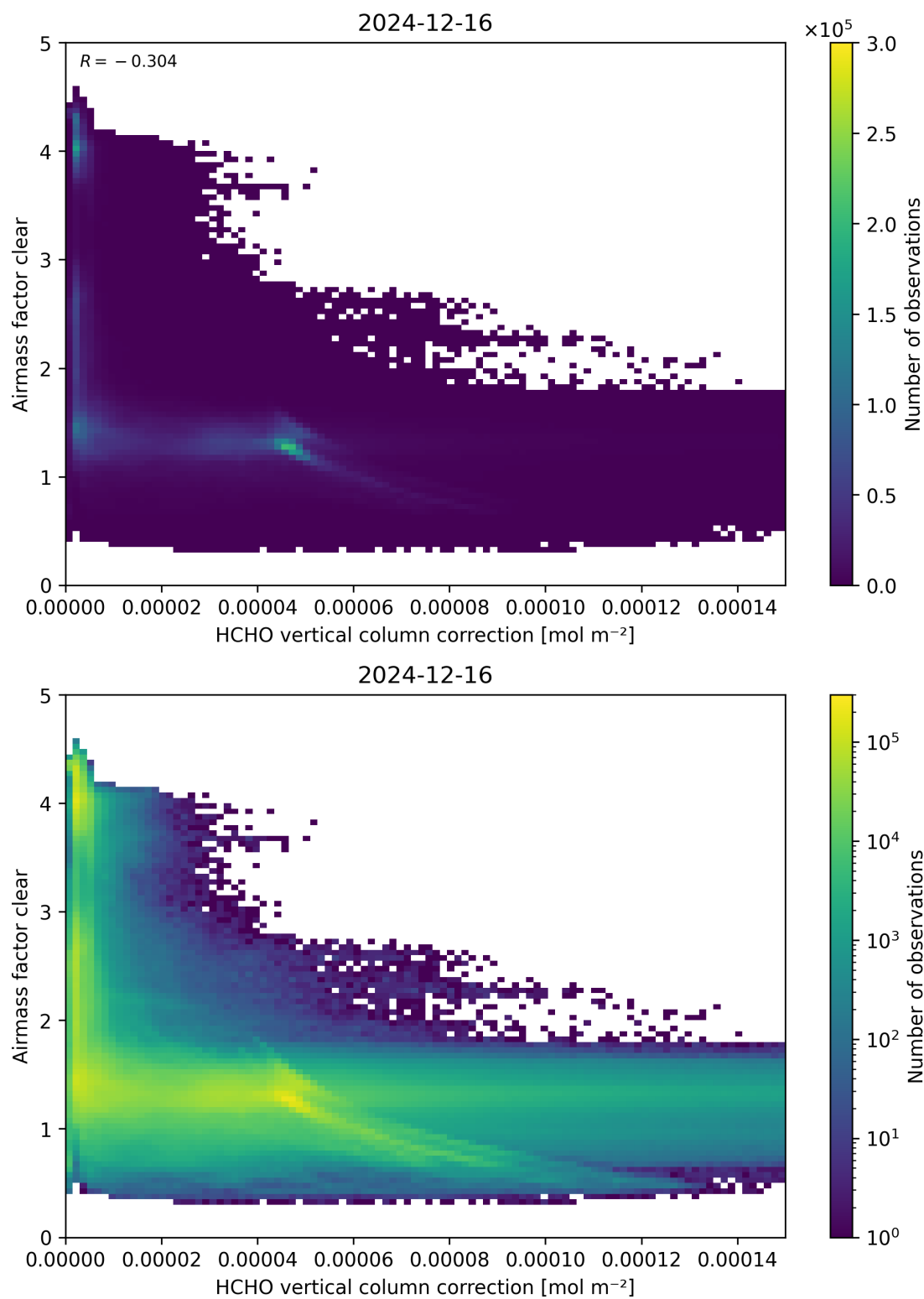
Figure 115: Scatter density plot of “HCHO vertical column correction” against “Airmass factor clear” for 2024-12-16 to 2024-12-17.
