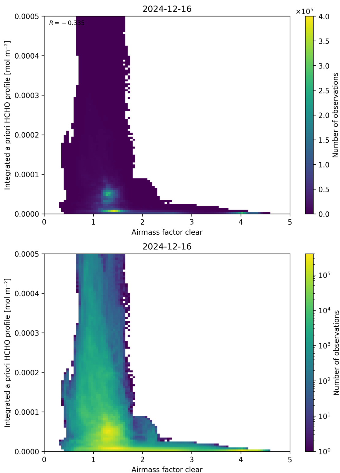
Figure 76: Scatter density plot of “Airmass factor clear” against “Integrated a priori HCHO profile” for 2024-12-16 to 2024-12-17.
