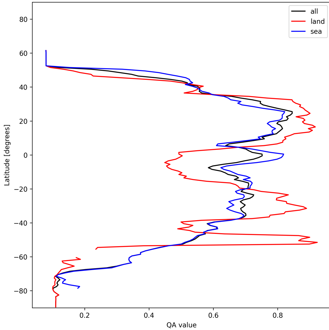
Figure 20: Zonal average of “QA value” for 2024-12-16 to 2024-12-17.
