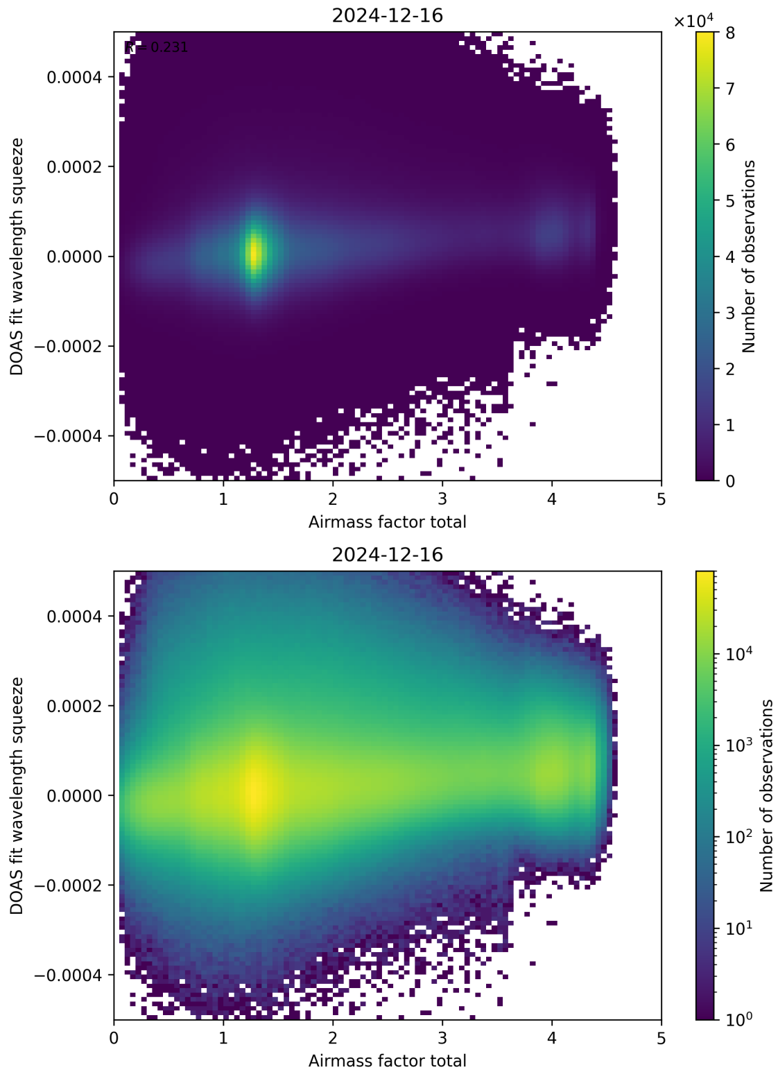
Figure 99: Scatter density plot of “Airmass factor total” against “DOAS fit wavelength squeeze” for 2024-12-16 to 2024-12-17.
