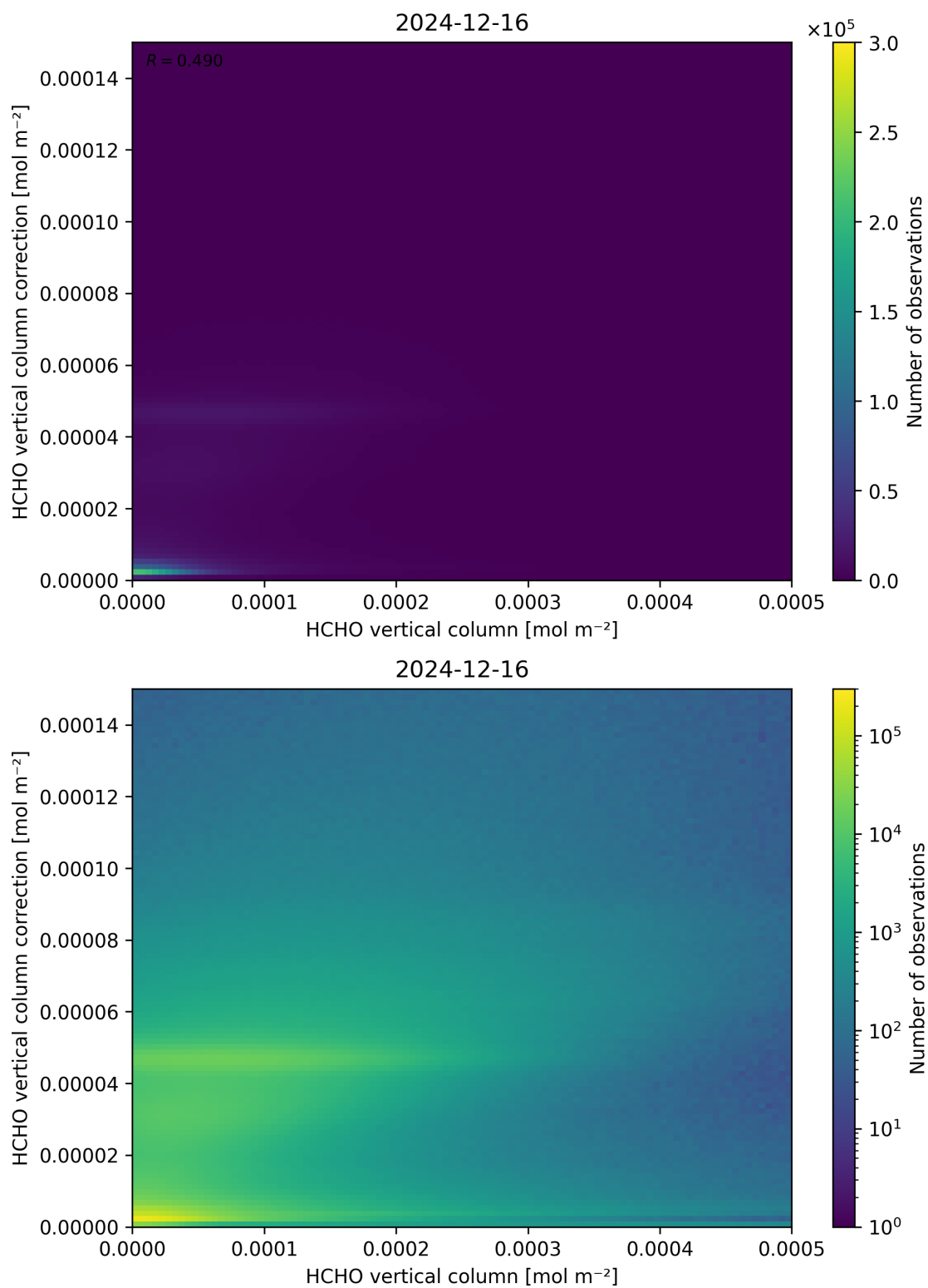
Figure 133: Scatter density plot of “HCHO vertical column” against “HCHO vertical column correction” for 2024-12-16 to 2024-12-17.
