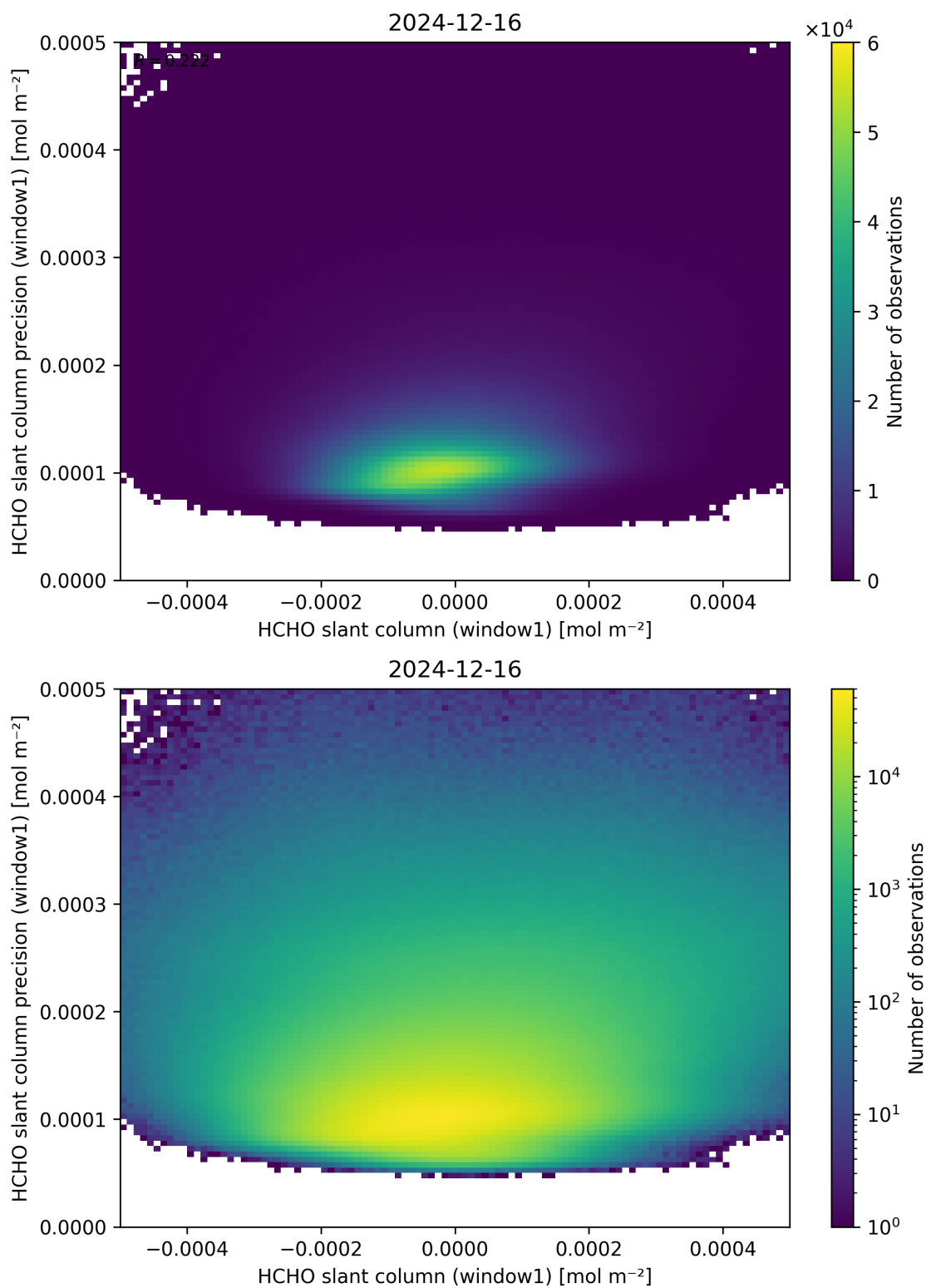
Figure 84: Scatter density plot of “HCHO slant column (window1)” against “HCHO slant column precision (window1)” for 2024-12-16 to 2024-12-17.
