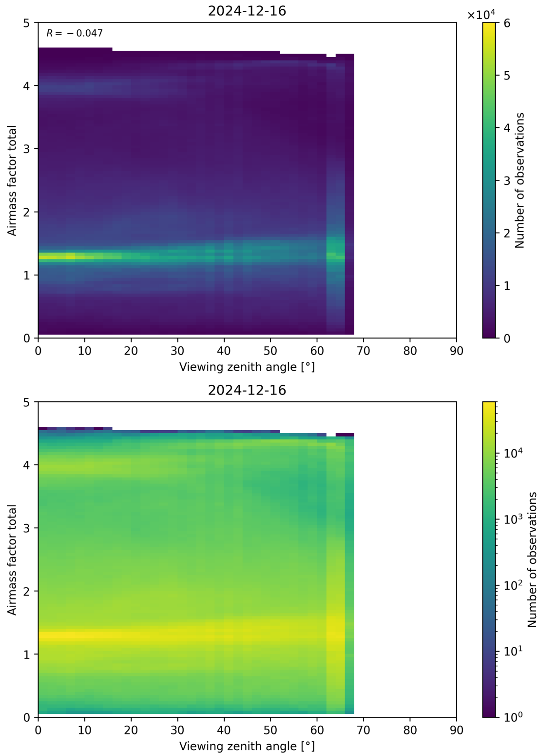
Figure 190: Scatter density plot of “Viewing zenith angle” against “Airmass factor total” for 2024-12-16 to 2024-12-17.
