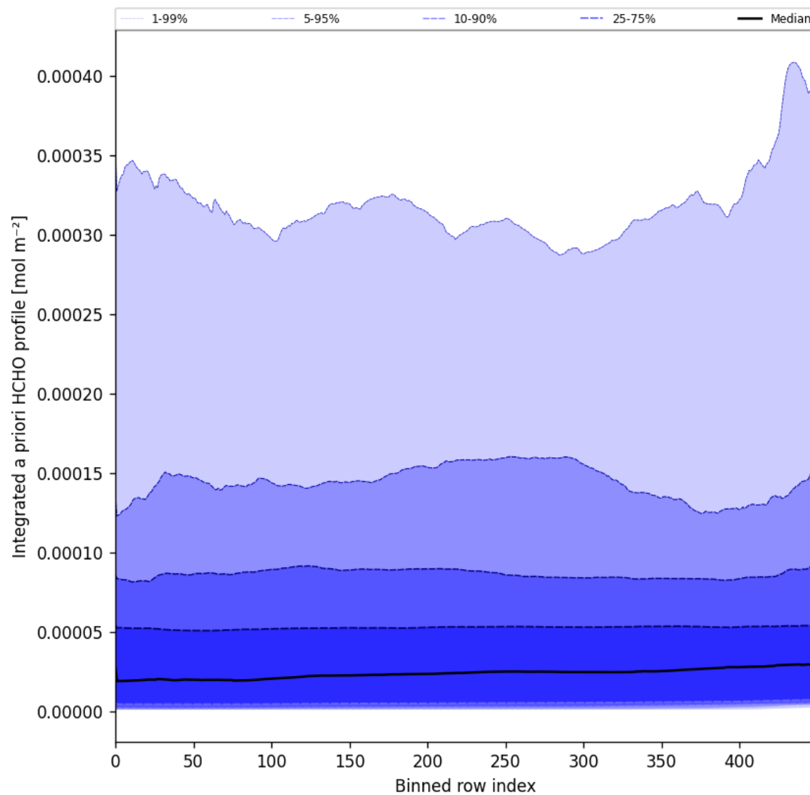
Figure 57: Along track statistics of “Integrated a priori HCHO profile” for 2024-12-16 to 2024-12-17
