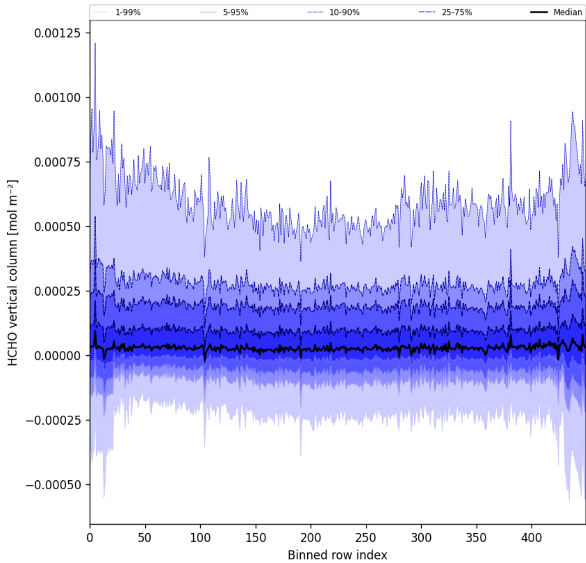
Figure 49: Along track statistics of “HCHO vertical column” for 2024-12-16 to 2024-12-17
