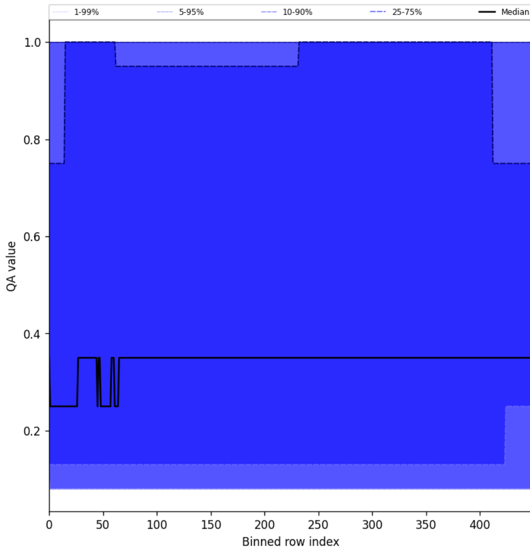
Figure 48: Along track statistics of “QA value” for 2024-12-16 to 2024-12-17
