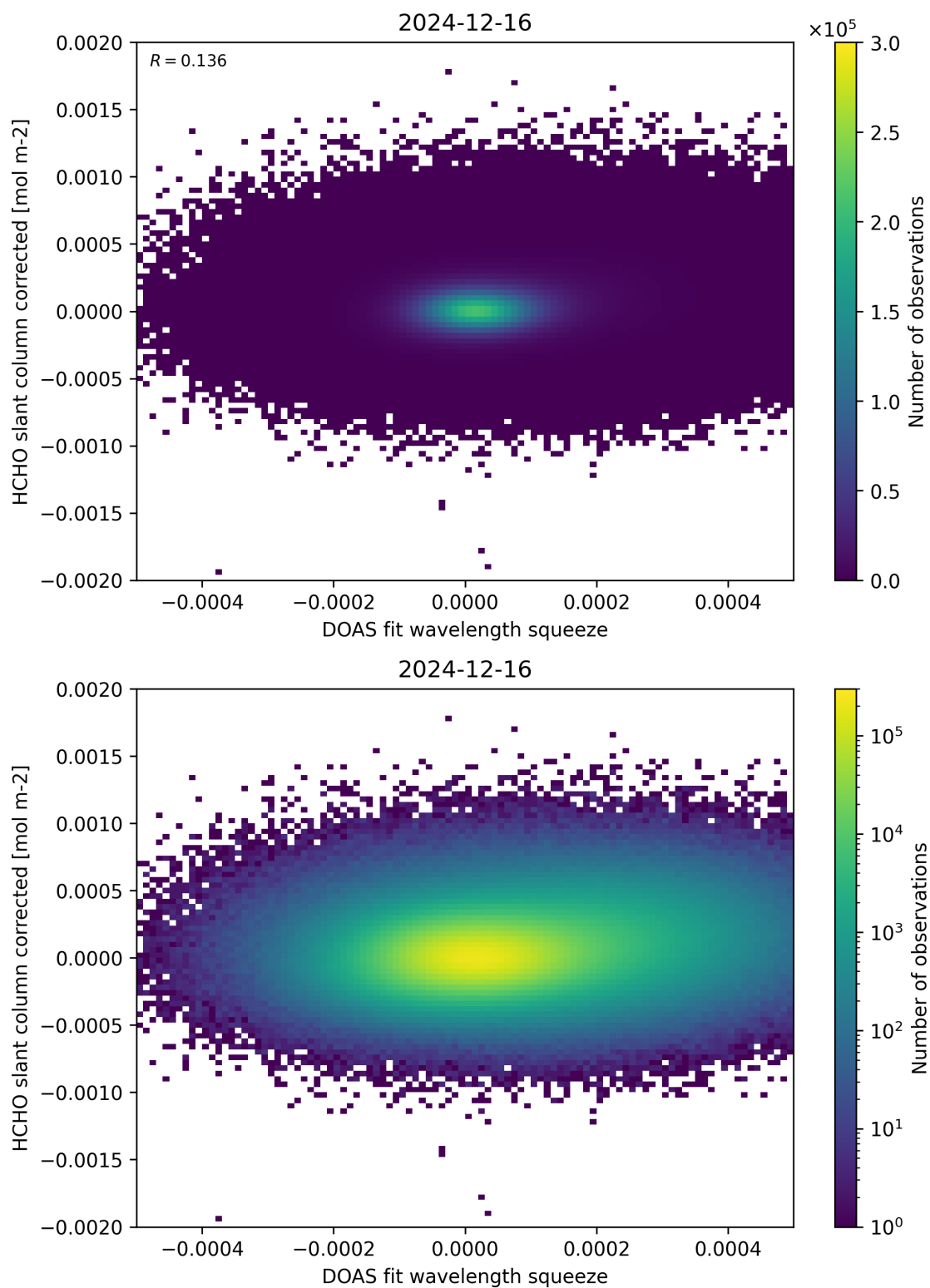
Figure 69: Scatter density plot of “DOAS fit wavelength squeeze” against “HCHO slant column corrected” for 2024-12-16 to 2024-12-17.
