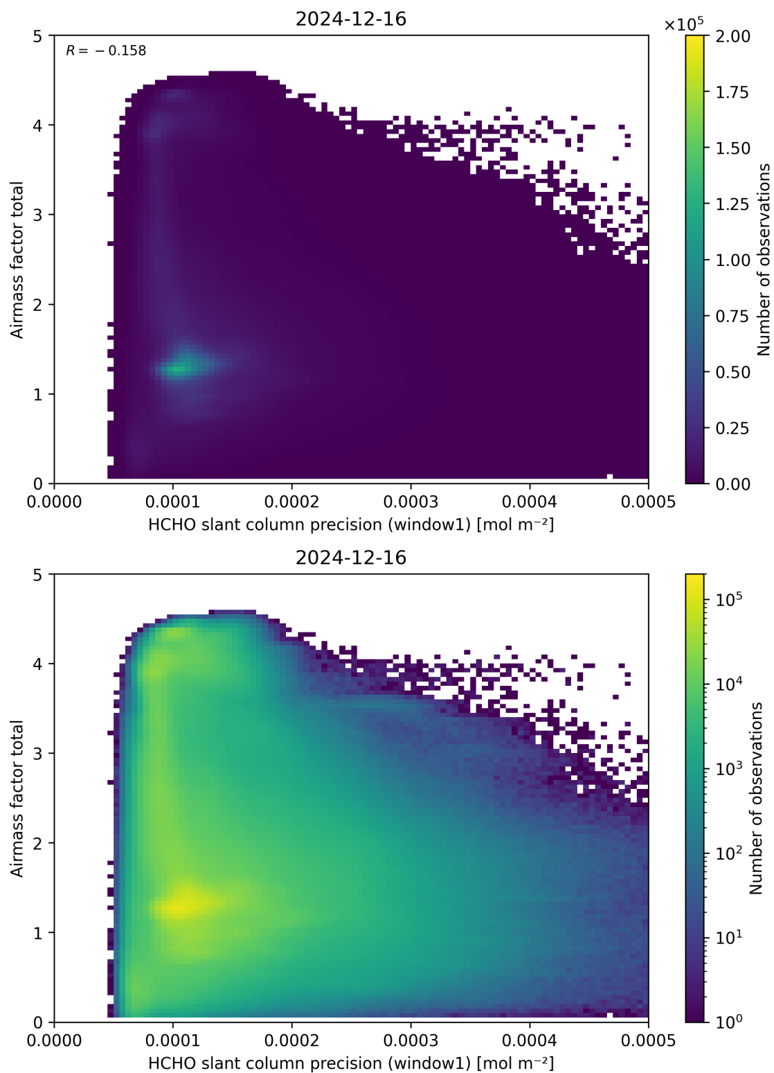
Figure 94: Scatter density plot of “HCHO slant column precision (window1)” against “Airmass factor total” for 2024-12-16 to 2024-12-17.
