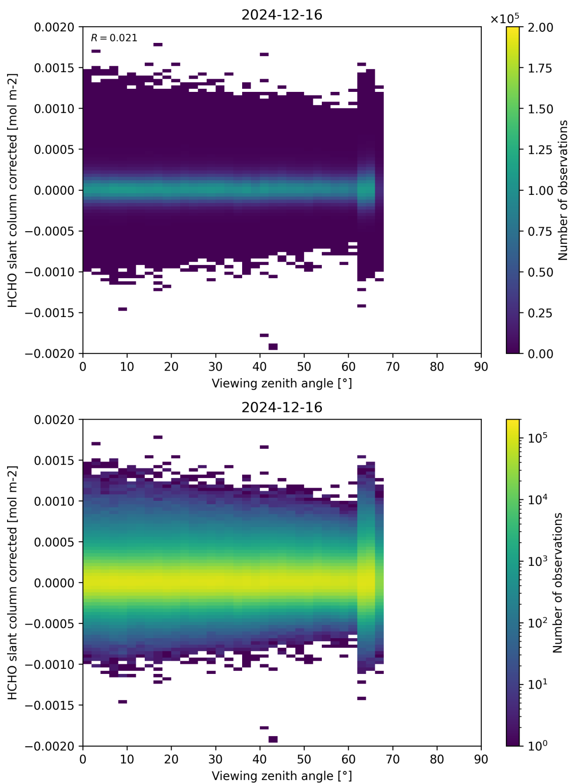
Figure 186: Scatter density plot of “Viewing zenith angle” against “HCHO slant column corrected” for 2024-12-16 to 2024-12-17.
