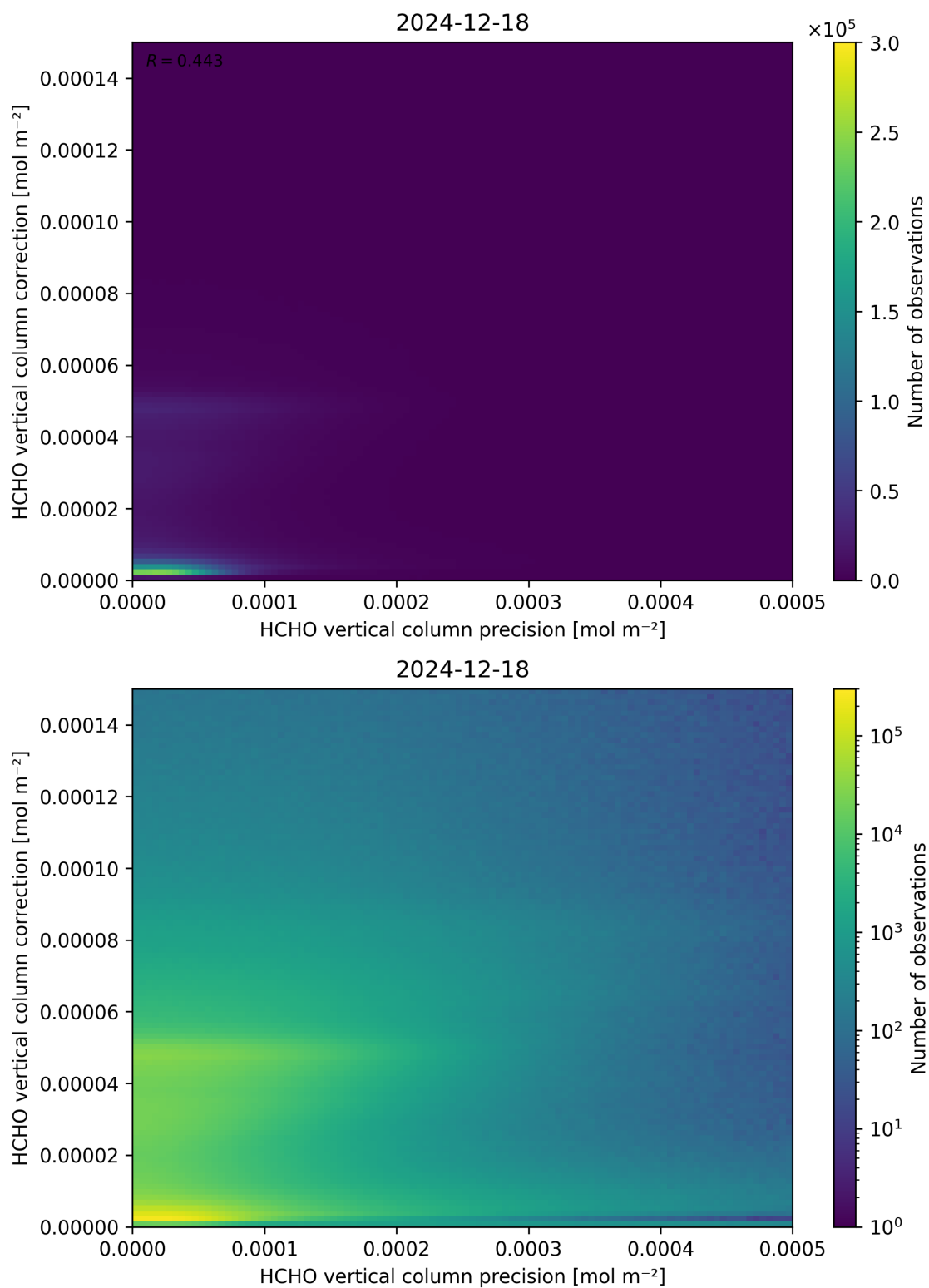
Figure 146: Scatter density plot of “HCHO vertical column precision” against “HCHO vertical column correction” for 2024-12-17 to 2024-12-19.
