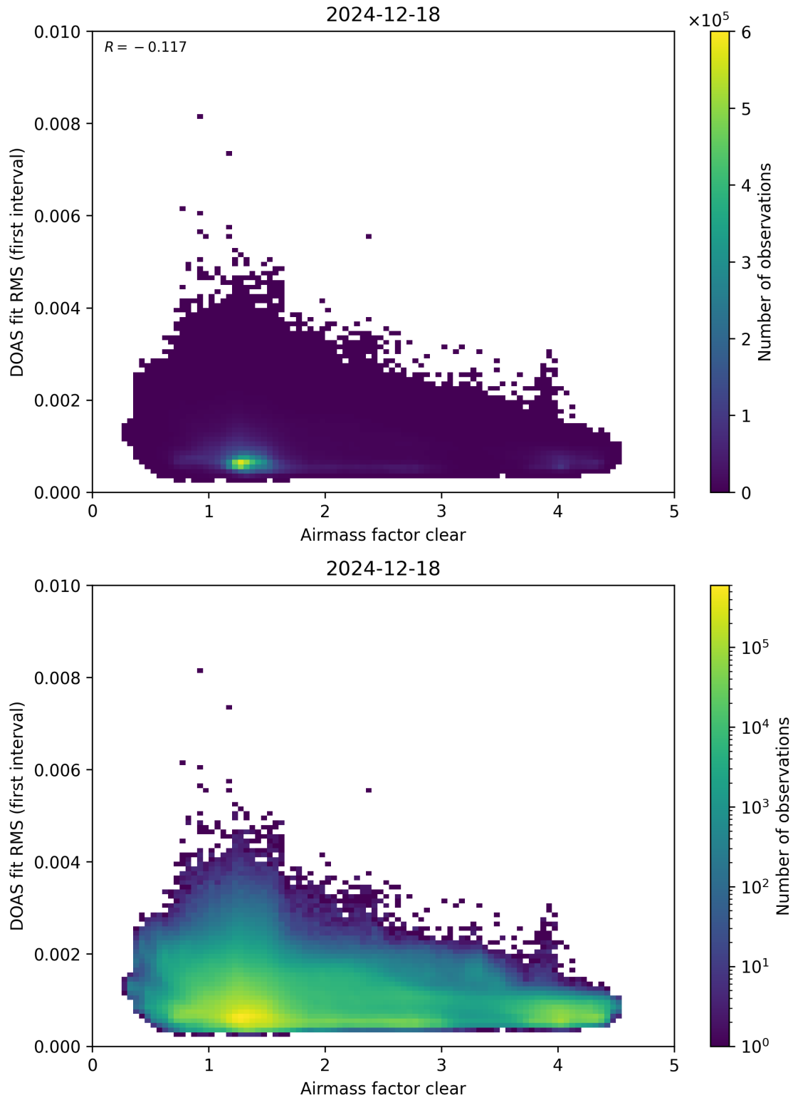
Figure 71: Scatter density plot of “Airmass factor clear” against “DOAS fit RMS (first interval)” for 2024-12-17 to 2024-12-19.
