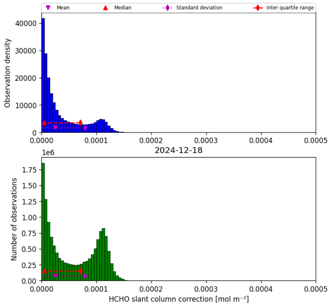
Figure 47: Histogram of “HCHO slant column correction” for 2024-12-17 to 2024-12-19
