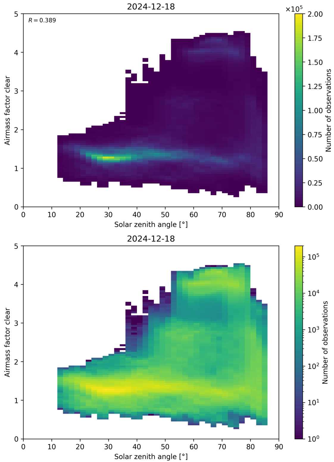
Figure 170: Scatter density plot of “Solar zenith angle” against “Airmass factor clear” for 2024-12-17 to 2024-12-19.
