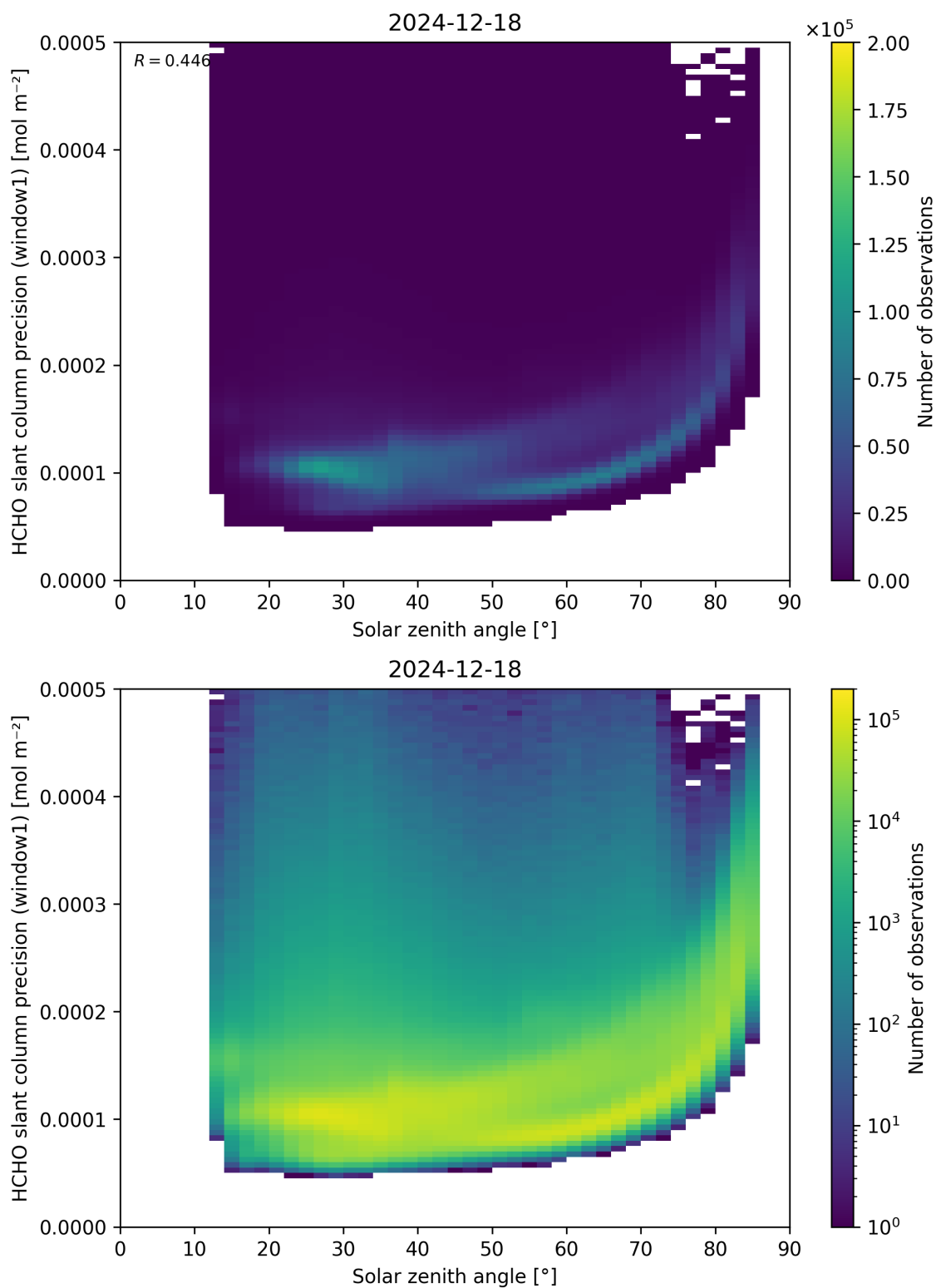
Figure 174: Scatter density plot of “Solar zenith angle” against “HCHO slant column precision (window1)” for 2024-12-17 to 2024-12-19.
