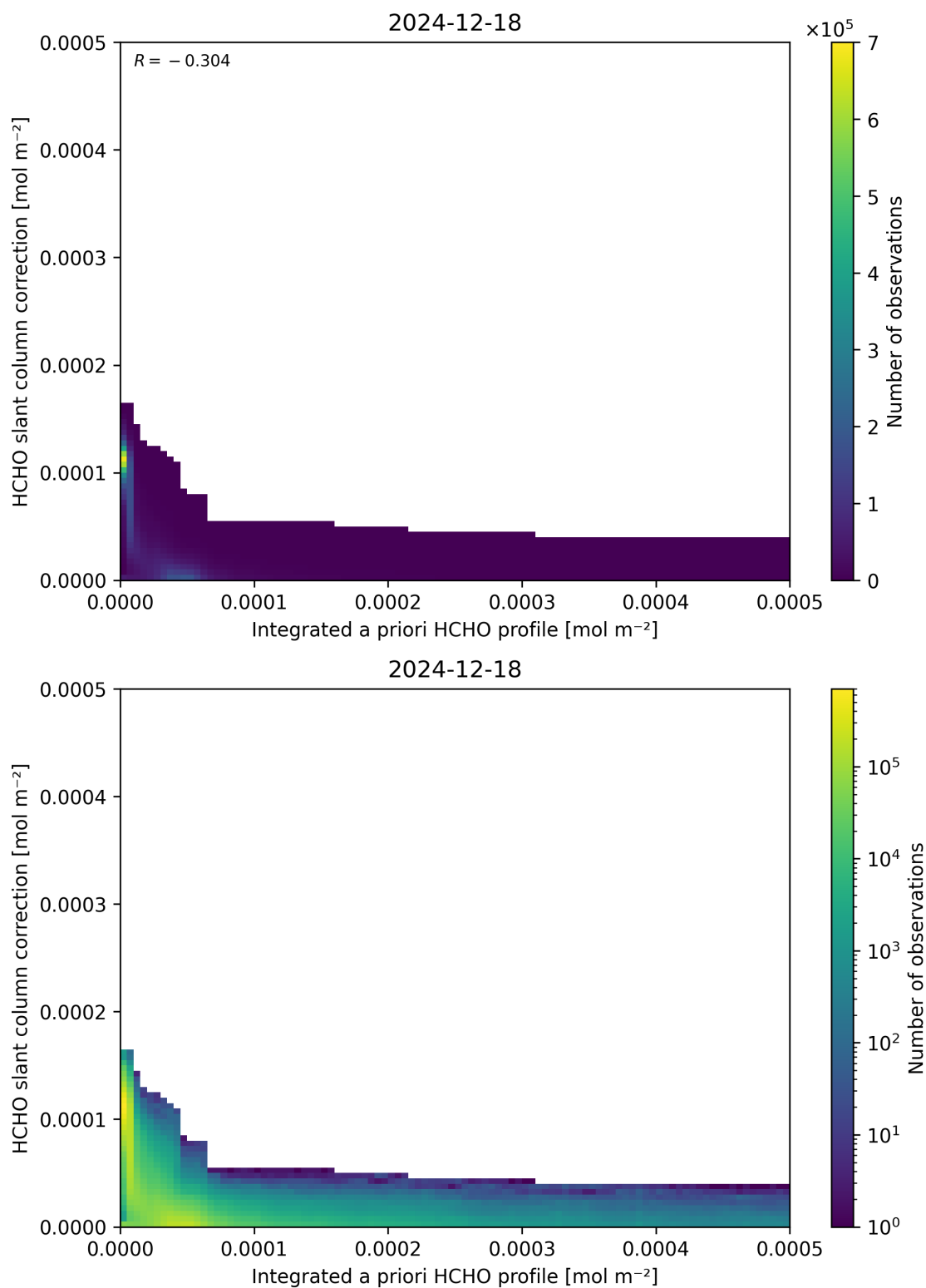
Figure 152: Scatter density plot of “Integrated a priori HCHO profile” against “HCHO slant column correction” for 2024-12-17 to 2024-12-19.
