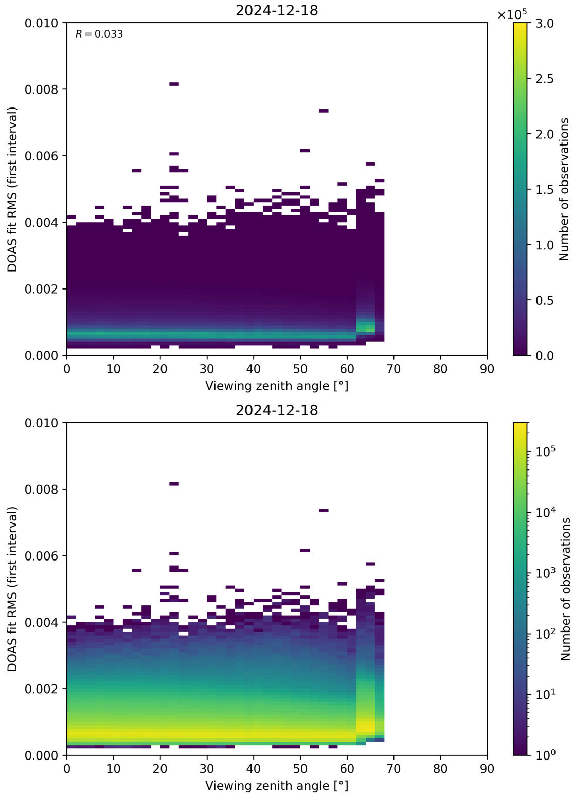
Figure 182: Scatter density plot of “Viewing zenith angle” against “DOAS fit RMS (first interval)” for 2024-12-17 to 2024-12-19.
