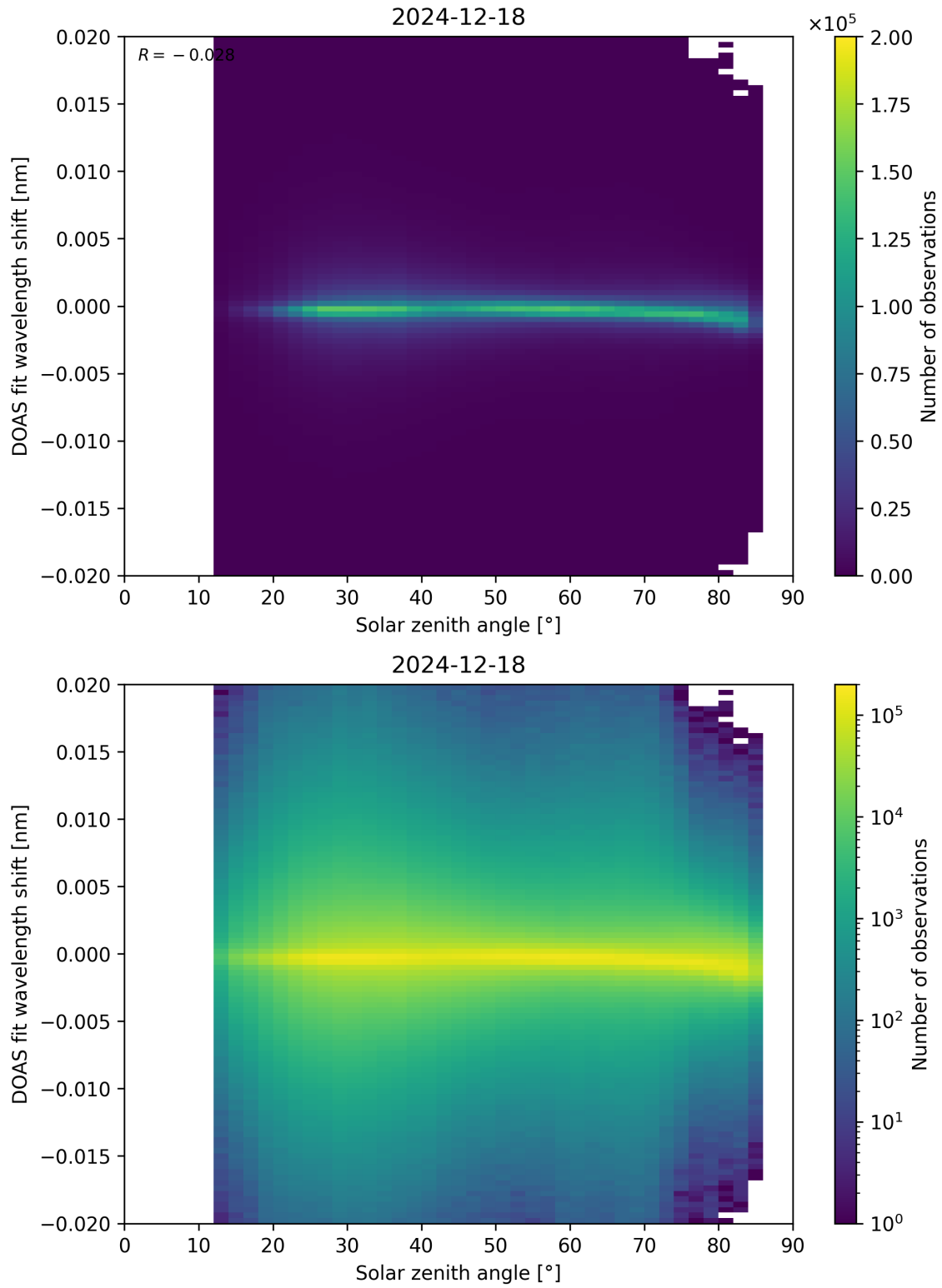
Figure 168: Scatter density plot of “Solar zenith angle” against “DOAS fit wavelength shift” for 2024-12-17 to 2024-12-19.
