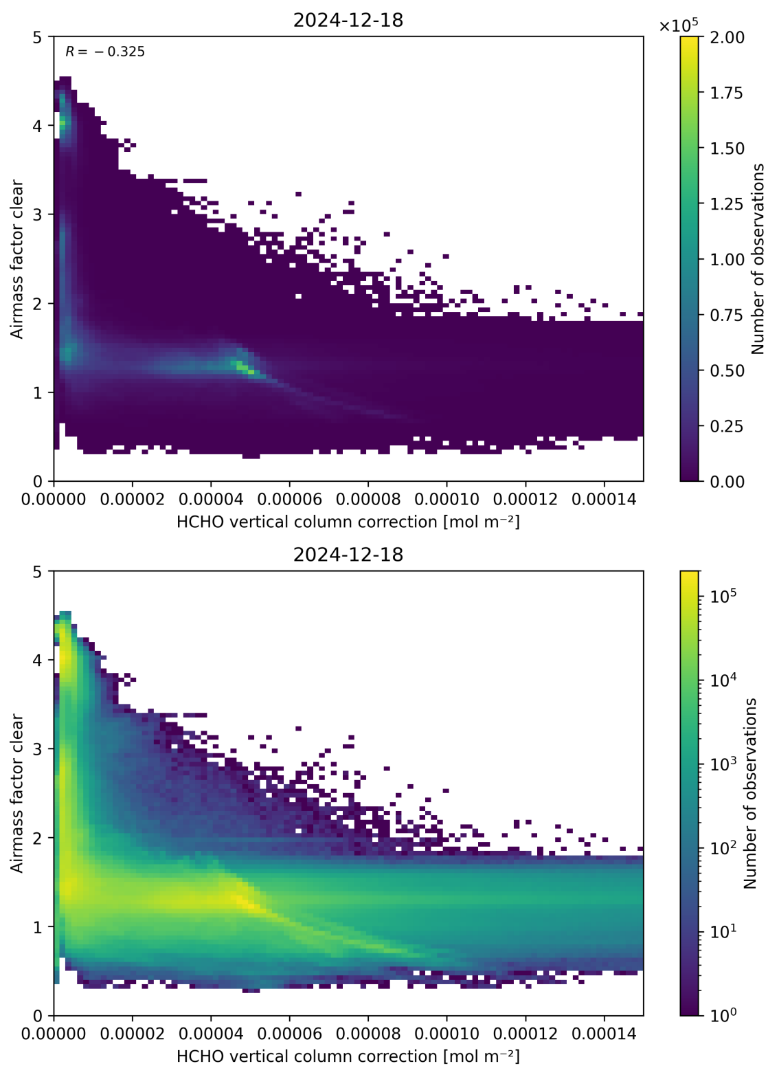
Figure 115: Scatter density plot of “HCHO vertical column correction” against “Airmass factor clear” for 2024-12-17 to 2024-12-19.
