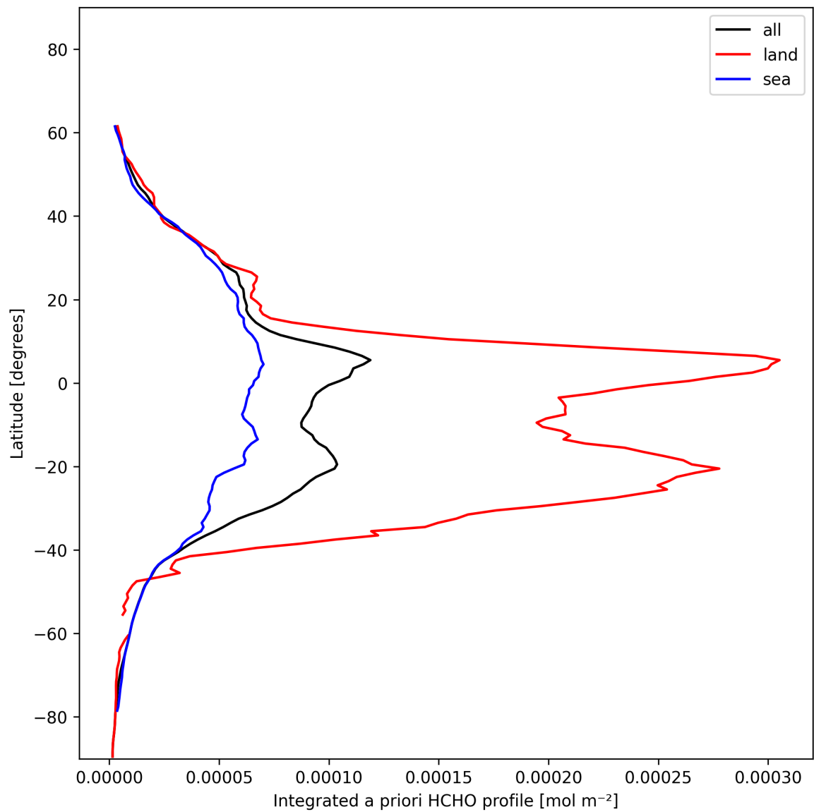
Figure 29: Zonal average of “Integrated a priori HCHO profile” for 2024-12-17 to 2024-12-19.
