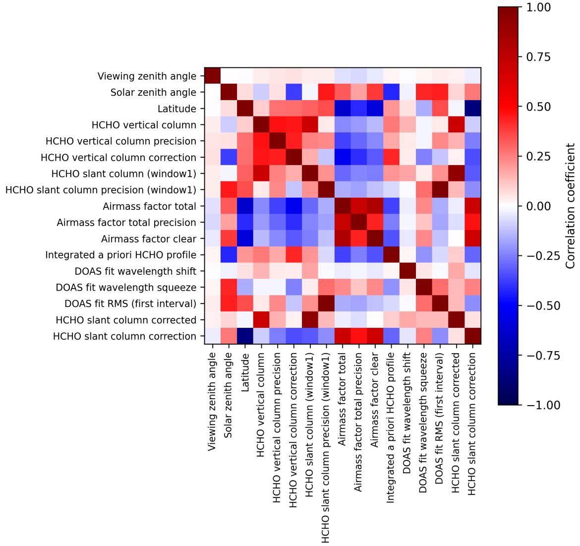
Figure 2: Map of correlation matrix for 2024-12-17 to 2024-12-19.
