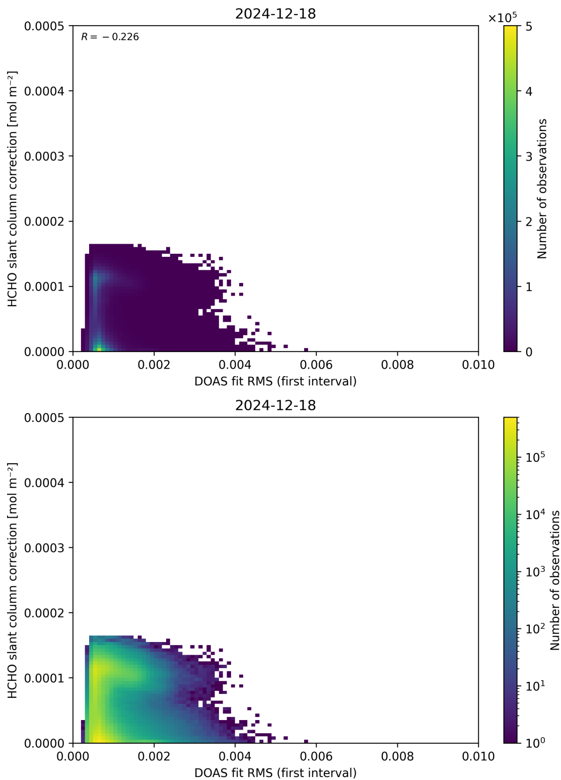
Figure 63: Scatter density plot of “DOAS fit RMS (first interval)” against “HCHO slant column correction” for 2024-12-17 to 2024-12-19.
