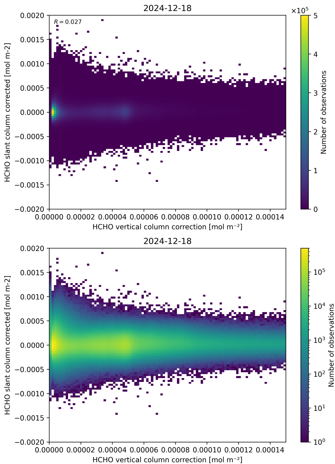
Figure 116: Scatter density plot of “HCHO vertical column correction” against “HCHO slant column corrected” for 2024-12-17 to 2024-12-19.
