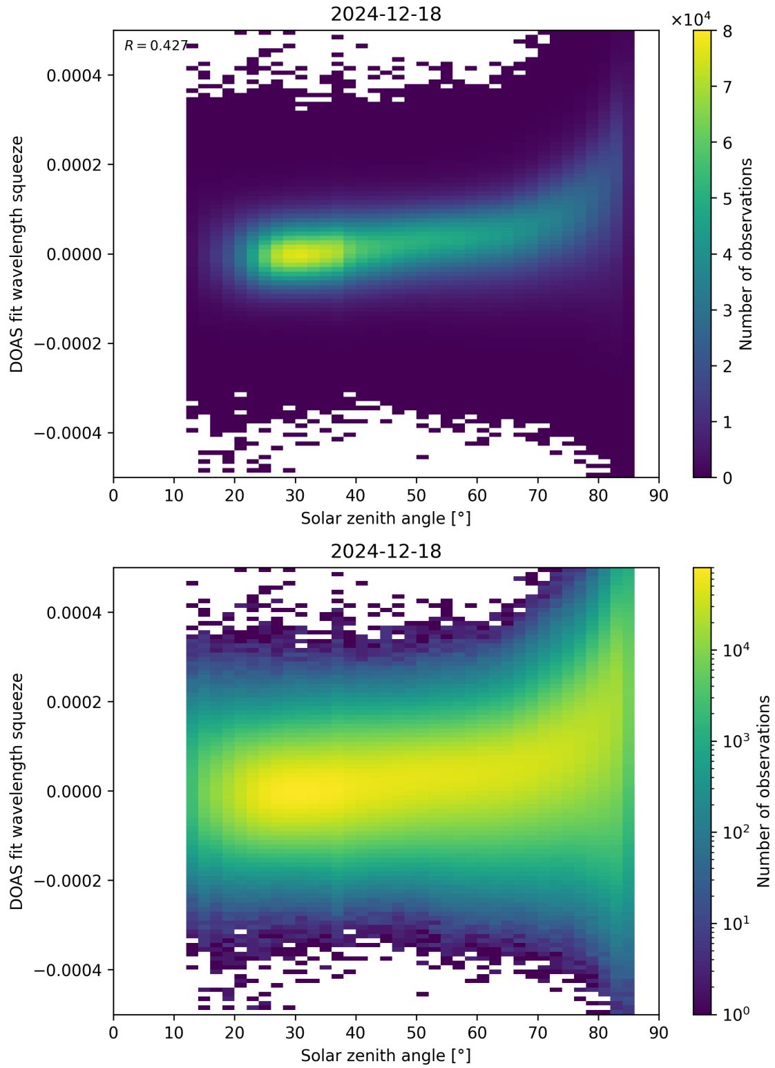
Figure 169: Scatter density plot of “Solar zenith angle” against “DOAS fit wavelength squeeze” for 2024-12-17 to 2024-12-19.
