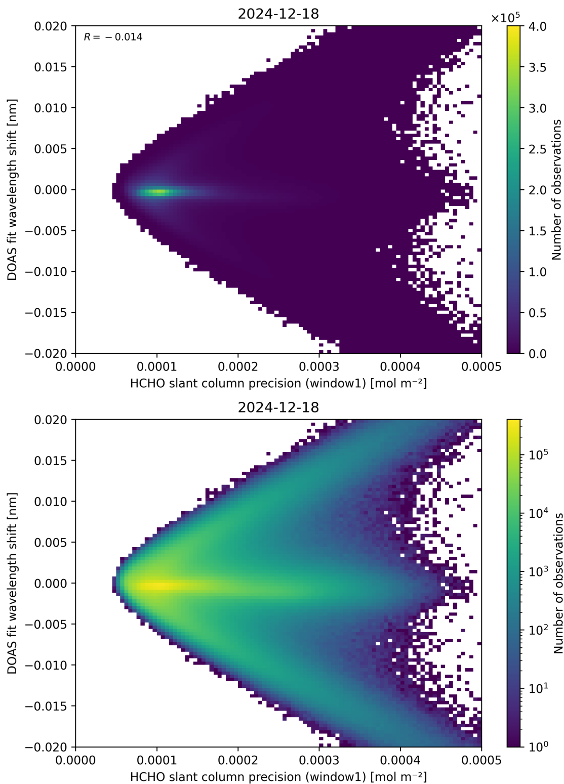
Figure 89: Scatter density plot of “HCHO slant column precision (window1)” against “DOAS fit wavelength shift” for 2024-12-17 to 2024-12-19.
