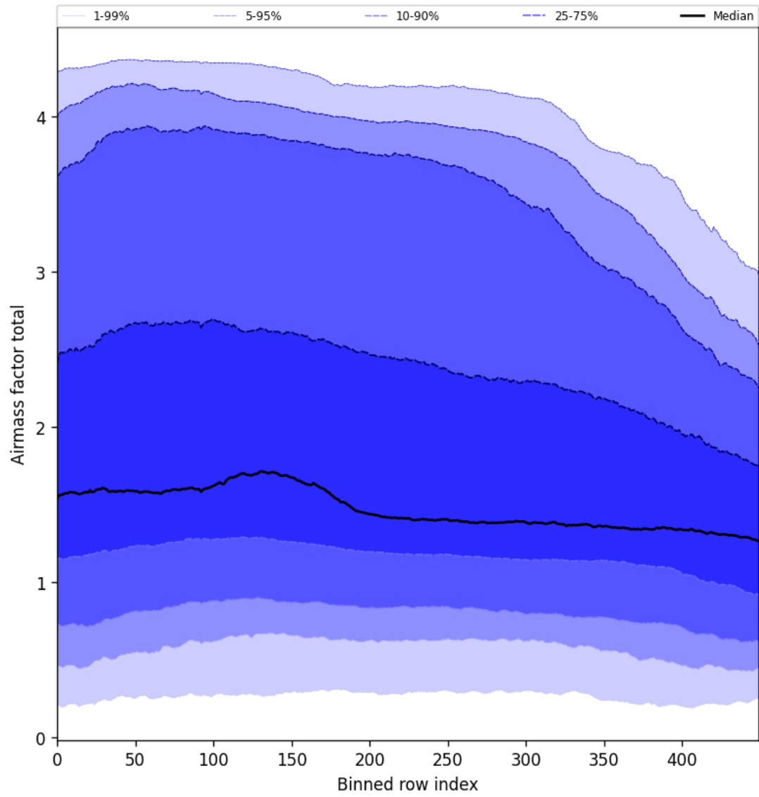
Figure 54: Along track statistics of “Airmass factor total” for 2024-12-17 to 2024-12-19
