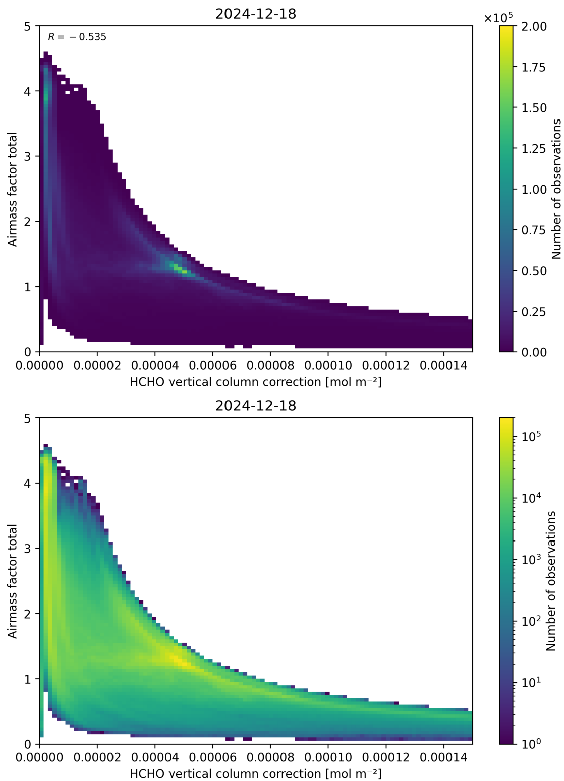
Figure 120: Scatter density plot of “HCHO vertical column correction” against “Airmass factor total” for 2024-12-17 to 2024-12-19.
