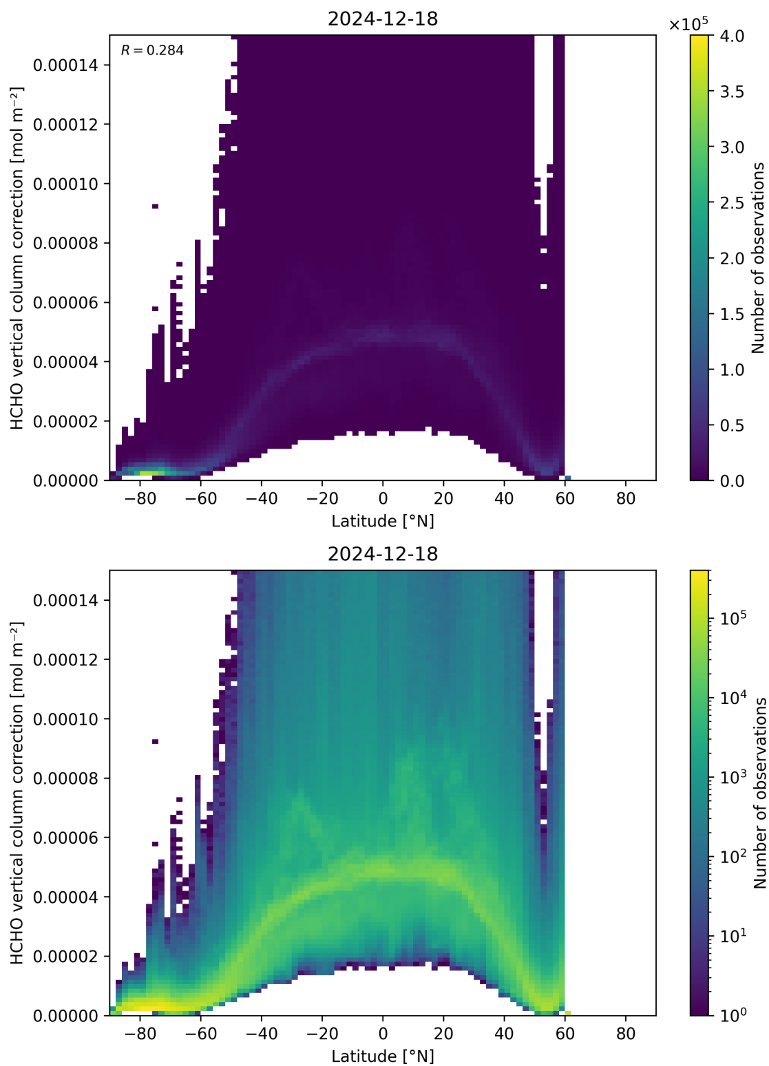
Figure 164: Scatter density plot of “Latitude” against “HCHO vertical column correction” for 2024-12-17 to 2024-12-19.
