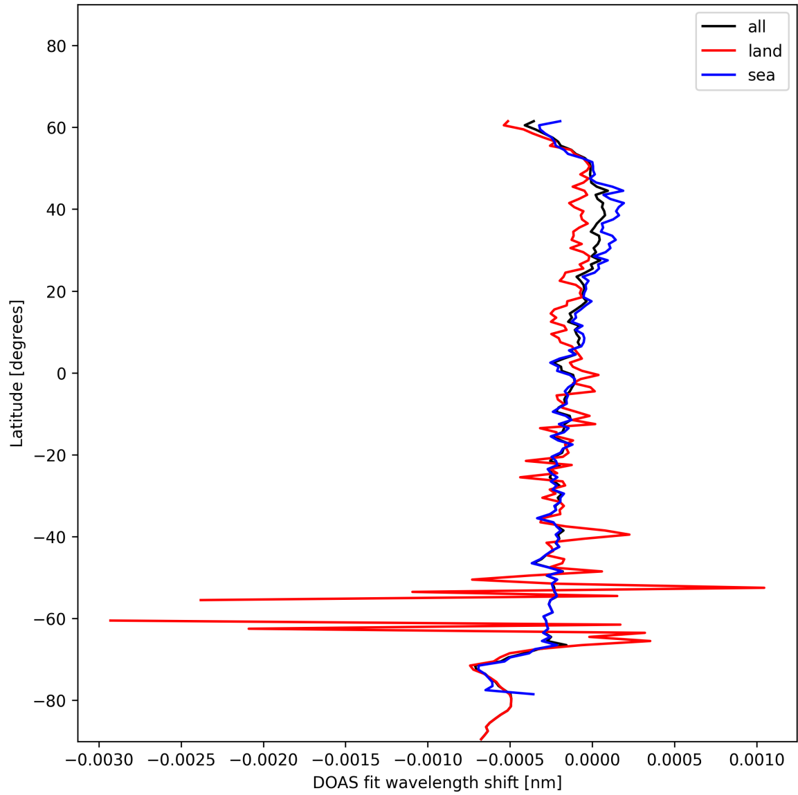
Figure 30: Zonal average of “DOAS fit wavelength shift” for 2024-12-17 to 2024-12-19.
