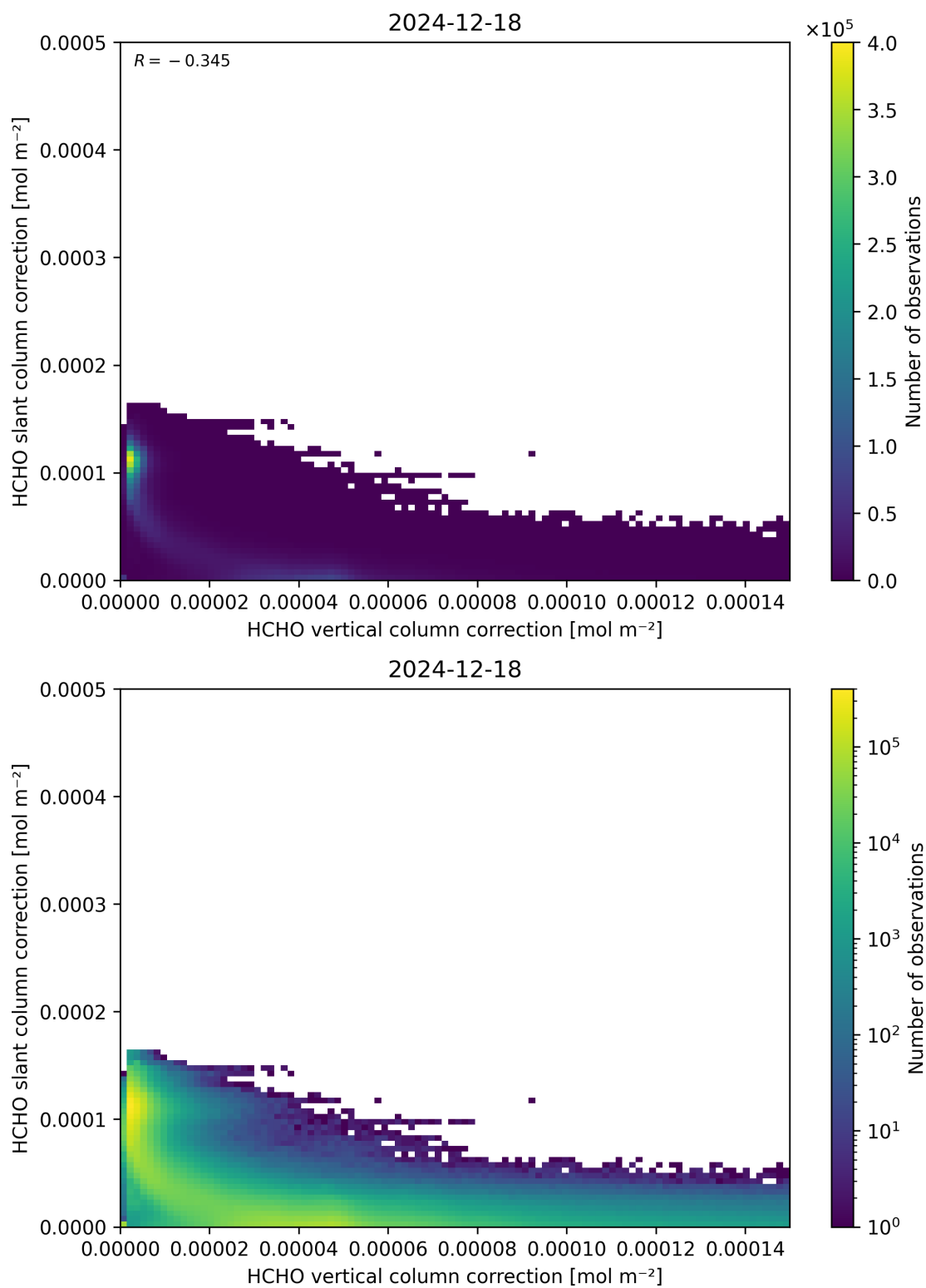
Figure 117: Scatter density plot of “HCHO vertical column correction” against “HCHO slant column correction” for 2024-12-17 to 2024-12-19.
