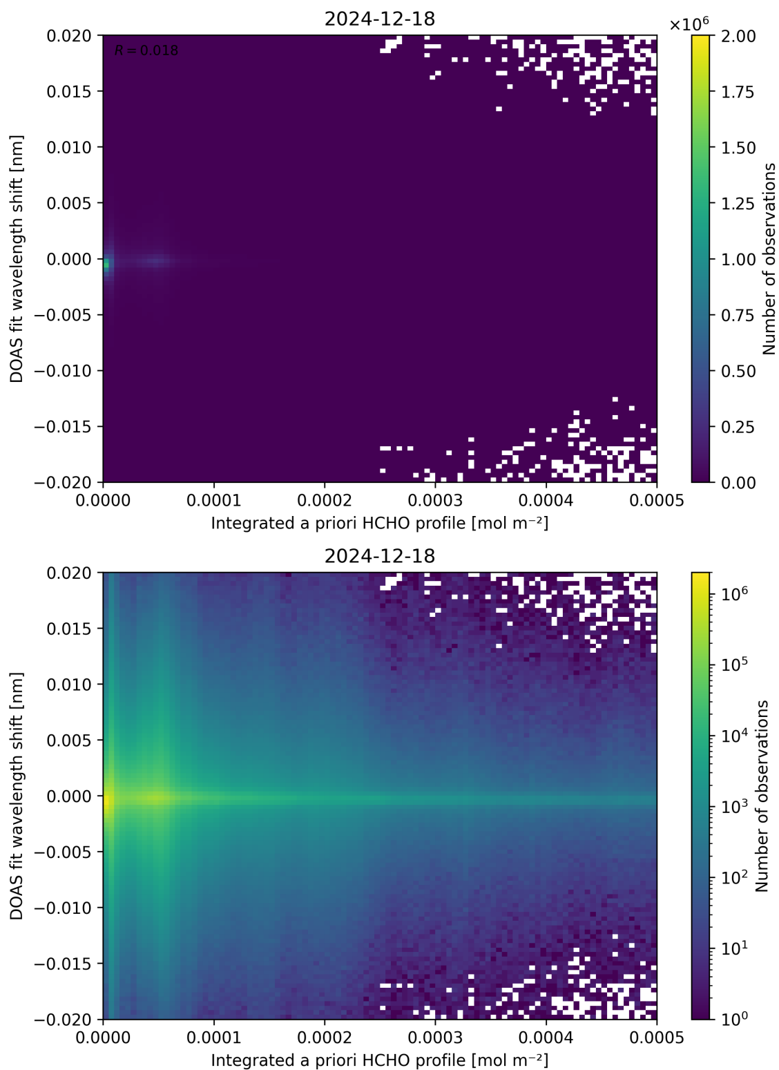
Figure 149: Scatter density plot of “Integrated a priori HCHO profile” against “DOAS fit wavelength shift” for 2024-12-17 to 2024-12-19.
