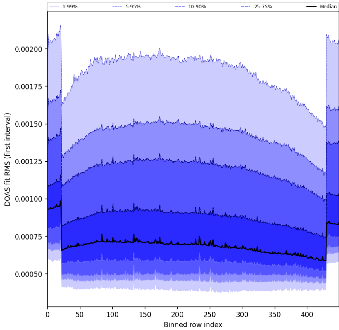
Figure 60: Along track statistics of “DOAS fit RMS (first interval)” for 2024-12-17 to 2024-12-19
