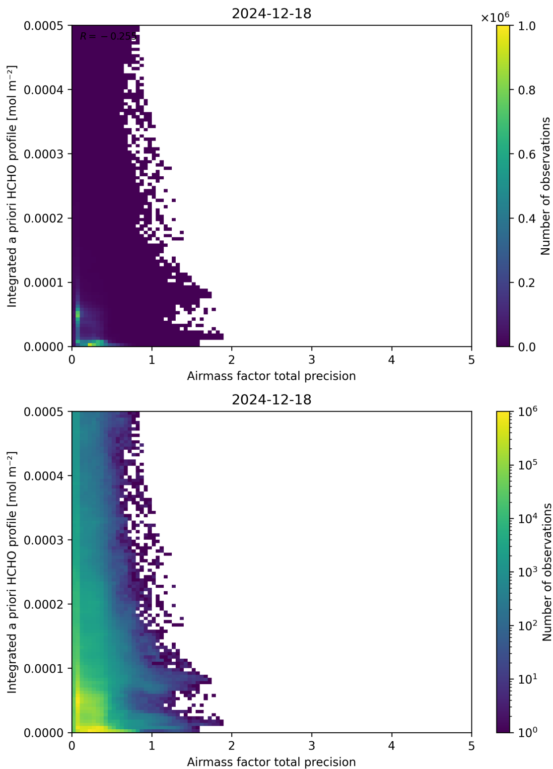
Figure 111: Scatter density plot of “Airmass factor total precision” against “Integrated a priori HCHO profile” for 2024-12-17 to 2024-12-19.
