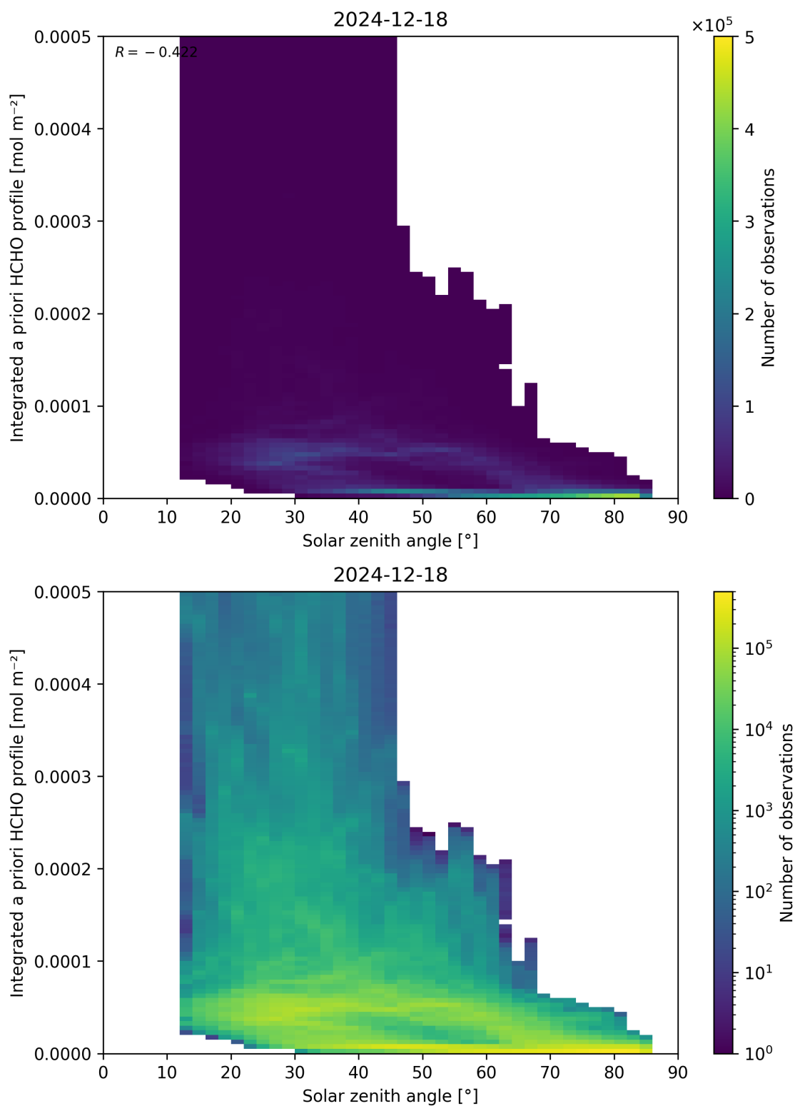
Figure 180: Scatter density plot of “Solar zenith angle” against “Integrated a priori HCHO profile” for 2024-12-17 to 2024-12-19.
