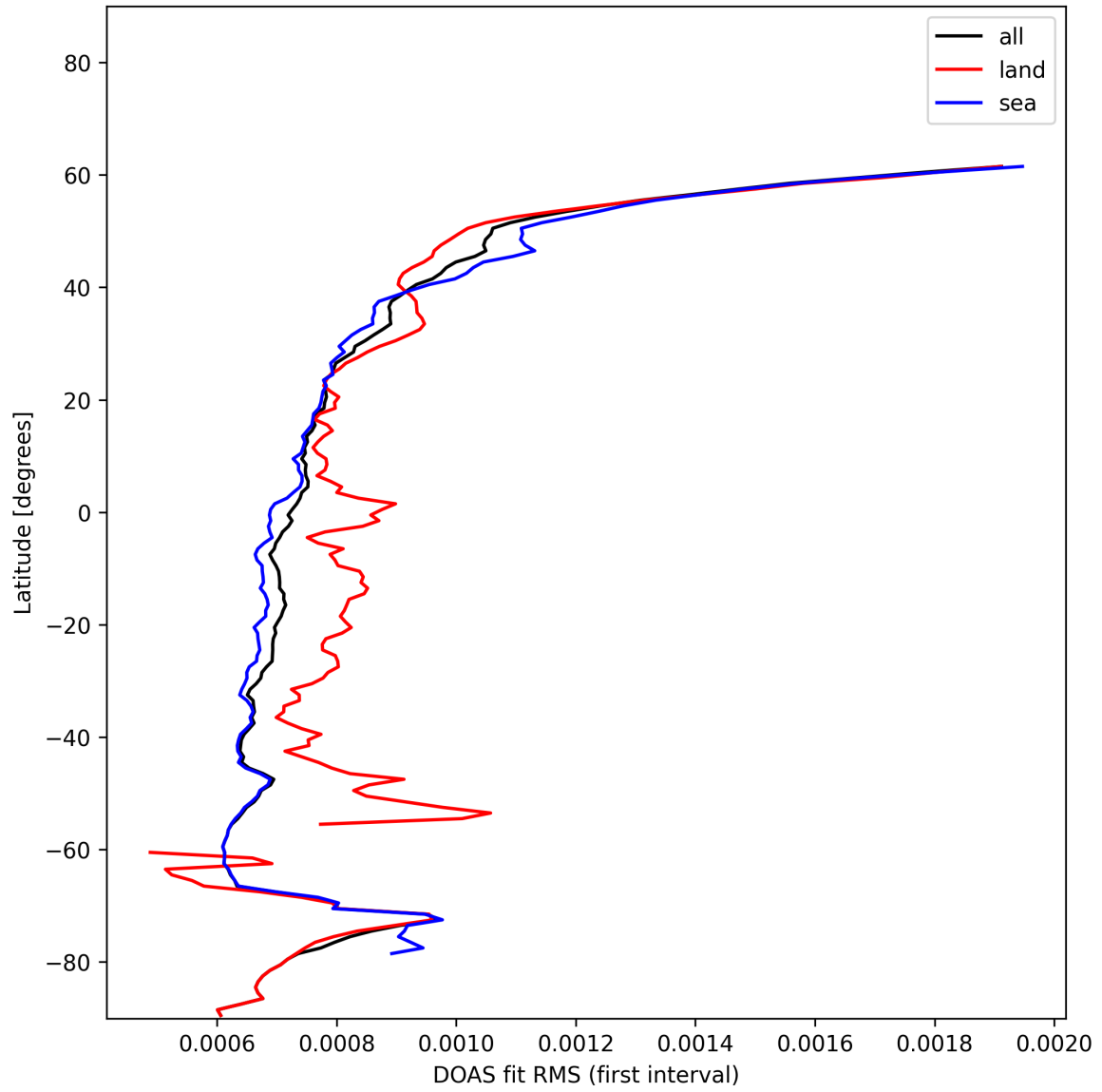
Figure 32: Zonal average of “DOAS fit RMS (first interval)” for 2024-12-17 to 2024-12-19.
