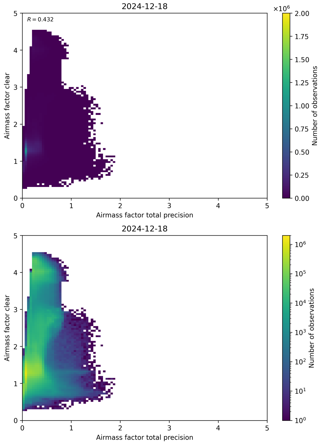
Figure 108: Scatter density plot of “Airmass factor total precision” against “Airmass factor clear” for 2024-12-17 to 2024-12-19.
