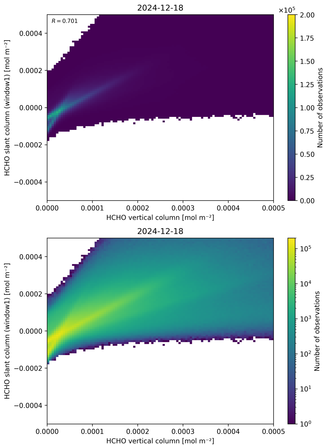
Figure 129: Scatter density plot of “HCHO vertical column” against “HCHO slant column (window1)” for 2024-12-17 to 2024-12-19.
