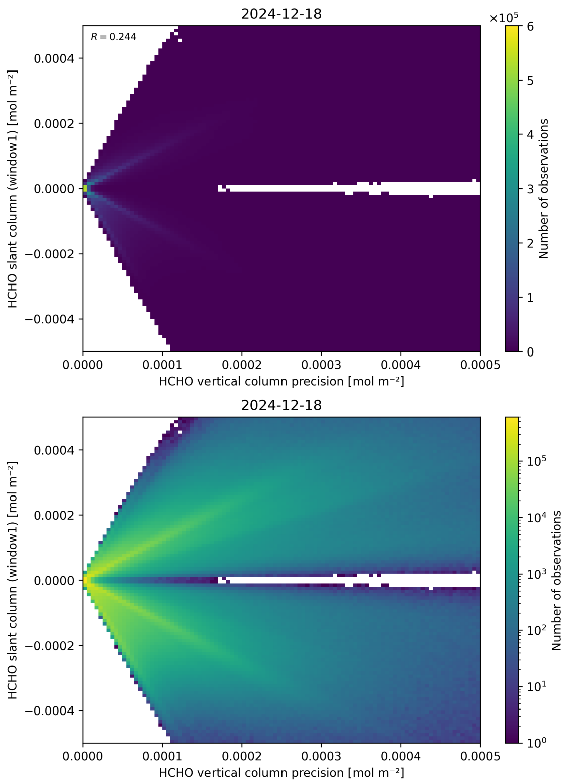
Figure 142: Scatter density plot of “HCHO vertical column precision” against “HCHO slant column (window1)” for 2024-12-17 to 2024-12-19.
