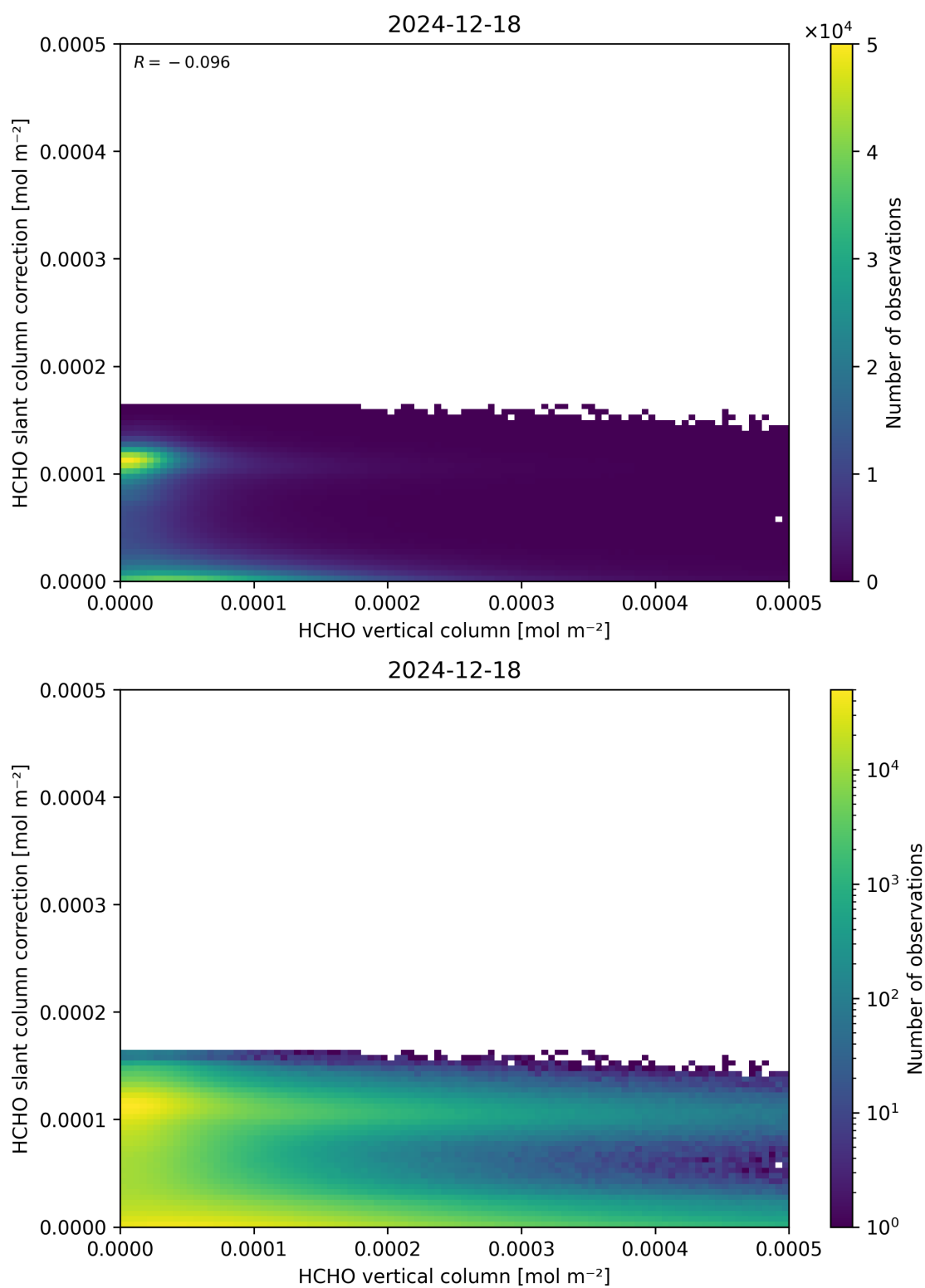
Figure 128: Scatter density plot of “HCHO vertical column” against “HCHO slant column correction” for 2024-12-17 to 2024-12-19.
