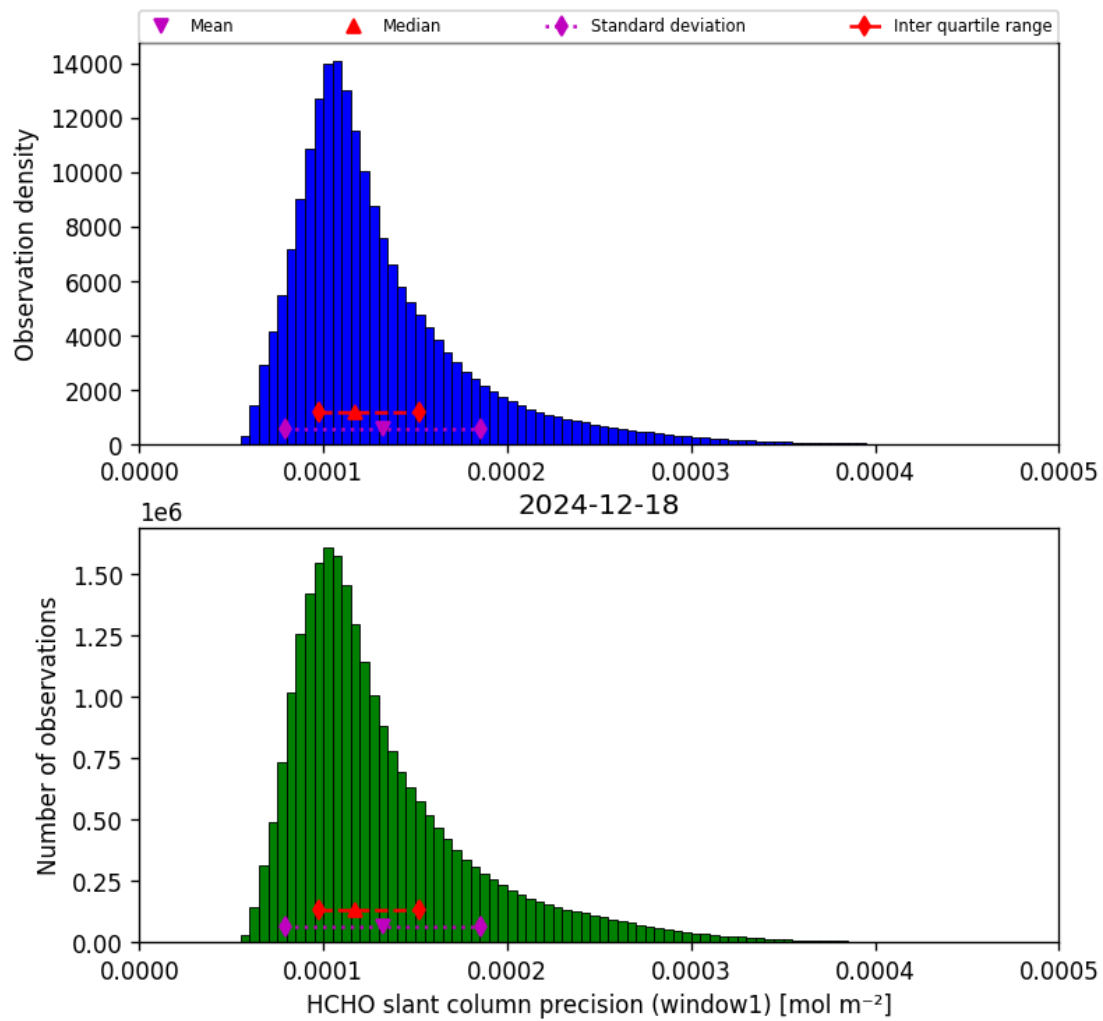
Figure 39: Histogram of “HCHO slant column precision (window1)” for 2024-12-17 to 2024-12-19
