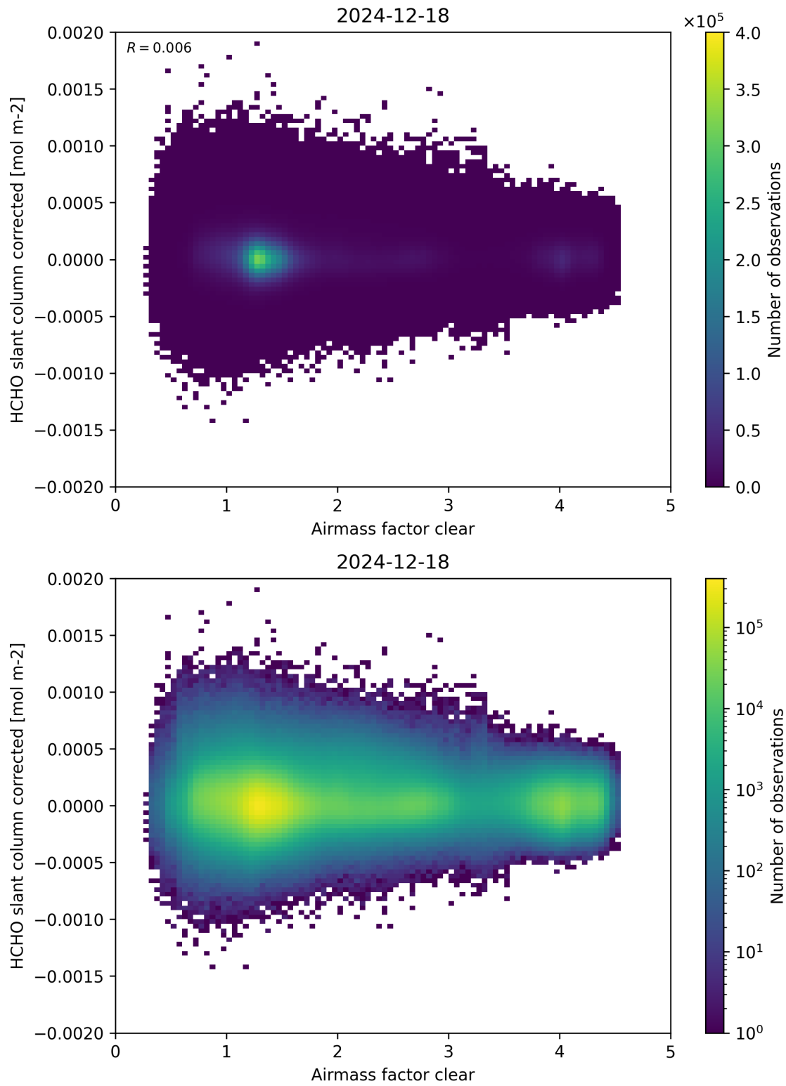
Figure 74: Scatter density plot of “Airmass factor clear” against “HCHO slant column corrected” for 2024-12-17 to 2024-12-19.
