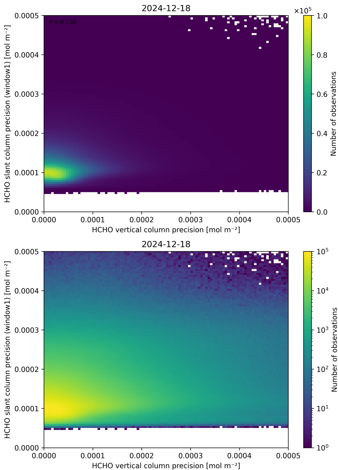
Figure 143: Scatter density plot of “HCHO vertical column precision” against “HCHO slant column precision (window1)” for 2024-12-17 to 2024-12-19.
