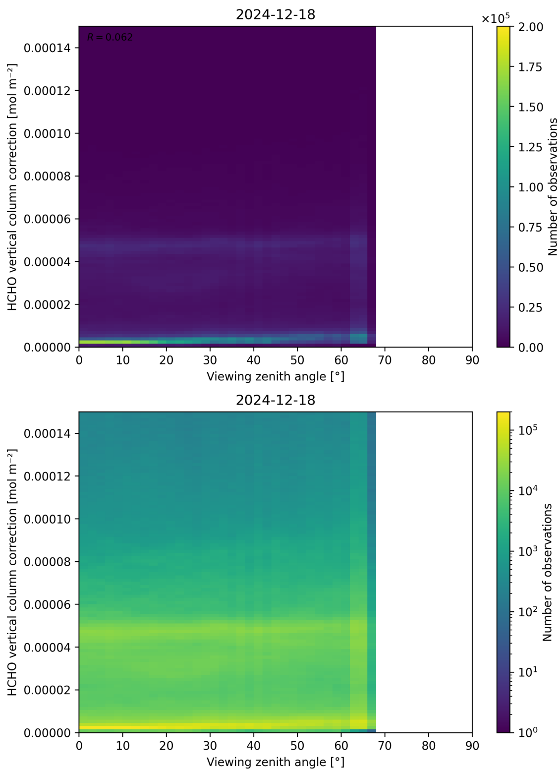
Figure 193: Scatter density plot of “Viewing zenith angle” against “HCHO vertical column correction” for 2024-12-17 to 2024-12-19.
