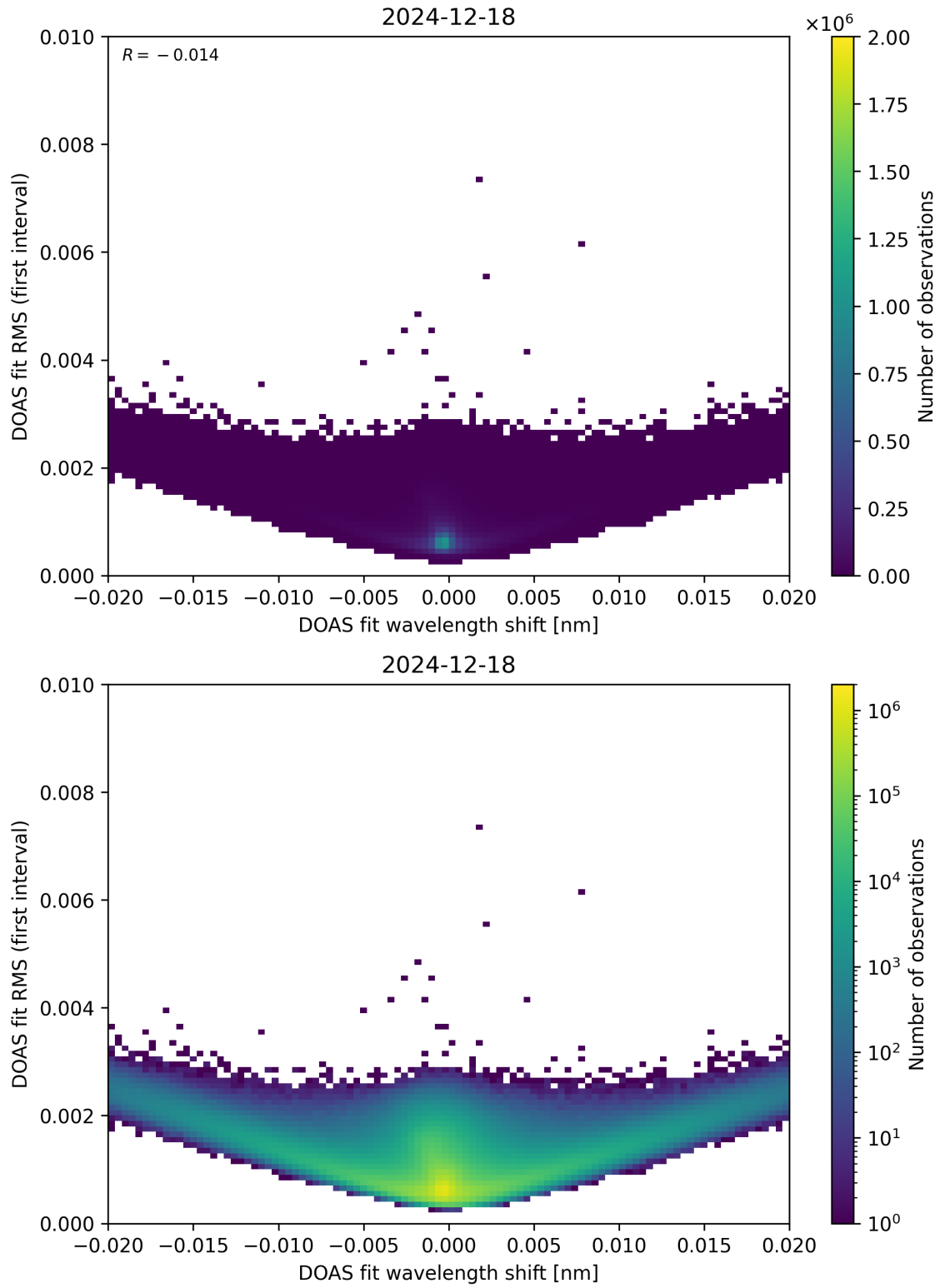
Figure 64: Scatter density plot of “DOAS fit wavelength shift” against “DOAS fit RMS (first interval)” for 2024-12-17 to 2024-12-19.
