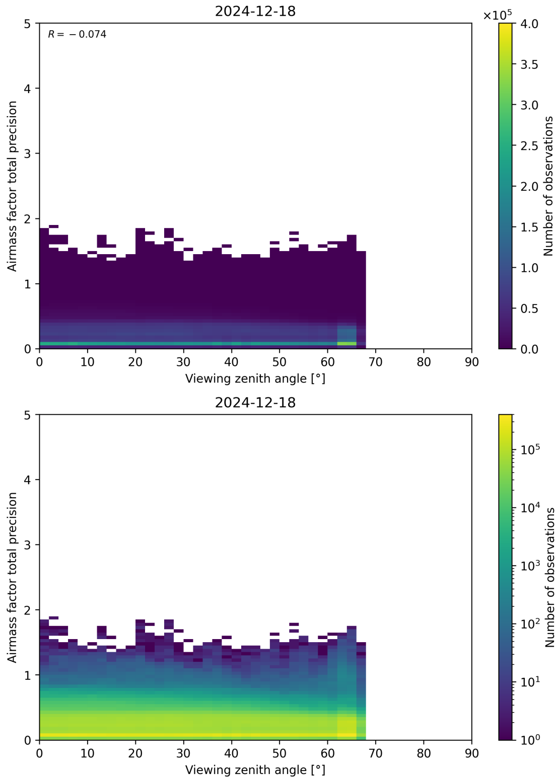
Figure 191: Scatter density plot of “Viewing zenith angle” against “Airmass factor total precision” for 2024-12-17 to 2024-12-19.
