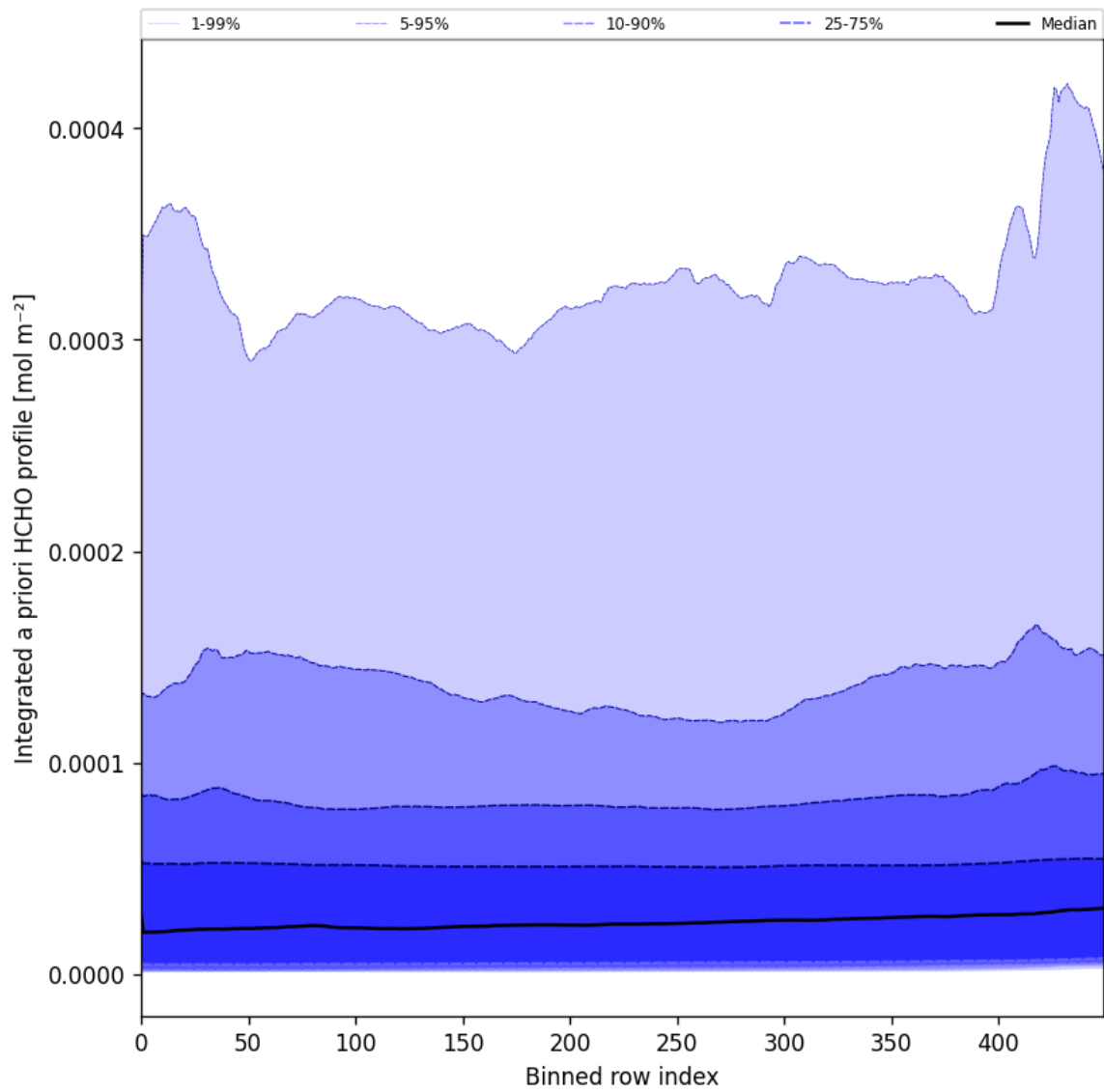
Figure 57: Along track statistics of "Integrated a priori HCHO profile" for 2024-12-17 to 2024-12-19
