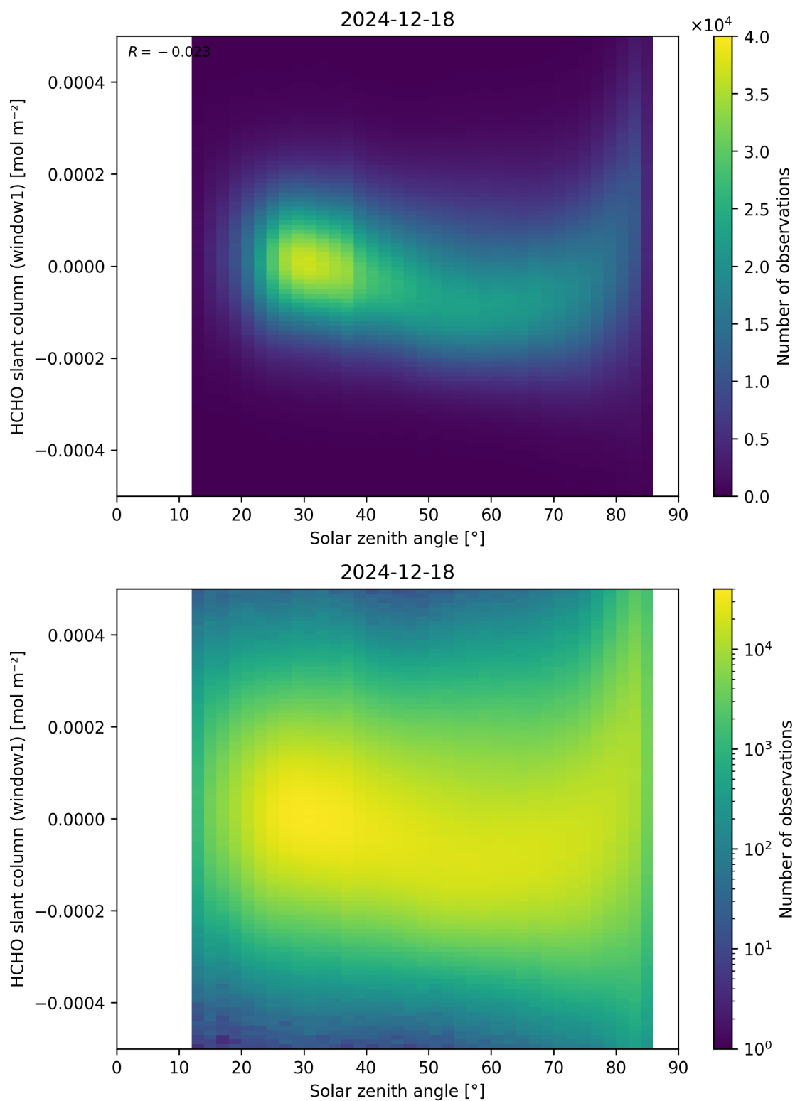
Figure 173: Scatter density plot of “Solar zenith angle” against “HCHO slant column (window1)” for 2024-12-17 to 2024-12-19.
