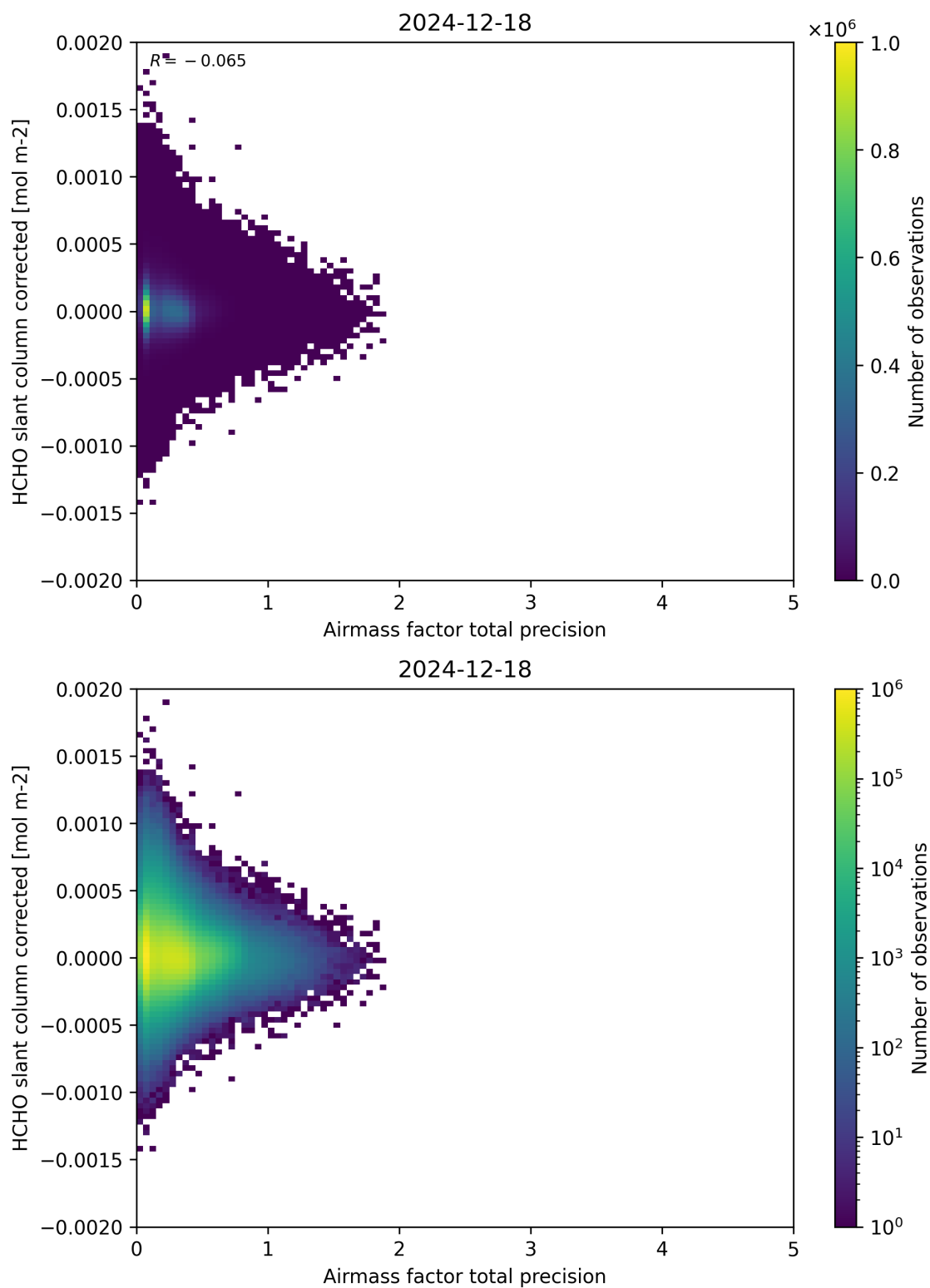
Figure 109: Scatter density plot of “Airmass factor total precision” against “HCHO slant column corrected” for 2024-12-17 to 2024-12-19.
