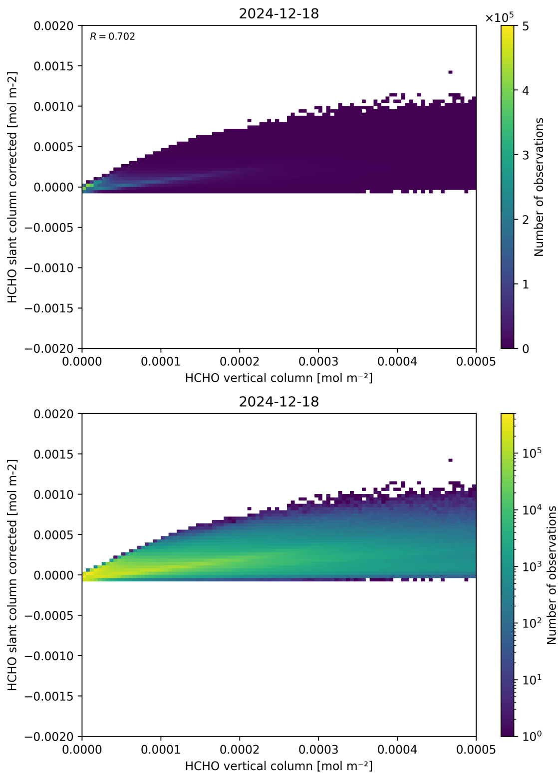
Figure 127: Scatter density plot of “HCHO vertical column” against “HCHO slant column corrected” for 2024-12-17 to 2024-12-19.
