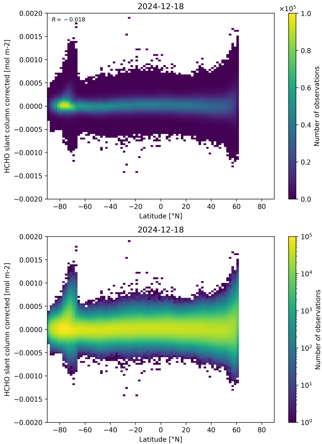
Figure 157: Scatter density plot of “Latitude” against “HCHO slant column corrected” for 2024-12-17 to 2024-12-19.
