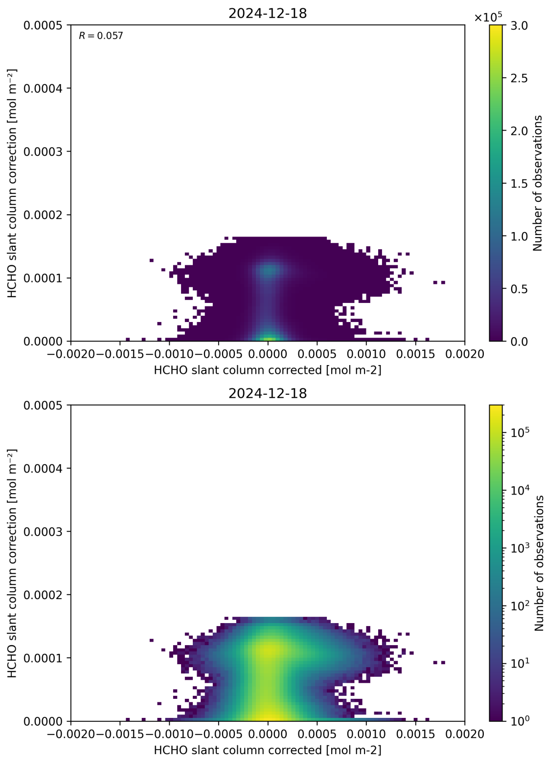
Figure 77: Scatter density plot of “HCHO slant column corrected” against “HCHO slant column correction” for 2024-12-17 to 2024-12-19.
