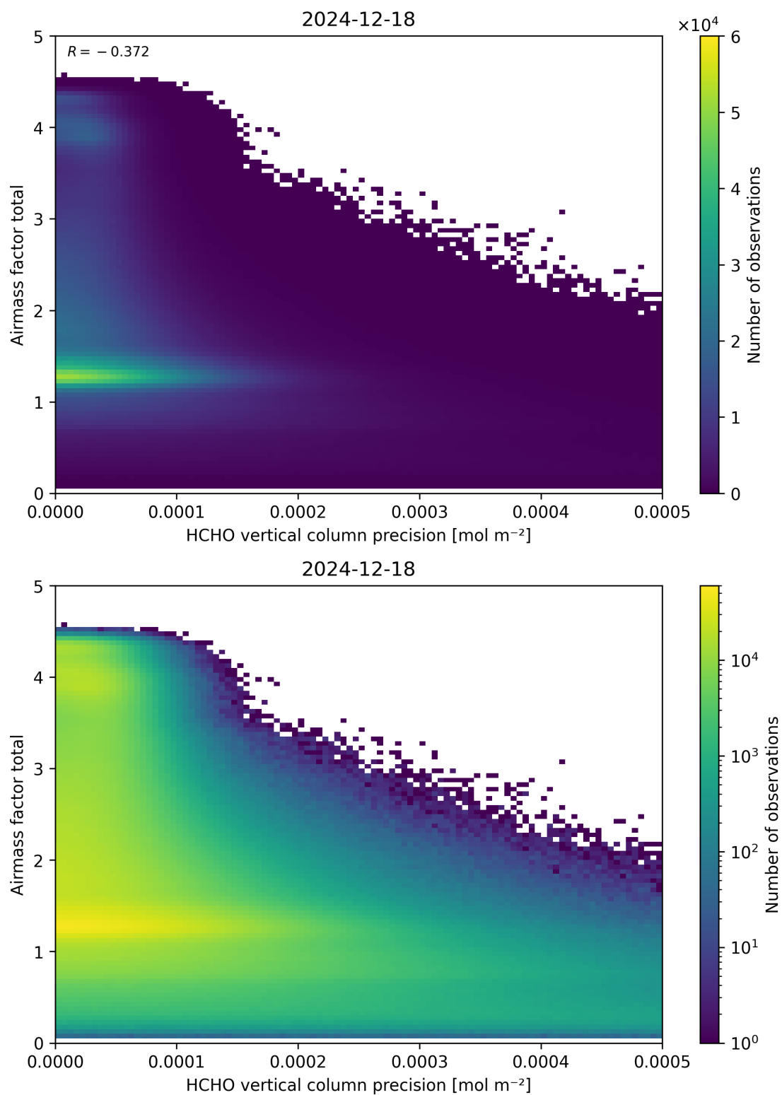
Figure 144: Scatter density plot of “HCHO vertical column precision” against “Airmass factor total” for 2024-12-17 to 2024-12-19.
