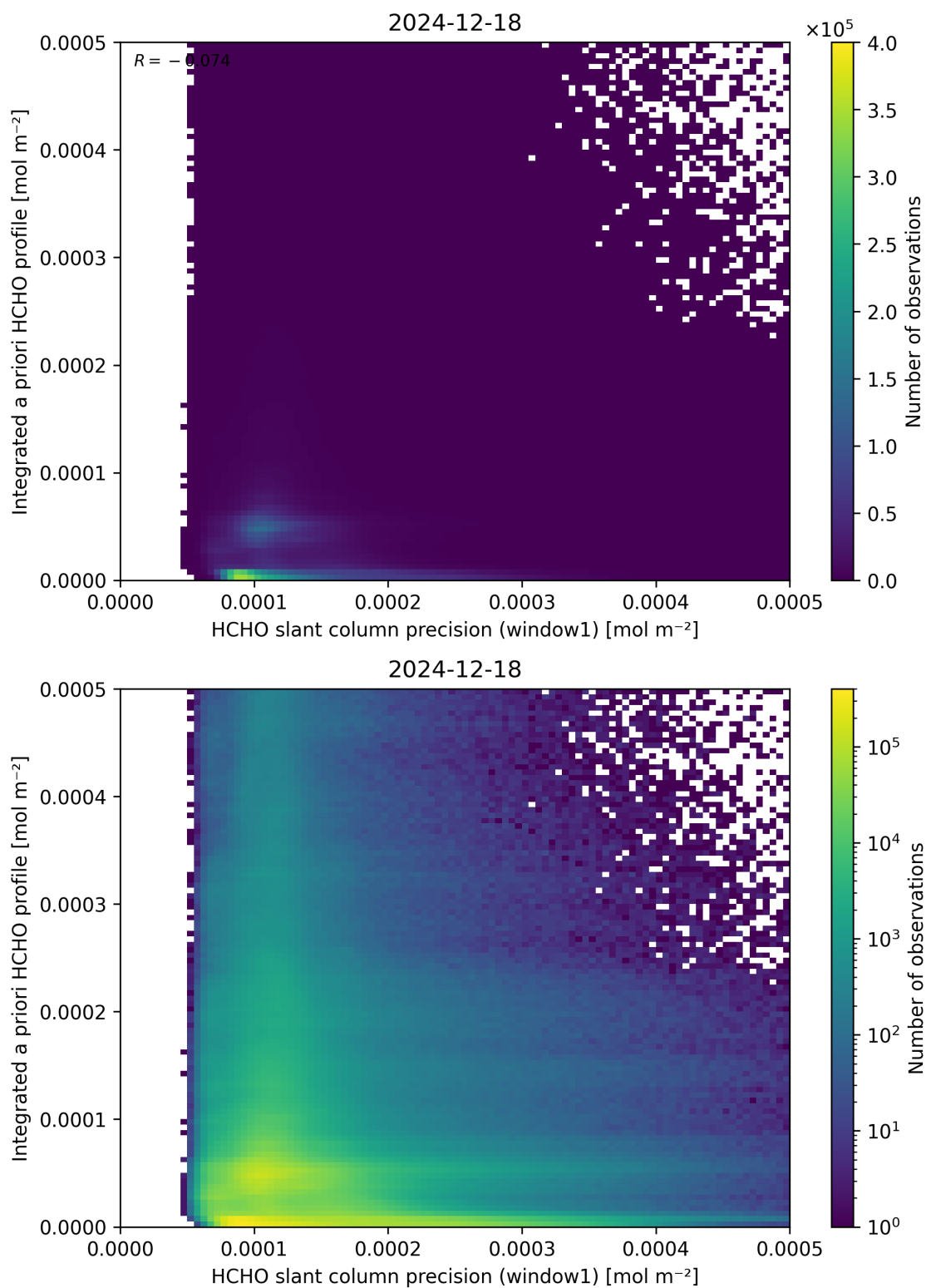
Figure 96: Scatter density plot of “HCHO slant column precision (window1)” against “Integrated a priori HCHO profile” for 2024-12-17 to 2024-12-19.
