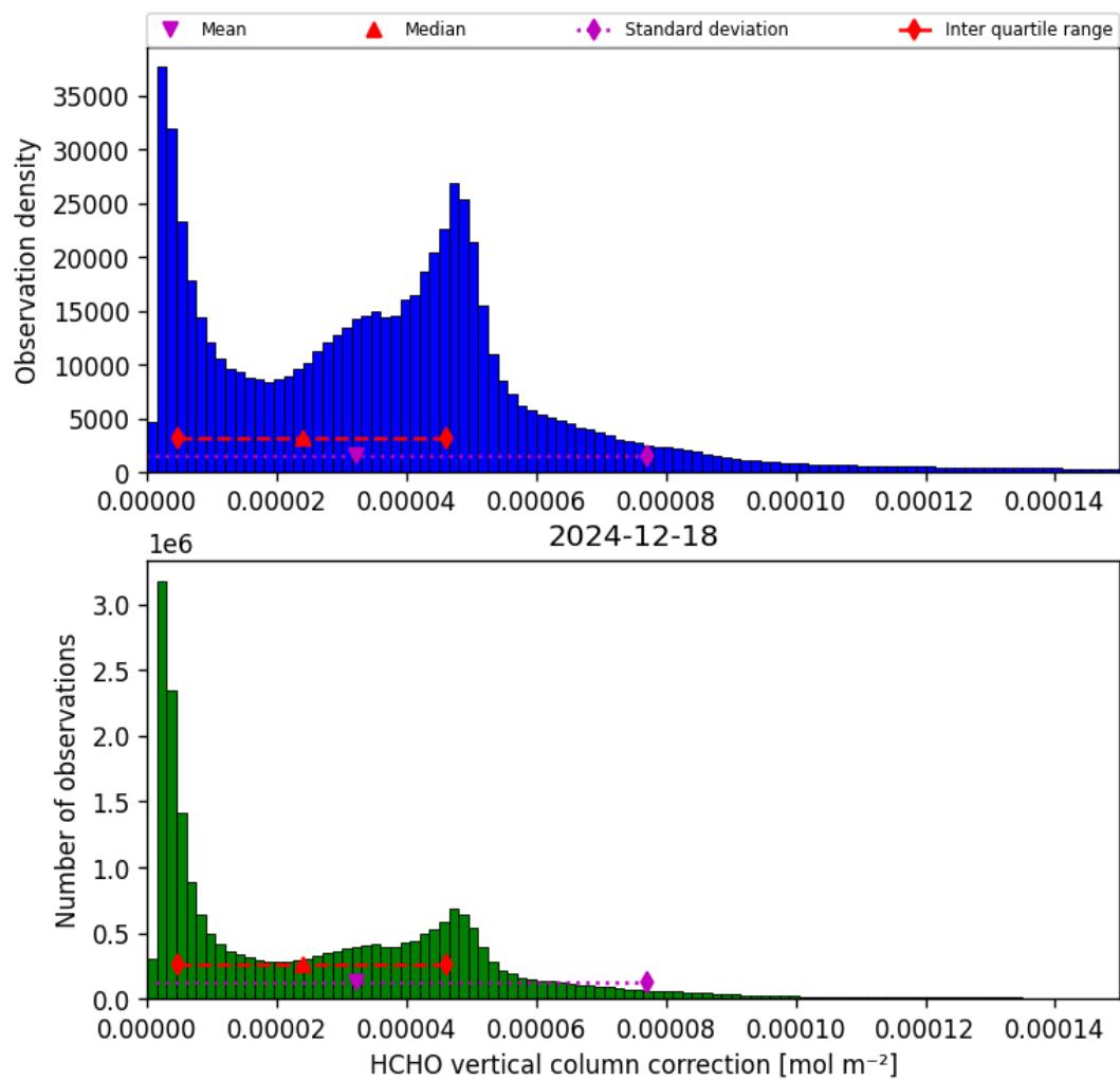
Figure 37: Histogram of “HCHO vertical column correction” for 2024-12-17 to 2024-12-19
