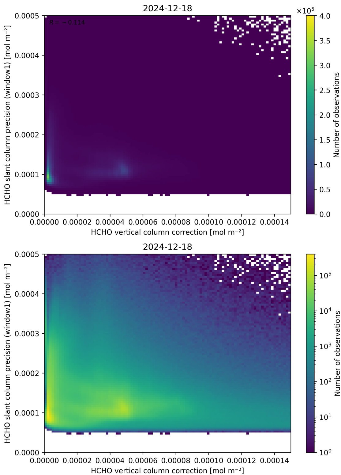
Figure 119: Scatter density plot of “HCHO vertical column correction” against “HCHO slant column precision (window1)” for 2024-12-17 to 2024-12-19.
