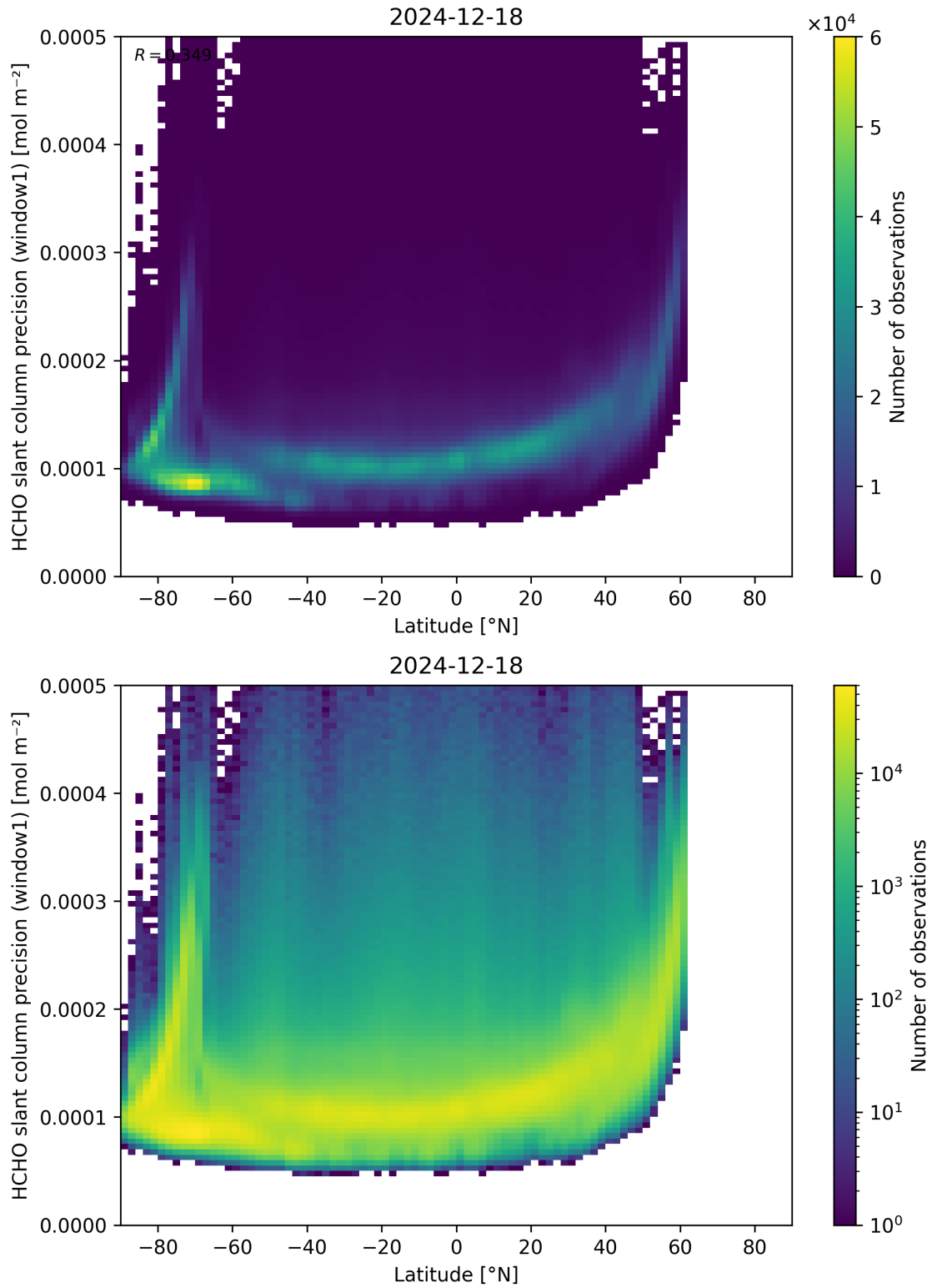
Figure 160: Scatter density plot of “Latitude” against “HCHO slant column precision (window1)” for 2024-12-17 to 2024-12-19.
