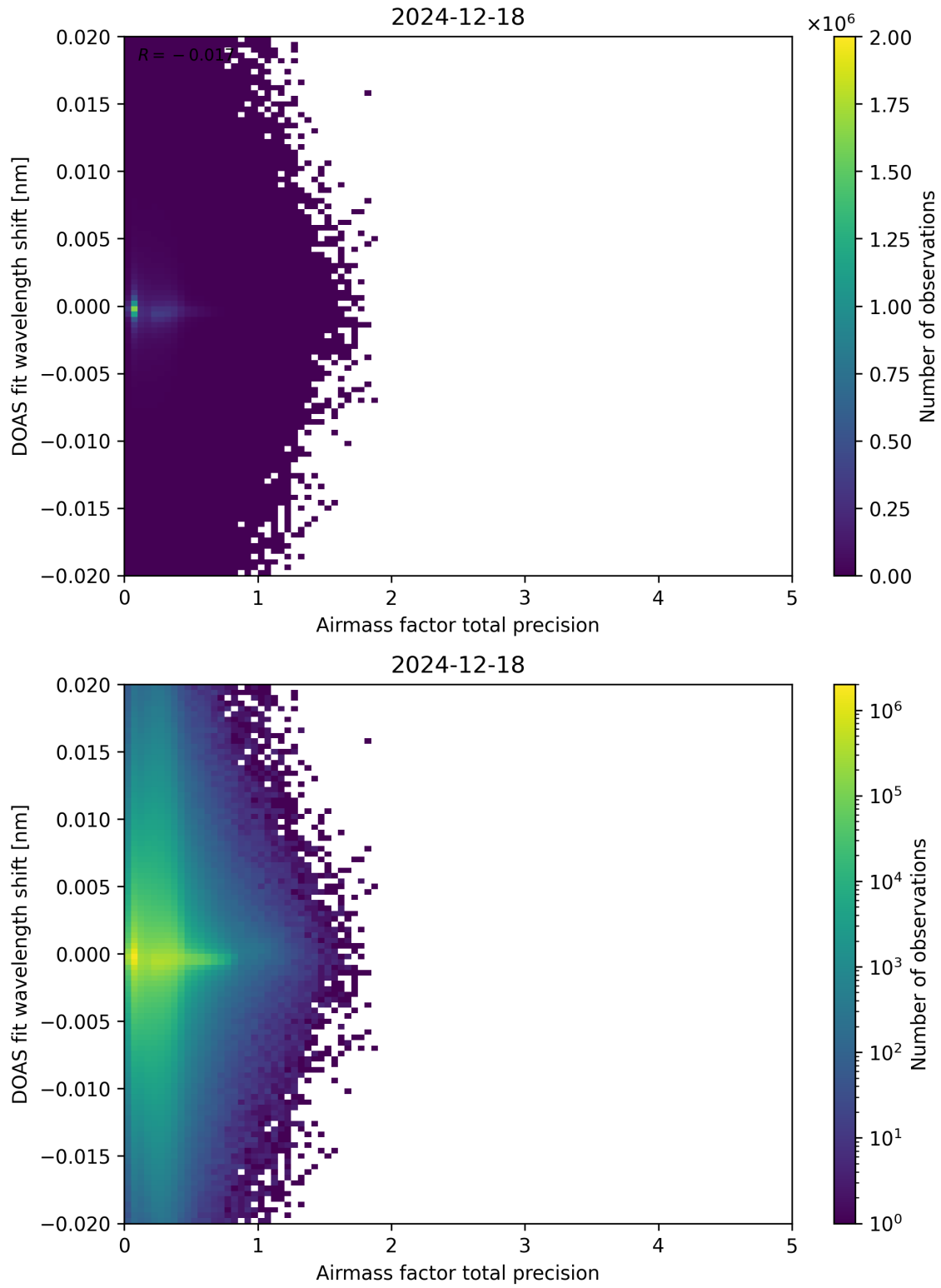
Figure 106: Scatter density plot of “Airmass factor total precision” against “DOAS fit wavelength shift” for 2024-12-17 to 2024-12-19.
