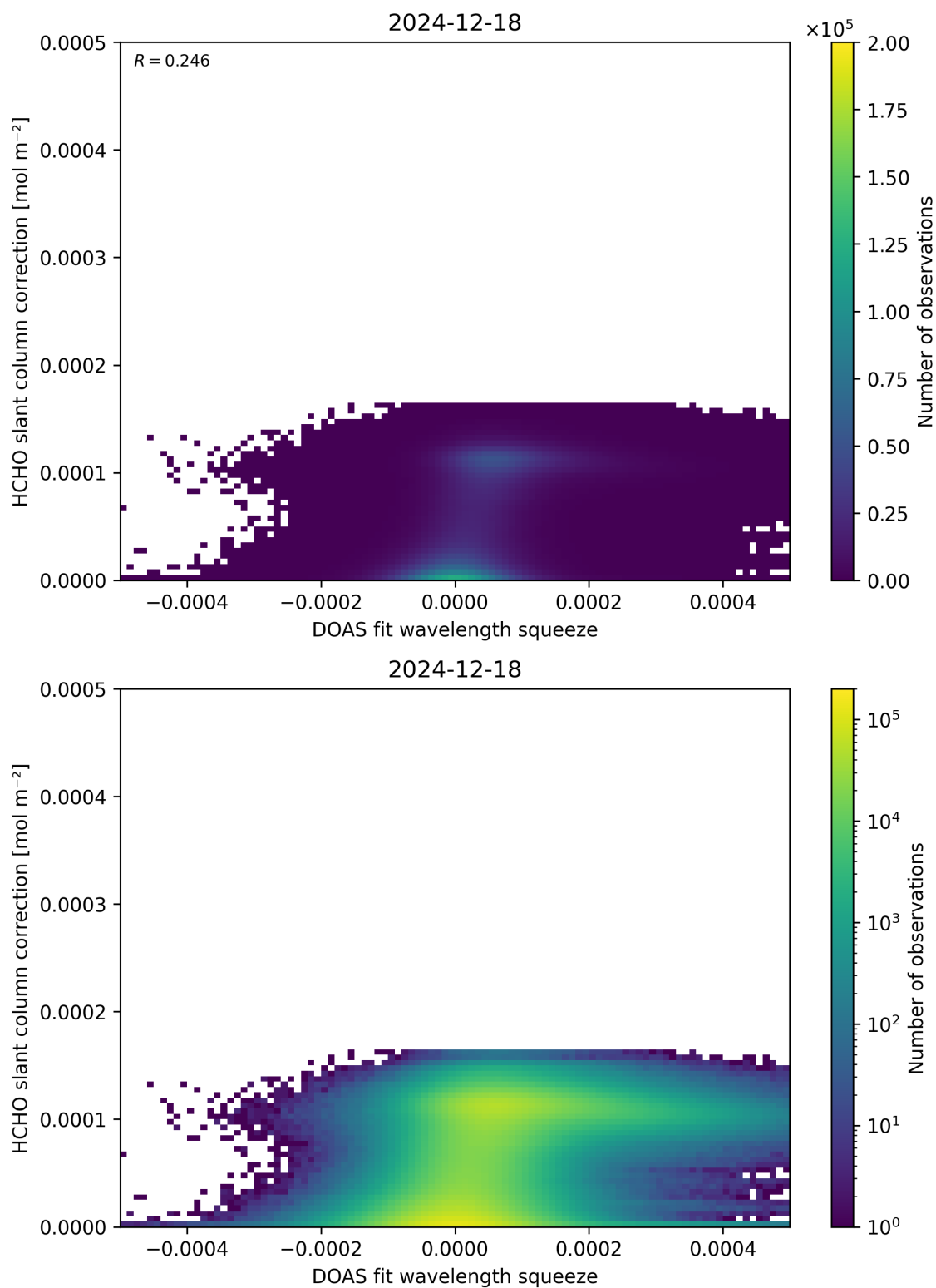
Figure 70: Scatter density plot of “DOAS fit wavelength squeeze” against “HCHO slant column correction” for 2024-12-17 to 2024-12-19.
