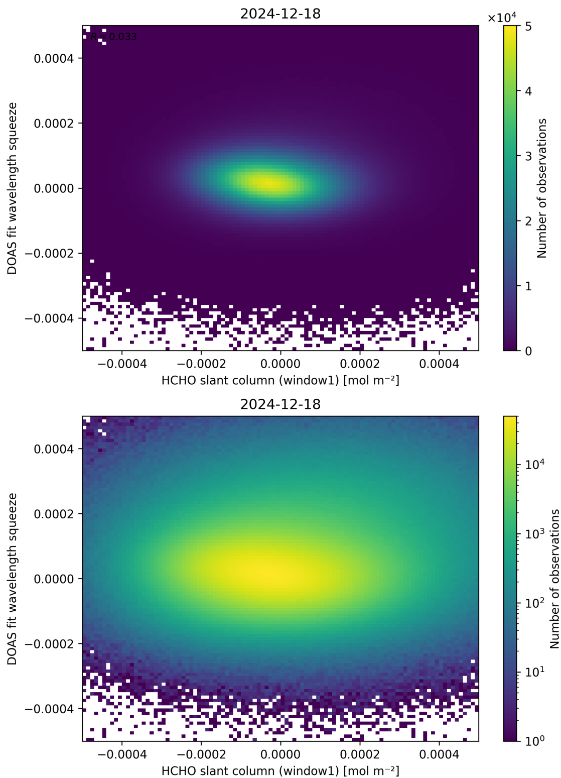
Figure 80: Scatter density plot of “HCHO slant column (window1)” against “DOAS fit wavelength squeeze” for 2024-12-17 to 2024-12-19.
