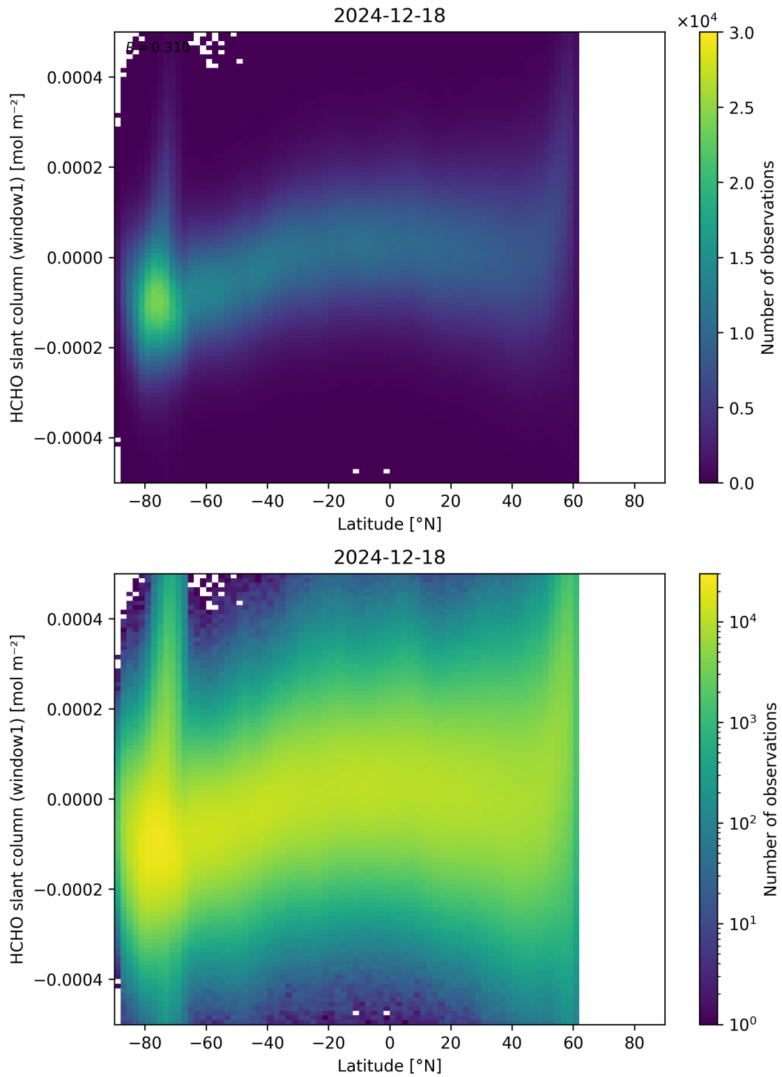
Figure 159: Scatter density plot of “Latitude” against “HCHO slant column (window1)” for 2024-12-17 to 2024-12-19.
