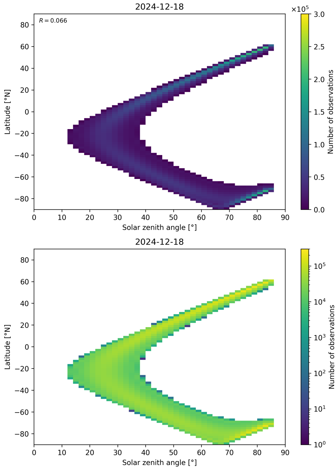
Figure 181: Scatter density plot of “Solar zenith angle” against “Latitude” for 2024-12-17 to 2024-12-19.
