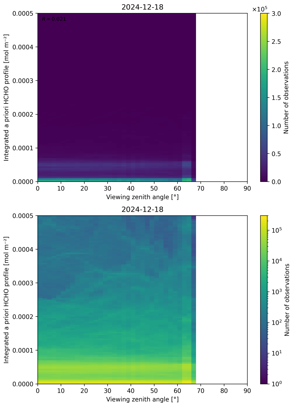
Figure 195: Scatter density plot of “Viewing zenith angle” against “Integrated a priori HCHO profile” for 2024-12-17 to 2024-12-19.
