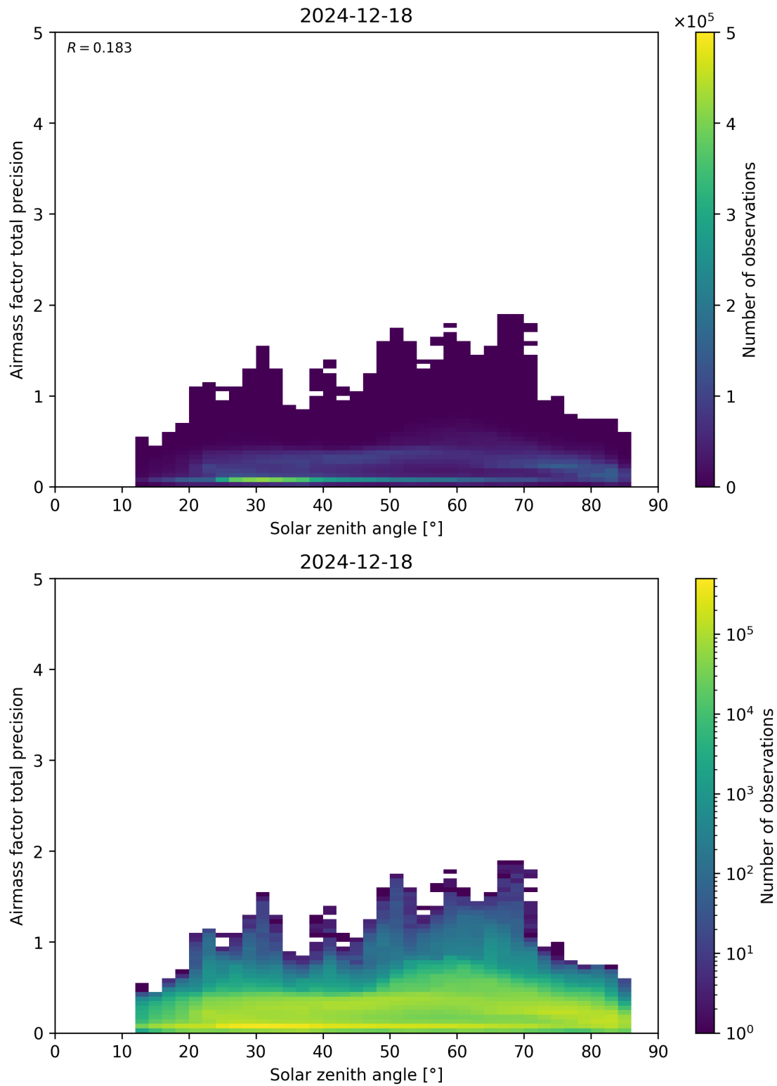
Figure 176: Scatter density plot of “Solar zenith angle” against “Airmass factor total precision” for 2024-12-17 to 2024-12-19.
