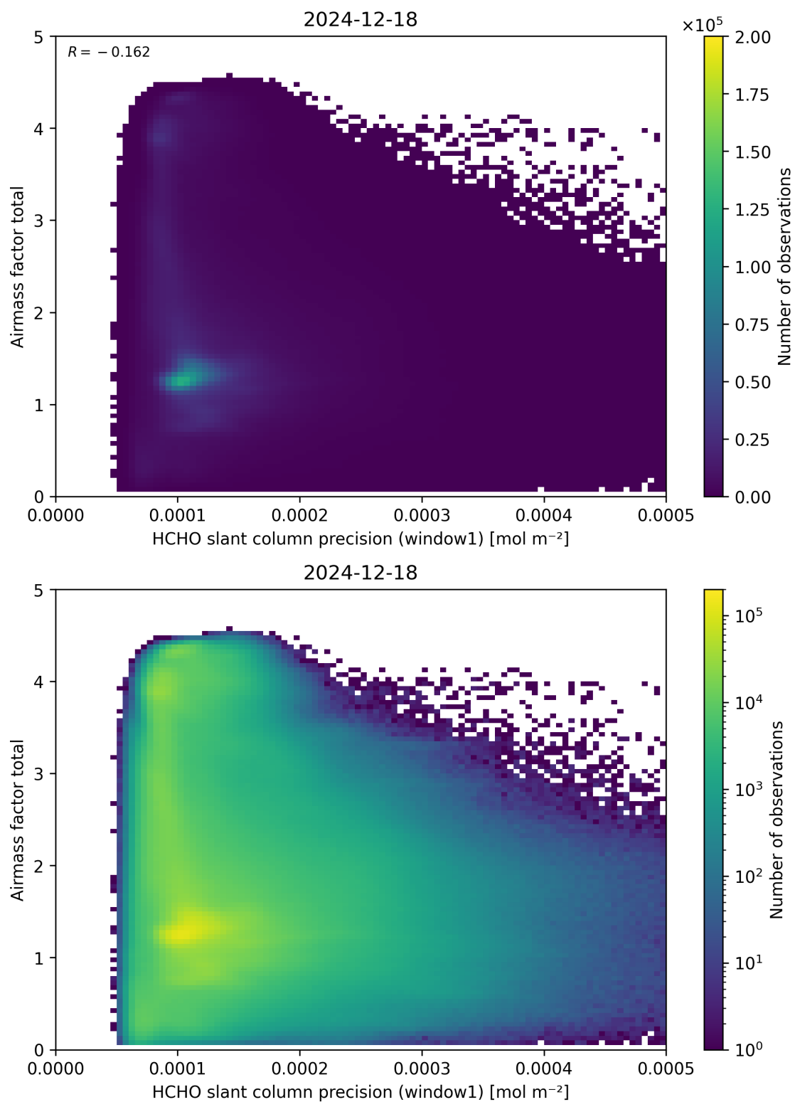
Figure 94: Scatter density plot of “HCHO slant column precision (window1)” against “Airmass factor total” for 2024-12-17 to 2024-12-19.
