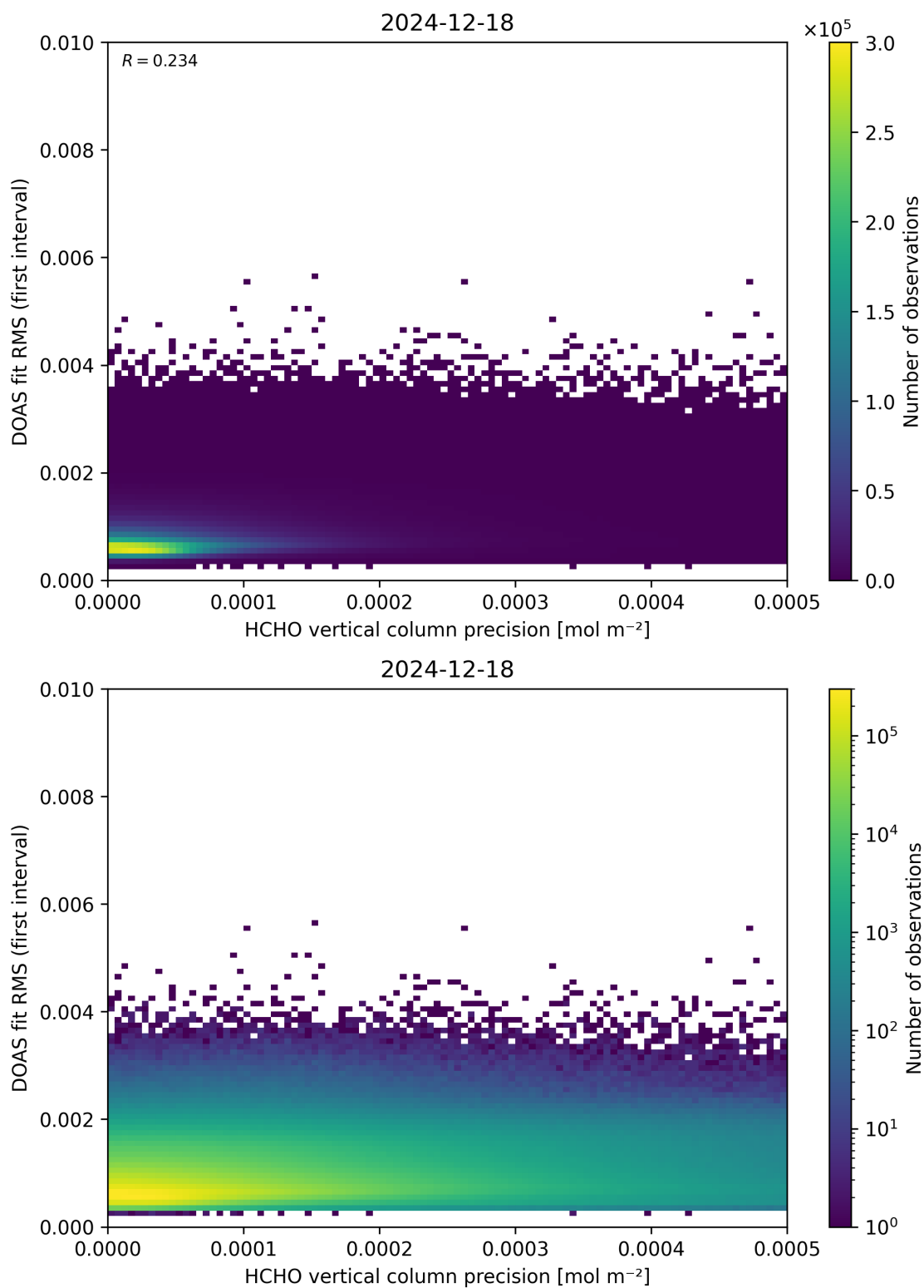
Figure 136: Scatter density plot of “HCHO vertical column precision” against “DOAS fit RMS (first interval)” for 2024-12-17 to 2024-12-19.
