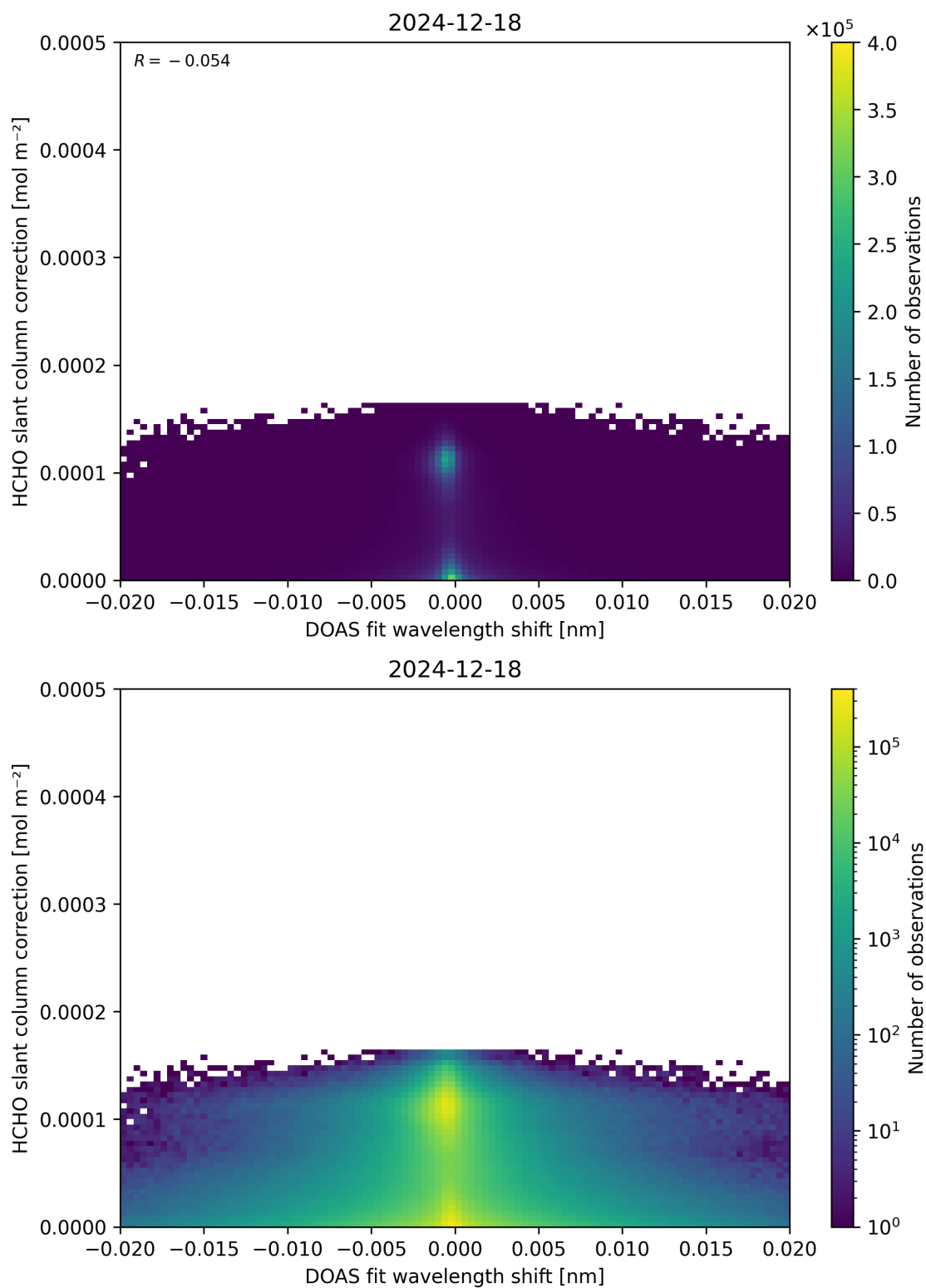
Figure 67: Scatter density plot of “DOAS fit wavelength shift” against “HCHO slant column correction” for 2024-12-17 to 2024-12-19.
