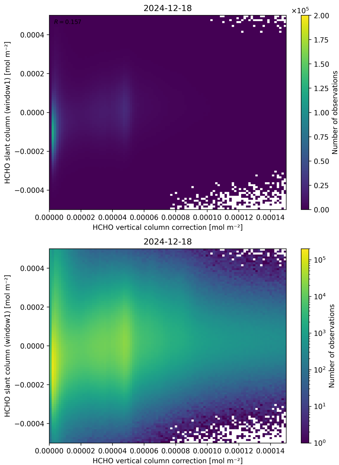
Figure 118: Scatter density plot of “HCHO vertical column correction” against “HCHO slant column (window1)” for 2024-12-17 to 2024-12-19.
