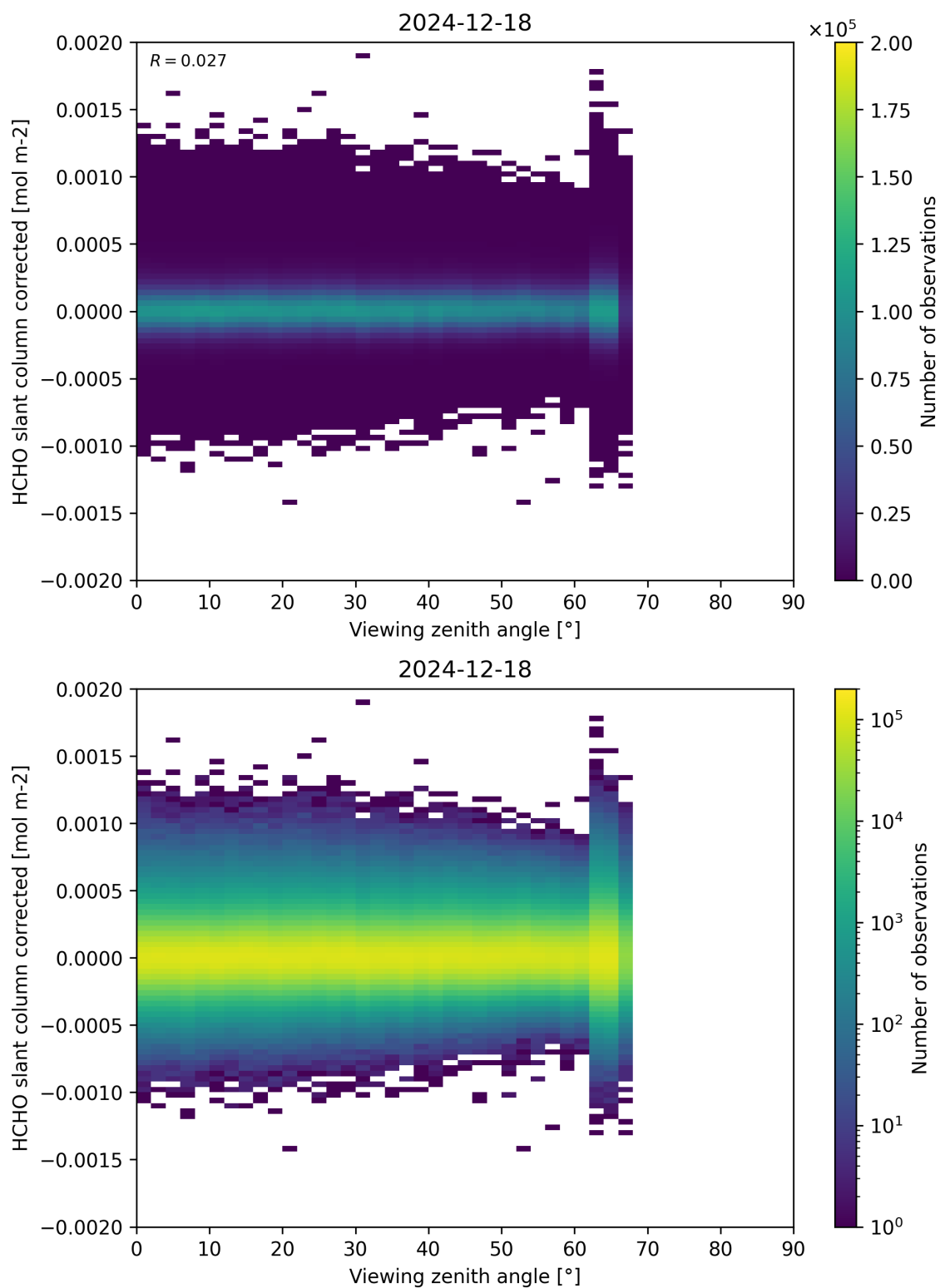
Figure 186: Scatter density plot of “Viewing zenith angle” against “HCHO slant column corrected” for 2024-12-17 to 2024-12-19.
