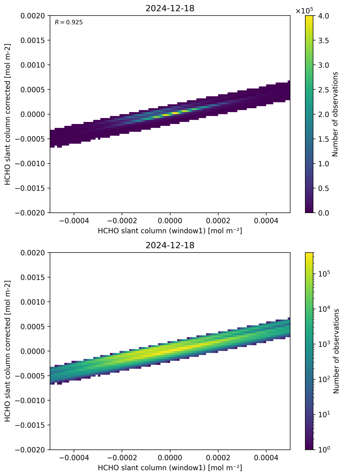
Figure 82: Scatter density plot of “HCHO slant column (window1)” against “HCHO slant column corrected” for 2024-12-17 to 2024-12-19.
