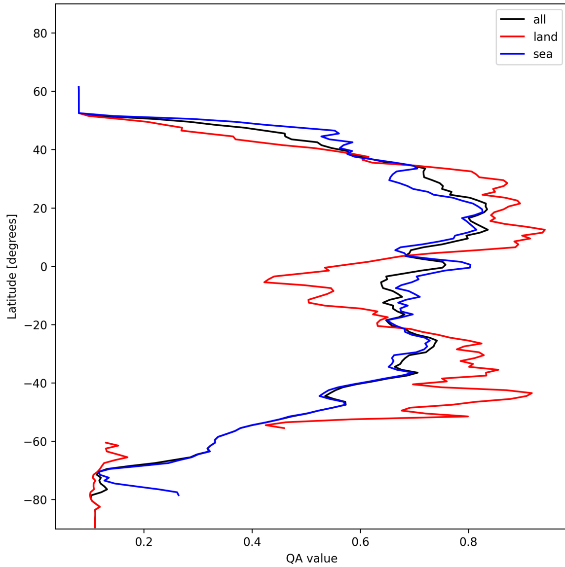
Figure 20: Zonal average of “QA value” for 2024-12-17 to 2024-12-19.
