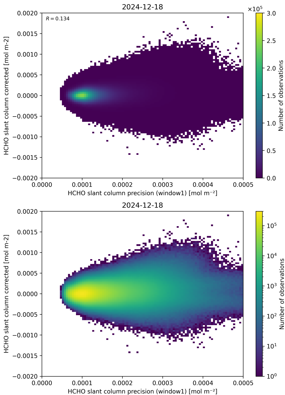
Figure 92: Scatter density plot of “HCHO slant column precision (window1)” against “HCHO slant column corrected” for 2024-12-17 to 2024-12-19.
