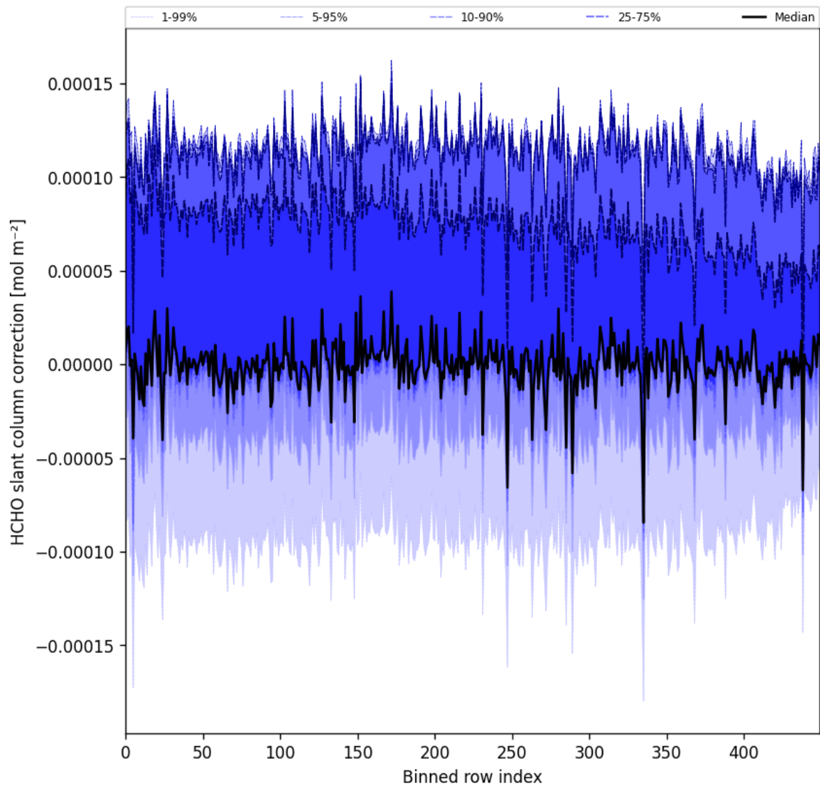
Figure 61: Along track statistics of “HCHO slant column correction” for 2024-12-17 to 2024-12-19
