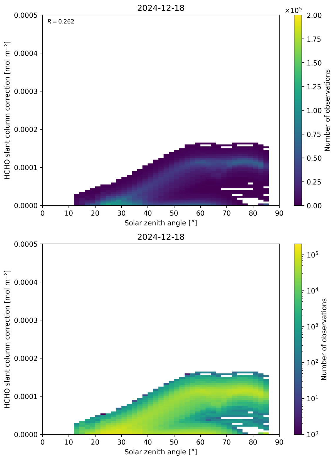
Figure 172: Scatter density plot of “Solar zenith angle” against “HCHO slant column correction” for 2024-12-17 to 2024-12-19.
