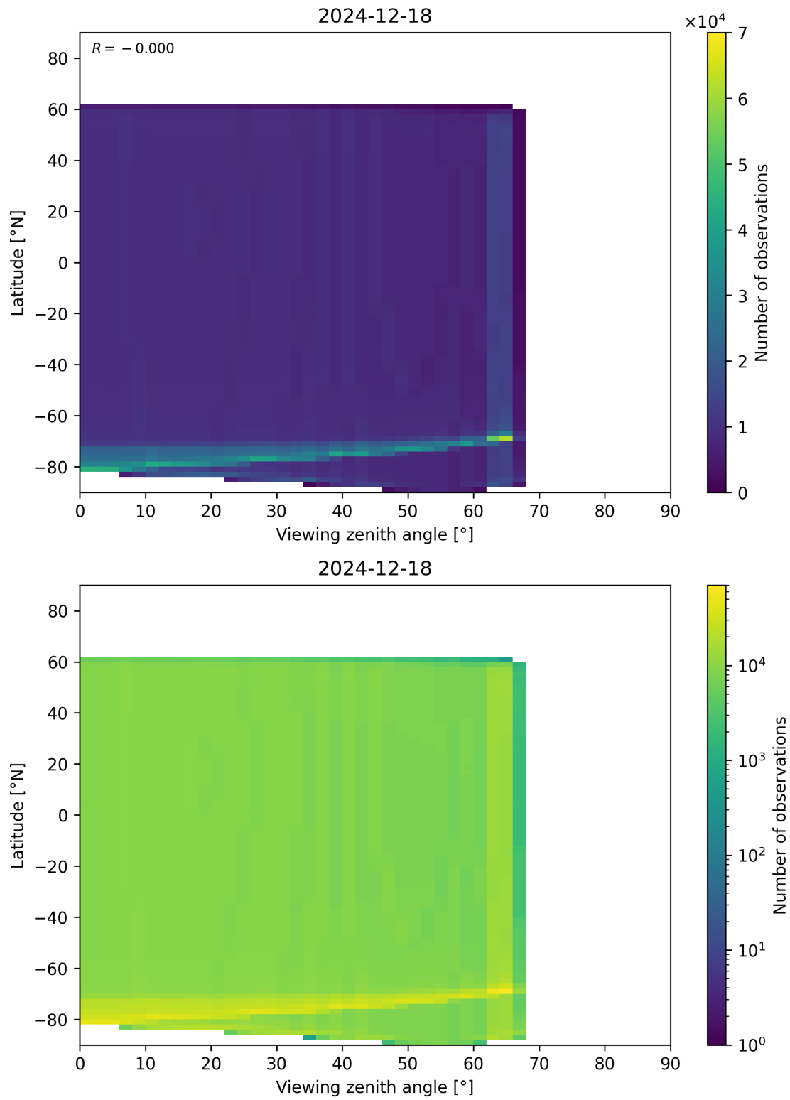
Figure 196: Scatter density plot of “Viewing zenith angle” against “Latitude” for 2024-12-17 to 2024-12-19.
