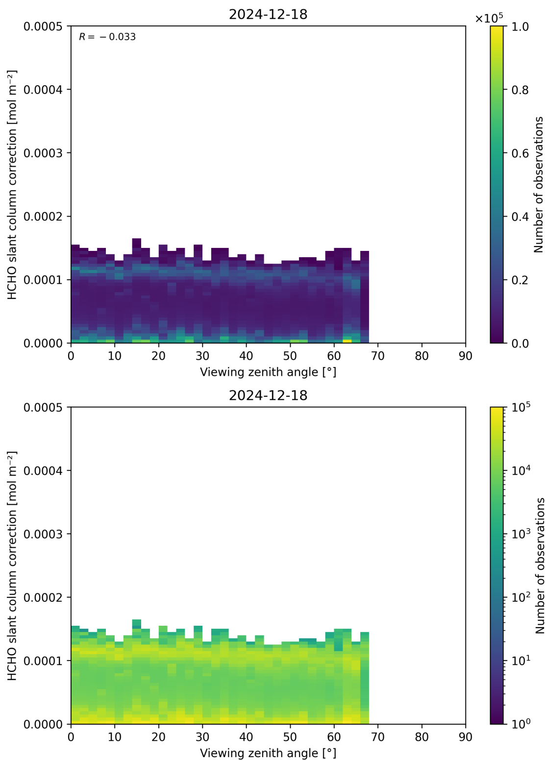
Figure 187: Scatter density plot of “Viewing zenith angle” against “HCHO slant column correction” for 2024-12-17 to 2024-12-19.
