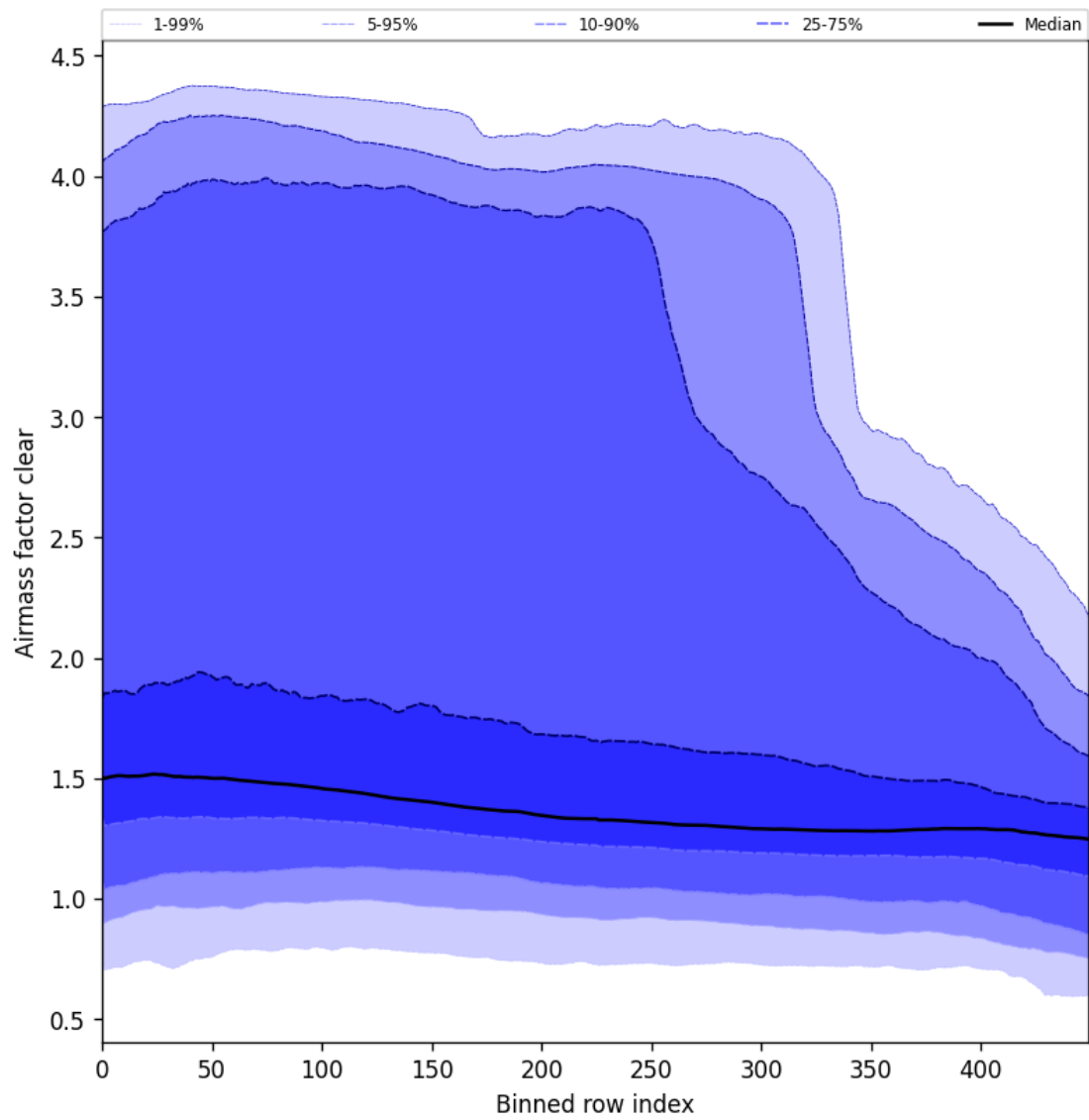
Figure 56: Along track statistics of “Airmass factor clear” for 2024-12-17 to 2024-12-19
