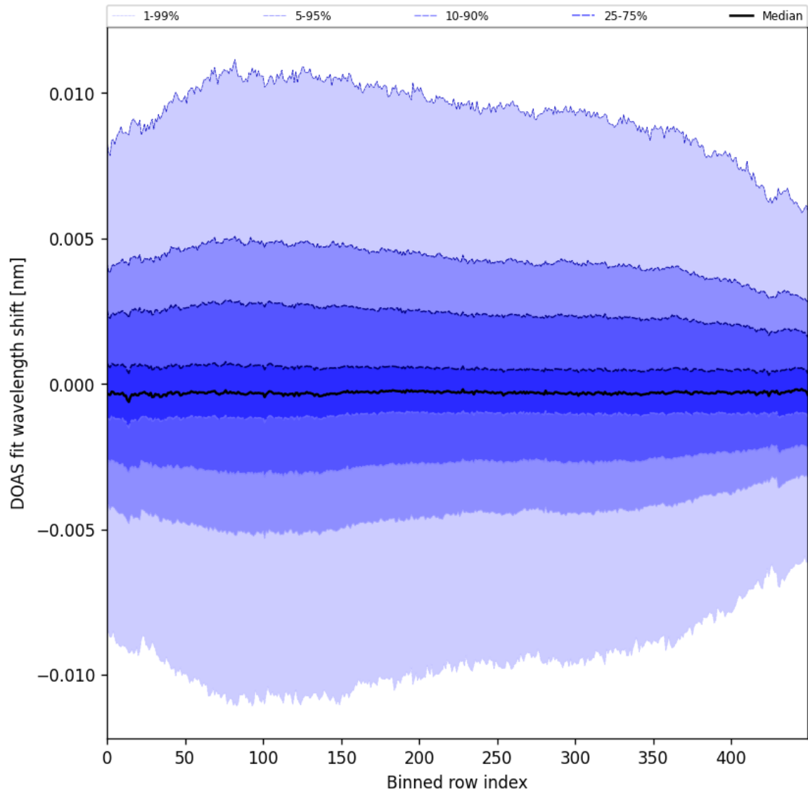
Figure 58: Along track statistics of “DOAS fit wavelength shift” for 2024-12-17 to 2024-12-19
