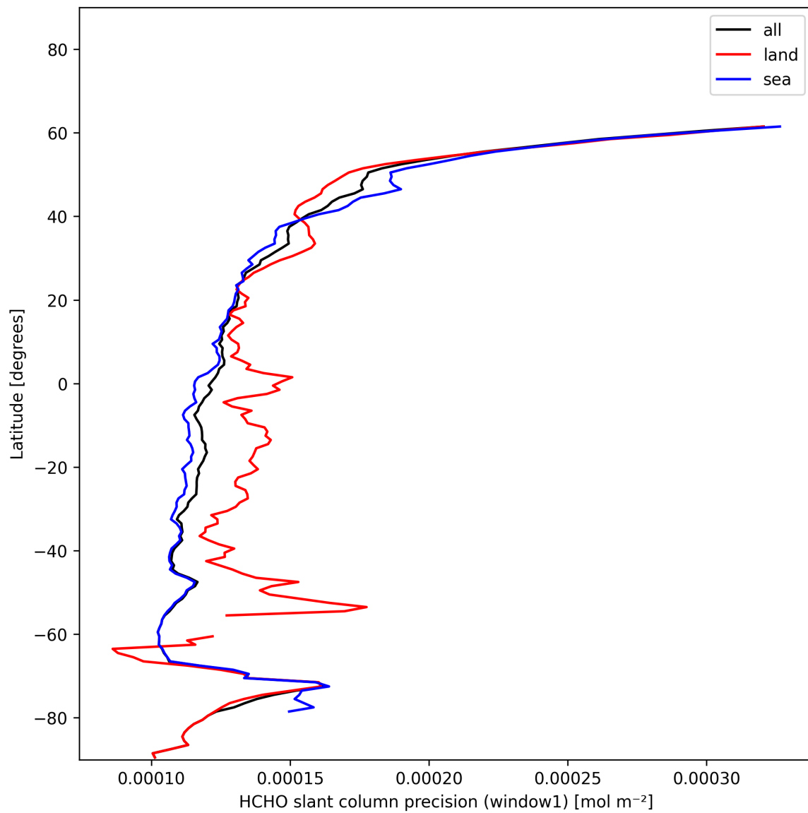
Figure 25: Zonal average of “HCHO slant column precision (window1)” for 2024-12-17 to 2024-12-19.
