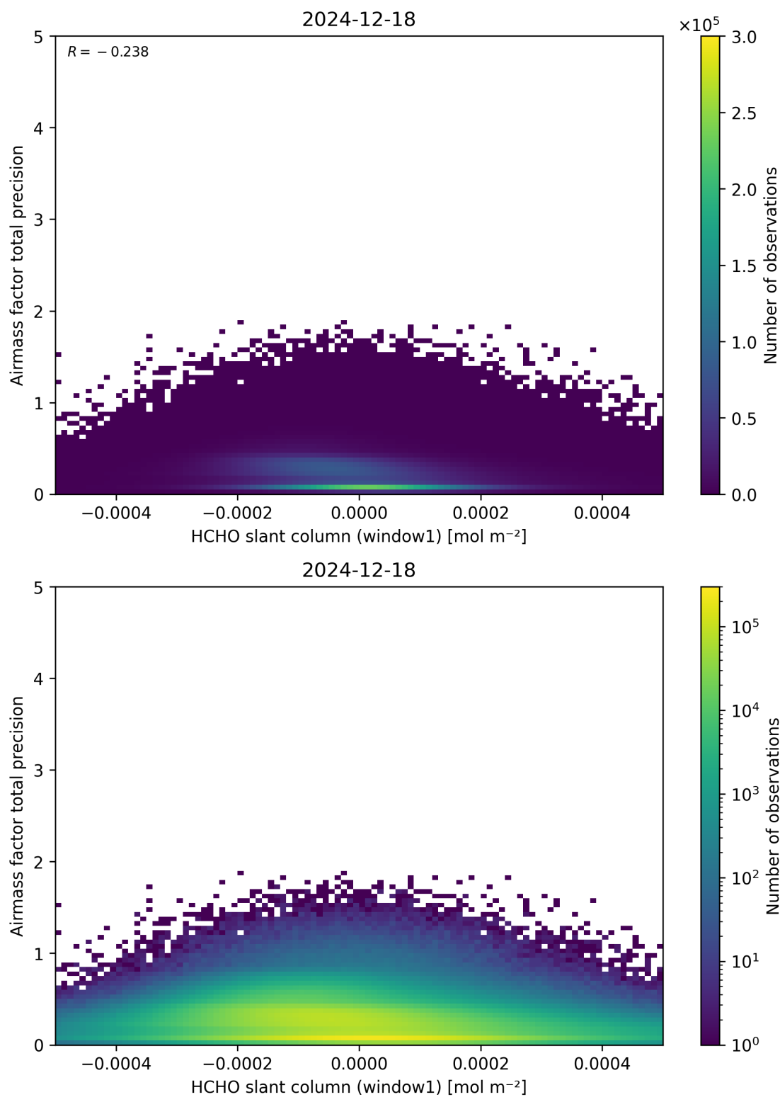
Figure 86: Scatter density plot of “HCHO slant column (window1)” against “Air mass factor total precision” for 2024-12-17 to 2024-12-19.
