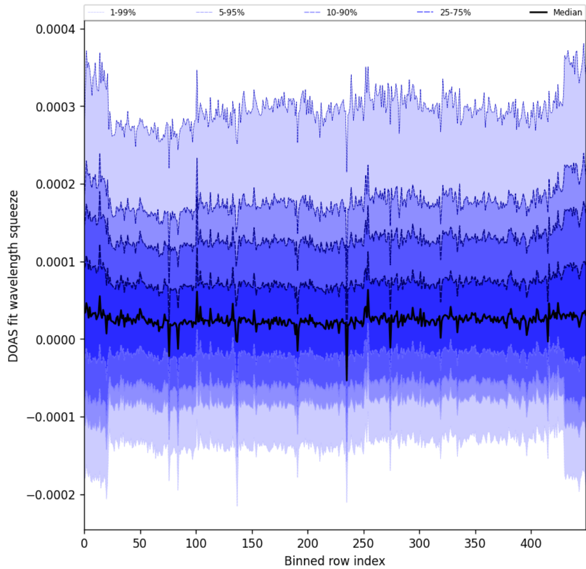
Figure 59: Along track statistics of “DOAS fit wavelength squeeze” for 2024-12-17 to 2024-12-19
