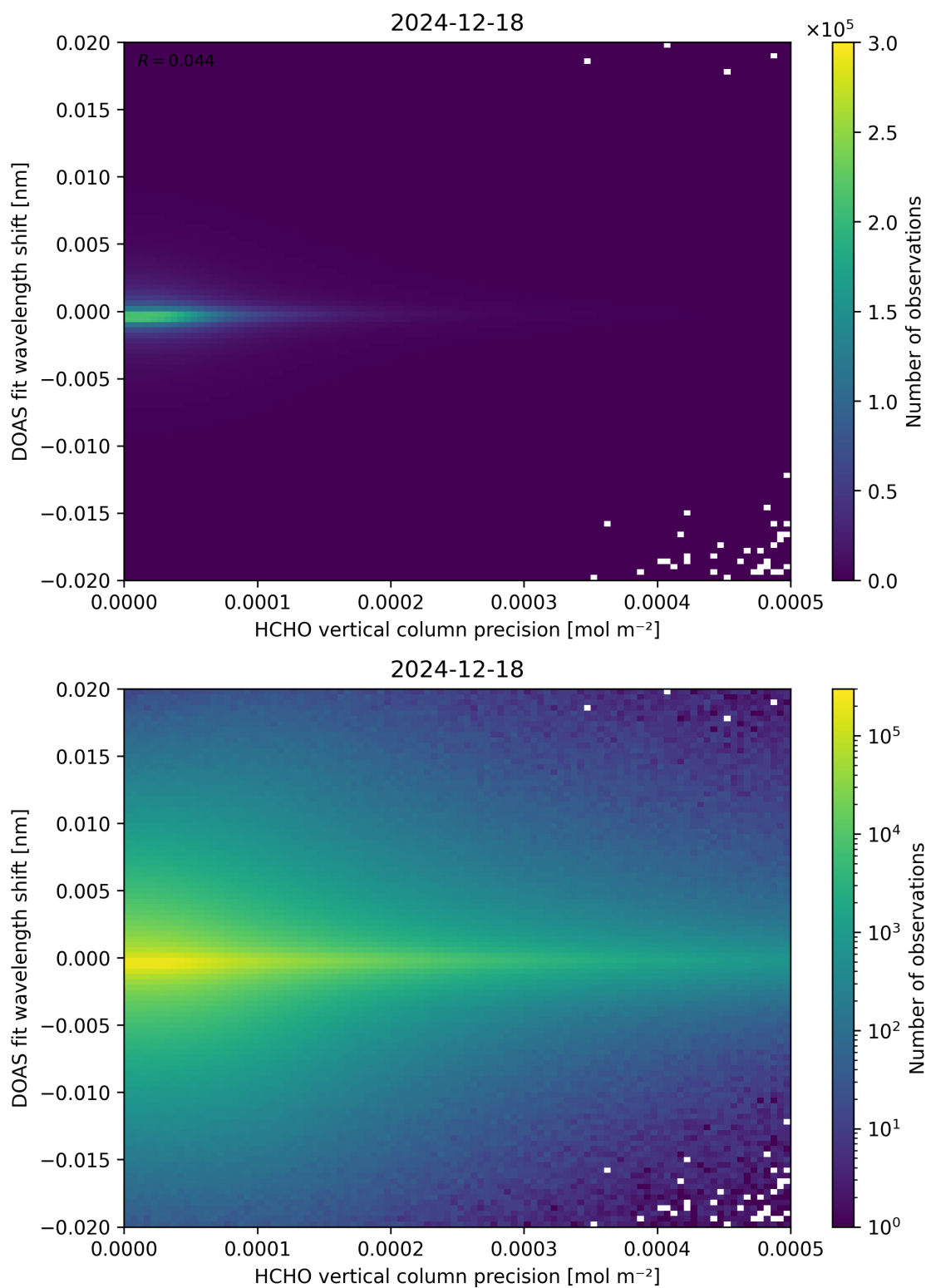
Figure 137: Scatter density plot of “HCHO vertical column precision” against “DOAS fit wavelength shift” for 2024-12-17 to 2024-12-19.
