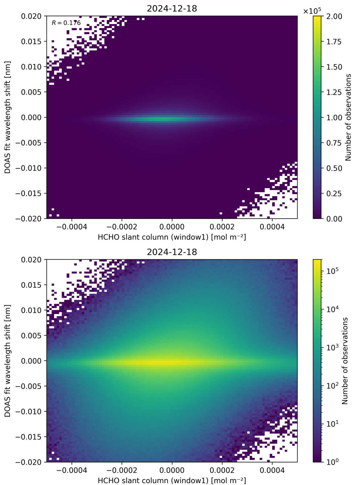
Figure 79: Scatter density plot of “HCHO slant column (window1)” against “DOAS fit wavelength shift” for 2024-12-17 to 2024-12-19.
