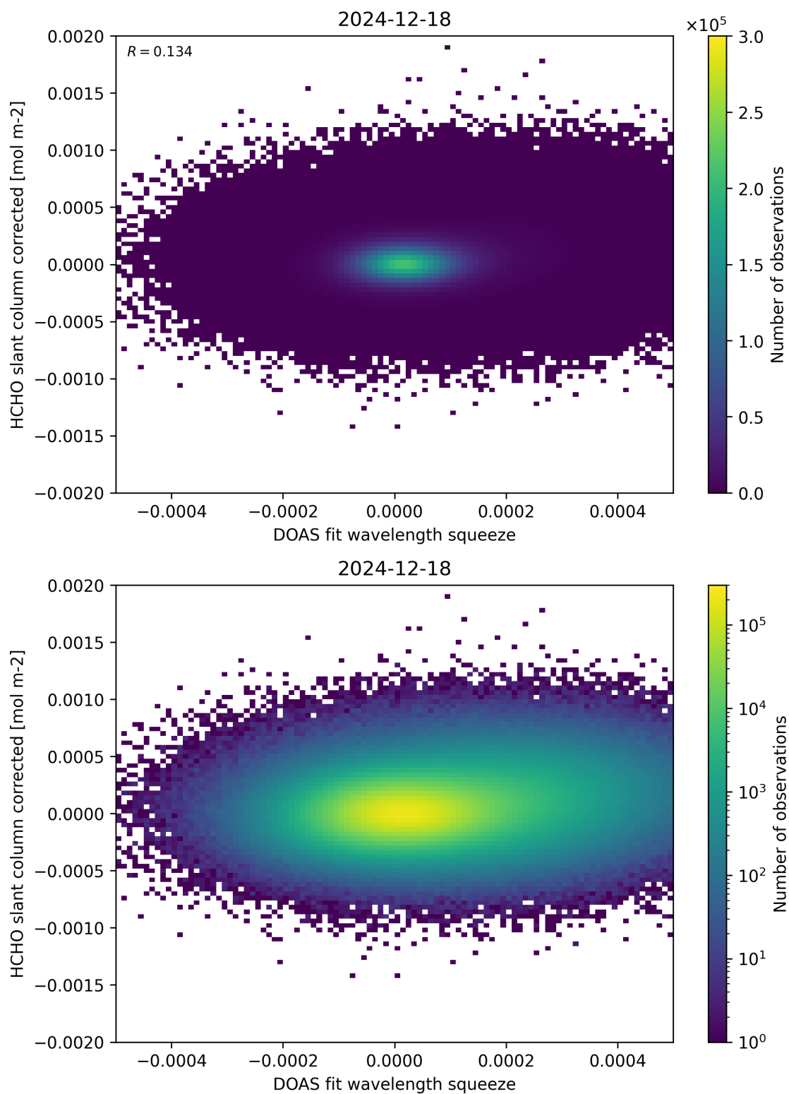
Figure 69: Scatter density plot of “DOAS fit wavelength squeeze” against “HCHO slant column corrected” for 2024-12-17 to 2024-12-19.
