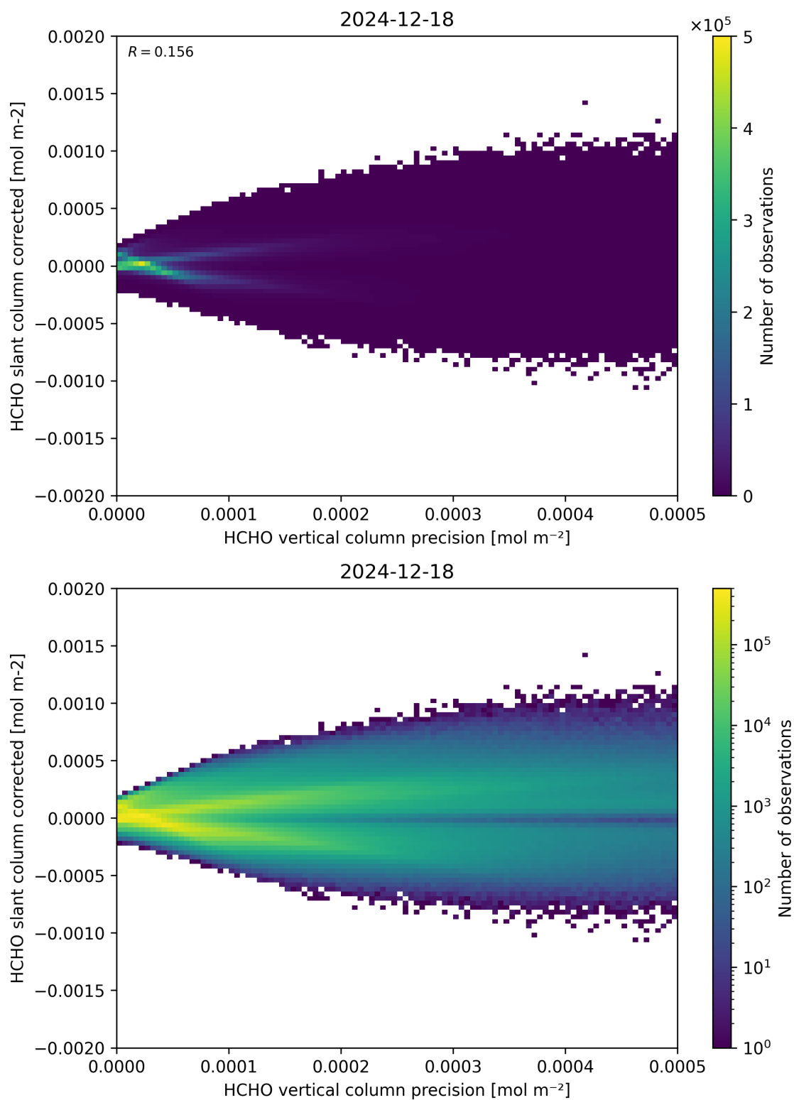
Figure 140: Scatter density plot of “HCHO vertical column precision” against “HCHO slant column corrected” for 2024-12-17 to 2024-12-19.
