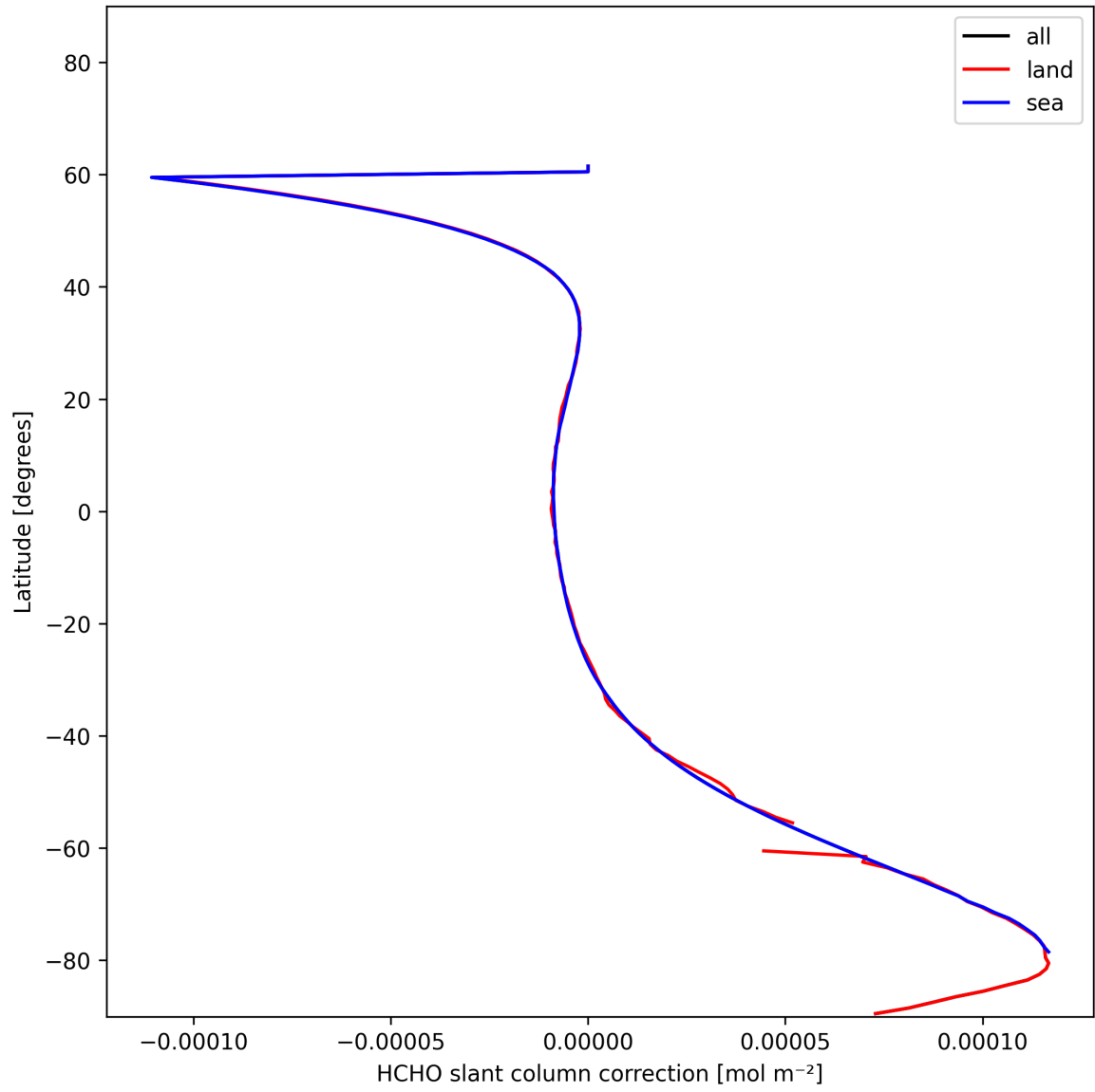
Figure 33: Zonal average of "HCHO slant column correction" for 2024-12-17 to 2024-12-19.
