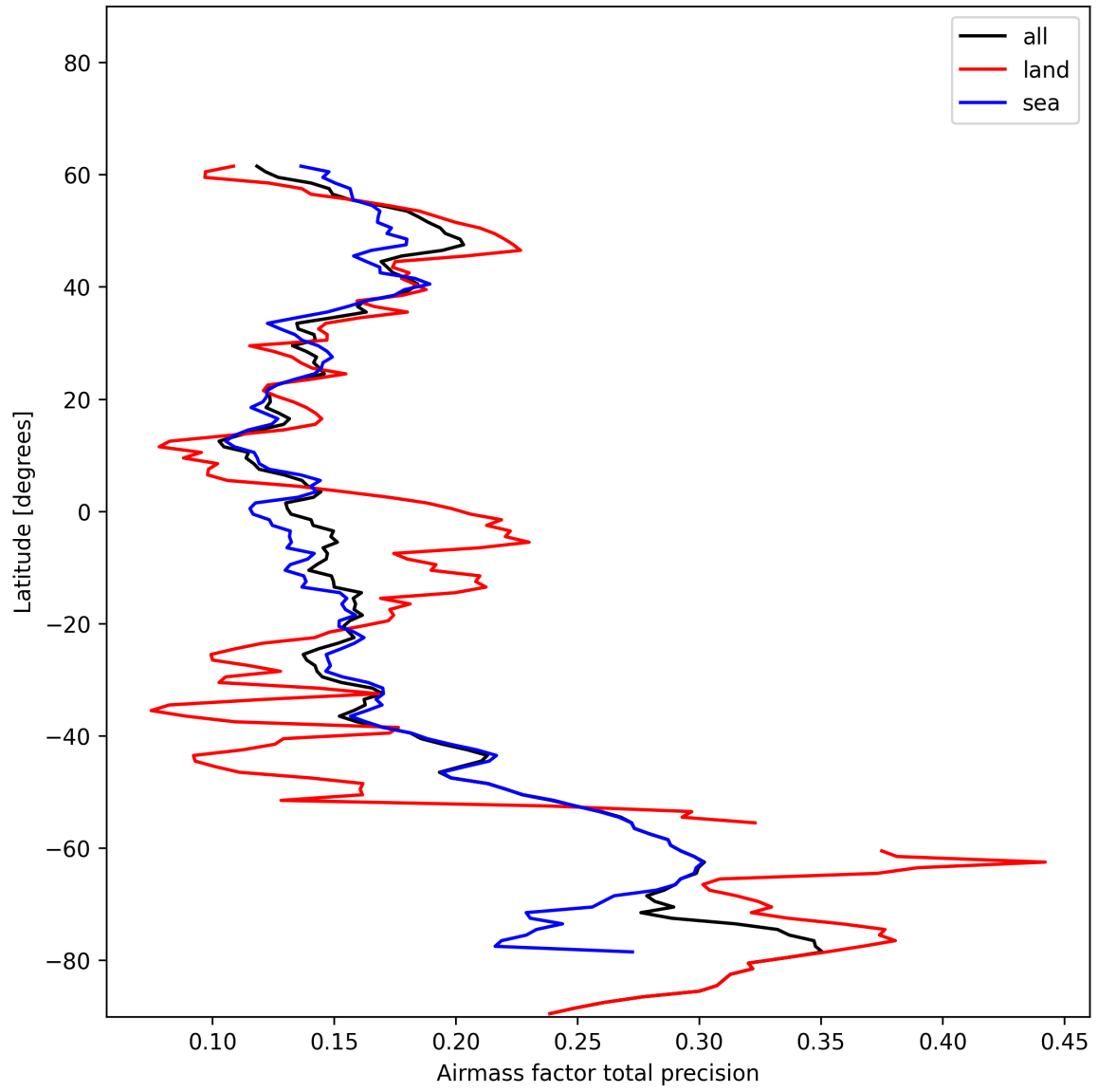
Figure 27: Zonal average of “Airmass factor total precision” for 2024-12-17 to 2024-12-19.
