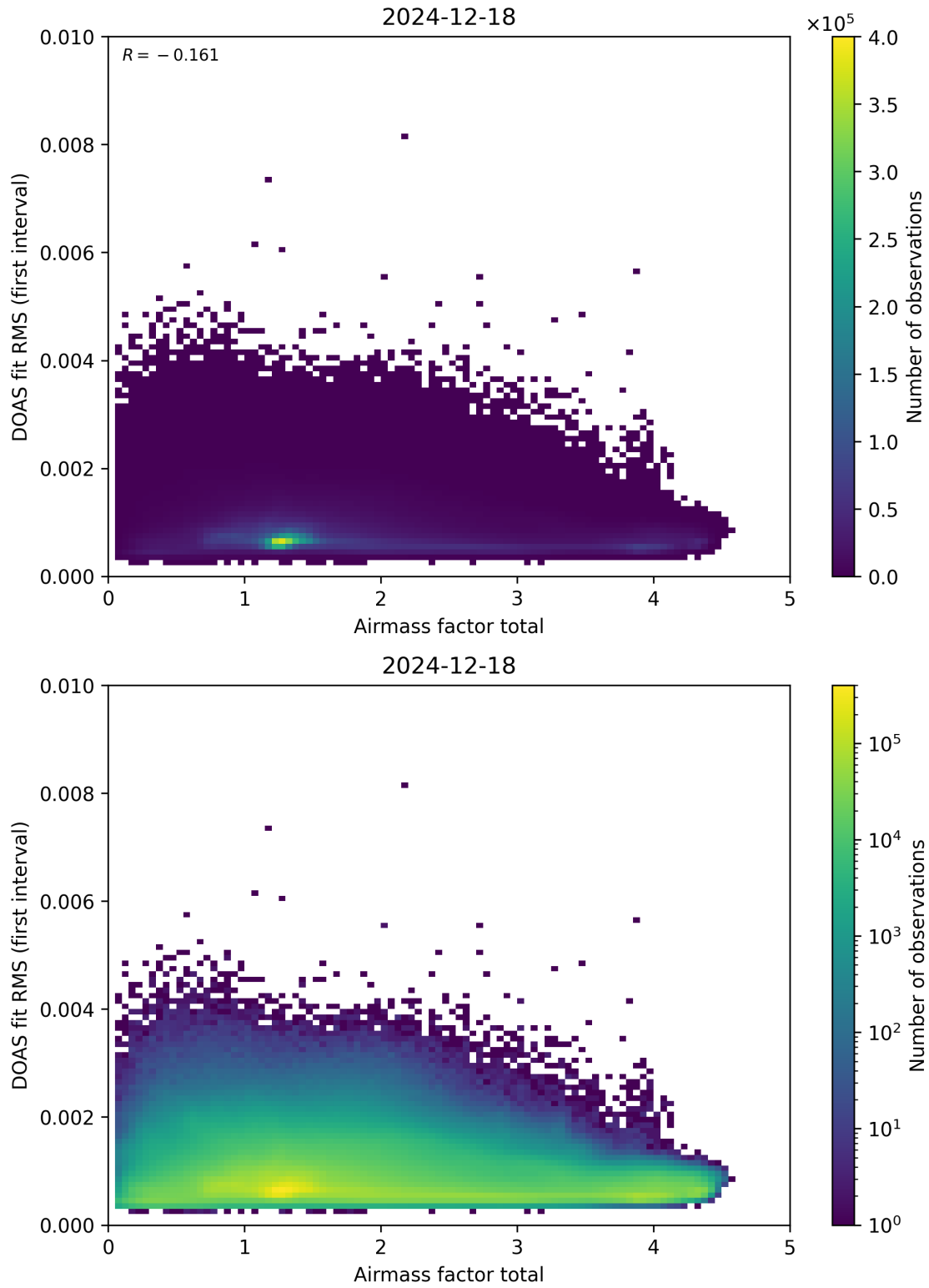
Figure 97: Scatter density plot of “Airmass factor total” against “DOAS fit RMS (first interval)” for 2024-12-17 to 2024-12-19.
