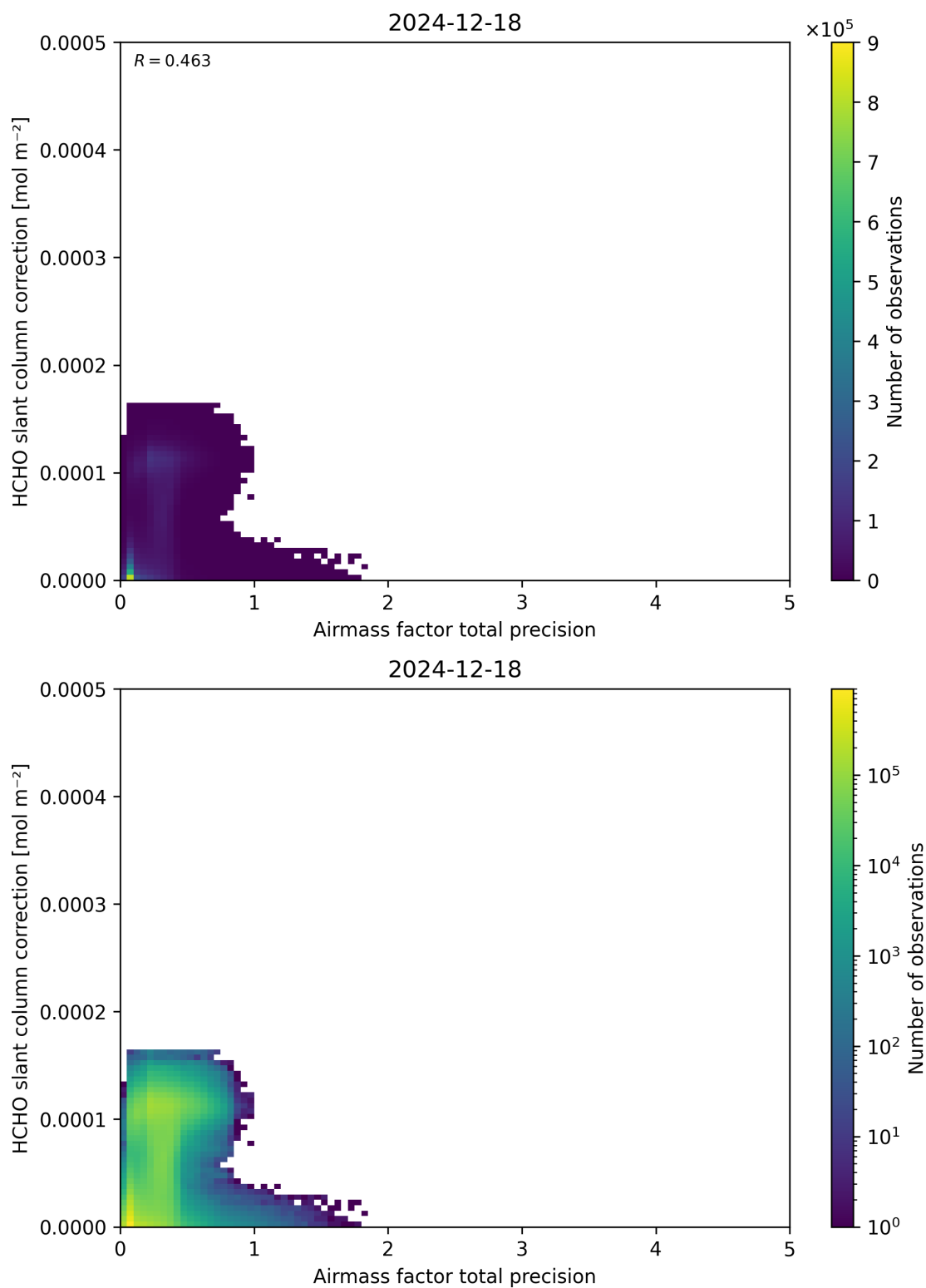
Figure 110: Scatter density plot of “Airmass factor total precision” against “HCHO slant column correction” for 2024-12-17 to 2024-12-19.
