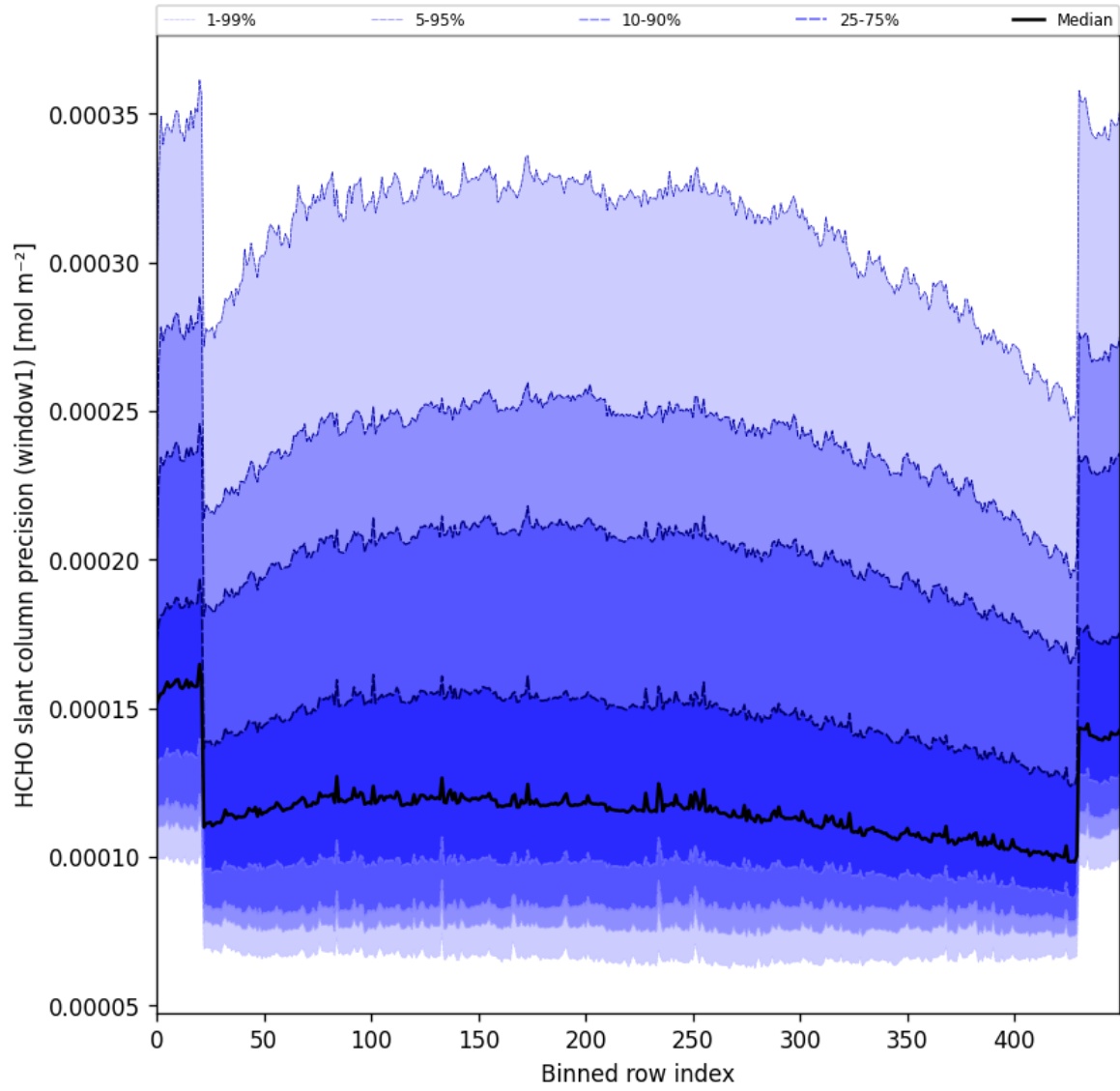
Figure 53: Along track statistics of “HCHO slant column precision (window1)” for 2024-12-17 to 2024-12-19
