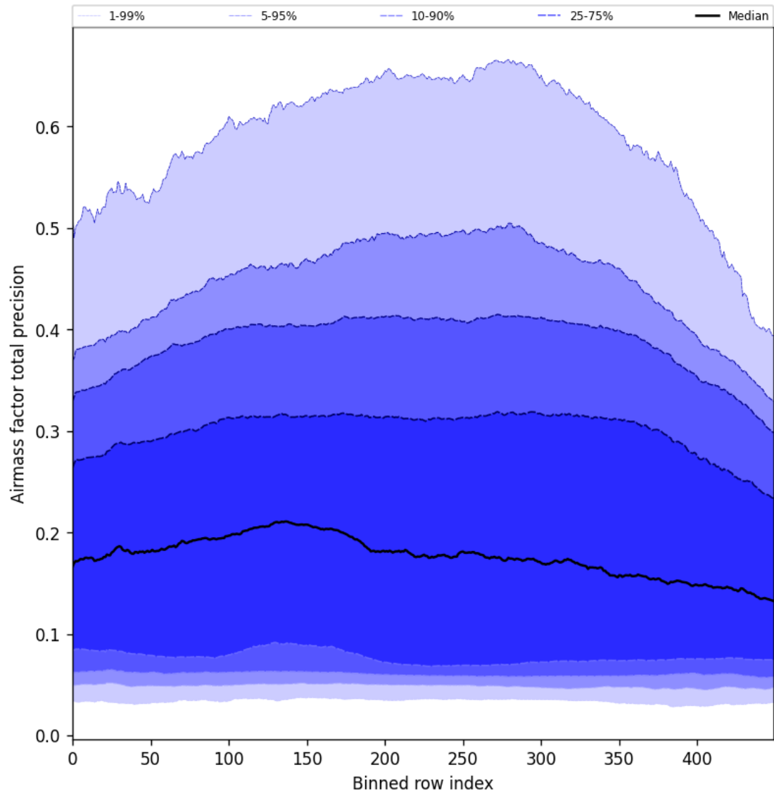
Figure 55: Along track statistics of “Airmass factor total precision” for 2024-12-17 to 2024-12-19
