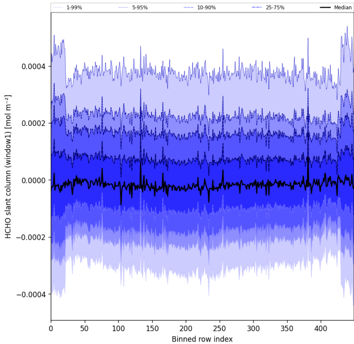
Figure 52: Along track statistics of “HCHO slant column (window1)” for 2024-12-17 to 2024-12-19
