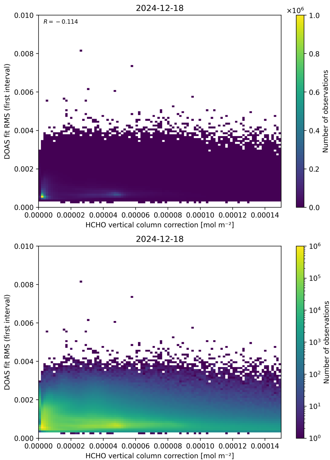
Figure 112: Scatter density plot of “HCHO vertical column correction” against “DOAS fit RMS (first interval)” for 2024-12-17 to 2024-12-19.
