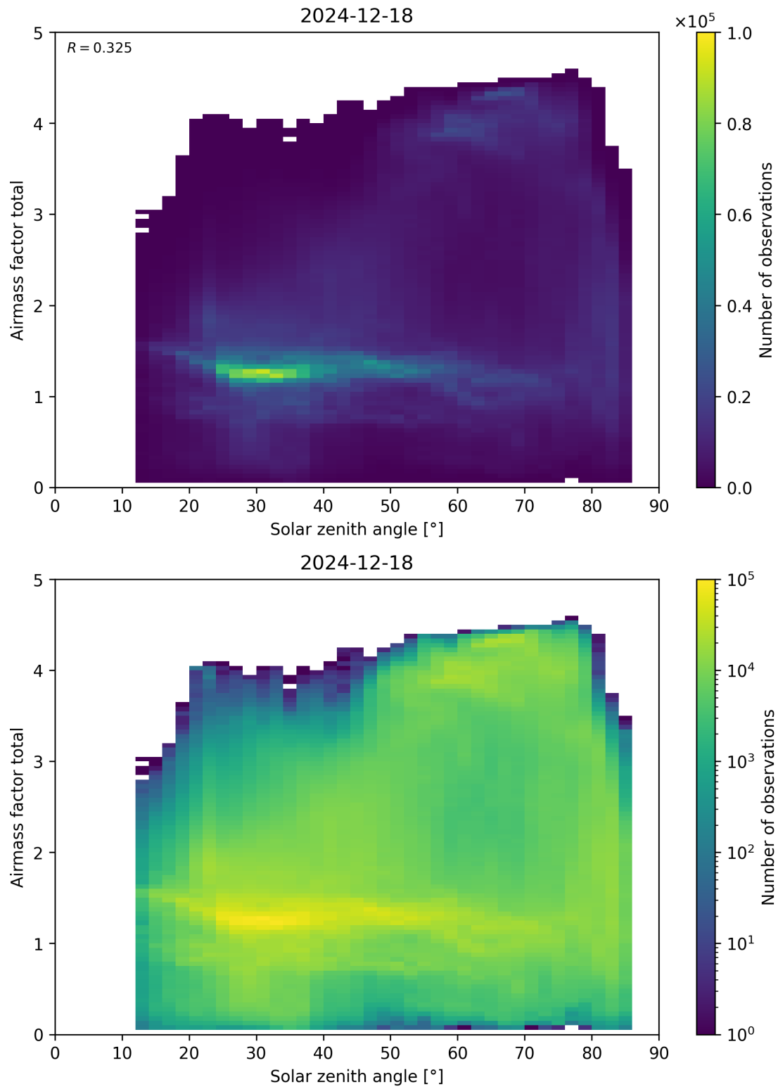
Figure 175: Scatter density plot of “Solar zenith angle” against “Airmass factor total” for 2024-12-17 to 2024-12-19.
