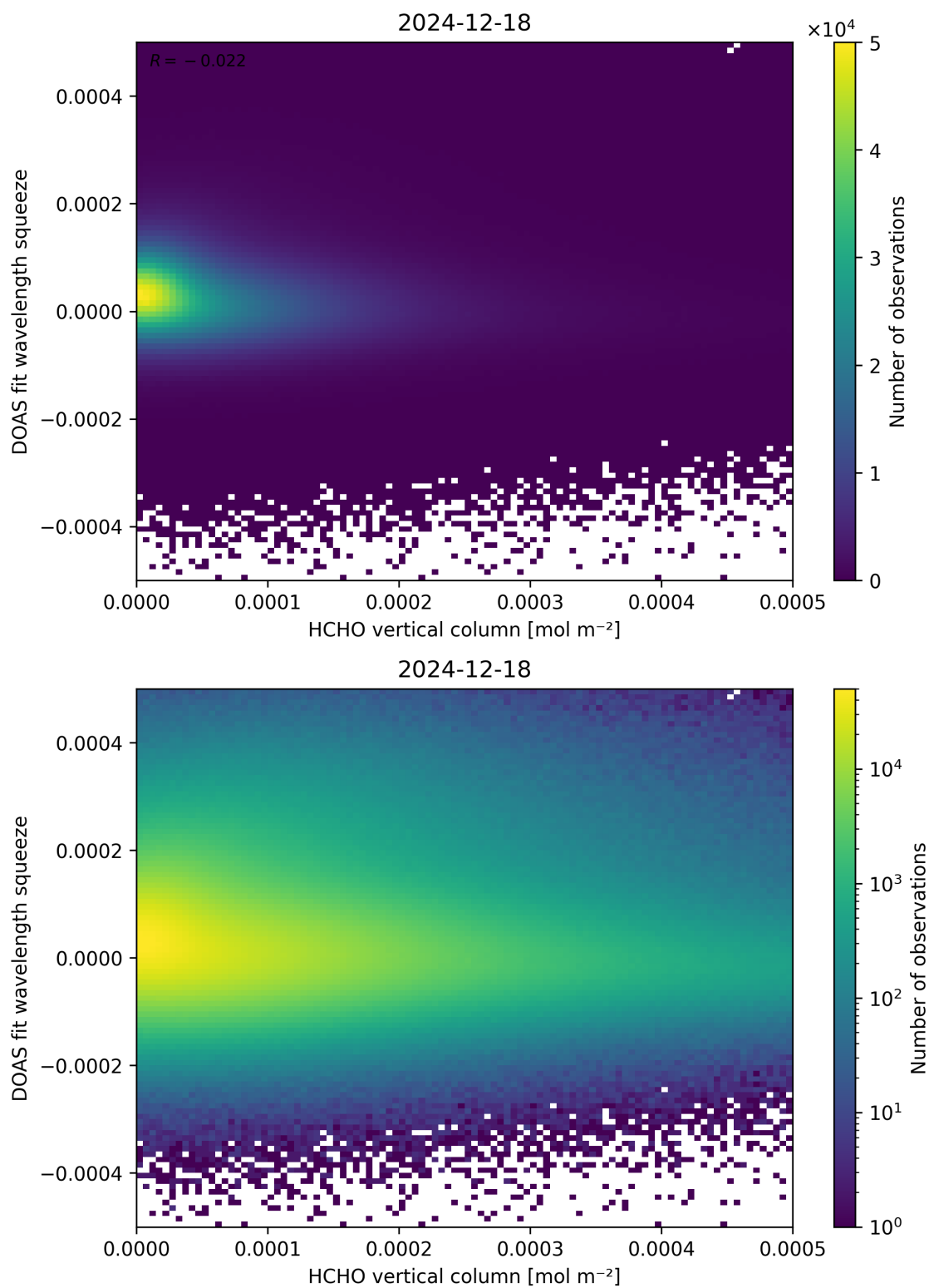
Figure 125: Scatter density plot of “HCHO vertical column” against “DOAS fit wavelength squeeze” for 2024-12-17 to 2024-12-19.
