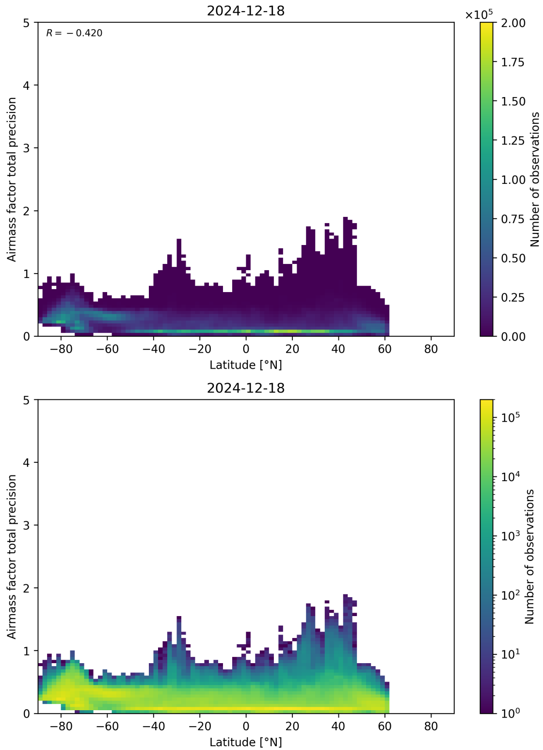
Figure 162: Scatter density plot of “Latitude” against “Airmass factor total precision” for 2024-12-17 to 2024-12-19.
