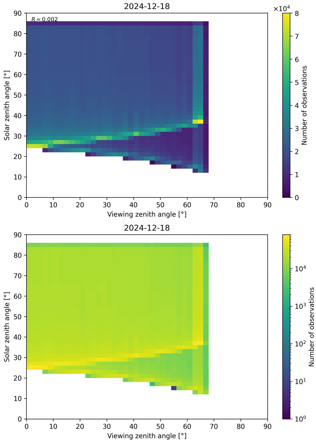
Figure 197: Scatter density plot of “Viewing zenith angle” against “Solar zenith angle” for 2024-12-17 to 2024-12-19.
