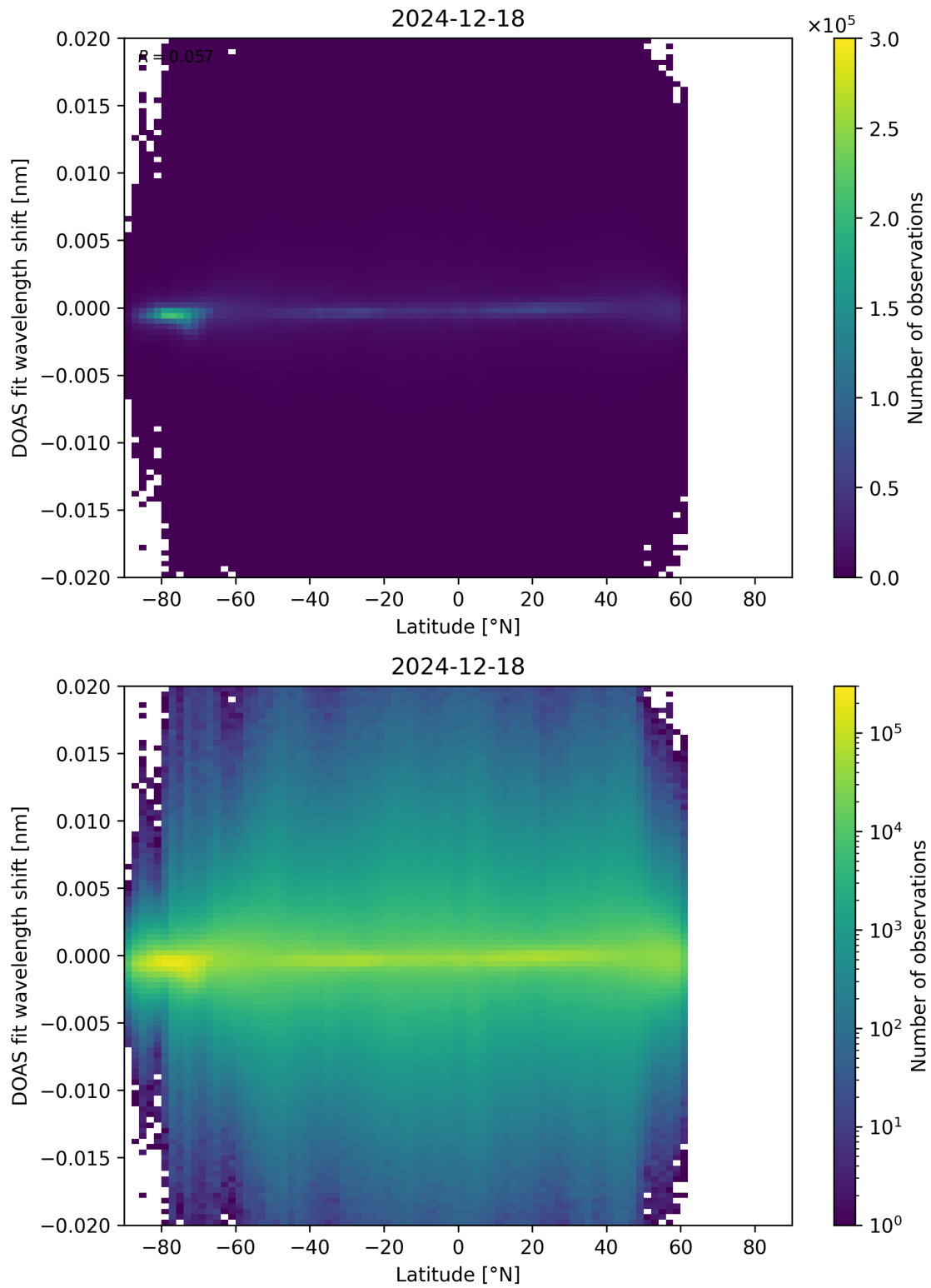
Figure 154: Scatter density plot of “Latitude” against “DOAS fit wavelength shift” for 2024-12-17 to 2024-12-19.
