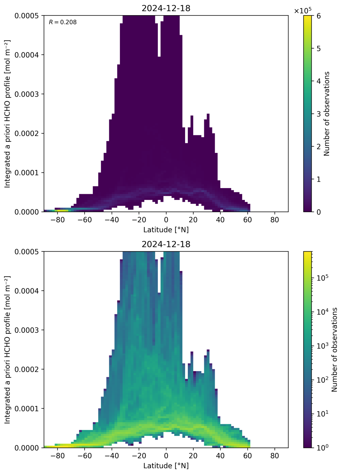
Figure 166: Scatter density plot of “Latitude” against “Integrated a priori HCHO profile” for 2024-12-17 to 2024-12-19.
