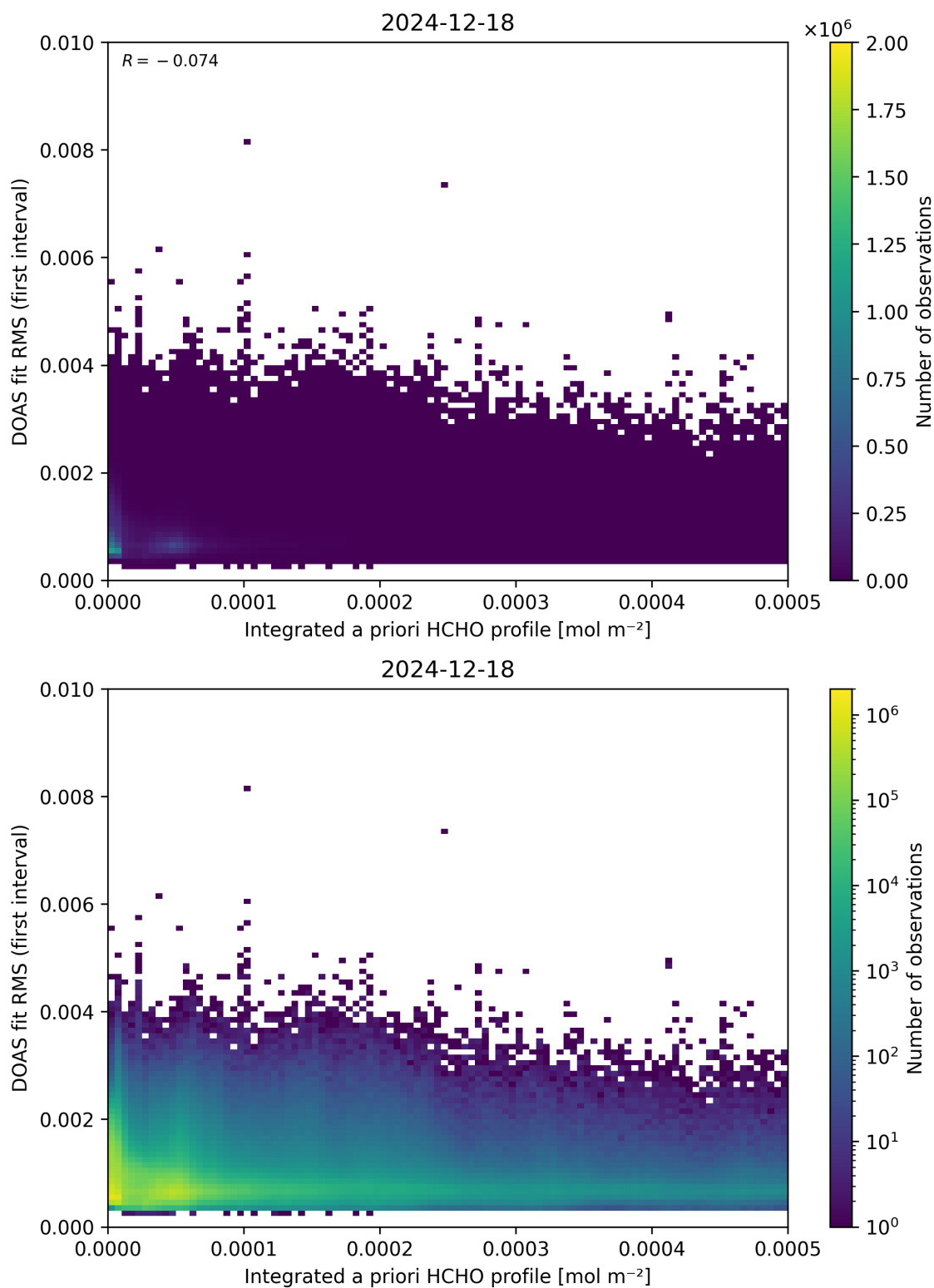
Figure 148: Scatter density plot of “Integrated a priori HCHO profile” against “DOAS fit RMS (first interval)” for 2024-12-17 to 2024-12-19.
