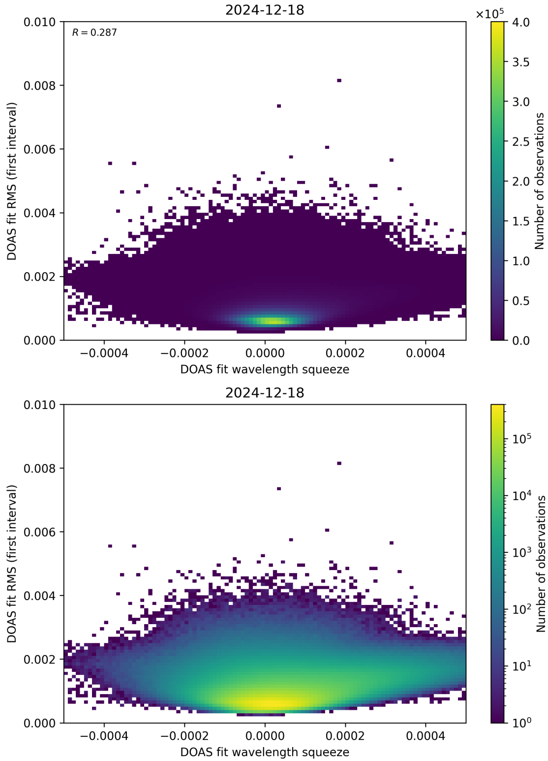
Figure 68: Scatter density plot of “DOAS fit wavelength squeeze” against “DOAS fit RMS (first interval)” for 2024-12-17 to 2024-12-19.
