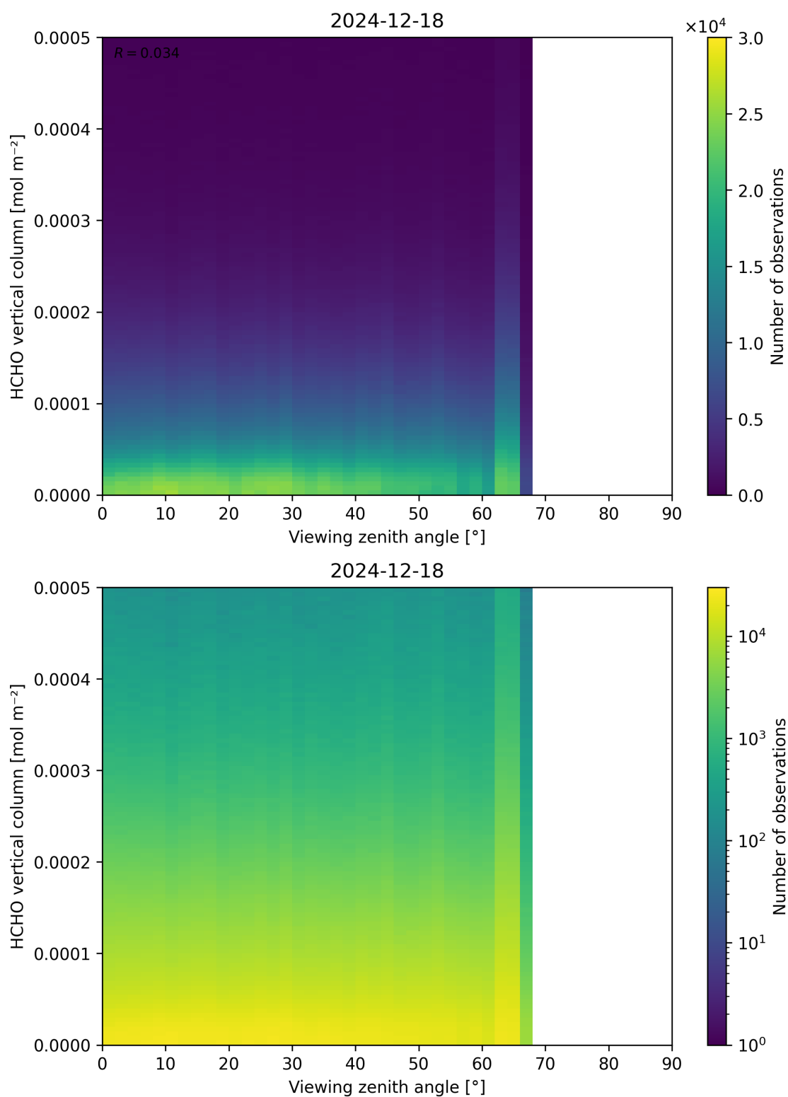
Figure 192: Scatter density plot of “Viewing zenith angle” against “HCHO vertical column” for 2024-12-17 to 2024-12-19.
