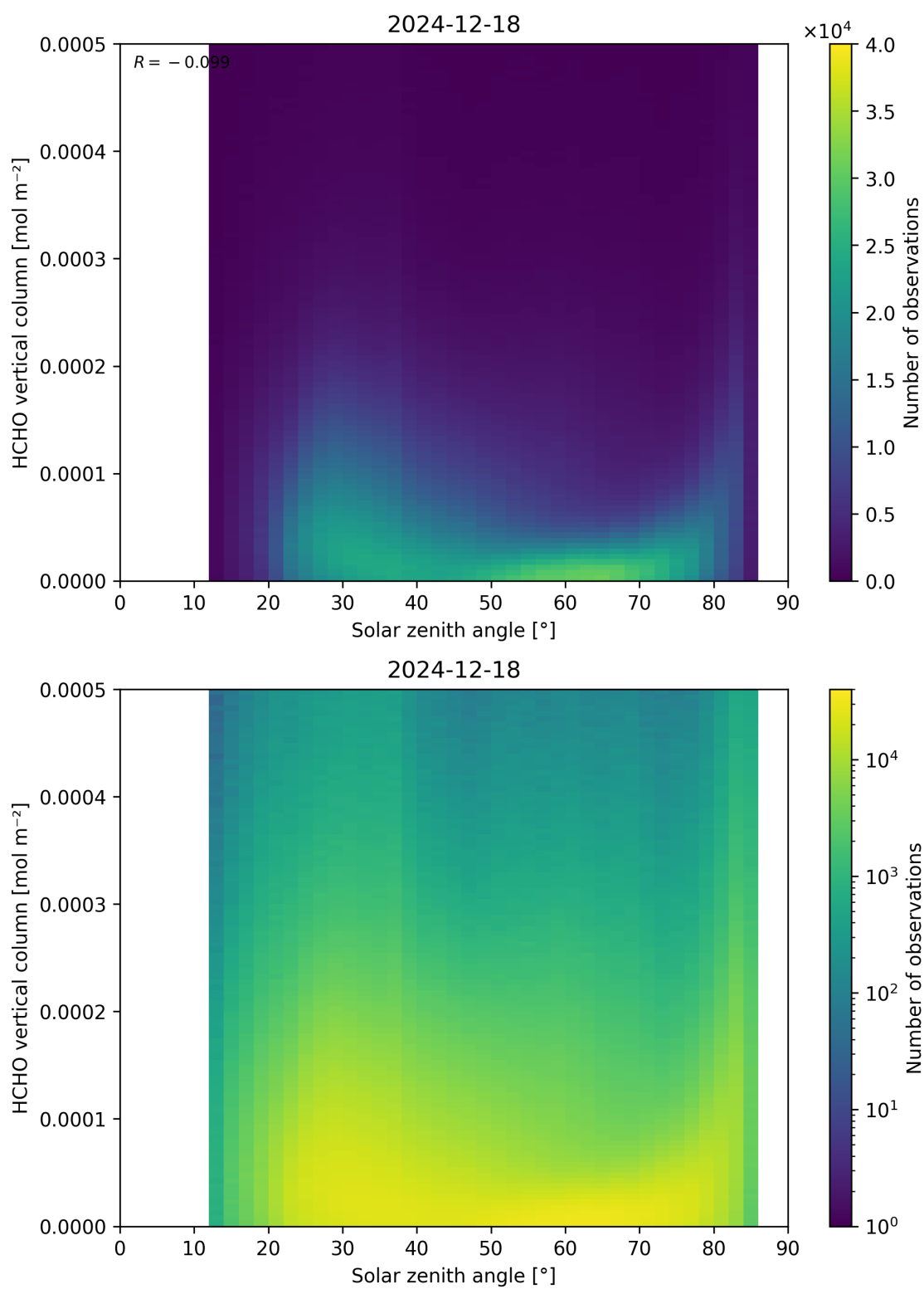
Figure 177: Scatter density plot of “Solar zenith angle” against “HCHO vertical column” for 2024-12-17 to 2024-12-19.
