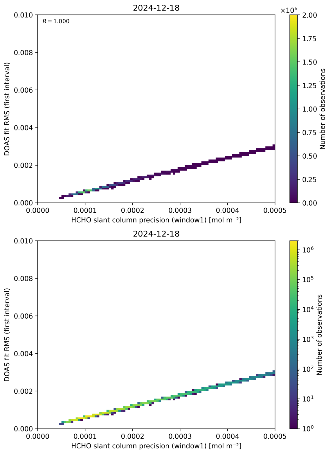
Figure 88: Scatter density plot of “HCHO slant column precision (window1)” against “DOAS fit RMS (first interval)” for 2024-12-17 to 2024-12-19.
