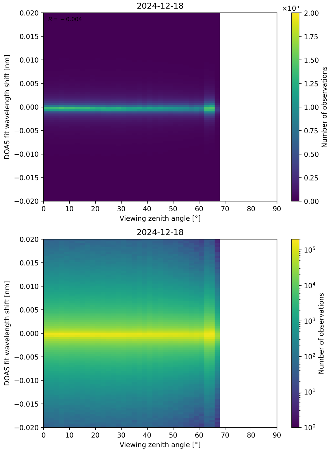
Figure 183: Scatter density plot of “Viewing zenith angle” against “DOAS fit wavelength shift” for 2024-12-17 to 2024-12-19.
