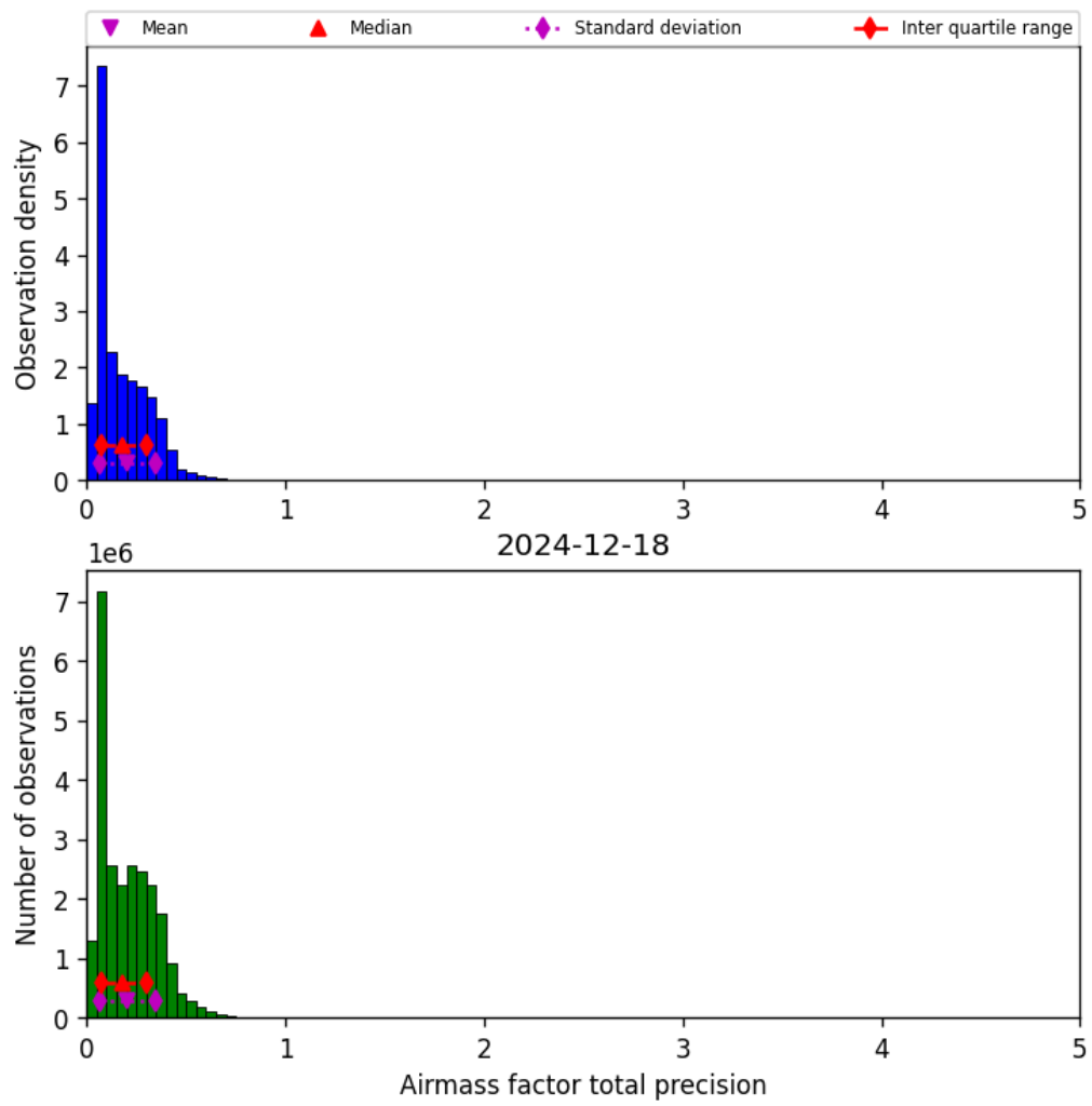
Figure 41: Histogram of “Airmass factor total precision” for 2024-12-17 to 2024-12-19
