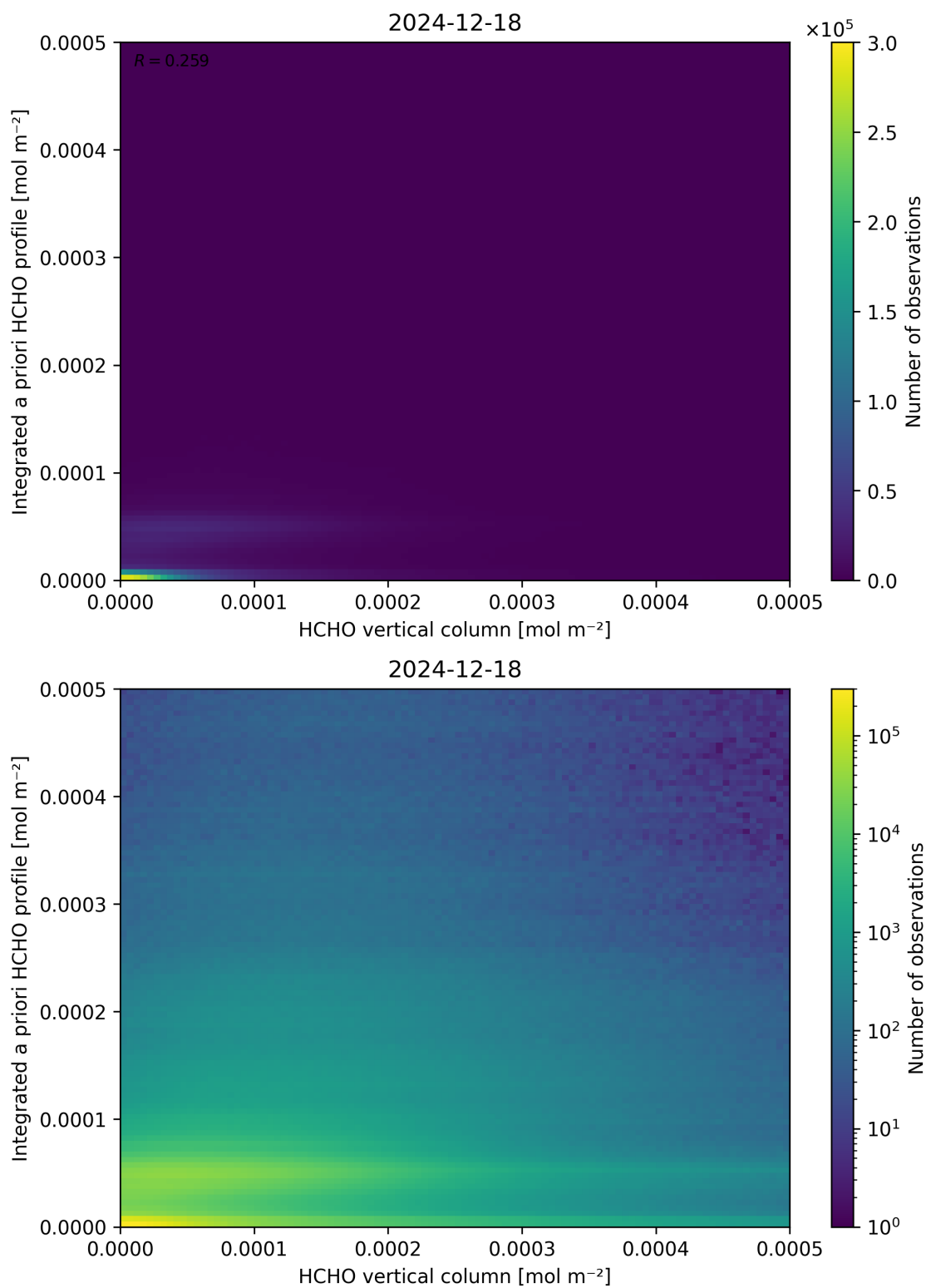
Figure 135: Scatter density plot of “HCHO vertical column” against “Integrated a priori HCHO profile” for 2024-12-17 to 2024-12-19.
