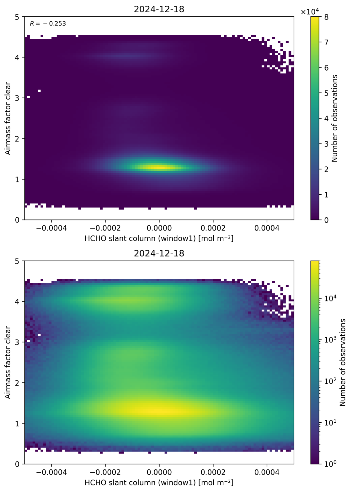
Figure 81: Scatter density plot of “HCHO slant column (window1)” against “Airmass factor clear” for 2024-12-17 to 2024-12-19.
