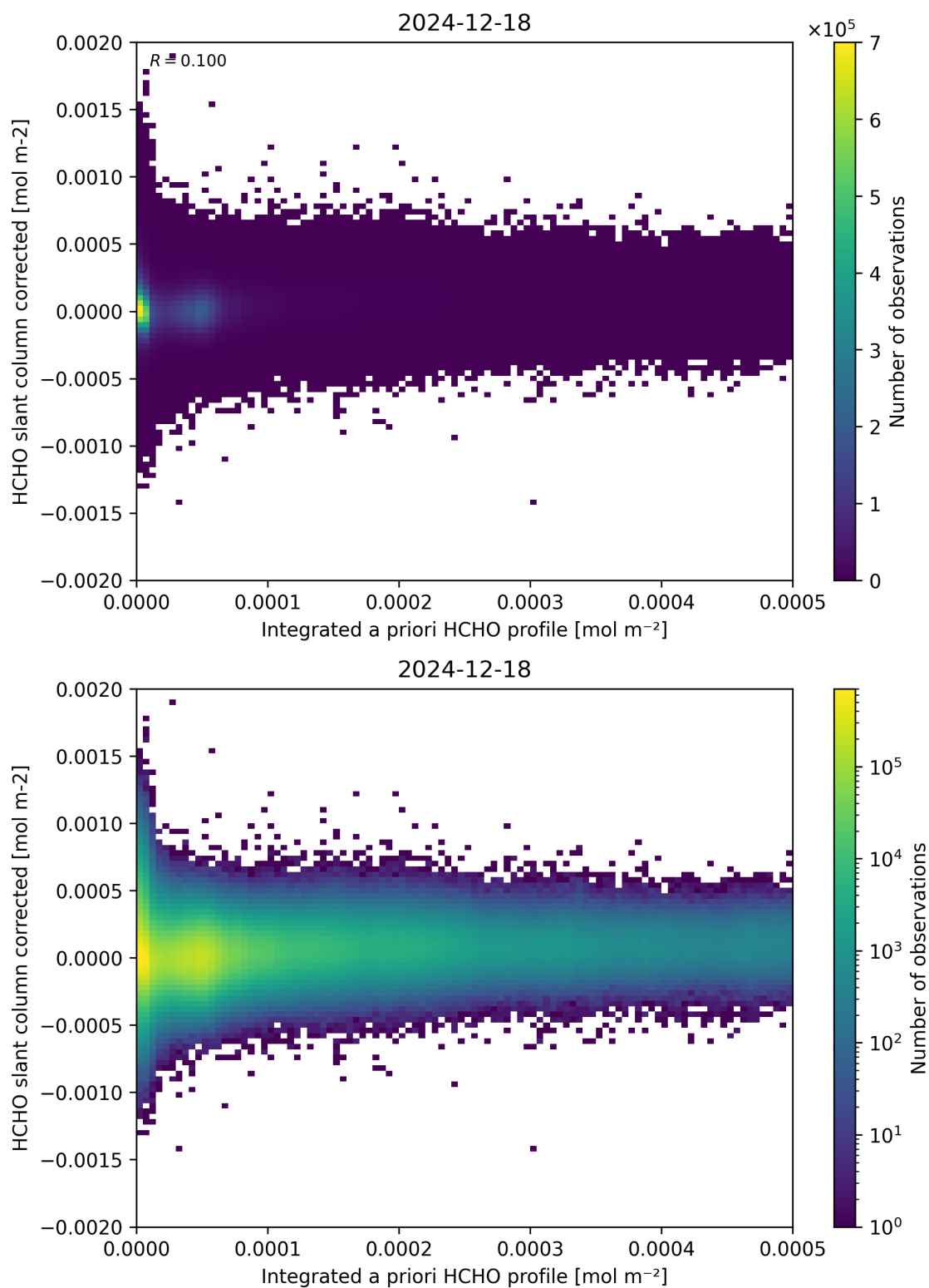
Figure 151: Scatter density plot of “Integrated a priori HCHO profile” against “HCHO slant column corrected” for 2024-12-17 to 2024-12-19.
