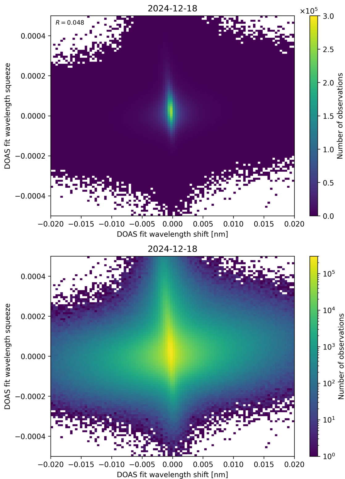
Figure 65: Scatter density plot of “DOAS fit wavelength shift” against “DOAS fit wavelength squeeze” for 2024-12-17 to 2024-12-19.
