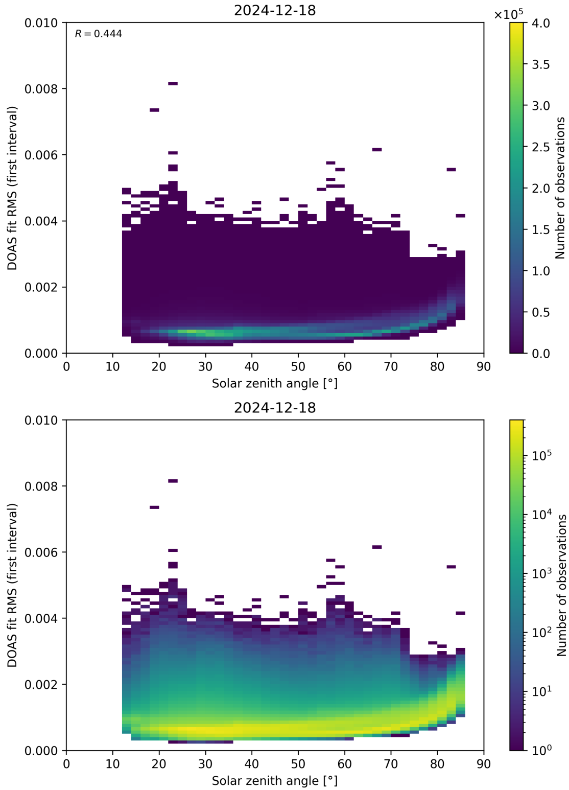
Figure 167: Scatter density plot of “Solar zenith angle” against “DOAS fit RMS (first interval)” for 2024-12-17 to 2024-12-19.
