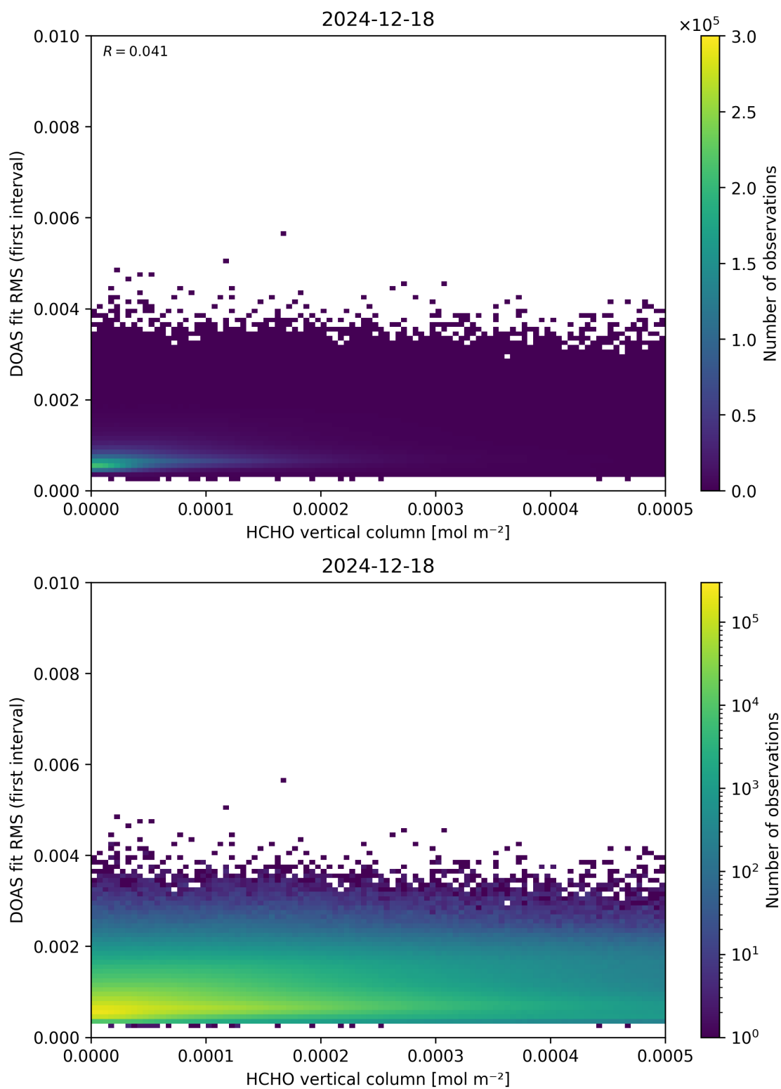
Figure 123: Scatter density plot of “HCHO vertical column” against “DOAS fit RMS (first interval)” for 2024-12-17 to 2024-12-19.
