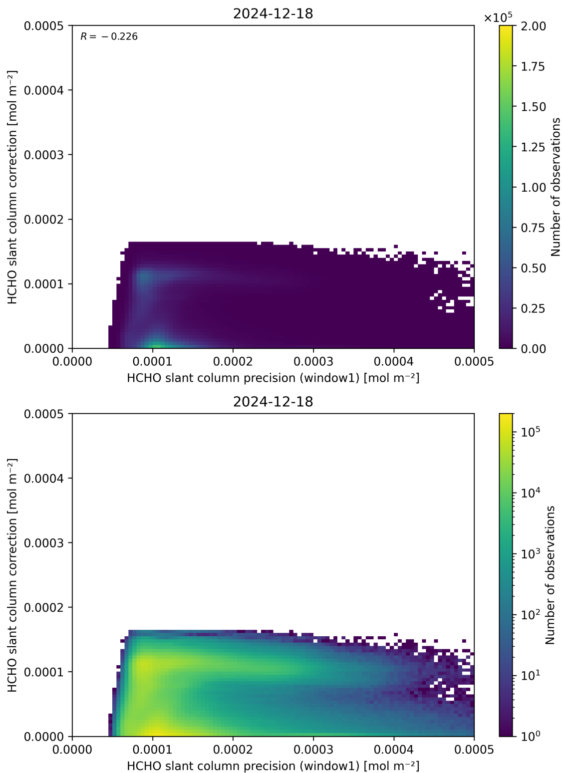
Figure 93: Scatter density plot of “HCHO slant column precision (window1)” against “HCHO slant column correction” for 2024-12-17 to 2024-12-19.
