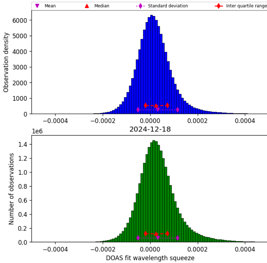
Figure 45: Histogram of “DOAS fit wavelength squeeze” for 2024-12-17 to 2024-12-19
