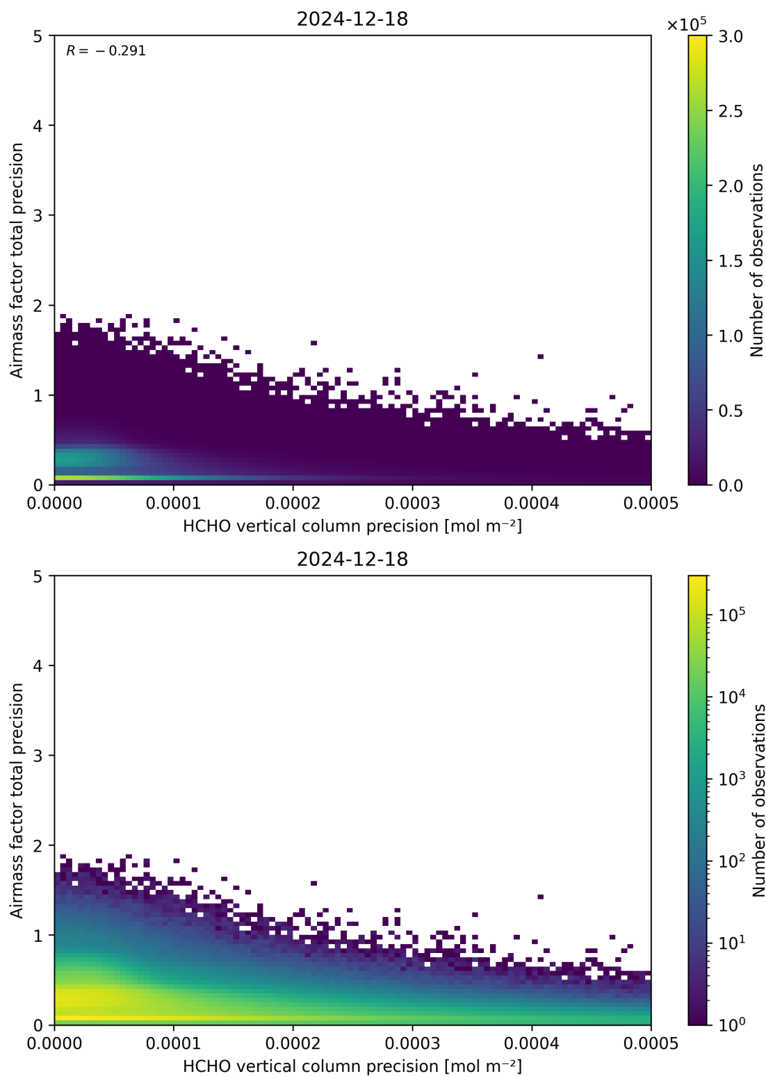
Figure 145: Scatter density plot of “HCHO vertical column precision” against “Airmass factor total precision” for 2024-12-17 to 2024-12-19.
