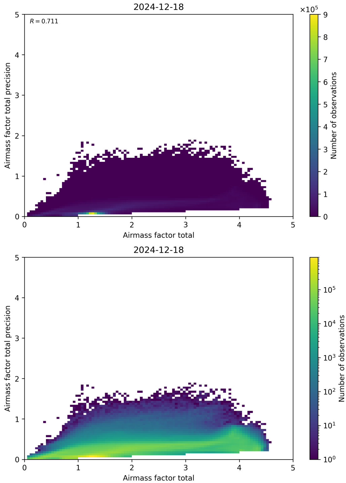
Figure 103: Scatter density plot of “Airmass factor total” against “Airmass factor total precision” for 2024-12-17 to 2024-12-19.
