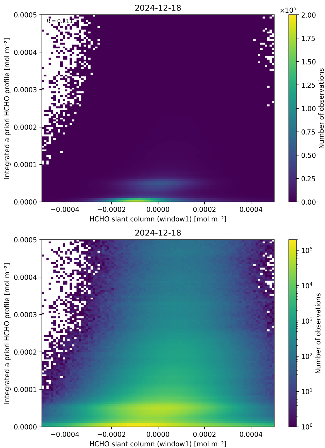
Figure 87: Scatter density plot of “HCHO slant column (window1)” against “Integrated a priori HCHO profile” for 2024-12-17 to 2024-12-19.
