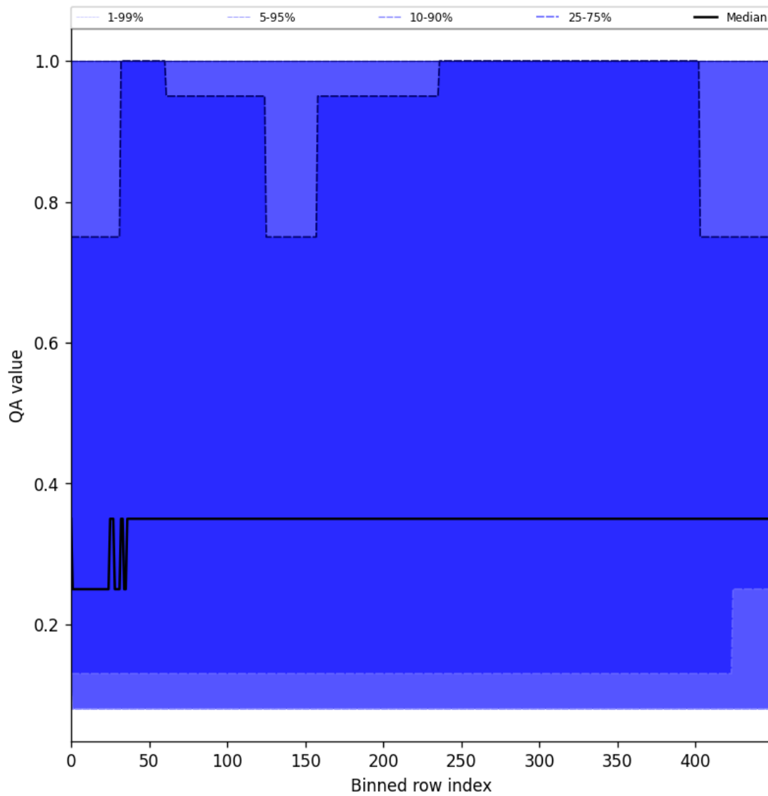
Figure 48: Along track statistics of “QA value” for 2024-12-17 to 2024-12-19
