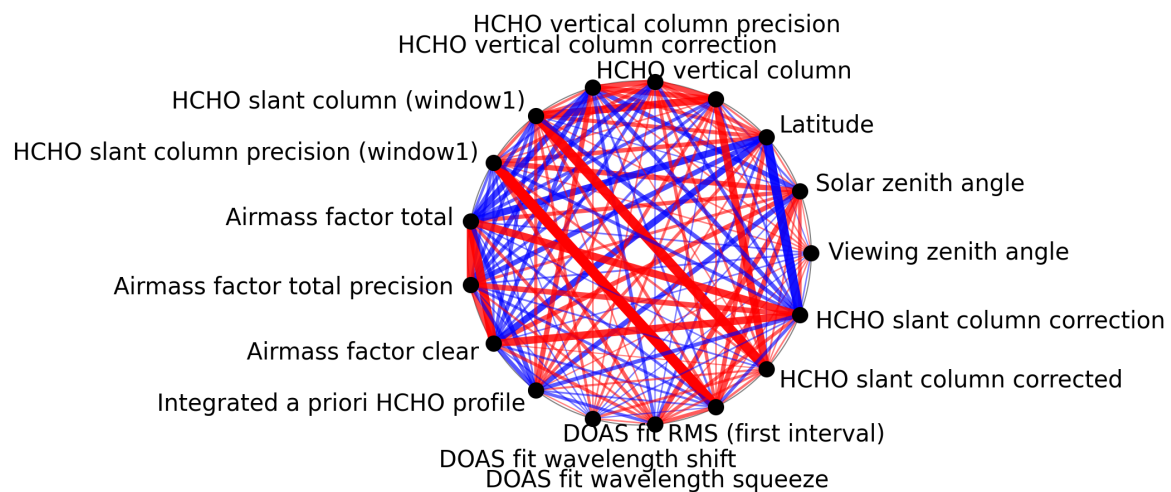
Figure 1: Map of correlation graph for 2024-12-17 to 2024-12-19.
