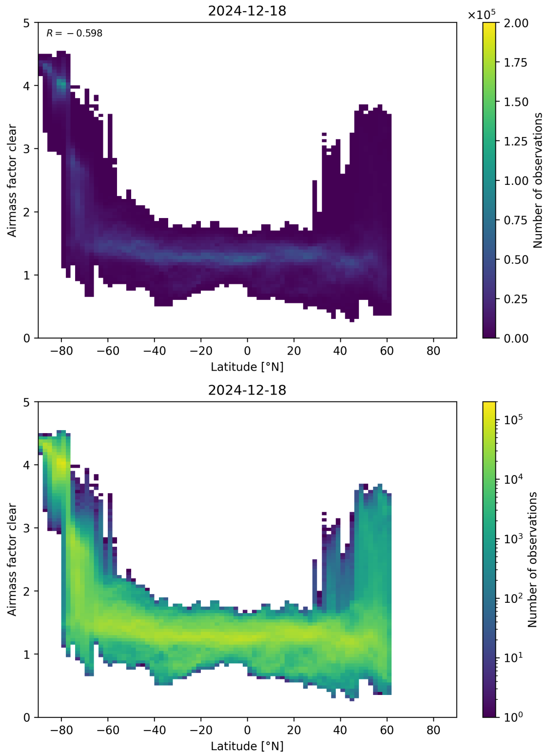
Figure 156: Scatter density plot of “Latitude” against “Airmass factor clear” for 2024-12-17 to 2024-12-19.
