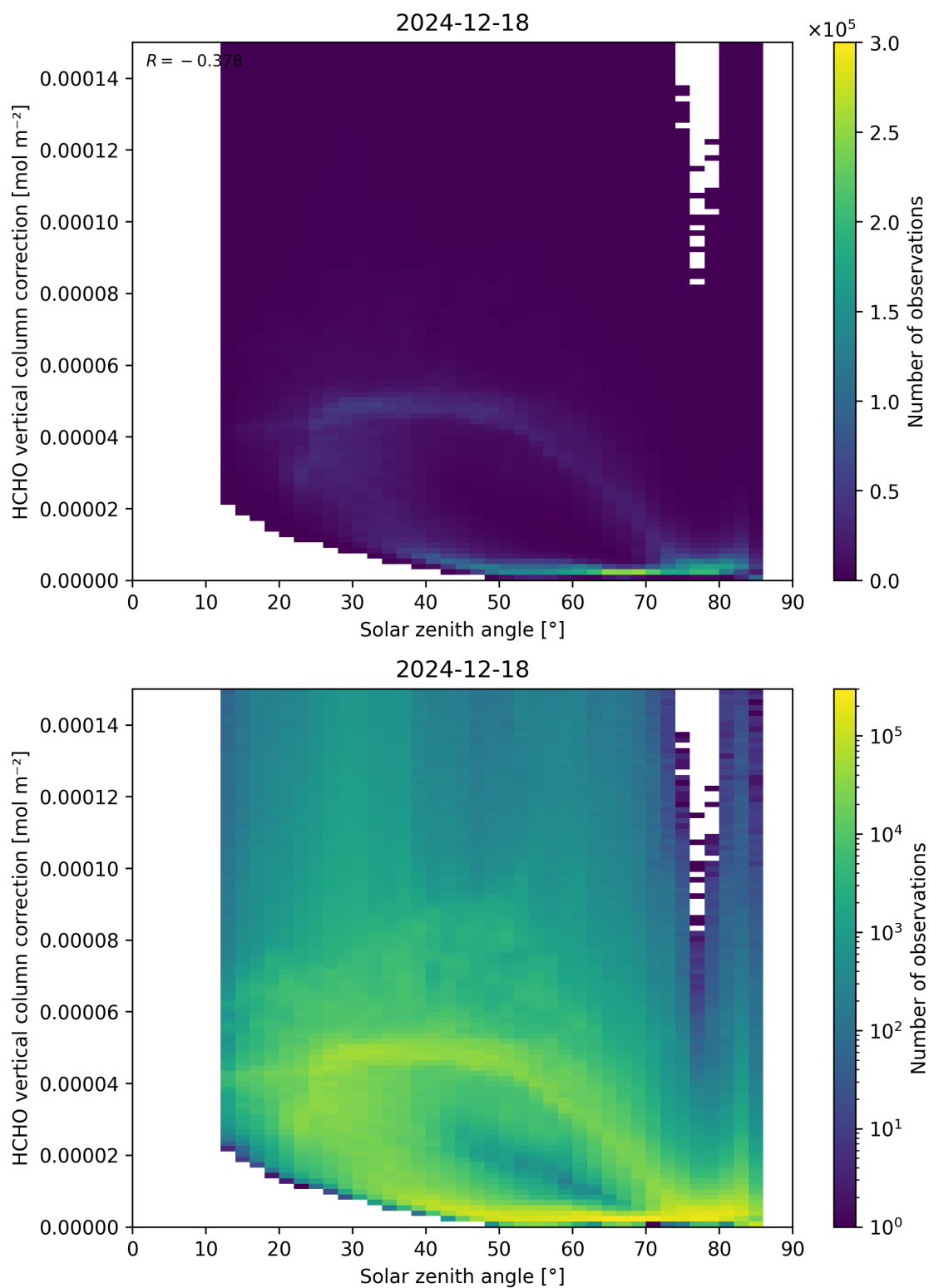
Figure 178: Scatter density plot of “Solar zenith angle” against “HCHO vertical column correction” for 2024-12-17 to 2024-12-19.
