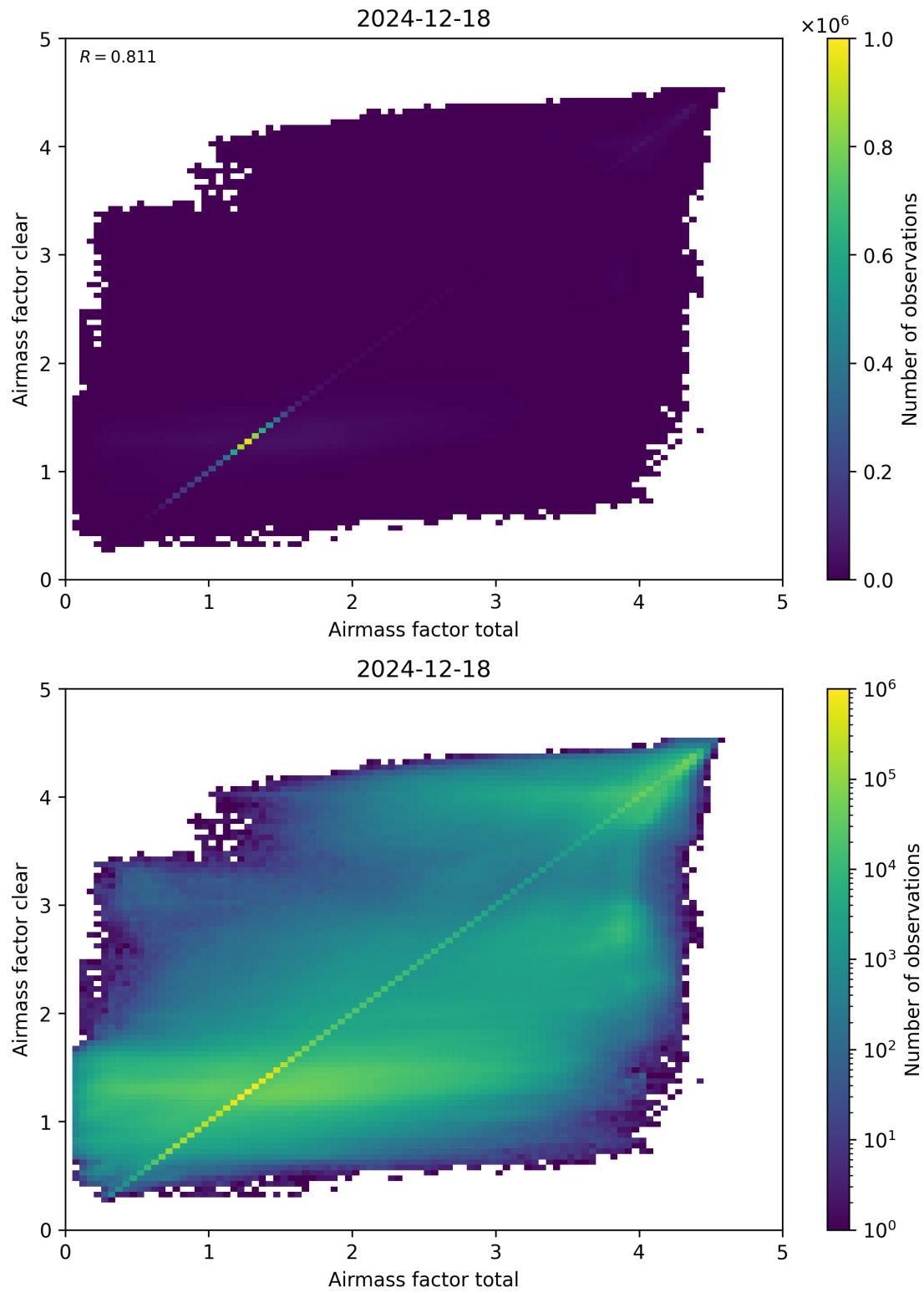
Figure 100: Scatter density plot of “Airmass factor total” against “Airmass factor clear” for 2024-12-17 to 2024-12-19.
