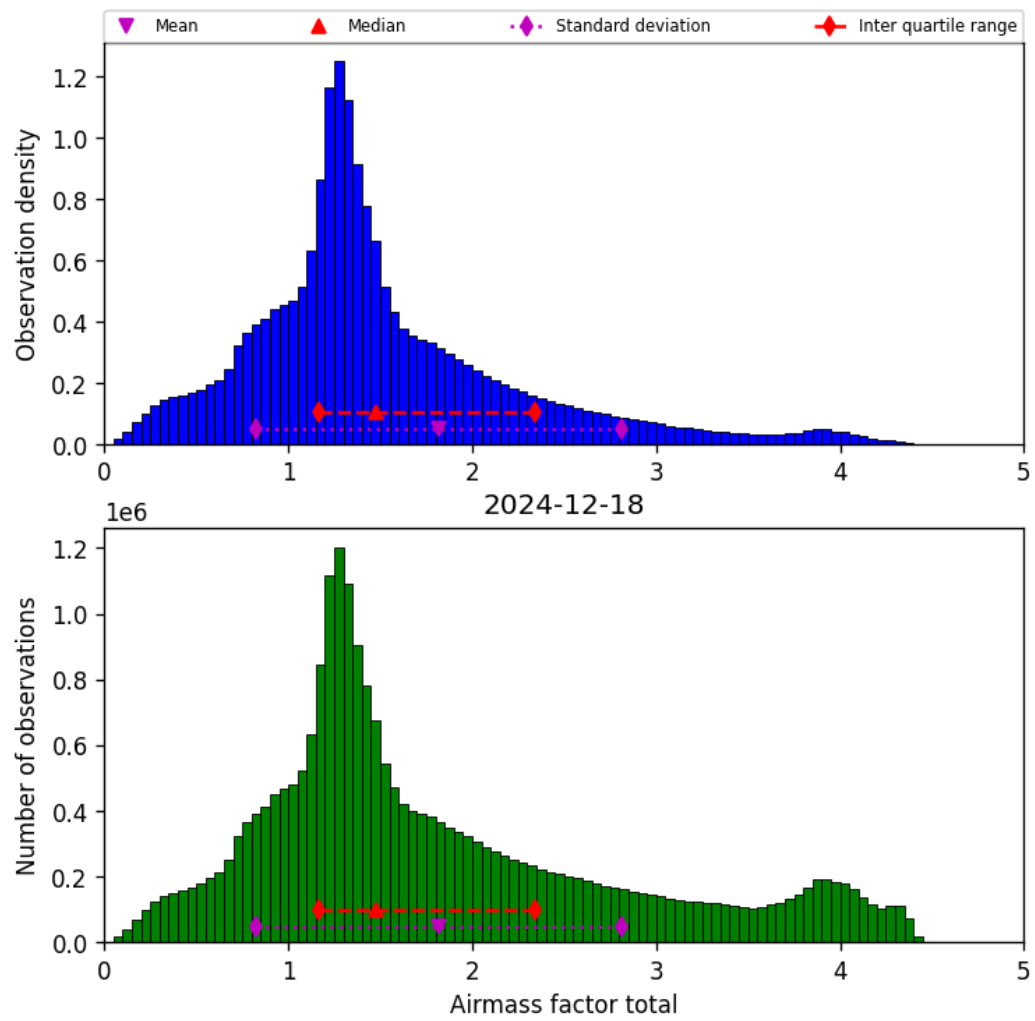
Figure 40: Histogram of “Airmass factor total” for 2024-12-17 to 2024-12-19
