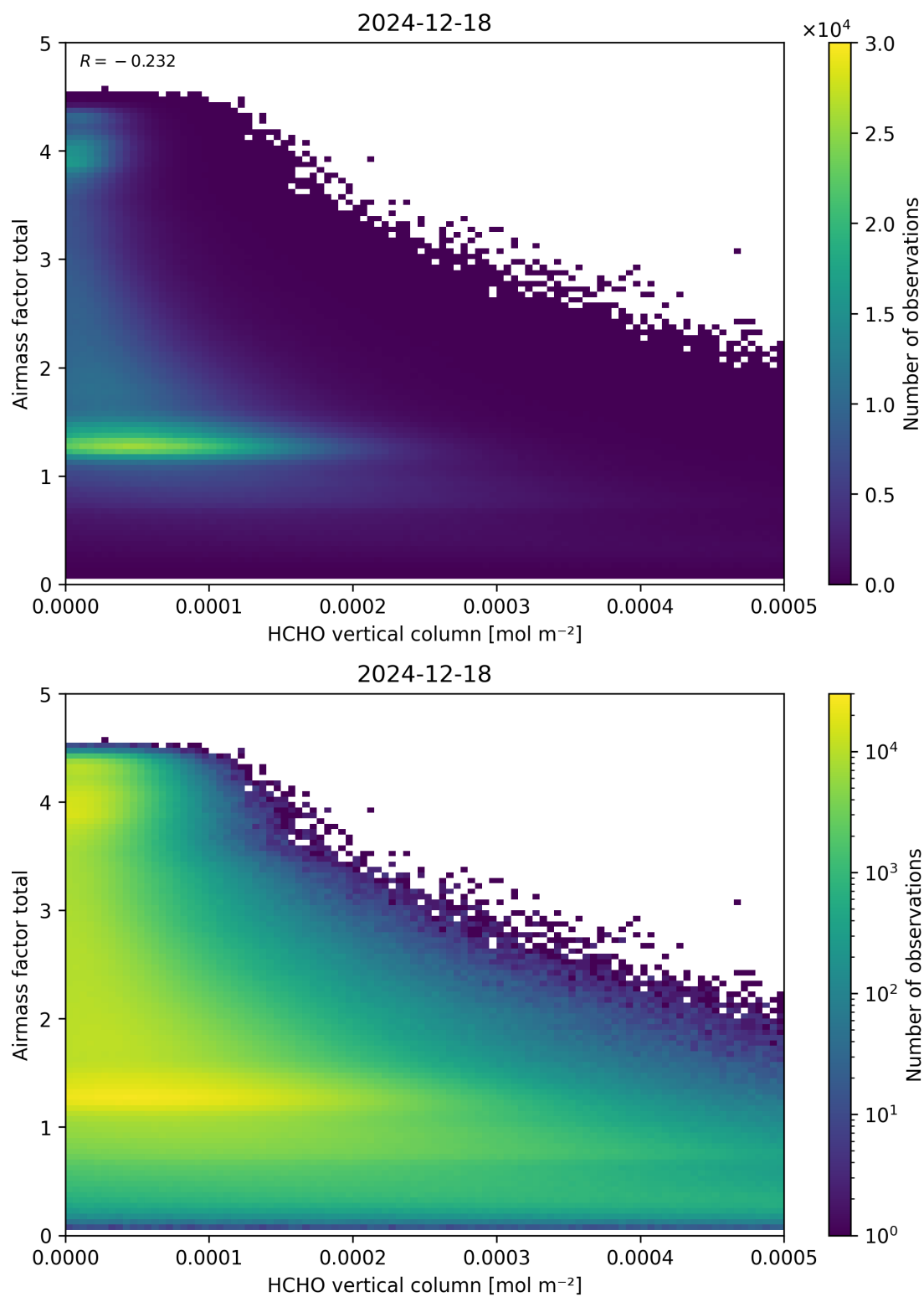
Figure 131: Scatter density plot of “HCHO vertical column” against “Airmass factor total” for 2024-12-17 to 2024-12-19.
