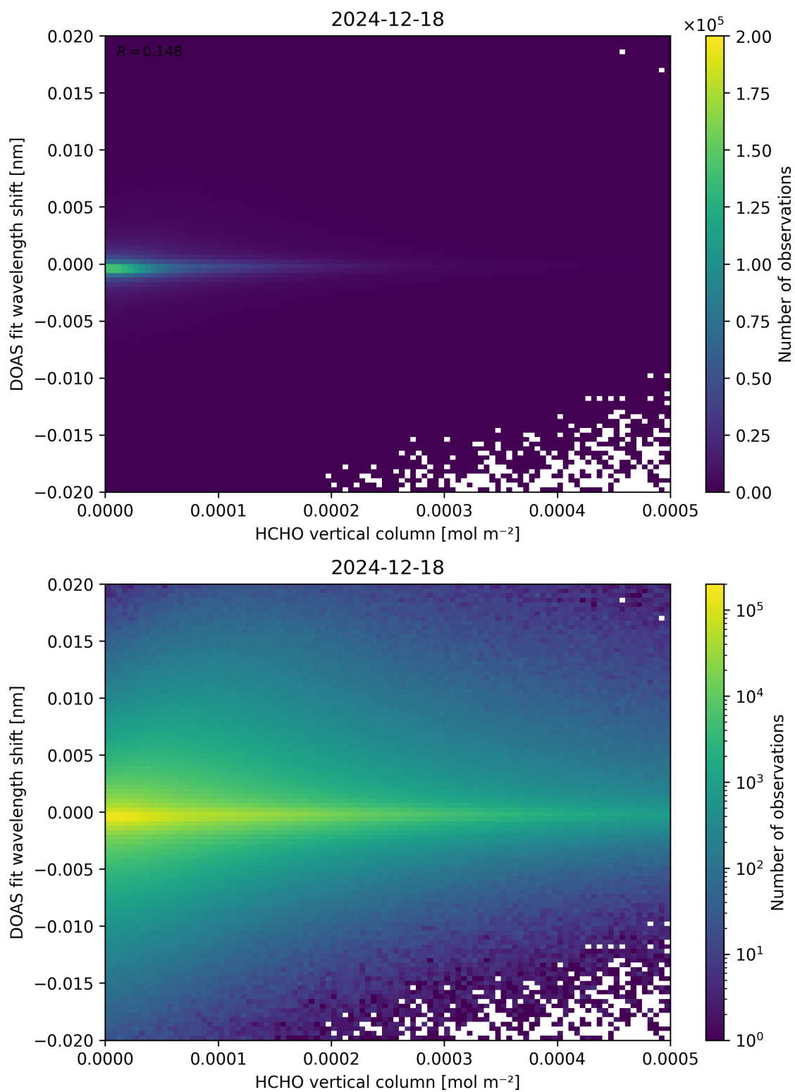
Figure 124: Scatter density plot of “HCHO vertical column” against “DOAS fit wavelength shift” for 2024-12-17 to 2024-12-19.
