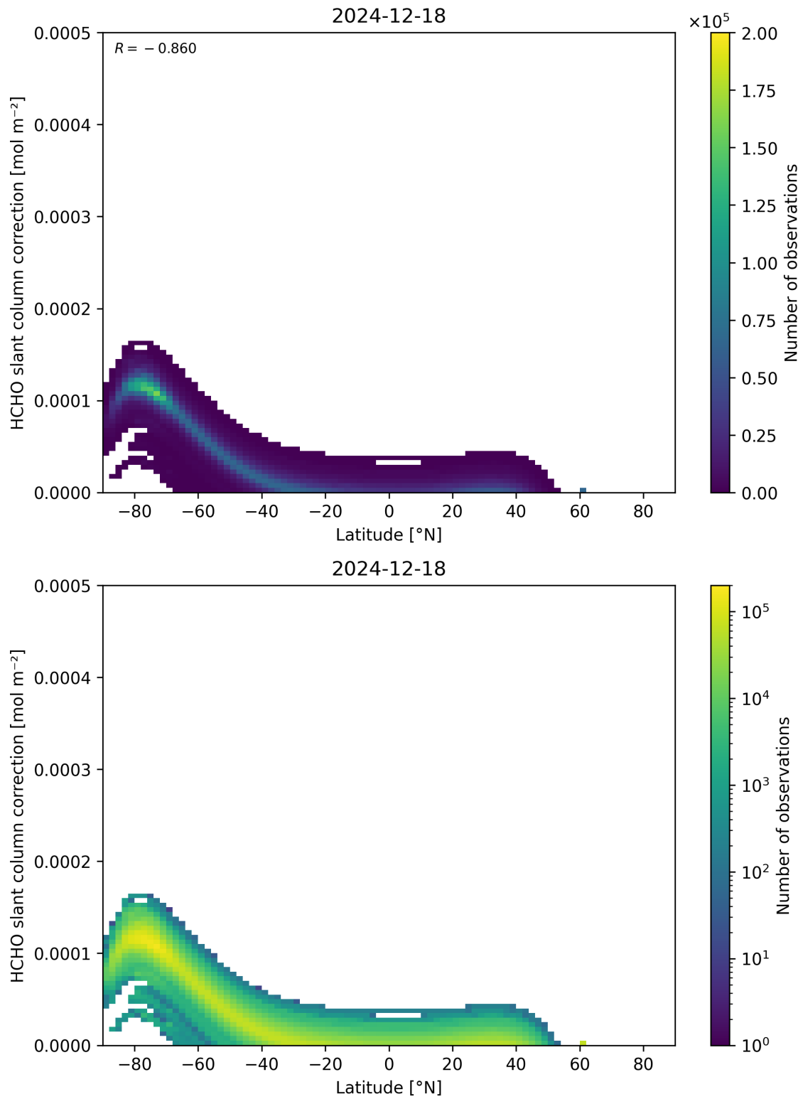
Figure 158: Scatter density plot of “Latitude” against “HCHO slant column correction” for 2024-12-17 to 2024-12-19.
