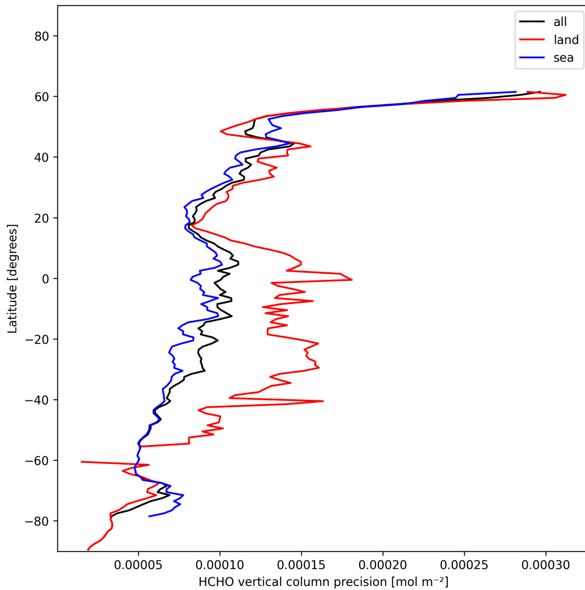
Figure 22: Zonal average of “HCHO vertical column precision” for 2024-12-17 to 2024-12-19.
