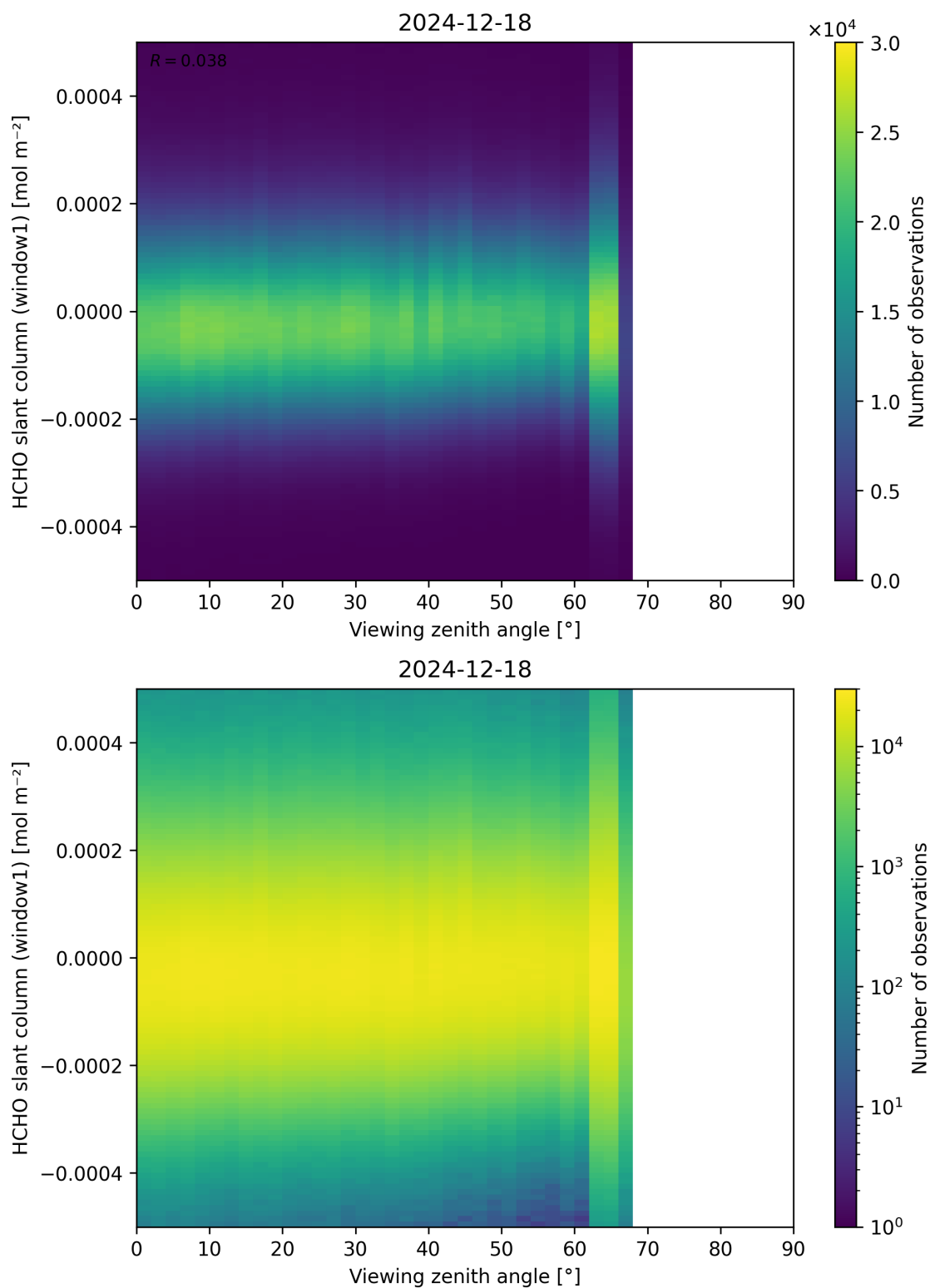
Figure 188: Scatter density plot of “Viewing zenith angle” against “HCHO slant column (window1)” for 2024-12-17 to 2024-12-19.
