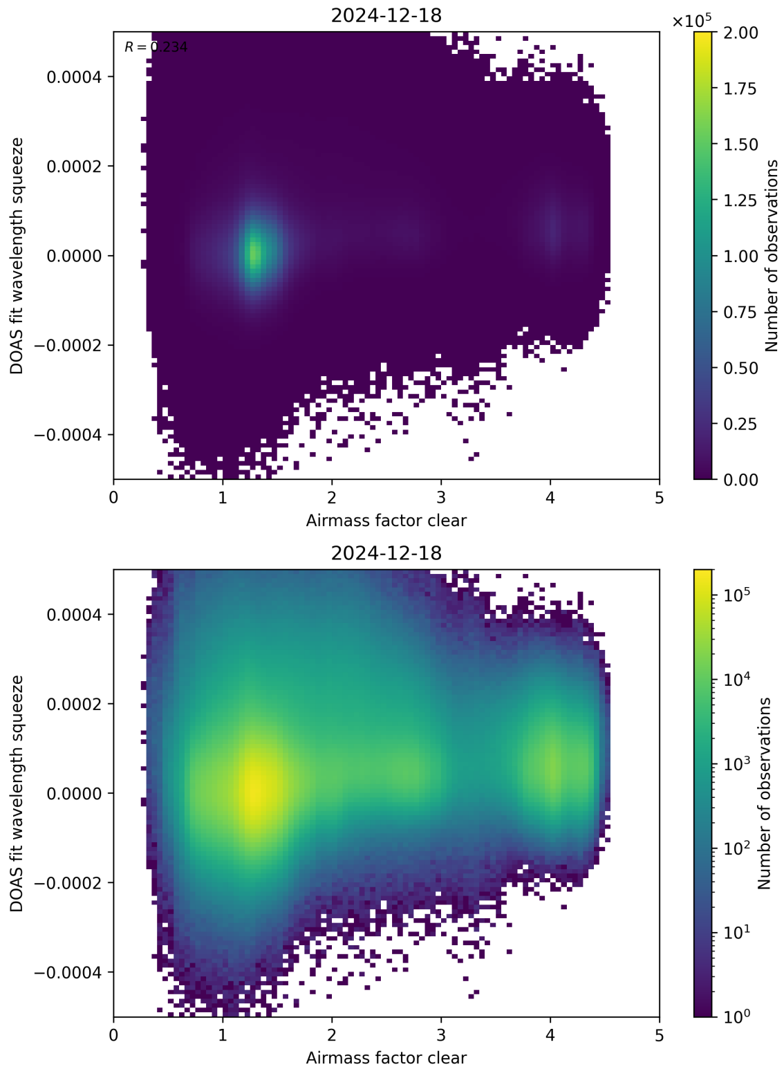
Figure 73: Scatter density plot of “Airmass factor clear” against “DOAS fit wavelength squeeze” for 2024-12-17 to 2024-12-19.
