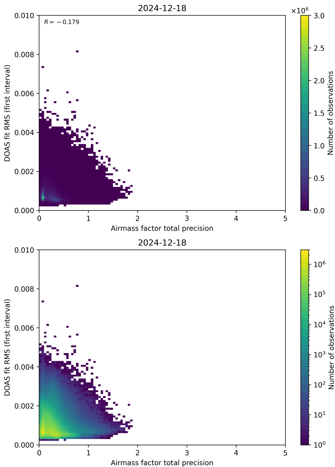
Figure 105: Scatter density plot of “Airmass factor total precision” against “DOAS fit RMS (first interval)” for 2024-12-17 to 2024-12-19.
