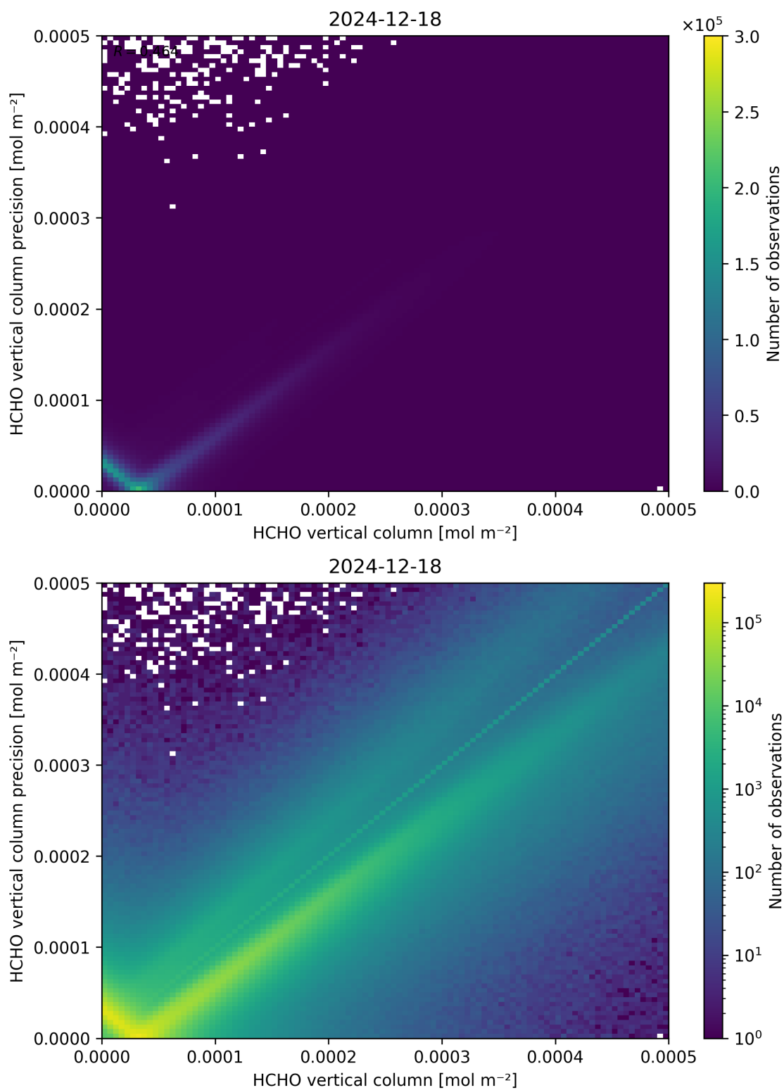
Figure 134: Scatter density plot of “HCHO vertical column” against “HCHO vertical column precision” for 2024-12-17 to 2024-12-19.
