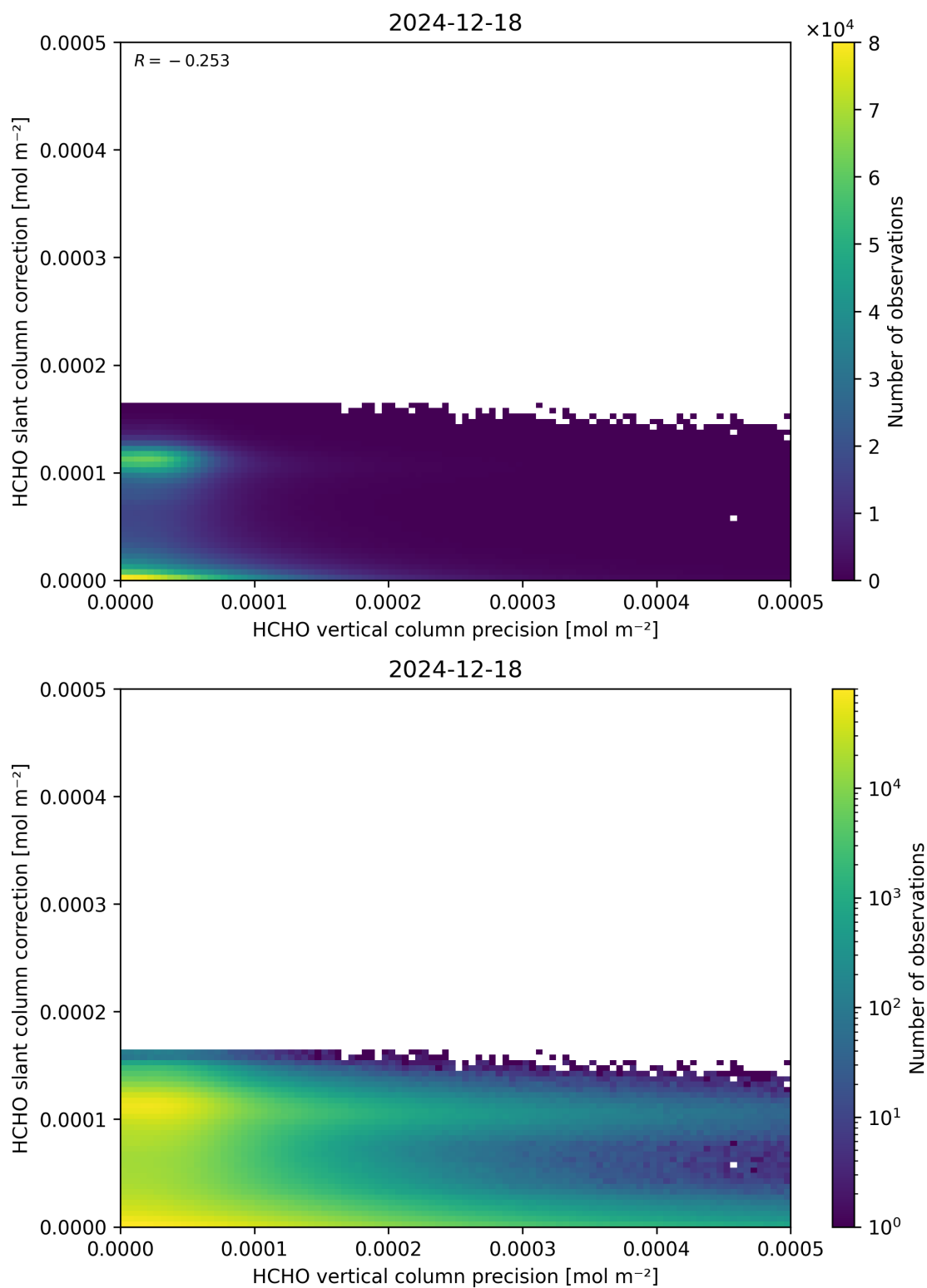
Figure 141: Scatter density plot of “HCHO vertical column precision” against “HCHO slant column correction” for 2024-12-17 to 2024-12-19.
