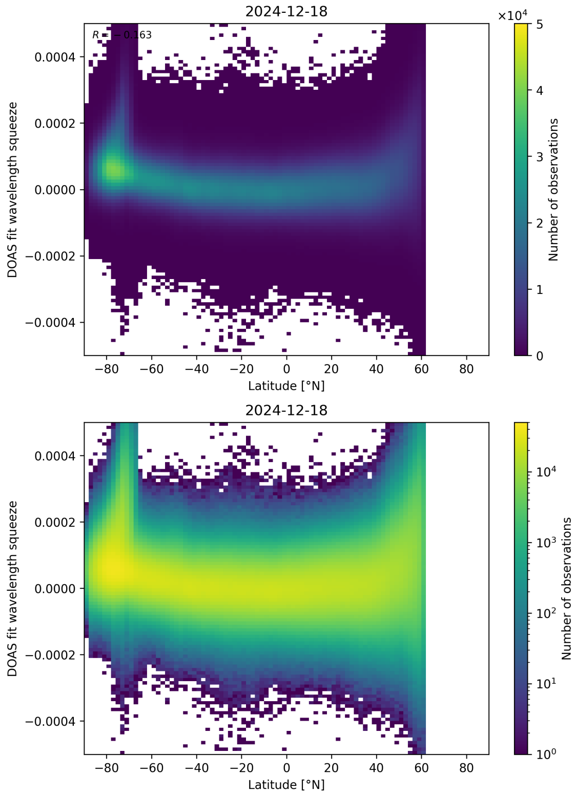
Figure 155: Scatter density plot of “Latitude” against “DOAS fit wavelength squeeze” for 2024-12-17 to 2024-12-19.
