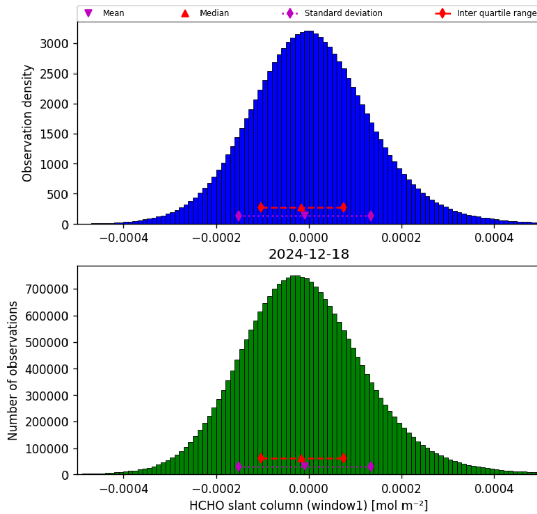
Figure 38: Histogram of “HCHO slant column (window1)” for 2024-12-17 to 2024-12-19
