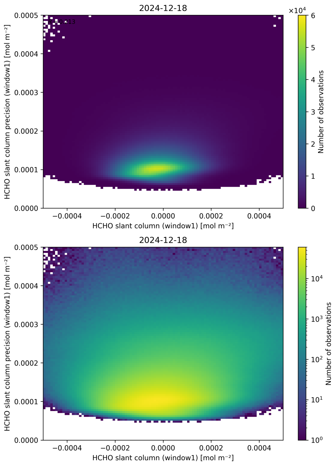
Figure 84: Scatter density plot of “HCHO slant column (window1)” against “HCHO slant column precision (window1)” for 2024-12-17 to 2024-12-19.
