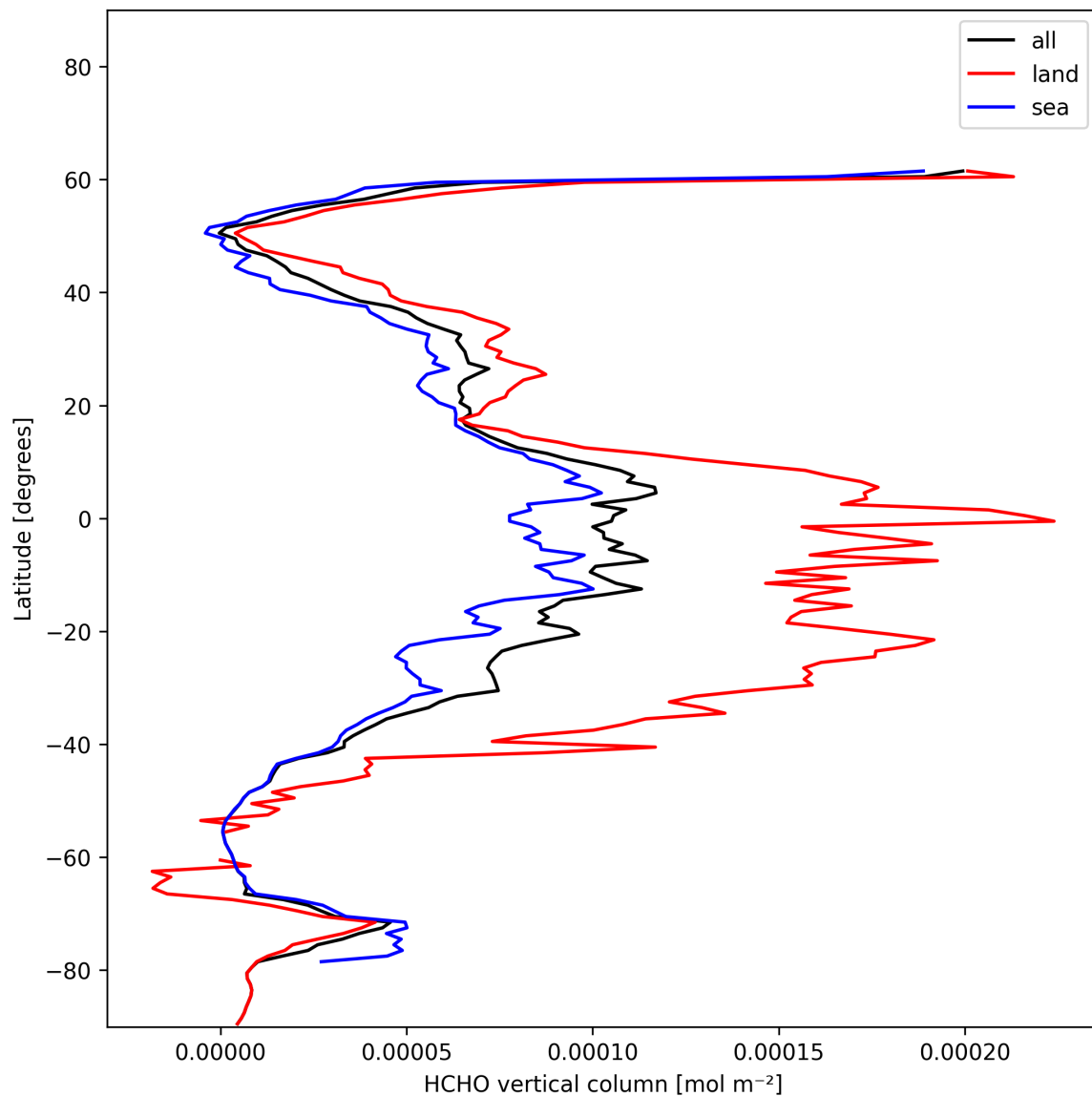
Figure 21: Zonal average of “HCHO vertical column” for 2024-12-17 to 2024-12-19.
