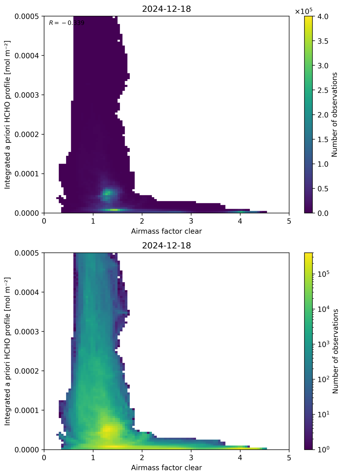
Figure 76: Scatter density plot of “Airmass factor clear” against “Integrated a priori HCHO profile” for 2024-12-17 to 2024-12-19.
