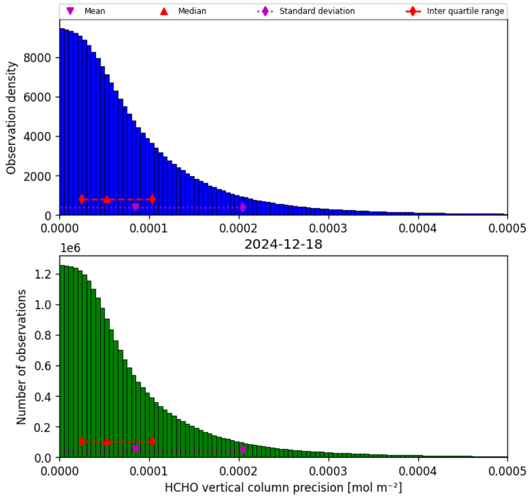
Figure 36: Histogram of “HCHO vertical column precision” for 2024-12-17 to 2024-12-19
