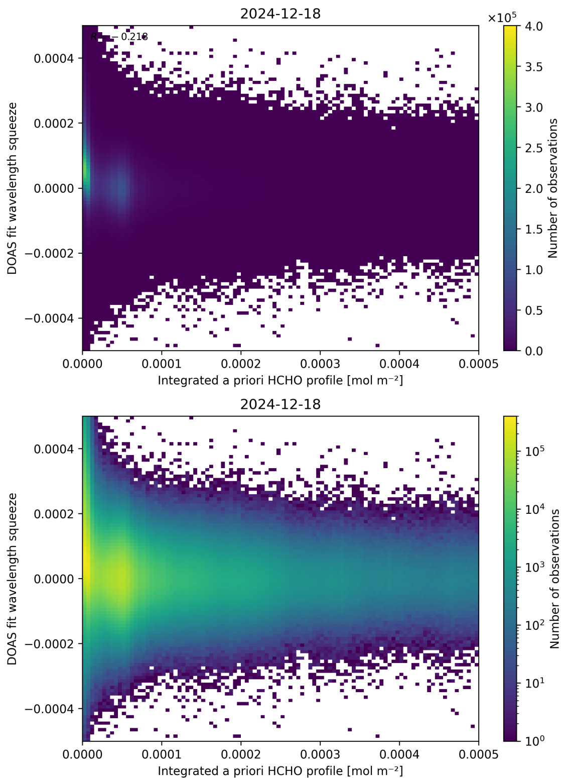
Figure 150: Scatter density plot of “Integrated a priori HCHO profile” against “DOAS fit wavelength squeeze” for 2024-12-17 to 2024-12-19.
