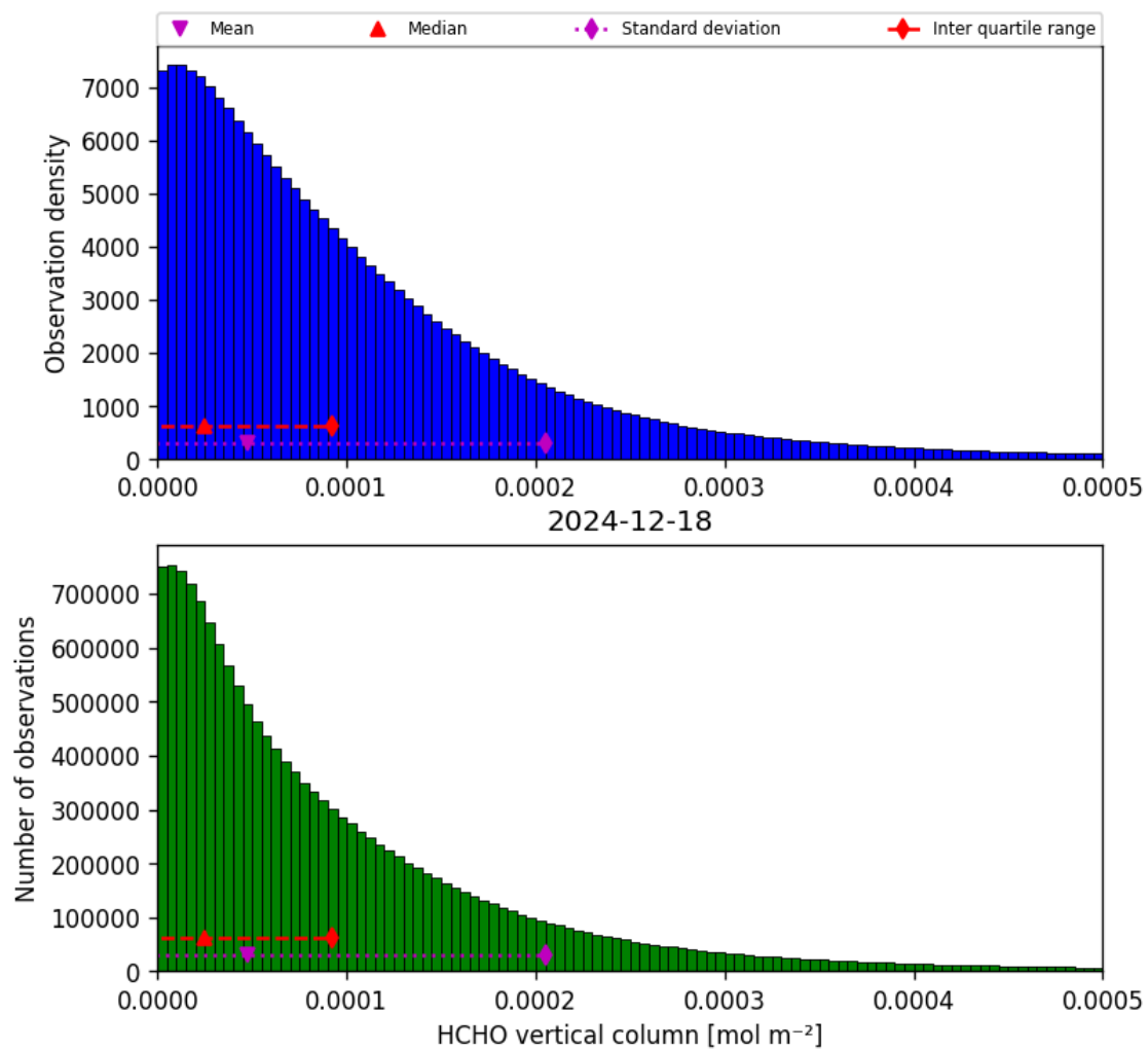
Figure 35: Histogram of “HCHO vertical column” for 2024-12-17 to 2024-12-19
