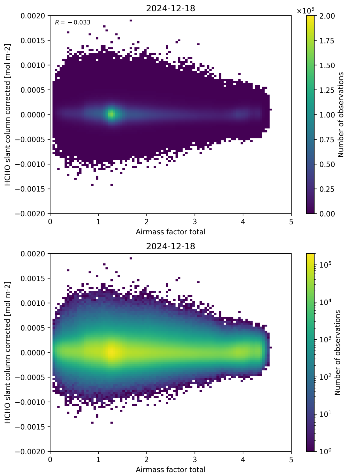
Figure 101: Scatter density plot of “Airmass factor total” against “HCHO slant column corrected” for 2024-12-17 to 2024-12-19.
