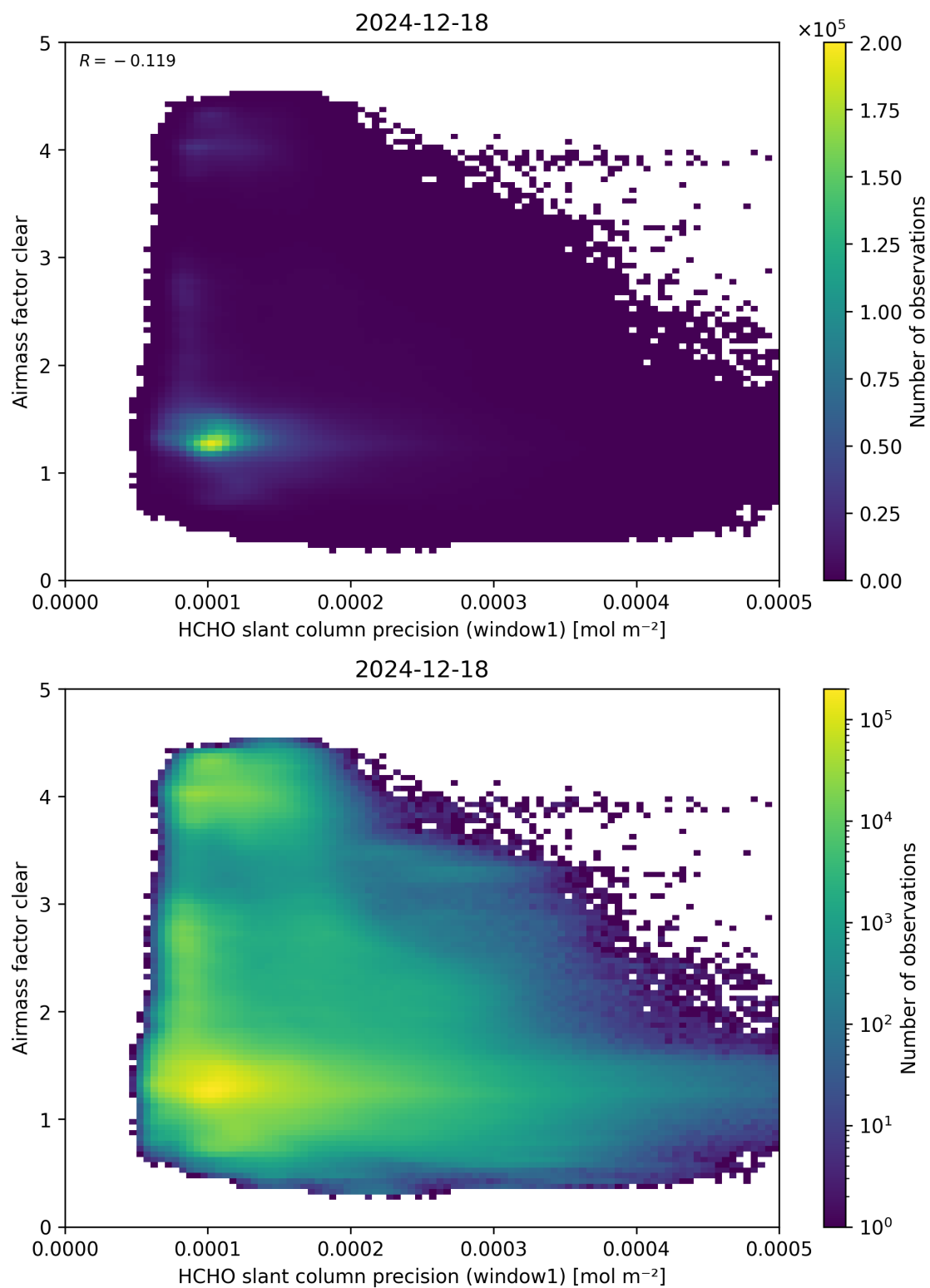
Figure 91: Scatter density plot of “HCHO slant column precision (window1)” against “Airmass factor clear” for 2024-12-17 to 2024-12-19.
