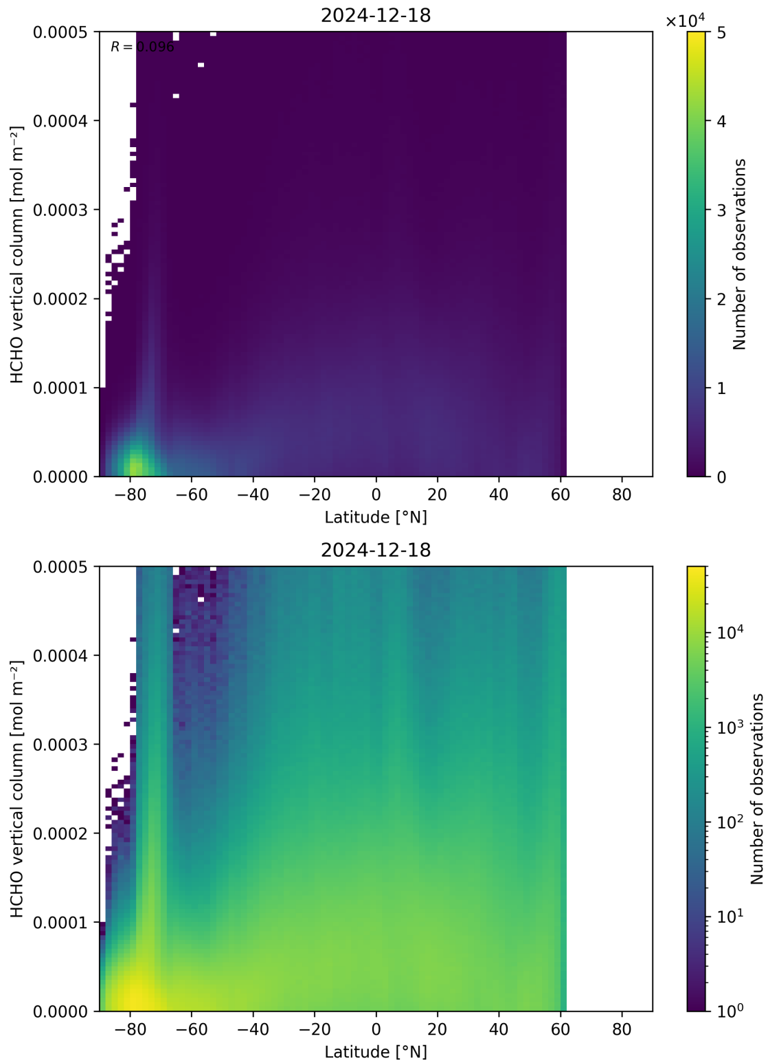
Figure 163: Scatter density plot of “Latitude” against “HCHO vertical column” for 2024-12-17 to 2024-12-19.
