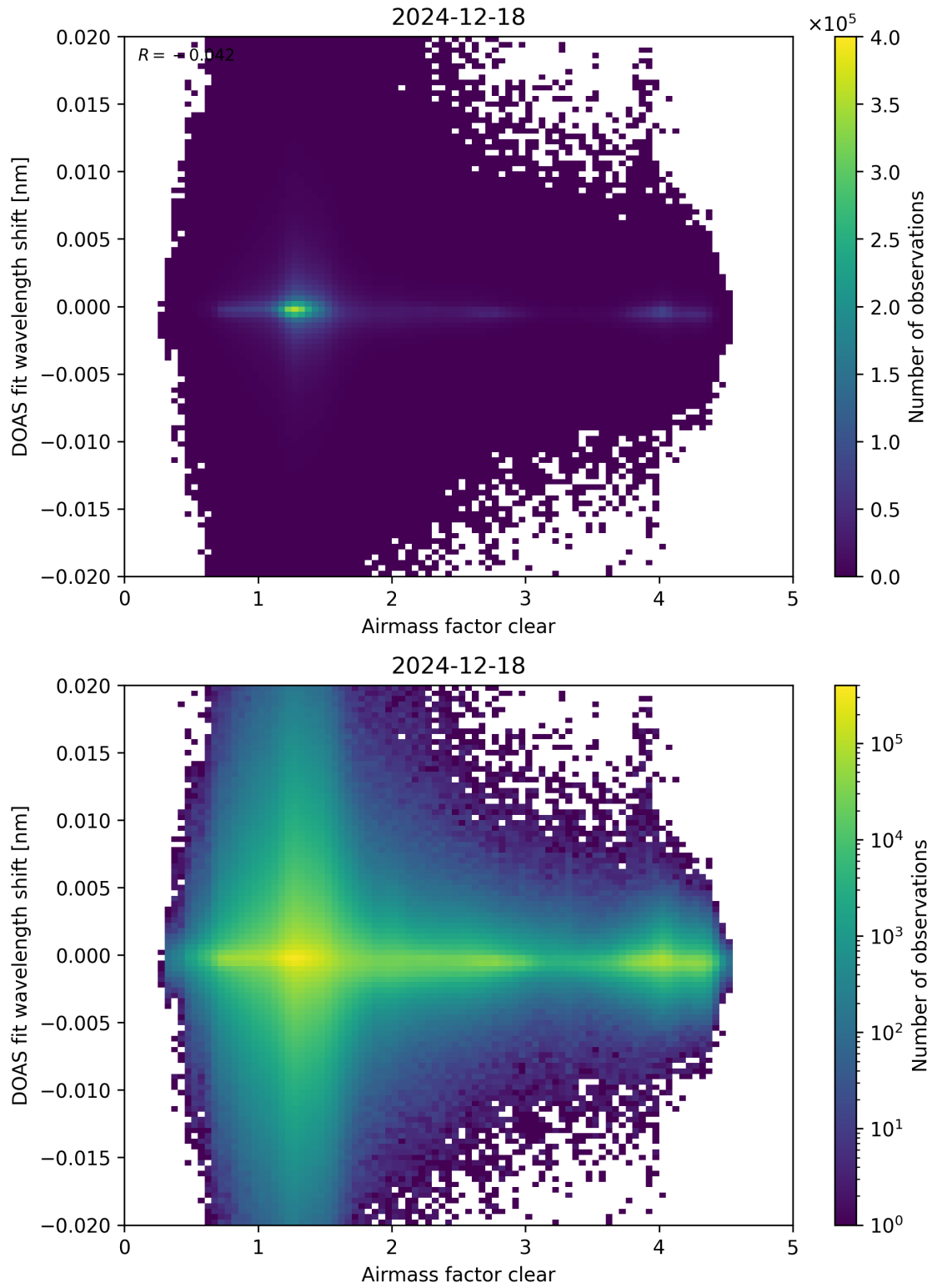
Figure 72: Scatter density plot of “Airmass factor clear” against “DOAS fit wavelength shift” for 2024-12-17 to 2024-12-19.
