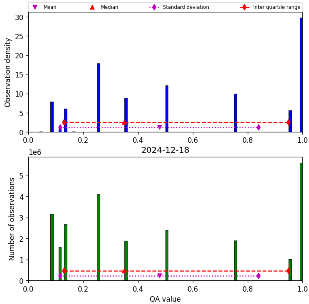
Figure 34: Histogram of “QA value” for 2024-12-17 to 2024-12-19
