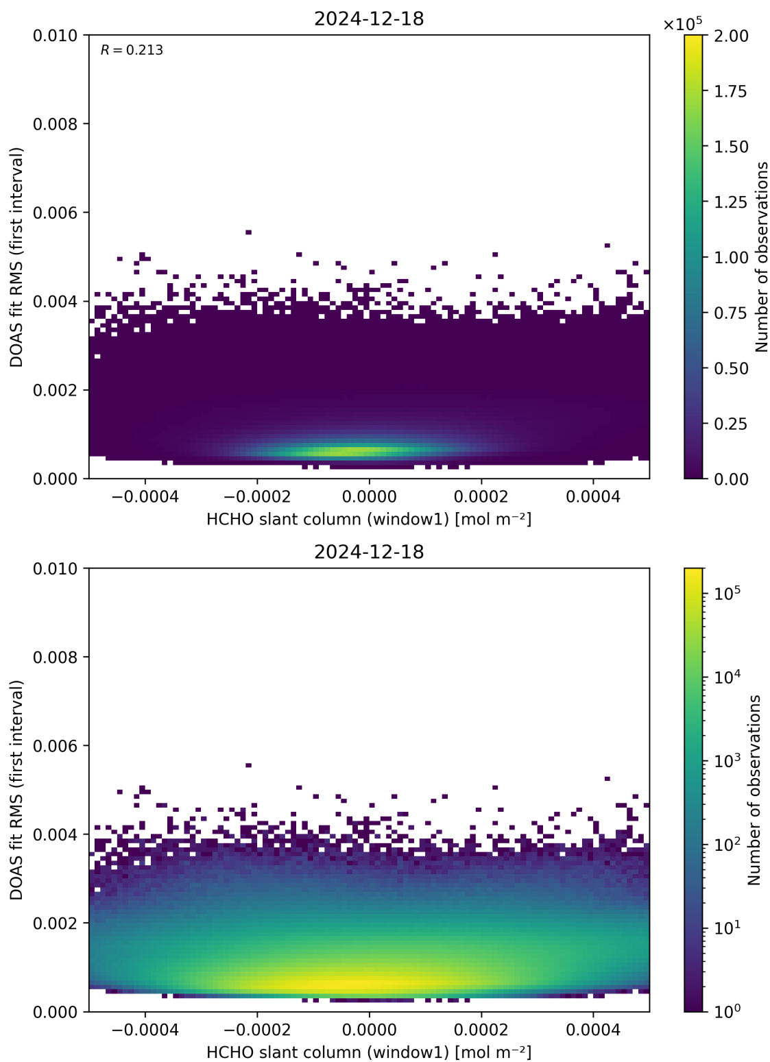
Figure 78: Scatter density plot of “HCHO slant column (window1)” against “DOAS fit RMS (first interval)” for 2024-12-17 to 2024-12-19.
