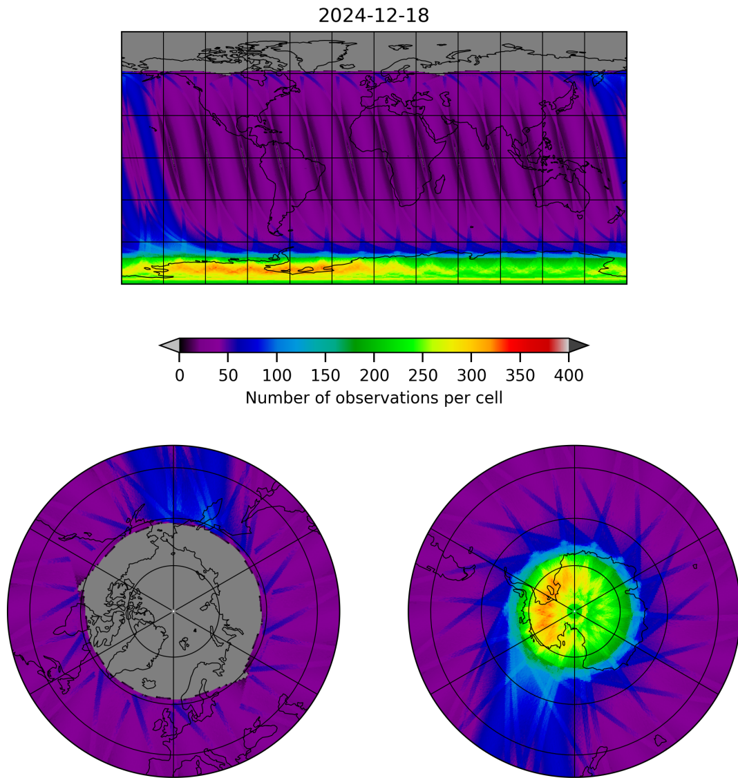
Figure 19: Map of the number of observations for 2024-12-17 to 2024-12-19
