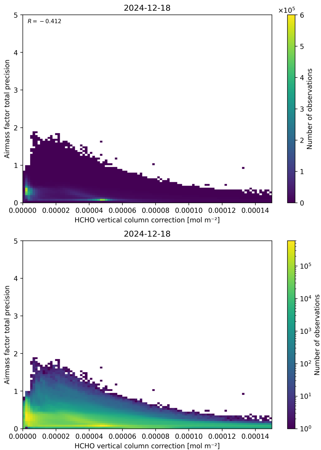
Figure 121: Scatter density plot of “HCHO vertical column correction” against “Airmass factor total precision” for 2024-12-17 to 2024-12-19.
