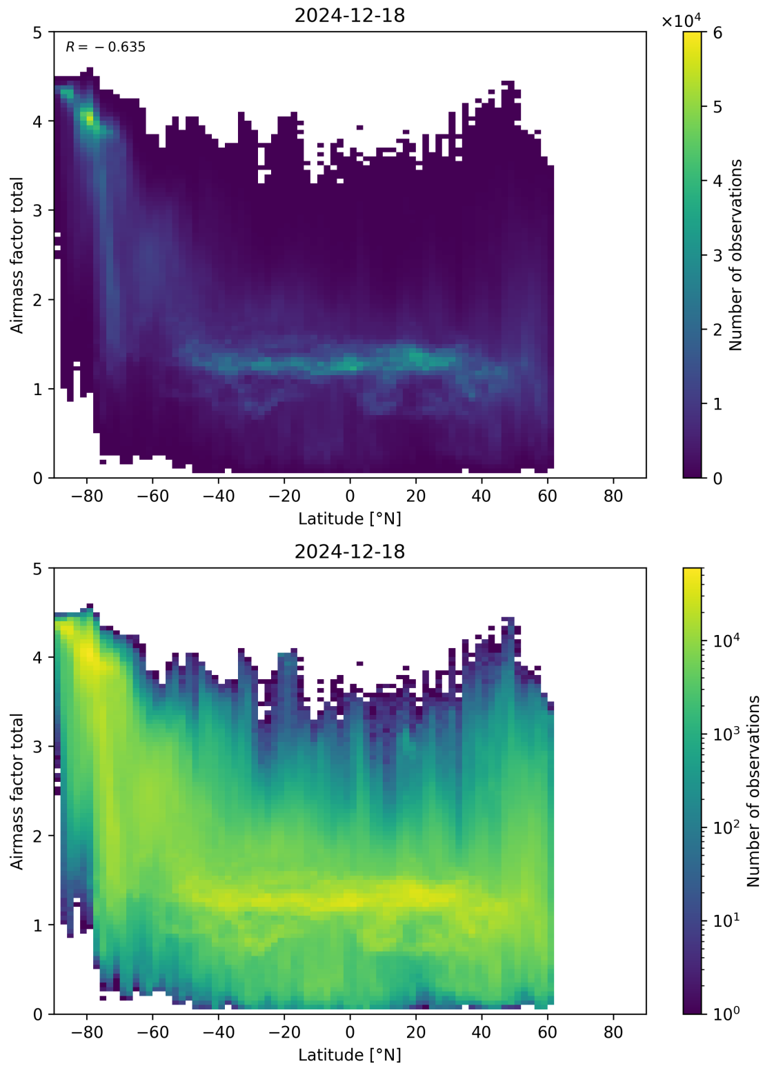
Figure 161: Scatter density plot of “Latitude” against “Airmass factor total” for 2024-12-17 to 2024-12-19.
