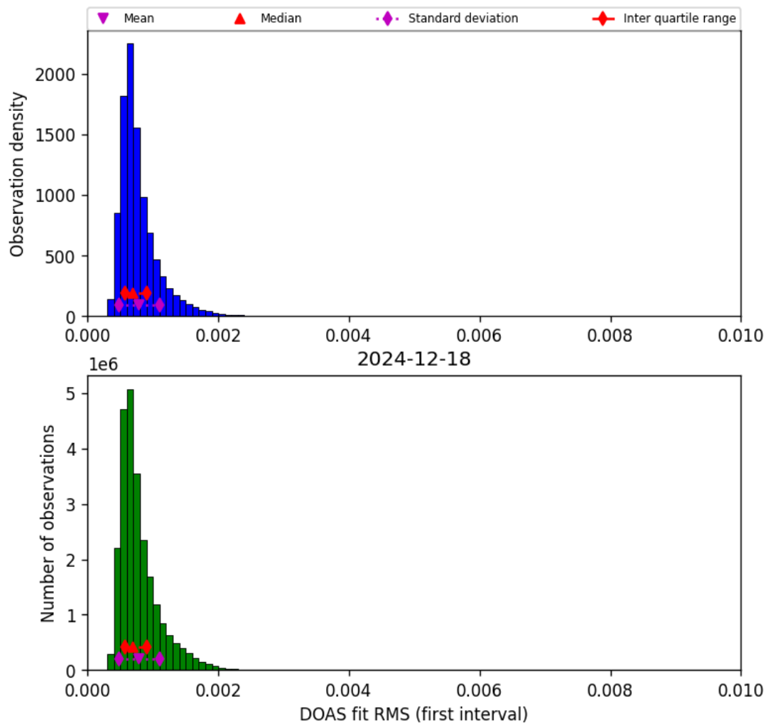
Figure 46: Histogram of “DOAS fit RMS (first interval)” for 2024-12-17 to 2024-12-19
