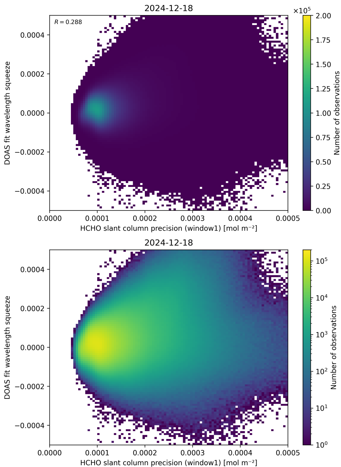
Figure 90: Scatter density plot of “HCHO slant column precision (window1)” against “DOAS fit wavelength squeeze” for 2024-12-17 to 2024-12-19.
