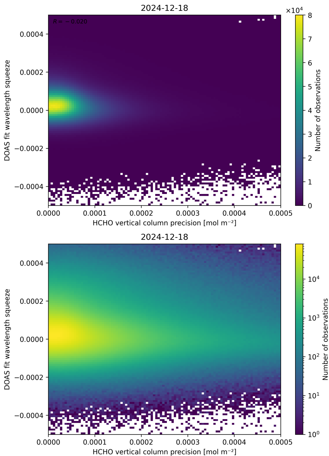
Figure 138: Scatter density plot of “HCHO vertical column precision” against “DOAS fit wavelength squeeze” for 2024-12-17 to 2024-12-19.
