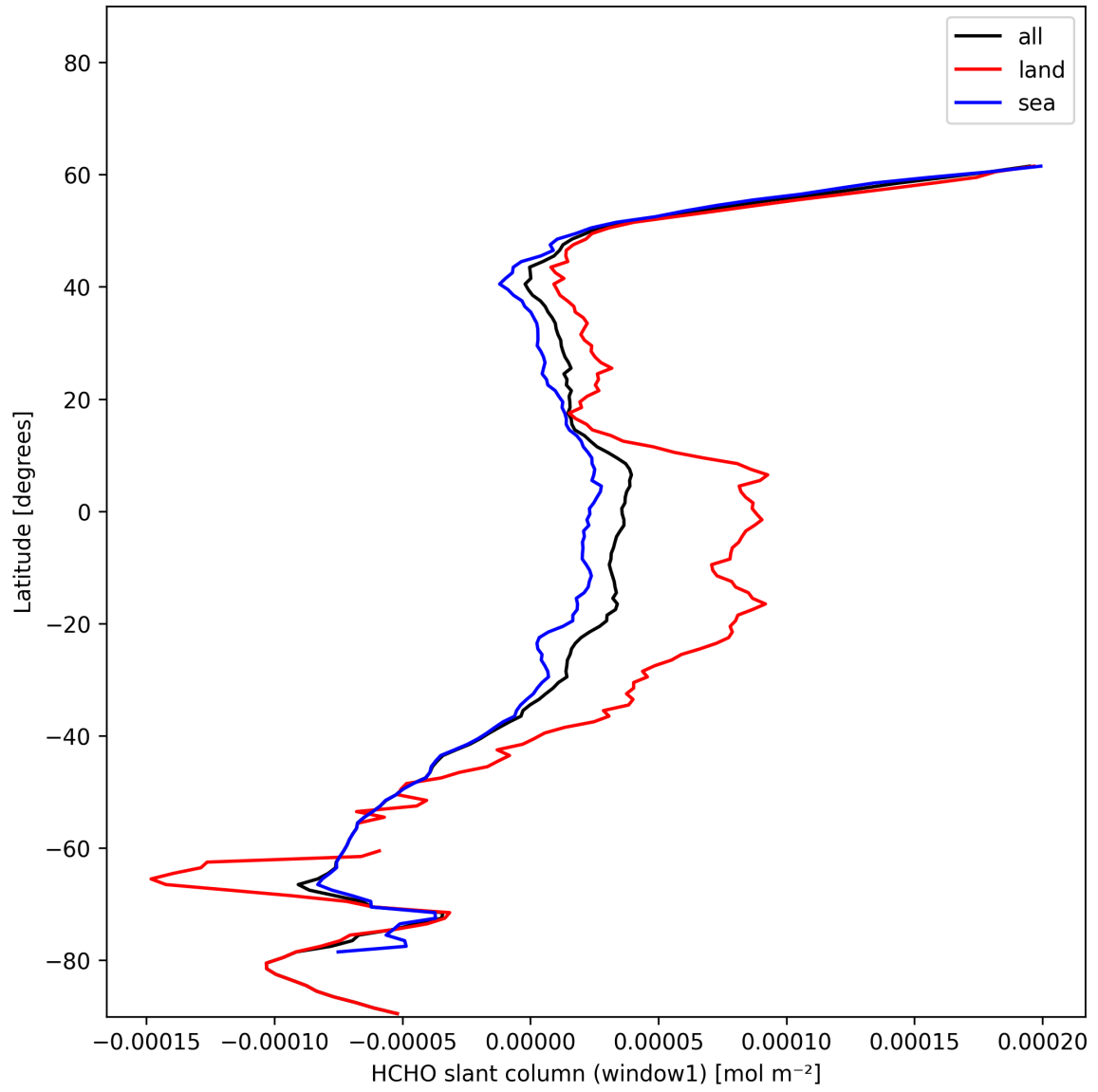
Figure 24: Zonal average of “HCHO slant column (window1)” for 2024-12-17 to 2024-12-19.
