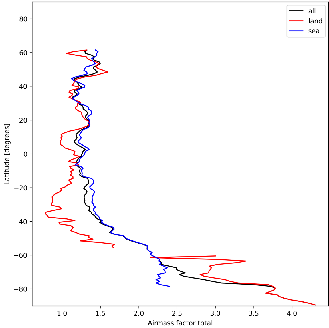
Figure 26: Zonal average of “Airmass factor total” for 2024-12-17 to 2024-12-19.
