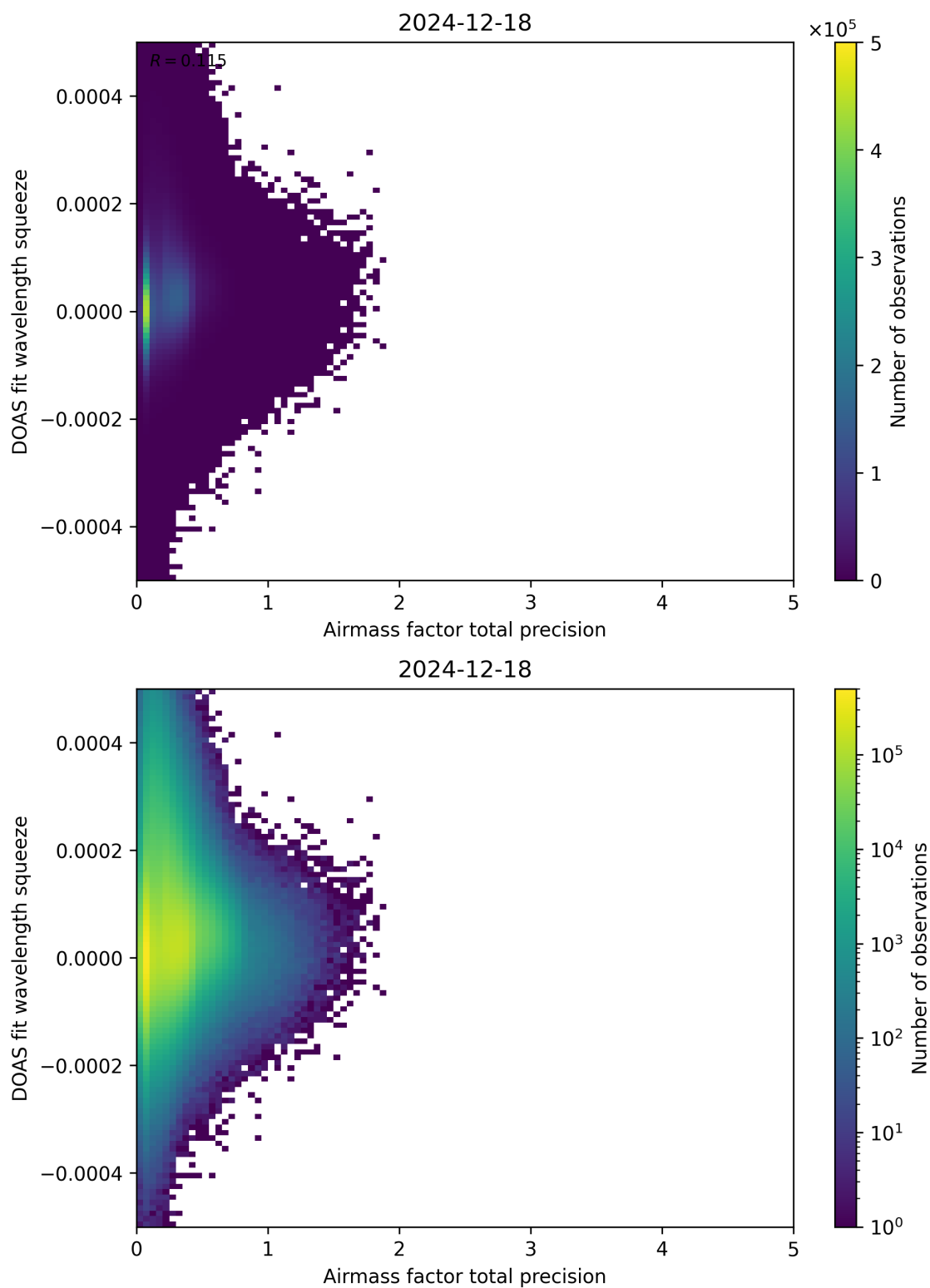
Figure 107: Scatter density plot of “Airmass factor total precision” against “DOAS fit wavelength squeeze” for 2024-12-17 to 2024-12-19.
