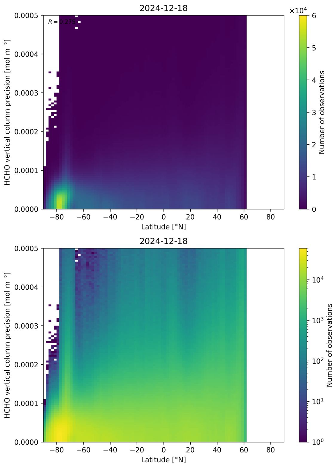
Figure 165: Scatter density plot of “Latitude” against “HCHO vertical column precision” for 2024-12-17 to 2024-12-19.
