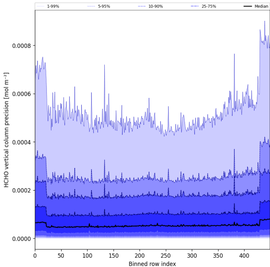
Figure 50: Along track statistics of “HCHO vertical column precision” for 2024-12-17 to 2024-12-19
