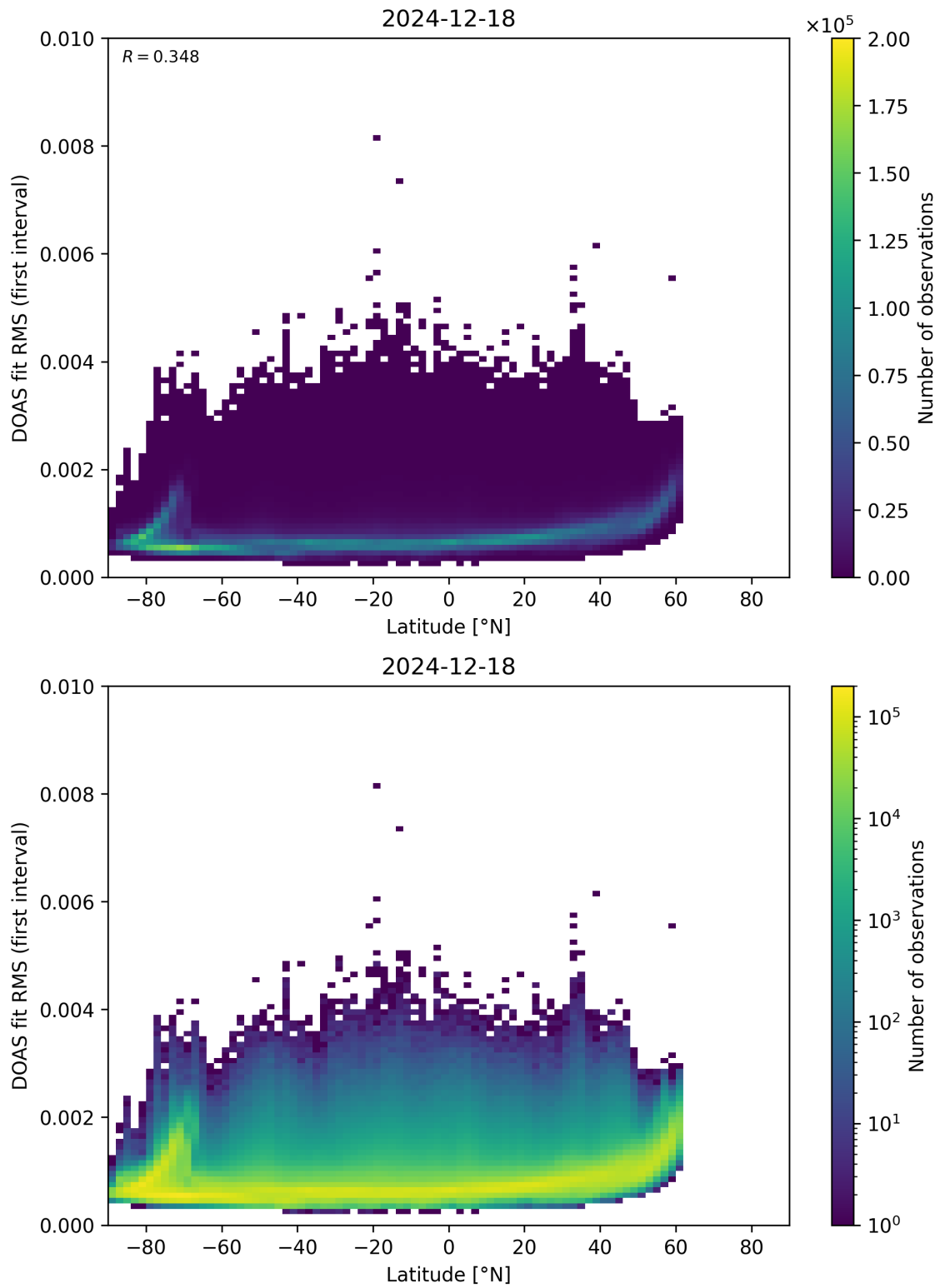
Figure 153: Scatter density plot of “Latitude” against “DOAS fit RMS (first interval)” for 2024-12-17 to 2024-12-19.
