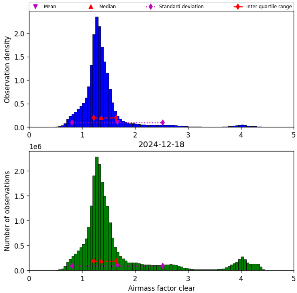
Figure 42: Histogram of “Airmass factor clear” for 2024-12-17 to 2024-12-19
