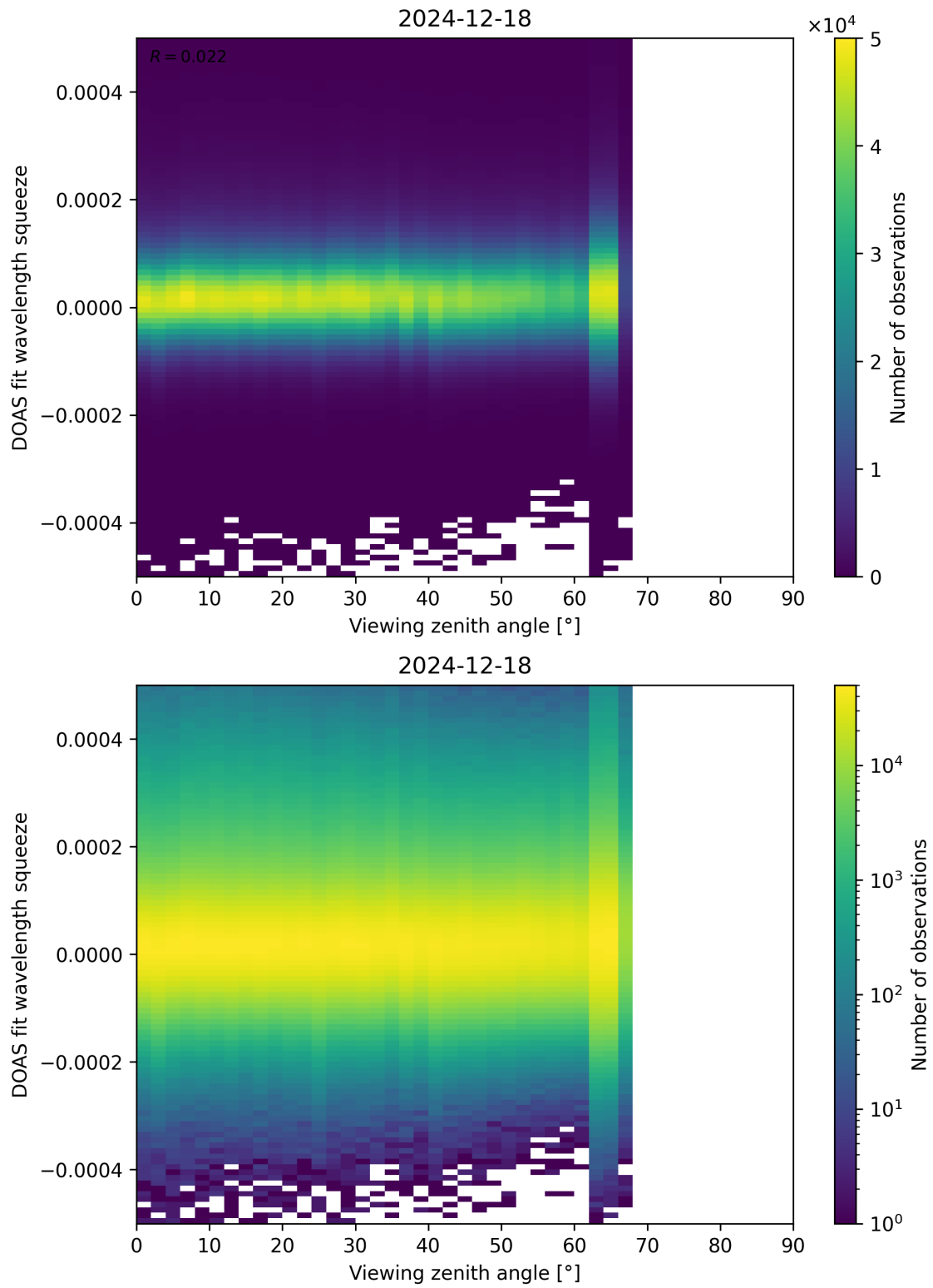
Figure 184: Scatter density plot of “Viewing zenith angle” against “DOAS fit wavelength squeeze” for 2024-12-17 to 2024-12-19.
