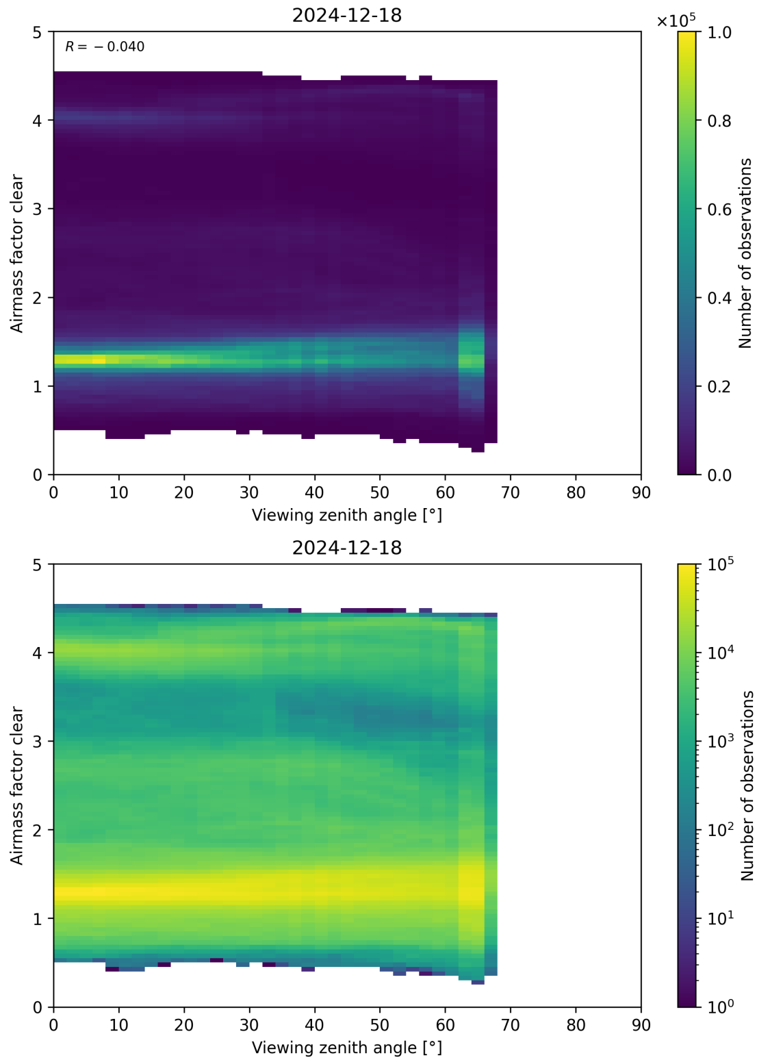
Figure 185: Scatter density plot of “Viewing zenith angle” against “Airmass factor clear” for 2024-12-17 to 2024-12-19.
