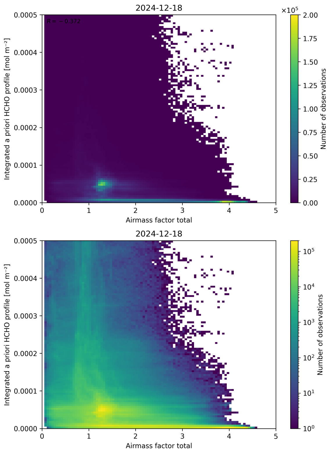
Figure 104: Scatter density plot of “Airmass factor total” against “Integrated a priori HCHO profile” for 2024-12-17 to 2024-12-19.
