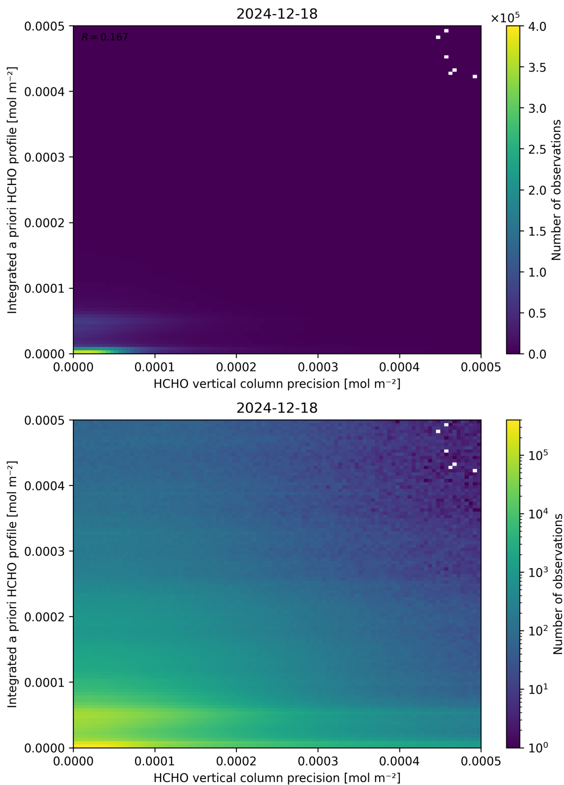
Figure 147: Scatter density plot of “HCHO vertical column precision” against “Integrated a priori HCHO profile” for 2024-12-17 to 2024-12-19.
