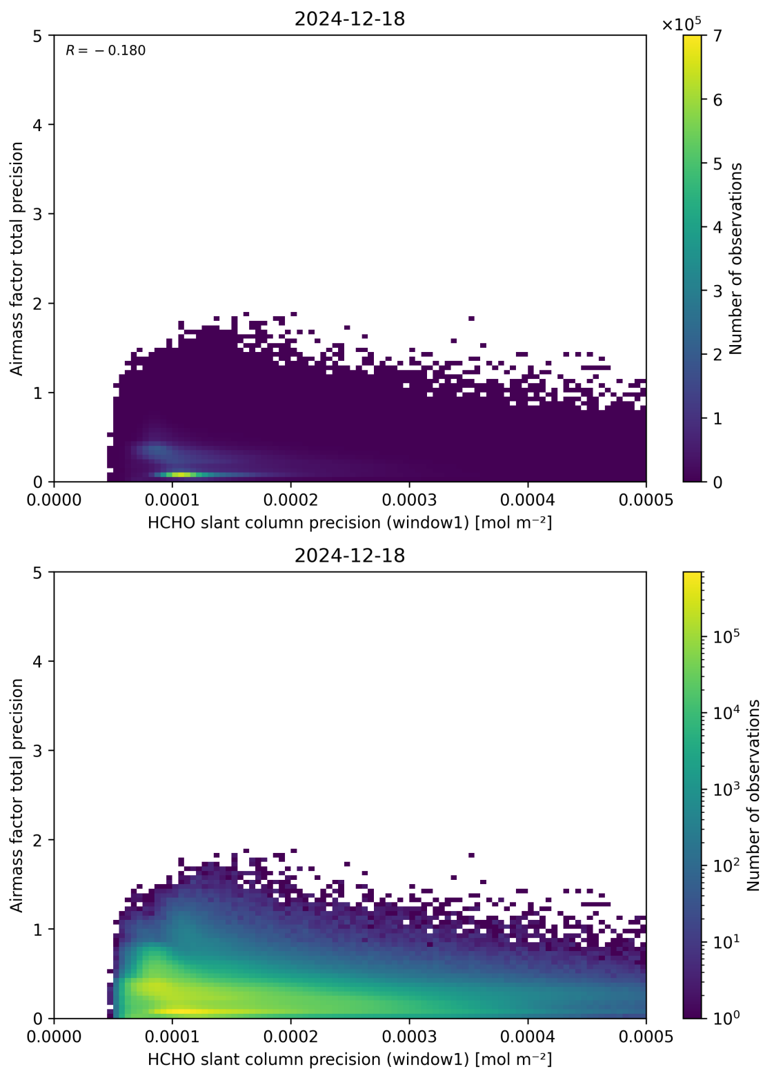
Figure 95: Scatter density plot of “HCHO slant column precision (window1)” against “Airmass factor total precision” for 2024-12-17 to 2024-12-19.
