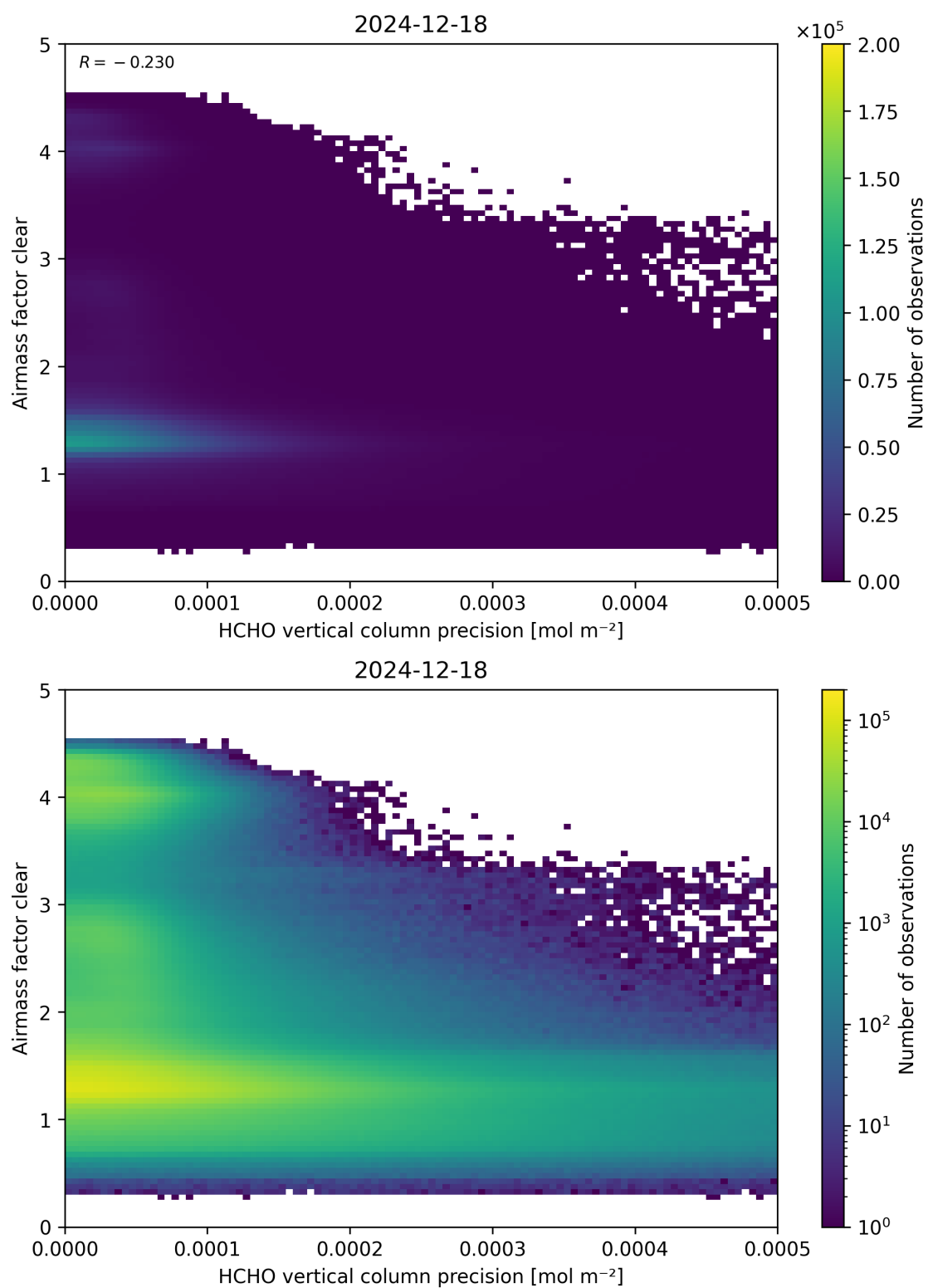
Figure 139: Scatter density plot of “HCHO vertical column precision” against “Airmass factor clear” for 2024-12-17 to 2024-12-19.
