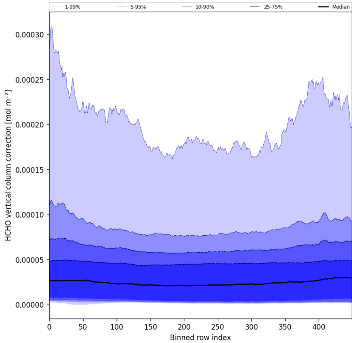
Figure 51: Along track statistics of “HCHO vertical column correction” for 2024-12-17 to 2024-12-19
