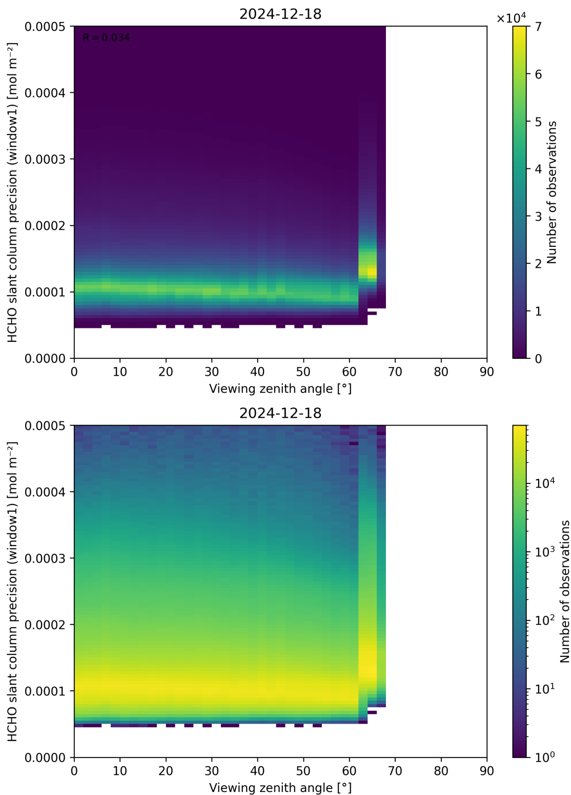
Figure 189: Scatter density plot of “Viewing zenith angle” against “HCHO slant column precision (window1)” for 2024-12-17 to 2024-12-19.
