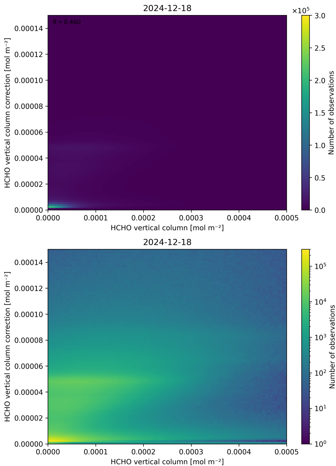
Figure 133: Scatter density plot of “HCHO vertical column” against “HCHO vertical column correction” for 2024-12-17 to 2024-12-19.
