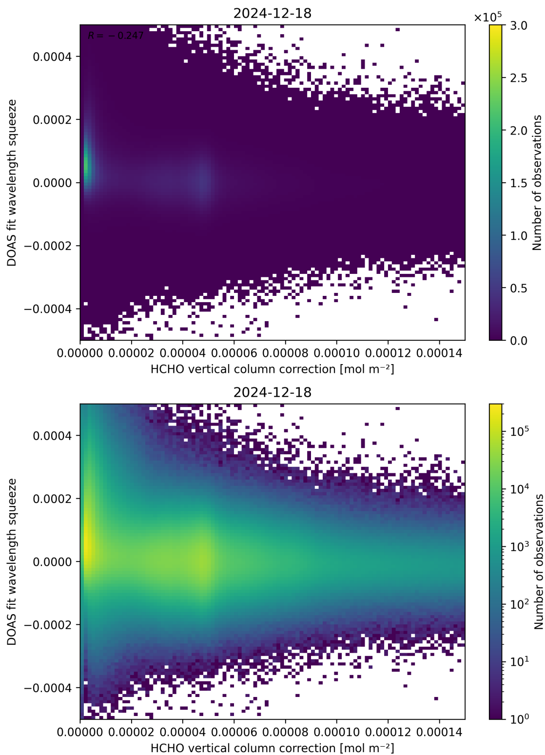
Figure 114: Scatter density plot of “HCHO vertical column correction” against “DOAS fit wavelength squeeze” for 2024-12-17 to 2024-12-19.
