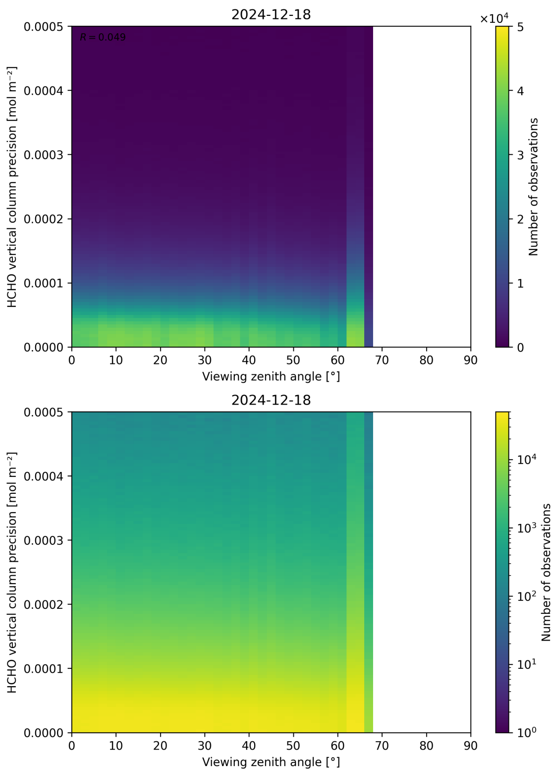
Figure 194: Scatter density plot of “Viewing zenith angle” against “HCHO vertical column precision” for 2024-12-17 to 2024-12-19.
