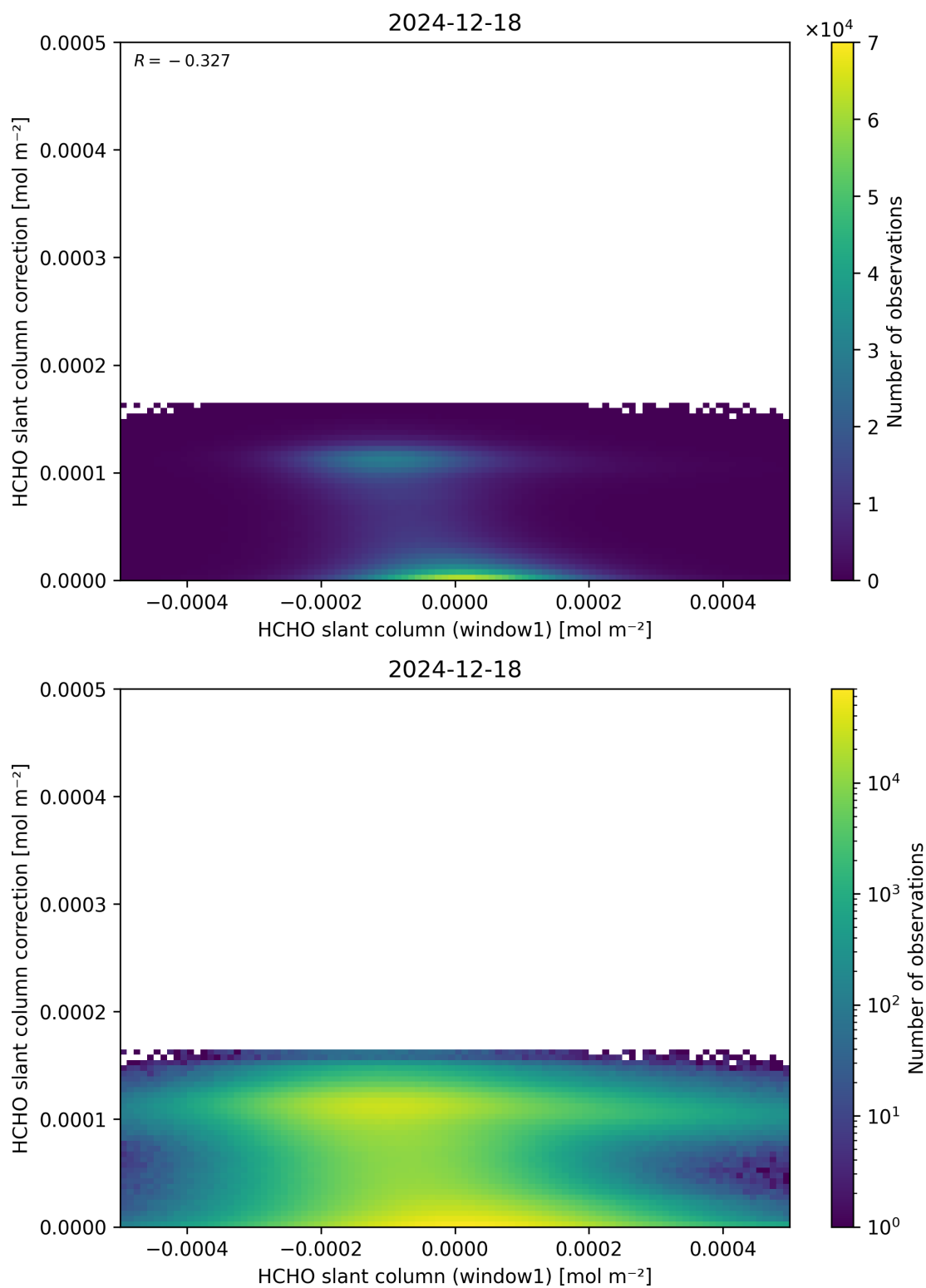
Figure 83: Scatter density plot of “HCHO slant column (window1)” against “HCHO slant column correction” for 2024-12-17 to 2024-12-19.
