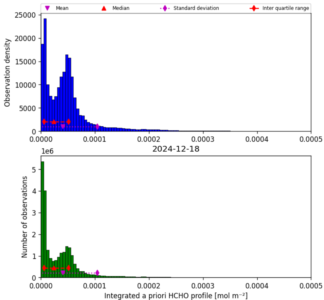
Figure 43: Histogram of “Integrated a priori HCHO profile” for 2024-12-17 to 2024-12-19
