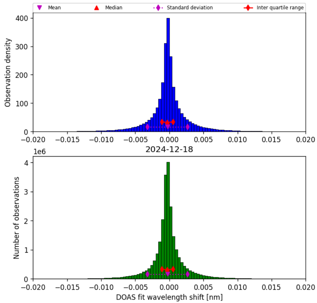
Figure 44: Histogram of “DOAS fit wavelength shift” for 2024-12-17 to 2024-12-19
