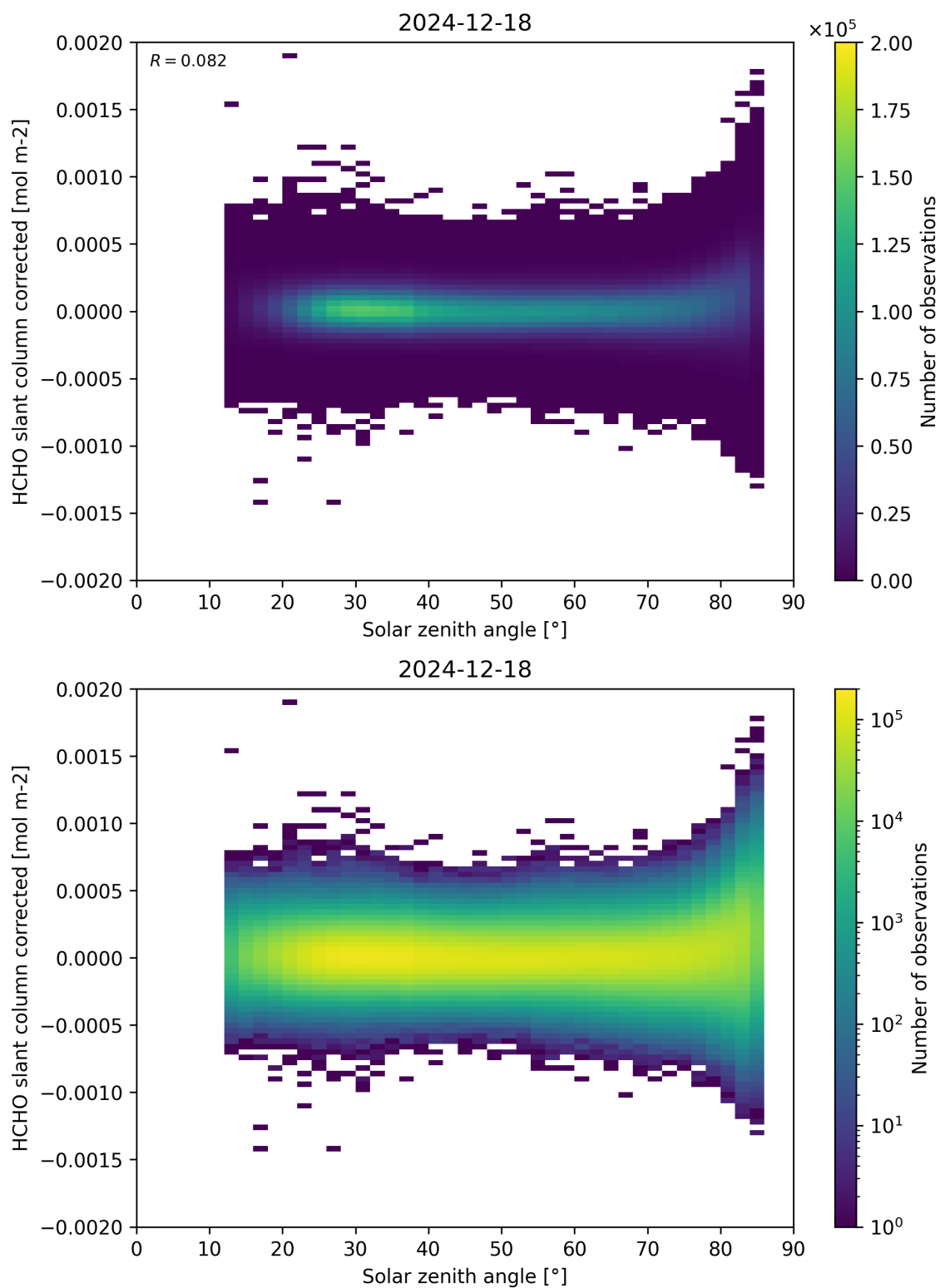
Figure 171: Scatter density plot of “Solar zenith angle” against “HCHO slant column corrected” for 2024-12-17 to 2024-12-19.
