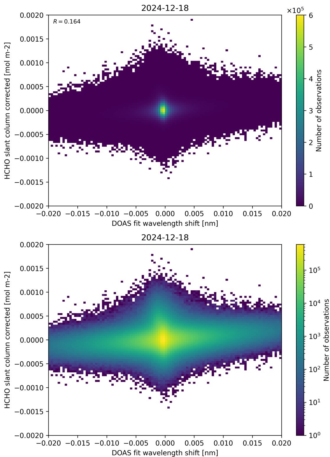
Figure 66: Scatter density plot of “DOAS fit wavelength shift” against “HCHO slant column corrected” for 2024-12-17 to 2024-12-19.
