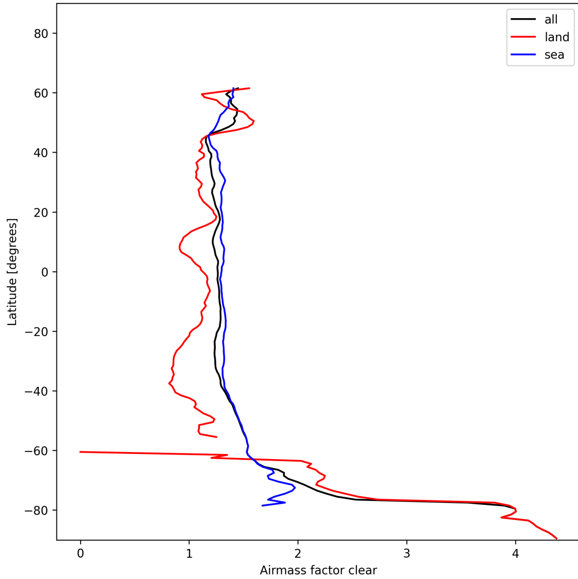
Figure 28: Zonal average of “Airmass factor clear” for 2024-12-17 to 2024-12-19.
