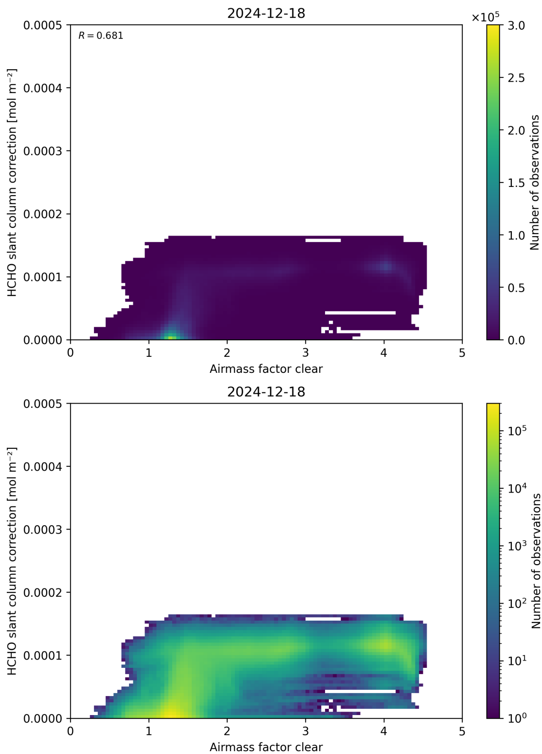
Figure 75: Scatter density plot of “Airmass factor clear” against “HCHO slant column correction” for 2024-12-17 to 2024-12-19.
