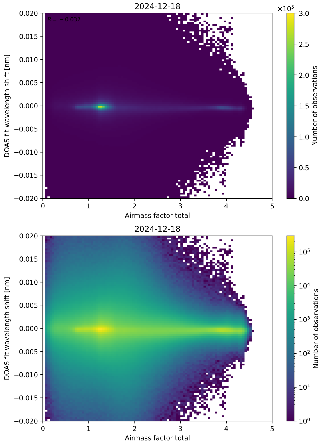
Figure 98: Scatter density plot of “Airmass factor total” against “DOAS fit wavelength shift” for 2024-12-17 to 2024-12-19.
