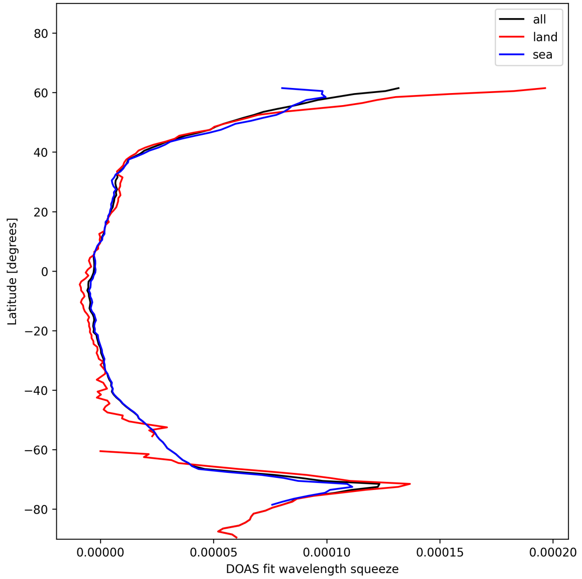
Figure 31: Zonal average of “DOAS fit wavelength squeeze” for 2024-12-17 to 2024-12-19.
