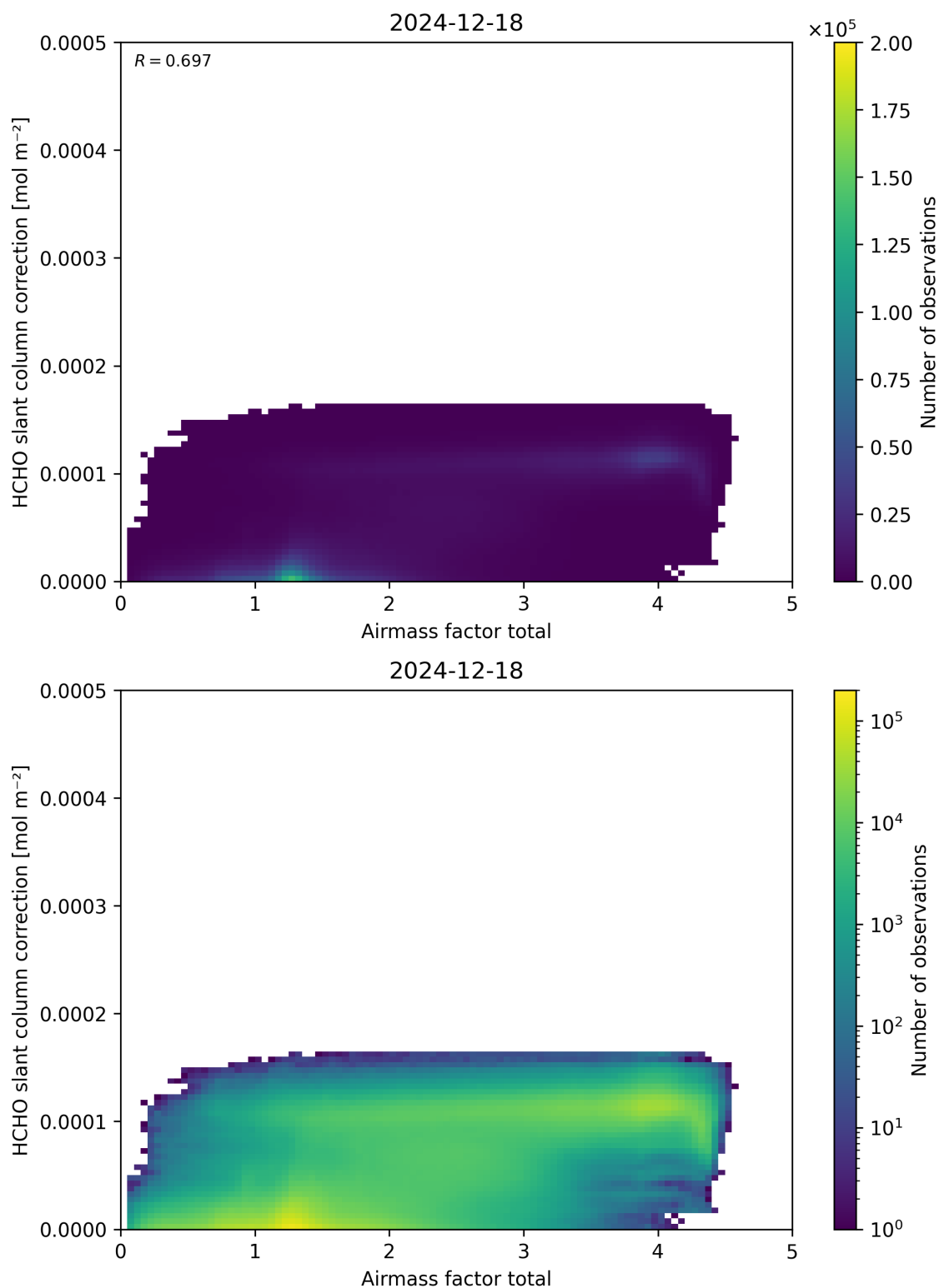
Figure 102: Scatter density plot of “Airmass factor total” against “HCHO slant column correction” for 2024-12-17 to 2024-12-19.
