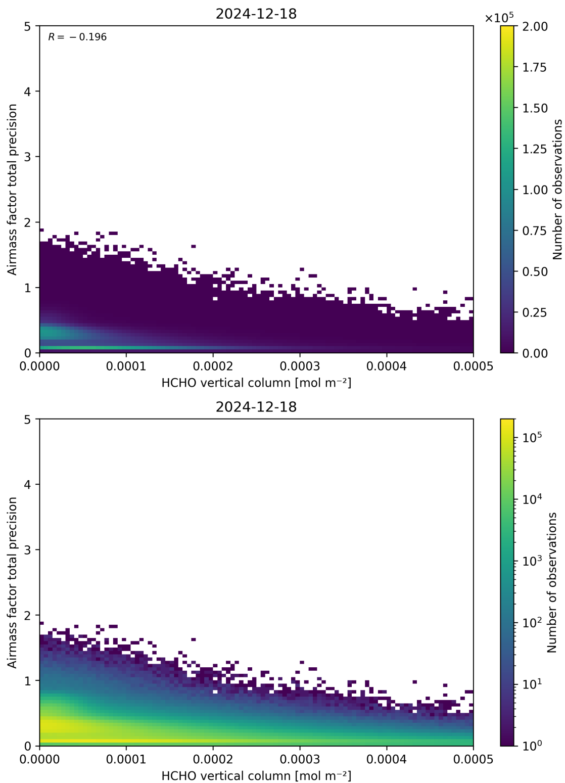
Figure 132: Scatter density plot of “HCHO vertical column” against “Airmass factor total precision” for 2024-12-17 to 2024-12-19.
