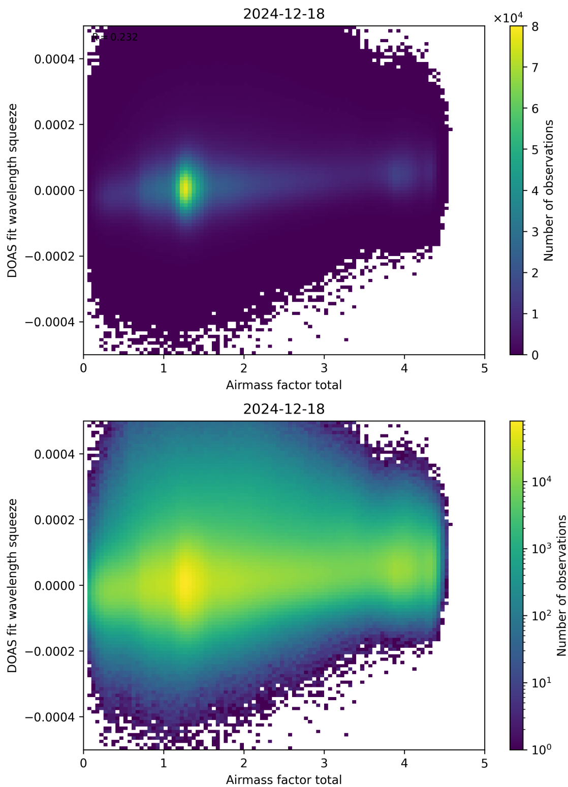
Figure 99: Scatter density plot of “Airmass factor total” against “DOAS fit wavelength squeeze” for 2024-12-17 to 2024-12-19.
