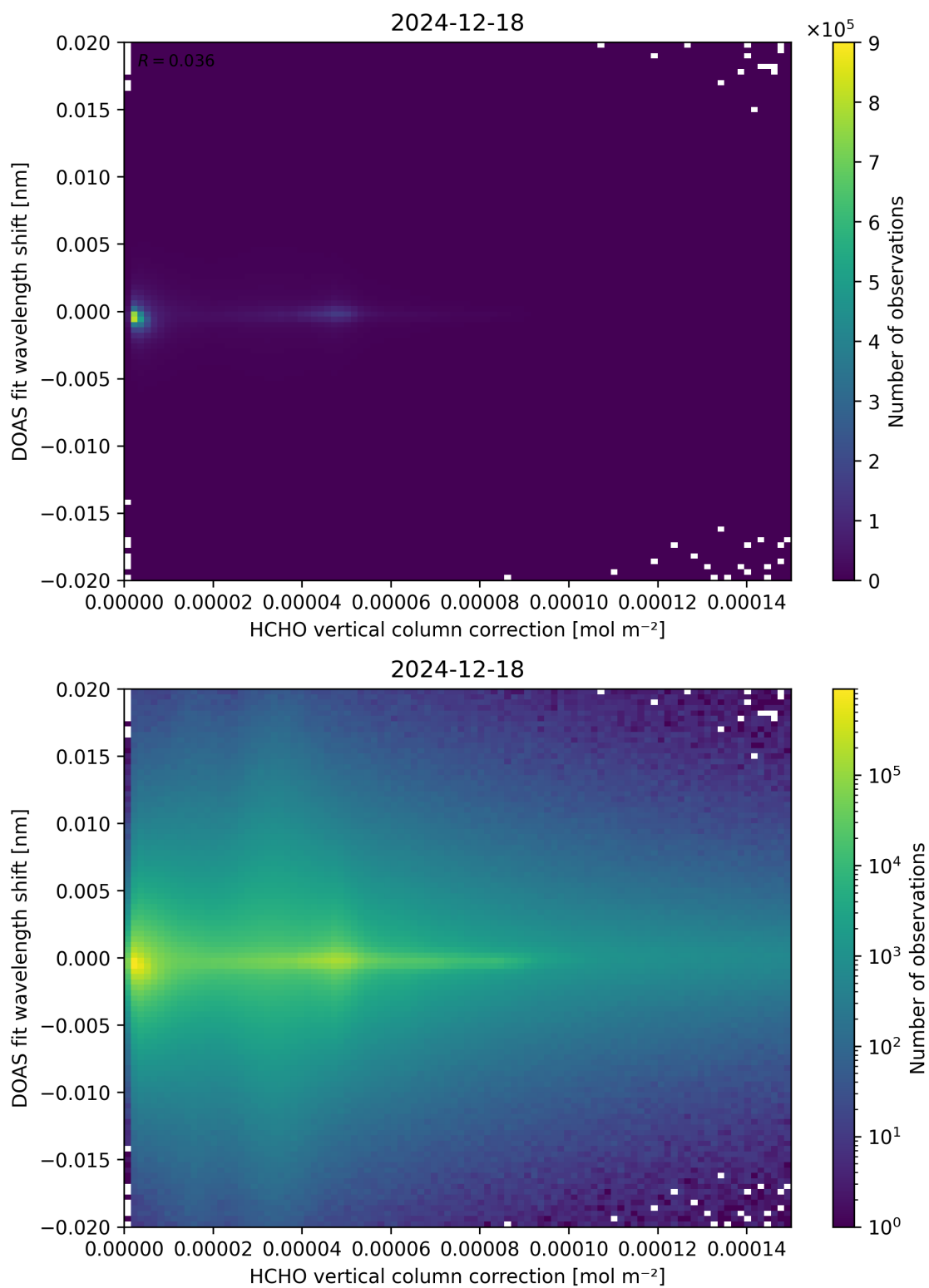
Figure 113: Scatter density plot of “HCHO vertical column correction” against “DOAS fit wavelength shift” for 2024-12-17 to 2024-12-19.
