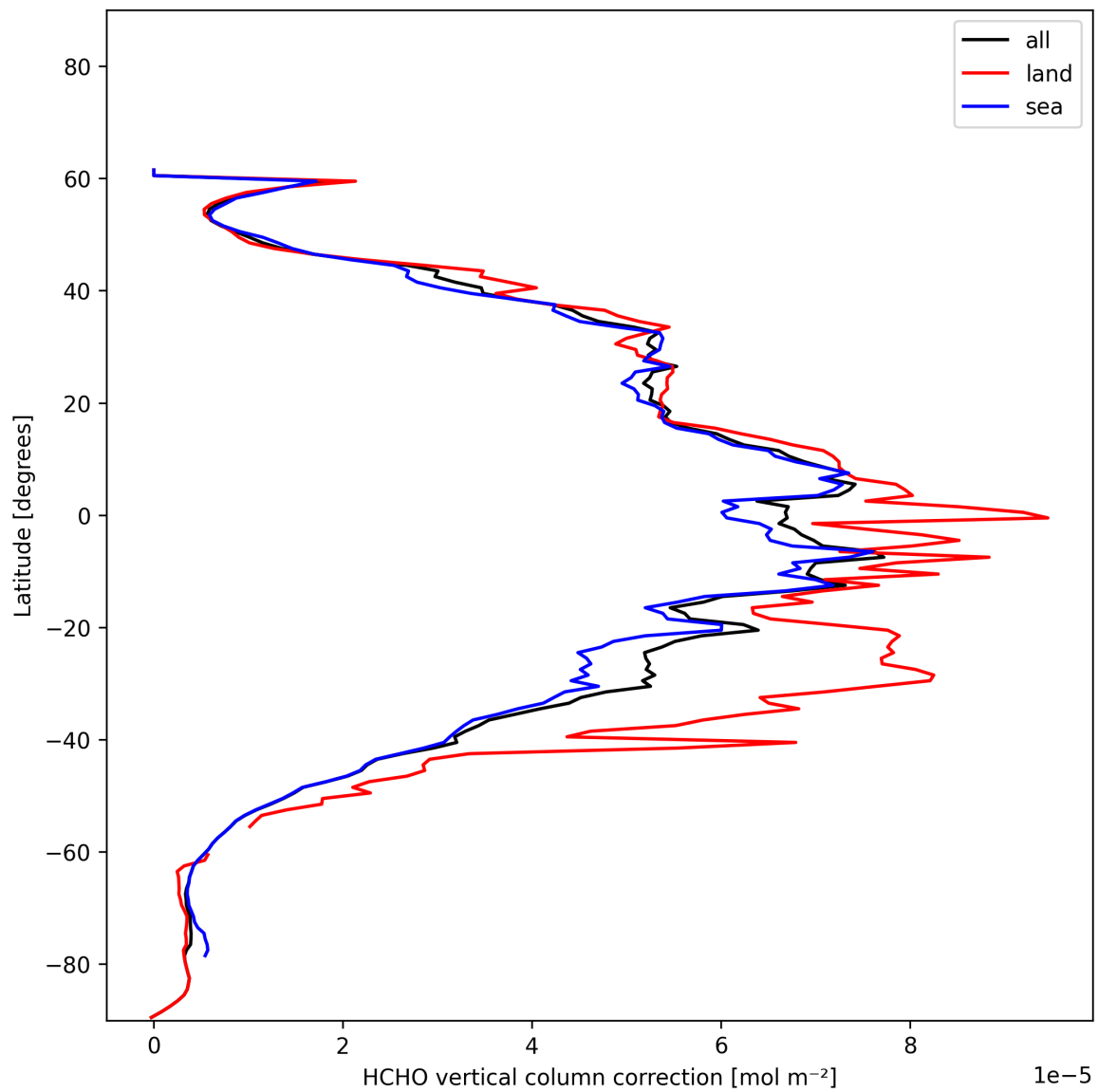
Figure 23: Zonal average of “HCHO vertical column correction” for 2024-12-17 to 2024-12-19.
