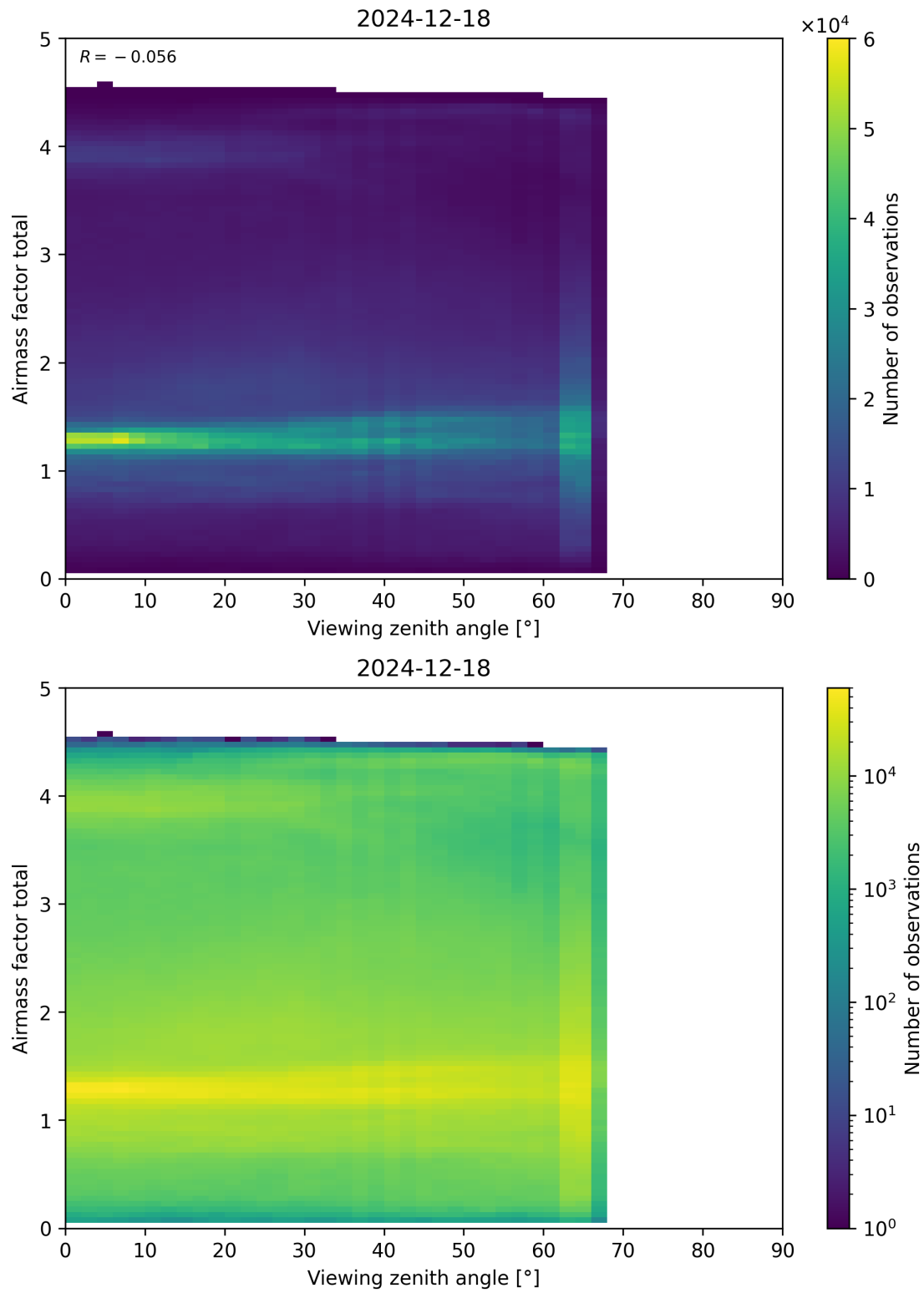
Figure 190: Scatter density plot of “Viewing zenith angle” against “Airmass factor total” for 2024-12-17 to 2024-12-19.
