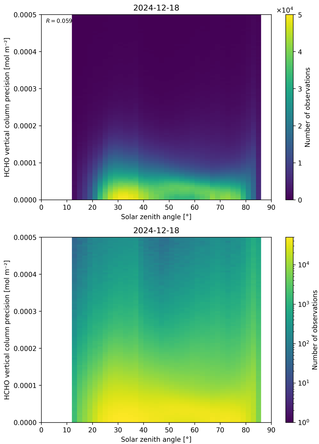
Figure 179: Scatter density plot of “Solar zenith angle” against “HCHO vertical column precision” for 2024-12-17 to 2024-12-19.
