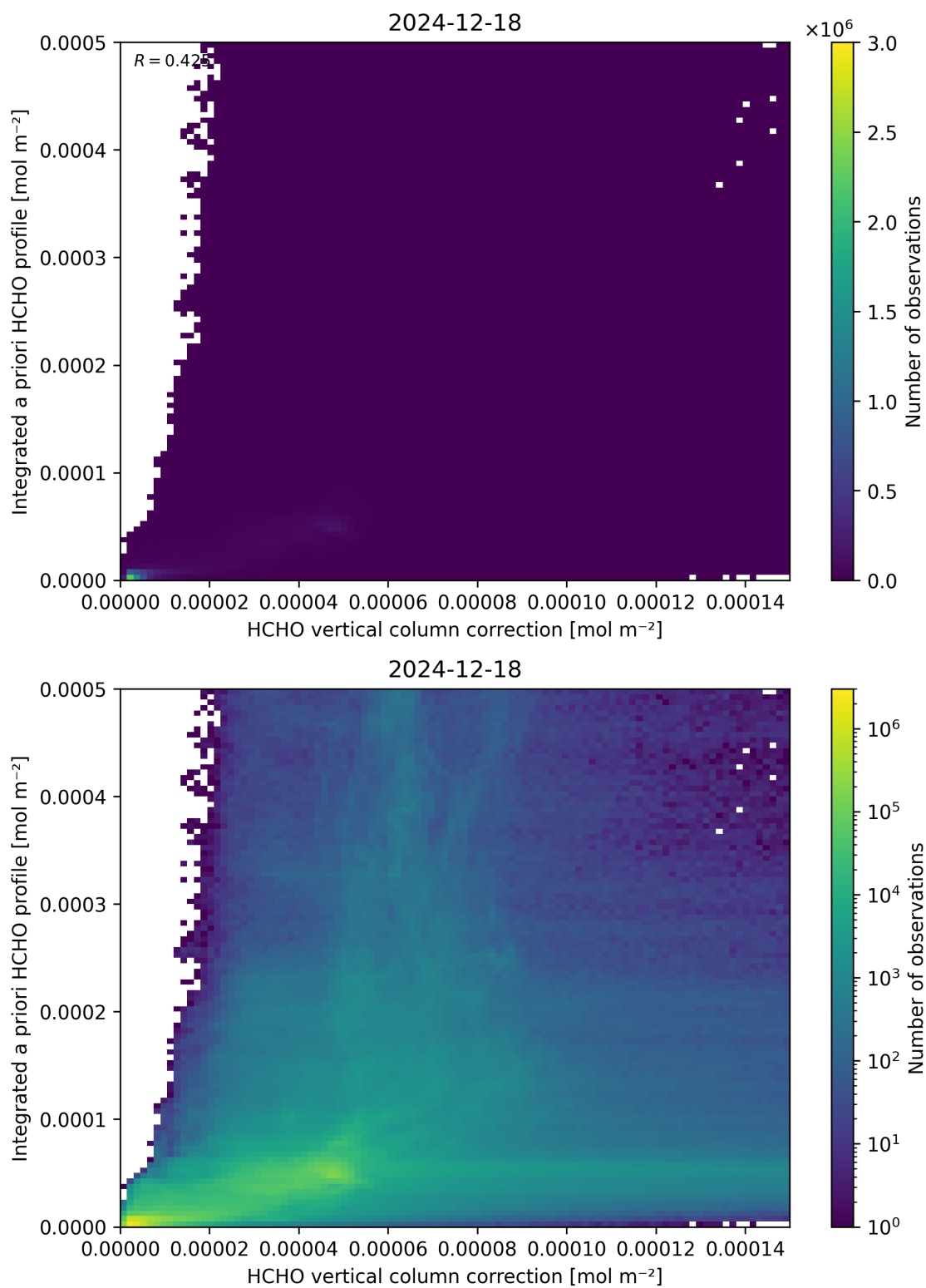
Figure 122: Scatter density plot of “HCHO vertical column correction” against “Integrated a priori HCHO profile” for 2024-12-17 to 2024-12-19.
