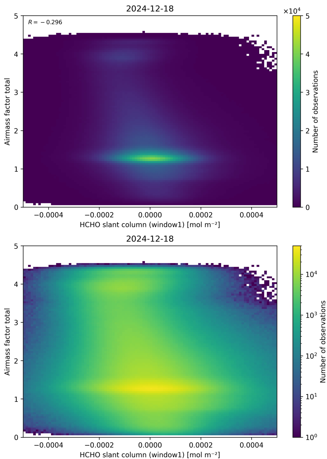
Figure 85: Scatter density plot of “HCHO slant column (window1)” against “Airmass factor total” for 2024-12-17 to 2024-12-19.
