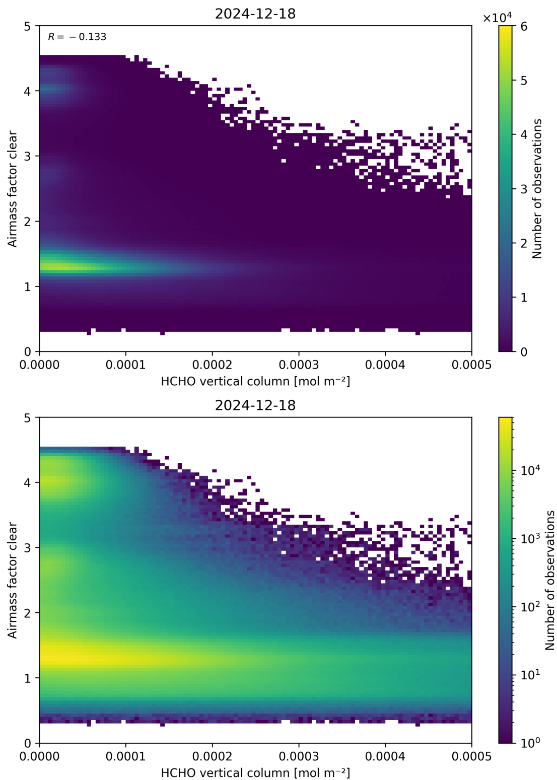
Figure 126: Scatter density plot of “HCHO vertical column” against “Airmass factor clear” for 2024-12-17 to 2024-12-19.
