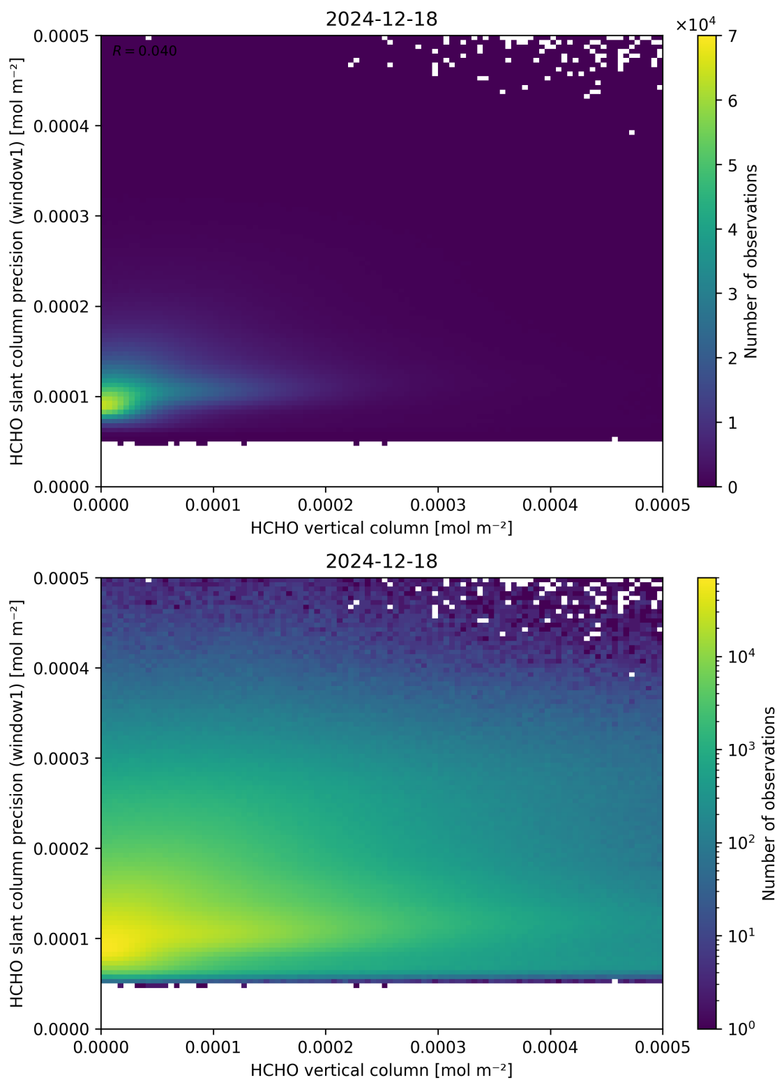
Figure 130: Scatter density plot of “HCHO vertical column” against “HCHO slant column precision (window1)” for 2024-12-17 to 2024-12-19.
