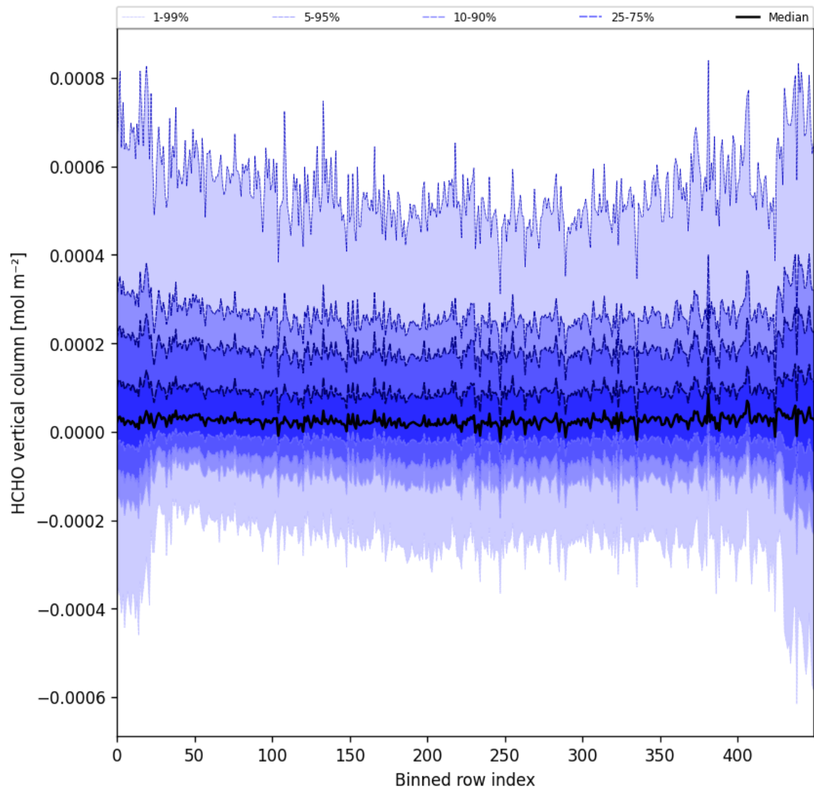
Figure 49: Along track statistics of “HCHO vertical column” for 2024-12-17 to 2024-12-19
