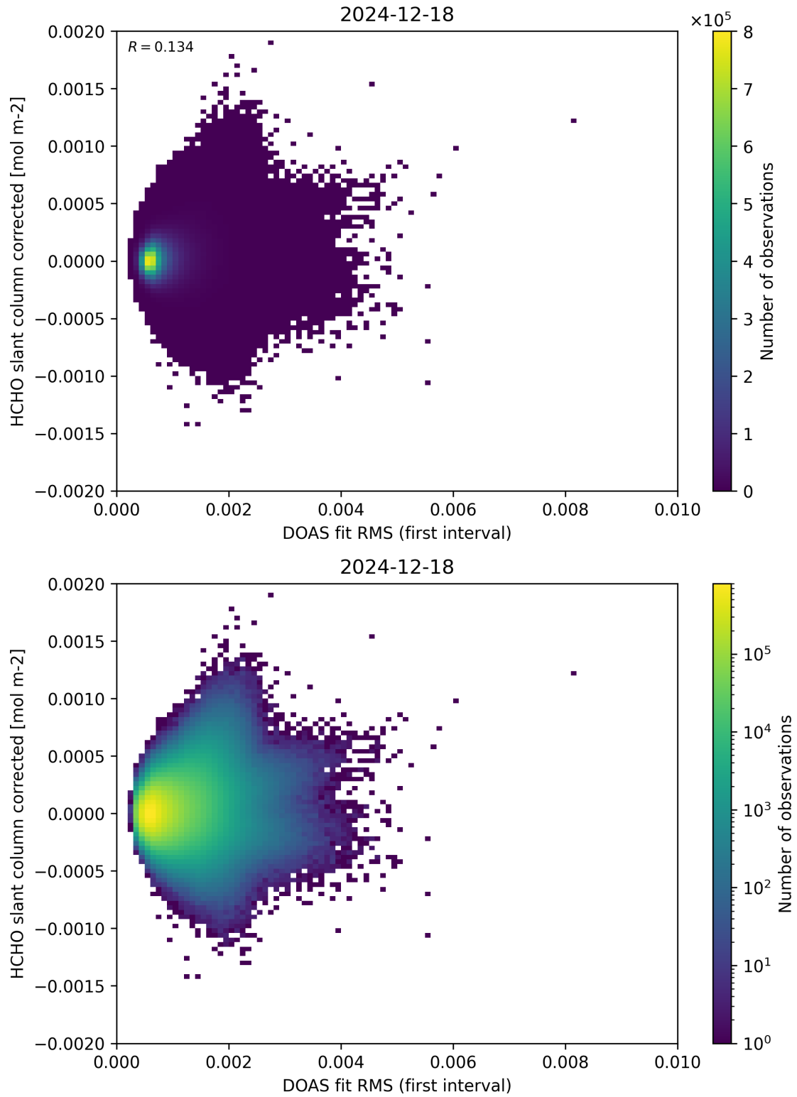
Figure 62: Scatter density plot of “DOAS fit RMS (first interval)” against “HCHO slant column corrected” for 2024-12-17 to 2024-12-19.
