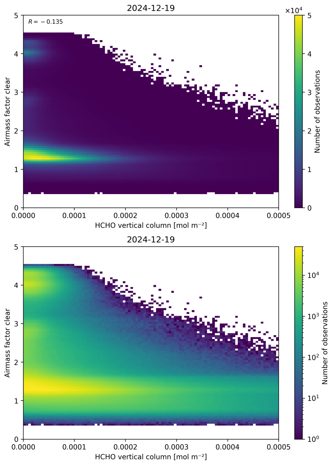
Figure 126: Scatter density plot of “HCHO vertical column” against “Airmass factor clear” for 2024-12-18 to 2024-12-20.
