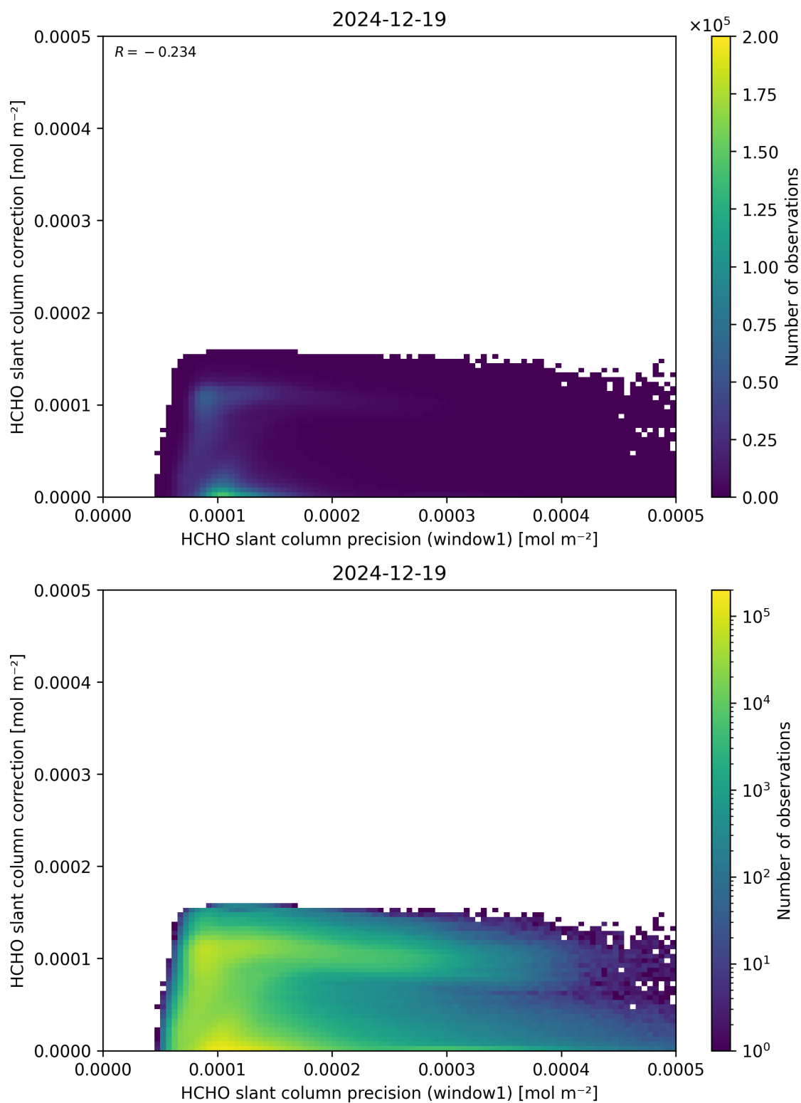
Figure 93: Scatter density plot of “HCHO slant column precision (window1)” against “HCHO slant column correction” for 2024-12-18 to 2024-12-20.
