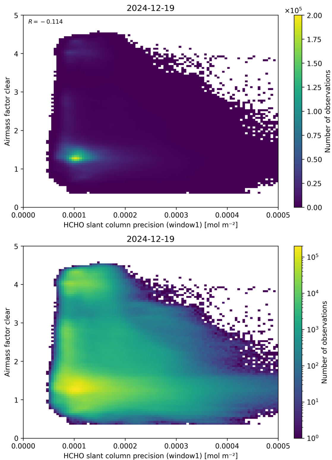
Figure 91: Scatter density plot of “HCHO slant column precision (window1)” against “Airmass factor clear” for 2024-12-18 to 2024-12-20.
