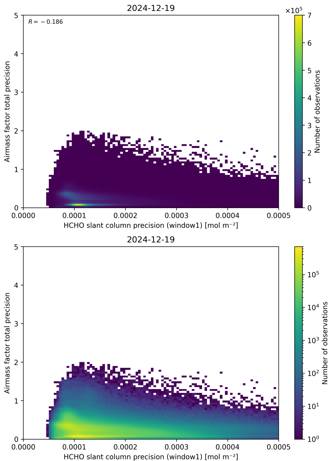
Figure 95: Scatter density plot of “HCHO slant column precision (window1)” against “Airmass factor total precision” for 2024-12-18 to 2024-12-20.
