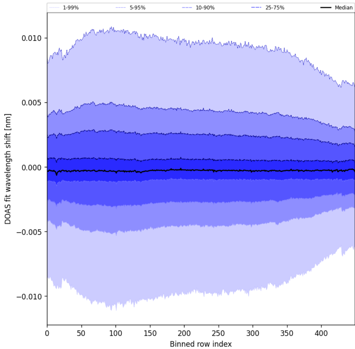
Figure 58: Along track statistics of “DOAS fit wavelength shift” for 2024-12-18 to 2024-12-20
