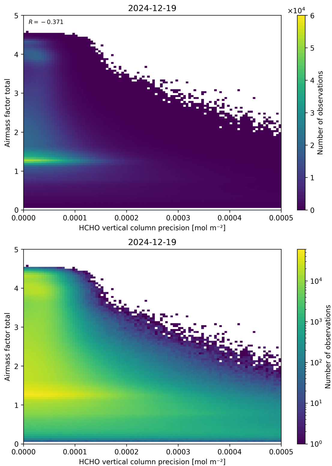
Figure 144: Scatter density plot of “HCHO vertical column precision” against “Airmass factor total” for 2024-12-18 to 2024-12-20.
