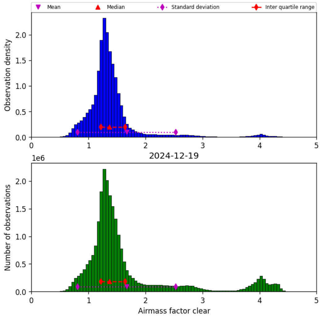
Figure 42: Histogram of “Airmass factor clear” for 2024-12-18 to 2024-12-20
