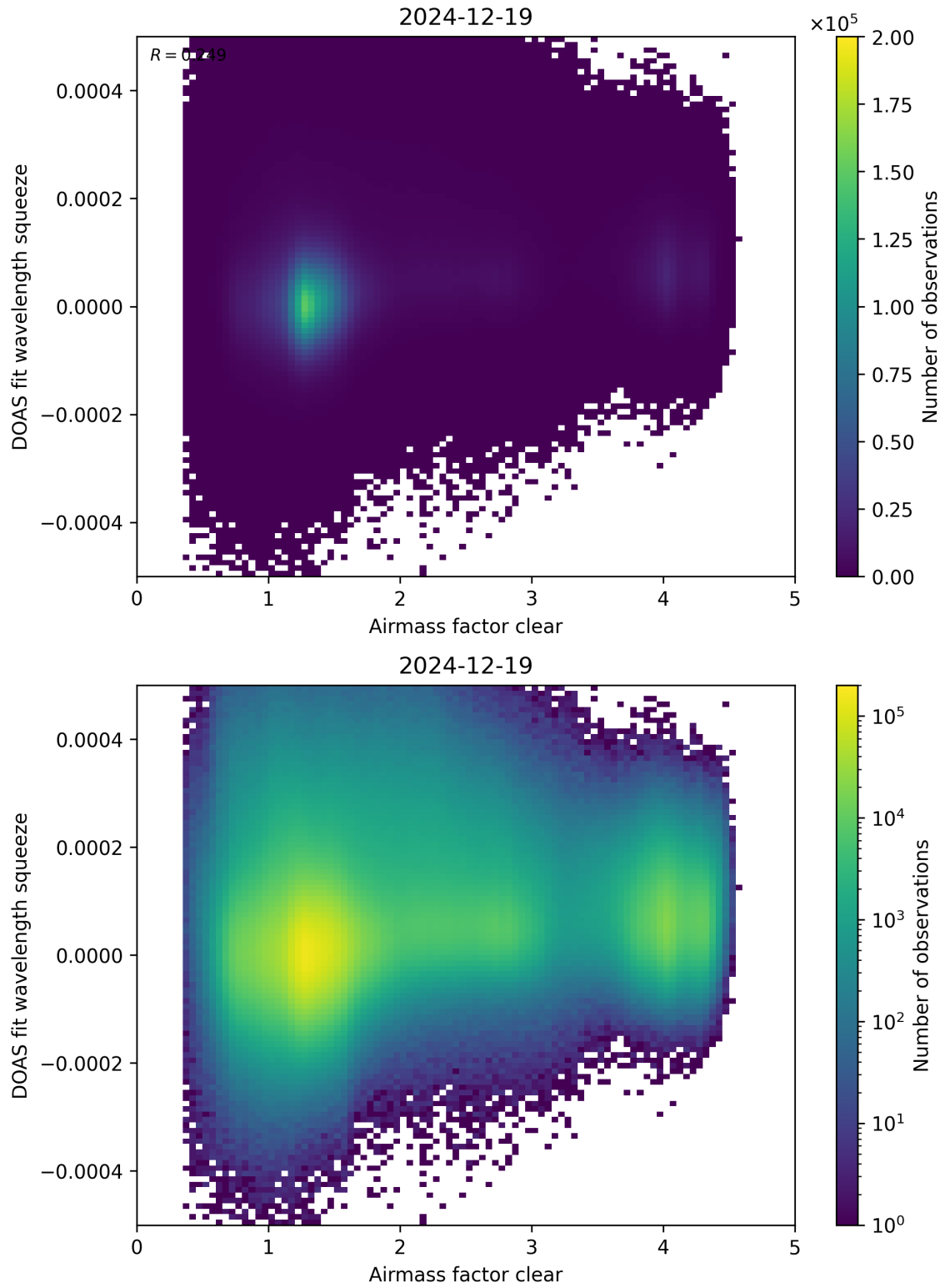
Figure 73: Scatter density plot of “Airmass factor clear” against “DOAS fit wavelength squeeze” for 2024-12-18 to 2024-12-20.
