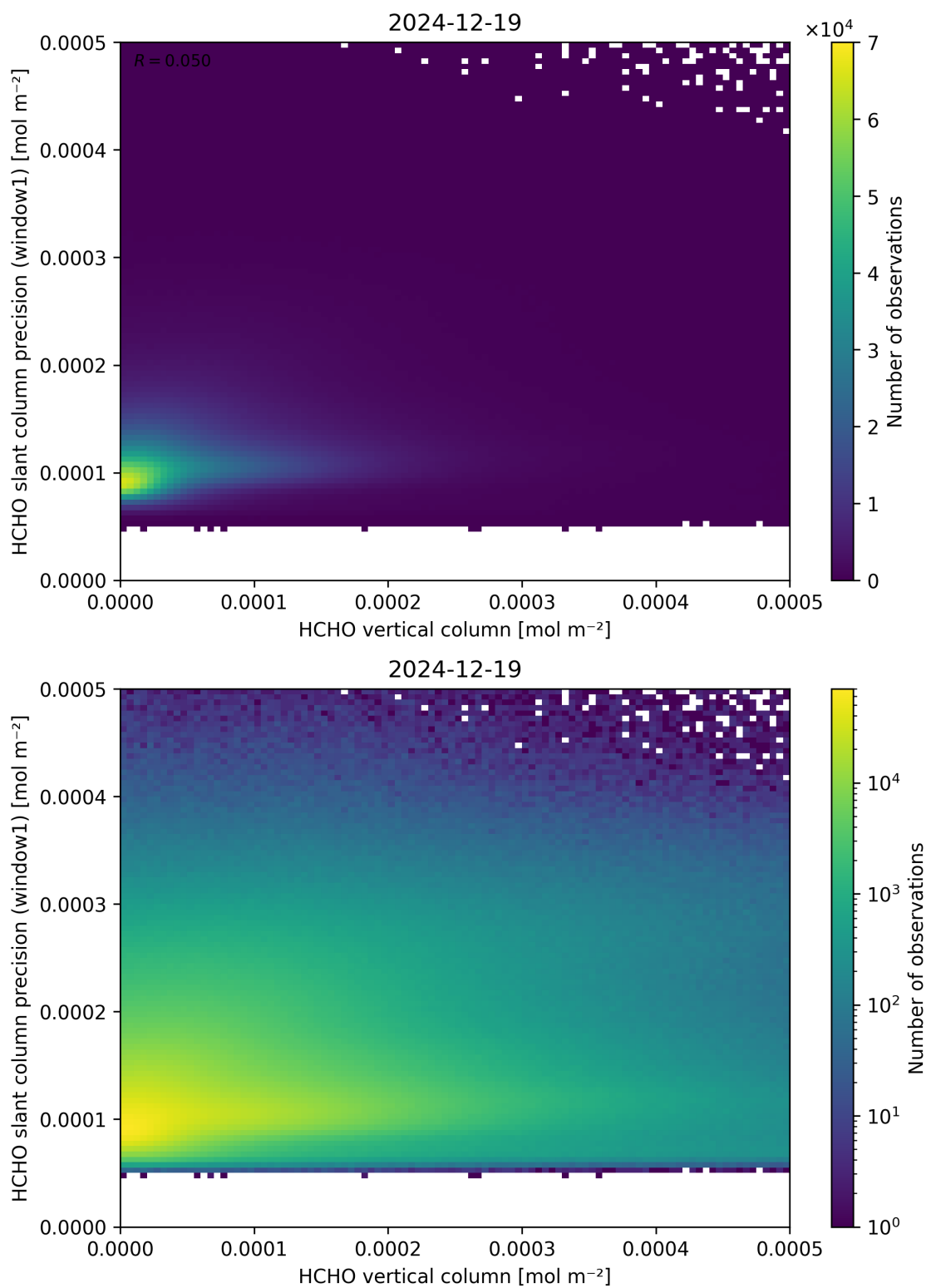
Figure 130: Scatter density plot of “HCHO vertical column” against “HCHO slant column precision (window1)” for 2024-12-18 to 2024-12-20.
