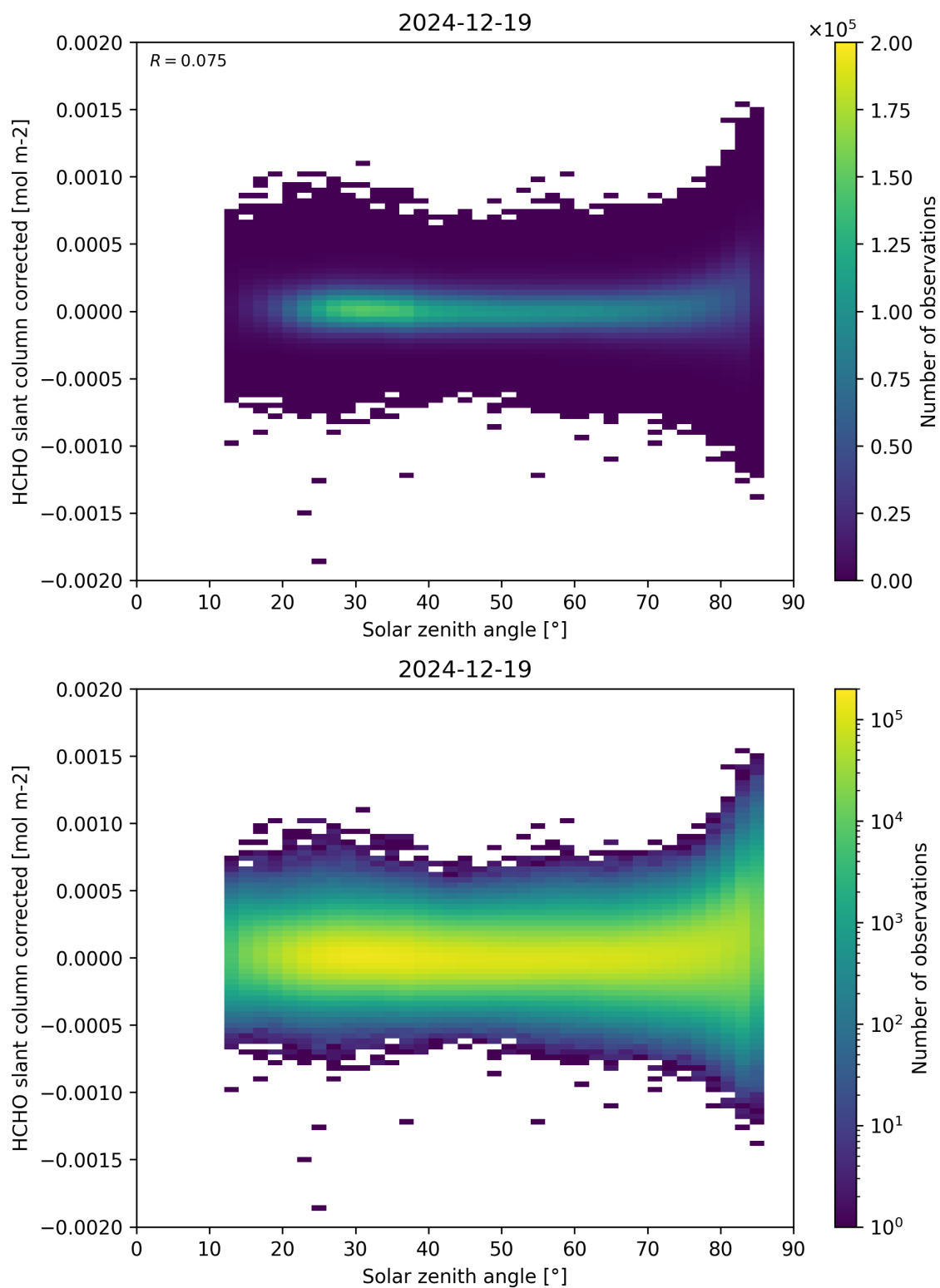
Figure 171: Scatter density plot of “Solar zenith angle” against “HCHO slant column corrected” for 2024-12-18 to 2024-12-20.
