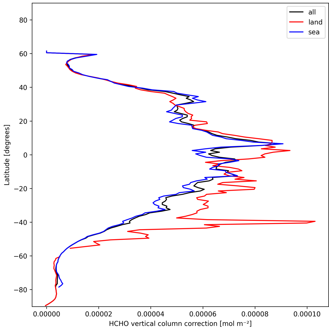
Figure 23: Zonal average of “HCHO vertical column correction” for 2024-12-18 to 2024-12-20.
