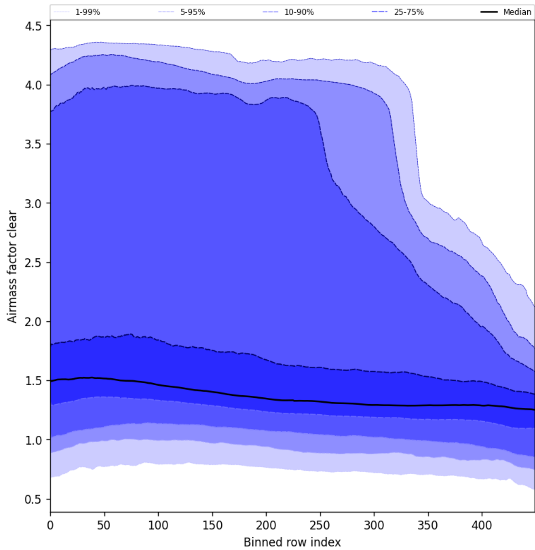
Figure 56: Along track statistics of “Air mass factor clear” for 2024-12-18 to 2024-12-20
