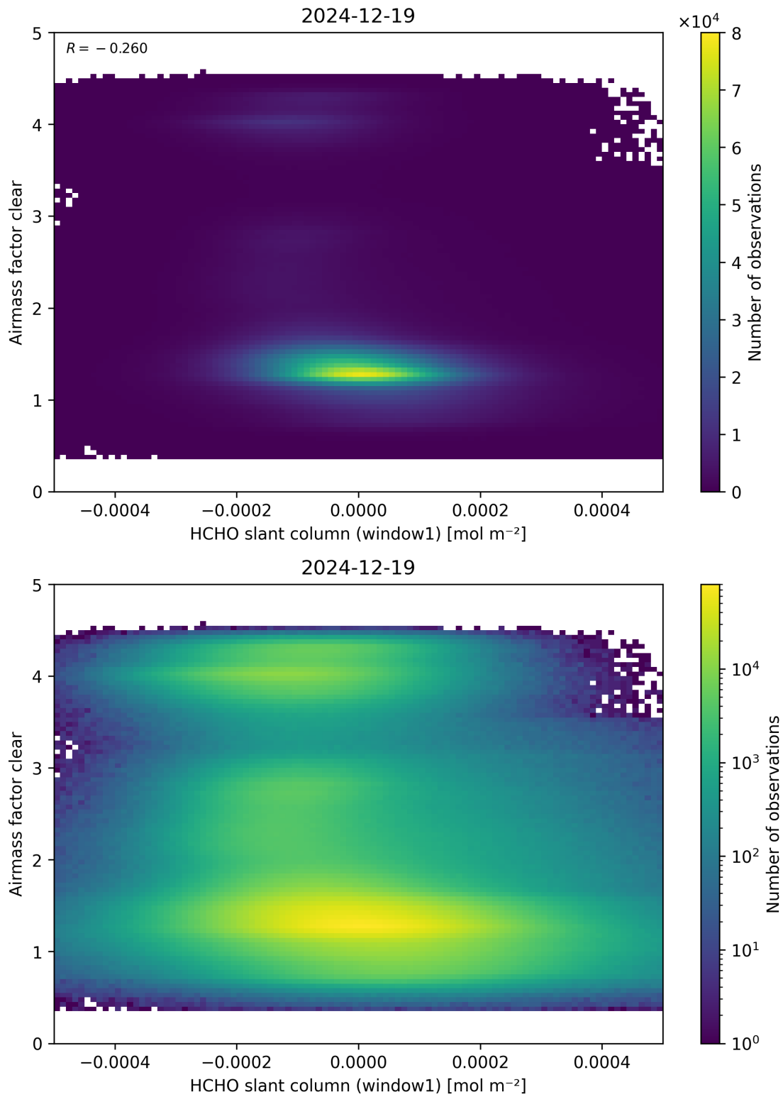
Figure 81: Scatter density plot of “HCHO slant column (window1)” against “Airmass factor clear” for 2024-12-18 to 2024-12-20.
