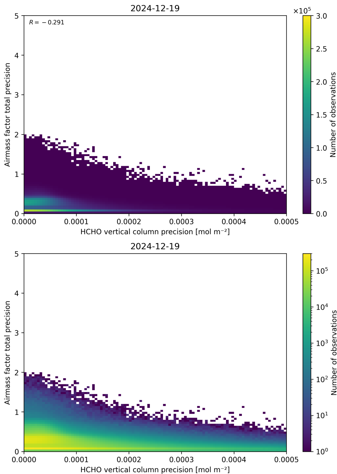
Figure 145: Scatter density plot of “HCHO vertical column precision” against “Airmass factor total precision” for 2024-12-18 to 2024-12-20.
