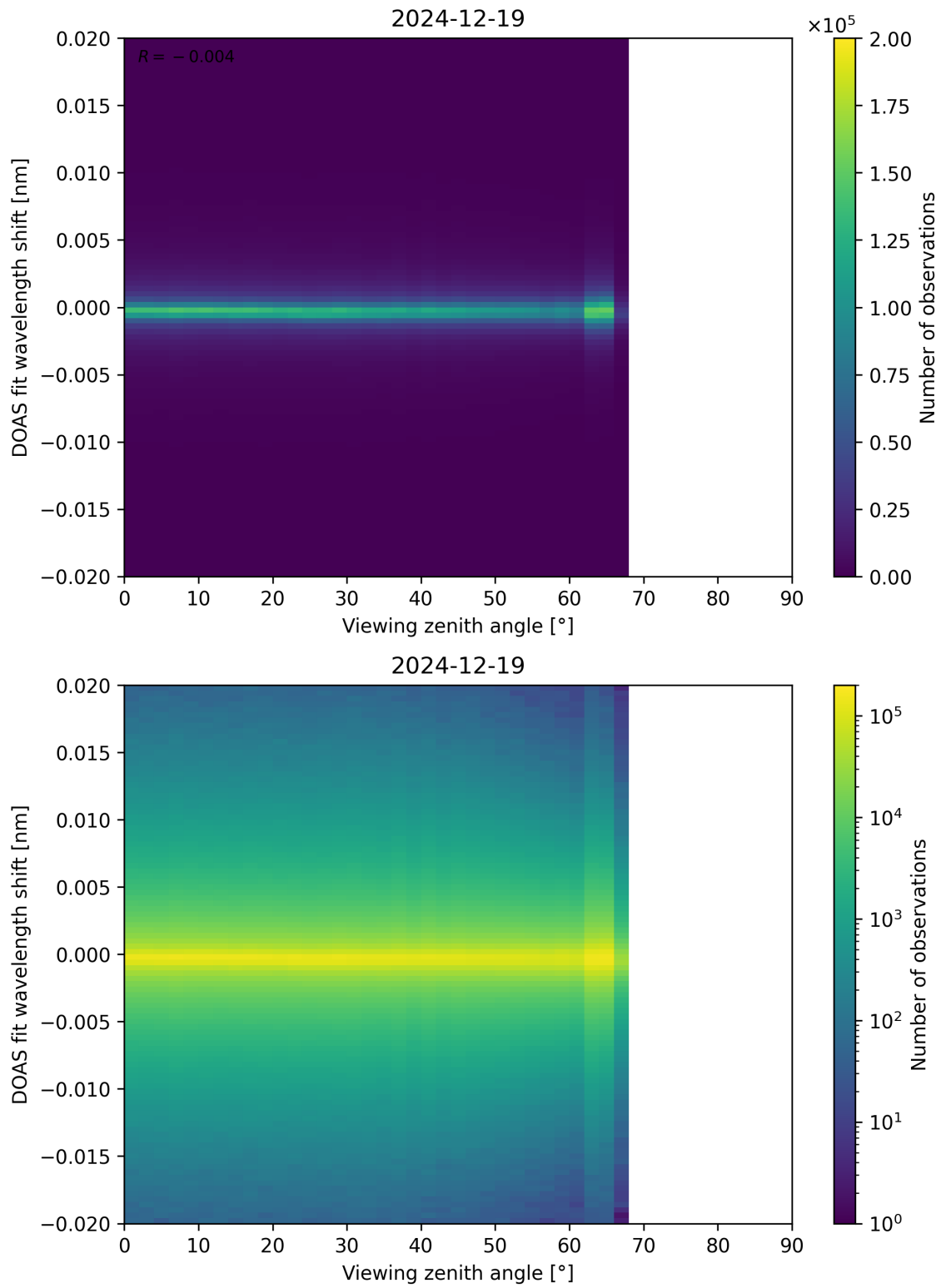
Figure 183: Scatter density plot of “Viewing zenith angle” against “DOAS fit wavelength shift” for 2024-12-18 to 2024-12-20.
