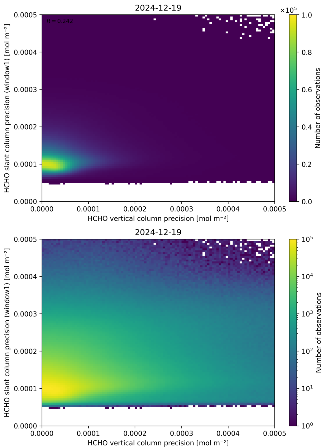
Figure 143: Scatter density plot of “HCHO vertical column precision” against “HCHO slant column precision (window1)” for 2024-12-18 to 2024-12-20.
