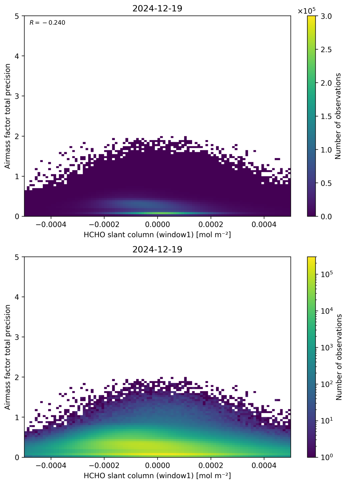
Figure 86: Scatter density plot of “HCHO slant column (window1)” against “Airmass factor total precision” for 2024-12-18 to 2024-12-20.
