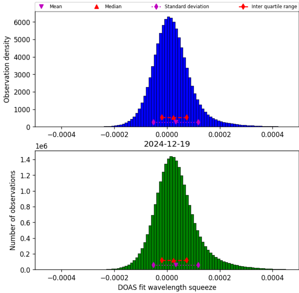
Figure 45: Histogram of “DOAS fit wavelength squeeze” for 2024-12-18 to 2024-12-20
