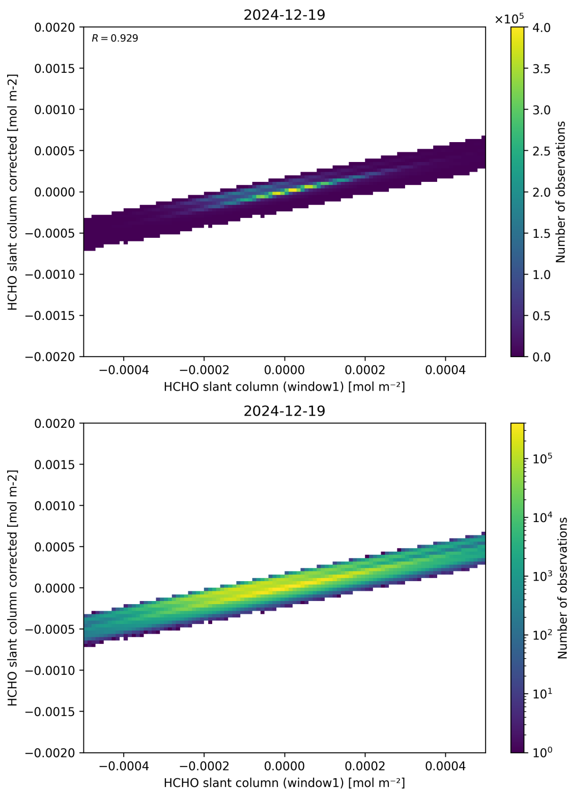
Figure 82: Scatter density plot of “HCHO slant column (window1)” against “HCHO slant column corrected” for 2024-12-18 to 2024-12-20.
