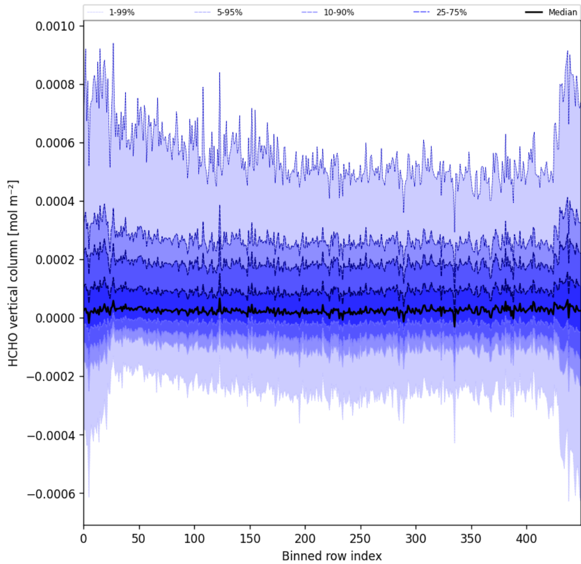
Figure 49: Along track statistics of “HCHO vertical column” for 2024-12-18 to 2024-12-20
