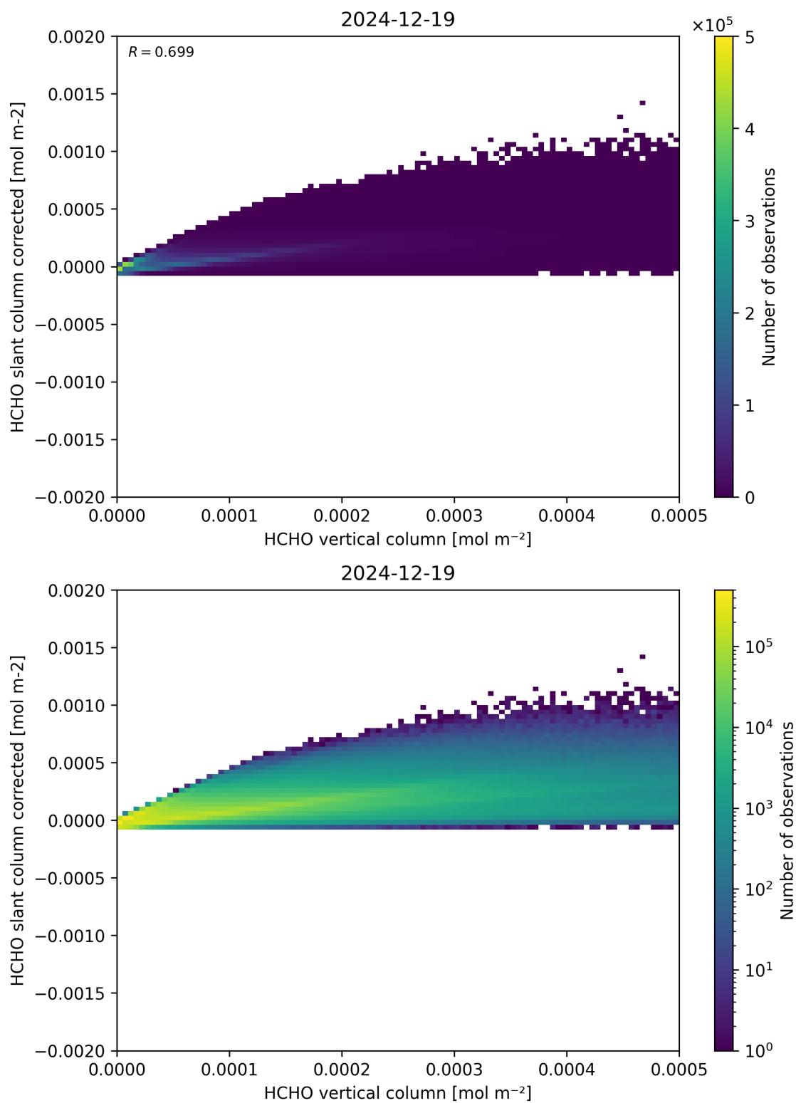
Figure 127: Scatter density plot of “HCHO vertical column” against “HCHO slant column corrected” for 2024-12-18 to 2024-12-20.
