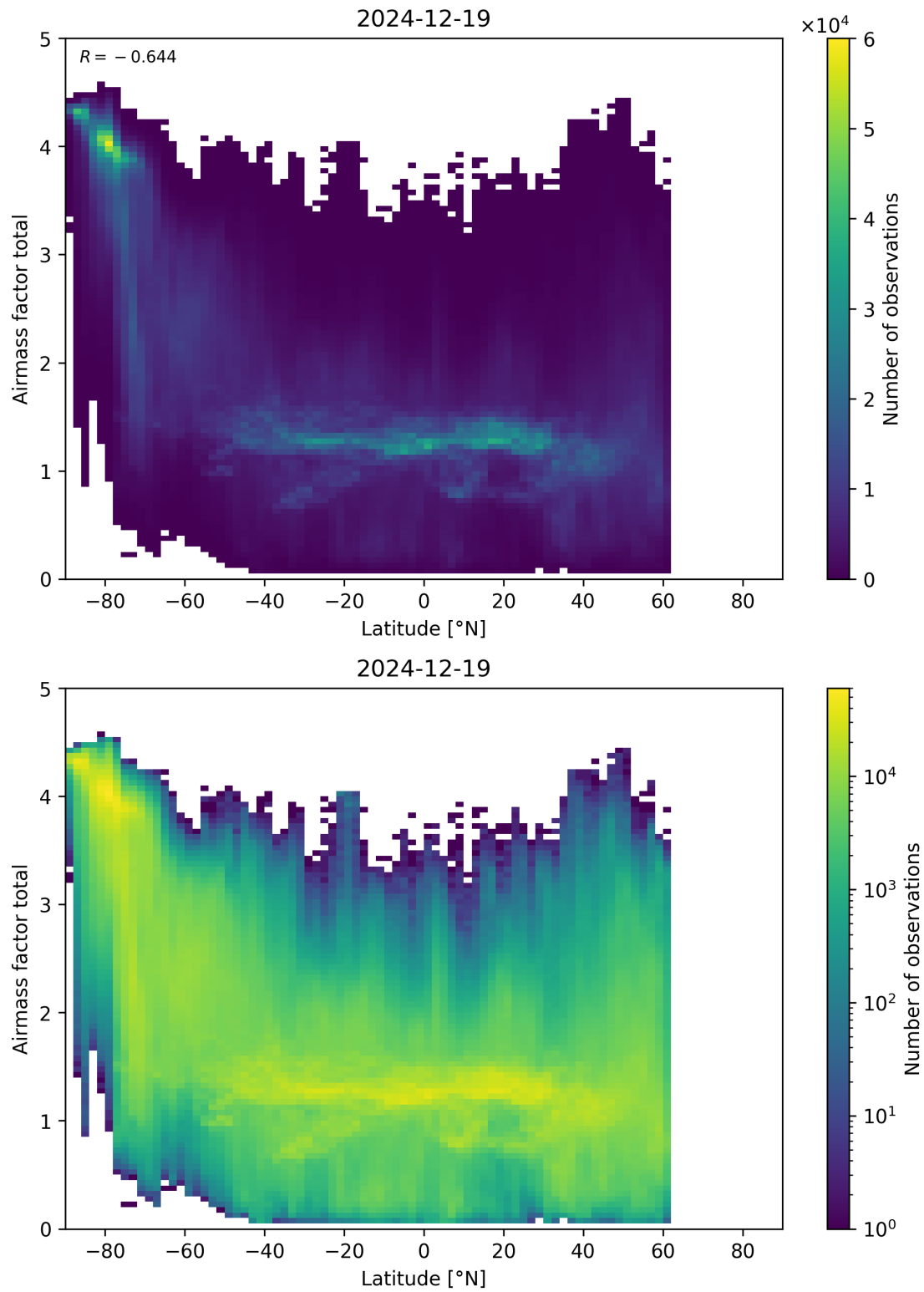
Figure 161: Scatter density plot of “Latitude” against “Airmass factor total” for 2024-12-18 to 2024-12-20.
