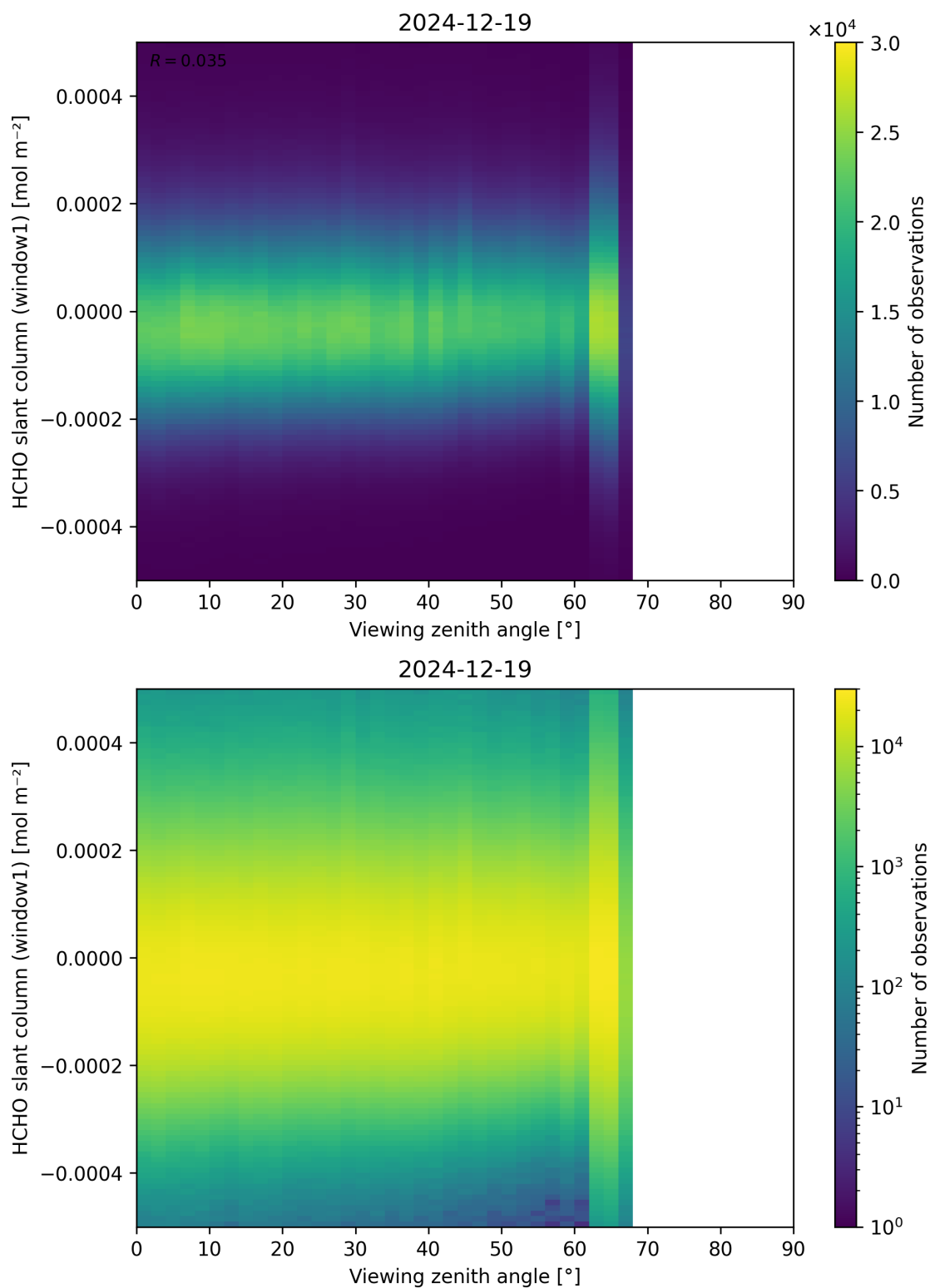
Figure 188: Scatter density plot of “Viewing zenith angle” against “HCHO slant column (window1)” for 2024-12-18 to 2024-12-20.
