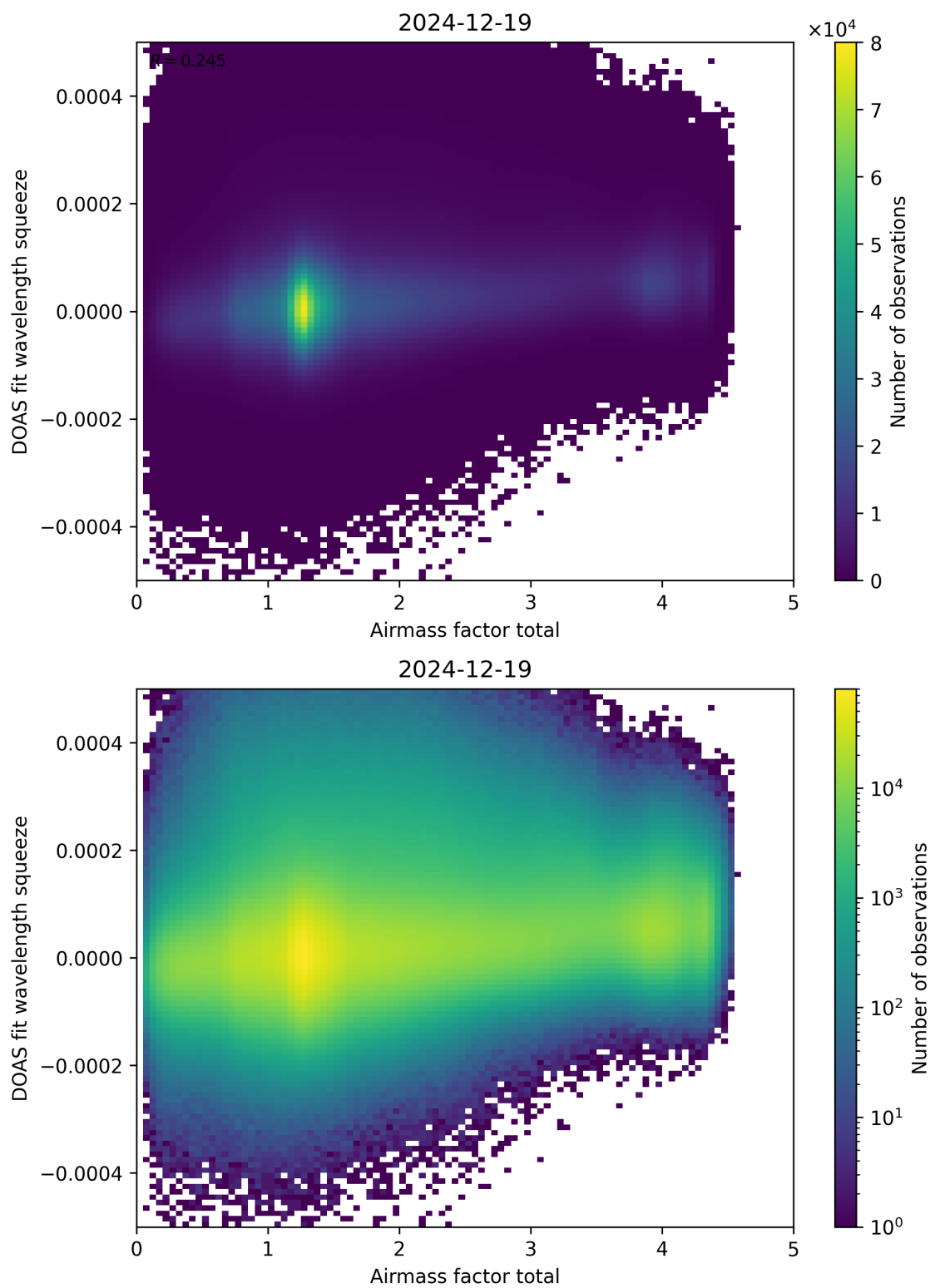
Figure 99: Scatter density plot of “Airmass factor total” against “DOAS fit wavelength squeeze” for 2024-12-18 to 2024-12-20.
