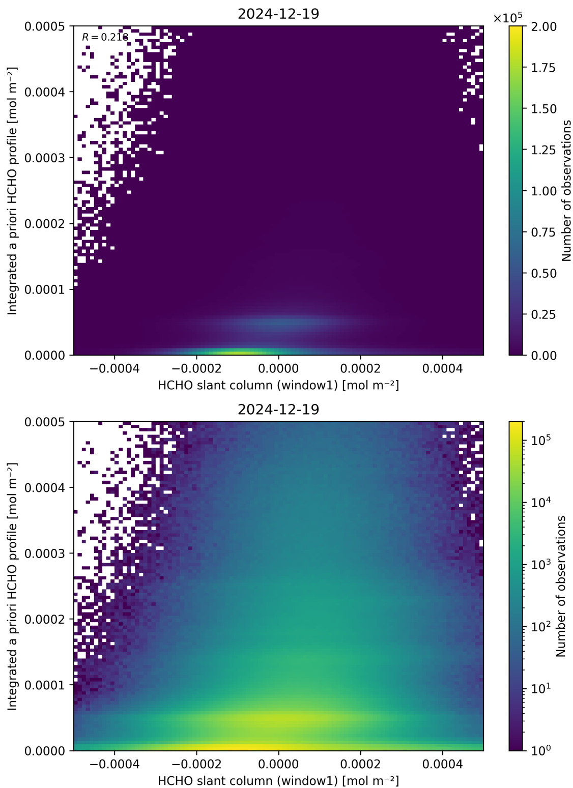
Figure 87: Scatter density plot of “HCHO slant column (window1)” against “Integrated a priori HCHO profile” for 2024-12-18 to 2024-12-20.
