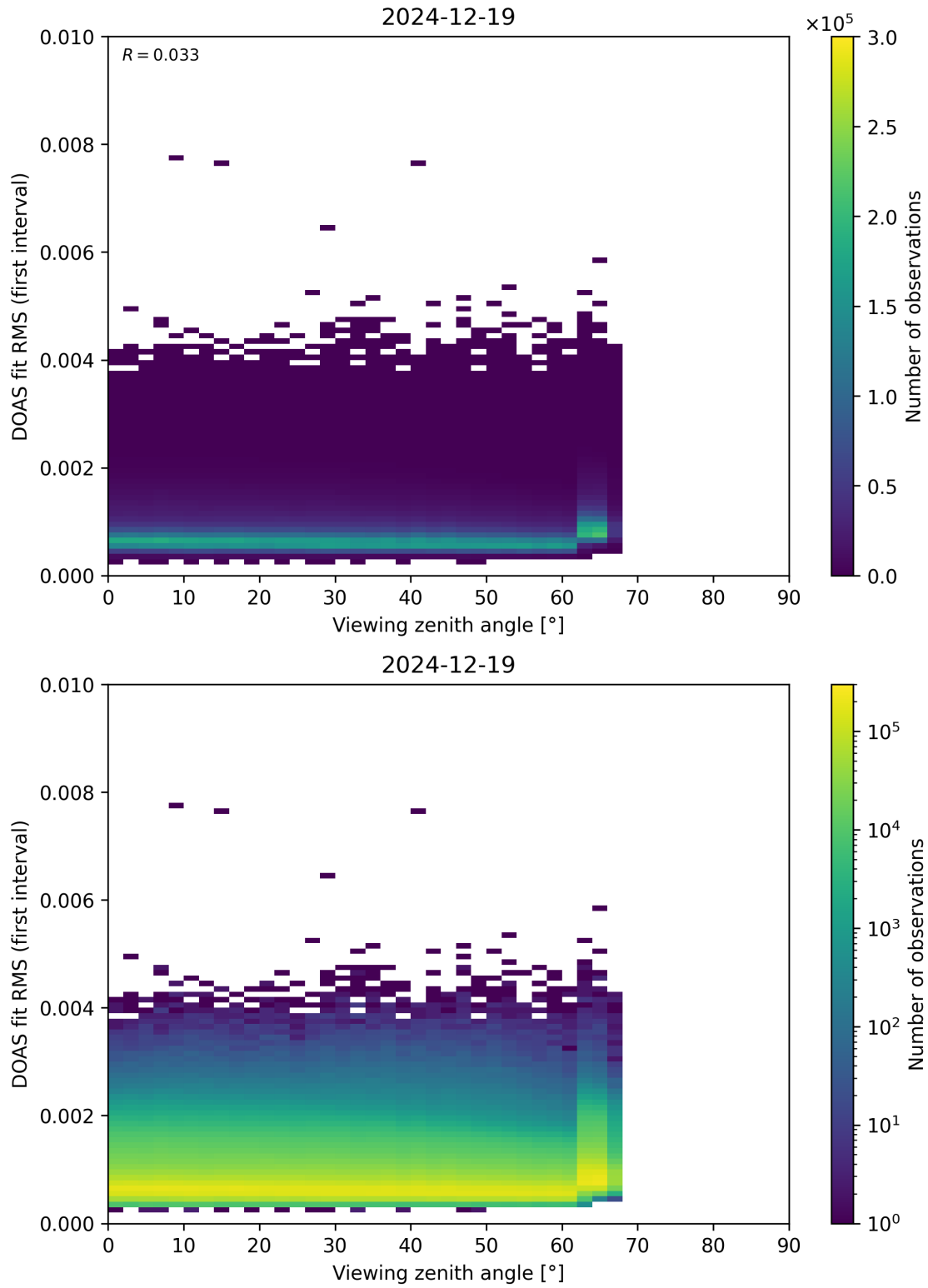
Figure 182: Scatter density plot of “Viewing zenith angle” against “DOAS fit RMS (first interval)” for 2024-12-18 to 2024-12-20.
