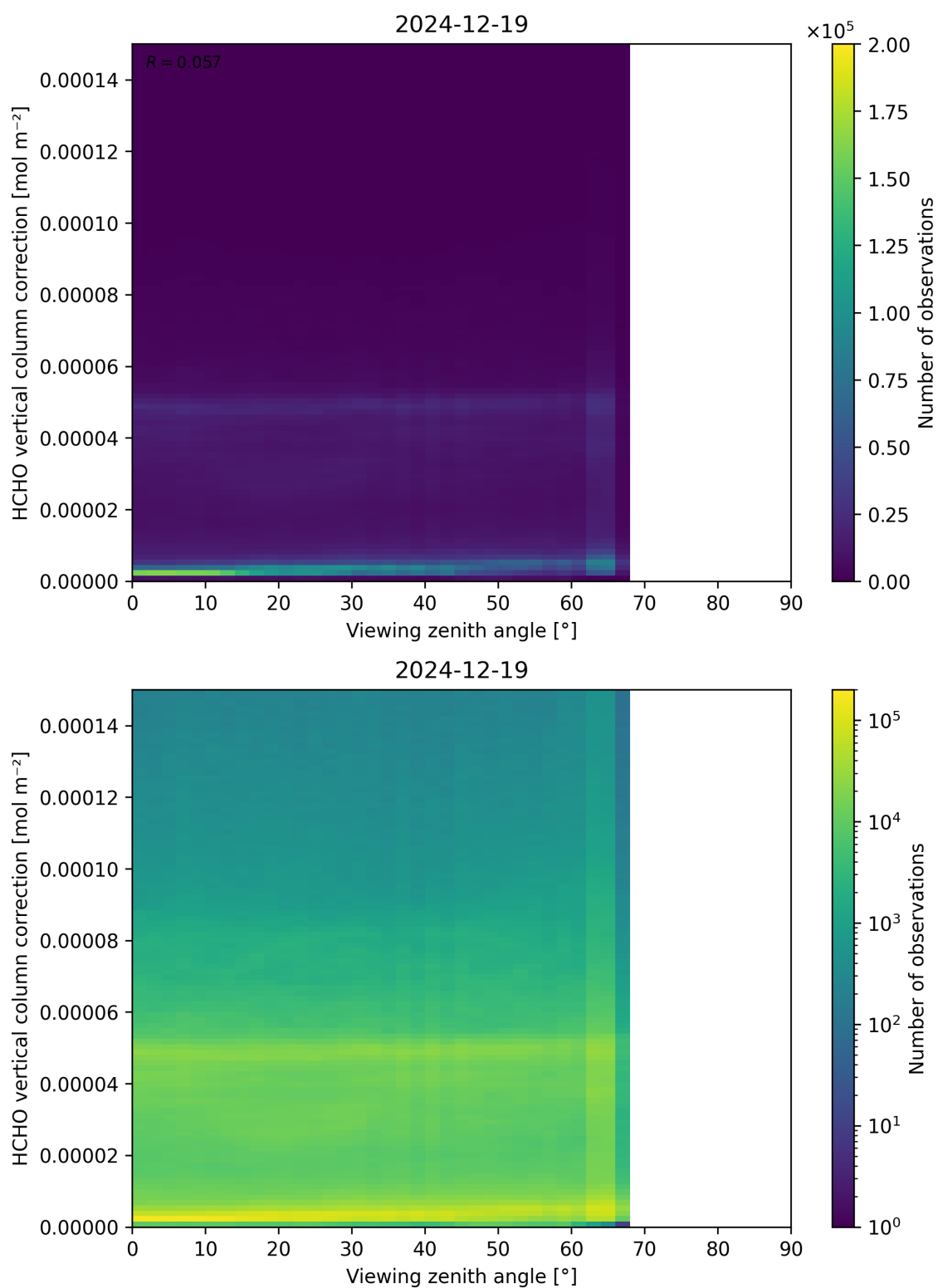
Figure 193: Scatter density plot of “Viewing zenith angle” against “HCHO vertical column correction” for 2024-12-18 to 2024-12-20.
