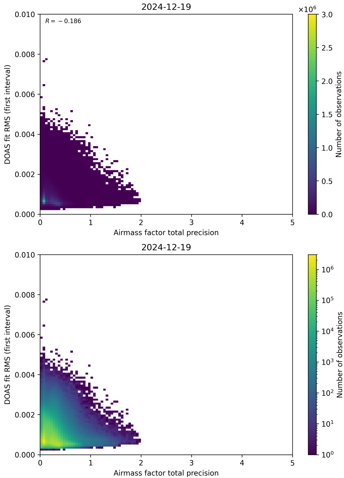
Figure 105: Scatter density plot of “Airmass factor total precision” against “DOAS fit RMS (first interval)” for 2024-12-18 to 2024-12-20.
