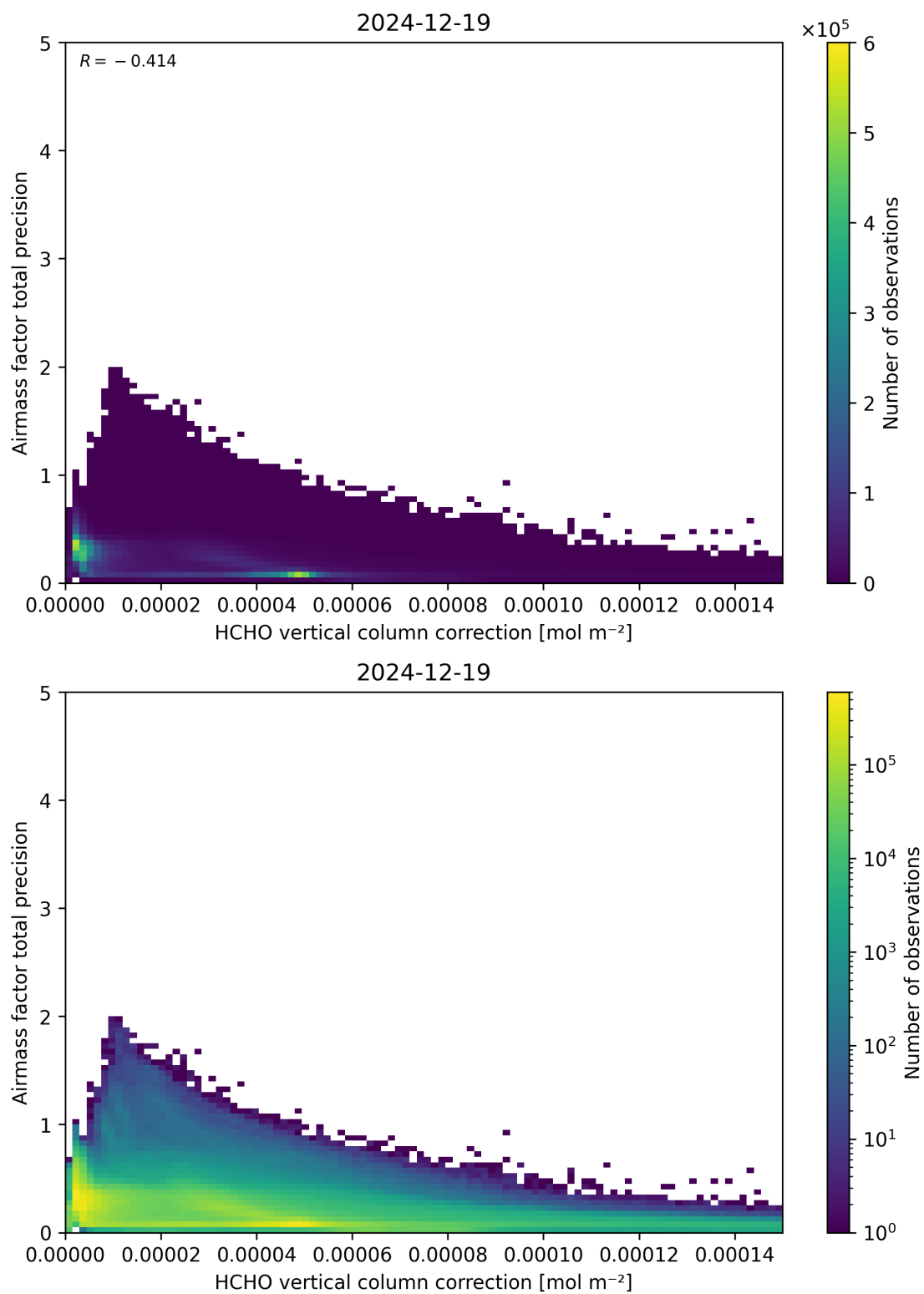
Figure 121: Scatter density plot of “HCHO vertical column correction” against “Airmass factor total precision” for 2024-12-18 to 2024-12-20.
