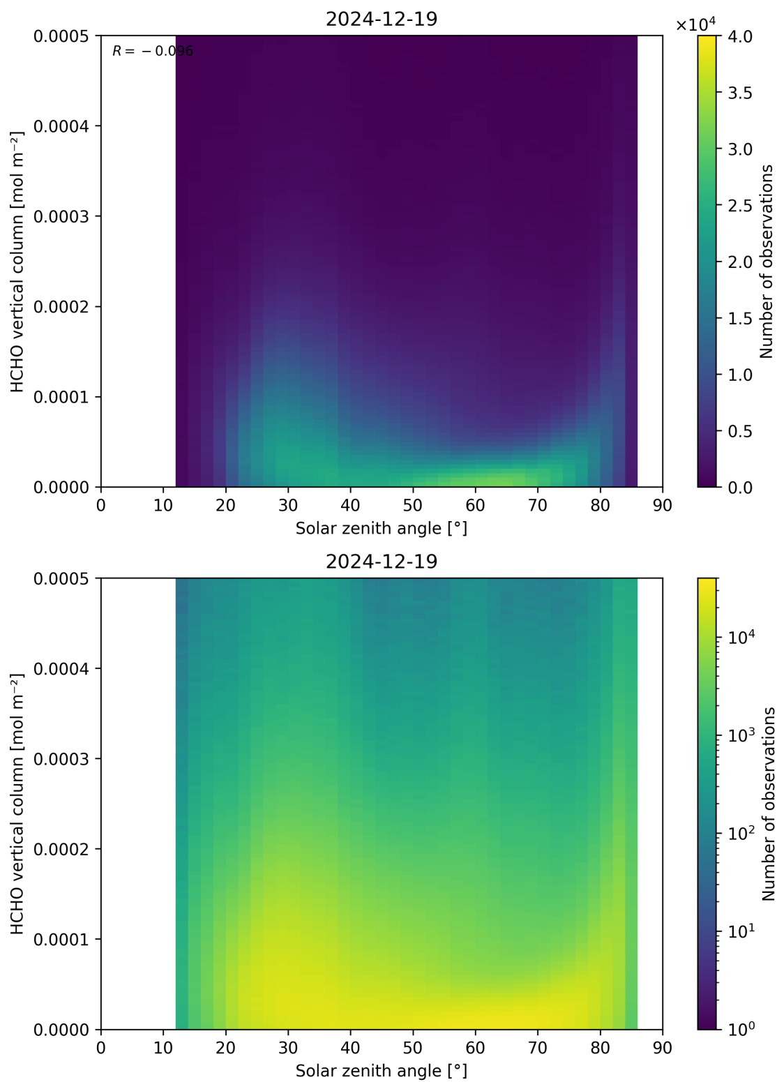
Figure 177: Scatter density plot of “Solar zenith angle” against “HCHO vertical column” for 2024-12-18 to 2024-12-20.
