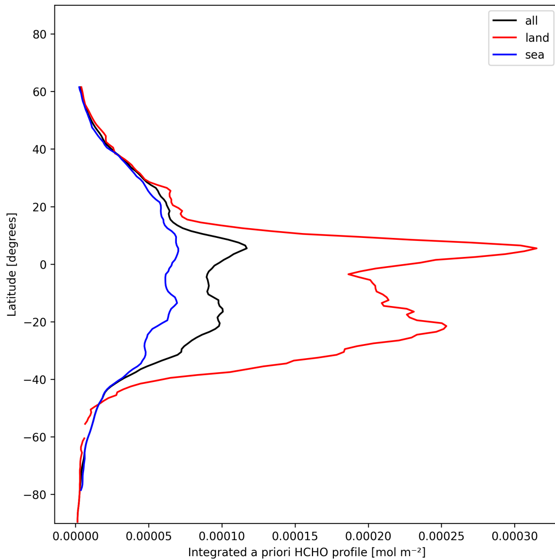
Figure 29: Zonal average of “Integrated a priori HCHO profile” for 2024-12-18 to 2024-12-20.
