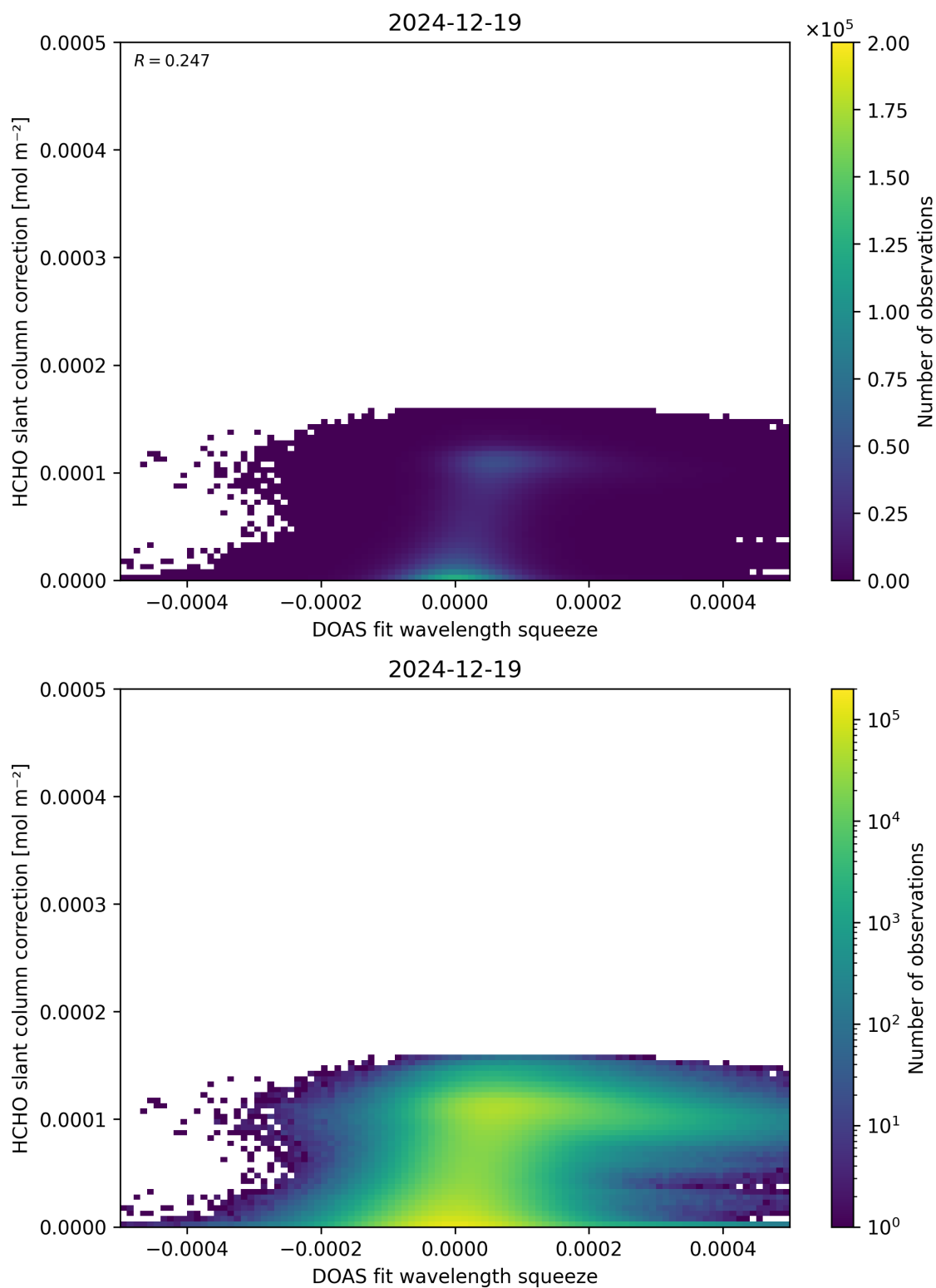
Figure 70: Scatter density plot of “DOAS fit wavelength squeeze” against “HCHO slant column correction” for 2024-12-18 to 2024-12-20.
