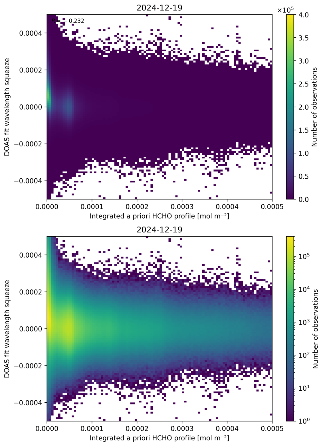
Figure 150: Scatter density plot of “Integrated a priori HCHO profile” against “DOAS fit wavelength squeeze” for 2024-12-18 to 2024-12-20.
