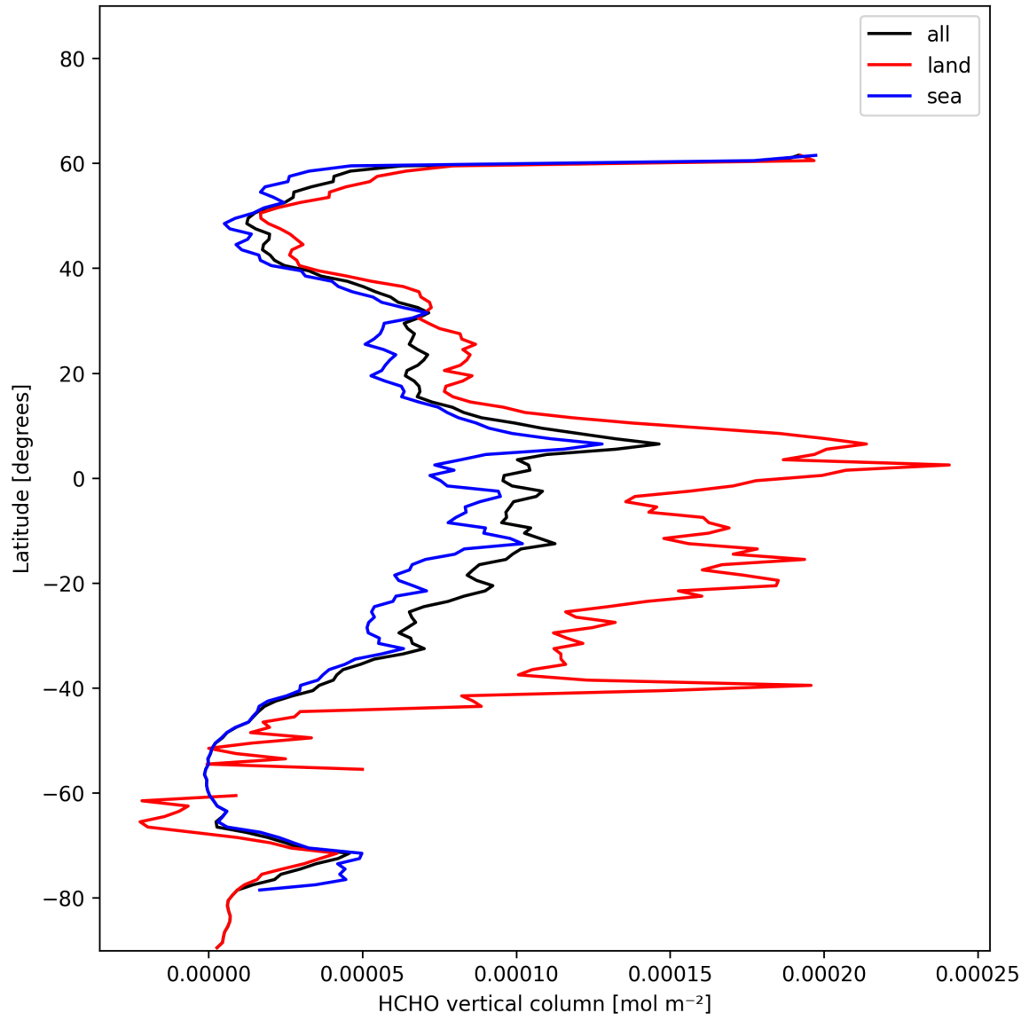
Figure 21: Zonal average of “HCHO vertical column” for 2024-12-18 to 2024-12-20.
