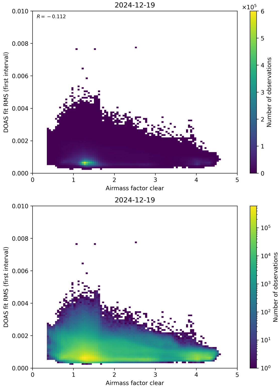
Figure 71: Scatter density plot of “Airmass factor clear” against “DOAS fit RMS (first interval)” for 2024-12-18 to 2024-12-20.
