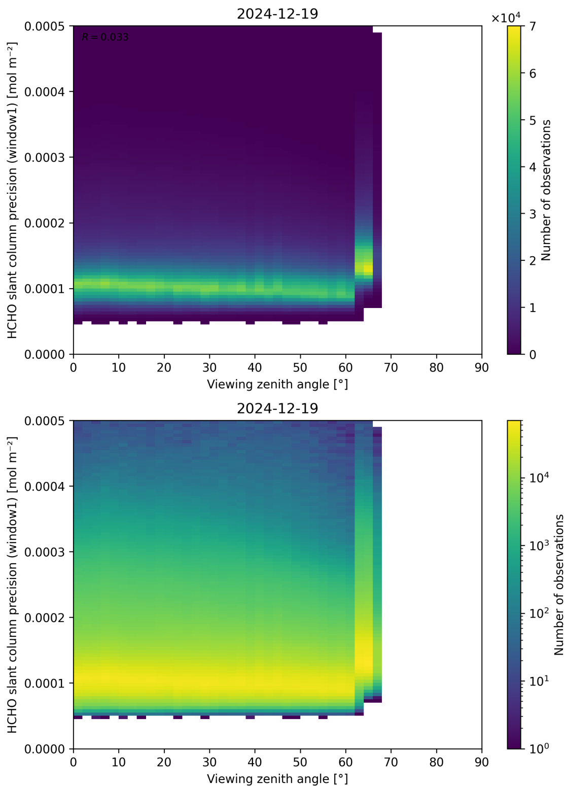
Figure 189: Scatter density plot of “Viewing zenith angle” against “HCHO slant column precision (window1)” for 2024-12-18 to 2024-12-20.
