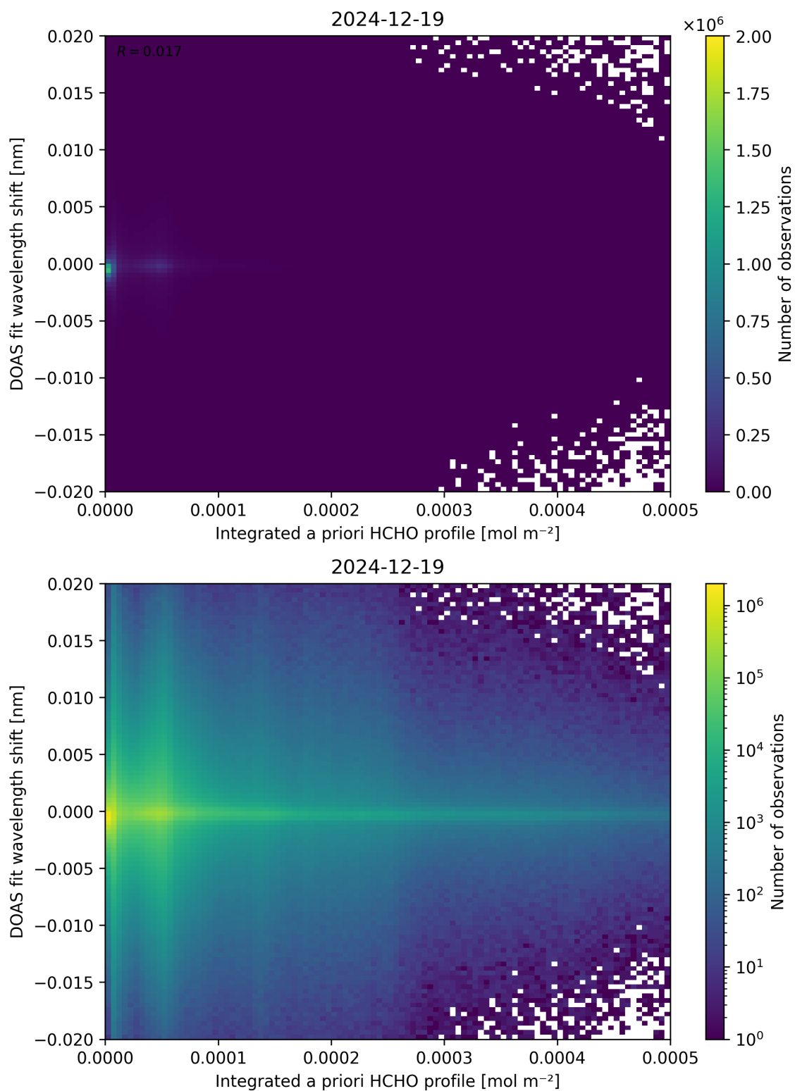
Figure 149: Scatter density plot of “Integrated a priori HCHO profile” against “DOAS fit wavelength shift” for 2024-12-18 to 2024-12-20.
