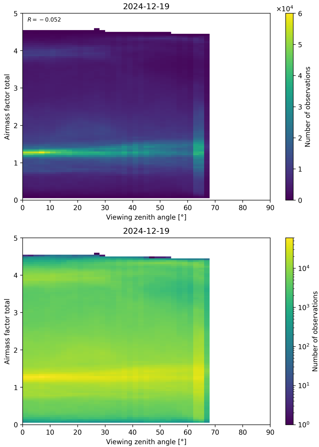
Figure 190: Scatter density plot of “Viewing zenith angle” against “Airmass factor total” for 2024-12-18 to 2024-12-20.
