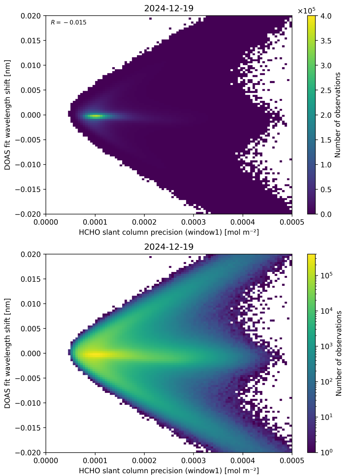
Figure 89: Scatter density plot of “HCHO slant column precision (window1)” against “DOAS fit wavelength shift” for 2024-12-18 to 2024-12-20.
