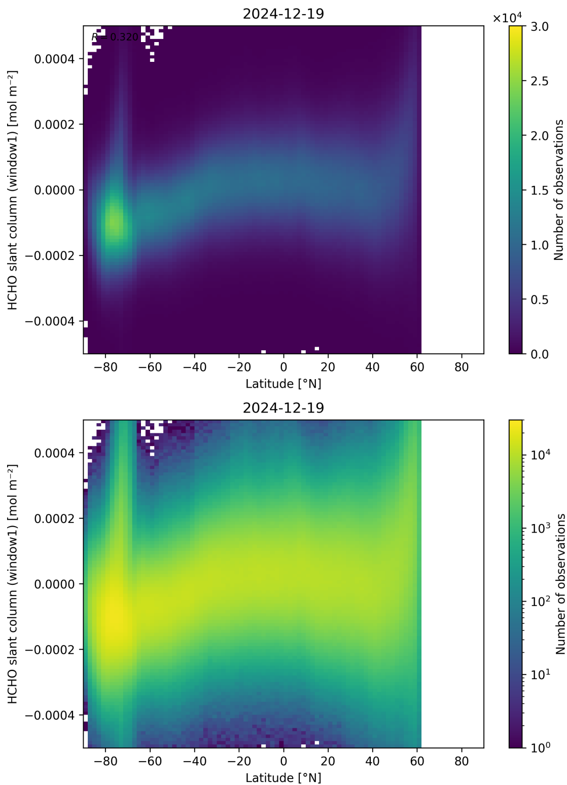
Figure 159: Scatter density plot of “Latitude” against “HCHO slant column (window1)” for 2024-12-18 to 2024-12-20.
