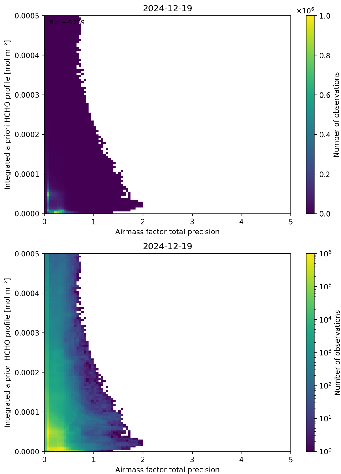
Figure 111: Scatter density plot of “Airmass factor total precision” against “Integrated a priori HCHO profile” for 2024-12-18 to 2024-12-20.
