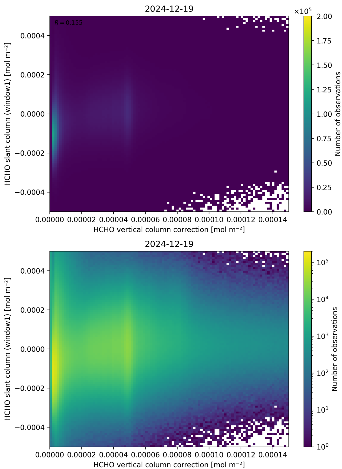
Figure 118: Scatter density plot of “HCHO vertical column correction” against “HCHO slant column (window1)” for 2024-12-18 to 2024-12-20.
