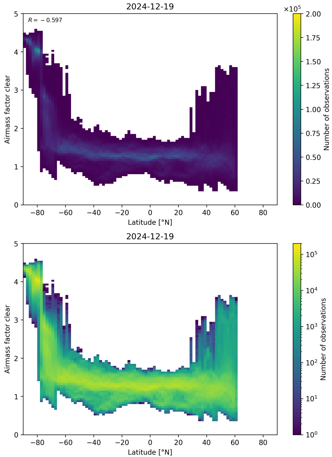
Figure 156: Scatter density plot of “Latitude” against “Airmass factor clear” for 2024-12-18 to 2024-12-20.
