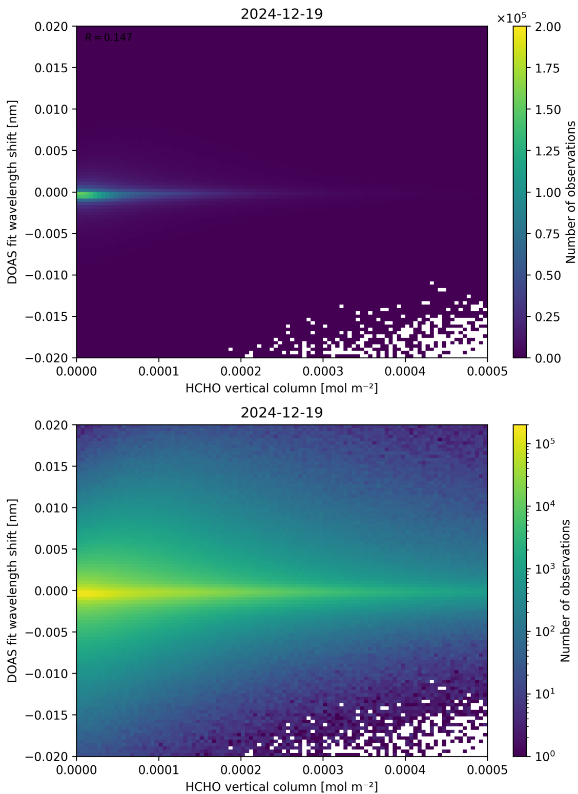
Figure 124: Scatter density plot of “HCHO vertical column” against “DOAS fit wavelength shift” for 2024-12-18 to 2024-12-20.
