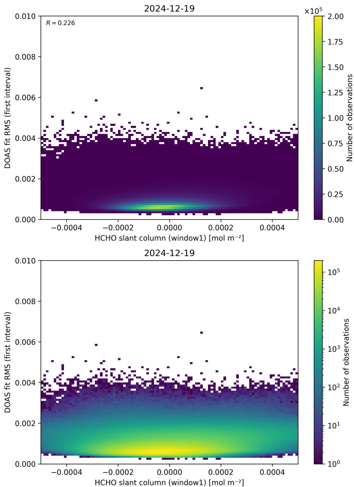
Figure 78: Scatter density plot of “HCHO slant column (window1)” against “DOAS fit RMS (first interval)” for 2024-12-18 to 2024-12-20.
