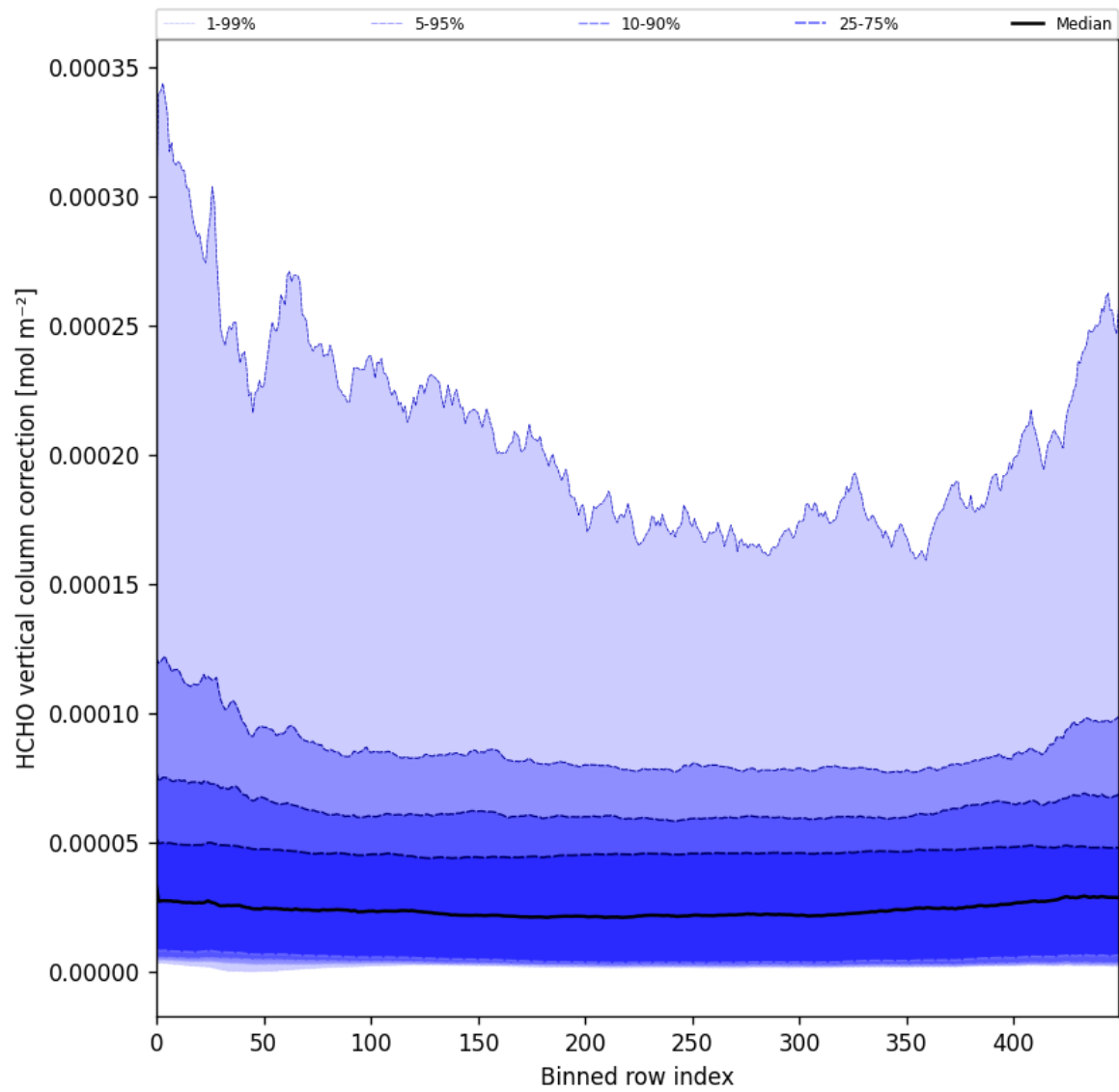
Figure 51: Along track statistics of “HCHO vertical column correction” for 2024-12-18 to 2024-12-20
