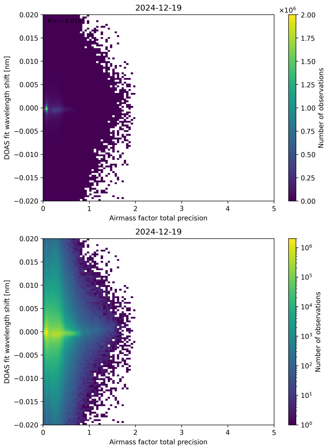
Figure 106: Scatter density plot of “Airmass factor total precision” against “DOAS fit wavelength shift” for 2024-12-18 to 2024-12-20.
