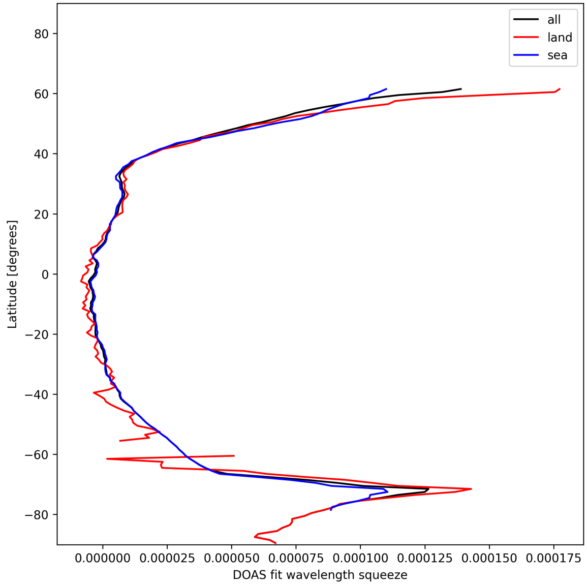
Figure 31: Zonal average of “DOAS fit wavelength squeeze” for 2024-12-18 to 2024-12-20.
