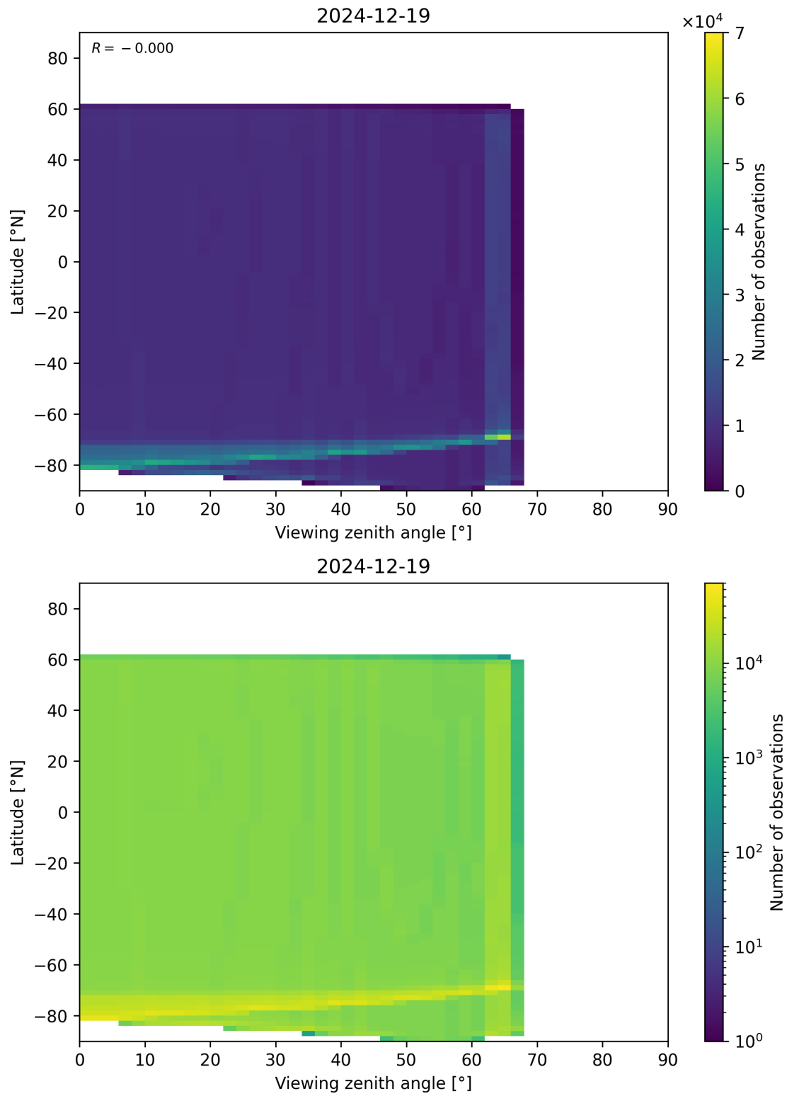
Figure 196: Scatter density plot of “Viewing zenith angle” against “Latitude” for 2024-12-18 to 2024-12-20.
