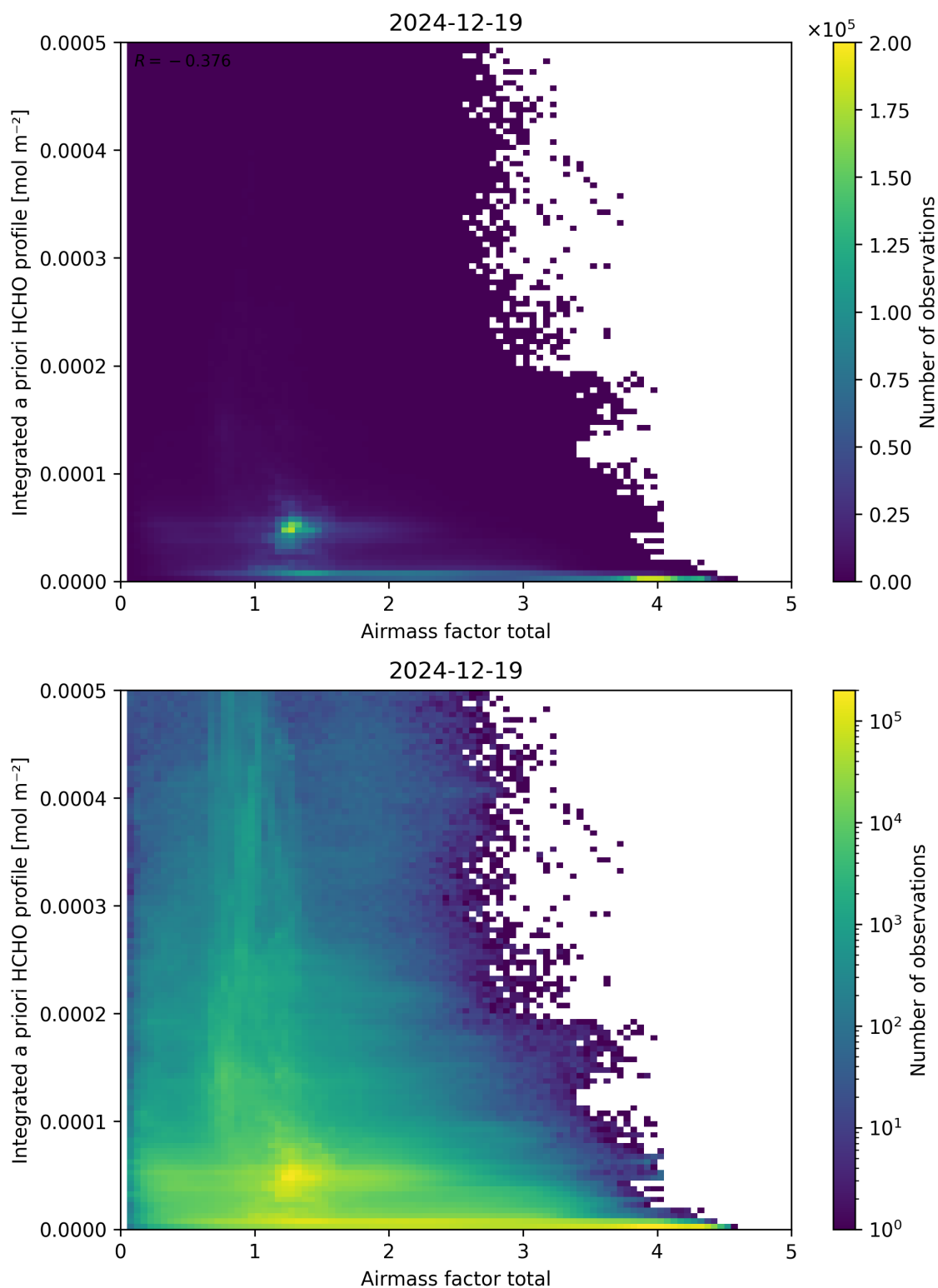
Figure 104: Scatter density plot of “Airmass factor total” against “Integrated a priori HCHO profile” for 2024-12-18 to 2024-12-20.
