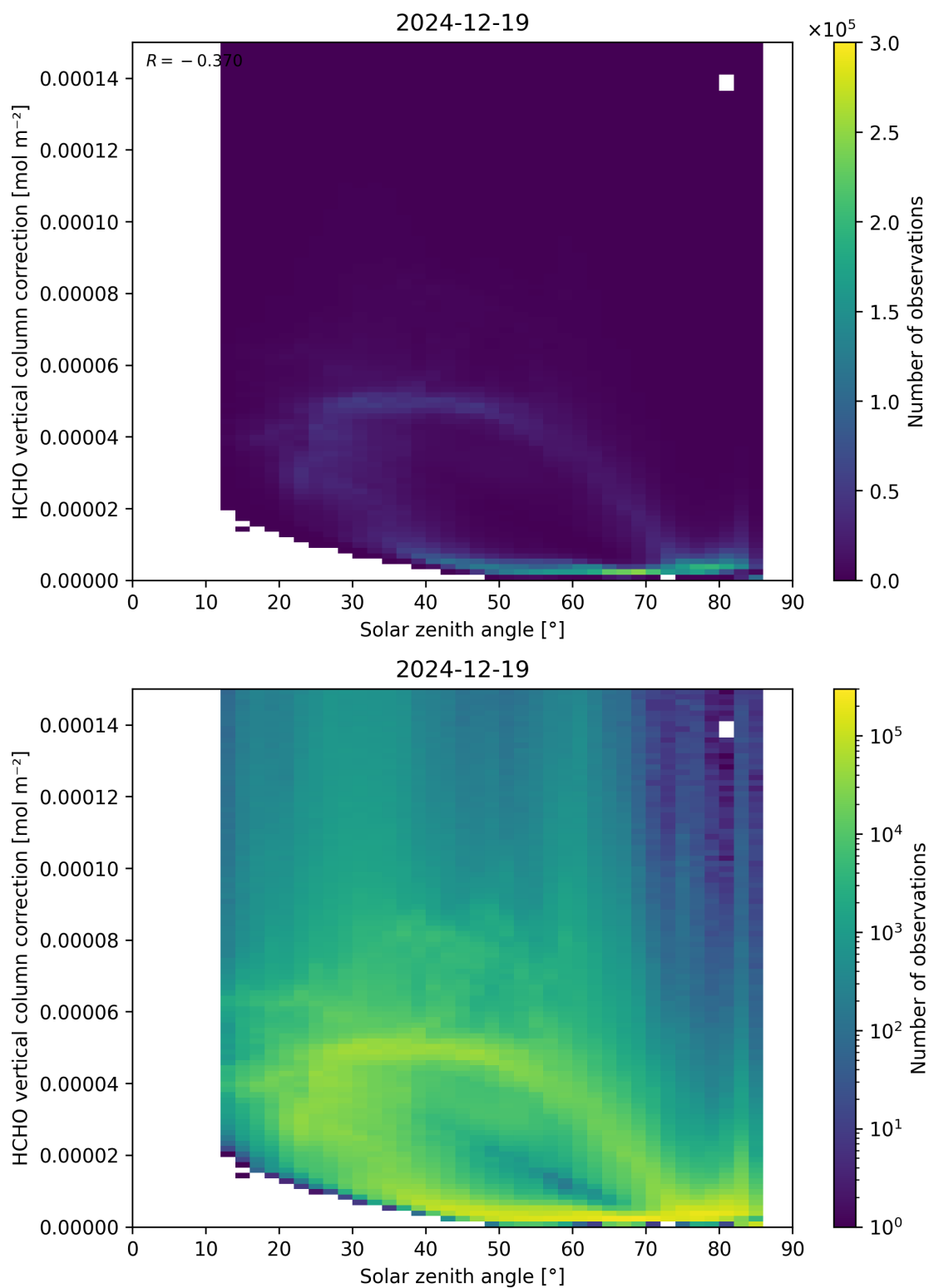
Figure 178: Scatter density plot of “Solar zenith angle” against “HCHO vertical column correction” for 2024-12-18 to 2024-12-20.
