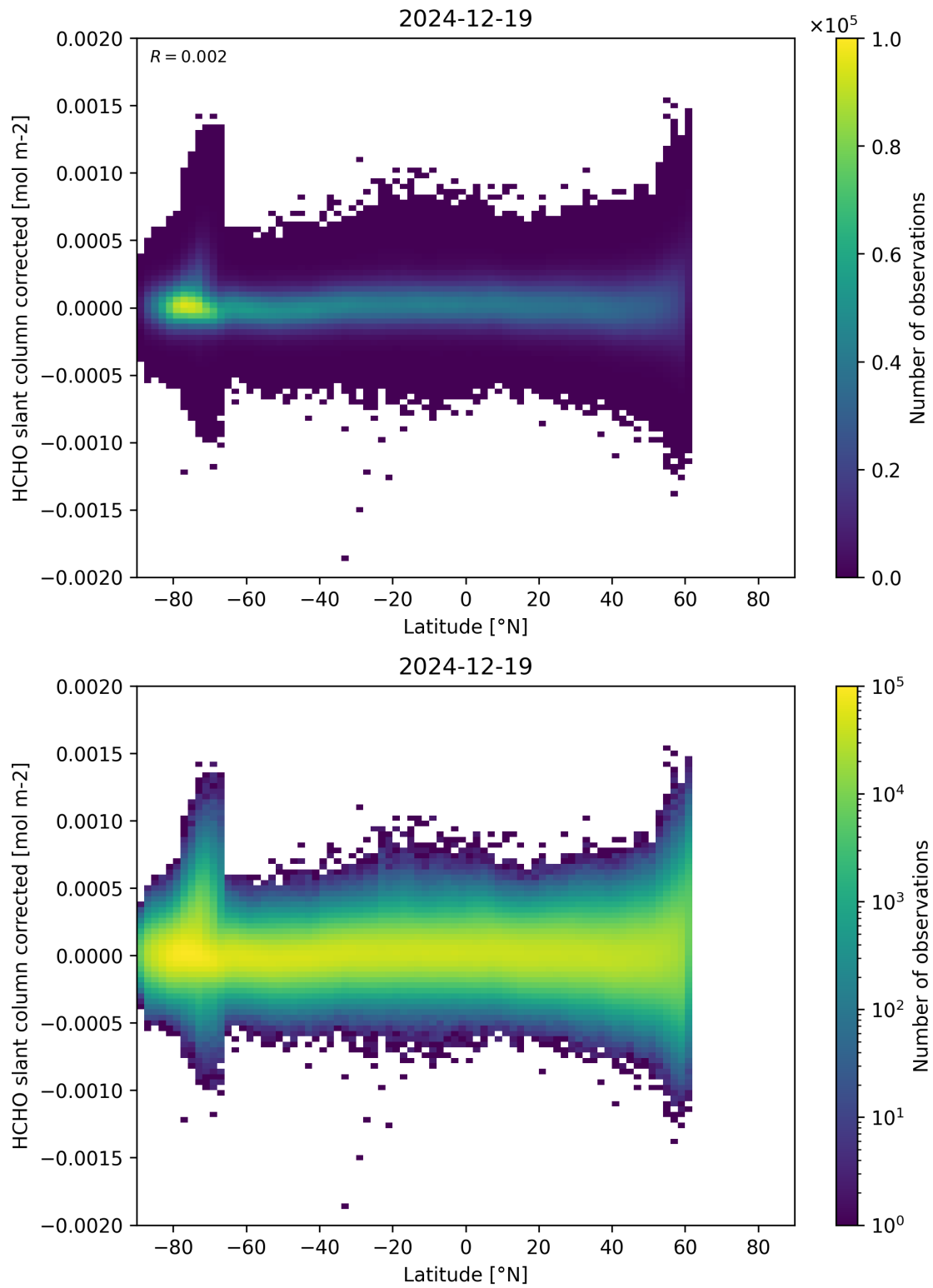
Figure 157: Scatter density plot of “Latitude” against “HCHO slant column corrected” for 2024-12-18 to 2024-12-20.
