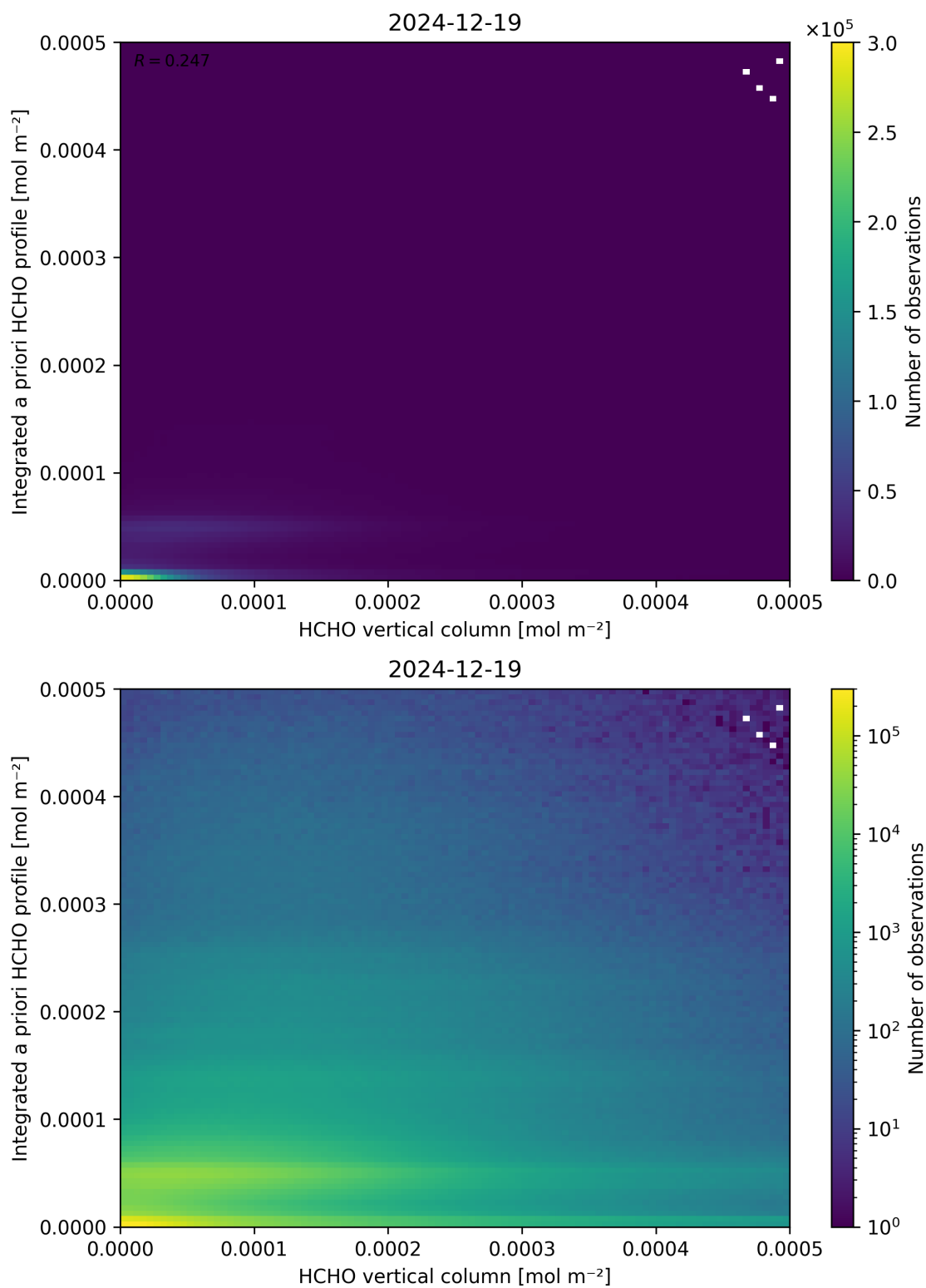
Figure 135: Scatter density plot of “HCHO vertical column” against “Integrated a priori HCHO profile” for 2024-12-18 to 2024-12-20.
