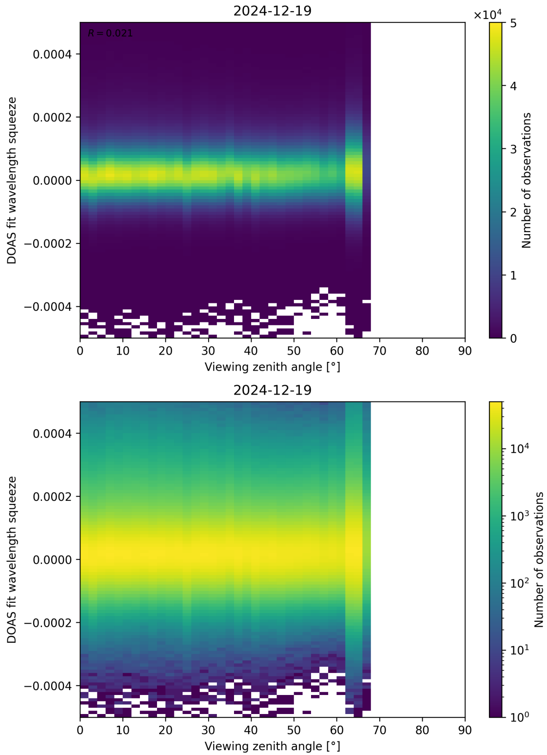
Figure 184: Scatter density plot of “Viewing zenith angle” against “DOAS fit wavelength squeeze” for 2024-12-18 to 2024-12-20.
