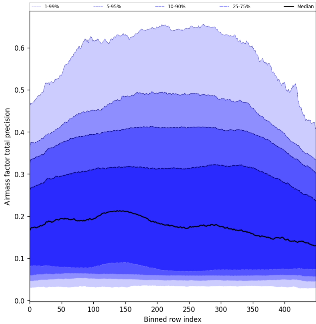
Figure 55: Along track statistics of “Airmass factor total precision” for 2024-12-18 to 2024-12-20
