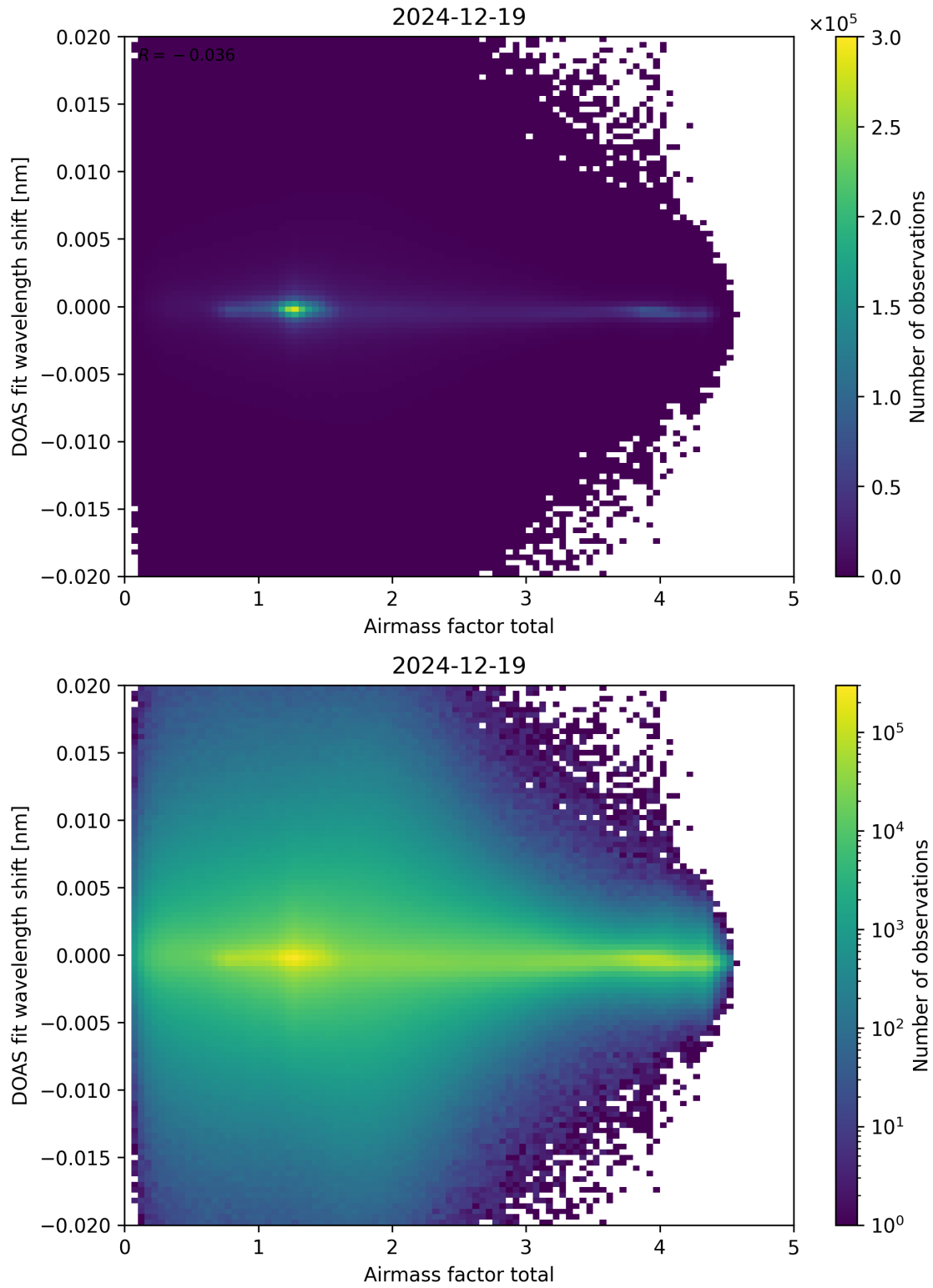
Figure 98: Scatter density plot of “Airmass factor total” against “DOAS fit wavelength shift” for 2024-12-18 to 2024-12-20.
