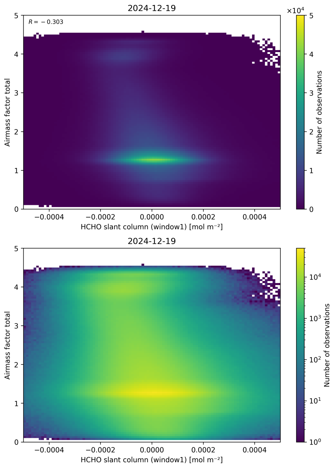
Figure 85: Scatter density plot of “HCHO slant column (window1)” against “Airmass factor total” for 2024-12-18 to 2024-12-20.
