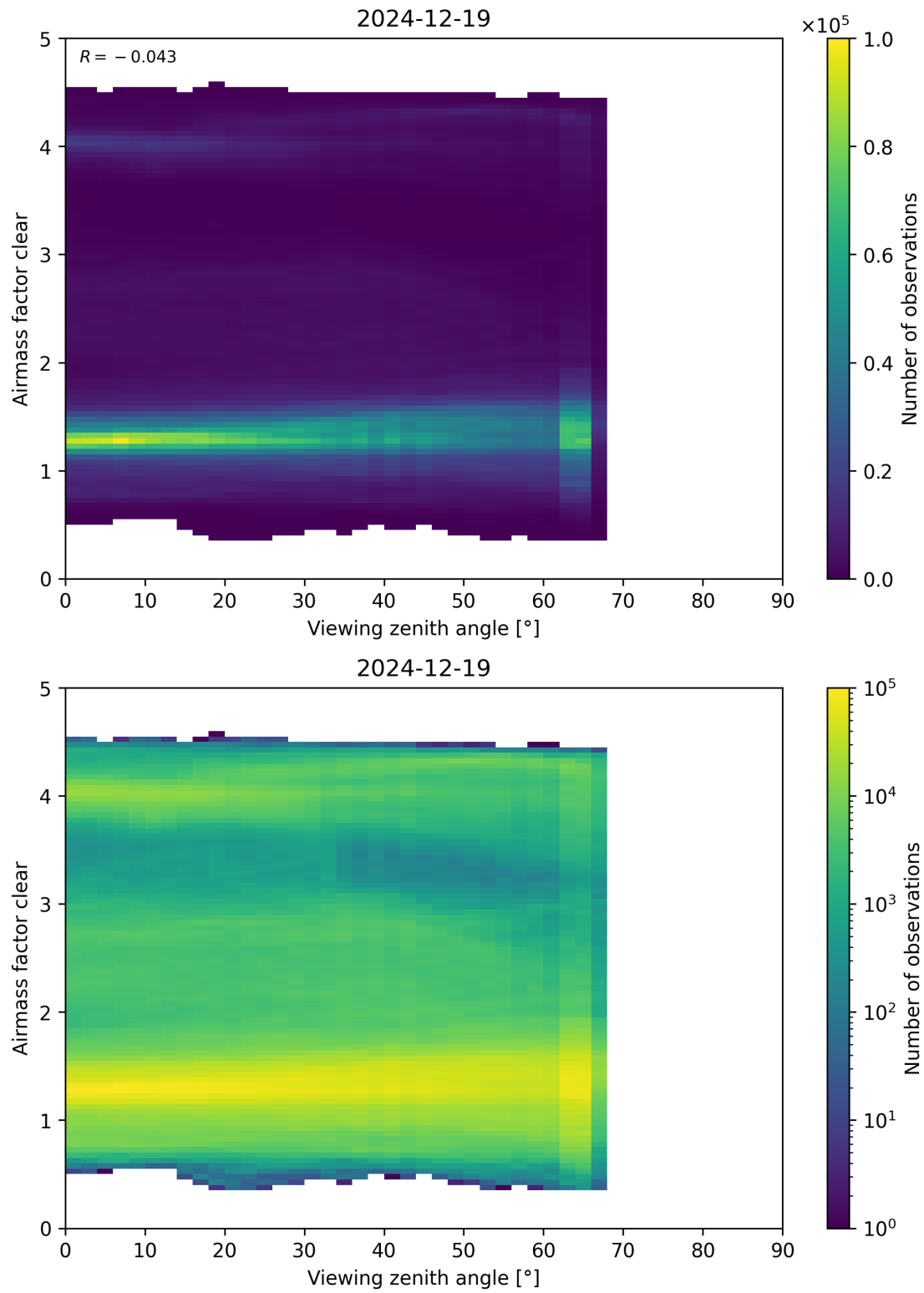
Figure 185: Scatter density plot of “Viewing zenith angle” against “Airmass factor clear” for 2024-12-18 to 2024-12-20.
