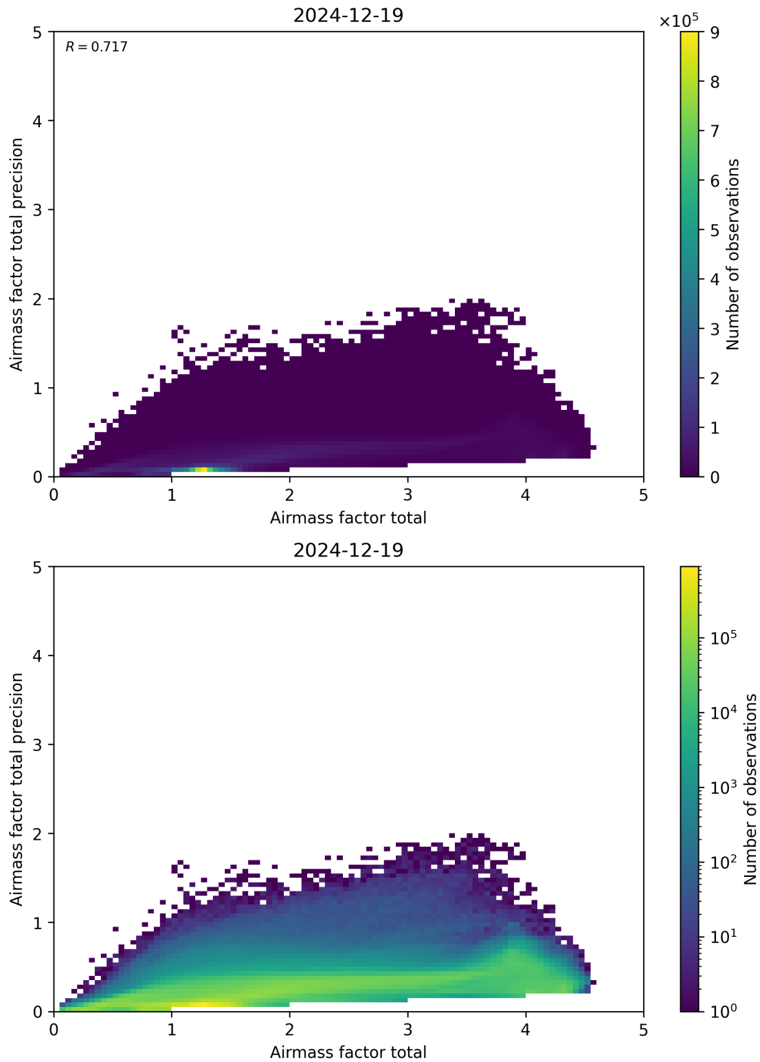
Figure 103: Scatter density plot of “Airmass factor total” against “Airmass factor total precision” for 2024-12-18 to 2024-12-20.
