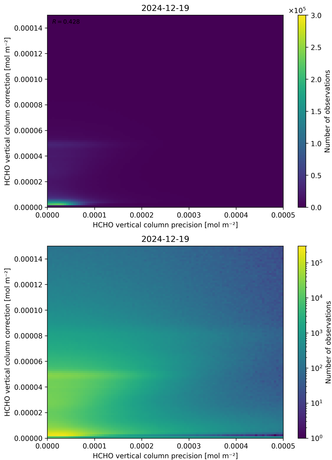
Figure 146: Scatter density plot of “HCHO vertical column precision” against “HCHO vertical column correction” for 2024-12-18 to 2024-12-20.
