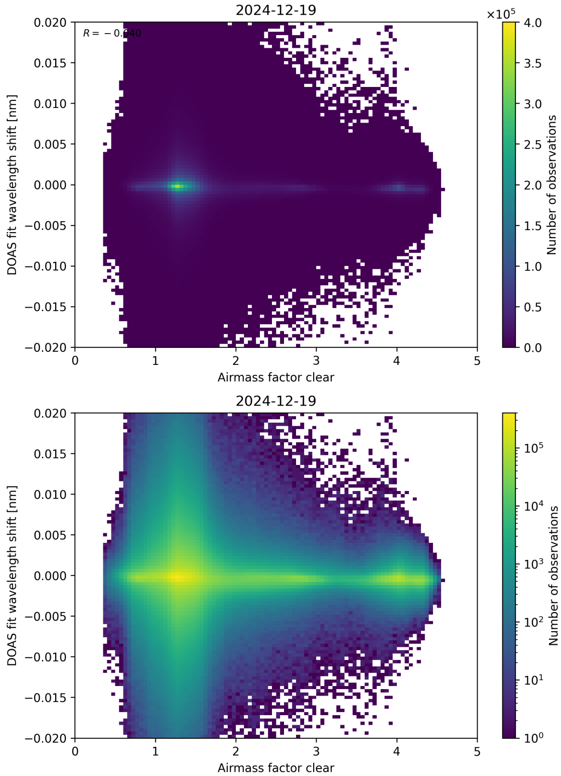
Figure 72: Scatter density plot of “Airmass factor clear” against “DOAS fit wavelength shift” for 2024-12-18 to 2024-12-20.
