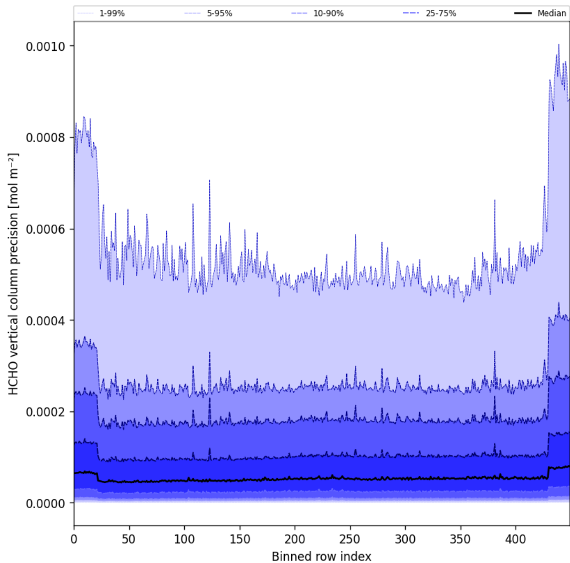
Figure 50: Along track statistics of “HCHO vertical column precision” for 2024-12-18 to 2024-12-20
