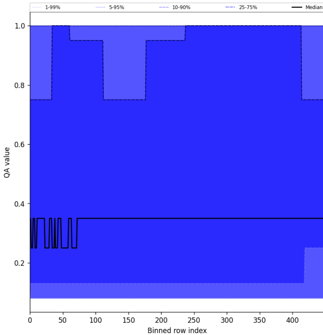
Figure 48: Along track statistics of “QA value” for 2024-12-18 to 2024-12-20
