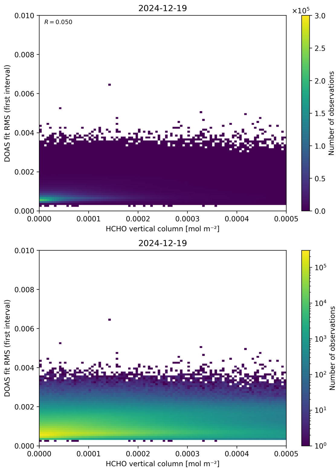
Figure 123: Scatter density plot of “HCHO vertical column” against “DOAS fit RMS (first interval)” for 2024-12-18 to 2024-12-20.
