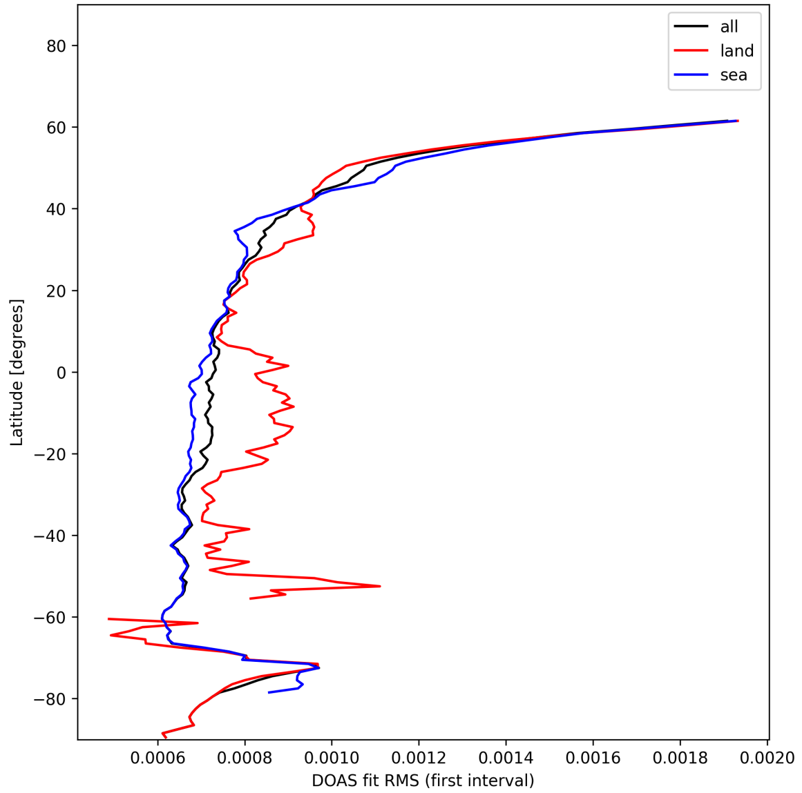
Figure 32: Zonal average of “DOAS fit RMS (first interval)” for 2024-12-18 to 2024-12-20.
