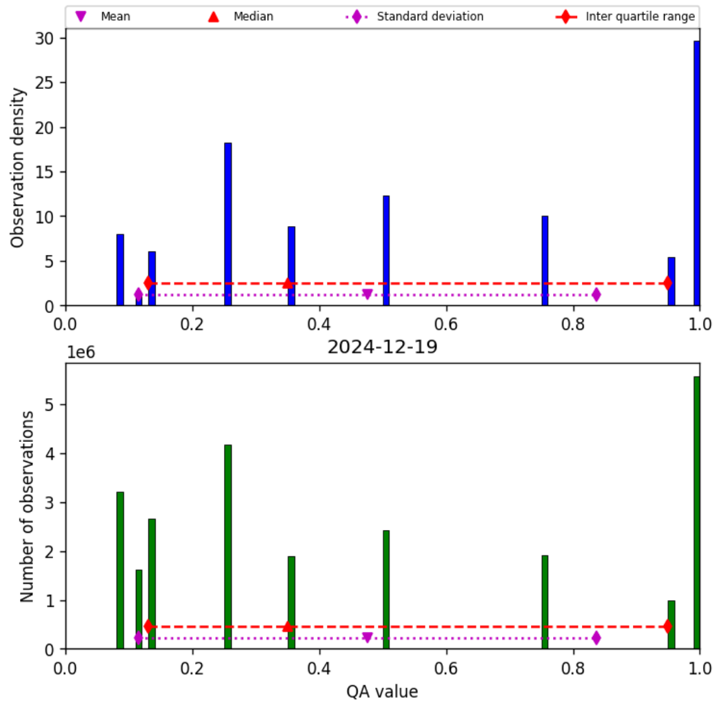
Figure 34: Histogram of “QA value” for 2024-12-18 to 2024-12-20
