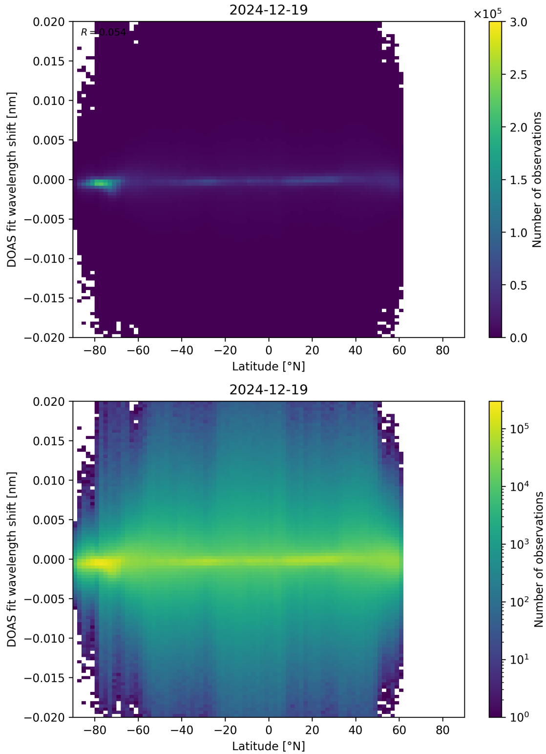
Figure 154: Scatter density plot of “Latitude” against “DOAS fit wavelength shift” for 2024-12-18 to 2024-12-20.
