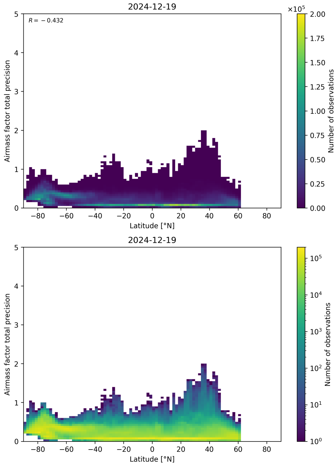
Figure 162: Scatter density plot of “Latitude” against “Airmass factor total precision” for 2024-12-18 to 2024-12-20.
