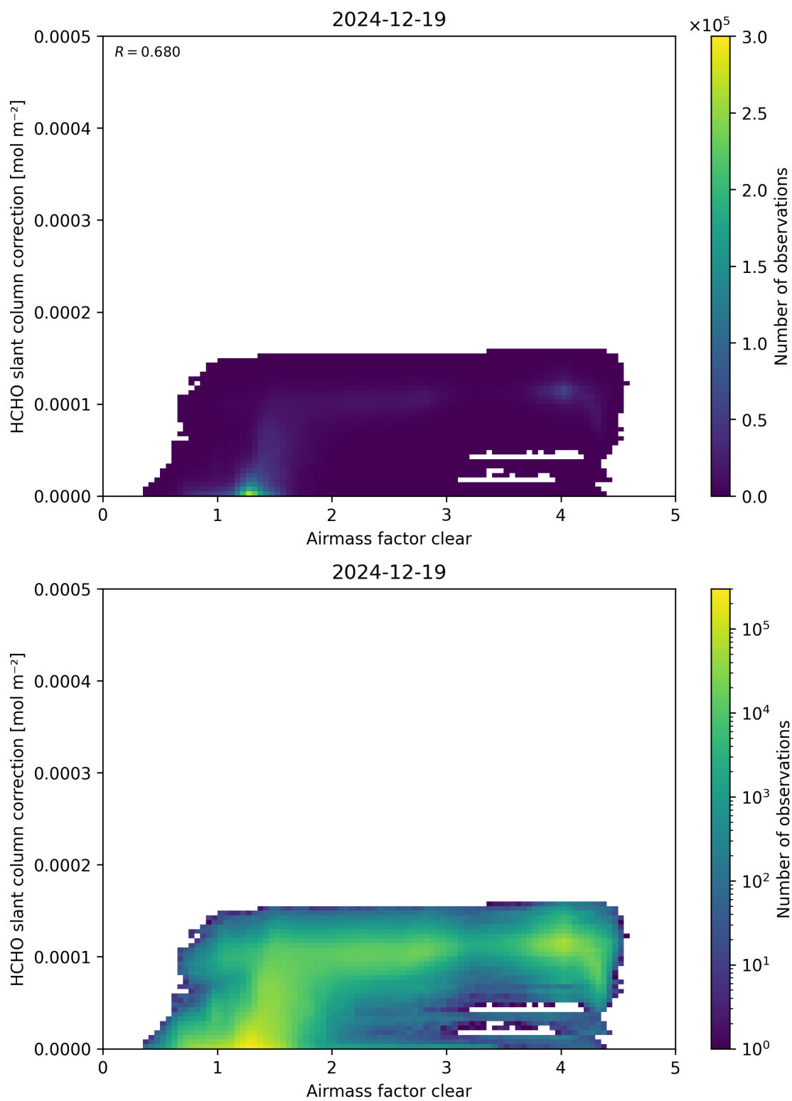
Figure 75: Scatter density plot of “Airmass factor clear” against “HCHO slant column correction” for 2024-12-18 to 2024-12-20.
