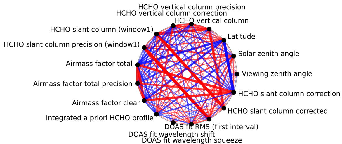
Figure 1: Map of correlation graph for 2024-12-18 to 2024-12-20.
