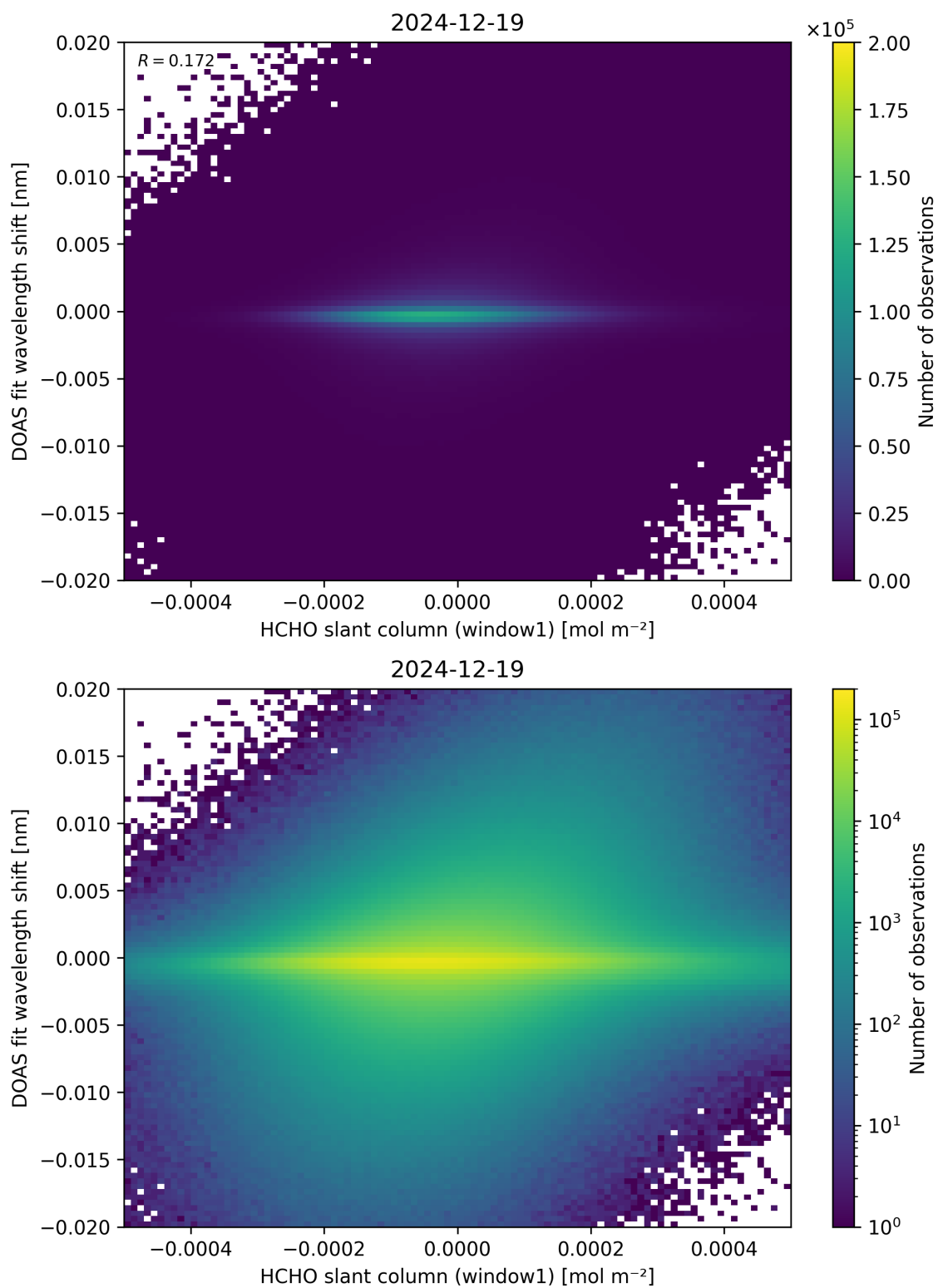
Figure 79: Scatter density plot of “HCHO slant column (window1)” against “DOAS fit wavelength shift” for 2024-12-18 to 2024-12-20.
