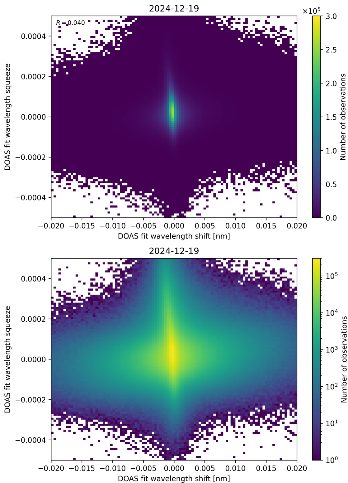
Figure 65: Scatter density plot of “DOAS fit wavelength shift” against “DOAS fit wavelength squeeze” for 2024-12-18 to 2024-12-20.
