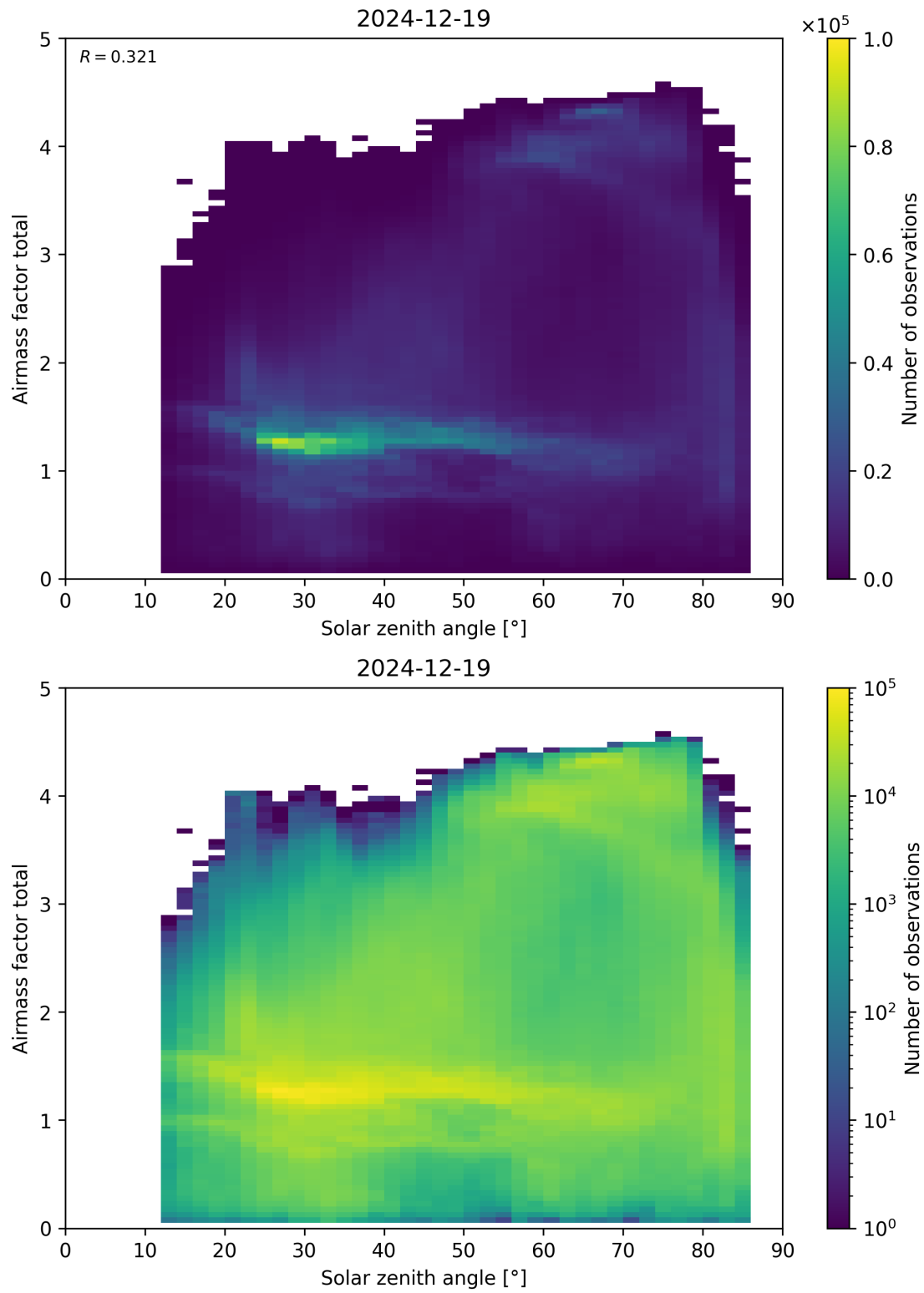
Figure 175: Scatter density plot of “Solar zenith angle” against “Airmass factor total” for 2024-12-18 to 2024-12-20.
