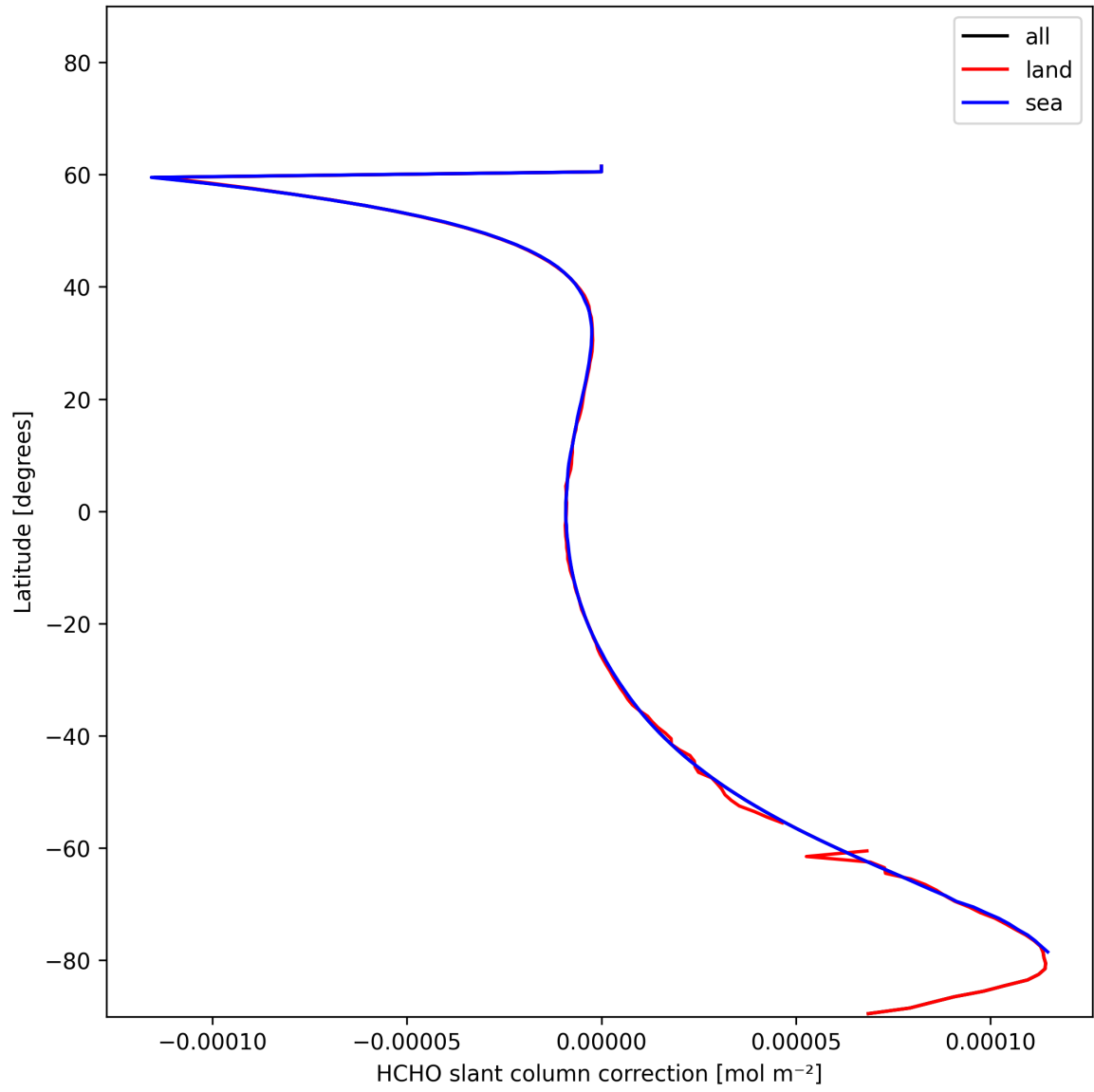
Figure 33: Zonal average of “HCHO slant column correction” for 2024-12-18 to 2024-12-20.
