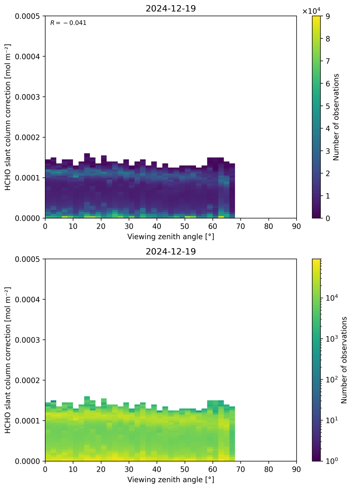
Figure 187: Scatter density plot of “Viewing zenith angle” against “HCHO slant column correction” for 2024-12-18 to 2024-12-20.
