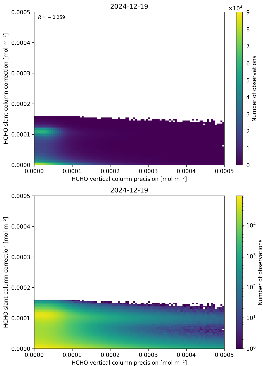
Figure 141: Scatter density plot of “HCHO vertical column precision” against “HCHO slant column correction” for 2024-12-18 to 2024-12-20.
