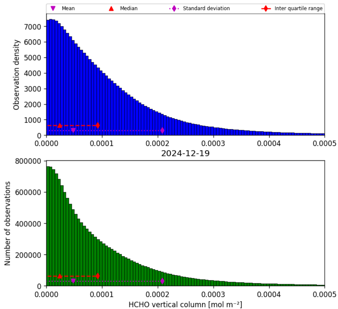
Figure 35: Histogram of “HCHO vertical column” for 2024-12-18 to 2024-12-20
