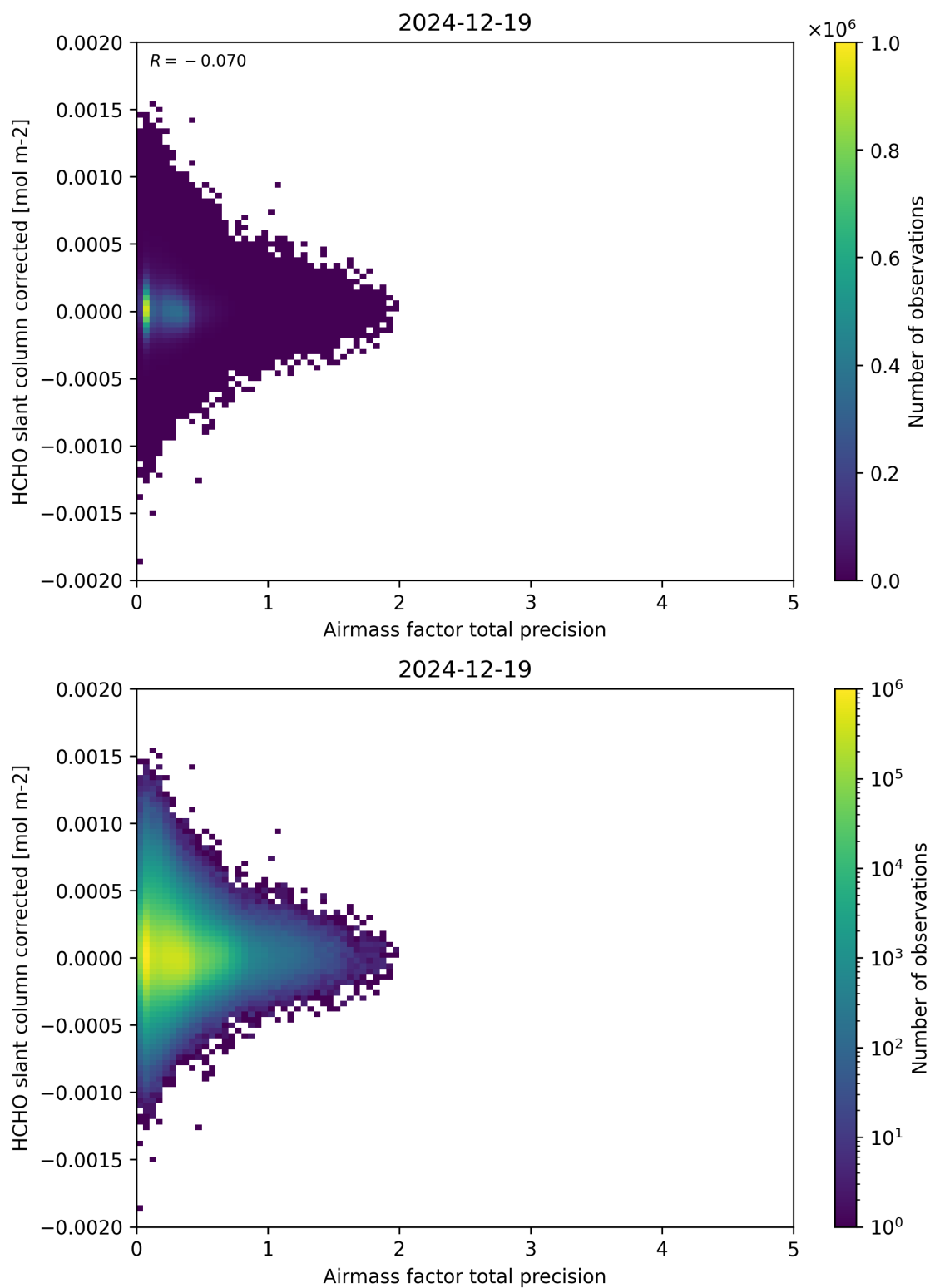
Figure 109: Scatter density plot of “Airmass factor total precision” against “HCHO slant column corrected” for 2024-12-18 to 2024-12-20.
