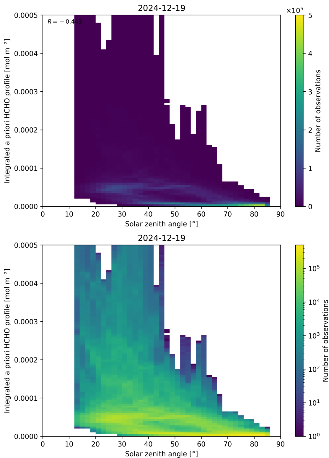
Figure 180: Scatter density plot of “Solar zenith angle” against “Integrated a priori HCHO profile” for 2024-12-18 to 2024-12-20.
