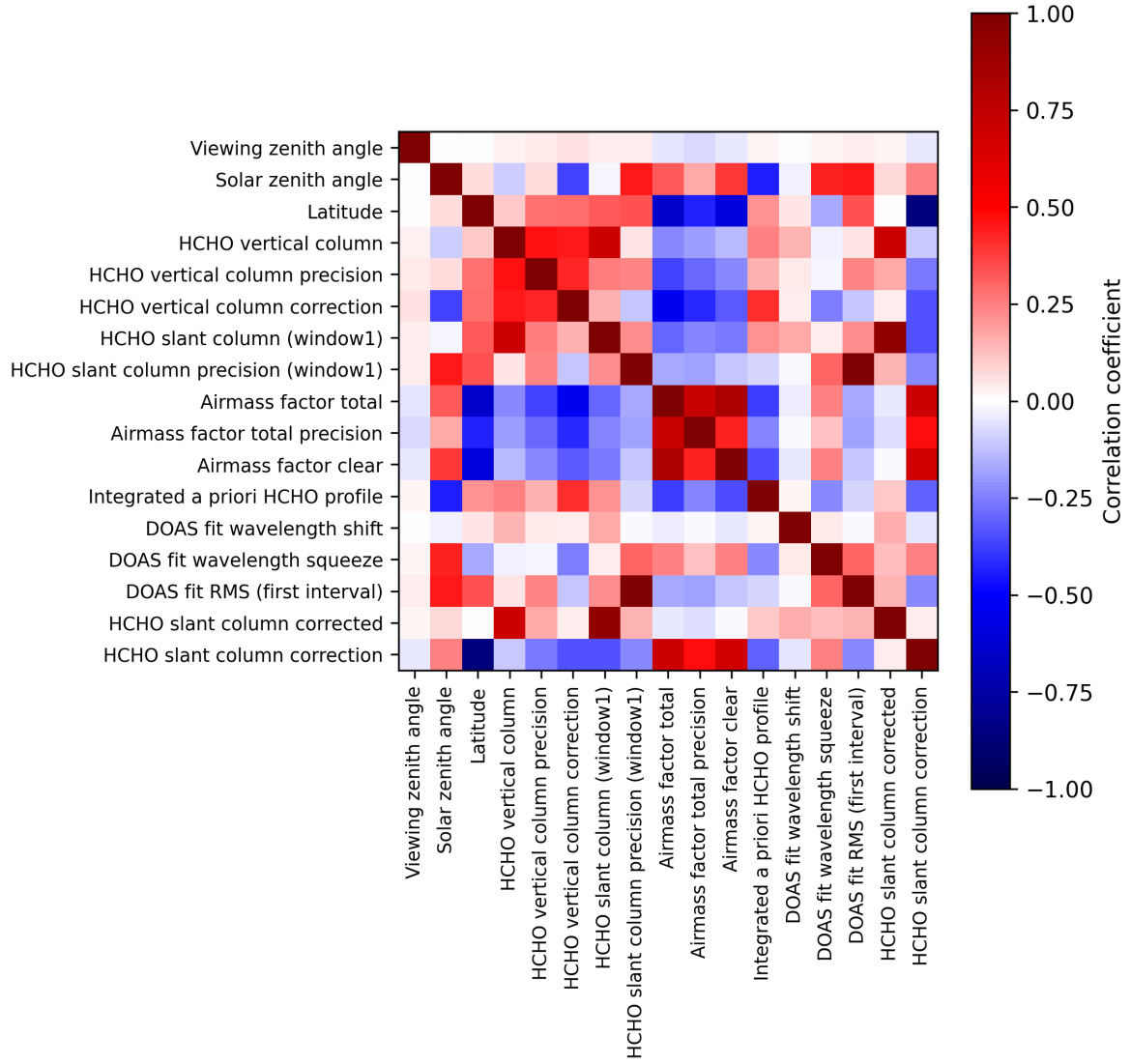
Figure 2: Map of correlation matrix for 2024-12-18 to 2024-12-20.
