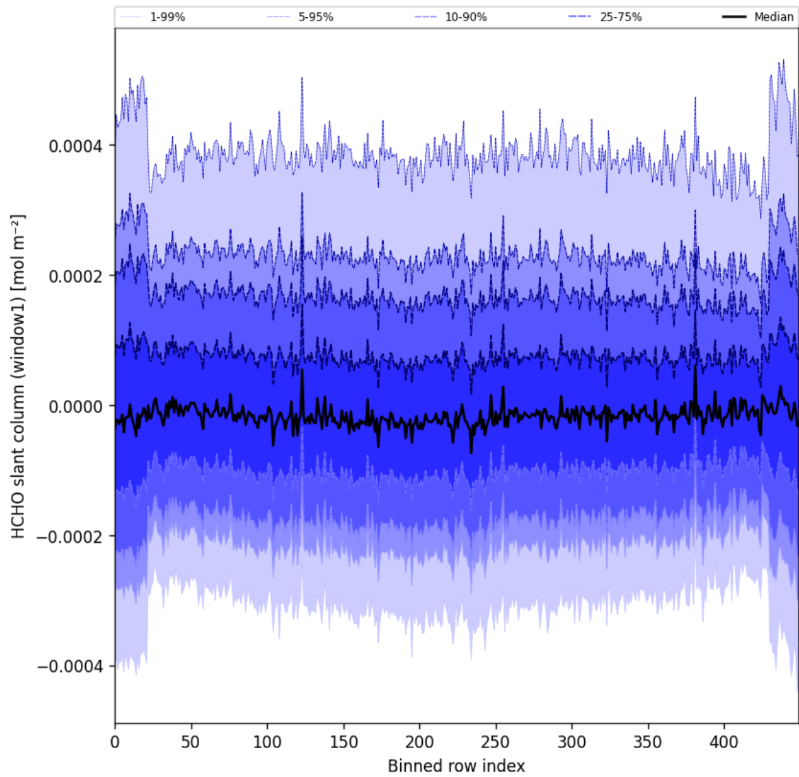
Figure 52: Along track statistics of “HCHO slant column (window1)” for 2024-12-18 to 2024-12-20
