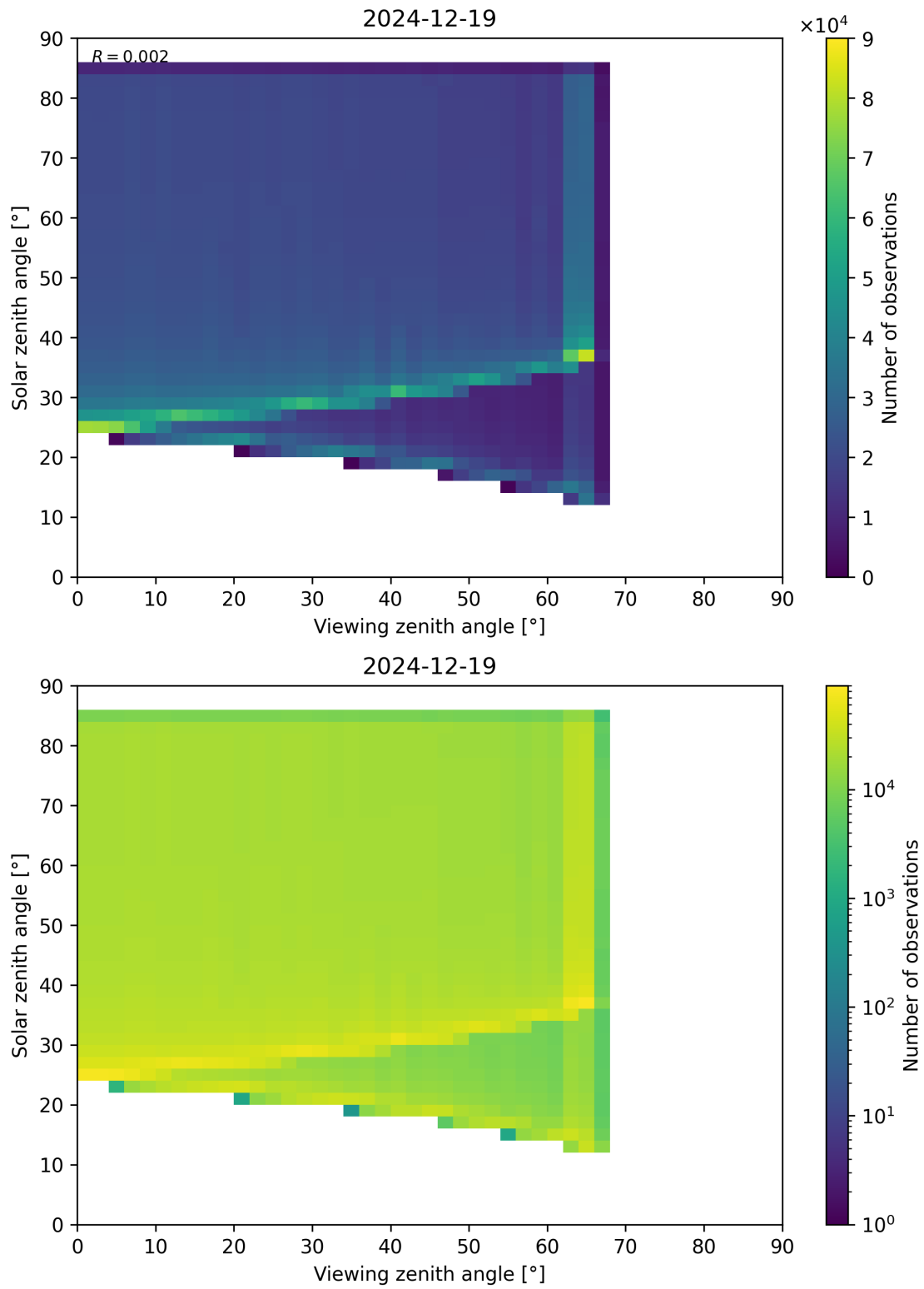
Figure 197: Scatter density plot of “Viewing zenith angle” against “Solar zenith angle” for 2024-12-18 to 2024-12-20.
