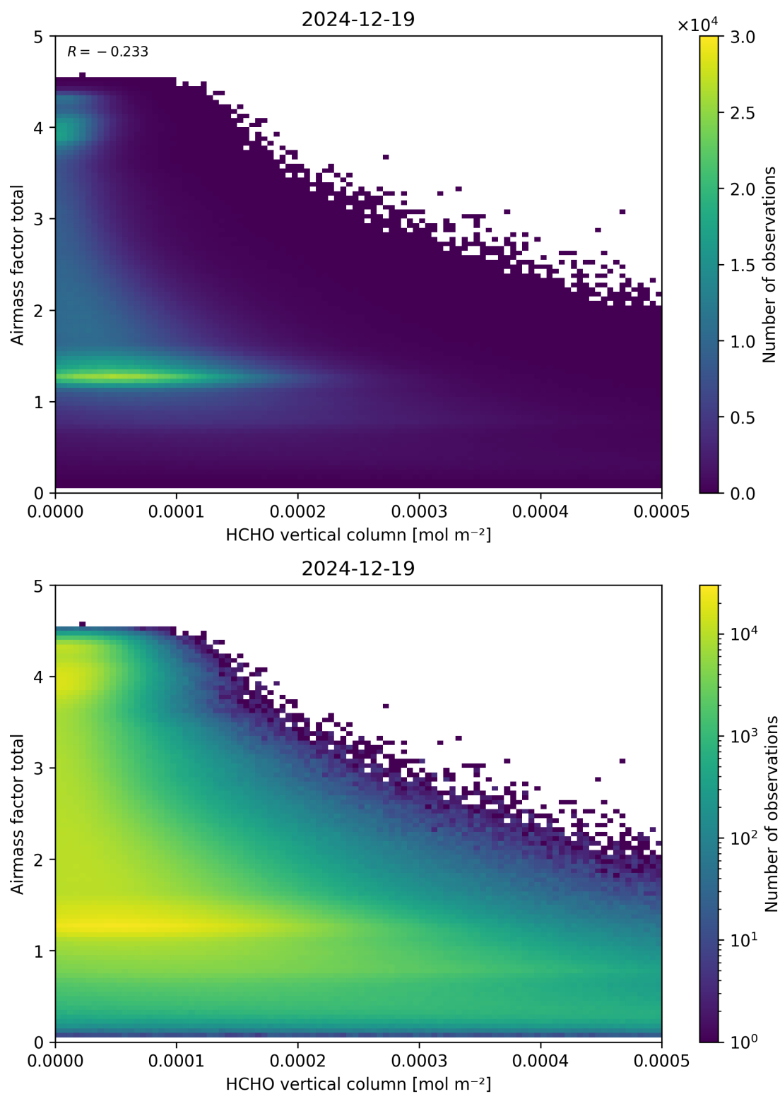
Figure 131: Scatter density plot of “HCHO vertical column” against “Airmass factor total” for 2024-12-18 to 2024-12-20.
