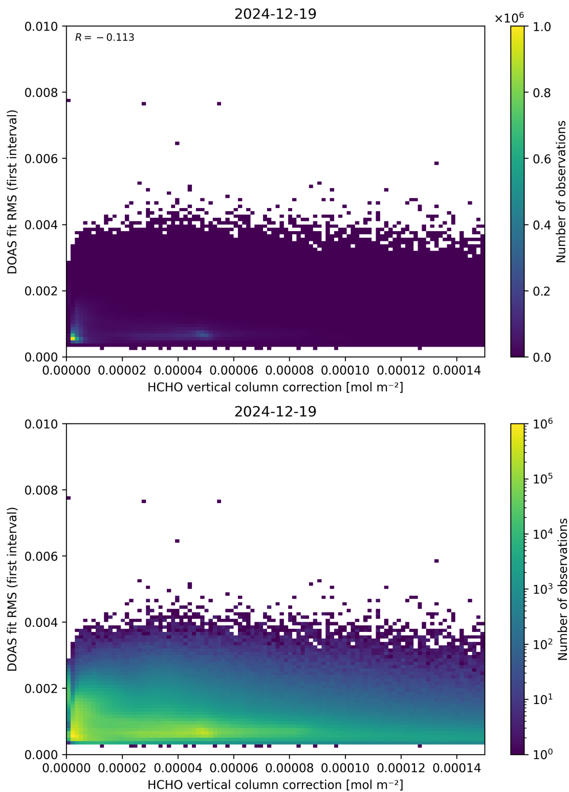
Figure 112: Scatter density plot of “HCHO vertical column correction” against “DOAS fit RMS (first interval)” for 2024-12-18 to 2024-12-20.
