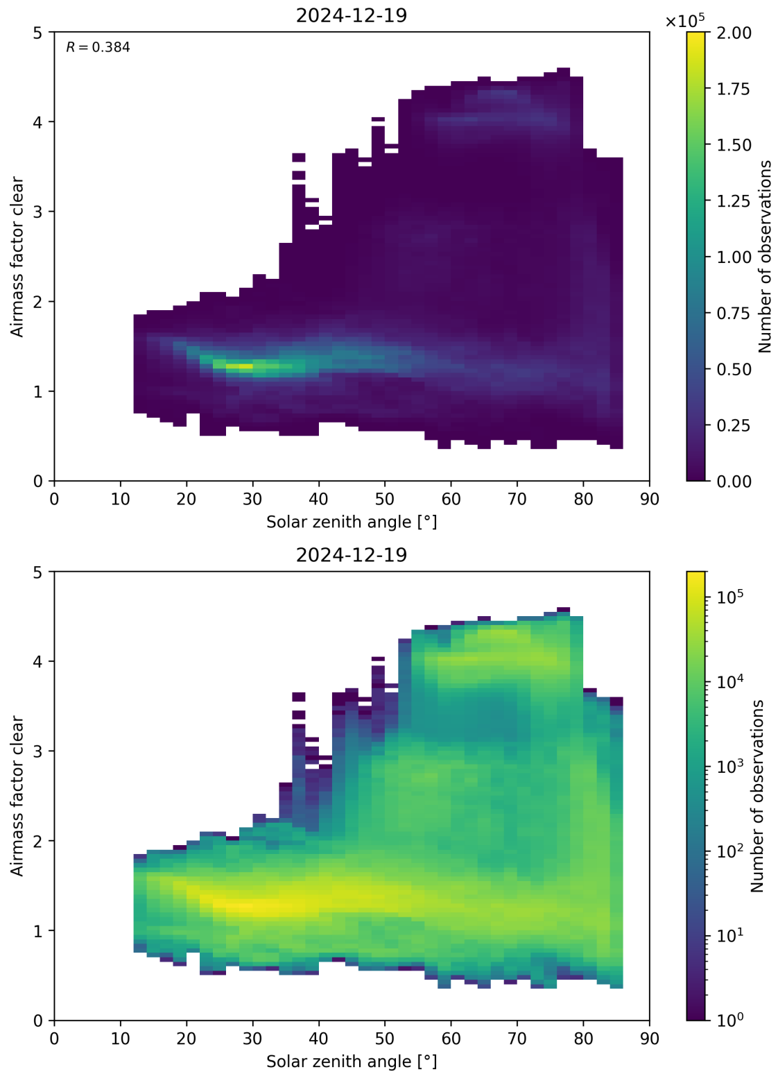
Figure 170: Scatter density plot of “Solar zenith angle” against “Airmass factor clear” for 2024-12-18 to 2024-12-20.
