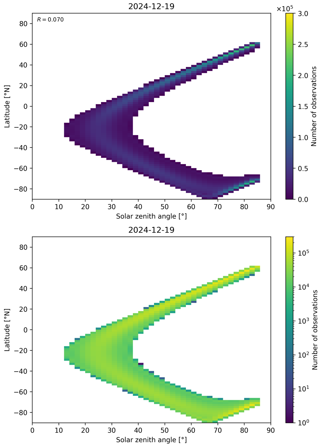
Figure 181: Scatter density plot of “Solar zenith angle” against “Latitude” for 2024-12-18 to 2024-12-20.
