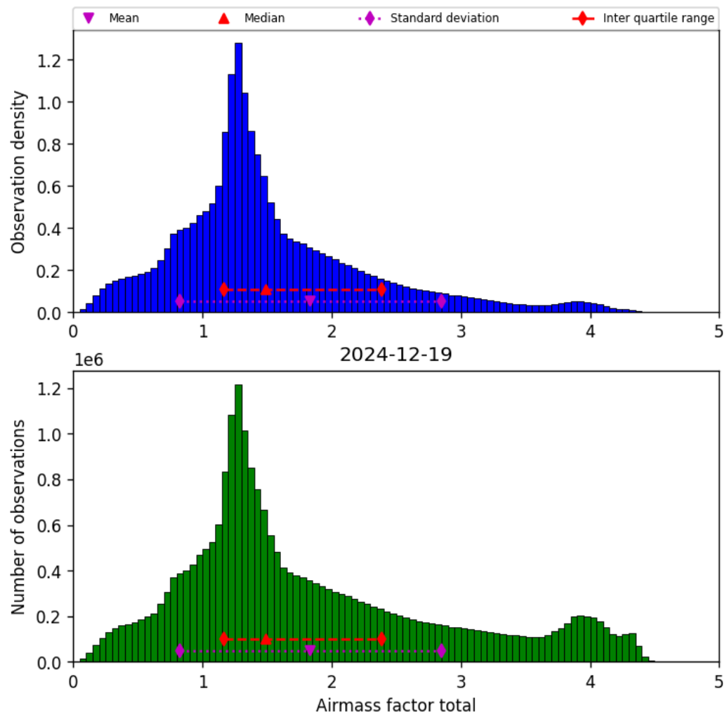
Figure 40: Histogram of “Airmass factor total” for 2024-12-18 to 2024-12-20
