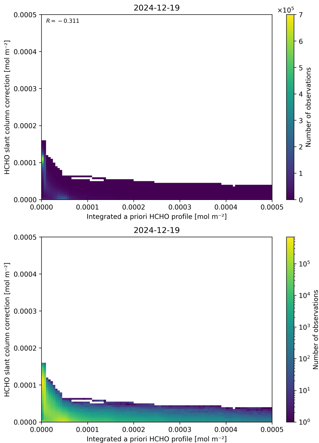
Figure 152: Scatter density plot of “Integrated a priori HCHO profile” against “HCHO slant column correction” for 2024-12-18 to 2024-12-20.
