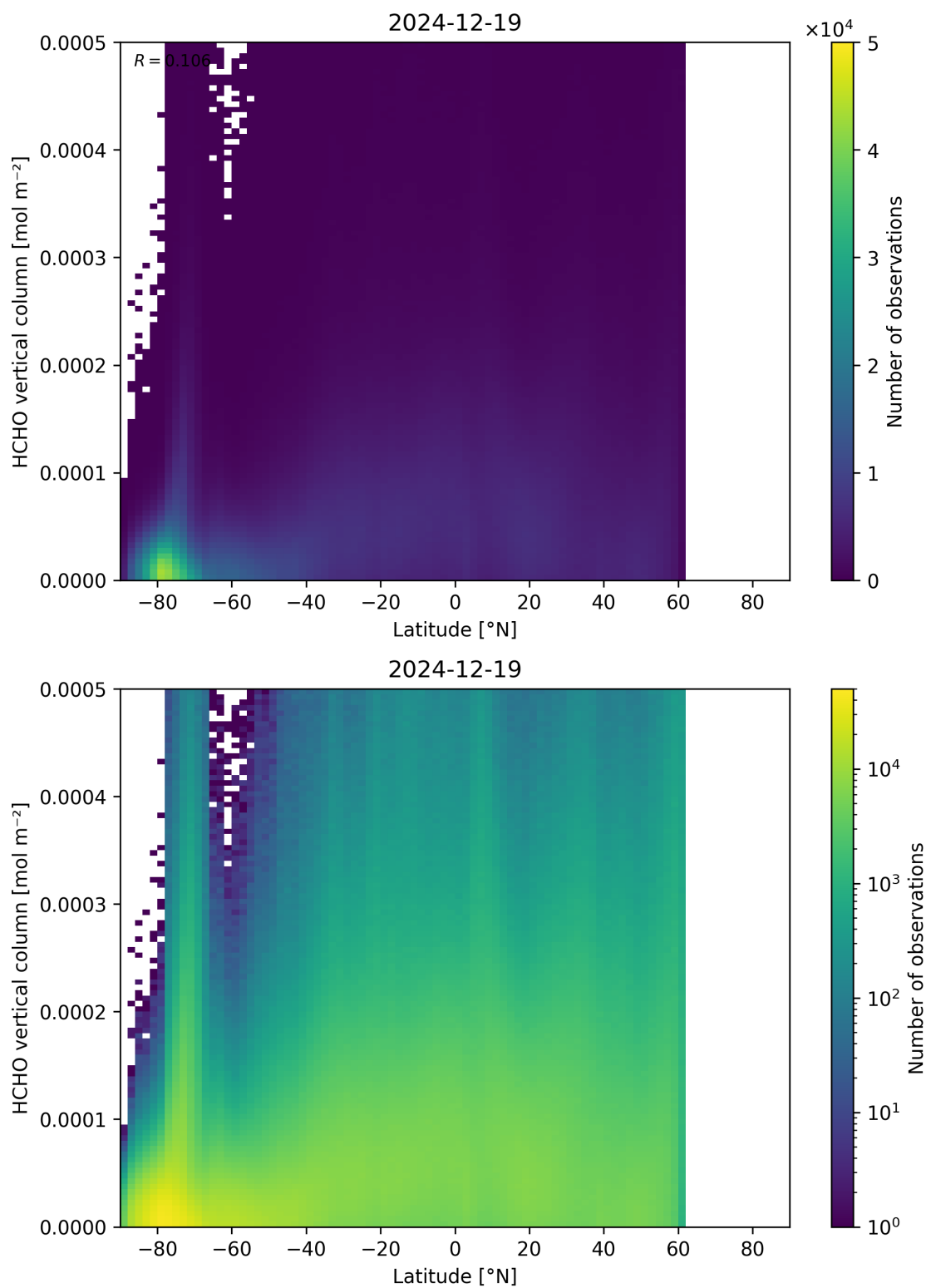
Figure 163: Scatter density plot of “Latitude” against “HCHO vertical column” for 2024-12-18 to 2024-12-20.
