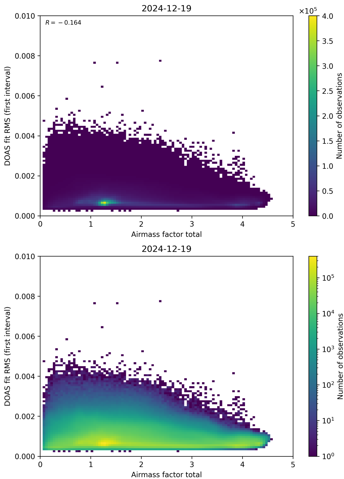
Figure 97: Scatter density plot of “Airmass factor total” against “DOAS fit RMS (first interval)” for 2024-12-18 to 2024-12-20.
