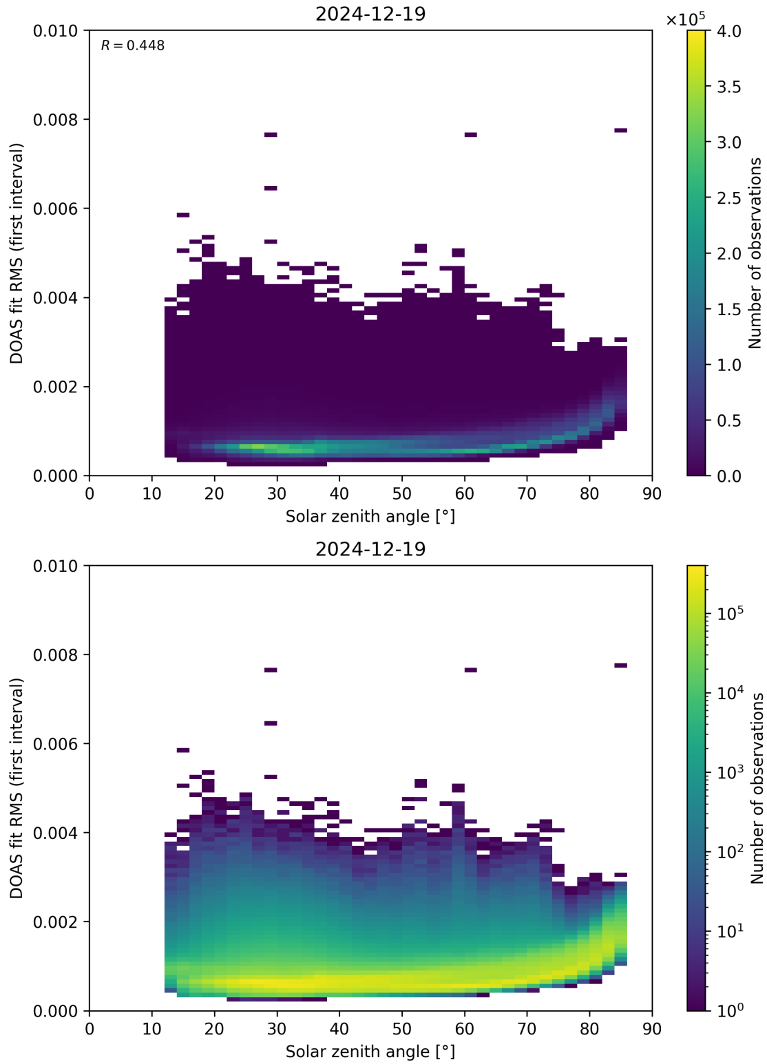
Figure 167: Scatter density plot of “Solar zenith angle” against “DOAS fit RMS (first interval)” for 2024-12-18 to 2024-12-20.
