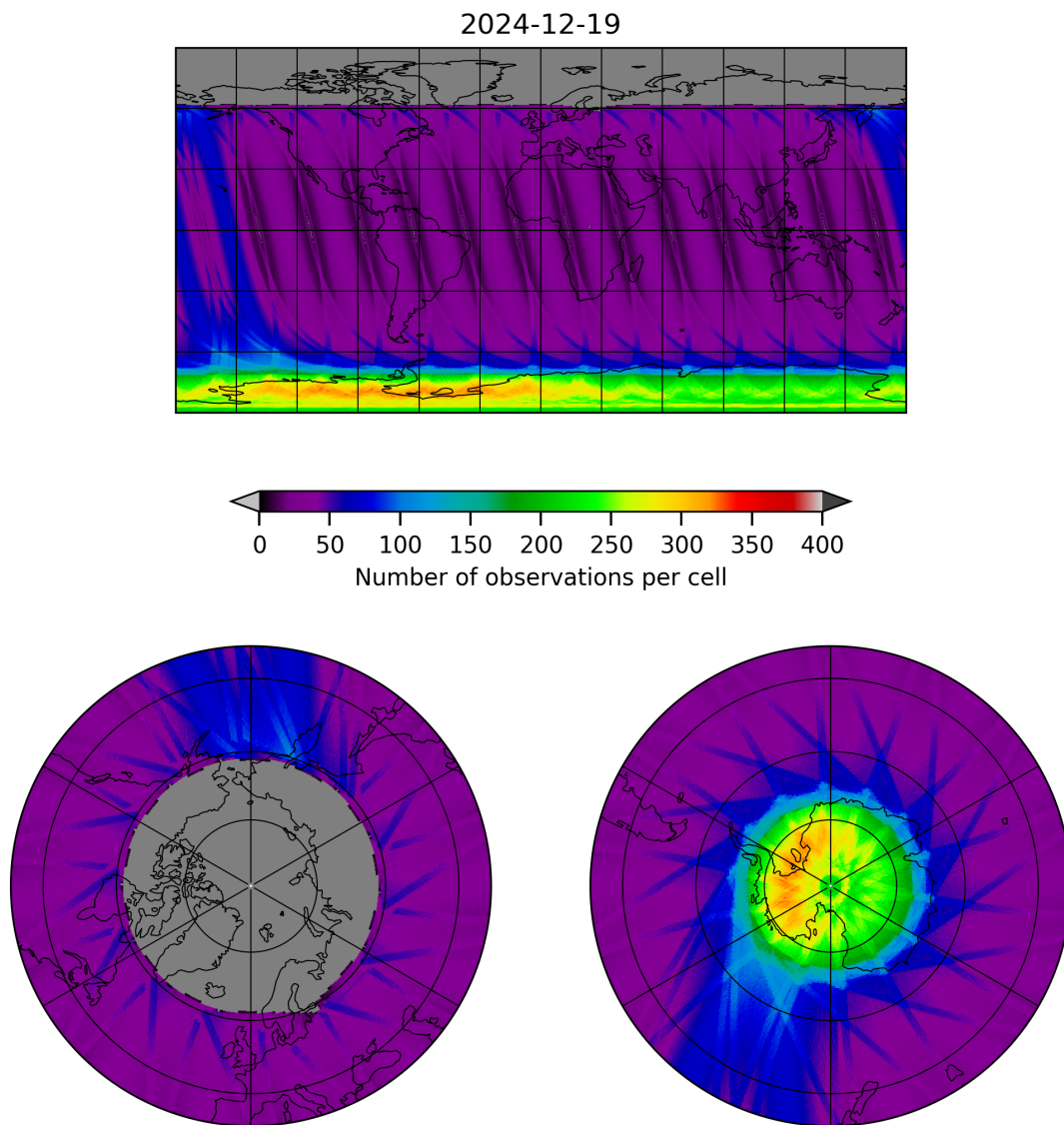
Figure 19: Map of the number of observations for 2024-12-18 to 2024-12-20
