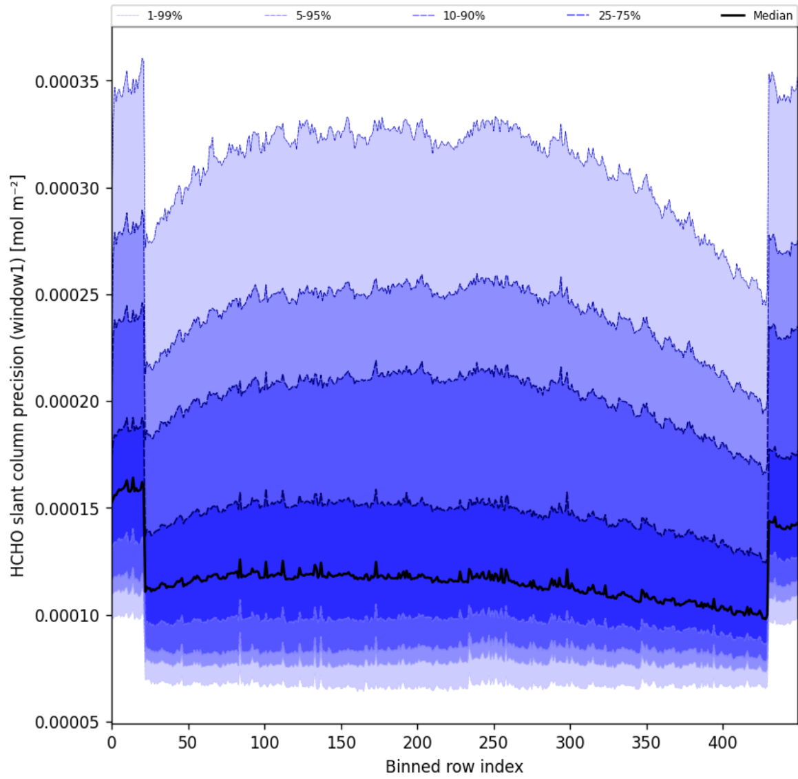
Figure 53: Along track statistics of “HCHO slant column precision (window1)” for 2024-12-18 to 2024-12-20
