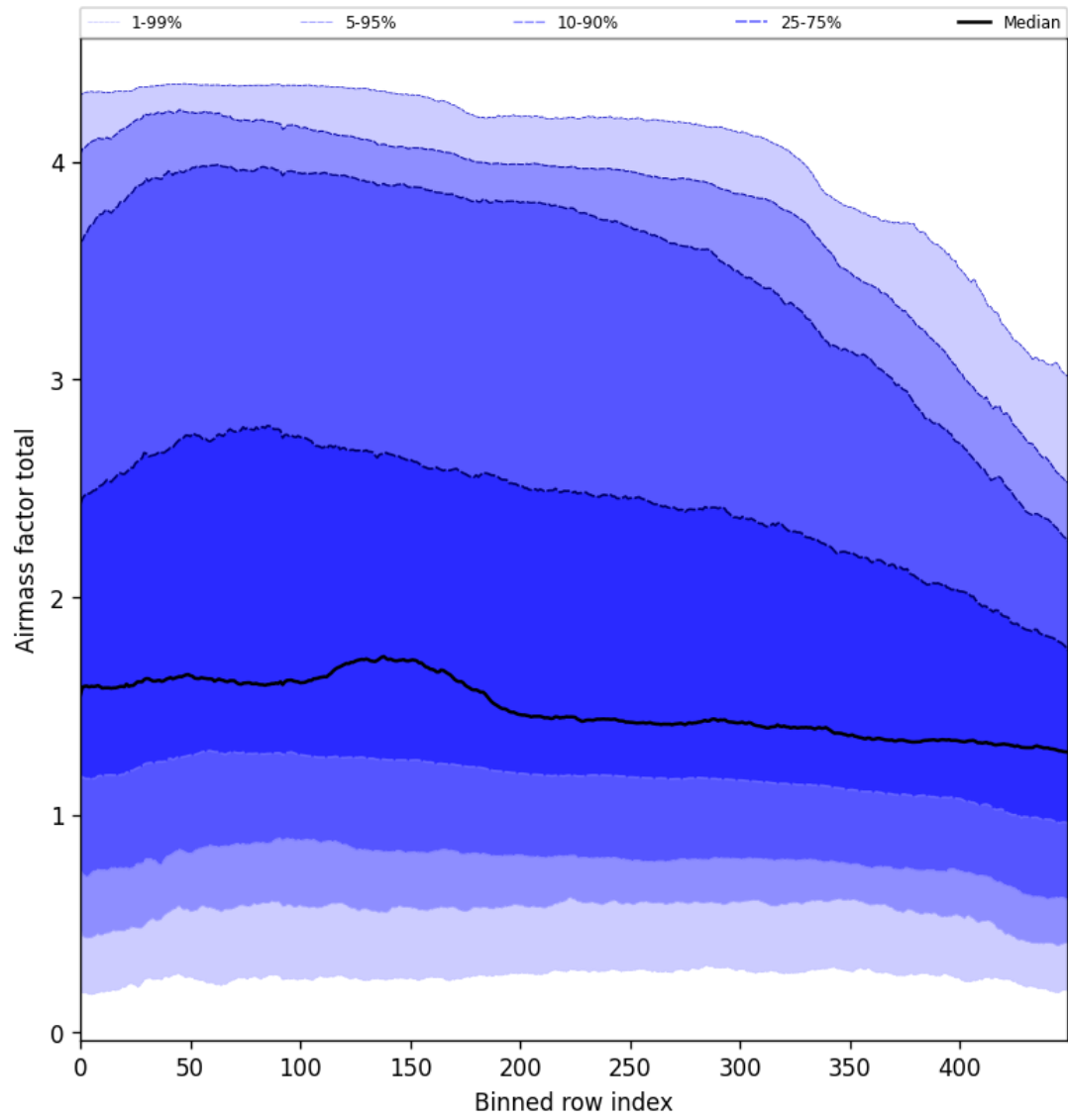
Figure 54: Along track statistics of “Airmass factor total” for 2024-12-18 to 2024-12-20
