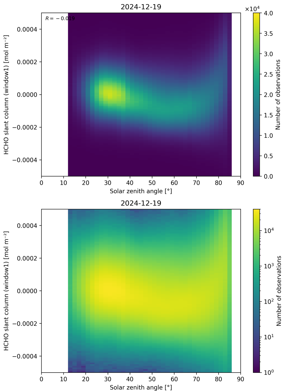
Figure 173: Scatter density plot of “Solar zenith angle” against “HCHO slant column (window1)” for 2024-12-18 to 2024-12-20.
