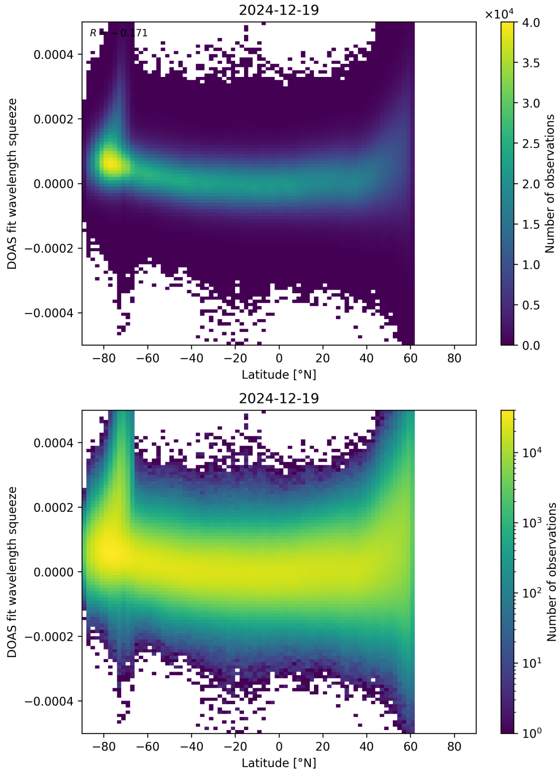
Figure 155: Scatter density plot of “Latitude” against “DOAS fit wavelength squeeze” for 2024-12-18 to 2024-12-20.
