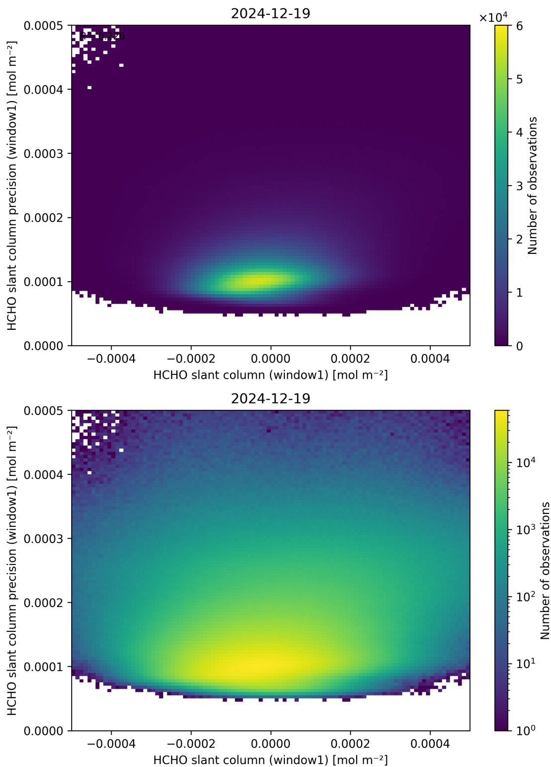
Figure 84: Scatter density plot of “HCHO slant column (window1)” against “HCHO slant column precision (window1)” for 2024-12-18 to 2024-12-20.
