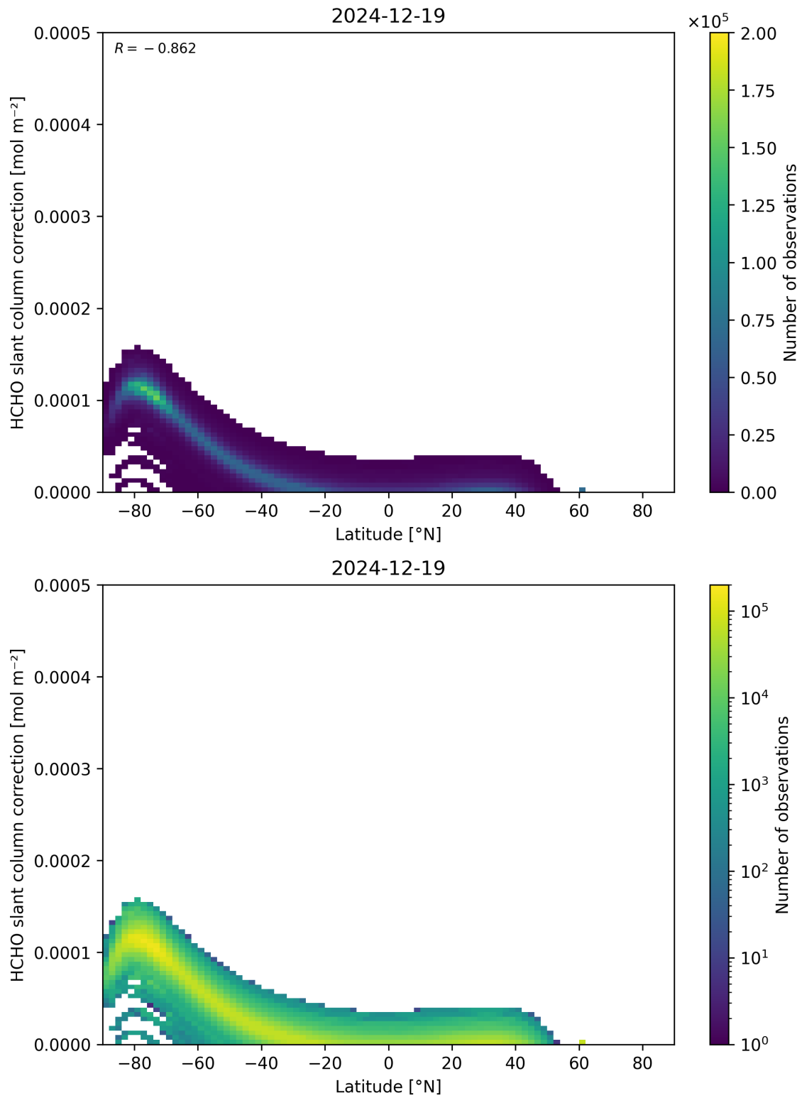
Figure 158: Scatter density plot of “Latitude” against “HCHO slant column correction” for 2024-12-18 to 2024-12-20.
