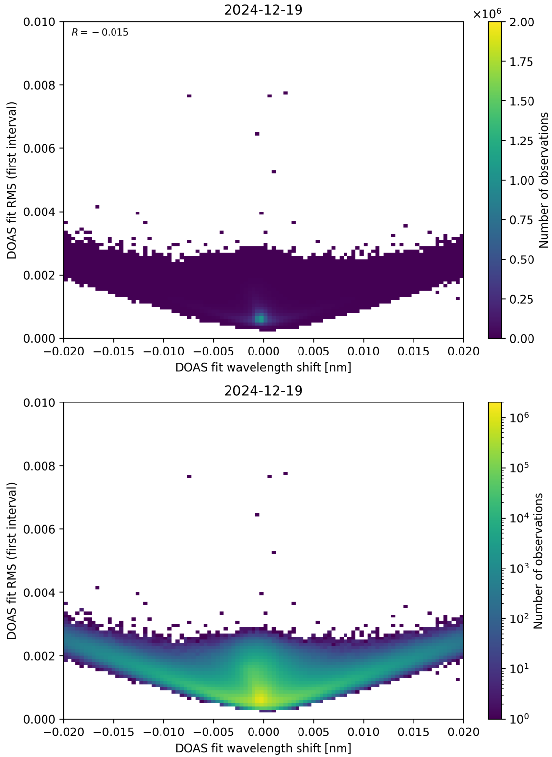
Figure 64: Scatter density plot of “DOAS fit wavelength shift” against “DOAS fit RMS (first interval)” for 2024-12-18 to 2024-12-20.
