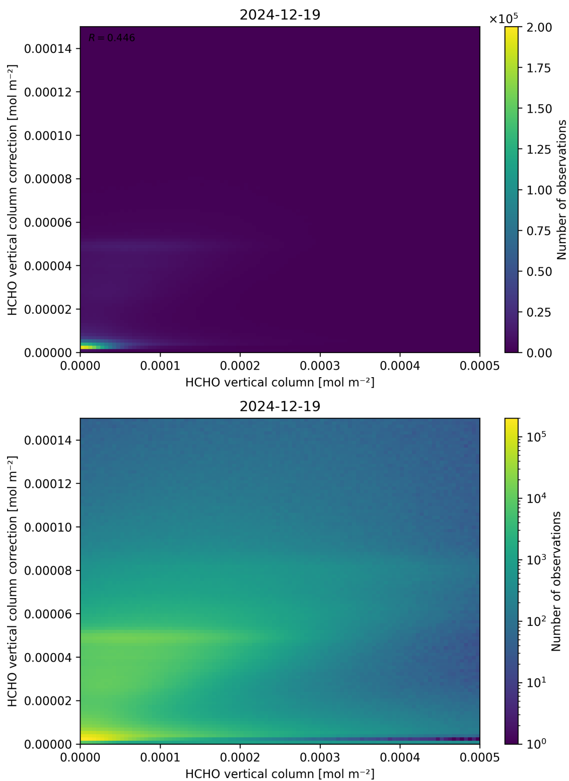
Figure 133: Scatter density plot of “HCHO vertical column” against “HCHO vertical column correction” for 2024-12-18 to 2024-12-20.
