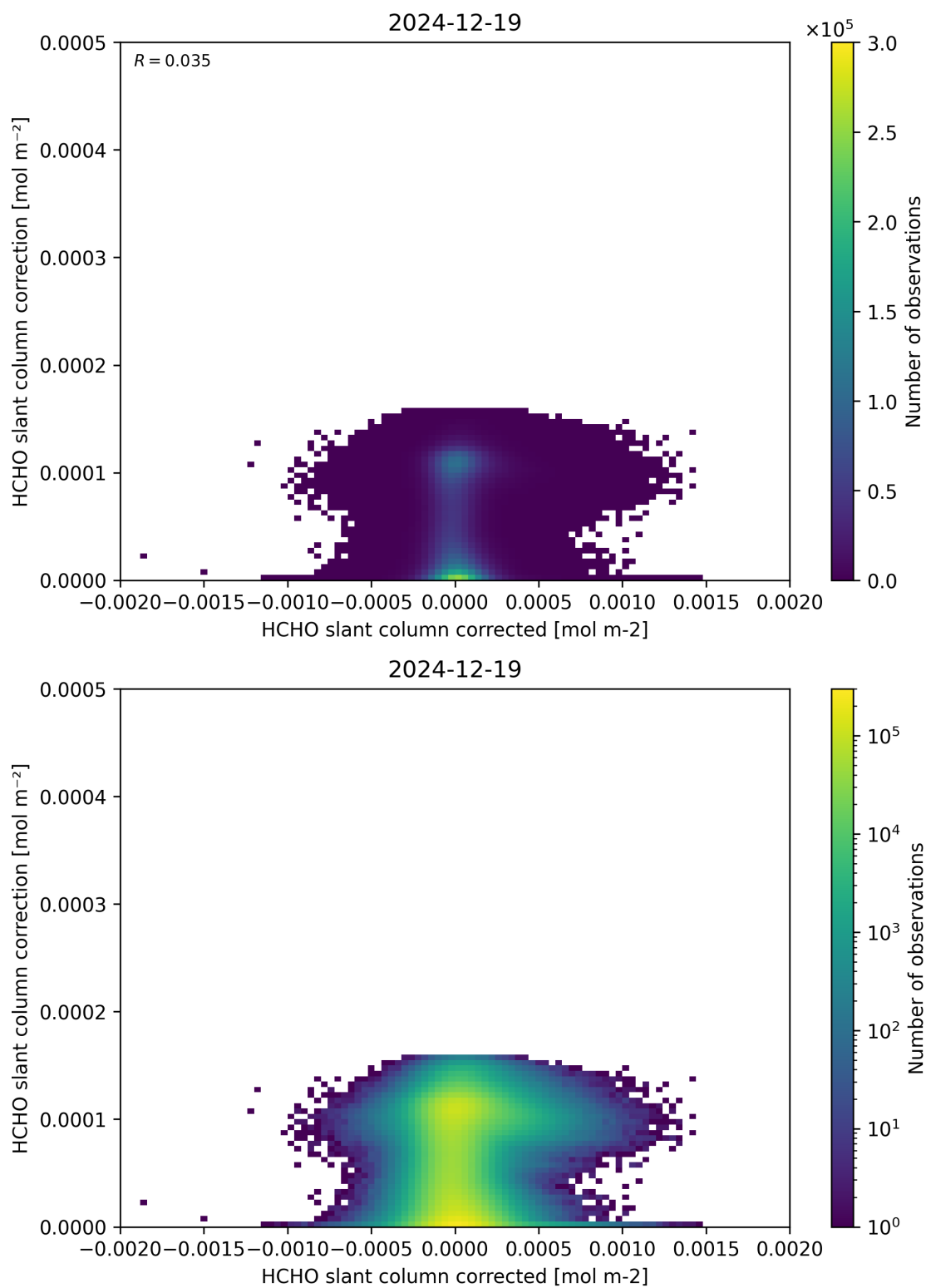
Figure 77: Scatter density plot of “HCHO slant column corrected” against “HCHO slant column correction” for 2024-12-18 to 2024-12-20.
