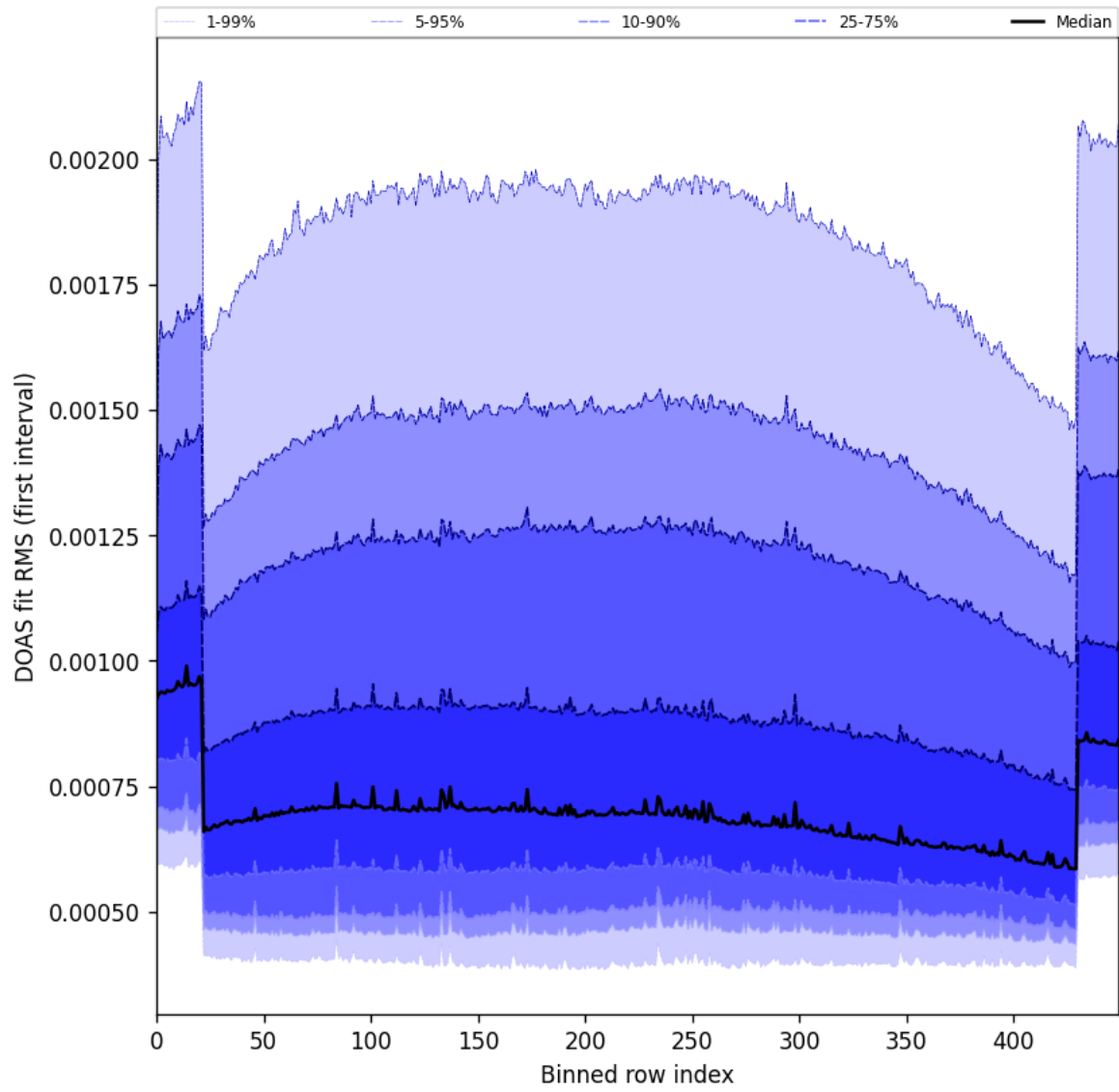
Figure 60: Along track statistics of “DOAS fit RMS (first interval)” for 2024-12-18 to 2024-12-20
