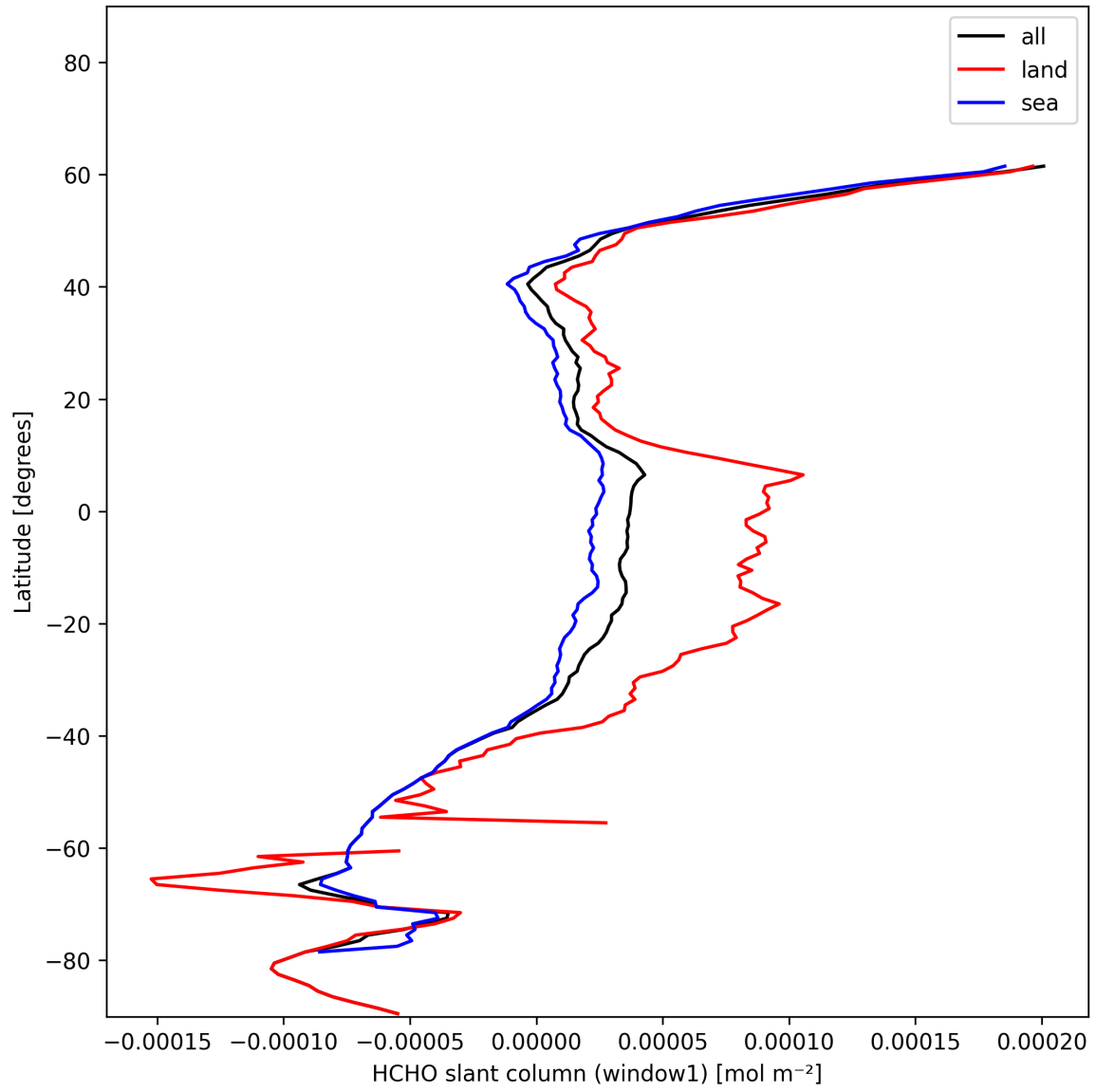
Figure 24: Zonal average of “HCHO slant column (window1)” for 2024-12-18 to 2024-12-20.
