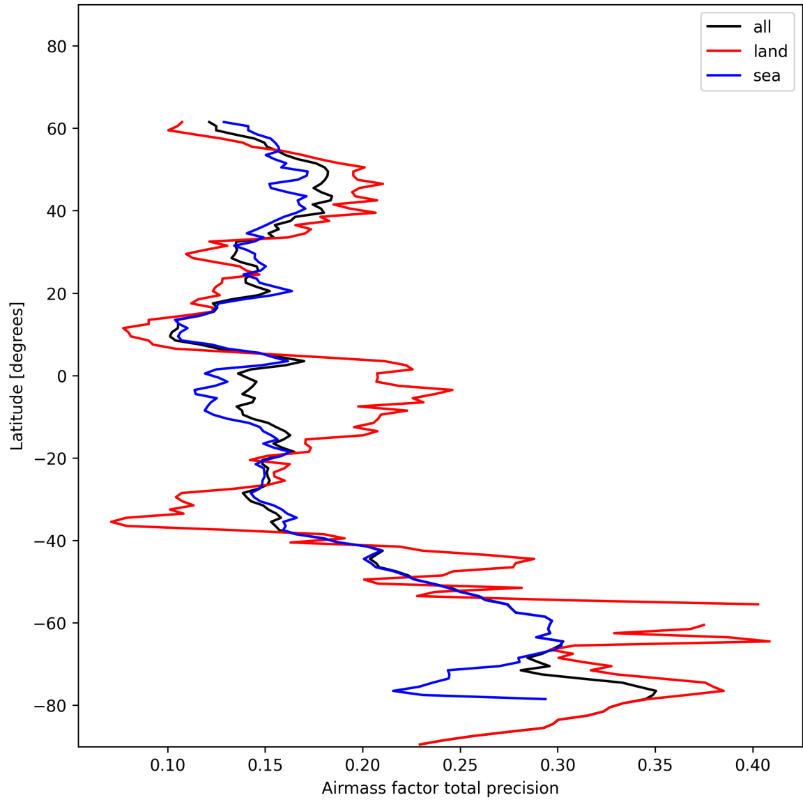
Figure 27: Zonal average of “Airmass factor total precision” for 2024-12-18 to 2024-12-20.
