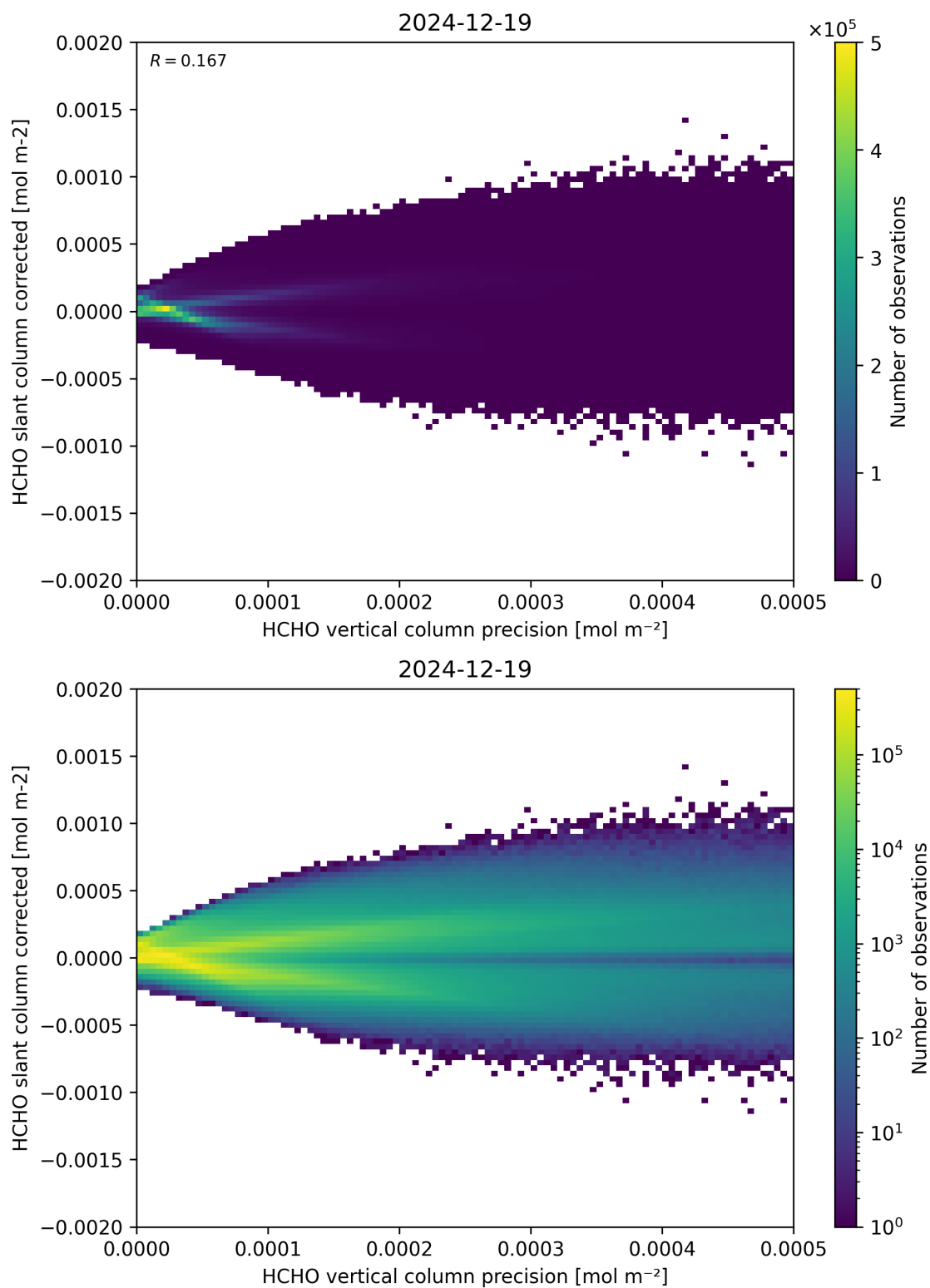
Figure 140: Scatter density plot of “HCHO vertical column precision” against “HCHO slant column corrected” for 2024-12-18 to 2024-12-20.
