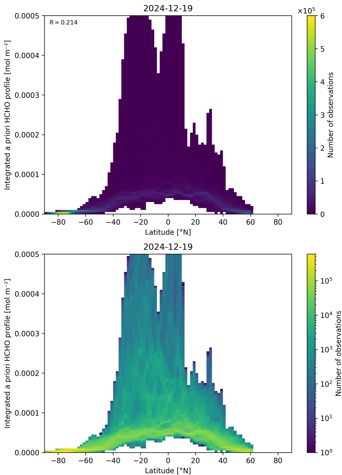
Figure 166: Scatter density plot of “Latitude” against “Integrated a priori HCHO profile” for 2024-12-18 to 2024-12-20.
