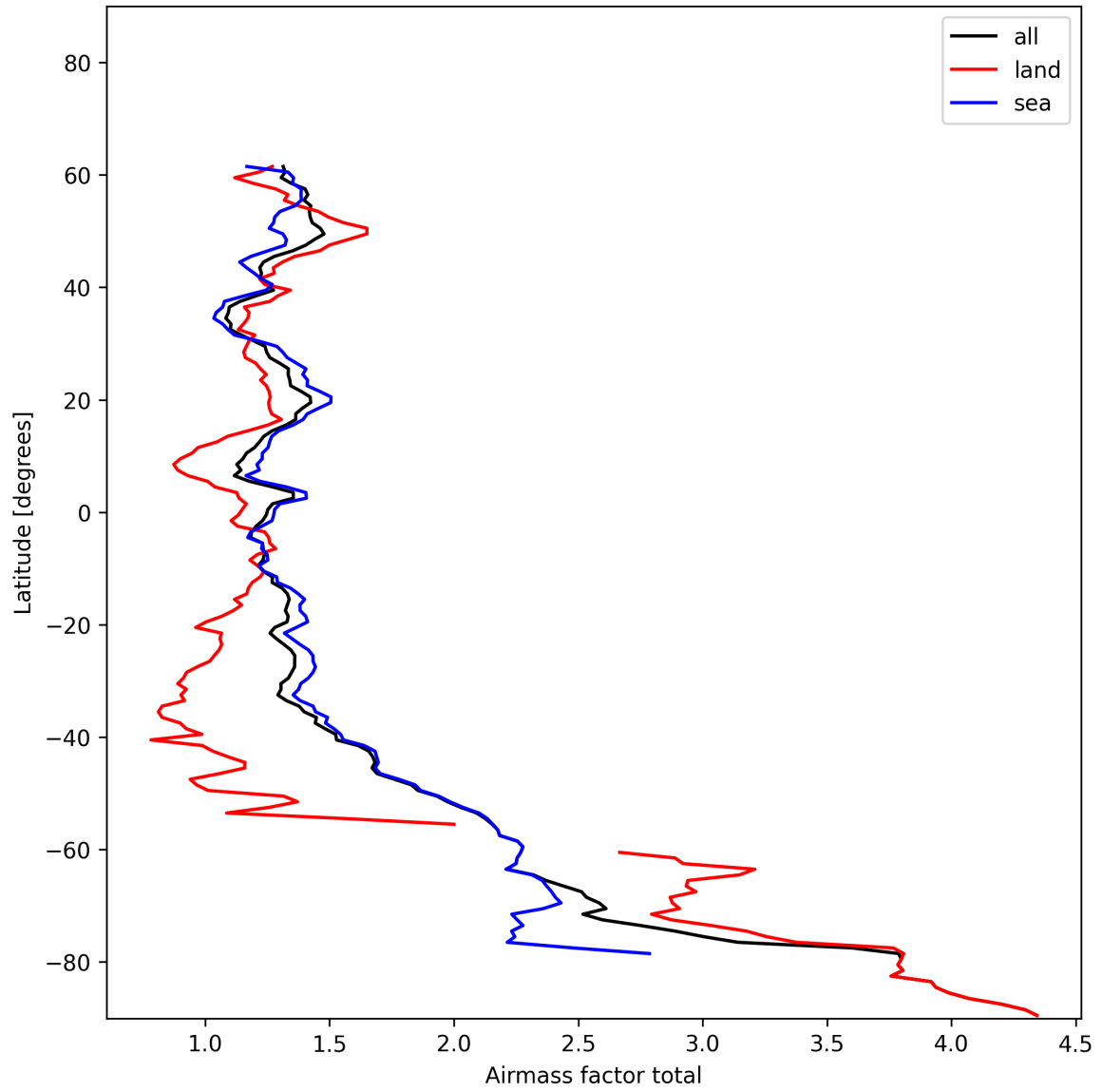
Figure 26: Zonal average of “Airmass factor total” for 2024-12-18 to 2024-12-20.
