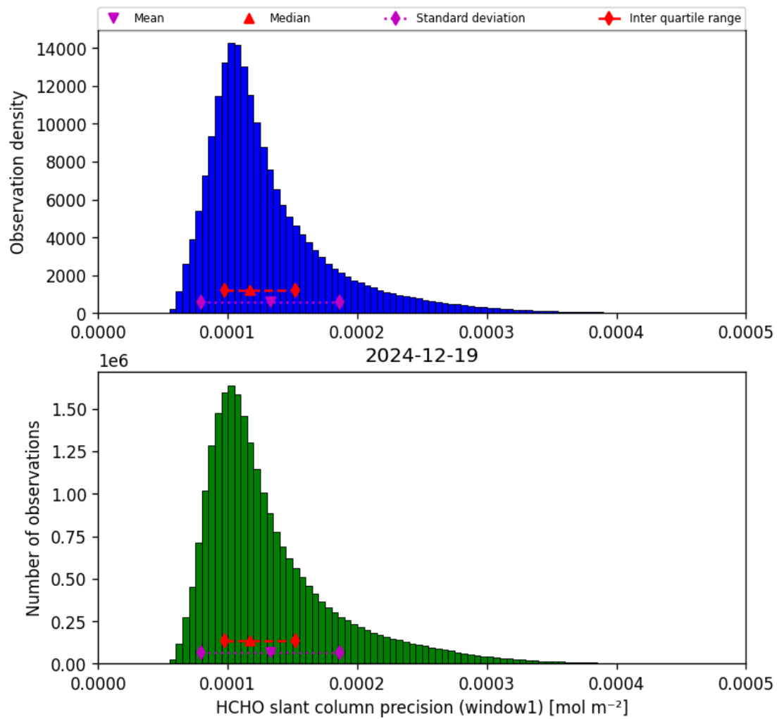
Figure 39: Histogram of “HCHO slant column precision (window1)” for 2024-12-18 to 2024-12-20
