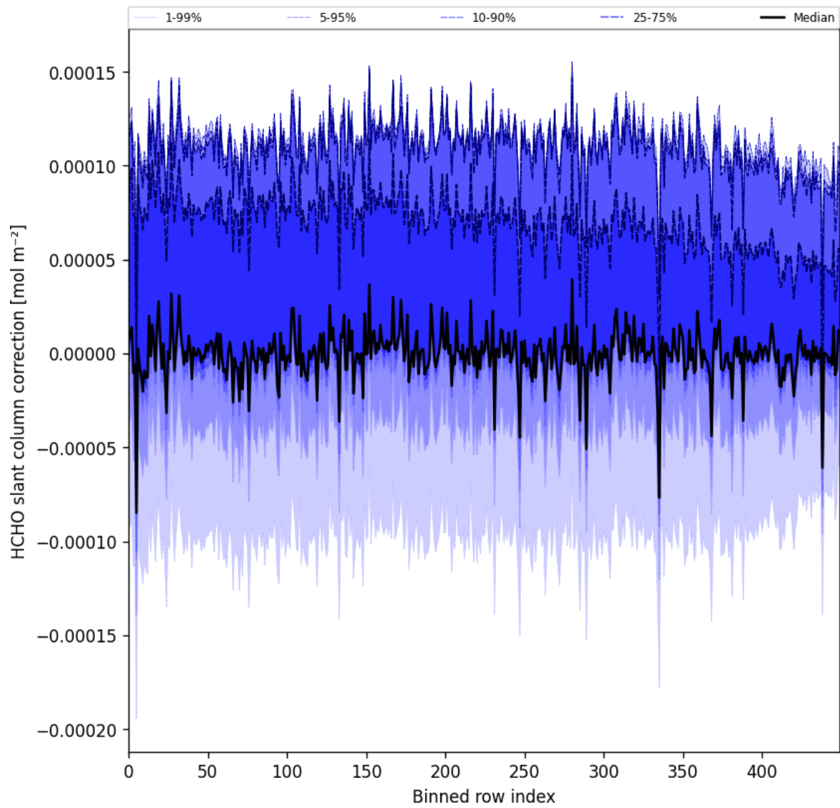
Figure 61: Along track statistics of “HCHO slant column correction” for 2024-12-18 to 2024-12-20
