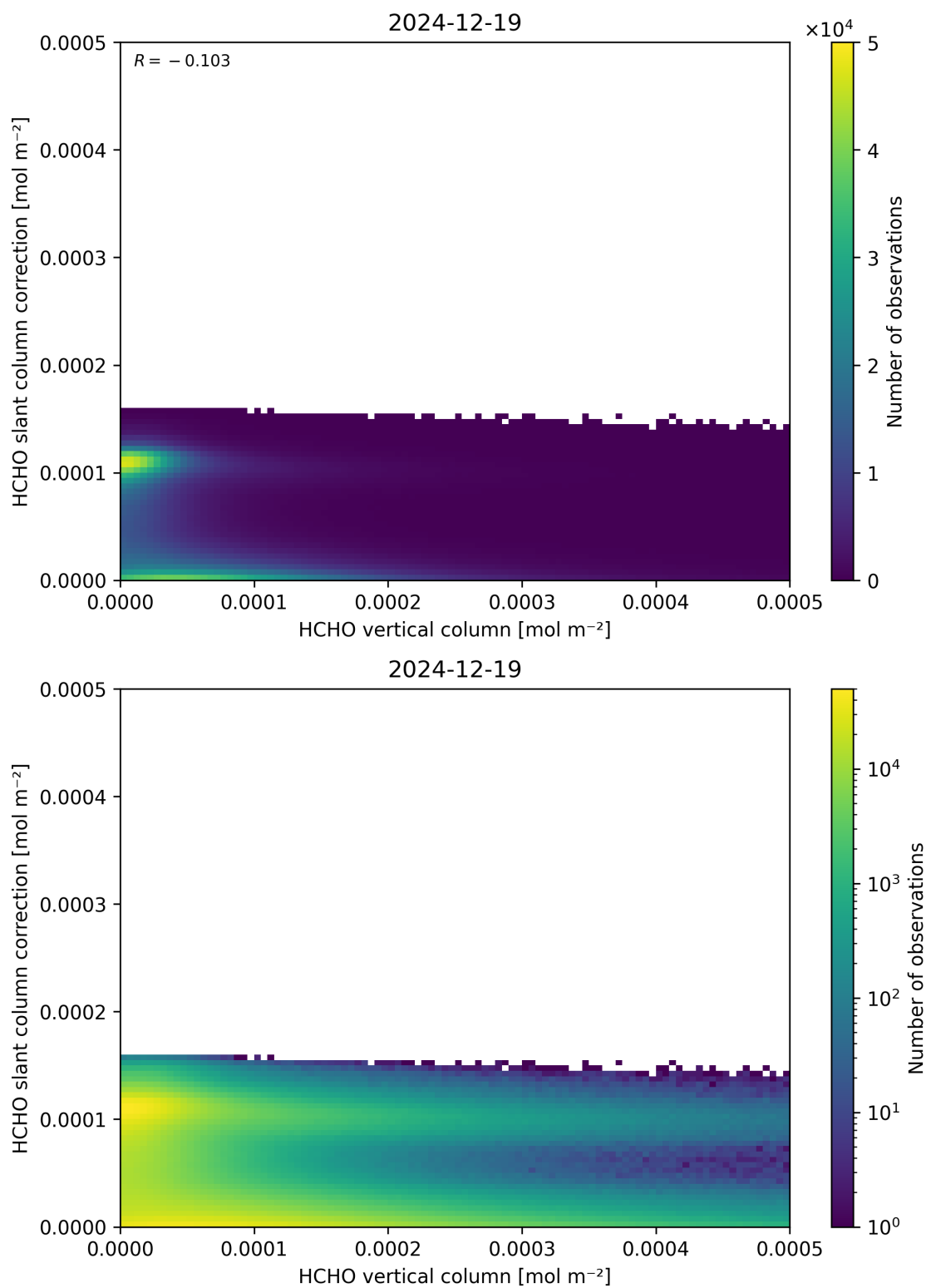
Figure 128: Scatter density plot of “HCHO vertical column” against “HCHO slant column correction” for 2024-12-18 to 2024-12-20.
