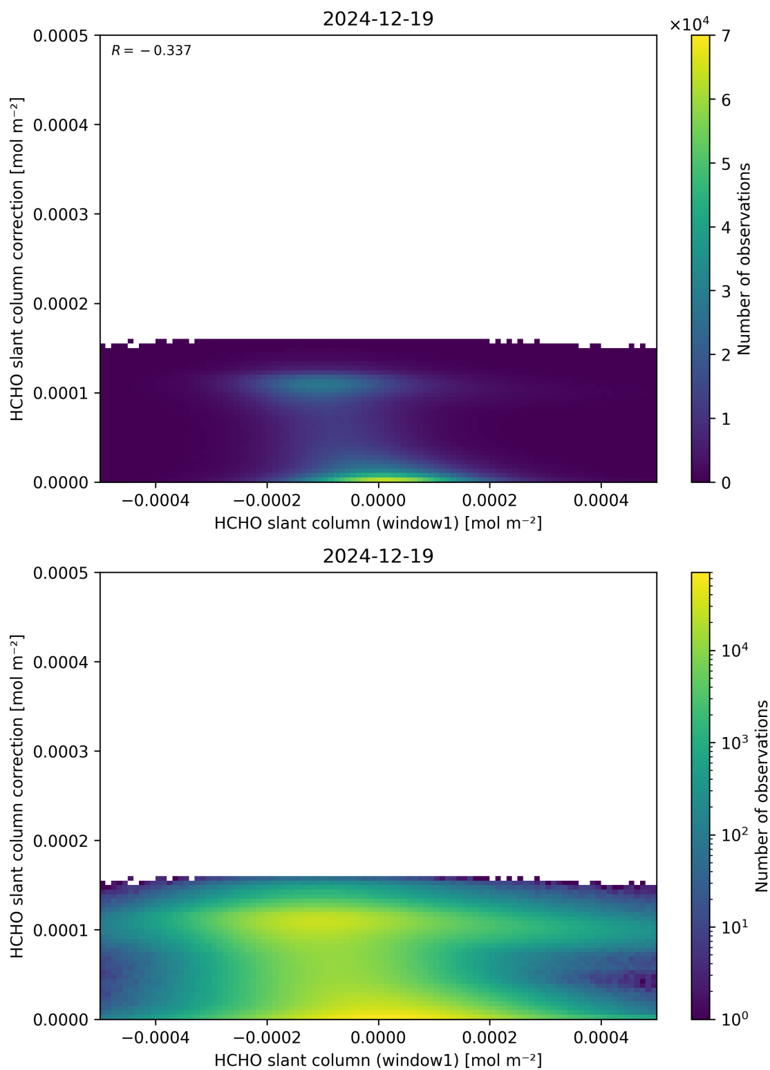
Figure 83: Scatter density plot of “HCHO slant column (window1)” against “HCHO slant column correction” for 2024-12-18 to 2024-12-20.
