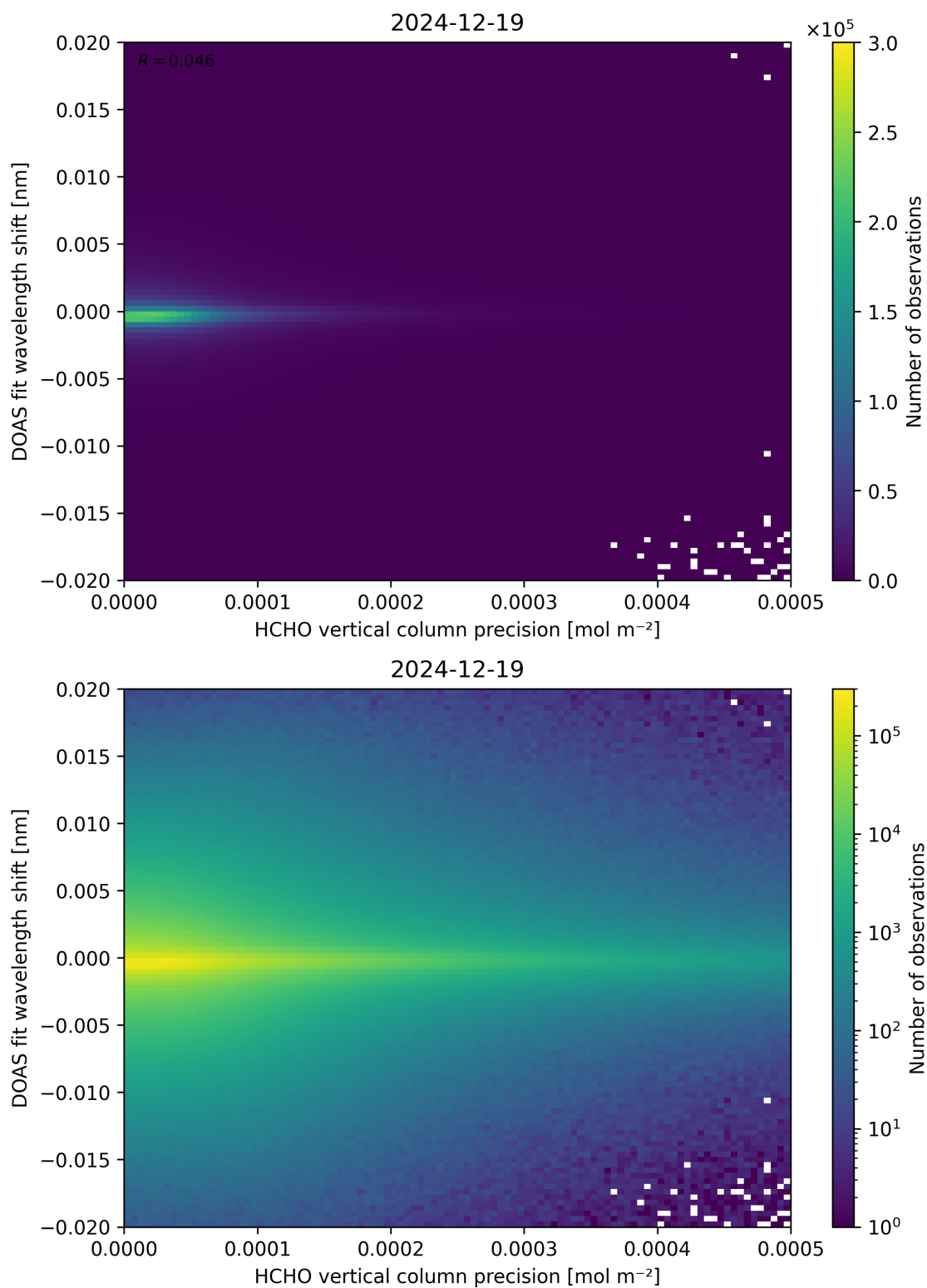
Figure 137: Scatter density plot of “HCHO vertical column precision” against “DOAS fit wavelength shift” for 2024-12-18 to 2024-12-20.
