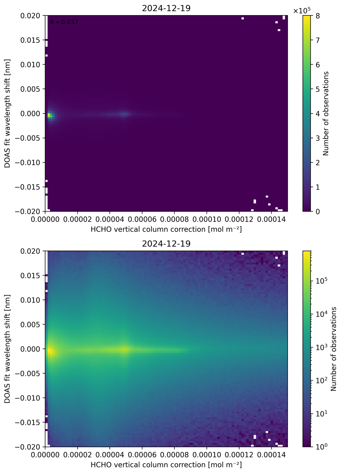
Figure 113: Scatter density plot of “HCHO vertical column correction” against “DOAS fit wavelength shift” for 2024-12-18 to 2024-12-20.
