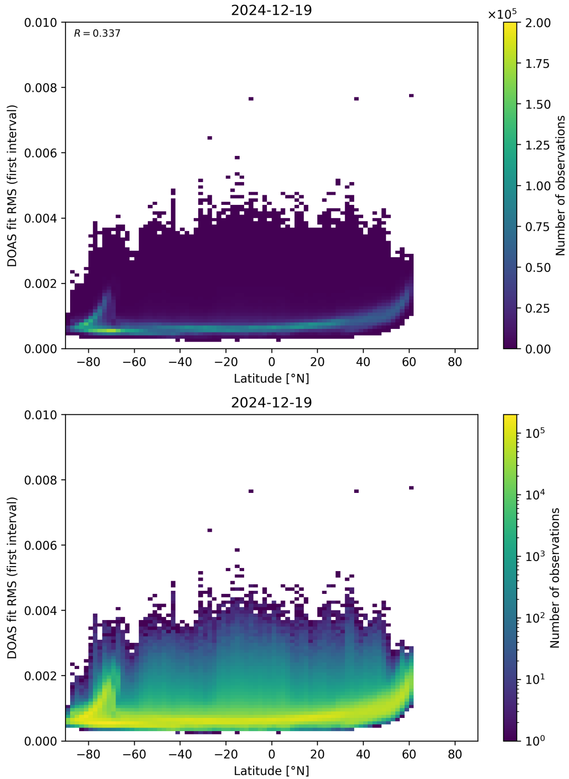
Figure 153: Scatter density plot of “Latitude” against “DOAS fit RMS (first interval)” for 2024-12-18 to 2024-12-20.
