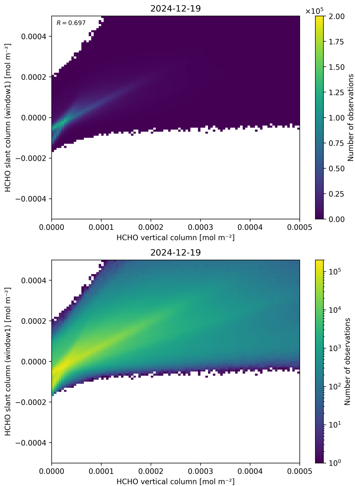
Figure 129: Scatter density plot of “HCHO vertical column” against “HCHO slant column (window1)” for 2024-12-18 to 2024-12-20.
