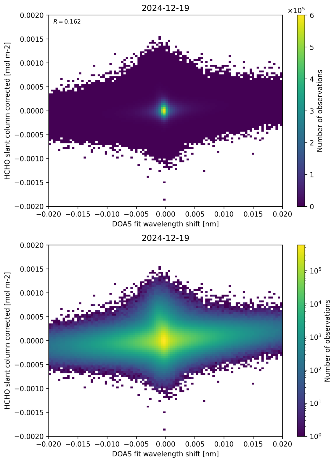
Figure 66: Scatter density plot of “DOAS fit wavelength shift” against “HCHO slant column corrected” for 2024-12-18 to 2024-12-20.
