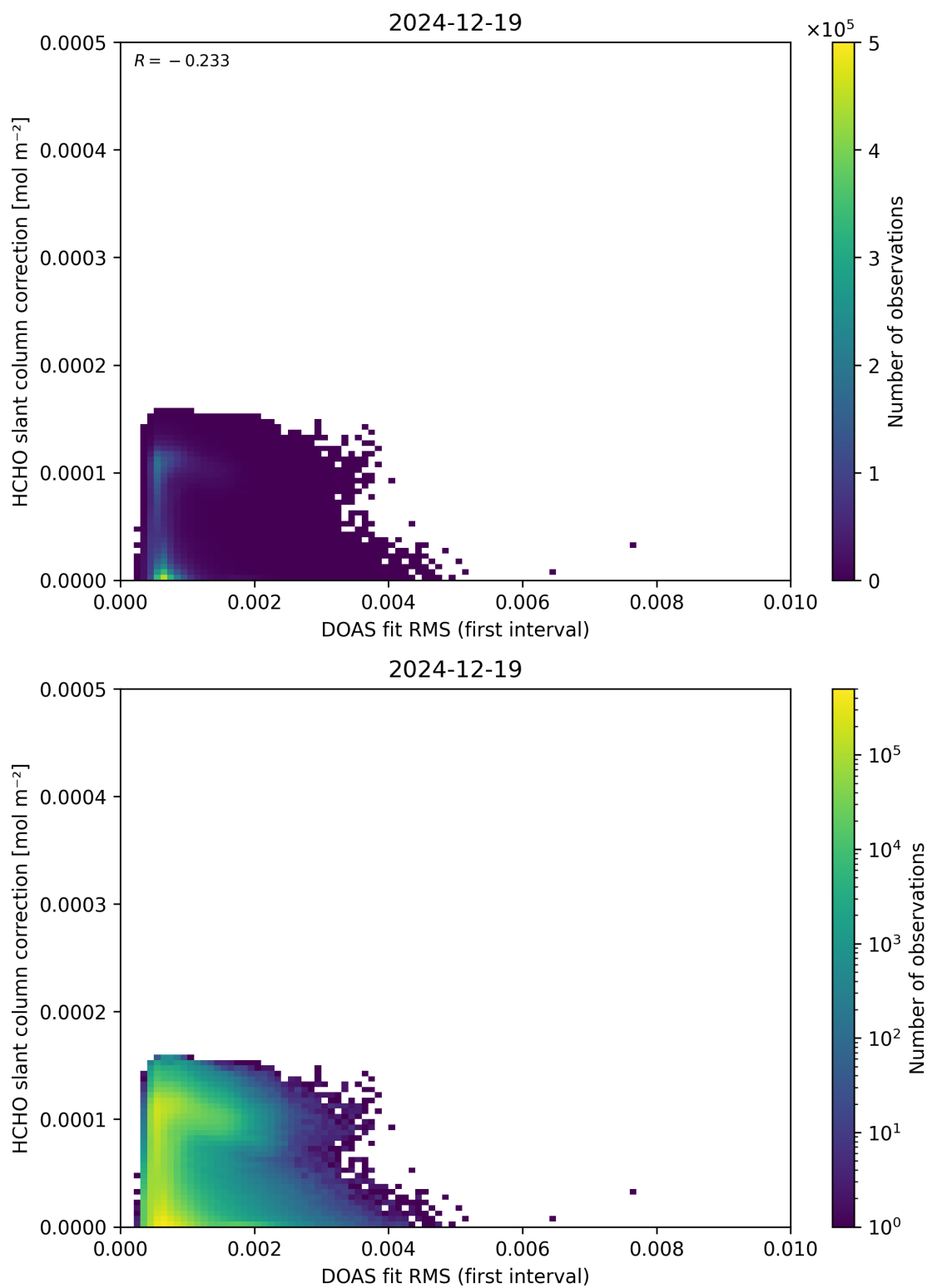
Figure 63: Scatter density plot of “DOAS fit RMS (first interval)” against “HCHO slant column correction” for 2024-12-18 to 2024-12-20.
