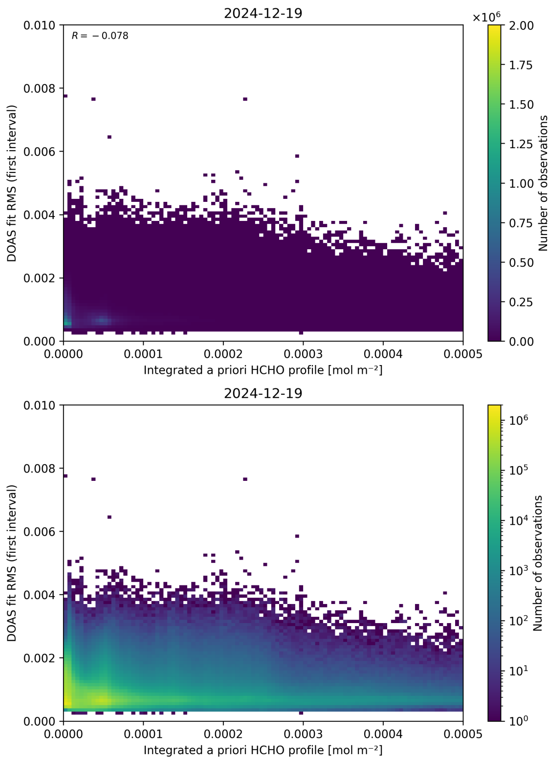
Figure 148: Scatter density plot of “Integrated a priori HCHO profile” against “DOAS fit RMS (first interval)” for 2024-12-18 to 2024-12-20.
