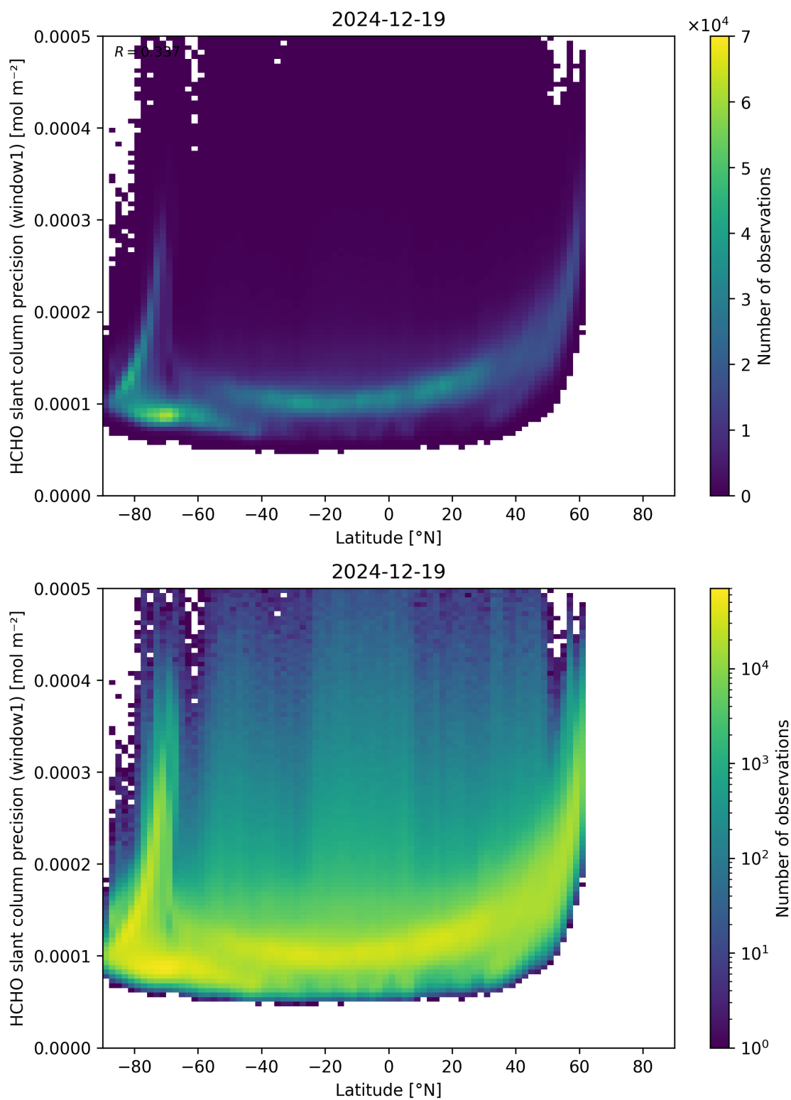
Figure 160: Scatter density plot of “Latitude” against “HCHO slant column precision (window1)” for 2024-12-18 to 2024-12-20.
