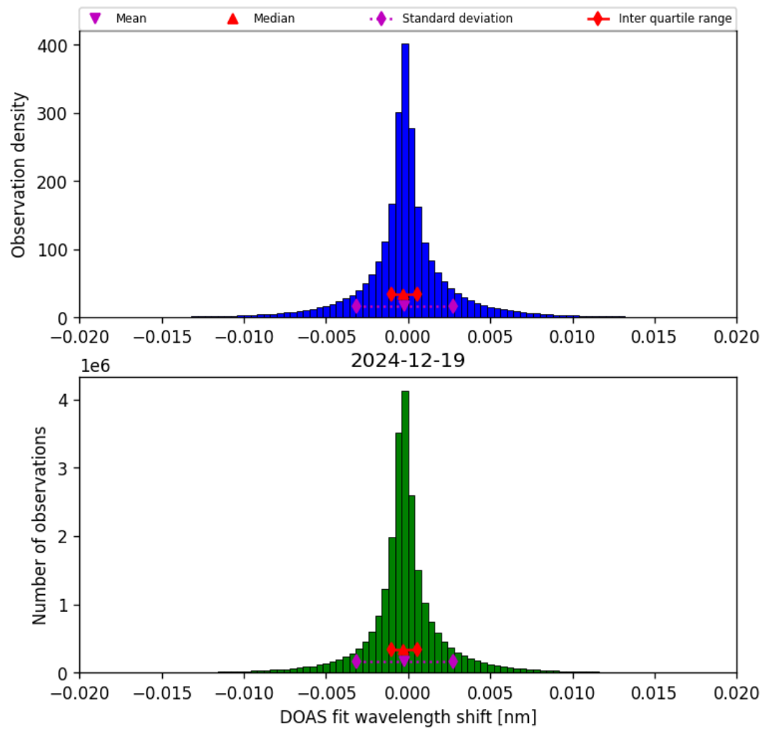
Figure 44: Histogram of “DOAS fit wavelength shift” for 2024-12-18 to 2024-12-20
