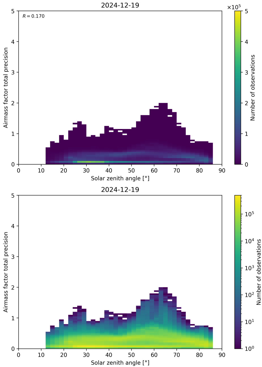
Figure 176: Scatter density plot of “Solar zenith angle” against “Airmass factor total precision” for 2024-12-18 to 2024-12-20.
