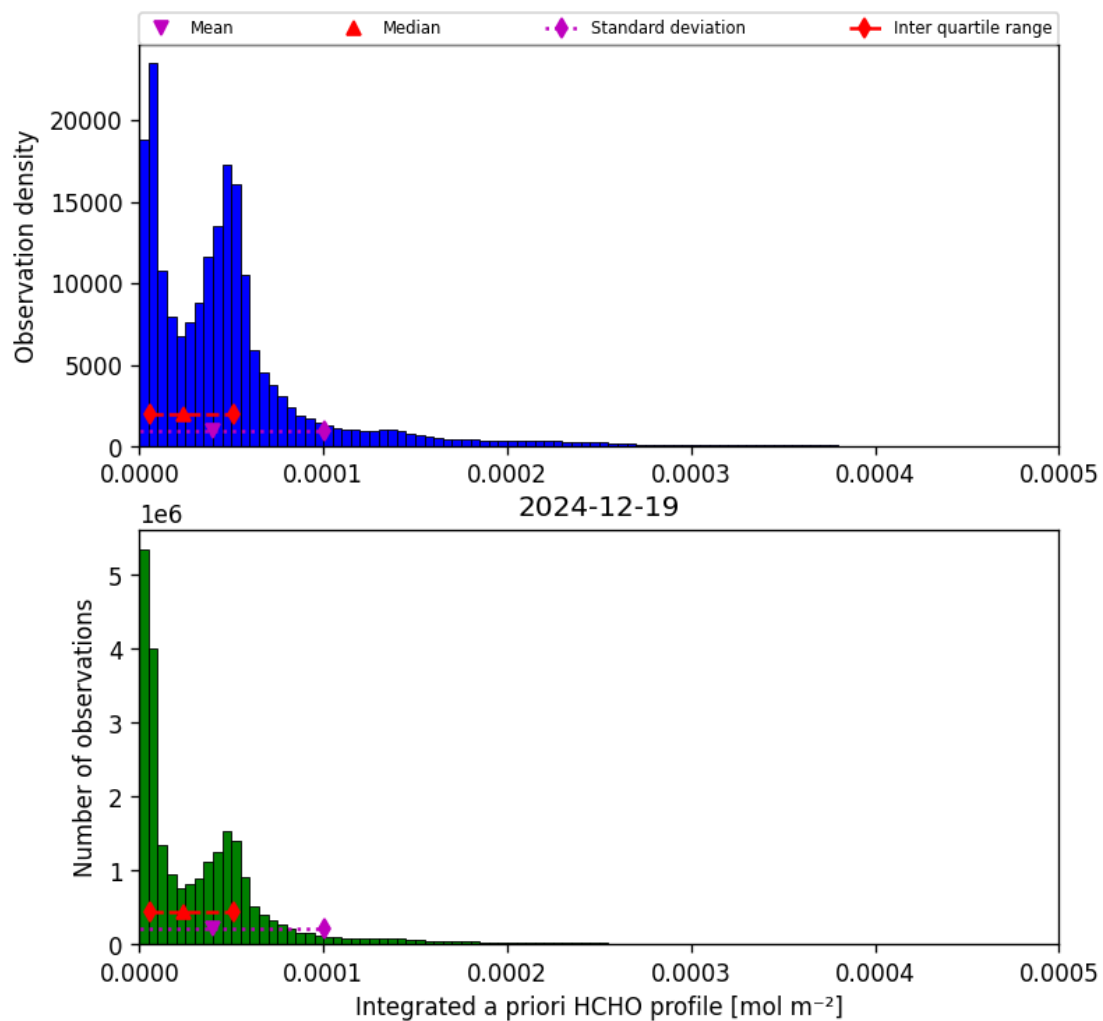
Figure 43: Histogram of “Integrated a priori HCHO profile” for 2024-12-18 to 2024-12-20
