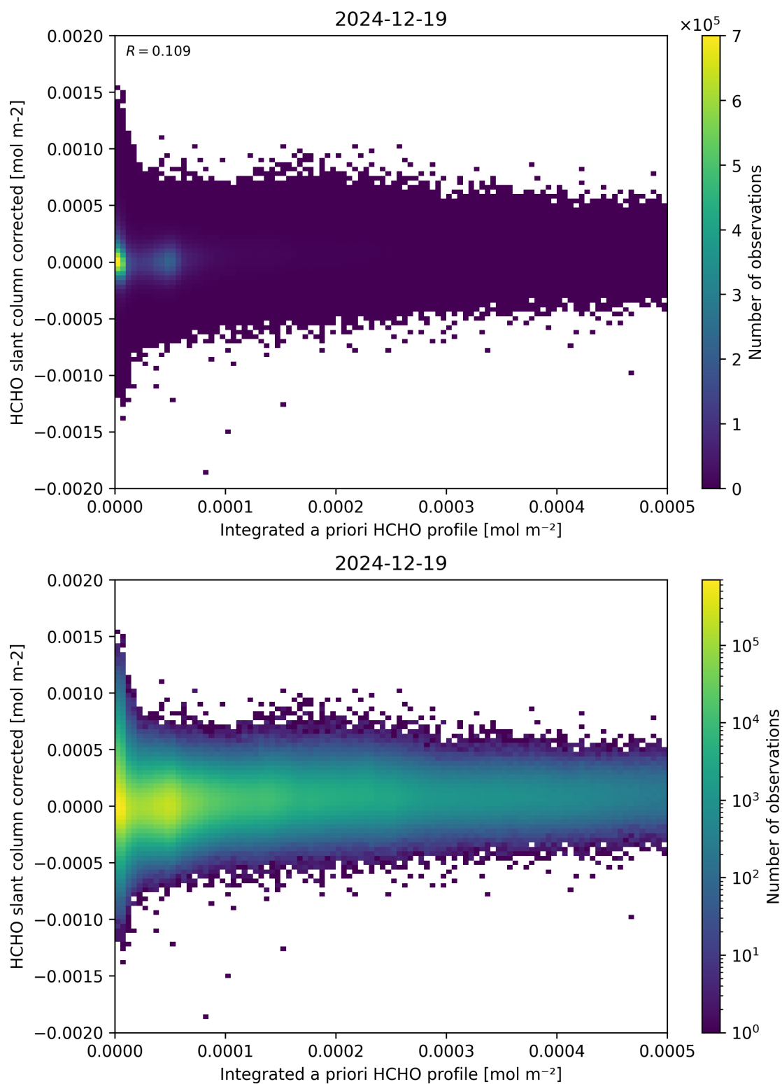
Figure 151: Scatter density plot of “Integrated a priori HCHO profile” against “HCHO slant column corrected” for 2024-12-18 to 2024-12-20.
