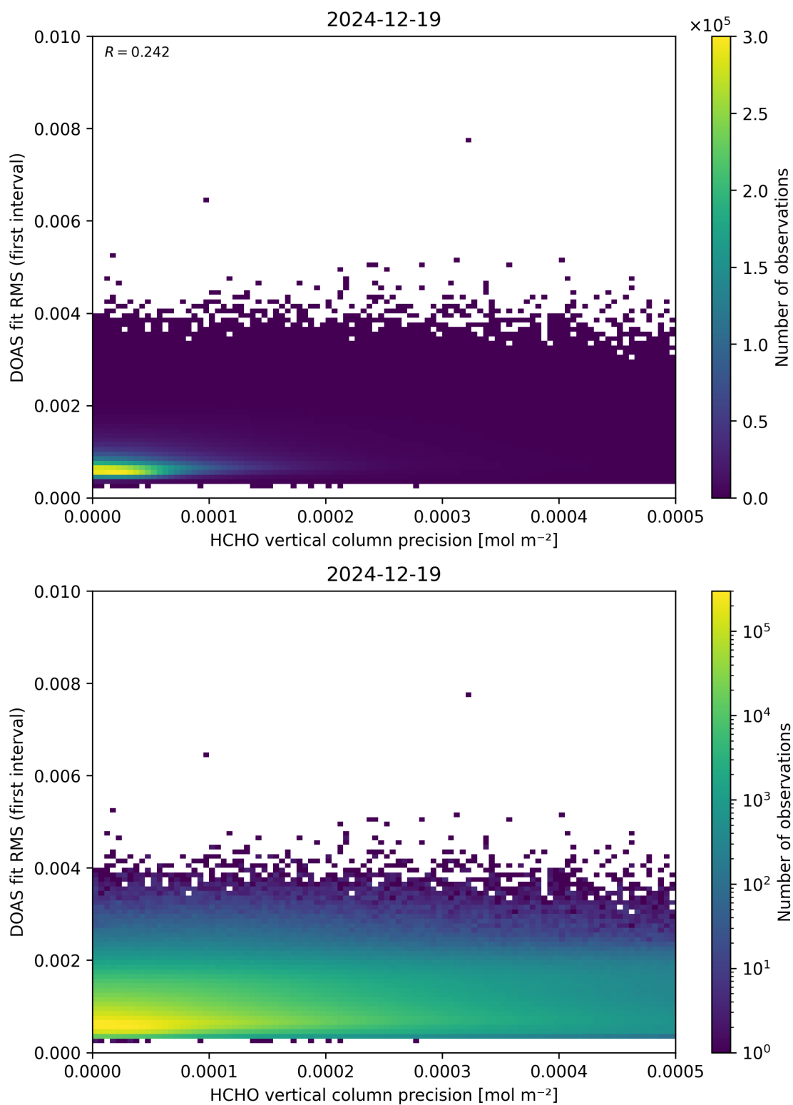
Figure 136: Scatter density plot of “HCHO vertical column precision” against “DOAS fit RMS (first interval)” for 2024-12-18 to 2024-12-20.
