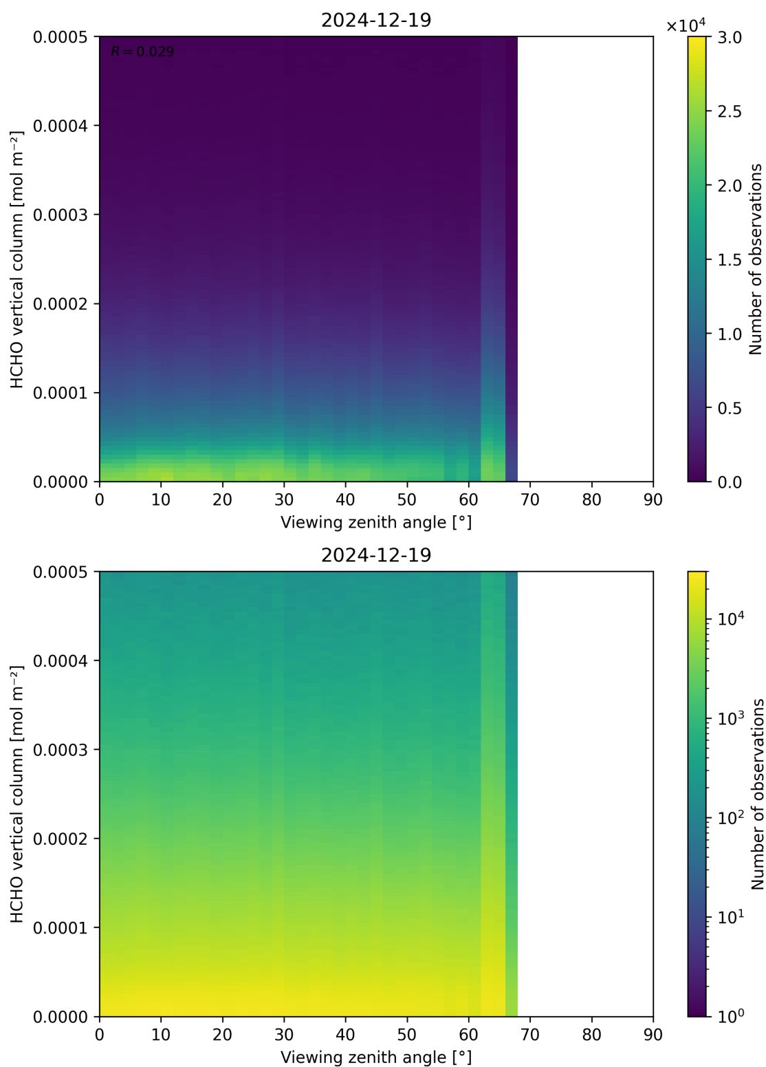
Figure 192: Scatter density plot of “Viewing zenith angle” against “HCHO vertical column” for 2024-12-18 to 2024-12-20.
