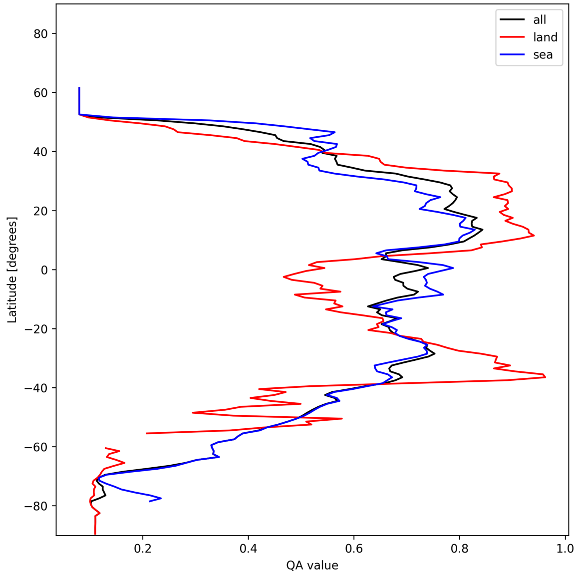
Figure 20: Zonal average of “QA value” for 2024-12-18 to 2024-12-20.
