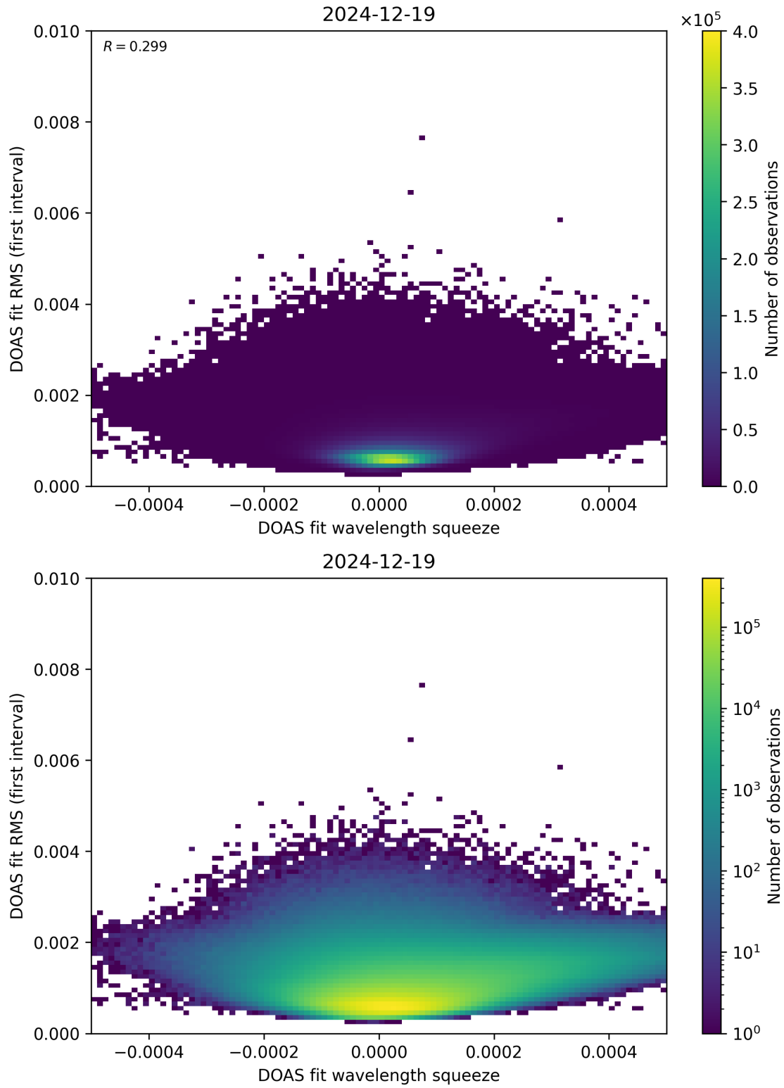
Figure 68: Scatter density plot of “DOAS fit wavelength squeeze” against “DOAS fit RMS (first interval)” for 2024-12-18 to 2024-12-20.
