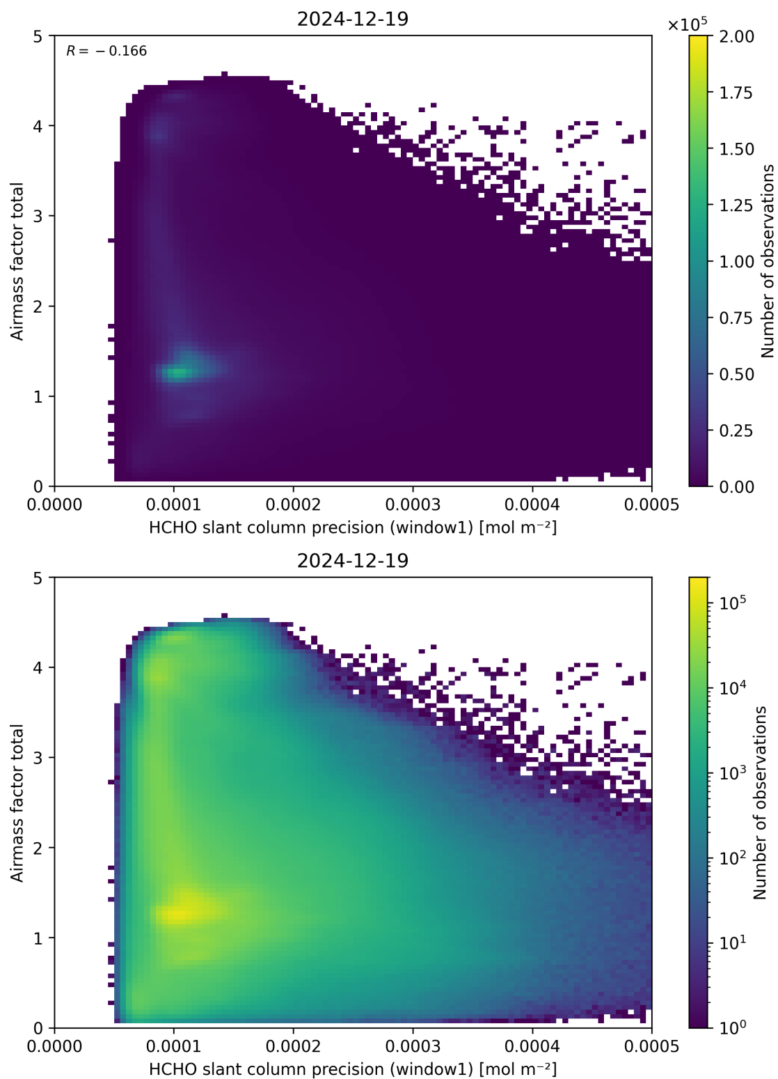
Figure 94: Scatter density plot of “HCHO slant column precision (window1)” against “Airmass factor total” for 2024-12-18 to 2024-12-20.
