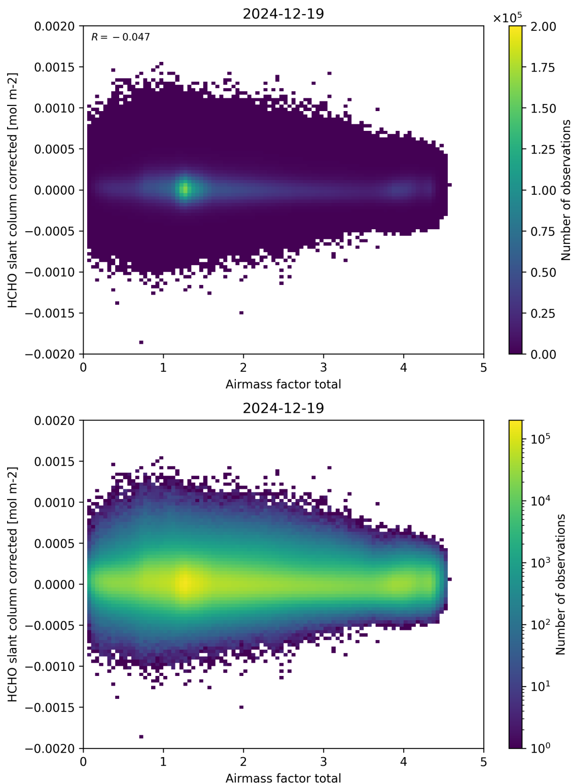
Figure 101: Scatter density plot of “Airmass factor total” against “HCHO slant column corrected” for 2024-12-18 to 2024-12-20.
