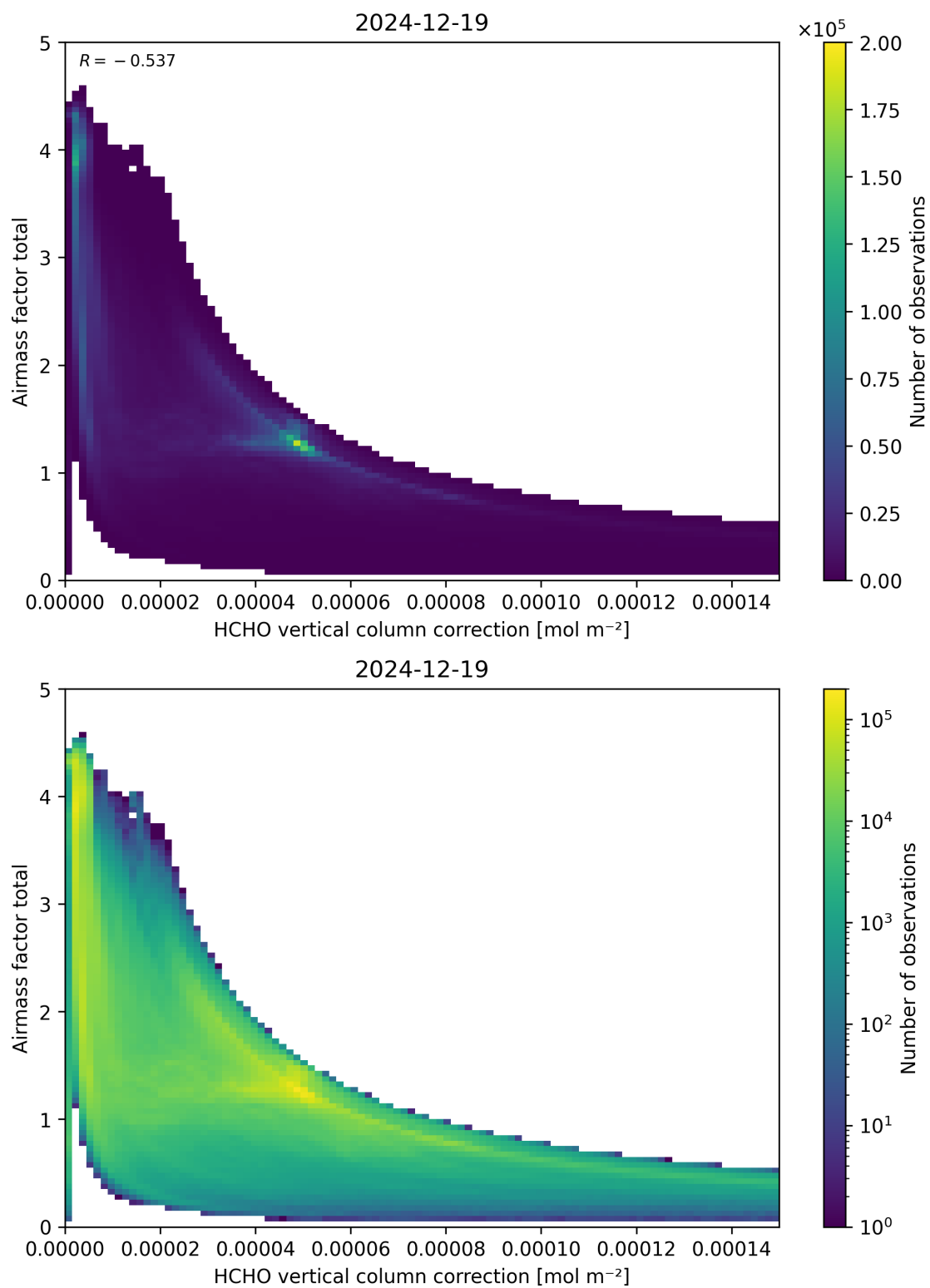
Figure 120: Scatter density plot of “HCHO vertical column correction” against “Airmass factor total” for 2024-12-18 to 2024-12-20.
