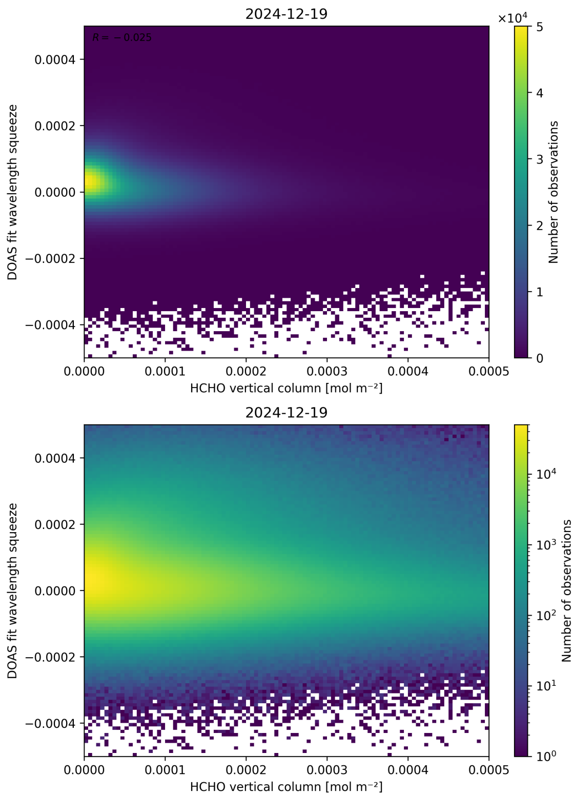
Figure 125: Scatter density plot of “HCHO vertical column” against “DOAS fit wavelength squeeze” for 2024-12-18 to 2024-12-20.
