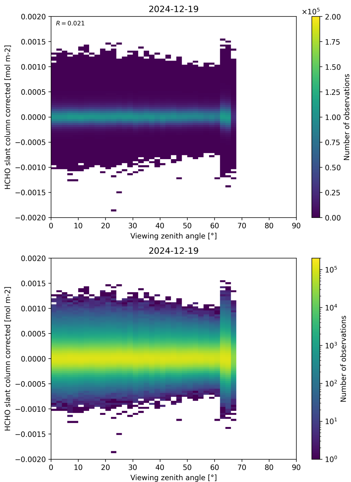
Figure 186: Scatter density plot of “Viewing zenith angle” against “HCHO slant column corrected” for 2024-12-18 to 2024-12-20.
