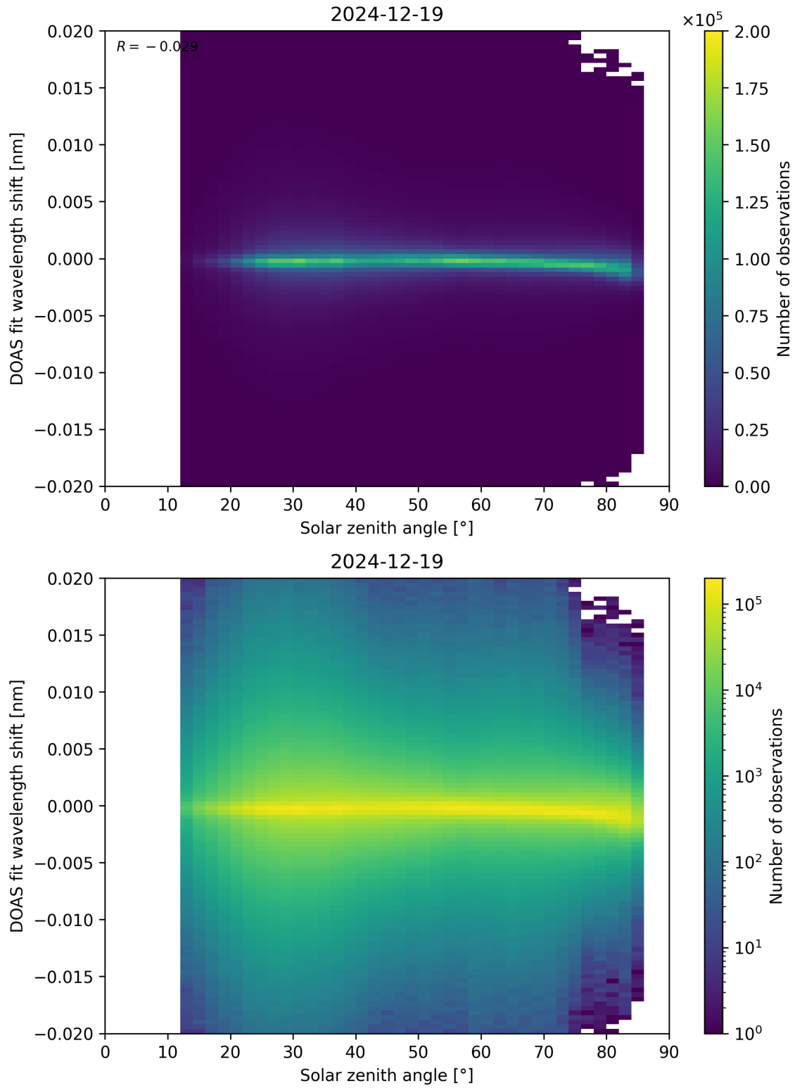
Figure 168: Scatter density plot of “Solar zenith angle” against “DOAS fit wavelength shift” for 2024-12-18 to 2024-12-20.
