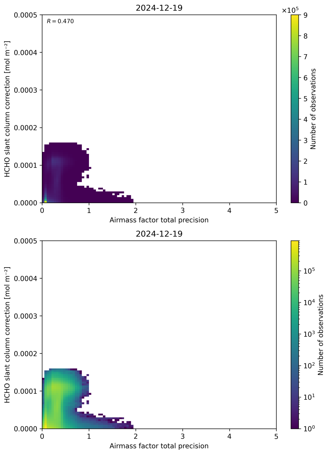
Figure 110: Scatter density plot of “Airmass factor total precision” against “HCHO slant column correction” for 2024-12-18 to 2024-12-20.
