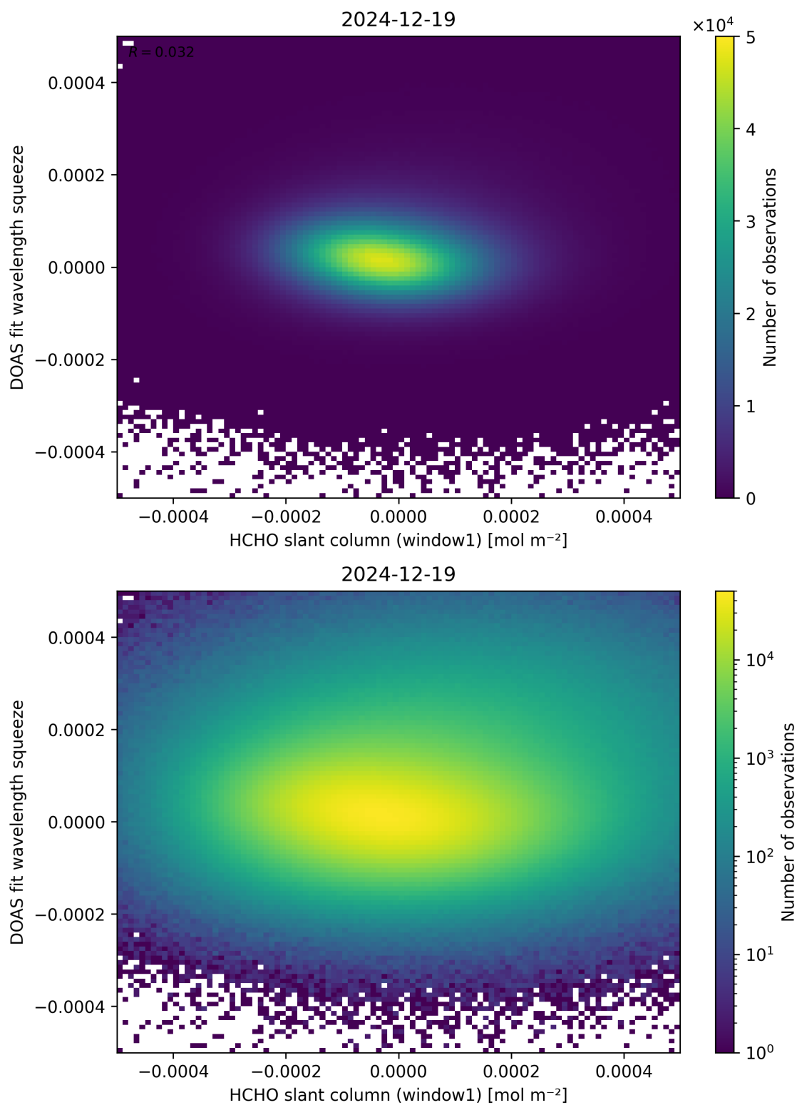
Figure 80: Scatter density plot of “HCHO slant column (window1)” against “DOAS fit wavelength squeeze” for 2024-12-18 to 2024-12-20.
