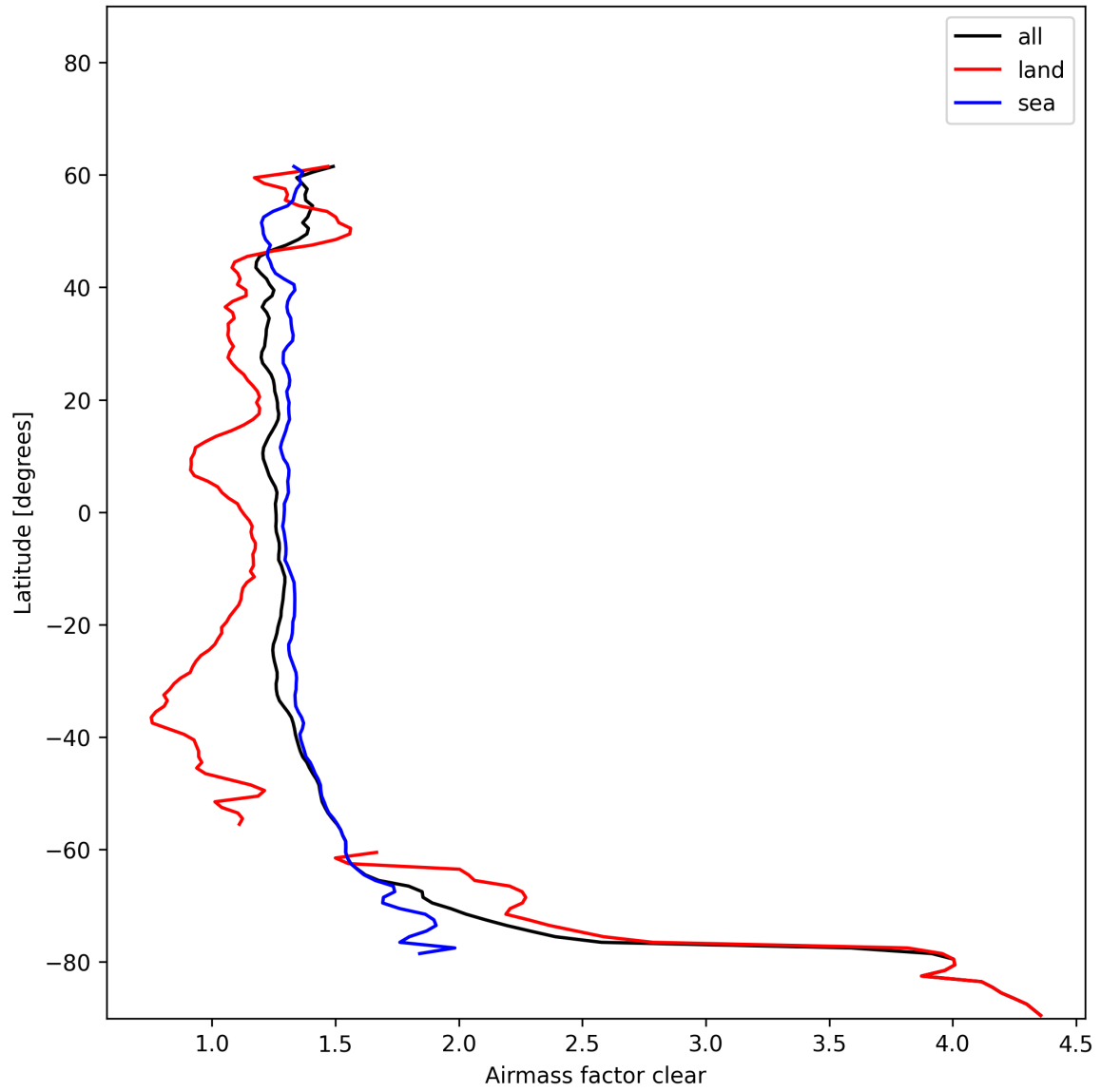
Figure 28: Zonal average of “Airmass factor clear” for 2024-12-18 to 2024-12-20.
