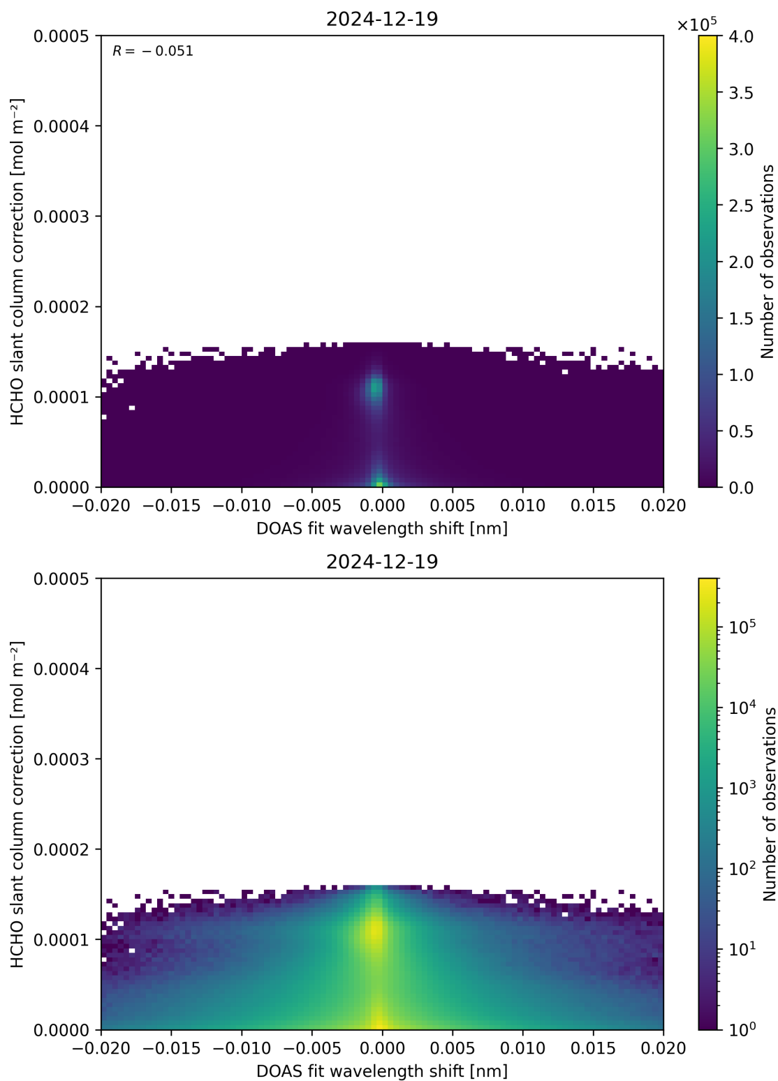
Figure 67: Scatter density plot of “DOAS fit wavelength shift” against “HCHO slant column correction” for 2024-12-18 to 2024-12-20.
