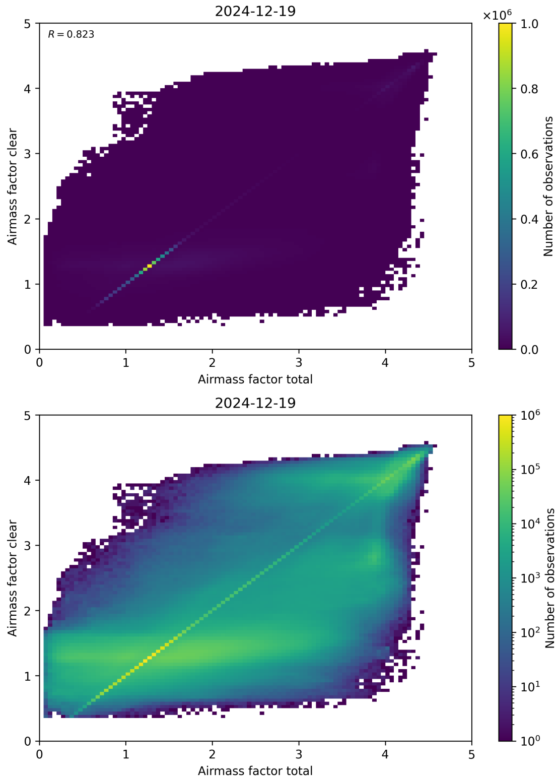
Figure 100: Scatter density plot of “Airmass factor total” against “Airmass factor clear” for 2024-12-18 to 2024-12-20.
