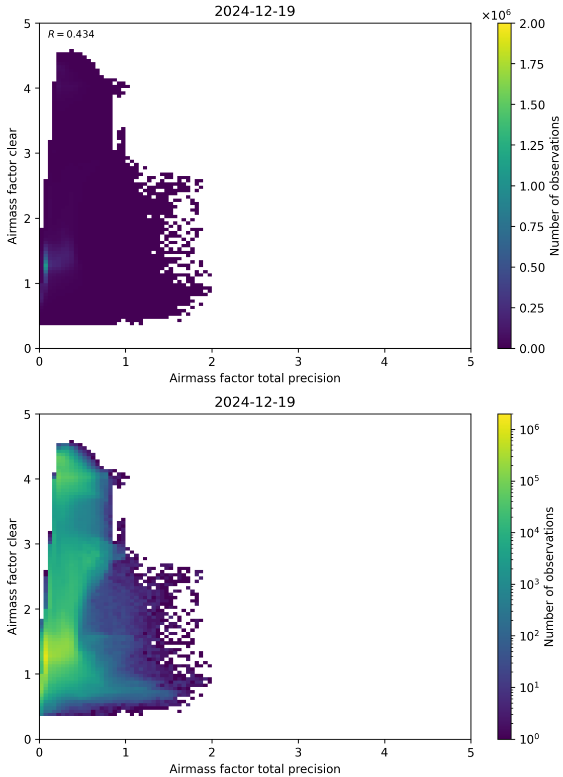
Figure 108: Scatter density plot of “Airmass factor total precision” against “Airmass factor clear” for 2024-12-18 to 2024-12-20.
