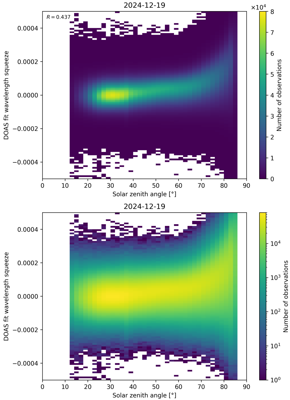
Figure 169: Scatter density plot of “Solar zenith angle” against “DOAS fit wavelength squeeze” for 2024-12-18 to 2024-12-20.
