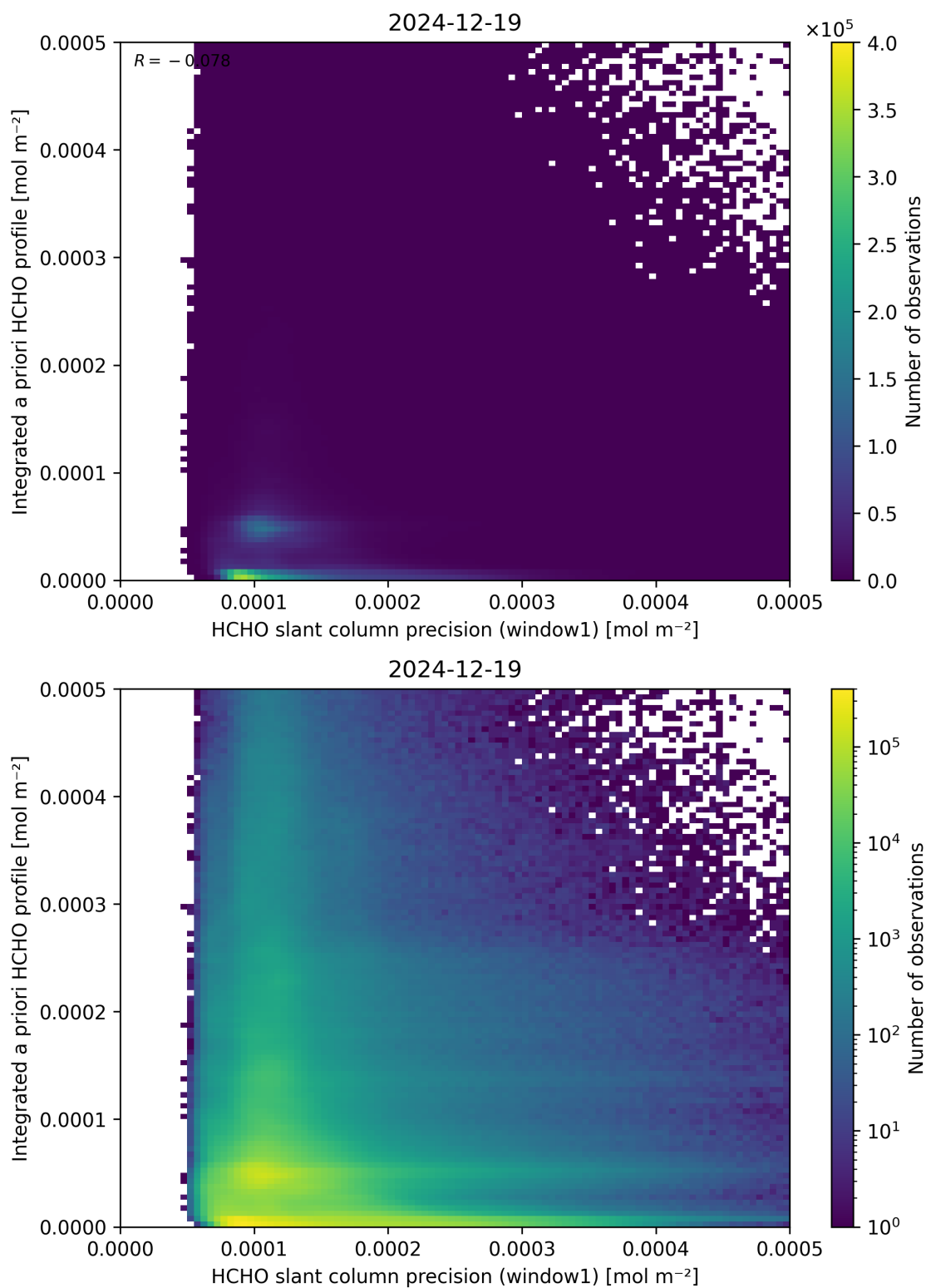
Figure 96: Scatter density plot of “HCHO slant column precision (window1)” against “Integrated a priori HCHO profile” for 2024-12-18 to 2024-12-20.
