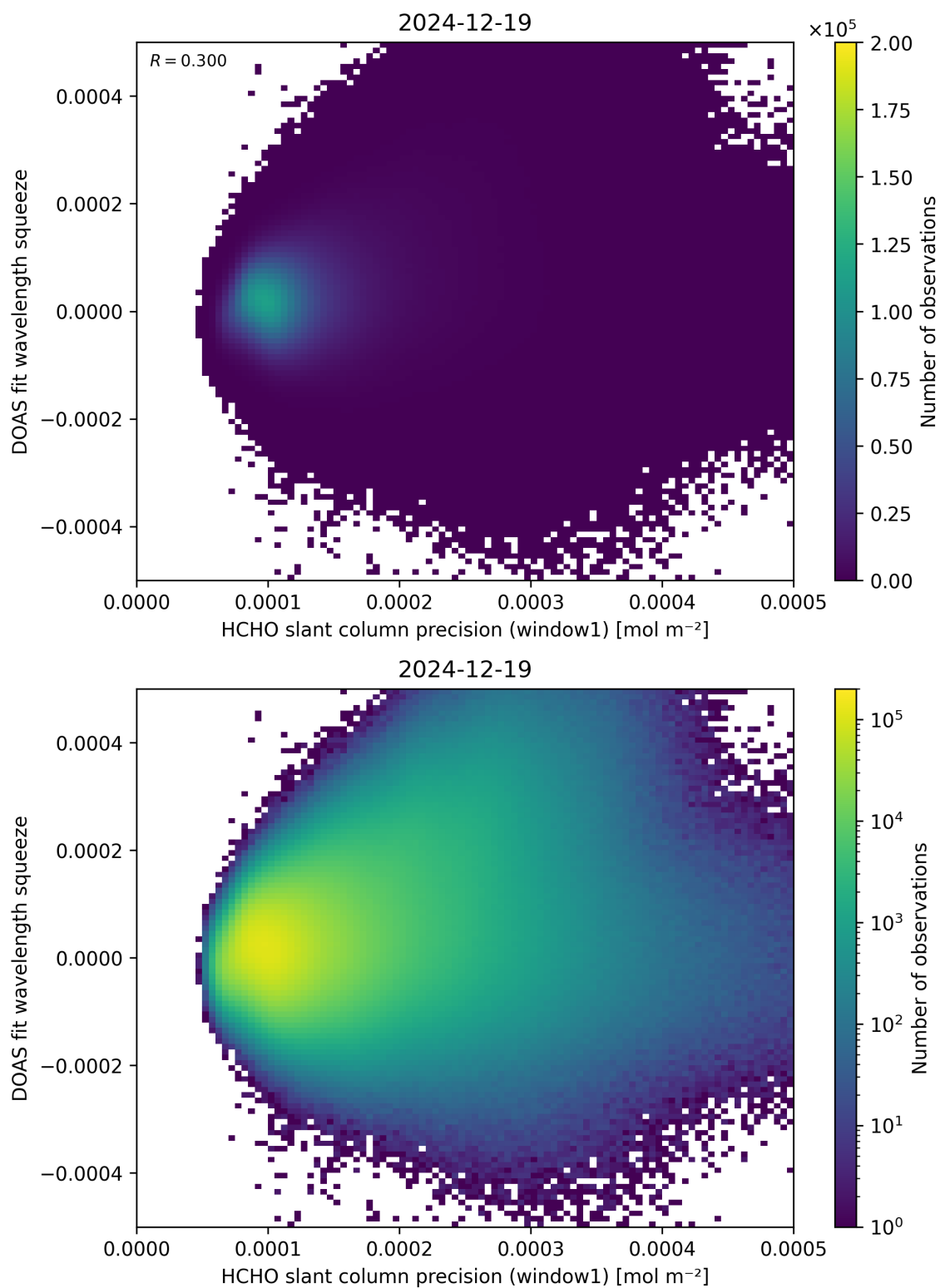
Figure 90: Scatter density plot of “HCHO slant column precision (window1)” against “DOAS fit wavelength squeeze” for 2024-12-18 to 2024-12-20.
