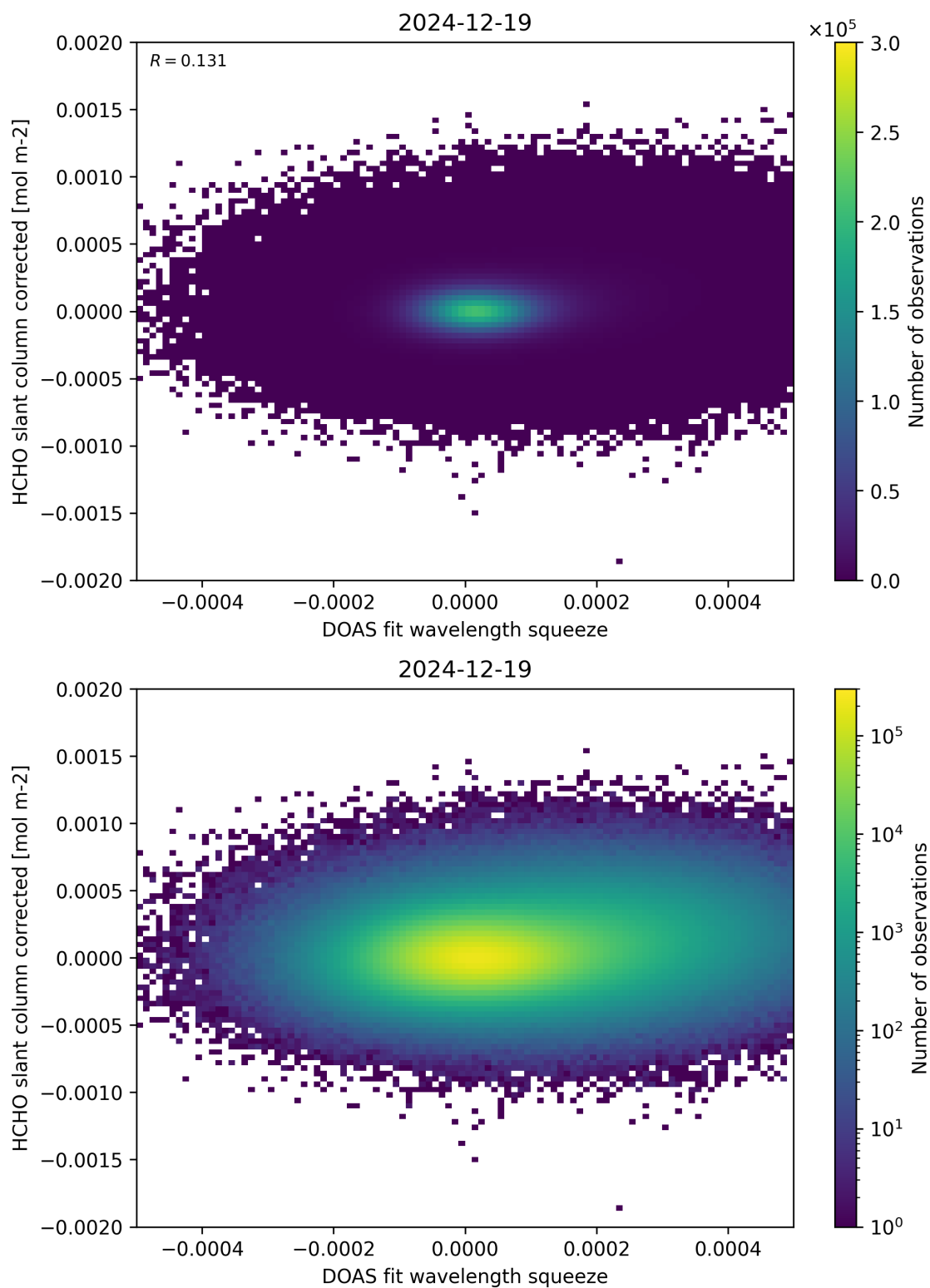
Figure 69: Scatter density plot of “DOAS fit wavelength squeeze” against “HCHO slant column corrected” for 2024-12-18 to 2024-12-20.
