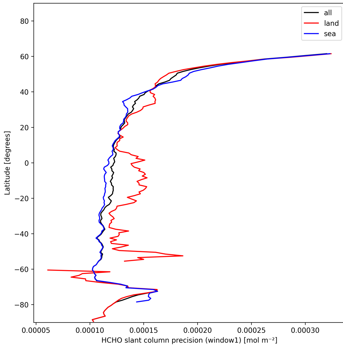
Figure 25: Zonal average of "HCHO slant column precision (window1)" for 2024-12-18 to 2024-12-20.
