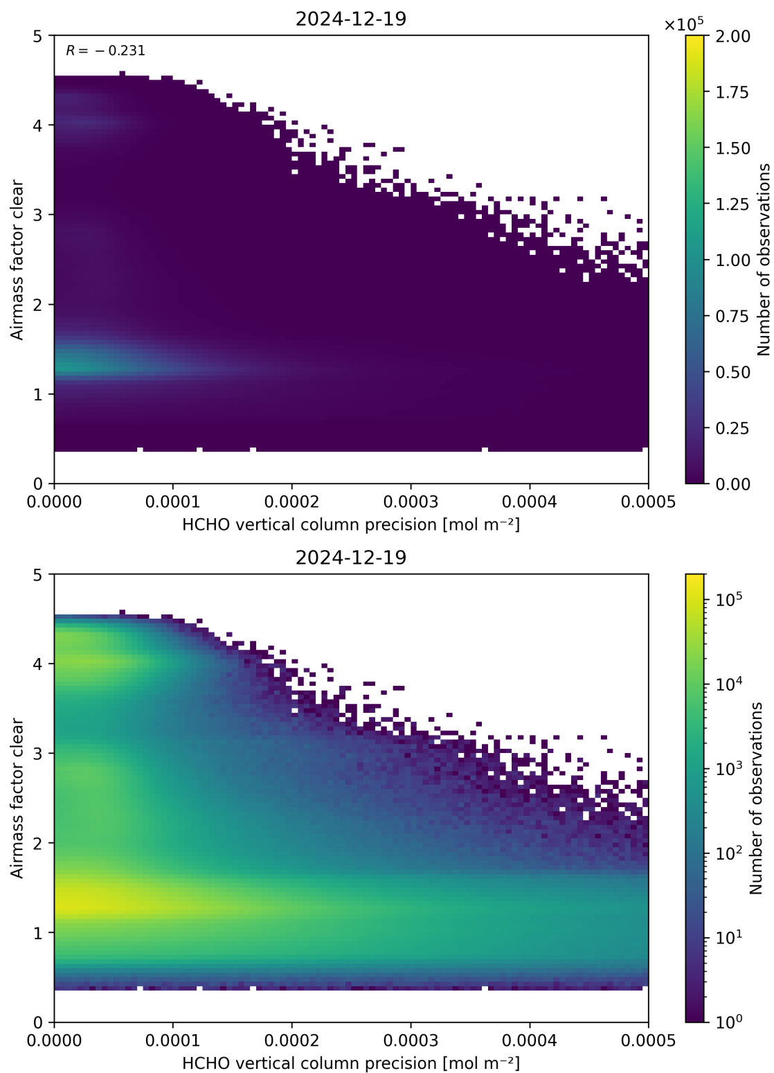
Figure 139: Scatter density plot of “HCHO vertical column precision” against “Airmass factor clear” for 2024-12-18 to 2024-12-20.
