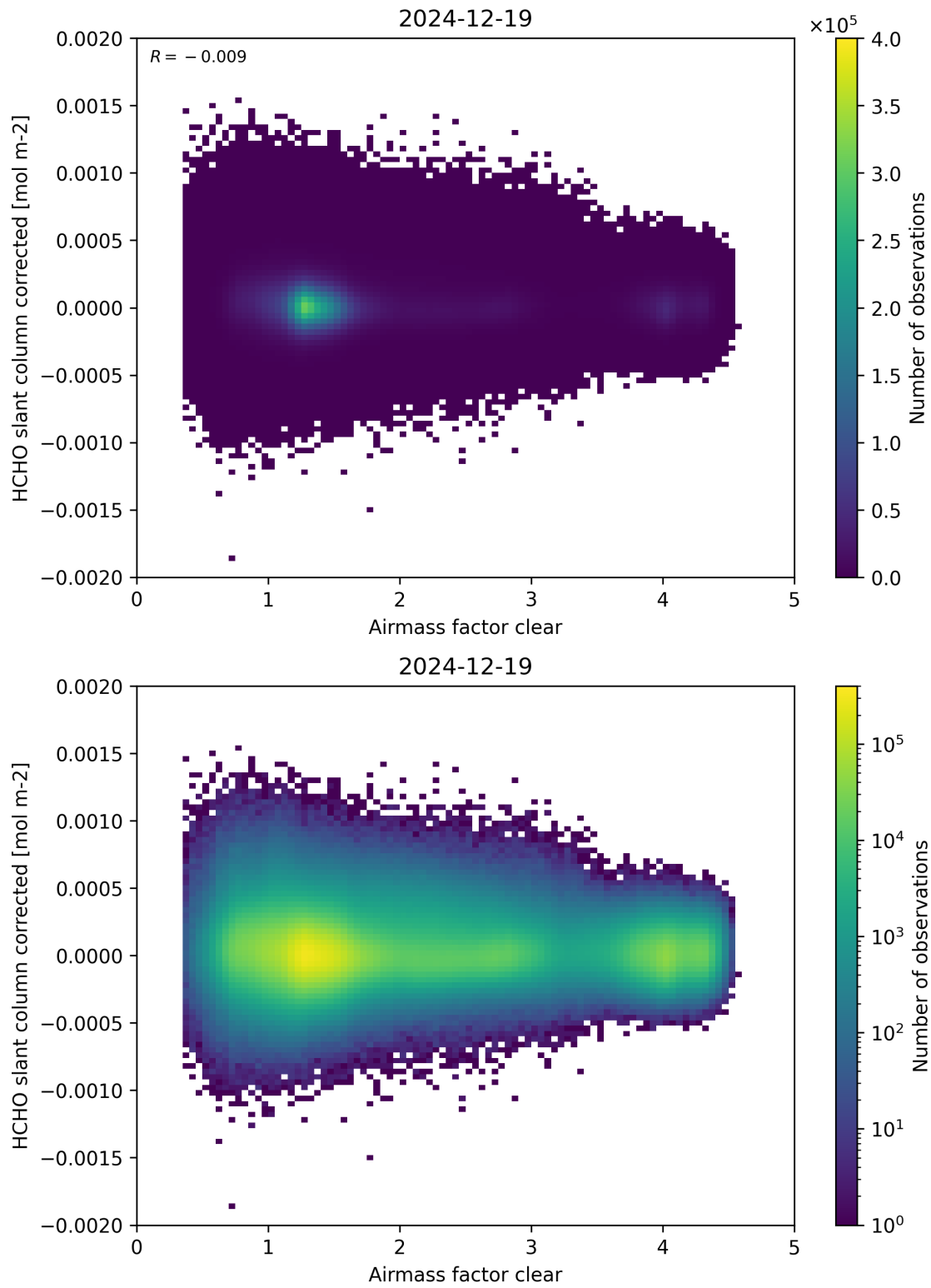
Figure 74: Scatter density plot of “Airmass factor clear” against “HCHO slant column corrected” for 2024-12-18 to 2024-12-20.
