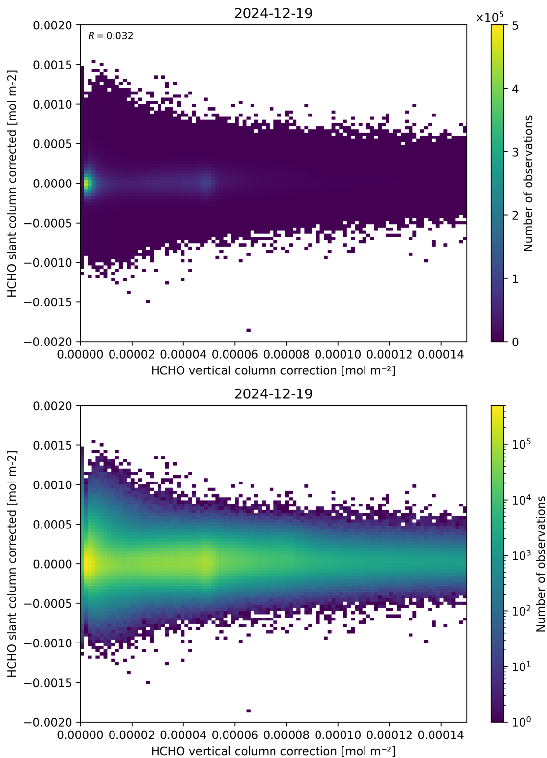
Figure 116: Scatter density plot of “HCHO vertical column correction” against “HCHO slant column corrected” for 2024-12-18 to 2024-12-20.
