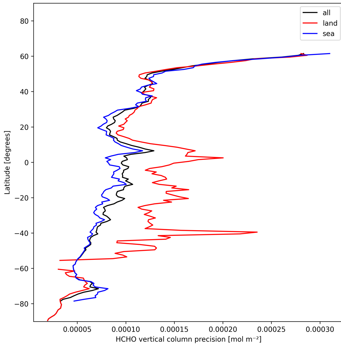
Figure 22: Zonal average of “HCHO vertical column precision” for 2024-12-18 to 2024-12-20.
