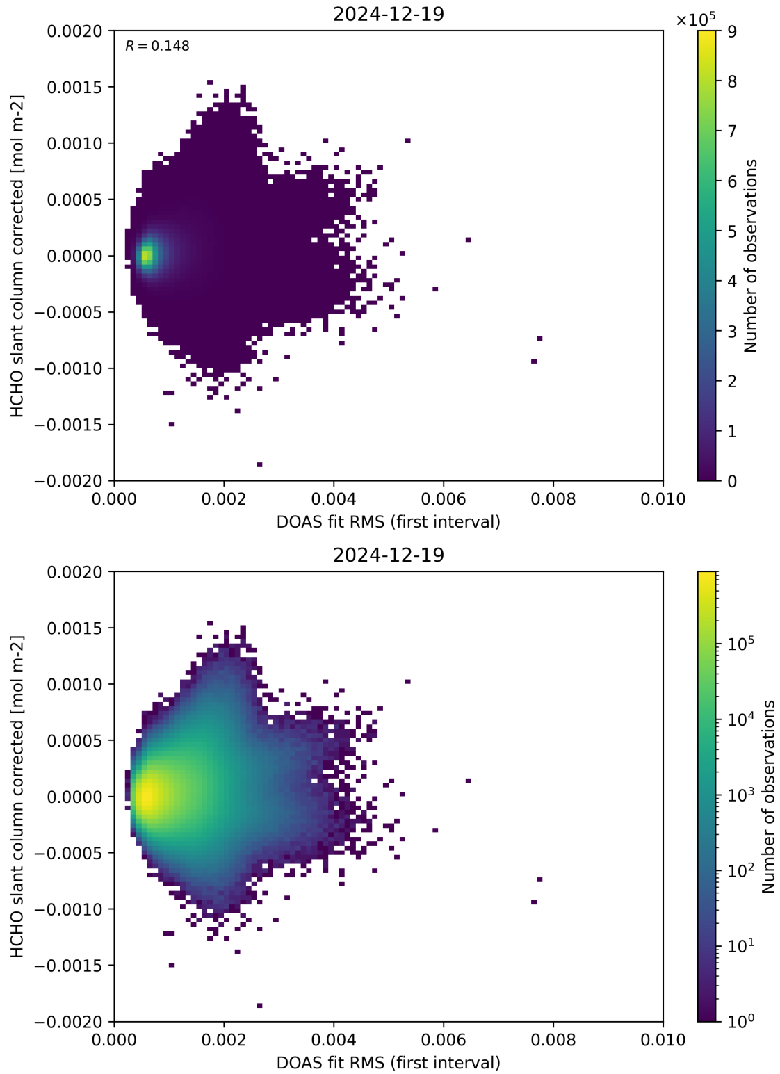
Figure 62: Scatter density plot of “DOAS fit RMS (first interval)” against “HCHO slant column corrected” for 2024-12-18 to 2024-12-20.
