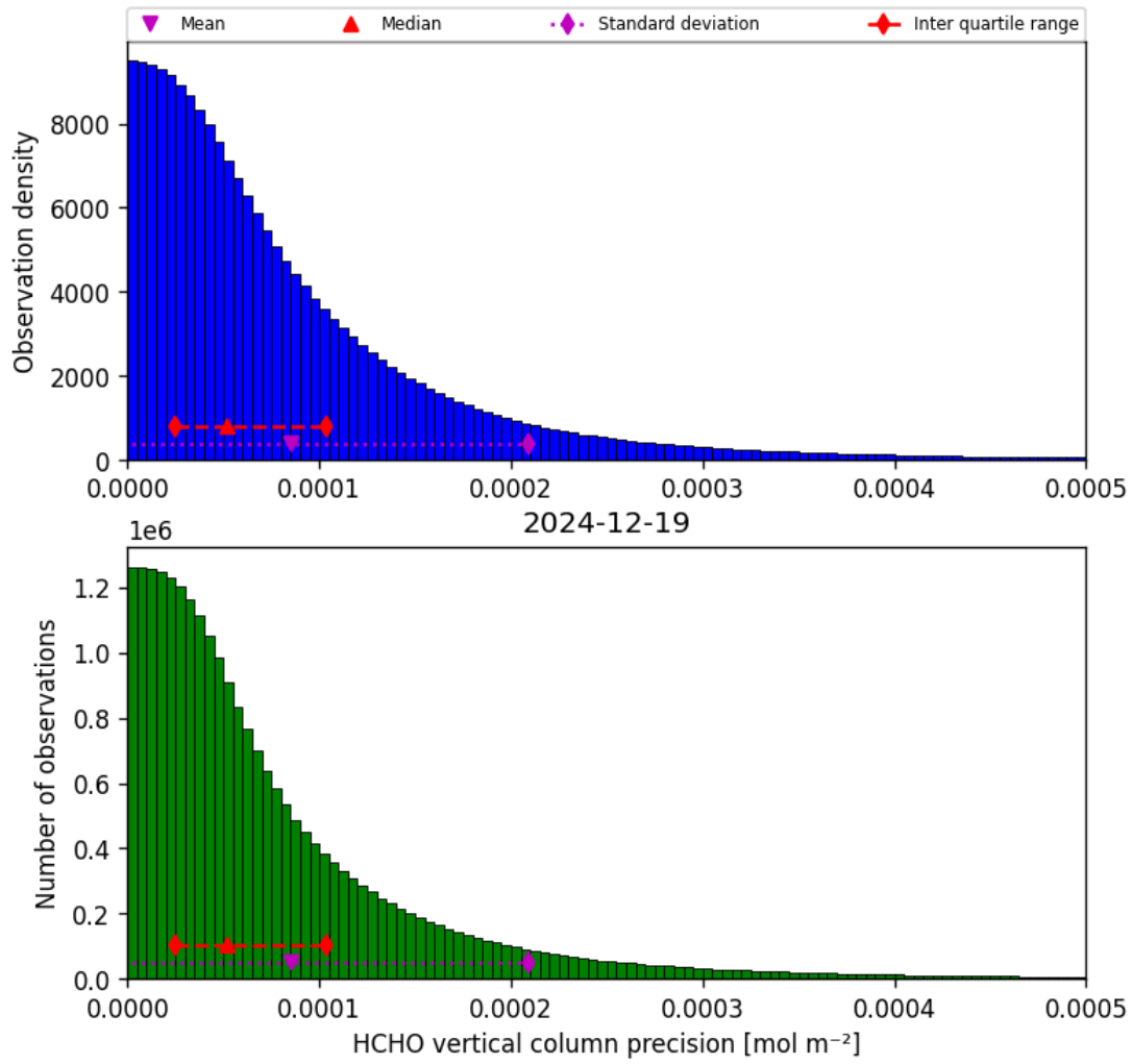
Figure 36: Histogram of “HCHO vertical column precision” for 2024-12-18 to 2024-12-20
