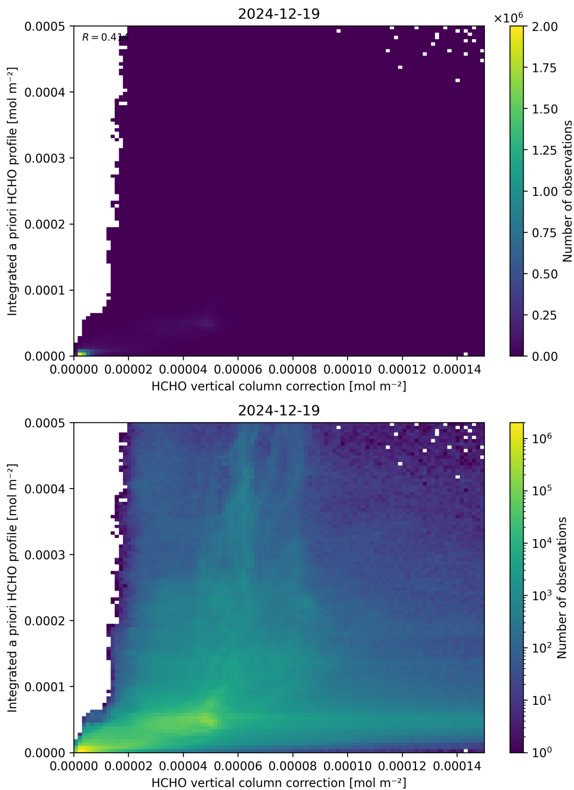
Figure 122: Scatter density plot of “HCHO vertical column correction” against “Integrated a priori HCHO profile” for 2024-12-18 to 2024-12-20.
