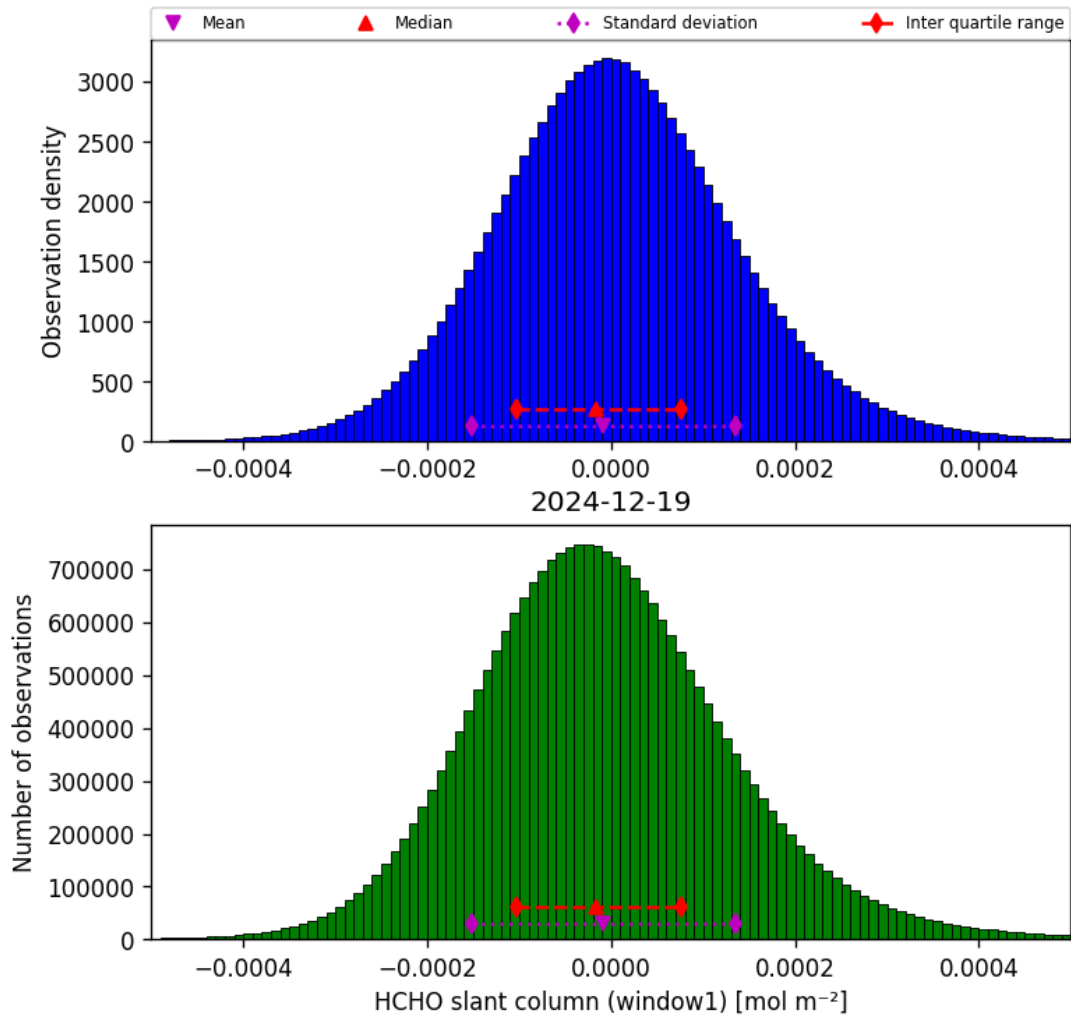
Figure 38: Histogram of “HCHO slant column (window1)” for 2024-12-18 to 2024-12-20
