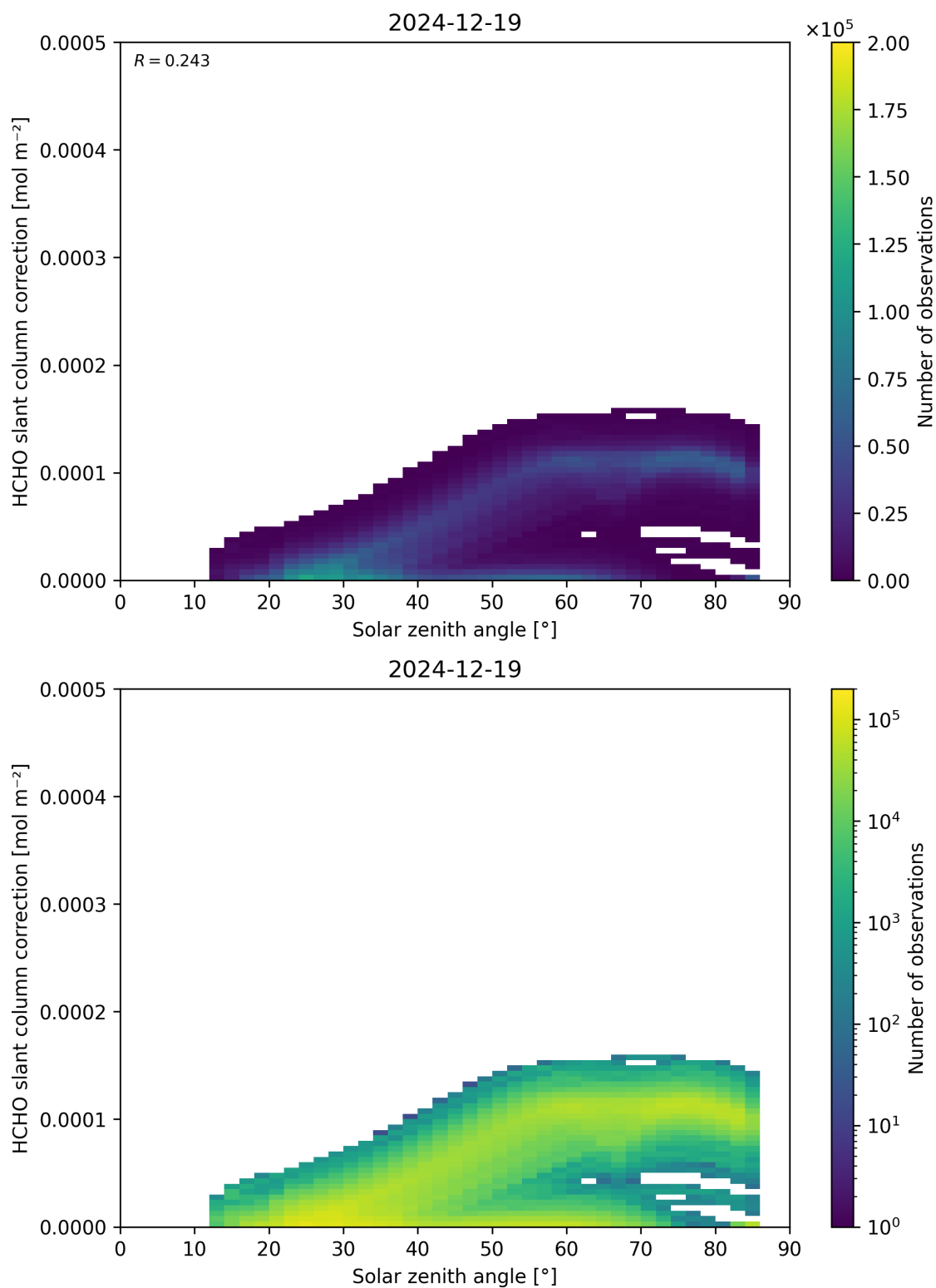
Figure 172: Scatter density plot of “Solar zenith angle” against “HCHO slant column correction” for 2024-12-18 to 2024-12-20.
