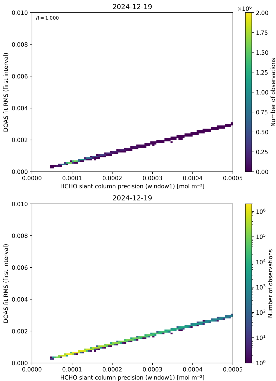
Figure 88: Scatter density plot of “HCHO slant column precision (window1)” against “DOAS fit RMS (first interval)” for 2024-12-18 to 2024-12-20.
