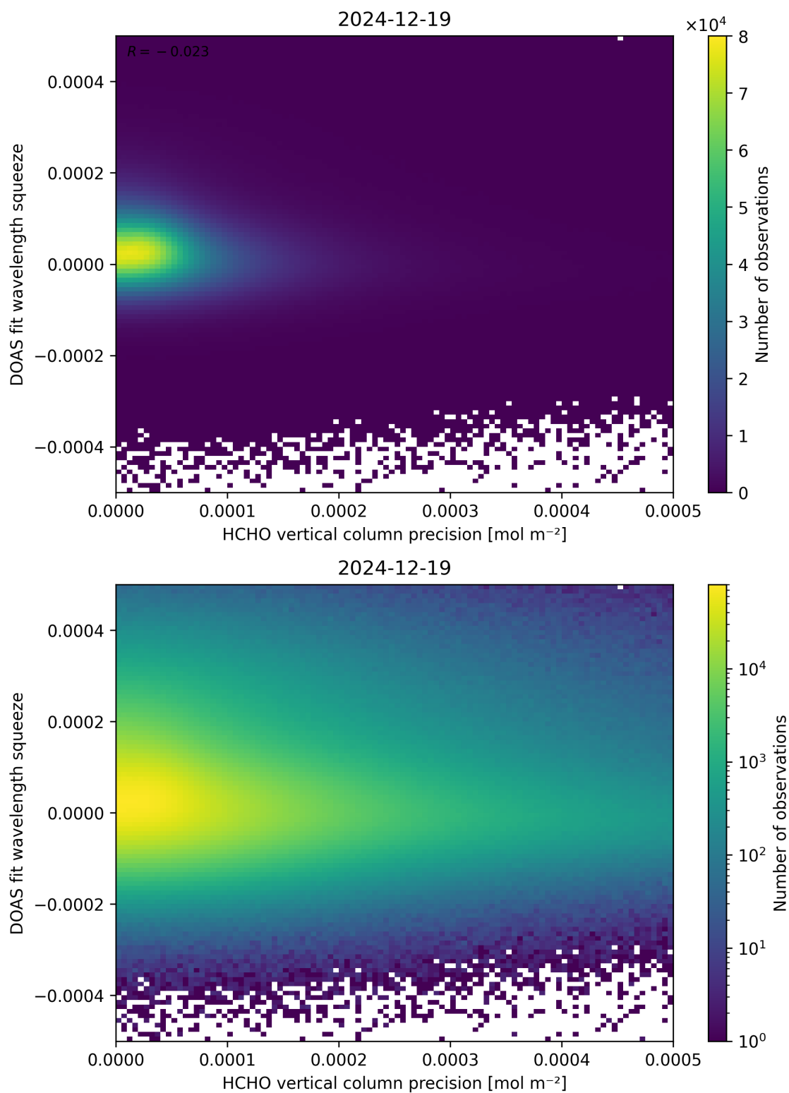
Figure 138: Scatter density plot of “HCHO vertical column precision” against “DOAS fit wavelength squeeze” for 2024-12-18 to 2024-12-20.
