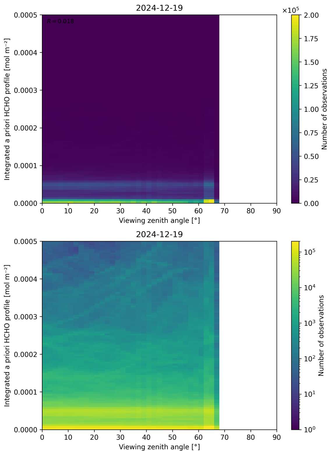
Figure 195: Scatter density plot of “Viewing zenith angle” against “Integrated a priori HCHO profile” for 2024-12-18 to 2024-12-20.
