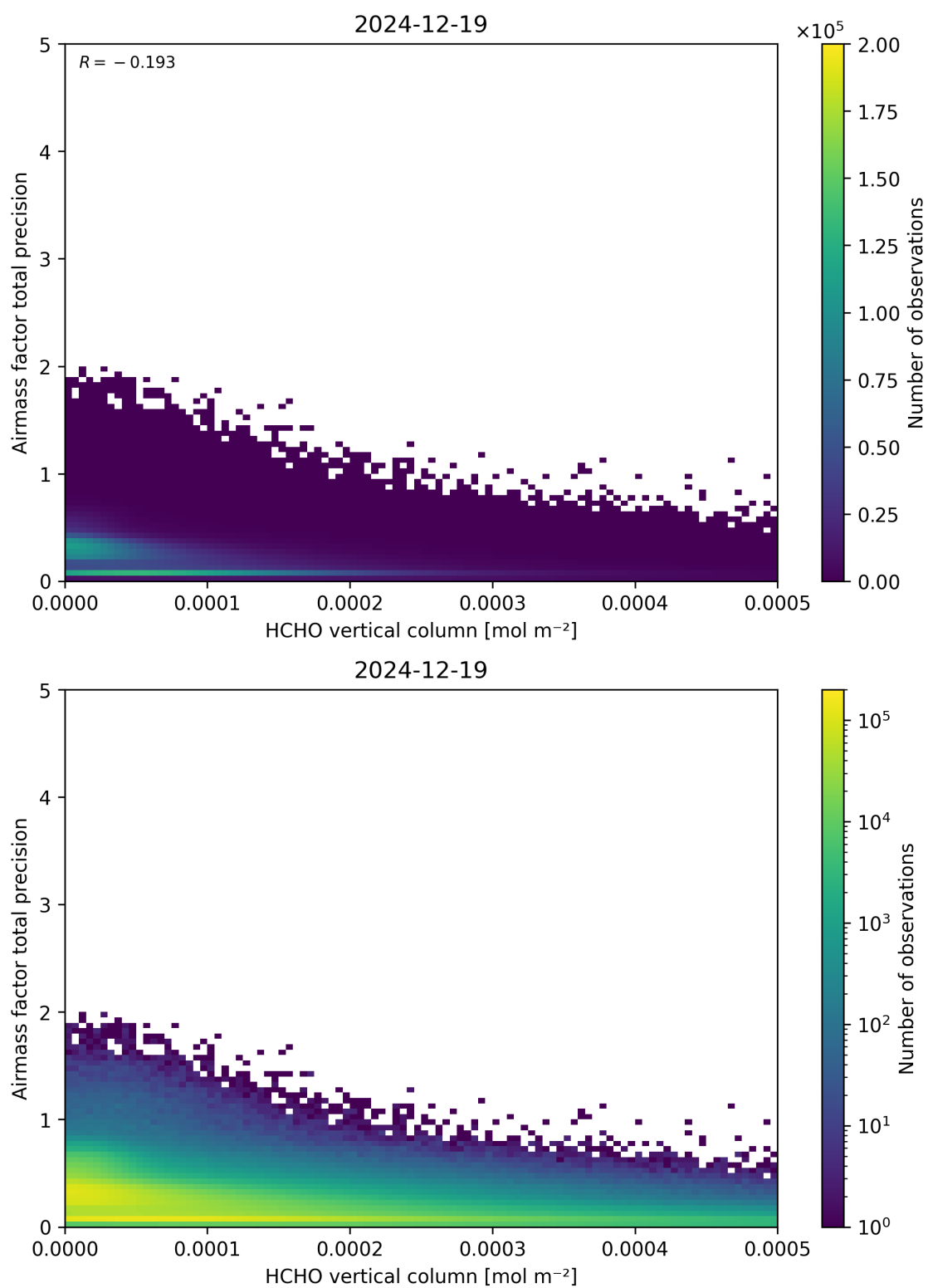
Figure 132: Scatter density plot of “HCHO vertical column” against “Airmass factor total precision” for 2024-12-18 to 2024-12-20.
