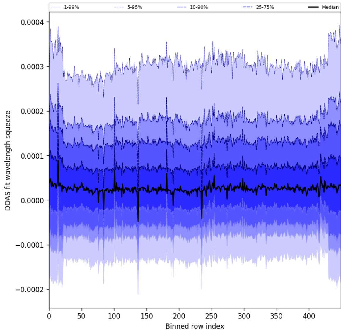
Figure 59: Along track statistics of “DOAS fit wavelength squeeze” for 2024-12-18 to 2024-12-20
