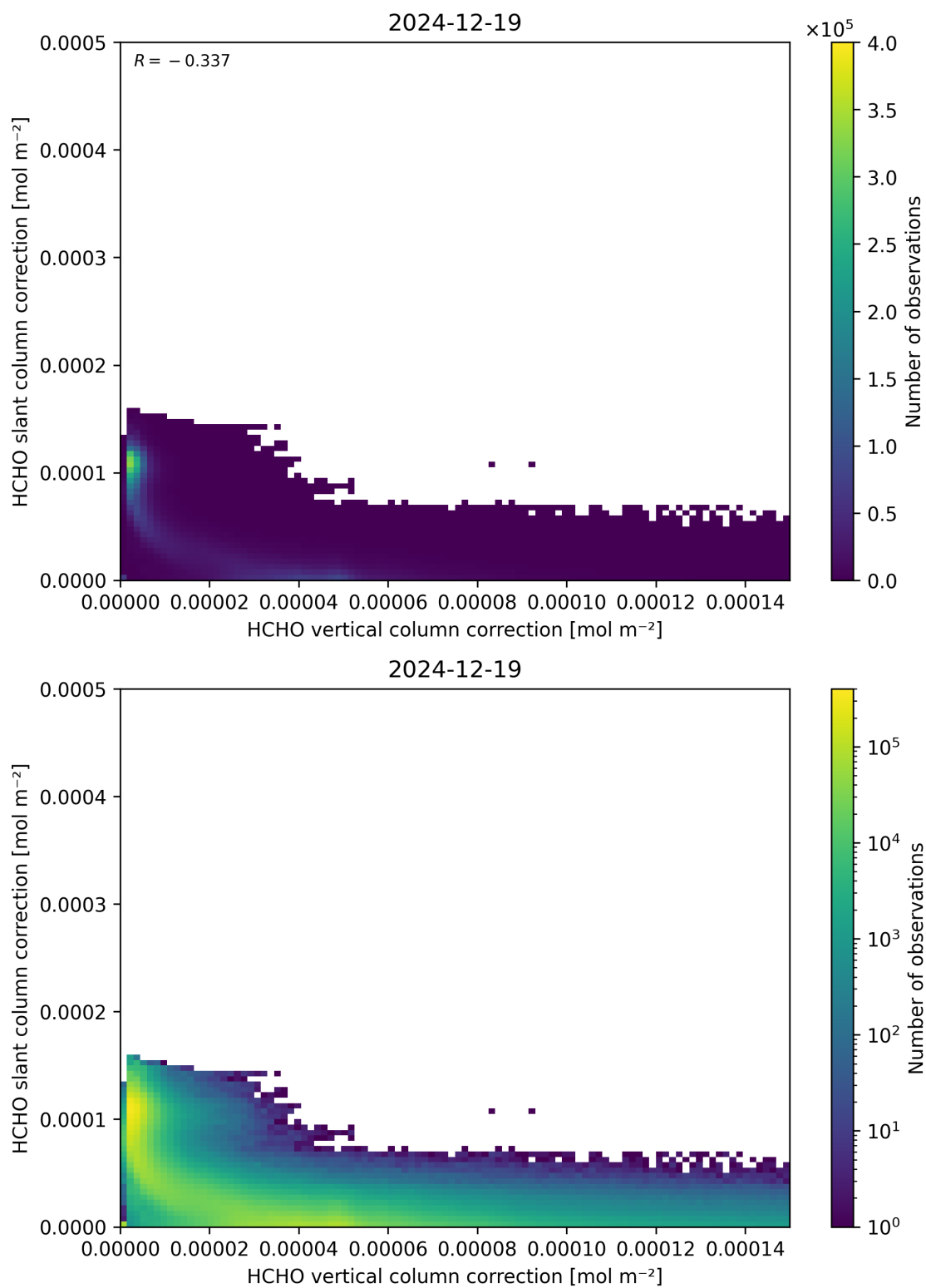
Figure 117: Scatter density plot of “HCHO vertical column correction” against “HCHO slant column correction” for 2024-12-18 to 2024-12-20.
