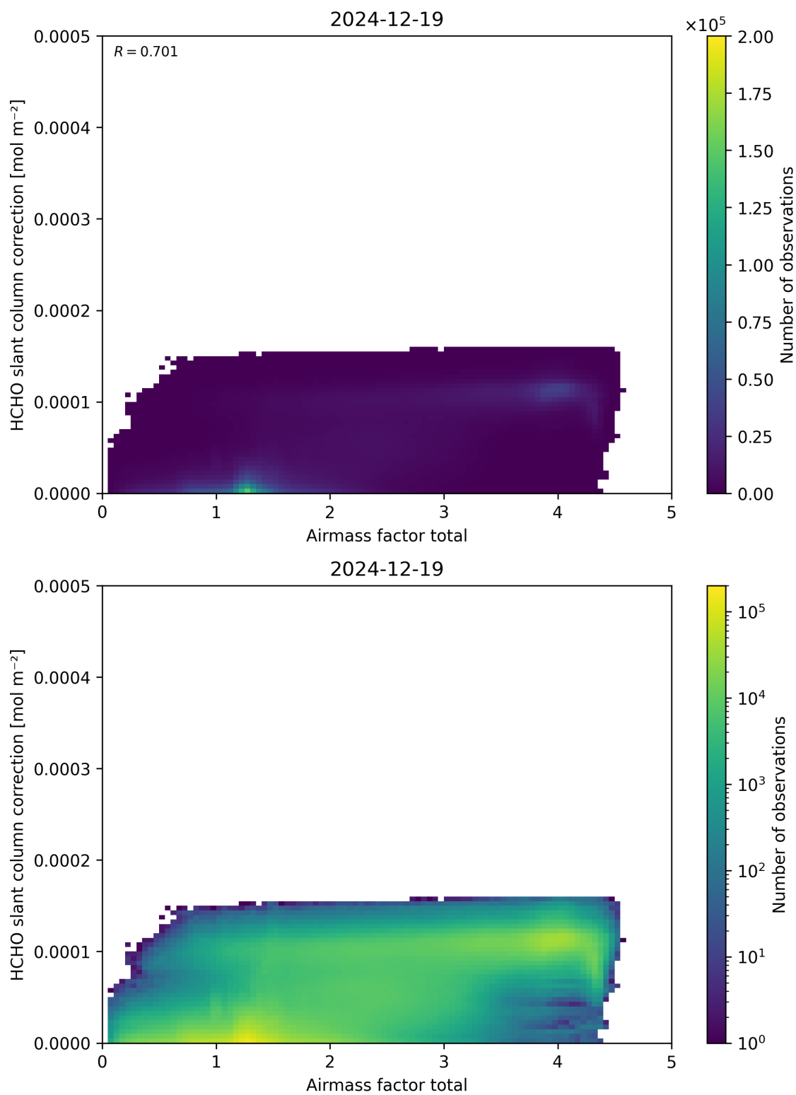
Figure 102: Scatter density plot of “Airmass factor total” against “HCHO slant column correction” for 2024-12-18 to 2024-12-20.
