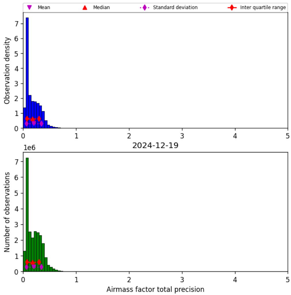
Figure 41: Histogram of “Airmass factor total precision” for 2024-12-18 to 2024-12-20
