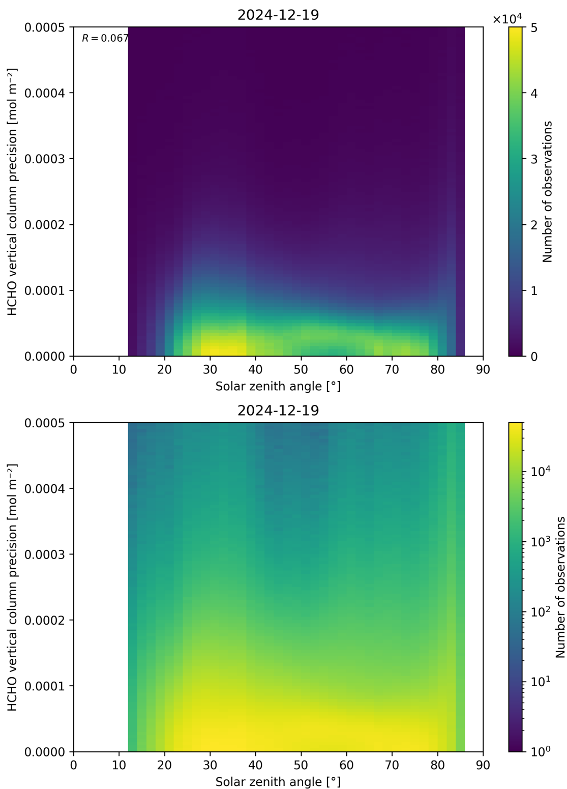
Figure 179: Scatter density plot of “Solar zenith angle” against “HCHO vertical column precision” for 2024-12-18 to 2024-12-20.
