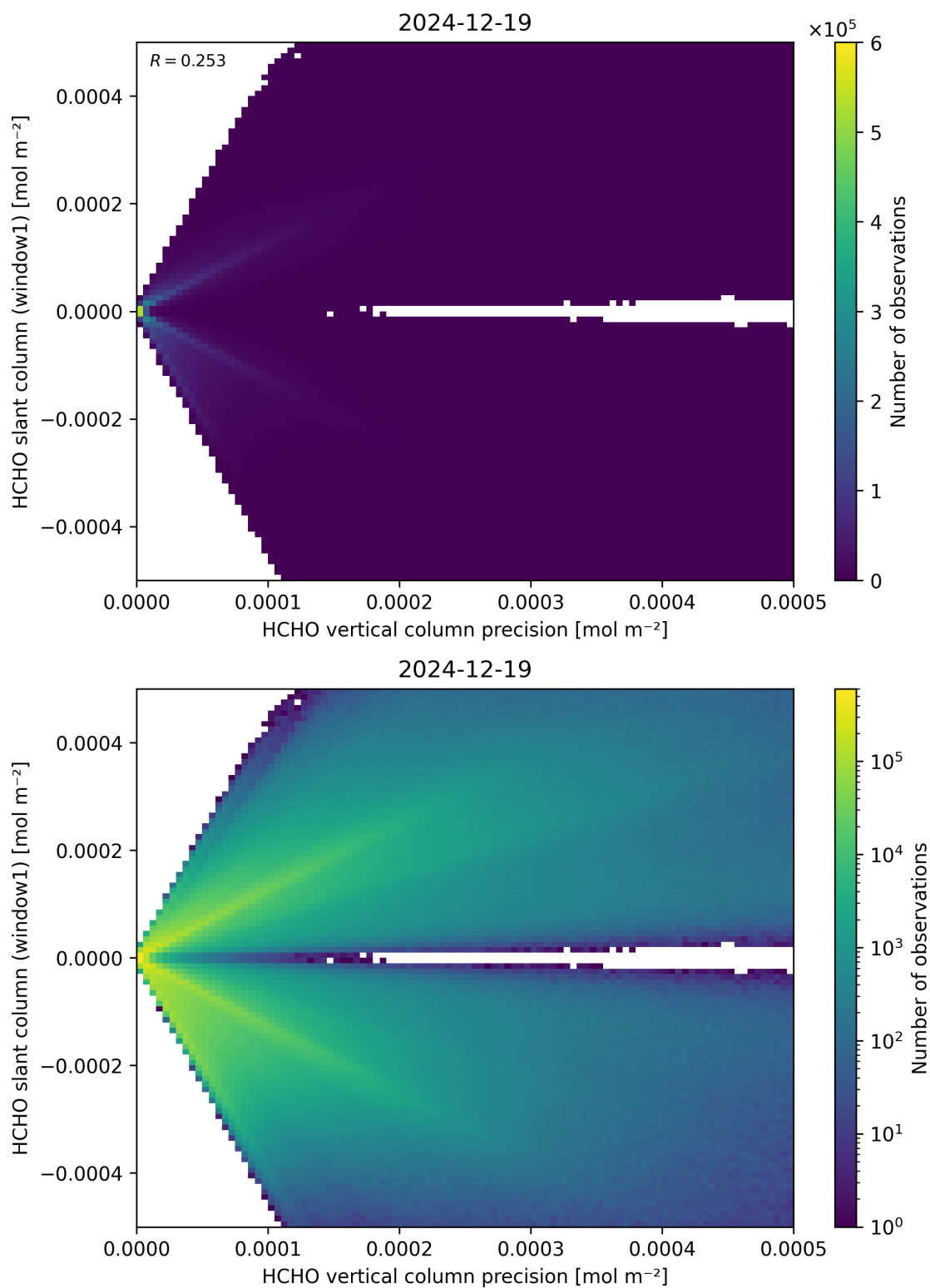
Figure 142: Scatter density plot of “HCHO vertical column precision” against “HCHO slant column (window1)” for 2024-12-18 to 2024-12-20.
