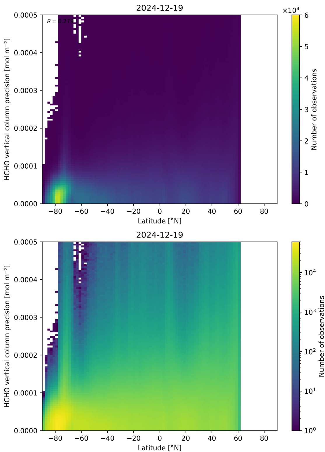
Figure 165: Scatter density plot of “Latitude” against “HCHO vertical column precision” for 2024-12-18 to 2024-12-20.
