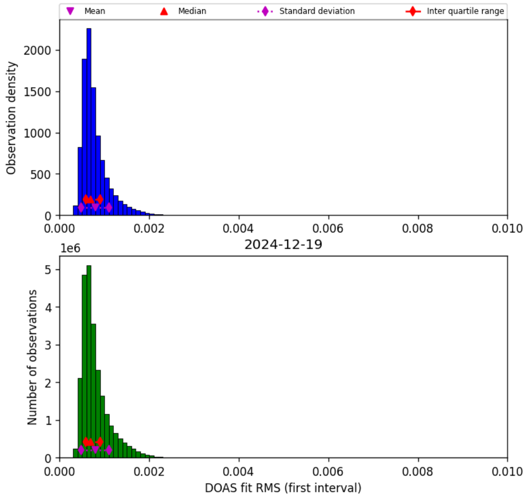
Figure 46: Histogram of “DOAS fit RMS (first interval)” for 2024-12-18 to 2024-12-20
