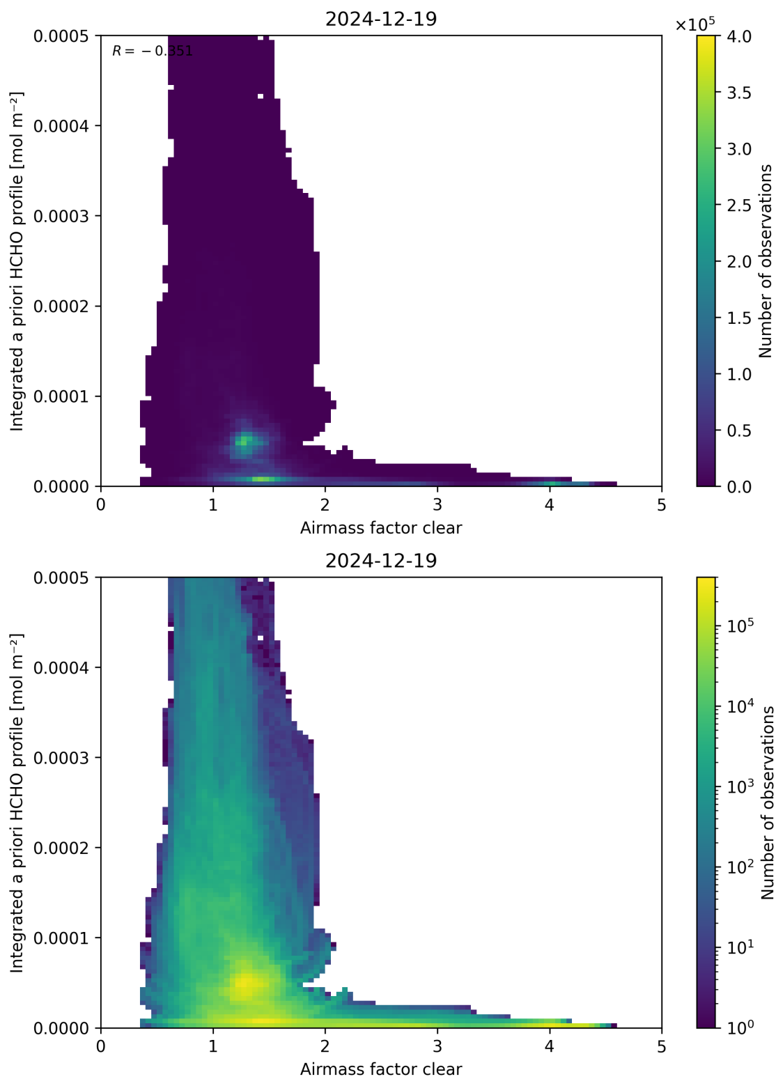
Figure 76: Scatter density plot of “Airmass factor clear” against “Integrated a priori HCHO profile” for 2024-12-18 to 2024-12-20.
