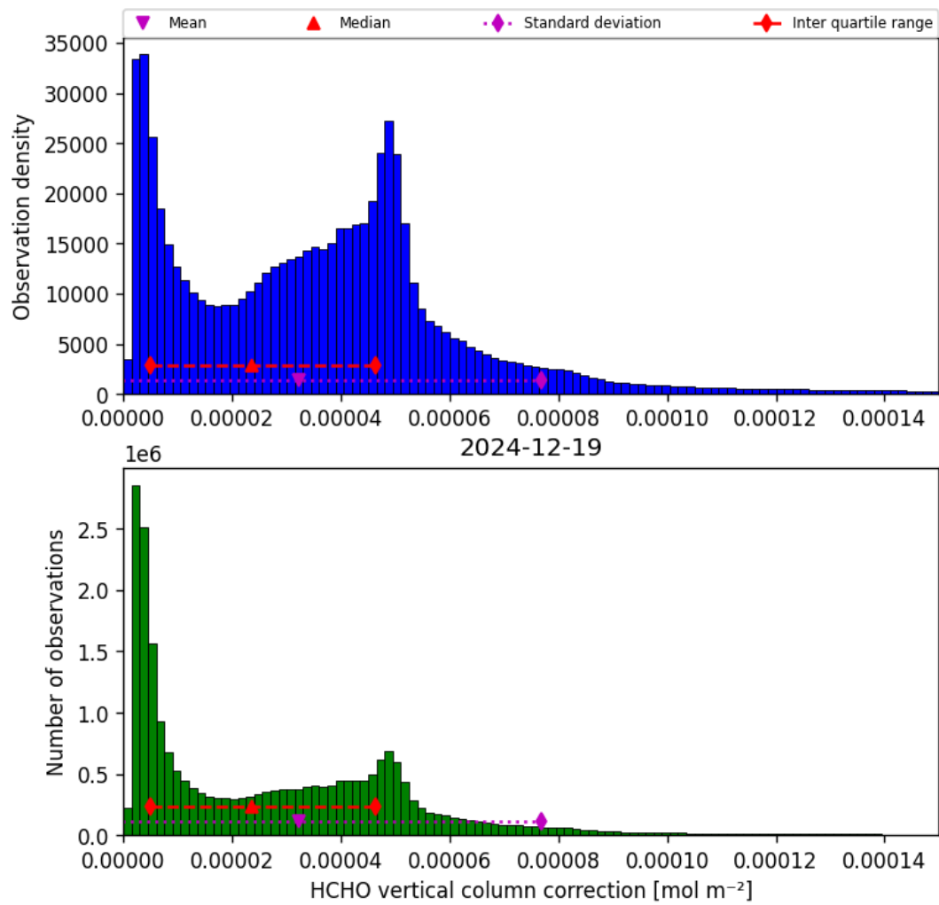
Figure 37: Histogram of “HCHO vertical column correction” for 2024-12-18 to 2024-12-20
