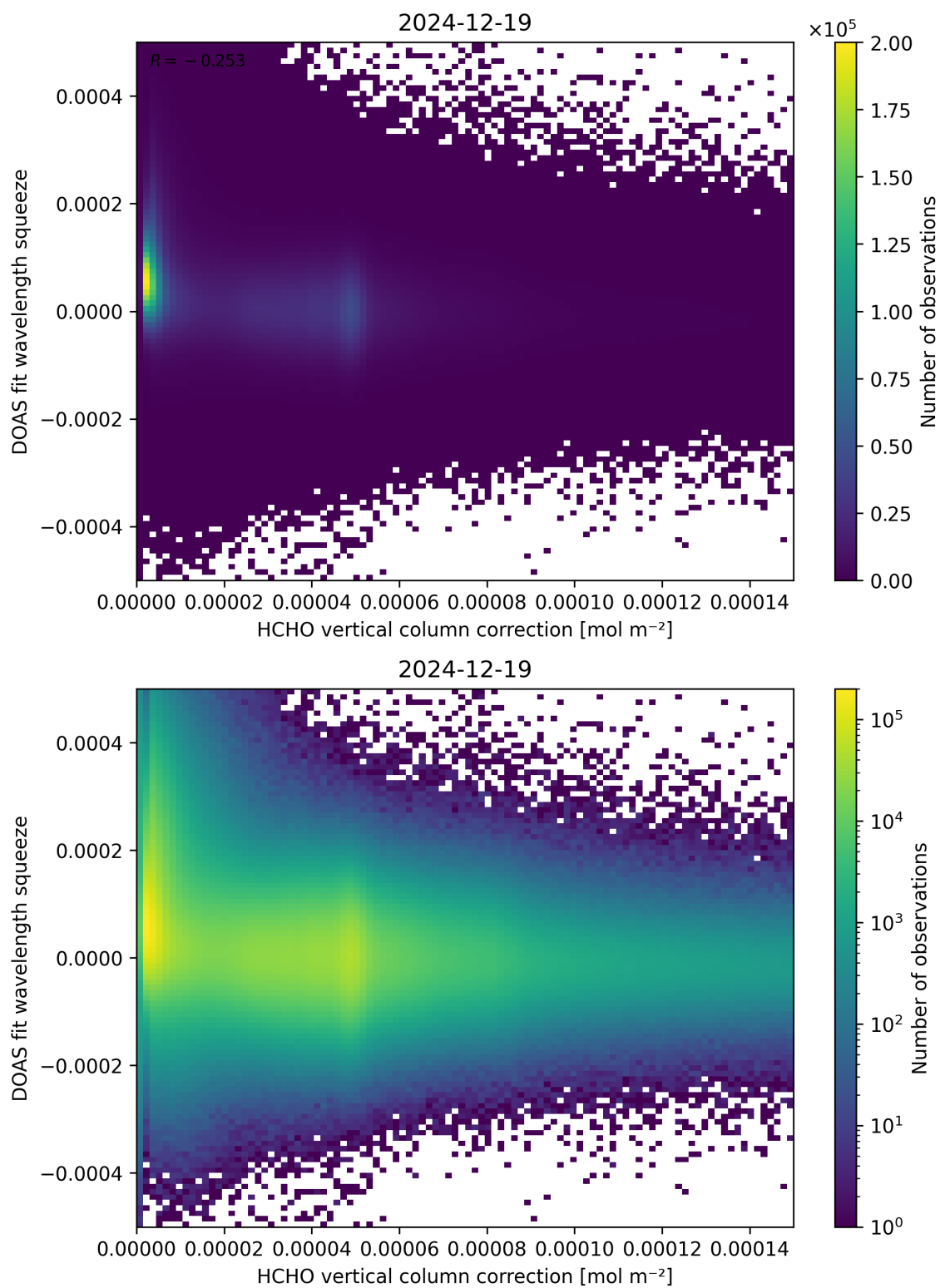
Figure 114: Scatter density plot of “HCHO vertical column correction” against “DOAS fit wavelength squeeze” for 2024-12-18 to 2024-12-20.
