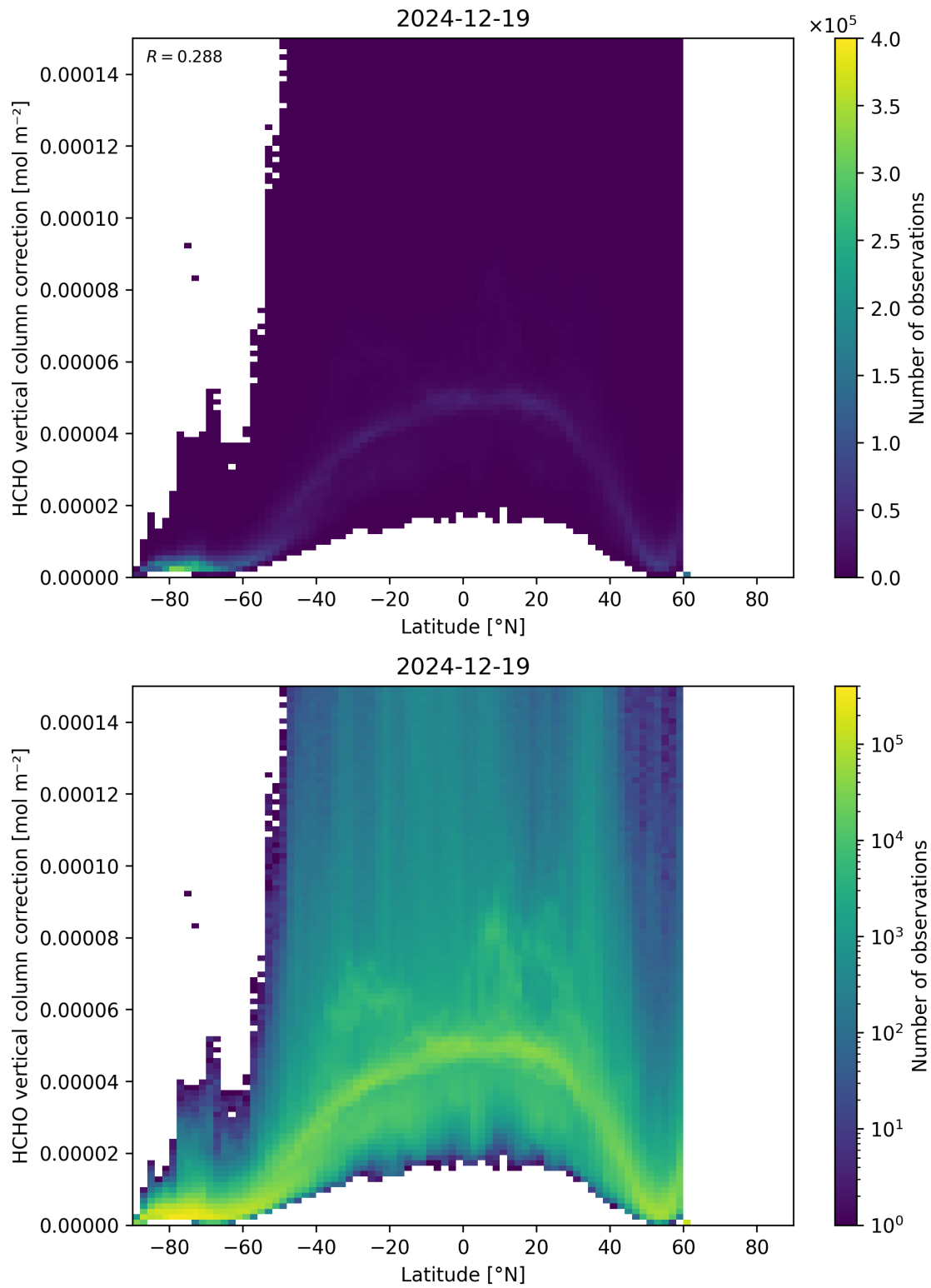
Figure 164: Scatter density plot of “Latitude” against “HCHO vertical column correction” for 2024-12-18 to 2024-12-20.
