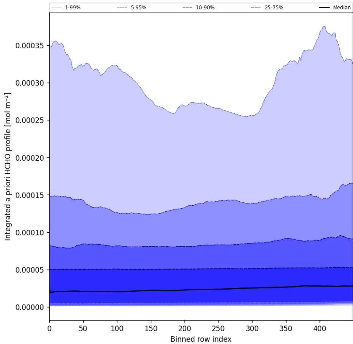
Figure 57: Along track statistics of "Integrated a priori HCHO profile" for 2024-12-18 to 2024-12-20
