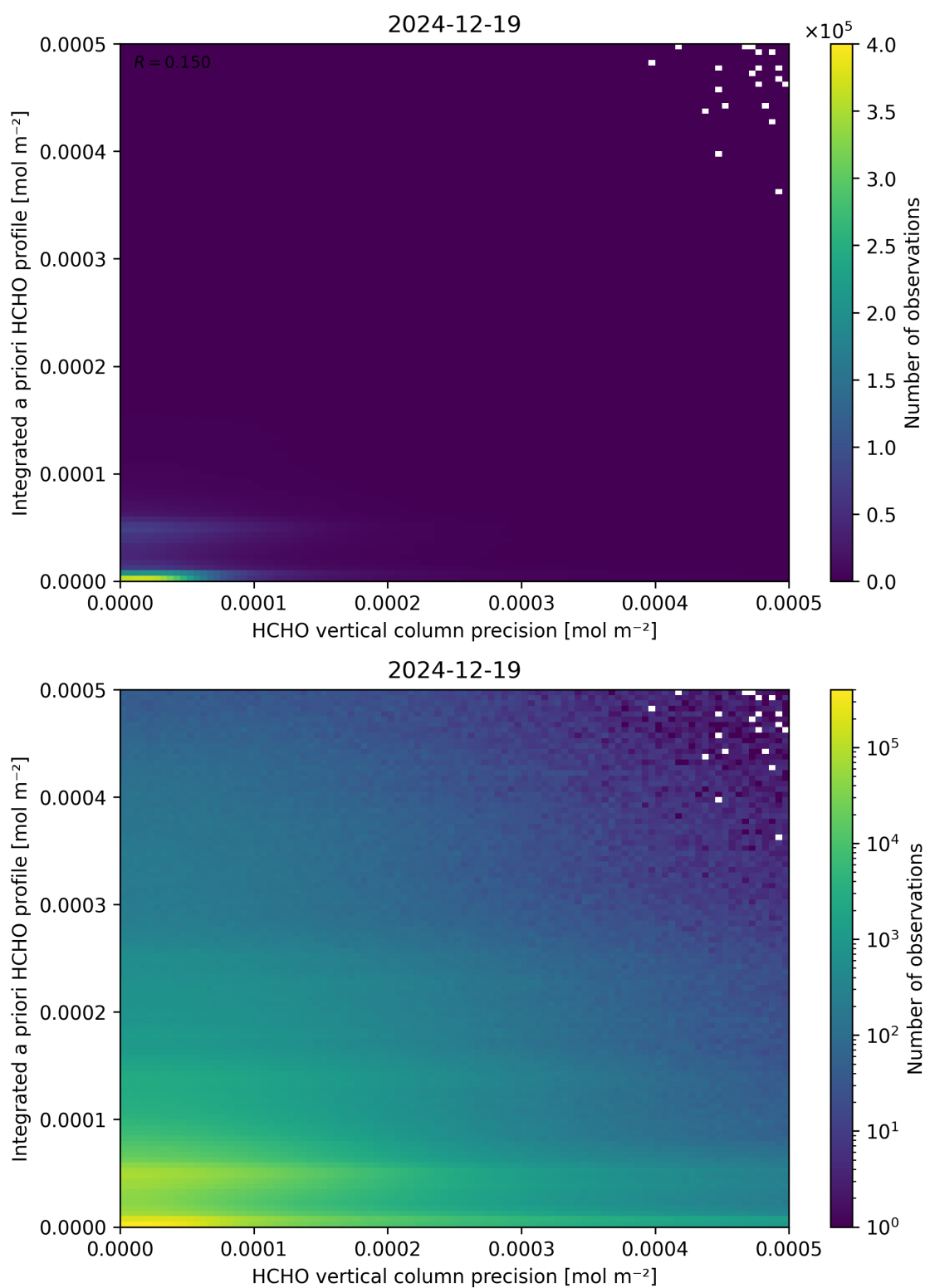
Figure 147: Scatter density plot of “HCHO vertical column precision” against “Integrated a priori HCHO profile” for 2024-12-18 to 2024-12-20.
