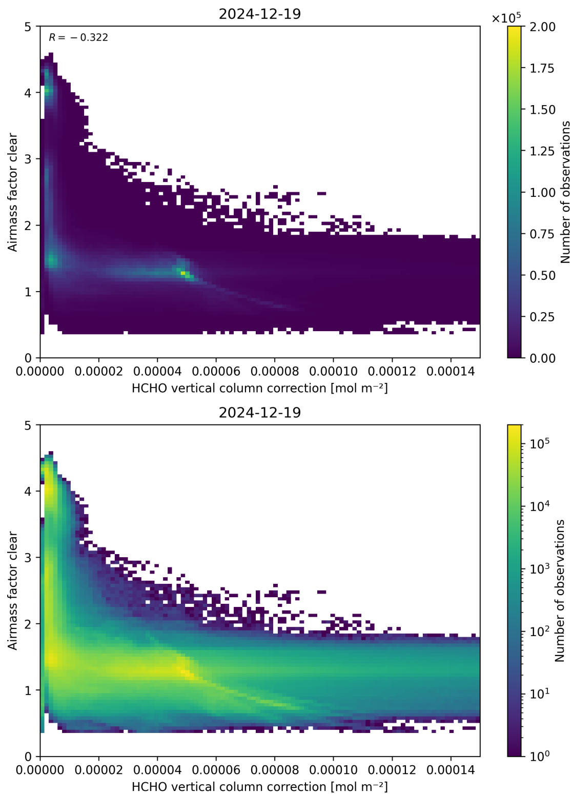
Figure 115: Scatter density plot of “HCHO vertical column correction” against “Airmass factor clear” for 2024-12-18 to 2024-12-20.
