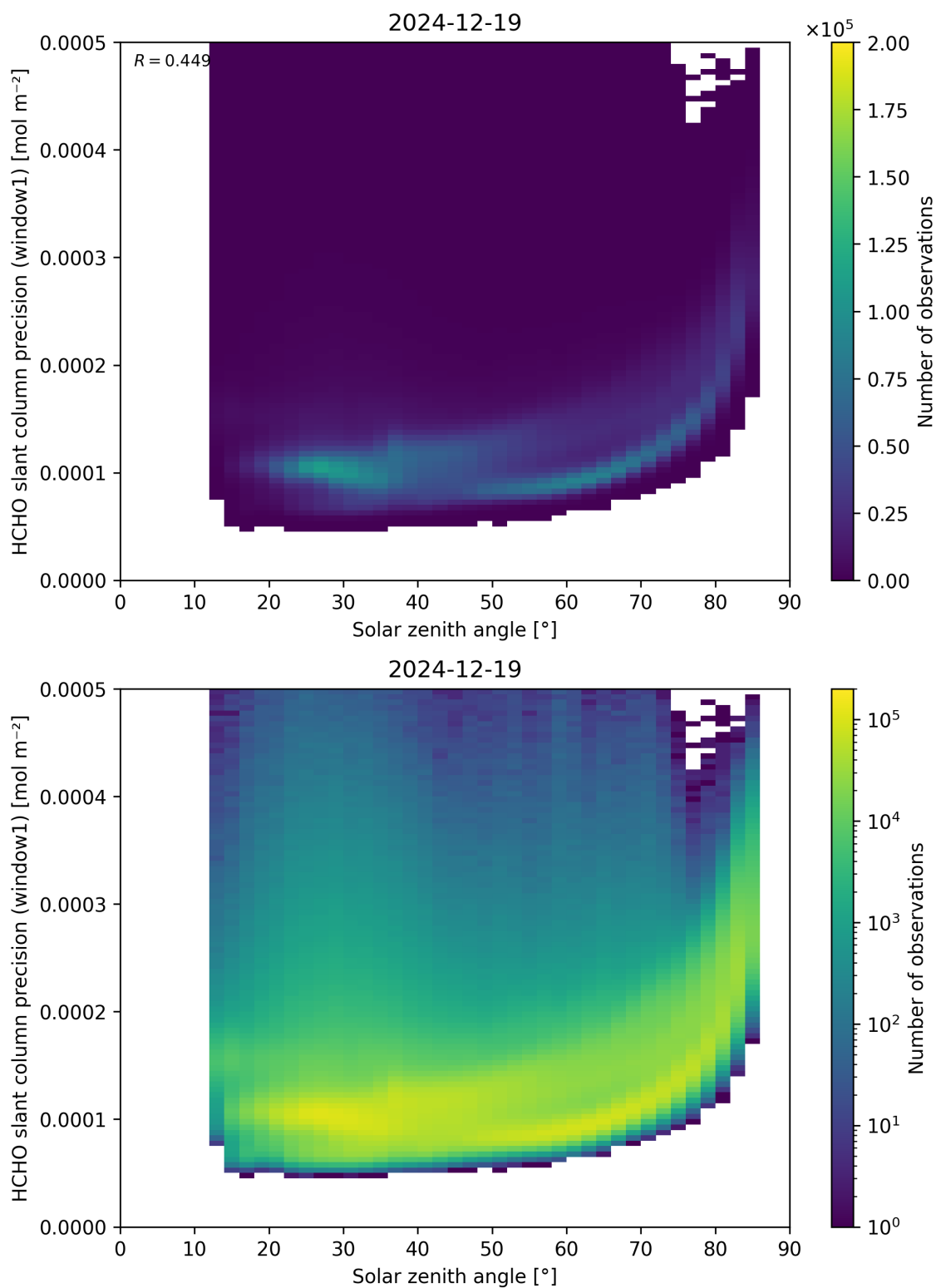
Figure 174: Scatter density plot of “Solar zenith angle” against “HCHO slant column precision (window1)” for 2024-12-18 to 2024-12-20.
