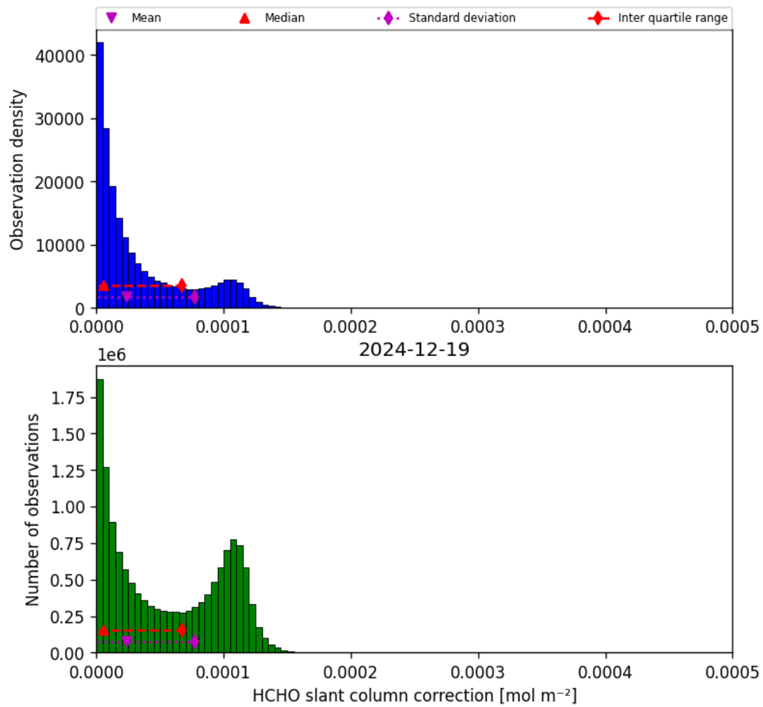
Figure 47: Histogram of “HCHO slant column correction” for 2024-12-18 to 2024-12-20
