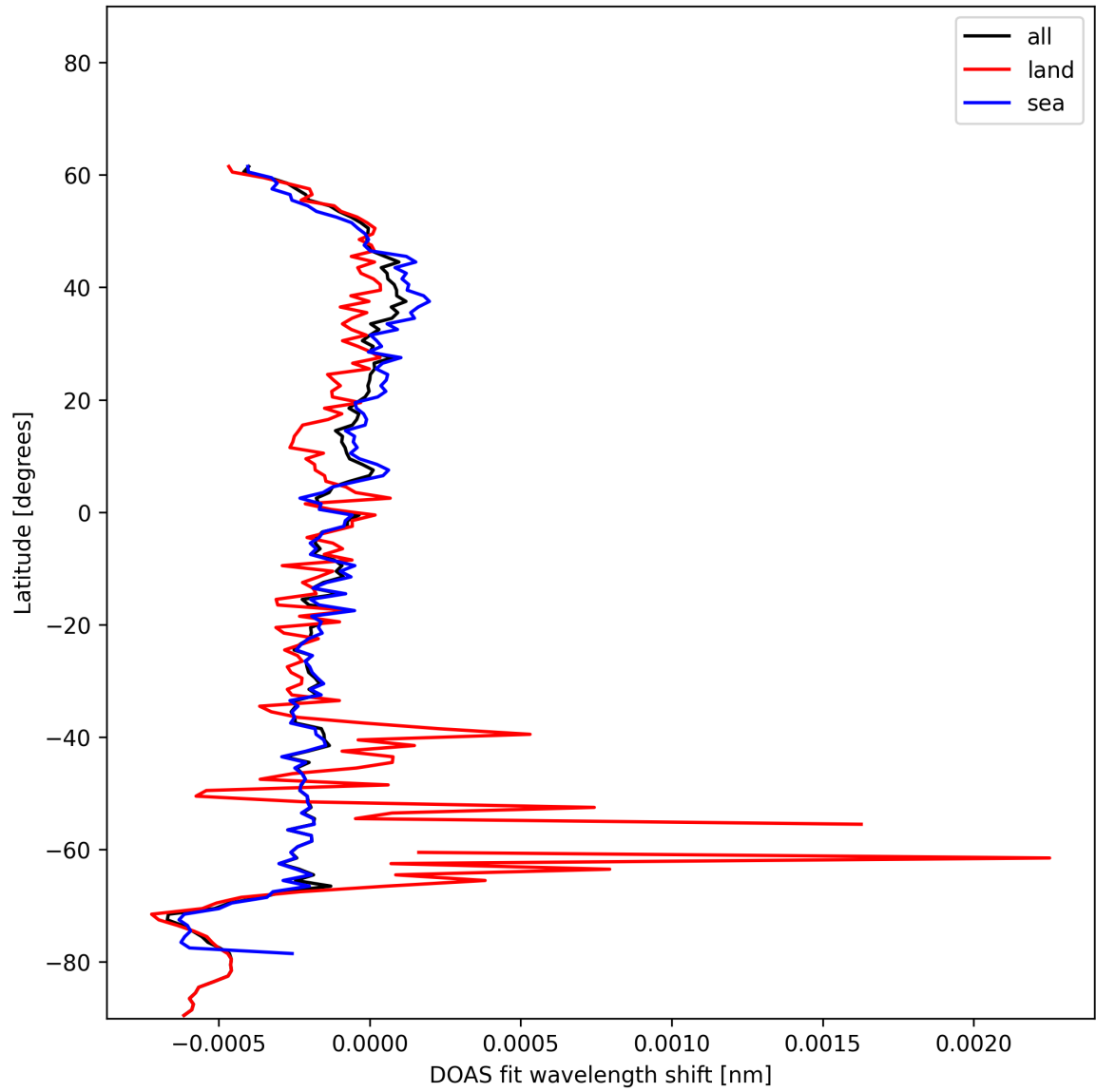
Figure 30: Zonal average of “DOAS fit wavelength shift” for 2024-12-18 to 2024-12-20.
