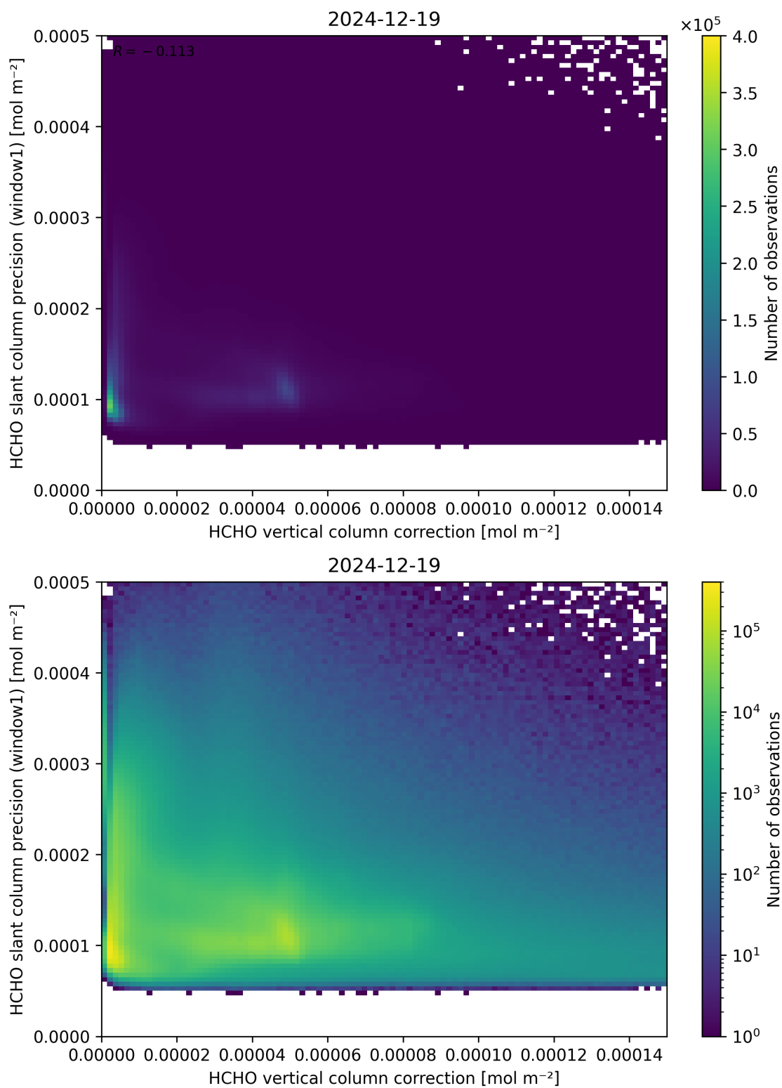
Figure 119: Scatter density plot of “HCHO vertical column correction” against “HCHO slant column precision (window1)” for 2024-12-18 to 2024-12-20.
