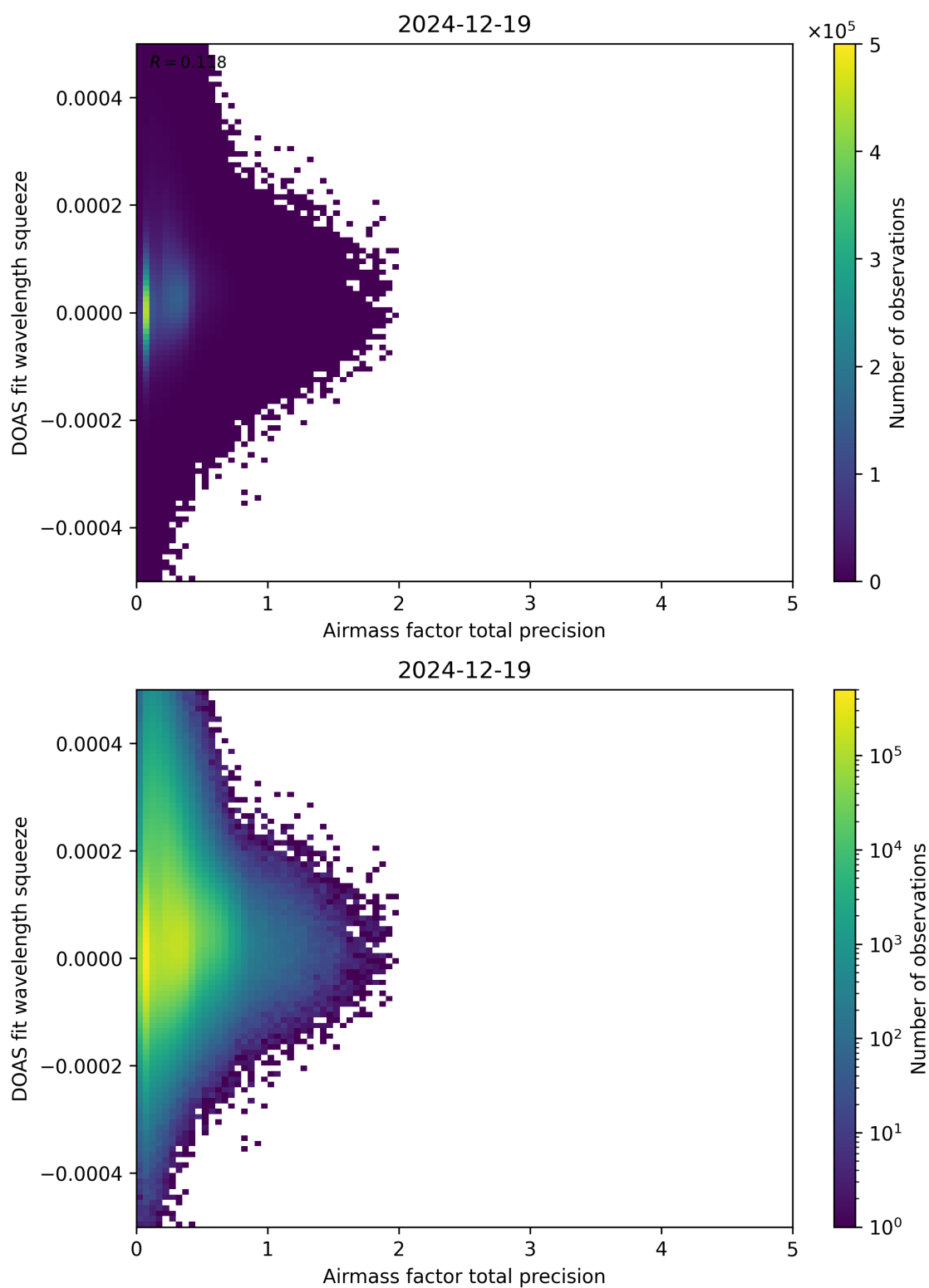
Figure 107: Scatter density plot of “Airmass factor total precision” against “DOAS fit wavelength squeeze” for 2024-12-18 to 2024-12-20.
