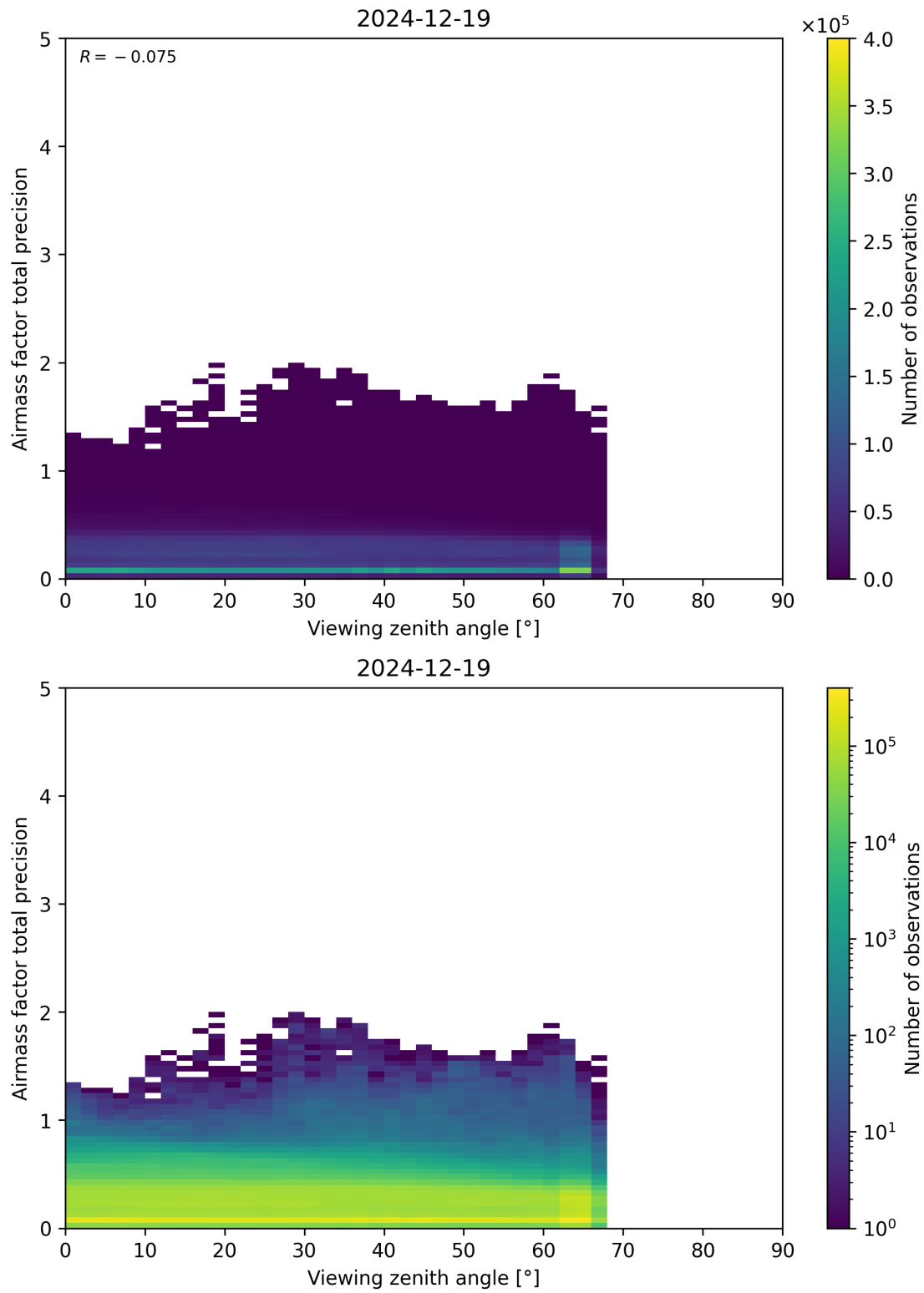
Figure 191: Scatter density plot of “Viewing zenith angle” against “Airmass factor total precision” for 2024-12-18 to 2024-12-20.
