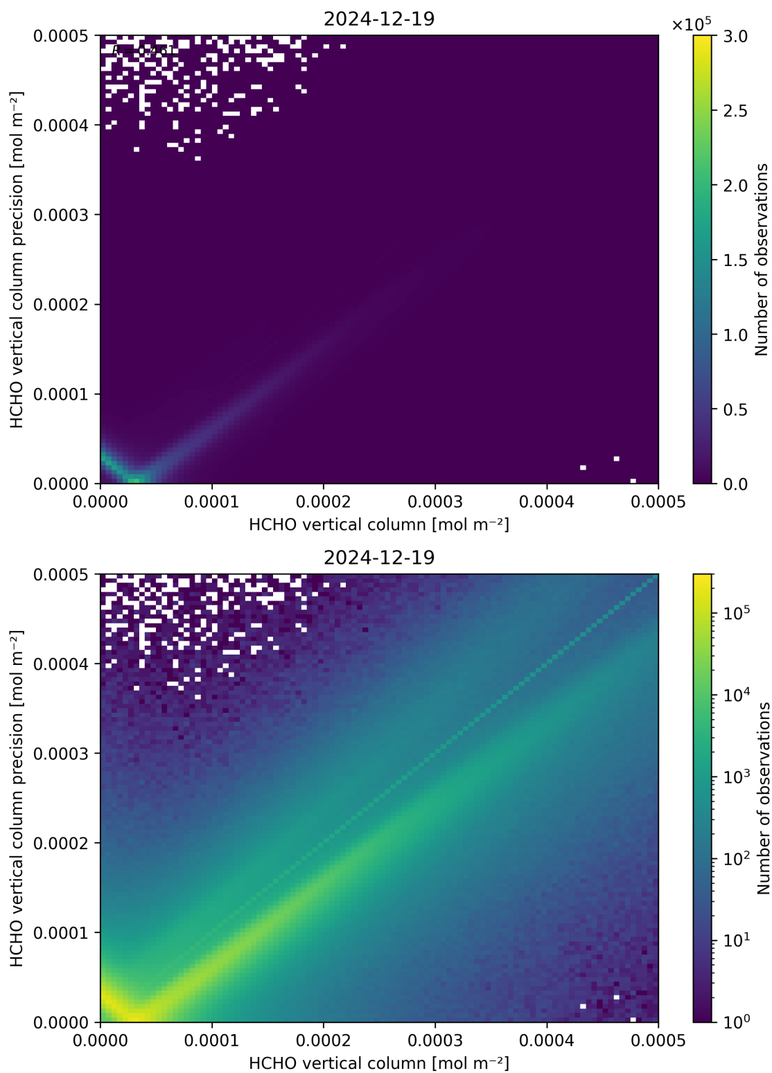
Figure 134: Scatter density plot of “HCHO vertical column” against “HCHO vertical column precision” for 2024-12-18 to 2024-12-20.
