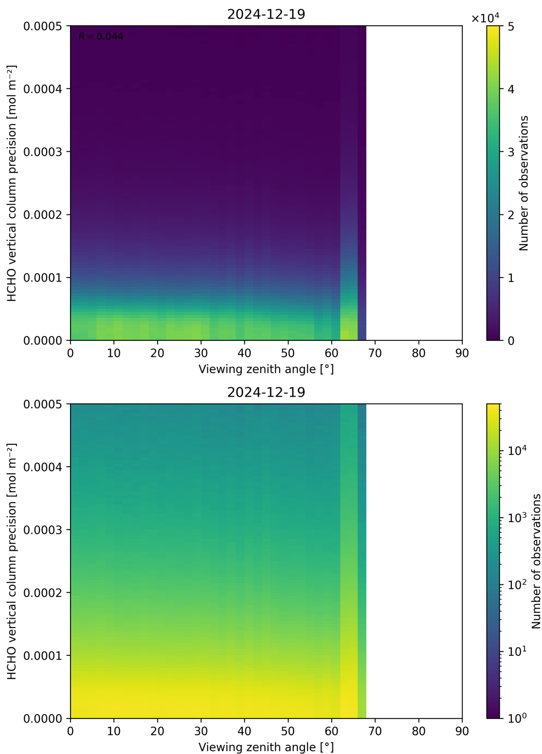
Figure 194: Scatter density plot of “Viewing zenith angle” against “HCHO vertical column precision” for 2024-12-18 to 2024-12-20.
