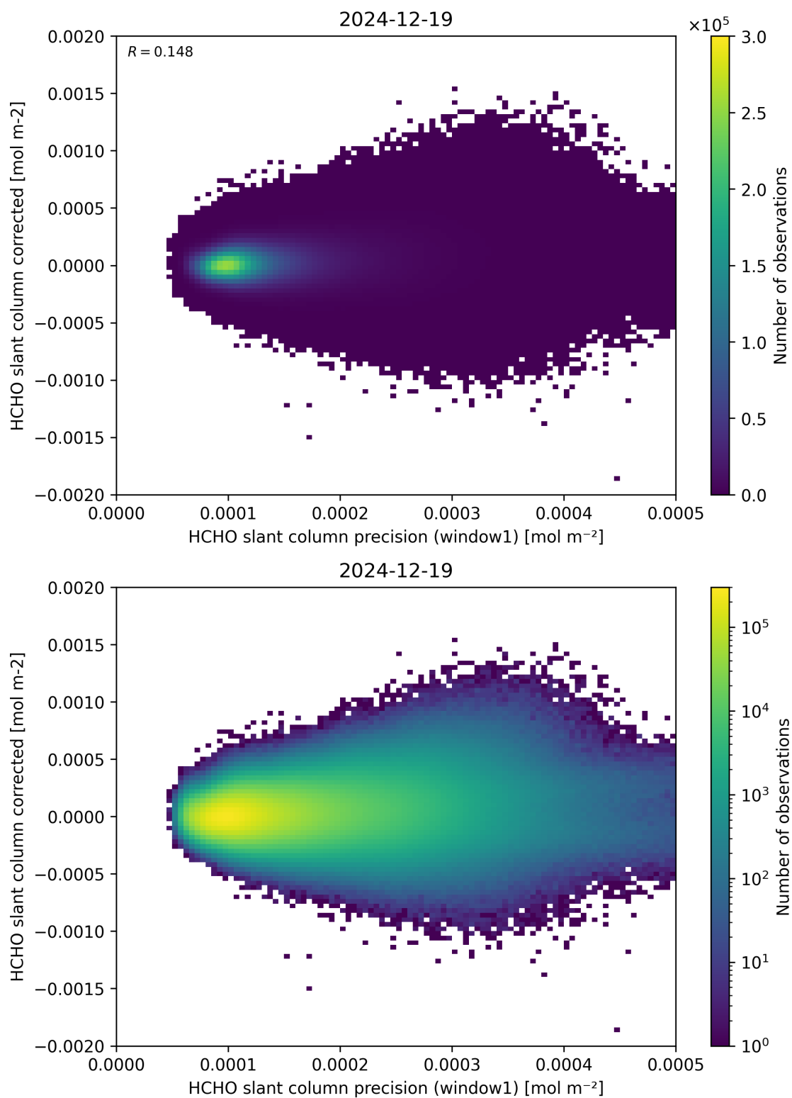
Figure 92: Scatter density plot of “HCHO slant column precision (window1)” against “HCHO slant column corrected” for 2024-12-18 to 2024-12-20.
