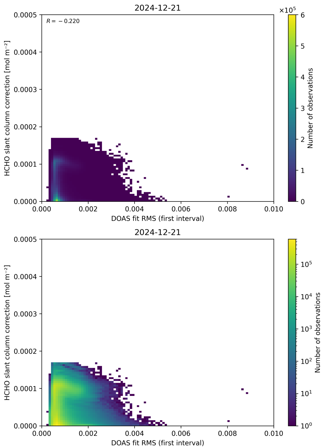
Figure 63: Scatter density plot of “DOAS fit RMS (first interval)” against “HCHO slant column correction” for 2024-12-20 to 2024-12-22.
