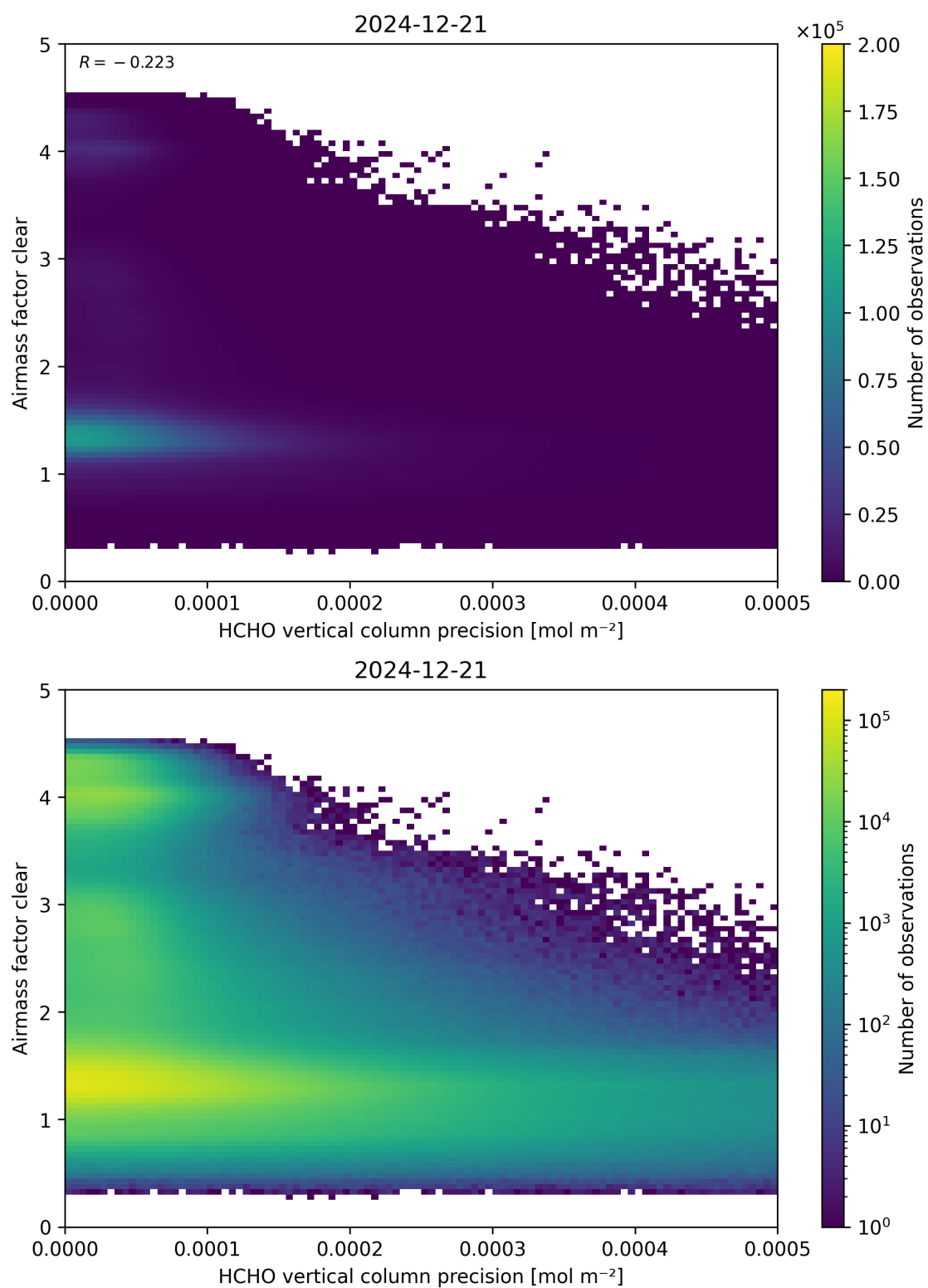
Figure 139: Scatter density plot of “HCHO vertical column precision” against “Airmass factor clear” for 2024-12-20 to 2024-12-22.
