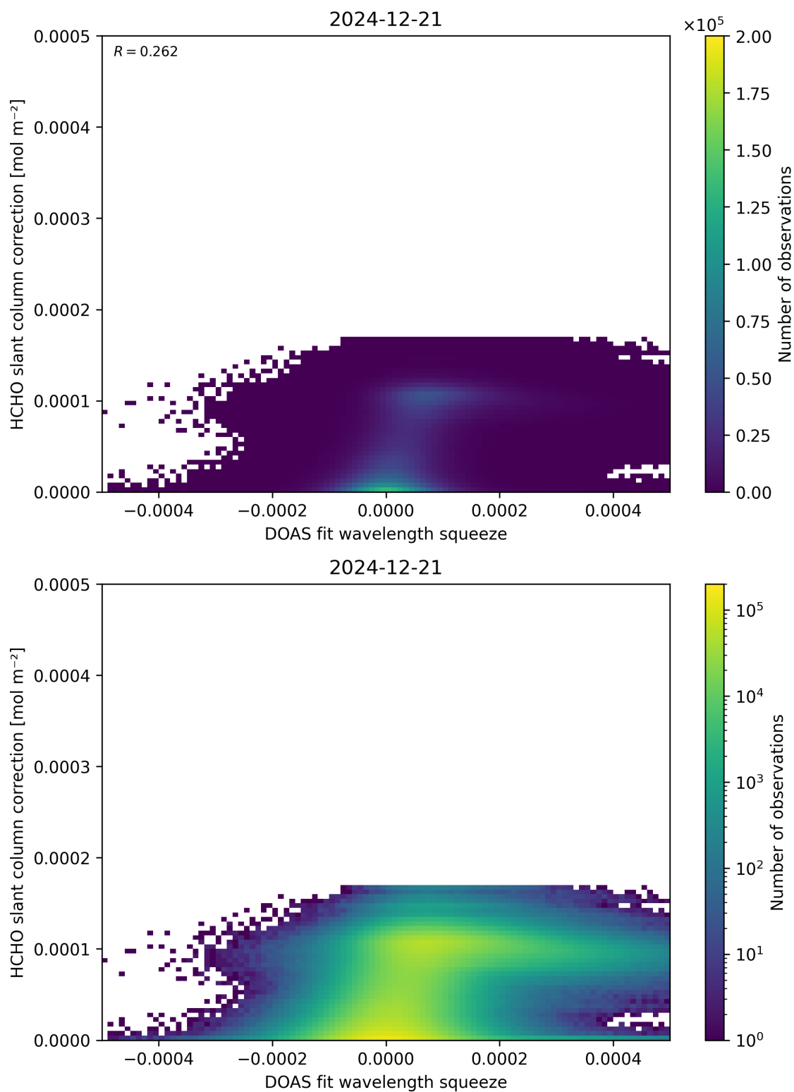
Figure 70: Scatter density plot of “DOAS fit wavelength squeeze” against “HCHO slant column correction” for 2024-12-20 to 2024-12-22.
