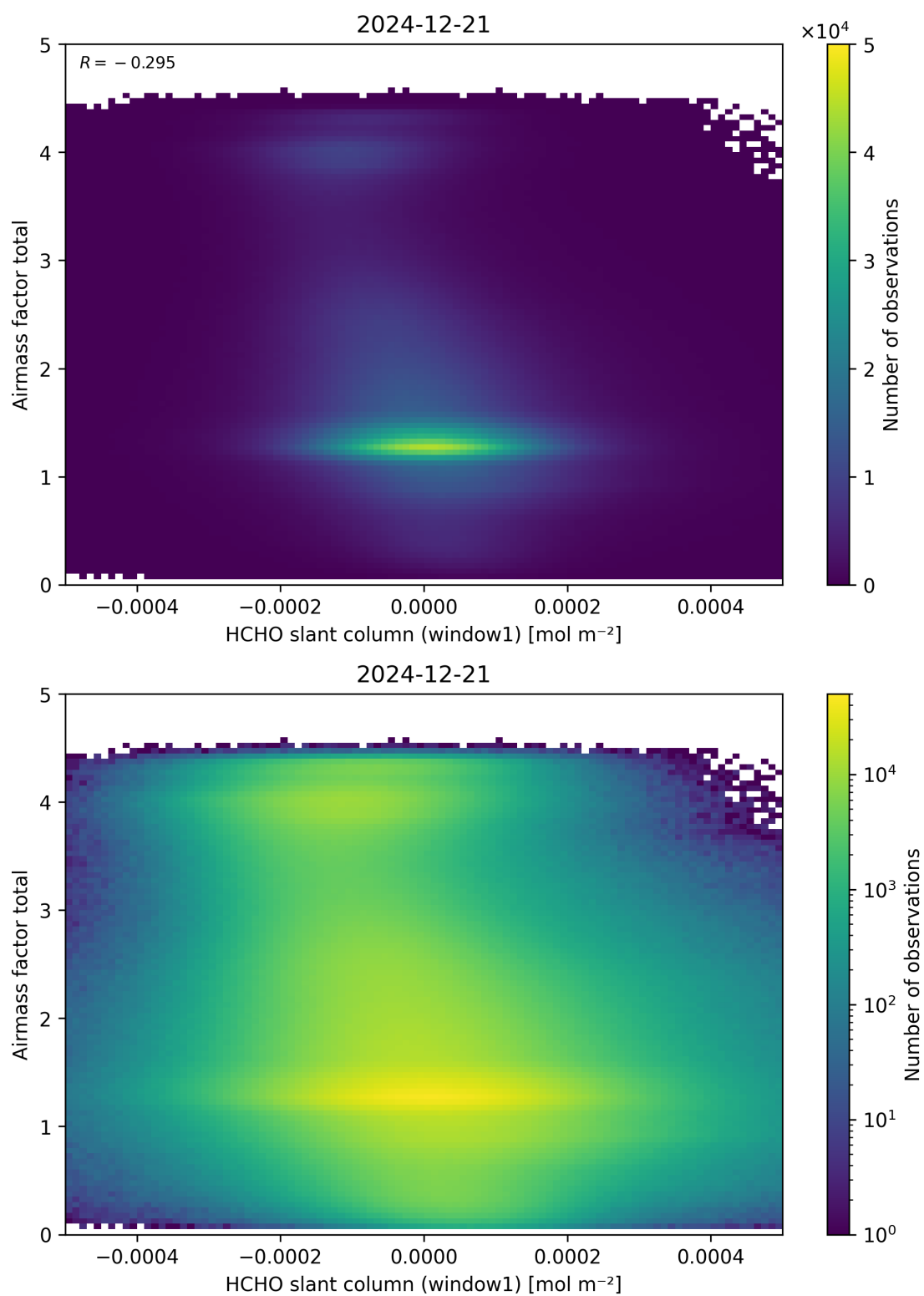
Figure 85: Scatter density plot of “HCHO slant column (window1)” against “Airmass factor total” for 2024-12-20 to 2024-12-22.
