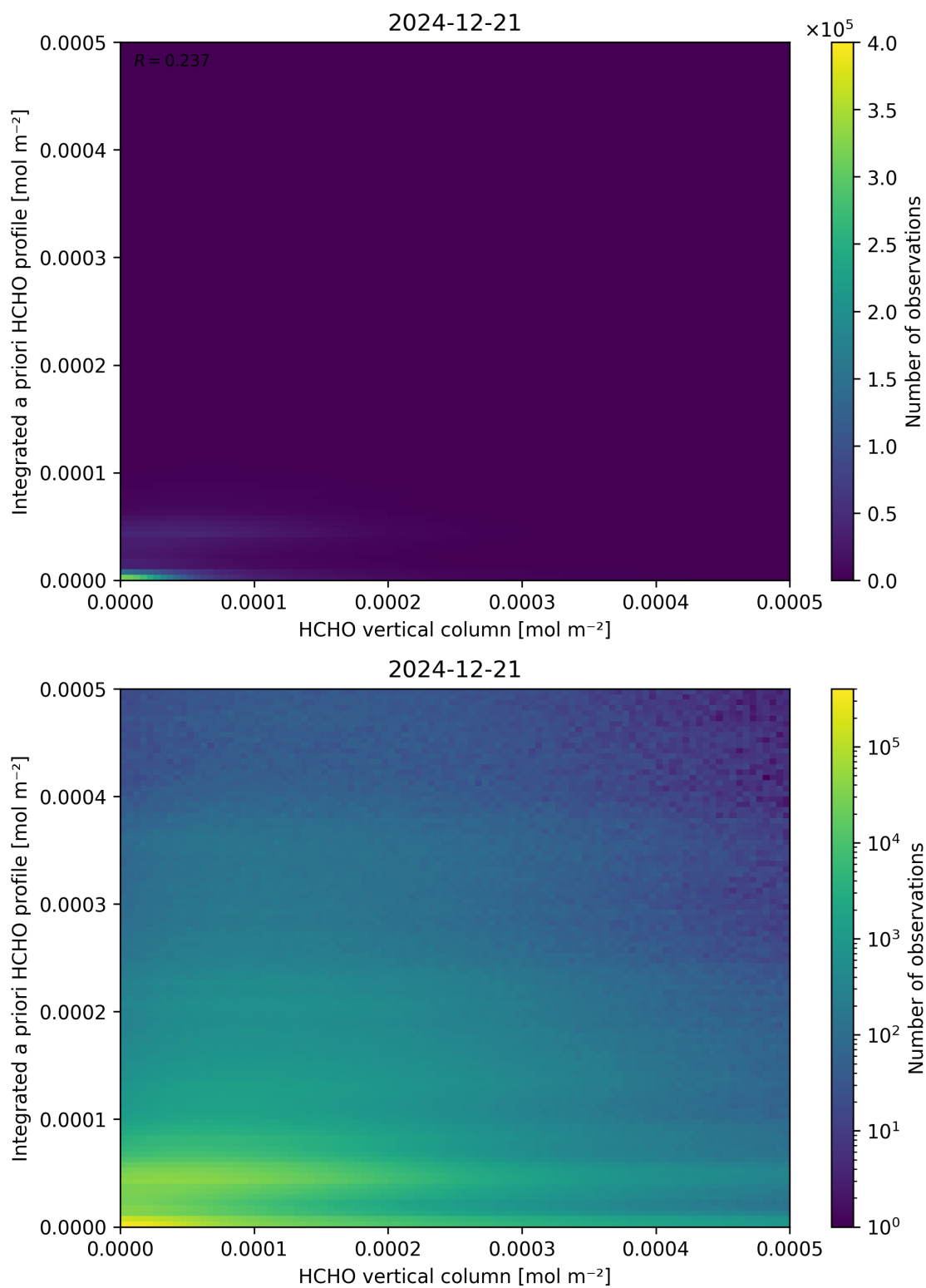
Figure 135: Scatter density plot of “HCHO vertical column” against “Integrated a priori HCHO profile” for 2024-12-20 to 2024-12-22.
