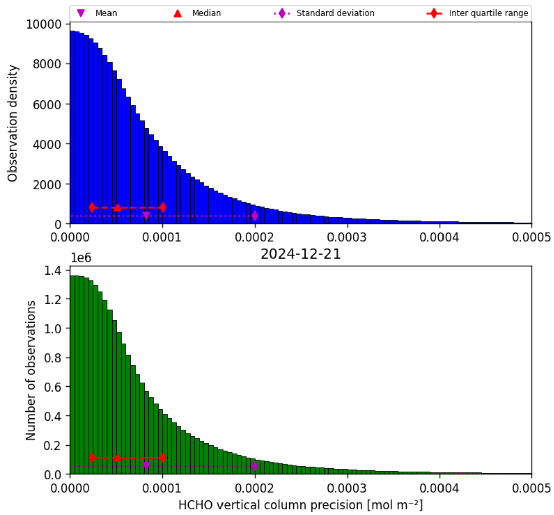
Figure 36: Histogram of “HCHO vertical column precision” for 2024-12-20 to 2024-12-22
