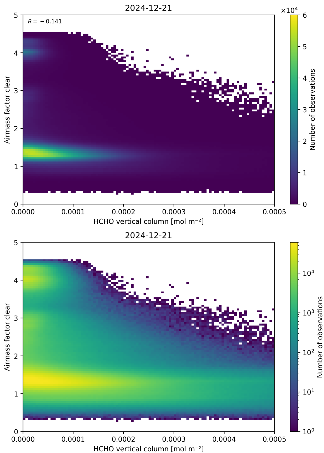
Figure 126: Scatter density plot of “HCHO vertical column” against “Airmass factor clear” for 2024-12-20 to 2024-12-22.
