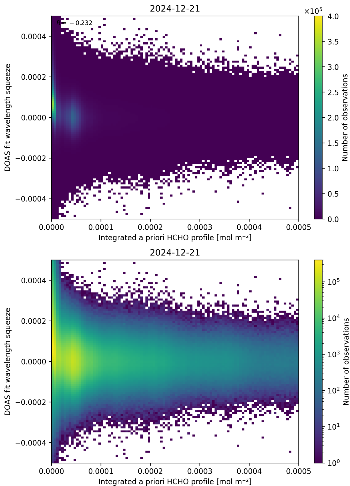
Figure 150: Scatter density plot of “Integrated a priori HCHO profile” against “DOAS fit wavelength squeeze” for 2024-12-20 to 2024-12-22.
