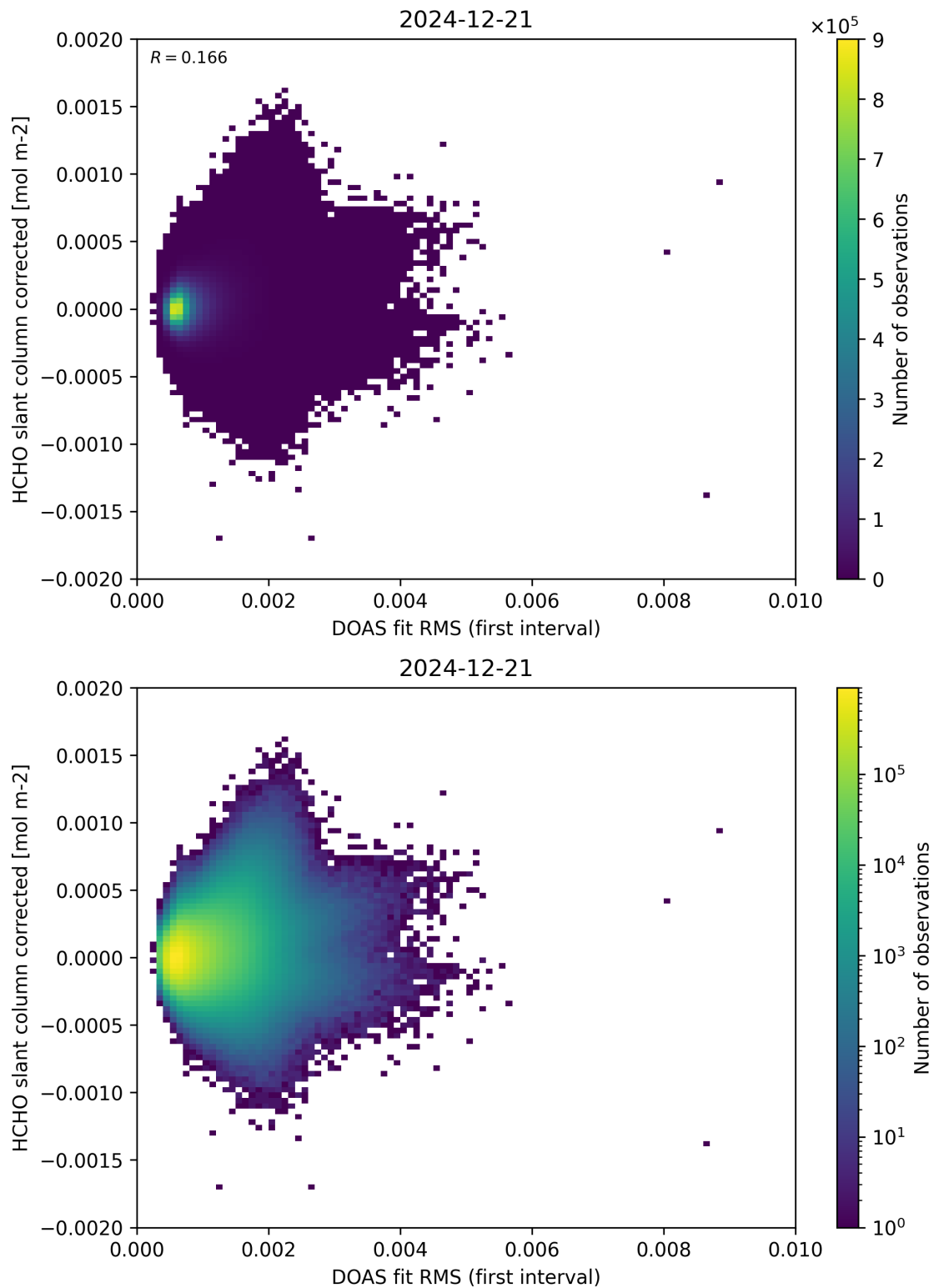
Figure 62: Scatter density plot of “DOAS fit RMS (first interval)” against “HCHO slant column corrected” for 2024-12-20 to 2024-12-22.
