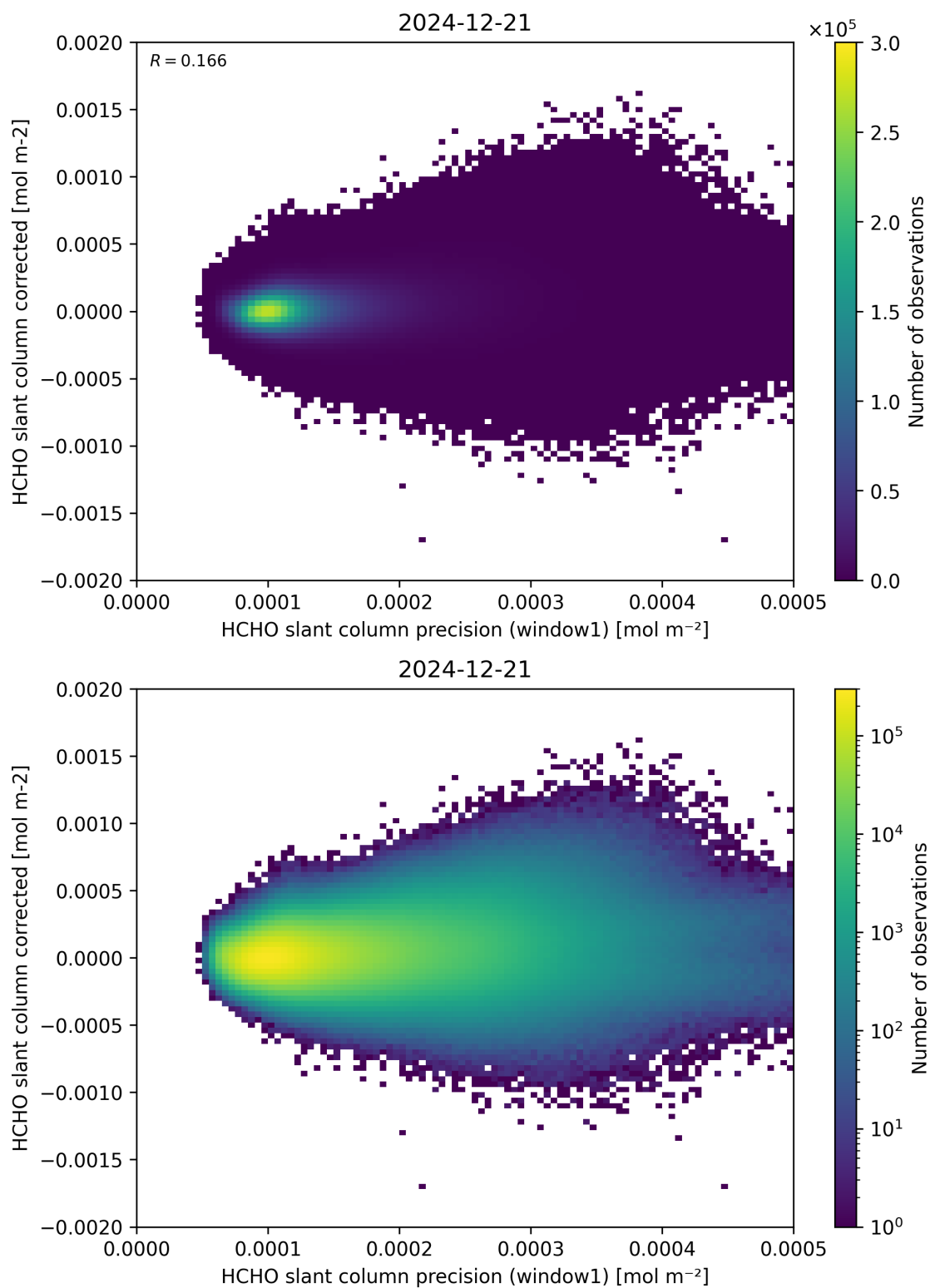
Figure 92: Scatter density plot of “HCHO slant column precision (window1)” against “HCHO slant column corrected” for 2024-12-20 to 2024-12-22.
