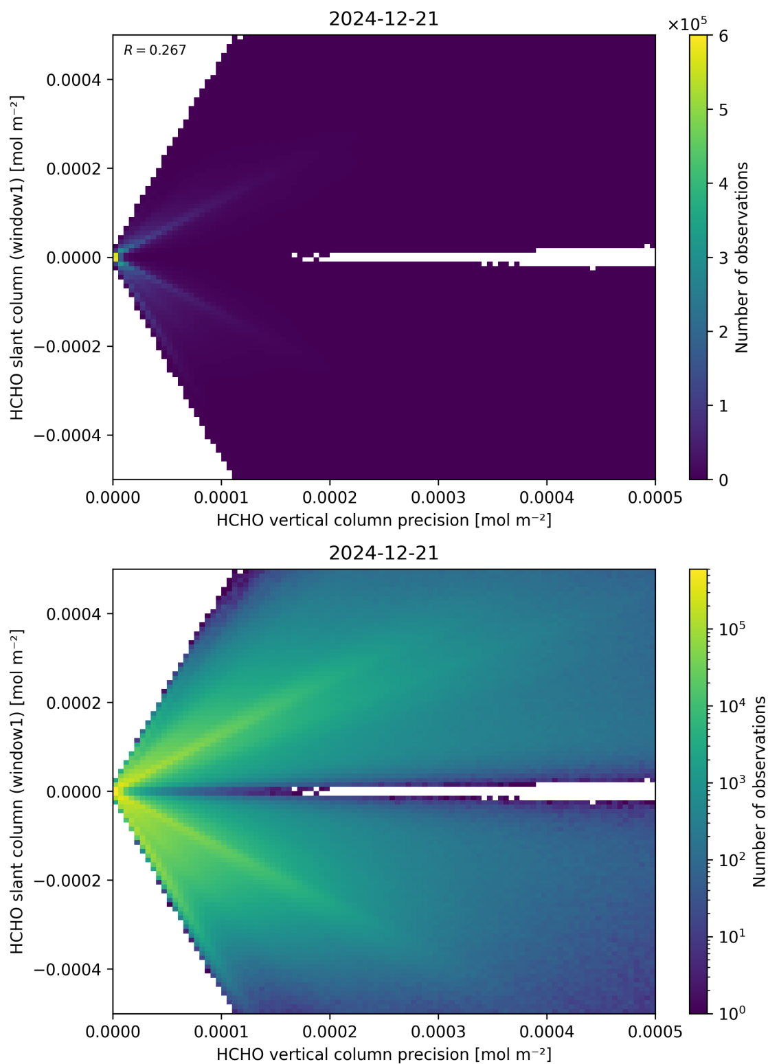
Figure 142: Scatter density plot of “HCHO vertical column precision” against “HCHO slant column (window1)” for 2024-12-20 to 2024-12-22.
