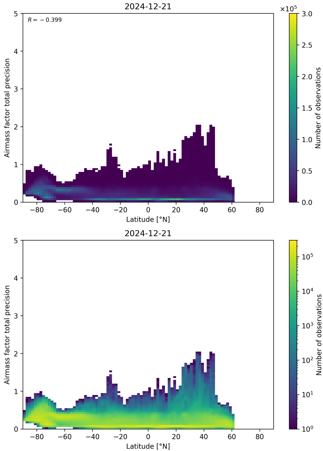
Figure 162: Scatter density plot of “Latitude” against “Airmass factor total precision” for 2024-12-20 to 2024-12-22.
