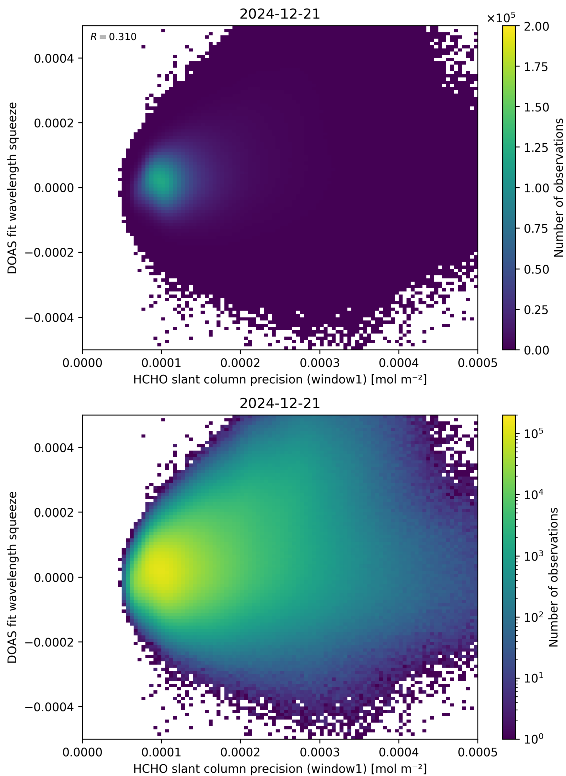
Figure 90: Scatter density plot of “HCHO slant column precision (window1)” against “DOAS fit wavelength squeeze” for 2024-12-20 to 2024-12-22.
