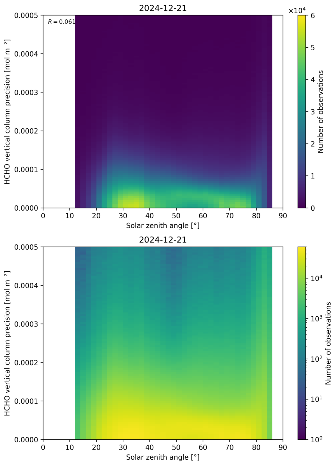
Figure 179: Scatter density plot of “Solar zenith angle” against “HCHO vertical column precision” for 2024-12-20 to 2024-12-22.
