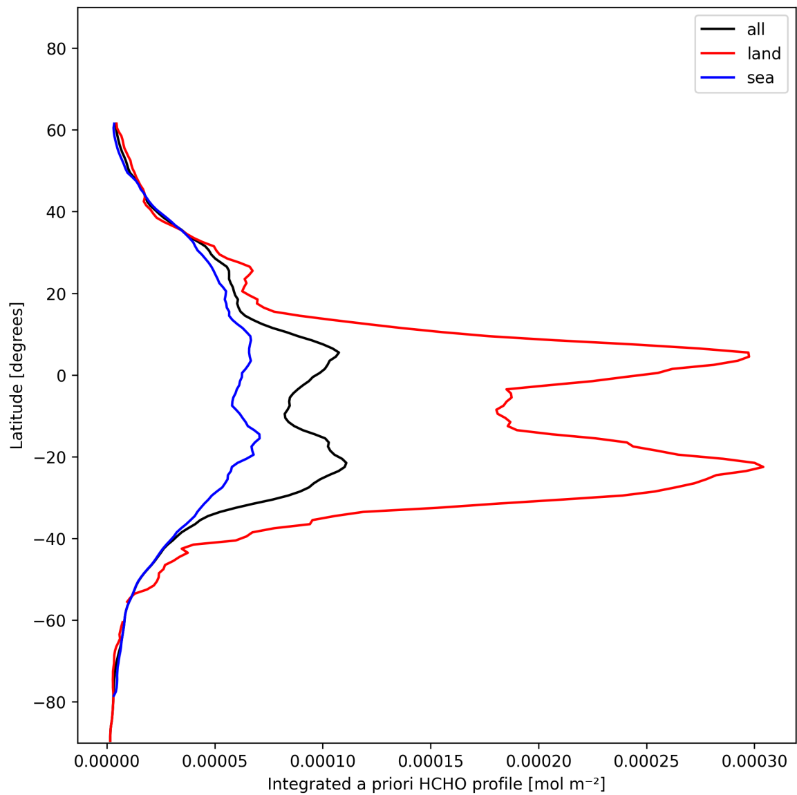
Figure 29: Zonal average of “Integrated a priori HCHO profile” for 2024-12-20 to 2024-12-22.
