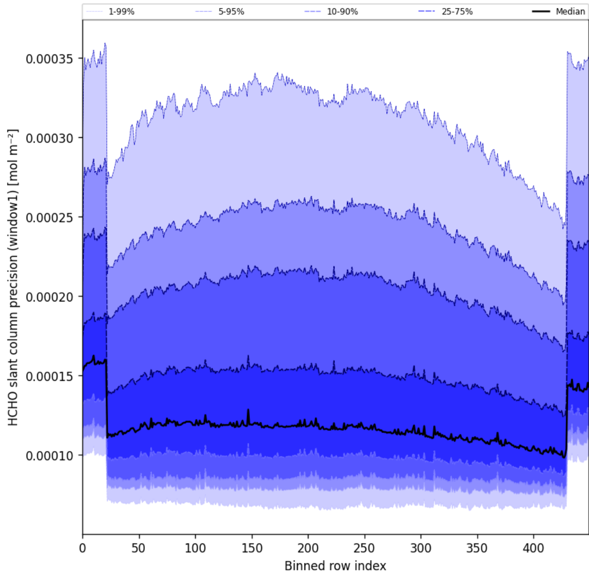
Figure 53: Along track statistics of “HCHO slant column precision (window1)” for 2024-12-20 to 2024-12-22
