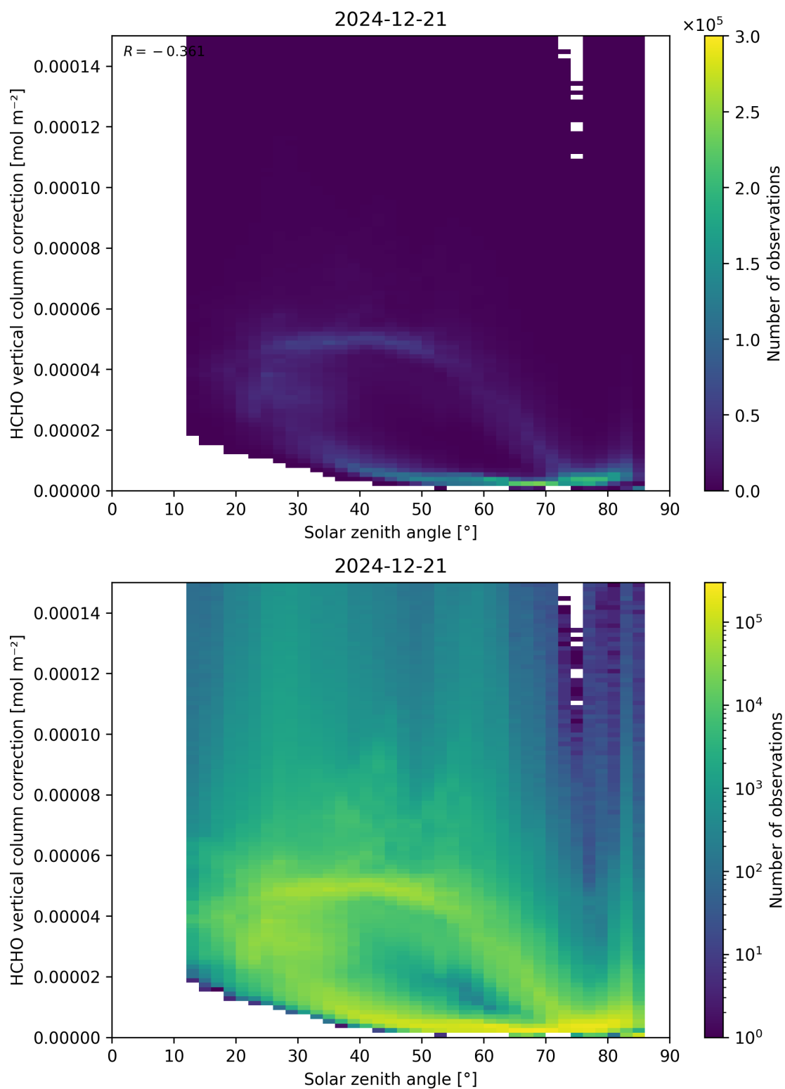
Figure 178: Scatter density plot of “Solar zenith angle” against “HCHO vertical column correction” for 2024-12-20 to 2024-12-22.
