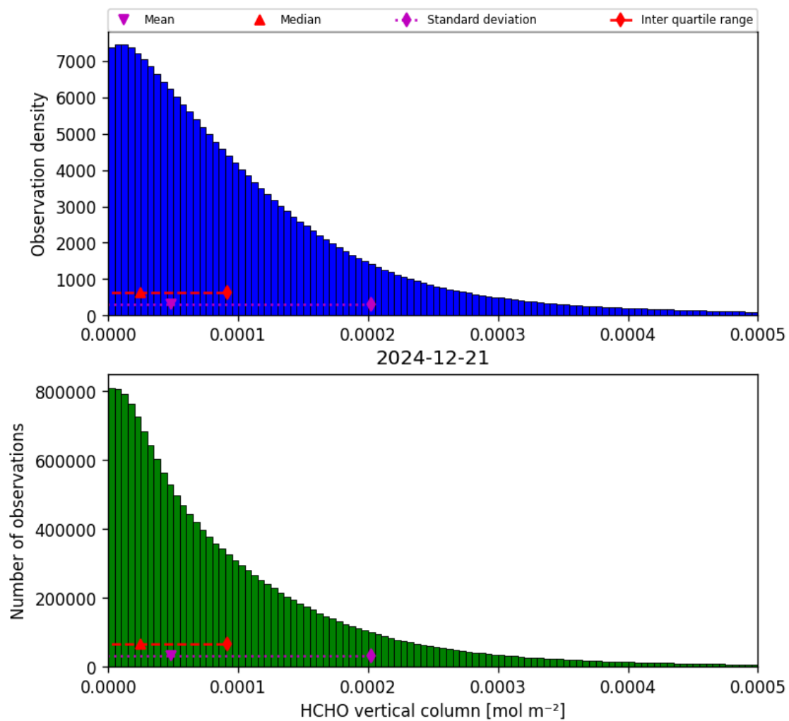
Figure 35: Histogram of “HCHO vertical column” for 2024-12-20 to 2024-12-22
