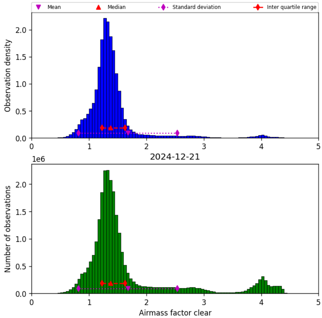
Figure 42: Histogram of “Airmass factor clear” for 2024-12-20 to 2024-12-22
