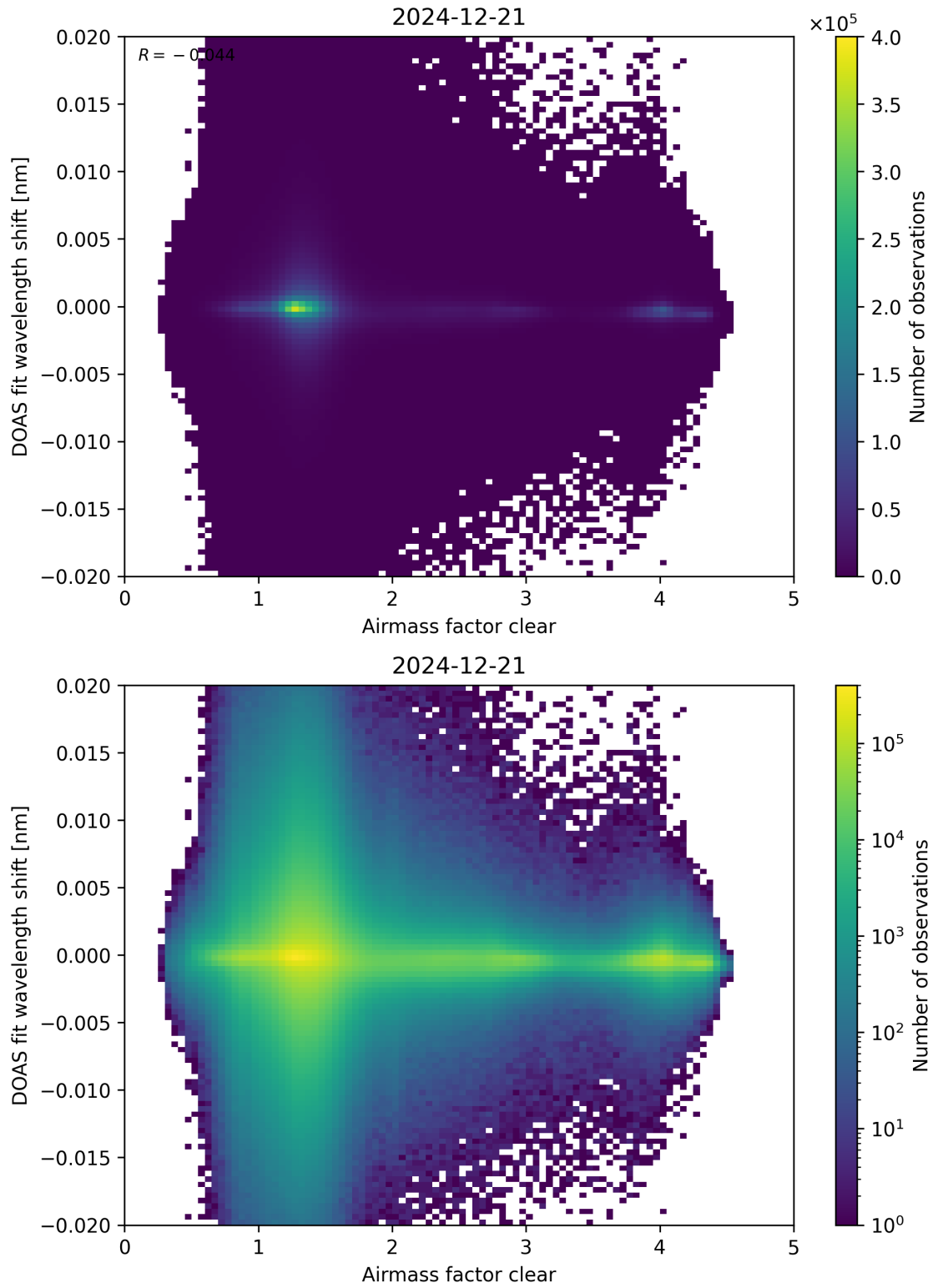
Figure 72: Scatter density plot of “Airmass factor clear” against “DOAS fit wavelength shift” for 2024-12-20 to 2024-12-22.
