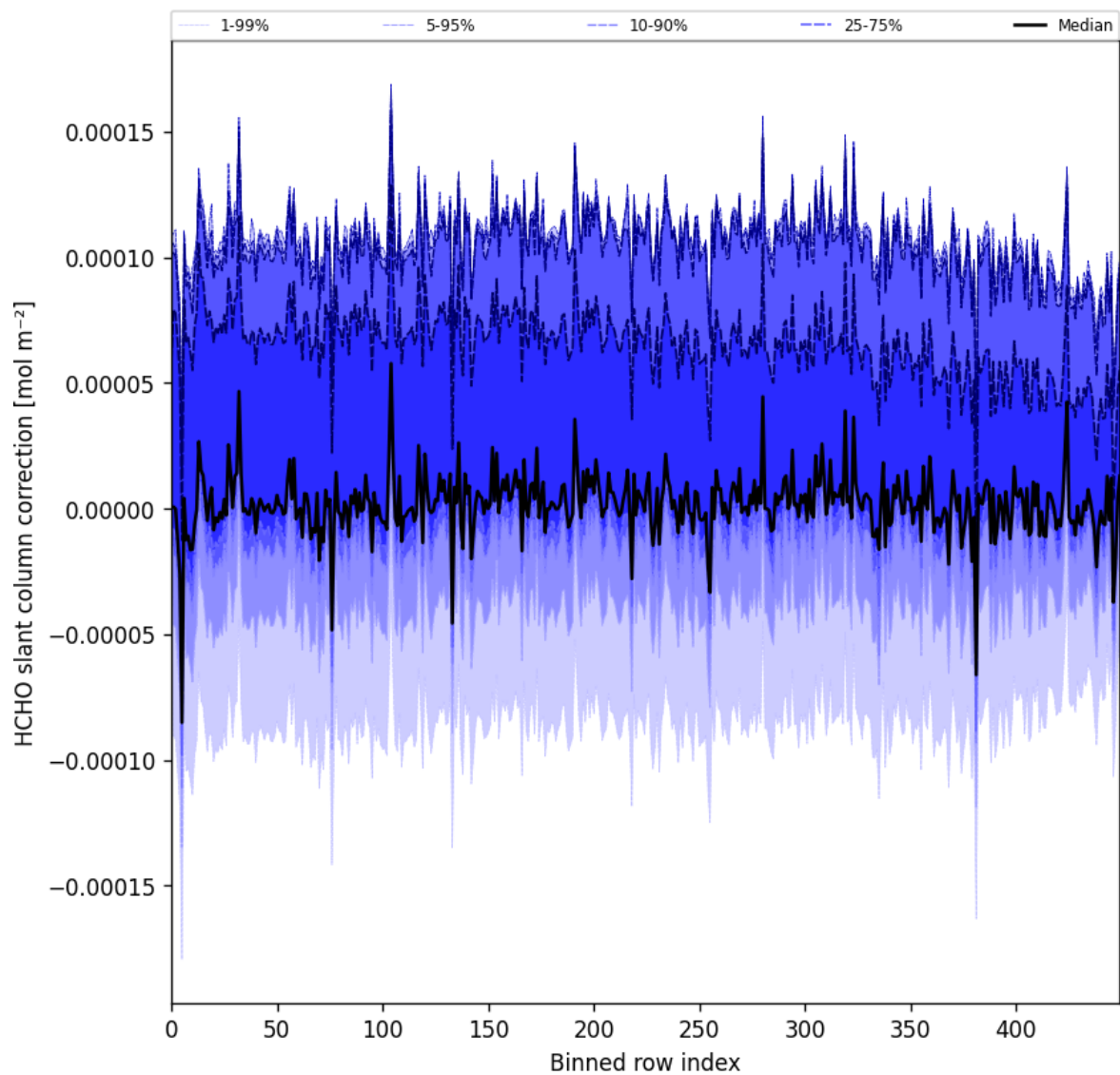
Figure 61: Along track statistics of “HCHO slant column correction” for 2024-12-20 to 2024-12-22
