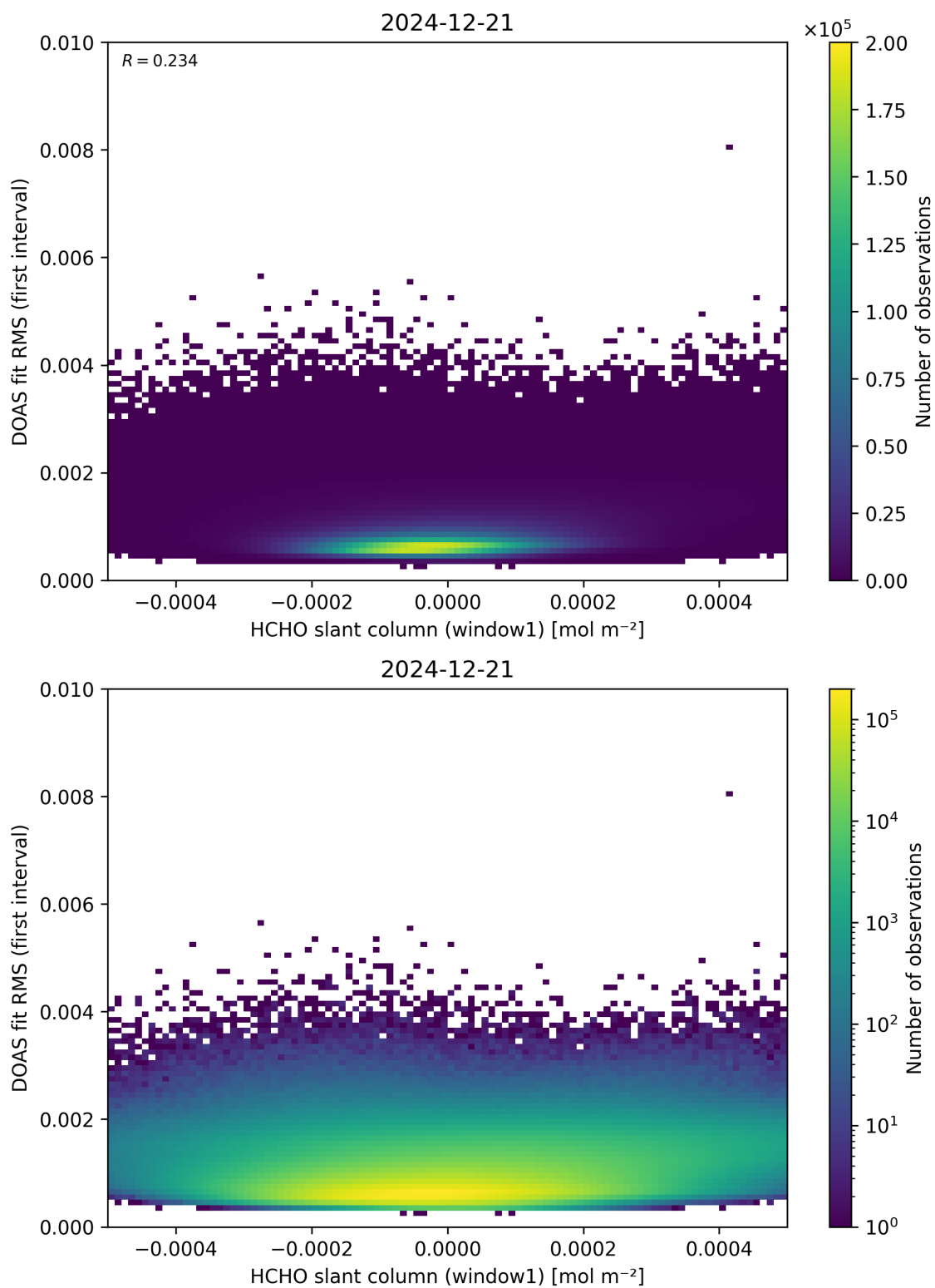
Figure 78: Scatter density plot of “HCHO slant column (window1)” against “DOAS fit RMS (first interval)” for 2024-12-20 to 2024-12-22.
