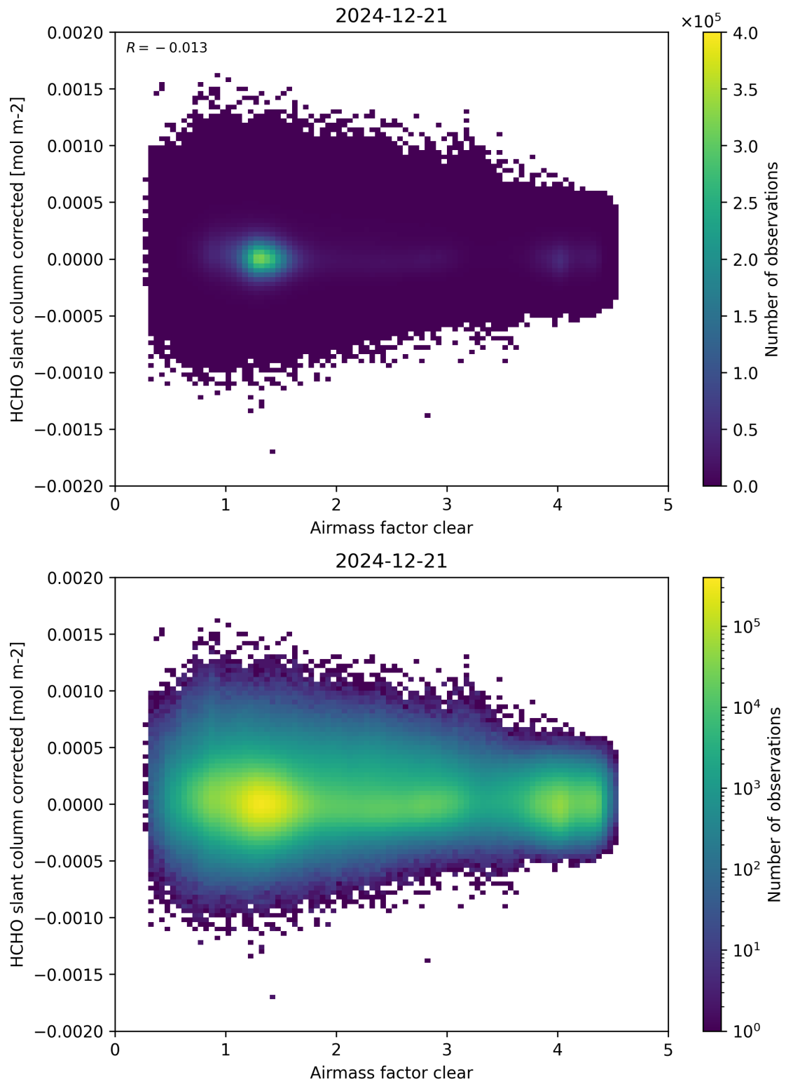
Figure 74: Scatter density plot of “Airmass factor clear” against “HCHO slant column corrected” for 2024-12-20 to 2024-12-22.
