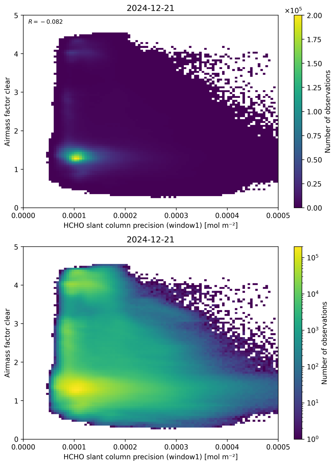
Figure 91: Scatter density plot of “HCHO slant column precision (window1)” against “Airmass factor clear” for 2024-12-20 to 2024-12-22.
