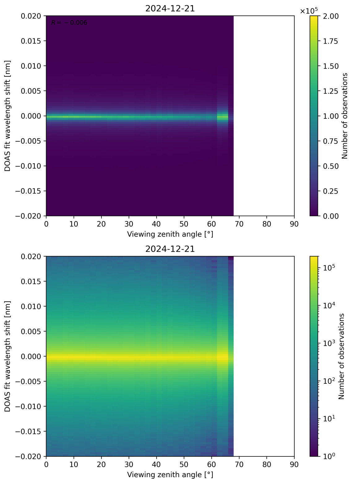
Figure 183: Scatter density plot of “Viewing zenith angle” against “DOAS fit wavelength shift” for 2024-12-20 to 2024-12-22.
