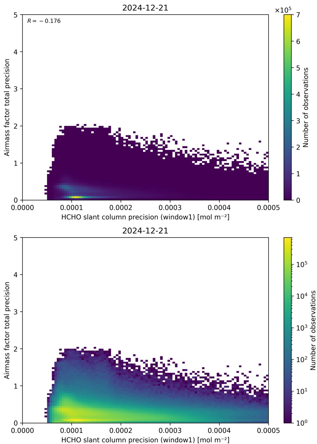
Figure 95: Scatter density plot of “HCHO slant column precision (window1)” against “Airmass factor total precision” for 2024-12-20 to 2024-12-22.
