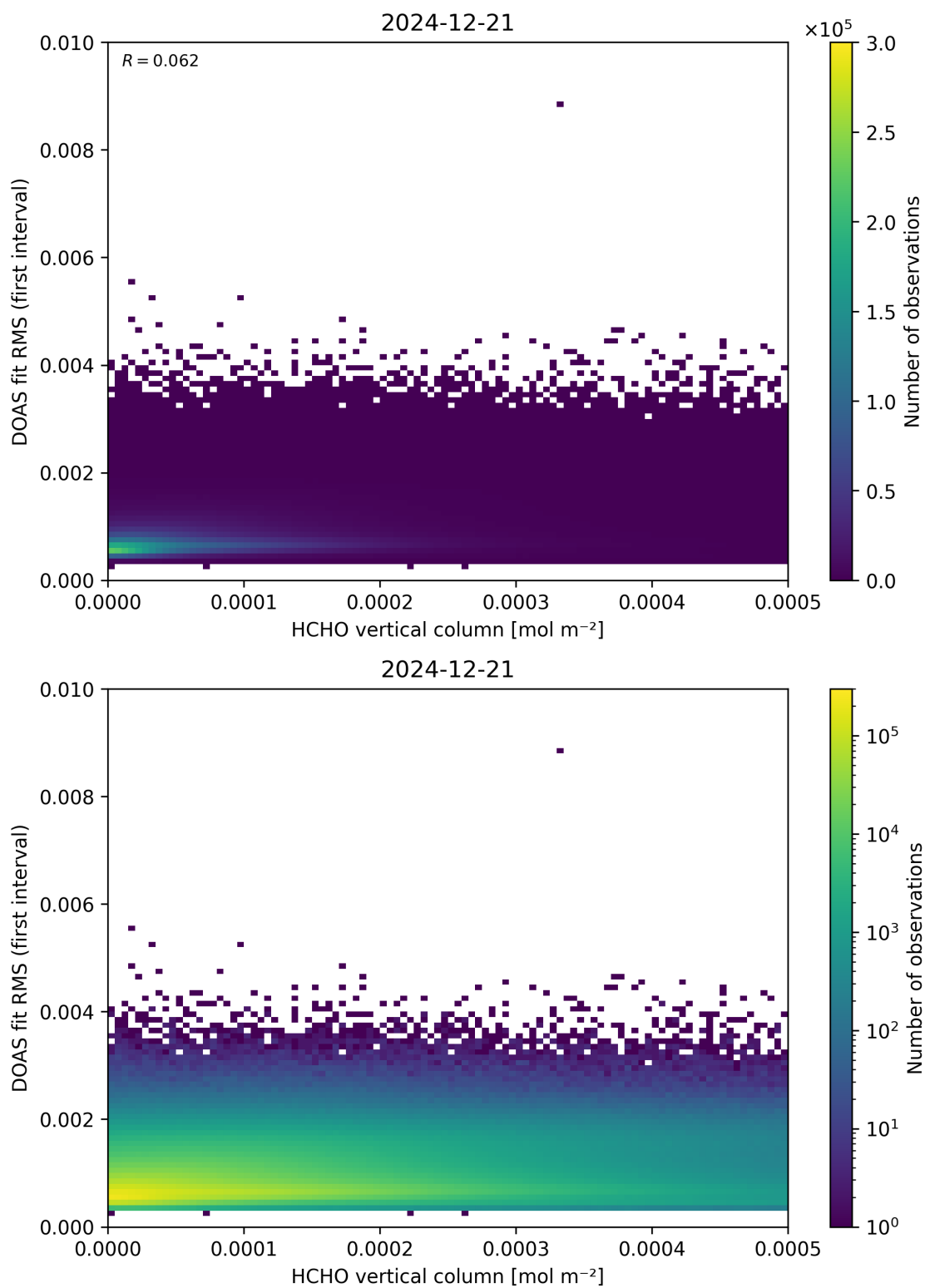
Figure 123: Scatter density plot of “HCHO vertical column” against “DOAS fit RMS (first interval)” for 2024-12-20 to 2024-12-22.
