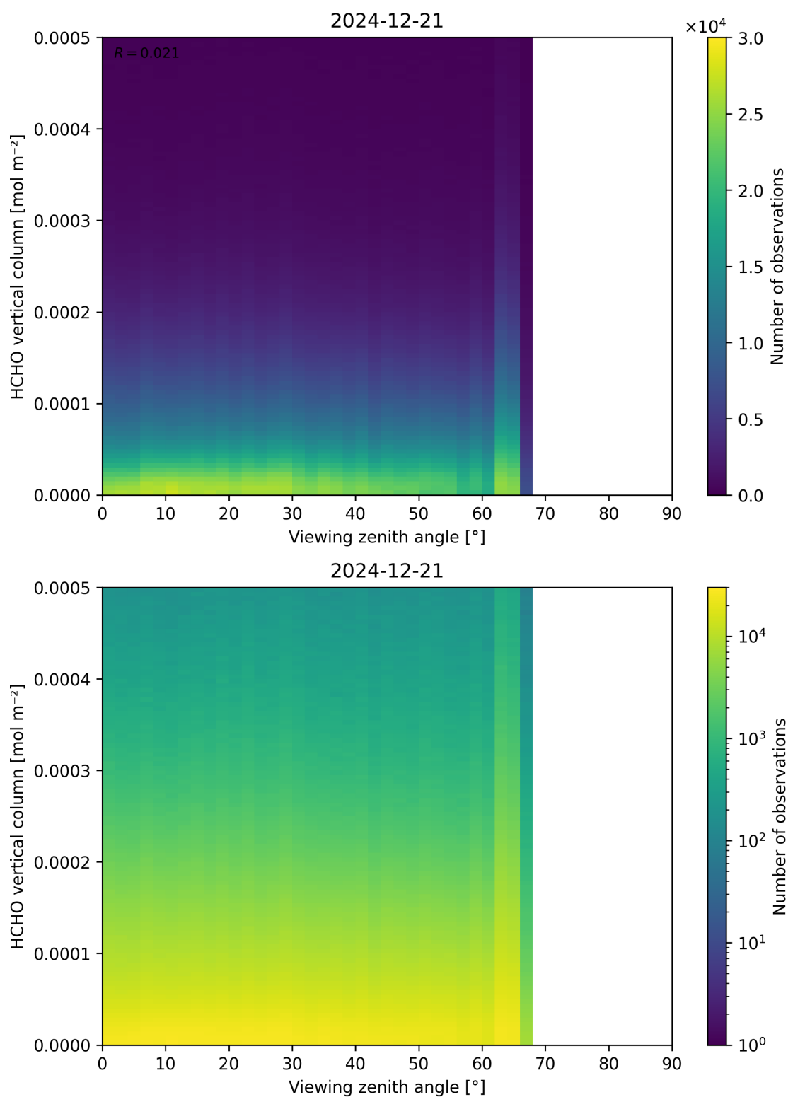
Figure 192: Scatter density plot of “Viewing zenith angle” against “HCHO vertical column” for 2024-12-20 to 2024-12-22.
