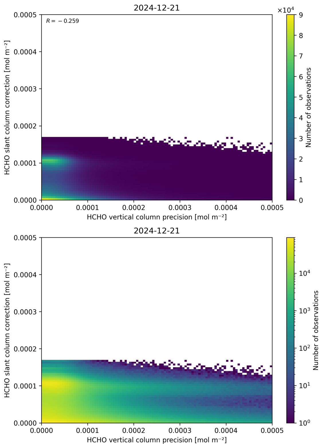
Figure 141: Scatter density plot of “HCHO vertical column precision” against “HCHO slant column correction” for 2024-12-20 to 2024-12-22.
