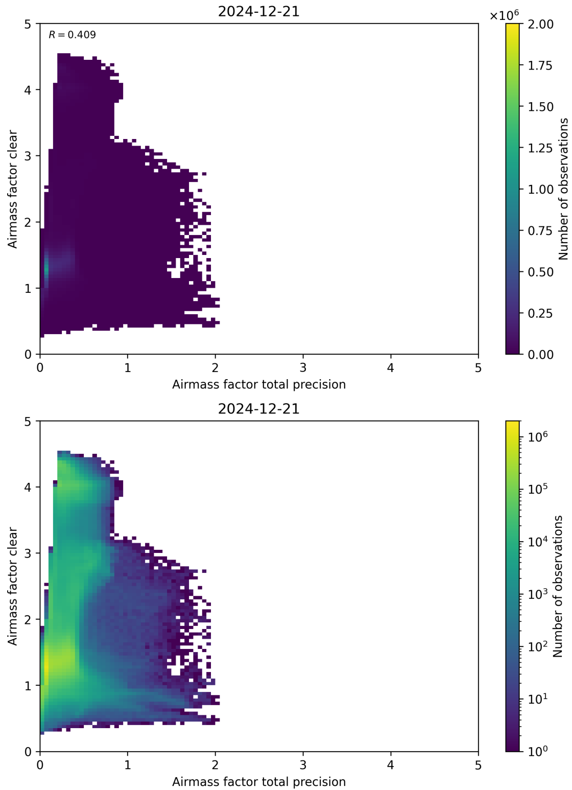
Figure 108: Scatter density plot of “Airmass factor total precision” against “Airmass factor clear” for 2024-12-20 to 2024-12-22.
