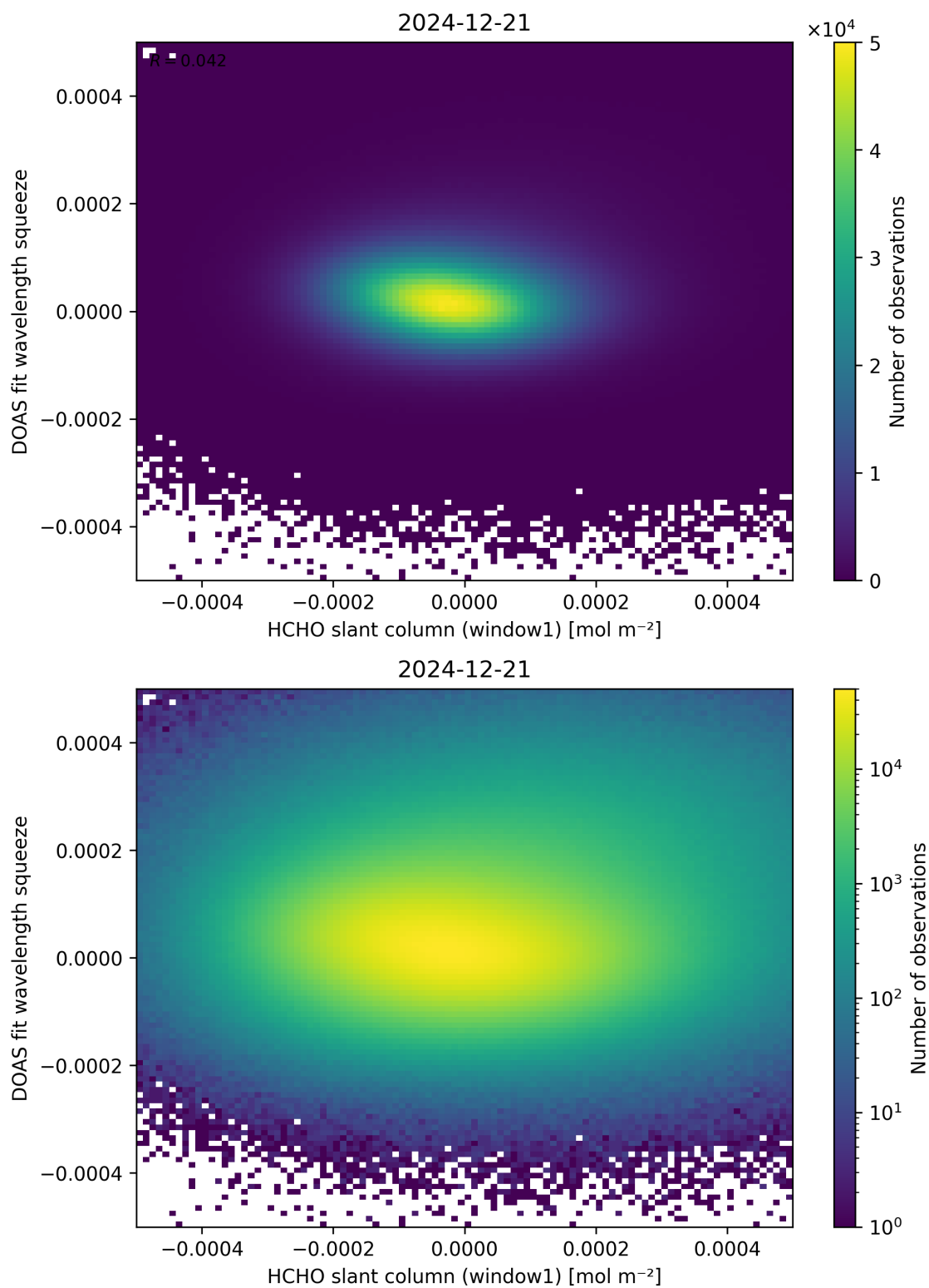
Figure 80: Scatter density plot of “HCHO slant column (window1)” against “DOAS fit wavelength squeeze” for 2024-12-20 to 2024-12-22.
