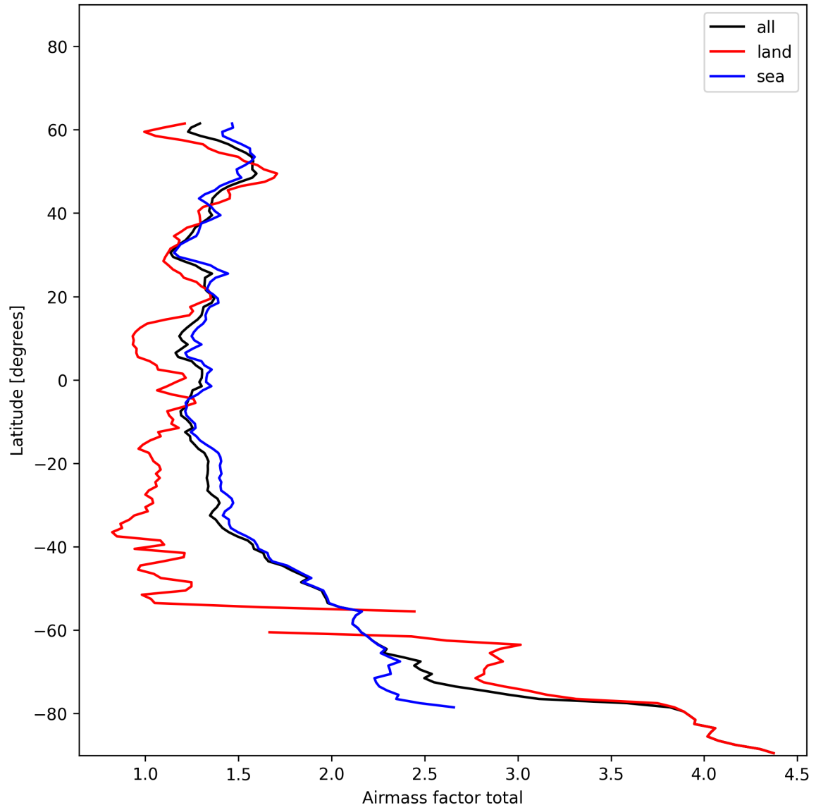
Figure 26: Zonal average of “Airmass factor total” for 2024-12-20 to 2024-12-22.
