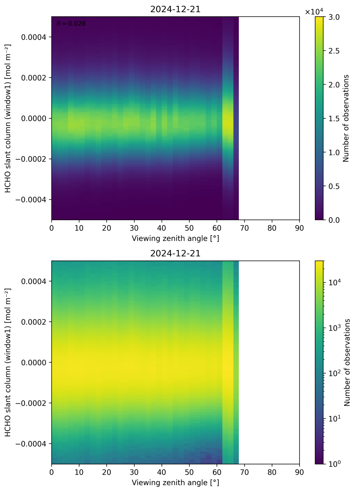
Figure 188: Scatter density plot of “Viewing zenith angle” against “HCHO slant column (window1)” for 2024-12-20 to 2024-12-22.
