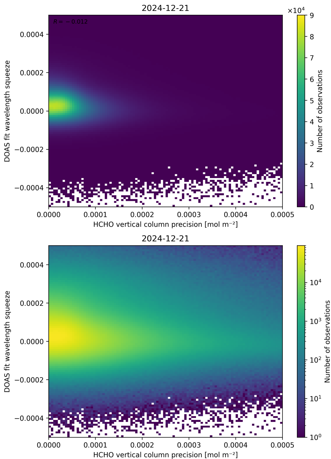
Figure 138: Scatter density plot of “HCHO vertical column precision” against “DOAS fit wavelength squeeze” for 2024-12-20 to 2024-12-22.
