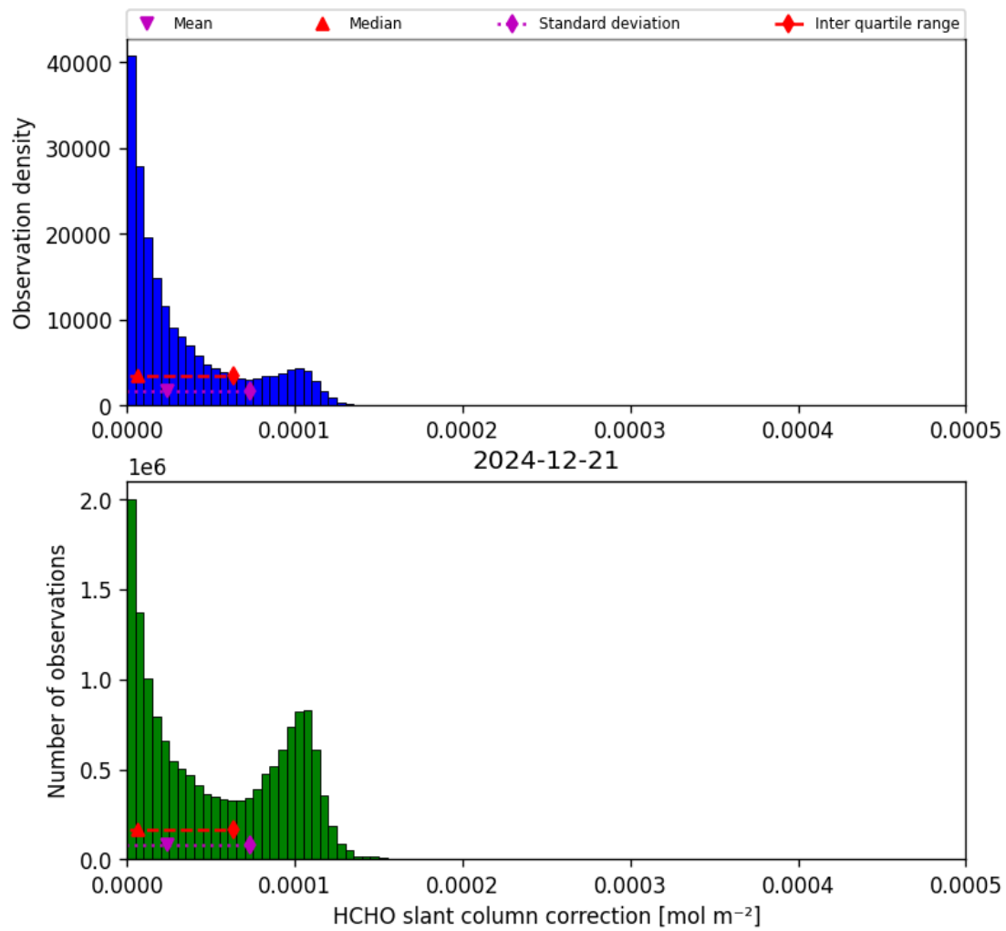
Figure 47: Histogram of “HCHO slant column correction” for 2024-12-20 to 2024-12-22
