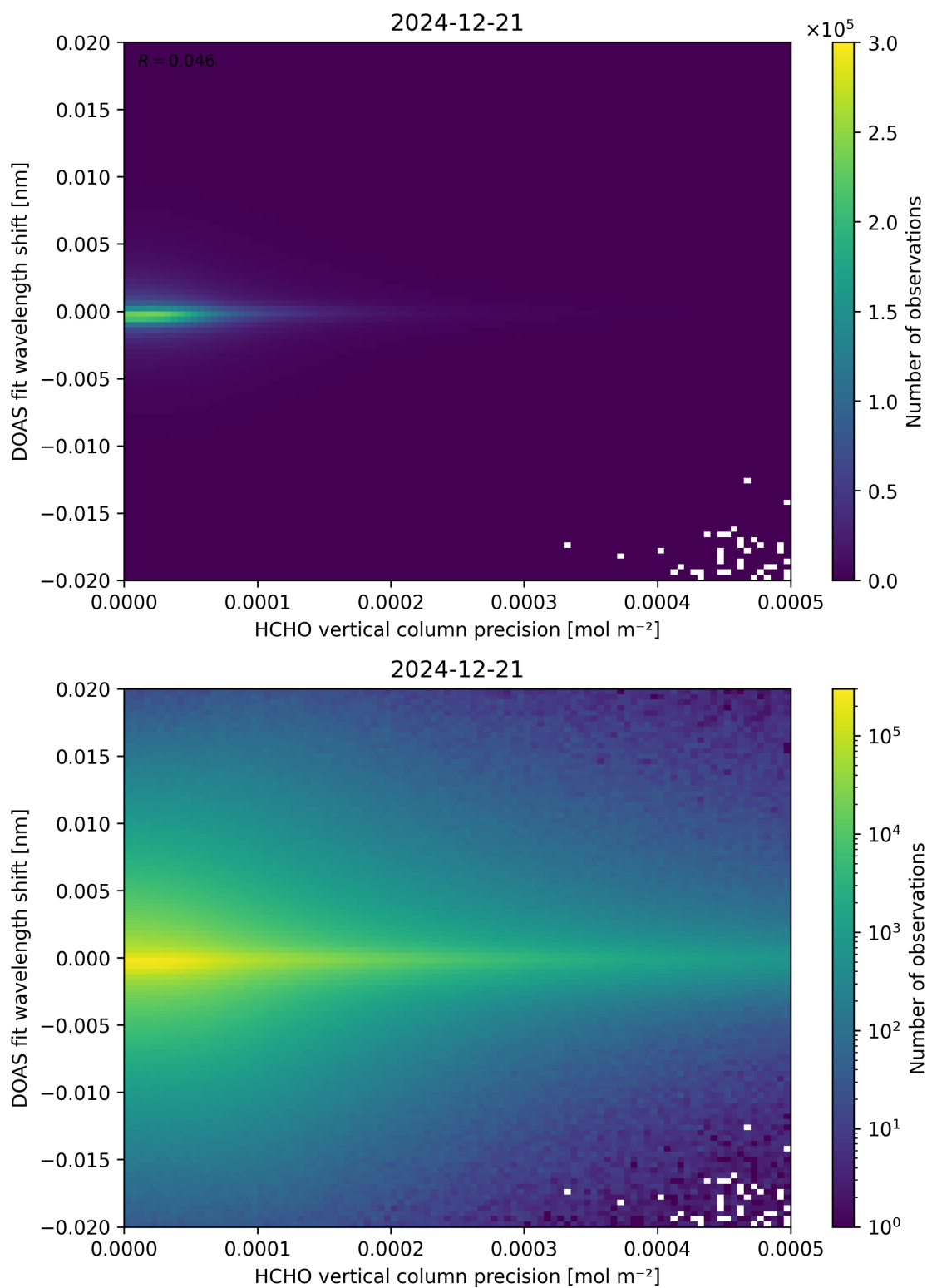
Figure 137: Scatter density plot of “HCHO vertical column precision” against “DOAS fit wavelength shift” for 2024-12-20 to 2024-12-22.
