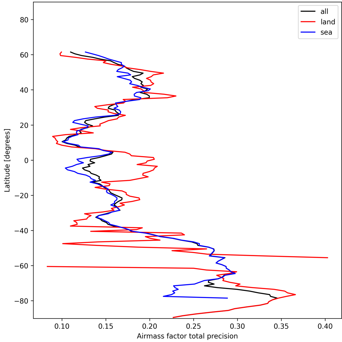
Figure 27: Zonal average of “Airmass factor total precision” for 2024-12-20 to 2024-12-22.
