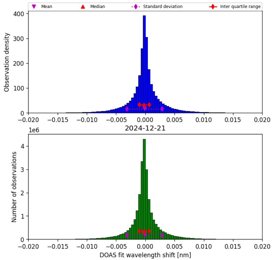
Figure 44: Histogram of “DOAS fit wavelength shift” for 2024-12-20 to 2024-12-22
