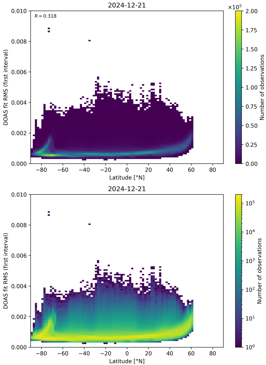
Figure 153: Scatter density plot of “Latitude” against “DOAS fit RMS (first interval)” for 2024-12-20 to 2024-12-22.
