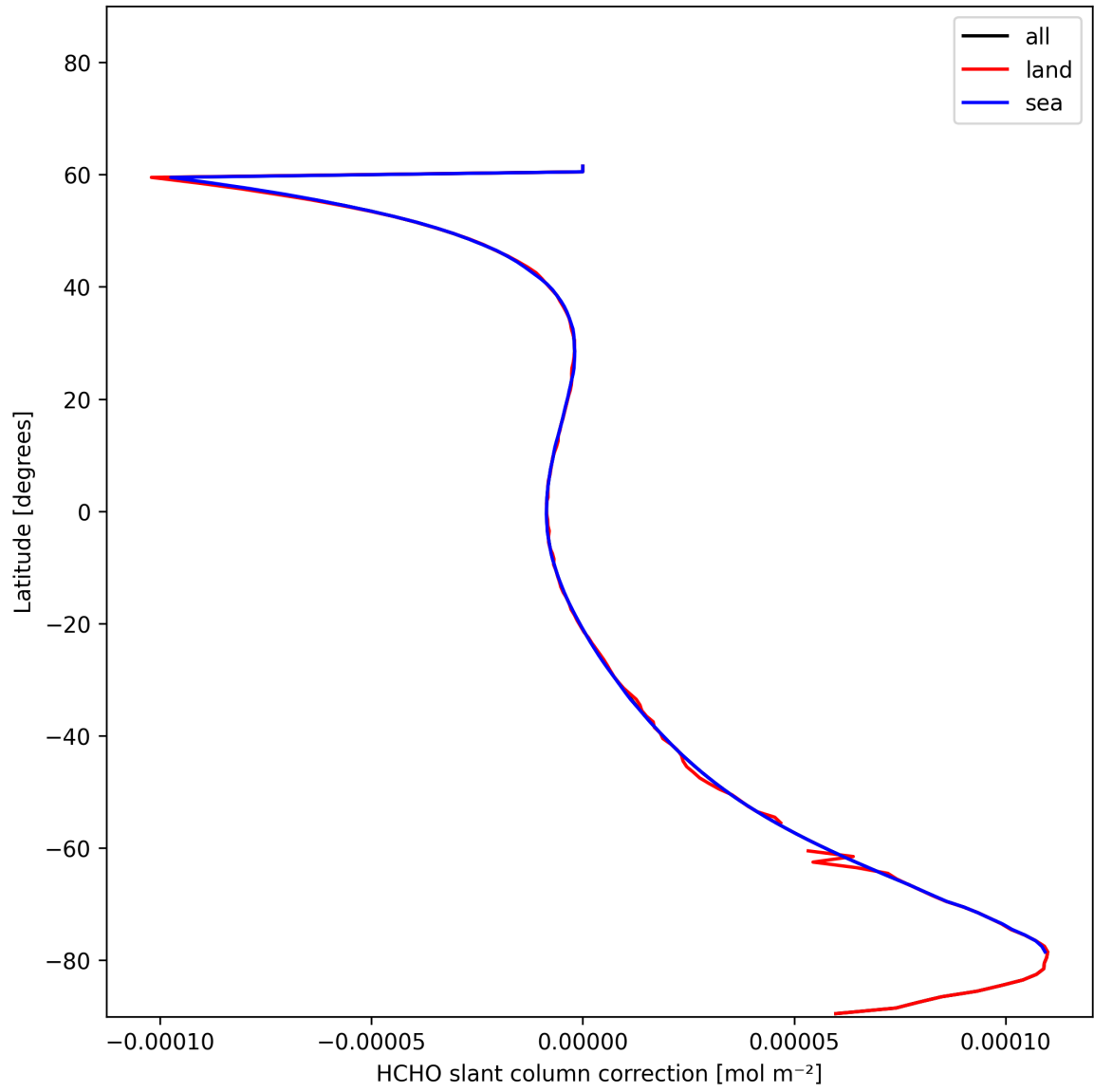
Figure 33: Zonal average of “HCHO slant column correction” for 2024-12-20 to 2024-12-22.
