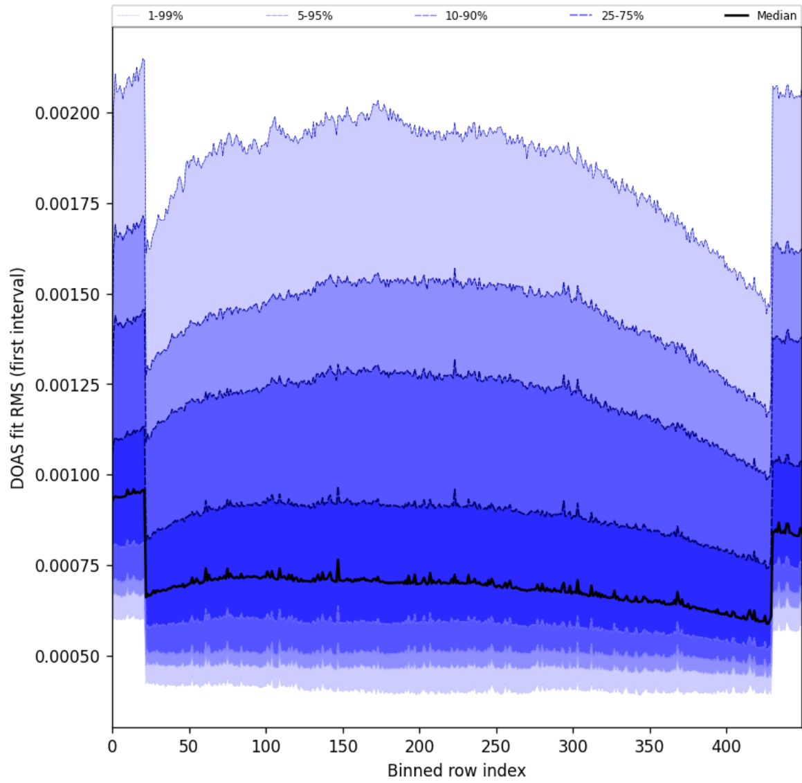
Figure 60: Along track statistics of “DOAS fit RMS (first interval)” for 2024-12-20 to 2024-12-22
