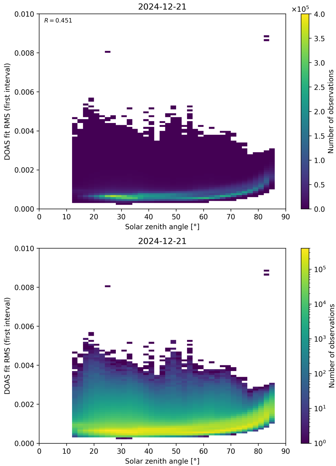
Figure 167: Scatter density plot of “Solar zenith angle” against “DOAS fit RMS (first interval)” for 2024-12-20 to 2024-12-22.
