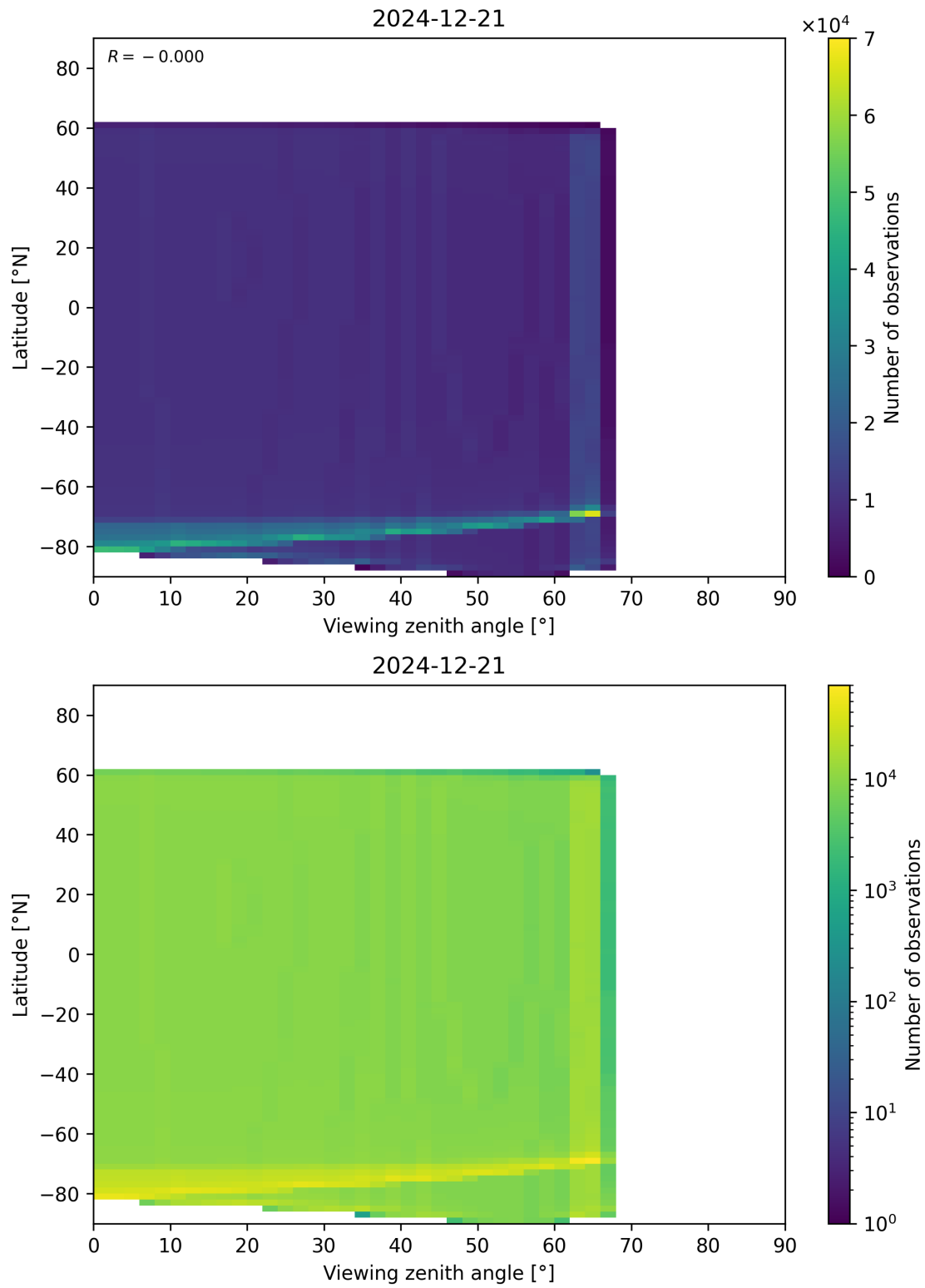
Figure 196: Scatter density plot of “Viewing zenith angle” against “Latitude” for 2024-12-20 to 2024-12-22.
