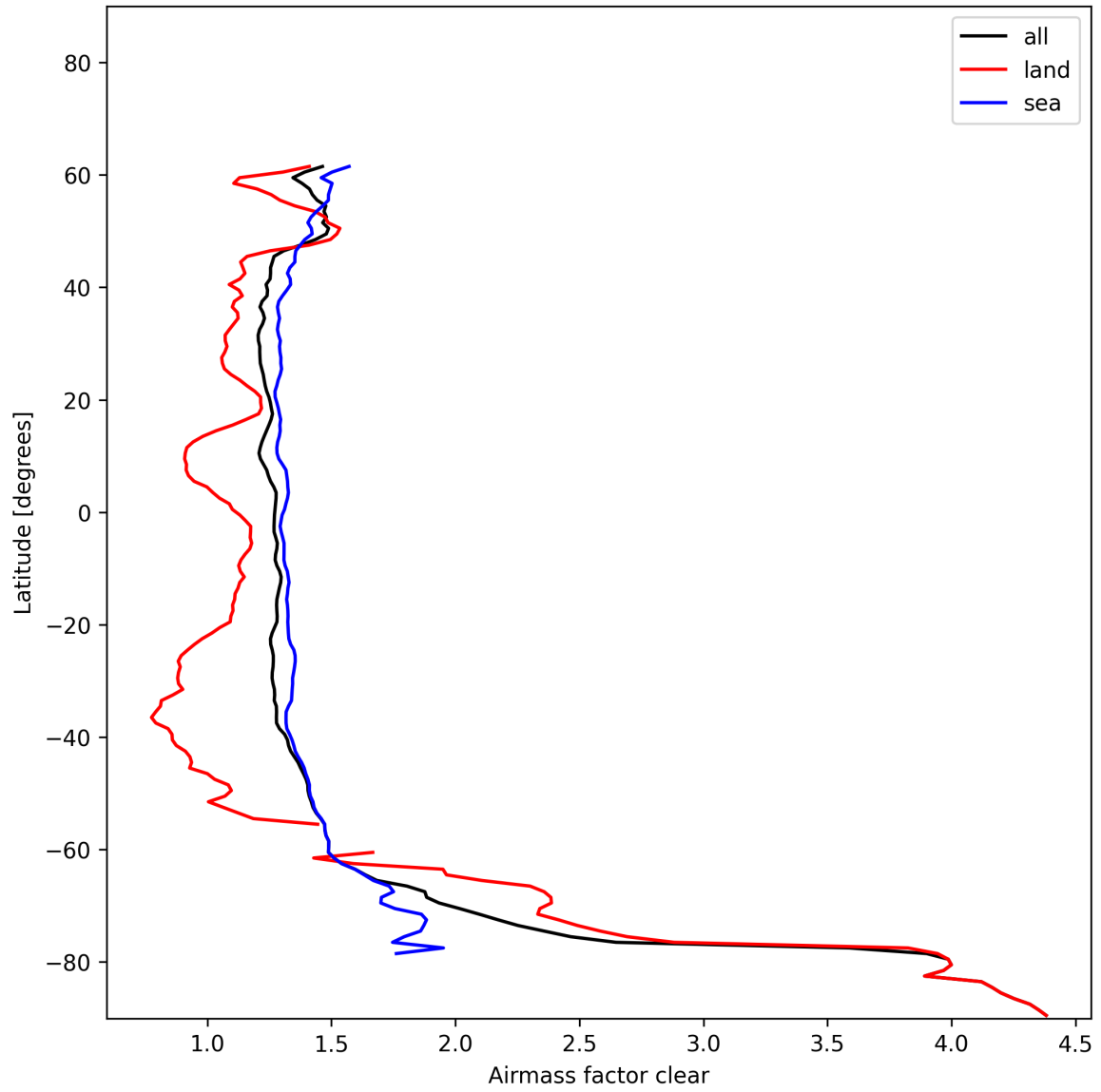
Figure 28: Zonal average of “Airmass factor clear” for 2024-12-20 to 2024-12-22.
