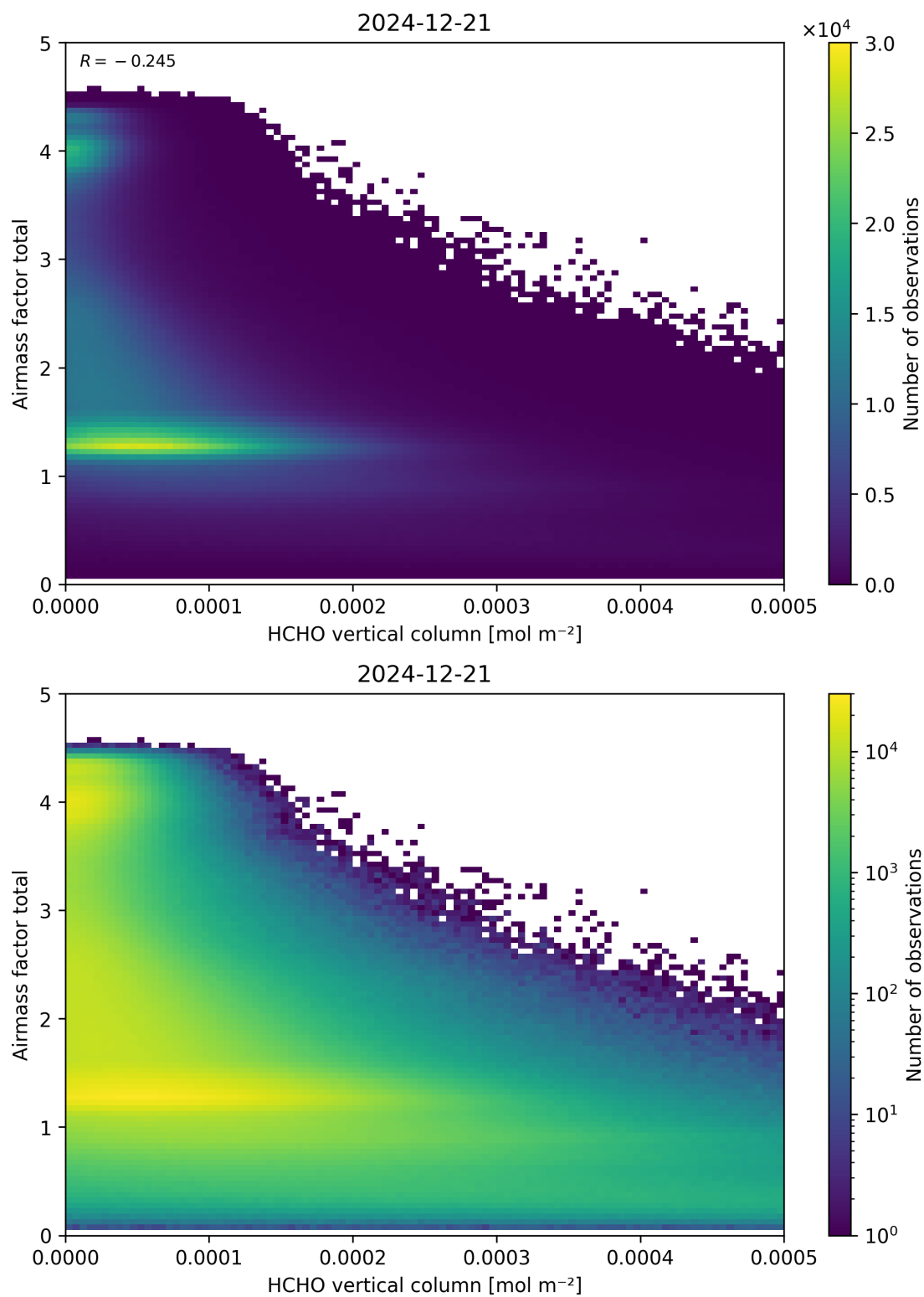
Figure 131: Scatter density plot of “HCHO vertical column” against “Airmass factor total” for 2024-12-20 to 2024-12-22.
