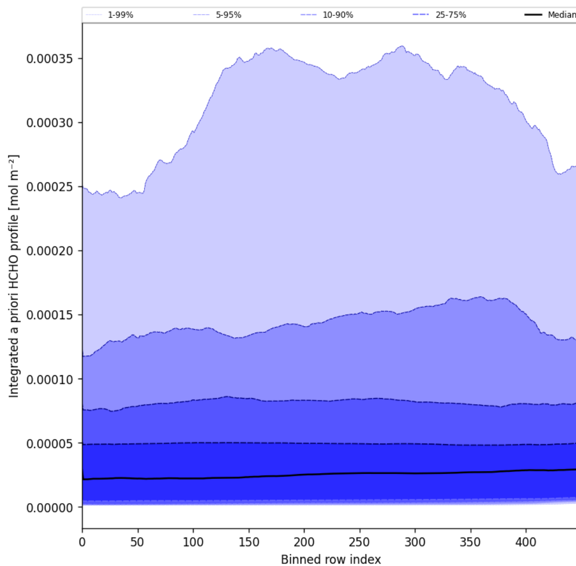
Figure 57: Along track statistics of “Integrated a priori HCHO profile” for 2024-12-20 to 2024-12-22
