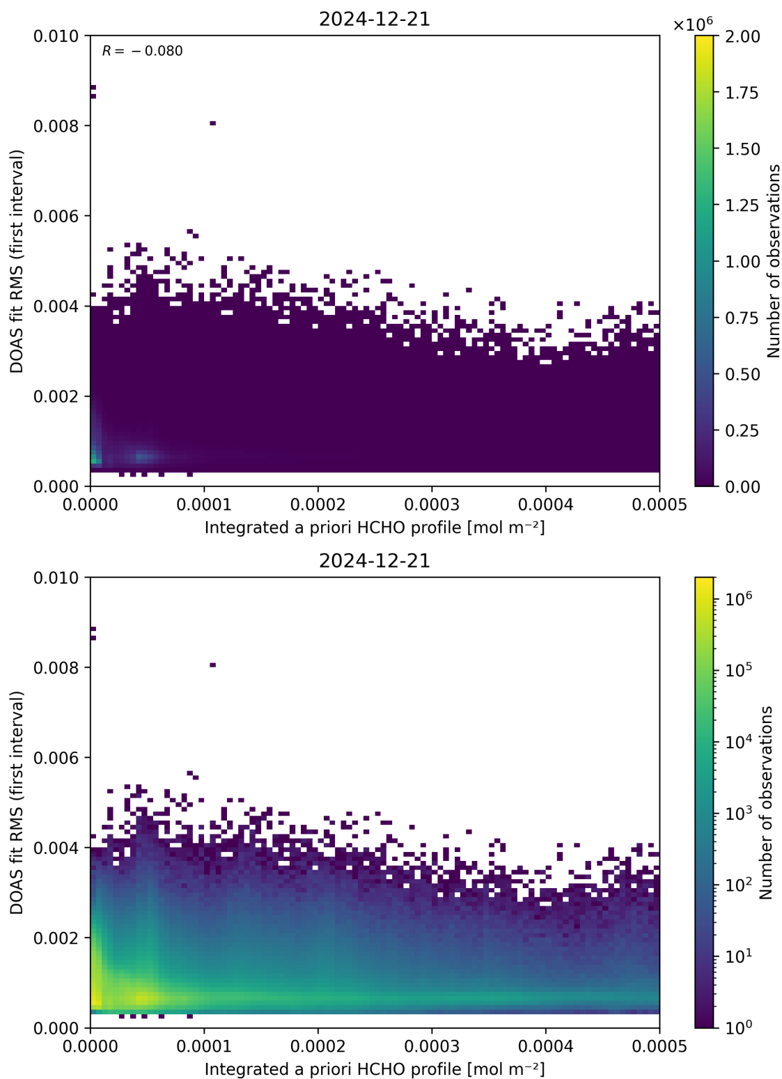
Figure 148: Scatter density plot of “Integrated a priori HCHO profile” against “DOAS fit RMS (first interval)” for 2024-12-20 to 2024-12-22.
