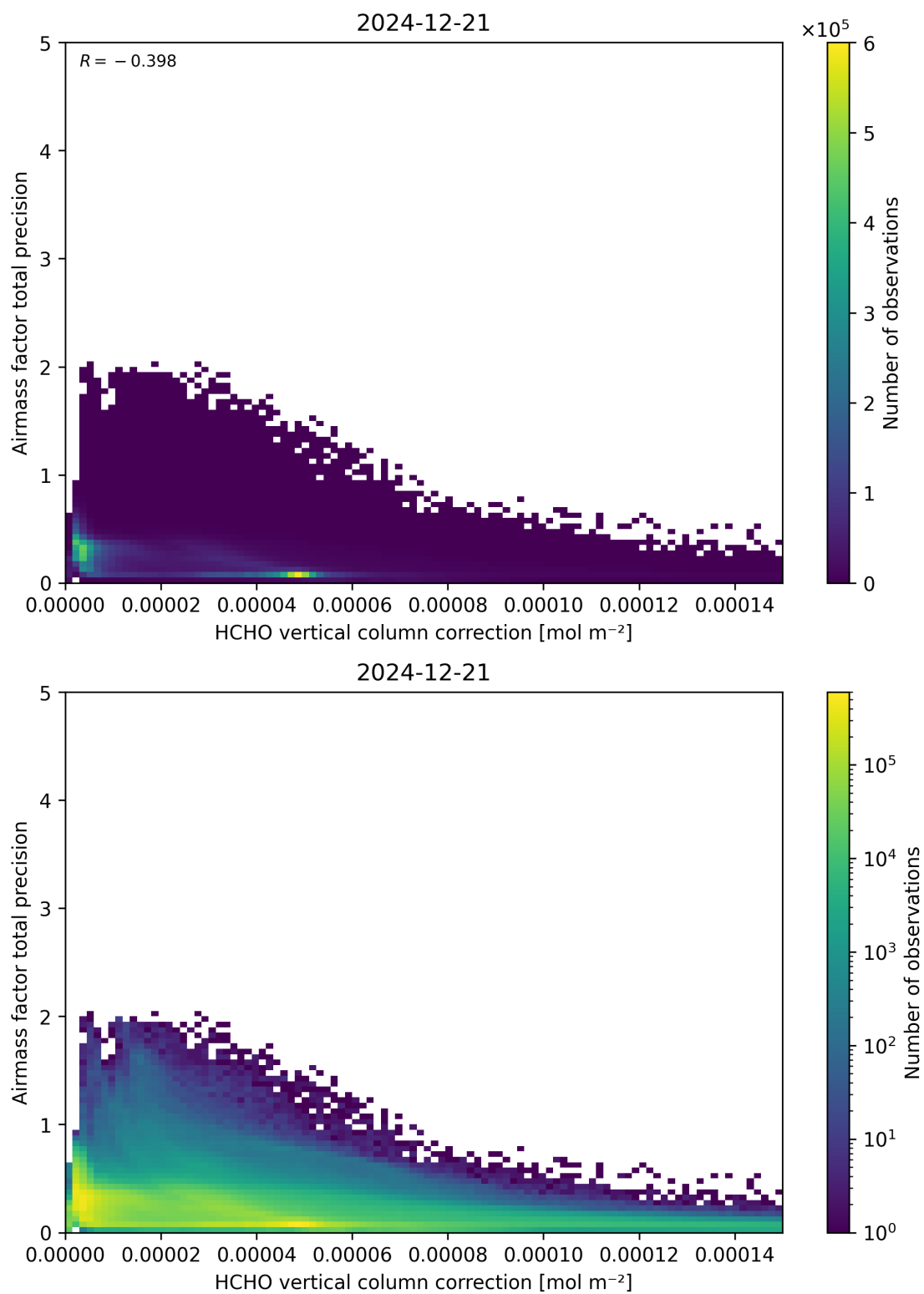
Figure 121: Scatter density plot of “HCHO vertical column correction” against “Airmass factor total precision” for 2024-12-20 to 2024-12-22.
