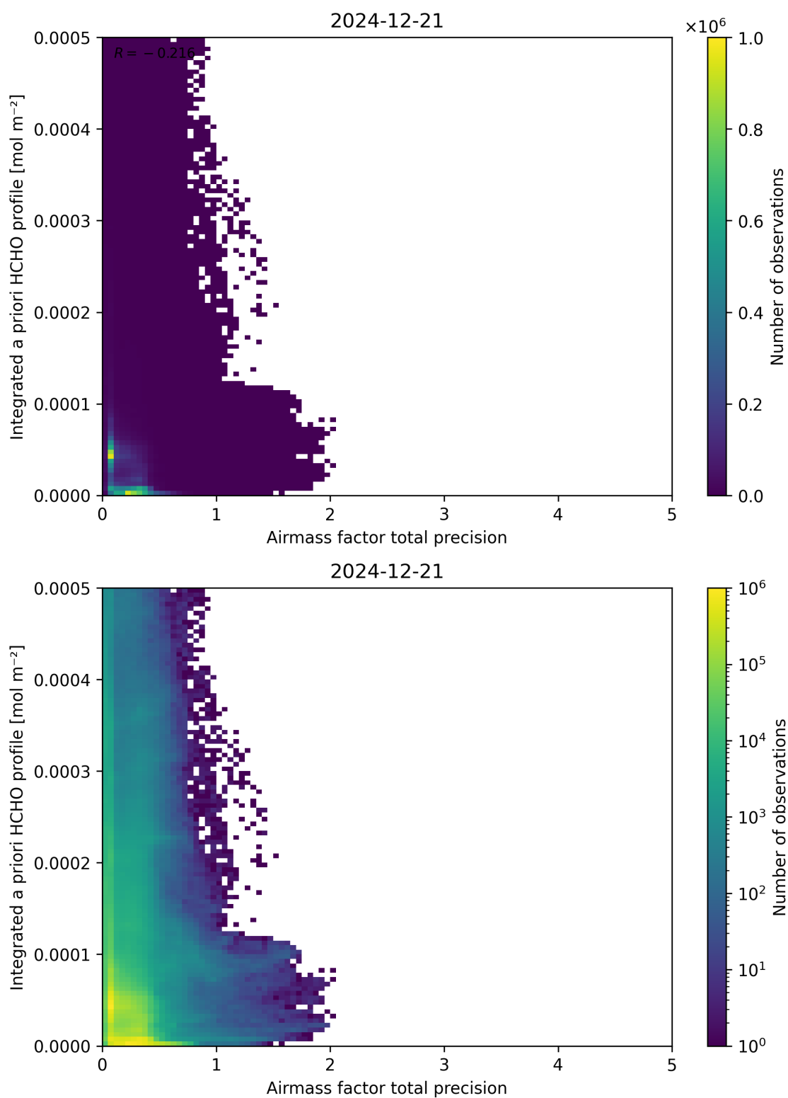
Figure 111: Scatter density plot of “Airmass factor total precision” against “Integrated a priori HCHO profile” for 2024-12-20 to 2024-12-22.
