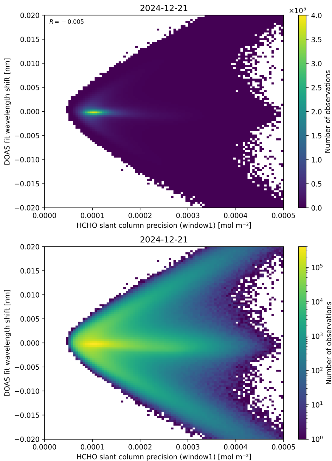
Figure 89: Scatter density plot of “HCHO slant column precision (window1)” against “DOAS fit wavelength shift” for 2024-12-20 to 2024-12-22.
