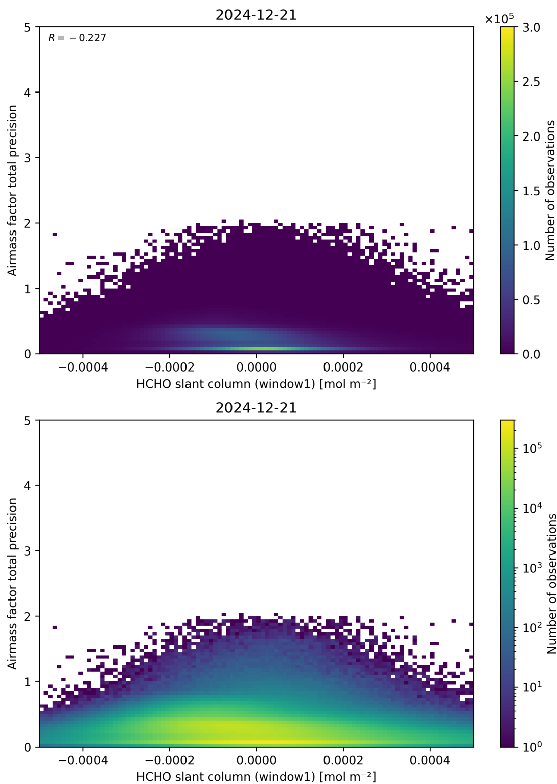
Figure 86: Scatter density plot of “HCHO slant column (window1)” against “Airmass factor total precision” for 2024-12-20 to 2024-12-22.
