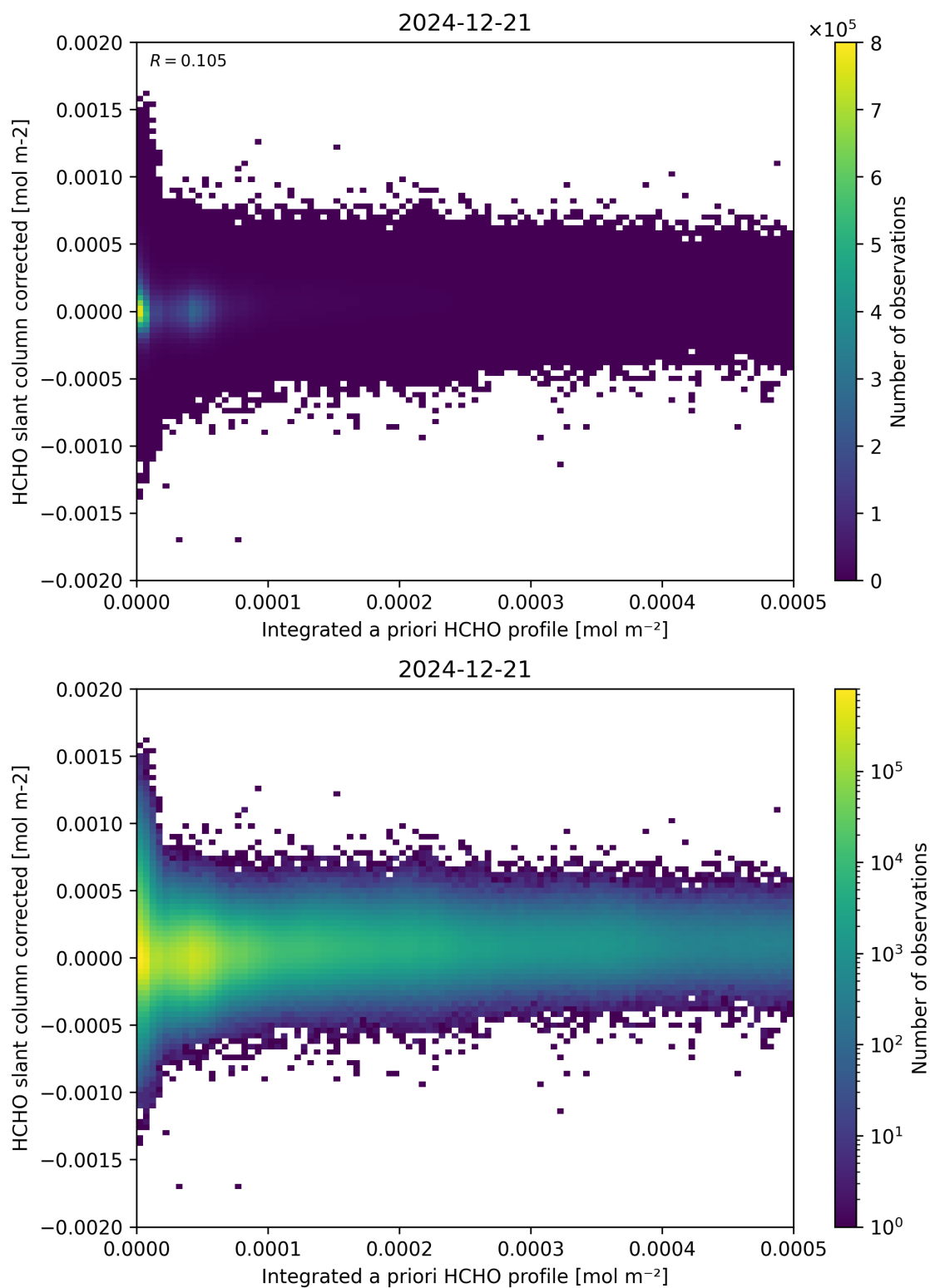
Figure 151: Scatter density plot of “Integrated a priori HCHO profile” against “HCHO slant column corrected” for 2024-12-20 to 2024-12-22.
