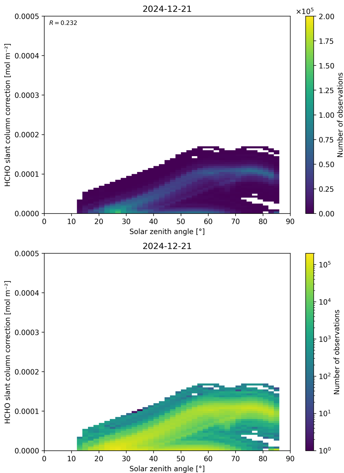
Figure 172: Scatter density plot of “Solar zenith angle” against “HCHO slant column correction” for 2024-12-20 to 2024-12-22.
