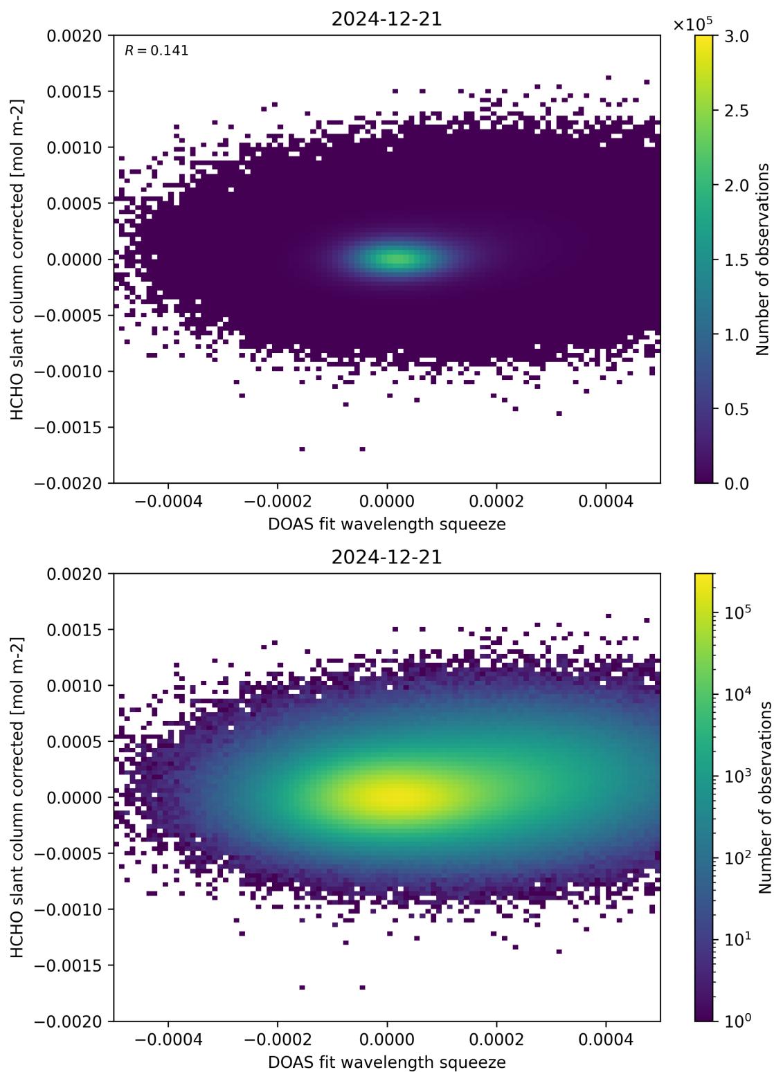
Figure 69: Scatter density plot of “DOAS fit wavelength squeeze” against “HCHO slant column corrected” for 2024-12-20 to 2024-12-22.
