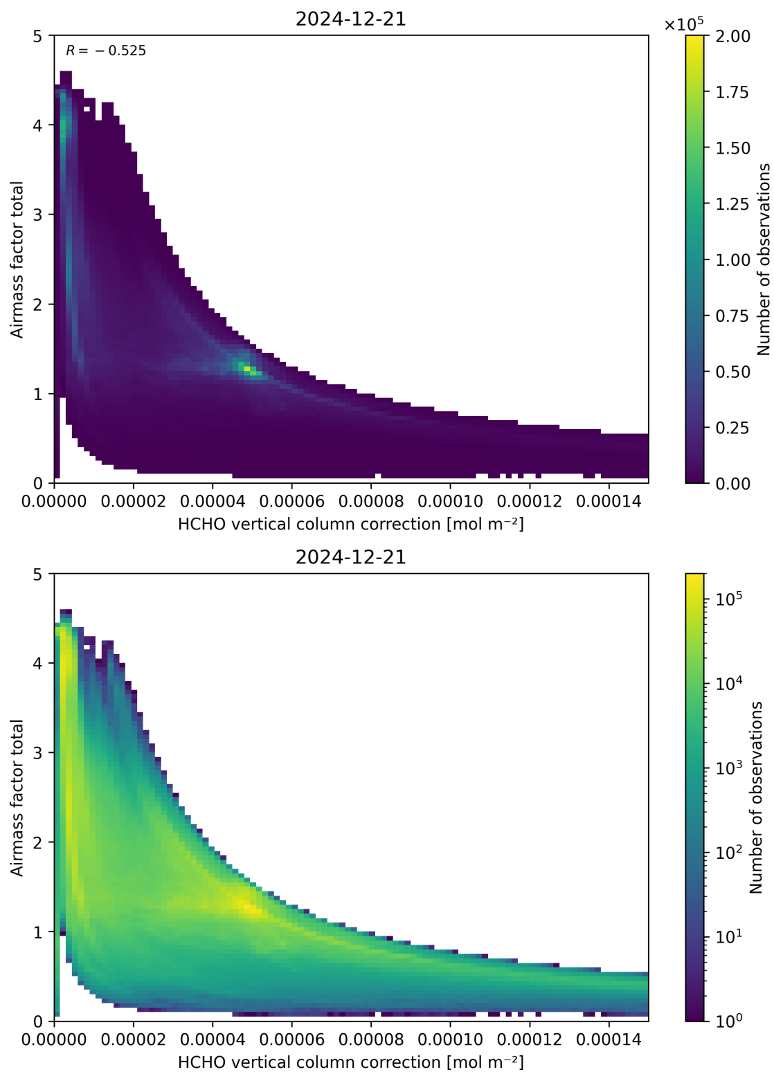
Figure 120: Scatter density plot of “HCHO vertical column correction” against “Airmass factor total” for 2024-12-20 to 2024-12-22.
