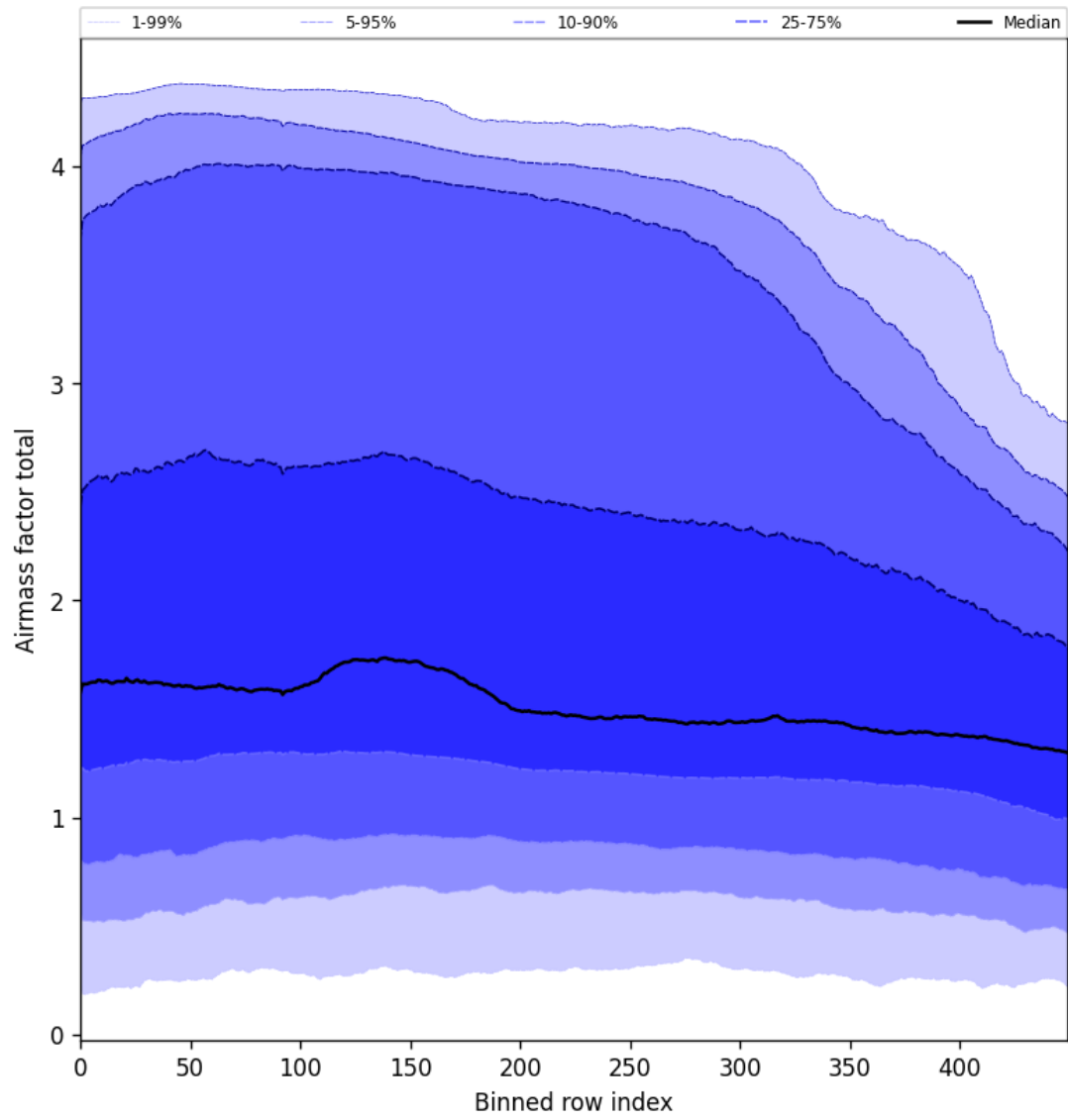
Figure 54: Along track statistics of “Airmass factor total” for 2024-12-20 to 2024-12-22
