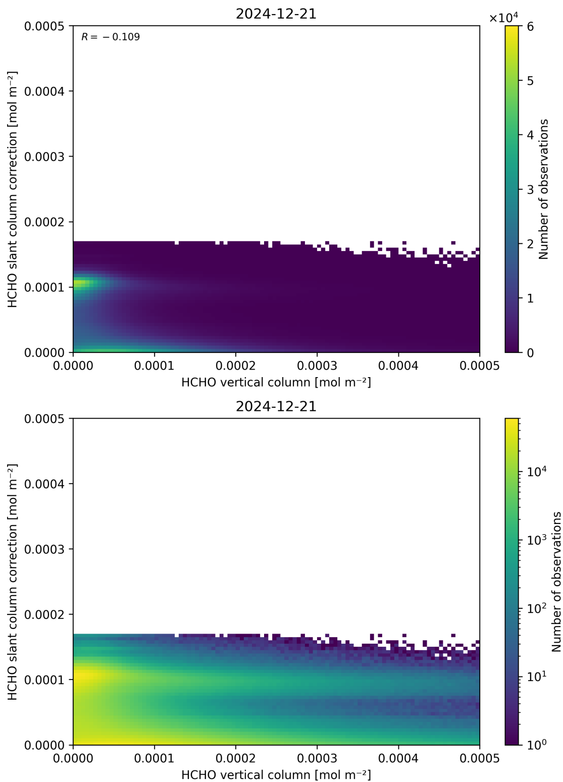
Figure 128: Scatter density plot of “HCHO vertical column” against “HCHO slant column correction” for 2024-12-20 to 2024-12-22.
