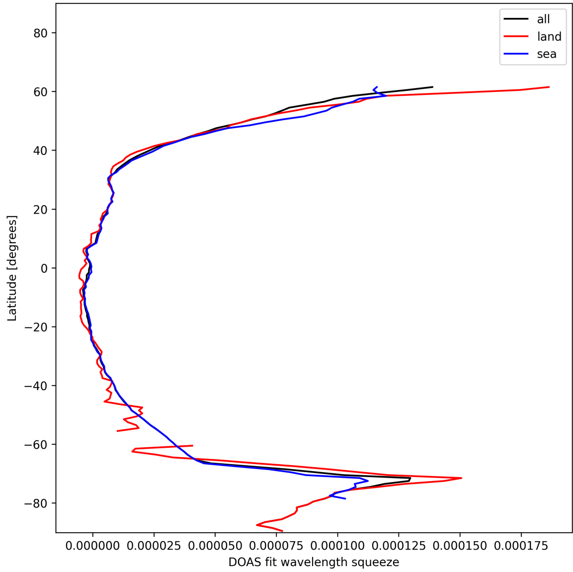
Figure 31: Zonal average of “DOAS fit wavelength squeeze” for 2024-12-20 to 2024-12-22.
