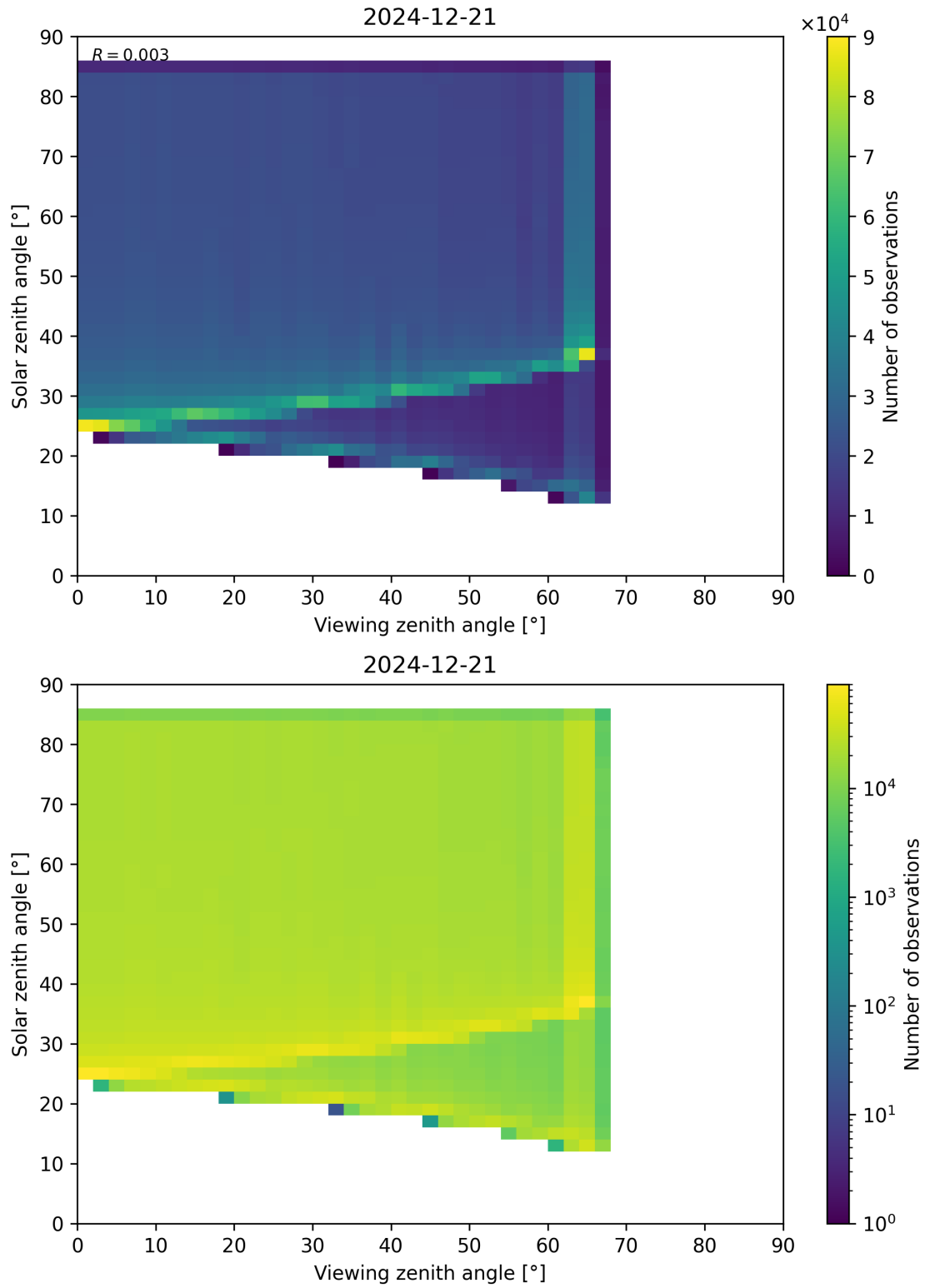
Figure 197: Scatter density plot of “Viewing zenith angle” against “Solar zenith angle” for 2024-12-20 to 2024-12-22.
