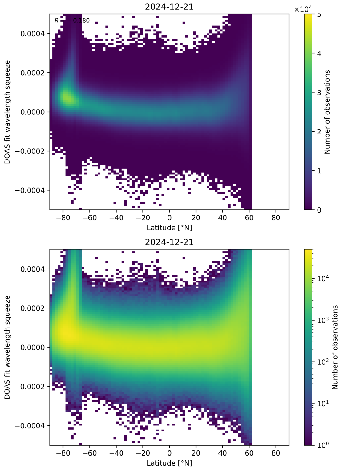
Figure 155: Scatter density plot of “Latitude” against “DOAS fit wavelength squeeze” for 2024-12-20 to 2024-12-22.
