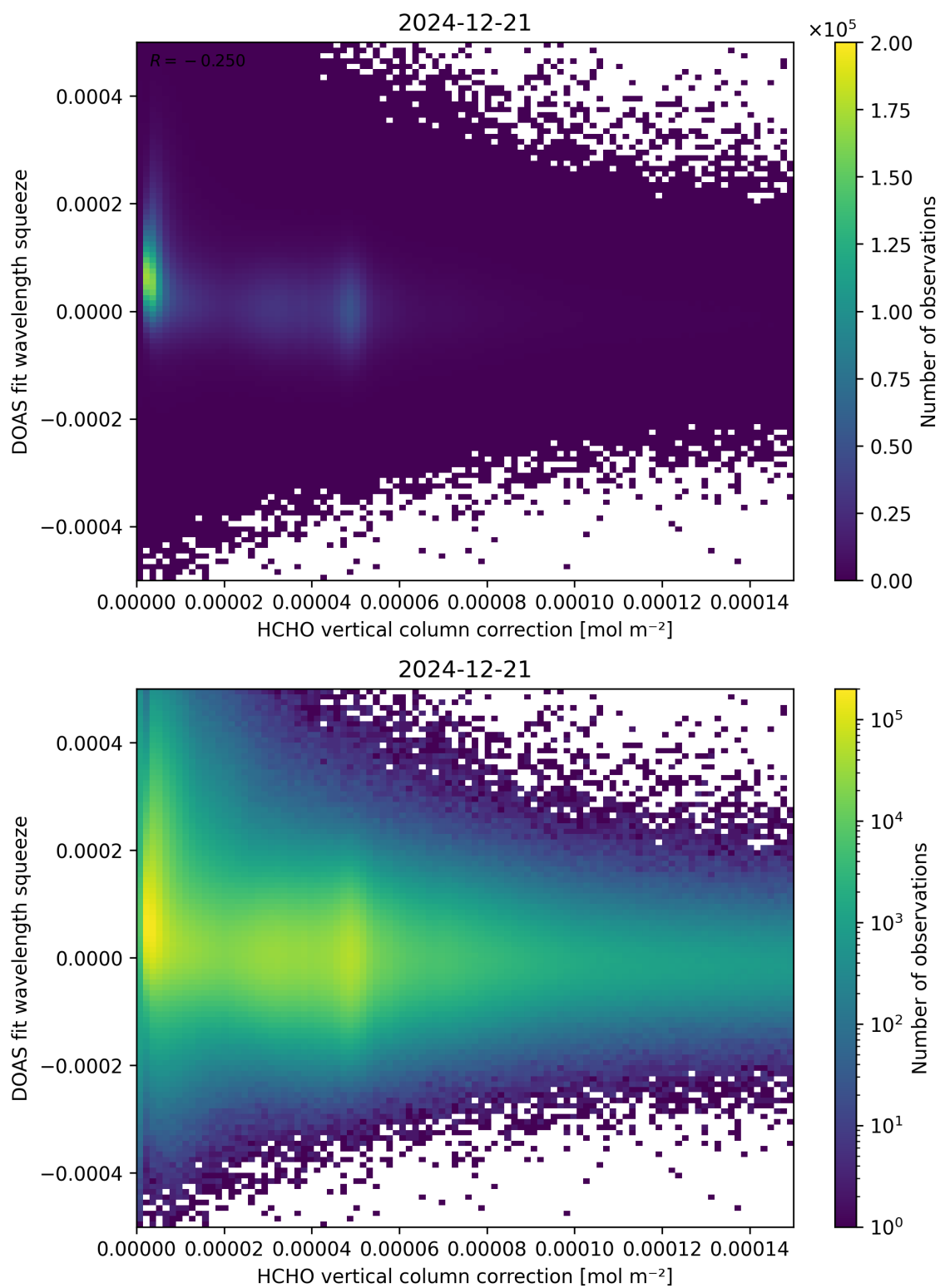
Figure 114: Scatter density plot of “HCHO vertical column correction” against “DOAS fit wavelength squeeze” for 2024-12-20 to 2024-12-22.
