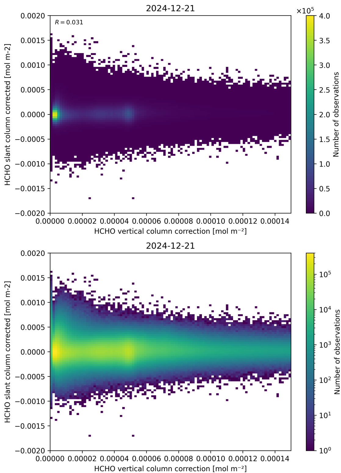
Figure 116: Scatter density plot of “HCHO vertical column correction” against “HCHO slant column corrected” for 2024-12-20 to 2024-12-22.
