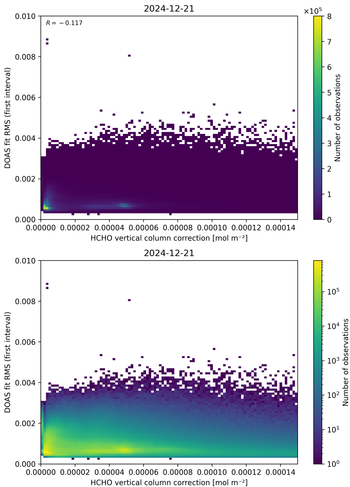
Figure 112: Scatter density plot of “HCHO vertical column correction” against “DOAS fit RMS (first interval)” for 2024-12-20 to 2024-12-22.
