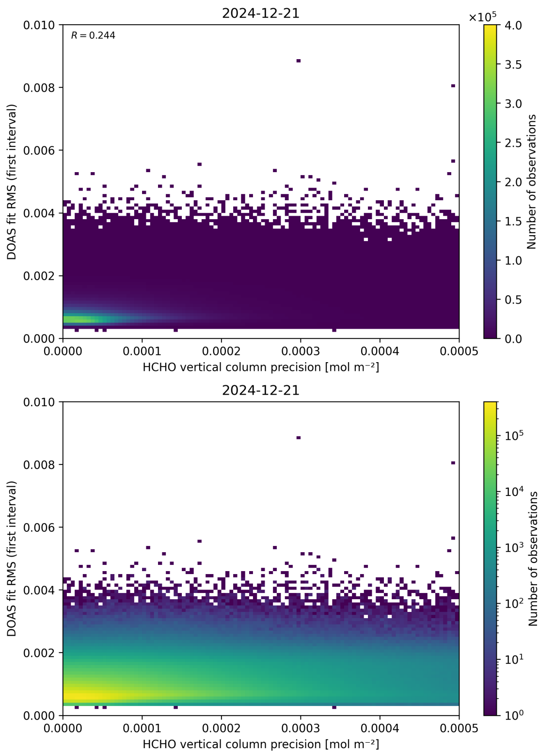
Figure 136: Scatter density plot of “HCHO vertical column precision” against “DOAS fit RMS (first interval)” for 2024-12-20 to 2024-12-22.
