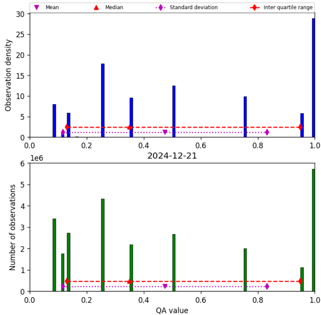
Figure 34: Histogram of “QA value” for 2024-12-20 to 2024-12-22
