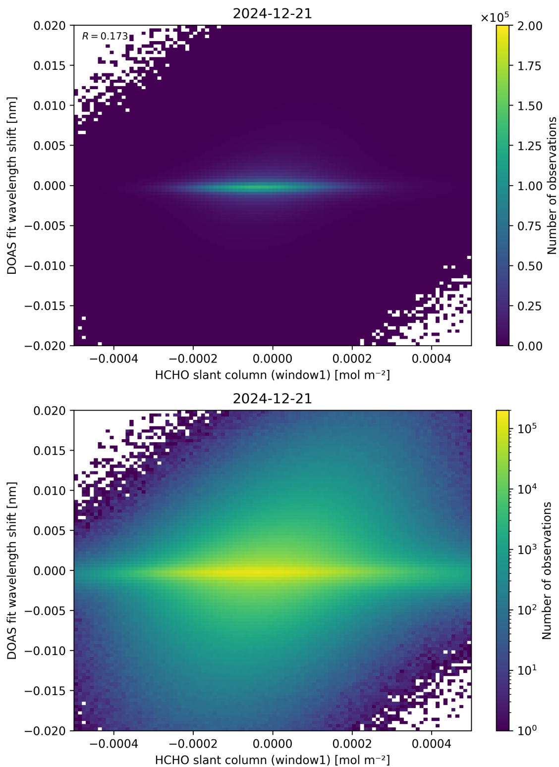
Figure 79: Scatter density plot of “HCHO slant column (window1)” against “DOAS fit wavelength shift” for 2024-12-20 to 2024-12-22.
