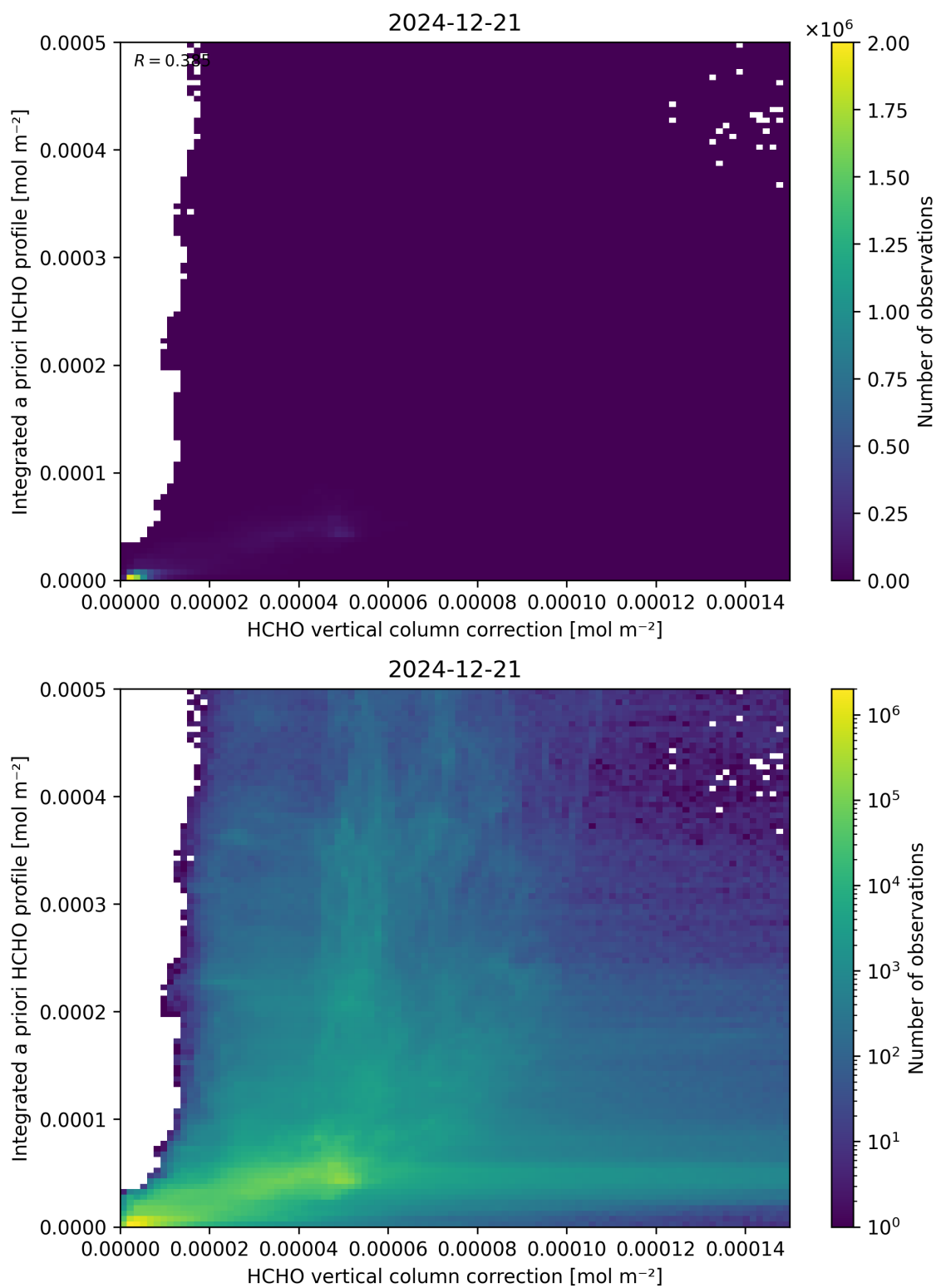
Figure 122: Scatter density plot of “HCHO vertical column correction” against “Integrated a priori HCHO profile” for 2024-12-20 to 2024-12-22.
