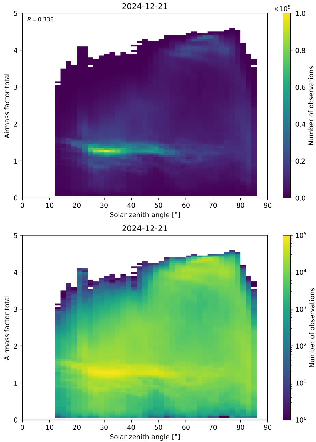
Figure 175: Scatter density plot of “Solar zenith angle” against “Airmass factor total” for 2024-12-20 to 2024-12-22.
