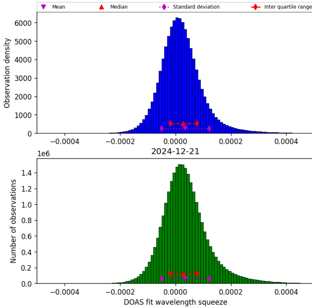
Figure 45: Histogram of “DOAS fit wavelength squeeze” for 2024-12-20 to 2024-12-22
