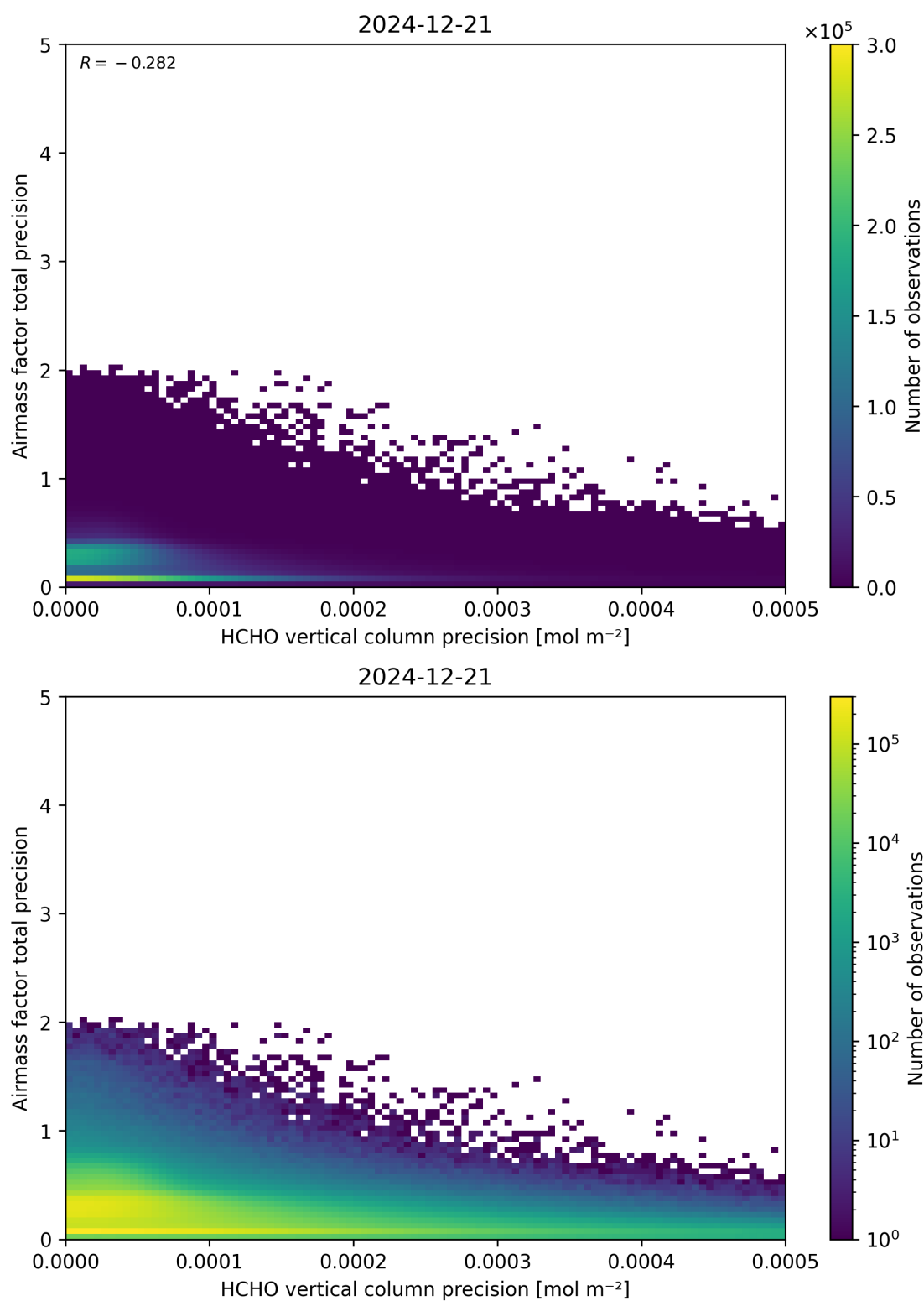
Figure 145: Scatter density plot of “HCHO vertical column precision” against “Airmass factor total precision” for 2024-12-20 to 2024-12-22.
