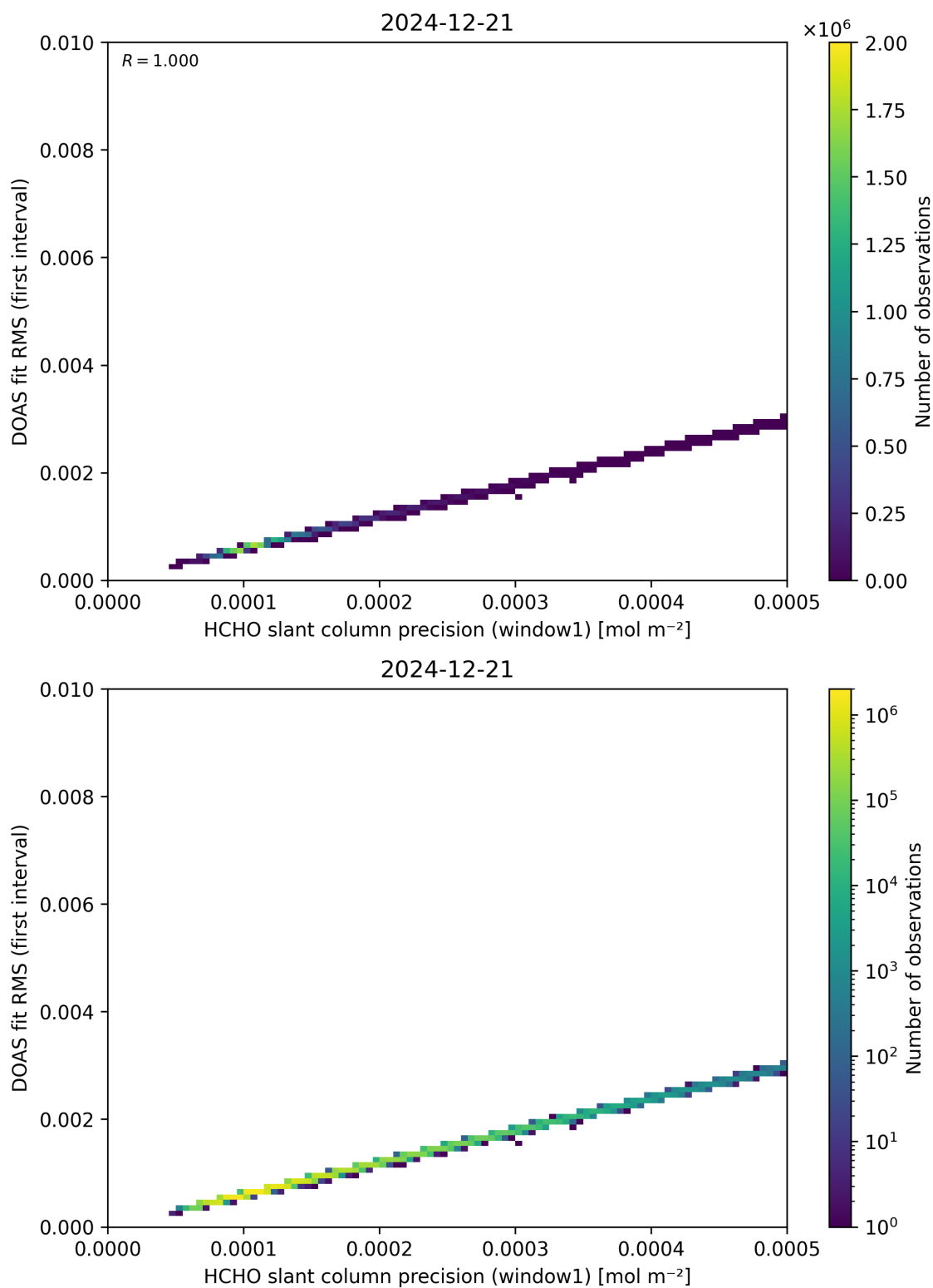
Figure 88: Scatter density plot of “HCHO slant column precision (window1)” against “DOAS fit RMS (first interval)” for 2024-12-20 to 2024-12-22.
