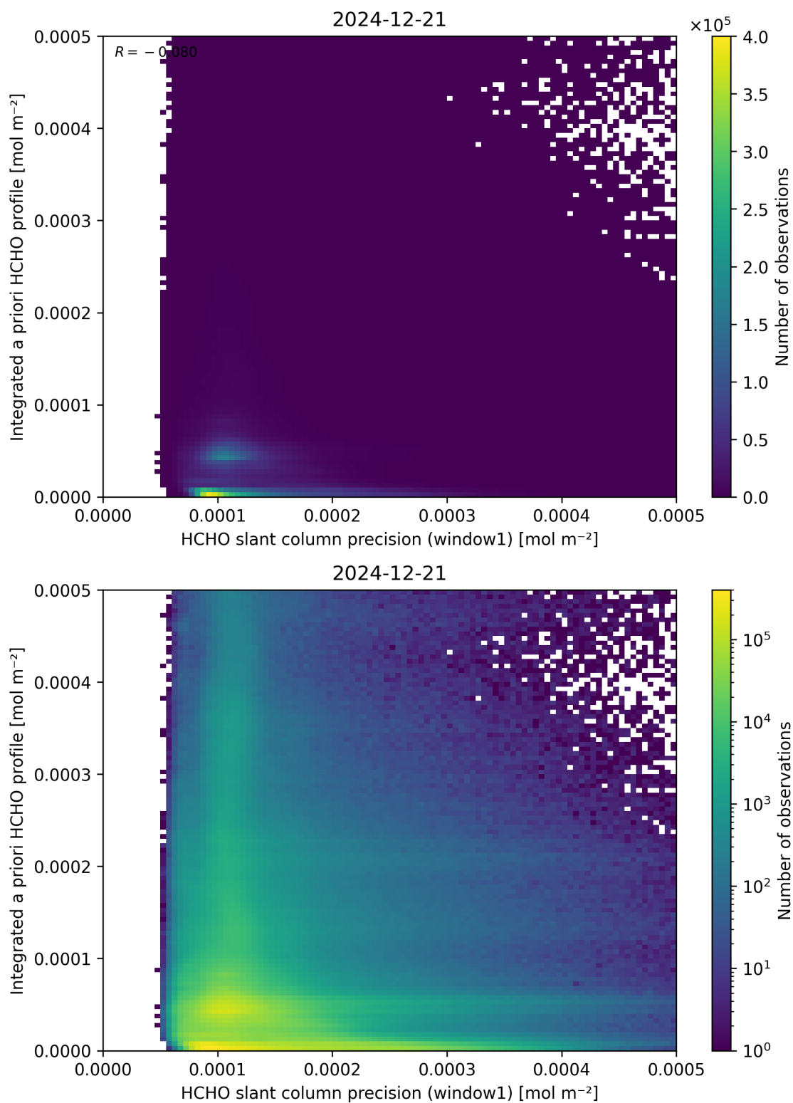
Figure 96: Scatter density plot of “HCHO slant column precision (window1)” against “Integrated a priori HCHO profile” for 2024-12-20 to 2024-12-22.
