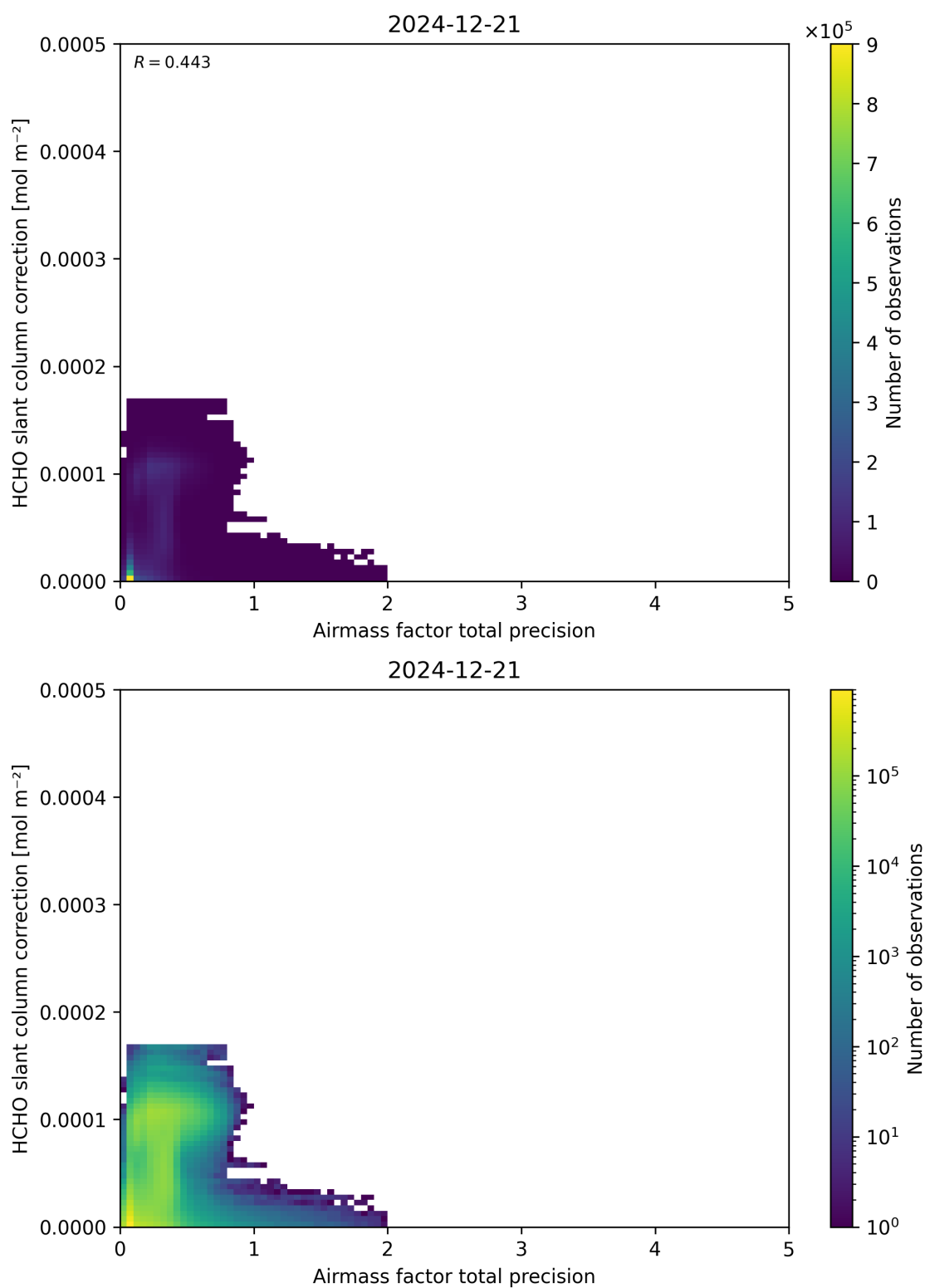
Figure 110: Scatter density plot of “Airmass factor total precision” against “HCHO slant column correction” for 2024-12-20 to 2024-12-22.
