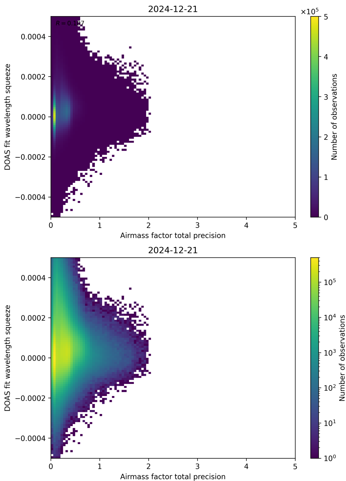
Figure 107: Scatter density plot of “Airmass factor total precision” against “DOAS fit wavelength squeeze” for 2024-12-20 to 2024-12-22.
