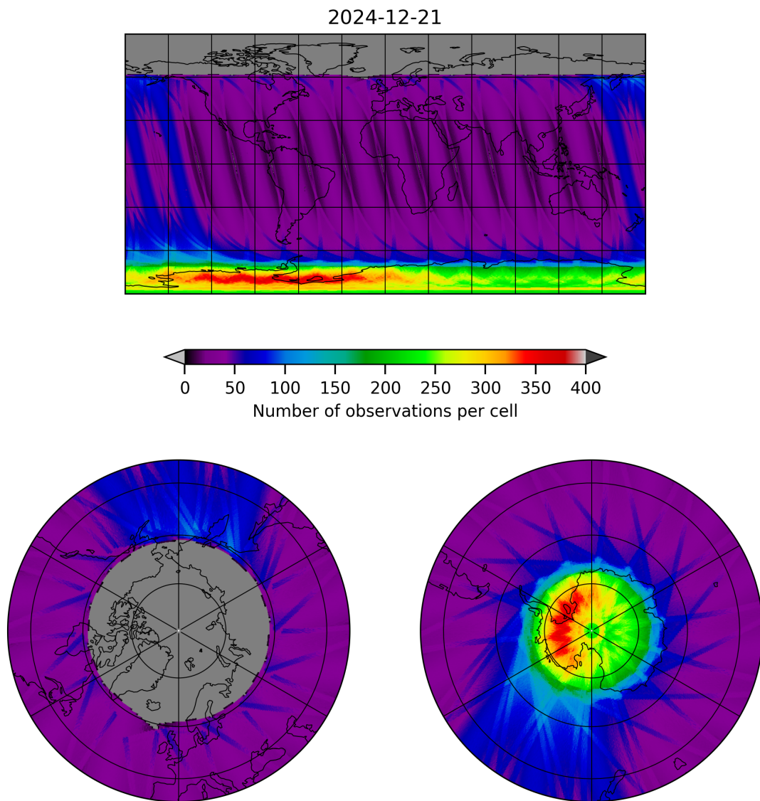
Figure 19: Map of the number of observations for 2024-12-20 to 2024-12-22
