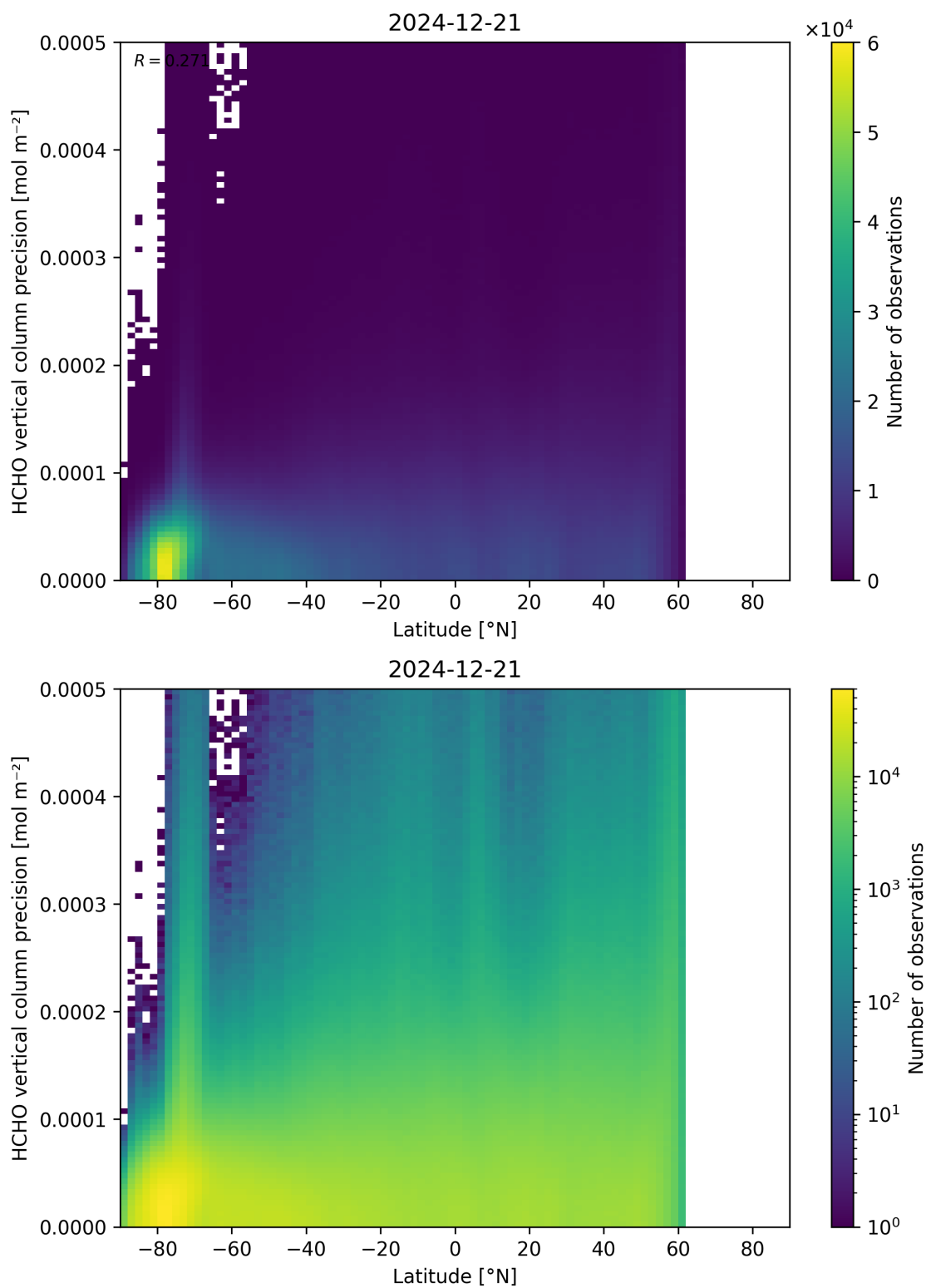
Figure 165: Scatter density plot of “Latitude” against “HCHO vertical column precision” for 2024-12-20 to 2024-12-22.
