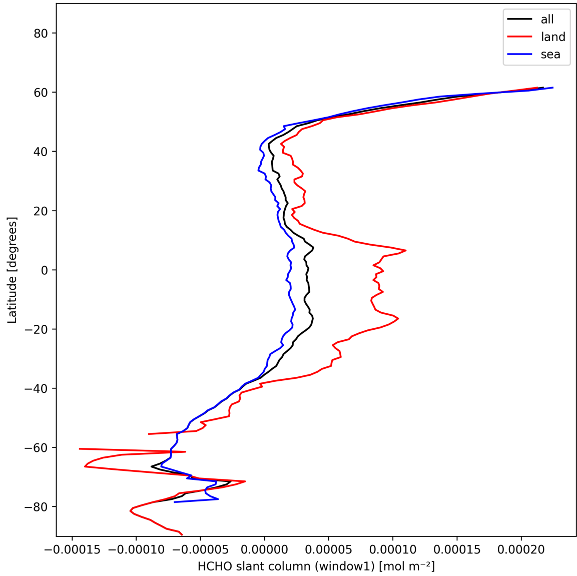
Figure 24: Zonal average of “HCHO slant column (window1)” for 2024-12-20 to 2024-12-22.
