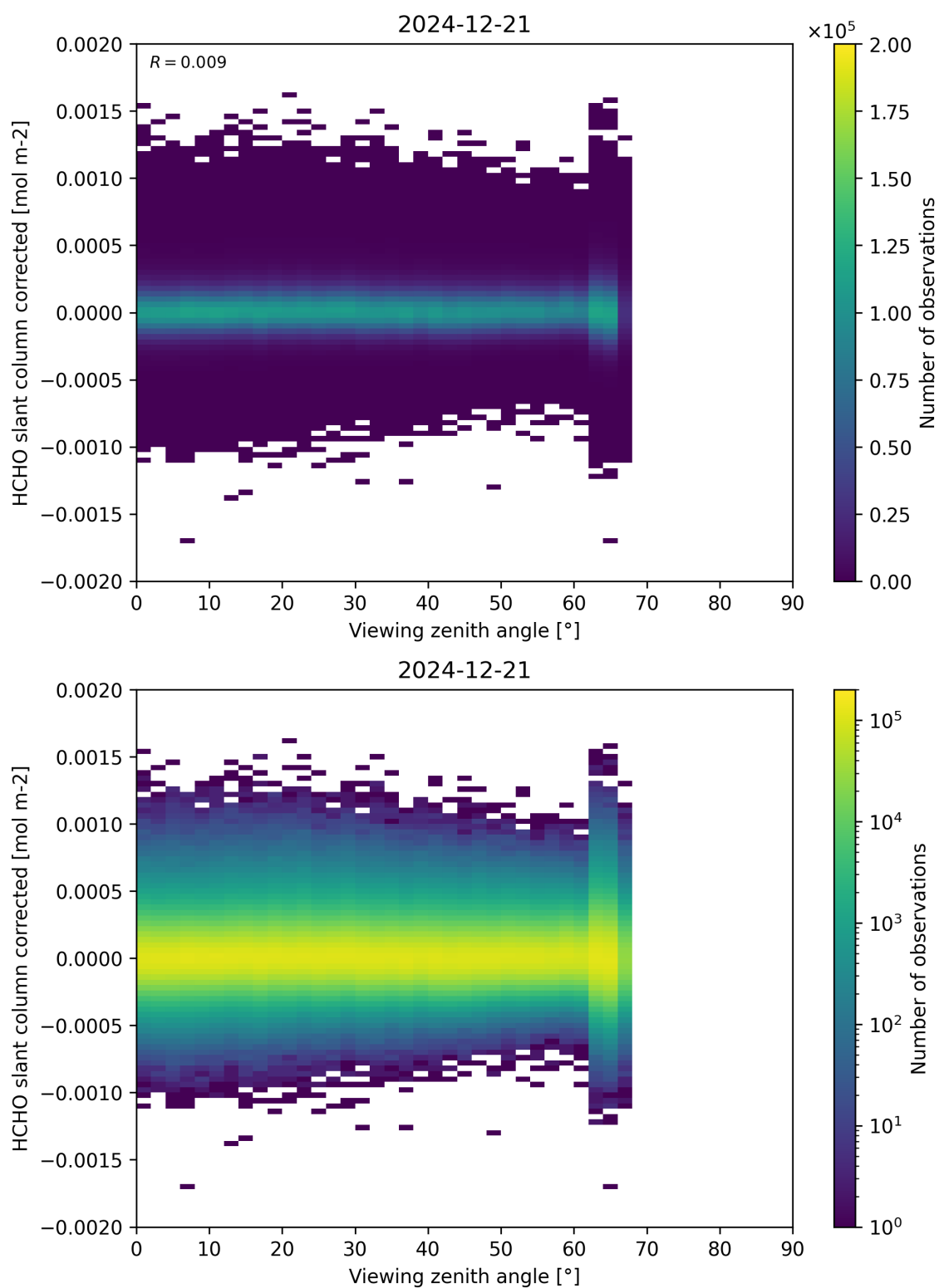
Figure 186: Scatter density plot of “Viewing zenith angle” against “HCHO slant column corrected” for 2024-12-20 to 2024-12-22.
