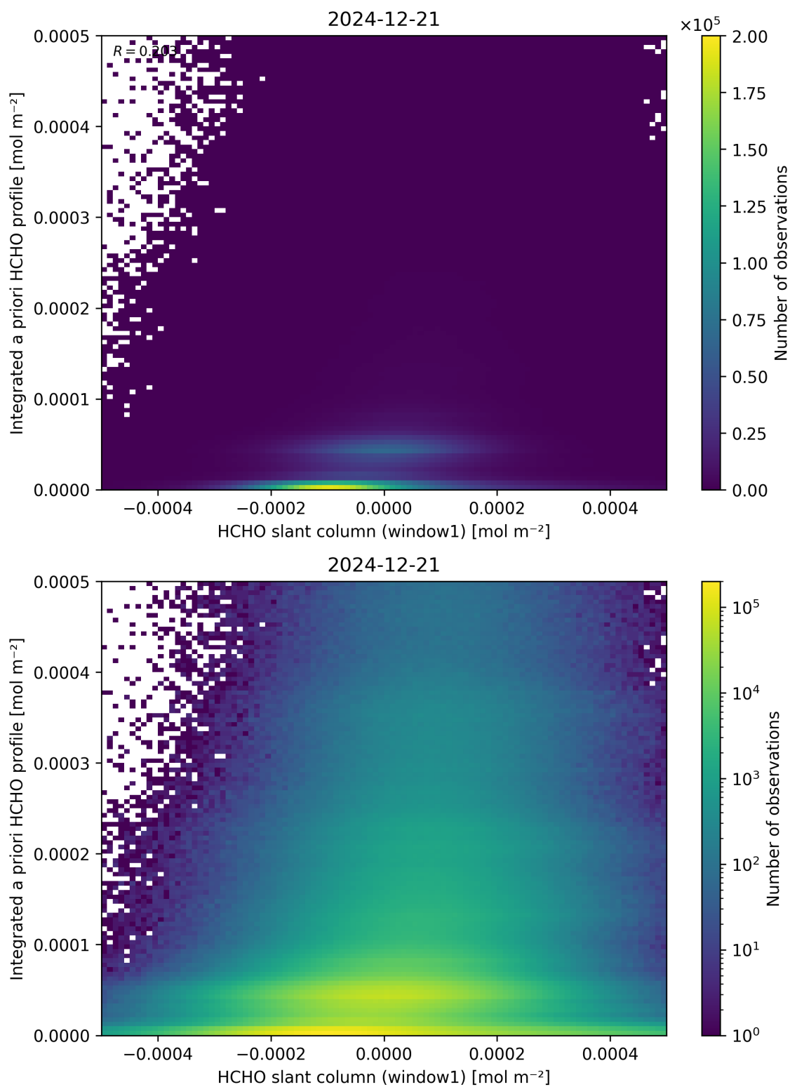
Figure 87: Scatter density plot of “HCHO slant column (window1)” against “Integrated a priori HCHO profile” for 2024-12-20 to 2024-12-22.
