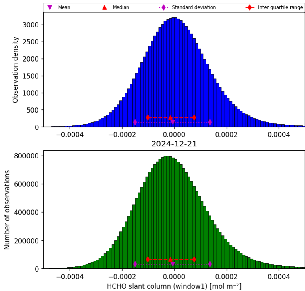
Figure 38: Histogram of “HCHO slant column (window1)” for 2024-12-20 to 2024-12-22
