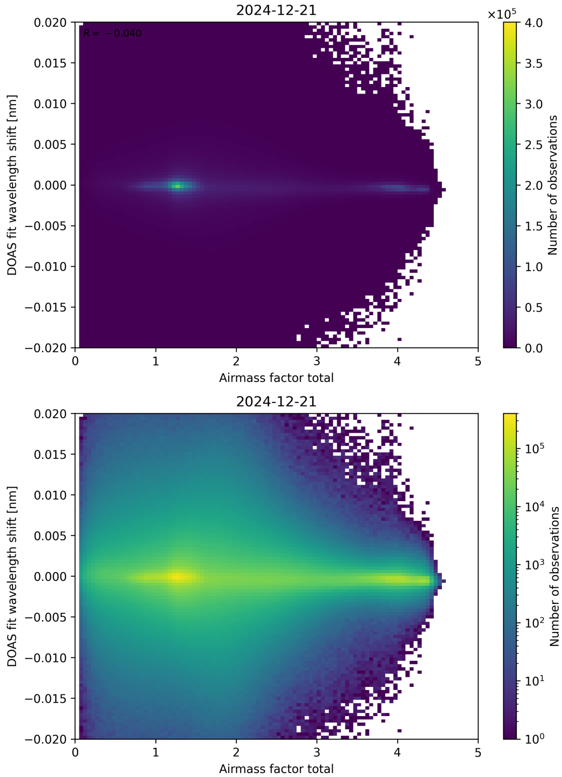
Figure 98: Scatter density plot of “Airmass factor total” against “DOAS fit wavelength shift” for 2024-12-20 to 2024-12-22.
