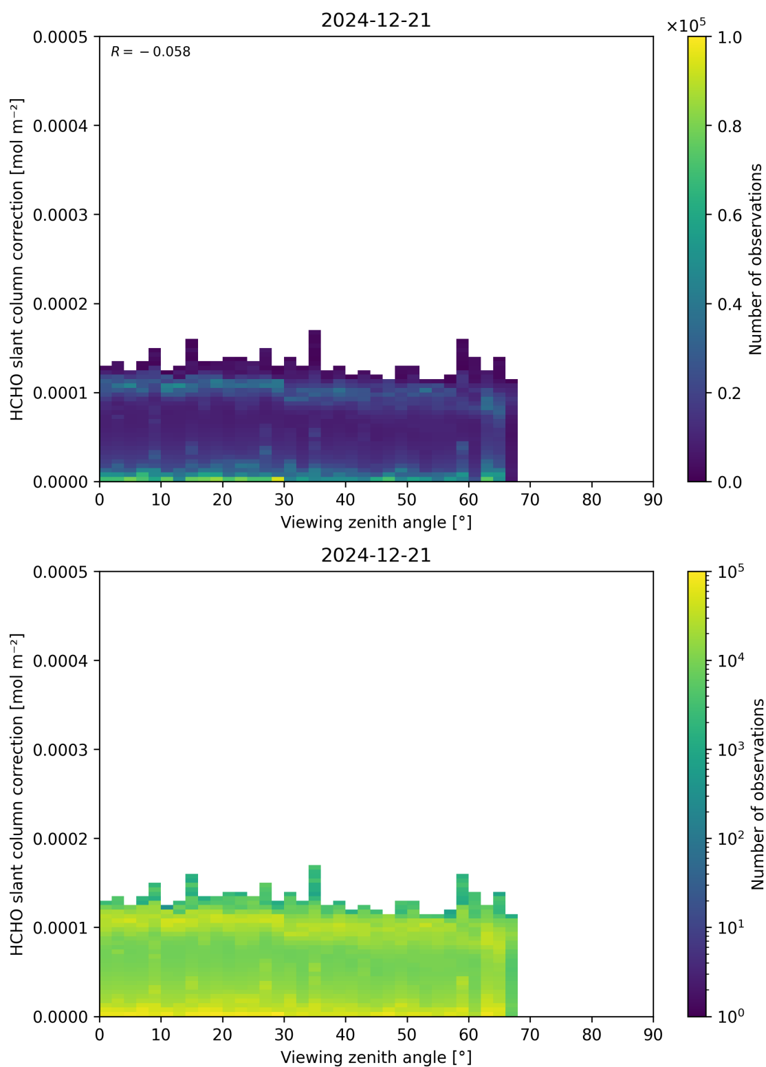
Figure 187: Scatter density plot of “Viewing zenith angle” against “HCHO slant column correction” for 2024-12-20 to 2024-12-22.
