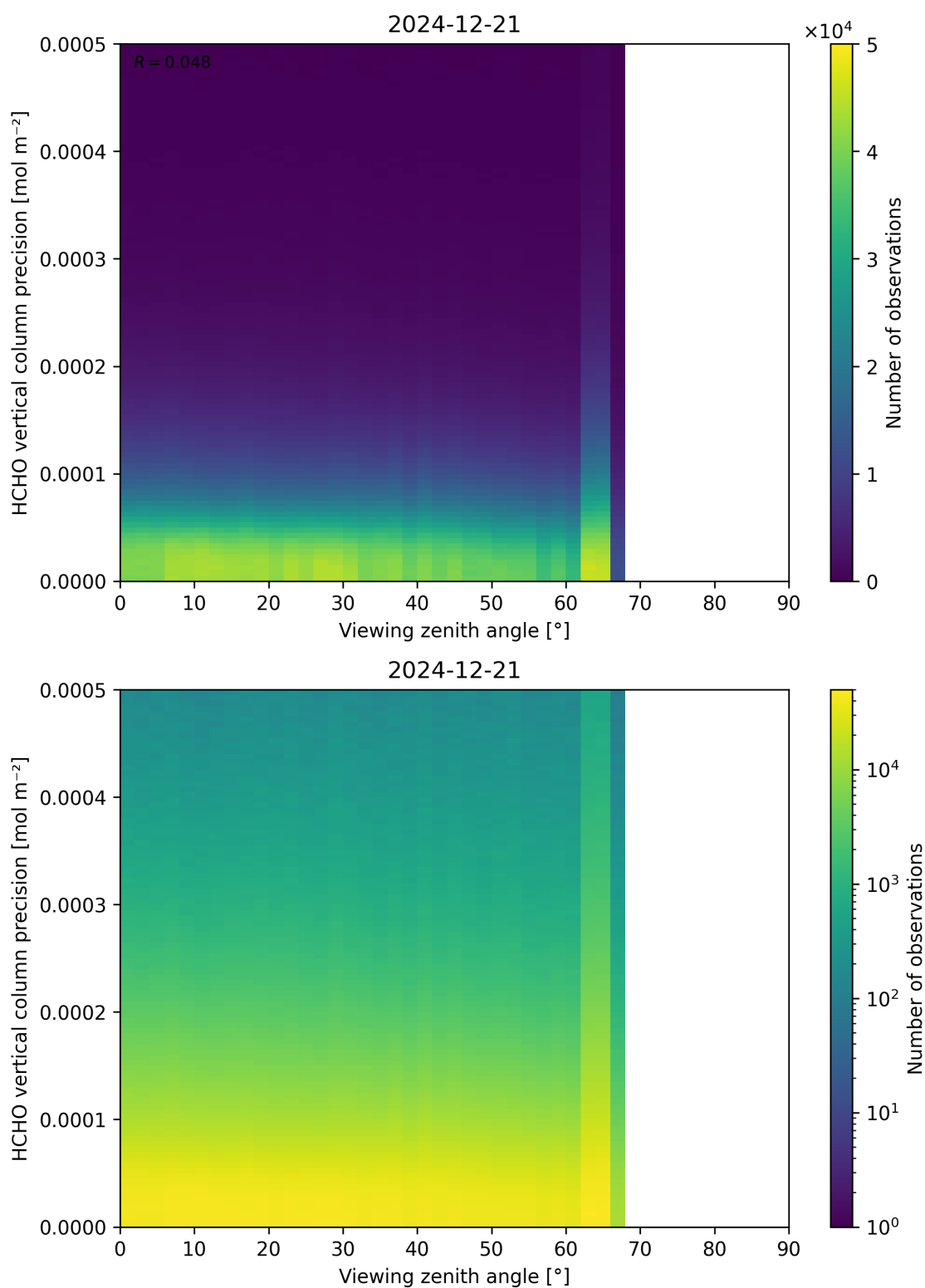
Figure 194: Scatter density plot of “Viewing zenith angle” against “HCHO vertical column precision” for 2024-12-20 to 2024-12-22.
