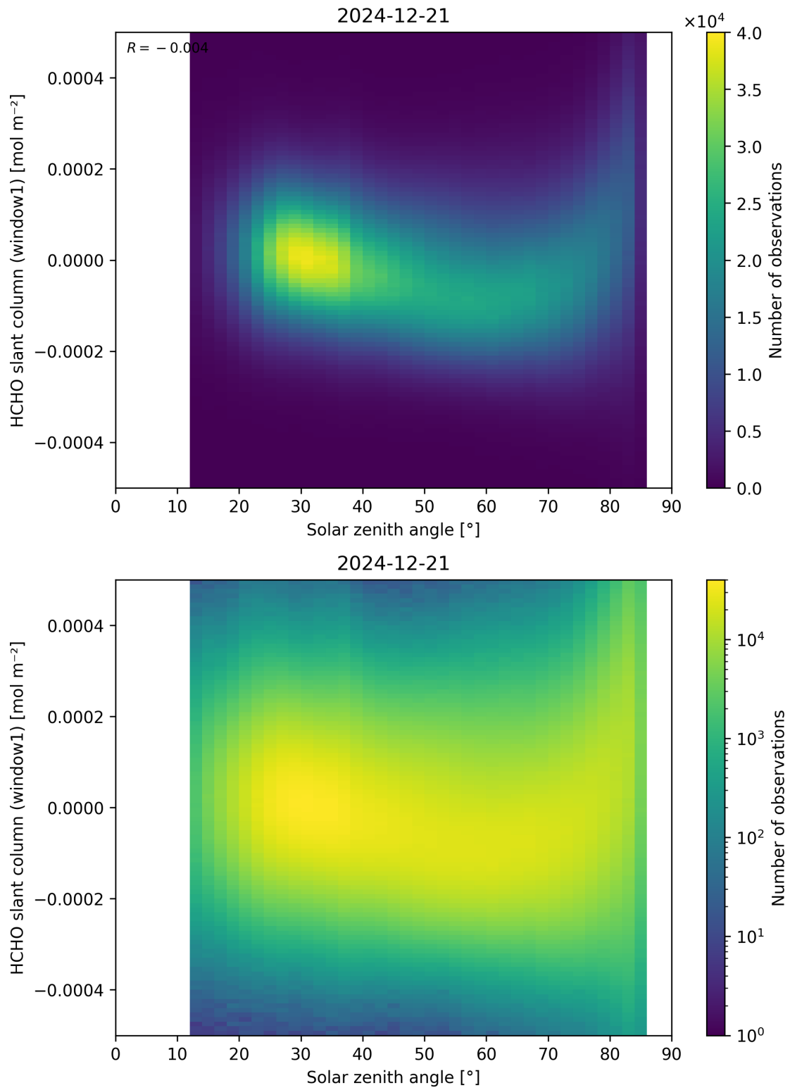
Figure 173: Scatter density plot of “Solar zenith angle” against “HCHO slant column (window1)” for 2024-12-20 to 2024-12-22.
