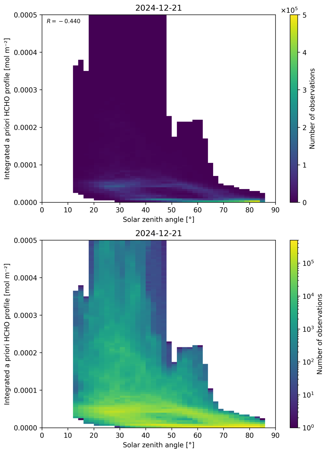
Figure 180: Scatter density plot of “Solar zenith angle” against “Integrated a priori HCHO profile” for 2024-12-20 to 2024-12-22.
