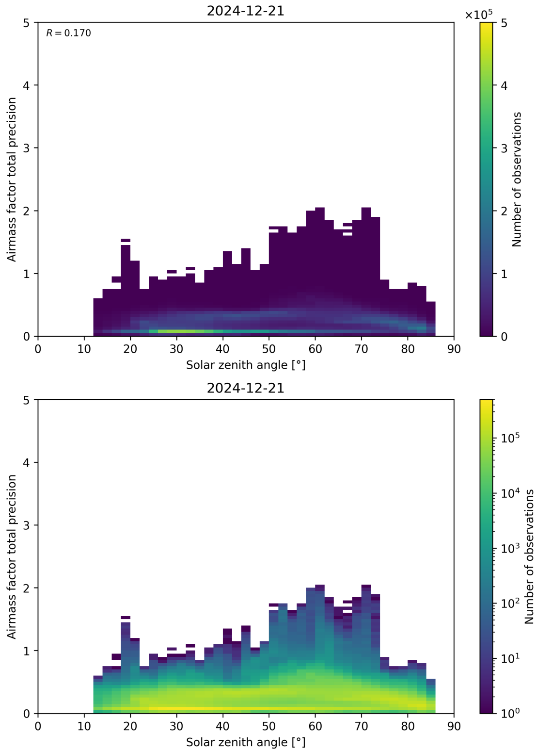
Figure 176: Scatter density plot of “Solar zenith angle” against “Airmass factor total precision” for 2024-12-20 to 2024-12-22.
