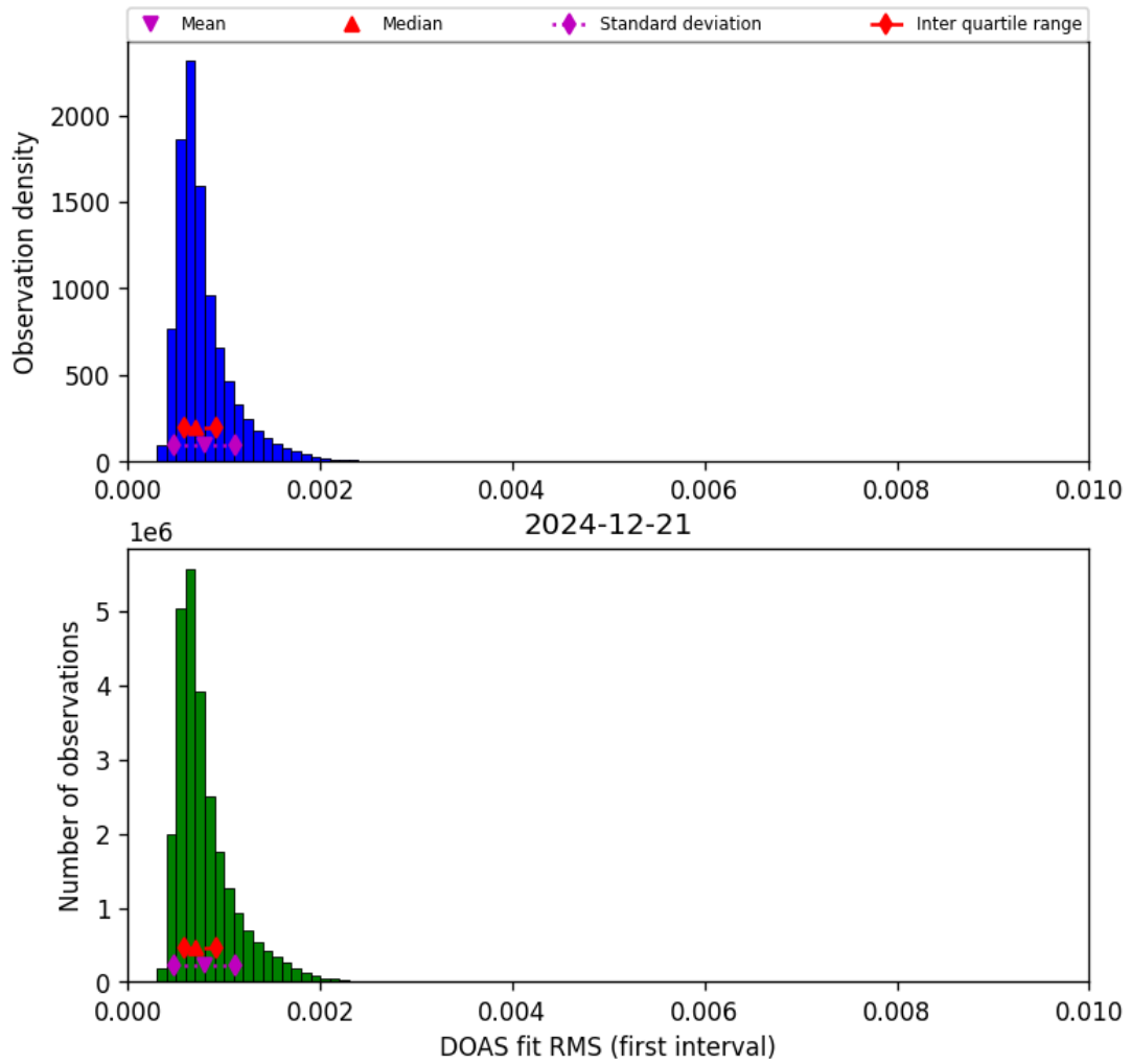
Figure 46: Histogram of “DOAS fit RMS (first interval)” for 2024-12-20 to 2024-12-22
