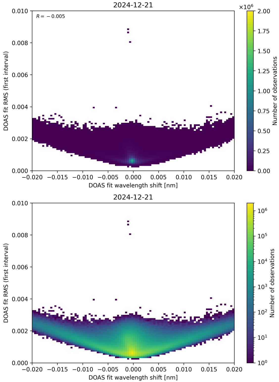
Figure 64: Scatter density plot of “DOAS fit wavelength shift” against “DOAS fit RMS (first interval)” for 2024-12-20 to 2024-12-22.
