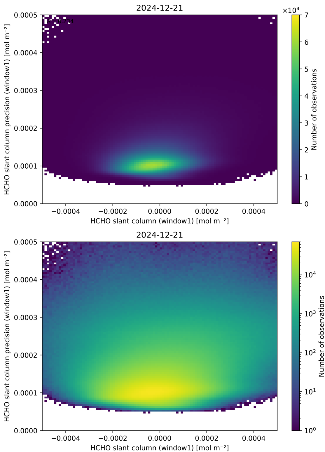
Figure 84: Scatter density plot of “HCHO slant column (window1)” against “HCHO slant column precision (window1)” for 2024-12-20 to 2024-12-22.
