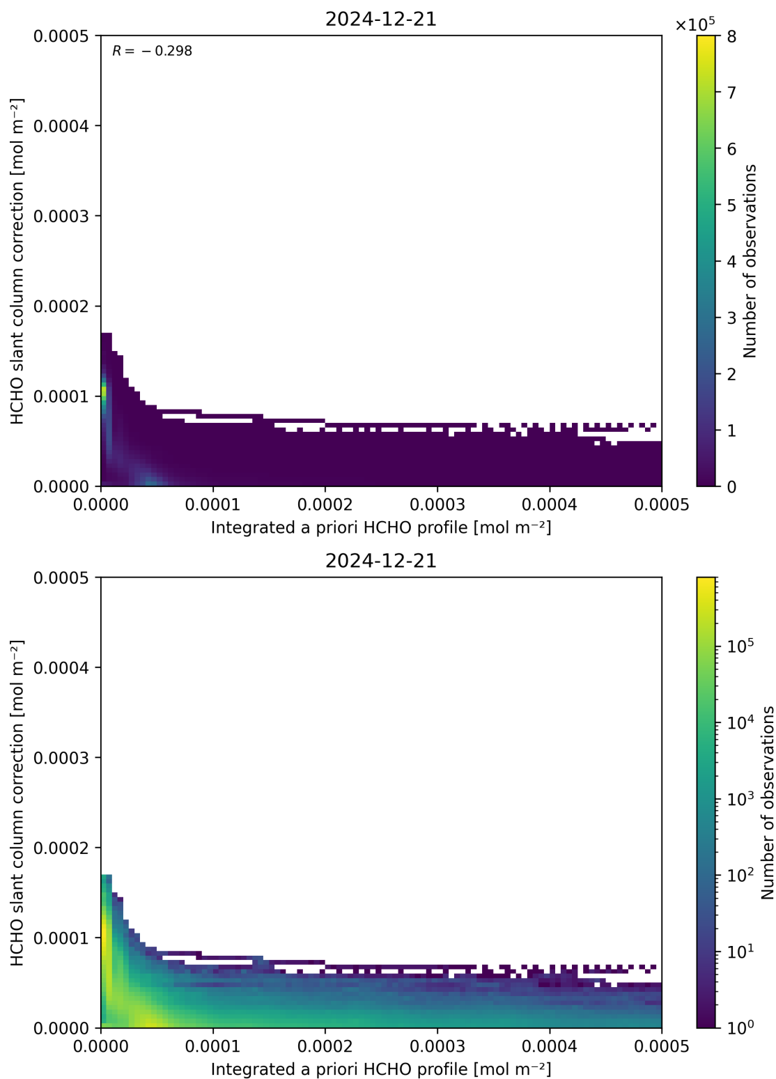
Figure 152: Scatter density plot of “Integrated a priori HCHO profile” against “HCHO slant column correction” for 2024-12-20 to 2024-12-22.
