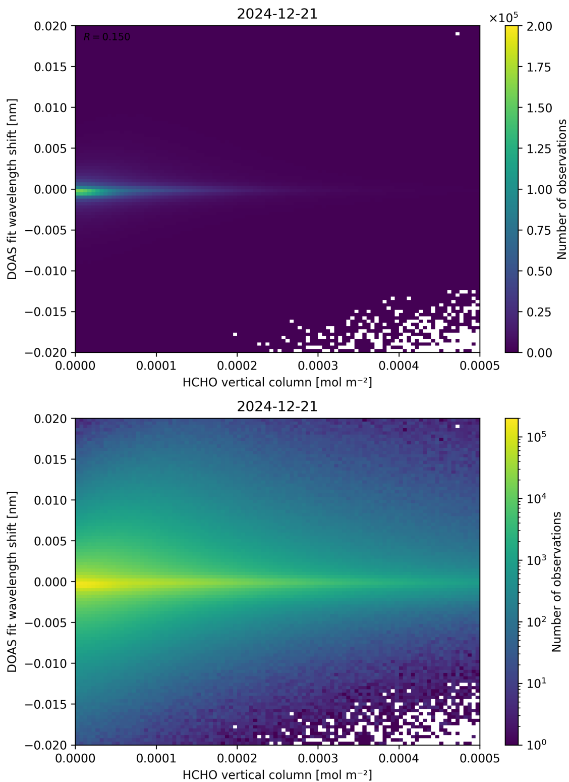
Figure 124: Scatter density plot of “HCHO vertical column” against “DOAS fit wavelength shift” for 2024-12-20 to 2024-12-22.
