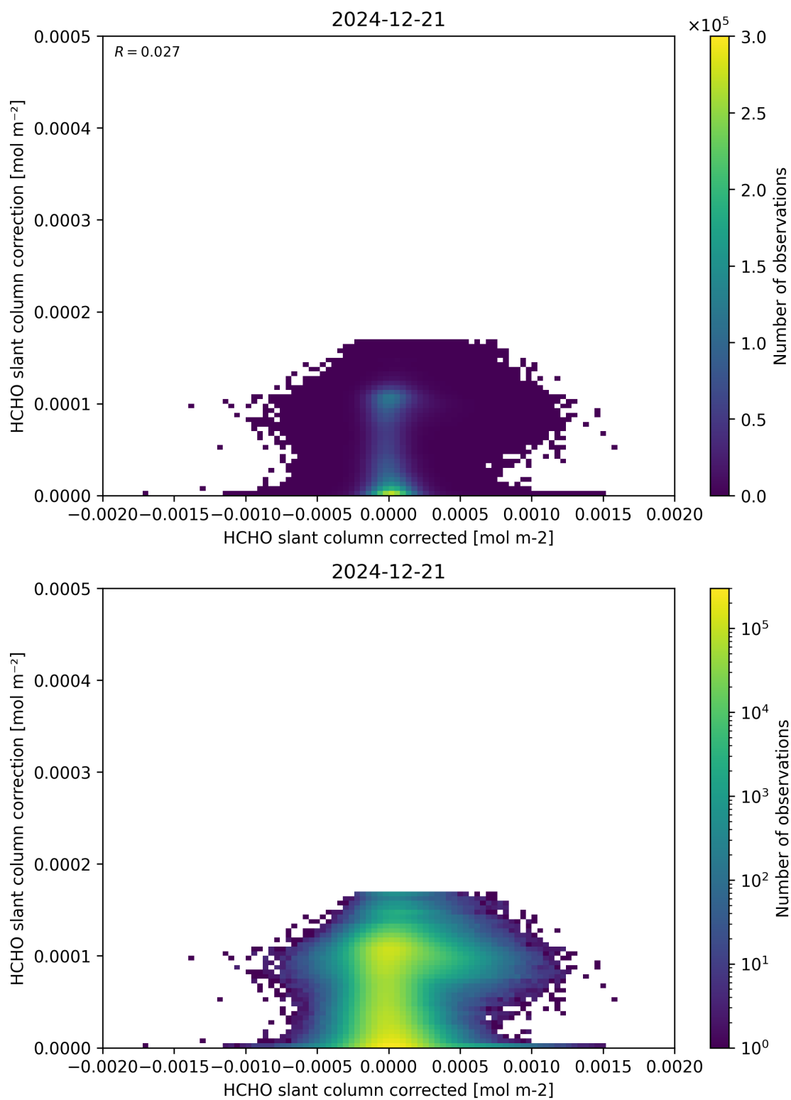
Figure 77: Scatter density plot of “HCHO slant column corrected” against “HCHO slant column correction” for 2024-12-20 to 2024-12-22.
