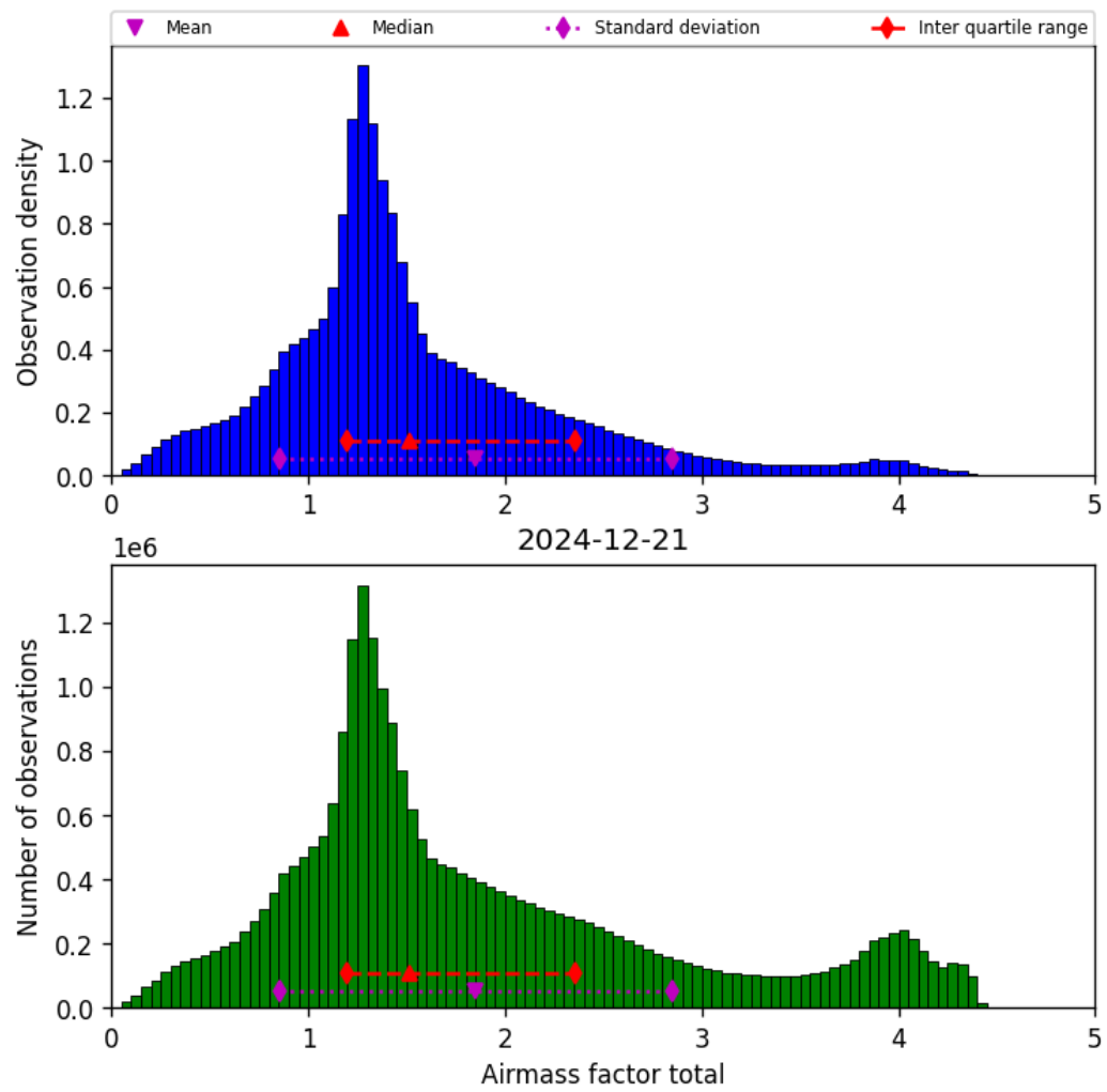
Figure 40: Histogram of “Airmass factor total” for 2024-12-20 to 2024-12-22
