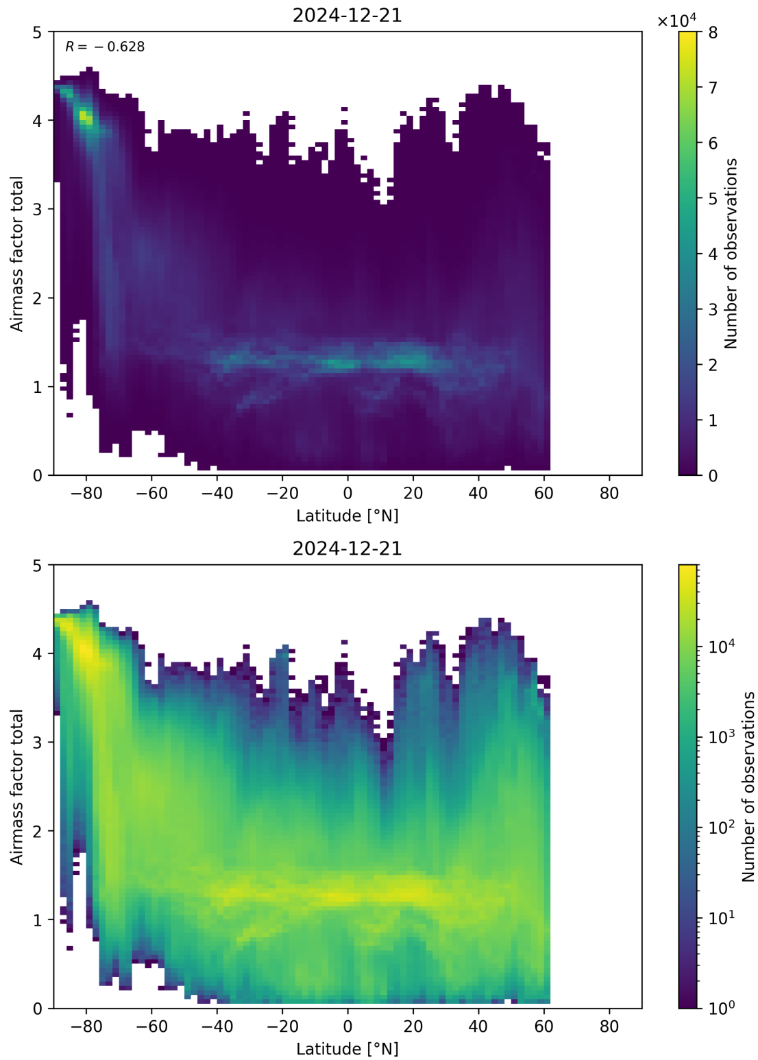
Figure 161: Scatter density plot of “Latitude” against “Airmass factor total” for 2024-12-20 to 2024-12-22.
