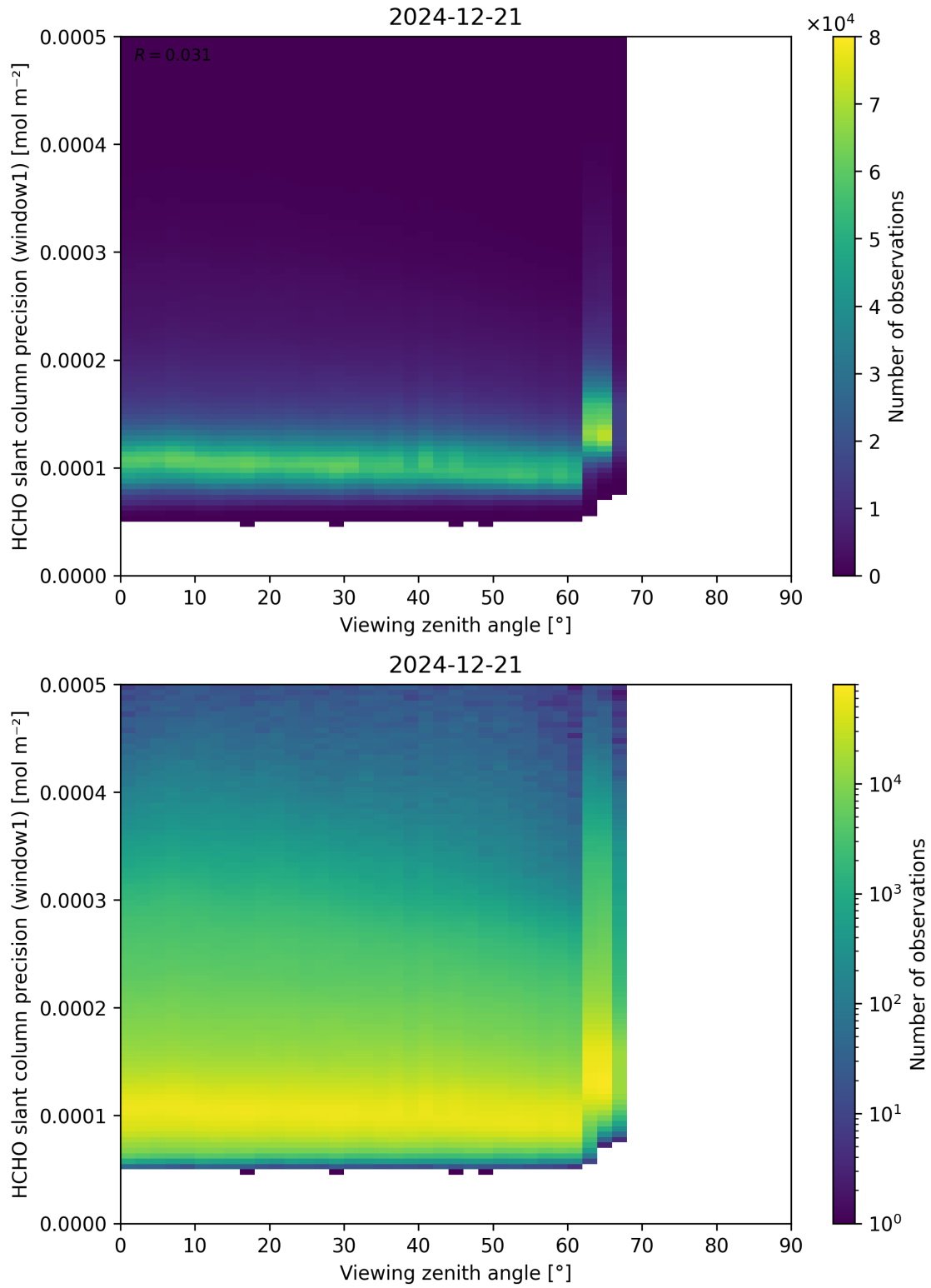
Figure 189: Scatter density plot of “Viewing zenith angle” against “HCHO slant column precision (window1)” for 2024-12-20 to 2024-12-22.
