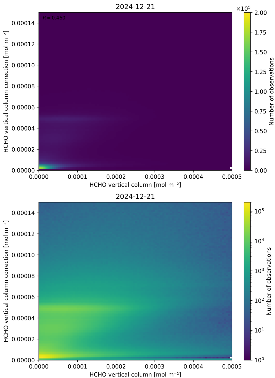
Figure 133: Scatter density plot of “HCHO vertical column” against “HCHO vertical column correction” for 2024-12-20 to 2024-12-22.
