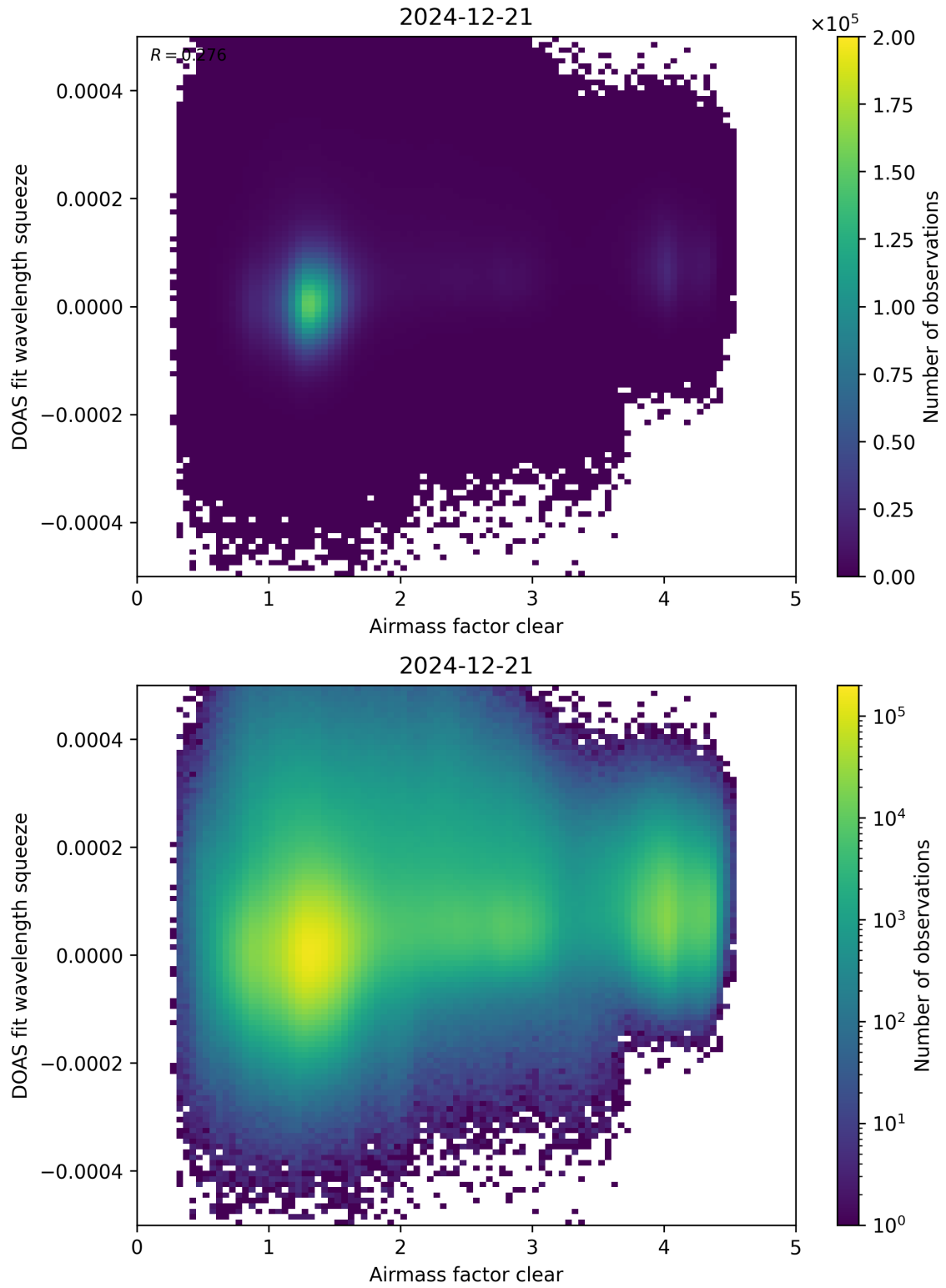
Figure 73: Scatter density plot of “Airmass factor clear” against “DOAS fit wavelength squeeze” for 2024-12-20 to 2024-12-22.
