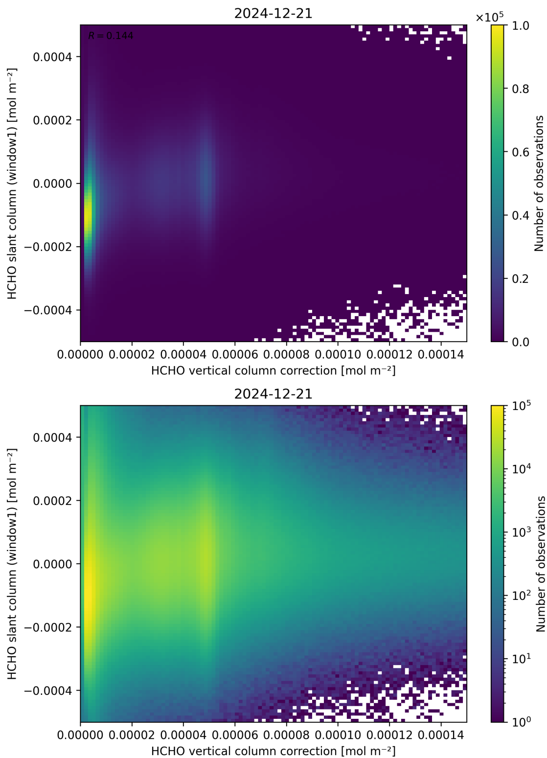
Figure 118: Scatter density plot of “HCHO vertical column correction” against “HCHO slant column (window1)” for 2024-12-20 to 2024-12-22.
