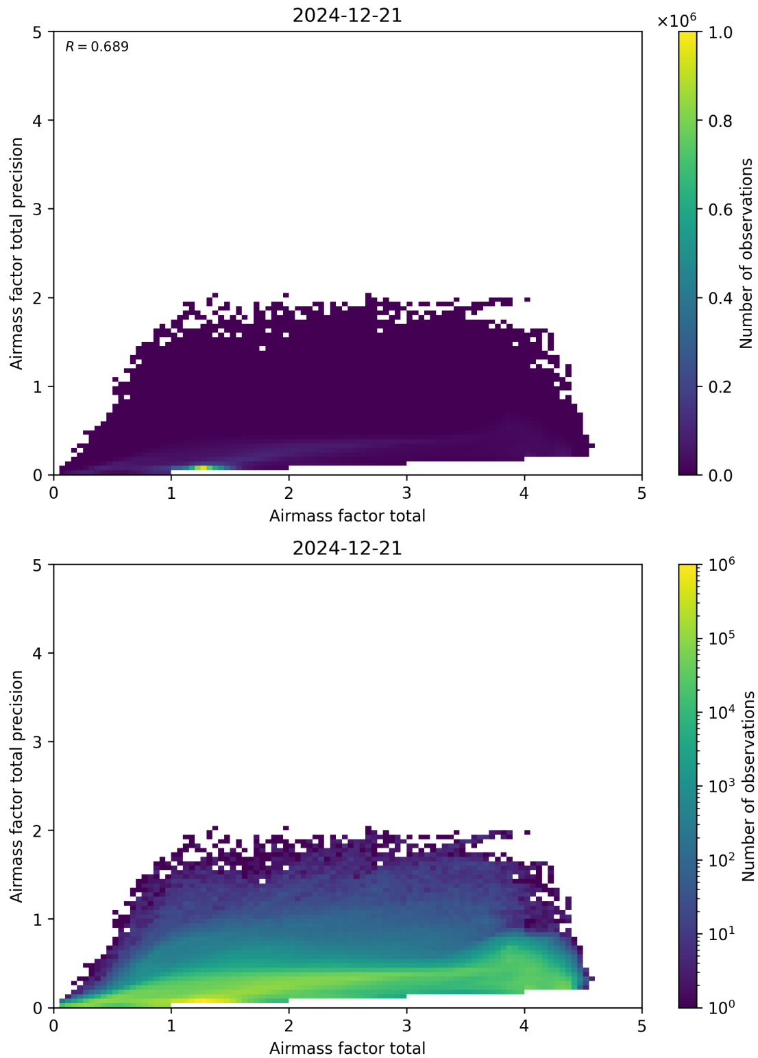
Figure 103: Scatter density plot of “Airmass factor total” against “Airmass factor total precision” for 2024-12-20 to 2024-12-22.
