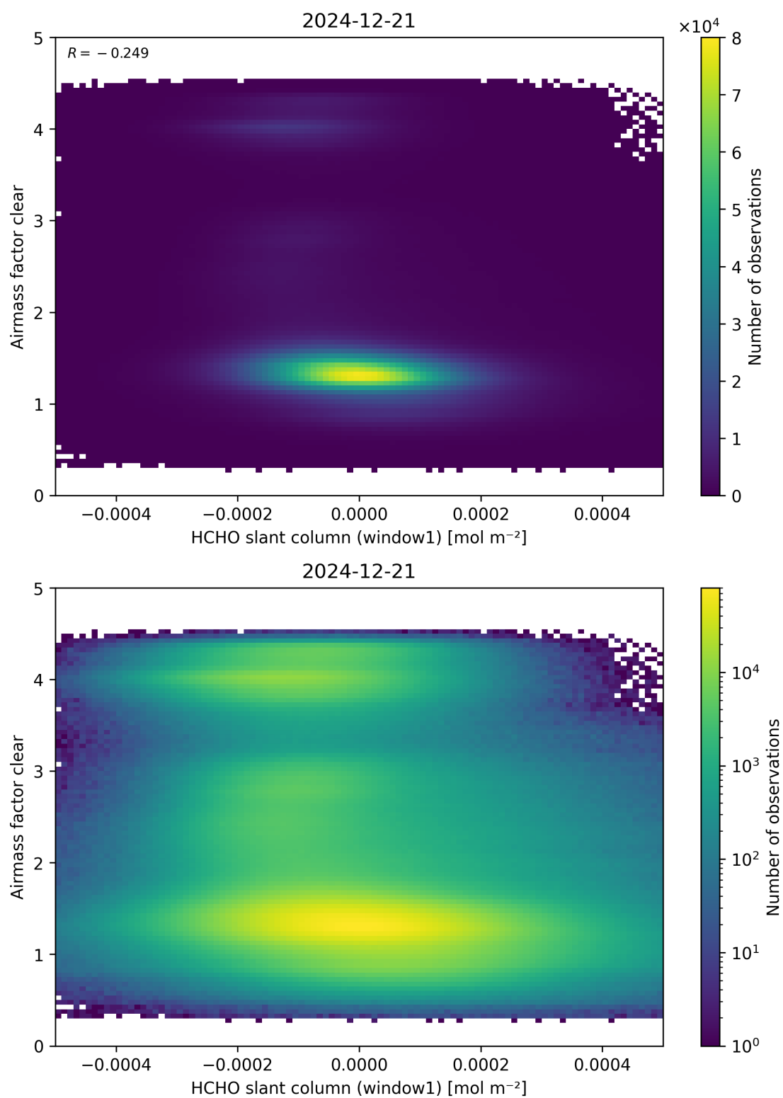
Figure 81: Scatter density plot of “HCHO slant column (window1)” against “Airmass factor clear” for 2024-12-20 to 2024-12-22.
