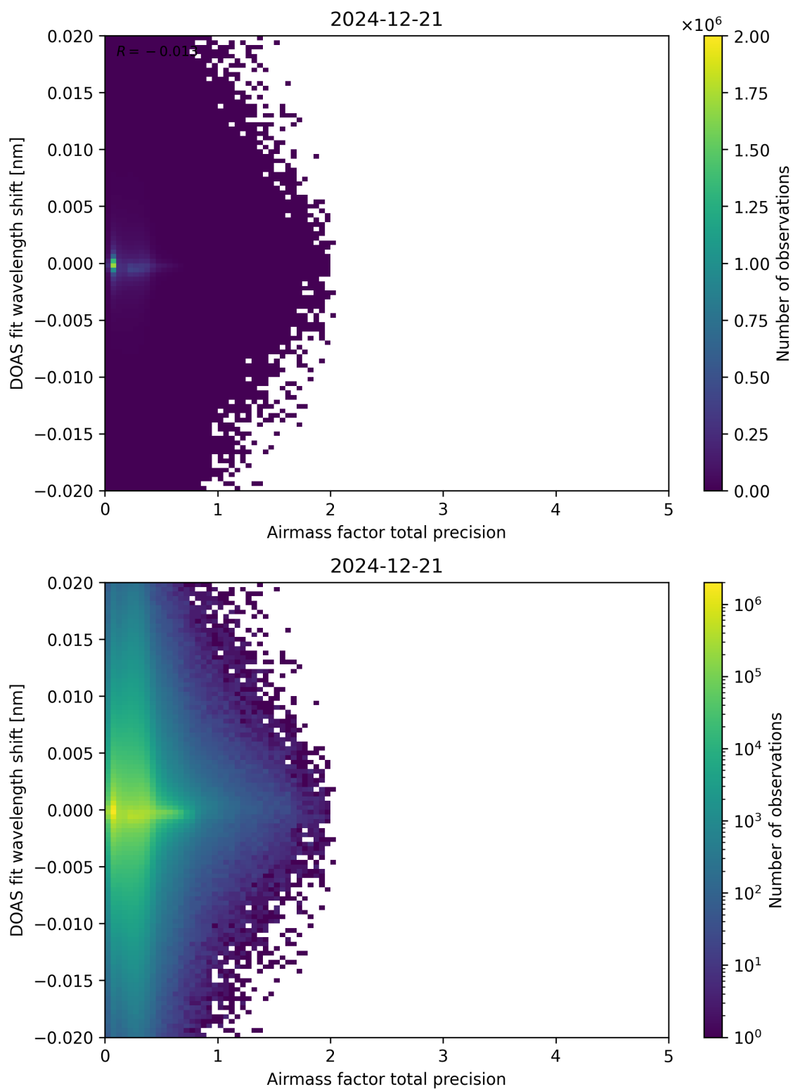
Figure 106: Scatter density plot of “Airmass factor total precision” against “DOAS fit wavelength shift” for 2024-12-20 to 2024-12-22.
