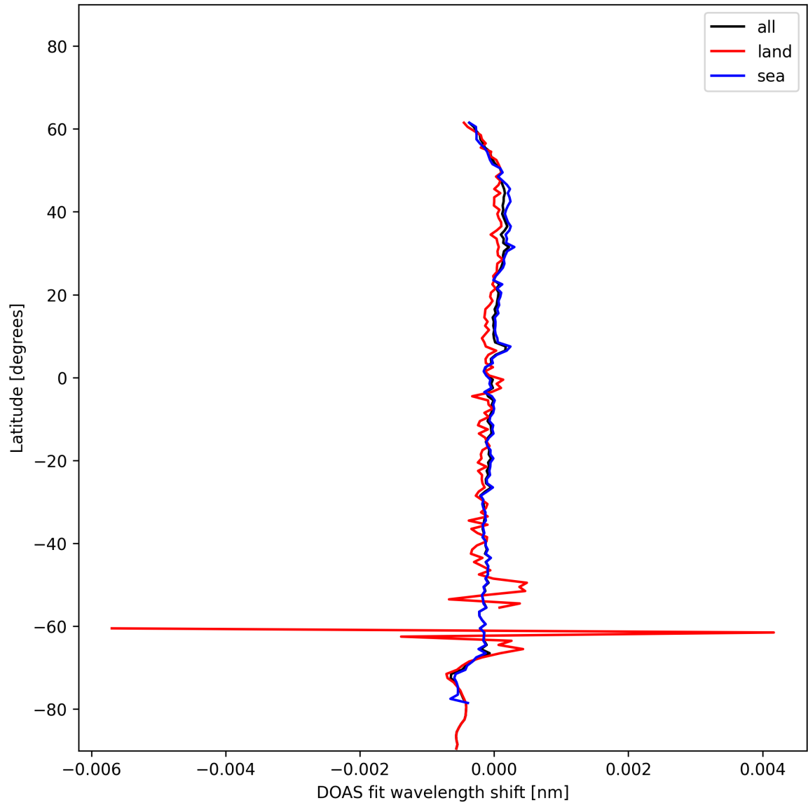
Figure 30: Zonal average of "DOAS fit wavelength shift" for 2024-12-20 to 2024-12-22.
