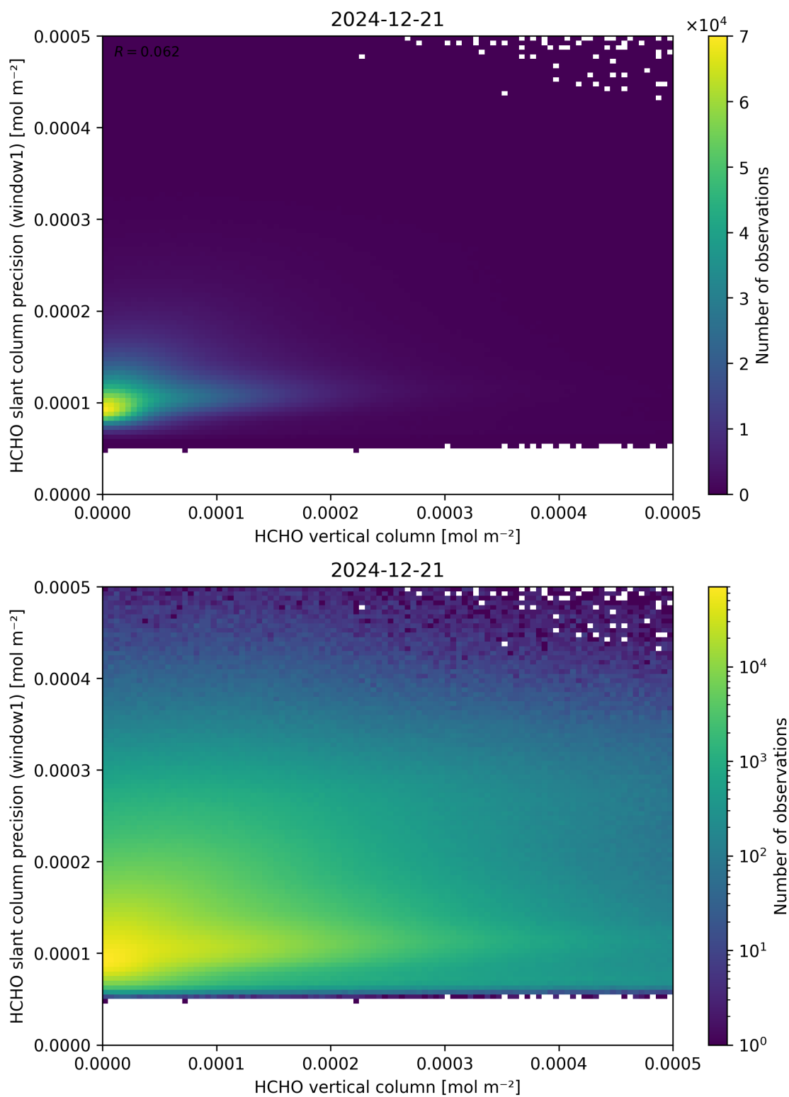
Figure 130: Scatter density plot of “HCHO vertical column” against “HCHO slant column precision (window1)” for 2024-12-20 to 2024-12-22.
