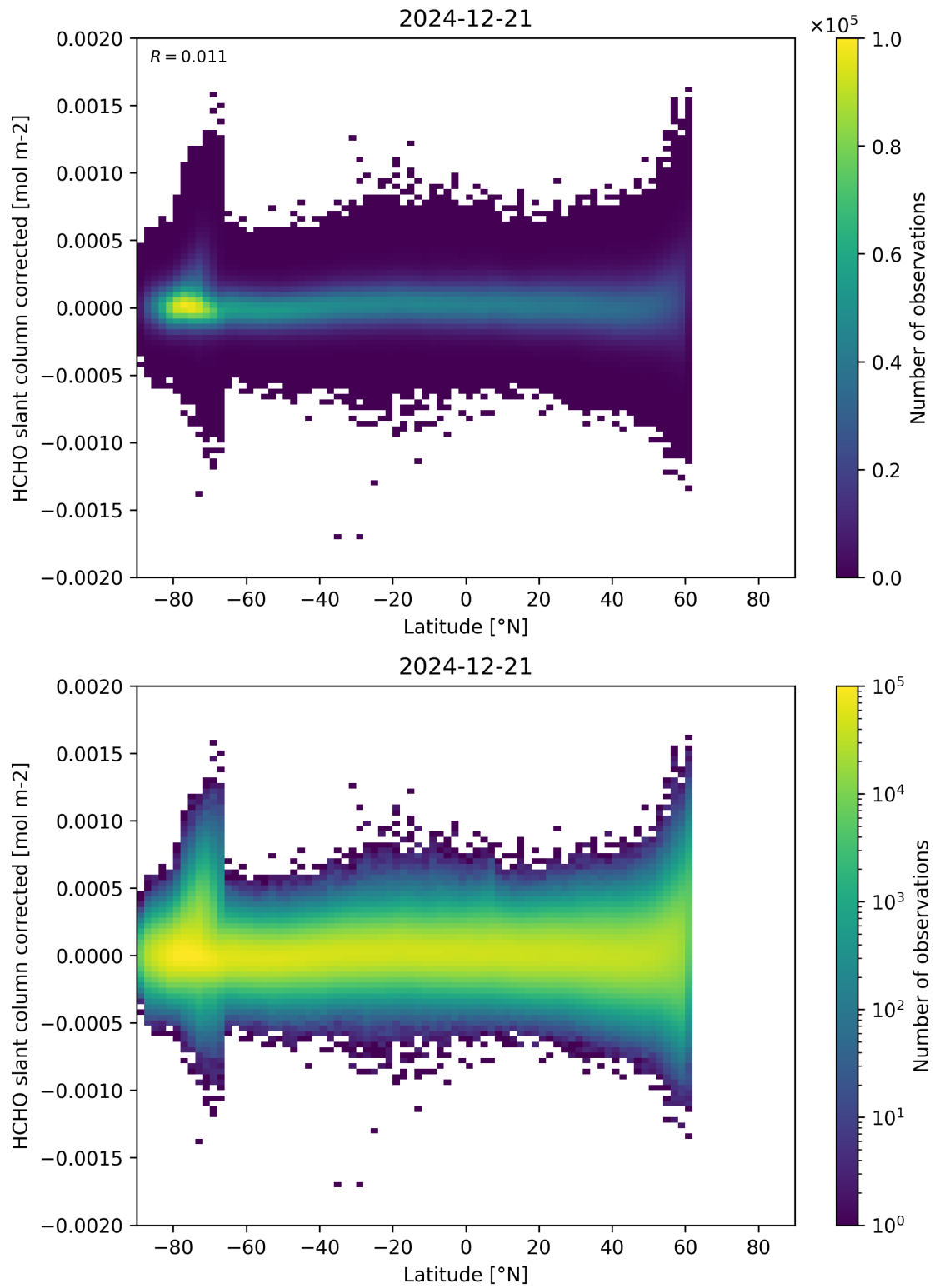
Figure 157: Scatter density plot of “Latitude” against “HCHO slant column corrected” for 2024-12-20 to 2024-12-22.
