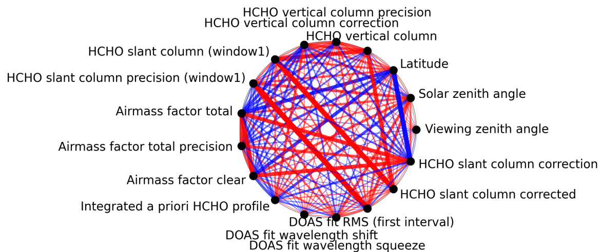
Figure 1: Map of correlation graph for 2024-12-20 to 2024-12-22.
