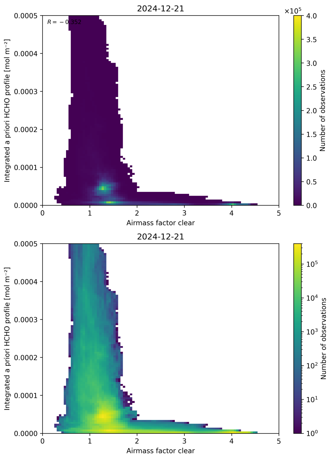
Figure 76: Scatter density plot of “Airmass factor clear” against “Integrated a priori HCHO profile” for 2024-12-20 to 2024-12-22.
