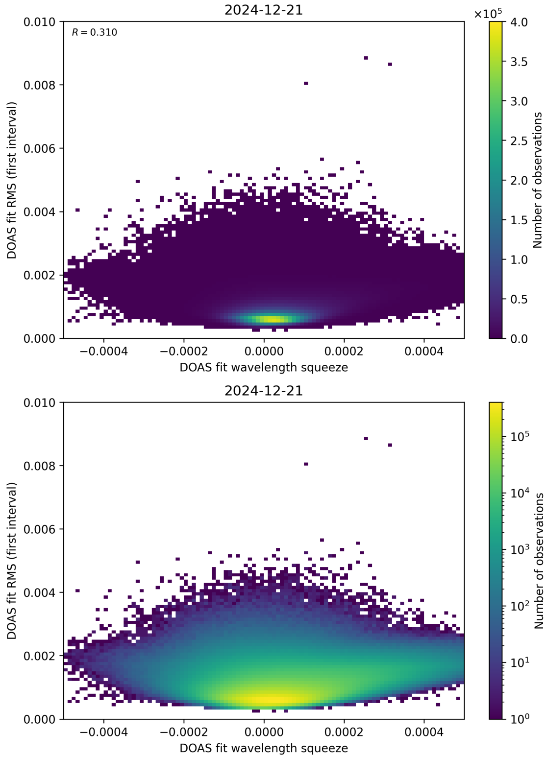
Figure 68: Scatter density plot of “DOAS fit wavelength squeeze” against “DOAS fit RMS (first interval)” for 2024-12-20 to 2024-12-22.
