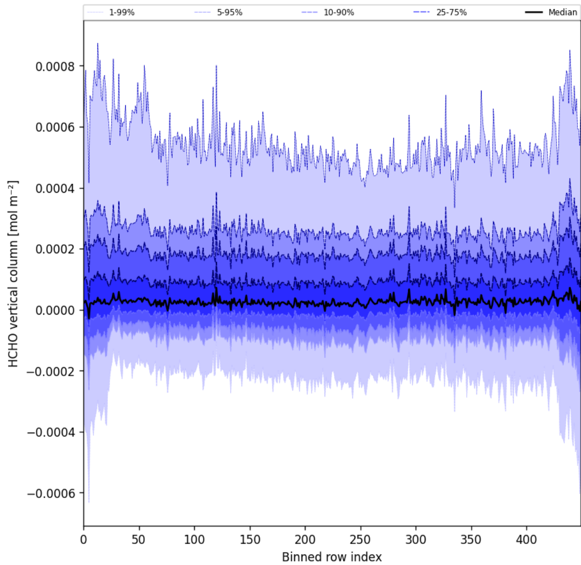
Figure 49: Along track statistics of “HCHO vertical column” for 2024-12-20 to 2024-12-22
