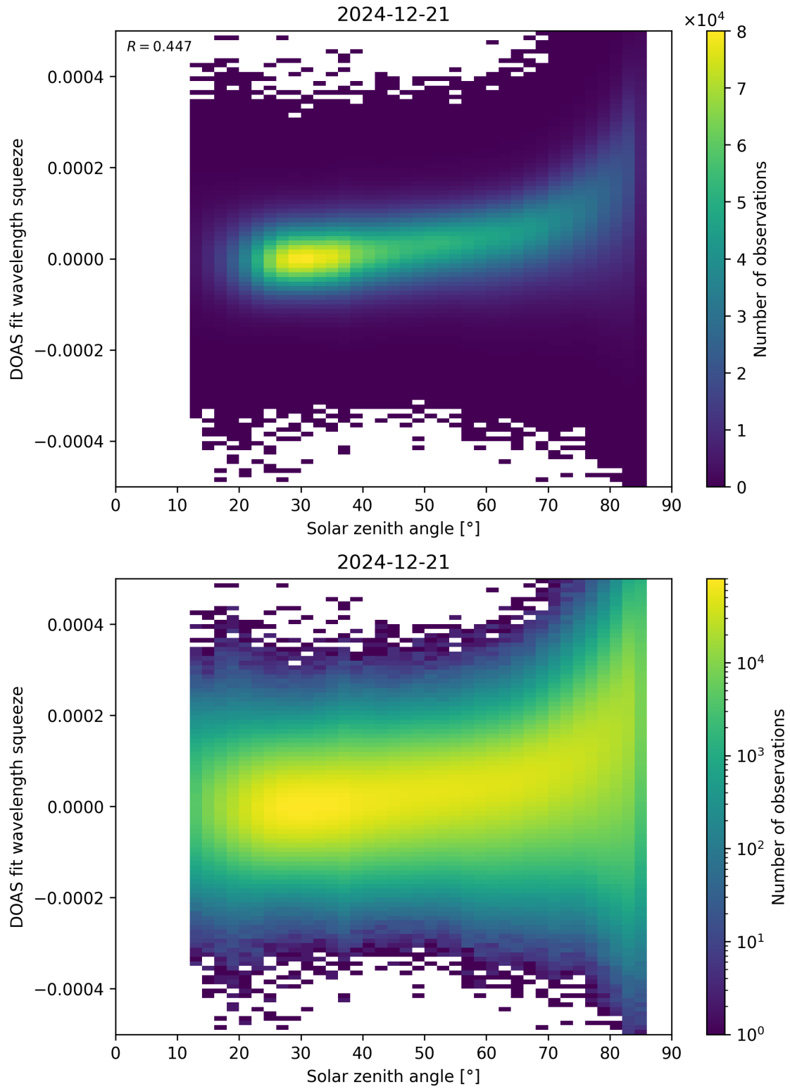
Figure 169: Scatter density plot of “Solar zenith angle” against “DOAS fit wavelength squeeze” for 2024-12-20 to 2024-12-22.
