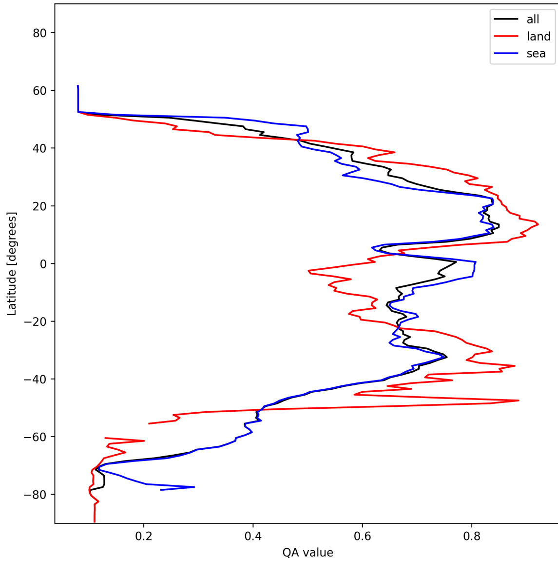
Figure 20: Zonal average of “QA value” for 2024-12-20 to 2024-12-22.
