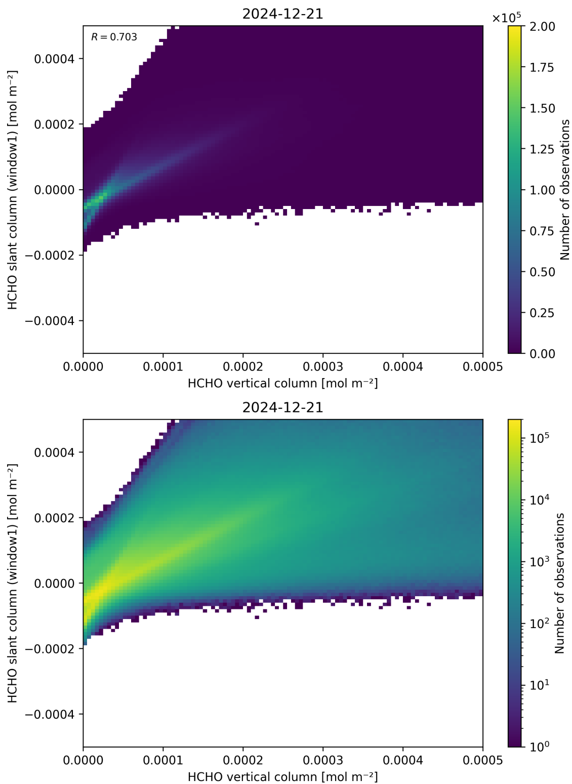
Figure 129: Scatter density plot of “HCHO vertical column” against “HCHO slant column (window1)” for 2024-12-20 to 2024-12-22.
