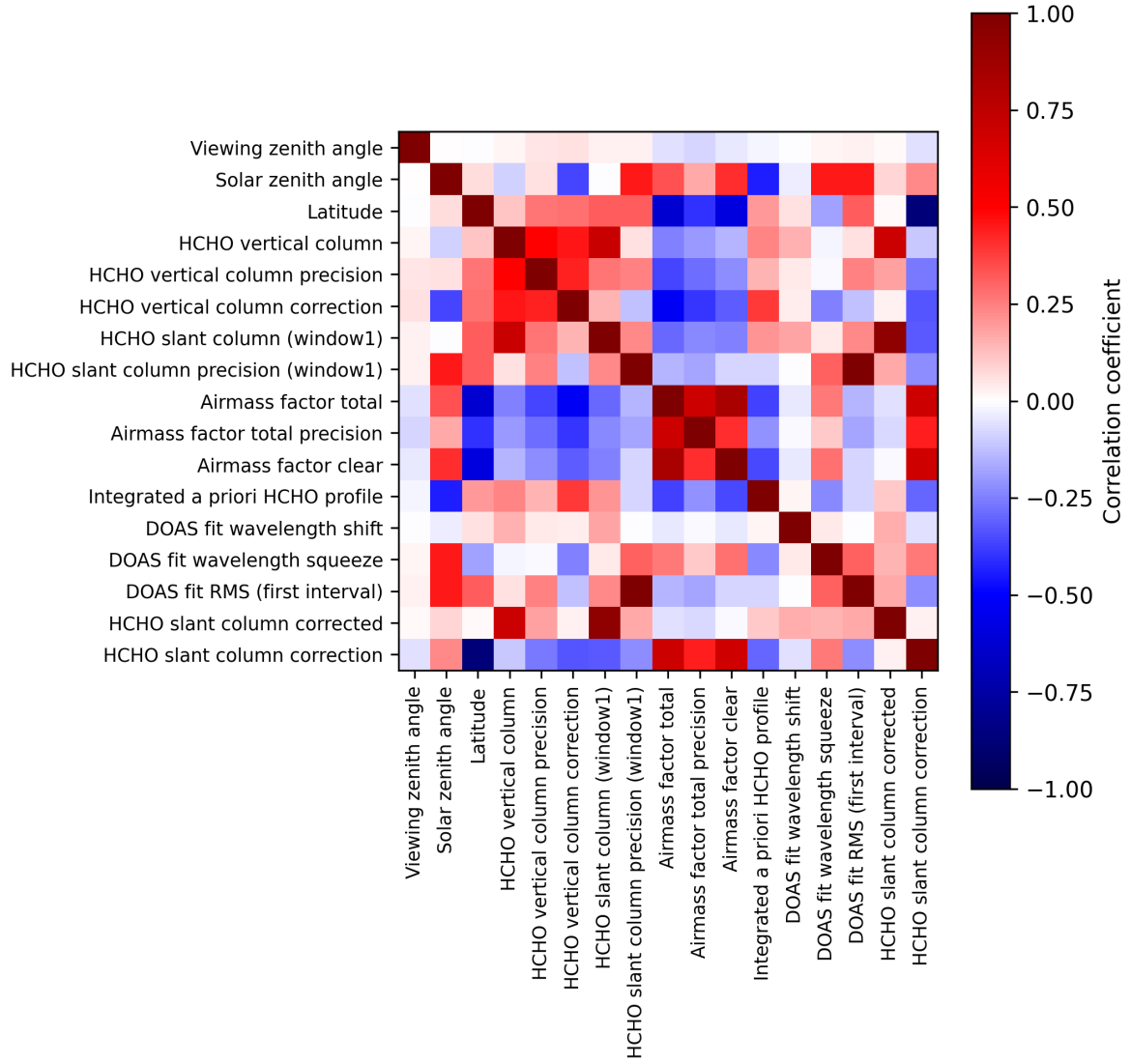
Figure 2: Map of correlation matrix for 2024-12-20 to 2024-12-22.
