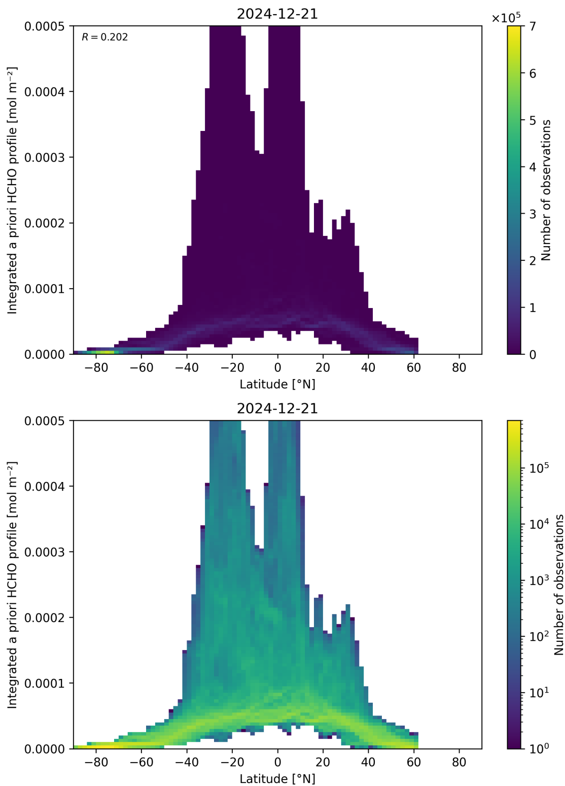
Figure 166: Scatter density plot of “Latitude” against “Integrated a priori HCHO profile” for 2024-12-20 to 2024-12-22.
