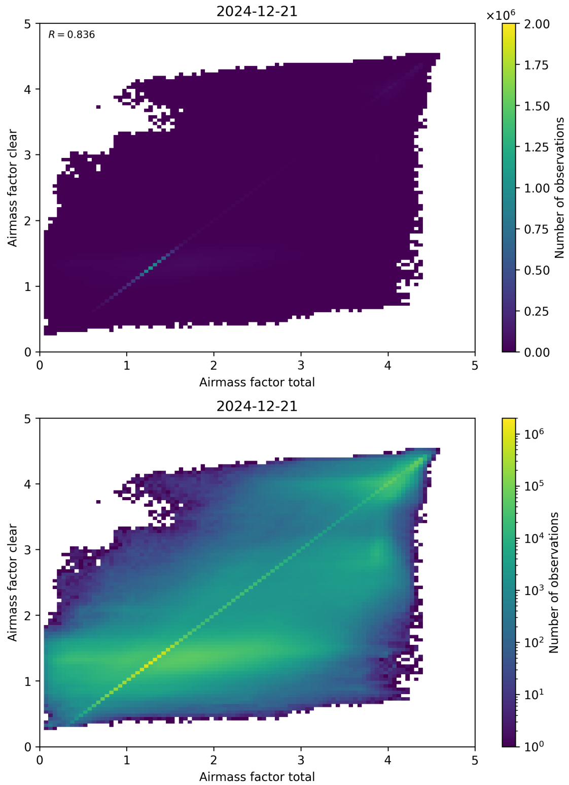
Figure 100: Scatter density plot of “Airmass factor total” against “Airmass factor clear” for 2024-12-20 to 2024-12-22.
