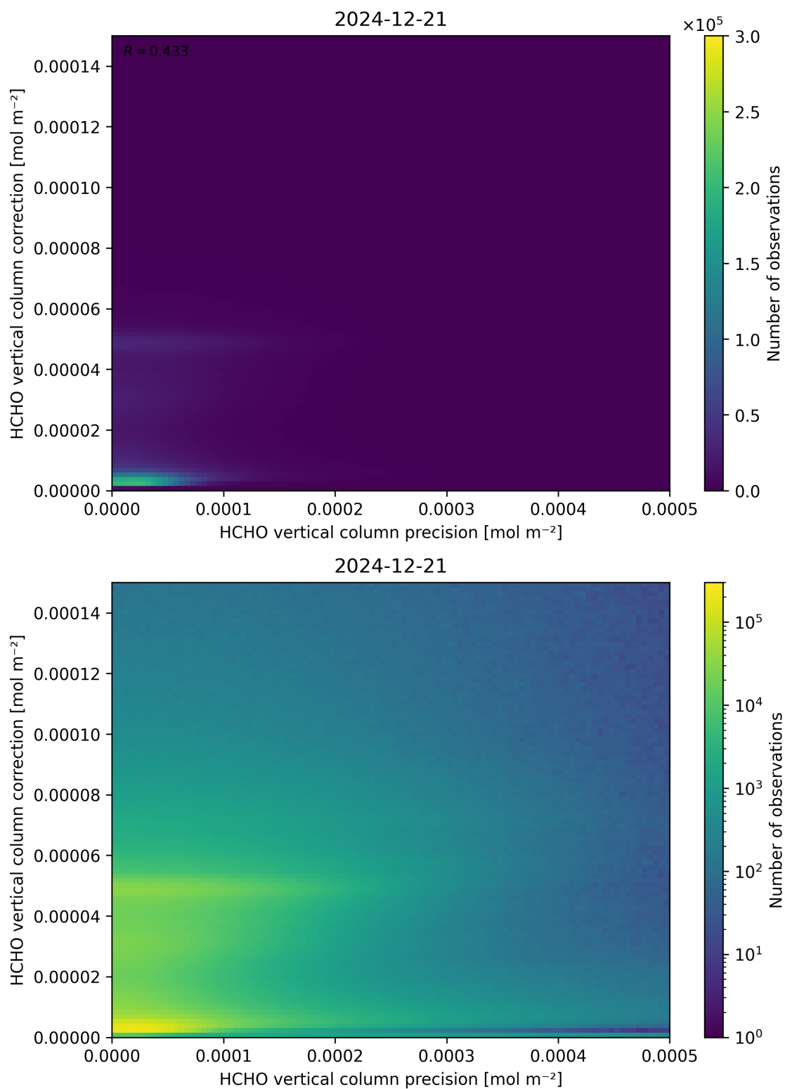
Figure 146: Scatter density plot of “HCHO vertical column precision” against “HCHO vertical column correction” for 2024-12-20 to 2024-12-22.
