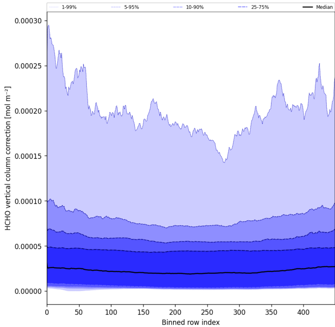
Figure 51: Along track statistics of “HCHO vertical column correction” for 2024-12-20 to 2024-12-22
