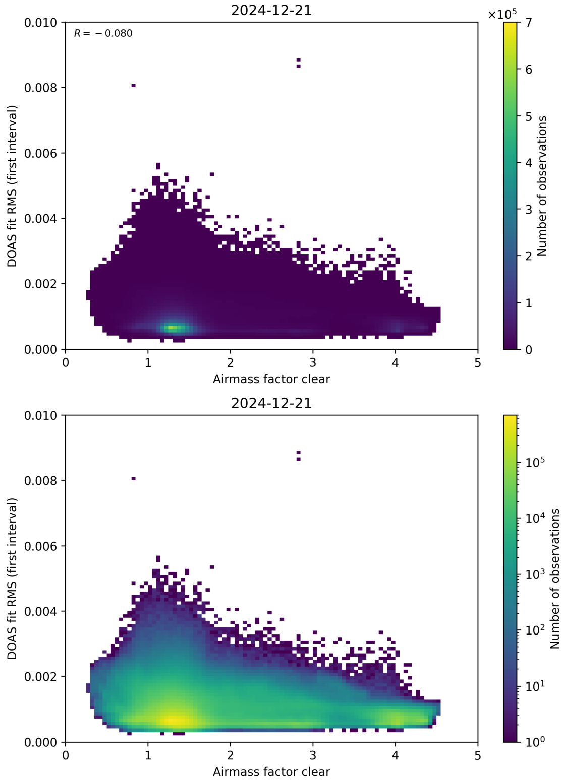
Figure 71: Scatter density plot of “Airmass factor clear” against “DOAS fit RMS (first interval)” for 2024-12-20 to 2024-12-22.
