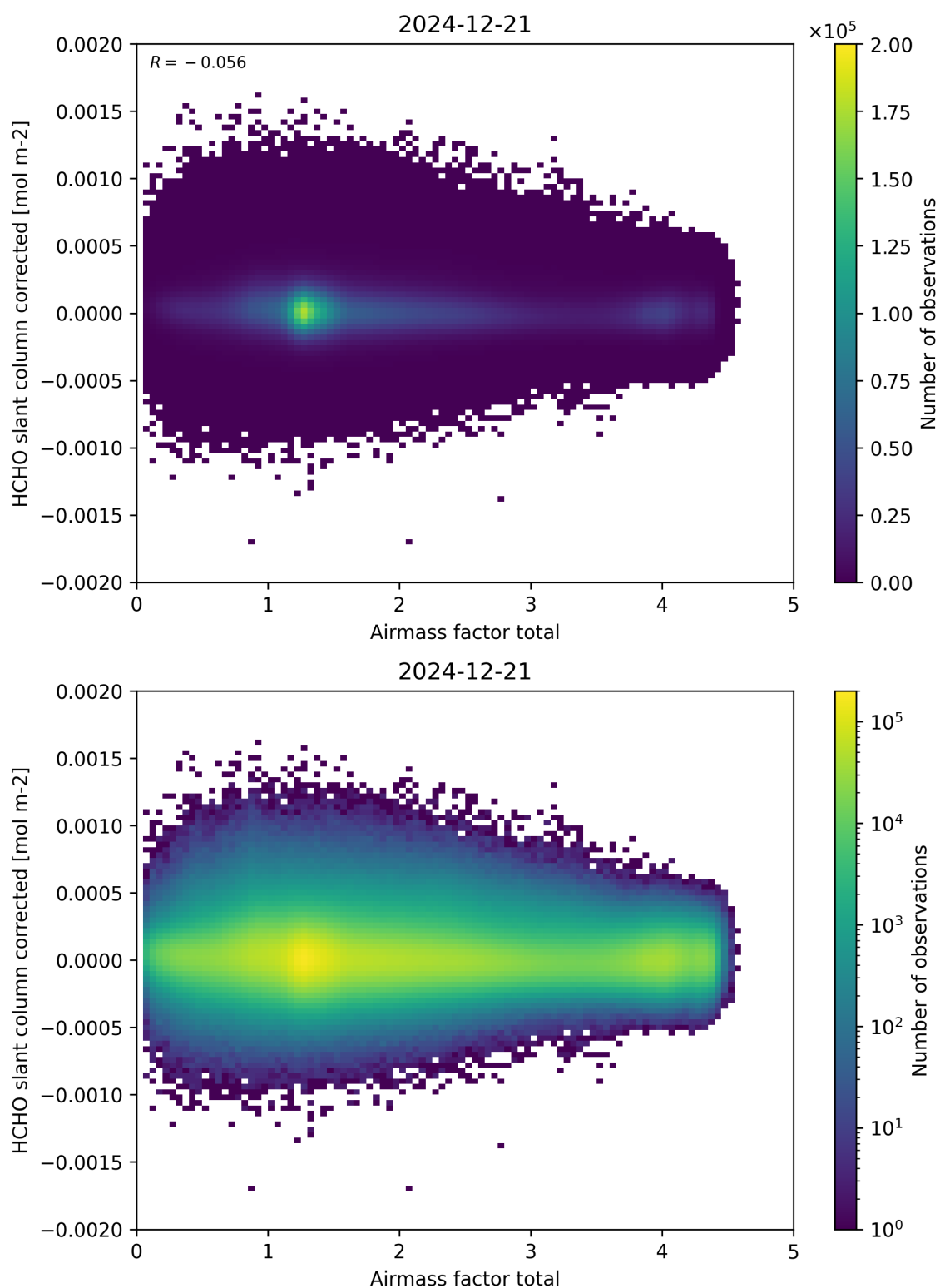
Figure 101: Scatter density plot of “Airmass factor total” against “HCHO slant column corrected” for 2024-12-20 to 2024-12-22.
