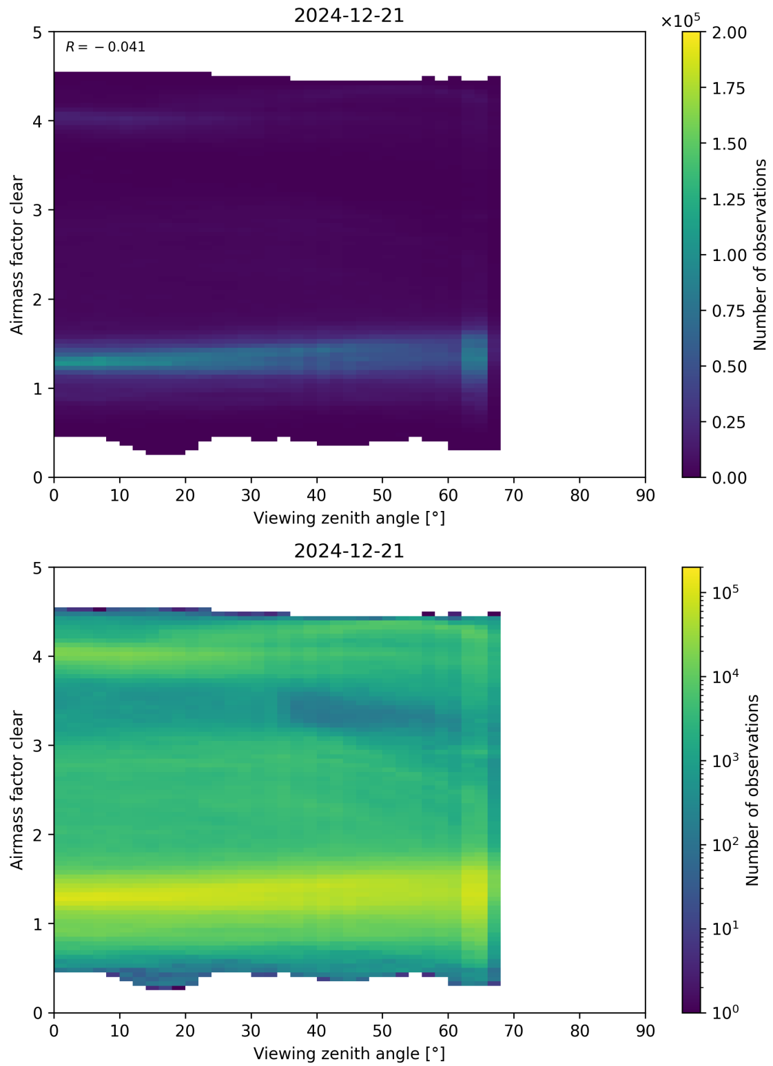
Figure 185: Scatter density plot of “Viewing zenith angle” against “Airmass factor clear” for 2024-12-20 to 2024-12-22.
