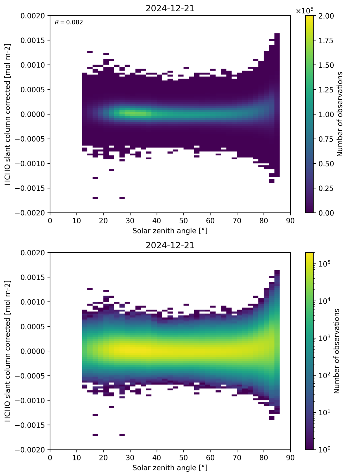
Figure 171: Scatter density plot of “Solar zenith angle” against “HCHO slant column corrected” for 2024-12-20 to 2024-12-22.
