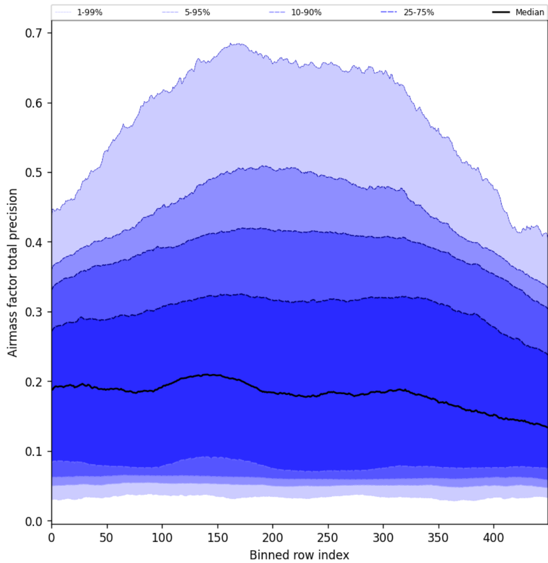
Figure 55: Along track statistics of “Airmass factor total precision” for 2024-12-20 to 2024-12-22
