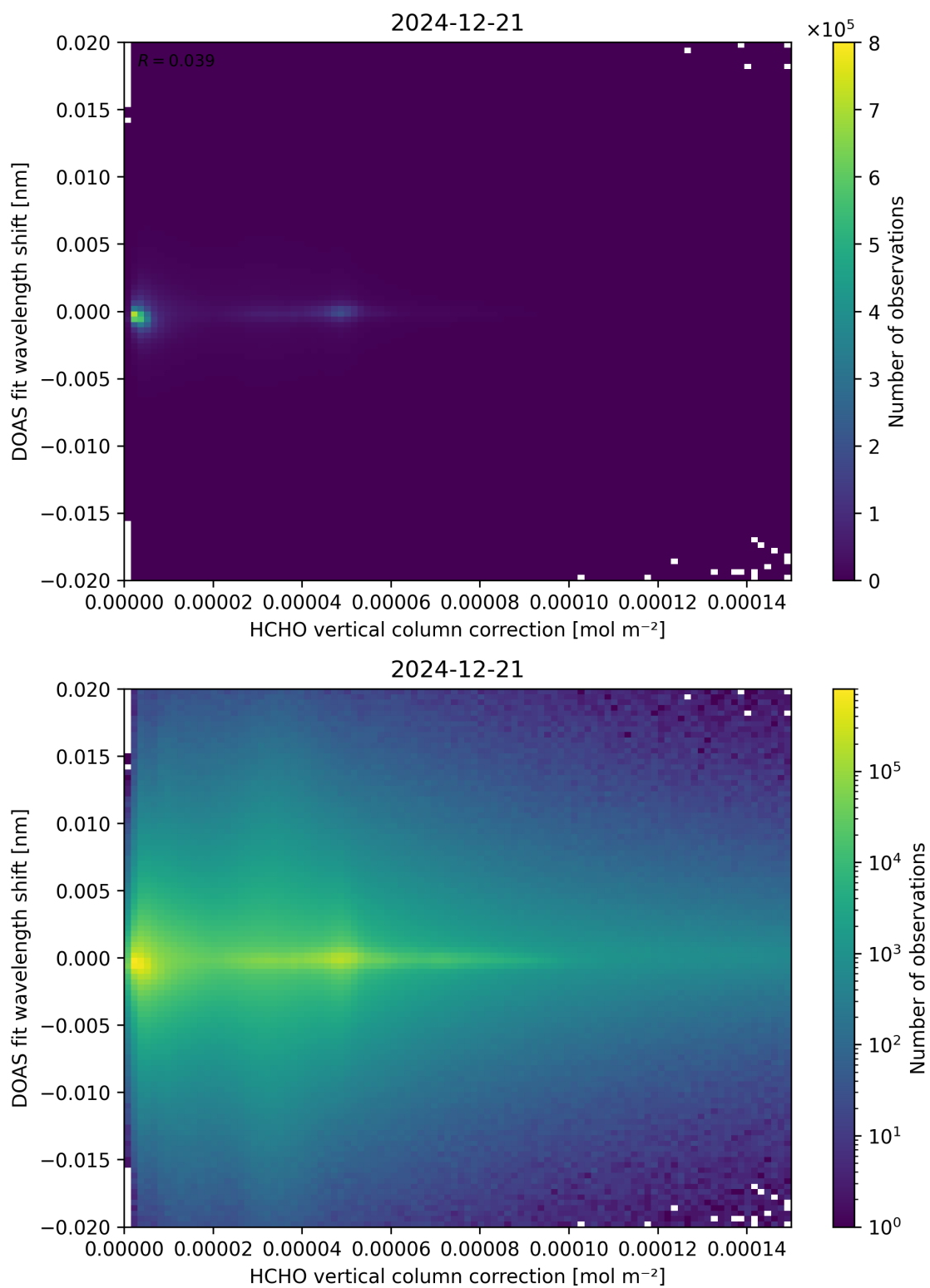
Figure 113: Scatter density plot of “HCHO vertical column correction” against “DOAS fit wavelength shift” for 2024-12-20 to 2024-12-22.
