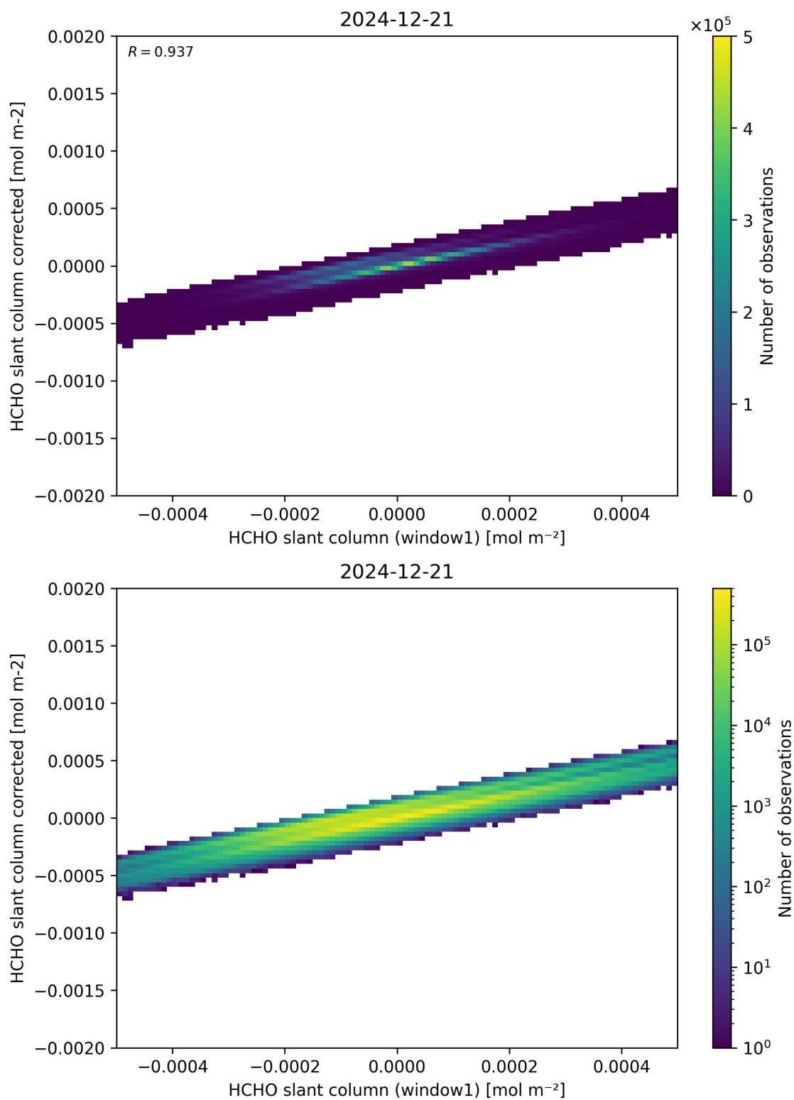
Figure 82: Scatter density plot of “HCHO slant column (window1)” against “HCHO slant column corrected” for 2024-12-20 to 2024-12-22.
