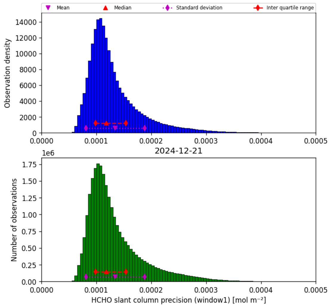
Figure 39: Histogram of “HCHO slant column precision (window1)” for 2024-12-20 to 2024-12-22
