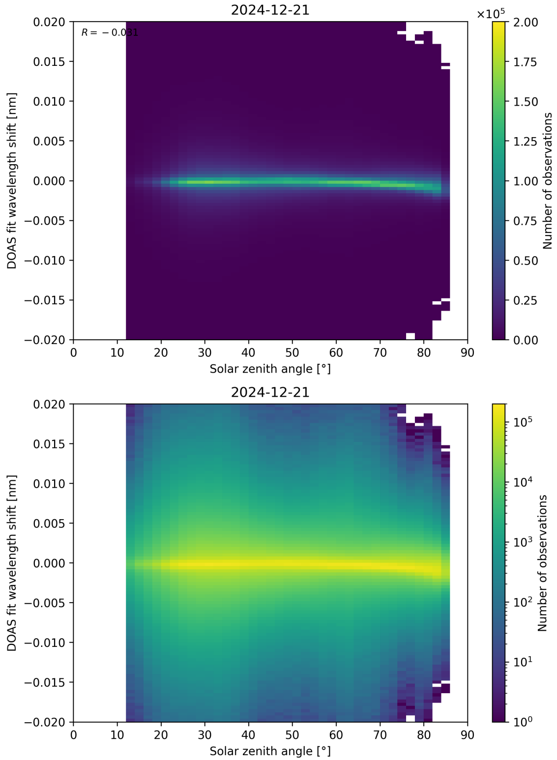
Figure 168: Scatter density plot of “Solar zenith angle” against “DOAS fit wavelength shift” for 2024-12-20 to 2024-12-22.
