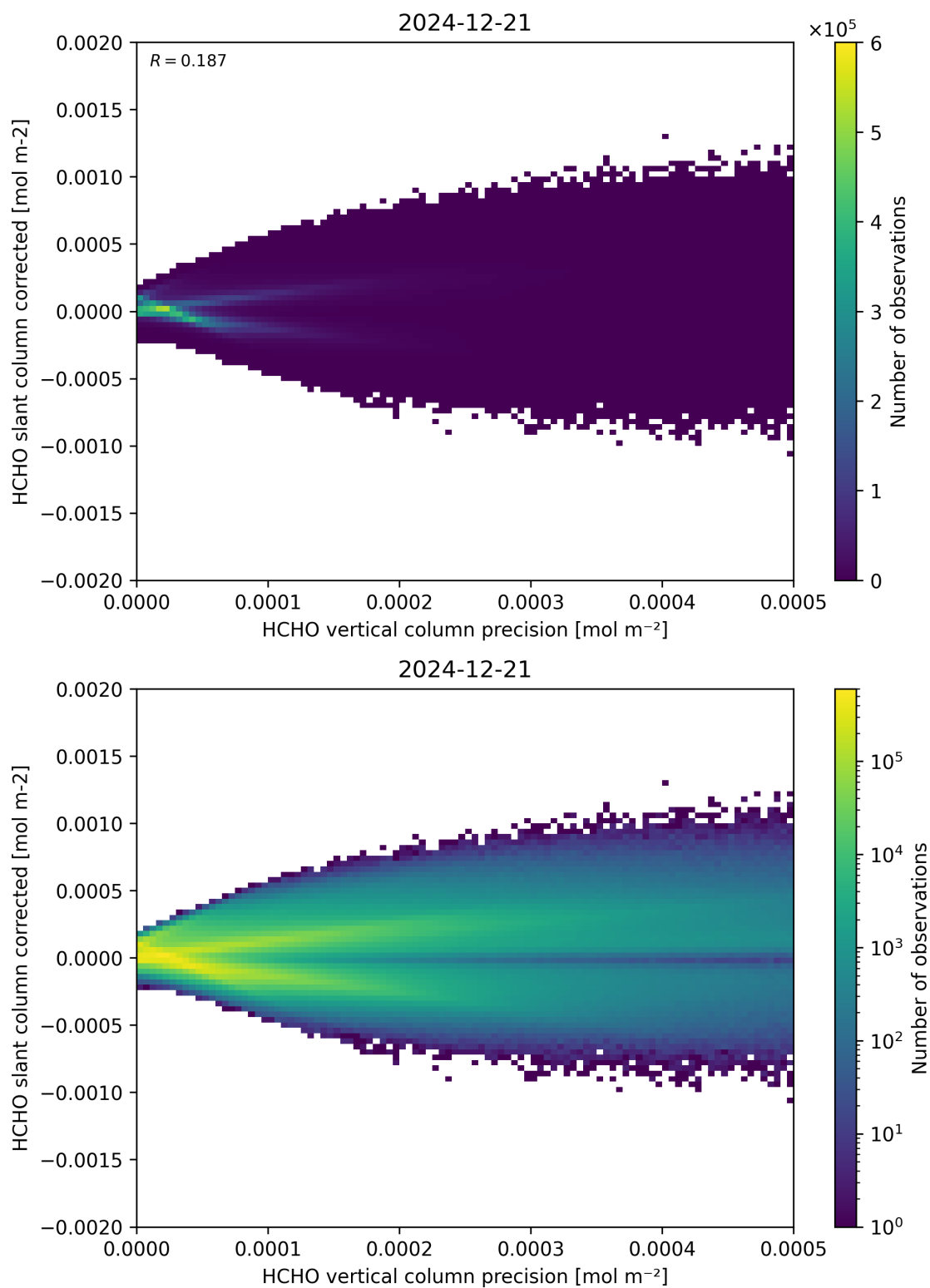
Figure 140: Scatter density plot of “HCHO vertical column precision” against “HCHO slant column corrected” for 2024-12-20 to 2024-12-22.
