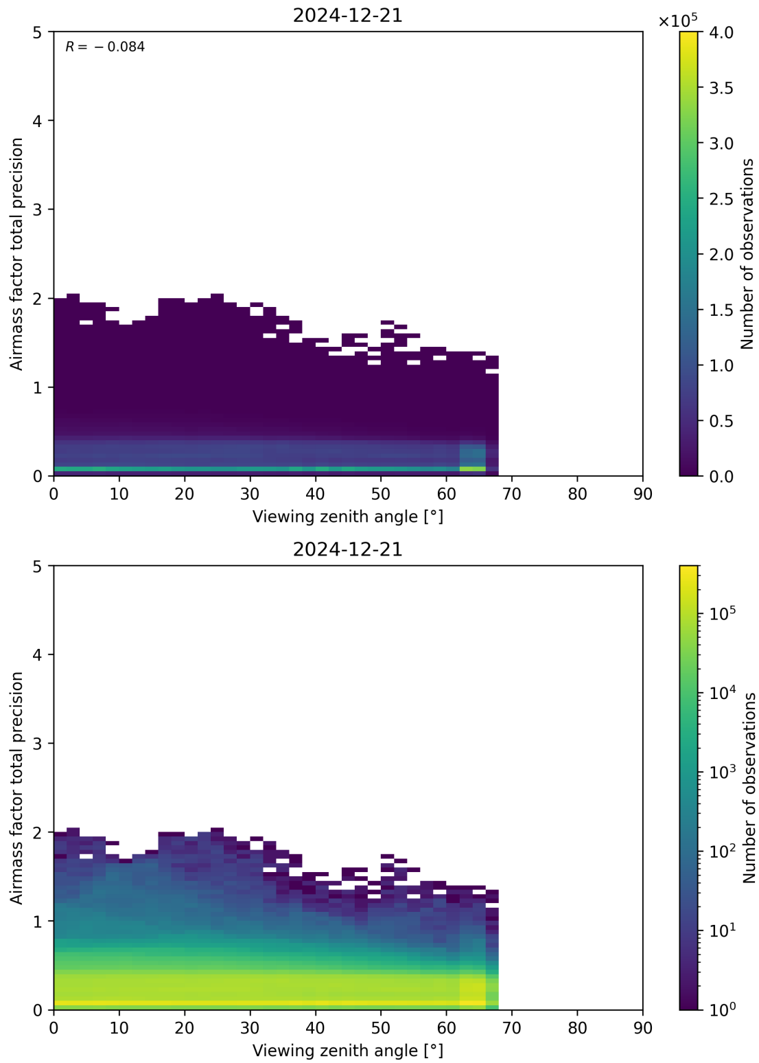
Figure 191: Scatter density plot of “Viewing zenith angle” against “Airmass factor total precision” for 2024-12-20 to 2024-12-22.
