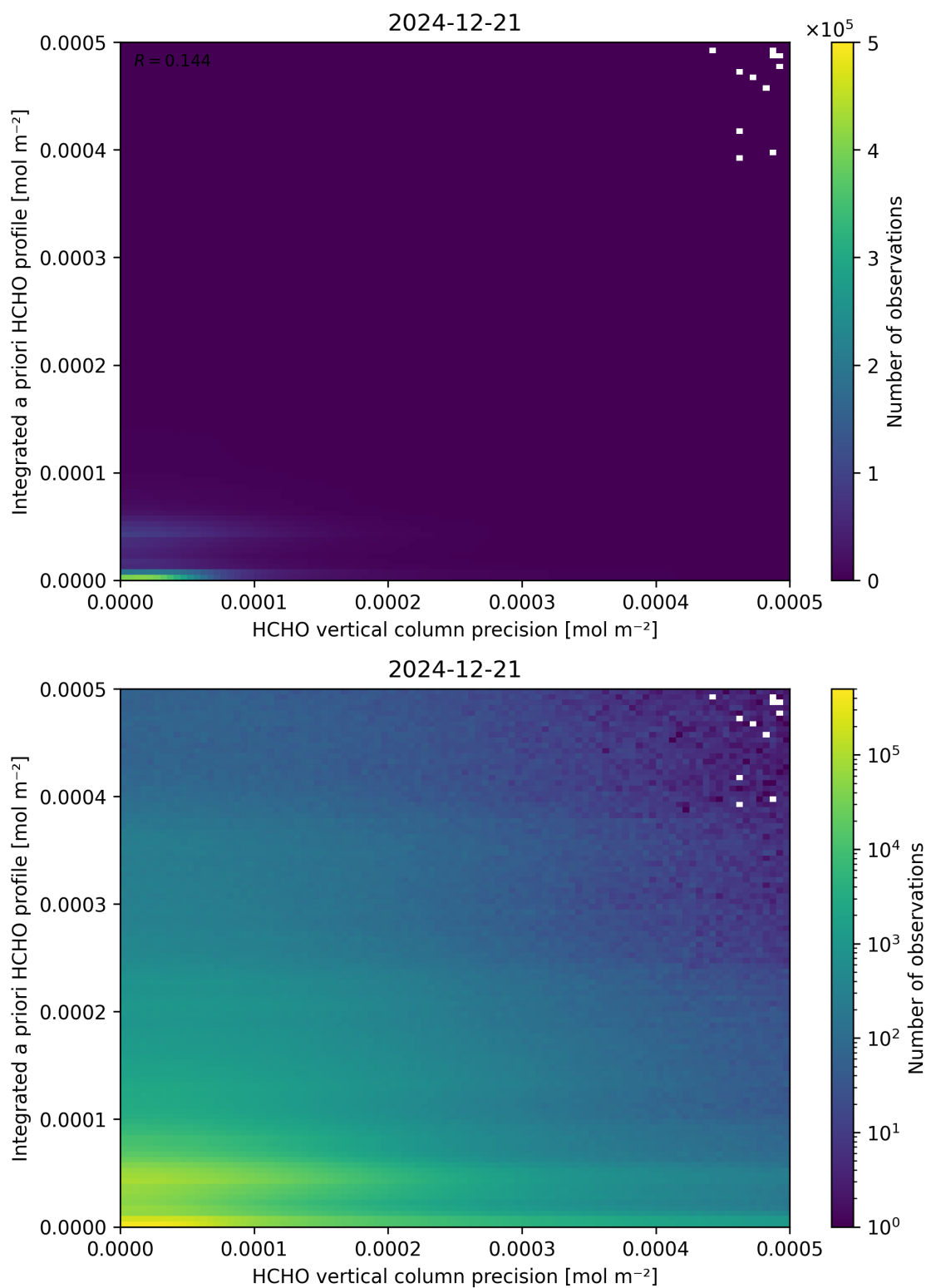
Figure 147: Scatter density plot of “HCHO vertical column precision” against “Integrated a priori HCHO profile” for 2024-12-20 to 2024-12-22.
