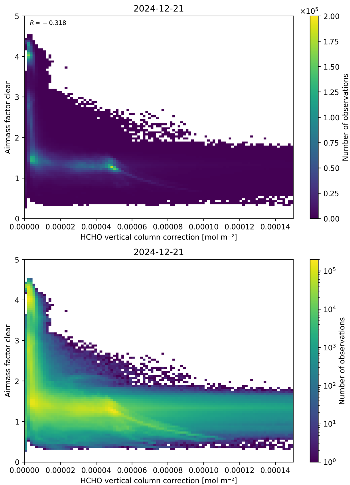
Figure 115: Scatter density plot of “HCHO vertical column correction” against “Airmass factor clear” for 2024-12-20 to 2024-12-22.
