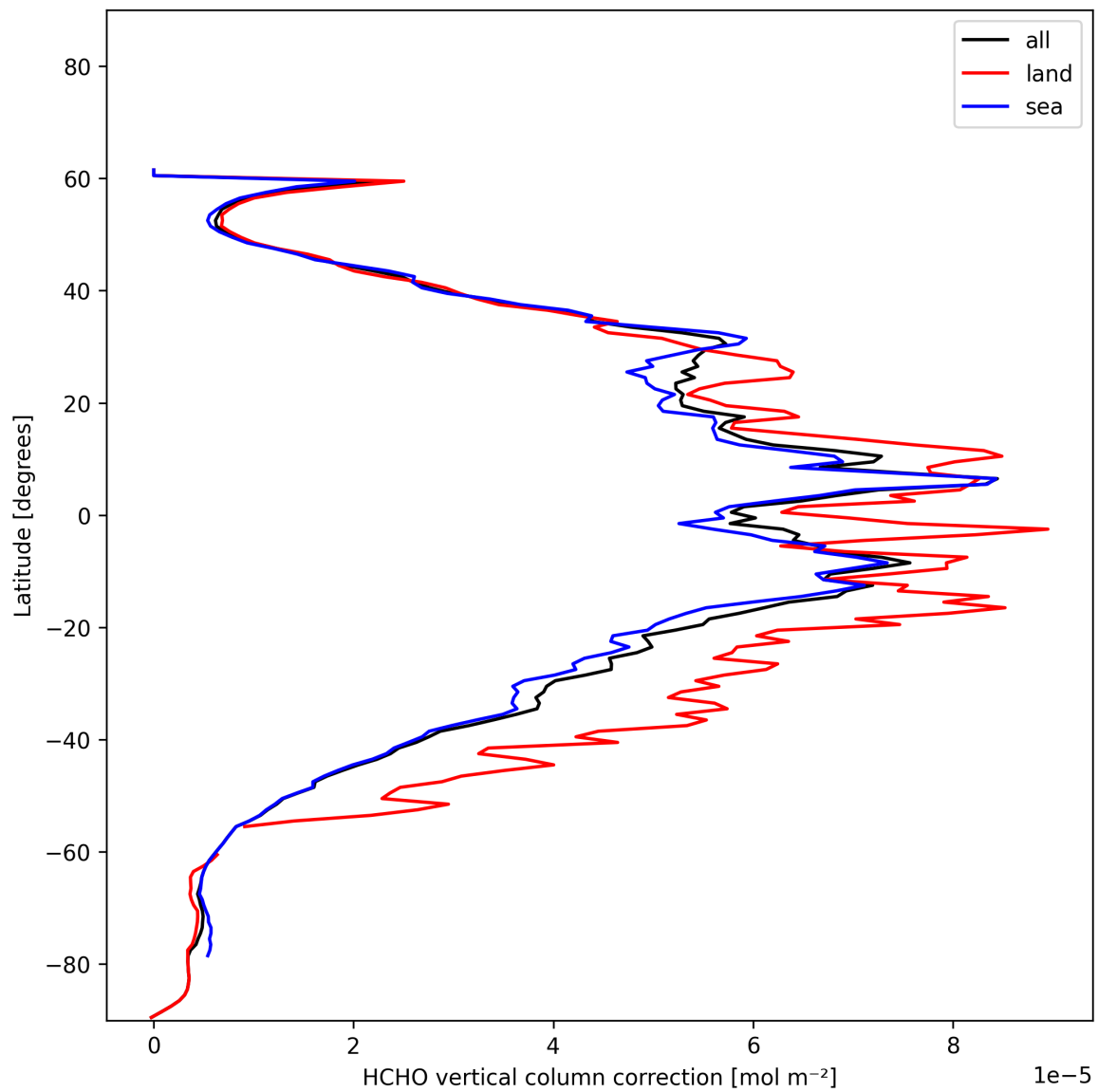
Figure 23: Zonal average of “HCHO vertical column correction” for 2024-12-20 to 2024-12-22.
