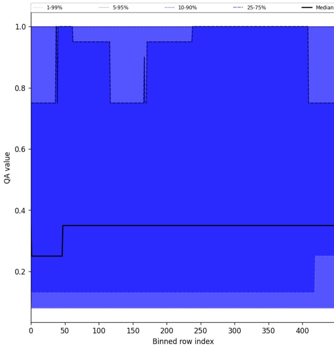
Figure 48: Along track statistics of “QA value” for 2024-12-20 to 2024-12-22
