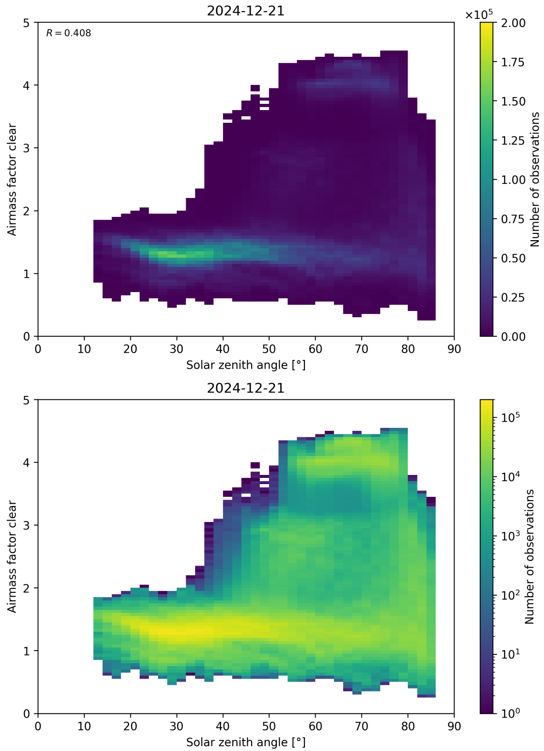
Figure 170: Scatter density plot of “Solar zenith angle” against “Airmass factor clear” for 2024-12-20 to 2024-12-22.
