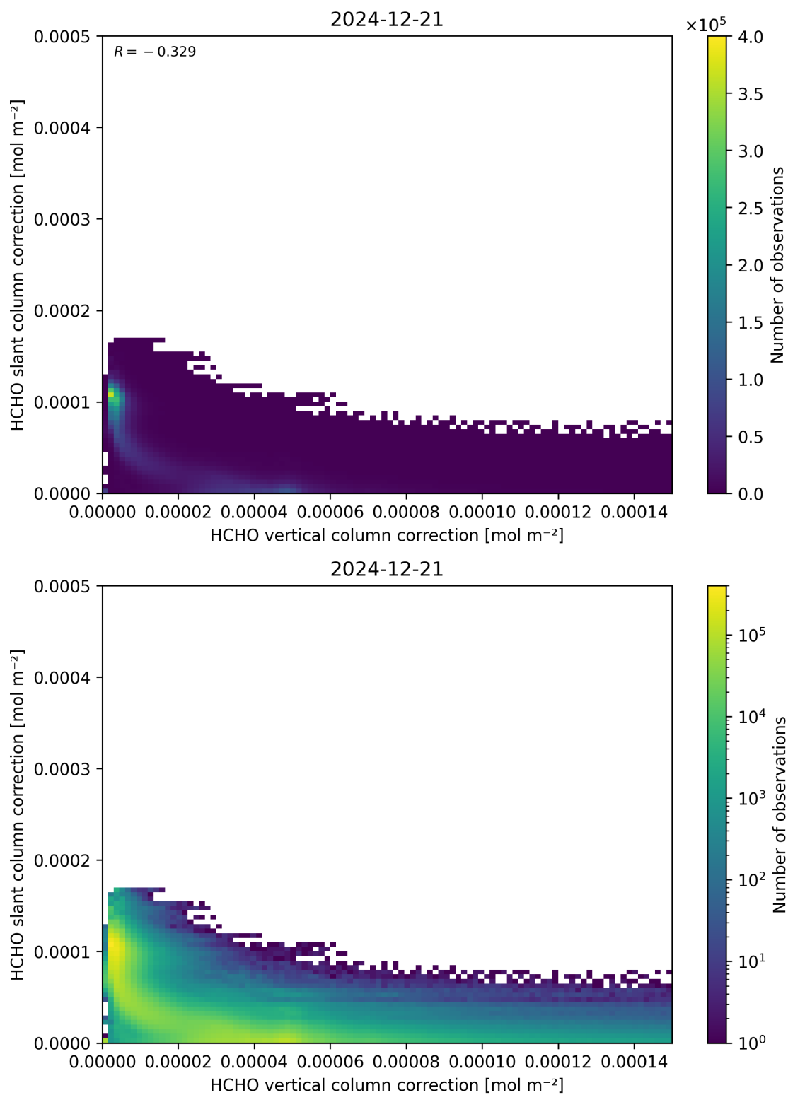
Figure 117: Scatter density plot of “HCHO vertical column correction” against “HCHO slant column correction” for 2024-12-20 to 2024-12-22.
