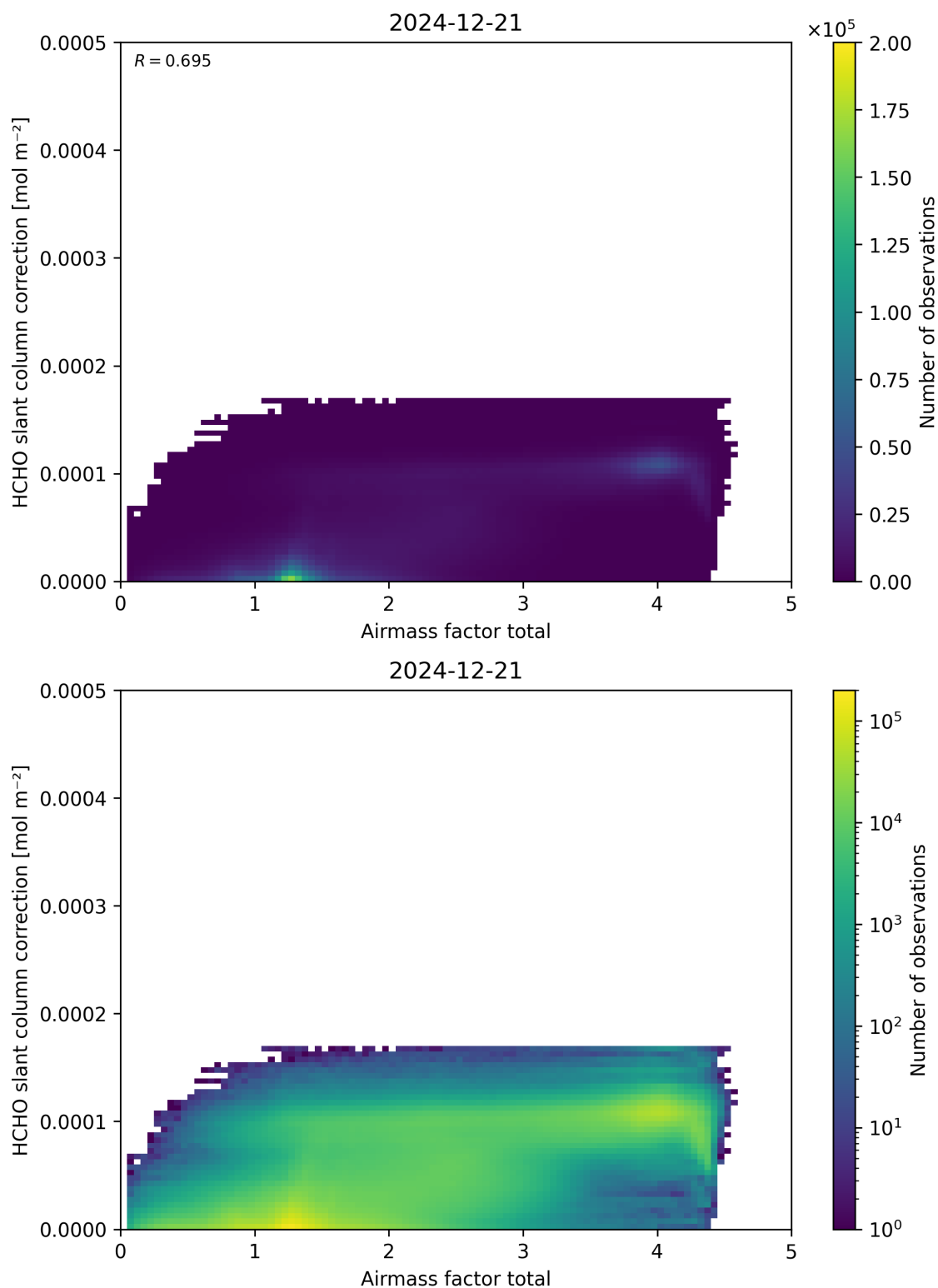
Figure 102: Scatter density plot of “Airmass factor total” against “HCHO slant column correction” for 2024-12-20 to 2024-12-22.
