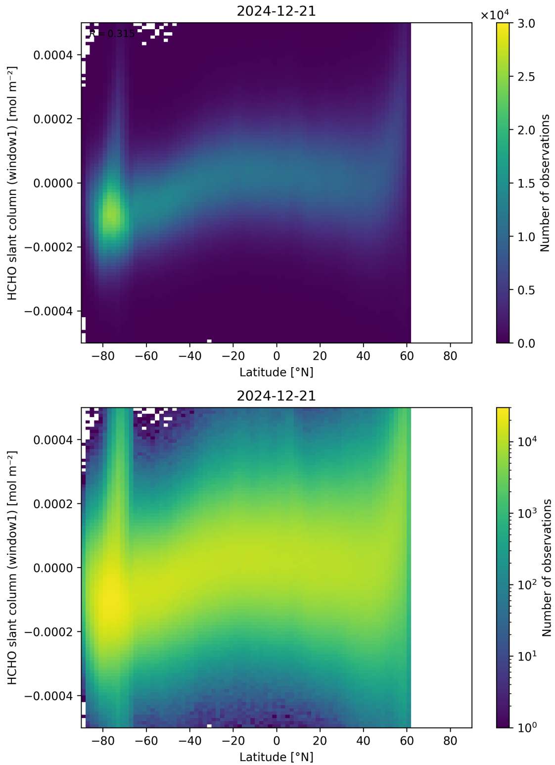
Figure 159: Scatter density plot of “Latitude” against “HCHO slant column (window1)” for 2024-12-20 to 2024-12-22.
