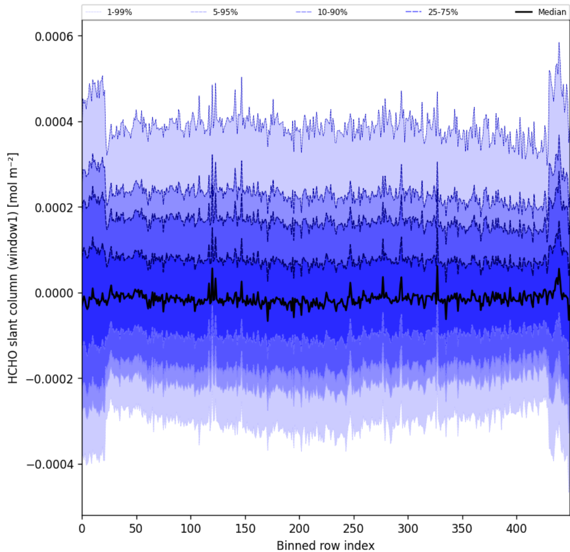
Figure 52: Along track statistics of “HCHO slant column (window1)” for 2024-12-20 to 2024-12-22
