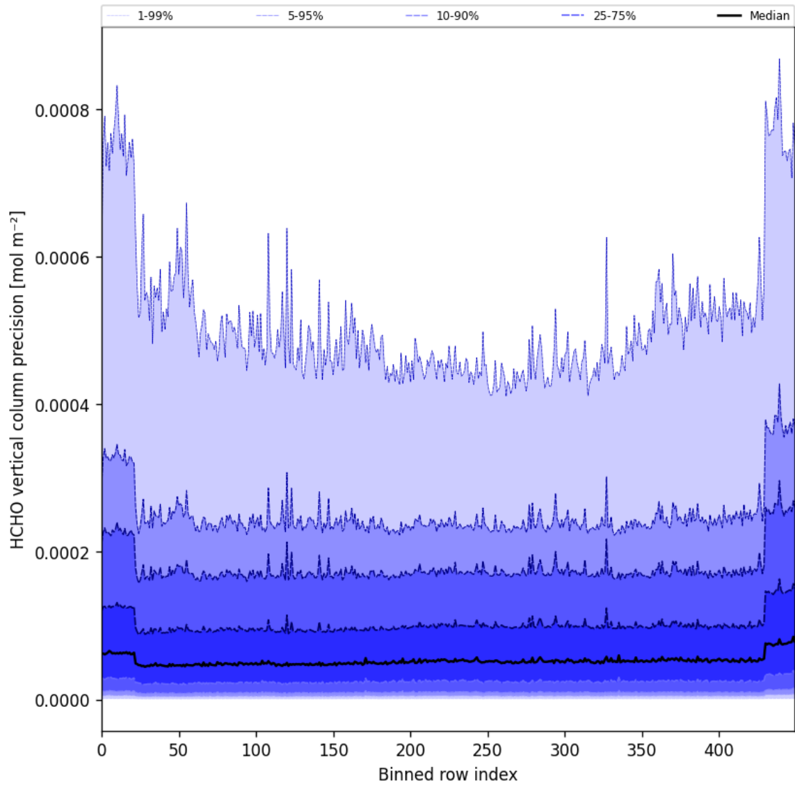
Figure 50: Along track statistics of “HCHO vertical column precision” for 2024-12-20 to 2024-12-22
