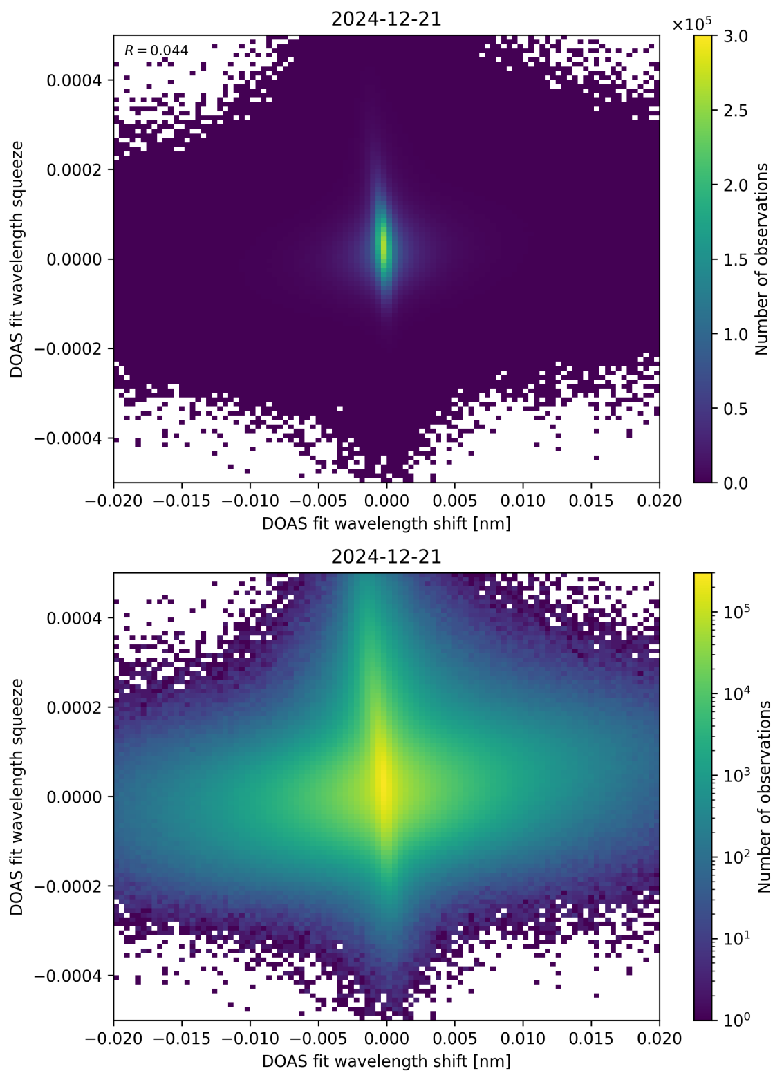
Figure 65: Scatter density plot of “DOAS fit wavelength shift” against “DOAS fit wavelength squeeze” for 2024-12-20 to 2024-12-22.
