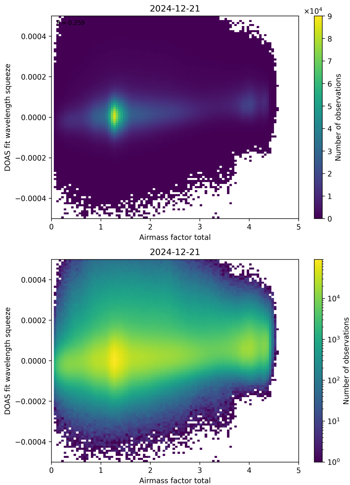
Figure 99: Scatter density plot of “Airmass factor total” against “DOAS fit wavelength squeeze” for 2024-12-20 to 2024-12-22.
