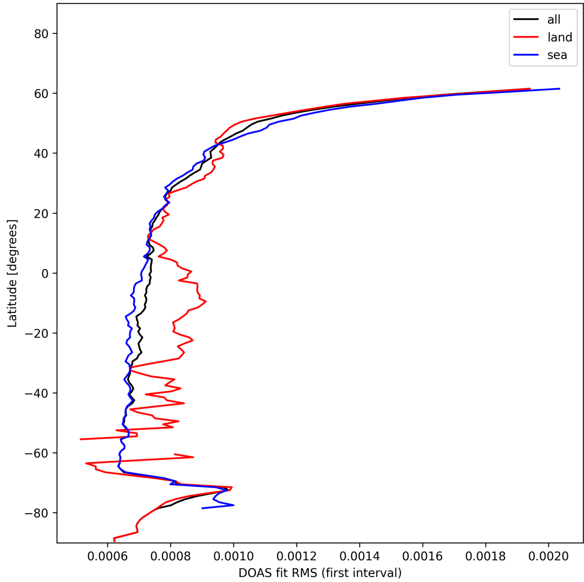
Figure 32: Zonal average of “DOAS fit RMS (first interval)” for 2024-12-20 to 2024-12-22.
