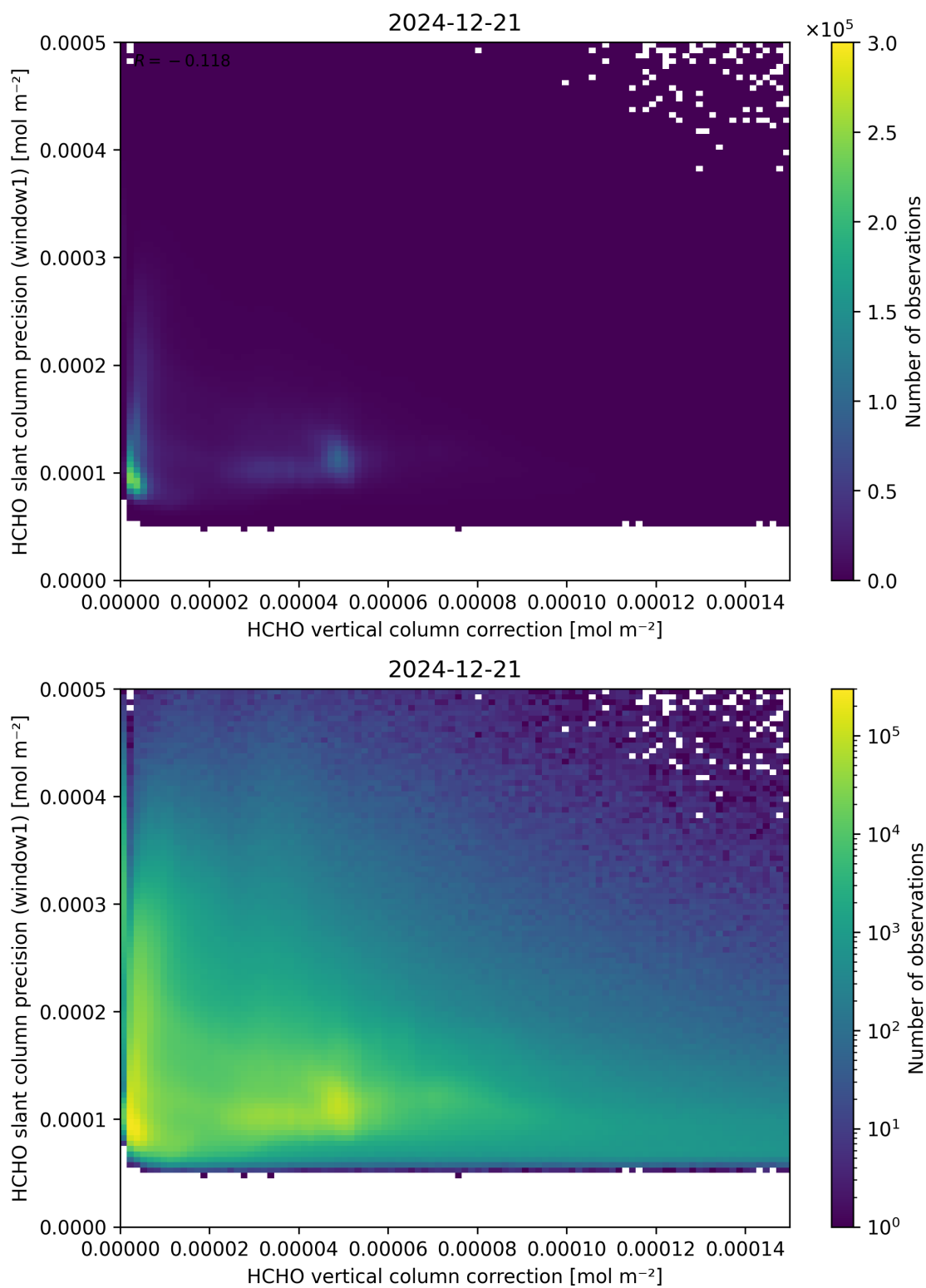
Figure 119: Scatter density plot of “HCHO vertical column correction” against “HCHO slant column precision (window1)” for 2024-12-20 to 2024-12-22.
