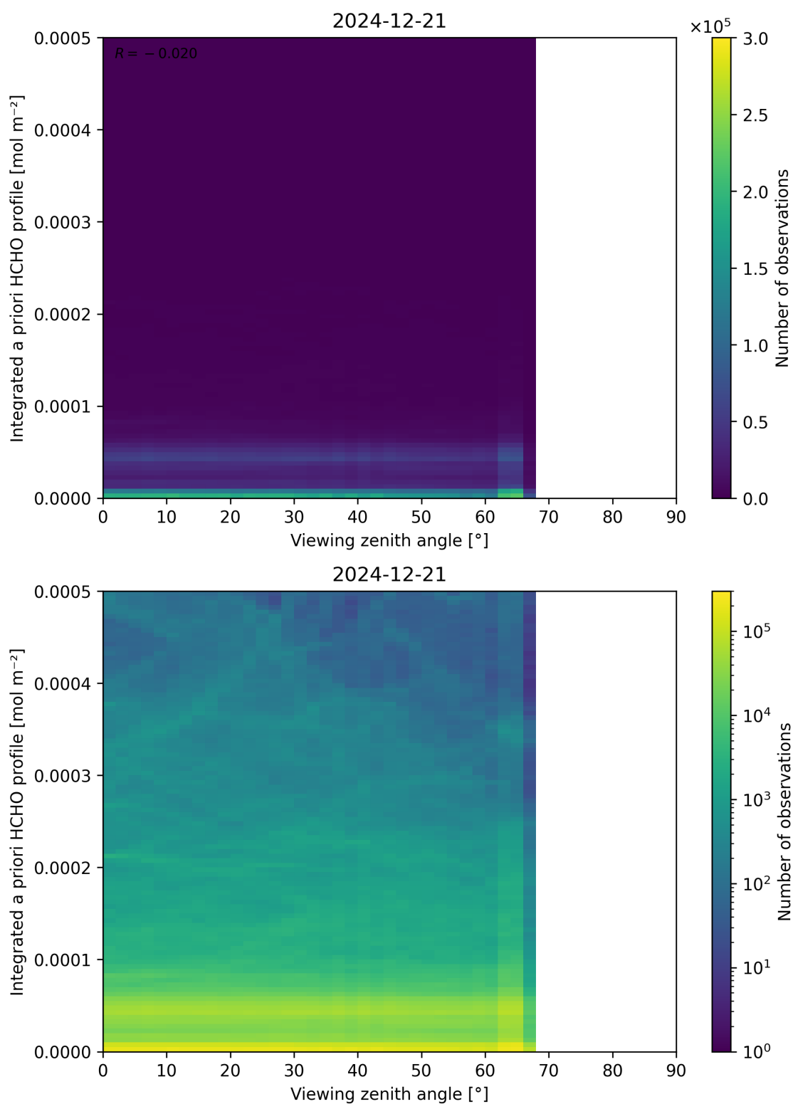
Figure 195: Scatter density plot of “Viewing zenith angle” against “Integrated a priori HCHO profile” for 2024-12-20 to 2024-12-22.
