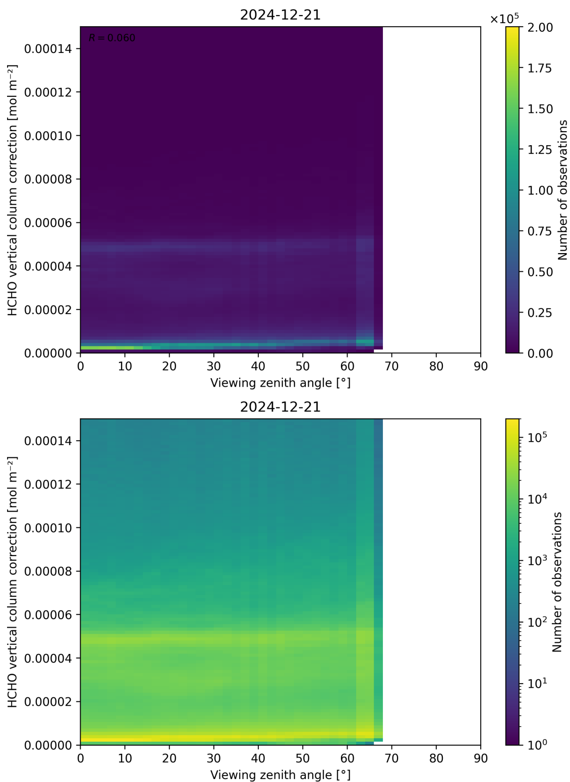
Figure 193: Scatter density plot of “Viewing zenith angle” against “HCHO vertical column correction” for 2024-12-20 to 2024-12-22.
