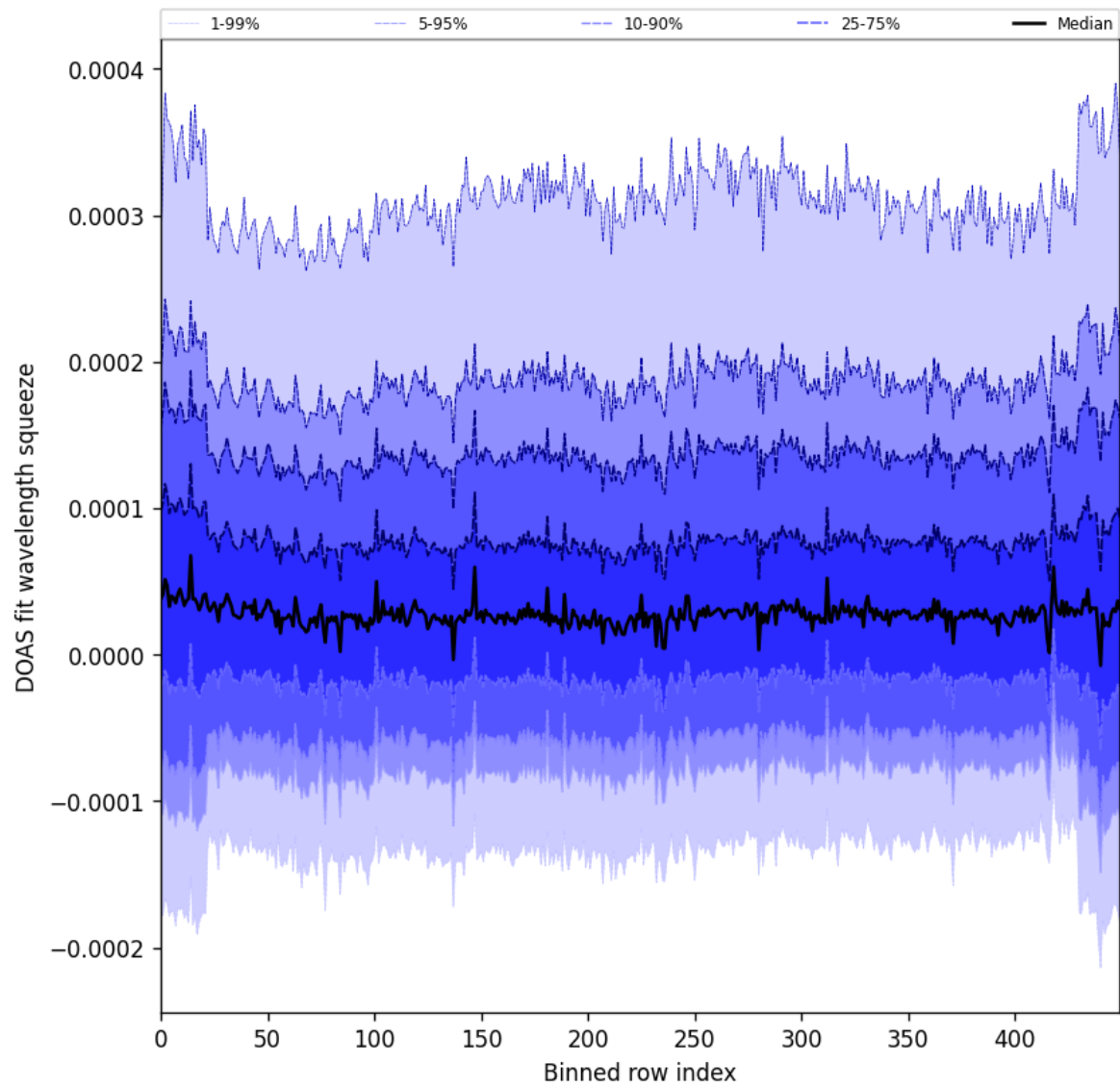
Figure 59: Along track statistics of “DOAS fit wavelength squeeze” for 2024-12-20 to 2024-12-22
