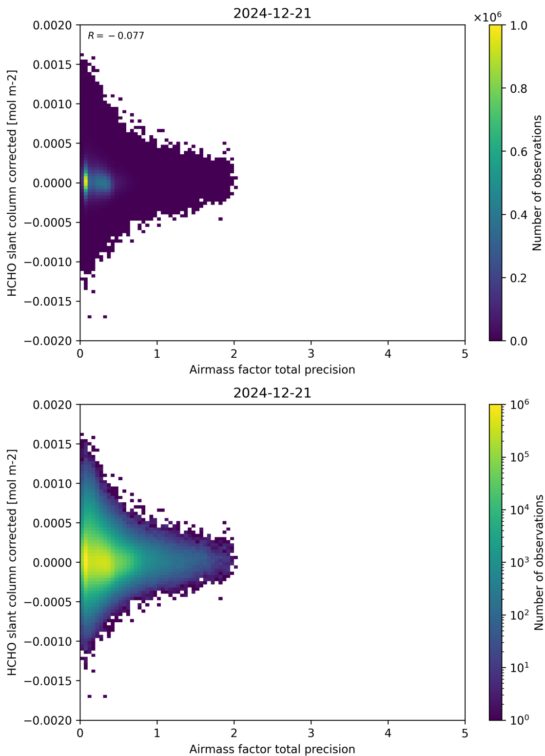
Figure 109: Scatter density plot of “Airmass factor total precision” against “HCHO slant column corrected” for 2024-12-20 to 2024-12-22.
