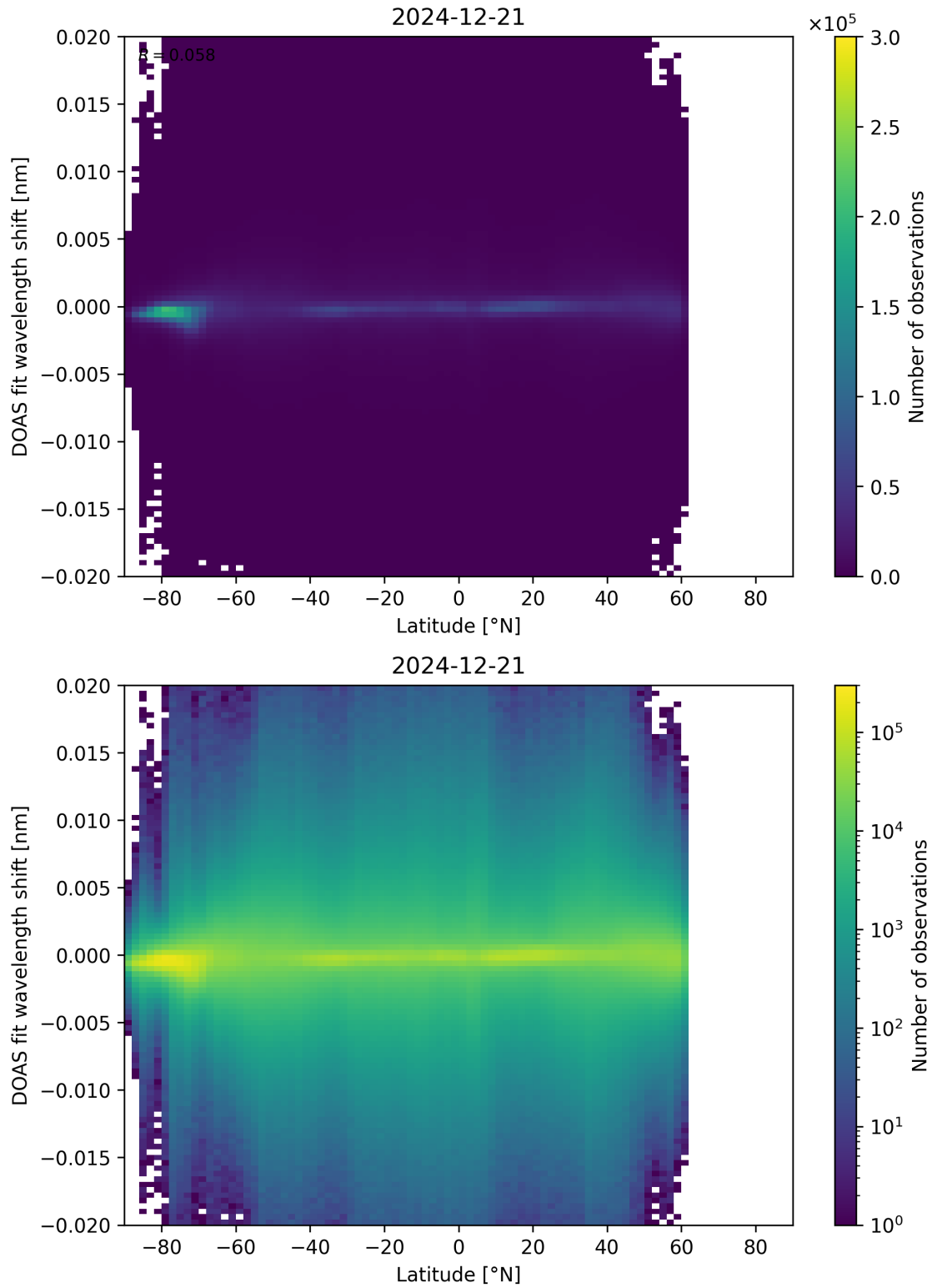
Figure 154: Scatter density plot of “Latitude” against “DOAS fit wavelength shift” for 2024-12-20 to 2024-12-22.
