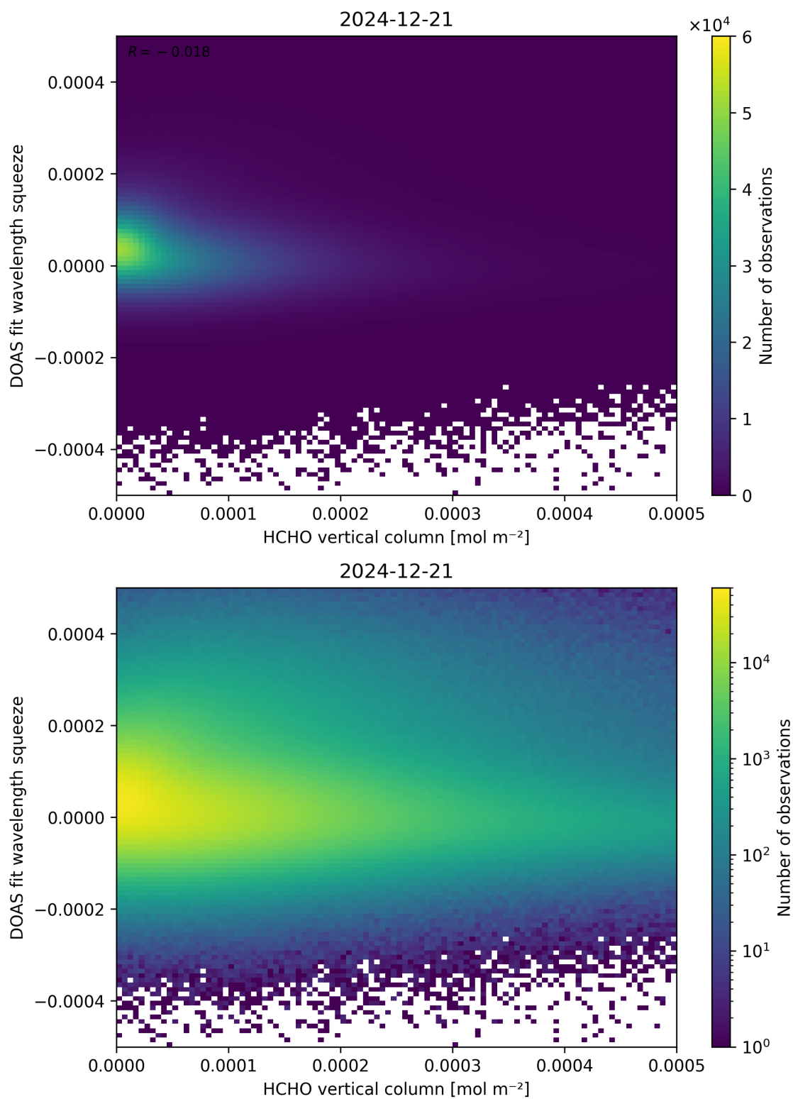
Figure 125: Scatter density plot of “HCHO vertical column” against “DOAS fit wavelength squeeze” for 2024-12-20 to 2024-12-22.
