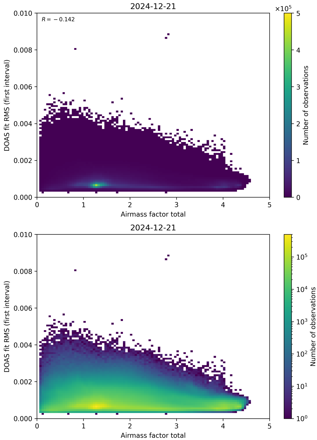
Figure 97: Scatter density plot of “Airmass factor total” against “DOAS fit RMS (first interval)” for 2024-12-20 to 2024-12-22.
