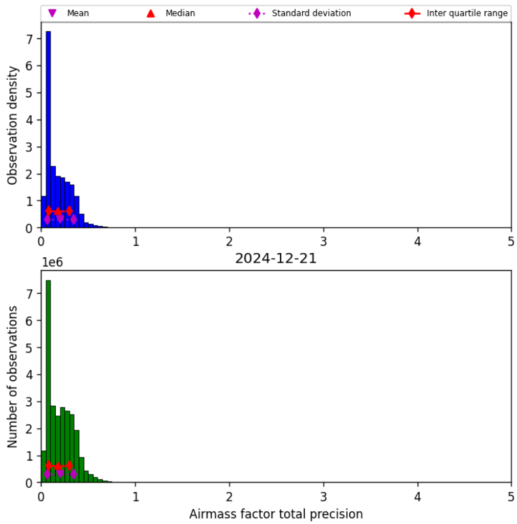
Figure 41: Histogram of “Airmass factor total precision” for 2024-12-20 to 2024-12-22
