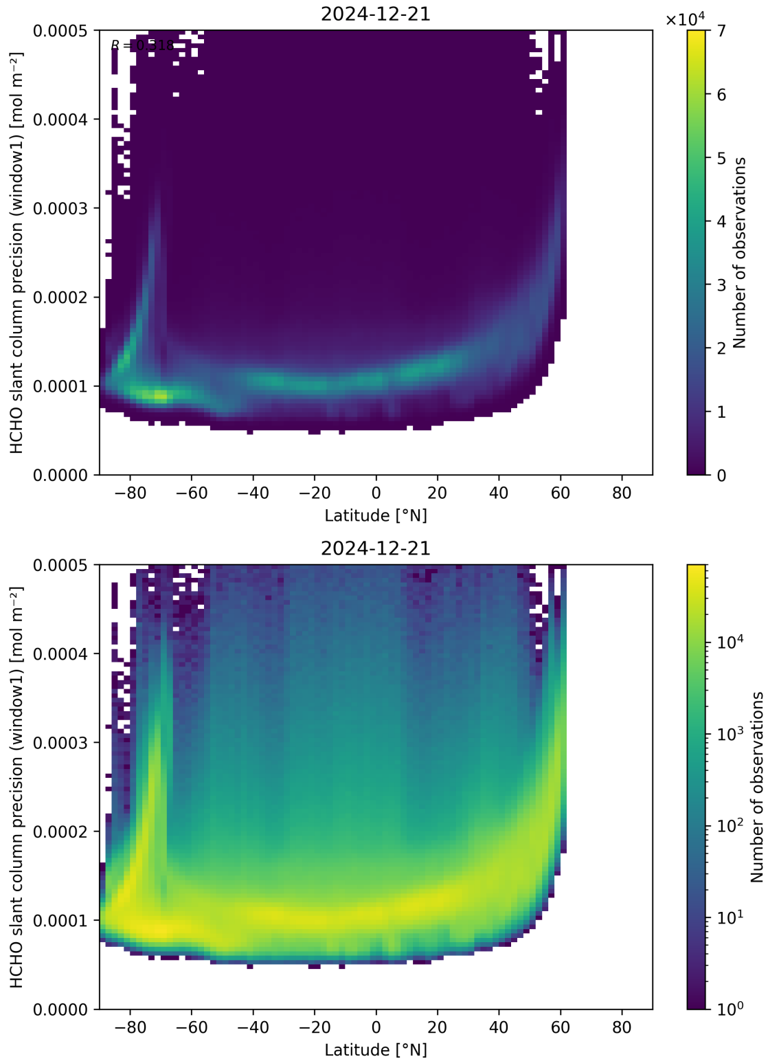
Figure 160: Scatter density plot of “Latitude” against “HCHO slant column precision (window1)” for 2024-12-20 to 2024-12-22.
