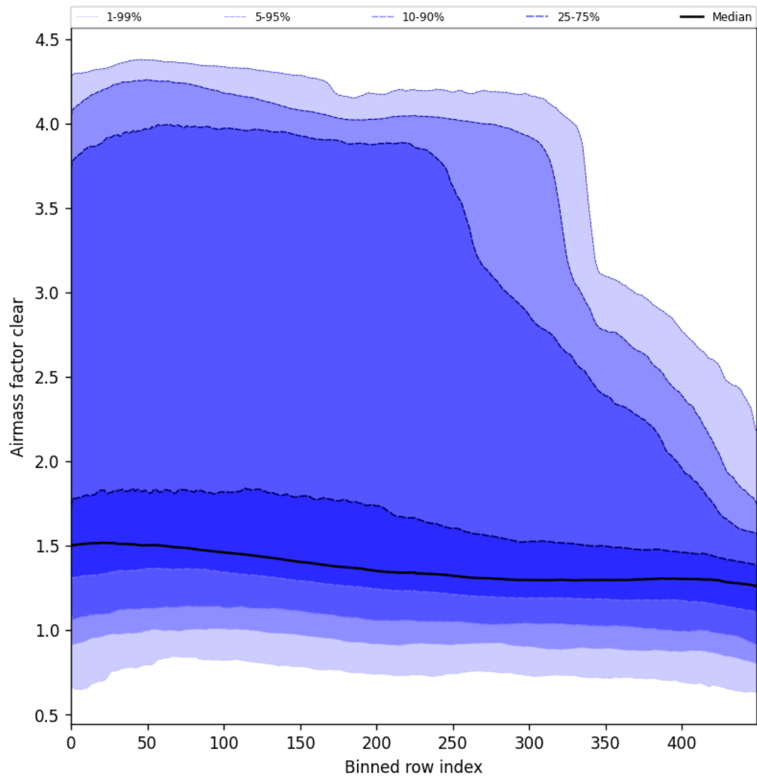
Figure 56: Along track statistics of “Airmass factor clear” for 2024-12-20 to 2024-12-22
