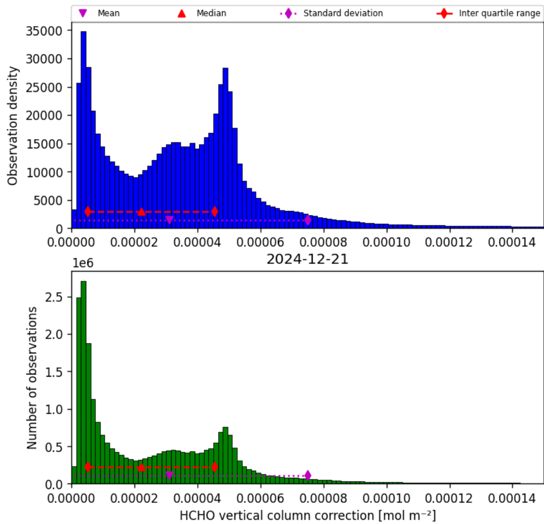
Figure 37: Histogram of “HCHO vertical column correction” for 2024-12-20 to 2024-12-22
