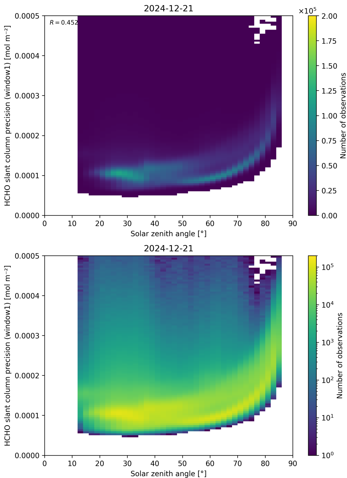
Figure 174: Scatter density plot of “Solar zenith angle” against “HCHO slant column precision (window1)” for 2024-12-20 to 2024-12-22.
