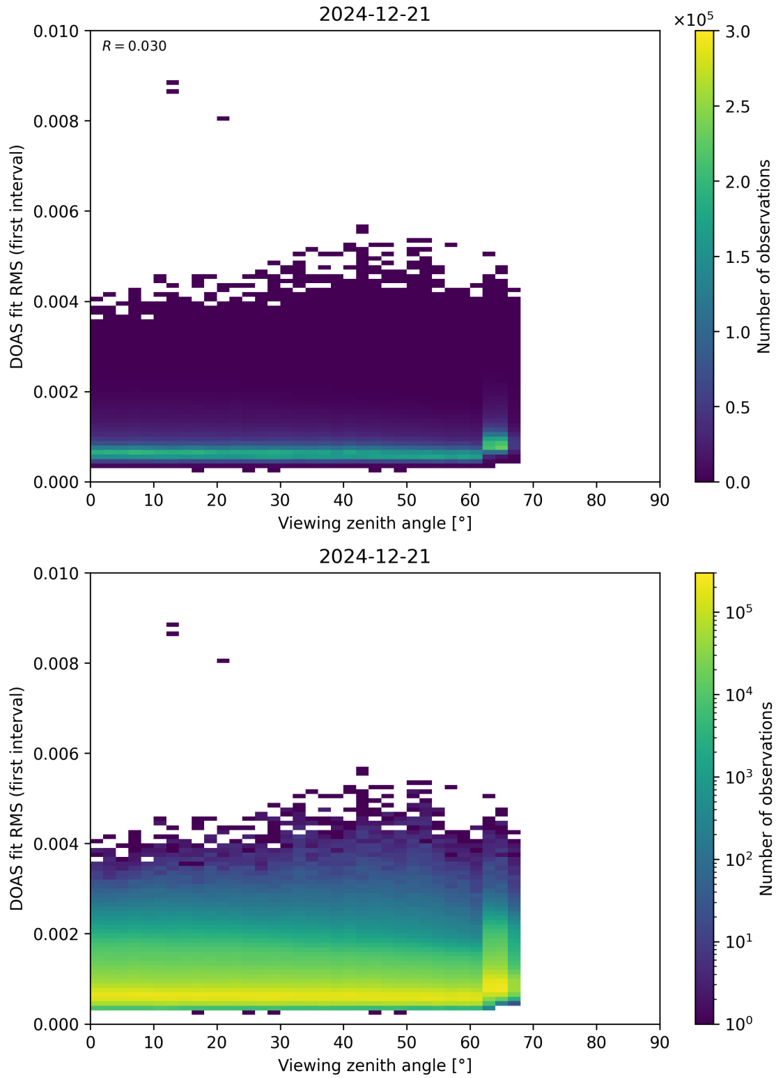
Figure 182: Scatter density plot of “Viewing zenith angle” against “DOAS fit RMS (first interval)” for 2024-12-20 to 2024-12-22.
