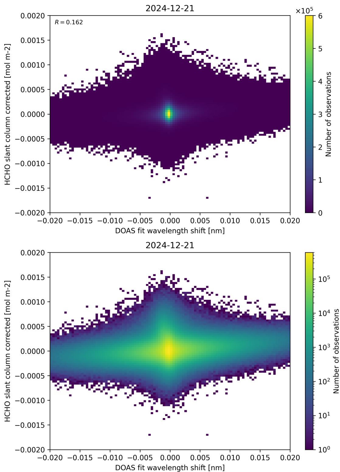
Figure 66: Scatter density plot of “DOAS fit wavelength shift” against “HCHO slant column corrected” for 2024-12-20 to 2024-12-22.
