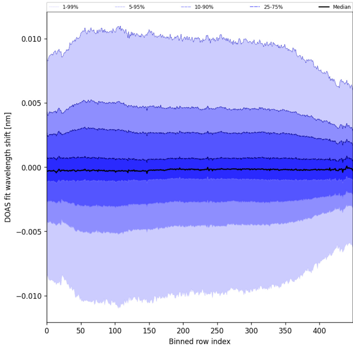
Figure 58: Along track statistics of “DOAS fit wavelength shift” for 2024-12-20 to 2024-12-22
