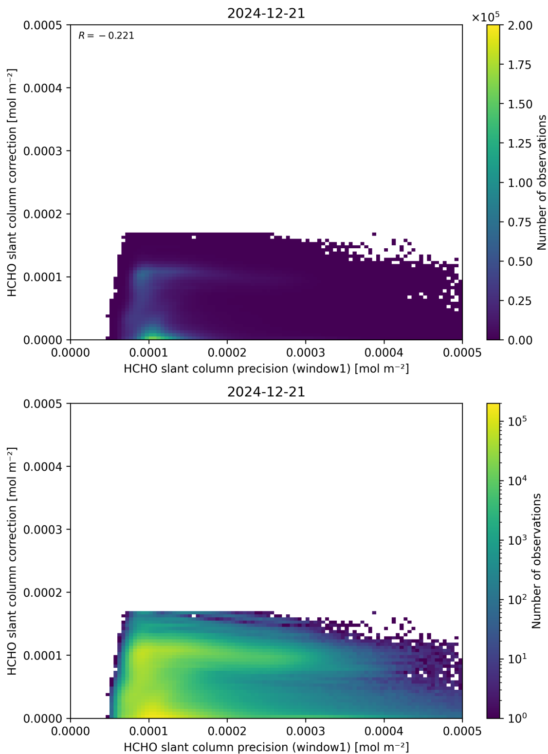
Figure 93: Scatter density plot of “HCHO slant column precision (window1)” against “HCHO slant column correction” for 2024-12-20 to 2024-12-22.
