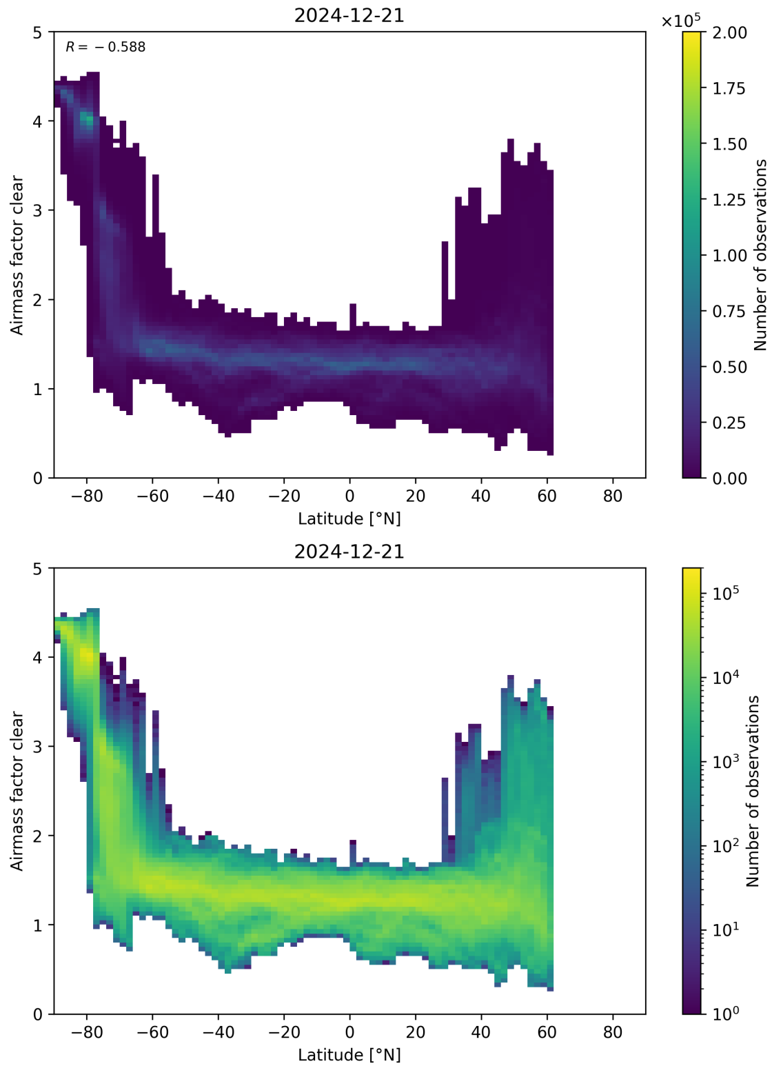
Figure 156: Scatter density plot of “Latitude” against “Airmass factor clear” for 2024-12-20 to 2024-12-22.
