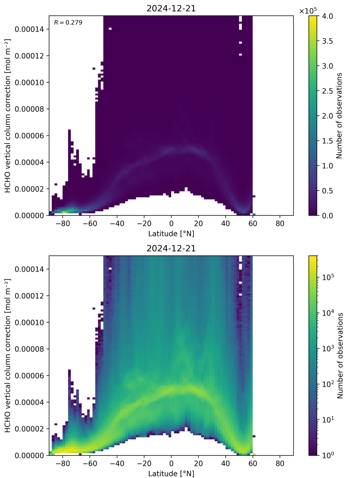
Figure 164: Scatter density plot of “Latitude” against “HCHO vertical column correction” for 2024-12-20 to 2024-12-22.
