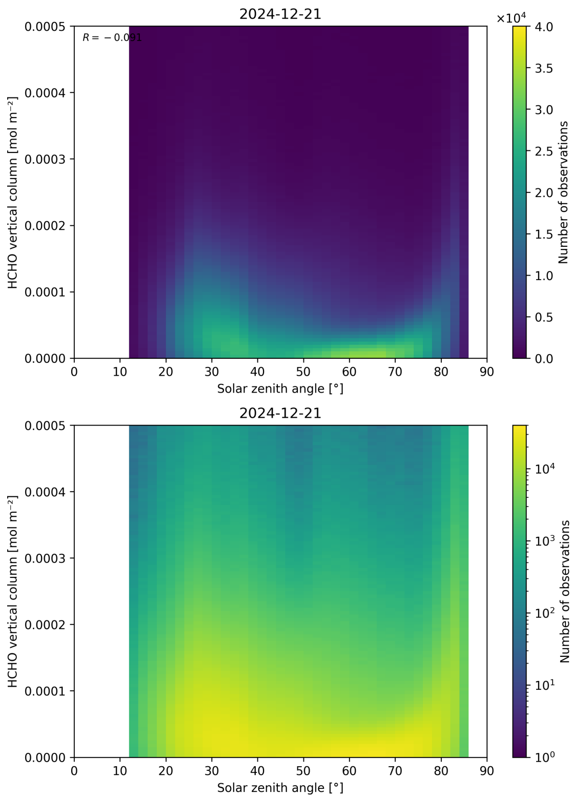
Figure 177: Scatter density plot of “Solar zenith angle” against “HCHO vertical column” for 2024-12-20 to 2024-12-22.
