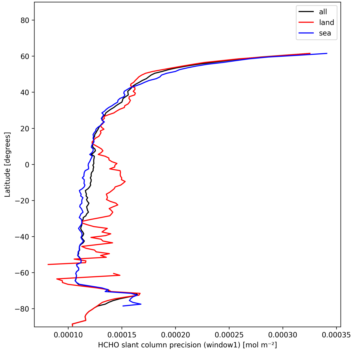
Figure 25: Zonal average of “HCHO slant column precision (window1)” for 2024-12-20 to 2024-12-22.
