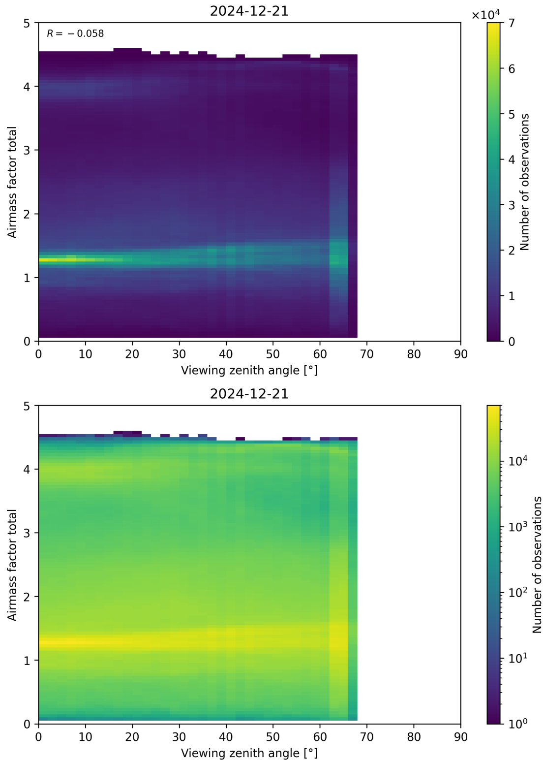
Figure 190: Scatter density plot of “Viewing zenith angle” against “Airmass factor total” for 2024-12-20 to 2024-12-22.
