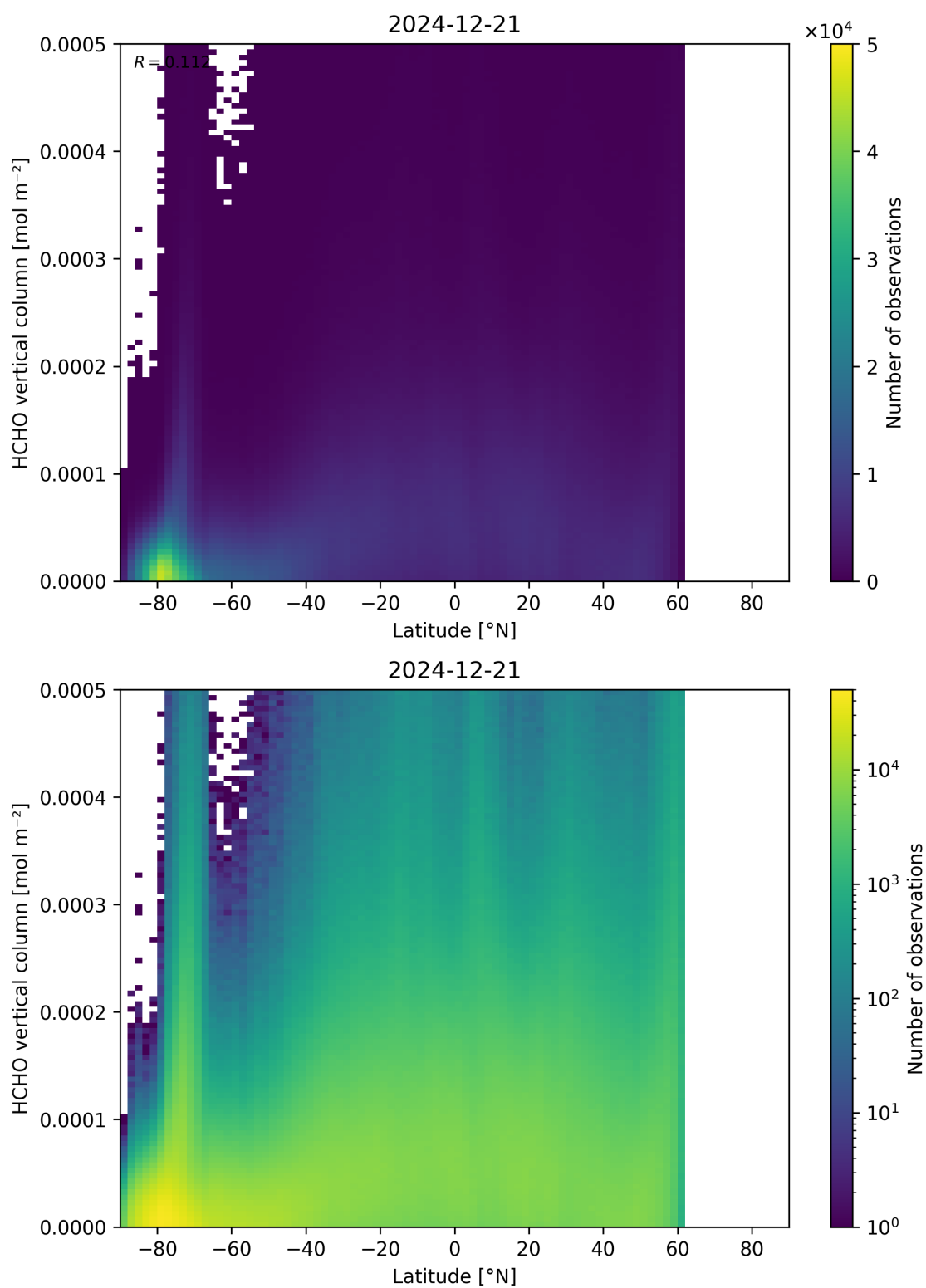
Figure 163: Scatter density plot of “Latitude” against “HCHO vertical column” for 2024-12-20 to 2024-12-22.
