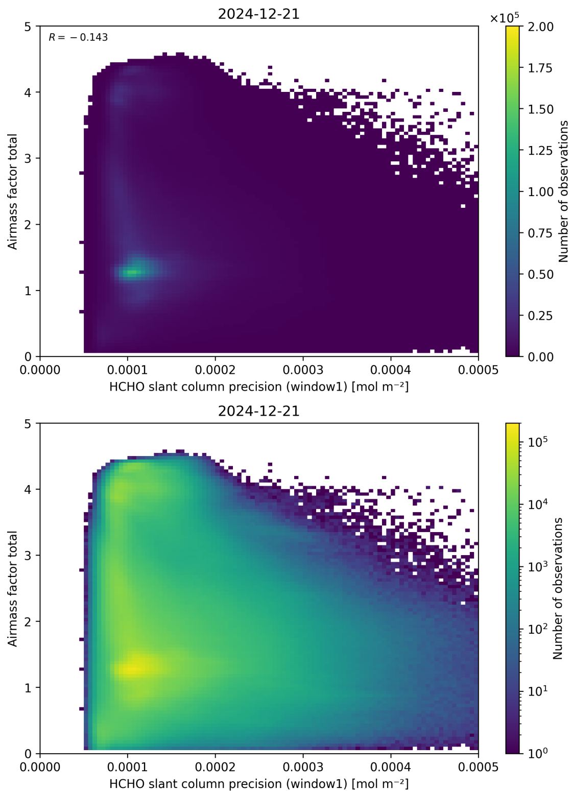
Figure 94: Scatter density plot of “HCHO slant column precision (window1)” against “Airmass factor total” for 2024-12-20 to 2024-12-22.
