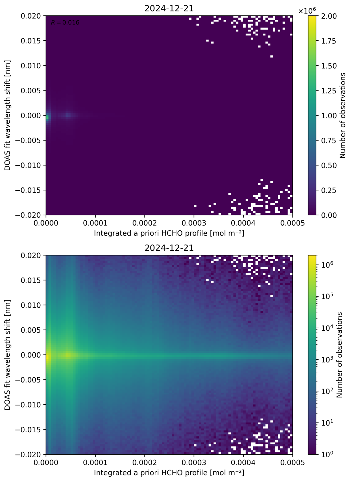
Figure 149: Scatter density plot of “Integrated a priori HCHO profile” against “DOAS fit wavelength shift” for 2024-12-20 to 2024-12-22.
