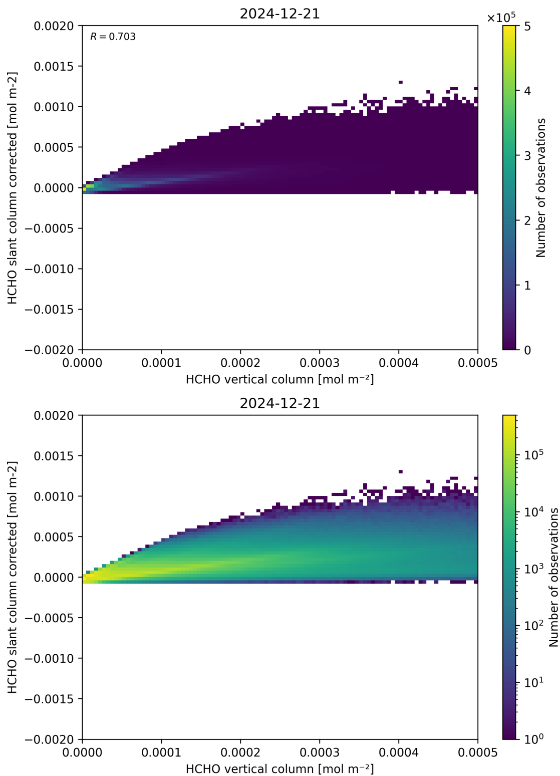
Figure 127: Scatter density plot of “HCHO vertical column” against “HCHO slant column corrected” for 2024-12-20 to 2024-12-22.
