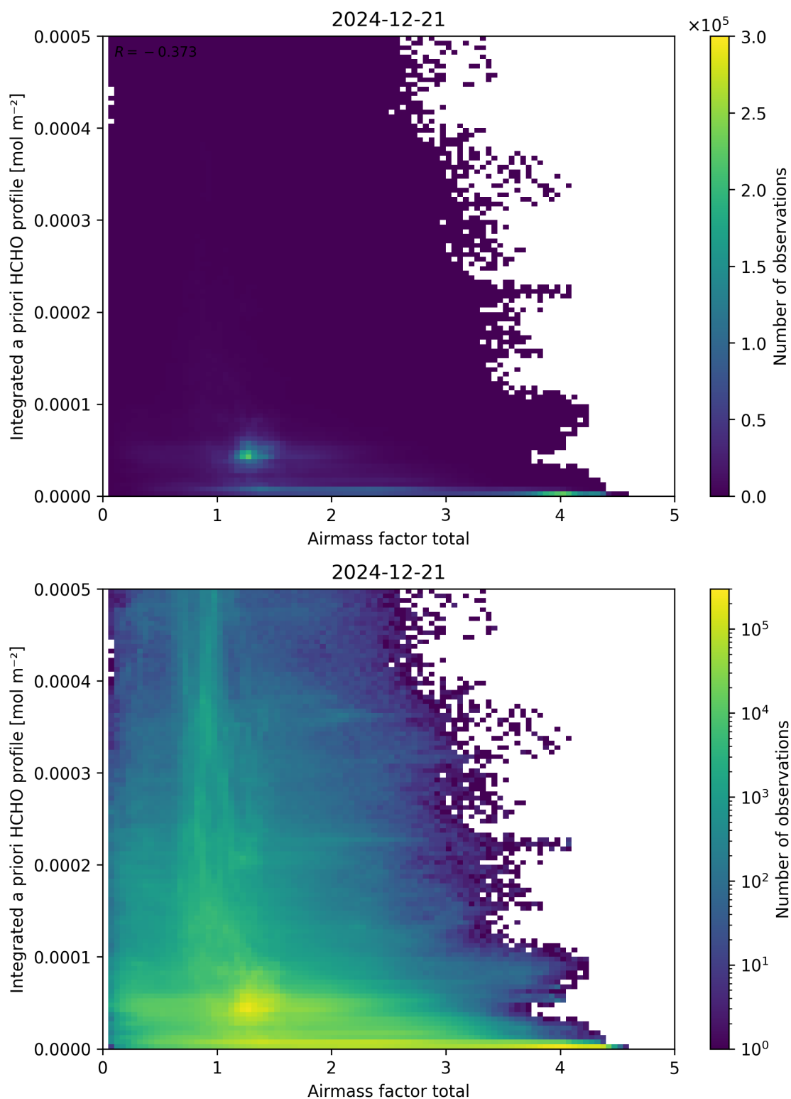
Figure 104: Scatter density plot of “Airmass factor total” against “Integrated a priori HCHO profile” for 2024-12-20 to 2024-12-22.
