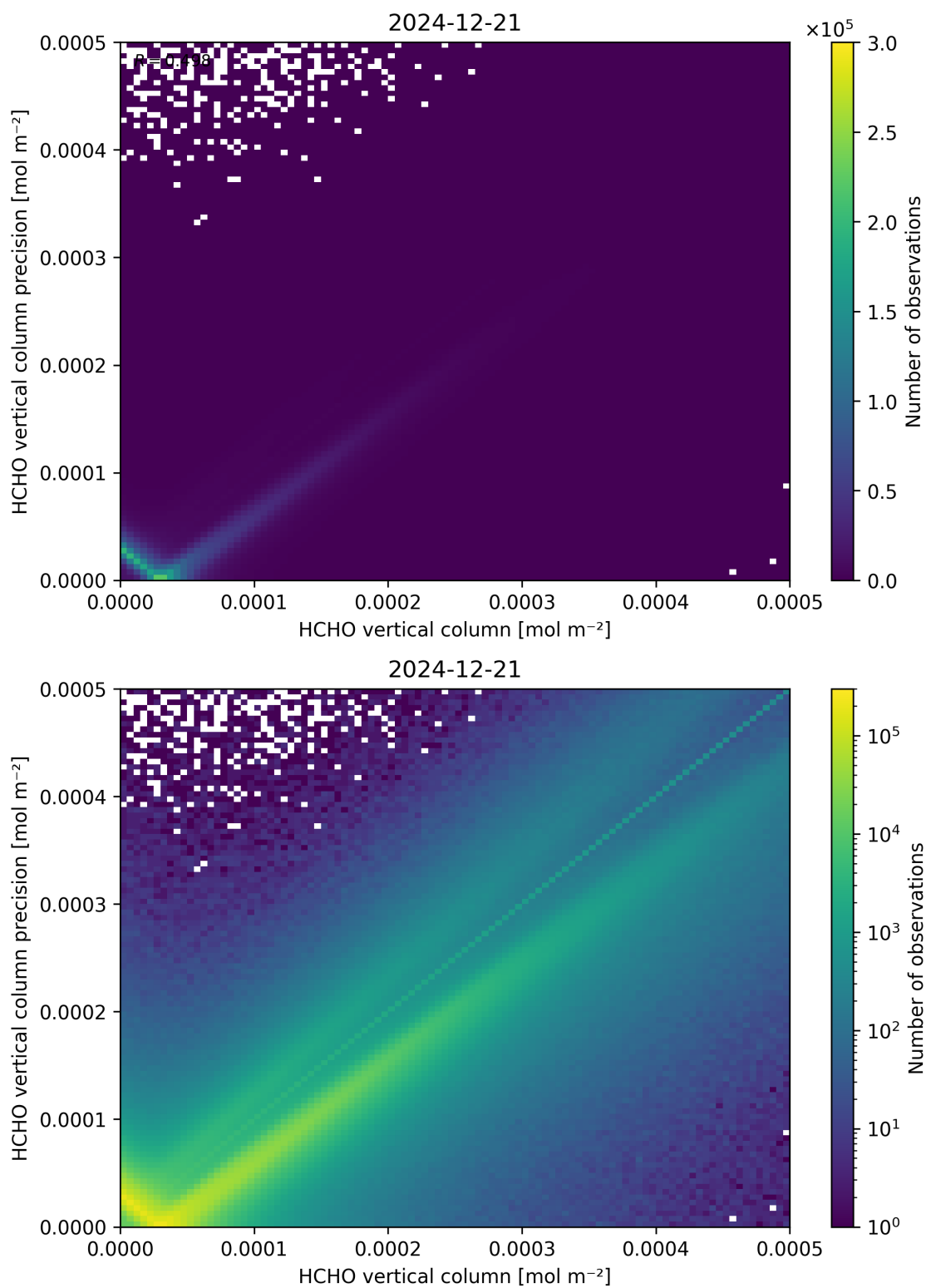
Figure 134: Scatter density plot of “HCHO vertical column” against “HCHO vertical column precision” for 2024-12-20 to 2024-12-22.
