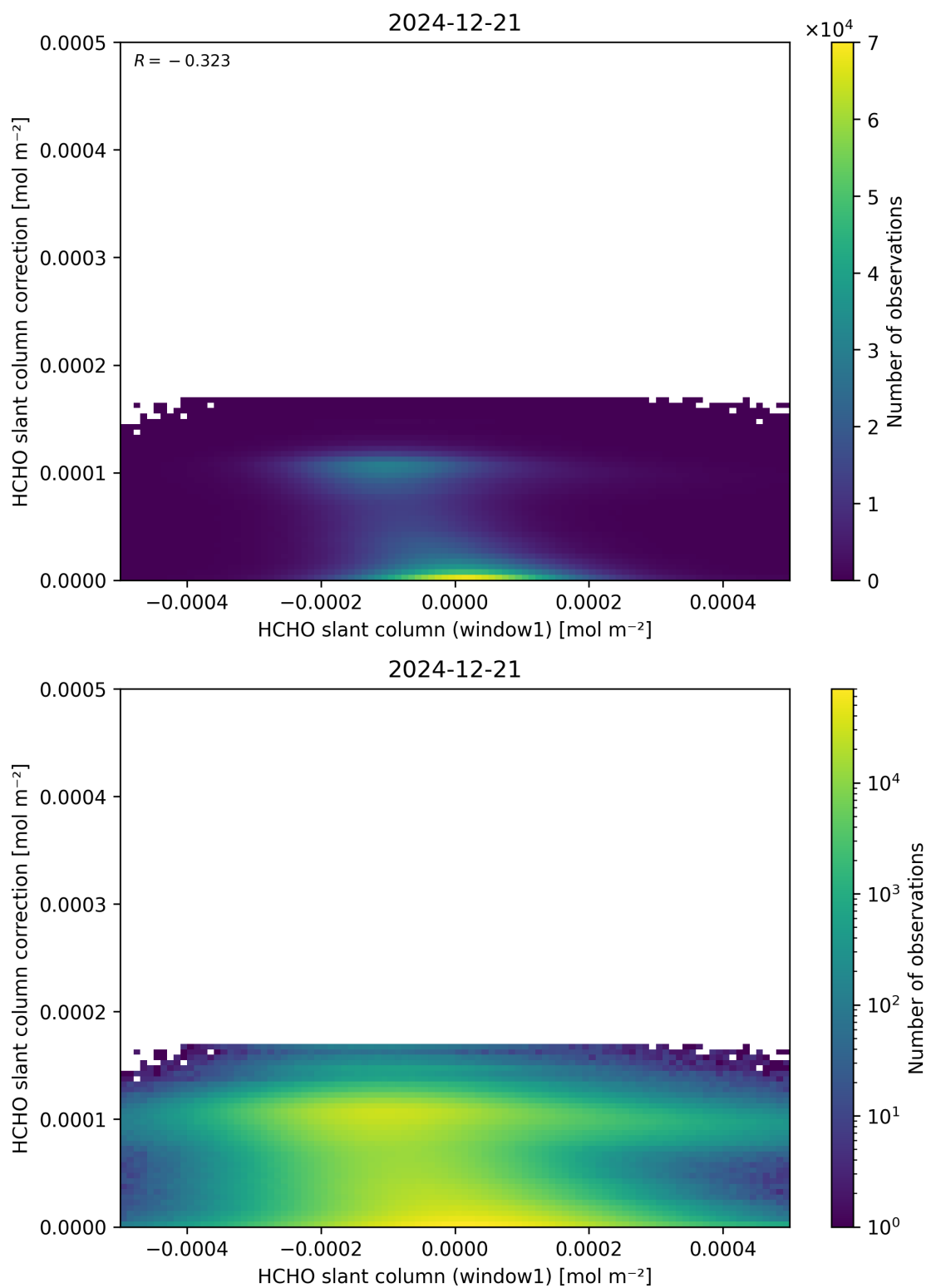
Figure 83: Scatter density plot of “HCHO slant column (window1)” against “HCHO slant column correction” for 2024-12-20 to 2024-12-22.
