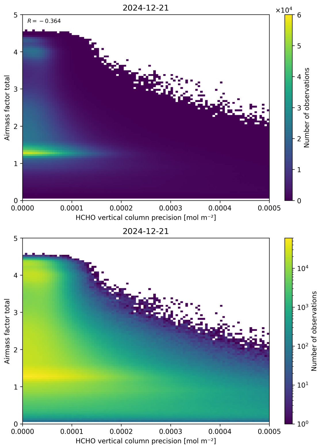
Figure 144: Scatter density plot of “HCHO vertical column precision” against “Airmass factor total” for 2024-12-20 to 2024-12-22.
