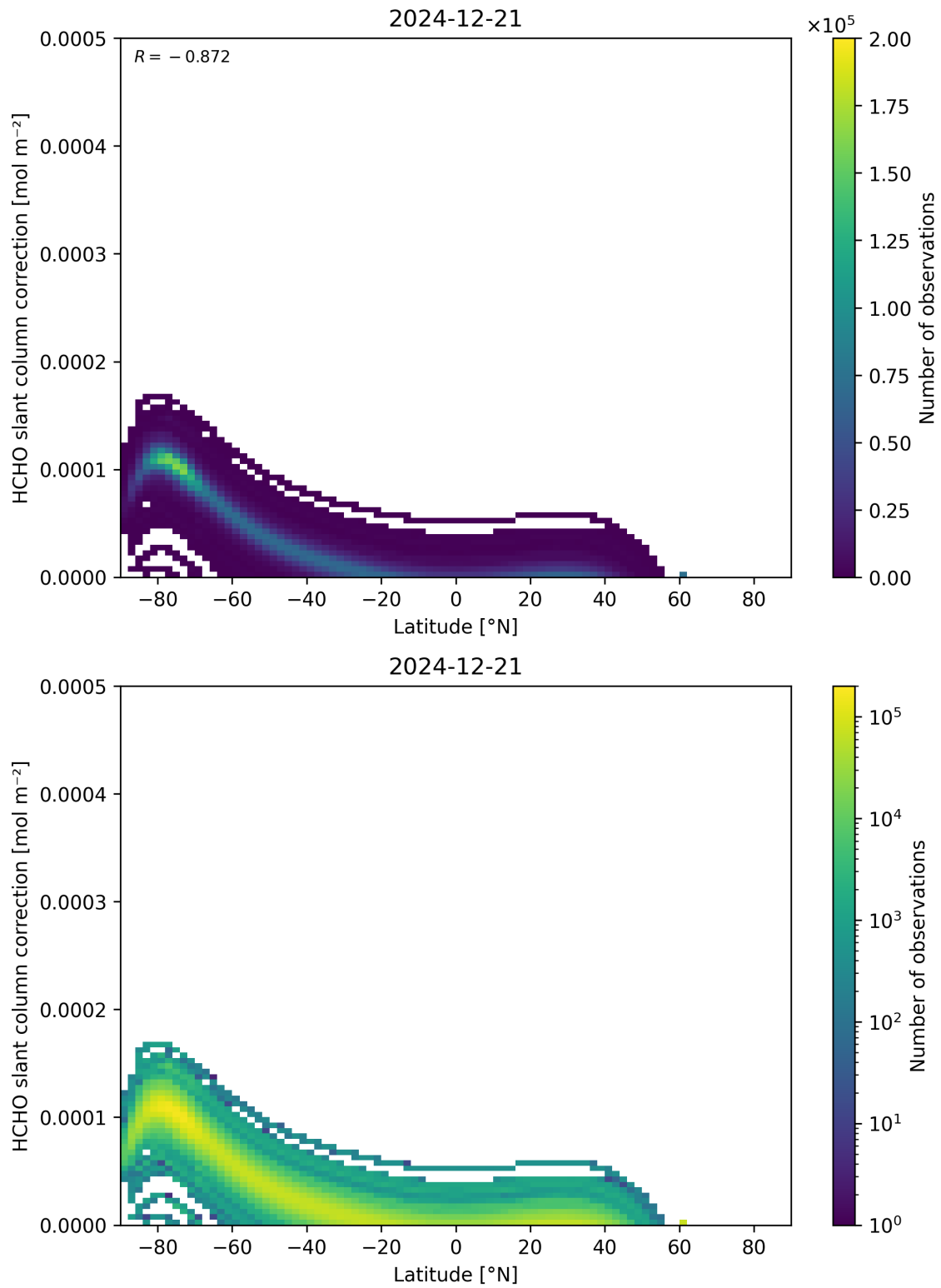
Figure 158: Scatter density plot of “Latitude” against “HCHO slant column correction” for 2024-12-20 to 2024-12-22.
