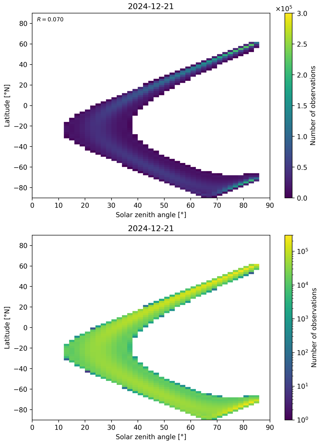
Figure 181: Scatter density plot of “Solar zenith angle” against “Latitude” for 2024-12-20 to 2024-12-22.
