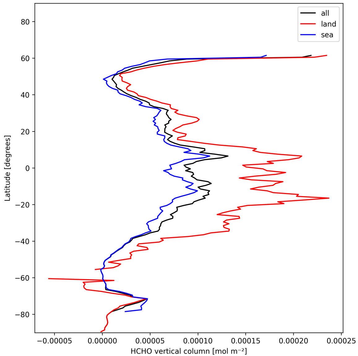
Figure 21: Zonal average of “HCHO vertical column” for 2024-12-20 to 2024-12-22.
