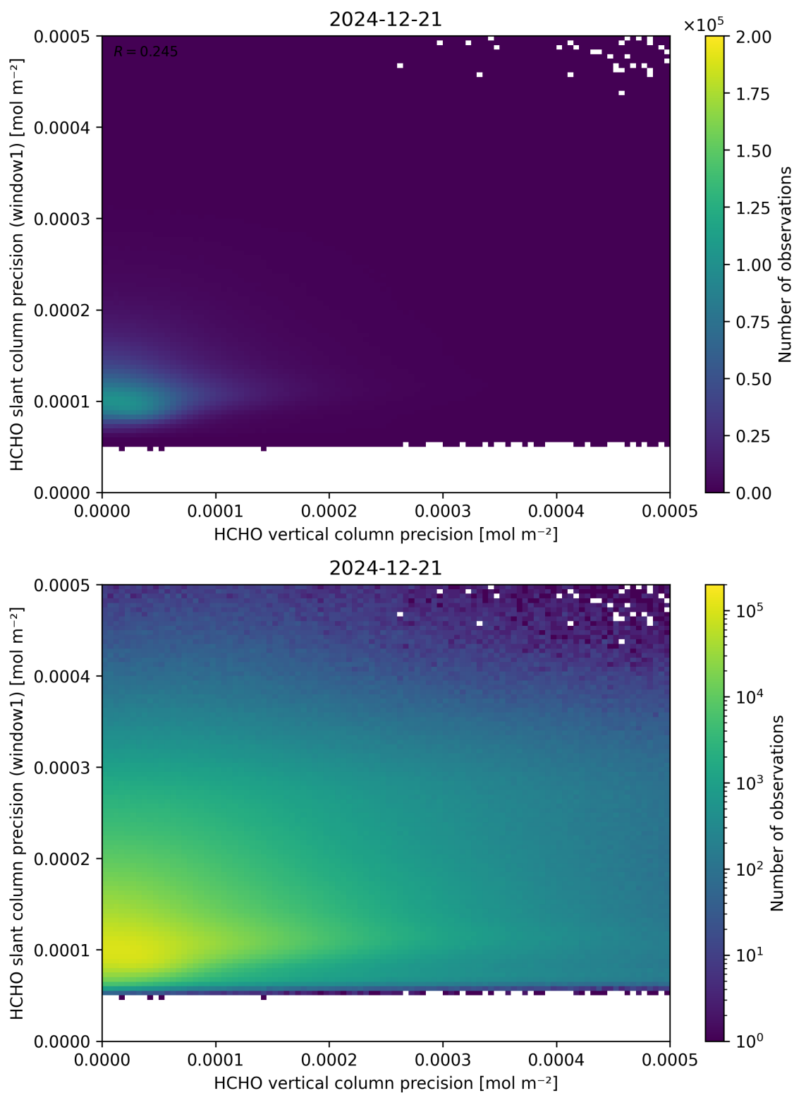
Figure 143: Scatter density plot of “HCHO vertical column precision” against “HCHO slant column precision (window1)” for 2024-12-20 to 2024-12-22.
