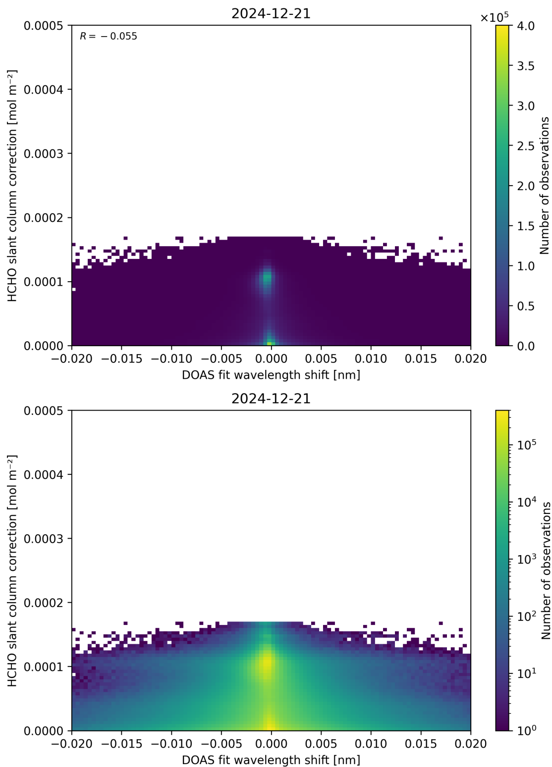
Figure 67: Scatter density plot of “DOAS fit wavelength shift” against “HCHO slant column correction” for 2024-12-20 to 2024-12-22.
