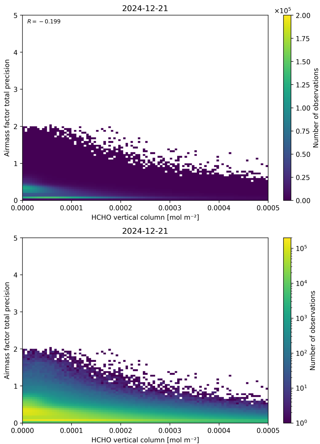
Figure 132: Scatter density plot of “HCHO vertical column” against “Airmass factor total precision” for 2024-12-20 to 2024-12-22.
