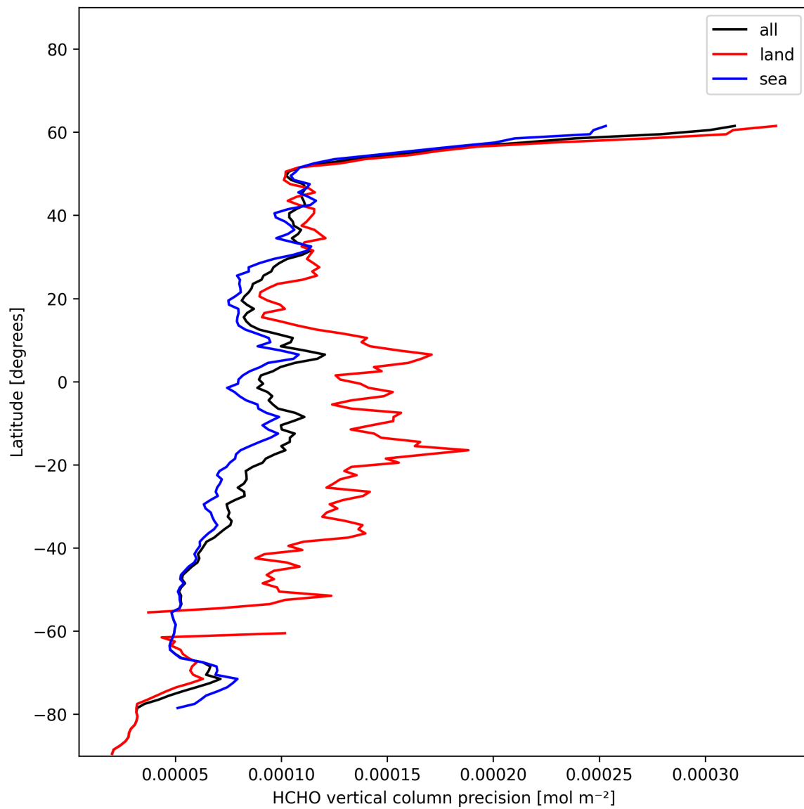
Figure 22: Zonal average of “HCHO vertical column precision” for 2024-12-20 to 2024-12-22.
