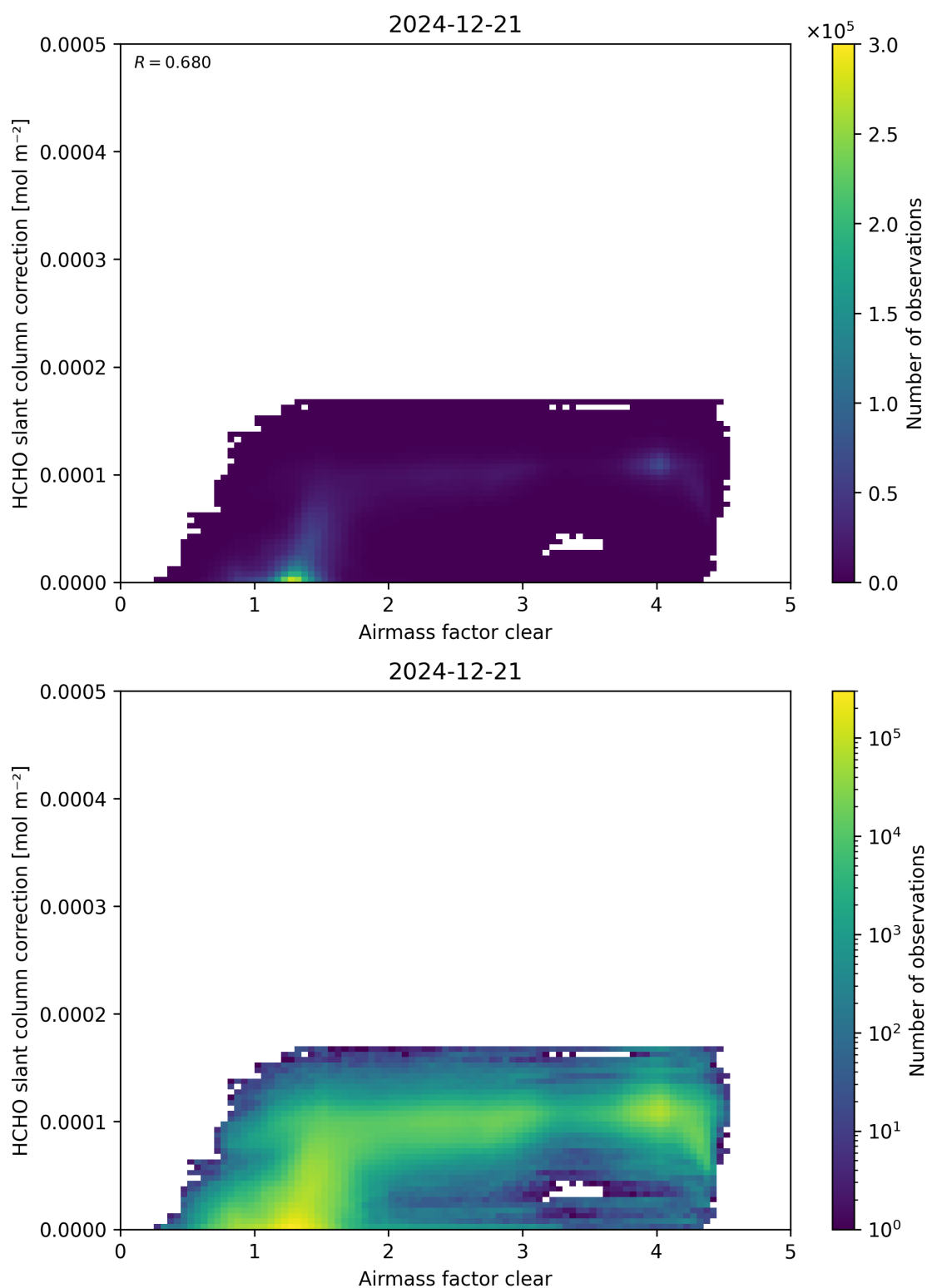
Figure 75: Scatter density plot of “Airmass factor clear” against “HCHO slant column correction” for 2024-12-20 to 2024-12-22.
