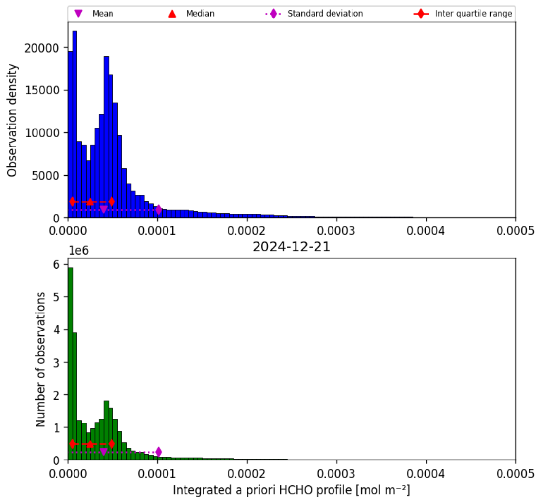
Figure 43: Histogram of “Integrated a priori HCHO profile” for 2024-12-20 to 2024-12-22
