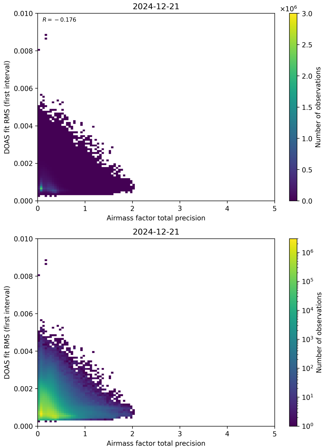
Figure 105: Scatter density plot of “Airmass factor total precision” against “DOAS fit RMS (first interval)” for 2024-12-20 to 2024-12-22.
