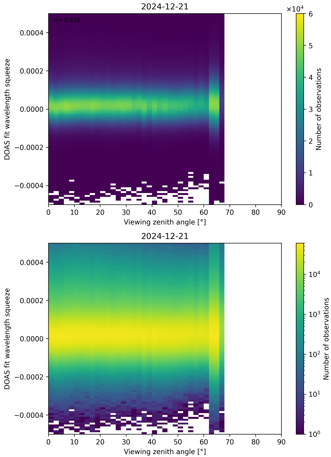
Figure 184: Scatter density plot of “Viewing zenith angle” against “DOAS fit wavelength squeeze” for 2024-12-20 to 2024-12-22.
