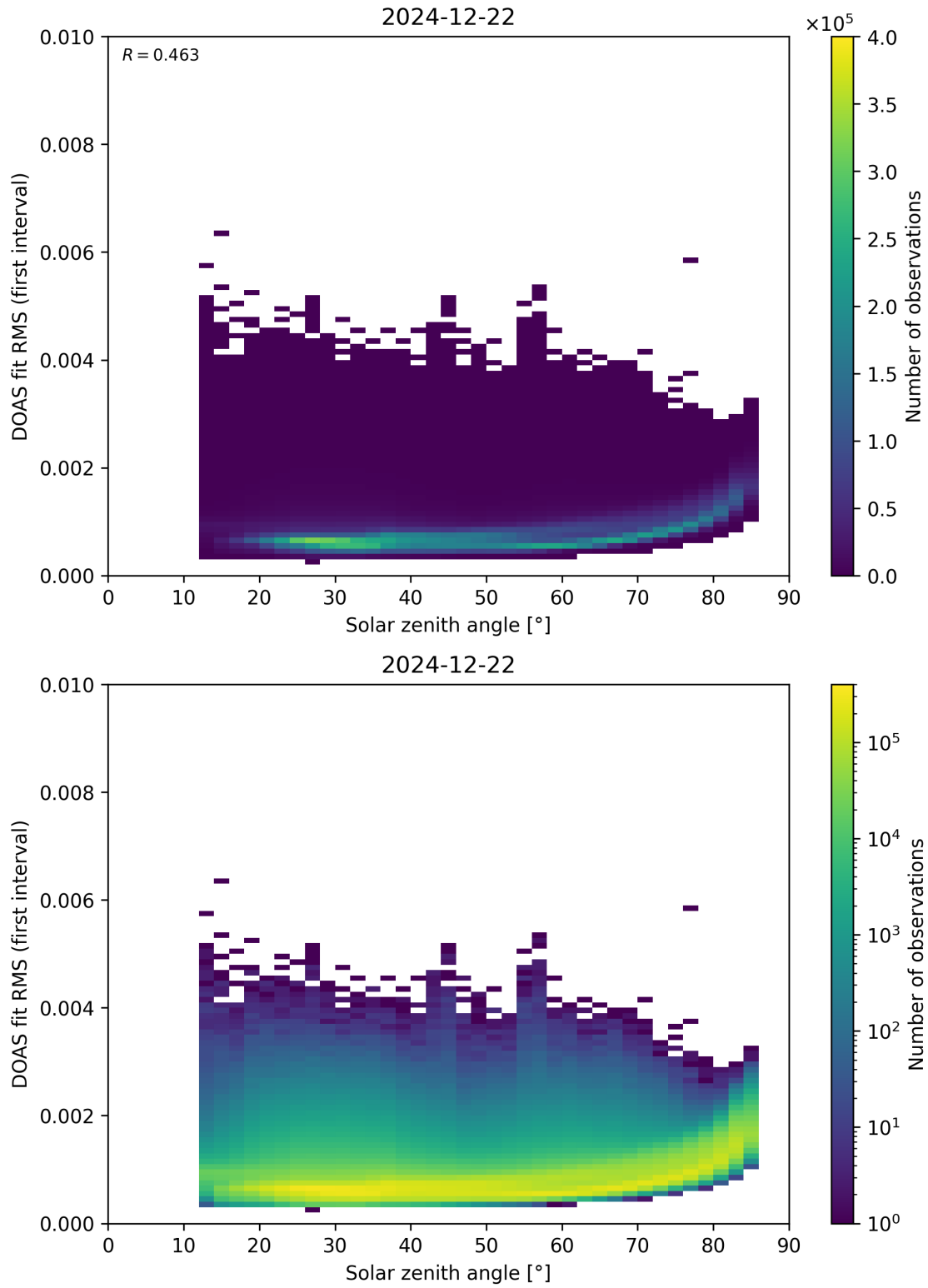
Figure 167: Scatter density plot of “Solar zenith angle” against “DOAS fit RMS (first interval)” for 2024-12-22 to 2024-12-23.
