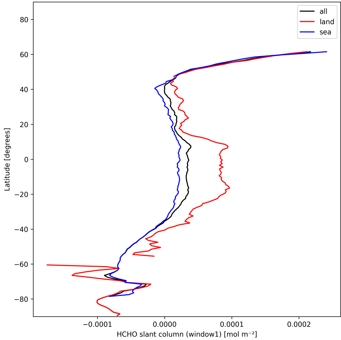
Figure 24: Zonal average of “HCHO slant column (window1)” for 2024-12-22 to 2024-12-23.
