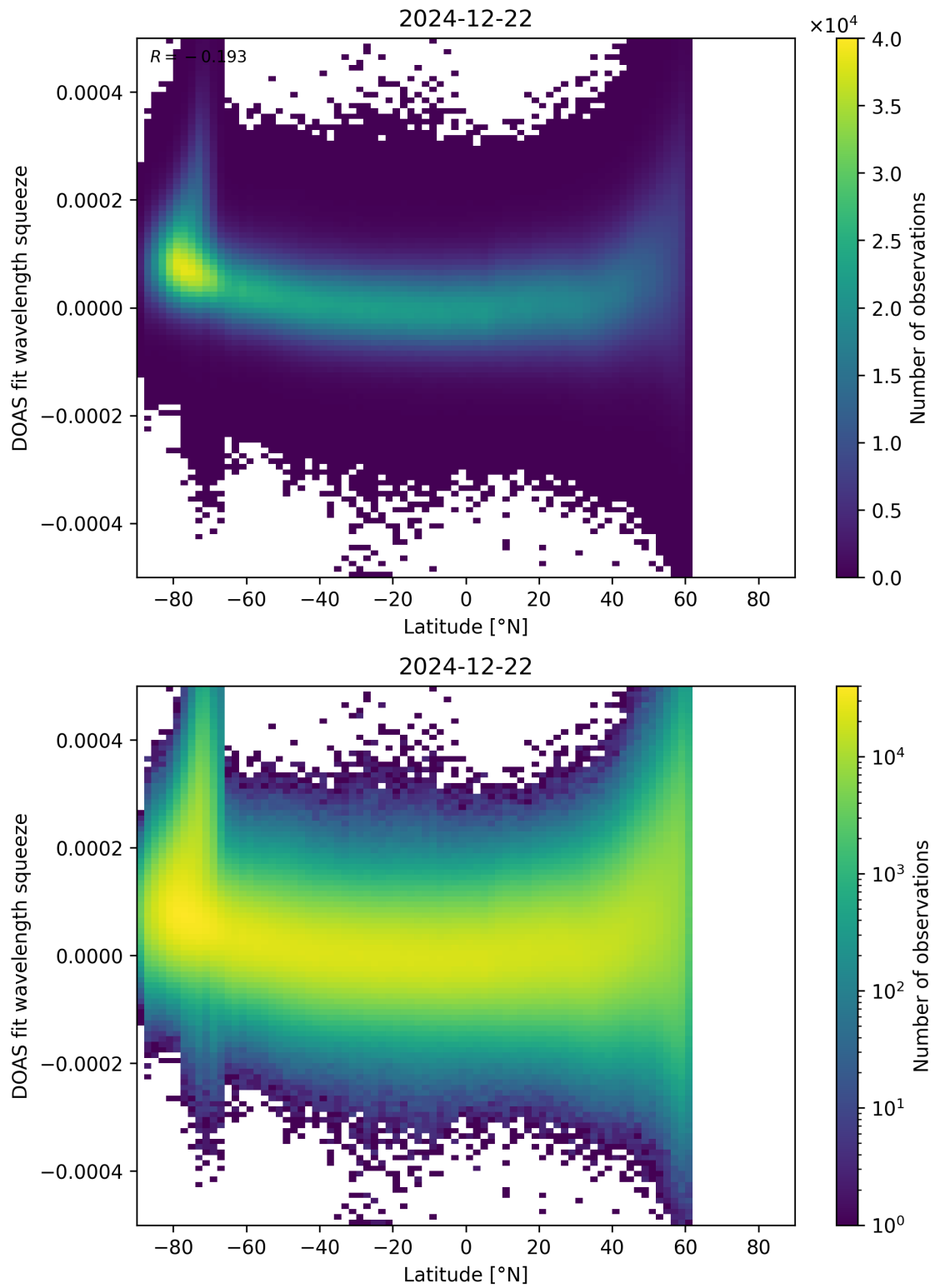
Figure 155: Scatter density plot of “Latitude” against “DOAS fit wavelength squeeze” for 2024-12-22 to 2024-12-23.
