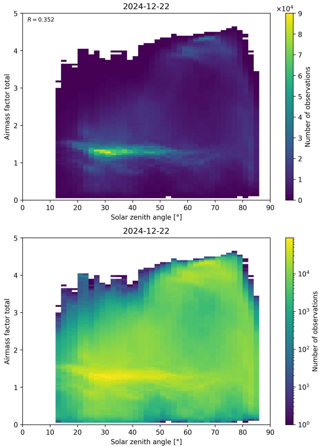
Figure 175: Scatter density plot of “Solar zenith angle” against “Airmass factor total” for 2024-12-22 to 2024-12-23.
