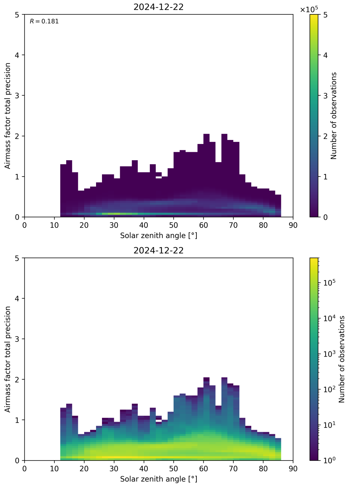
Figure 176: Scatter density plot of “Solar zenith angle” against “Airmass factor total precision” for 2024-12-22 to 2024-12-23.
