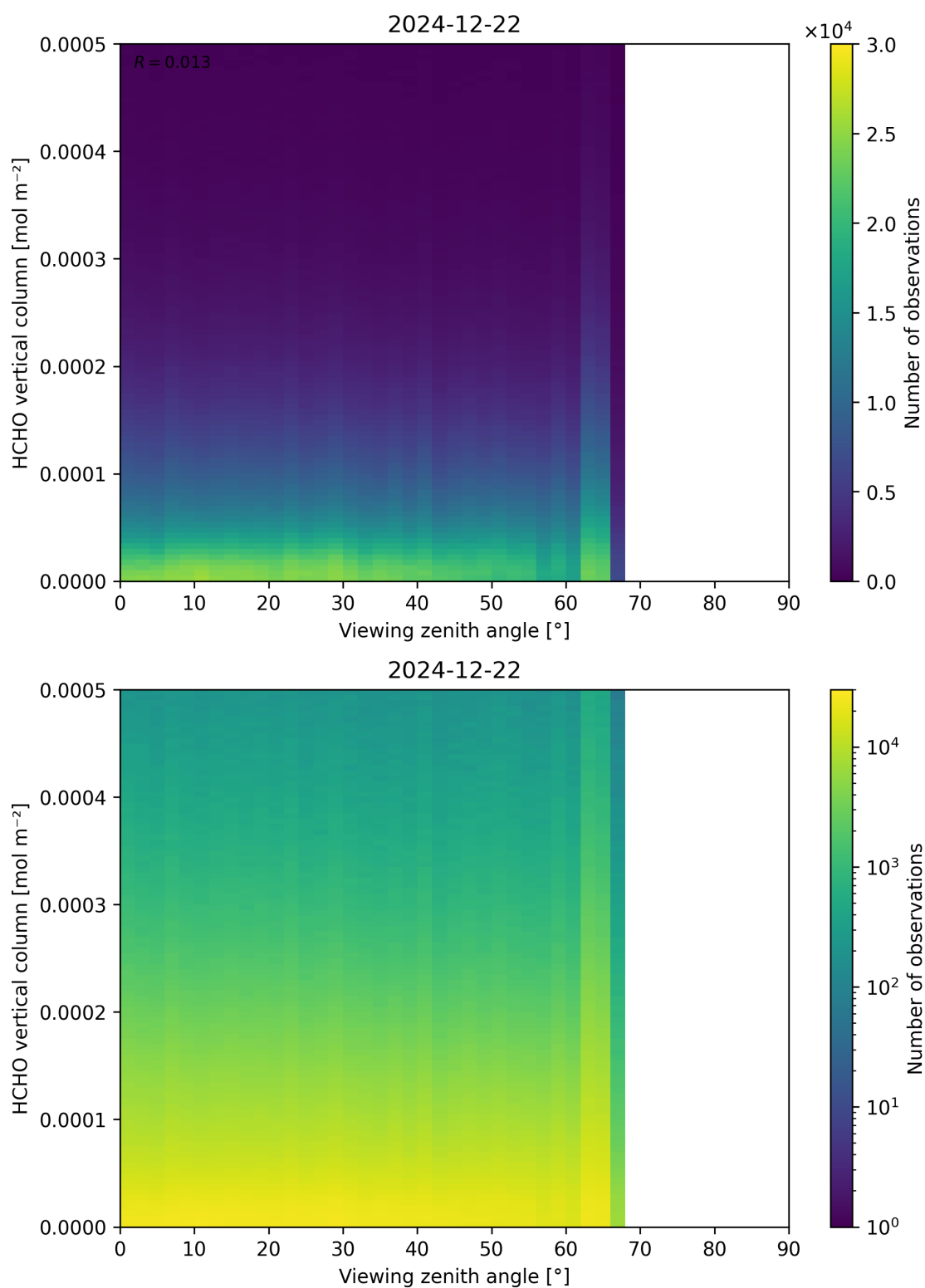
Figure 192: Scatter density plot of “Viewing zenith angle” against “HCHO vertical column” for 2024-12-22 to 2024-12-23.
