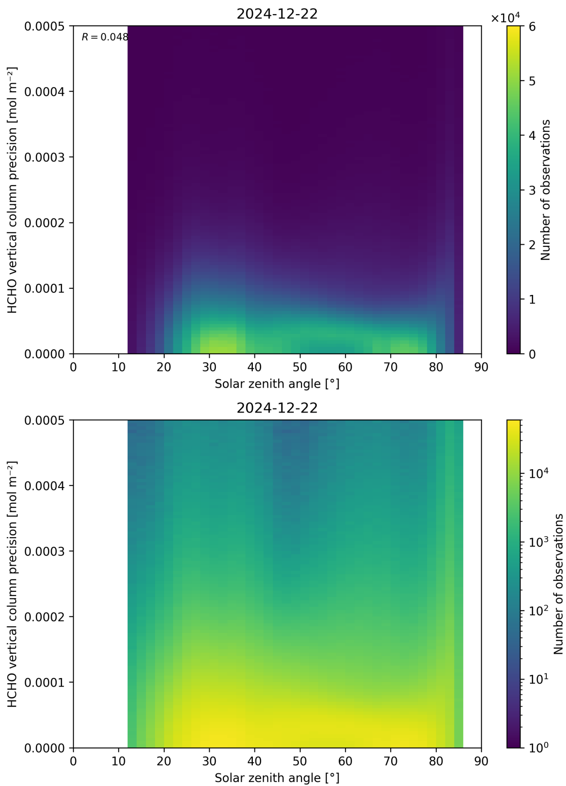
Figure 179: Scatter density plot of “Solar zenith angle” against “HCHO vertical column precision” for 2024-12-22 to 2024-12-23.
