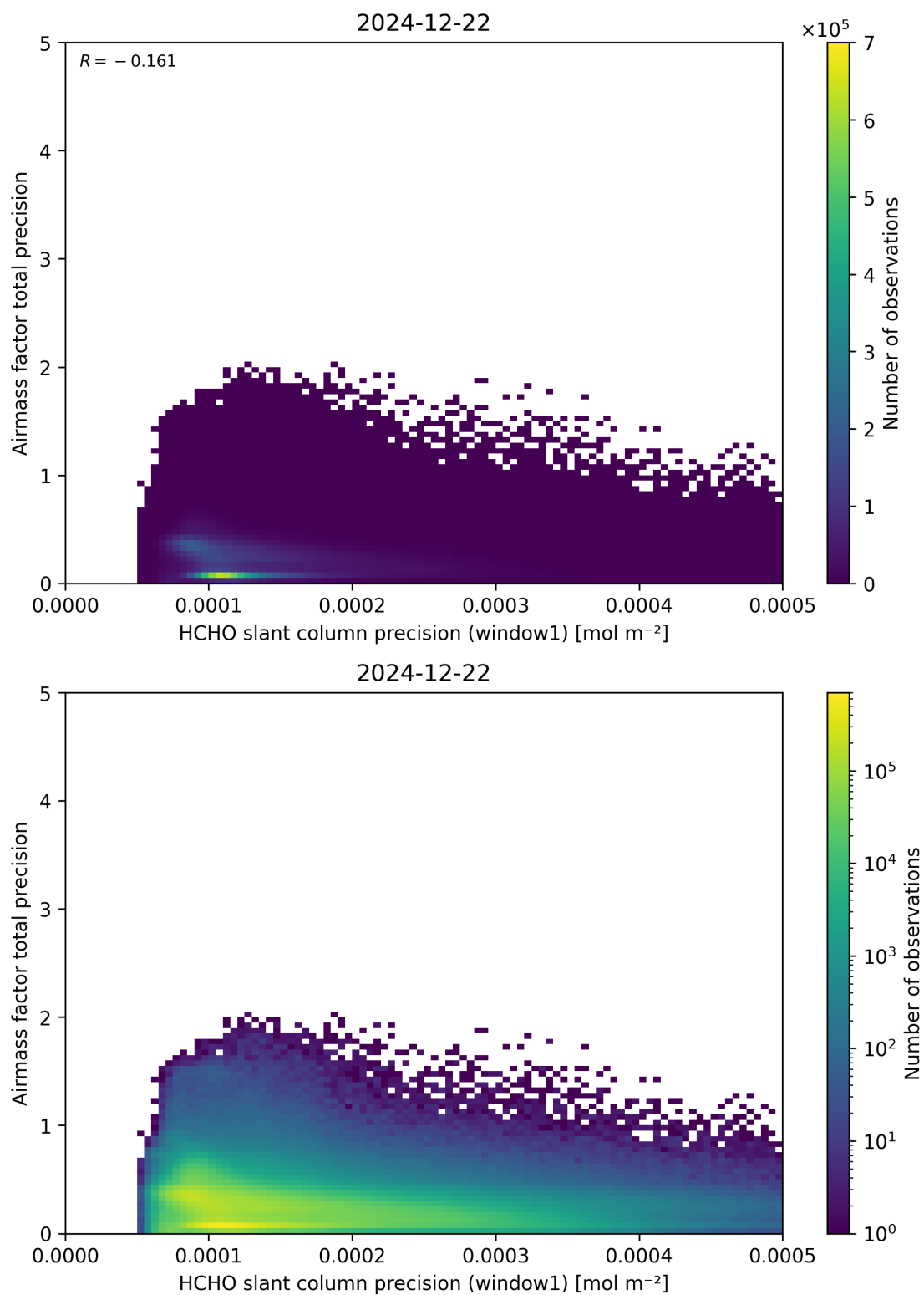
Figure 95: Scatter density plot of “HCHO slant column precision (window1)” against “Airmass factor total precision” for 2024-12-22 to 2024-12-23.
