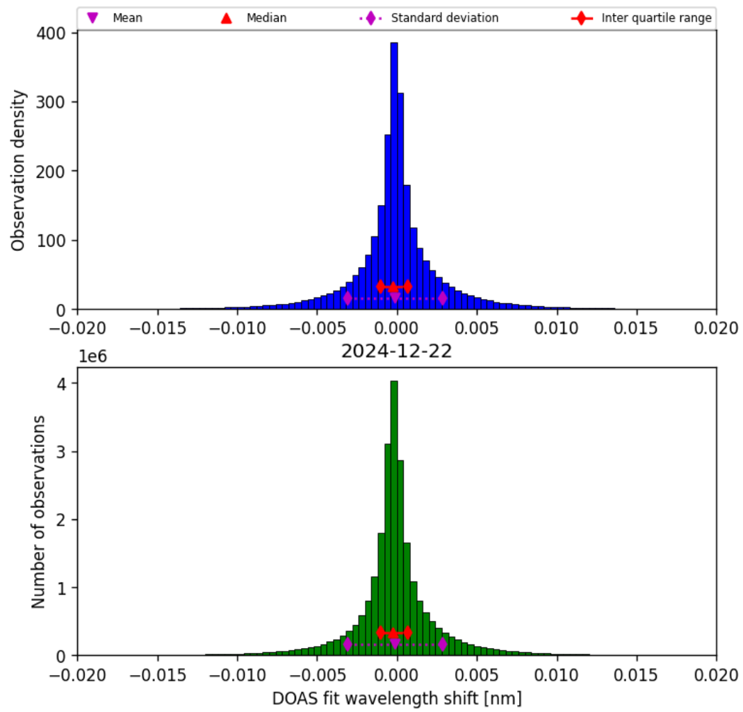
Figure 44: Histogram of “DOAS fit wavelength shift” for 2024-12-22 to 2024-12-23
