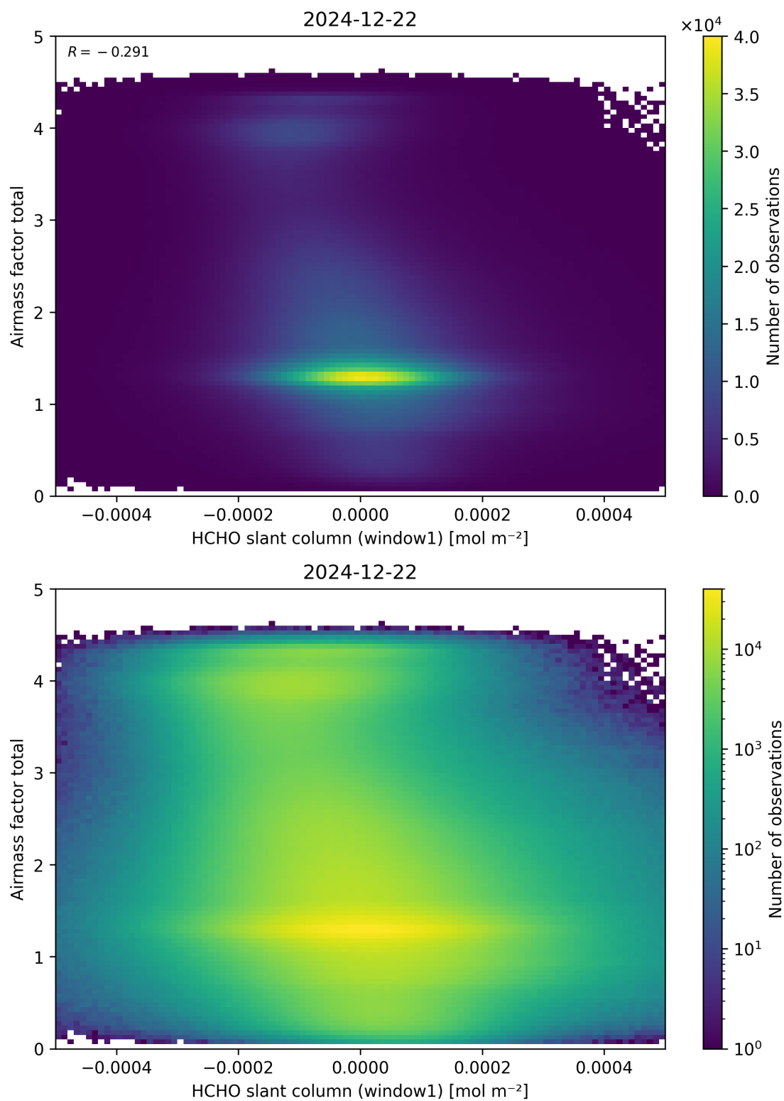
Figure 85: Scatter density plot of “HCHO slant column (window1)” against “Airmass factor total” for 2024-12-22 to 2024-12-23.
