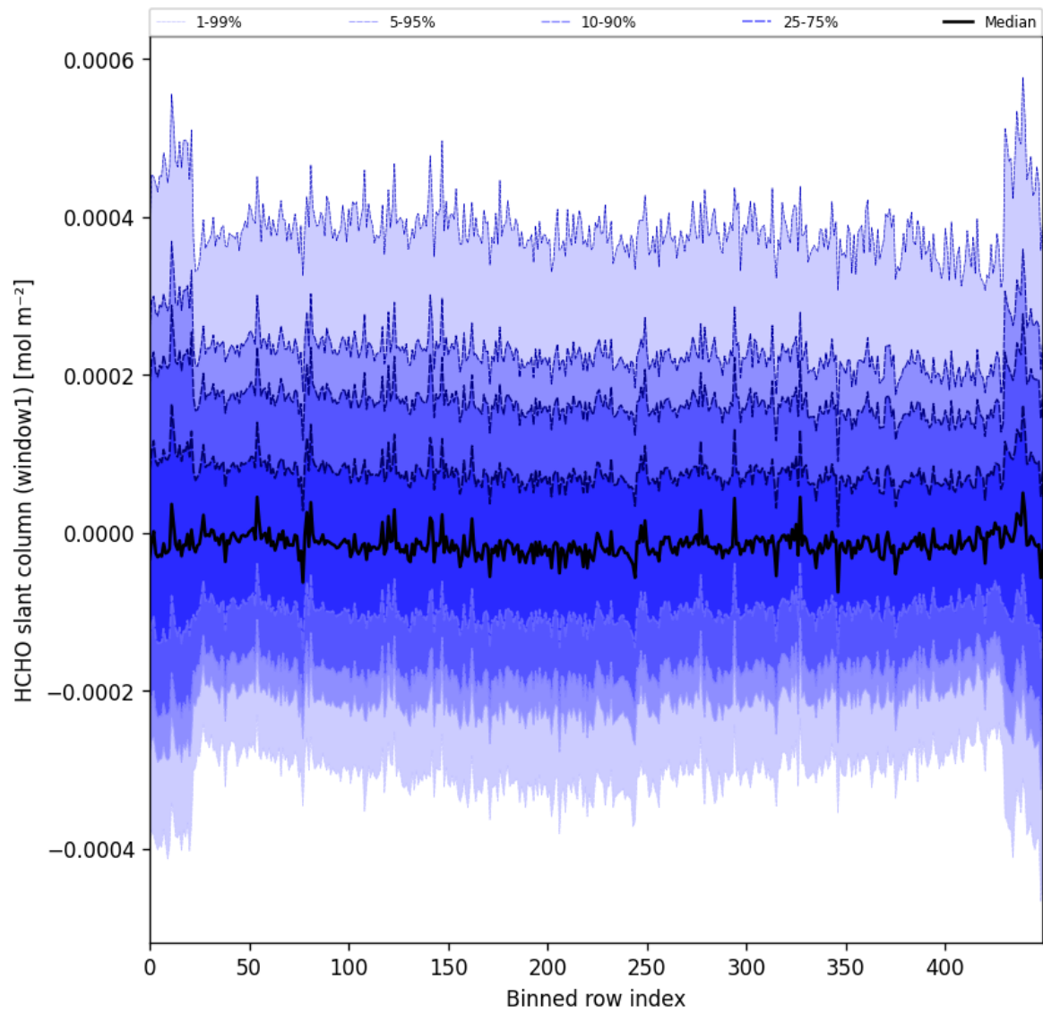
Figure 52: Along track statistics of “HCHO slant column (window1)” for 2024-12-22 to 2024-12-23
