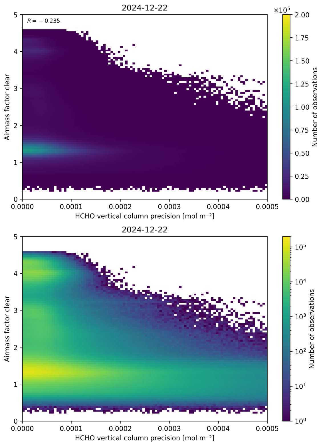
Figure 139: Scatter density plot of “HCHO vertical column precision” against “Airmass factor clear” for 2024-12-22 to 2024-12-23.
