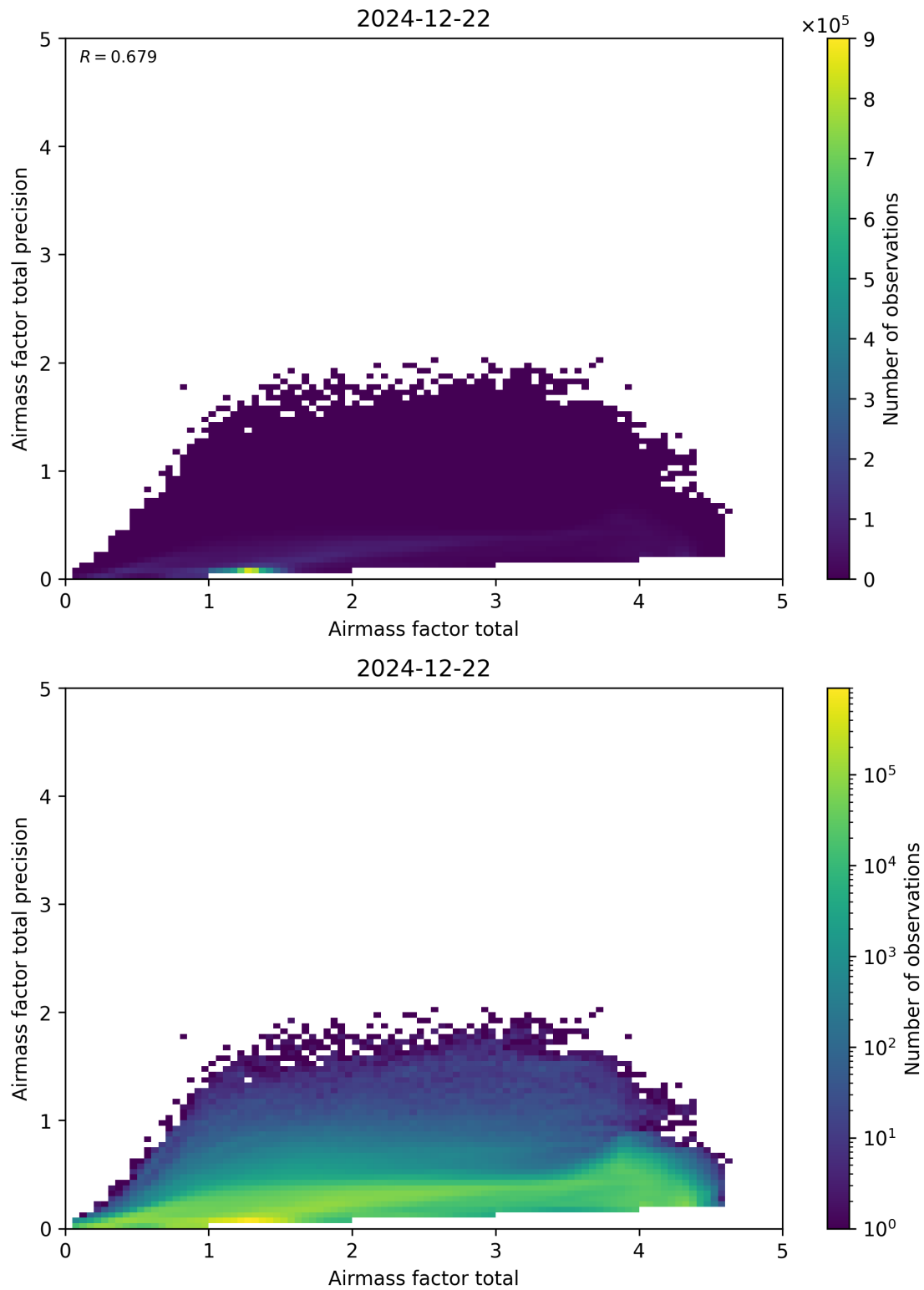
Figure 103: Scatter density plot of “Airmass factor total” against “Airmass factor total precision” for 2024-12-22 to 2024-12-23.
