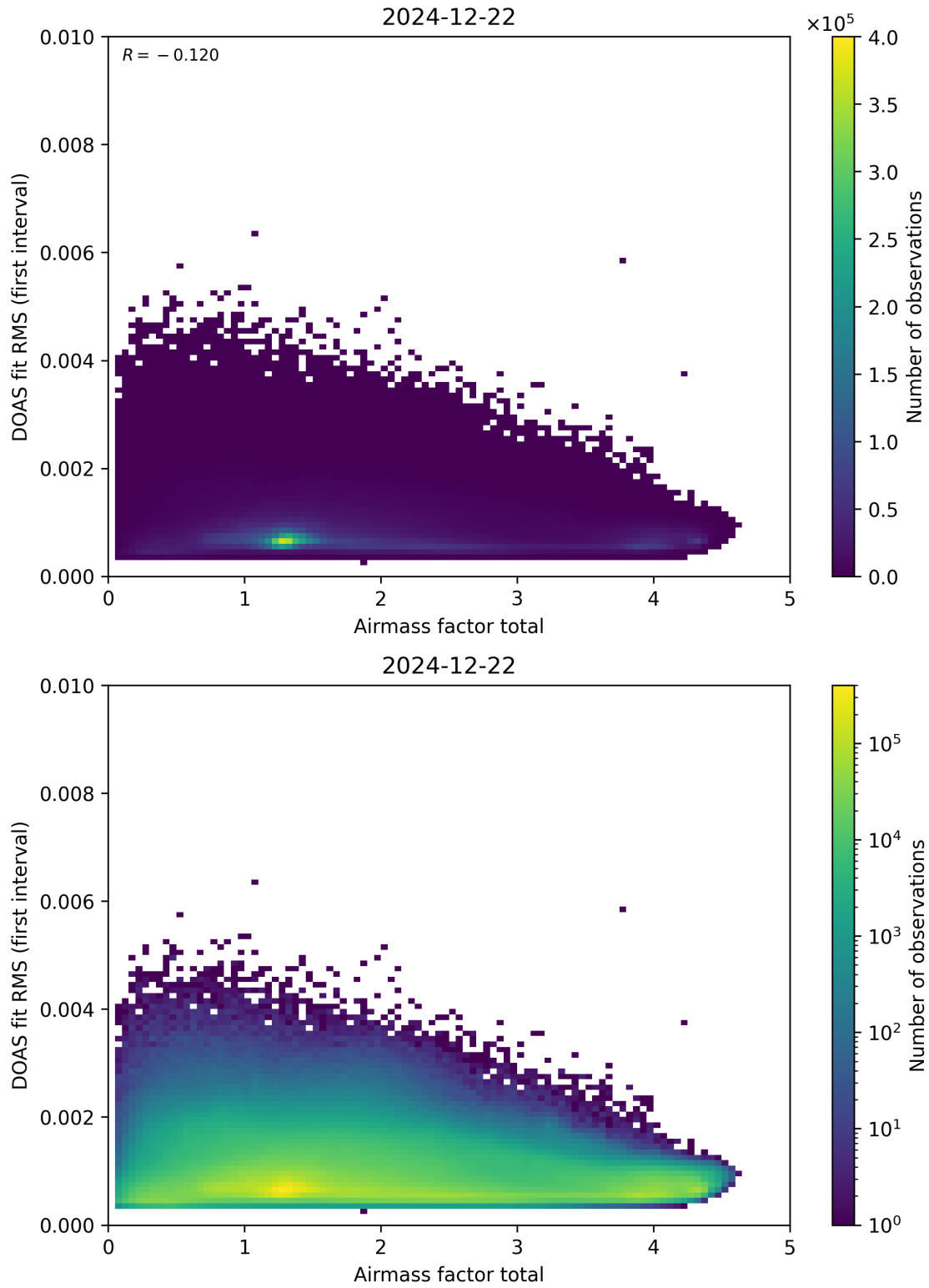
Figure 97: Scatter density plot of “Airmass factor total” against “DOAS fit RMS (first interval)” for 2024-12-22 to 2024-12-23.
