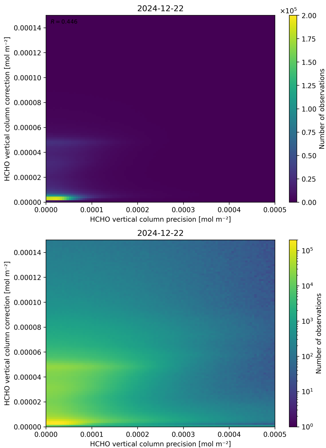
Figure 146: Scatter density plot of “HCHO vertical column precision” against “HCHO vertical column correction” for 2024-12-22 to 2024-12-23.
