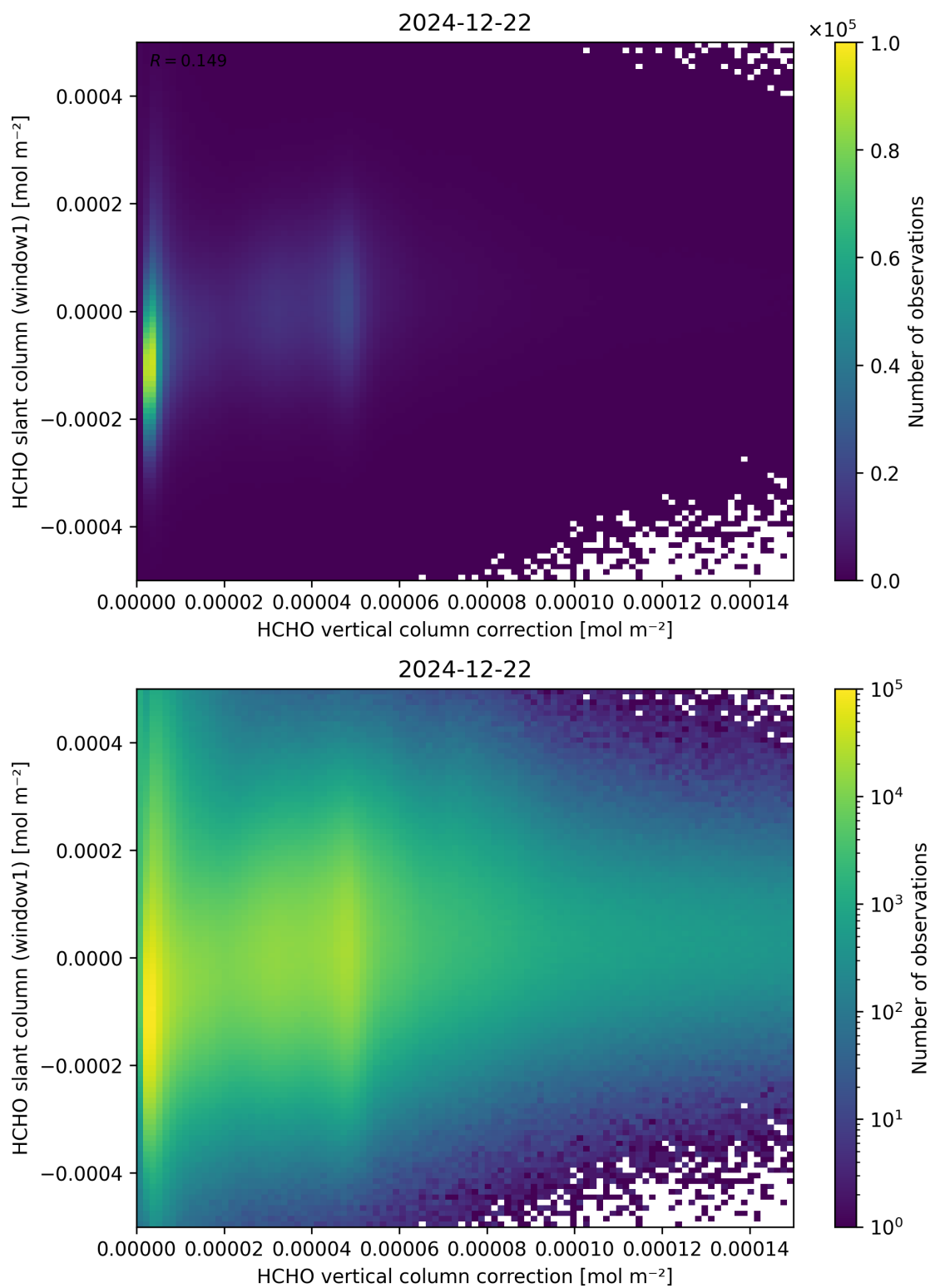
Figure 118: Scatter density plot of “HCHO vertical column correction” against “HCHO slant column (window1)” for 2024-12-22 to 2024-12-23.
