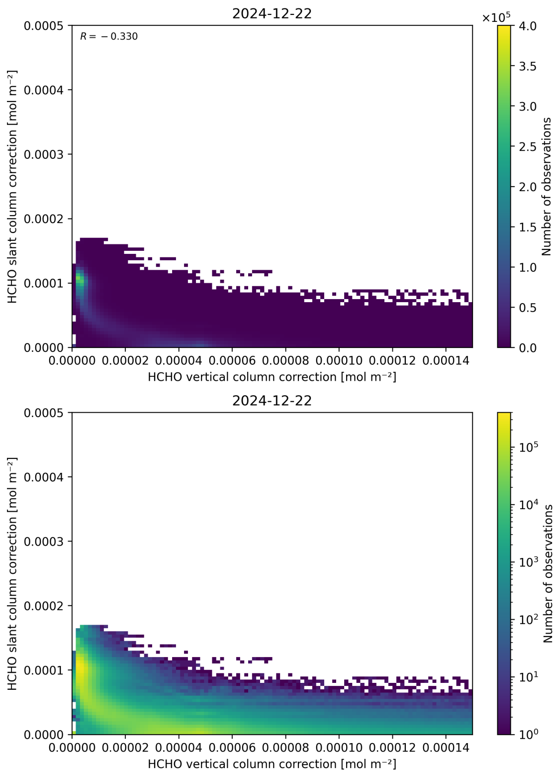
Figure 117: Scatter density plot of “HCHO vertical column correction” against “HCHO slant column correction” for 2024-12-22 to 2024-12-23.
