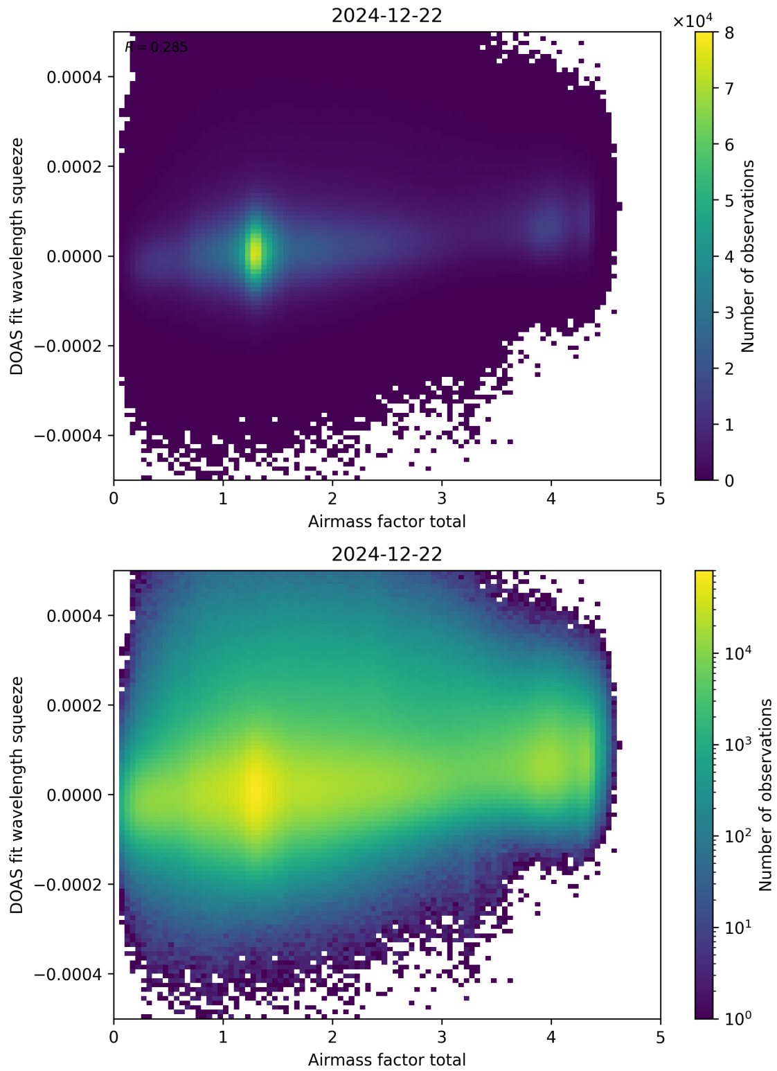
Figure 99: Scatter density plot of “Airmass factor total” against “DOAS fit wavelength squeeze” for 2024-12-22 to 2024-12-23.
