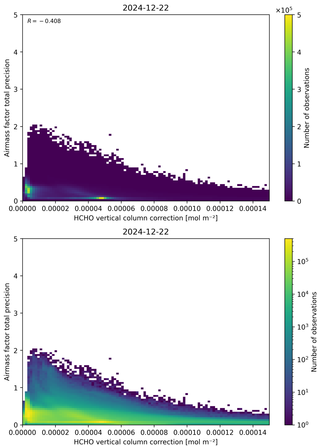
Figure 121: Scatter density plot of “HCHO vertical column correction” against “Airmass factor total precision” for 2024-12-22 to 2024-12-23.
