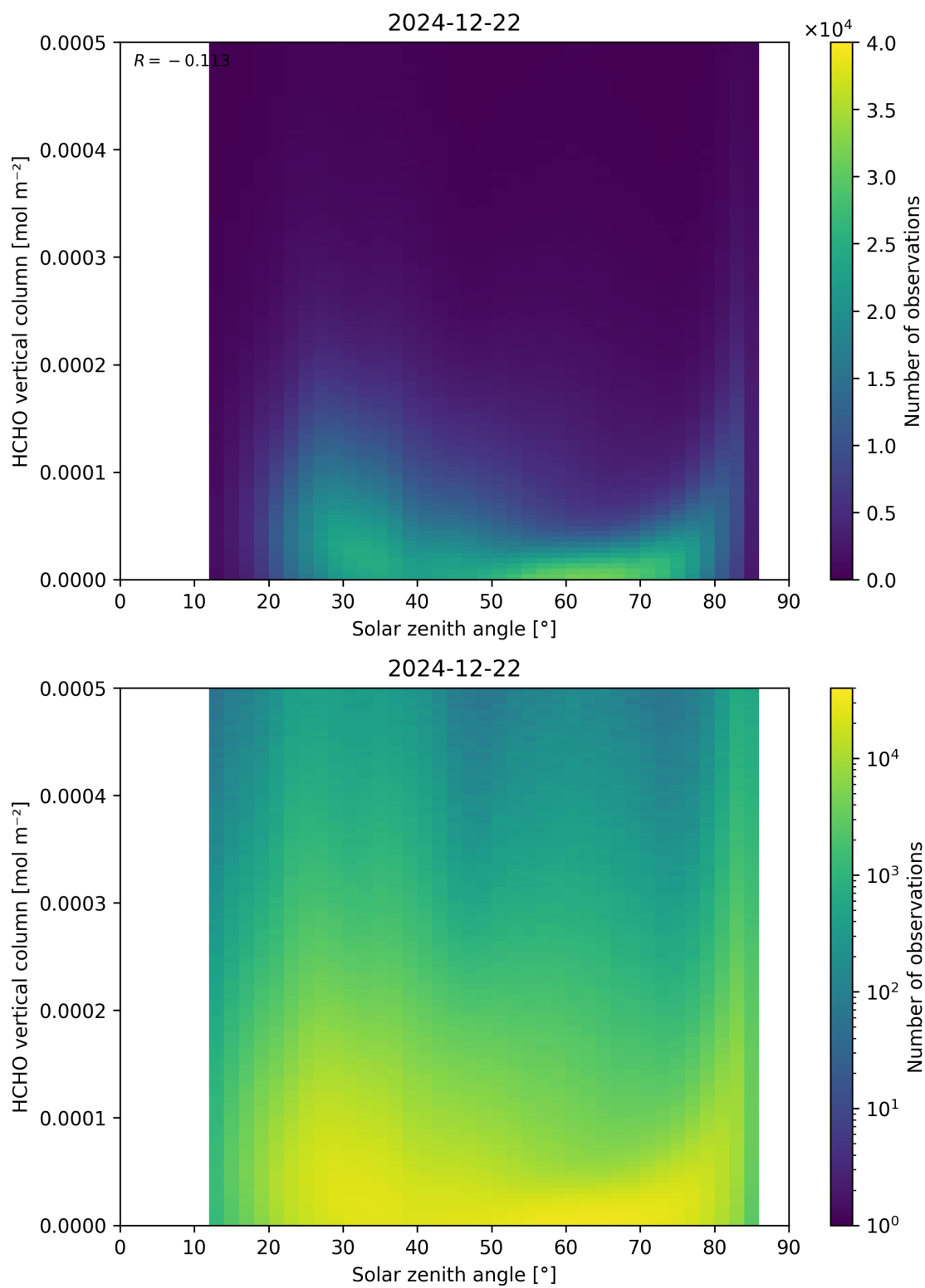
Figure 177: Scatter density plot of “Solar zenith angle” against “HCHO vertical column” for 2024-12-22 to 2024-12-23.
