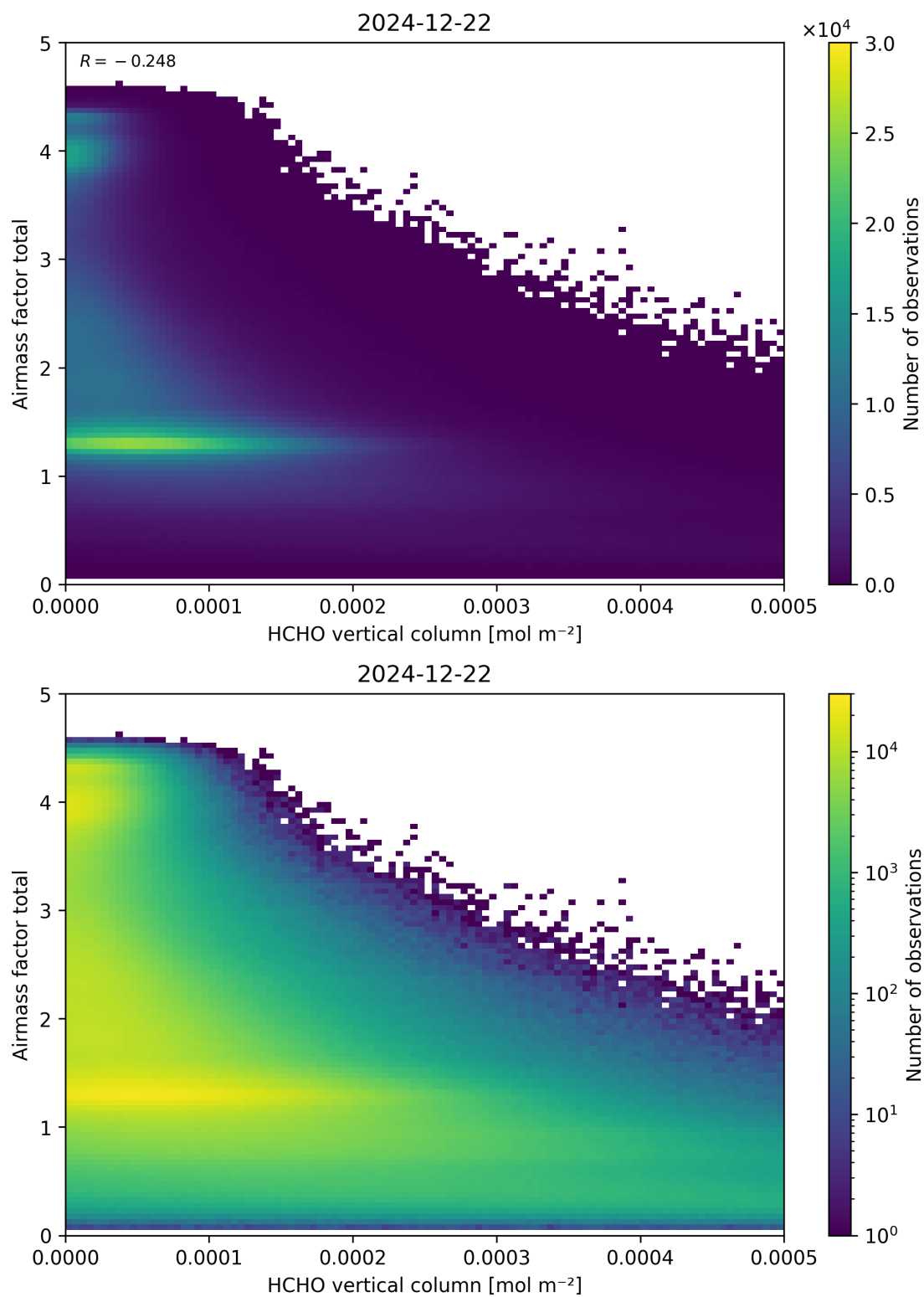
Figure 131: Scatter density plot of “HCHO vertical column” against “Airmass factor total” for 2024-12-22 to 2024-12-23.
