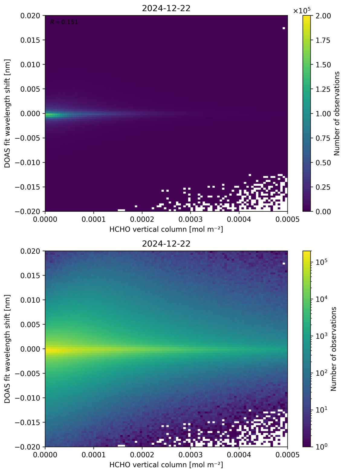
Figure 124: Scatter density plot of “HCHO vertical column” against “DOAS fit wavelength shift” for 2024-12-22 to 2024-12-23.
