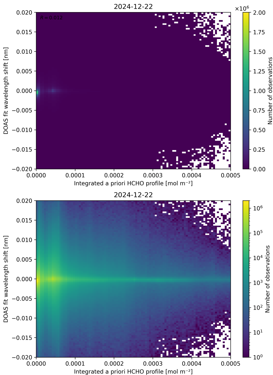
Figure 149: Scatter density plot of “Integrated a priori HCHO profile” against “DOAS fit wavelength shift” for 2024-12-22 to 2024-12-23.
