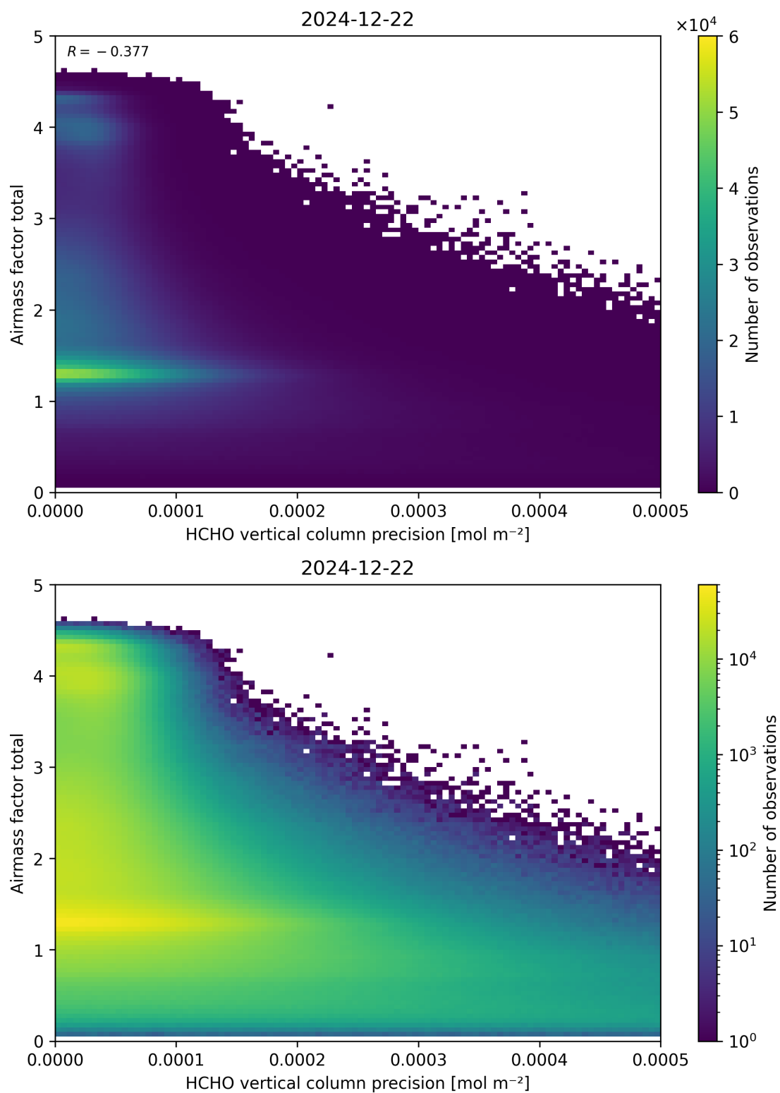
Figure 144: Scatter density plot of “HCHO vertical column precision” against “Airmass factor total” for 2024-12-22 to 2024-12-23.
