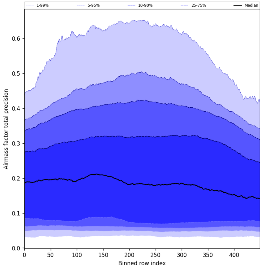
Figure 55: Along track statistics of “Airmass factor total precision” for 2024-12-22 to 2024-12-23
