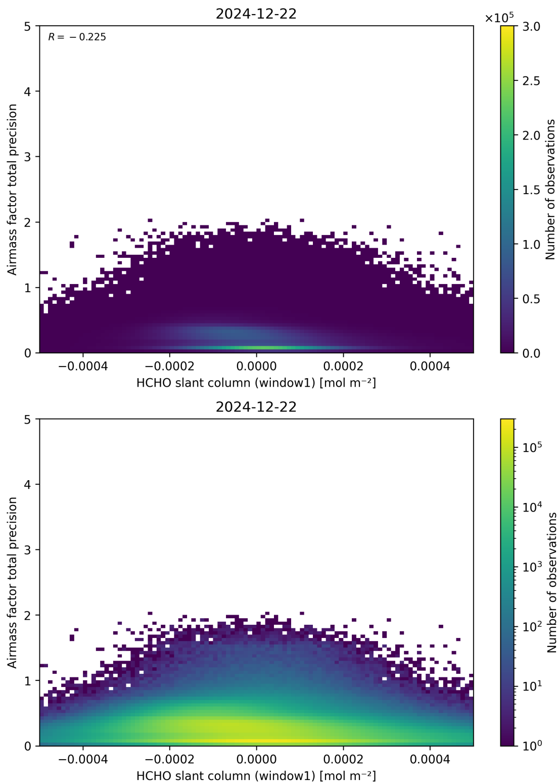
Figure 86: Scatter density plot of “HCHO slant column (window1)” against “Airmass factor total precision” for 2024-12-22 to 2024-12-23.
