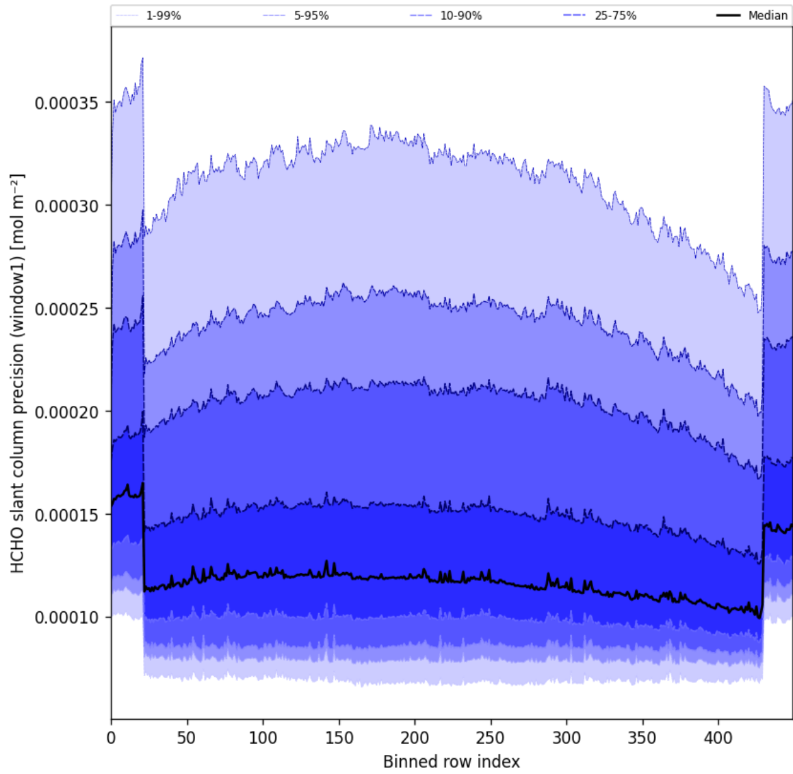
Figure 53: Along track statistics of “HCHO slant column precision (window1)” for 2024-12-22 to 2024-12-23
