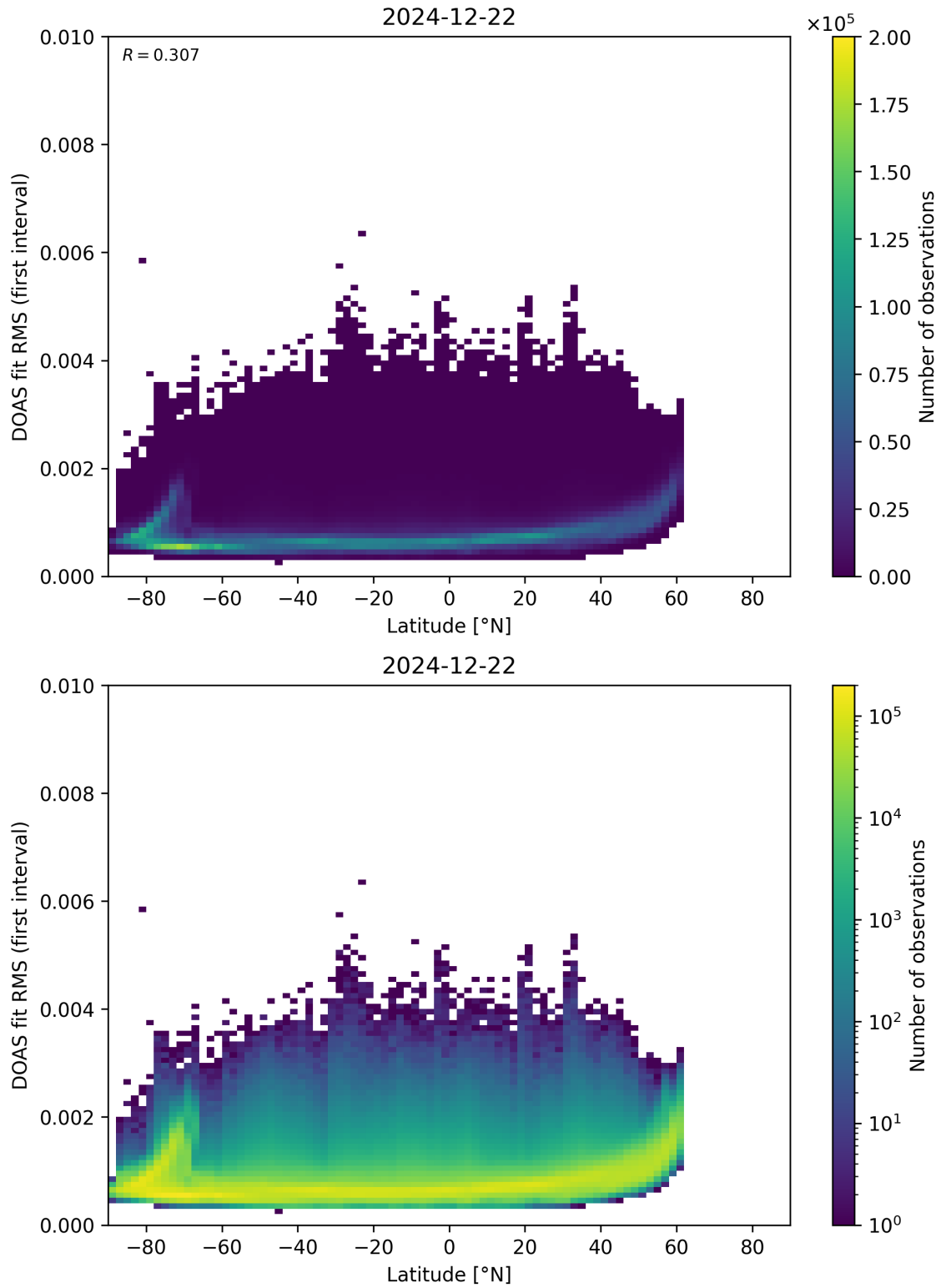
Figure 153: Scatter density plot of “Latitude” against “DOAS fit RMS (first interval)” for 2024-12-22 to 2024-12-23.
