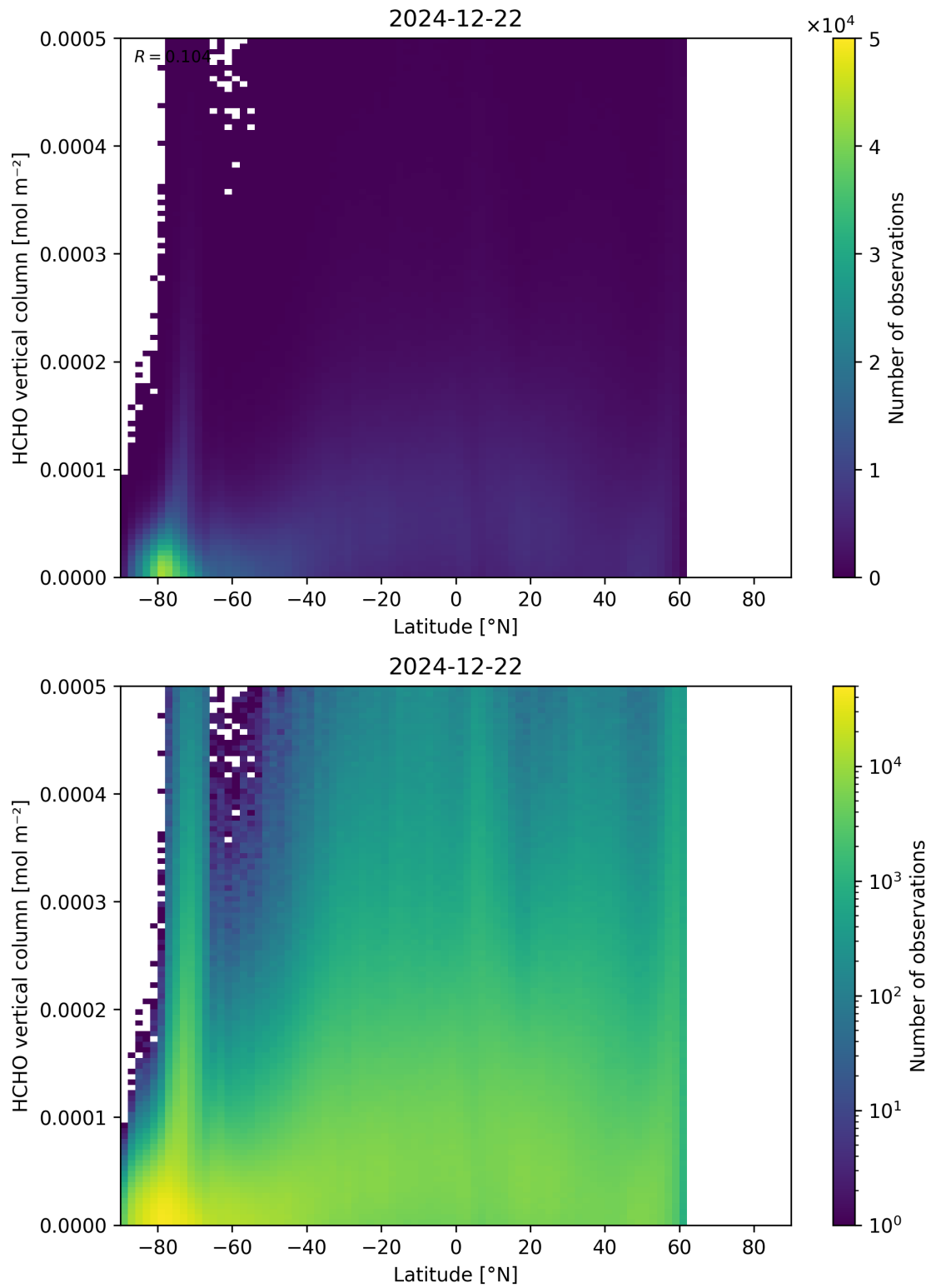
Figure 163: Scatter density plot of “Latitude” against “HCHO vertical column” for 2024-12-22 to 2024-12-23.
