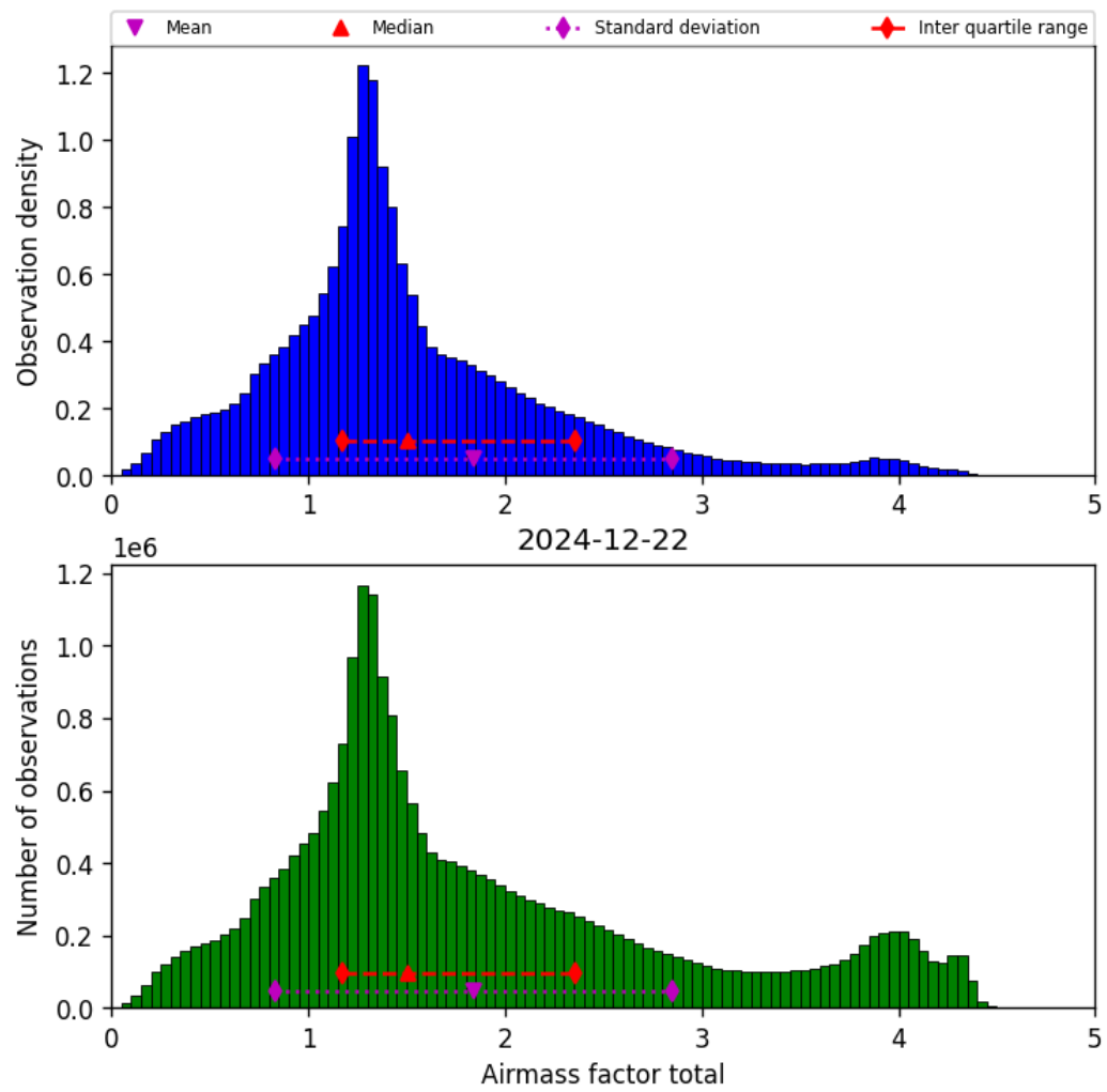
Figure 40: Histogram of “Airmass factor total” for 2024-12-22 to 2024-12-23
