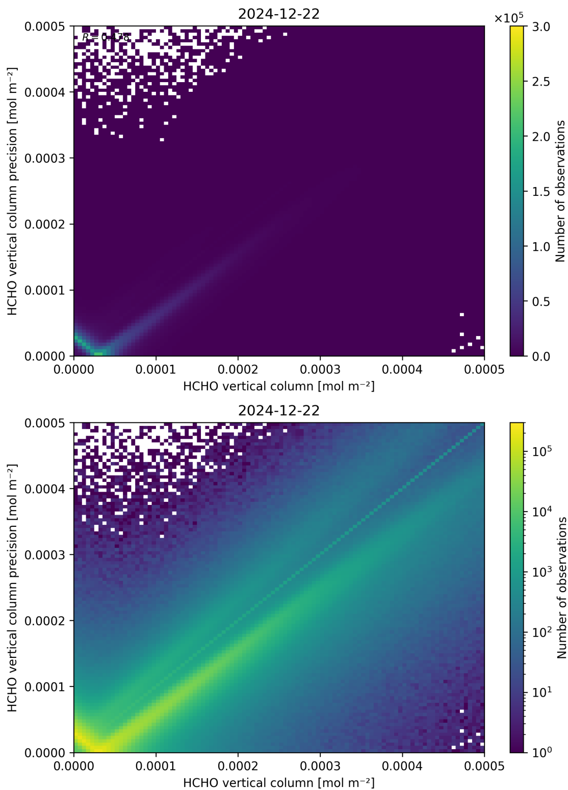
Figure 134: Scatter density plot of “HCHO vertical column” against “HCHO vertical column precision” for 2024-12-22 to 2024-12-23.
