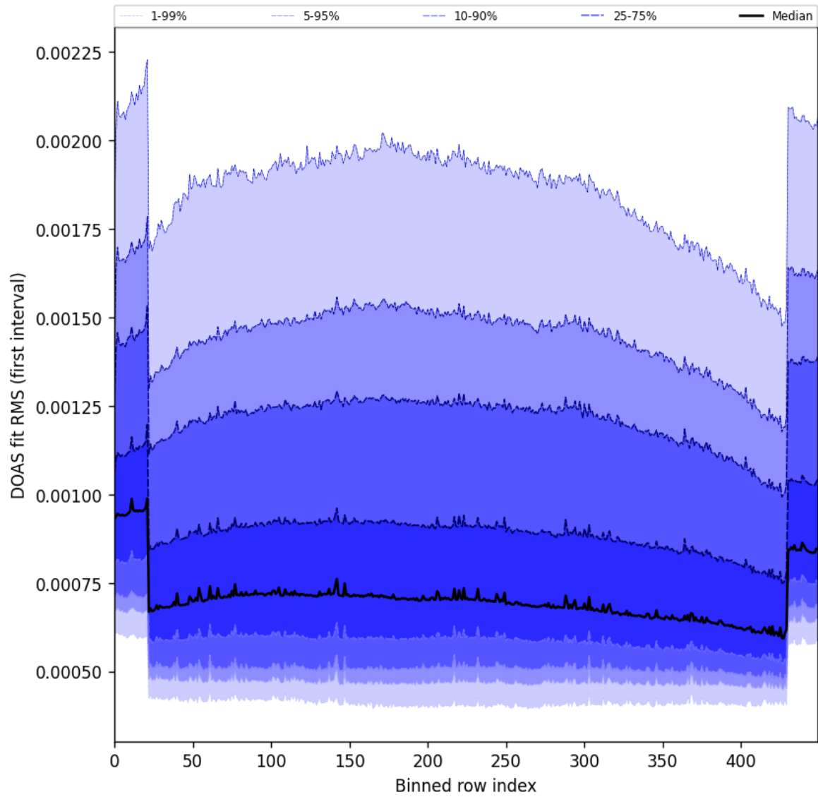
Figure 60: Along track statistics of “DOAS fit RMS (first interval)” for 2024-12-22 to 2024-12-23
