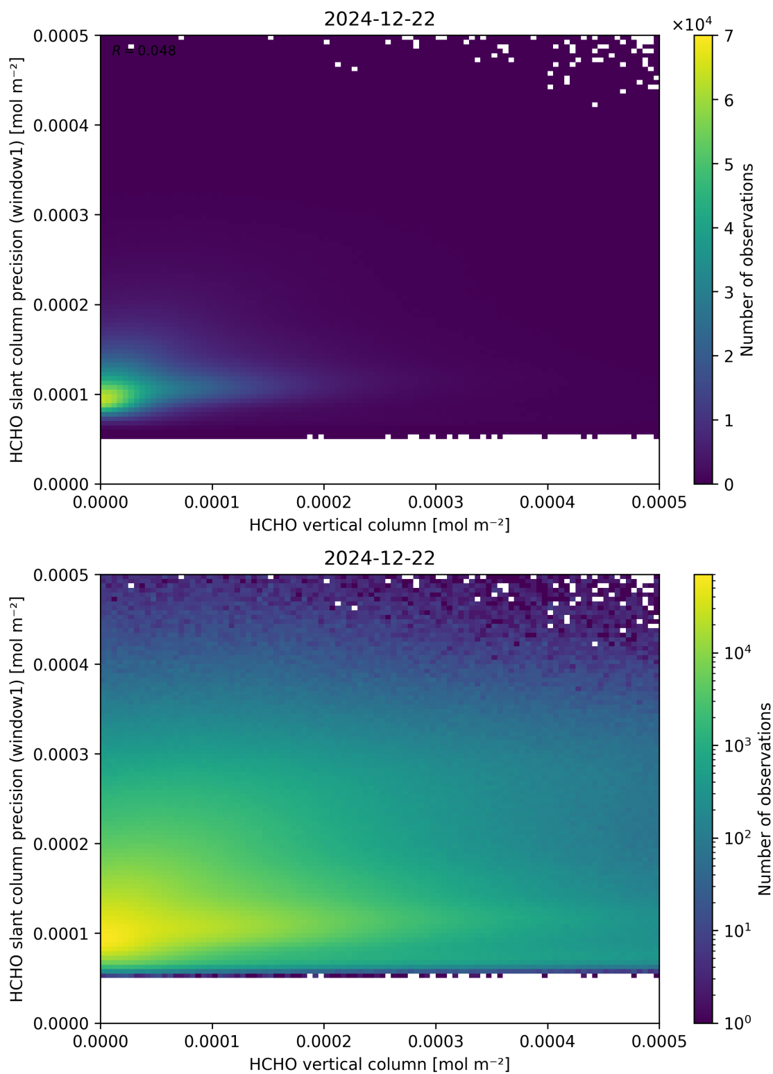
Figure 130: Scatter density plot of “HCHO vertical column” against “HCHO slant column precision (window1)” for 2024-12-22 to 2024-12-23.
