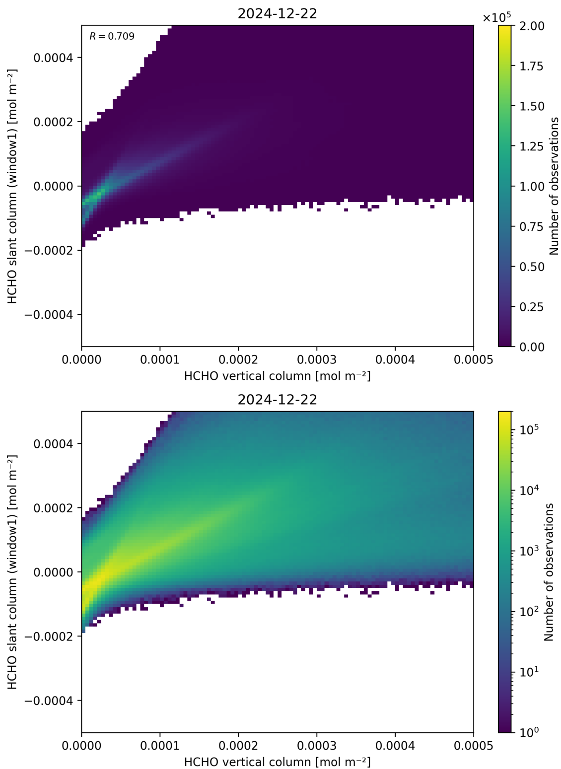
Figure 129: Scatter density plot of “HCHO vertical column” against “HCHO slant column (window1)” for 2024-12-22 to 2024-12-23.
