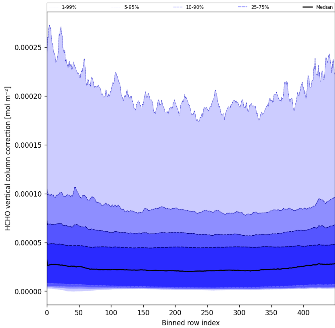
Figure 51: Along track statistics of “HCHO vertical column correction” for 2024-12-22 to 2024-12-23
