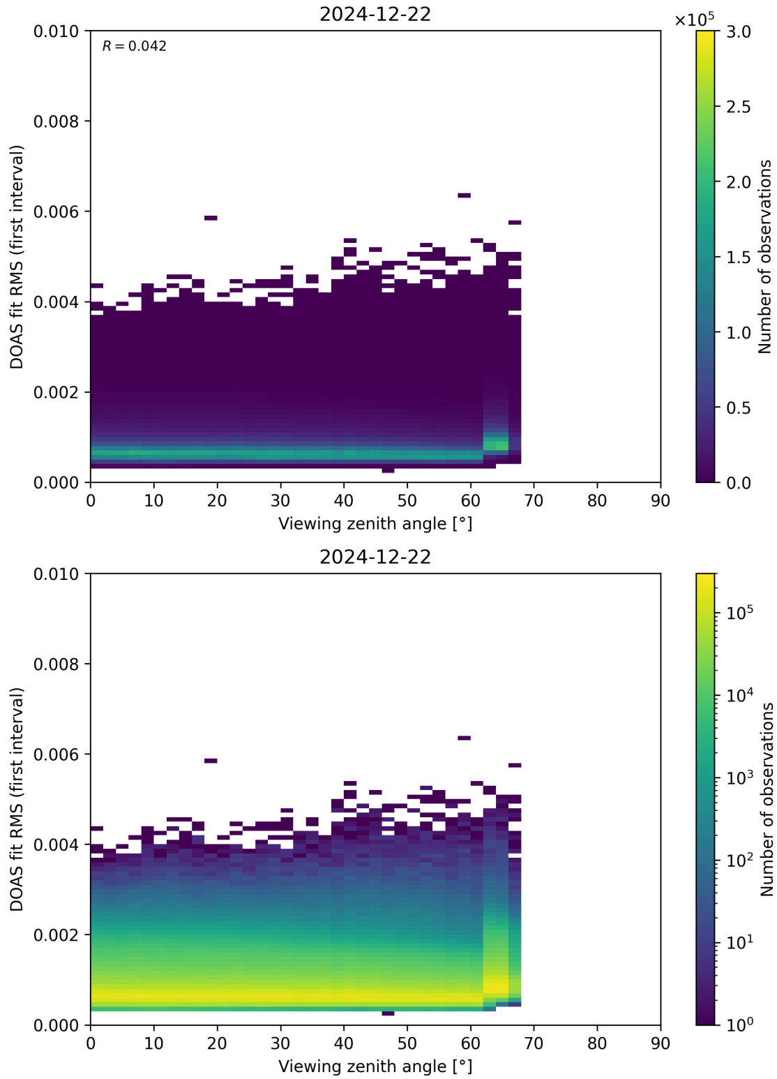
Figure 182: Scatter density plot of “Viewing zenith angle” against “DOAS fit RMS (first interval)” for 2024-12-22 to 2024-12-23.
