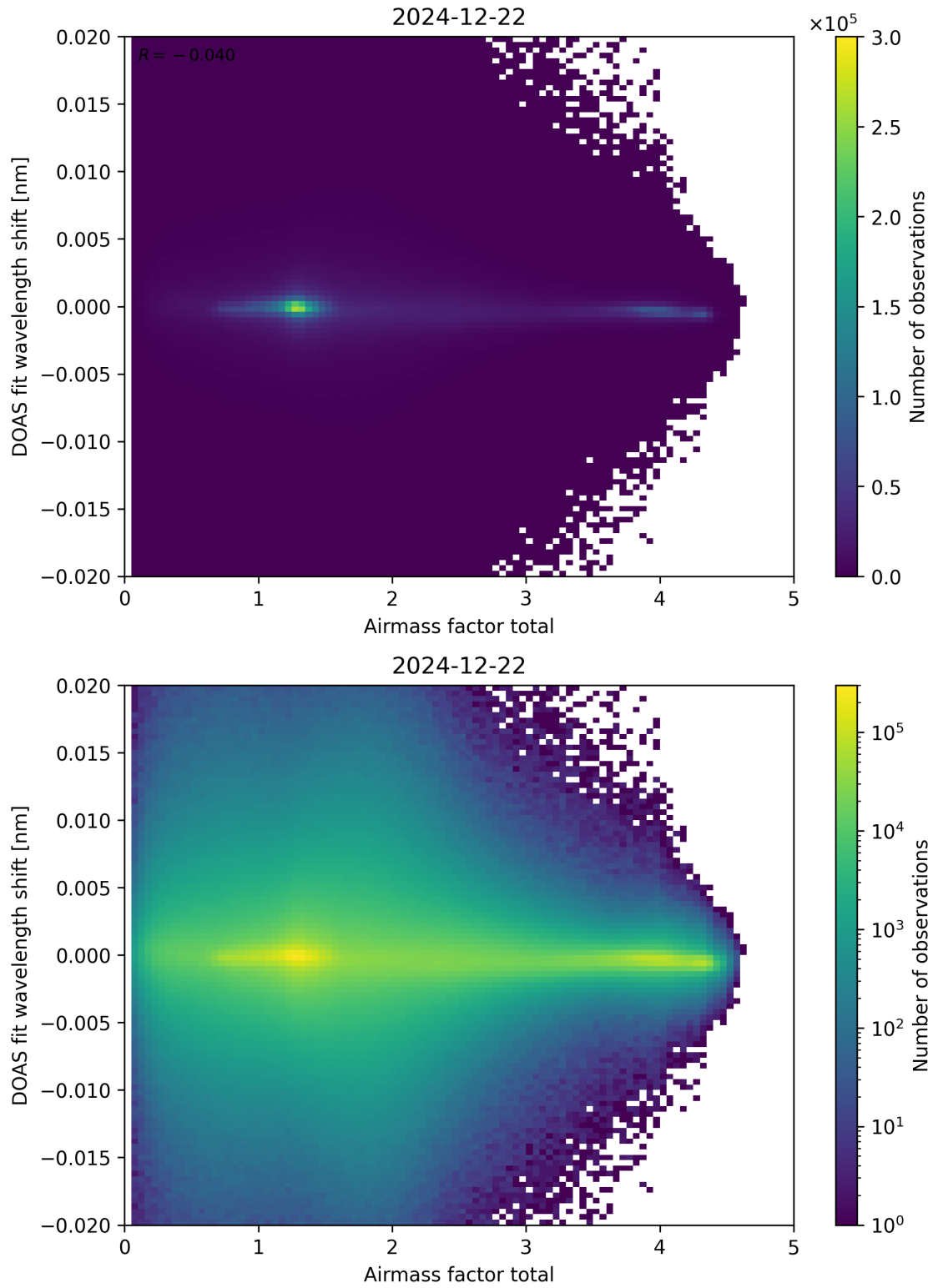
Figure 98: Scatter density plot of “Airmass factor total” against “DOAS fit wavelength shift” for 2024-12-22 to 2024-12-23.
