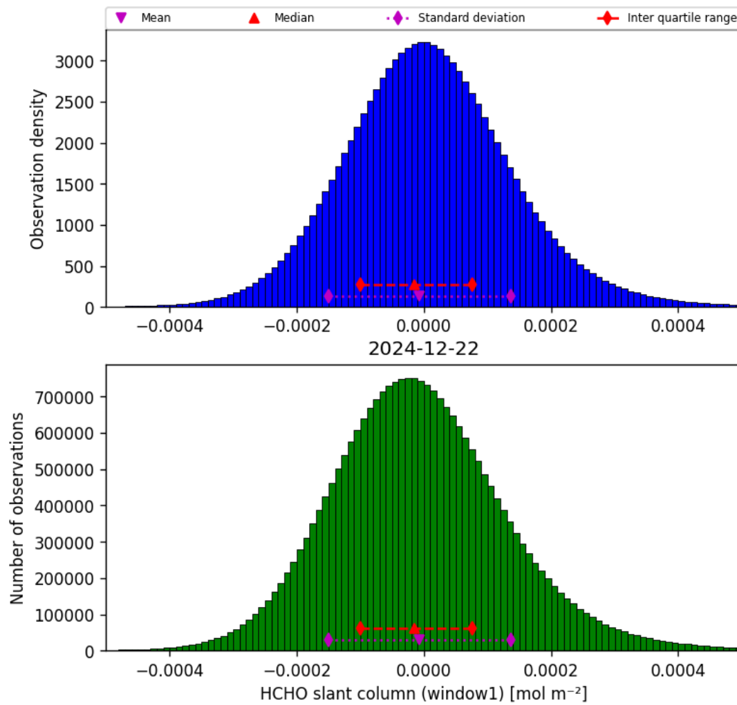
Figure 38: Histogram of “HCHO slant column (window1)” for 2024-12-22 to 2024-12-23
