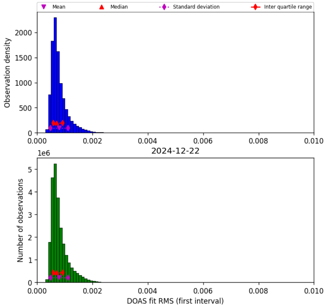
Figure 46: Histogram of “DOAS fit RMS (first interval)” for 2024-12-22 to 2024-12-23
