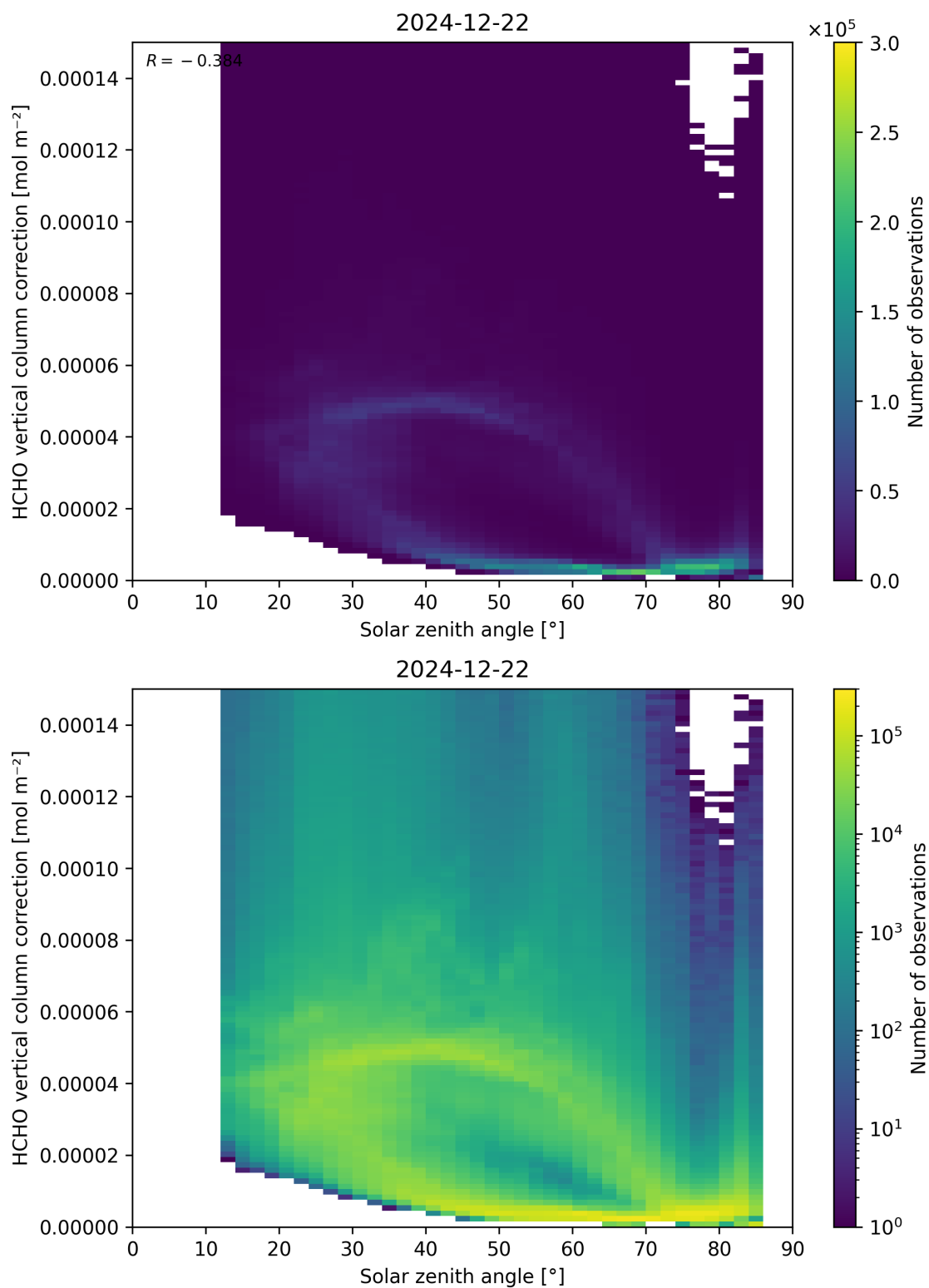
Figure 178: Scatter density plot of “Solar zenith angle” against “HCHO vertical column correction” for 2024-12-22 to 2024-12-23.
