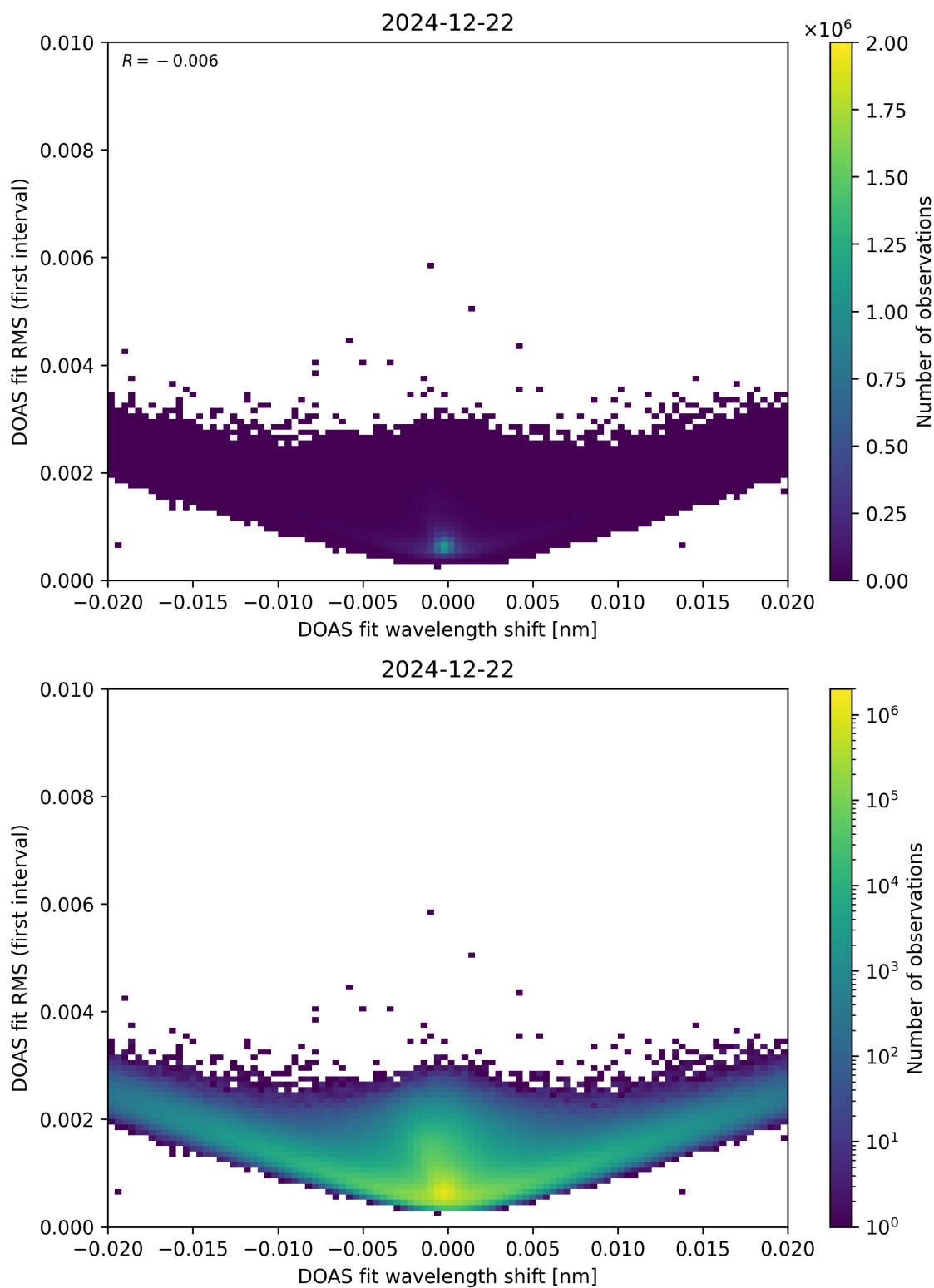
Figure 64: Scatter density plot of “DOAS fit wavelength shift” against “DOAS fit RMS (first interval)” for 2024-12-22 to 2024-12-23.
