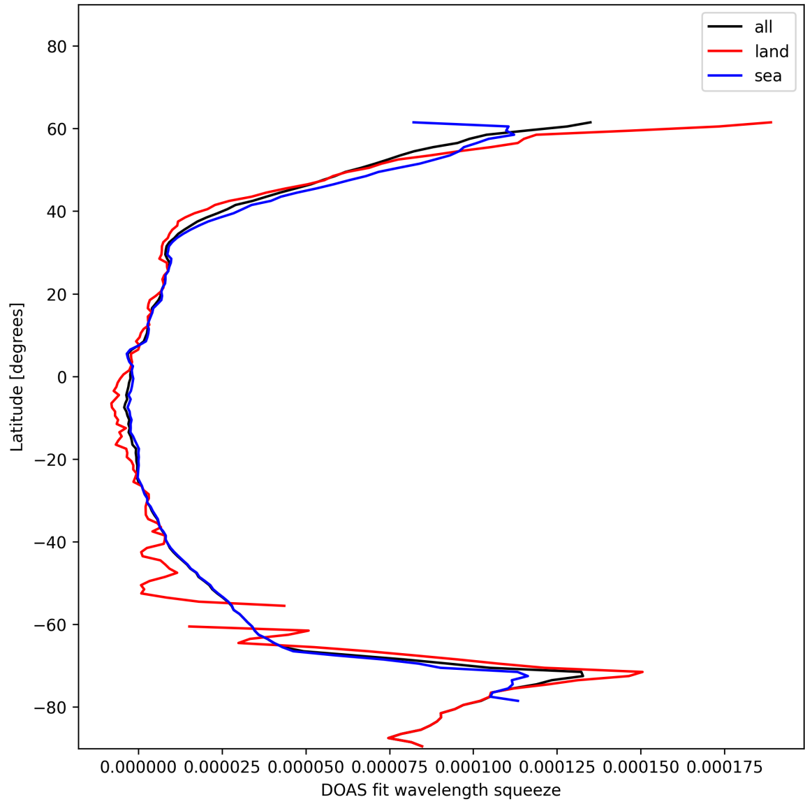
Figure 31: Zonal average of “DOAS fit wavelength squeeze” for 2024-12-22 to 2024-12-23.
