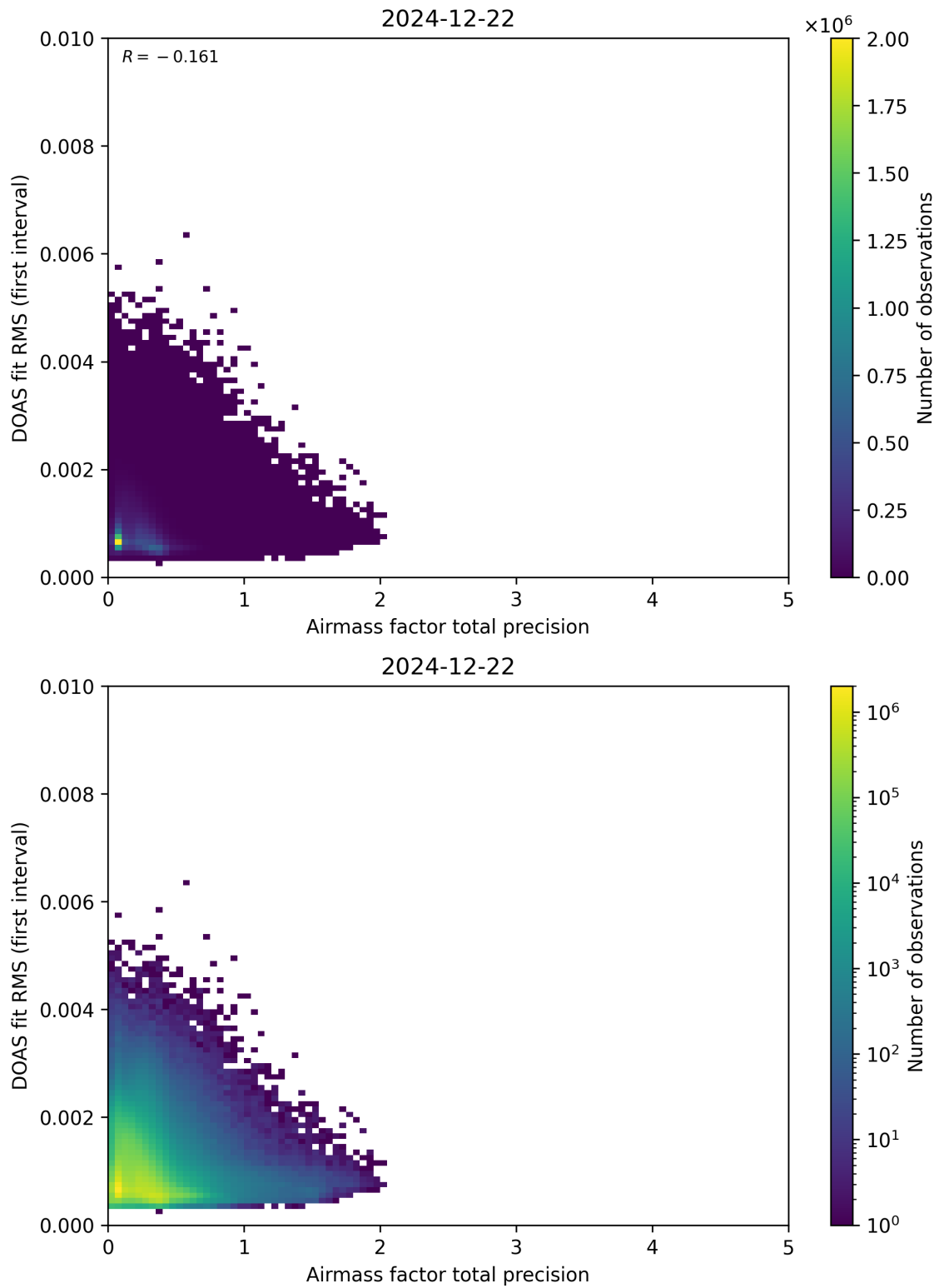
Figure 105: Scatter density plot of “Airmass factor total precision” against “DOAS fit RMS (first interval)” for 2024-12-22 to 2024-12-23.
