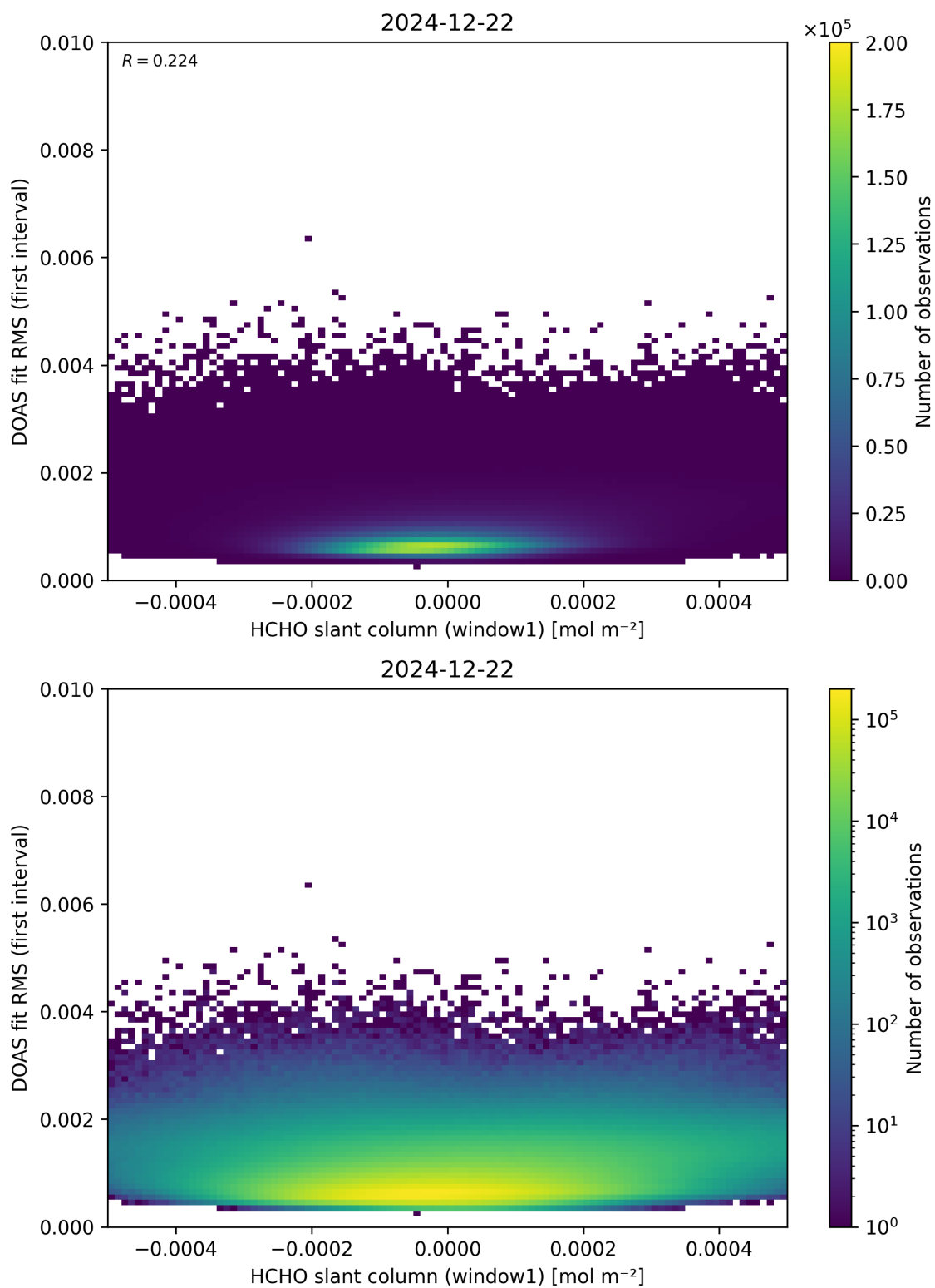
Figure 78: Scatter density plot of “HCHO slant column (window1)” against “DOAS fit RMS (first interval)” for 2024-12-22 to 2024-12-23.
