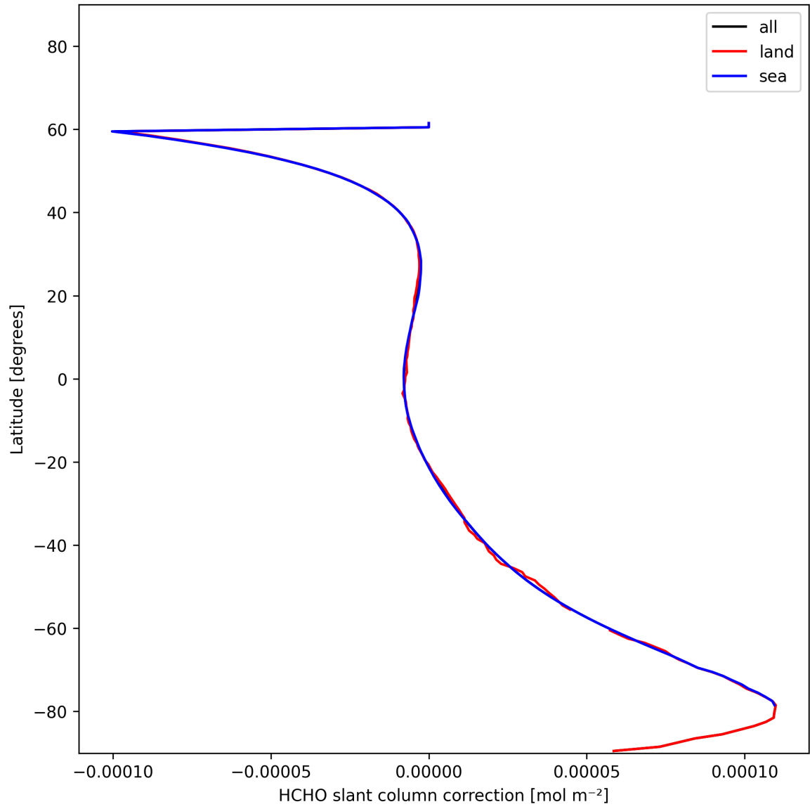
Figure 33: Zonal average of “HCHO slant column correction” for 2024-12-22 to 2024-12-23.
