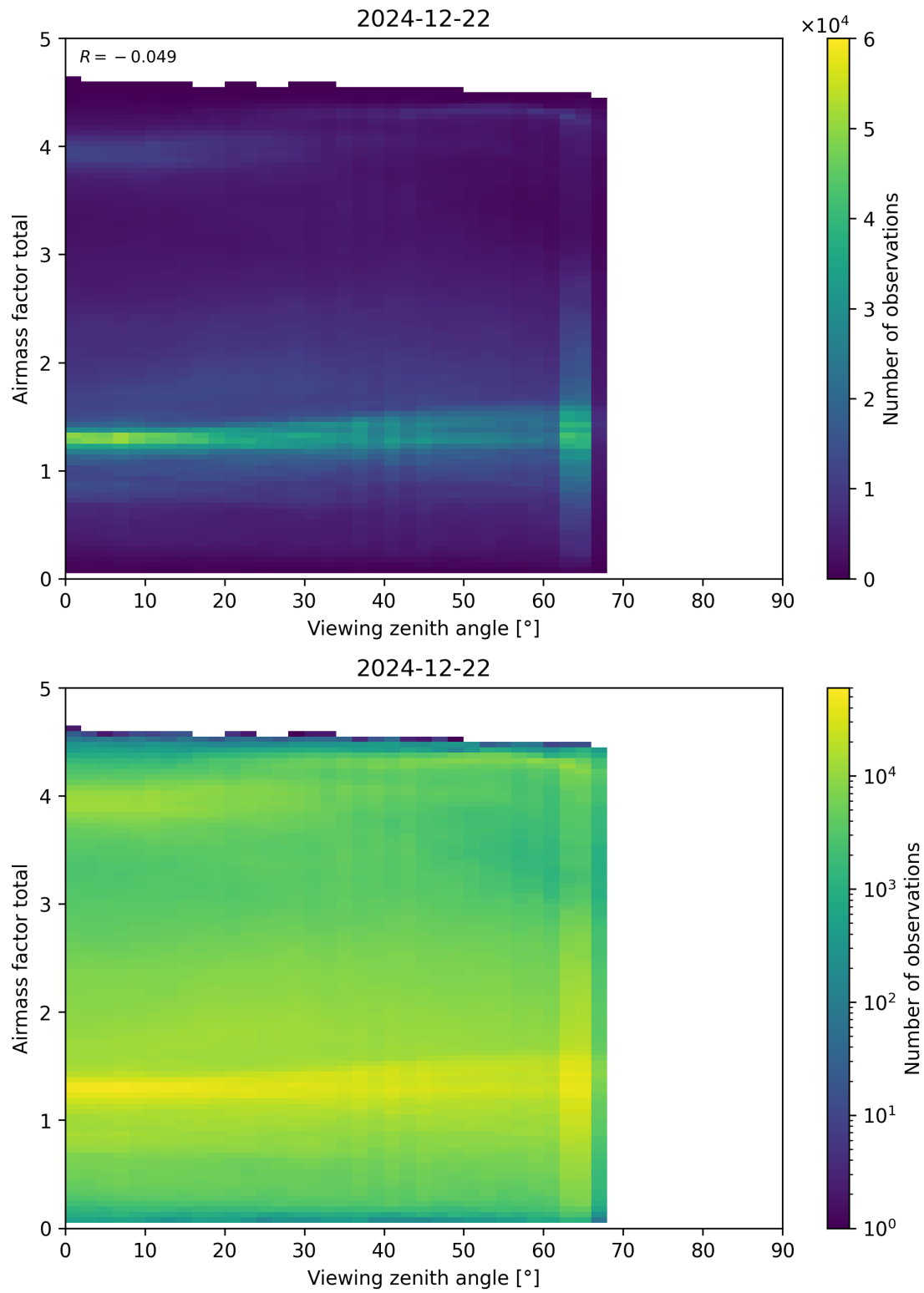
Figure 190: Scatter density plot of “Viewing zenith angle” against “Airmass factor total” for 2024-12-22 to 2024-12-23.
