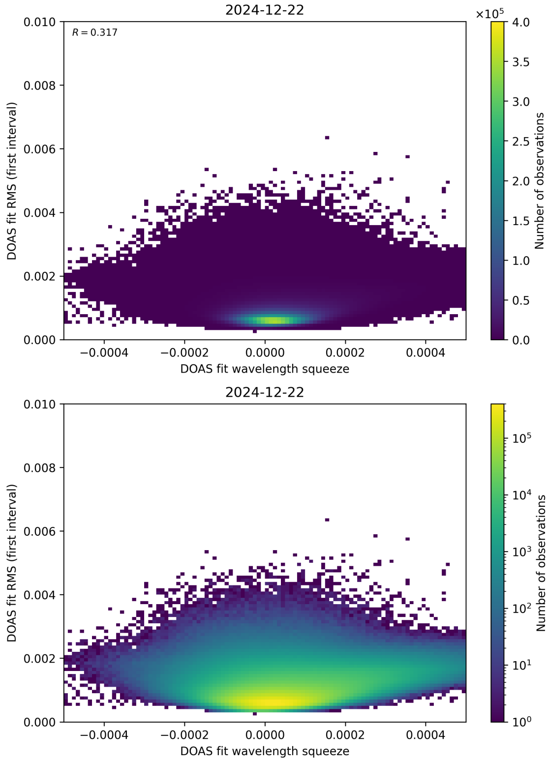
Figure 68: Scatter density plot of “DOAS fit wavelength squeeze” against “DOAS fit RMS (first interval)” for 2024-12-22 to 2024-12-23.
