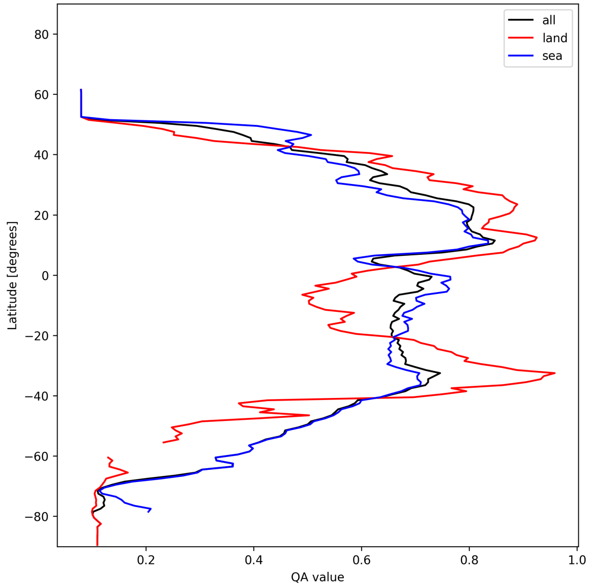
Figure 20: Zonal average of “QA value” for 2024-12-22 to 2024-12-23.
