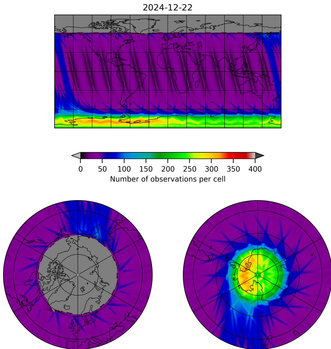
Figure 19: Map of the number of observations for 2024-12-22 to 2024-12-23
