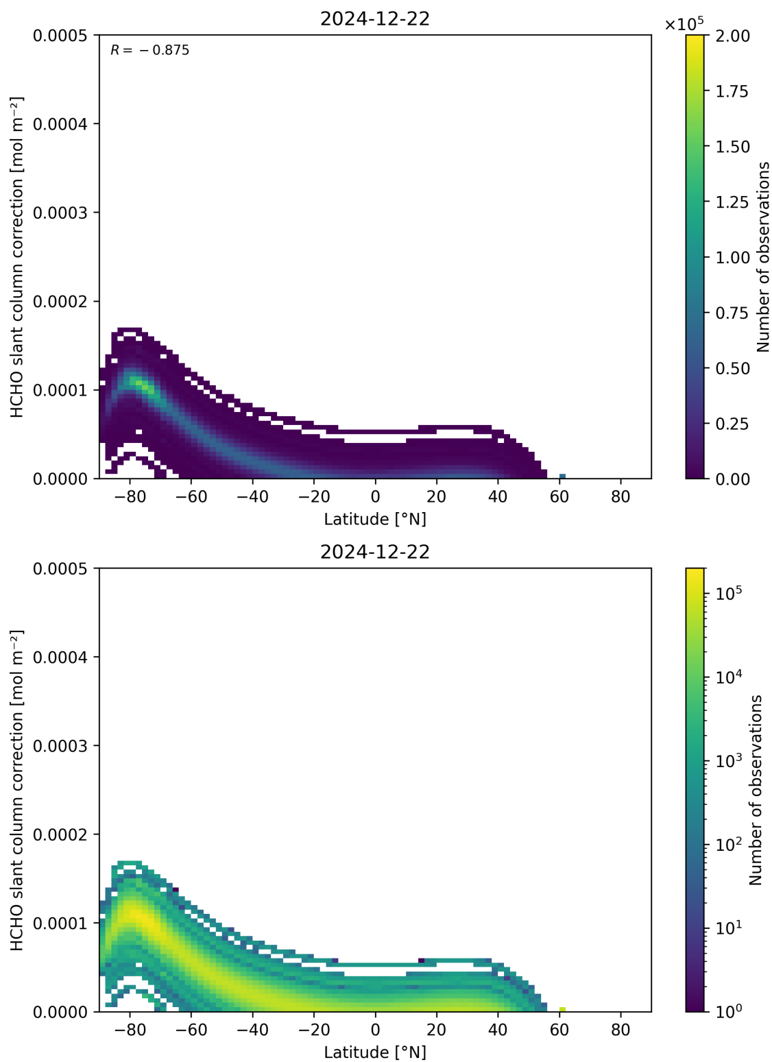
Figure 158: Scatter density plot of “Latitude” against “HCHO slant column correction” for 2024-12-22 to 2024-12-23.
