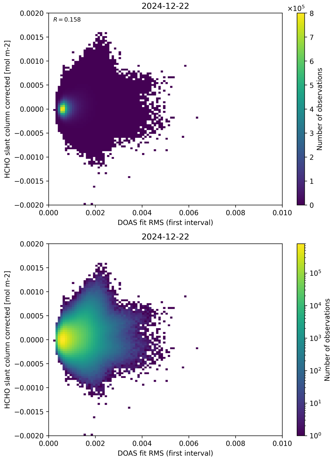
Figure 62: Scatter density plot of “DOAS fit RMS (first interval)” against “HCHO slant column corrected” for 2024-12-22 to 2024-12-23.
