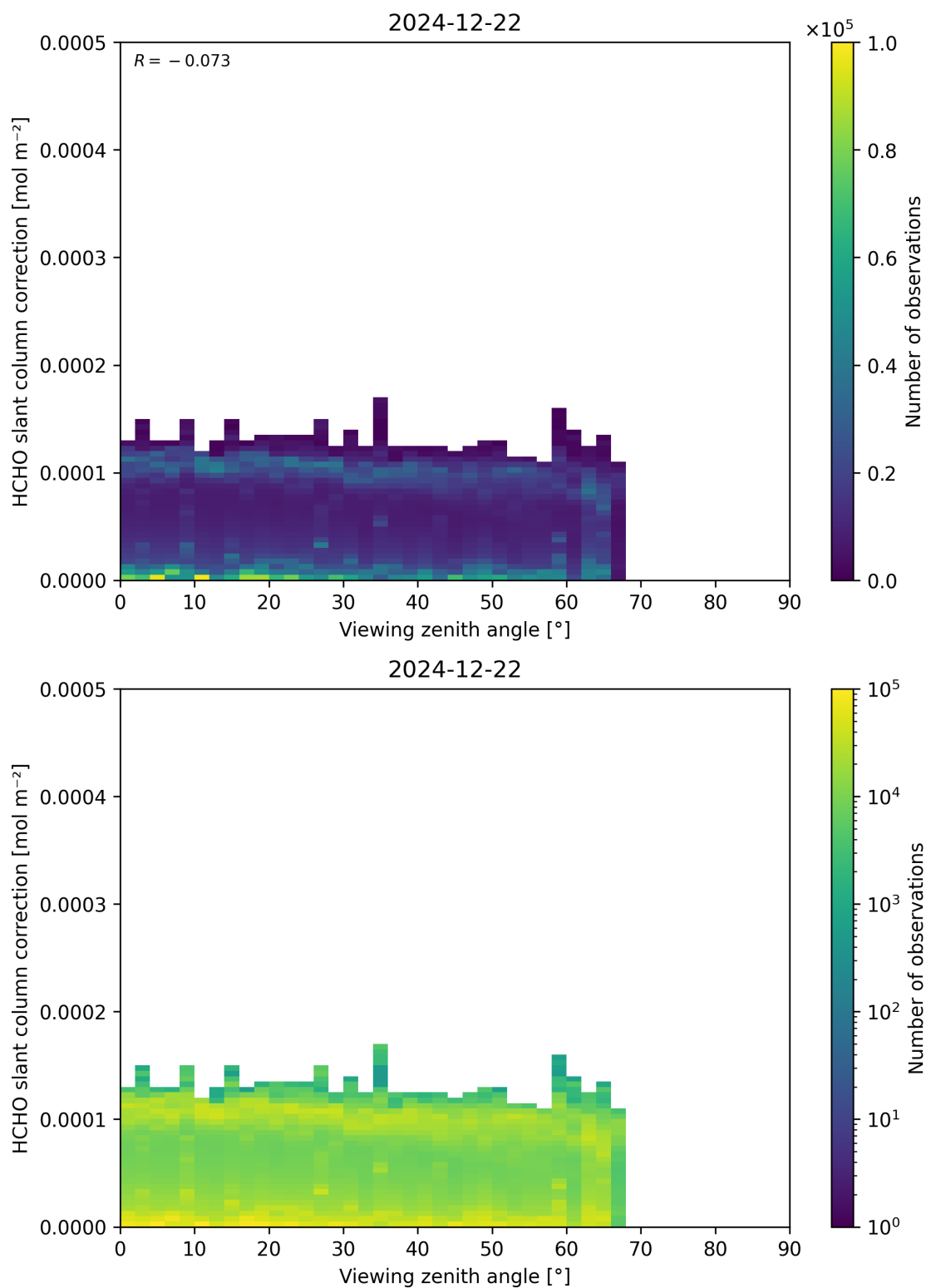
Figure 187: Scatter density plot of “Viewing zenith angle” against “HCHO slant column correction” for 2024-12-22 to 2024-12-23.
