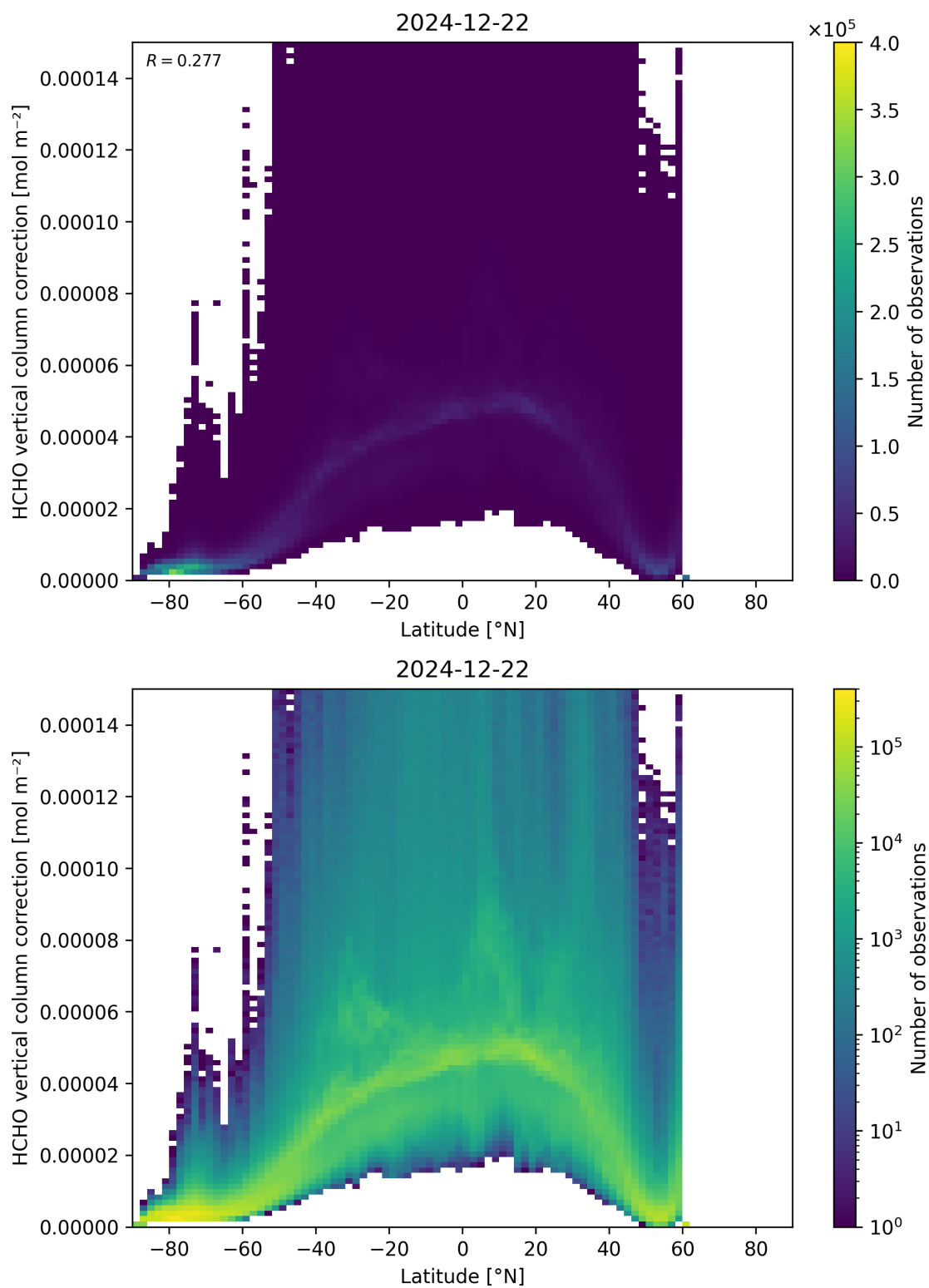
Figure 164: Scatter density plot of “Latitude” against “HCHO vertical column correction” for 2024-12-22 to 2024-12-23.
