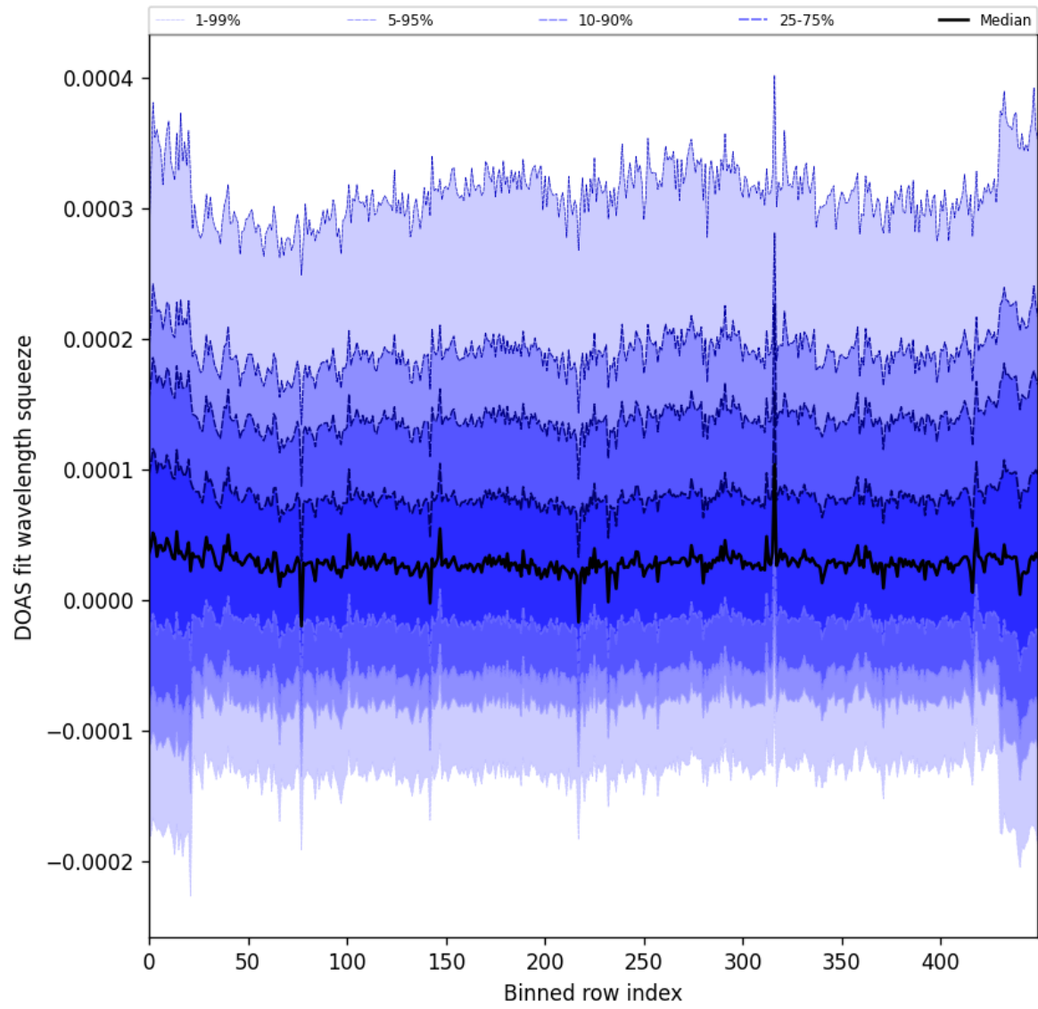
Figure 59: Along track statistics of “DOAS fit wavelength squeeze” for 2024-12-22 to 2024-12-23
