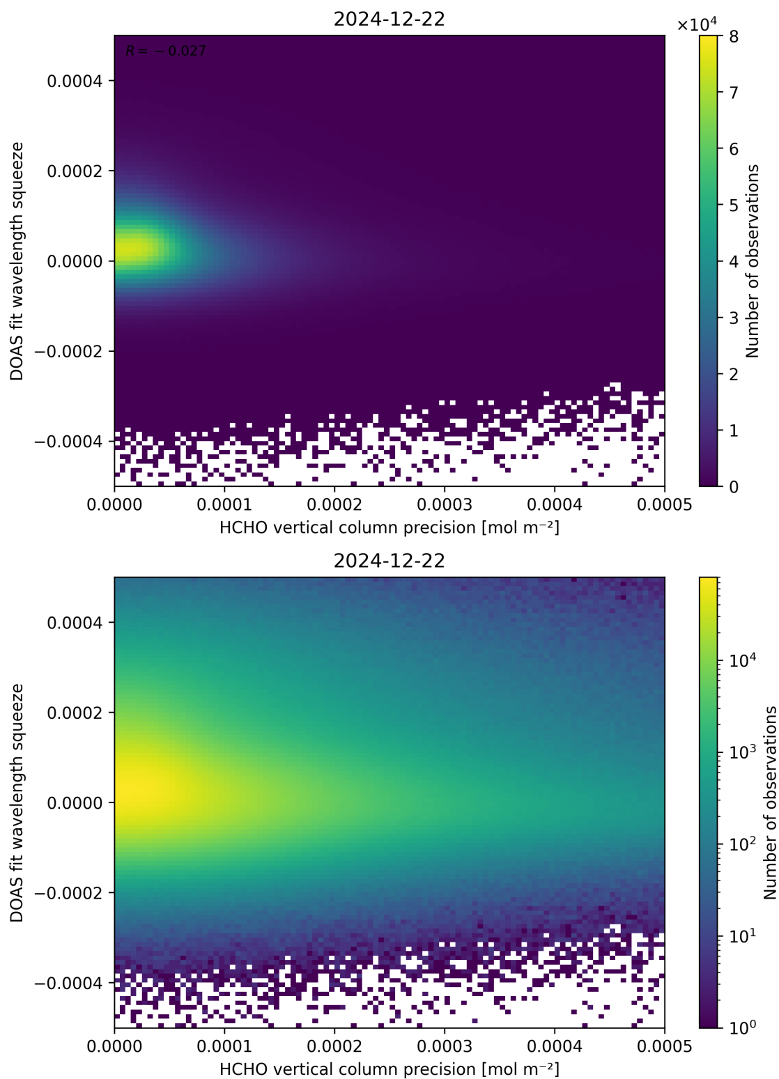
Figure 138: Scatter density plot of “HCHO vertical column precision” against “DOAS fit wavelength squeeze” for 2024-12-22 to 2024-12-23.
