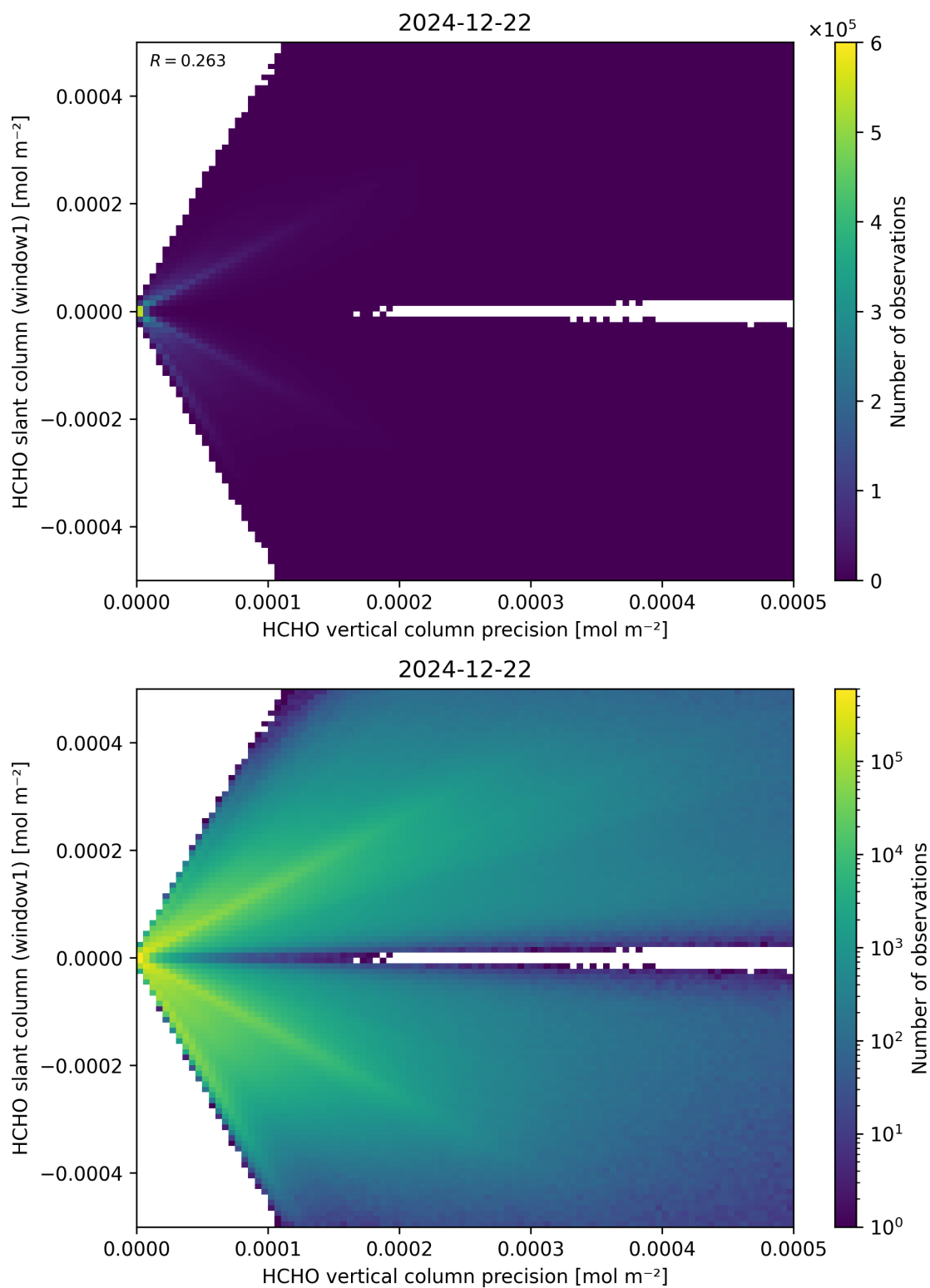
Figure 142: Scatter density plot of “HCHO vertical column precision” against “HCHO slant column (window1)” for 2024-12-22 to 2024-12-23.
