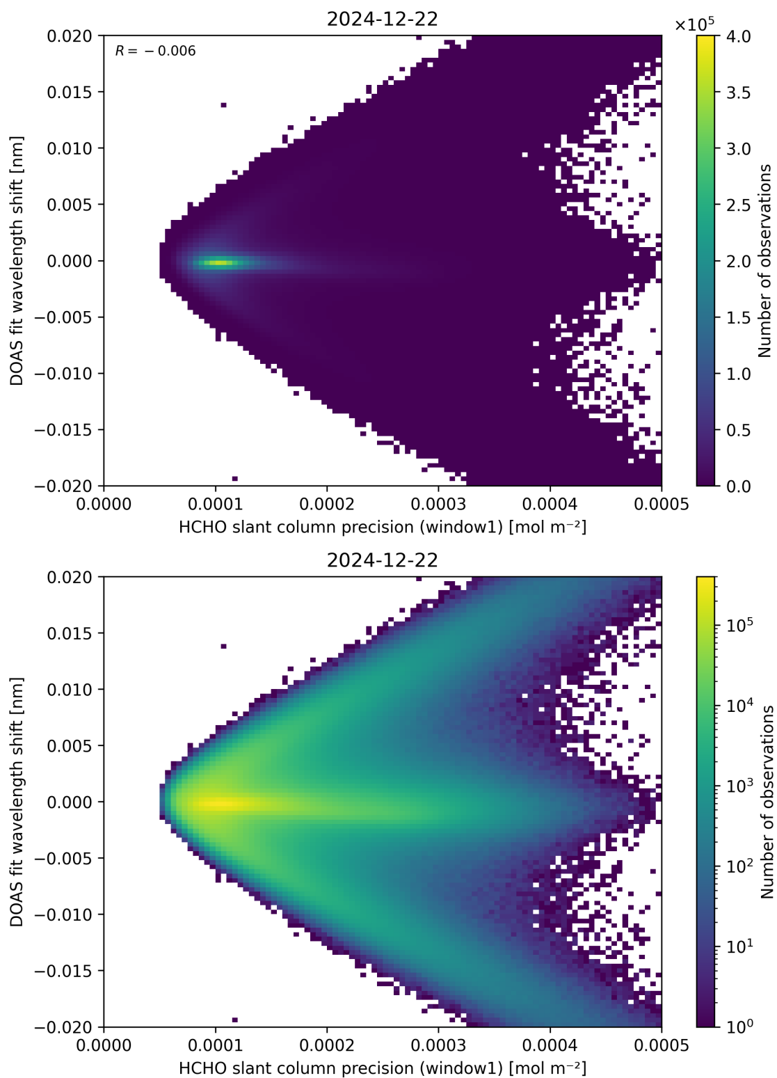
Figure 89: Scatter density plot of “HCHO slant column precision (window1)” against “DOAS fit wavelength shift” for 2024-12-22 to 2024-12-23.
