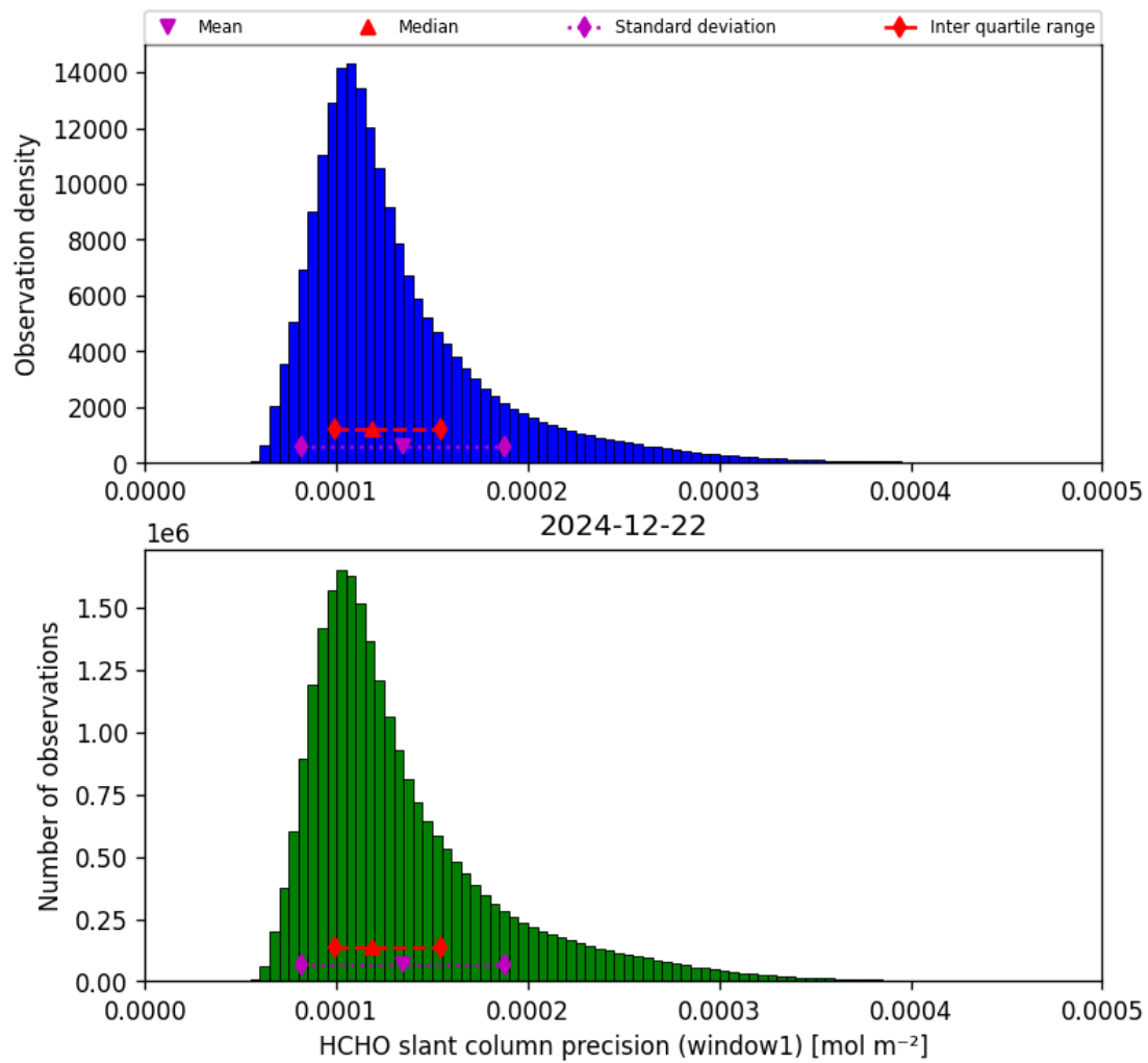
Figure 39: Histogram of “HCHO slant column precision (window1)” for 2024-12-22 to 2024-12-23
