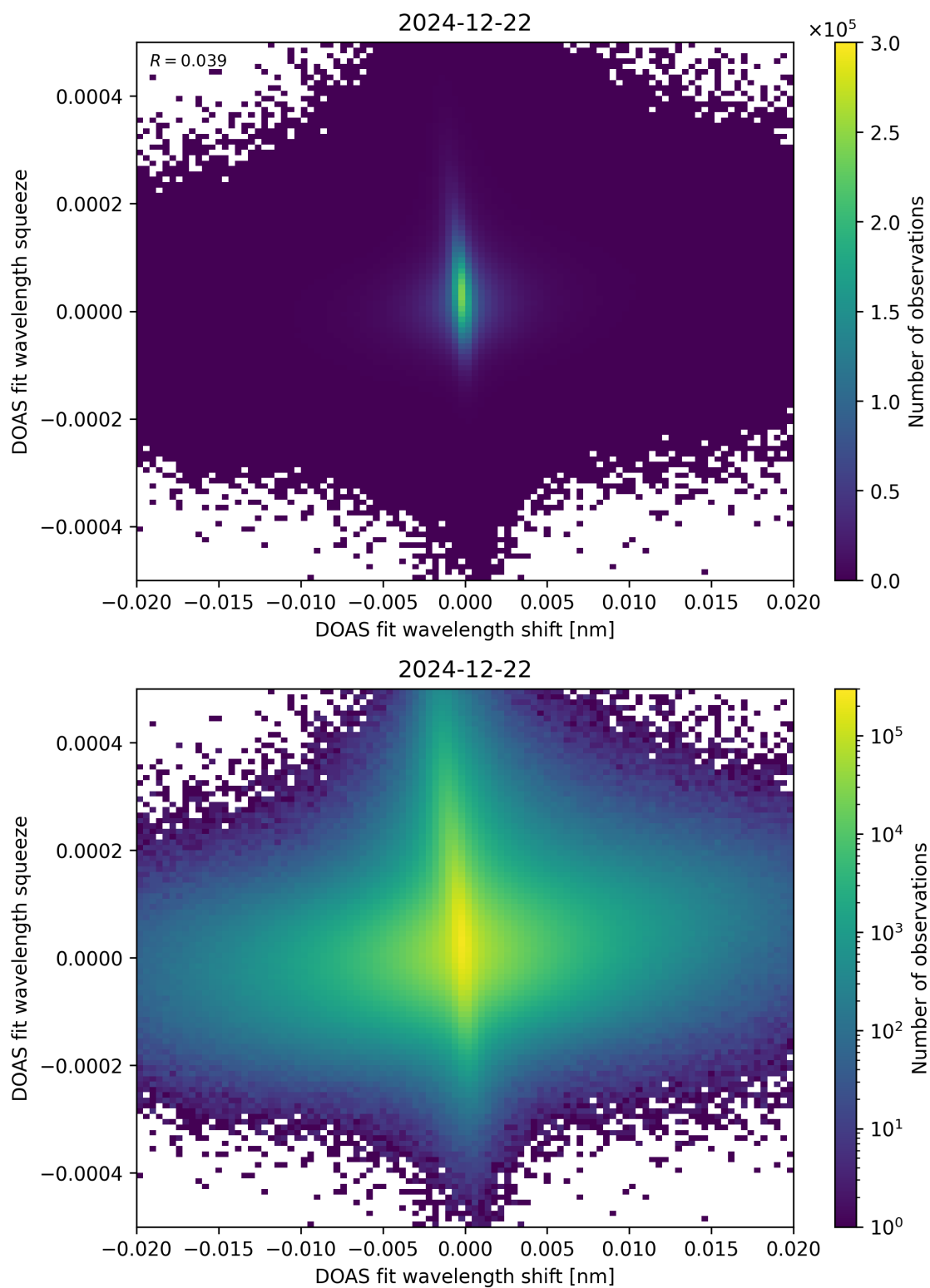
Figure 65: Scatter density plot of “DOAS fit wavelength shift” against “DOAS fit wavelength squeeze” for 2024-12-22 to 2024-12-23.
