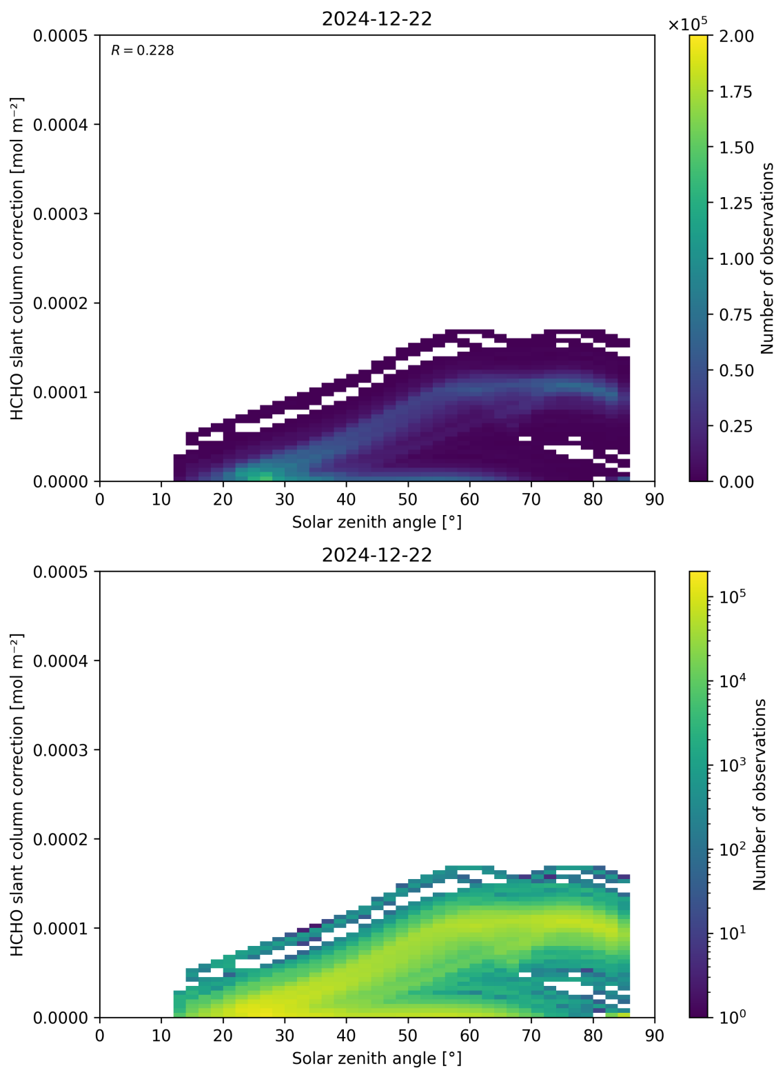
Figure 172: Scatter density plot of “Solar zenith angle” against “HCHO slant column correction” for 2024-12-22 to 2024-12-23.
