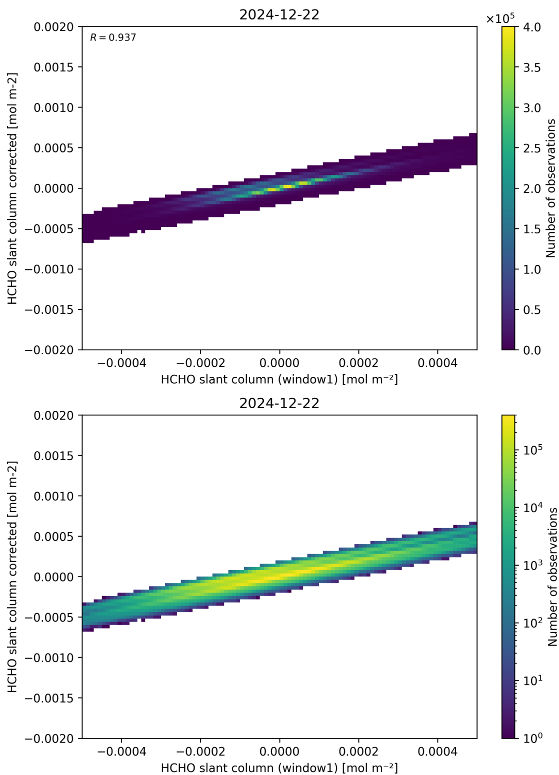
Figure 82: Scatter density plot of “HCHO slant column (window1)” against “HCHO slant column corrected” for 2024-12-22 to 2024-12-23.
