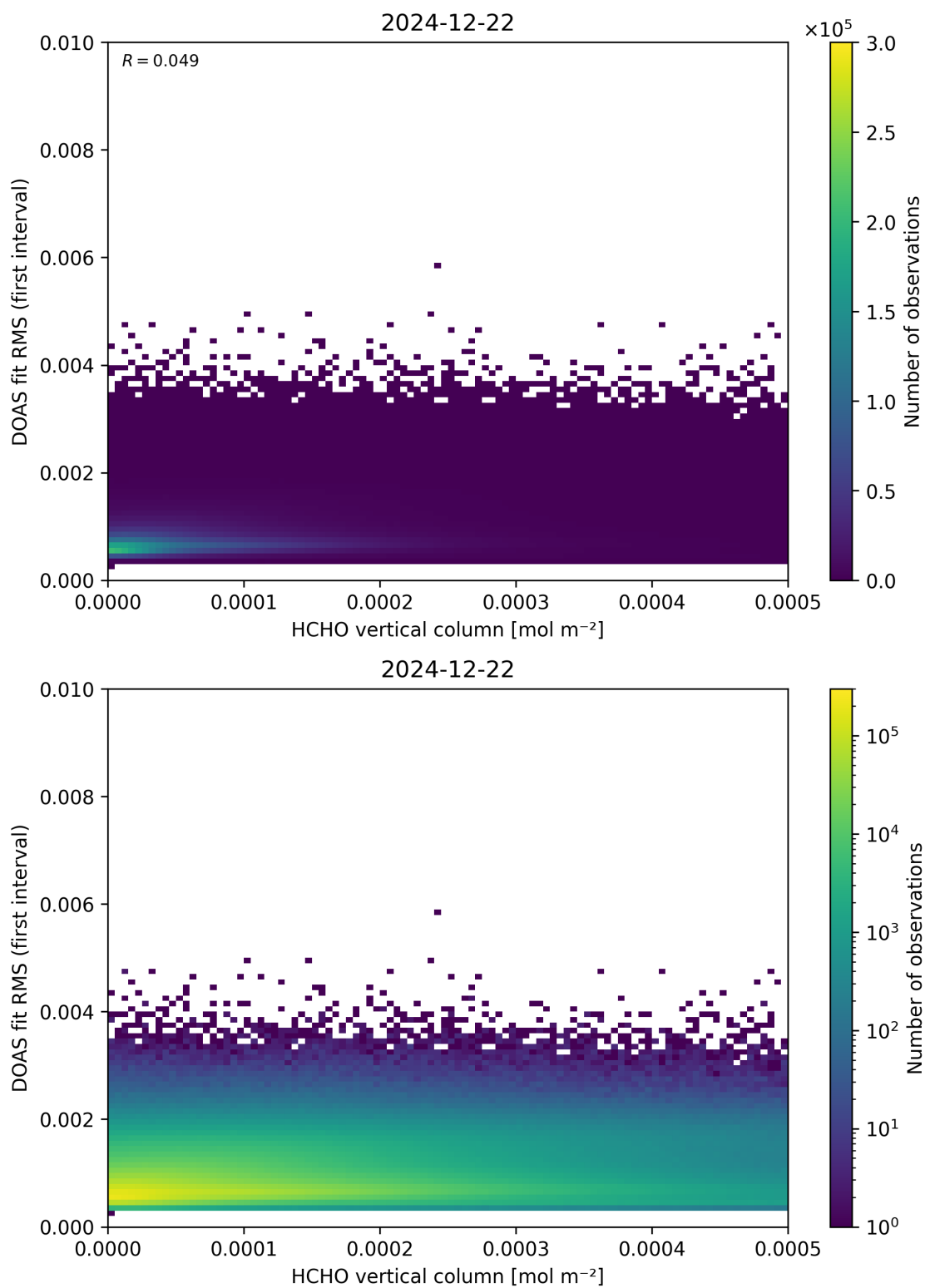
Figure 123: Scatter density plot of “HCHO vertical column” against “DOAS fit RMS (first interval)” for 2024-12-22 to 2024-12-23.
