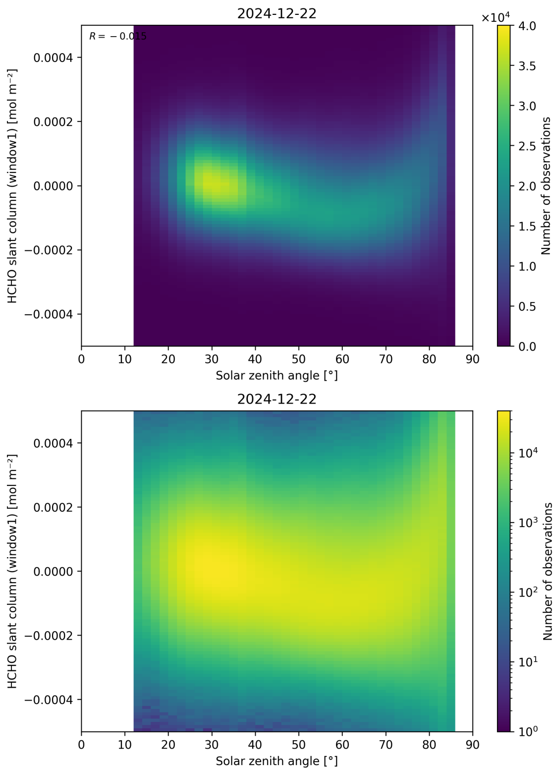
Figure 173: Scatter density plot of “Solar zenith angle” against “HCHO slant column (window1)” for 2024-12-22 to 2024-12-23.
