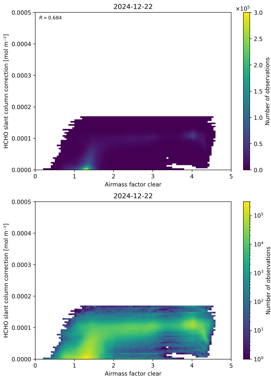
Figure 75: Scatter density plot of “Airmass factor clear” against “HCHO slant column correction” for 2024-12-22 to 2024-12-23.
