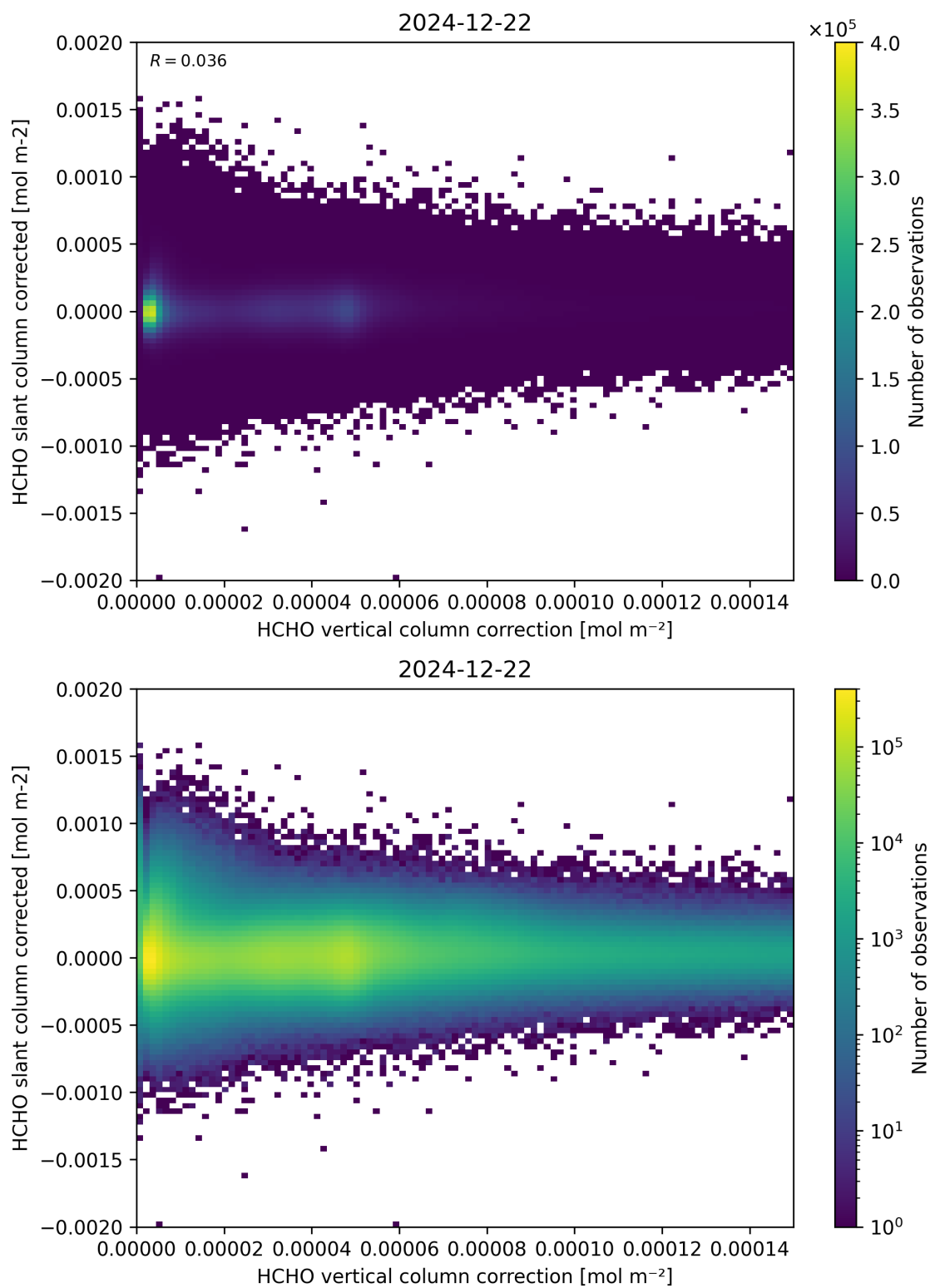
Figure 116: Scatter density plot of “HCHO vertical column correction” against “HCHO slant column corrected” for 2024-12-22 to 2024-12-23.
