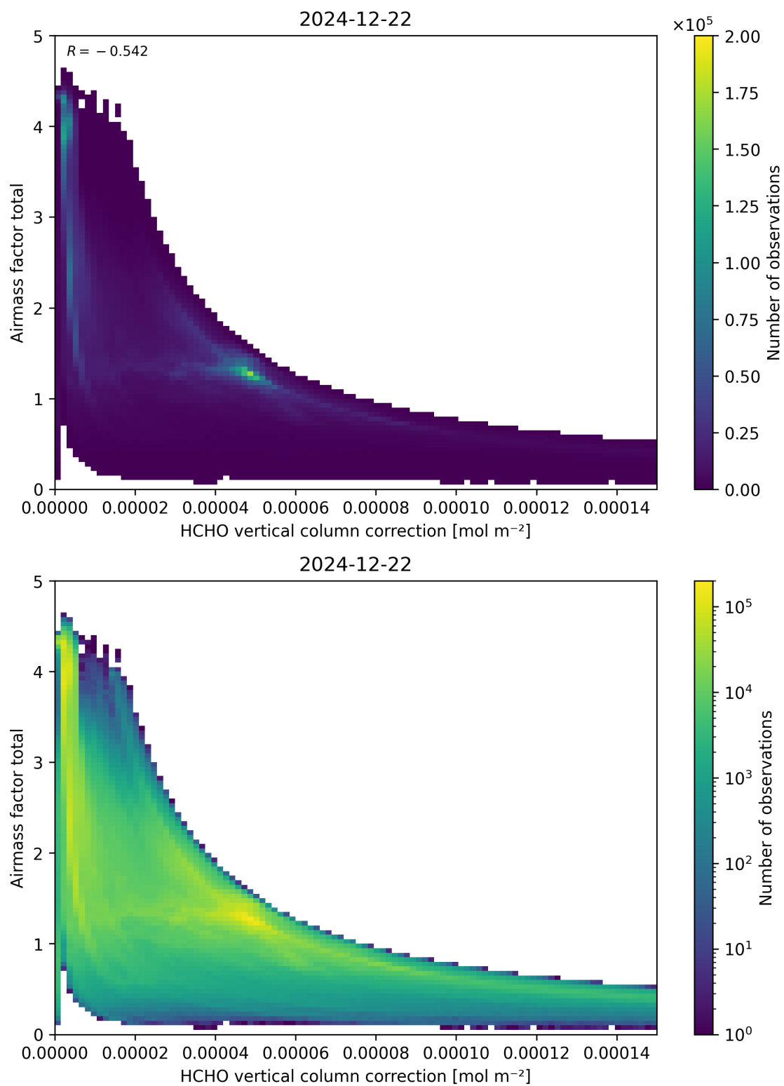
Figure 120: Scatter density plot of “HCHO vertical column correction” against “Airmass factor total” for 2024-12-22 to 2024-12-23.
