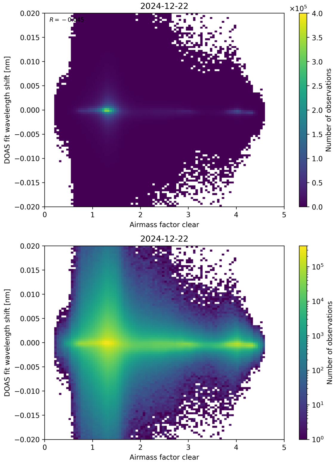
Figure 72: Scatter density plot of “Airmass factor clear” against “DOAS fit wavelength shift” for 2024-12-22 to 2024-12-23.
