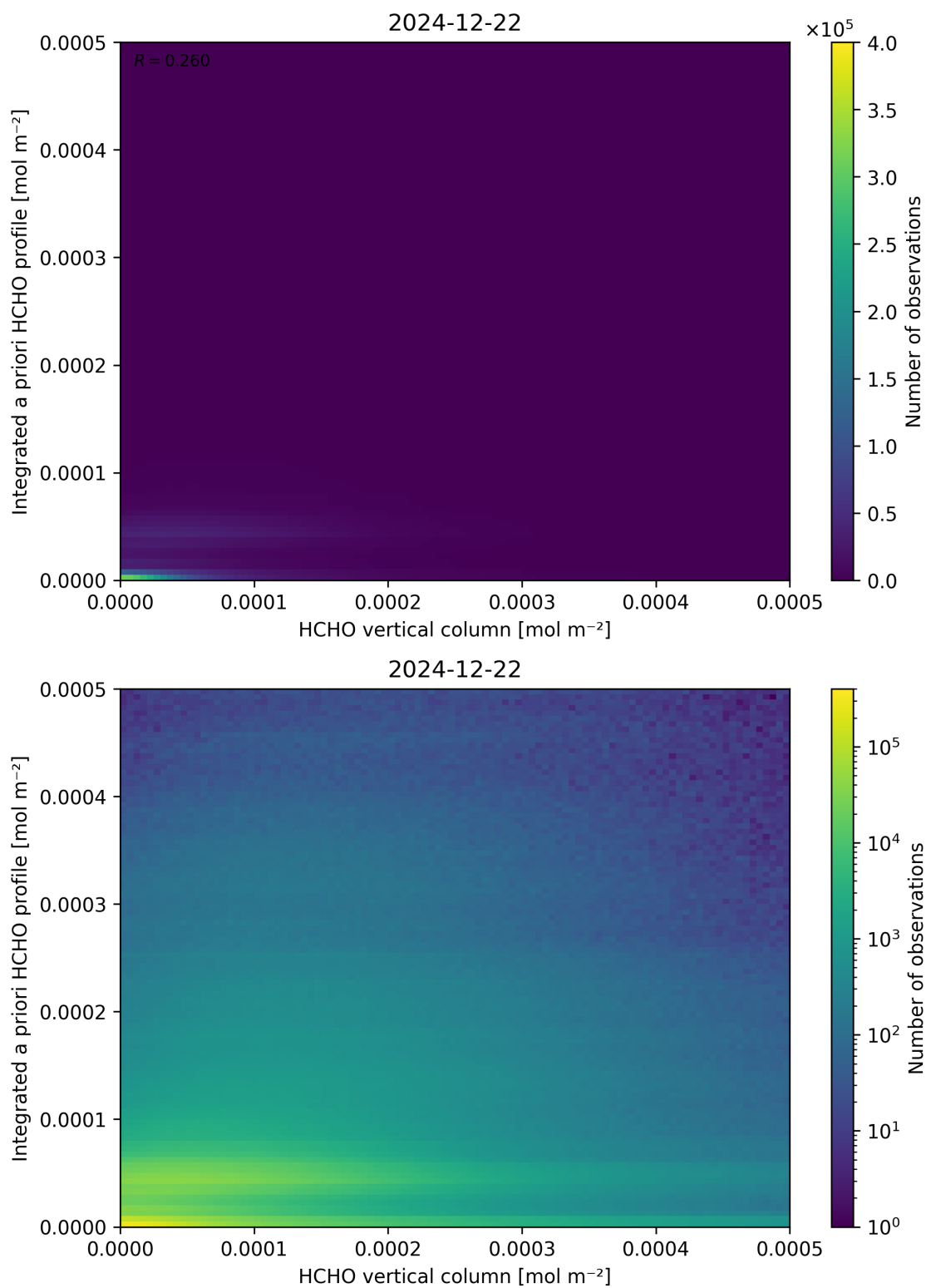
Figure 135: Scatter density plot of “HCHO vertical column” against “Integrated a priori HCHO profile” for 2024-12-22 to 2024-12-23.
