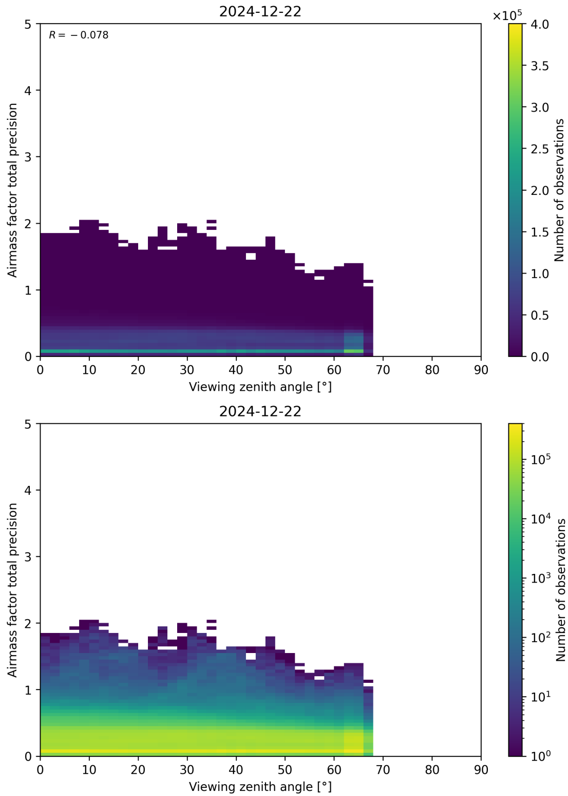
Figure 191: Scatter density plot of “Viewing zenith angle” against “Airmass factor total precision” for 2024-12-22 to 2024-12-23.
