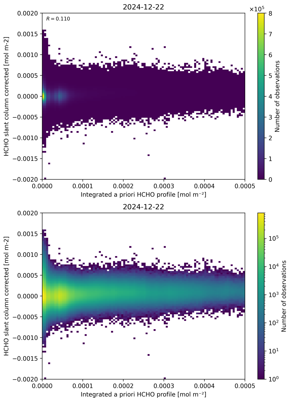
Figure 151: Scatter density plot of “Integrated a priori HCHO profile” against “HCHO slant column corrected” for 2024-12-22 to 2024-12-23.
