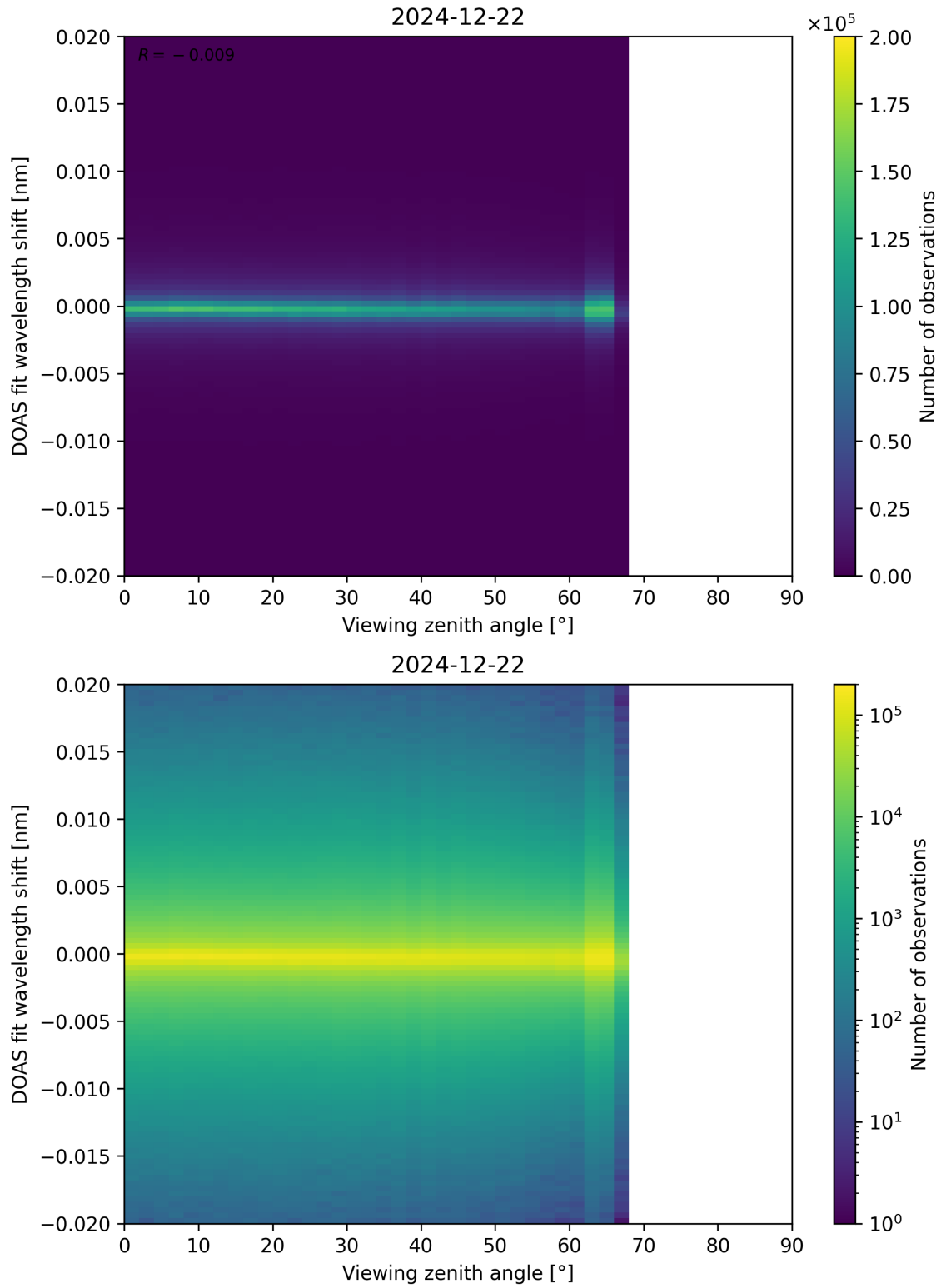
Figure 183: Scatter density plot of “Viewing zenith angle” against “DOAS fit wavelength shift” for 2024-12-22 to 2024-12-23.
