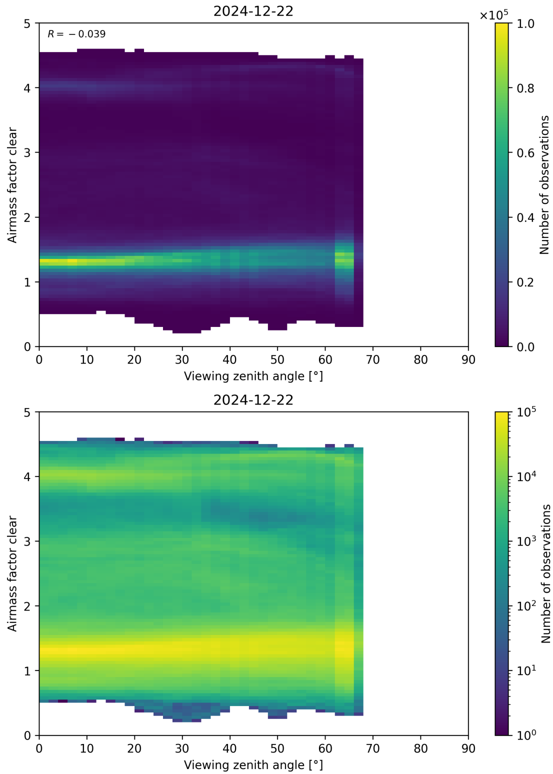
Figure 185: Scatter density plot of “Viewing zenith angle” against “Airmass factor clear” for 2024-12-22 to 2024-12-23.
