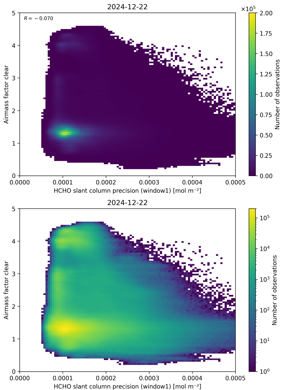
Figure 91: Scatter density plot of “HCHO slant column precision (window1)” against “Airmass factor clear” for 2024-12-22 to 2024-12-23.
