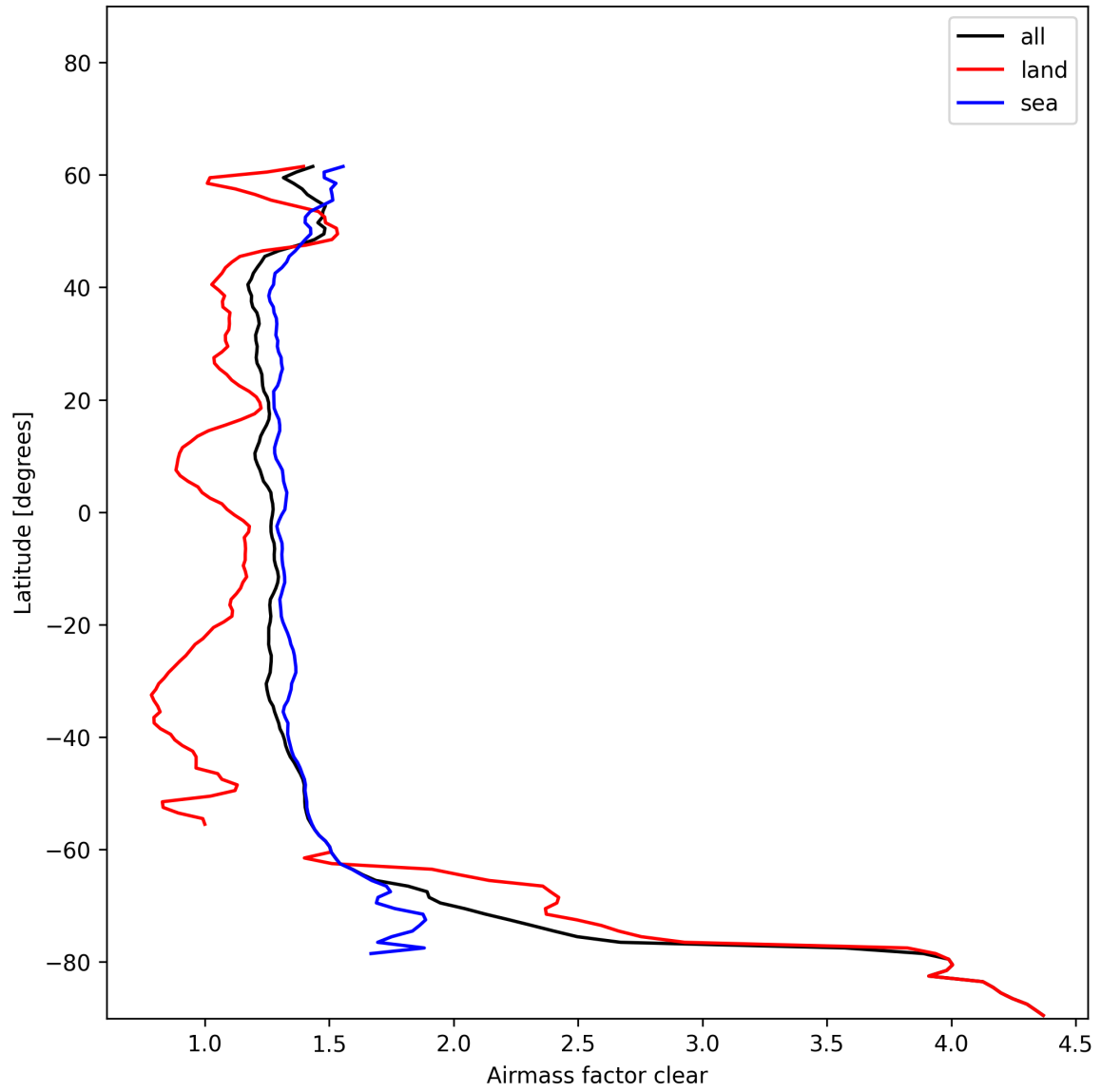
Figure 28: Zonal average of “Airmass factor clear” for 2024-12-22 to 2024-12-23.
