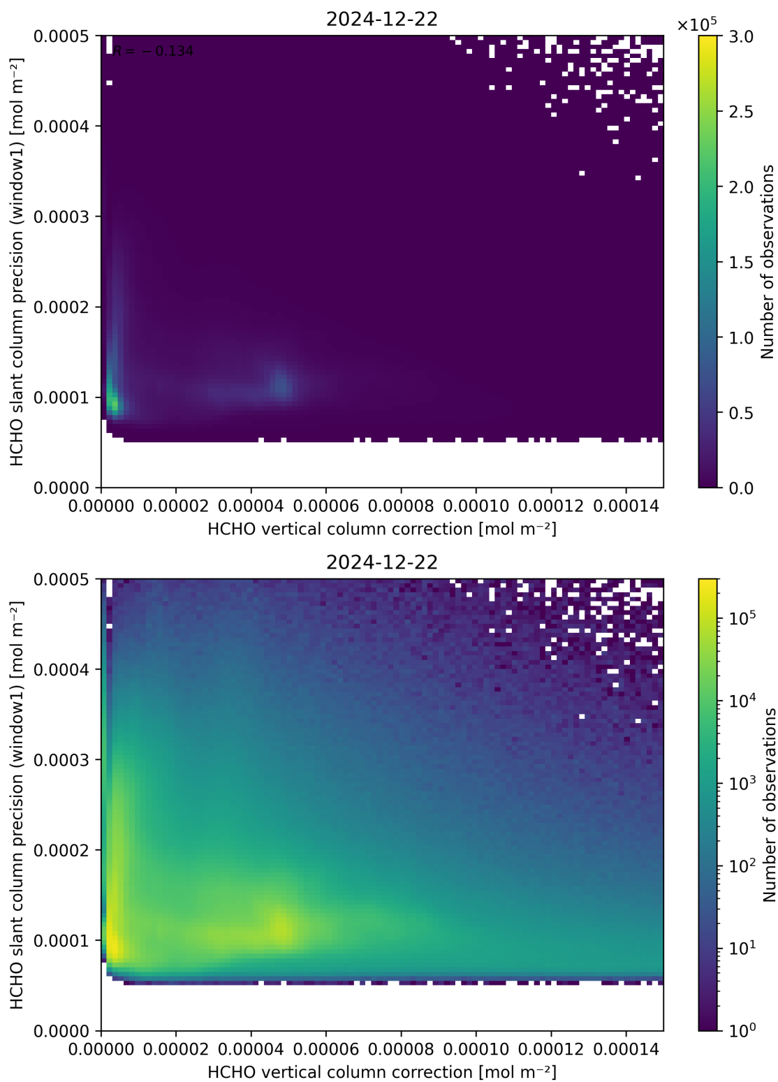
Figure 119: Scatter density plot of “HCHO vertical column correction” against “HCHO slant column precision (window1)” for 2024-12-22 to 2024-12-23.
