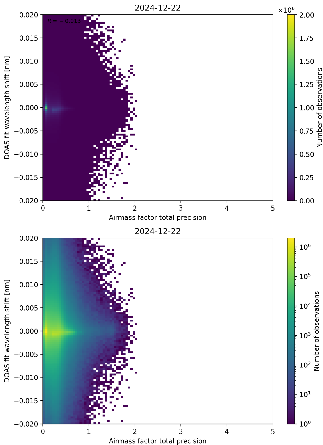
Figure 106: Scatter density plot of “Airmass factor total precision” against “DOAS fit wavelength shift” for 2024-12-22 to 2024-12-23.
