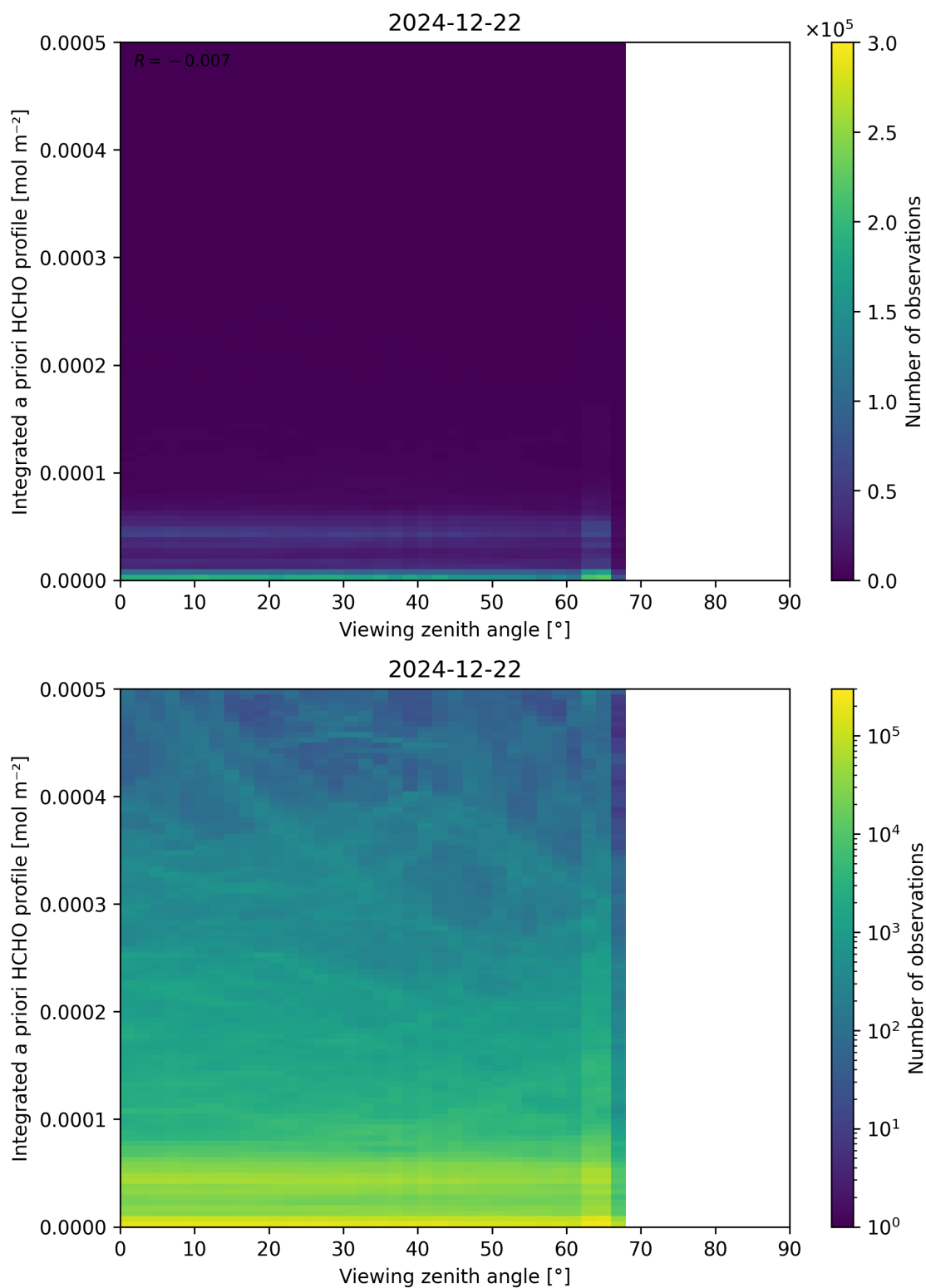
Figure 195: Scatter density plot of “Viewing zenith angle” against “Integrated a priori HCHO profile” for 2024-12-22 to 2024-12-23.
