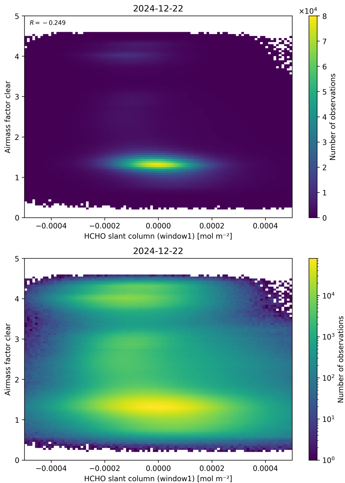
Figure 81: Scatter density plot of “HCHO slant column (window1)” against “Airmass factor clear” for 2024-12-22 to 2024-12-23.
