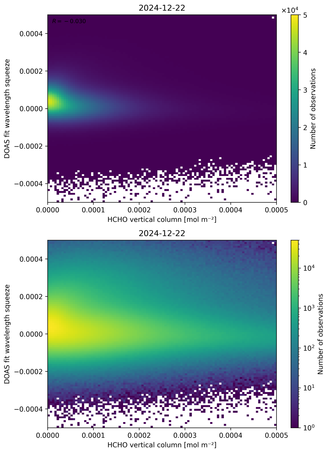
Figure 125: Scatter density plot of “HCHO vertical column” against “DOAS fit wavelength squeeze” for 2024-12-22 to 2024-12-23.
