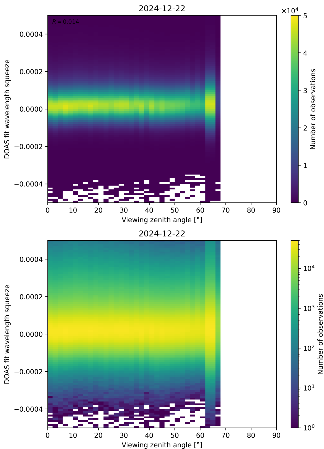
Figure 184: Scatter density plot of “Viewing zenith angle” against “DOAS fit wavelength squeeze” for 2024-12-22 to 2024-12-23.
