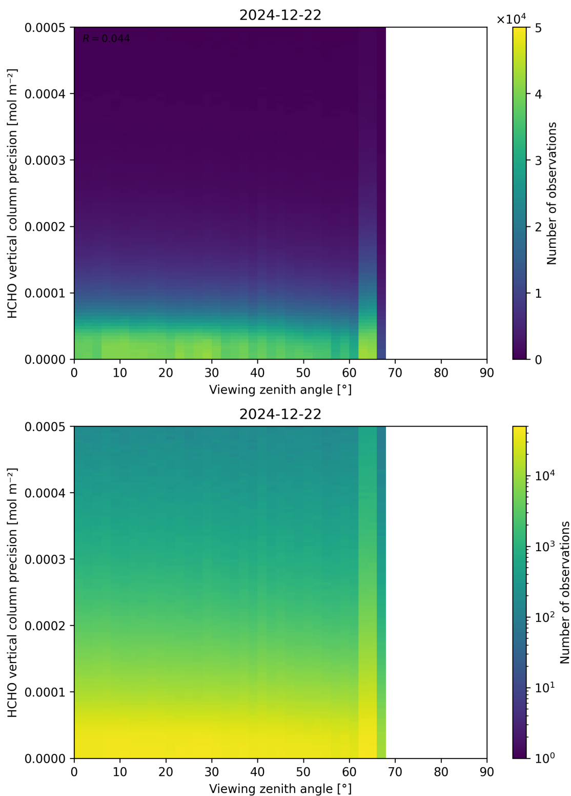
Figure 194: Scatter density plot of “Viewing zenith angle” against “HCHO vertical column precision” for 2024-12-22 to 2024-12-23.
