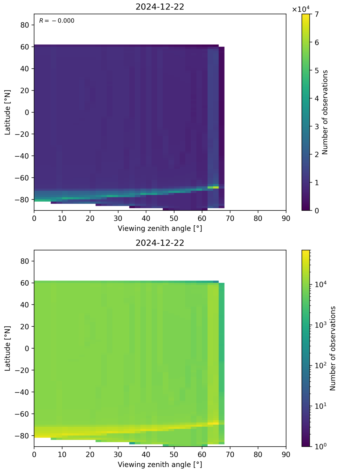
Figure 196: Scatter density plot of “Viewing zenith angle” against “Latitude” for 2024-12-22 to 2024-12-23.
