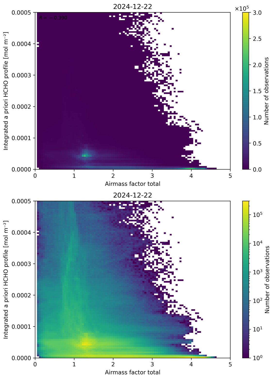
Figure 104: Scatter density plot of “Airmass factor total” against “Integrated a priori HCHO profile” for 2024-12-22 to 2024-12-23.
