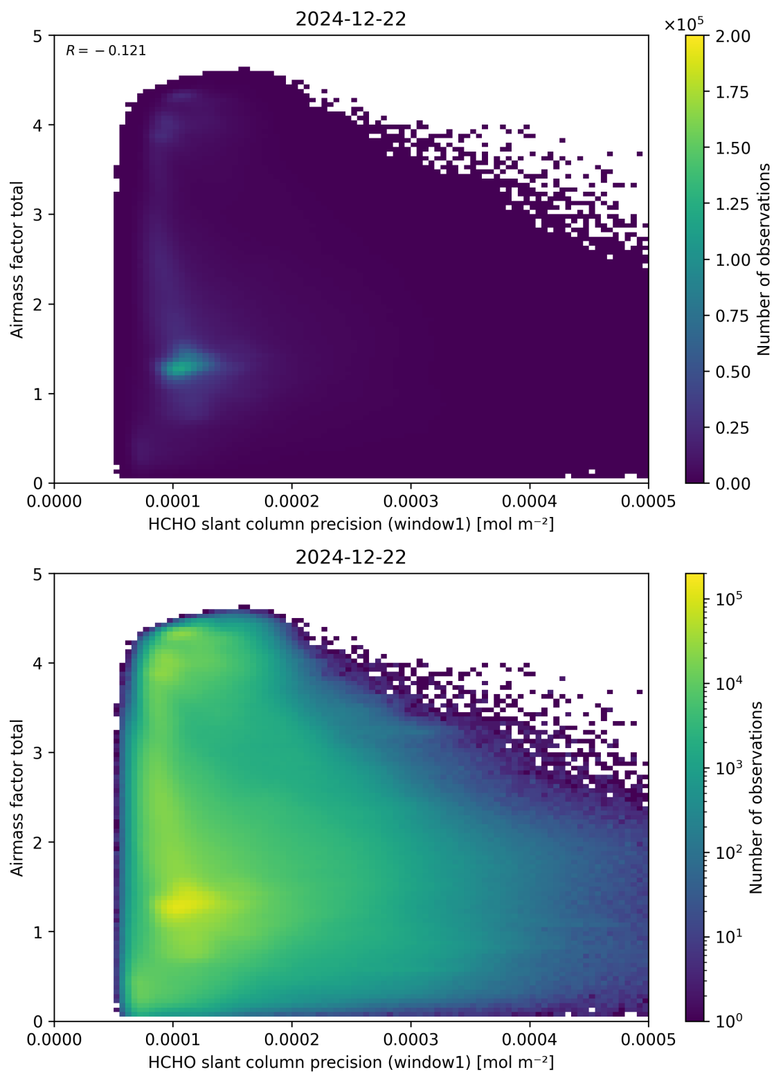
Figure 94: Scatter density plot of “HCHO slant column precision (window1)” against “Airmass factor total” for 2024-12-22 to 2024-12-23.
