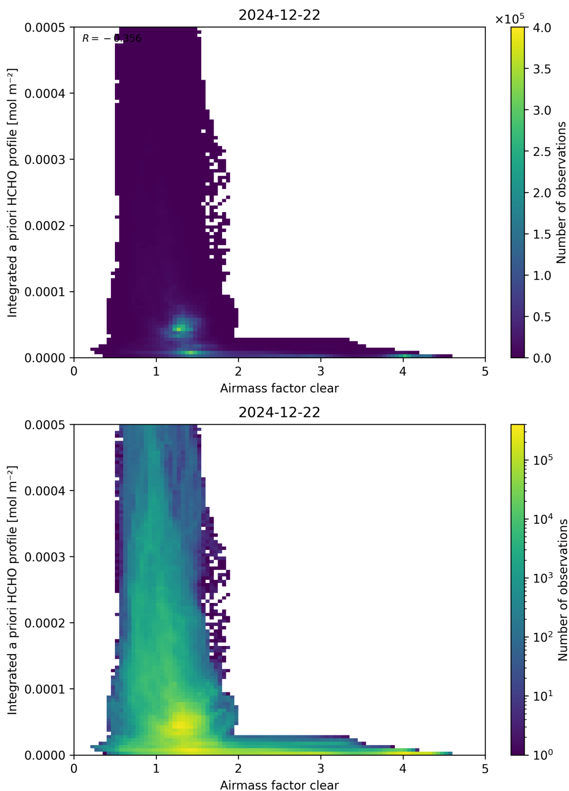
Figure 76: Scatter density plot of “Airmass factor clear” against “Integrated a priori HCHO profile” for 2024-12-22 to 2024-12-23.
