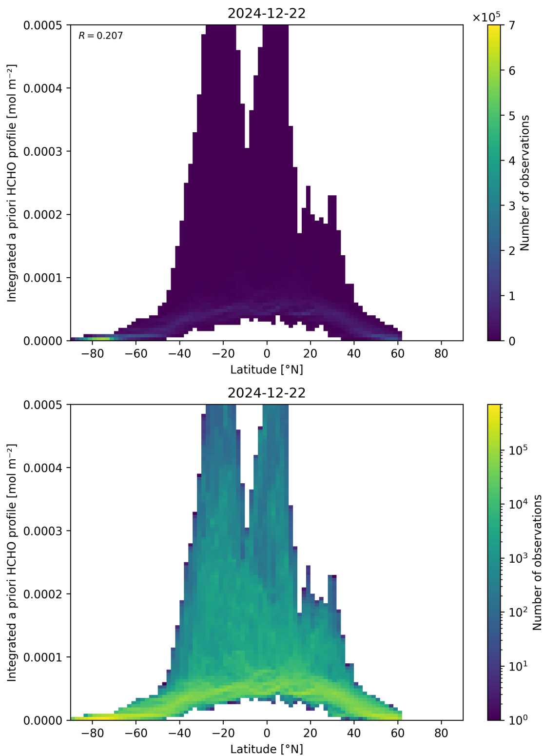
Figure 166: Scatter density plot of “Latitude” against “Integrated a priori HCHO profile” for 2024-12-22 to 2024-12-23.
