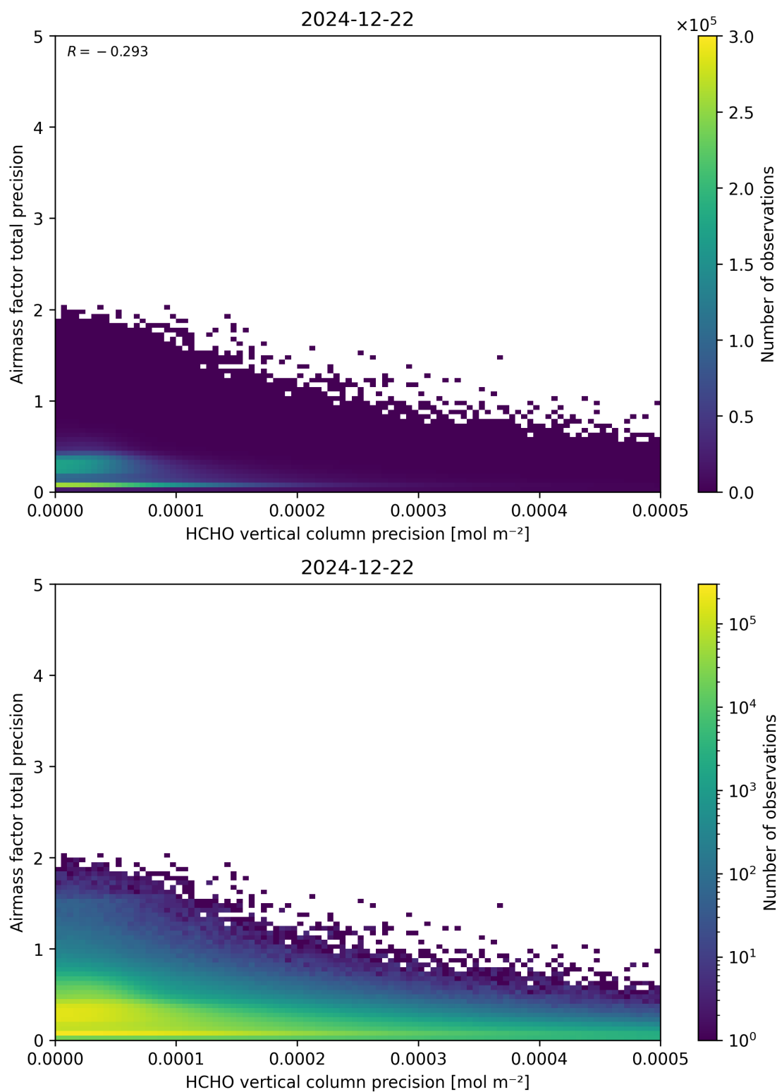
Figure 145: Scatter density plot of “HCHO vertical column precision” against “Airmass factor total precision” for 2024-12-22 to 2024-12-23.
