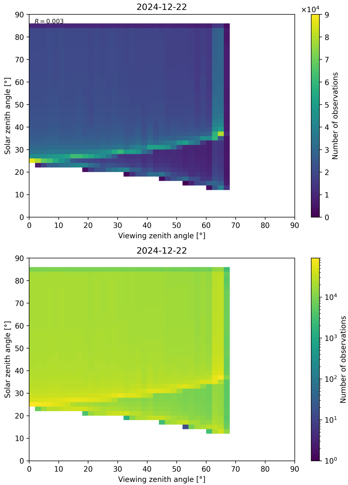
Figure 197: Scatter density plot of “Viewing zenith angle” against “Solar zenith angle” for 2024-12-22 to 2024-12-23.
