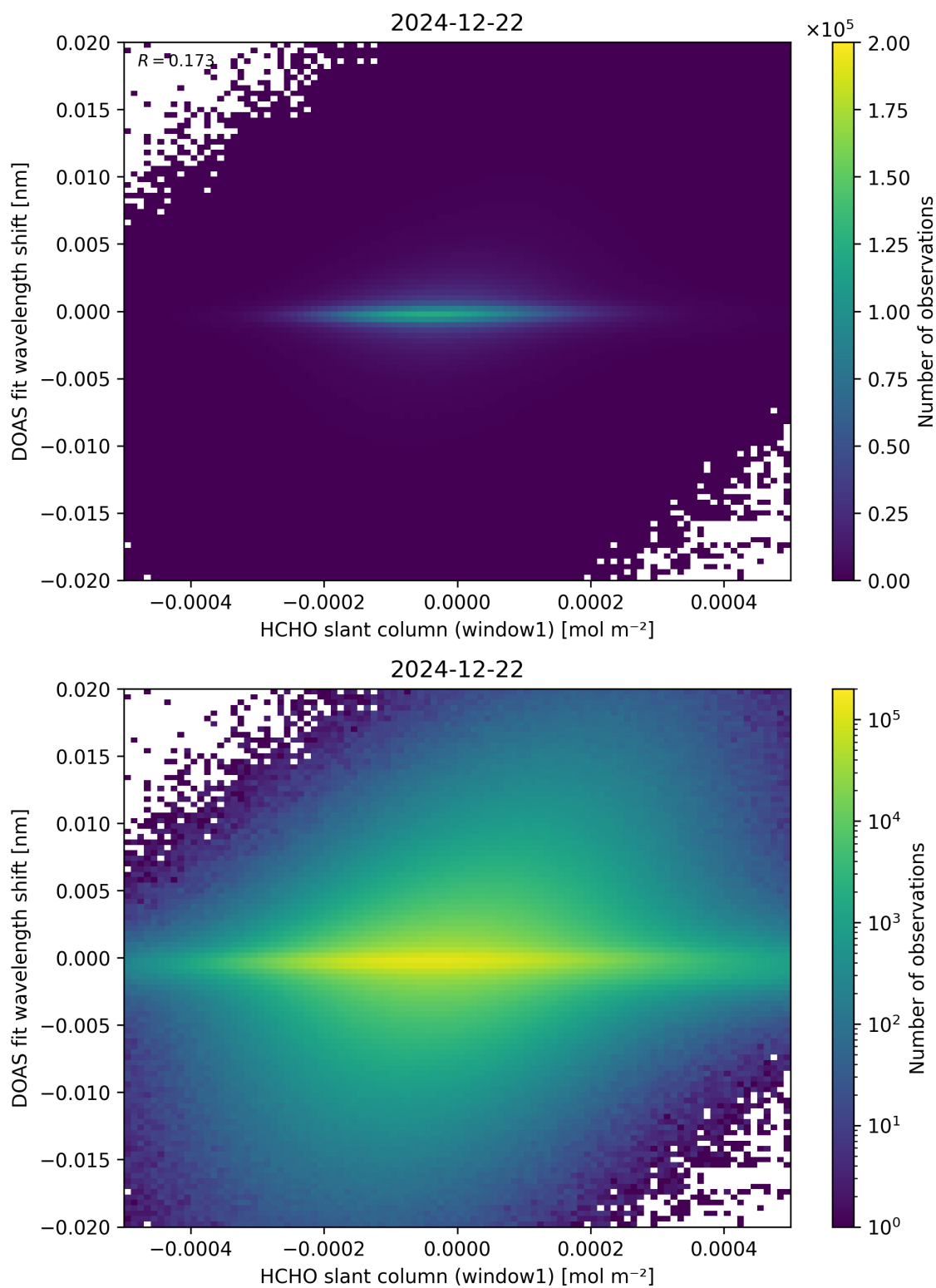
Figure 79: Scatter density plot of “HCHO slant column (window1)” against “DOAS fit wavelength shift” for 2024-12-22 to 2024-12-23.
