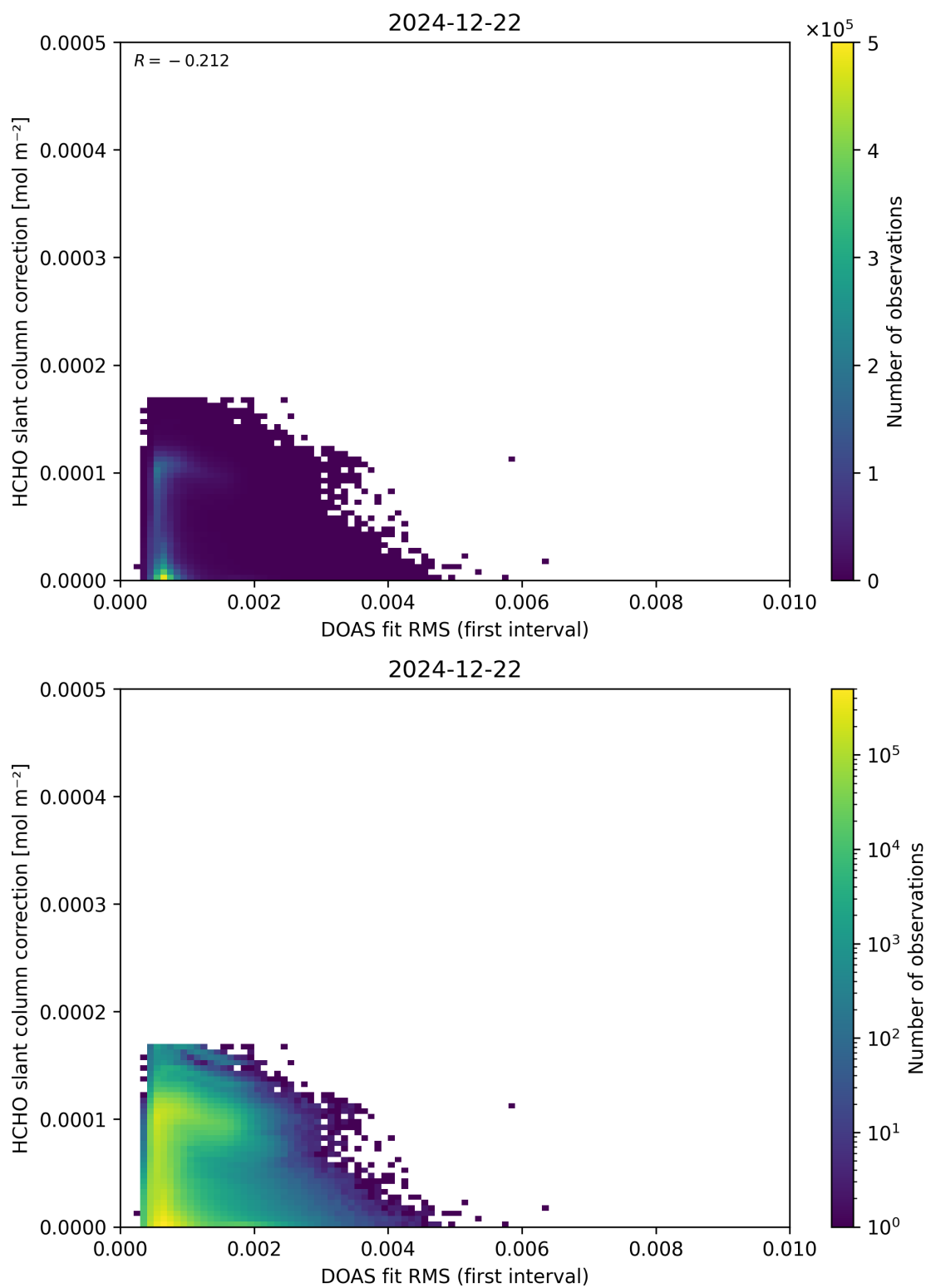
Figure 63: Scatter density plot of “DOAS fit RMS (first interval)” against “HCHO slant column correction” for 2024-12-22 to 2024-12-23.
