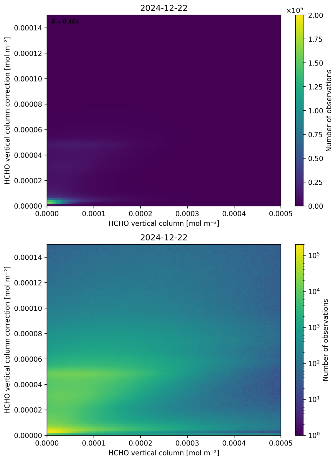
Figure 133: Scatter density plot of “HCHO vertical column” against “HCHO vertical column correction” for 2024-12-22 to 2024-12-23.
