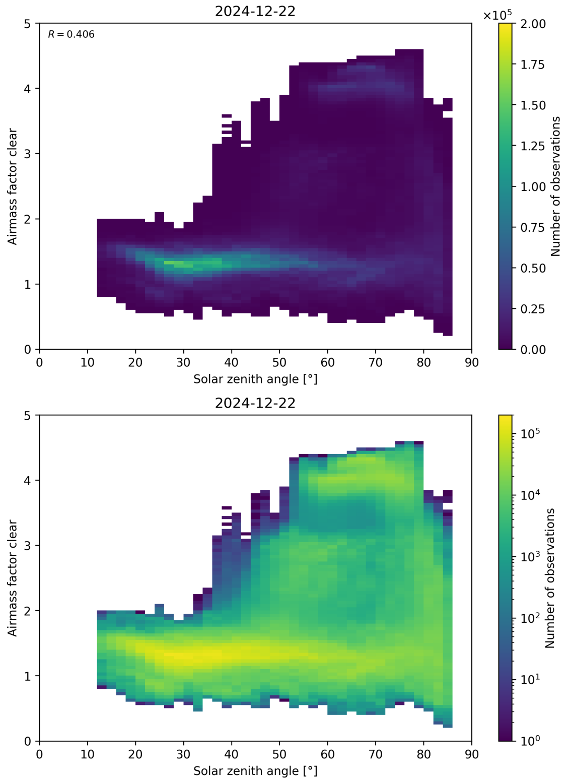
Figure 170: Scatter density plot of “Solar zenith angle” against “Airmass factor clear” for 2024-12-22 to 2024-12-23.
