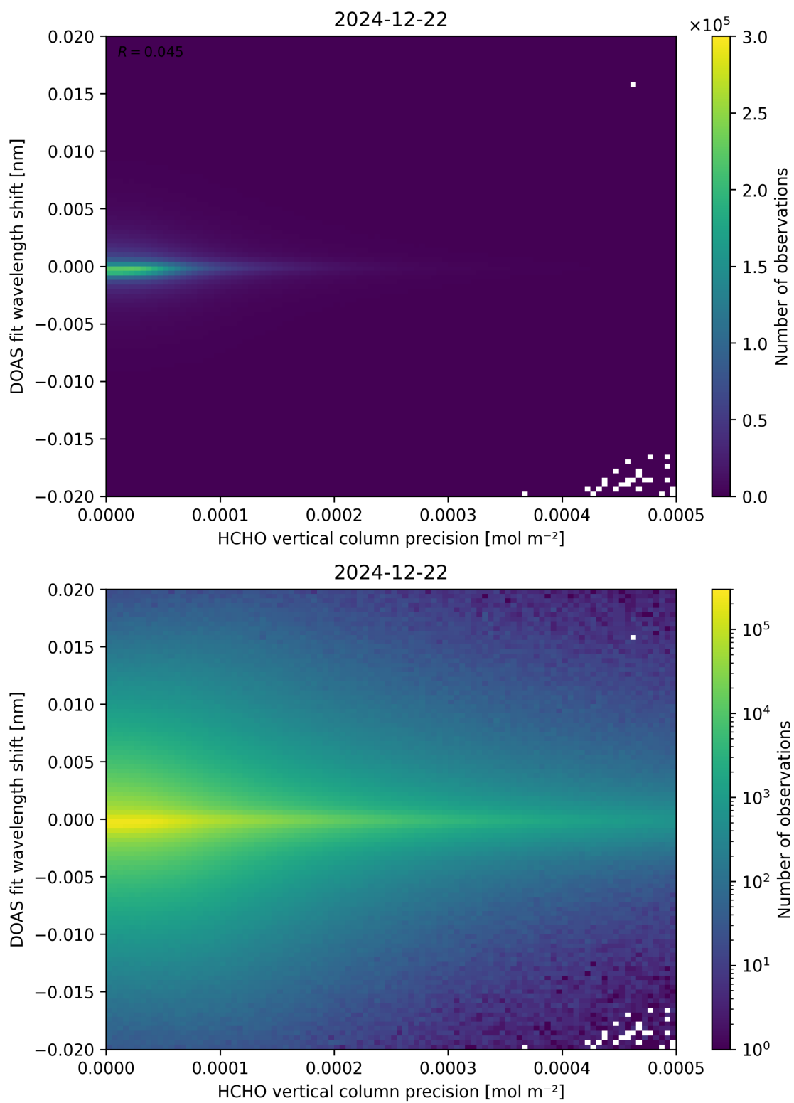
Figure 137: Scatter density plot of “HCHO vertical column precision” against “DOAS fit wavelength shift” for 2024-12-22 to 2024-12-23.
