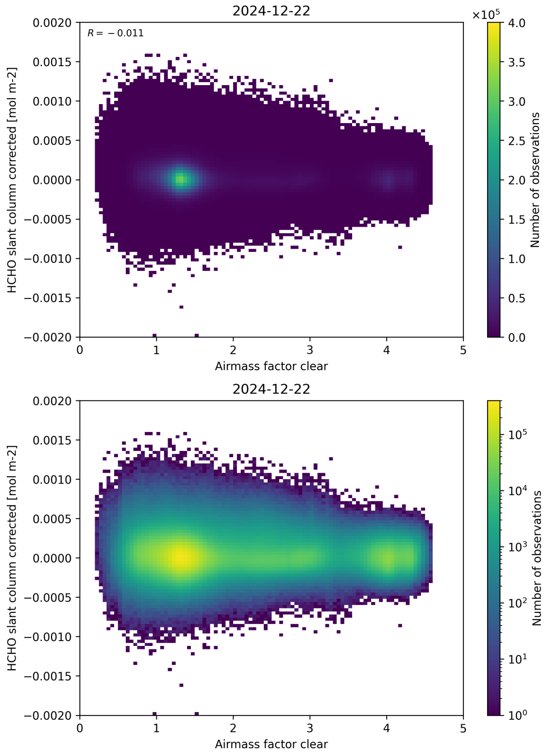
Figure 74: Scatter density plot of “Airmass factor clear” against “HCHO slant column corrected” for 2024-12-22 to 2024-12-23.
