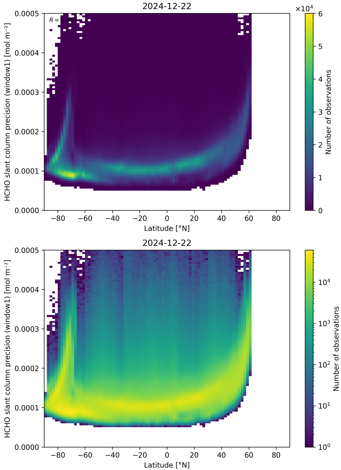
Figure 160: Scatter density plot of “Latitude” against “HCHO slant column precision (window1)” for 2024-12-22 to 2024-12-23.
