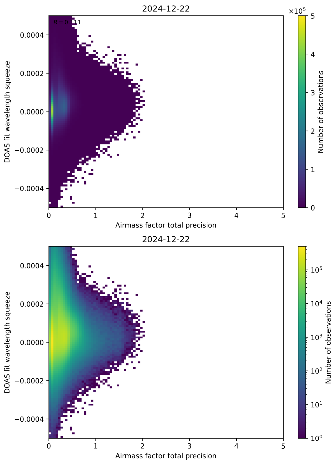
Figure 107: Scatter density plot of “Airmass factor total precision” against “DOAS fit wavelength squeeze” for 2024-12-22 to 2024-12-23.
