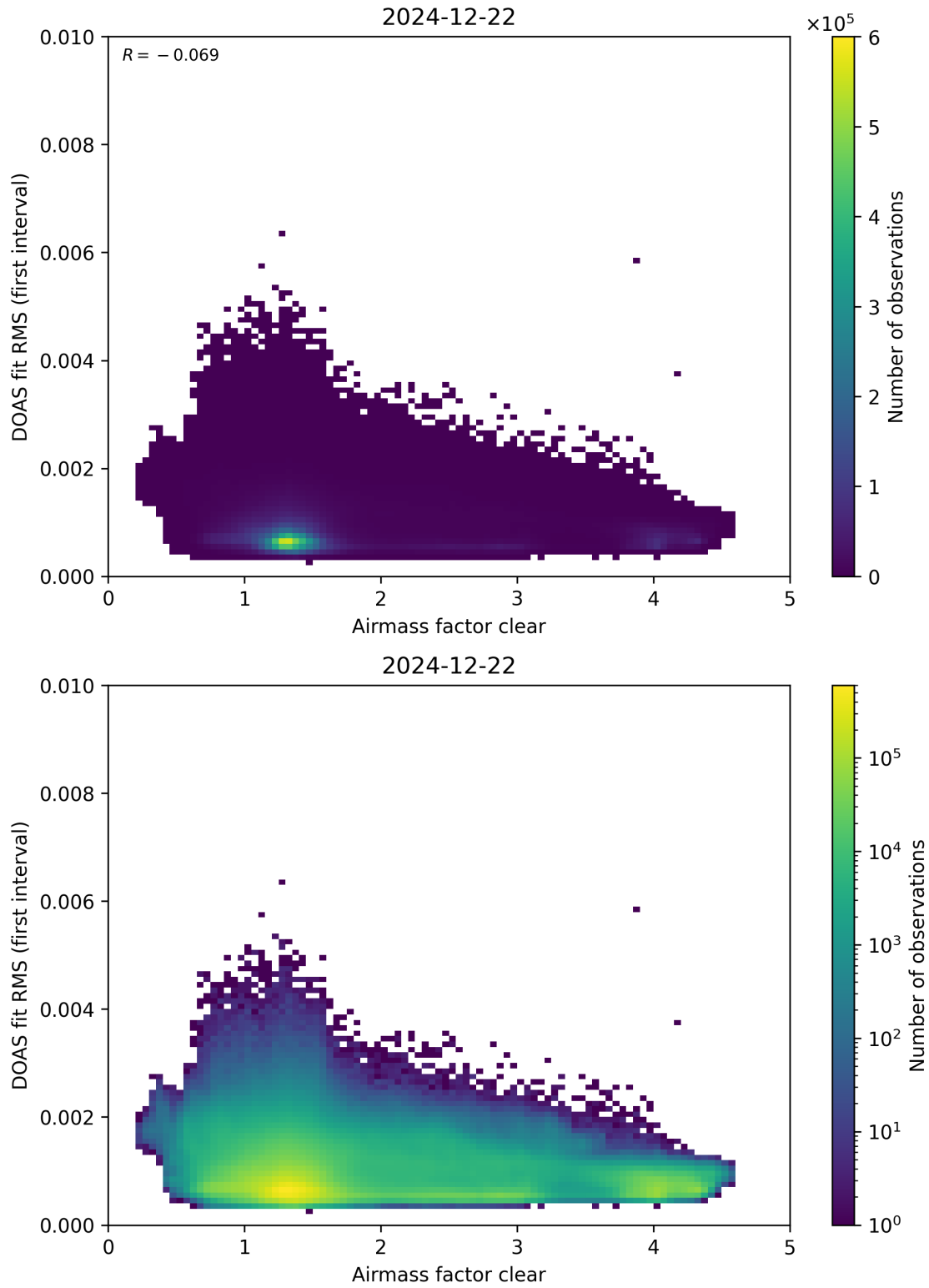
Figure 71: Scatter density plot of “Airmass factor clear” against “DOAS fit RMS (first interval)” for 2024-12-22 to 2024-12-23.
