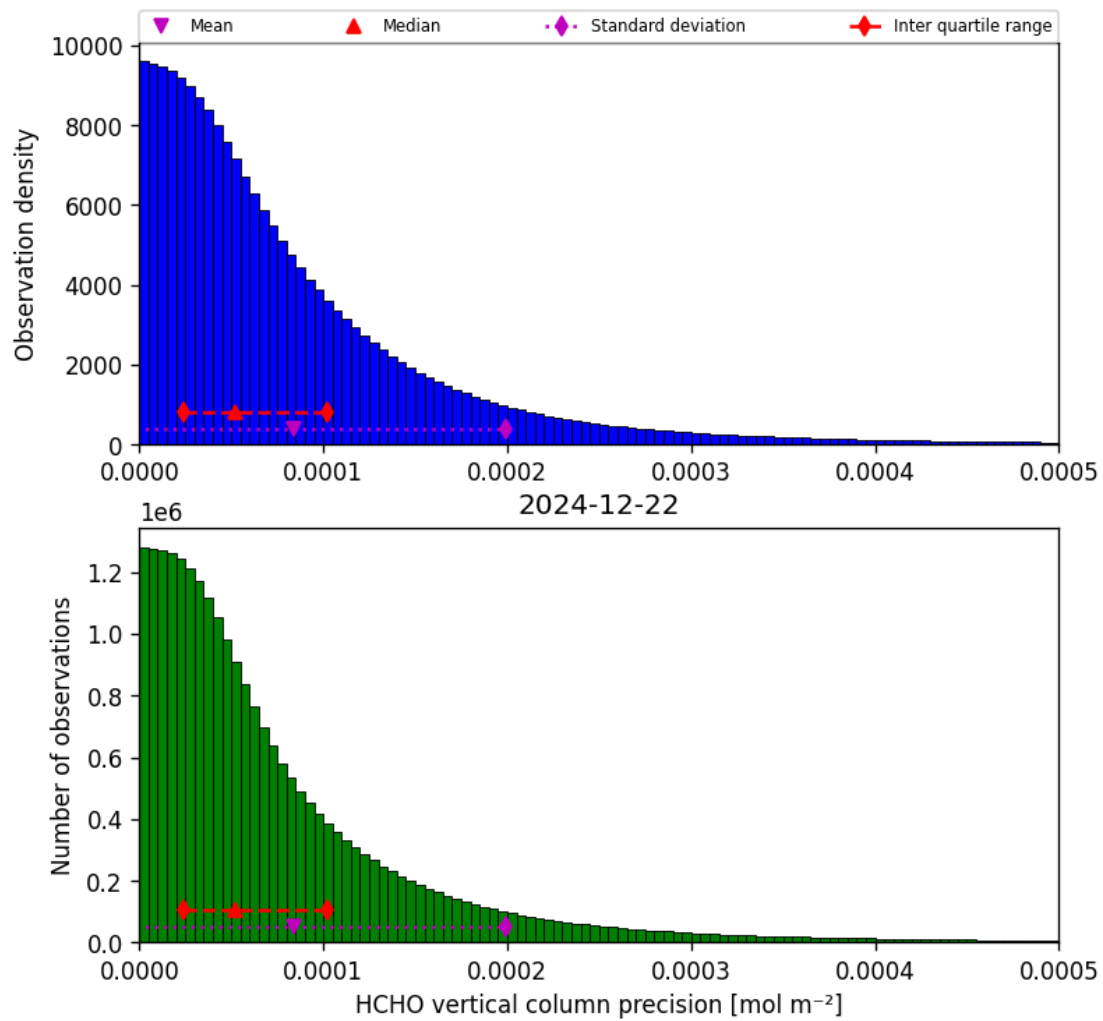
Figure 36: Histogram of “HCHO vertical column precision” for 2024-12-22 to 2024-12-23
