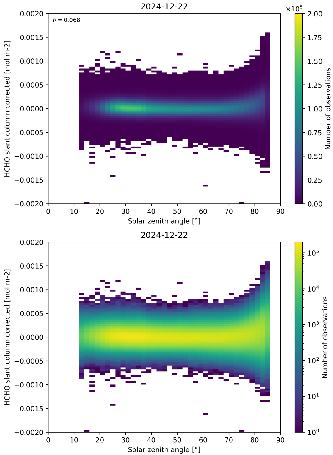
Figure 171: Scatter density plot of “Solar zenith angle” against “HCHO slant column corrected” for 2024-12-22 to 2024-12-23.
