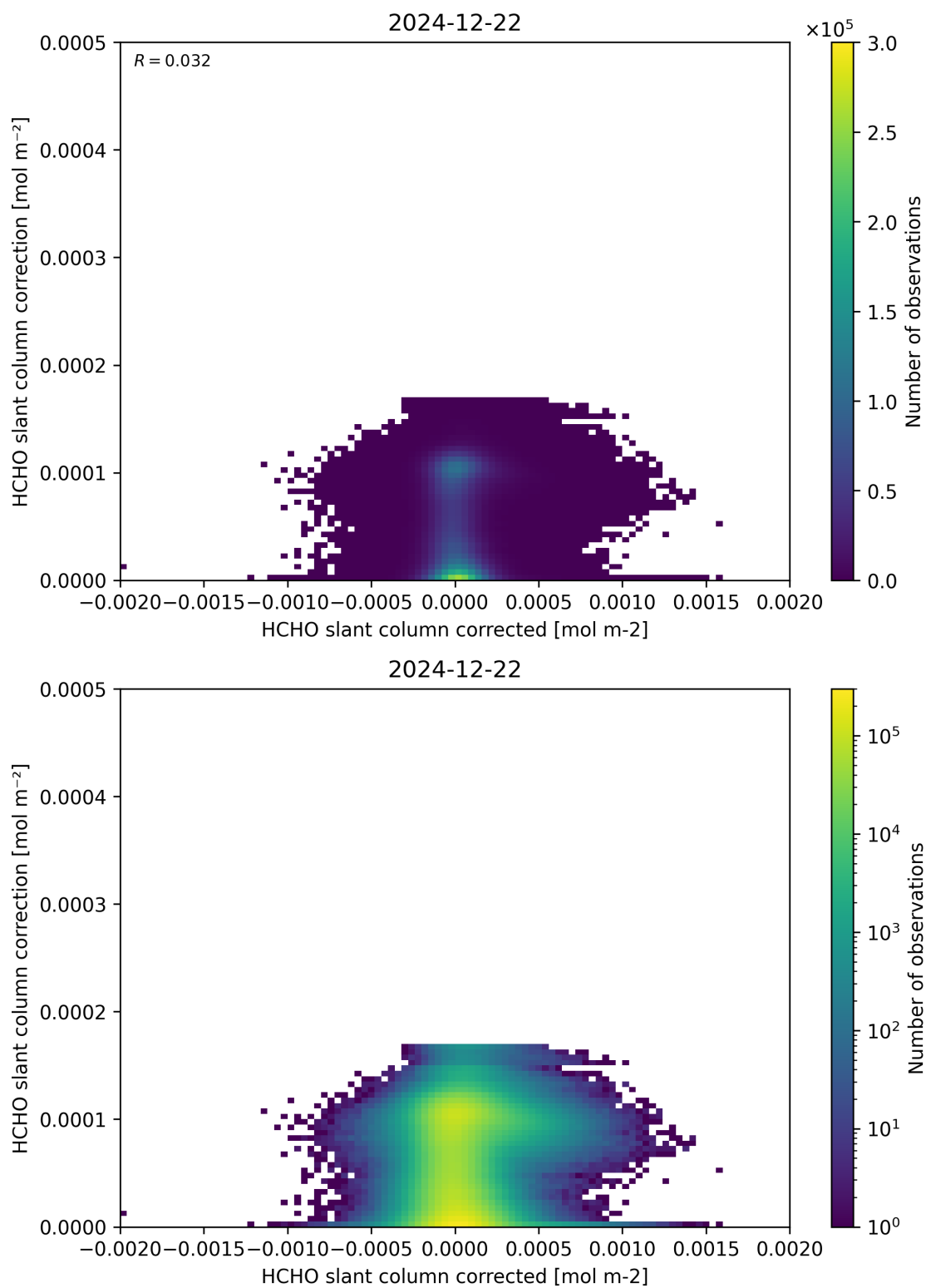
Figure 77: Scatter density plot of “HCHO slant column corrected” against “HCHO slant column correction” for 2024-12-22 to 2024-12-23.
