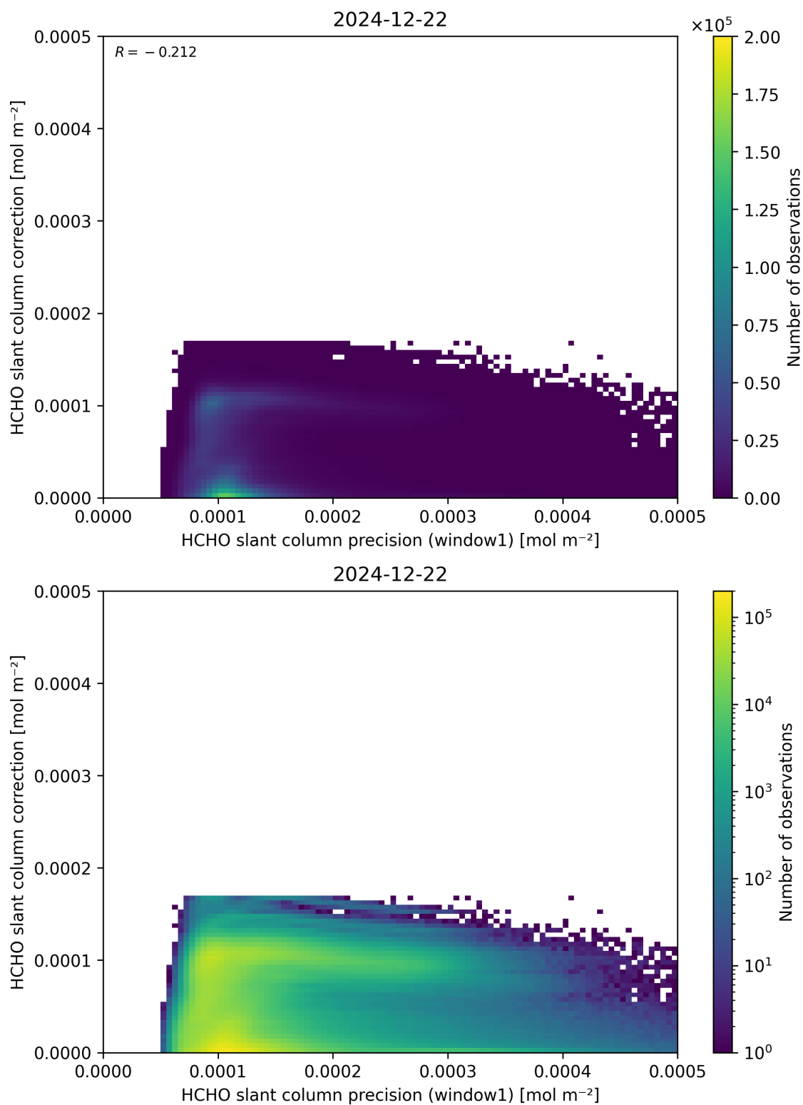
Figure 93: Scatter density plot of “HCHO slant column precision (window1)” against “HCHO slant column correction” for 2024-12-22 to 2024-12-23.
