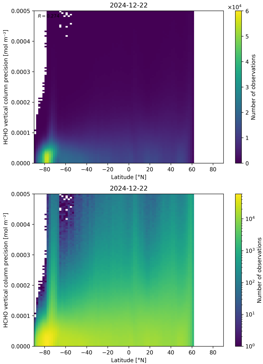
Figure 165: Scatter density plot of “Latitude” against “HCHO vertical column precision” for 2024-12-22 to 2024-12-23.
