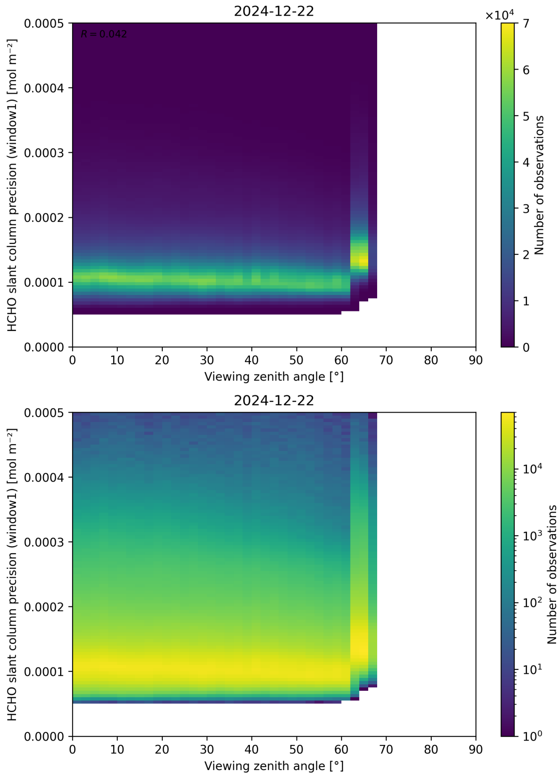
Figure 189: Scatter density plot of “Viewing zenith angle” against “HCHO slant column precision (window1)” for 2024-12-22 to 2024-12-23.
