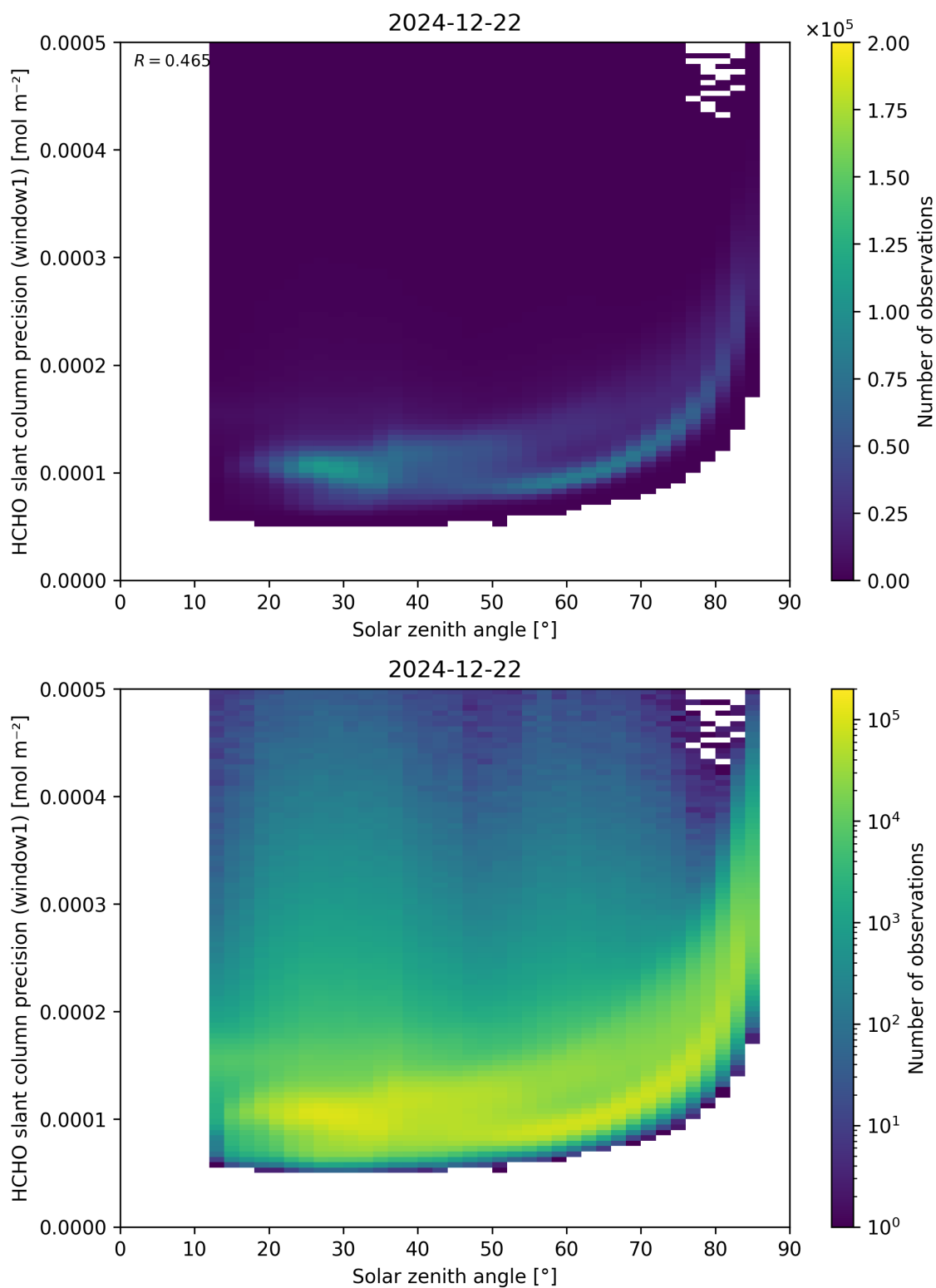
Figure 174: Scatter density plot of “Solar zenith angle” against “HCHO slant column precision (window1)” for 2024-12-22 to 2024-12-23.
