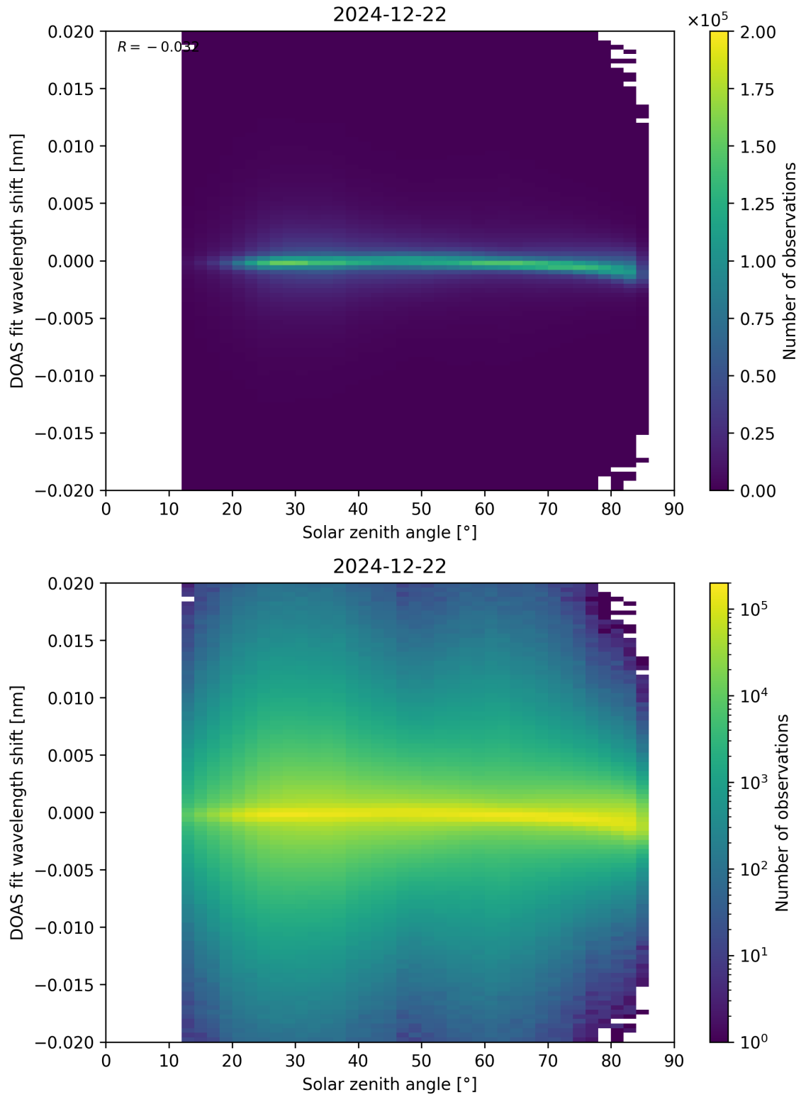
Figure 168: Scatter density plot of “Solar zenith angle” against “DOAS fit wavelength shift” for 2024-12-22 to 2024-12-23.
