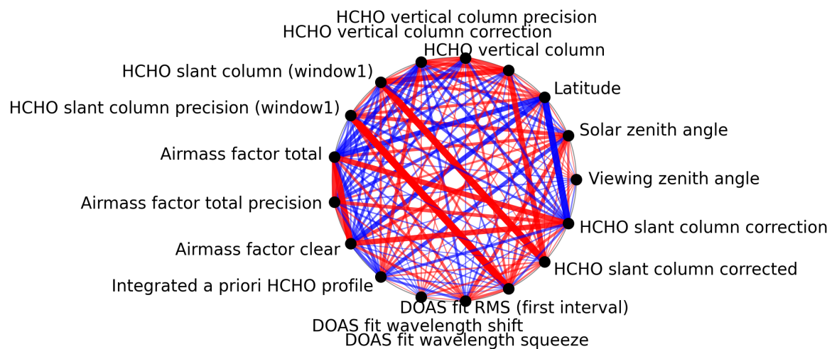
Figure 1: Map of correlation graph for 2024-12-22 to 2024-12-23.
