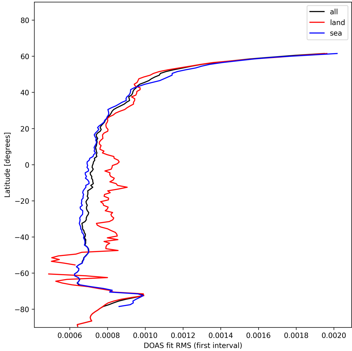
Figure 32: Zonal average of “DOAS fit RMS (first interval)” for 2024-12-22 to 2024-12-23.
