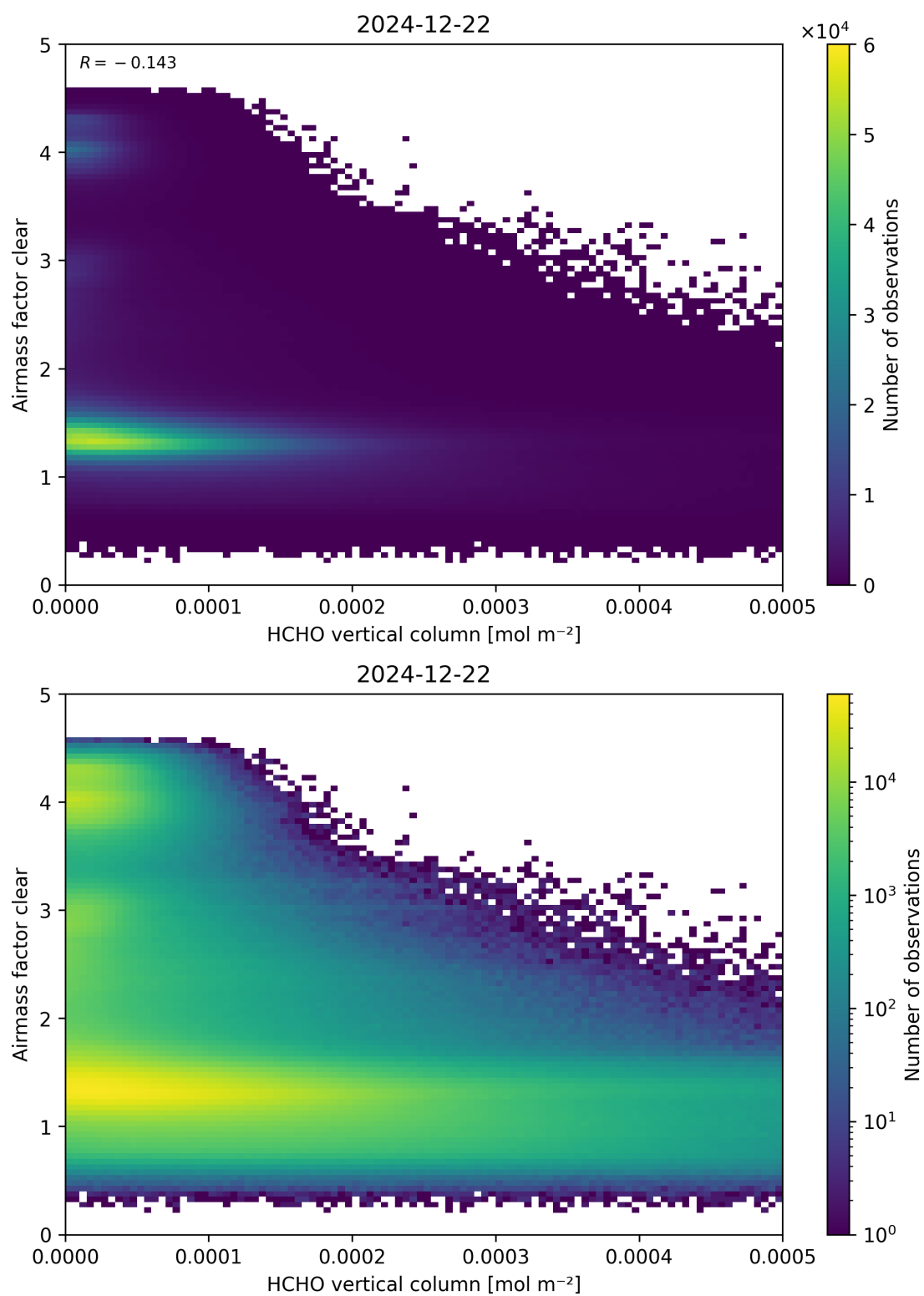
Figure 126: Scatter density plot of “HCHO vertical column” against “Airmass factor clear” for 2024-12-22 to 2024-12-23.
