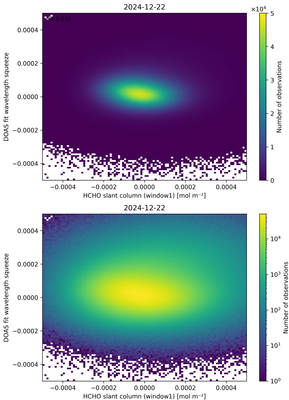
Figure 80: Scatter density plot of “HCHO slant column (window1)” against “DOAS fit wavelength squeeze” for 2024-12-22 to 2024-12-23.
