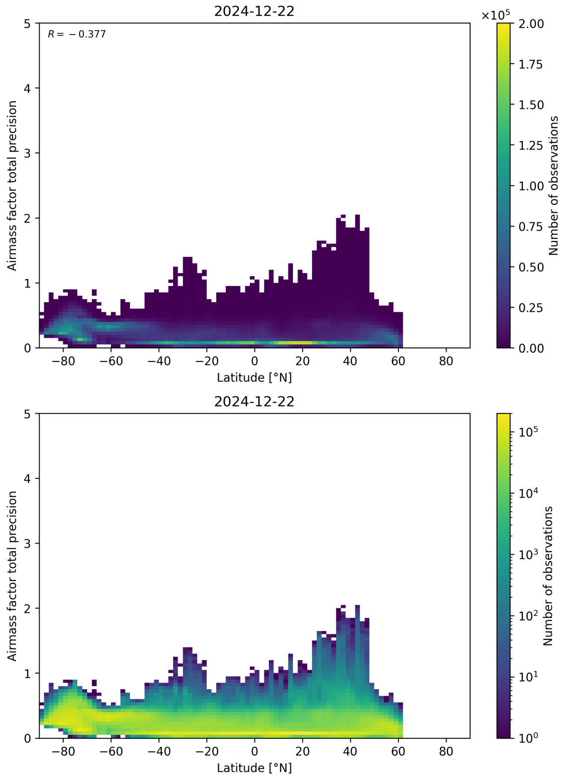
Figure 162: Scatter density plot of “Latitude” against “Airmass factor total precision” for 2024-12-22 to 2024-12-23.
