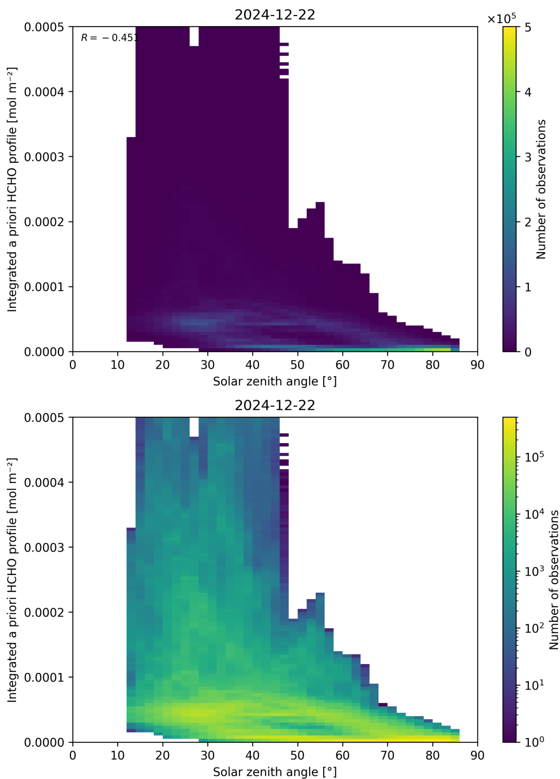
Figure 180: Scatter density plot of “Solar zenith angle” against “Integrated a priori HCHO profile” for 2024-12-22 to 2024-12-23.
