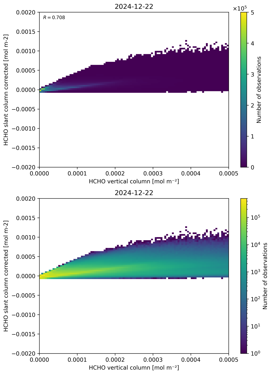
Figure 127: Scatter density plot of “HCHO vertical column” against “HCHO slant column corrected” for 2024-12-22 to 2024-12-23.
