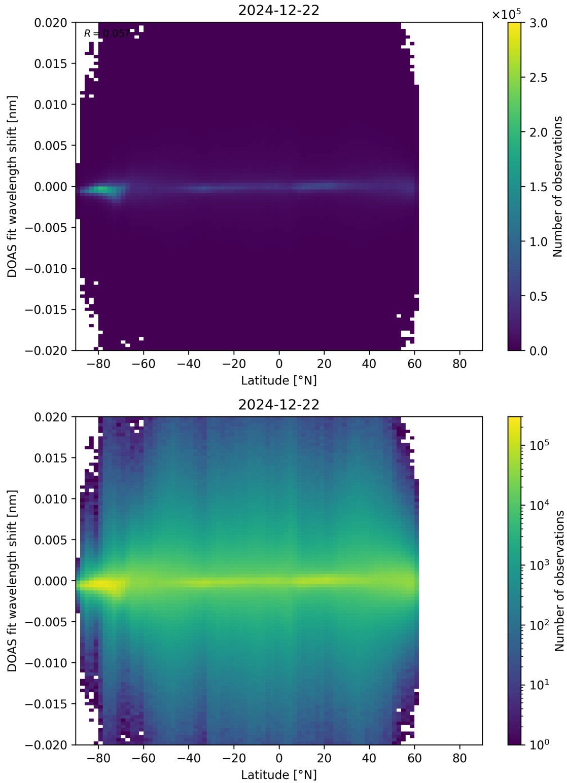
Figure 154: Scatter density plot of “Latitude” against “DOAS fit wavelength shift” for 2024-12-22 to 2024-12-23.
