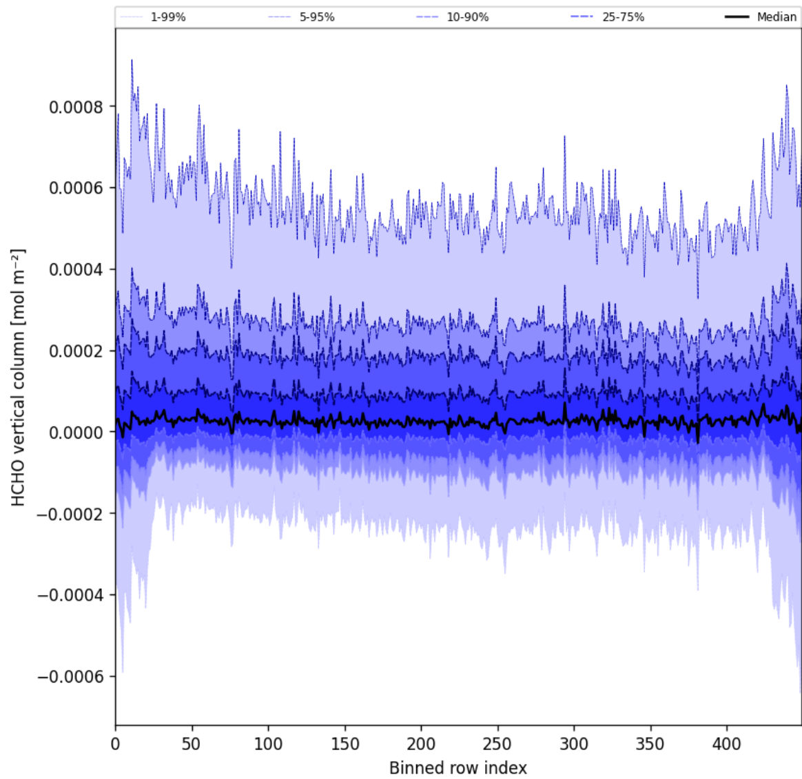
Figure 49: Along track statistics of “HCHO vertical column” for 2024-12-22 to 2024-12-23
