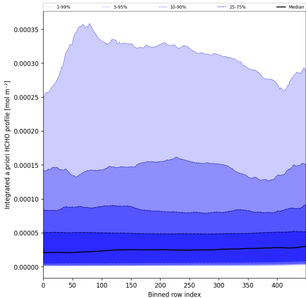
Figure 57: Along track statistics of "Integrated a priori HCHO profile" for 2024-12-22 to 2024-12-23
