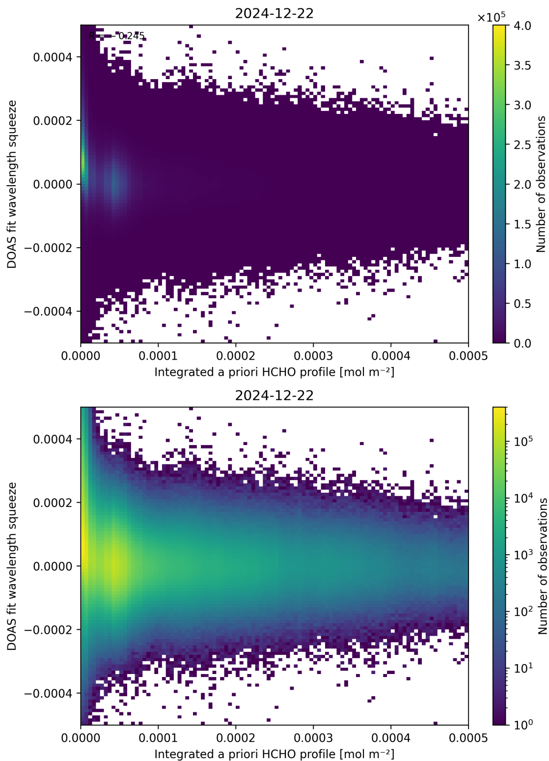
Figure 150: Scatter density plot of “Integrated a priori HCHO profile” against “DOAS fit wavelength squeeze” for 2024-12-22 to 2024-12-23.
