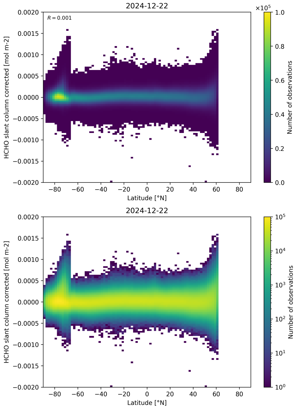
Figure 157: Scatter density plot of “Latitude” against “HCHO slant column corrected” for 2024-12-22 to 2024-12-23.
