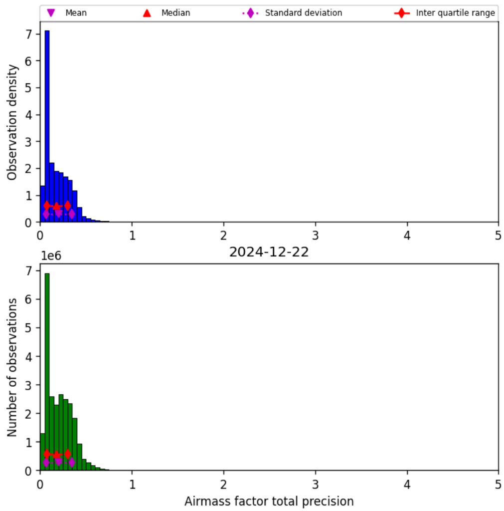
Figure 41: Histogram of “Airmass factor total precision” for 2024-12-22 to 2024-12-23
