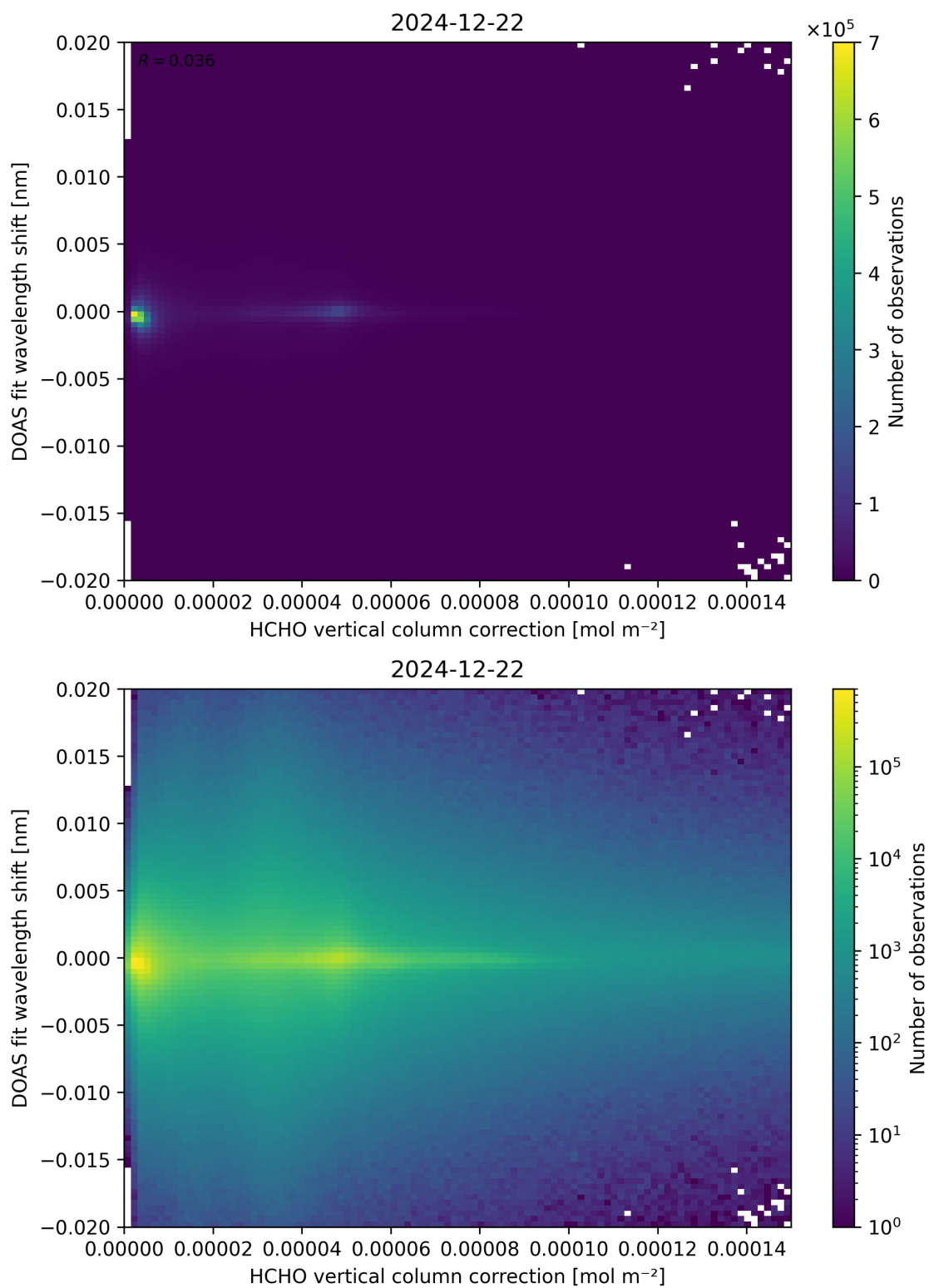
Figure 113: Scatter density plot of “HCHO vertical column correction” against “DOAS fit wavelength shift” for 2024-12-22 to 2024-12-23.
