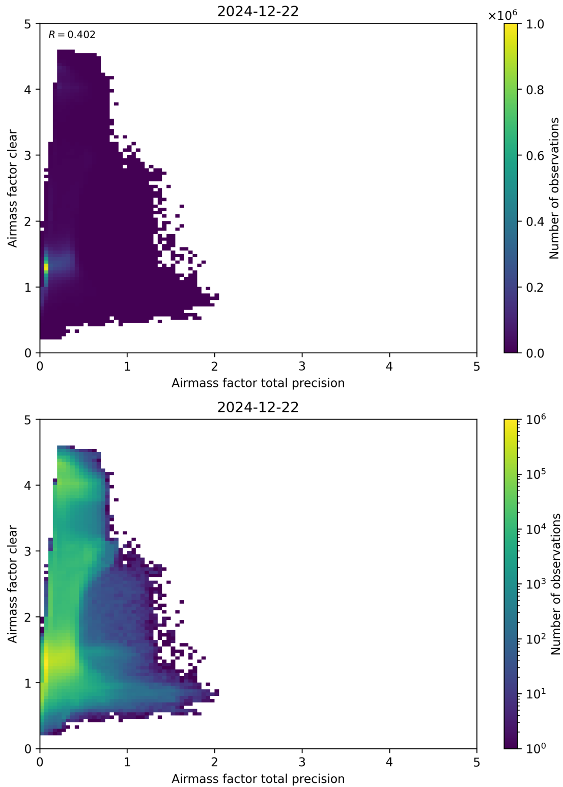
Figure 108: Scatter density plot of “Airmass factor total precision” against “Airmass factor clear” for 2024-12-22 to 2024-12-23.
