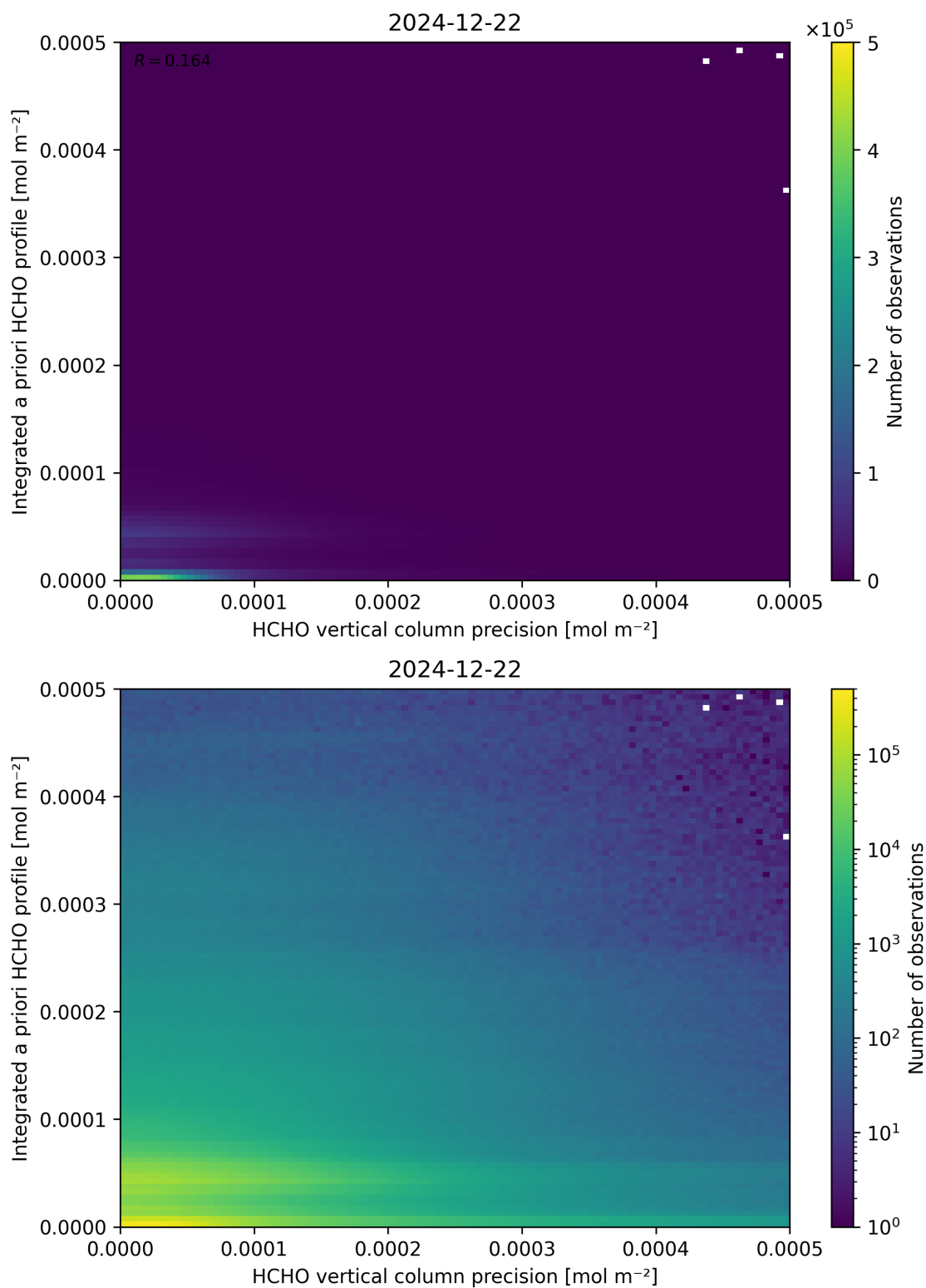
Figure 147: Scatter density plot of “HCHO vertical column precision” against “Integrated a priori HCHO profile” for 2024-12-22 to 2024-12-23.
