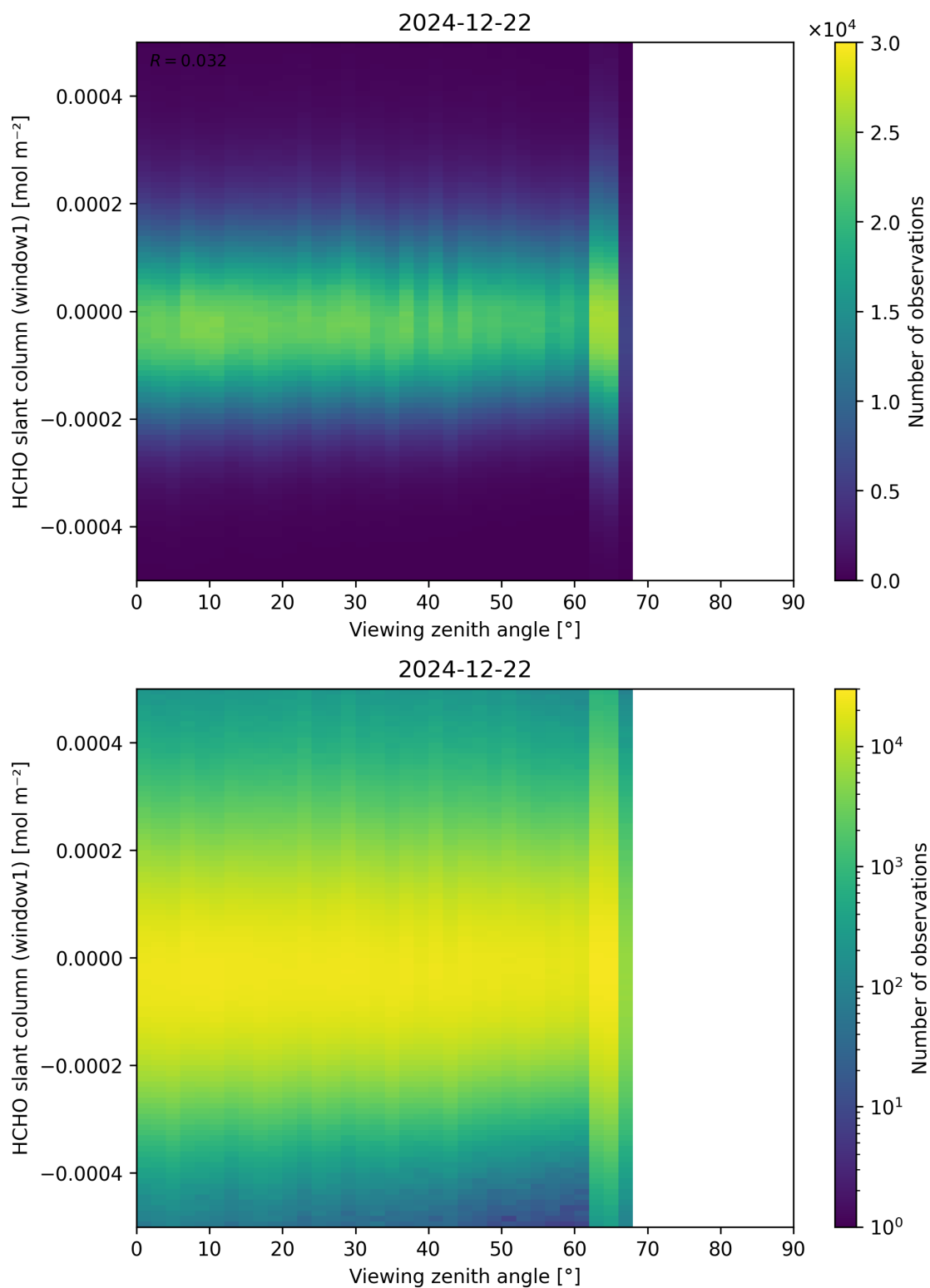
Figure 188: Scatter density plot of “Viewing zenith angle” against “HCHO slant column (window1)” for 2024-12-22 to 2024-12-23.
