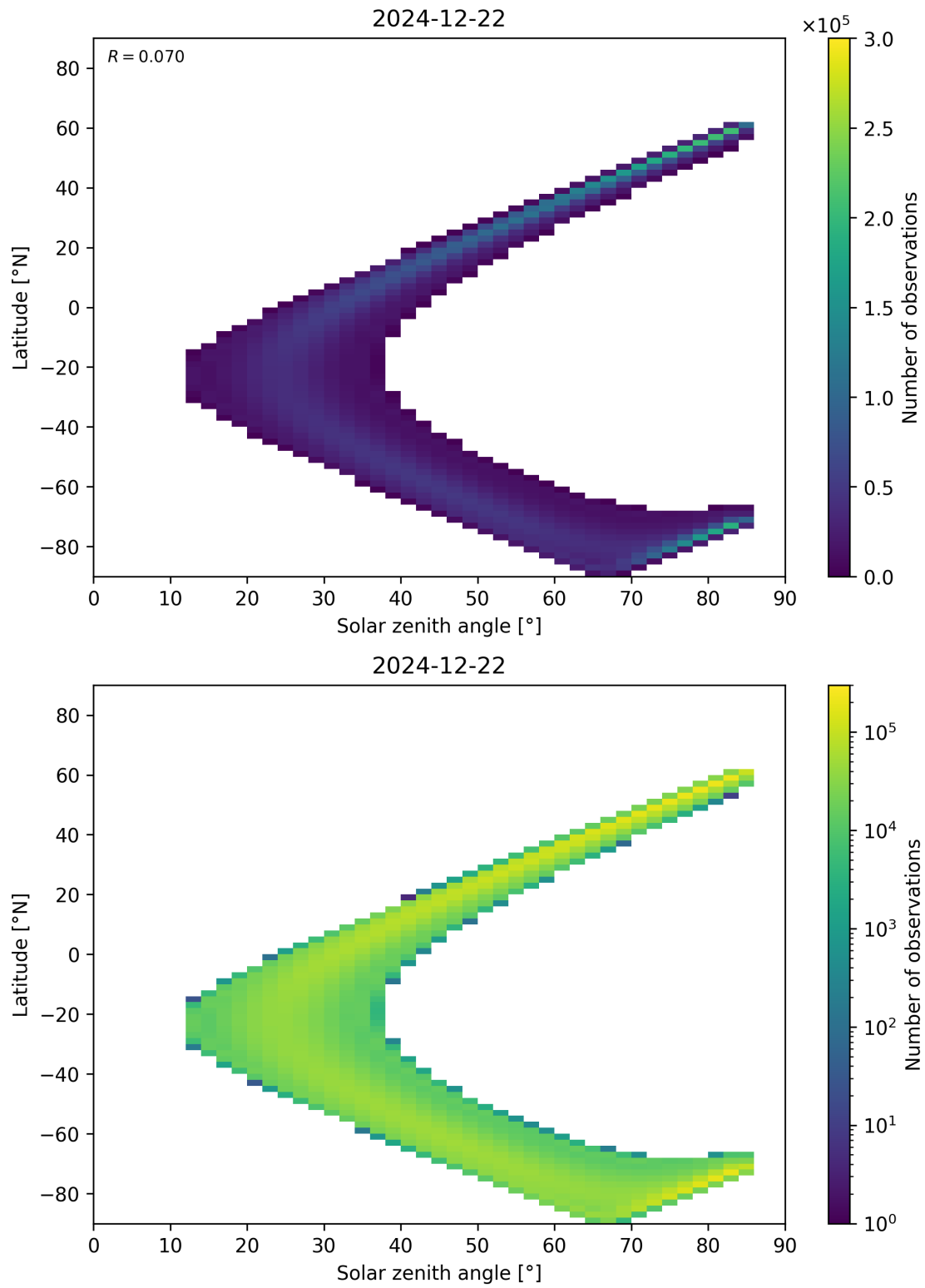
Figure 181: Scatter density plot of “Solar zenith angle” against “Latitude” for 2024-12-22 to 2024-12-23.
