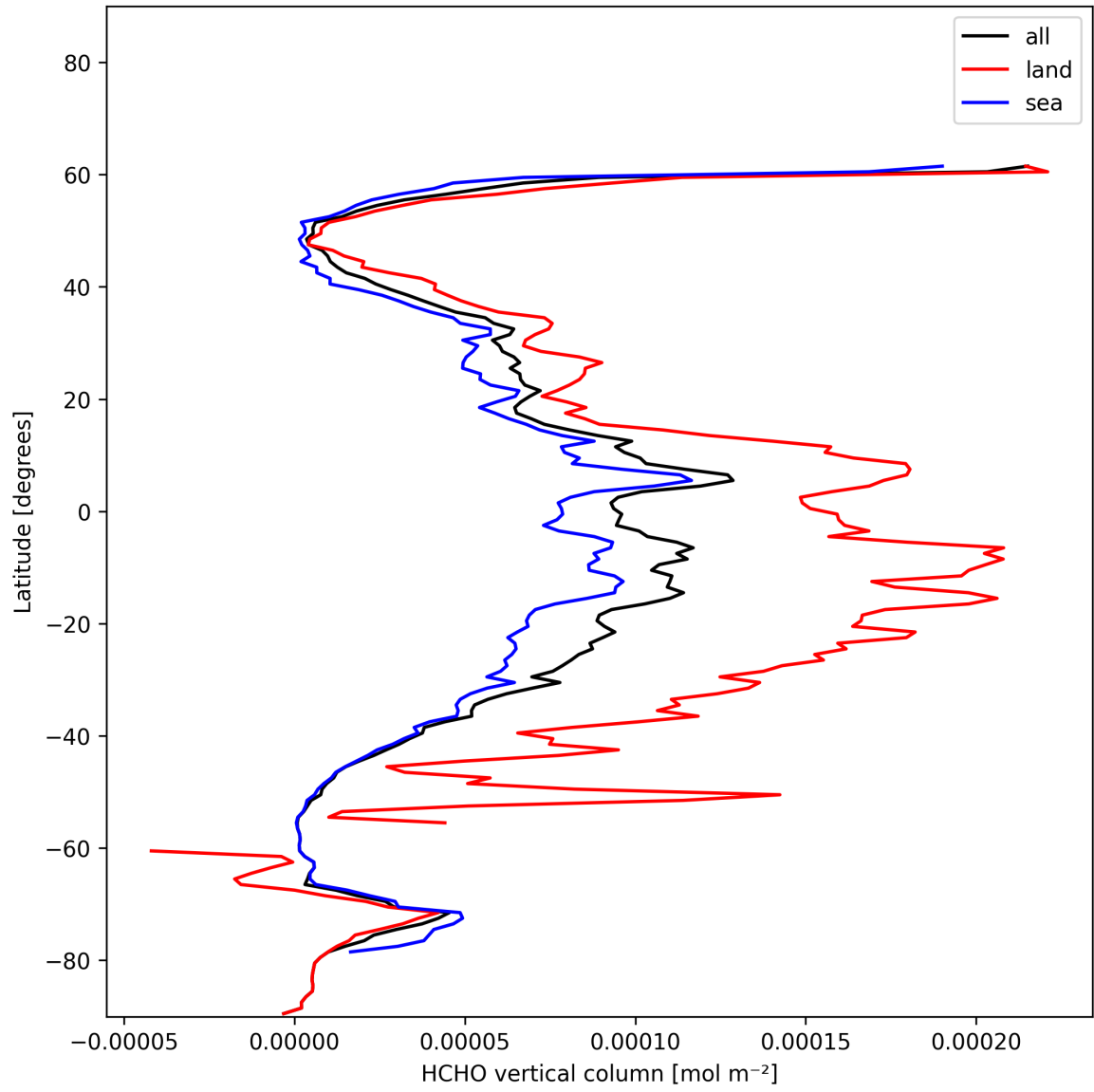
Figure 21: Zonal average of “HCHO vertical column” for 2024-12-22 to 2024-12-23.
