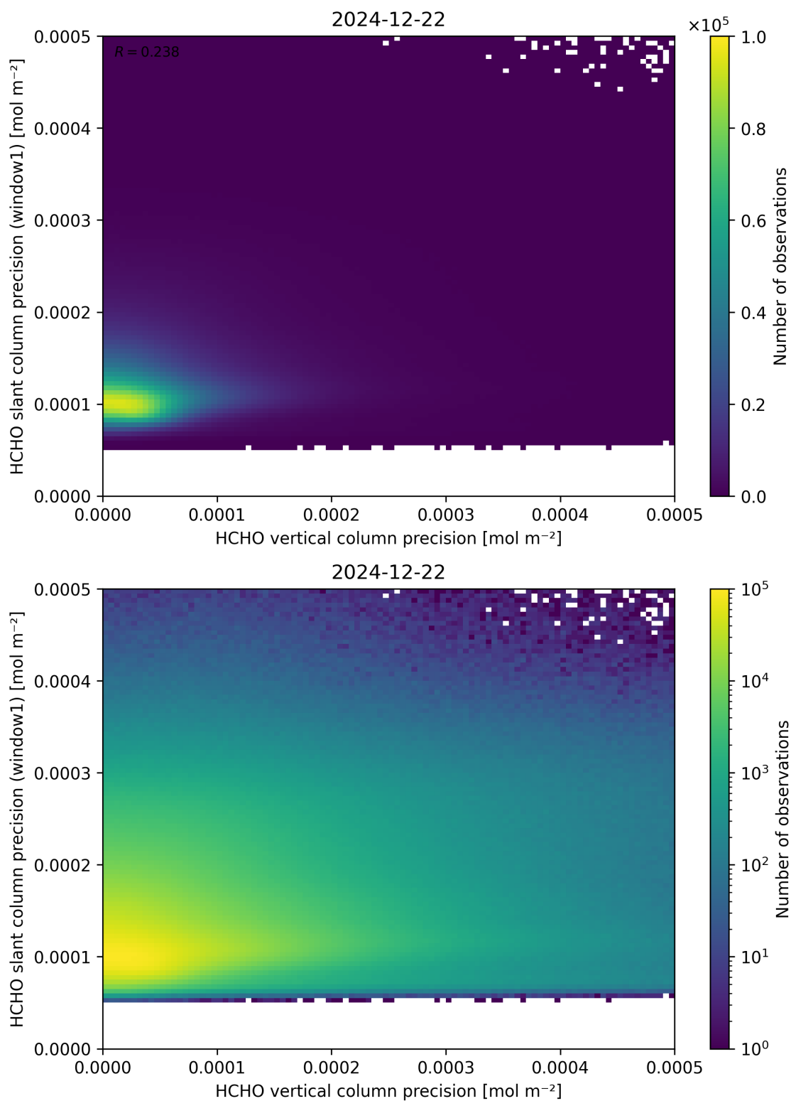
Figure 143: Scatter density plot of “HCHO vertical column precision” against “HCHO slant column precision (window1)” for 2024-12-22 to 2024-12-23.
