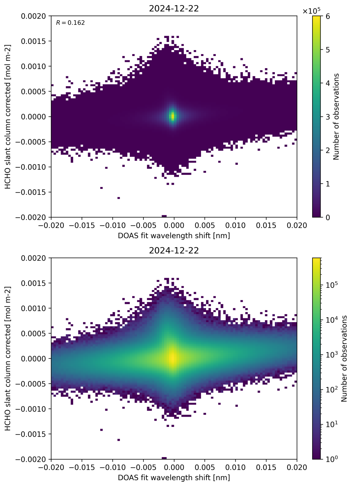
Figure 66: Scatter density plot of “DOAS fit wavelength shift” against “HCHO slant column corrected” for 2024-12-22 to 2024-12-23.
