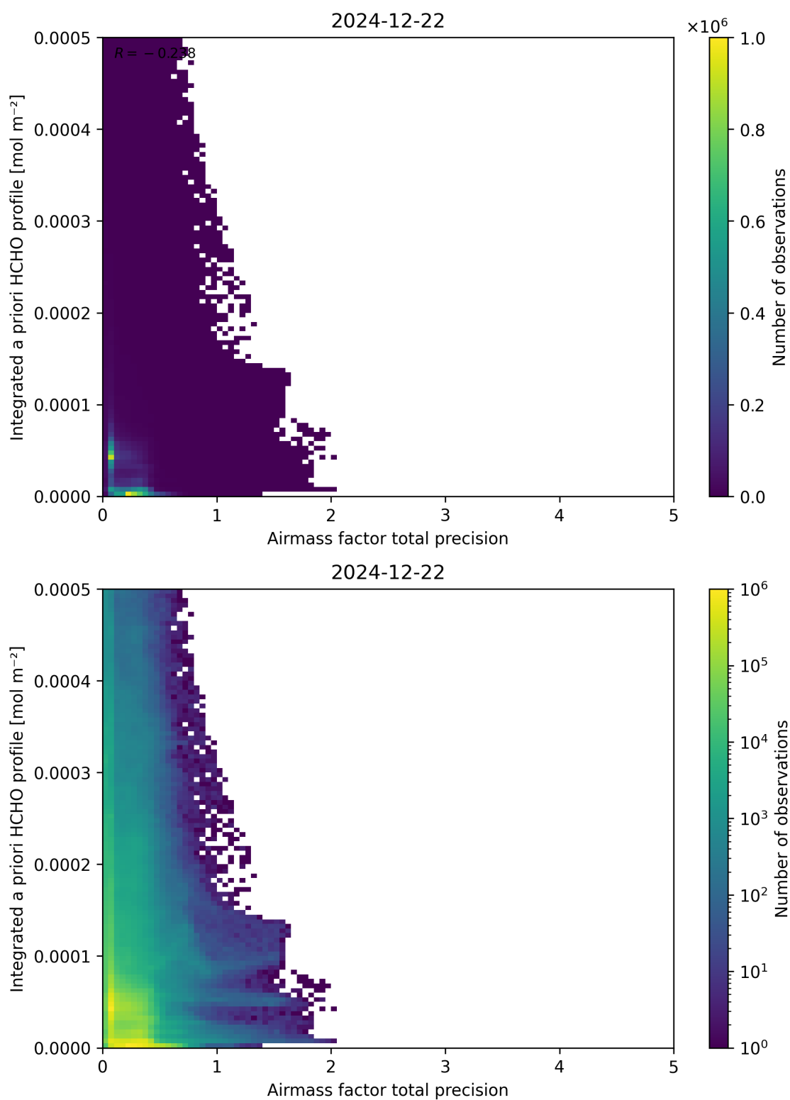
Figure 111: Scatter density plot of “Airmass factor total precision” against “Integrated a priori HCHO profile” for 2024-12-22 to 2024-12-23.
