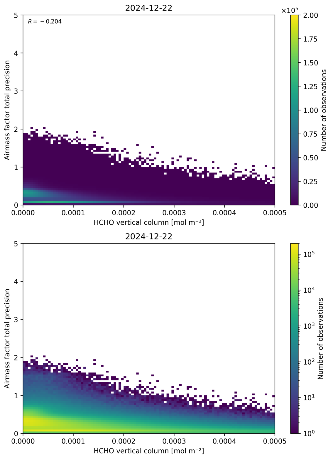
Figure 132: Scatter density plot of “HCHO vertical column” against “Airmass factor total precision” for 2024-12-22 to 2024-12-23.
