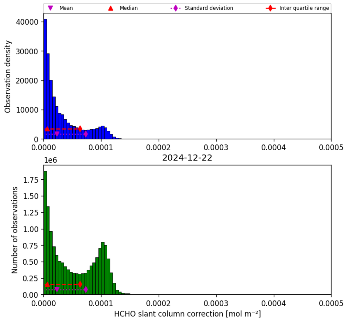
Figure 47: Histogram of “HCHO slant column correction” for 2024-12-22 to 2024-12-23
