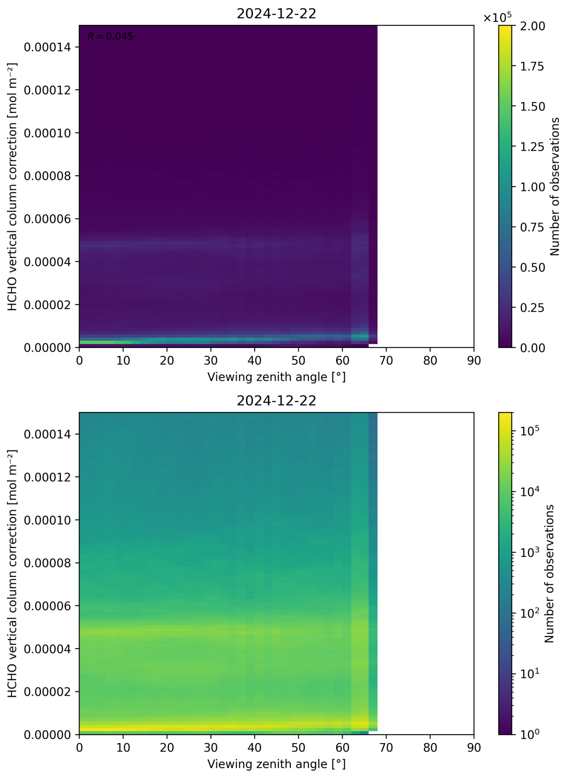
Figure 193: Scatter density plot of “Viewing zenith angle” against “HCHO vertical column correction” for 2024-12-22 to 2024-12-23.
