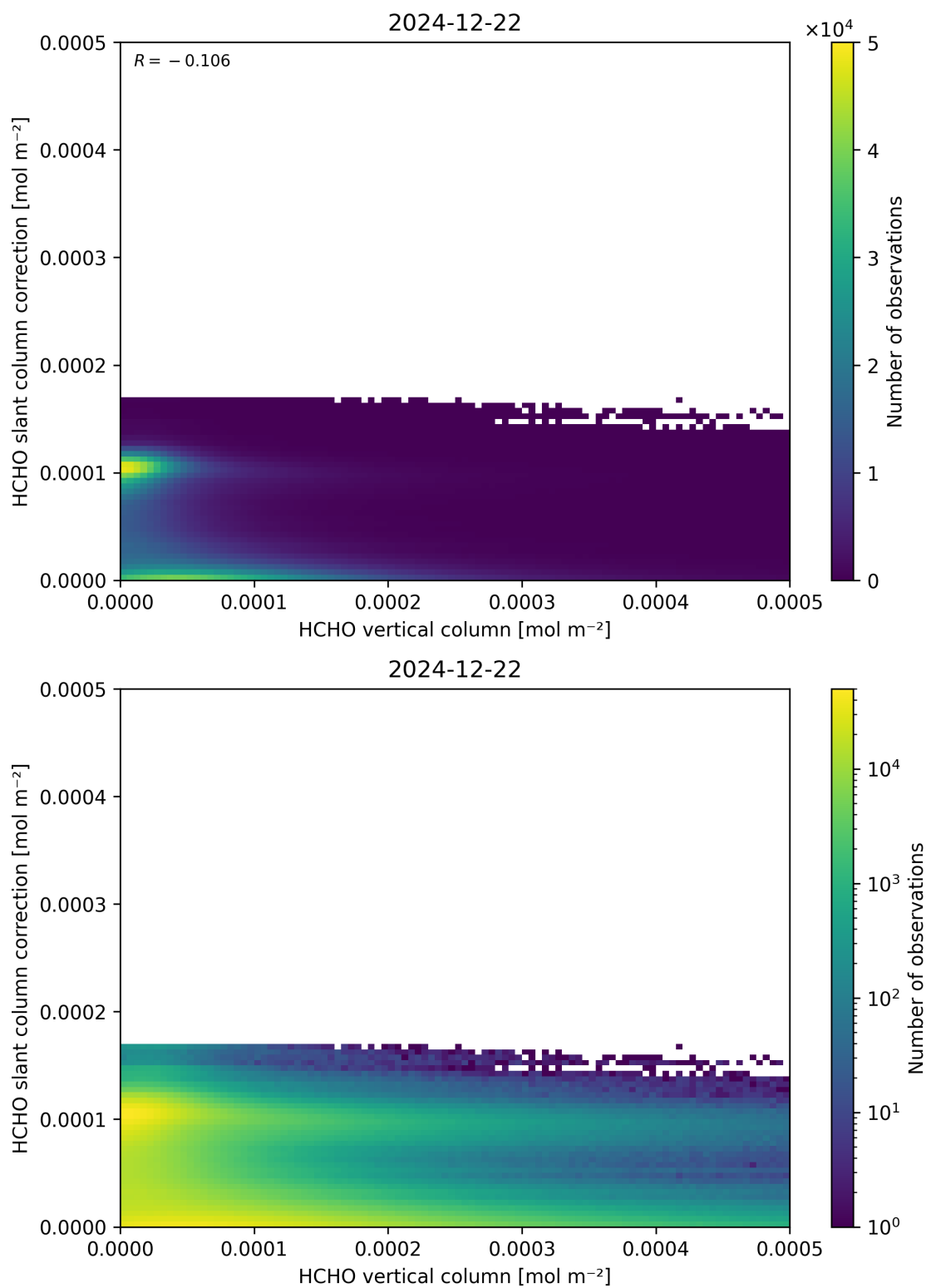
Figure 128: Scatter density plot of “HCHO vertical column” against “HCHO slant column correction” for 2024-12-22 to 2024-12-23.
