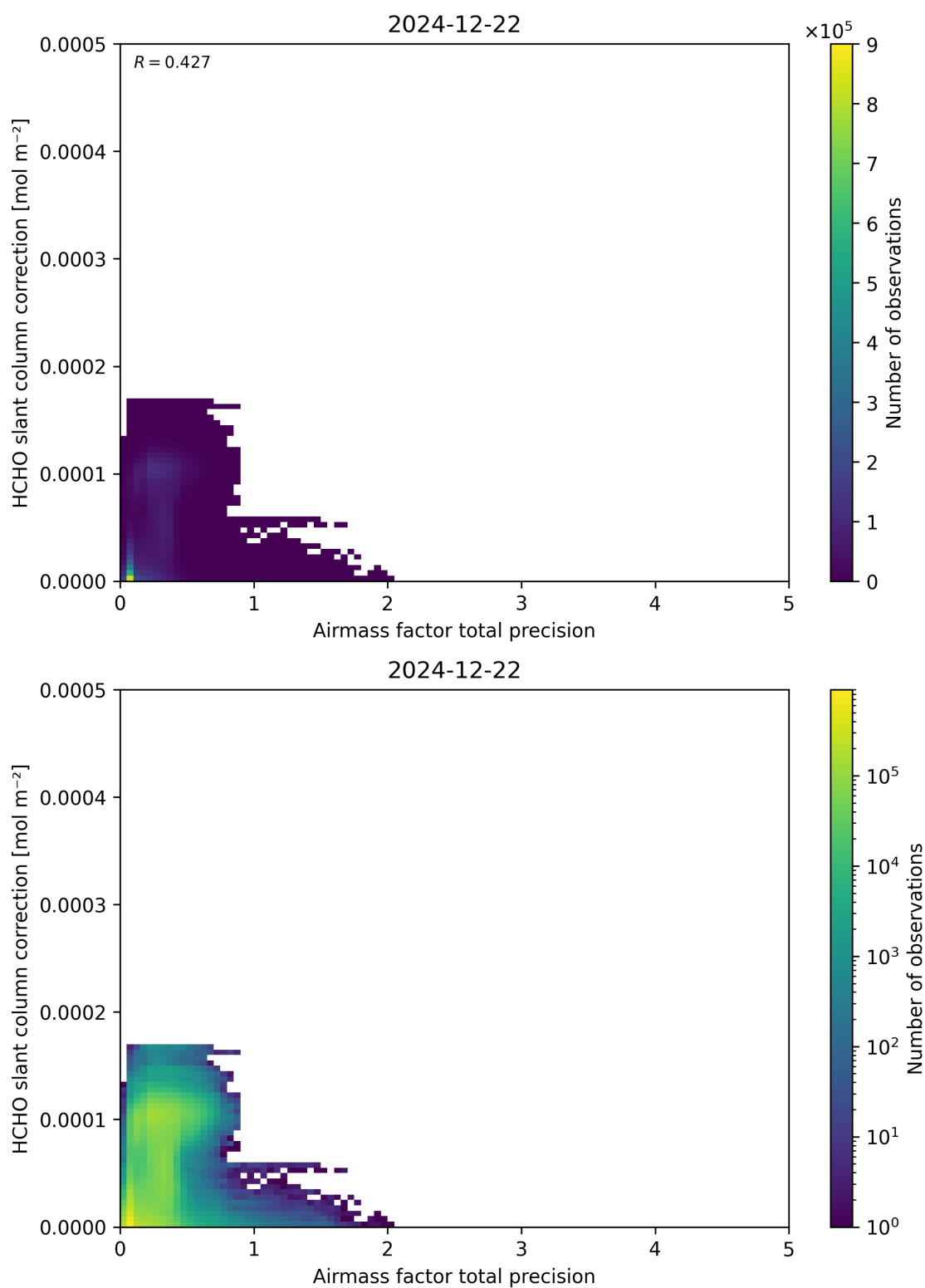
Figure 110: Scatter density plot of “Airmass factor total precision” against “HCHO slant column correction” for 2024-12-22 to 2024-12-23.
