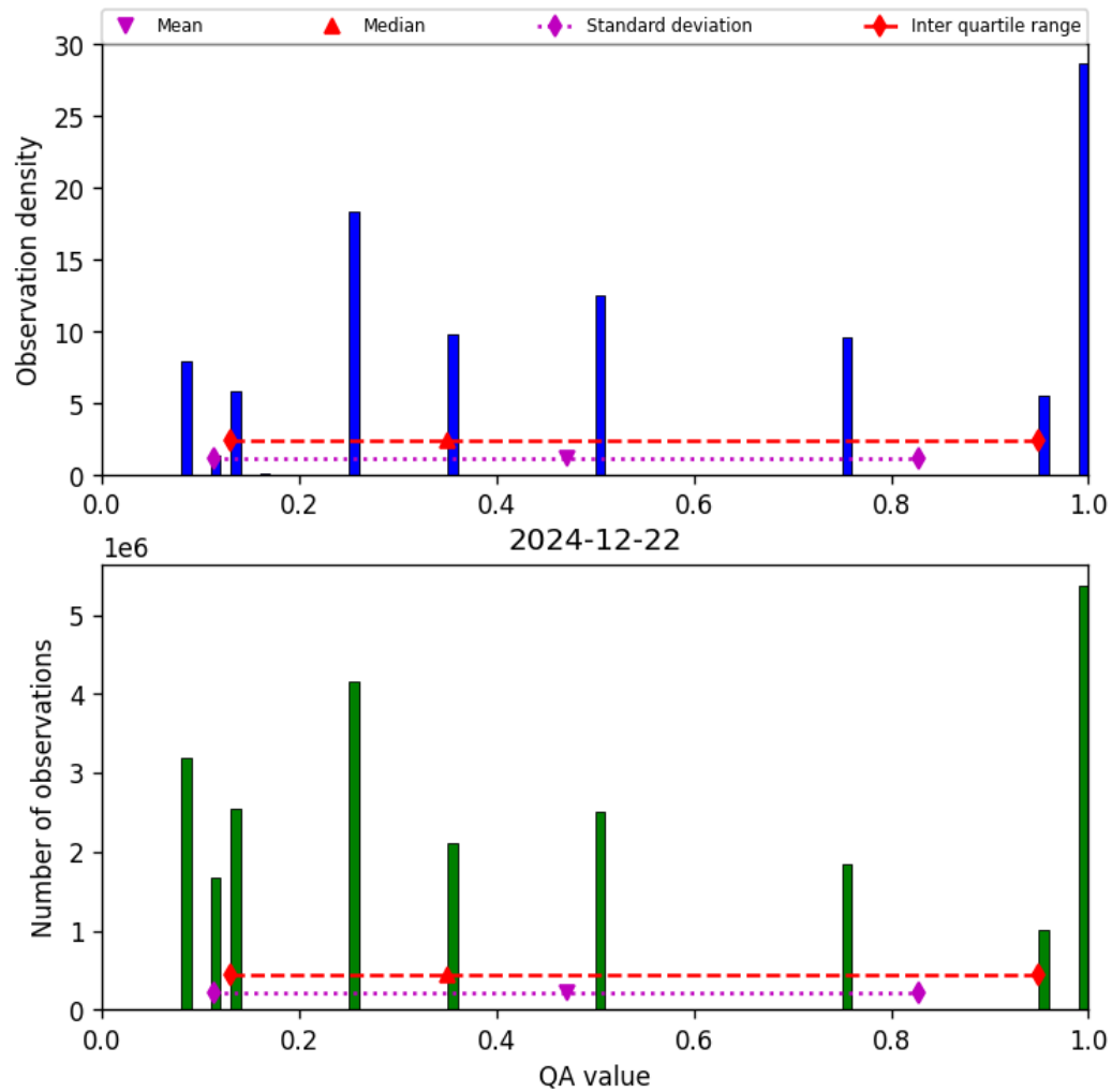
Figure 34: Histogram of “QA value” for 2024-12-22 to 2024-12-23
