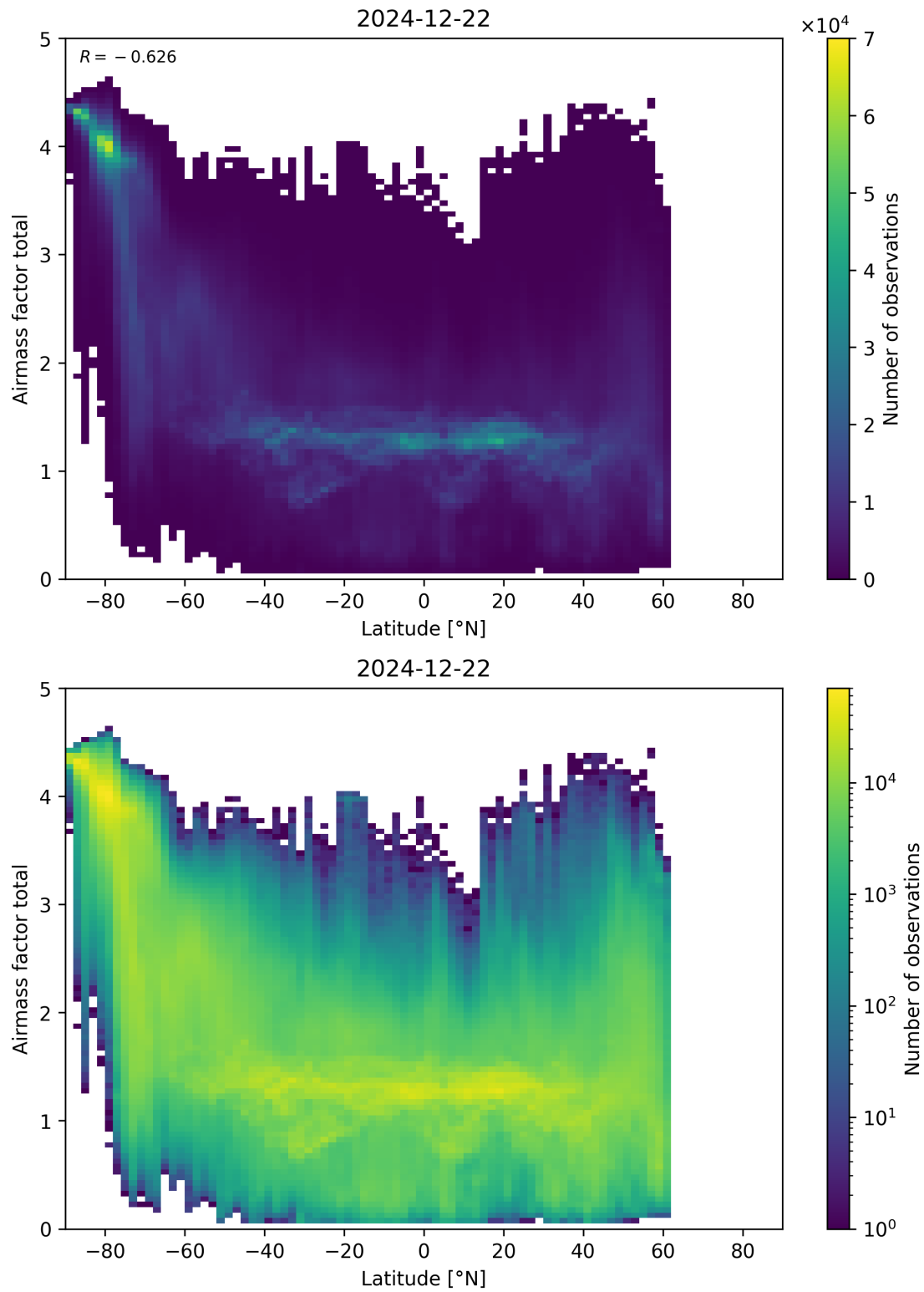
Figure 161: Scatter density plot of “Latitude” against “Airmass factor total” for 2024-12-22 to 2024-12-23.
