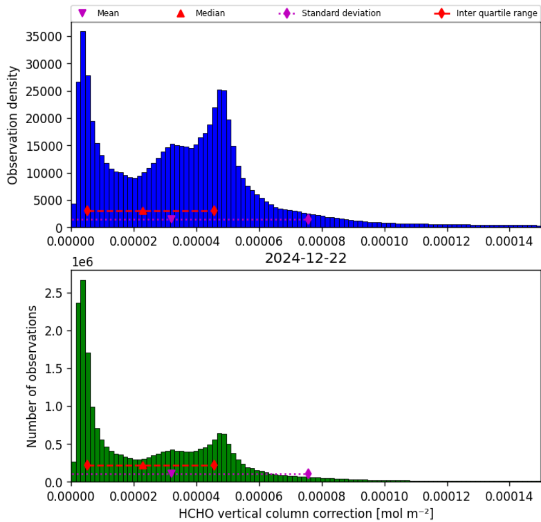
Figure 37: Histogram of “HCHO vertical column correction” for 2024-12-22 to 2024-12-23
