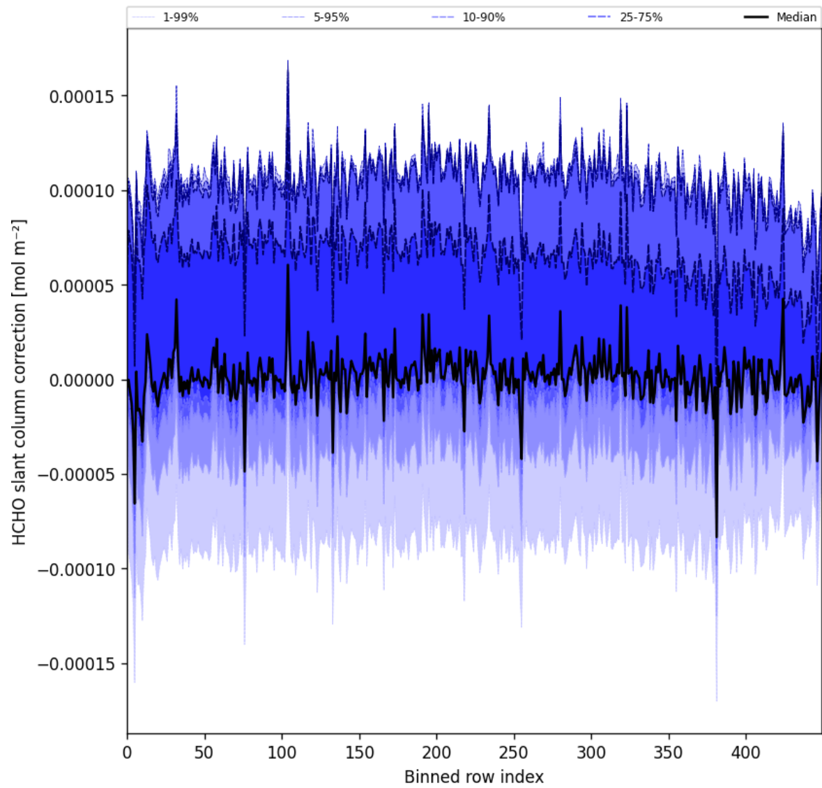
Figure 61: Along track statistics of “HCHO slant column correction” for 2024-12-22 to 2024-12-23
