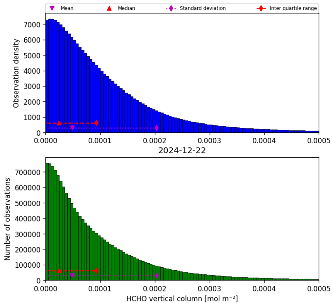
Figure 35: Histogram of “HCHO vertical column” for 2024-12-22 to 2024-12-23
