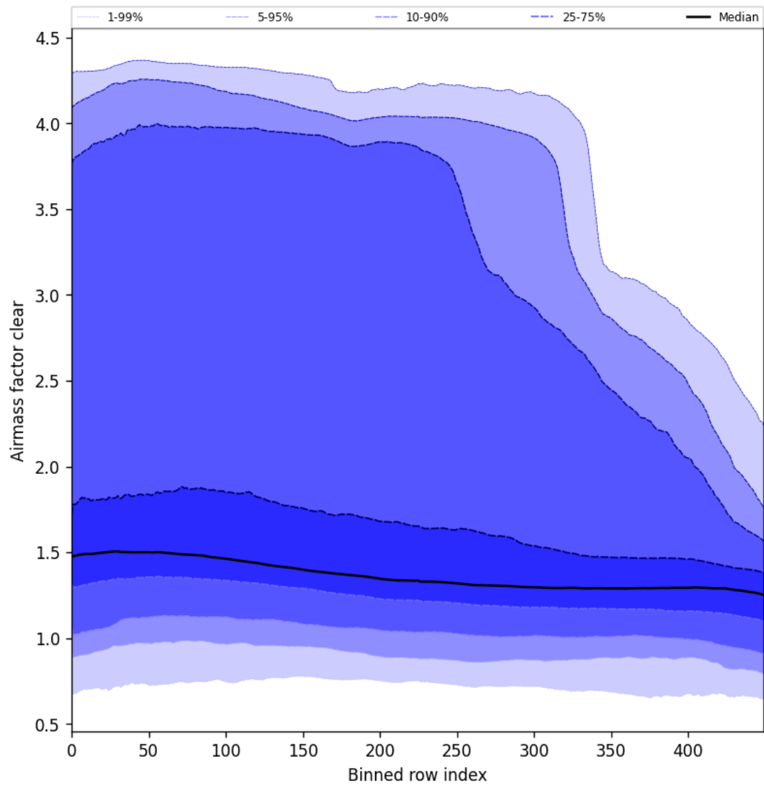
Figure 56: Along track statistics of “Air mass factor clear” for 2024-12-22 to 2024-12-23
