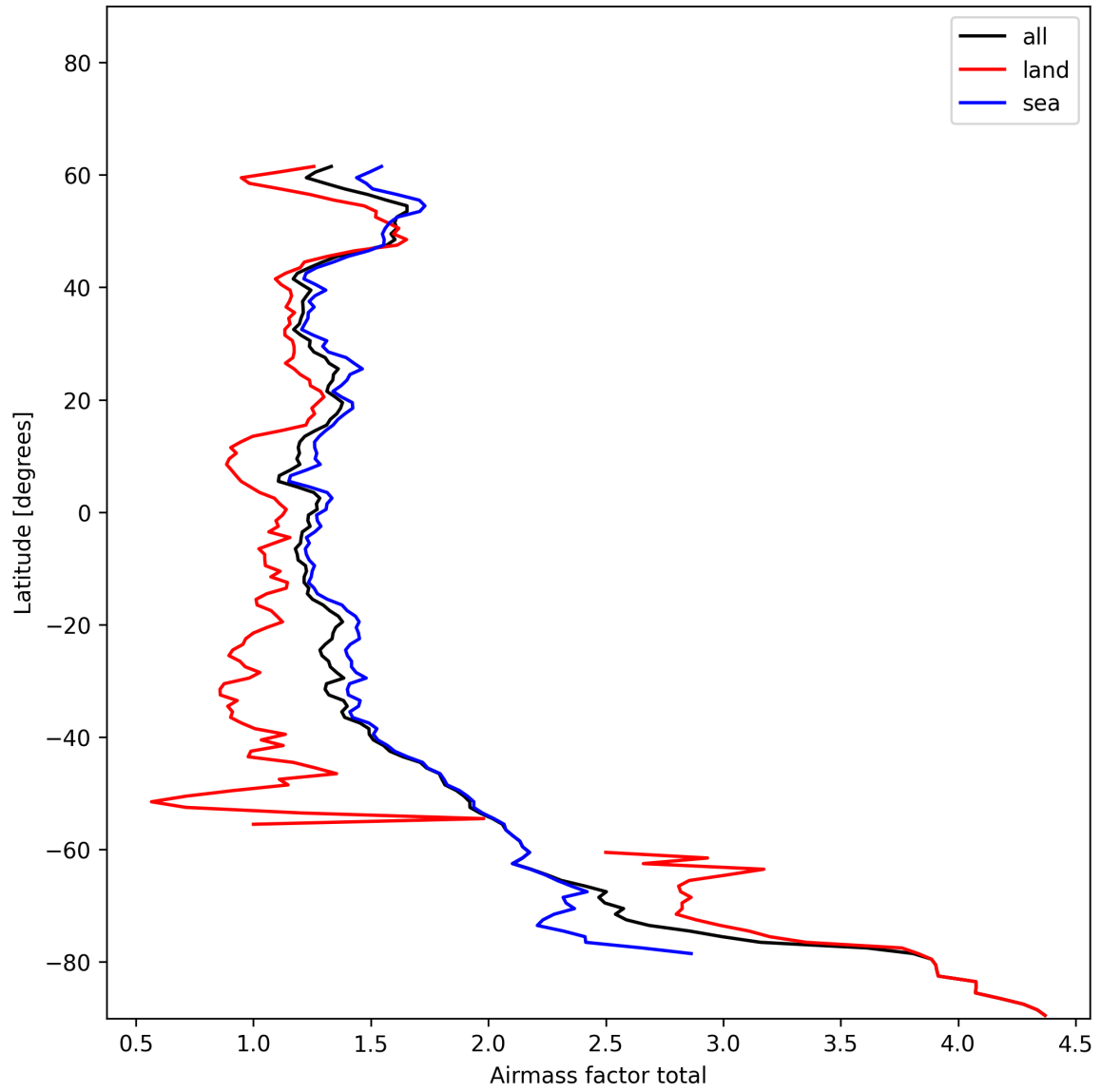
Figure 26: Zonal average of “Airmass factor total” for 2024-12-22 to 2024-12-23.
