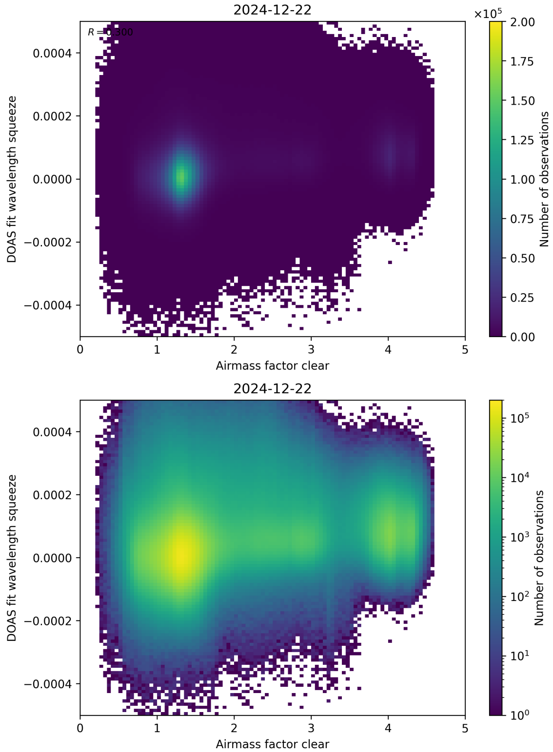
Figure 73: Scatter density plot of “Airmass factor clear” against “DOAS fit wavelength squeeze” for 2024-12-22 to 2024-12-23.
