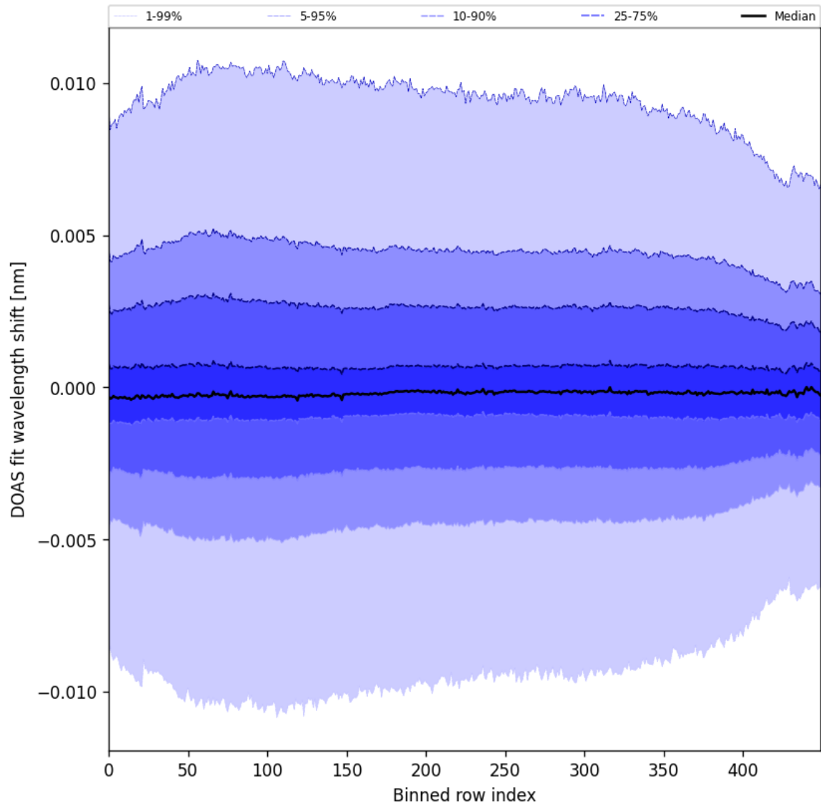
Figure 58: Along track statistics of “DOAS fit wavelength shift” for 2024-12-22 to 2024-12-23
