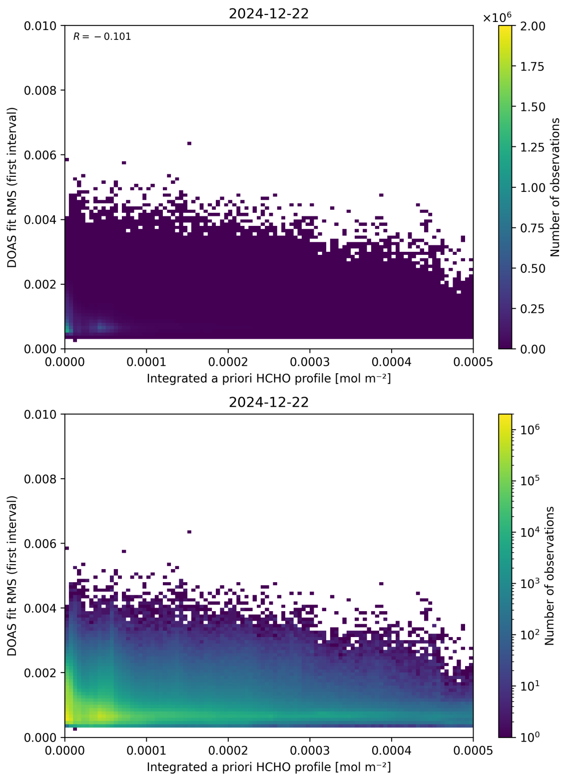
Figure 148: Scatter density plot of “Integrated a priori HCHO profile” against “DOAS fit RMS (first interval)” for 2024-12-22 to 2024-12-23.
