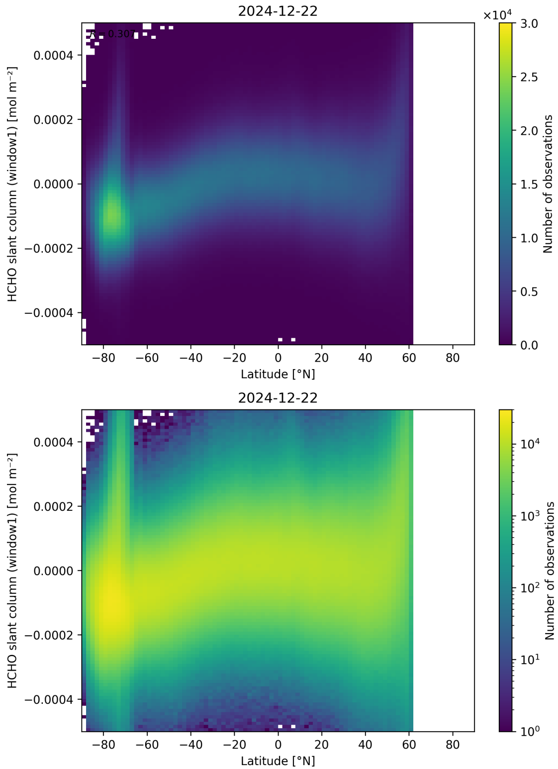
Figure 159: Scatter density plot of “Latitude” against “HCHO slant column (window1)” for 2024-12-22 to 2024-12-23.
