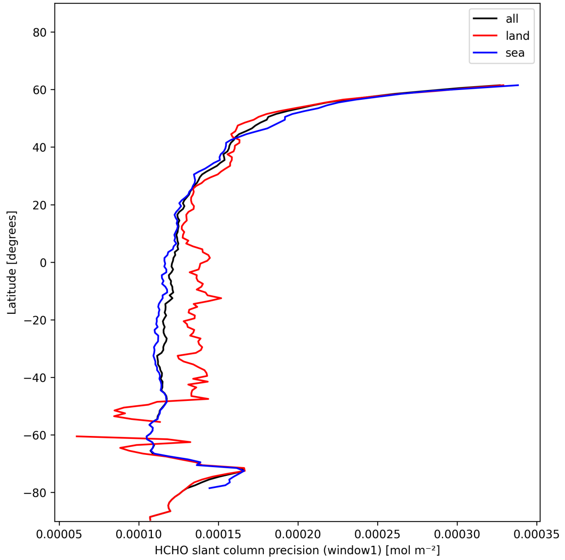
Figure 25: Zonal average of “HCHO slant column precision (window1)” for 2024-12-22 to 2024-12-23.
