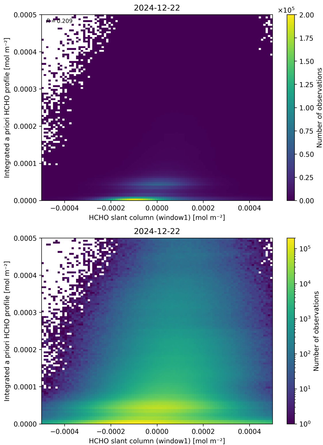
Figure 87: Scatter density plot of “HCHO slant column (window1)” against “Integrated a priori HCHO profile” for 2024-12-22 to 2024-12-23.
