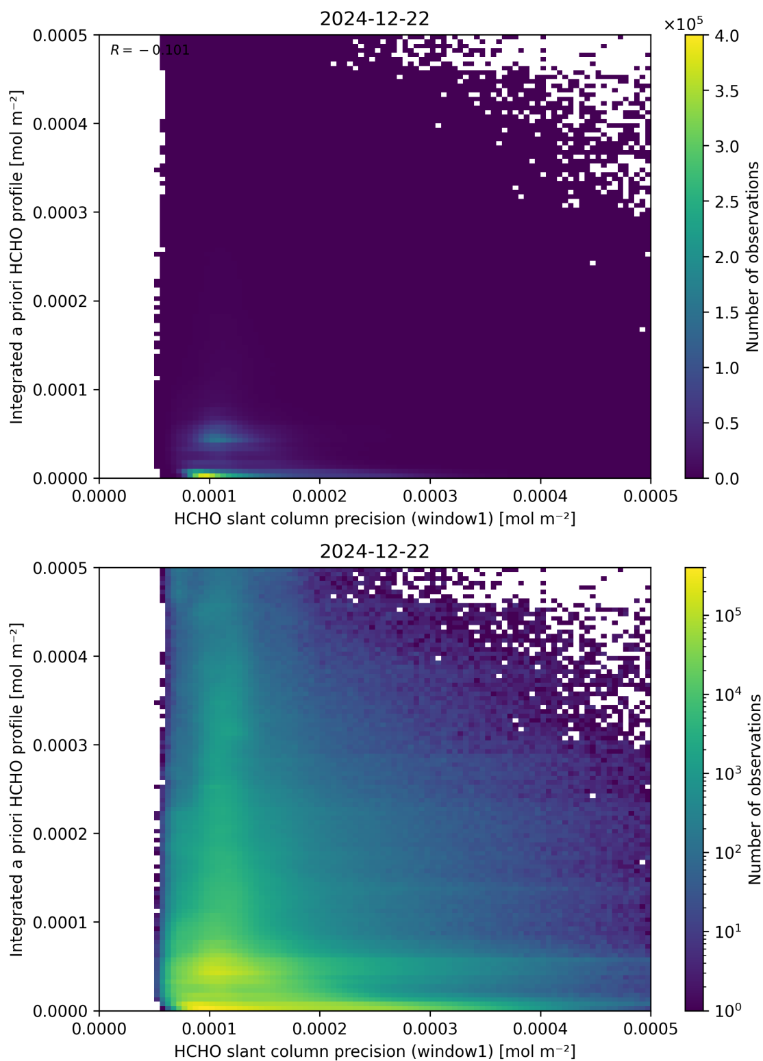
Figure 96: Scatter density plot of “HCHO slant column precision (window1)” against “Integrated a priori HCHO profile” for 2024-12-22 to 2024-12-23.
