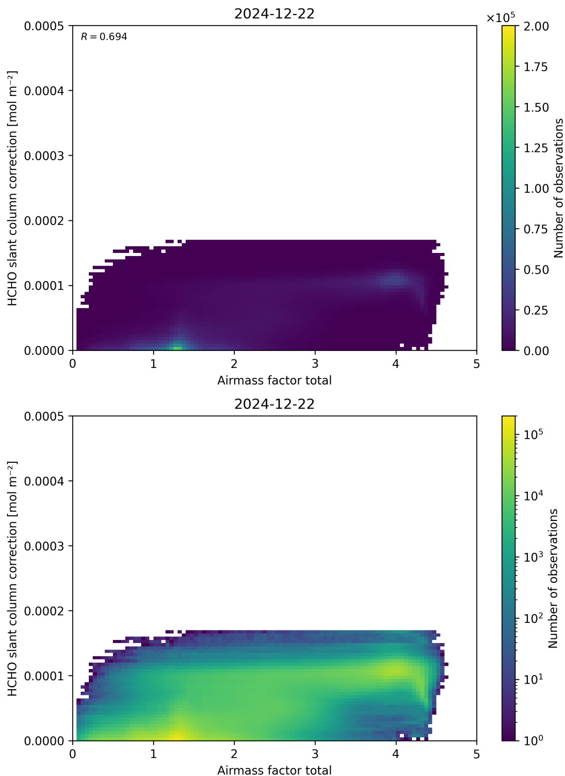
Figure 102: Scatter density plot of “Airmass factor total” against “HCHO slant column correction” for 2024-12-22 to 2024-12-23.
