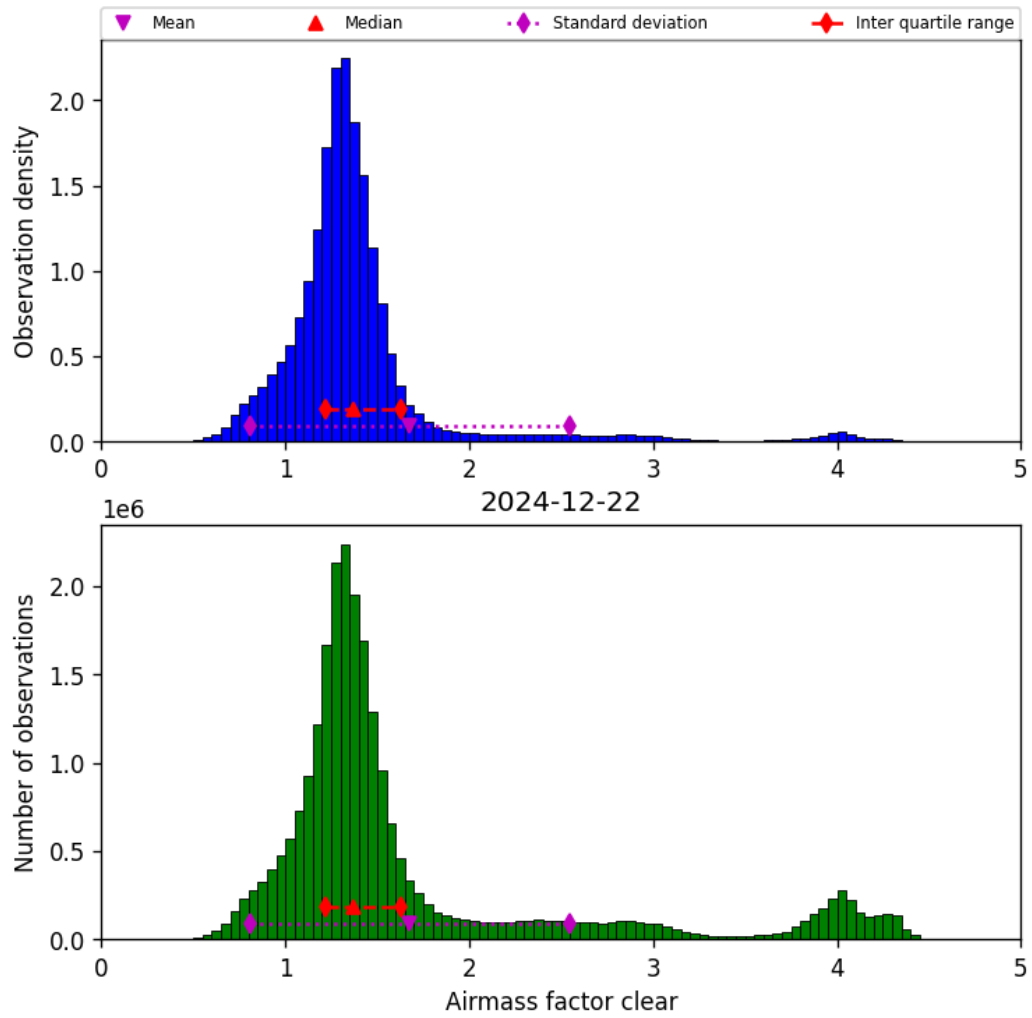
Figure 42: Histogram of “Airmass factor clear” for 2024-12-22 to 2024-12-23
