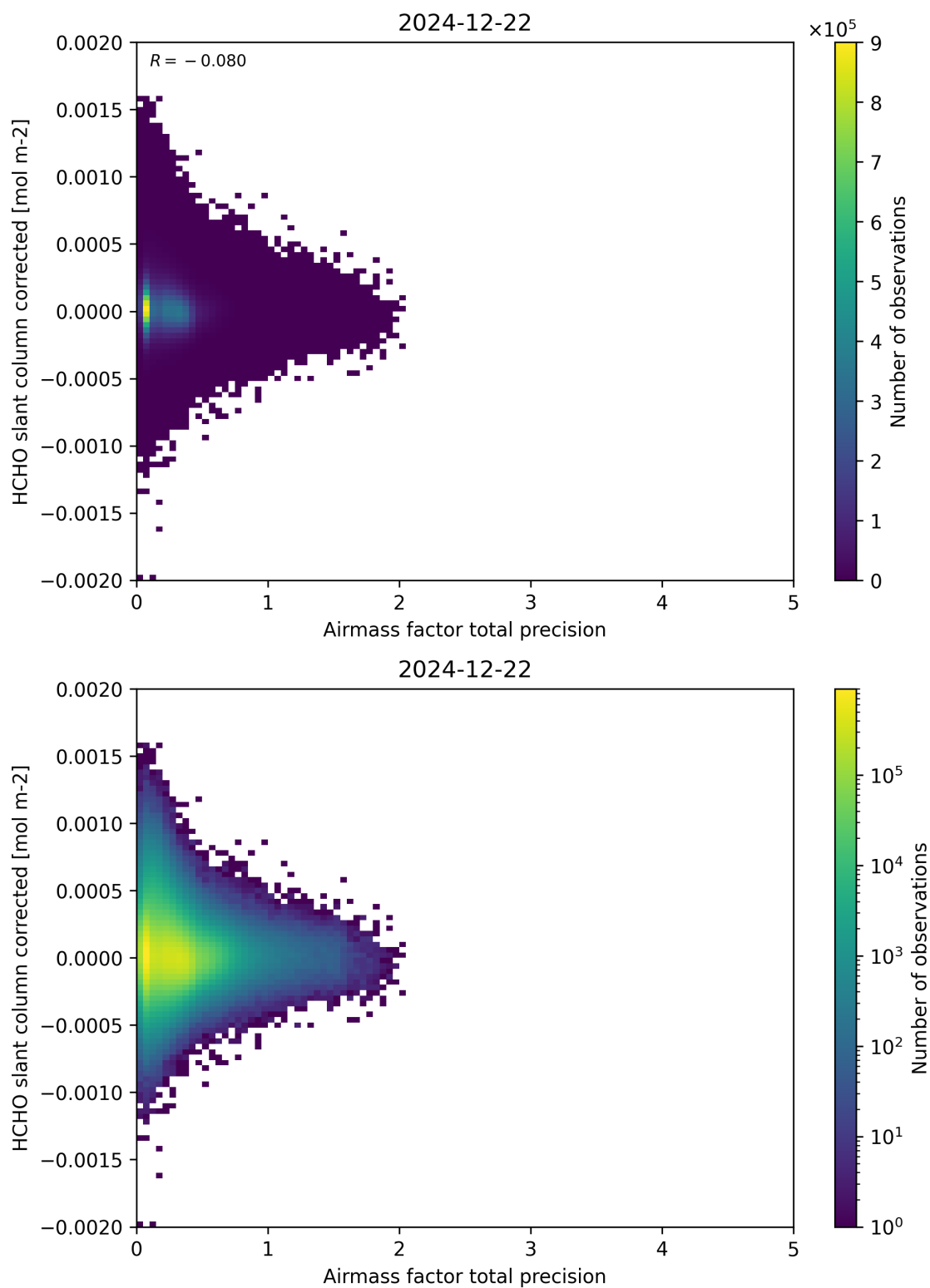
Figure 109: Scatter density plot of “Airmass factor total precision” against “HCHO slant column corrected” for 2024-12-22 to 2024-12-23.
