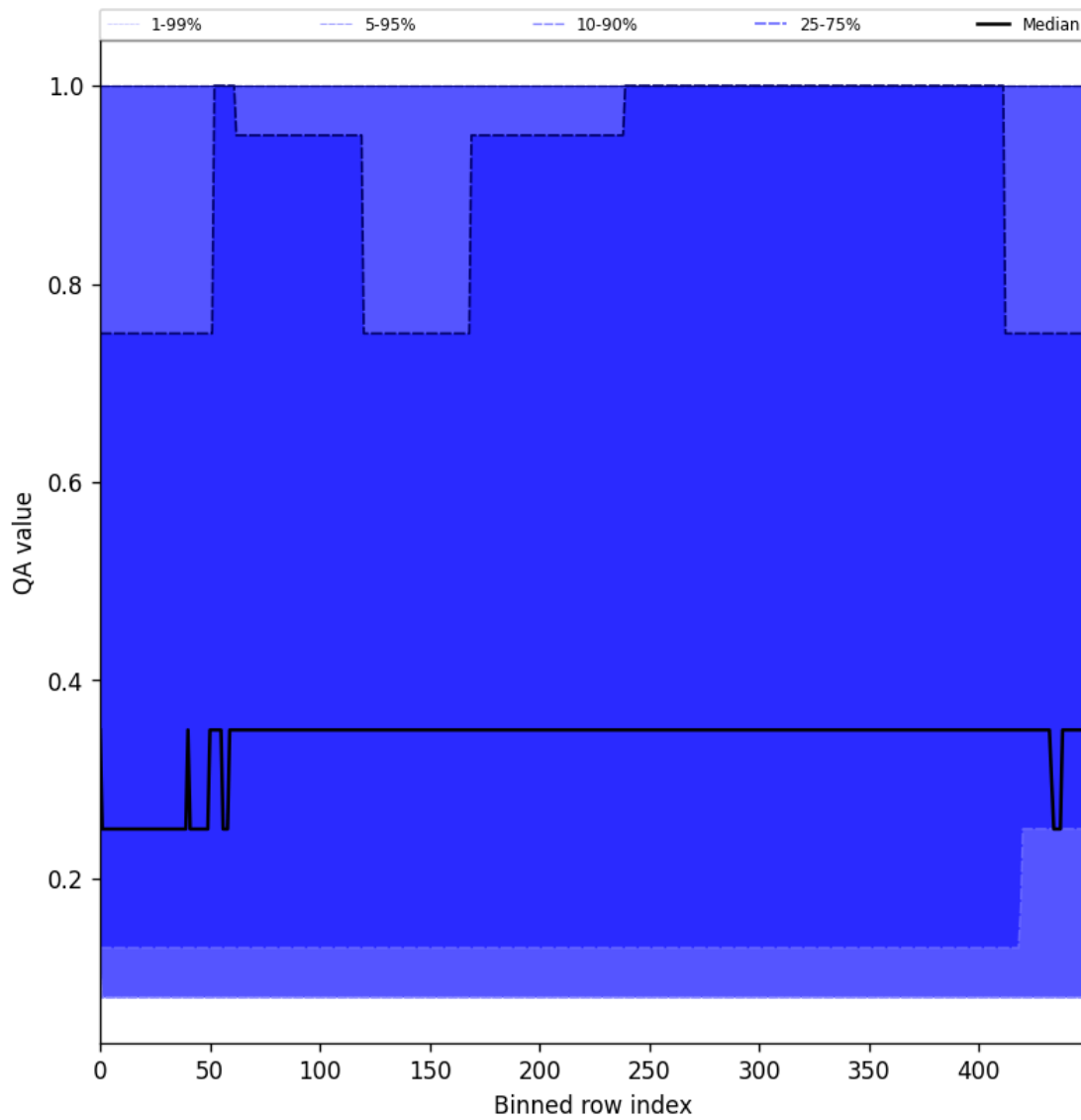
Figure 48: Along track statistics of “QA value” for 2024-12-22 to 2024-12-23
