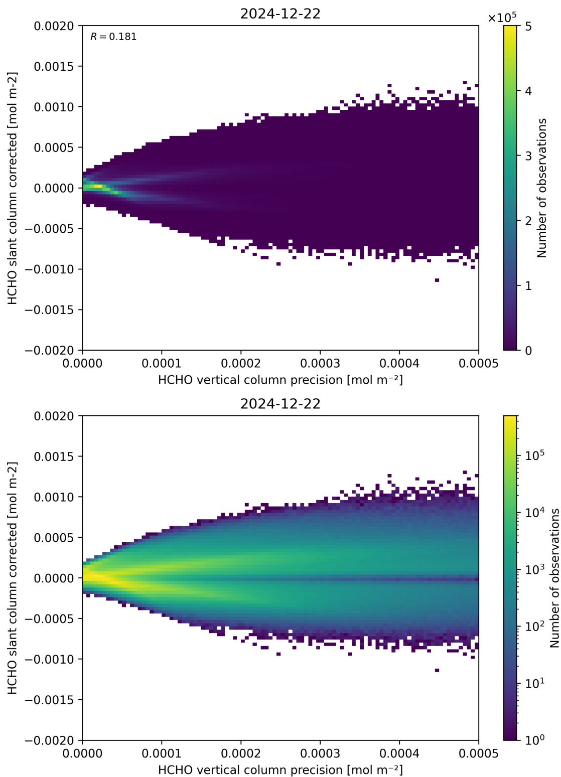
Figure 140: Scatter density plot of “HCHO vertical column precision” against “HCHO slant column corrected” for 2024-12-22 to 2024-12-23.
