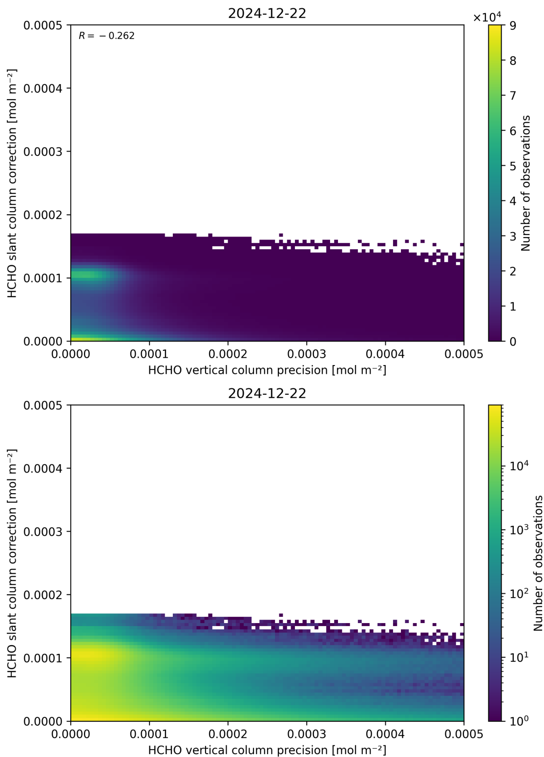
Figure 141: Scatter density plot of “HCHO vertical column precision” against “HCHO slant column correction” for 2024-12-22 to 2024-12-23.
