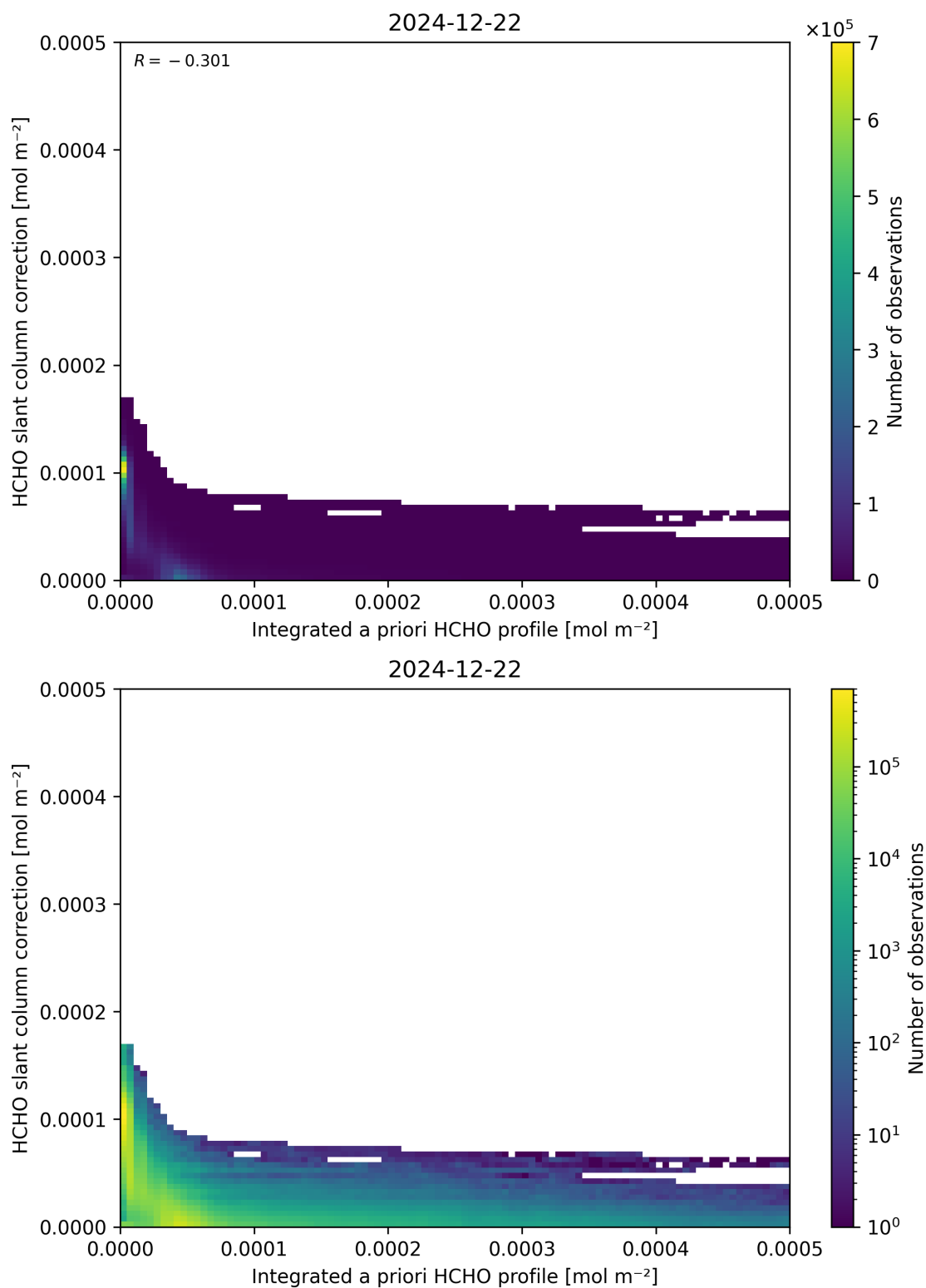
Figure 152: Scatter density plot of “Integrated a priori HCHO profile” against “HCHO slant column correction” for 2024-12-22 to 2024-12-23.
