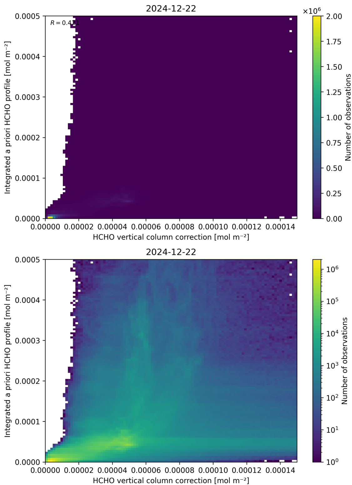
Figure 122: Scatter density plot of “HCHO vertical column correction” against “Integrated a priori HCHO profile” for 2024-12-22 to 2024-12-23.
