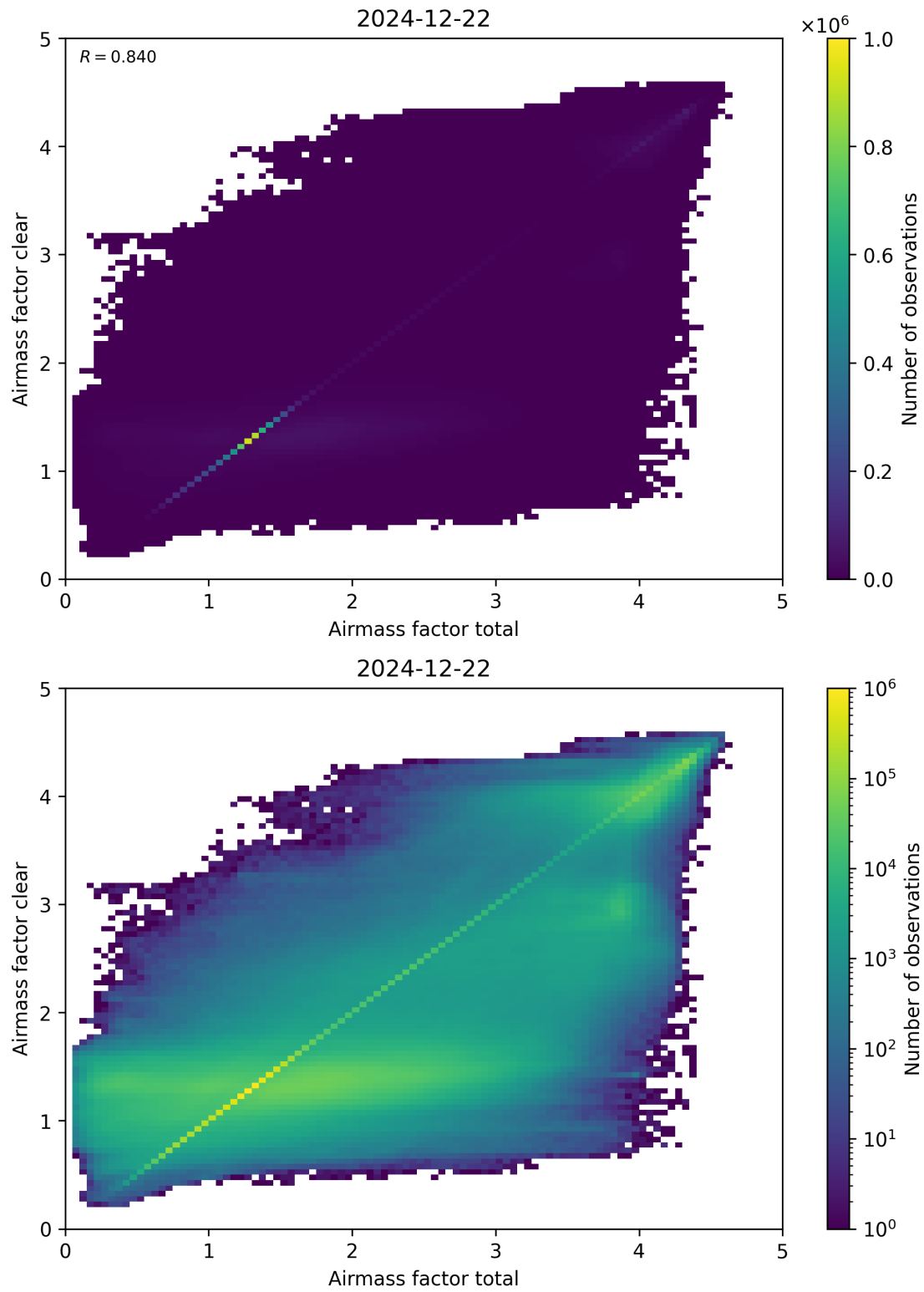
Figure 100: Scatter density plot of “Airmass factor total” against “Airmass factor clear” for 2024-12-22 to 2024-12-23.
