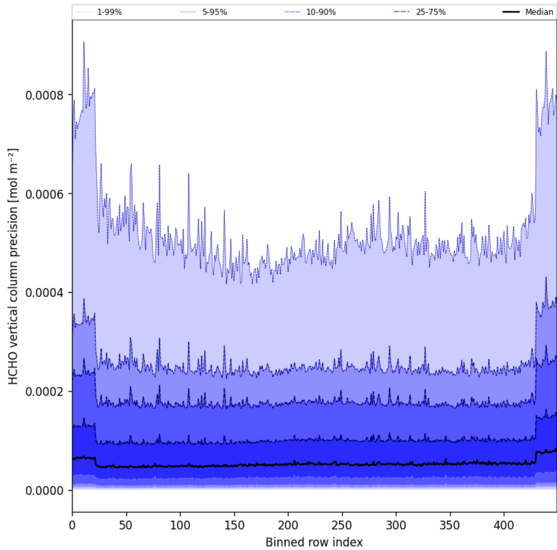
Figure 50: Along track statistics of “HCHO vertical column precision” for 2024-12-22 to 2024-12-23
