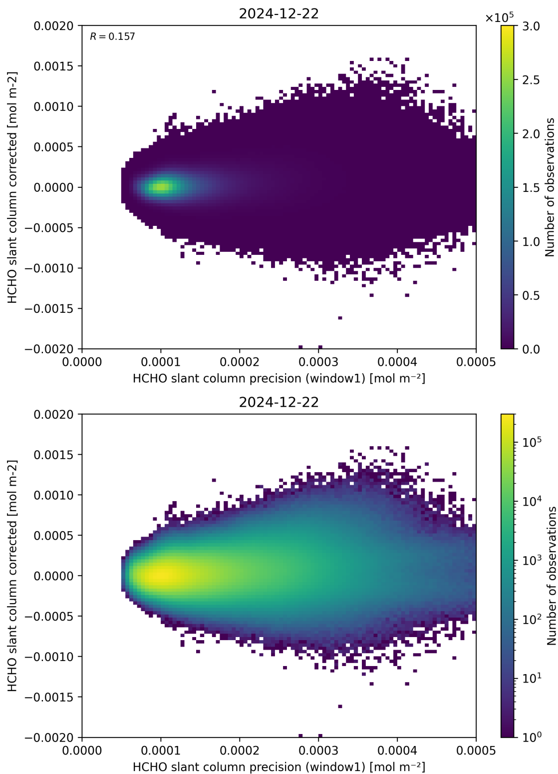
Figure 92: Scatter density plot of “HCHO slant column precision (window1)” against “HCHO slant column corrected” for 2024-12-22 to 2024-12-23.
