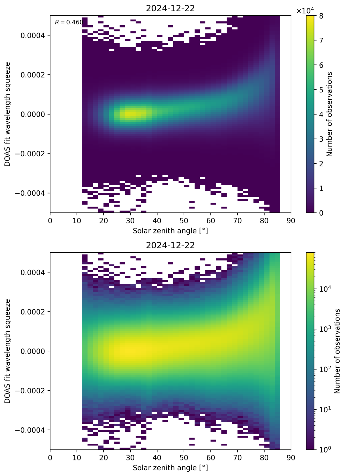
Figure 169: Scatter density plot of “Solar zenith angle” against “DOAS fit wavelength squeeze” for 2024-12-22 to 2024-12-23.
