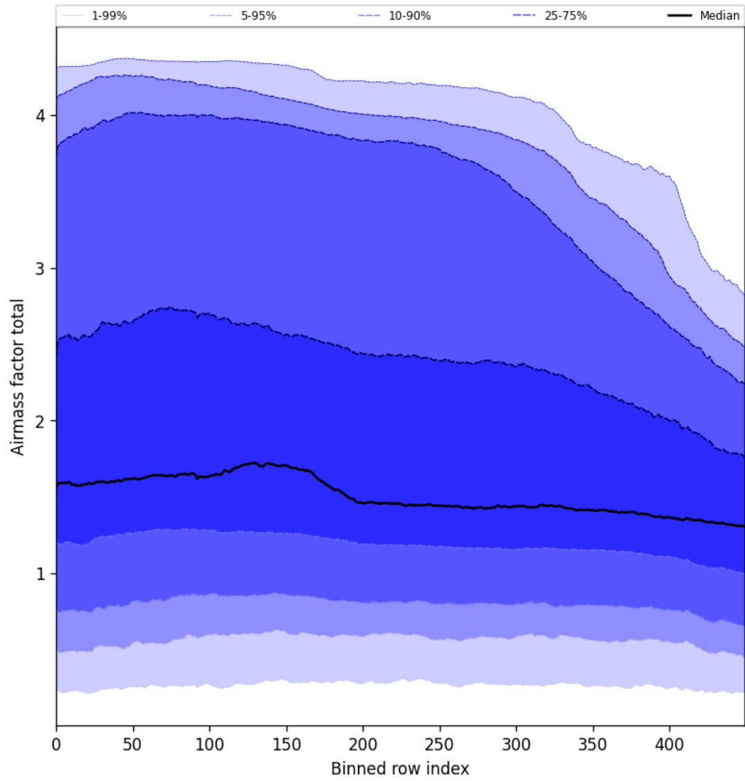
Figure 54: Along track statistics of “Airmass factor total” for 2024-12-22 to 2024-12-23
