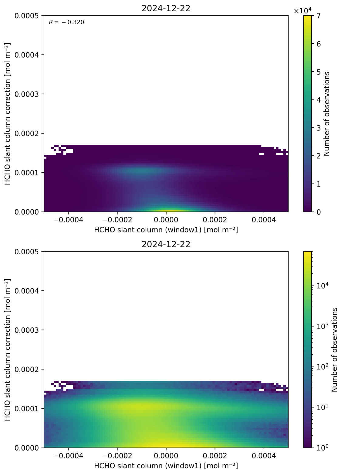
Figure 83: Scatter density plot of “HCHO slant column (window1)” against “HCHO slant column correction” for 2024-12-22 to 2024-12-23.
