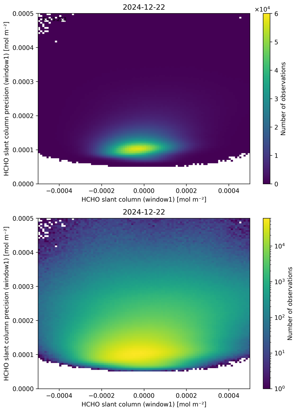
Figure 84: Scatter density plot of “HCHO slant column (window1)” against “HCHO slant column precision (window1)” for 2024-12-22 to 2024-12-23.
