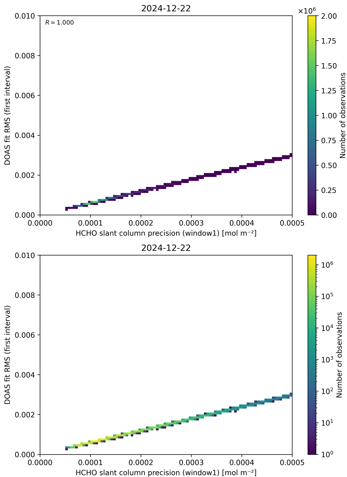
Figure 88: Scatter density plot of “HCHO slant column precision (window1)” against “DOAS fit RMS (first interval)” for 2024-12-22 to 2024-12-23.
