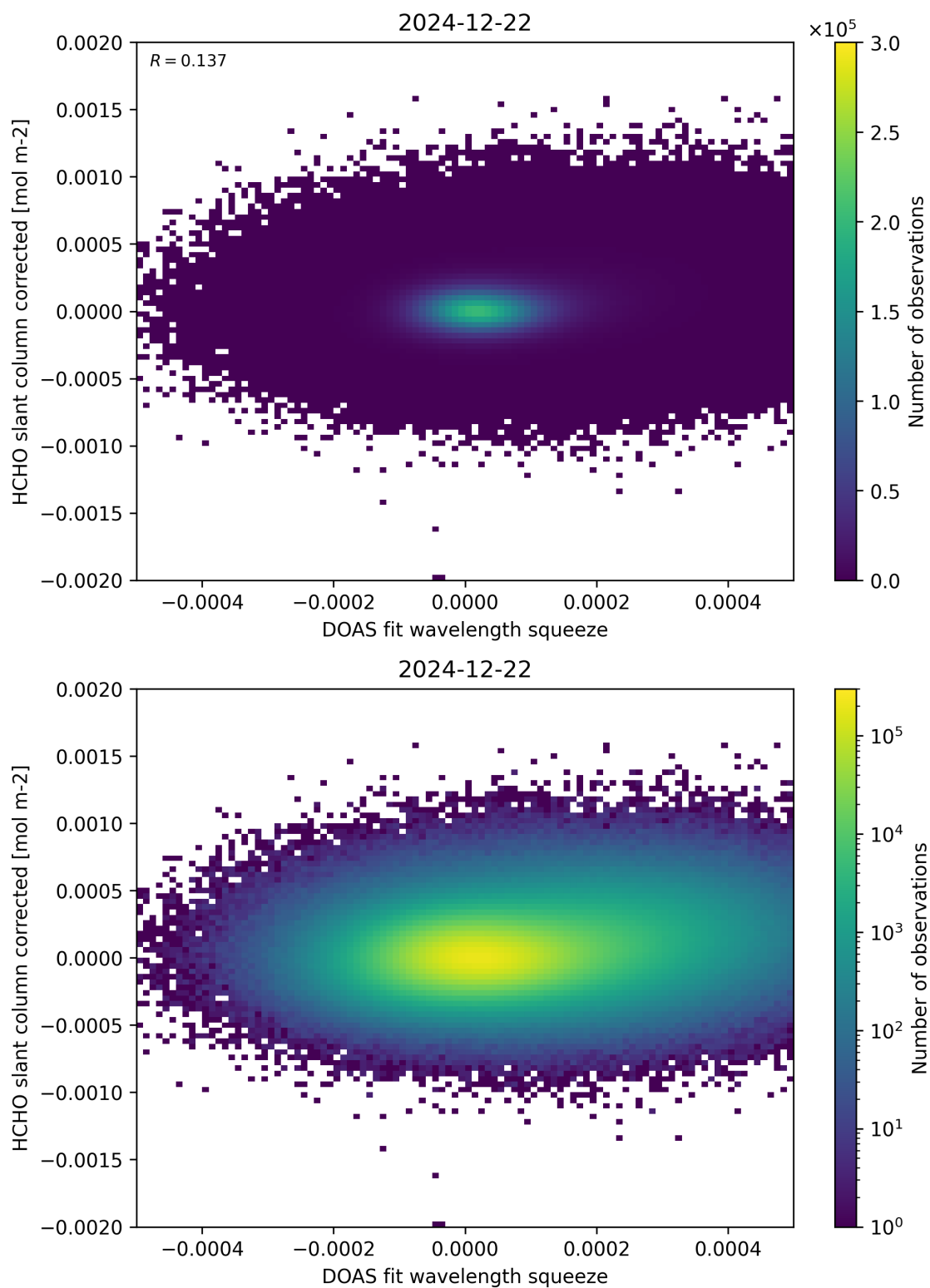
Figure 69: Scatter density plot of “DOAS fit wavelength squeeze” against “HCHO slant column corrected” for 2024-12-22 to 2024-12-23.
