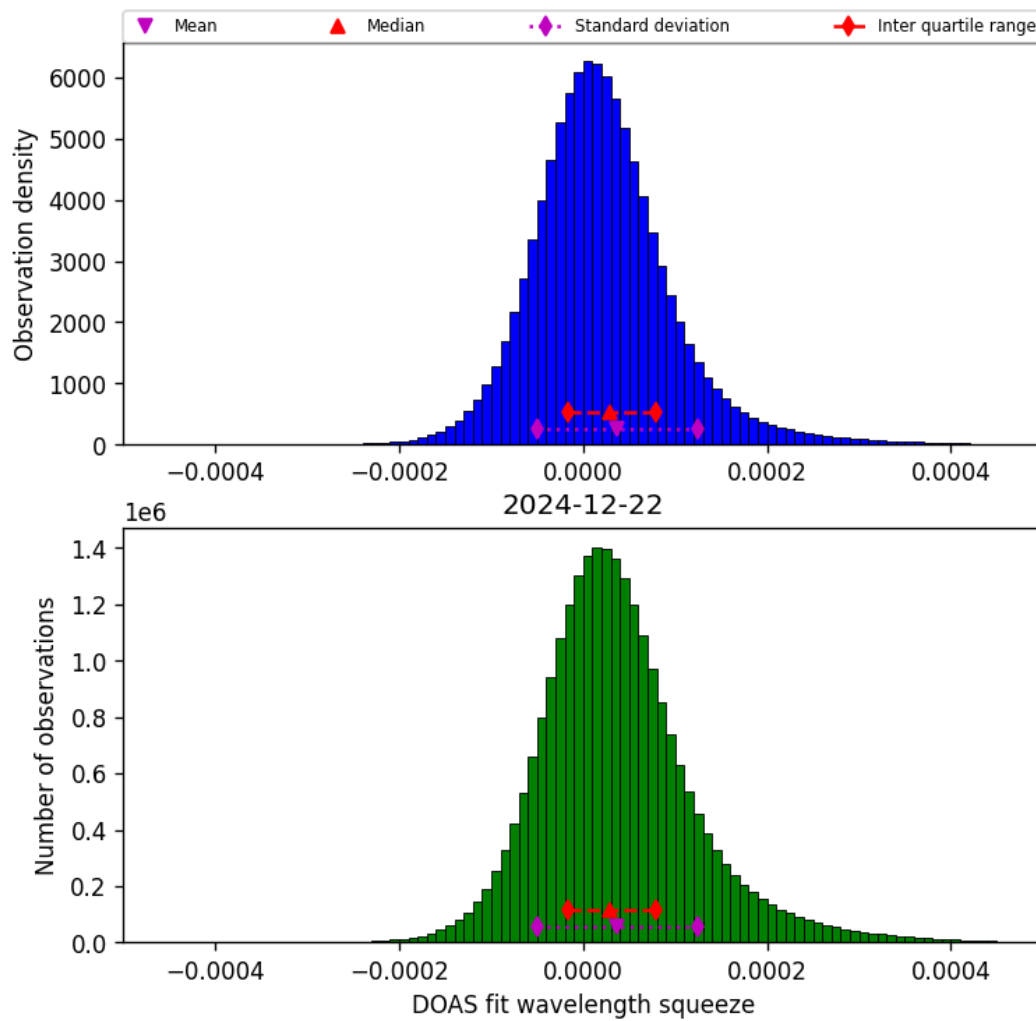
Figure 45: Histogram of “DOAS fit wavelength squeeze” for 2024-12-22 to 2024-12-23
