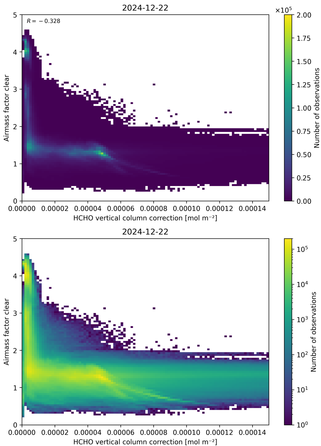
Figure 115: Scatter density plot of “HCHO vertical column correction” against “Airmass factor clear” for 2024-12-22 to 2024-12-23.
