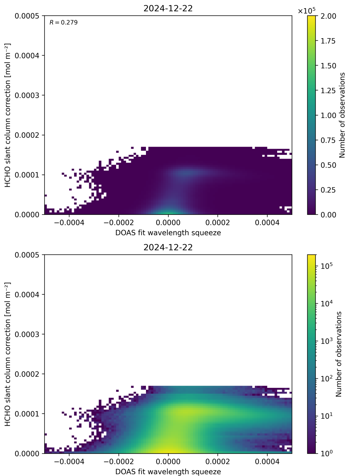
Figure 70: Scatter density plot of “DOAS fit wavelength squeeze” against “HCHO slant column correction” for 2024-12-22 to 2024-12-23.
