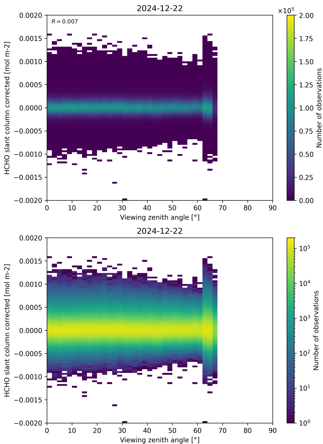
Figure 186: Scatter density plot of “Viewing zenith angle” against “HCHO slant column corrected” for 2024-12-22 to 2024-12-23.
