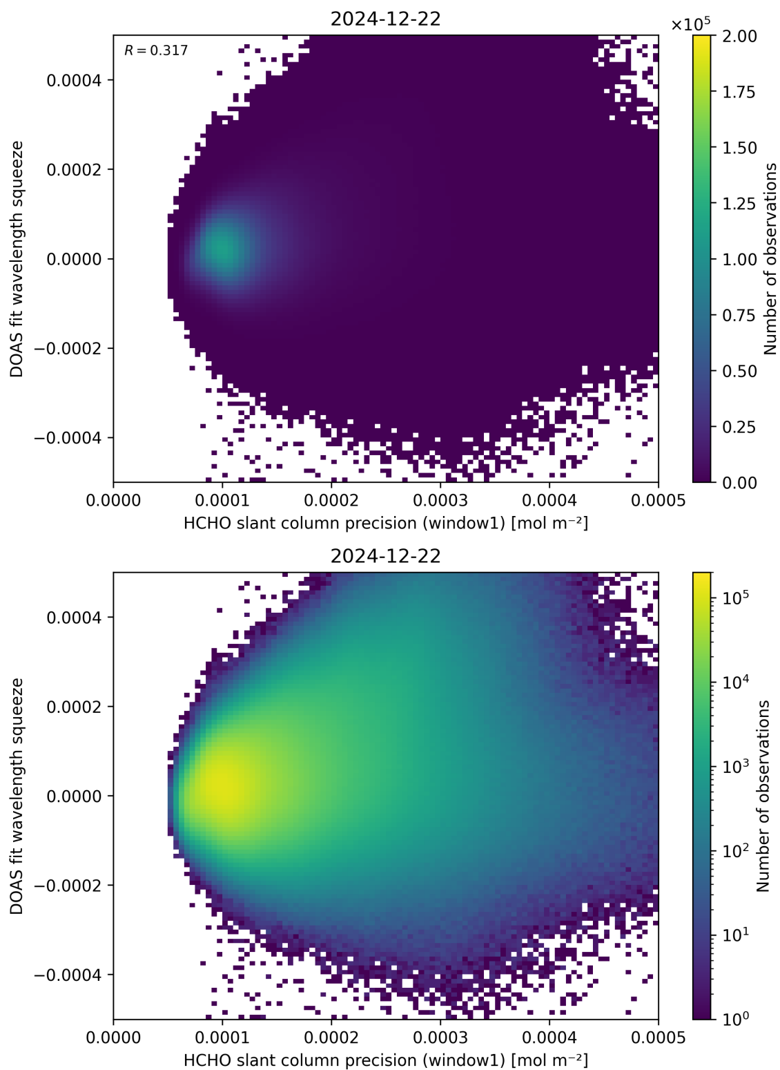
Figure 90: Scatter density plot of “HCHO slant column precision (window1)” against “DOAS fit wavelength squeeze” for 2024-12-22 to 2024-12-23.
