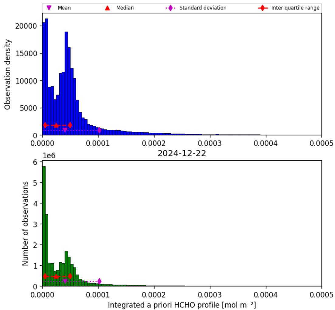
Figure 43: Histogram of “Integrated a priori HCHO profile” for 2024-12-22 to 2024-12-23
