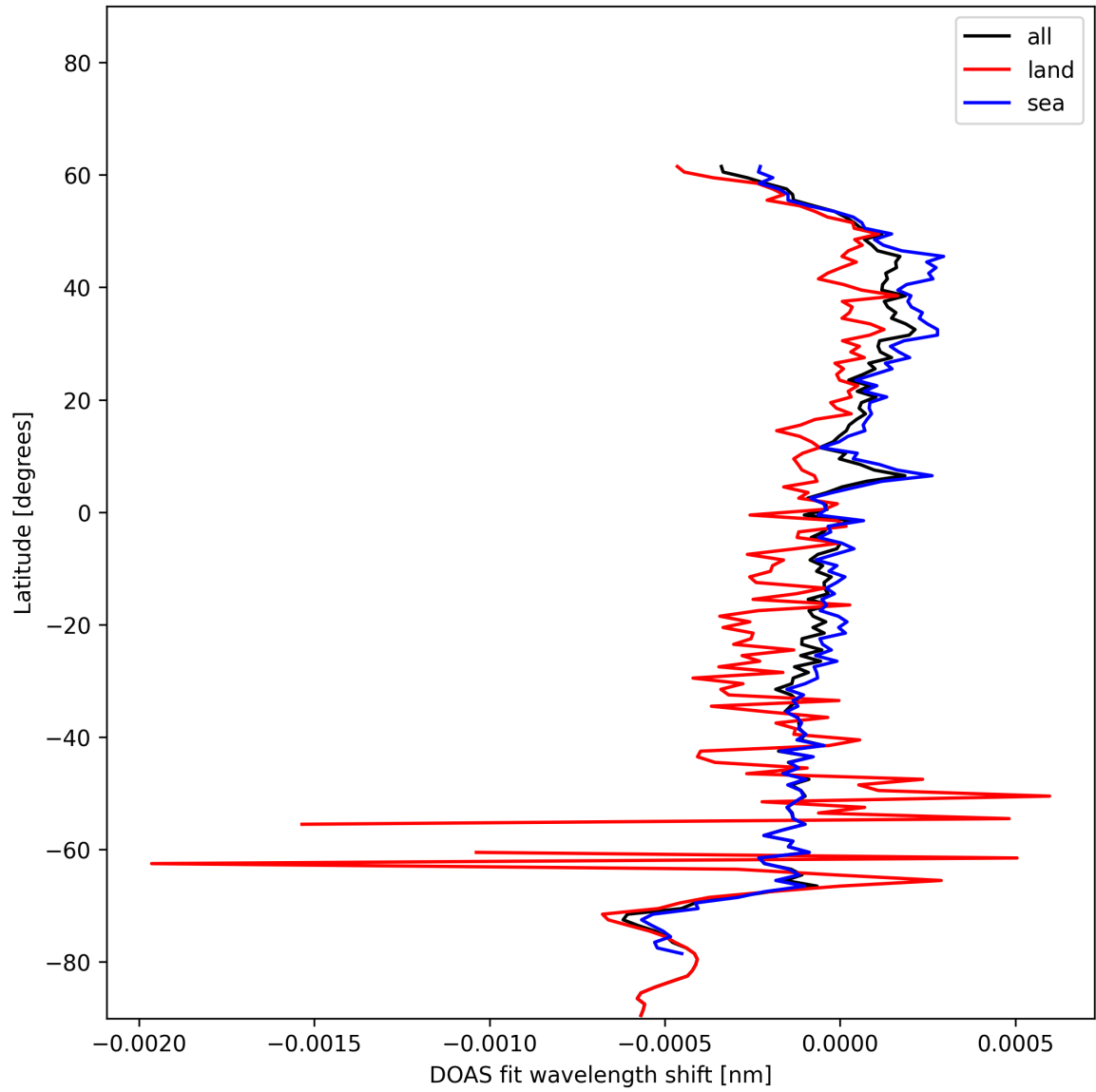
Figure 30: Zonal average of “DOAS fit wavelength shift” for 2024-12-22 to 2024-12-23.
