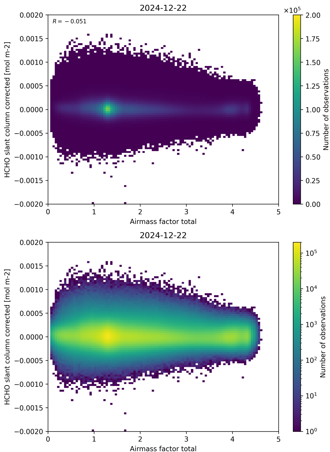
Figure 101: Scatter density plot of “Airmass factor total” against “HCHO slant column corrected” for 2024-12-22 to 2024-12-23.
