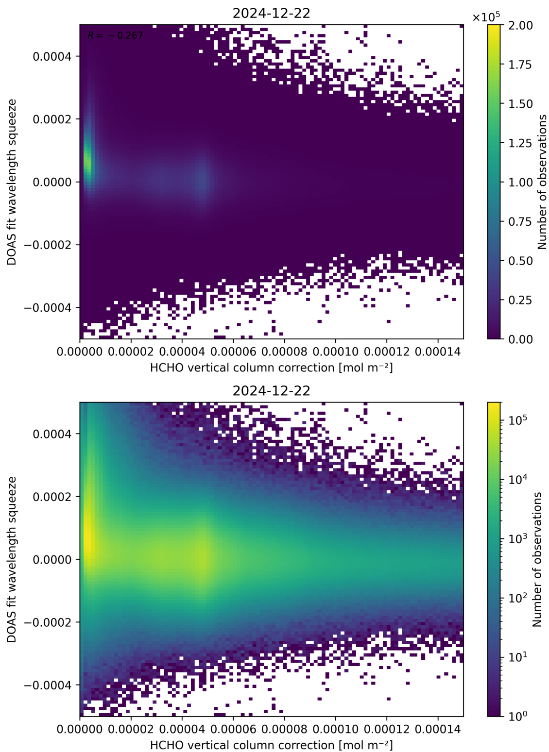
Figure 114: Scatter density plot of “HCHO vertical column correction” against “DOAS fit wavelength squeeze” for 2024-12-22 to 2024-12-23.
