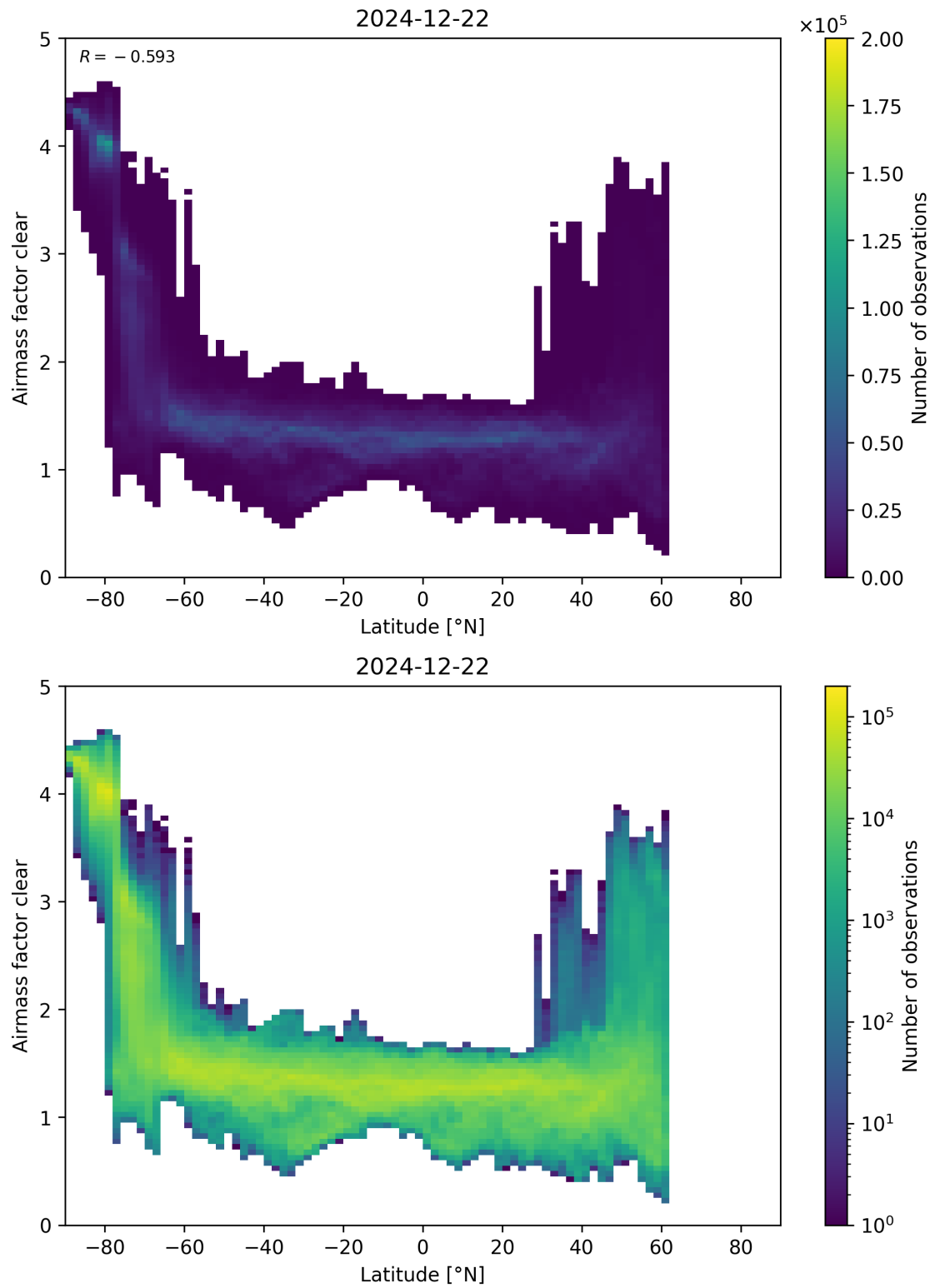
Figure 156: Scatter density plot of “Latitude” against “Airmass factor clear” for 2024-12-22 to 2024-12-23.
