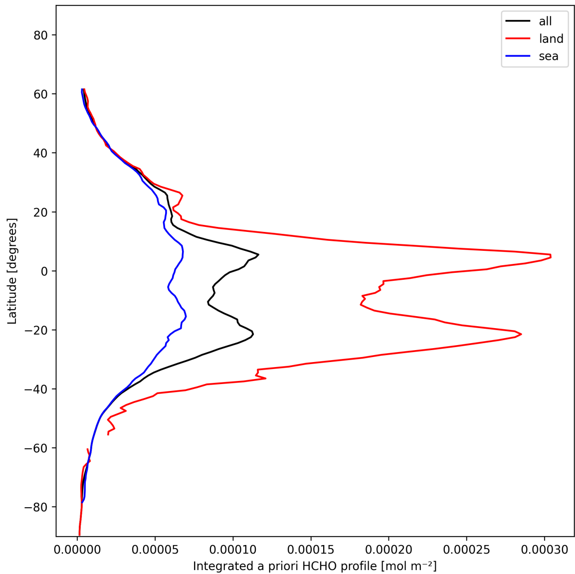
Figure 29: Zonal average of “Integrated a priori HCHO profile” for 2024-12-22 to 2024-12-23.
