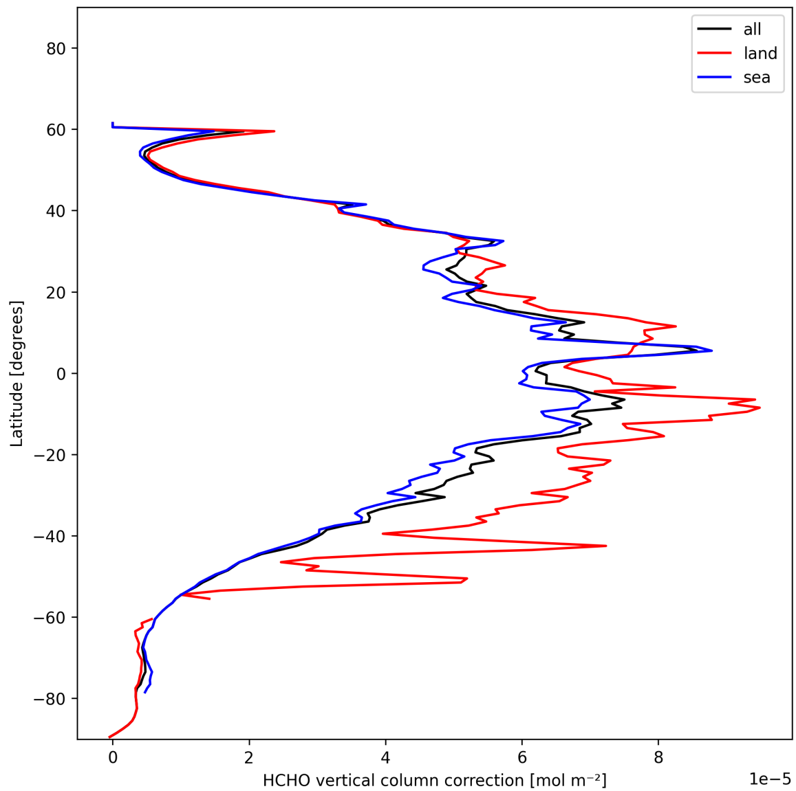
Figure 23: Zonal average of “HCHO vertical column correction” for 2024-12-22 to 2024-12-23.
