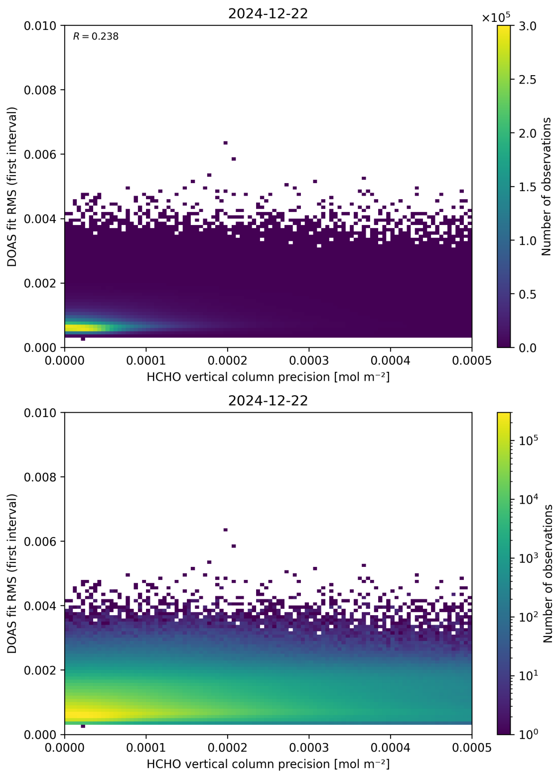
Figure 136: Scatter density plot of “HCHO vertical column precision” against “DOAS fit RMS (first interval)” for 2024-12-22 to 2024-12-23.
