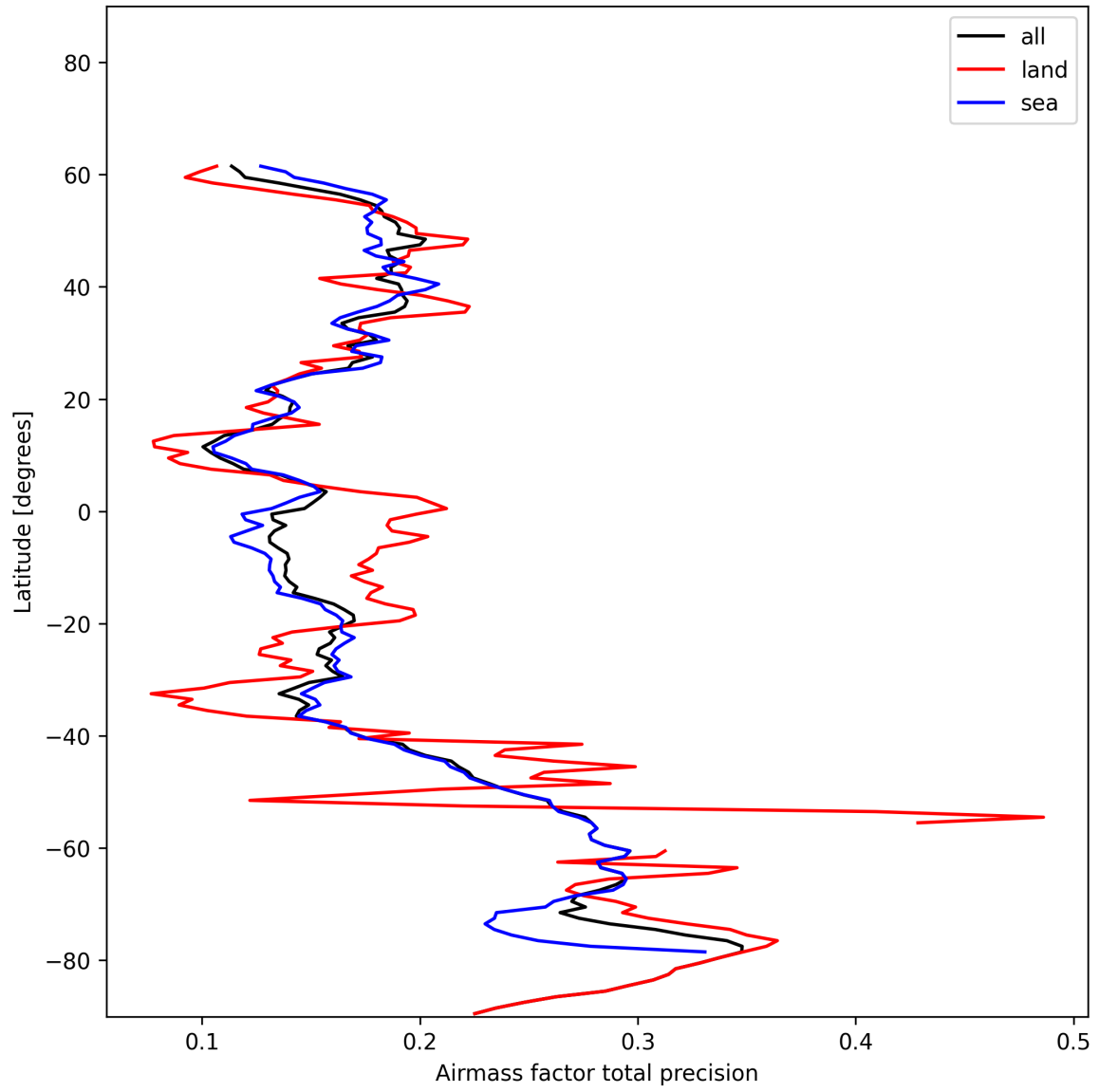
Figure 27: Zonal average of “Airmass factor total precision” for 2024-12-22 to 2024-12-23.
