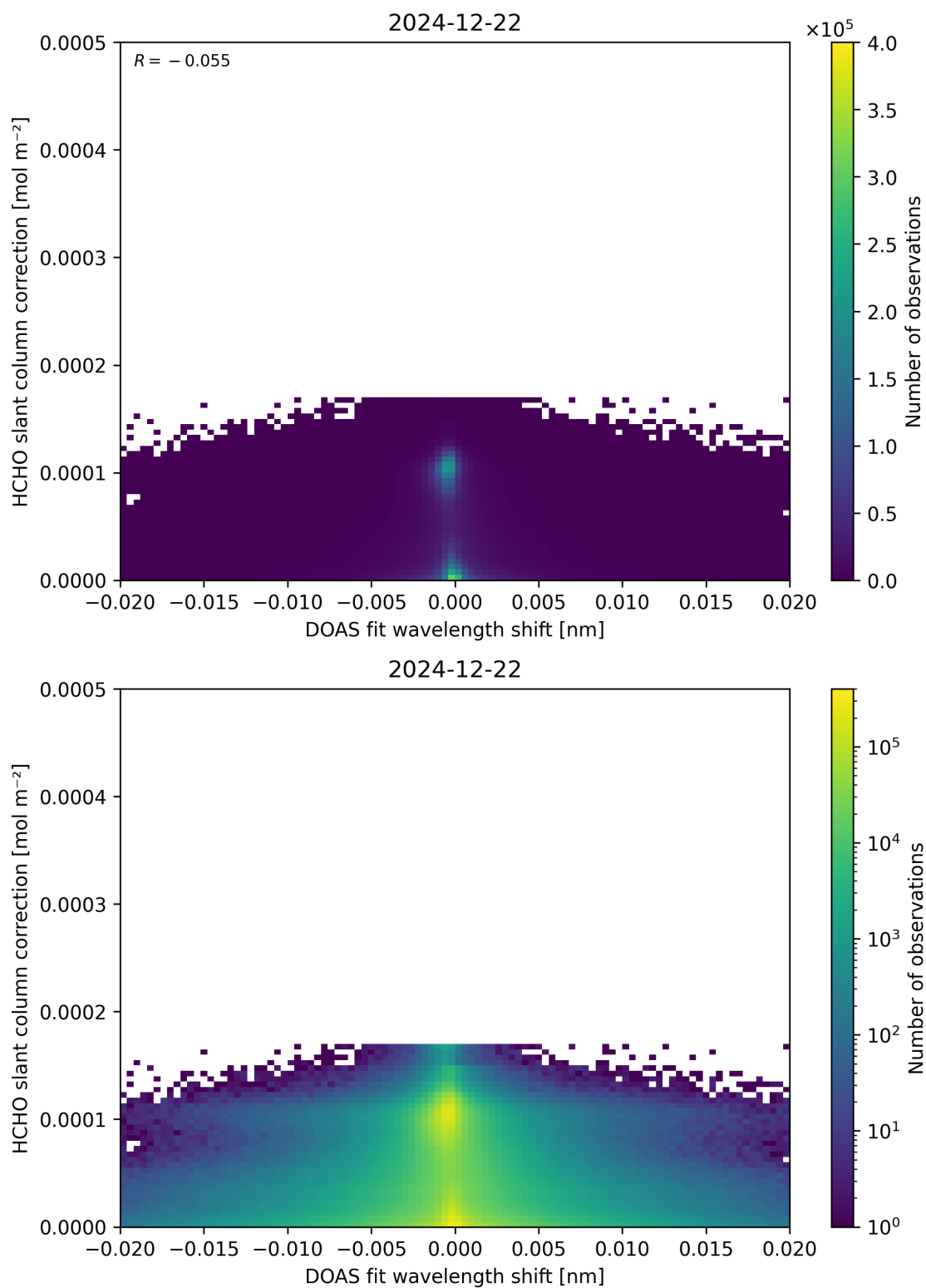
Figure 67: Scatter density plot of “DOAS fit wavelength shift” against “HCHO slant column correction” for 2024-12-22 to 2024-12-23.
