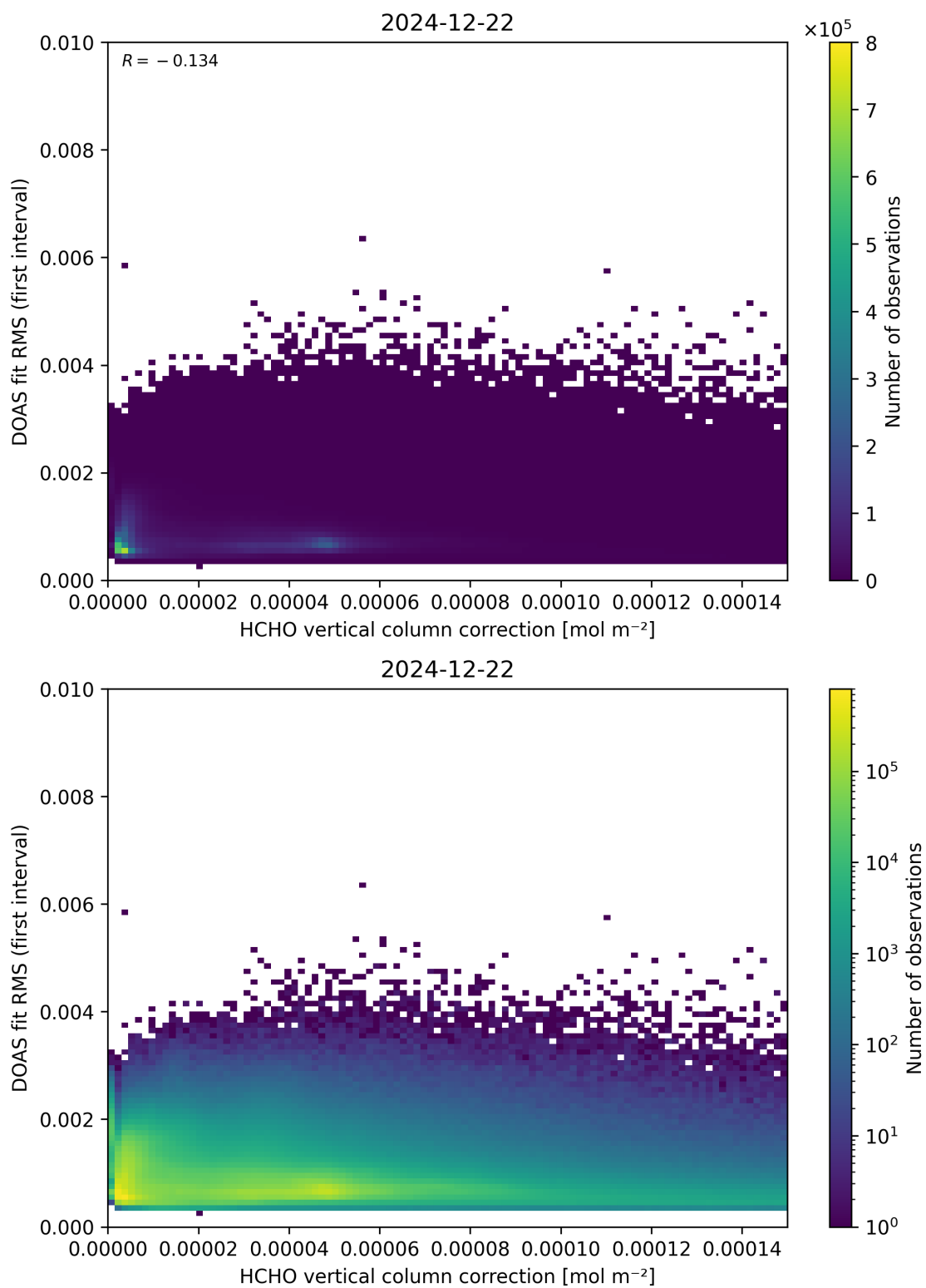
Figure 112: Scatter density plot of “HCHO vertical column correction” against “DOAS fit RMS (first interval)” for 2024-12-22 to 2024-12-23.
