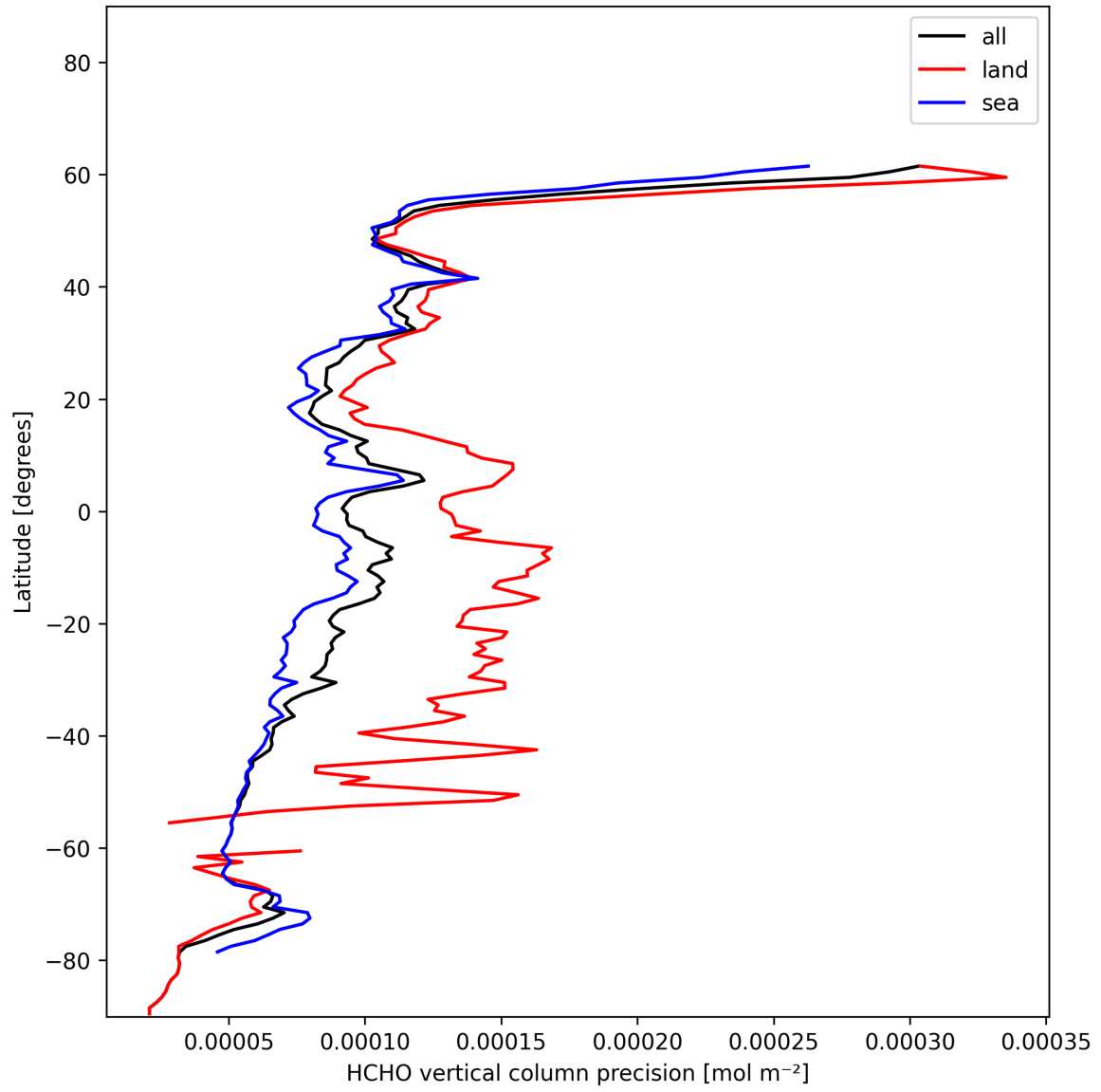
Figure 22: Zonal average of “HCHO vertical column precision” for 2024-12-22 to 2024-12-23.
