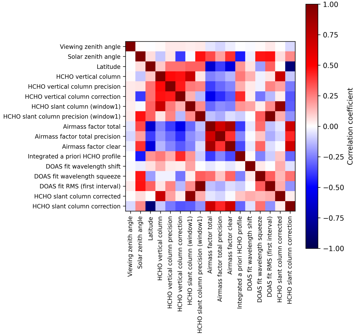
Figure 2: Map of correlation matrix for 2024-12-22 to 2024-12-23.
