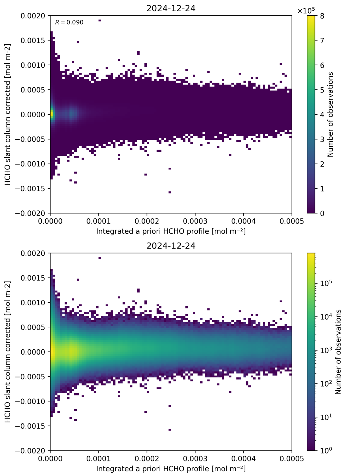
Figure 151: Scatter density plot of “Integrated a priori HCHO profile” against “HCHO slant column corrected” for 2024-12-23 to 2024-12-25.
