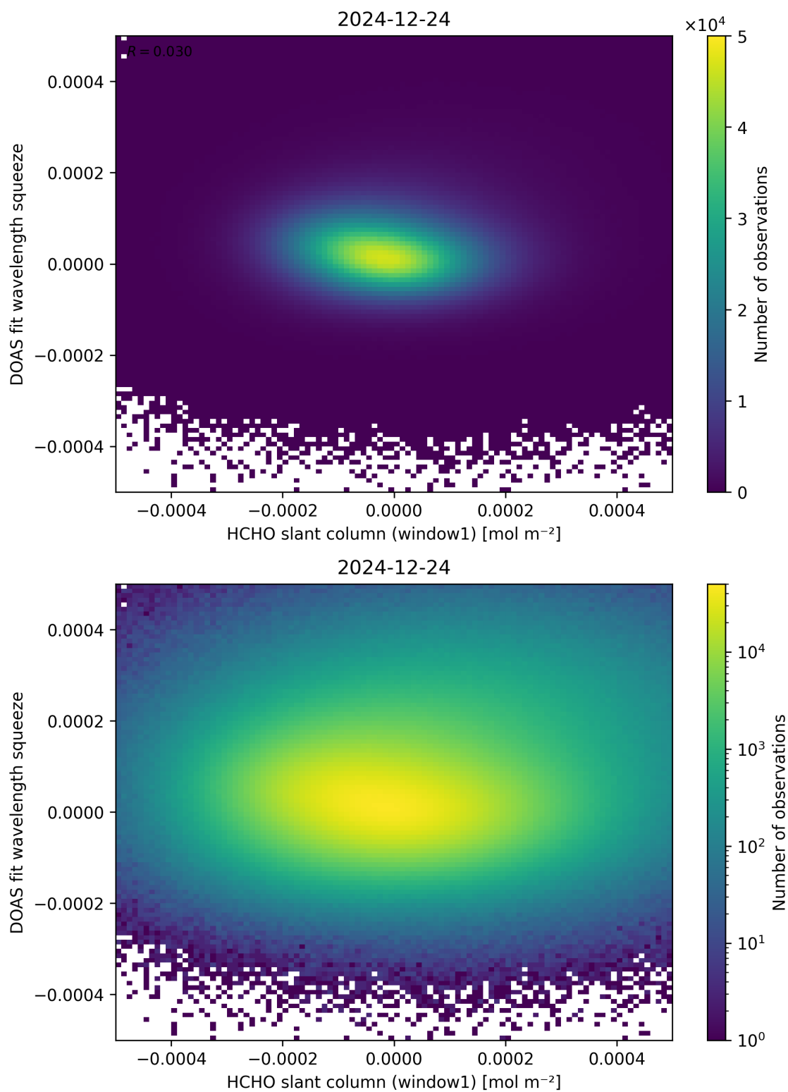
Figure 80: Scatter density plot of “HCHO slant column (window1)” against “DOAS fit wavelength squeeze” for 2024-12-23 to 2024-12-25.
