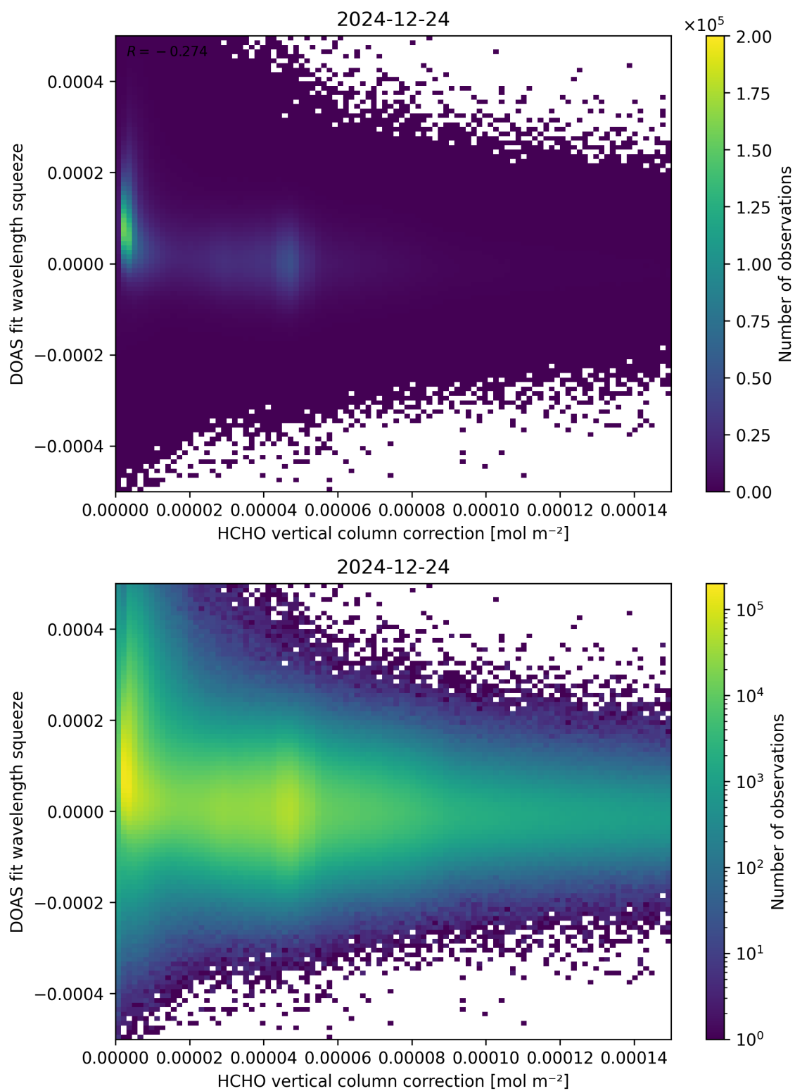
Figure 114: Scatter density plot of “HCHO vertical column correction” against “DOAS fit wavelength squeeze” for 2024-12-23 to 2024-12-25.
