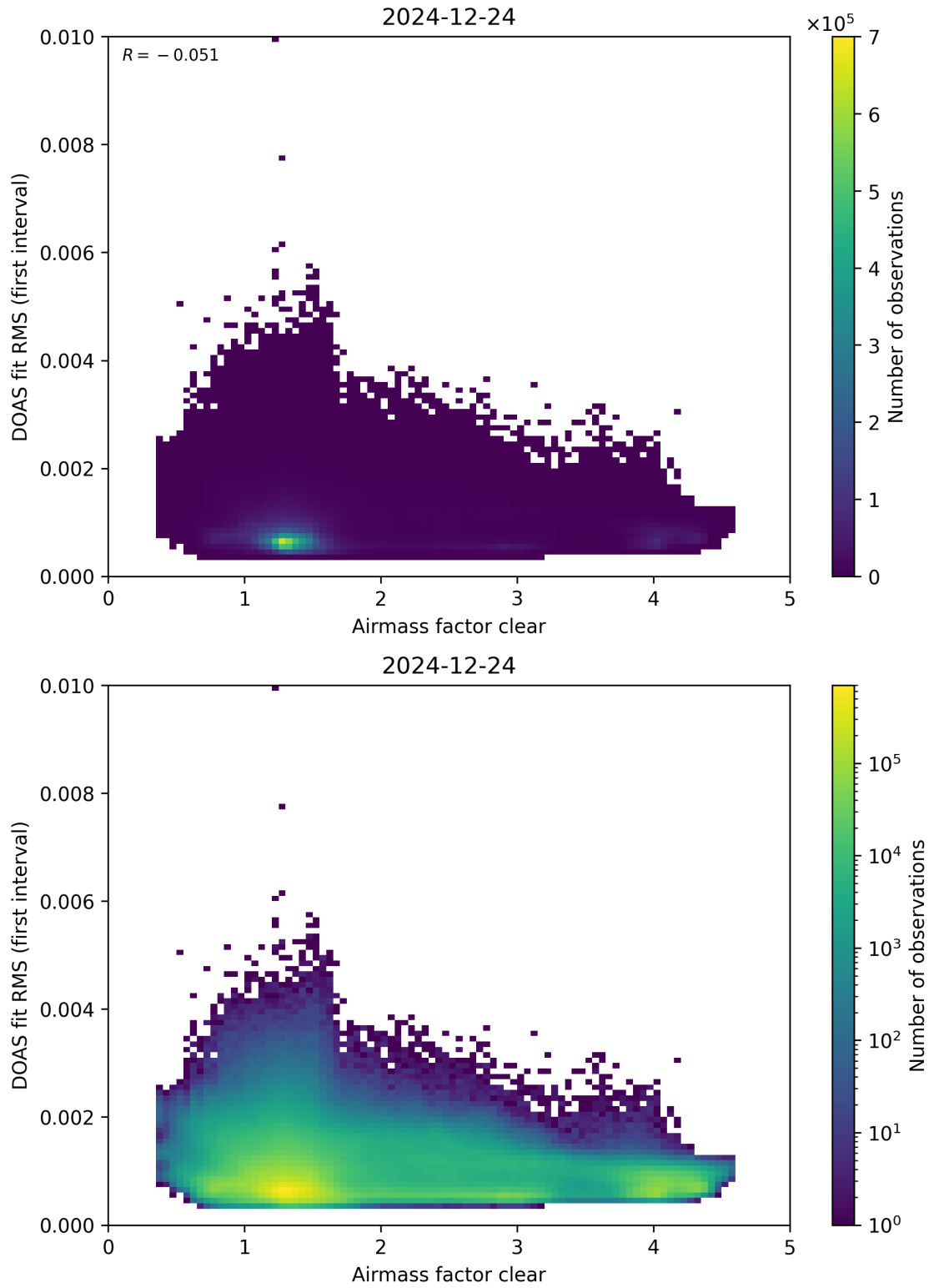
Figure 71: Scatter density plot of “Airmass factor clear” against “DOAS fit RMS (first interval)” for 2024-12-23 to 2024-12-25.
