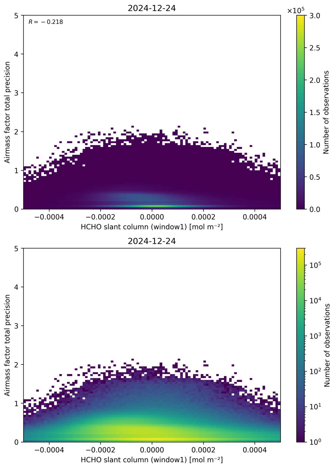
Figure 86: Scatter density plot of “HCHO slant column (window1)” against “Airmass factor total precision” for 2024-12-23 to 2024-12-25.
