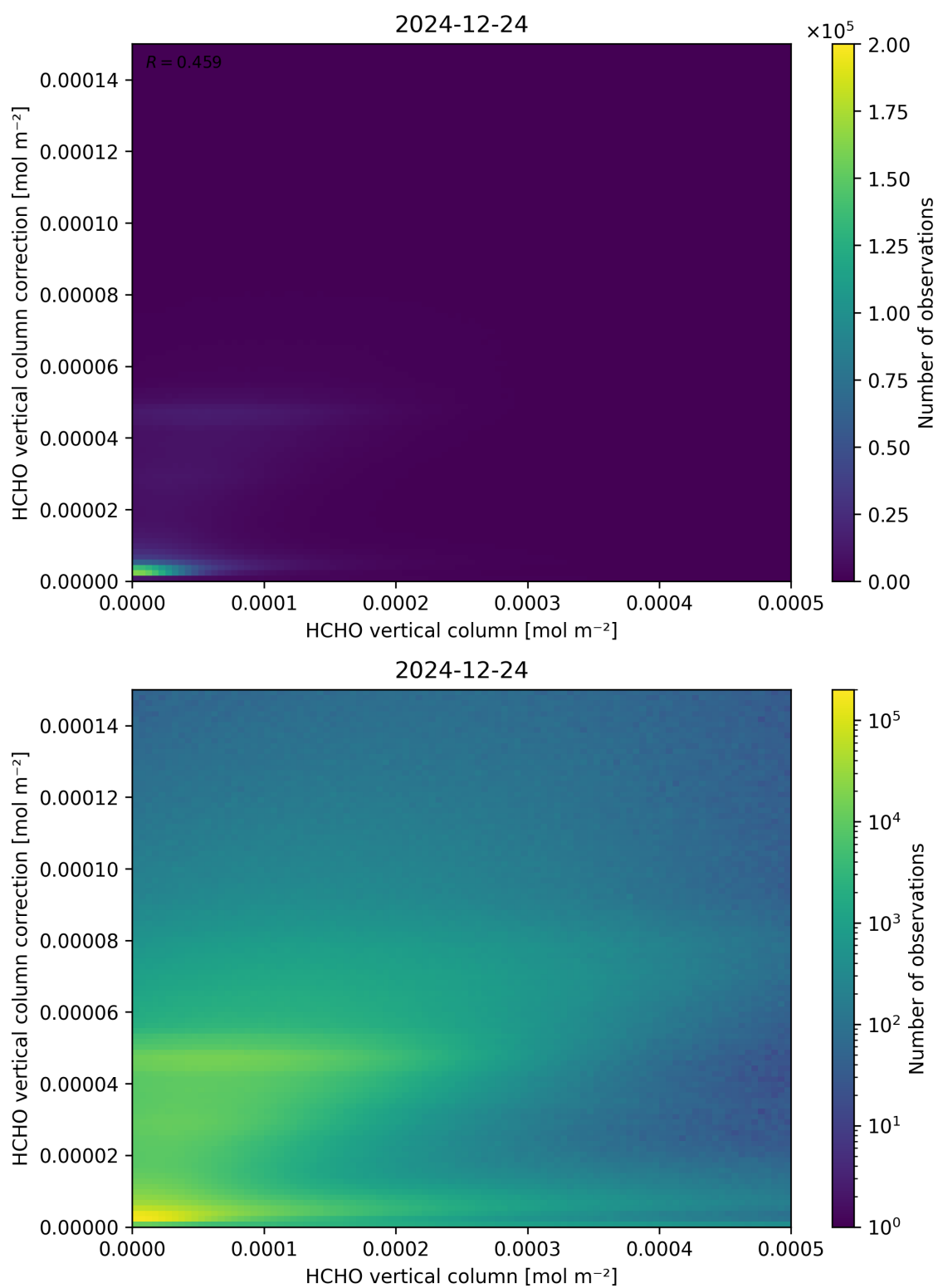
Figure 133: Scatter density plot of “HCHO vertical column” against “HCHO vertical column correction” for 2024-12-23 to 2024-12-25.
