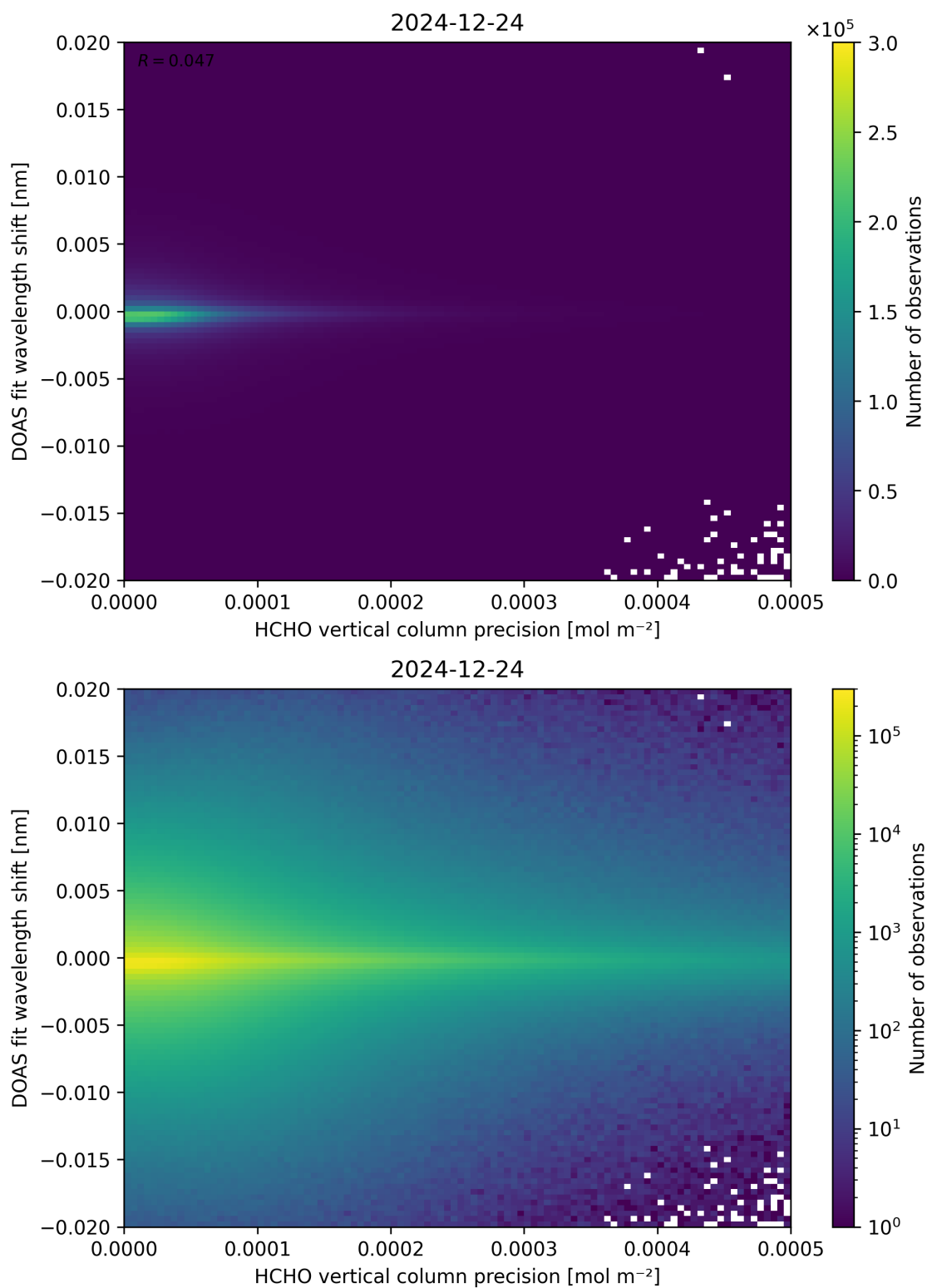
Figure 137: Scatter density plot of “HCHO vertical column precision” against “DOAS fit wavelength shift” for 2024-12-23 to 2024-12-25.
