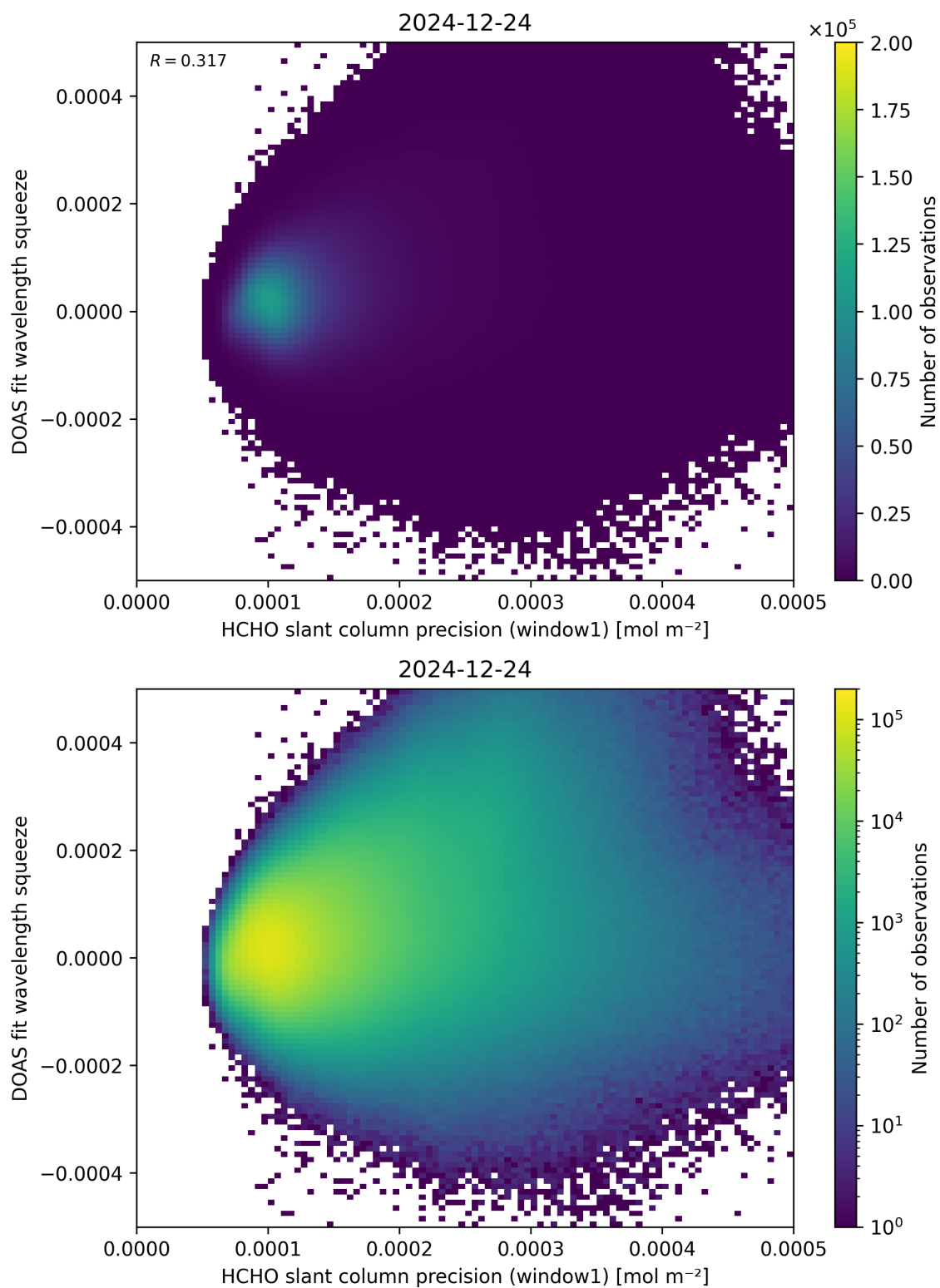
Figure 90: Scatter density plot of “HCHO slant column precision (window1)” against “DOAS fit wavelength squeeze” for 2024-12-23 to 2024-12-25.
