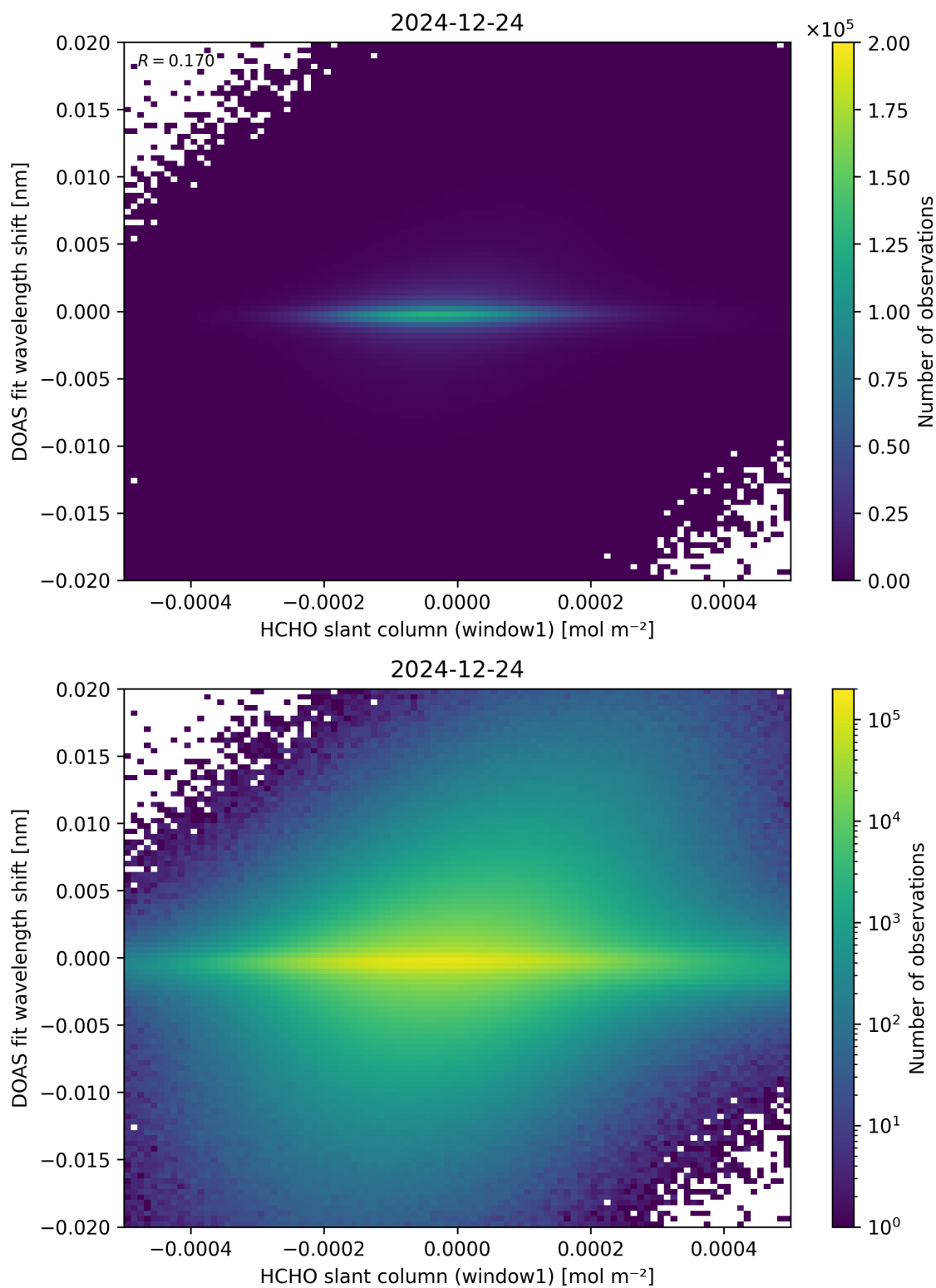
Figure 79: Scatter density plot of “HCHO slant column (window1)” against “DOAS fit wavelength shift” for 2024-12-23 to 2024-12-25.
