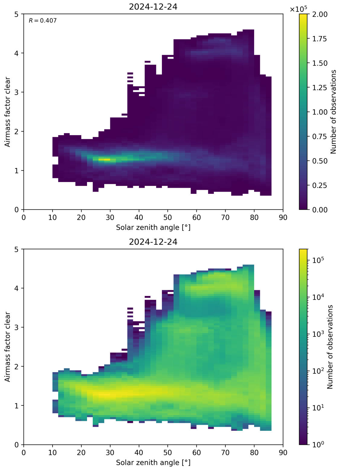
Figure 170: Scatter density plot of “Solar zenith angle” against “Airmass factor clear” for 2024-12-23 to 2024-12-25.
