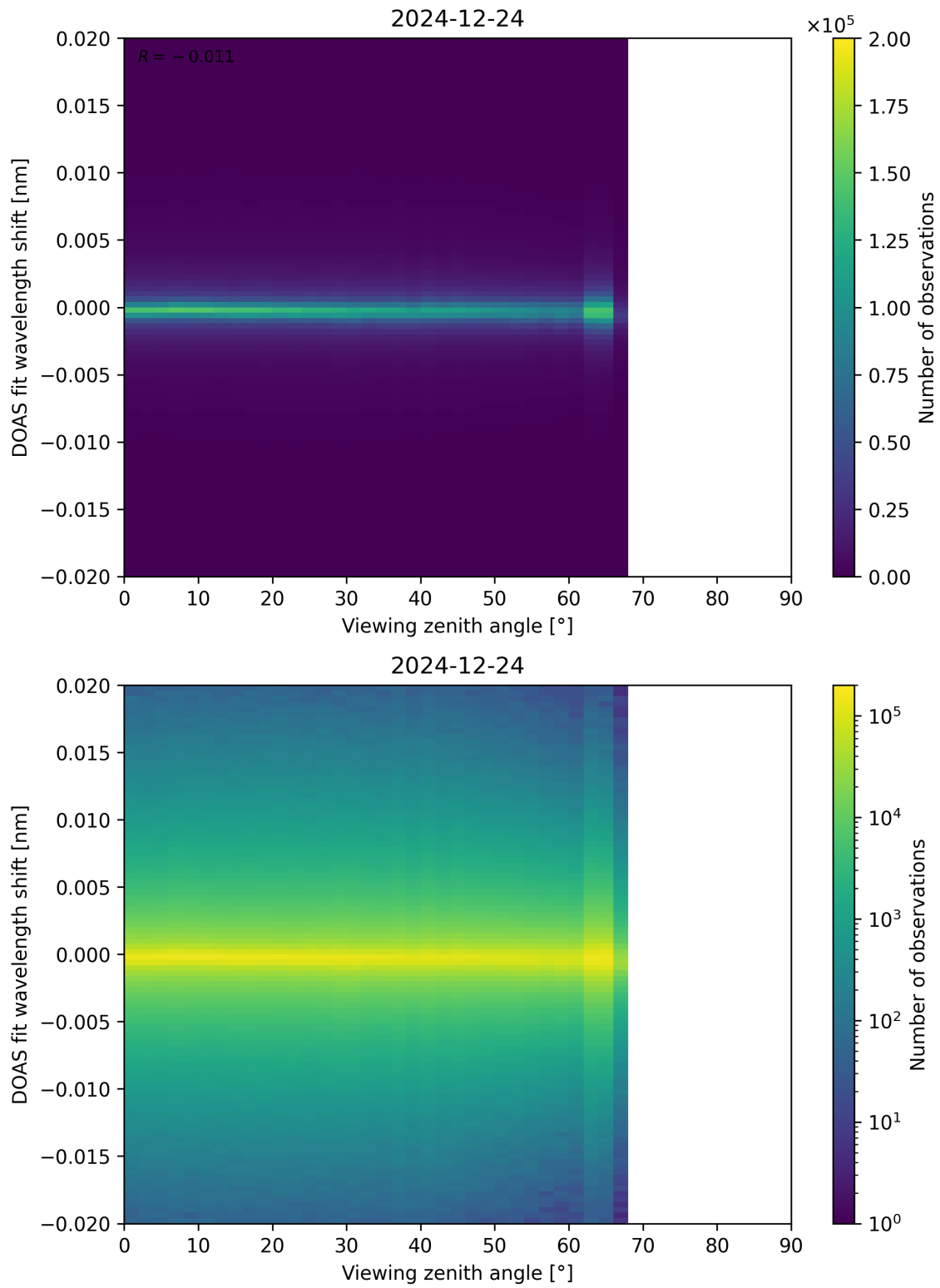
Figure 183: Scatter density plot of “Viewing zenith angle” against “DOAS fit wavelength shift” for 2024-12-23 to 2024-12-25.
