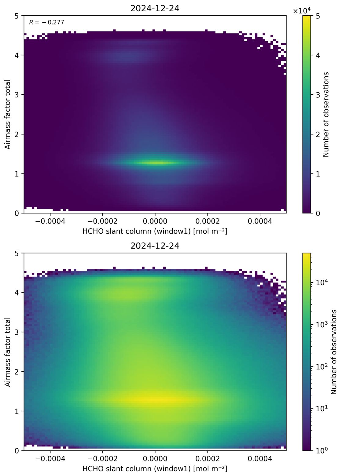
Figure 85: Scatter density plot of “HCHO slant column (window1)” against “Airmass factor total” for 2024-12-23 to 2024-12-25.
