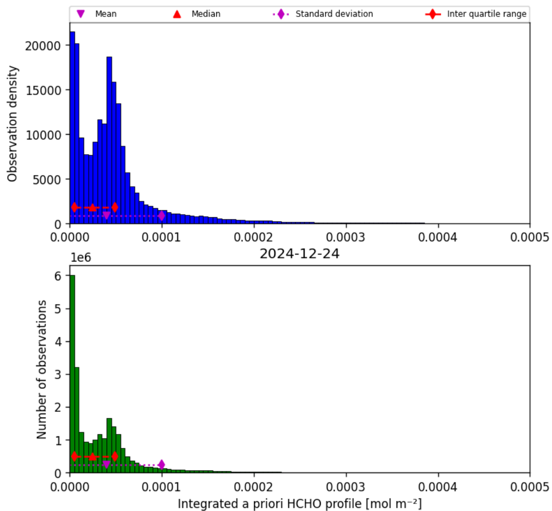
Figure 43: Histogram of “Integrated a priori HCHO profile” for 2024-12-23 to 2024-12-25
