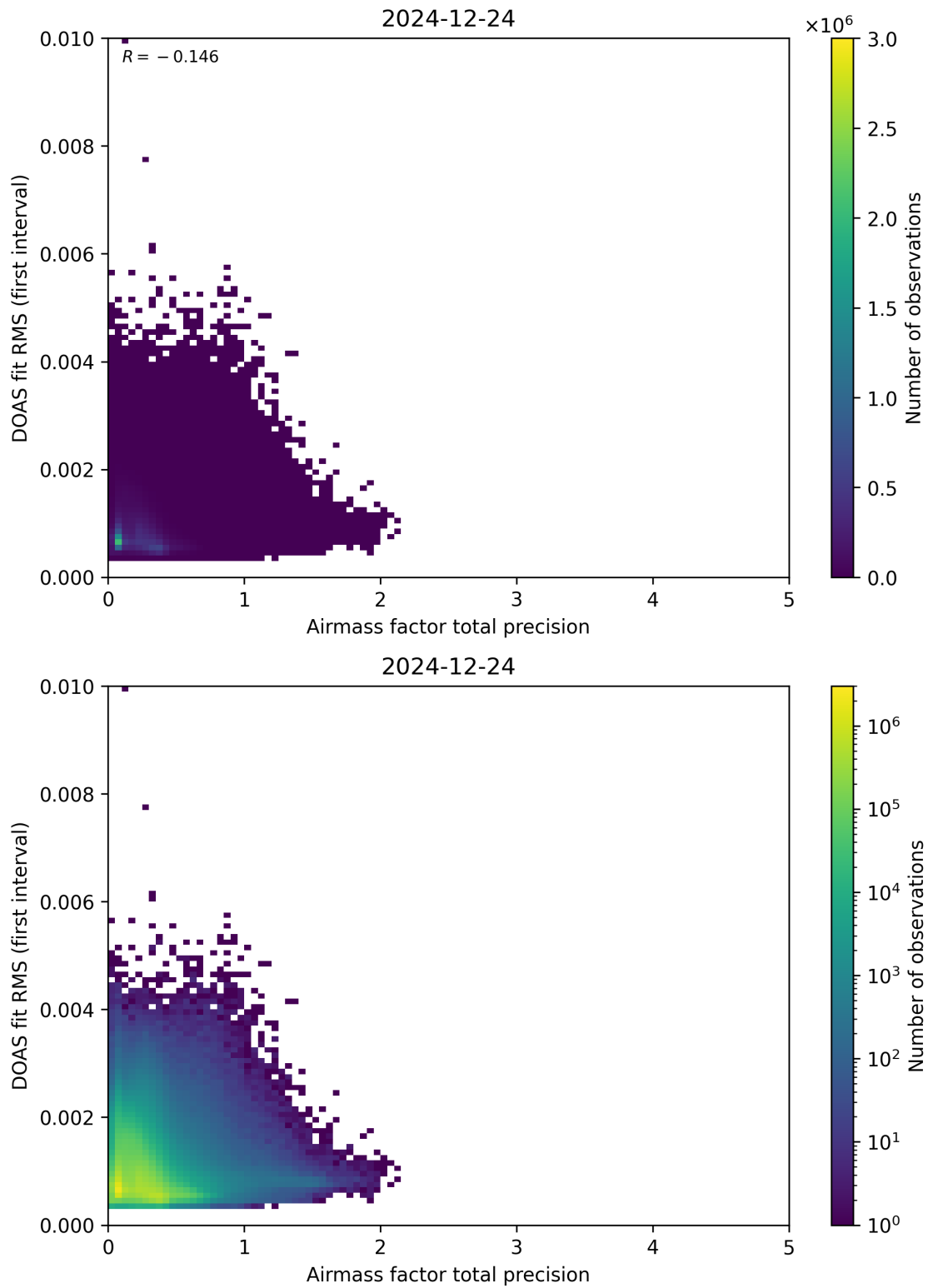
Figure 105: Scatter density plot of “Airmass factor total precision” against “DOAS fit RMS (first interval)” for 2024-12-23 to 2024-12-25.
