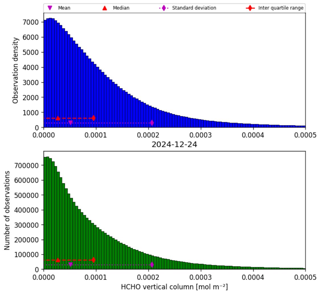
Figure 35: Histogram of “HCHO vertical column” for 2024-12-23 to 2024-12-25
