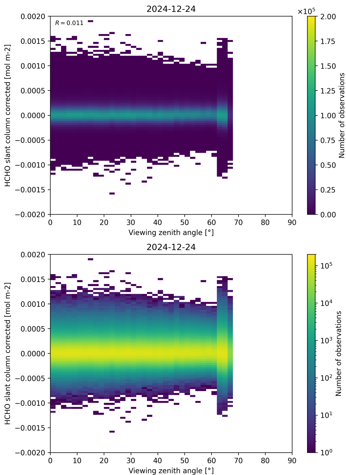
Figure 186: Scatter density plot of “Viewing zenith angle” against “HCHO slant column corrected” for 2024-12-23 to 2024-12-25.
