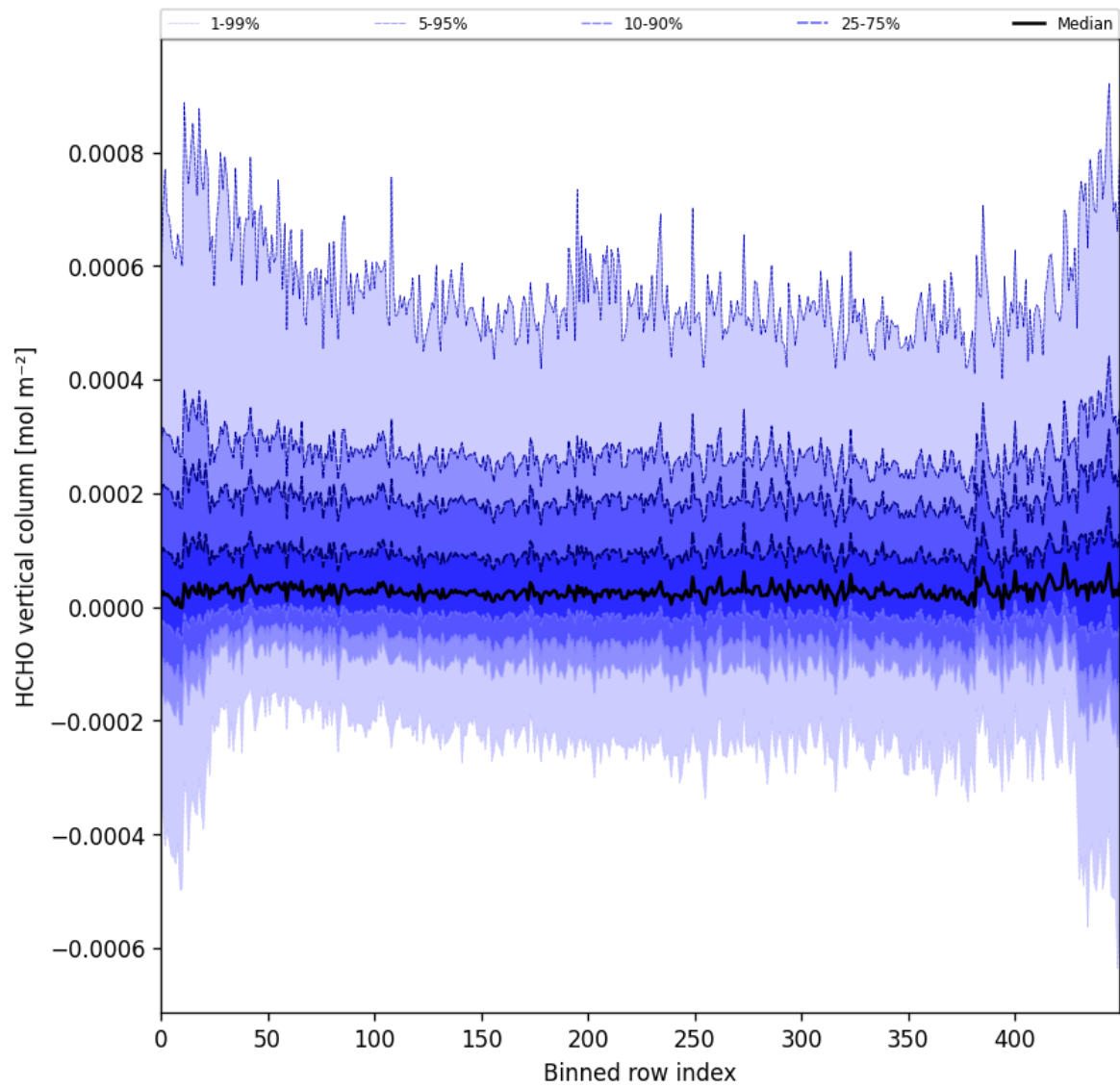
Figure 49: Along track statistics of “HCHO vertical column” for 2024-12-23 to 2024-12-25
