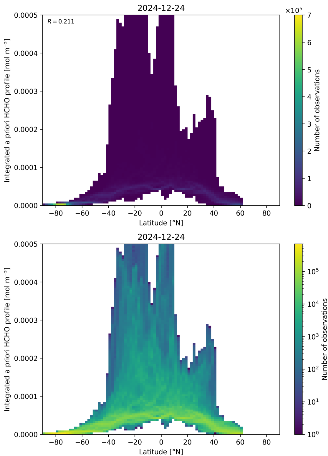
Figure 166: Scatter density plot of “Latitude” against “Integrated a priori HCHO profile” for 2024-12-23 to 2024-12-25.
