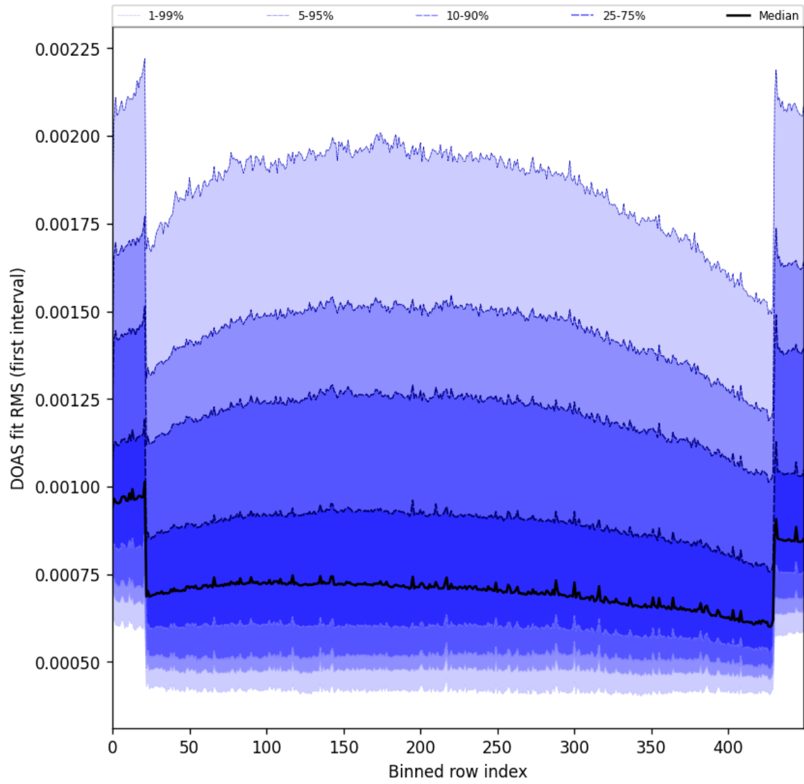
Figure 60: Along track statistics of “DOAS fit RMS (first interval)” for 2024-12-23 to 2024-12-25
