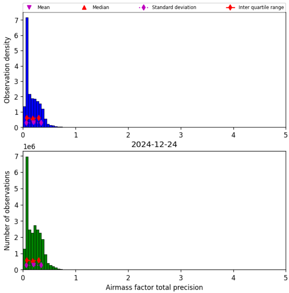
Figure 41: Histogram of “Airmass factor total precision” for 2024-12-23 to 2024-12-25
