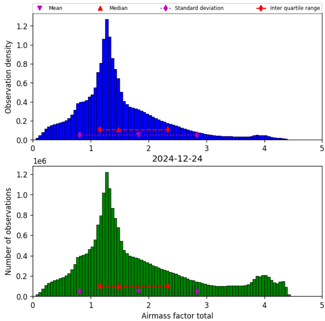
Figure 40: Histogram of “Airmass factor total” for 2024-12-23 to 2024-12-25
