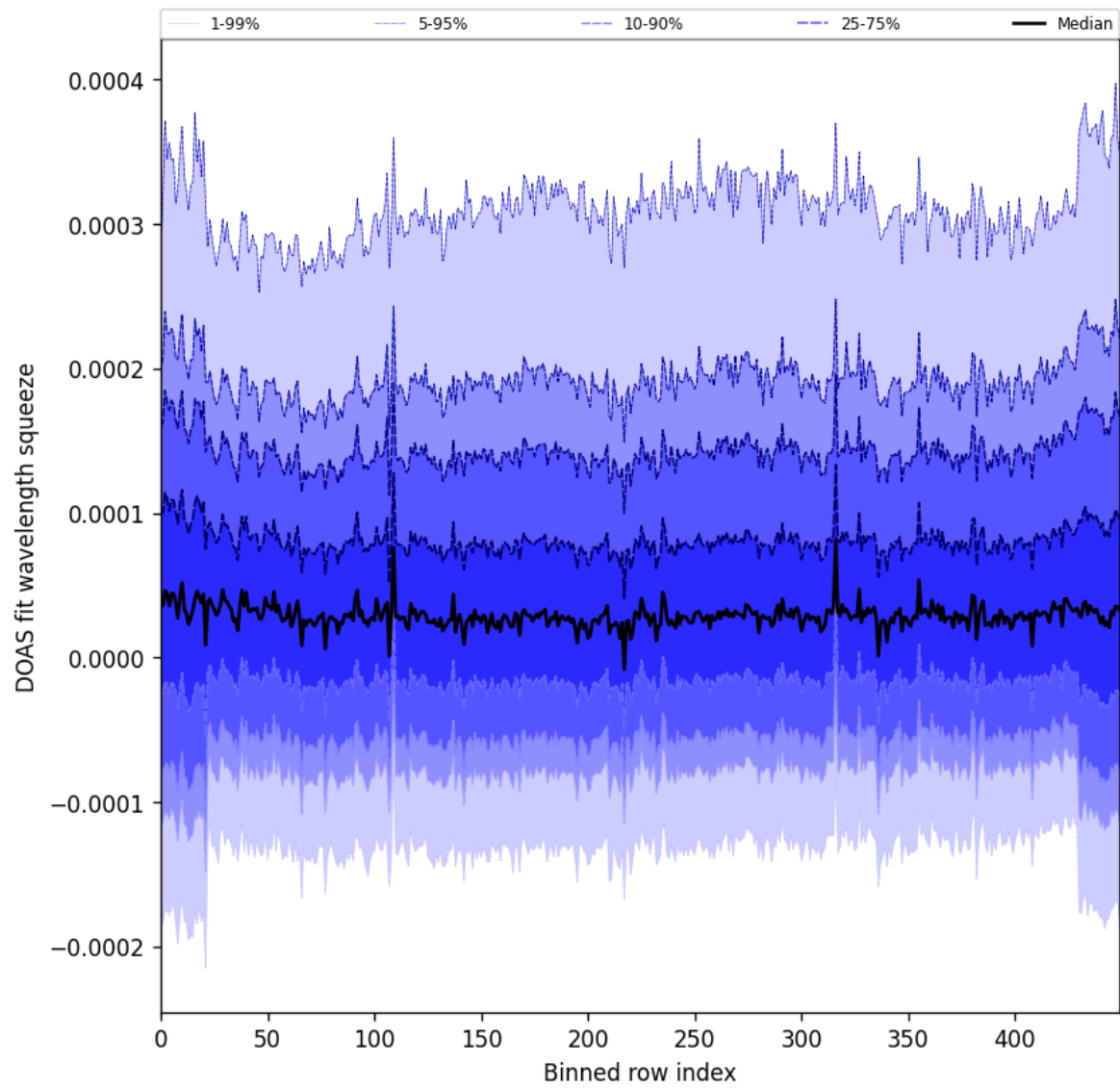
Figure 59: Along track statistics of “DOAS fit wavelength squeeze” for 2024-12-23 to 2024-12-25
