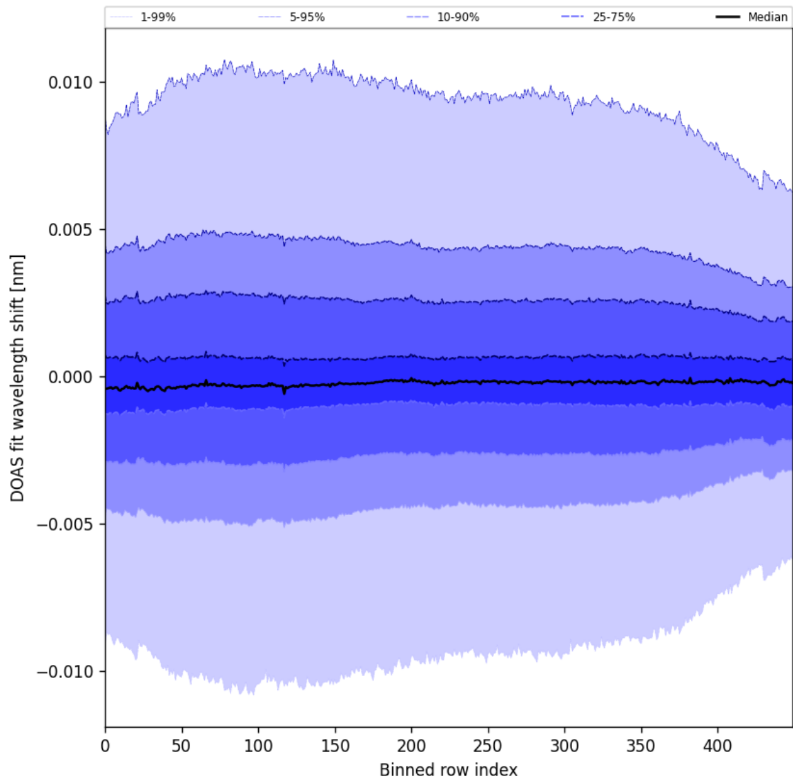
Figure 58: Along track statistics of “DOAS fit wavelength shift” for 2024-12-23 to 2024-12-25
