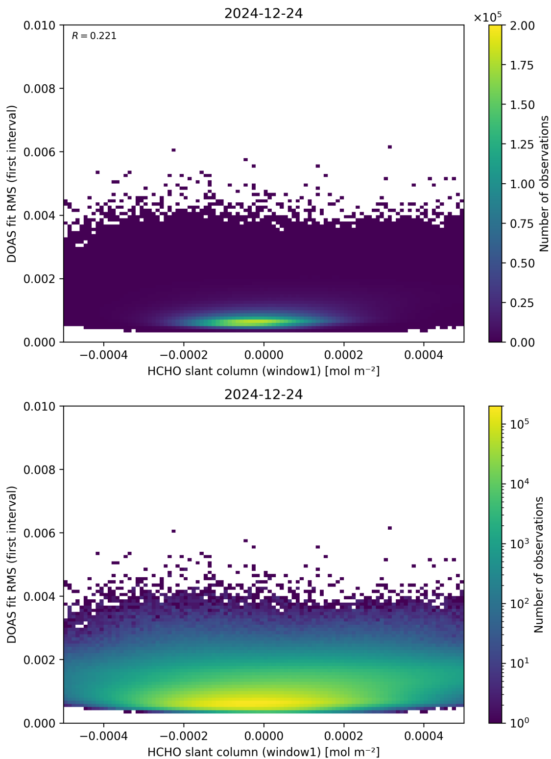
Figure 78: Scatter density plot of “HCHO slant column (window1)” against “DOAS fit RMS (first interval)” for 2024-12-23 to 2024-12-25.
