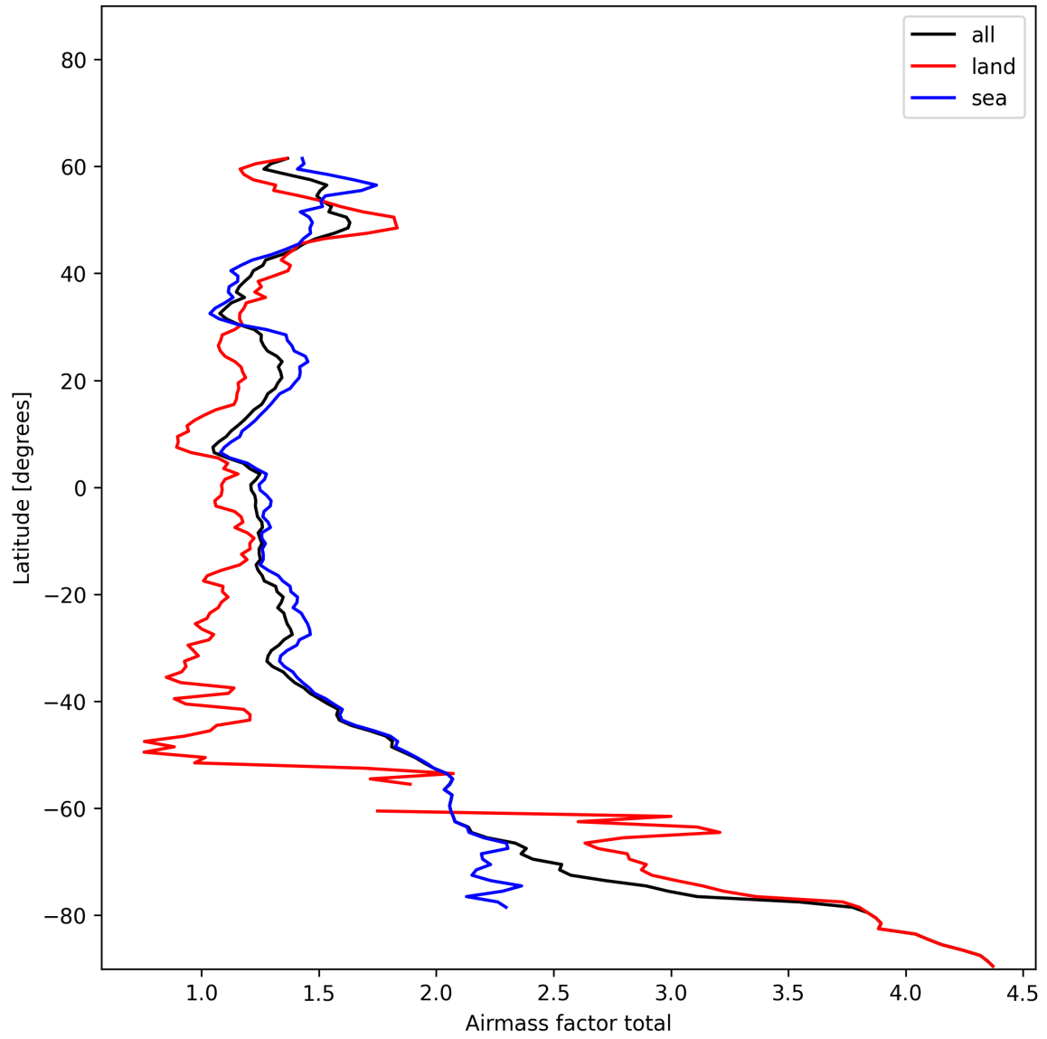
Figure 26: Zonal average of “Airmass factor total” for 2024-12-23 to 2024-12-25.
