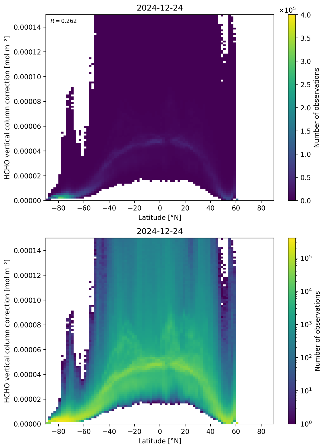
Figure 164: Scatter density plot of “Latitude” against “HCHO vertical column correction” for 2024-12-23 to 2024-12-25.
