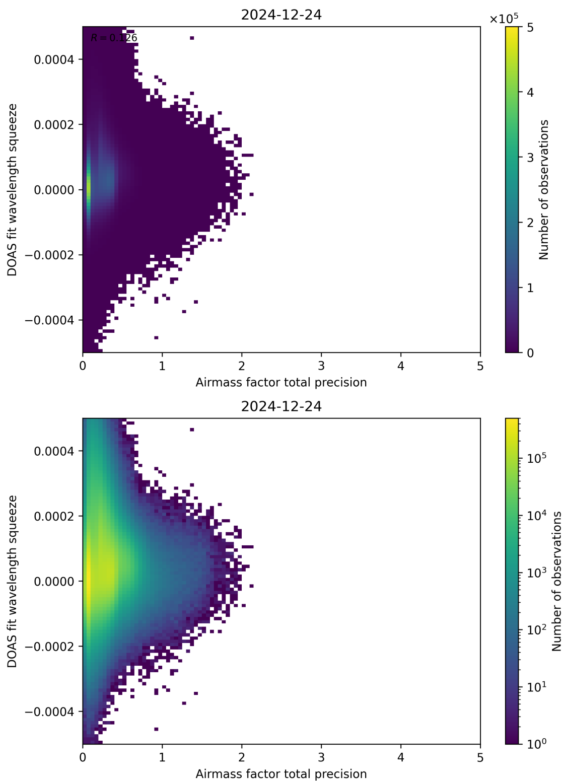
Figure 107: Scatter density plot of “Airmass factor total precision” against “DOAS fit wavelength squeeze” for 2024-12-23 to 2024-12-25.
