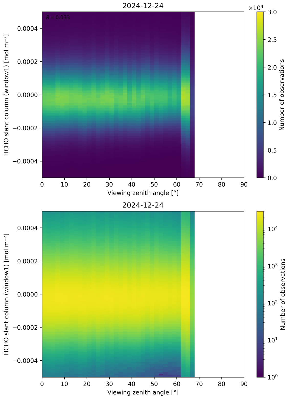
Figure 188: Scatter density plot of “Viewing zenith angle” against “HCHO slant column (window1)” for 2024-12-23 to 2024-12-25.
