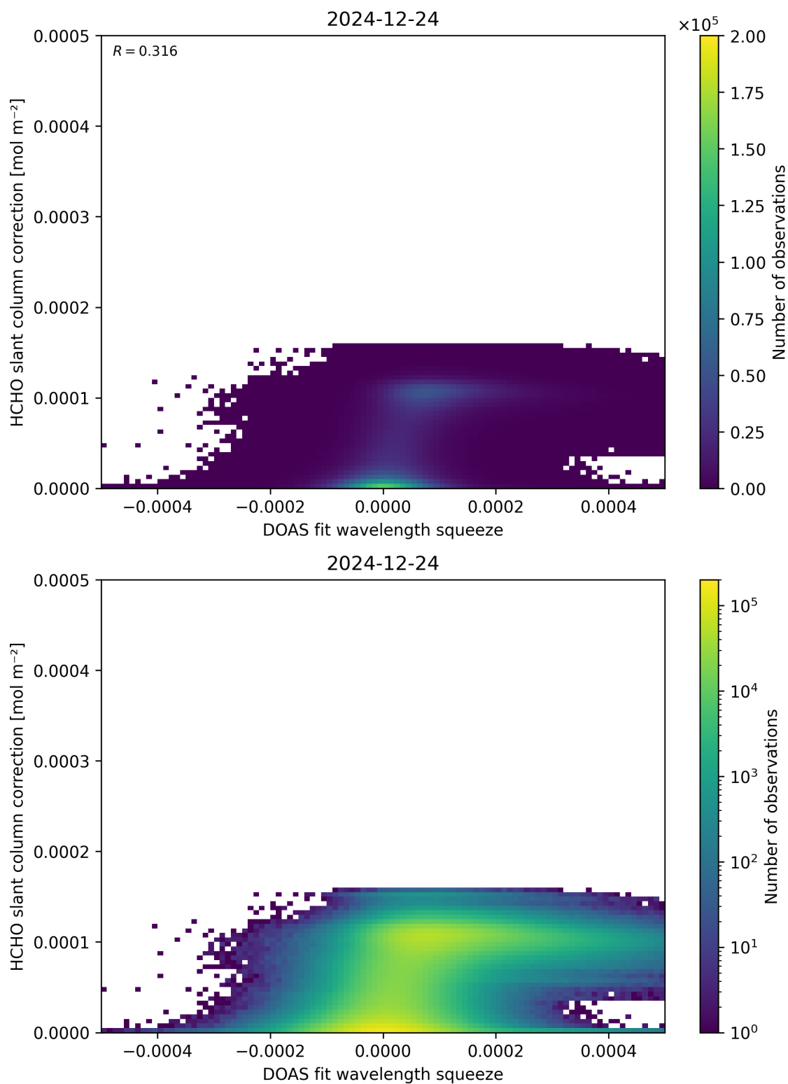
Figure 70: Scatter density plot of “DOAS fit wavelength squeeze” against “HCHO slant column correction” for 2024-12-23 to 2024-12-25.
