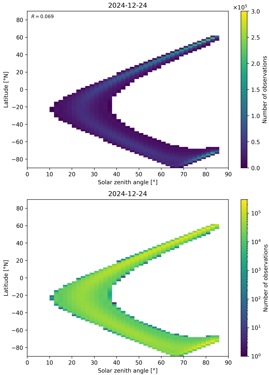
Figure 181: Scatter density plot of “Solar zenith angle” against “Latitude” for 2024-12-23 to 2024-12-25.
