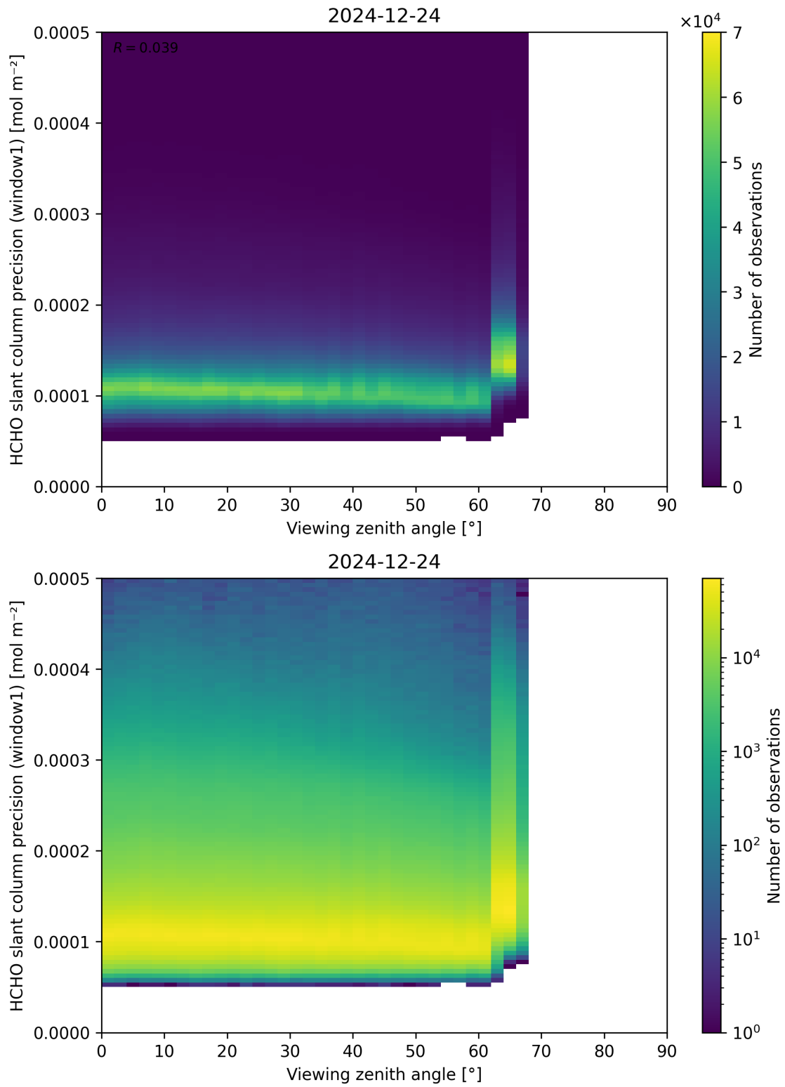
Figure 189: Scatter density plot of “Viewing zenith angle” against “HCHO slant column precision (window1)” for 2024-12-23 to 2024-12-25.
