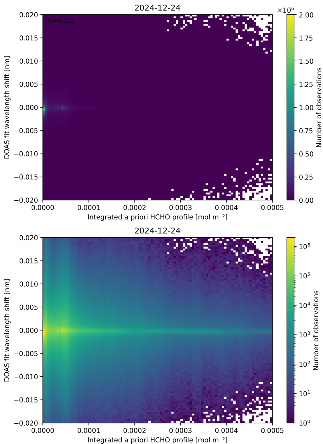
Figure 149: Scatter density plot of “Integrated a priori HCHO profile” against “DOAS fit wavelength shift” for 2024-12-23 to 2024-12-25.
