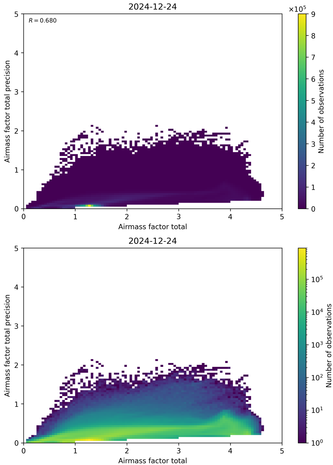
Figure 103: Scatter density plot of “Airmass factor total” against “Airmass factor total precision” for 2024-12-23 to 2024-12-25.
