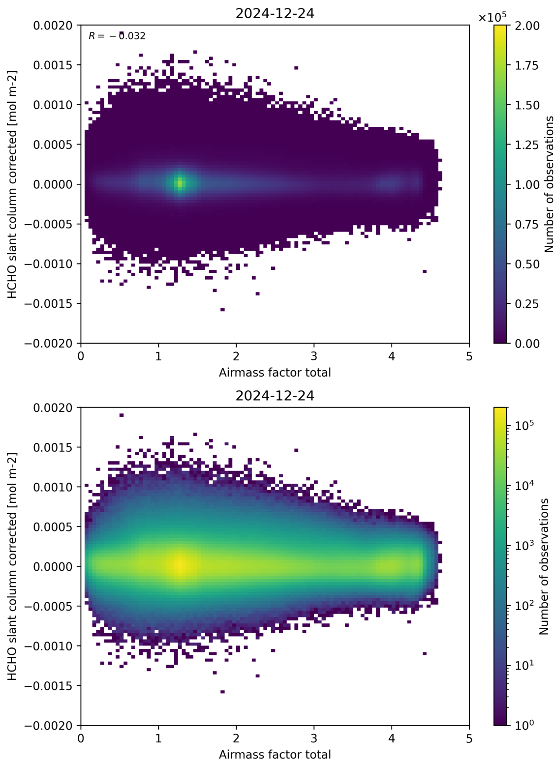
Figure 101: Scatter density plot of “Airmass factor total” against “HCHO slant column corrected” for 2024-12-23 to 2024-12-25.
