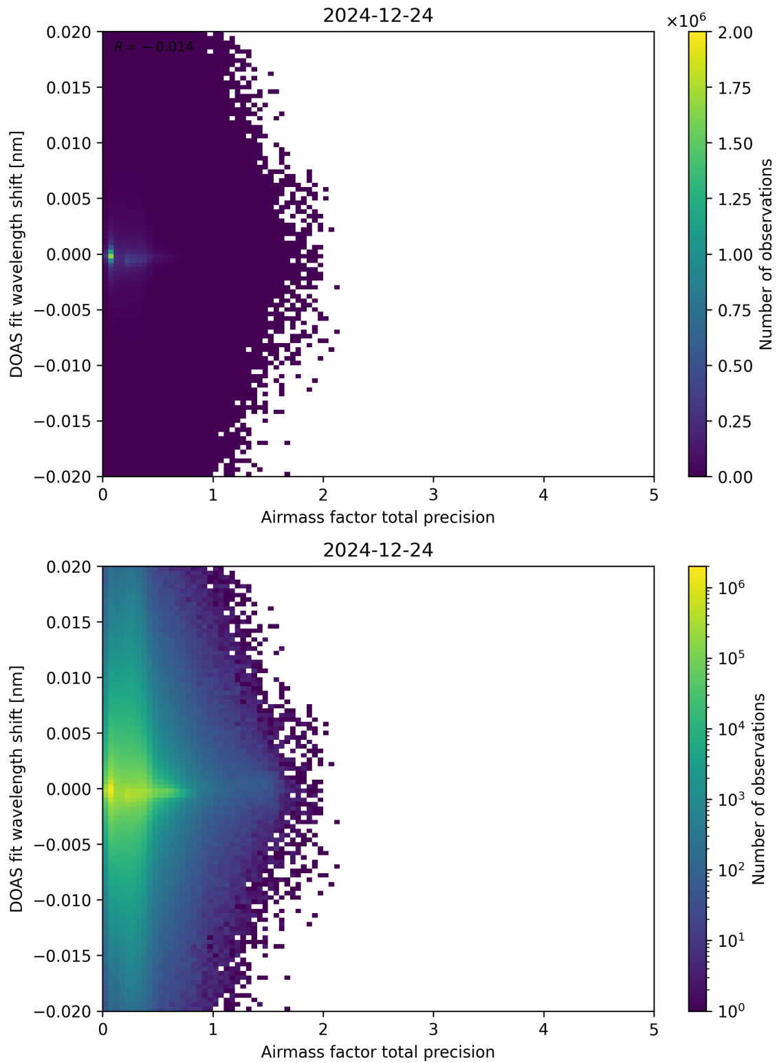
Figure 106: Scatter density plot of “Airmass factor total precision” against “DOAS fit wavelength shift” for 2024-12-23 to 2024-12-25.
