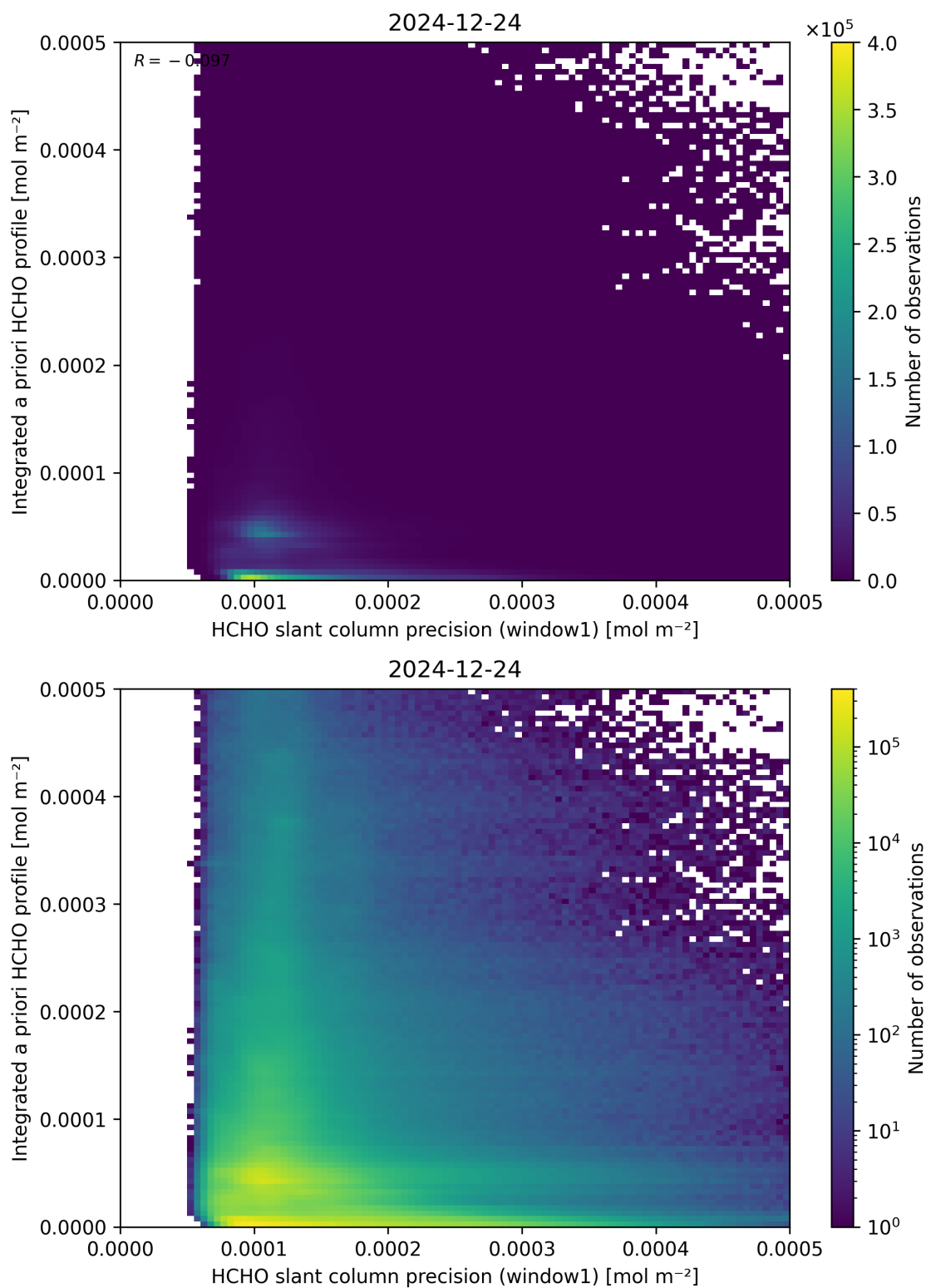
Figure 96: Scatter density plot of “HCHO slant column precision (window1)” against “Integrated a priori HCHO profile” for 2024-12-23 to 2024-12-25.
