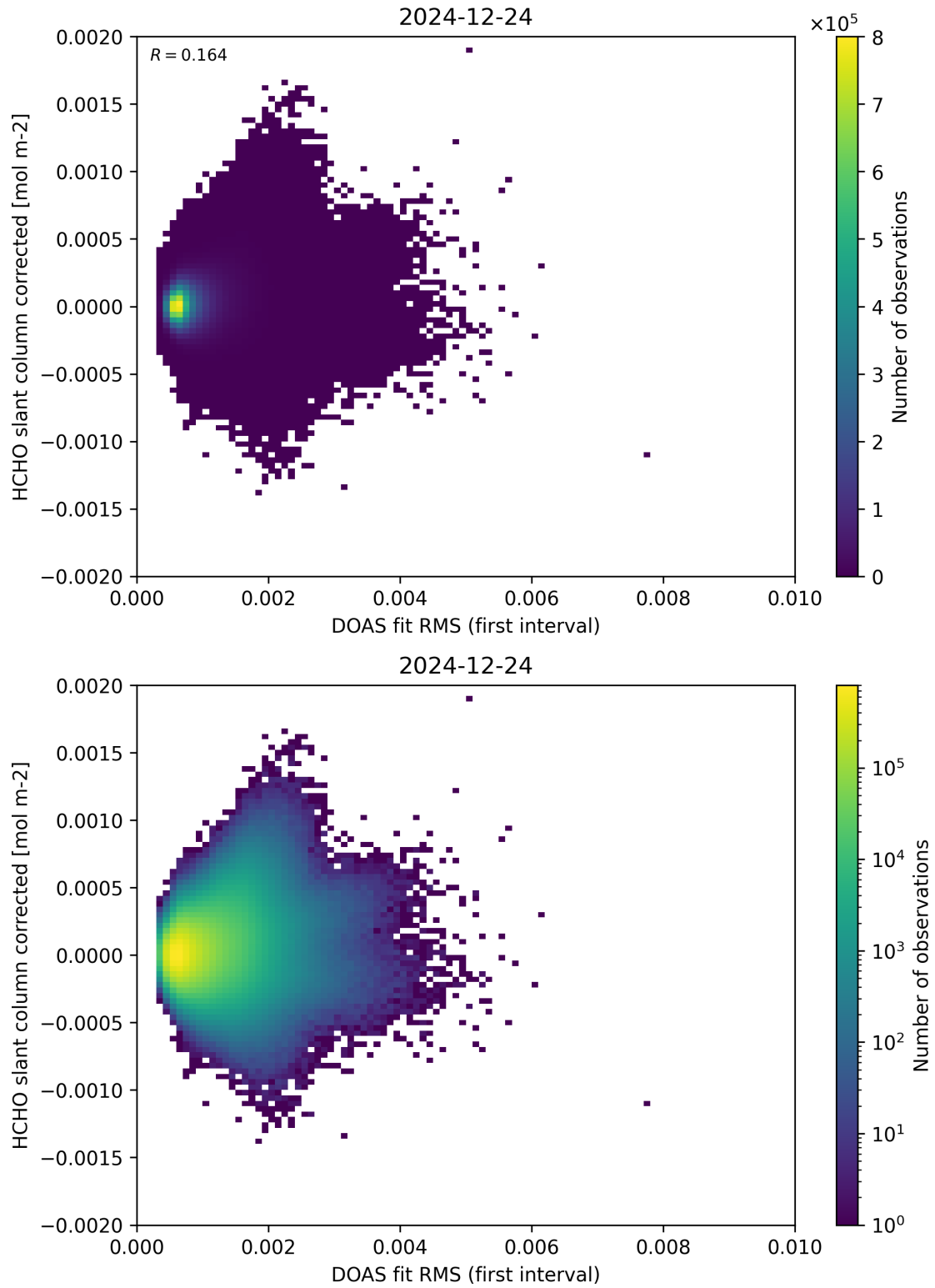
Figure 62: Scatter density plot of “DOAS fit RMS (first interval)” against “HCHO slant column corrected” for 2024-12-23 to 2024-12-25.
