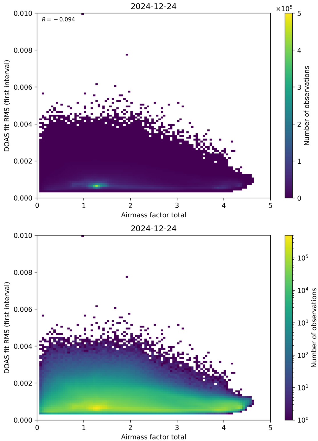
Figure 97: Scatter density plot of “Airmass factor total” against “DOAS fit RMS (first interval)” for 2024-12-23 to 2024-12-25.
