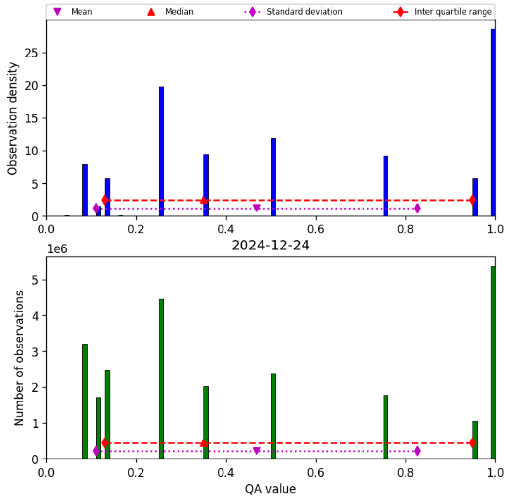
Figure 34: Histogram of “QA value” for 2024-12-23 to 2024-12-25
