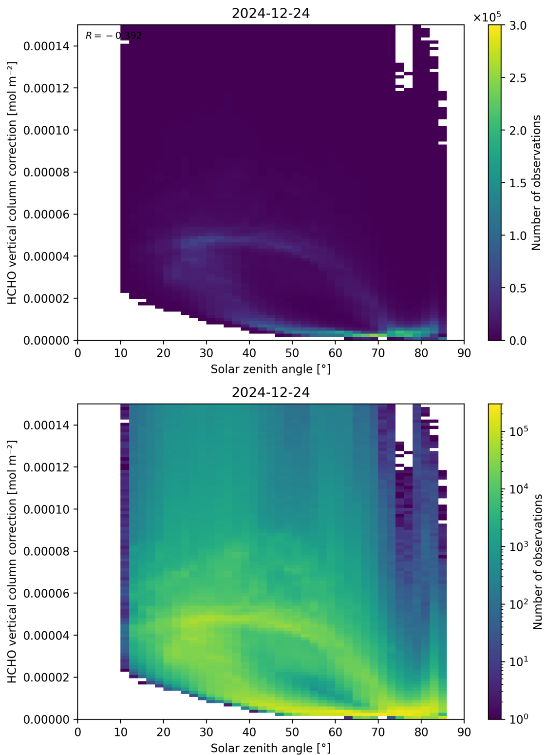
Figure 178: Scatter density plot of “Solar zenith angle” against “HCHO vertical column correction” for 2024-12-23 to 2024-12-25.
