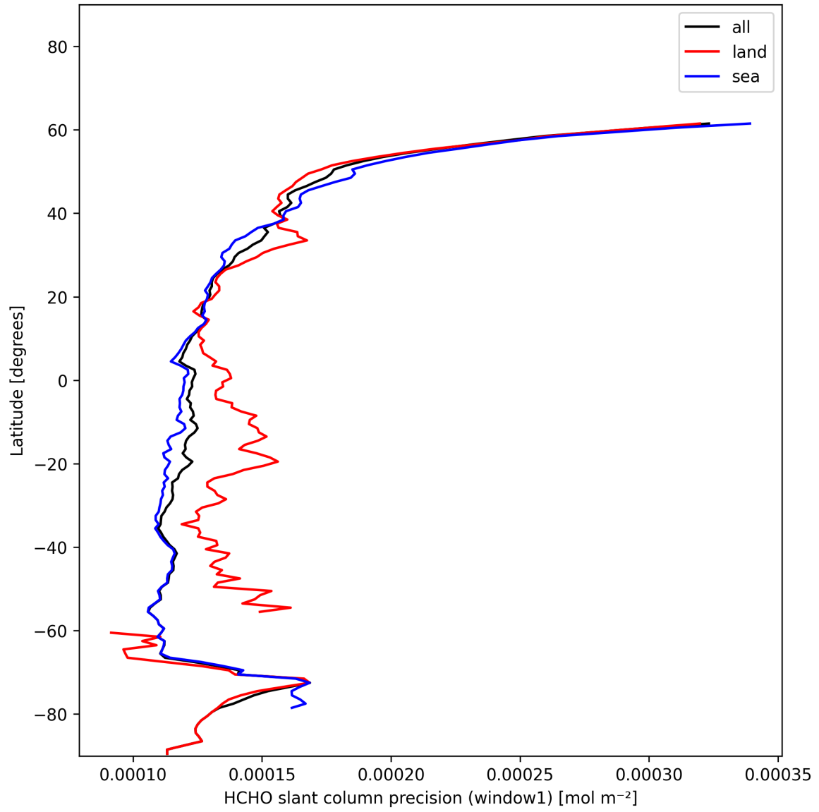
Figure 25: Zonal average of “HCHO slant column precision (window1)” for 2024-12-23 to 2024-12-25.
