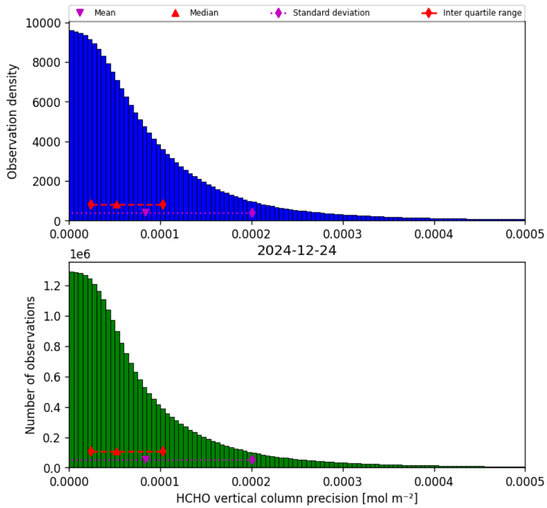
Figure 36: Histogram of “HCHO vertical column precision” for 2024-12-23 to 2024-12-25
