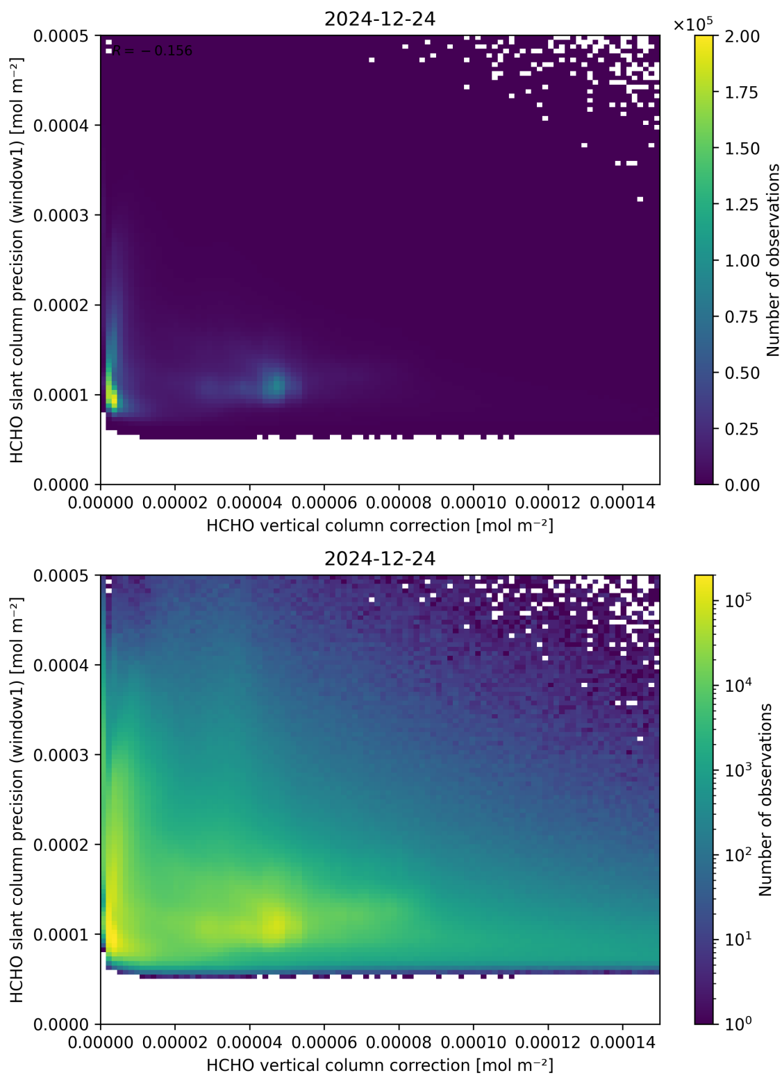
Figure 119: Scatter density plot of “HCHO vertical column correction” against “HCHO slant column precision (window1)” for 2024-12-23 to 2024-12-25.
