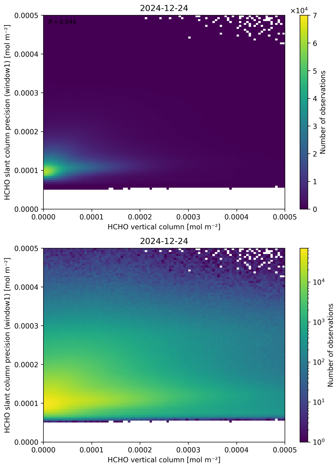
Figure 130: Scatter density plot of “HCHO vertical column” against “HCHO slant column precision (window1)” for 2024-12-23 to 2024-12-25.
