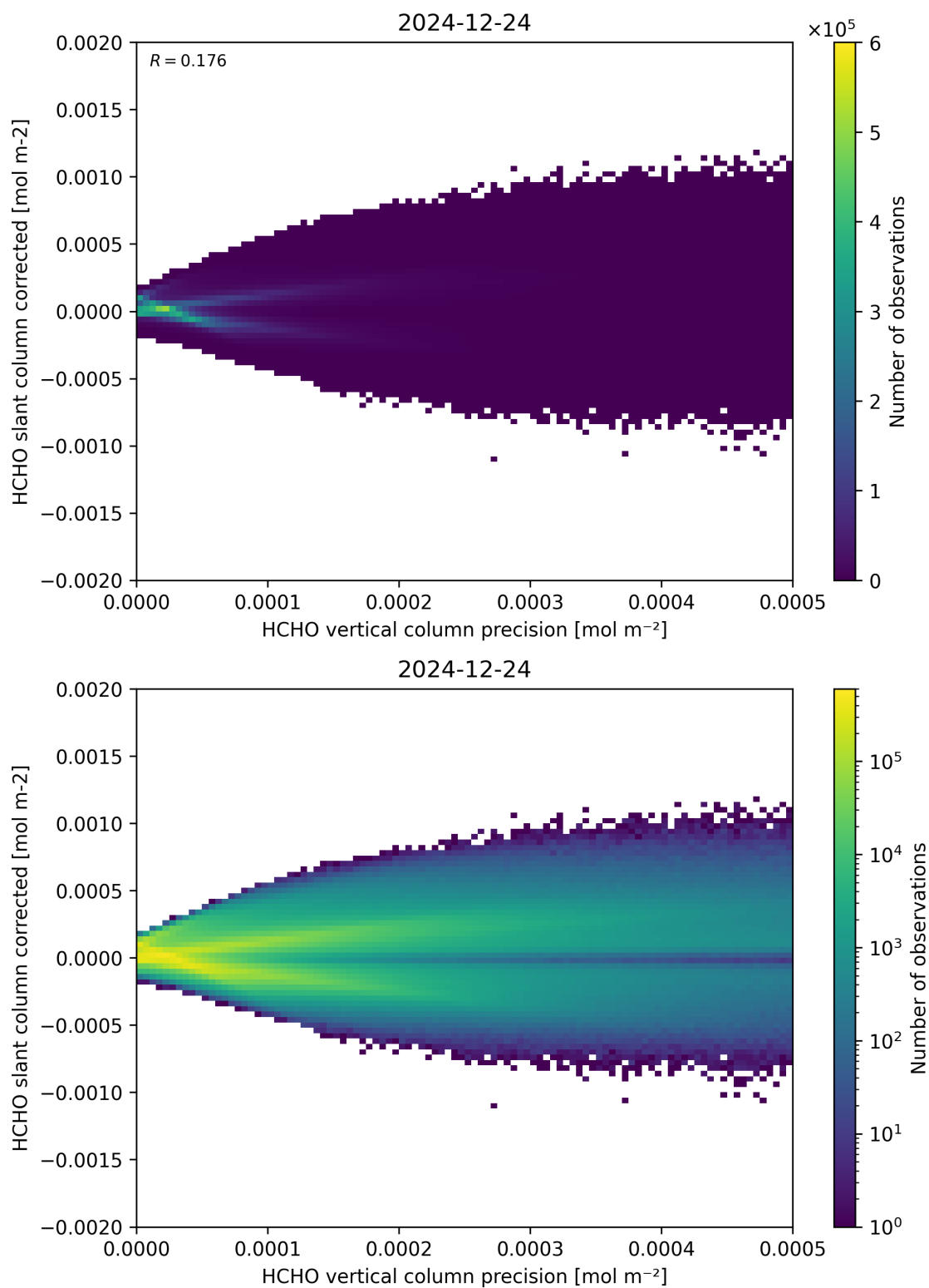
Figure 140: Scatter density plot of “HCHO vertical column precision” against “HCHO slant column corrected” for 2024-12-23 to 2024-12-25.
