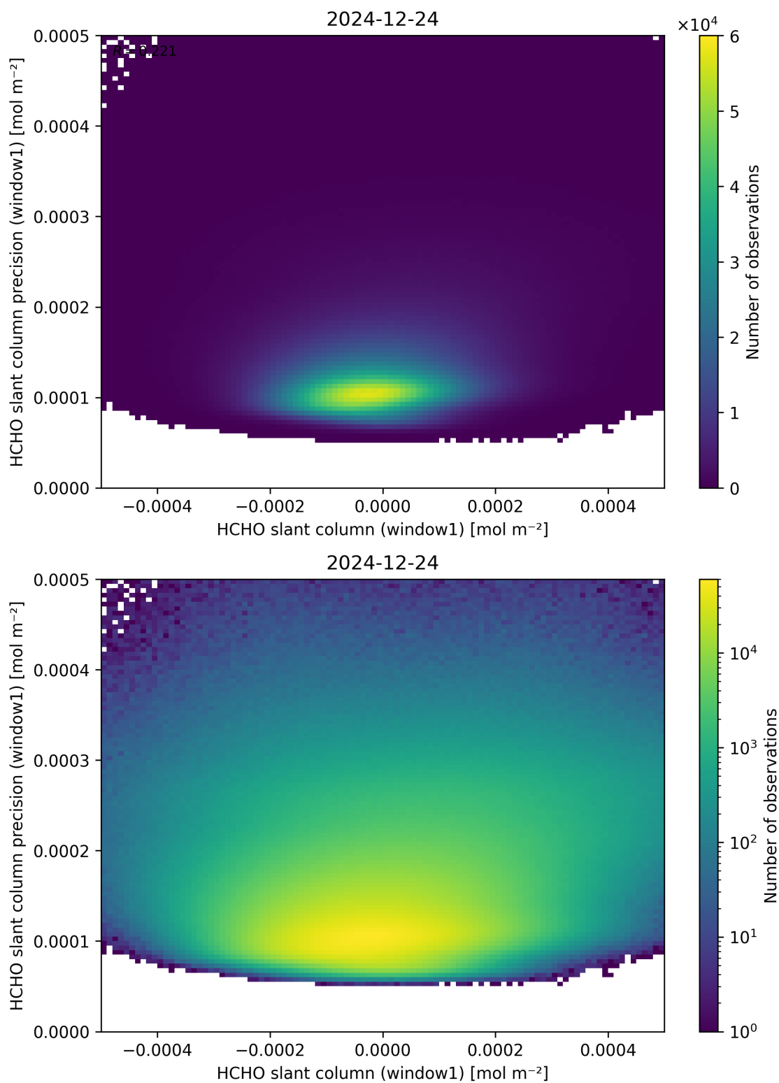
Figure 84: Scatter density plot of “HCHO slant column (window1)” against “HCHO slant column precision (window1)” for 2024-12-23 to 2024-12-25.
