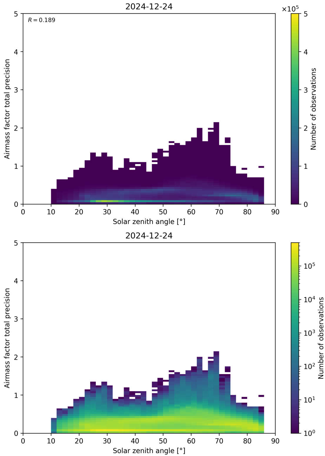
Figure 176: Scatter density plot of “Solar zenith angle” against “Airmass factor total precision” for 2024-12-23 to 2024-12-25.
