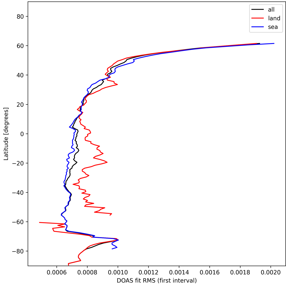
Figure 32: Zonal average of “DOAS fit RMS (first interval)” for 2024-12-23 to 2024-12-25.
