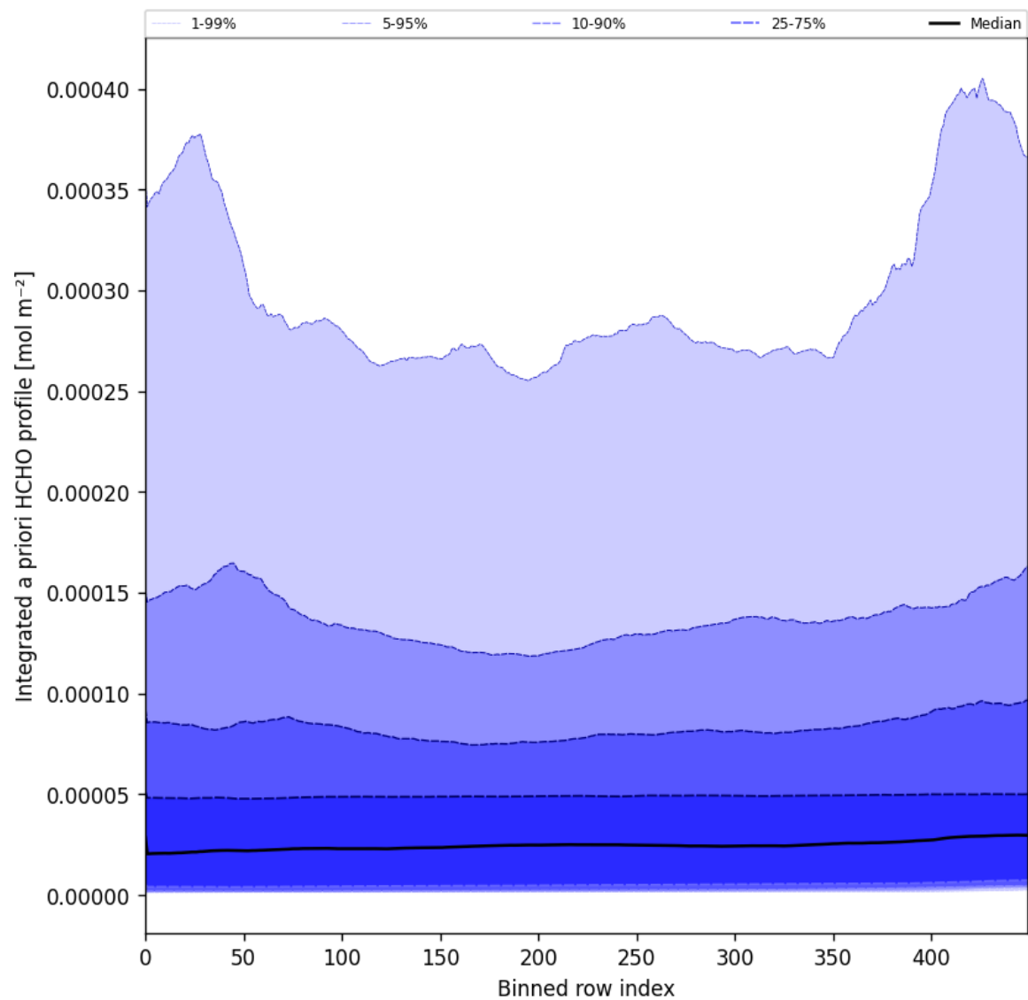
Figure 57: Along track statistics of "Integrated a priori HCHO profile" for 2024-12-23 to 2024-12-25
