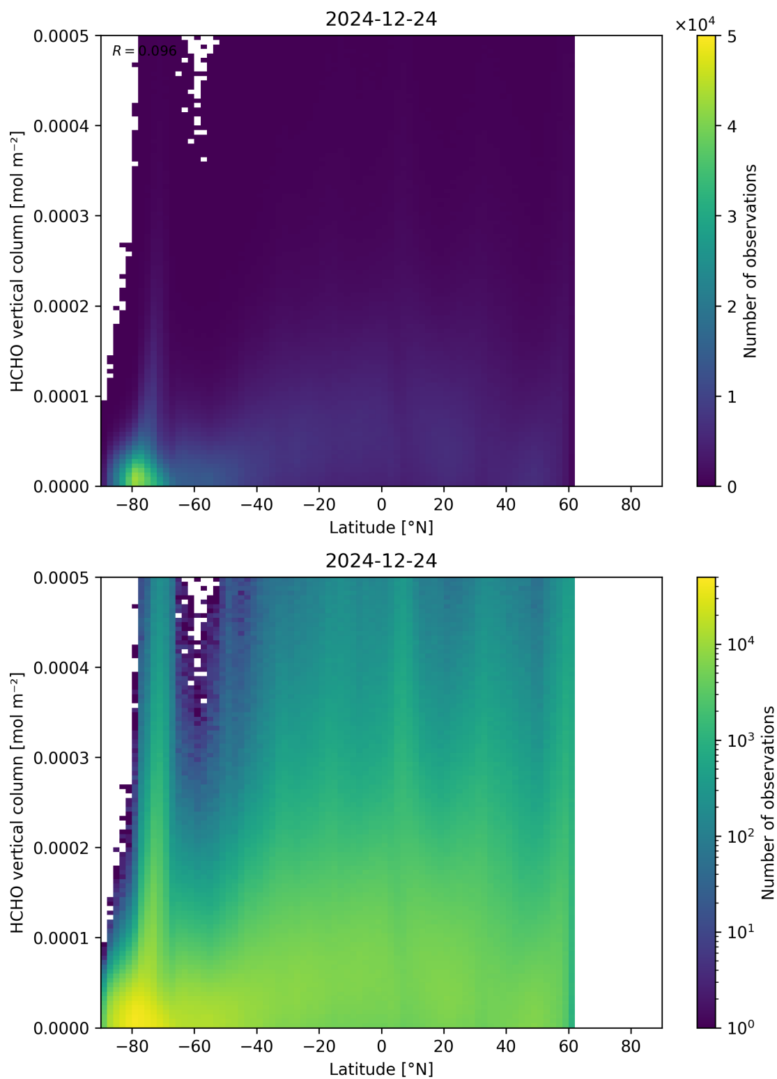
Figure 163: Scatter density plot of “Latitude” against “HCHO vertical column” for 2024-12-23 to 2024-12-25.
