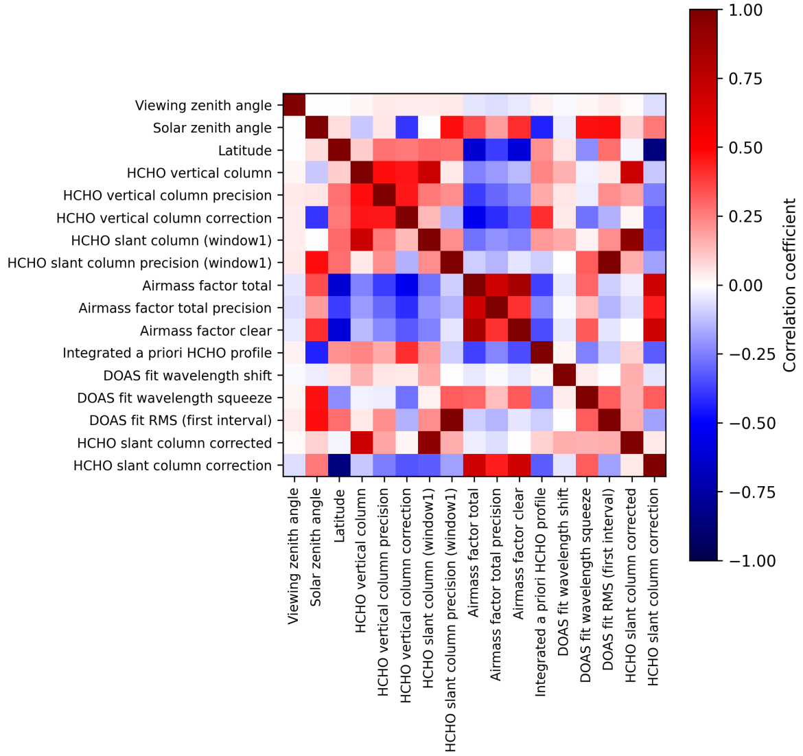
Figure 2: Map of correlation matrix for 2024-12-23 to 2024-12-25.
