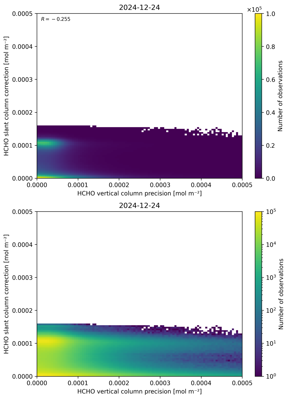
Figure 141: Scatter density plot of “HCHO vertical column precision” against “HCHO slant column correction” for 2024-12-23 to 2024-12-25.
