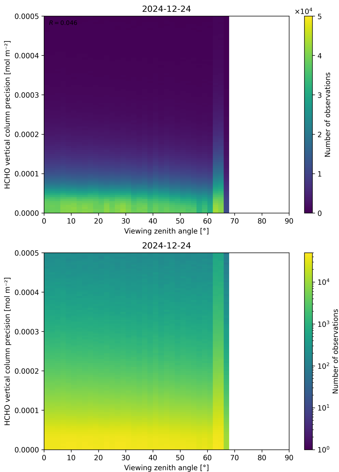
Figure 194: Scatter density plot of “Viewing zenith angle” against “HCHO vertical column precision” for 2024-12-23 to 2024-12-25.
