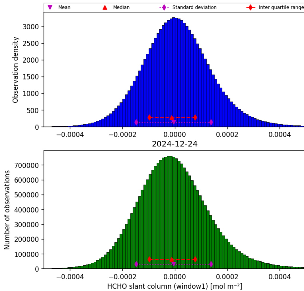
Figure 38: Histogram of “HCHO slant column (window1)” for 2024-12-23 to 2024-12-25
