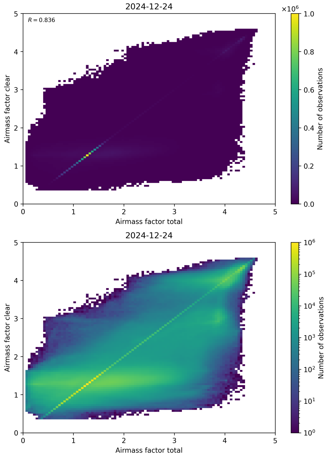
Figure 100: Scatter density plot of “Airmass factor total” against “Airmass factor clear” for 2024-12-23 to 2024-12-25.
