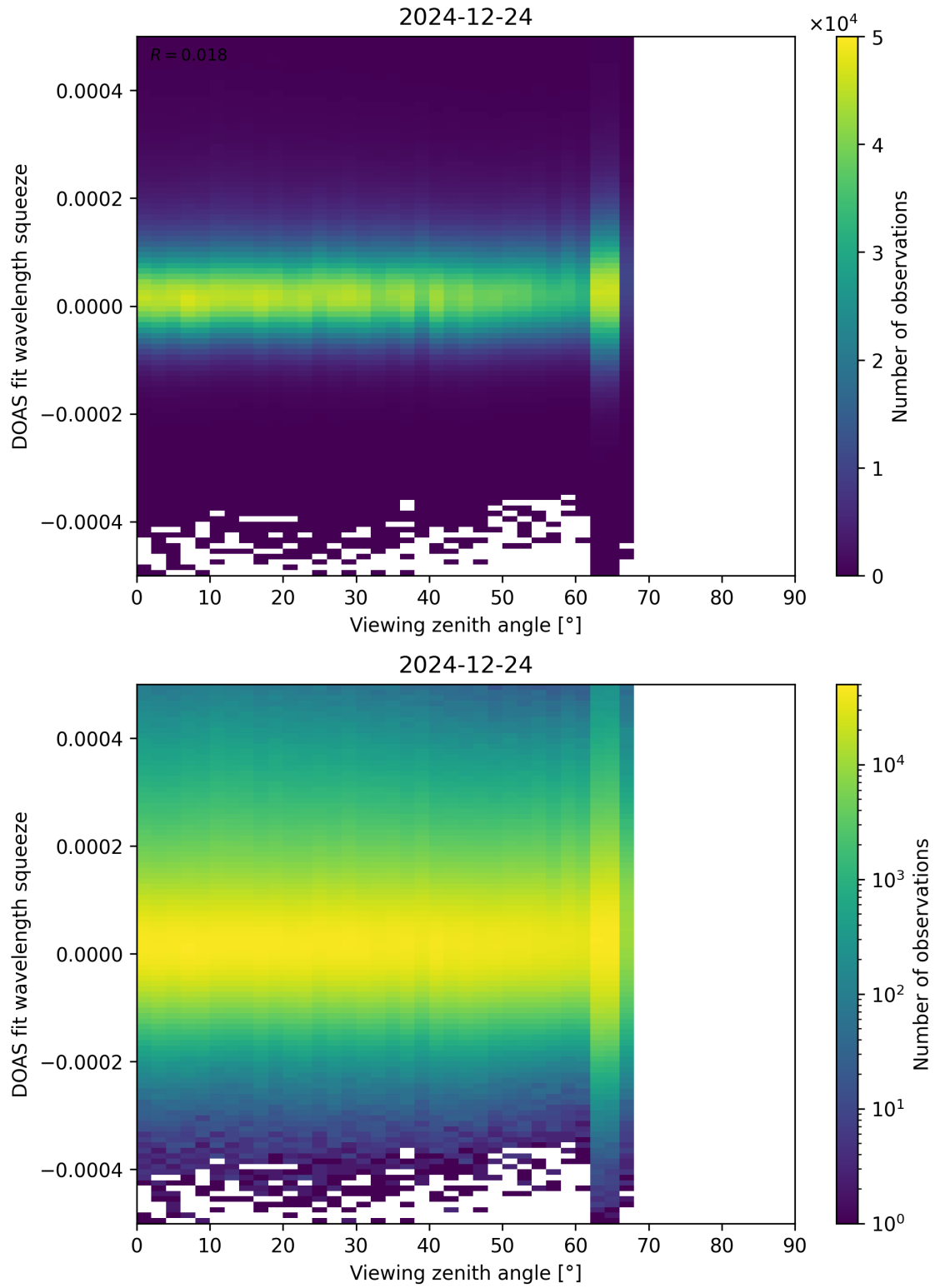
Figure 184: Scatter density plot of “Viewing zenith angle” against “DOAS fit wavelength squeeze” for 2024-12-23 to 2024-12-25.
