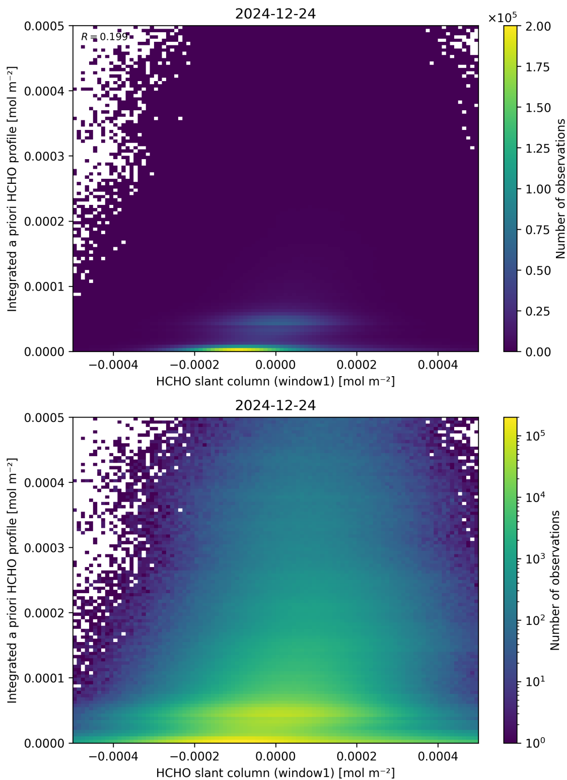
Figure 87: Scatter density plot of “HCHO slant column (window1)” against “Integrated a priori HCHO profile” for 2024-12-23 to 2024-12-25.
