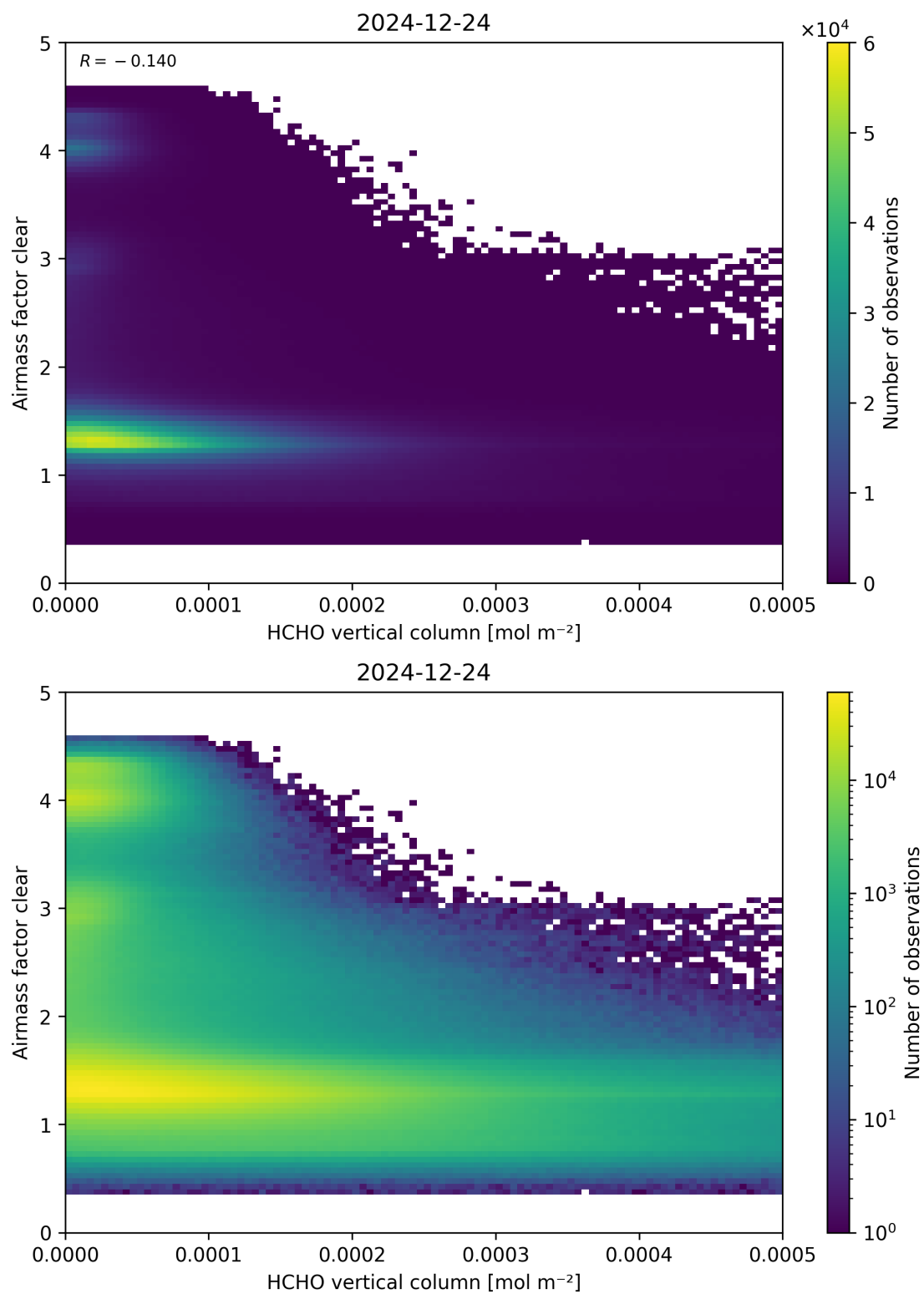
Figure 126: Scatter density plot of “HCHO vertical column” against “Airmass factor clear” for 2024-12-23 to 2024-12-25.
