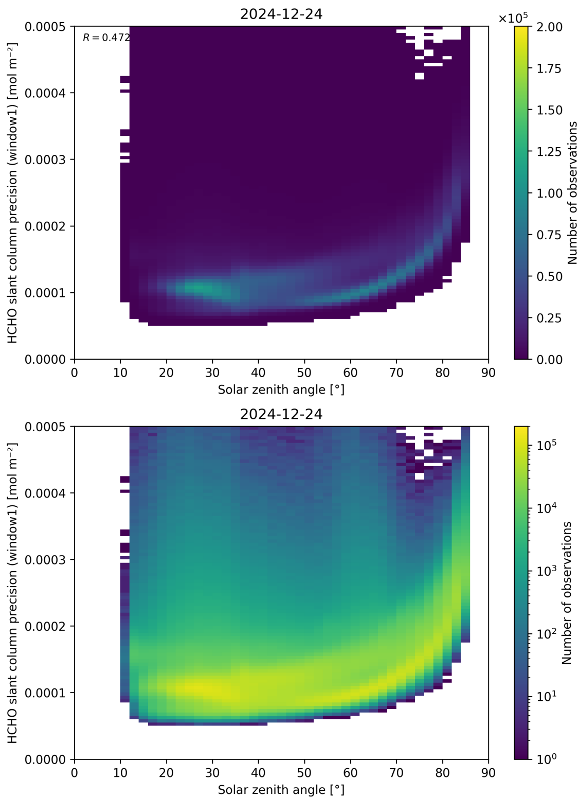
Figure 174: Scatter density plot of “Solar zenith angle” against “HCHO slant column precision (window1)” for 2024-12-23 to 2024-12-25.
