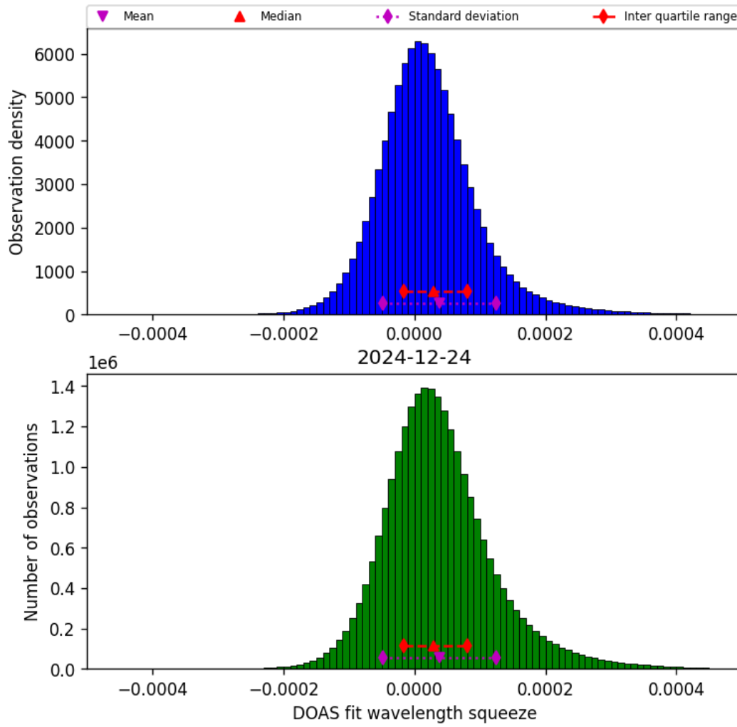
Figure 45: Histogram of “DOAS fit wavelength squeeze” for 2024-12-23 to 2024-12-25
