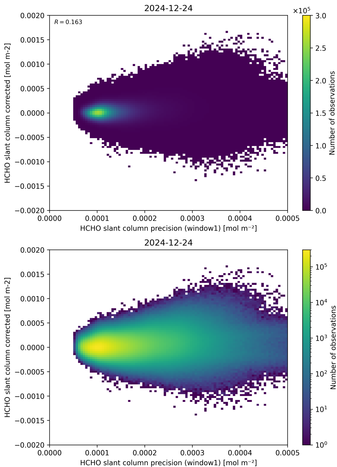
Figure 92: Scatter density plot of “HCHO slant column precision (window1)” against “HCHO slant column corrected” for 2024-12-23 to 2024-12-25.
