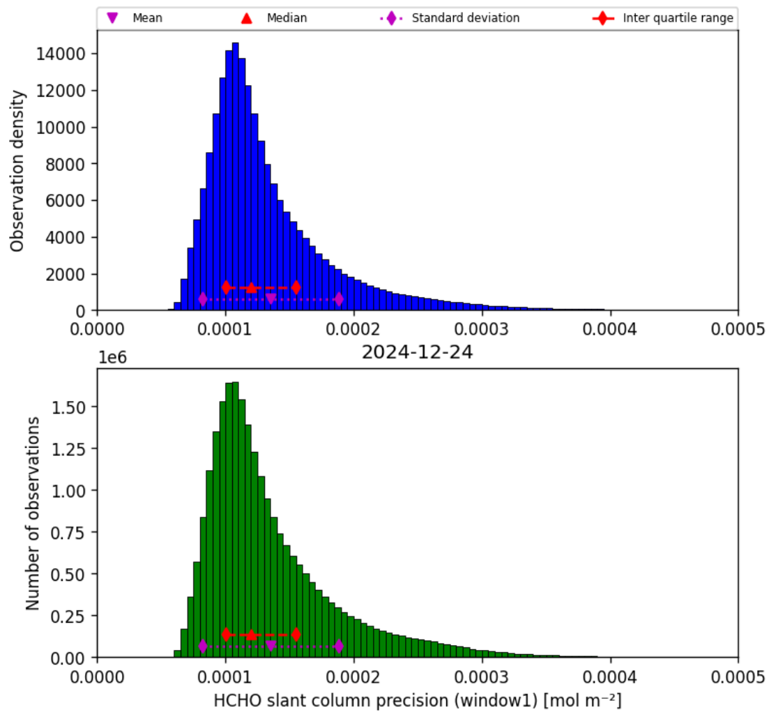
Figure 39: Histogram of “HCHO slant column precision (window1)” for 2024-12-23 to 2024-12-25
