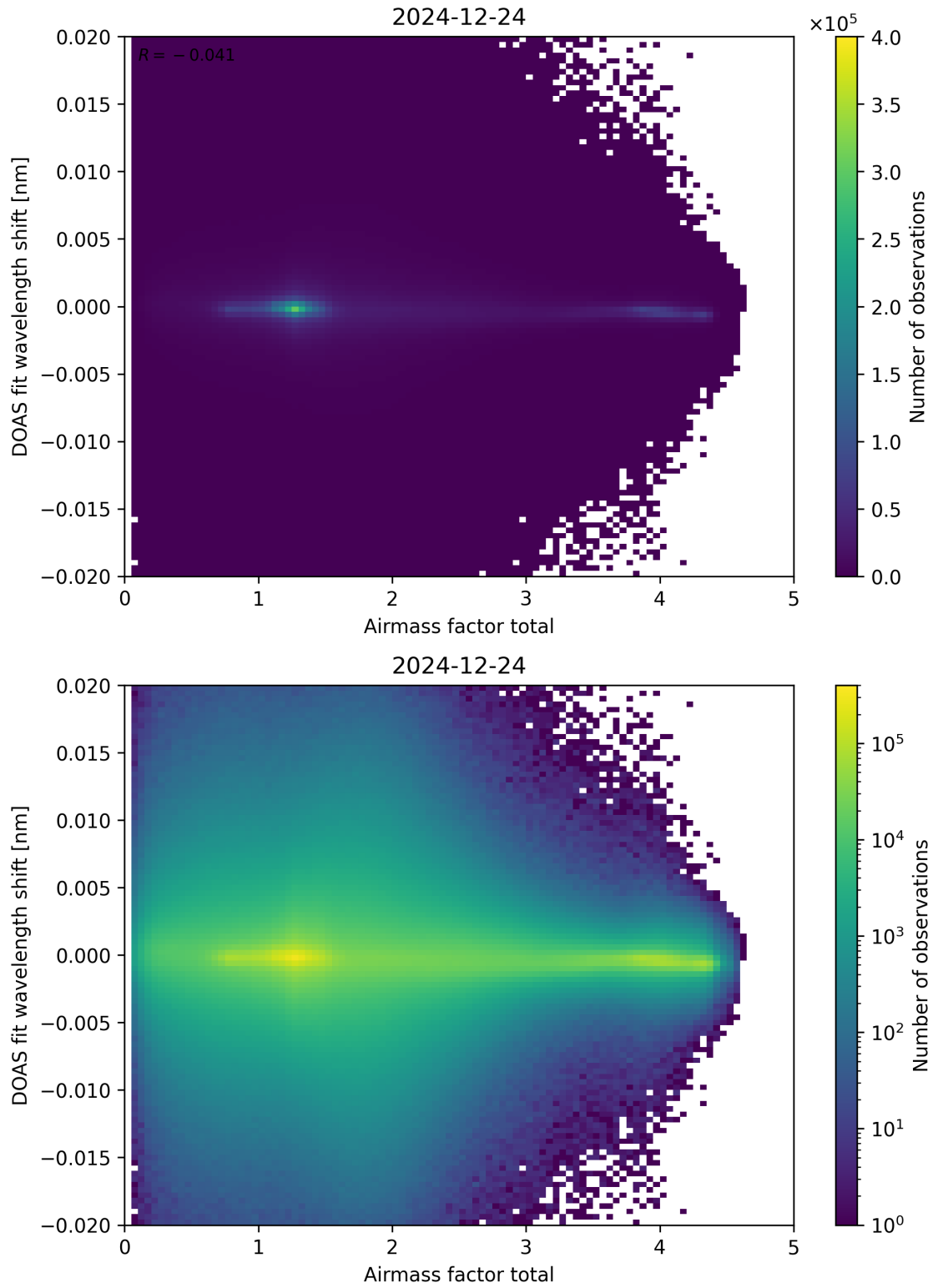
Figure 98: Scatter density plot of “Airmass factor total” against “DOAS fit wavelength shift” for 2024-12-23 to 2024-12-25.
