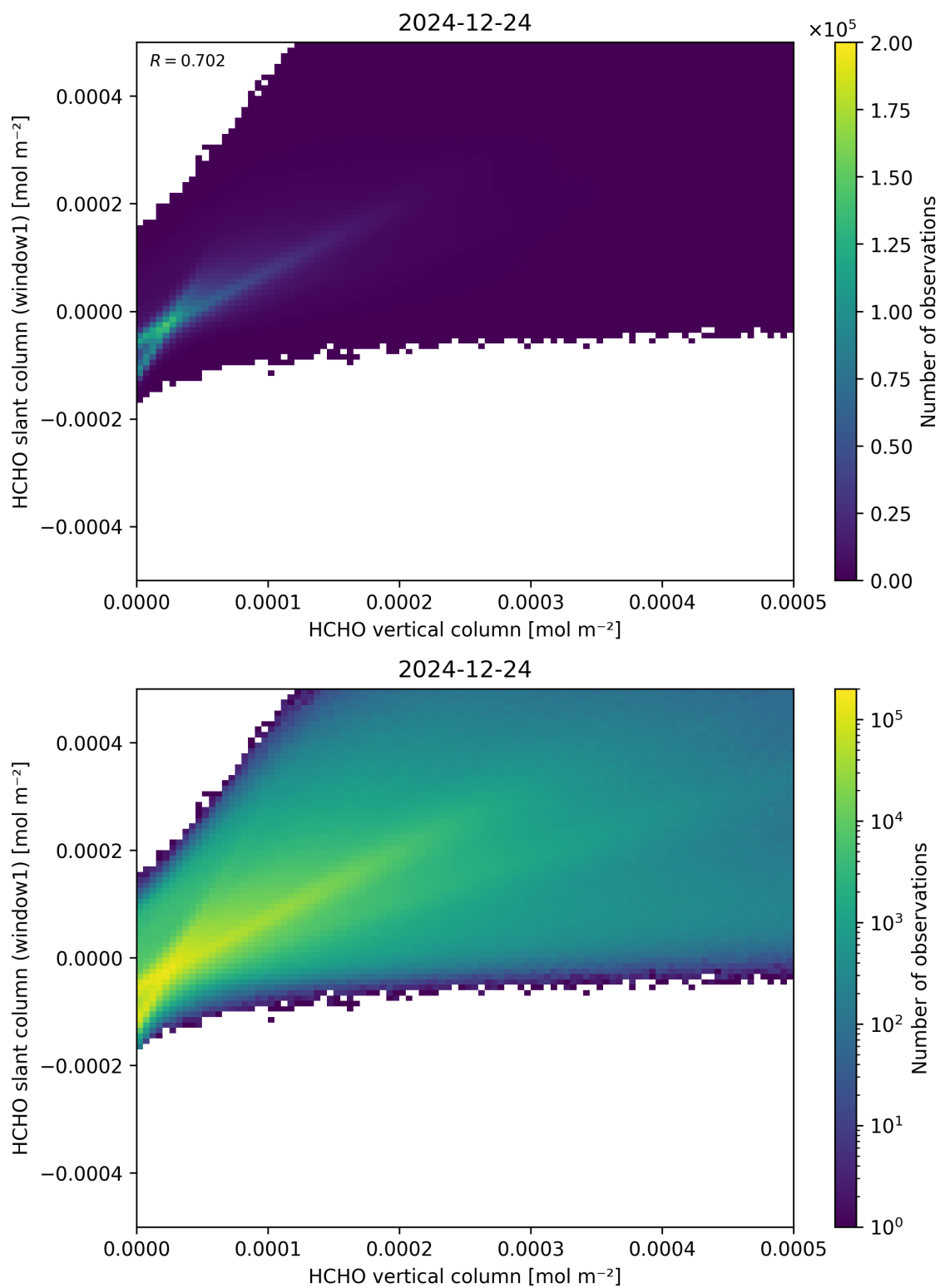
Figure 129: Scatter density plot of “HCHO vertical column” against “HCHO slant column (window1)” for 2024-12-23 to 2024-12-25.
