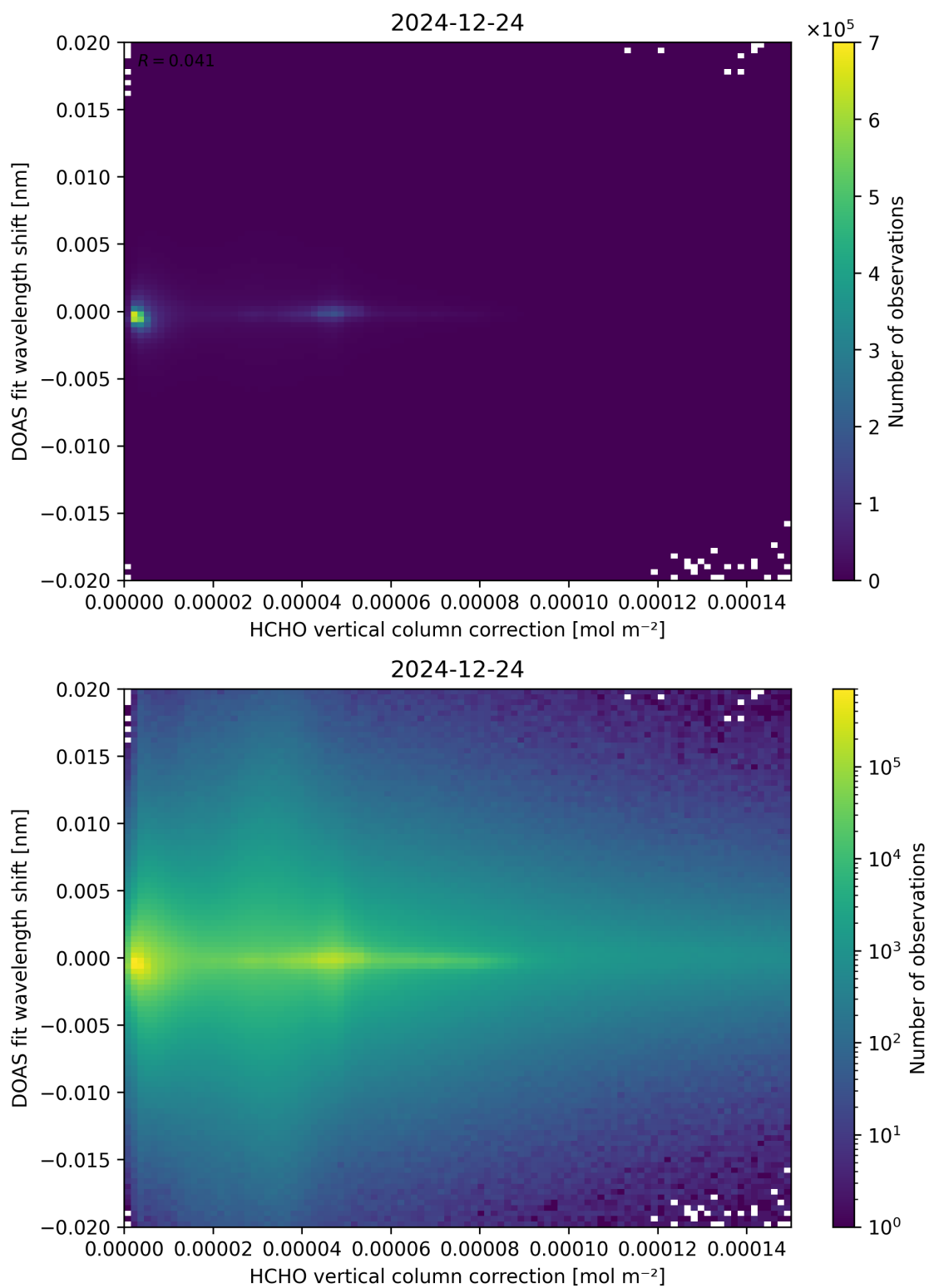
Figure 113: Scatter density plot of “HCHO vertical column correction” against “DOAS fit wavelength shift” for 2024-12-23 to 2024-12-25.
