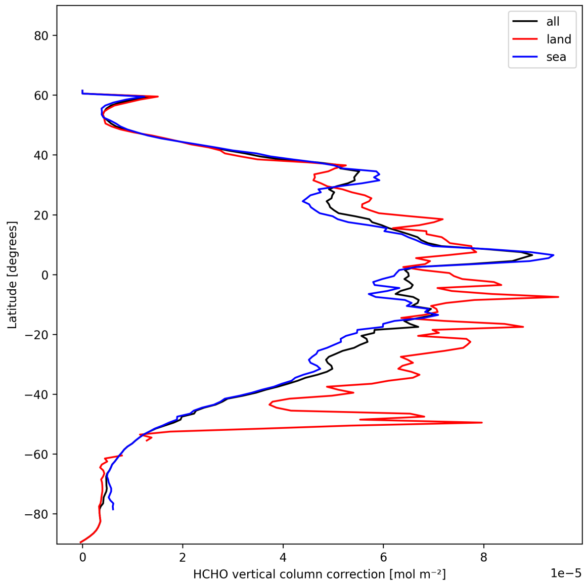
Figure 23: Zonal average of “HCHO vertical column correction” for 2024-12-23 to 2024-12-25.
