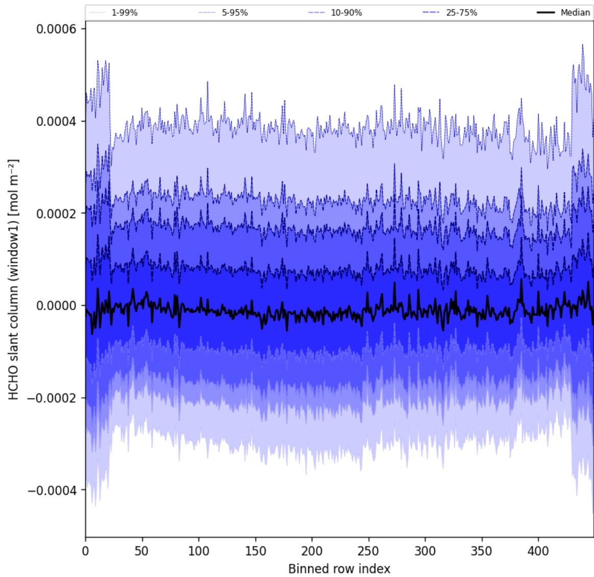
Figure 52: Along track statistics of “HCHO slant column (window1)” for 2024-12-23 to 2024-12-25
