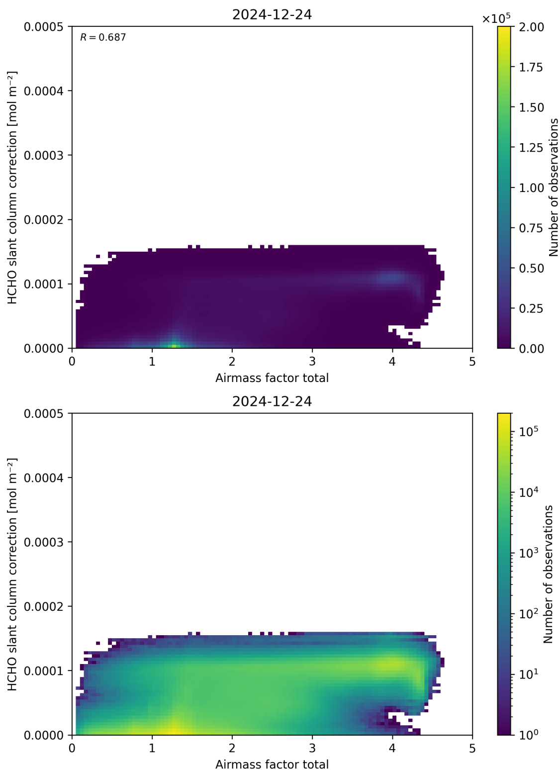
Figure 102: Scatter density plot of “Airmass factor total” against “HCHO slant column correction” for 2024-12-23 to 2024-12-25.
