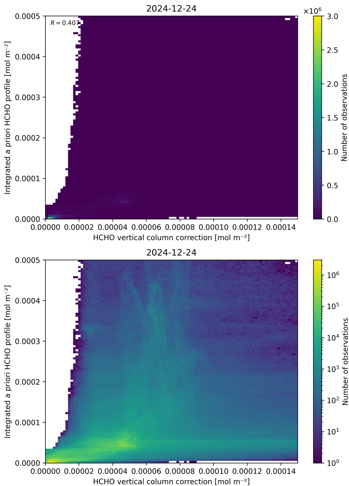
Figure 122: Scatter density plot of “HCHO vertical column correction” against “Integrated a priori HCHO profile” for 2024-12-23 to 2024-12-25.
