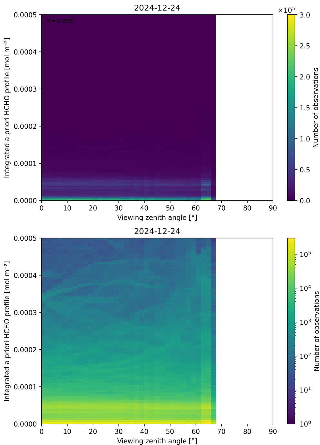
Figure 195: Scatter density plot of “Viewing zenith angle” against “Integrated a priori HCHO profile” for 2024-12-23 to 2024-12-25.
