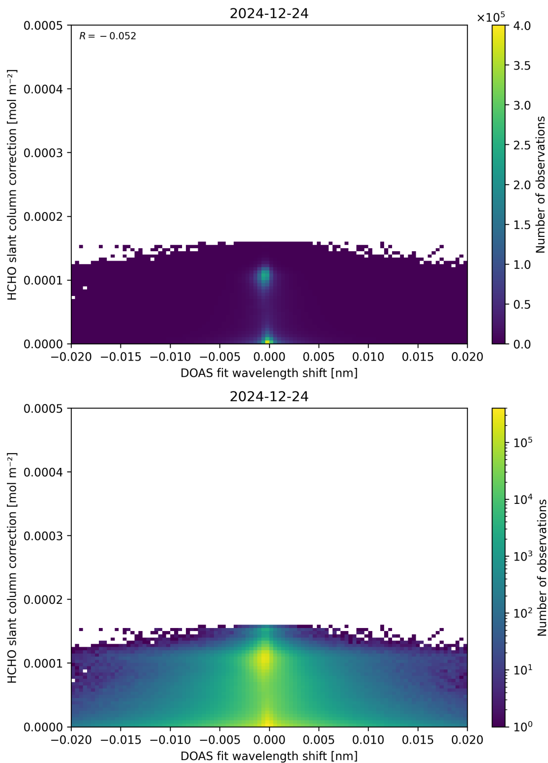
Figure 67: Scatter density plot of “DOAS fit wavelength shift” against “HCHO slant column correction” for 2024-12-23 to 2024-12-25.
