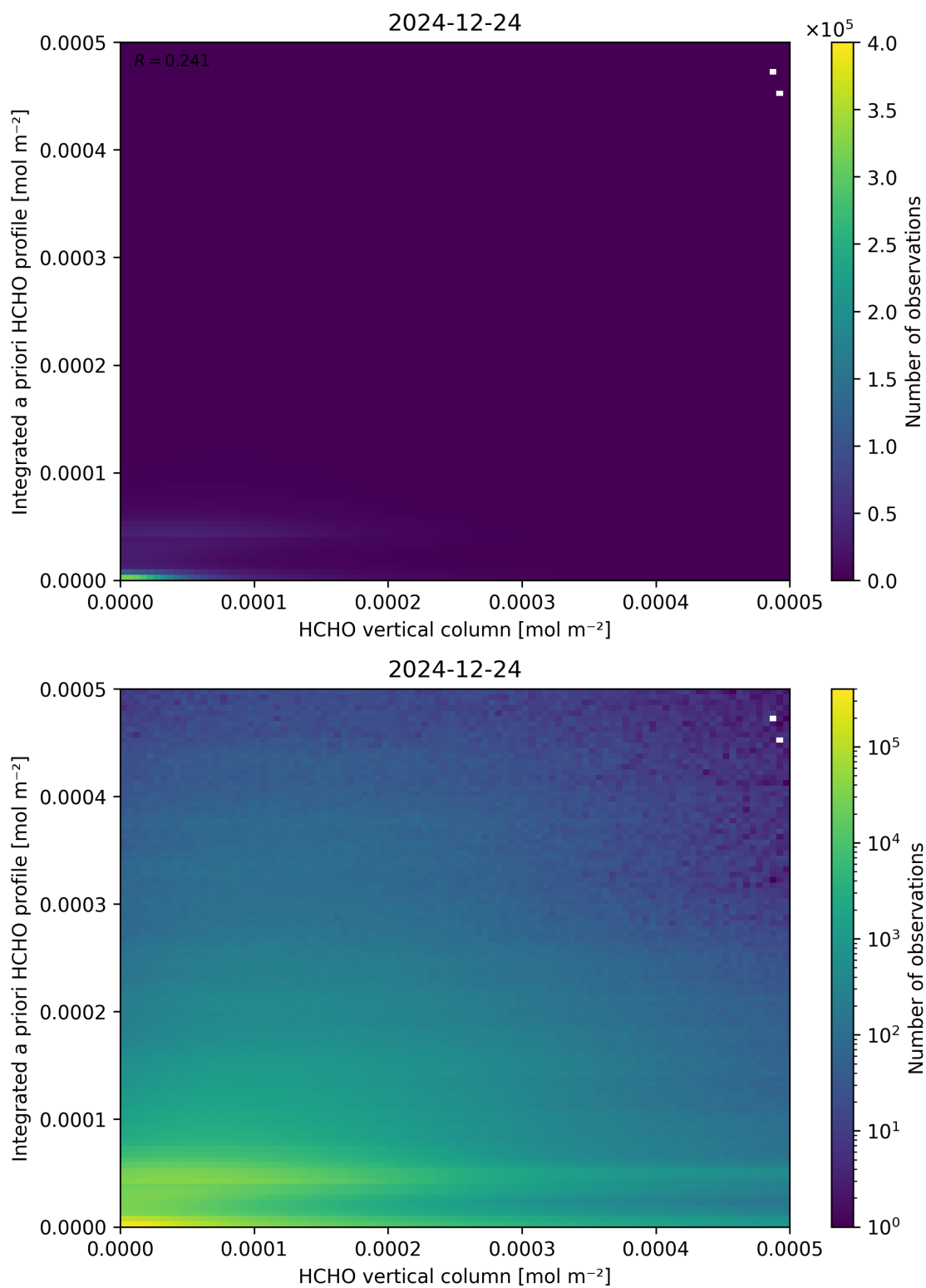
Figure 135: Scatter density plot of “HCHO vertical column” against “Integrated a priori HCHO profile” for 2024-12-23 to 2024-12-25.
