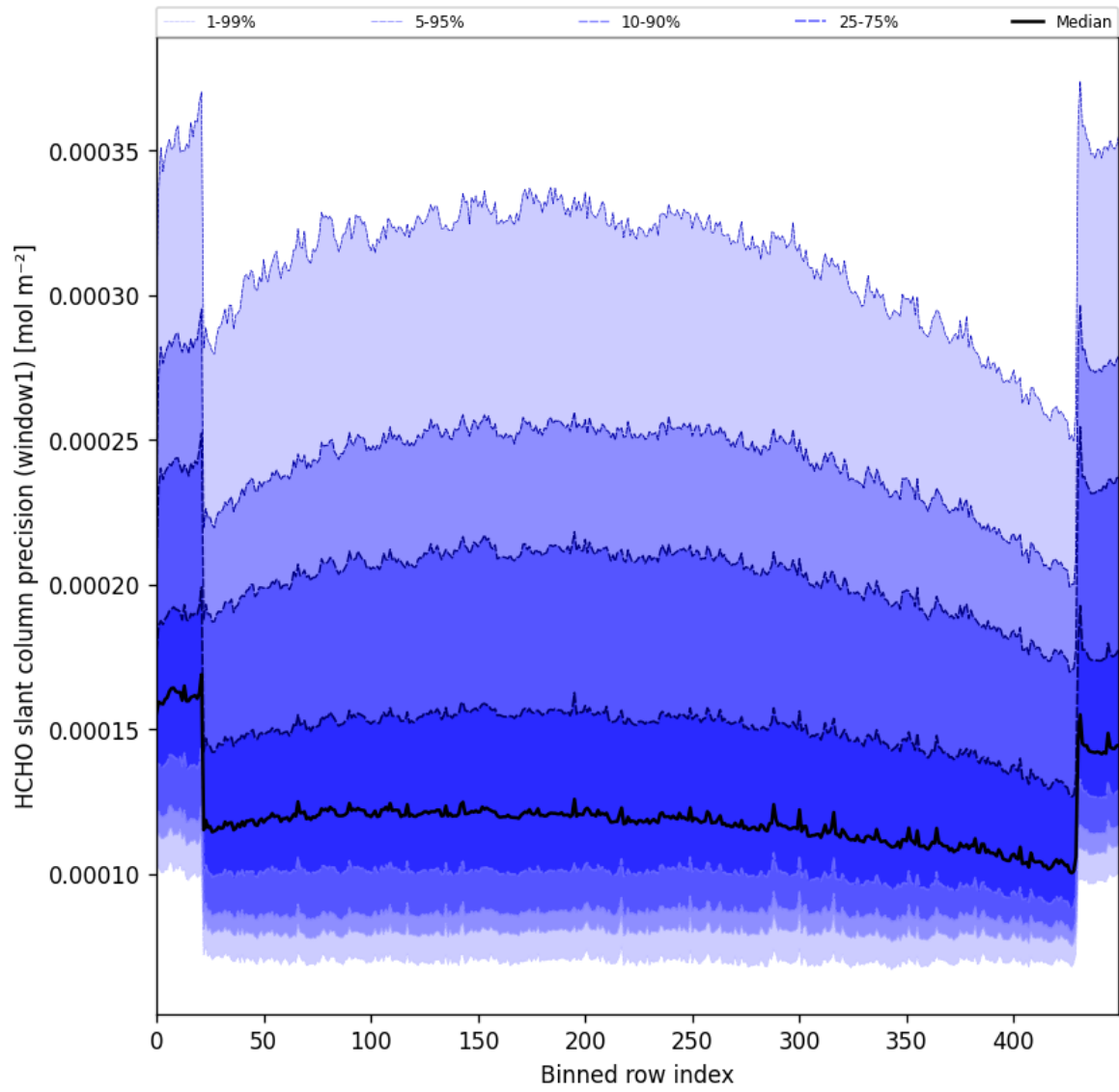
Figure 53: Along track statistics of “HCHO slant column precision (window1)” for 2024-12-23 to 2024-12-25
