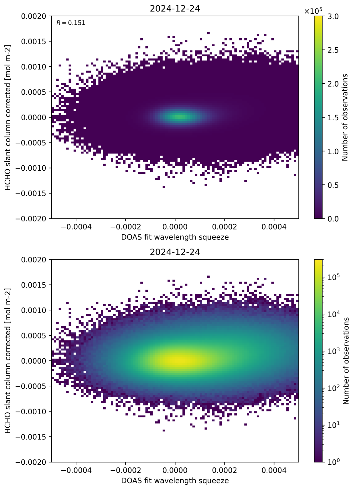
Figure 69: Scatter density plot of “DOAS fit wavelength squeeze” against “HCHO slant column corrected” for 2024-12-23 to 2024-12-25.
