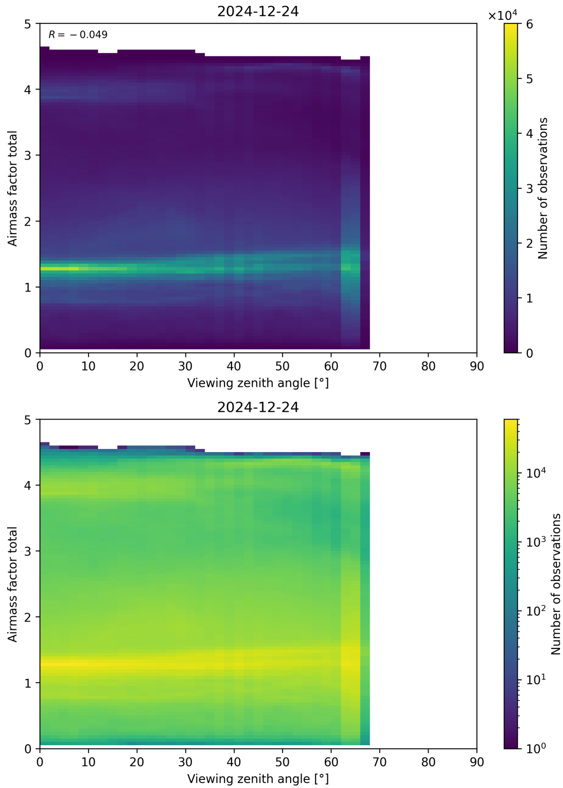
Figure 190: Scatter density plot of “Viewing zenith angle” against “Airmass factor total” for 2024-12-23 to 2024-12-25.
