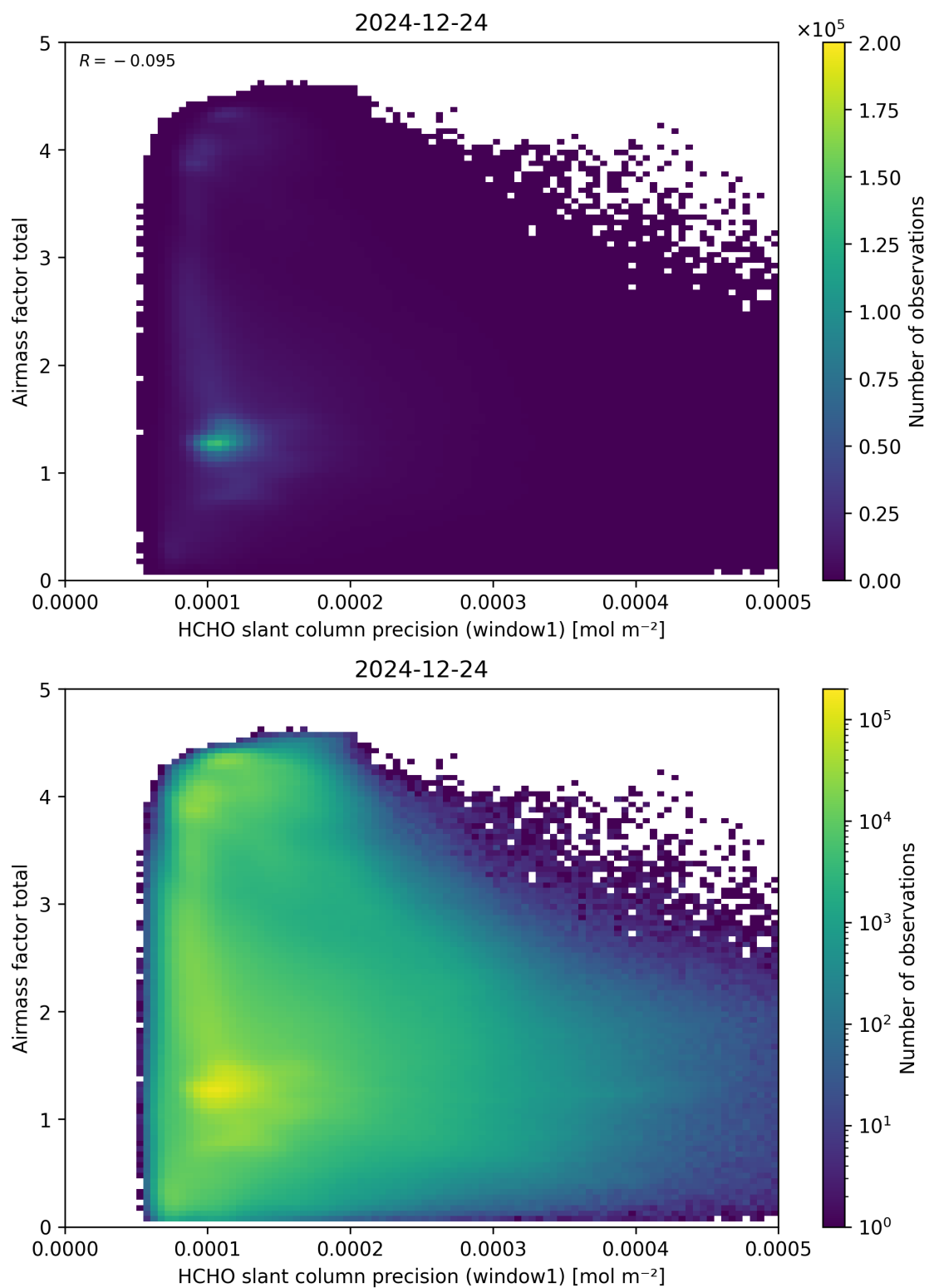
Figure 94: Scatter density plot of “HCHO slant column precision (window1)” against “Airmass factor total” for 2024-12-23 to 2024-12-25.
