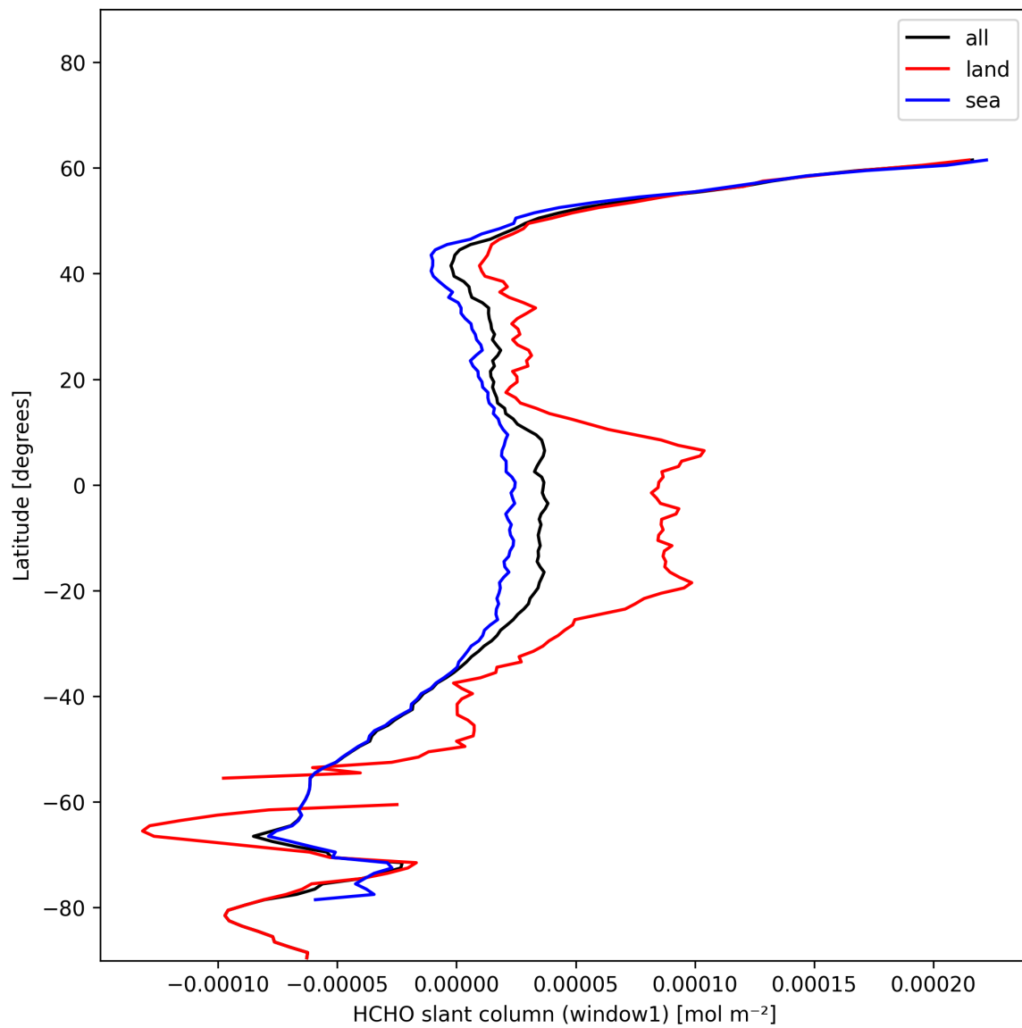
Figure 24: Zonal average of “HCHO slant column (window1)” for 2024-12-23 to 2024-12-25.
