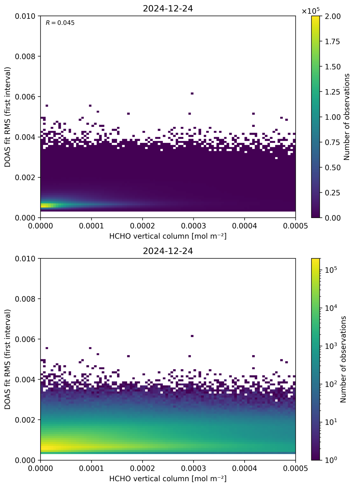
Figure 123: Scatter density plot of “HCHO vertical column” against “DOAS fit RMS (first interval)” for 2024-12-23 to 2024-12-25.
