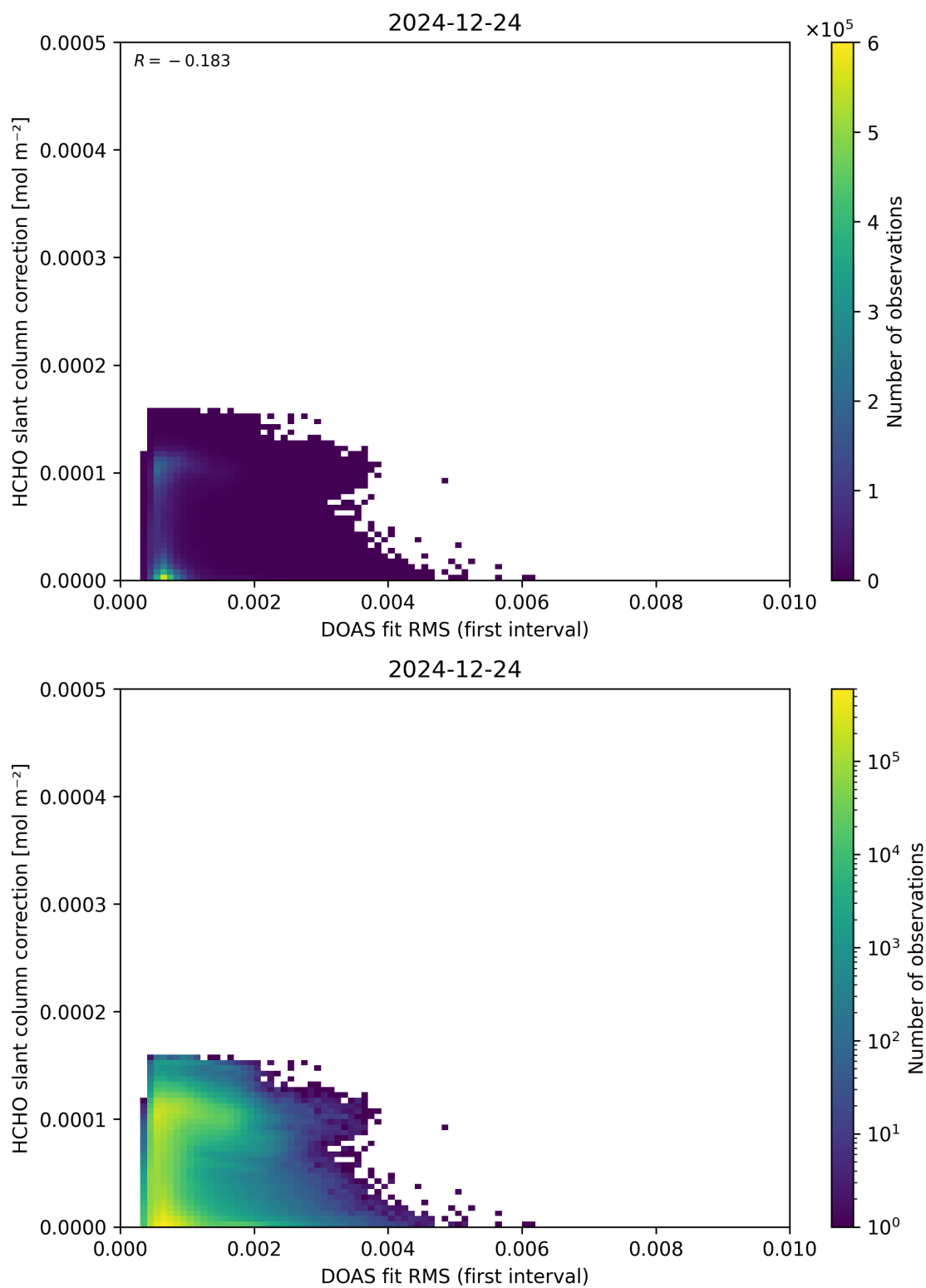
Figure 63: Scatter density plot of “DOAS fit RMS (first interval)” against “HCHO slant column correction” for 2024-12-23 to 2024-12-25.
