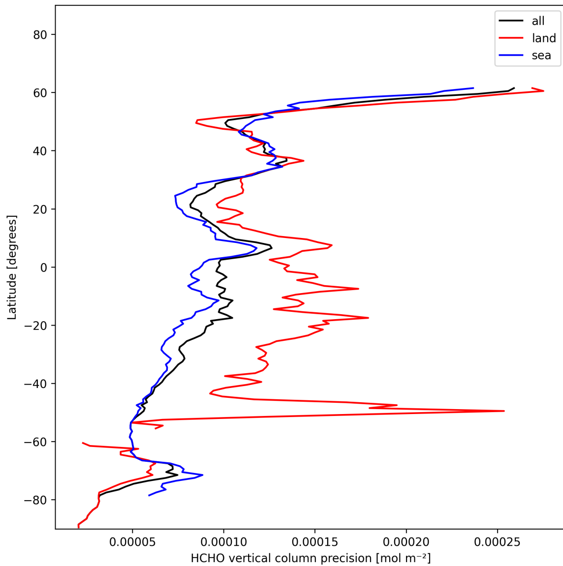
Figure 22: Zonal average of “HCHO vertical column precision” for 2024-12-23 to 2024-12-25.
