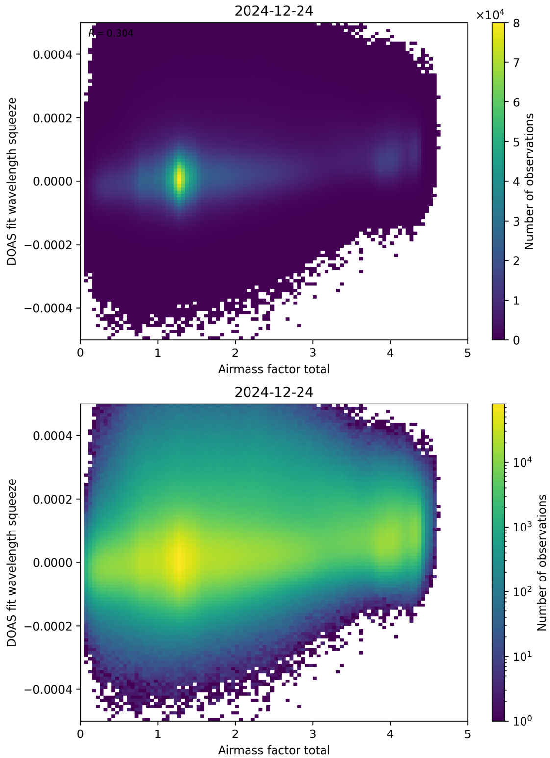
Figure 99: Scatter density plot of “Airmass factor total” against “DOAS fit wavelength squeeze” for 2024-12-23 to 2024-12-25.
