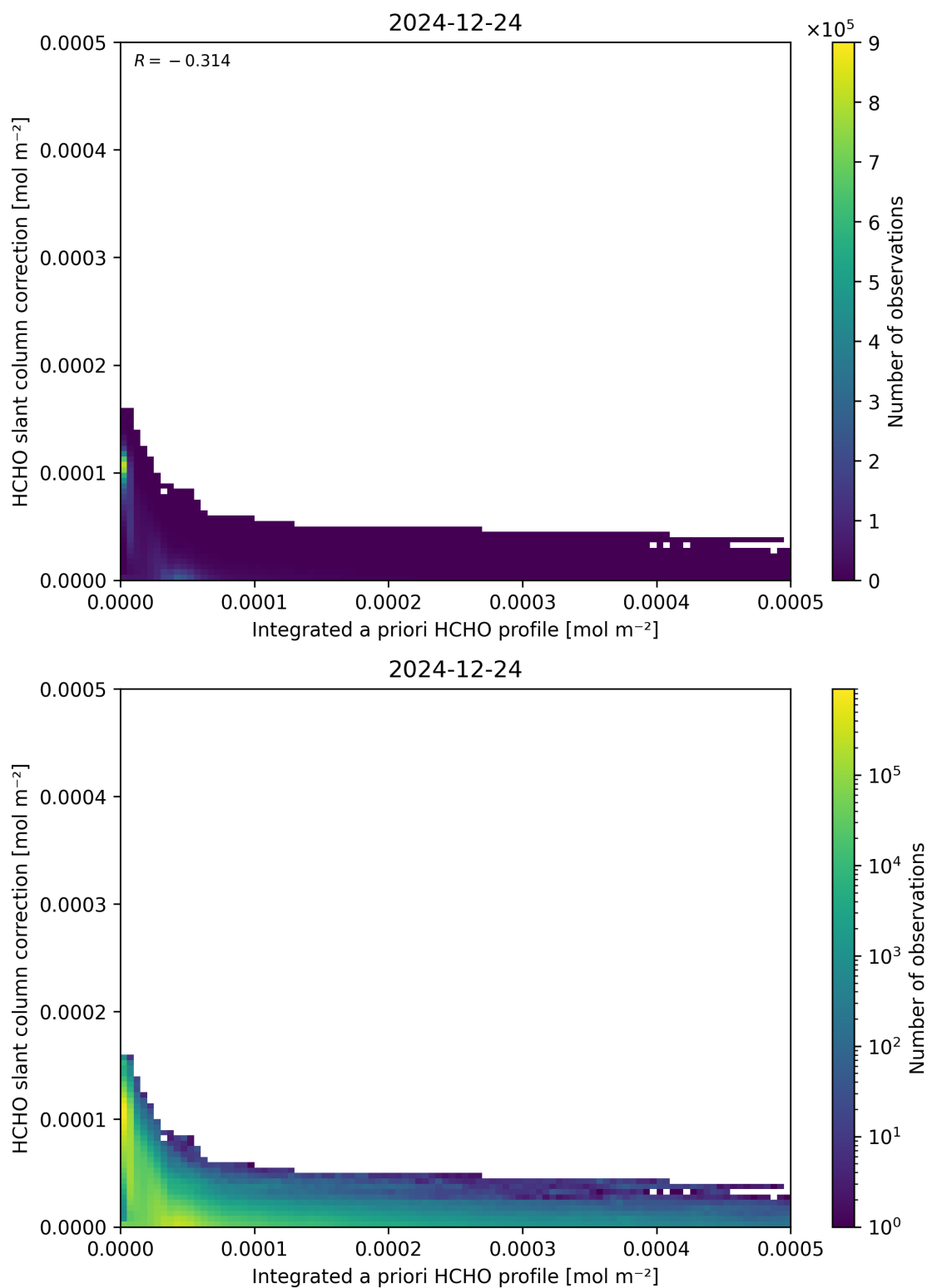
Figure 152: Scatter density plot of “Integrated a priori HCHO profile” against “HCHO slant column correction” for 2024-12-23 to 2024-12-25.
