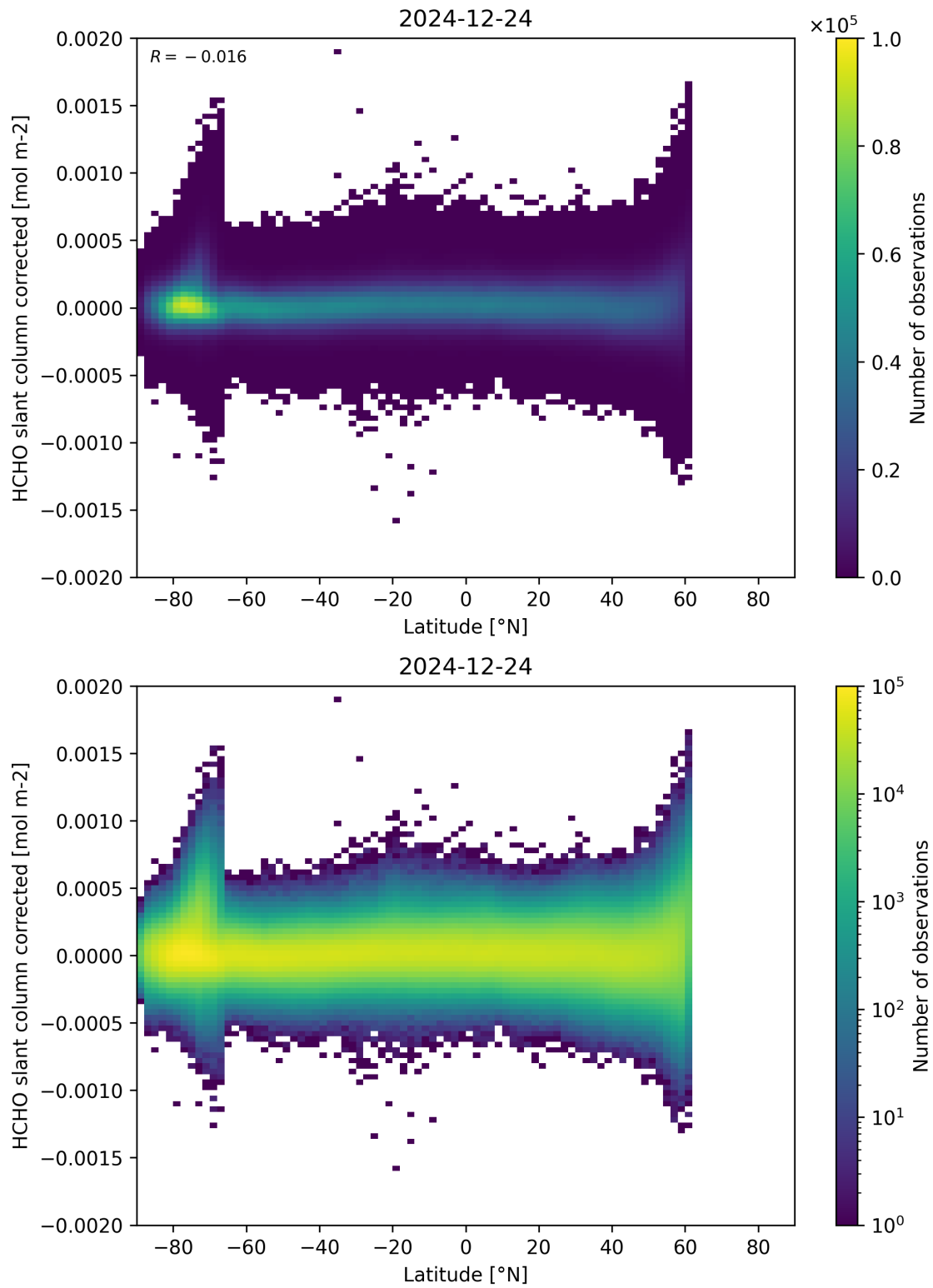
Figure 157: Scatter density plot of “Latitude” against “HCHO slant column corrected” for 2024-12-23 to 2024-12-25.
