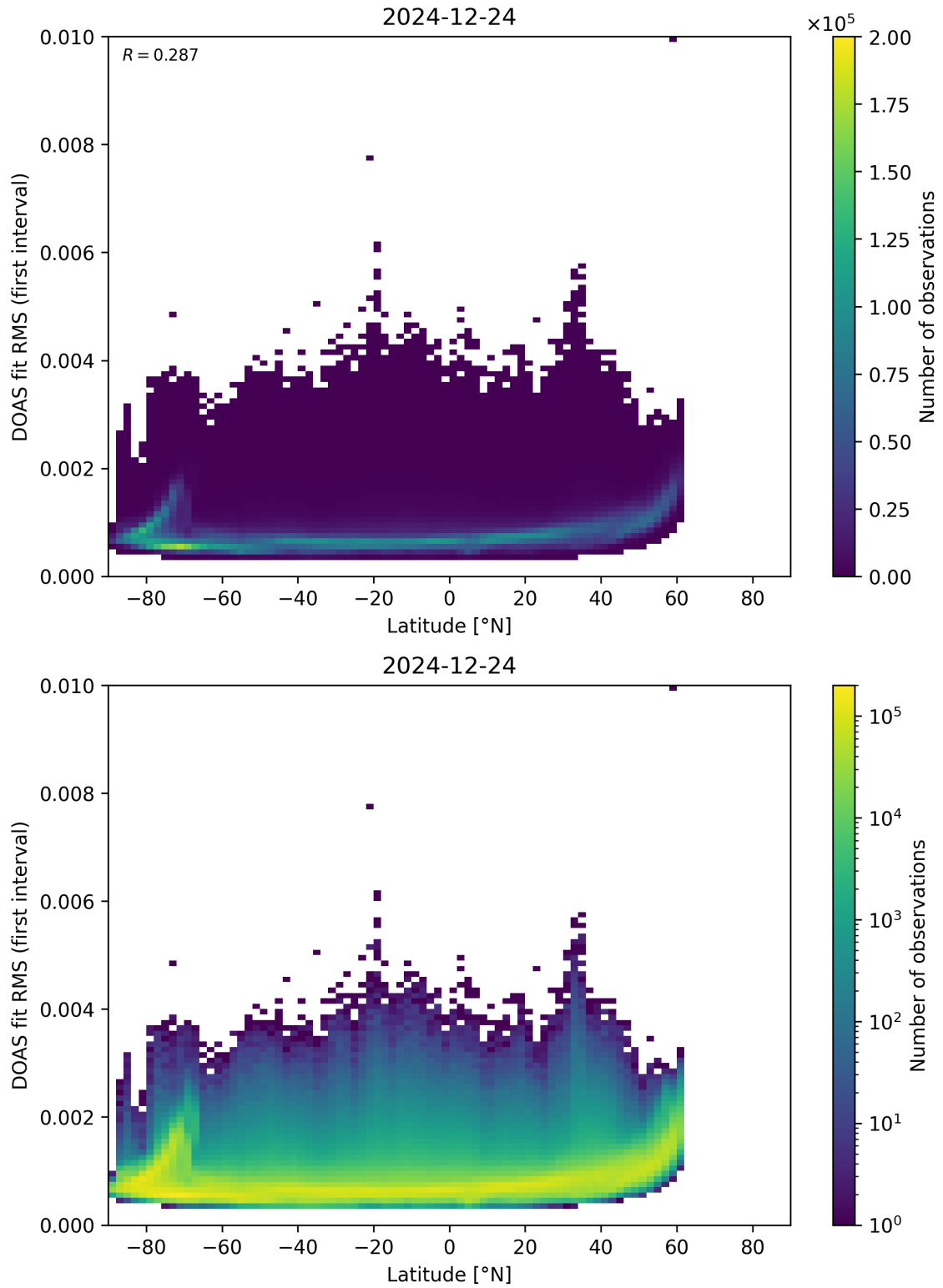
Figure 153: Scatter density plot of “Latitude” against “DOAS fit RMS (first interval)” for 2024-12-23 to 2024-12-25.
