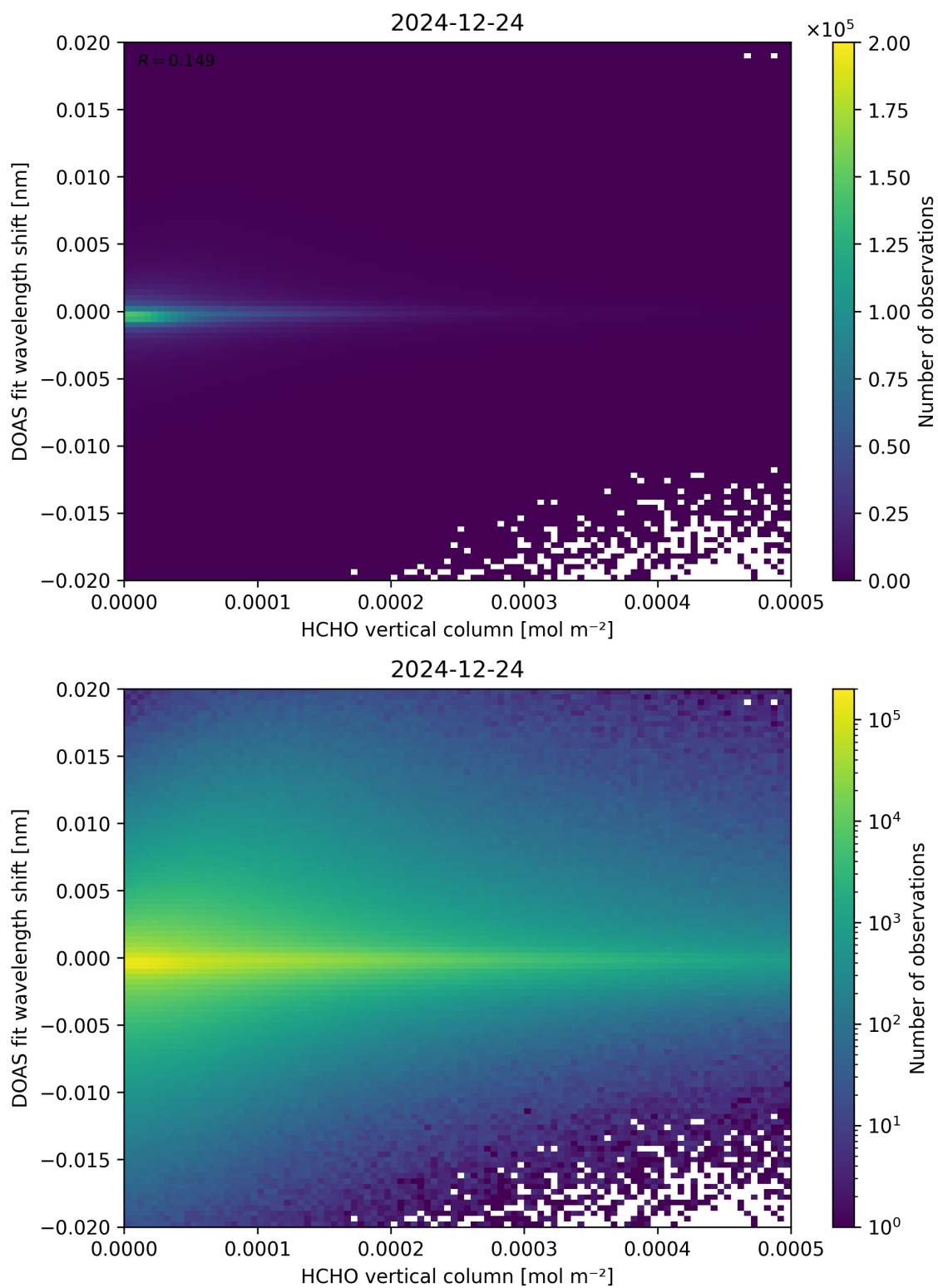
Figure 124: Scatter density plot of “HCHO vertical column” against “DOAS fit wavelength shift” for 2024-12-23 to 2024-12-25.
