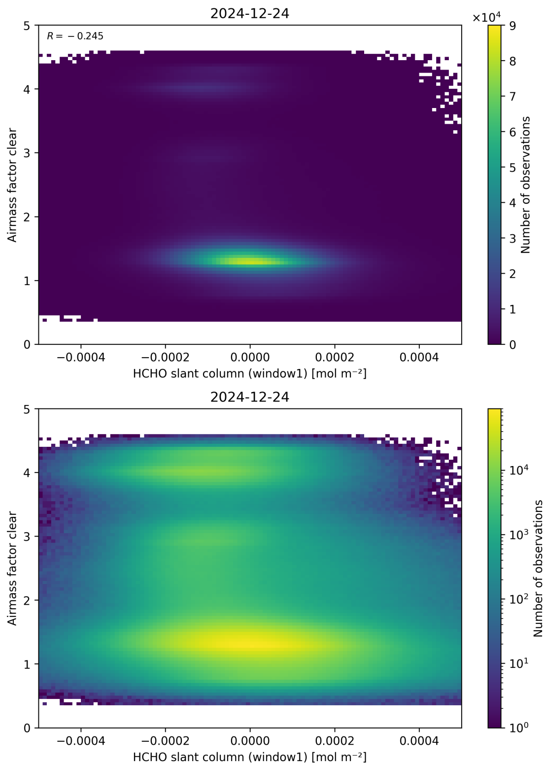
Figure 81: Scatter density plot of “HCHO slant column (window1)” against “Airmass factor clear” for 2024-12-23 to 2024-12-25.
