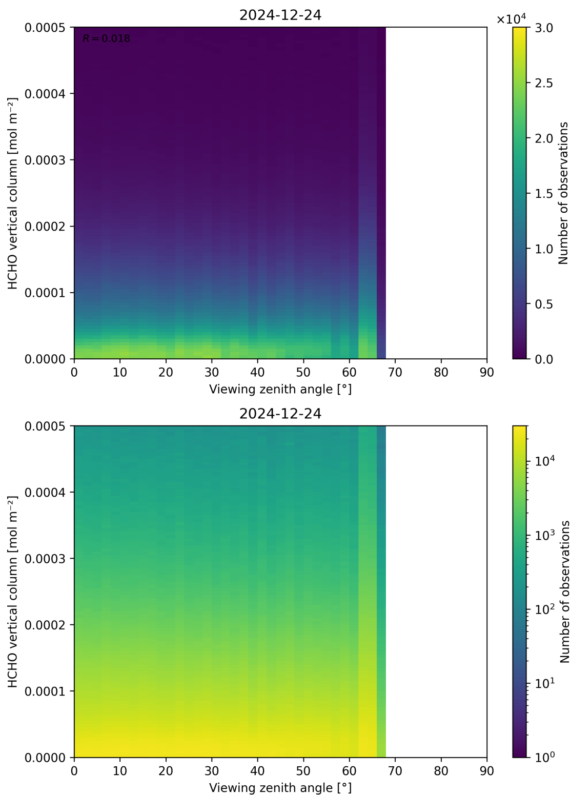
Figure 192: Scatter density plot of “Viewing zenith angle” against “HCHO vertical column” for 2024-12-23 to 2024-12-25.
