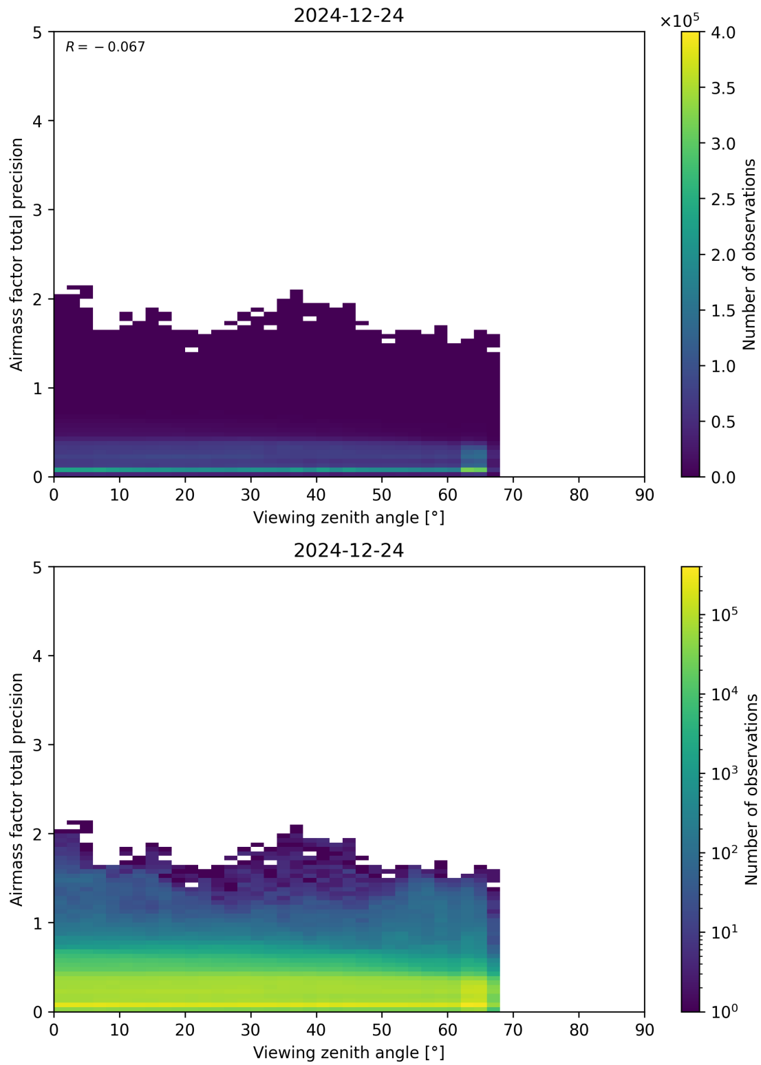
Figure 191: Scatter density plot of “Viewing zenith angle” against “Airmass factor total precision” for 2024-12-23 to 2024-12-25.
