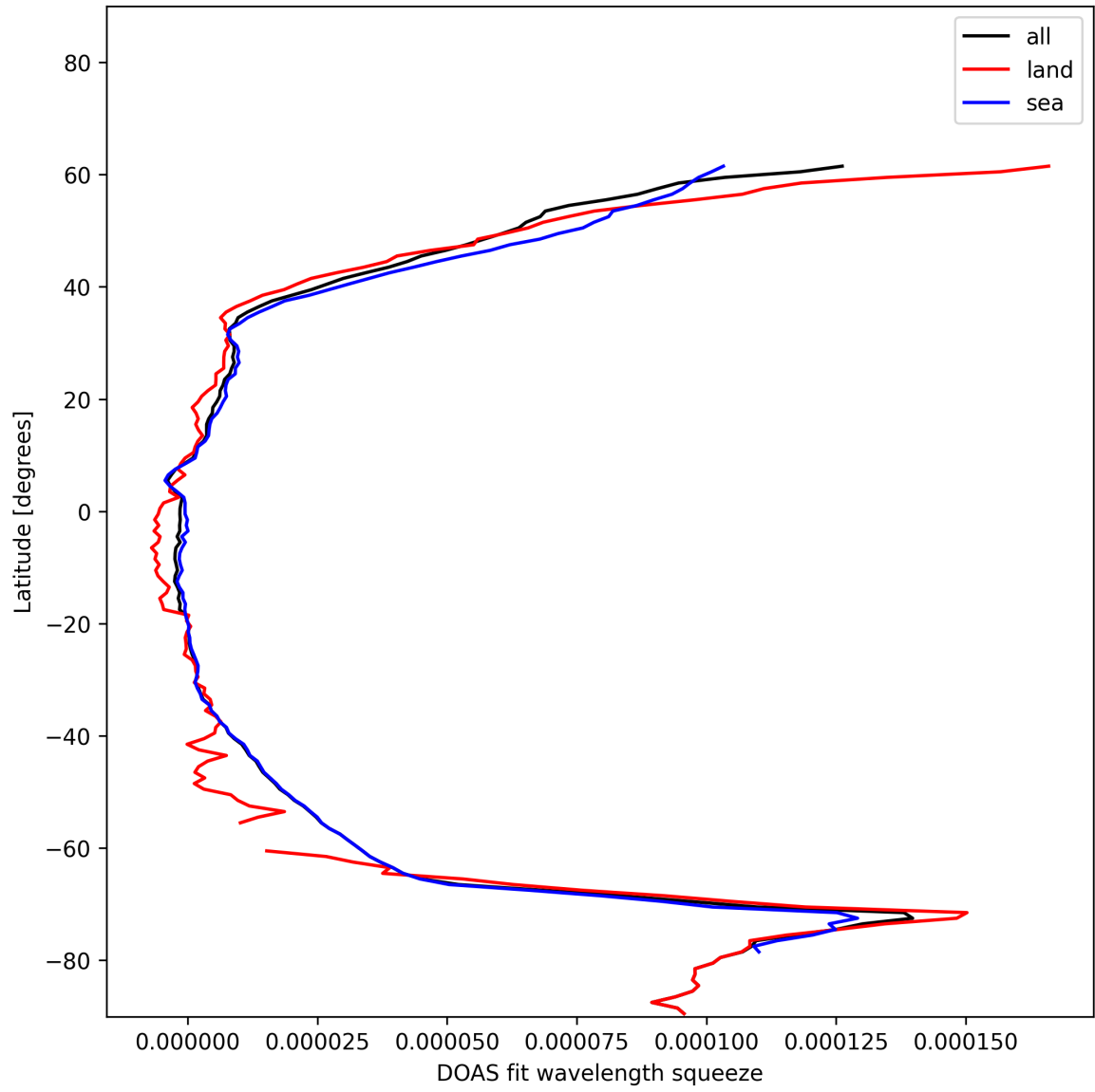
Figure 31: Zonal average of “DOAS fit wavelength squeeze” for 2024-12-23 to 2024-12-25.
