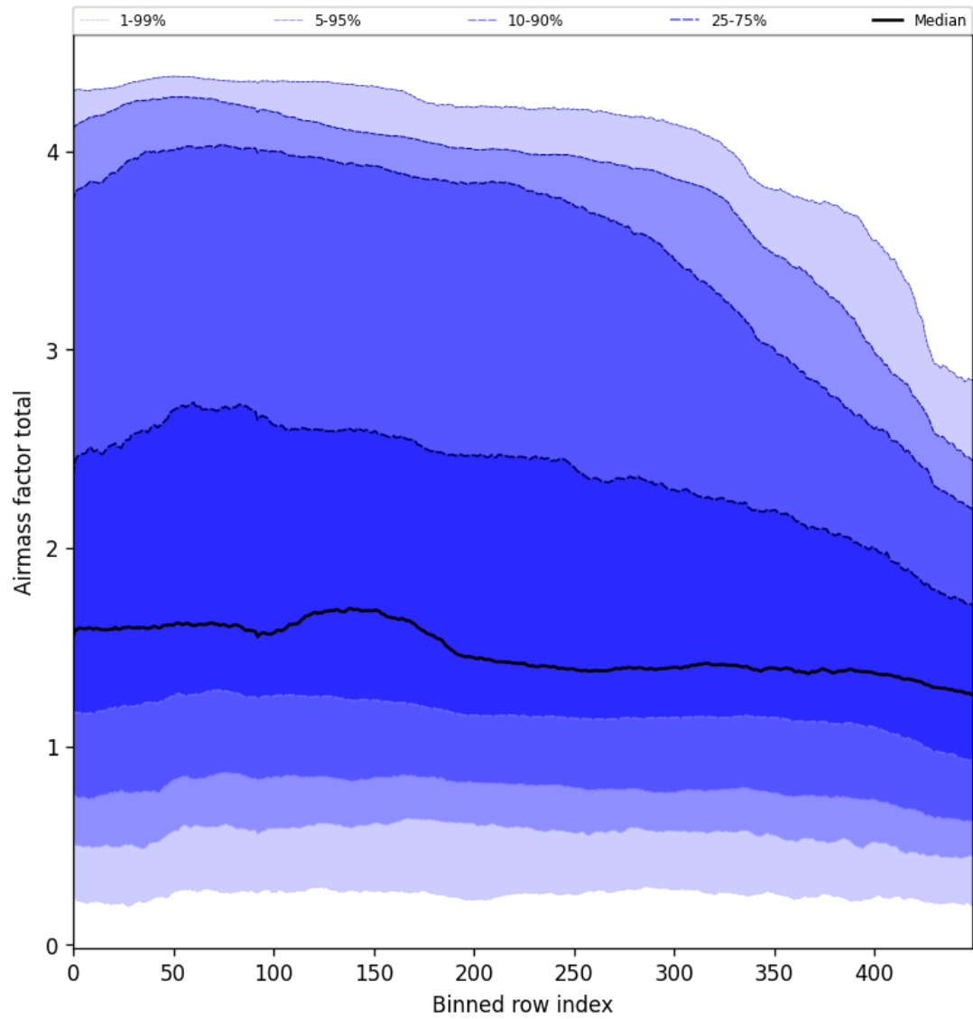
Figure 54: Along track statistics of “Airmass factor total” for 2024-12-23 to 2024-12-25
