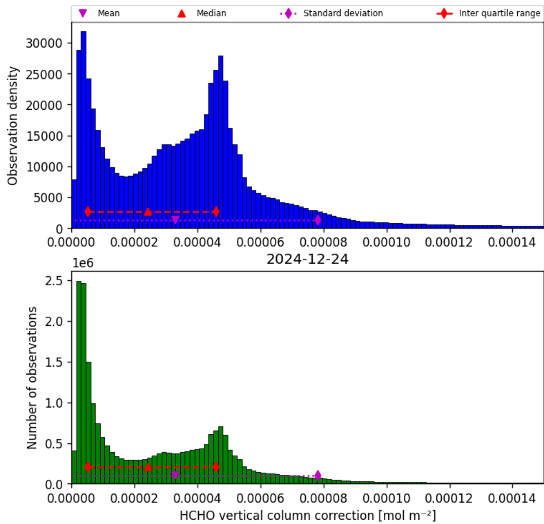
Figure 37: Histogram of “HCHO vertical column correction” for 2024-12-23 to 2024-12-25
