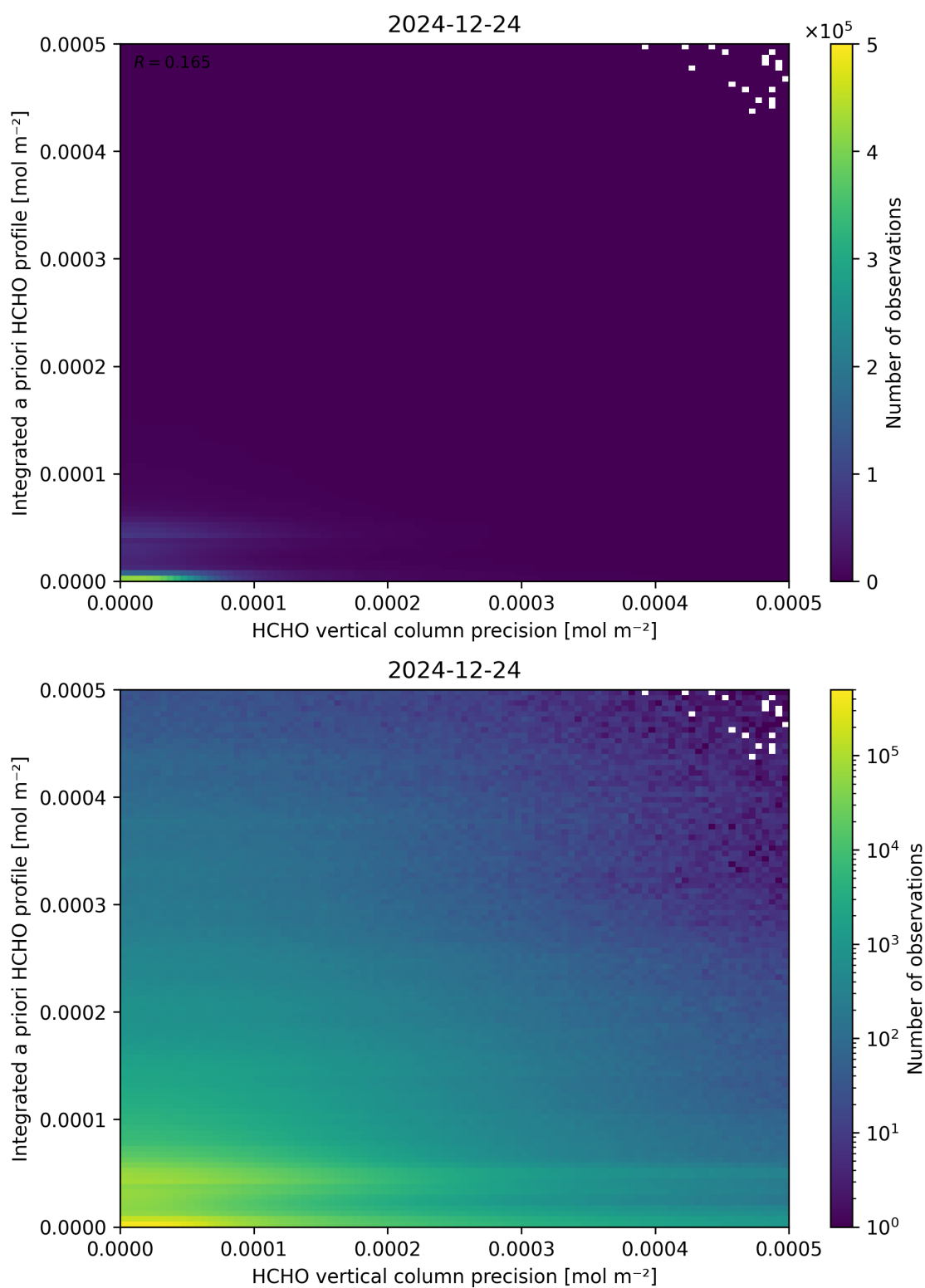
Figure 147: Scatter density plot of “HCHO vertical column precision” against “Integrated a priori HCHO profile” for 2024-12-23 to 2024-12-25.
