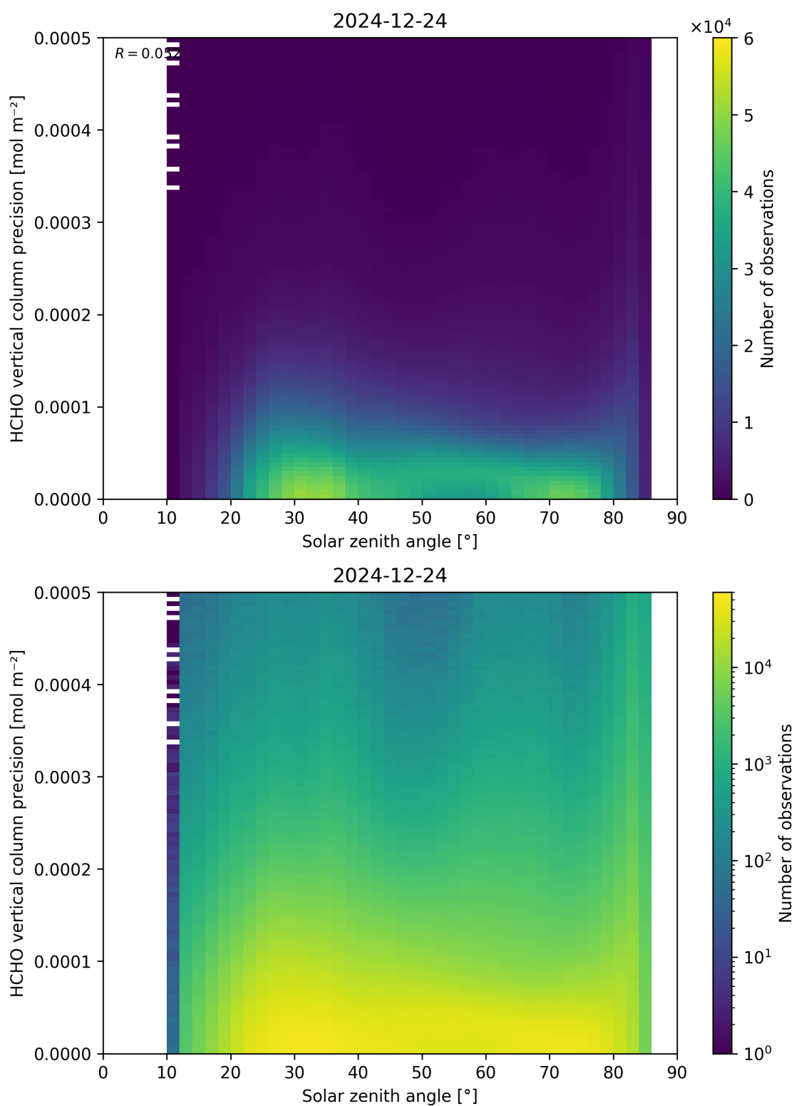
Figure 179: Scatter density plot of “Solar zenith angle” against “HCHO vertical column precision” for 2024-12-23 to 2024-12-25.
