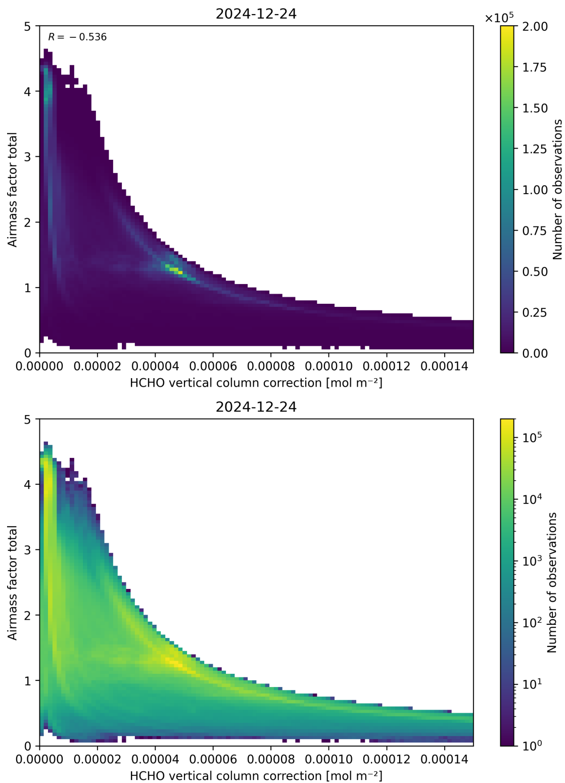
Figure 120: Scatter density plot of “HCHO vertical column correction” against “Airmass factor total” for 2024-12-23 to 2024-12-25.
