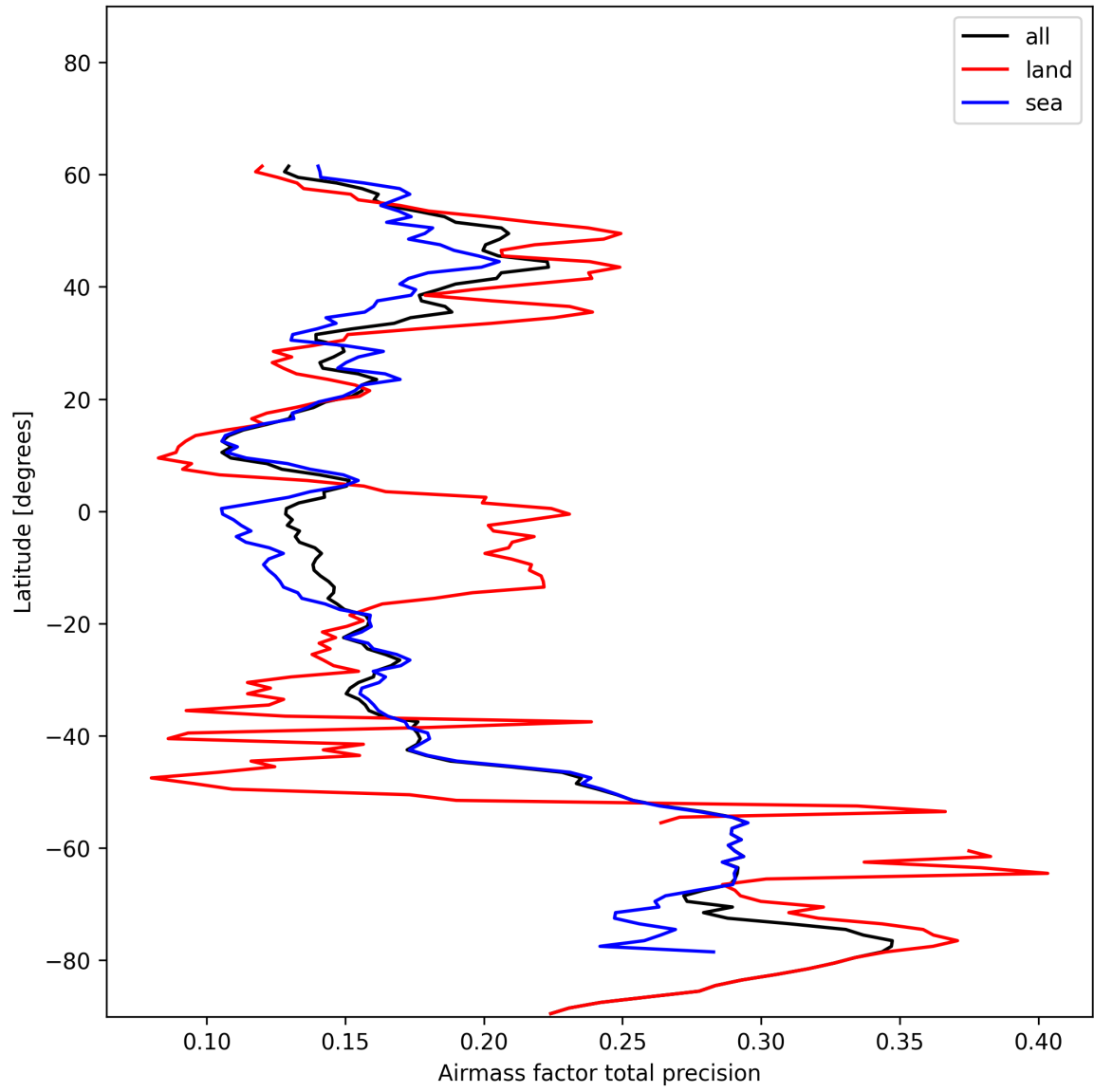
Figure 27: Zonal average of “Airmass factor total precision” for 2024-12-23 to 2024-12-25.
