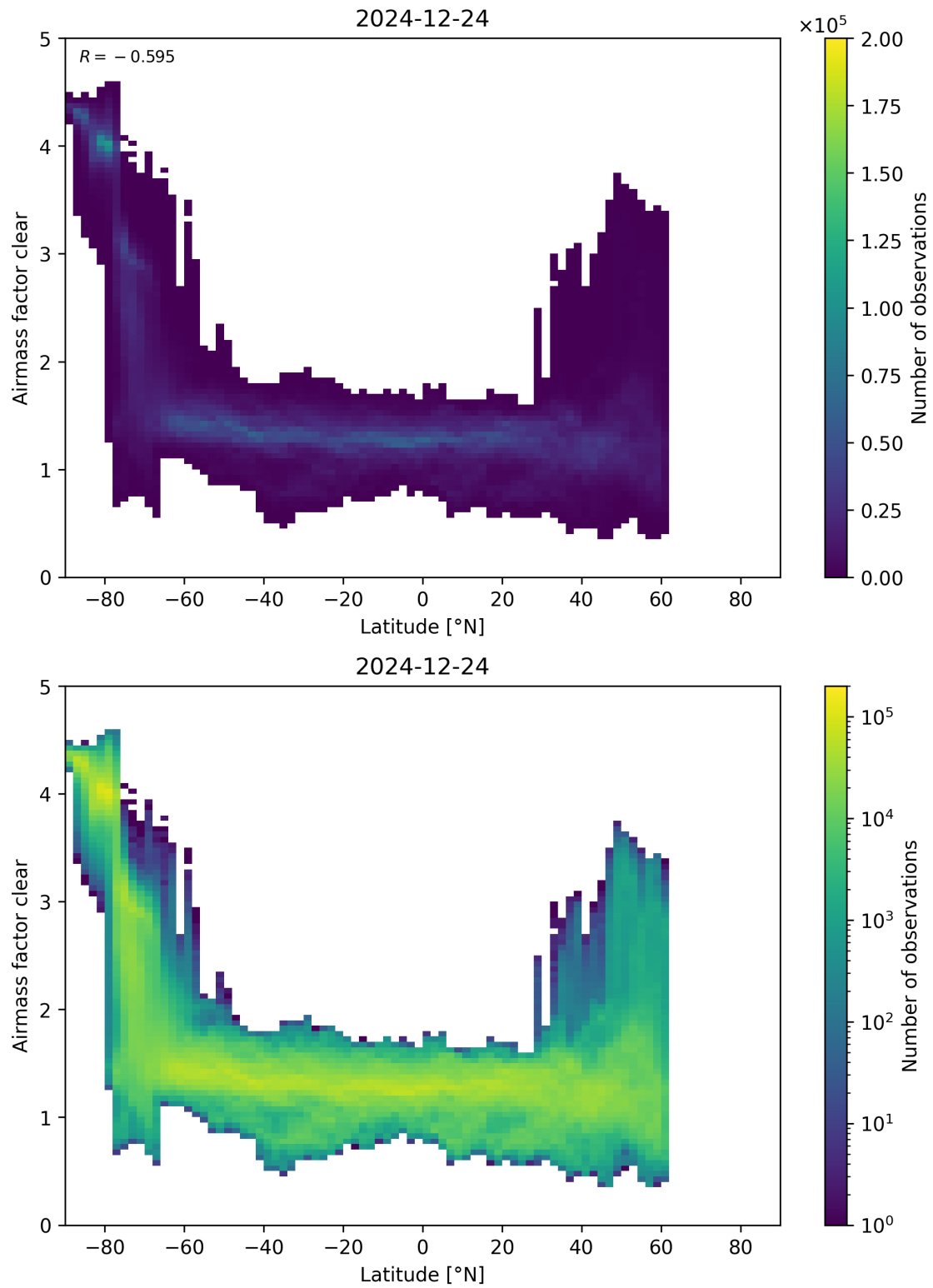
Figure 156: Scatter density plot of “Latitude” against “Airmass factor clear” for 2024-12-23 to 2024-12-25.
