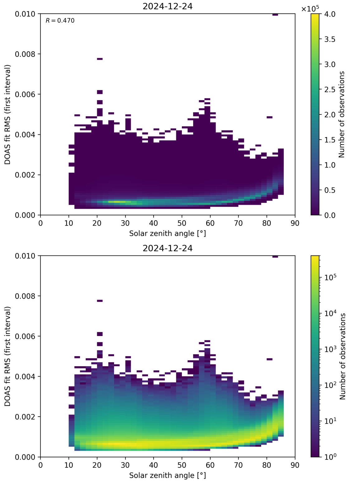
Figure 167: Scatter density plot of “Solar zenith angle” against “DOAS fit RMS (first interval)” for 2024-12-23 to 2024-12-25.
