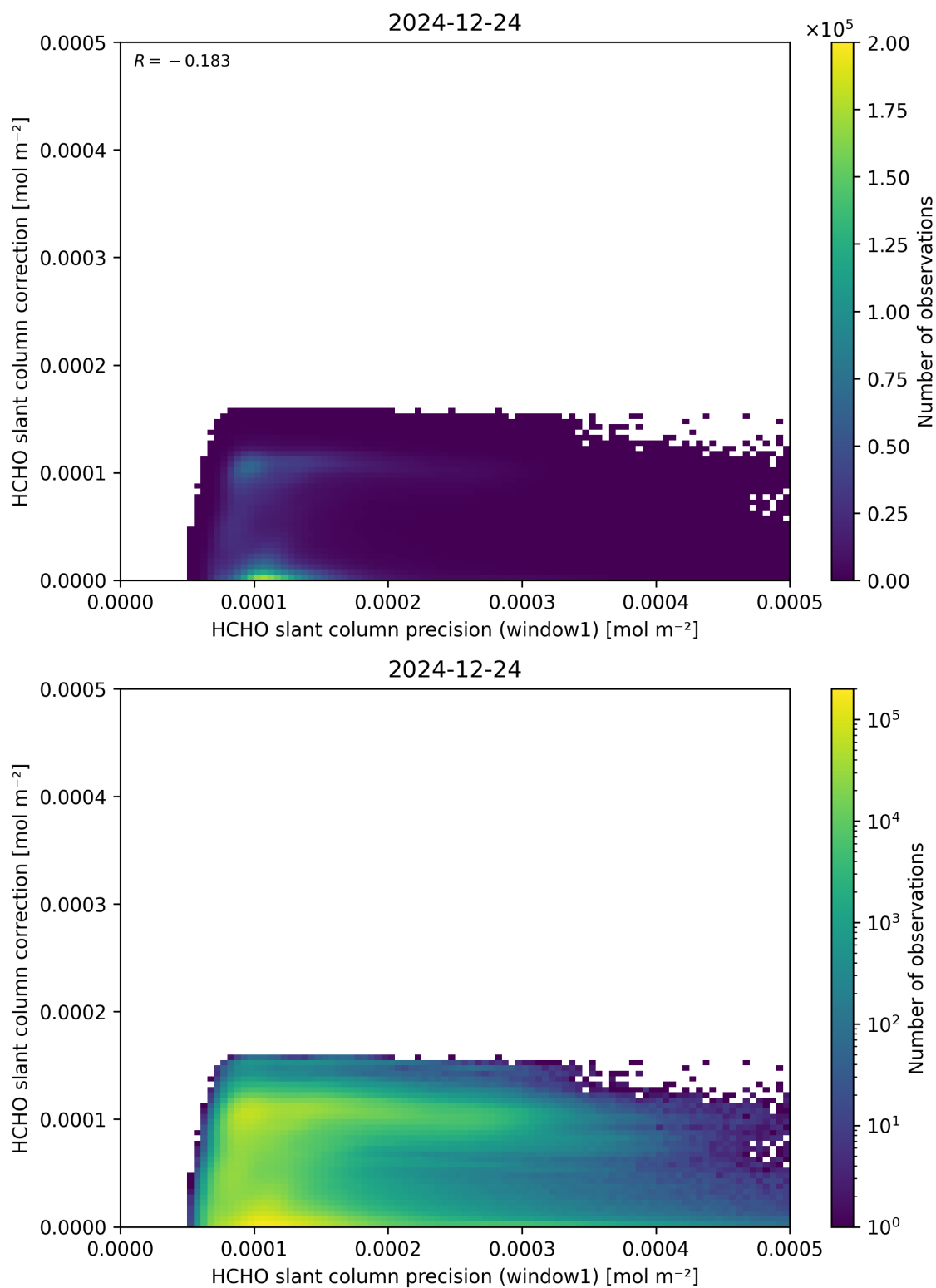
Figure 93: Scatter density plot of “HCHO slant column precision (window1)” against “HCHO slant column correction” for 2024-12-23 to 2024-12-25.
