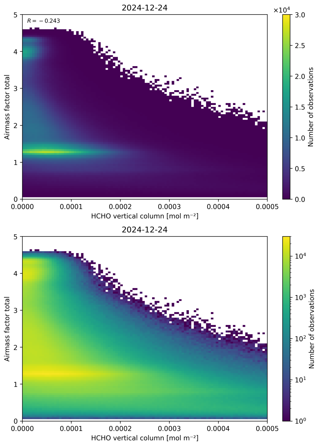
Figure 131: Scatter density plot of “HCHO vertical column” against “Airmass factor total” for 2024-12-23 to 2024-12-25.
