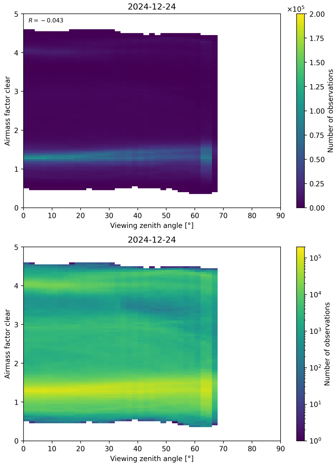
Figure 185: Scatter density plot of “Viewing zenith angle” against “Airmass factor clear” for 2024-12-23 to 2024-12-25.
