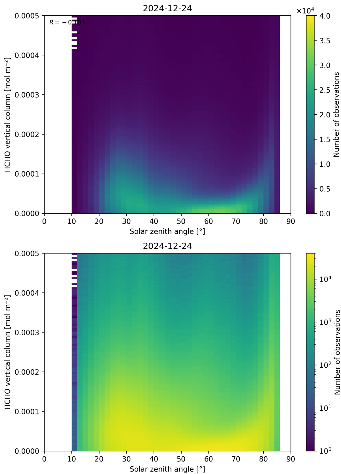
Figure 177: Scatter density plot of “Solar zenith angle” against “HCHO vertical column” for 2024-12-23 to 2024-12-25.
