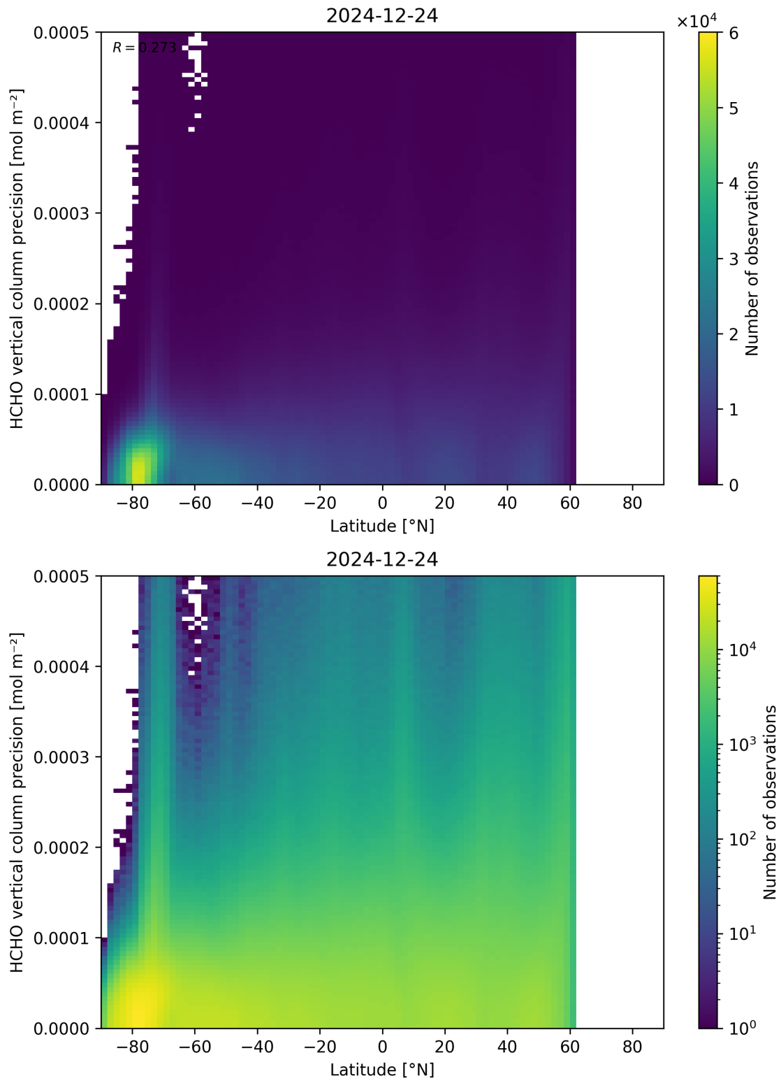
Figure 165: Scatter density plot of “Latitude” against “HCHO vertical column precision” for 2024-12-23 to 2024-12-25.
