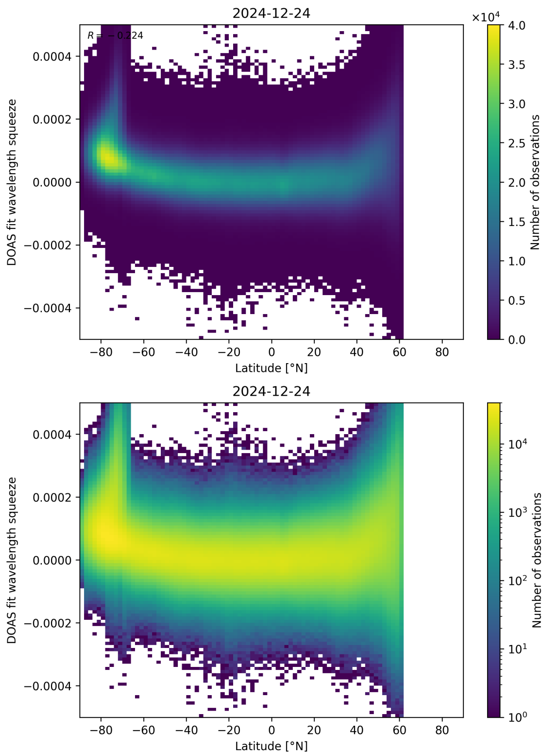
Figure 155: Scatter density plot of “Latitude” against “DOAS fit wavelength squeeze” for 2024-12-23 to 2024-12-25.
