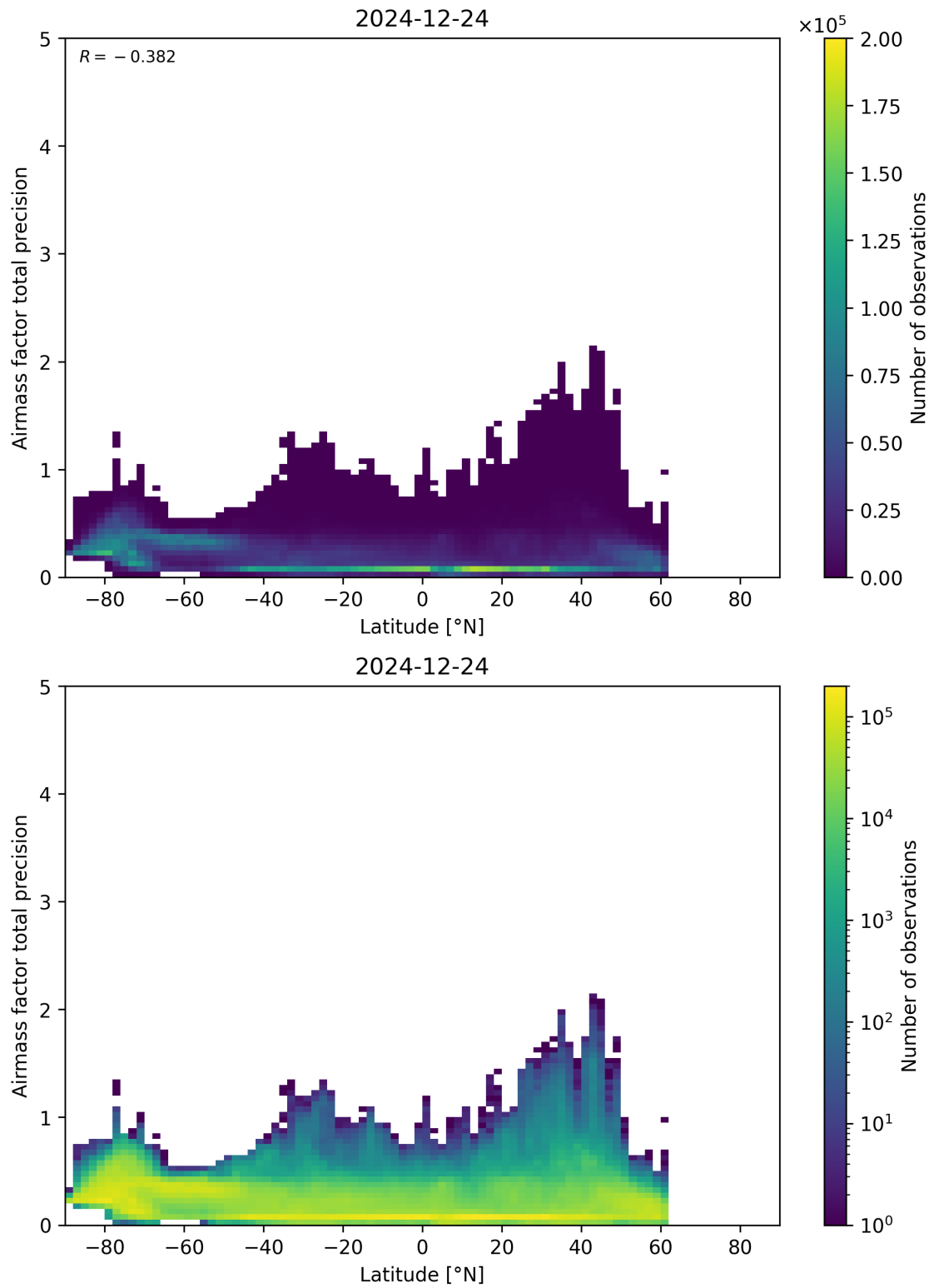
Figure 162: Scatter density plot of “Latitude” against “Airmass factor total precision” for 2024-12-23 to 2024-12-25.
