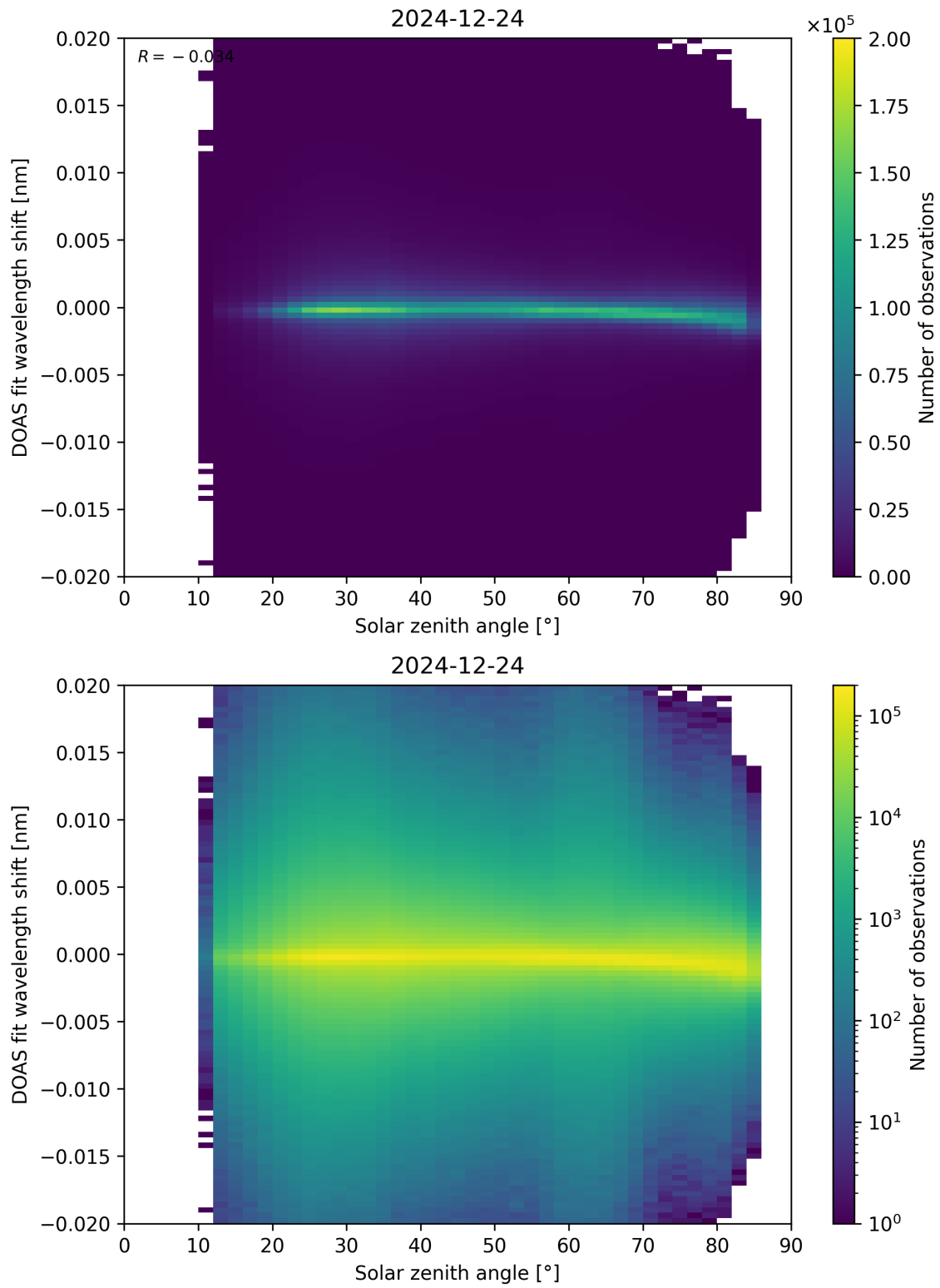
Figure 168: Scatter density plot of “Solar zenith angle” against “DOAS fit wavelength shift” for 2024-12-23 to 2024-12-25.
