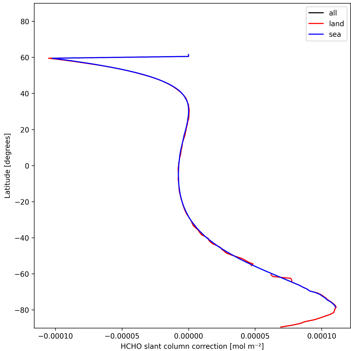
Figure 33: Zonal average of “HCHO slant column correction” for 2024-12-23 to 2024-12-25.
