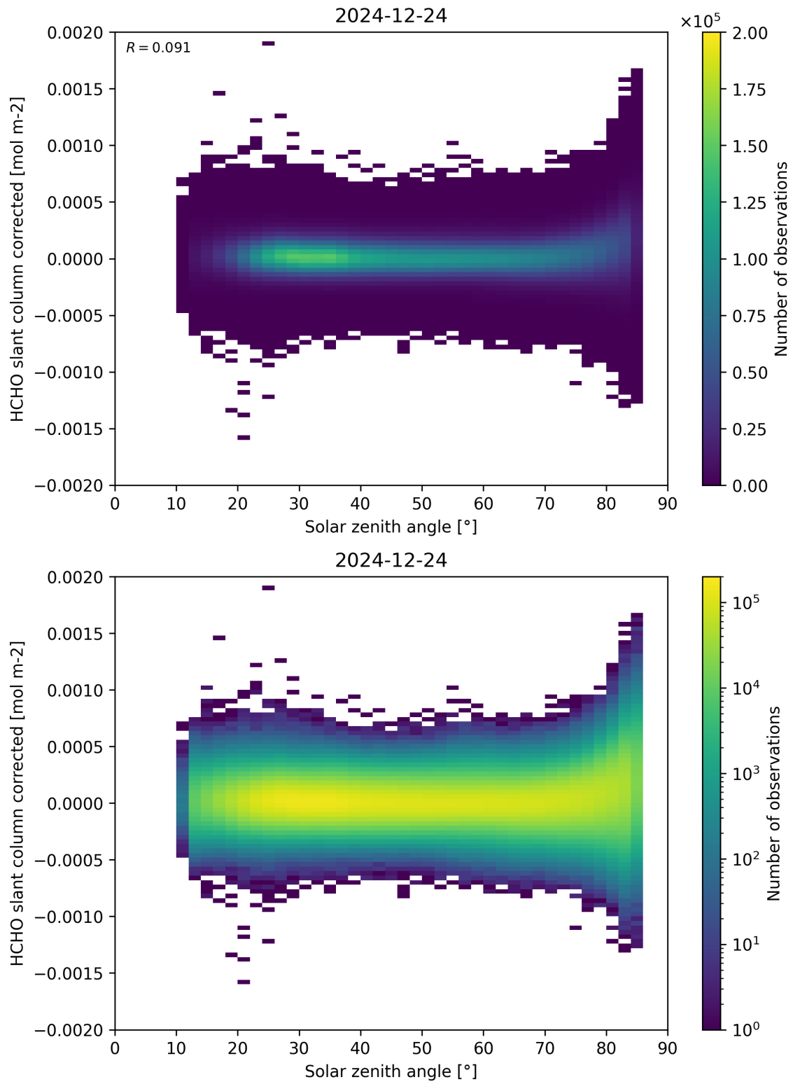
Figure 171: Scatter density plot of “Solar zenith angle” against “HCHO slant column corrected” for 2024-12-23 to 2024-12-25.
