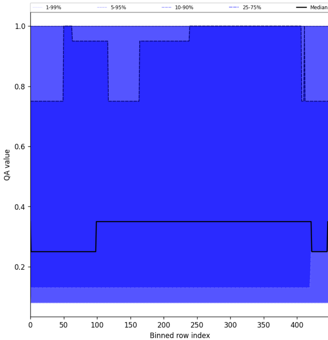
Figure 48: Along track statistics of “QA value” for 2024-12-23 to 2024-12-25
