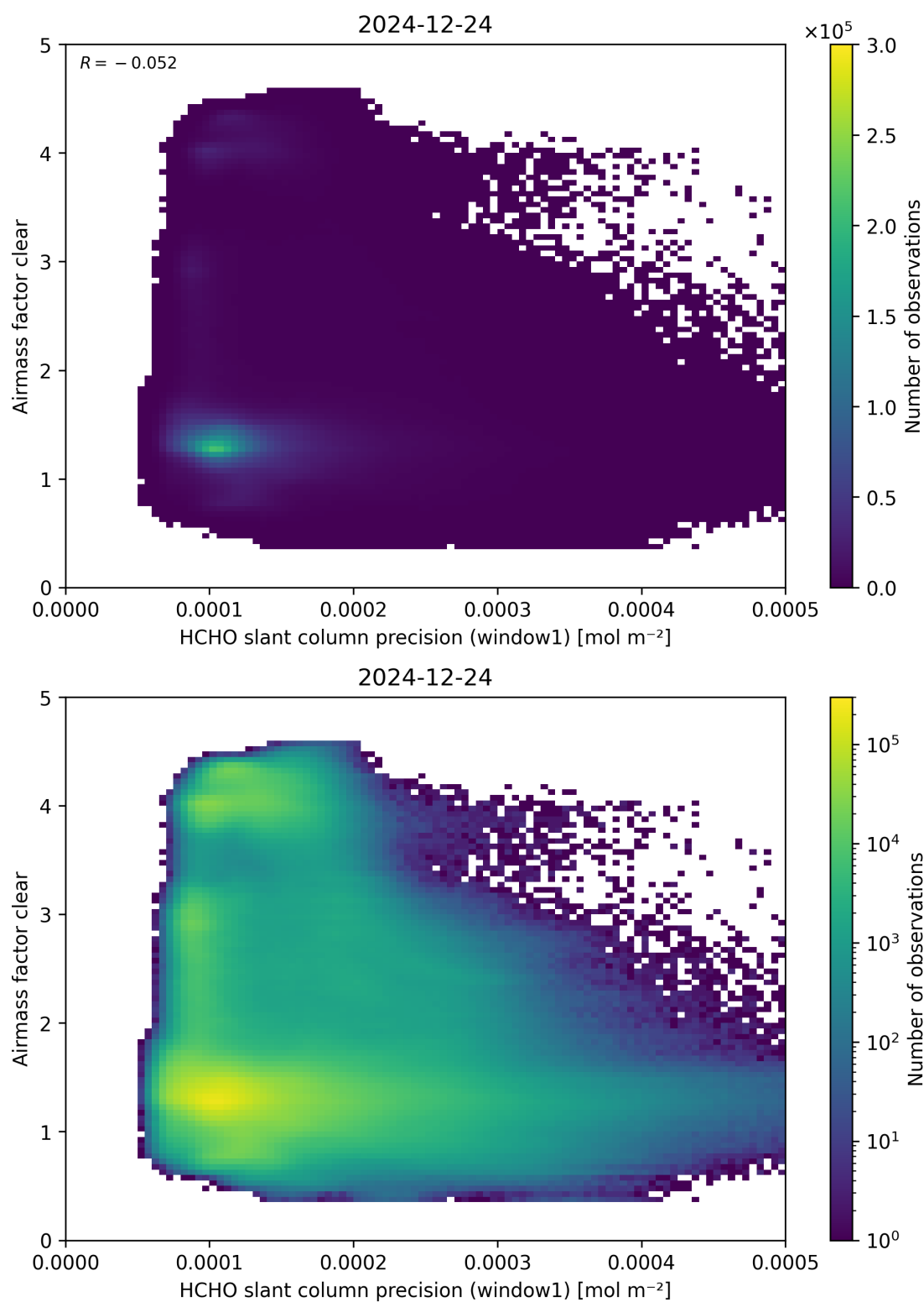
Figure 91: Scatter density plot of “HCHO slant column precision (window1)” against “Airmass factor clear” for 2024-12-23 to 2024-12-25.
