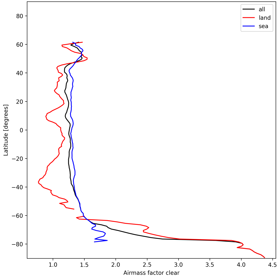
Figure 28: Zonal average of “Airmass factor clear” for 2024-12-23 to 2024-12-25.
