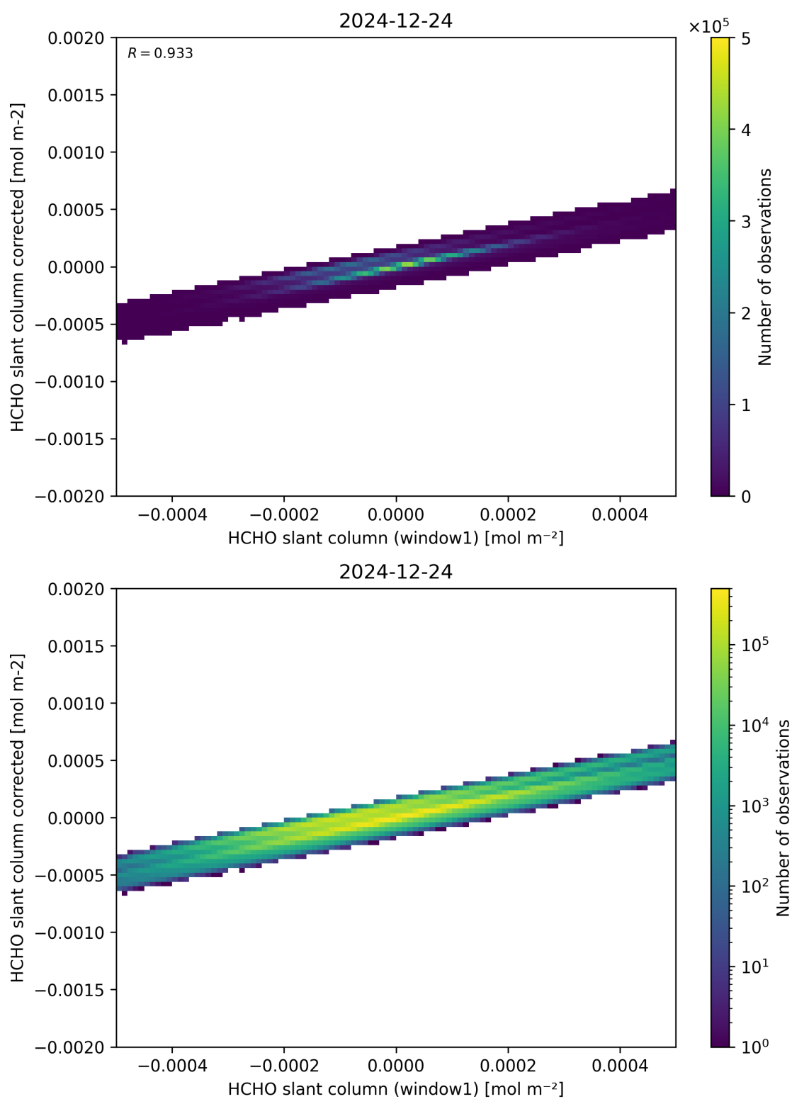
Figure 82: Scatter density plot of “HCHO slant column (window1)” against “HCHO slant column corrected” for 2024-12-23 to 2024-12-25.
