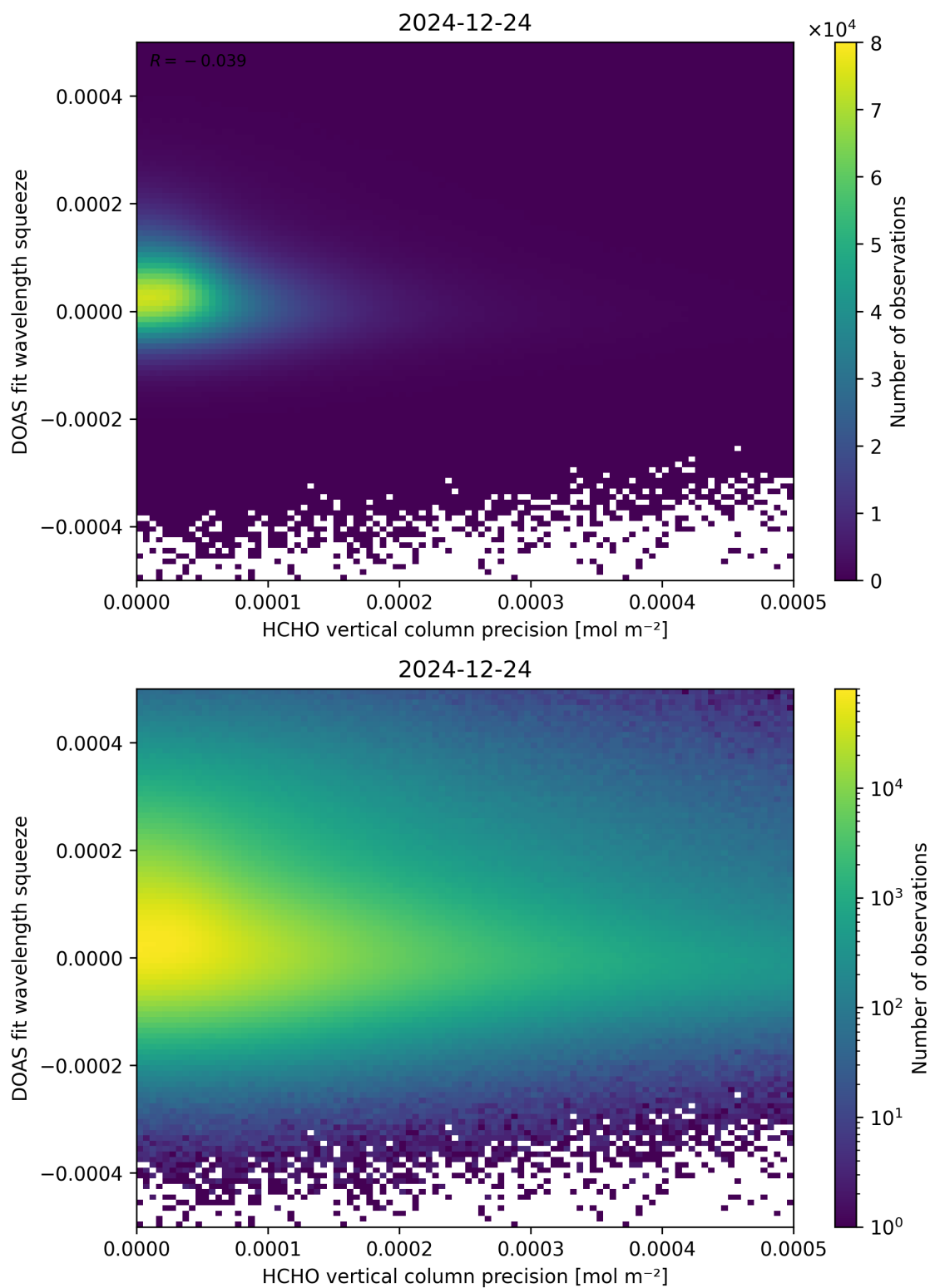
Figure 138: Scatter density plot of “HCHO vertical column precision” against “DOAS fit wavelength squeeze” for 2024-12-23 to 2024-12-25.
