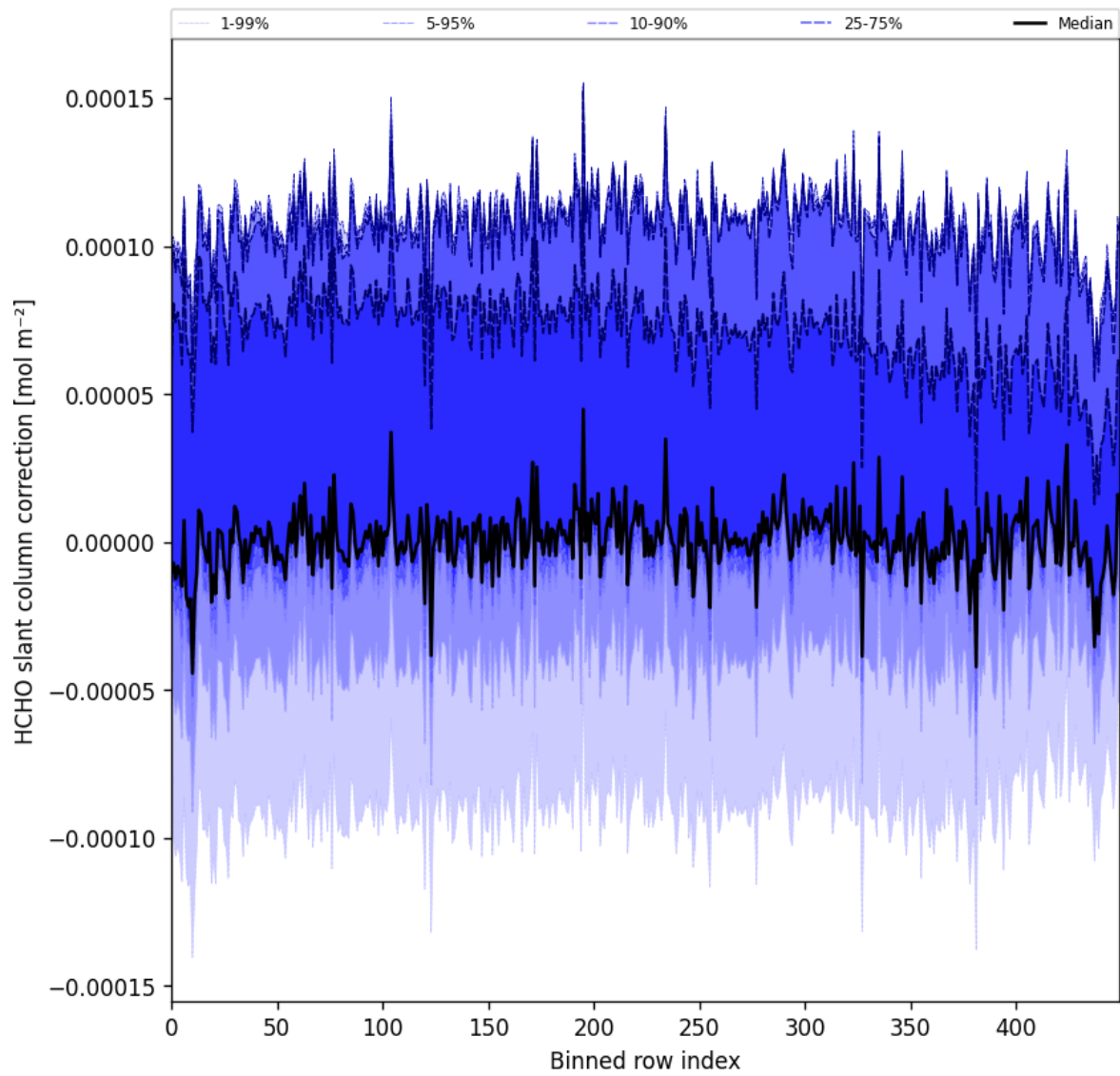
Figure 61: Along track statistics of “HCHO slant column correction” for 2024-12-23 to 2024-12-25
