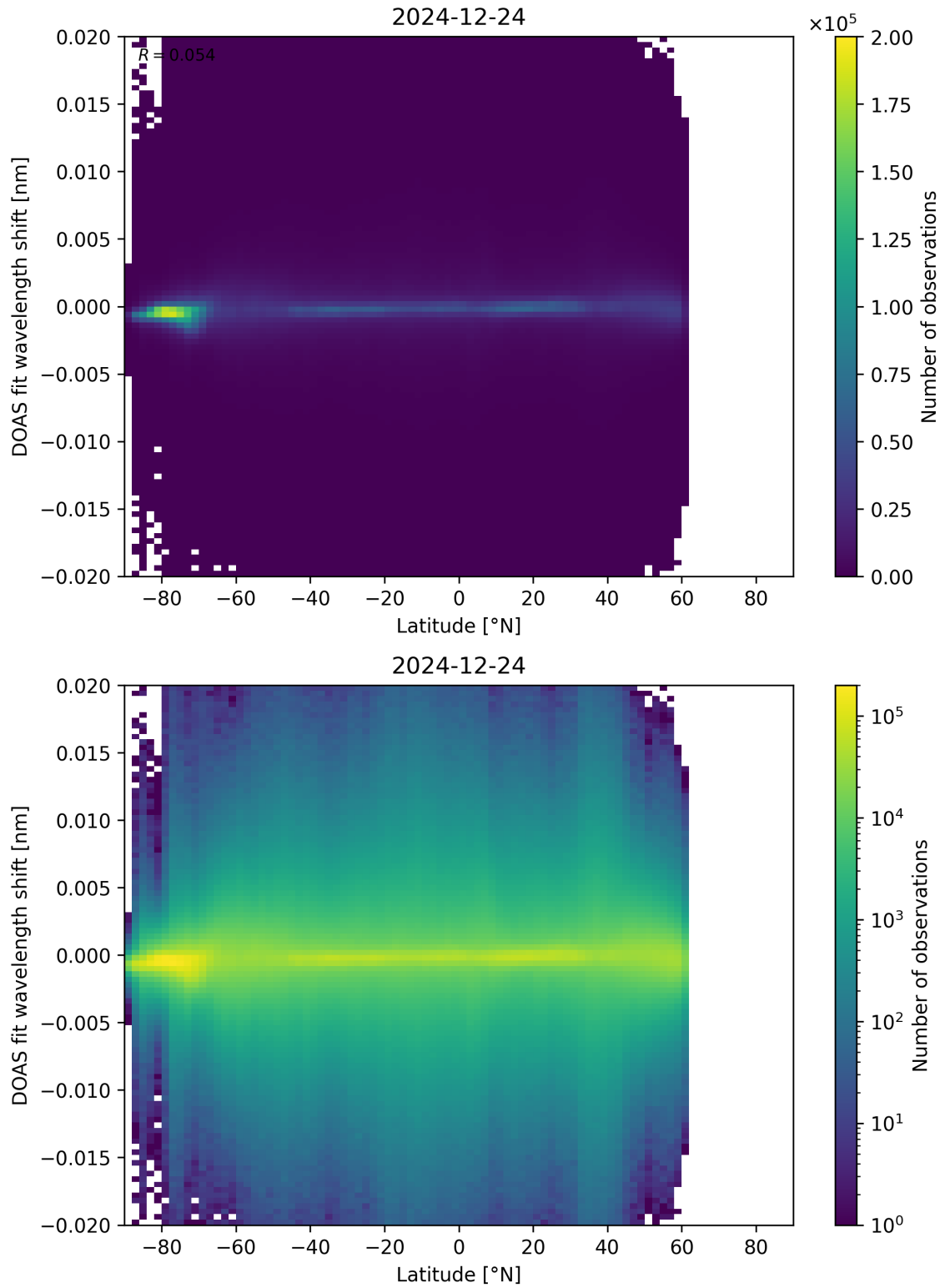
Figure 154: Scatter density plot of “Latitude” against “DOAS fit wavelength shift” for 2024-12-23 to 2024-12-25.
