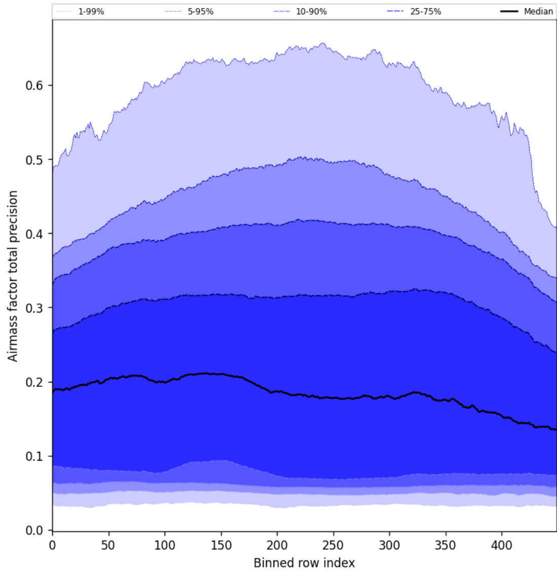
Figure 55: Along track statistics of “Airmass factor total precision” for 2024-12-23 to 2024-12-25
