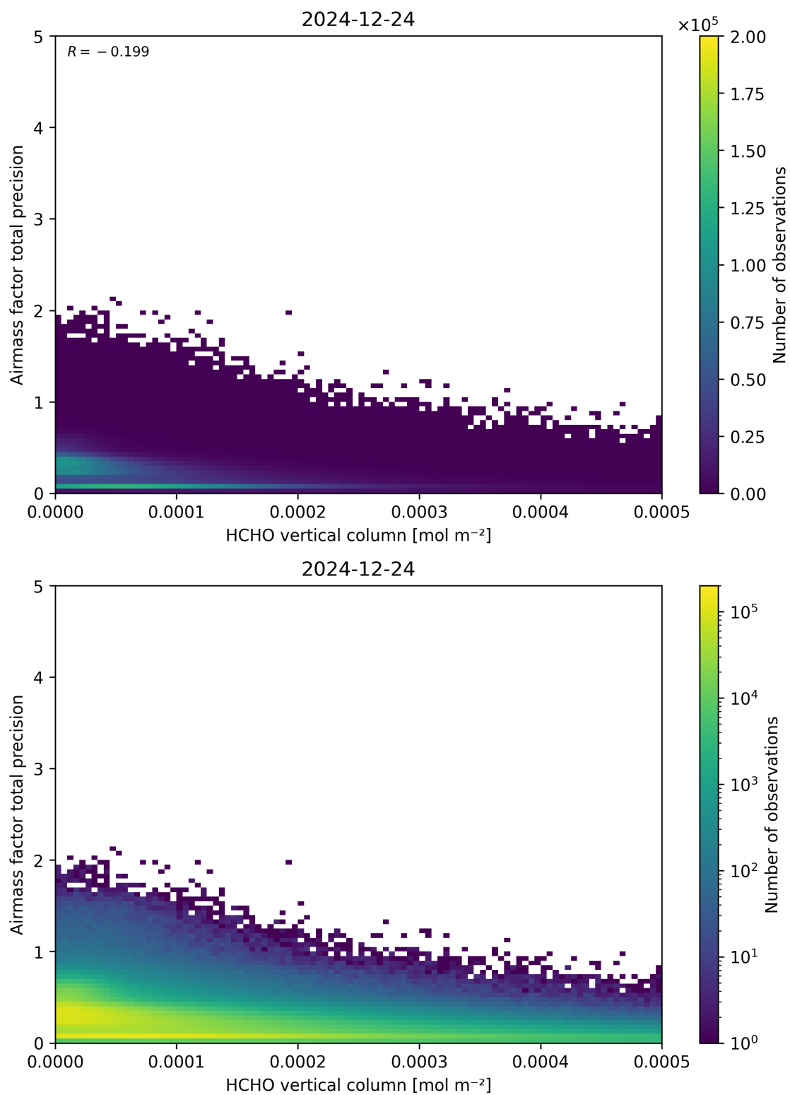
Figure 132: Scatter density plot of “HCHO vertical column” against “Airmass factor total precision” for 2024-12-23 to 2024-12-25.
