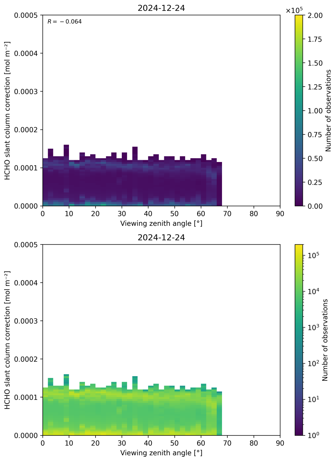
Figure 187: Scatter density plot of “Viewing zenith angle” against “HCHO slant column correction” for 2024-12-23 to 2024-12-25.
