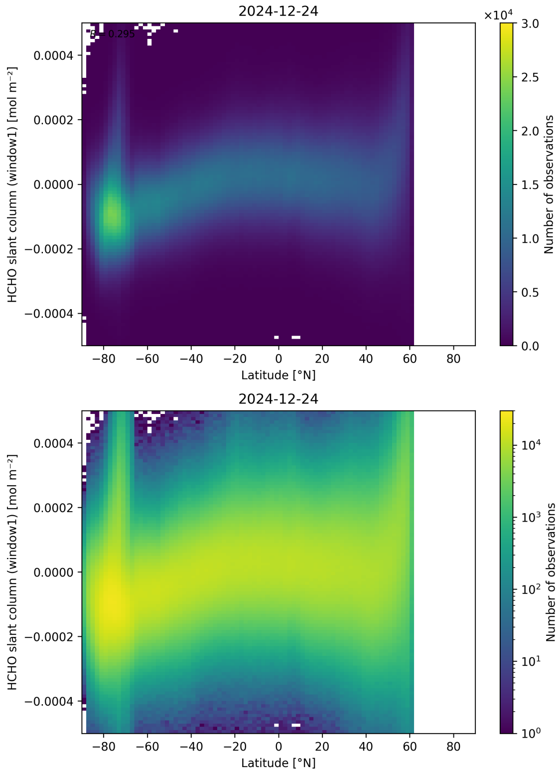
Figure 159: Scatter density plot of “Latitude” against “HCHO slant column (window1)” for 2024-12-23 to 2024-12-25.
