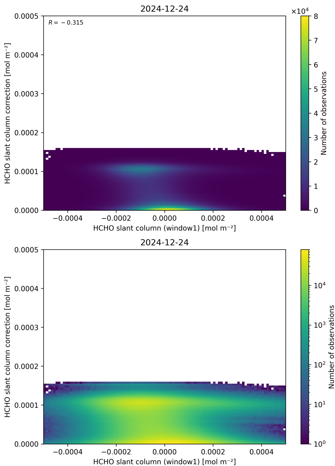
Figure 83: Scatter density plot of “HCHO slant column (window1)” against “HCHO slant column correction” for 2024-12-23 to 2024-12-25.
