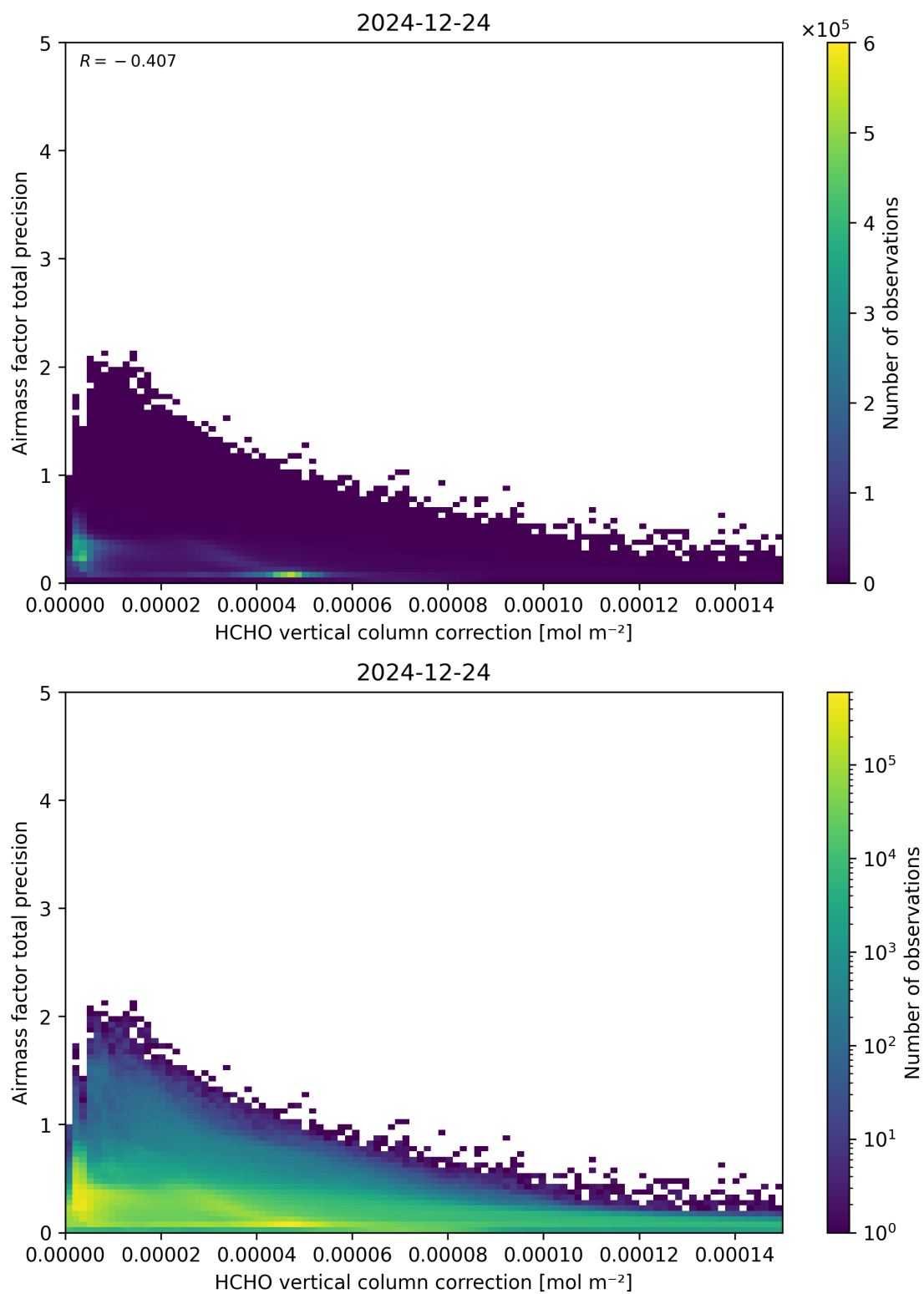
Figure 121: Scatter density plot of “HCHO vertical column correction” against “Airmass factor total precision” for 2024-12-23 to 2024-12-25.
