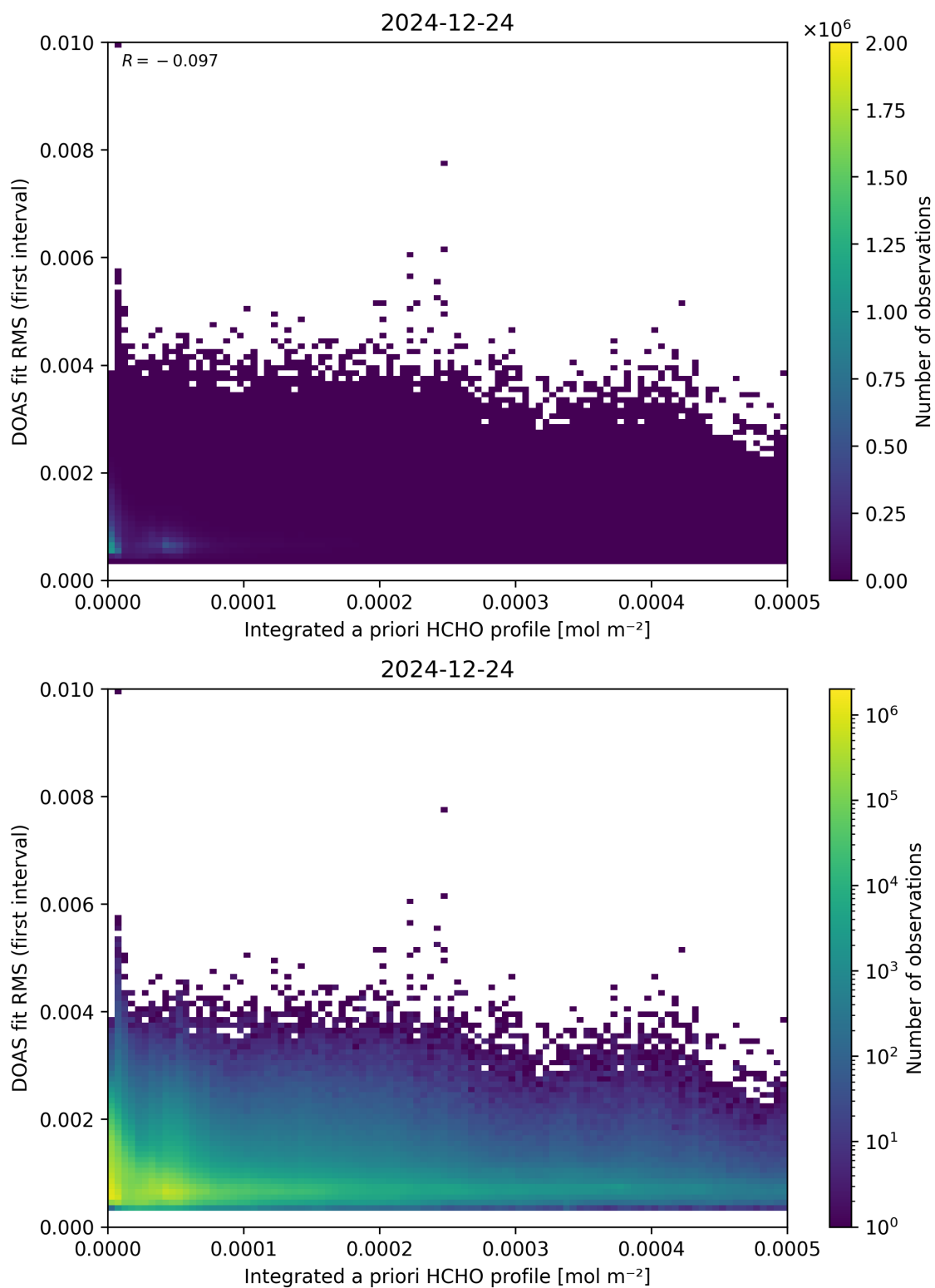
Figure 148: Scatter density plot of “Integrated a priori HCHO profile” against “DOAS fit RMS (first interval)” for 2024-12-23 to 2024-12-25.
