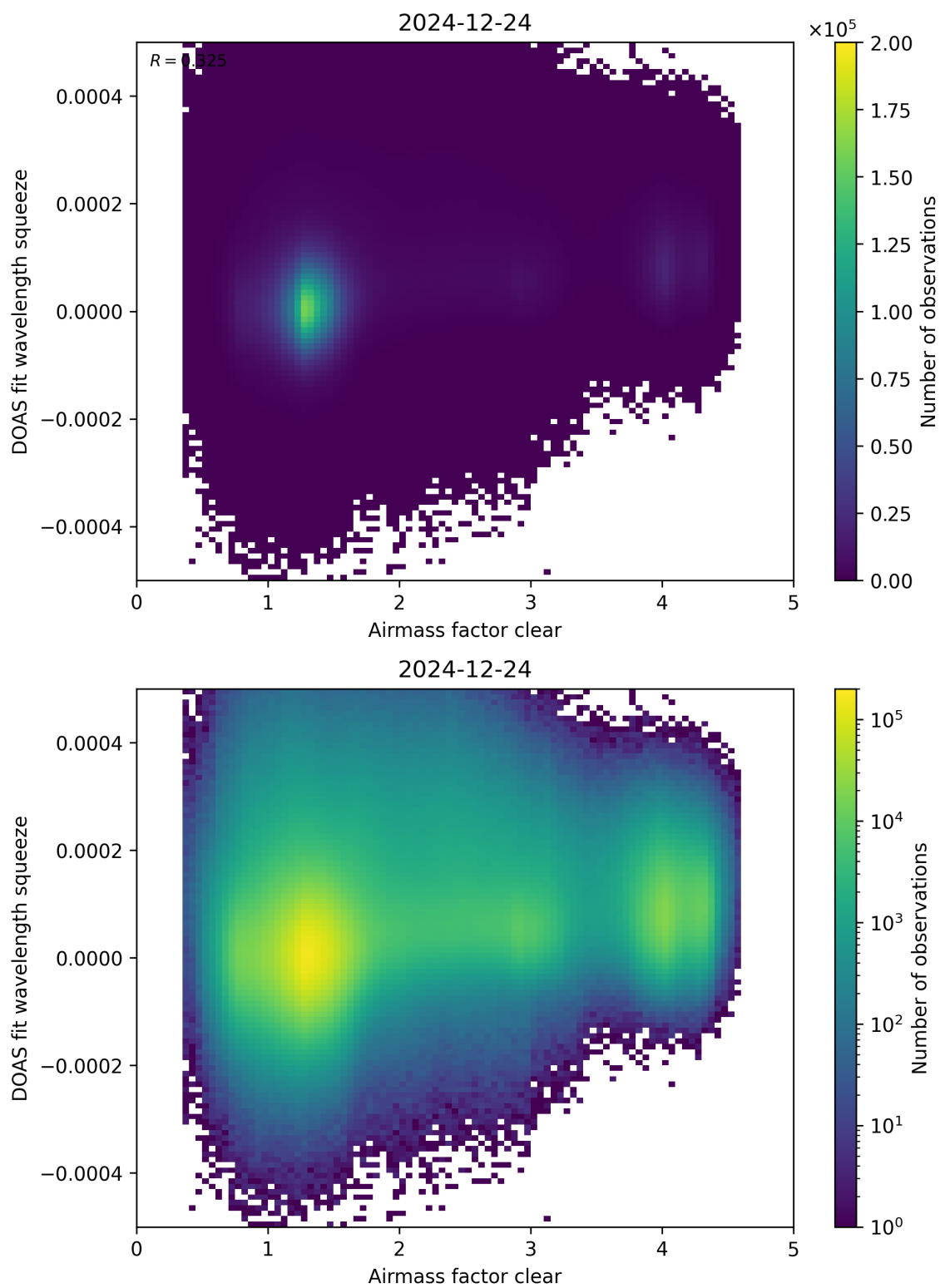
Figure 73: Scatter density plot of “Airmass factor clear” against “DOAS fit wavelength squeeze” for 2024-12-23 to 2024-12-25.
