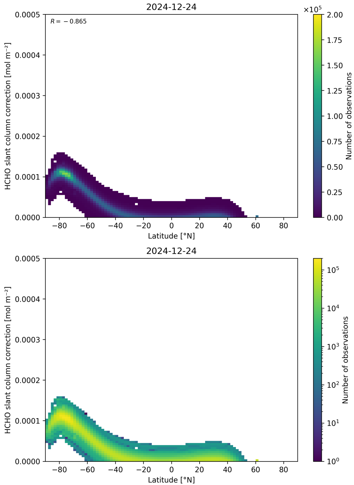
Figure 158: Scatter density plot of “Latitude” against “HCHO slant column correction” for 2024-12-23 to 2024-12-25.
