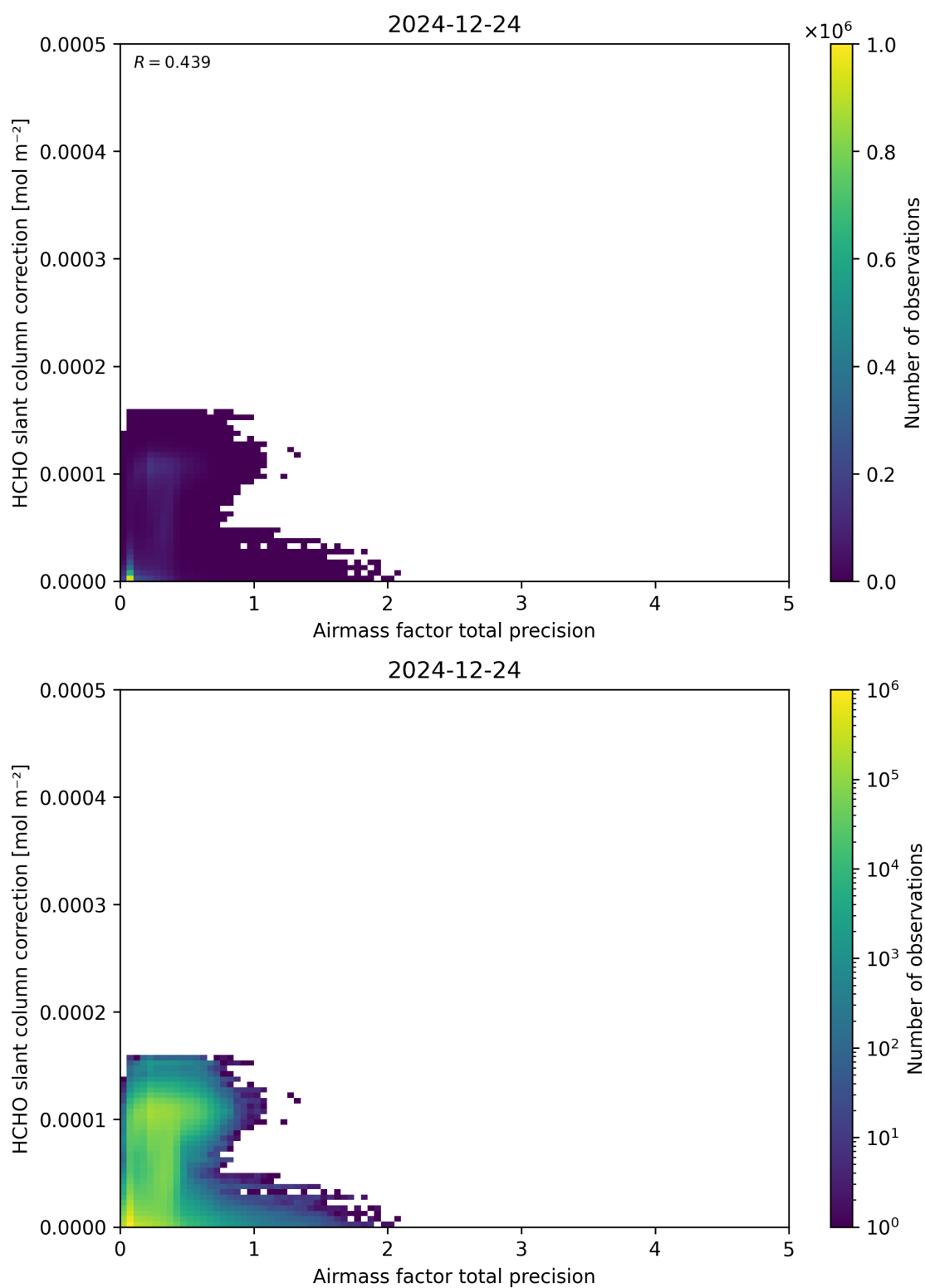
Figure 110: Scatter density plot of “Airmass factor total precision” against “HCHO slant column correction” for 2024-12-23 to 2024-12-25.
