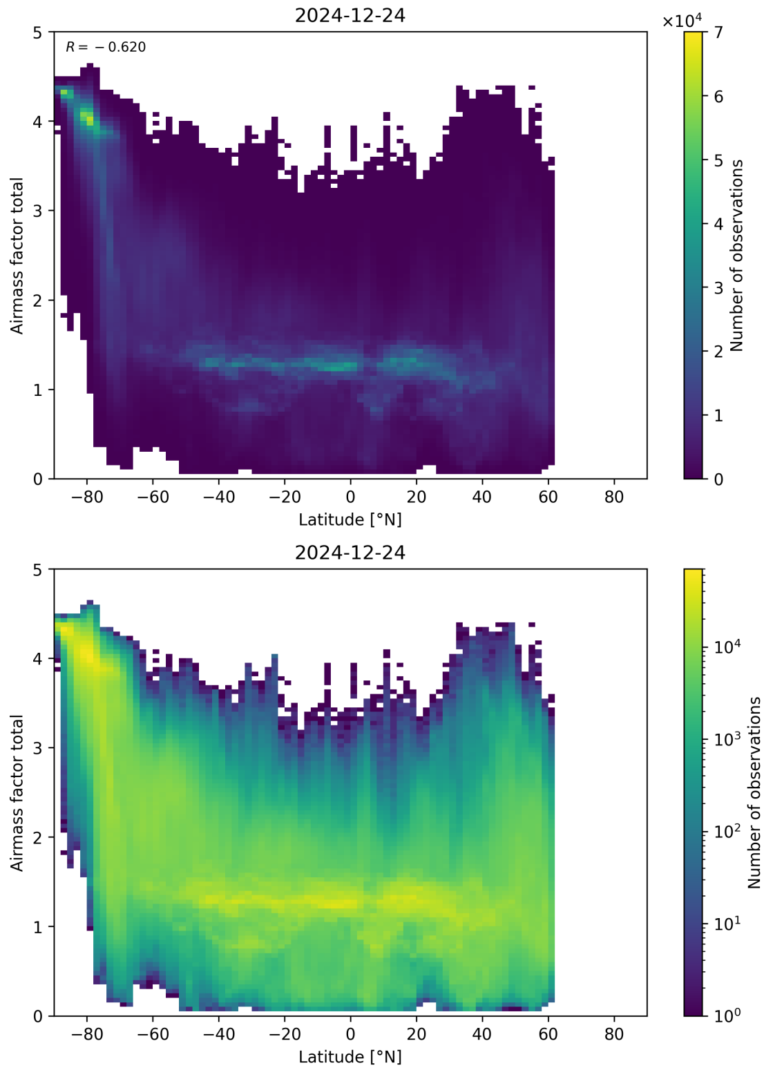
Figure 161: Scatter density plot of “Latitude” against “Airmass factor total” for 2024-12-23 to 2024-12-25.
