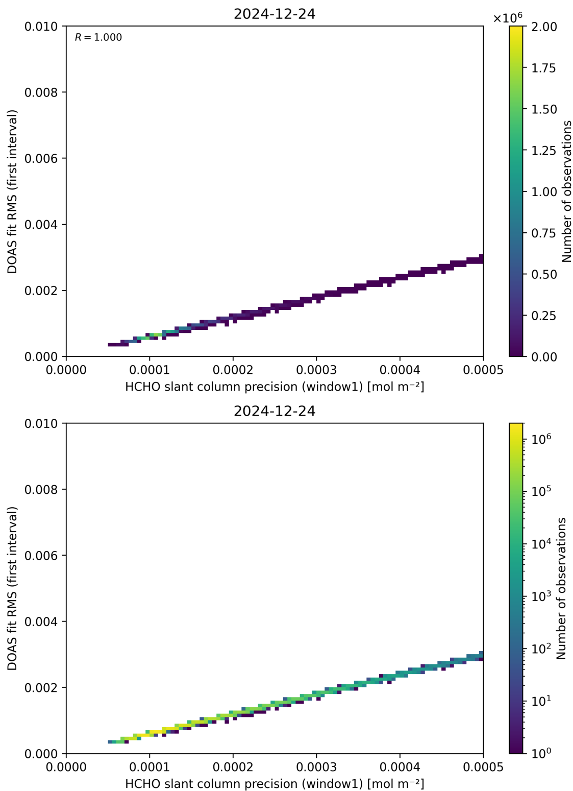
Figure 88: Scatter density plot of “HCHO slant column precision (window1)” against “DOAS fit RMS (first interval)” for 2024-12-23 to 2024-12-25.
