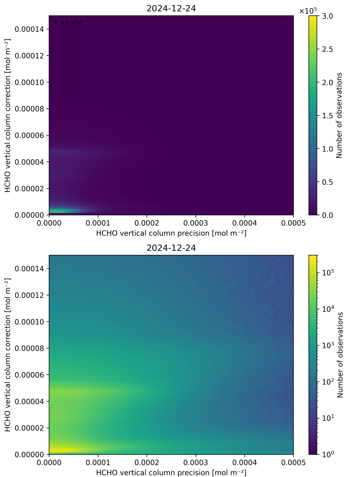
Figure 146: Scatter density plot of “HCHO vertical column precision” against “HCHO vertical column correction” for 2024-12-23 to 2024-12-25.
