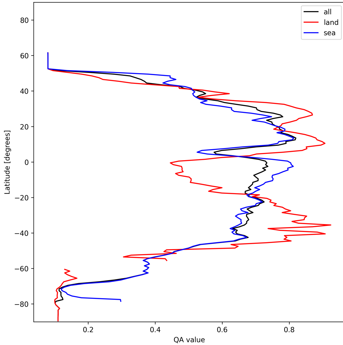
Figure 20: Zonal average of “QA value” for 2024-12-23 to 2024-12-25.
