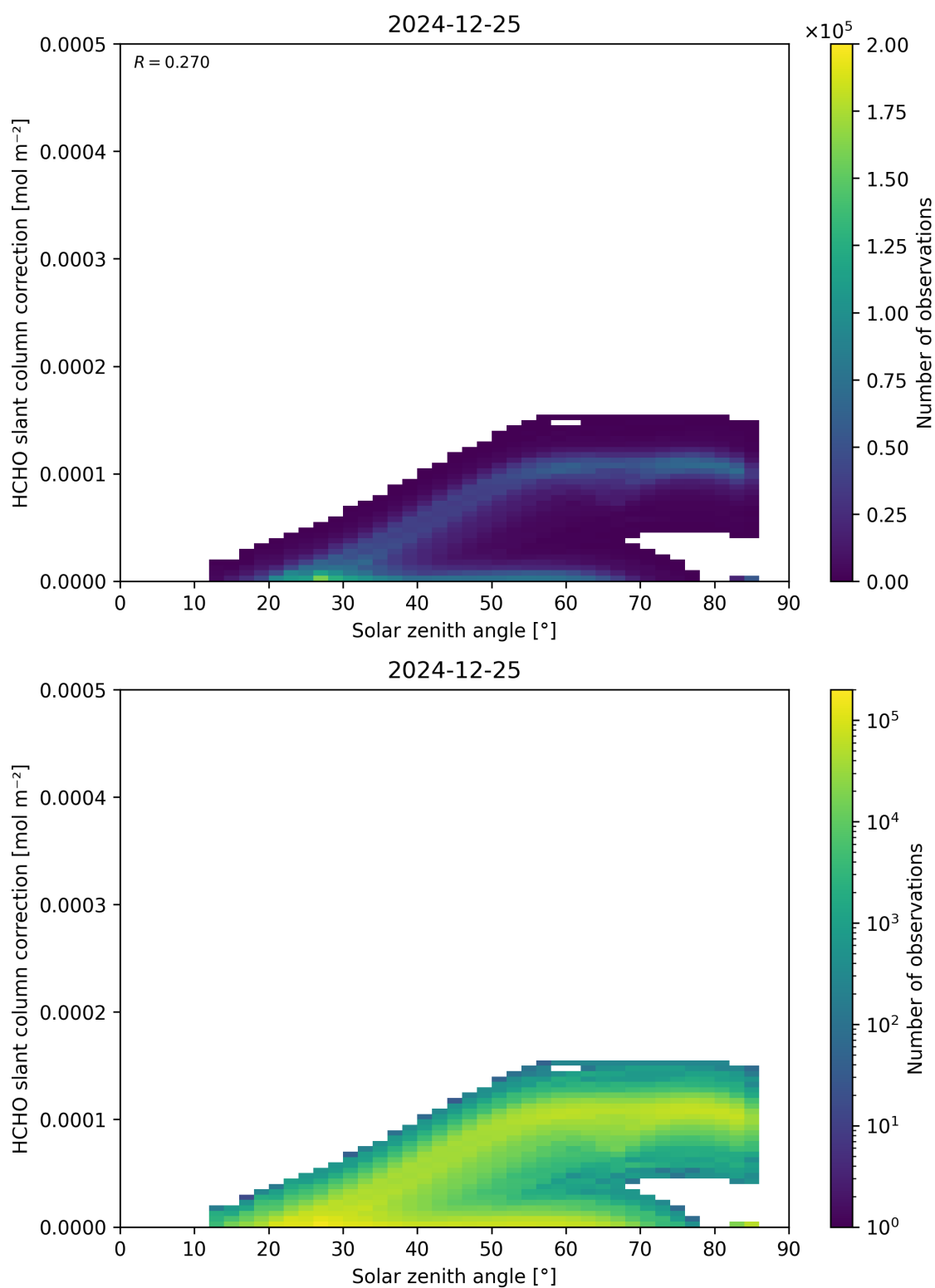
Figure 172: Scatter density plot of “Solar zenith angle” against “HCHO slant column correction” for 2024-12-24 to 2024-12-26.
