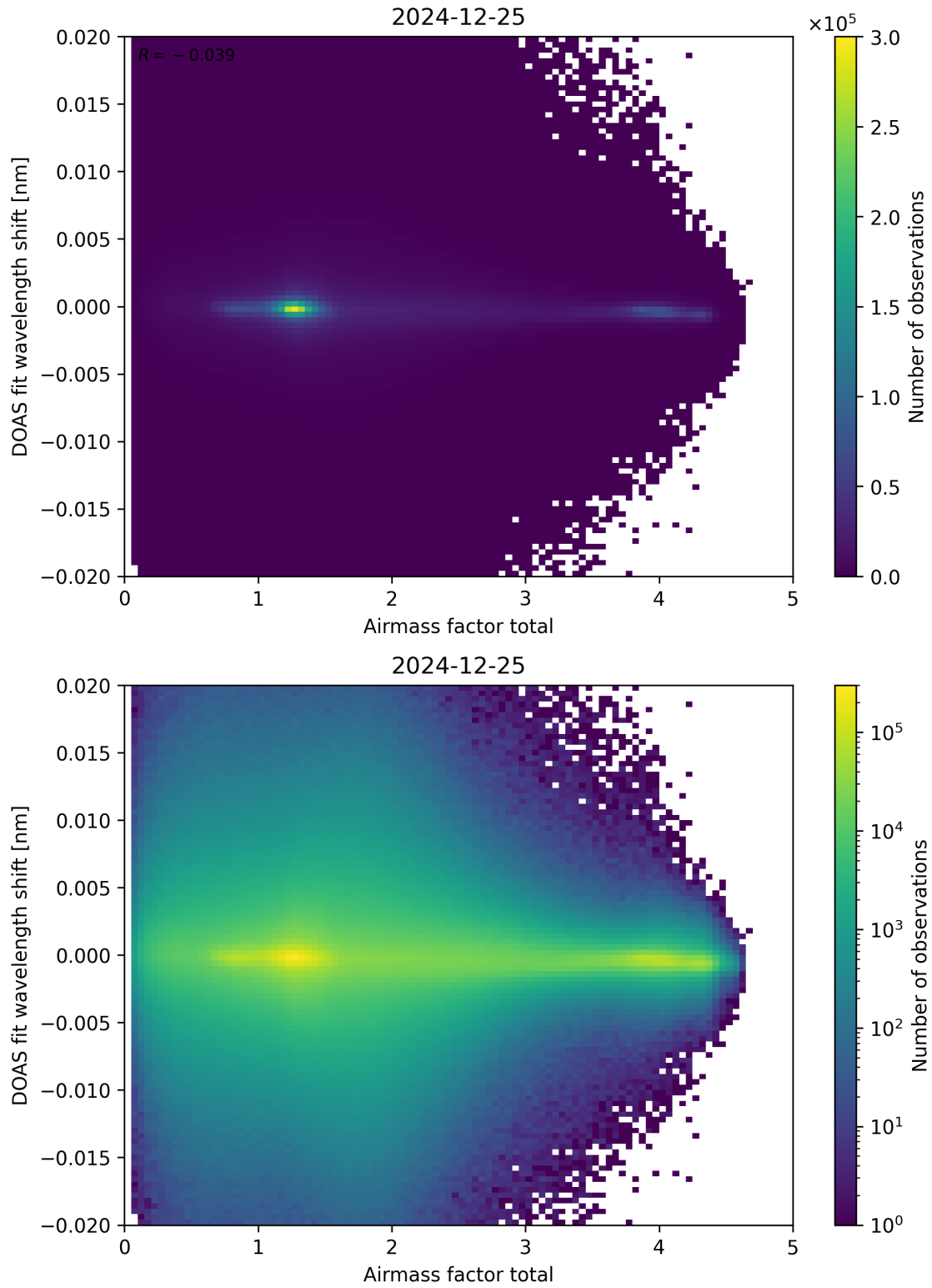
Figure 98: Scatter density plot of “Airmass factor total” against “DOAS fit wavelength shift” for 2024-12-24 to 2024-12-26.
