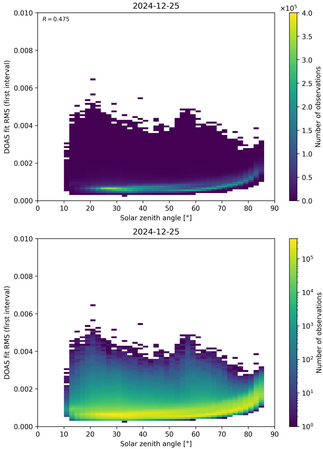
Figure 167: Scatter density plot of “Solar zenith angle” against “DOAS fit RMS (first interval)” for 2024-12-24 to 2024-12-26.
