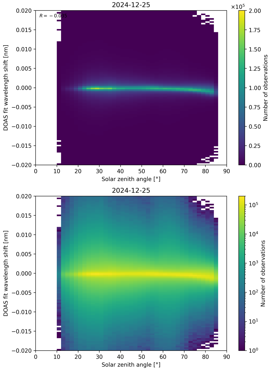
Figure 168: Scatter density plot of “Solar zenith angle” against “DOAS fit wavelength shift” for 2024-12-24 to 2024-12-26.
