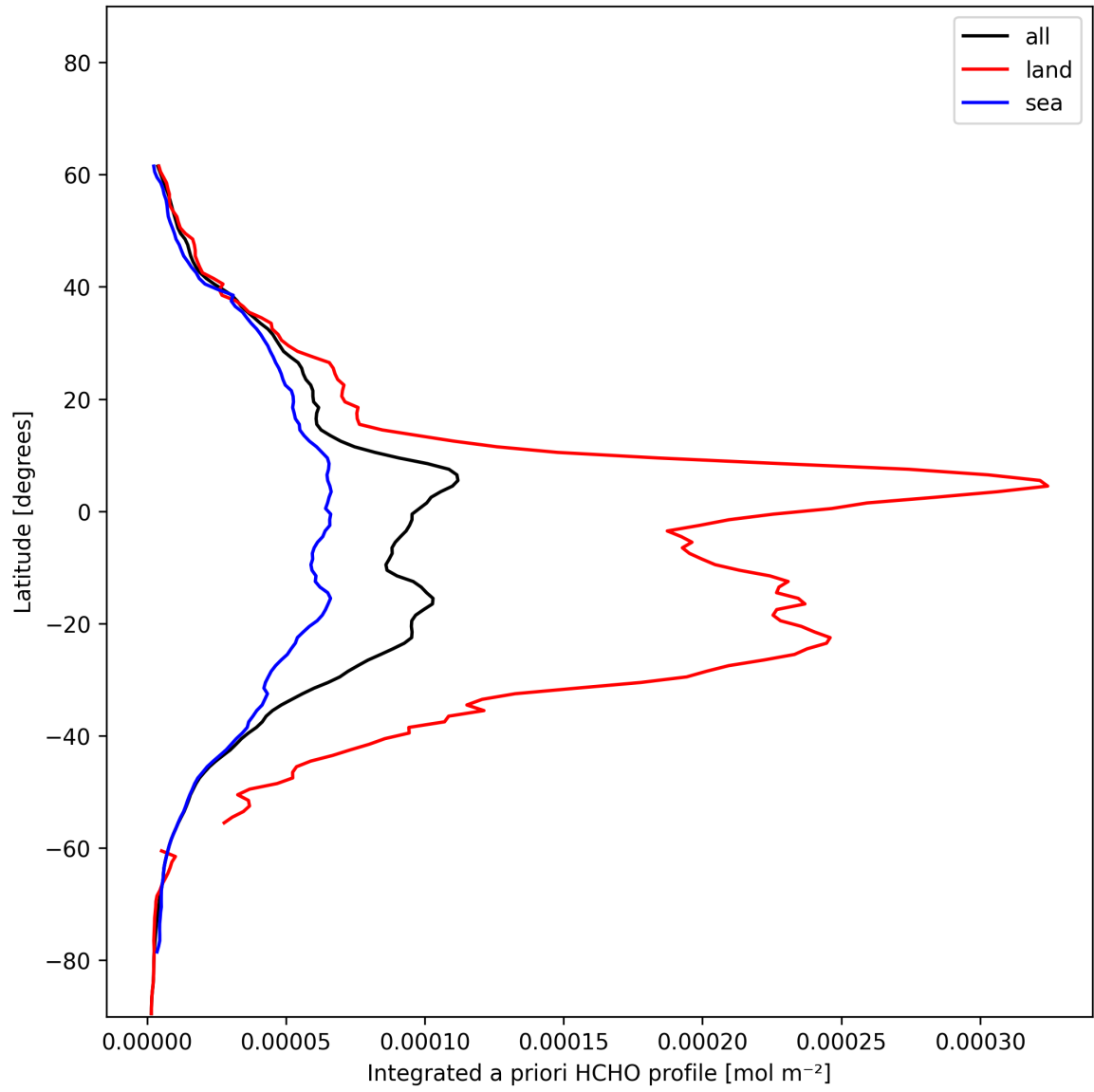
Figure 29: Zonal average of “Integrated a priori HCHO profile” for 2024-12-24 to 2024-12-26.
