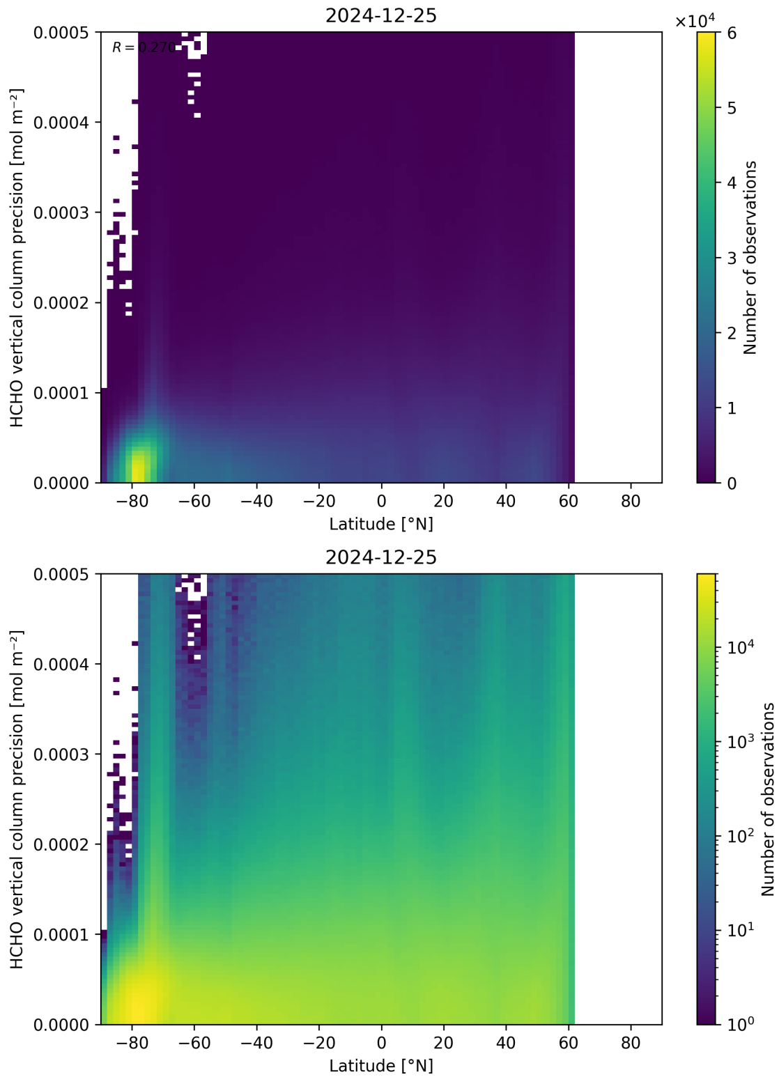
Figure 165: Scatter density plot of “Latitude” against “HCHO vertical column precision” for 2024-12-24 to 2024-12-26.
