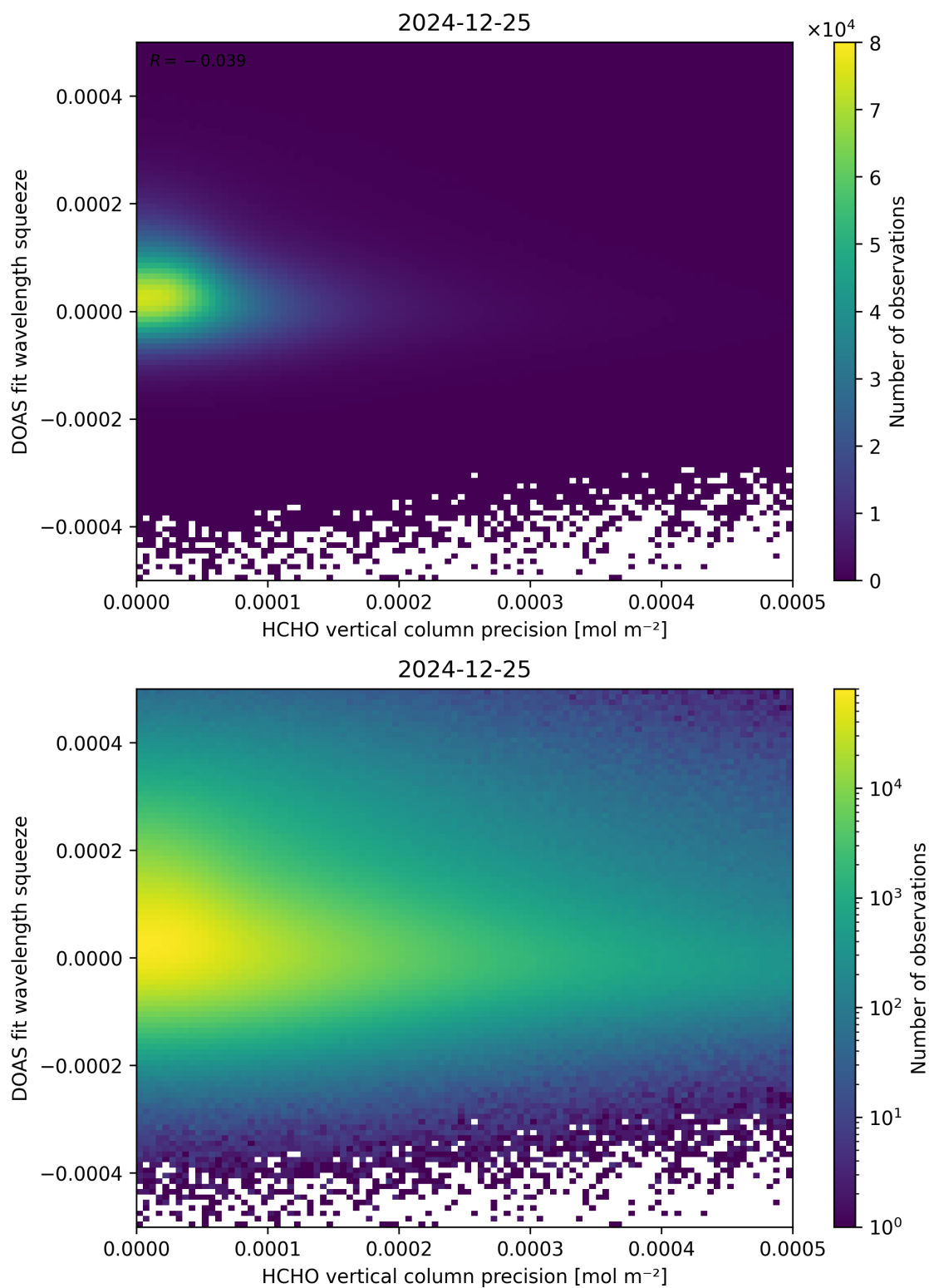
Figure 138: Scatter density plot of “HCHO vertical column precision” against “DOAS fit wavelength squeeze” for 2024-12-24 to 2024-12-26.
