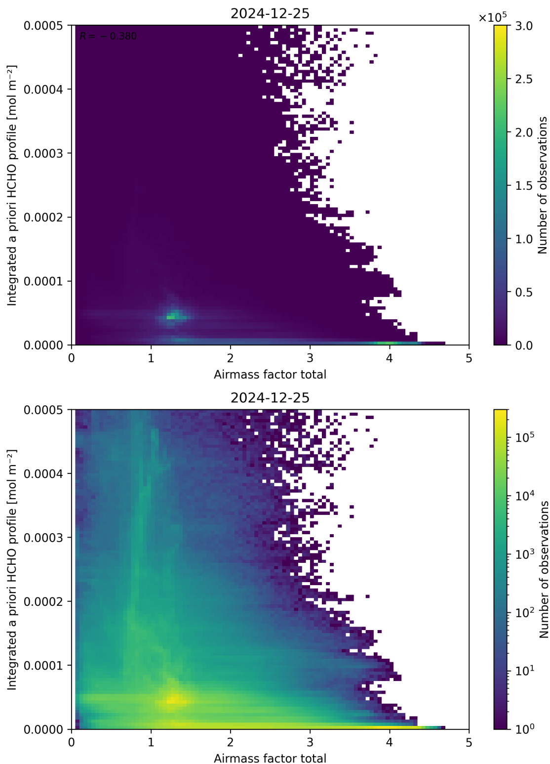
Figure 104: Scatter density plot of “Airmass factor total” against “Integrated a priori HCHO profile” for 2024-12-24 to 2024-12-26.
