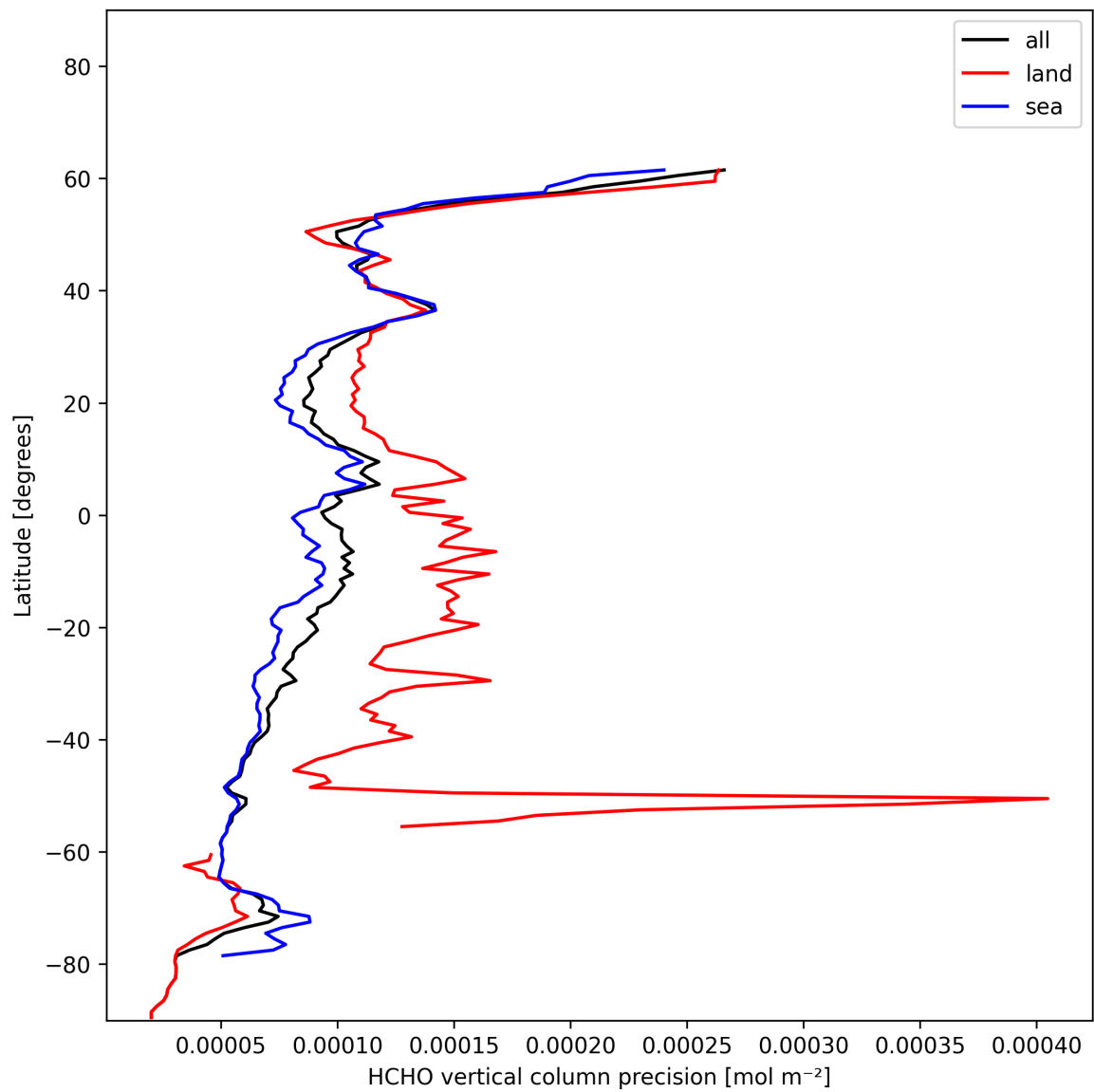
Figure 22: Zonal average of “HCHO vertical column precision” for 2024-12-24 to 2024-12-26.
