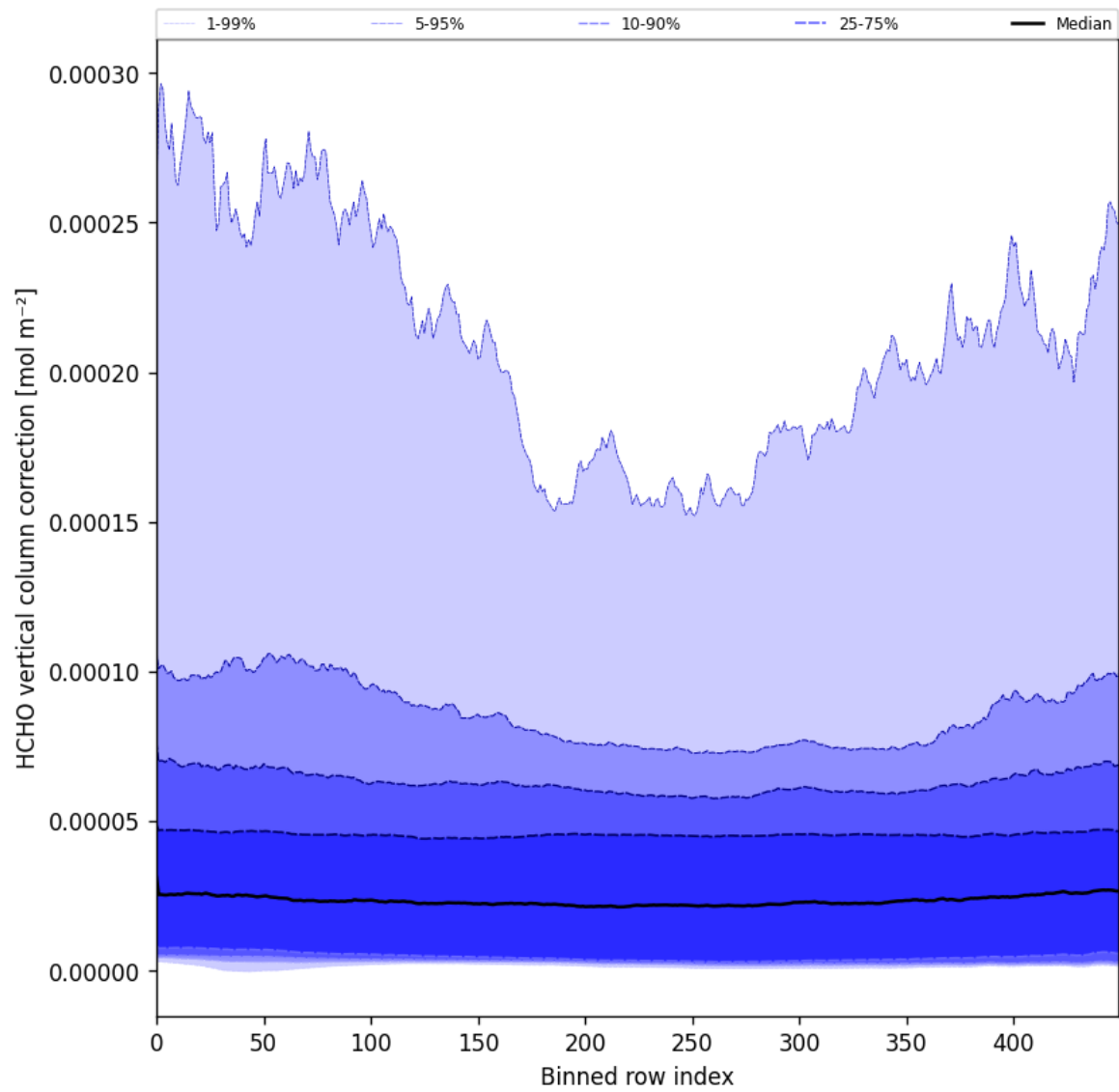
Figure 51: Along track statistics of “HCHO vertical column correction” for 2024-12-24 to 2024-12-26
