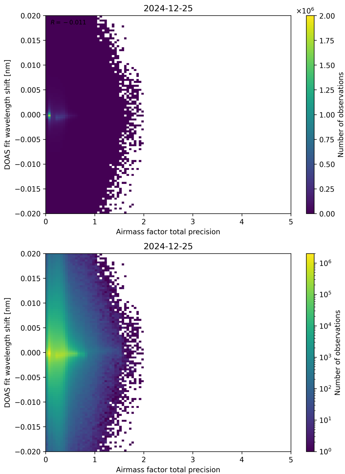
Figure 106: Scatter density plot of “Airmass factor total precision” against “DOAS fit wavelength shift” for 2024-12-24 to 2024-12-26.
