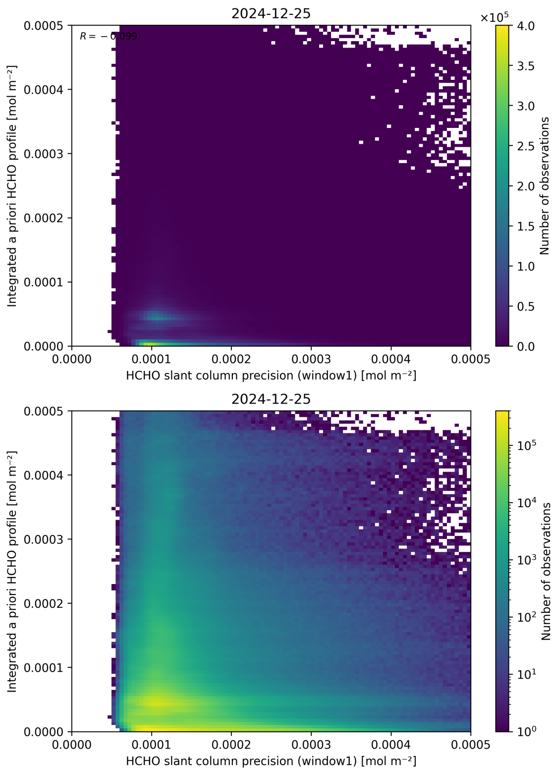
Figure 96: Scatter density plot of “HCHO slant column precision (window1)” against “Integrated a priori HCHO profile” for 2024-12-24 to 2024-12-26.
