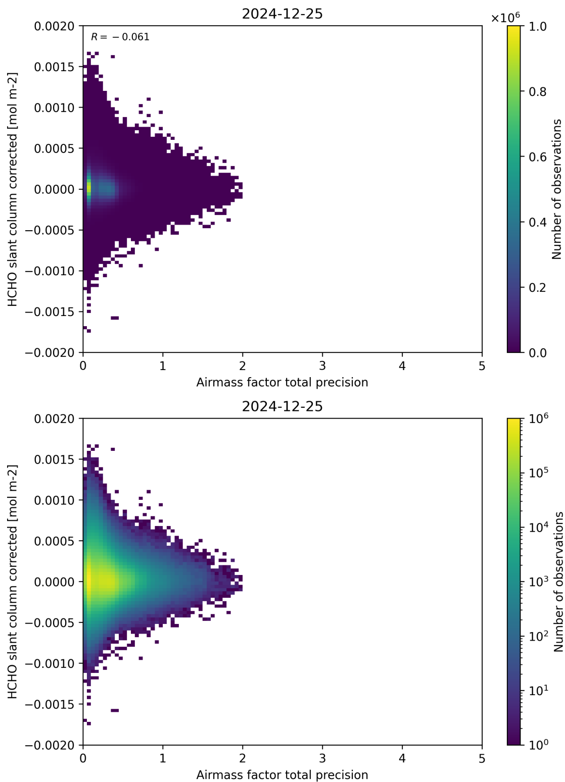
Figure 109: Scatter density plot of “Airmass factor total precision” against “HCHO slant column corrected” for 2024-12-24 to 2024-12-26.
