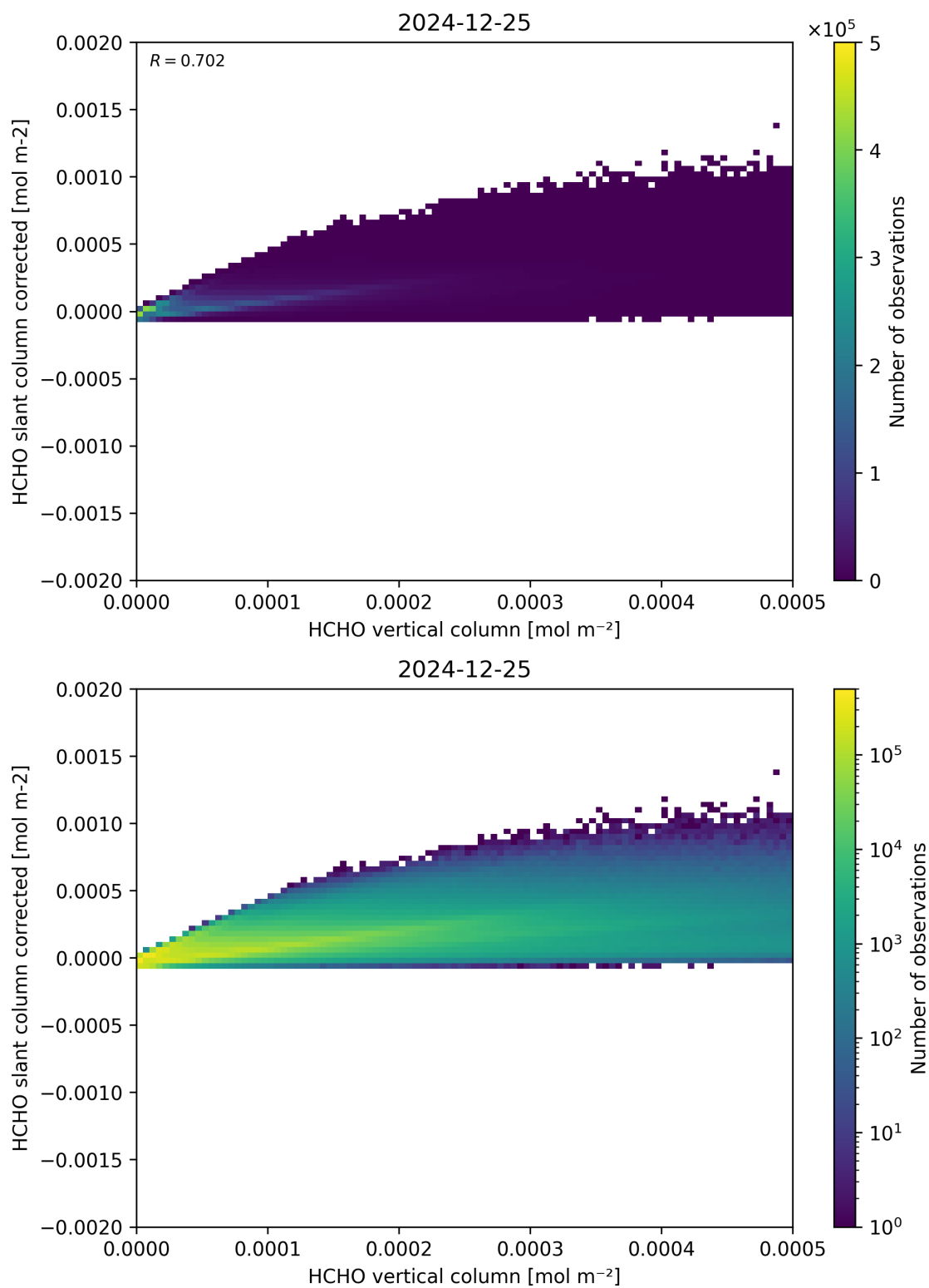
Figure 127: Scatter density plot of “HCHO vertical column” against “HCHO slant column corrected” for 2024-12-24 to 2024-12-26.
