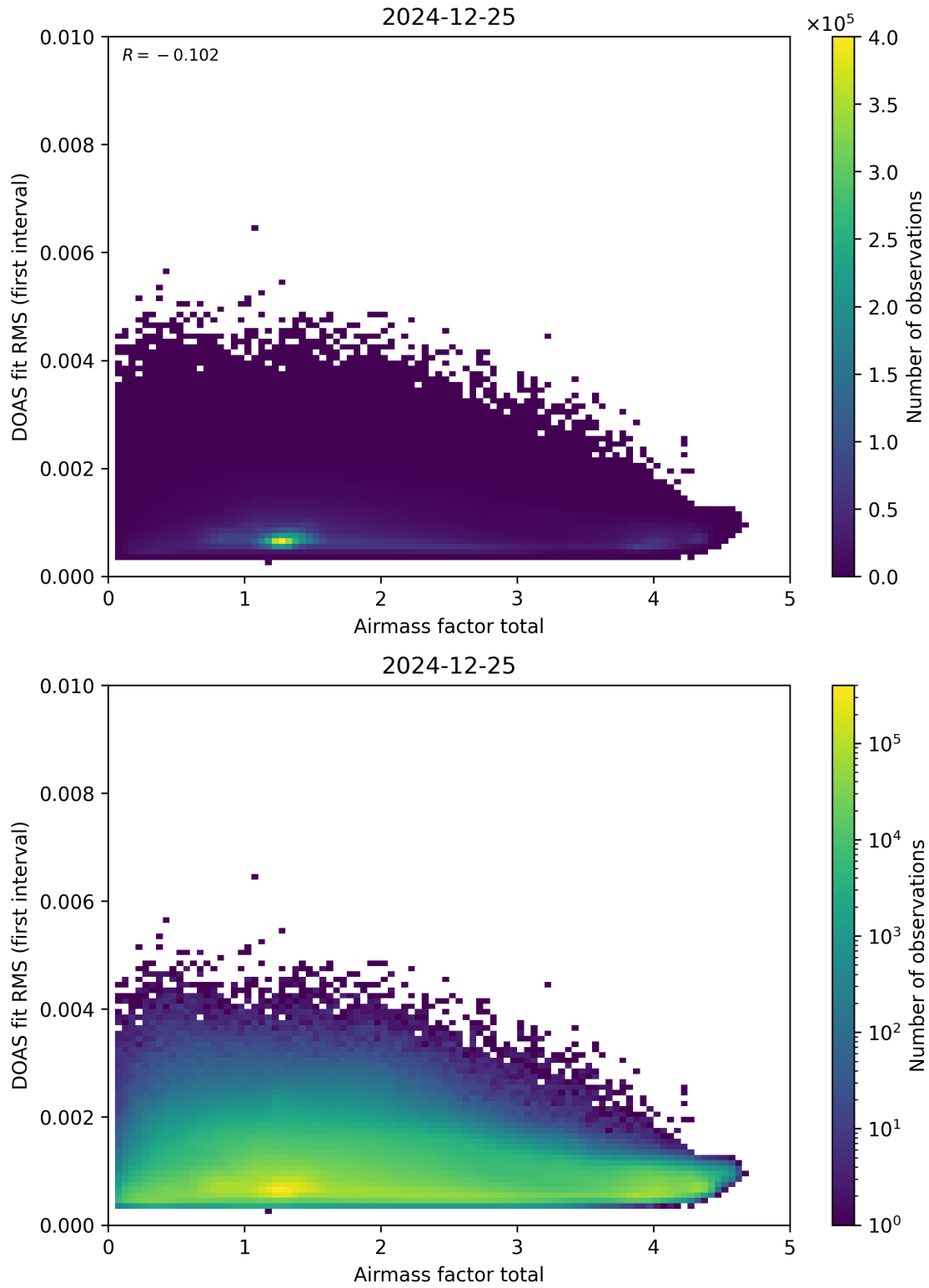
Figure 97: Scatter density plot of “Airmass factor total” against “DOAS fit RMS (first interval)” for 2024-12-24 to 2024-12-26.
