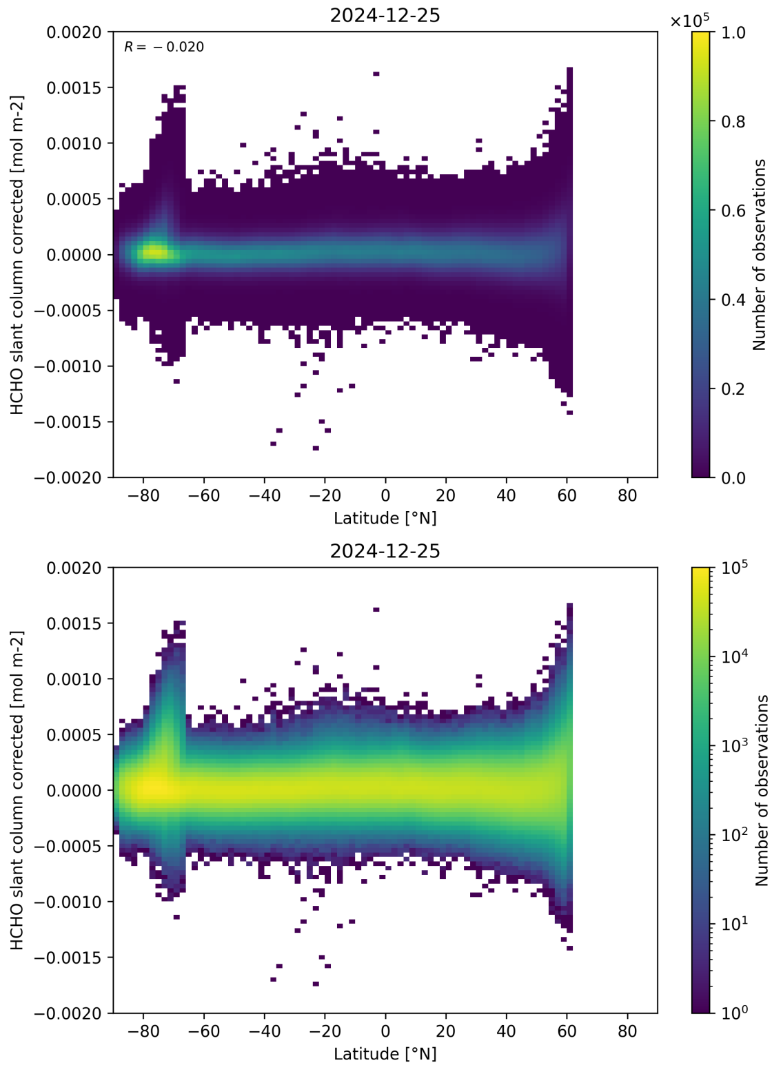
Figure 157: Scatter density plot of “Latitude” against “HCHO slant column corrected” for 2024-12-24 to 2024-12-26.
