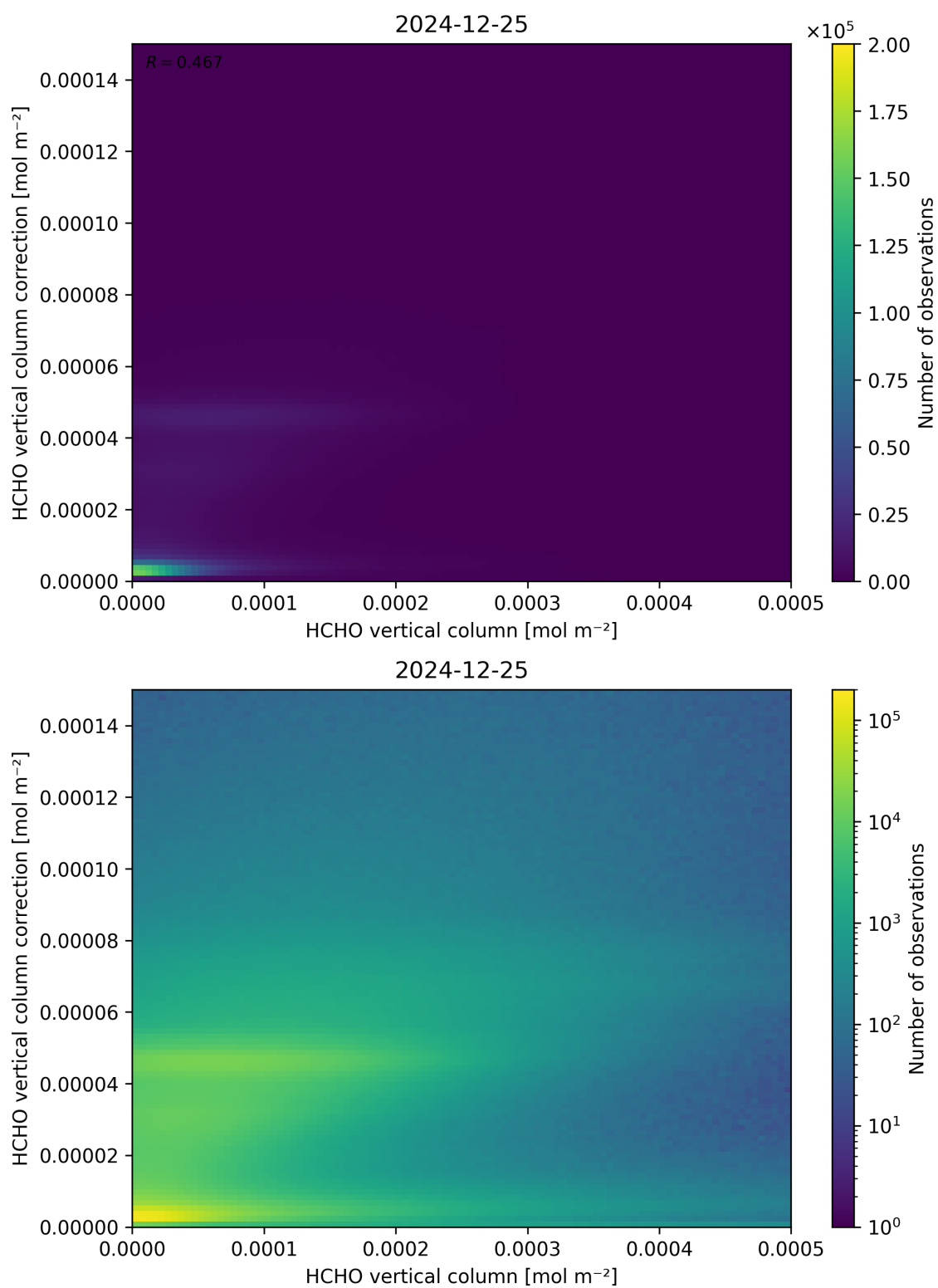
Figure 133: Scatter density plot of “HCHO vertical column” against “HCHO vertical column correction” for 2024-12-24 to 2024-12-26.
