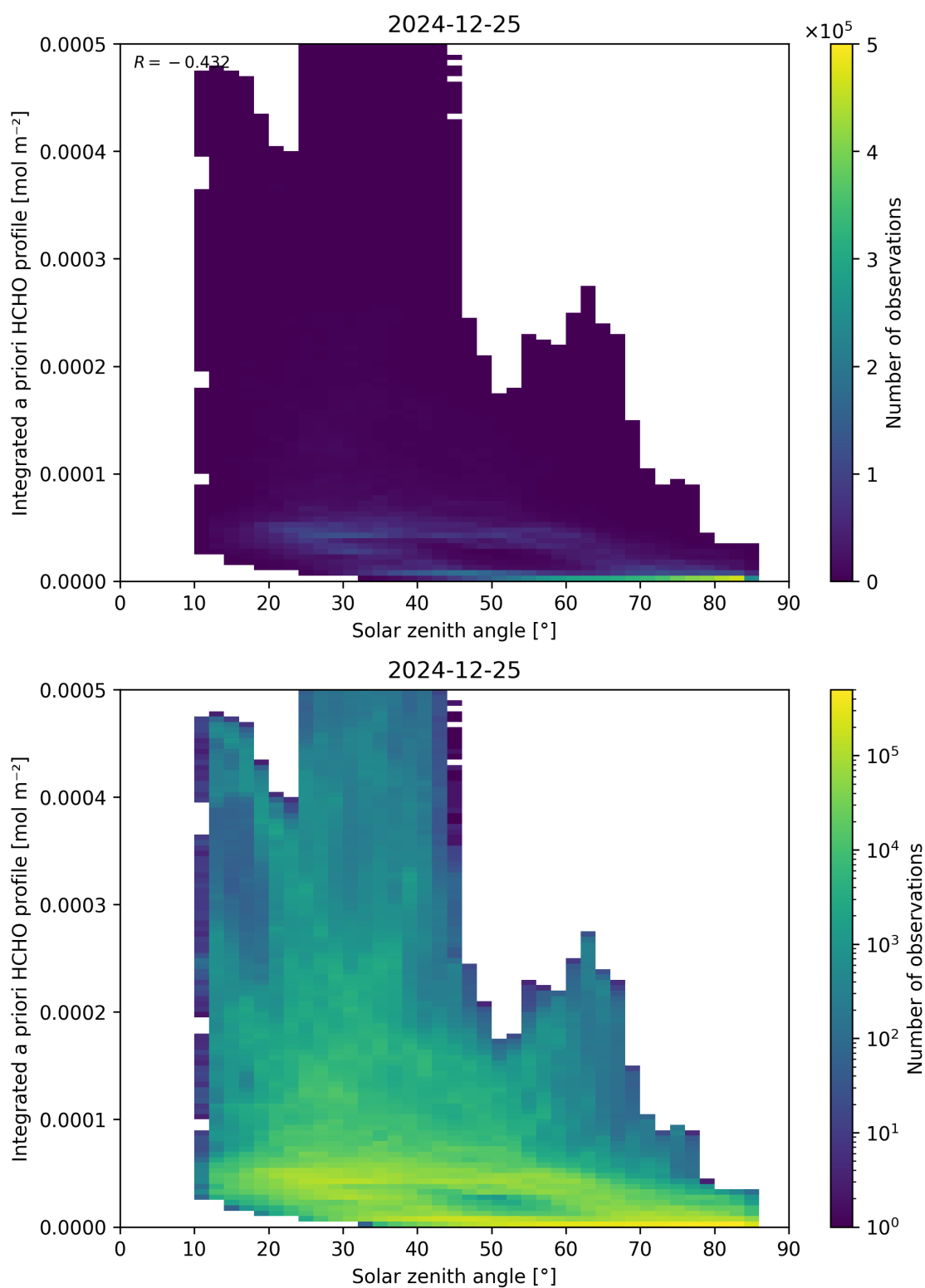
Figure 180: Scatter density plot of “Solar zenith angle” against “Integrated a priori HCHO profile” for 2024-12-24 to 2024-12-26.
