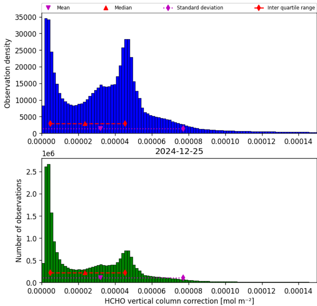
Figure 37: Histogram of “HCHO vertical column correction” for 2024-12-24 to 2024-12-26
