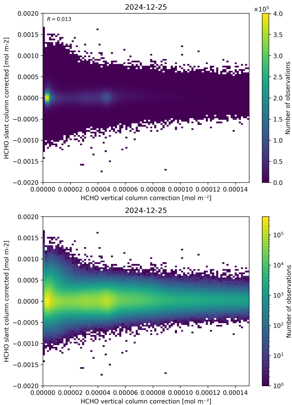
Figure 116: Scatter density plot of “HCHO vertical column correction” against “HCHO slant column corrected” for 2024-12-24 to 2024-12-26.
