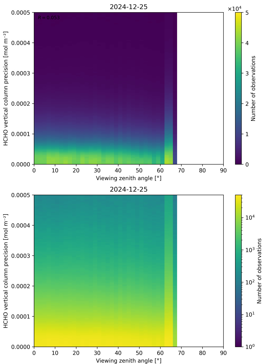
Figure 194: Scatter density plot of “Viewing zenith angle” against “HCHO vertical column precision” for 2024-12-24 to 2024-12-26.
