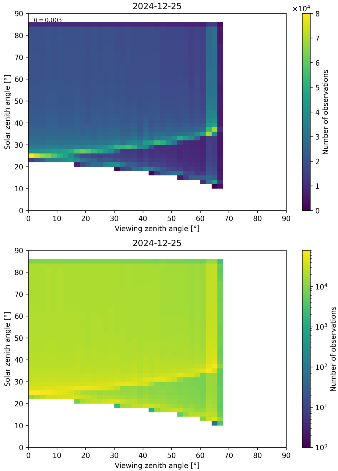
Figure 197: Scatter density plot of “Viewing zenith angle” against “Solar zenith angle” for 2024-12-24 to 2024-12-26.
