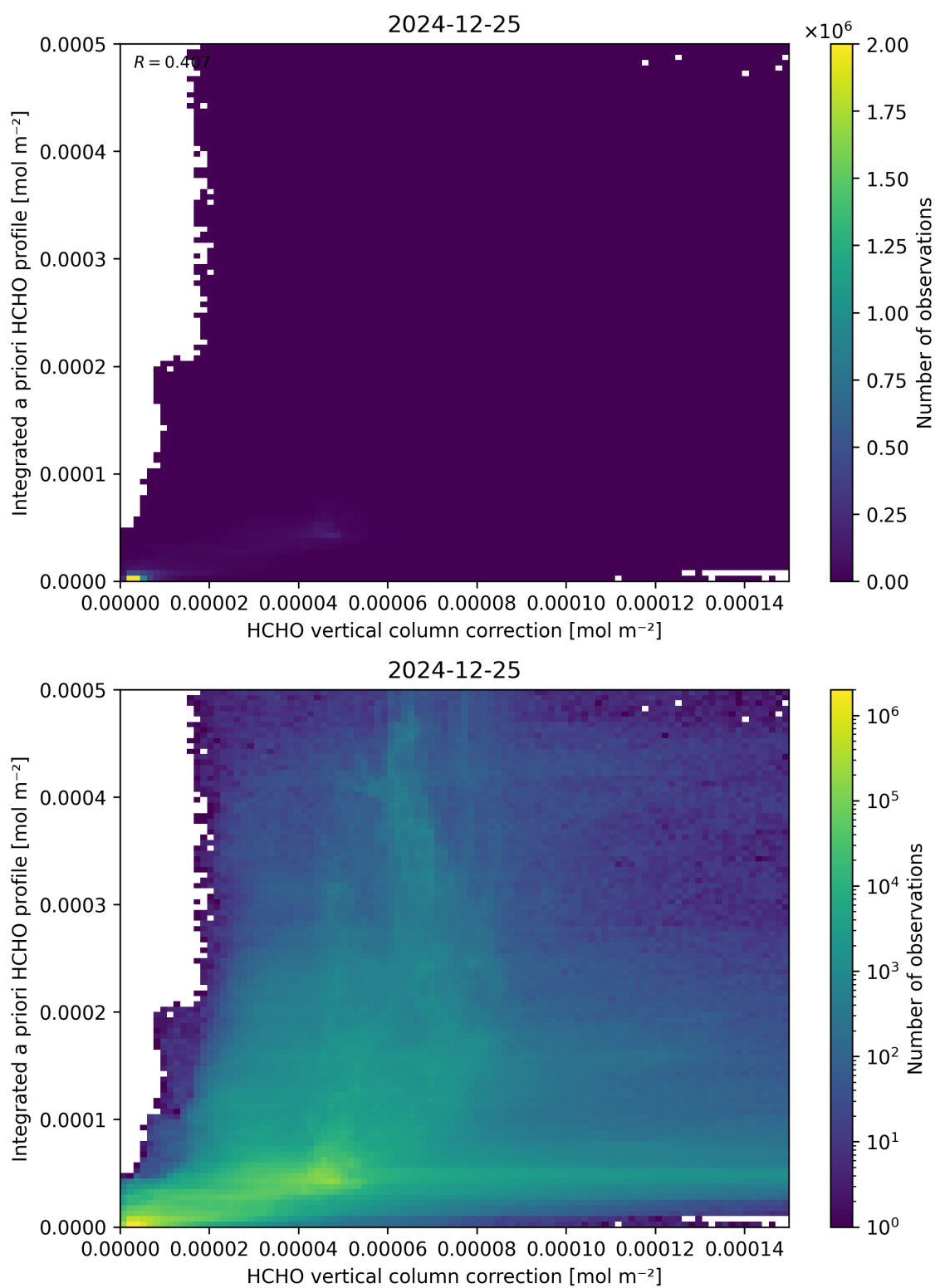
Figure 122: Scatter density plot of “HCHO vertical column correction” against “Integrated a priori HCHO profile” for 2024-12-24 to 2024-12-26.
