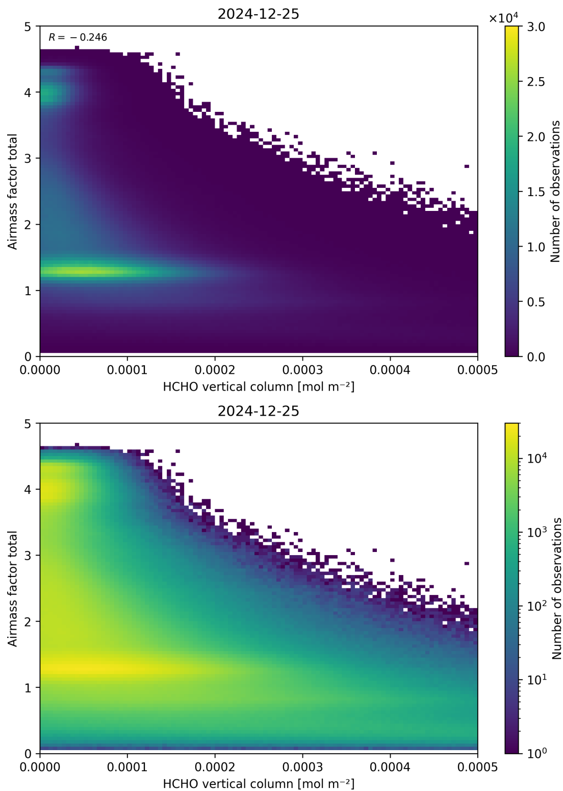
Figure 131: Scatter density plot of “HCHO vertical column” against “Airmass factor total” for 2024-12-24 to 2024-12-26.
