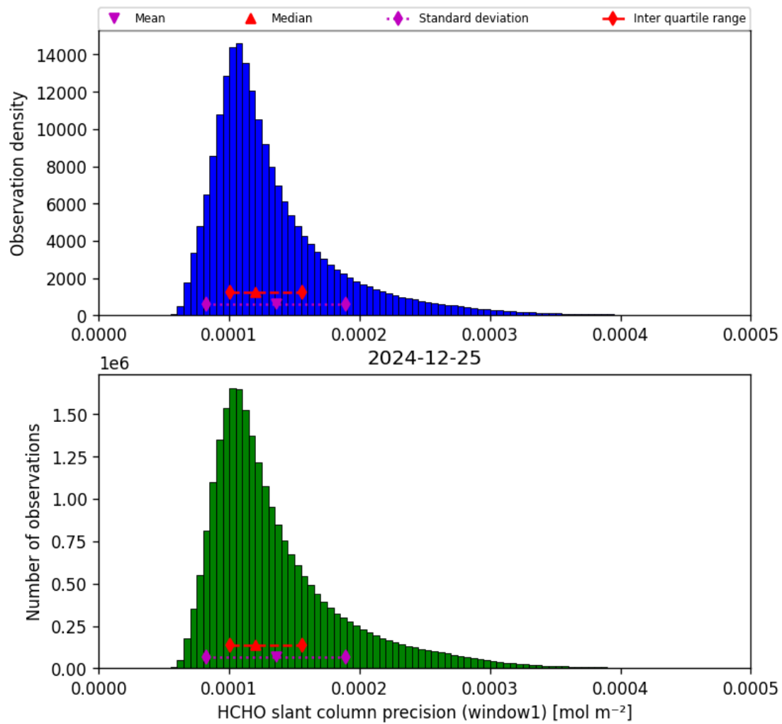
Figure 39: Histogram of “HCHO slant column precision (window1)” for 2024-12-24 to 2024-12-26
