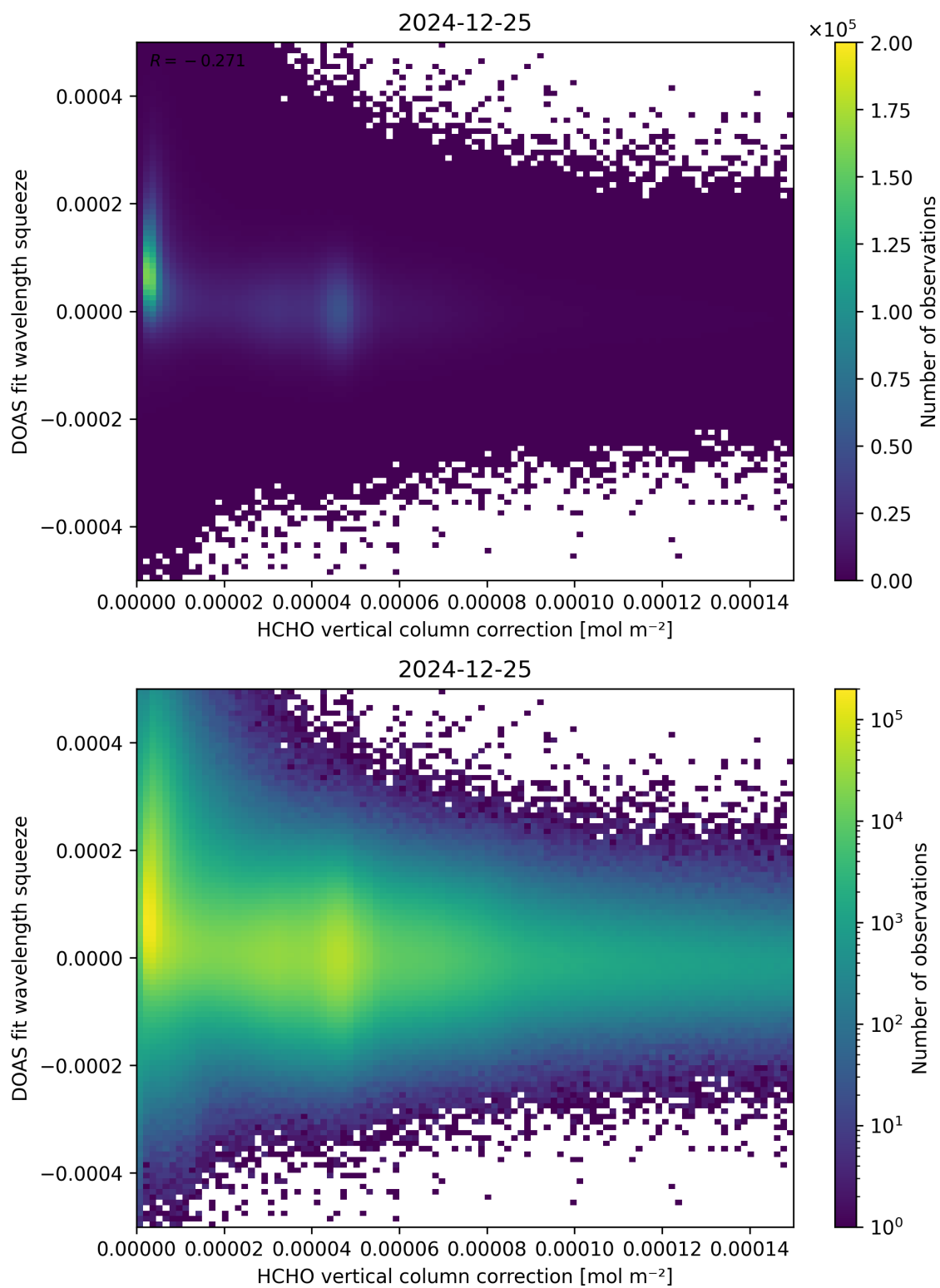
Figure 114: Scatter density plot of “HCHO vertical column correction” against “DOAS fit wavelength squeeze” for 2024-12-24 to 2024-12-26.
