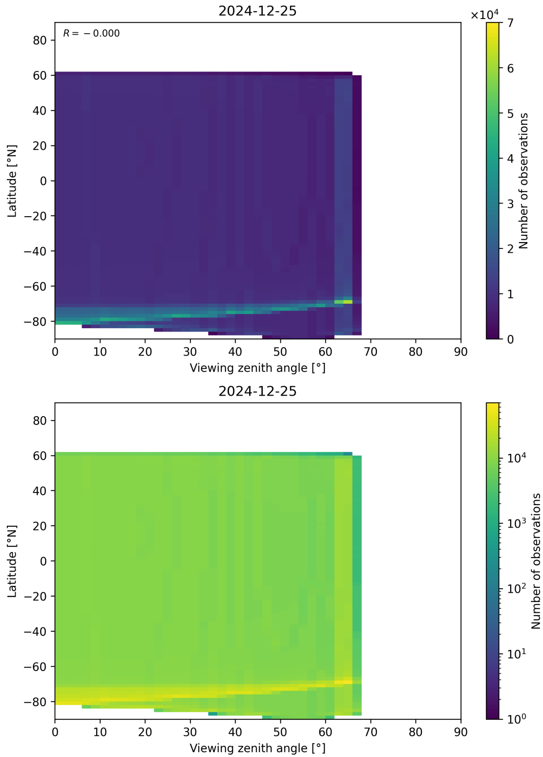
Figure 196: Scatter density plot of “Viewing zenith angle” against “Latitude” for 2024-12-24 to 2024-12-26.
