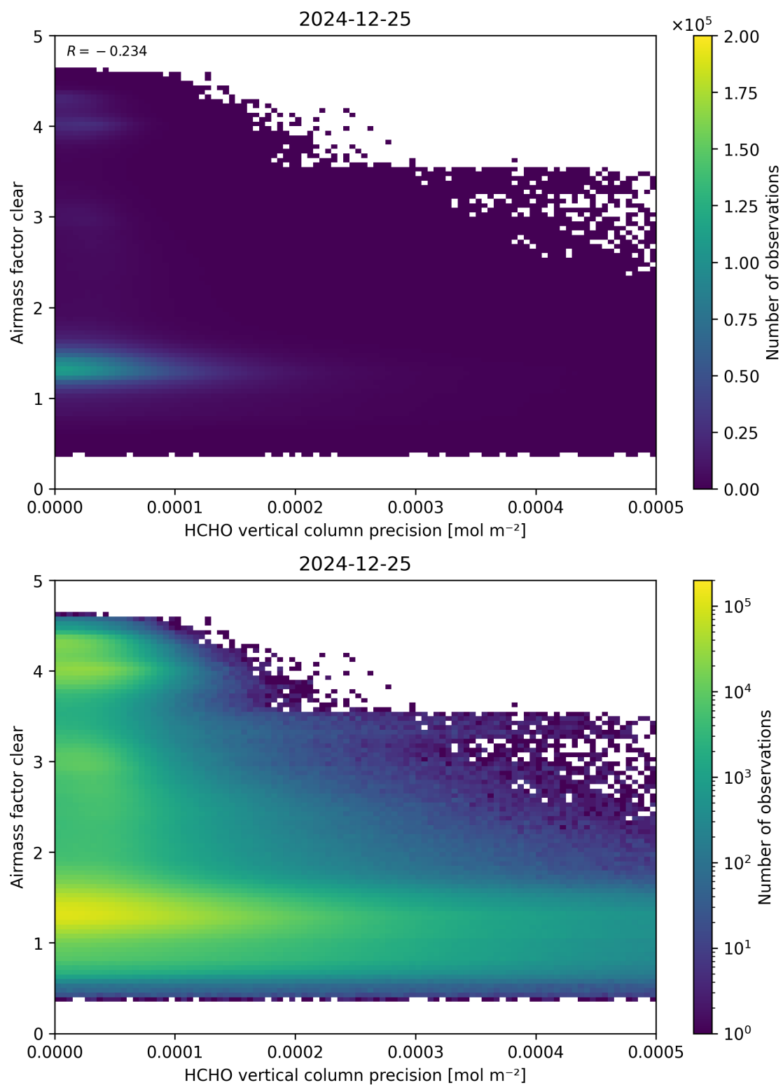
Figure 139: Scatter density plot of “HCHO vertical column precision” against “Airmass factor clear” for 2024-12-24 to 2024-12-26.
