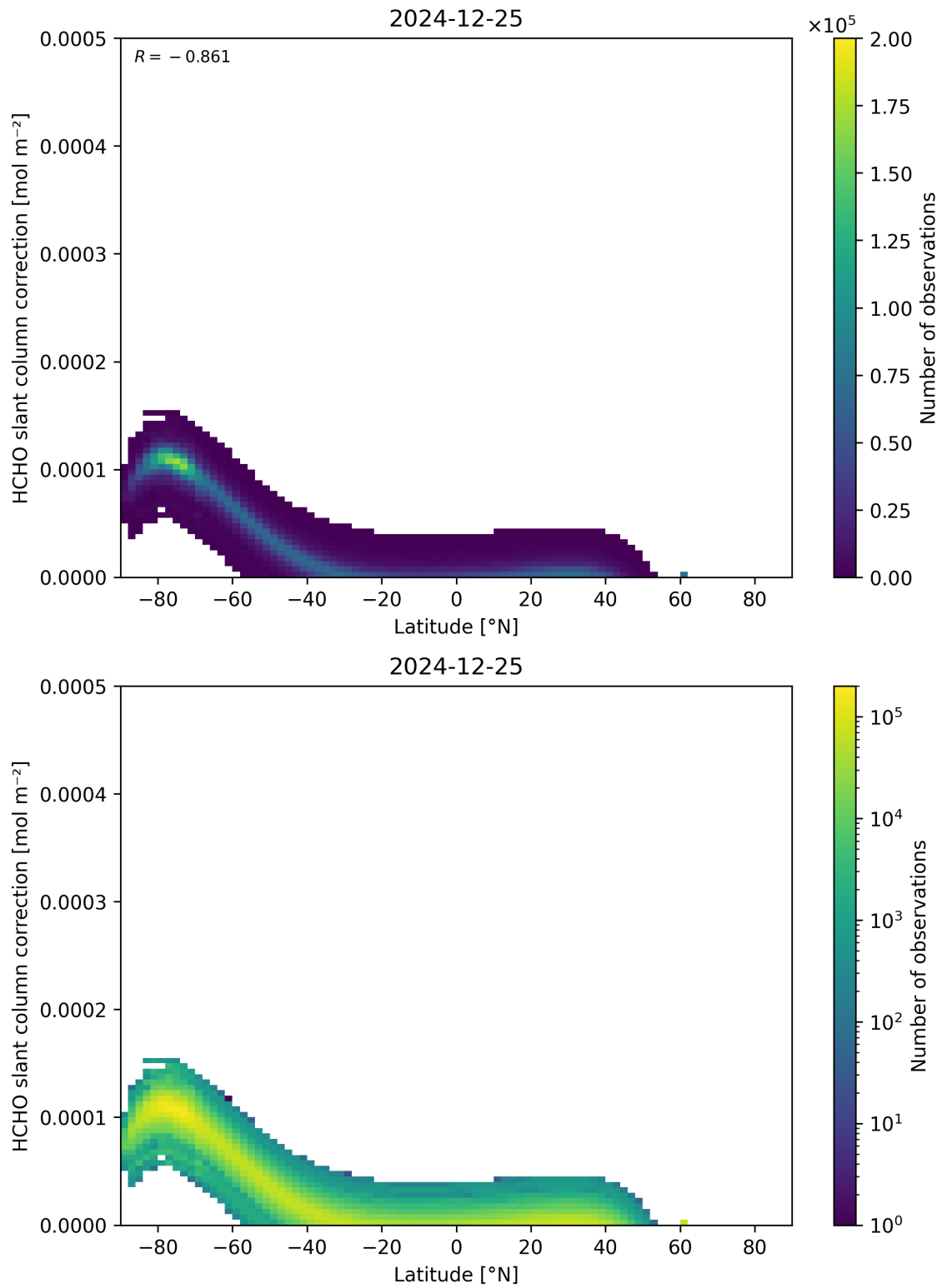
Figure 158: Scatter density plot of “Latitude” against “HCHO slant column correction” for 2024-12-24 to 2024-12-26.
