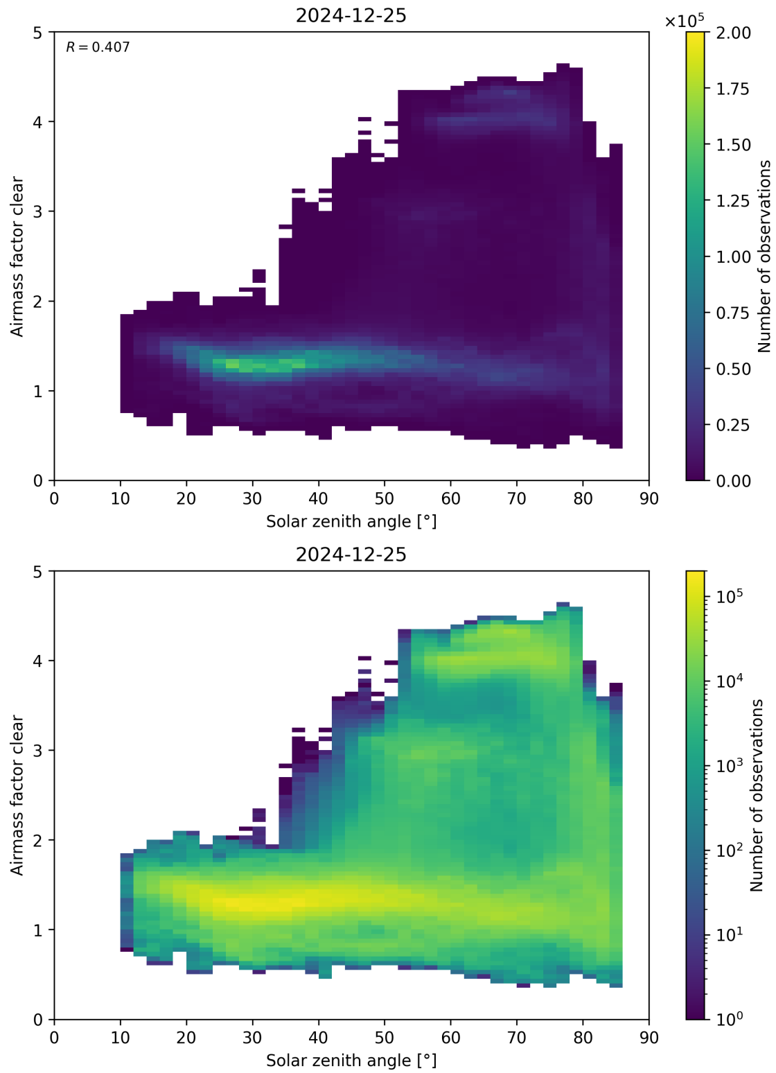
Figure 170: Scatter density plot of “Solar zenith angle” against “Airmass factor clear” for 2024-12-24 to 2024-12-26.
