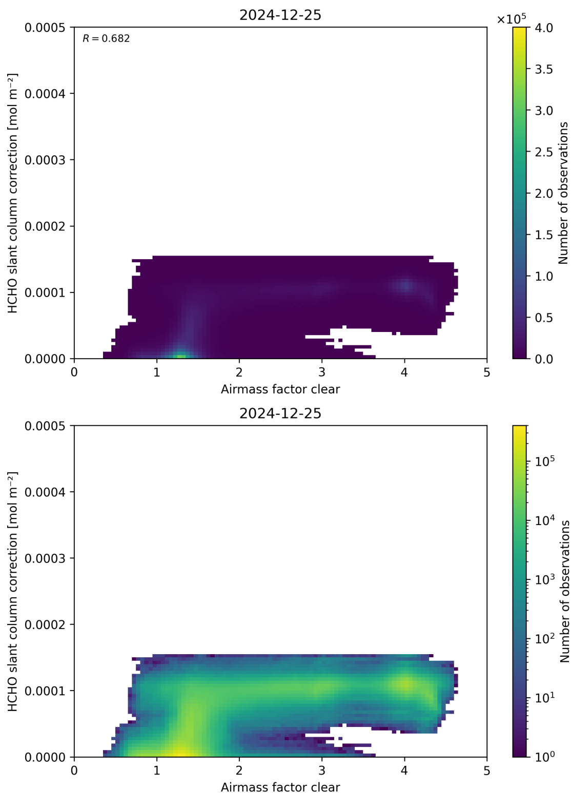
Figure 75: Scatter density plot of “Airmass factor clear” against “HCHO slant column correction” for 2024-12-24 to 2024-12-26.
