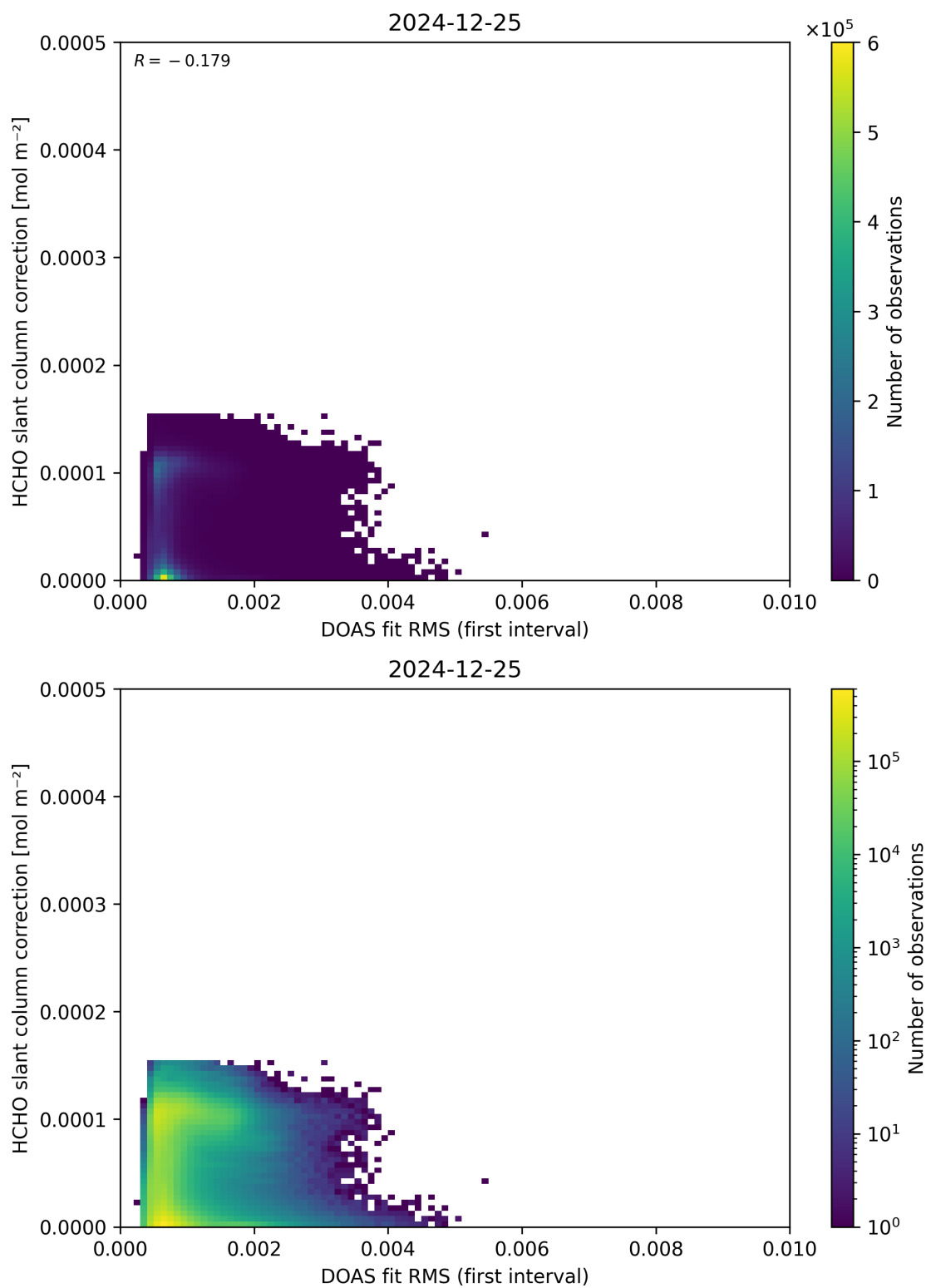
Figure 63: Scatter density plot of “DOAS fit RMS (first interval)” against “HCHO slant column correction” for 2024-12-24 to 2024-12-26.
