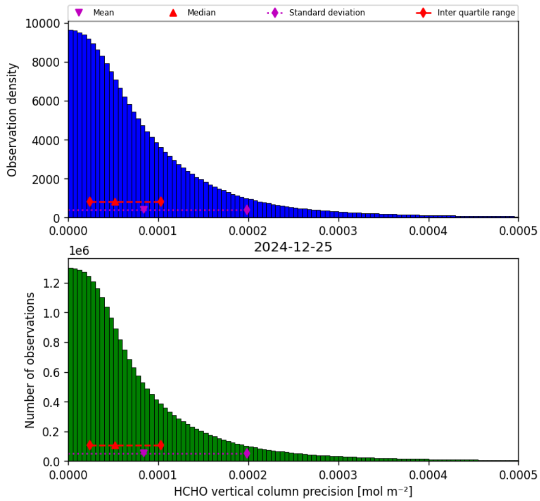
Figure 36: Histogram of “HCHO vertical column precision” for 2024-12-24 to 2024-12-26
