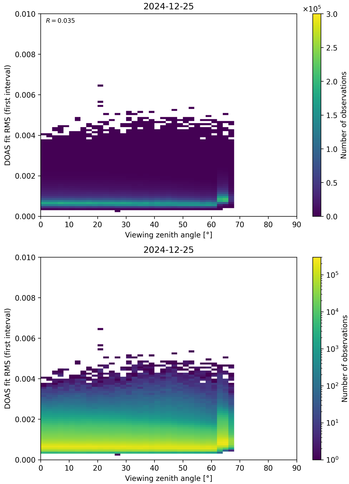
Figure 182: Scatter density plot of “Viewing zenith angle” against “DOAS fit RMS (first interval)” for 2024-12-24 to 2024-12-26.
