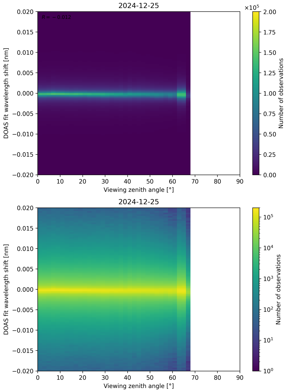
Figure 183: Scatter density plot of “Viewing zenith angle” against “DOAS fit wavelength shift” for 2024-12-24 to 2024-12-26.
