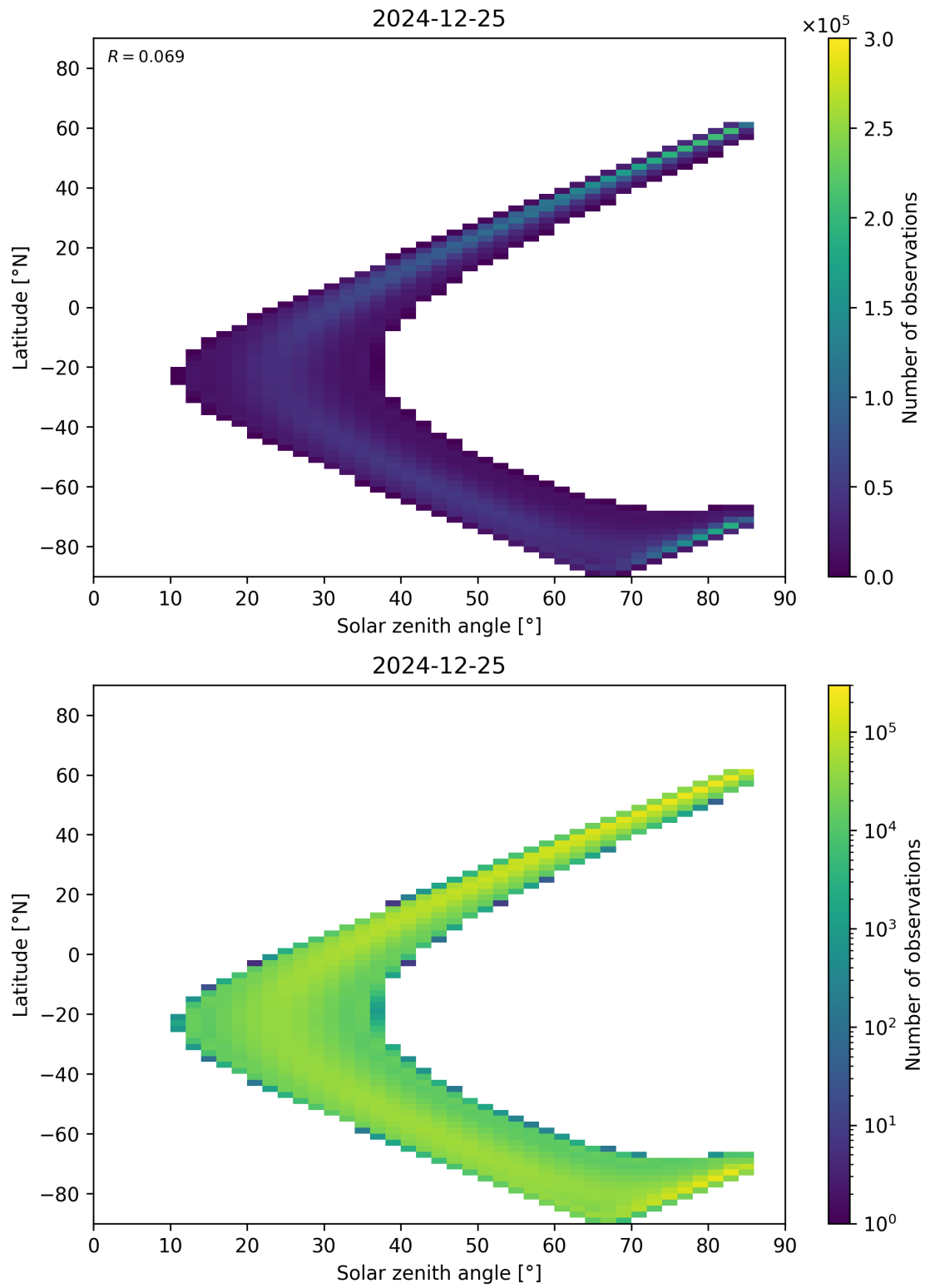
Figure 181: Scatter density plot of “Solar zenith angle” against “Latitude” for 2024-12-24 to 2024-12-26.
