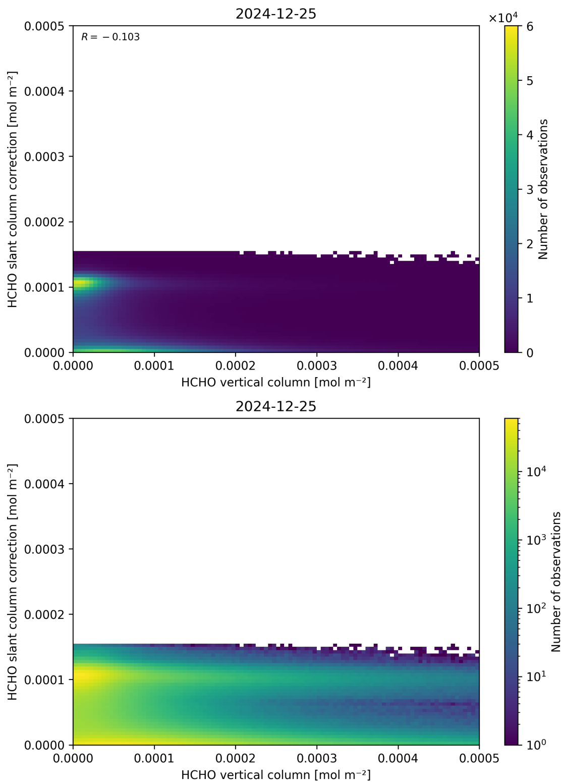
Figure 128: Scatter density plot of “HCHO vertical column” against “HCHO slant column correction” for 2024-12-24 to 2024-12-26.
