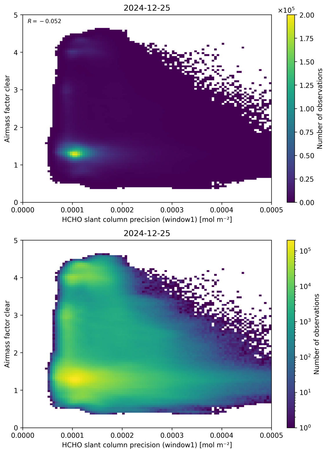
Figure 91: Scatter density plot of “HCHO slant column precision (window1)” against “Airmass factor clear” for 2024-12-24 to 2024-12-26.
