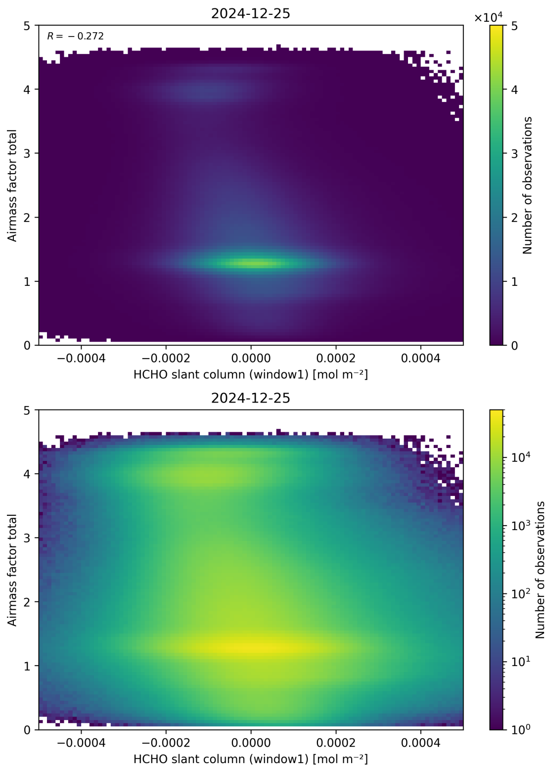
Figure 85: Scatter density plot of “HCHO slant column (window1)” against “Airmass factor total” for 2024-12-24 to 2024-12-26.
