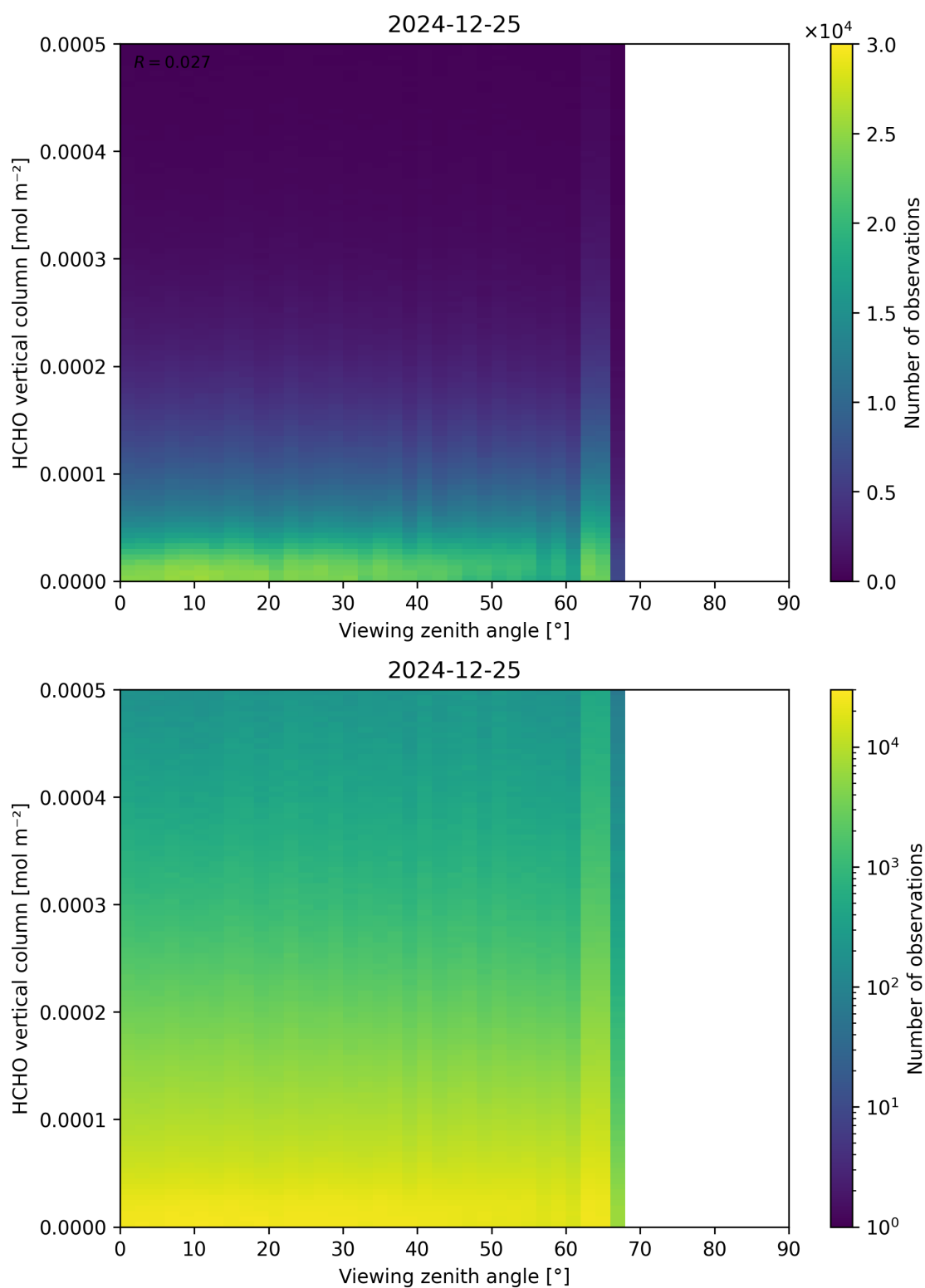
Figure 192: Scatter density plot of “Viewing zenith angle” against “HCHO vertical column” for 2024-12-24 to 2024-12-26.
