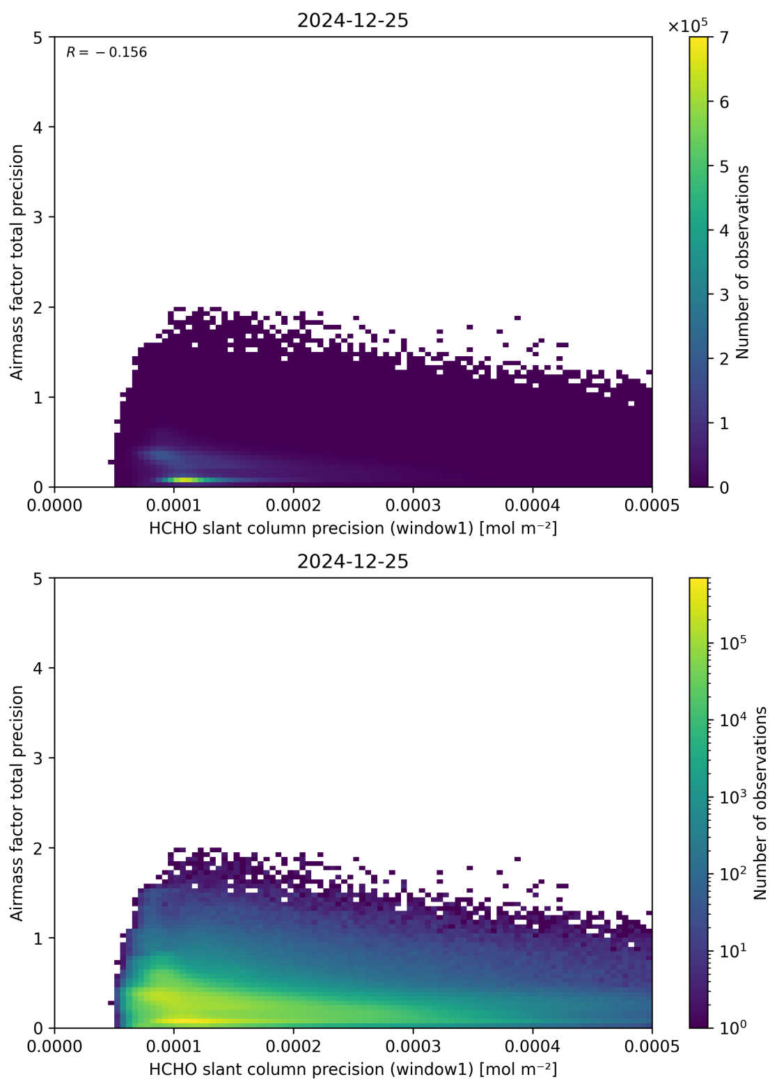
Figure 95: Scatter density plot of “HCHO slant column precision (window1)” against “Airmass factor total precision” for 2024-12-24 to 2024-12-26.
