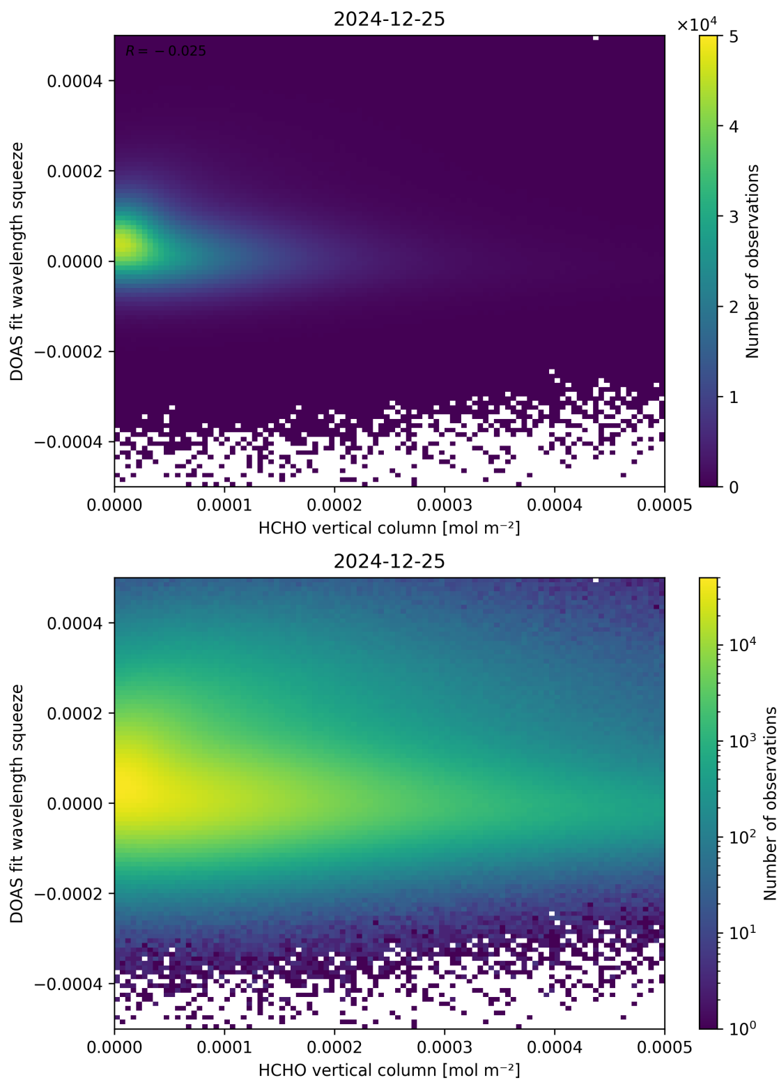
Figure 125: Scatter density plot of “HCHO vertical column” against “DOAS fit wavelength squeeze” for 2024-12-24 to 2024-12-26.
