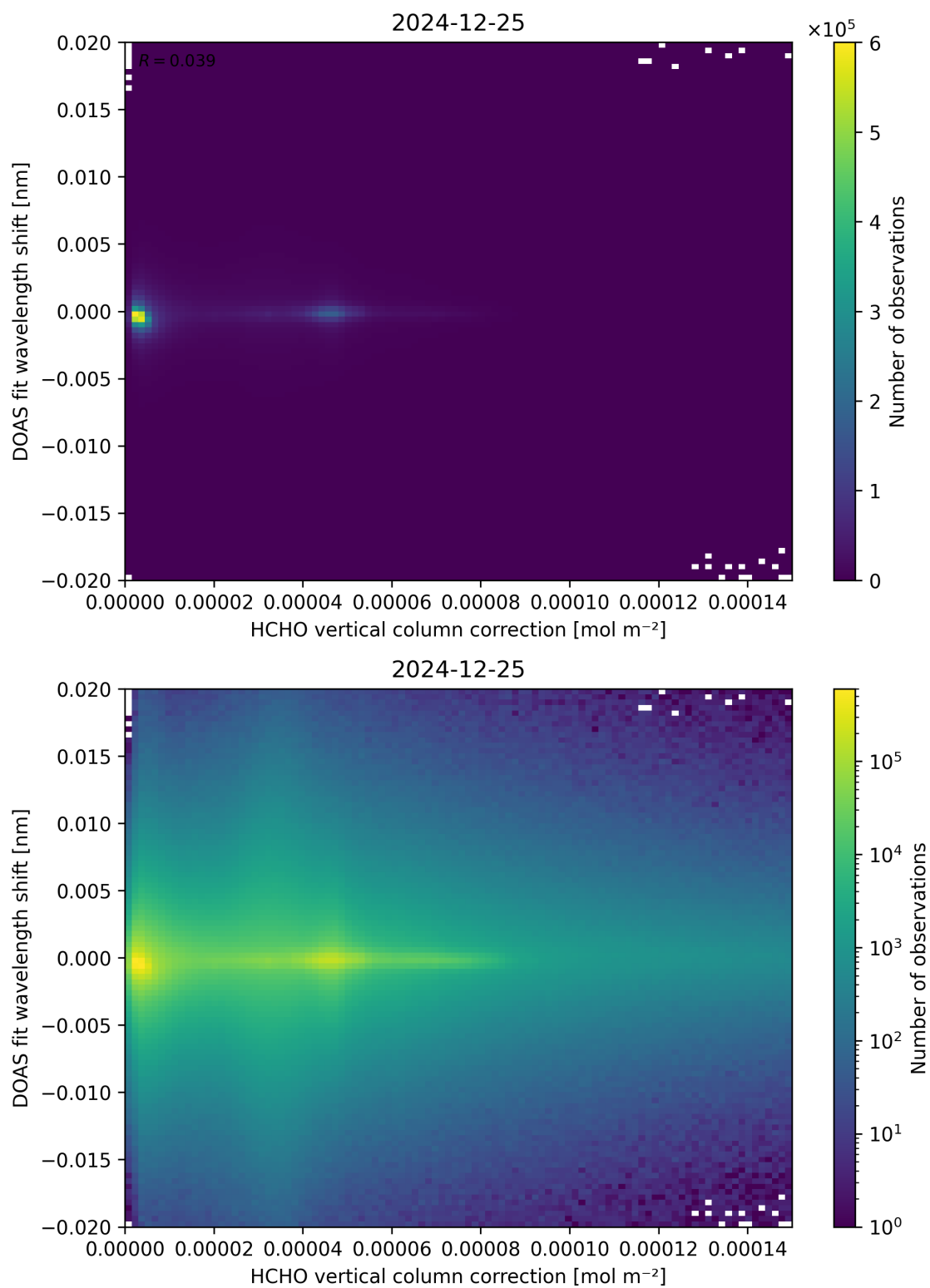
Figure 113: Scatter density plot of “HCHO vertical column correction” against “DOAS fit wavelength shift” for 2024-12-24 to 2024-12-26.
