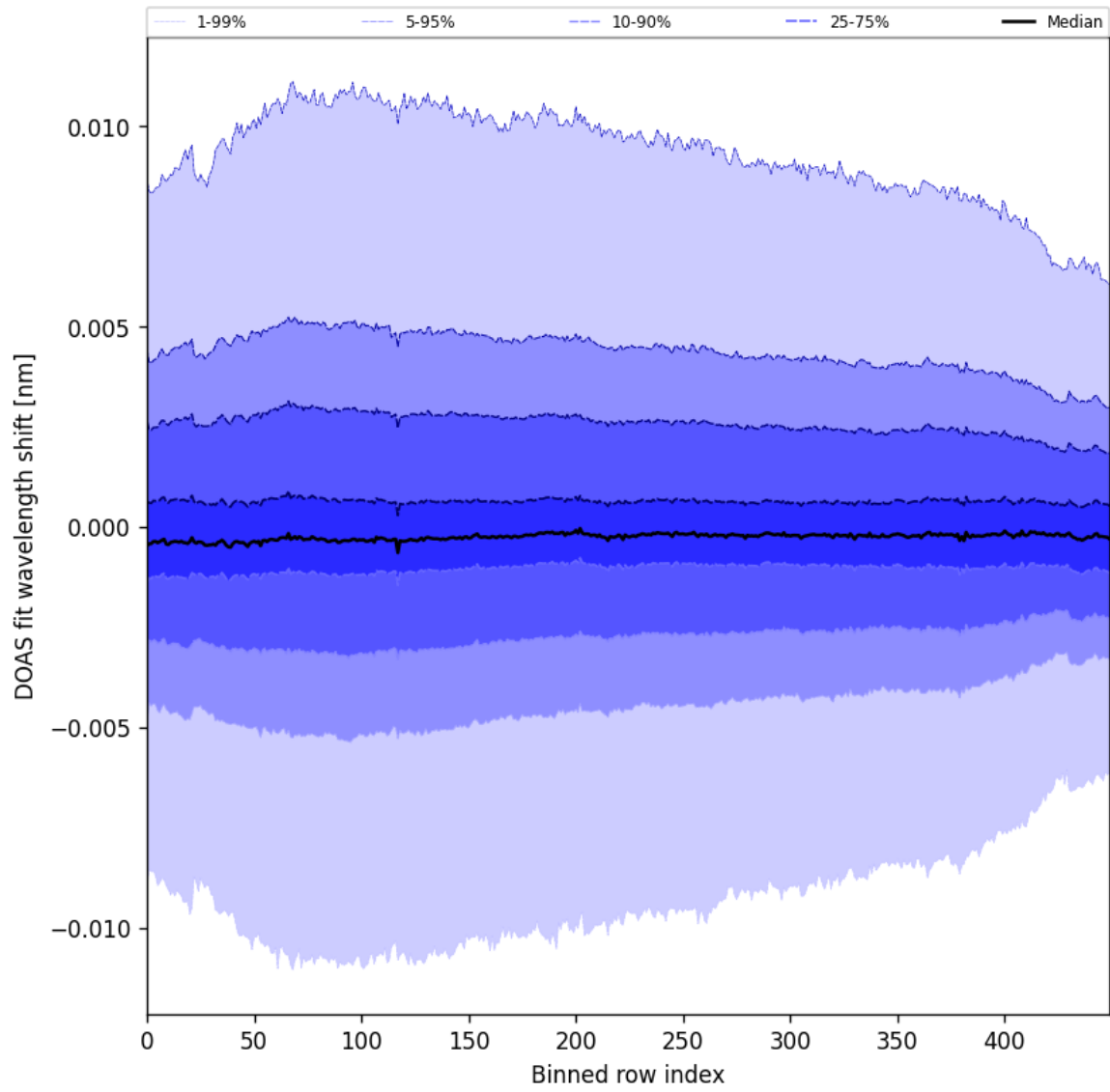
Figure 58: Along track statistics of “DOAS fit wavelength shift” for 2024-12-24 to 2024-12-26
