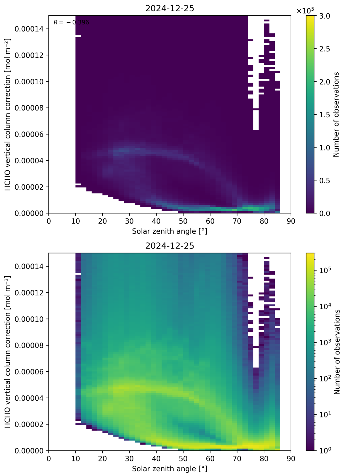
Figure 178: Scatter density plot of “Solar zenith angle” against “HCHO vertical column correction” for 2024-12-24 to 2024-12-26.
