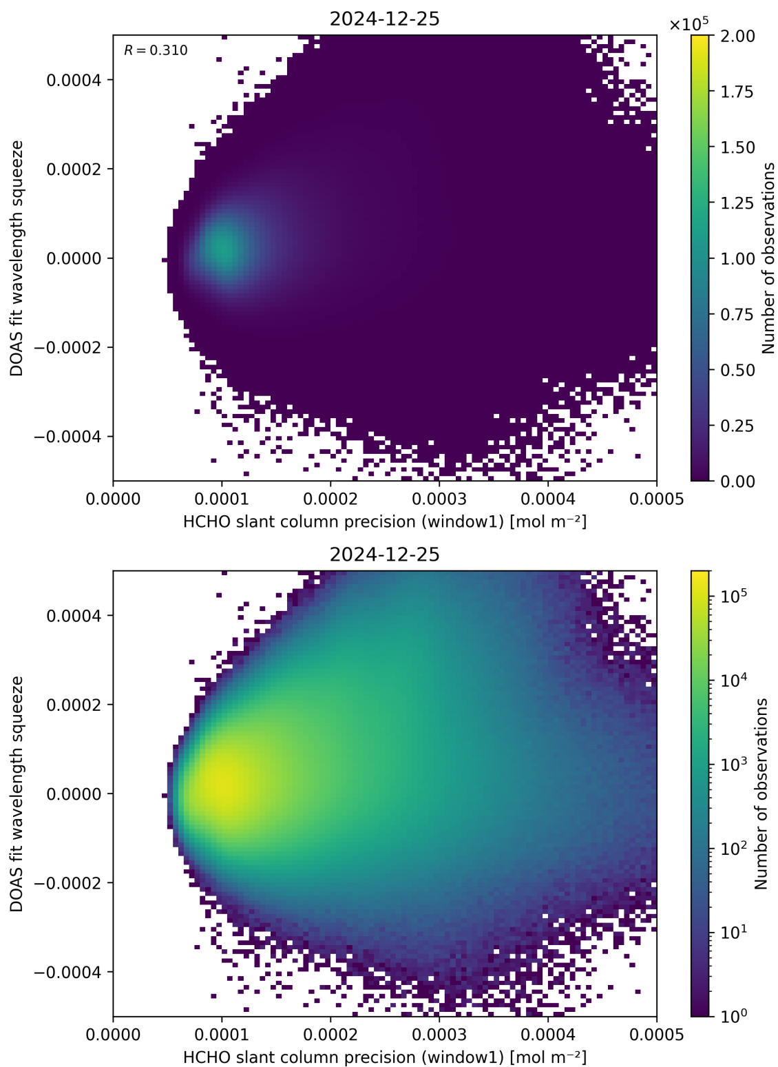
Figure 90: Scatter density plot of “HCHO slant column precision (window1)” against “DOAS fit wavelength squeeze” for 2024-12-24 to 2024-12-26.
