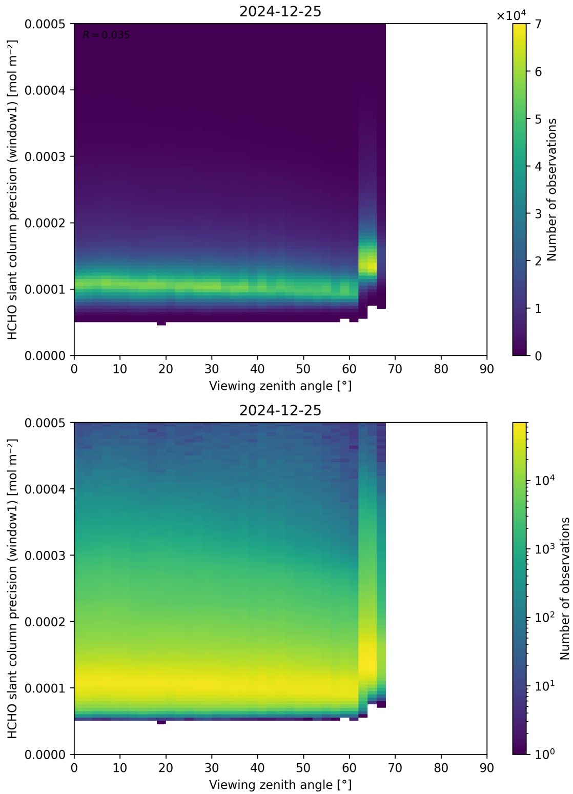
Figure 189: Scatter density plot of “Viewing zenith angle” against “HCHO slant column precision (window1)” for 2024-12-24 to 2024-12-26.
