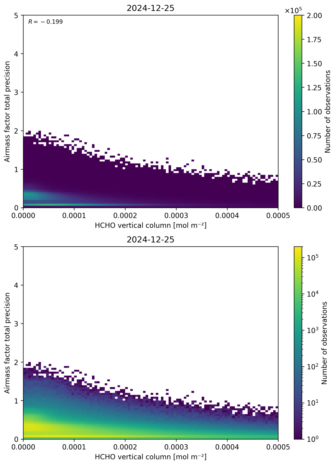
Figure 132: Scatter density plot of “HCHO vertical column” against “Airmass factor total precision” for 2024-12-24 to 2024-12-26.
