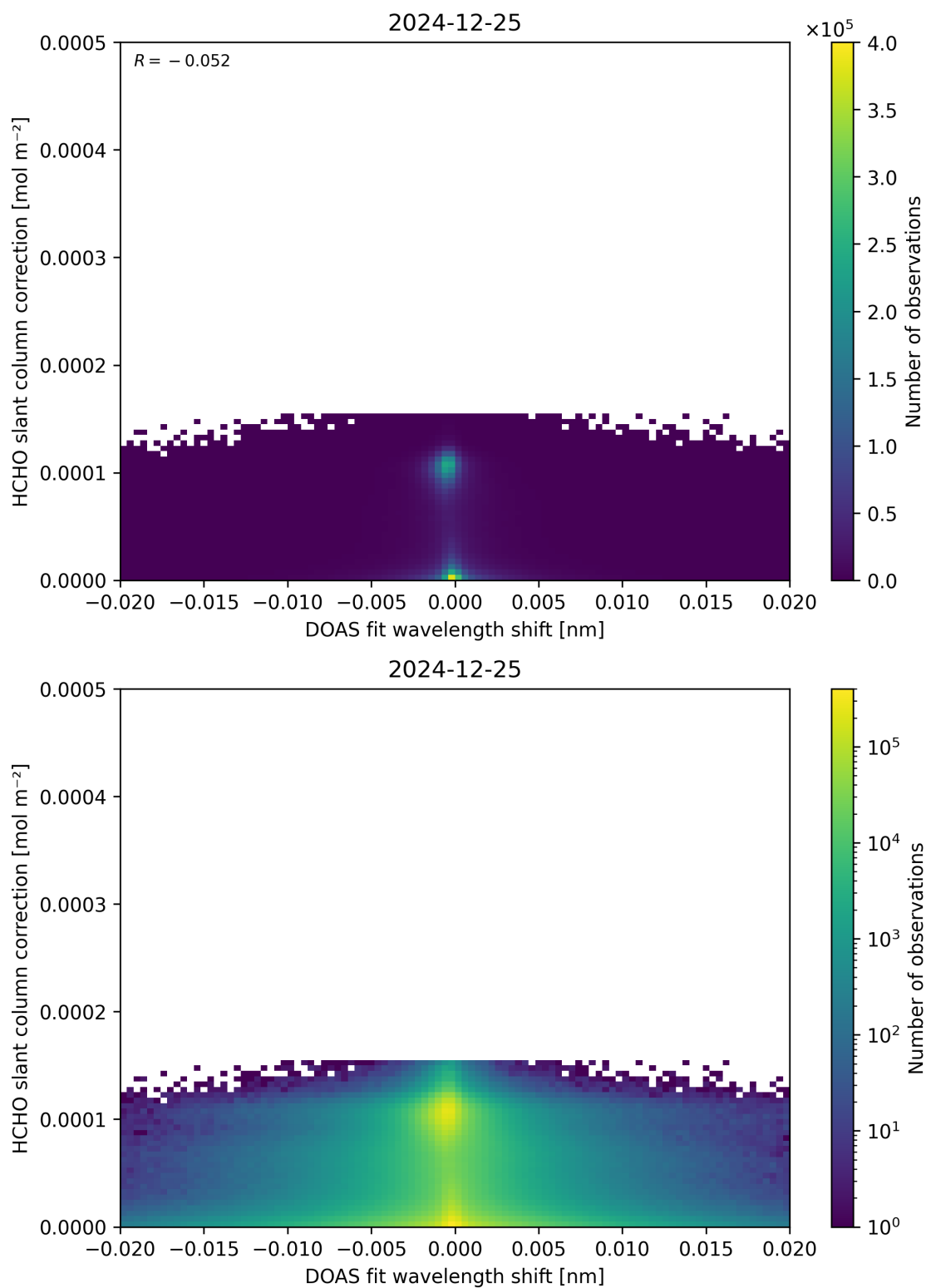
Figure 67: Scatter density plot of “DOAS fit wavelength shift” against “HCHO slant column correction” for 2024-12-24 to 2024-12-26.
