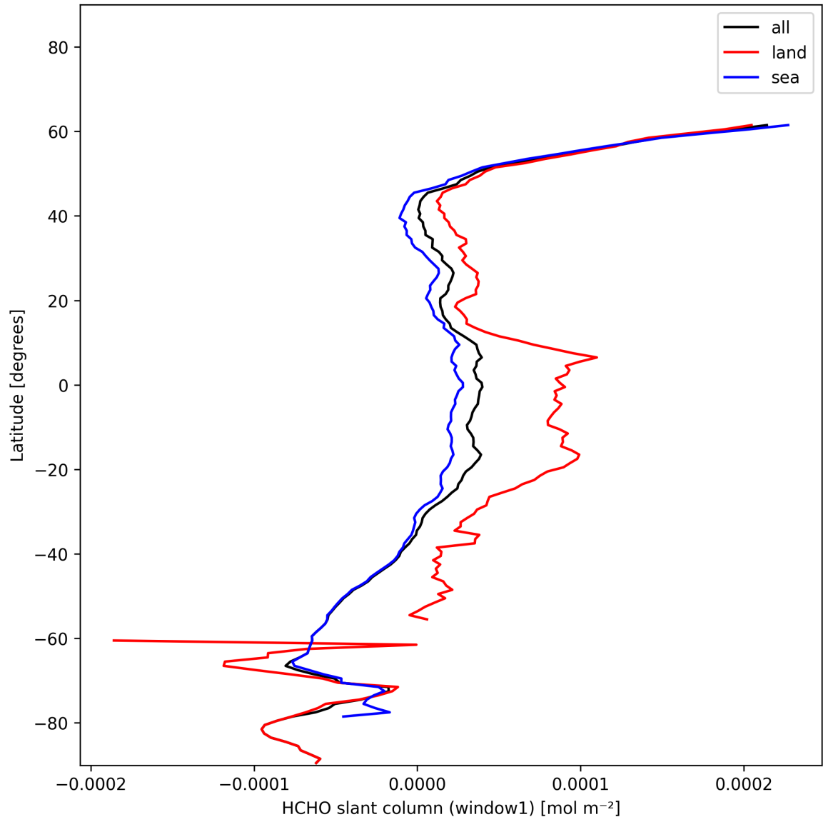
Figure 24: Zonal average of “HCHO slant column (window1)” for 2024-12-24 to 2024-12-26.
