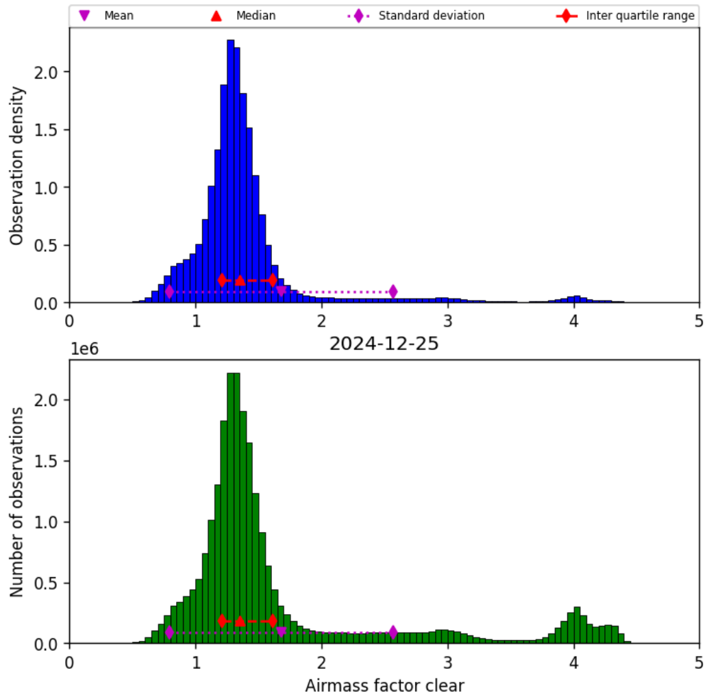
Figure 42: Histogram of “Airmass factor clear” for 2024-12-24 to 2024-12-26
