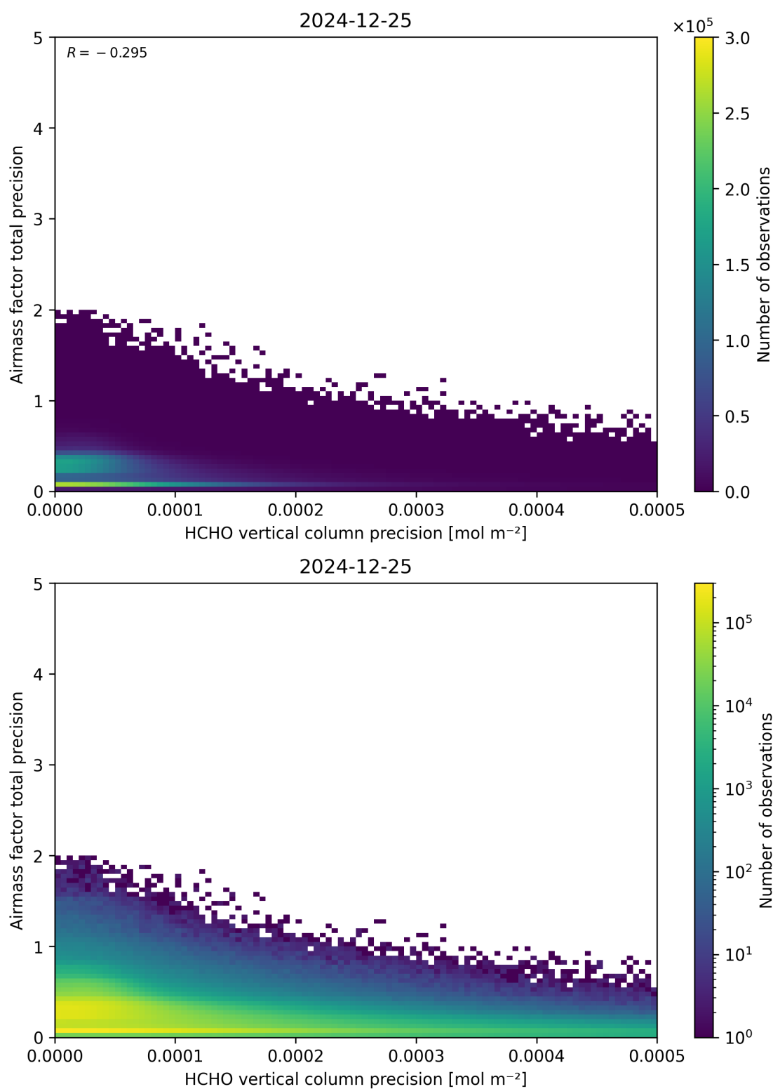
Figure 145: Scatter density plot of “HCHO vertical column precision” against “Airmass factor total precision” for 2024-12-24 to 2024-12-26.
