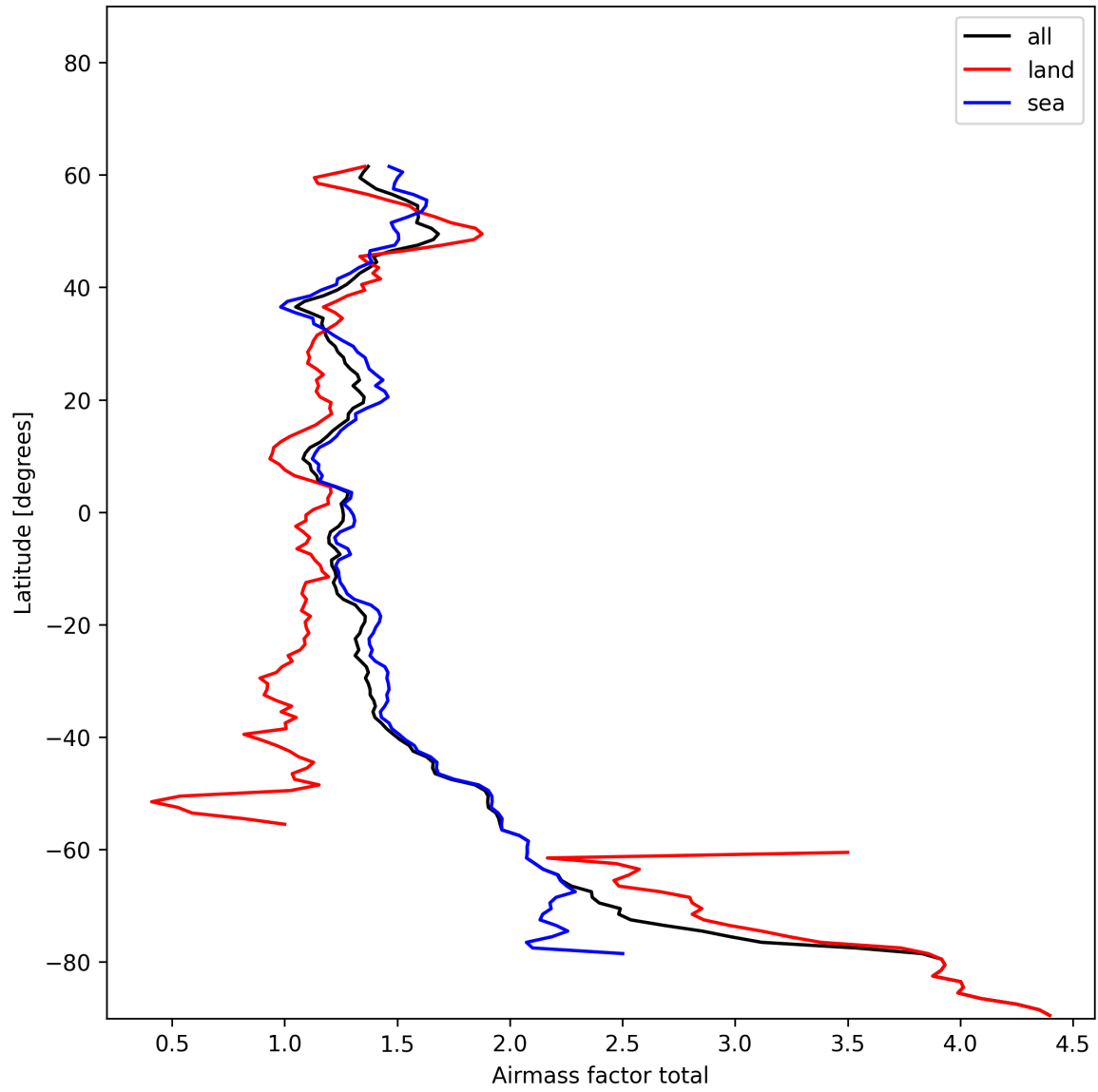
Figure 26: Zonal average of “Airmass factor total” for 2024-12-24 to 2024-12-26.
