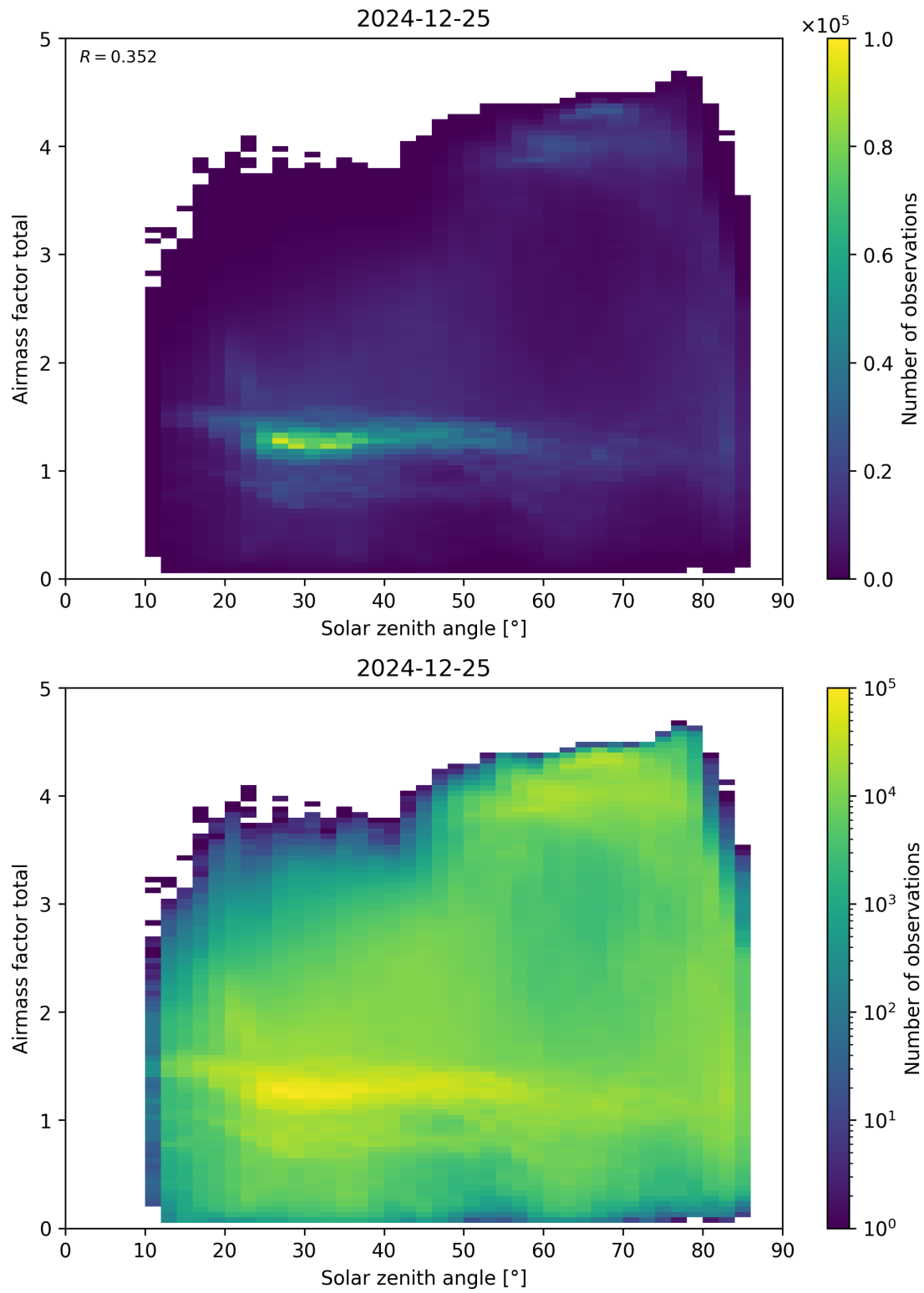
Figure 175: Scatter density plot of “Solar zenith angle” against “Airmass factor total” for 2024-12-24 to 2024-12-26.
