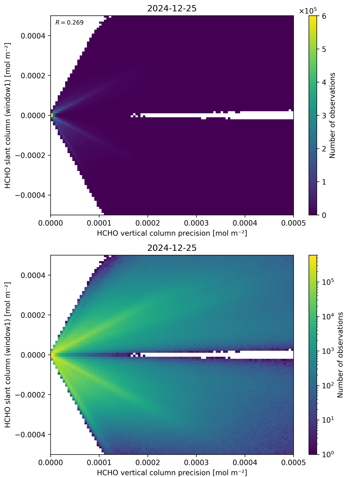
Figure 142: Scatter density plot of “HCHO vertical column precision” against “HCHO slant column (window1)” for 2024-12-24 to 2024-12-26.
