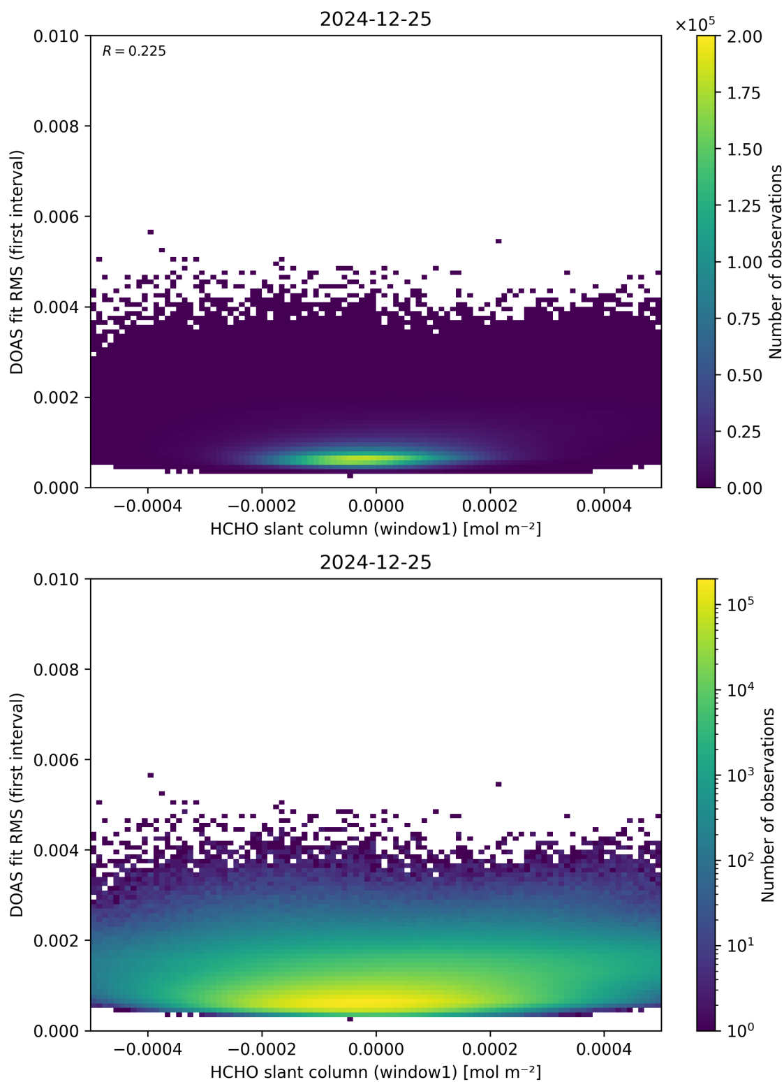
Figure 78: Scatter density plot of “HCHO slant column (window1)” against “DOAS fit RMS (first interval)” for 2024-12-24 to 2024-12-26.
