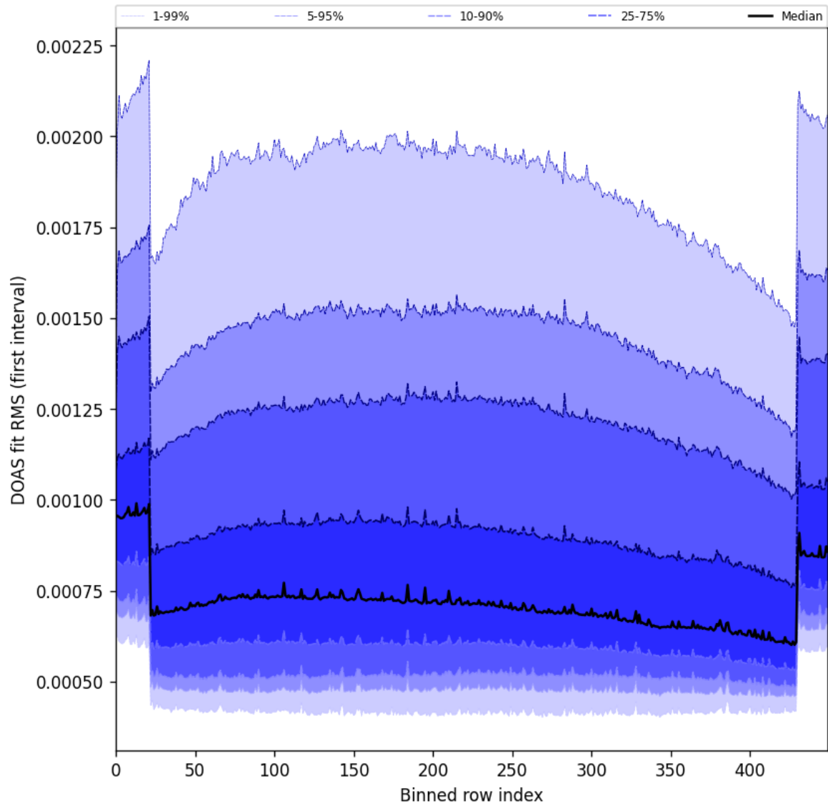
Figure 60: Along track statistics of “DOAS fit RMS (first interval)” for 2024-12-24 to 2024-12-26
