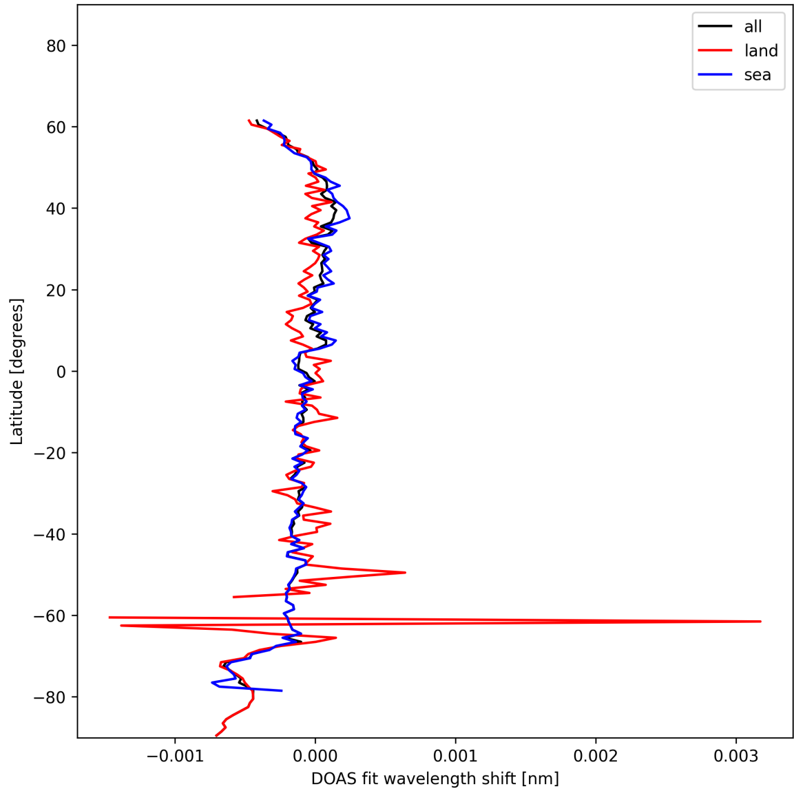
Figure 30: Zonal average of “DOAS fit wavelength shift” for 2024-12-24 to 2024-12-26.
