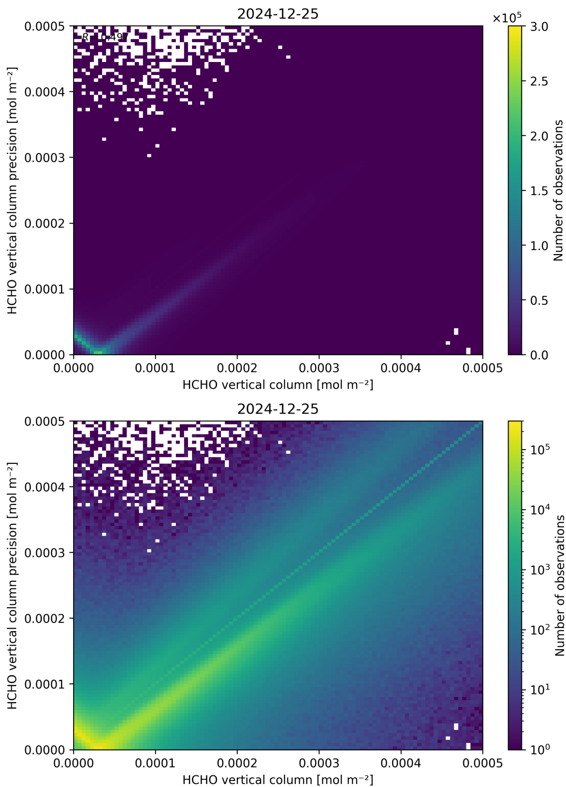
Figure 134: Scatter density plot of “HCHO vertical column” against “HCHO vertical column precision” for 2024-12-24 to 2024-12-26.
