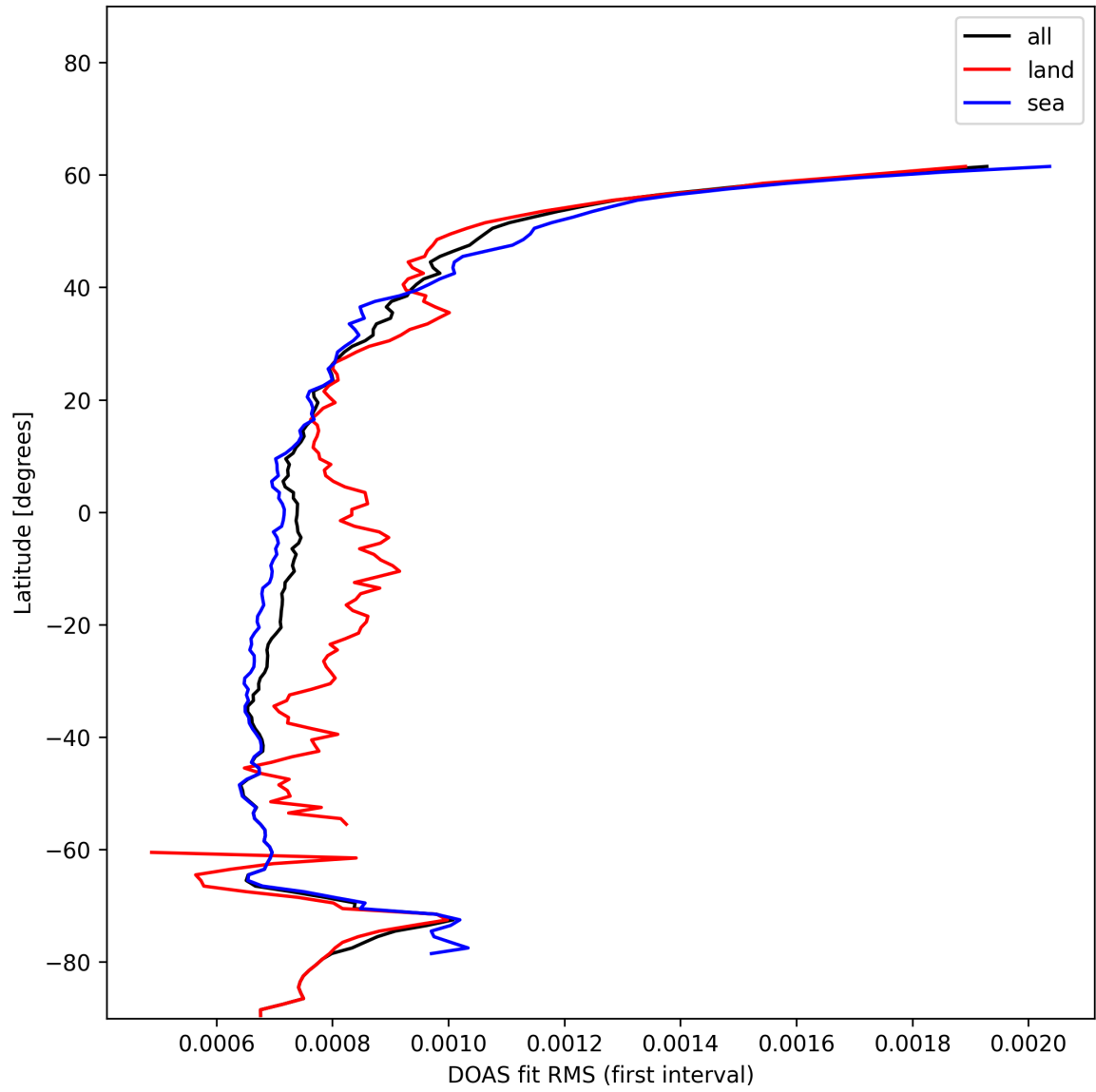
Figure 32: Zonal average of “DOAS fit RMS (first interval)” for 2024-12-24 to 2024-12-26.
