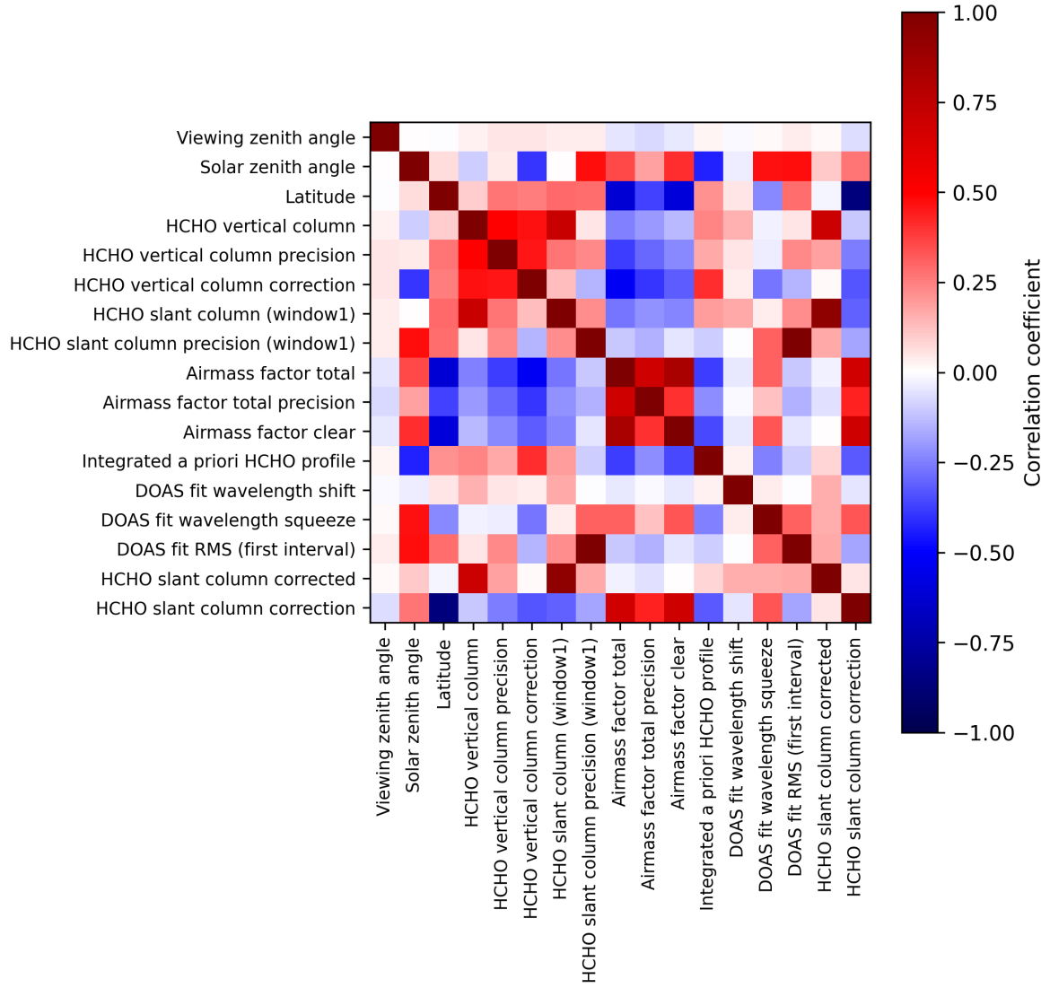
Figure 2: Map of correlation matrix for 2024-12-24 to 2024-12-26.
