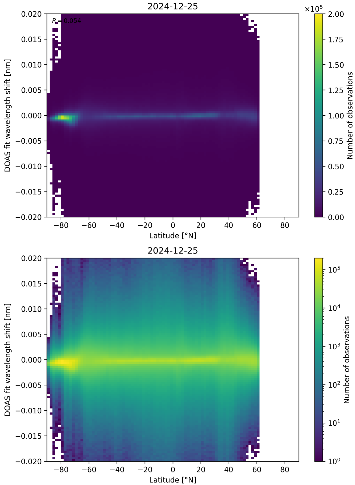
Figure 154: Scatter density plot of “Latitude” against “DOAS fit wavelength shift” for 2024-12-24 to 2024-12-26.
