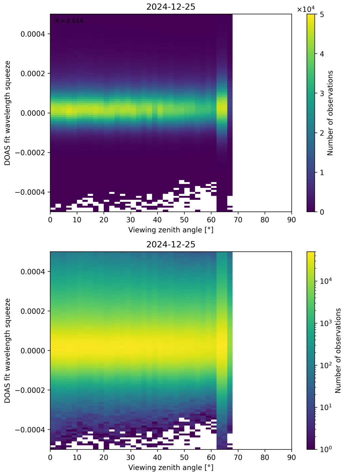
Figure 184: Scatter density plot of “Viewing zenith angle” against “DOAS fit wavelength squeeze” for 2024-12-24 to 2024-12-26.
