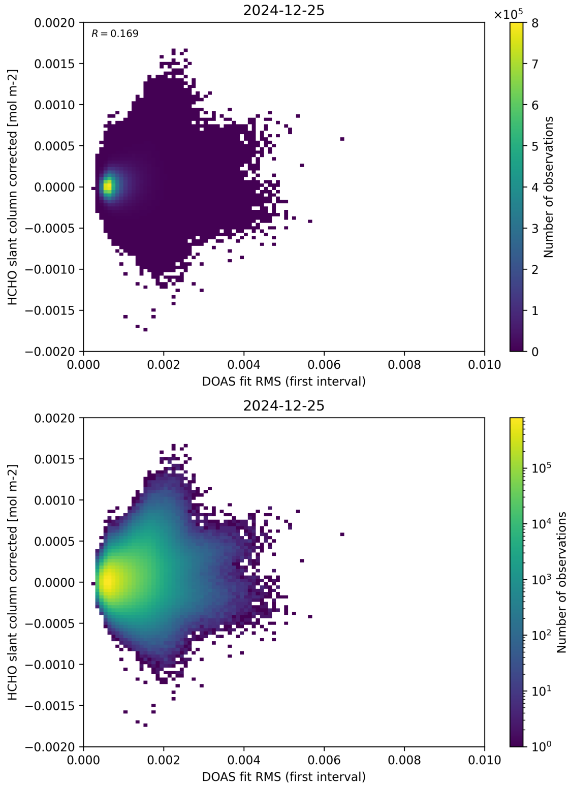
Figure 62: Scatter density plot of “DOAS fit RMS (first interval)” against “HCHO slant column corrected” for 2024-12-24 to 2024-12-26.
