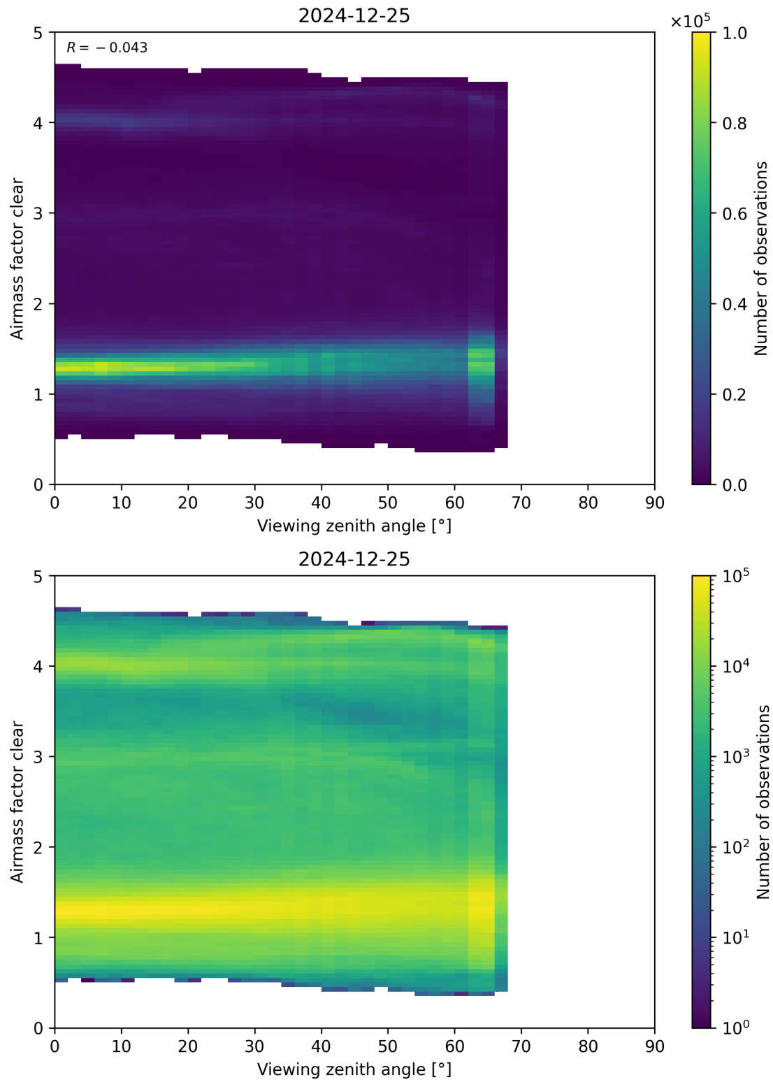
Figure 185: Scatter density plot of “Viewing zenith angle” against “Airmass factor clear” for 2024-12-24 to 2024-12-26.
