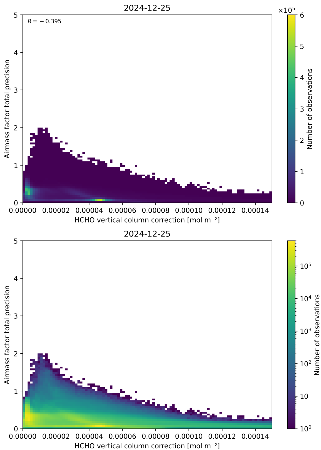
Figure 121: Scatter density plot of “HCHO vertical column correction” against “Airmass factor total precision” for 2024-12-24 to 2024-12-26.
