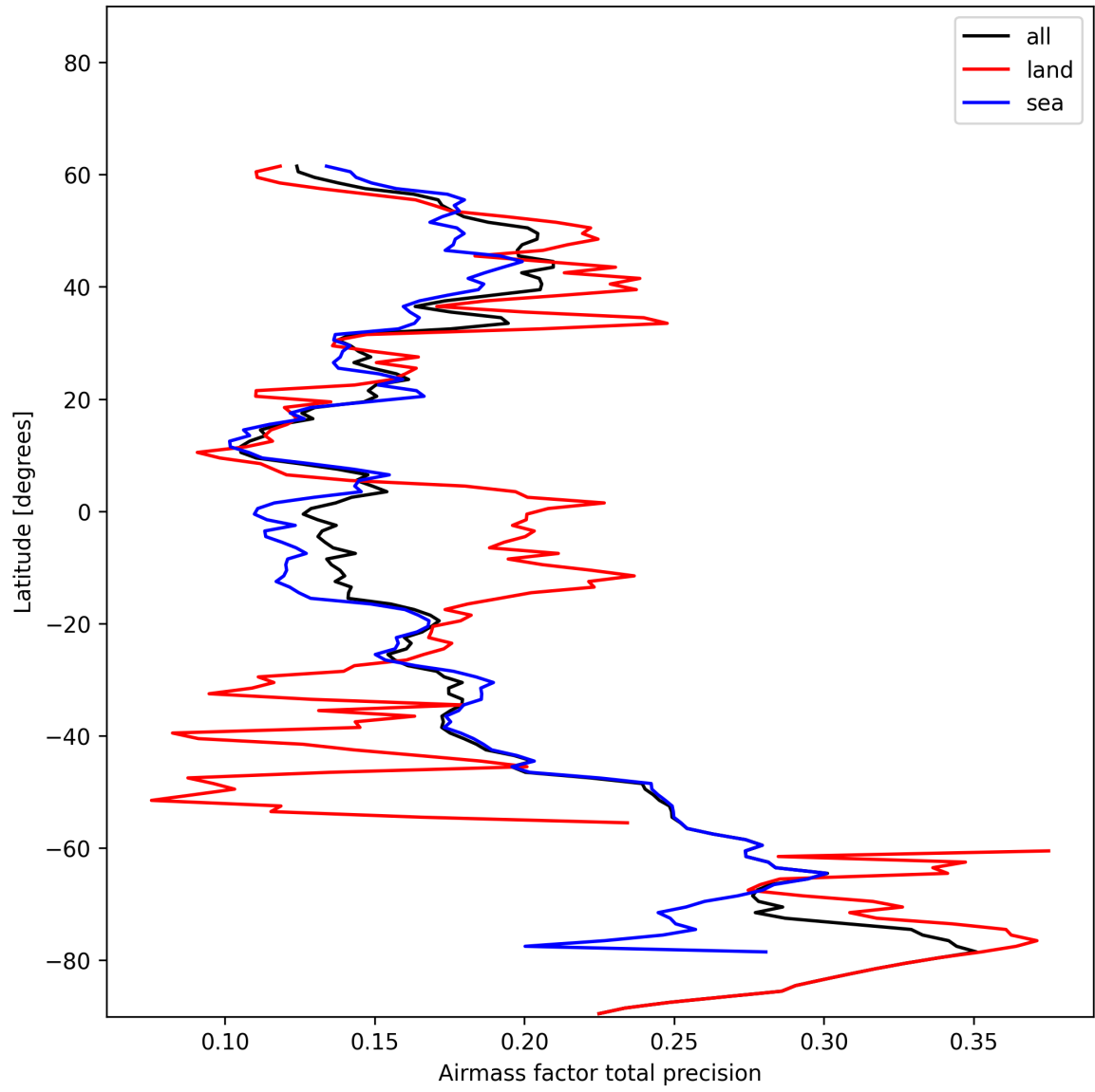
Figure 27: Zonal average of “Airmass factor total precision” for 2024-12-24 to 2024-12-26.
