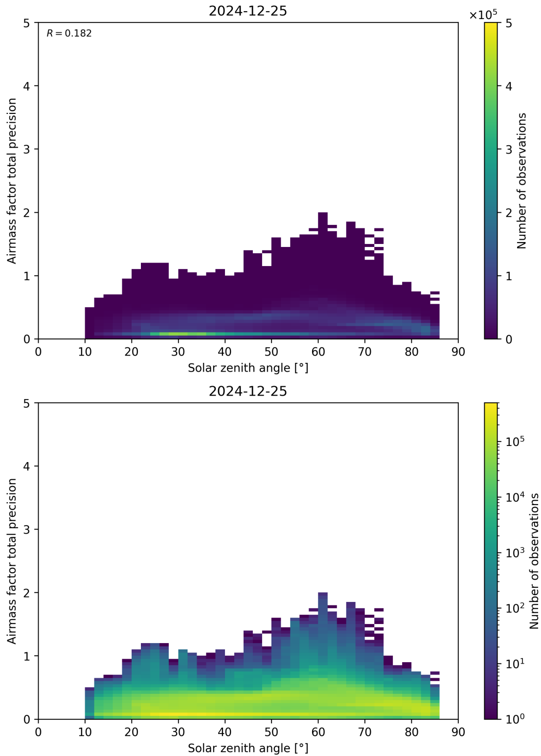
Figure 176: Scatter density plot of “Solar zenith angle” against “Airmass factor total precision” for 2024-12-24 to 2024-12-26.
