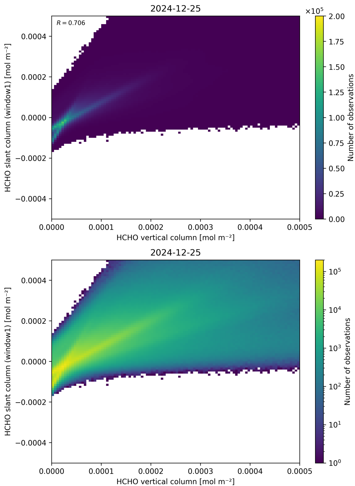
Figure 129: Scatter density plot of “HCHO vertical column” against “HCHO slant column (window1)” for 2024-12-24 to 2024-12-26.
