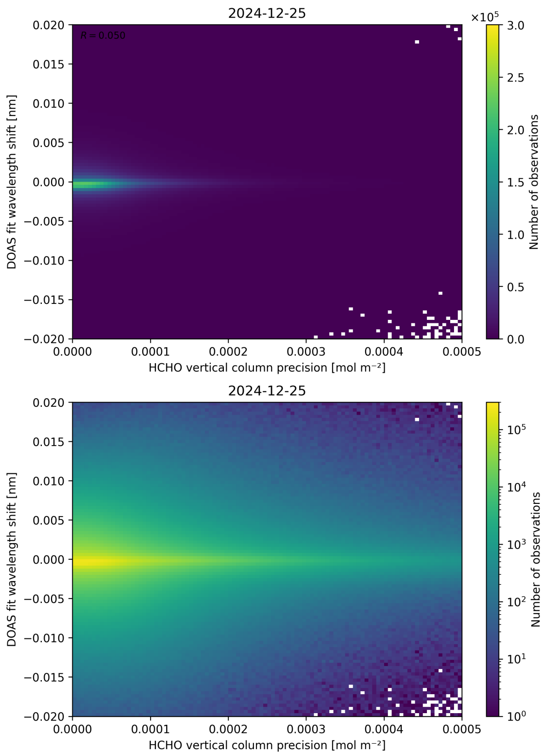
Figure 137: Scatter density plot of “HCHO vertical column precision” against “DOAS fit wavelength shift” for 2024-12-24 to 2024-12-26.
