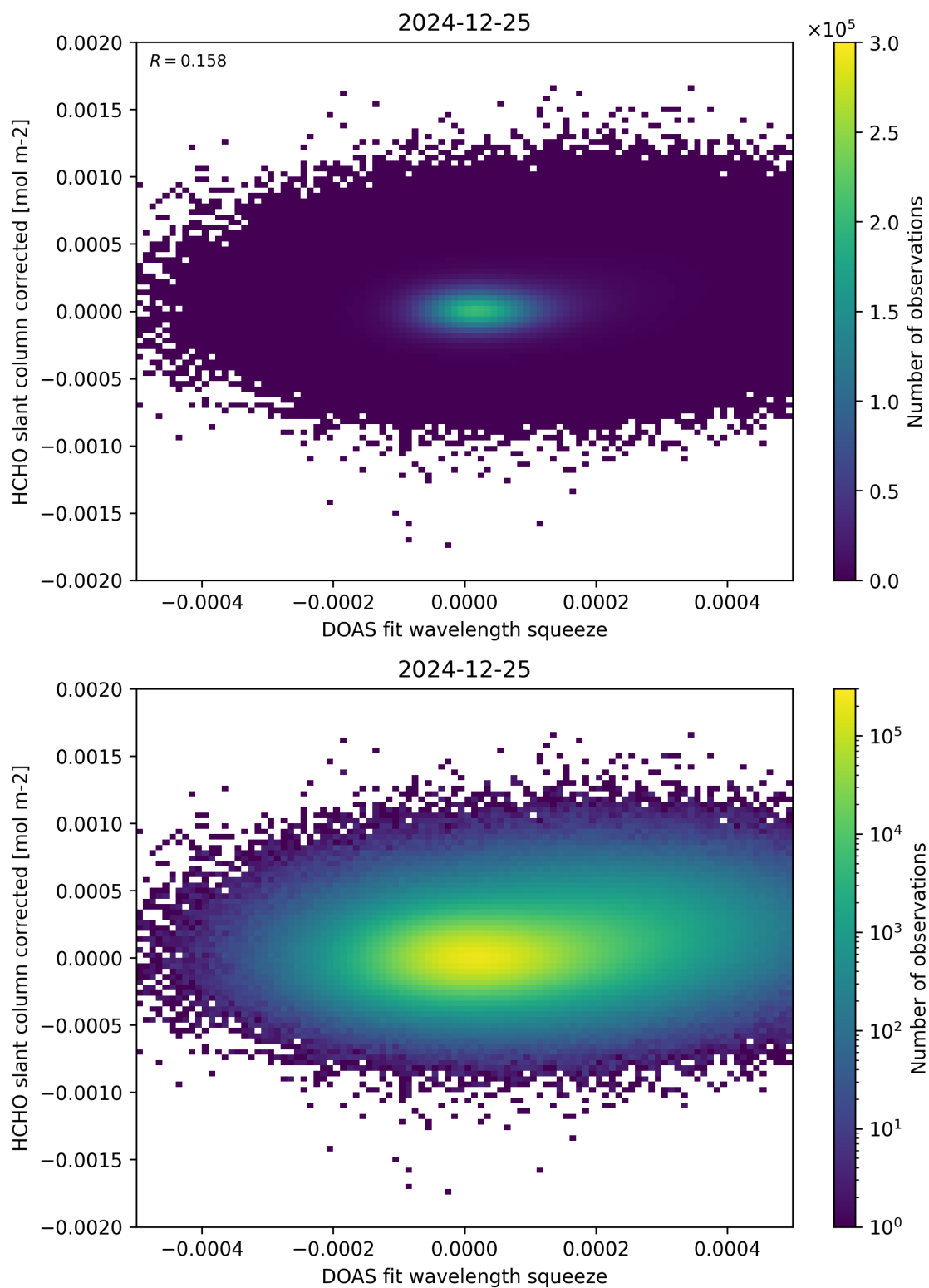
Figure 69: Scatter density plot of “DOAS fit wavelength squeeze” against “HCHO slant column corrected” for 2024-12-24 to 2024-12-26.
