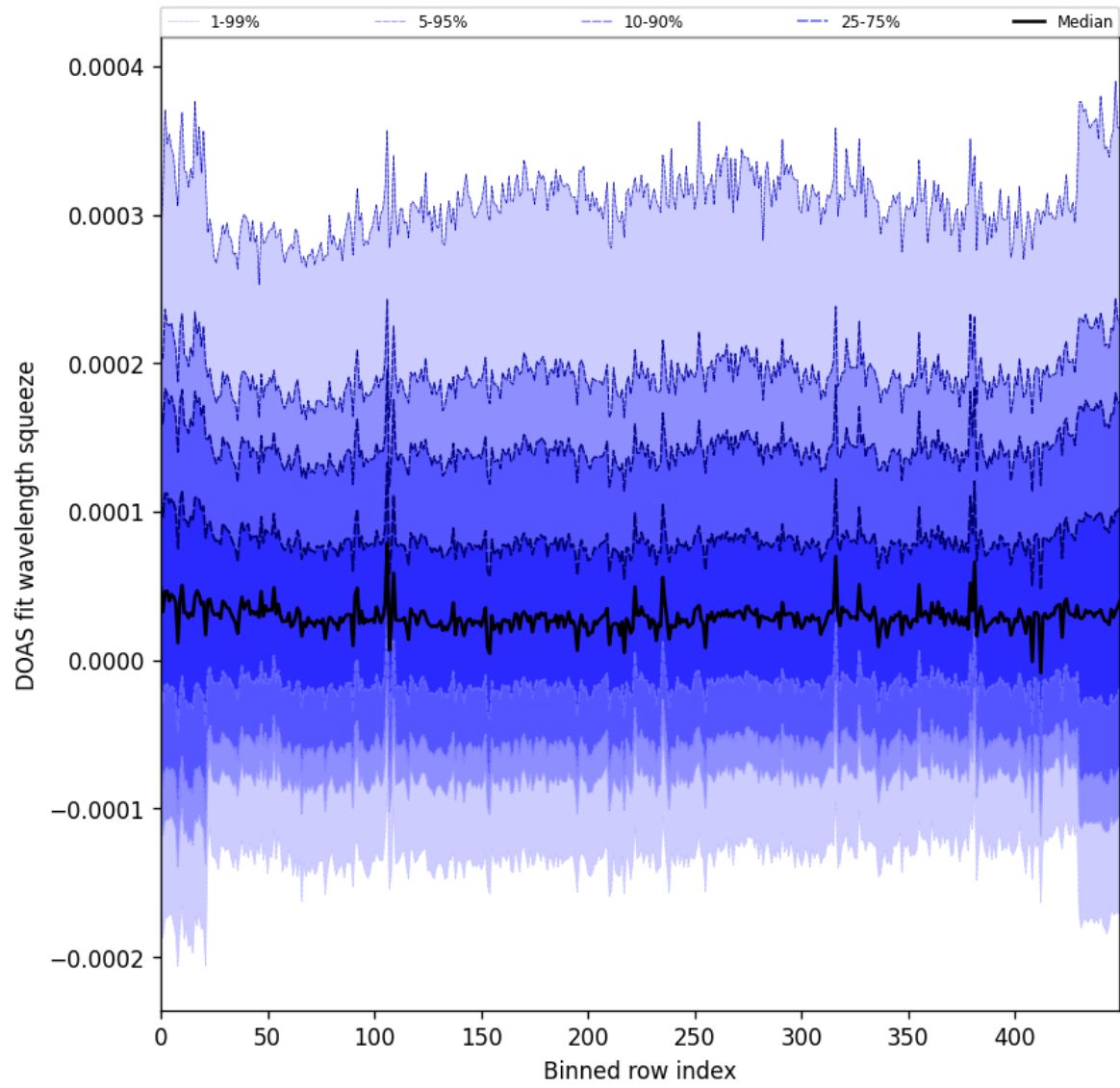
Figure 59: Along track statistics of “DOAS fit wavelength squeeze” for 2024-12-24 to 2024-12-26
