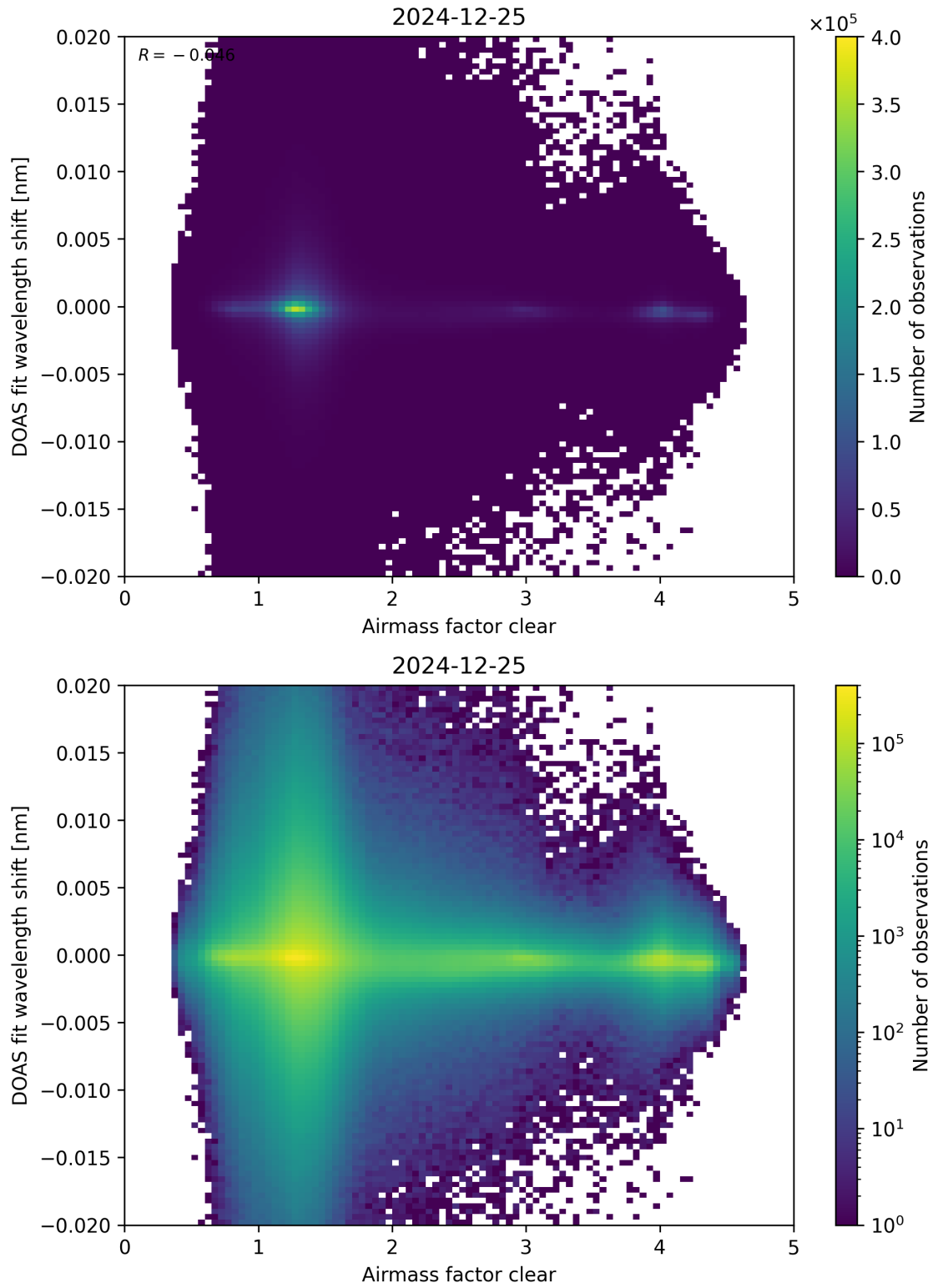
Figure 72: Scatter density plot of “Airmass factor clear” against “DOAS fit wavelength shift” for 2024-12-24 to 2024-12-26.
