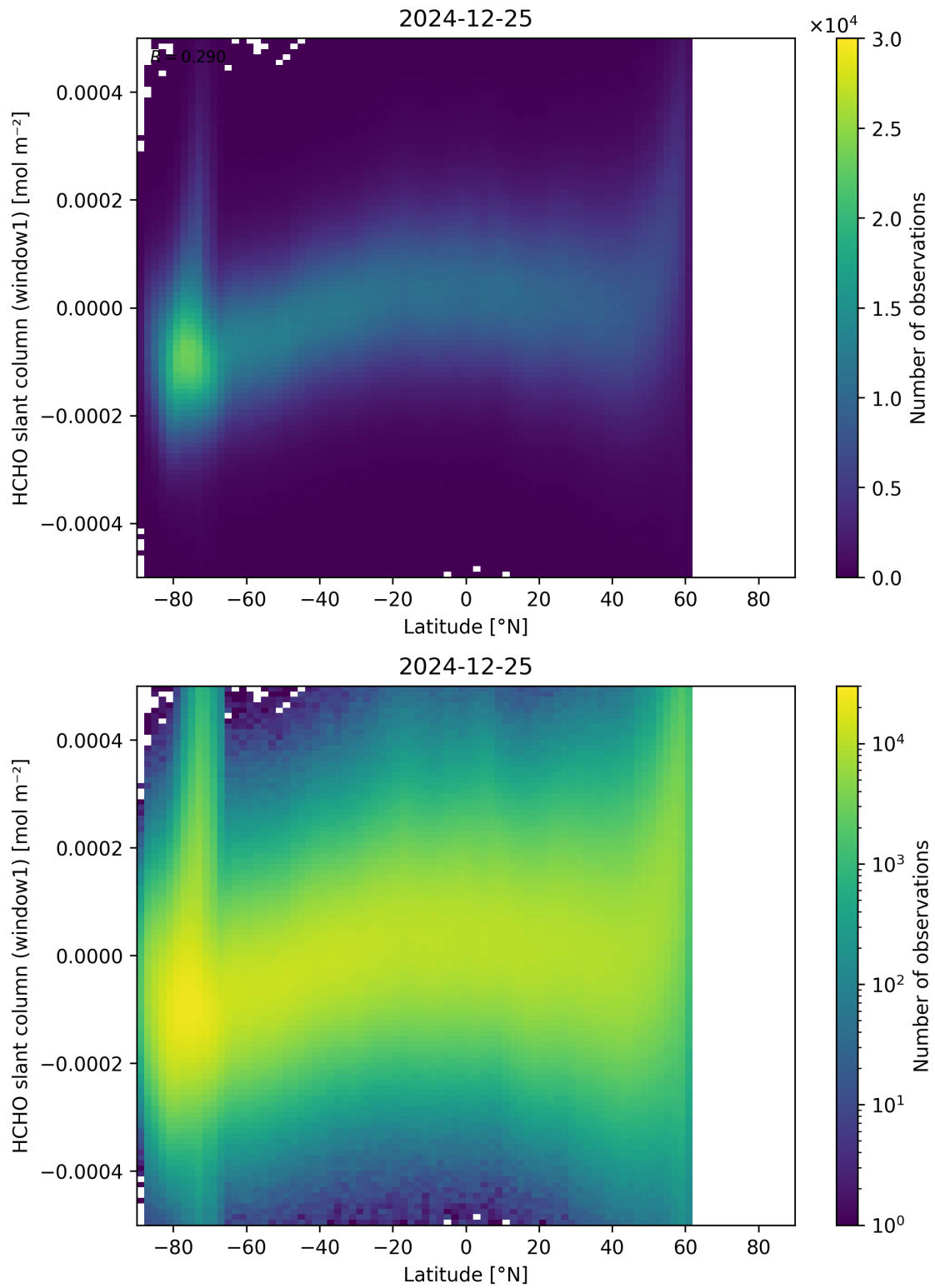
Figure 159: Scatter density plot of “Latitude” against “HCHO slant column (window1)” for 2024-12-24 to 2024-12-26.
