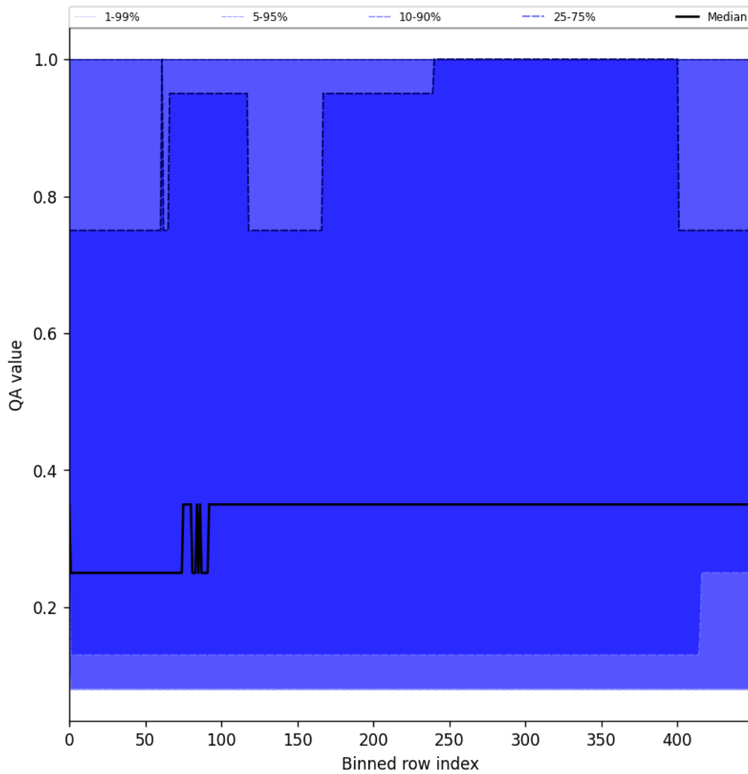
Figure 48: Along track statistics of “QA value” for 2024-12-24 to 2024-12-26
