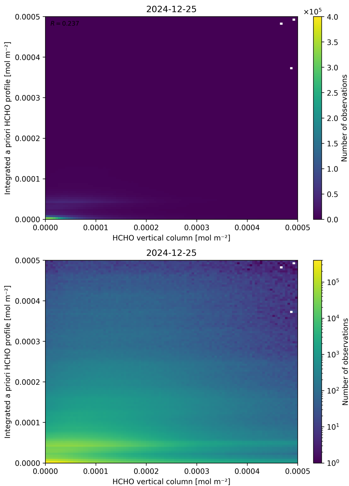
Figure 135: Scatter density plot of “HCHO vertical column” against “Integrated a priori HCHO profile” for 2024-12-24 to 2024-12-26.
