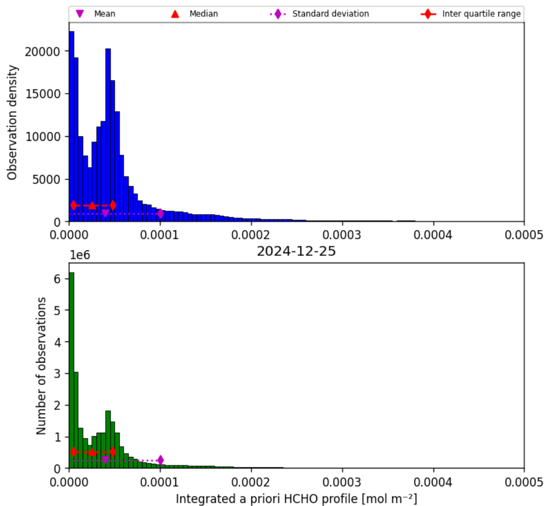
Figure 43: Histogram of “Integrated a priori HCHO profile” for 2024-12-24 to 2024-12-26
