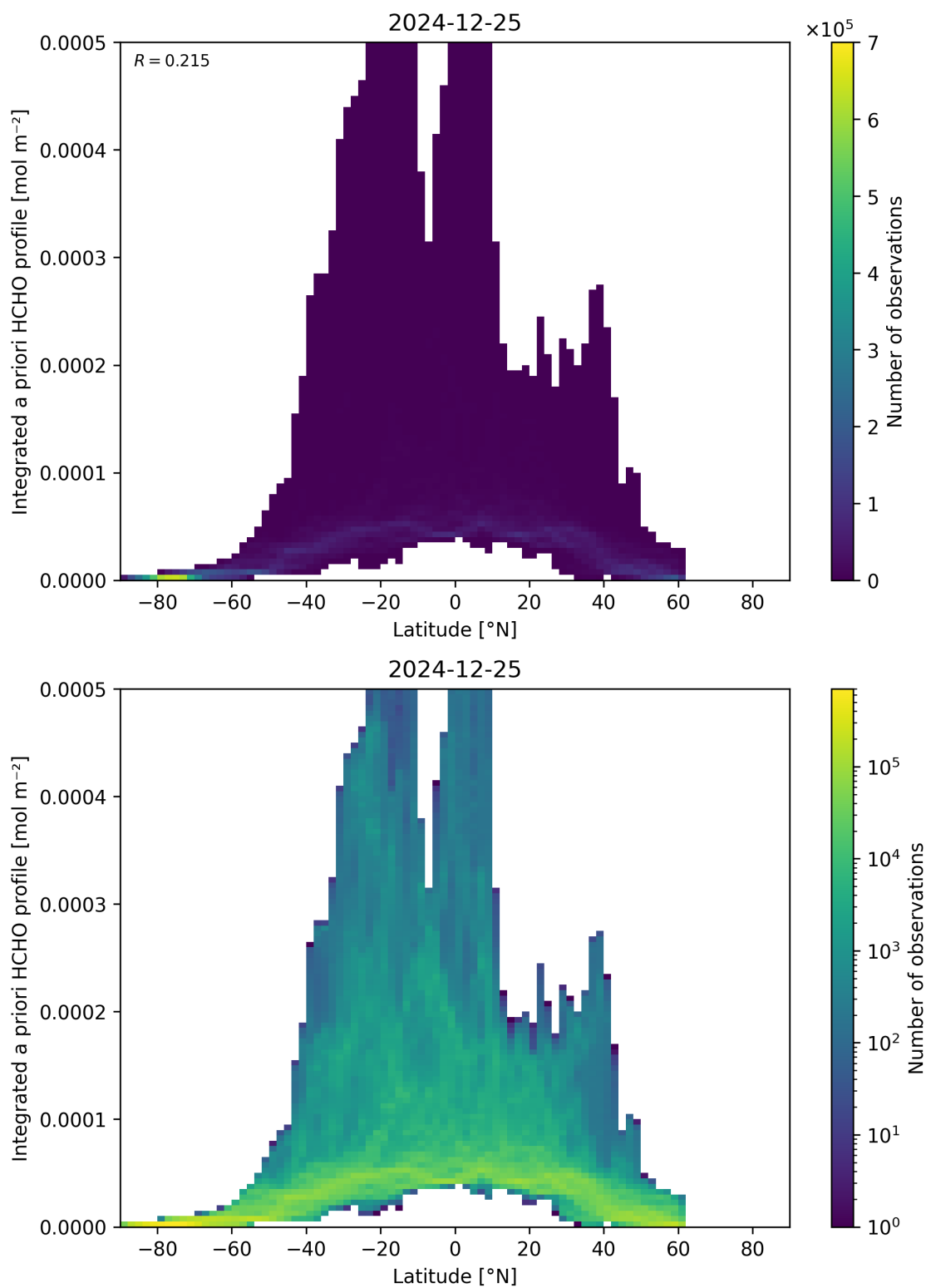
Figure 166: Scatter density plot of “Latitude” against “Integrated a priori HCHO profile” for 2024-12-24 to 2024-12-26.
