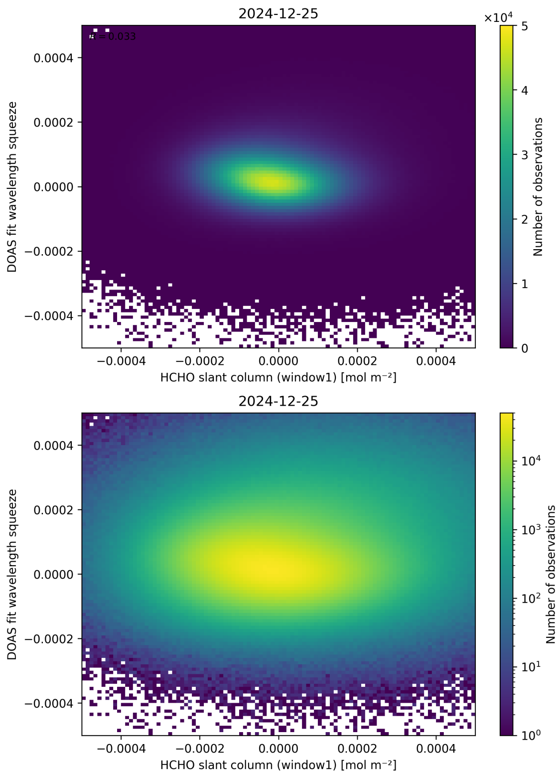
Figure 80: Scatter density plot of “HCHO slant column (window1)” against “DOAS fit wavelength squeeze” for 2024-12-24 to 2024-12-26.
