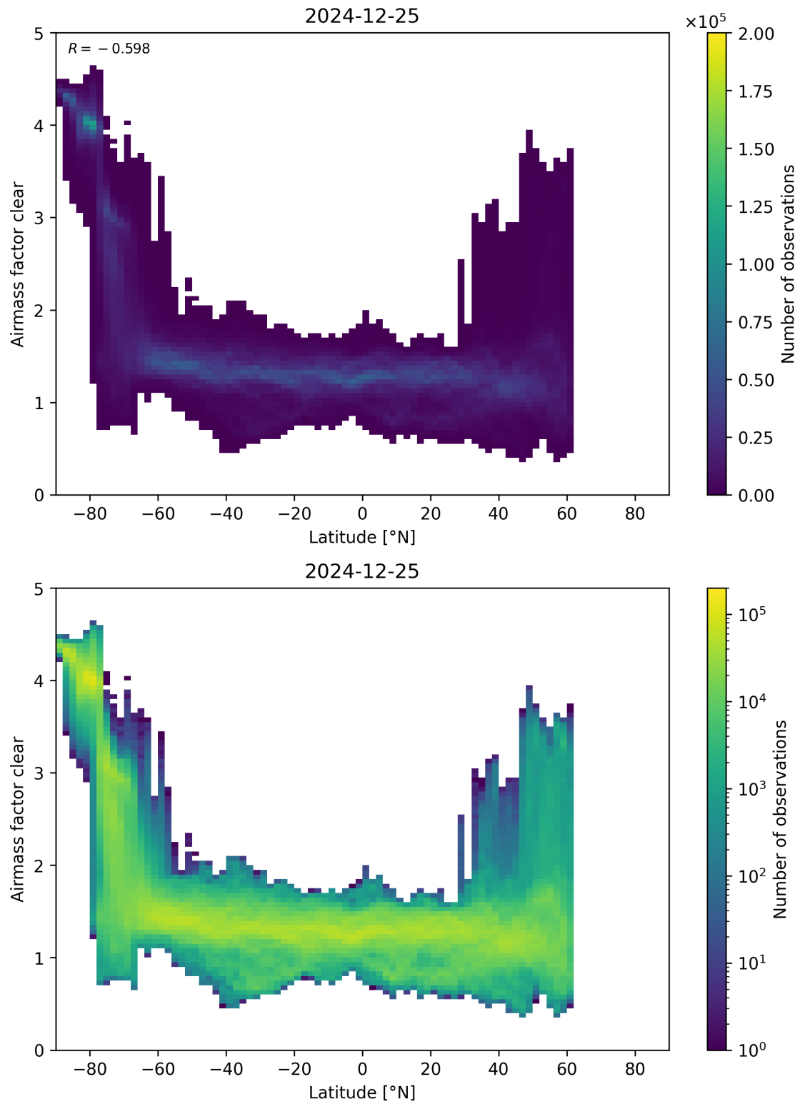
Figure 156: Scatter density plot of “Latitude” against “Airmass factor clear” for 2024-12-24 to 2024-12-26.
