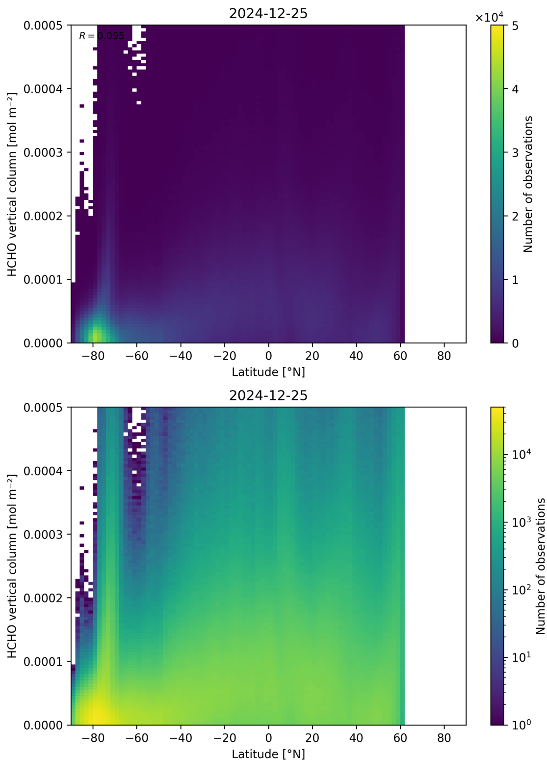
Figure 163: Scatter density plot of “Latitude” against “HCHO vertical column” for 2024-12-24 to 2024-12-26.
