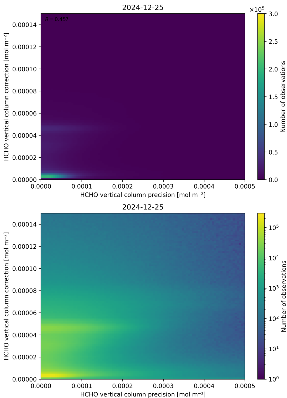
Figure 146: Scatter density plot of “HCHO vertical column precision” against “HCHO vertical column correction” for 2024-12-24 to 2024-12-26.
