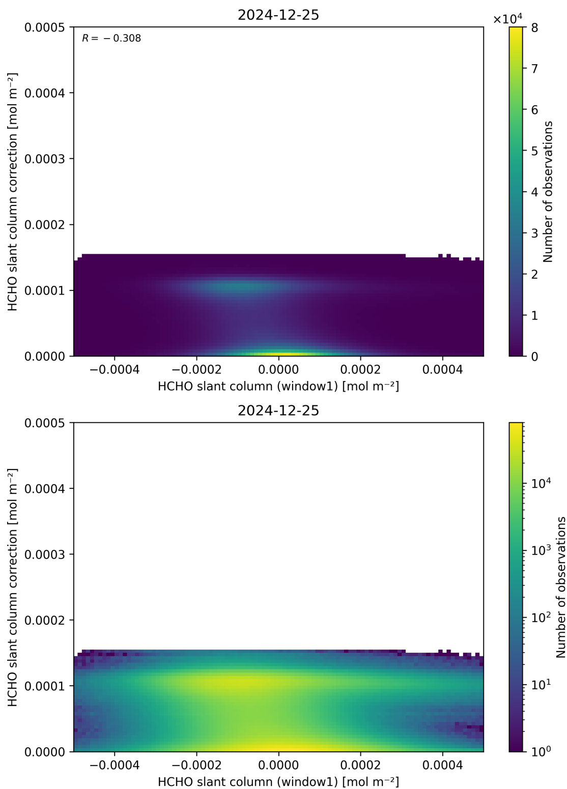
Figure 83: Scatter density plot of “HCHO slant column (window1)” against “HCHO slant column correction” for 2024-12-24 to 2024-12-26.
