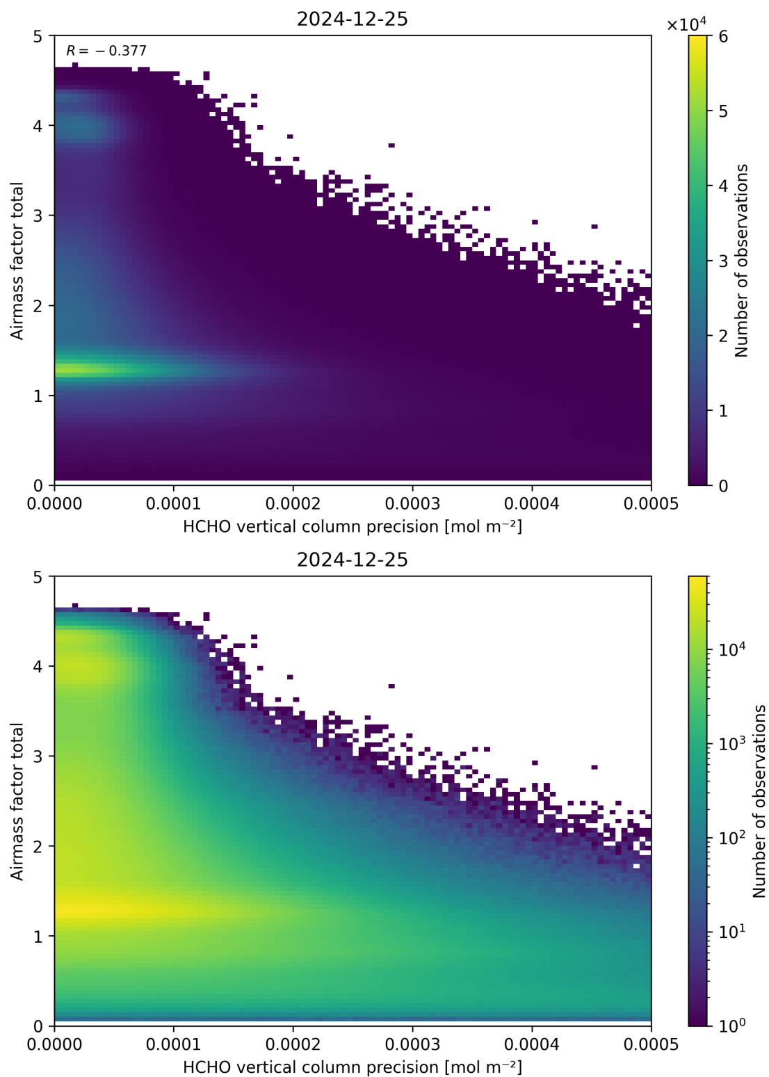
Figure 144: Scatter density plot of “HCHO vertical column precision” against “Airmass factor total” for 2024-12-24 to 2024-12-26.
