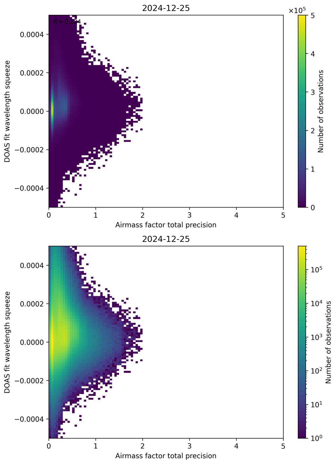
Figure 107: Scatter density plot of “Airmass factor total precision” against “DOAS fit wavelength squeeze” for 2024-12-24 to 2024-12-26.
