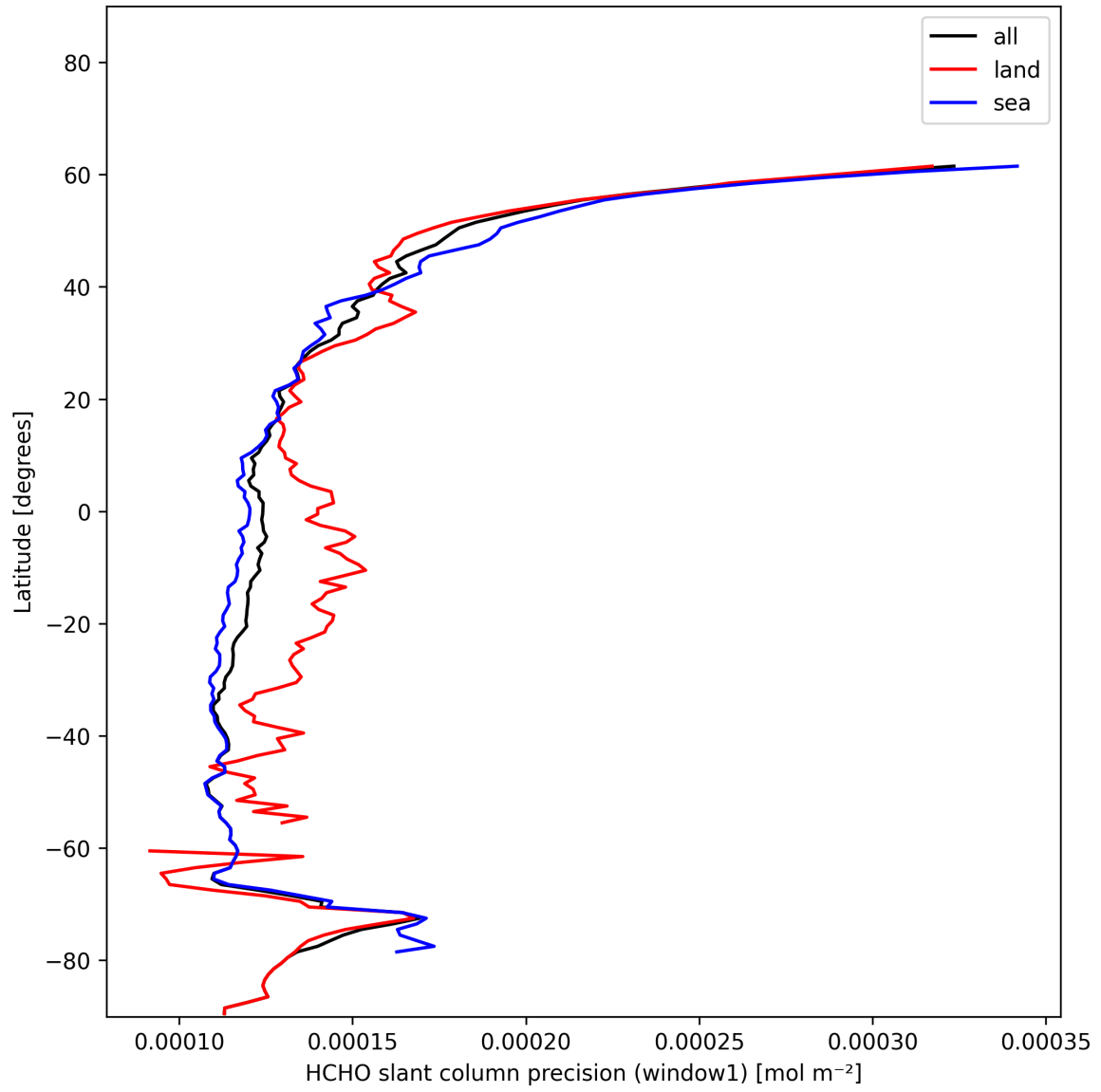
Figure 25: Zonal average of “HCHO slant column precision (window1)” for 2024-12-24 to 2024-12-26.
