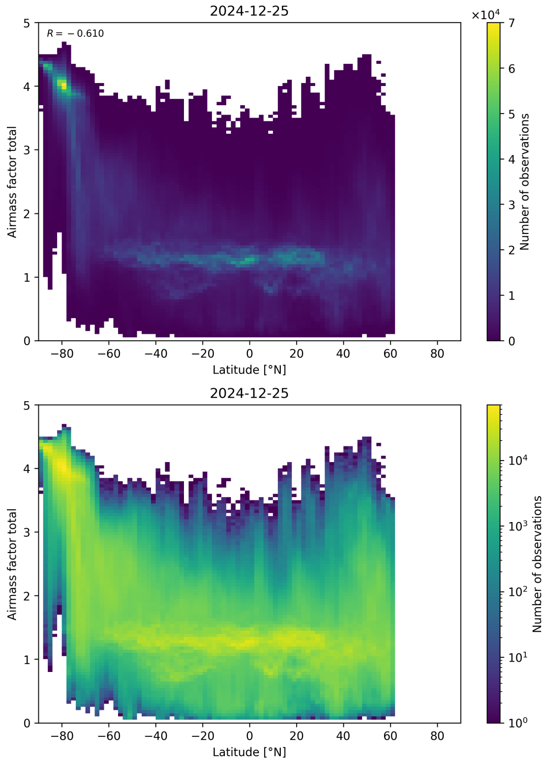
Figure 161: Scatter density plot of “Latitude” against “Airmass factor total” for 2024-12-24 to 2024-12-26.
