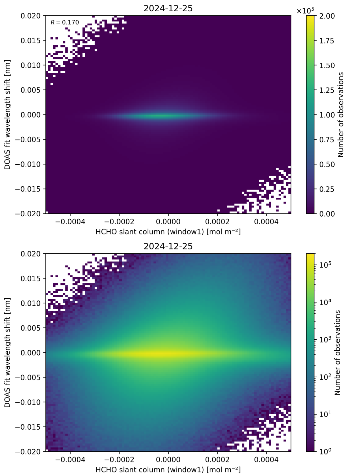
Figure 79: Scatter density plot of “HCHO slant column (window1)” against “DOAS fit wavelength shift” for 2024-12-24 to 2024-12-26.
