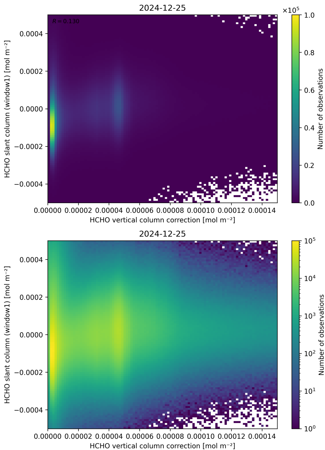
Figure 118: Scatter density plot of “HCHO vertical column correction” against “HCHO slant column (window1)” for 2024-12-24 to 2024-12-26.
