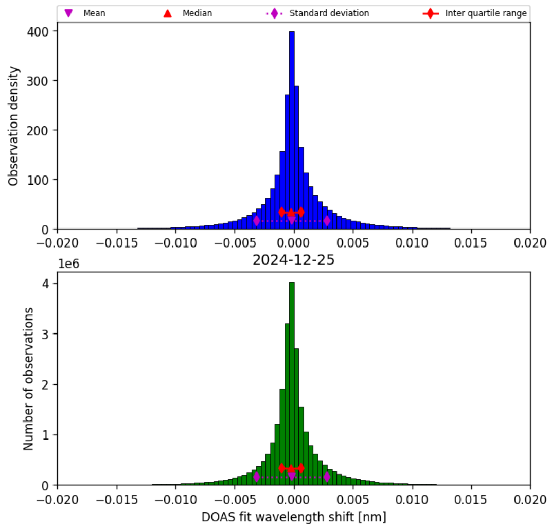
Figure 44: Histogram of “DOAS fit wavelength shift” for 2024-12-24 to 2024-12-26
