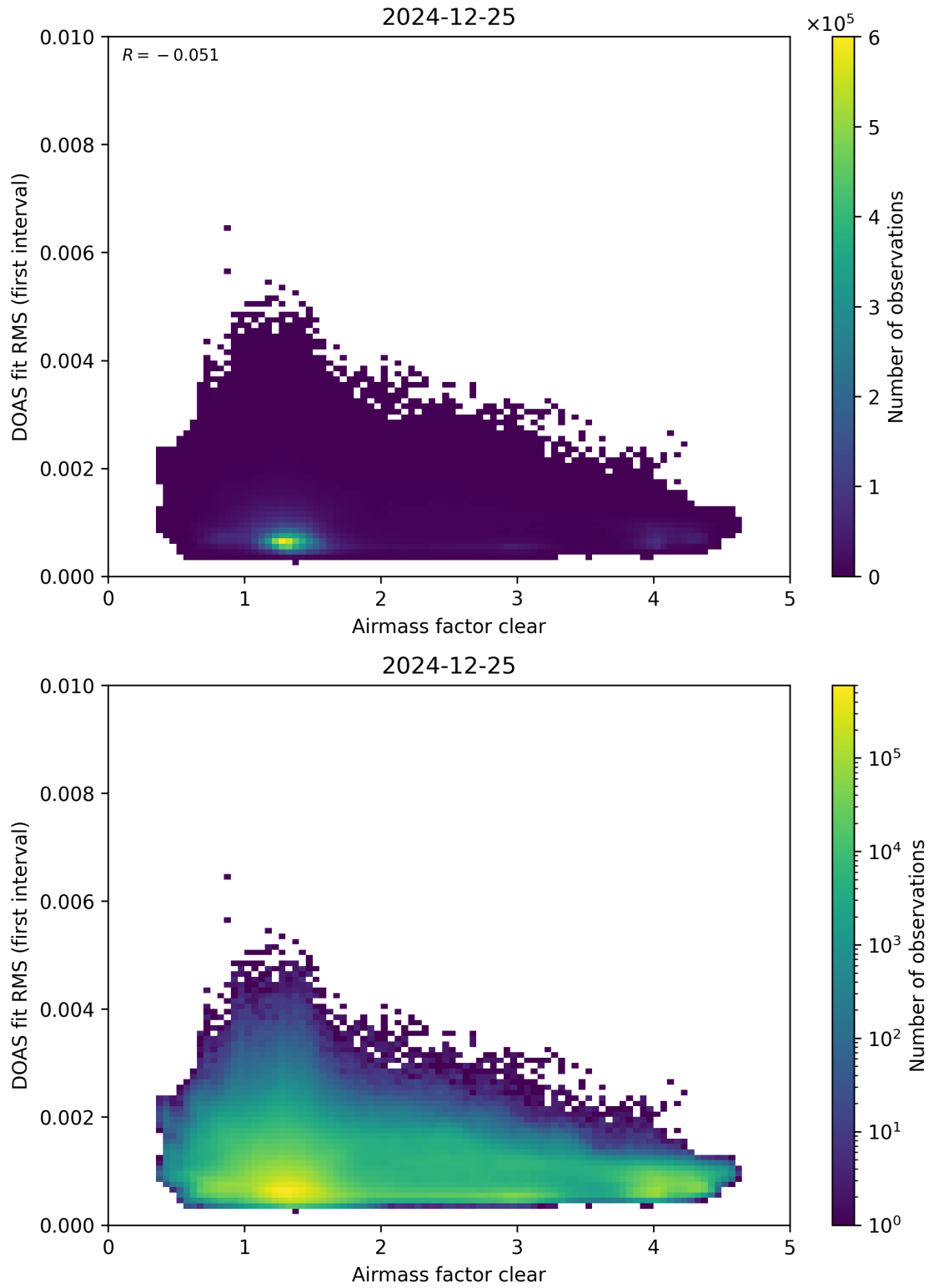
Figure 71: Scatter density plot of “Airmass factor clear” against “DOAS fit RMS (first interval)” for 2024-12-24 to 2024-12-26.
