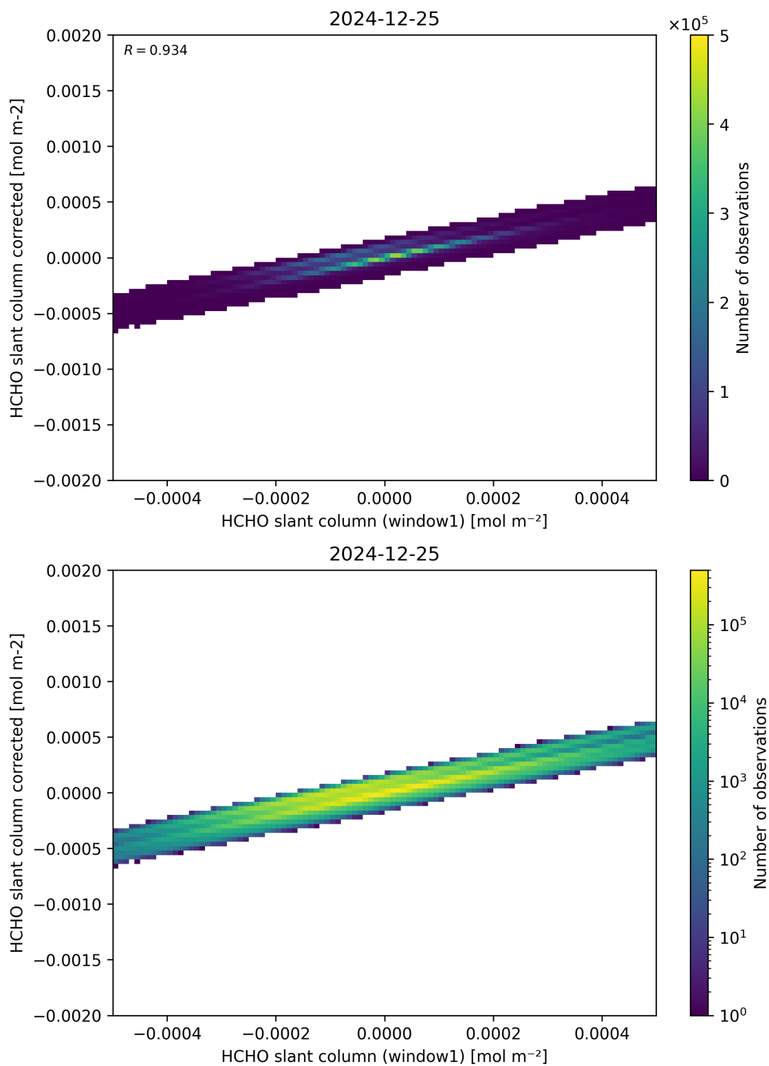
Figure 82: Scatter density plot of “HCHO slant column (window1)” against “HCHO slant column corrected” for 2024-12-24 to 2024-12-26.
