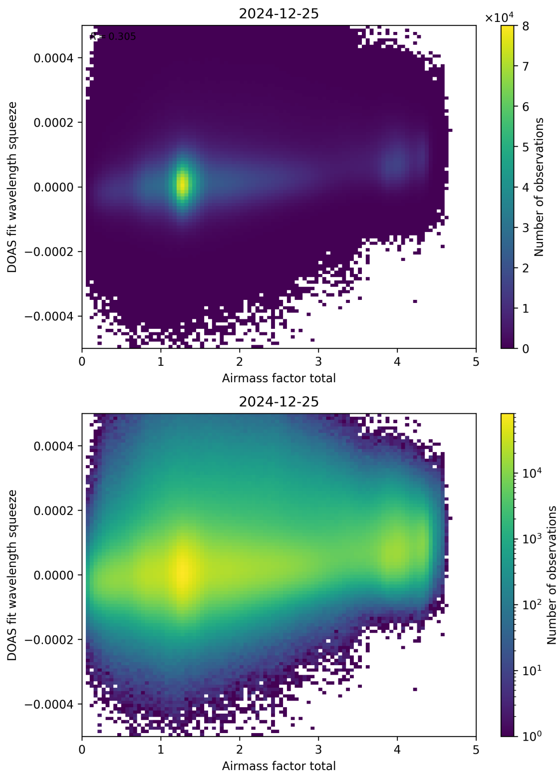
Figure 99: Scatter density plot of “Airmass factor total” against “DOAS fit wavelength squeeze” for 2024-12-24 to 2024-12-26.
