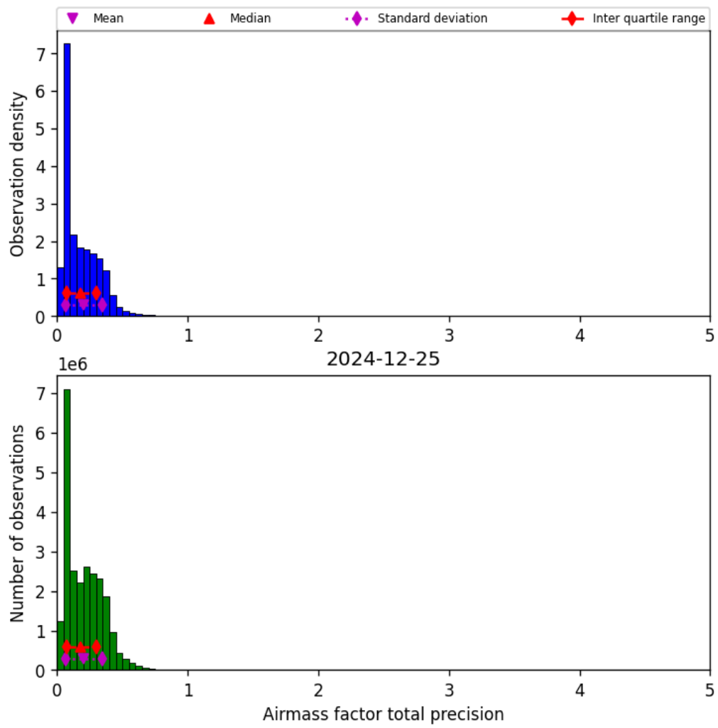
Figure 41: Histogram of “Airmass factor total precision” for 2024-12-24 to 2024-12-26
