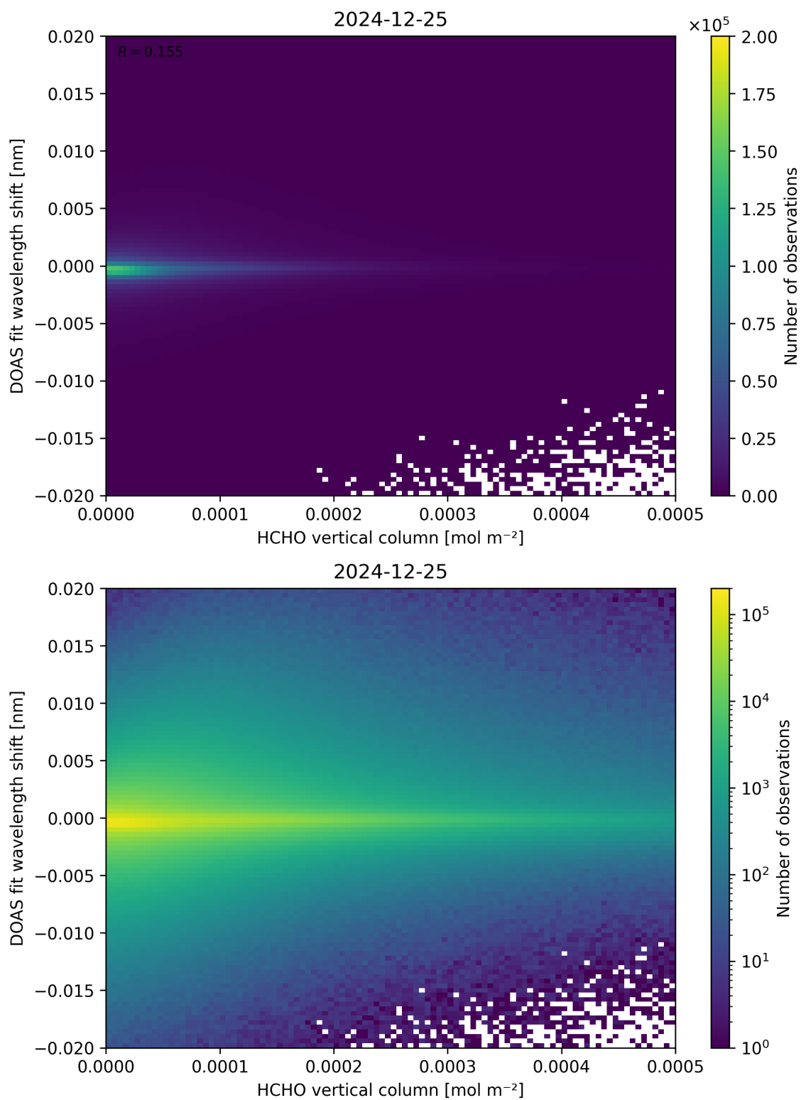
Figure 124: Scatter density plot of “HCHO vertical column” against “DOAS fit wavelength shift” for 2024-12-24 to 2024-12-26.
