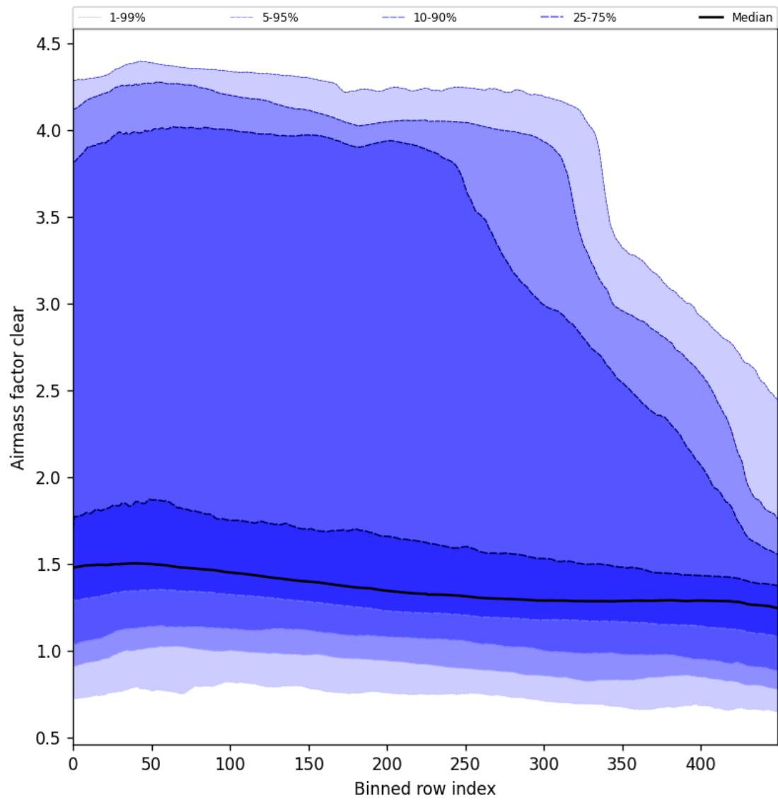
Figure 56: Along track statistics of “Airmass factor clear” for 2024-12-24 to 2024-12-26
