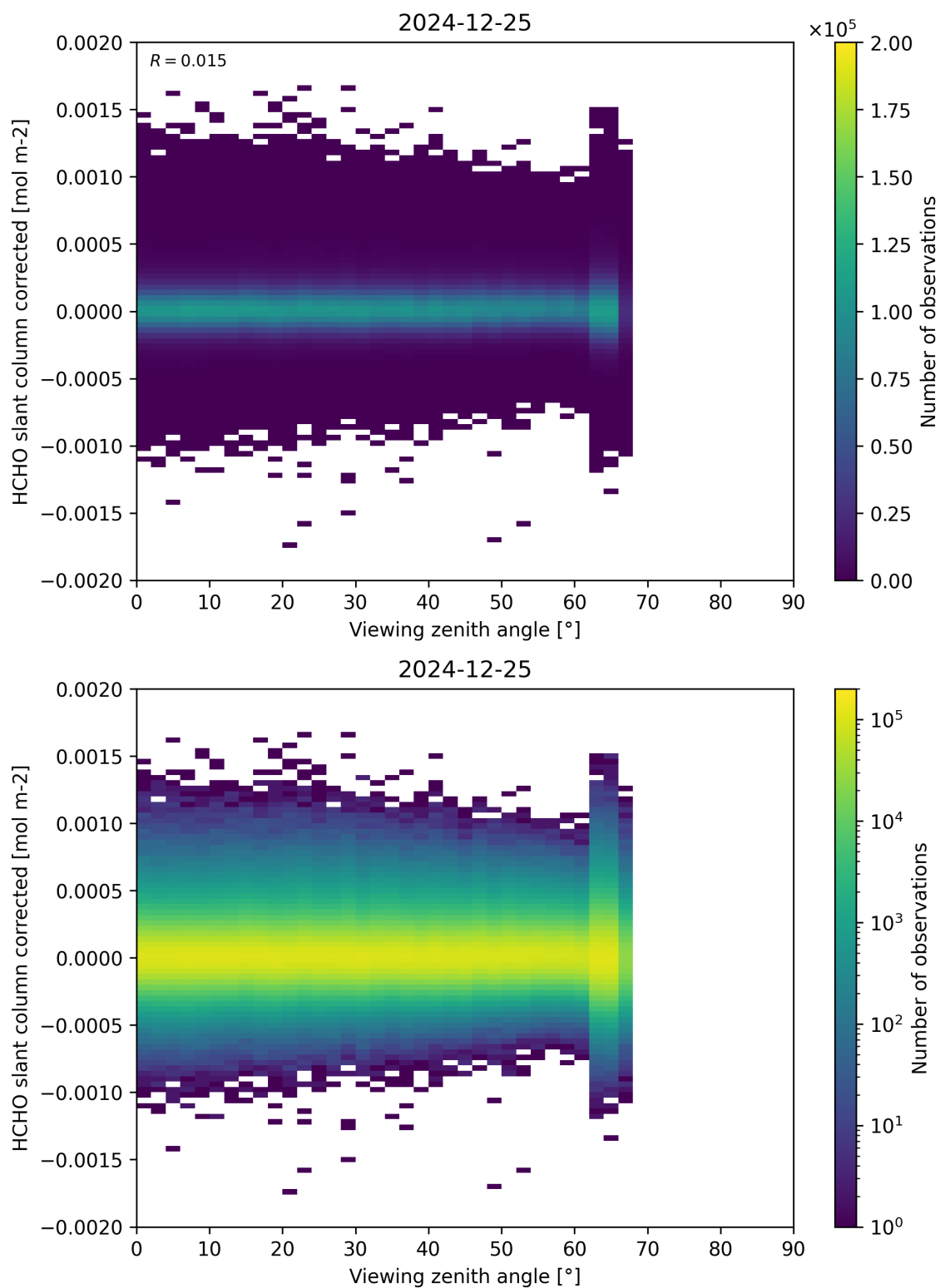
Figure 186: Scatter density plot of “Viewing zenith angle” against “HCHO slant column corrected” for 2024-12-24 to 2024-12-26.
