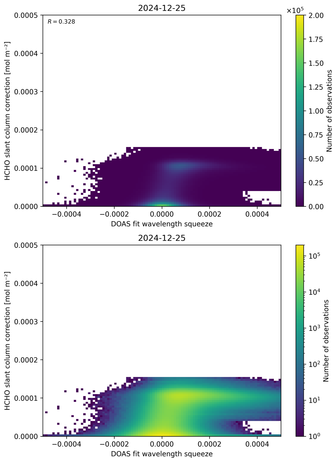
Figure 70: Scatter density plot of “DOAS fit wavelength squeeze” against “HCHO slant column correction” for 2024-12-24 to 2024-12-26.
