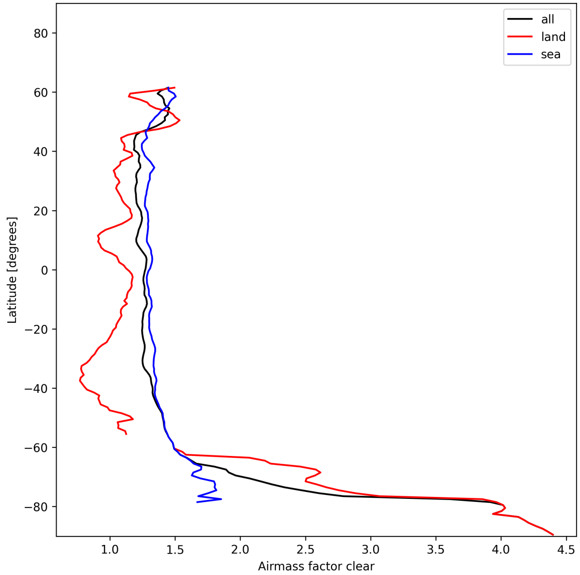
Figure 28: Zonal average of “Airmass factor clear” for 2024-12-24 to 2024-12-26.
