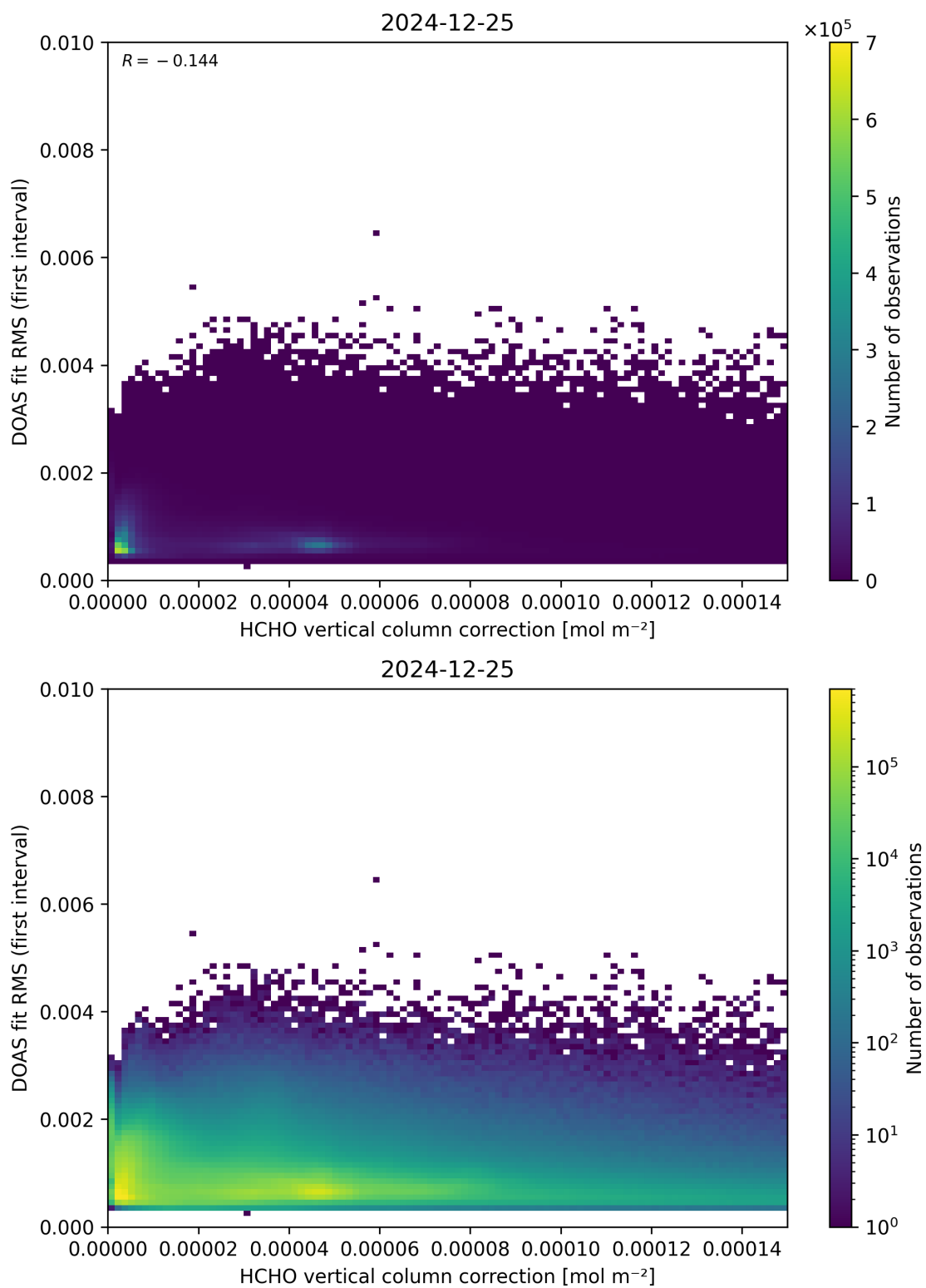
Figure 112: Scatter density plot of “HCHO vertical column correction” against “DOAS fit RMS (first interval)” for 2024-12-24 to 2024-12-26.
