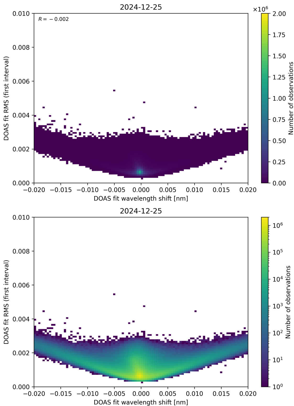
Figure 64: Scatter density plot of “DOAS fit wavelength shift” against “DOAS fit RMS (first interval)” for 2024-12-24 to 2024-12-26.
