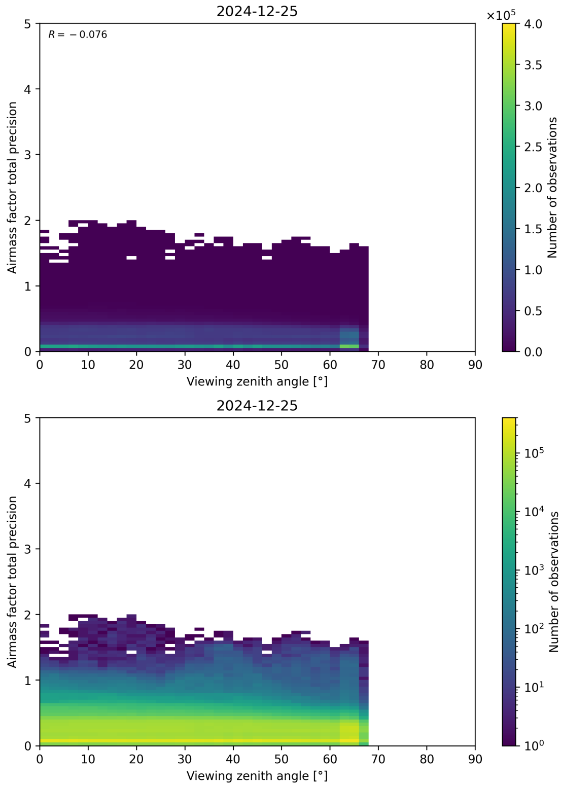
Figure 191: Scatter density plot of “Viewing zenith angle” against “Airmass factor total precision” for 2024-12-24 to 2024-12-26.
