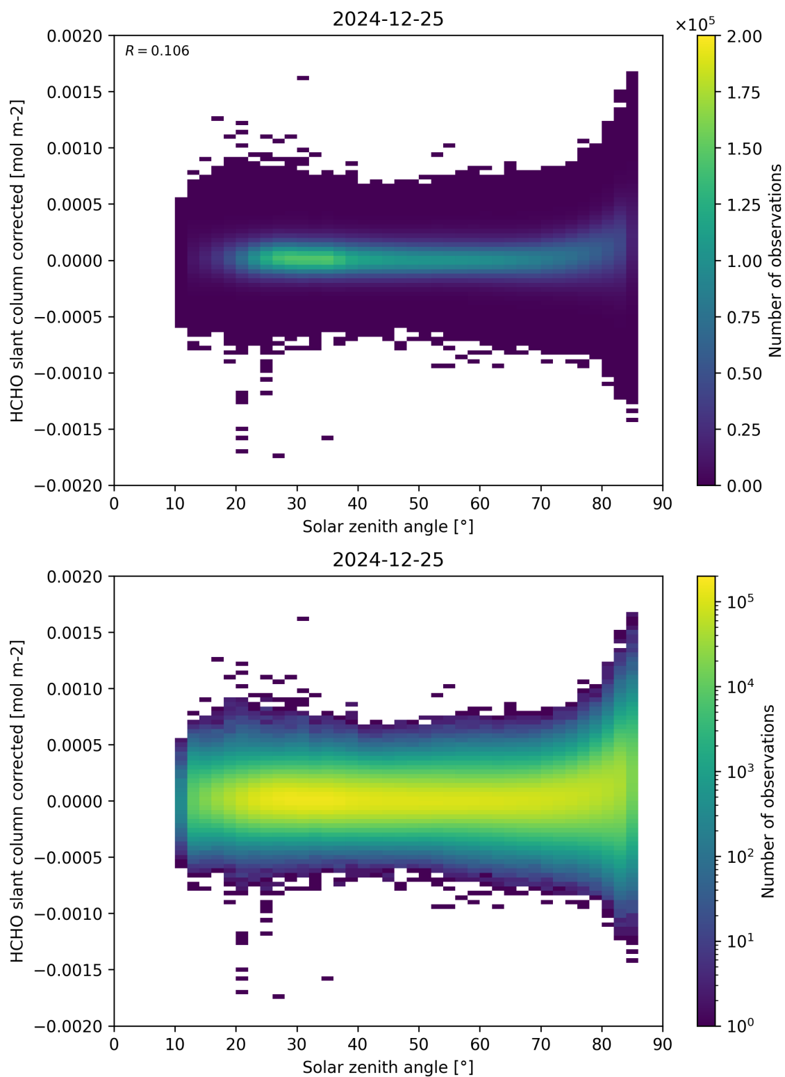
Figure 171: Scatter density plot of “Solar zenith angle” against “HCHO slant column corrected” for 2024-12-24 to 2024-12-26.
