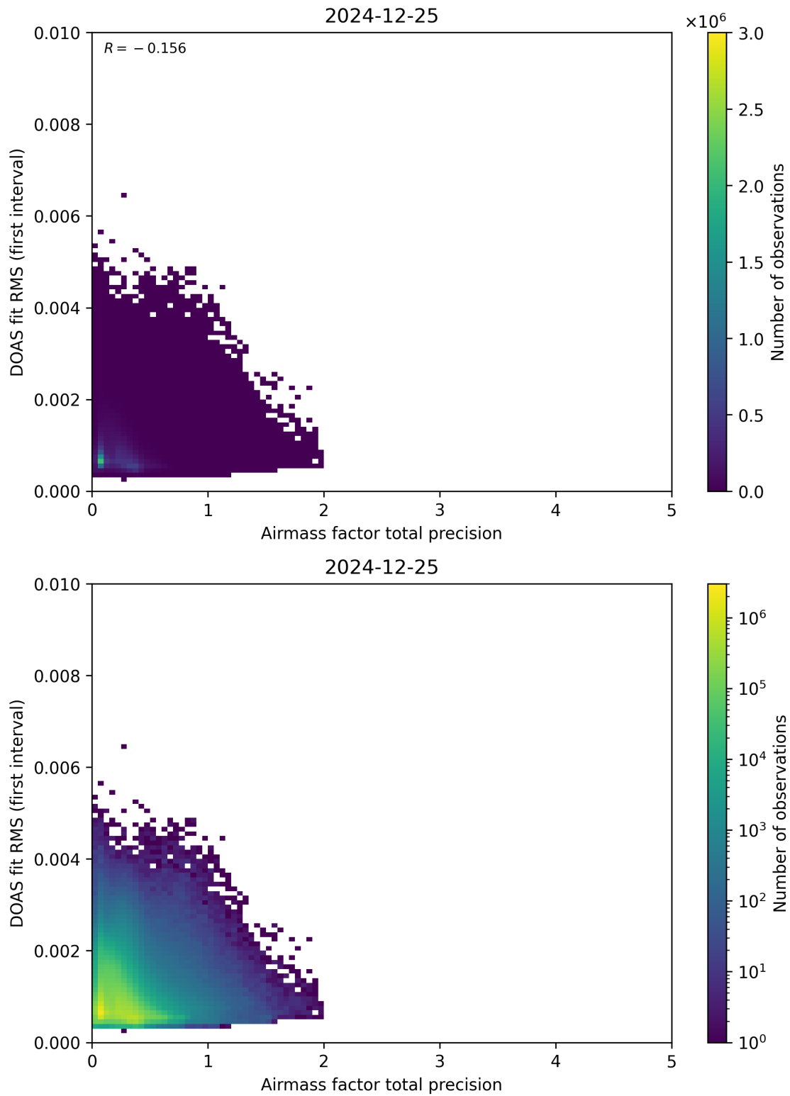
Figure 105: Scatter density plot of “Airmass factor total precision” against “DOAS fit RMS (first interval)” for 2024-12-24 to 2024-12-26.
