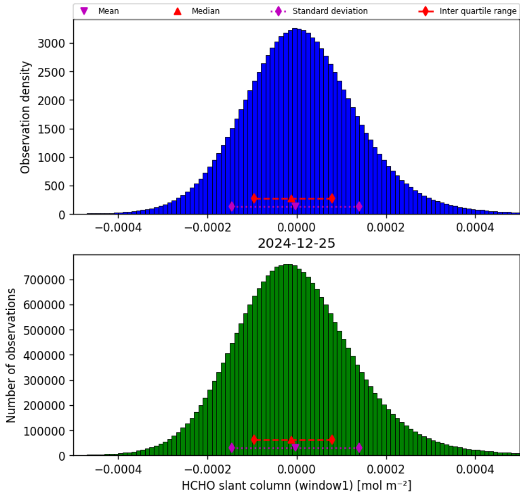
Figure 38: Histogram of “HCHO slant column (window1)” for 2024-12-24 to 2024-12-26
