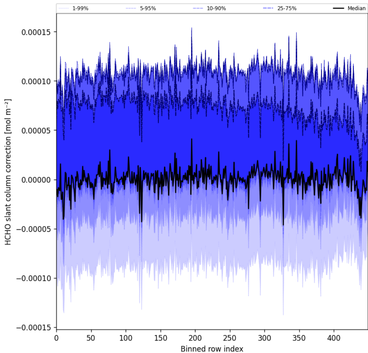
Figure 61: Along track statistics of “HCHO slant column correction” for 2024-12-24 to 2024-12-26
