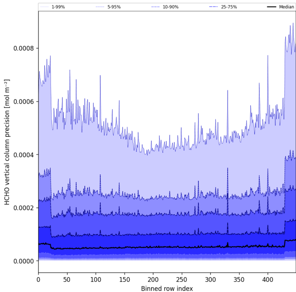
Figure 50: Along track statistics of “HCHO vertical column precision” for 2024-12-24 to 2024-12-26
