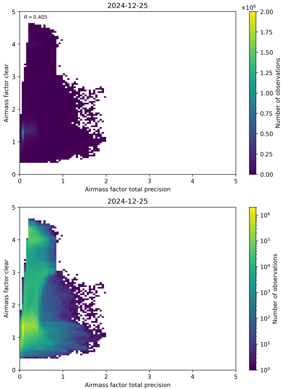
Figure 108: Scatter density plot of “Airmass factor total precision” against “Airmass factor clear” for 2024-12-24 to 2024-12-26.
