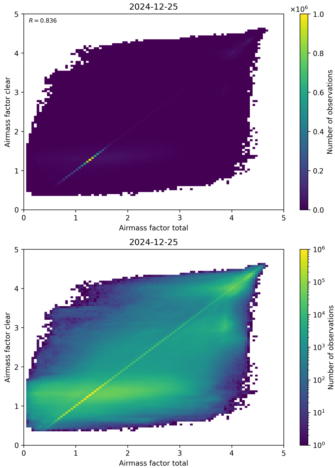
Figure 100: Scatter density plot of “Airmass factor total” against “Airmass factor clear” for 2024-12-24 to 2024-12-26.
