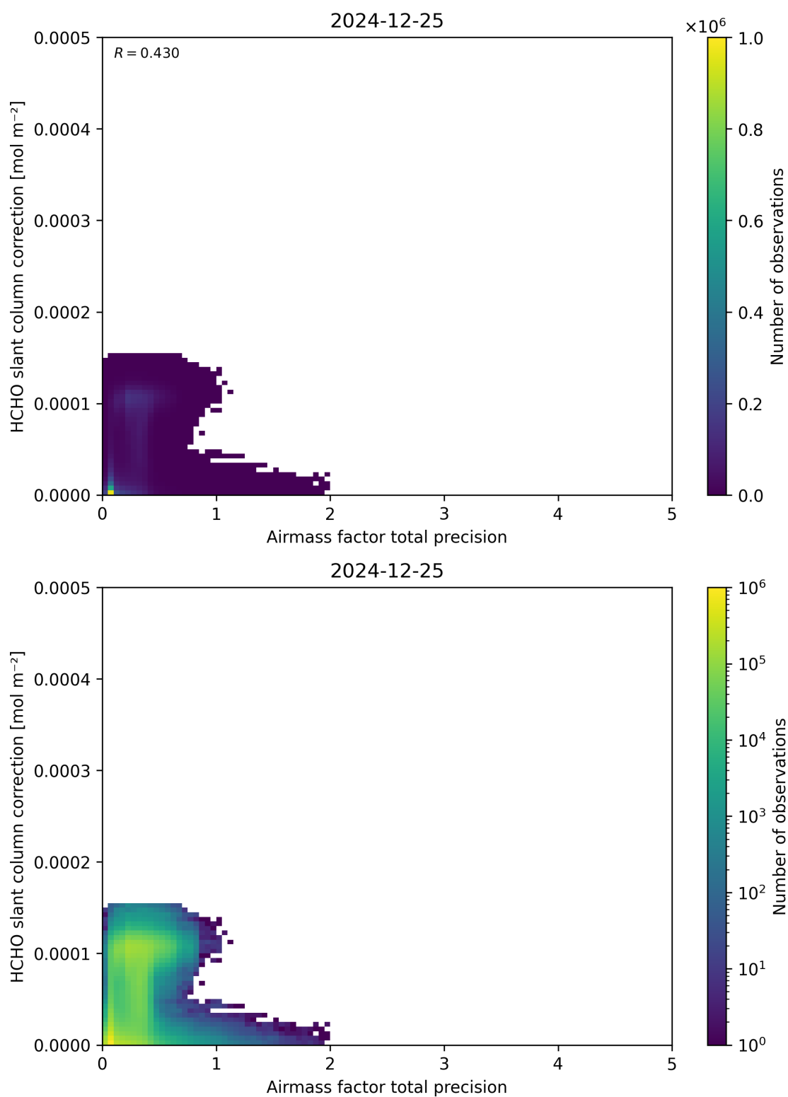
Figure 110: Scatter density plot of “Airmass factor total precision” against “HCHO slant column correction” for 2024-12-24 to 2024-12-26.
