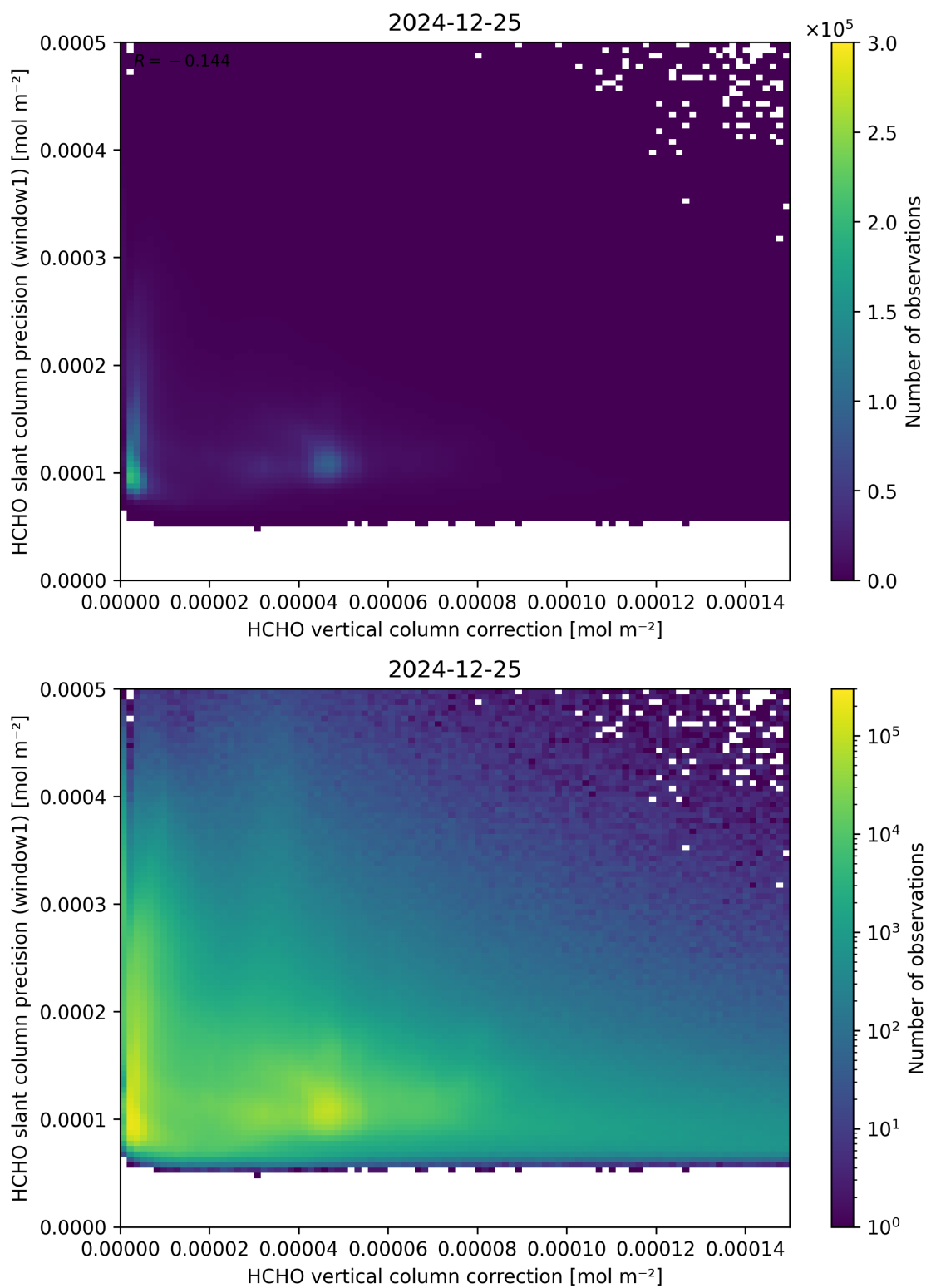
Figure 119: Scatter density plot of “HCHO vertical column correction” against “HCHO slant column precision (window1)” for 2024-12-24 to 2024-12-26.
