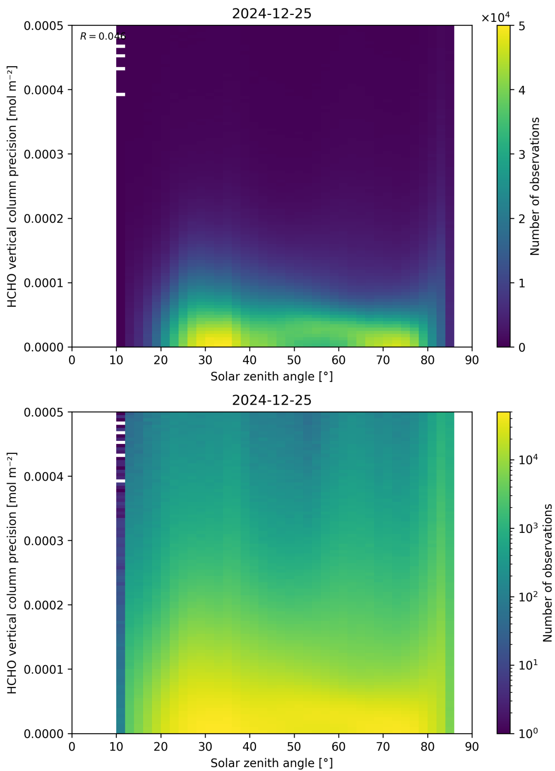
Figure 179: Scatter density plot of “Solar zenith angle” against “HCHO vertical column precision” for 2024-12-24 to 2024-12-26.
