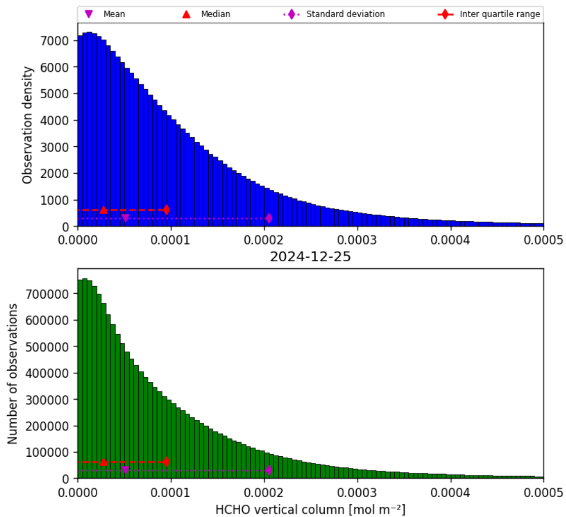
Figure 35: Histogram of “HCHO vertical column” for 2024-12-24 to 2024-12-26
