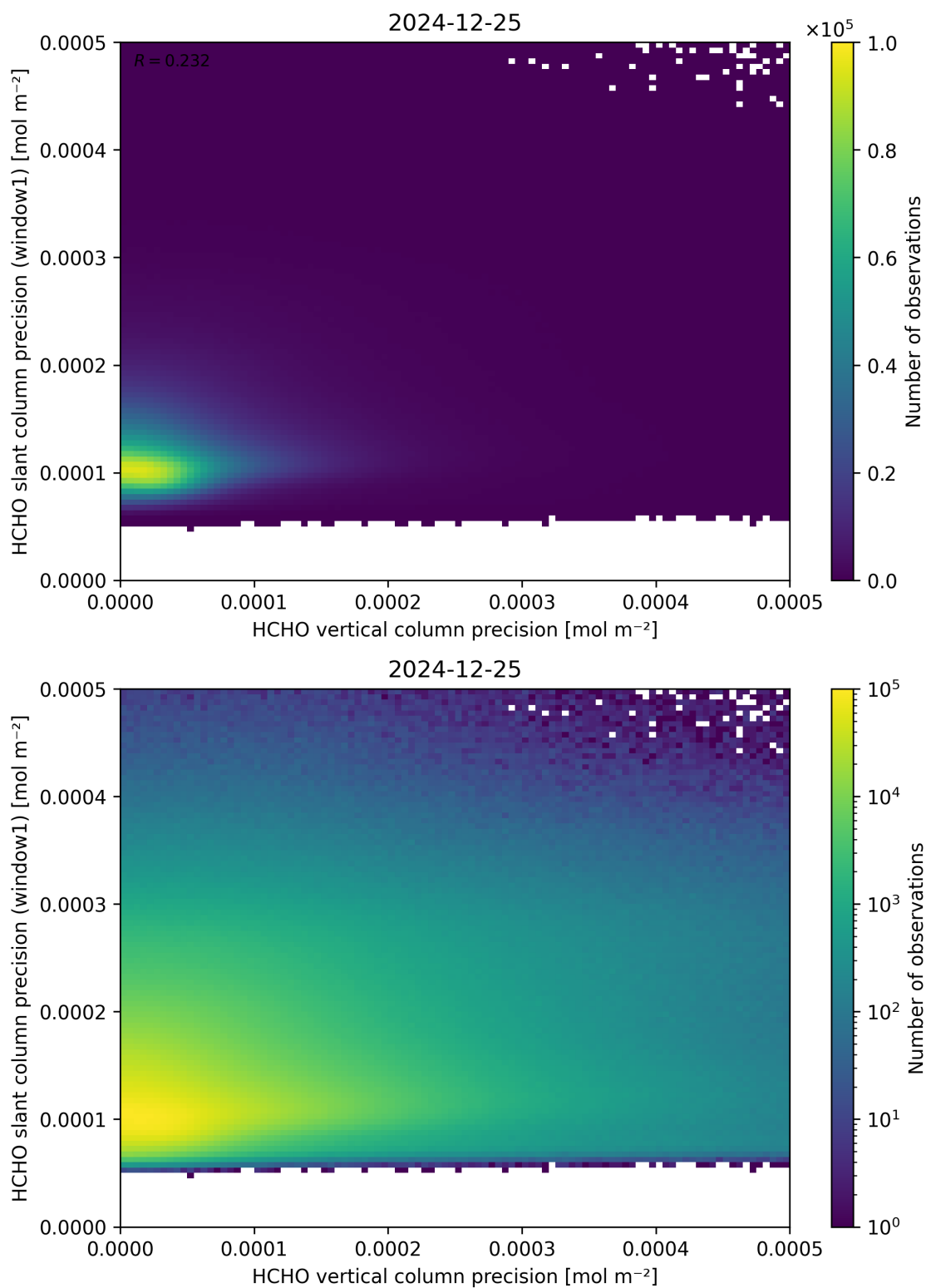
Figure 143: Scatter density plot of “HCHO vertical column precision” against “HCHO slant column precision (window1)” for 2024-12-24 to 2024-12-26.
