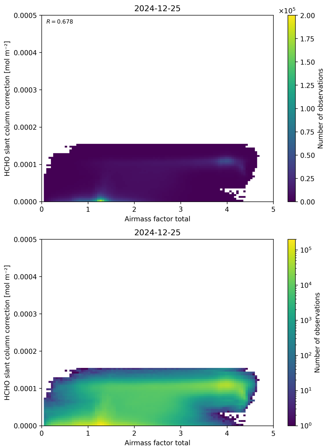
Figure 102: Scatter density plot of “Airmass factor total” against “HCHO slant column correction” for 2024-12-24 to 2024-12-26.
