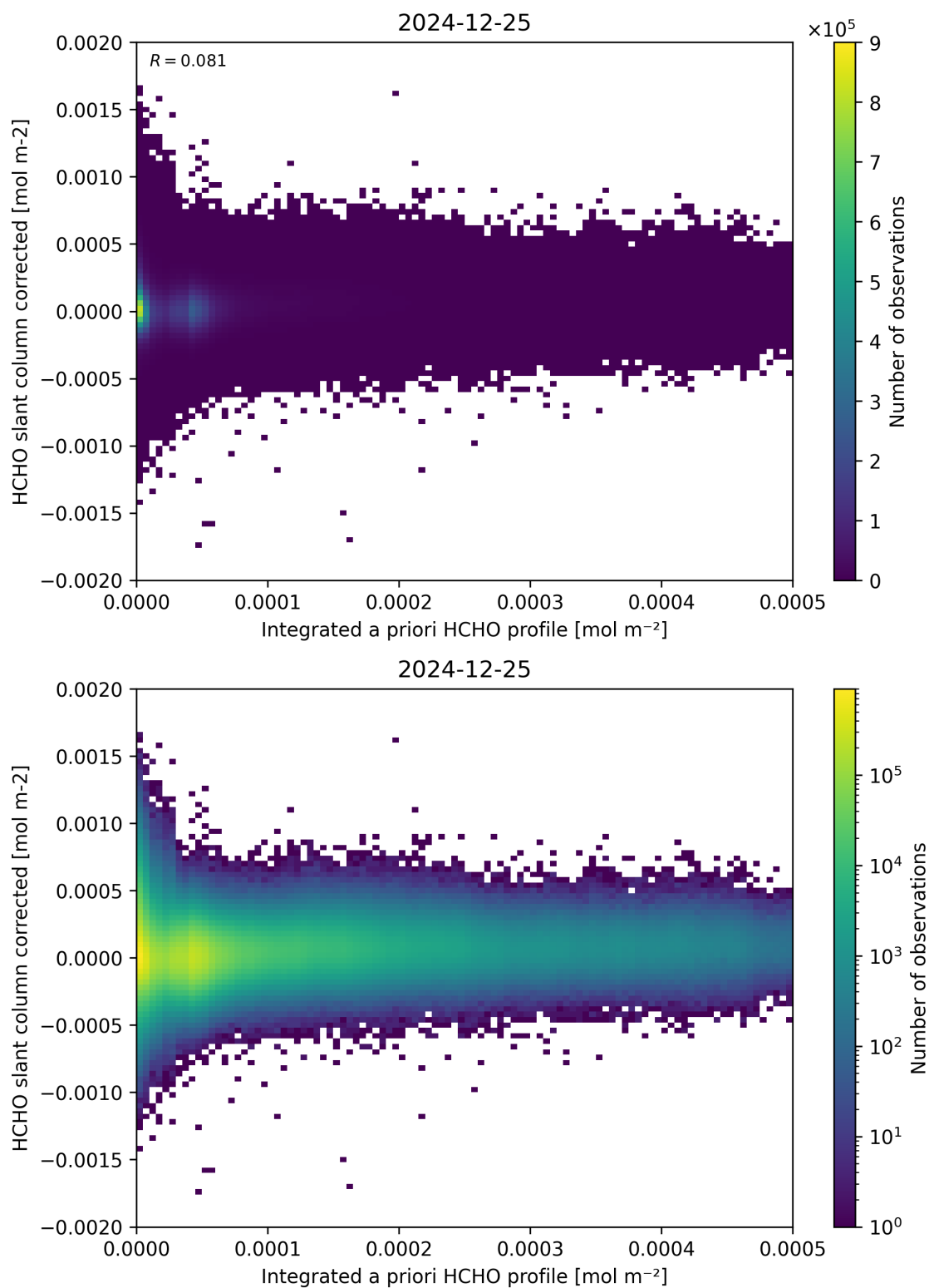
Figure 151: Scatter density plot of “Integrated a priori HCHO profile” against “HCHO slant column corrected” for 2024-12-24 to 2024-12-26.
