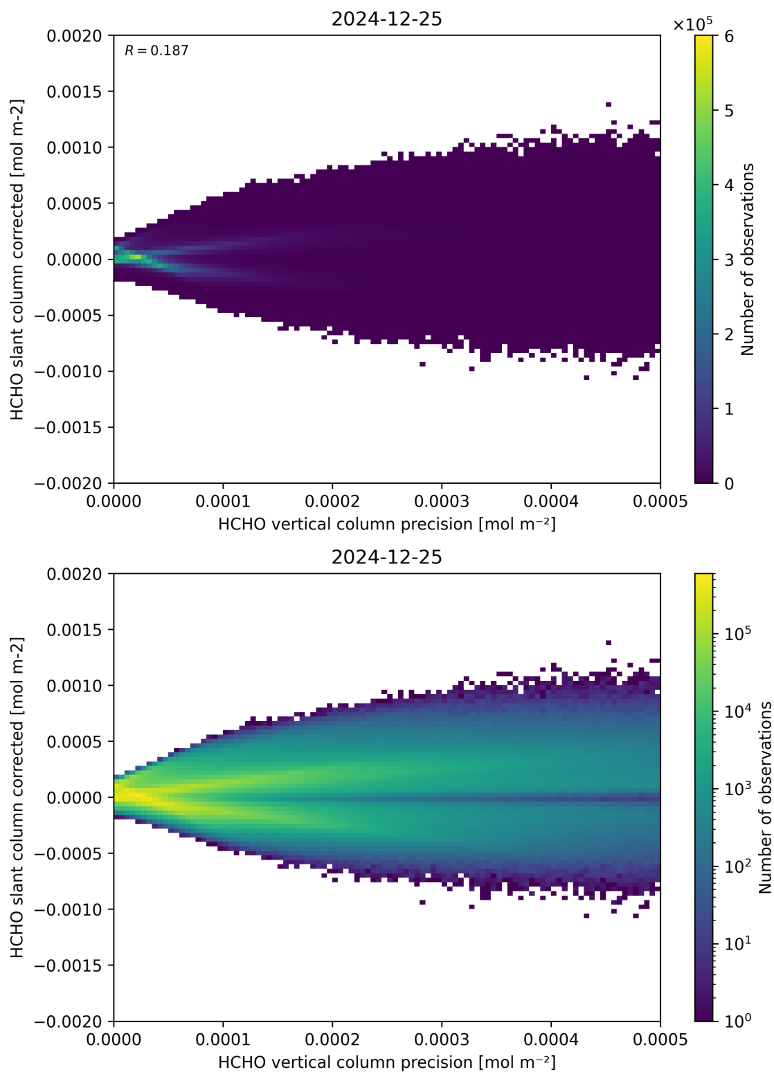
Figure 140: Scatter density plot of “HCHO vertical column precision” against “HCHO slant column corrected” for 2024-12-24 to 2024-12-26.
