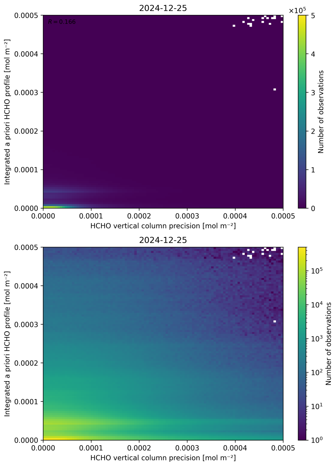
Figure 147: Scatter density plot of “HCHO vertical column precision” against “Integrated a priori HCHO profile” for 2024-12-24 to 2024-12-26.
