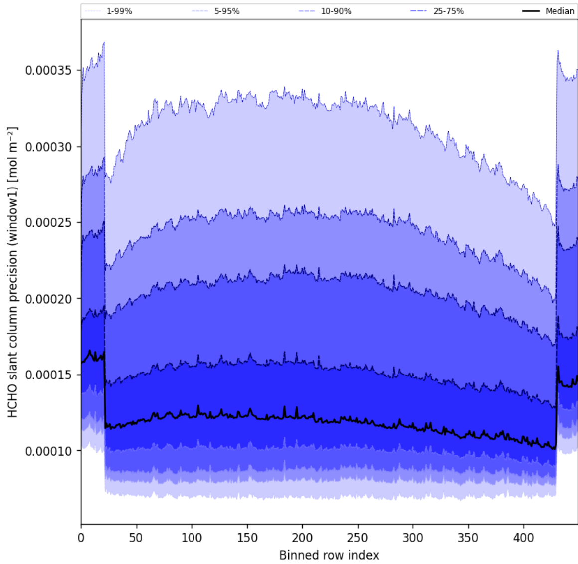
Figure 53: Along track statistics of “HCHO slant column precision (window1)” for 2024-12-24 to 2024-12-26
