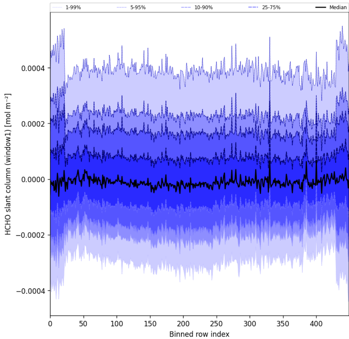
Figure 52: Along track statistics of “HCHO slant column (window1)” for 2024-12-24 to 2024-12-26
