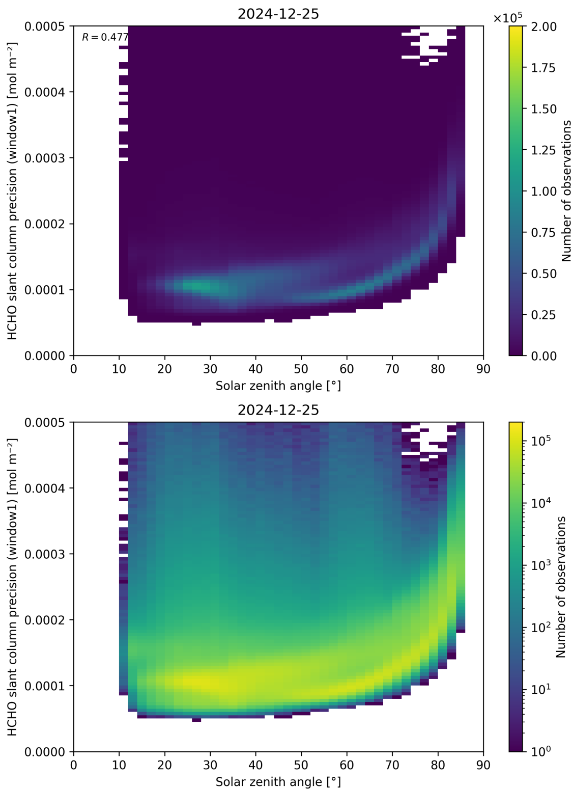
Figure 174: Scatter density plot of “Solar zenith angle” against “HCHO slant column precision (window1)” for 2024-12-24 to 2024-12-26.
