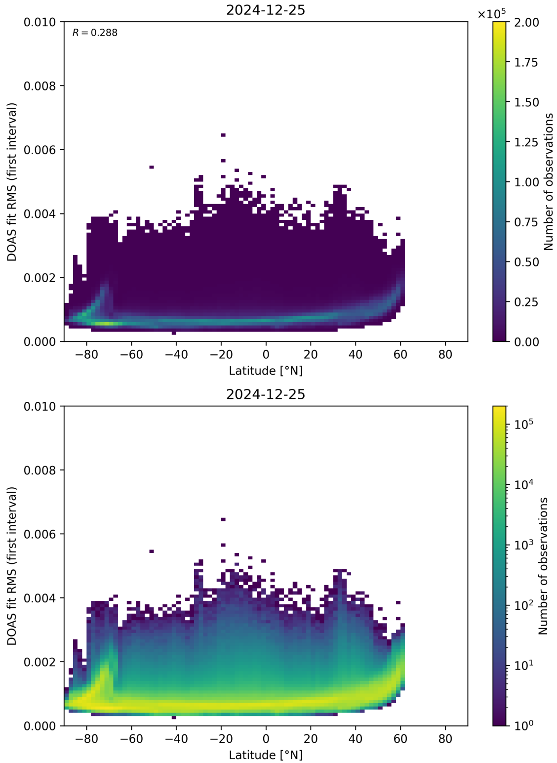
Figure 153: Scatter density plot of “Latitude” against “DOAS fit RMS (first interval)” for 2024-12-24 to 2024-12-26.
