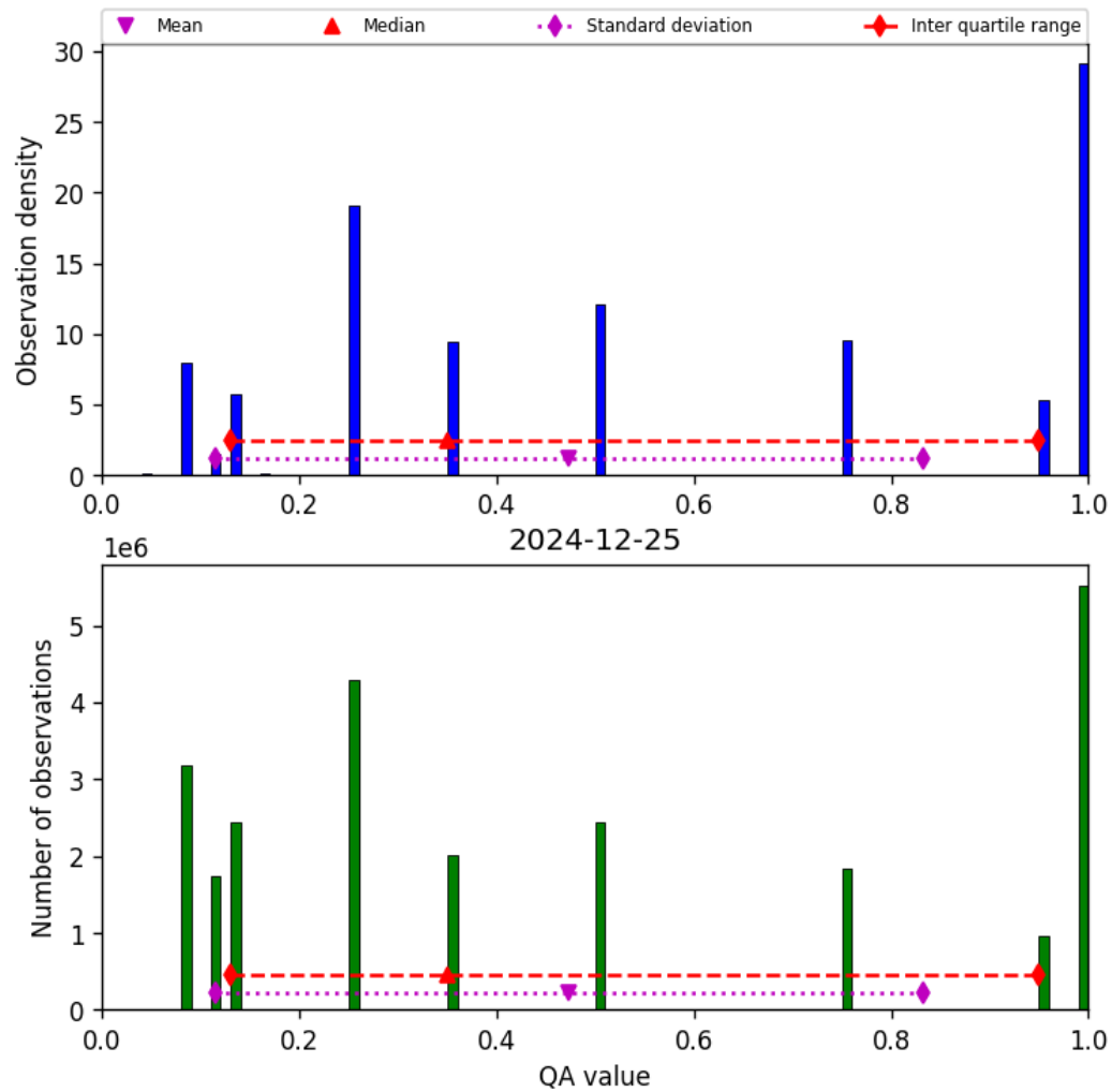
Figure 34: Histogram of “QA value” for 2024-12-24 to 2024-12-26
