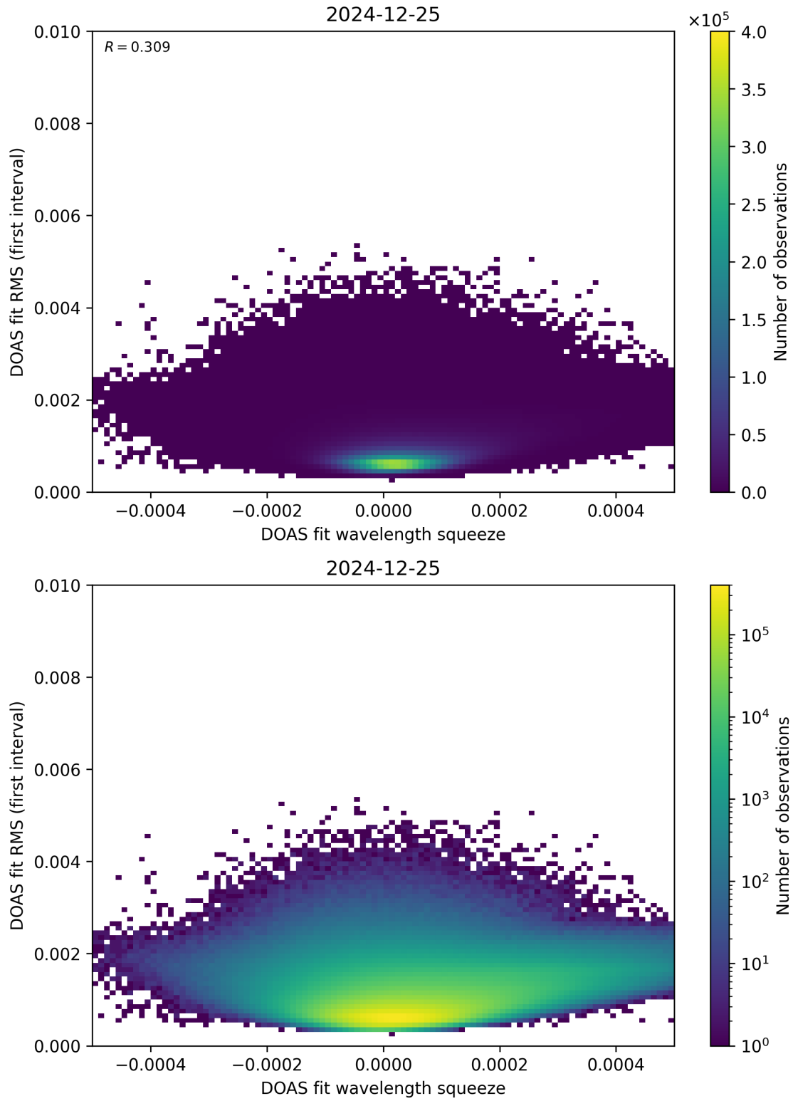
Figure 68: Scatter density plot of “DOAS fit wavelength squeeze” against “DOAS fit RMS (first interval)” for 2024-12-24 to 2024-12-26.
