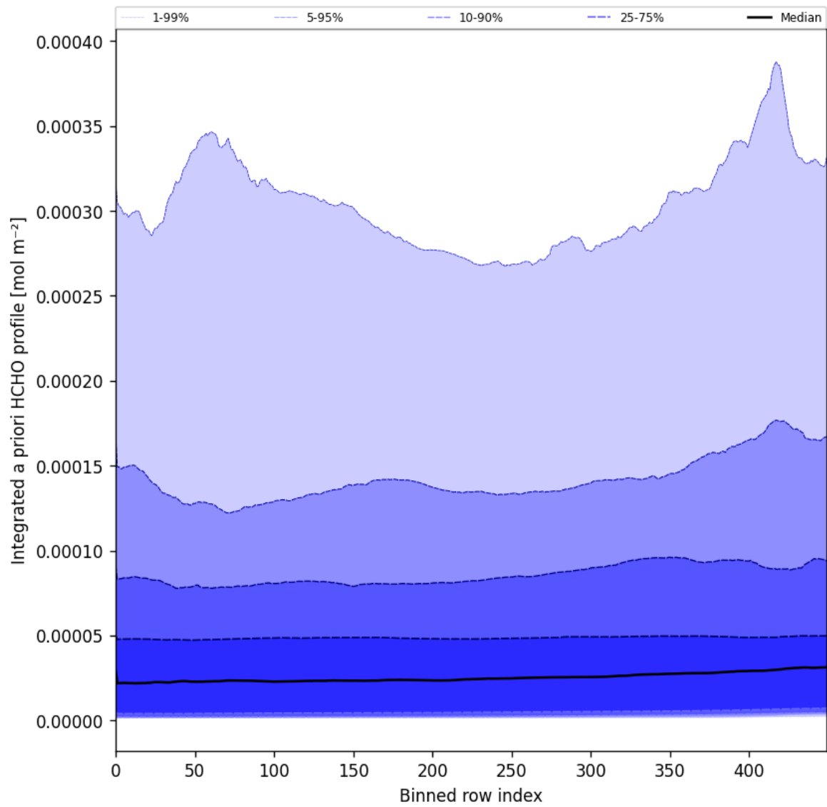
Figure 57: Along track statistics of "Integrated a priori HCHO profile" for 2024-12-24 to 2024-12-26
