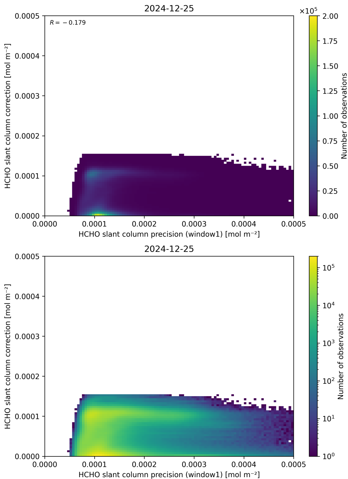
Figure 93: Scatter density plot of “HCHO slant column precision (window1)” against “HCHO slant column correction” for 2024-12-24 to 2024-12-26.
