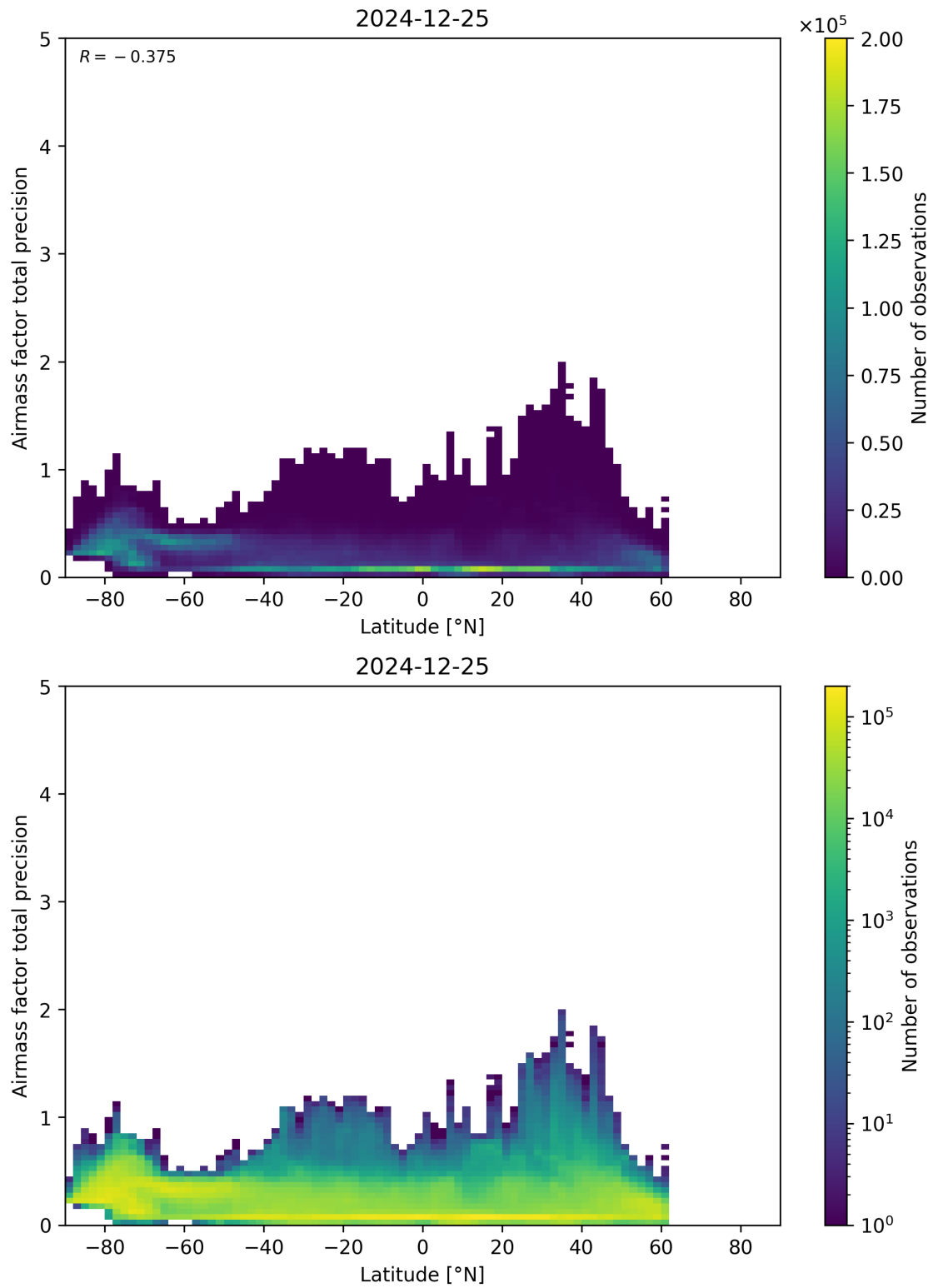
Figure 162: Scatter density plot of “Latitude” against “Airmass factor total precision” for 2024-12-24 to 2024-12-26.
