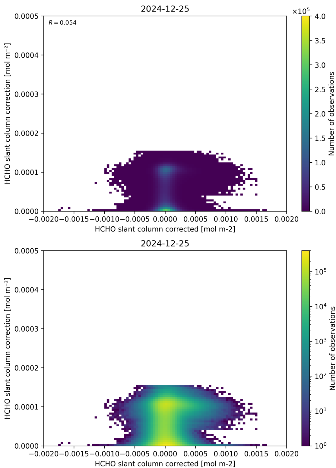
Figure 77: Scatter density plot of “HCHO slant column corrected” against “HCHO slant column correction” for 2024-12-24 to 2024-12-26.
