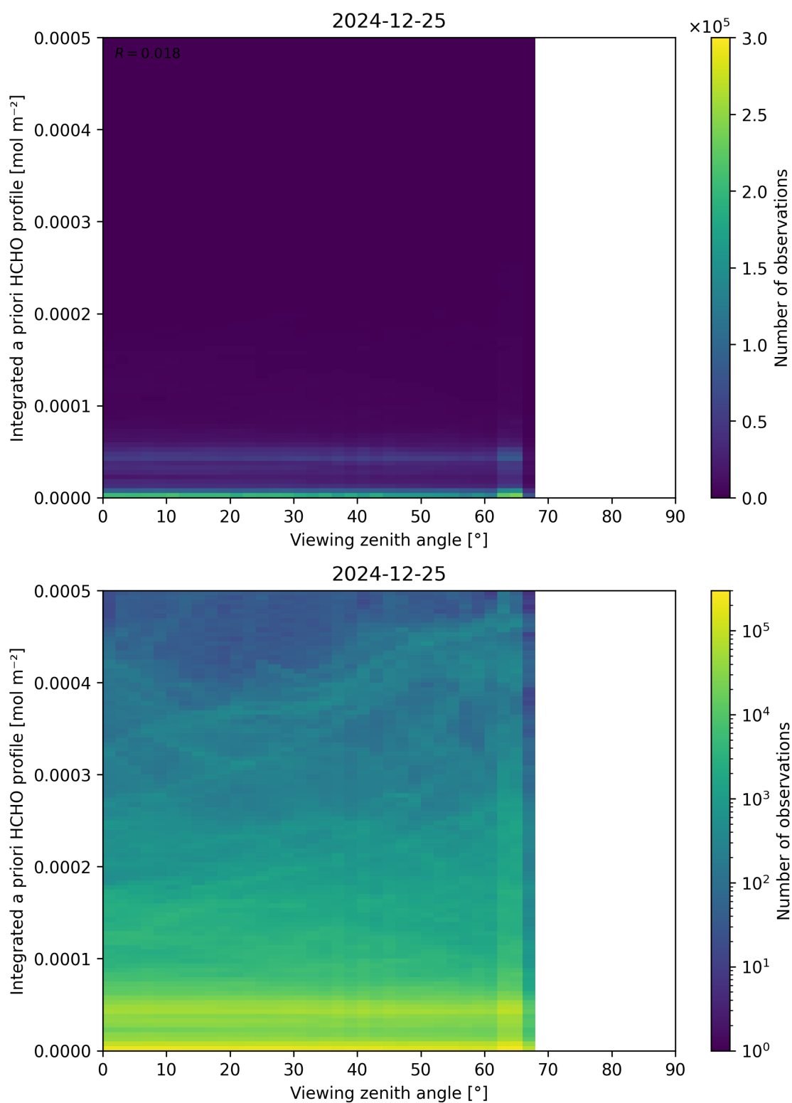
Figure 195: Scatter density plot of “Viewing zenith angle” against “Integrated a priori HCHO profile” for 2024-12-24 to 2024-12-26.
