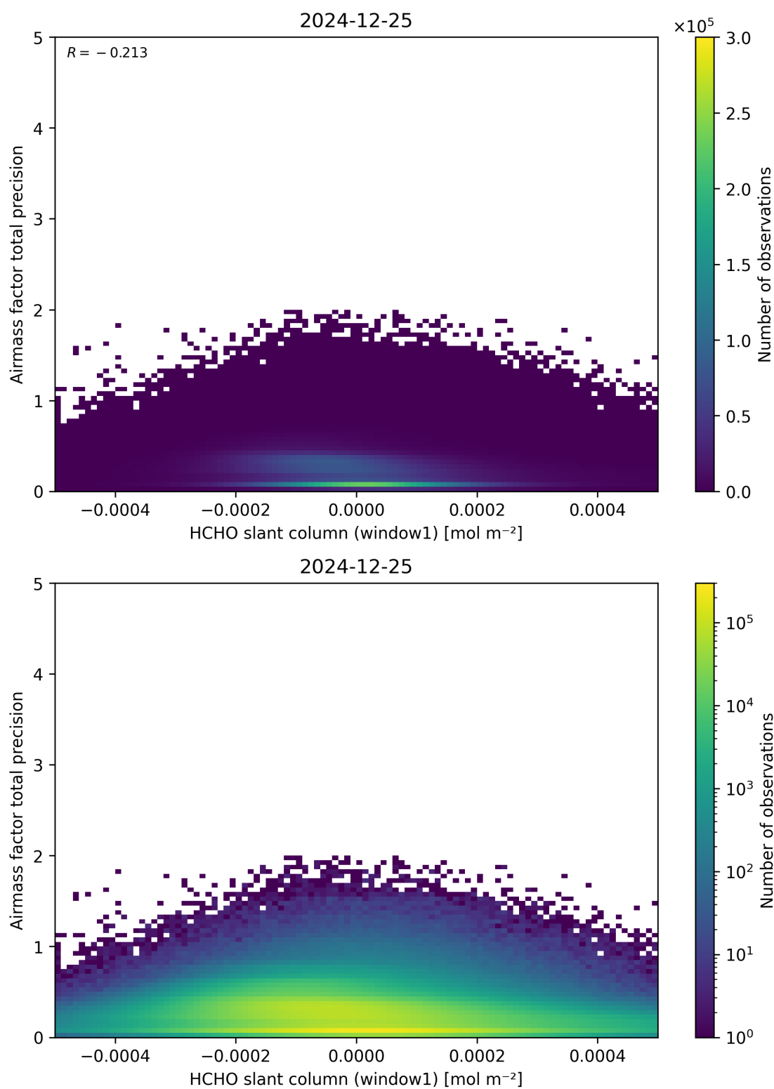
Figure 86: Scatter density plot of “HCHO slant column (window1)” against “Airmass factor total precision” for 2024-12-24 to 2024-12-26.
