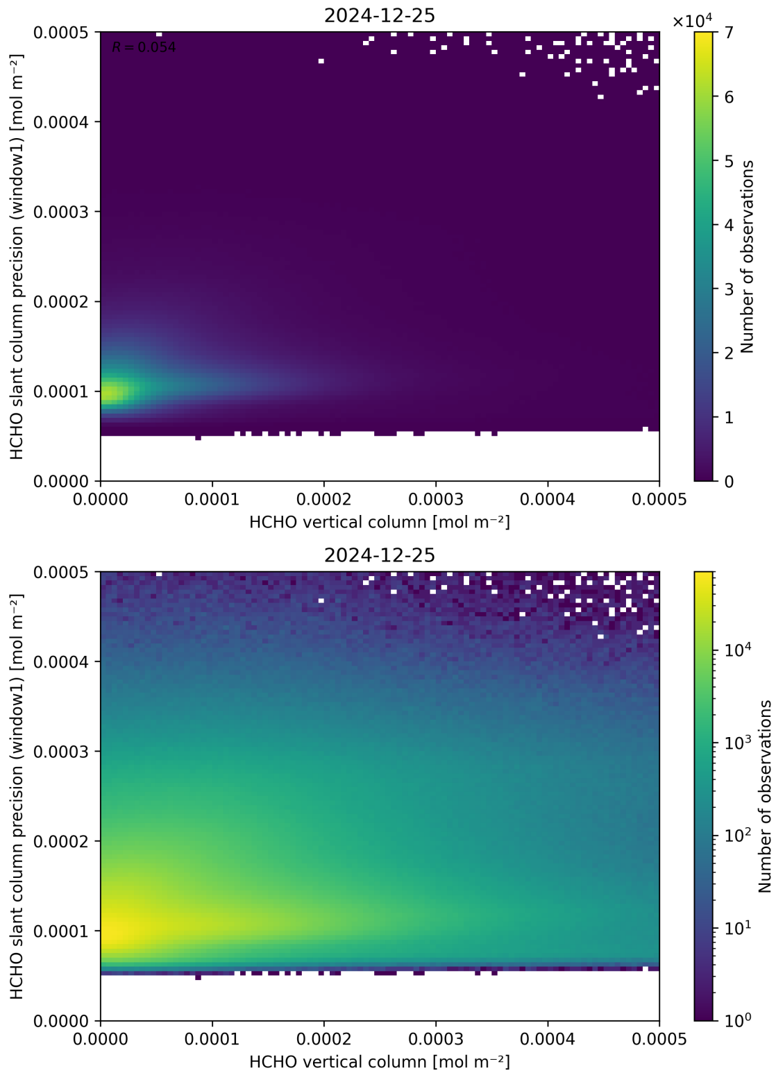
Figure 130: Scatter density plot of “HCHO vertical column” against “HCHO slant column precision (window1)” for 2024-12-24 to 2024-12-26.
