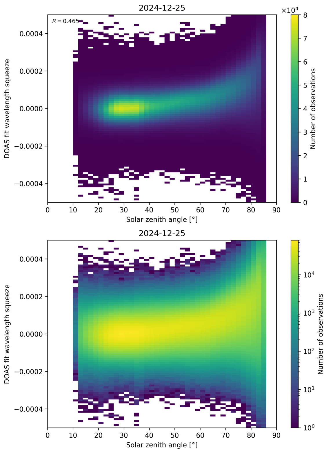
Figure 169: Scatter density plot of “Solar zenith angle” against “DOAS fit wavelength squeeze” for 2024-12-24 to 2024-12-26.
