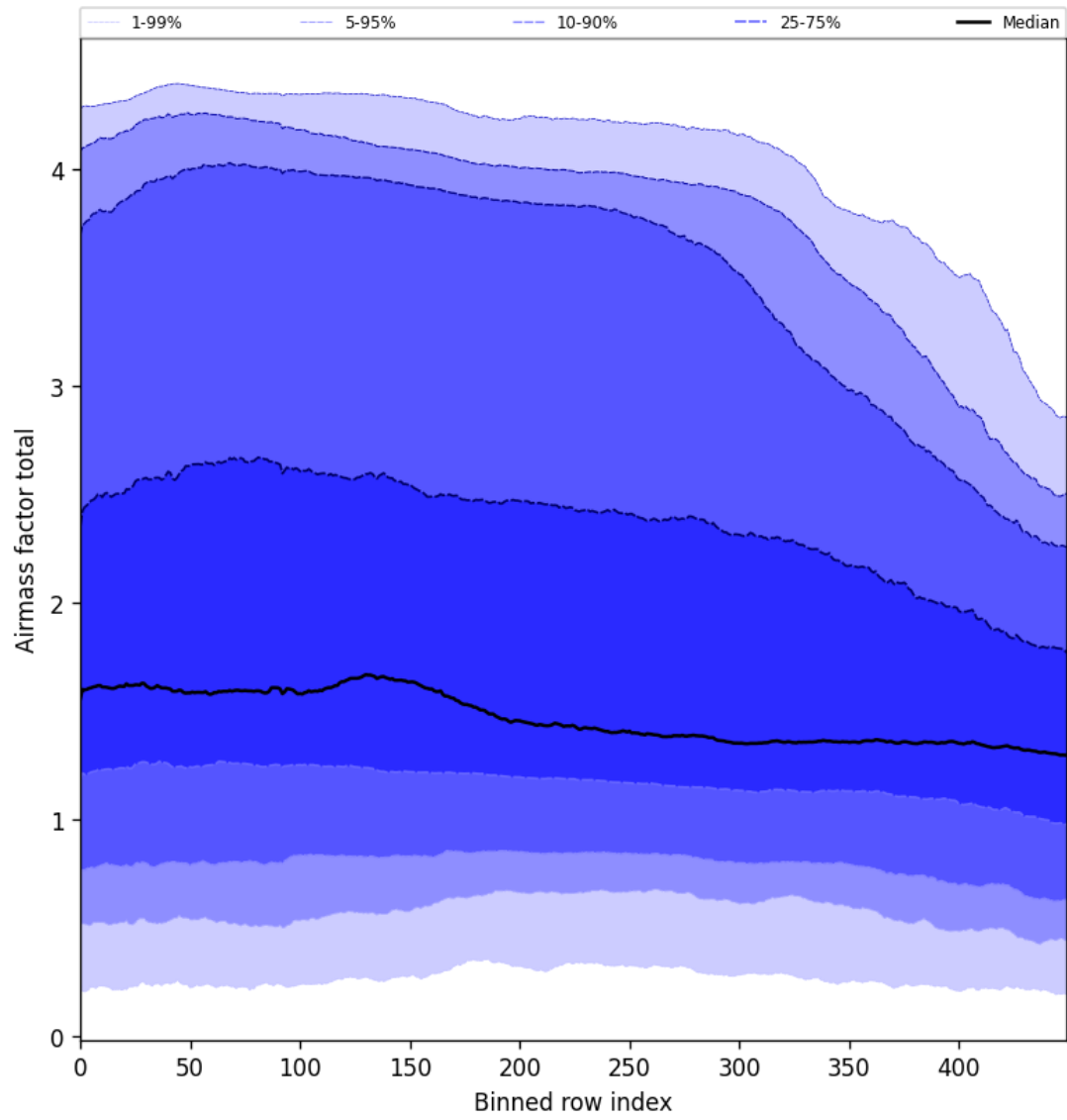
Figure 54: Along track statistics of “Airmass factor total” for 2024-12-24 to 2024-12-26
