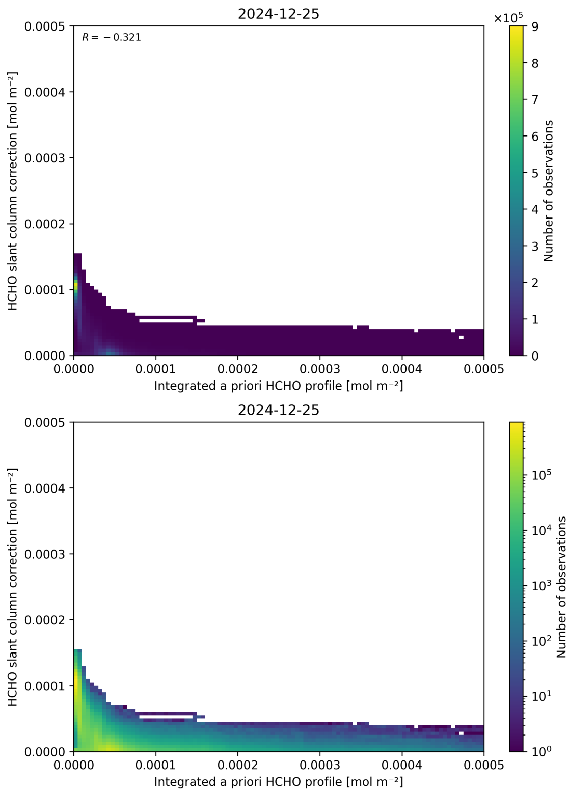
Figure 152: Scatter density plot of “Integrated a priori HCHO profile” against “HCHO slant column correction” for 2024-12-24 to 2024-12-26.
