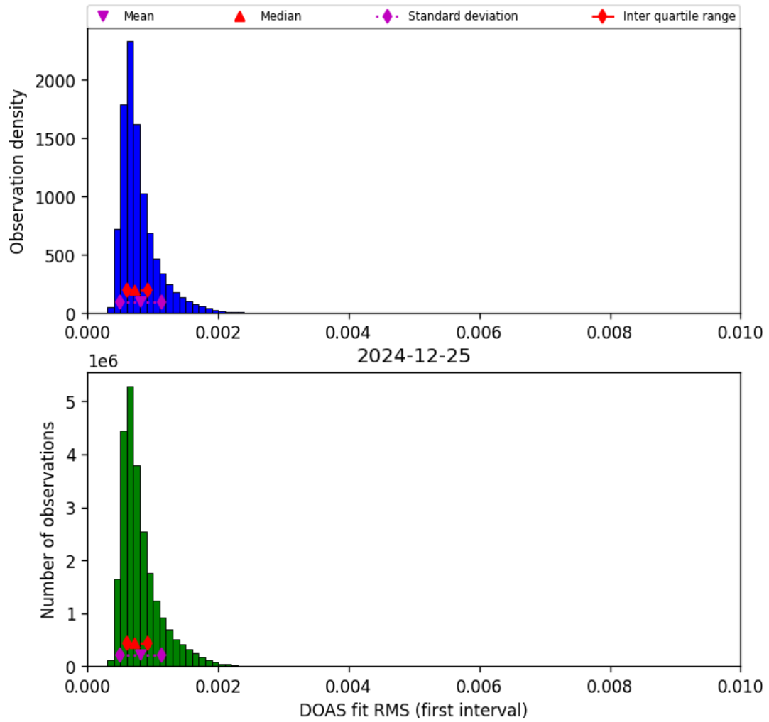
Figure 46: Histogram of “DOAS fit RMS (first interval)” for 2024-12-24 to 2024-12-26
