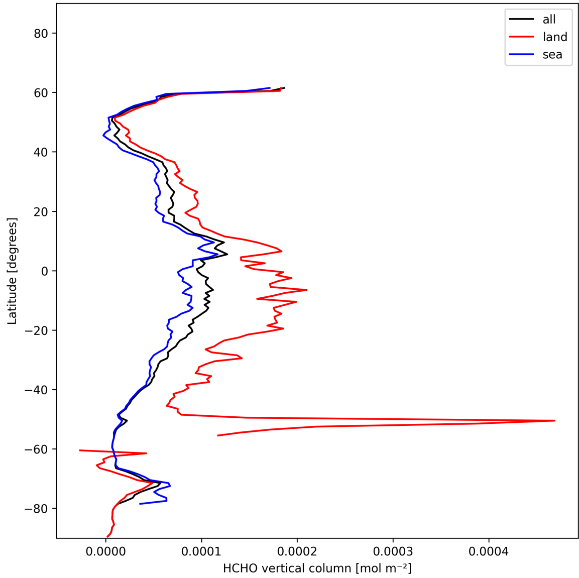
Figure 21: Zonal average of “HCHO vertical column” for 2024-12-24 to 2024-12-26.
