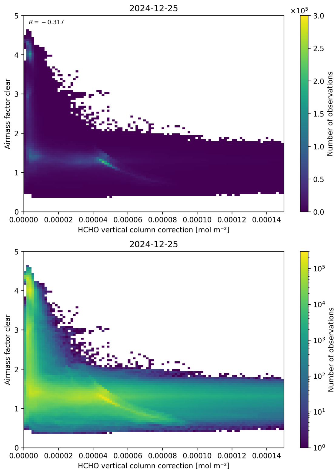
Figure 115: Scatter density plot of “HCHO vertical column correction” against “Airmass factor clear” for 2024-12-24 to 2024-12-26.
