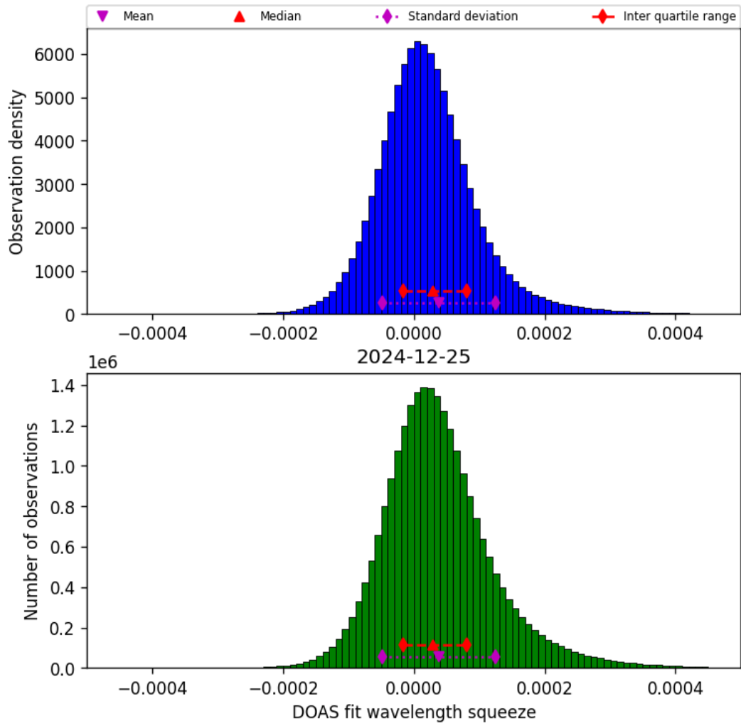
Figure 45: Histogram of “DOAS fit wavelength squeeze” for 2024-12-24 to 2024-12-26
