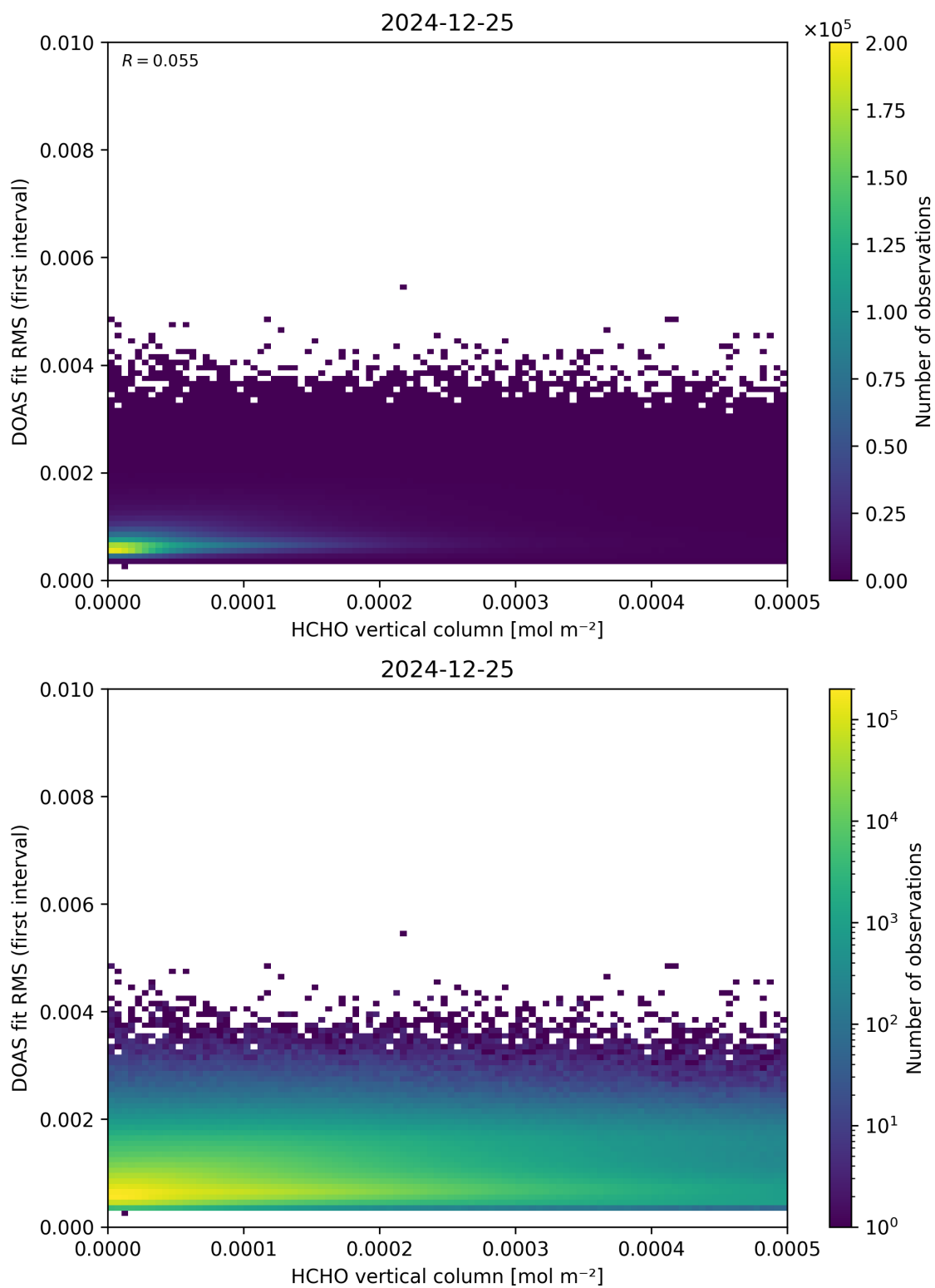
Figure 123: Scatter density plot of “HCHO vertical column” against “DOAS fit RMS (first interval)” for 2024-12-24 to 2024-12-26.
