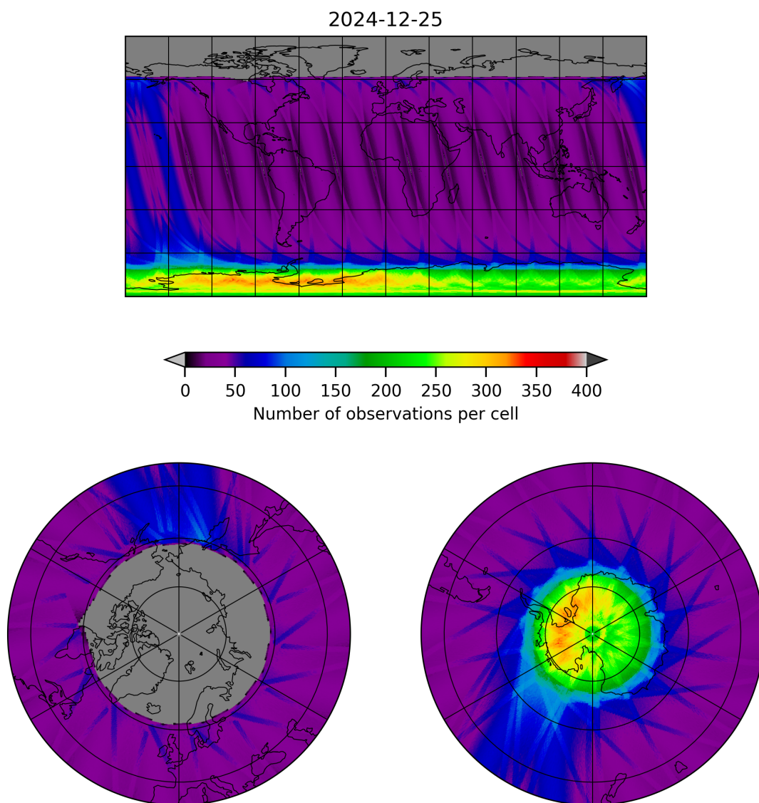
Figure 19: Map of the number of observations for 2024-12-24 to 2024-12-26
