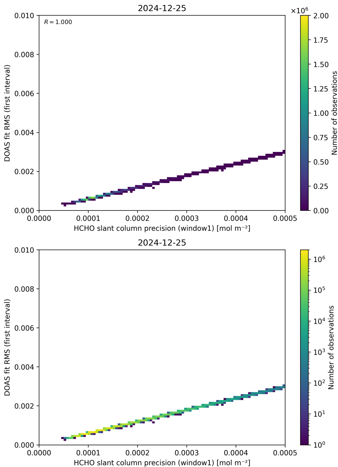
Figure 88: Scatter density plot of “HCHO slant column precision (window1)” against “DOAS fit RMS (first interval)” for 2024-12-24 to 2024-12-26.
