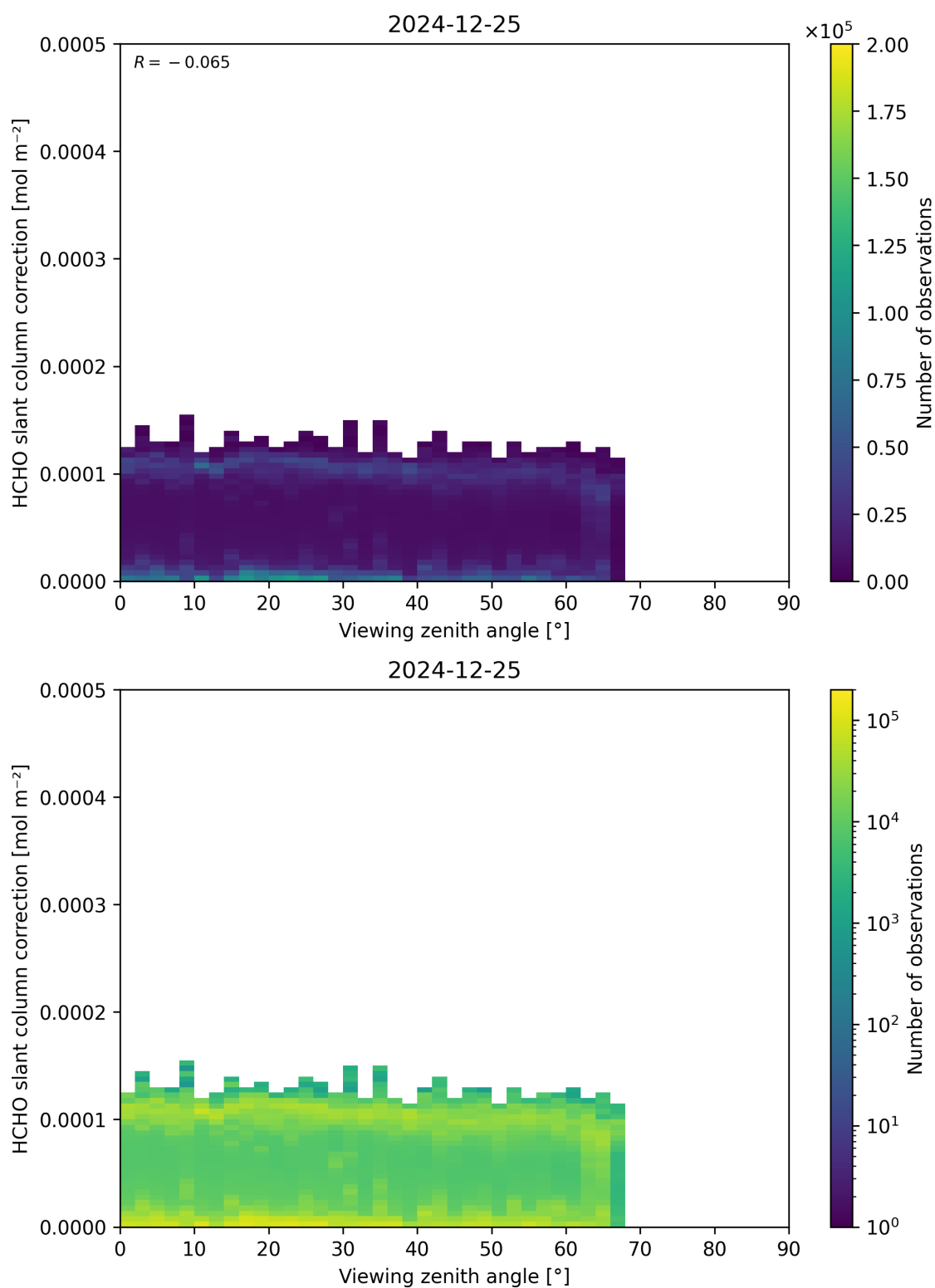
Figure 187: Scatter density plot of “Viewing zenith angle” against “HCHO slant column correction” for 2024-12-24 to 2024-12-26.
