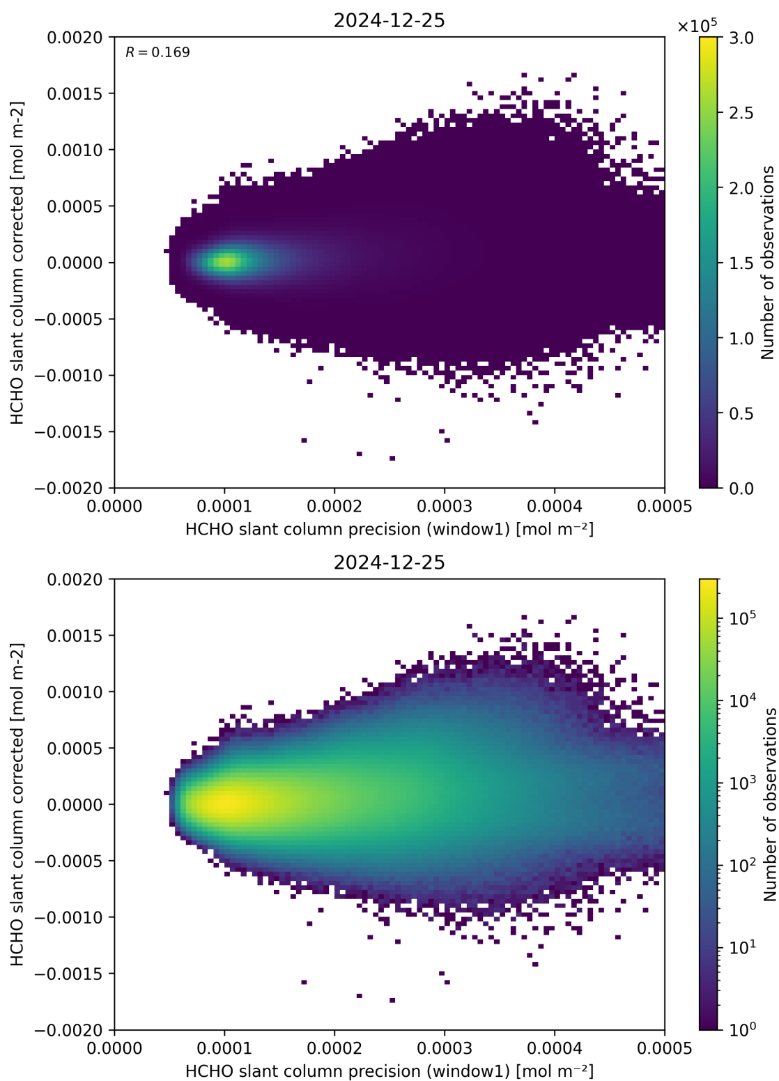
Figure 92: Scatter density plot of “HCHO slant column precision (window1)” against “HCHO slant column corrected” for 2024-12-24 to 2024-12-26.
