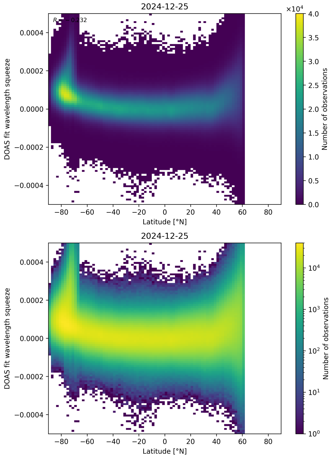
Figure 155: Scatter density plot of “Latitude” against “DOAS fit wavelength squeeze” for 2024-12-24 to 2024-12-26.
