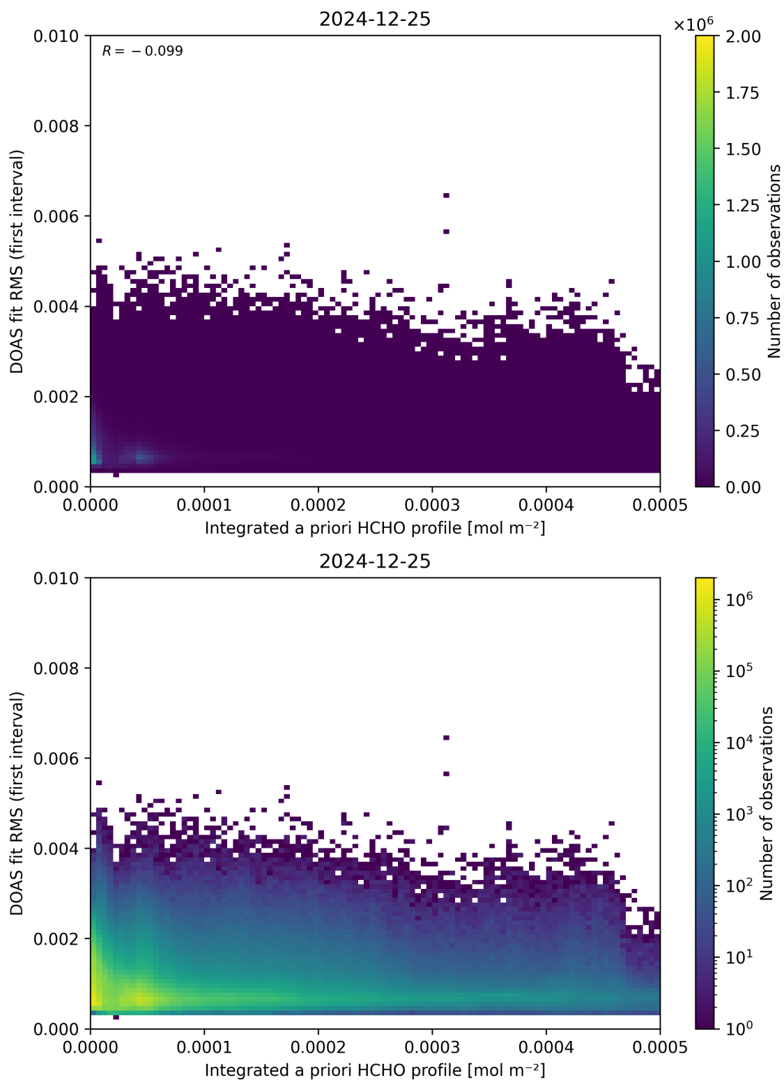
Figure 148: Scatter density plot of “Integrated a priori HCHO profile” against “DOAS fit RMS (first interval)” for 2024-12-24 to 2024-12-26.
