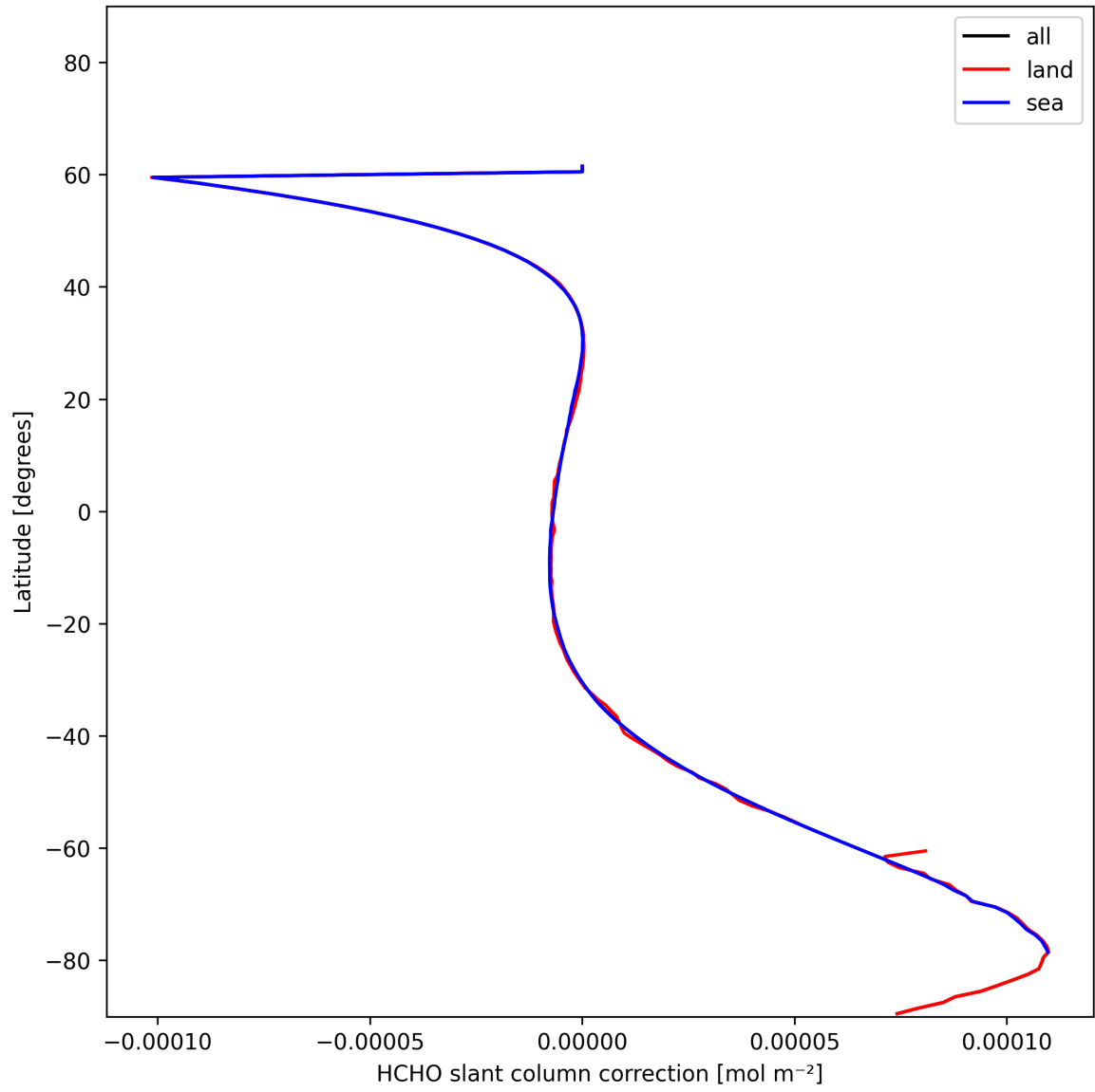
Figure 33: Zonal average of “HCHO slant column correction” for 2024-12-24 to 2024-12-26.
