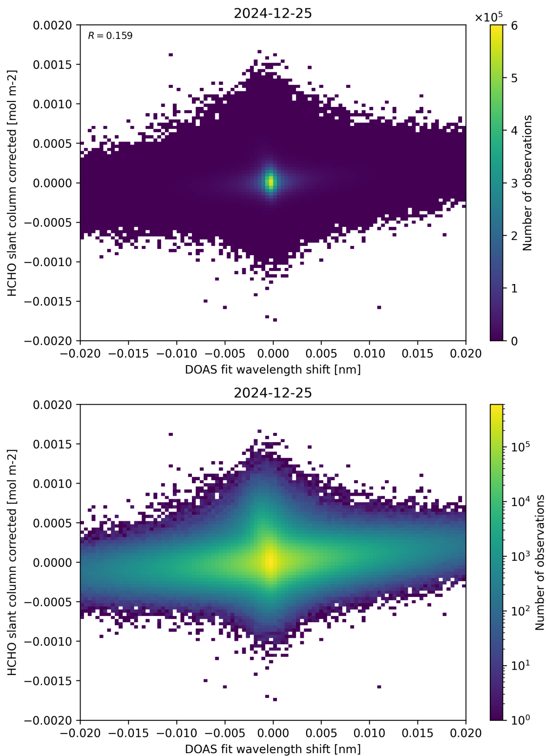
Figure 66: Scatter density plot of “DOAS fit wavelength shift” against “HCHO slant column corrected” for 2024-12-24 to 2024-12-26.
