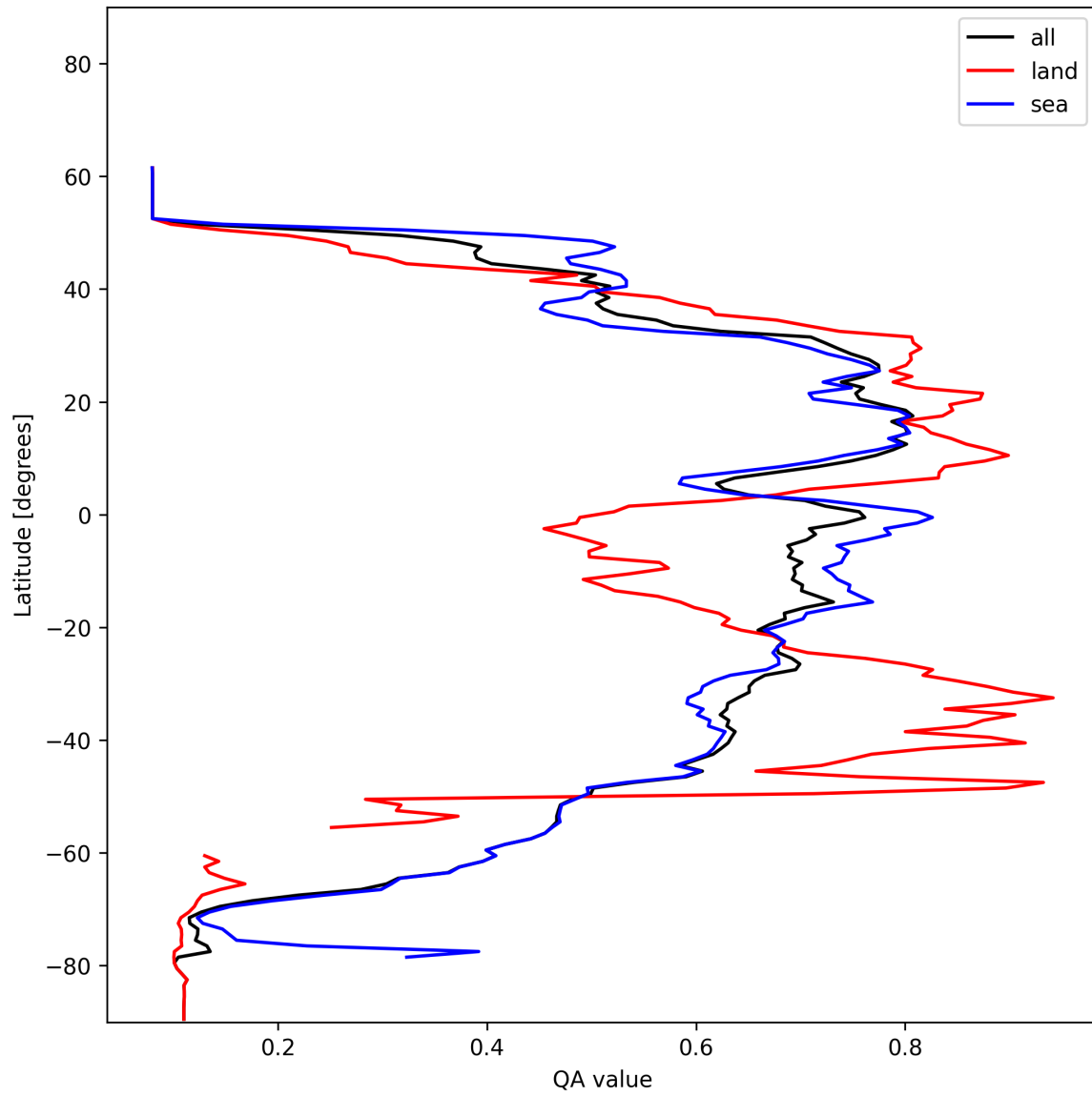
Figure 20: Zonal average of “QA value” for 2024-12-24 to 2024-12-26.
