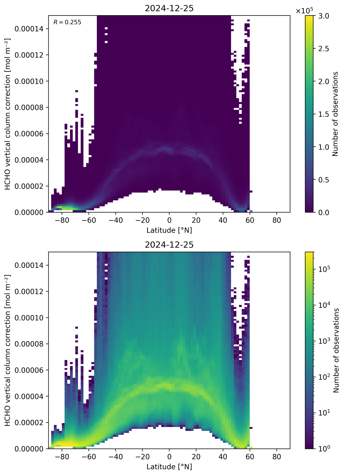
Figure 164: Scatter density plot of “Latitude” against “HCHO vertical column correction” for 2024-12-24 to 2024-12-26.
