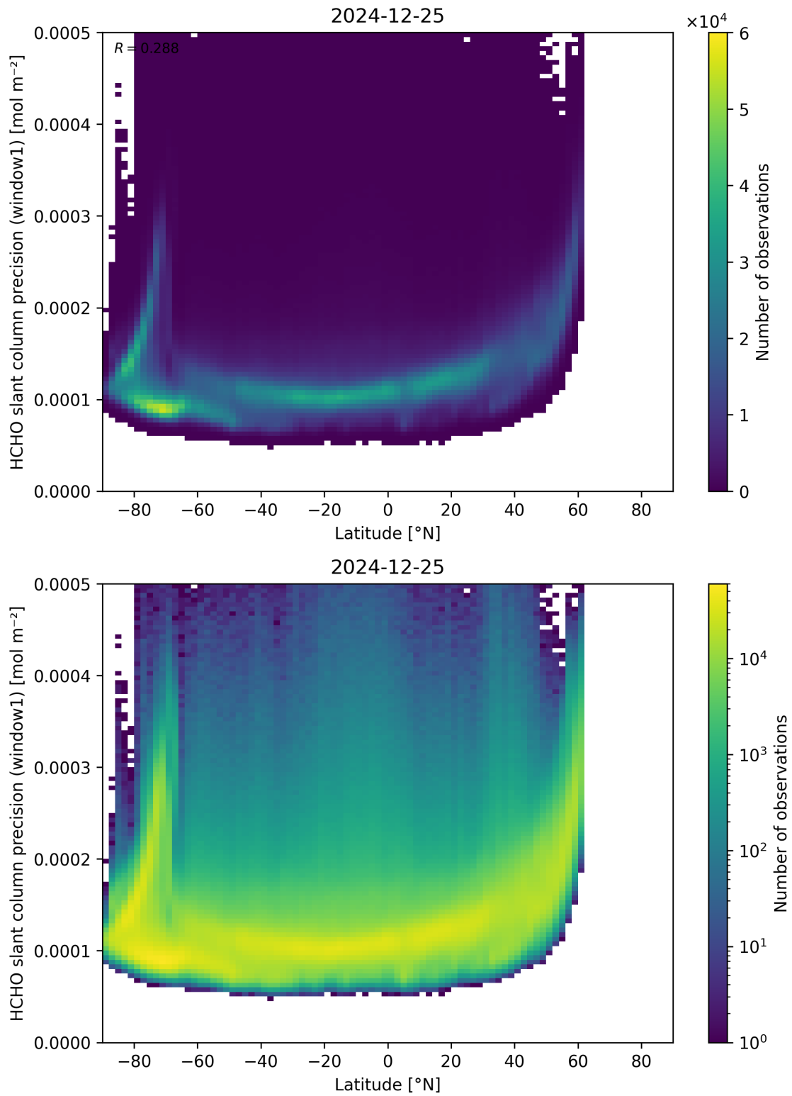
Figure 160: Scatter density plot of “Latitude” against “HCHO slant column precision (window1)” for 2024-12-24 to 2024-12-26.
