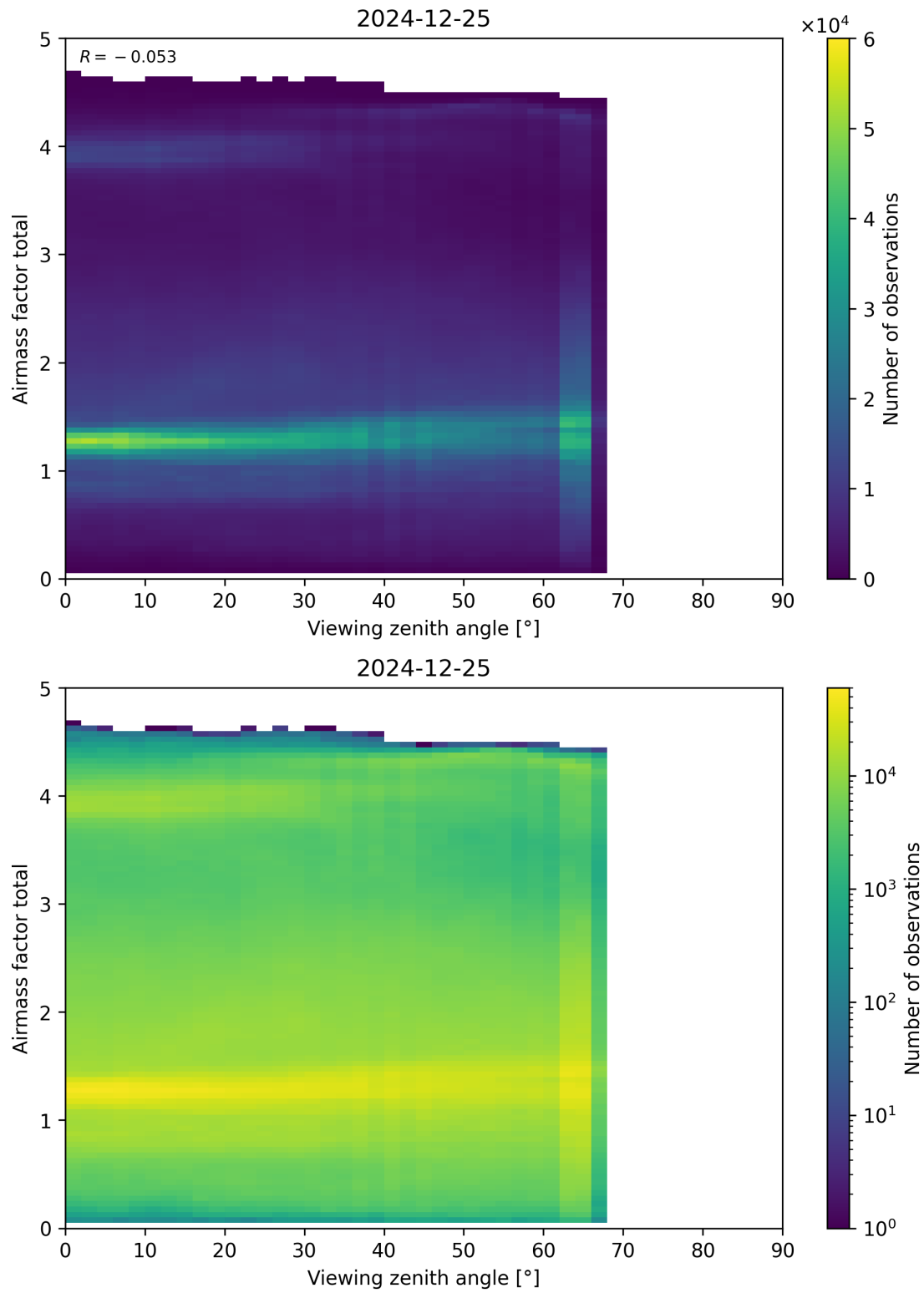
Figure 190: Scatter density plot of “Viewing zenith angle” against “Airmass factor total” for 2024-12-24 to 2024-12-26.
