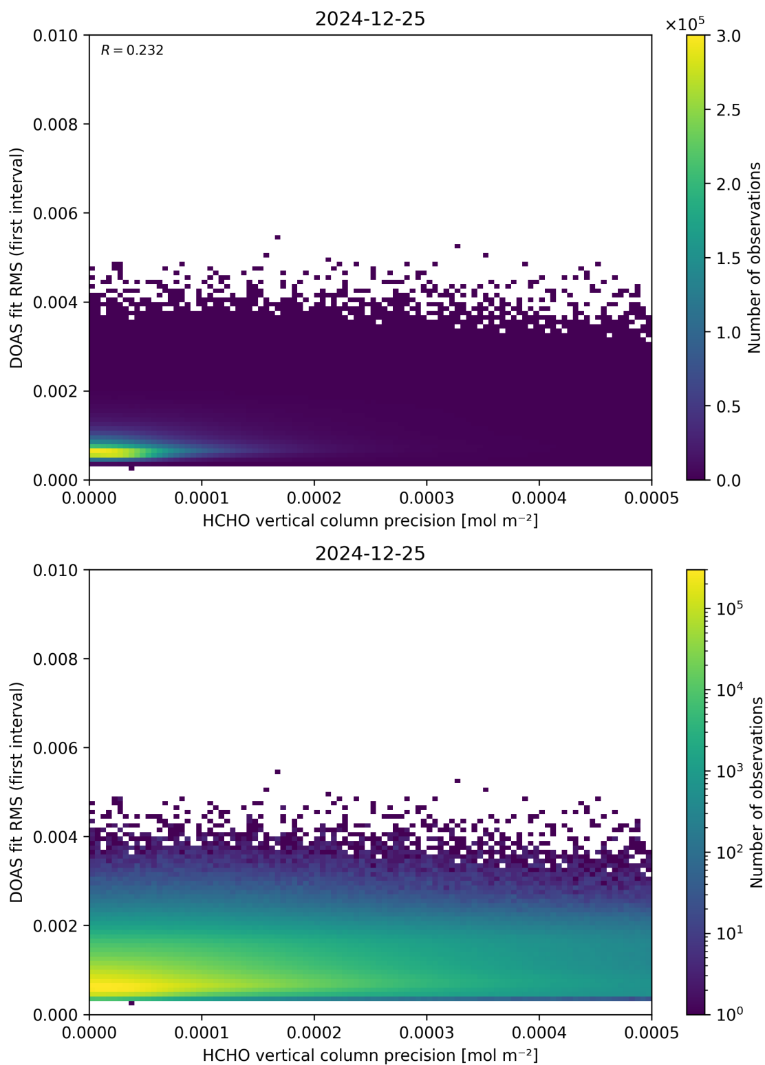
Figure 136: Scatter density plot of “HCHO vertical column precision” against “DOAS fit RMS (first interval)” for 2024-12-24 to 2024-12-26.
