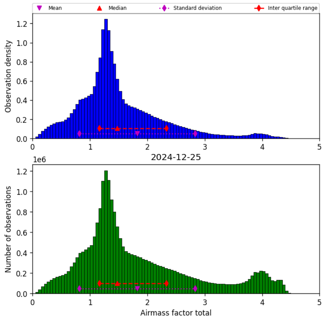
Figure 40: Histogram of “Airmass factor total” for 2024-12-24 to 2024-12-26
