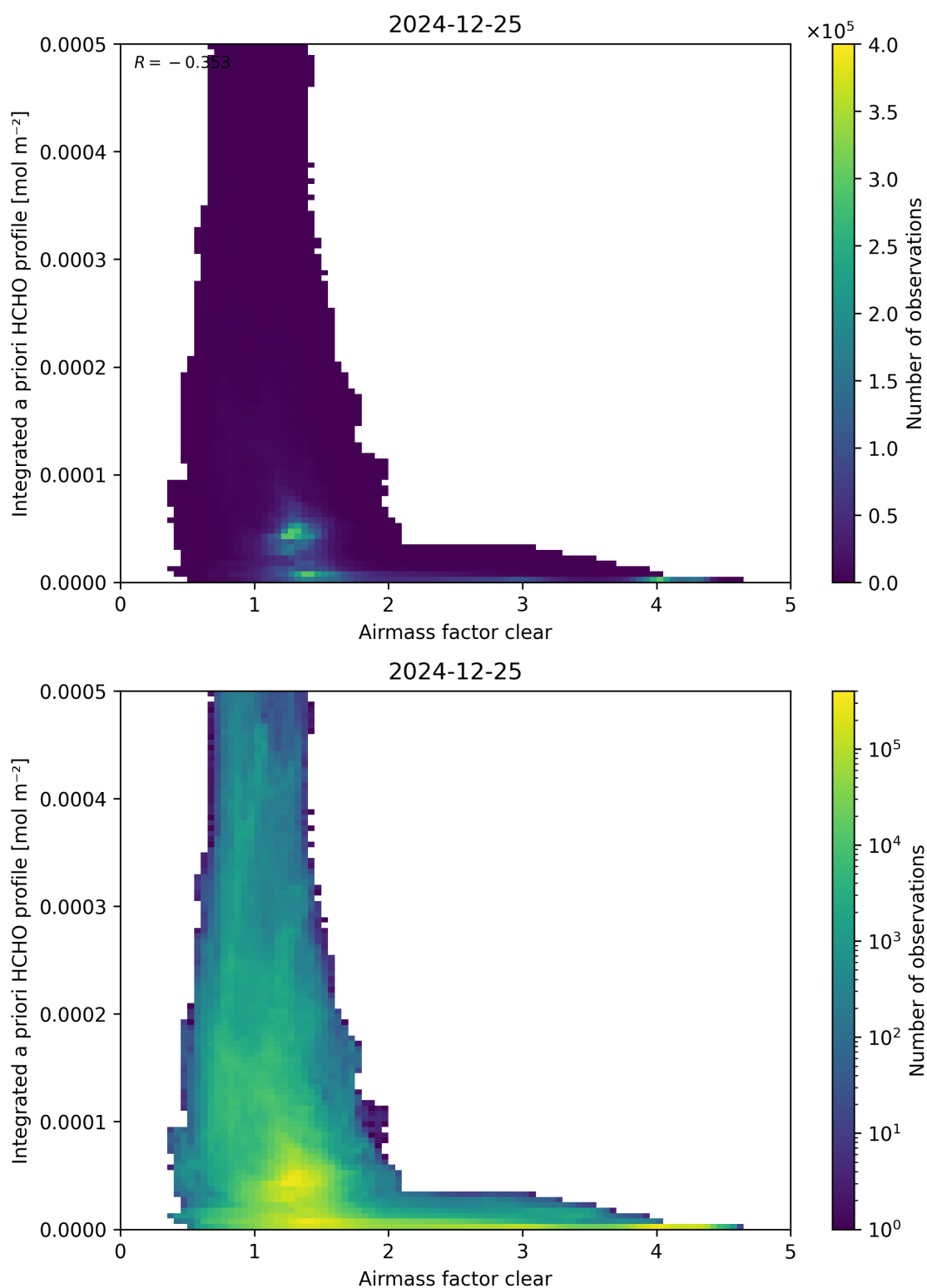
Figure 76: Scatter density plot of “Airmass factor clear” against “Integrated a priori HCHO profile” for 2024-12-24 to 2024-12-26.
