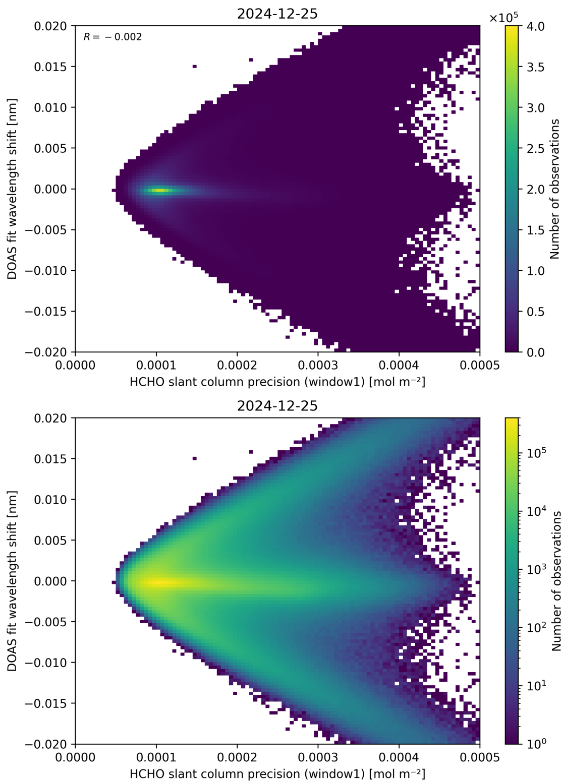
Figure 89: Scatter density plot of “HCHO slant column precision (window1)” against “DOAS fit wavelength shift” for 2024-12-24 to 2024-12-26.
