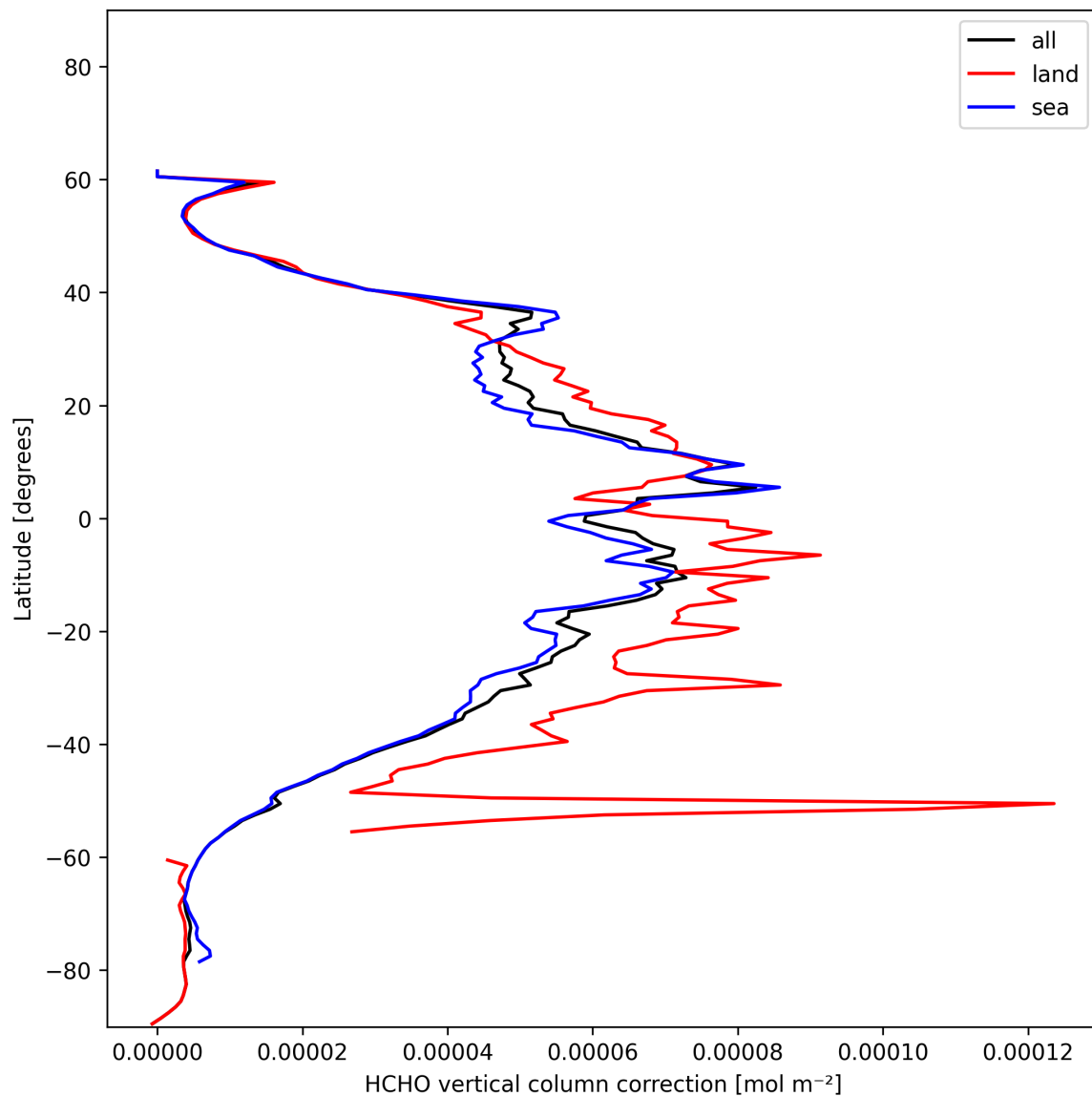
Figure 23: Zonal average of “HCHO vertical column correction” for 2024-12-24 to 2024-12-26.
