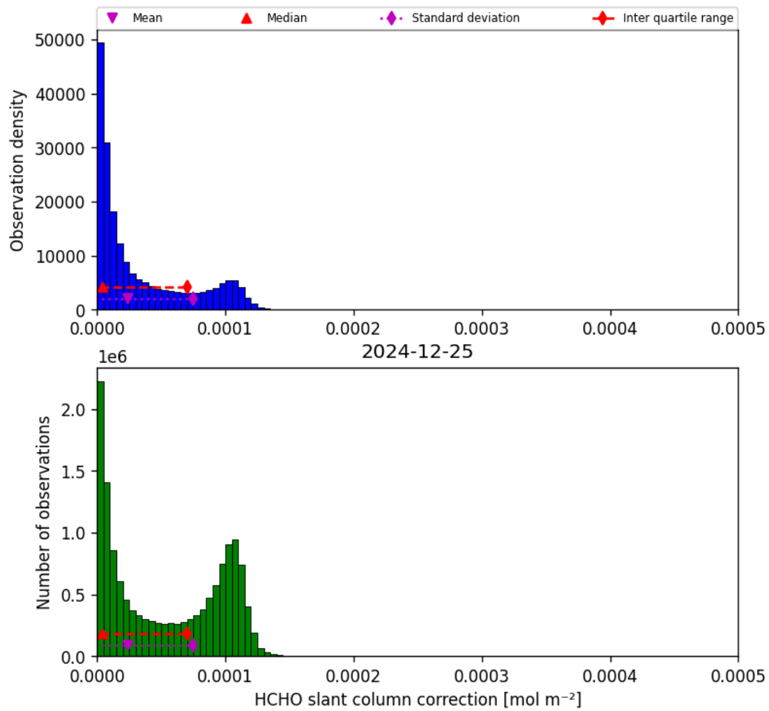
Figure 47: Histogram of “HCHO slant column correction” for 2024-12-24 to 2024-12-26
