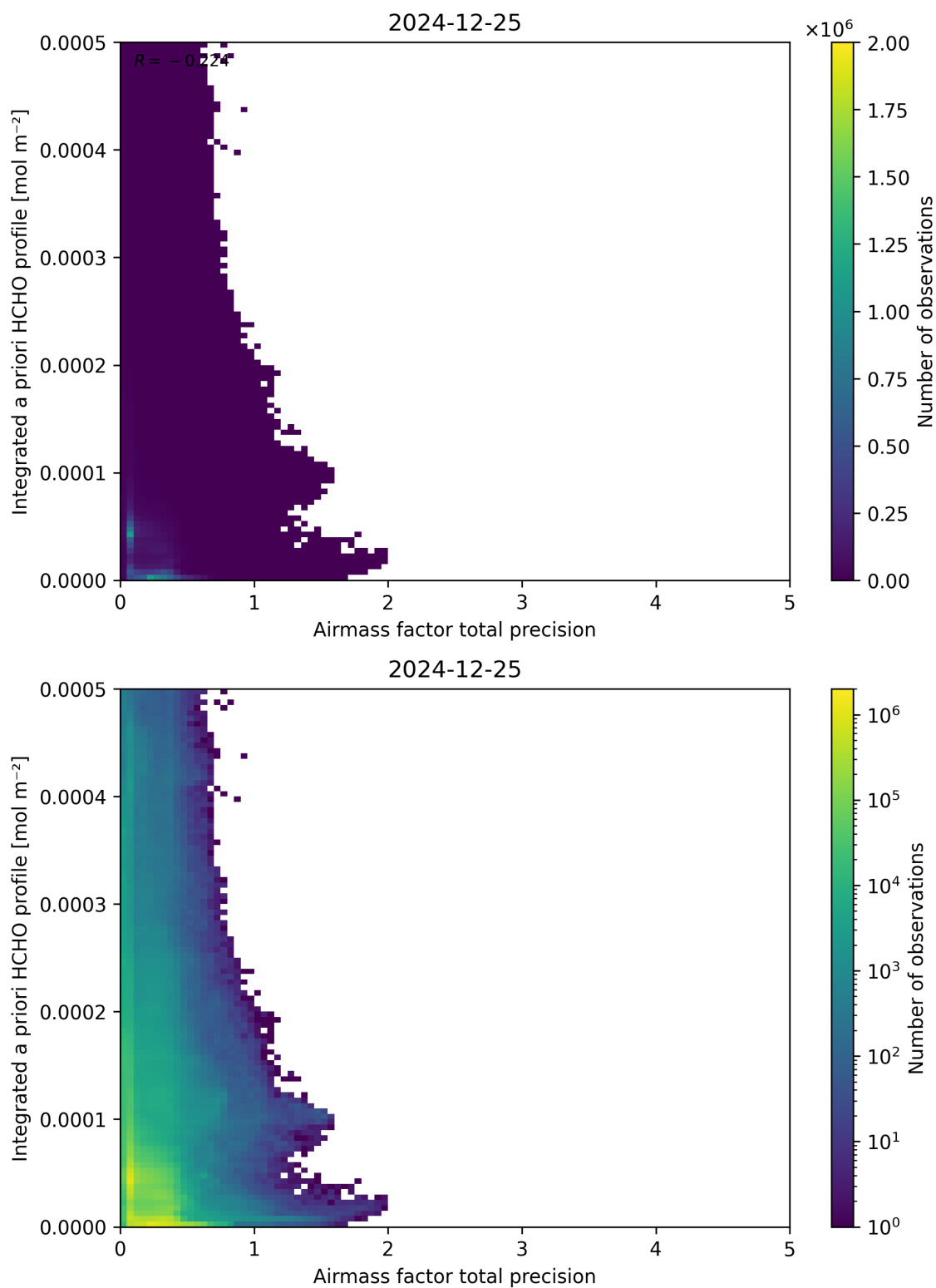
Figure 111: Scatter density plot of “Airmass factor total precision” against “Integrated a priori HCHO profile” for 2024-12-24 to 2024-12-26.
