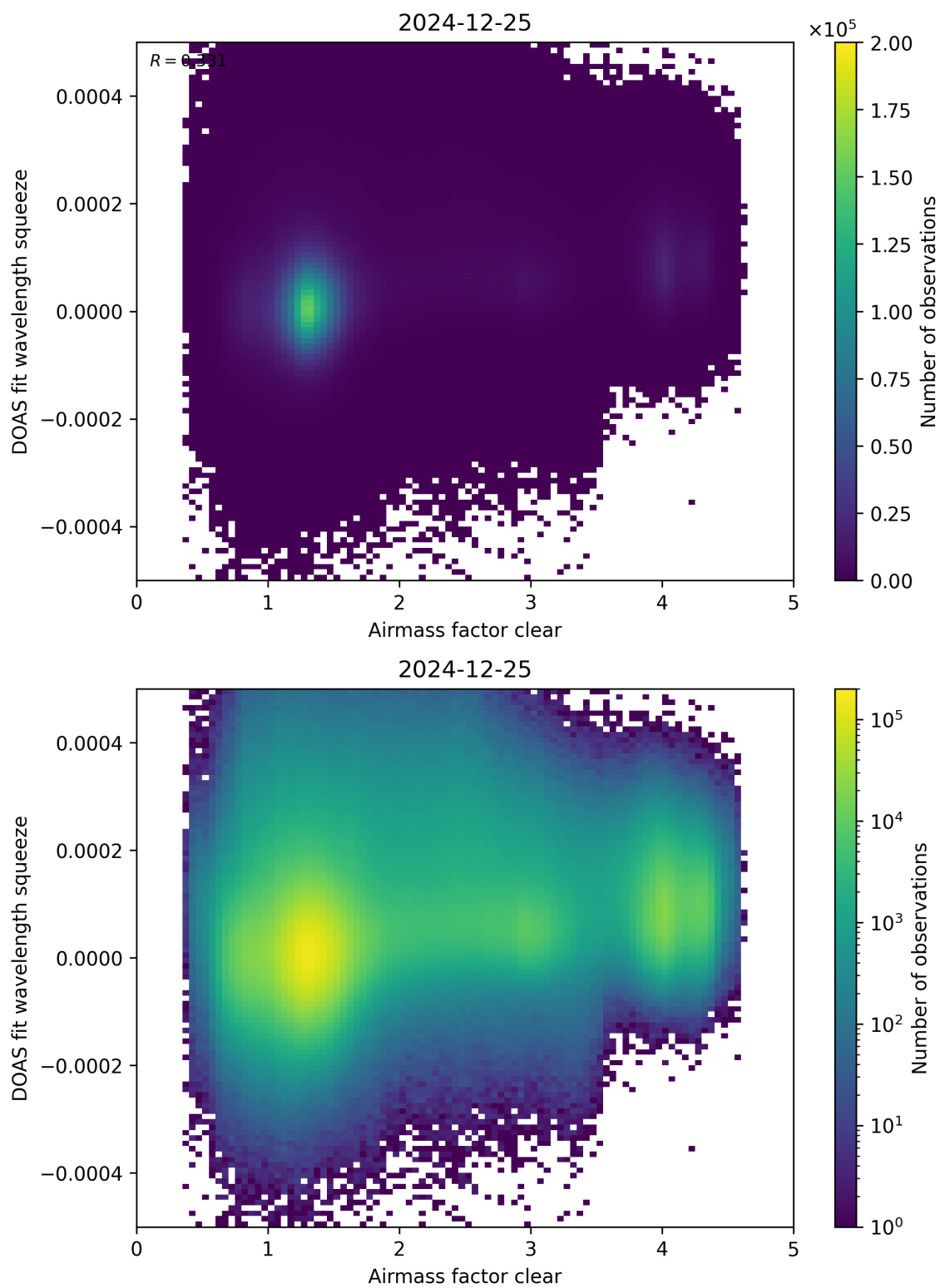
Figure 73: Scatter density plot of “Airmass factor clear” against “DOAS fit wavelength squeeze” for 2024-12-24 to 2024-12-26.
