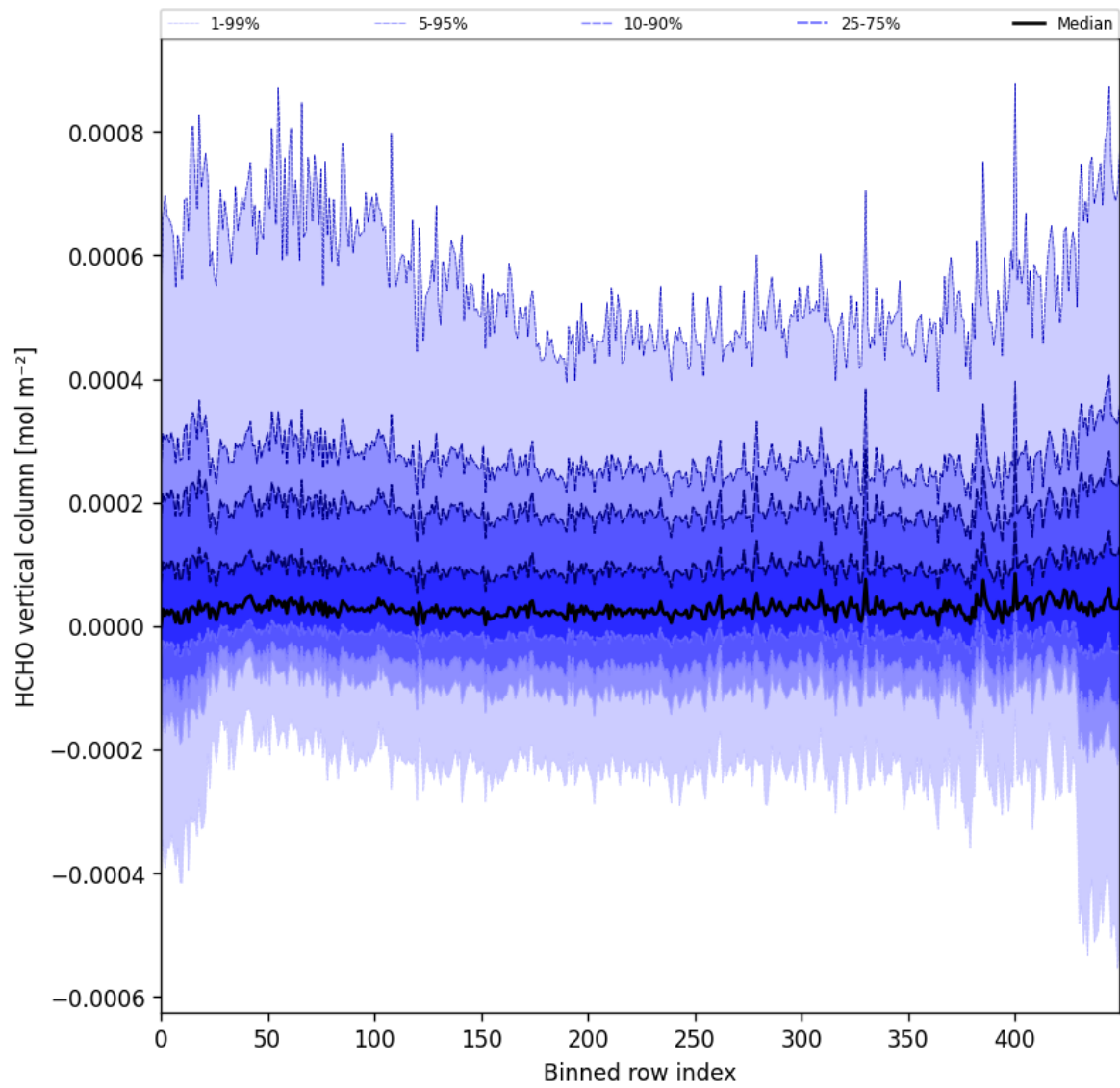
Figure 49: Along track statistics of “HCHO vertical column” for 2024-12-24 to 2024-12-26
