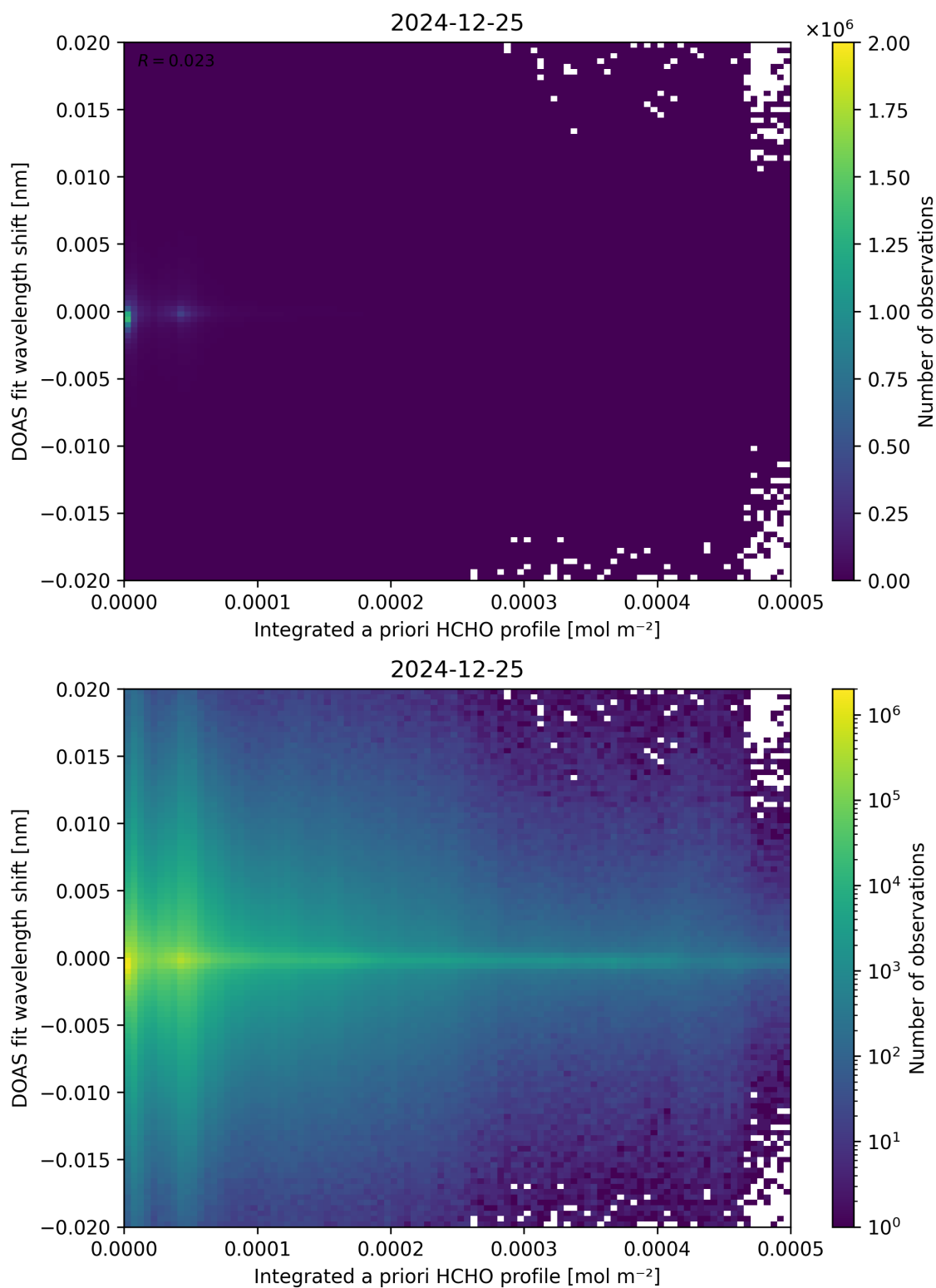
Figure 149: Scatter density plot of “Integrated a priori HCHO profile” against “DOAS fit wavelength shift” for 2024-12-24 to 2024-12-26.
