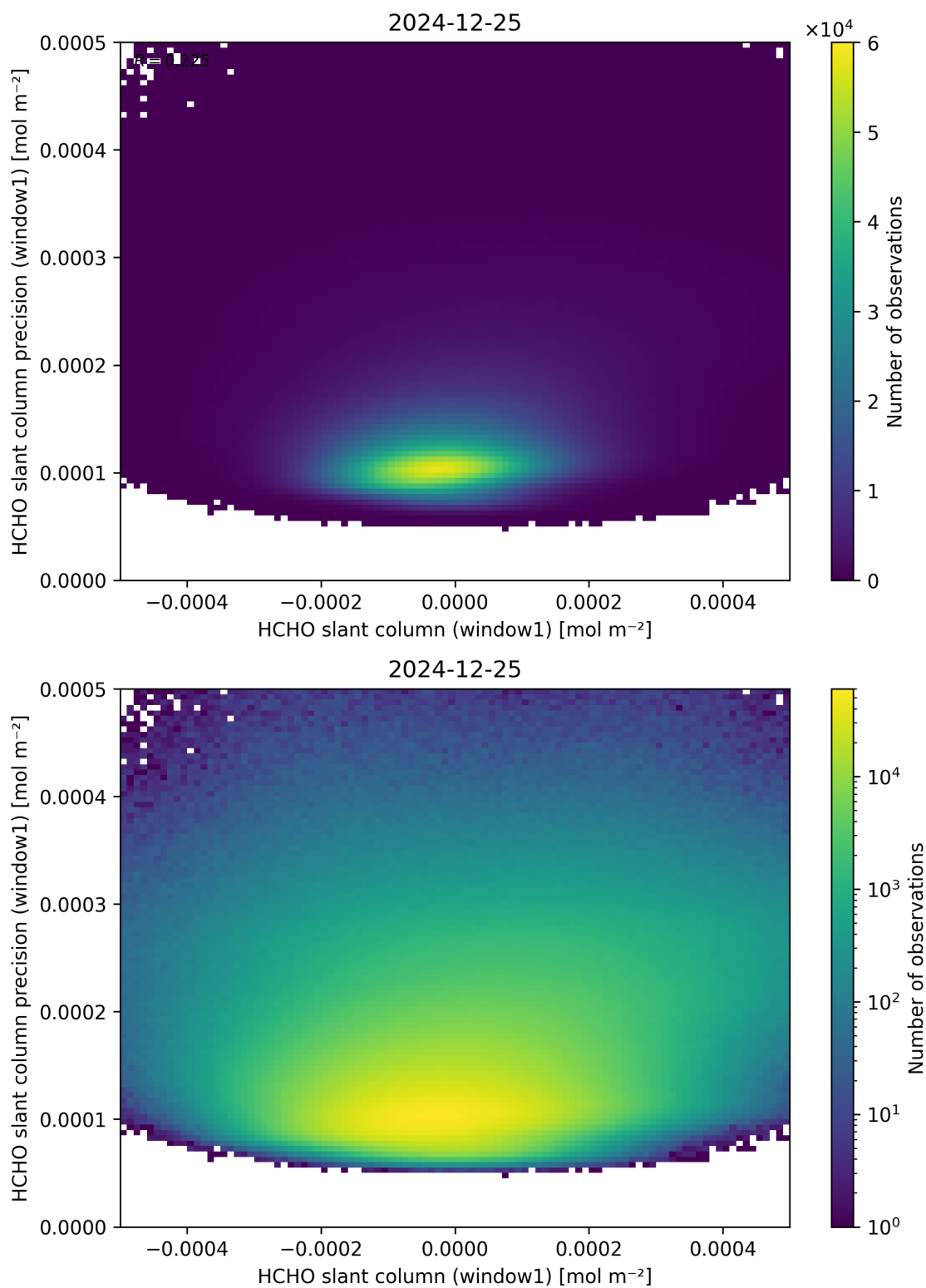
Figure 84: Scatter density plot of “HCHO slant column (window1)” against “HCHO slant column precision (window1)” for 2024-12-24 to 2024-12-26.
