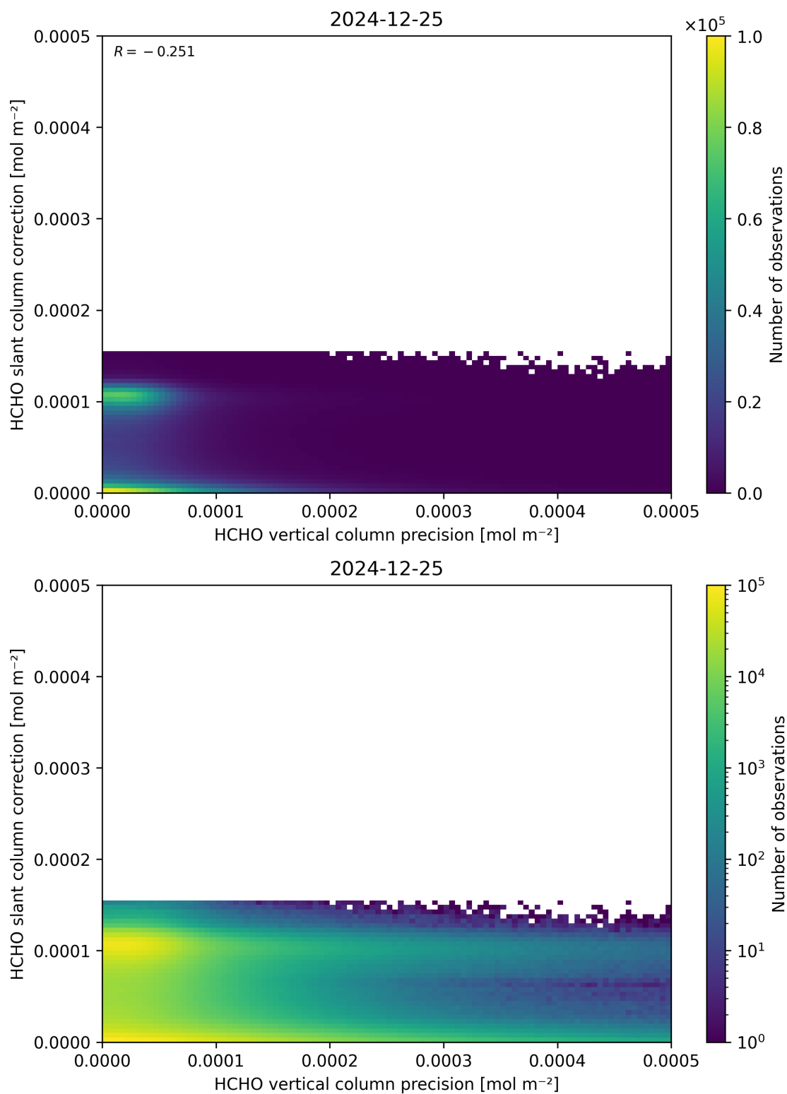
Figure 141: Scatter density plot of “HCHO vertical column precision” against “HCHO slant column correction” for 2024-12-24 to 2024-12-26.
