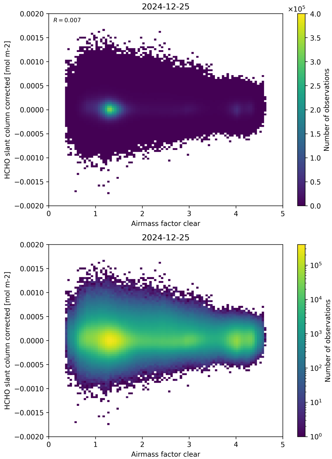
Figure 74: Scatter density plot of “Airmass factor clear” against “HCHO slant column corrected” for 2024-12-24 to 2024-12-26.
