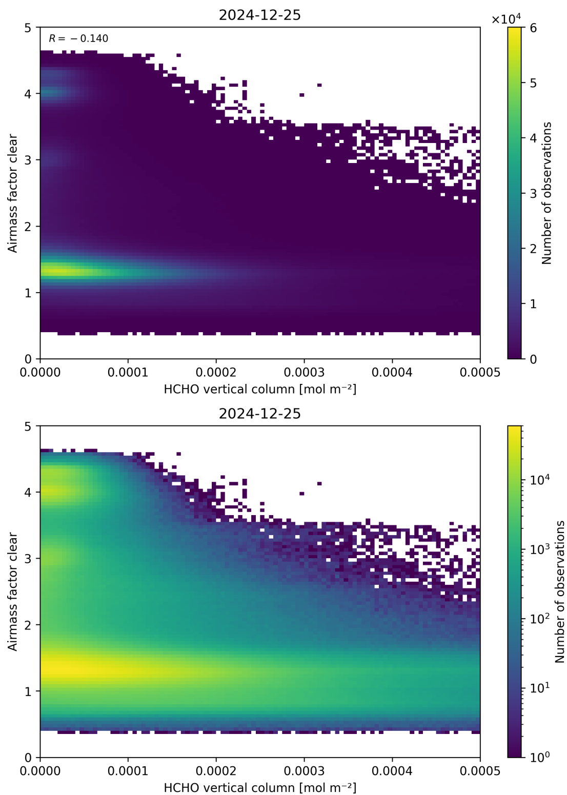
Figure 126: Scatter density plot of “HCHO vertical column” against “Airmass factor clear” for 2024-12-24 to 2024-12-26.
