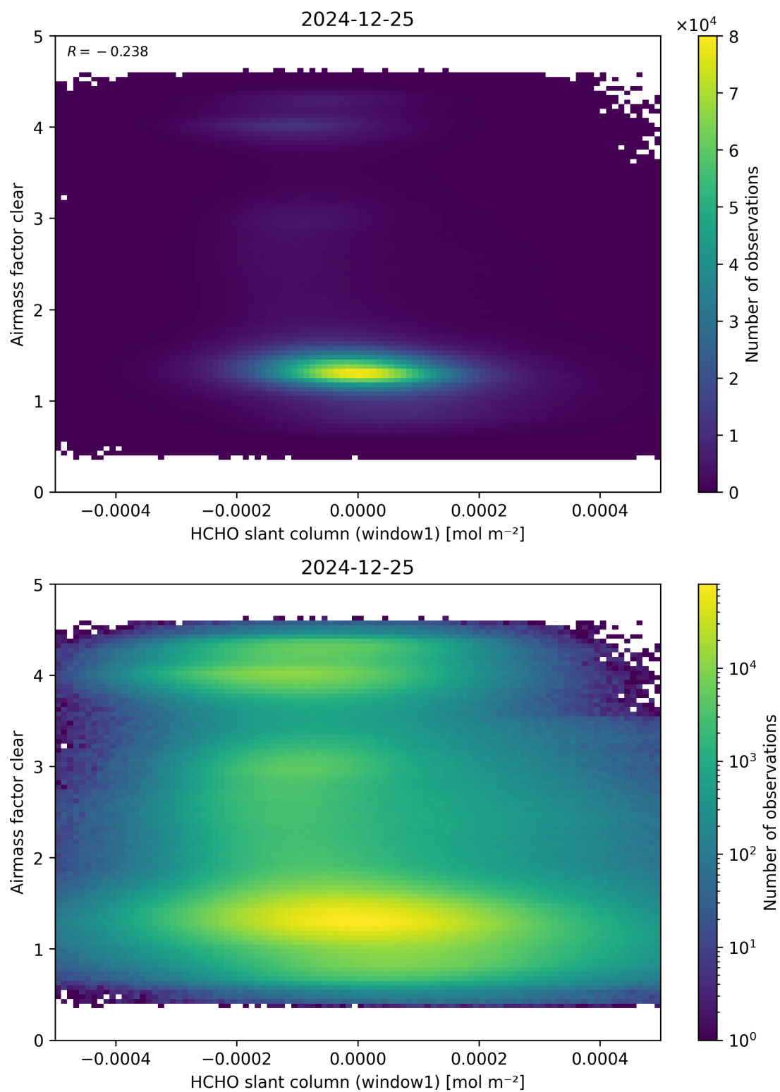
Figure 81: Scatter density plot of “HCHO slant column (window1)” against “Airmass factor clear” for 2024-12-24 to 2024-12-26.
