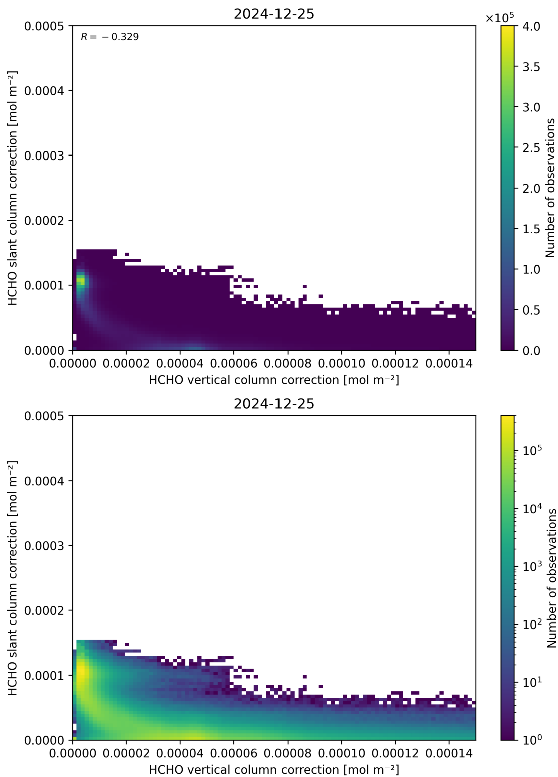
Figure 117: Scatter density plot of “HCHO vertical column correction” against “HCHO slant column correction” for 2024-12-24 to 2024-12-26.
