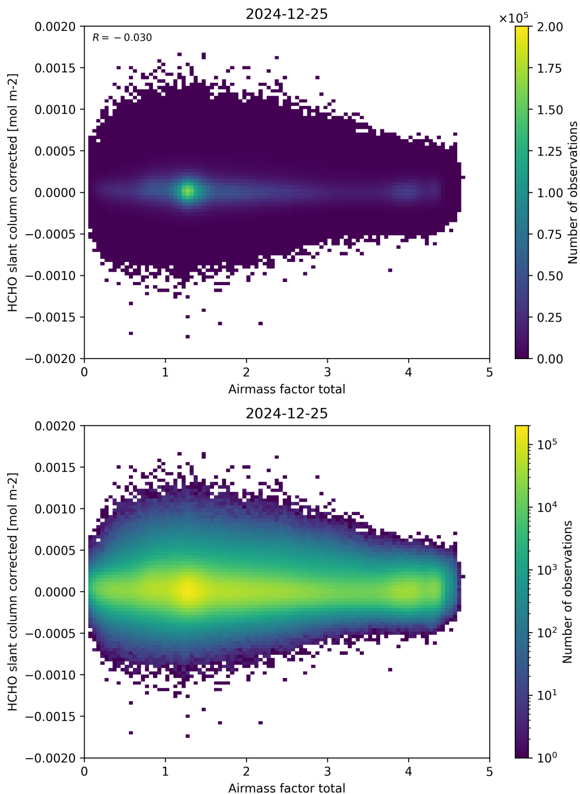
Figure 101: Scatter density plot of “Airmass factor total” against “HCHO slant column corrected” for 2024-12-24 to 2024-12-26.
