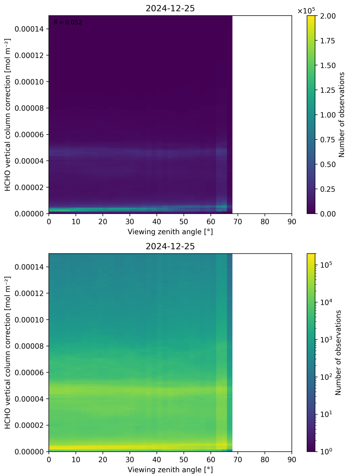
Figure 193: Scatter density plot of “Viewing zenith angle” against “HCHO vertical column correction” for 2024-12-24 to 2024-12-26.
