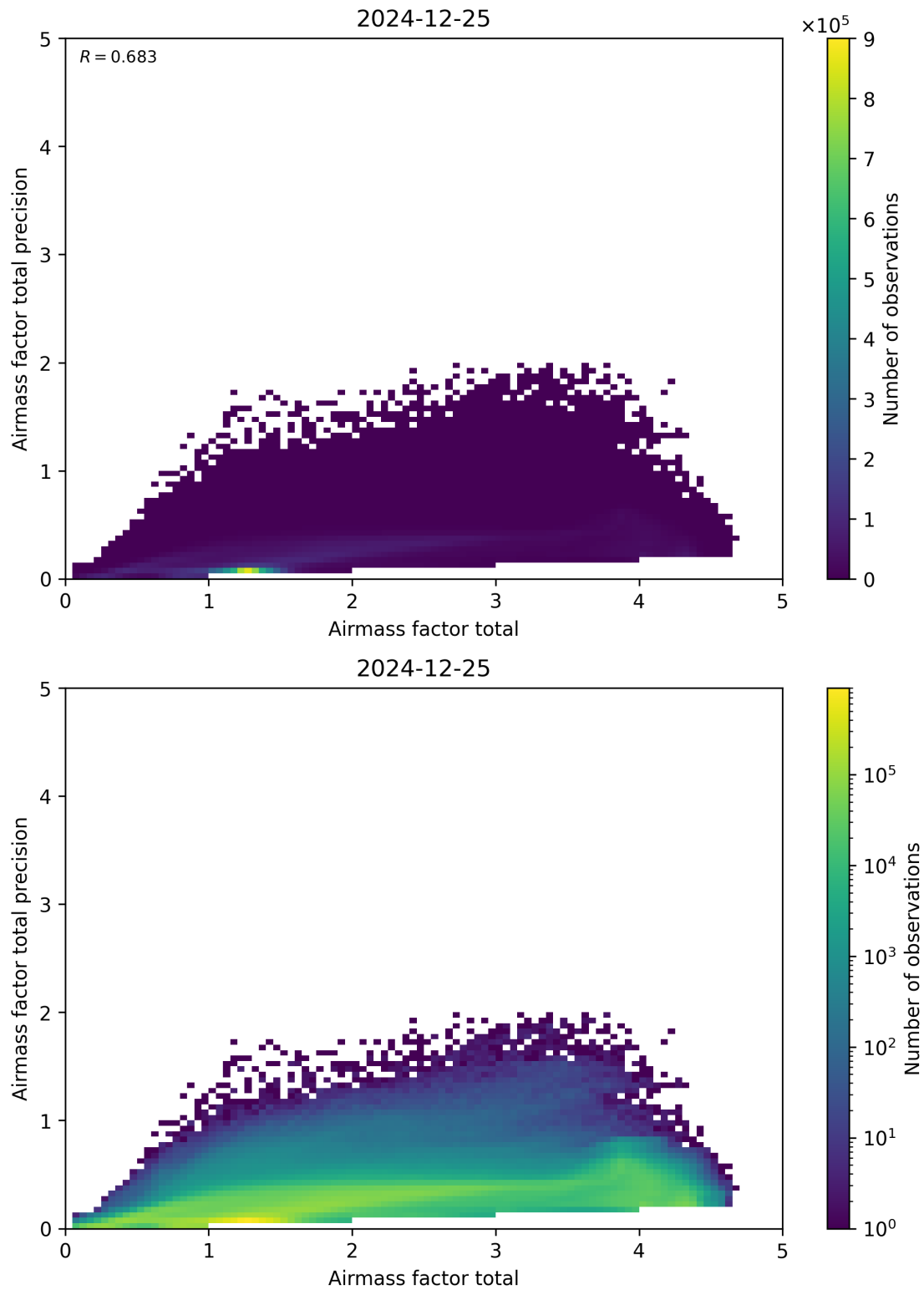
Figure 103: Scatter density plot of “Airmass factor total” against “Airmass factor total precision” for 2024-12-24 to 2024-12-26.
