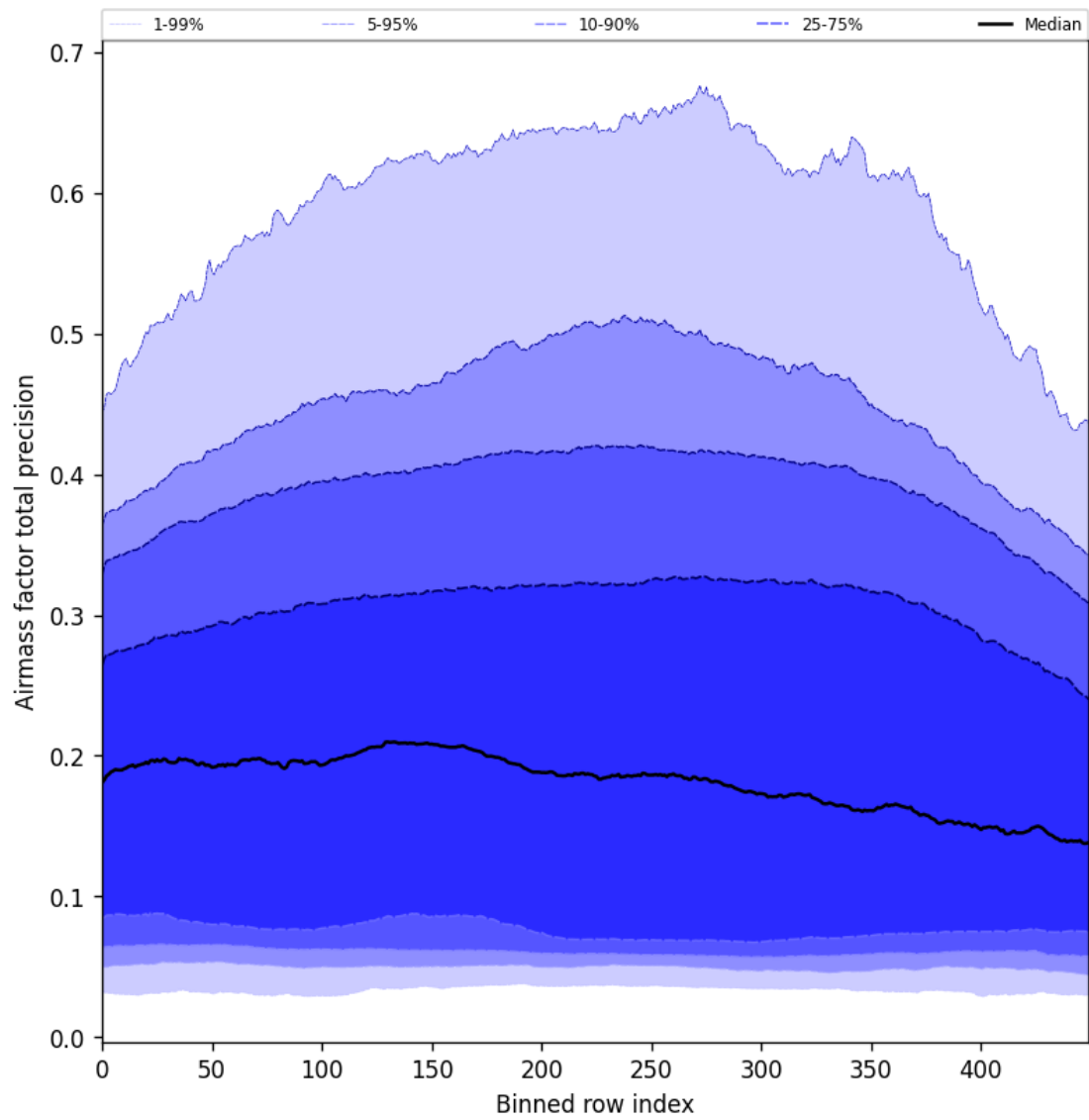
Figure 55: Along track statistics of “Airmass factor total precision” for 2024-12-24 to 2024-12-26
