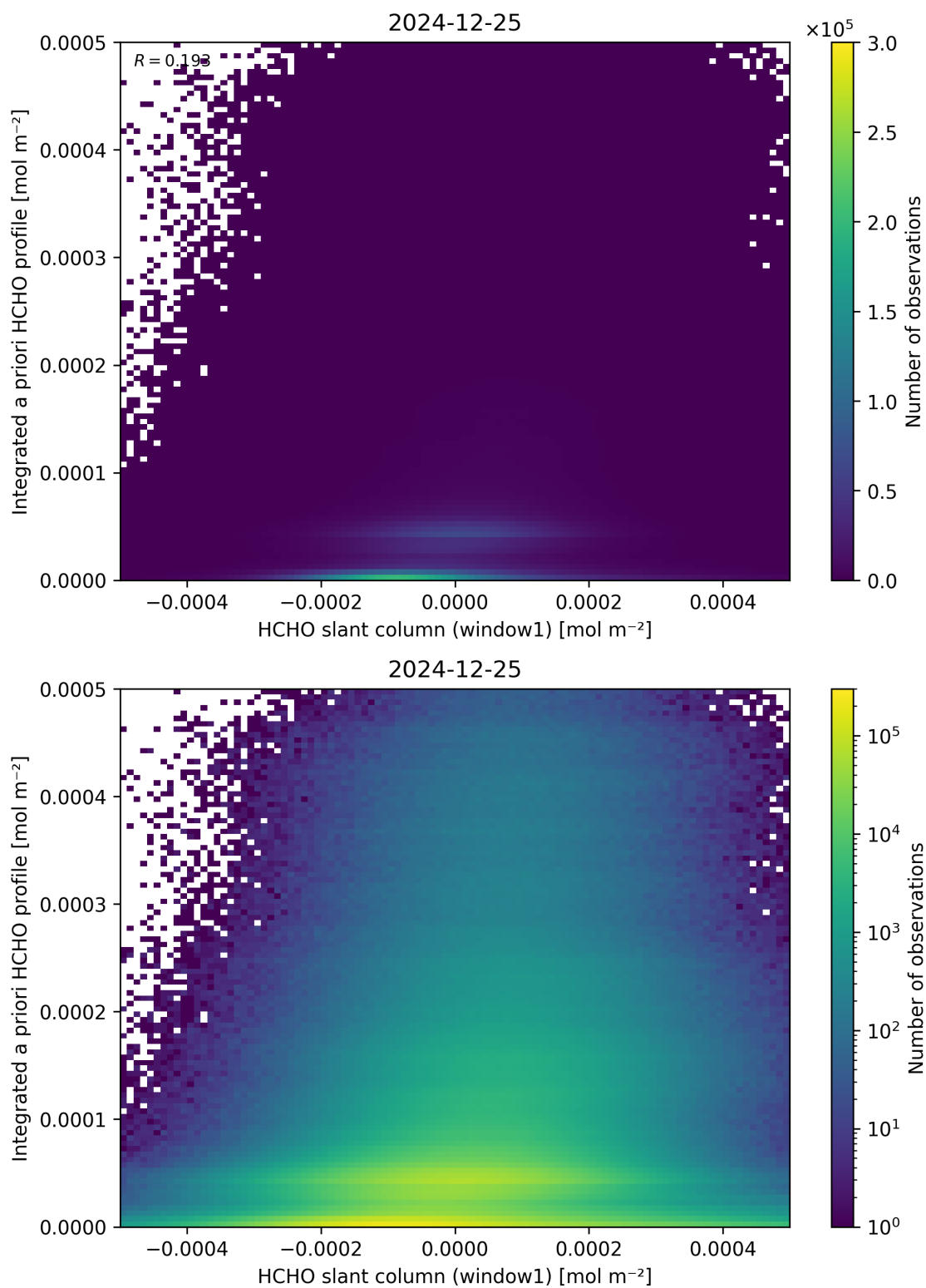
Figure 87: Scatter density plot of “HCHO slant column (window1)” against “Integrated a priori HCHO profile” for 2024-12-24 to 2024-12-26.
