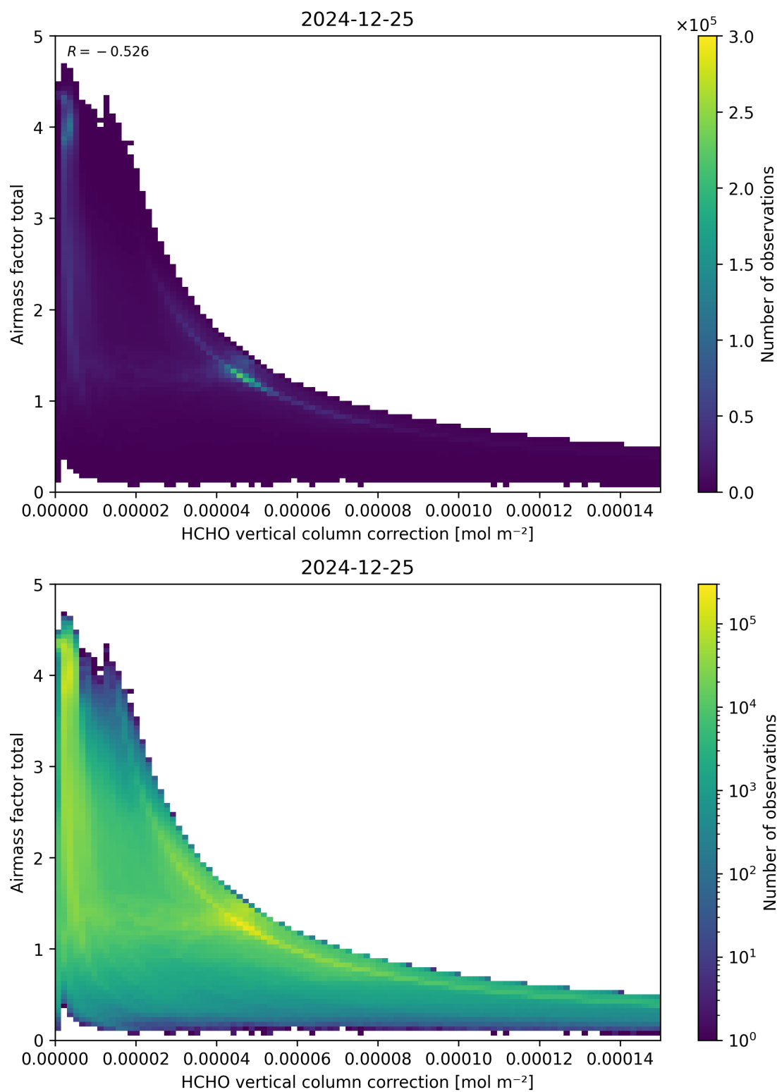
Figure 120: Scatter density plot of “HCHO vertical column correction” against “Airmass factor total” for 2024-12-24 to 2024-12-26.
