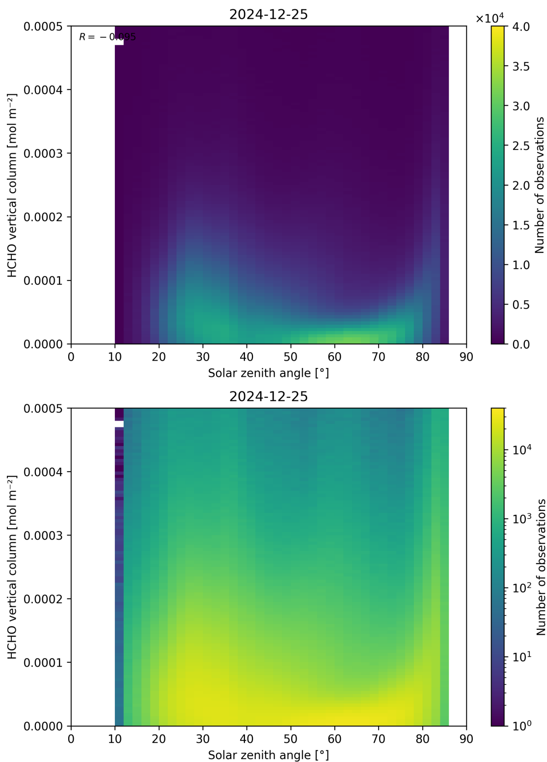
Figure 177: Scatter density plot of “Solar zenith angle” against “HCHO vertical column” for 2024-12-24 to 2024-12-26.
