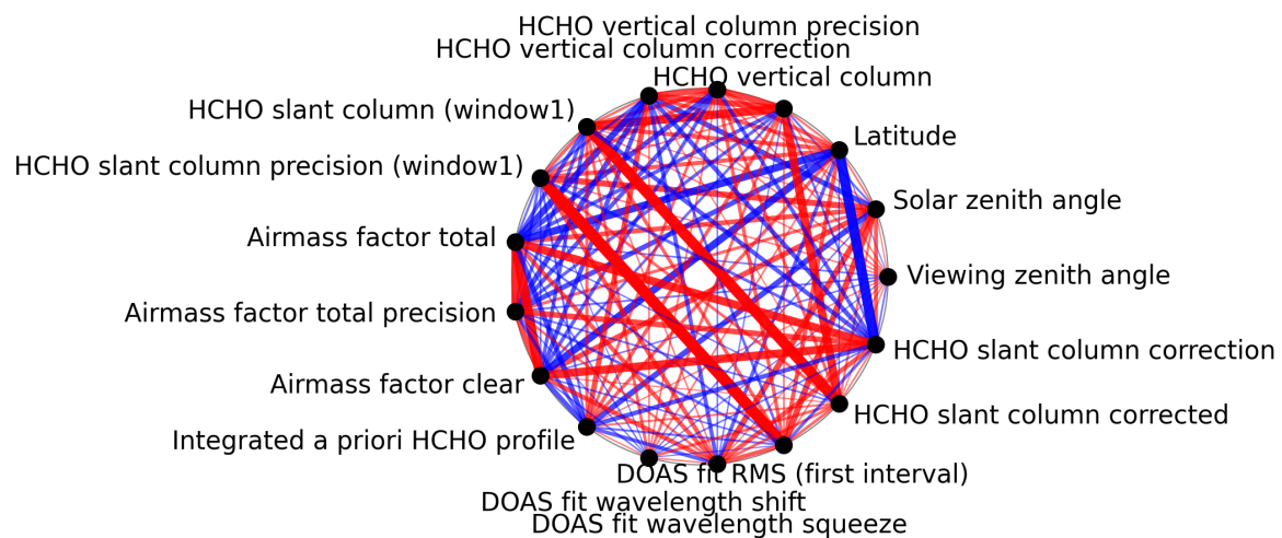
Figure 1: Map of correlation graph for 2024-12-24 to 2024-12-26.
