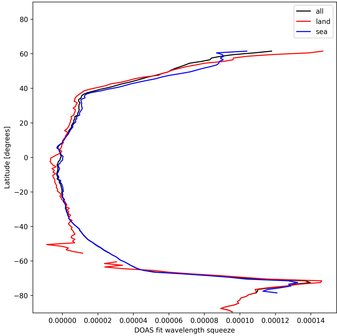
Figure 31: Zonal average of “DOAS fit wavelength squeeze” for 2024-12-24 to 2024-12-26.
