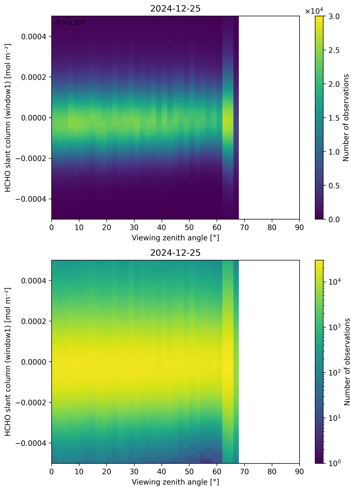
Figure 188: Scatter density plot of “Viewing zenith angle” against “HCHO slant column (window1)” for 2024-12-24 to 2024-12-26.
