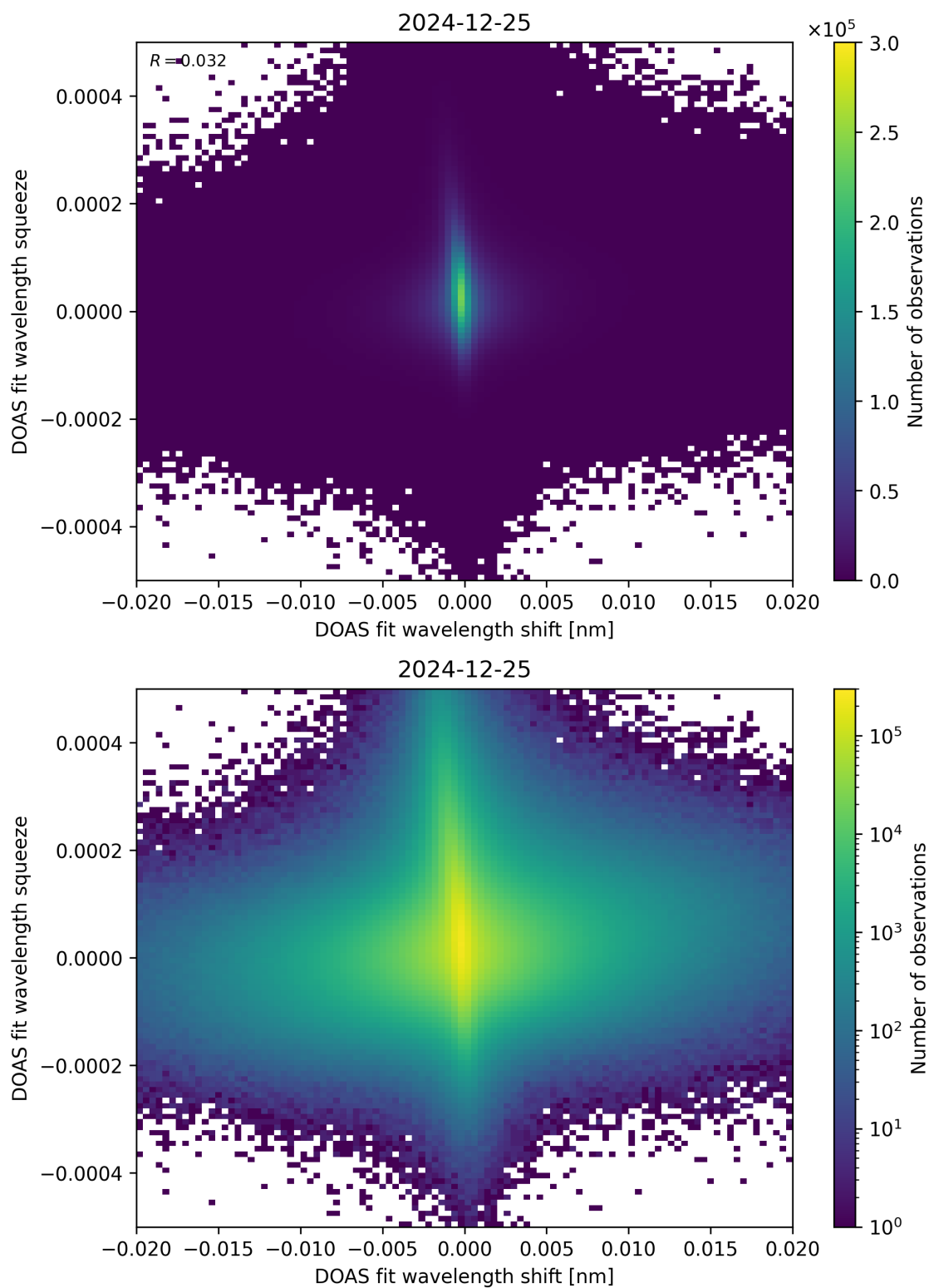
Figure 65: Scatter density plot of “DOAS fit wavelength shift” against “DOAS fit wavelength squeeze” for 2024-12-24 to 2024-12-26.
