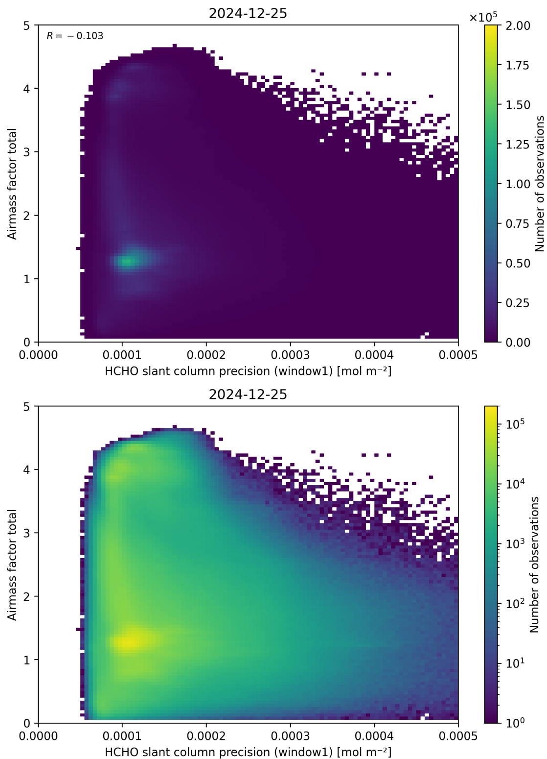
Figure 94: Scatter density plot of “HCHO slant column precision (window1)” against “Airmass factor total” for 2024-12-24 to 2024-12-26.
