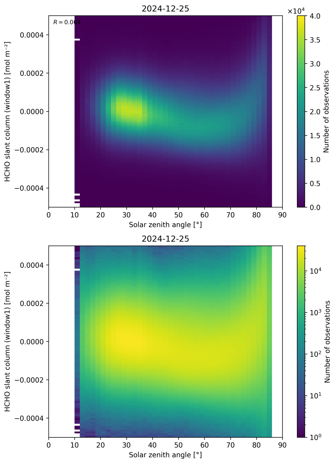
Figure 173: Scatter density plot of “Solar zenith angle” against “HCHO slant column (window1)” for 2024-12-24 to 2024-12-26.
