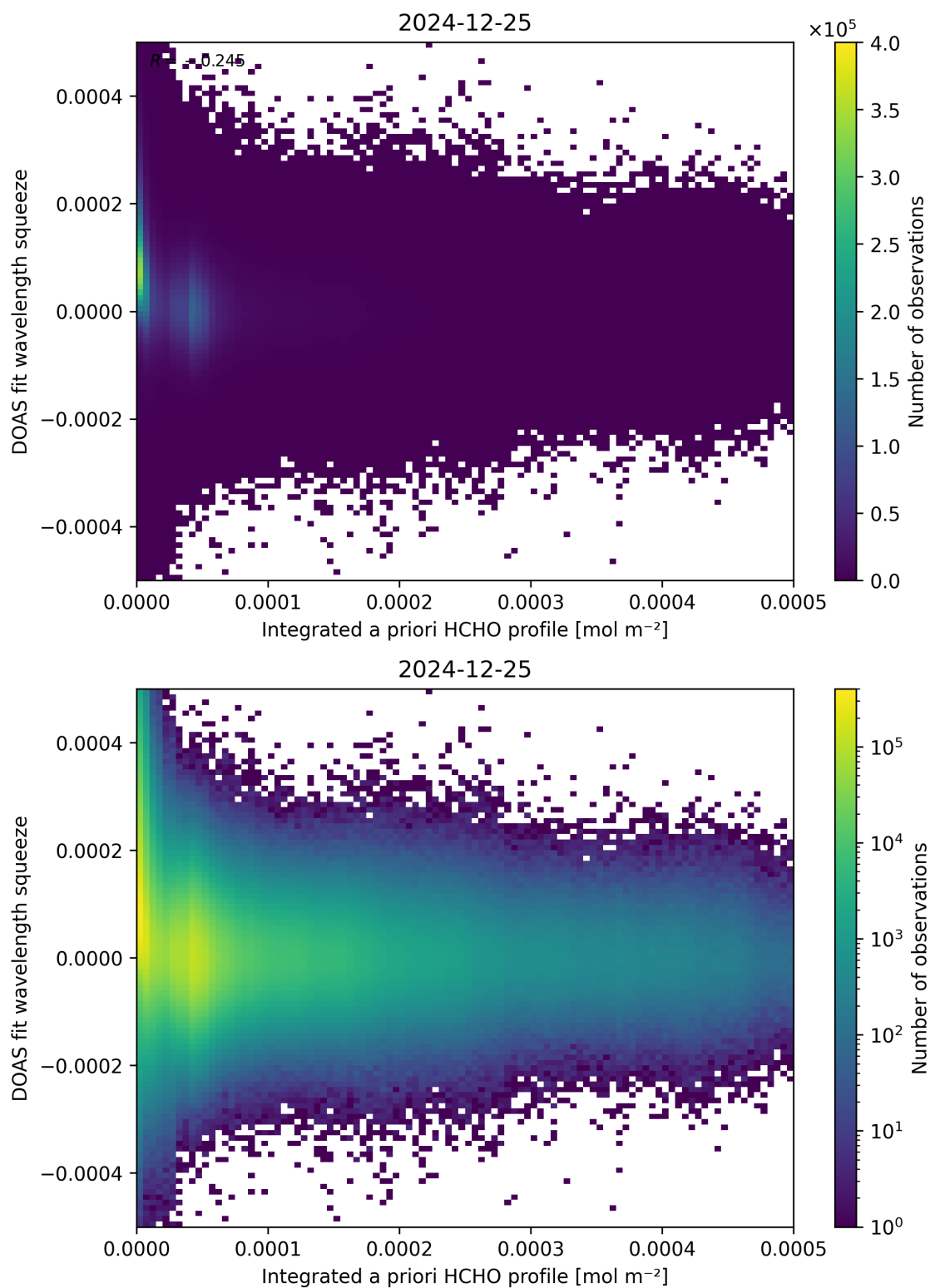
Figure 150: Scatter density plot of “Integrated a priori HCHO profile” against “DOAS fit wavelength squeeze” for 2024-12-24 to 2024-12-26.
