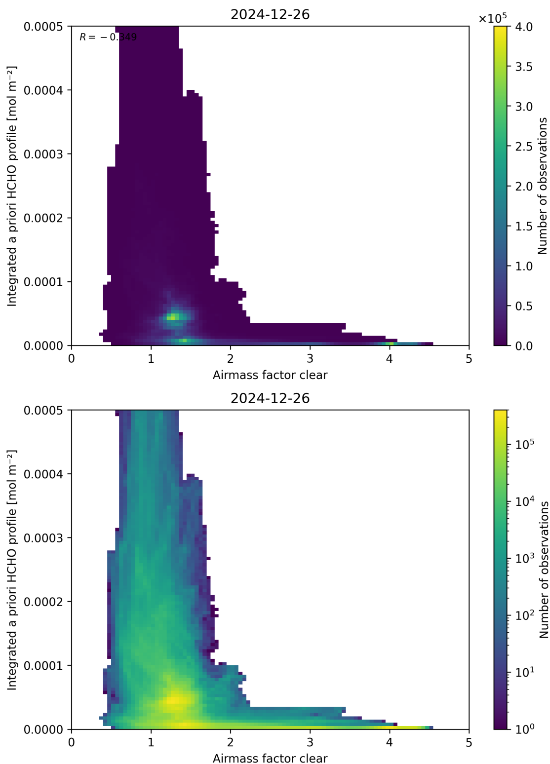
Figure 76: Scatter density plot of “Airmass factor clear” against “Integrated a priori HCHO profile” for 2024-12-25 to 2024-12-27.
