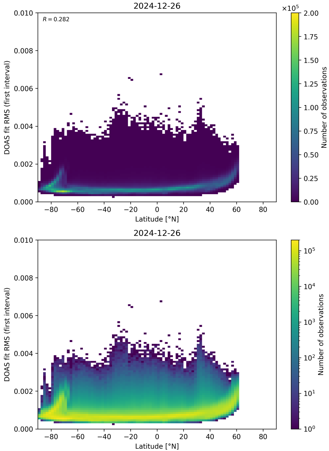
Figure 153: Scatter density plot of “Latitude” against “DOAS fit RMS (first interval)” for 2024-12-25 to 2024-12-27.
