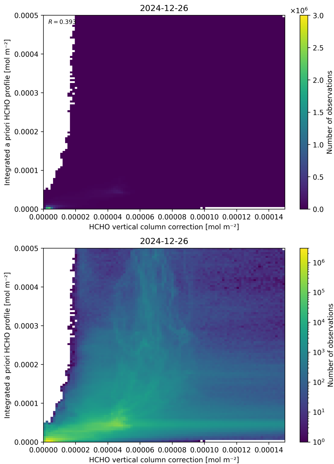
Figure 122: Scatter density plot of “HCHO vertical column correction” against “Integrated a priori HCHO profile” for 2024-12-25 to 2024-12-27.
