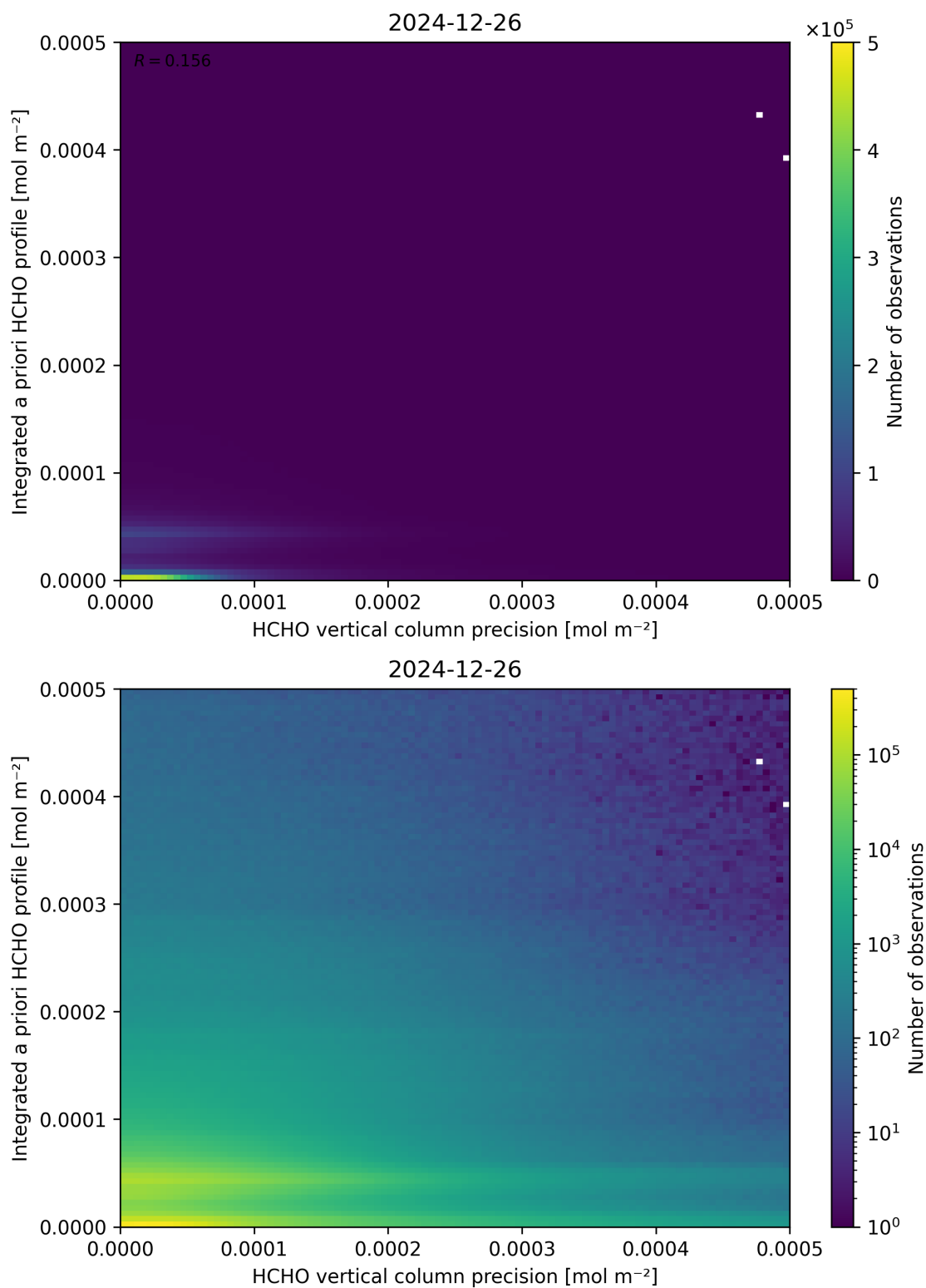
Figure 147: Scatter density plot of “HCHO vertical column precision” against “Integrated a priori HCHO profile” for 2024-12-25 to 2024-12-27.
