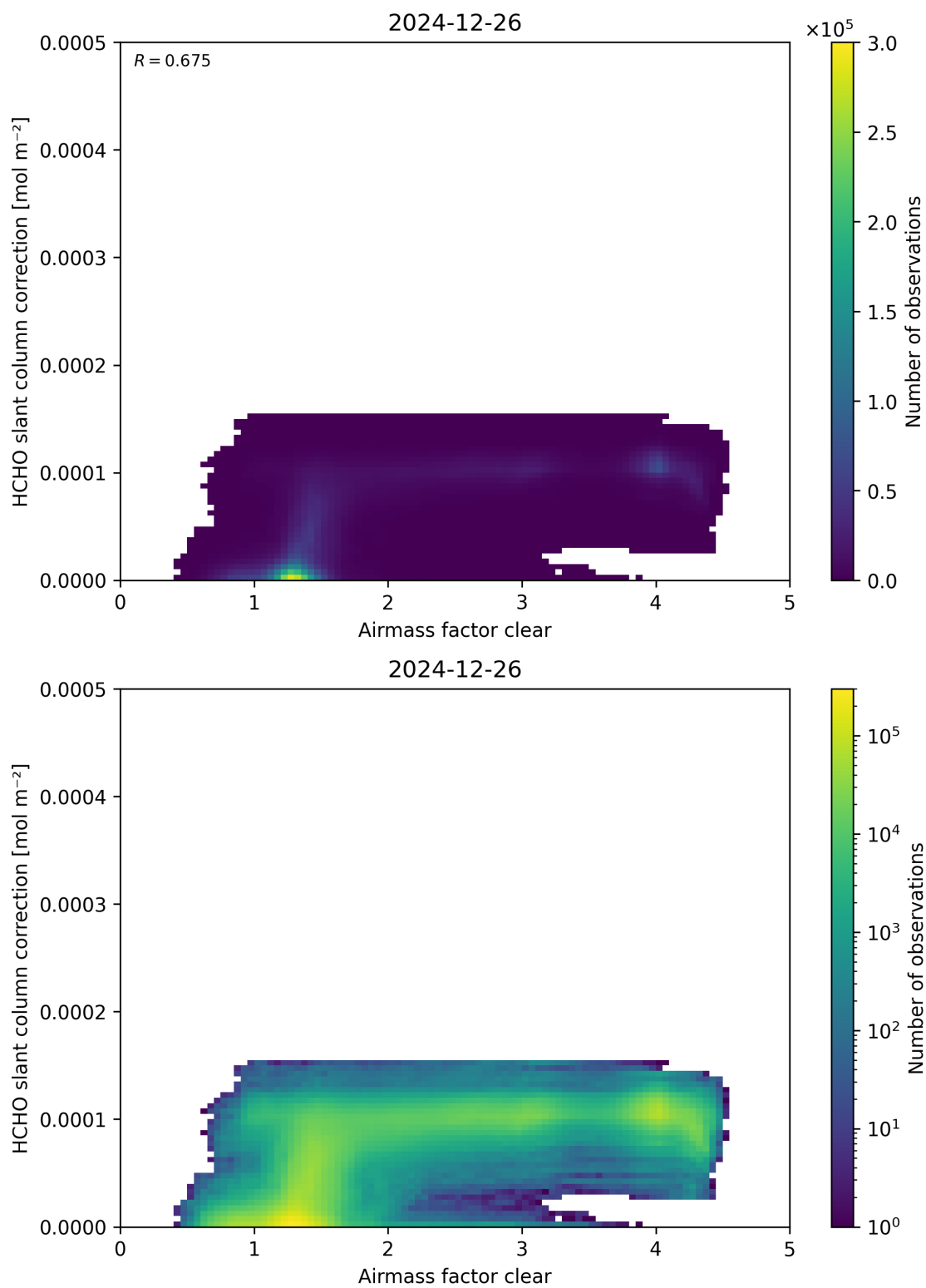
Figure 75: Scatter density plot of “Airmass factor clear” against “HCHO slant column correction” for 2024-12-25 to 2024-12-27.
