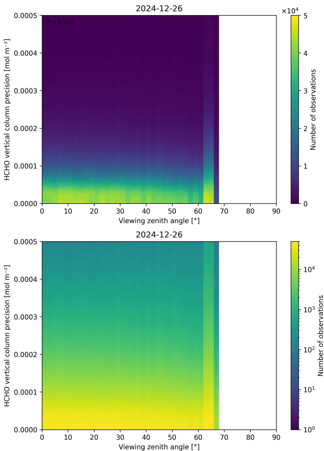
Figure 194: Scatter density plot of “Viewing zenith angle” against “HCHO vertical column precision” for 2024-12-25 to 2024-12-27.
