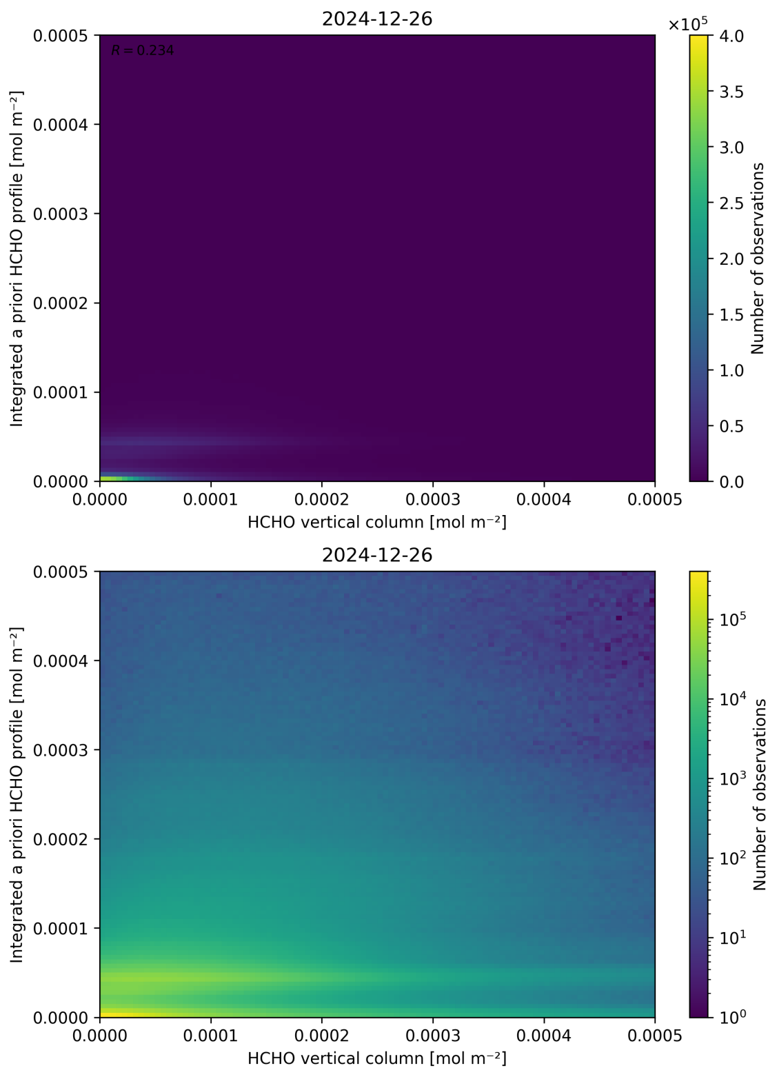
Figure 135: Scatter density plot of “HCHO vertical column” against “Integrated a priori HCHO profile” for 2024-12-25 to 2024-12-27.
