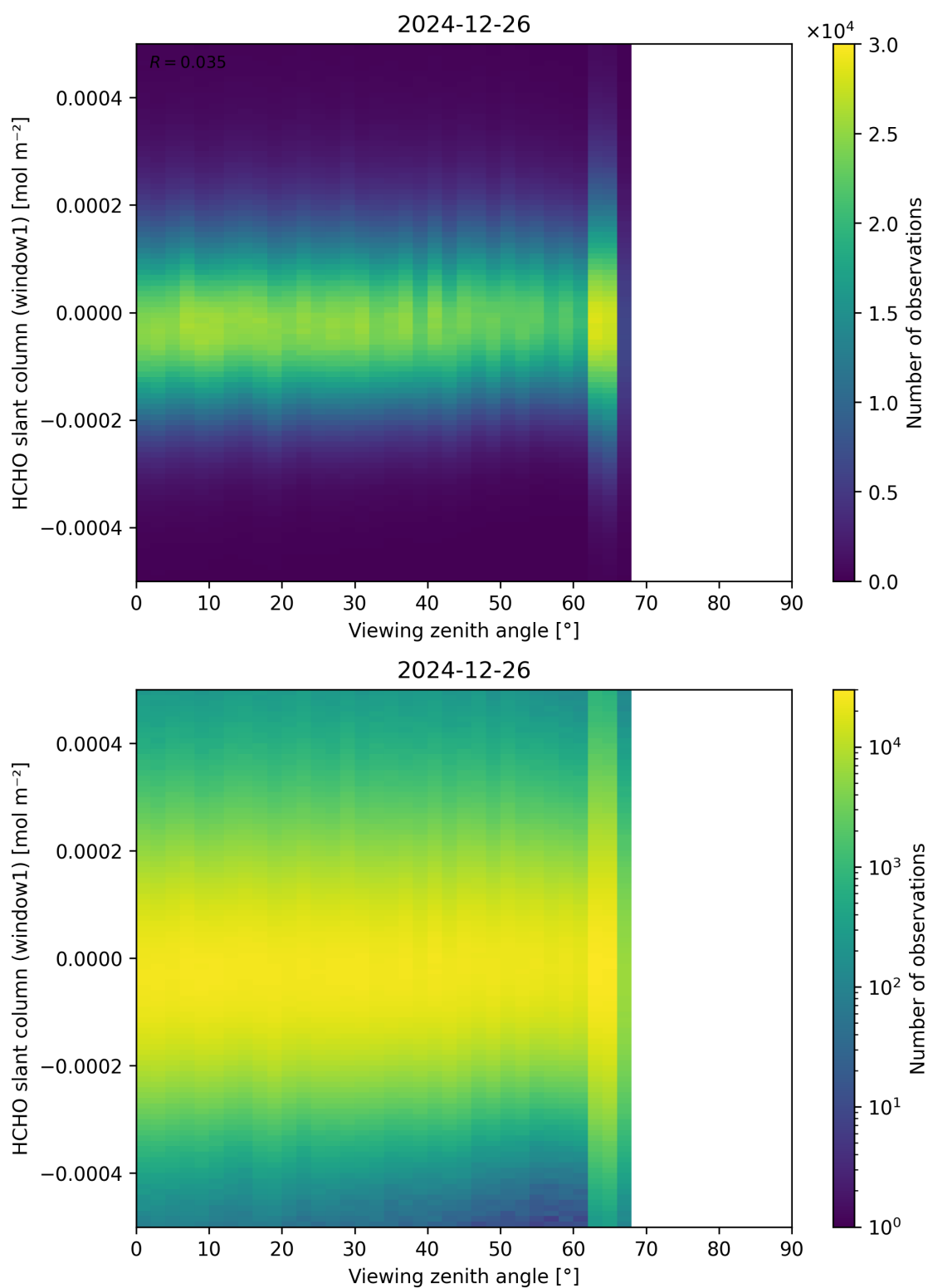
Figure 188: Scatter density plot of “Viewing zenith angle” against “HCHO slant column (window1)” for 2024-12-25 to 2024-12-27.
