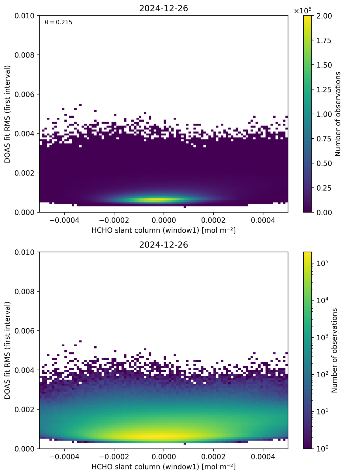
Figure 78: Scatter density plot of “HCHO slant column (window1)” against “DOAS fit RMS (first interval)” for 2024-12-25 to 2024-12-27.
