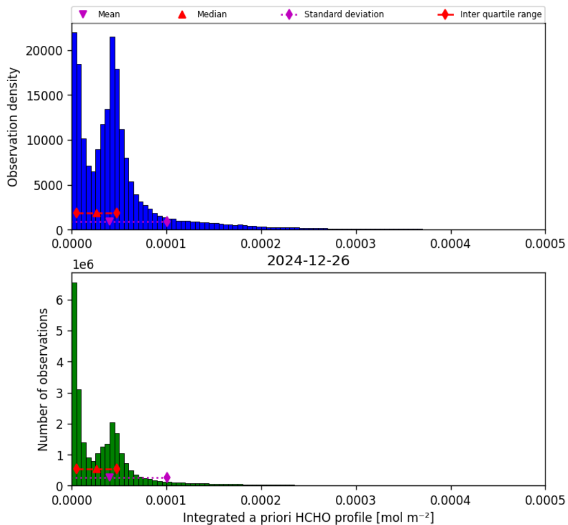
Figure 43: Histogram of “Integrated a priori HCHO profile” for 2024-12-25 to 2024-12-27
