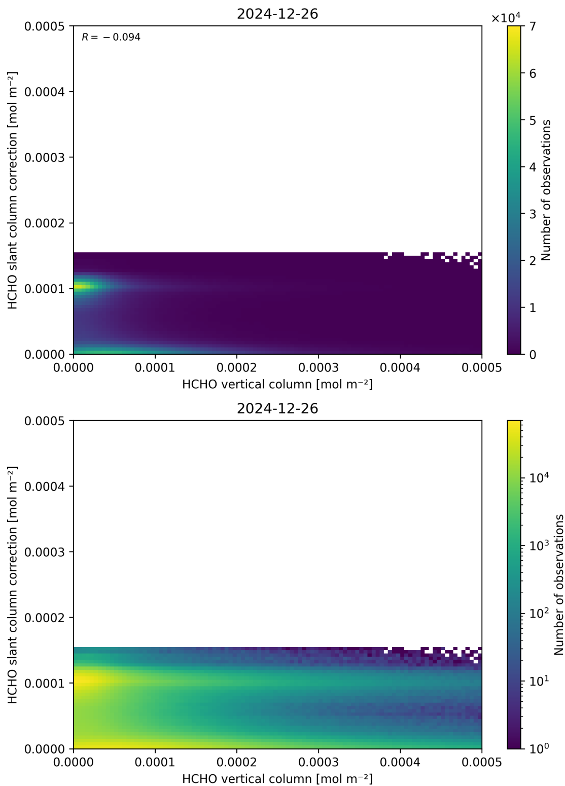
Figure 128: Scatter density plot of “HCHO vertical column” against “HCHO slant column correction” for 2024-12-25 to 2024-12-27.
