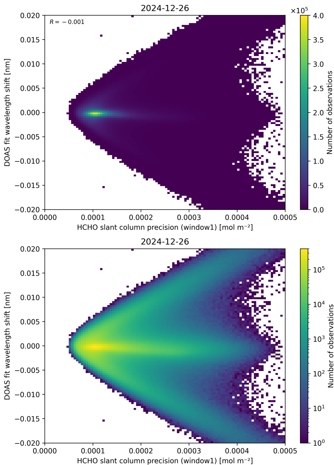
Figure 89: Scatter density plot of “HCHO slant column precision (window1)” against “DOAS fit wavelength shift” for 2024-12-25 to 2024-12-27.
