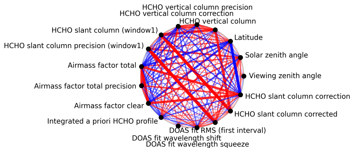
Figure 1: Map of correlation graph for 2024-12-25 to 2024-12-27.
