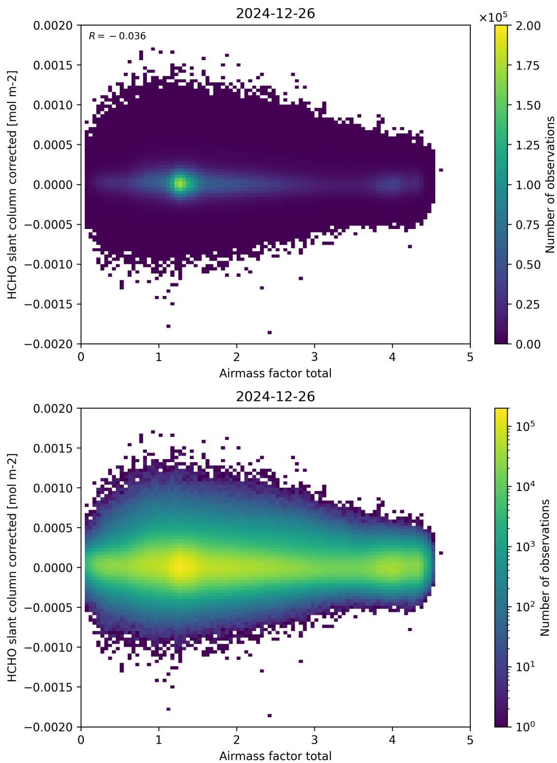
Figure 101: Scatter density plot of “Airmass factor total” against “HCHO slant column corrected” for 2024-12-25 to 2024-12-27.
