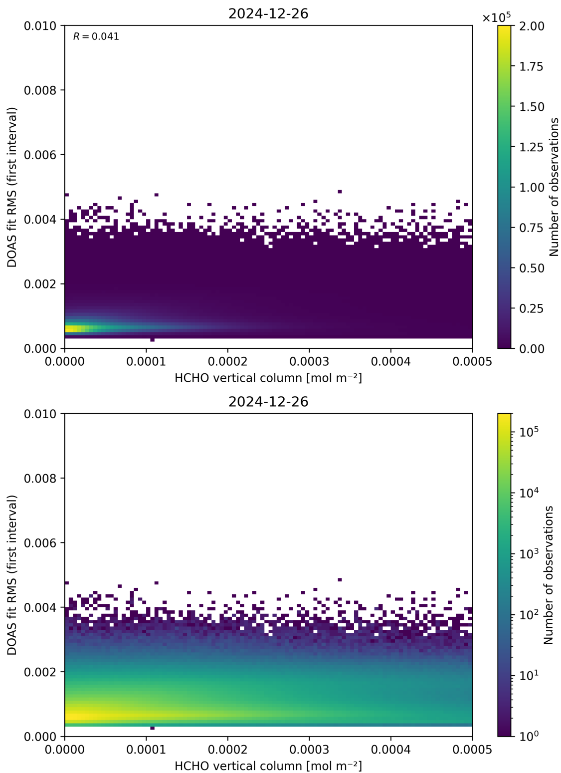
Figure 123: Scatter density plot of “HCHO vertical column” against “DOAS fit RMS (first interval)” for 2024-12-25 to 2024-12-27.
