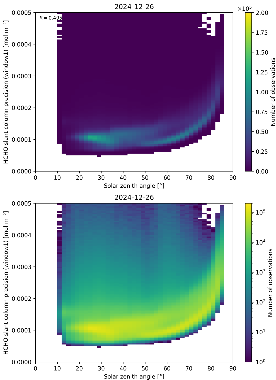
Figure 174: Scatter density plot of “Solar zenith angle” against “HCHO slant column precision (window1)” for 2024-12-25 to 2024-12-27.
