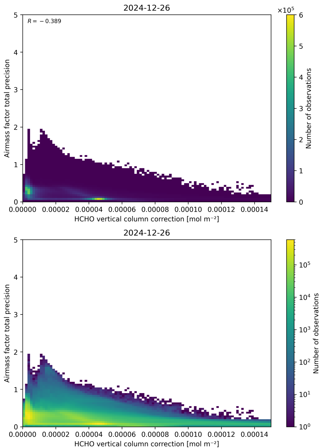
Figure 121: Scatter density plot of “HCHO vertical column correction” against “Airmass factor total precision” for 2024-12-25 to 2024-12-27.
