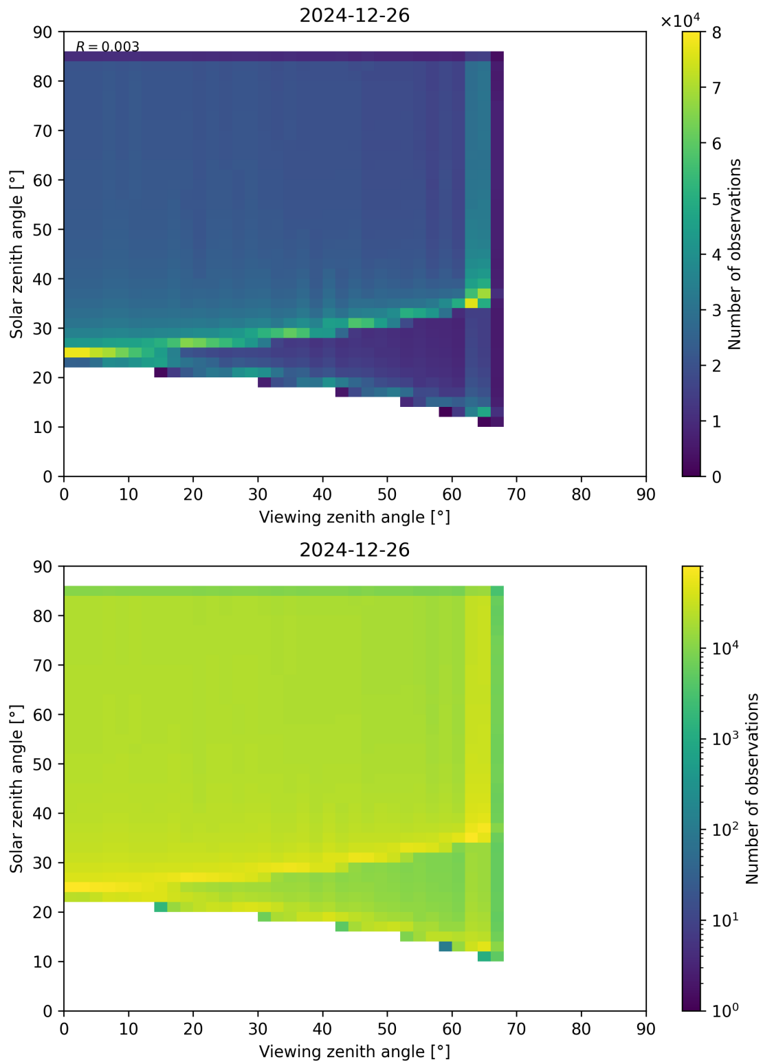
Figure 197: Scatter density plot of “Viewing zenith angle” against “Solar zenith angle” for 2024-12-25 to 2024-12-27.
