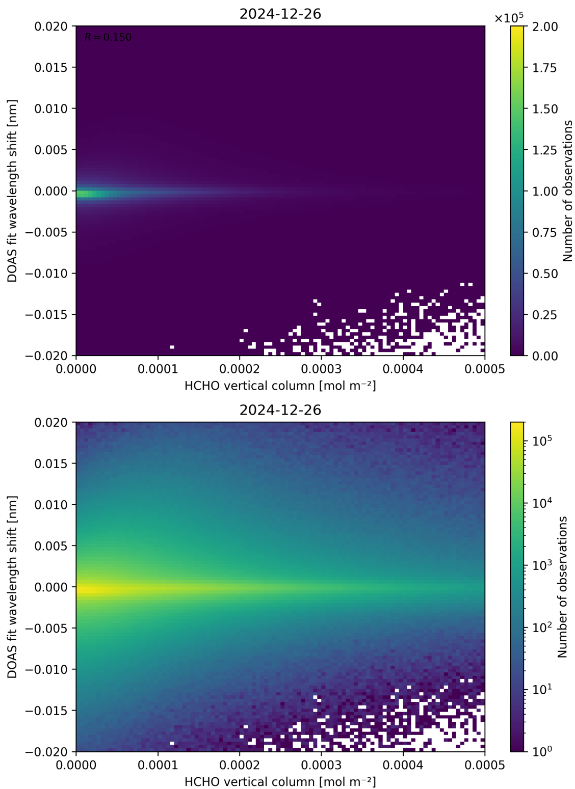
Figure 124: Scatter density plot of “HCHO vertical column” against “DOAS fit wavelength shift” for 2024-12-25 to 2024-12-27.
