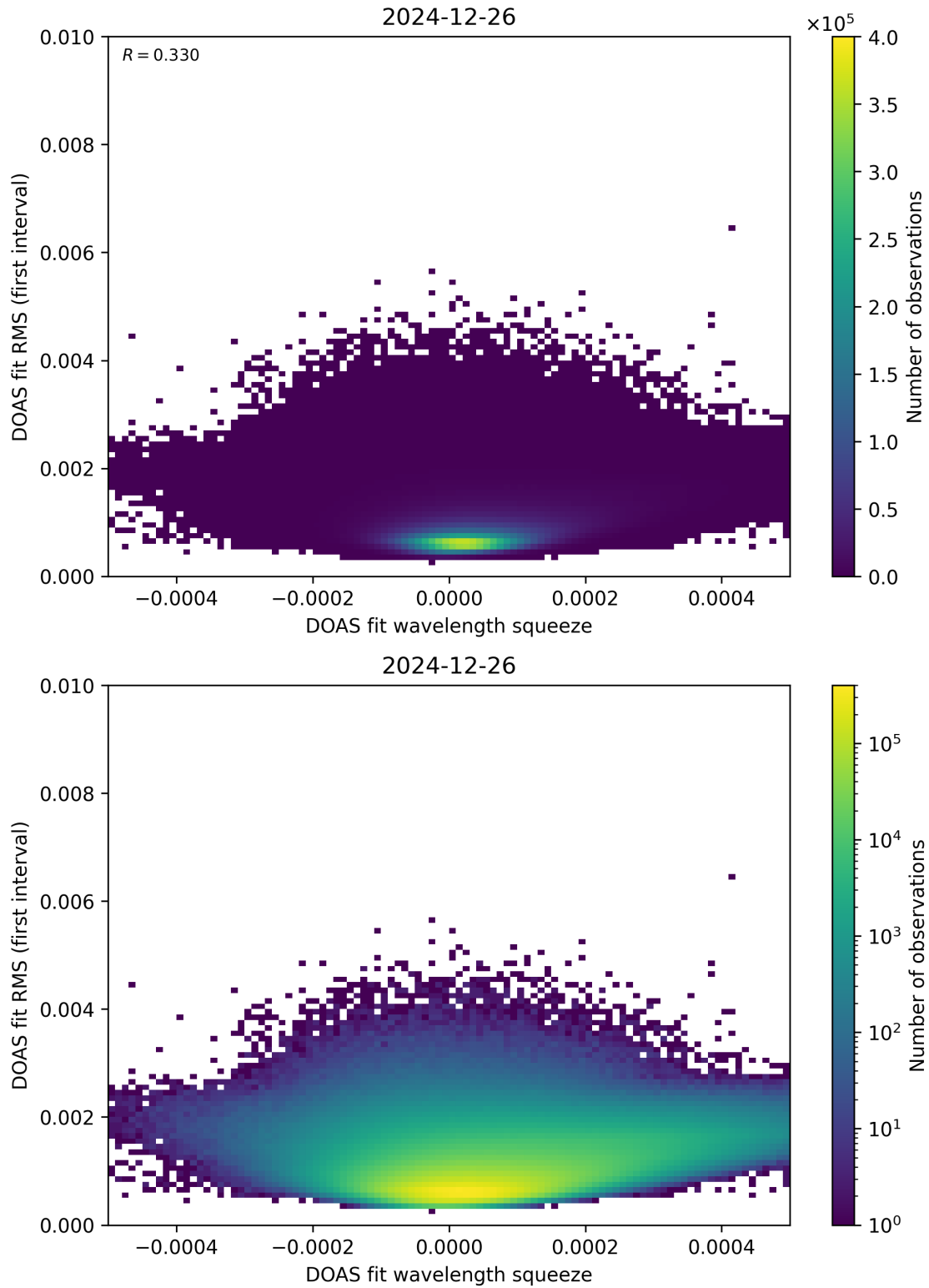
Figure 68: Scatter density plot of “DOAS fit wavelength squeeze” against “DOAS fit RMS (first interval)” for 2024-12-25 to 2024-12-27.
