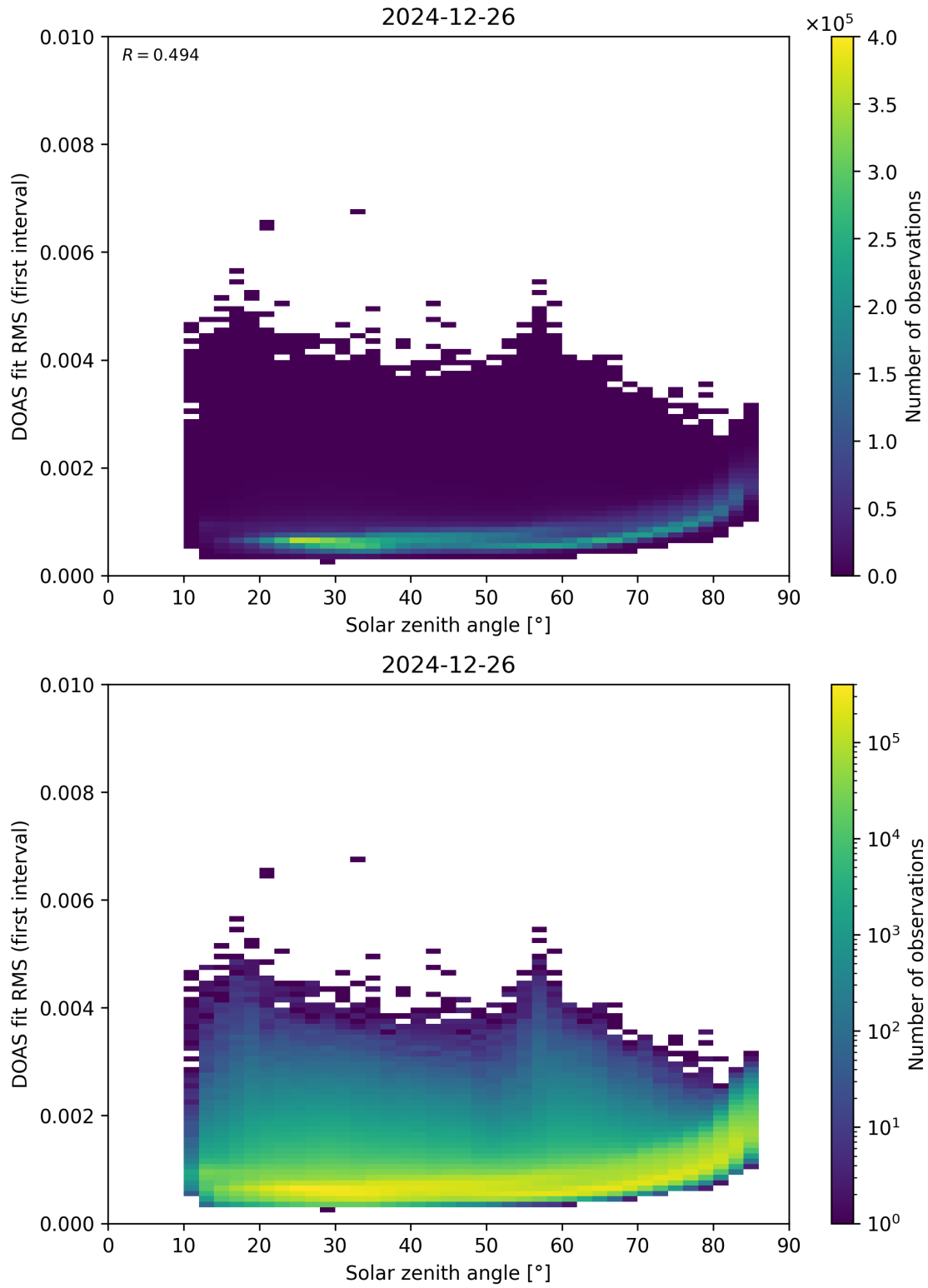
Figure 167: Scatter density plot of “Solar zenith angle” against “DOAS fit RMS (first interval)” for 2024-12-25 to 2024-12-27.
