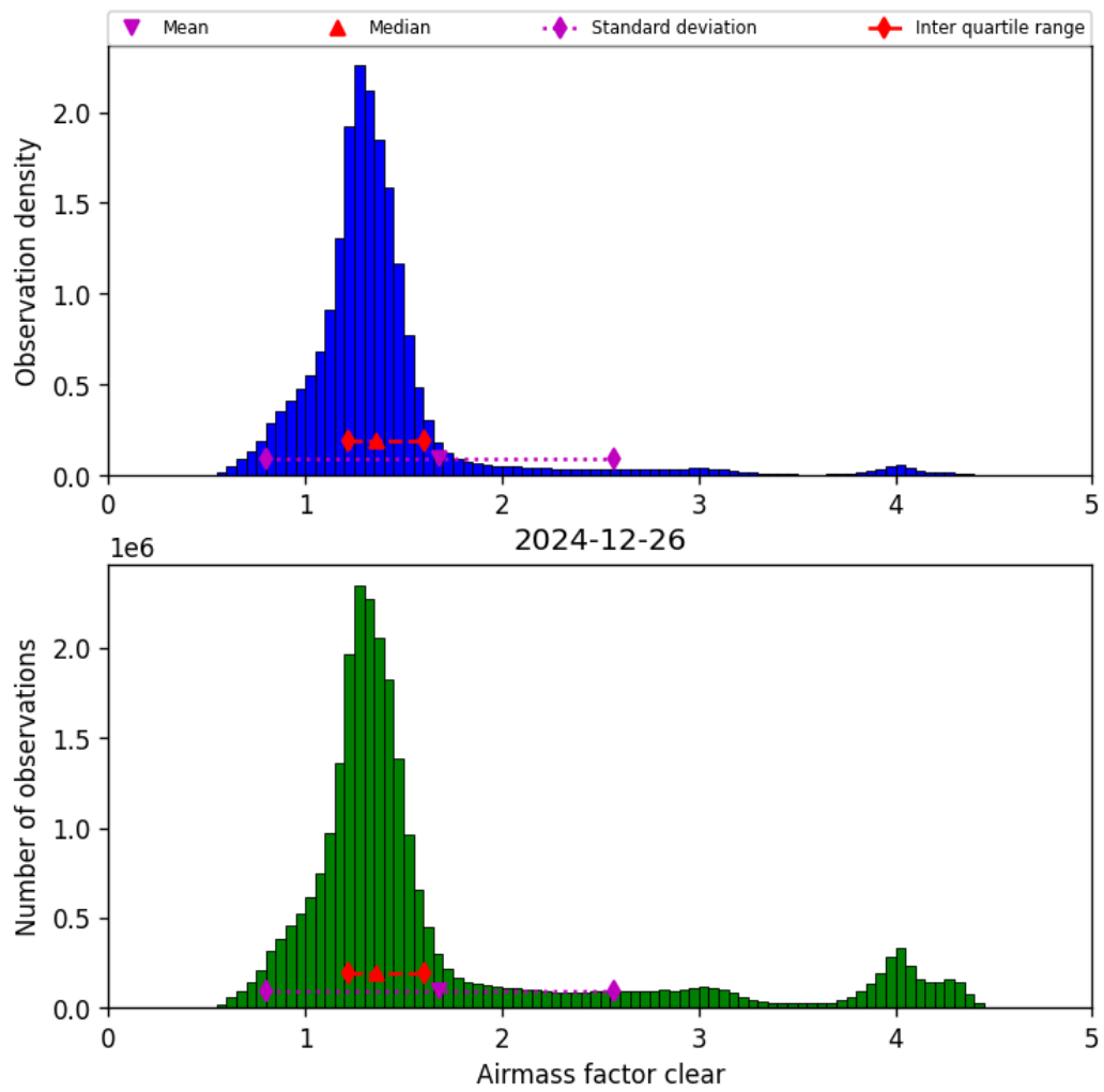
Figure 42: Histogram of “Airmass factor clear” for 2024-12-25 to 2024-12-27
