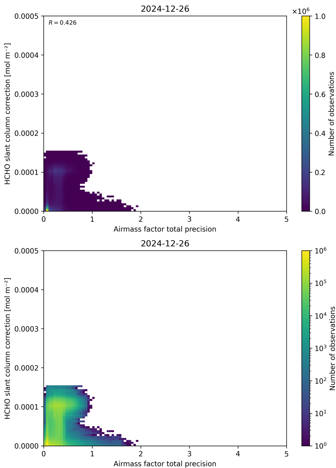
Figure 110: Scatter density plot of “Airmass factor total precision” against “HCHO slant column correction” for 2024-12-25 to 2024-12-27.
