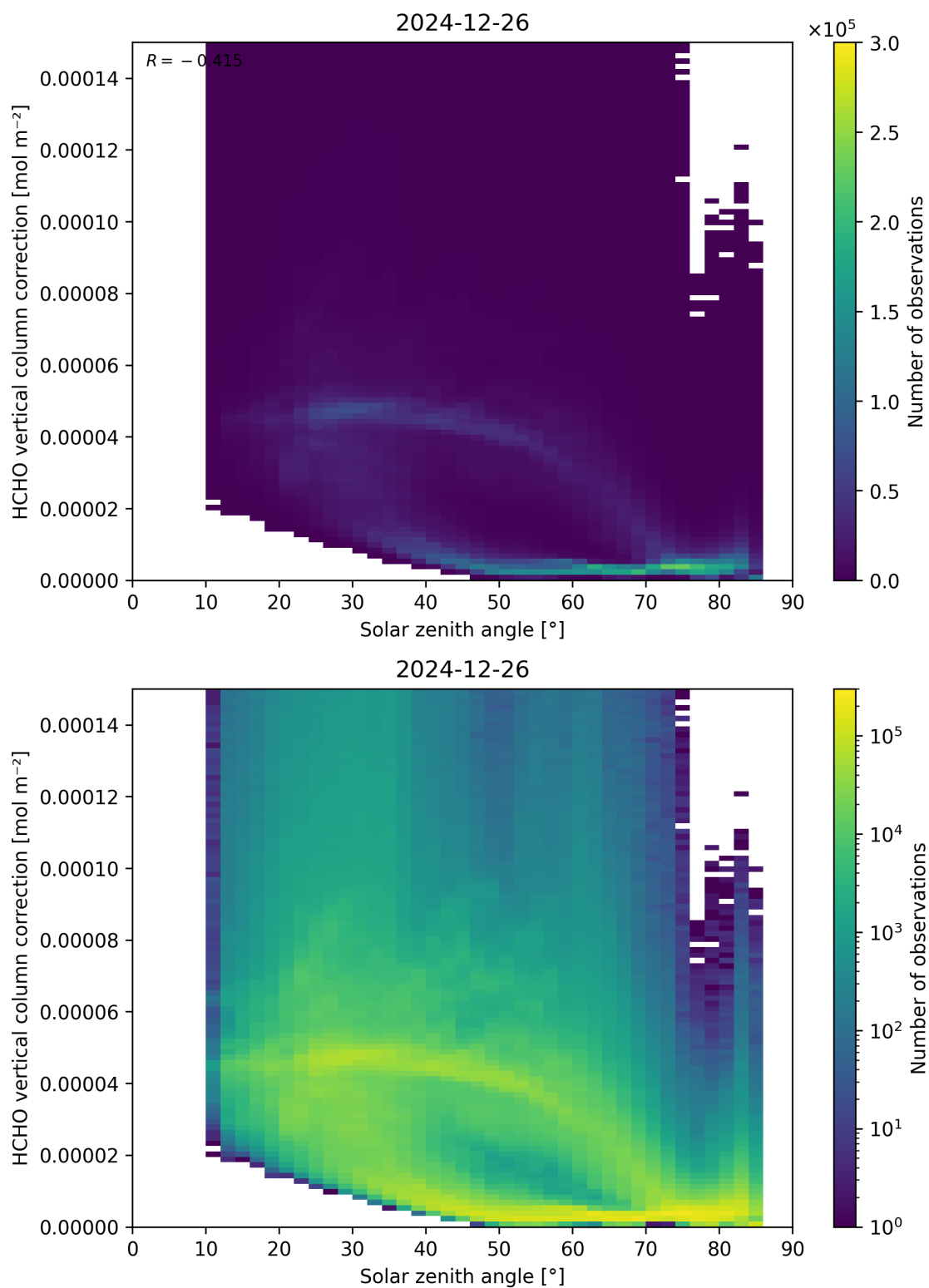
Figure 178: Scatter density plot of “Solar zenith angle” against “HCHO vertical column correction” for 2024-12-25 to 2024-12-27.
