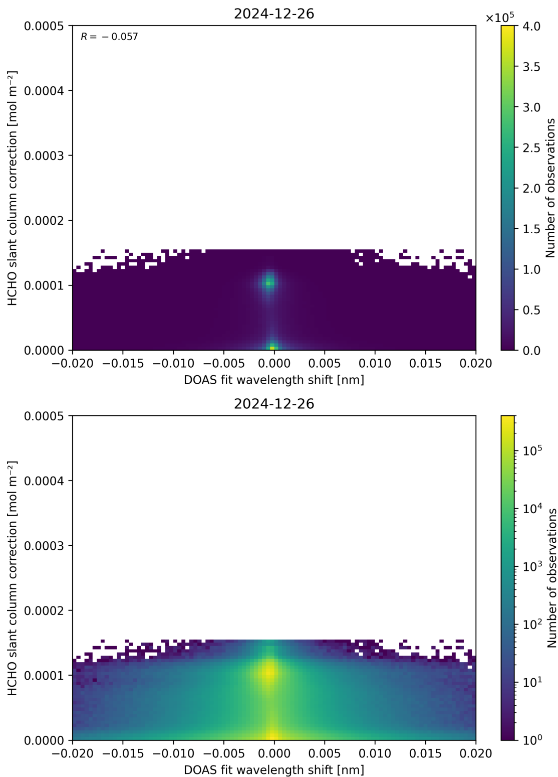
Figure 67: Scatter density plot of “DOAS fit wavelength shift” against “HCHO slant column correction” for 2024-12-25 to 2024-12-27.
