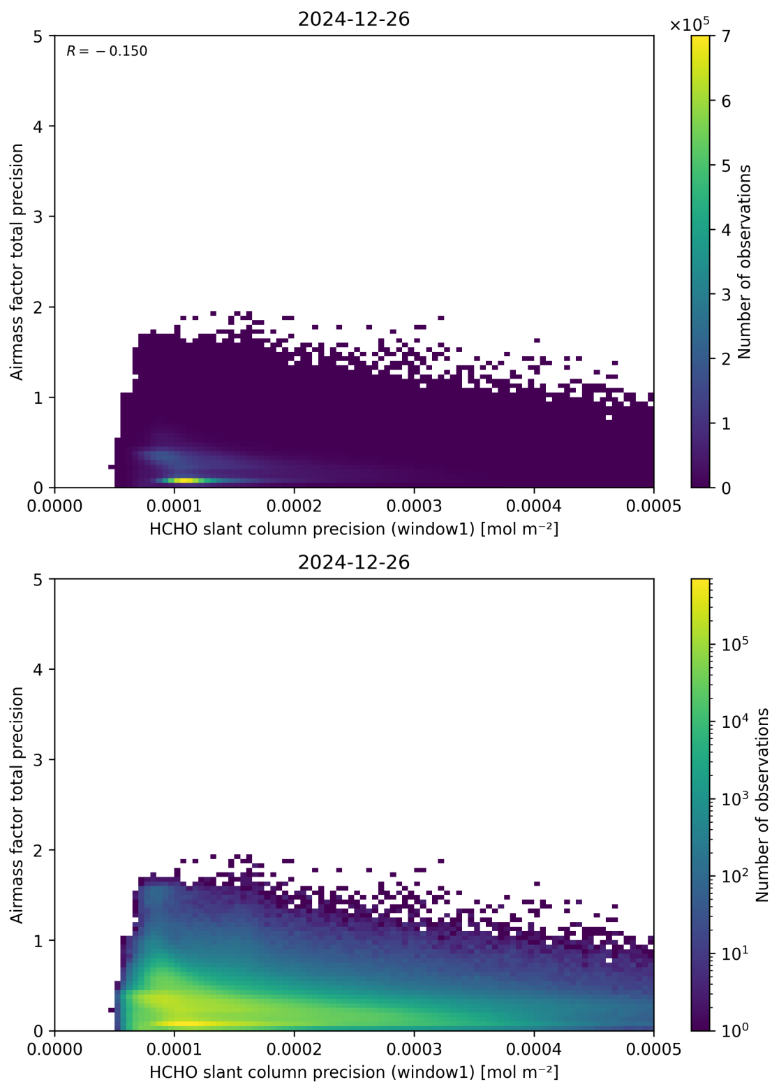
Figure 95: Scatter density plot of “HCHO slant column precision (window1)” against “Airmass factor total precision” for 2024-12-25 to 2024-12-27.
