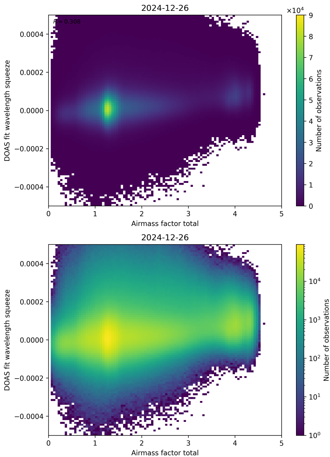
Figure 99: Scatter density plot of “Airmass factor total” against “DOAS fit wavelength squeeze” for 2024-12-25 to 2024-12-27.
