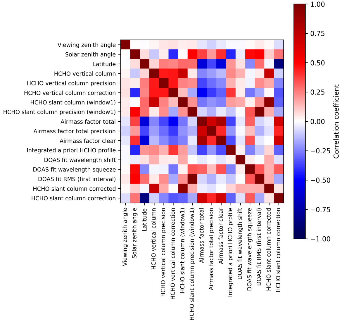
Figure 2: Map of correlation matrix for 2024-12-25 to 2024-12-27.
