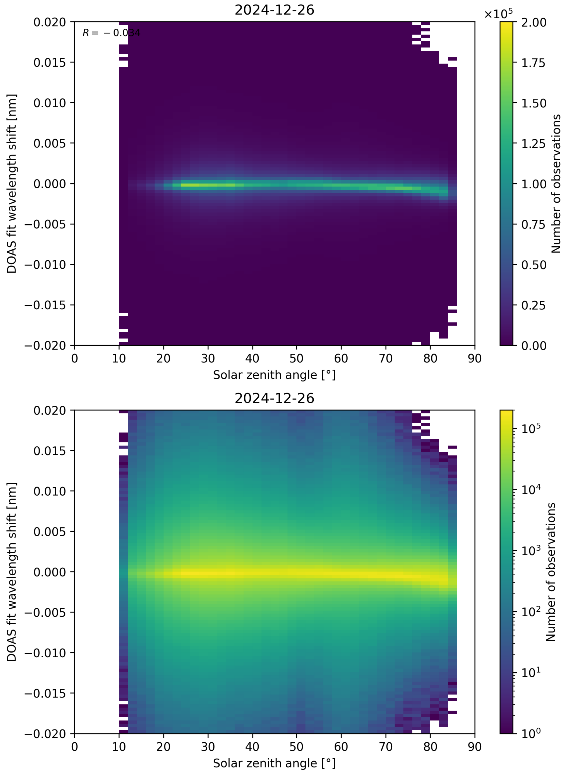
Figure 168: Scatter density plot of “Solar zenith angle” against “DOAS fit wavelength shift” for 2024-12-25 to 2024-12-27.
