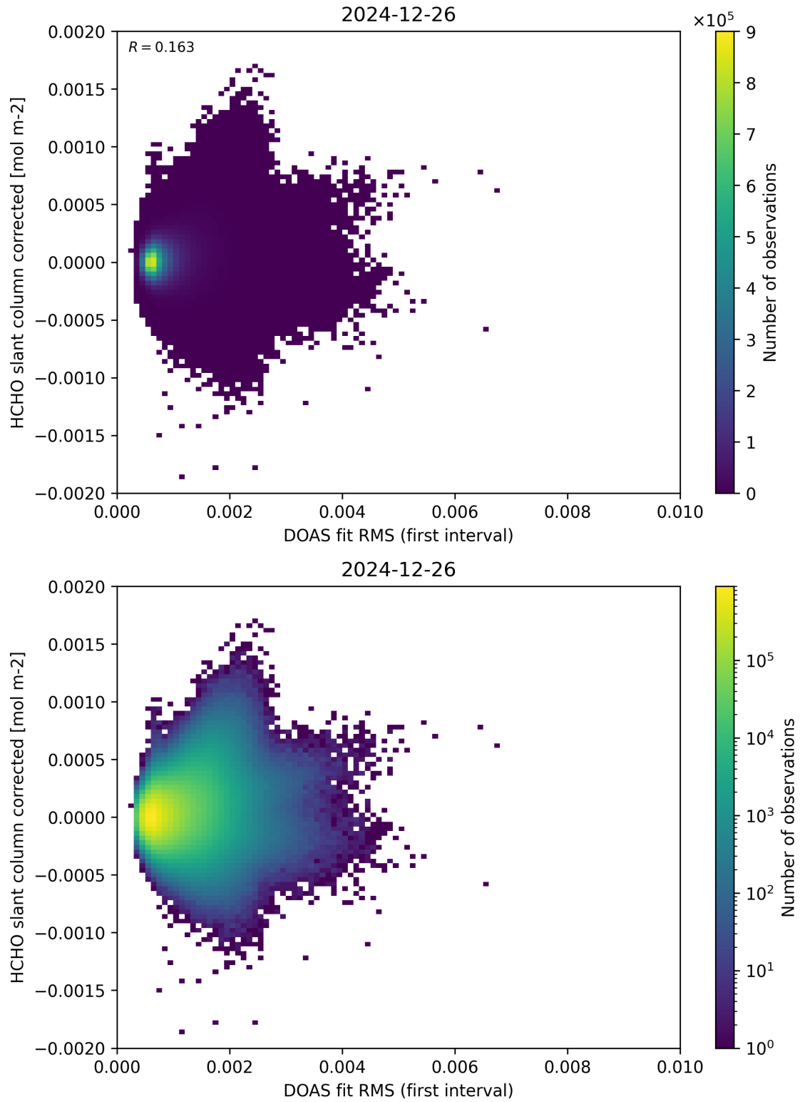
Figure 62: Scatter density plot of “DOAS fit RMS (first interval)” against “HCHO slant column corrected” for 2024-12-25 to 2024-12-27.
