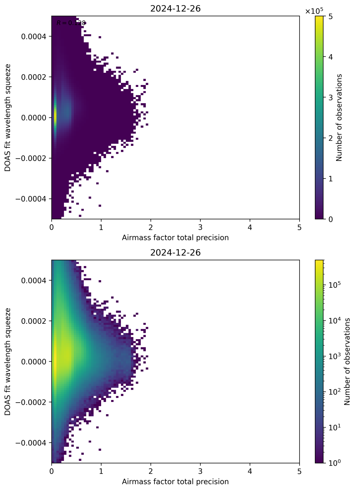
Figure 107: Scatter density plot of “Airmass factor total precision” against “DOAS fit wavelength squeeze” for 2024-12-25 to 2024-12-27.
