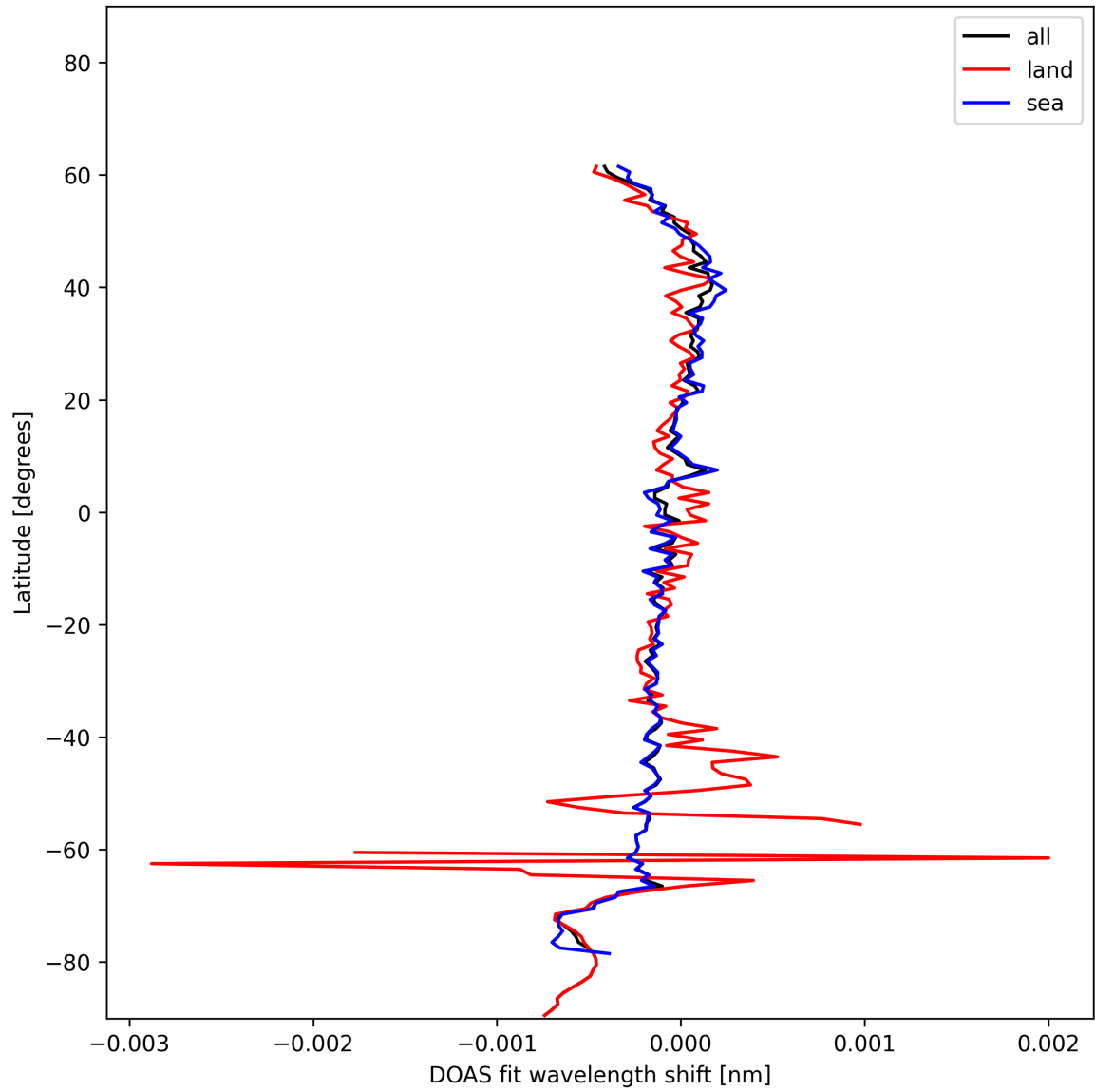
Figure 30: Zonal average of “DOAS fit wavelength shift” for 2024-12-25 to 2024-12-27.
