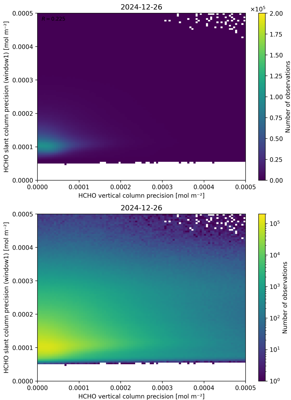
Figure 143: Scatter density plot of “HCHO vertical column precision” against “HCHO slant column precision (window1)” for 2024-12-25 to 2024-12-27.
