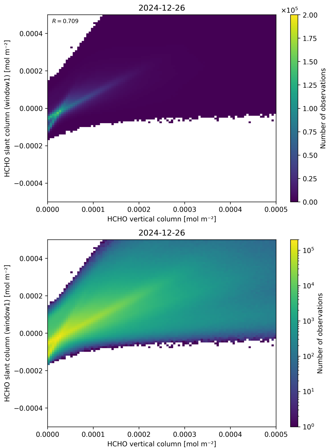
Figure 129: Scatter density plot of “HCHO vertical column” against “HCHO slant column (window1)” for 2024-12-25 to 2024-12-27.
