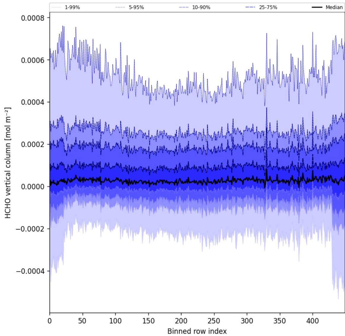
Figure 49: Along track statistics of “HCHO vertical column” for 2024-12-25 to 2024-12-27
