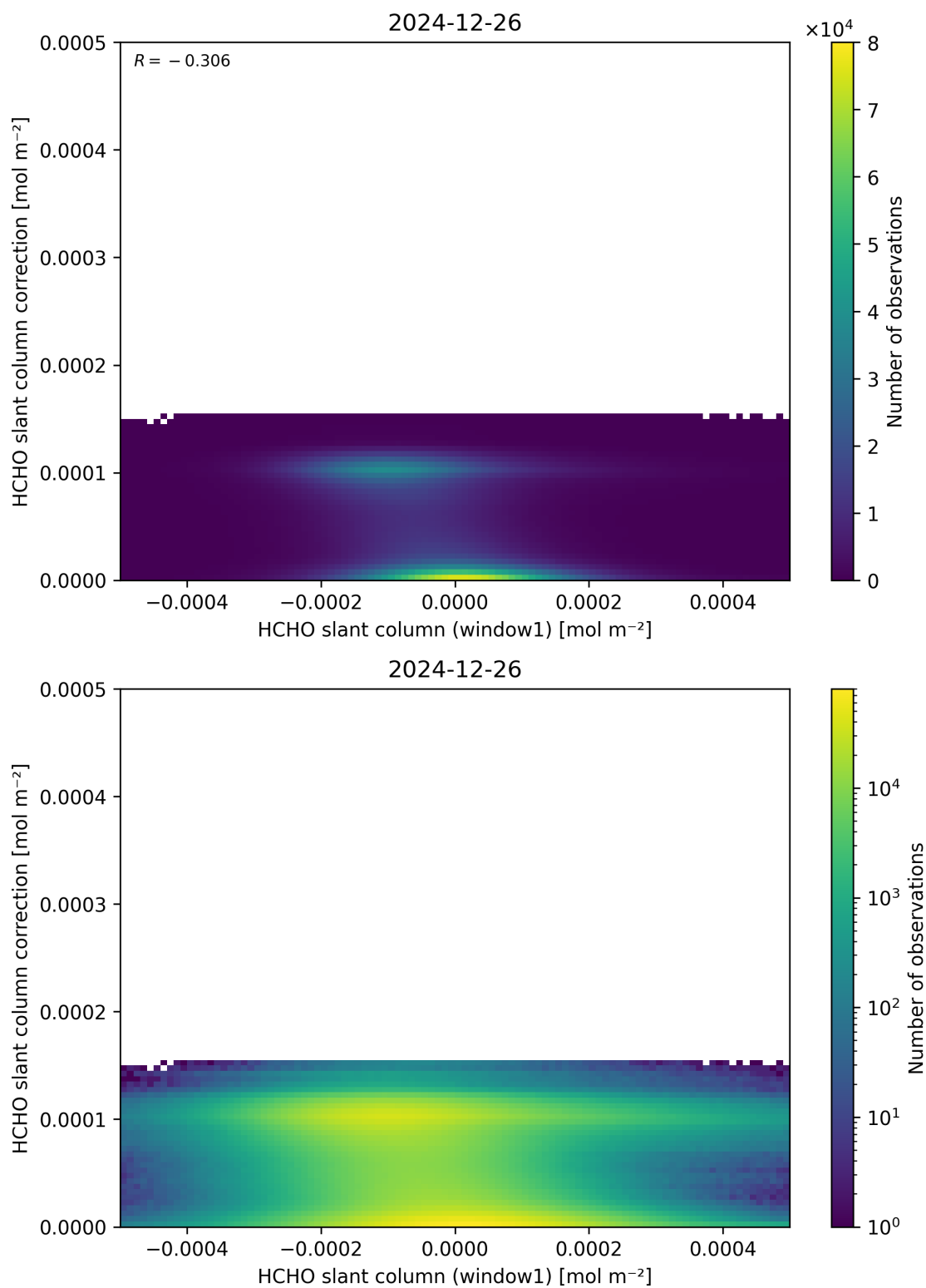
Figure 83: Scatter density plot of “HCHO slant column (window1)” against “HCHO slant column correction” for 2024-12-25 to 2024-12-27.
