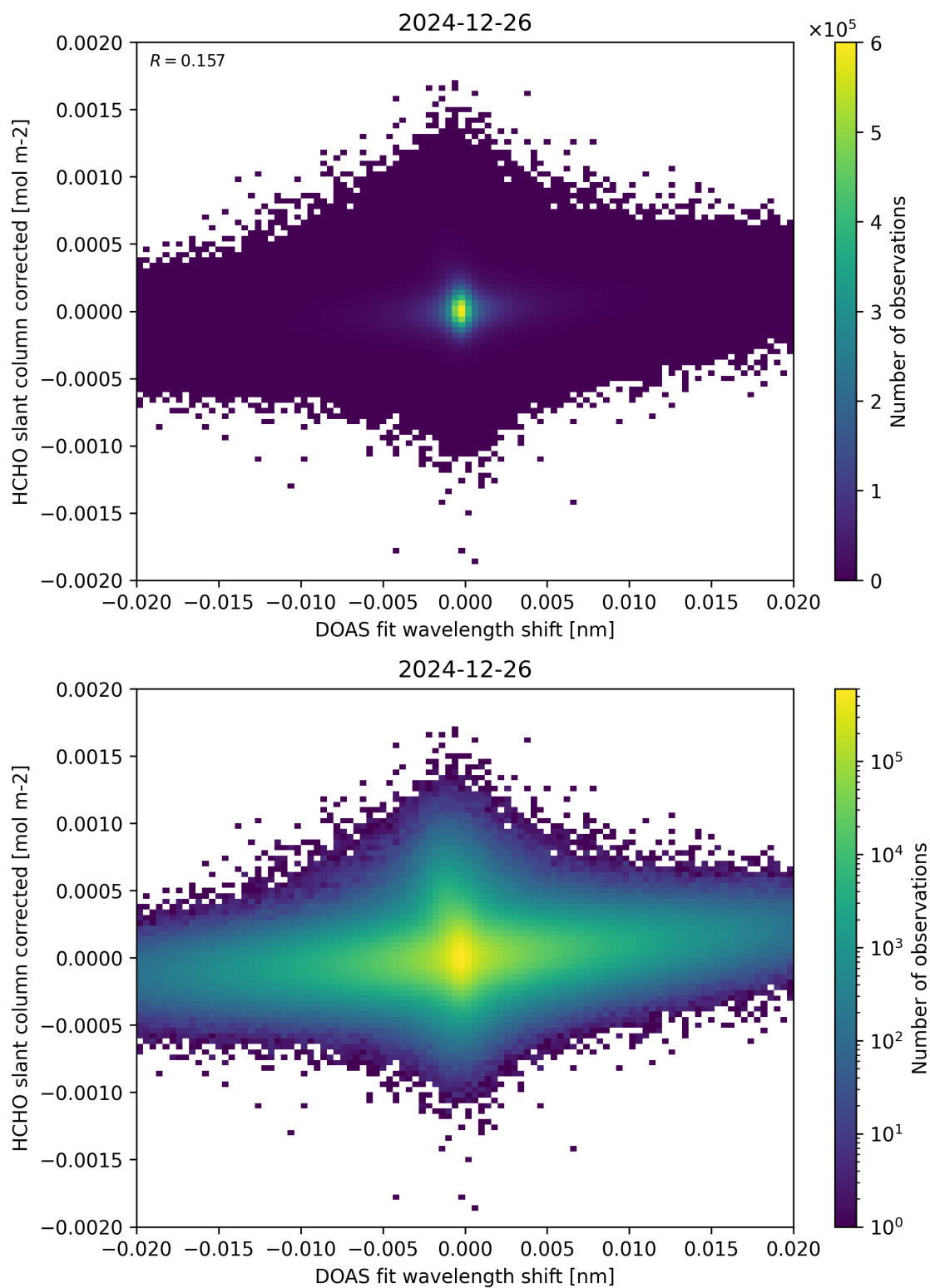
Figure 66: Scatter density plot of “DOAS fit wavelength shift” against “HCHO slant column corrected” for 2024-12-25 to 2024-12-27.
