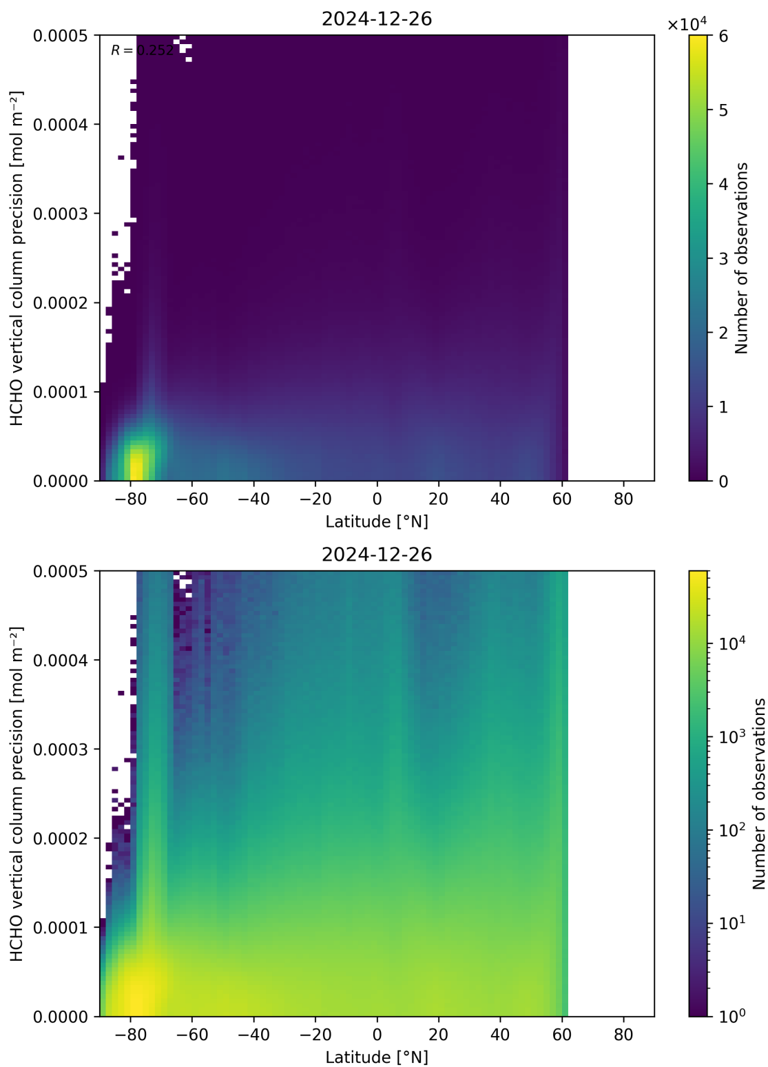
Figure 165: Scatter density plot of “Latitude” against “HCHO vertical column precision” for 2024-12-25 to 2024-12-27.
