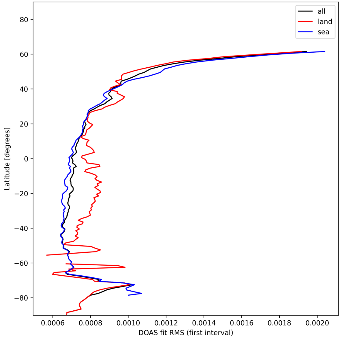
Figure 32: Zonal average of “DOAS fit RMS (first interval)” for 2024-12-25 to 2024-12-27.
