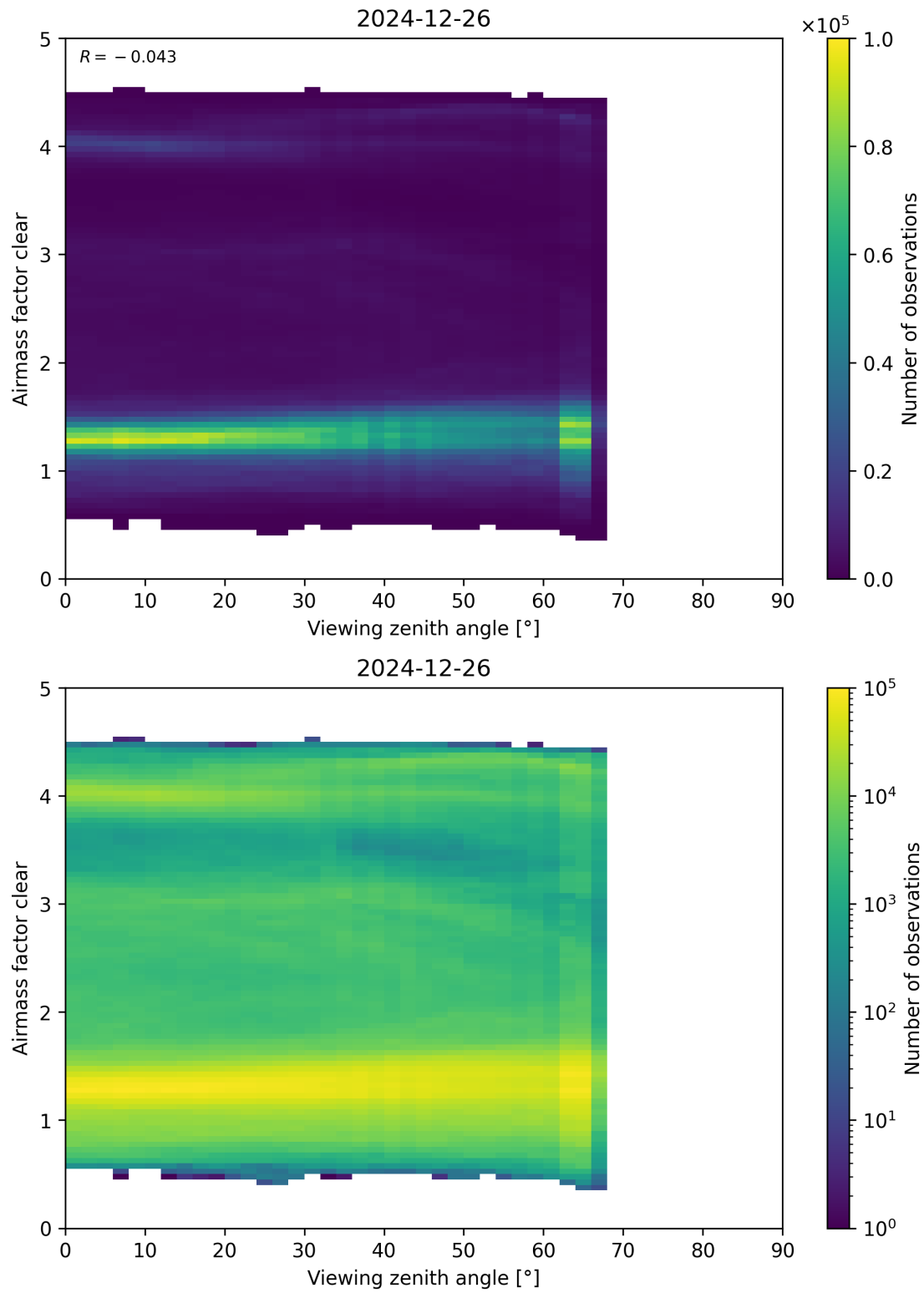
Figure 185: Scatter density plot of “Viewing zenith angle” against “Airmass factor clear” for 2024-12-25 to 2024-12-27.
