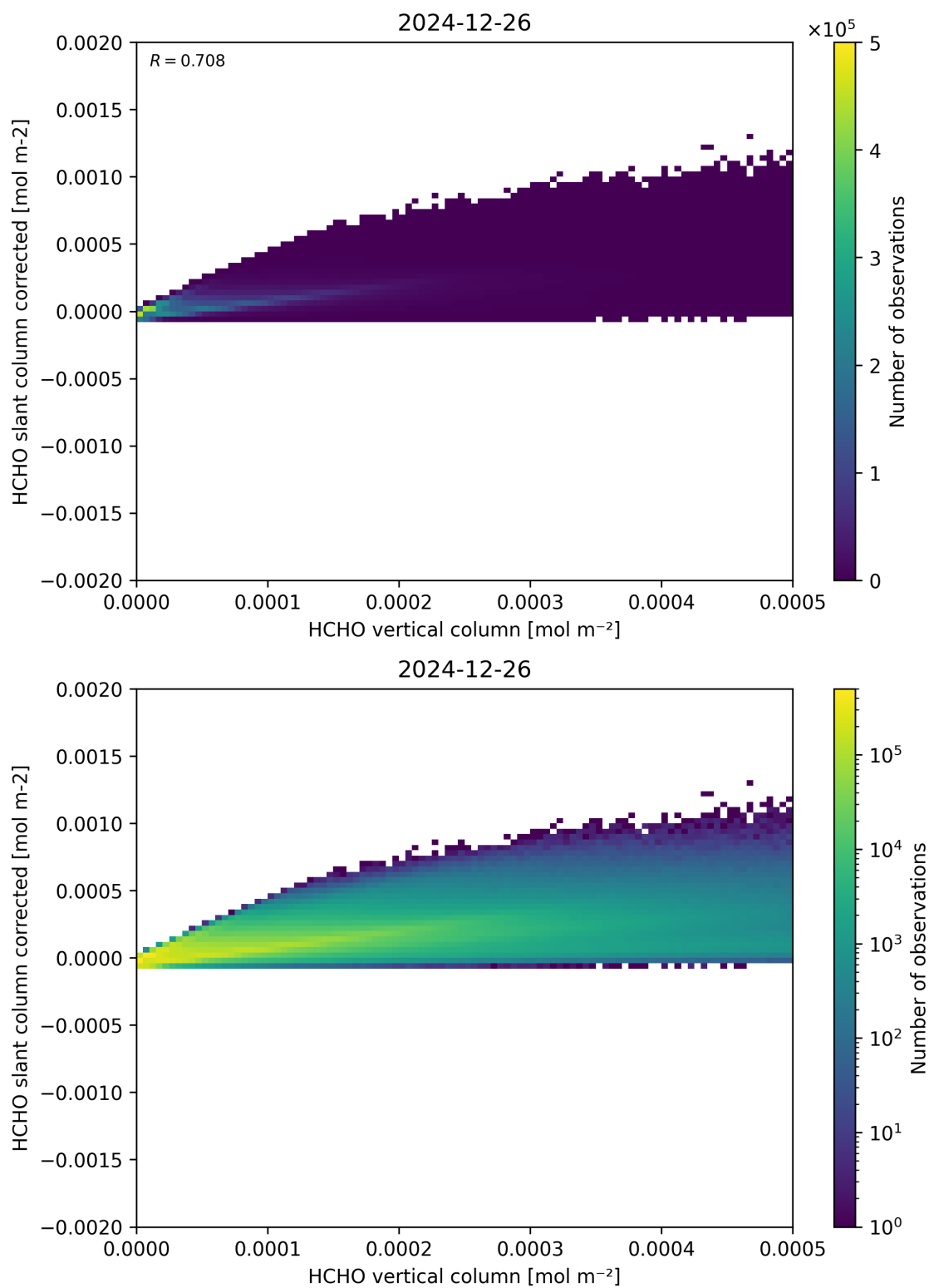
Figure 127: Scatter density plot of “HCHO vertical column” against “HCHO slant column corrected” for 2024-12-25 to 2024-12-27.
