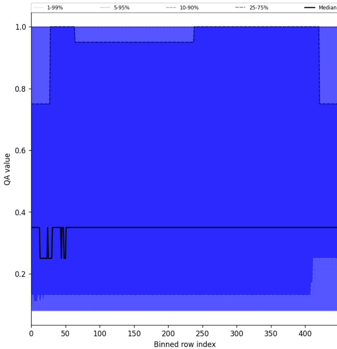
Figure 48: Along track statistics of “QA value” for 2024-12-25 to 2024-12-27
