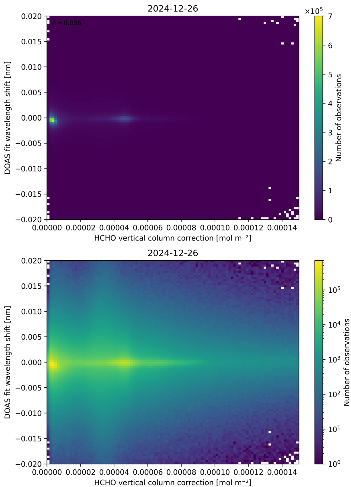
Figure 113: Scatter density plot of “HCHO vertical column correction” against “DOAS fit wavelength shift” for 2024-12-25 to 2024-12-27.
