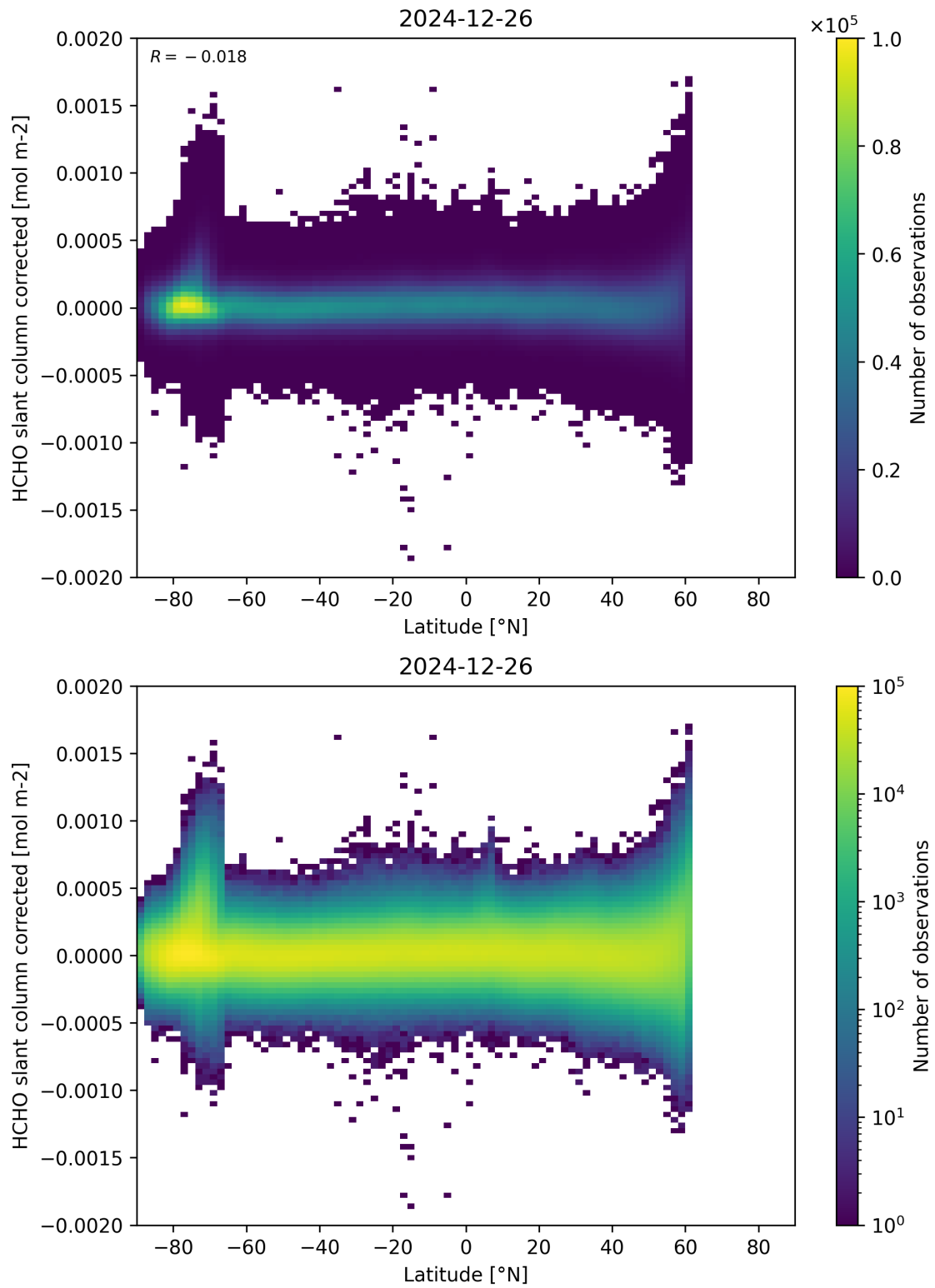
Figure 157: Scatter density plot of “Latitude” against “HCHO slant column corrected” for 2024-12-25 to 2024-12-27.
