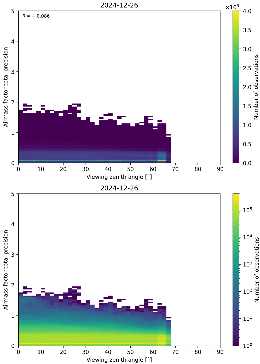
Figure 191: Scatter density plot of “Viewing zenith angle” against “Airmass factor total precision” for 2024-12-25 to 2024-12-27.
