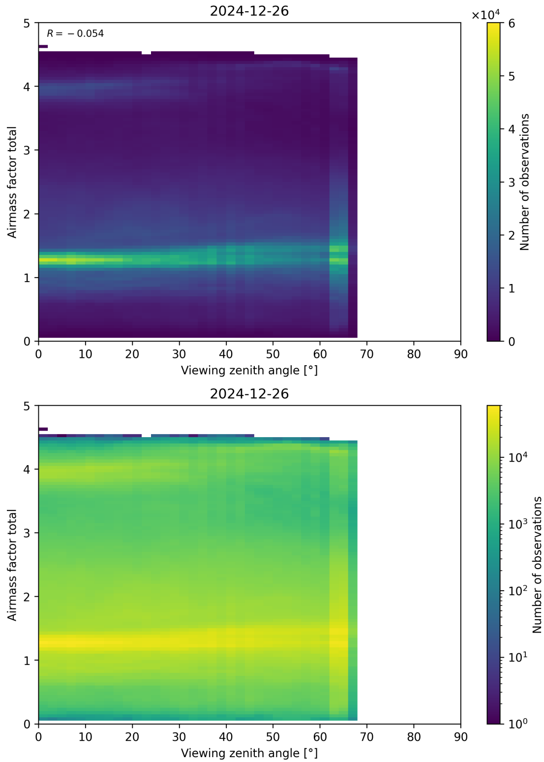
Figure 190: Scatter density plot of “Viewing zenith angle” against “Airmass factor total” for 2024-12-25 to 2024-12-27.
