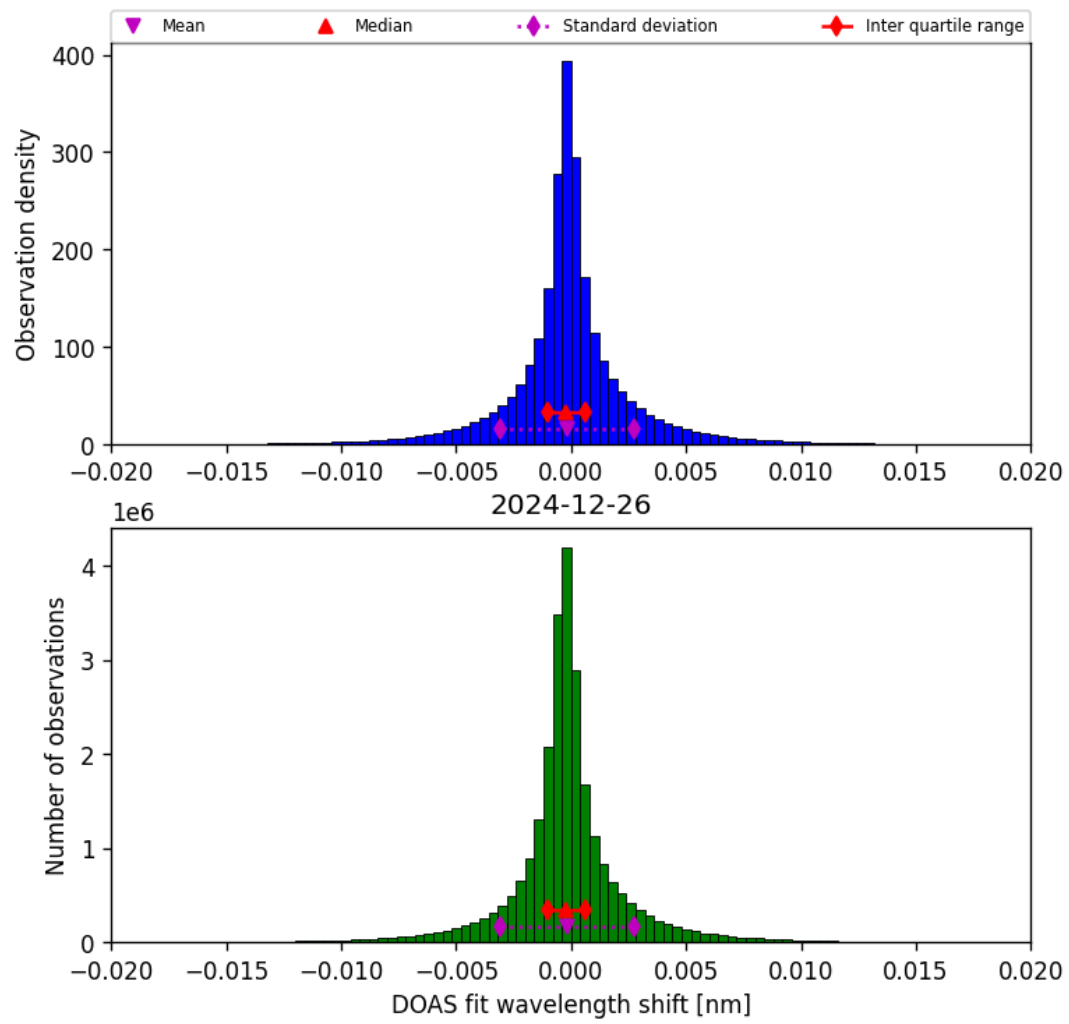
Figure 44: Histogram of “DOAS fit wavelength shift” for 2024-12-25 to 2024-12-27
