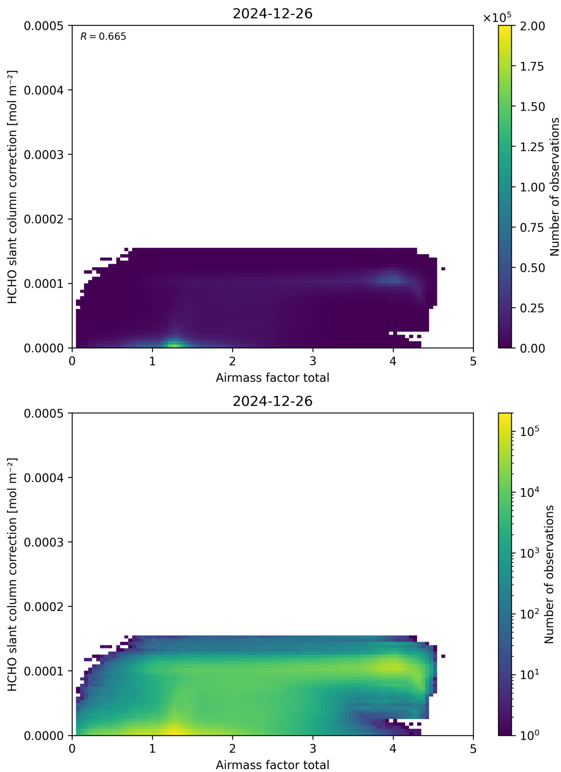
Figure 102: Scatter density plot of “Airmass factor total” against “HCHO slant column correction” for 2024-12-25 to 2024-12-27.
