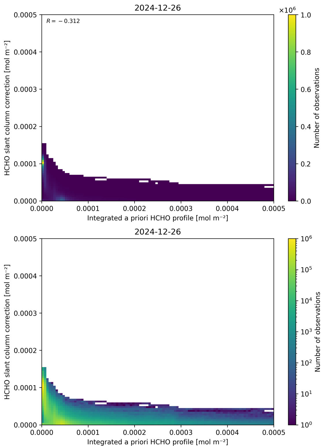
Figure 152: Scatter density plot of “Integrated a priori HCHO profile” against “HCHO slant column correction” for 2024-12-25 to 2024-12-27.
