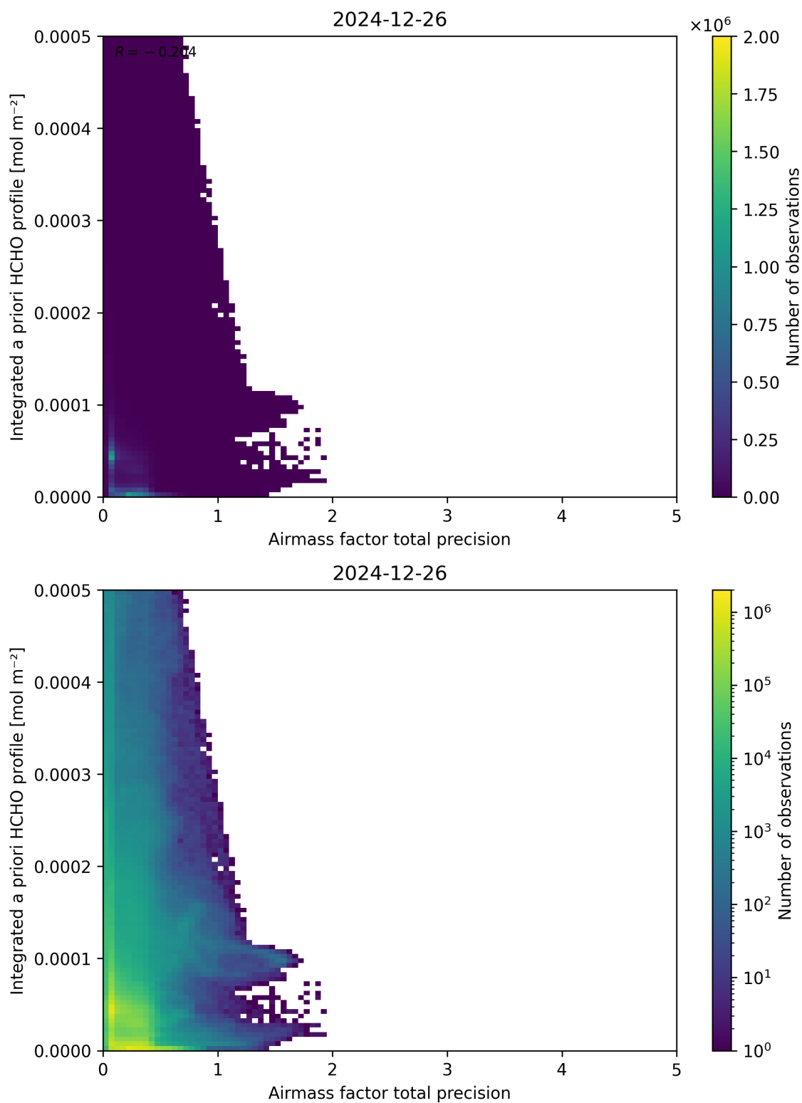
Figure 111: Scatter density plot of “Airmass factor total precision” against “Integrated a priori HCHO profile” for 2024-12-25 to 2024-12-27.
