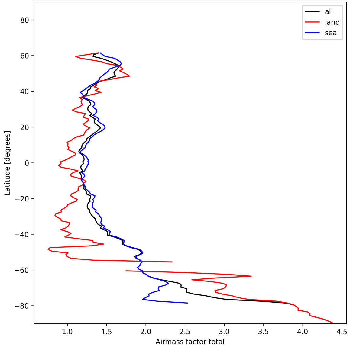
Figure 26: Zonal average of “Airmass factor total” for 2024-12-25 to 2024-12-27.
