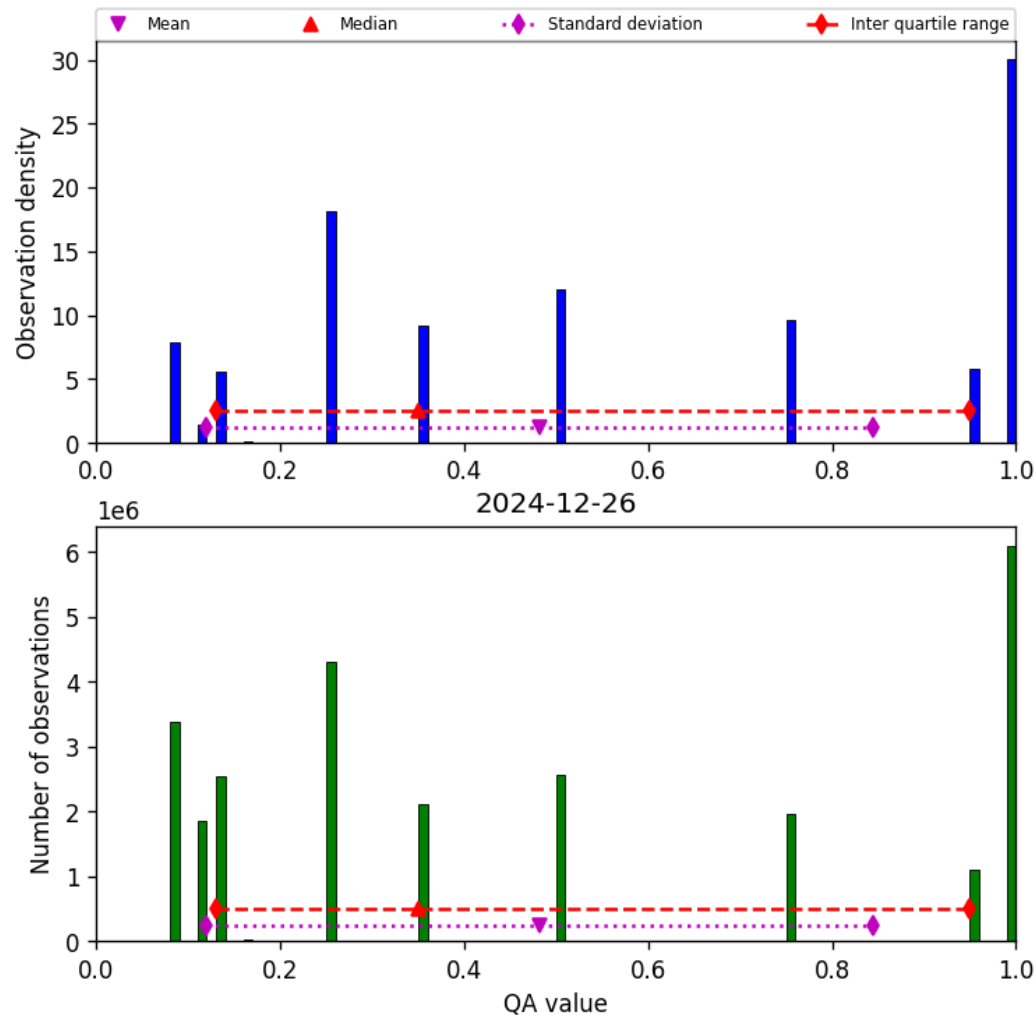
Figure 34: Histogram of “QA value” for 2024-12-25 to 2024-12-27
