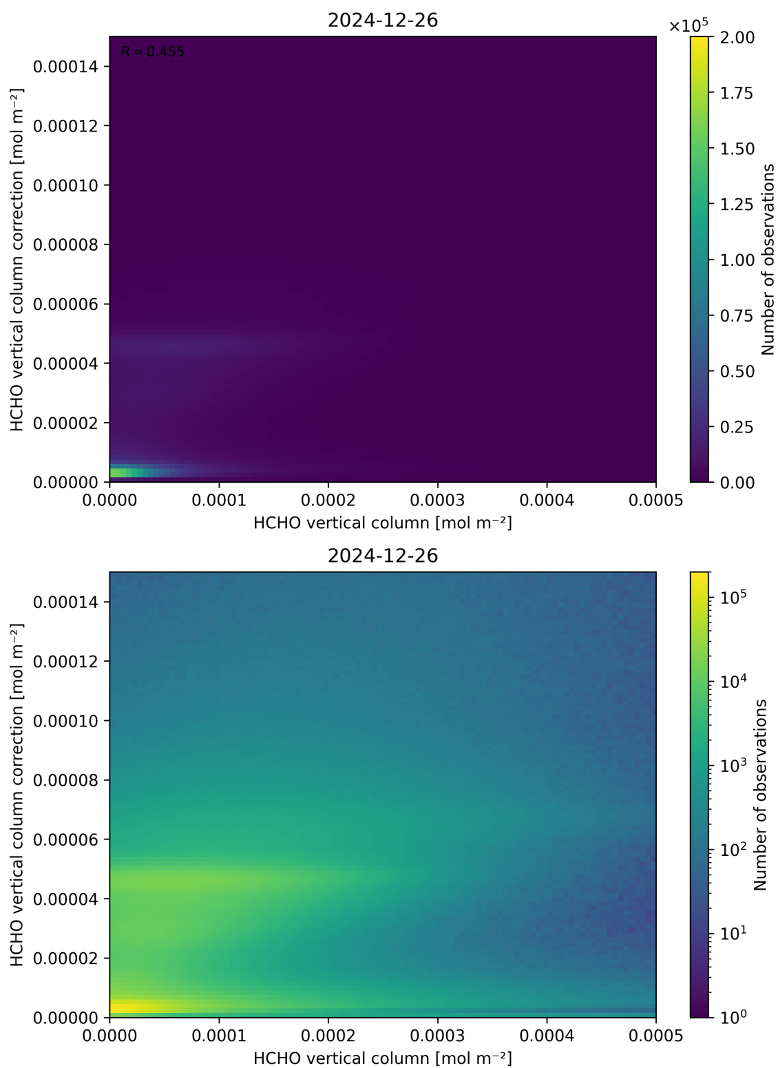
Figure 133: Scatter density plot of “HCHO vertical column” against “HCHO vertical column correction” for 2024-12-25 to 2024-12-27.
