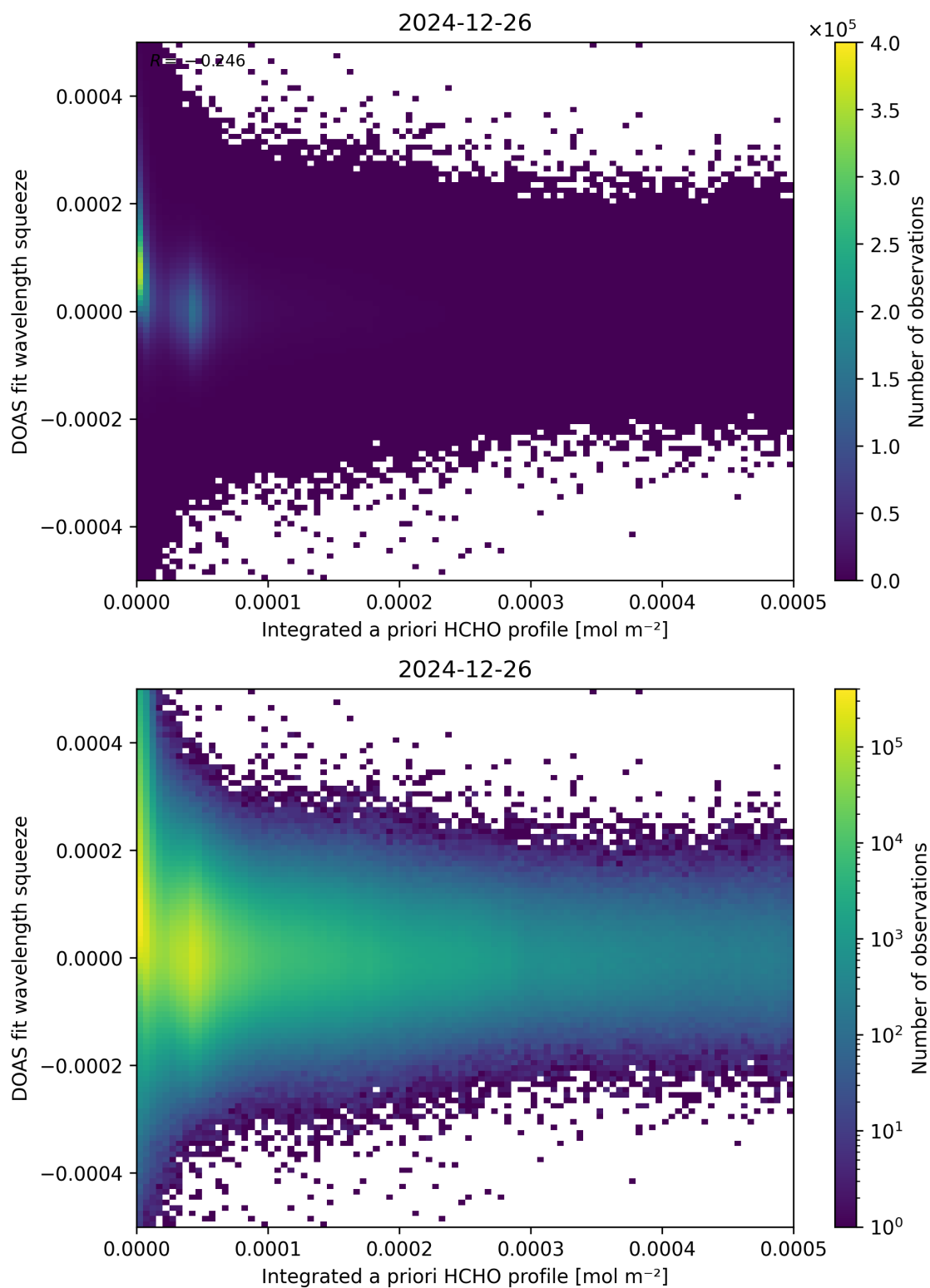
Figure 150: Scatter density plot of “Integrated a priori HCHO profile” against “DOAS fit wavelength squeeze” for 2024-12-25 to 2024-12-27.
