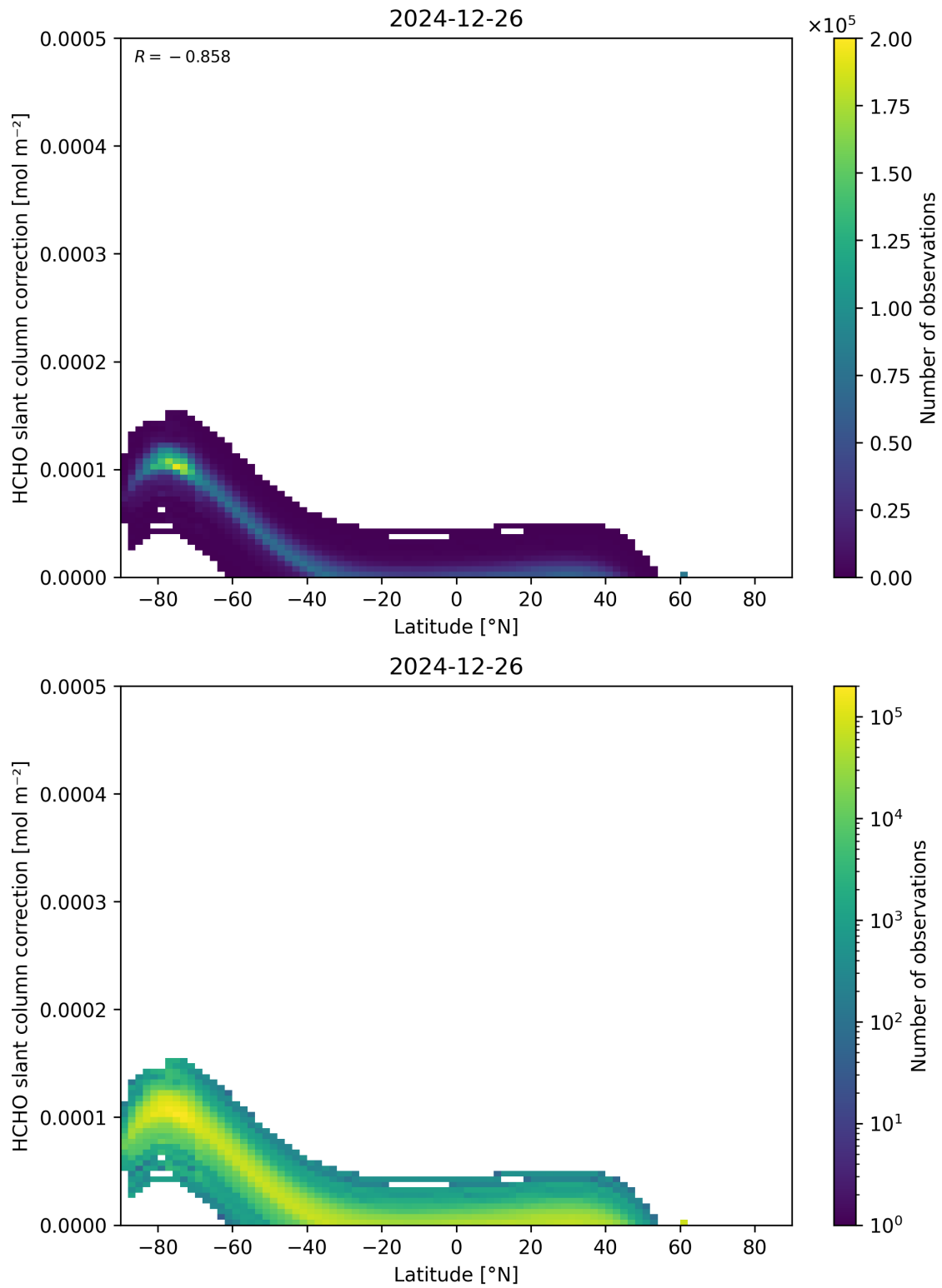
Figure 158: Scatter density plot of “Latitude” against “HCHO slant column correction” for 2024-12-25 to 2024-12-27.
