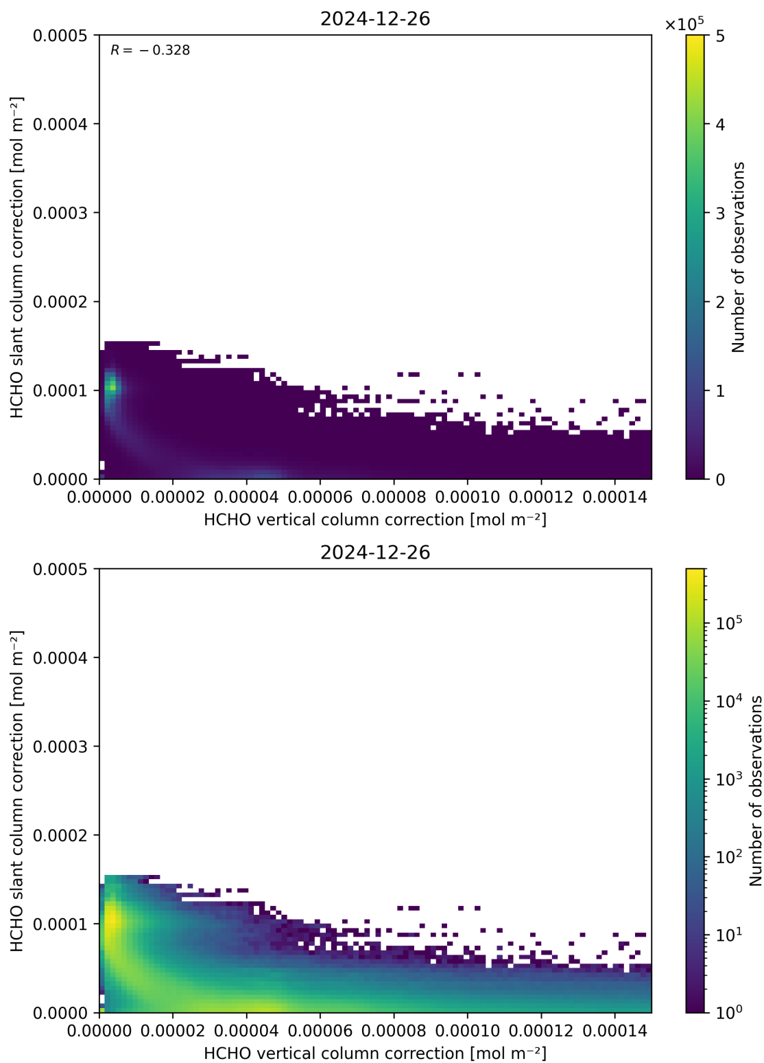
Figure 117: Scatter density plot of “HCHO vertical column correction” against “HCHO slant column correction” for 2024-12-25 to 2024-12-27.
