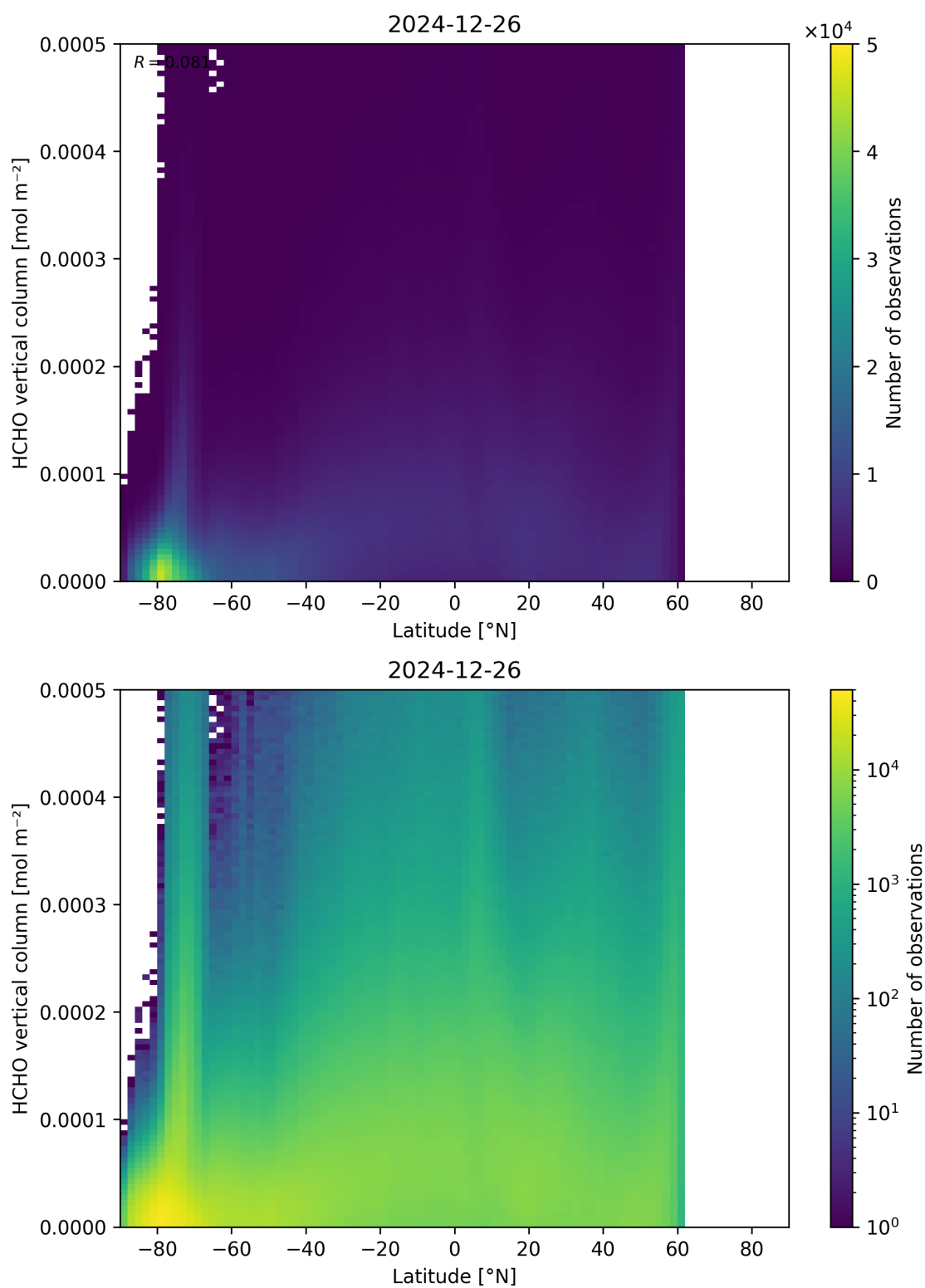
Figure 163: Scatter density plot of “Latitude” against “HCHO vertical column” for 2024-12-25 to 2024-12-27.
