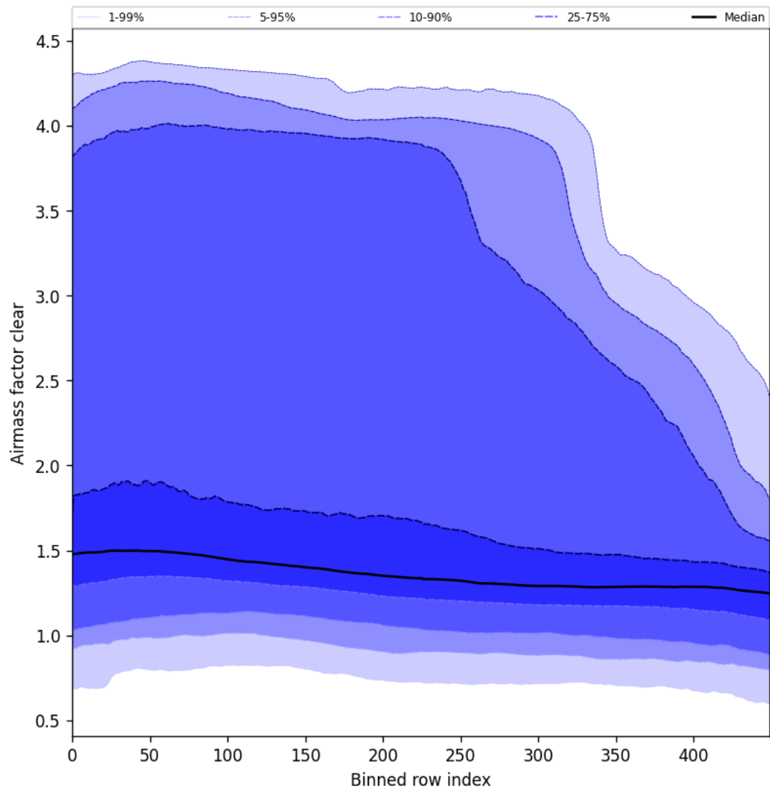
Figure 56: Along track statistics of “Airmass factor clear” for 2024-12-25 to 2024-12-27
