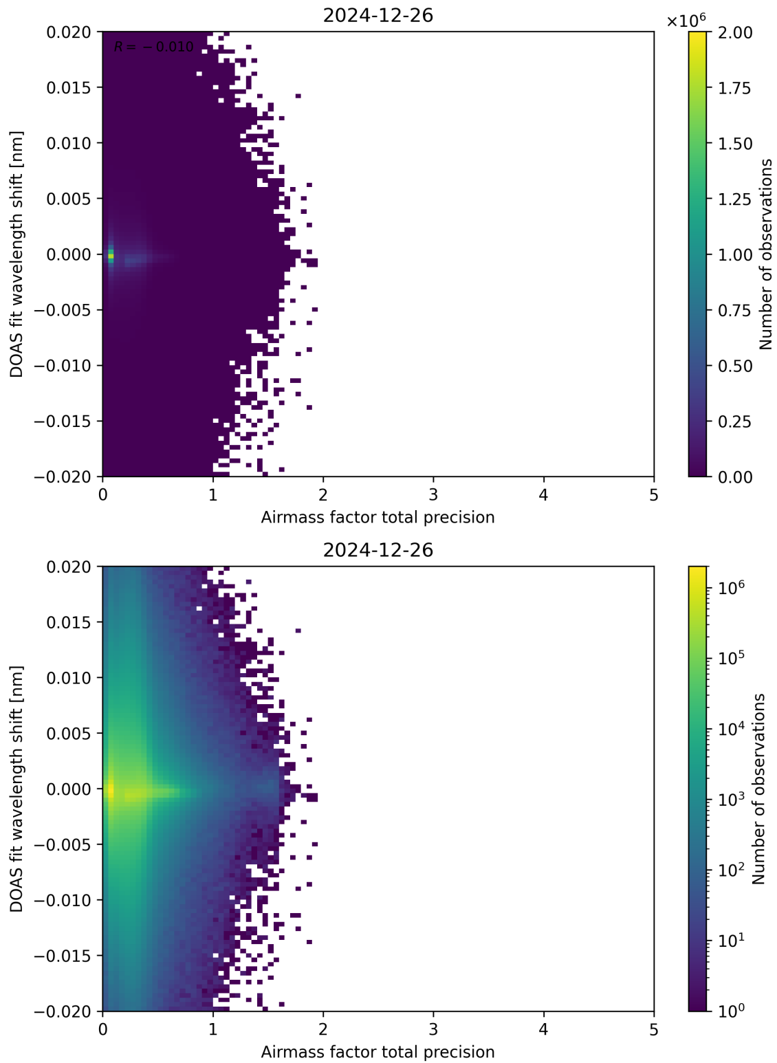
Figure 106: Scatter density plot of “Airmass factor total precision” against “DOAS fit wavelength shift” for 2024-12-25 to 2024-12-27.
