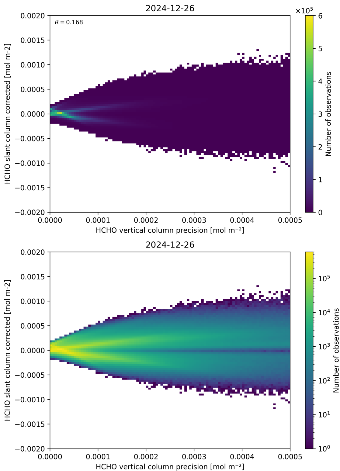
Figure 140: Scatter density plot of “HCHO vertical column precision” against “HCHO slant column corrected” for 2024-12-25 to 2024-12-27.
