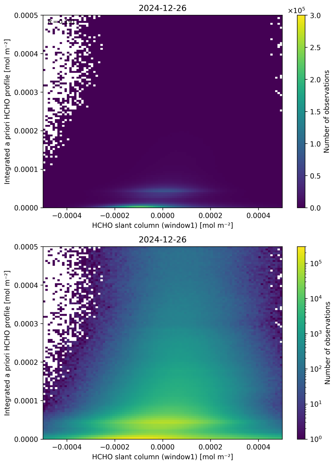
Figure 87: Scatter density plot of “HCHO slant column (window1)” against “Integrated a priori HCHO profile” for 2024-12-25 to 2024-12-27.
