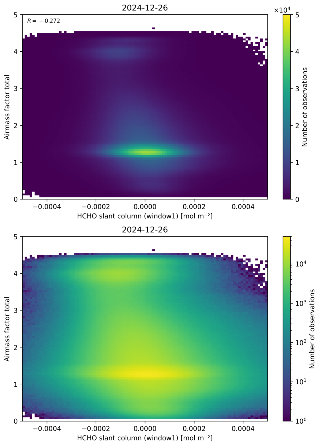
Figure 85: Scatter density plot of “HCHO slant column (window1)” against “Airmass factor total” for 2024-12-25 to 2024-12-27.
