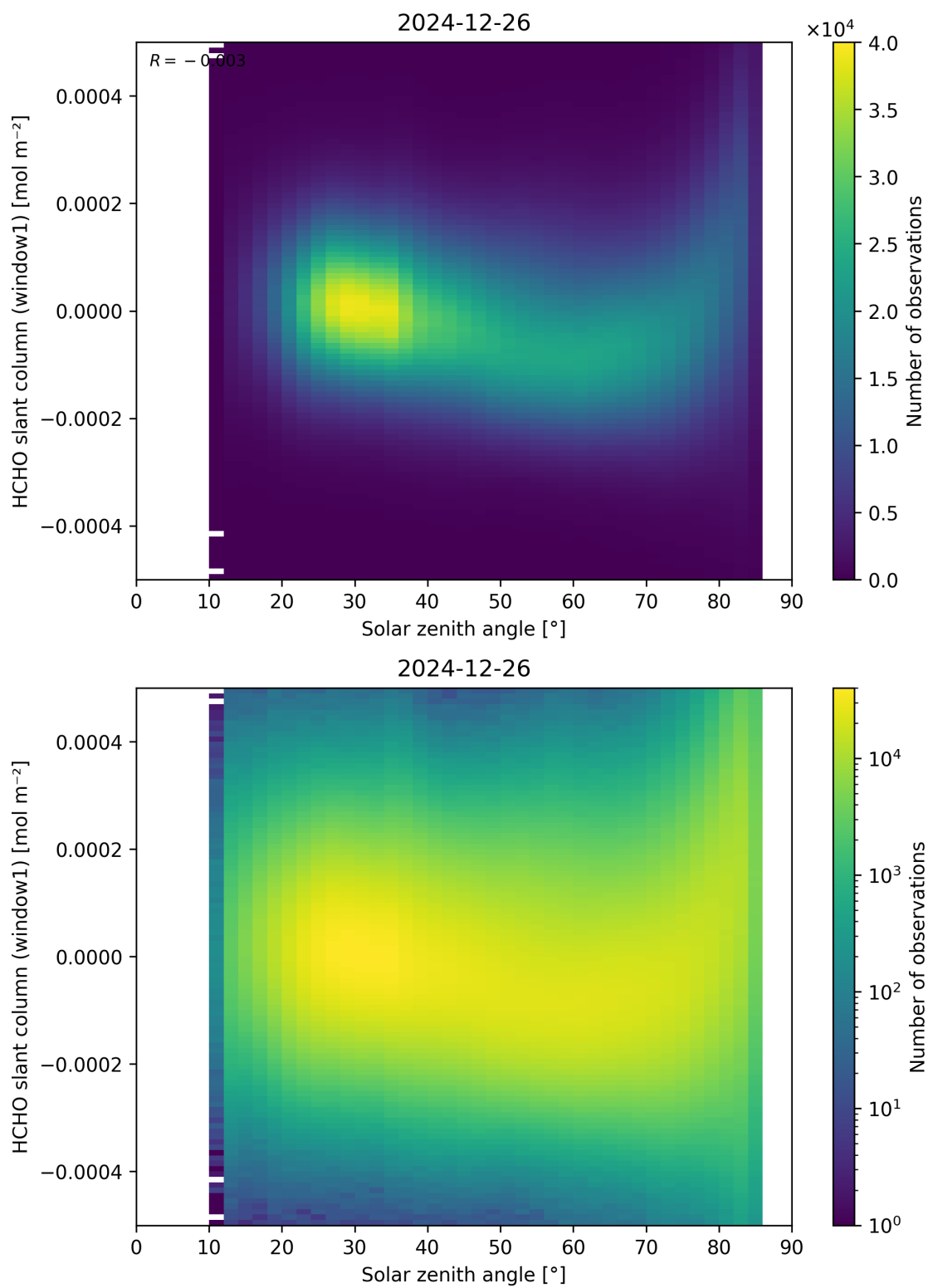
Figure 173: Scatter density plot of “Solar zenith angle” against “HCHO slant column (window1)” for 2024-12-25 to 2024-12-27.
