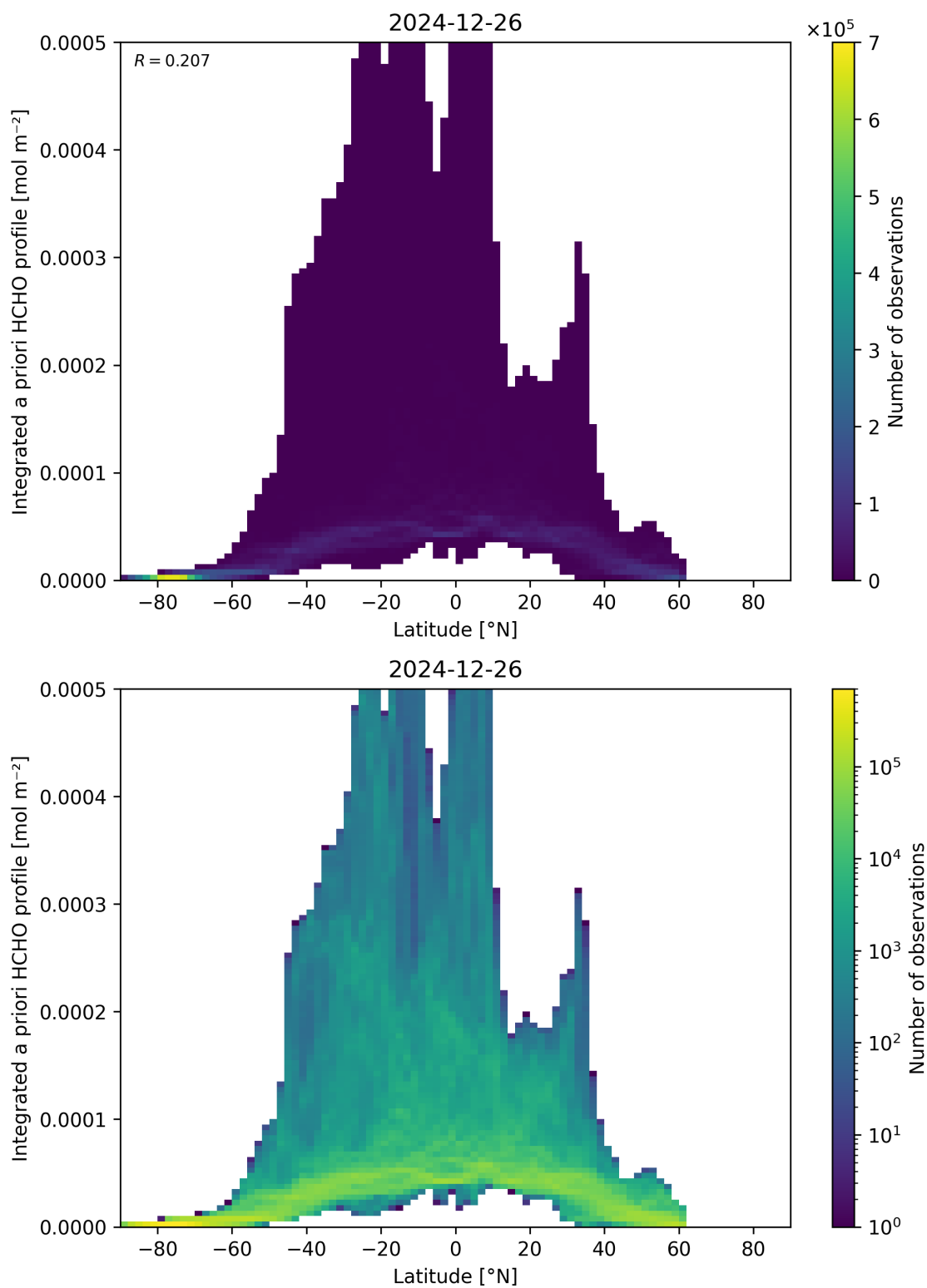
Figure 166: Scatter density plot of “Latitude” against “Integrated a priori HCHO profile” for 2024-12-25 to 2024-12-27.
