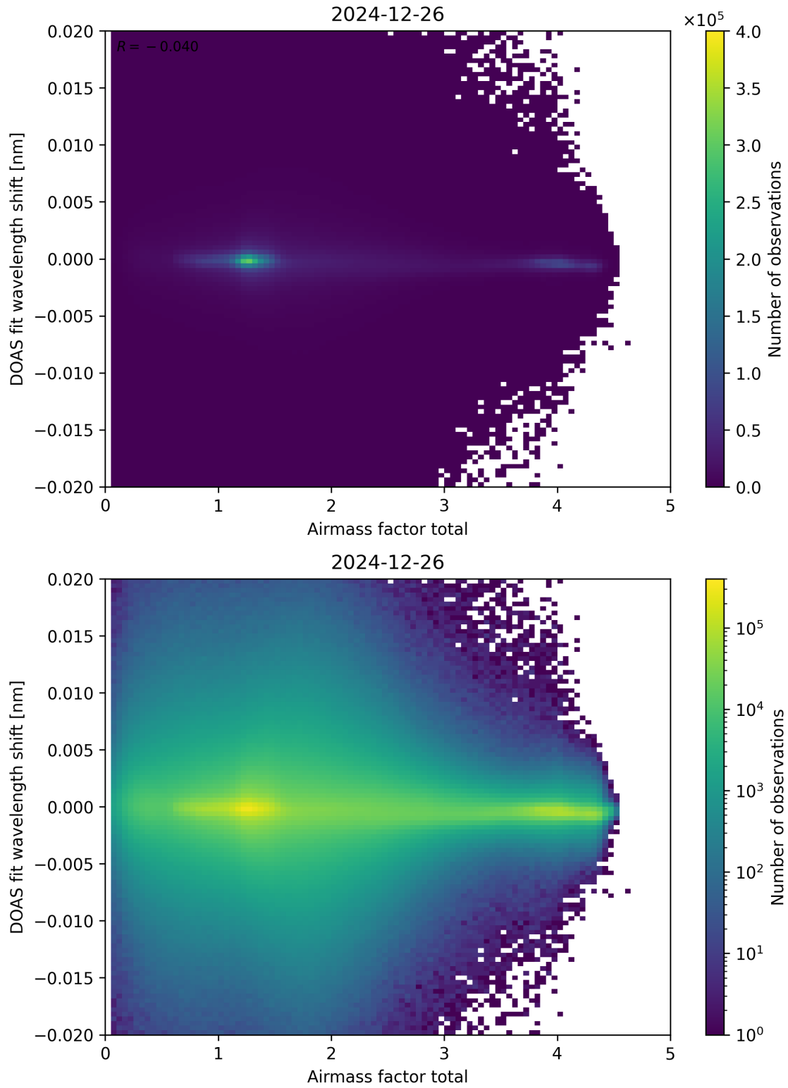
Figure 98: Scatter density plot of “Airmass factor total” against “DOAS fit wavelength shift” for 2024-12-25 to 2024-12-27.
