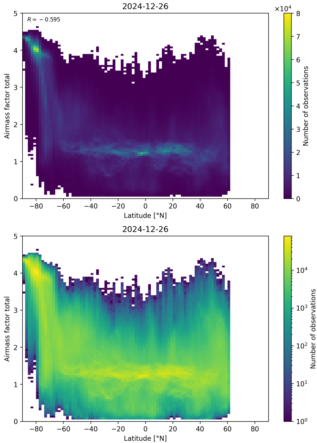
Figure 161: Scatter density plot of “Latitude” against “Airmass factor total” for 2024-12-25 to 2024-12-27.
