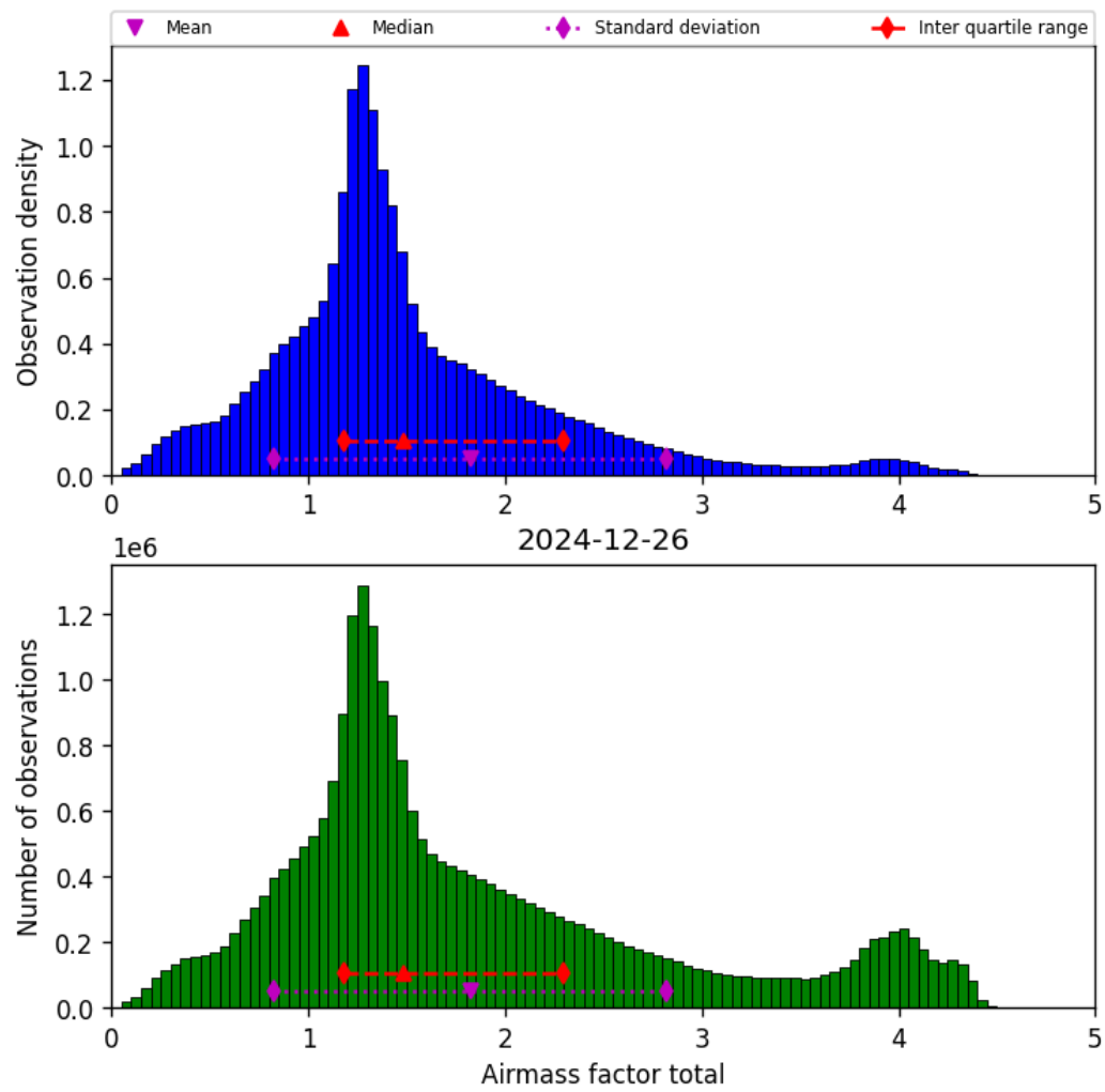
Figure 40: Histogram of “Airmass factor total” for 2024-12-25 to 2024-12-27
