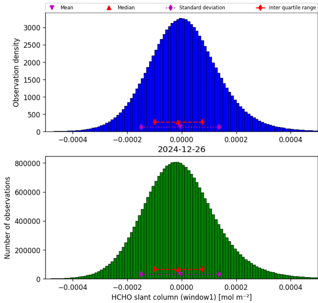
Figure 38: Histogram of “HCHO slant column (window1)” for 2024-12-25 to 2024-12-27
