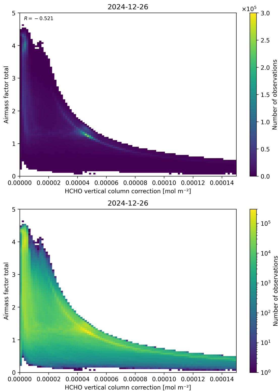
Figure 120: Scatter density plot of “HCHO vertical column correction” against “Airmass factor total” for 2024-12-25 to 2024-12-27.
