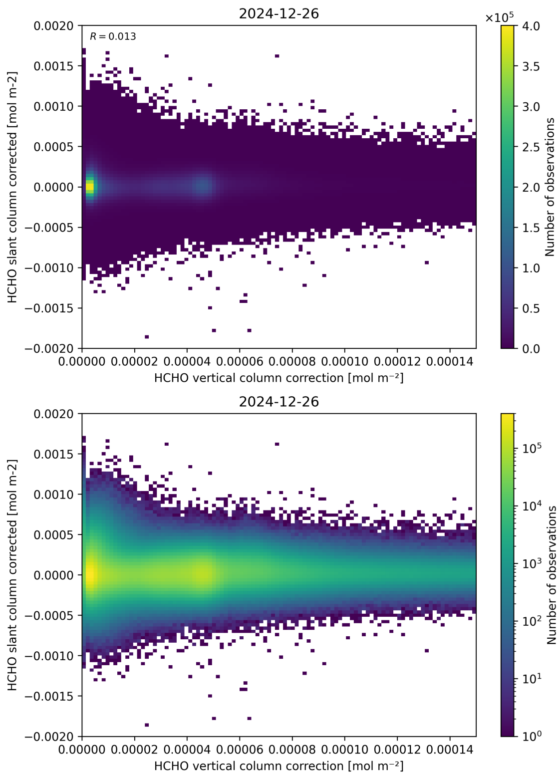
Figure 116: Scatter density plot of “HCHO vertical column correction” against “HCHO slant column corrected” for 2024-12-25 to 2024-12-27.
