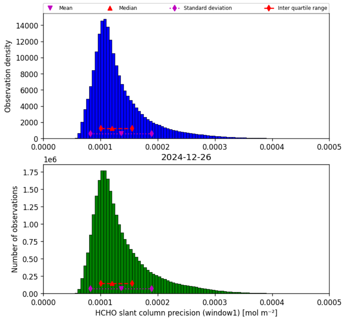
Figure 39: Histogram of “HCHO slant column precision (window1)” for 2024-12-25 to 2024-12-27
