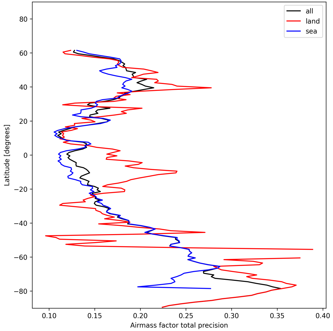
Figure 27: Zonal average of “Airmass factor total precision” for 2024-12-25 to 2024-12-27.
