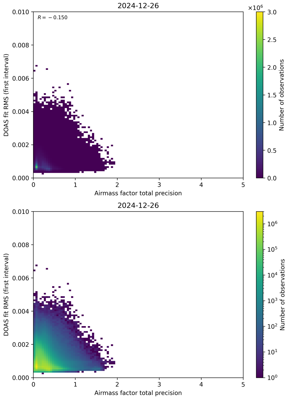
Figure 105: Scatter density plot of “Airmass factor total precision” against “DOAS fit RMS (first interval)” for 2024-12-25 to 2024-12-27.
