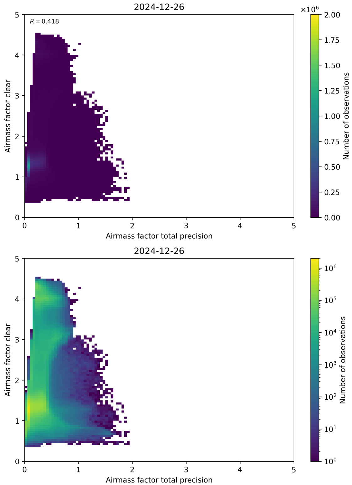
Figure 108: Scatter density plot of “Airmass factor total precision” against “Airmass factor clear” for 2024-12-25 to 2024-12-27.
