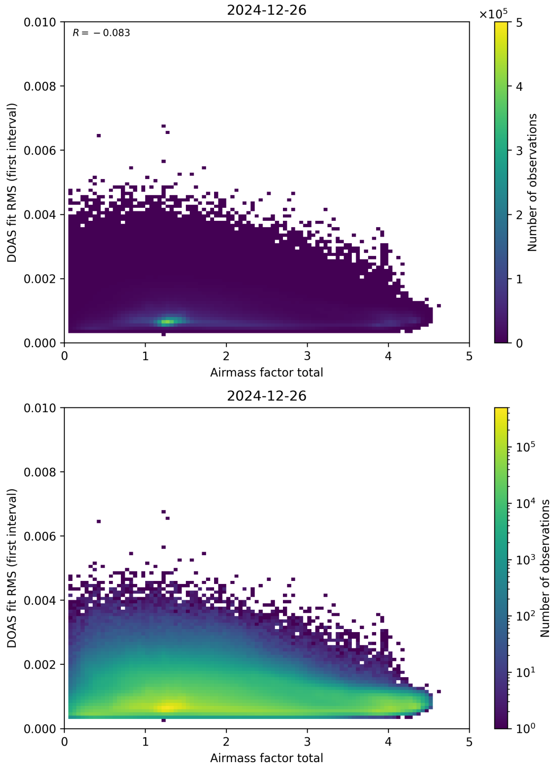
Figure 97: Scatter density plot of “Airmass factor total” against “DOAS fit RMS (first interval)” for 2024-12-25 to 2024-12-27.
