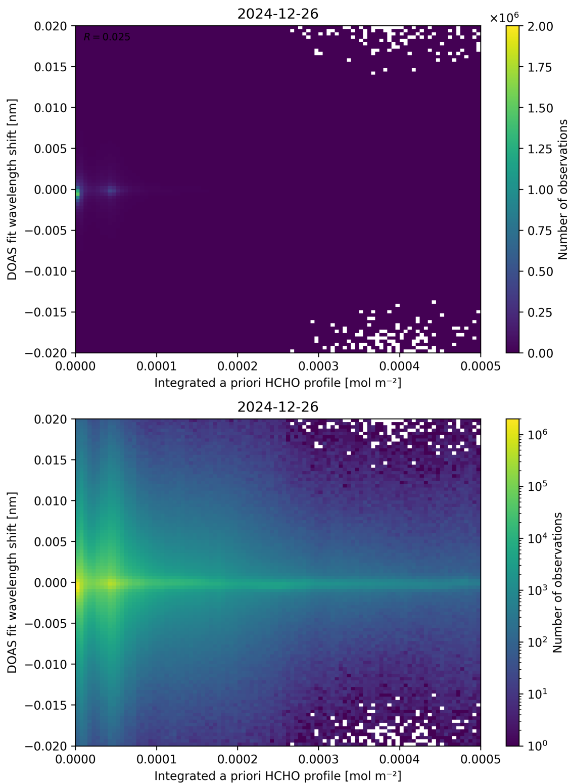
Figure 149: Scatter density plot of “Integrated a priori HCHO profile” against “DOAS fit wavelength shift” for 2024-12-25 to 2024-12-27.
