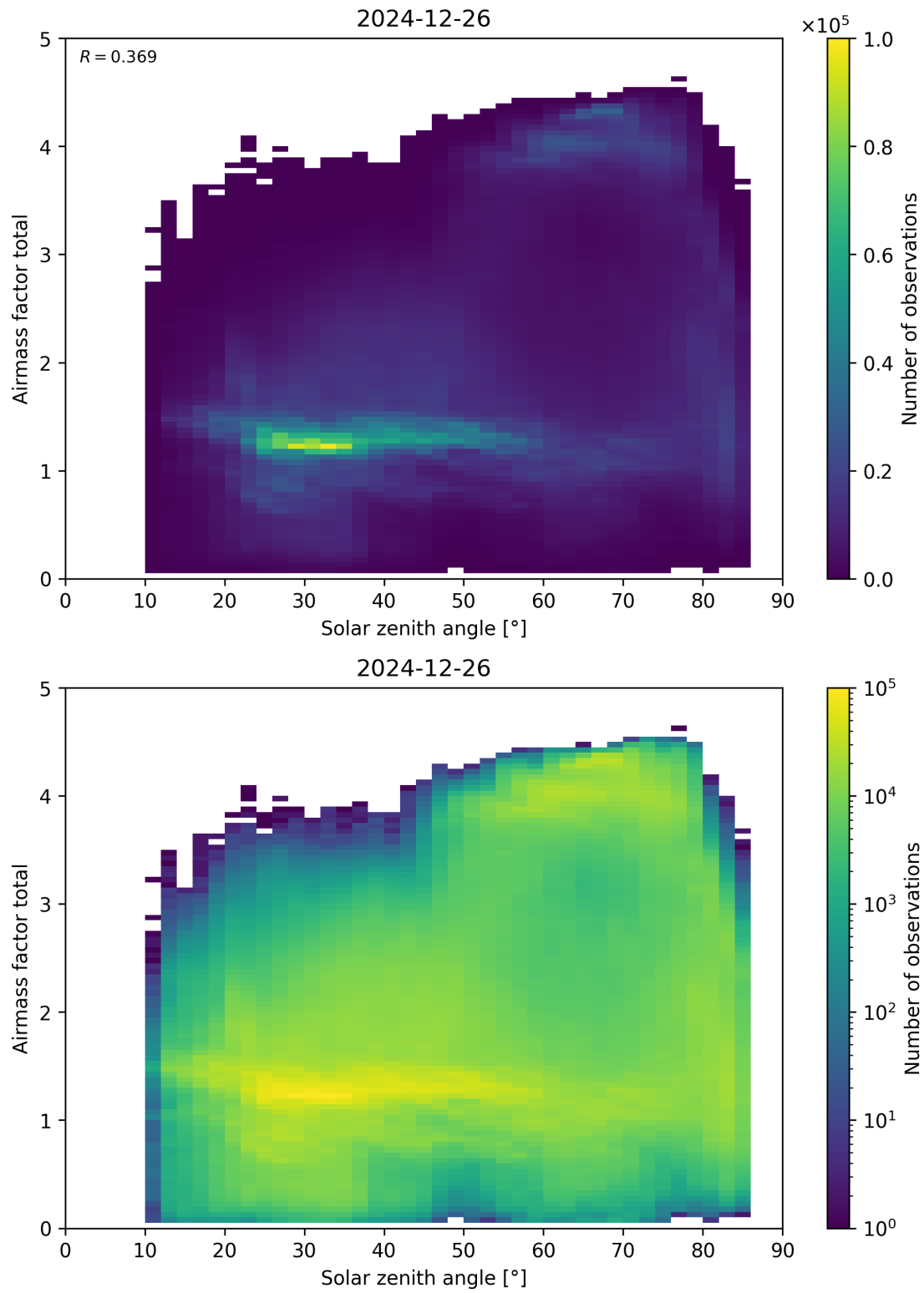
Figure 175: Scatter density plot of “Solar zenith angle” against “Airmass factor total” for 2024-12-25 to 2024-12-27.
