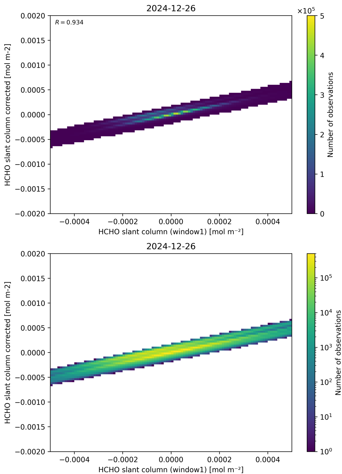
Figure 82: Scatter density plot of “HCHO slant column (window1)” against “HCHO slant column corrected” for 2024-12-25 to 2024-12-27.
