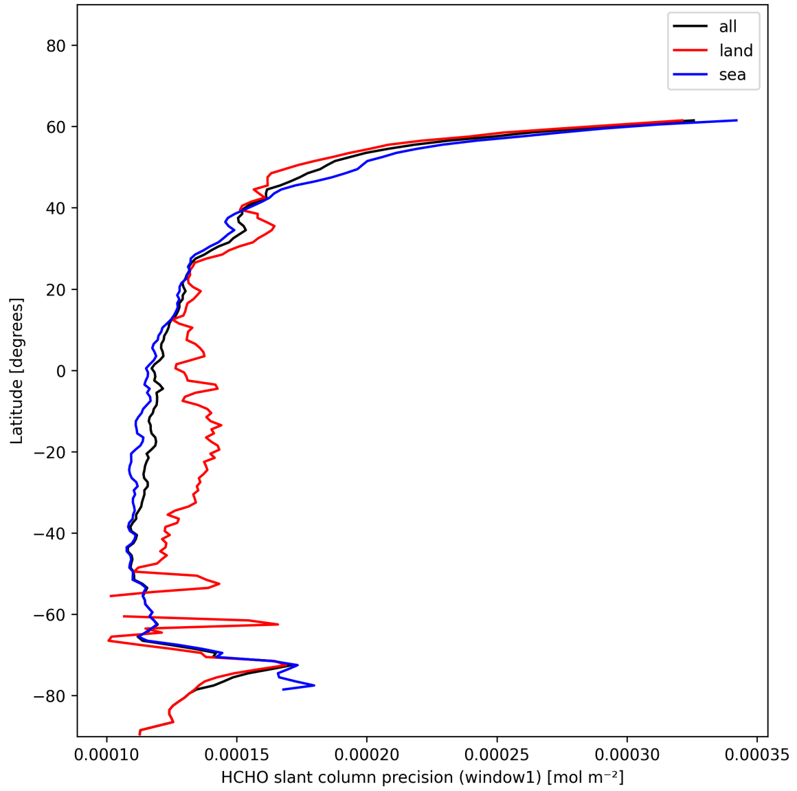
Figure 25: Zonal average of “HCHO slant column precision (window1)” for 2024-12-25 to 2024-12-27.
