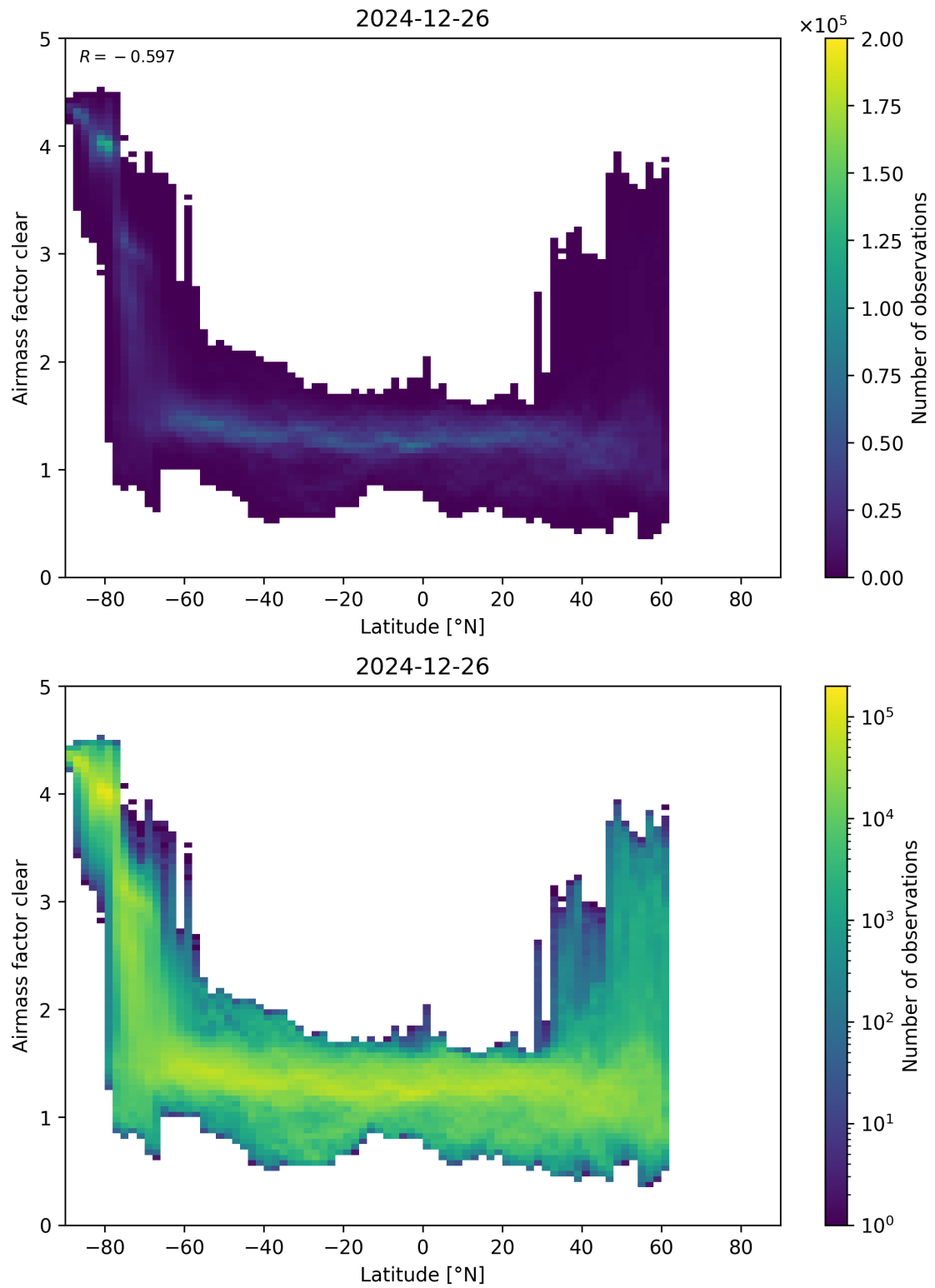
Figure 156: Scatter density plot of “Latitude” against “Airmass factor clear” for 2024-12-25 to 2024-12-27.
