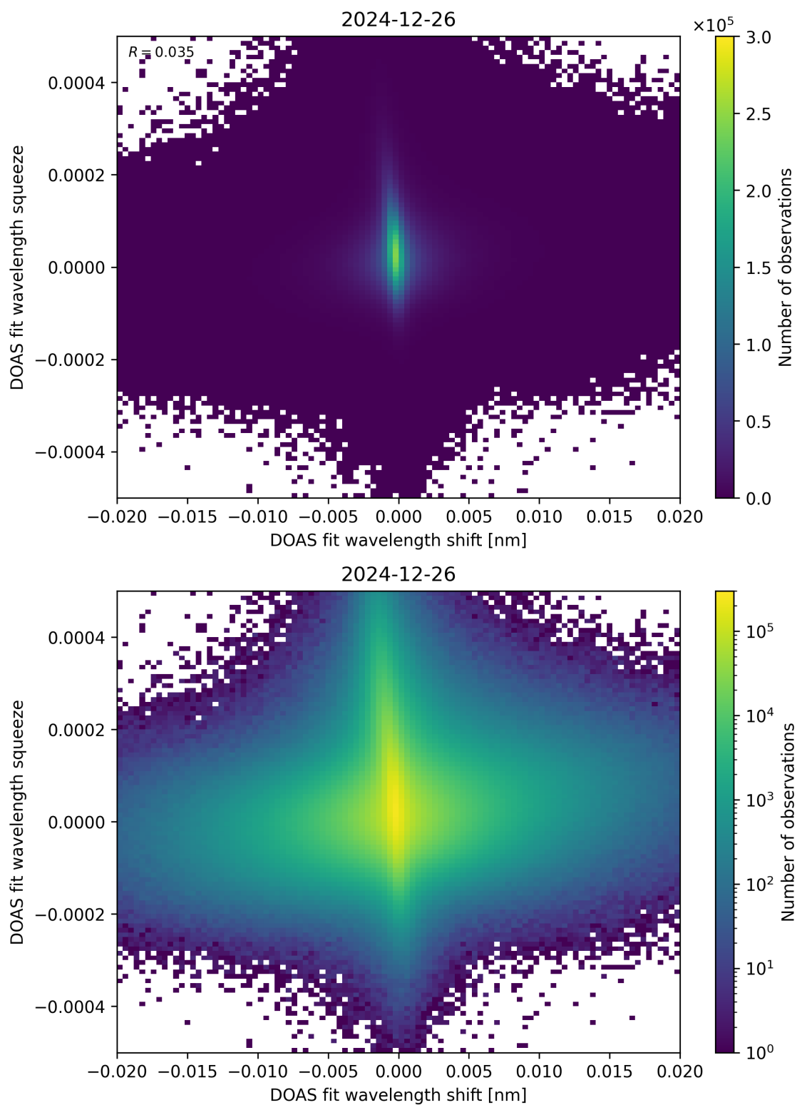
Figure 65: Scatter density plot of “DOAS fit wavelength shift” against “DOAS fit wavelength squeeze” for 2024-12-25 to 2024-12-27.
