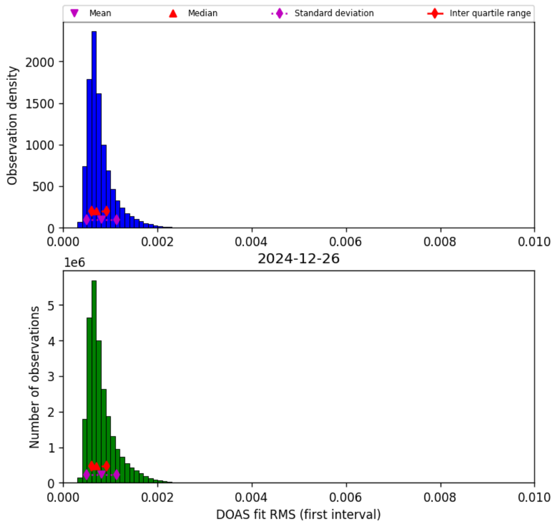
Figure 46: Histogram of “DOAS fit RMS (first interval)” for 2024-12-25 to 2024-12-27
