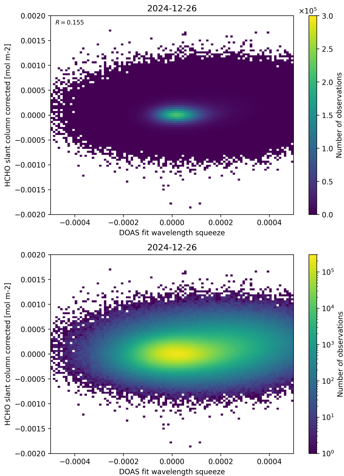
Figure 69: Scatter density plot of “DOAS fit wavelength squeeze” against “HCHO slant column corrected” for 2024-12-25 to 2024-12-27.
