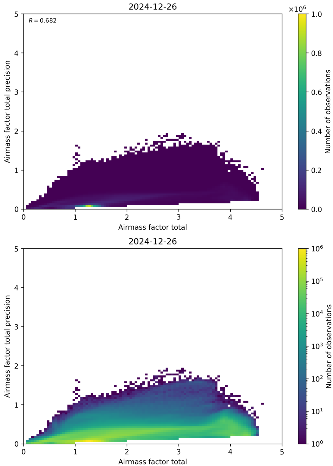
Figure 103: Scatter density plot of “Airmass factor total” against “Airmass factor total precision” for 2024-12-25 to 2024-12-27.
