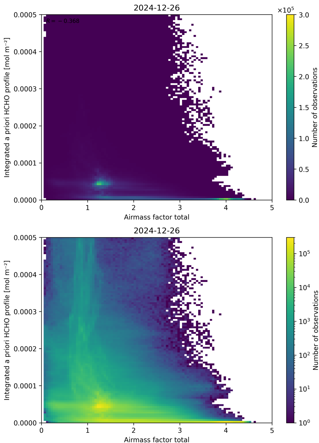
Figure 104: Scatter density plot of “Airmass factor total” against “Integrated a priori HCHO profile” for 2024-12-25 to 2024-12-27.
