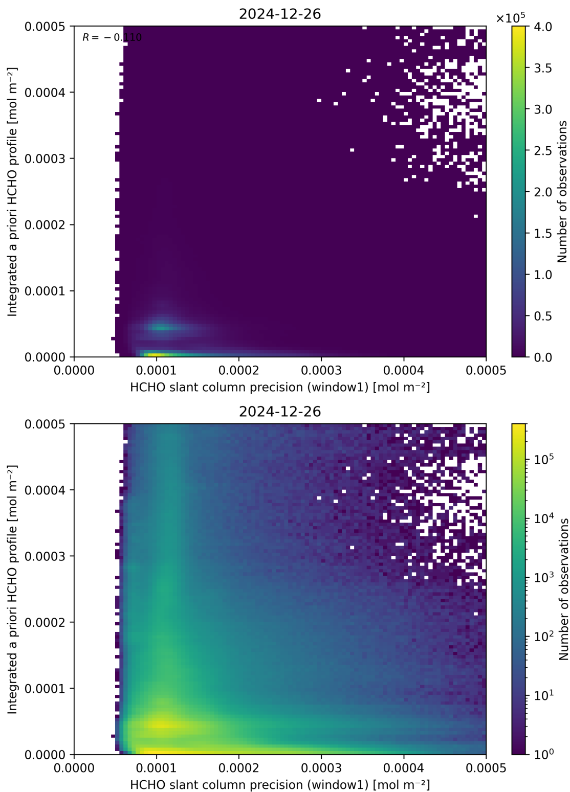
Figure 96: Scatter density plot of “HCHO slant column precision (window1)” against “Integrated a priori HCHO profile” for 2024-12-25 to 2024-12-27.
