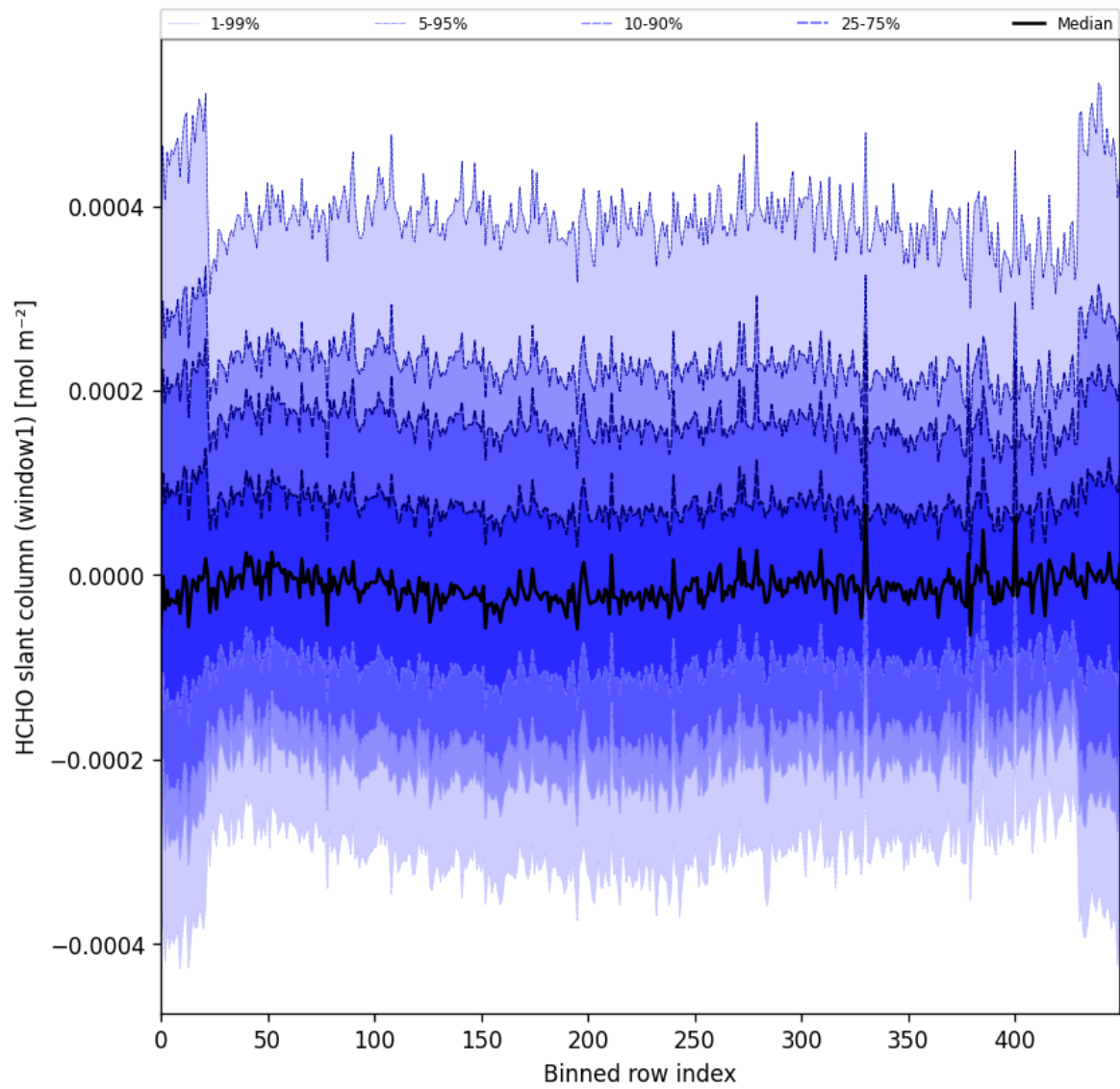
Figure 52: Along track statistics of “HCHO slant column (window1)” for 2024-12-25 to 2024-12-27
