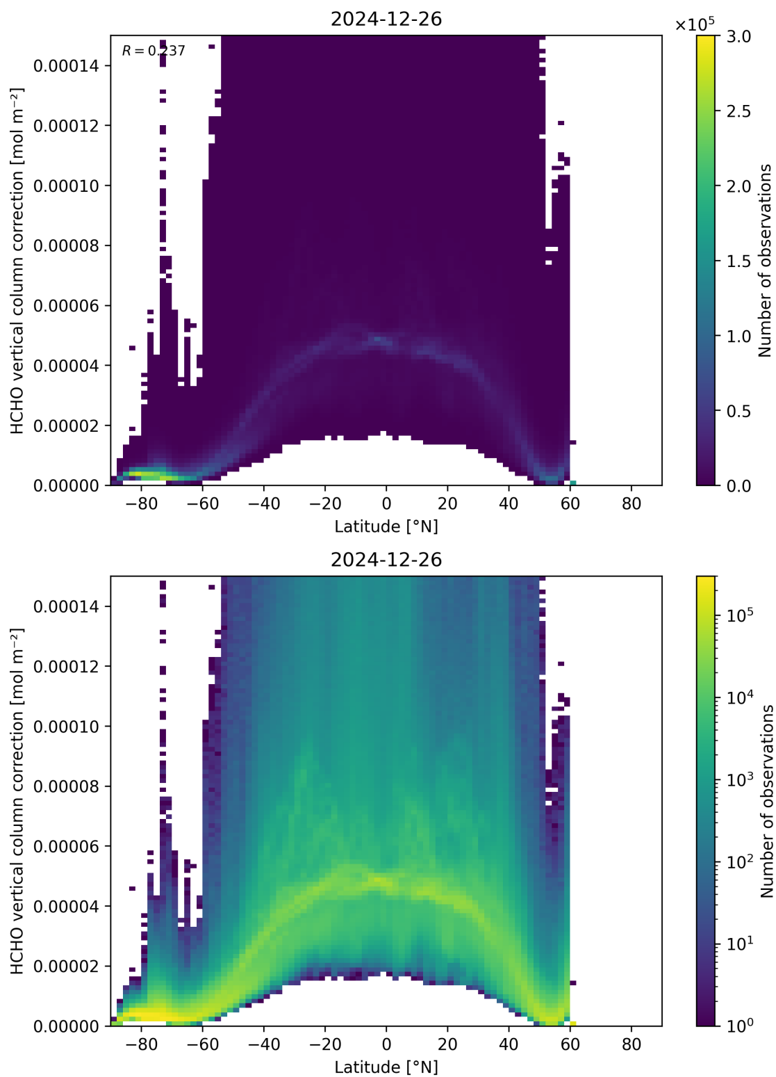
Figure 164: Scatter density plot of “Latitude” against “HCHO vertical column correction” for 2024-12-25 to 2024-12-27.
