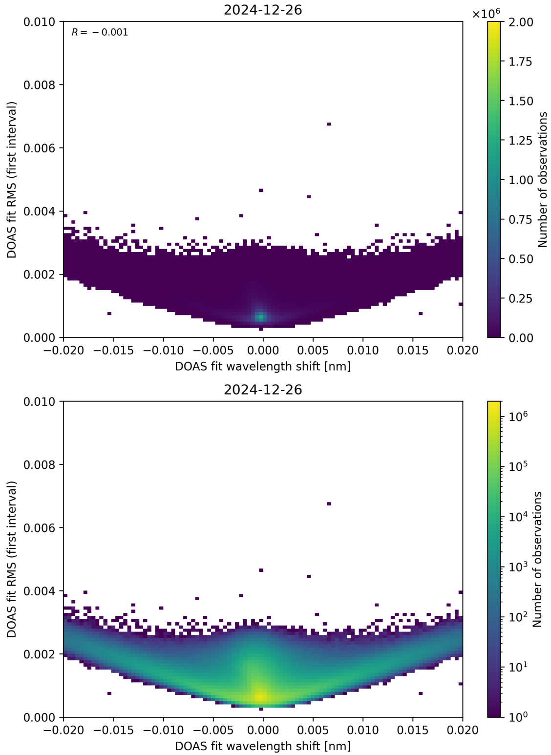
Figure 64: Scatter density plot of “DOAS fit wavelength shift” against “DOAS fit RMS (first interval)” for 2024-12-25 to 2024-12-27.
