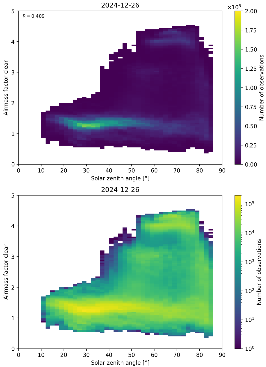
Figure 170: Scatter density plot of “Solar zenith angle” against “Airmass factor clear” for 2024-12-25 to 2024-12-27.
