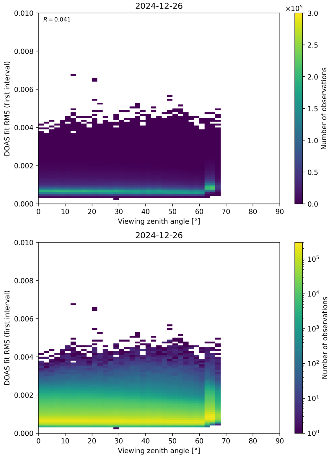
Figure 182: Scatter density plot of “Viewing zenith angle” against “DOAS fit RMS (first interval)” for 2024-12-25 to 2024-12-27.
