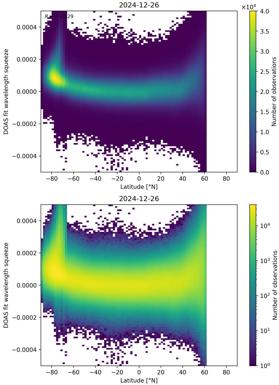
Figure 155: Scatter density plot of “Latitude” against “DOAS fit wavelength squeeze” for 2024-12-25 to 2024-12-27.
