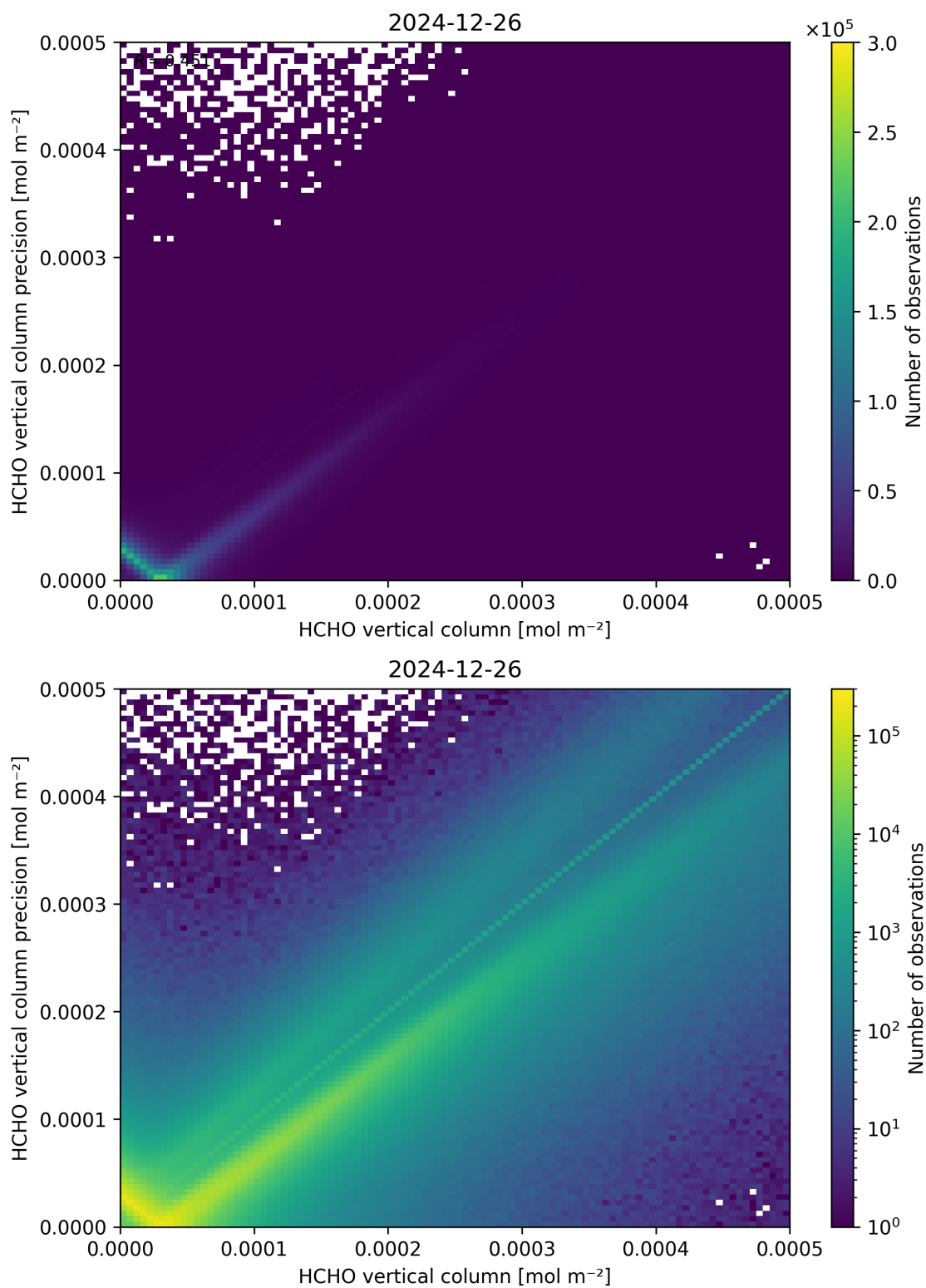
Figure 134: Scatter density plot of “HCHO vertical column” against “HCHO vertical column precision” for 2024-12-25 to 2024-12-27.
