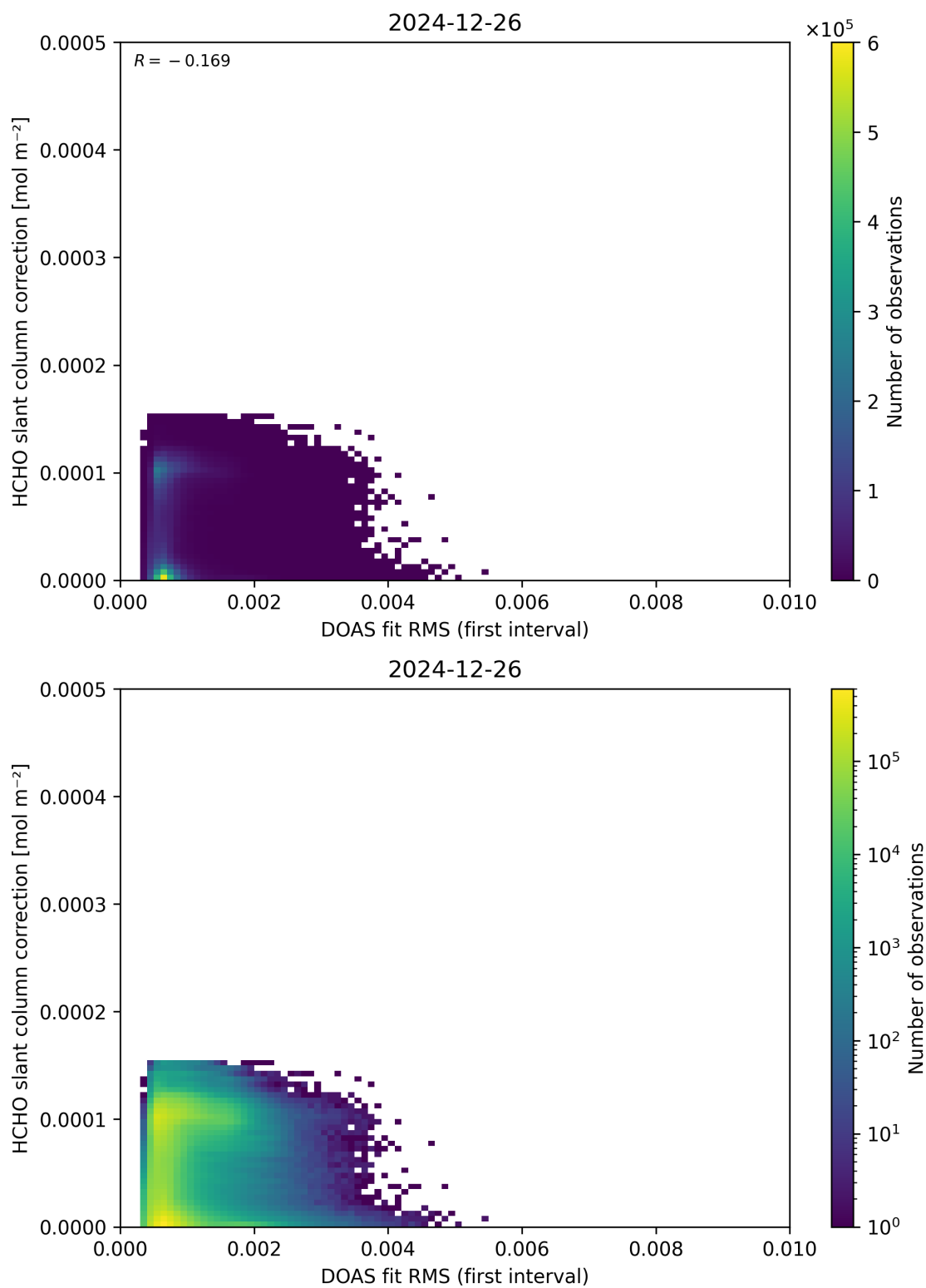
Figure 63: Scatter density plot of “DOAS fit RMS (first interval)” against “HCHO slant column correction” for 2024-12-25 to 2024-12-27.
