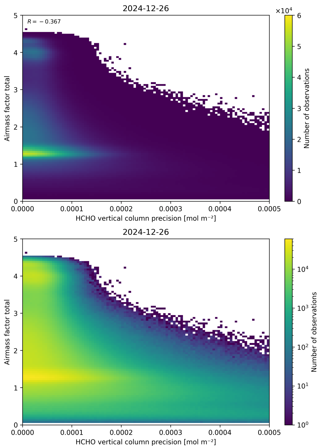
Figure 144: Scatter density plot of “HCHO vertical column precision” against “Airmass factor total” for 2024-12-25 to 2024-12-27.
