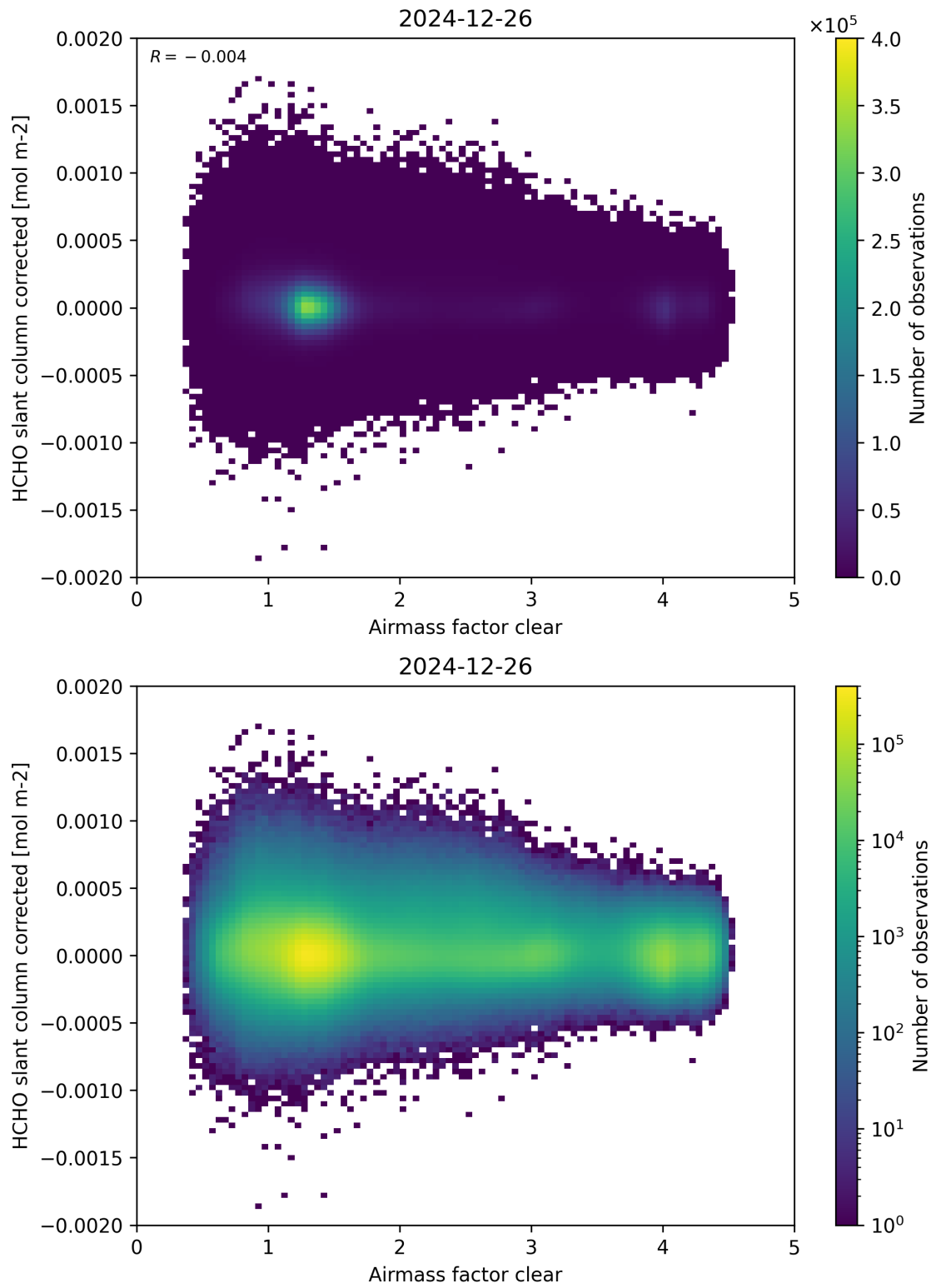
Figure 74: Scatter density plot of “Airmass factor clear” against “HCHO slant column corrected” for 2024-12-25 to 2024-12-27.
