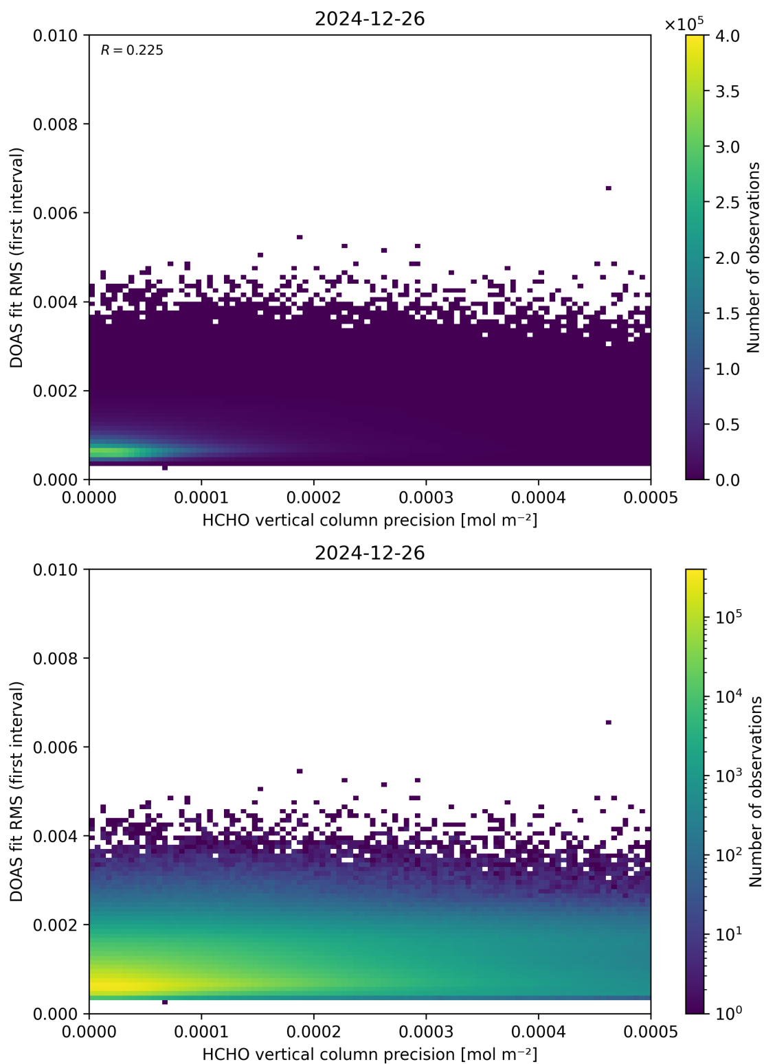
Figure 136: Scatter density plot of “HCHO vertical column precision” against “DOAS fit RMS (first interval)” for 2024-12-25 to 2024-12-27.
