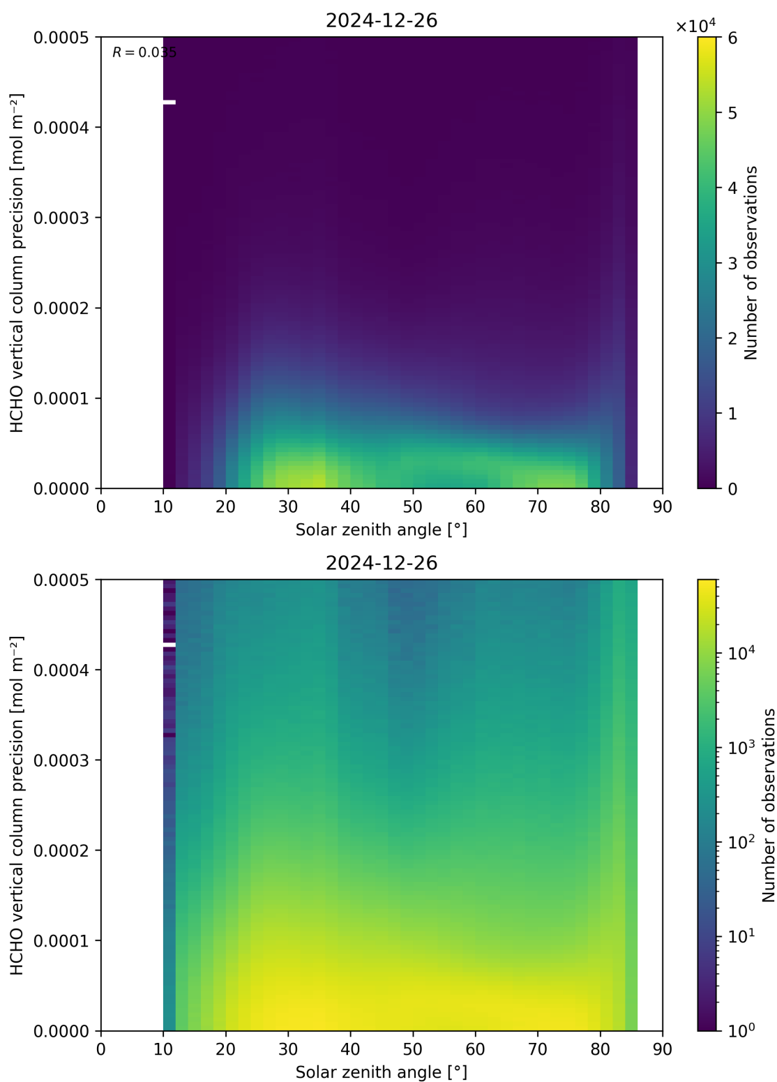
Figure 179: Scatter density plot of “Solar zenith angle” against “HCHO vertical column precision” for 2024-12-25 to 2024-12-27.
