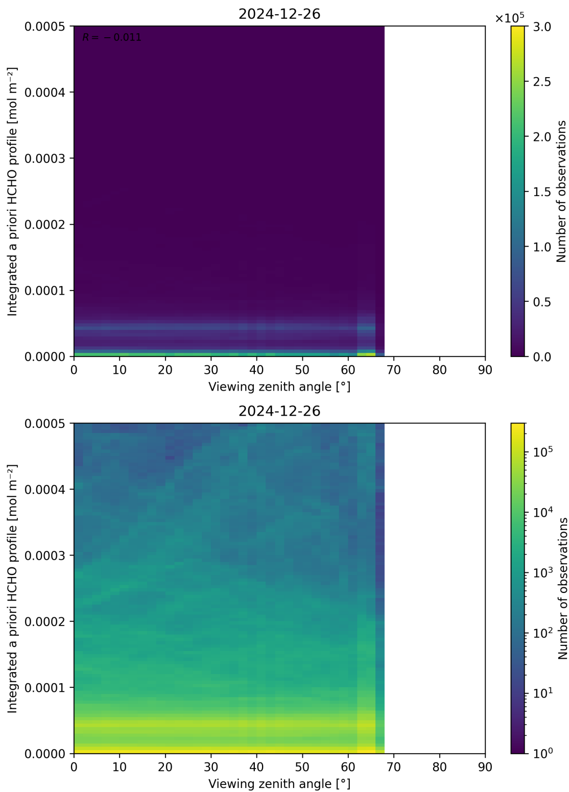
Figure 195: Scatter density plot of “Viewing zenith angle” against “Integrated a priori HCHO profile” for 2024-12-25 to 2024-12-27.
