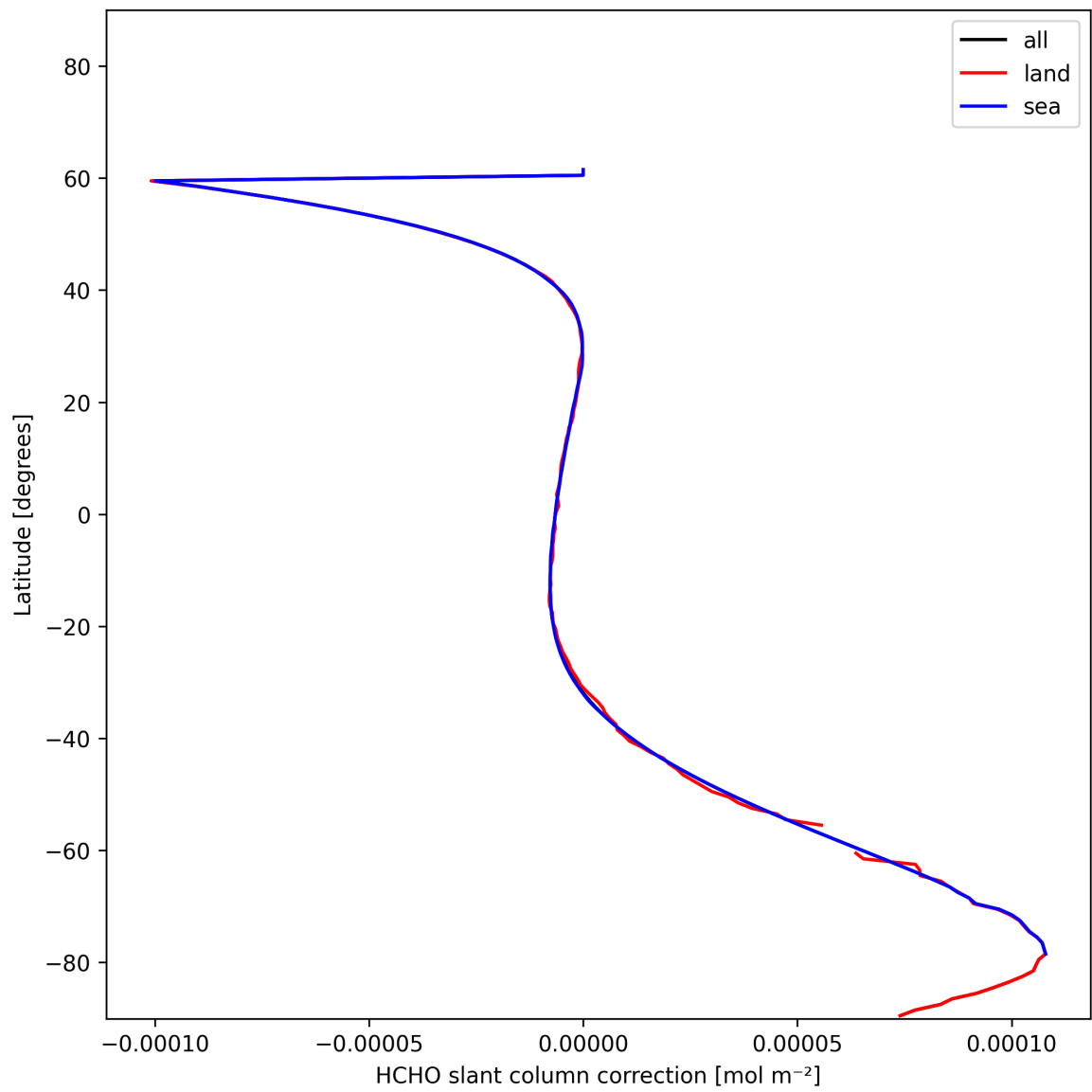
Figure 33: Zonal average of “HCHO slant column correction” for 2024-12-25 to 2024-12-27.
