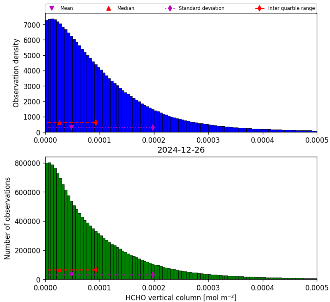
Figure 35: Histogram of “HCHO vertical column” for 2024-12-25 to 2024-12-27
