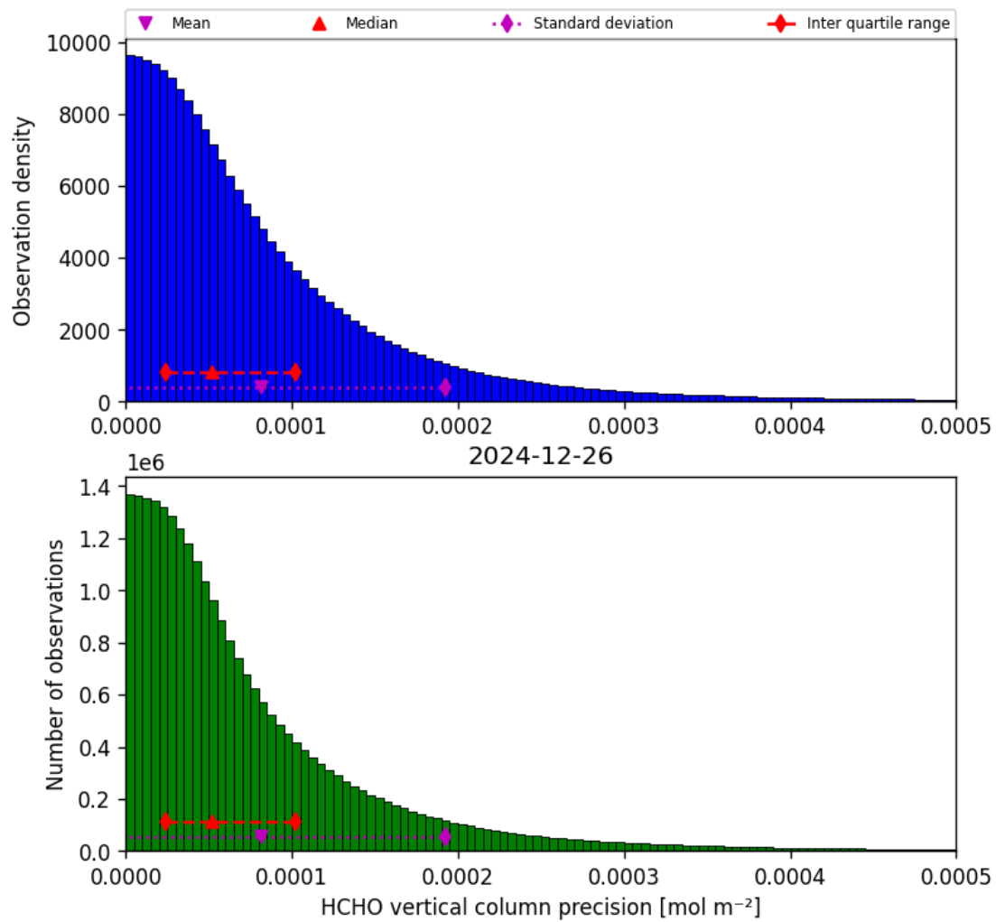
Figure 36: Histogram of “HCHO vertical column precision” for 2024-12-25 to 2024-12-27
