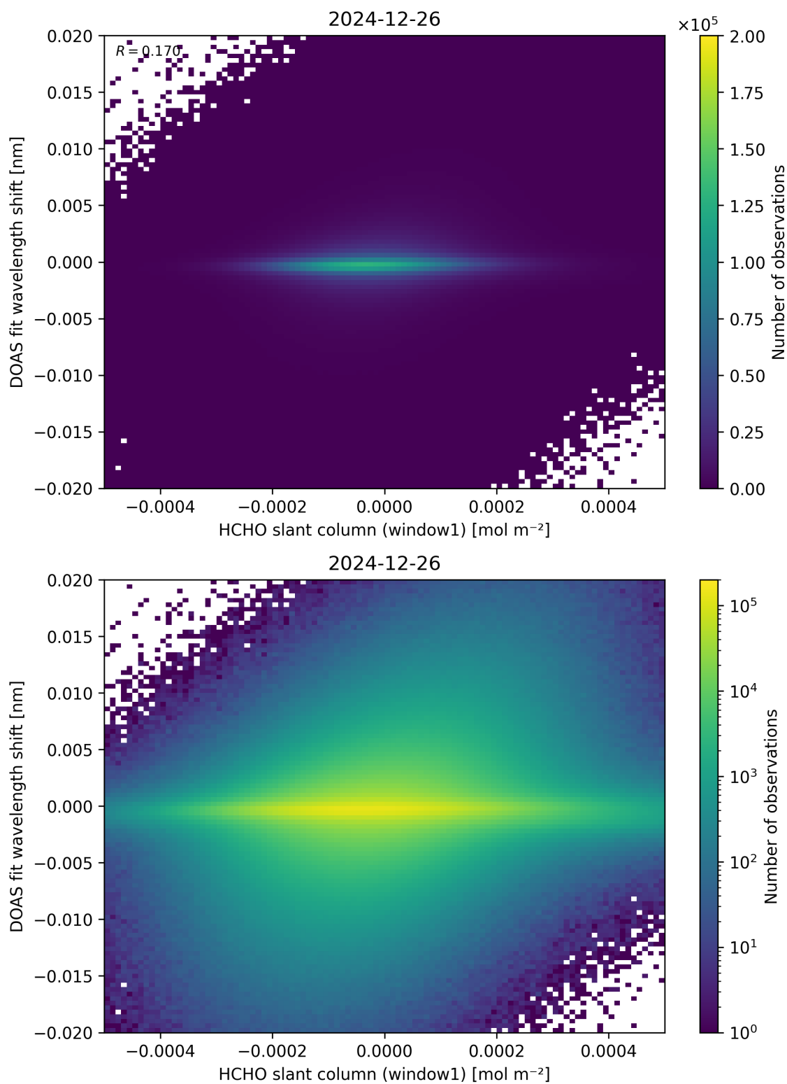
Figure 79: Scatter density plot of “HCHO slant column (window1)” against “DOAS fit wavelength shift” for 2024-12-25 to 2024-12-27.
