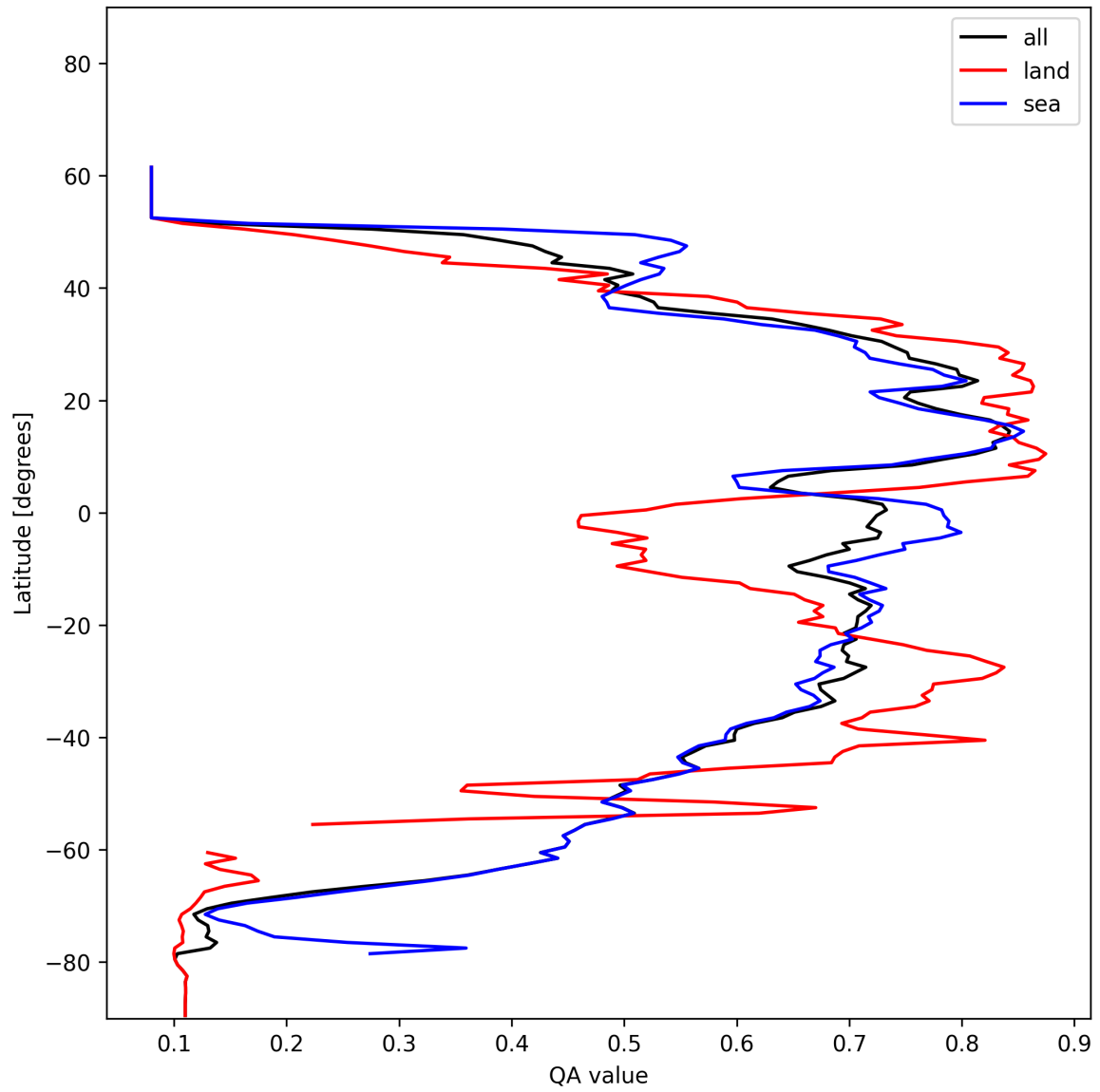
Figure 20: Zonal average of “QA value” for 2024-12-25 to 2024-12-27.
