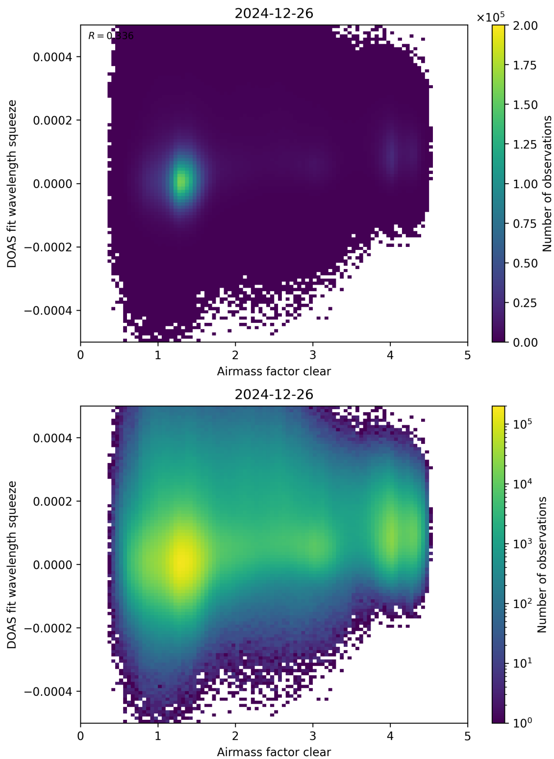
Figure 73: Scatter density plot of “Airmass factor clear” against “DOAS fit wavelength squeeze” for 2024-12-25 to 2024-12-27.
