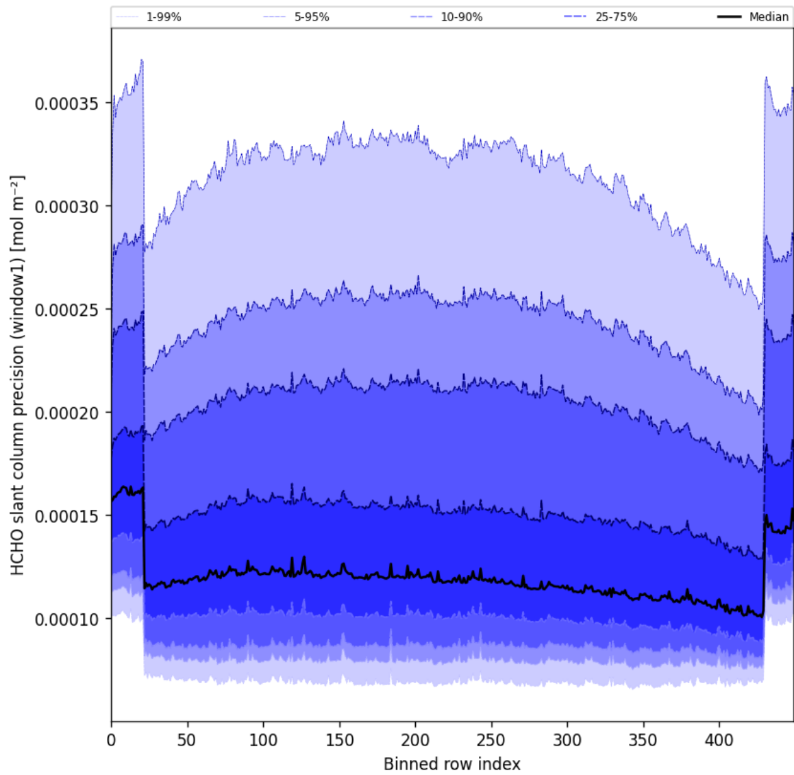
Figure 53: Along track statistics of “HCHO slant column precision (window1)” for 2024-12-25 to 2024-12-27
