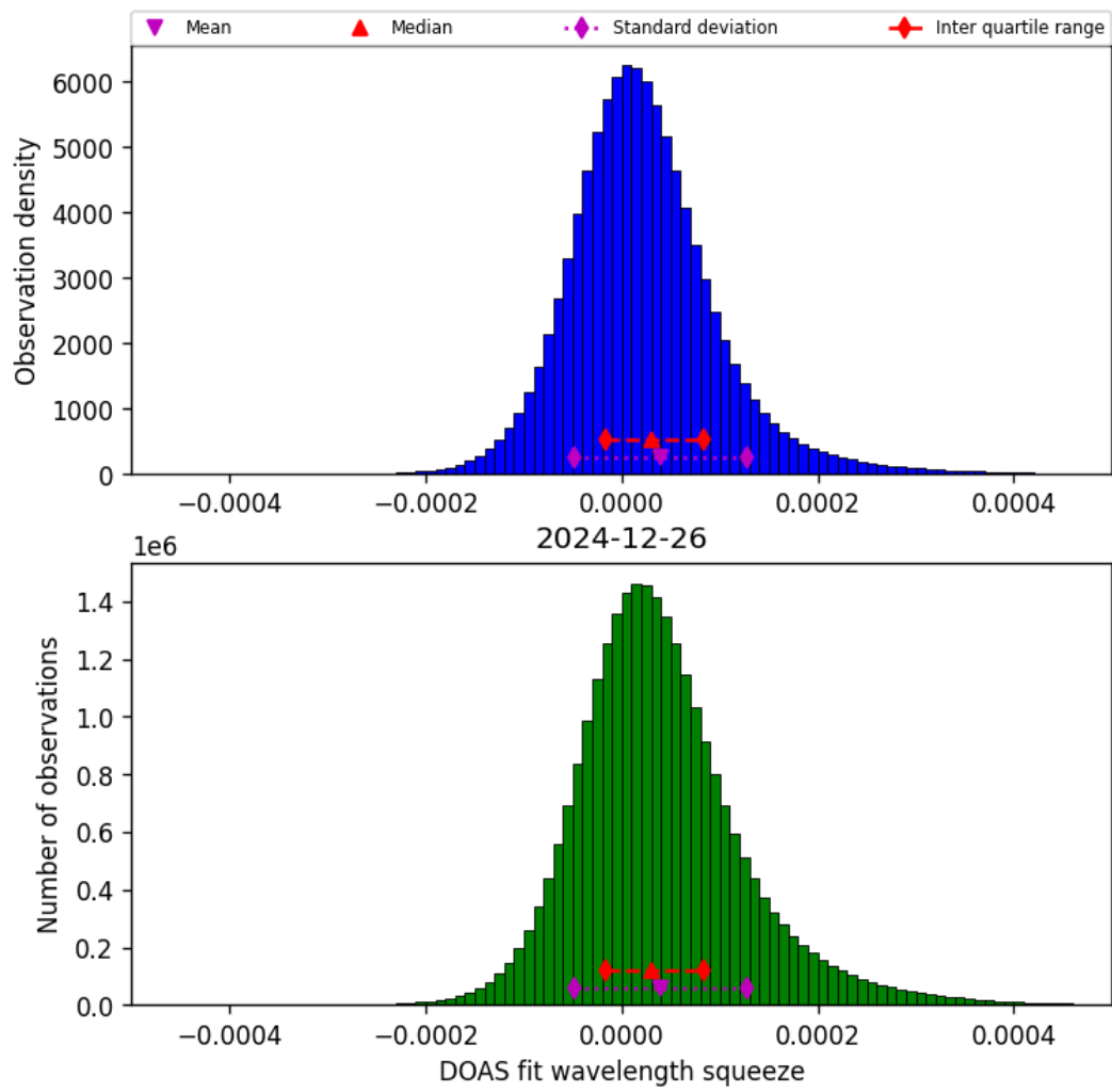
Figure 45: Histogram of “DOAS fit wavelength squeeze” for 2024-12-25 to 2024-12-27
