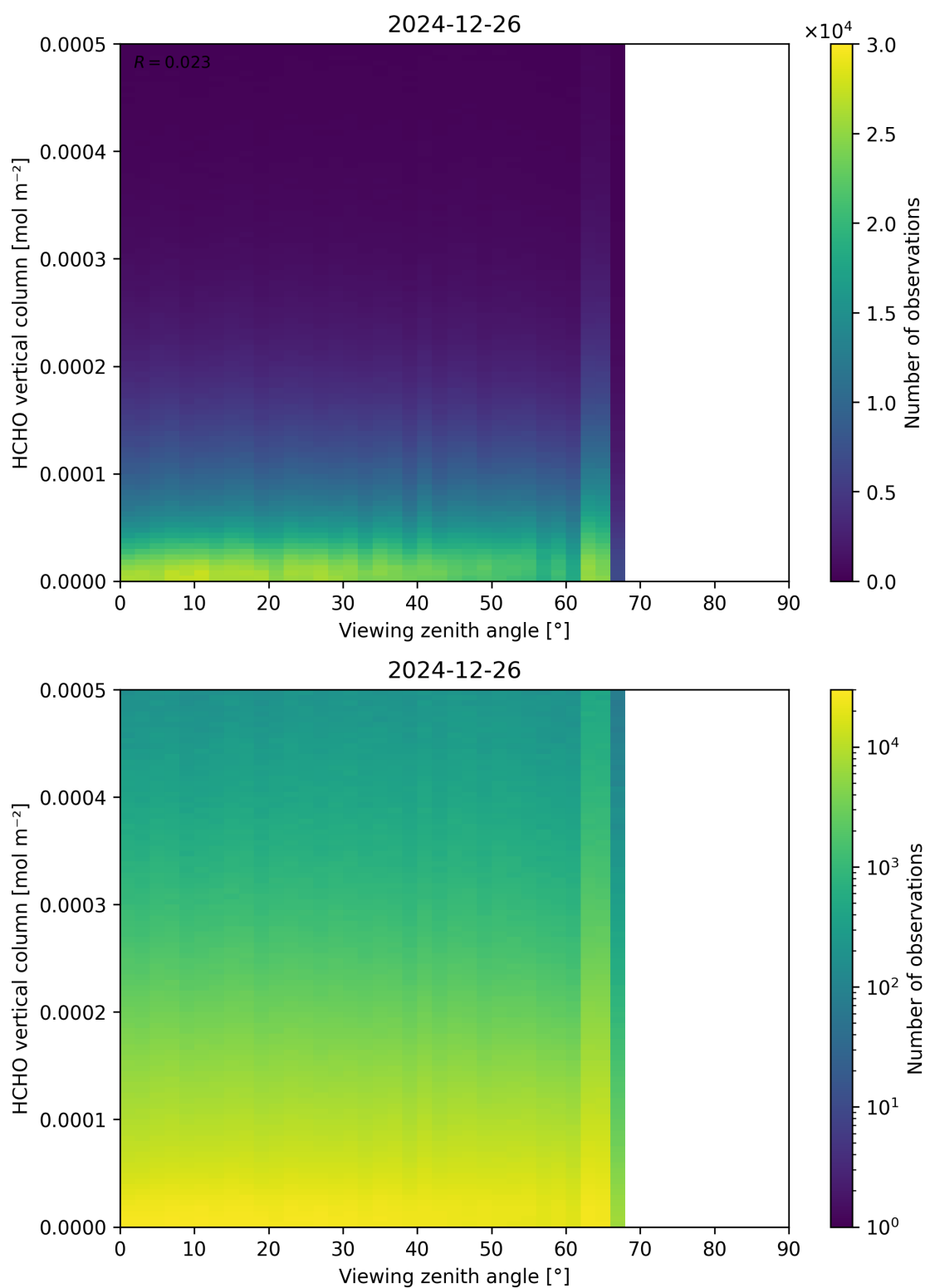
Figure 192: Scatter density plot of “Viewing zenith angle” against “HCHO vertical column” for 2024-12-25 to 2024-12-27.
