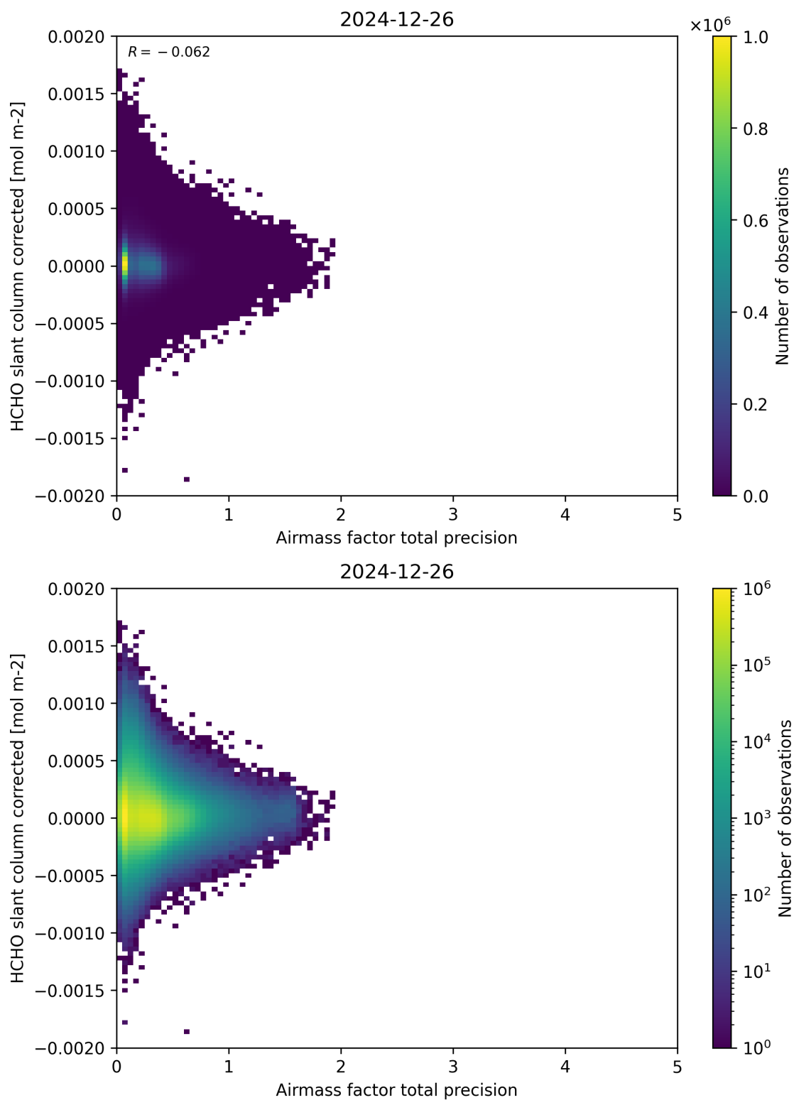
Figure 109: Scatter density plot of “Airmass factor total precision” against “HCHO slant column corrected” for 2024-12-25 to 2024-12-27.
