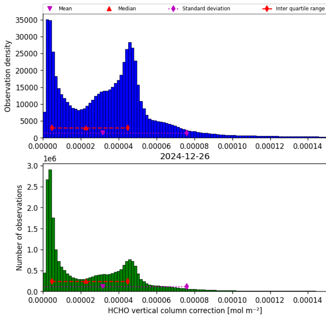
Figure 37: Histogram of “HCHO vertical column correction” for 2024-12-25 to 2024-12-27
