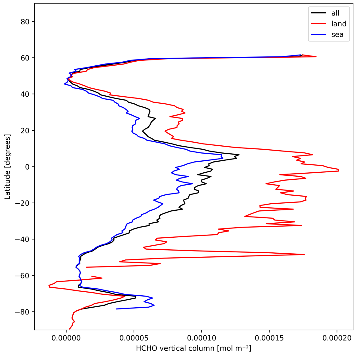
Figure 21: Zonal average of “HCHO vertical column” for 2024-12-25 to 2024-12-27.
