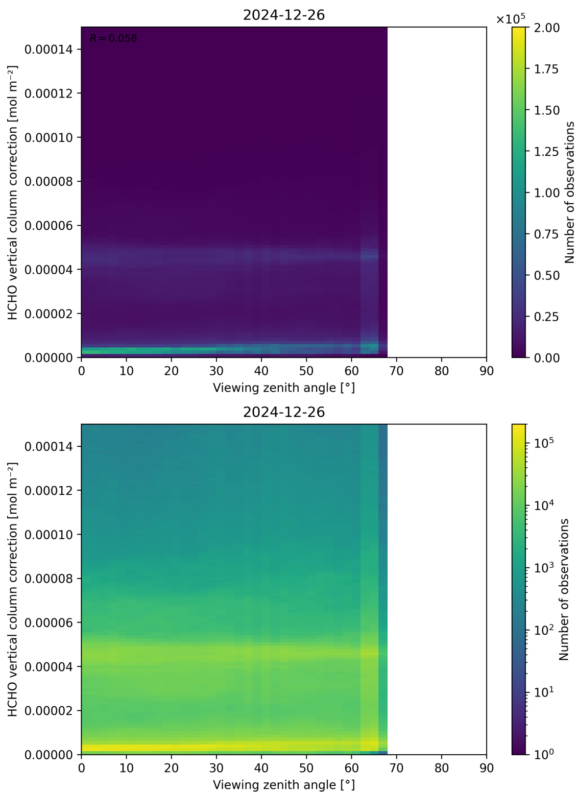
Figure 193: Scatter density plot of “Viewing zenith angle” against “HCHO vertical column correction” for 2024-12-25 to 2024-12-27.
