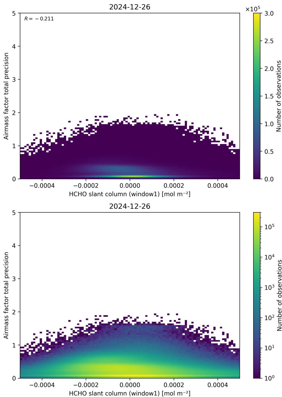
Figure 86: Scatter density plot of “HCHO slant column (window1)” against “Airmass factor total precision” for 2024-12-25 to 2024-12-27.
