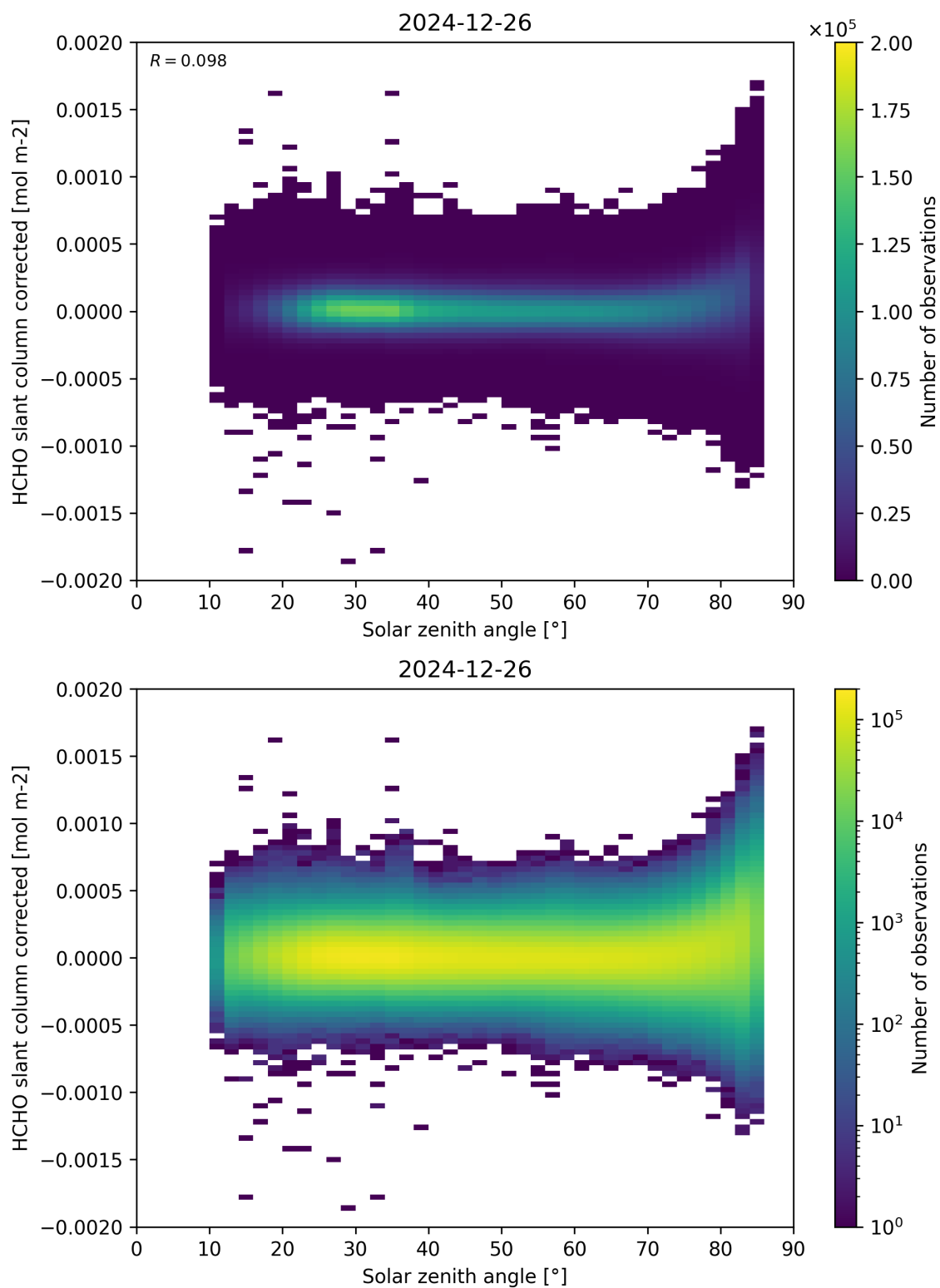
Figure 171: Scatter density plot of “Solar zenith angle” against “HCHO slant column corrected” for 2024-12-25 to 2024-12-27.
