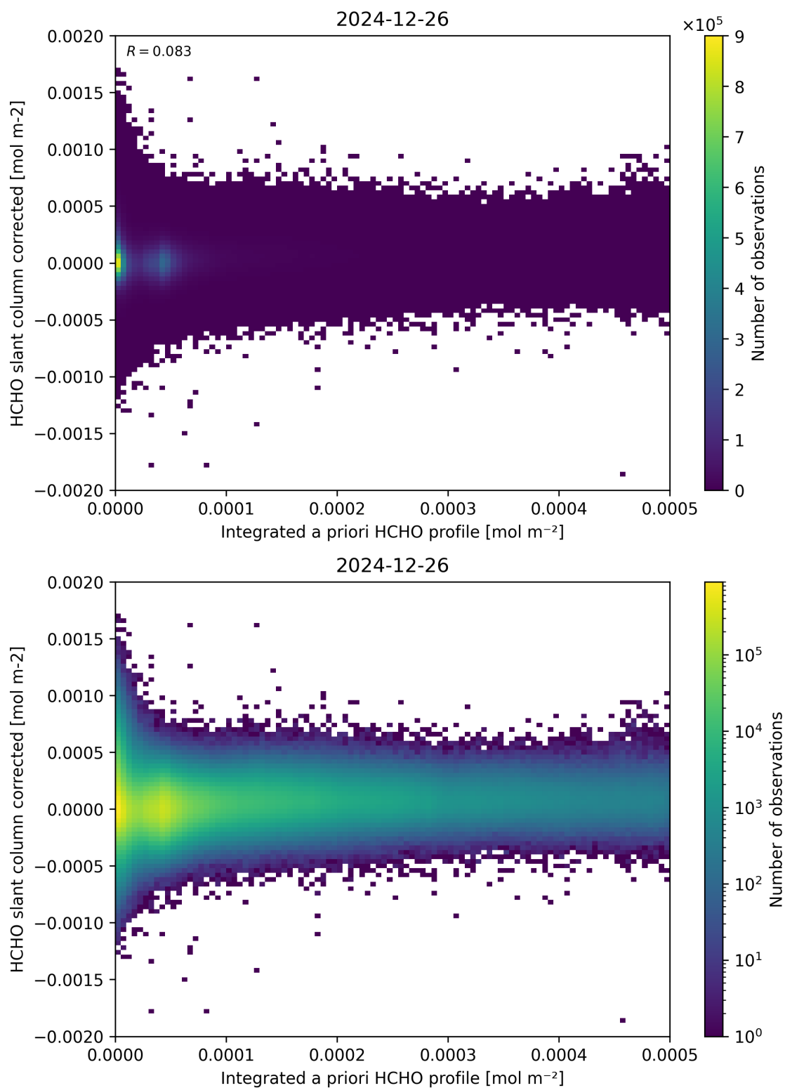
Figure 151: Scatter density plot of “Integrated a priori HCHO profile” against “HCHO slant column corrected” for 2024-12-25 to 2024-12-27.
