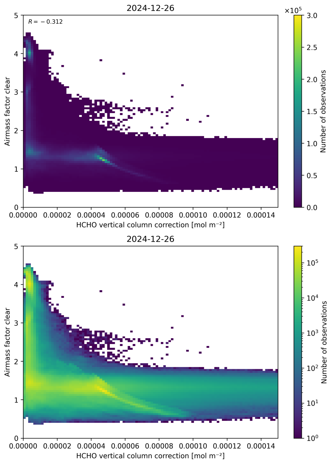
Figure 115: Scatter density plot of “HCHO vertical column correction” against “Airmass factor clear” for 2024-12-25 to 2024-12-27.
