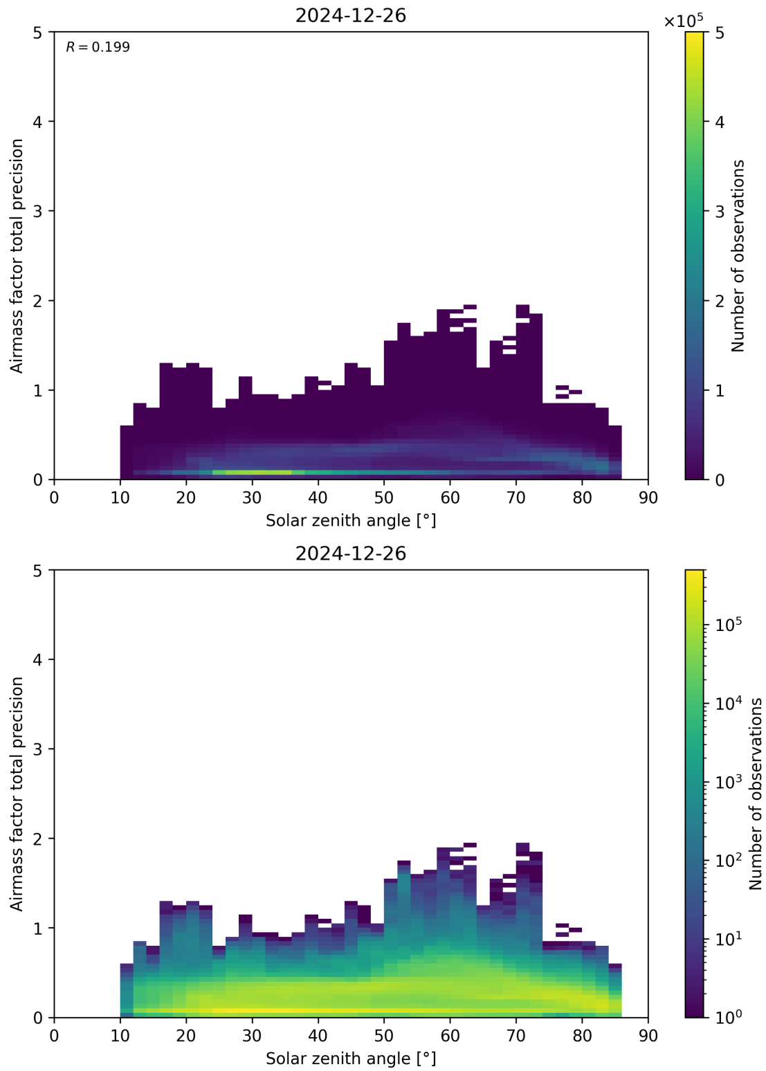
Figure 176: Scatter density plot of “Solar zenith angle” against “Airmass factor total precision” for 2024-12-25 to 2024-12-27.
