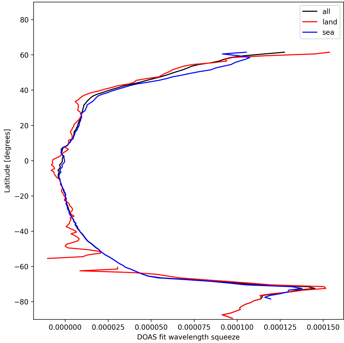
Figure 31: Zonal average of “DOAS fit wavelength squeeze” for 2024-12-25 to 2024-12-27.
