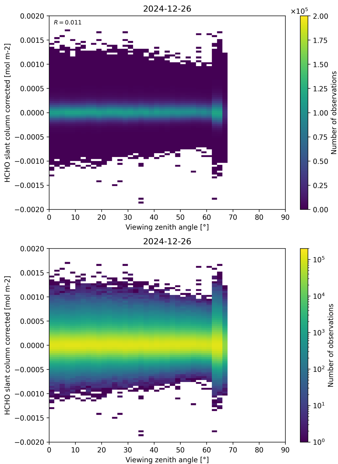
Figure 186: Scatter density plot of “Viewing zenith angle” against “HCHO slant column corrected” for 2024-12-25 to 2024-12-27.
