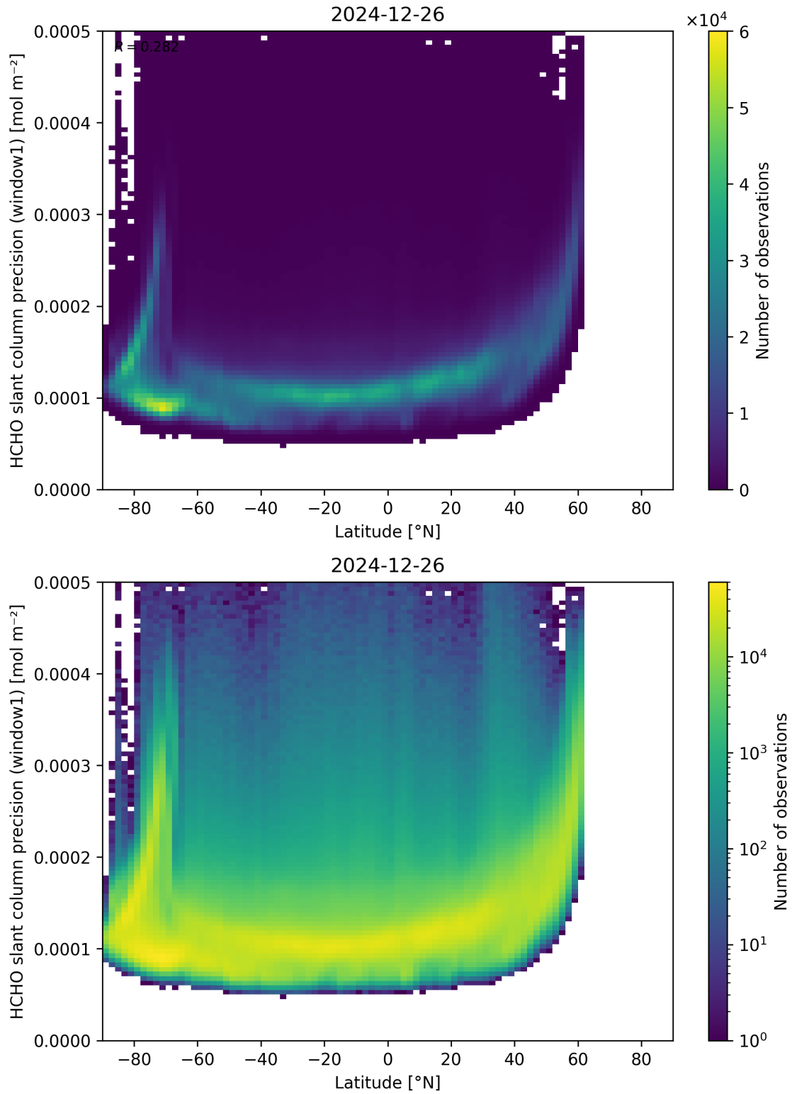
Figure 160: Scatter density plot of “Latitude” against “HCHO slant column precision (window1)” for 2024-12-25 to 2024-12-27.
