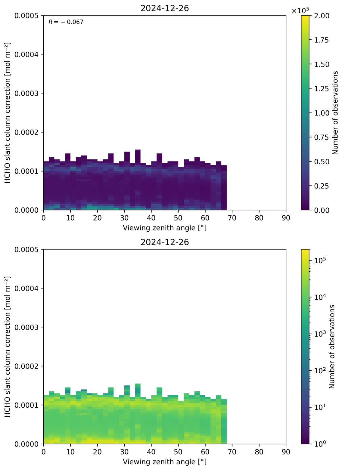
Figure 187: Scatter density plot of “Viewing zenith angle” against “HCHO slant column correction” for 2024-12-25 to 2024-12-27.
