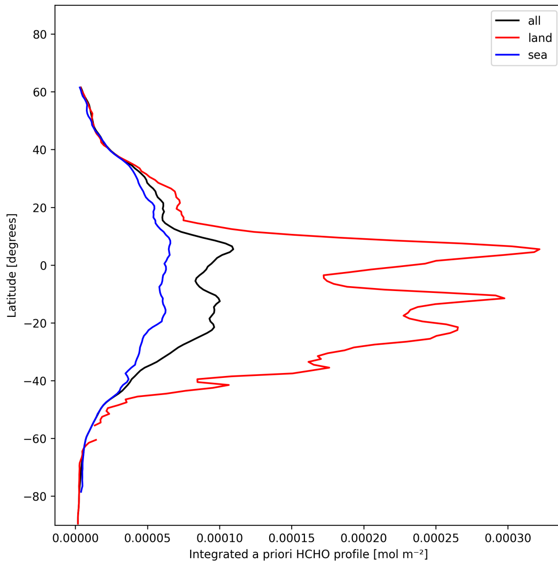
Figure 29: Zonal average of “Integrated a priori HCHO profile” for 2024-12-25 to 2024-12-27.
