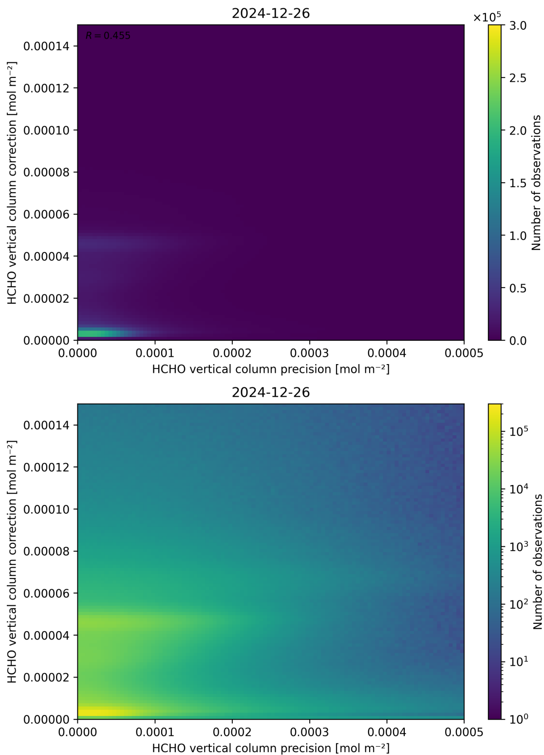
Figure 146: Scatter density plot of “HCHO vertical column precision” against “HCHO vertical column correction” for 2024-12-25 to 2024-12-27.
