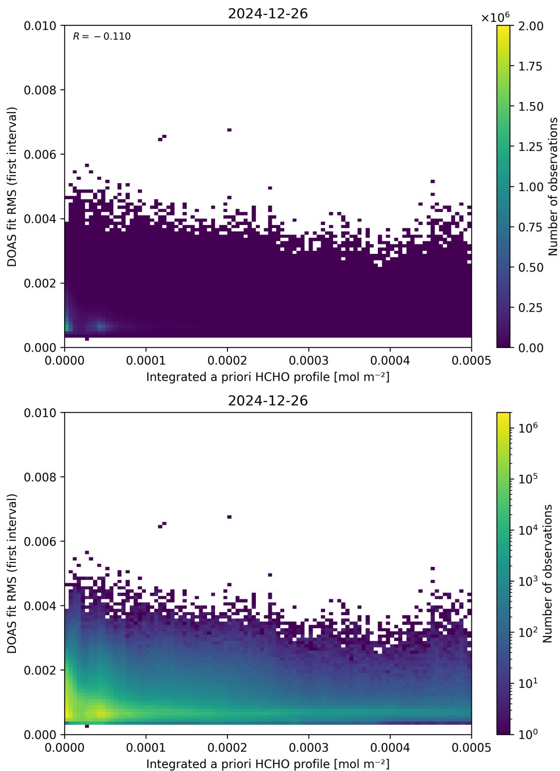
Figure 148: Scatter density plot of “Integrated a priori HCHO profile” against “DOAS fit RMS (first interval)” for 2024-12-25 to 2024-12-27.
