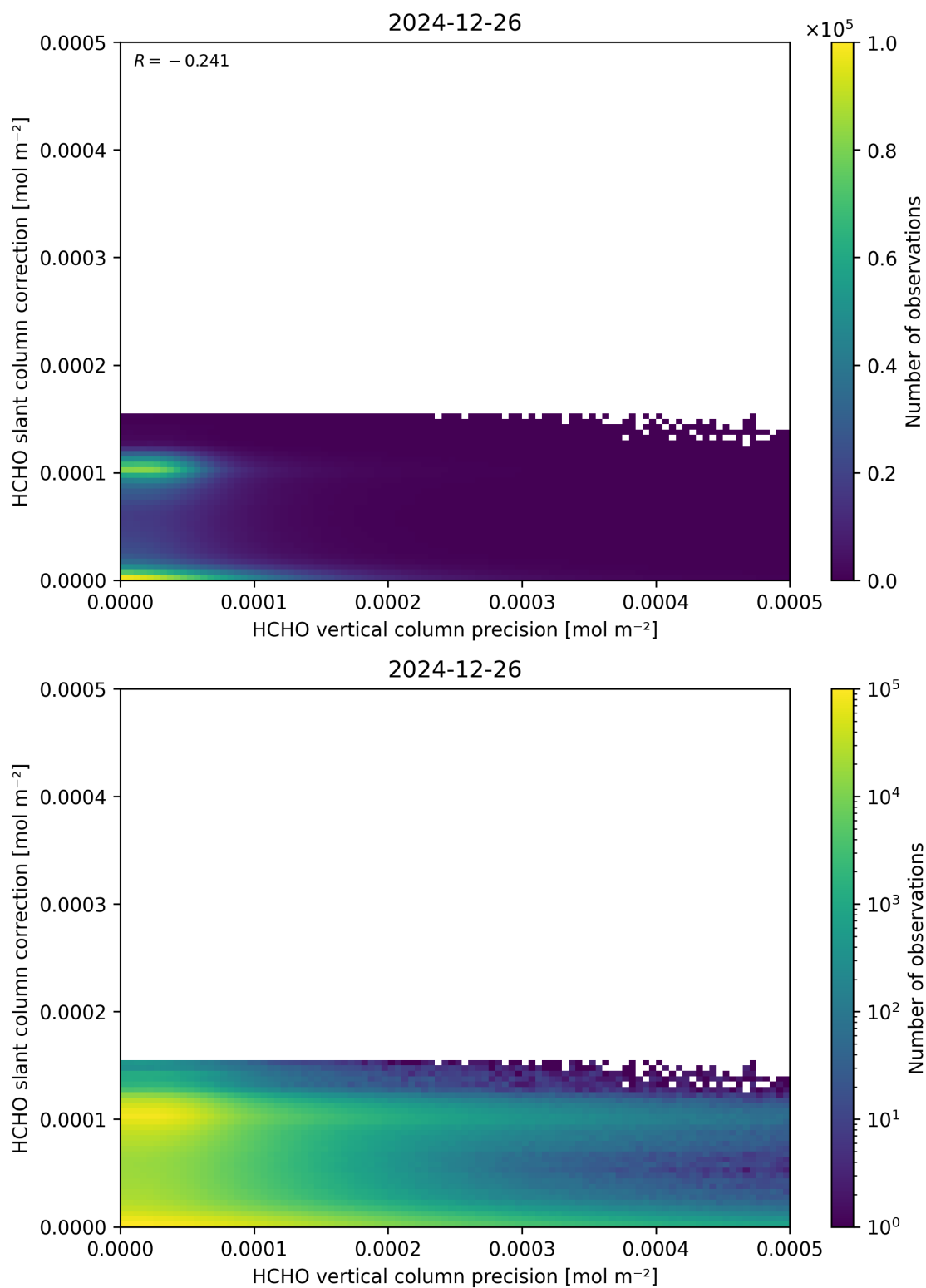
Figure 141: Scatter density plot of “HCHO vertical column precision” against “HCHO slant column correction” for 2024-12-25 to 2024-12-27.
