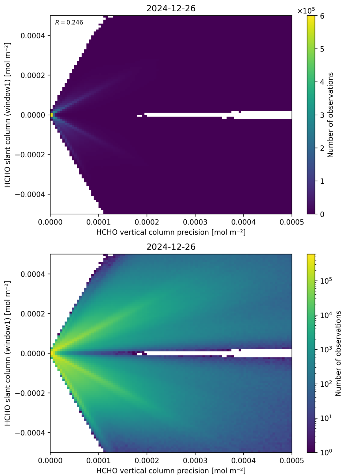
Figure 142: Scatter density plot of “HCHO vertical column precision” against “HCHO slant column (window1)” for 2024-12-25 to 2024-12-27.
