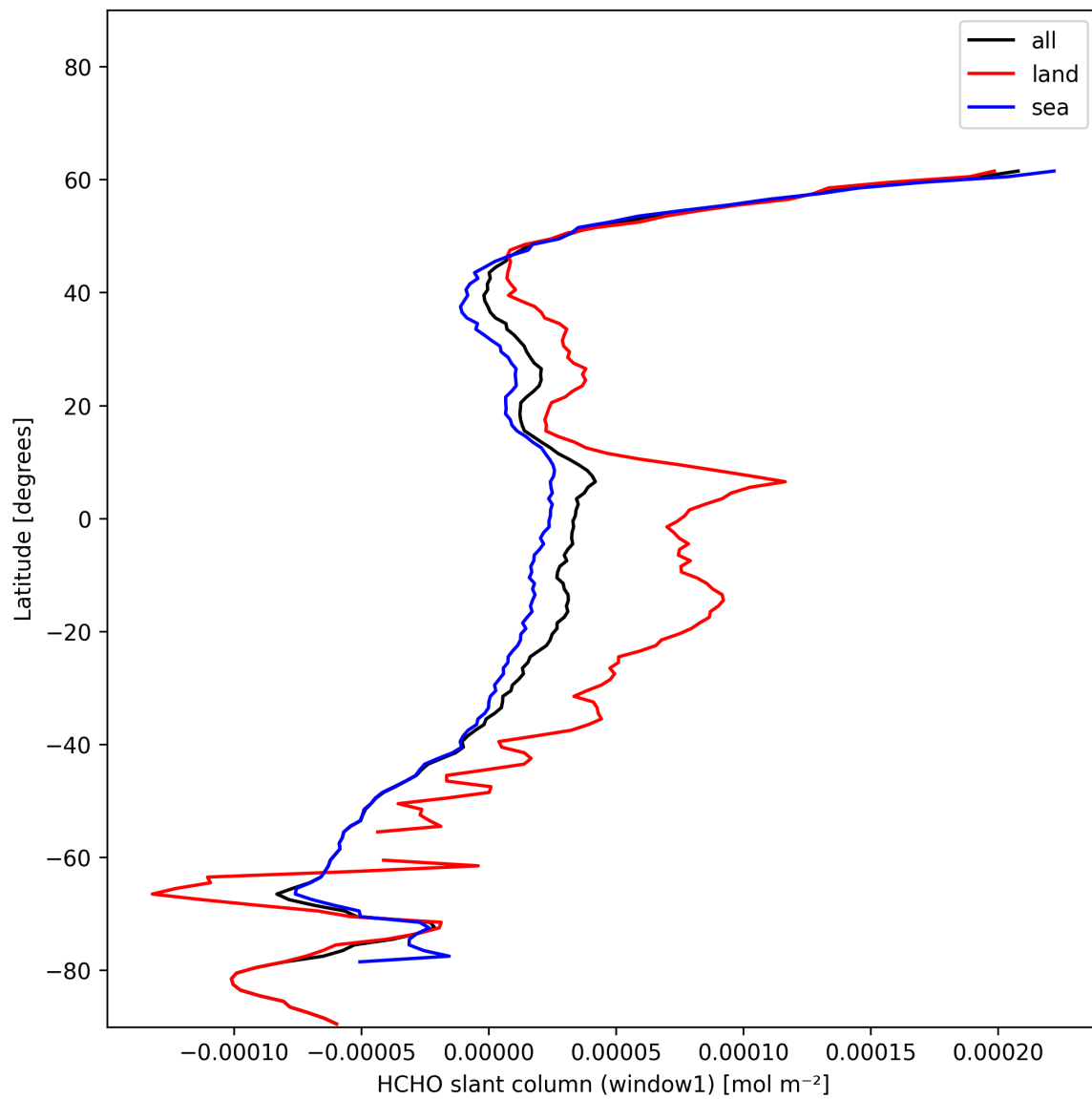
Figure 24: Zonal average of “HCHO slant column (window1)” for 2024-12-25 to 2024-12-27.
