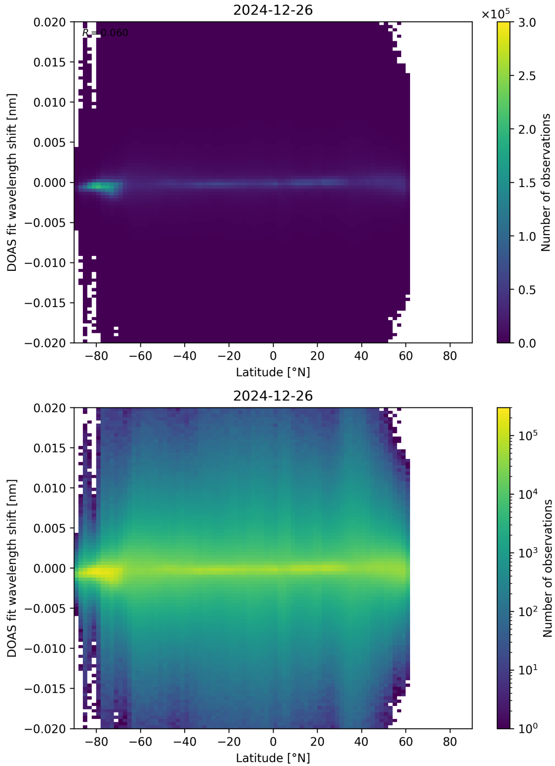
Figure 154: Scatter density plot of “Latitude” against “DOAS fit wavelength shift” for 2024-12-25 to 2024-12-27.
