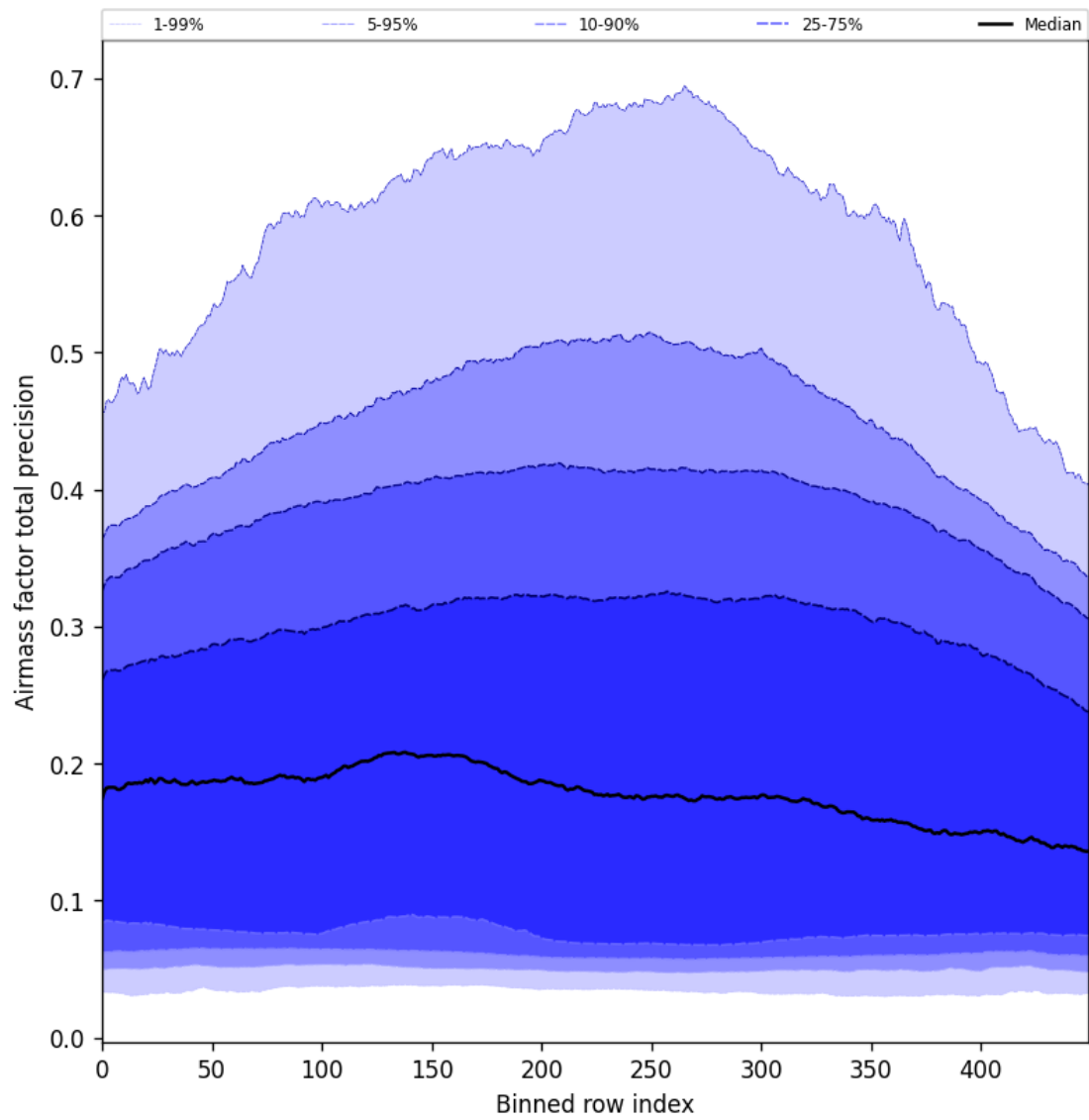
Figure 55: Along track statistics of “Airmass factor total precision” for 2024-12-25 to 2024-12-27
