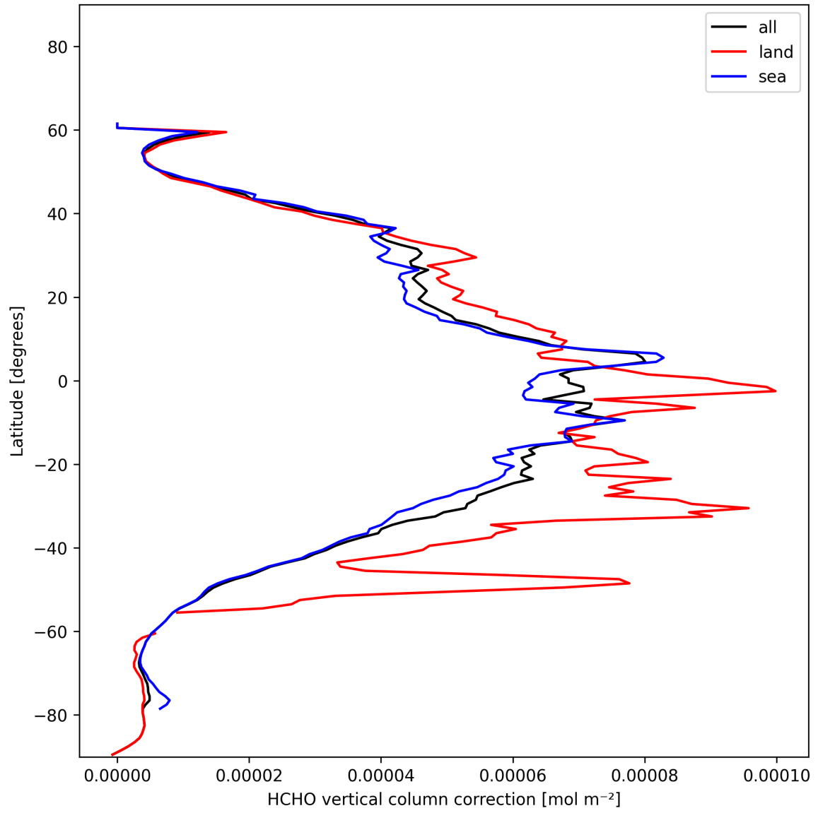
Figure 23: Zonal average of “HCHO vertical column correction” for 2024-12-25 to 2024-12-27.
