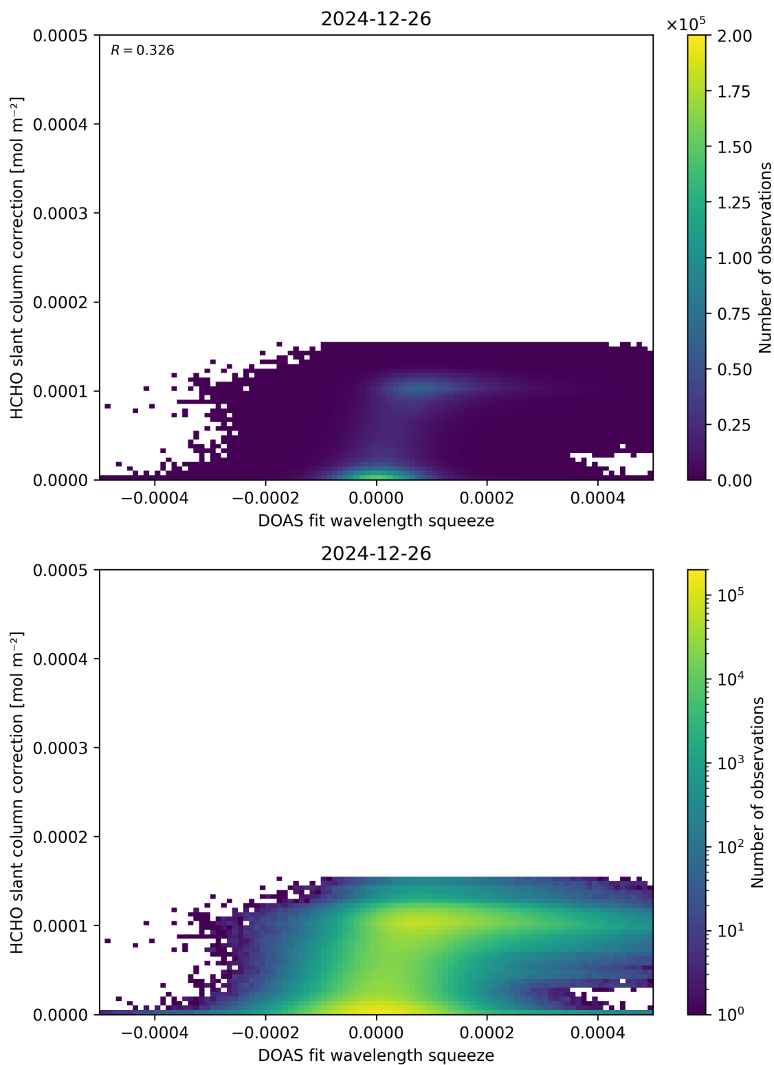
Figure 70: Scatter density plot of “DOAS fit wavelength squeeze” against “HCHO slant column correction” for 2024-12-25 to 2024-12-27.
