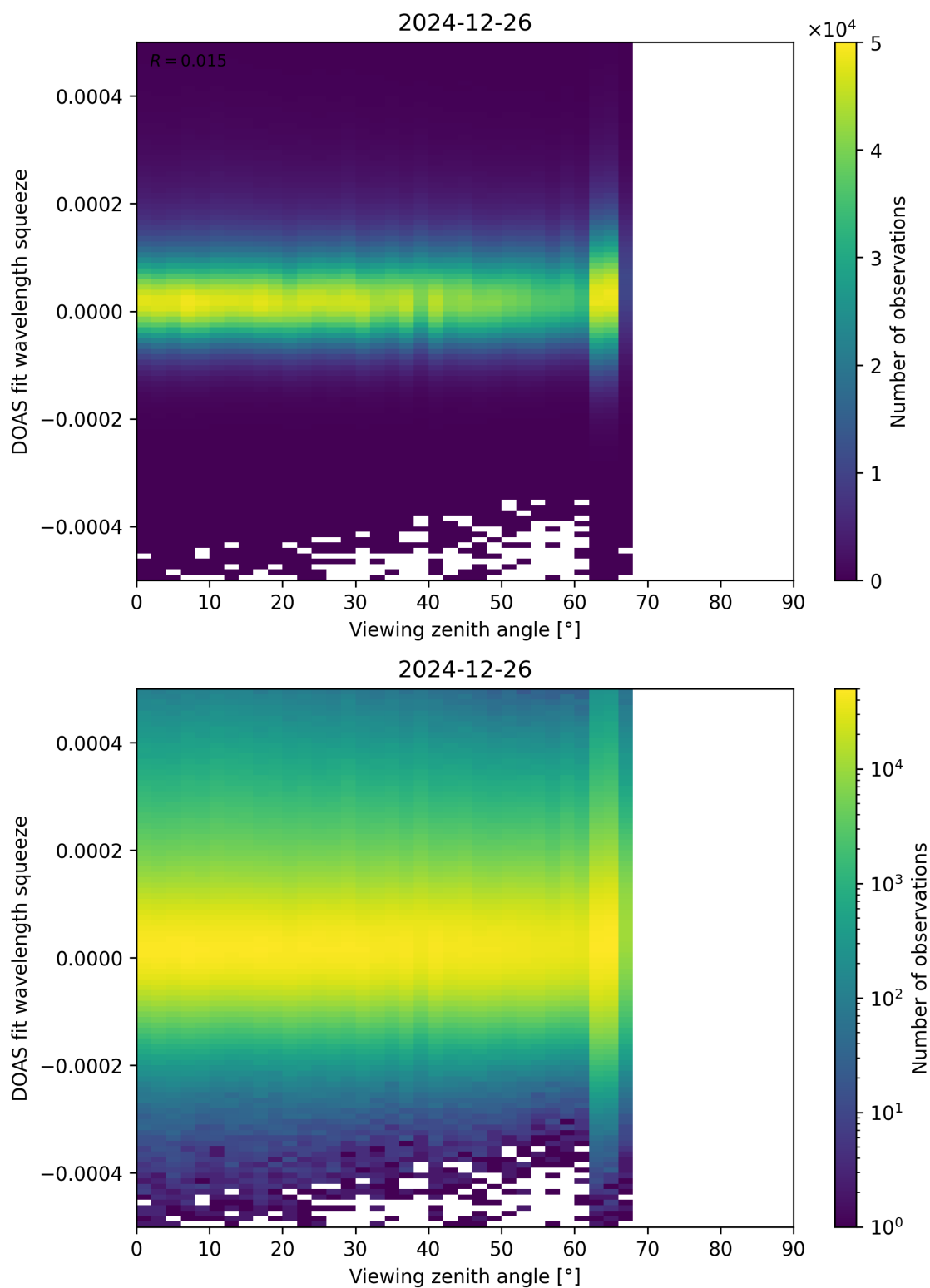
Figure 184: Scatter density plot of “Viewing zenith angle” against “DOAS fit wavelength squeeze” for 2024-12-25 to 2024-12-27.
