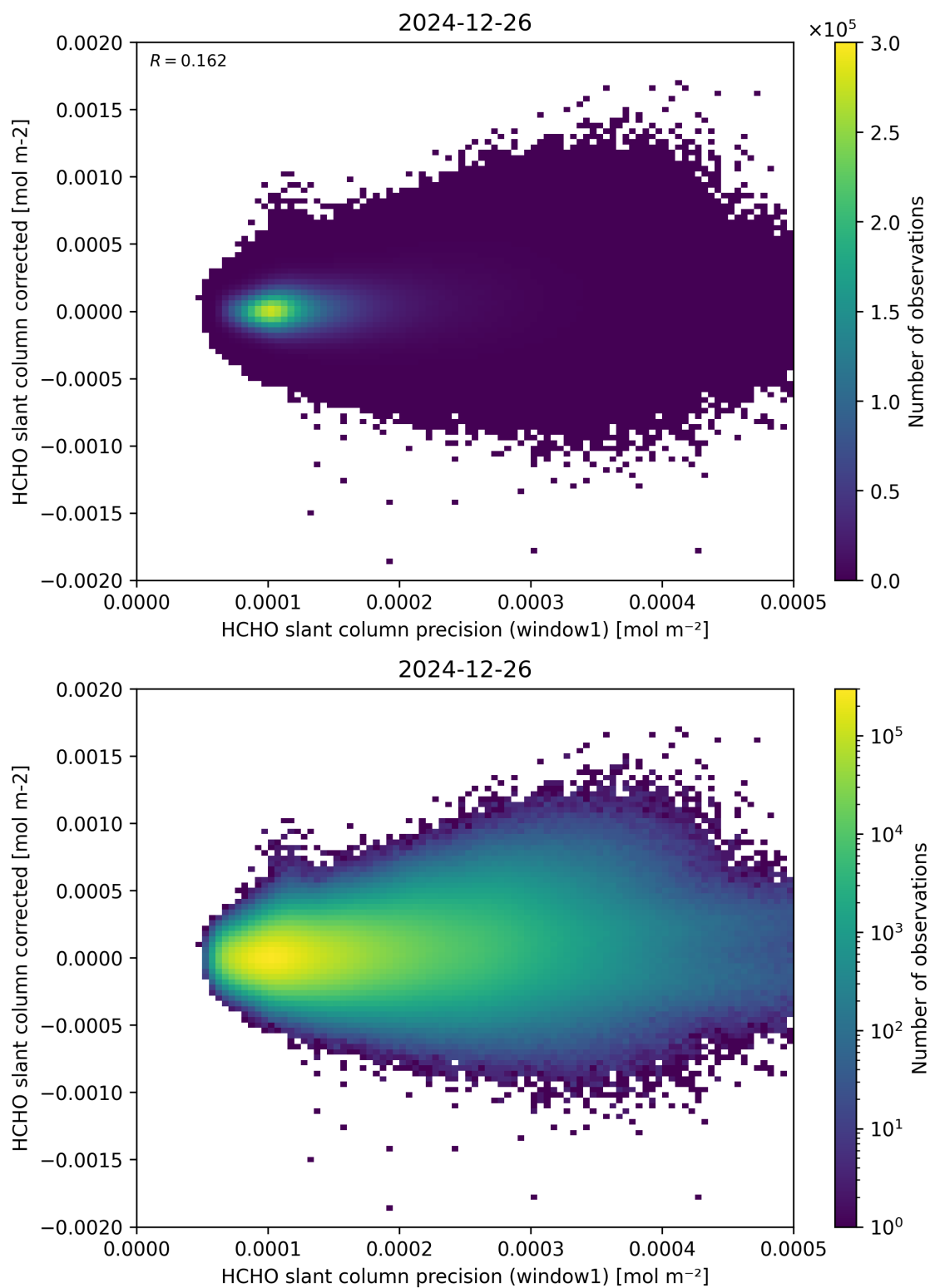
Figure 92: Scatter density plot of “HCHO slant column precision (window1)” against “HCHO slant column corrected” for 2024-12-25 to 2024-12-27.
