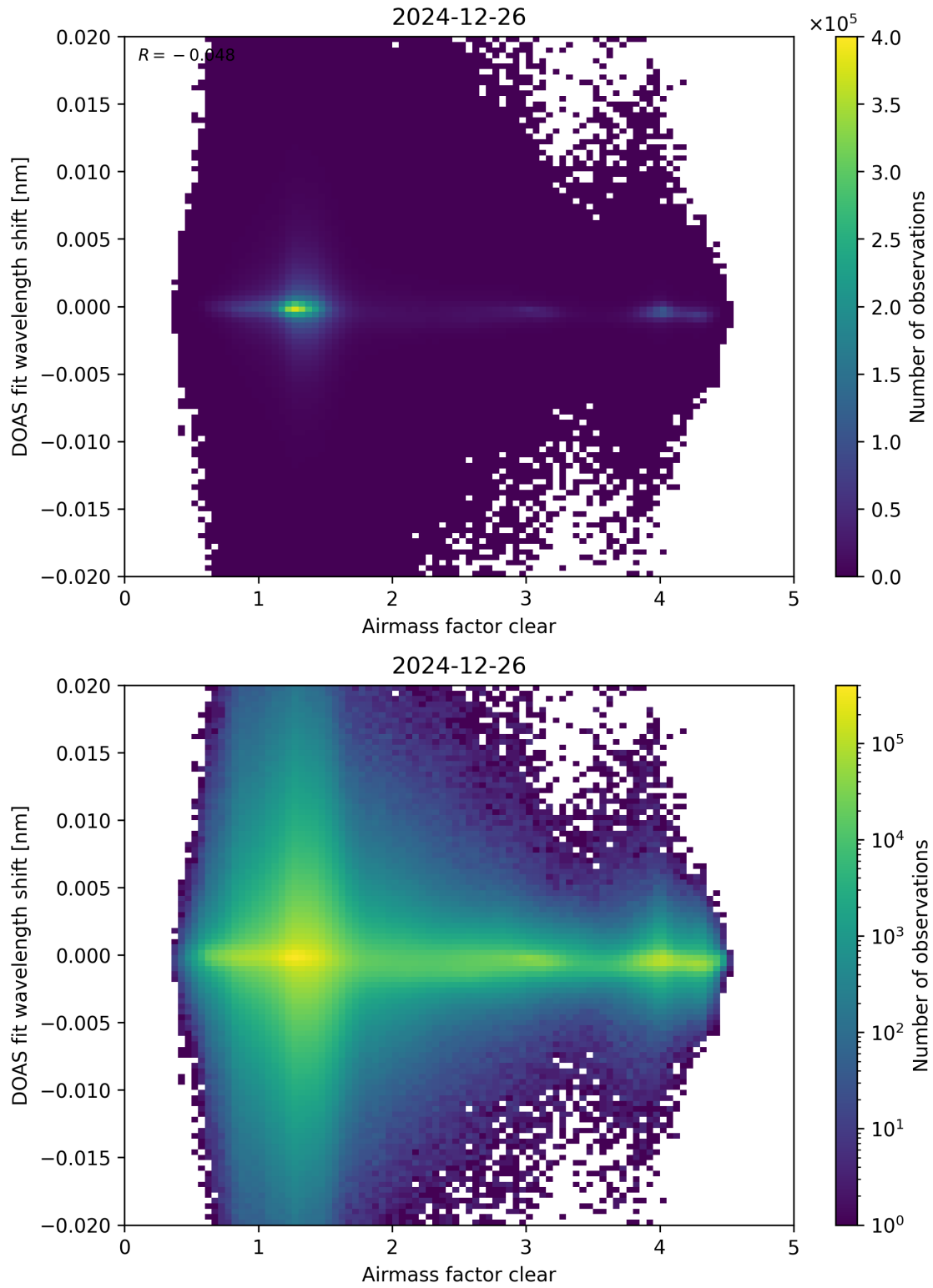
Figure 72: Scatter density plot of “Airmass factor clear” against “DOAS fit wavelength shift” for 2024-12-25 to 2024-12-27.
