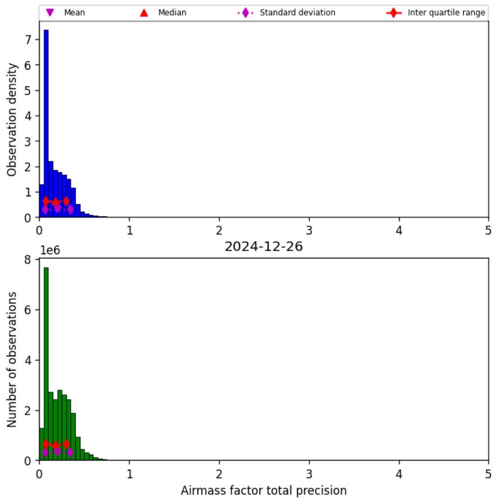
Figure 41: Histogram of “Airmass factor total precision” for 2024-12-25 to 2024-12-27
