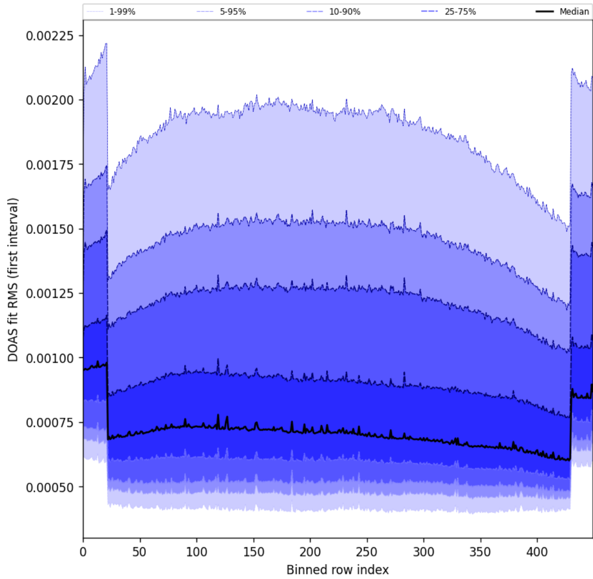
Figure 60: Along track statistics of “DOAS fit RMS (first interval)” for 2024-12-25 to 2024-12-27
