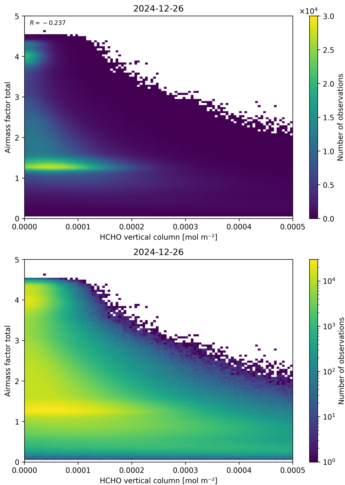
Figure 131: Scatter density plot of “HCHO vertical column” against “Airmass factor total” for 2024-12-25 to 2024-12-27.
