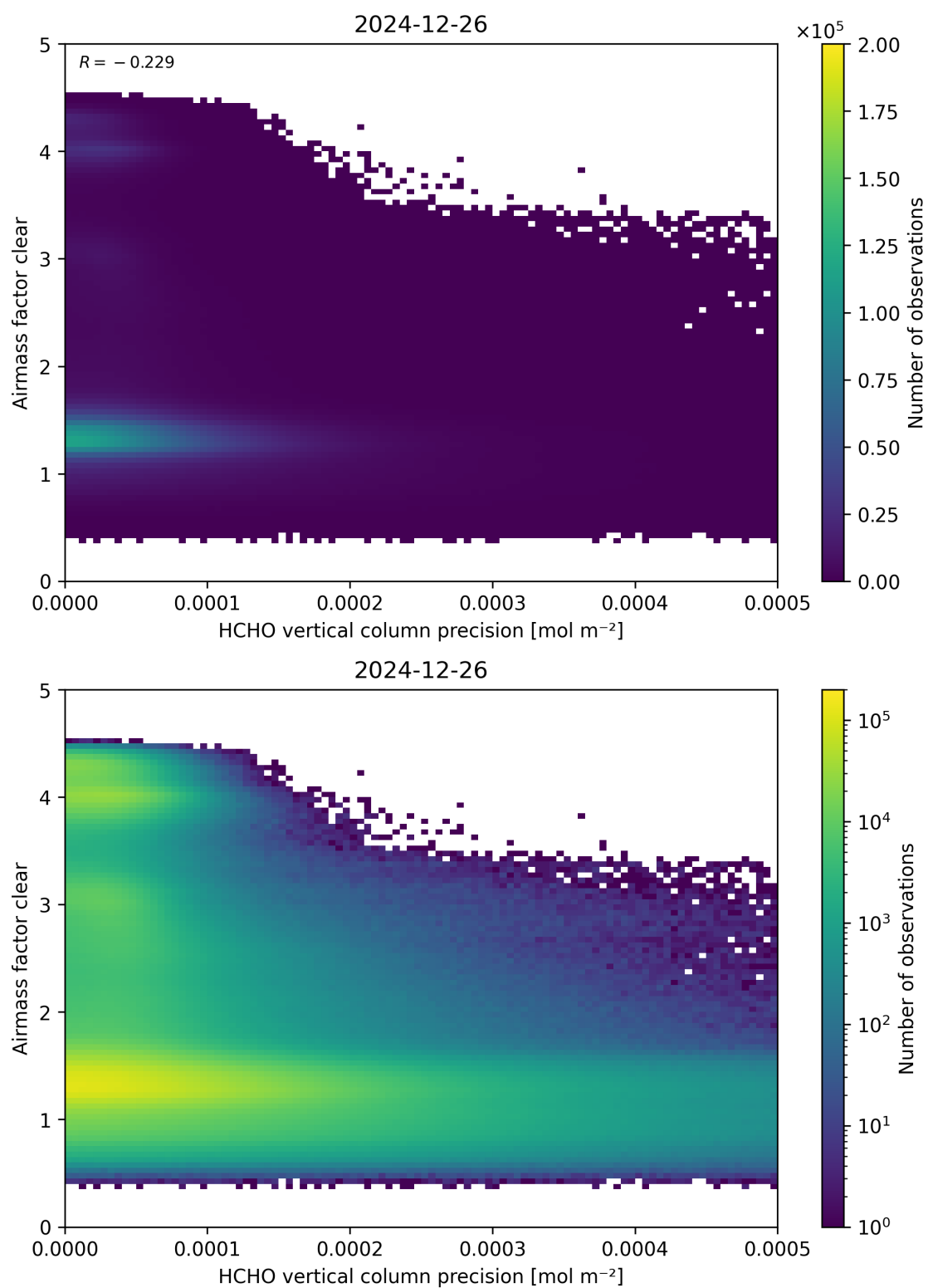
Figure 139: Scatter density plot of “HCHO vertical column precision” against “Airmass factor clear” for 2024-12-25 to 2024-12-27.
