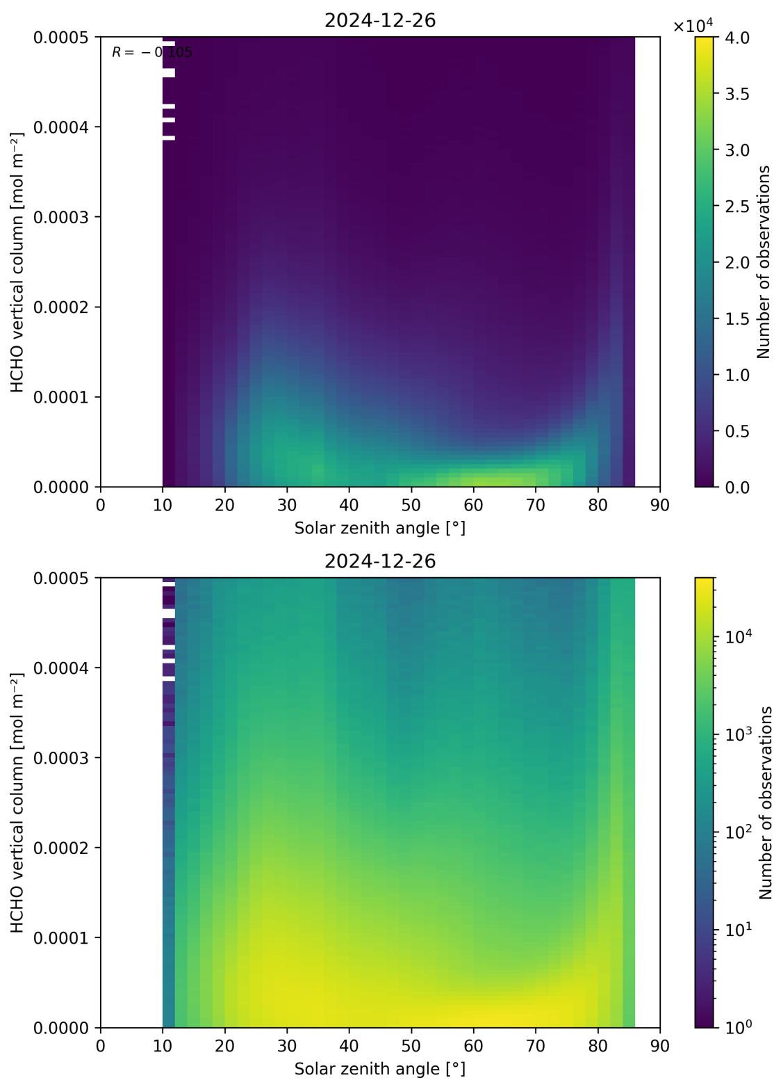
Figure 177: Scatter density plot of “Solar zenith angle” against “HCHO vertical column” for 2024-12-25 to 2024-12-27.
