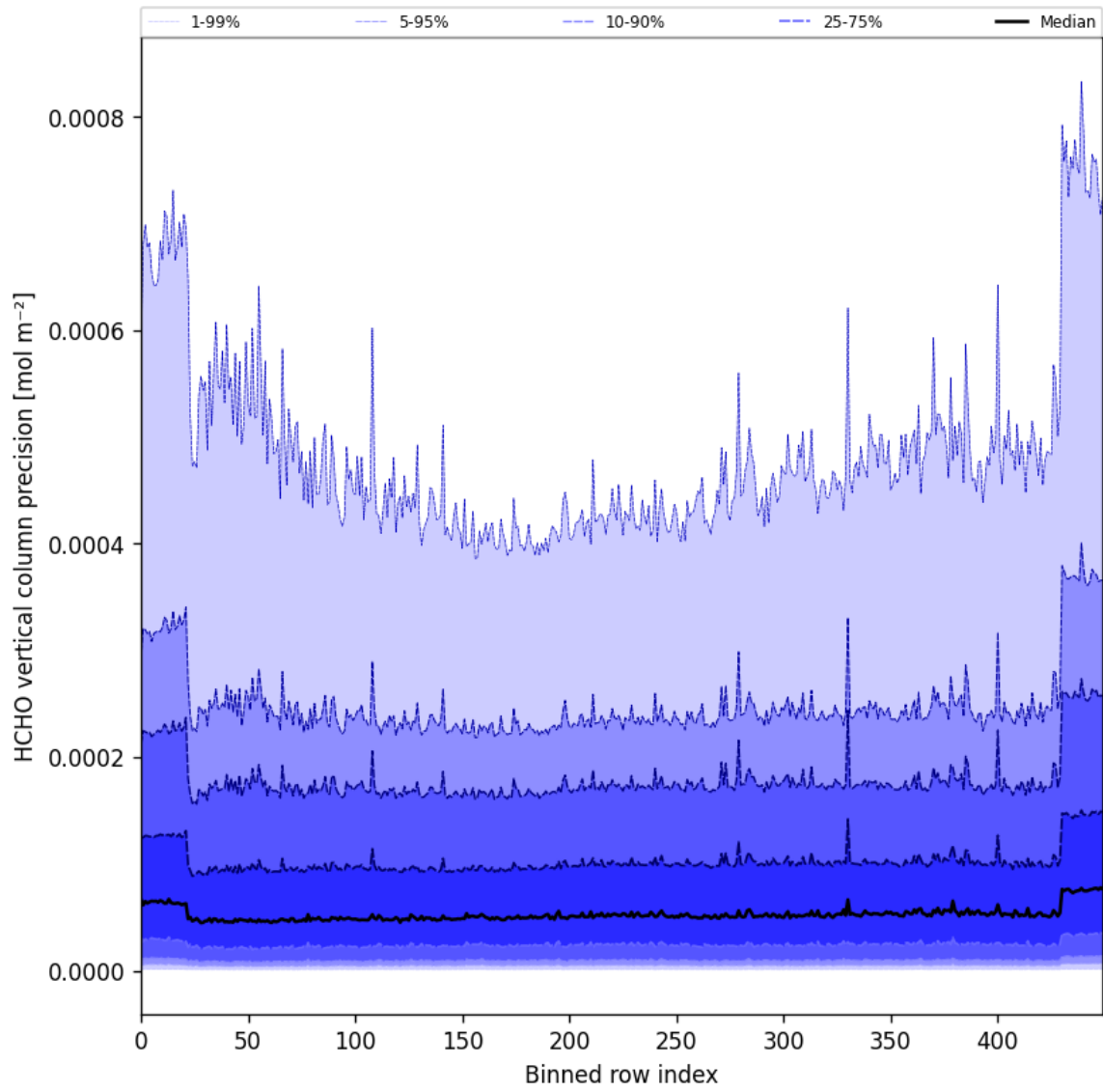
Figure 50: Along track statistics of “HCHO vertical column precision” for 2024-12-25 to 2024-12-27
