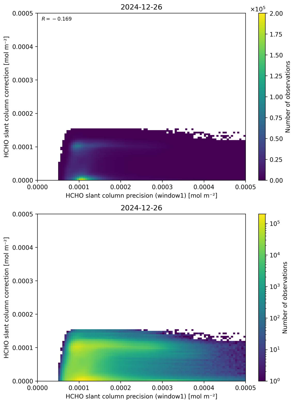
Figure 93: Scatter density plot of “HCHO slant column precision (window1)” against “HCHO slant column correction” for 2024-12-25 to 2024-12-27.
