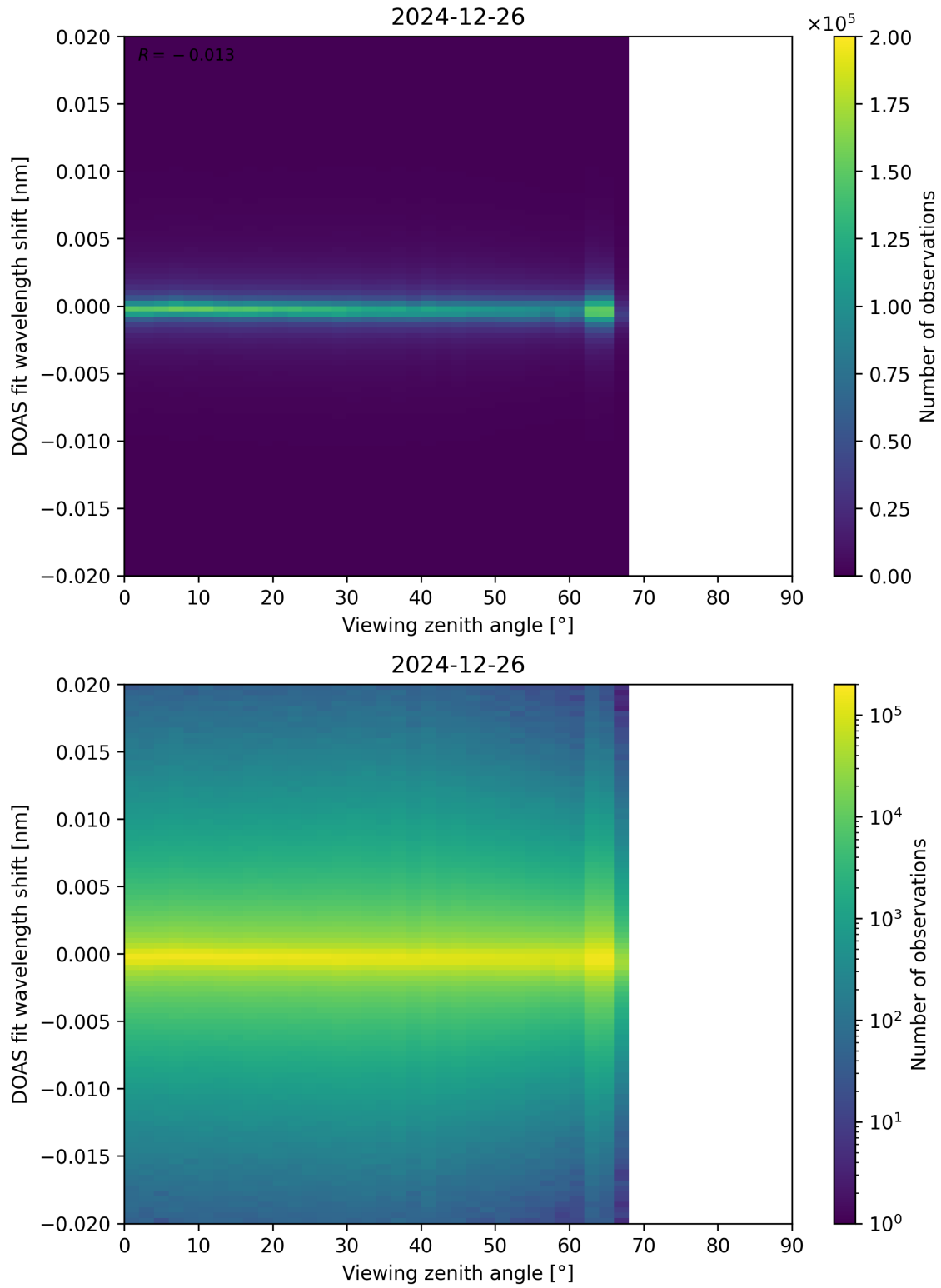
Figure 183: Scatter density plot of “Viewing zenith angle” against “DOAS fit wavelength shift” for 2024-12-25 to 2024-12-27.
