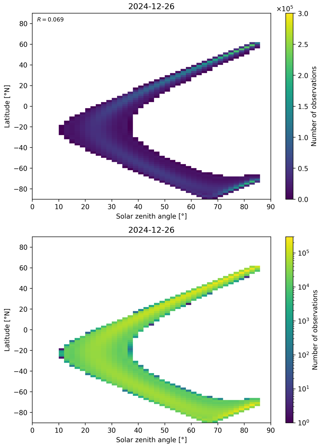
Figure 181: Scatter density plot of “Solar zenith angle” against “Latitude” for 2024-12-25 to 2024-12-27.
