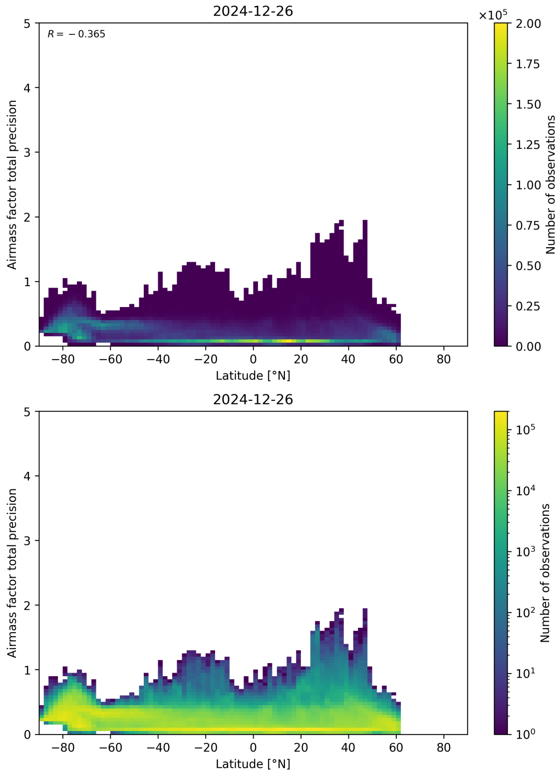
Figure 162: Scatter density plot of “Latitude” against “Airmass factor total precision” for 2024-12-25 to 2024-12-27.
