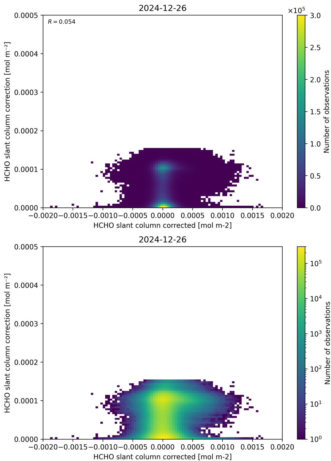
Figure 77: Scatter density plot of “HCHO slant column corrected” against “HCHO slant column correction” for 2024-12-25 to 2024-12-27.
