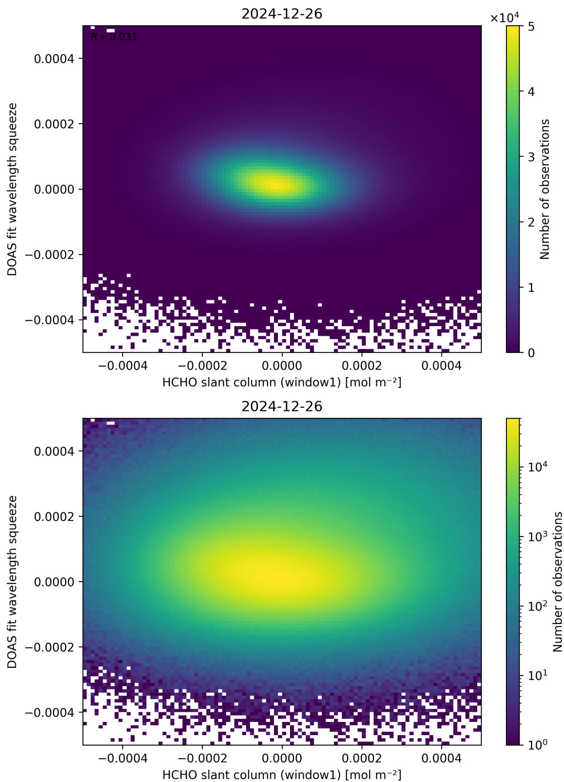
Figure 80: Scatter density plot of “HCHO slant column (window1)” against “DOAS fit wavelength squeeze” for 2024-12-25 to 2024-12-27.
