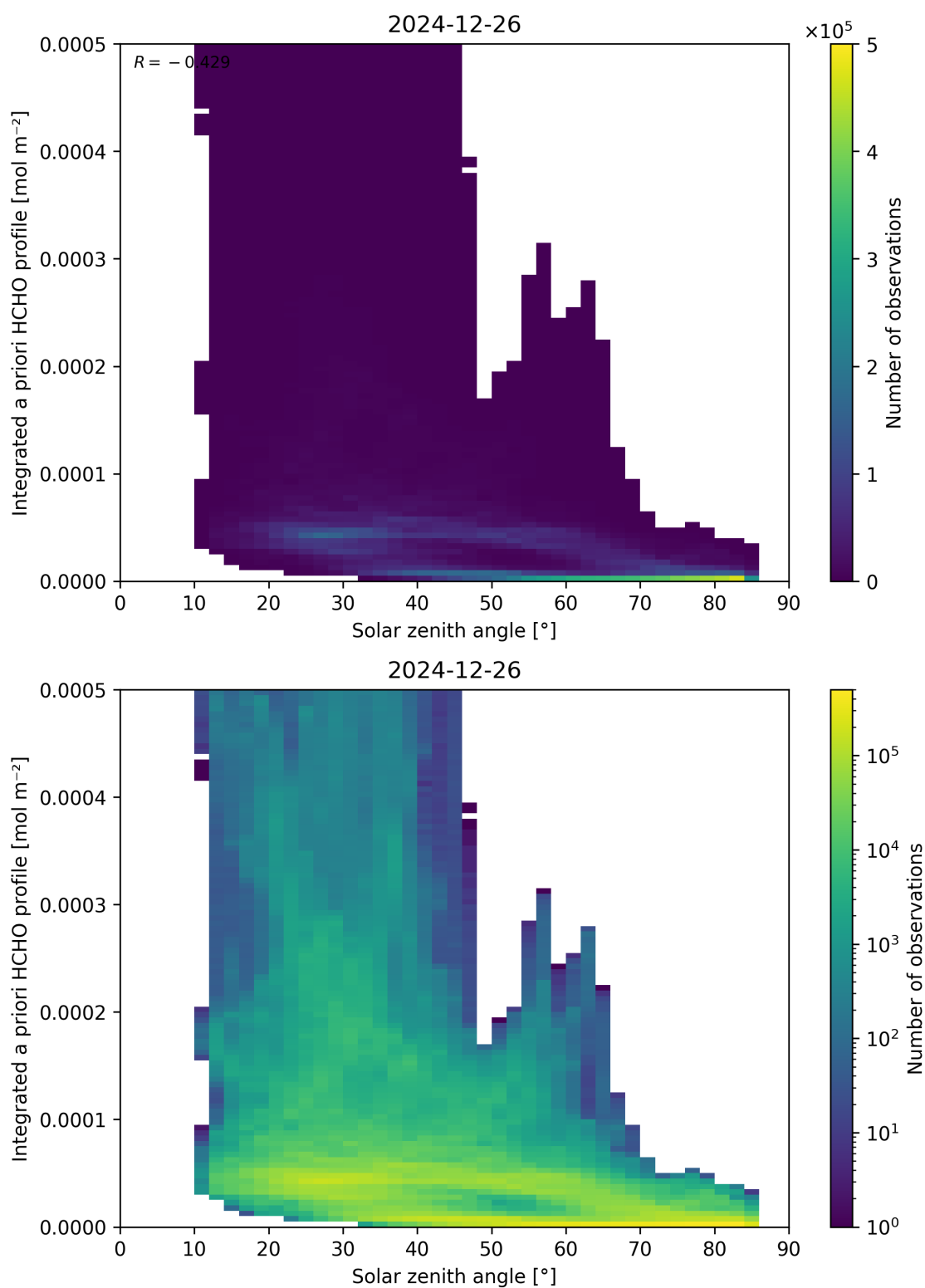
Figure 180: Scatter density plot of “Solar zenith angle” against “Integrated a priori HCHO profile” for 2024-12-25 to 2024-12-27.
