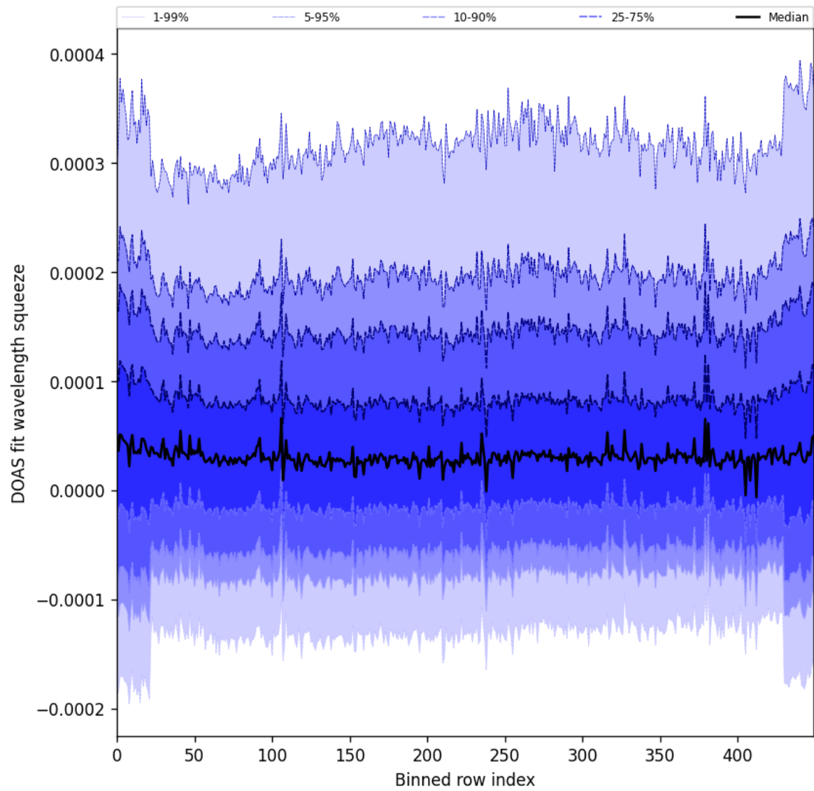
Figure 59: Along track statistics of “DOAS fit wavelength squeeze” for 2024-12-25 to 2024-12-27
