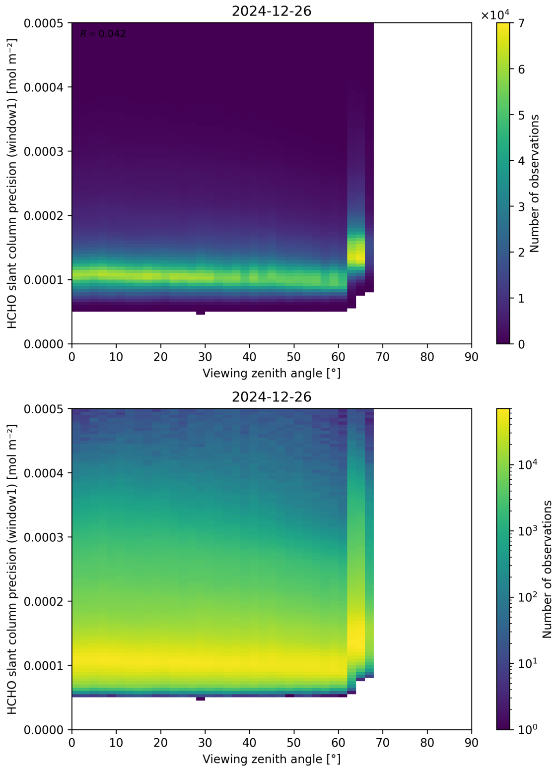
Figure 189: Scatter density plot of “Viewing zenith angle” against “HCHO slant column precision (window1)” for 2024-12-25 to 2024-12-27.
