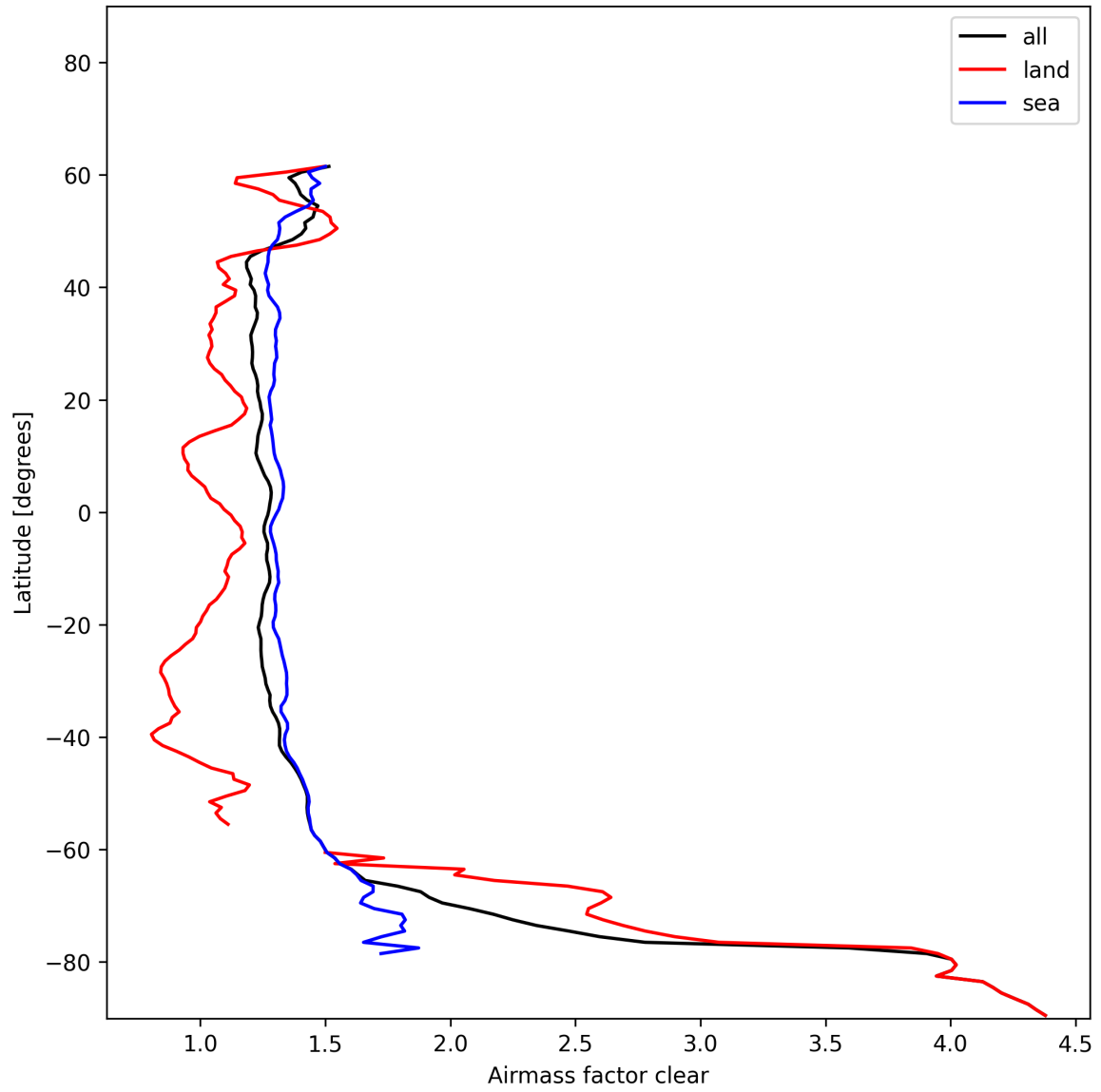
Figure 28: Zonal average of “Airmass factor clear” for 2024-12-25 to 2024-12-27.
