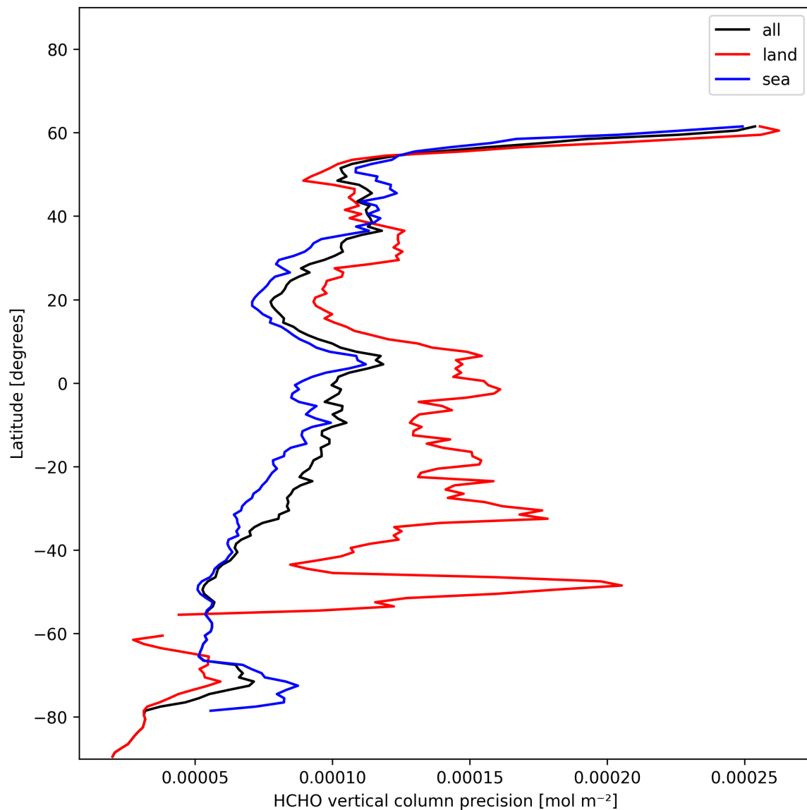
Figure 22: Zonal average of “HCHO vertical column precision” for 2024-12-25 to 2024-12-27.
