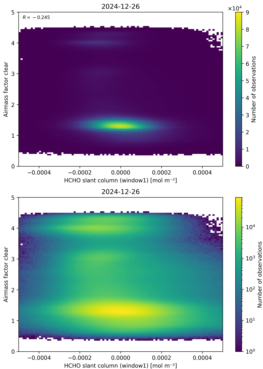
Figure 81: Scatter density plot of “HCHO slant column (window1)” against “Airmass factor clear” for 2024-12-25 to 2024-12-27.
