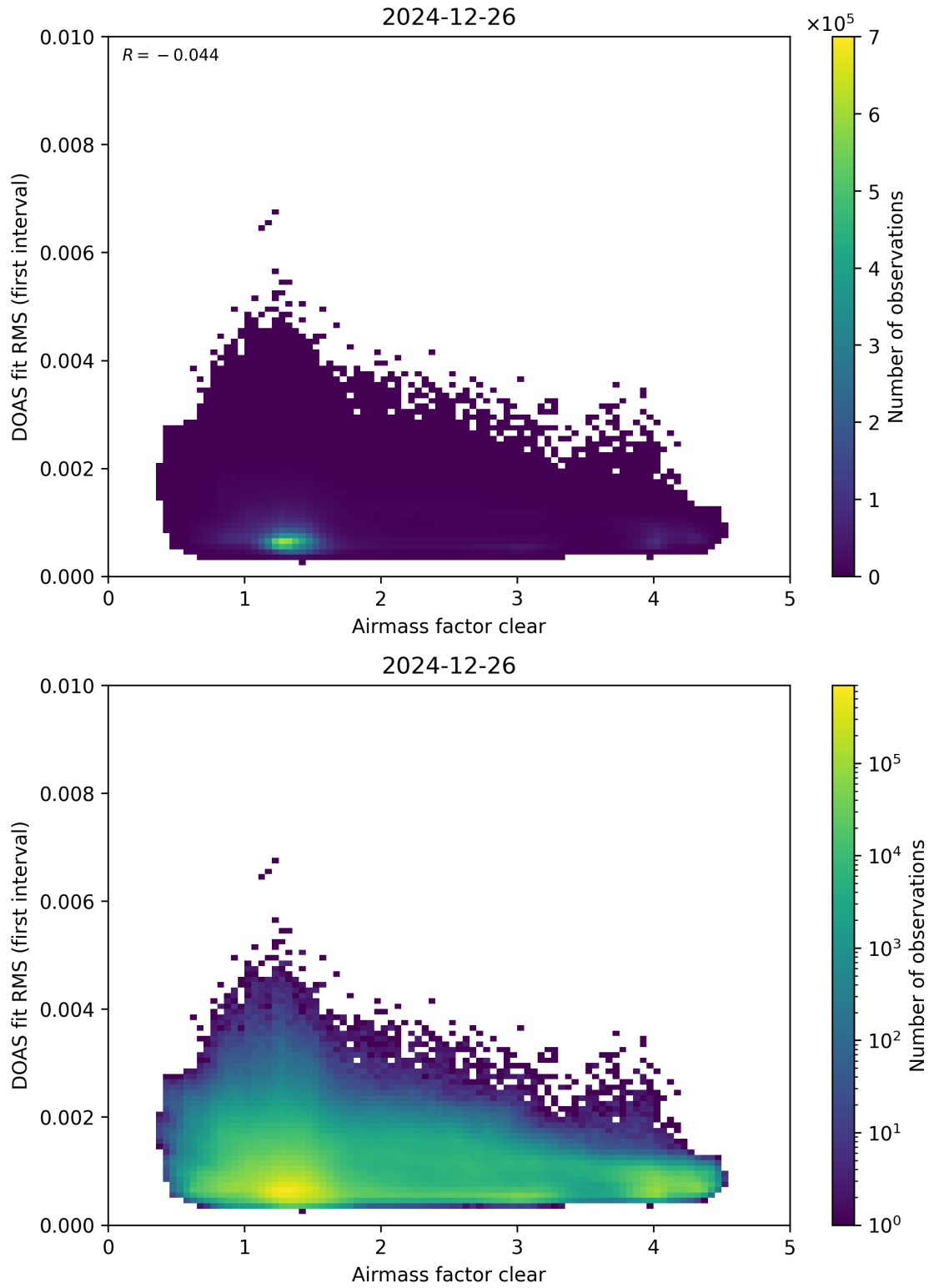
Figure 71: Scatter density plot of “Airmass factor clear” against “DOAS fit RMS (first interval)” for 2024-12-25 to 2024-12-27.
