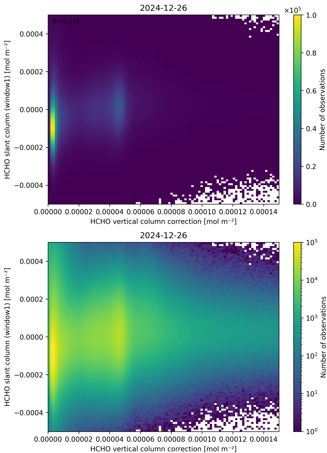
Figure 118: Scatter density plot of “HCHO vertical column correction” against “HCHO slant column (window1)” for 2024-12-25 to 2024-12-27.
