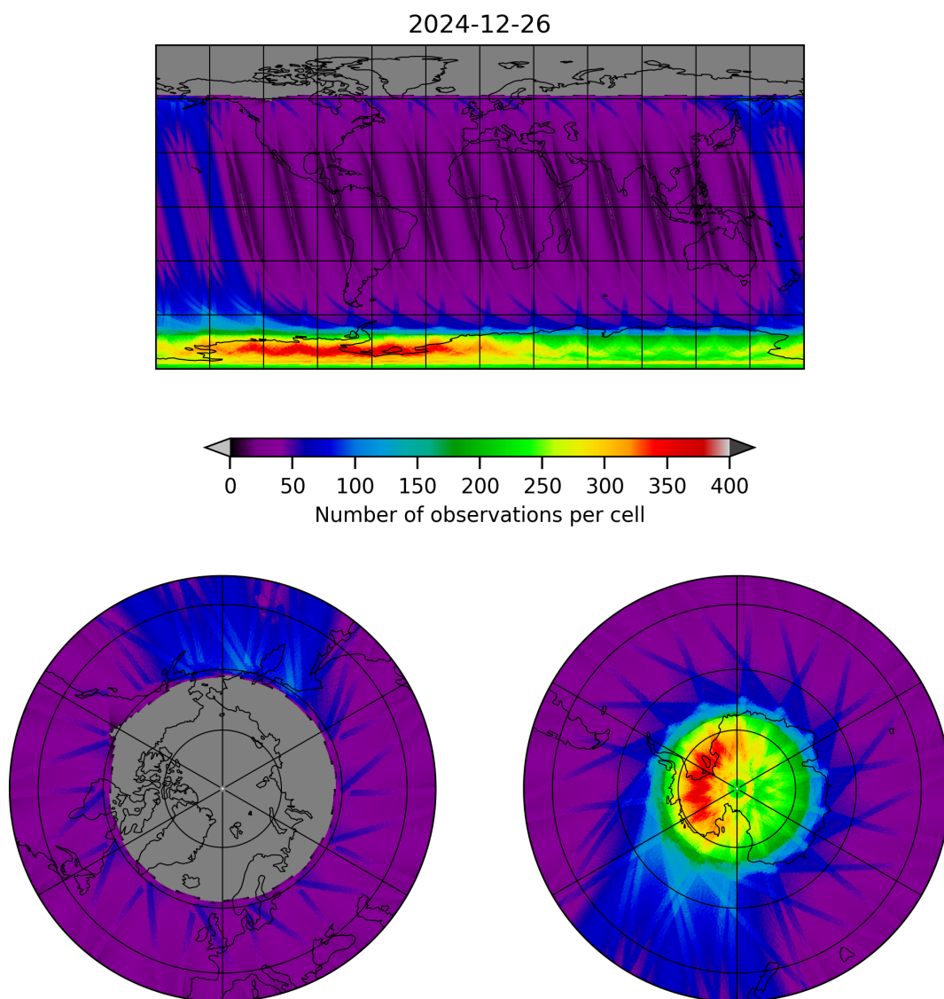
Figure 19: Map of the number of observations for 2024-12-25 to 2024-12-27
