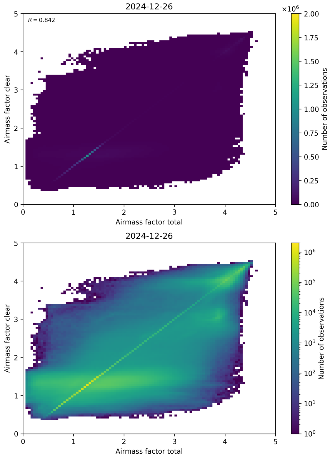
Figure 100: Scatter density plot of “Airmass factor total” against “Airmass factor clear” for 2024-12-25 to 2024-12-27.
