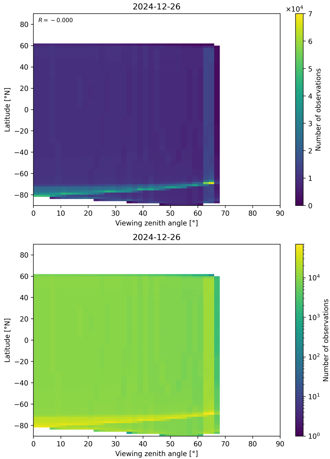
Figure 196: Scatter density plot of “Viewing zenith angle” against “Latitude” for 2024-12-25 to 2024-12-27.
