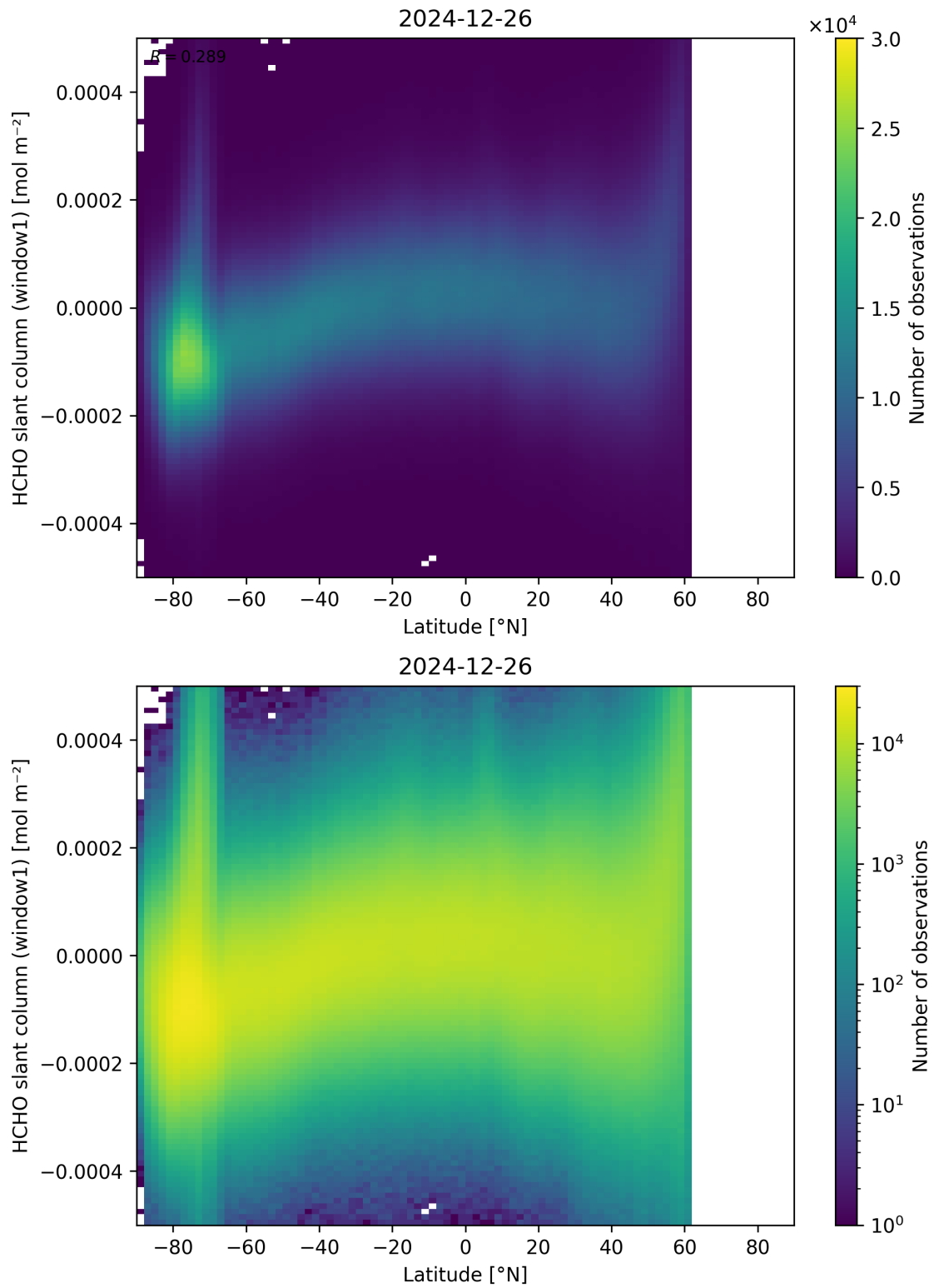
Figure 159: Scatter density plot of “Latitude” against “HCHO slant column (window1)” for 2024-12-25 to 2024-12-27.
