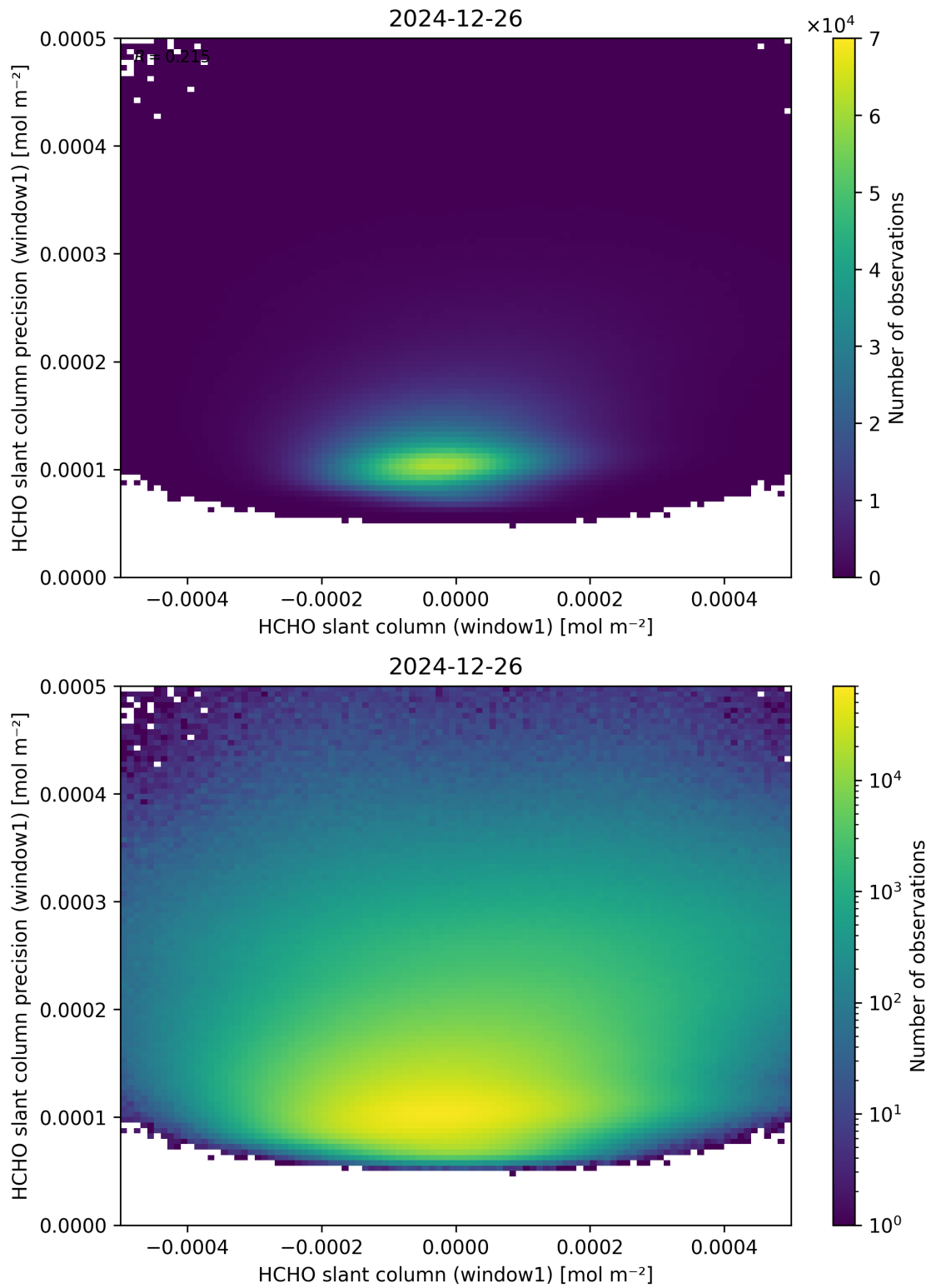
Figure 84: Scatter density plot of “HCHO slant column (window1)” against “HCHO slant column precision (window1)” for 2024-12-25 to 2024-12-27.
