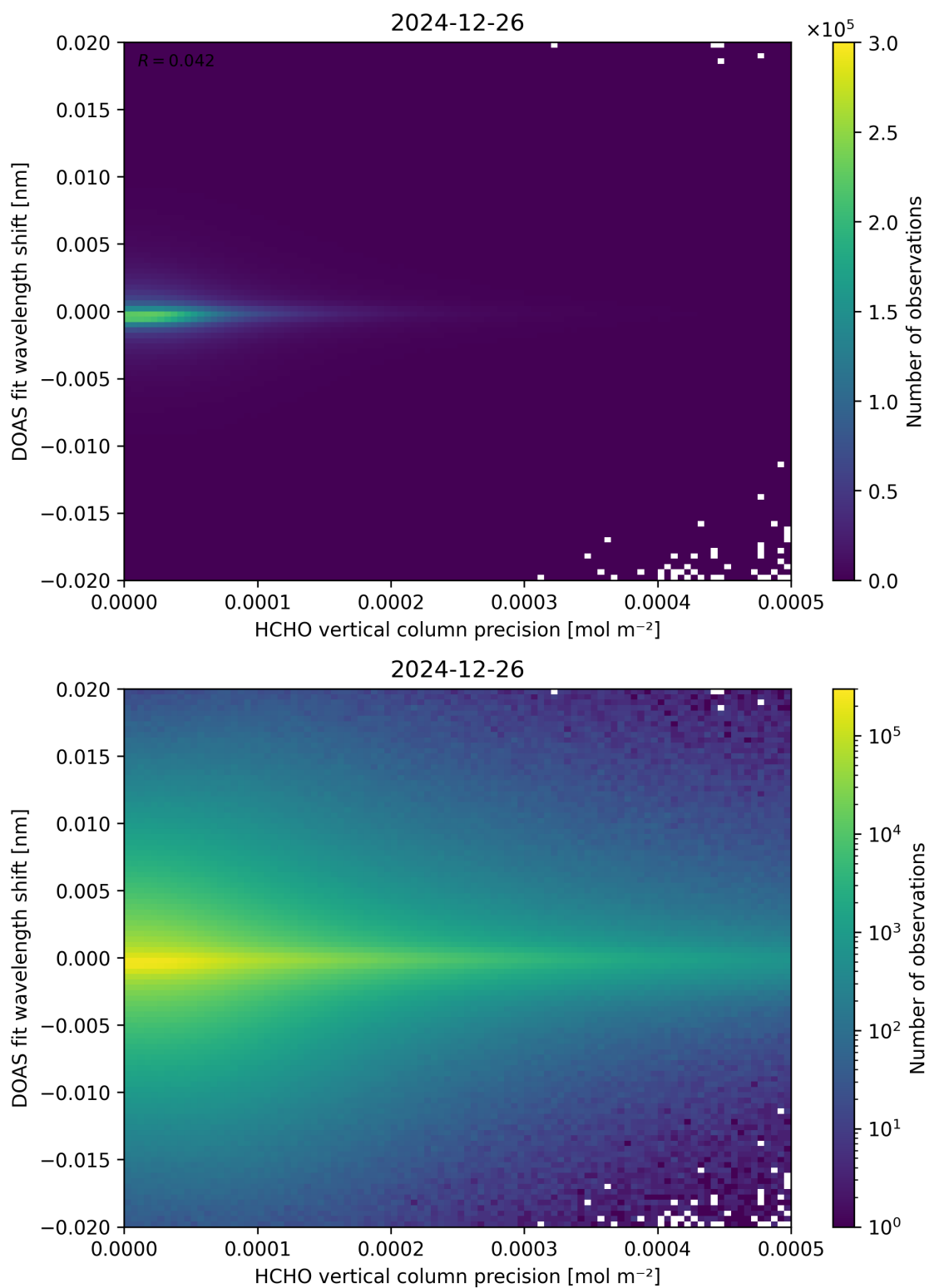
Figure 137: Scatter density plot of “HCHO vertical column precision” against “DOAS fit wavelength shift” for 2024-12-25 to 2024-12-27.
