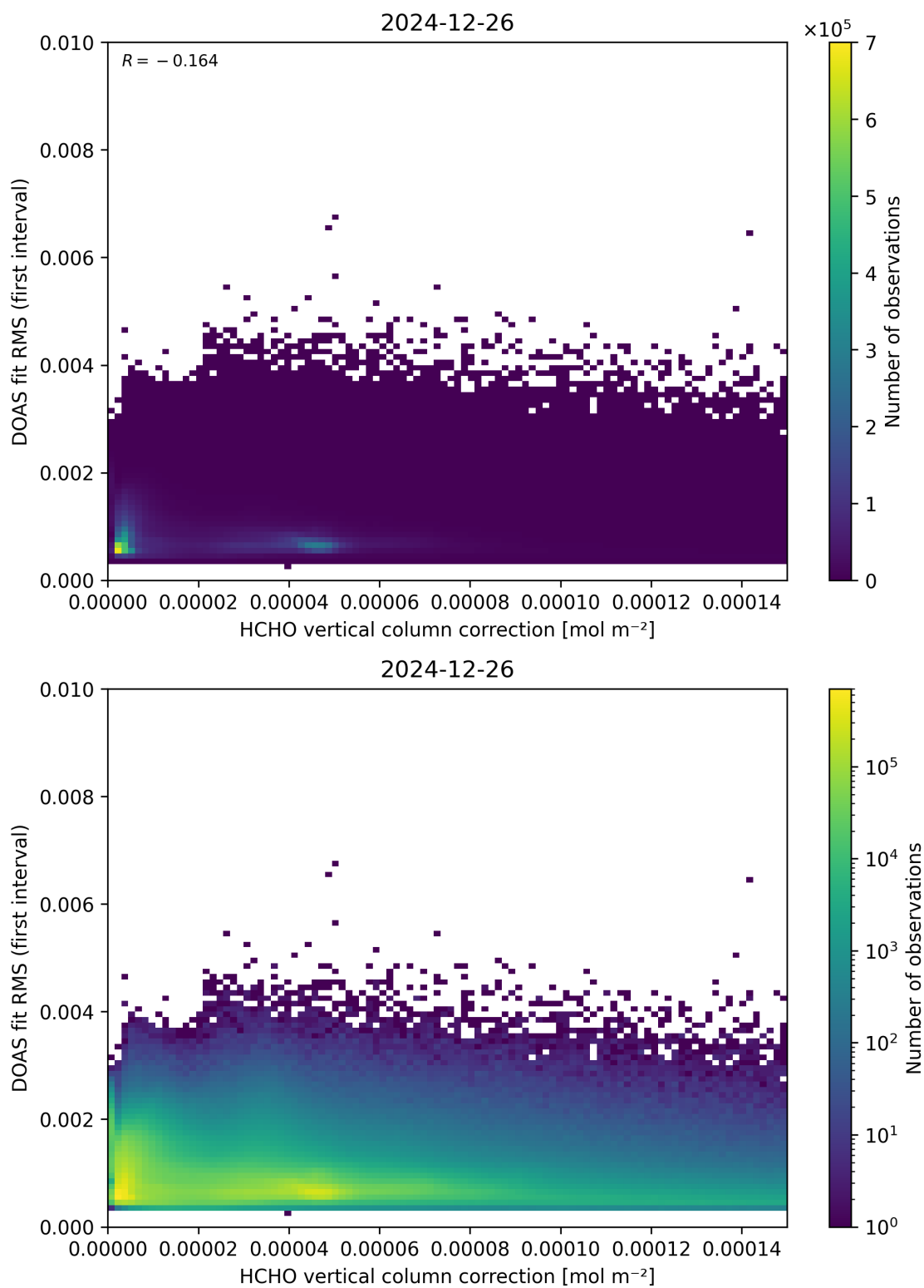
Figure 112: Scatter density plot of “HCHO vertical column correction” against “DOAS fit RMS (first interval)” for 2024-12-25 to 2024-12-27.
