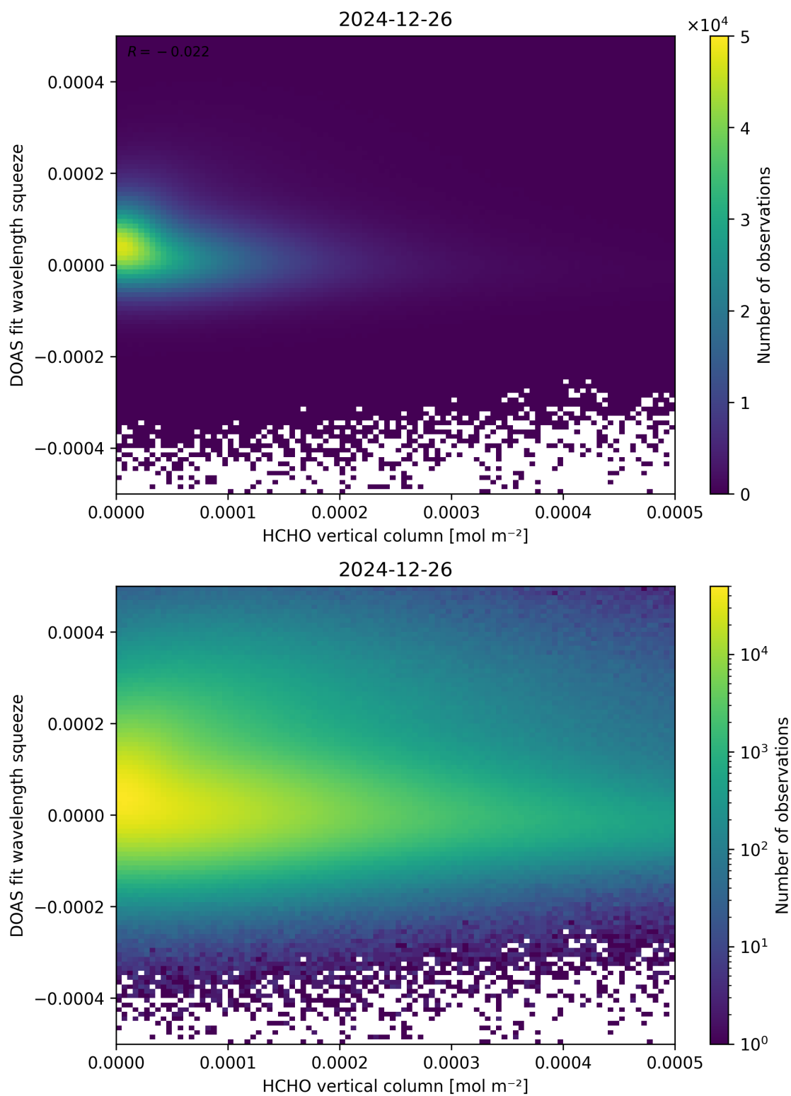
Figure 125: Scatter density plot of “HCHO vertical column” against “DOAS fit wavelength squeeze” for 2024-12-25 to 2024-12-27.
