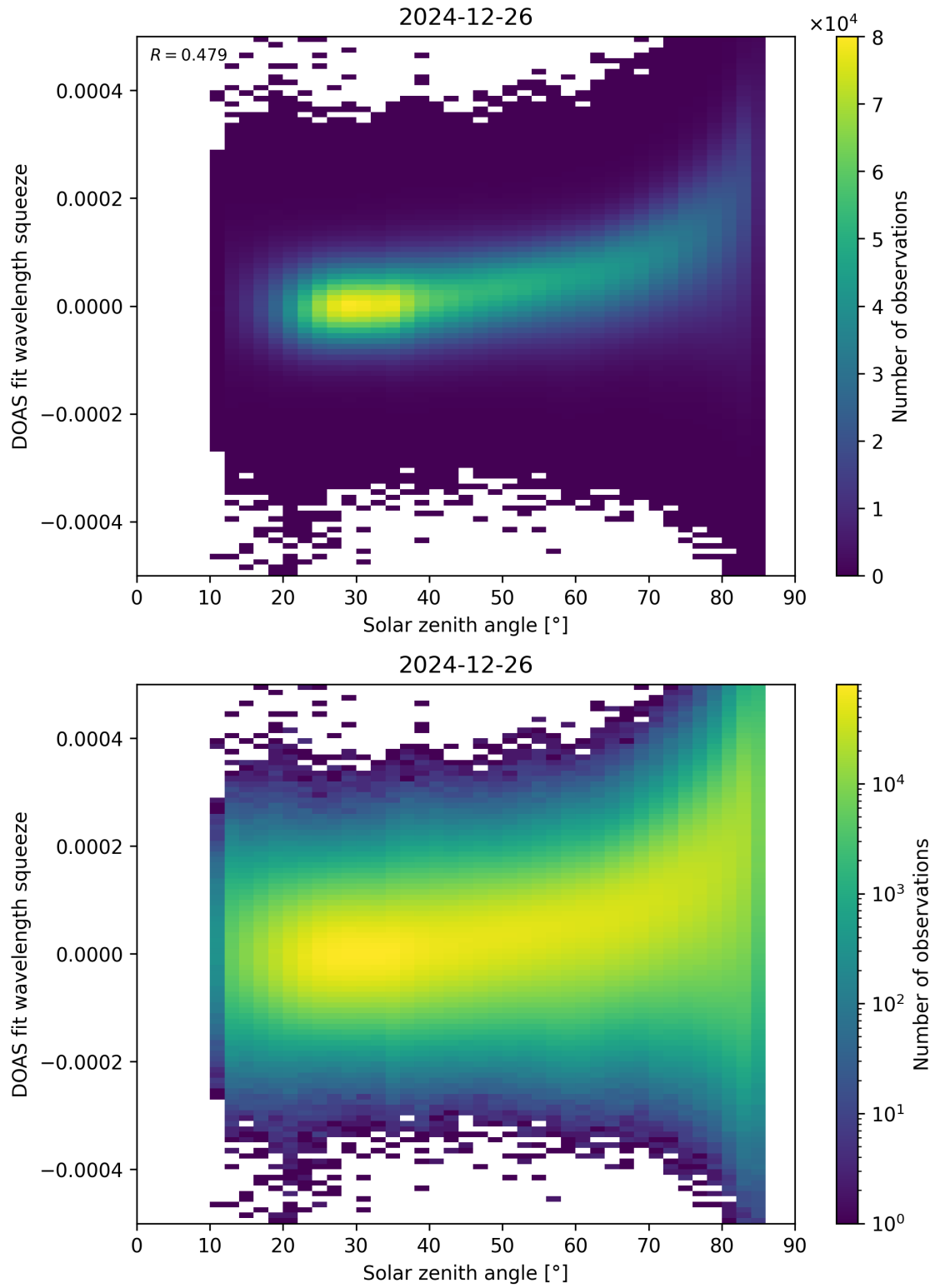
Figure 169: Scatter density plot of “Solar zenith angle” against “DOAS fit wavelength squeeze” for 2024-12-25 to 2024-12-27.
