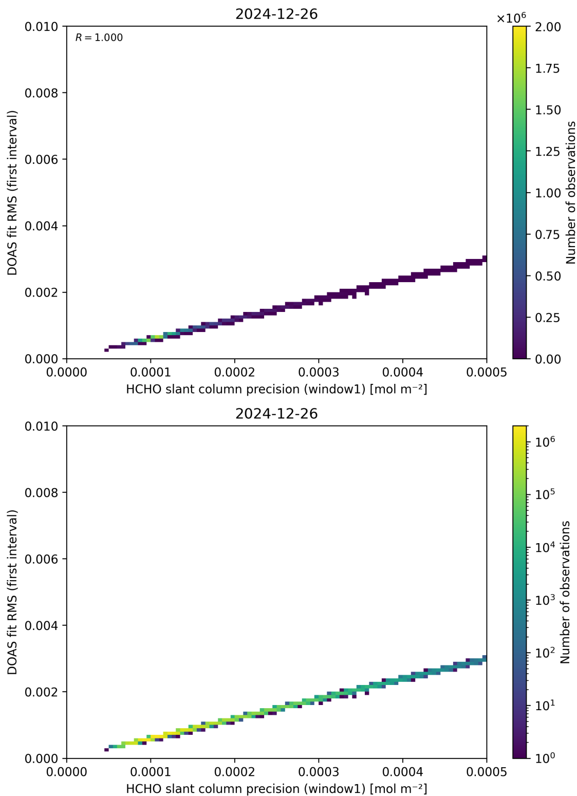
Figure 88: Scatter density plot of “HCHO slant column precision (window1)” against “DOAS fit RMS (first interval)” for 2024-12-25 to 2024-12-27.
