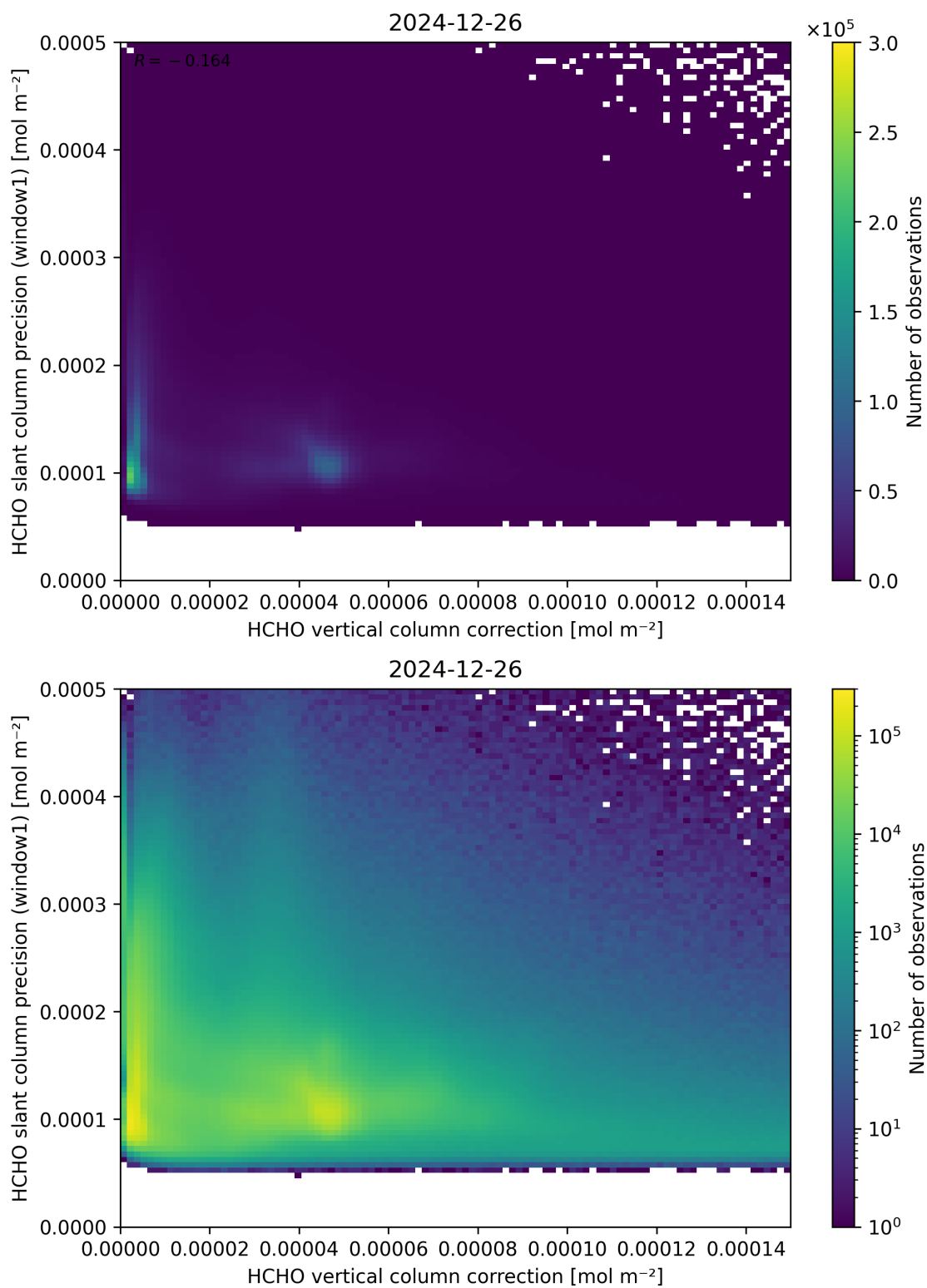
Figure 119: Scatter density plot of “HCHO vertical column correction” against “HCHO slant column precision (window1)” for 2024-12-25 to 2024-12-27.
