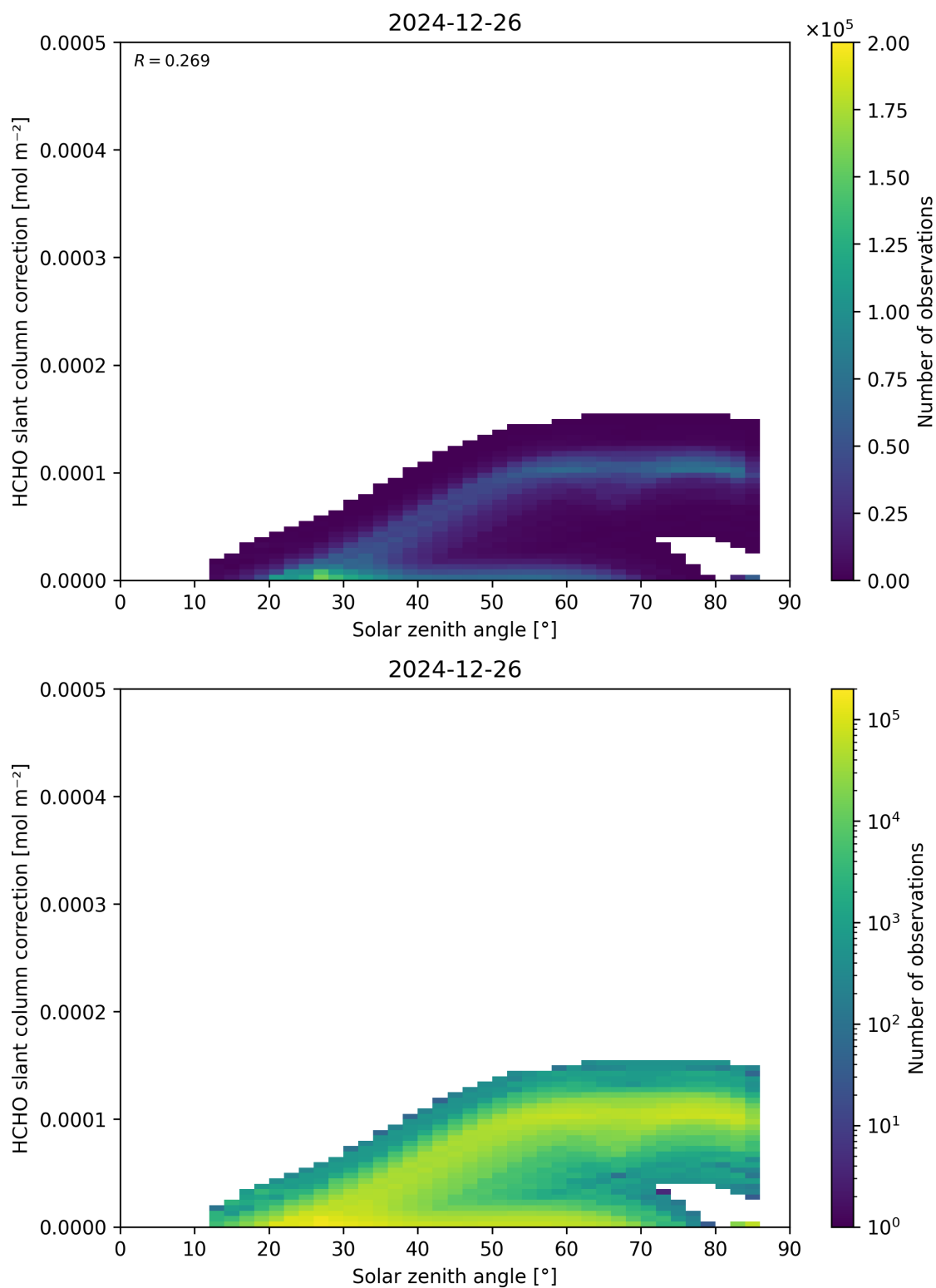
Figure 172: Scatter density plot of “Solar zenith angle” against “HCHO slant column correction” for 2024-12-25 to 2024-12-27.
