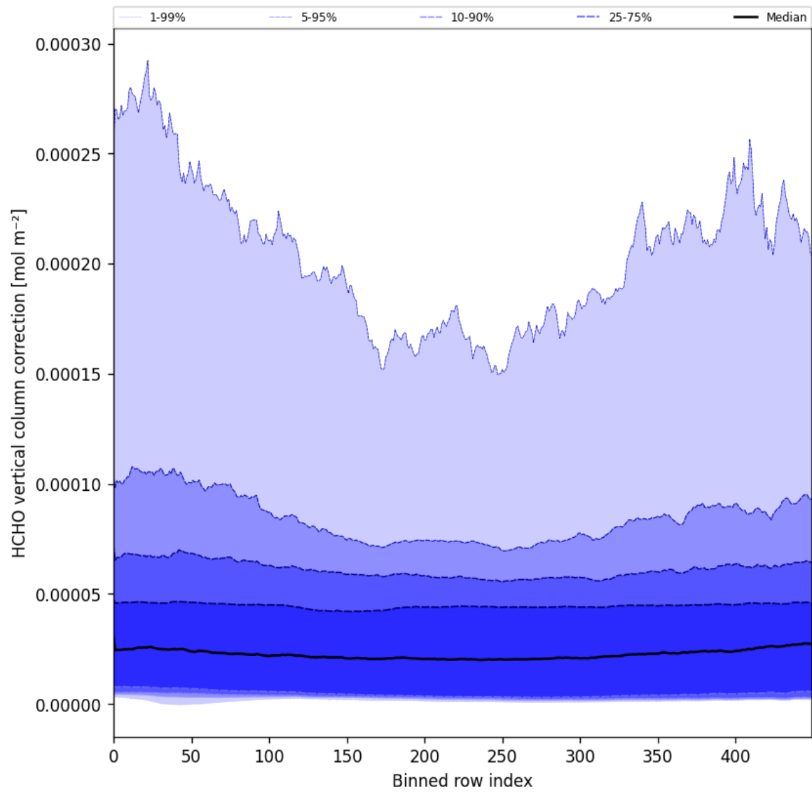
Figure 51: Along track statistics of “HCHO vertical column correction” for 2024-12-25 to 2024-12-27
