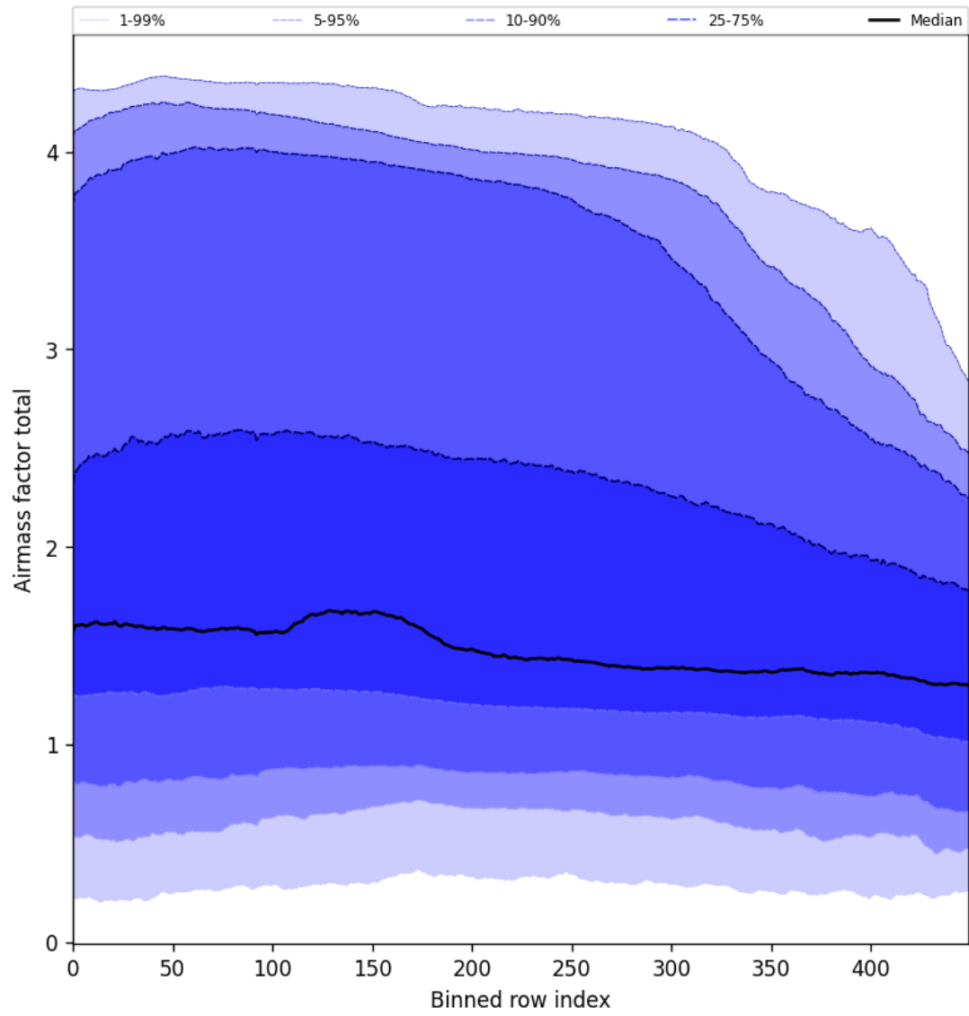
Figure 54: Along track statistics of “Airmass factor total” for 2024-12-25 to 2024-12-27
