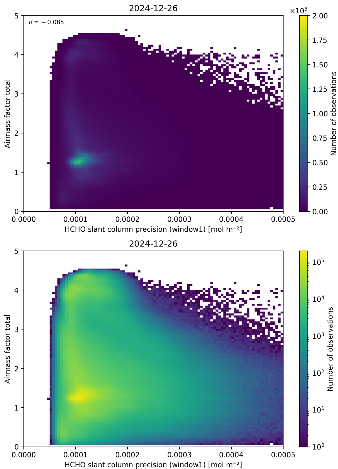
Figure 94: Scatter density plot of “HCHO slant column precision (window1)” against “Airmass factor total” for 2024-12-25 to 2024-12-27.
