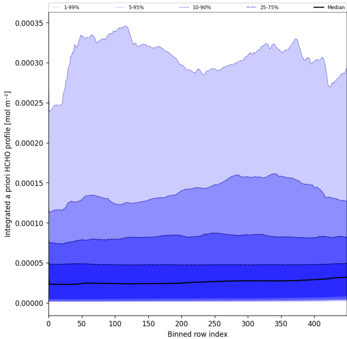
Figure 57: Along track statistics of “Integrated a priori HCHO profile” for 2024-12-25 to 2024-12-27
