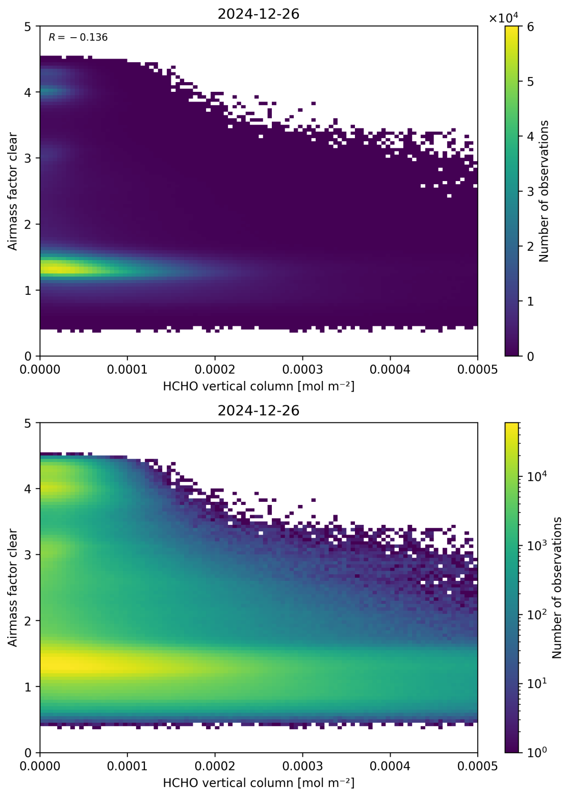
Figure 126: Scatter density plot of “HCHO vertical column” against “Airmass factor clear” for 2024-12-25 to 2024-12-27.
