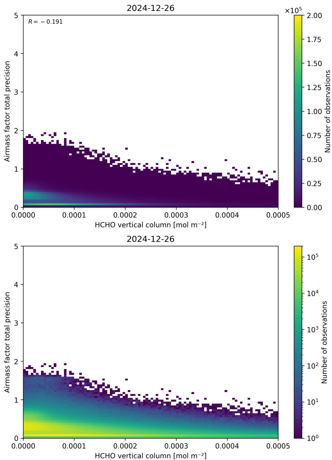
Figure 132: Scatter density plot of “HCHO vertical column” against “Airmass factor total precision” for 2024-12-25 to 2024-12-27.
