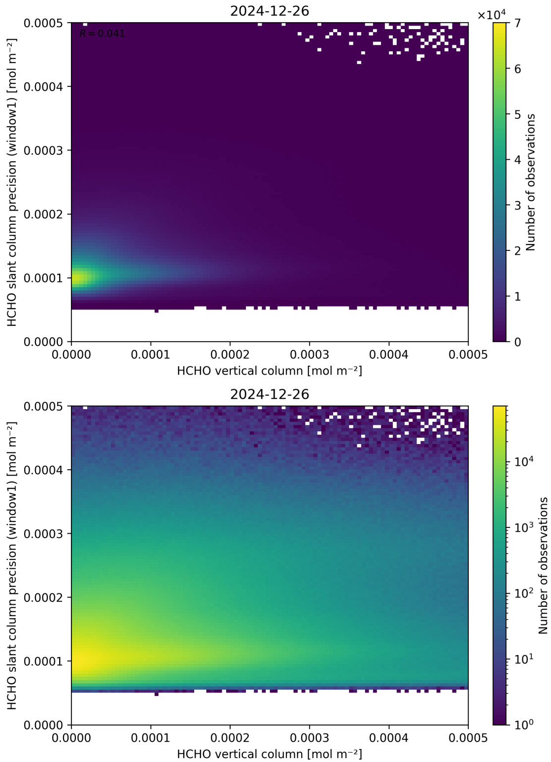
Figure 130: Scatter density plot of “HCHO vertical column” against “HCHO slant column precision (window1)” for 2024-12-25 to 2024-12-27.
