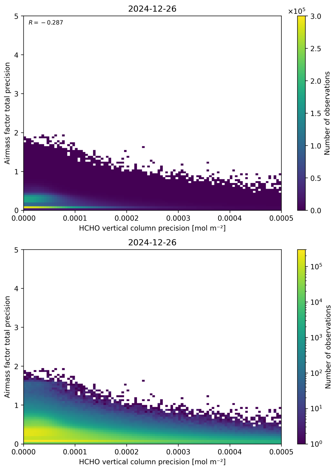
Figure 145: Scatter density plot of “HCHO vertical column precision” against “Airmass factor total precision” for 2024-12-25 to 2024-12-27.
