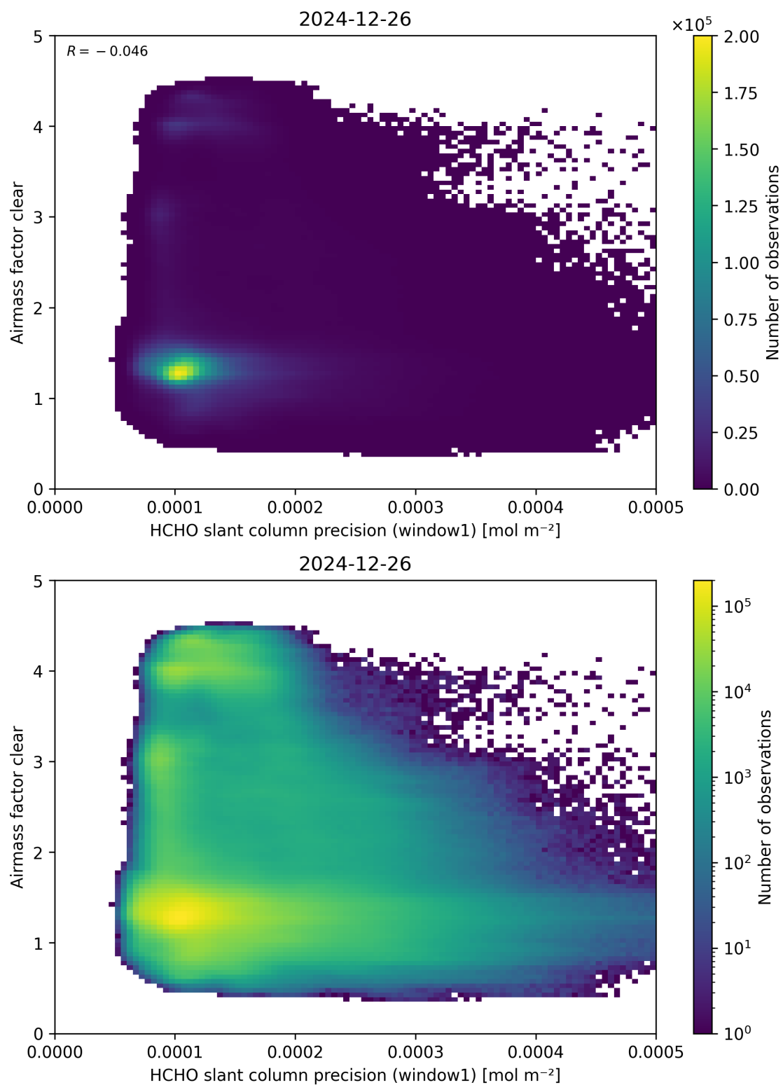
Figure 91: Scatter density plot of “HCHO slant column precision (window1)” against “Airmass factor clear” for 2024-12-25 to 2024-12-27.
