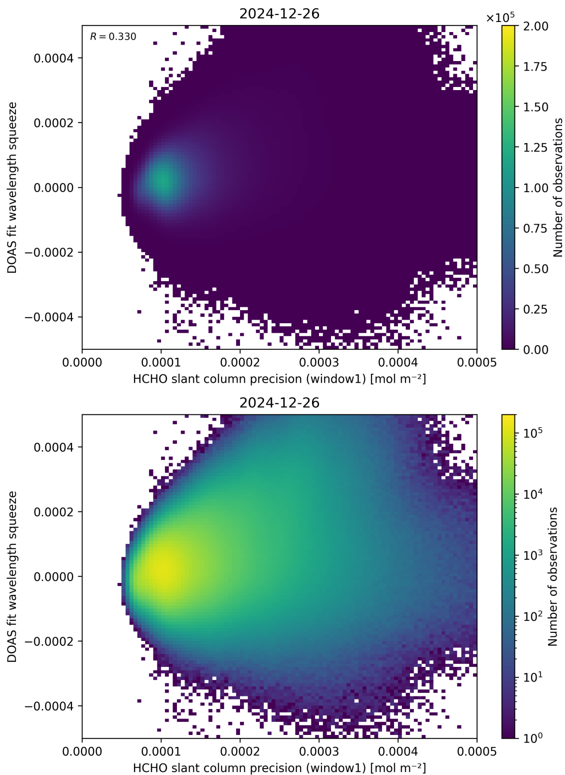
Figure 90: Scatter density plot of “HCHO slant column precision (window1)” against “DOAS fit wavelength squeeze” for 2024-12-25 to 2024-12-27.
