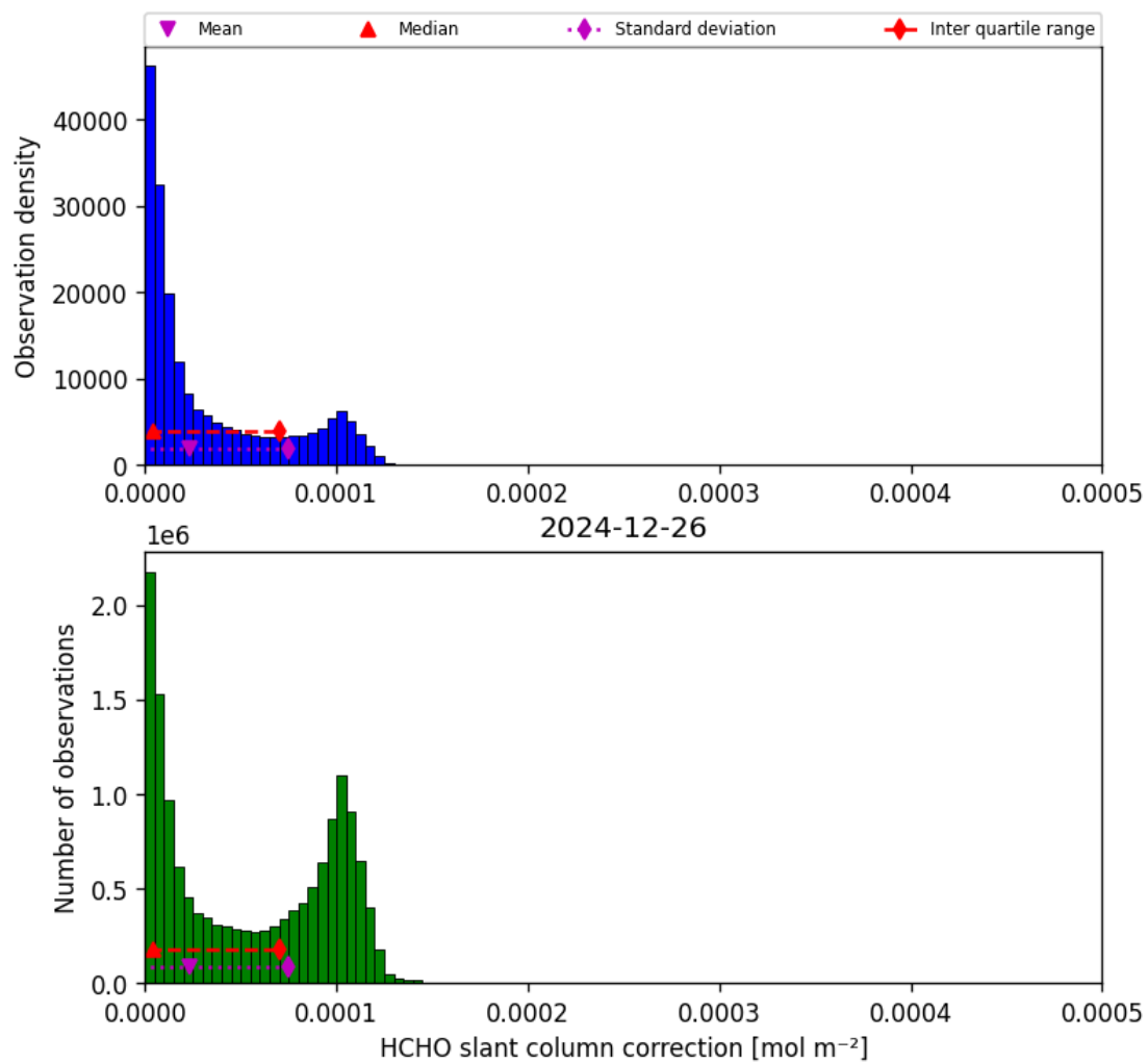
Figure 47: Histogram of “HCHO slant column correction” for 2024-12-25 to 2024-12-27
