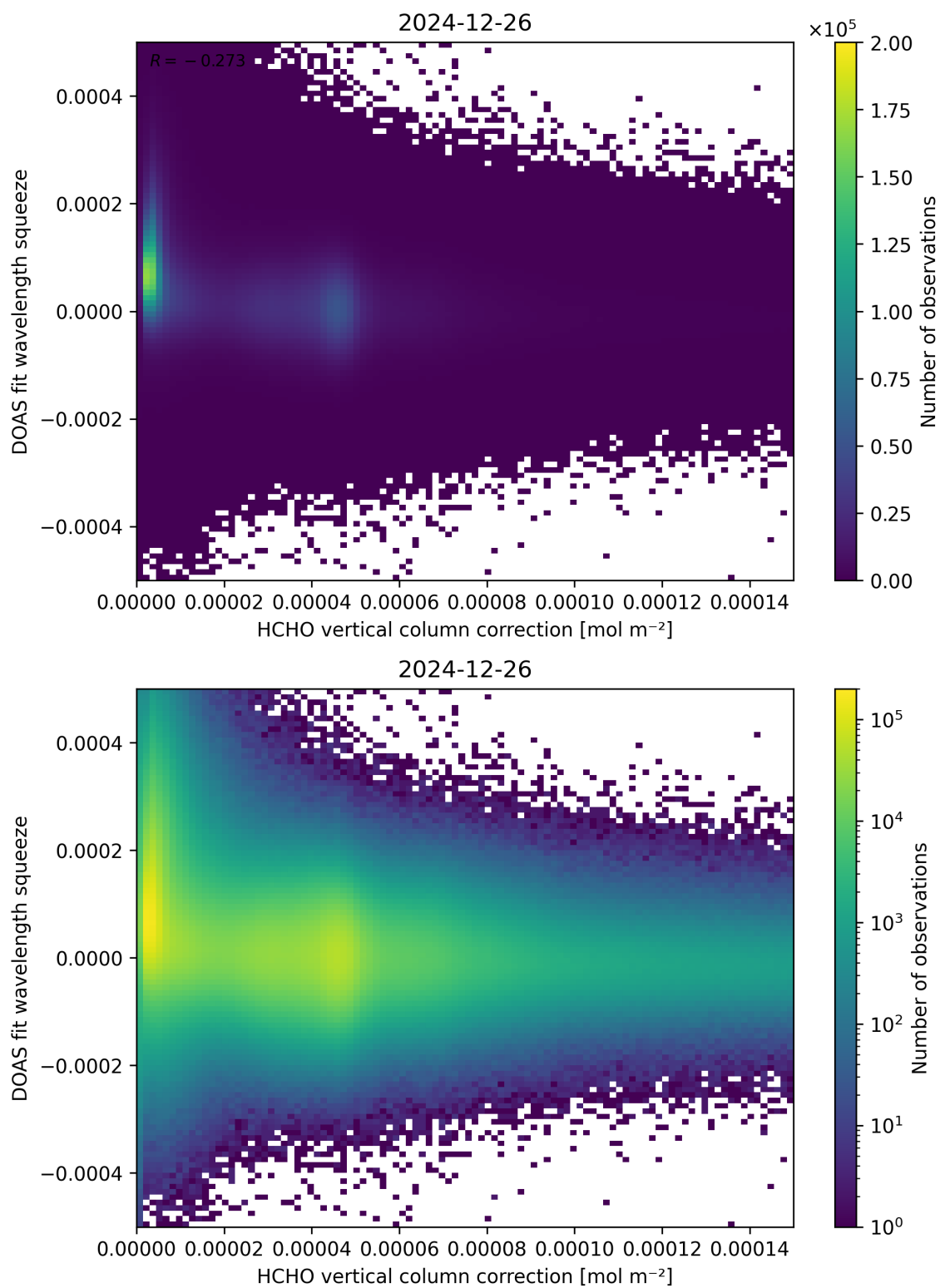
Figure 114: Scatter density plot of “HCHO vertical column correction” against “DOAS fit wavelength squeeze” for 2024-12-25 to 2024-12-27.
