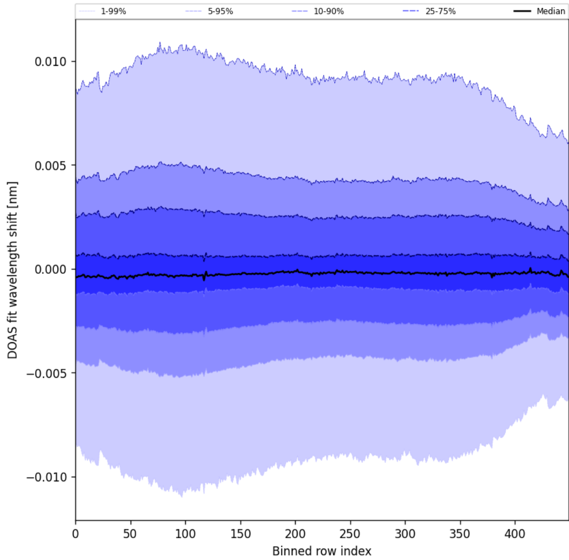
Figure 58: Along track statistics of “DOAS fit wavelength shift” for 2024-12-25 to 2024-12-27
