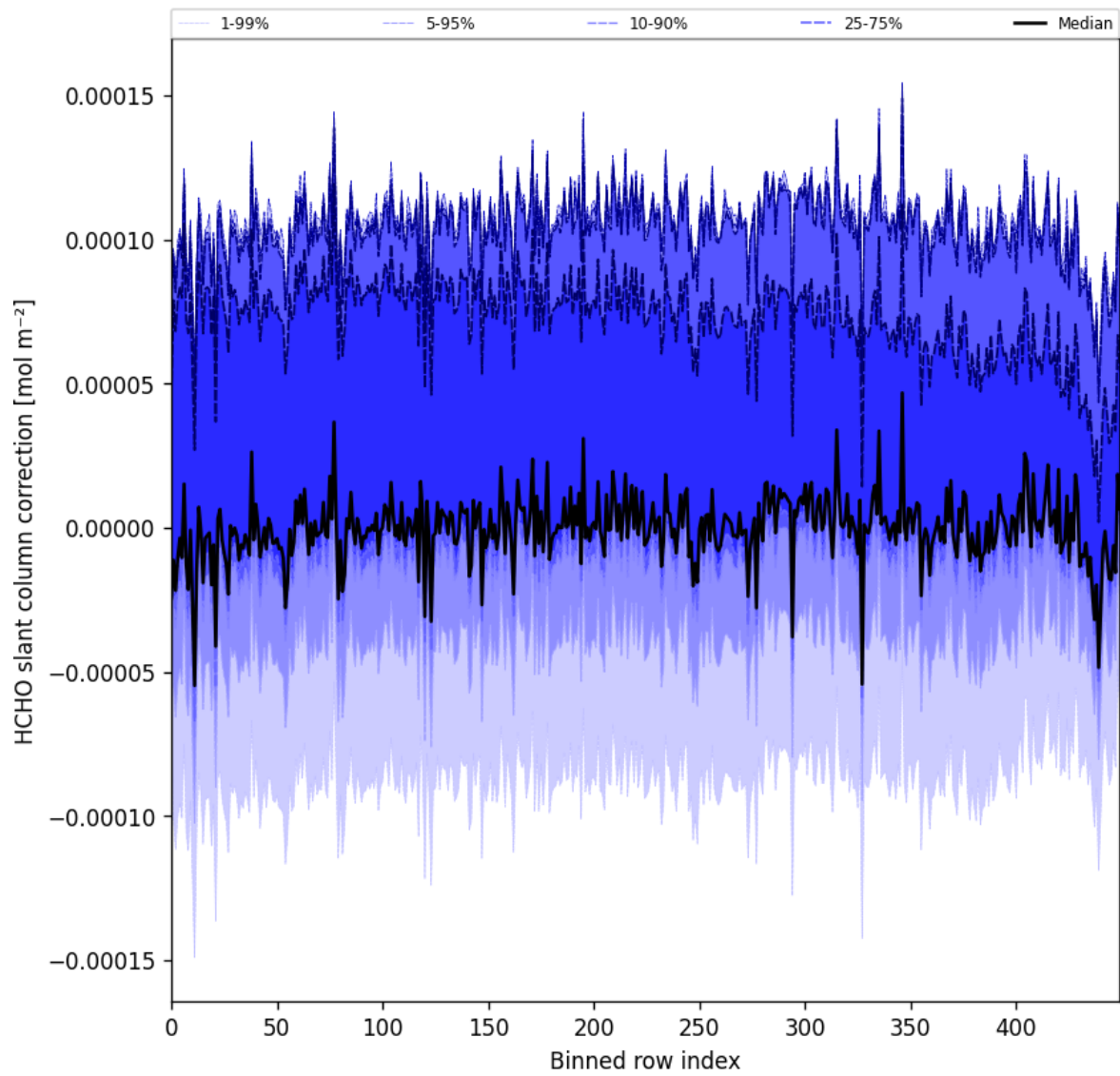
Figure 61: Along track statistics of “HCHO slant column correction” for 2024-12-25 to 2024-12-27
