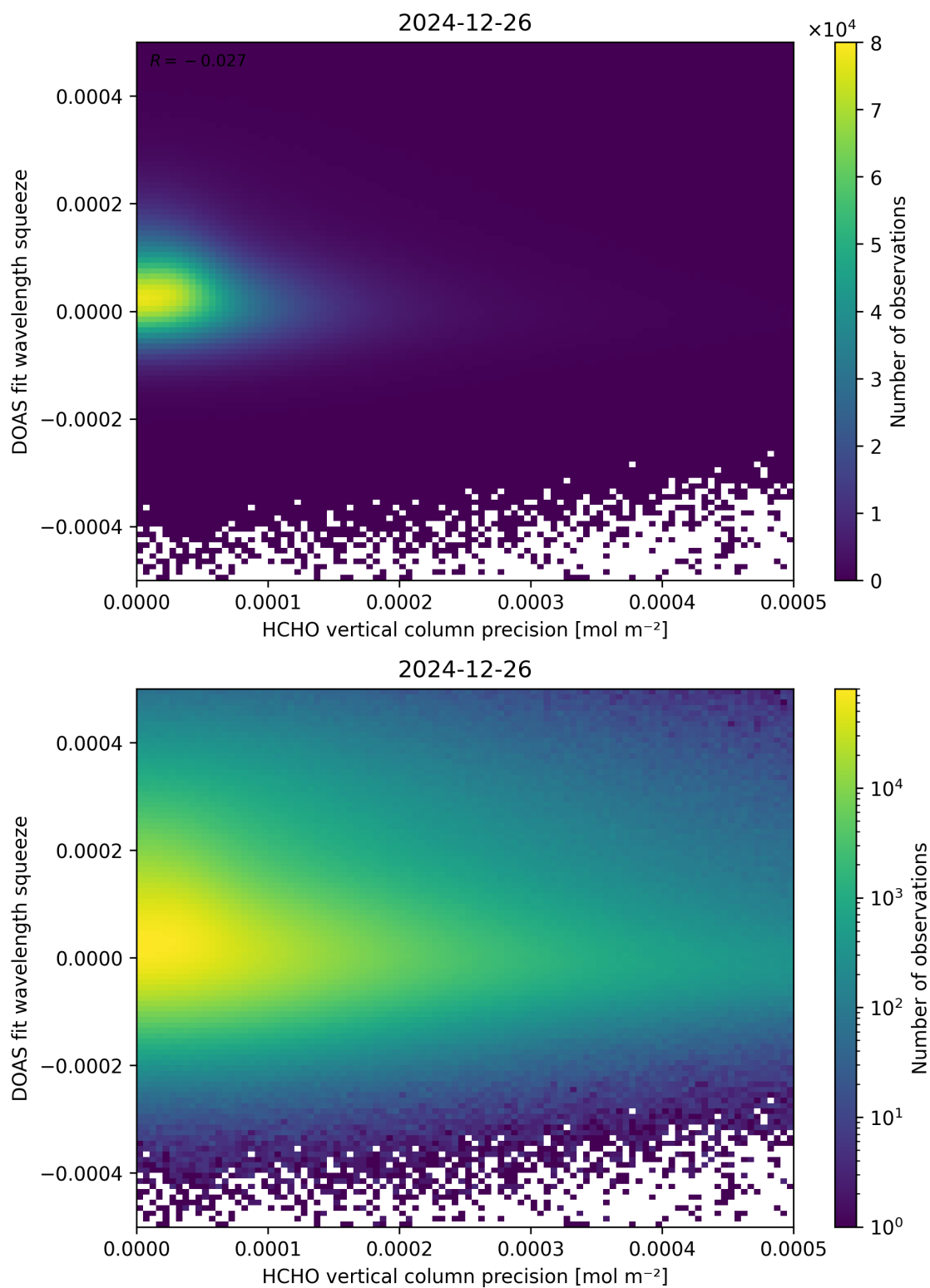
Figure 138: Scatter density plot of “HCHO vertical column precision” against “DOAS fit wavelength squeeze” for 2024-12-25 to 2024-12-27.
