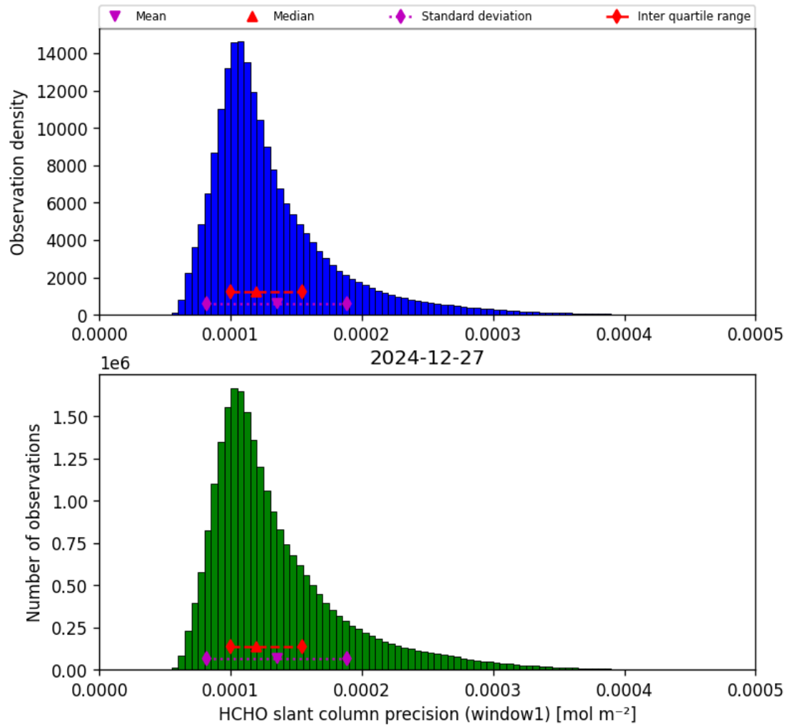
Figure 39: Histogram of “HCHO slant column precision (window1)” for 2024-12-27 to 2024-12-28
