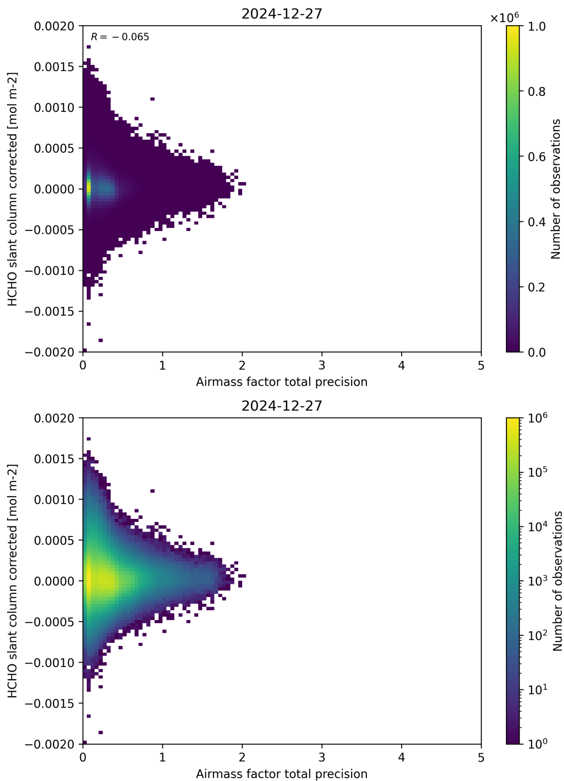
Figure 109: Scatter density plot of “Airmass factor total precision” against “HCHO slant column corrected” for 2024-12-27 to 2024-12-28.
