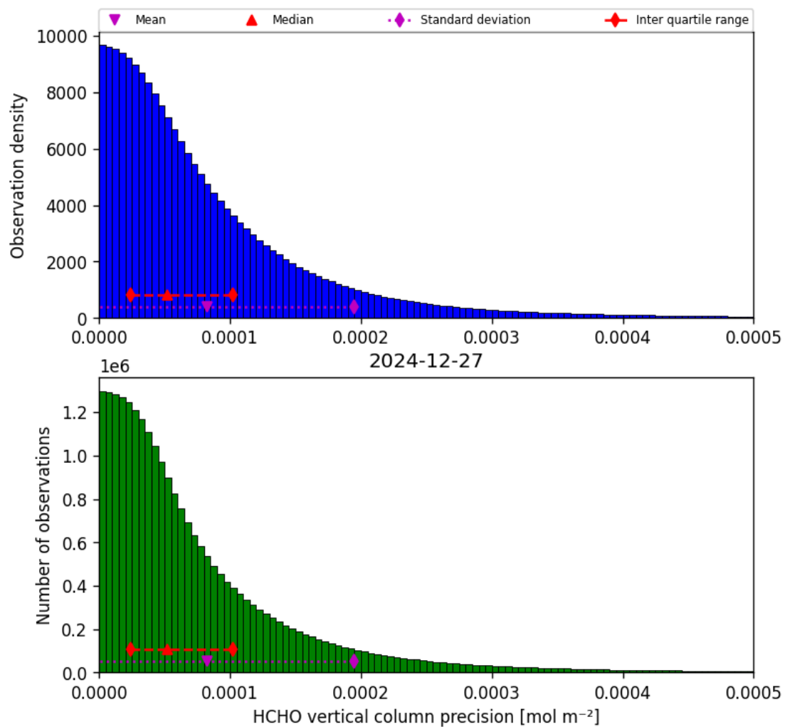
Figure 36: Histogram of “HCHO vertical column precision” for 2024-12-27 to 2024-12-28
