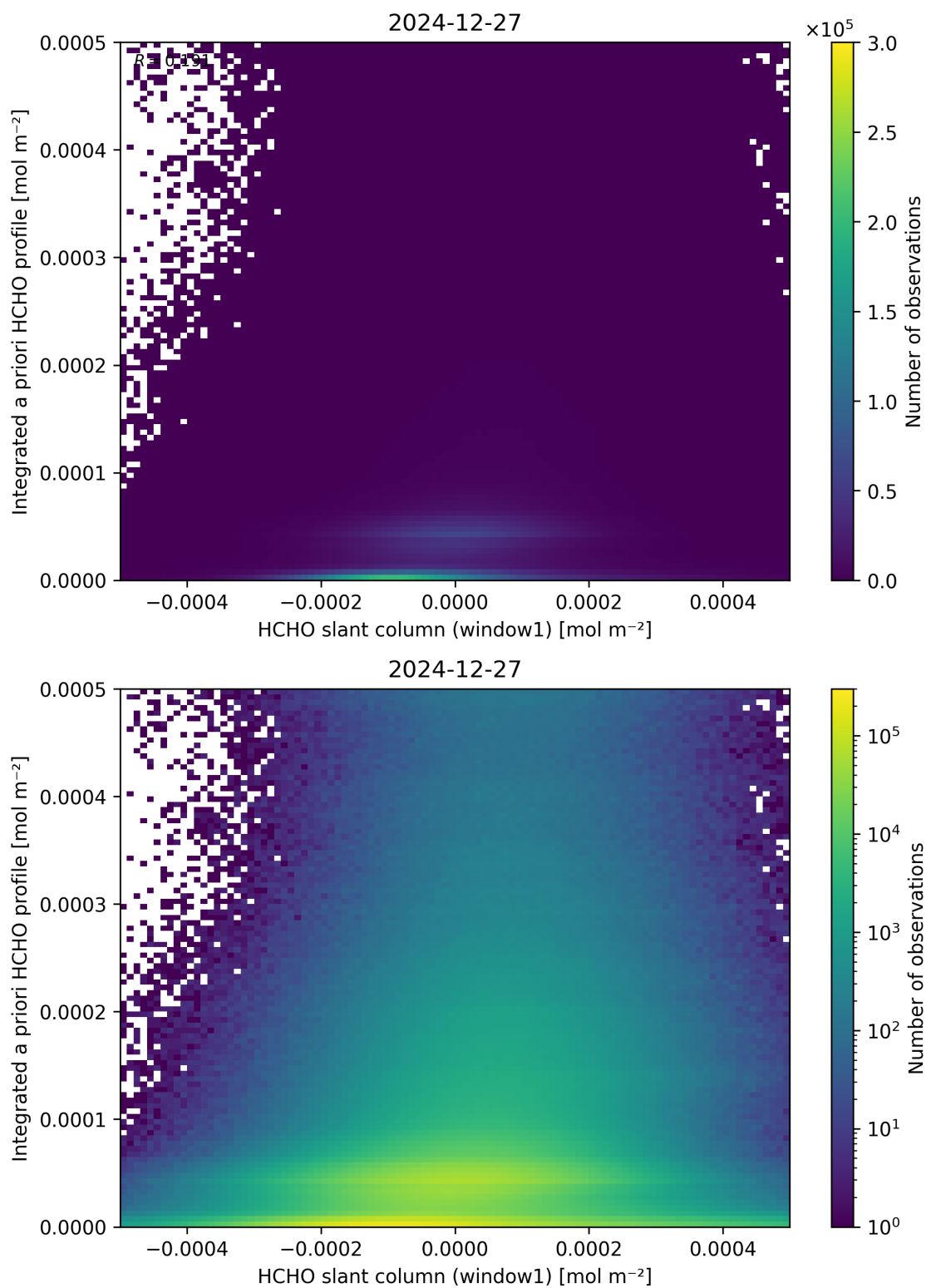
Figure 87: Scatter density plot of “HCHO slant column (window1)” against “Integrated a priori HCHO profile” for 2024-12-27 to 2024-12-28.
