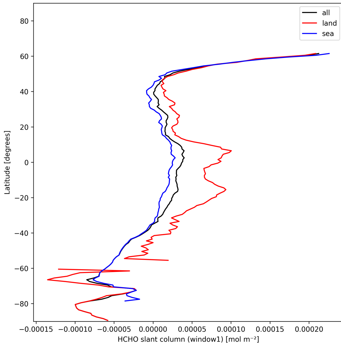
Figure 24: Zonal average of “HCHO slant column (window1)” for 2024-12-27 to 2024-12-28.
