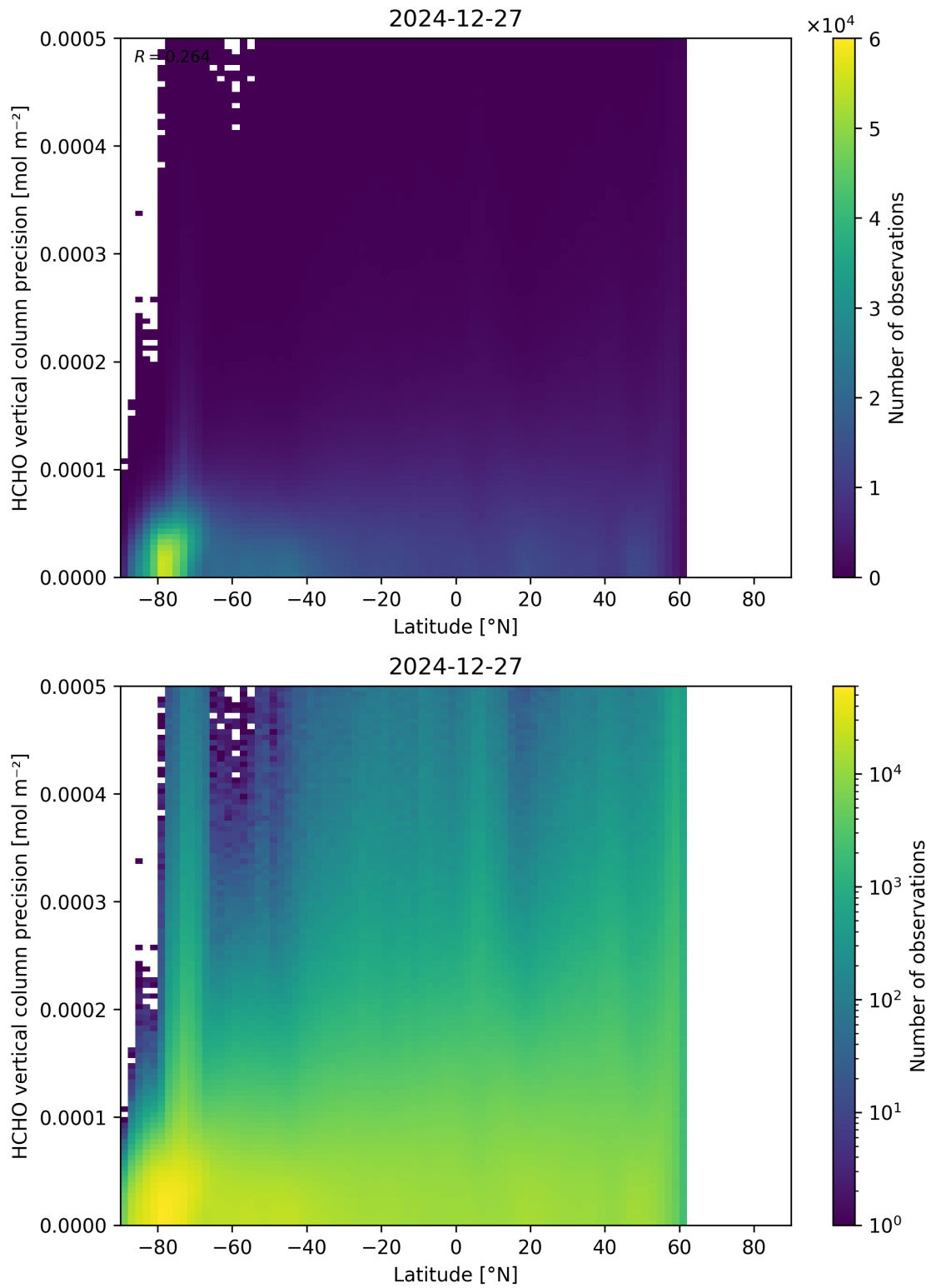
Figure 165: Scatter density plot of “Latitude” against “HCHO vertical column precision” for 2024-12-27 to 2024-12-28.
