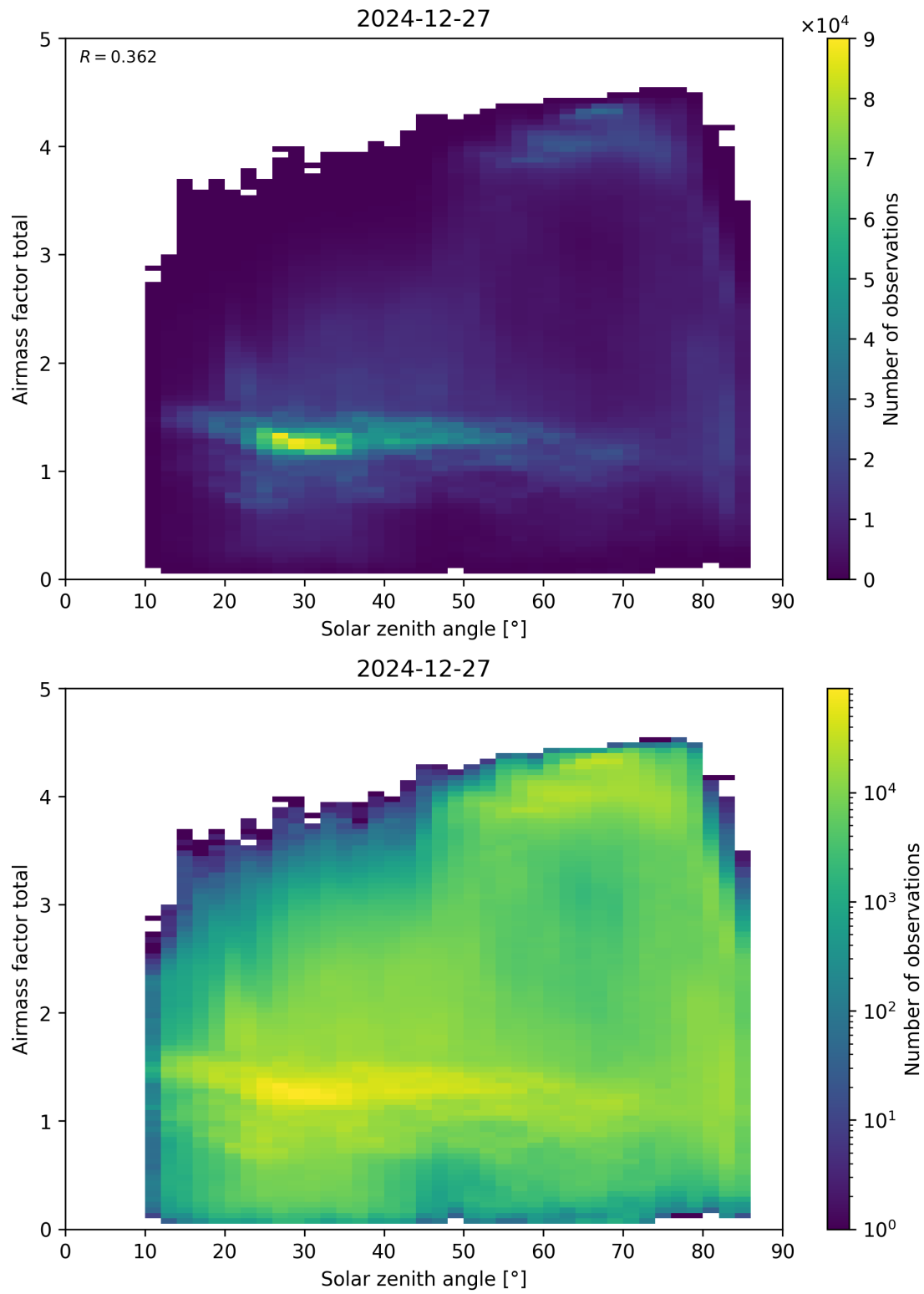
Figure 175: Scatter density plot of “Solar zenith angle” against “Airmass factor total” for 2024-12-27 to 2024-12-28.
