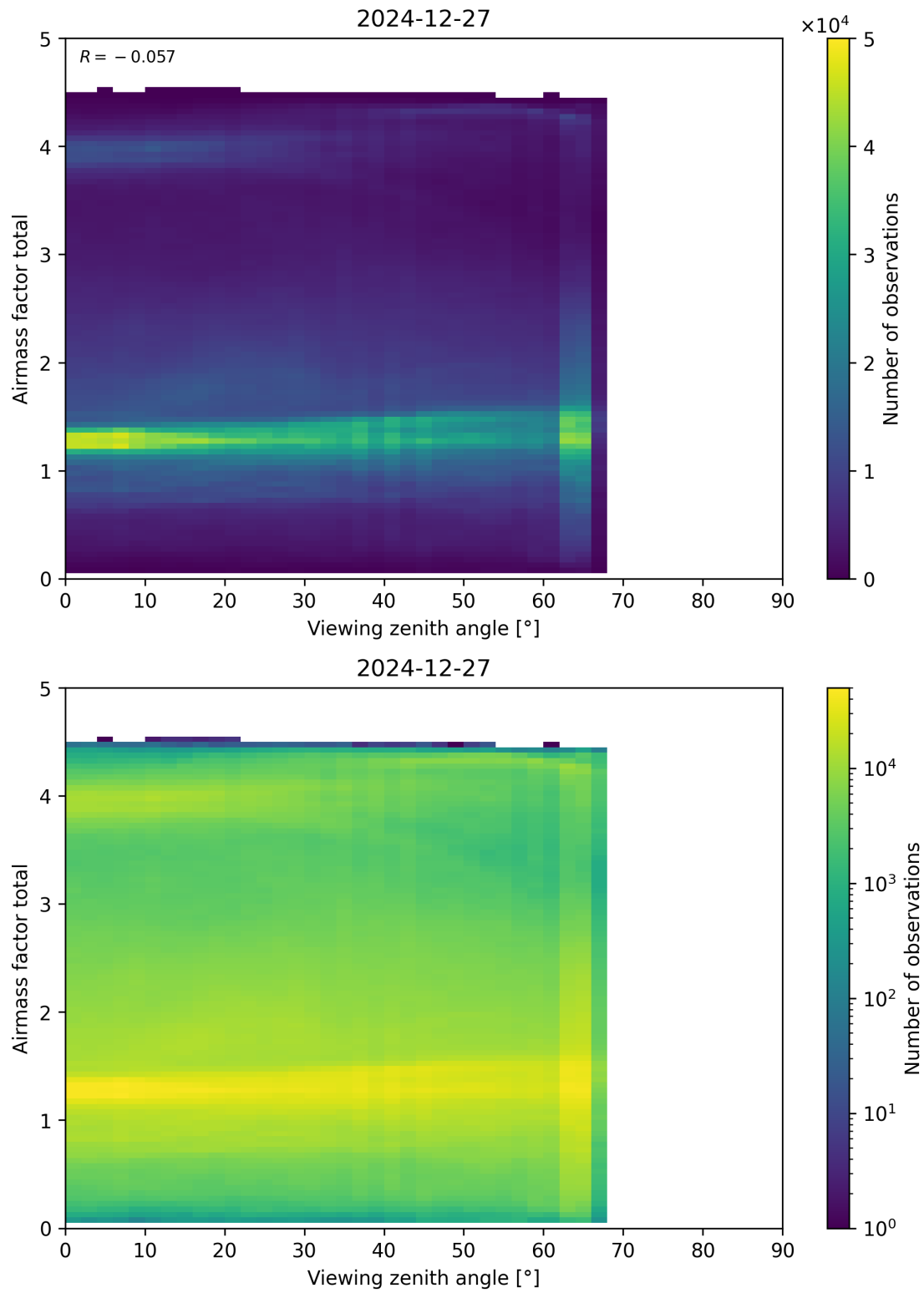
Figure 190: Scatter density plot of “Viewing zenith angle” against “Airmass factor total” for 2024-12-27 to 2024-12-28.
