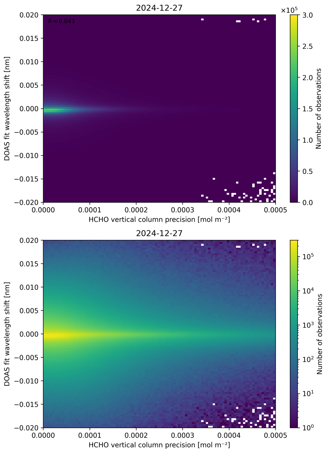
Figure 137: Scatter density plot of “HCHO vertical column precision” against “DOAS fit wavelength shift” for 2024-12-27 to 2024-12-28.
