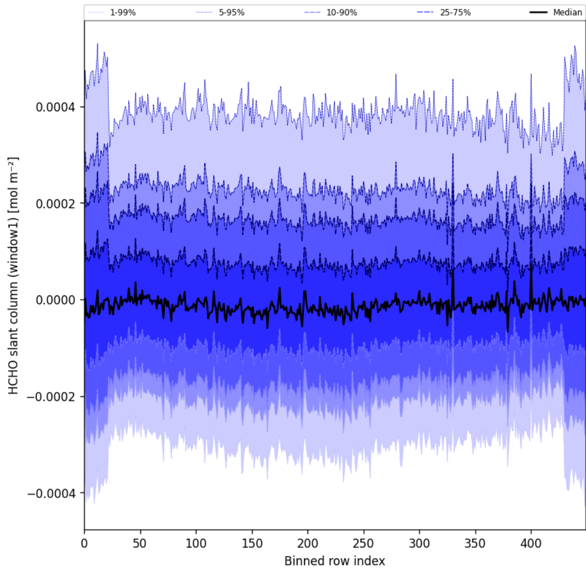
Figure 52: Along track statistics of “HCHO slant column (window1)” for 2024-12-27 to 2024-12-28
