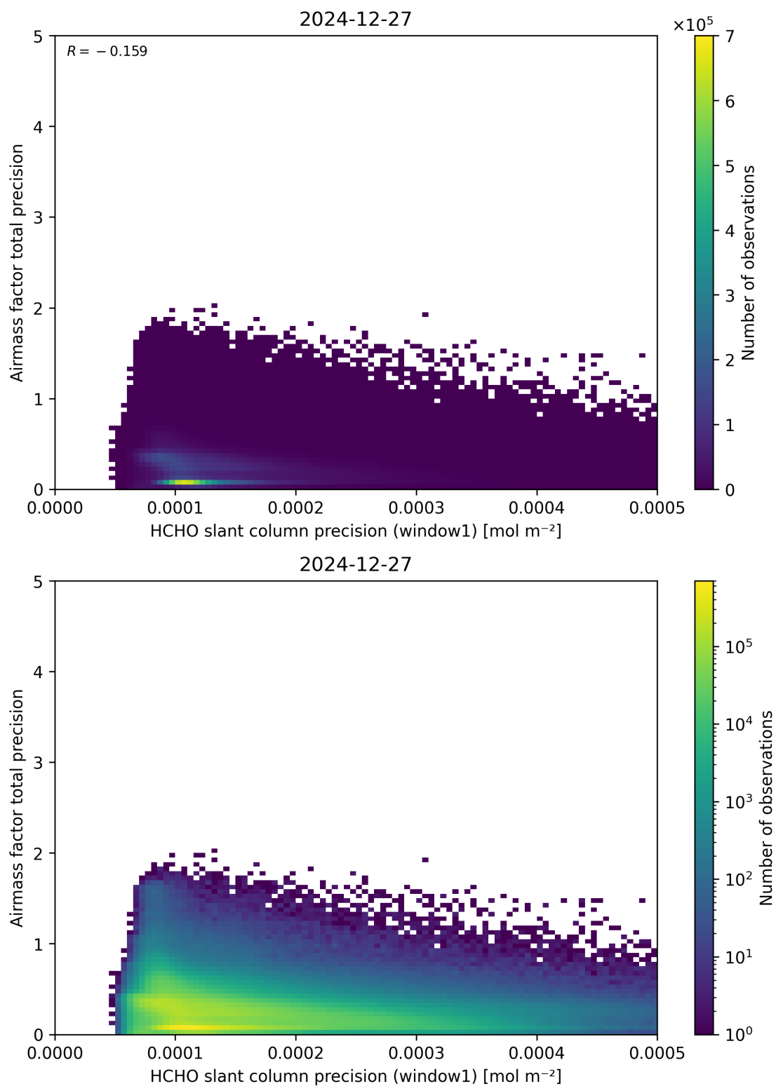
Figure 95: Scatter density plot of “HCHO slant column precision (window1)” against “Airmass factor total precision” for 2024-12-27 to 2024-12-28.
