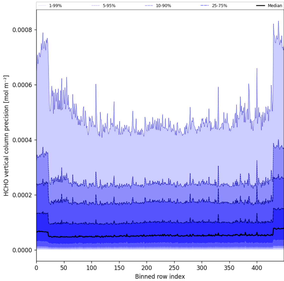
Figure 50: Along track statistics of “HCHO vertical column precision” for 2024-12-27 to 2024-12-28
