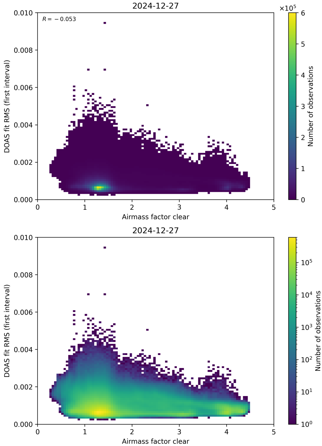
Figure 71: Scatter density plot of “Airmass factor clear” against “DOAS fit RMS (first interval)” for 2024-12-27 to 2024-12-28.
