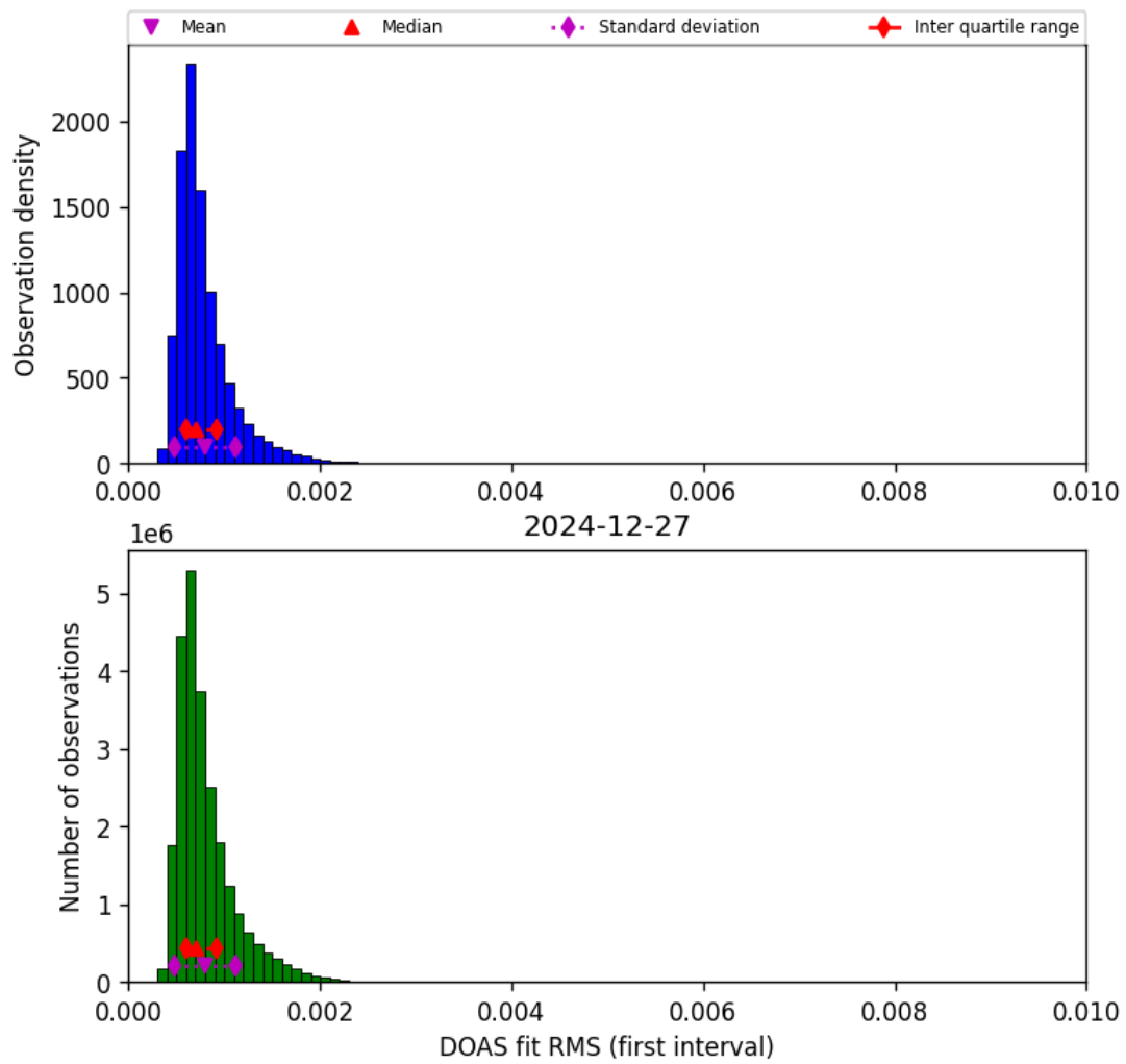
Figure 46: Histogram of “DOAS fit RMS (first interval)” for 2024-12-27 to 2024-12-28
