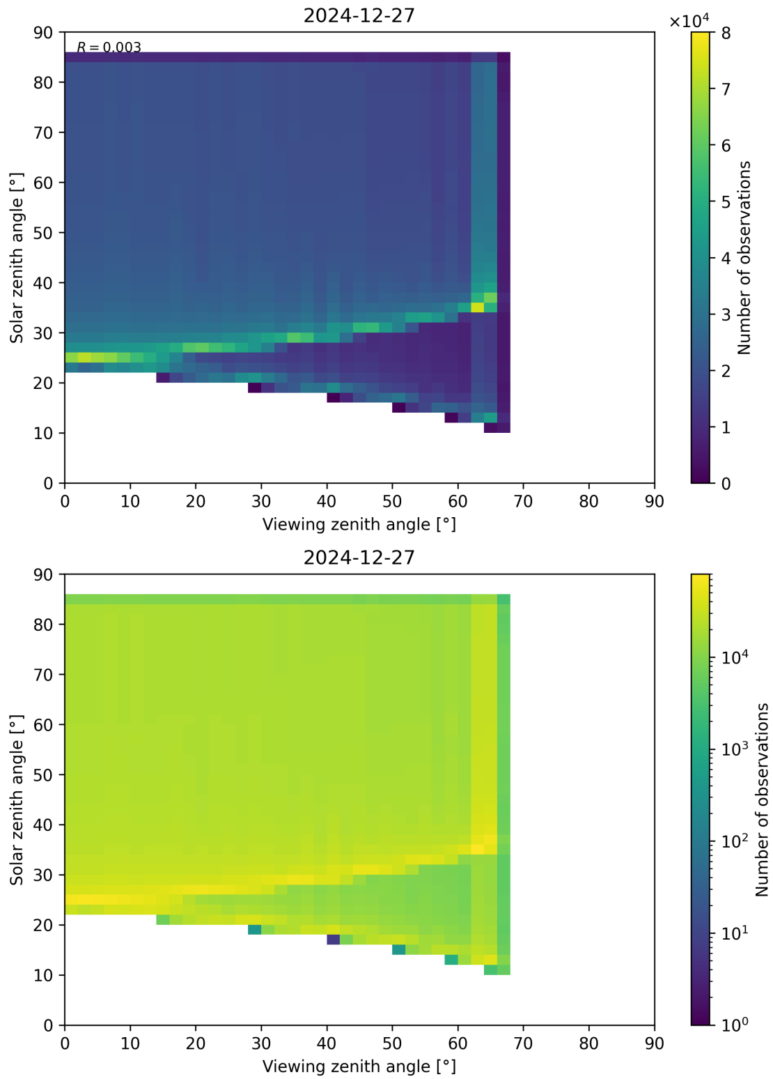
Figure 197: Scatter density plot of “Viewing zenith angle” against “Solar zenith angle” for 2024-12-27 to 2024-12-28.
