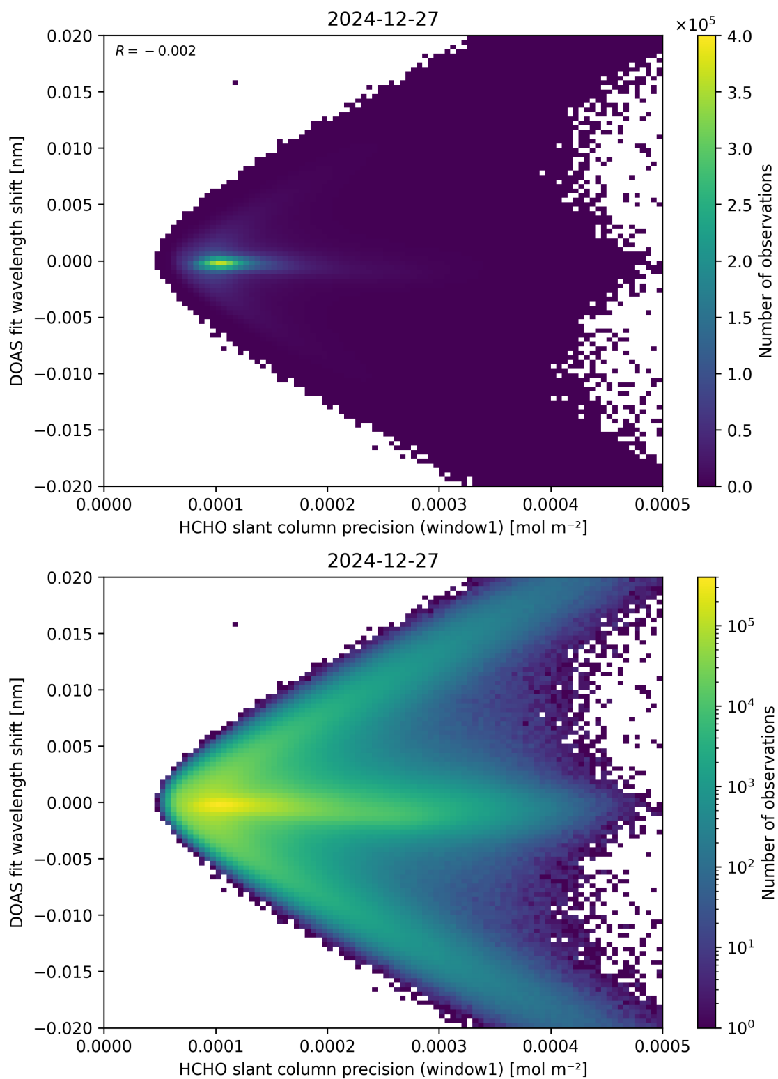
Figure 89: Scatter density plot of “HCHO slant column precision (window1)” against “DOAS fit wavelength shift” for 2024-12-27 to 2024-12-28.
