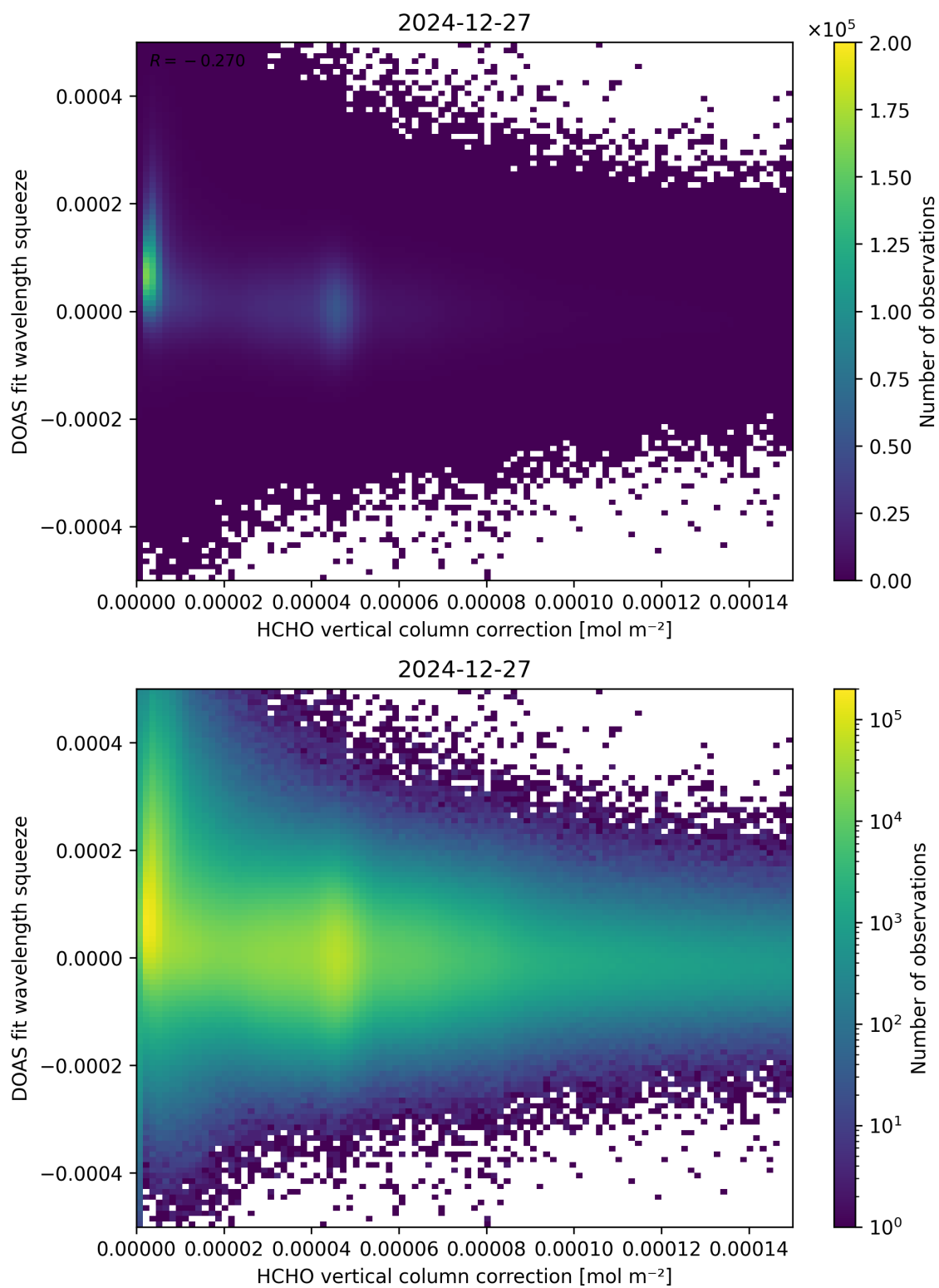
Figure 114: Scatter density plot of “HCHO vertical column correction” against “DOAS fit wavelength squeeze” for 2024-12-27 to 2024-12-28.
