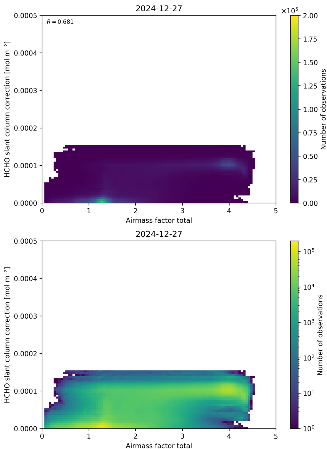
Figure 102: Scatter density plot of “Airmass factor total” against “HCHO slant column correction” for 2024-12-27 to 2024-12-28.
