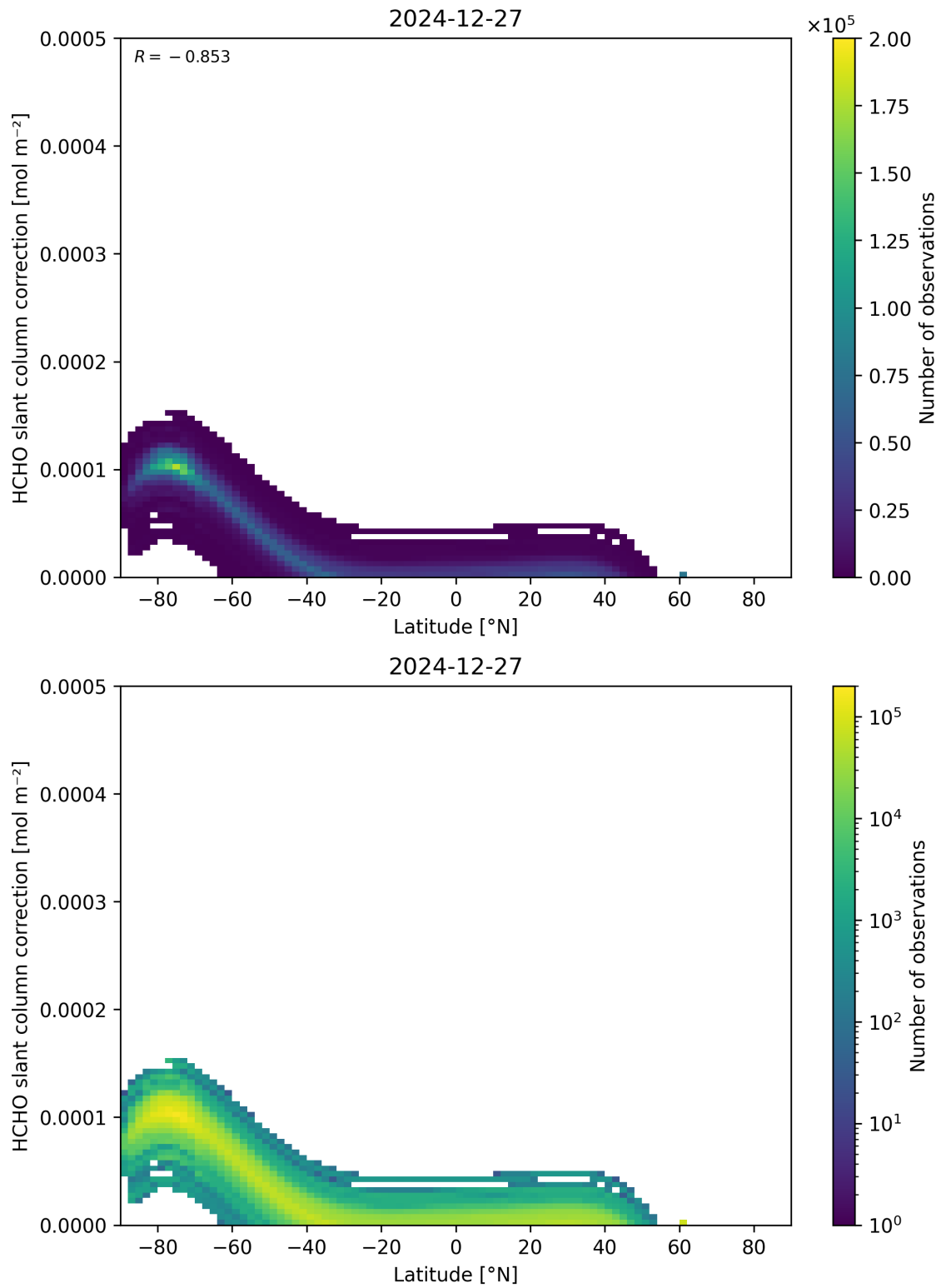
Figure 158: Scatter density plot of “Latitude” against “HCHO slant column correction” for 2024-12-27 to 2024-12-28.
