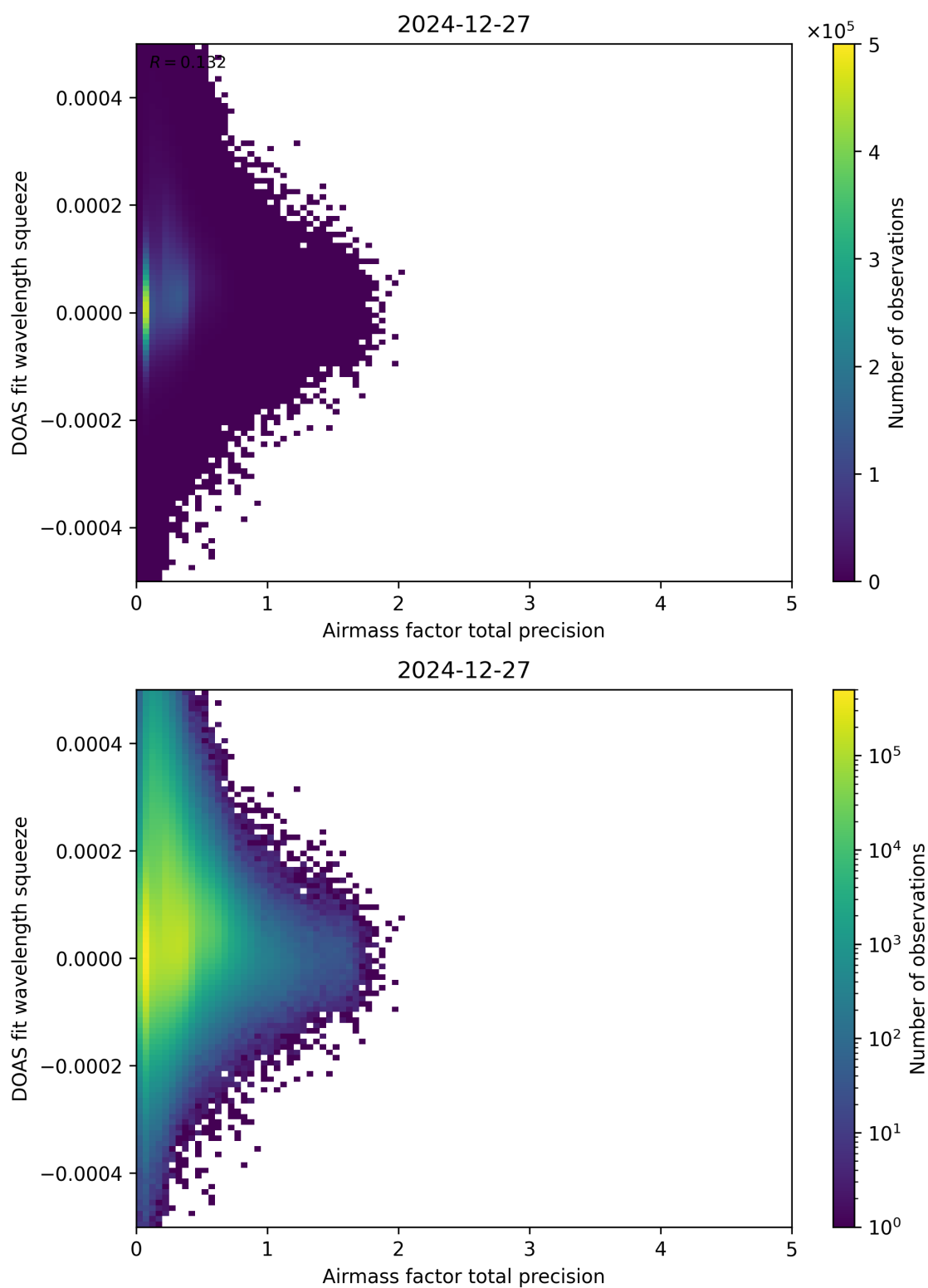
Figure 107: Scatter density plot of “Airmass factor total precision” against “DOAS fit wavelength squeeze” for 2024-12-27 to 2024-12-28.
