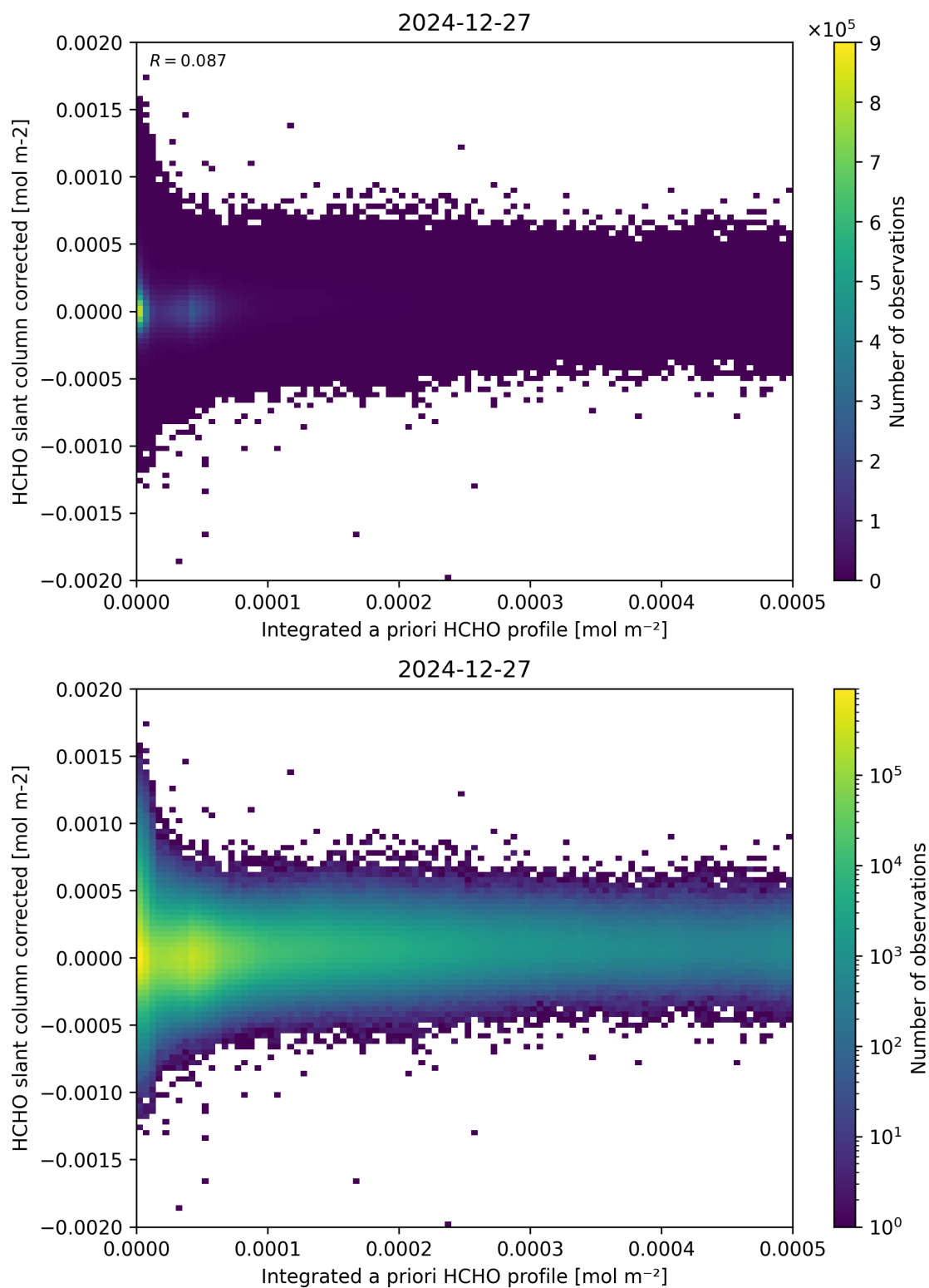
Figure 151: Scatter density plot of “Integrated a priori HCHO profile” against “HCHO slant column corrected” for 2024-12-27 to 2024-12-28.
