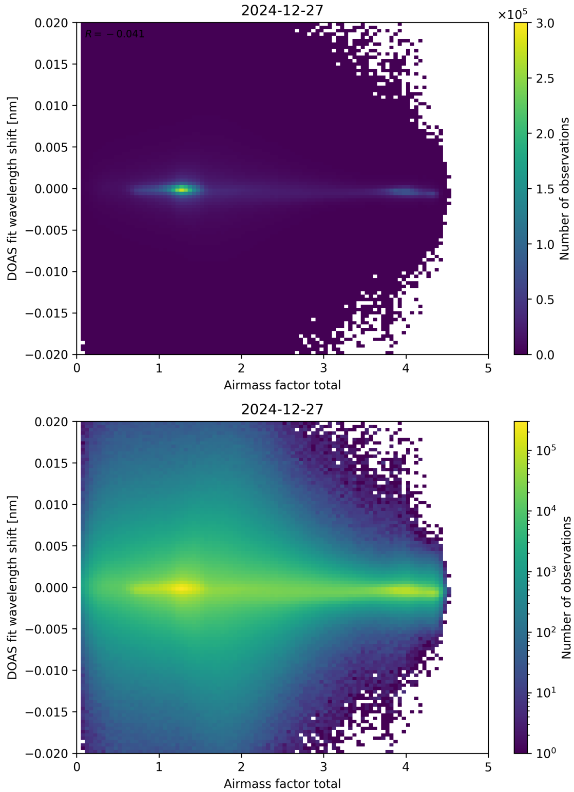
Figure 98: Scatter density plot of “Airmass factor total” against “DOAS fit wavelength shift” for 2024-12-27 to 2024-12-28.
