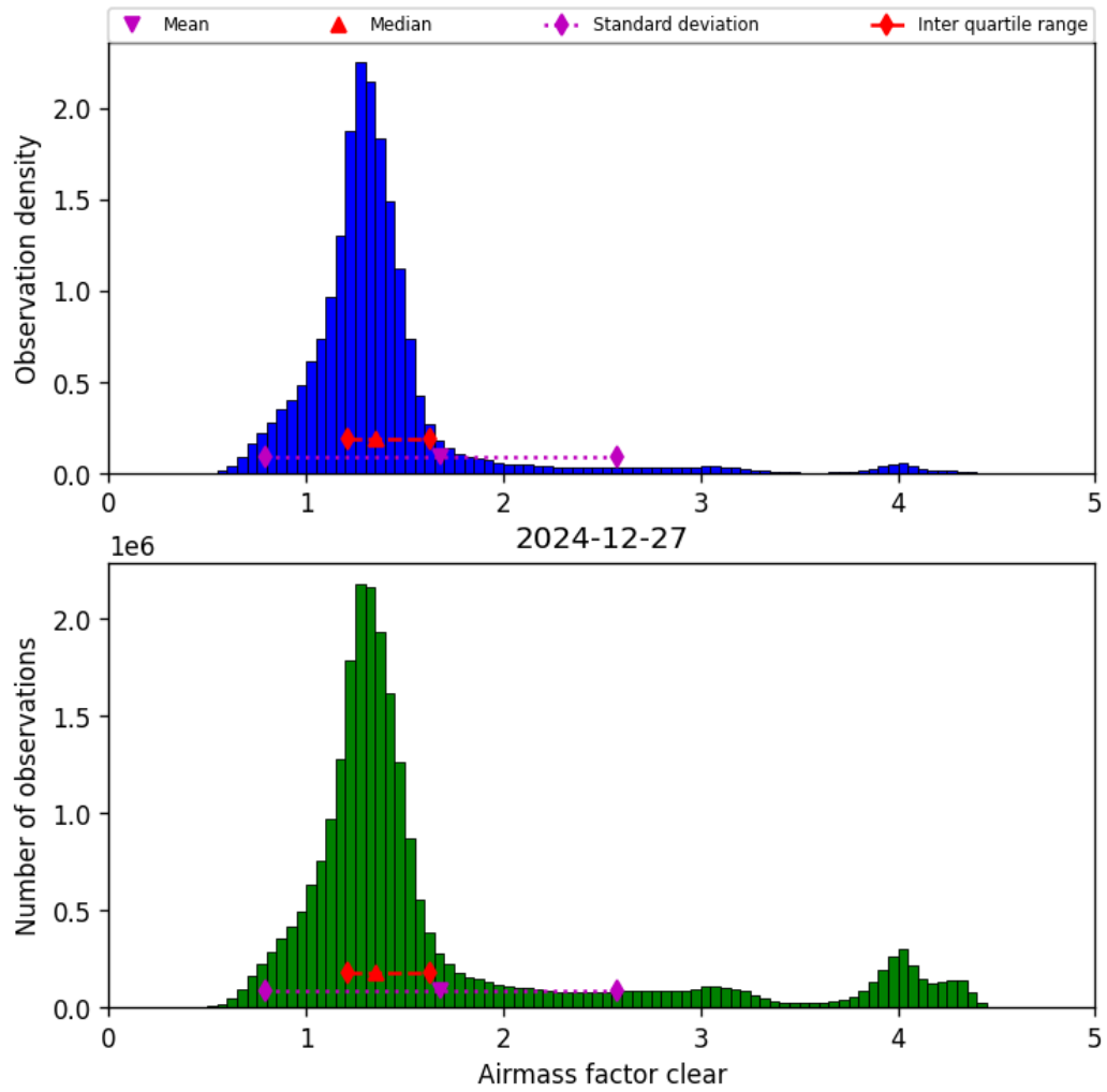
Figure 42: Histogram of “Airmass factor clear” for 2024-12-27 to 2024-12-28
