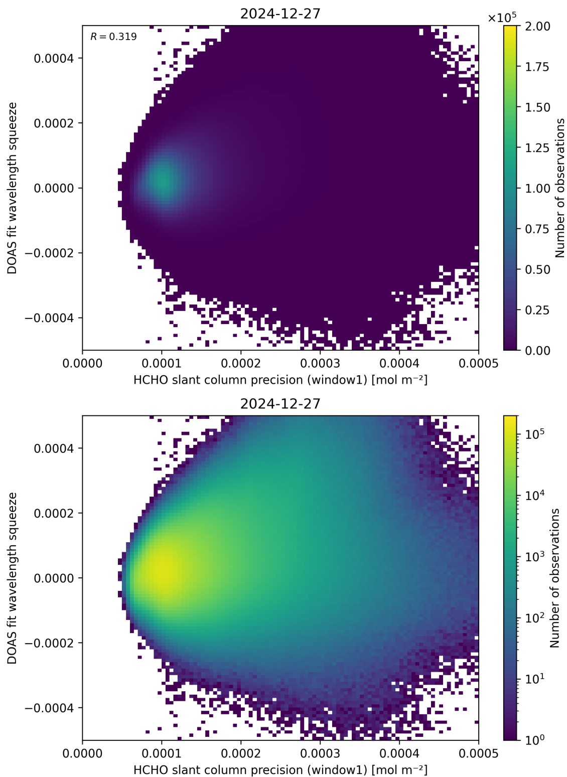
Figure 90: Scatter density plot of “HCHO slant column precision (window1)” against “DOAS fit wavelength squeeze” for 2024-12-27 to 2024-12-28.
