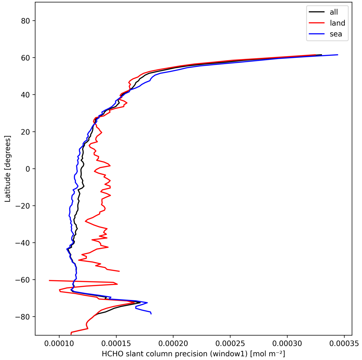
Figure 25: Zonal average of “HCHO slant column precision (window1)” for 2024-12-27 to 2024-12-28.
