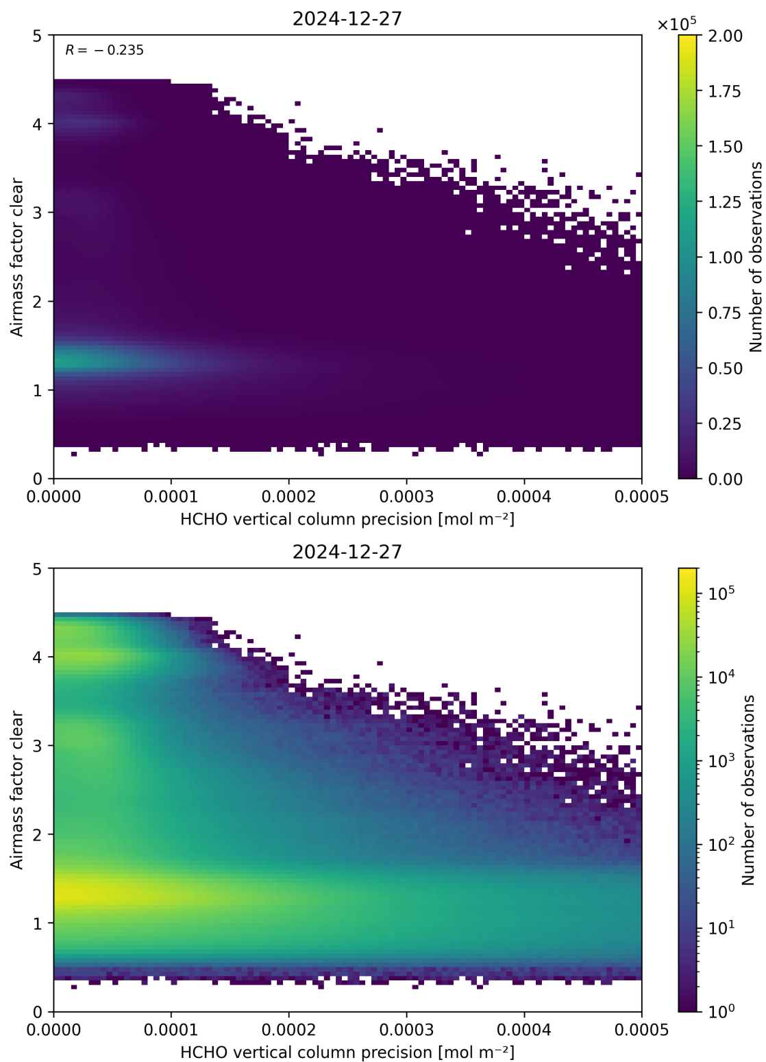
Figure 139: Scatter density plot of “HCHO vertical column precision” against “Airmass factor clear” for 2024-12-27 to 2024-12-28.
