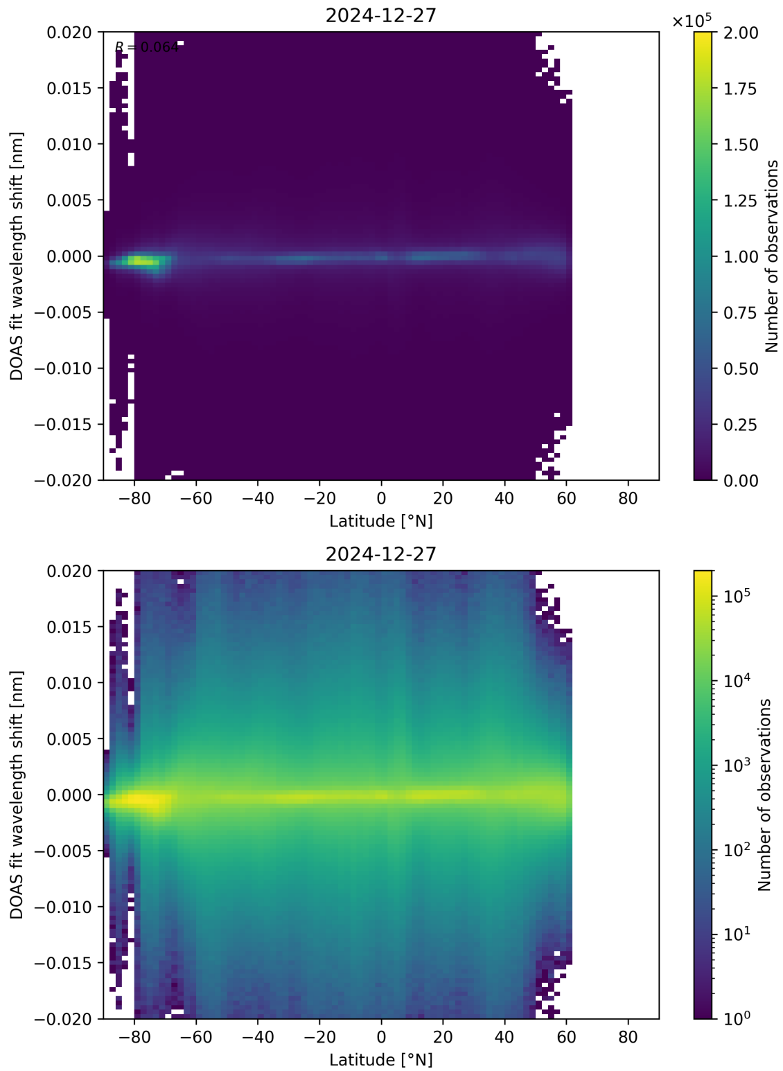
Figure 154: Scatter density plot of “Latitude” against “DOAS fit wavelength shift” for 2024-12-27 to 2024-12-28.
