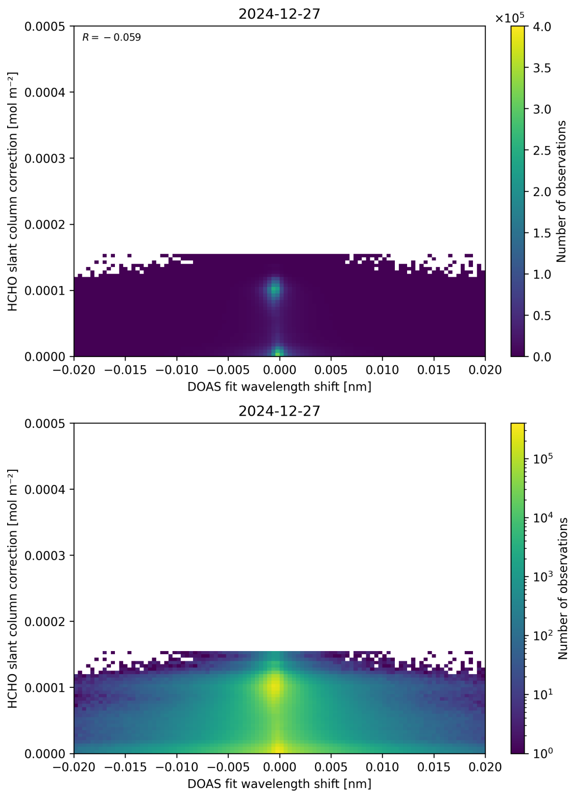
Figure 67: Scatter density plot of “DOAS fit wavelength shift” against “HCHO slant column correction” for 2024-12-27 to 2024-12-28.
