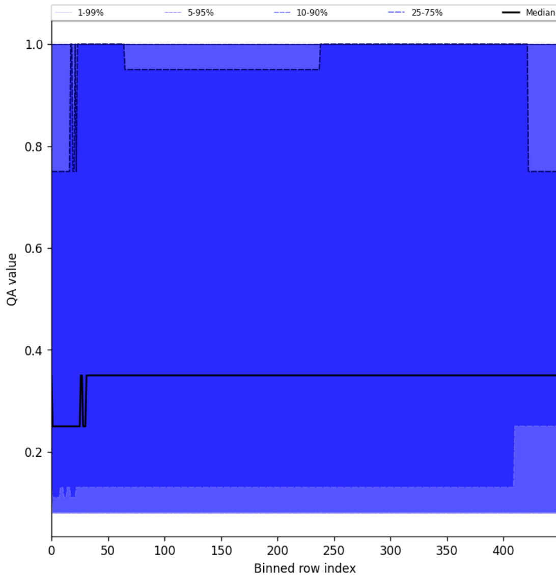
Figure 48: Along track statistics of “QA value” for 2024-12-27 to 2024-12-28
