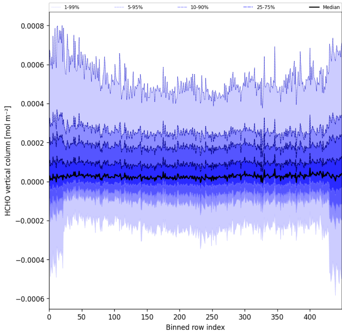
Figure 49: Along track statistics of “HCHO vertical column” for 2024-12-27 to 2024-12-28
