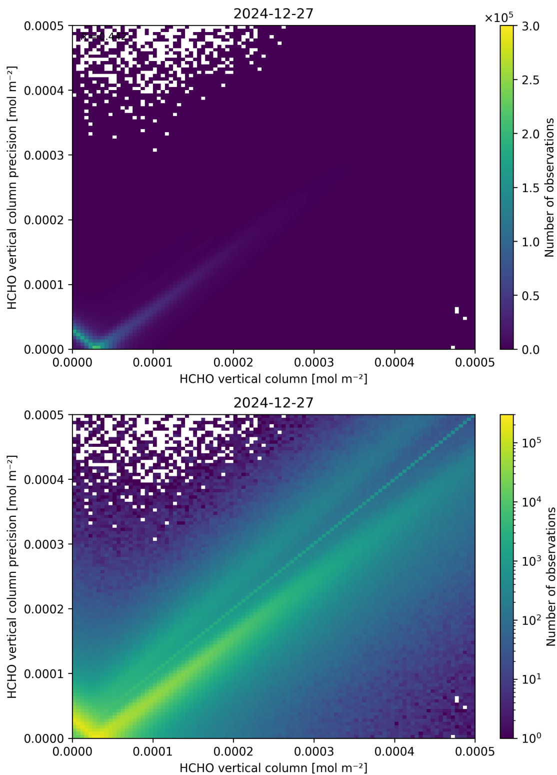
Figure 134: Scatter density plot of “HCHO vertical column” against “HCHO vertical column precision” for 2024-12-27 to 2024-12-28.
