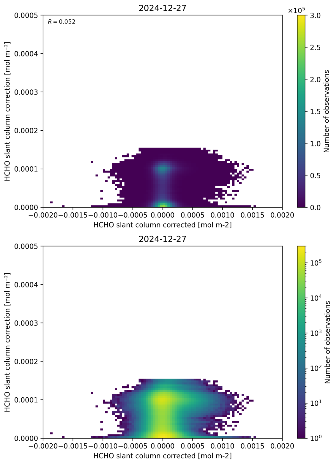
Figure 77: Scatter density plot of “HCHO slant column corrected” against “HCHO slant column correction” for 2024-12-27 to 2024-12-28.
