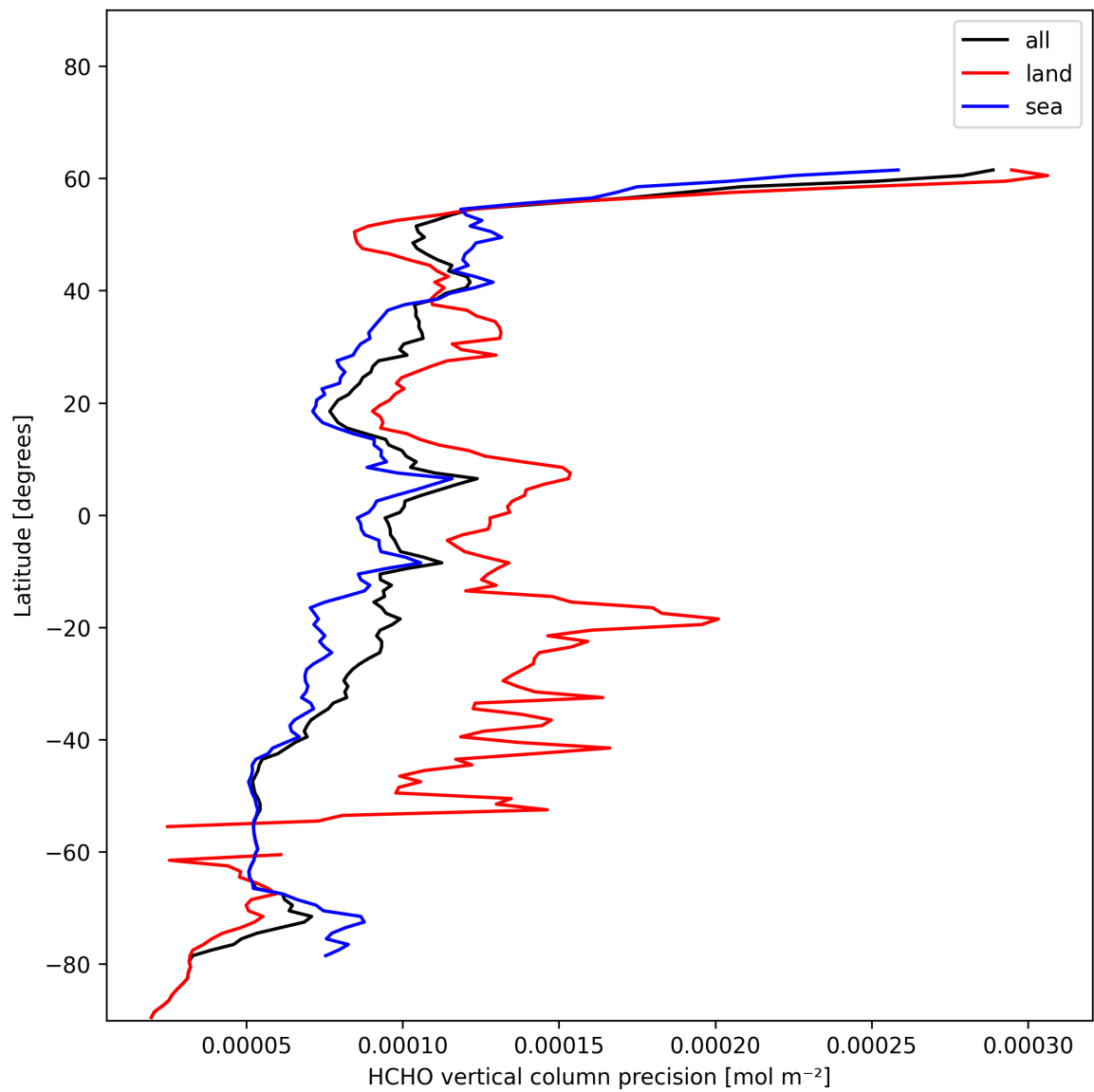
Figure 22: Zonal average of “HCHO vertical column precision” for 2024-12-27 to 2024-12-28.
