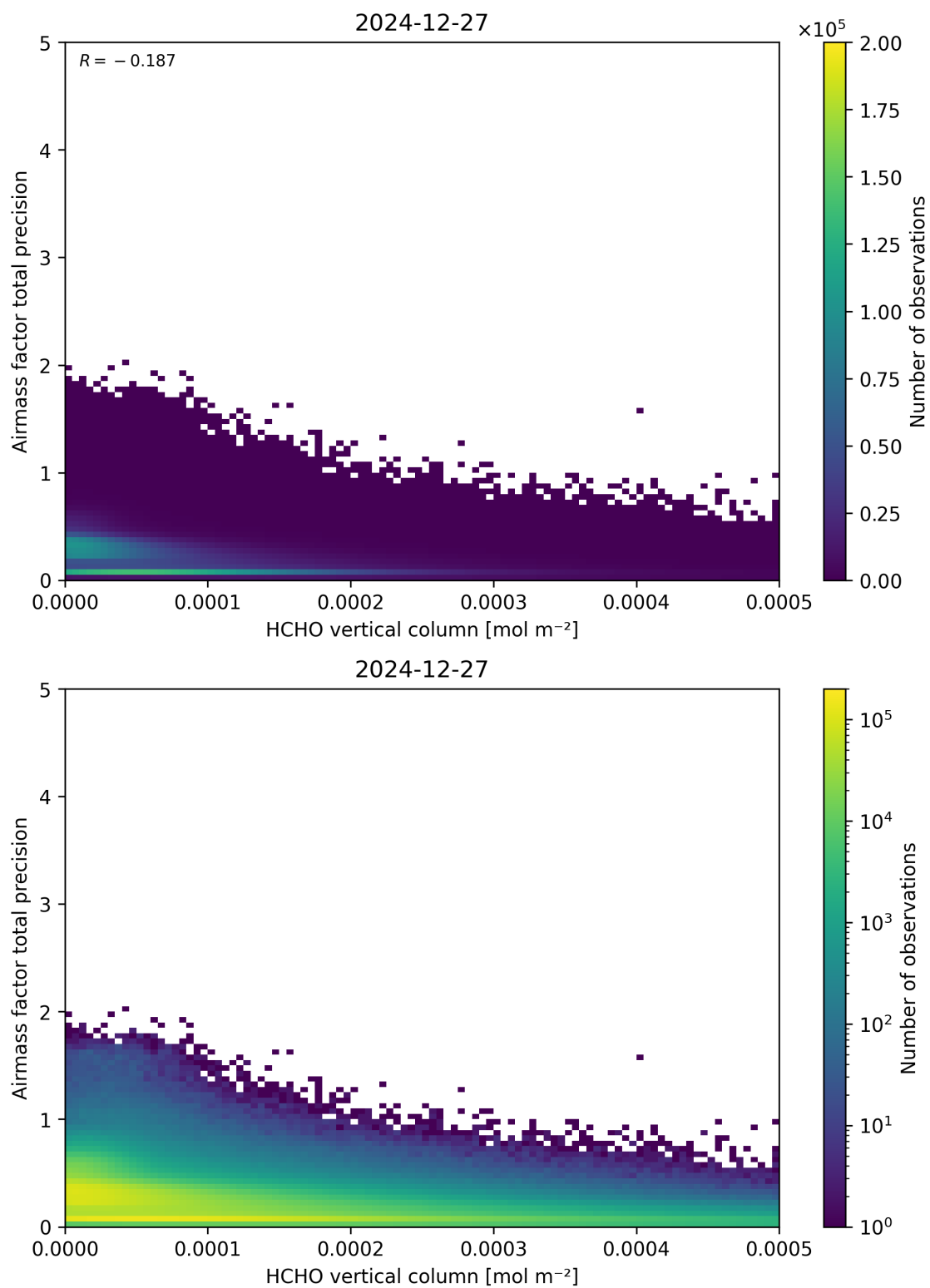
Figure 132: Scatter density plot of “HCHO vertical column” against “Airmass factor total precision” for 2024-12-27 to 2024-12-28.
