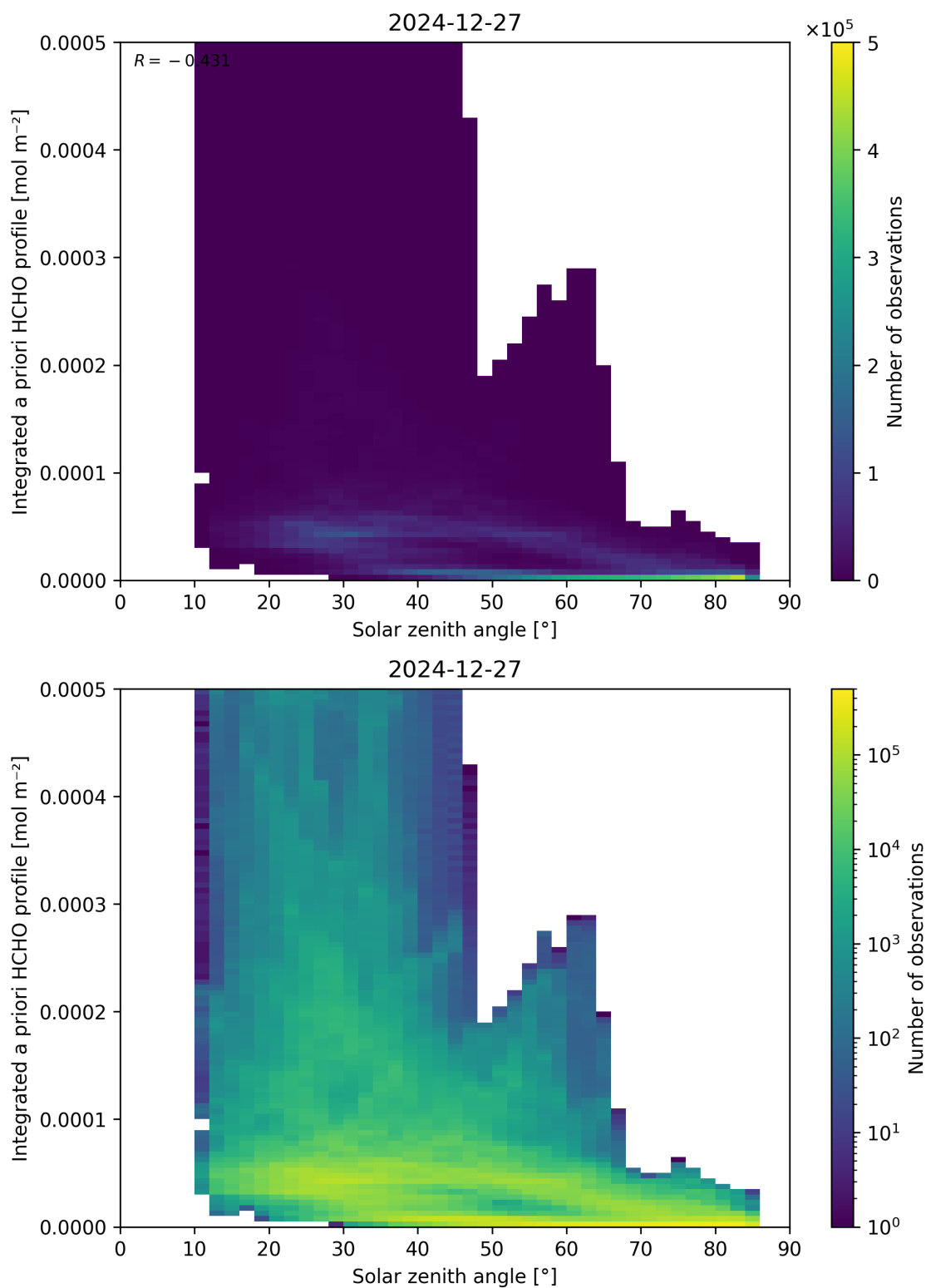
Figure 180: Scatter density plot of “Solar zenith angle” against “Integrated a priori HCHO profile” for 2024-12-27 to 2024-12-28.
