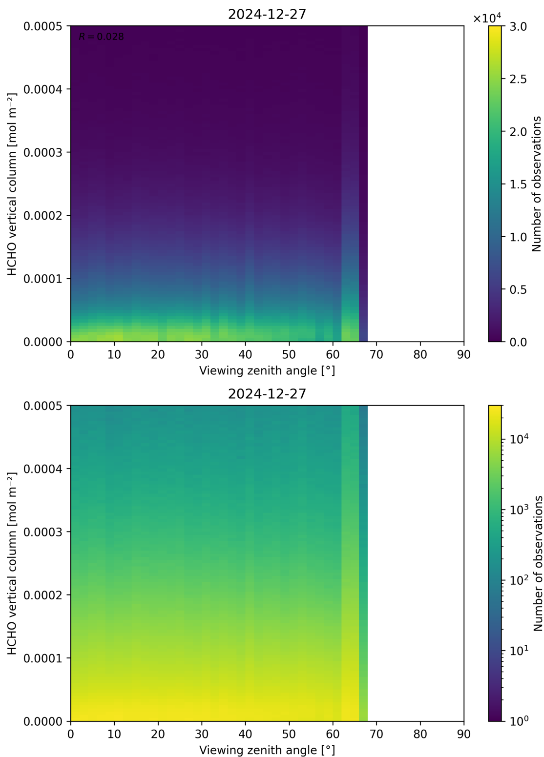
Figure 192: Scatter density plot of “Viewing zenith angle” against “HCHO vertical column” for 2024-12-27 to 2024-12-28.
