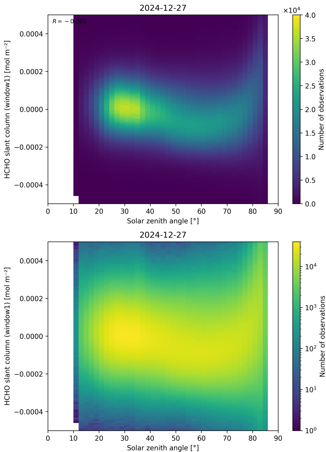
Figure 173: Scatter density plot of “Solar zenith angle” against “HCHO slant column (window1)” for 2024-12-27 to 2024-12-28.
