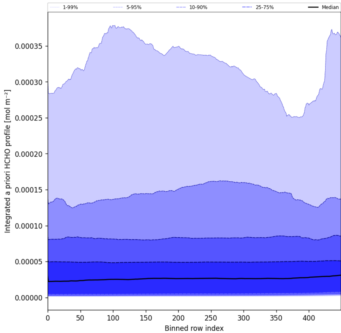
Figure 57: Along track statistics of “Integrated a priori HCHO profile” for 2024-12-27 to 2024-12-28
