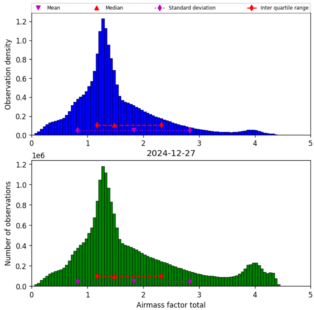
Figure 40: Histogram of “Airmass factor total” for 2024-12-27 to 2024-12-28
