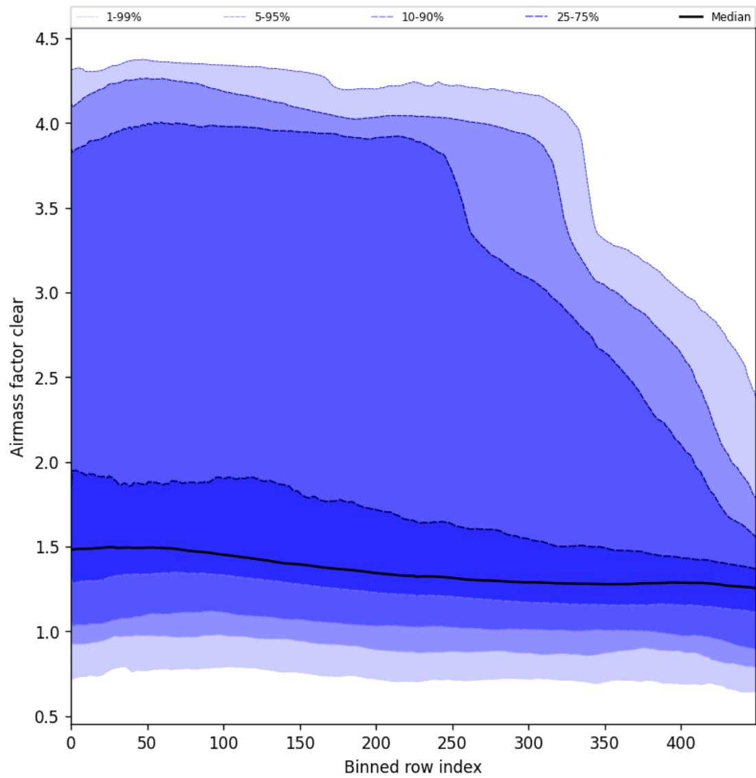
Figure 56: Along track statistics of “Air mass factor clear” for 2024-12-27 to 2024-12-28
