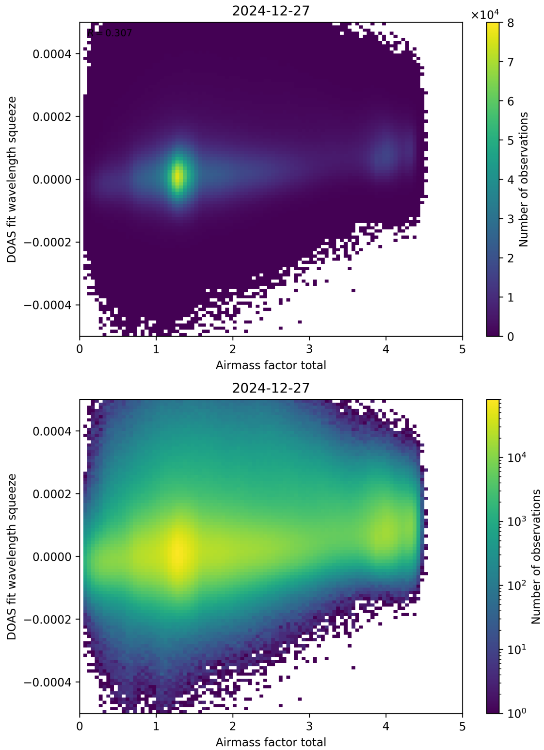
Figure 99: Scatter density plot of “Airmass factor total” against “DOAS fit wavelength squeeze” for 2024-12-27 to 2024-12-28.
