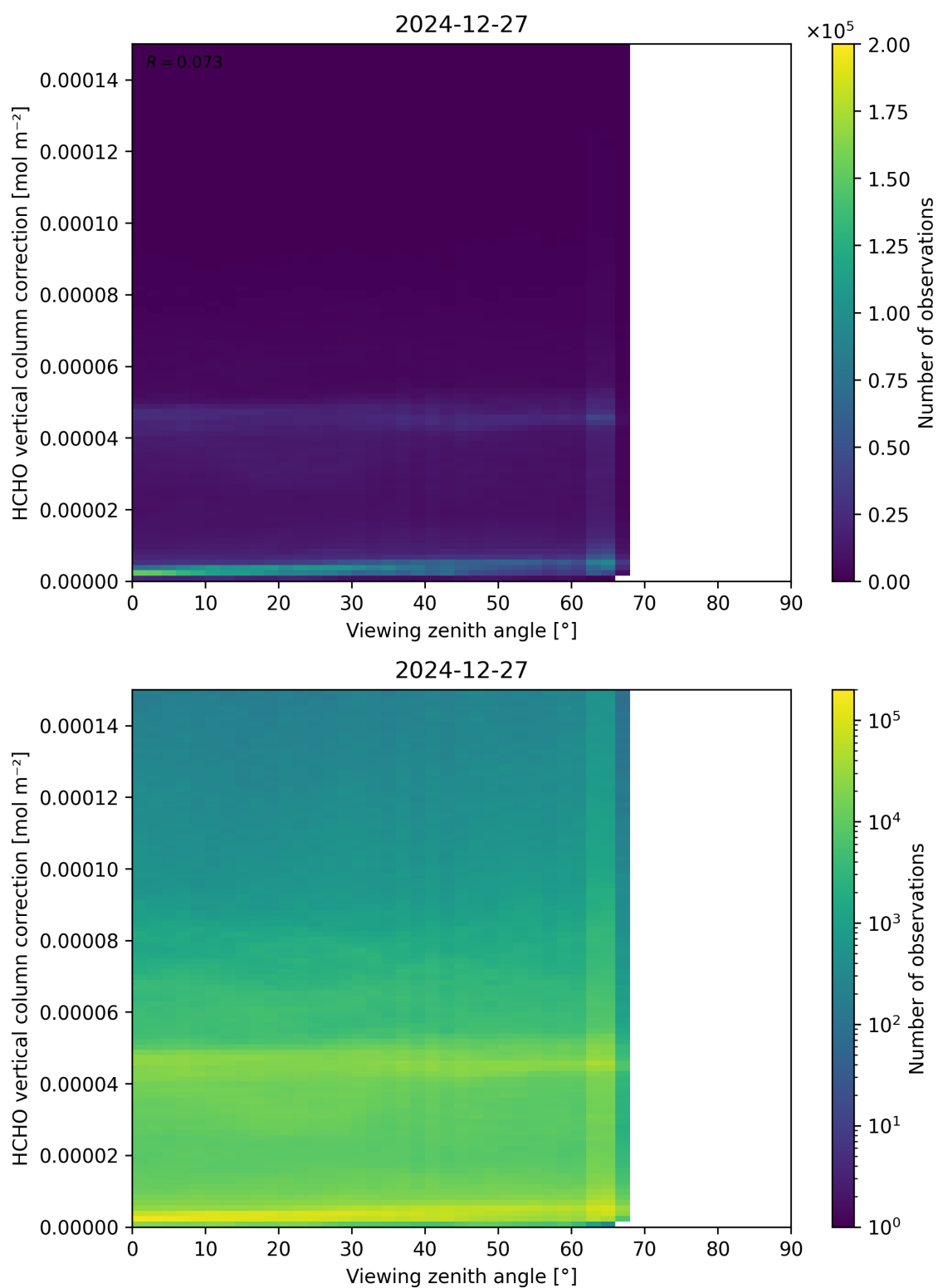
Figure 193: Scatter density plot of “Viewing zenith angle” against “HCHO vertical column correction” for 2024-12-27 to 2024-12-28.
