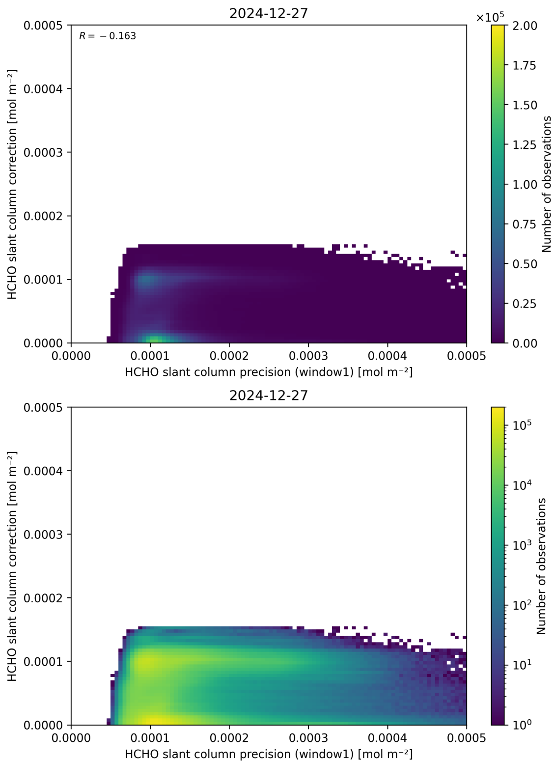
Figure 93: Scatter density plot of “HCHO slant column precision (window1)” against “HCHO slant column correction” for 2024-12-27 to 2024-12-28.
