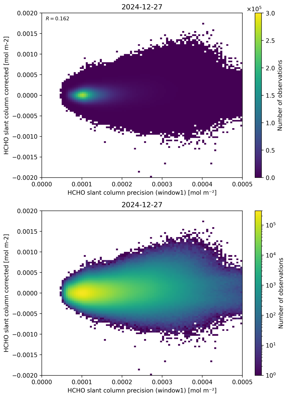
Figure 92: Scatter density plot of “HCHO slant column precision (window1)” against “HCHO slant column corrected” for 2024-12-27 to 2024-12-28.
