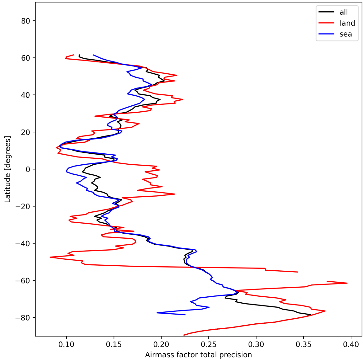
Figure 27: Zonal average of “Airmass factor total precision” for 2024-12-27 to 2024-12-28.
