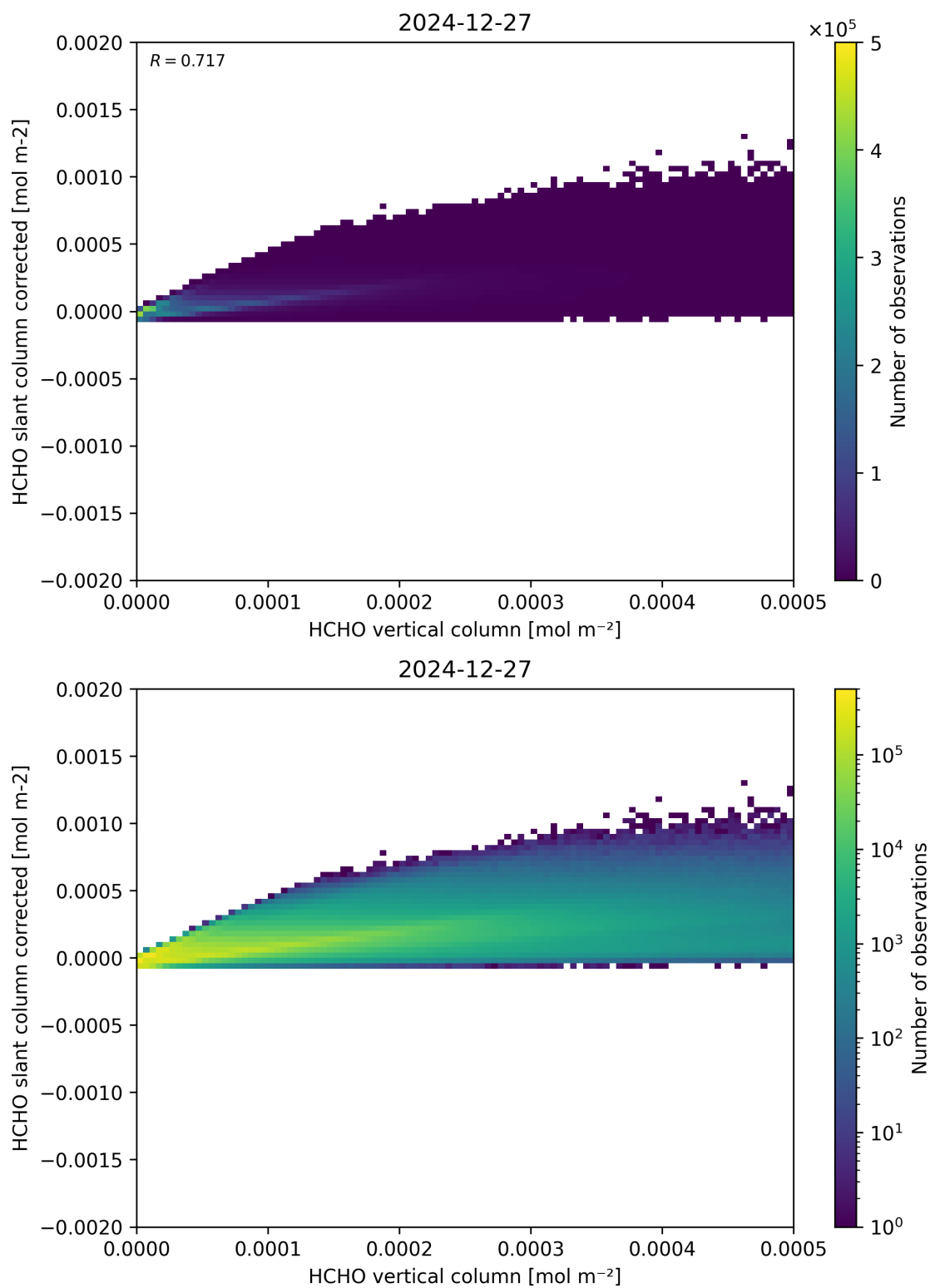
Figure 127: Scatter density plot of “HCHO vertical column” against “HCHO slant column corrected” for 2024-12-27 to 2024-12-28.
