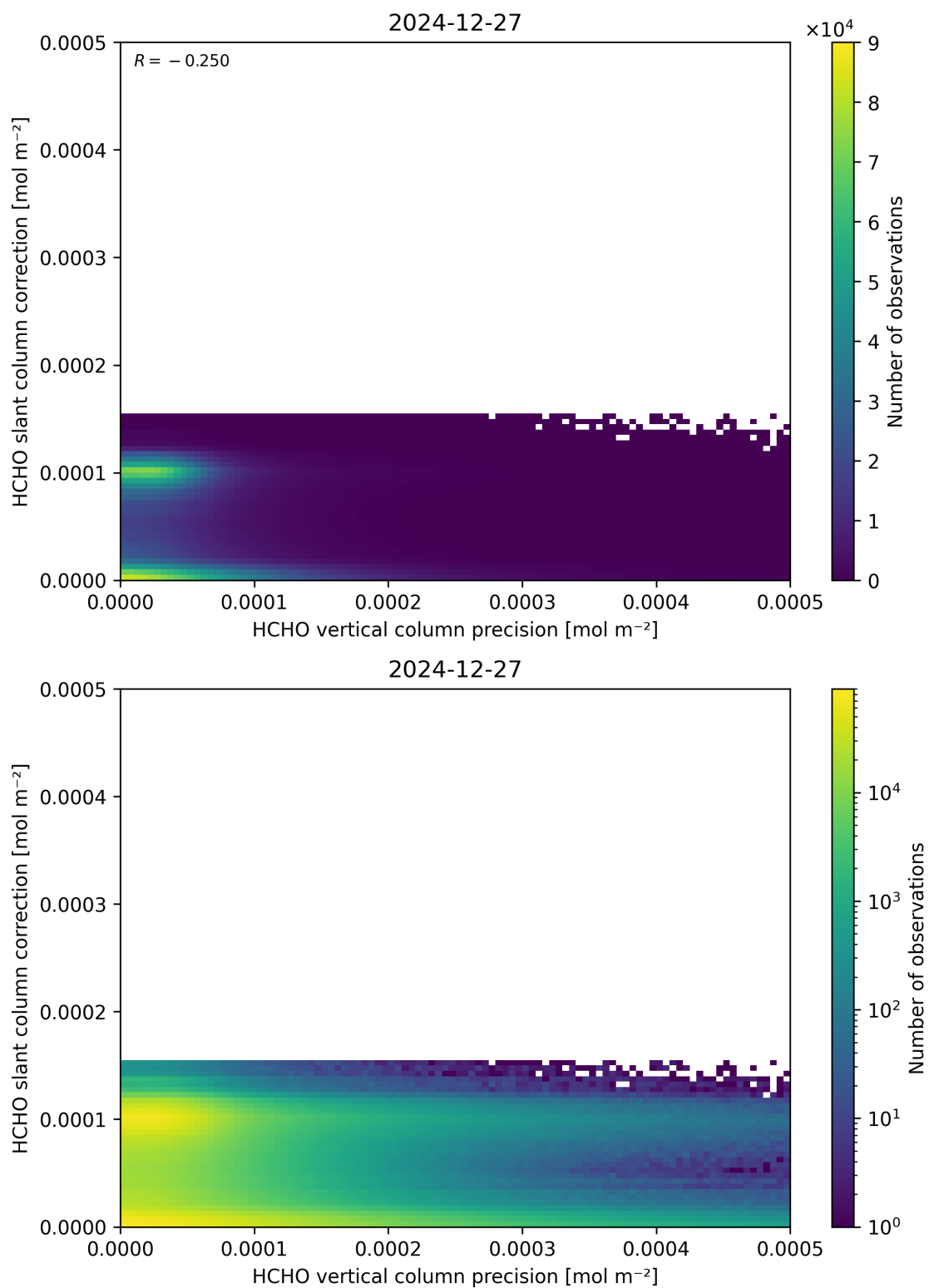
Figure 141: Scatter density plot of “HCHO vertical column precision” against “HCHO slant column correction” for 2024-12-27 to 2024-12-28.
