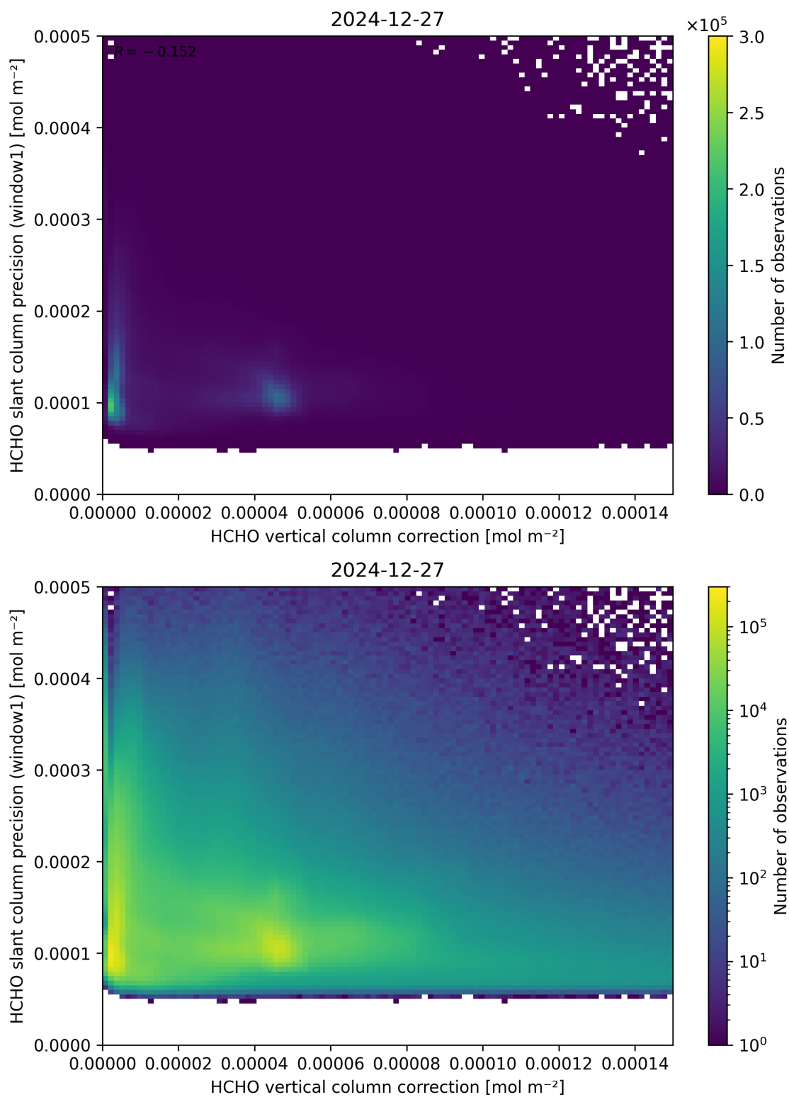
Figure 119: Scatter density plot of “HCHO vertical column correction” against “HCHO slant column precision (window1)” for 2024-12-27 to 2024-12-28.
