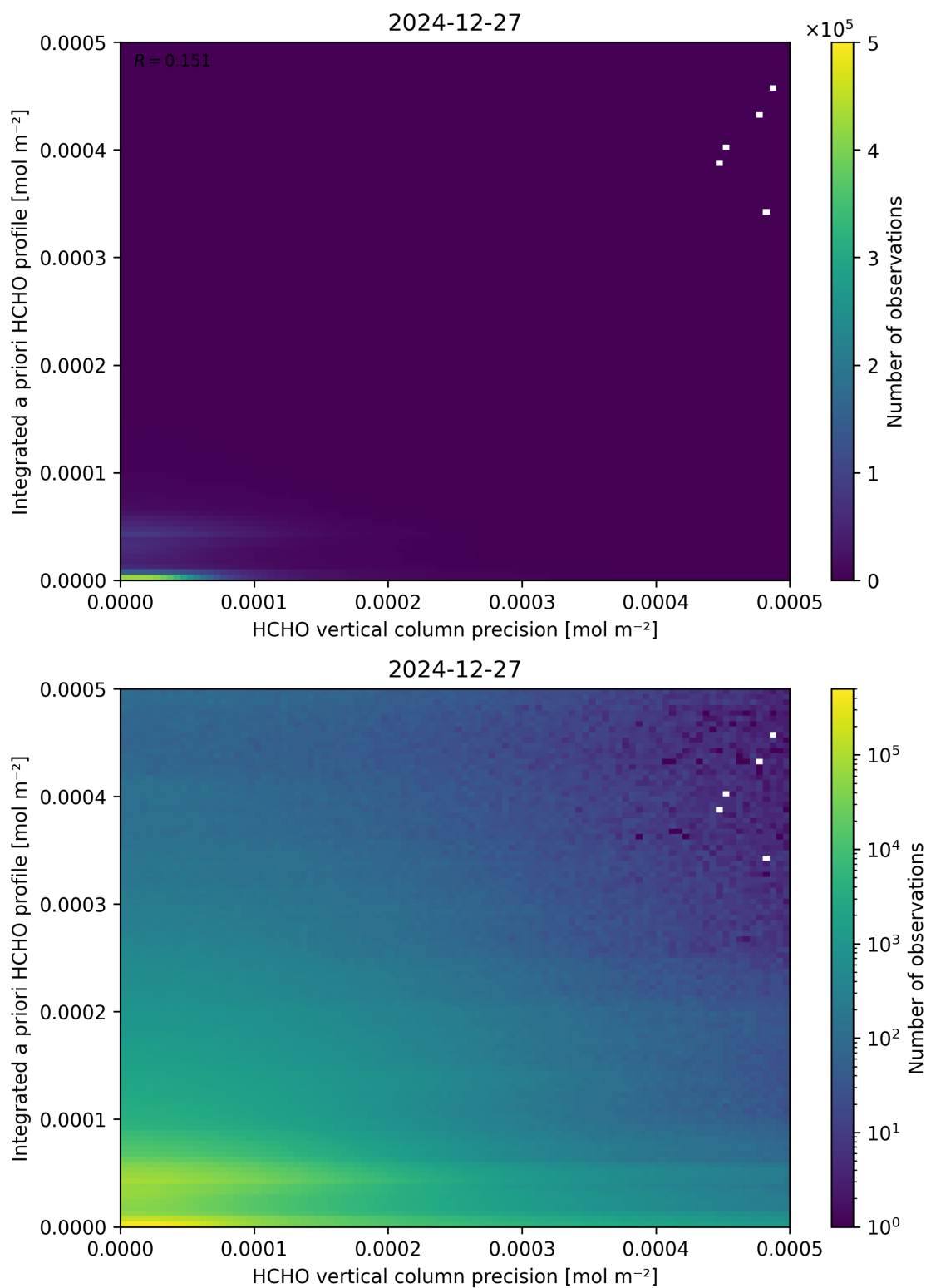
Figure 147: Scatter density plot of “HCHO vertical column precision” against “Integrated a priori HCHO profile” for 2024-12-27 to 2024-12-28.
