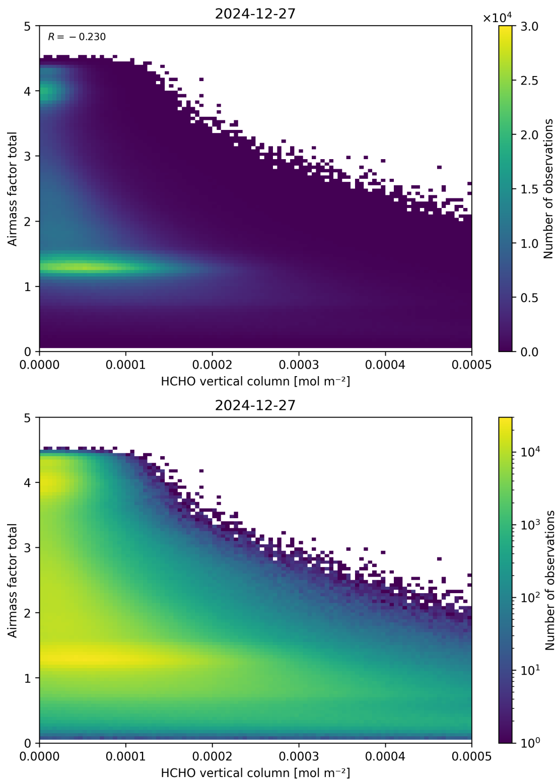
Figure 131: Scatter density plot of “HCHO vertical column” against “Airmass factor total” for 2024-12-27 to 2024-12-28.
