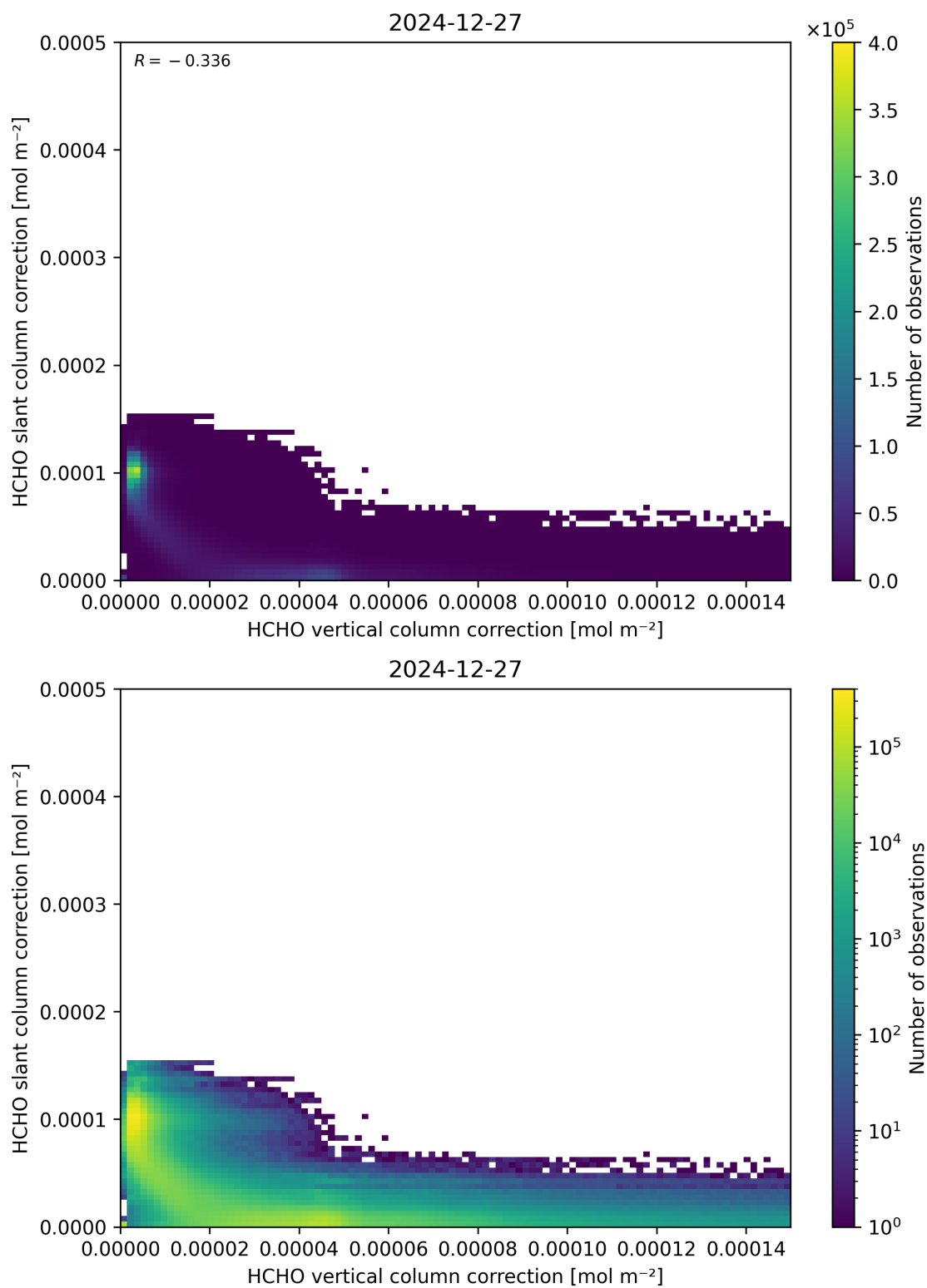
Figure 117: Scatter density plot of “HCHO vertical column correction” against “HCHO slant column correction” for 2024-12-27 to 2024-12-28.
