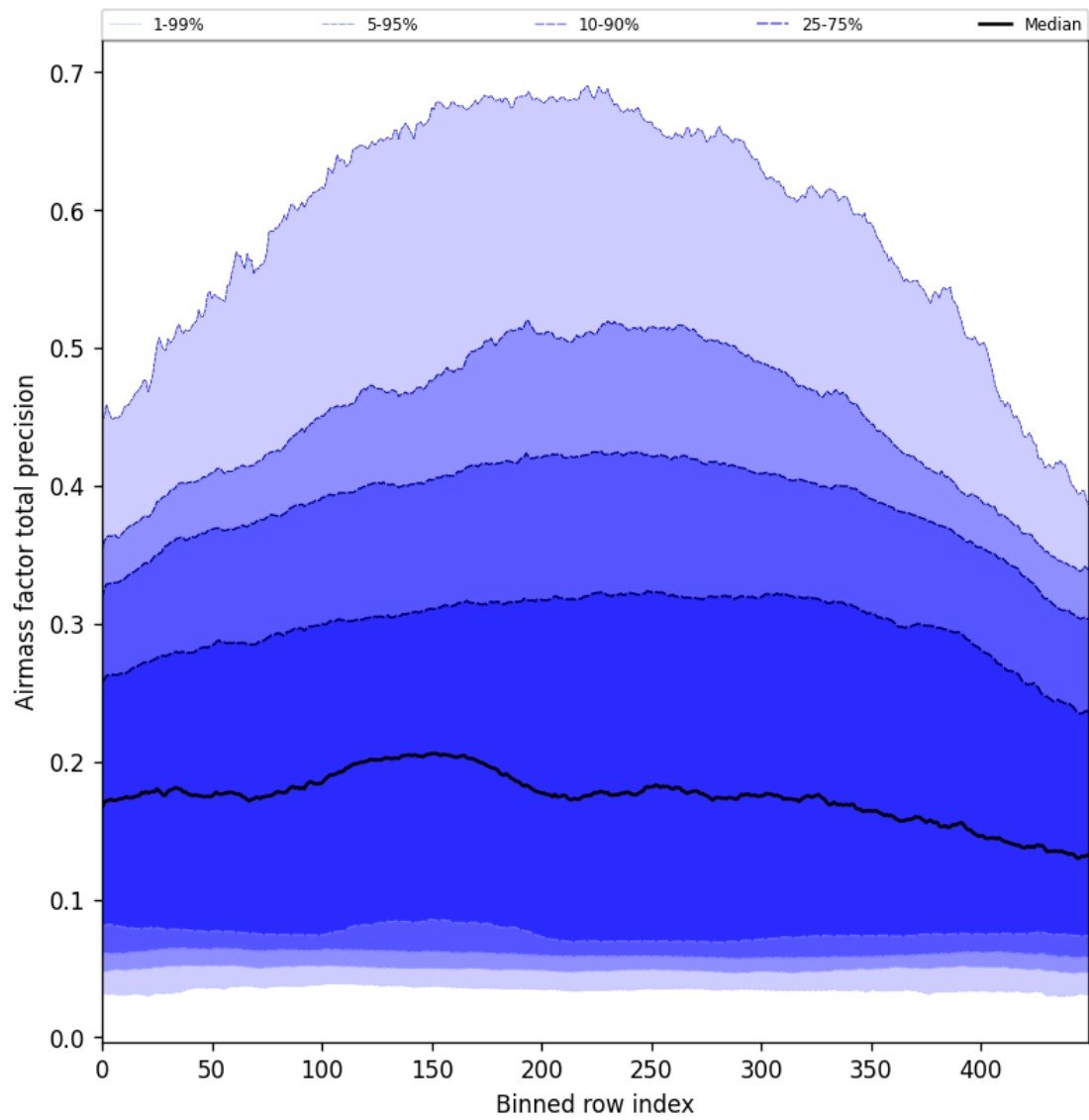
Figure 55: Along track statistics of “Airmass factor total precision” for 2024-12-27 to 2024-12-28
