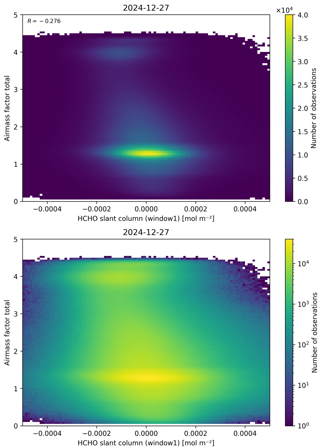
Figure 85: Scatter density plot of “HCHO slant column (window1)” against “Airmass factor total” for 2024-12-27 to 2024-12-28.
