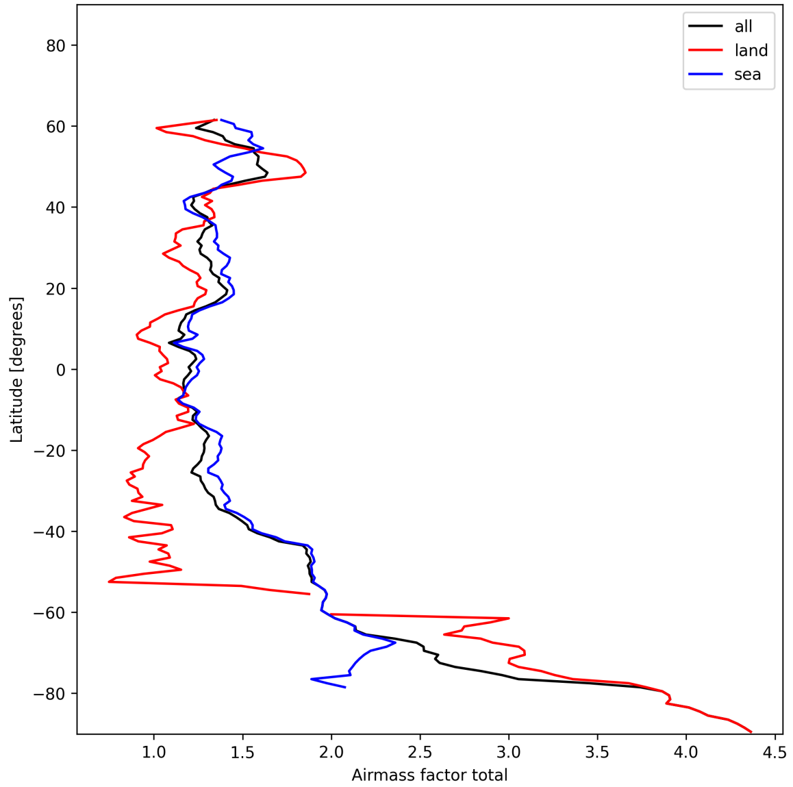
Figure 26: Zonal average of “Airmass factor total” for 2024-12-27 to 2024-12-28.
