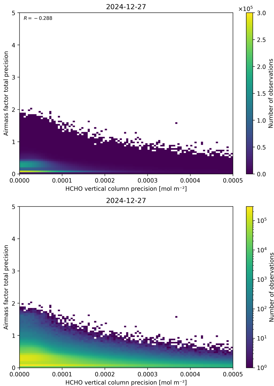
Figure 145: Scatter density plot of “HCHO vertical column precision” against “Airmass factor total precision” for 2024-12-27 to 2024-12-28.
