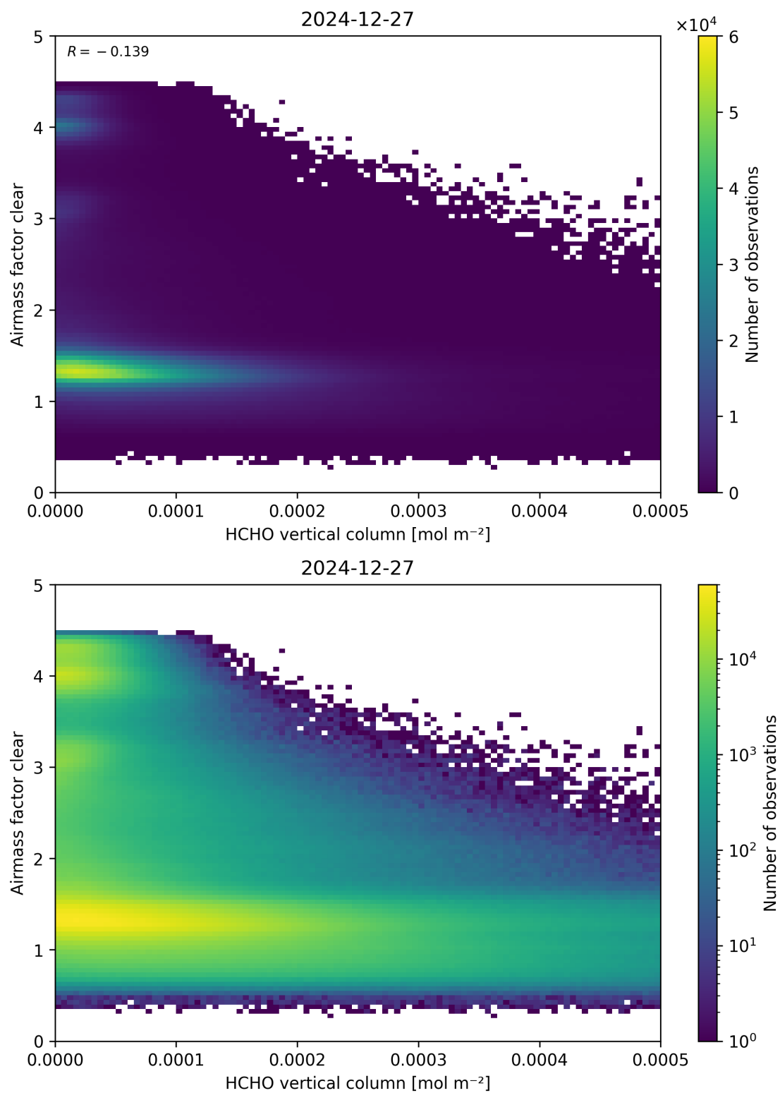
Figure 126: Scatter density plot of “HCHO vertical column” against “Airmass factor clear” for 2024-12-27 to 2024-12-28.
