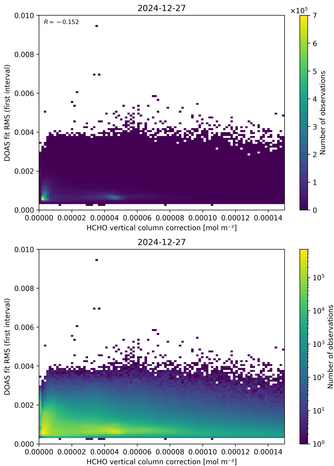
Figure 112: Scatter density plot of “HCHO vertical column correction” against “DOAS fit RMS (first interval)” for 2024-12-27 to 2024-12-28.
