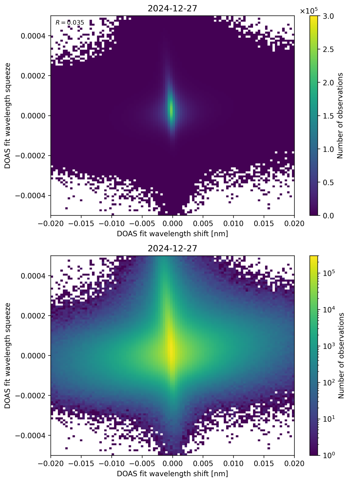
Figure 65: Scatter density plot of “DOAS fit wavelength shift” against “DOAS fit wavelength squeeze” for 2024-12-27 to 2024-12-28.
