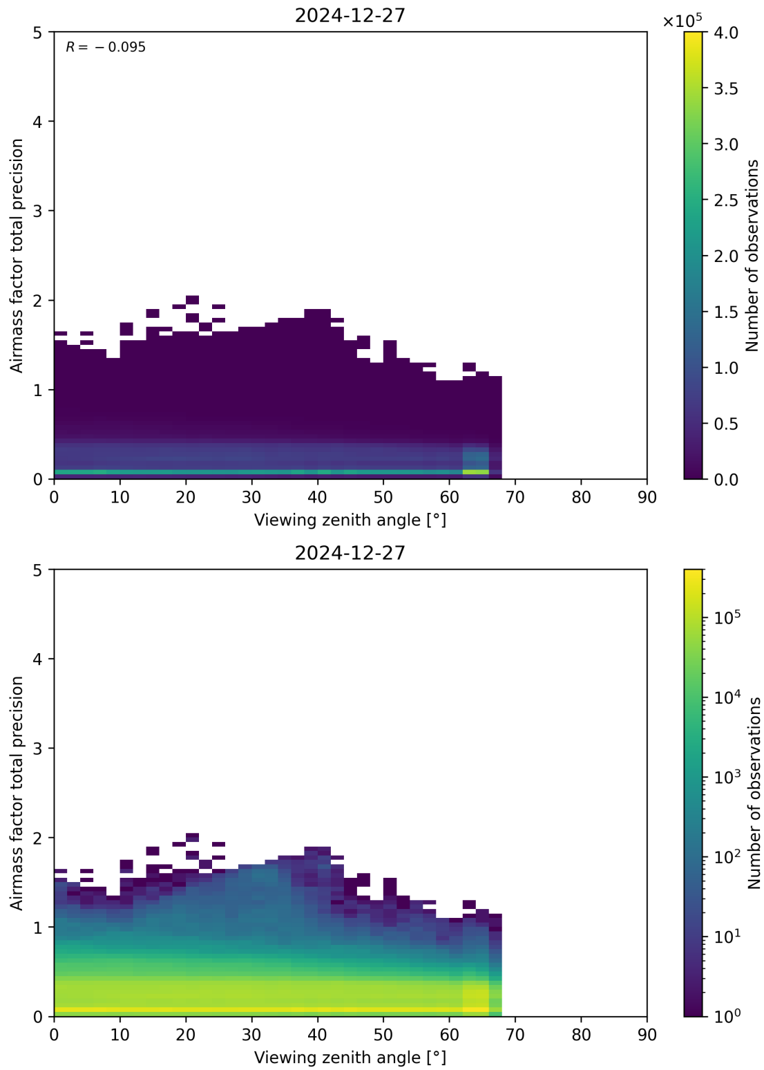
Figure 191: Scatter density plot of “Viewing zenith angle” against “Airmass factor total precision” for 2024-12-27 to 2024-12-28.
