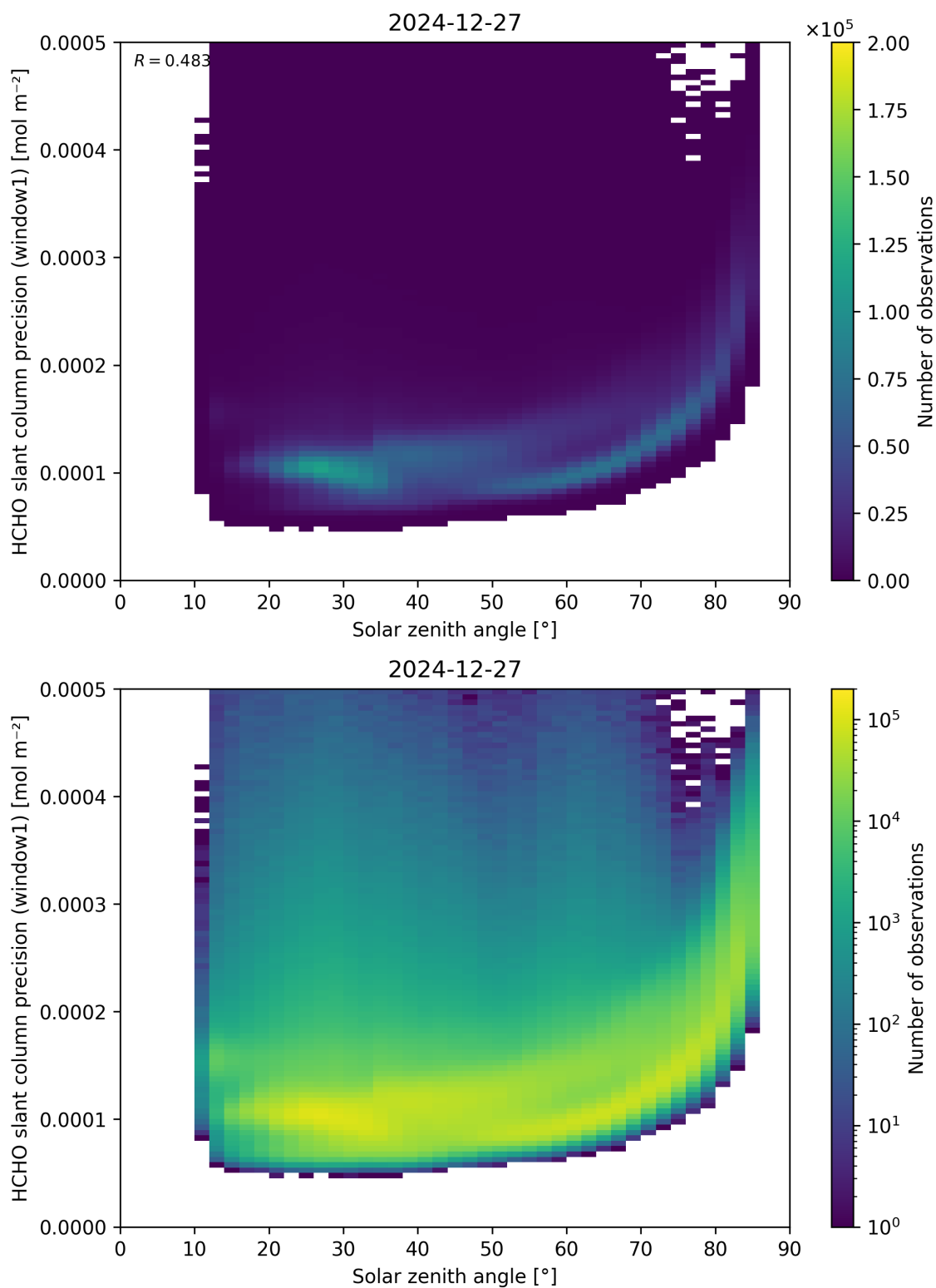
Figure 174: Scatter density plot of “Solar zenith angle” against “HCHO slant column precision (window1)” for 2024-12-27 to 2024-12-28.
