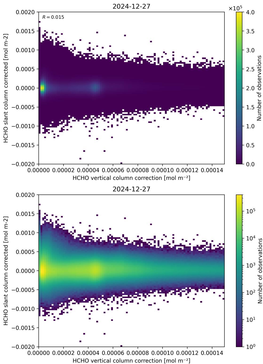
Figure 116: Scatter density plot of “HCHO vertical column correction” against “HCHO slant column corrected” for 2024-12-27 to 2024-12-28.
