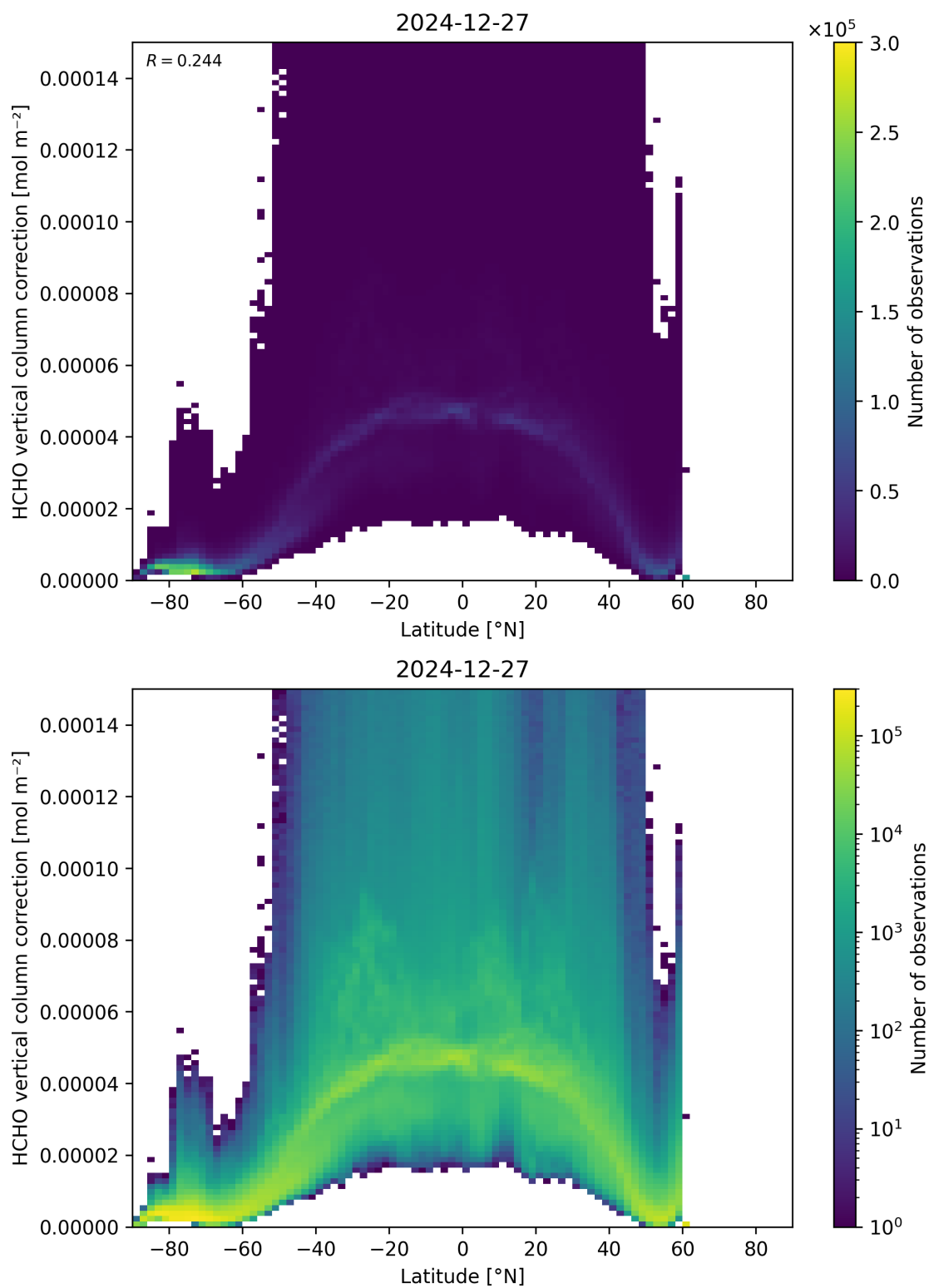
Figure 164: Scatter density plot of “Latitude” against “HCHO vertical column correction” for 2024-12-27 to 2024-12-28.
