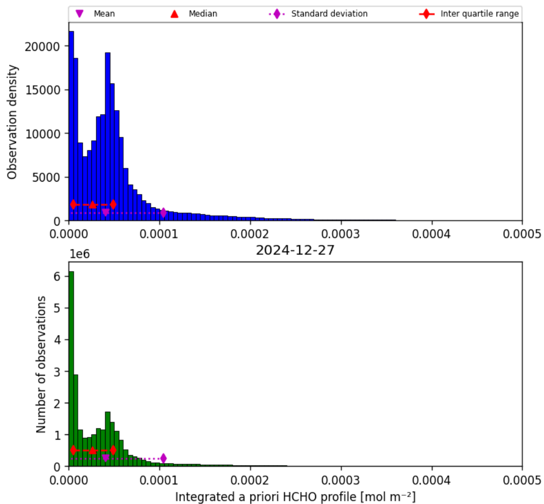
Figure 43: Histogram of “Integrated a priori HCHO profile” for 2024-12-27 to 2024-12-28
