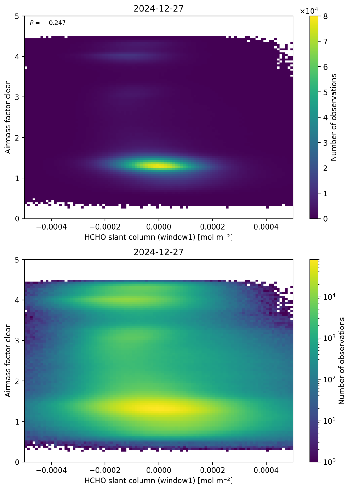
Figure 81: Scatter density plot of “HCHO slant column (window1)” against “Airmass factor clear” for 2024-12-27 to 2024-12-28.
