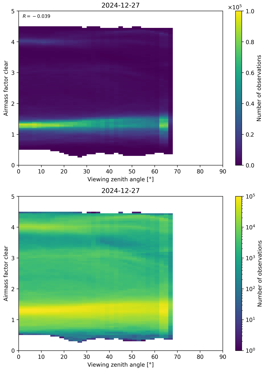
Figure 185: Scatter density plot of “Viewing zenith angle” against “Airmass factor clear” for 2024-12-27 to 2024-12-28.
