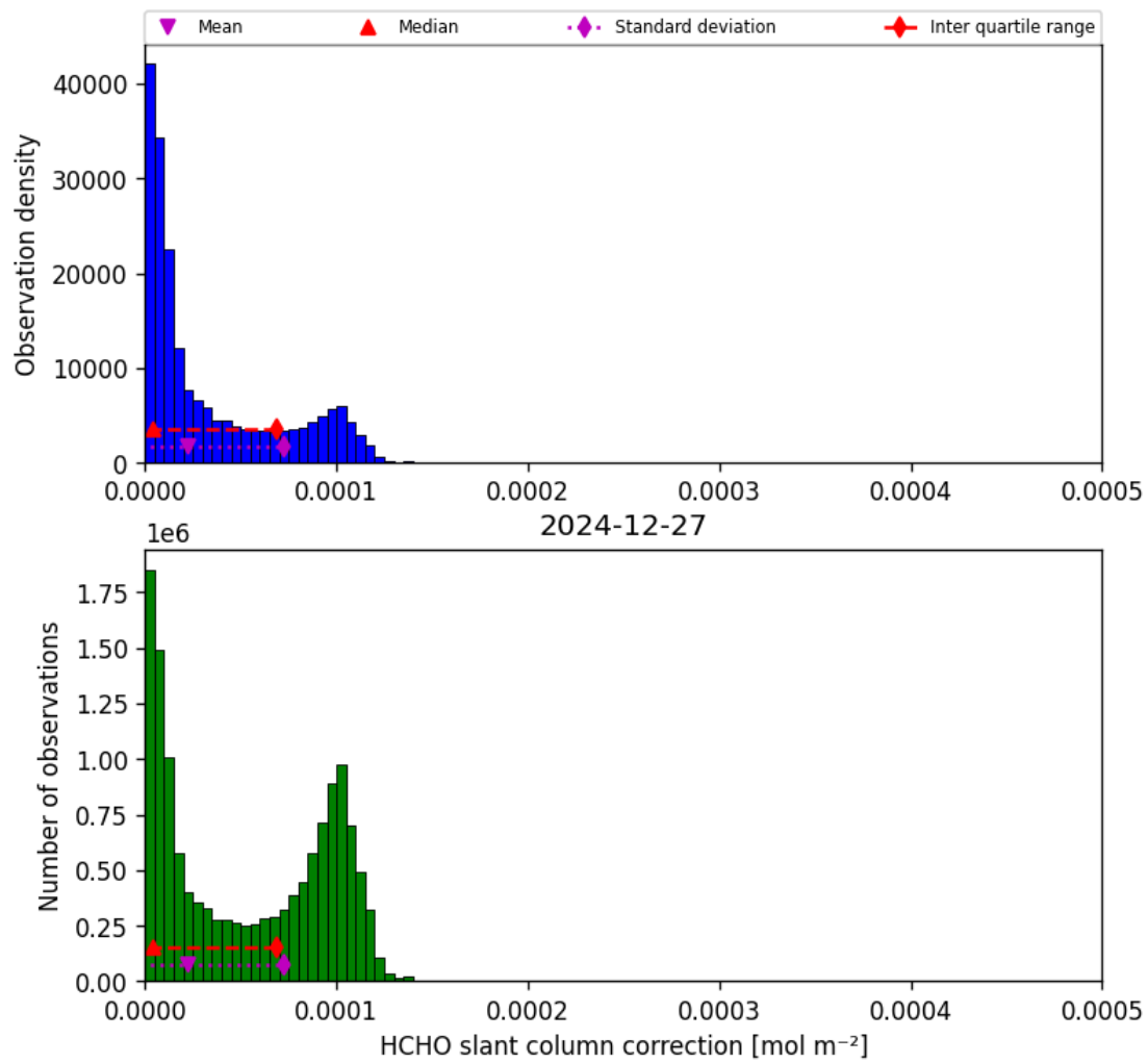
Figure 47: Histogram of “HCHO slant column correction” for 2024-12-27 to 2024-12-28
