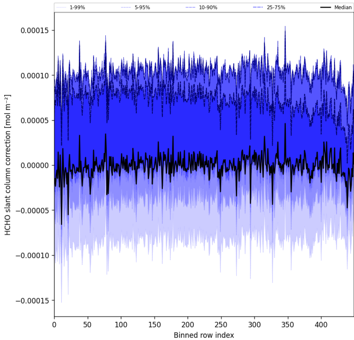
Figure 61: Along track statistics of “HCHO slant column correction” for 2024-12-27 to 2024-12-28
