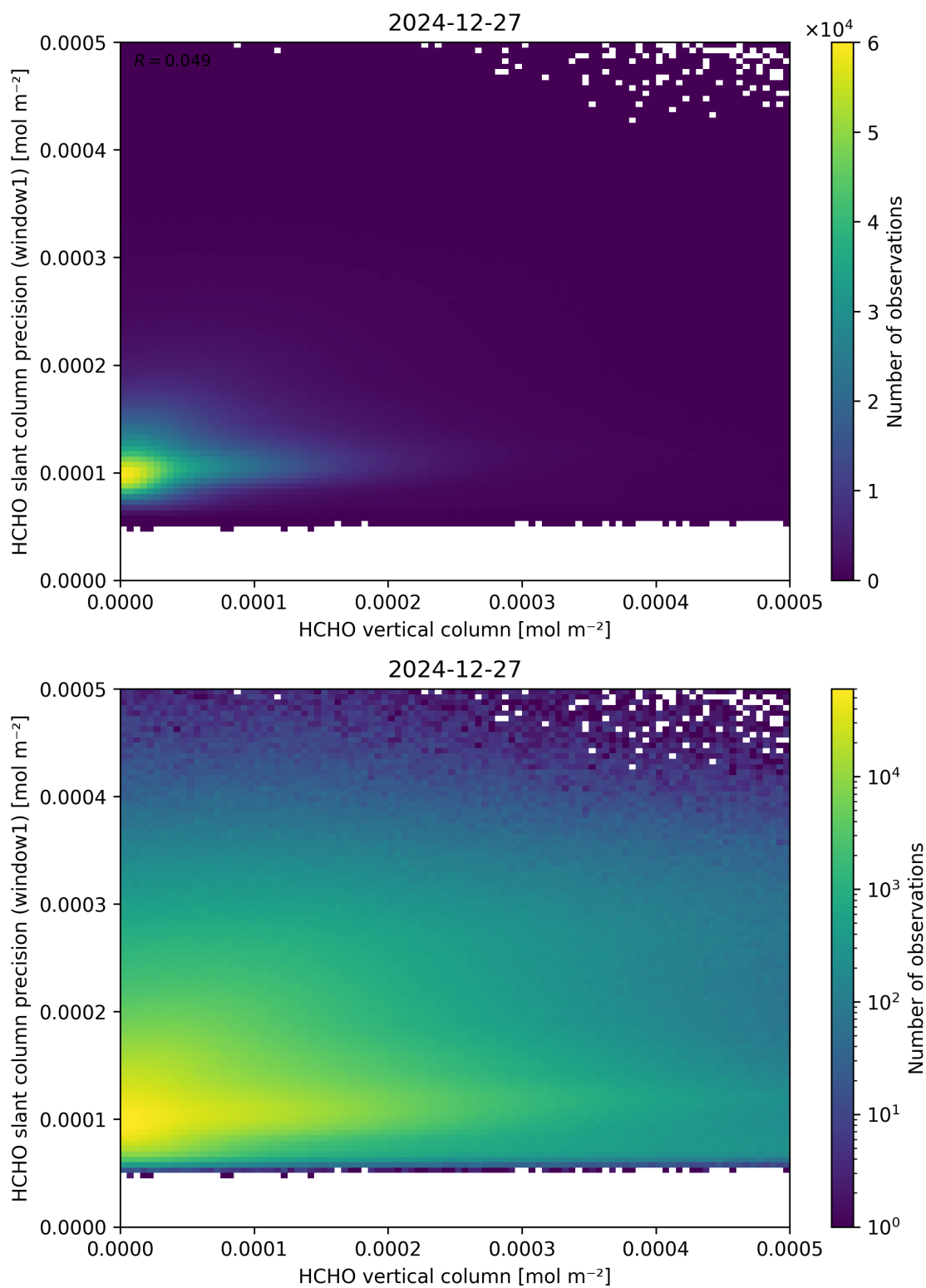
Figure 130: Scatter density plot of “HCHO vertical column” against “HCHO slant column precision (window1)” for 2024-12-27 to 2024-12-28.
