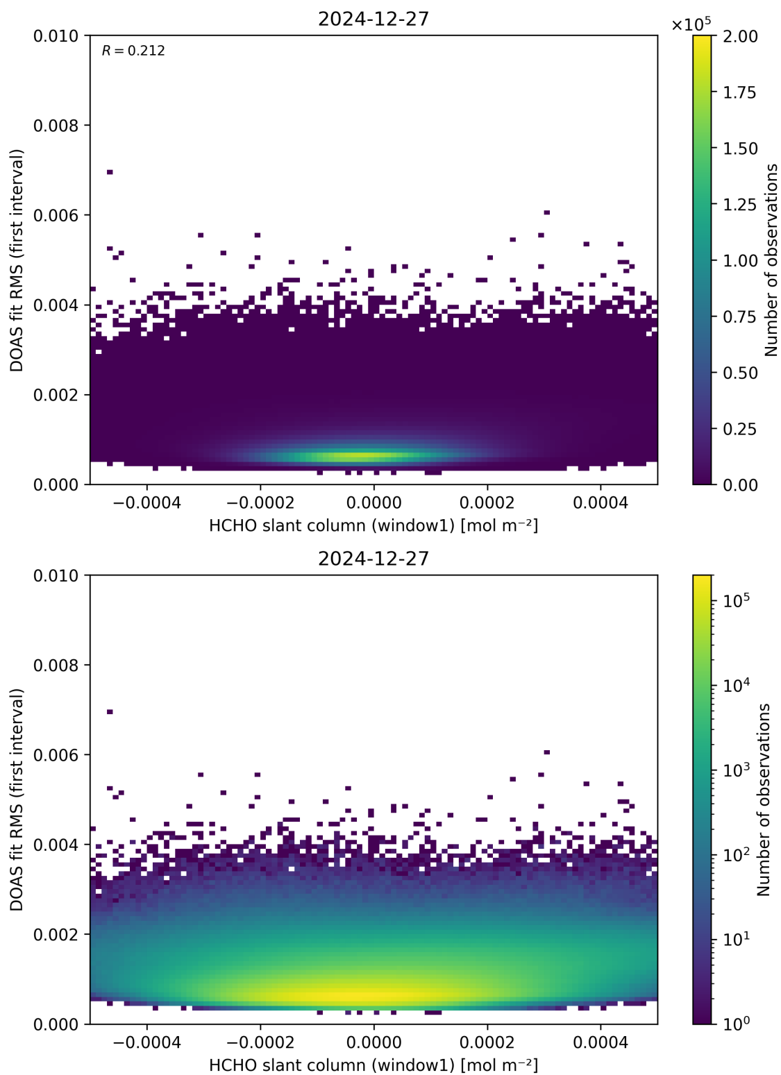
Figure 78: Scatter density plot of “HCHO slant column (window1)” against “DOAS fit RMS (first interval)” for 2024-12-27 to 2024-12-28.
