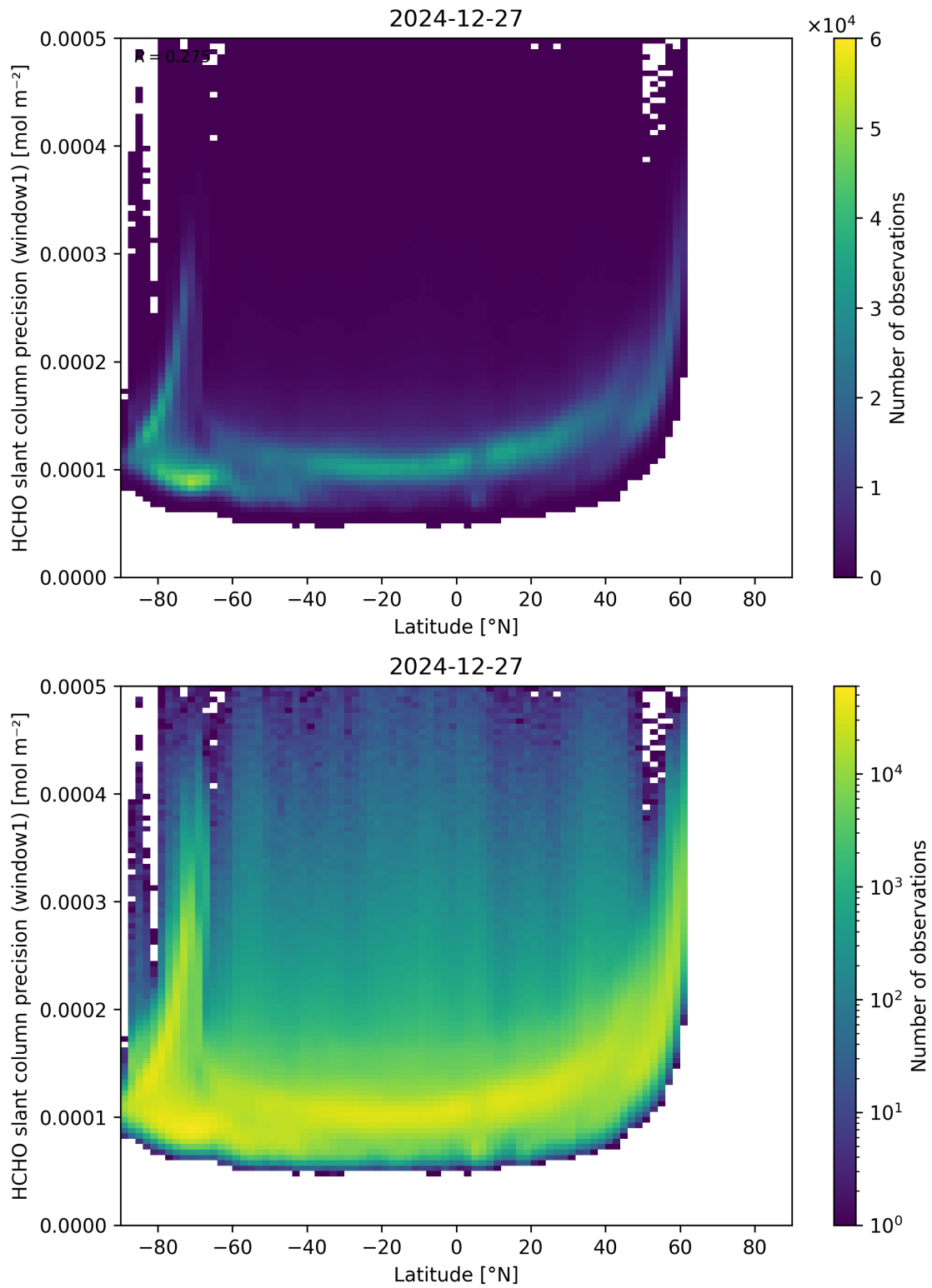
Figure 160: Scatter density plot of “Latitude” against “HCHO slant column precision (window1)” for 2024-12-27 to 2024-12-28.
