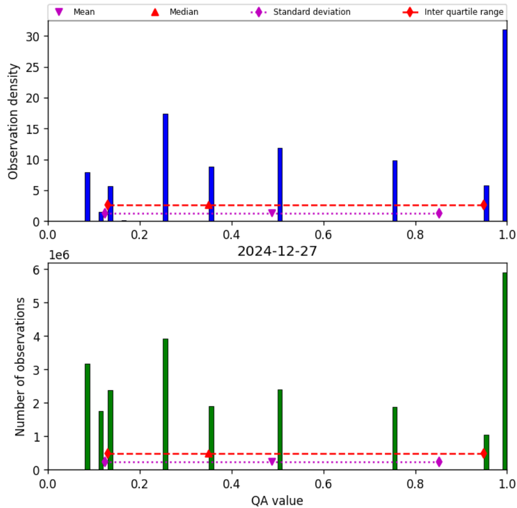
Figure 34: Histogram of “QA value” for 2024-12-27 to 2024-12-28
