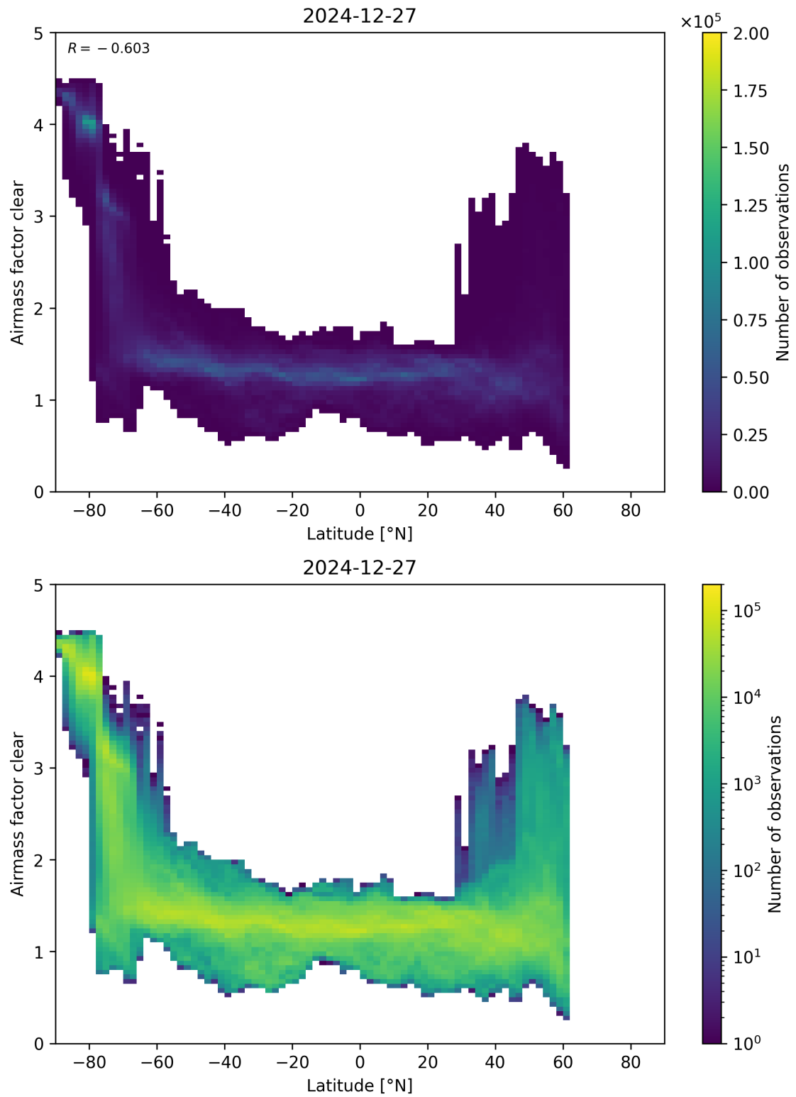
Figure 156: Scatter density plot of “Latitude” against “Airmass factor clear” for 2024-12-27 to 2024-12-28.
