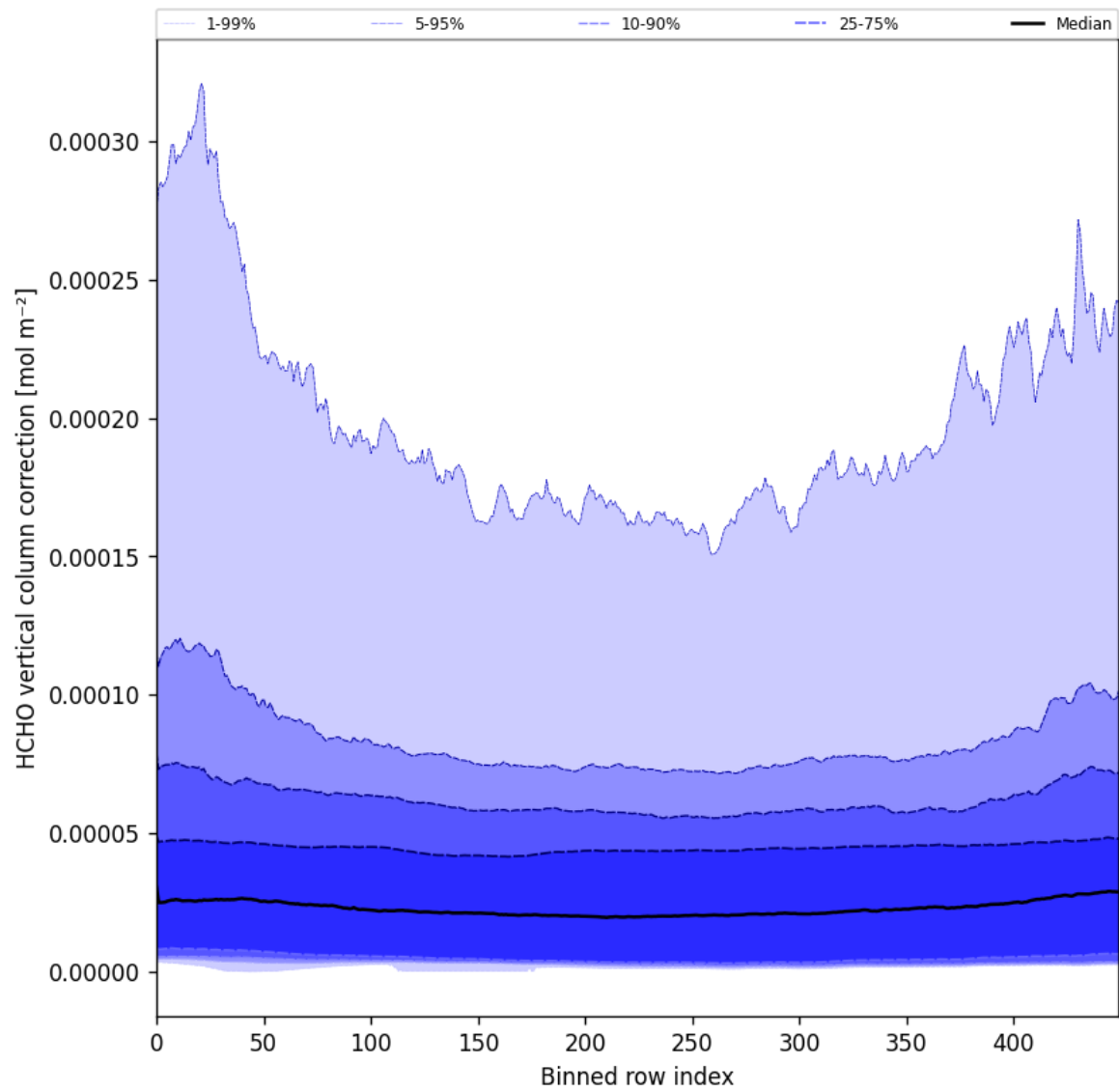
Figure 51: Along track statistics of “HCHO vertical column correction” for 2024-12-27 to 2024-12-28
