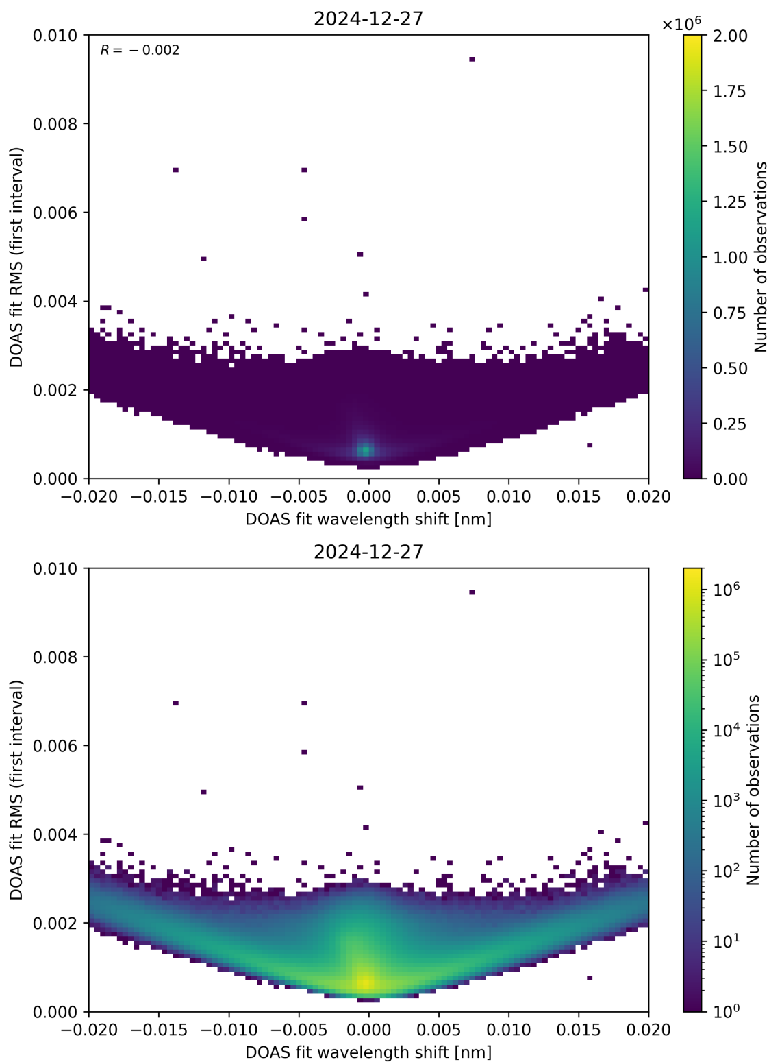
Figure 64: Scatter density plot of “DOAS fit wavelength shift” against “DOAS fit RMS (first interval)” for 2024-12-27 to 2024-12-28.
