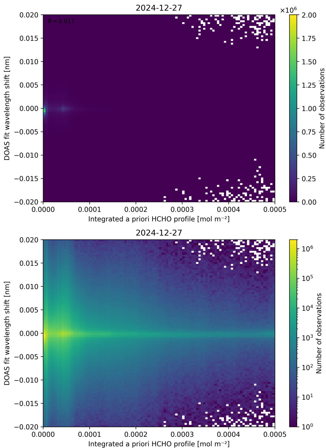
Figure 149: Scatter density plot of “Integrated a priori HCHO profile” against “DOAS fit wavelength shift” for 2024-12-27 to 2024-12-28.
