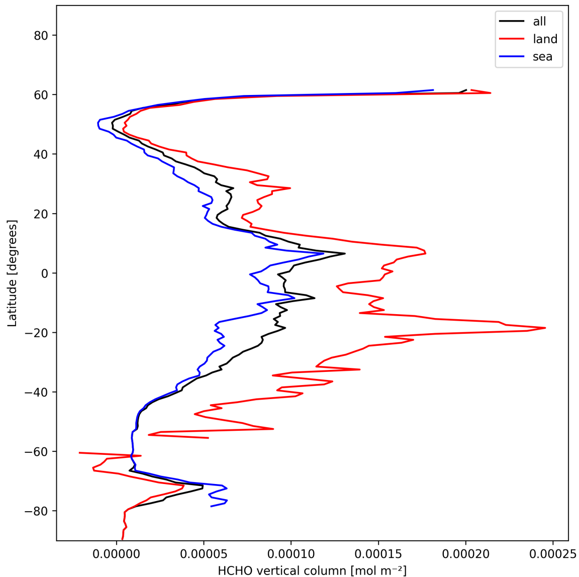
Figure 21: Zonal average of “HCHO vertical column” for 2024-12-27 to 2024-12-28.
