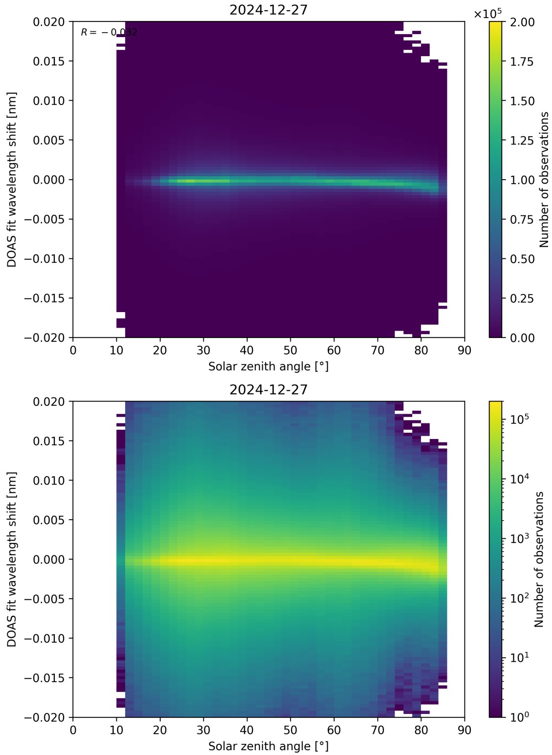
Figure 168: Scatter density plot of “Solar zenith angle” against “DOAS fit wavelength shift” for 2024-12-27 to 2024-12-28.
