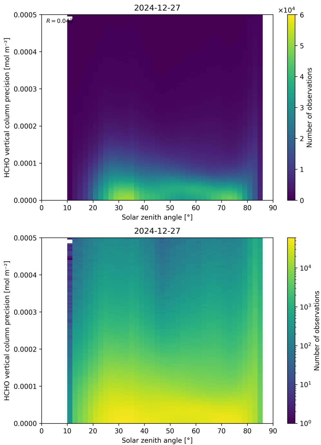
Figure 179: Scatter density plot of “Solar zenith angle” against “HCHO vertical column precision” for 2024-12-27 to 2024-12-28.
