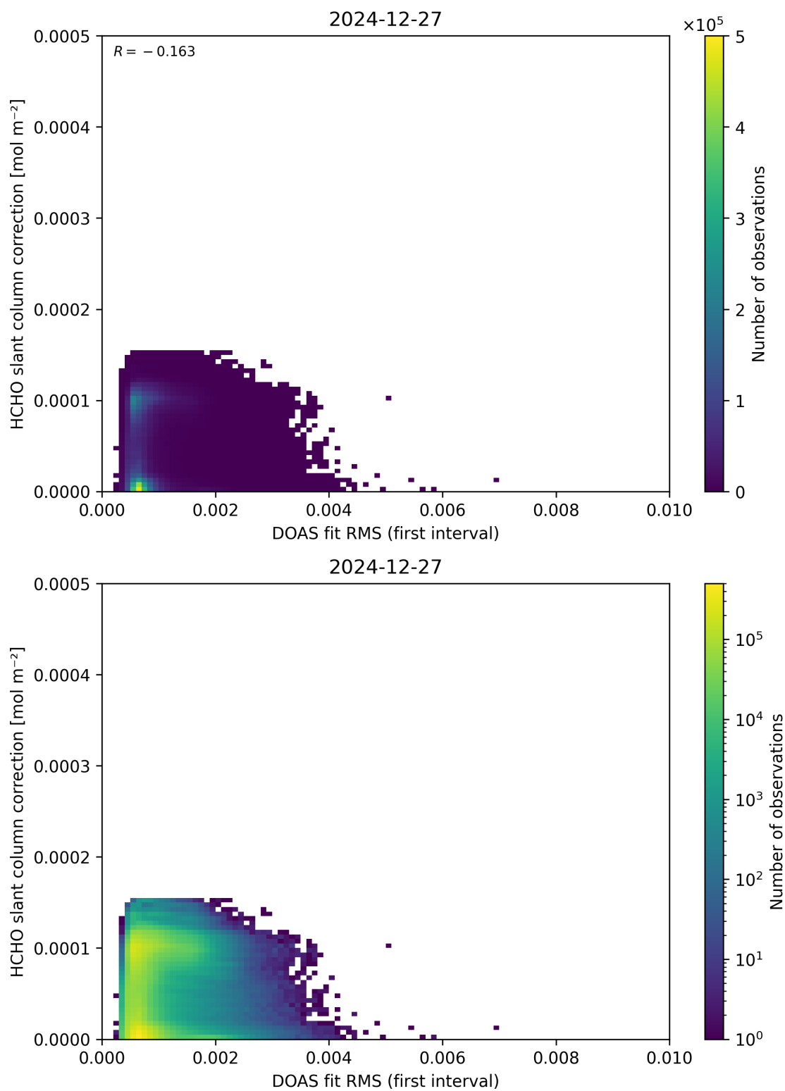
Figure 63: Scatter density plot of “DOAS fit RMS (first interval)” against “HCHO slant column correction” for 2024-12-27 to 2024-12-28.
