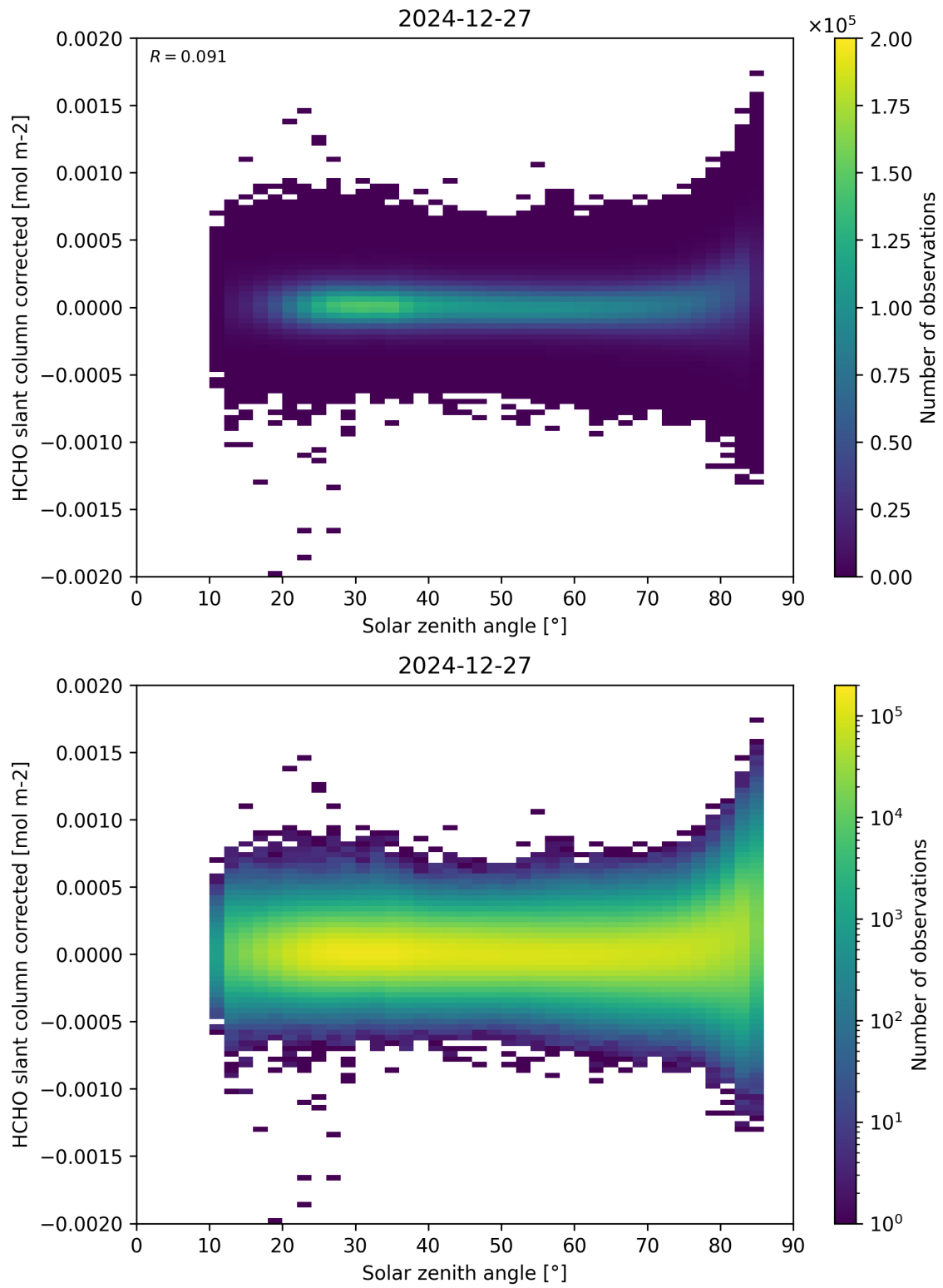
Figure 171: Scatter density plot of “Solar zenith angle” against “HCHO slant column corrected” for 2024-12-27 to 2024-12-28.
