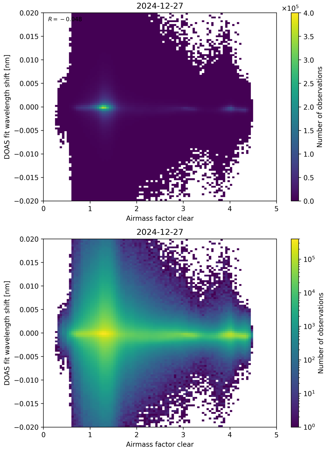
Figure 72: Scatter density plot of “Airmass factor clear” against “DOAS fit wavelength shift” for 2024-12-27 to 2024-12-28.
