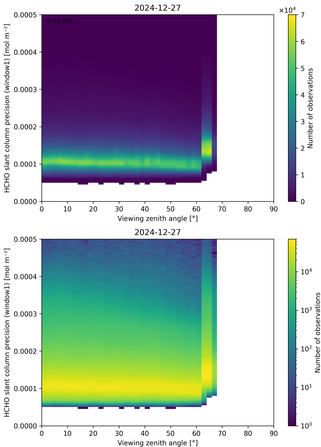
Figure 189: Scatter density plot of “Viewing zenith angle” against “HCHO slant column precision (window1)” for 2024-12-27 to 2024-12-28.
