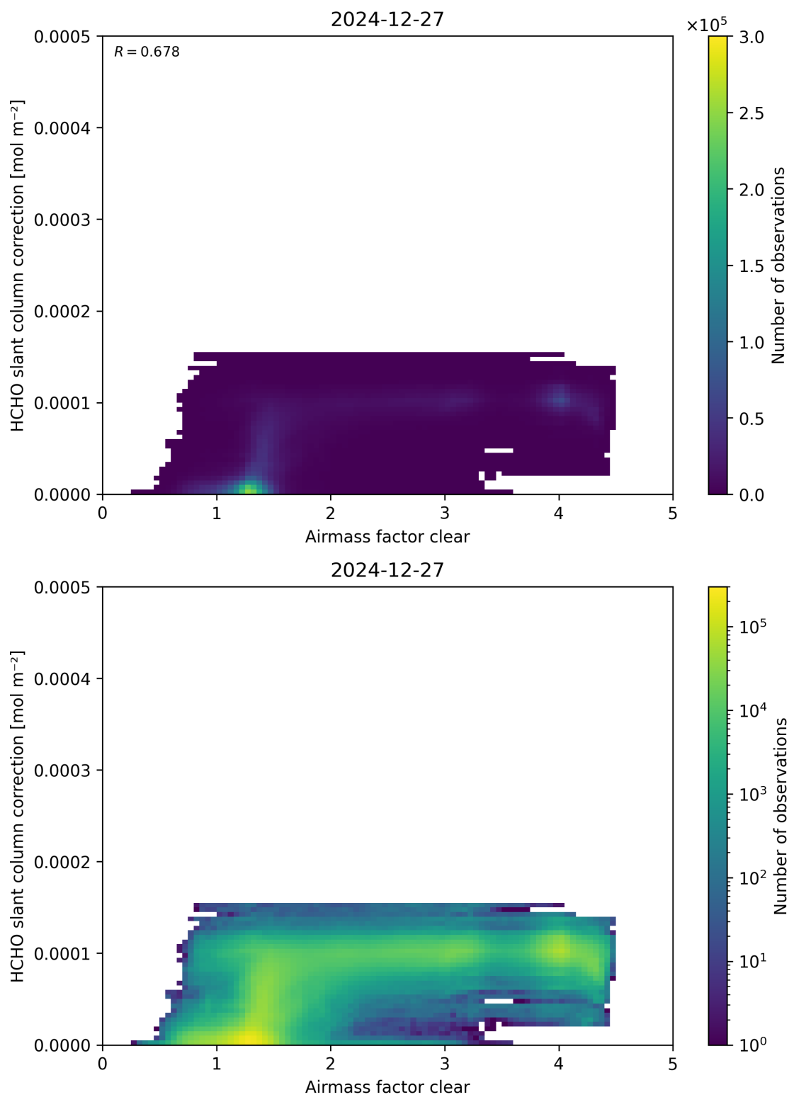
Figure 75: Scatter density plot of “Airmass factor clear” against “HCHO slant column correction” for 2024-12-27 to 2024-12-28.
