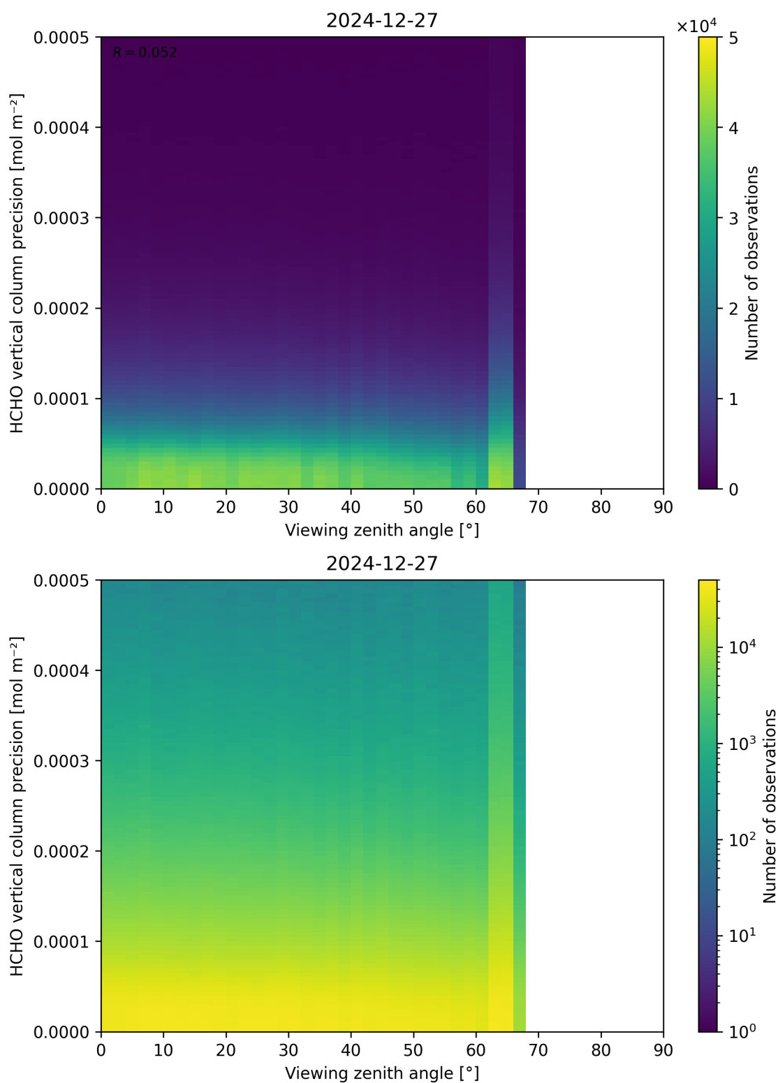
Figure 194: Scatter density plot of “Viewing zenith angle” against “HCHO vertical column precision” for 2024-12-27 to 2024-12-28.
