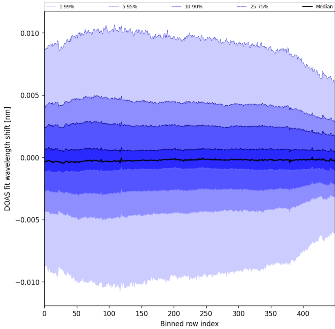
Figure 58: Along track statistics of “DOAS fit wavelength shift” for 2024-12-27 to 2024-12-28
