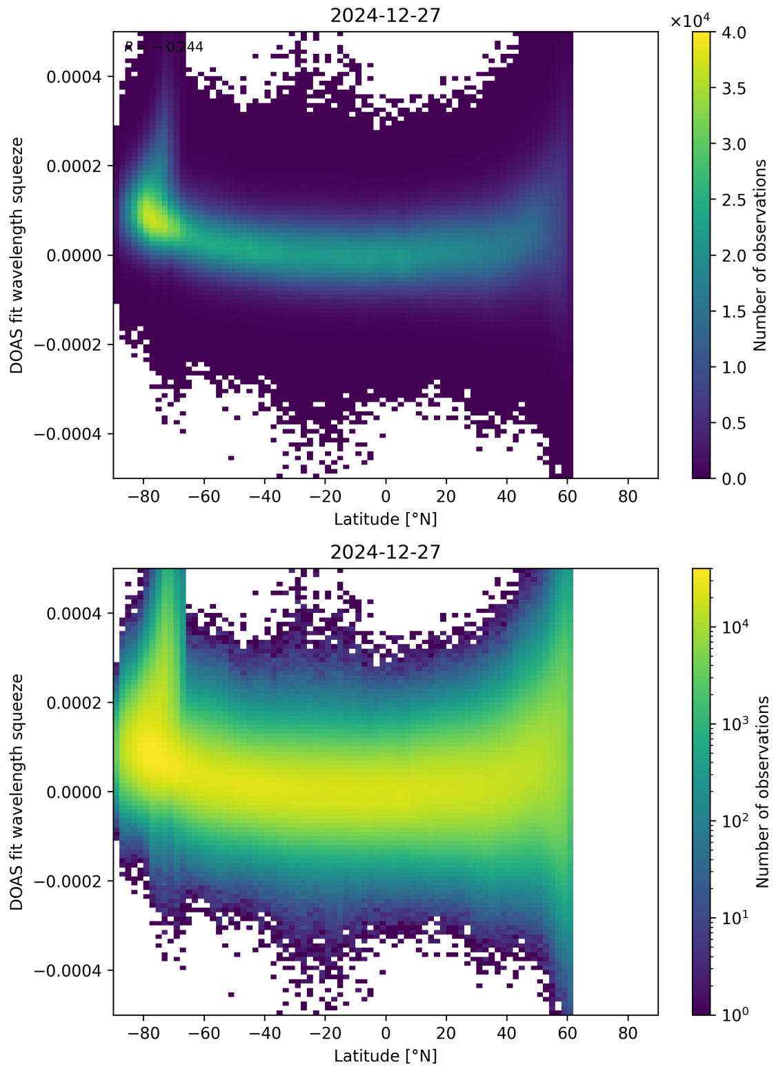
Figure 155: Scatter density plot of “Latitude” against “DOAS fit wavelength squeeze” for 2024-12-27 to 2024-12-28.
