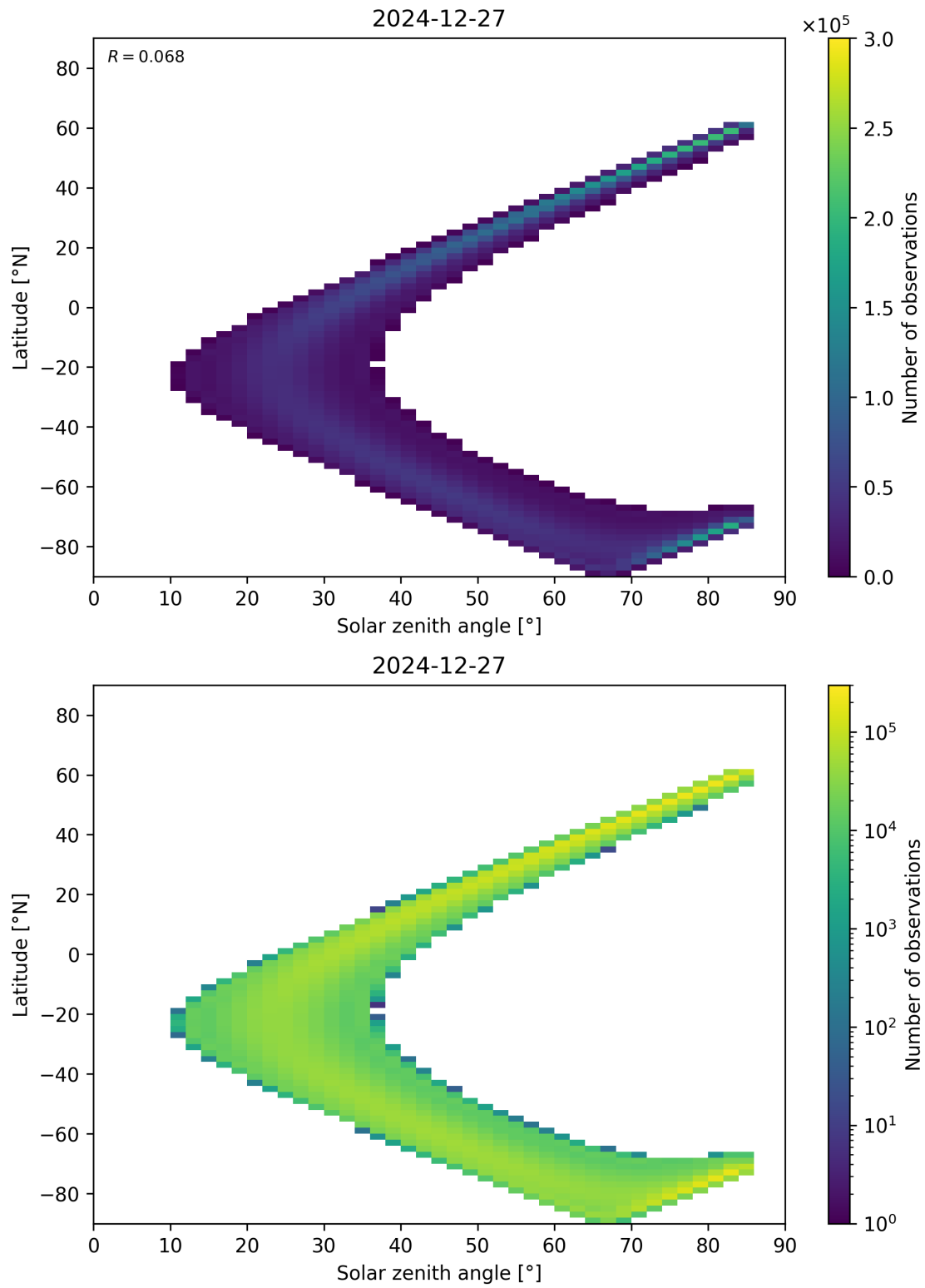
Figure 181: Scatter density plot of “Solar zenith angle” against “Latitude” for 2024-12-27 to 2024-12-28.
