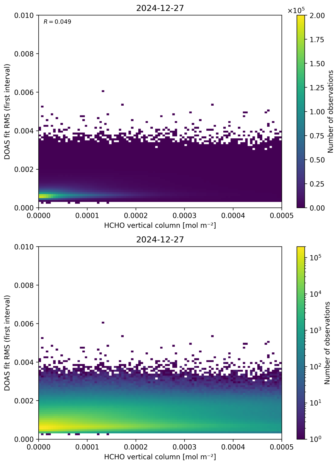
Figure 123: Scatter density plot of “HCHO vertical column” against “DOAS fit RMS (first interval)” for 2024-12-27 to 2024-12-28.
