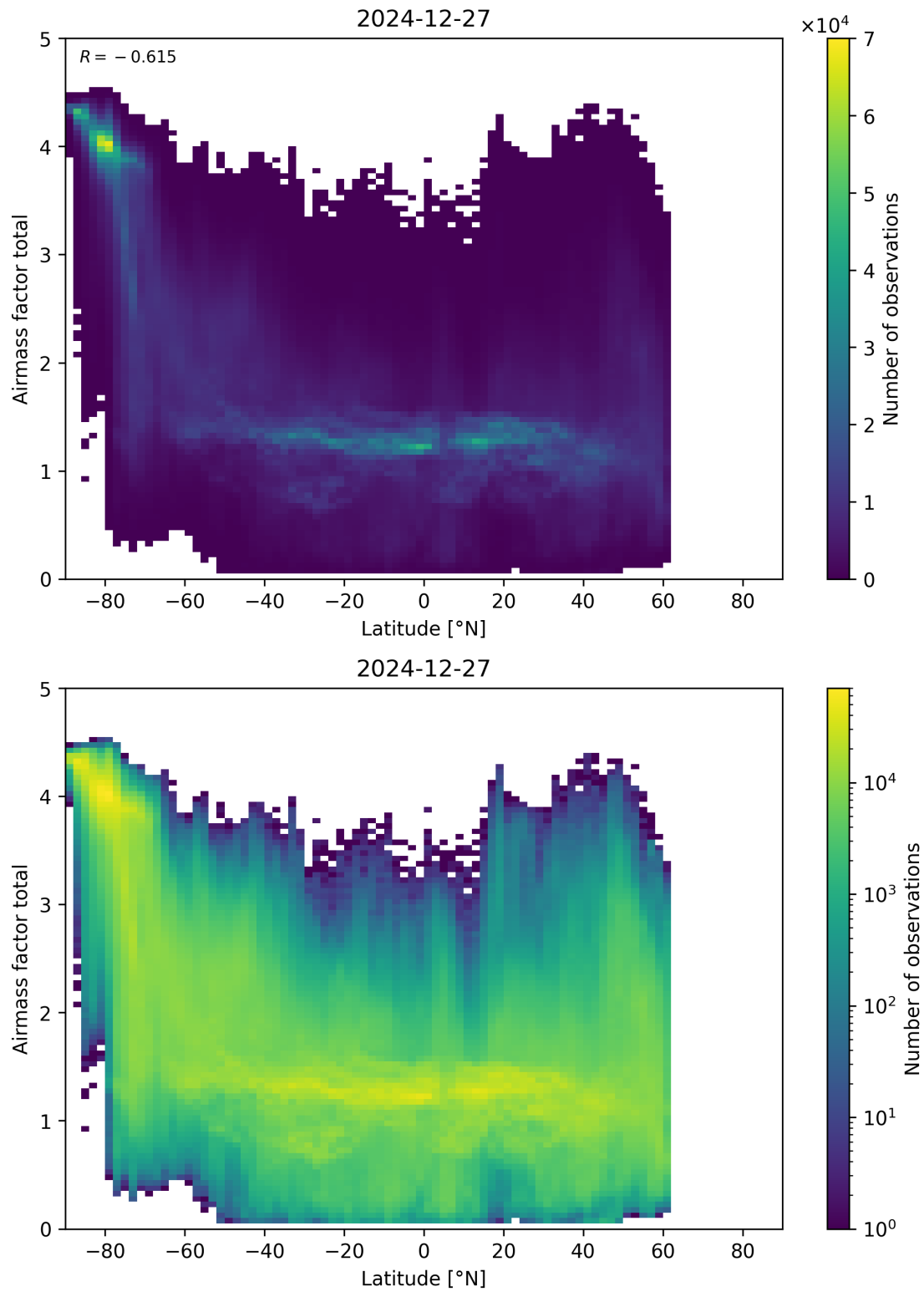
Figure 161: Scatter density plot of “Latitude” against “Airmass factor total” for 2024-12-27 to 2024-12-28.
