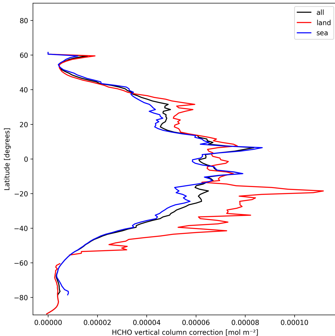
Figure 23: Zonal average of “HCHO vertical column correction” for 2024-12-27 to 2024-12-28.
