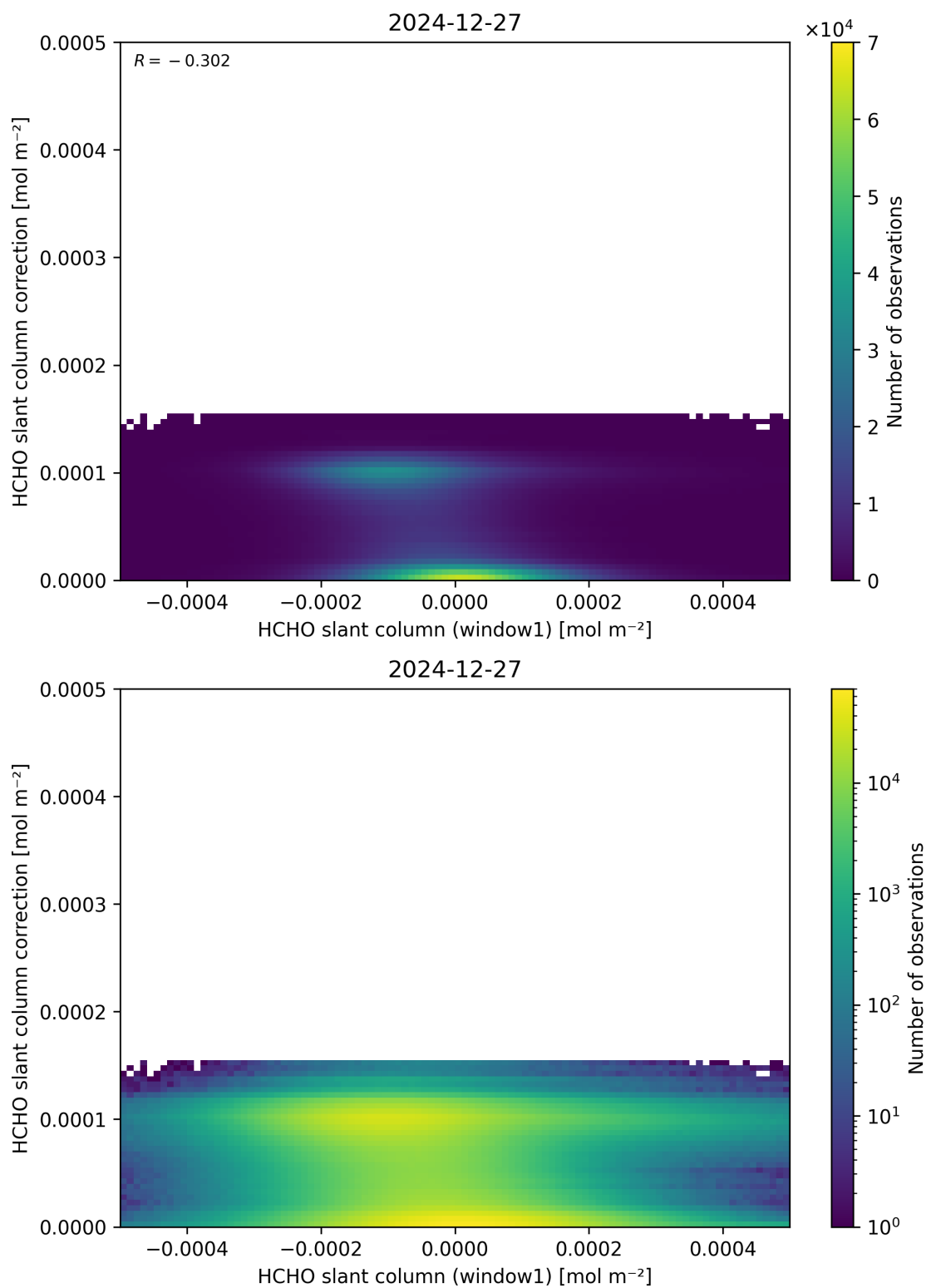
Figure 83: Scatter density plot of “HCHO slant column (window1)” against “HCHO slant column correction” for 2024-12-27 to 2024-12-28.
