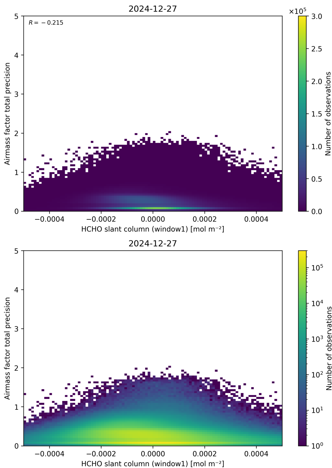
Figure 86: Scatter density plot of “HCHO slant column (window1)” against “Airmass factor total precision” for 2024-12-27 to 2024-12-28.
