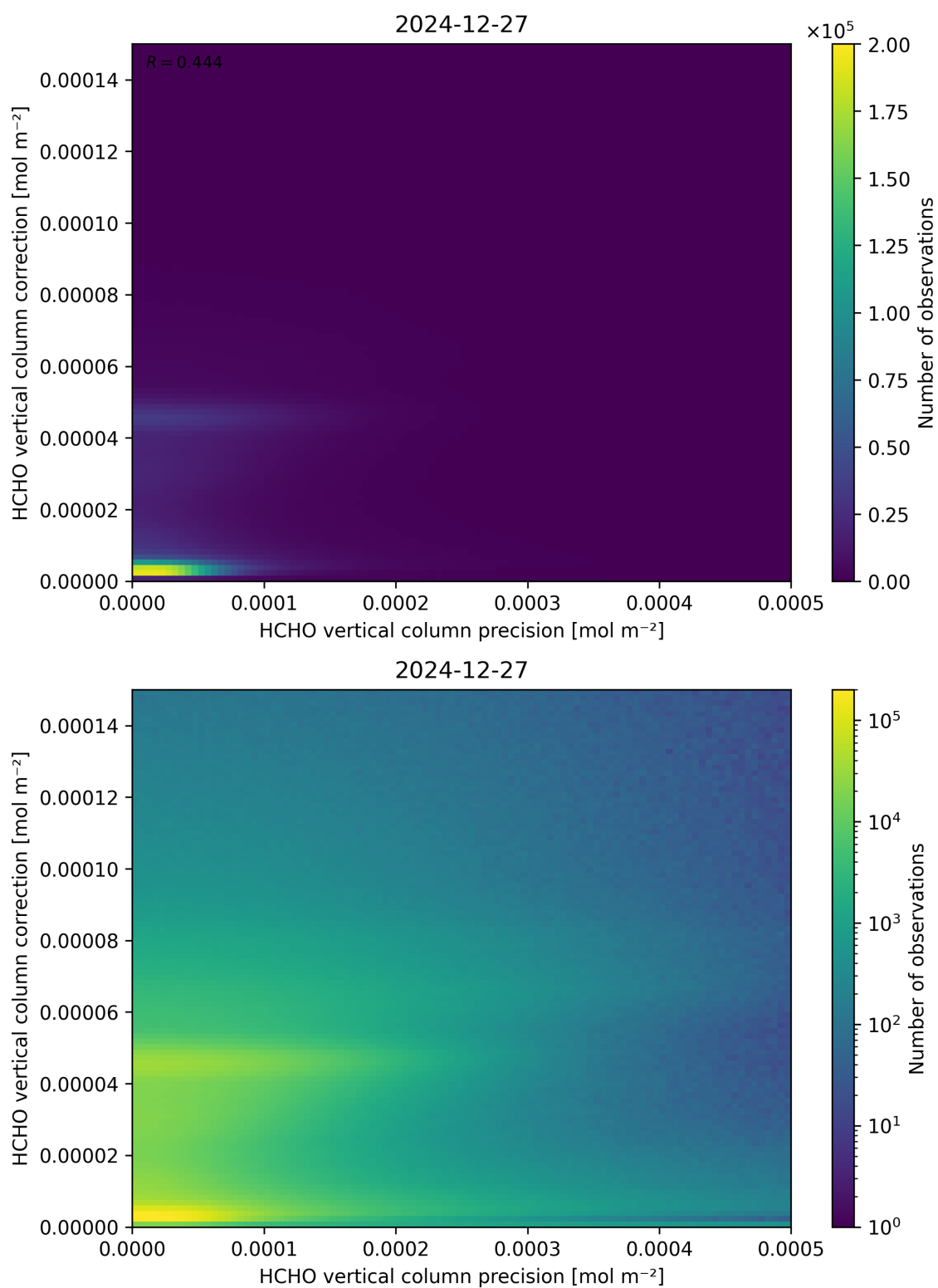
Figure 146: Scatter density plot of “HCHO vertical column precision” against “HCHO vertical column correction” for 2024-12-27 to 2024-12-28.
