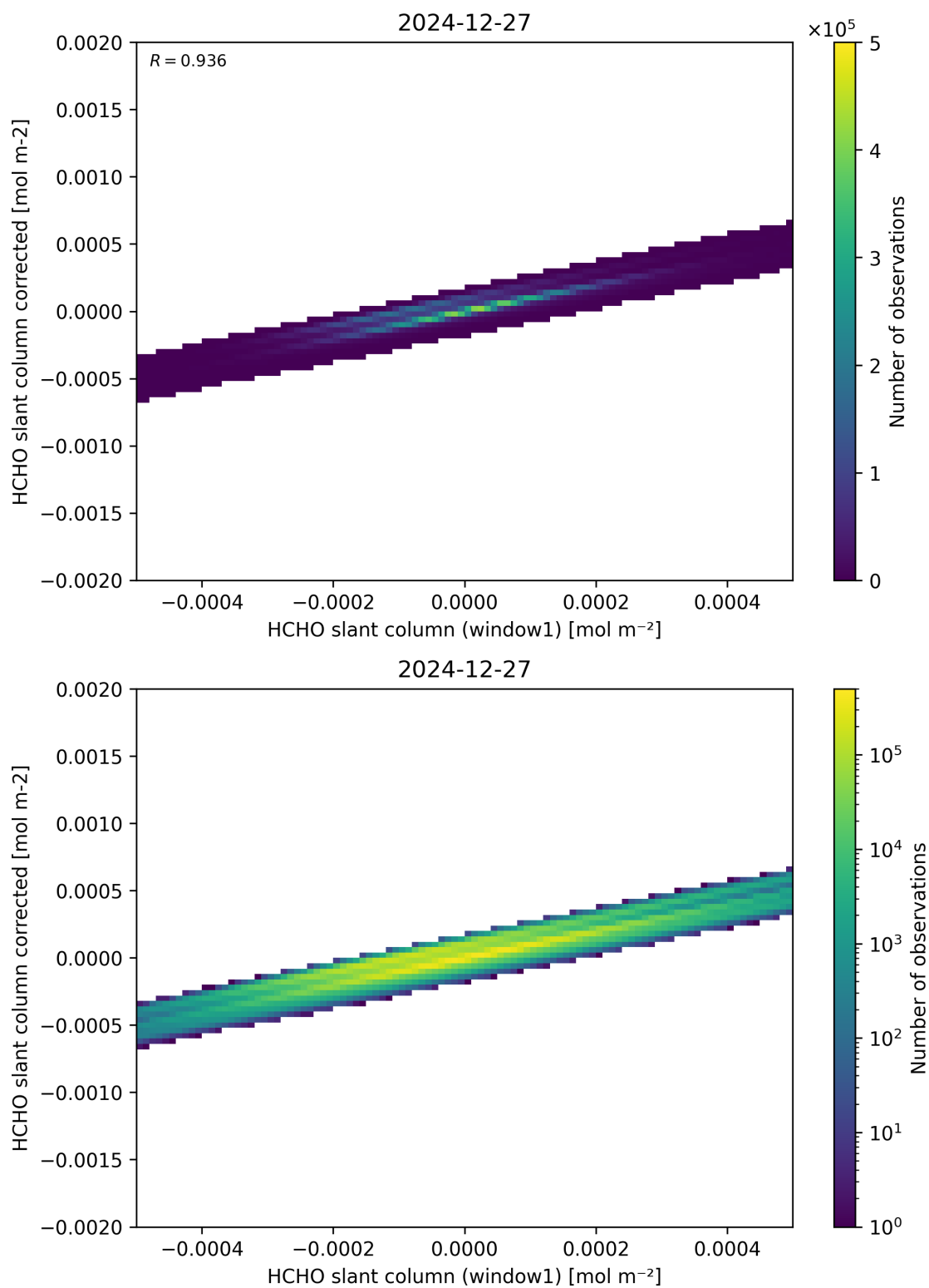
Figure 82: Scatter density plot of “HCHO slant column (window1)” against “HCHO slant column corrected” for 2024-12-27 to 2024-12-28.
