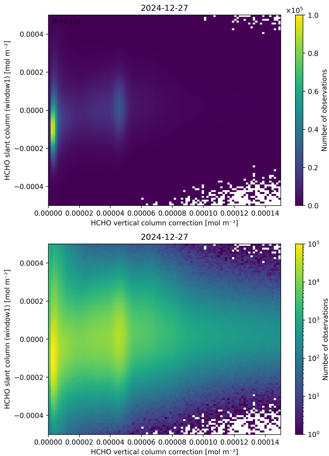
Figure 118: Scatter density plot of “HCHO vertical column correction” against “HCHO slant column (window1)” for 2024-12-27 to 2024-12-28.
