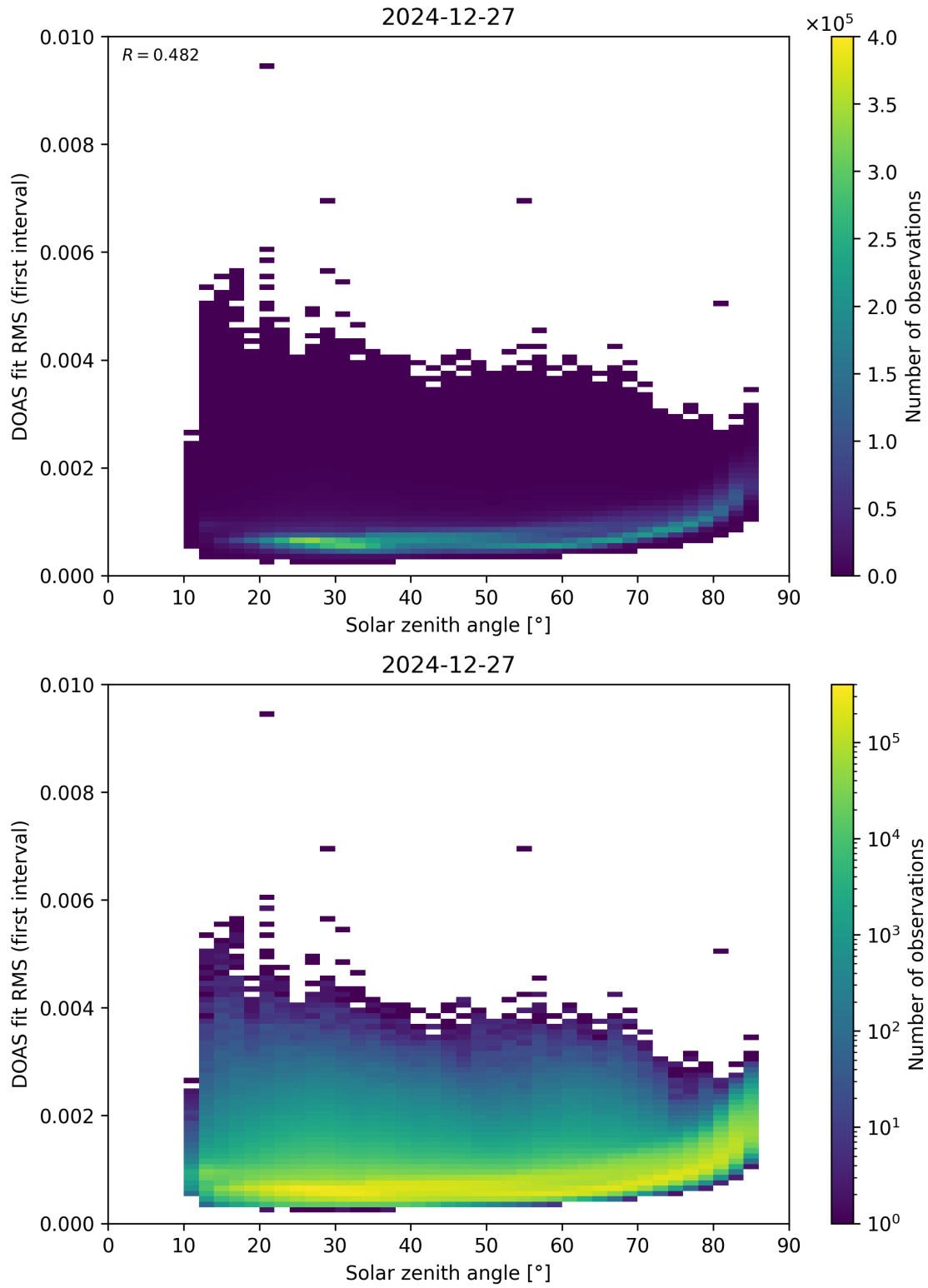
Figure 167: Scatter density plot of “Solar zenith angle” against “DOAS fit RMS (first interval)” for 2024-12-27 to 2024-12-28.
