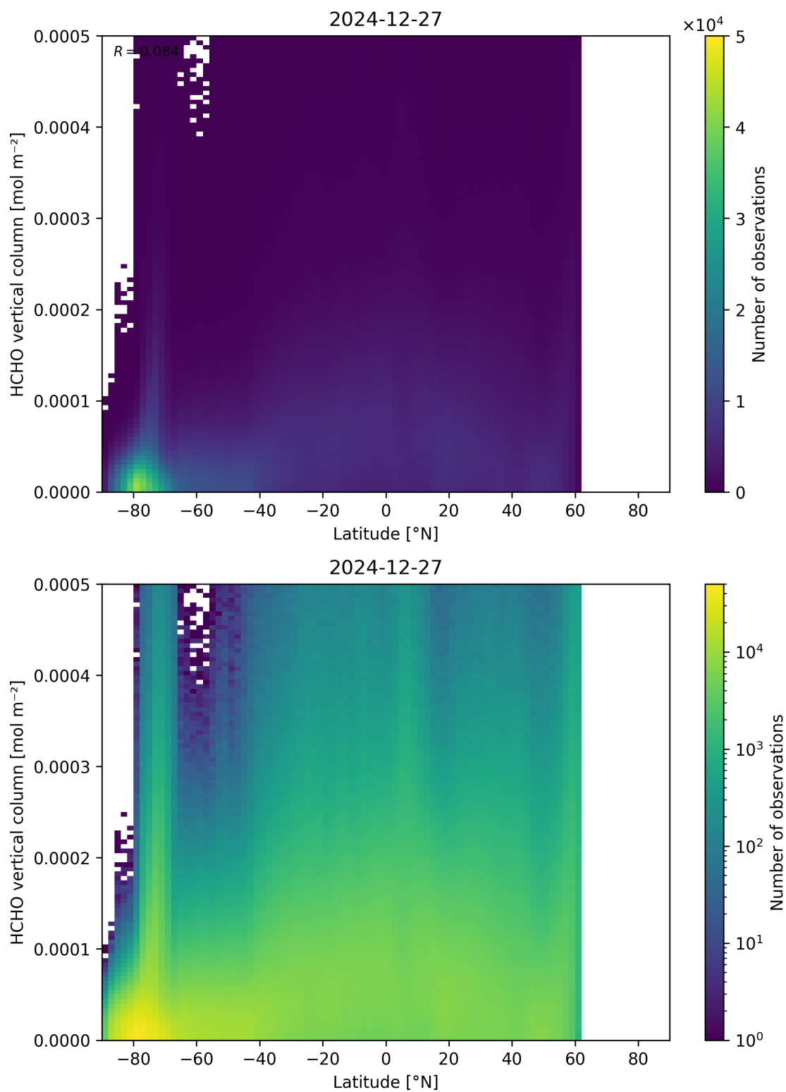
Figure 163: Scatter density plot of “Latitude” against “HCHO vertical column” for 2024-12-27 to 2024-12-28.
