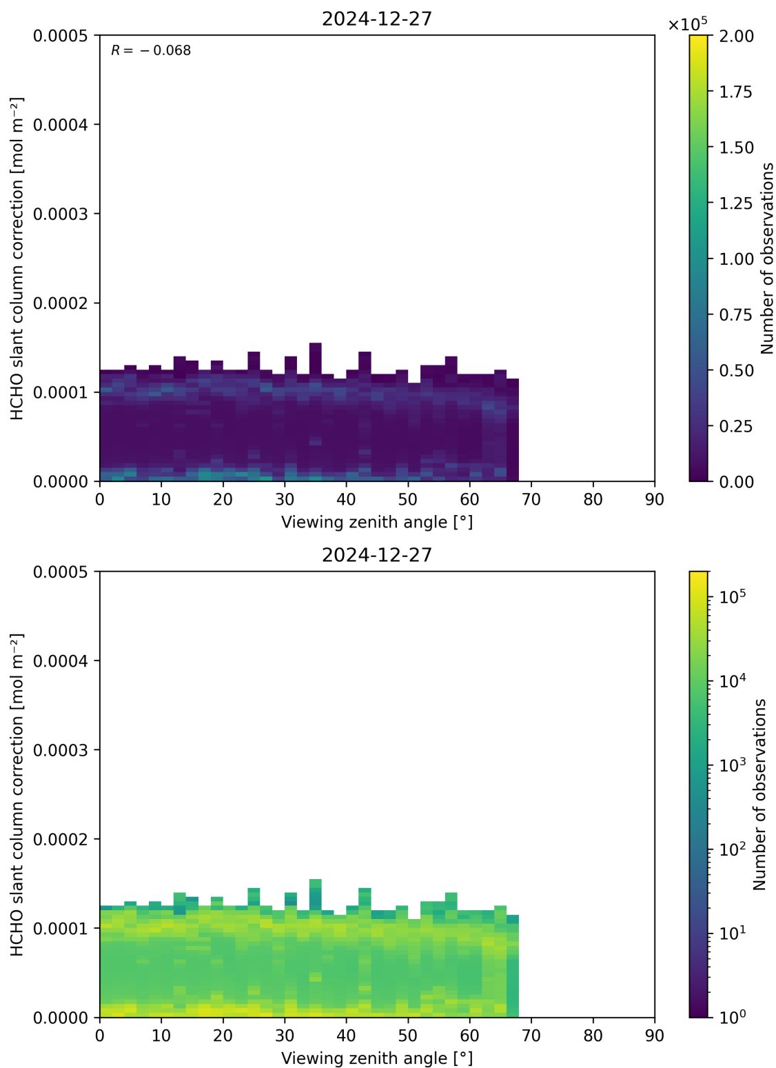
Figure 187: Scatter density plot of “Viewing zenith angle” against “HCHO slant column correction” for 2024-12-27 to 2024-12-28.
