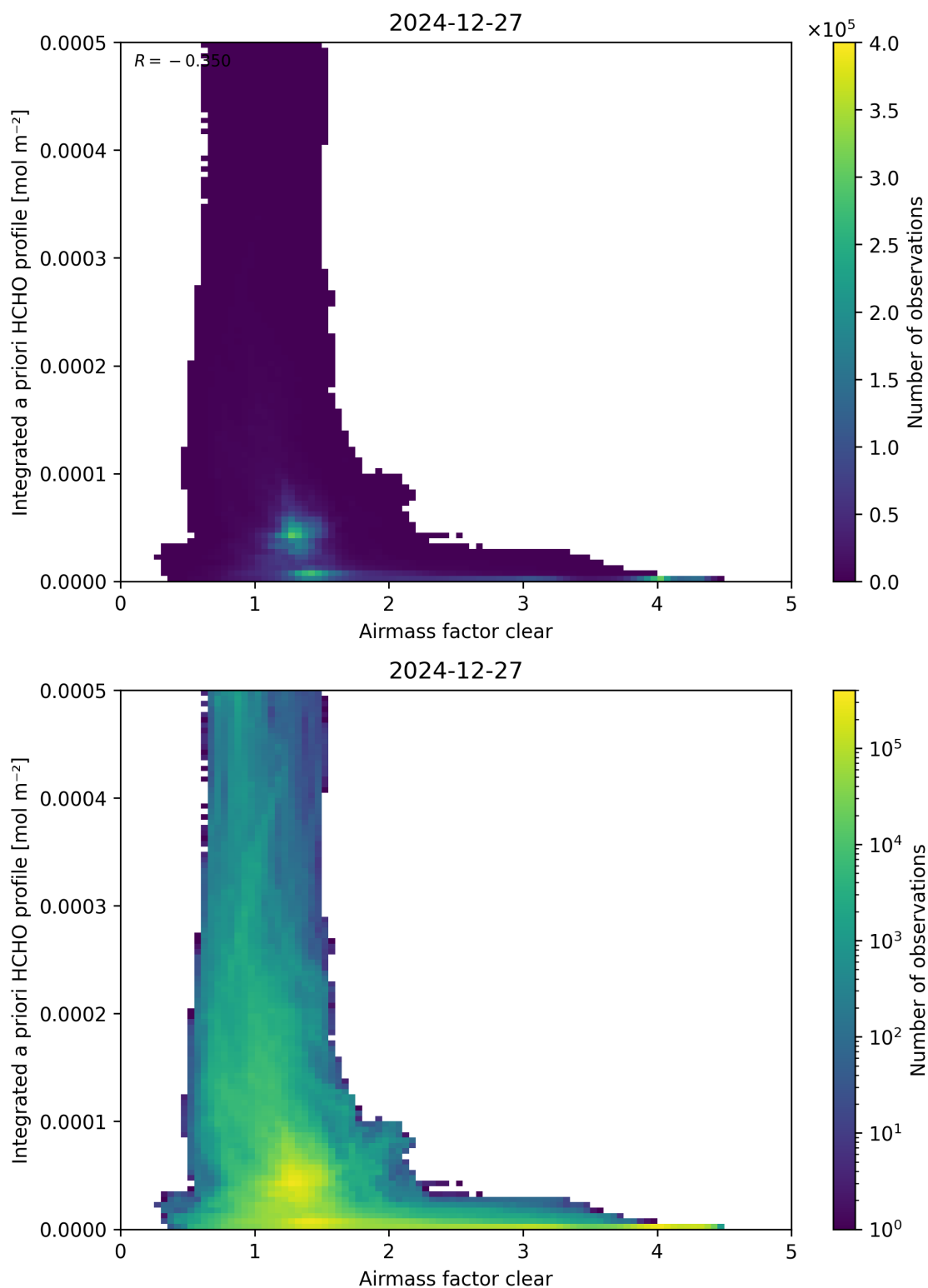
Figure 76: Scatter density plot of “Airmass factor clear” against “Integrated a priori HCHO profile” for 2024-12-27 to 2024-12-28.
