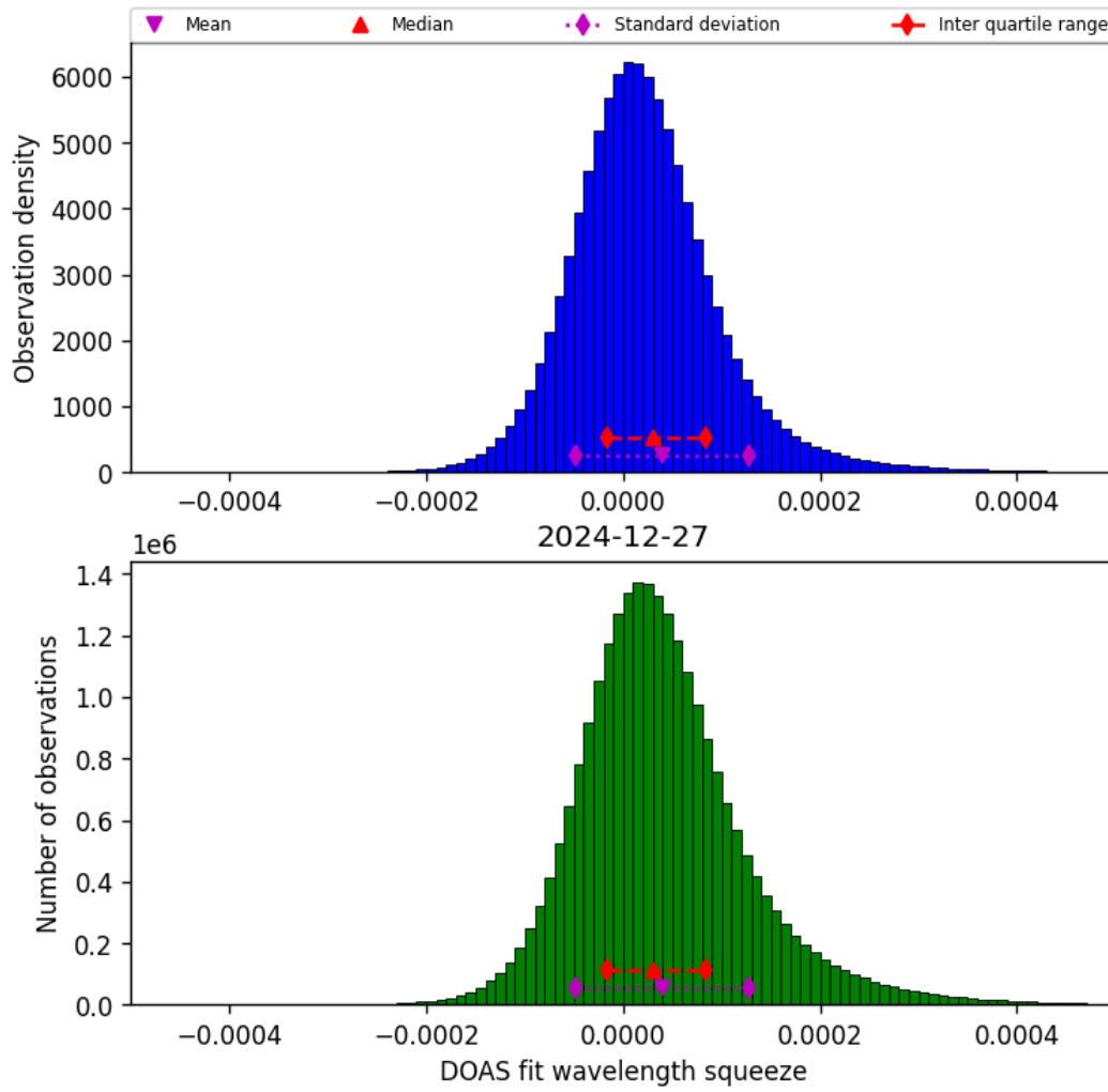
Figure 45: Histogram of “DOAS fit wavelength squeeze” for 2024-12-27 to 2024-12-28
