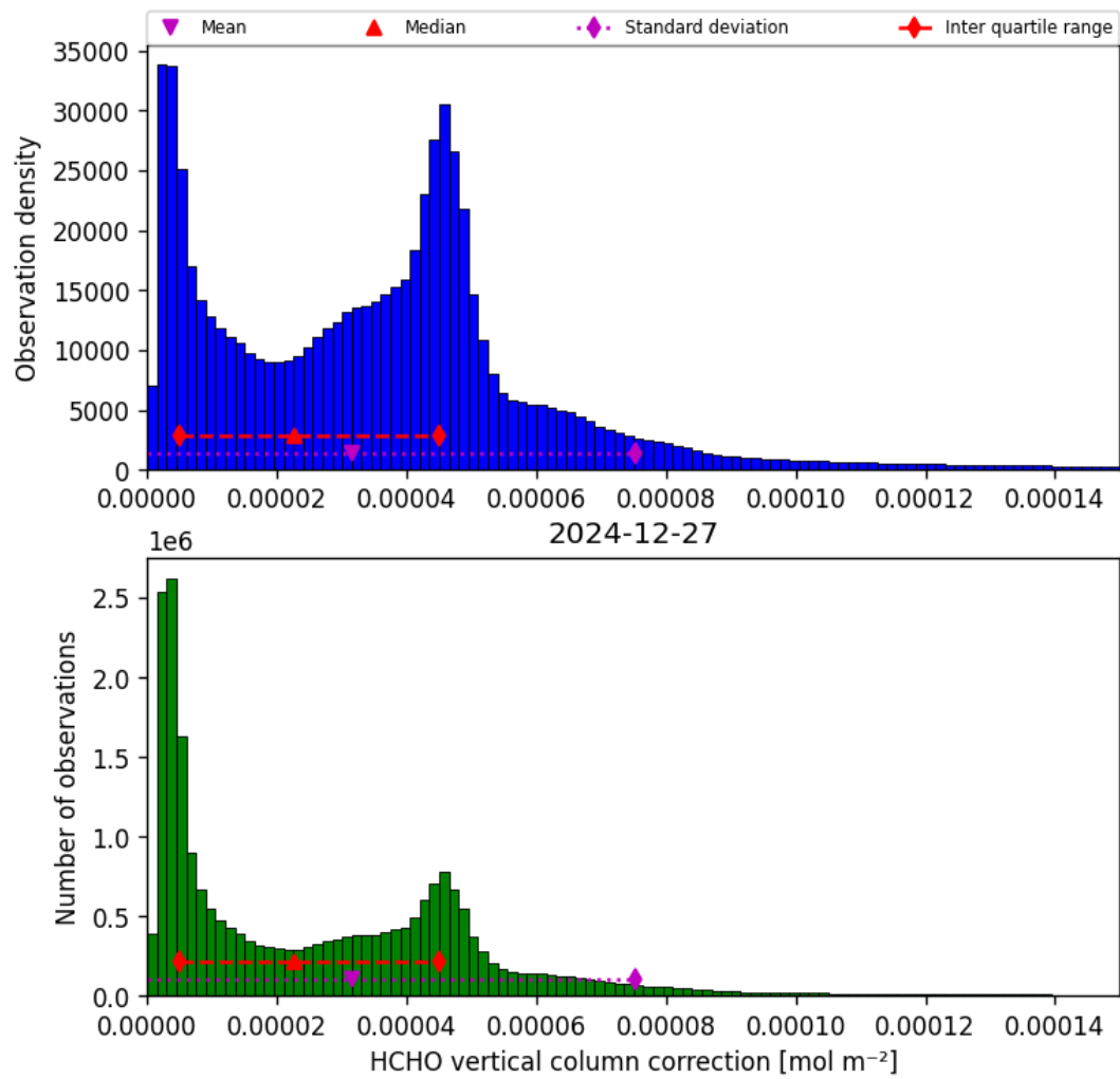
Figure 37: Histogram of “HCHO vertical column correction” for 2024-12-27 to 2024-12-28
