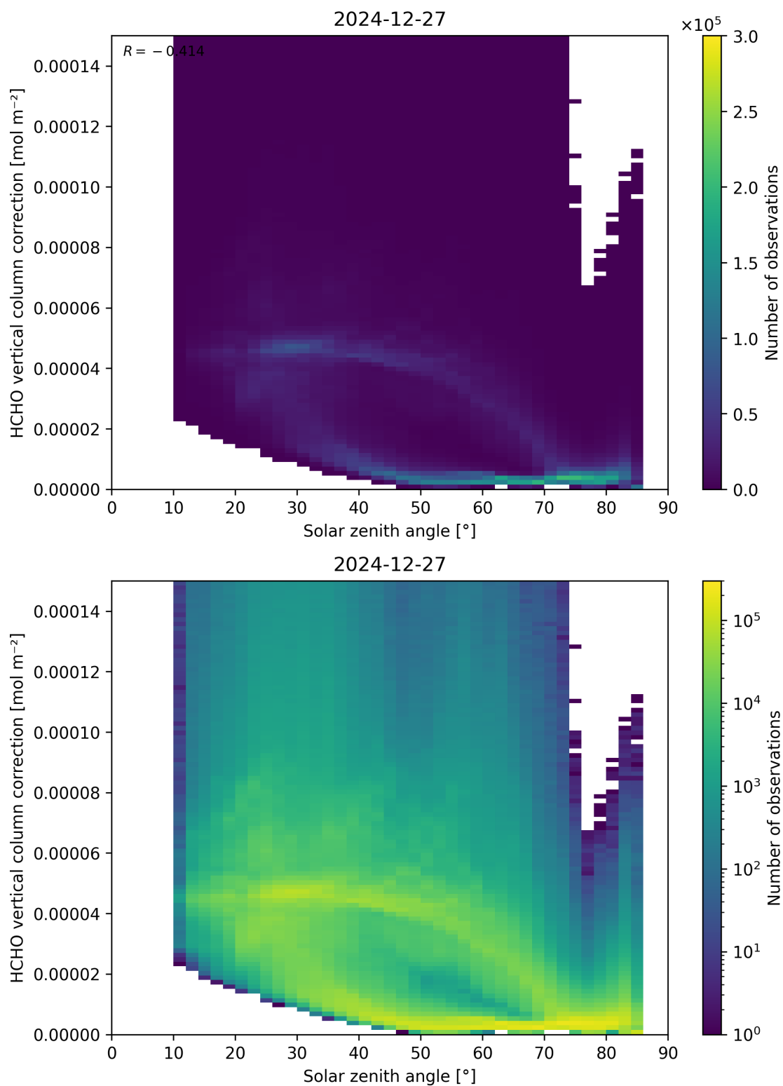
Figure 178: Scatter density plot of “Solar zenith angle” against “HCHO vertical column correction” for 2024-12-27 to 2024-12-28.
