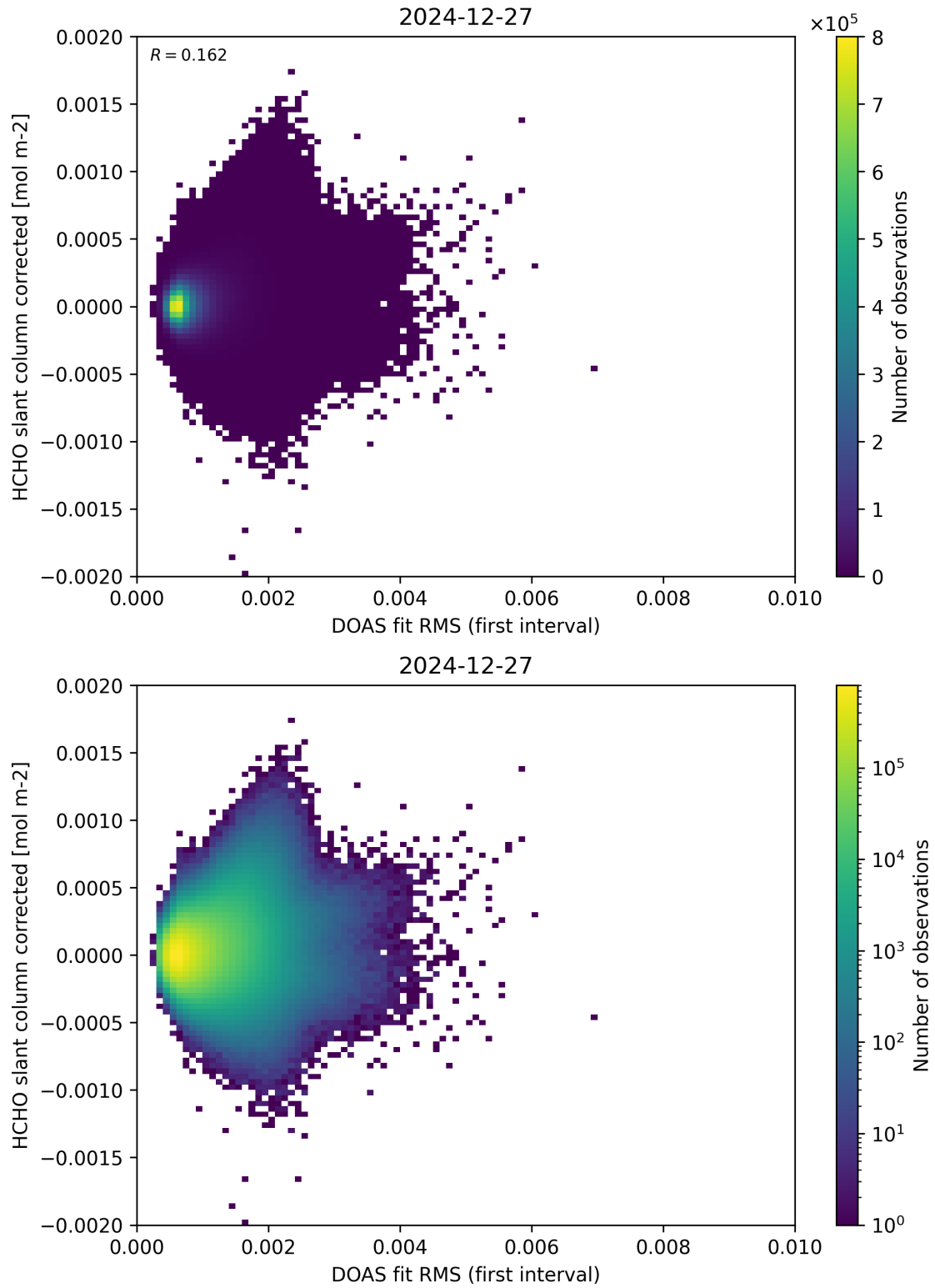
Figure 62: Scatter density plot of “DOAS fit RMS (first interval)” against “HCHO slant column corrected” for 2024-12-27 to 2024-12-28.
