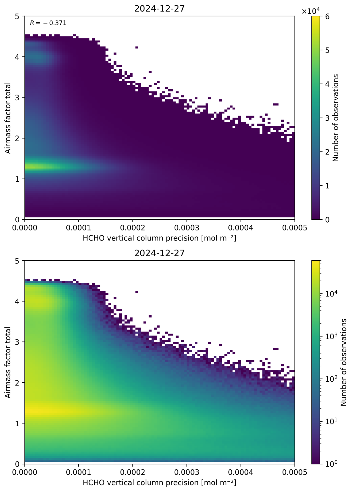
Figure 144: Scatter density plot of “HCHO vertical column precision” against “Airmass factor total” for 2024-12-27 to 2024-12-28.
