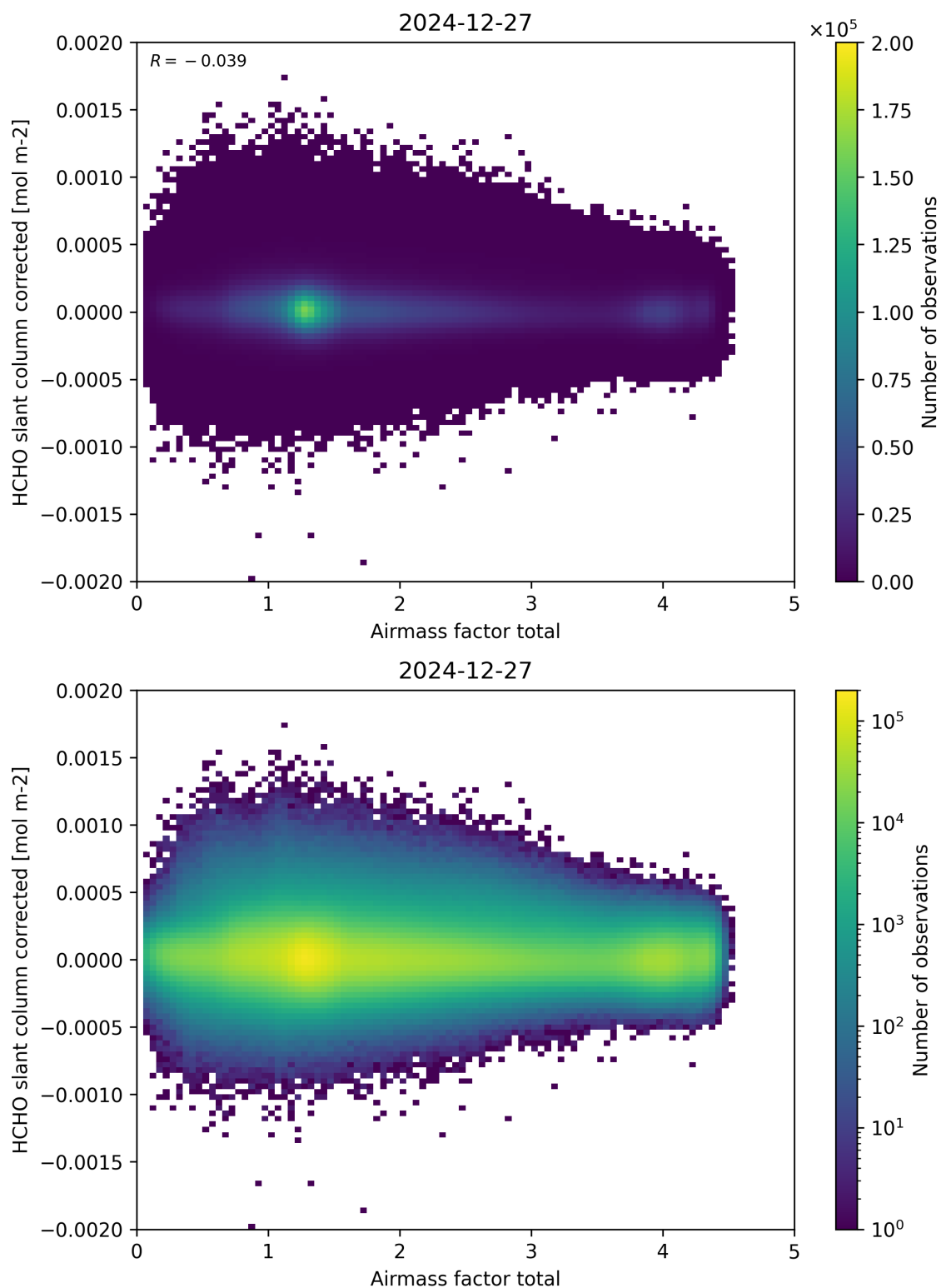
Figure 101: Scatter density plot of “Airmass factor total” against “HCHO slant column corrected” for 2024-12-27 to 2024-12-28.
