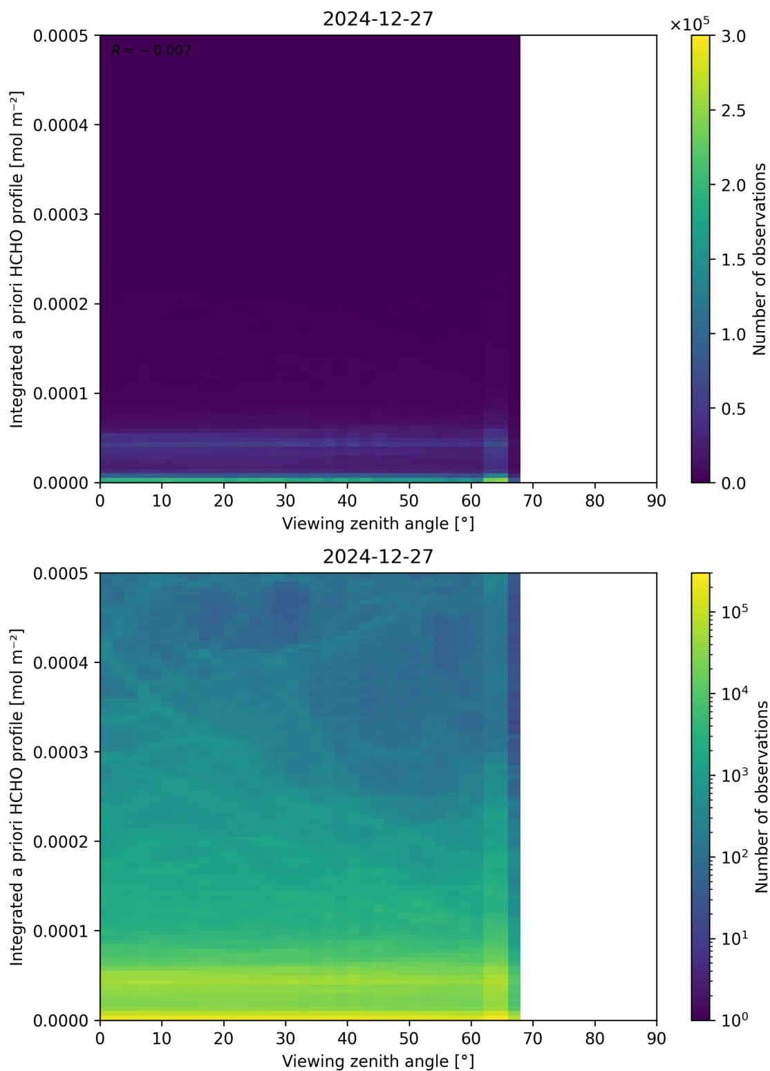
Figure 195: Scatter density plot of “Viewing zenith angle” against “Integrated a priori HCHO profile” for 2024-12-27 to 2024-12-28.
