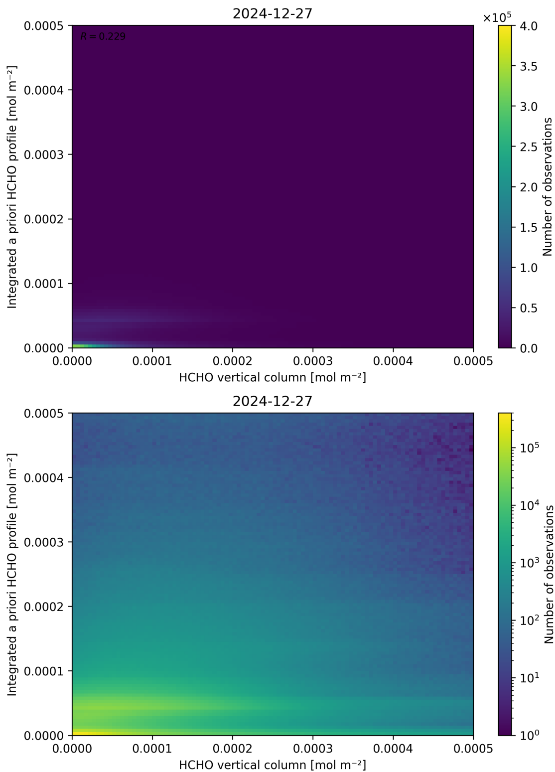
Figure 135: Scatter density plot of “HCHO vertical column” against “Integrated a priori HCHO profile” for 2024-12-27 to 2024-12-28.
