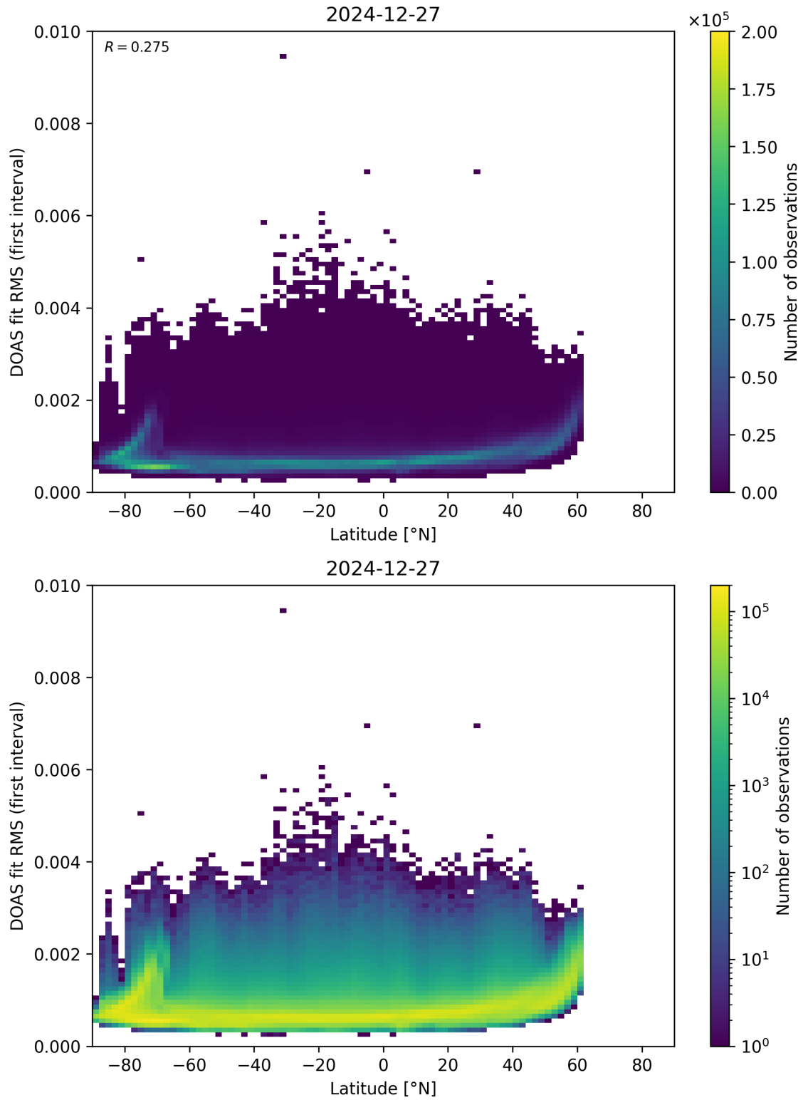
Figure 153: Scatter density plot of “Latitude” against “DOAS fit RMS (first interval)” for 2024-12-27 to 2024-12-28.
