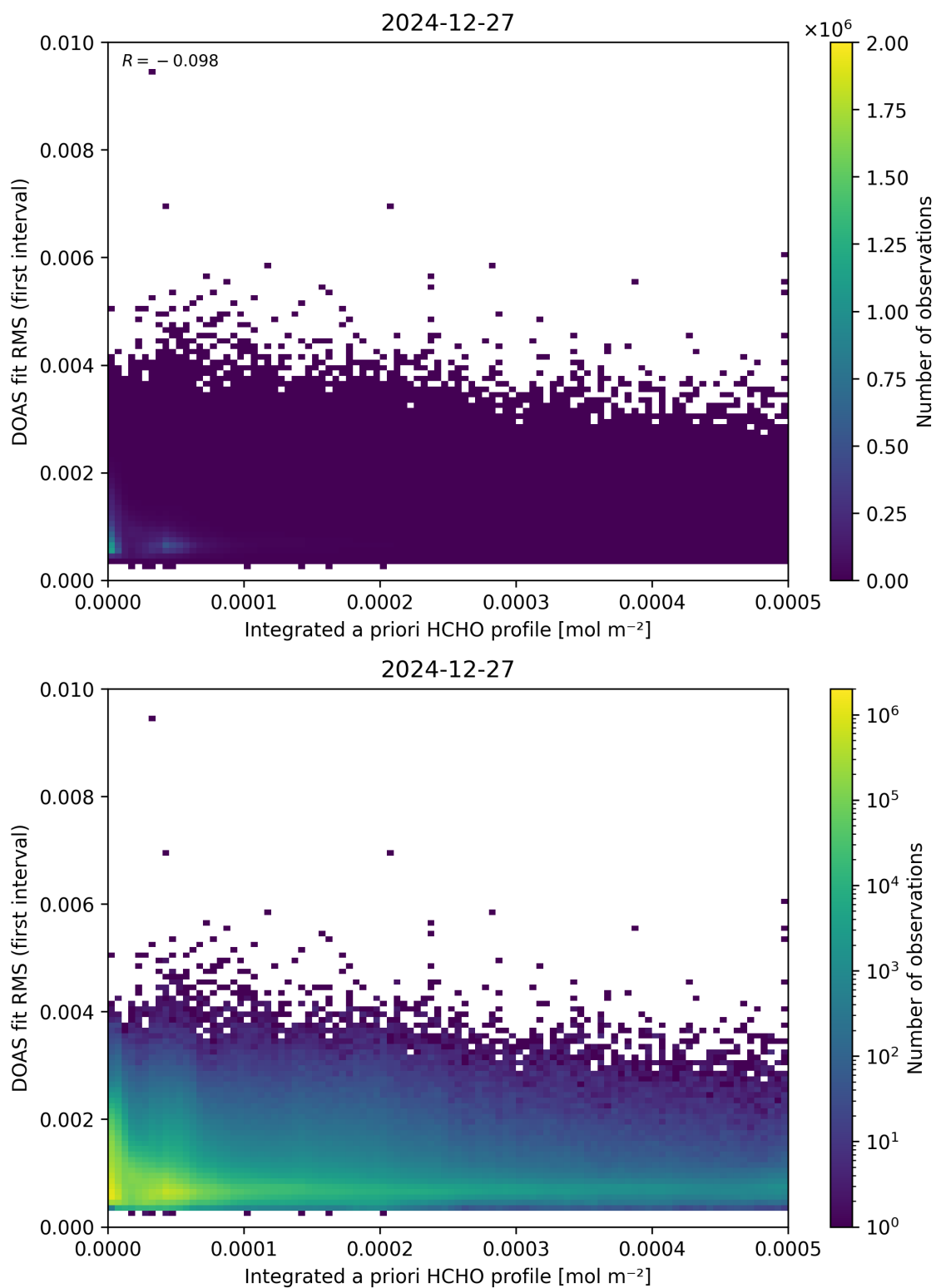
Figure 148: Scatter density plot of “Integrated a priori HCHO profile” against “DOAS fit RMS (first interval)” for 2024-12-27 to 2024-12-28.
