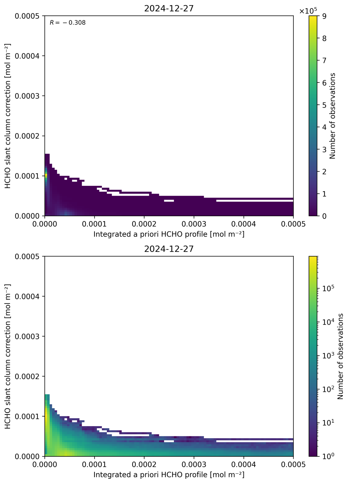
Figure 152: Scatter density plot of “Integrated a priori HCHO profile” against “HCHO slant column correction” for 2024-12-27 to 2024-12-28.
