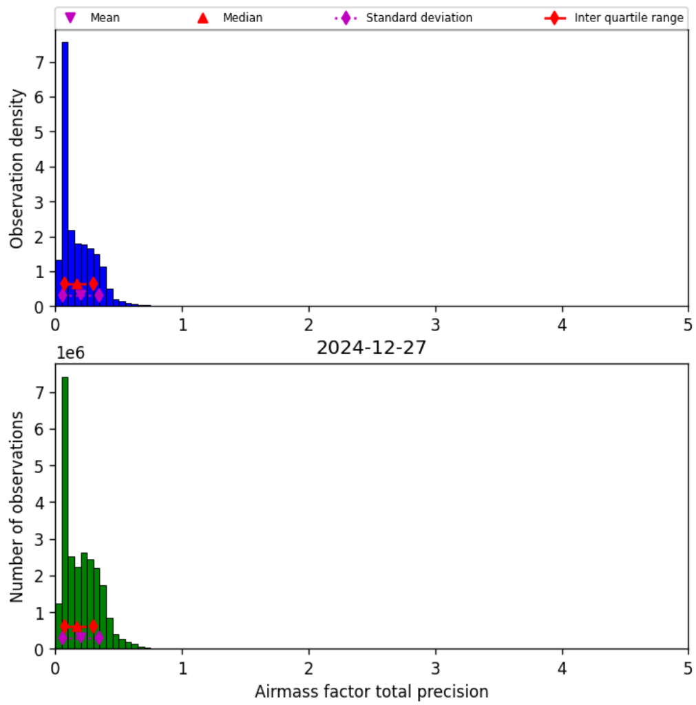
Figure 41: Histogram of “Airmass factor total precision” for 2024-12-27 to 2024-12-28
