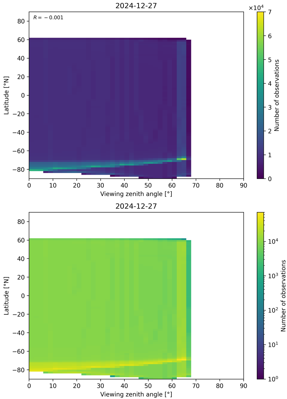
Figure 196: Scatter density plot of “Viewing zenith angle” against “Latitude” for 2024-12-27 to 2024-12-28.
