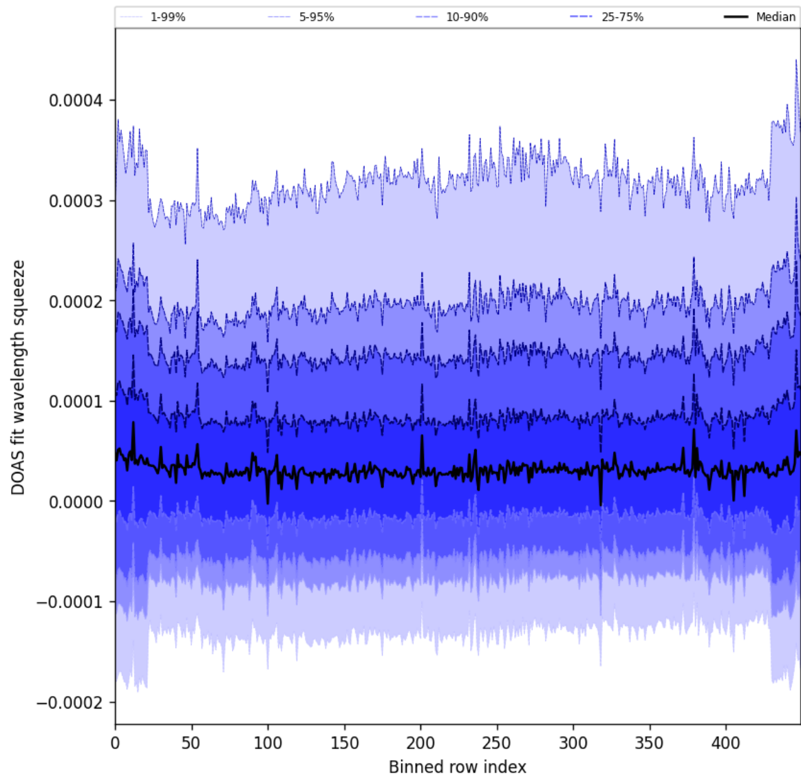
Figure 59: Along track statistics of “DOAS fit wavelength squeeze” for 2024-12-27 to 2024-12-28
