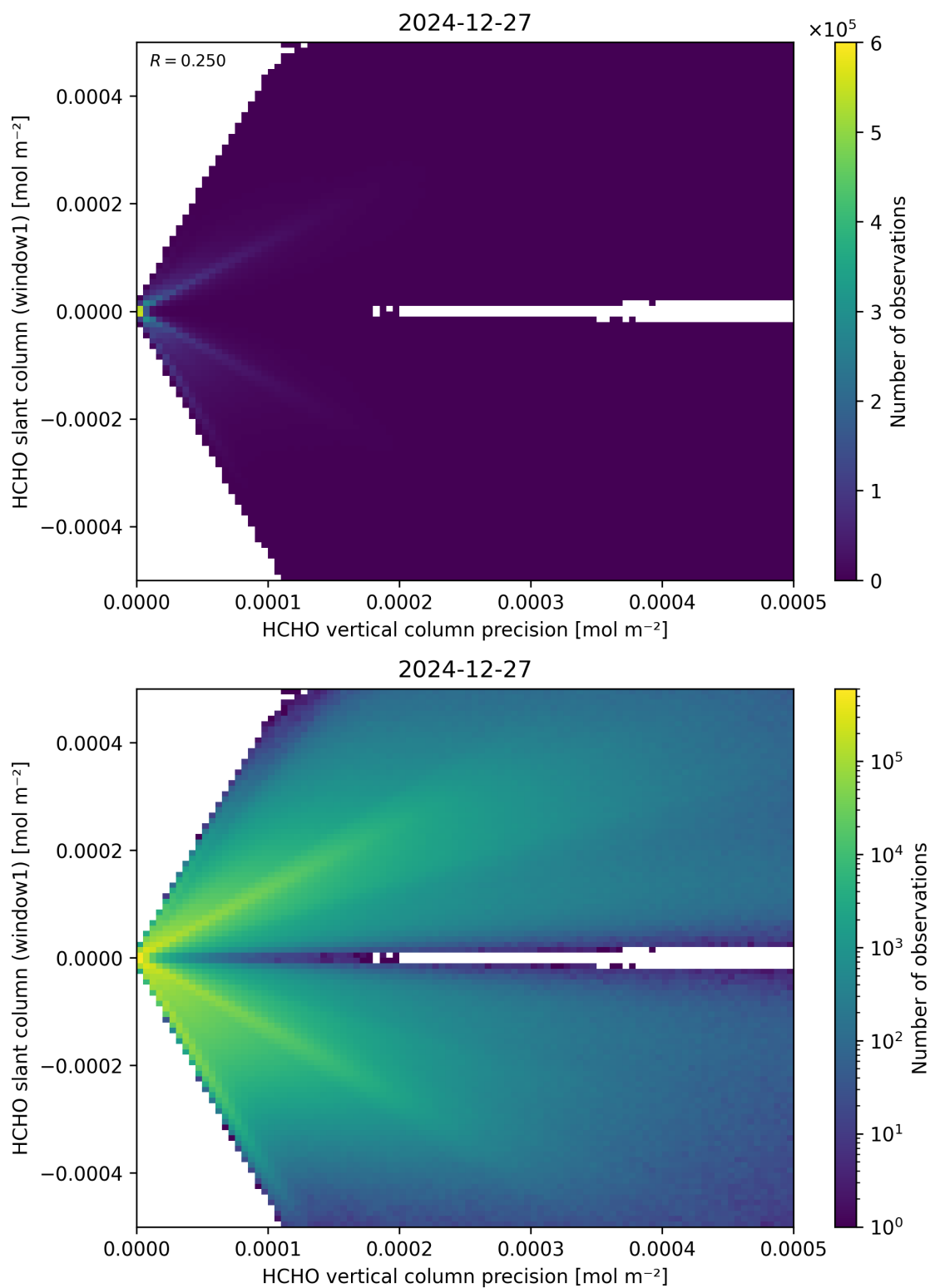
Figure 142: Scatter density plot of “HCHO vertical column precision” against “HCHO slant column (window1)” for 2024-12-27 to 2024-12-28.
