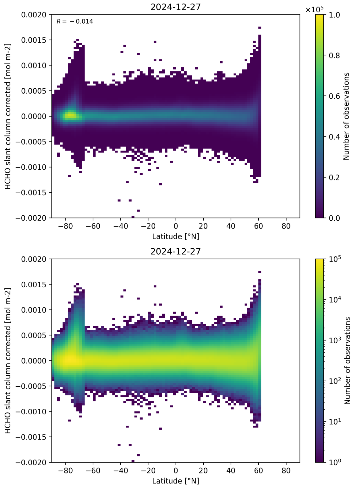
Figure 157: Scatter density plot of “Latitude” against “HCHO slant column corrected” for 2024-12-27 to 2024-12-28.
