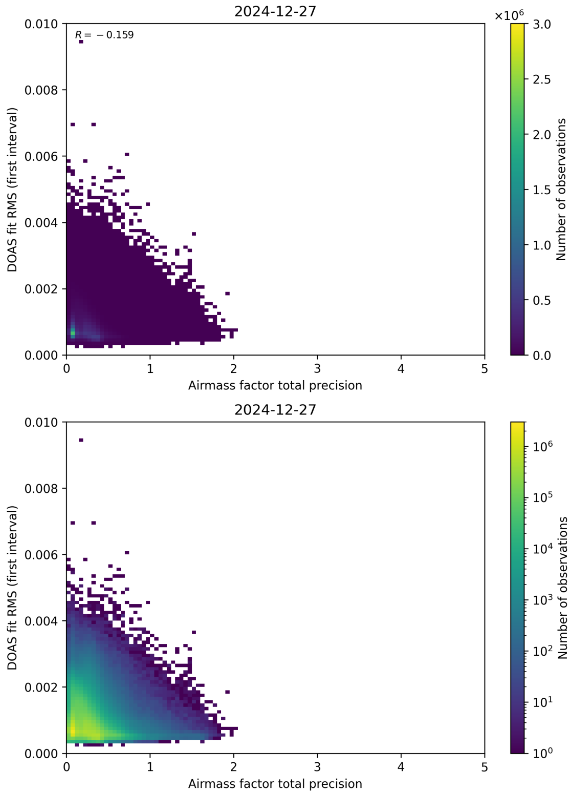
Figure 105: Scatter density plot of “Airmass factor total precision” against “DOAS fit RMS (first interval)” for 2024-12-27 to 2024-12-28.
