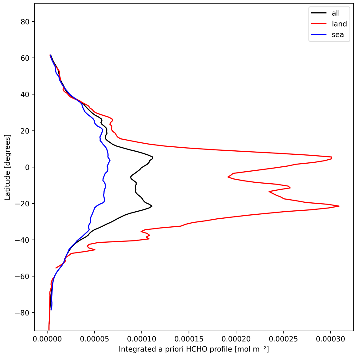
Figure 29: Zonal average of “Integrated a priori HCHO profile” for 2024-12-27 to 2024-12-28.
