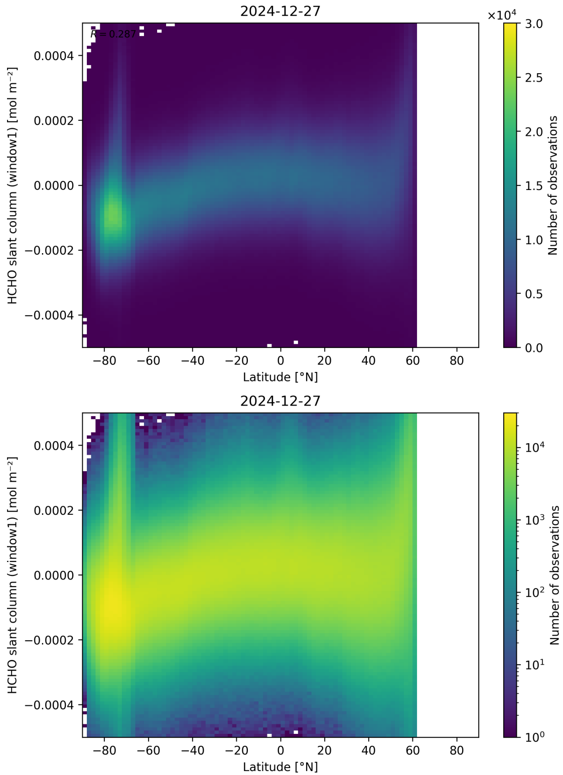
Figure 159: Scatter density plot of “Latitude” against “HCHO slant column (window1)” for 2024-12-27 to 2024-12-28.
