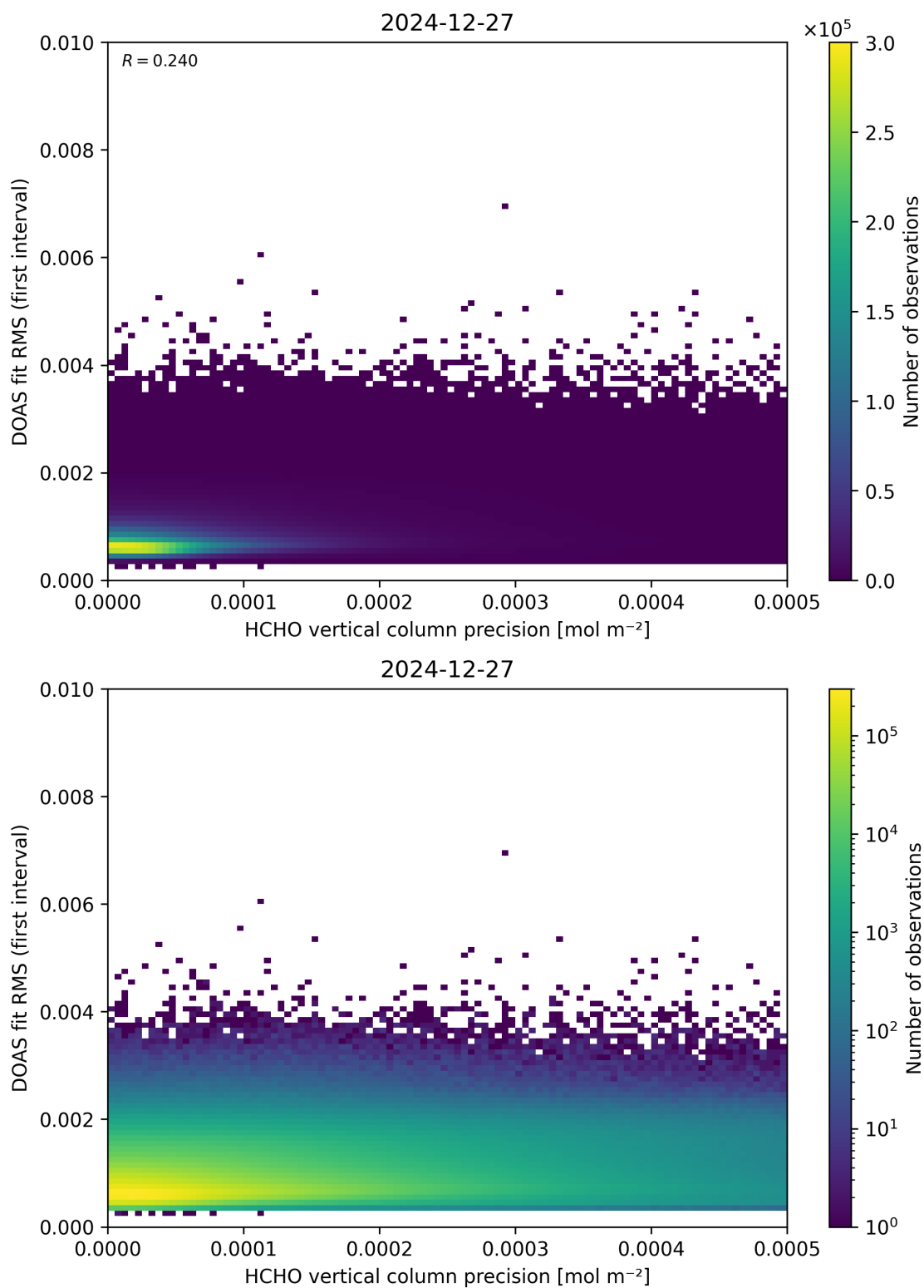
Figure 136: Scatter density plot of “HCHO vertical column precision” against “DOAS fit RMS (first interval)” for 2024-12-27 to 2024-12-28.
