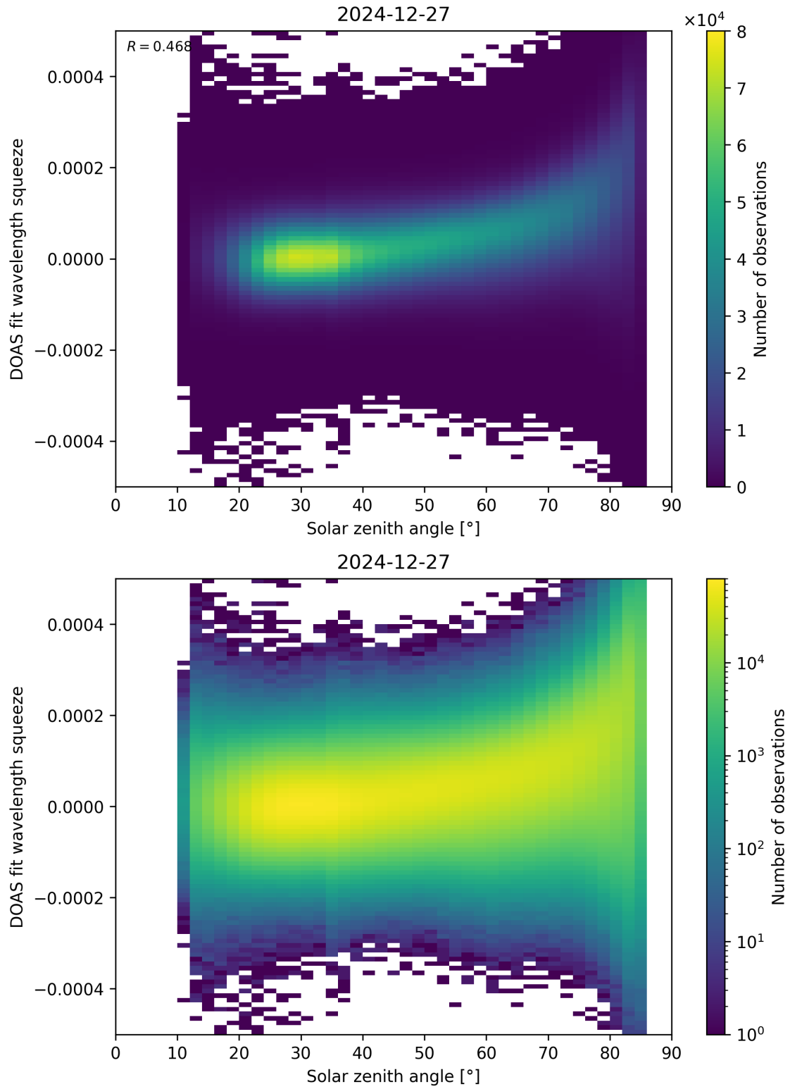
Figure 169: Scatter density plot of “Solar zenith angle” against “DOAS fit wavelength squeeze” for 2024-12-27 to 2024-12-28.
