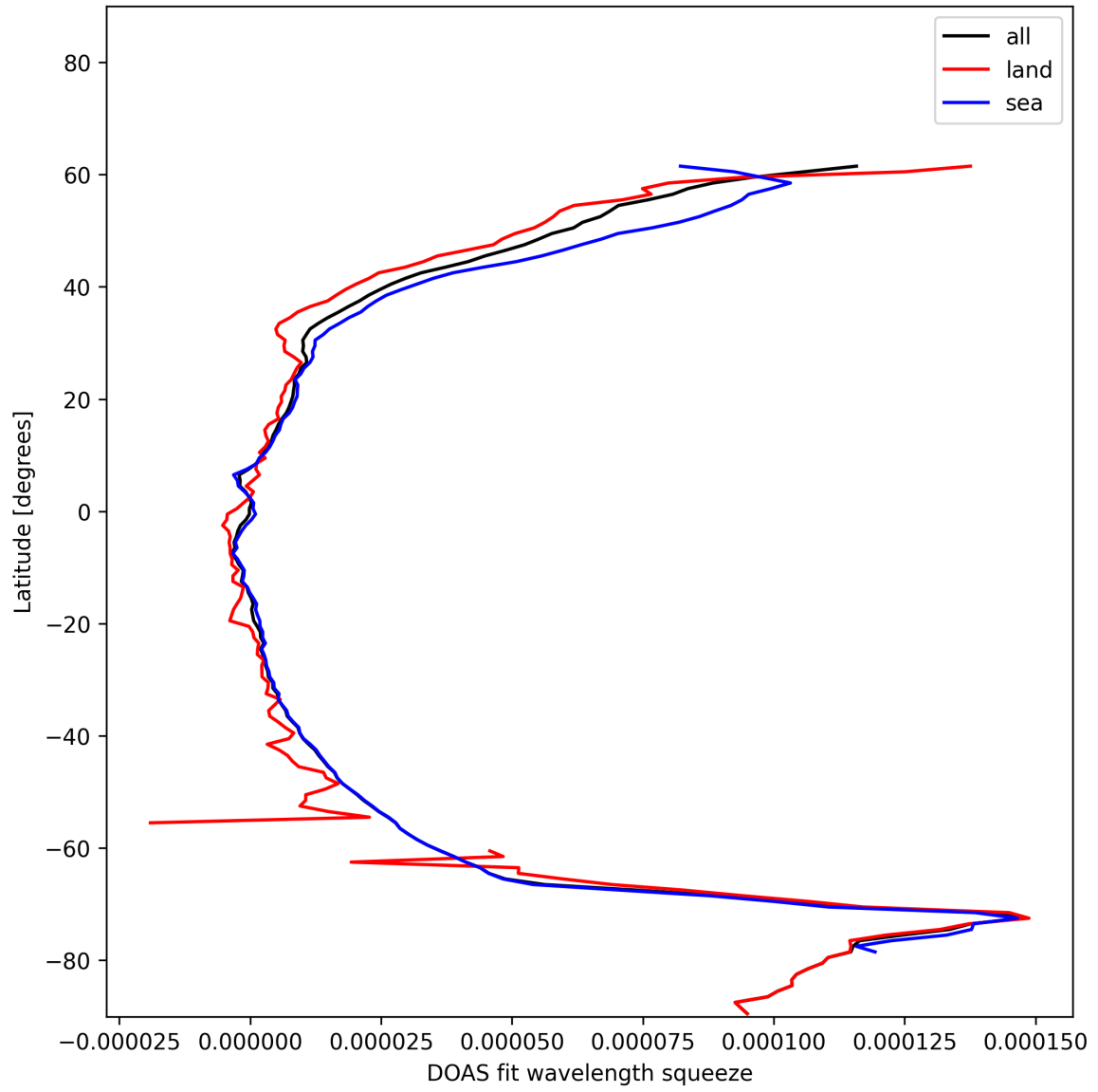
Figure 31: Zonal average of “DOAS fit wavelength squeeze” for 2024-12-27 to 2024-12-28.
