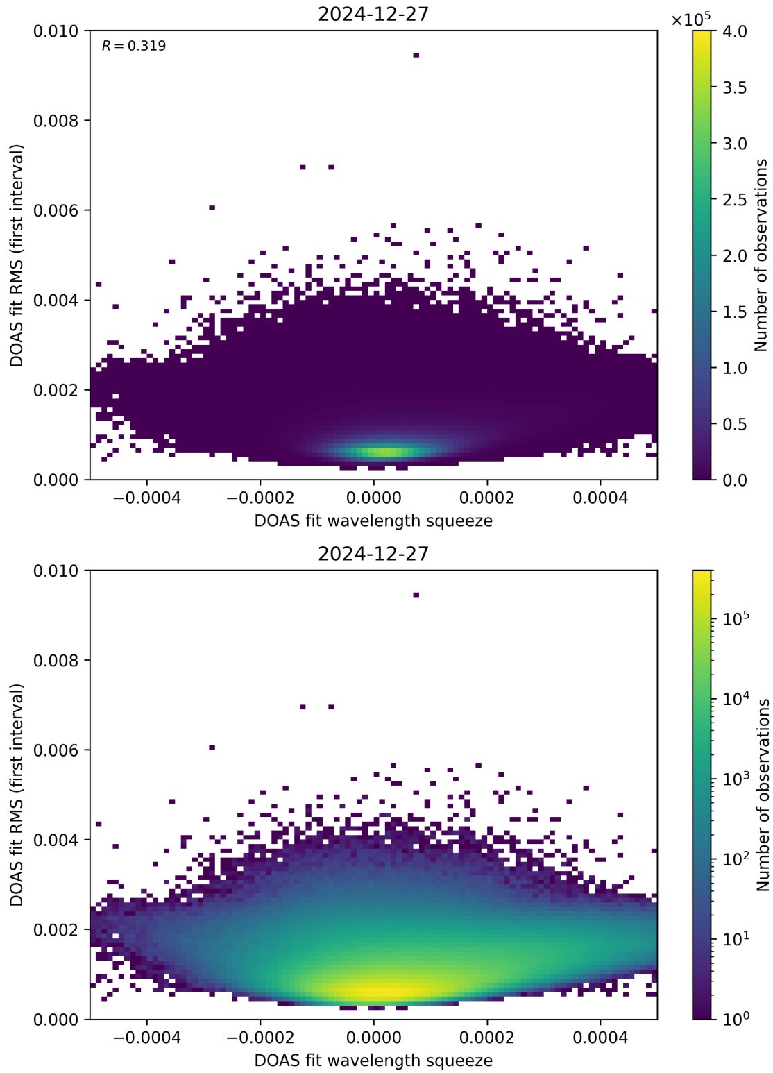
Figure 68: Scatter density plot of “DOAS fit wavelength squeeze” against “DOAS fit RMS (first interval)” for 2024-12-27 to 2024-12-28.
