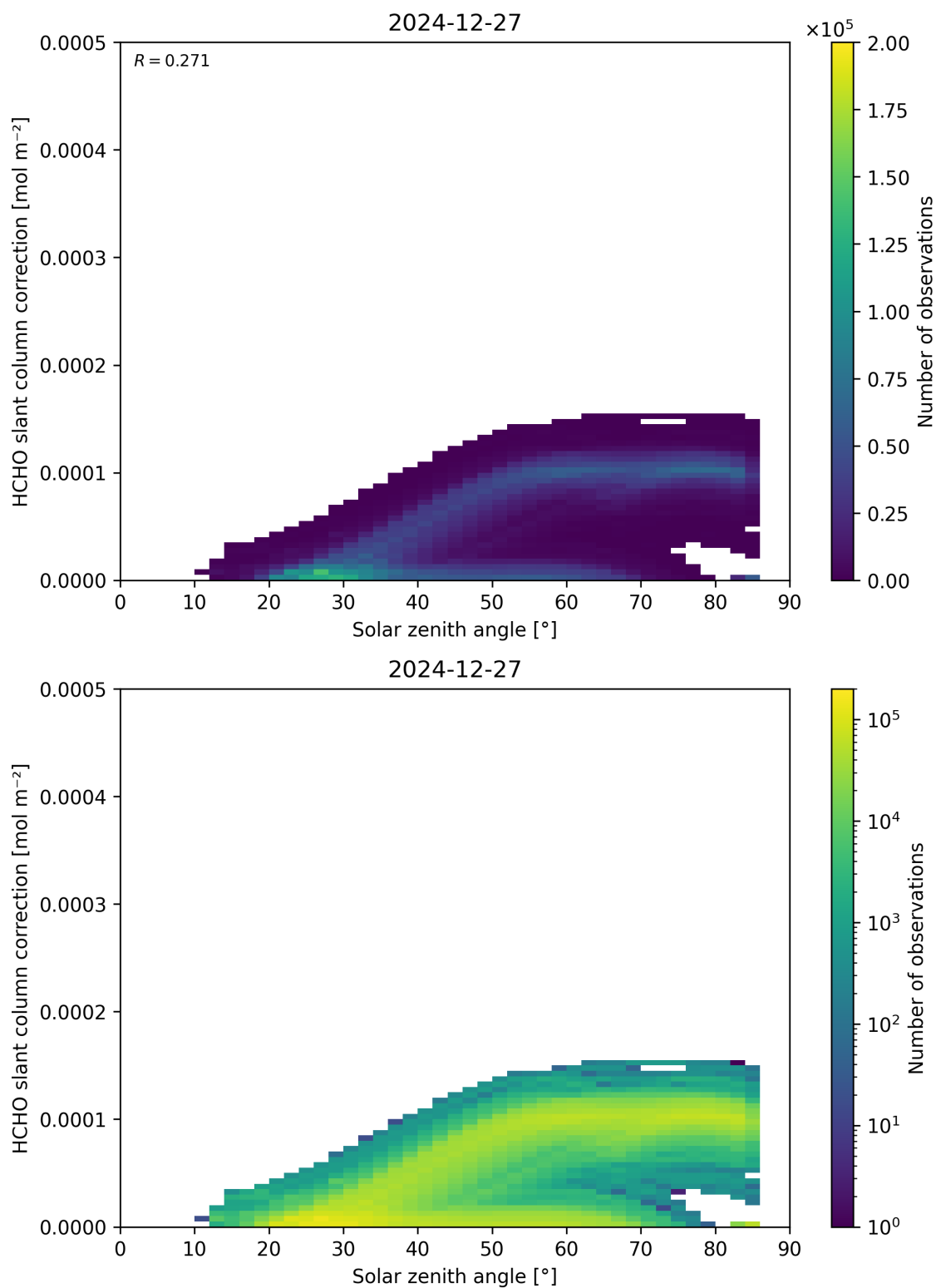
Figure 172: Scatter density plot of “Solar zenith angle” against “HCHO slant column correction” for 2024-12-27 to 2024-12-28.
