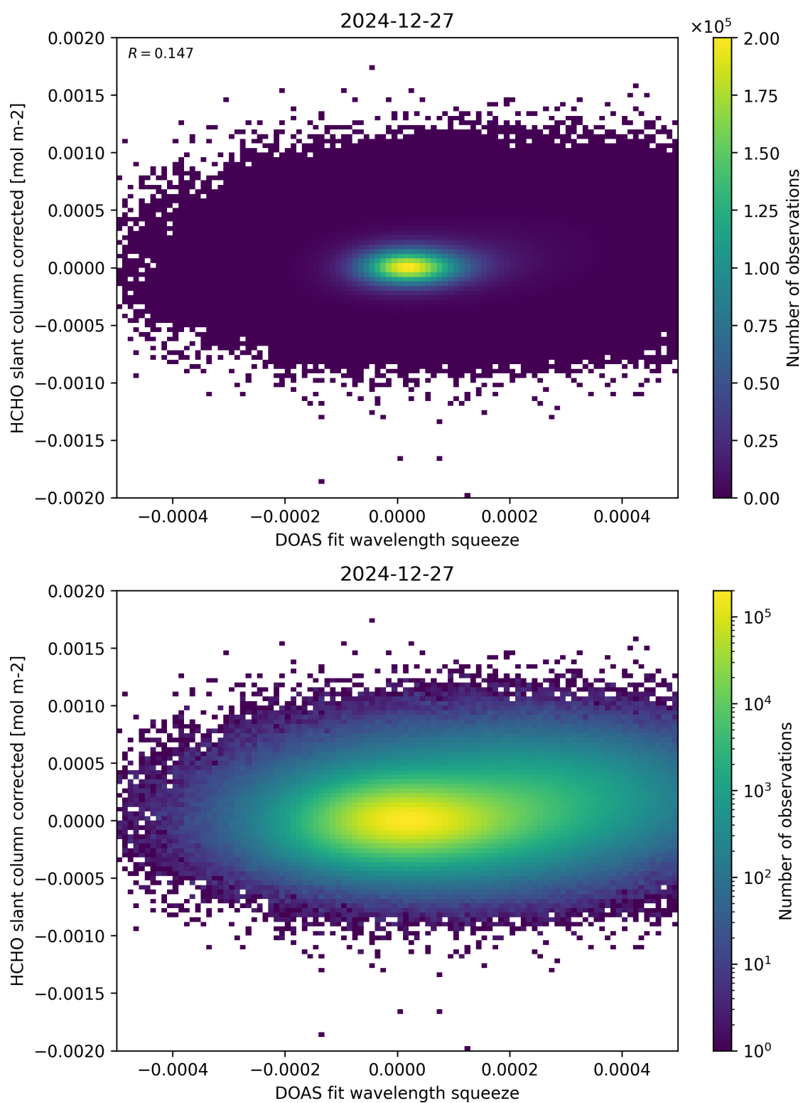
Figure 69: Scatter density plot of “DOAS fit wavelength squeeze” against “HCHO slant column corrected” for 2024-12-27 to 2024-12-28.
