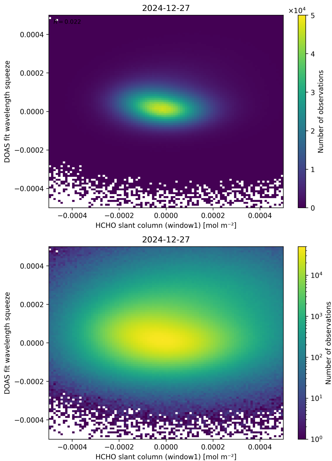
Figure 80: Scatter density plot of “HCHO slant column (window1)” against “DOAS fit wavelength squeeze” for 2024-12-27 to 2024-12-28.
