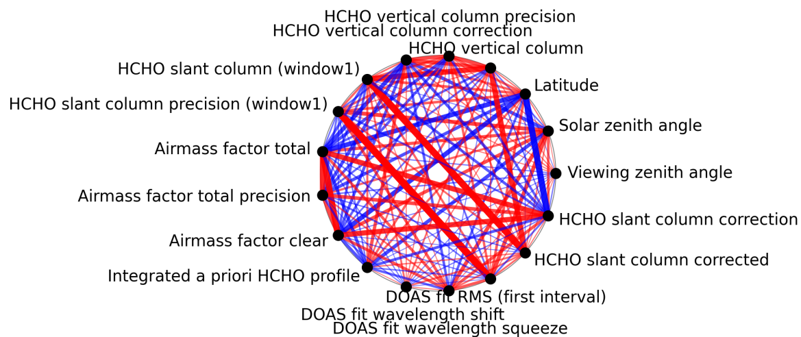
Figure 1: Map of correlation graph for 2024-12-27 to 2024-12-28.
