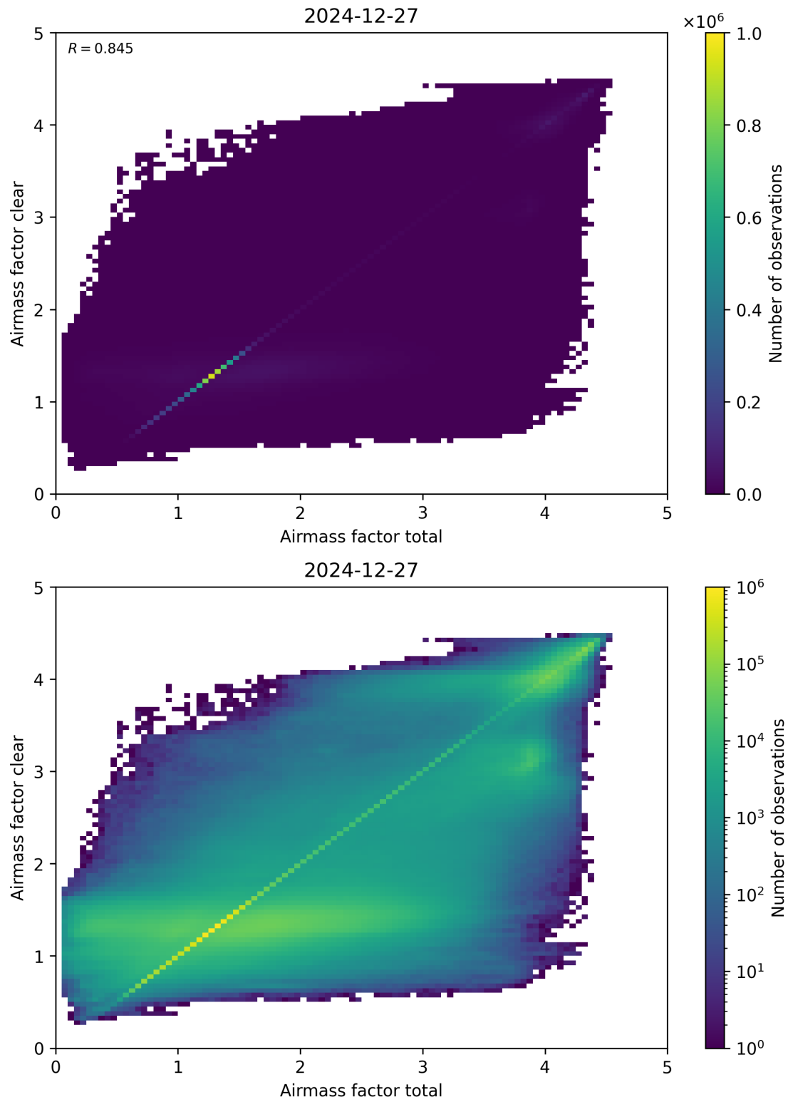
Figure 100: Scatter density plot of “Airmass factor total” against “Airmass factor clear” for 2024-12-27 to 2024-12-28.
