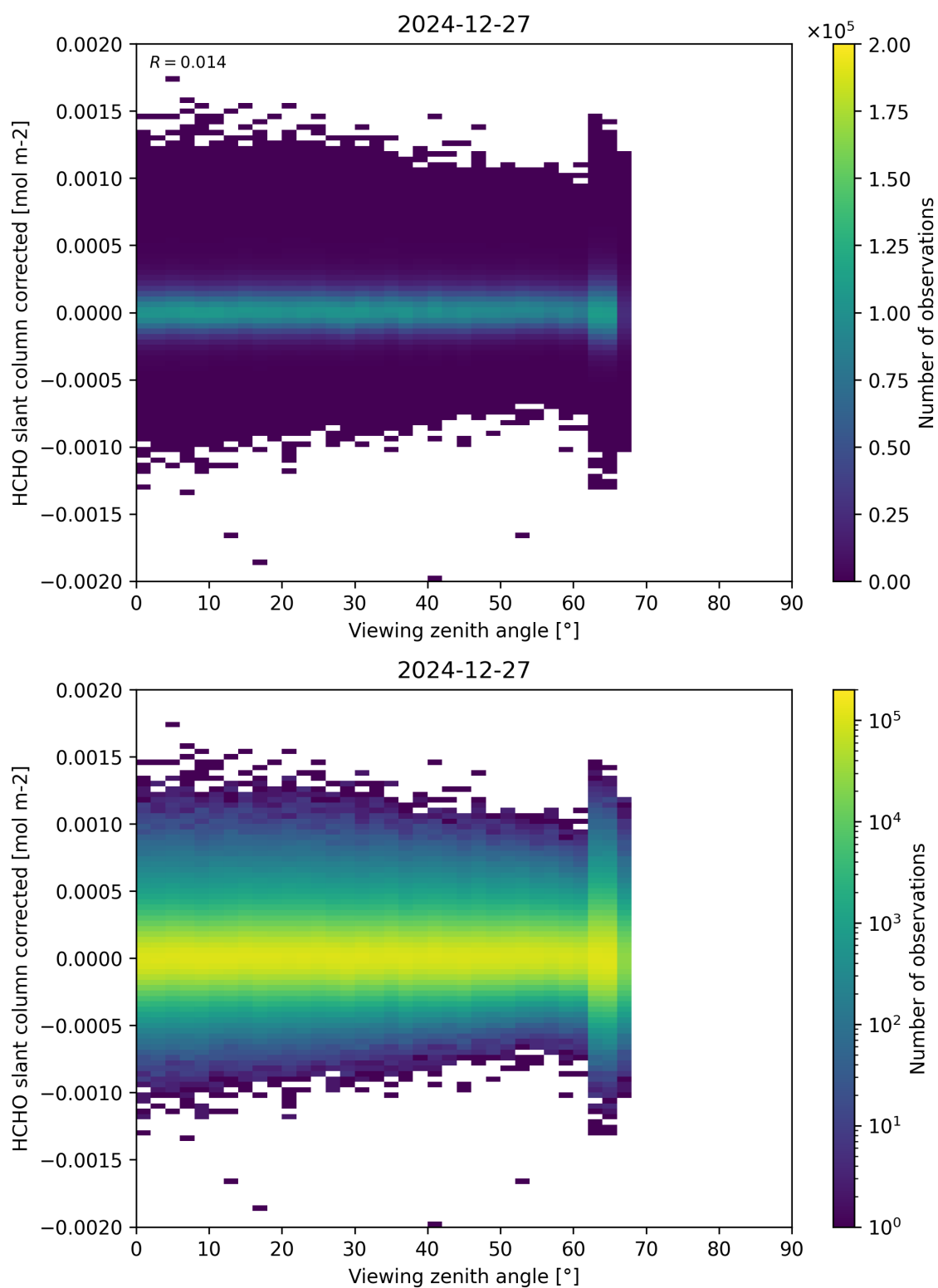
Figure 186: Scatter density plot of “Viewing zenith angle” against “HCHO slant column corrected” for 2024-12-27 to 2024-12-28.
