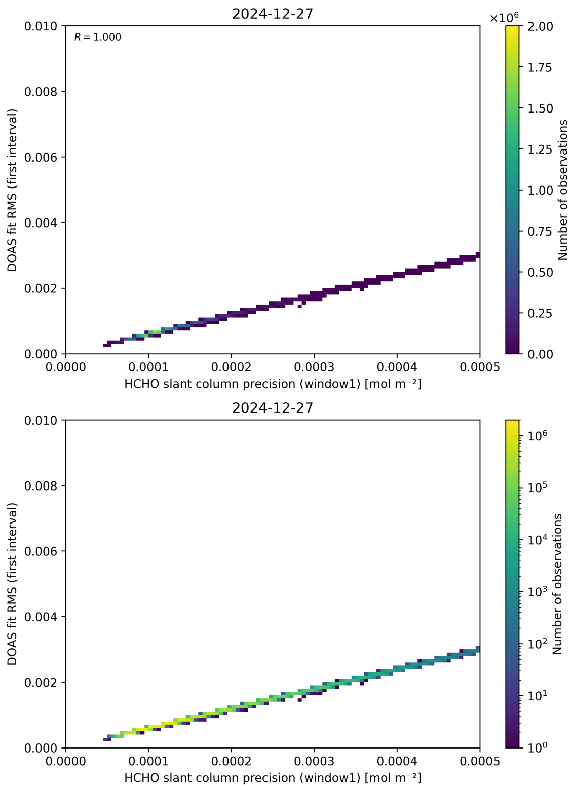
Figure 88: Scatter density plot of “HCHO slant column precision (window1)” against “DOAS fit RMS (first interval)” for 2024-12-27 to 2024-12-28.
