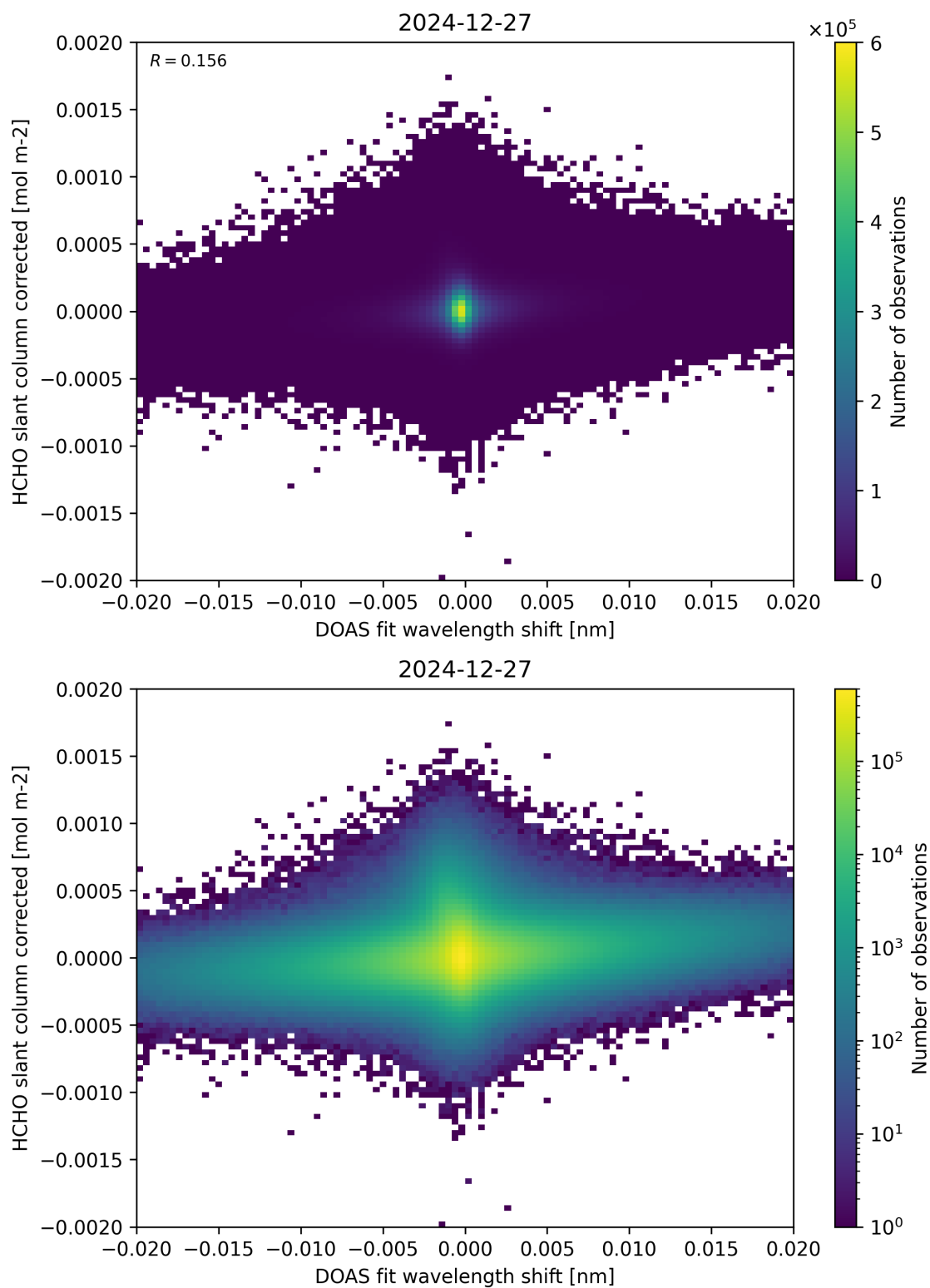
Figure 66: Scatter density plot of “DOAS fit wavelength shift” against “HCHO slant column corrected” for 2024-12-27 to 2024-12-28.
