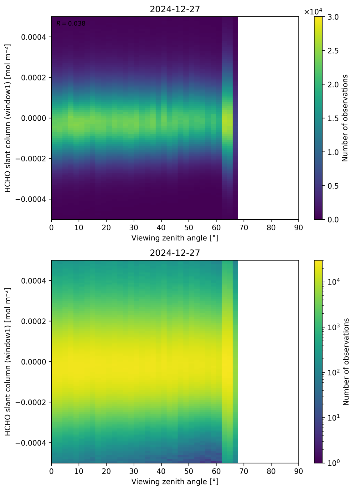
Figure 188: Scatter density plot of “Viewing zenith angle” against “HCHO slant column (window1)” for 2024-12-27 to 2024-12-28.
