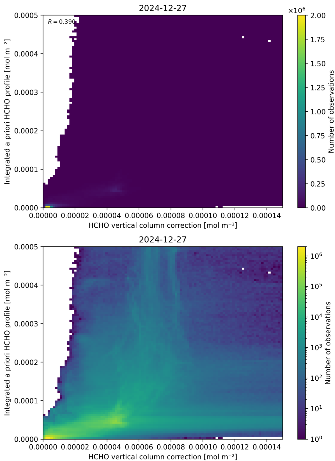
Figure 122: Scatter density plot of “HCHO vertical column correction” against “Integrated a priori HCHO profile” for 2024-12-27 to 2024-12-28.
