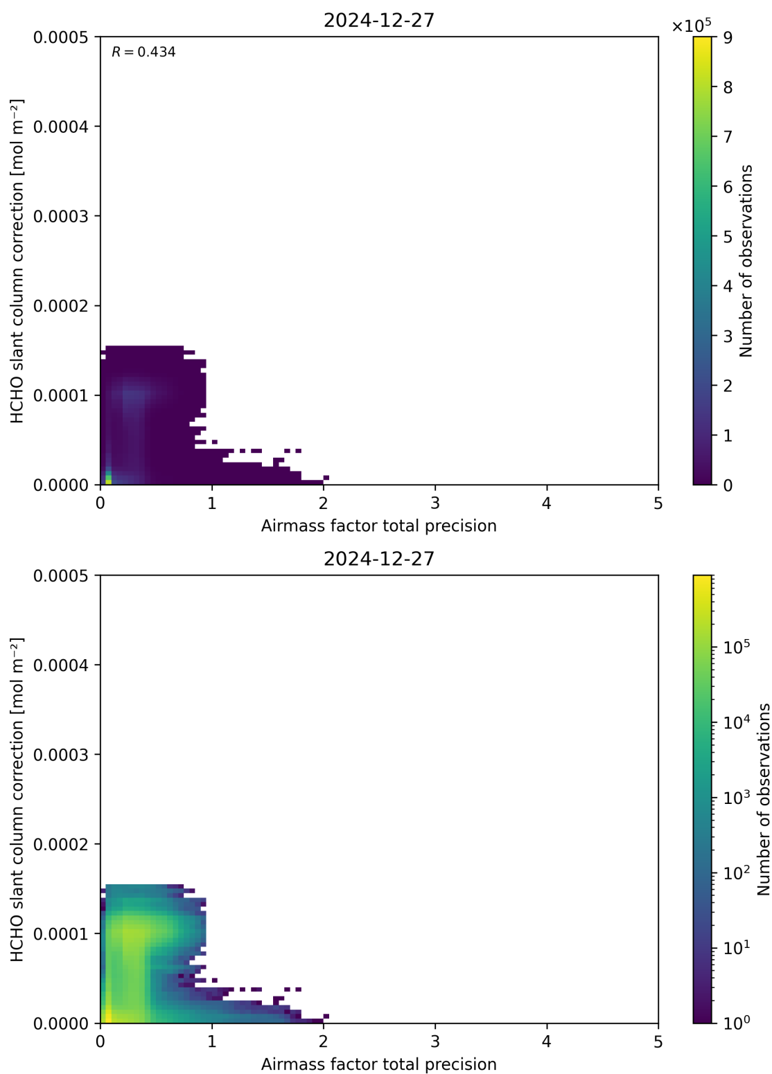
Figure 110: Scatter density plot of “Airmass factor total precision” against “HCHO slant column correction” for 2024-12-27 to 2024-12-28.
