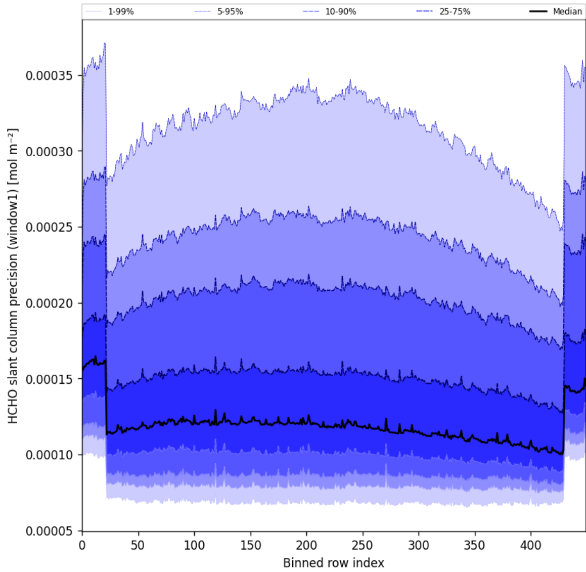
Figure 53: Along track statistics of “HCHO slant column precision (window1)” for 2024-12-27 to 2024-12-28
