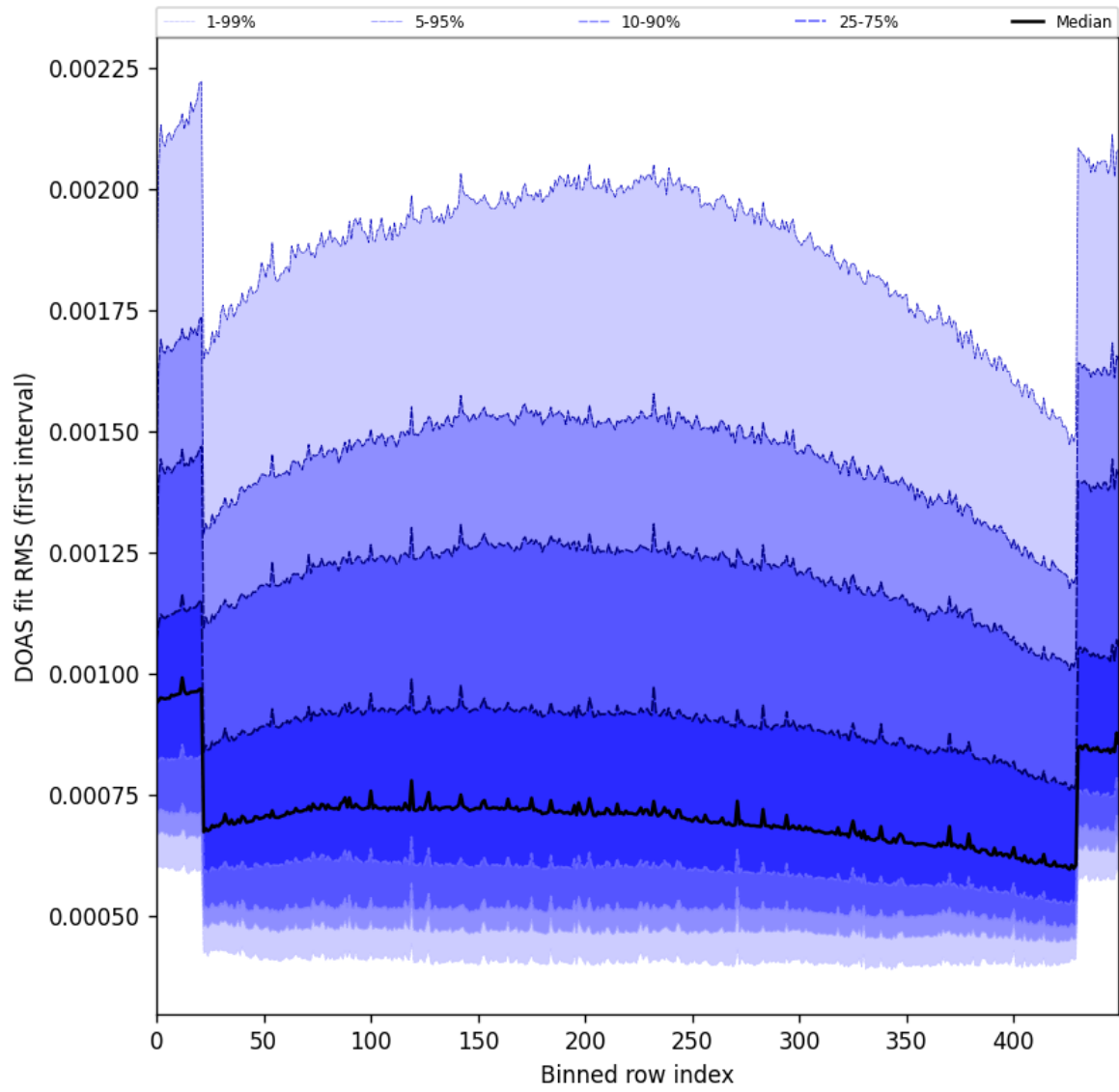
Figure 60: Along track statistics of “DOAS fit RMS (first interval)” for 2024-12-27 to 2024-12-28
