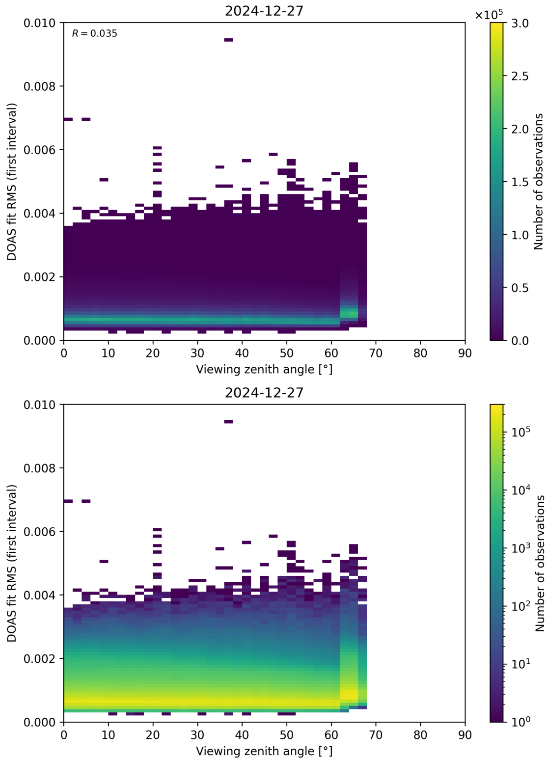
Figure 182: Scatter density plot of “Viewing zenith angle” against “DOAS fit RMS (first interval)” for 2024-12-27 to 2024-12-28.
