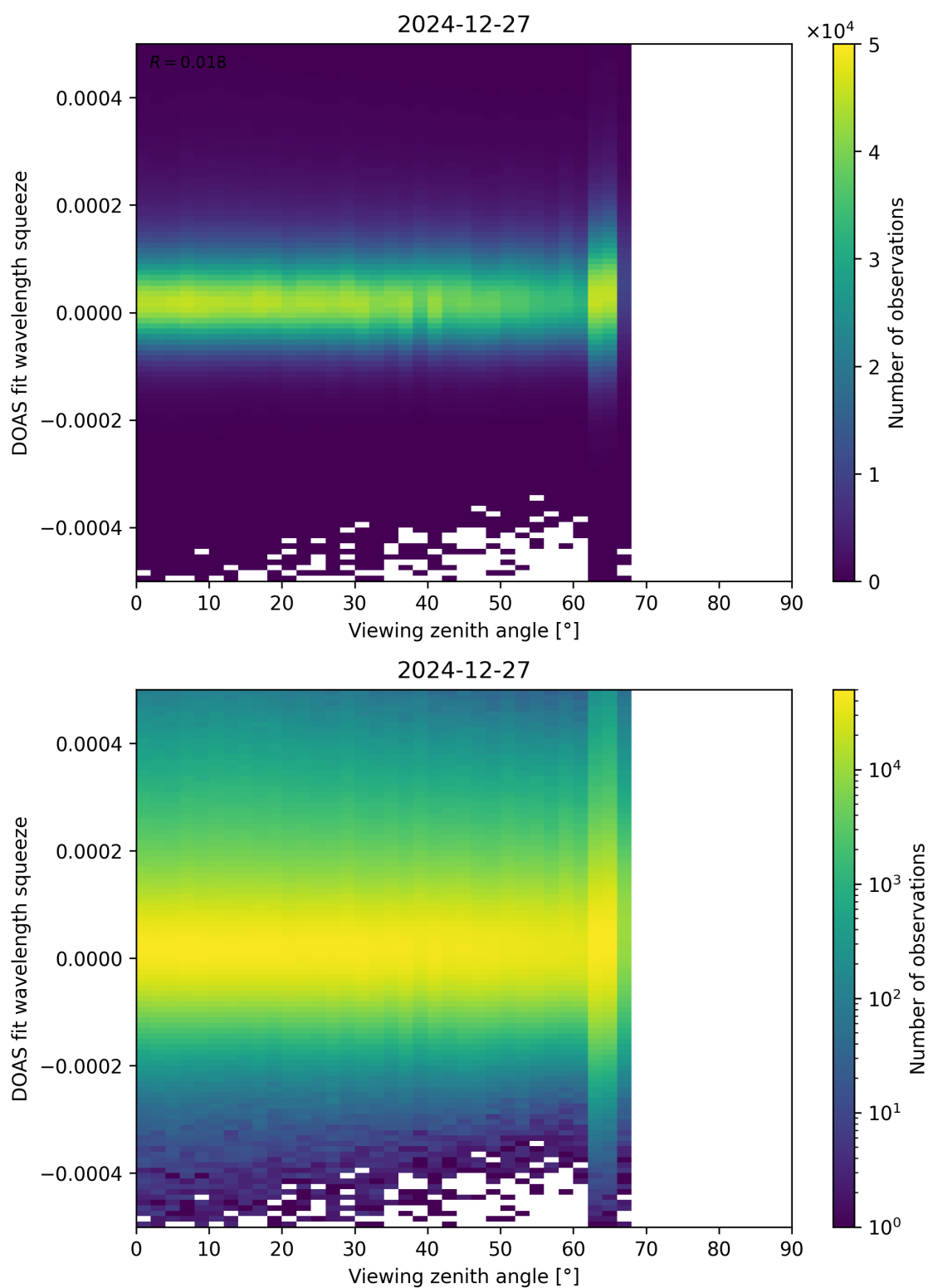
Figure 184: Scatter density plot of “Viewing zenith angle” against “DOAS fit wavelength squeeze” for 2024-12-27 to 2024-12-28.
