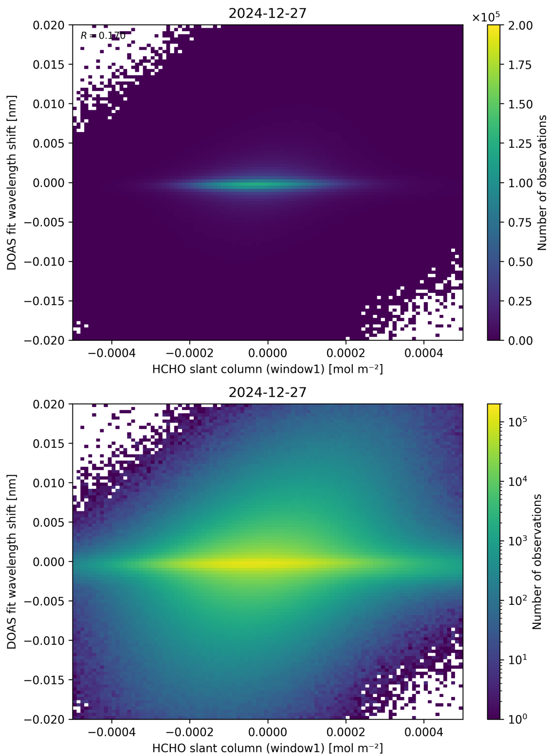
Figure 79: Scatter density plot of “HCHO slant column (window1)” against “DOAS fit wavelength shift” for 2024-12-27 to 2024-12-28.
