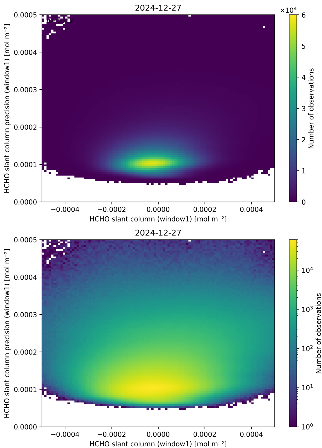
Figure 84: Scatter density plot of “HCHO slant column (window1)” against “HCHO slant column precision (window1)” for 2024-12-27 to 2024-12-28.
