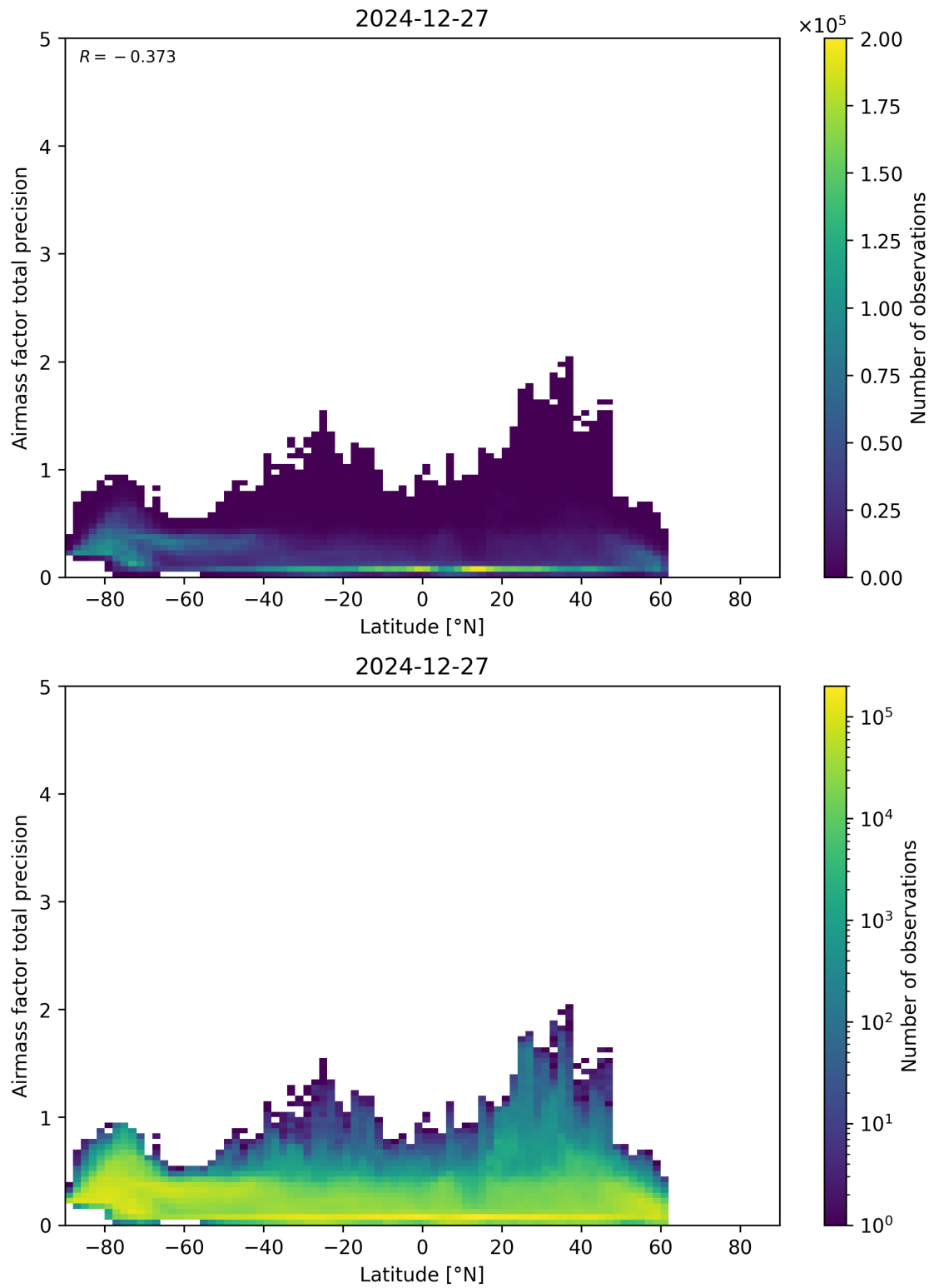
Figure 162: Scatter density plot of “Latitude” against “Airmass factor total precision” for 2024-12-27 to 2024-12-28.
