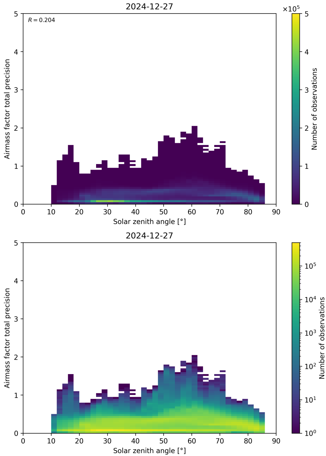
Figure 176: Scatter density plot of “Solar zenith angle” against “Airmass factor total precision” for 2024-12-27 to 2024-12-28.
