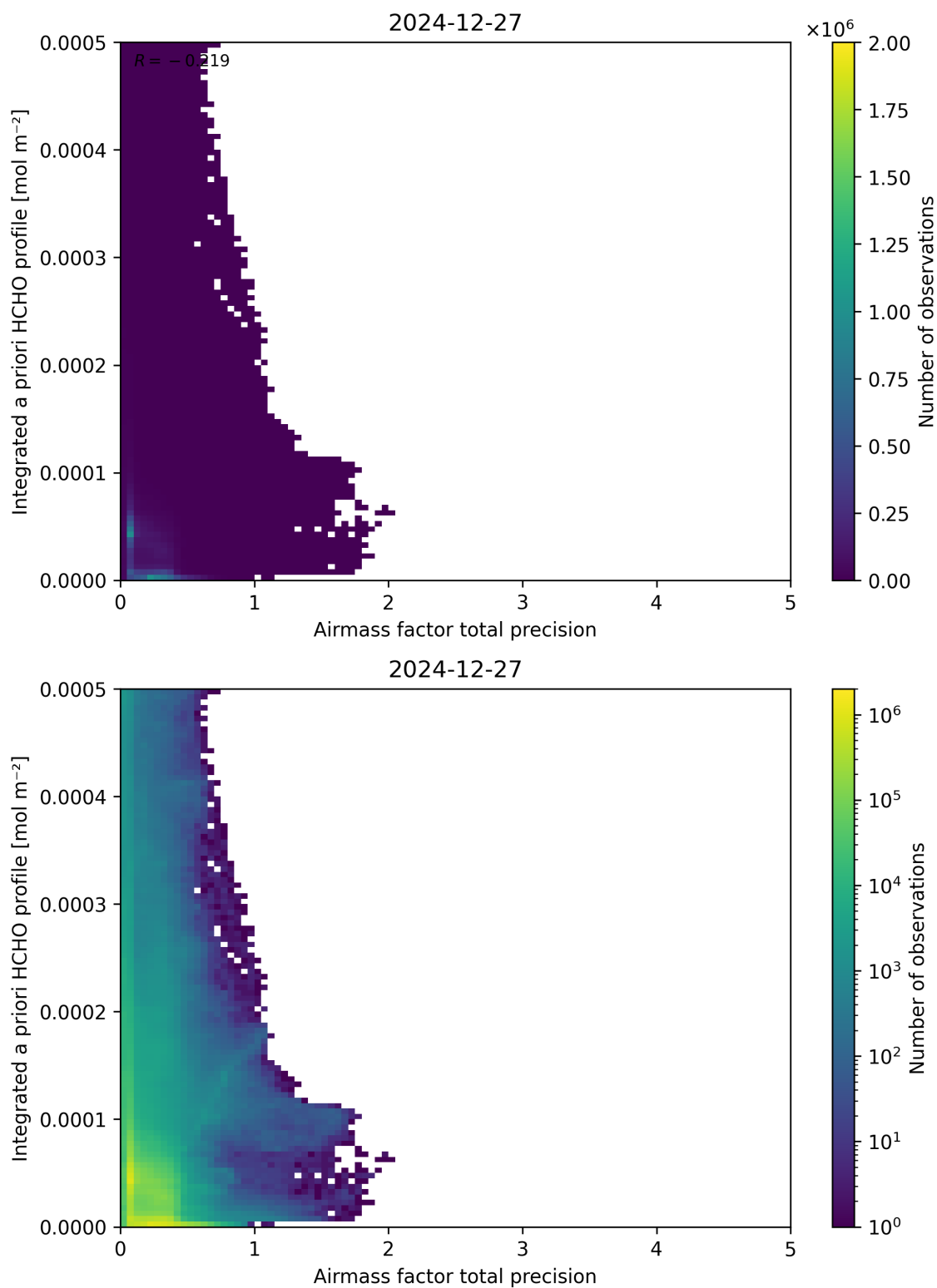
Figure 111: Scatter density plot of “Airmass factor total precision” against “Integrated a priori HCHO profile” for 2024-12-27 to 2024-12-28.
