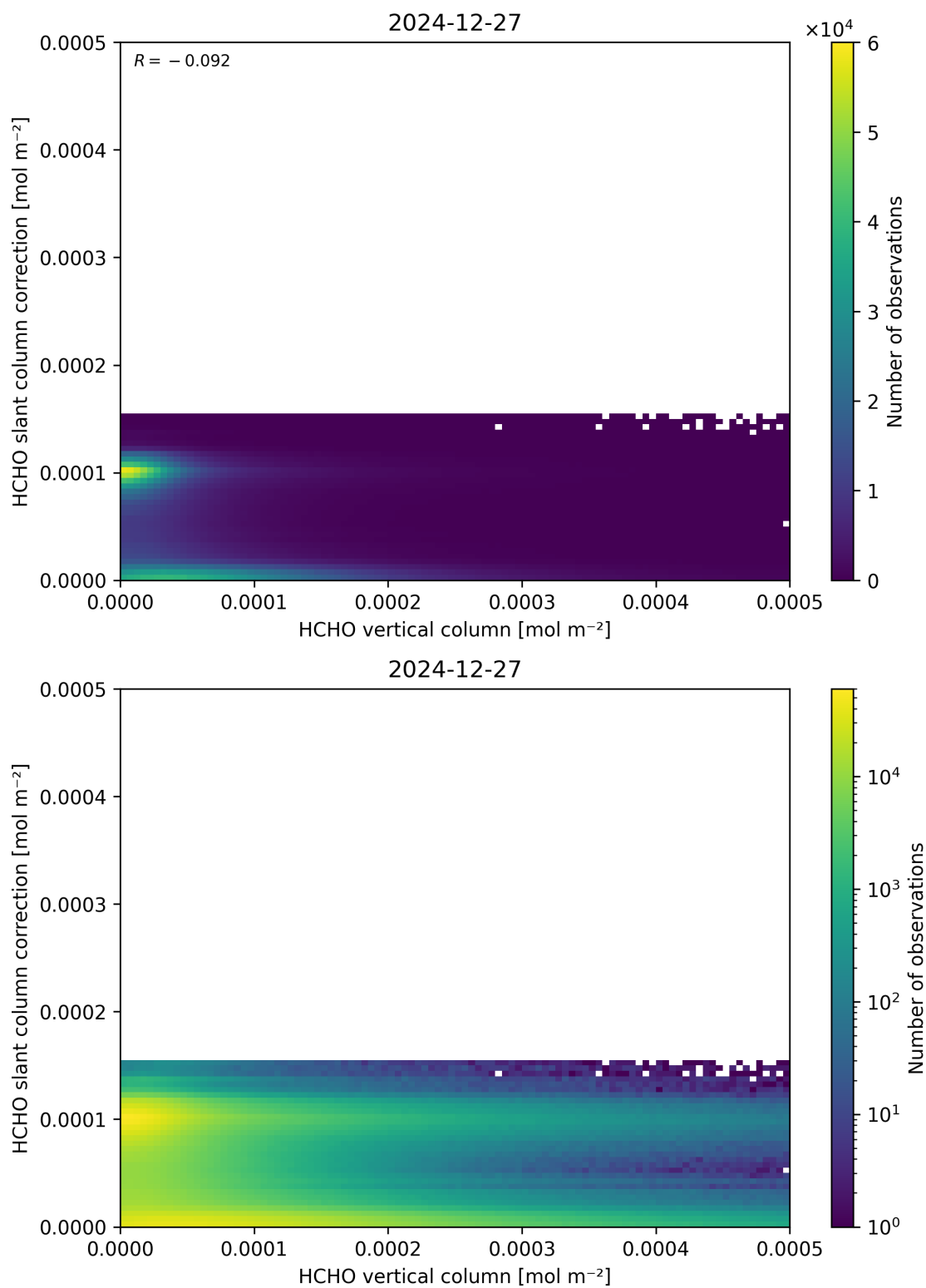
Figure 128: Scatter density plot of “HCHO vertical column” against “HCHO slant column correction” for 2024-12-27 to 2024-12-28.
