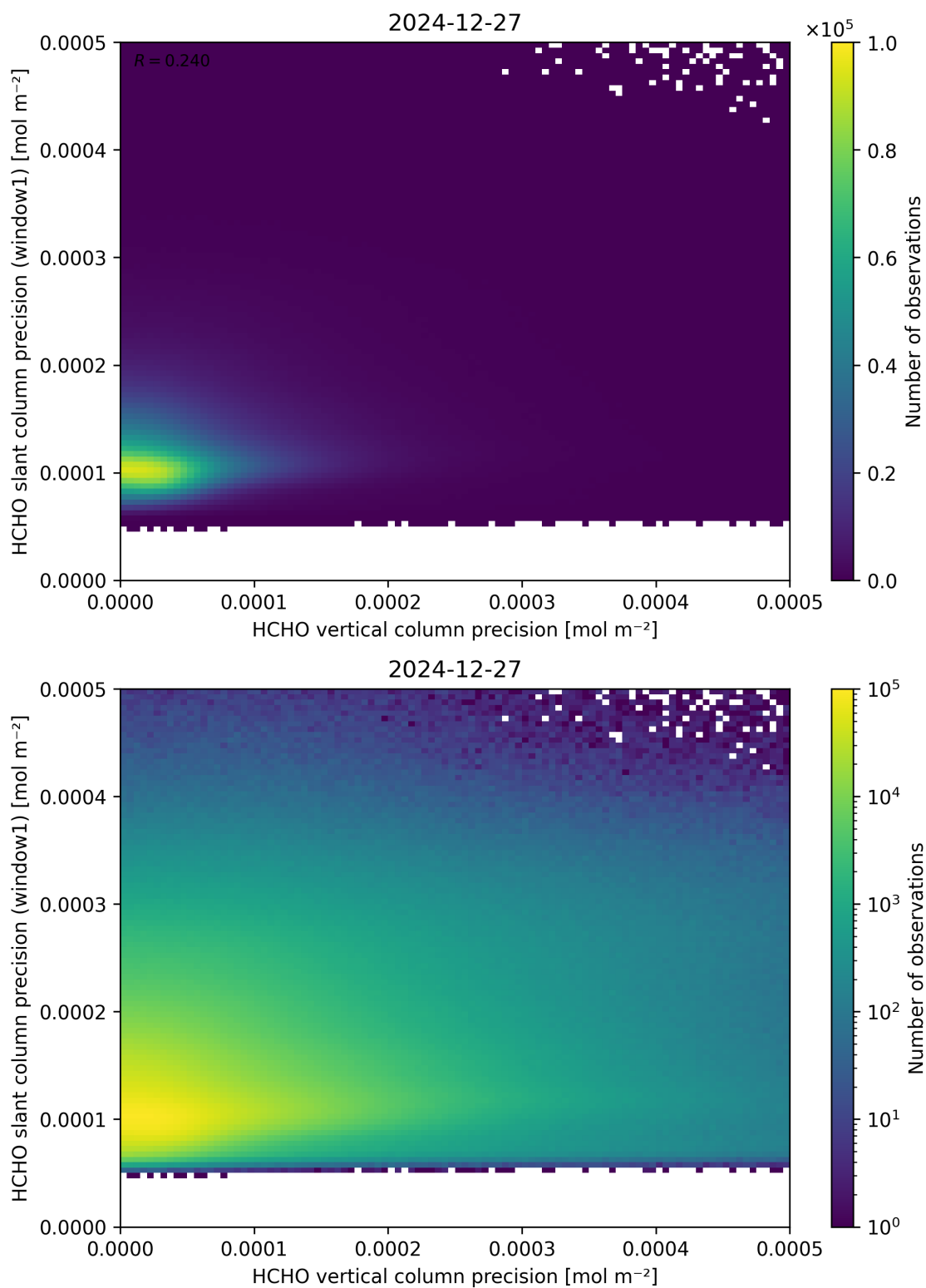
Figure 143: Scatter density plot of “HCHO vertical column precision” against “HCHO slant column precision (window1)” for 2024-12-27 to 2024-12-28.
