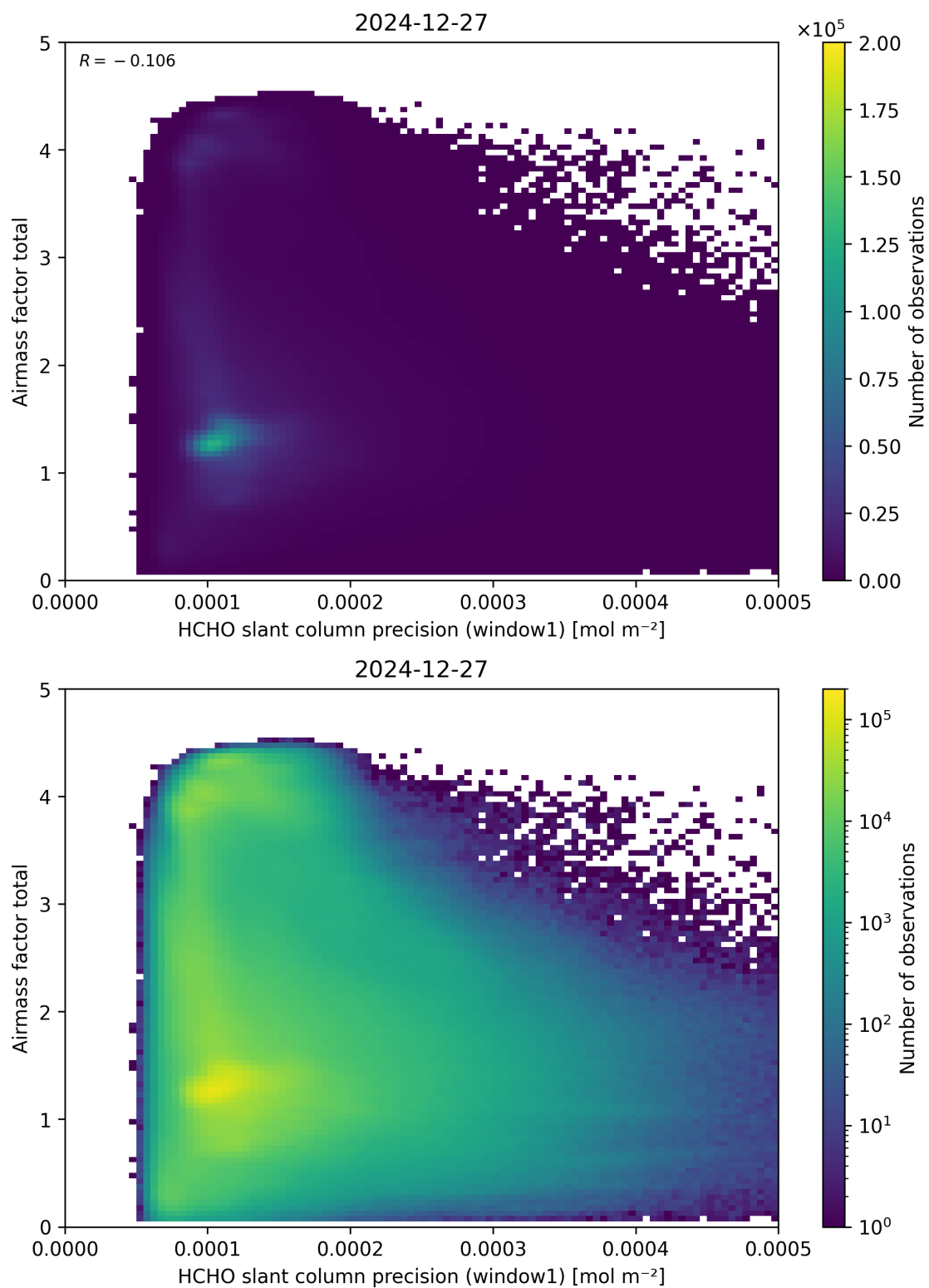
Figure 94: Scatter density plot of “HCHO slant column precision (window1)” against “Airmass factor total” for 2024-12-27 to 2024-12-28.
