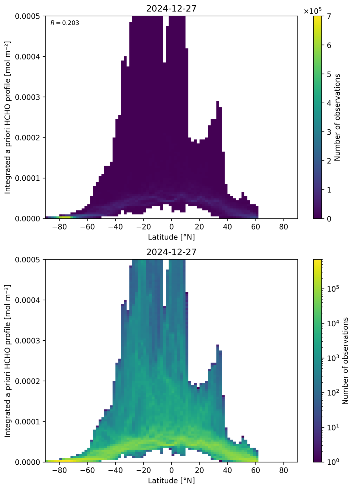
Figure 166: Scatter density plot of “Latitude” against “Integrated a priori HCHO profile” for 2024-12-27 to 2024-12-28.
