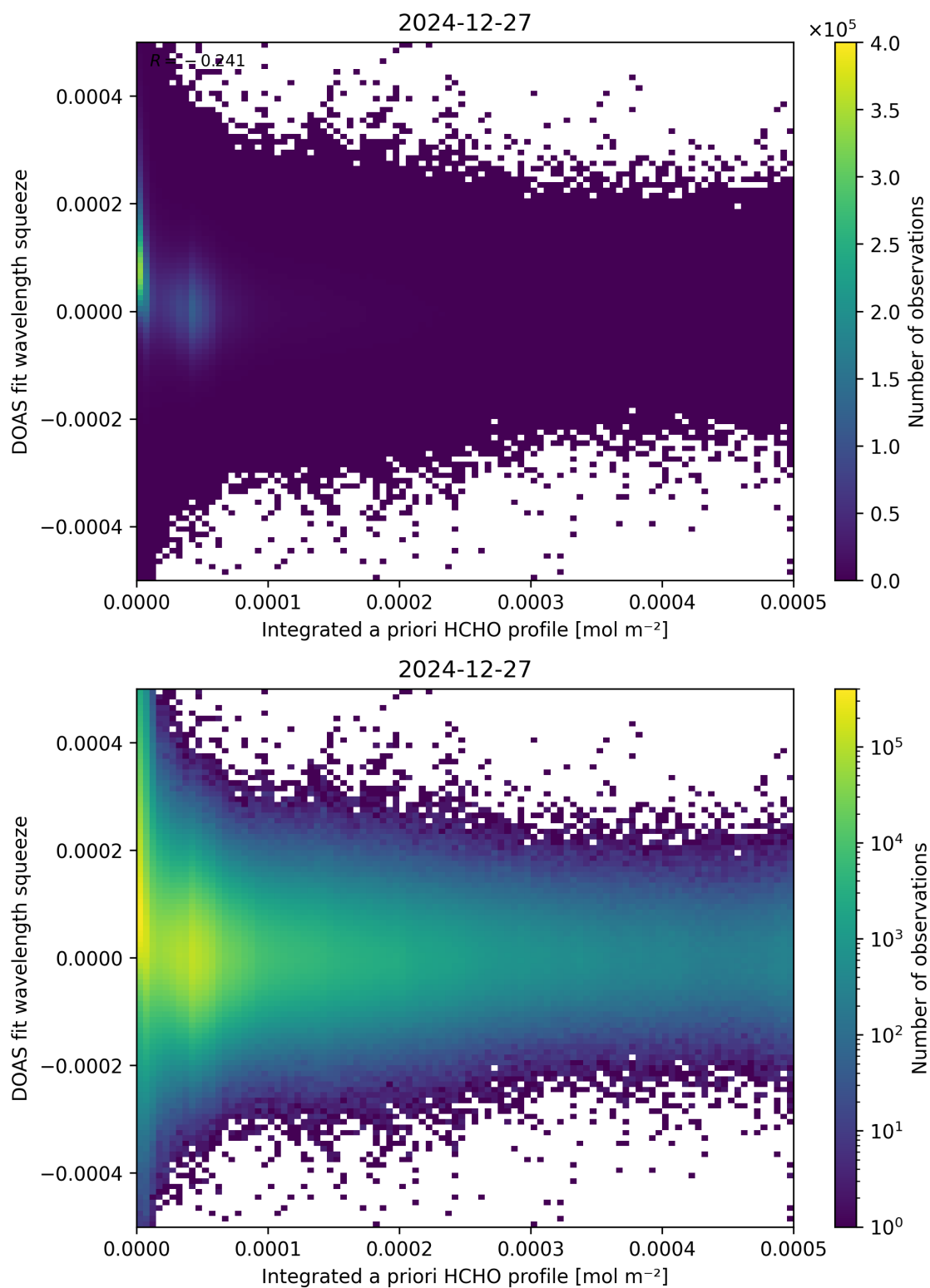
Figure 150: Scatter density plot of “Integrated a priori HCHO profile” against “DOAS fit wavelength squeeze” for 2024-12-27 to 2024-12-28.
