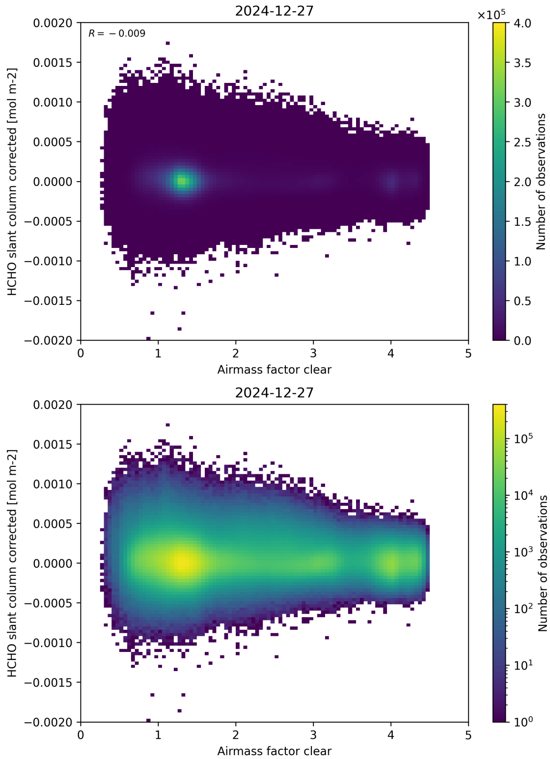
Figure 74: Scatter density plot of “Airmass factor clear” against “HCHO slant column corrected” for 2024-12-27 to 2024-12-28.
