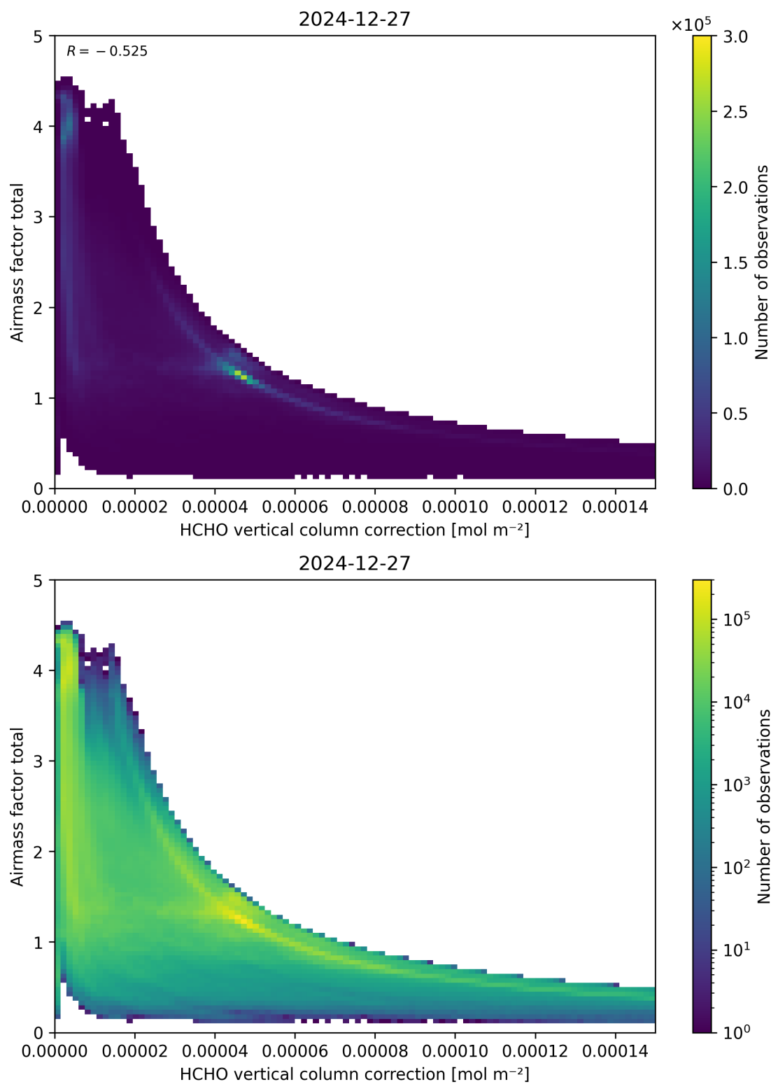
Figure 120: Scatter density plot of “HCHO vertical column correction” against “Airmass factor total” for 2024-12-27 to 2024-12-28.
