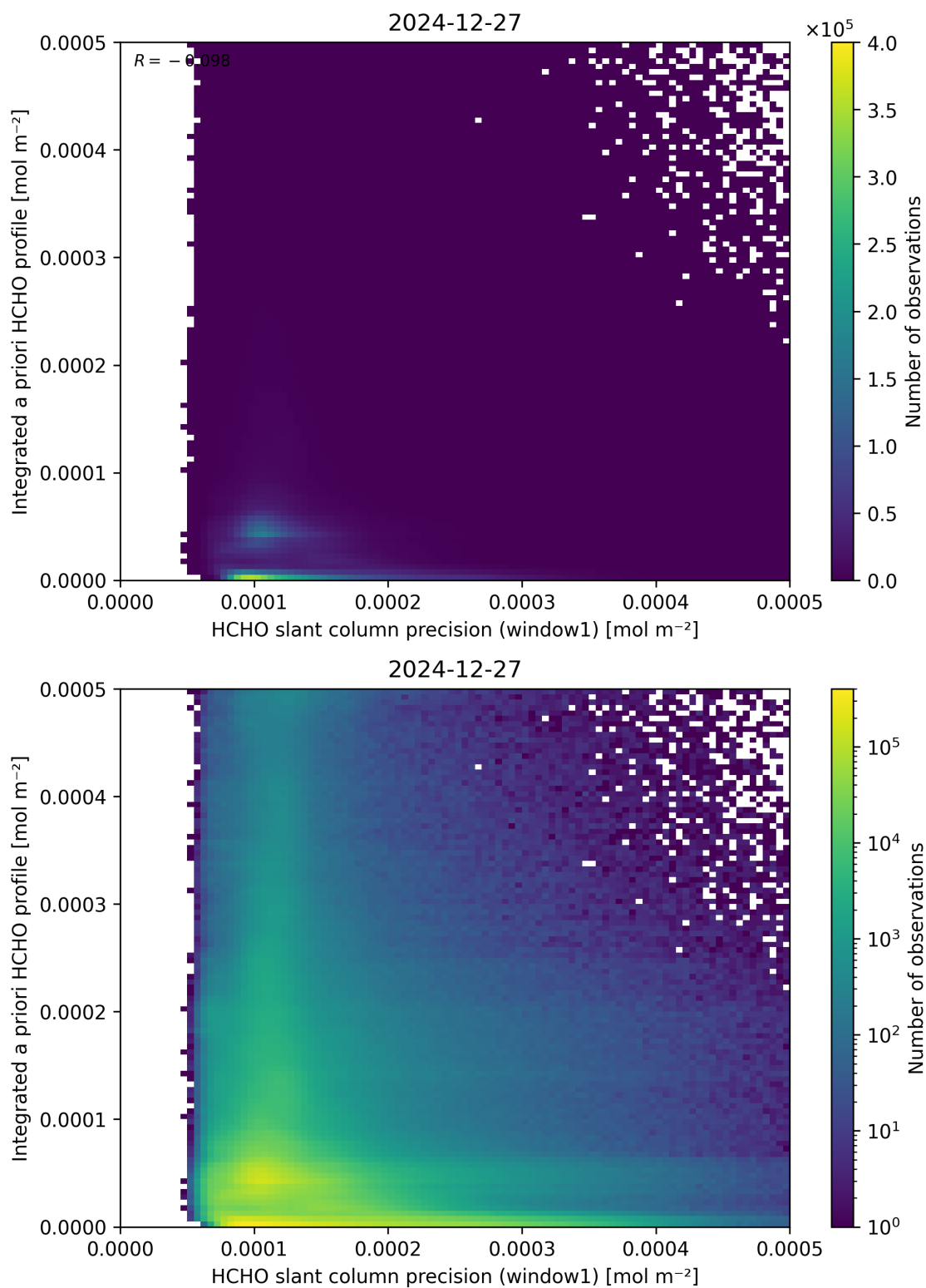
Figure 96: Scatter density plot of “HCHO slant column precision (window1)” against “Integrated a priori HCHO profile” for 2024-12-27 to 2024-12-28.
