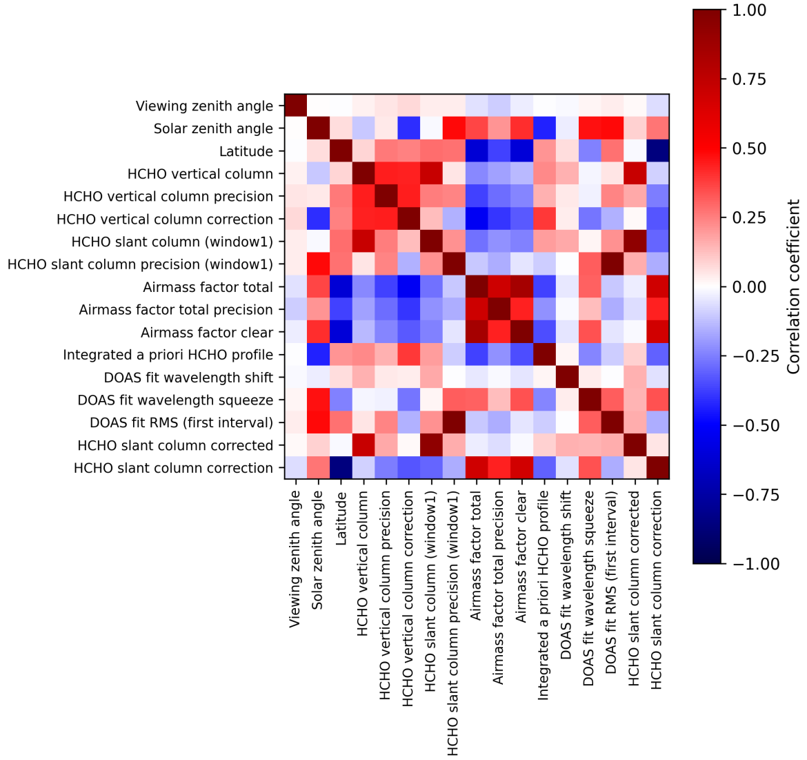
Figure 2: Map of correlation matrix for 2024-12-27 to 2024-12-28.
