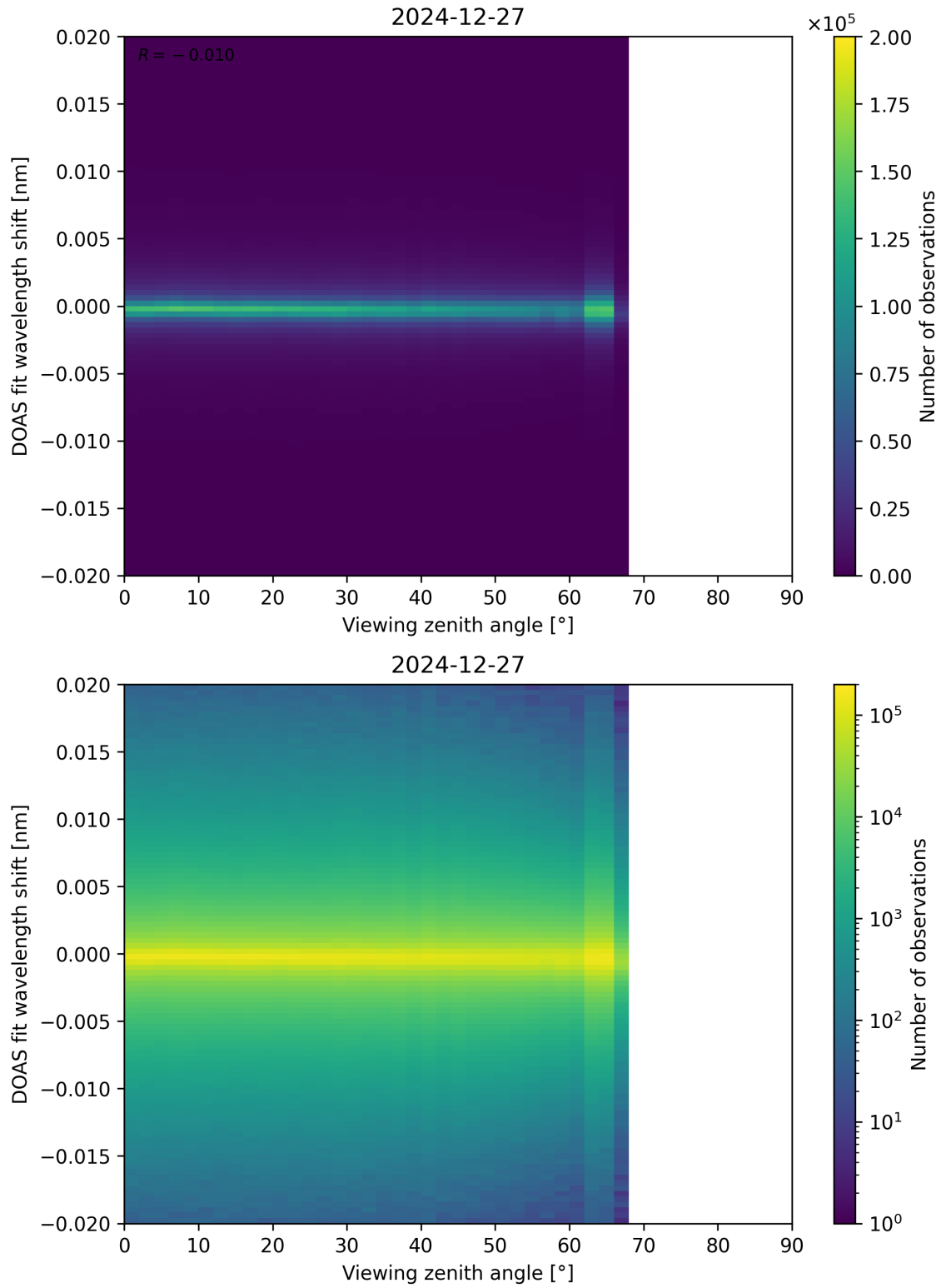
Figure 183: Scatter density plot of “Viewing zenith angle” against “DOAS fit wavelength shift” for 2024-12-27 to 2024-12-28.
