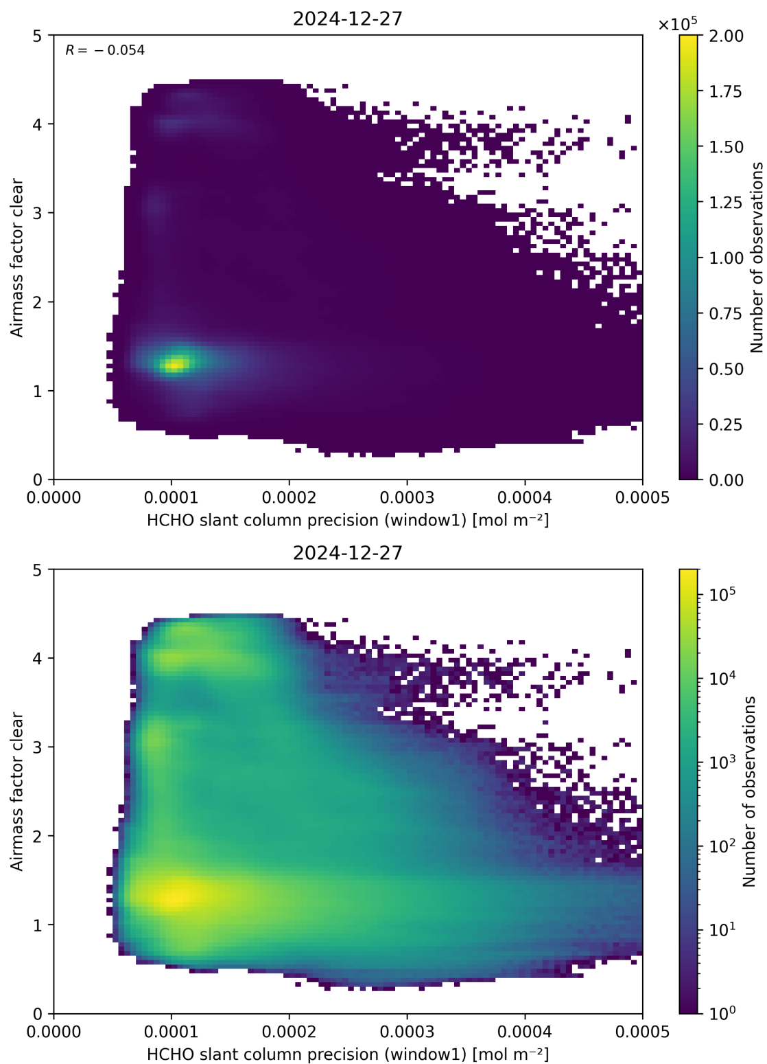
Figure 91: Scatter density plot of “HCHO slant column precision (window1)” against “Airmass factor clear” for 2024-12-27 to 2024-12-28.
