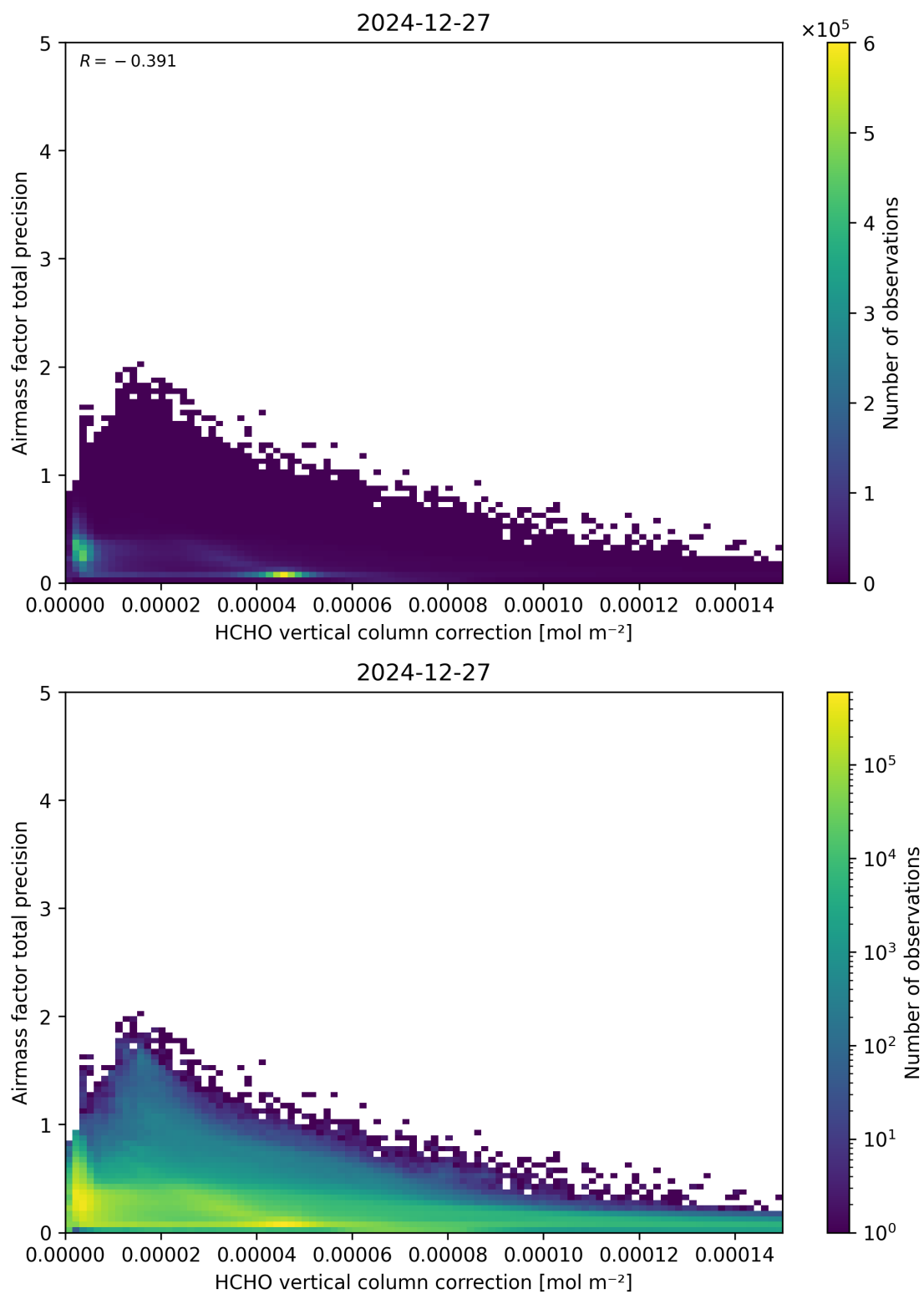
Figure 121: Scatter density plot of “HCHO vertical column correction” against “Airmass factor total precision” for 2024-12-27 to 2024-12-28.
