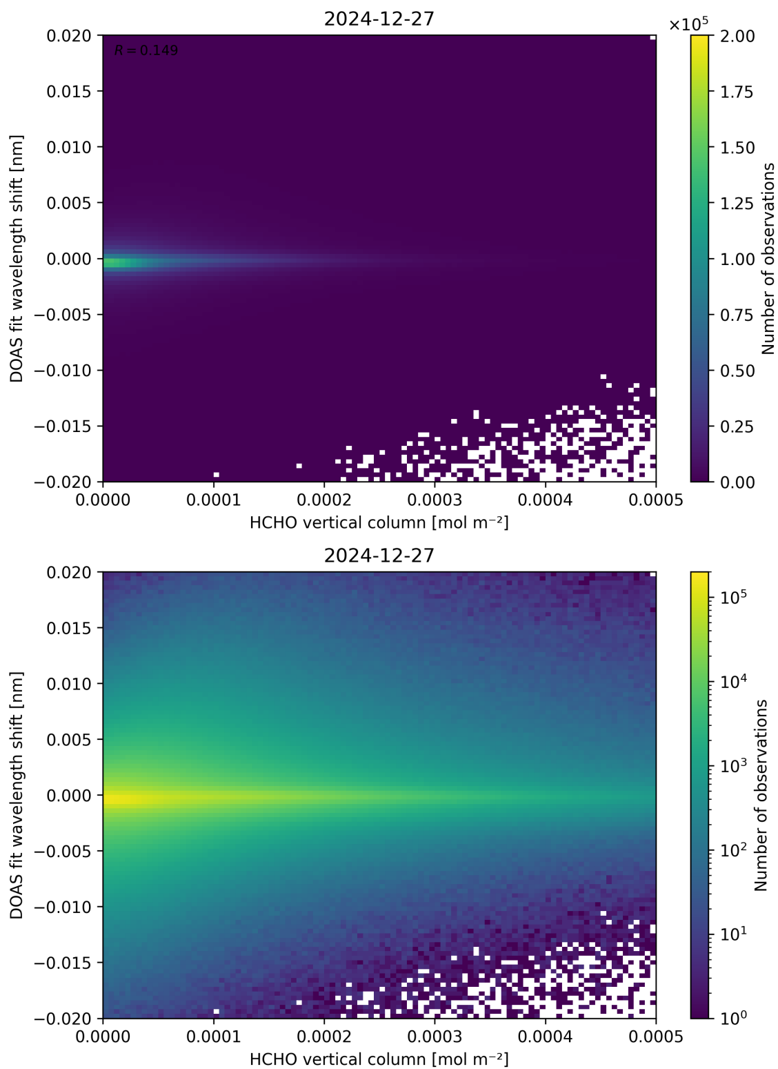
Figure 124: Scatter density plot of “HCHO vertical column” against “DOAS fit wavelength shift” for 2024-12-27 to 2024-12-28.
