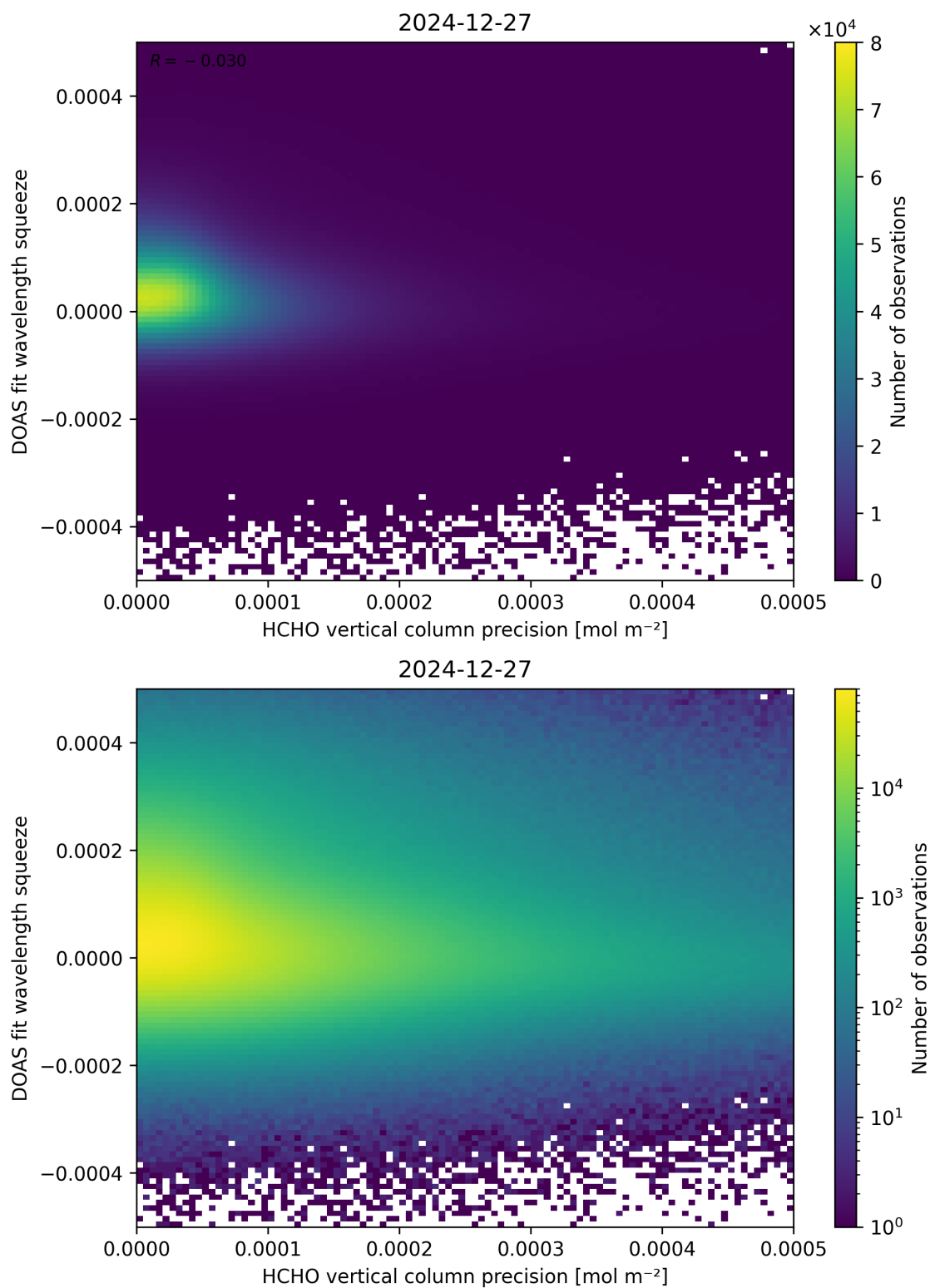
Figure 138: Scatter density plot of “HCHO vertical column precision” against “DOAS fit wavelength squeeze” for 2024-12-27 to 2024-12-28.
