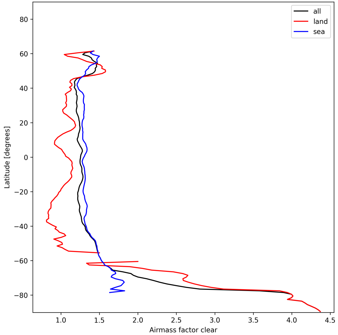
Figure 28: Zonal average of “Airmass factor clear” for 2024-12-27 to 2024-12-28.
