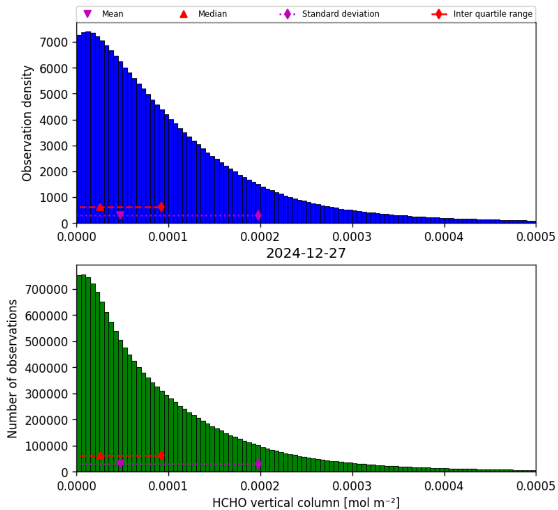
Figure 35: Histogram of “HCHO vertical column” for 2024-12-27 to 2024-12-28
