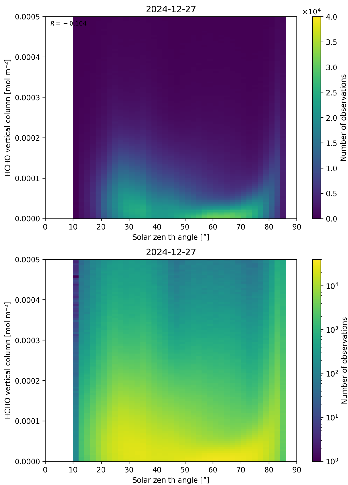
Figure 177: Scatter density plot of “Solar zenith angle” against “HCHO vertical column” for 2024-12-27 to 2024-12-28.
