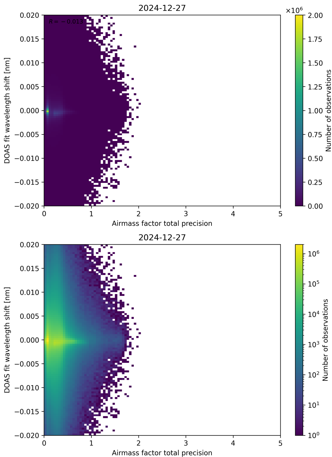
Figure 106: Scatter density plot of “Airmass factor total precision” against “DOAS fit wavelength shift” for 2024-12-27 to 2024-12-28.
