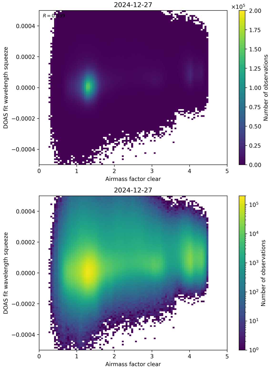
Figure 73: Scatter density plot of “Airmass factor clear” against “DOAS fit wavelength squeeze” for 2024-12-27 to 2024-12-28.
