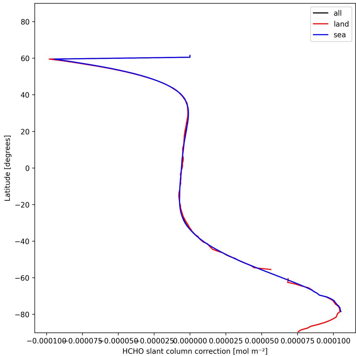
Figure 33: Zonal average of “HCHO slant column correction” for 2024-12-27 to 2024-12-28.
