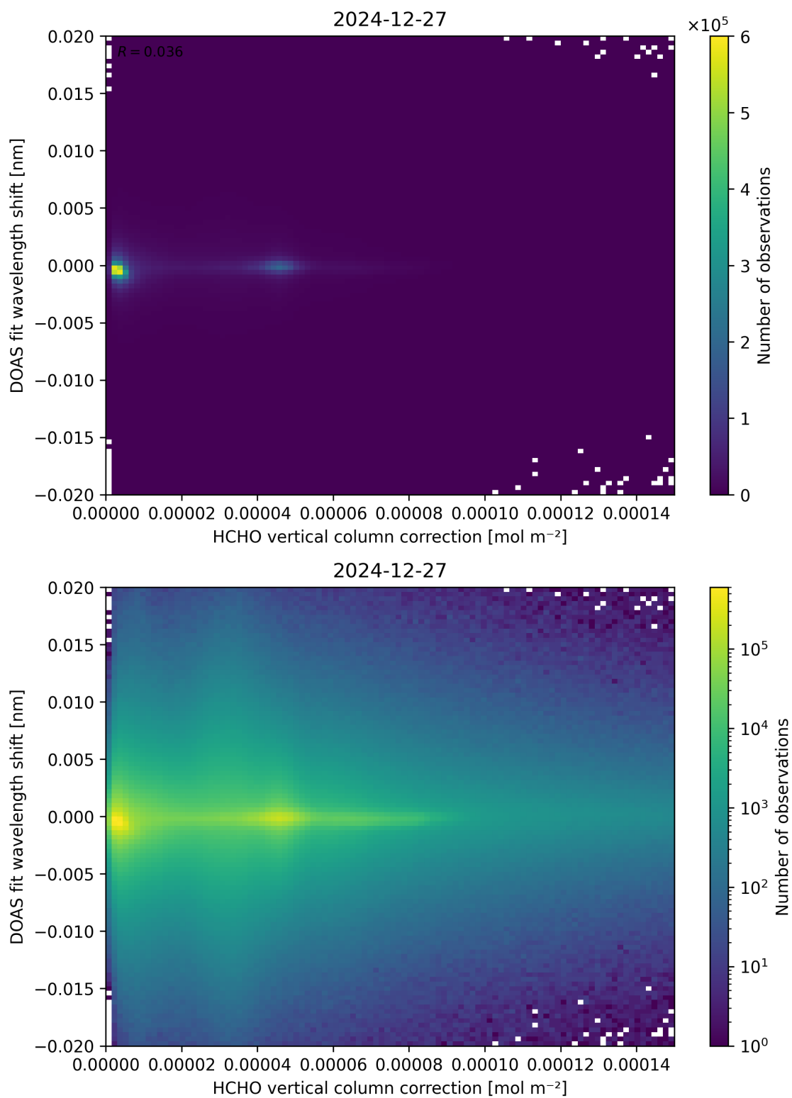
Figure 113: Scatter density plot of “HCHO vertical column correction” against “DOAS fit wavelength shift” for 2024-12-27 to 2024-12-28.
