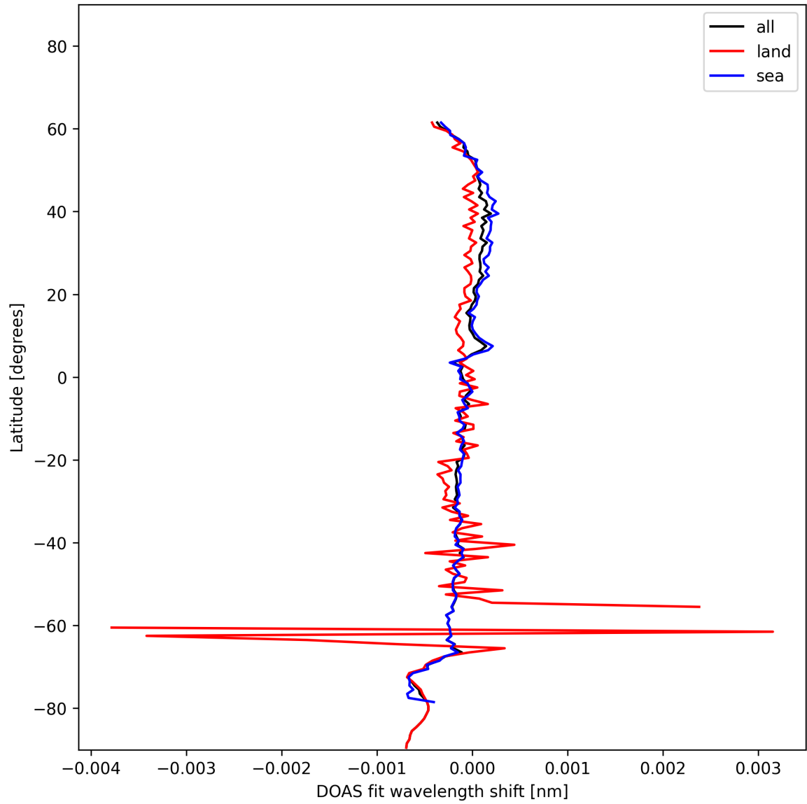
Figure 30: Zonal average of "DOAS fit wavelength shift" for 2024-12-27 to 2024-12-28.
