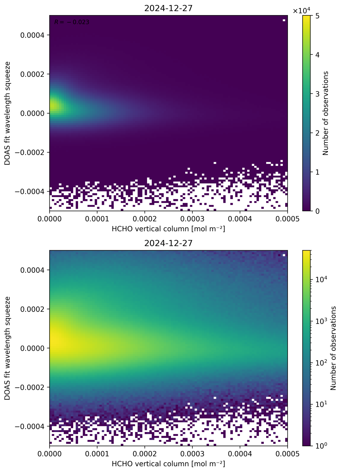
Figure 125: Scatter density plot of “HCHO vertical column” against “DOAS fit wavelength squeeze” for 2024-12-27 to 2024-12-28.
