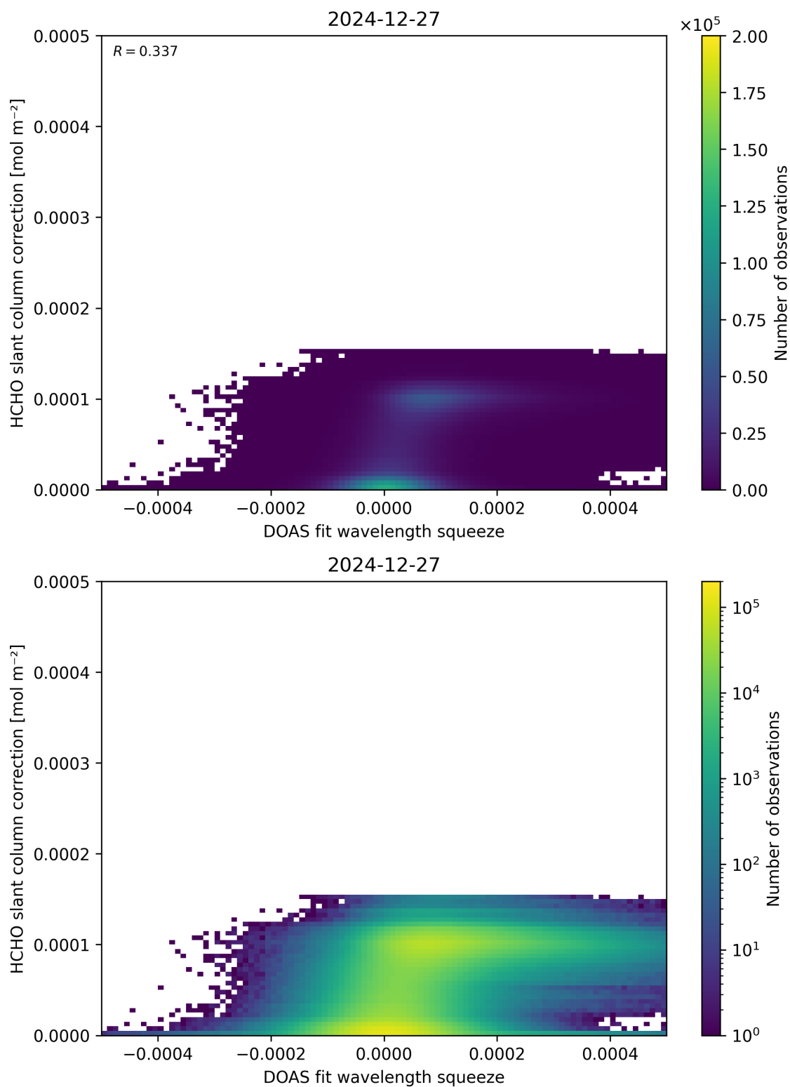
Figure 70: Scatter density plot of “DOAS fit wavelength squeeze” against “HCHO slant column correction” for 2024-12-27 to 2024-12-28.
