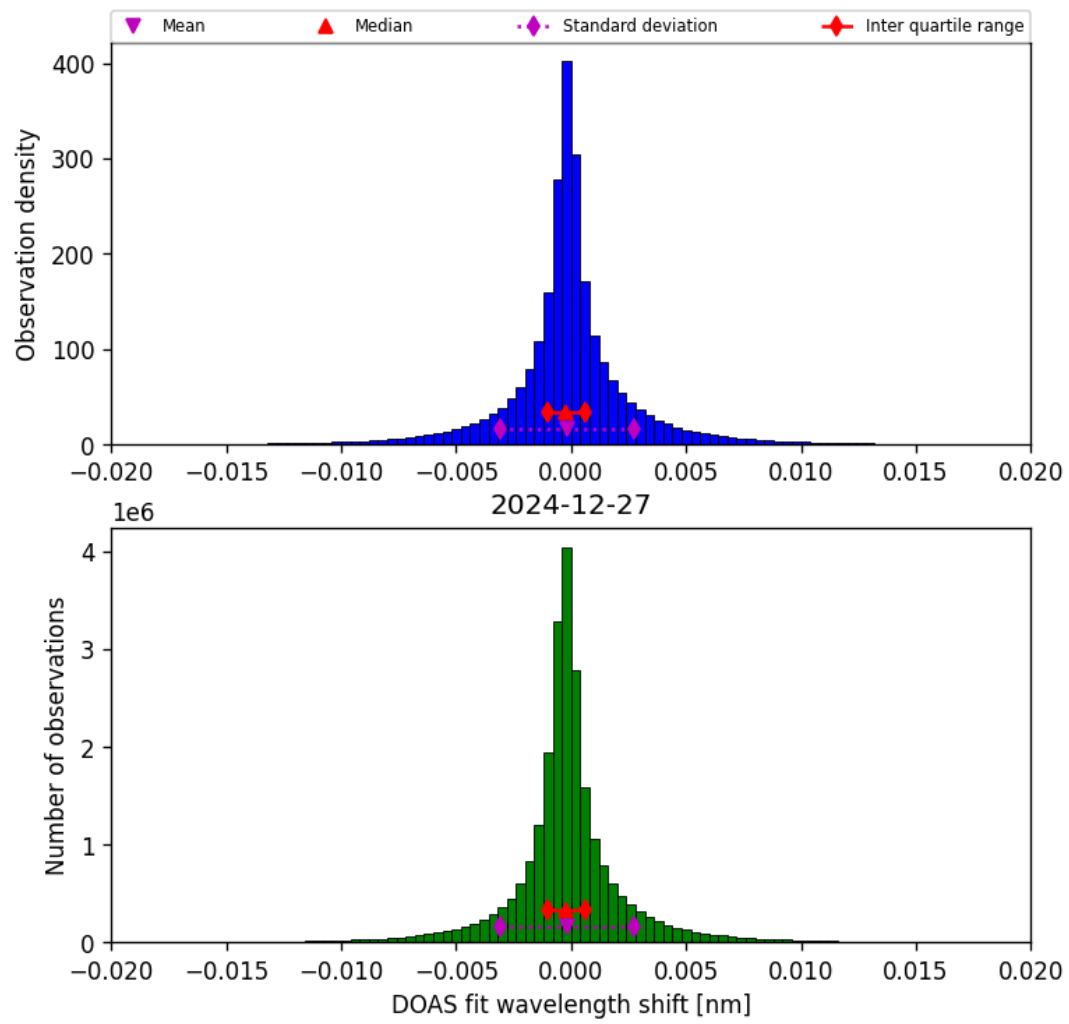
Figure 44: Histogram of “DOAS fit wavelength shift” for 2024-12-27 to 2024-12-28
