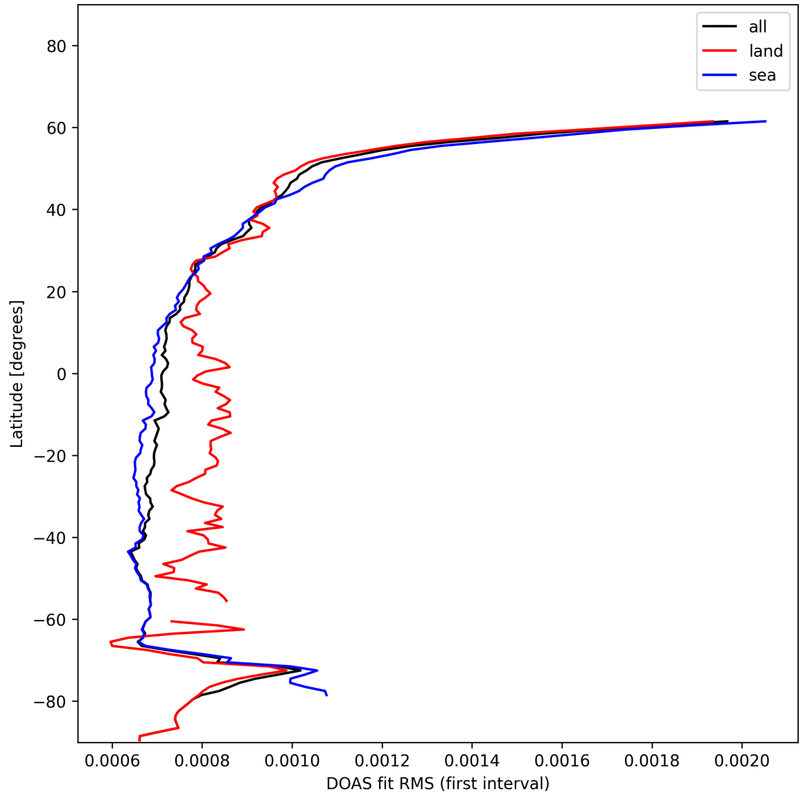
Figure 32: Zonal average of “DOAS fit RMS (first interval)” for 2024-12-27 to 2024-12-28.
