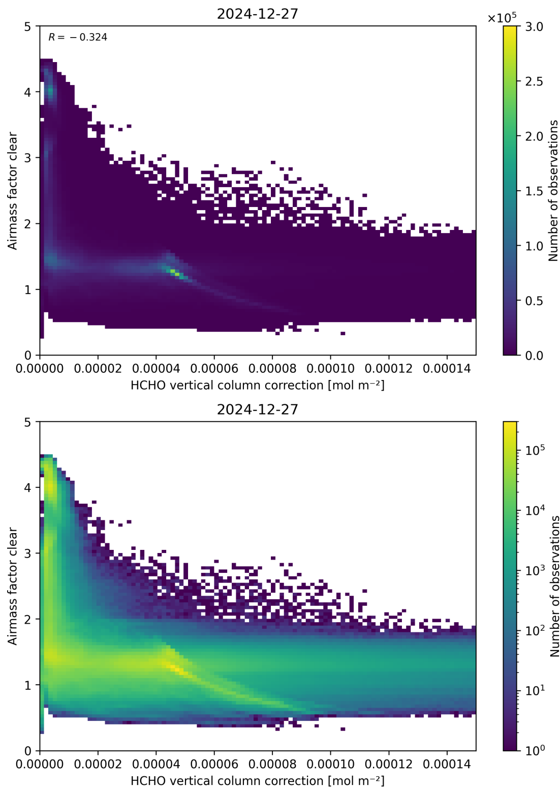
Figure 115: Scatter density plot of “HCHO vertical column correction” against “Airmass factor clear” for 2024-12-27 to 2024-12-28.
