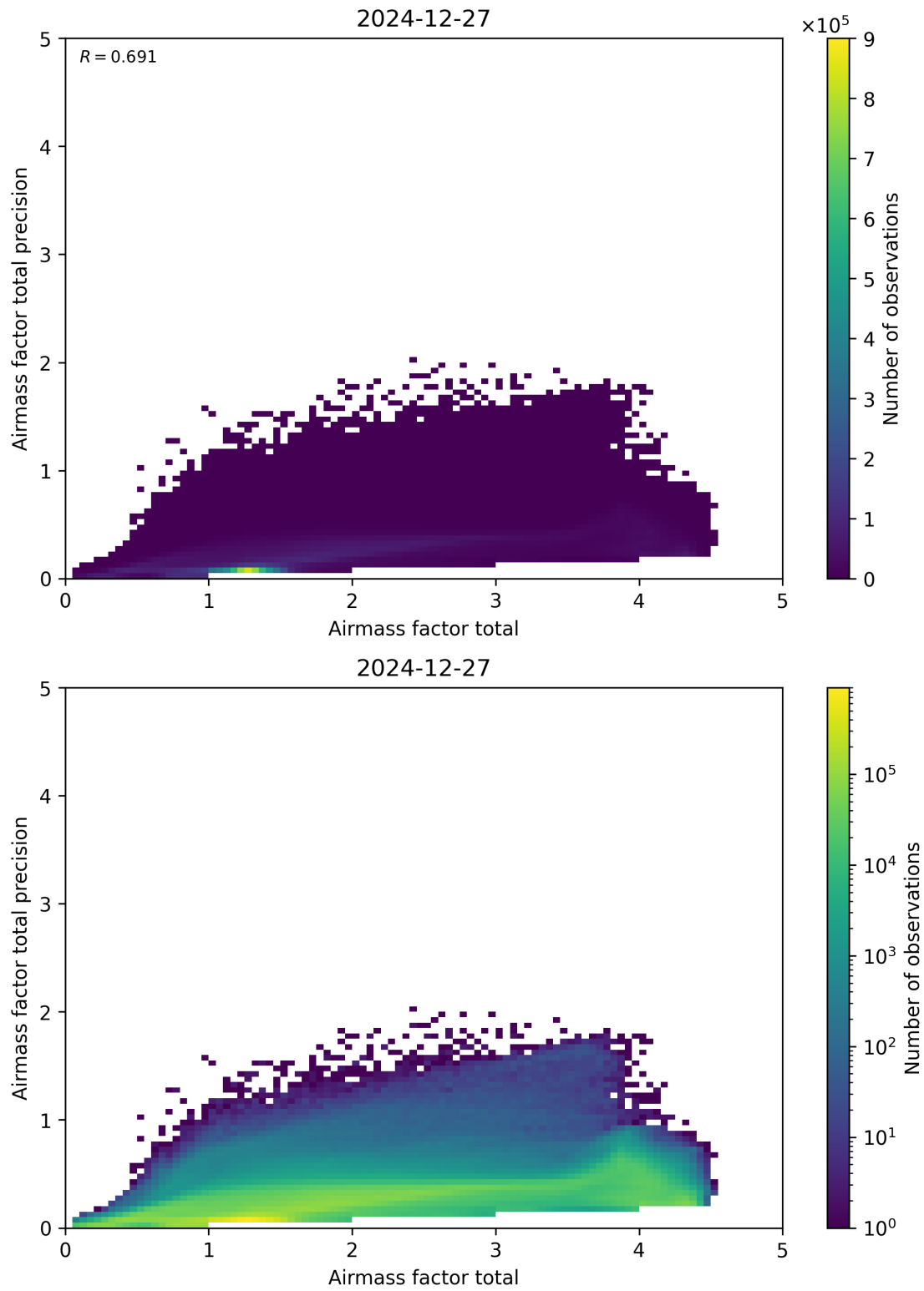
Figure 103: Scatter density plot of “Airmass factor total” against “Airmass factor total precision” for 2024-12-27 to 2024-12-28.
