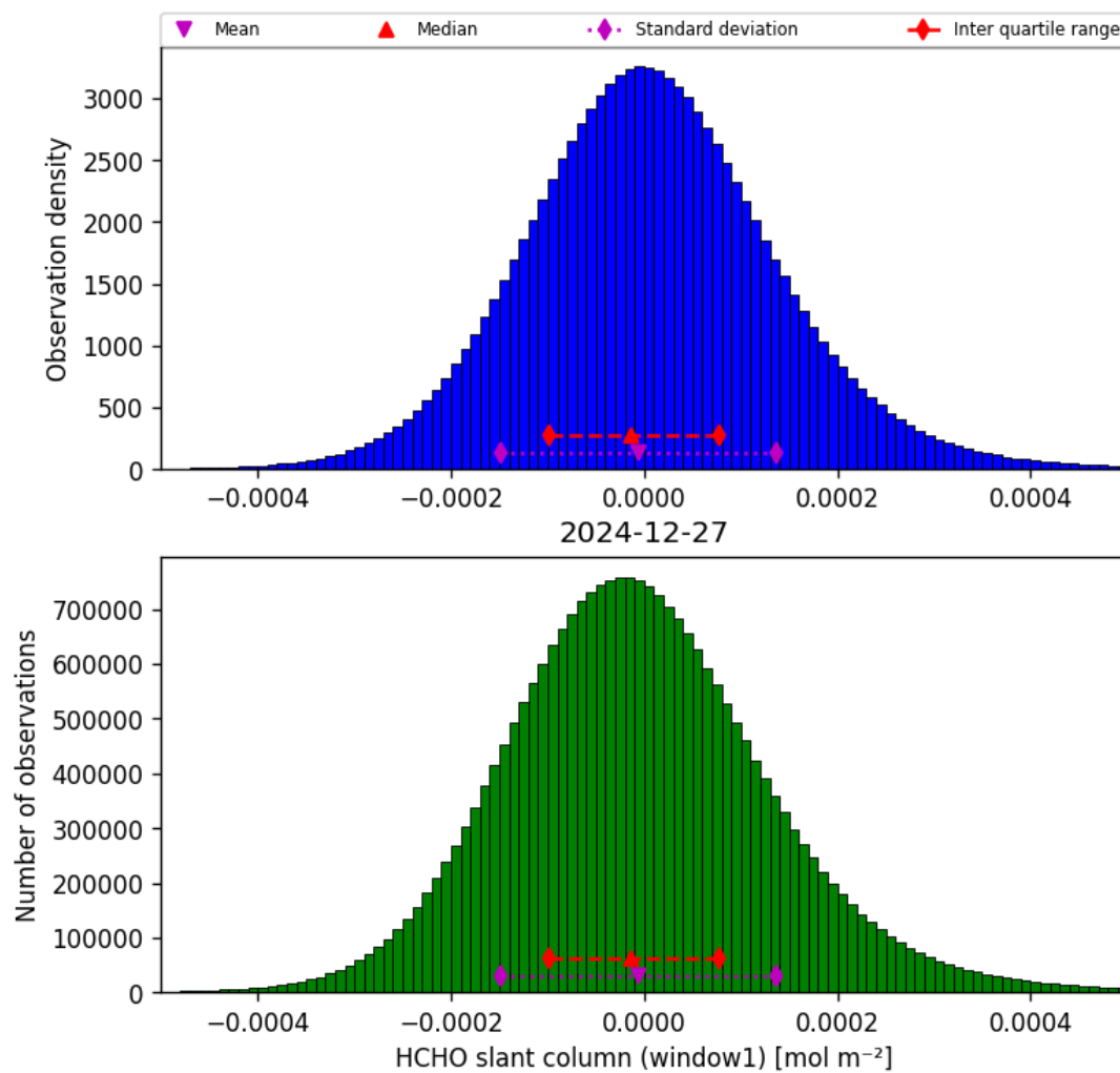
Figure 38: Histogram of “HCHO slant column (window1)” for 2024-12-27 to 2024-12-28
