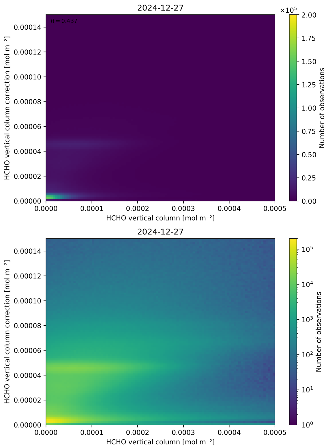
Figure 133: Scatter density plot of “HCHO vertical column” against “HCHO vertical column correction” for 2024-12-27 to 2024-12-28.
