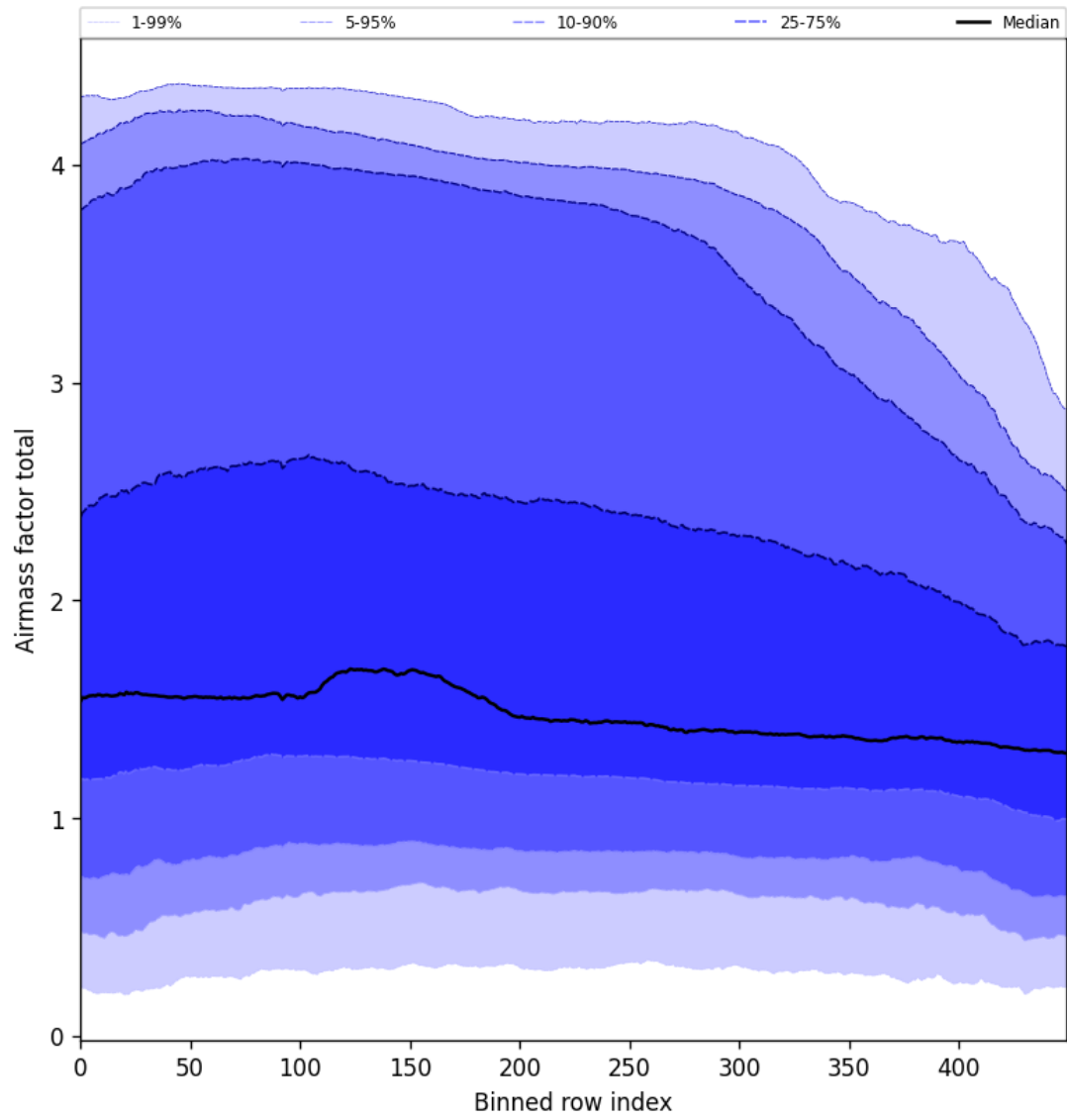
Figure 54: Along track statistics of “Airmass factor total” for 2024-12-27 to 2024-12-28
