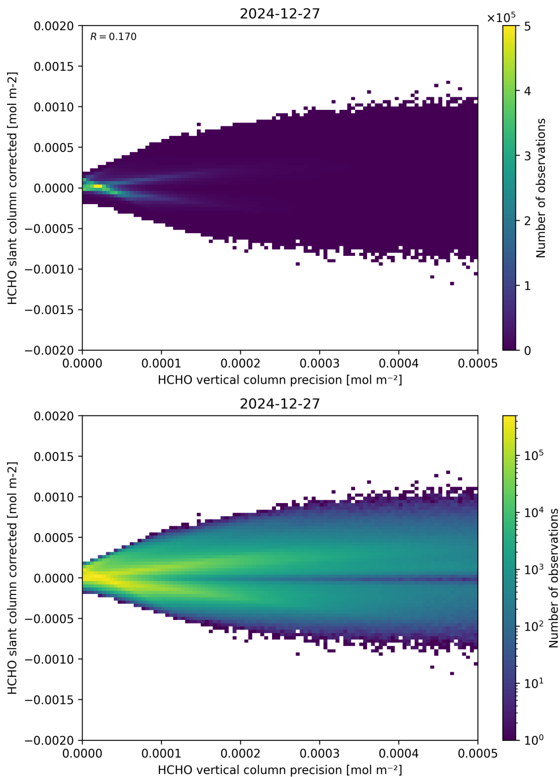
Figure 140: Scatter density plot of “HCHO vertical column precision” against “HCHO slant column corrected” for 2024-12-27 to 2024-12-28.
