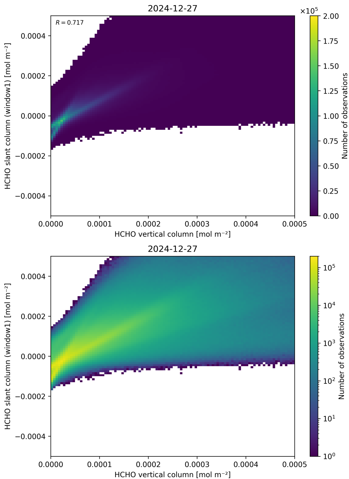
Figure 129: Scatter density plot of “HCHO vertical column” against “HCHO slant column (window1)” for 2024-12-27 to 2024-12-28.
