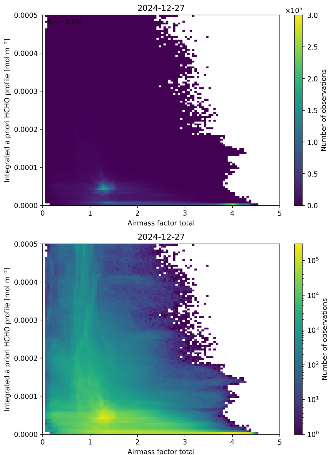
Figure 104: Scatter density plot of “Airmass factor total” against “Integrated a priori HCHO profile” for 2024-12-27 to 2024-12-28.
