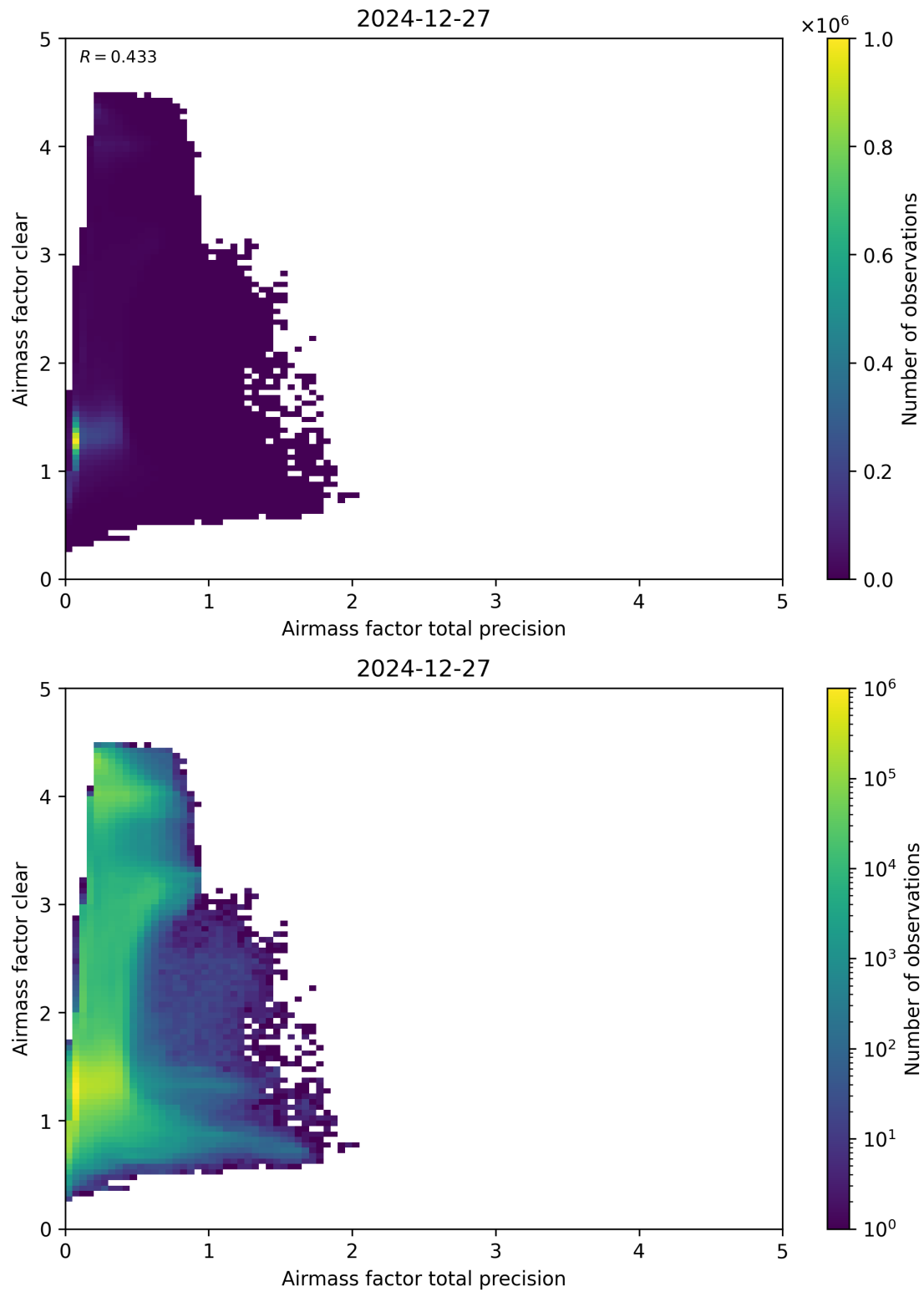
Figure 108: Scatter density plot of “Airmass factor total precision” against “Airmass factor clear” for 2024-12-27 to 2024-12-28.
