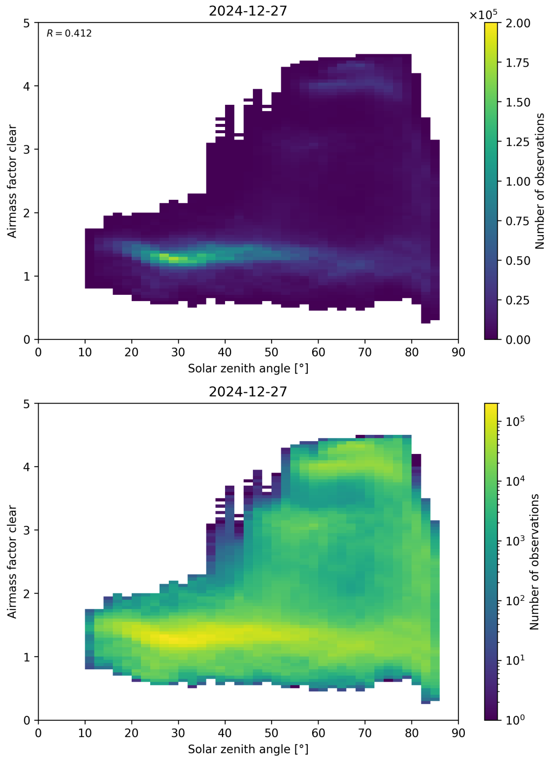
Figure 170: Scatter density plot of “Solar zenith angle” against “Airmass factor clear” for 2024-12-27 to 2024-12-28.
