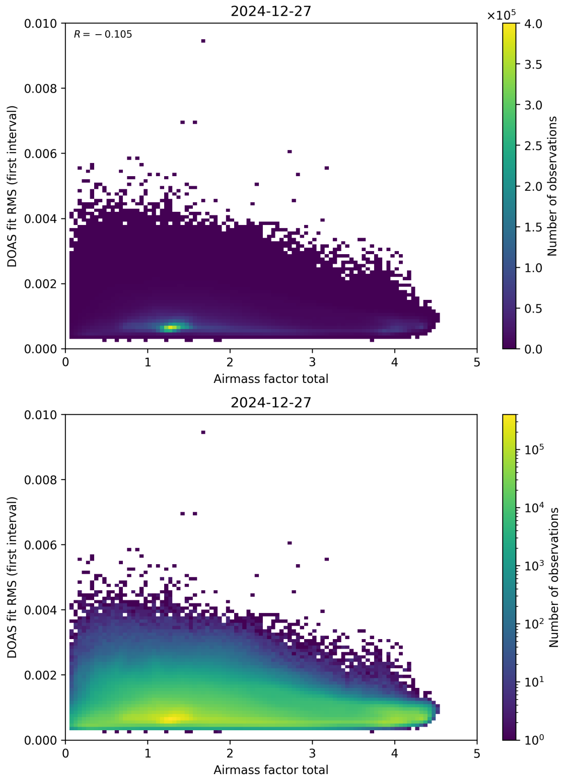
Figure 97: Scatter density plot of “Airmass factor total” against “DOAS fit RMS (first interval)” for 2024-12-27 to 2024-12-28.
