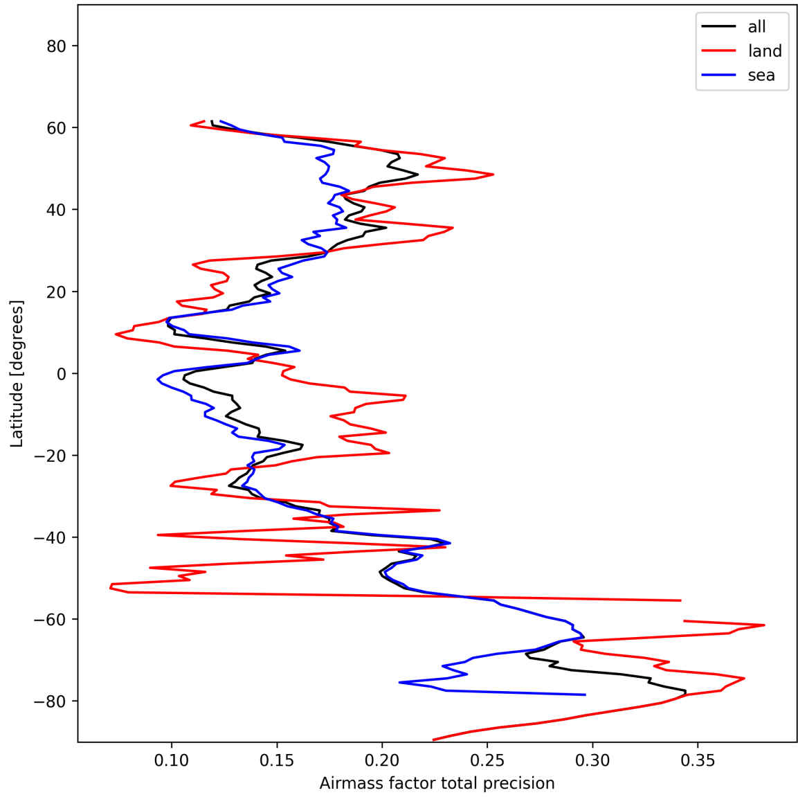
Figure 27: Zonal average of “Airmass factor total precision” for 2024-12-27 to 2024-12-29.
