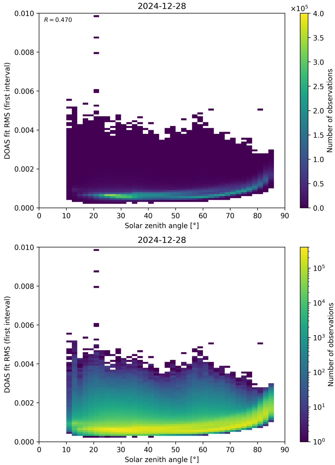
Figure 167: Scatter density plot of “Solar zenith angle” against “DOAS fit RMS (first interval)” for 2024-12-27 to 2024-12-29.
