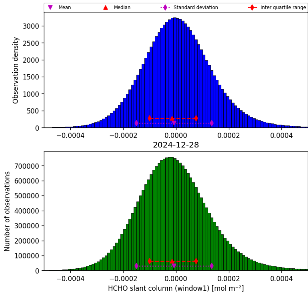
Figure 38: Histogram of “HCHO slant column (window1)” for 2024-12-27 to 2024-12-29
