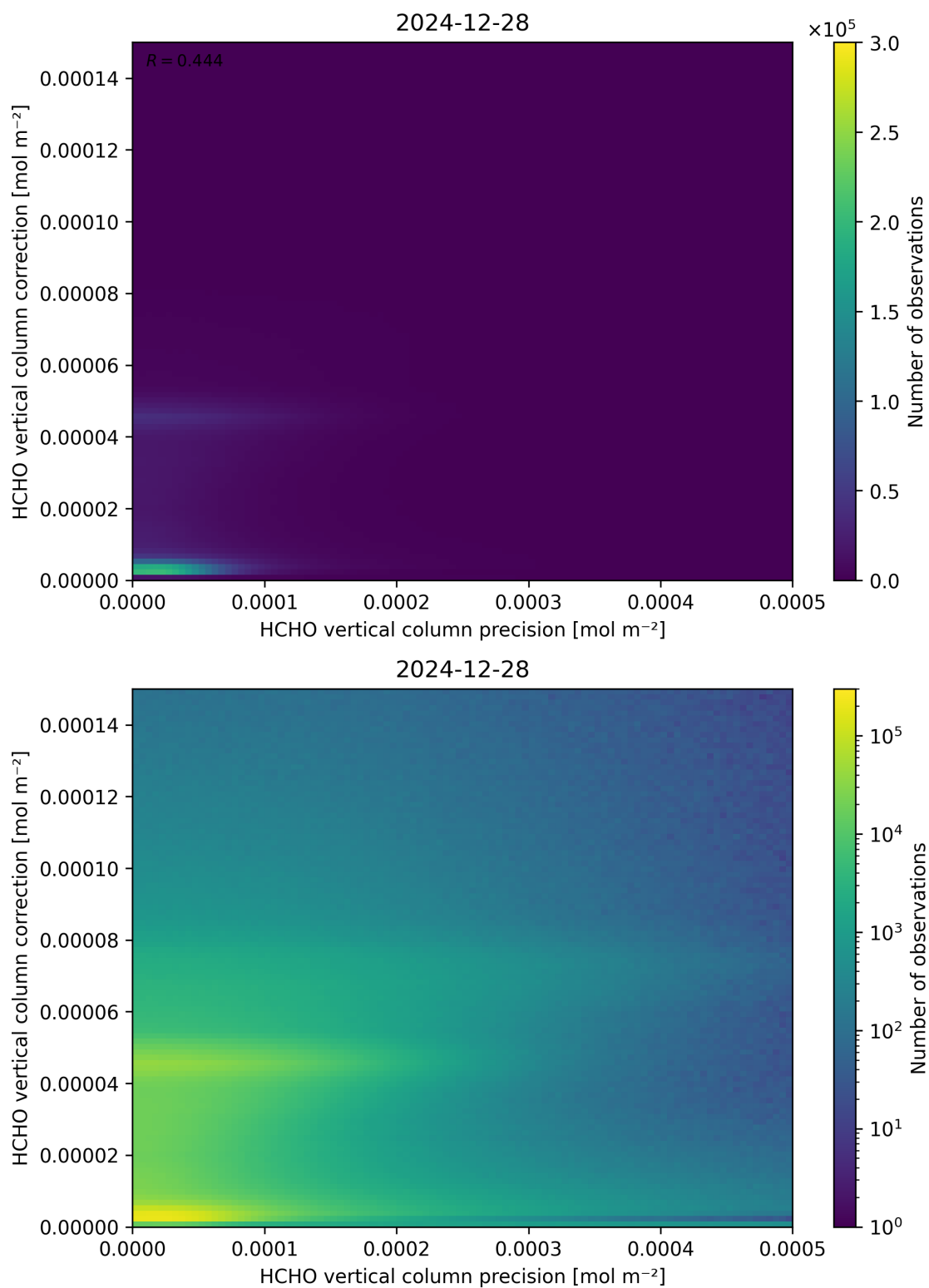
Figure 146: Scatter density plot of “HCHO vertical column precision” against “HCHO vertical column correction” for 2024-12-27 to 2024-12-29.
