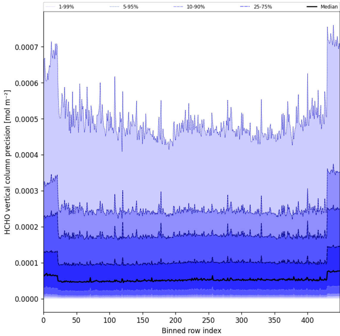
Figure 50: Along track statistics of “HCHO vertical column precision” for 2024-12-27 to 2024-12-29
