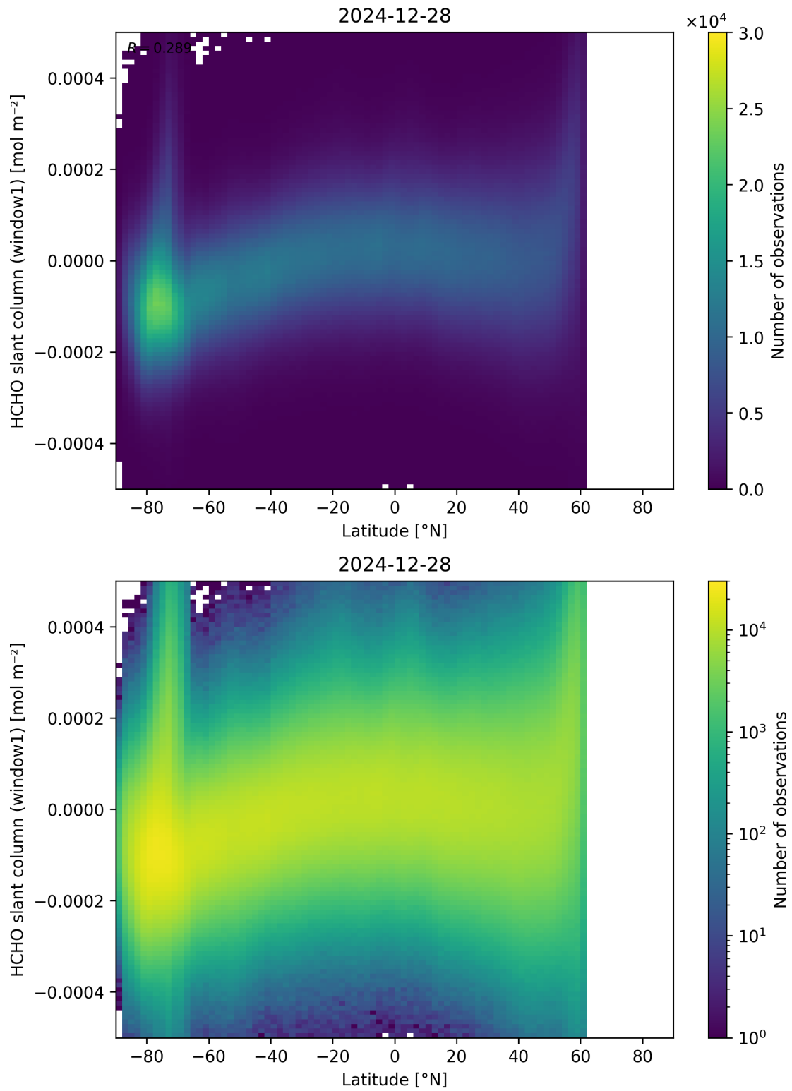
Figure 159: Scatter density plot of “Latitude” against “HCHO slant column (window1)” for 2024-12-27 to 2024-12-29.
