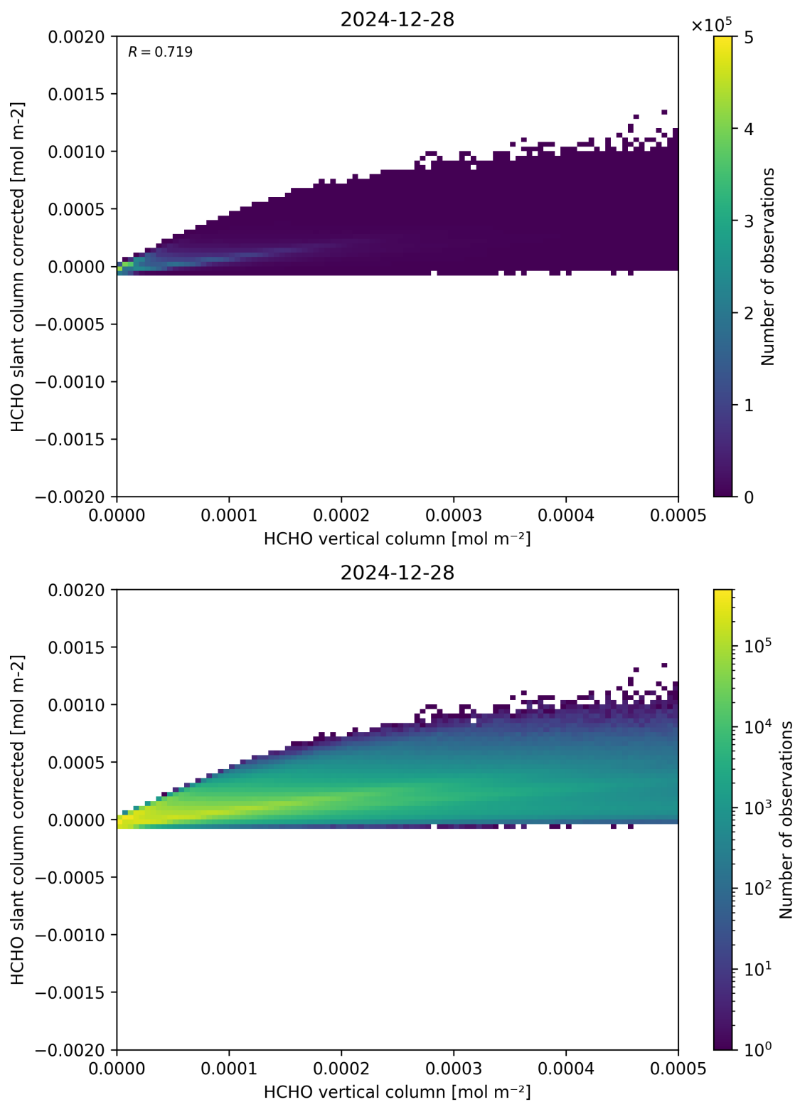
Figure 127: Scatter density plot of “HCHO vertical column” against “HCHO slant column corrected” for 2024-12-27 to 2024-12-29.
