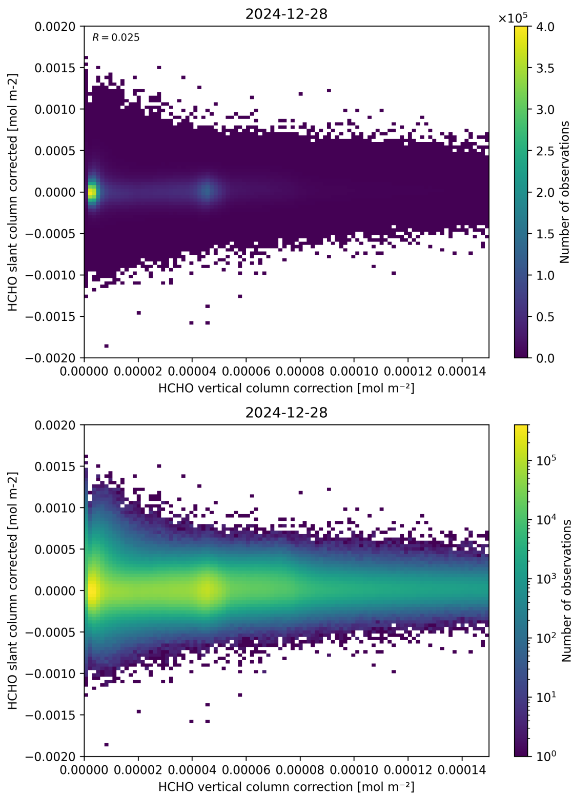
Figure 116: Scatter density plot of “HCHO vertical column correction” against “HCHO slant column corrected” for 2024-12-27 to 2024-12-29.
