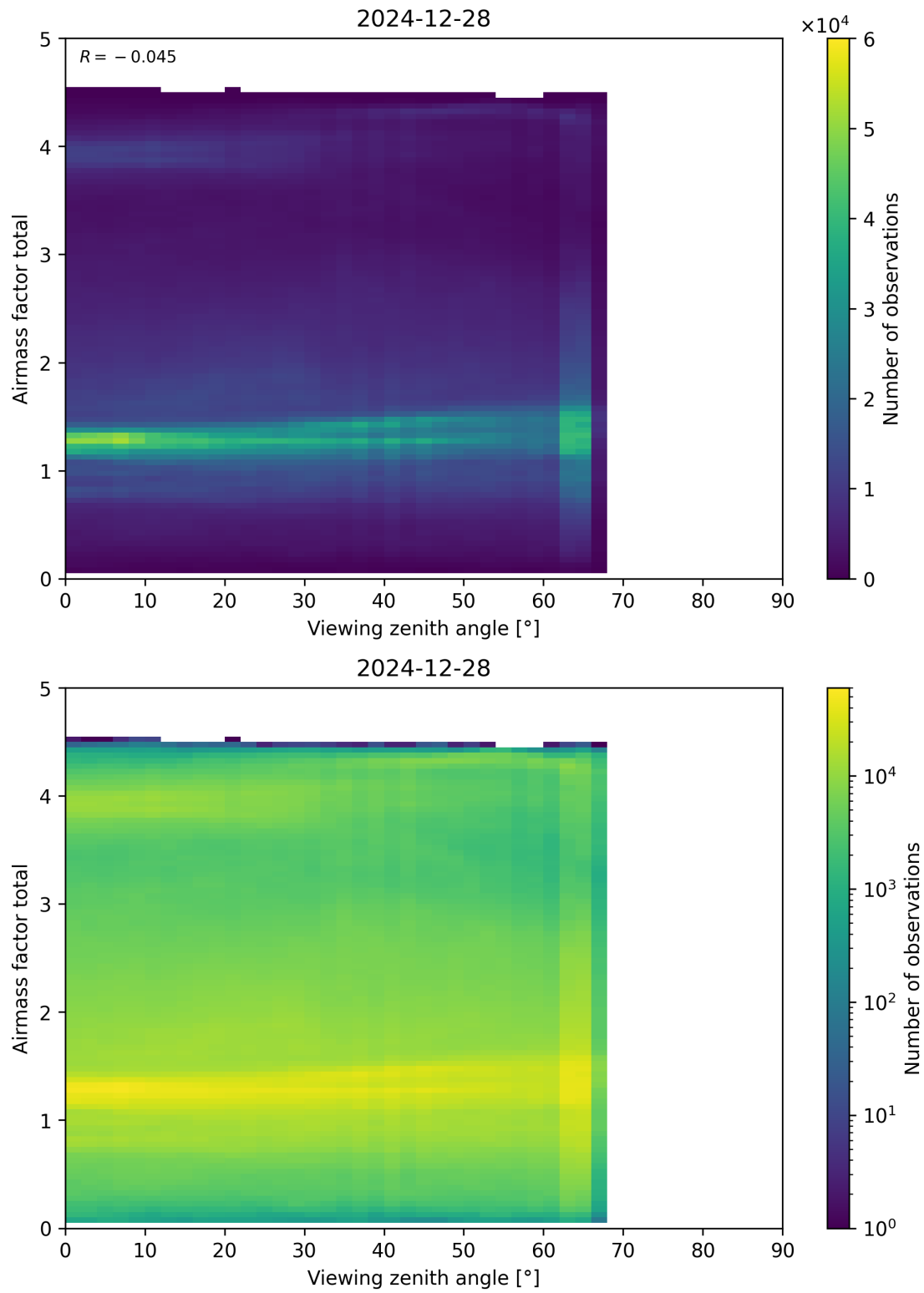
Figure 190: Scatter density plot of “Viewing zenith angle” against “Airmass factor total” for 2024-12-27 to 2024-12-29.
