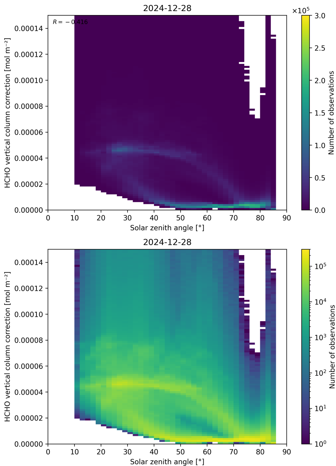
Figure 178: Scatter density plot of “Solar zenith angle” against “HCHO vertical column correction” for 2024-12-27 to 2024-12-29.
