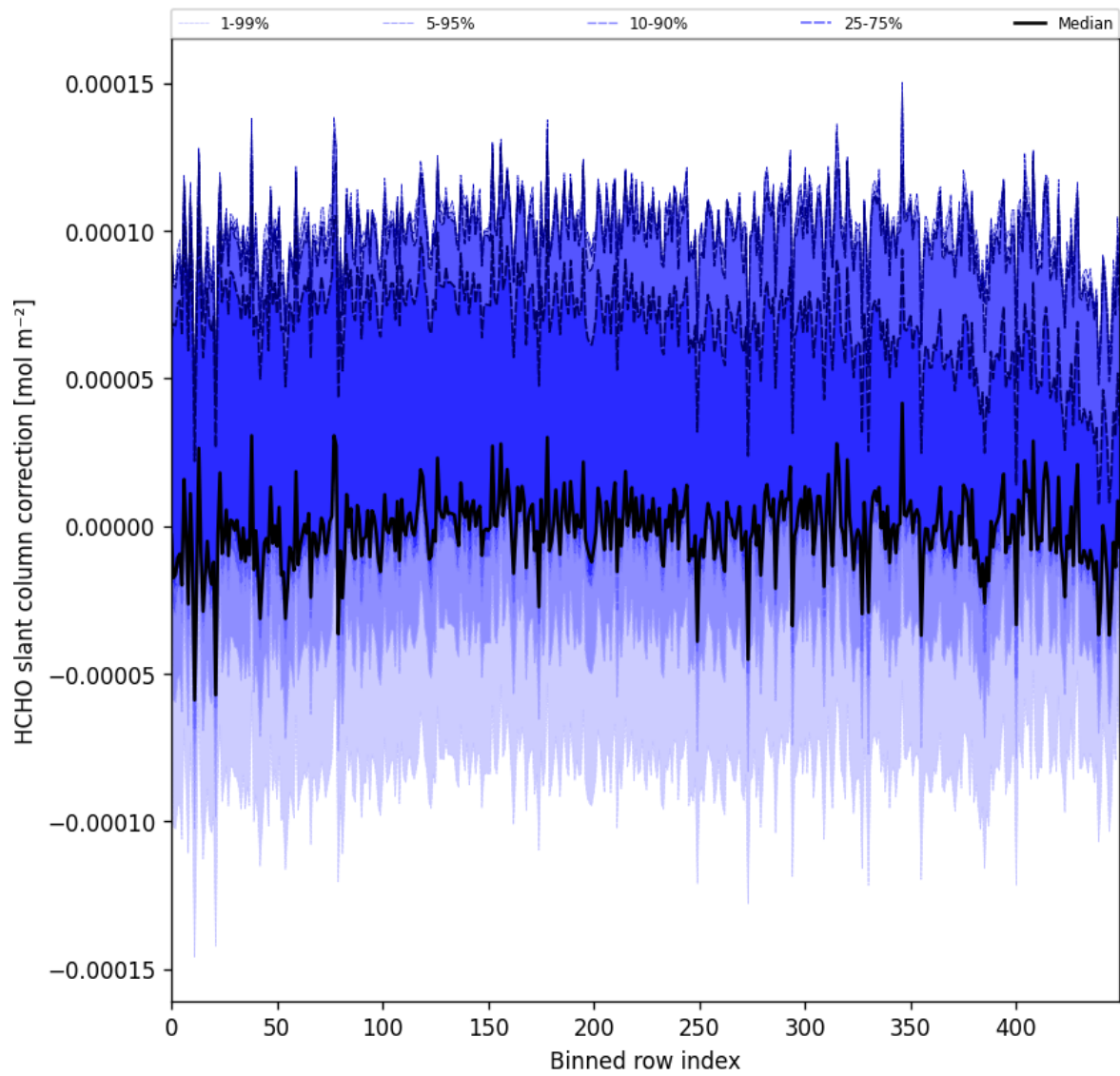
Figure 61: Along track statistics of “HCHO slant column correction” for 2024-12-27 to 2024-12-29
