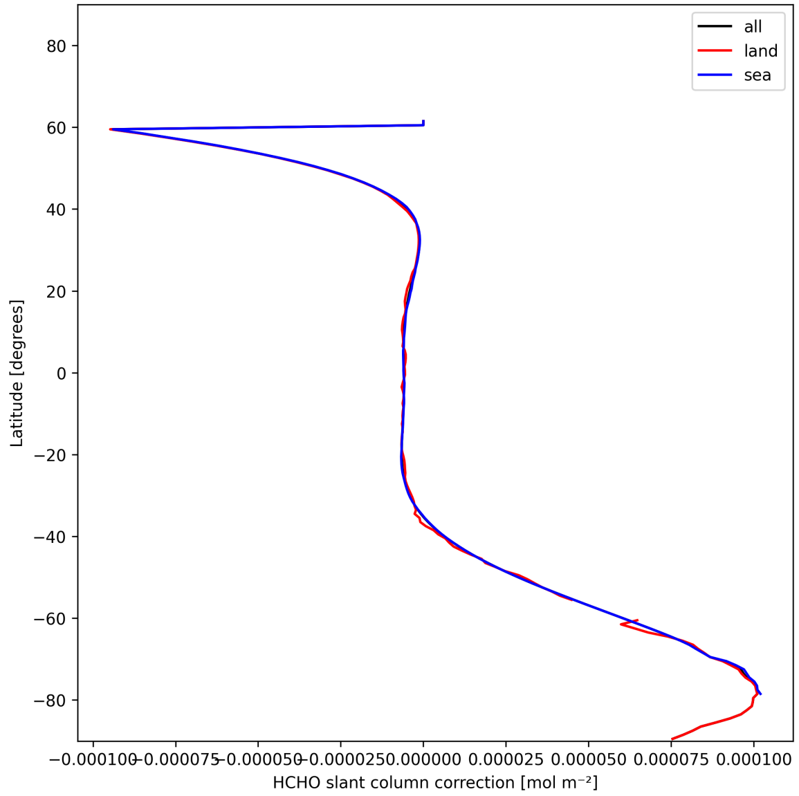
Figure 33: Zonal average of “HCHO slant column correction” for 2024-12-27 to 2024-12-29.
