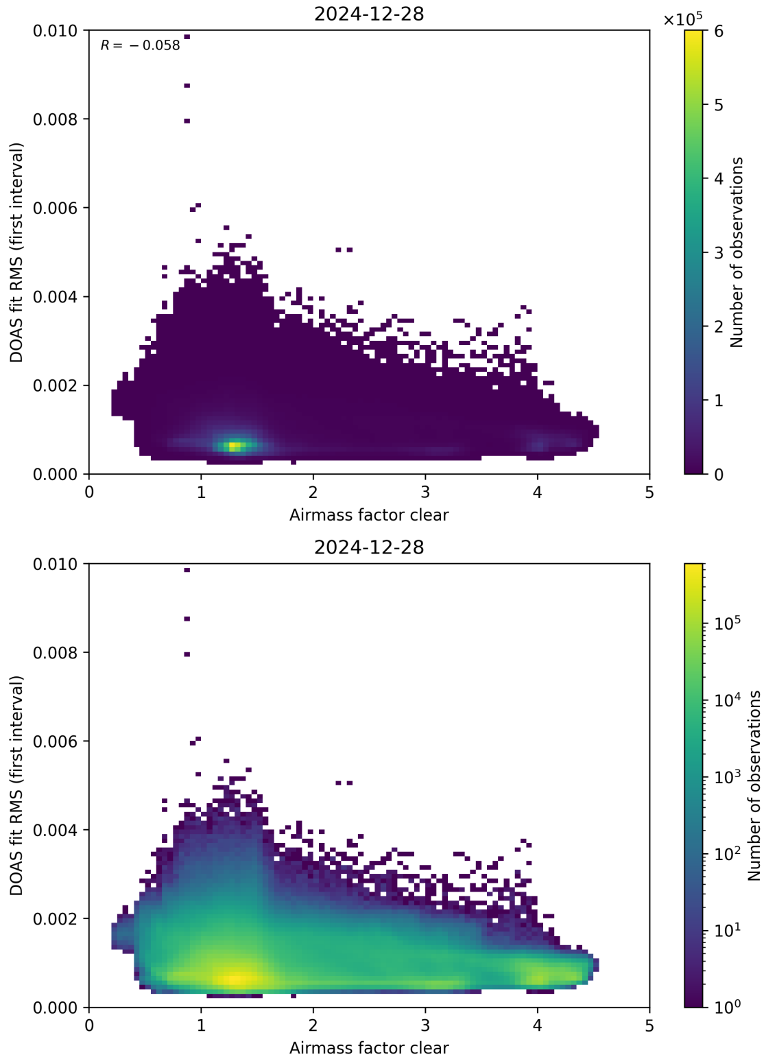
Figure 71: Scatter density plot of “Airmass factor clear” against “DOAS fit RMS (first interval)” for 2024-12-27 to 2024-12-29.
