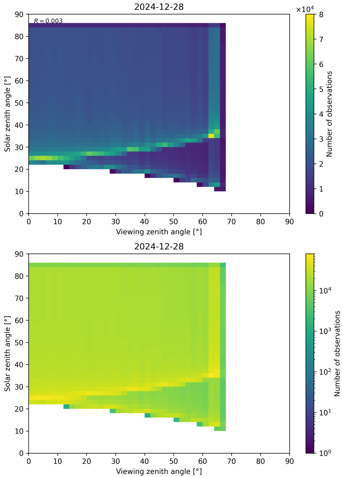
Figure 197: Scatter density plot of “Viewing zenith angle” against “Solar zenith angle” for 2024-12-27 to 2024-12-29.
