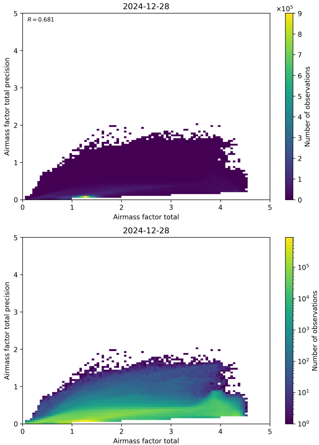
Figure 103: Scatter density plot of “Airmass factor total” against “Airmass factor total precision” for 2024-12-27 to 2024-12-29.
