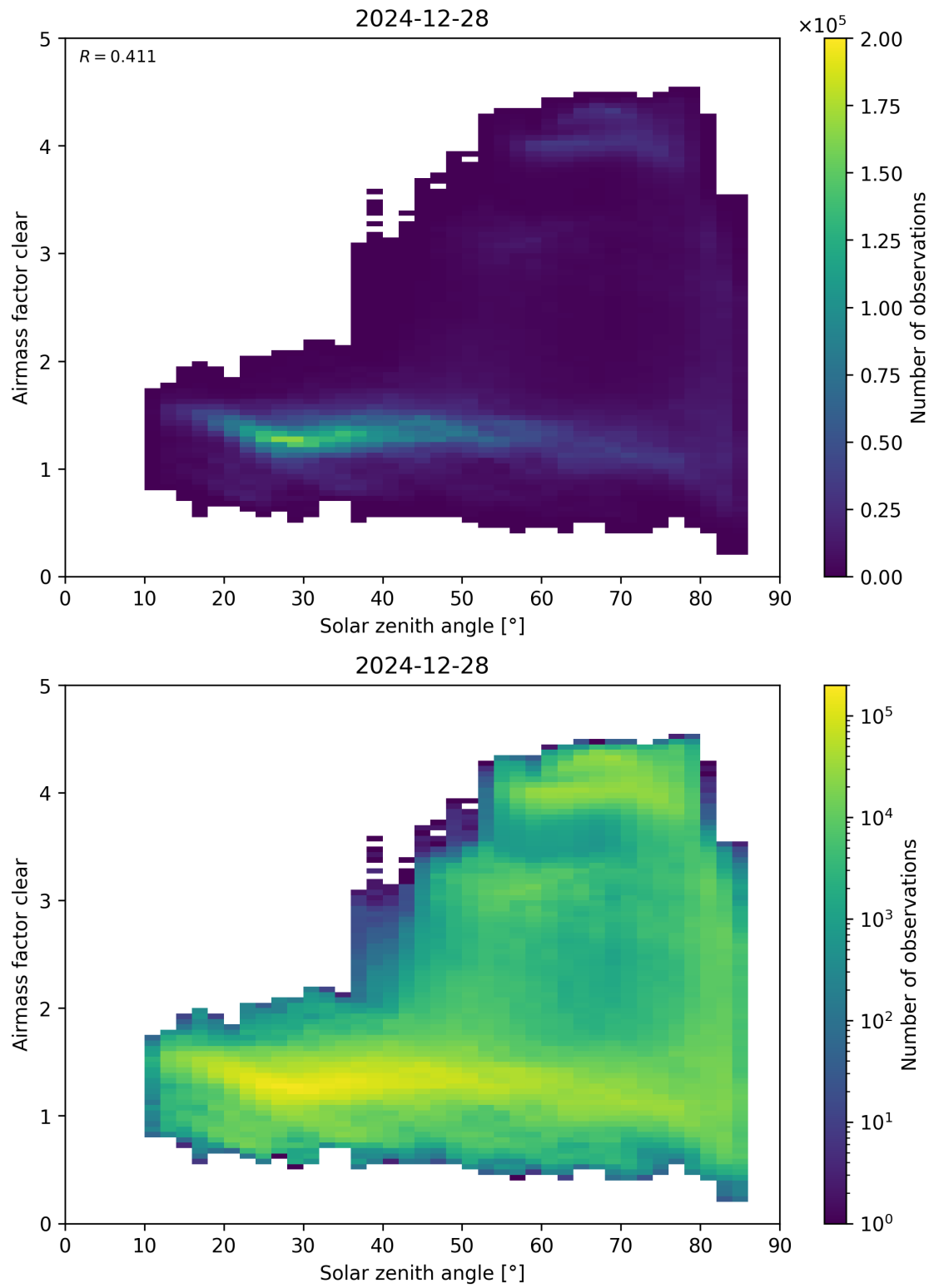
Figure 170: Scatter density plot of “Solar zenith angle” against “Airmass factor clear” for 2024-12-27 to 2024-12-29.
