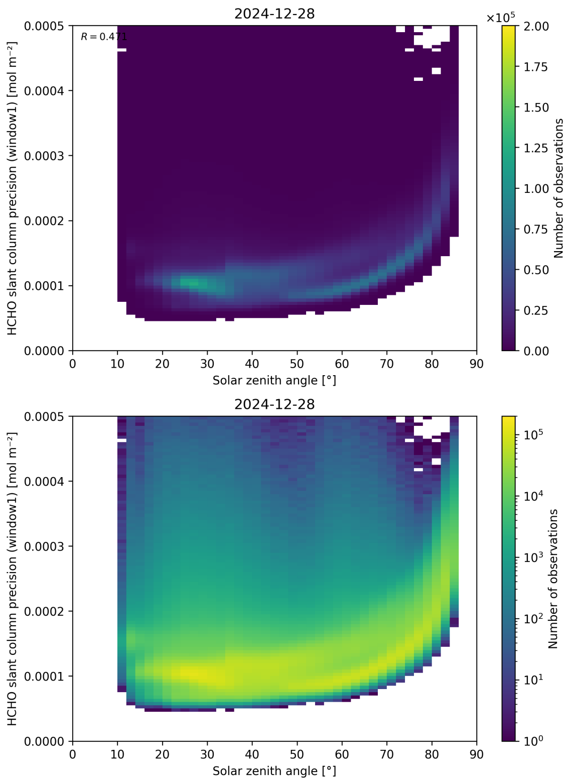
Figure 174: Scatter density plot of “Solar zenith angle” against “HCHO slant column precision (window1)” for 2024-12-27 to 2024-12-29.
