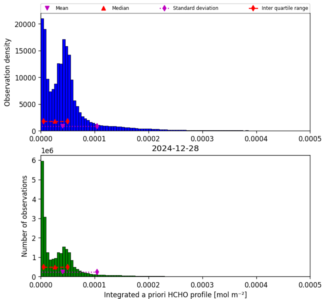
Figure 43: Histogram of “Integrated a priori HCHO profile” for 2024-12-27 to 2024-12-29
