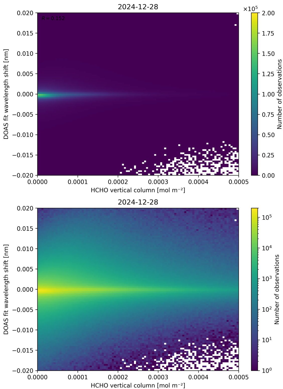
Figure 124: Scatter density plot of “HCHO vertical column” against “DOAS fit wavelength shift” for 2024-12-27 to 2024-12-29.
