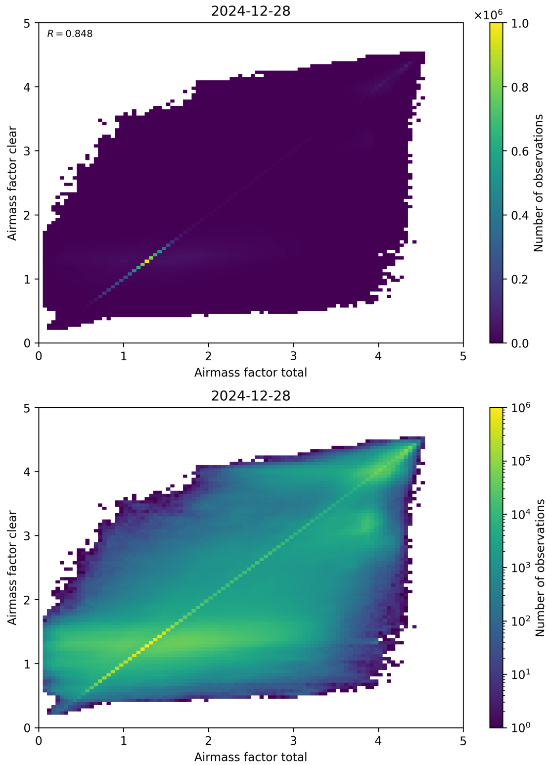
Figure 100: Scatter density plot of “Airmass factor total” against “Airmass factor clear” for 2024-12-27 to 2024-12-29.
