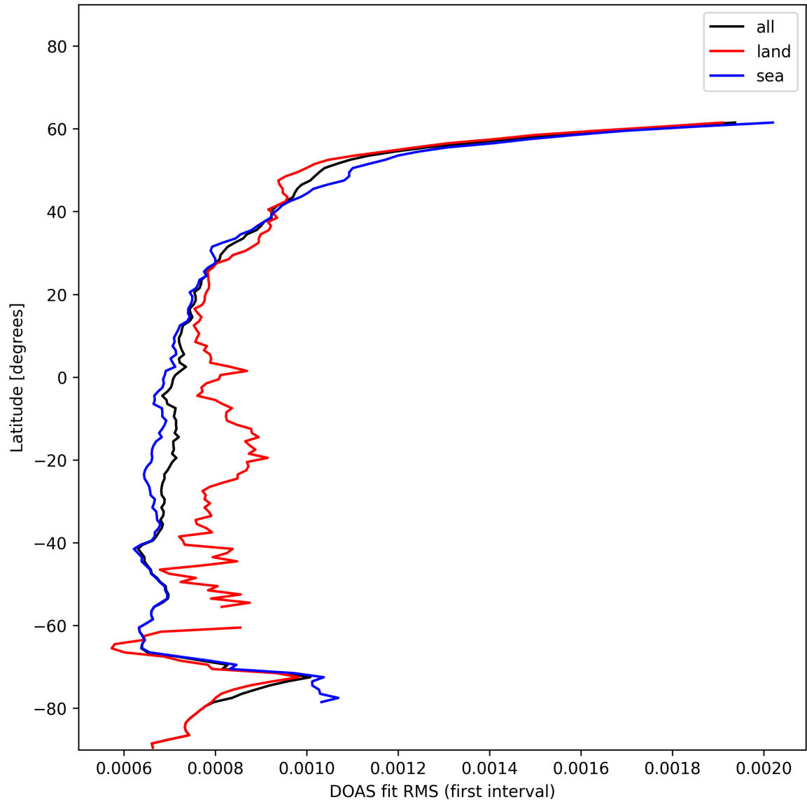
Figure 32: Zonal average of "DOAS fit RMS (first interval)" for 2024-12-27 to 2024-12-29.
