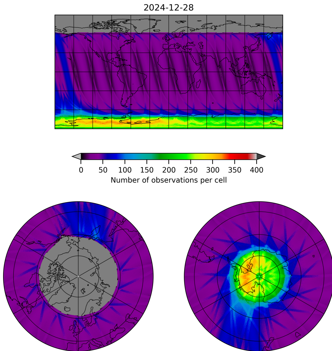
Figure 19: Map of the number of observations for 2024-12-27 to 2024-12-29
