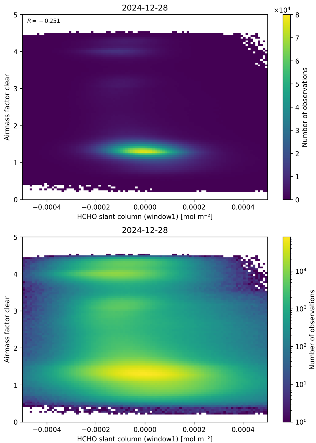
Figure 81: Scatter density plot of “HCHO slant column (window1)” against “Airmass factor clear” for 2024-12-27 to 2024-12-29.
