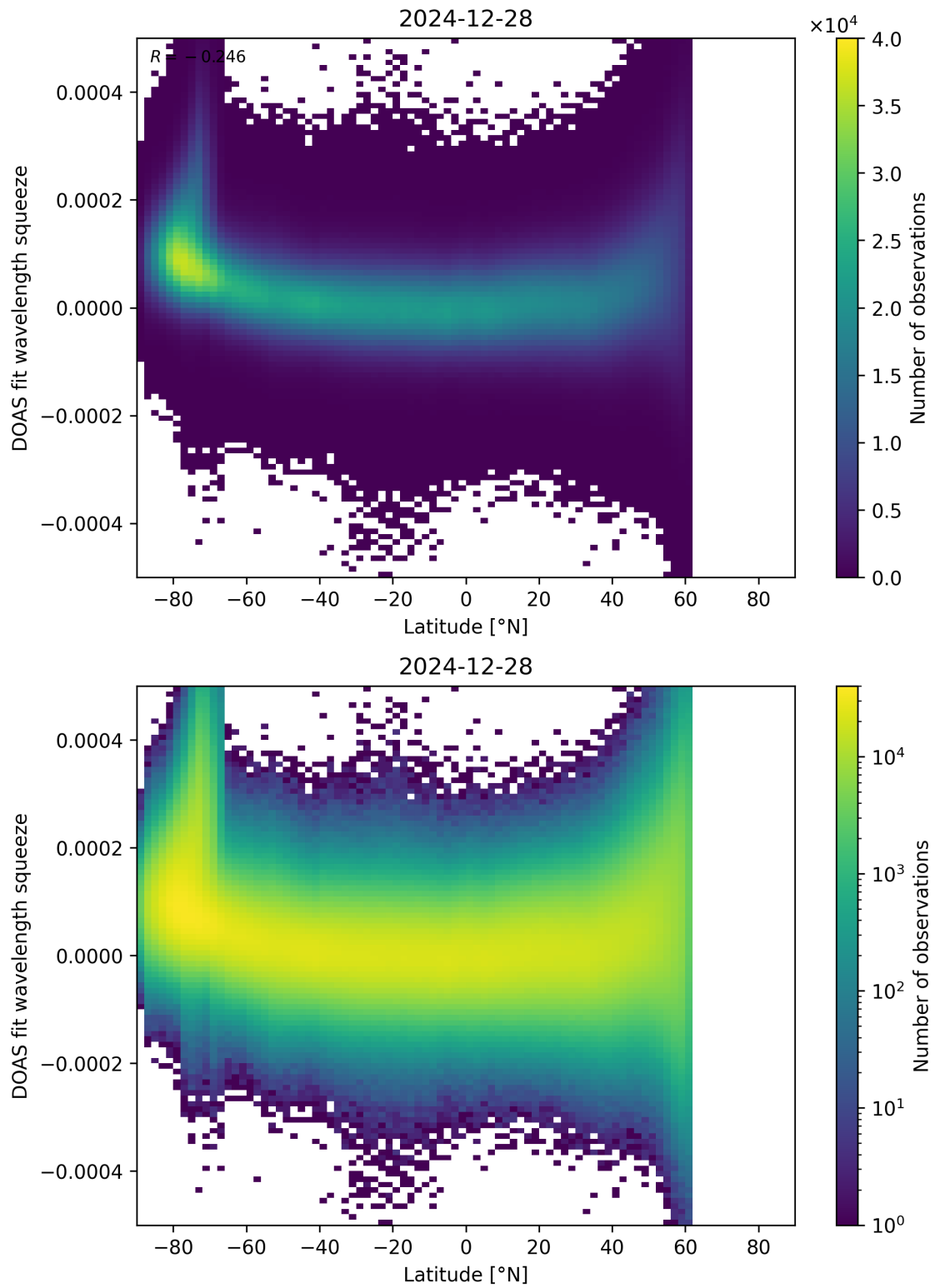
Figure 155: Scatter density plot of “Latitude” against “DOAS fit wavelength squeeze” for 2024-12-27 to 2024-12-29.
