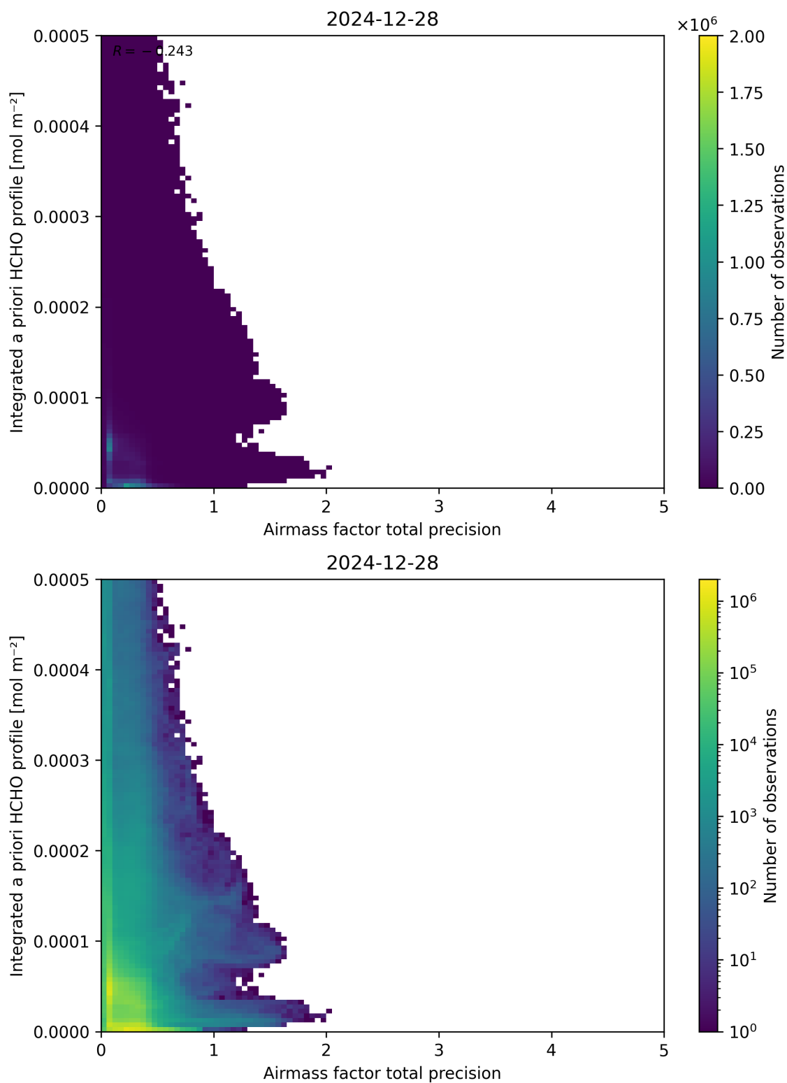
Figure 111: Scatter density plot of “Airmass factor total precision” against “Integrated a priori HCHO profile” for 2024-12-27 to 2024-12-29.
