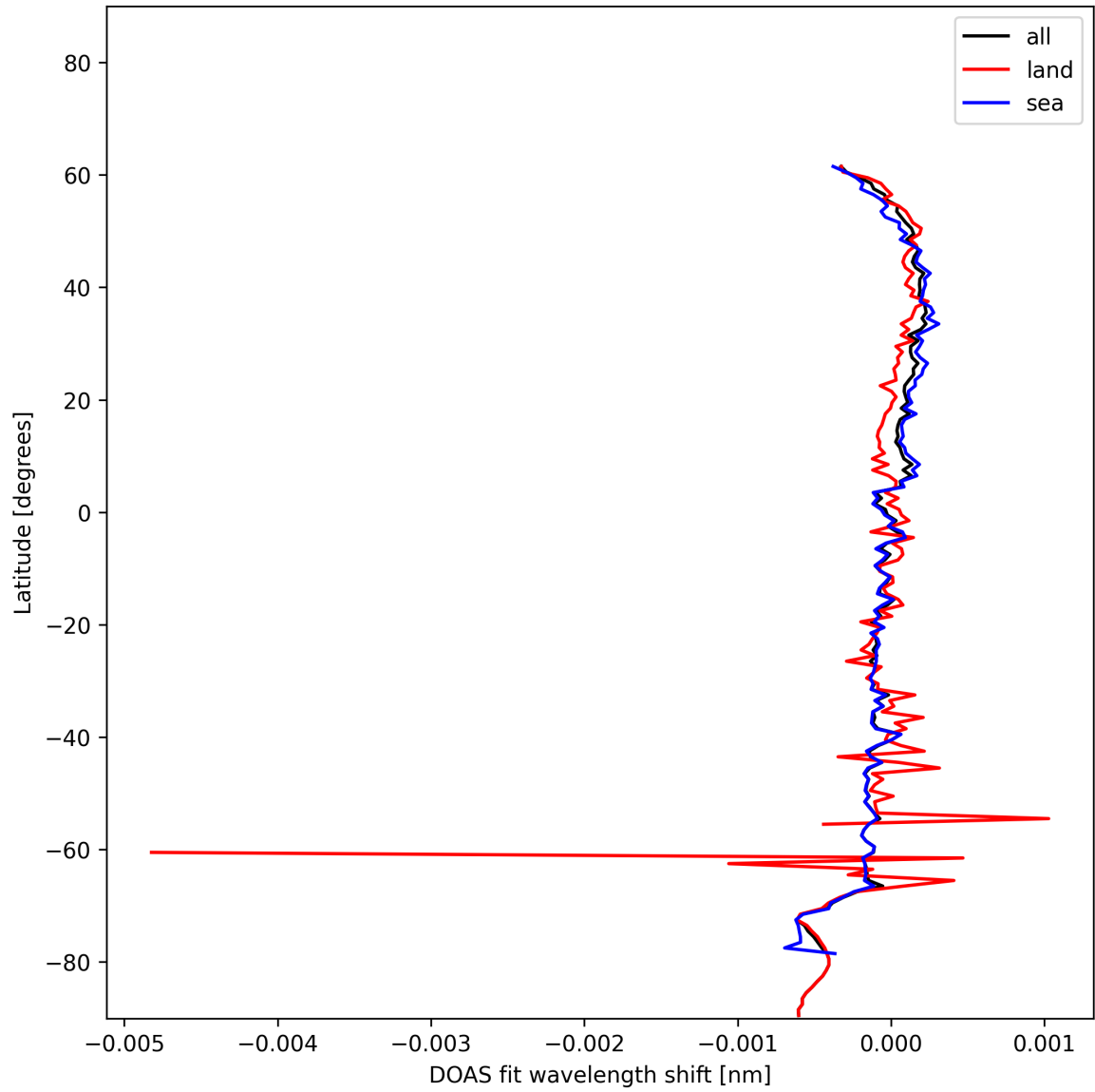
Figure 30: Zonal average of "DOAS fit wavelength shift" for 2024-12-27 to 2024-12-29.
