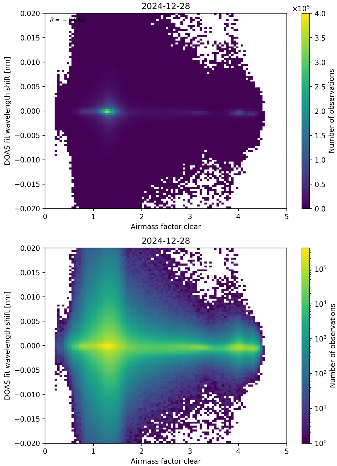
Figure 72: Scatter density plot of “Airmass factor clear” against “DOAS fit wavelength shift” for 2024-12-27 to 2024-12-29.
