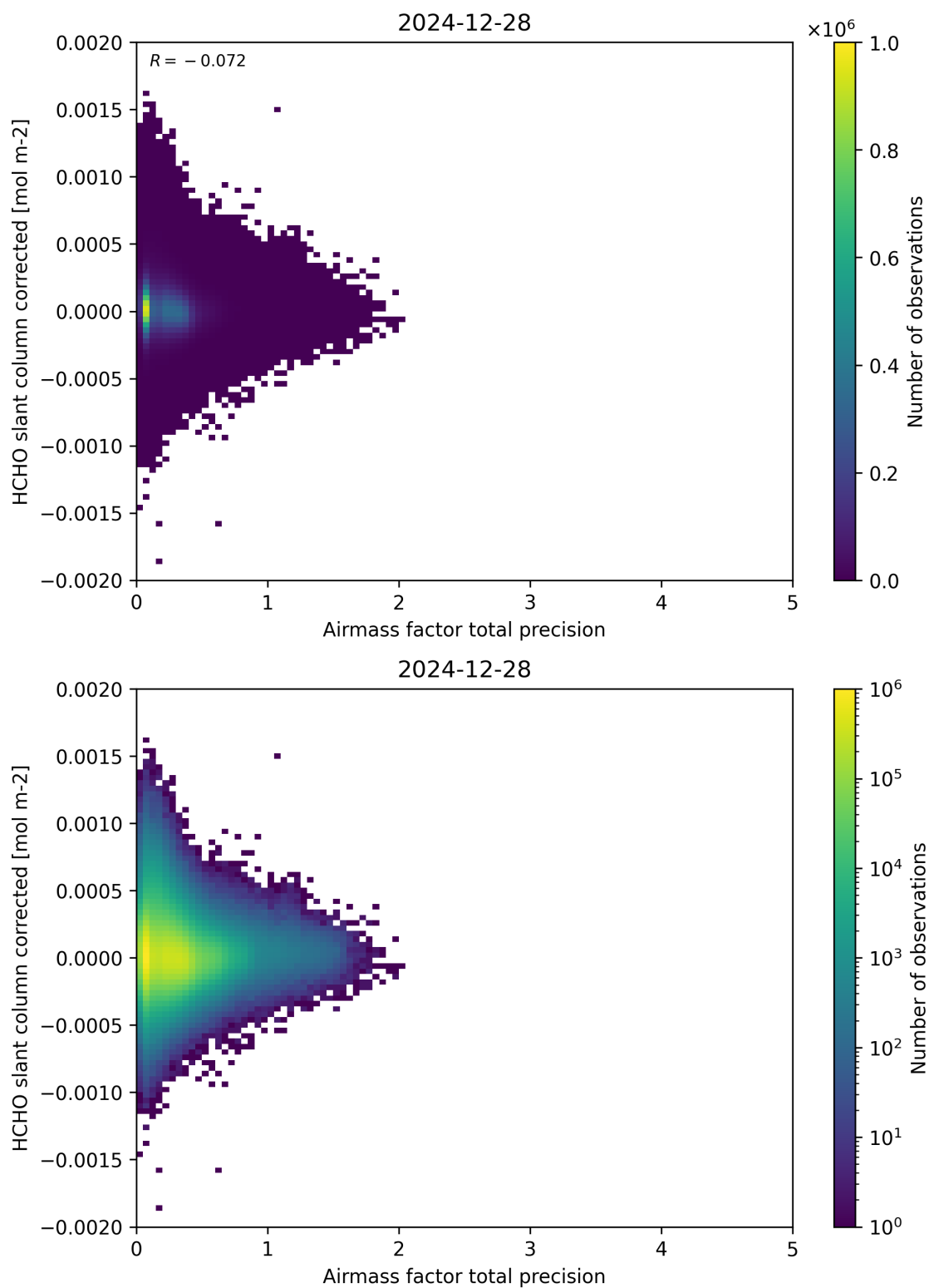
Figure 109: Scatter density plot of “Airmass factor total precision” against “HCHO slant column corrected” for 2024-12-27 to 2024-12-29.
