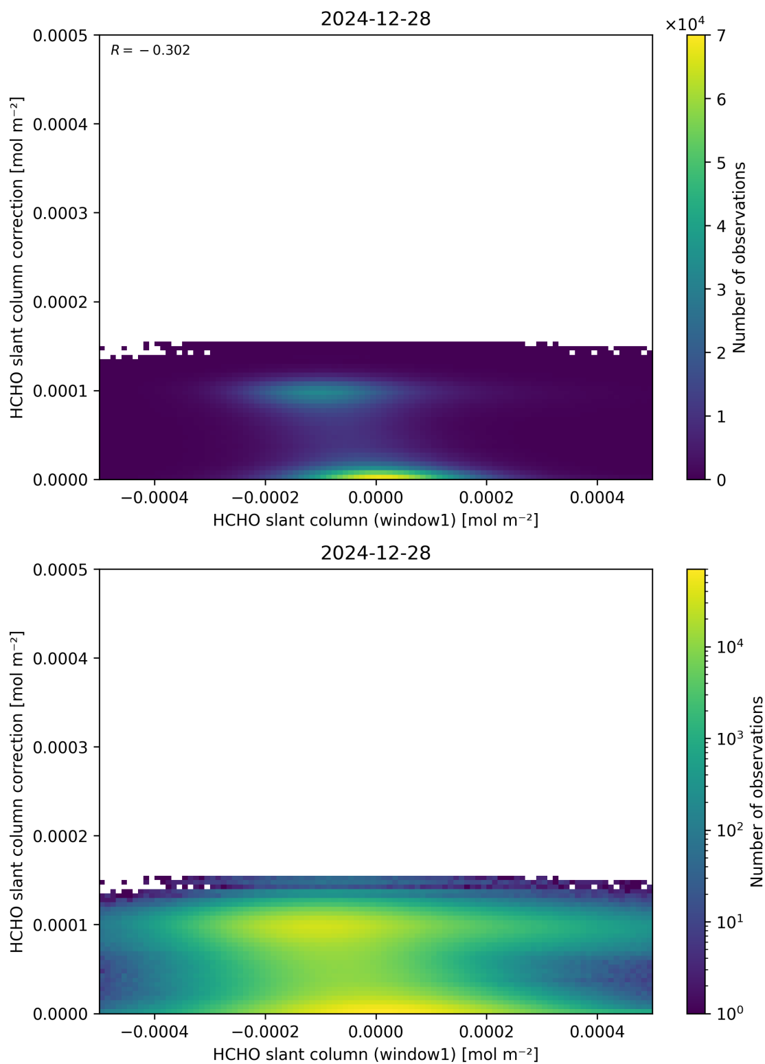
Figure 83: Scatter density plot of “HCHO slant column (window1)” against “HCHO slant column correction” for 2024-12-27 to 2024-12-29.
