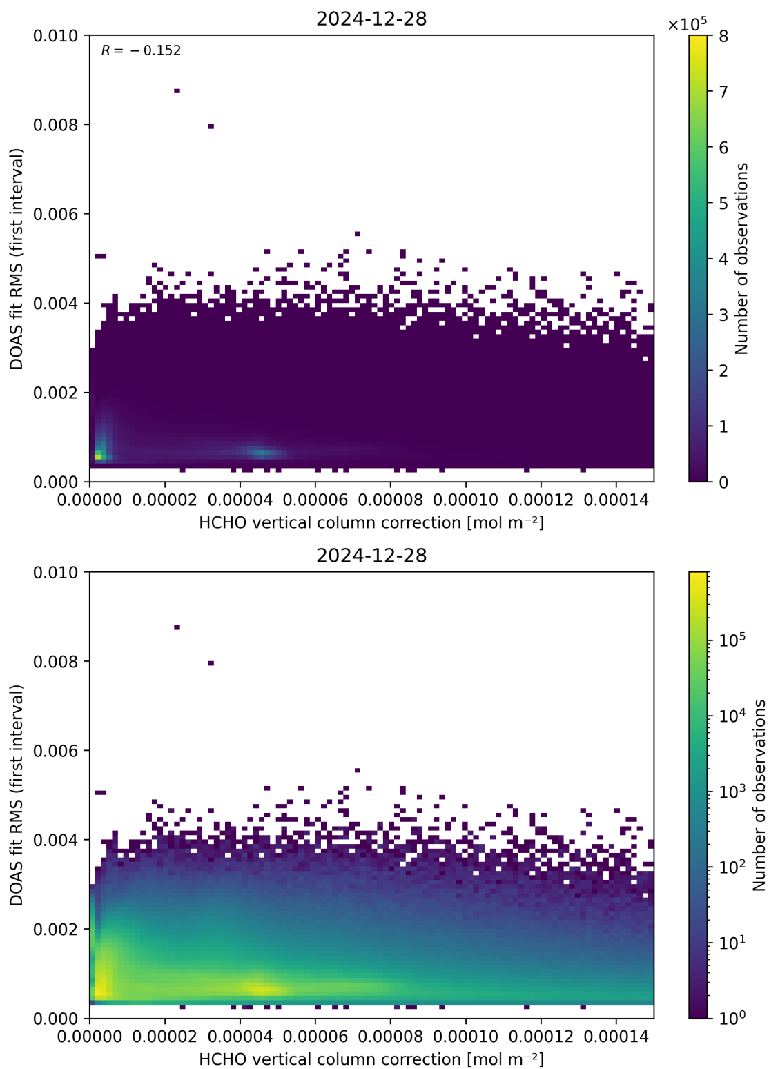
Figure 112: Scatter density plot of “HCHO vertical column correction” against “DOAS fit RMS (first interval)” for 2024-12-27 to 2024-12-29.
