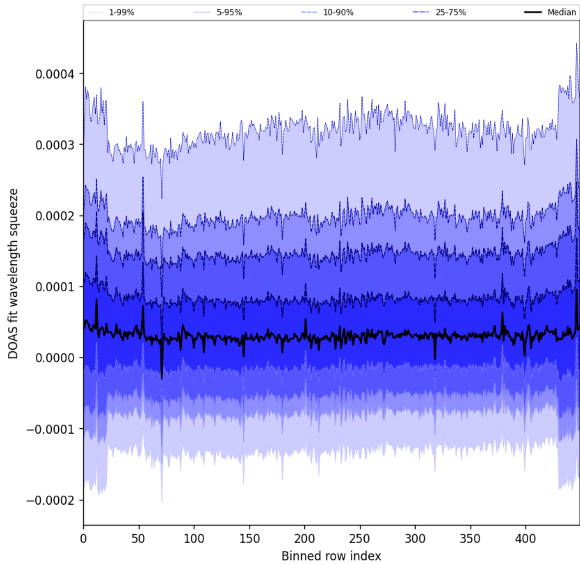
Figure 59: Along track statistics of “DOAS fit wavelength squeeze” for 2024-12-27 to 2024-12-29
