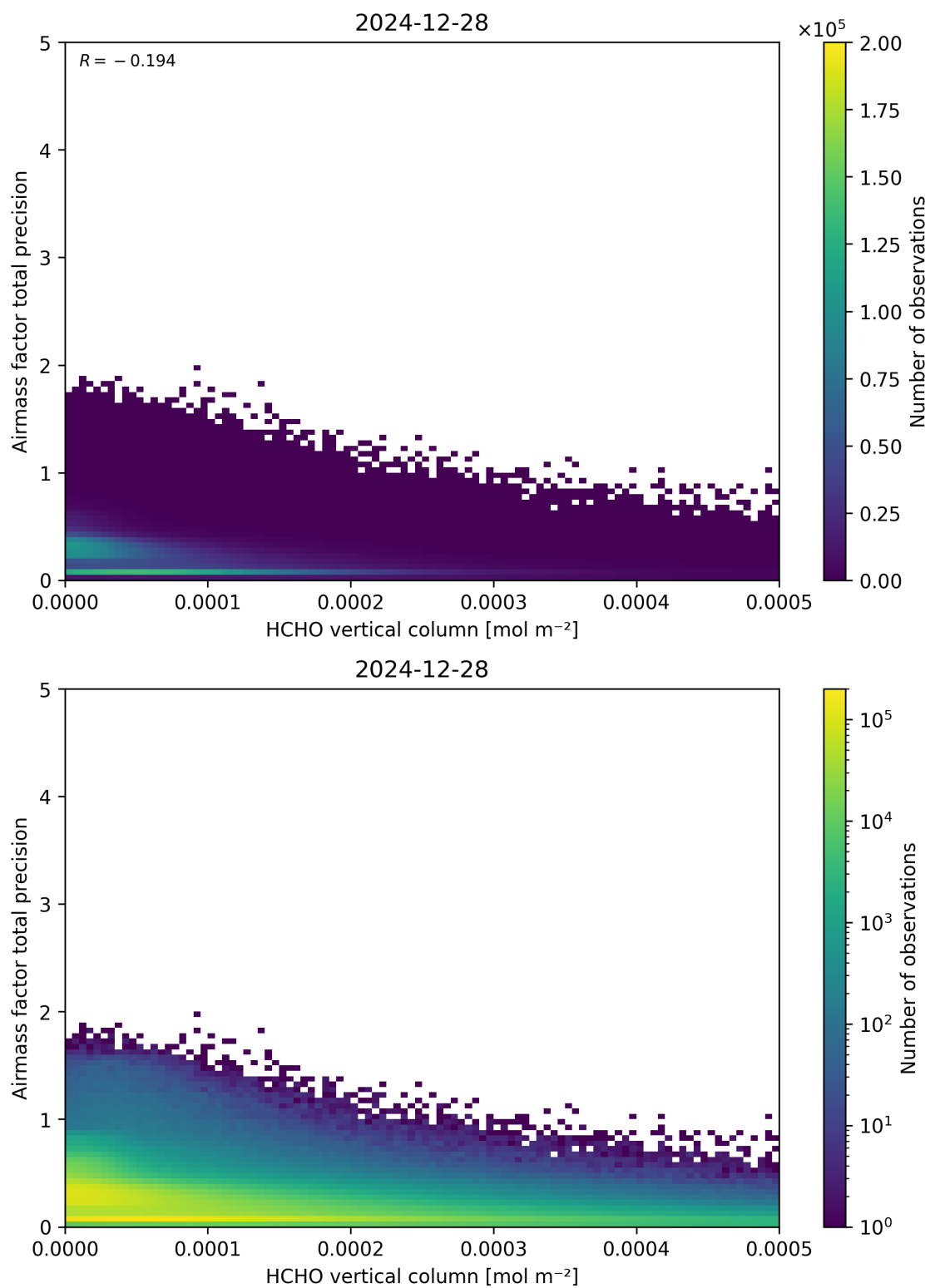
Figure 132: Scatter density plot of “HCHO vertical column” against “Airmass factor total precision” for 2024-12-27 to 2024-12-29.
