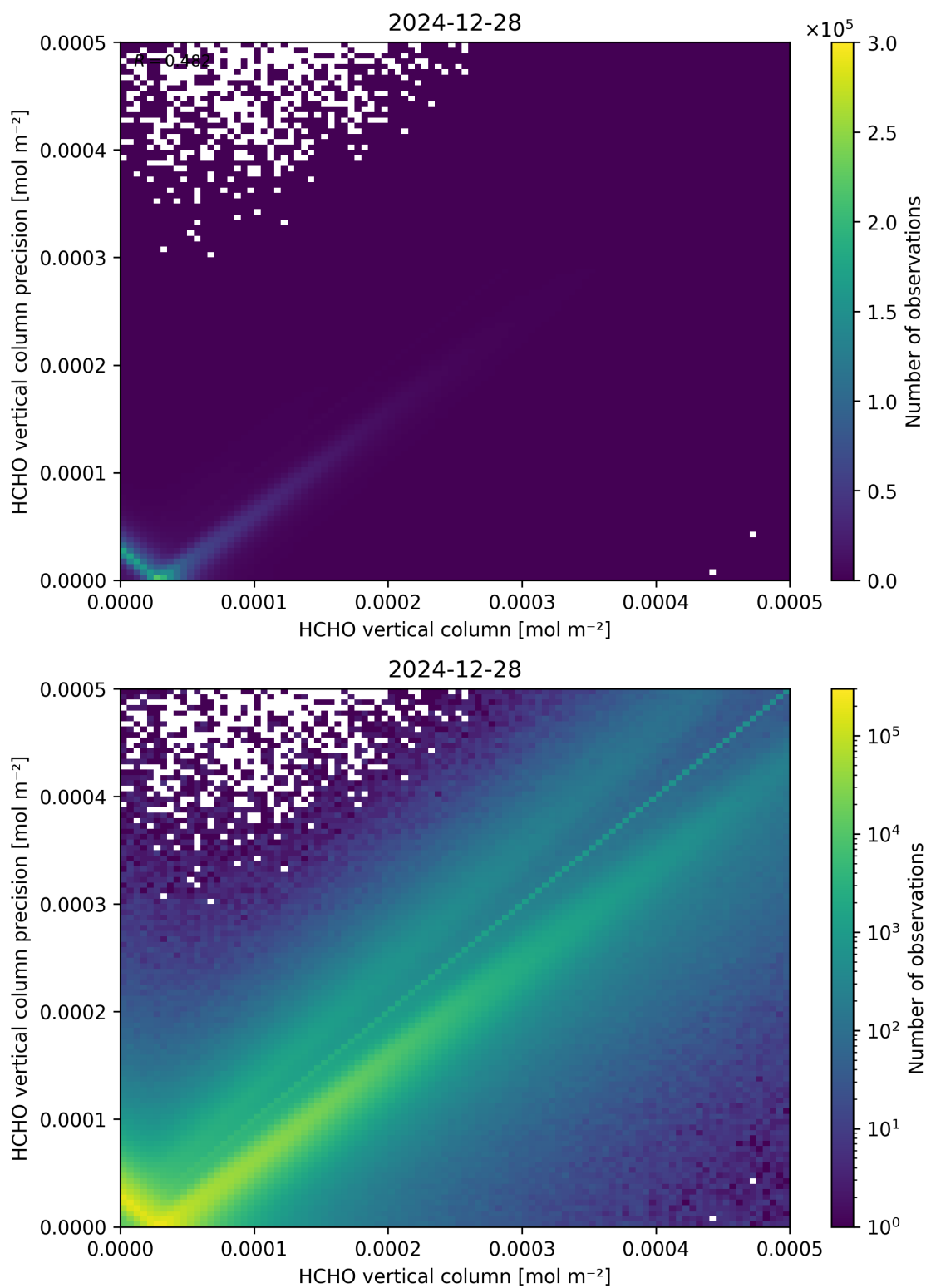
Figure 134: Scatter density plot of “HCHO vertical column” against “HCHO vertical column precision” for 2024-12-27 to 2024-12-29.
