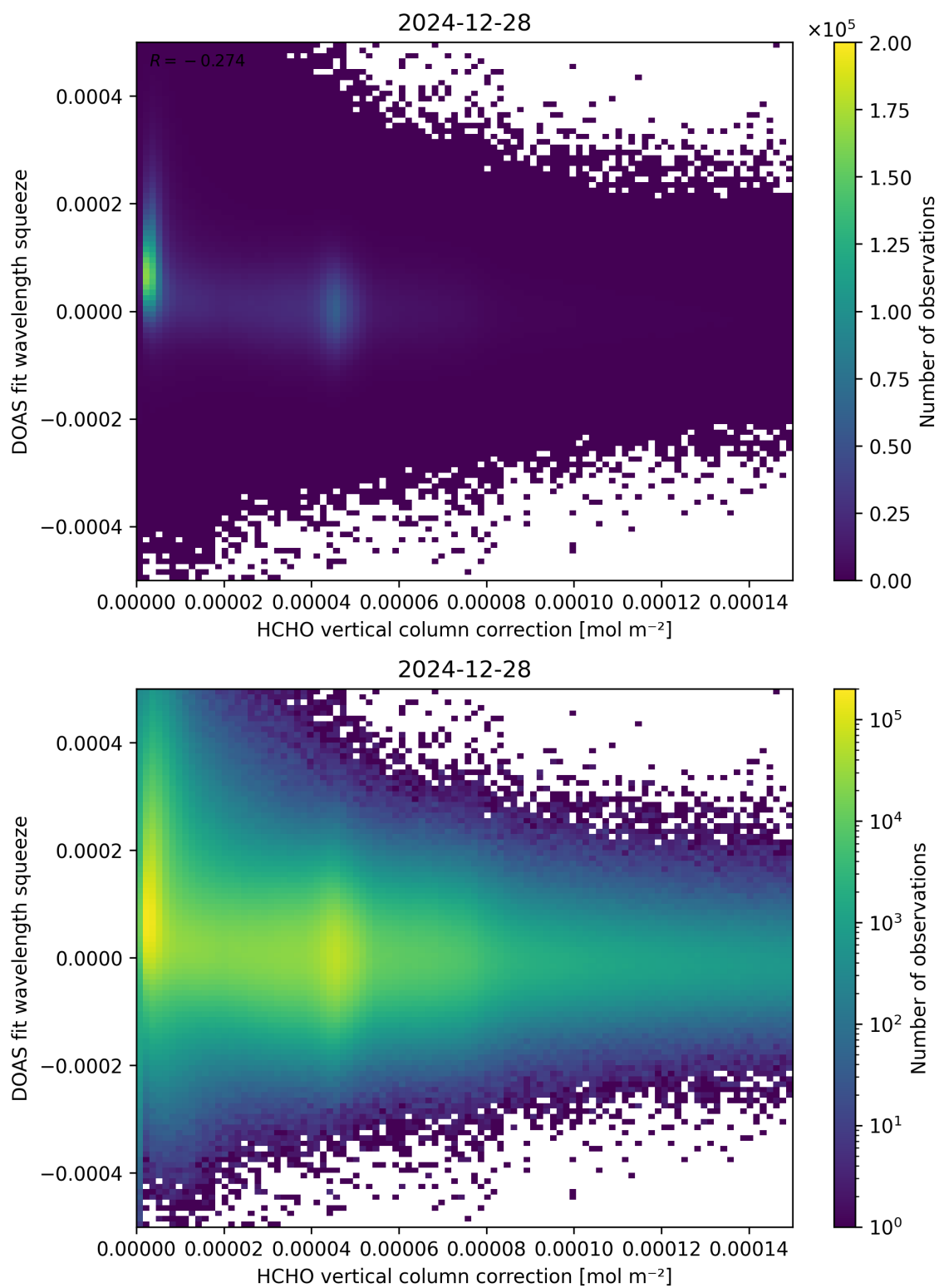
Figure 114: Scatter density plot of “HCHO vertical column correction” against “DOAS fit wavelength squeeze” for 2024-12-27 to 2024-12-29.
