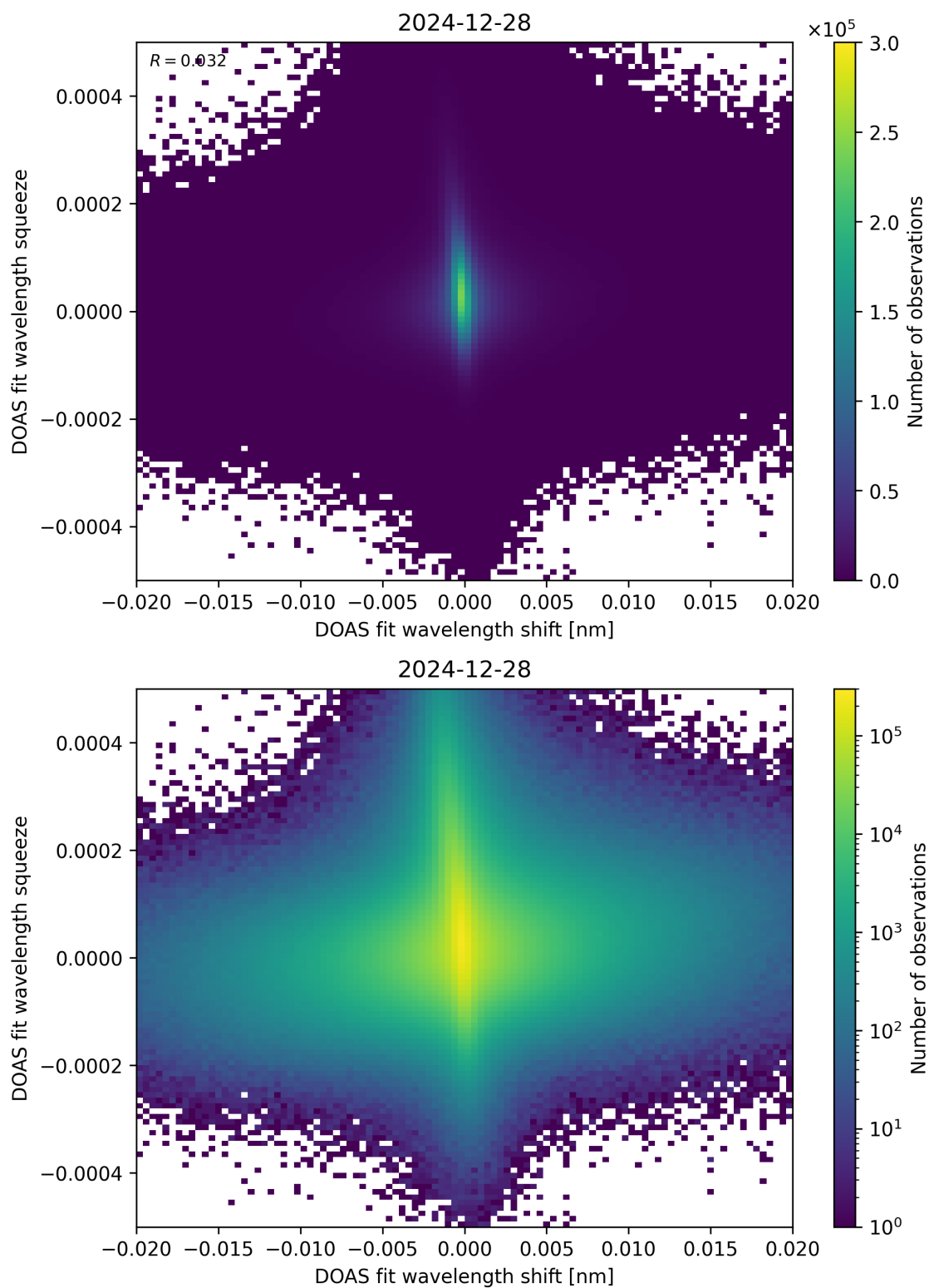
Figure 65: Scatter density plot of “DOAS fit wavelength shift” against “DOAS fit wavelength squeeze” for 2024-12-27 to 2024-12-29.
