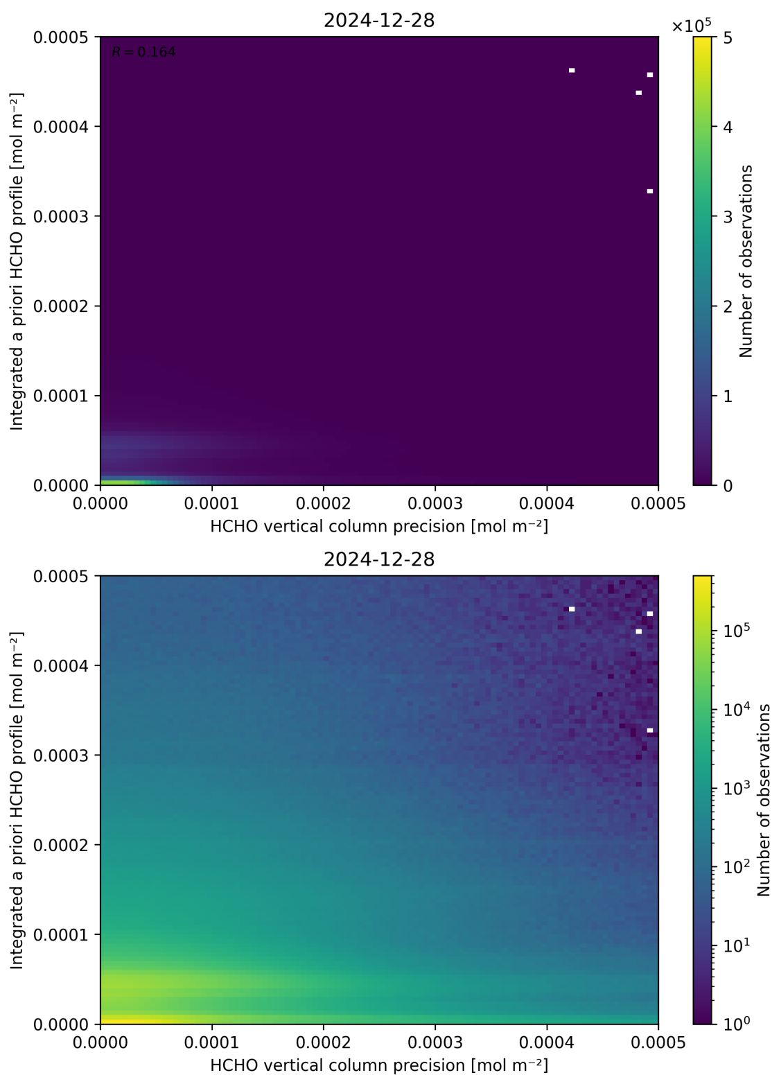
Figure 147: Scatter density plot of “HCHO vertical column precision” against “Integrated a priori HCHO profile” for 2024-12-27 to 2024-12-29.
