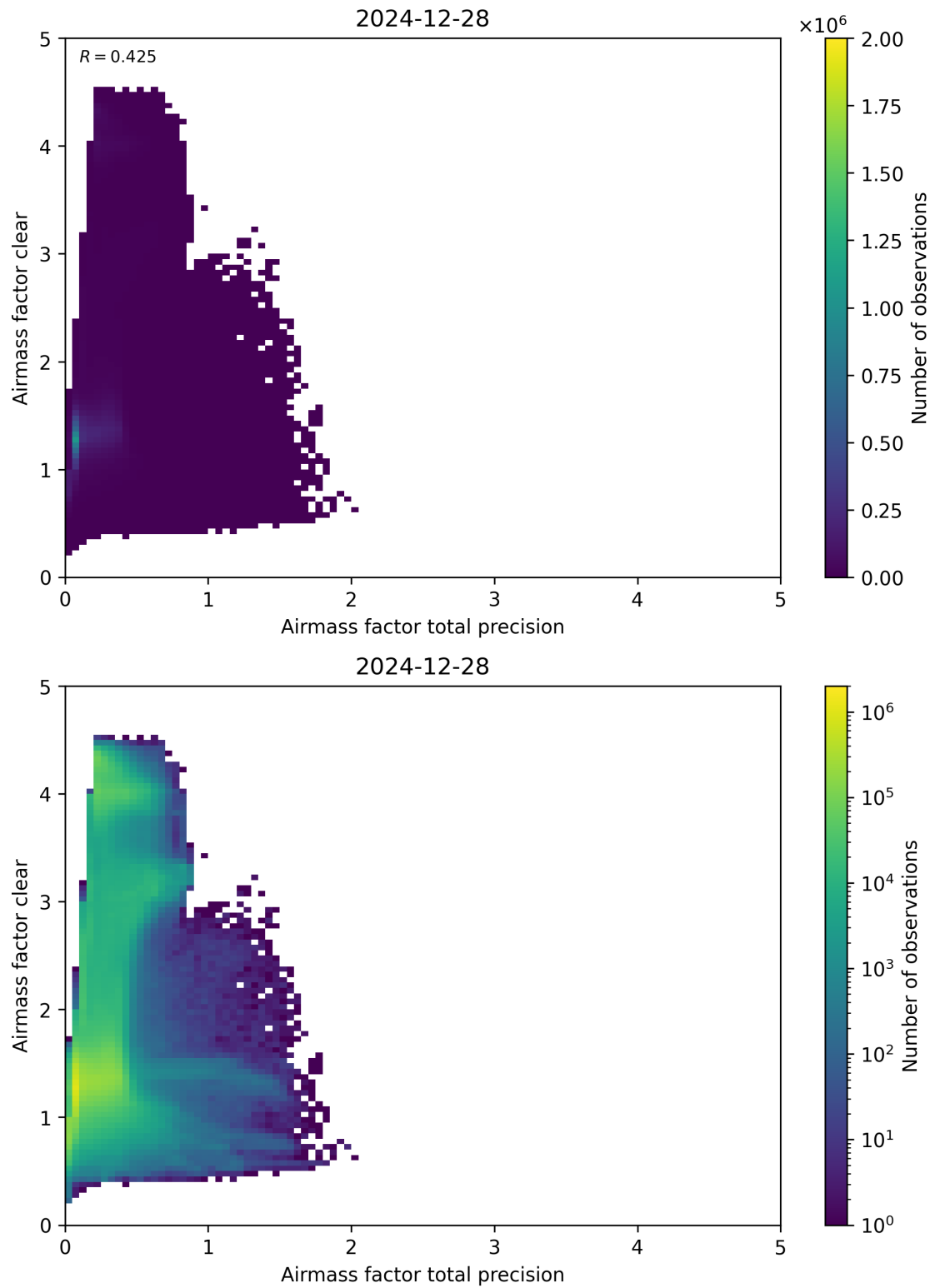
Figure 108: Scatter density plot of “Airmass factor total precision” against “Airmass factor clear” for 2024-12-27 to 2024-12-29.
