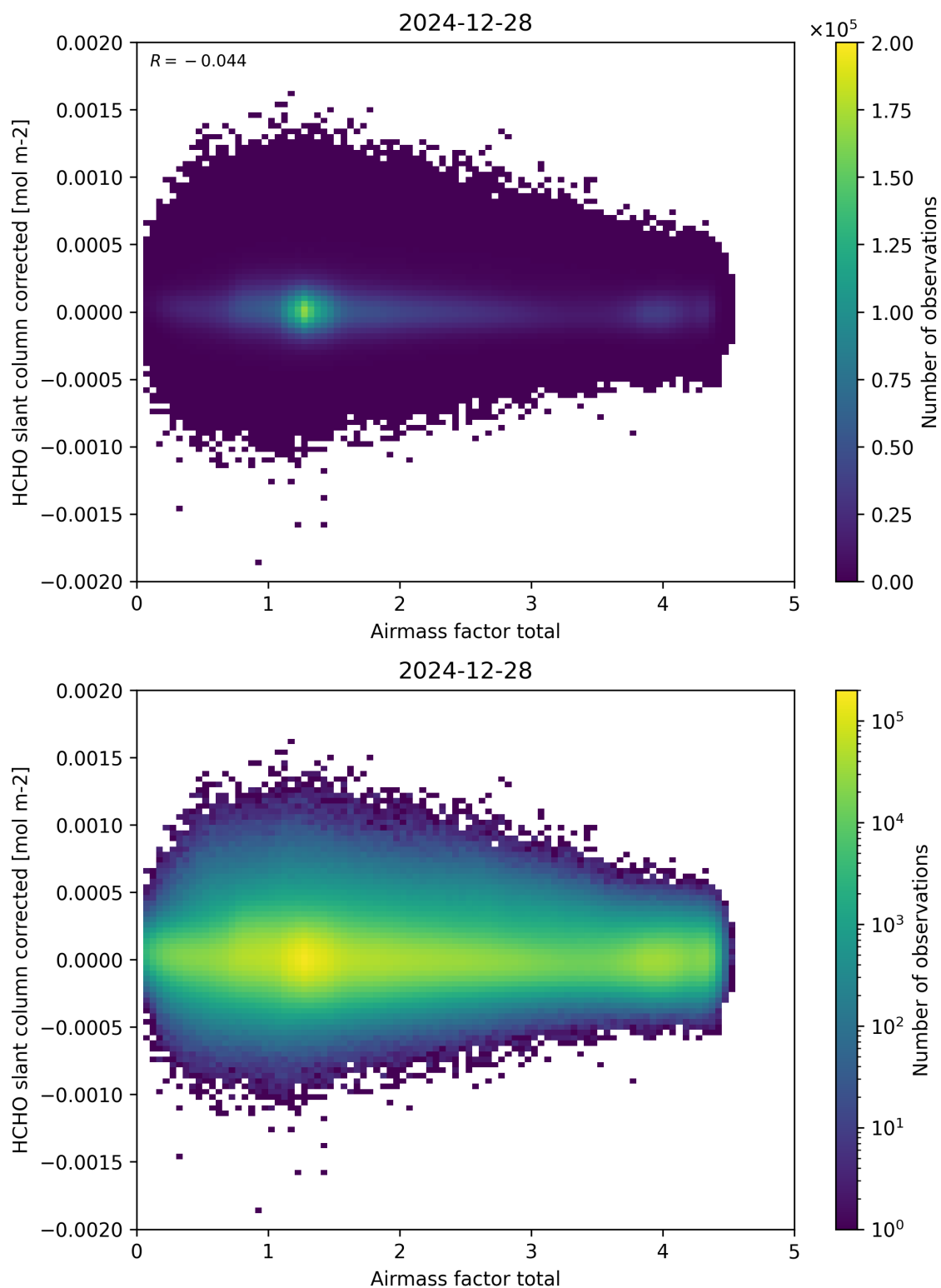
Figure 101: Scatter density plot of “Airmass factor total” against “HCHO slant column corrected” for 2024-12-27 to 2024-12-29.
