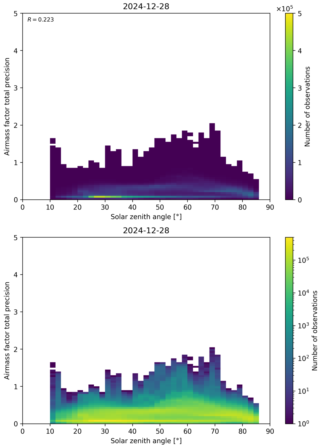
Figure 176: Scatter density plot of “Solar zenith angle” against “Airmass factor total precision” for 2024-12-27 to 2024-12-29.
