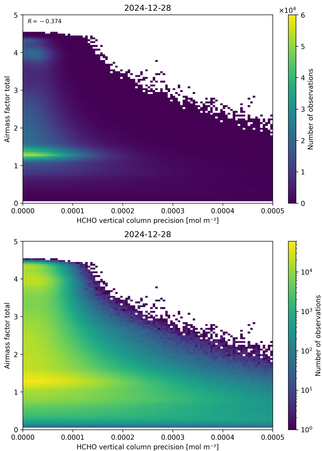
Figure 144: Scatter density plot of “HCHO vertical column precision” against “Airmass factor total” for 2024-12-27 to 2024-12-29.
