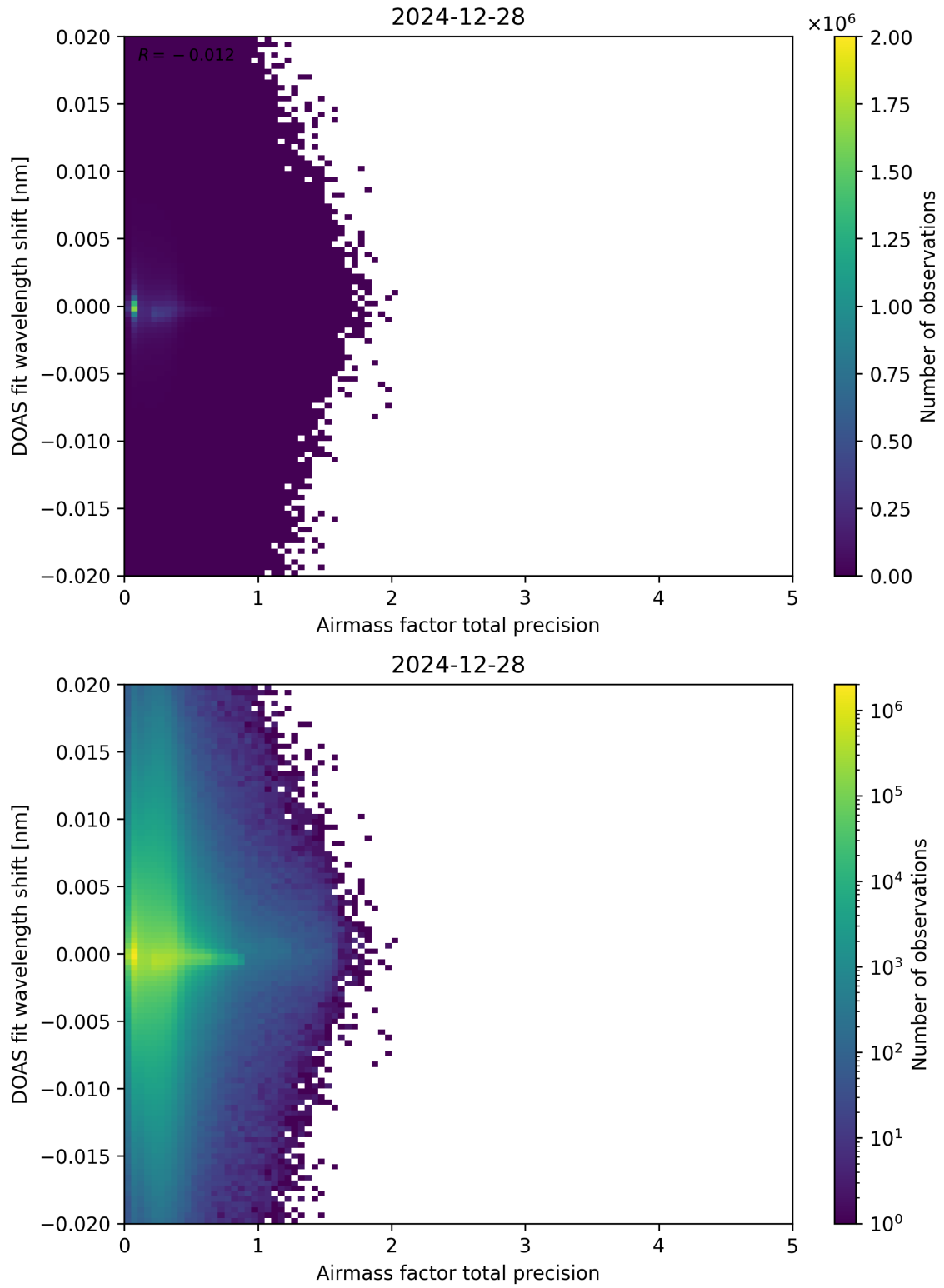
Figure 106: Scatter density plot of “Airmass factor total precision” against “DOAS fit wavelength shift” for 2024-12-27 to 2024-12-29.
