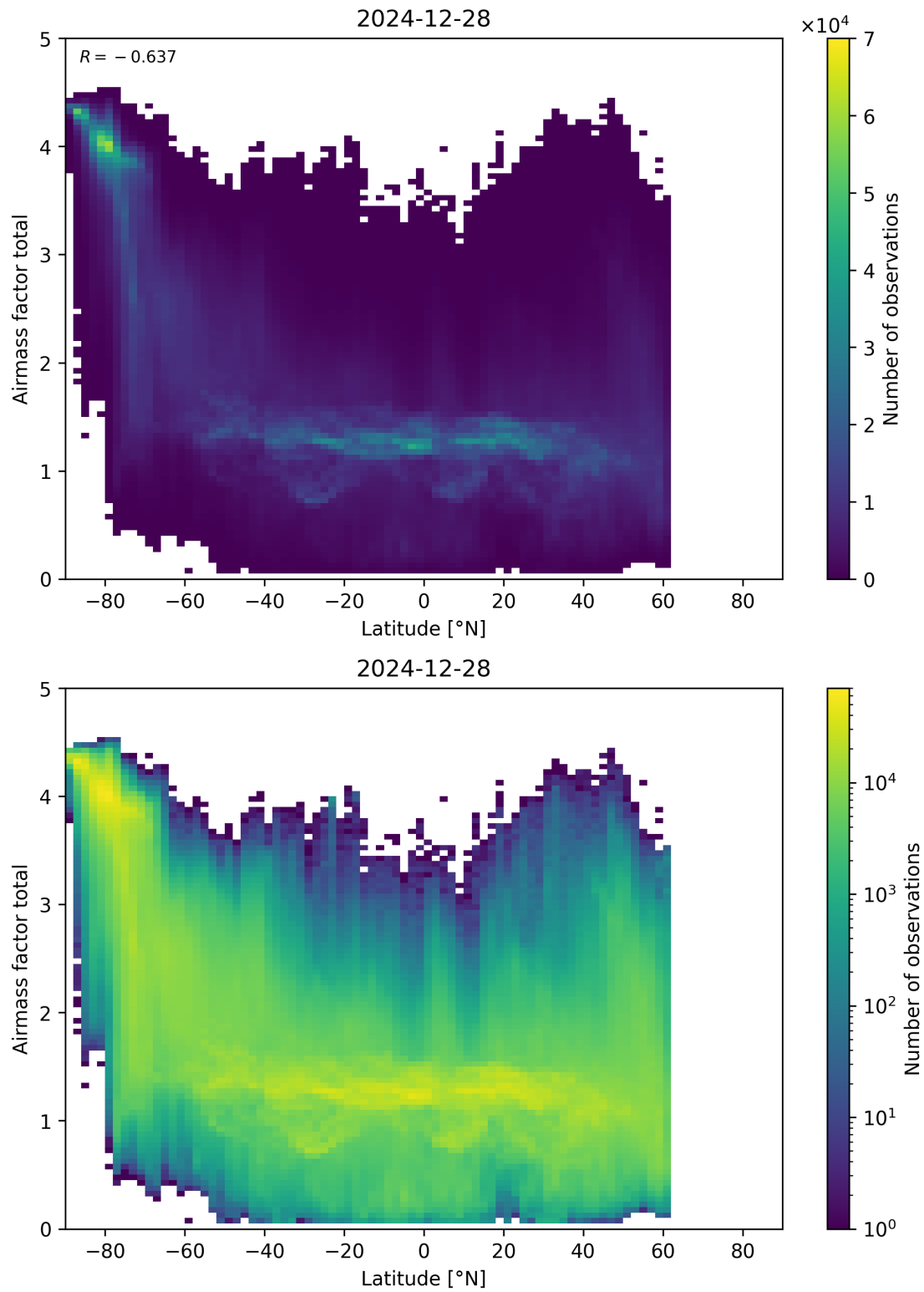
Figure 161: Scatter density plot of “Latitude” against “Airmass factor total” for 2024-12-27 to 2024-12-29.
