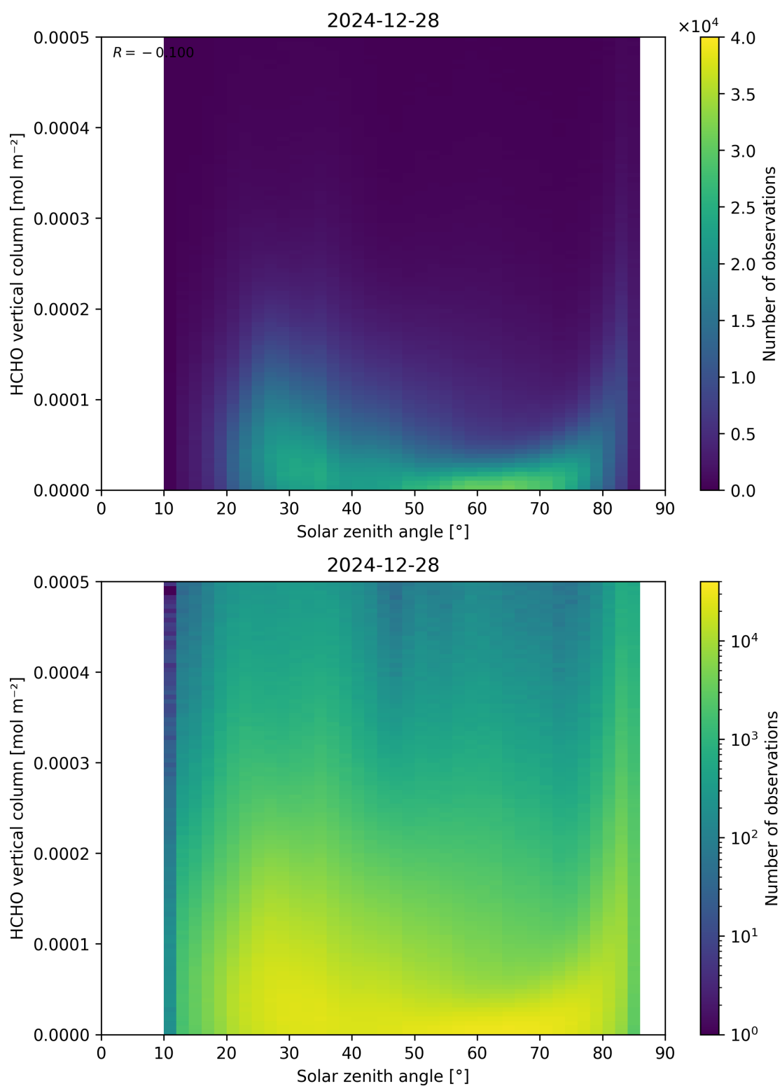
Figure 177: Scatter density plot of “Solar zenith angle” against “HCHO vertical column” for 2024-12-27 to 2024-12-29.
