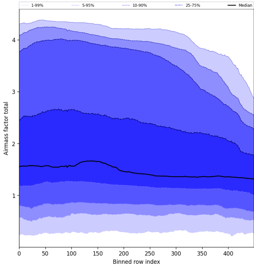
Figure 54: Along track statistics of “Airmass factor total” for 2024-12-27 to 2024-12-29
