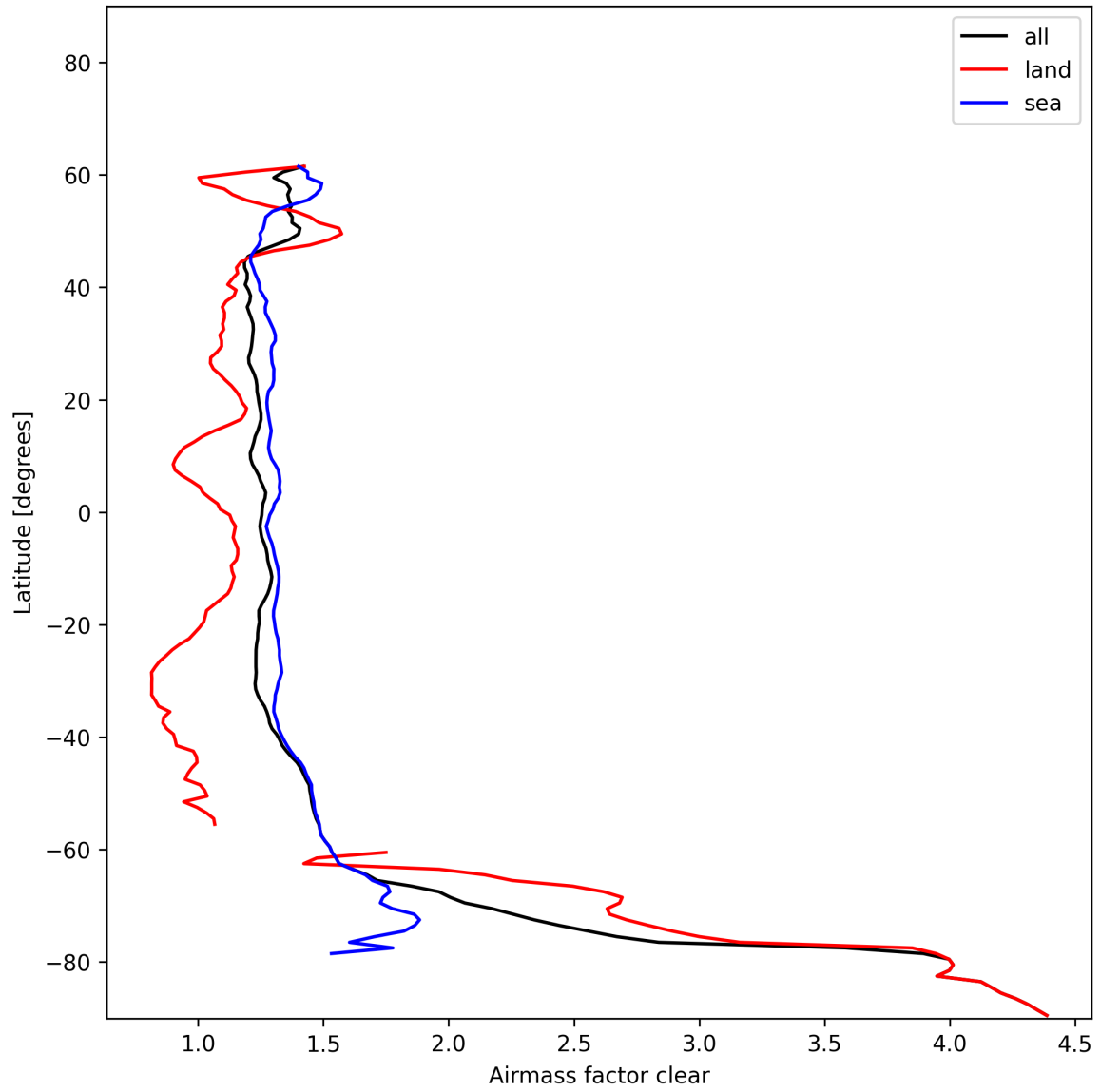
Figure 28: Zonal average of “Airmass factor clear” for 2024-12-27 to 2024-12-29.
