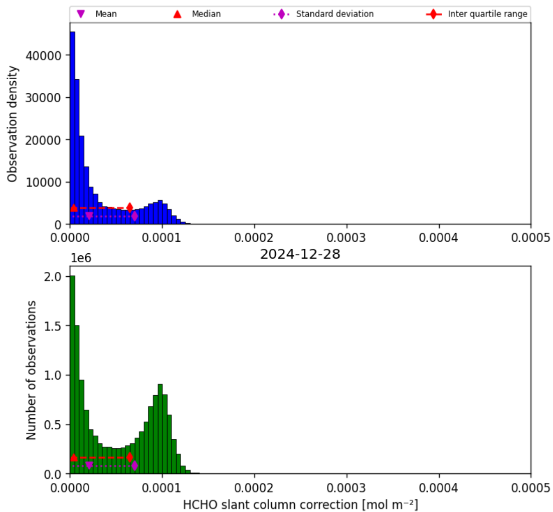
Figure 47: Histogram of “HCHO slant column correction” for 2024-12-27 to 2024-12-29
