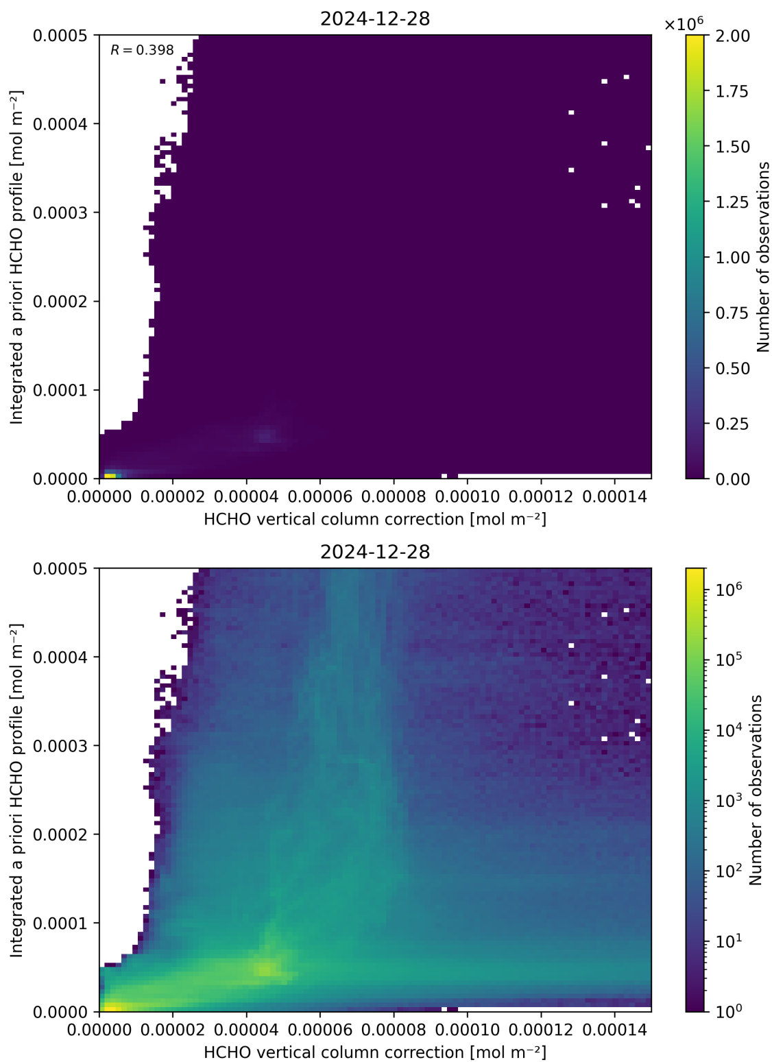
Figure 122: Scatter density plot of “HCHO vertical column correction” against “Integrated a priori HCHO profile” for 2024-12-27 to 2024-12-29.
