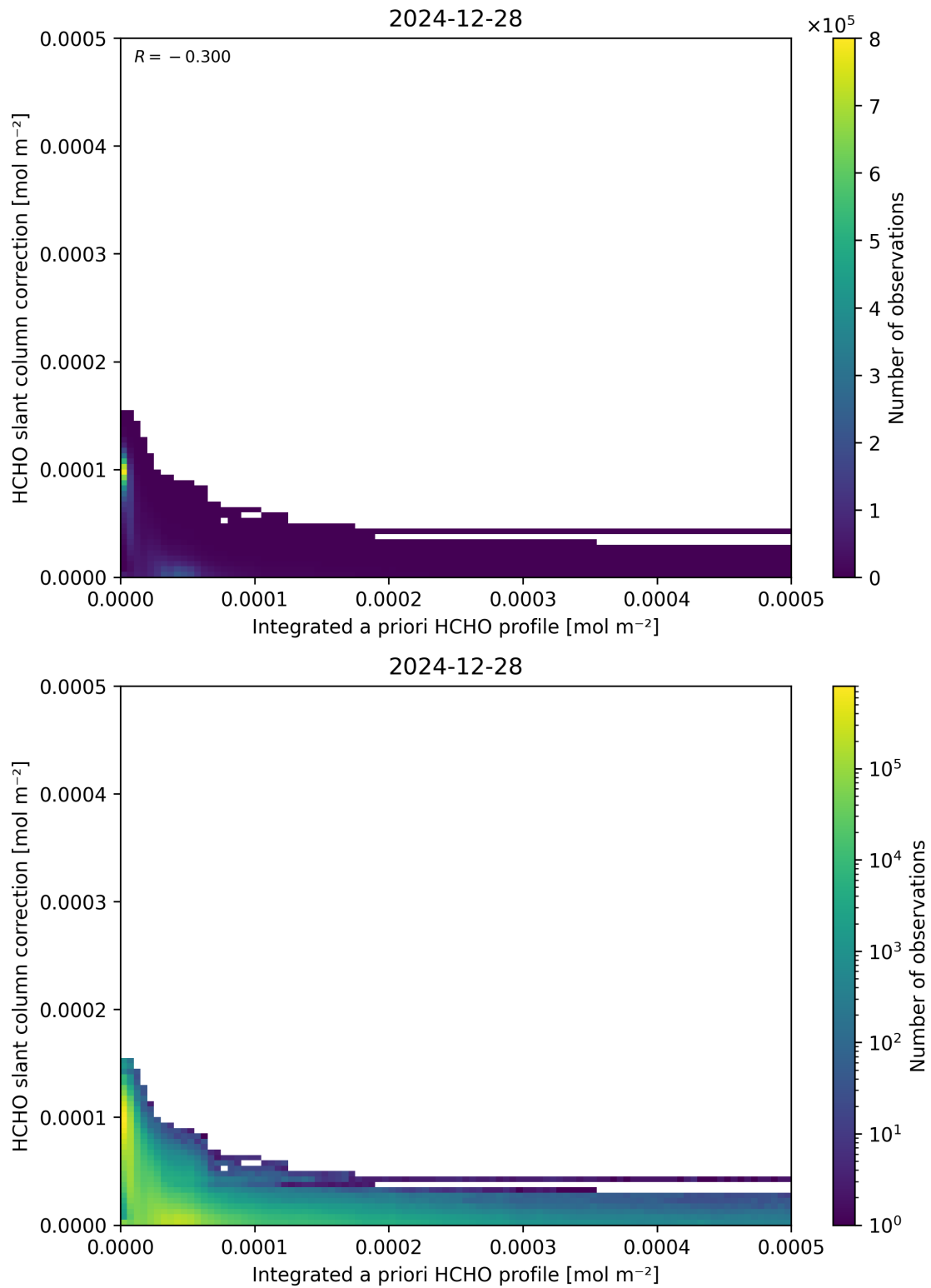
Figure 152: Scatter density plot of “Integrated a priori HCHO profile” against “HCHO slant column correction” for 2024-12-27 to 2024-12-29.
