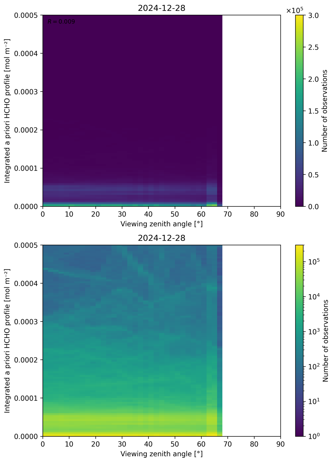
Figure 195: Scatter density plot of “Viewing zenith angle” against “Integrated a priori HCHO profile” for 2024-12-27 to 2024-12-29.
