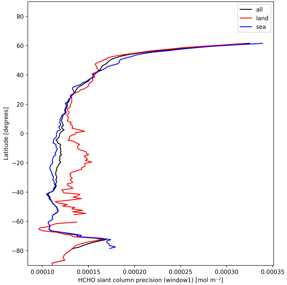
Figure 25: Zonal average of “HCHO slant column precision (window1)” for 2024-12-27 to 2024-12-29.
