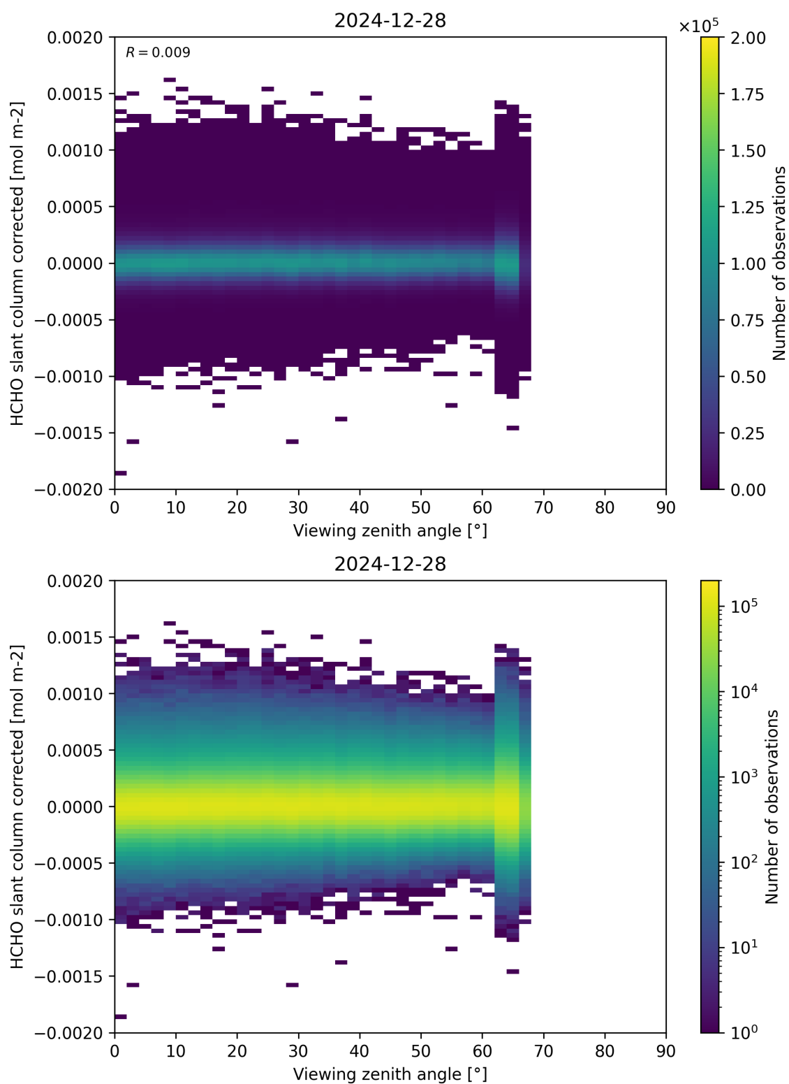
Figure 186: Scatter density plot of “Viewing zenith angle” against “HCHO slant column corrected” for 2024-12-27 to 2024-12-29.
