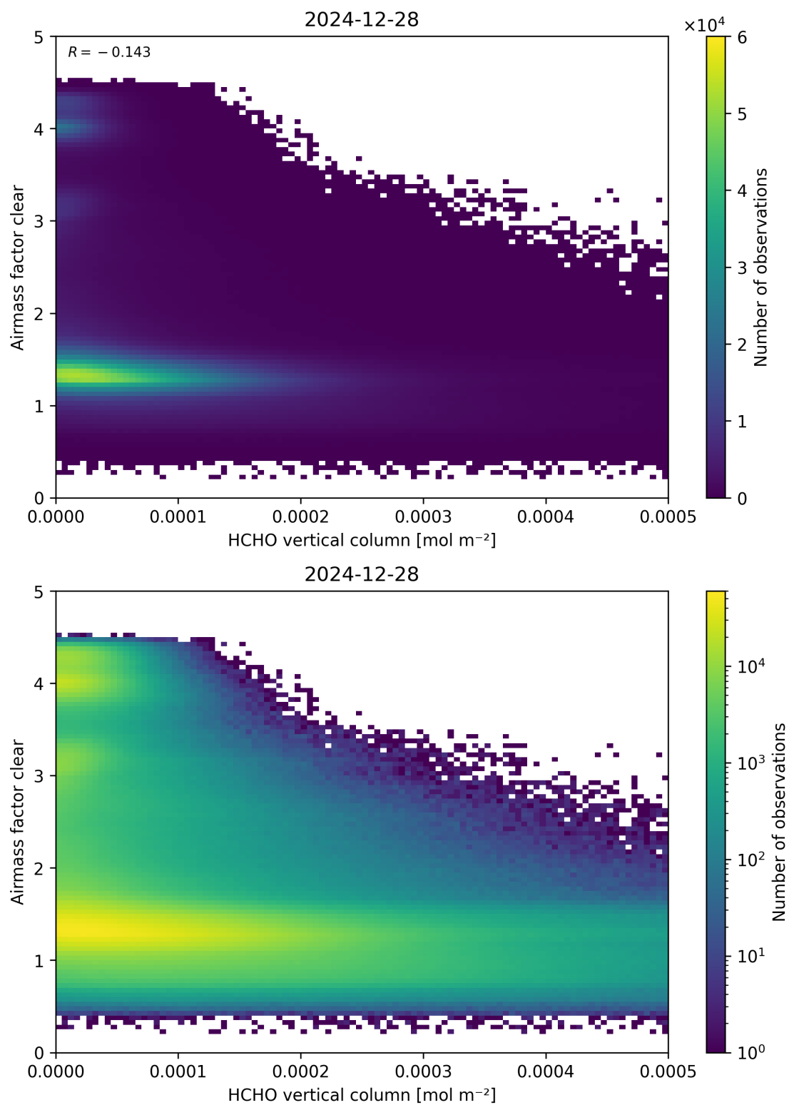
Figure 126: Scatter density plot of “HCHO vertical column” against “Airmass factor clear” for 2024-12-27 to 2024-12-29.
