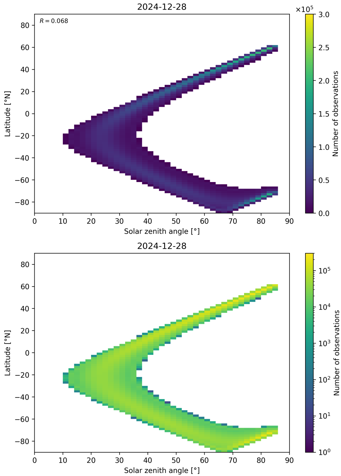
Figure 181: Scatter density plot of “Solar zenith angle” against “Latitude” for 2024-12-27 to 2024-12-29.
