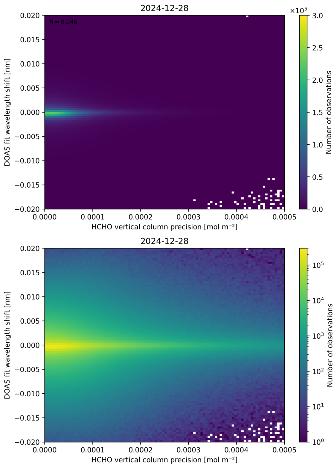
Figure 137: Scatter density plot of “HCHO vertical column precision” against “DOAS fit wavelength shift” for 2024-12-27 to 2024-12-29.
