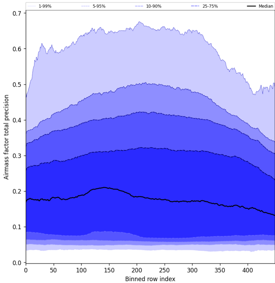
Figure 55: Along track statistics of “Airmass factor total precision” for 2024-12-27 to 2024-12-29
