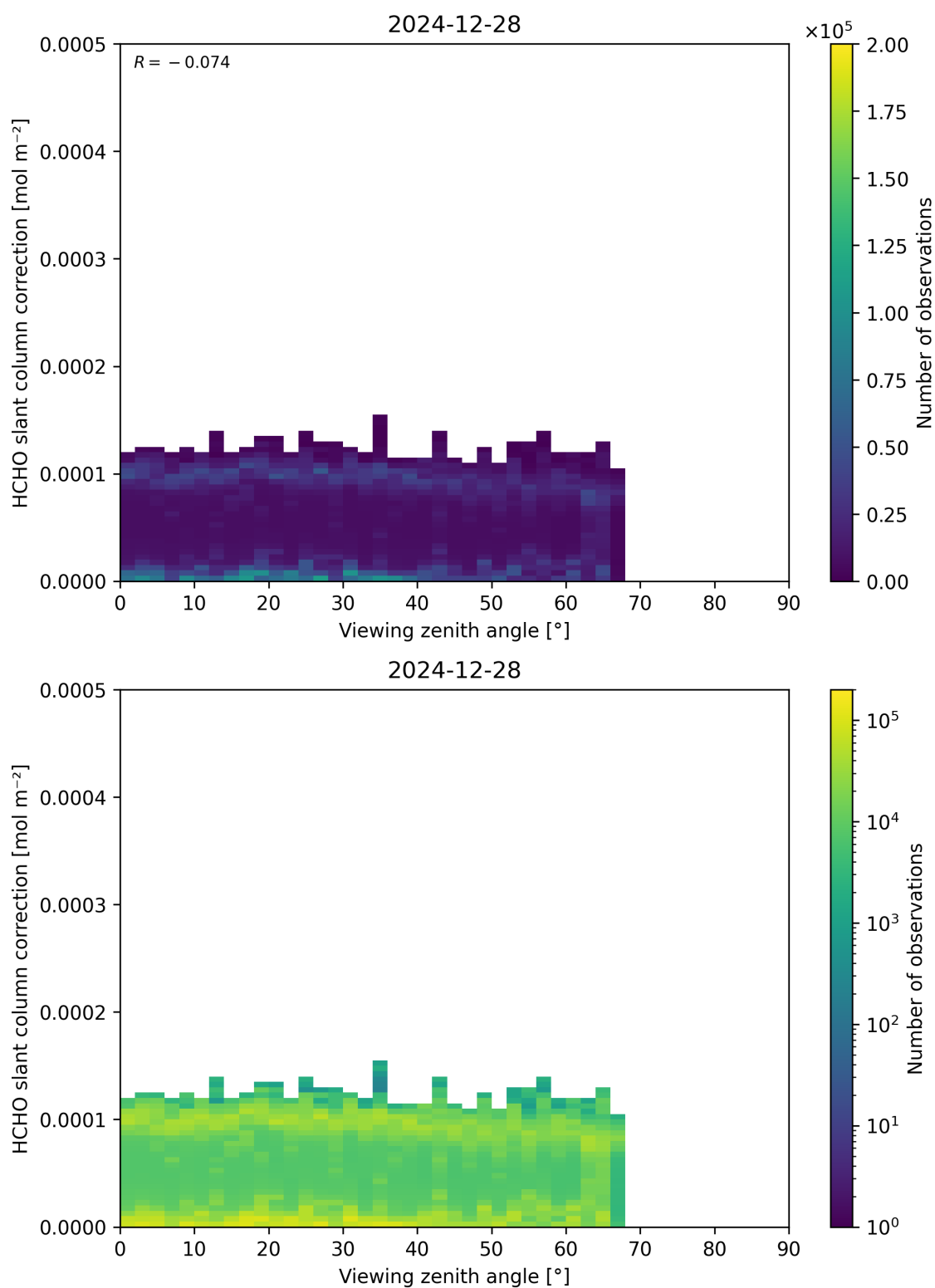
Figure 187: Scatter density plot of “Viewing zenith angle” against “HCHO slant column correction” for 2024-12-27 to 2024-12-29.
