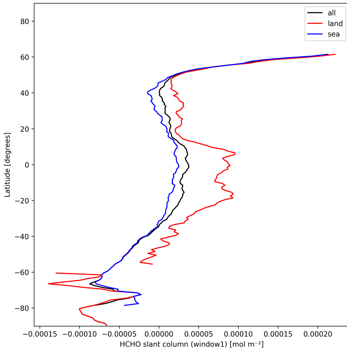
Figure 24: Zonal average of “HCHO slant column (window1)” for 2024-12-27 to 2024-12-29.
