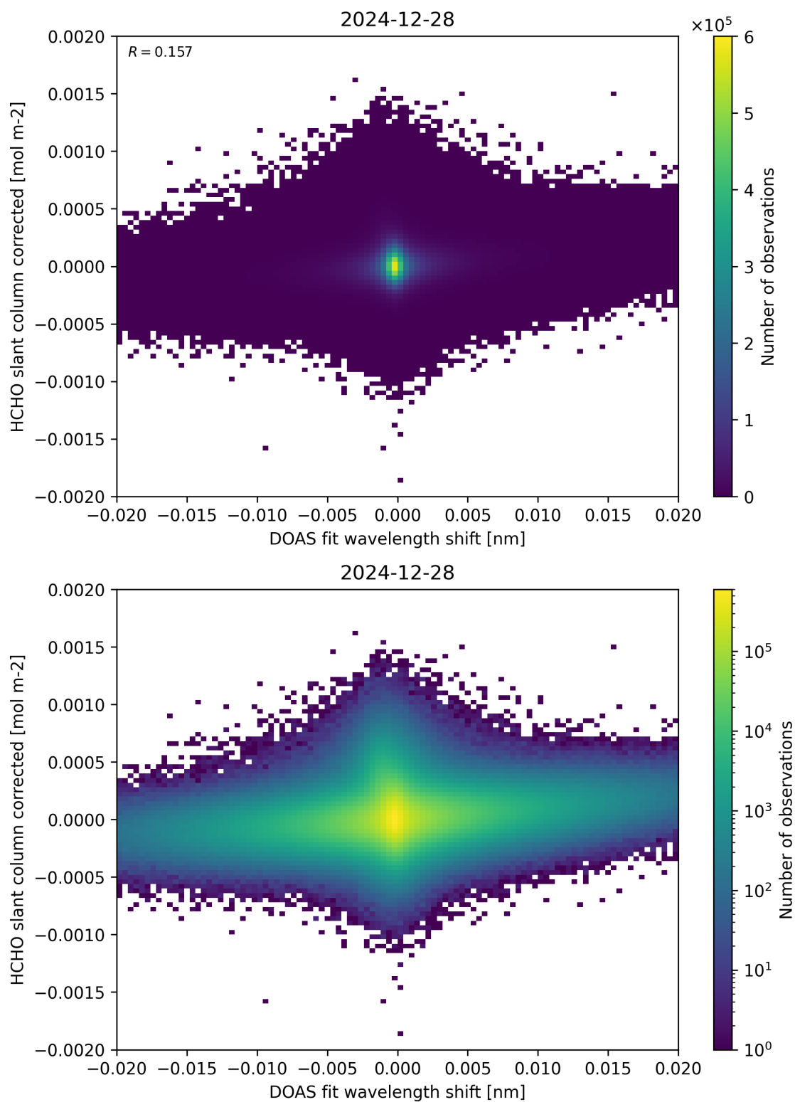
Figure 66: Scatter density plot of “DOAS fit wavelength shift” against “HCHO slant column corrected” for 2024-12-27 to 2024-12-29.
