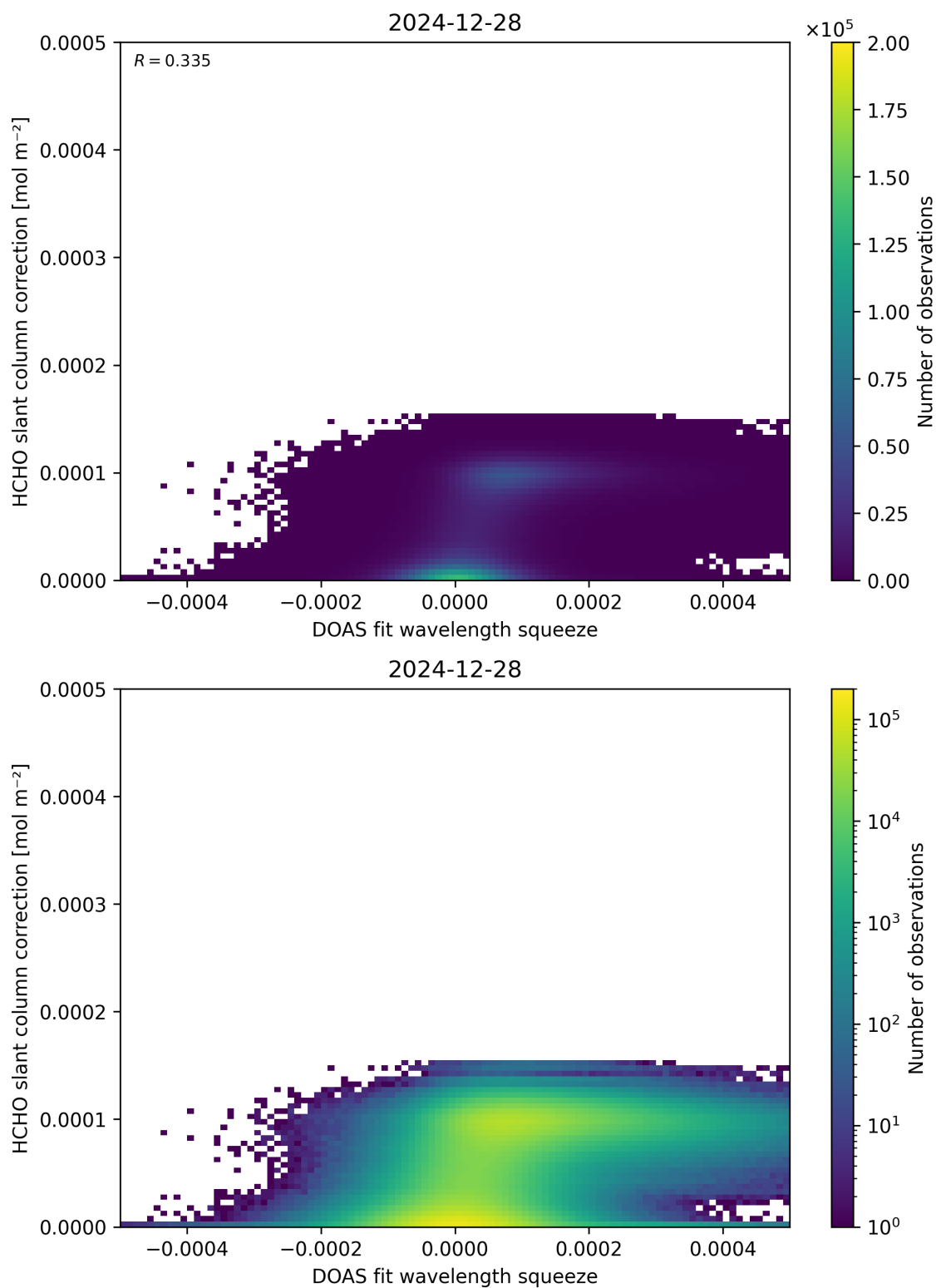
Figure 70: Scatter density plot of “DOAS fit wavelength squeeze” against “HCHO slant column correction” for 2024-12-27 to 2024-12-29.
