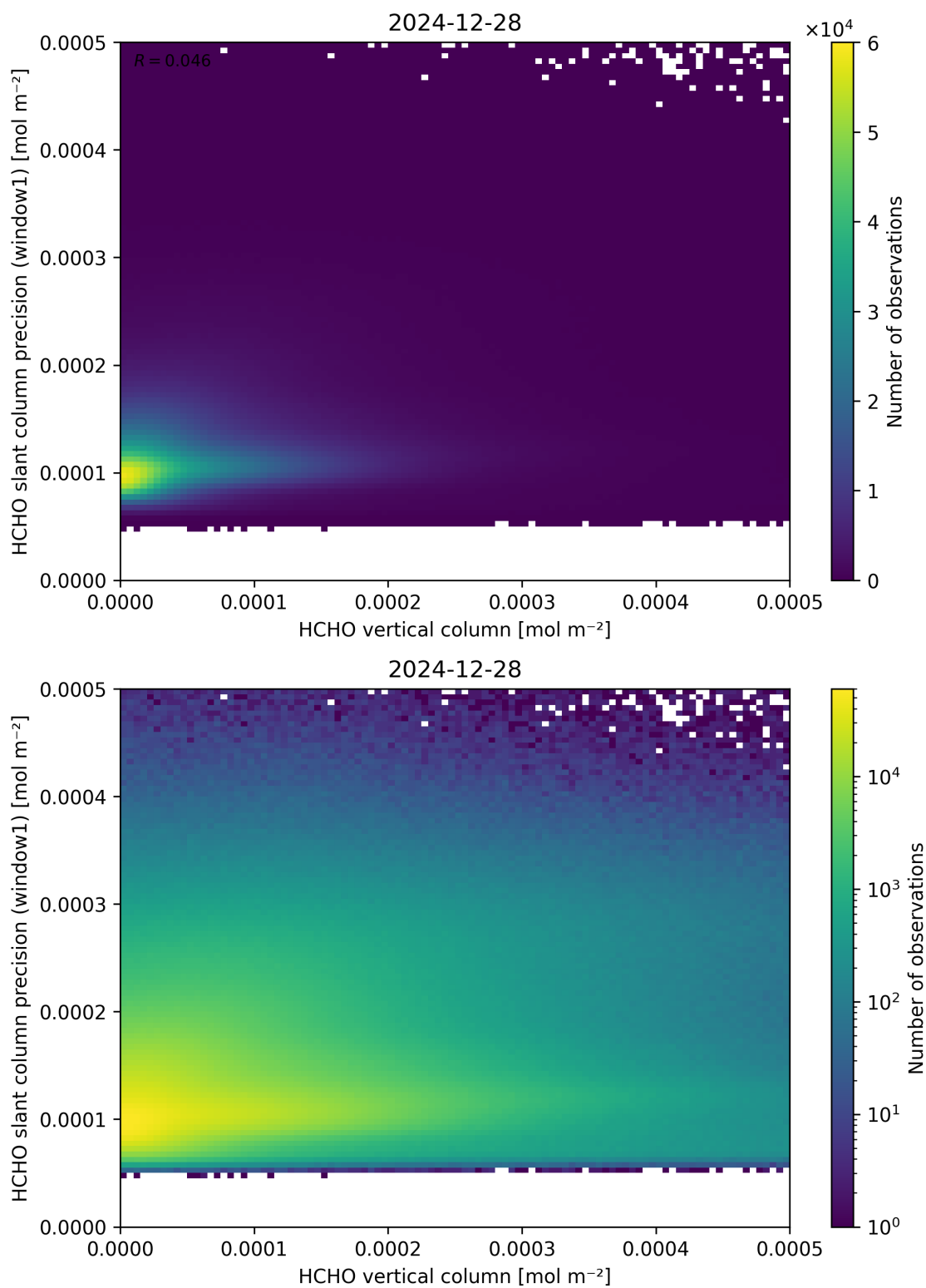
Figure 130: Scatter density plot of “HCHO vertical column” against “HCHO slant column precision (window1)” for 2024-12-27 to 2024-12-29.
