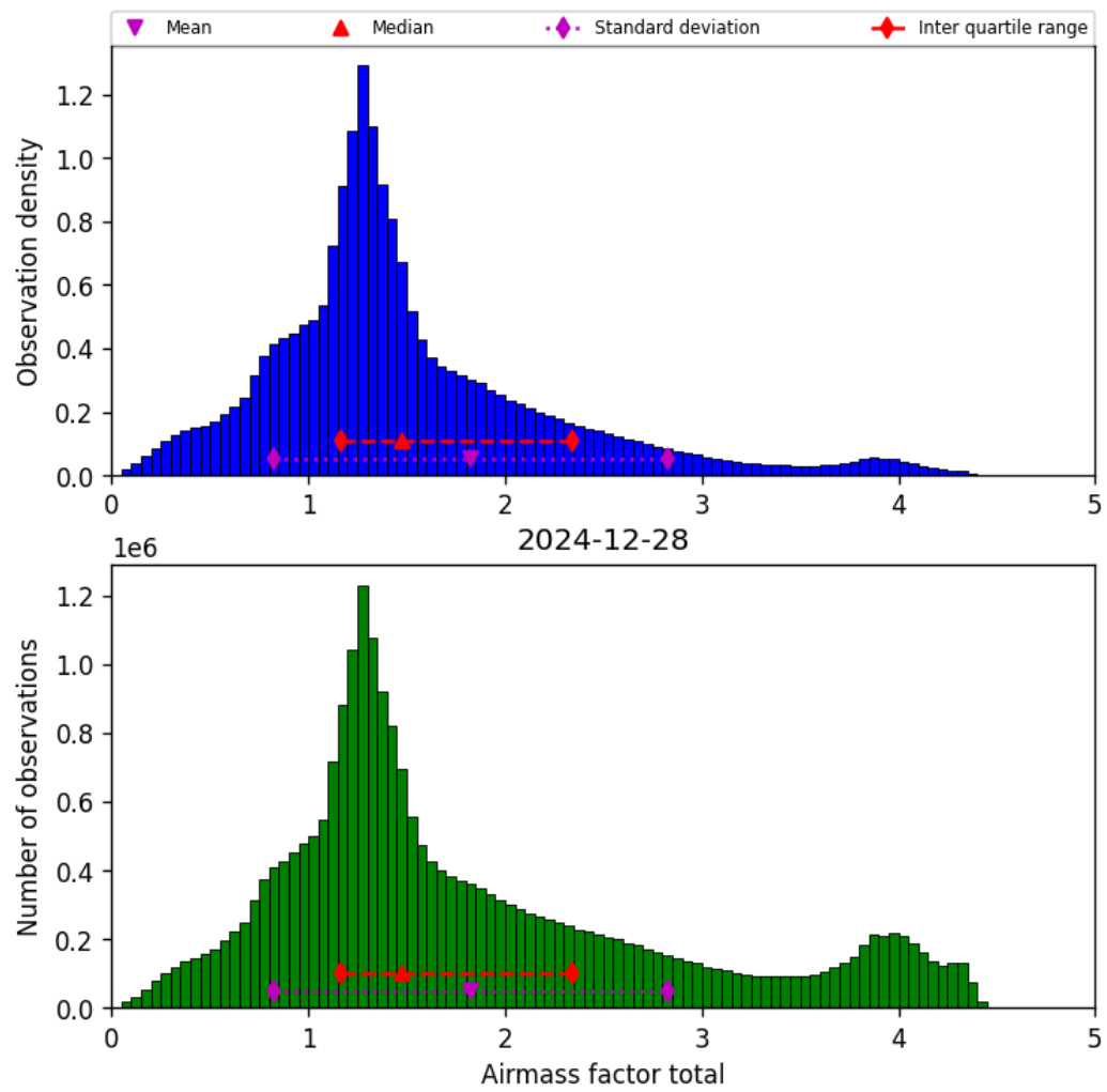
Figure 40: Histogram of “Airmass factor total” for 2024-12-27 to 2024-12-29
