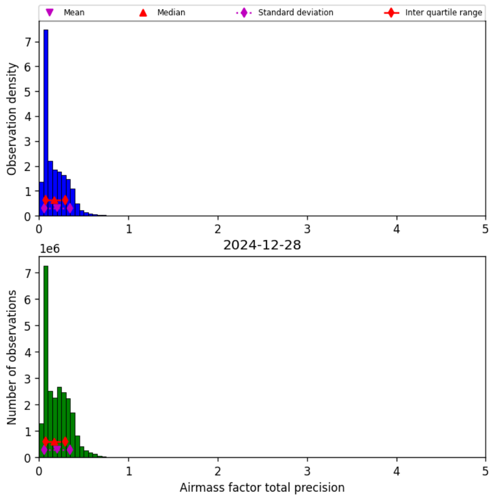
Figure 41: Histogram of “Airmass factor total precision” for 2024-12-27 to 2024-12-29
