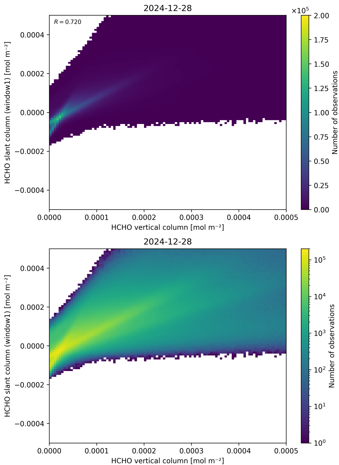
Figure 129: Scatter density plot of “HCHO vertical column” against “HCHO slant column (window1)” for 2024-12-27 to 2024-12-29.
