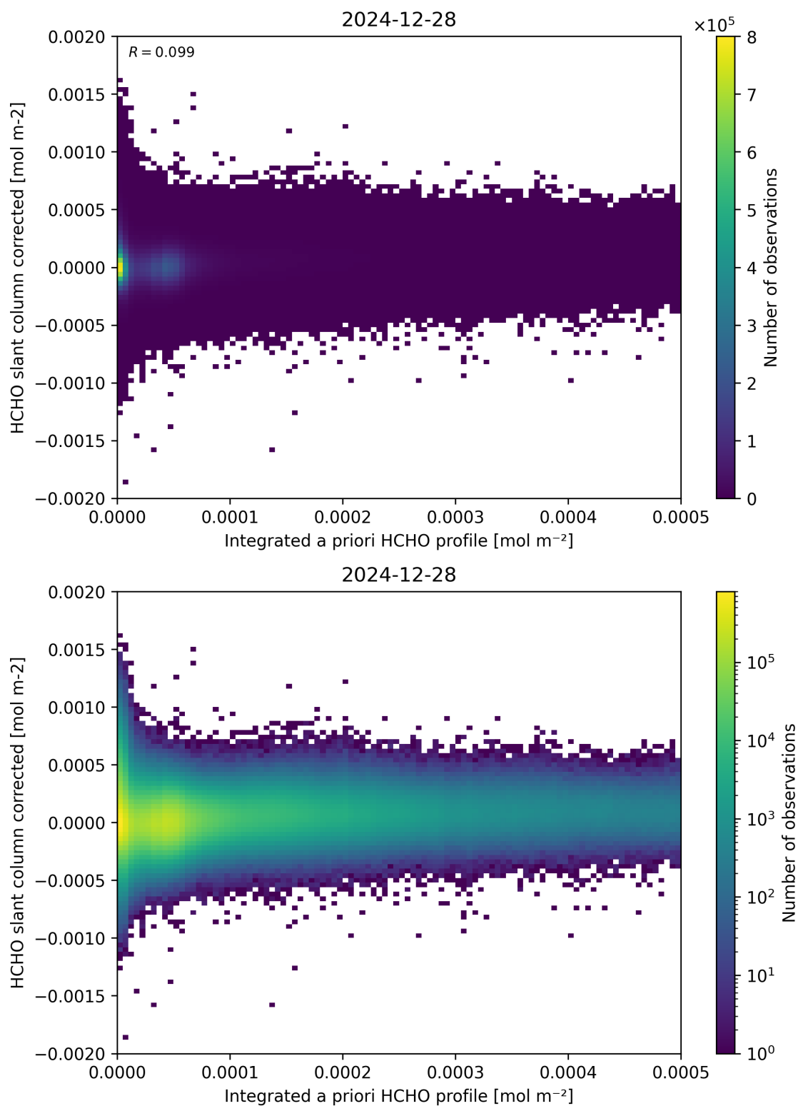
Figure 151: Scatter density plot of “Integrated a priori HCHO profile” against “HCHO slant column corrected” for 2024-12-27 to 2024-12-29.
