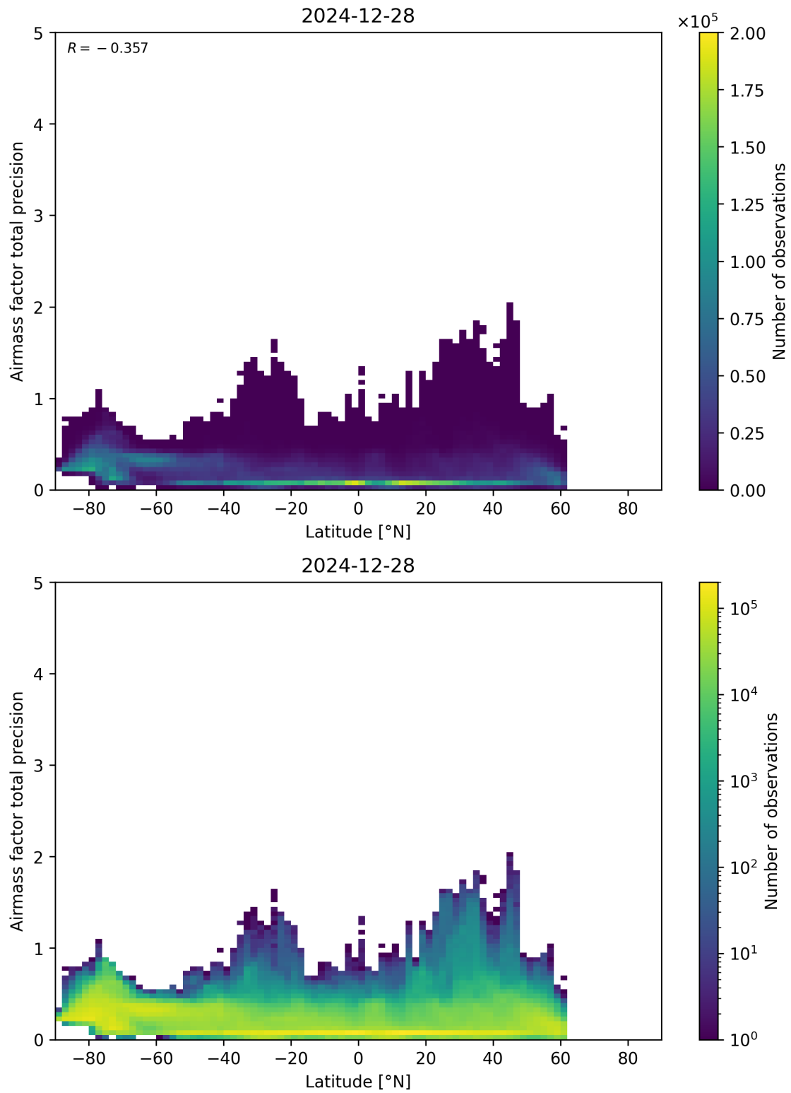
Figure 162: Scatter density plot of “Latitude” against “Airmass factor total precision” for 2024-12-27 to 2024-12-29.
