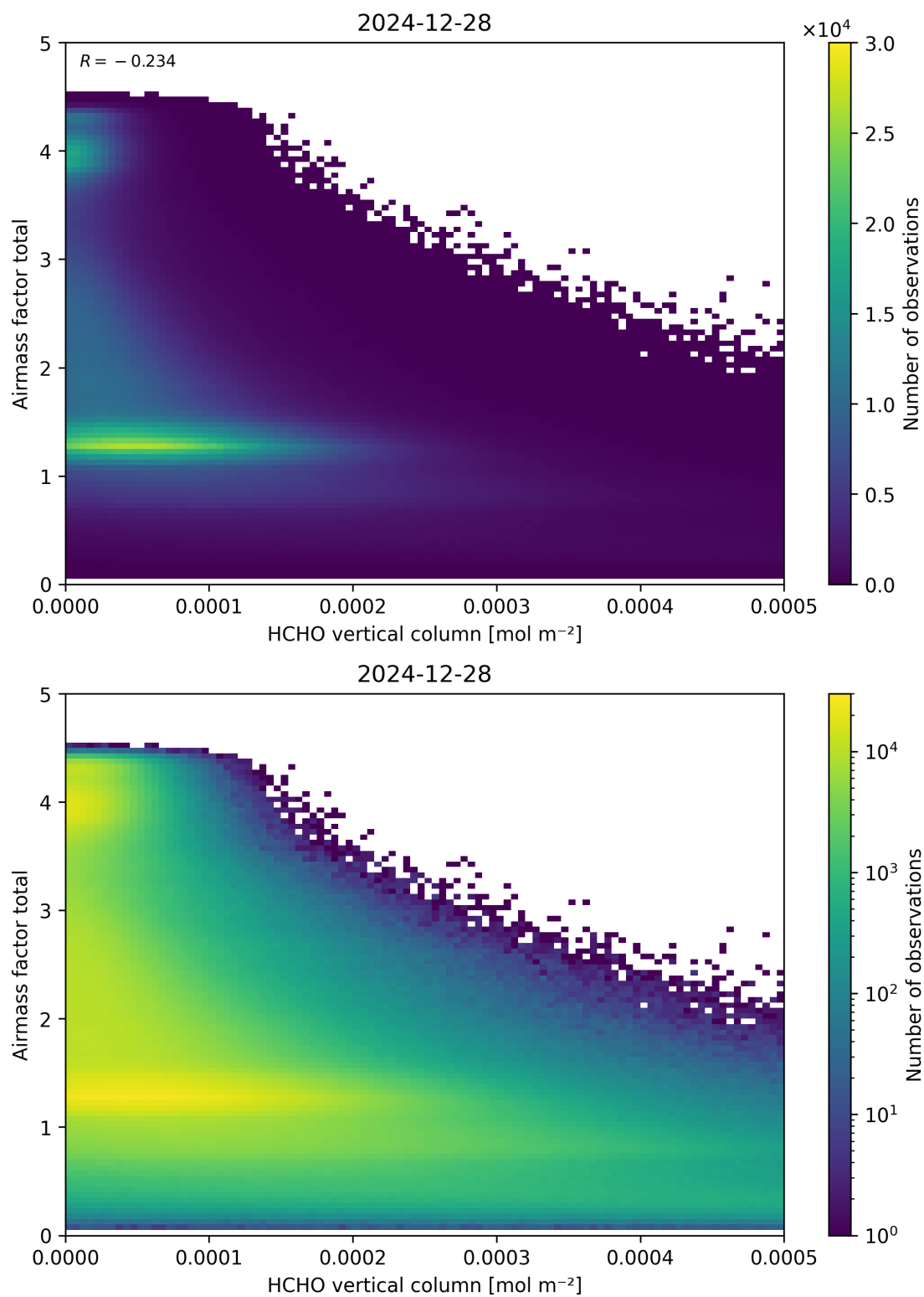
Figure 131: Scatter density plot of “HCHO vertical column” against “Airmass factor total” for 2024-12-27 to 2024-12-29.
