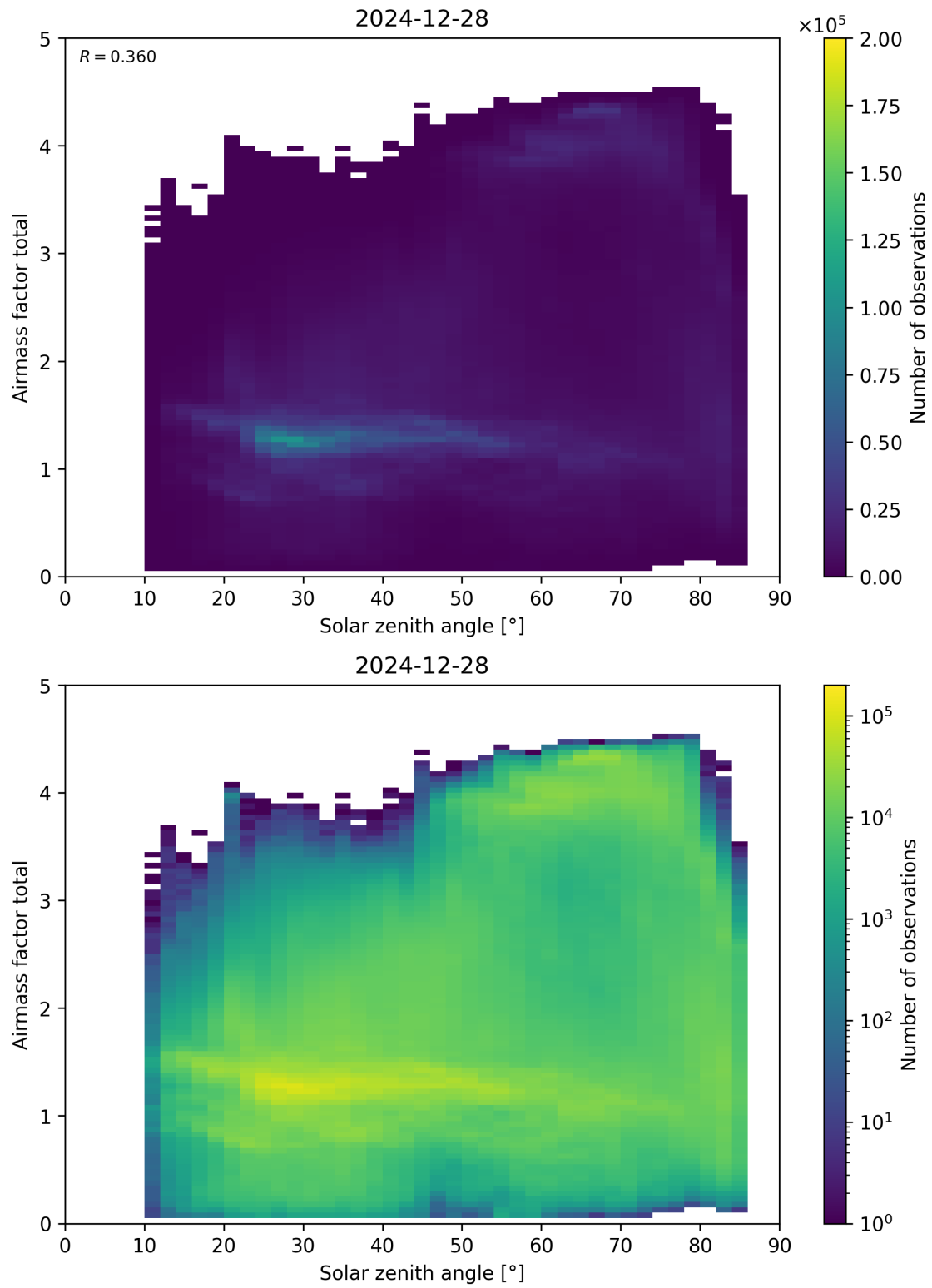
Figure 175: Scatter density plot of “Solar zenith angle” against “Airmass factor total” for 2024-12-27 to 2024-12-29.
