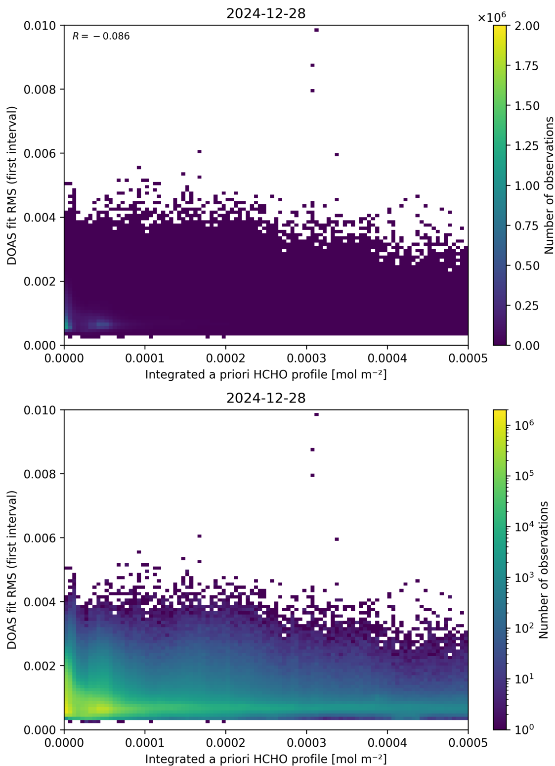
Figure 148: Scatter density plot of “Integrated a priori HCHO profile” against “DOAS fit RMS (first interval)” for 2024-12-27 to 2024-12-29.
