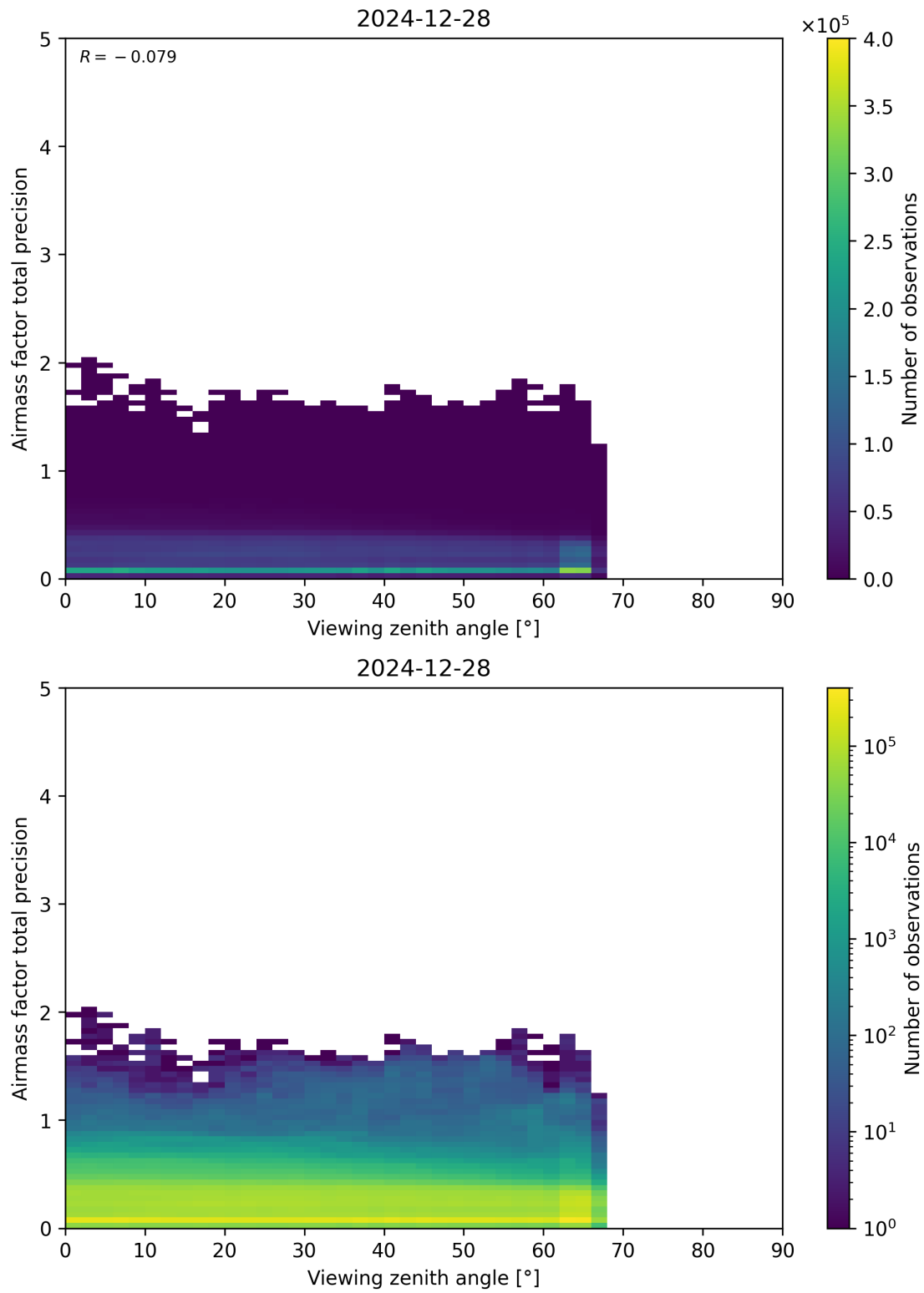
Figure 191: Scatter density plot of “Viewing zenith angle” against “Airmass factor total precision” for 2024-12-27 to 2024-12-29.
