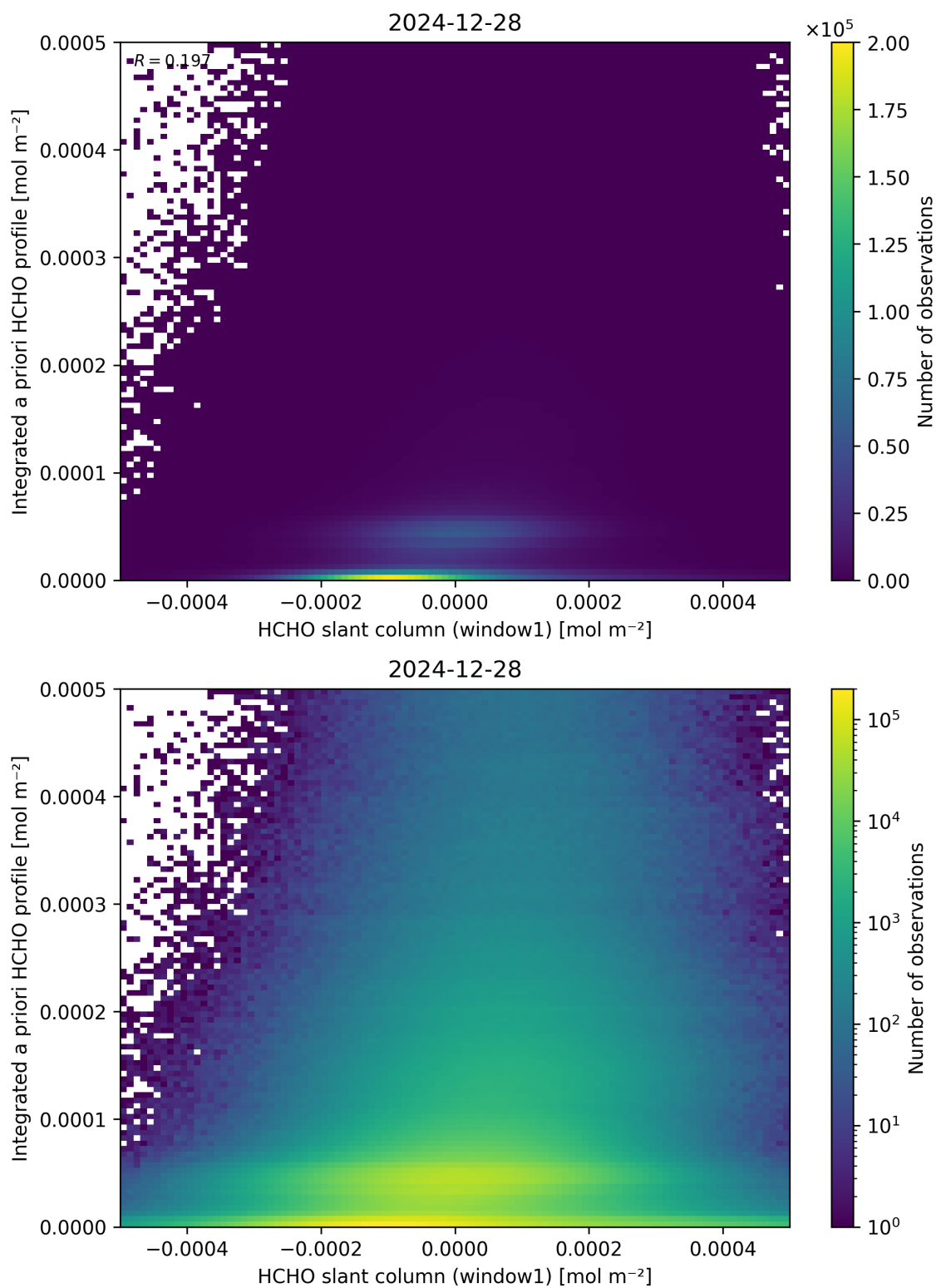
Figure 87: Scatter density plot of “HCHO slant column (window1)” against “Integrated a priori HCHO profile” for 2024-12-27 to 2024-12-29.
