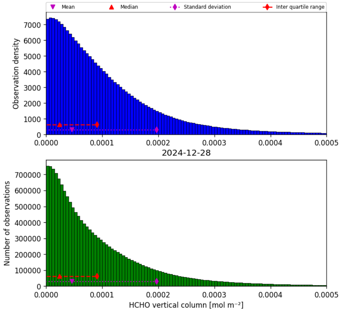
Figure 35: Histogram of “HCHO vertical column” for 2024-12-27 to 2024-12-29
