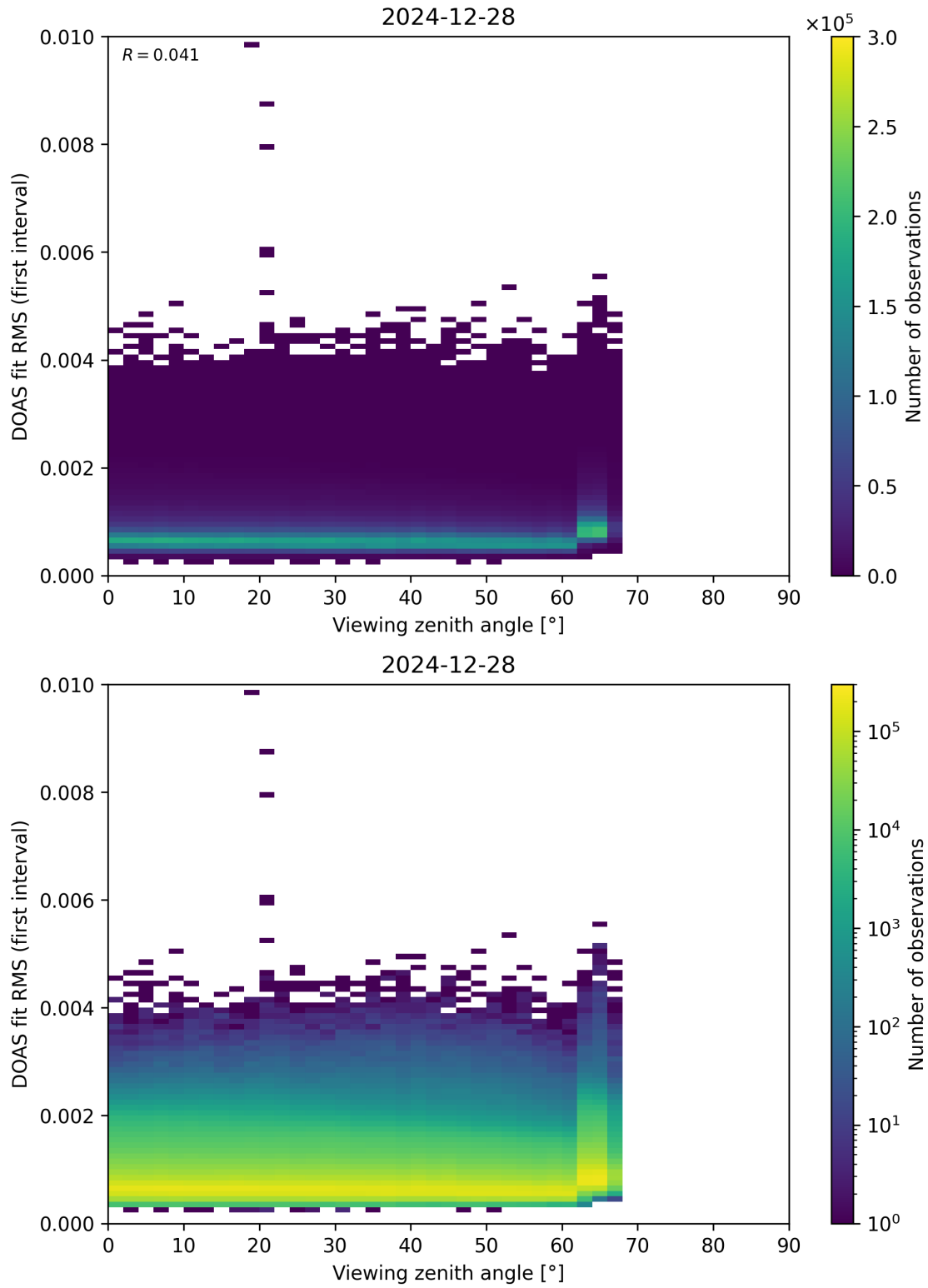
Figure 182: Scatter density plot of “Viewing zenith angle” against “DOAS fit RMS (first interval)” for 2024-12-27 to 2024-12-29.
