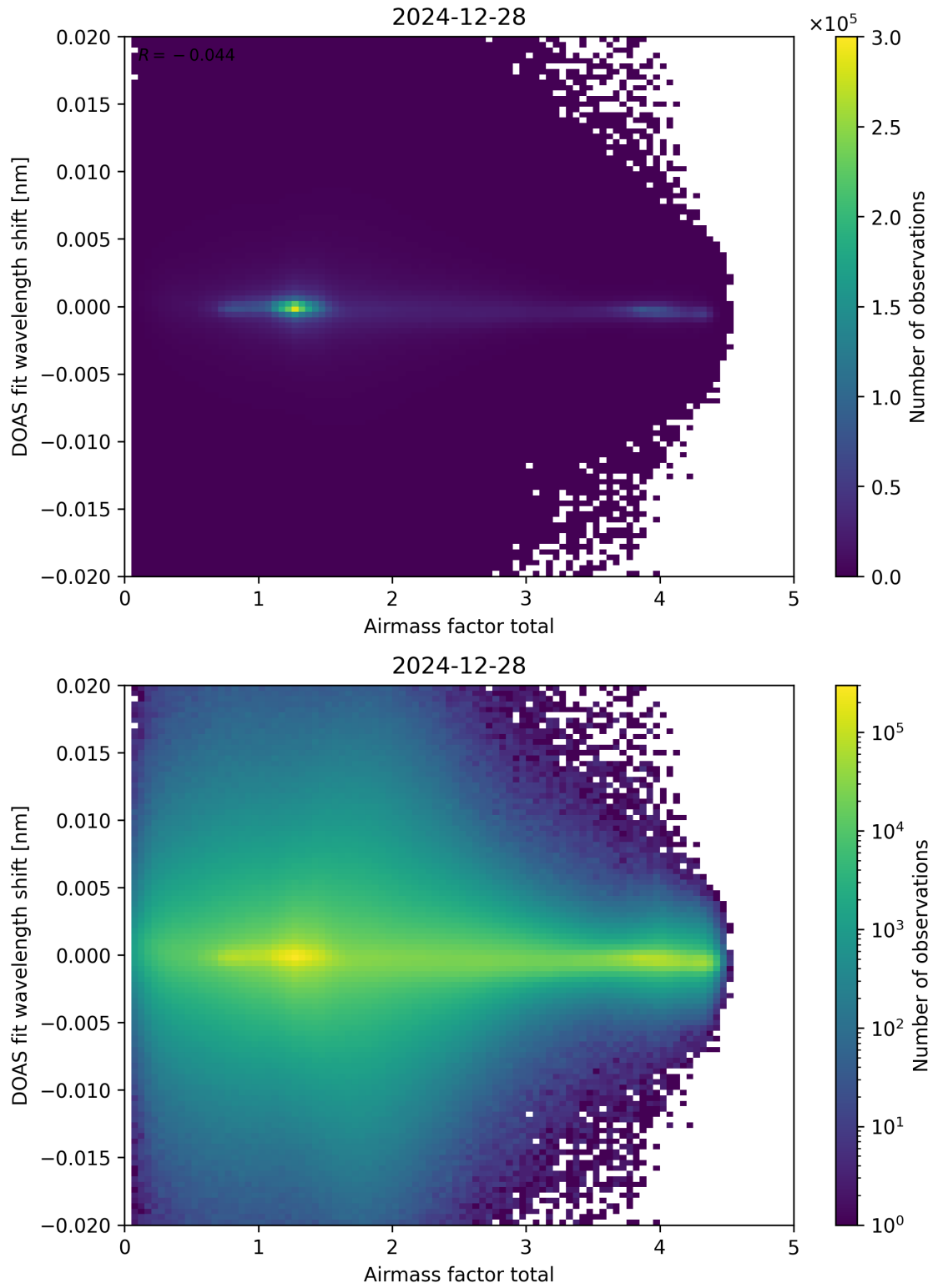
Figure 98: Scatter density plot of “Airmass factor total” against “DOAS fit wavelength shift” for 2024-12-27 to 2024-12-29.
