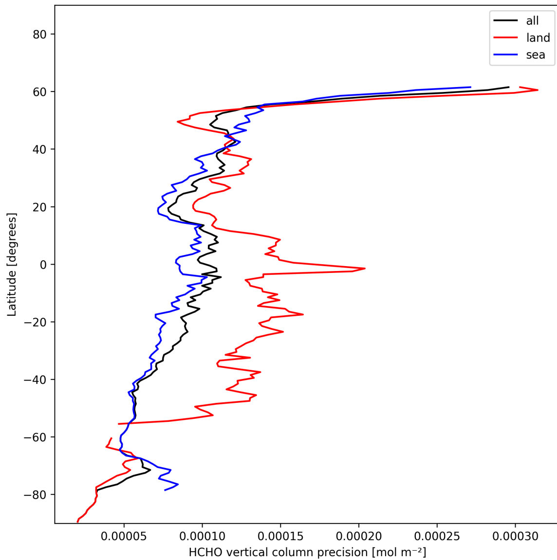
Figure 22: Zonal average of “HCHO vertical column precision” for 2024-12-27 to 2024-12-29.
