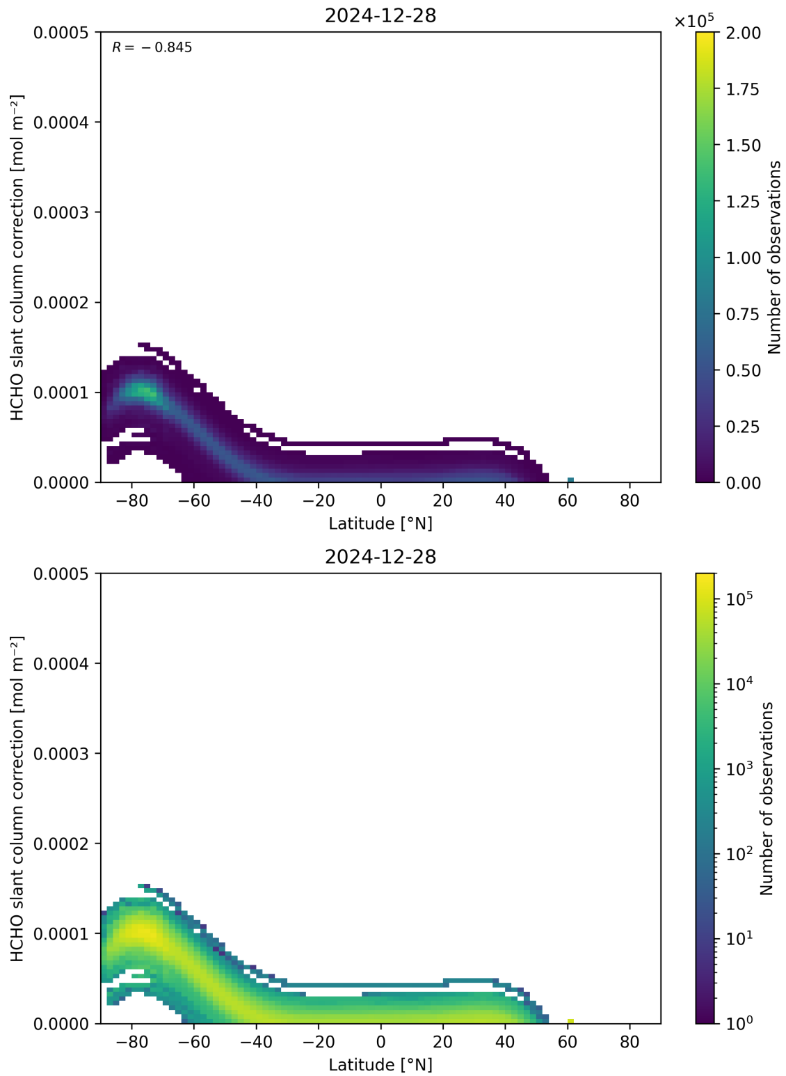
Figure 158: Scatter density plot of “Latitude” against “HCHO slant column correction” for 2024-12-27 to 2024-12-29.
