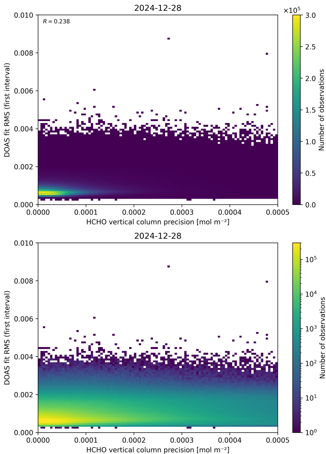
Figure 136: Scatter density plot of “HCHO vertical column precision” against “DOAS fit RMS (first interval)” for 2024-12-27 to 2024-12-29.
