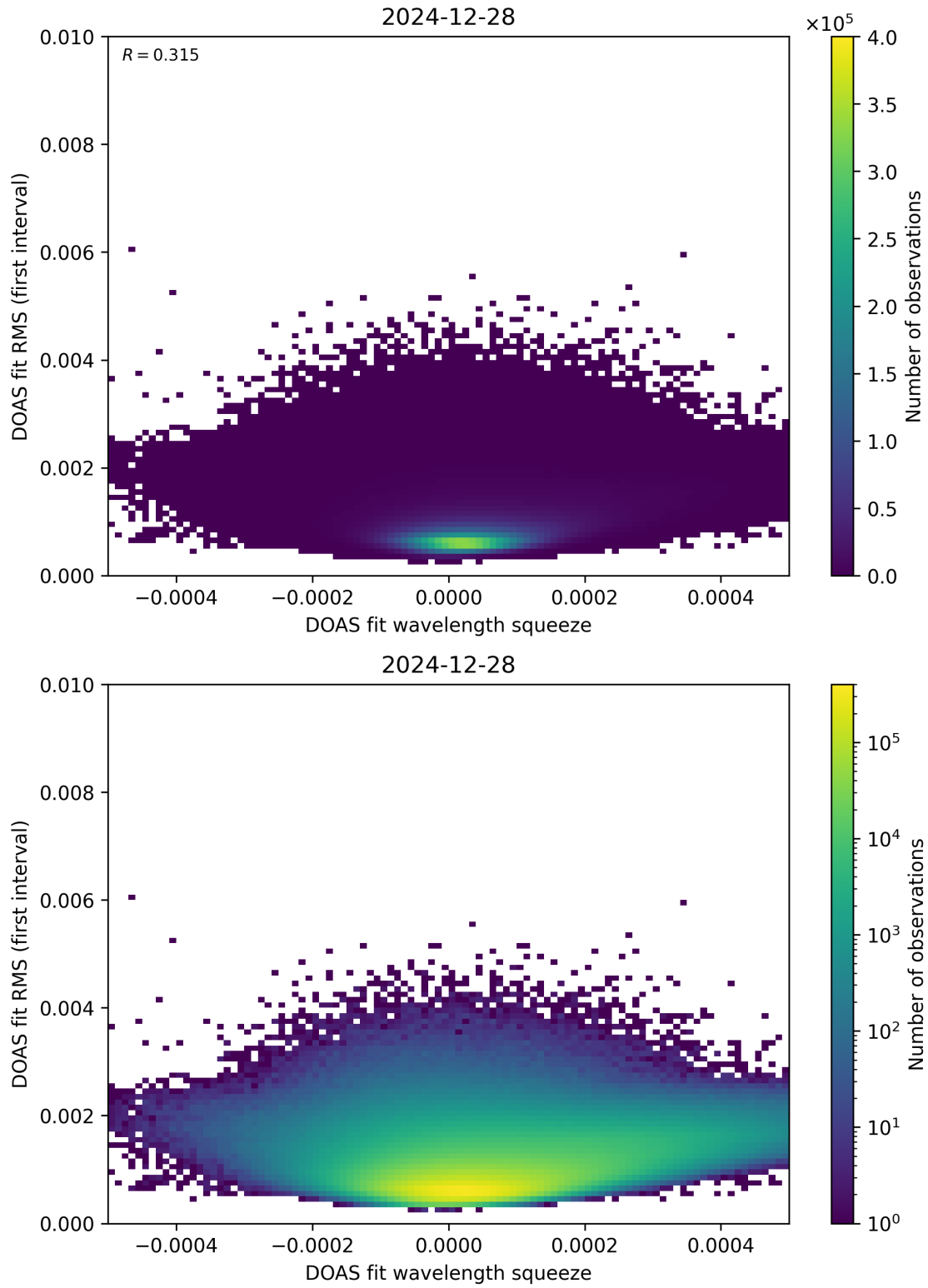
Figure 68: Scatter density plot of “DOAS fit wavelength squeeze” against “DOAS fit RMS (first interval)” for 2024-12-27 to 2024-12-29.
