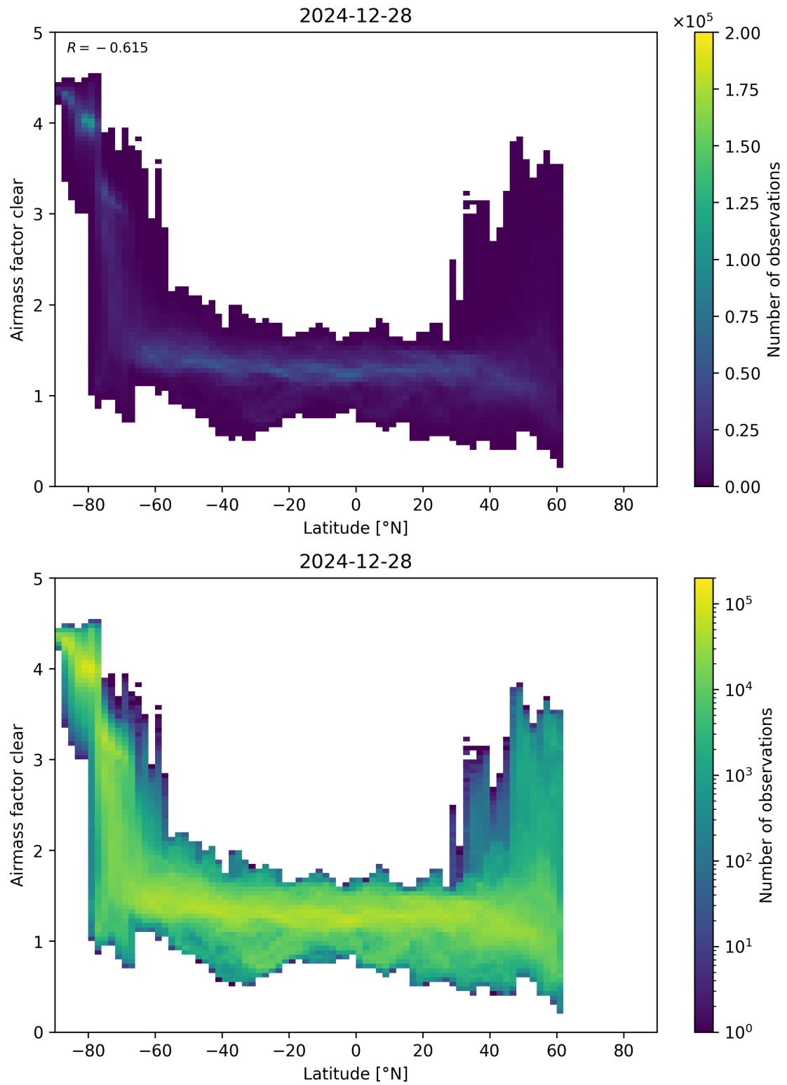
Figure 156: Scatter density plot of “Latitude” against “Airmass factor clear” for 2024-12-27 to 2024-12-29.
