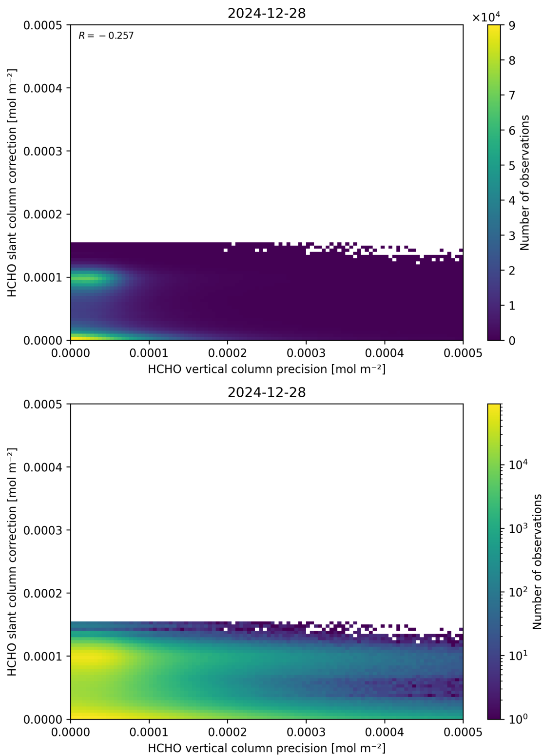
Figure 141: Scatter density plot of “HCHO vertical column precision” against “HCHO slant column correction” for 2024-12-27 to 2024-12-29.
