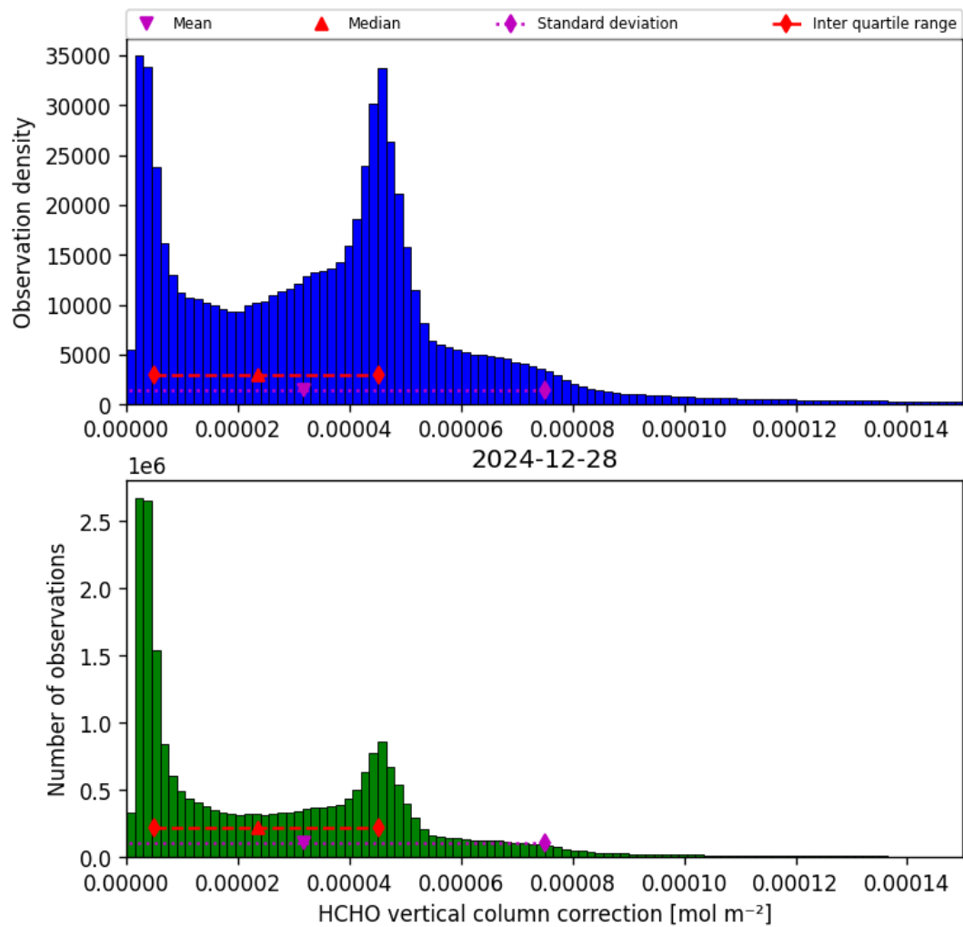
Figure 37: Histogram of “HCHO vertical column correction” for 2024-12-27 to 2024-12-29
