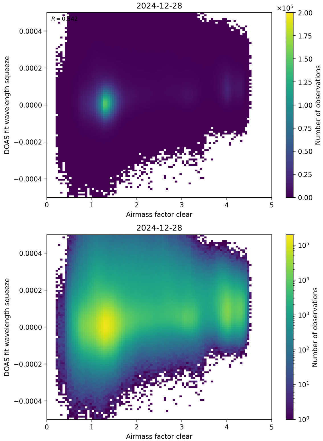
Figure 73: Scatter density plot of “Airmass factor clear” against “DOAS fit wavelength squeeze” for 2024-12-27 to 2024-12-29.
