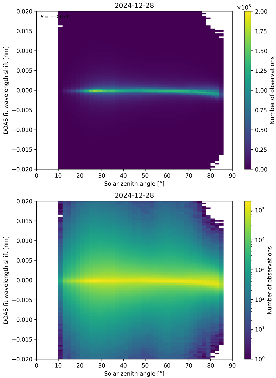
Figure 168: Scatter density plot of “Solar zenith angle” against “DOAS fit wavelength shift” for 2024-12-27 to 2024-12-29.
