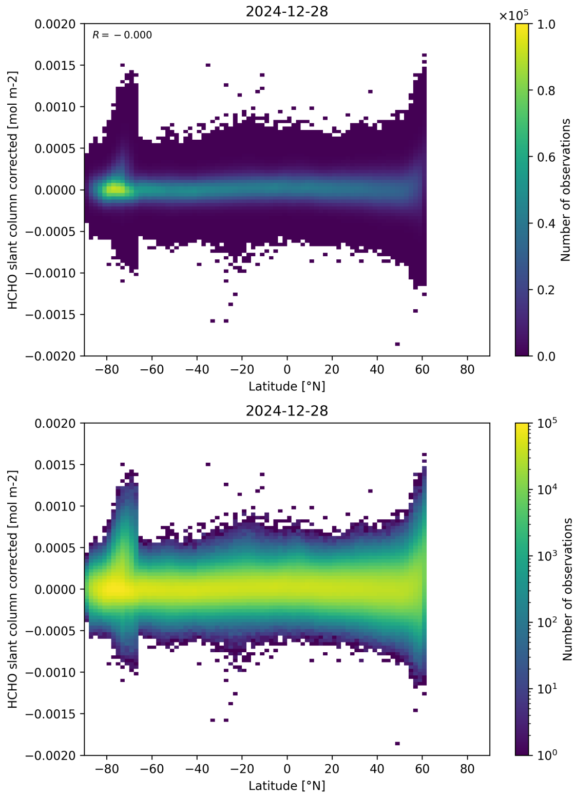
Figure 157: Scatter density plot of “Latitude” against “HCHO slant column corrected” for 2024-12-27 to 2024-12-29.
