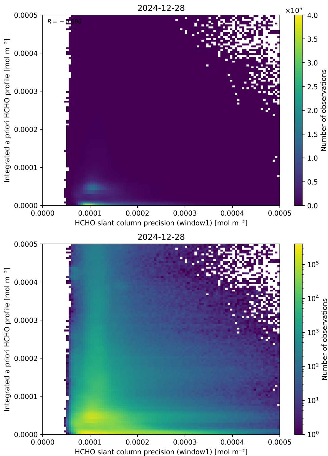
Figure 96: Scatter density plot of “HCHO slant column precision (window1)” against “Integrated a priori HCHO profile” for 2024-12-27 to 2024-12-29.
