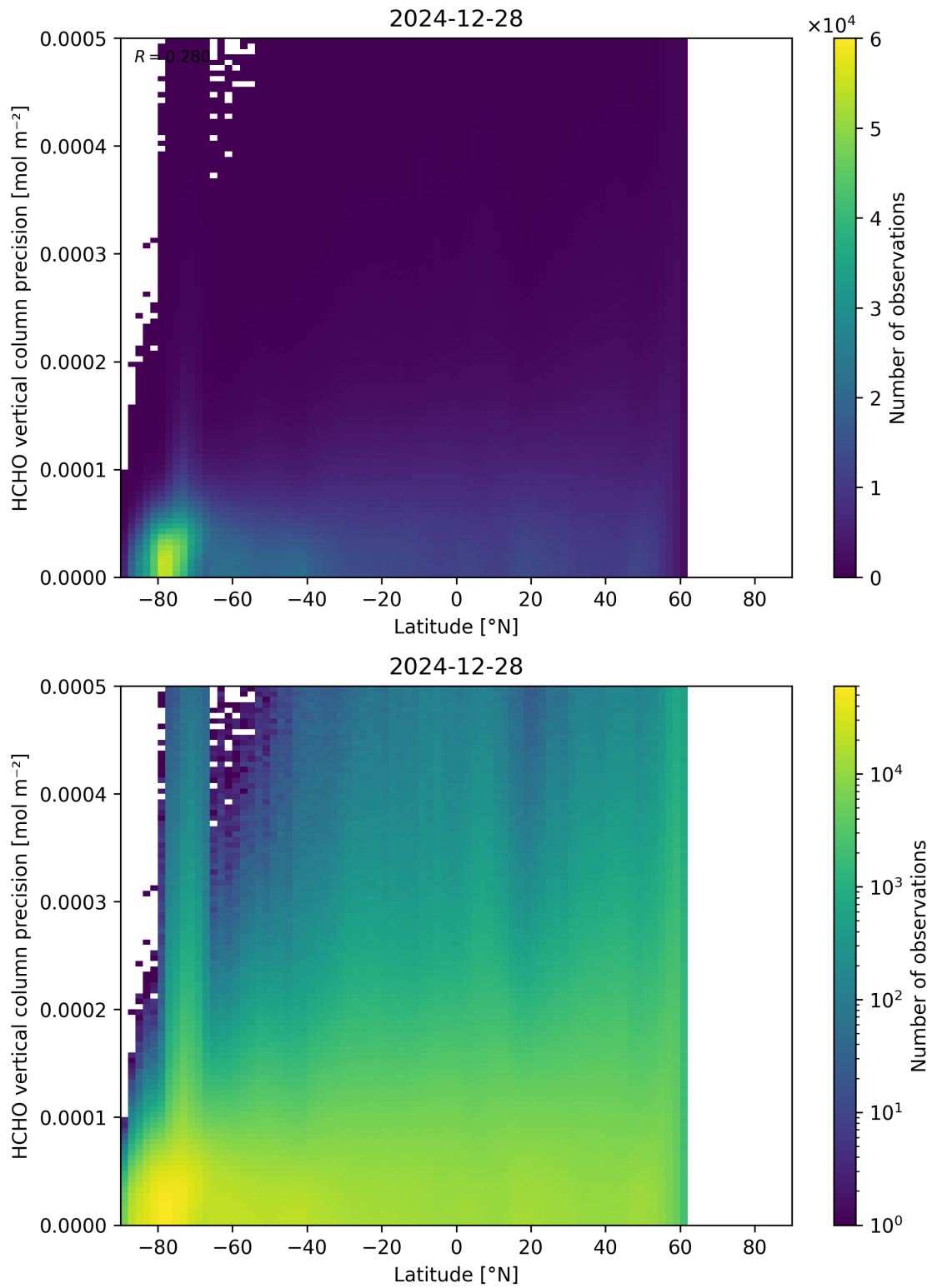
Figure 165: Scatter density plot of “Latitude” against “HCHO vertical column precision” for 2024-12-27 to 2024-12-29.
