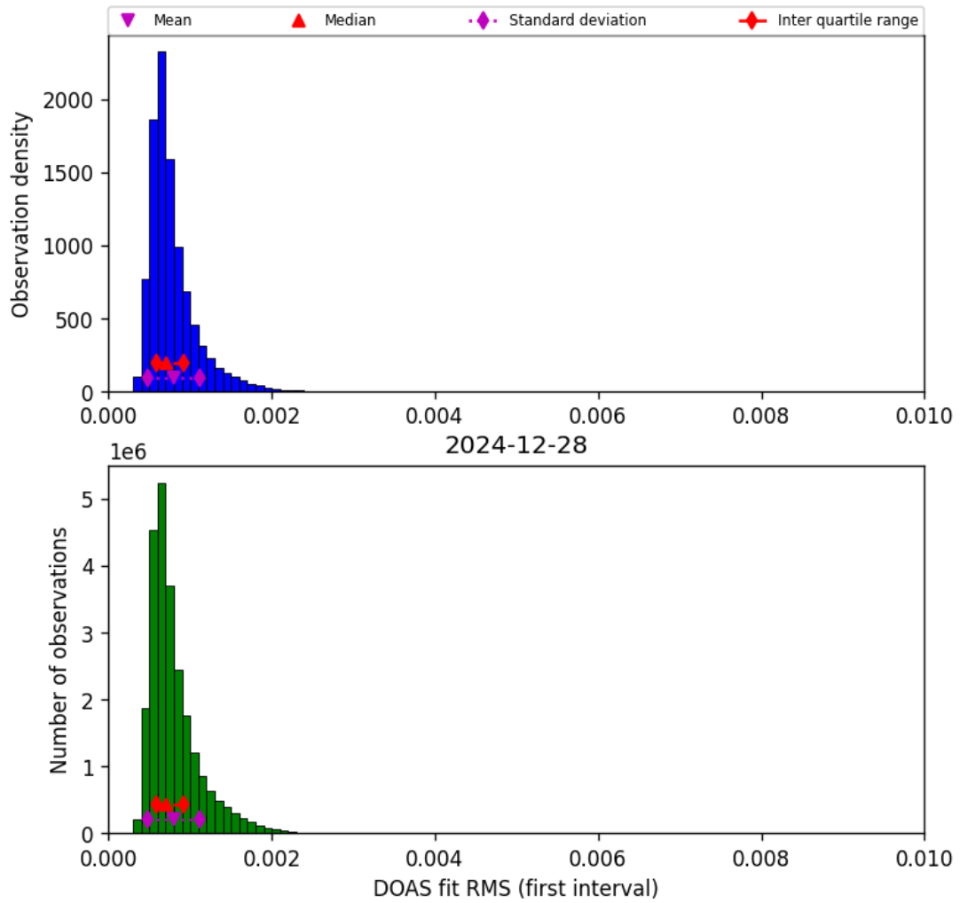
Figure 46: Histogram of “DOAS fit RMS (first interval)” for 2024-12-27 to 2024-12-29
