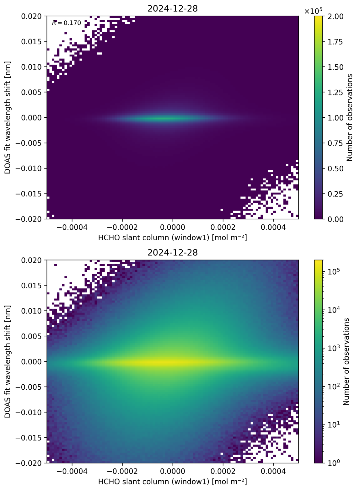
Figure 79: Scatter density plot of “HCHO slant column (window1)” against “DOAS fit wavelength shift” for 2024-12-27 to 2024-12-29.
