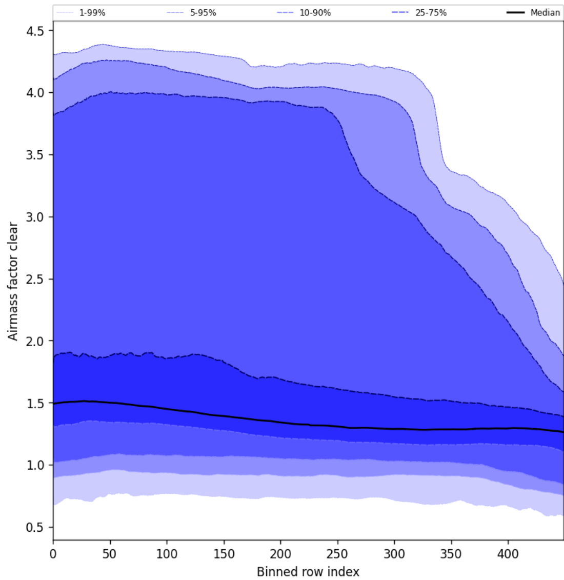
Figure 56: Along track statistics of “Air mass factor clear” for 2024-12-27 to 2024-12-29
