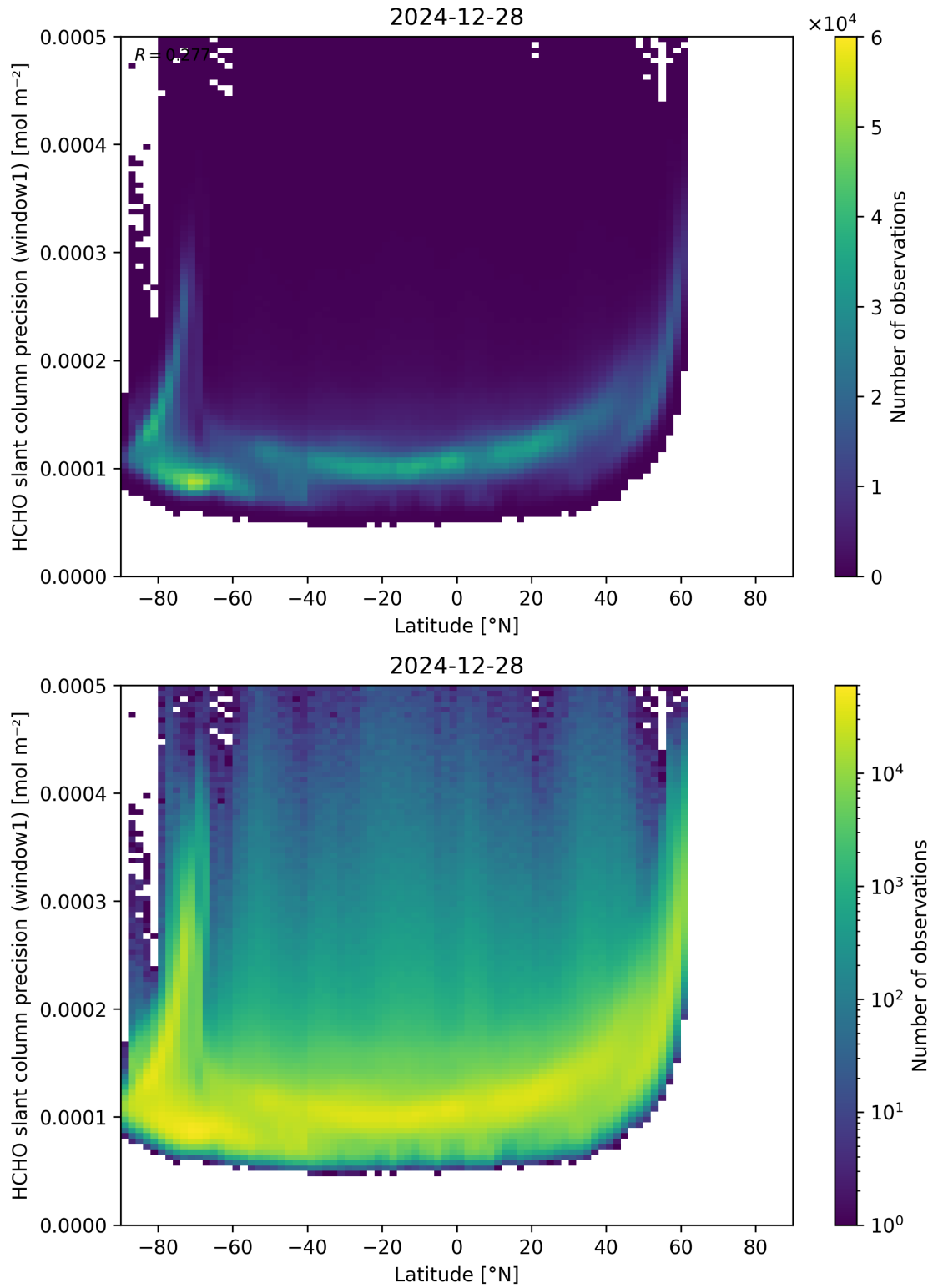
Figure 160: Scatter density plot of “Latitude” against “HCHO slant column precision (window1)” for 2024-12-27 to 2024-12-29.
