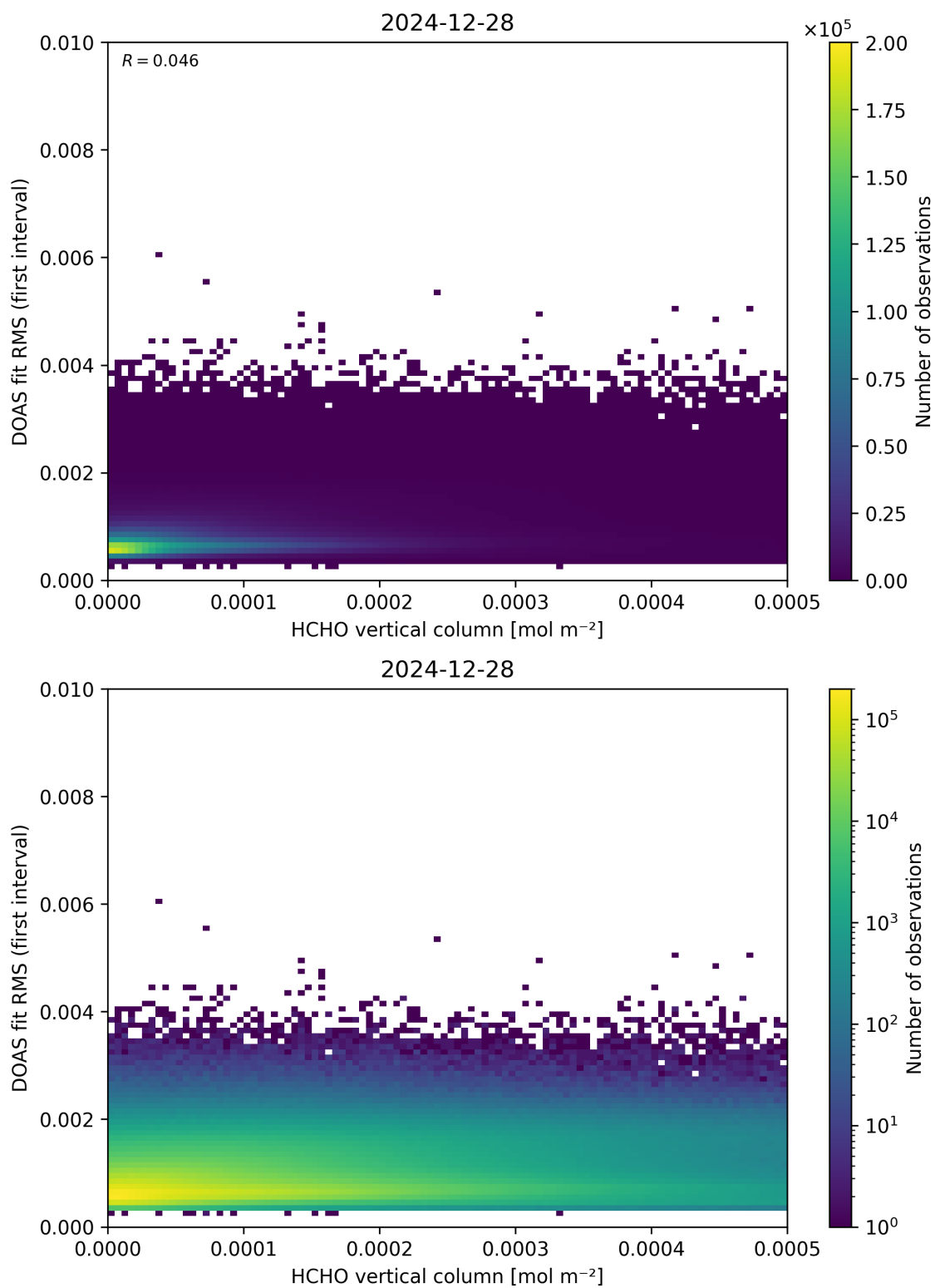
Figure 123: Scatter density plot of “HCHO vertical column” against “DOAS fit RMS (first interval)” for 2024-12-27 to 2024-12-29.
