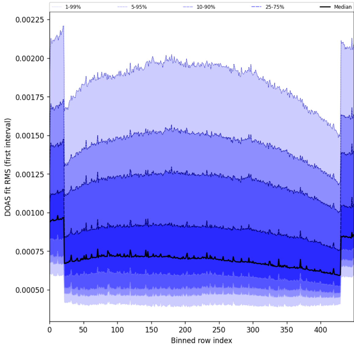
Figure 60: Along track statistics of “DOAS fit RMS (first interval)” for 2024-12-27 to 2024-12-29
