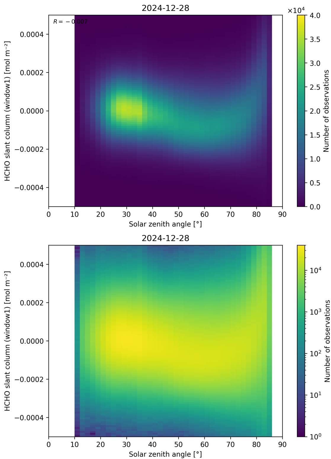
Figure 173: Scatter density plot of “Solar zenith angle” against “HCHO slant column (window1)” for 2024-12-27 to 2024-12-29.
