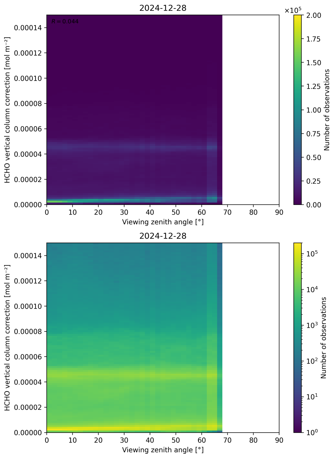
Figure 193: Scatter density plot of “Viewing zenith angle” against “HCHO vertical column correction” for 2024-12-27 to 2024-12-29.
