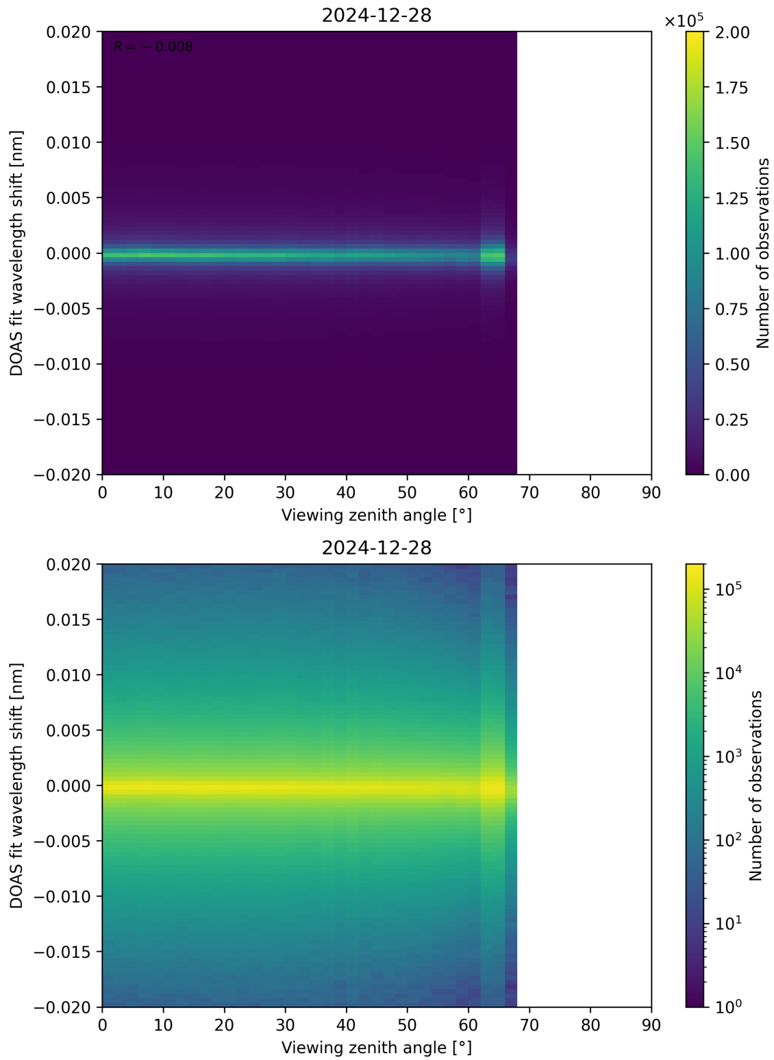
Figure 183: Scatter density plot of “Viewing zenith angle” against “DOAS fit wavelength shift” for 2024-12-27 to 2024-12-29.
