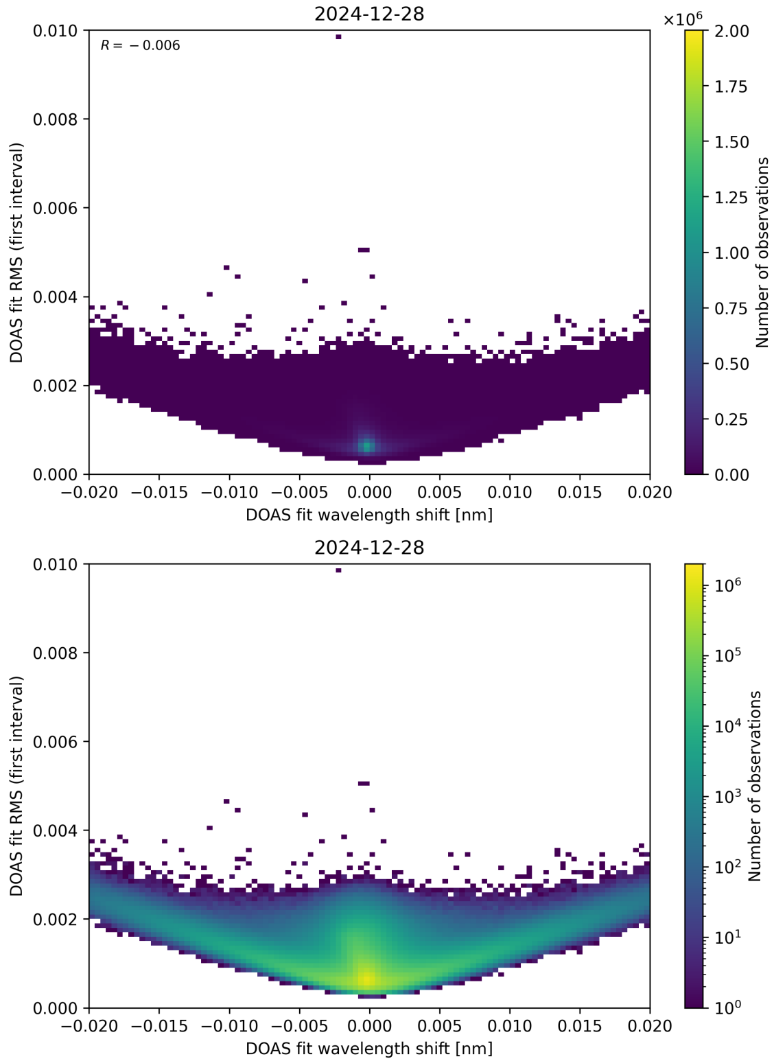
Figure 64: Scatter density plot of “DOAS fit wavelength shift” against “DOAS fit RMS (first interval)” for 2024-12-27 to 2024-12-29.
