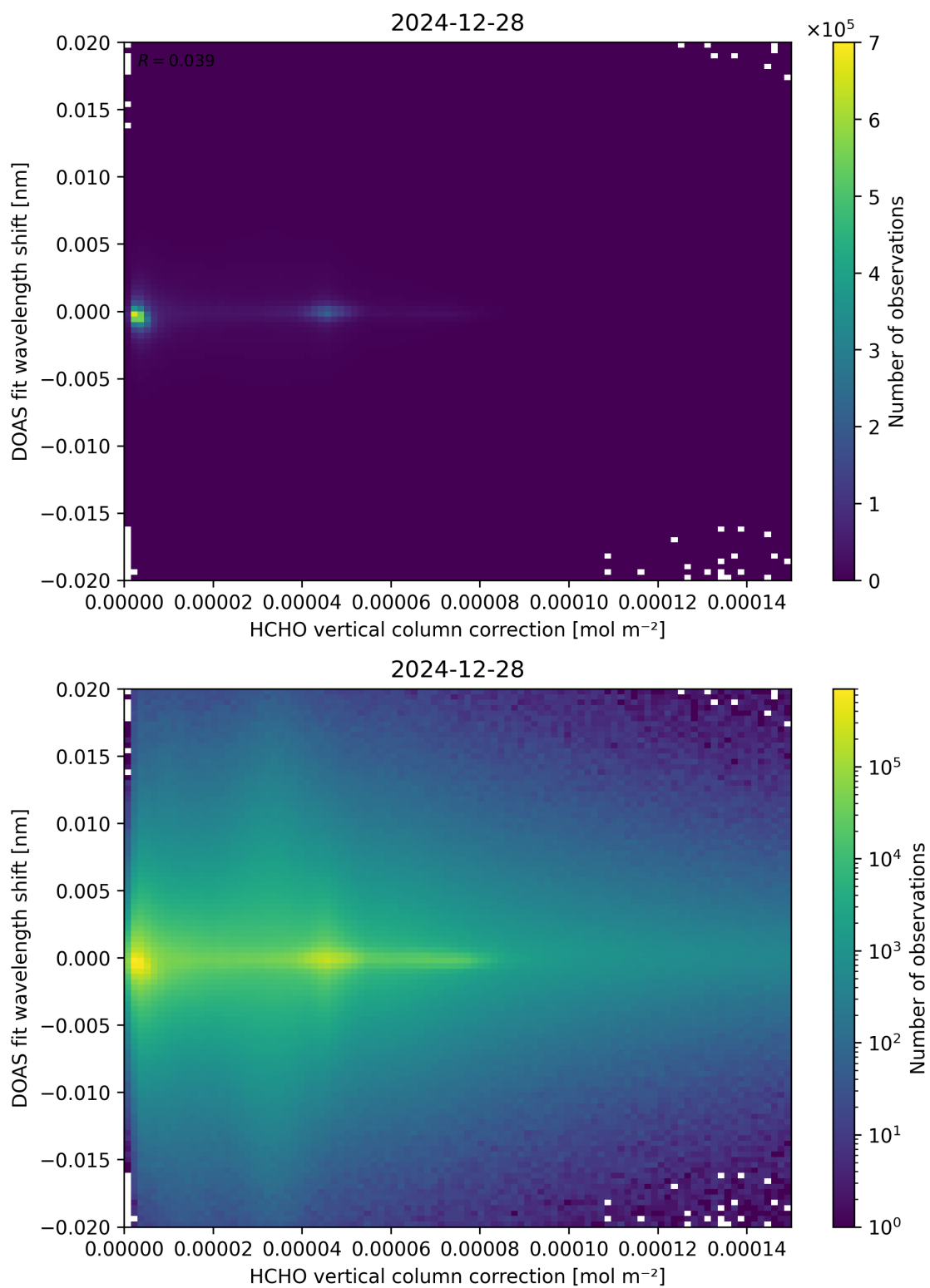
Figure 113: Scatter density plot of “HCHO vertical column correction” against “DOAS fit wavelength shift” for 2024-12-27 to 2024-12-29.
