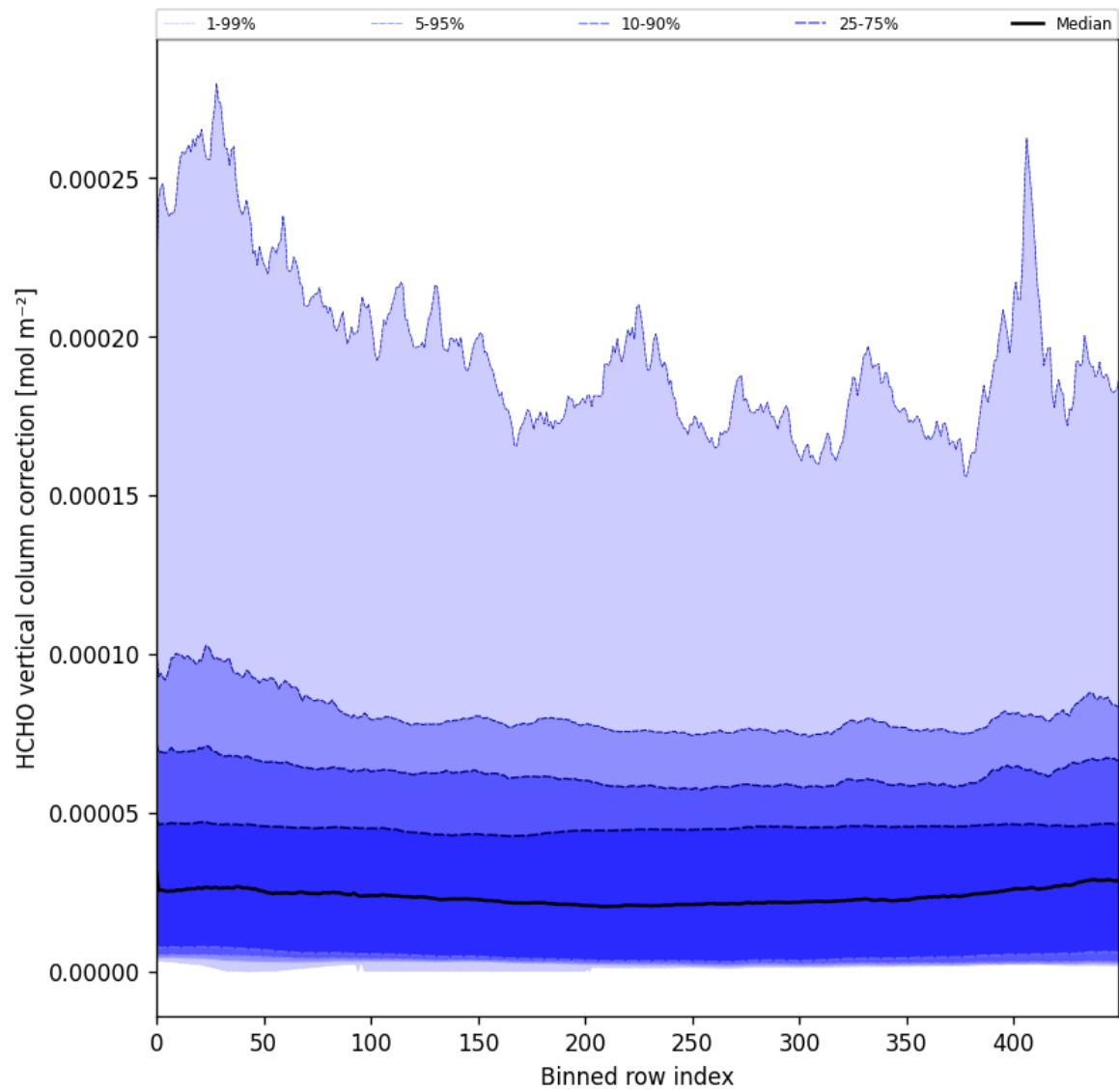
Figure 51: Along track statistics of “HCHO vertical column correction” for 2024-12-27 to 2024-12-29
