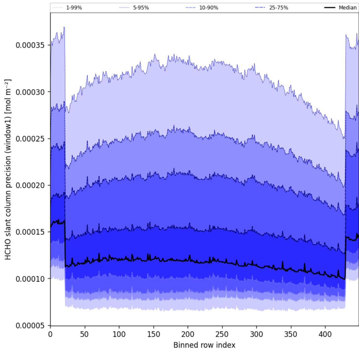
Figure 53: Along track statistics of “HCHO slant column precision (window1)” for 2024-12-27 to 2024-12-29
