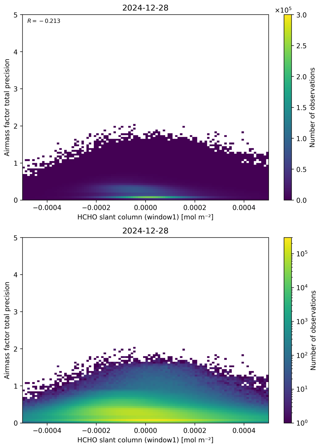
Figure 86: Scatter density plot of “HCHO slant column (window1)” against “Airmass factor total precision” for 2024-12-27 to 2024-12-29.
