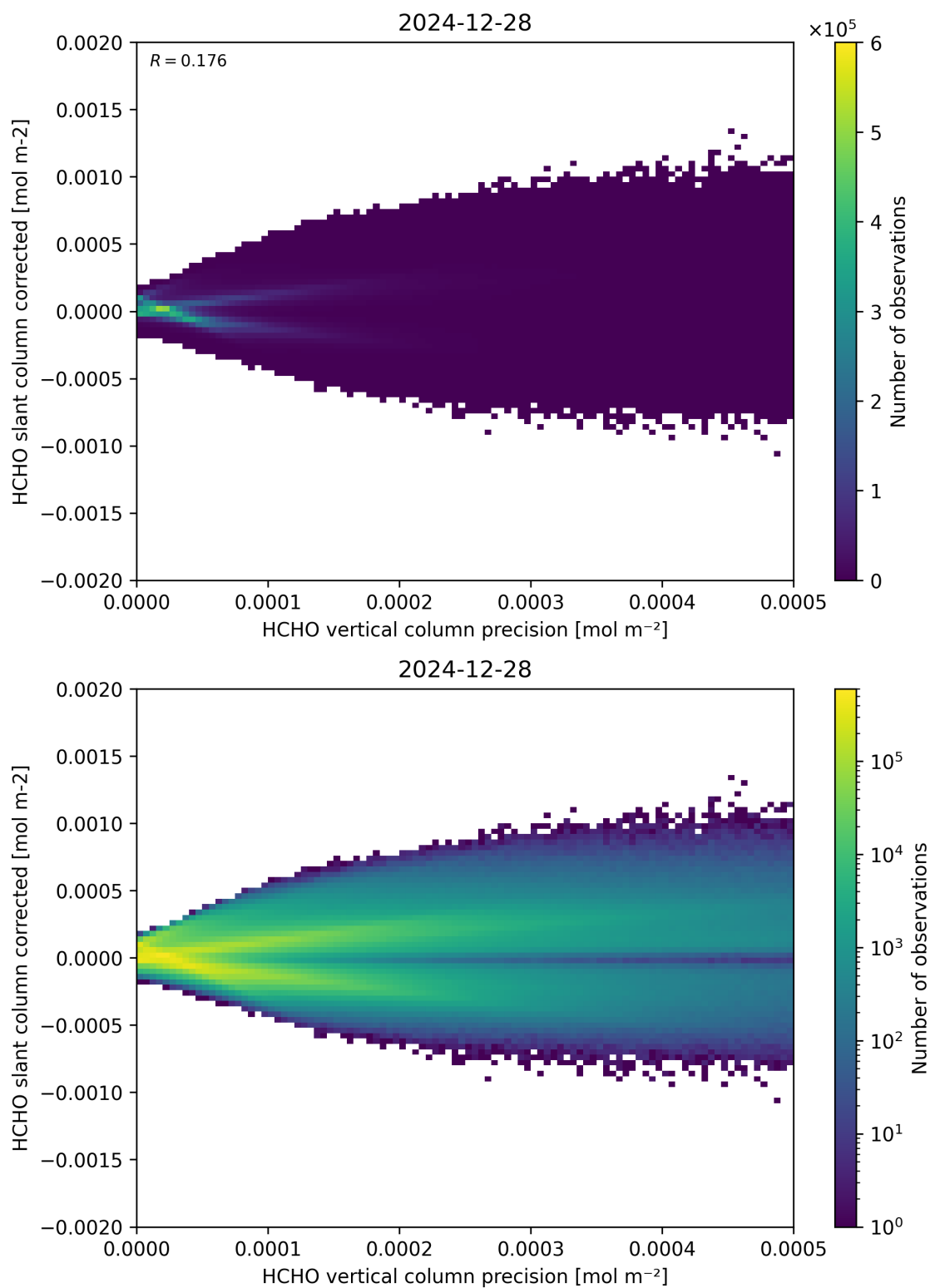
Figure 140: Scatter density plot of “HCHO vertical column precision” against “HCHO slant column corrected” for 2024-12-27 to 2024-12-29.
