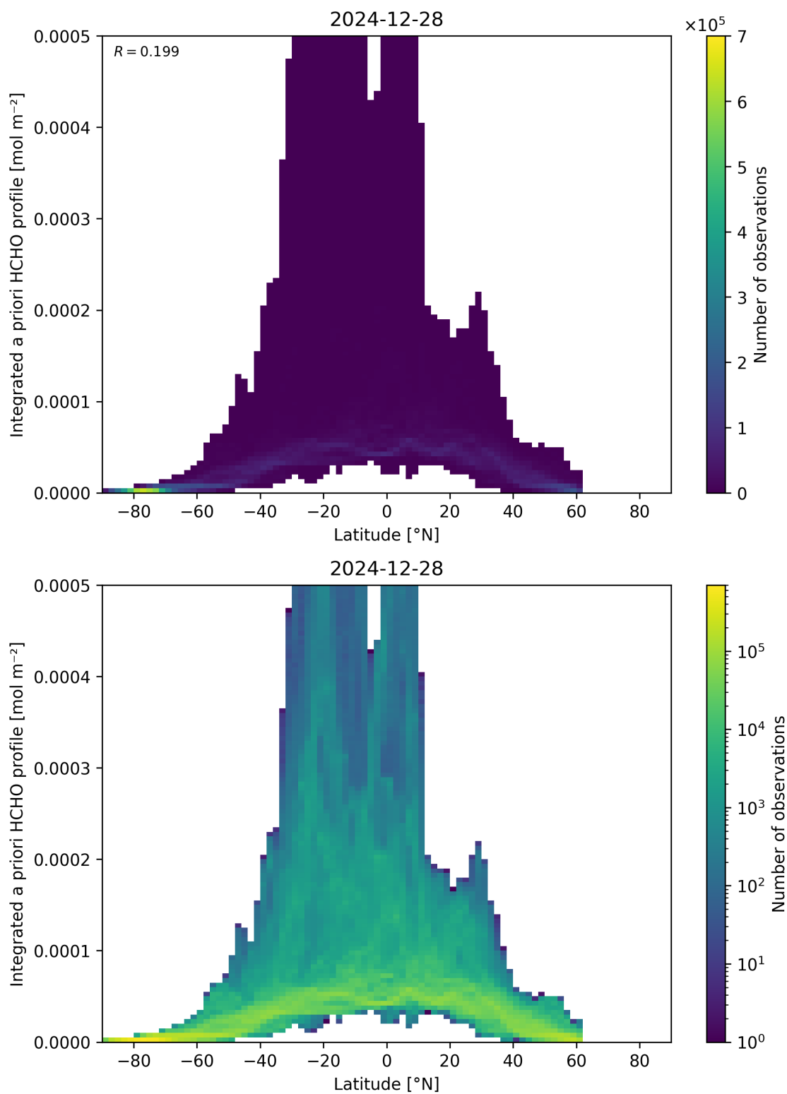
Figure 166: Scatter density plot of “Latitude” against “Integrated a priori HCHO profile” for 2024-12-27 to 2024-12-29.
