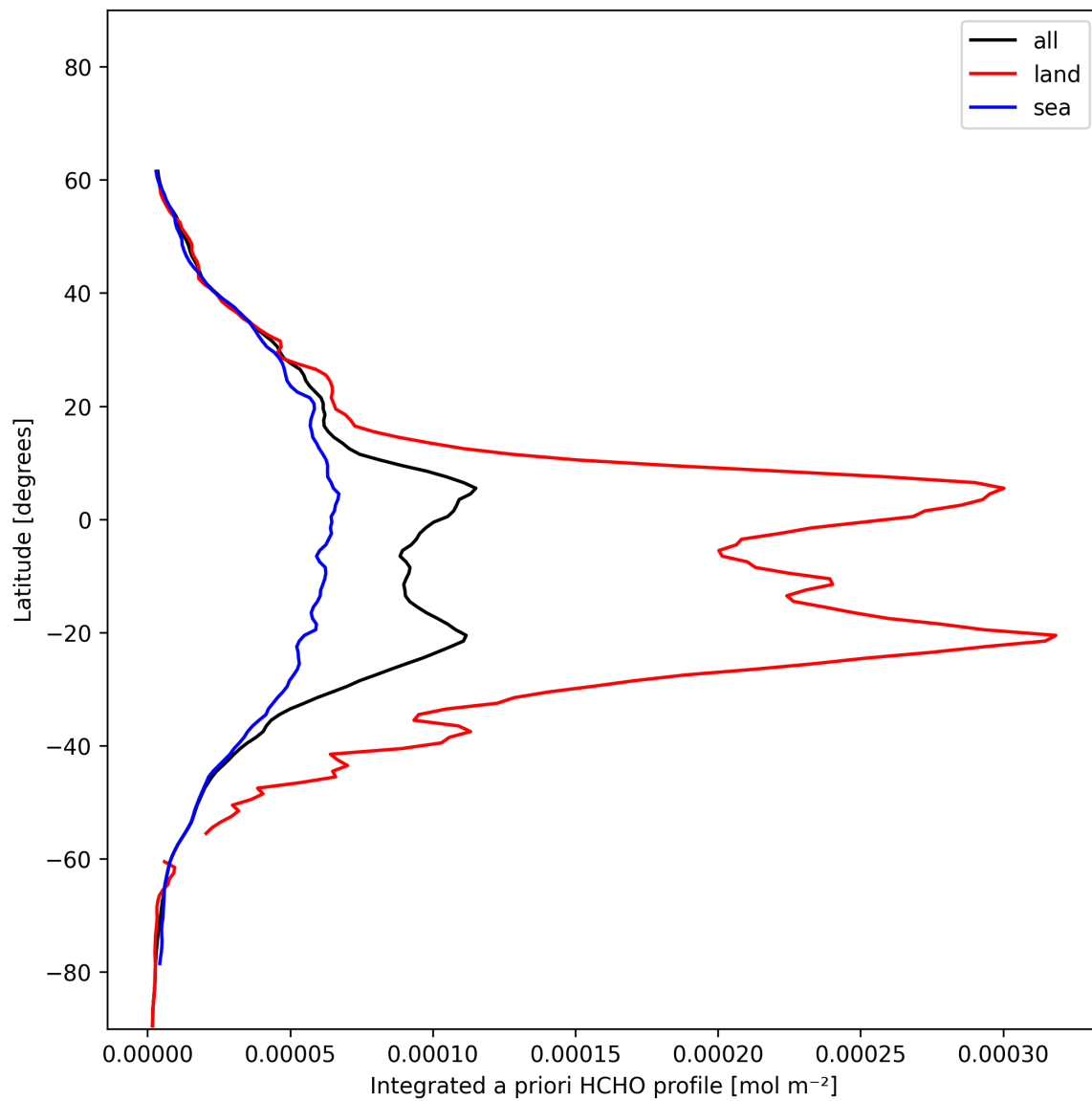
Figure 29: Zonal average of “Integrated a priori HCHO profile” for 2024-12-27 to 2024-12-29.
