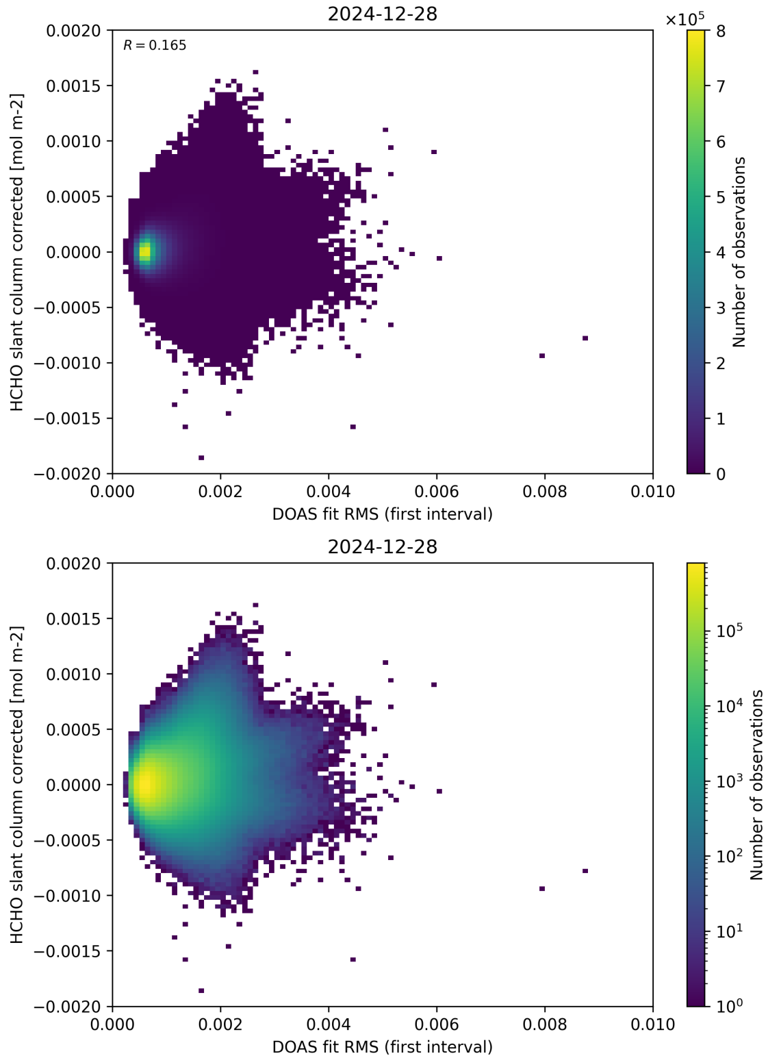
Figure 62: Scatter density plot of “DOAS fit RMS (first interval)” against “HCHO slant column corrected” for 2024-12-27 to 2024-12-29.
