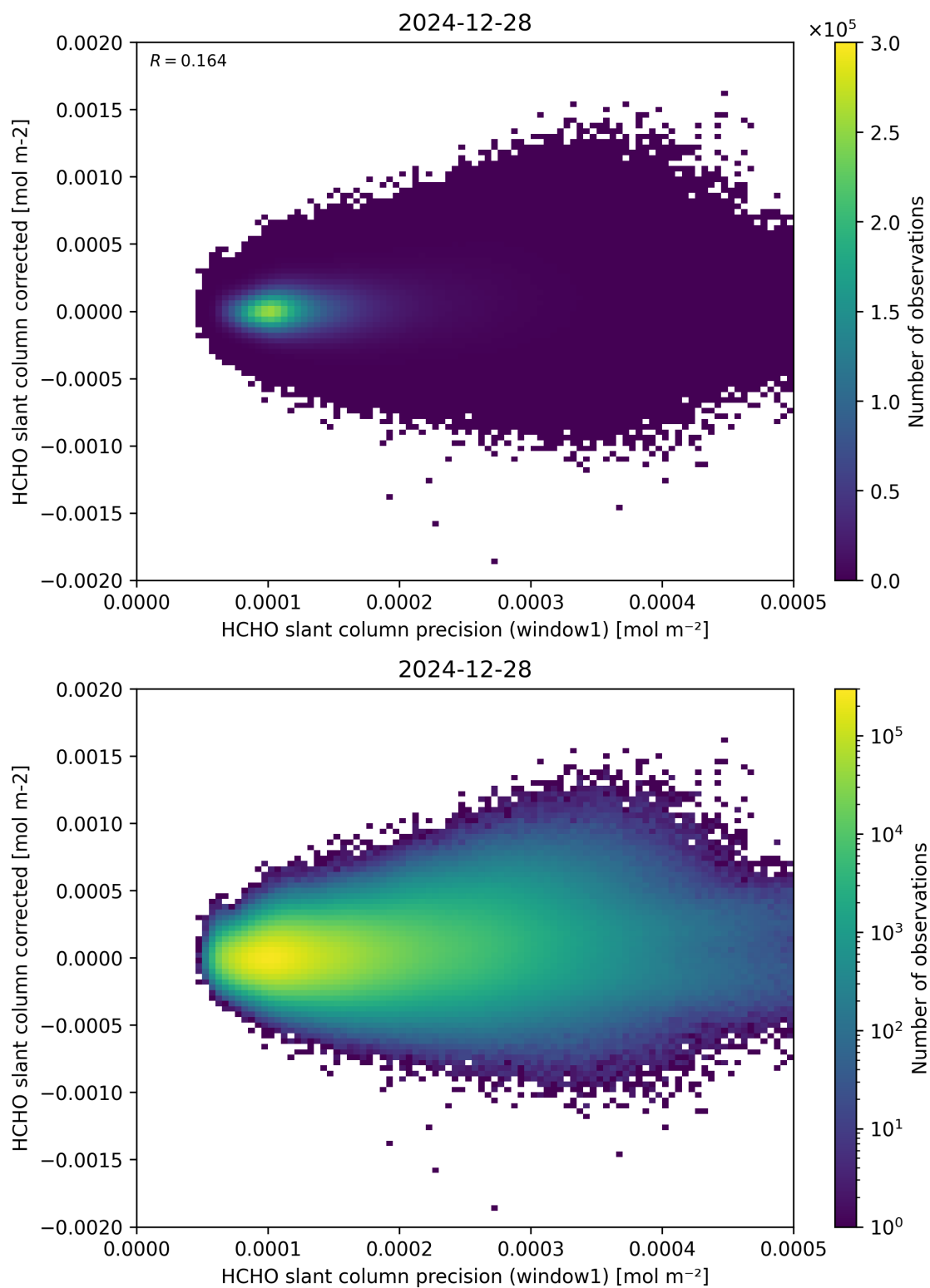
Figure 92: Scatter density plot of “HCHO slant column precision (window1)” against “HCHO slant column corrected” for 2024-12-27 to 2024-12-29.
