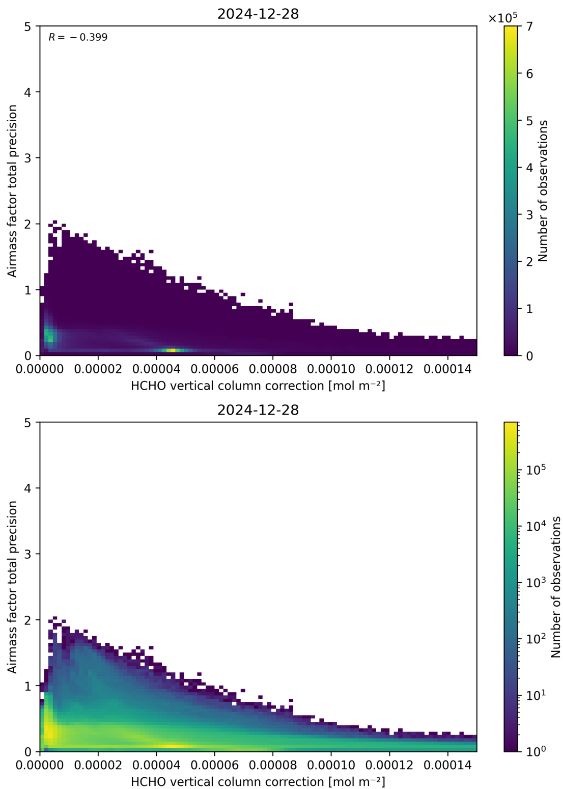
Figure 121: Scatter density plot of “HCHO vertical column correction” against “Airmass factor total precision” for 2024-12-27 to 2024-12-29.
