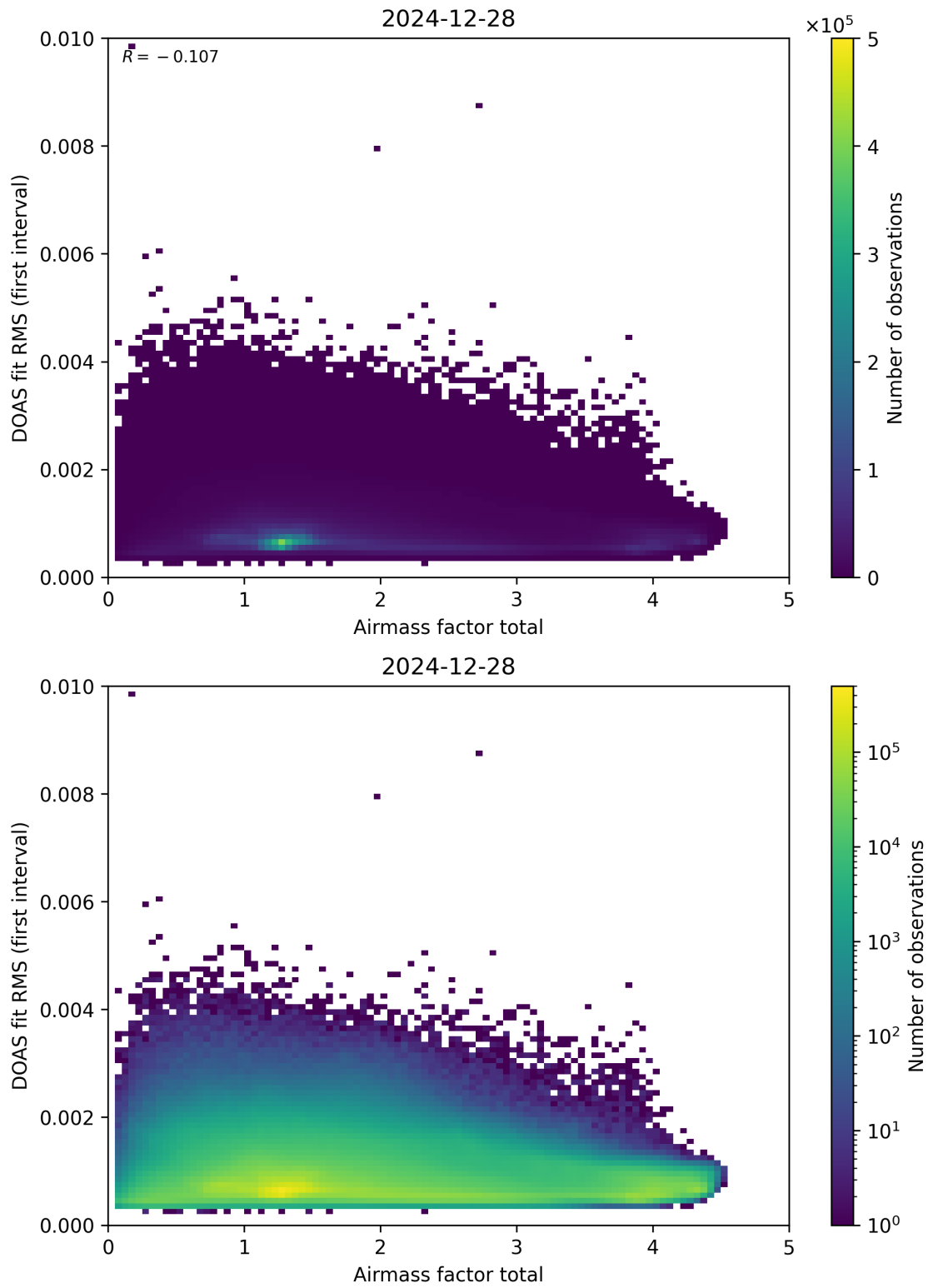
Figure 97: Scatter density plot of “Airmass factor total” against “DOAS fit RMS (first interval)” for 2024-12-27 to 2024-12-29.
