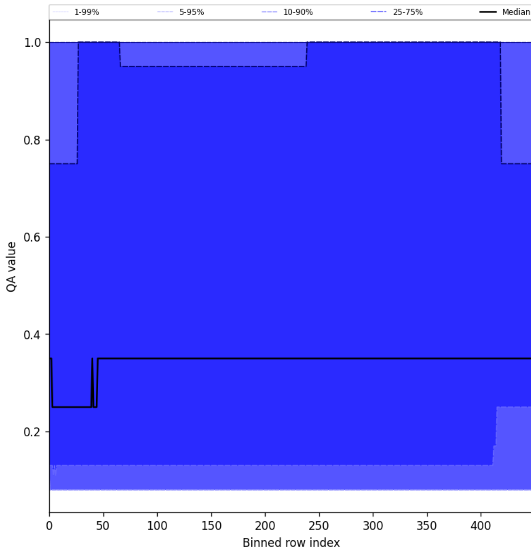
Figure 48: Along track statistics of “QA value” for 2024-12-27 to 2024-12-29
