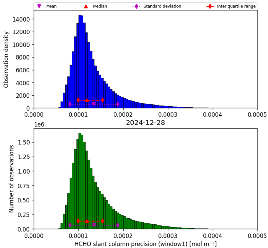
Figure 39: Histogram of “HCHO slant column precision (window1)” for 2024-12-27 to 2024-12-29
