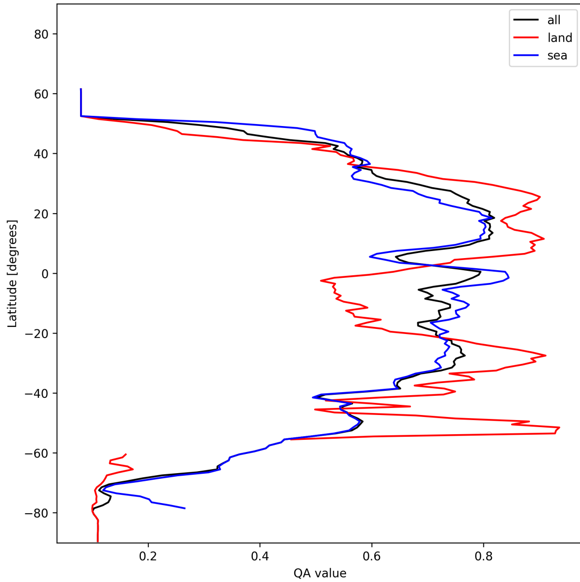
Figure 20: Zonal average of “QA value” for 2024-12-27 to 2024-12-29.
