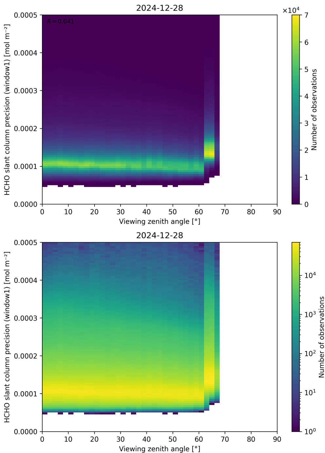
Figure 189: Scatter density plot of “Viewing zenith angle” against “HCHO slant column precision (window1)” for 2024-12-27 to 2024-12-29.
