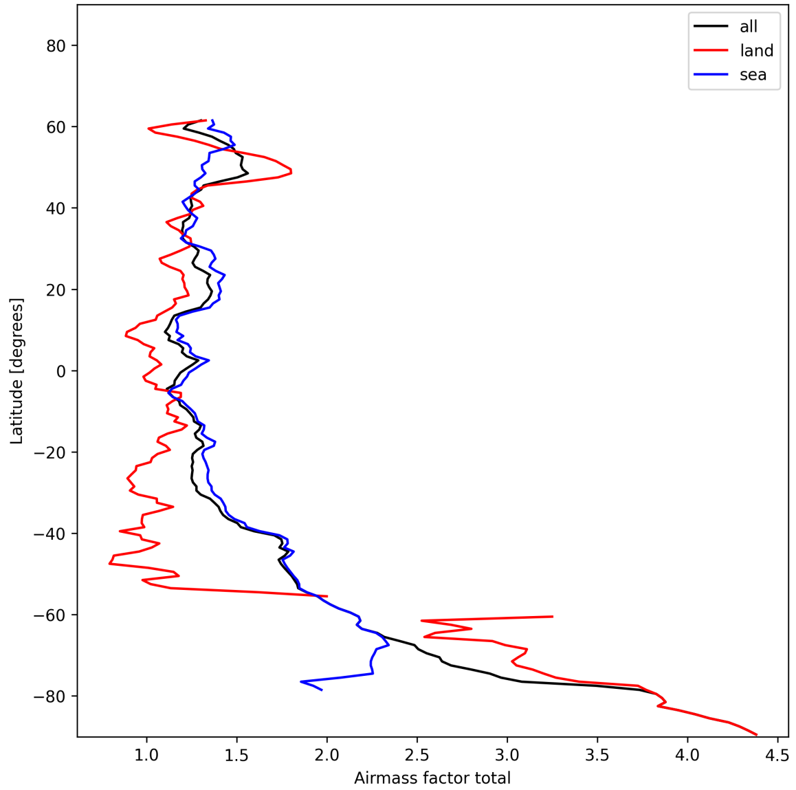
Figure 26: Zonal average of “Airmass factor total” for 2024-12-27 to 2024-12-29.
