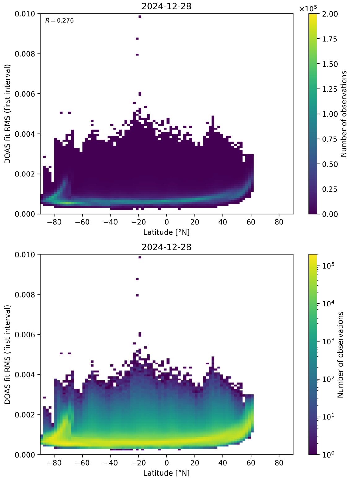
Figure 153: Scatter density plot of “Latitude” against “DOAS fit RMS (first interval)” for 2024-12-27 to 2024-12-29.
