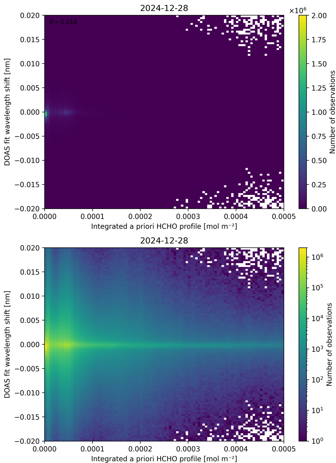
Figure 149: Scatter density plot of “Integrated a priori HCHO profile” against “DOAS fit wavelength shift” for 2024-12-27 to 2024-12-29.
