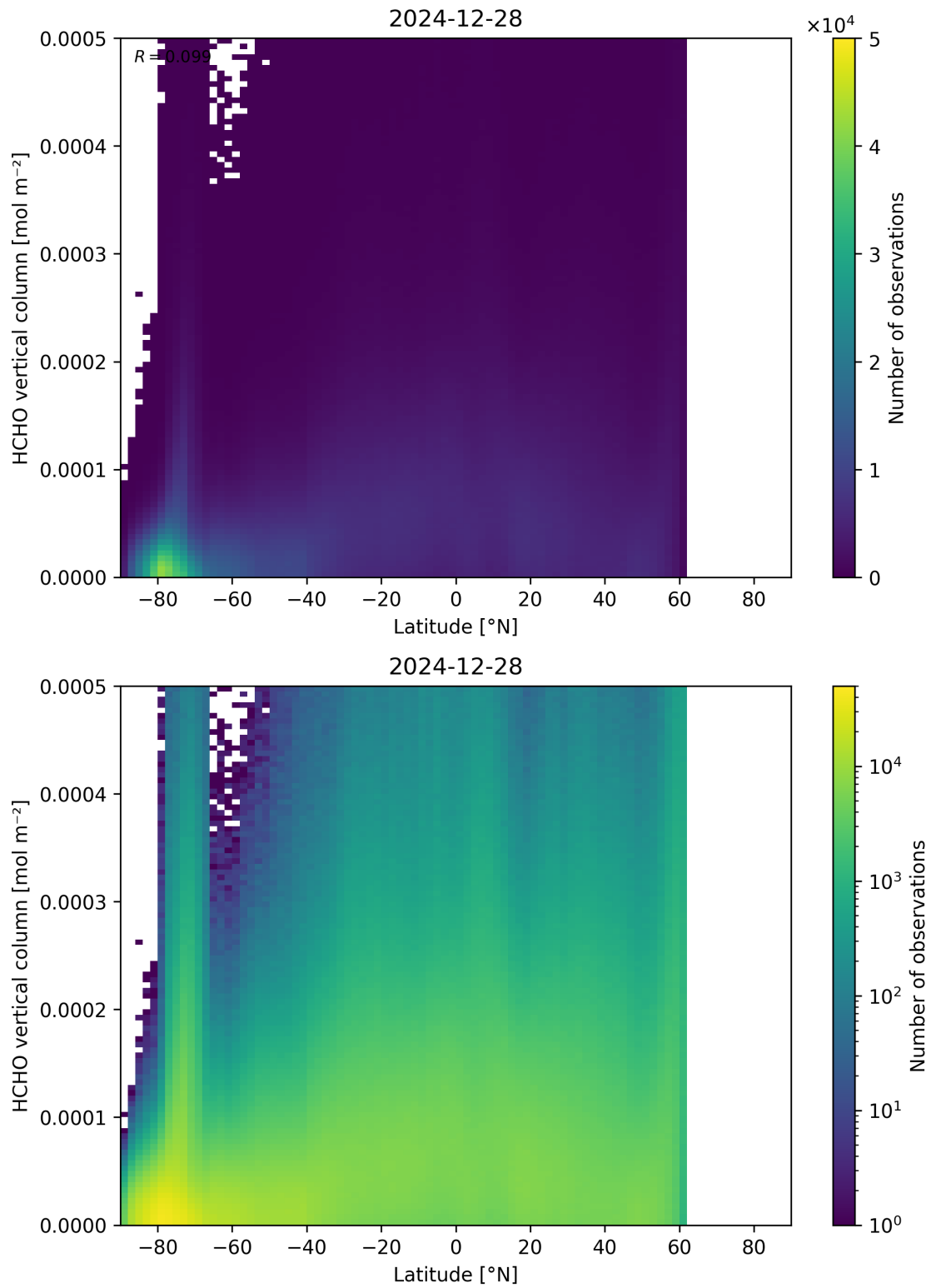
Figure 163: Scatter density plot of “Latitude” against “HCHO vertical column” for 2024-12-27 to 2024-12-29.
