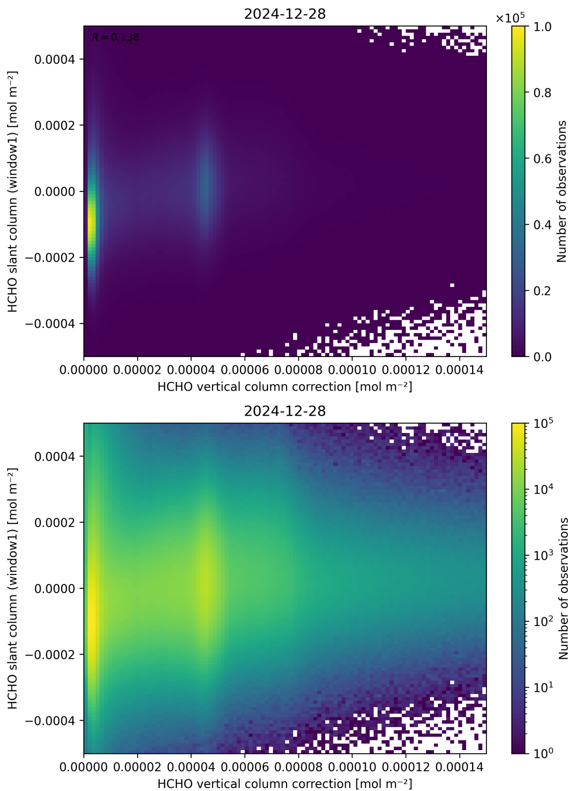
Figure 118: Scatter density plot of “HCHO vertical column correction” against “HCHO slant column (window1)” for 2024-12-27 to 2024-12-29.
