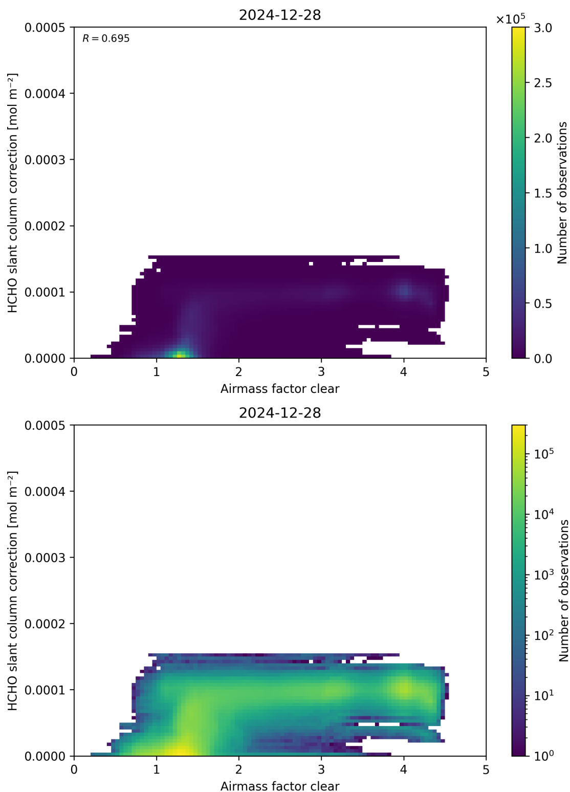
Figure 75: Scatter density plot of “Airmass factor clear” against “HCHO slant column correction” for 2024-12-27 to 2024-12-29.
