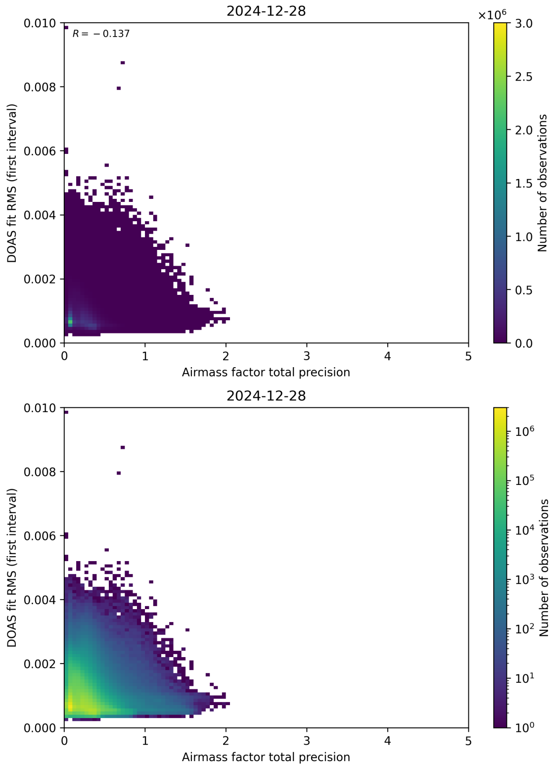
Figure 105: Scatter density plot of “Airmass factor total precision” against “DOAS fit RMS (first interval)” for 2024-12-27 to 2024-12-29.
