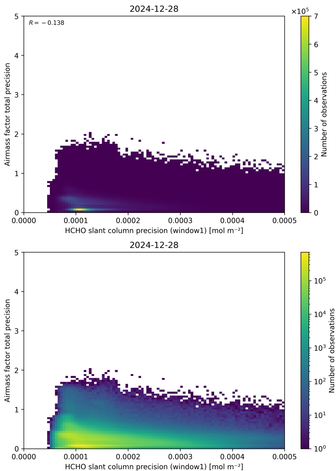
Figure 95: Scatter density plot of “HCHO slant column precision (window1)” against “Airmass factor total precision” for 2024-12-27 to 2024-12-29.
