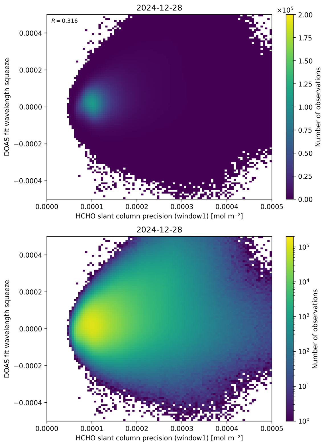
Figure 90: Scatter density plot of “HCHO slant column precision (window1)” against “DOAS fit wavelength squeeze” for 2024-12-27 to 2024-12-29.
