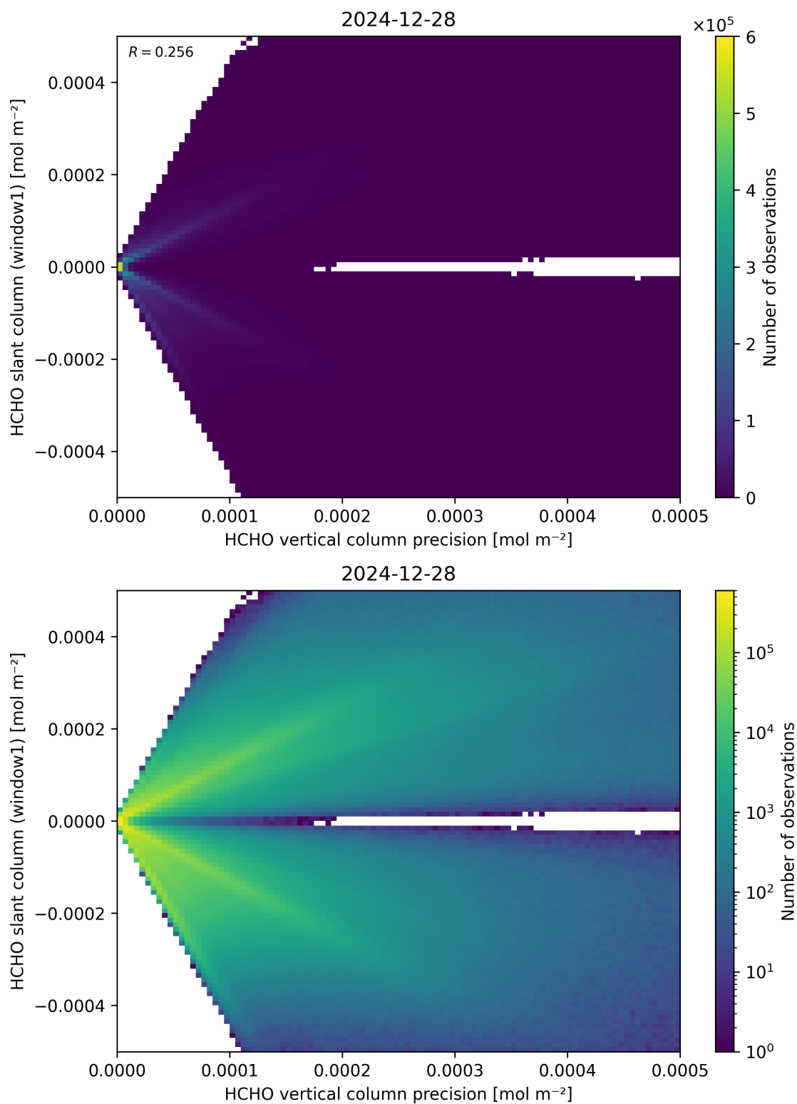
Figure 142: Scatter density plot of “HCHO vertical column precision” against “HCHO slant column (window1)” for 2024-12-27 to 2024-12-29.
