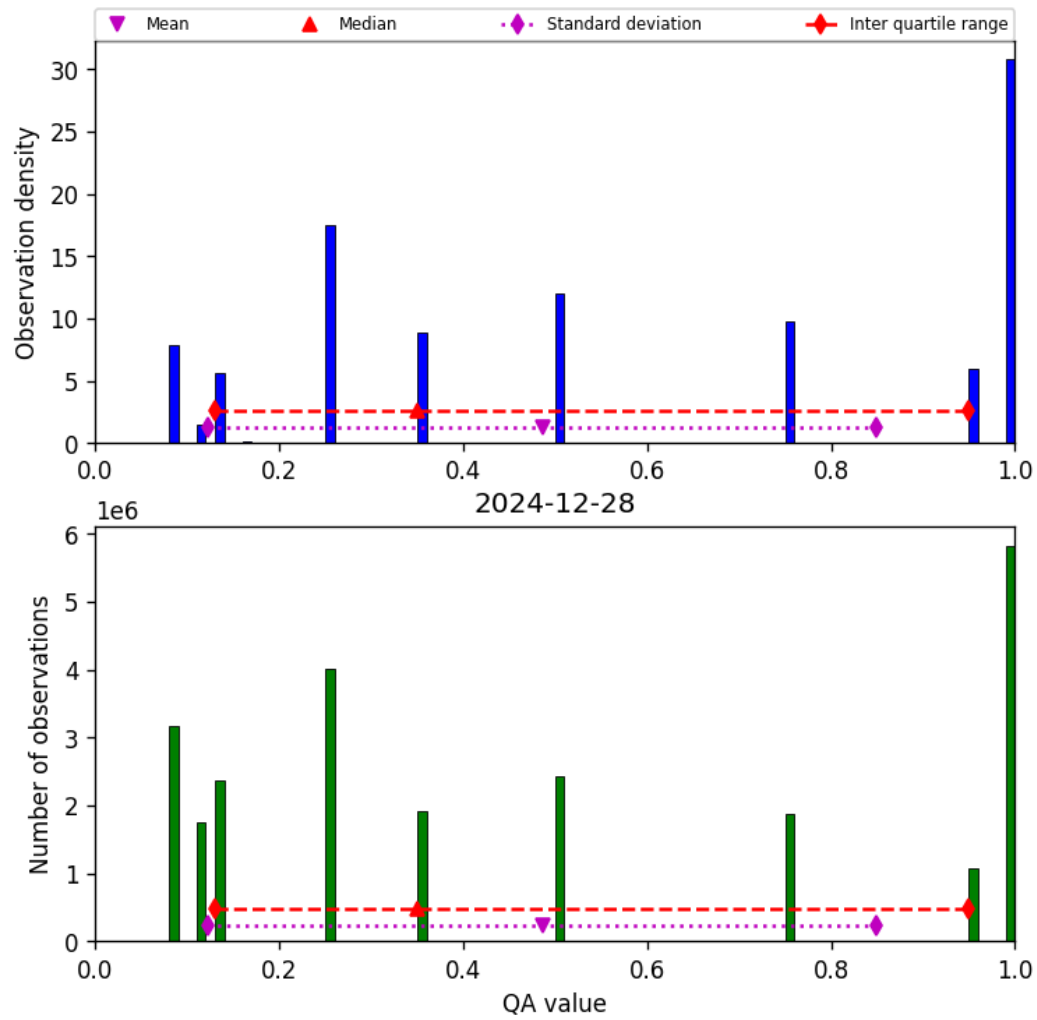
Figure 34: Histogram of “QA value” for 2024-12-27 to 2024-12-29
