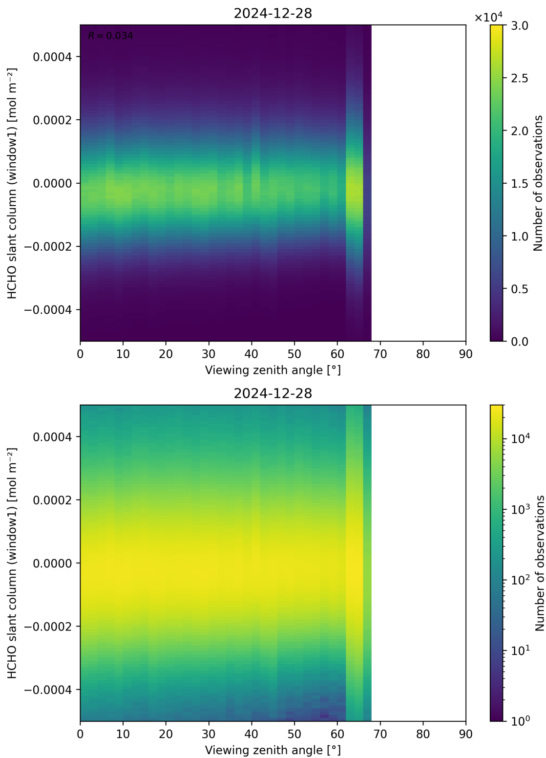
Figure 188: Scatter density plot of “Viewing zenith angle” against “HCHO slant column (window1)” for 2024-12-27 to 2024-12-29.
