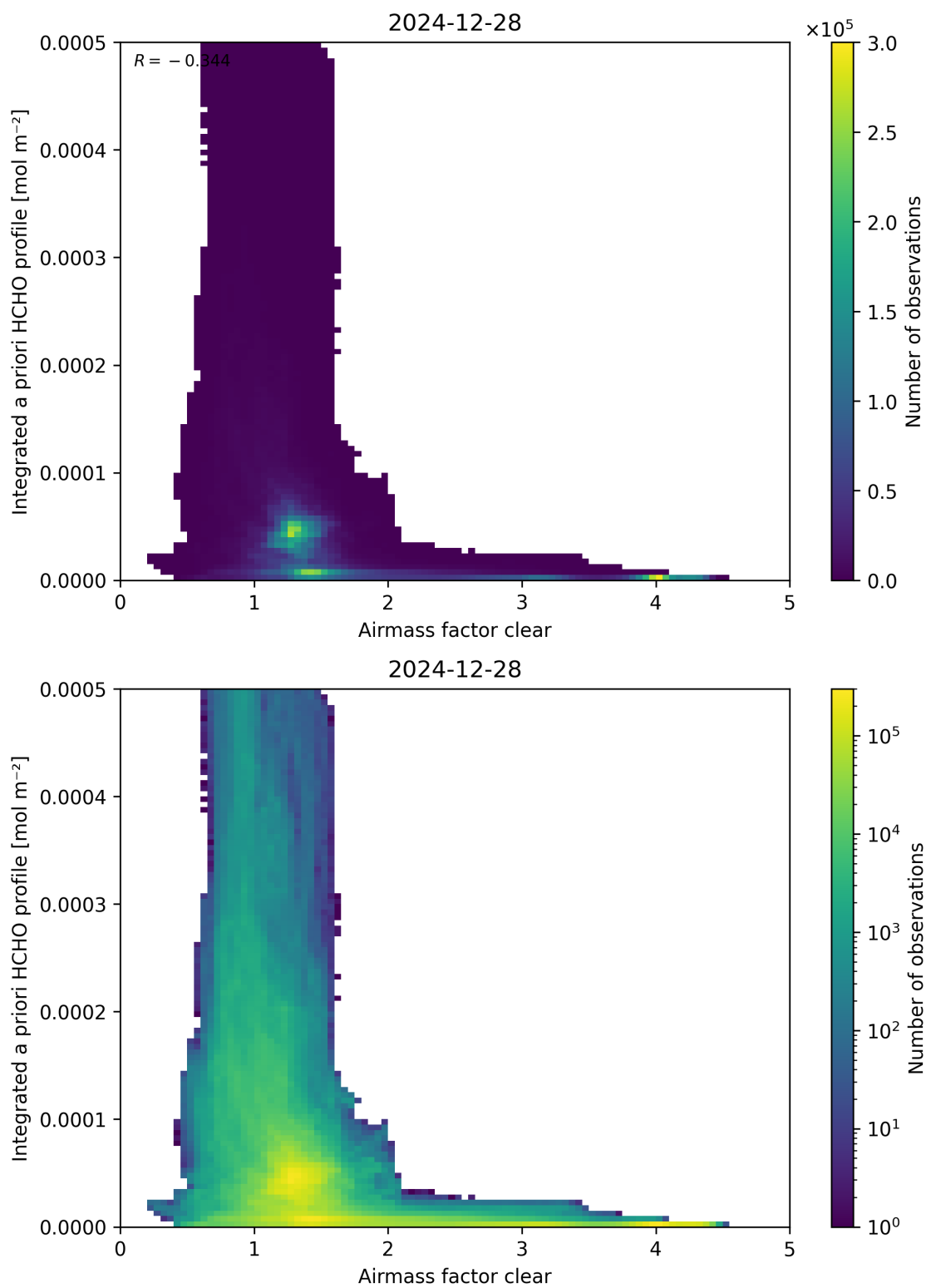
Figure 76: Scatter density plot of “Airmass factor clear” against “Integrated a priori HCHO profile” for 2024-12-27 to 2024-12-29.
