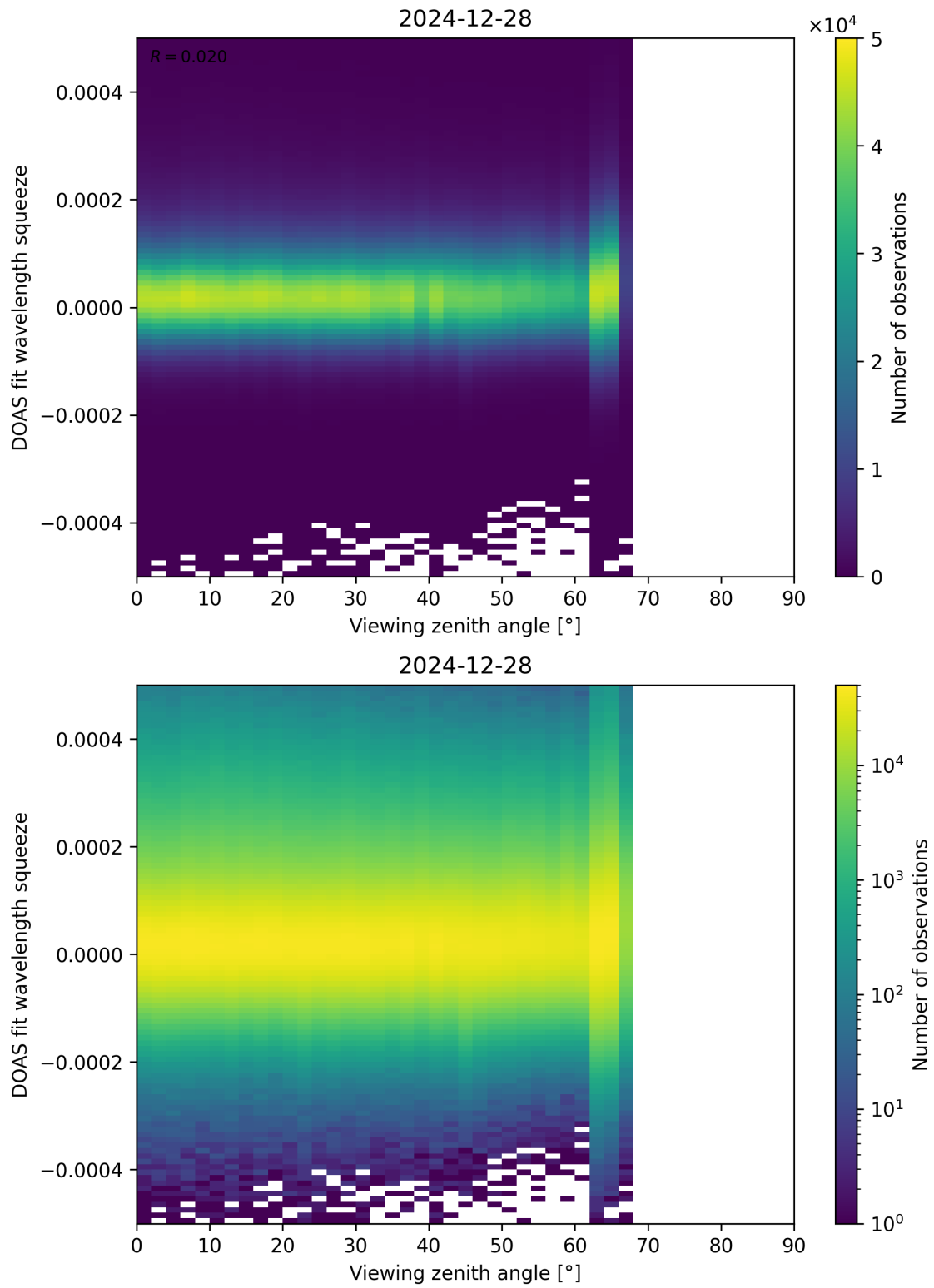
Figure 184: Scatter density plot of “Viewing zenith angle” against “DOAS fit wavelength squeeze” for 2024-12-27 to 2024-12-29.
