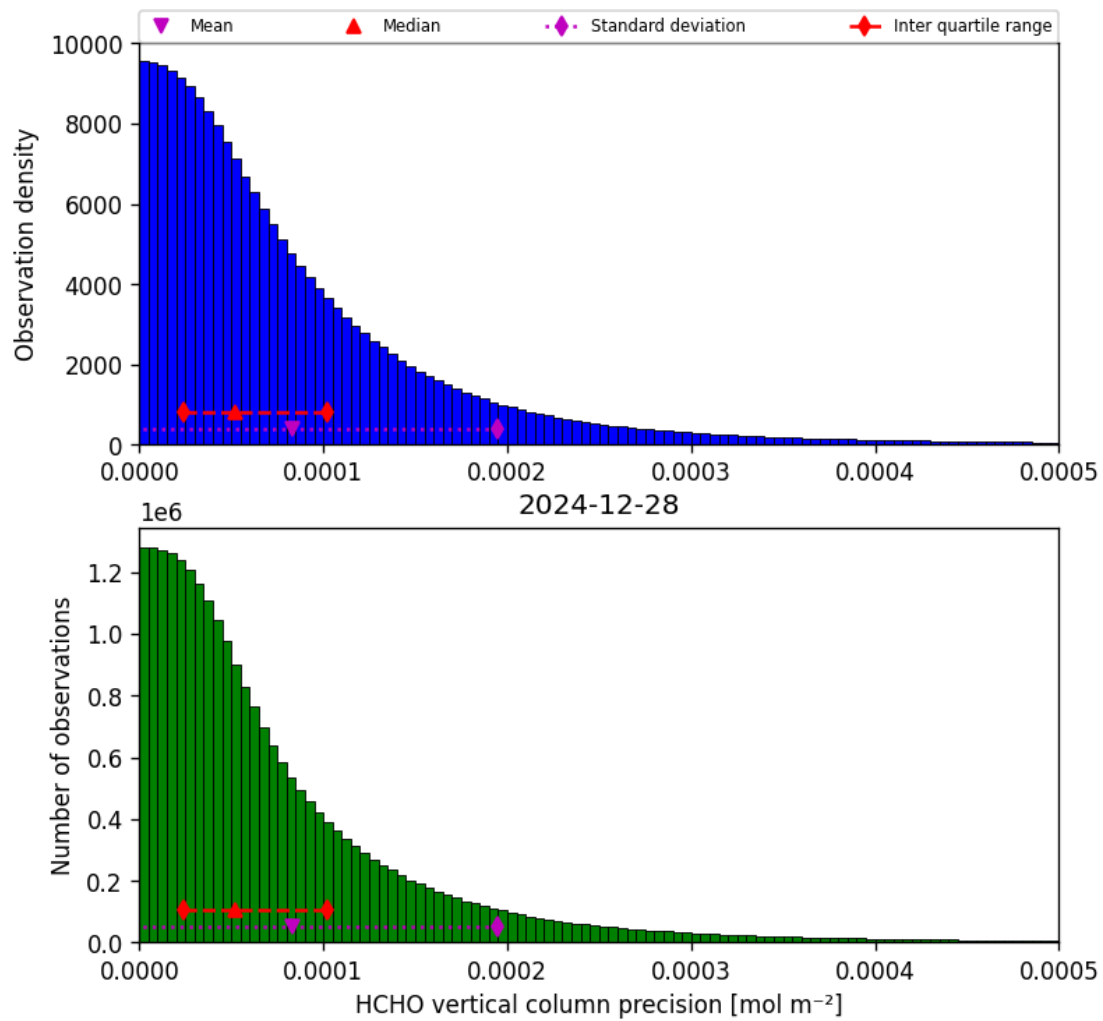
Figure 36: Histogram of “HCHO vertical column precision” for 2024-12-27 to 2024-12-29
