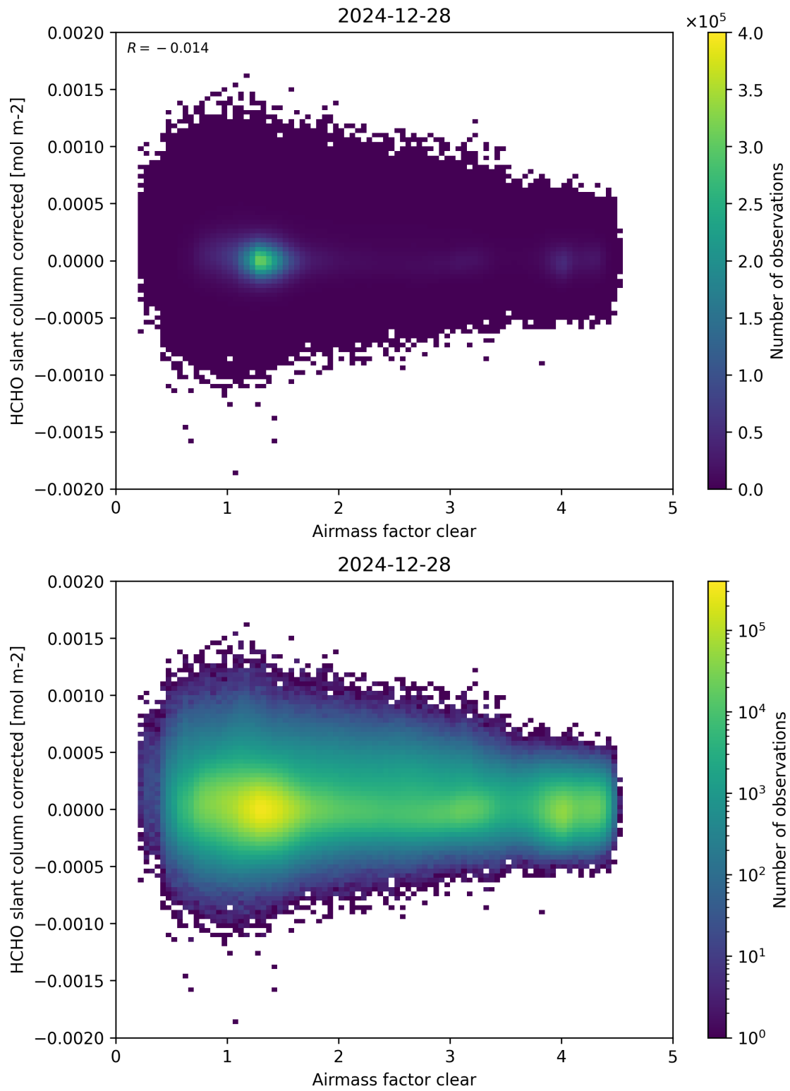
Figure 74: Scatter density plot of “Airmass factor clear” against “HCHO slant column corrected” for 2024-12-27 to 2024-12-29.
