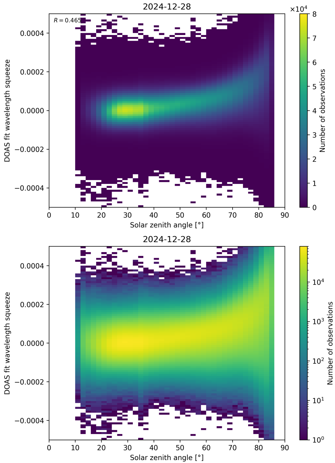
Figure 169: Scatter density plot of “Solar zenith angle” against “DOAS fit wavelength squeeze” for 2024-12-27 to 2024-12-29.
