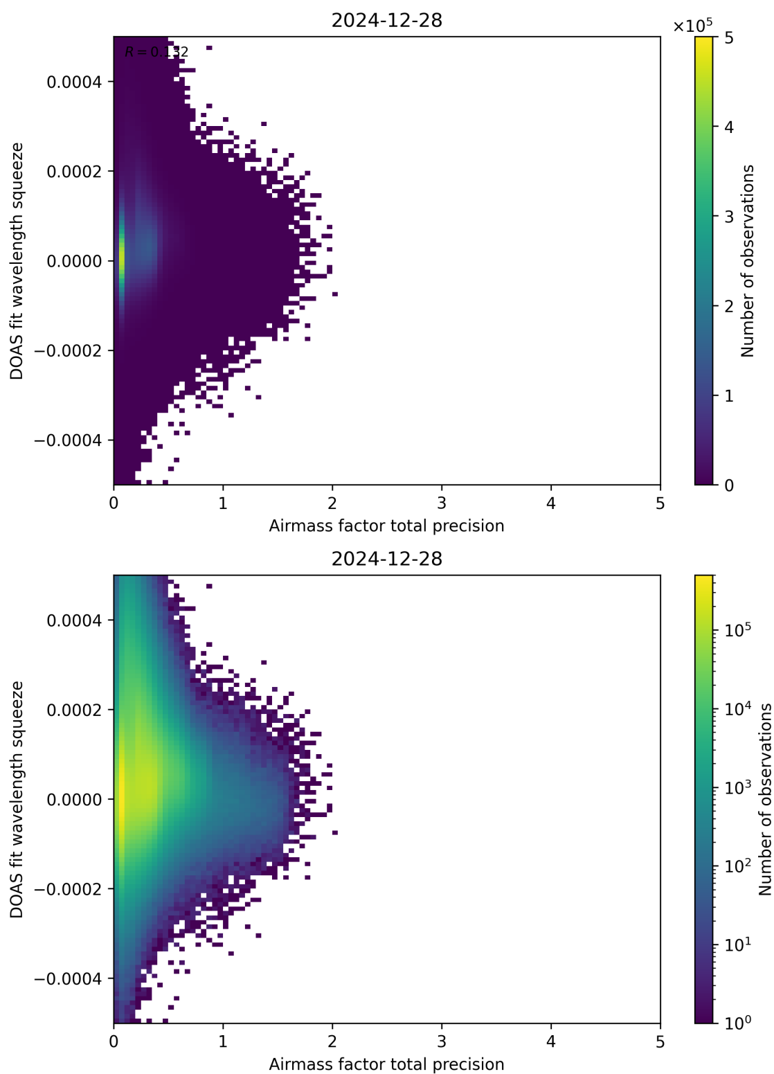
Figure 107: Scatter density plot of “Airmass factor total precision” against “DOAS fit wavelength squeeze” for 2024-12-27 to 2024-12-29.
