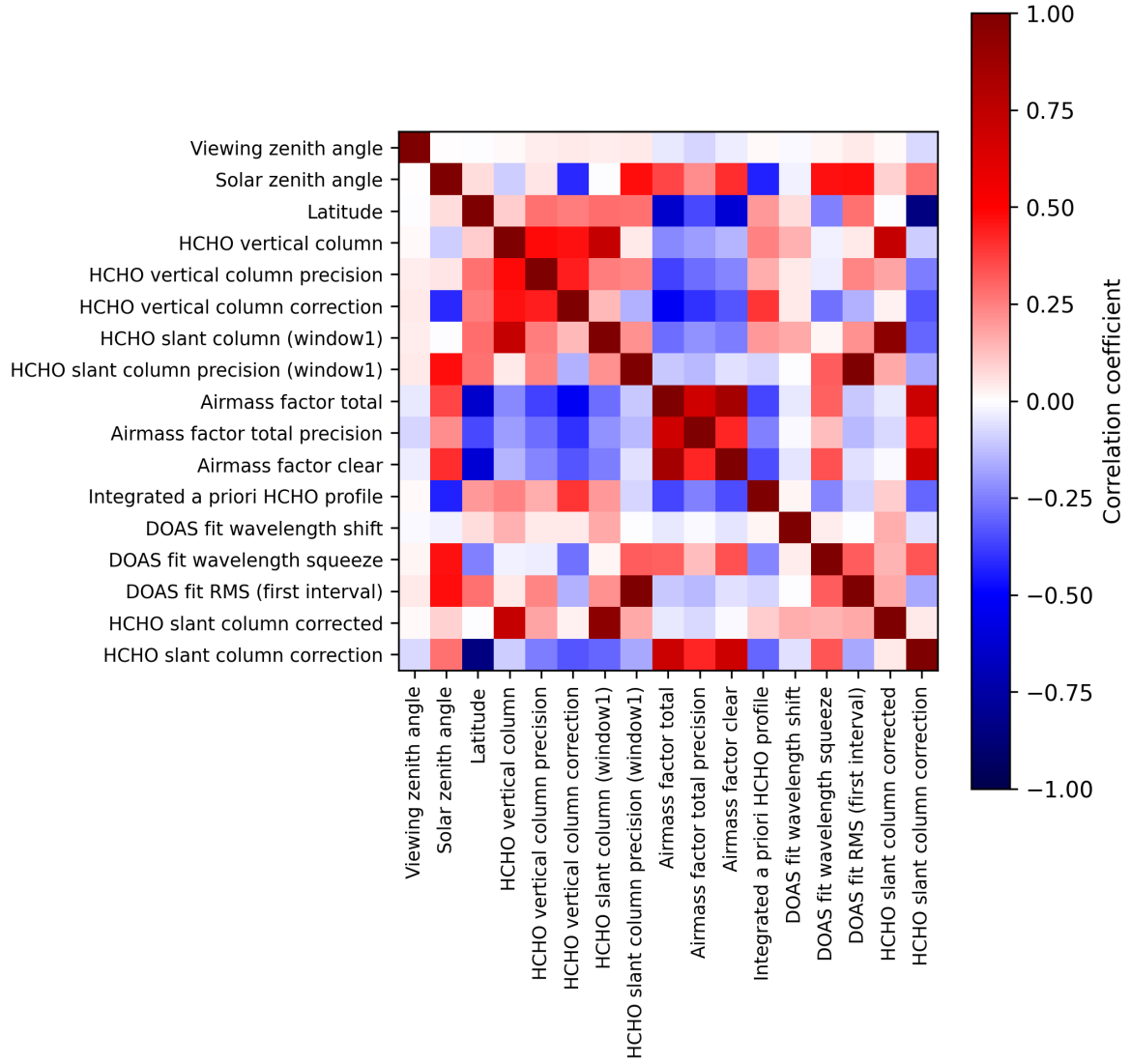
Figure 2: Map of correlation matrix for 2024-12-27 to 2024-12-29.
