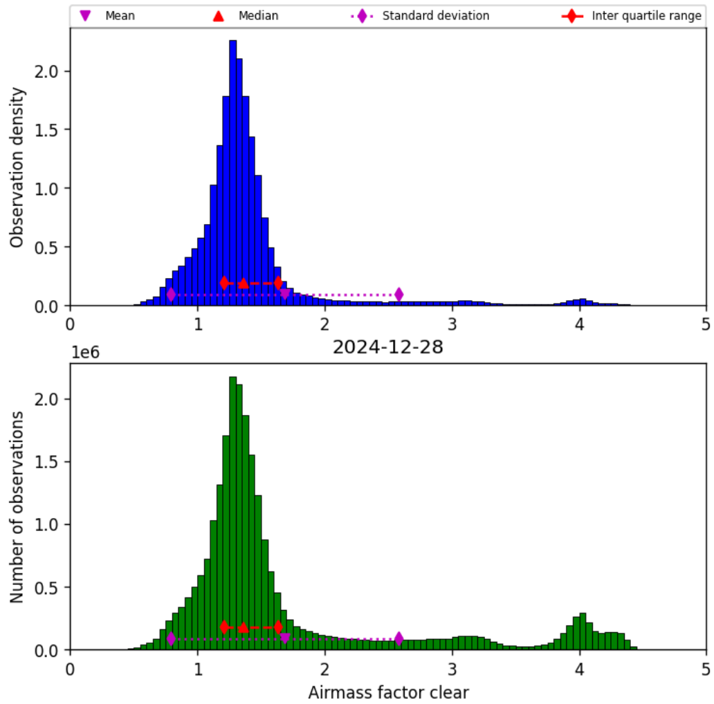
Figure 42: Histogram of “Airmass factor clear” for 2024-12-27 to 2024-12-29
