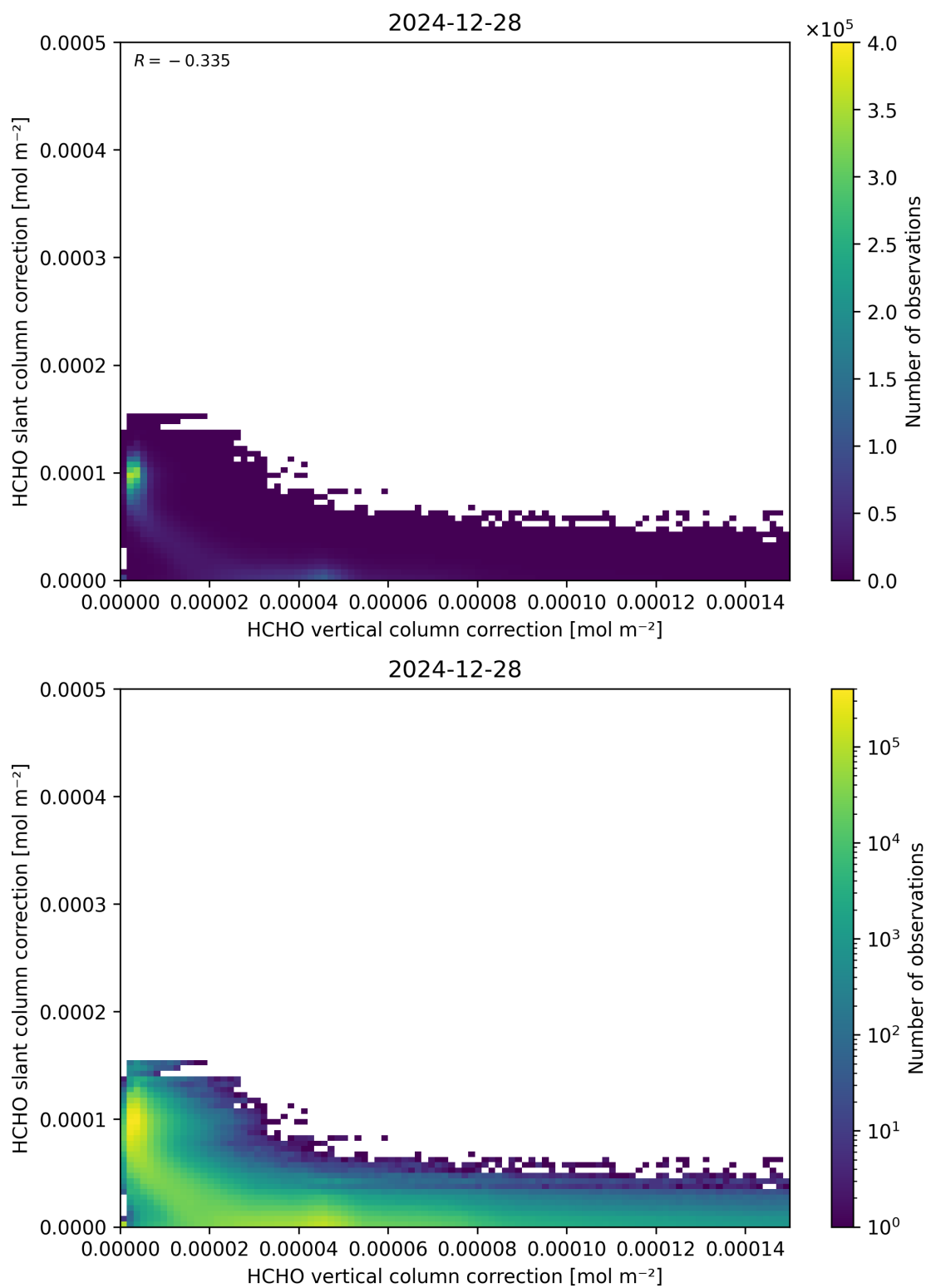
Figure 117: Scatter density plot of “HCHO vertical column correction” against “HCHO slant column correction” for 2024-12-27 to 2024-12-29.
