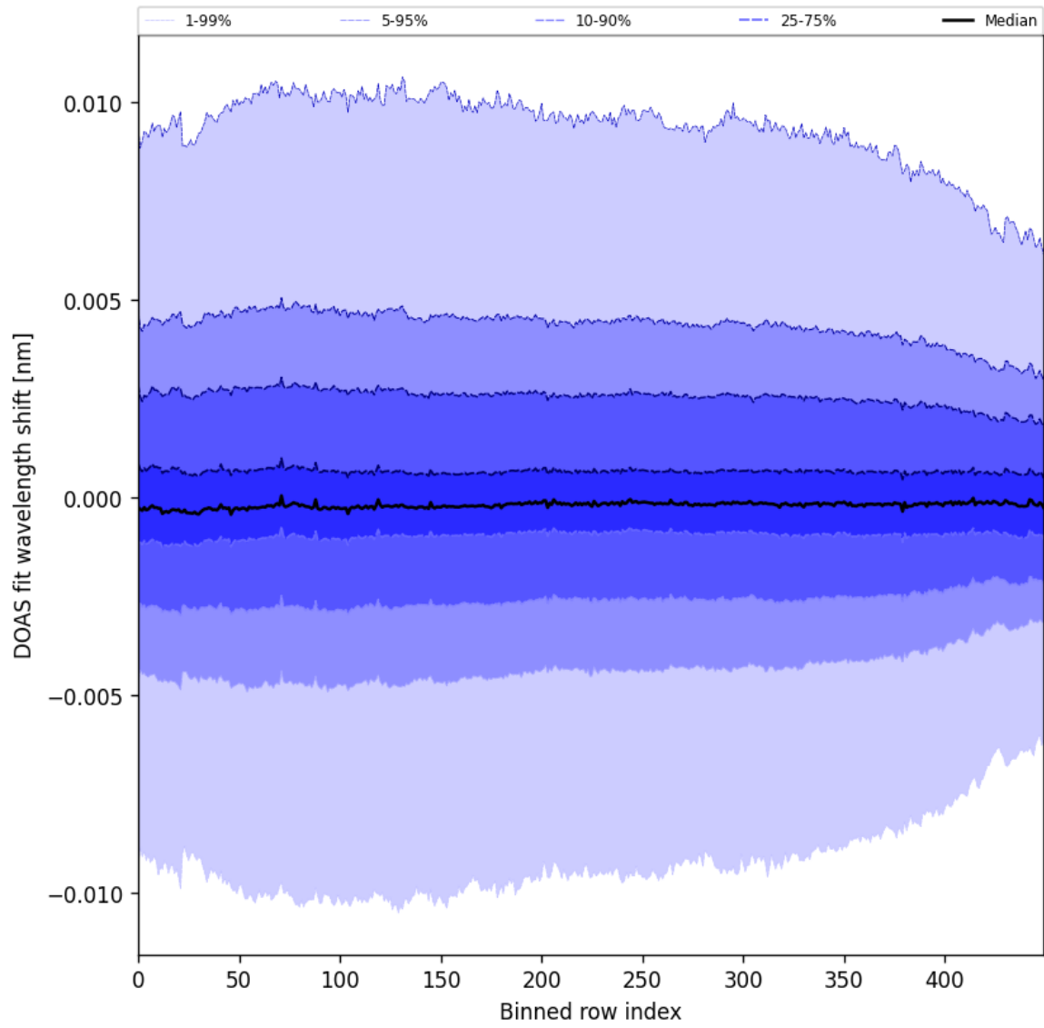
Figure 58: Along track statistics of “DOAS fit wavelength shift” for 2024-12-27 to 2024-12-29
