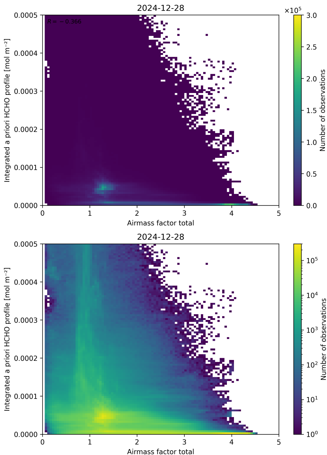
Figure 104: Scatter density plot of “Airmass factor total” against “Integrated a priori HCHO profile” for 2024-12-27 to 2024-12-29.
