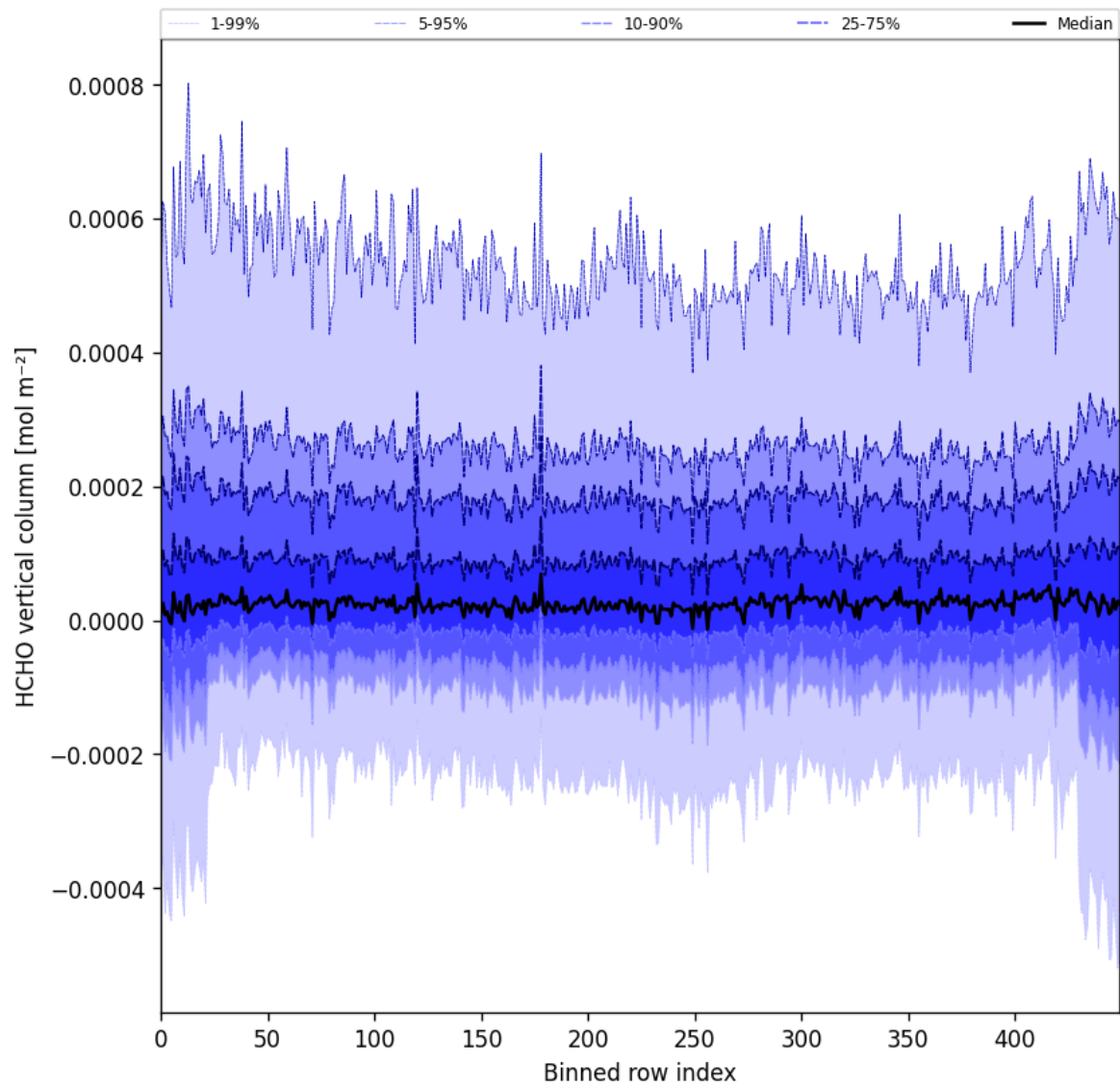
Figure 49: Along track statistics of “HCHO vertical column” for 2024-12-27 to 2024-12-29
