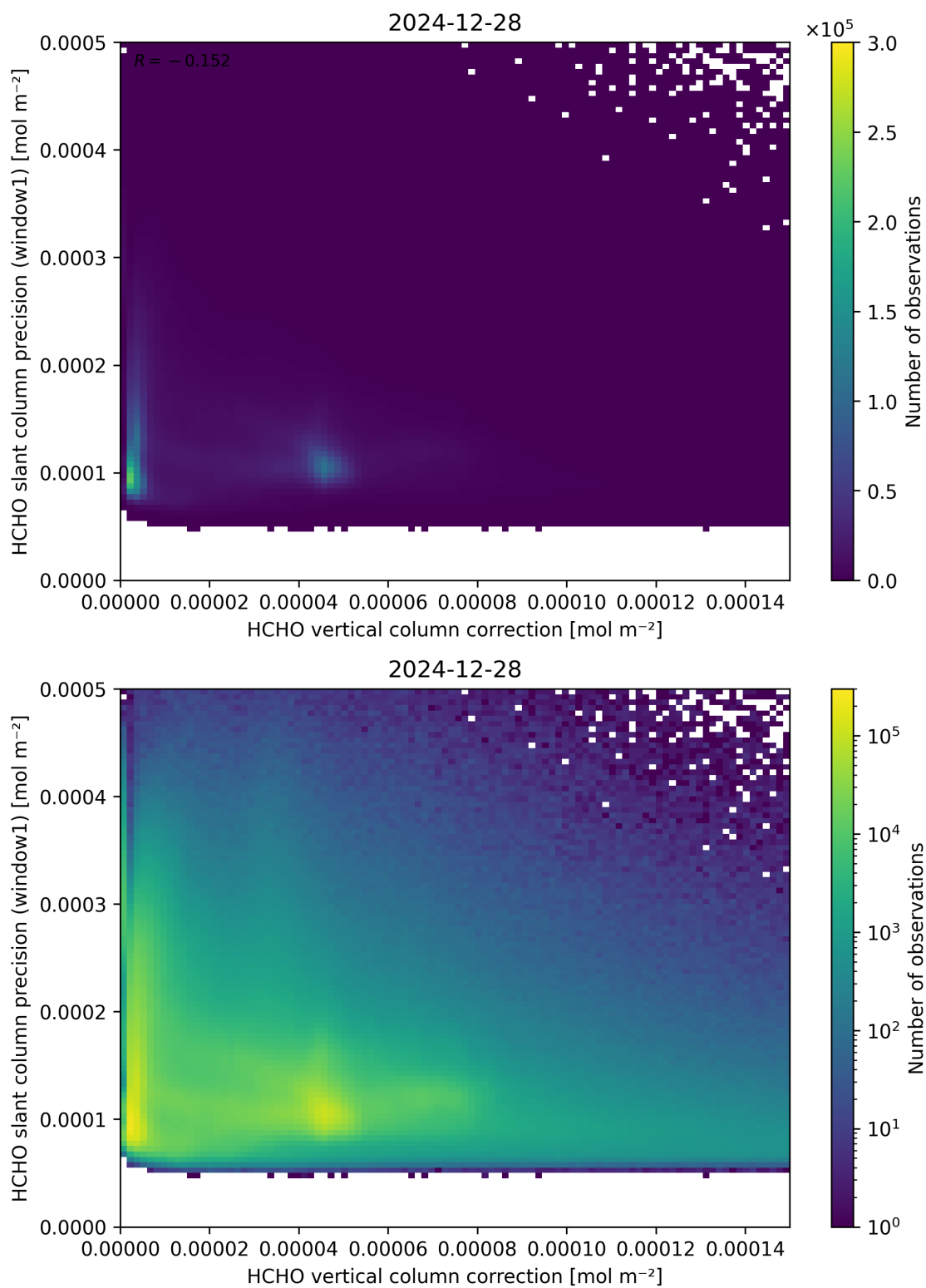
Figure 119: Scatter density plot of “HCHO vertical column correction” against “HCHO slant column precision (window1)” for 2024-12-27 to 2024-12-29.
