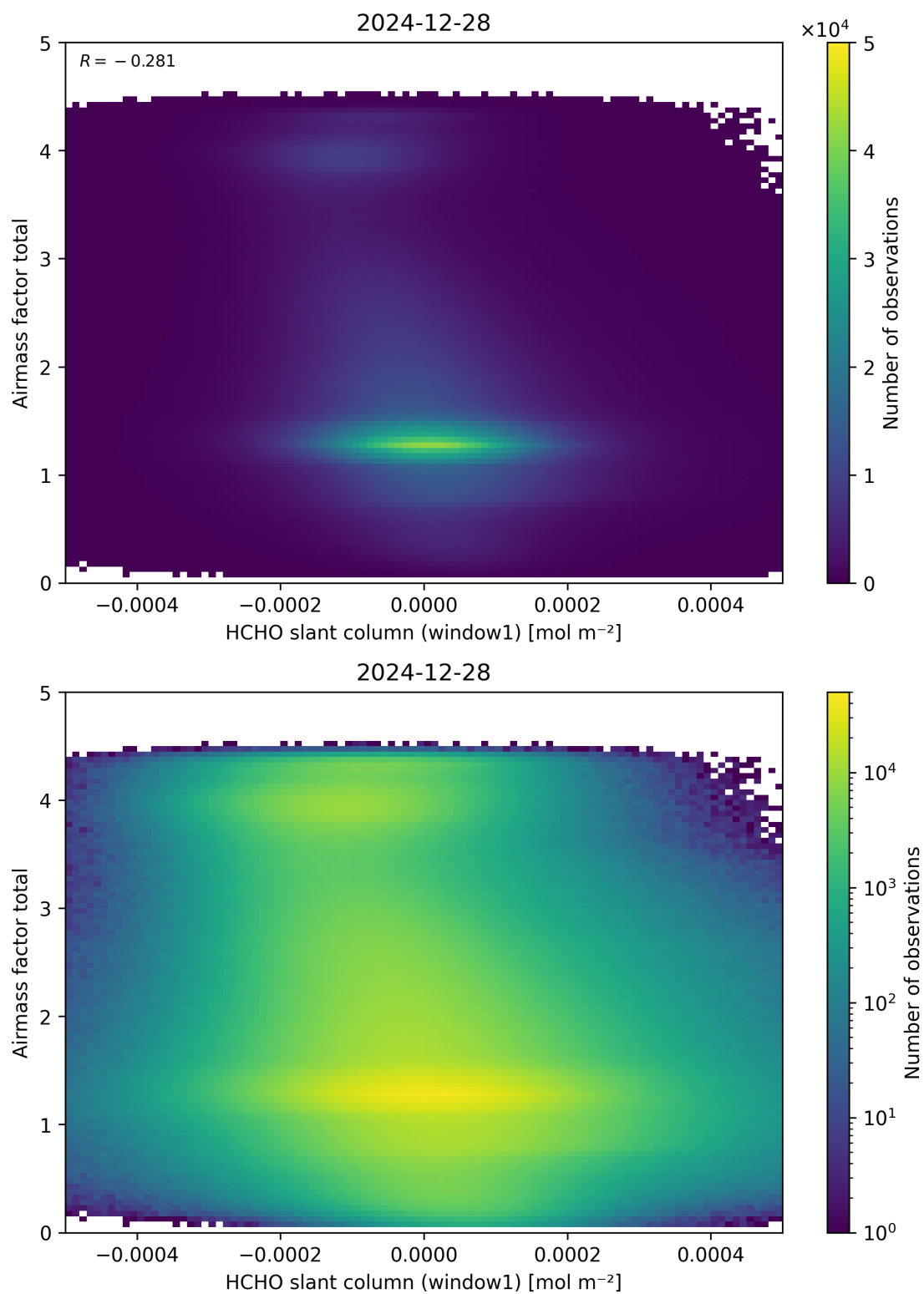
Figure 85: Scatter density plot of “HCHO slant column (window1)” against “Airmass factor total” for 2024-12-27 to 2024-12-29.
