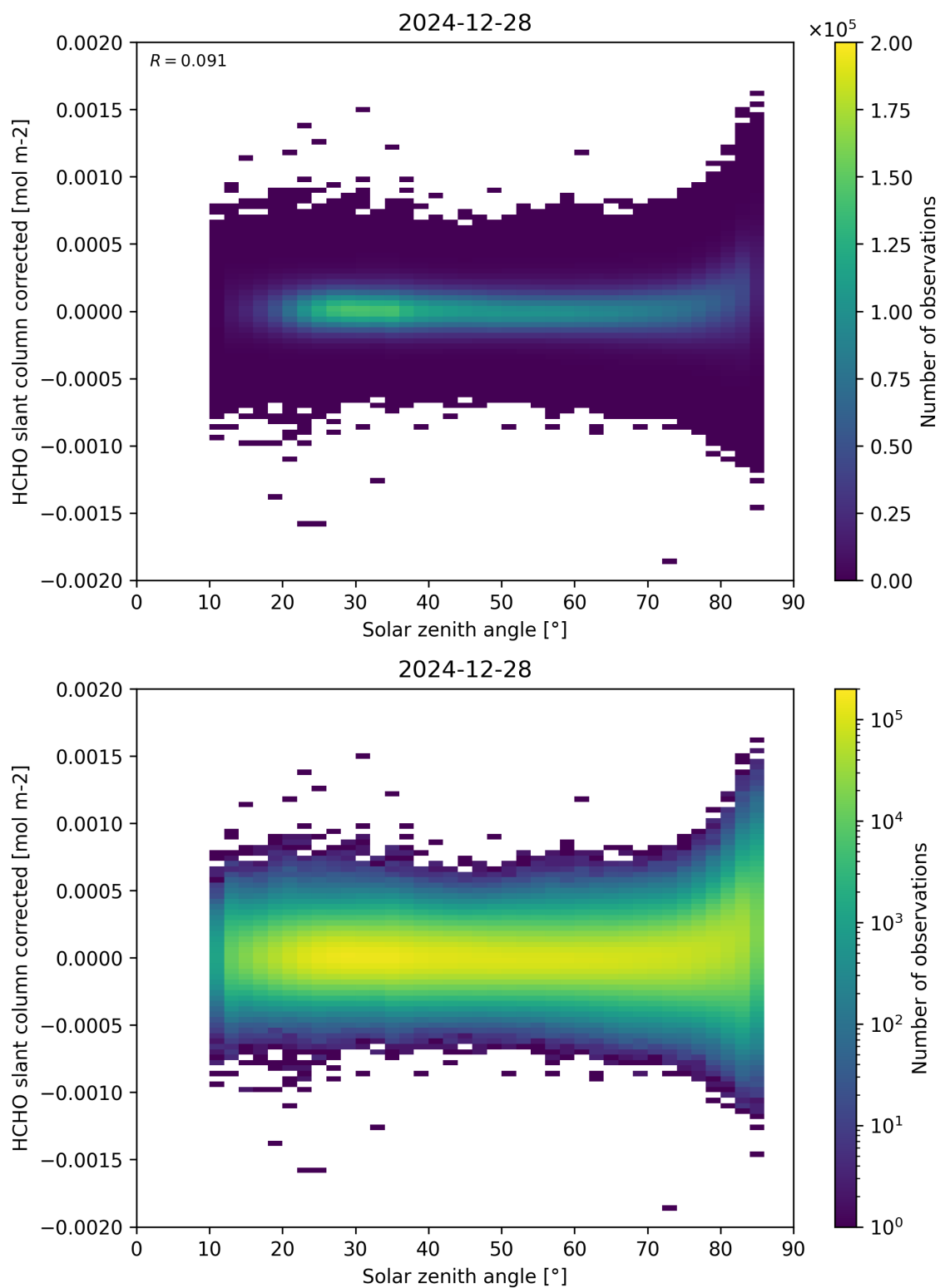
Figure 171: Scatter density plot of “Solar zenith angle” against “HCHO slant column corrected” for 2024-12-27 to 2024-12-29.
