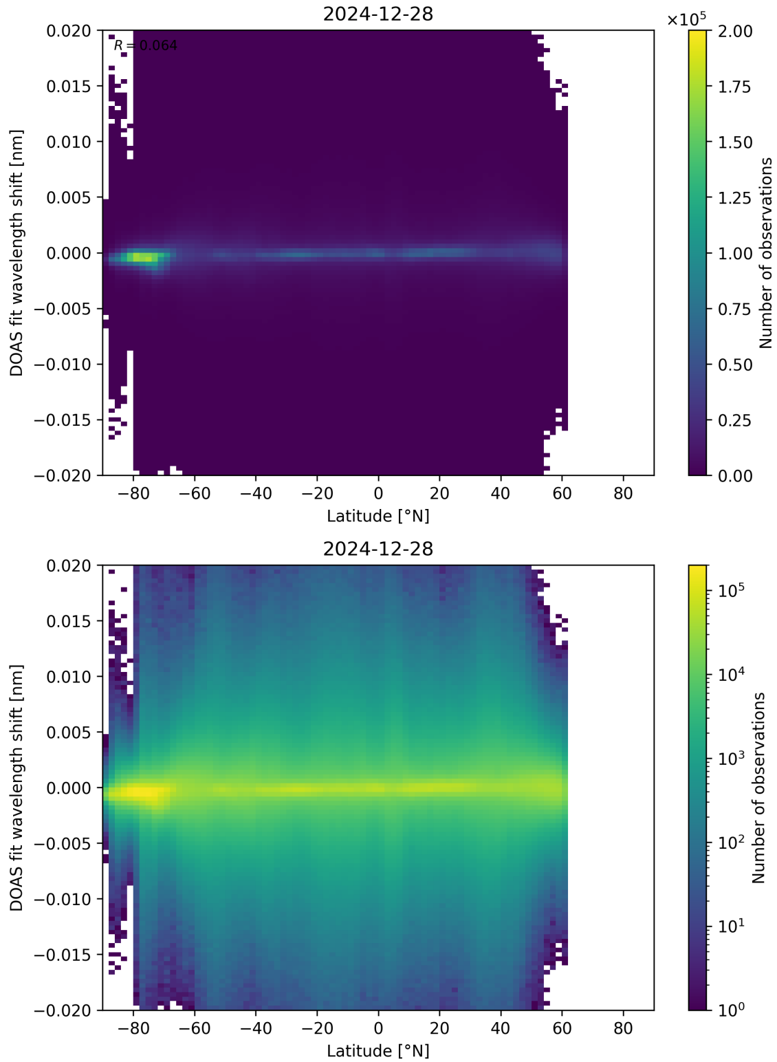
Figure 154: Scatter density plot of “Latitude” against “DOAS fit wavelength shift” for 2024-12-27 to 2024-12-29.
