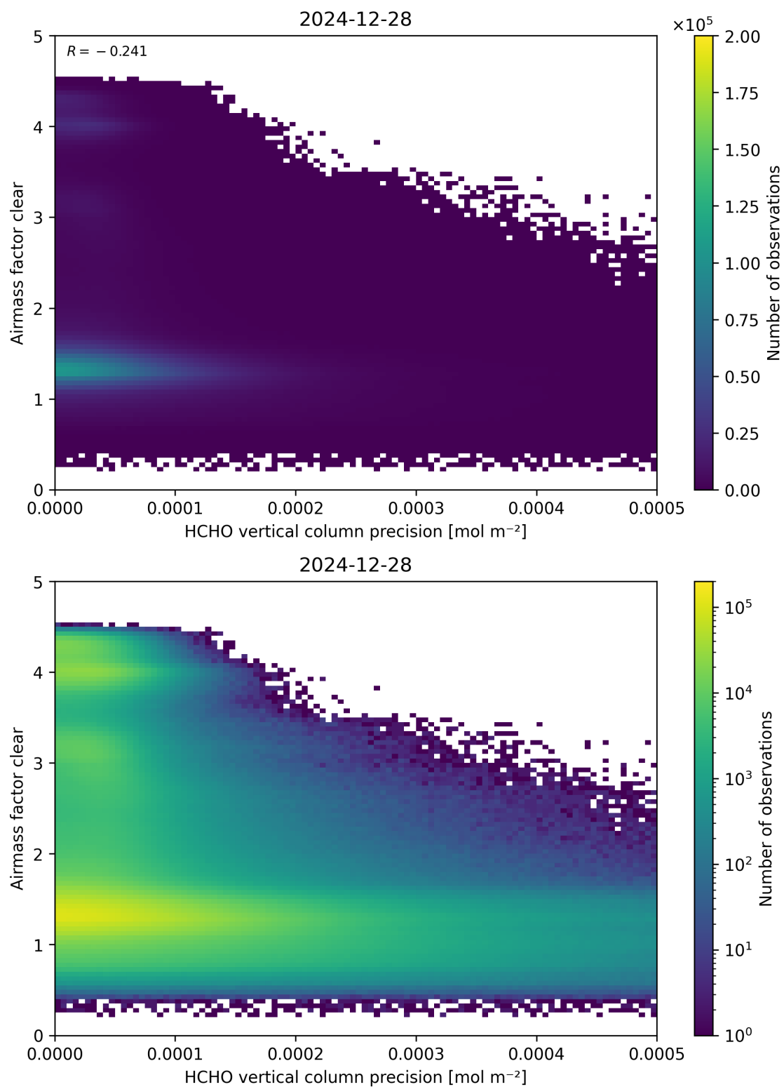
Figure 139: Scatter density plot of “HCHO vertical column precision” against “Airmass factor clear” for 2024-12-27 to 2024-12-29.
