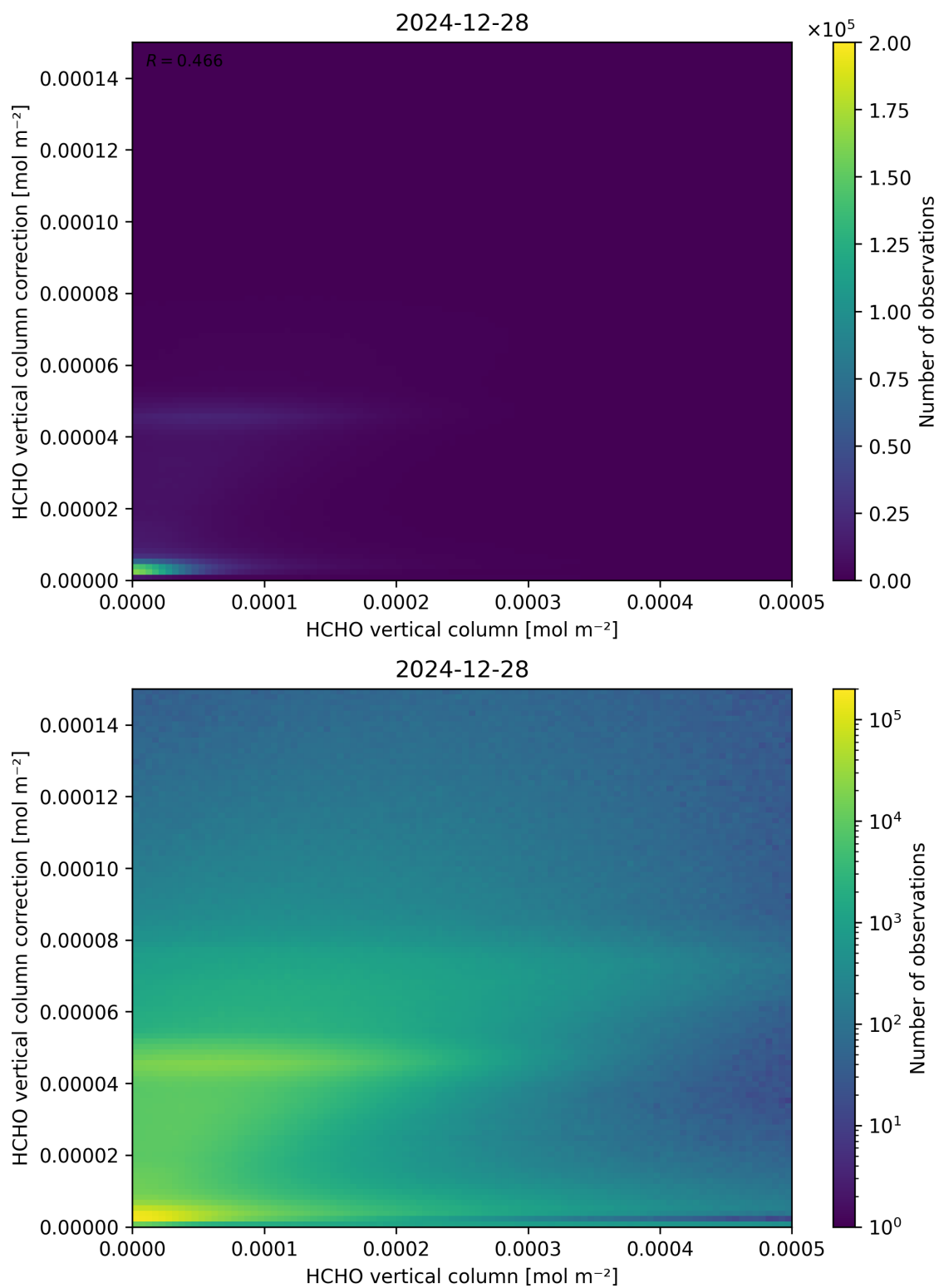
Figure 133: Scatter density plot of “HCHO vertical column” against “HCHO vertical column correction” for 2024-12-27 to 2024-12-29.
