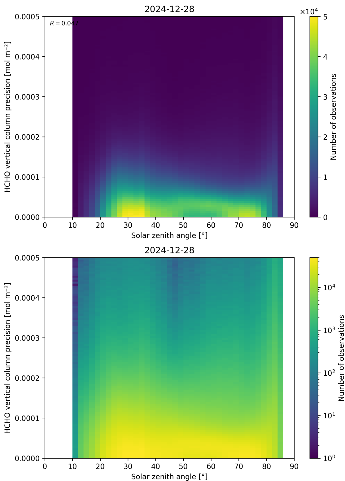
Figure 179: Scatter density plot of “Solar zenith angle” against “HCHO vertical column precision” for 2024-12-27 to 2024-12-29.
