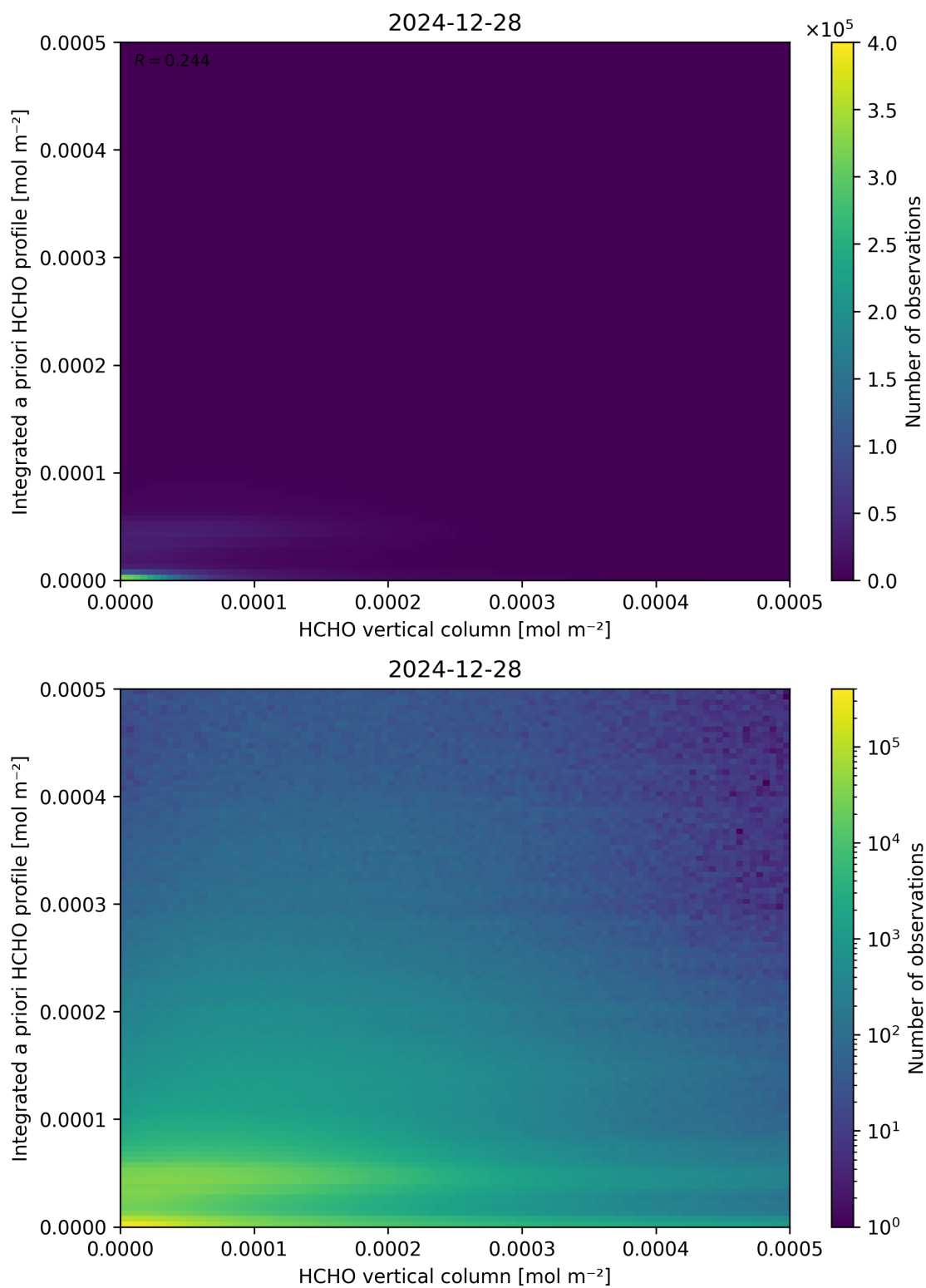
Figure 135: Scatter density plot of “HCHO vertical column” against “Integrated a priori HCHO profile” for 2024-12-27 to 2024-12-29.
