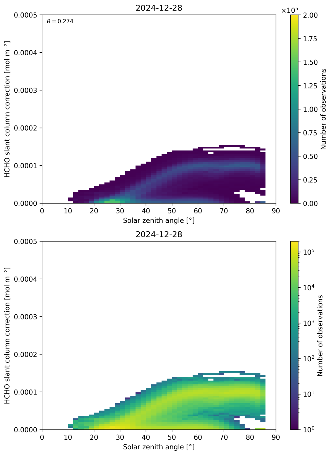
Figure 172: Scatter density plot of “Solar zenith angle” against “HCHO slant column correction” for 2024-12-27 to 2024-12-29.
