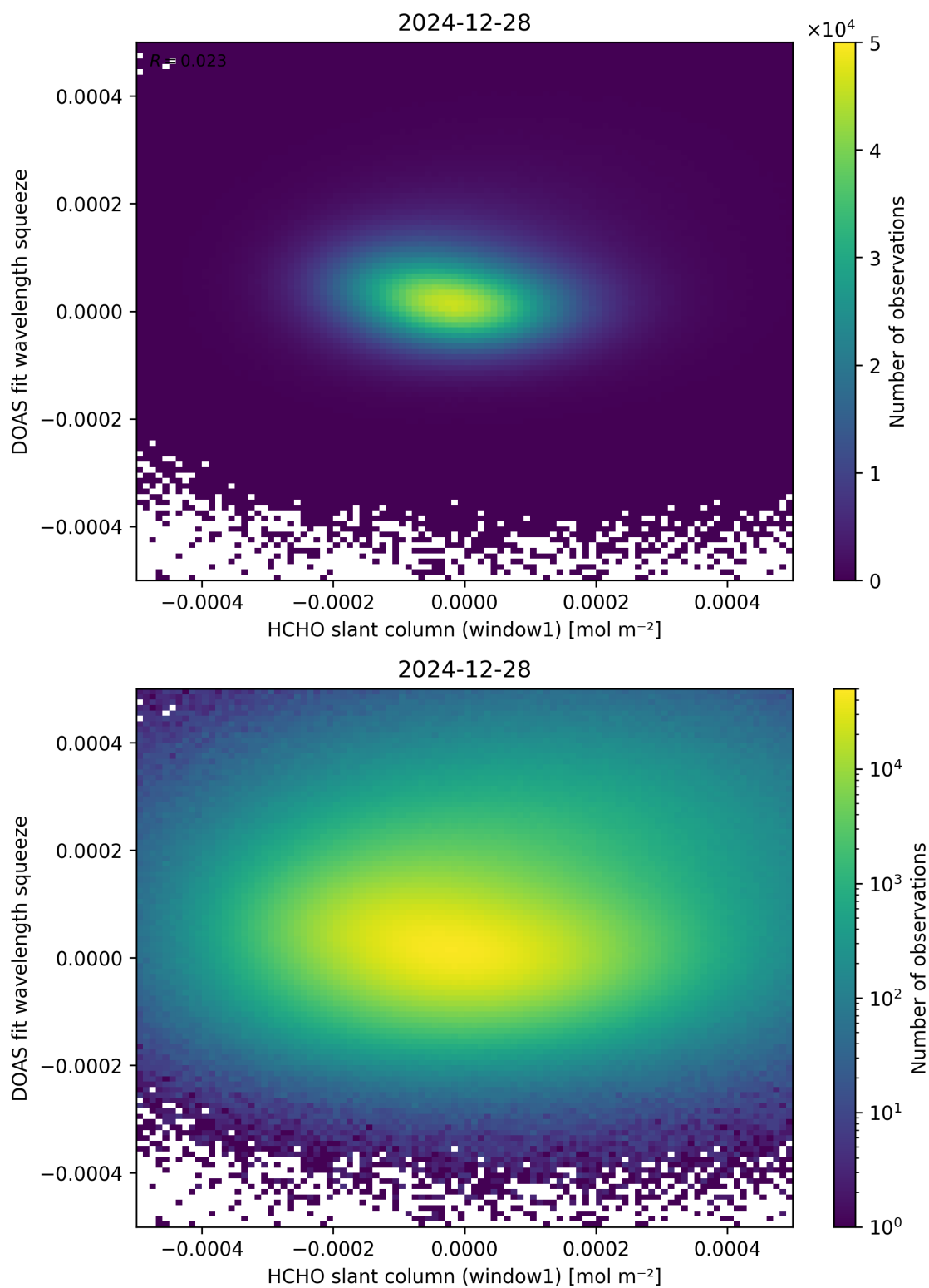
Figure 80: Scatter density plot of “HCHO slant column (window1)” against “DOAS fit wavelength squeeze” for 2024-12-27 to 2024-12-29.
