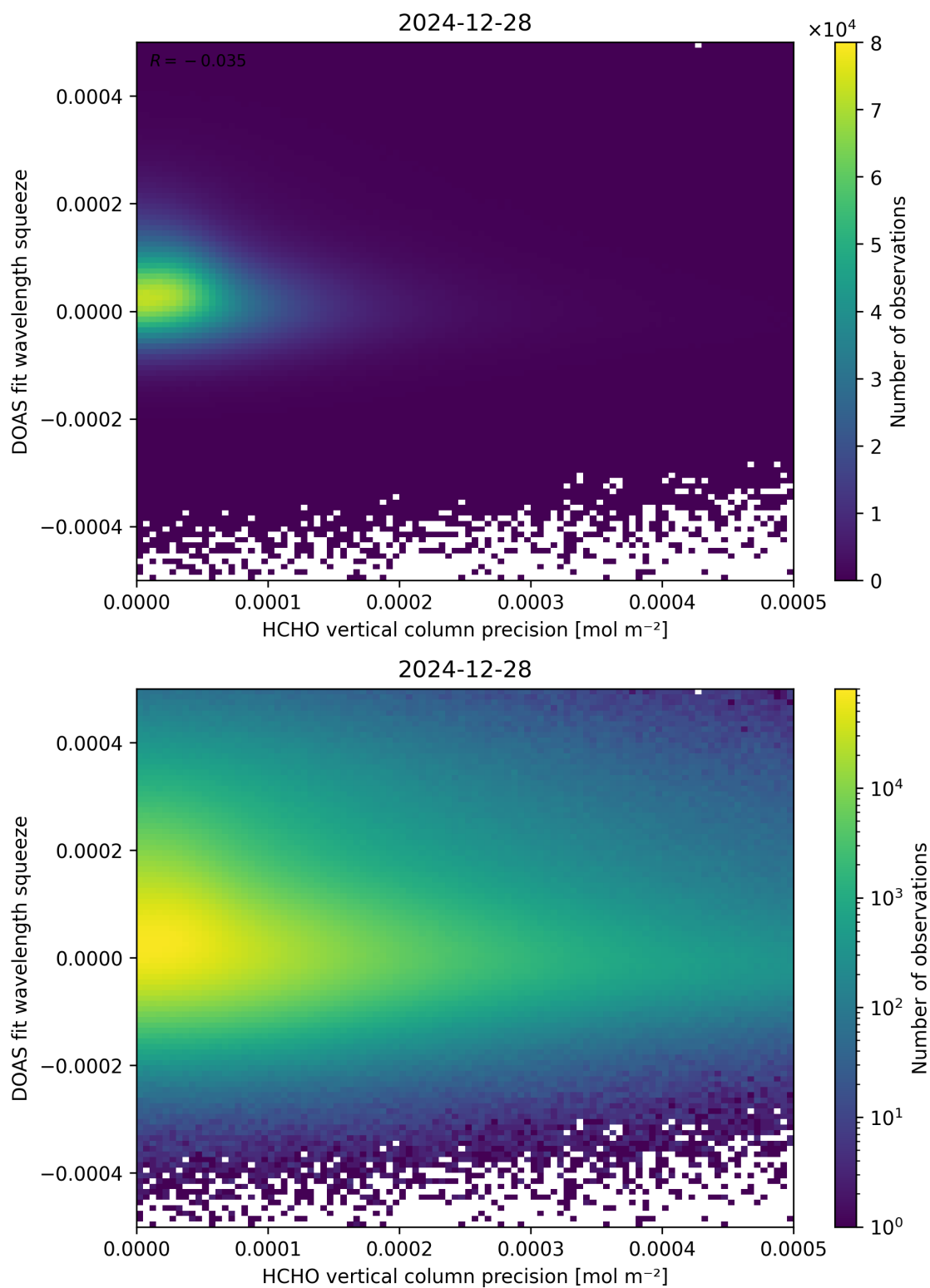
Figure 138: Scatter density plot of “HCHO vertical column precision” against “DOAS fit wavelength squeeze” for 2024-12-27 to 2024-12-29.
