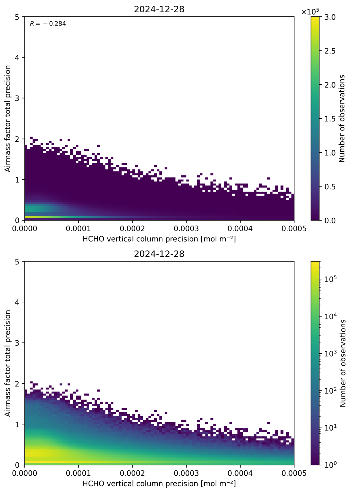
Figure 145: Scatter density plot of “HCHO vertical column precision” against “Airmass factor total precision” for 2024-12-27 to 2024-12-29.
