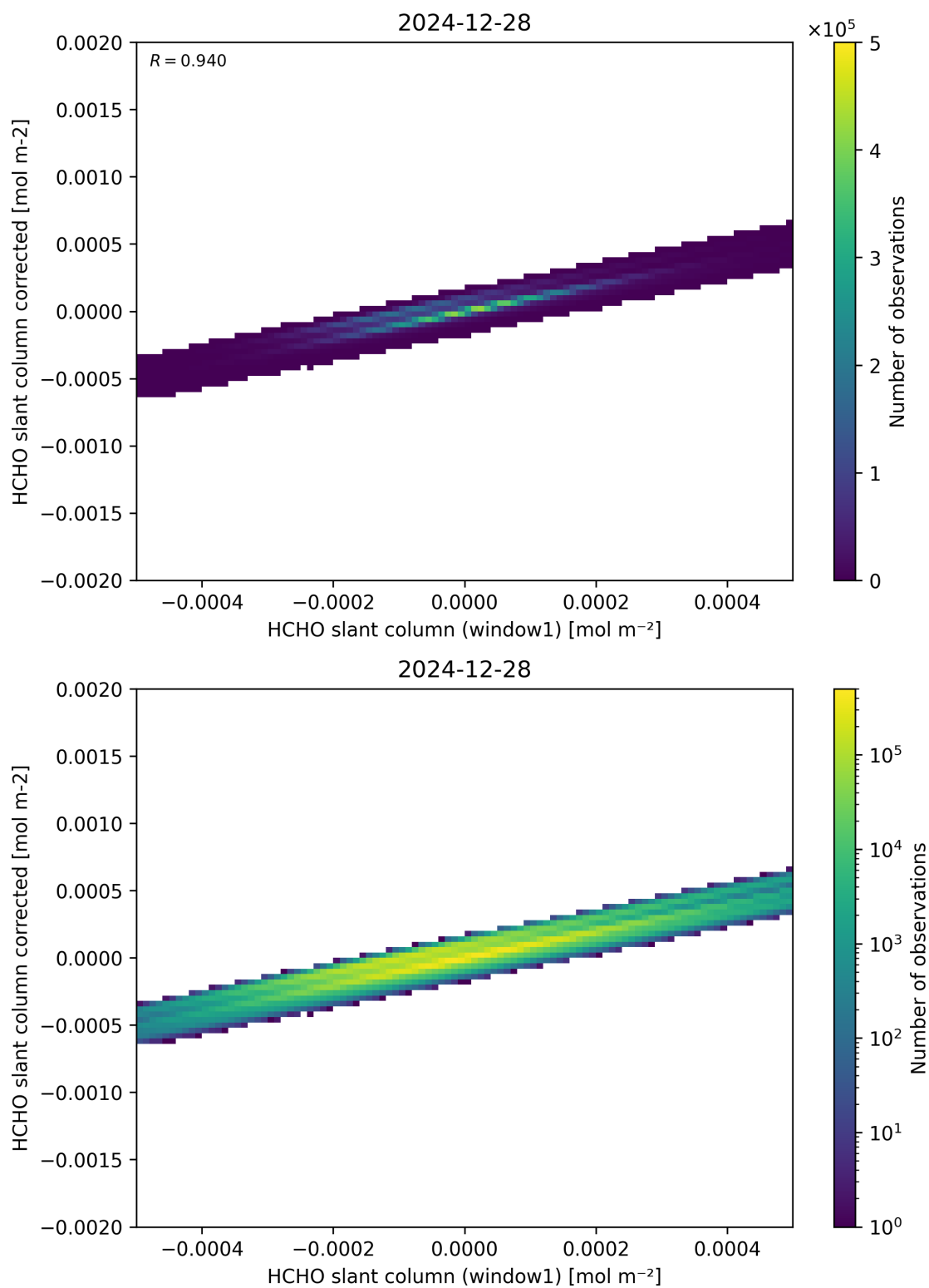
Figure 82: Scatter density plot of “HCHO slant column (window1)” against “HCHO slant column corrected” for 2024-12-27 to 2024-12-29.
