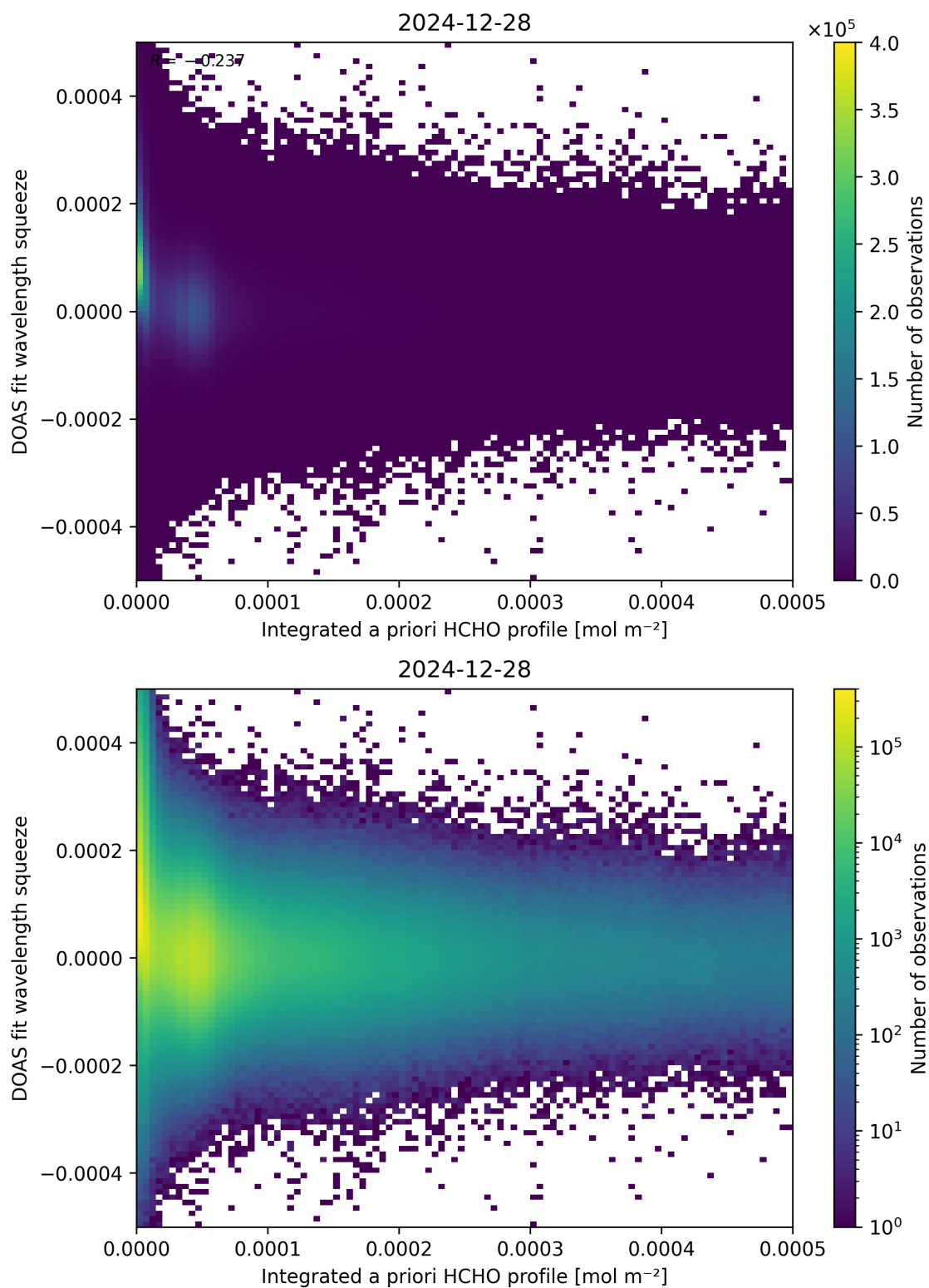
Figure 150: Scatter density plot of “Integrated a priori HCHO profile” against “DOAS fit wavelength squeeze” for 2024-12-27 to 2024-12-29.
