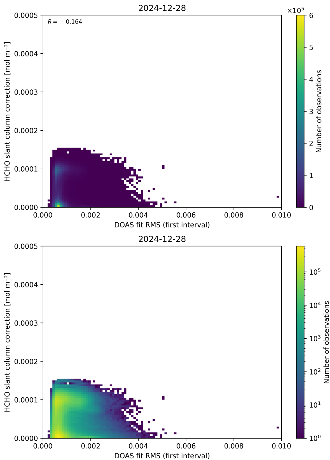
Figure 63: Scatter density plot of “DOAS fit RMS (first interval)” against “HCHO slant column correction” for 2024-12-27 to 2024-12-29.
