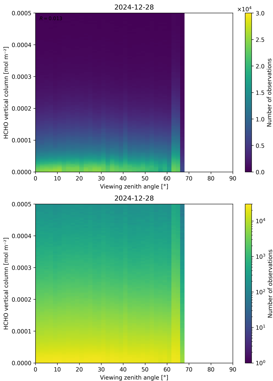
Figure 192: Scatter density plot of “Viewing zenith angle” against “HCHO vertical column” for 2024-12-27 to 2024-12-29.
