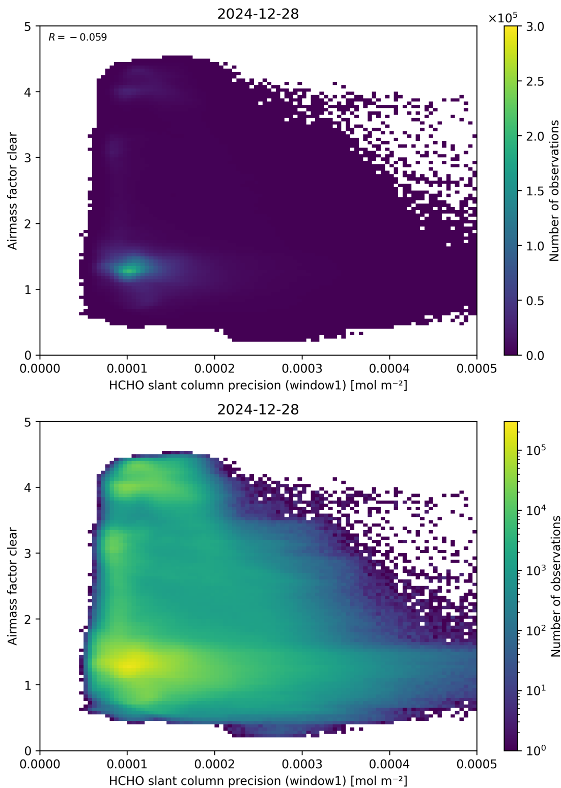
Figure 91: Scatter density plot of “HCHO slant column precision (window1)” against “Airmass factor clear” for 2024-12-27 to 2024-12-29.
