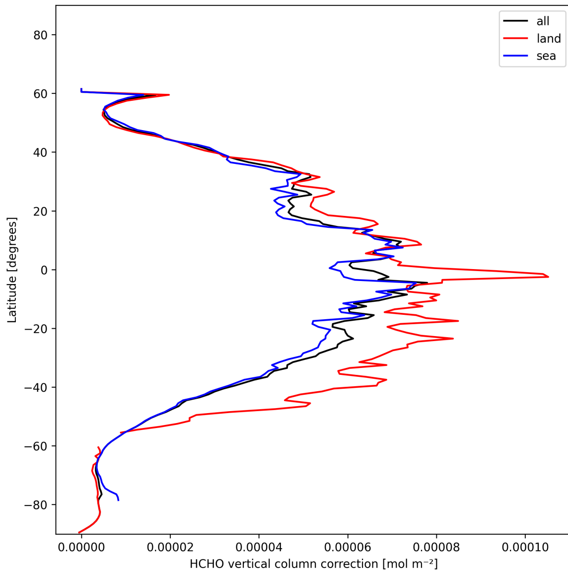
Figure 23: Zonal average of “HCHO vertical column correction” for 2024-12-27 to 2024-12-29.
