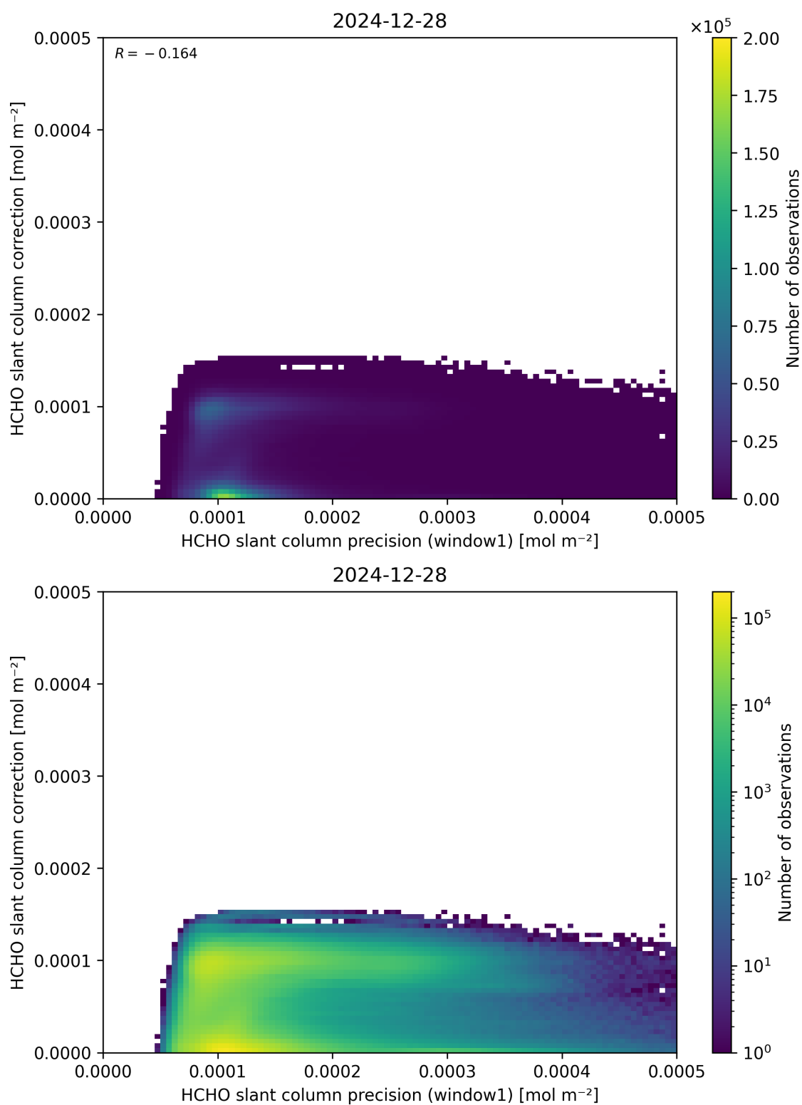
Figure 93: Scatter density plot of “HCHO slant column precision (window1)” against “HCHO slant column correction” for 2024-12-27 to 2024-12-29.
