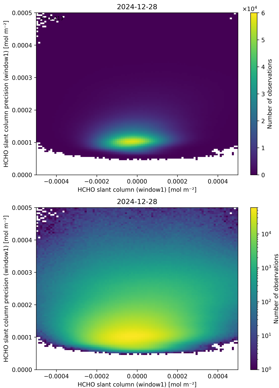
Figure 84: Scatter density plot of “HCHO slant column (window1)” against “HCHO slant column precision (window1)” for 2024-12-27 to 2024-12-29.
