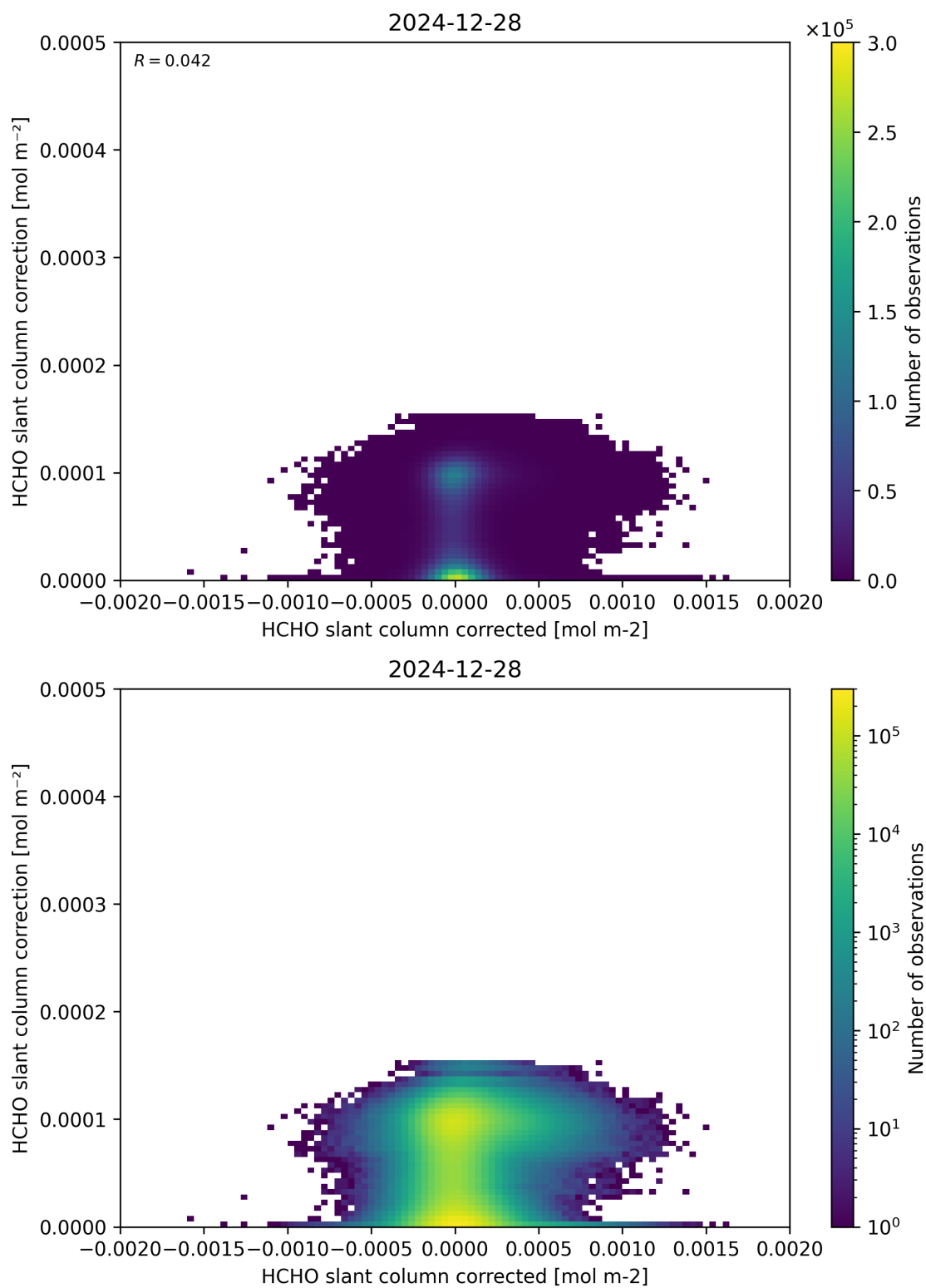
Figure 77: Scatter density plot of “HCHO slant column corrected” against “HCHO slant column correction” for 2024-12-27 to 2024-12-29.
