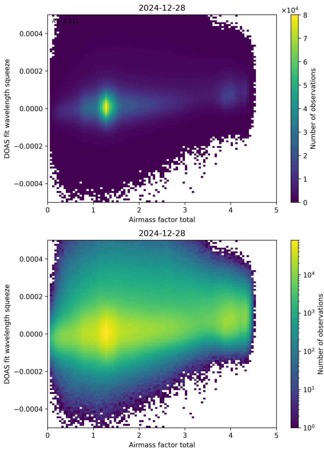
Figure 99: Scatter density plot of “Airmass factor total” against “DOAS fit wavelength squeeze” for 2024-12-27 to 2024-12-29.
