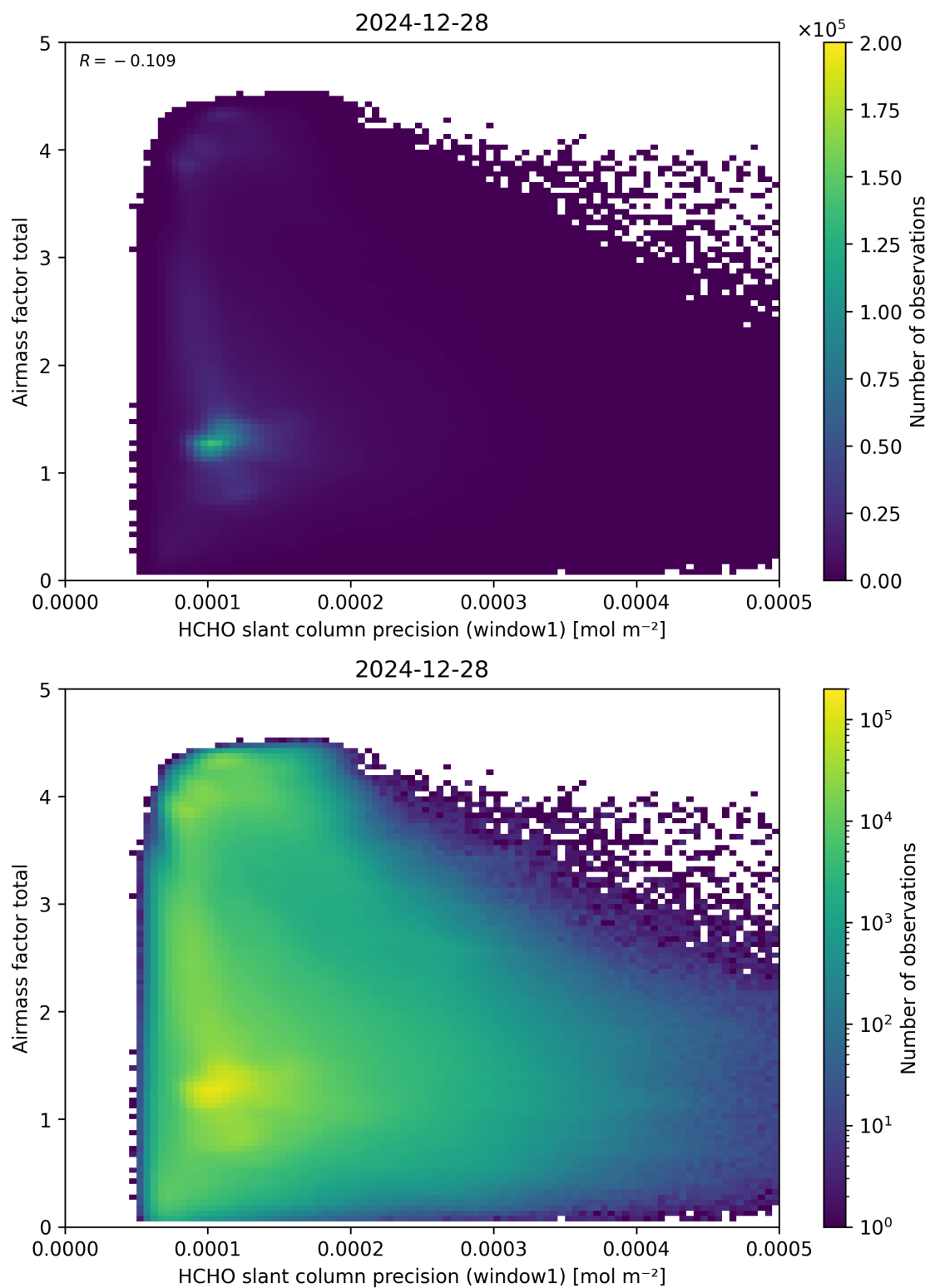
Figure 94: Scatter density plot of “HCHO slant column precision (window1)” against “Airmass factor total” for 2024-12-27 to 2024-12-29.
