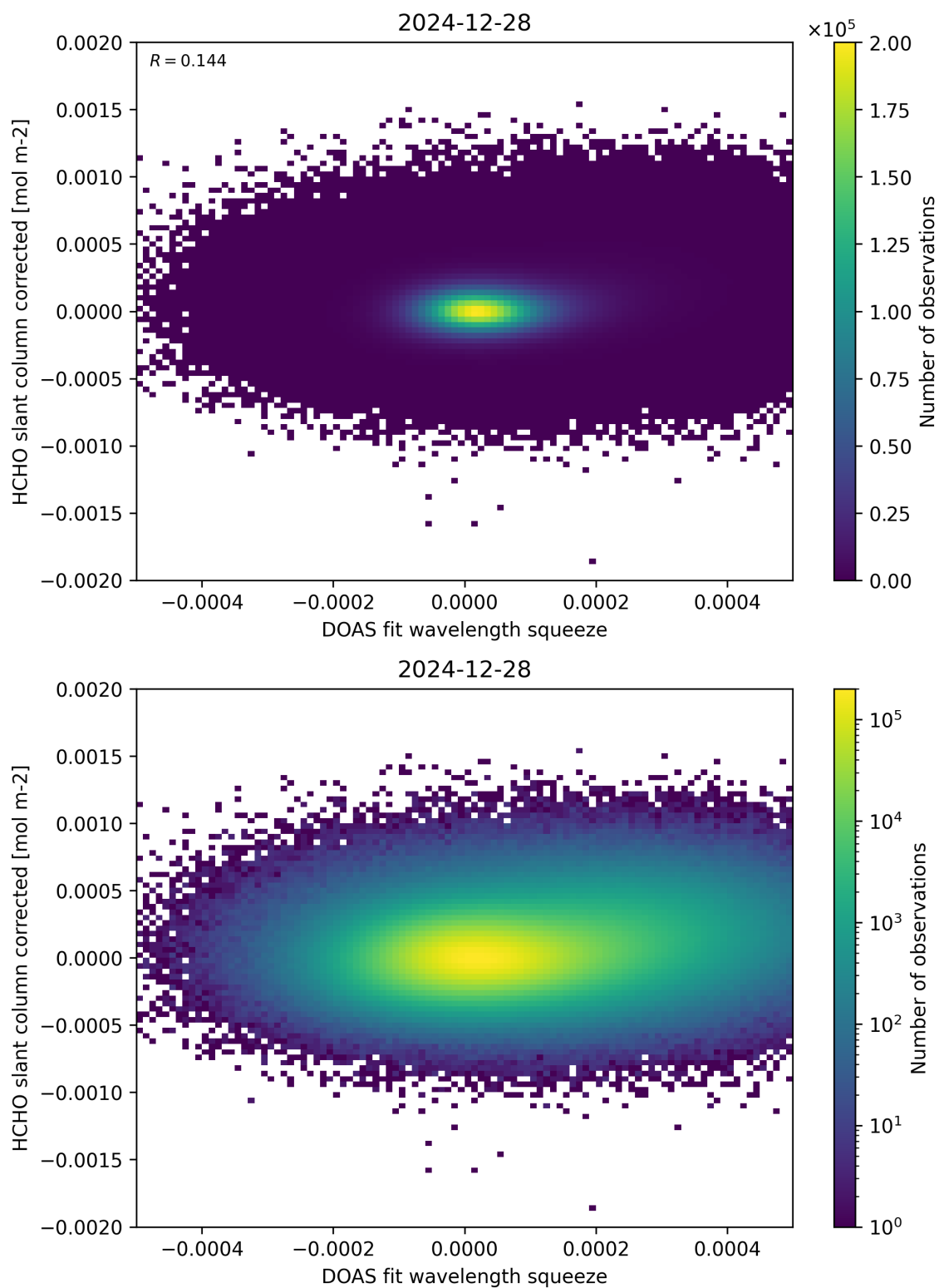
Figure 69: Scatter density plot of “DOAS fit wavelength squeeze” against “HCHO slant column corrected” for 2024-12-27 to 2024-12-29.
