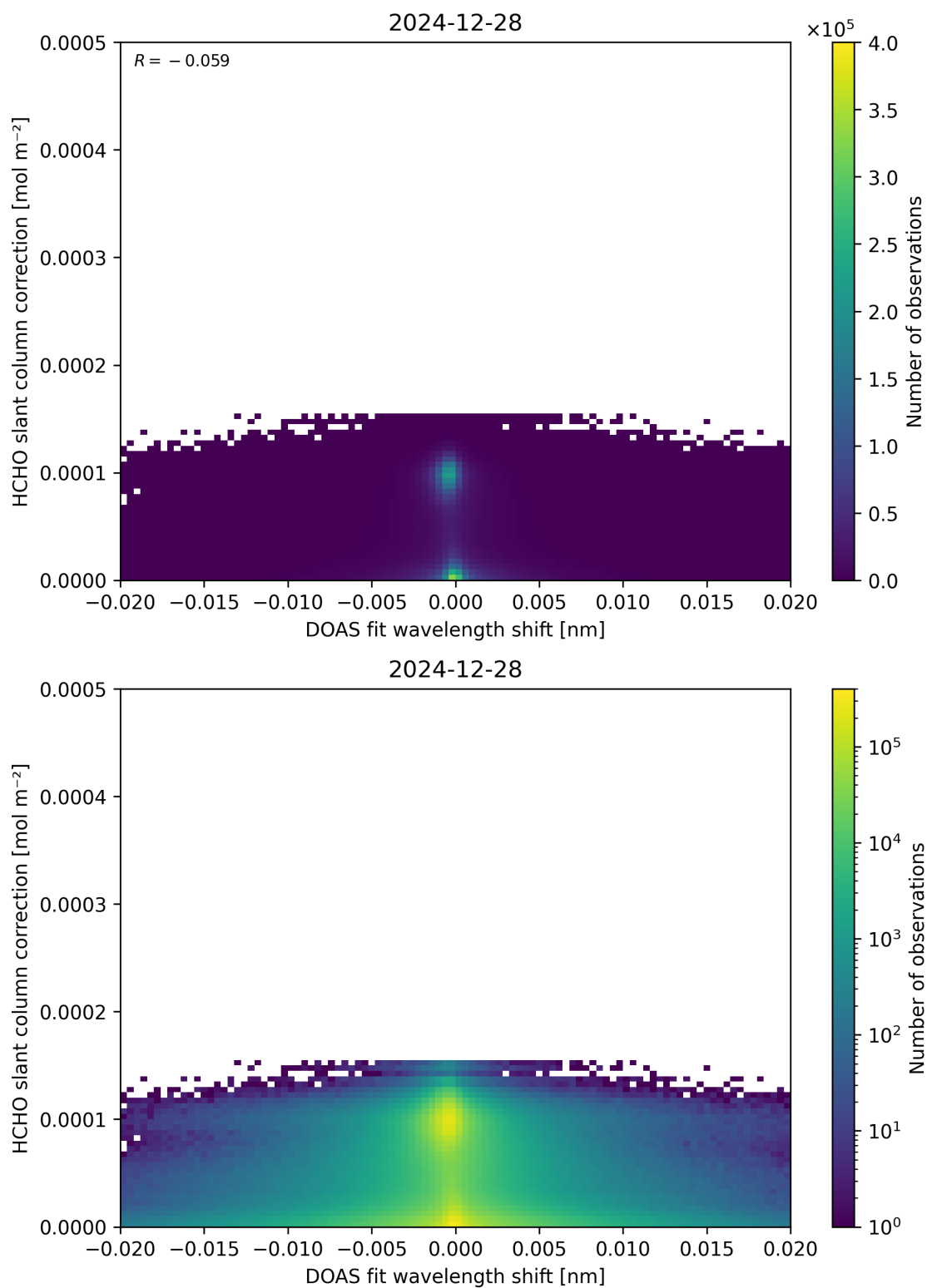
Figure 67: Scatter density plot of “DOAS fit wavelength shift” against “HCHO slant column correction” for 2024-12-27 to 2024-12-29.
