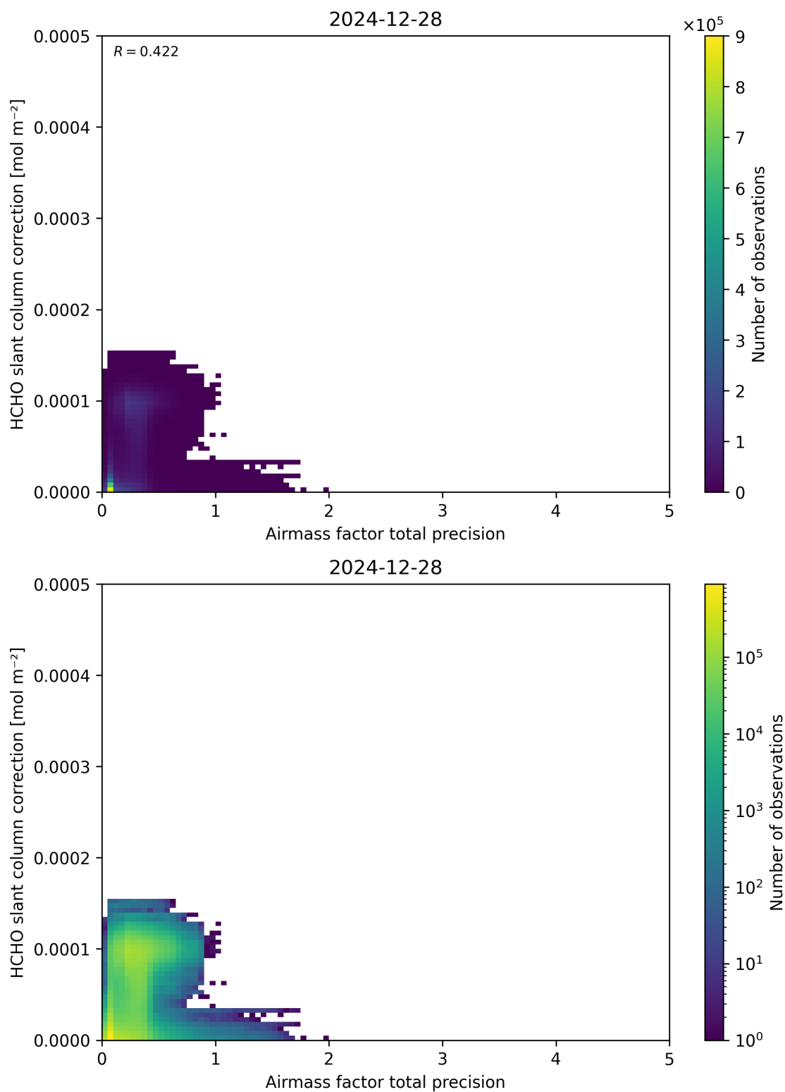
Figure 110: Scatter density plot of “Airmass factor total precision” against “HCHO slant column correction” for 2024-12-27 to 2024-12-29.
