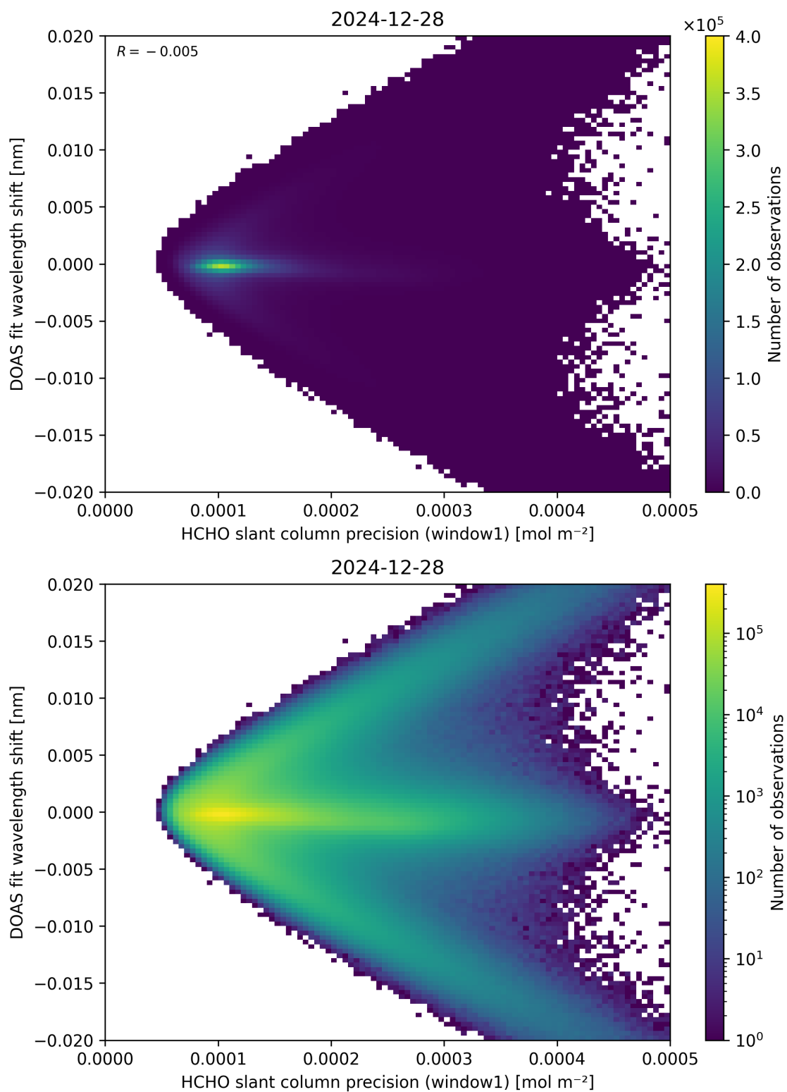
Figure 89: Scatter density plot of “HCHO slant column precision (window1)” against “DOAS fit wavelength shift” for 2024-12-27 to 2024-12-29.
