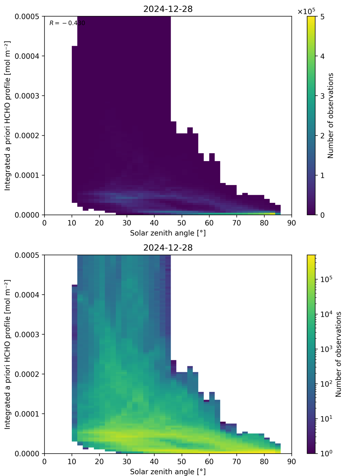
Figure 180: Scatter density plot of “Solar zenith angle” against “Integrated a priori HCHO profile” for 2024-12-27 to 2024-12-29.
