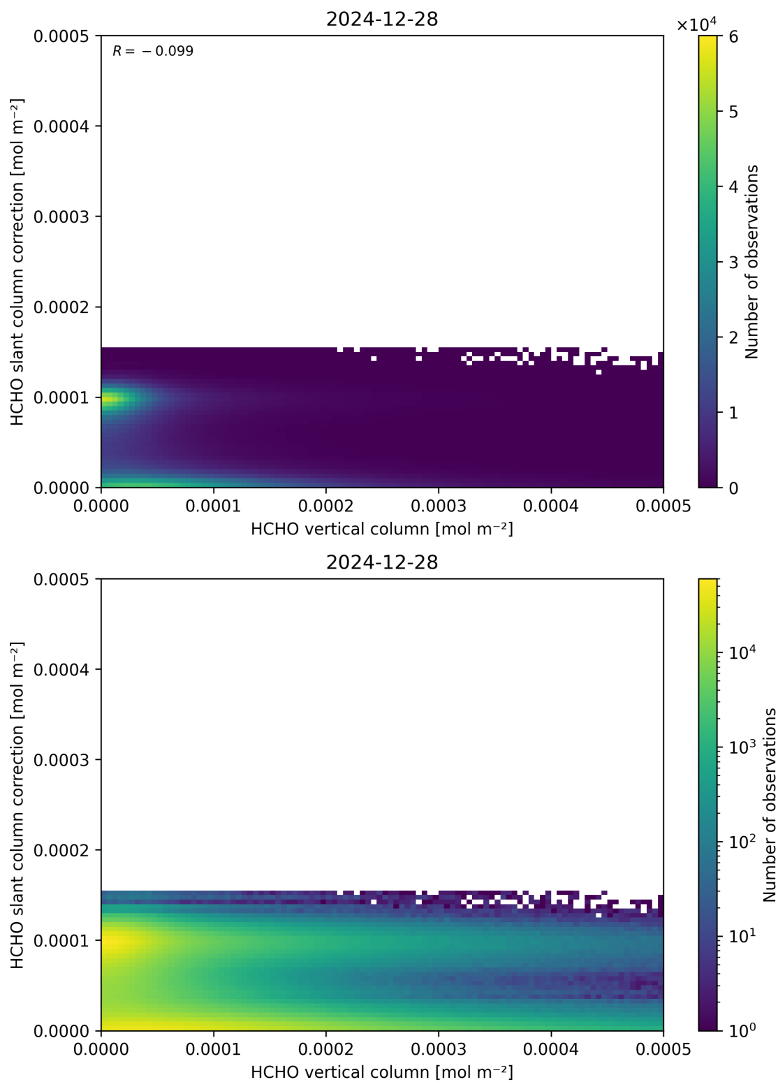
Figure 128: Scatter density plot of “HCHO vertical column” against “HCHO slant column correction” for 2024-12-27 to 2024-12-29.
