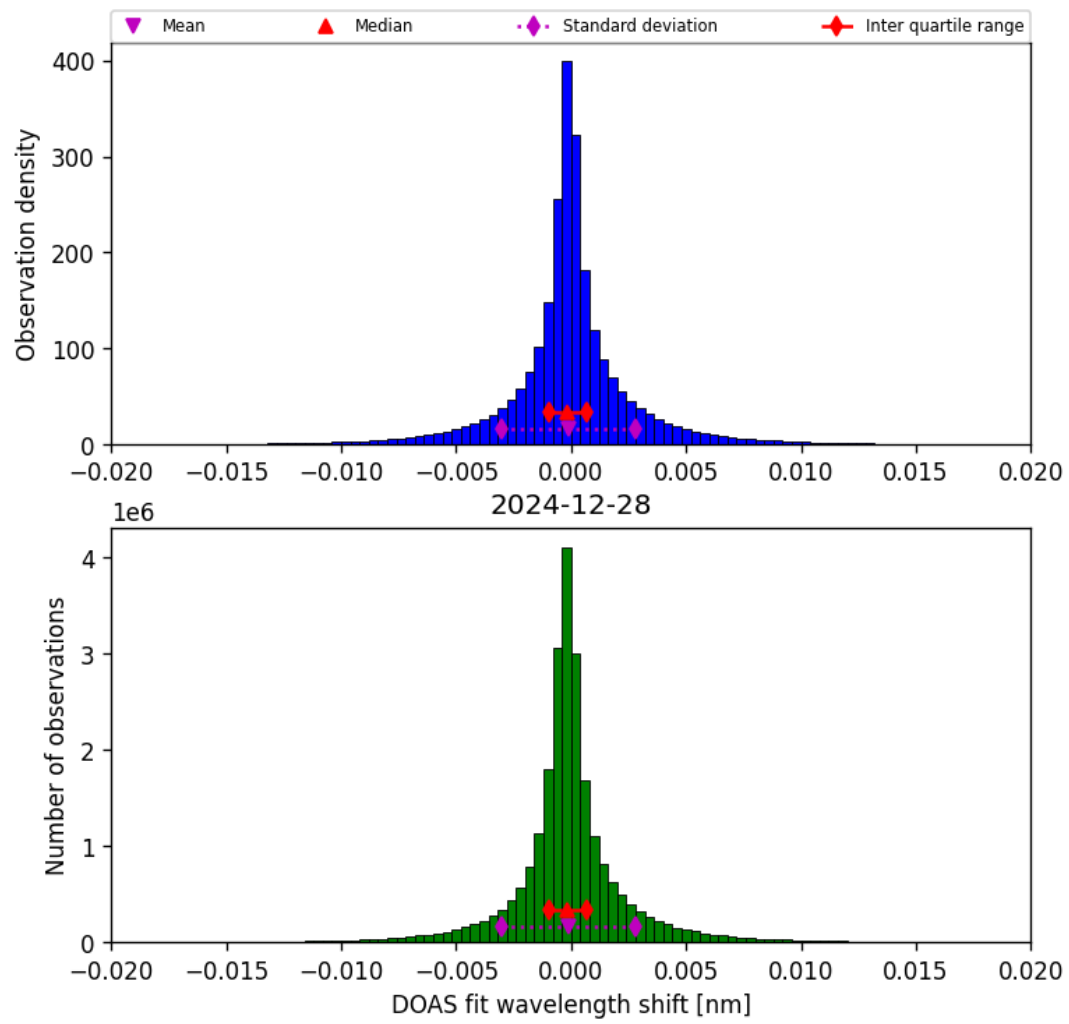
Figure 44: Histogram of “DOAS fit wavelength shift” for 2024-12-27 to 2024-12-29
