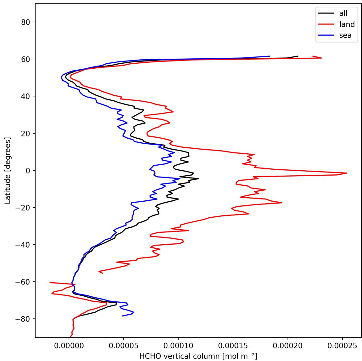
Figure 21: Zonal average of “HCHO vertical column” for 2024-12-27 to 2024-12-29.
