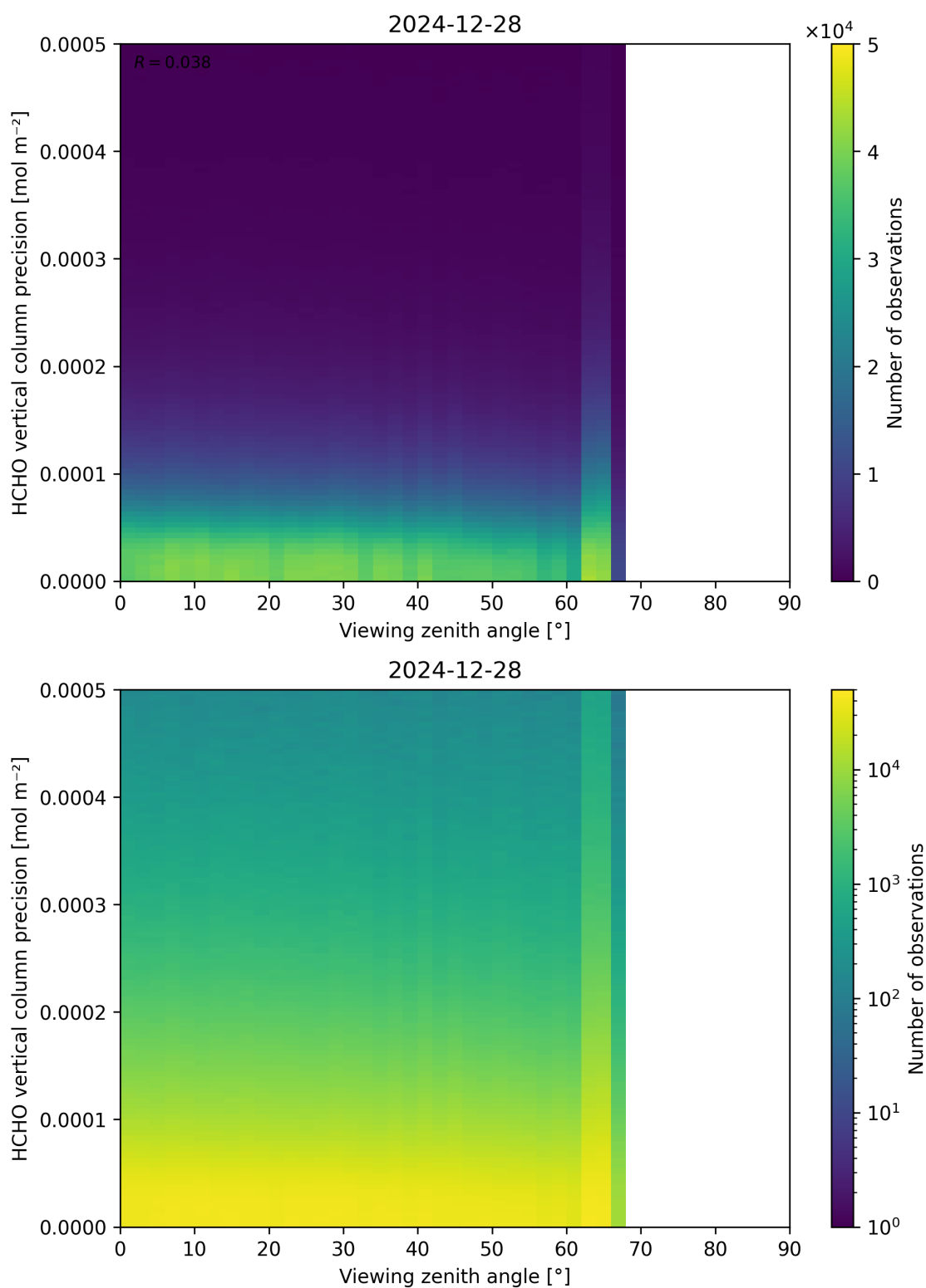
Figure 194: Scatter density plot of “Viewing zenith angle” against “HCHO vertical column precision” for 2024-12-27 to 2024-12-29.
