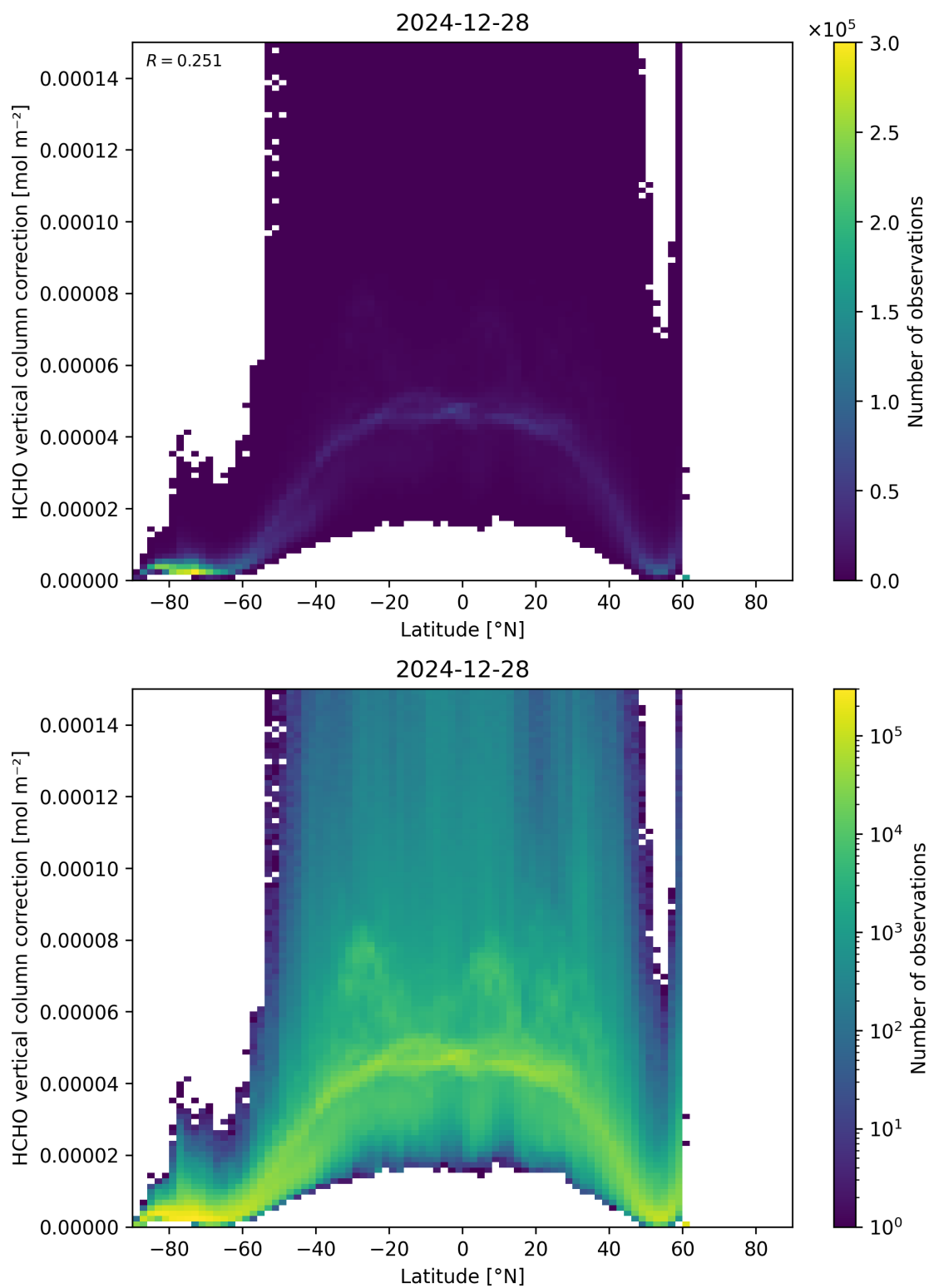
Figure 164: Scatter density plot of “Latitude” against “HCHO vertical column correction” for 2024-12-27 to 2024-12-29.
