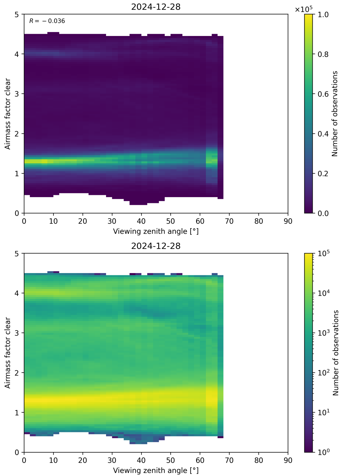
Figure 185: Scatter density plot of “Viewing zenith angle” against “Airmass factor clear” for 2024-12-27 to 2024-12-29.
