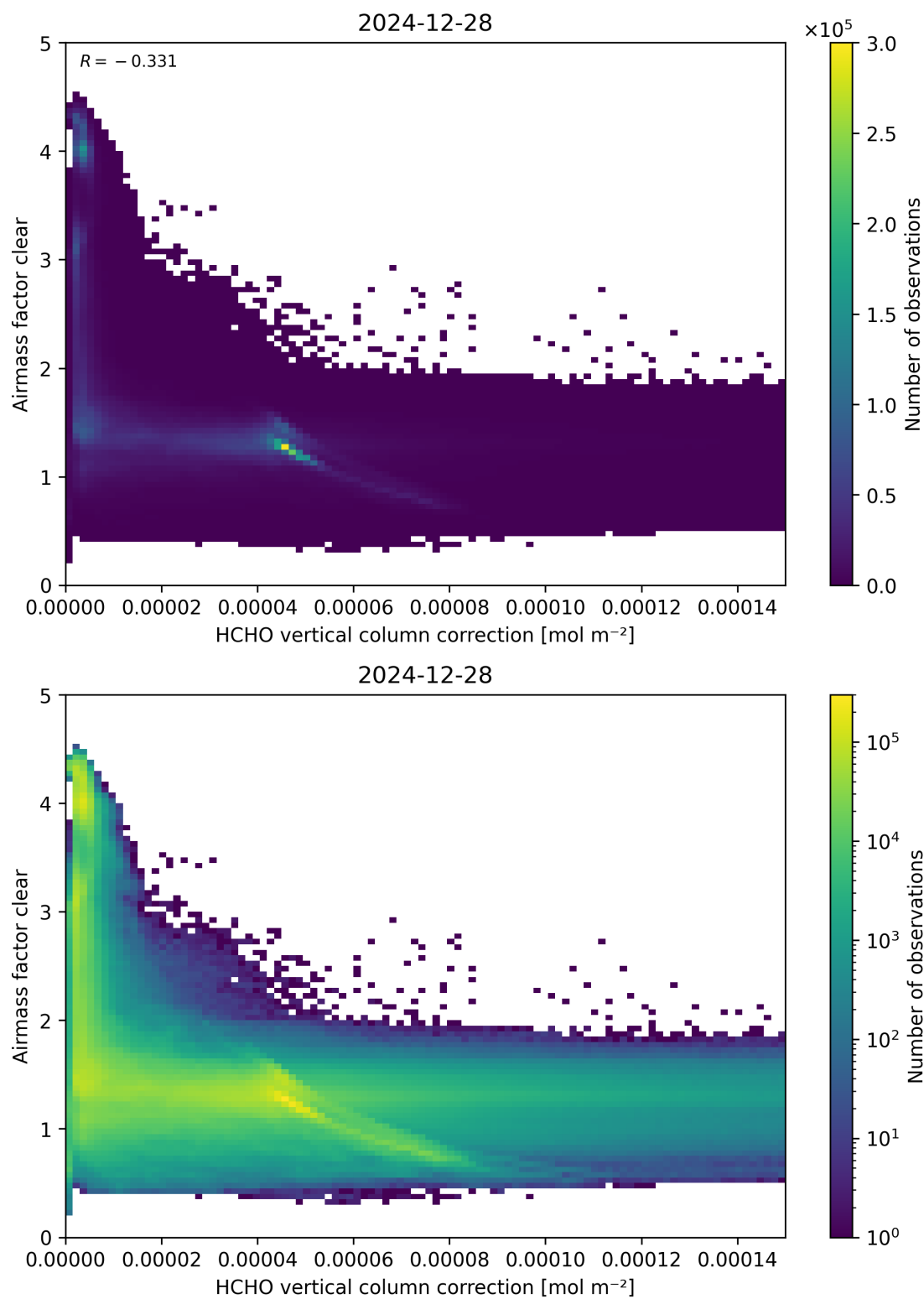
Figure 115: Scatter density plot of “HCHO vertical column correction” against “Airmass factor clear” for 2024-12-27 to 2024-12-29.
