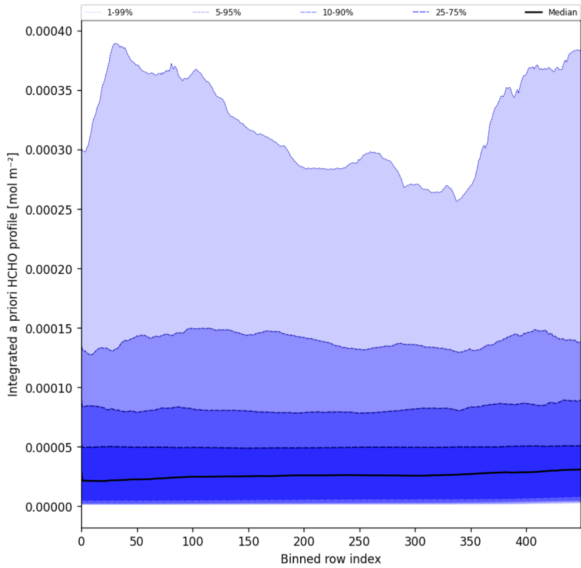
Figure 57: Along track statistics of "Integrated a priori HCHO profile" for 2024-12-27 to 2024-12-29
