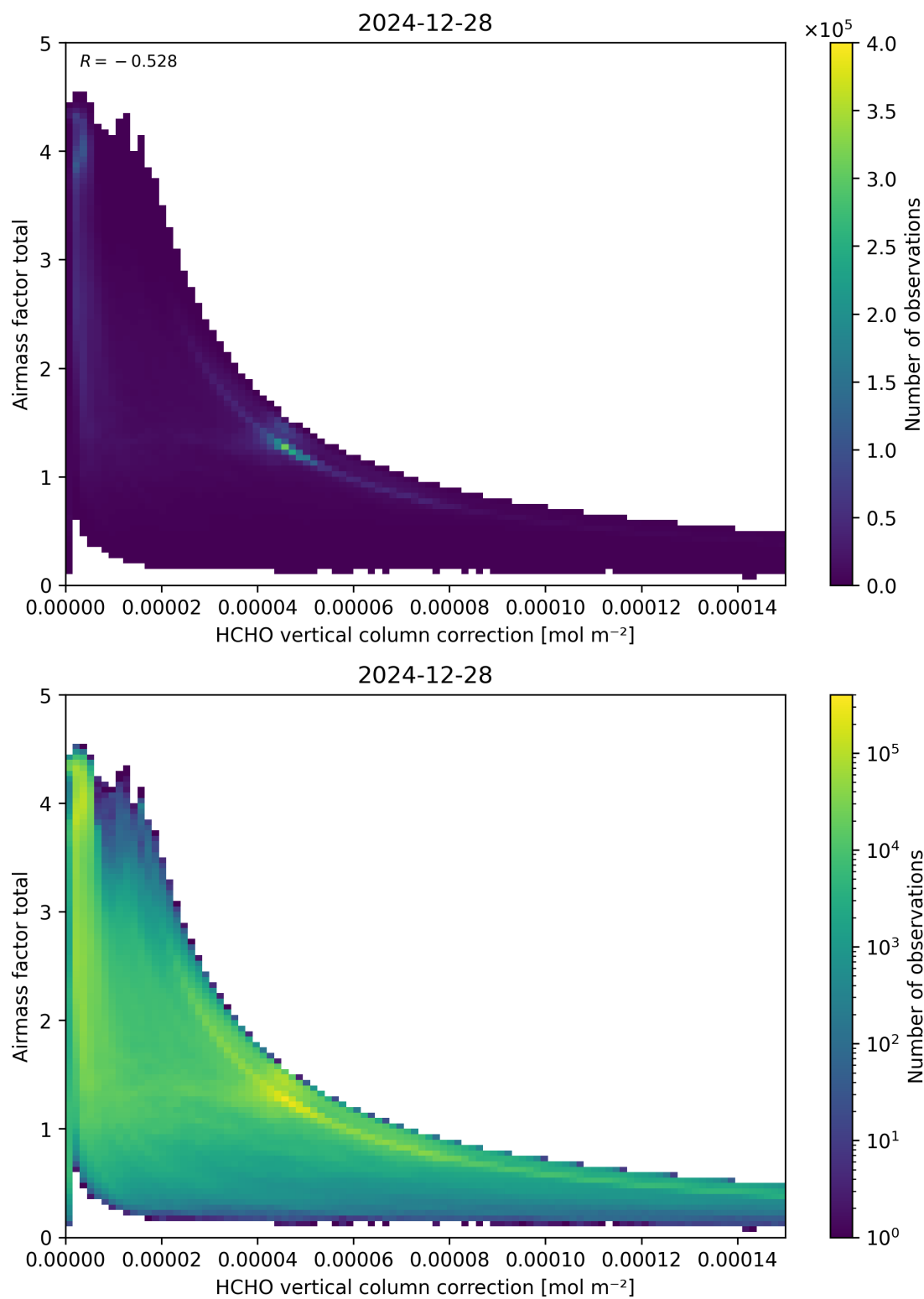
Figure 120: Scatter density plot of “HCHO vertical column correction” against “Airmass factor total” for 2024-12-27 to 2024-12-29.
