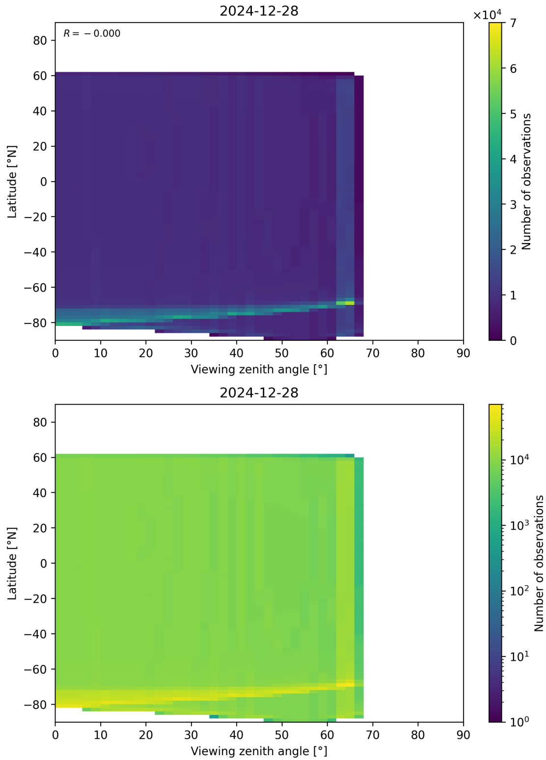
Figure 196: Scatter density plot of “Viewing zenith angle” against “Latitude” for 2024-12-27 to 2024-12-29.
