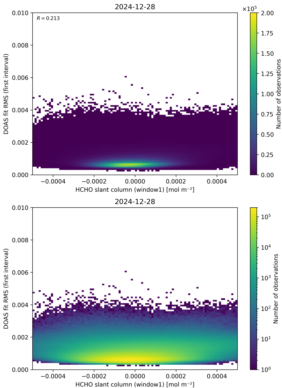
Figure 78: Scatter density plot of “HCHO slant column (window1)” against “DOAS fit RMS (first interval)” for 2024-12-27 to 2024-12-29.
