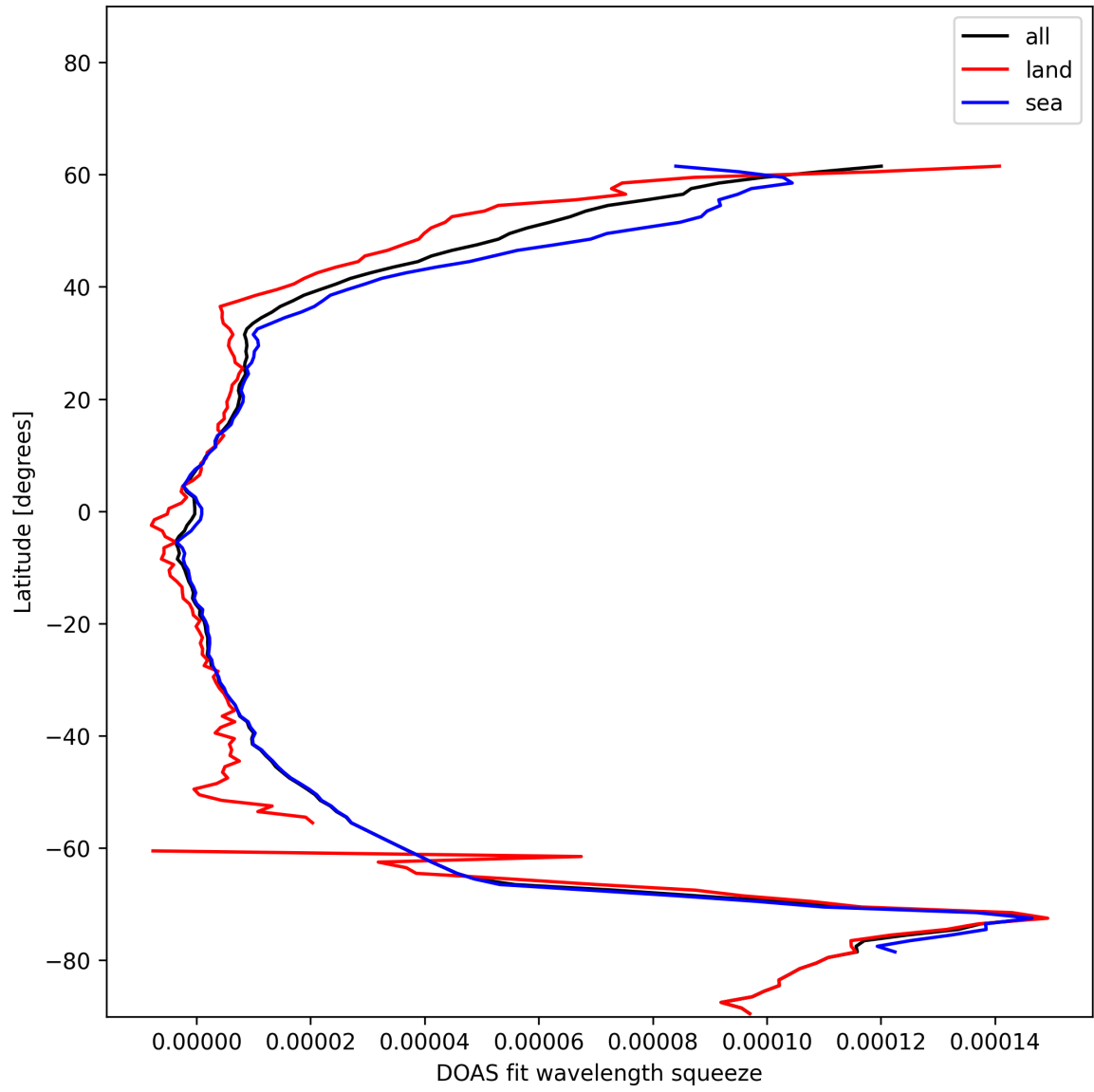
Figure 31: Zonal average of “DOAS fit wavelength squeeze” for 2024-12-27 to 2024-12-29.
