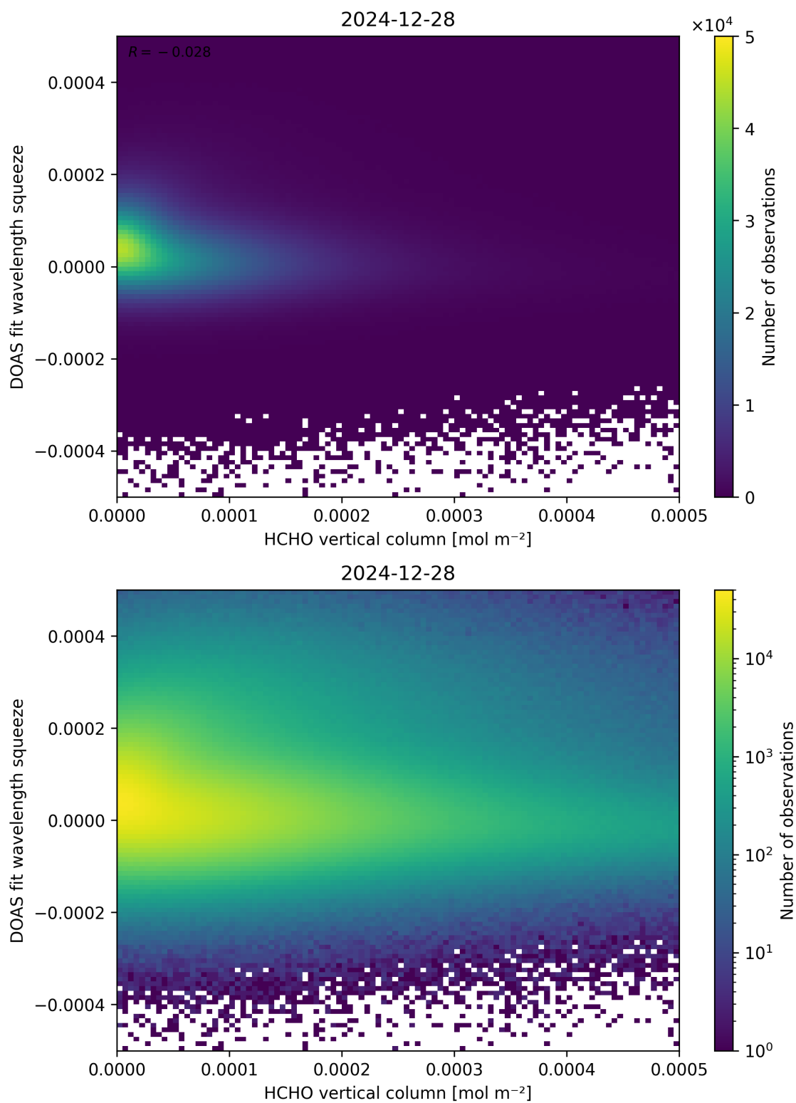
Figure 125: Scatter density plot of “HCHO vertical column” against “DOAS fit wavelength squeeze” for 2024-12-27 to 2024-12-29.
