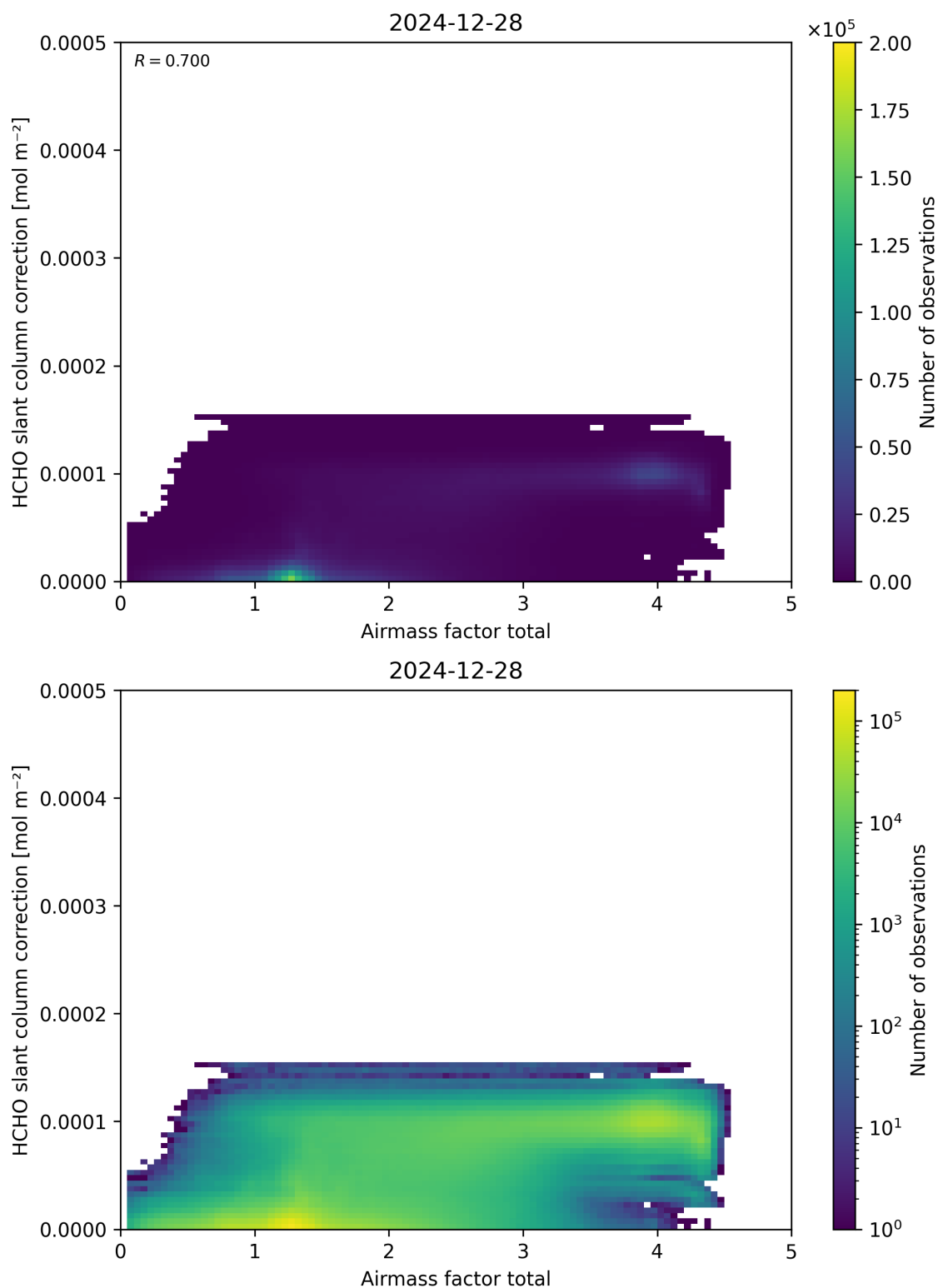
Figure 102: Scatter density plot of “Airmass factor total” against “HCHO slant column correction” for 2024-12-27 to 2024-12-29.
