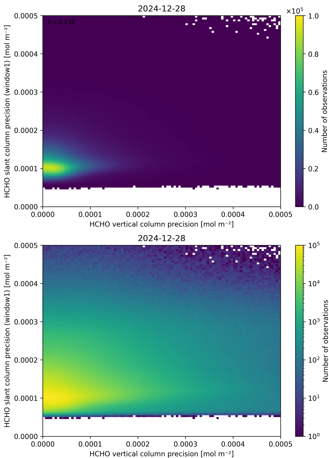
Figure 143: Scatter density plot of “HCHO vertical column precision” against “HCHO slant column precision (window1)” for 2024-12-27 to 2024-12-29.
