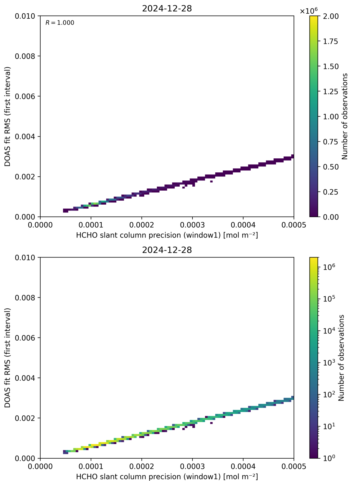
Figure 88: Scatter density plot of “HCHO slant column precision (window1)” against “DOAS fit RMS (first interval)” for 2024-12-27 to 2024-12-29.
