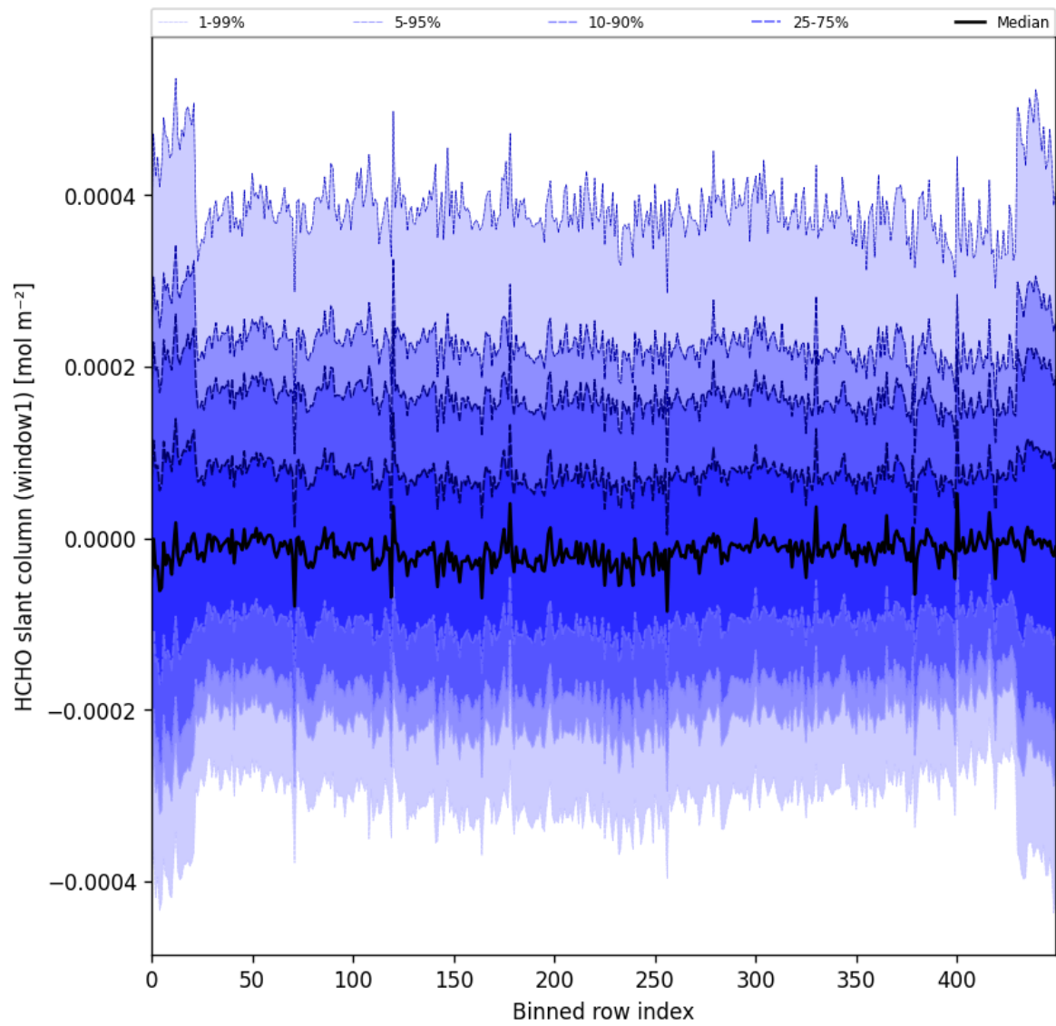
Figure 52: Along track statistics of “HCHO slant column (window1)” for 2024-12-27 to 2024-12-29
