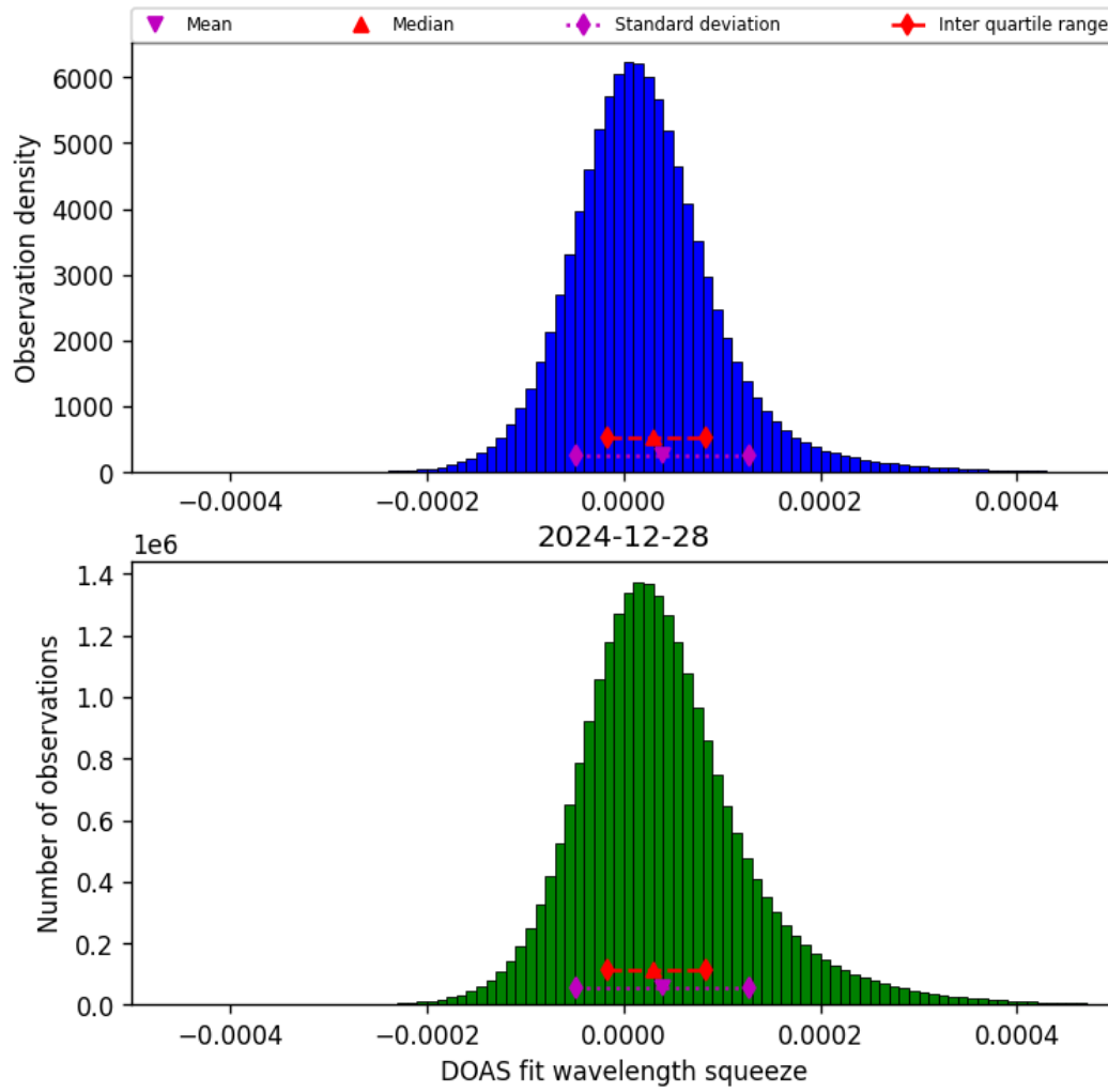
Figure 45: Histogram of “DOAS fit wavelength squeeze” for 2024-12-27 to 2024-12-29
