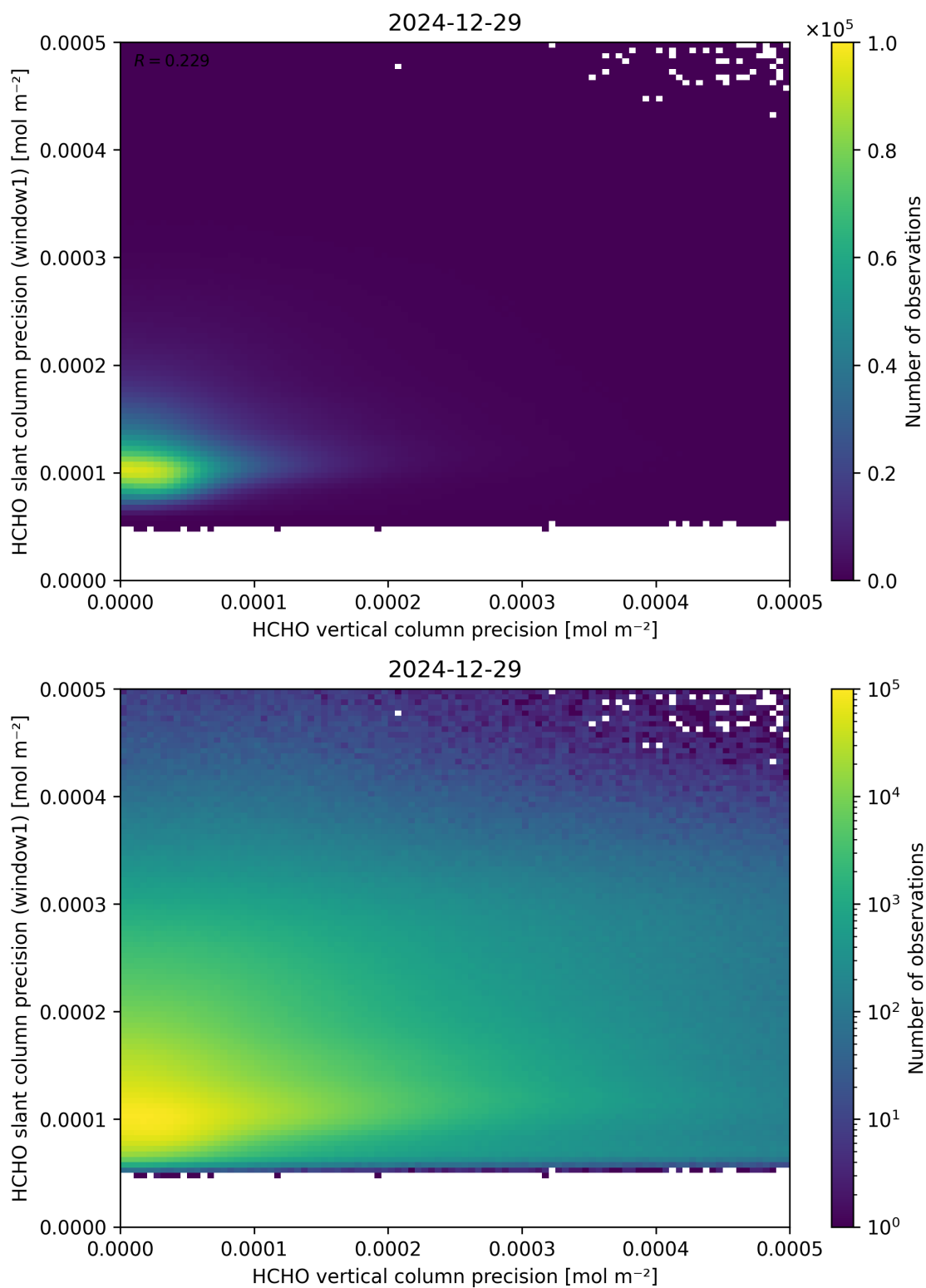
Figure 143: Scatter density plot of “HCHO vertical column precision” against “HCHO slant column precision (window1)” for 2024-12-28 to 2024-12-30.
