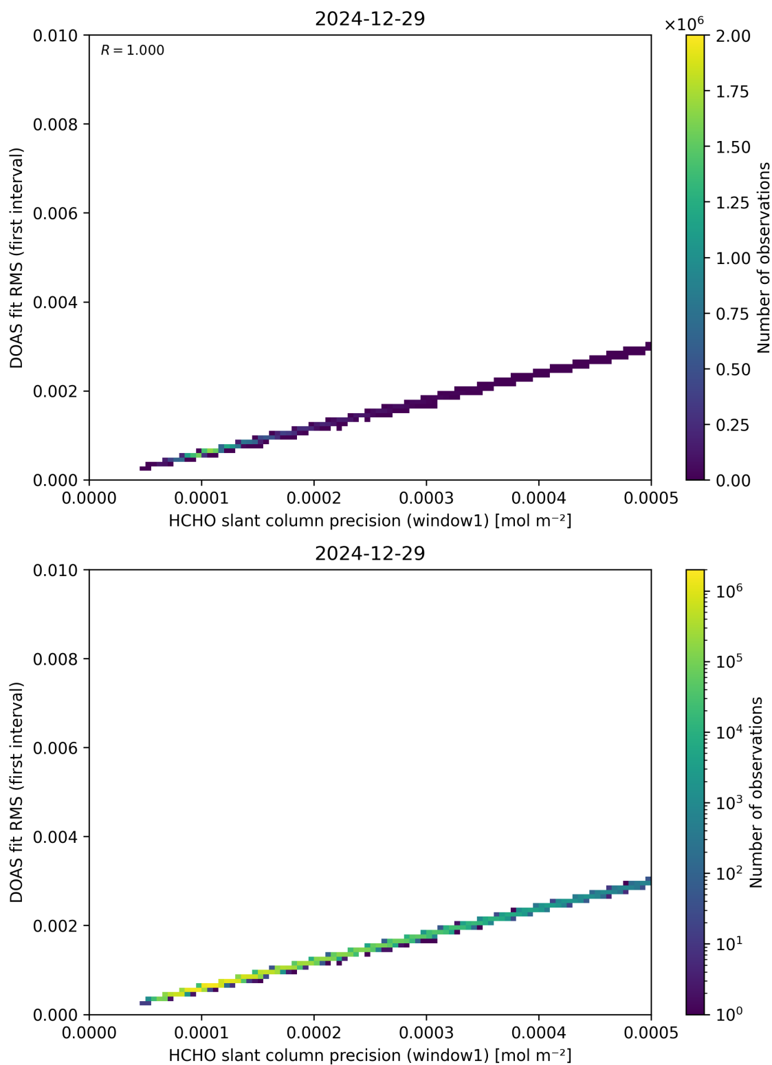
Figure 88: Scatter density plot of “HCHO slant column precision (window1)” against “DOAS fit RMS (first interval)” for 2024-12-28 to 2024-12-30.
