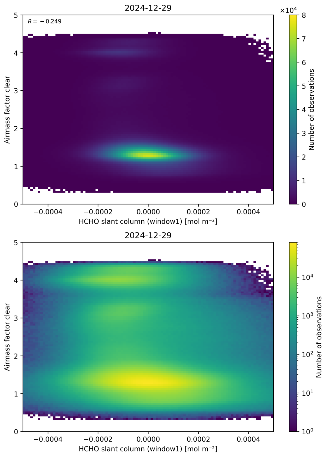
Figure 81: Scatter density plot of “HCHO slant column (window1)” against “Airmass factor clear” for 2024-12-28 to 2024-12-30.
