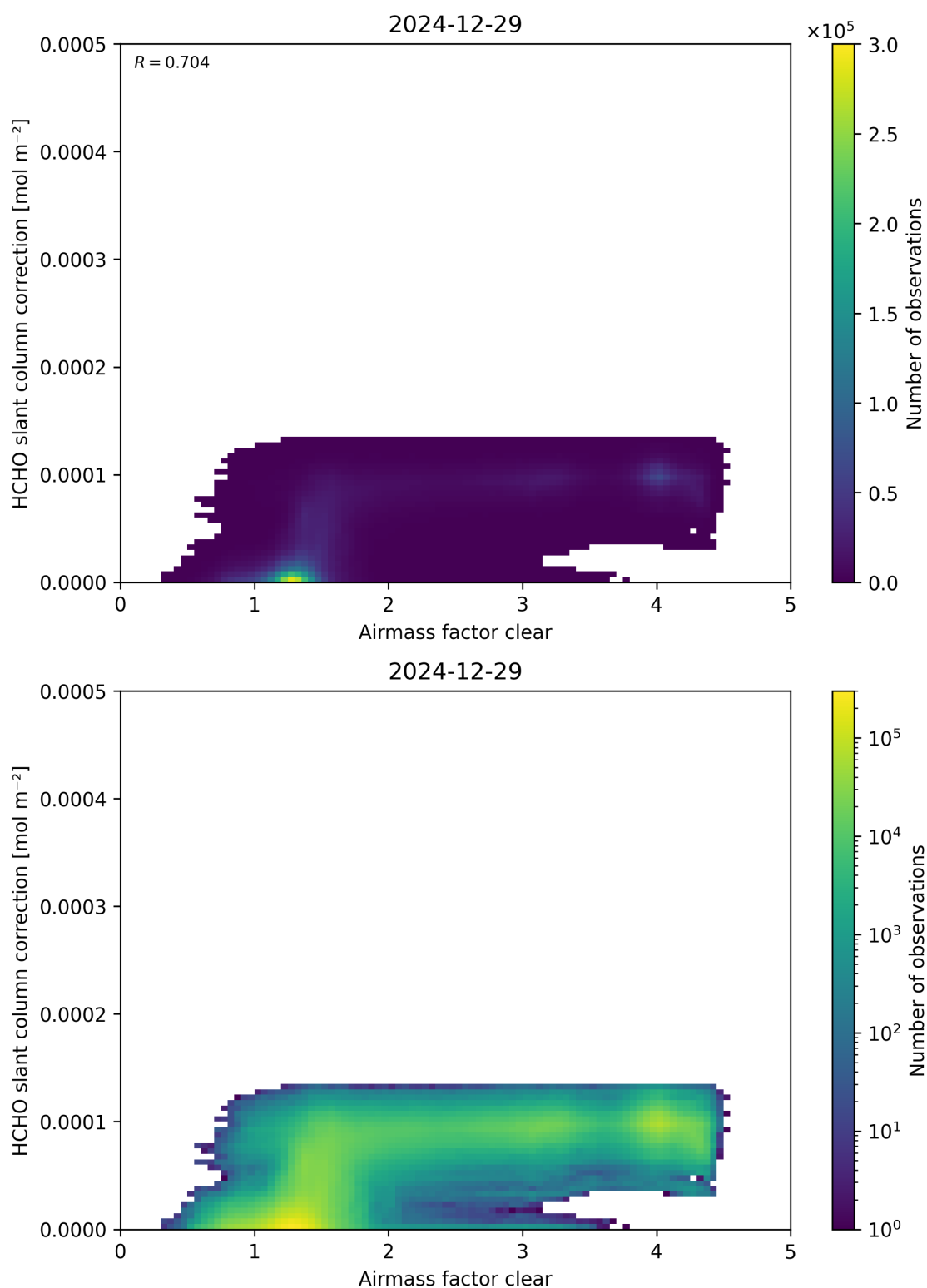
Figure 75: Scatter density plot of “Airmass factor clear” against “HCHO slant column correction” for 2024-12-28 to 2024-12-30.
