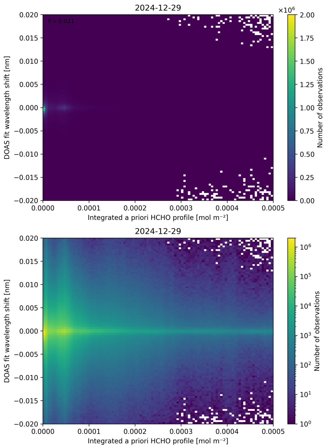
Figure 149: Scatter density plot of “Integrated a priori HCHO profile” against “DOAS fit wavelength shift” for 2024-12-28 to 2024-12-30.
