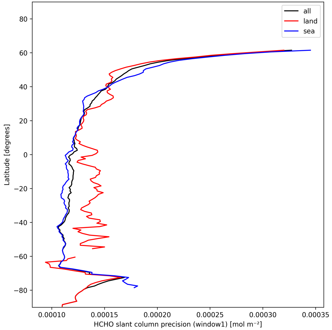
Figure 25: Zonal average of “HCHO slant column precision (window1)” for 2024-12-28 to 2024-12-30.
