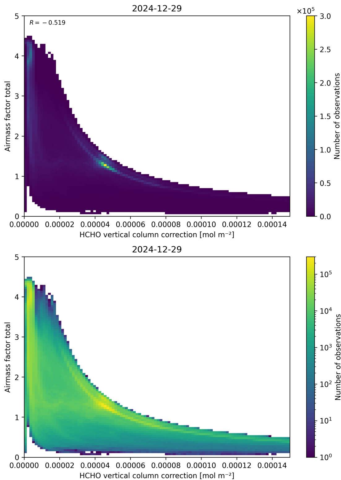
Figure 120: Scatter density plot of “HCHO vertical column correction” against “Airmass factor total” for 2024-12-28 to 2024-12-30.
