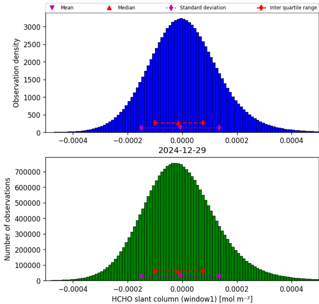
Figure 38: Histogram of “HCHO slant column (window1)” for 2024-12-28 to 2024-12-30
