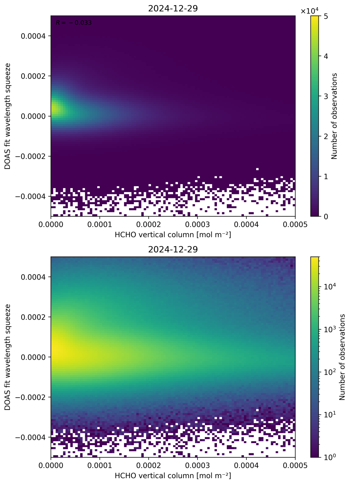
Figure 125: Scatter density plot of “HCHO vertical column” against “DOAS fit wavelength squeeze” for 2024-12-28 to 2024-12-30.
