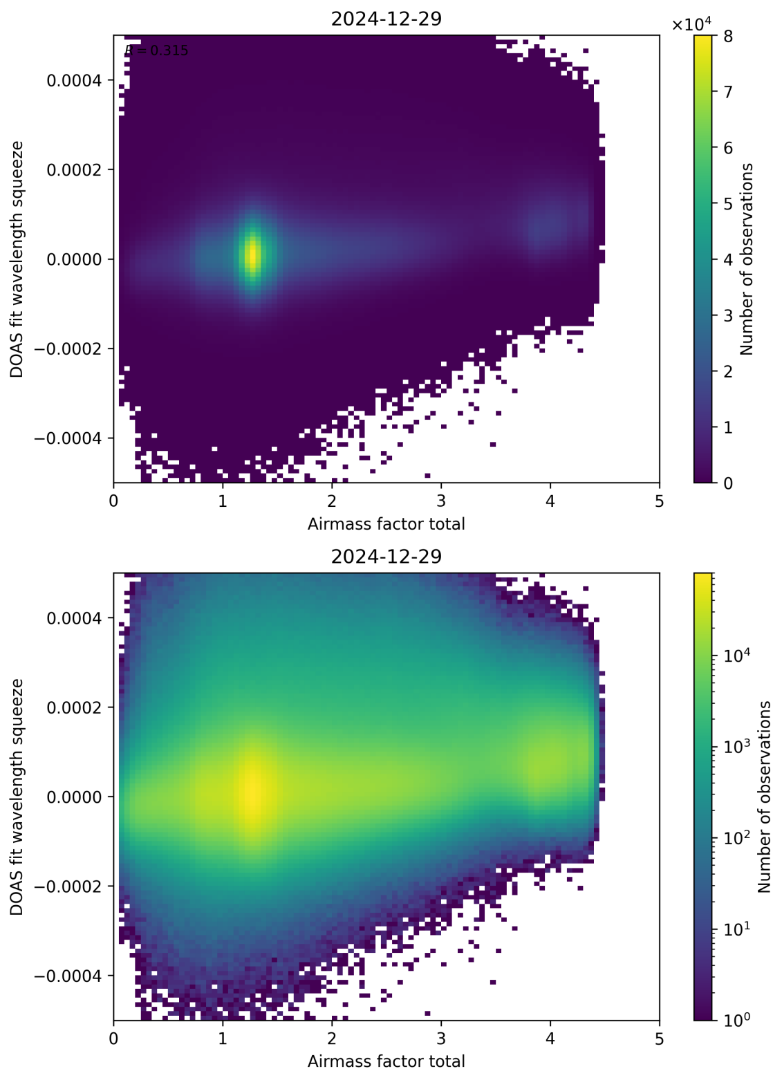
Figure 99: Scatter density plot of “Airmass factor total” against “DOAS fit wavelength squeeze” for 2024-12-28 to 2024-12-30.
