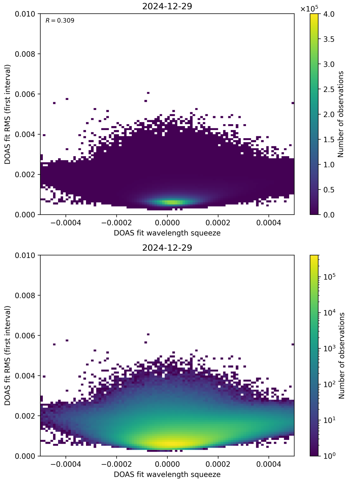
Figure 68: Scatter density plot of “DOAS fit wavelength squeeze” against “DOAS fit RMS (first interval)” for 2024-12-28 to 2024-12-30.
