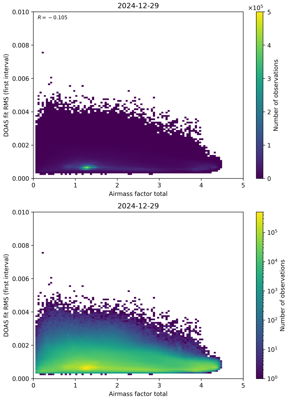
Figure 97: Scatter density plot of “Airmass factor total” against “DOAS fit RMS (first interval)” for 2024-12-28 to 2024-12-30.
