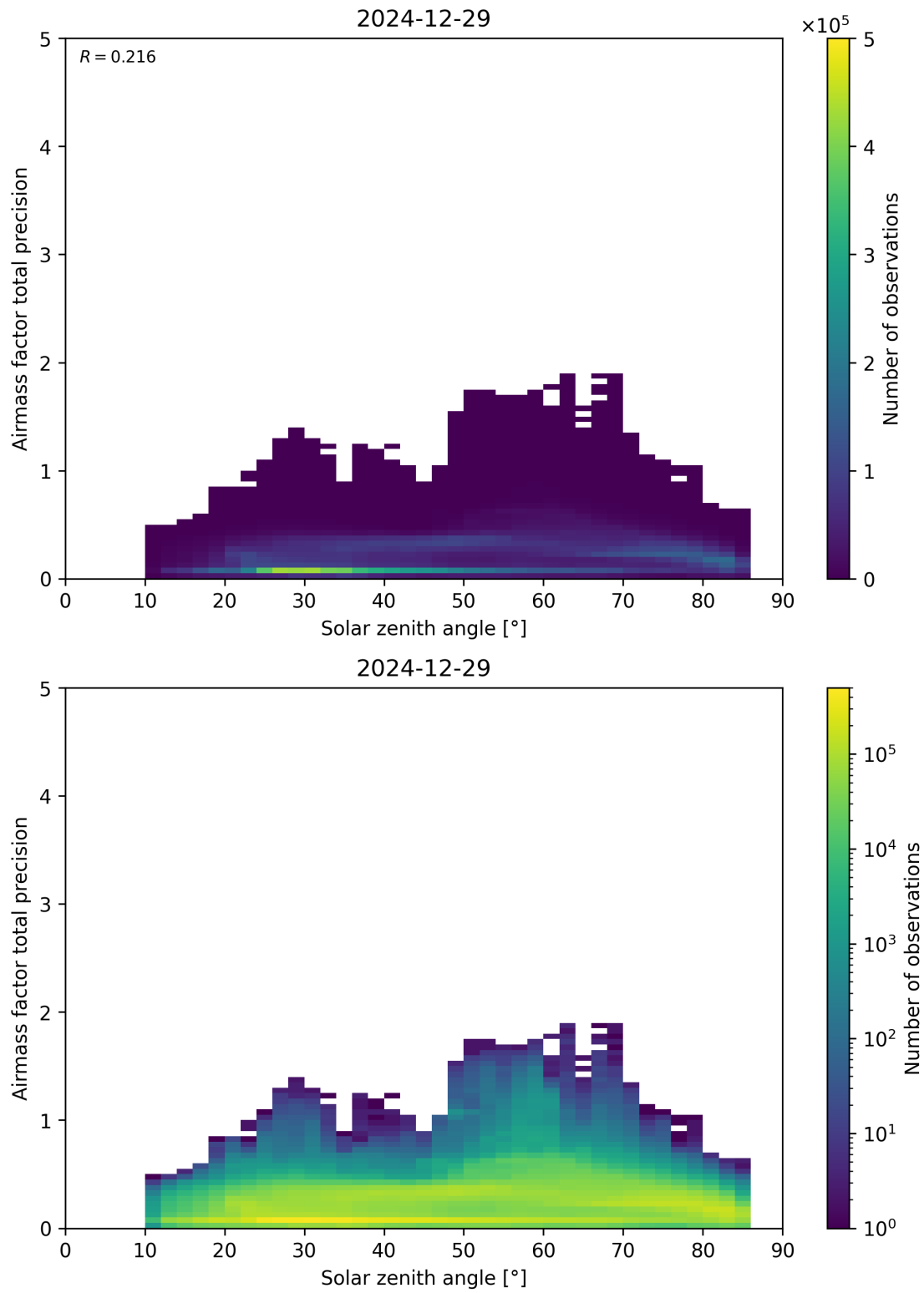
Figure 176: Scatter density plot of “Solar zenith angle” against “Airmass factor total precision” for 2024-12-28 to 2024-12-30.
