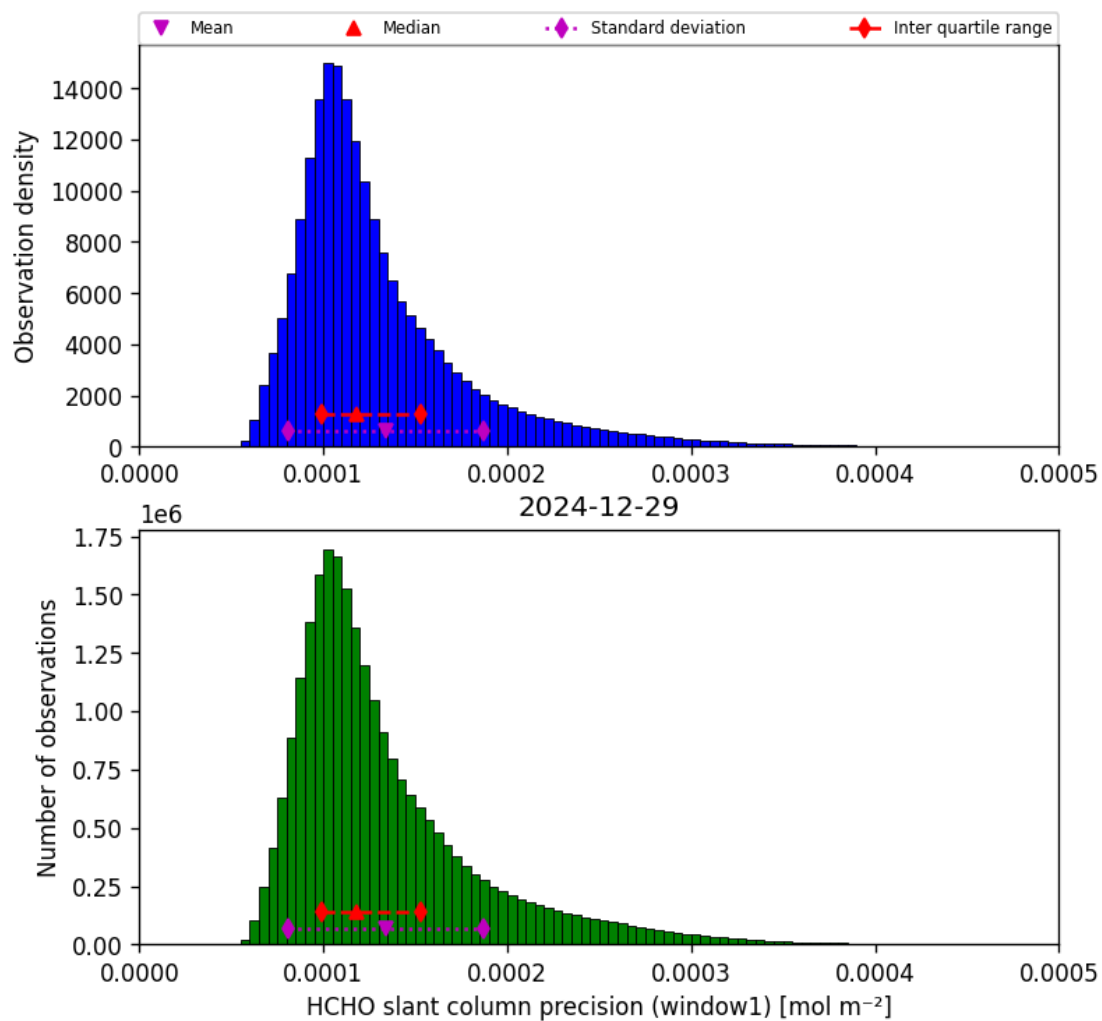
Figure 39: Histogram of “HCHO slant column precision (window1)” for 2024-12-28 to 2024-12-30
