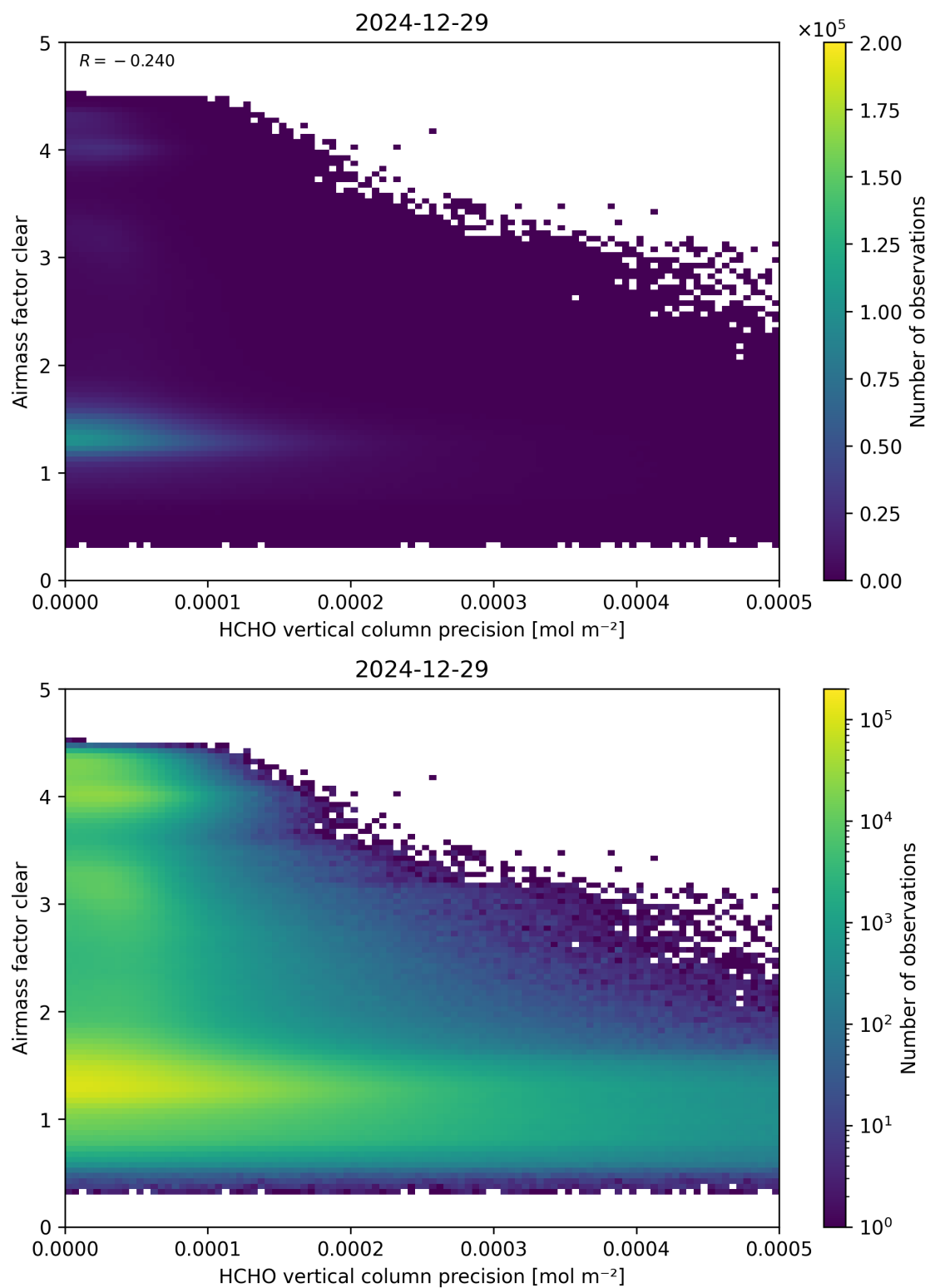
Figure 139: Scatter density plot of “HCHO vertical column precision” against “Airmass factor clear” for 2024-12-28 to 2024-12-30.
