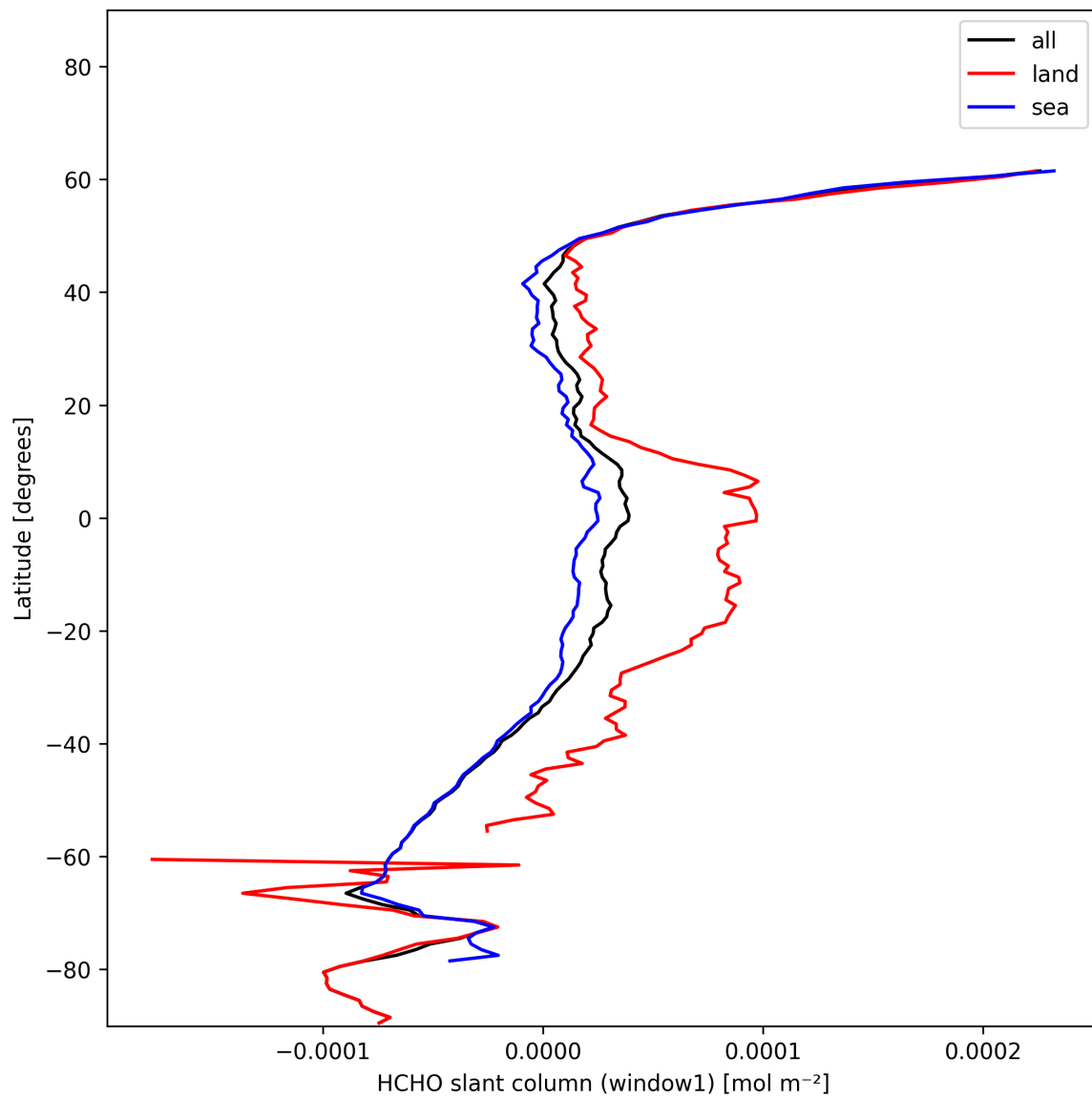
Figure 24: Zonal average of “HCHO slant column (window1)” for 2024-12-28 to 2024-12-30.
