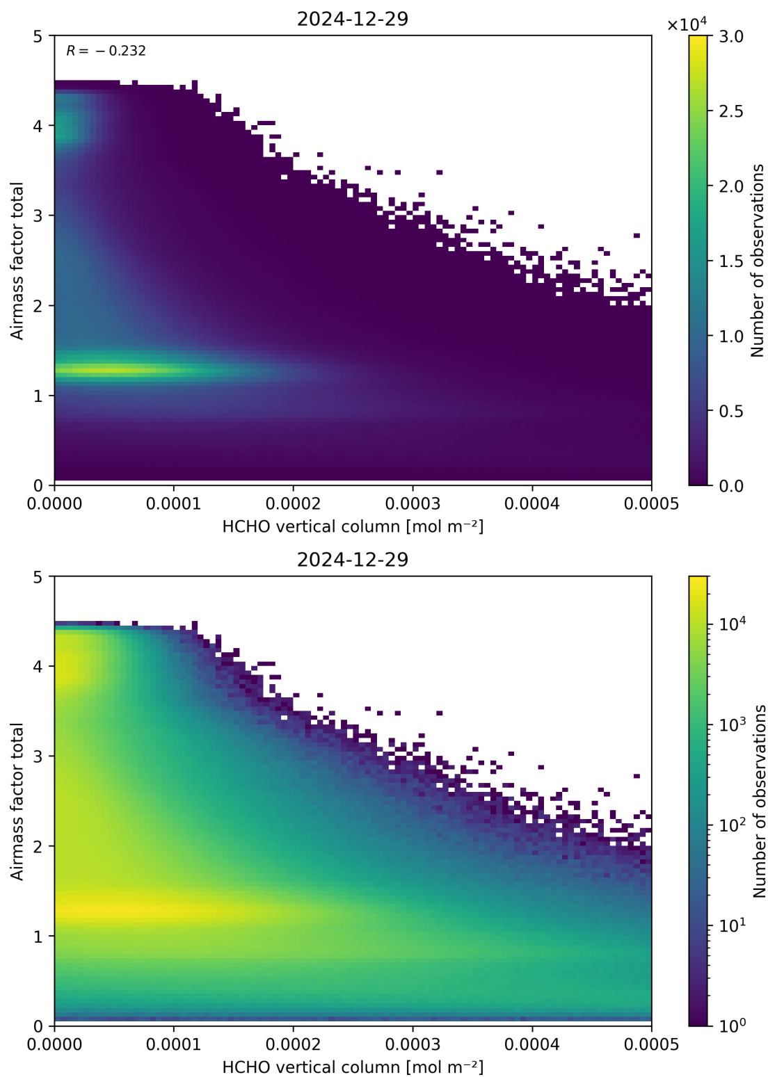
Figure 131: Scatter density plot of “HCHO vertical column” against “Airmass factor total” for 2024-12-28 to 2024-12-30.
