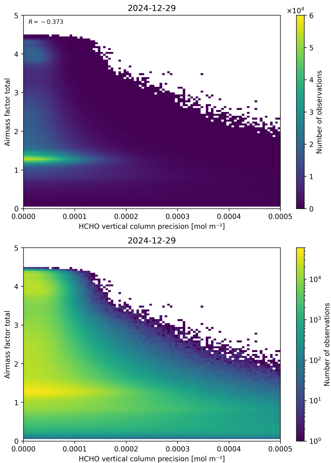
Figure 144: Scatter density plot of “HCHO vertical column precision” against “Airmass factor total” for 2024-12-28 to 2024-12-30.
