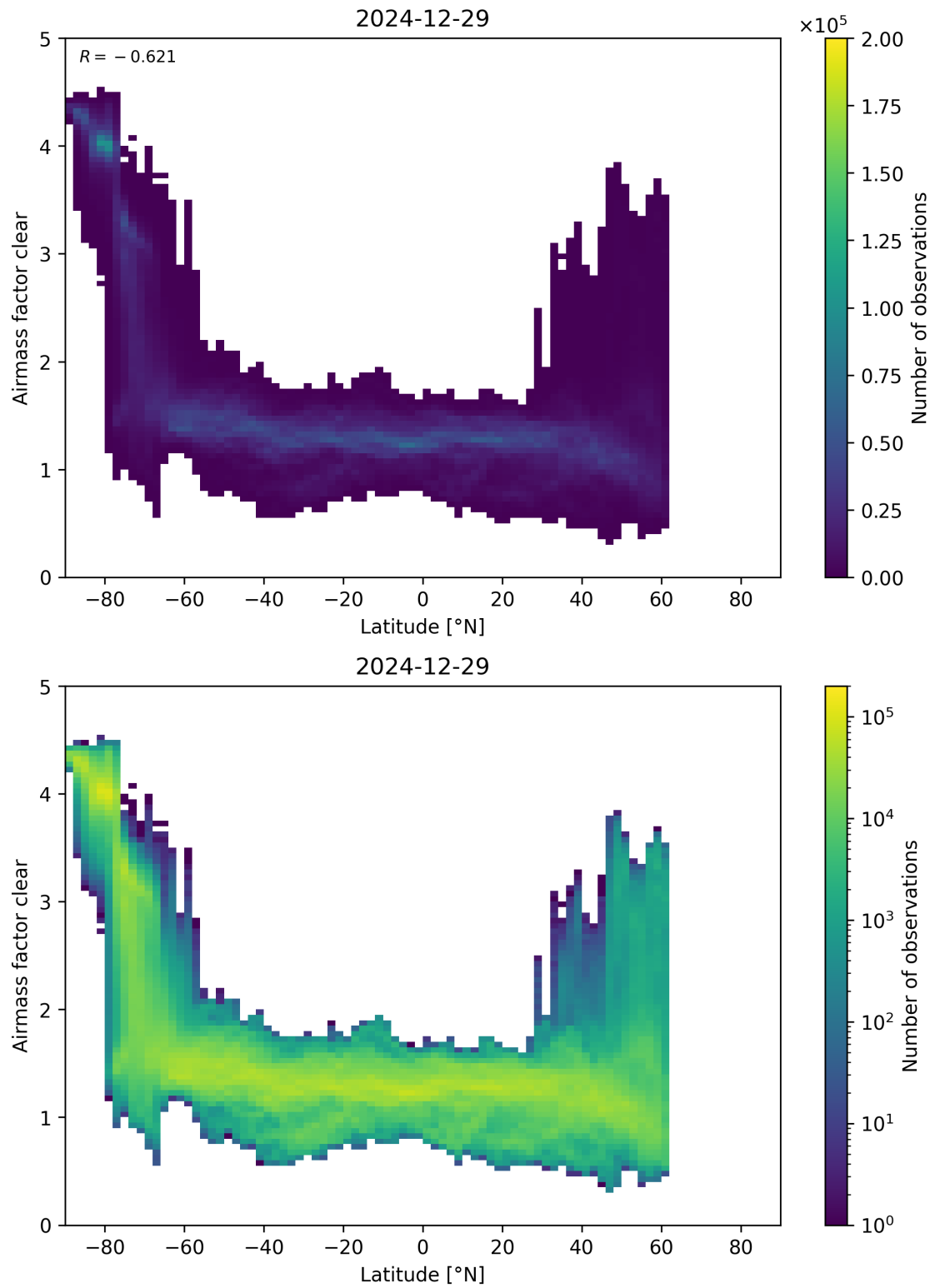
Figure 156: Scatter density plot of “Latitude” against “Airmass factor clear” for 2024-12-28 to 2024-12-30.
