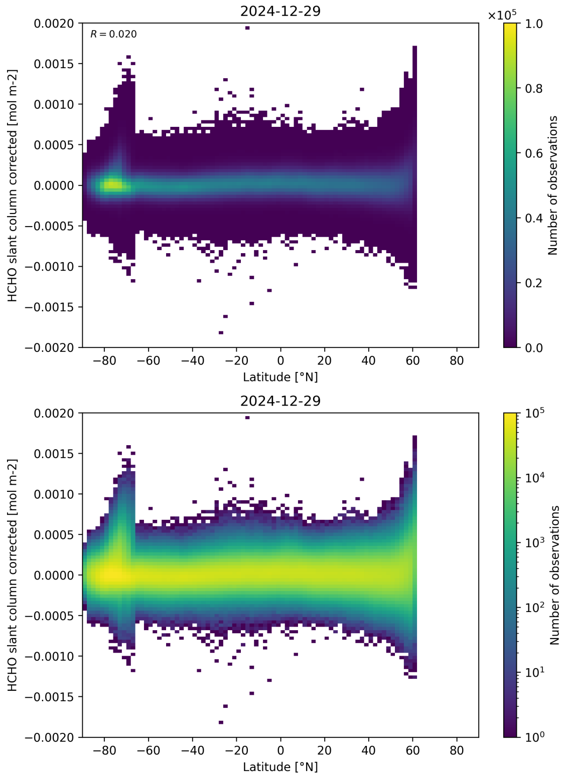
Figure 157: Scatter density plot of “Latitude” against “HCHO slant column corrected” for 2024-12-28 to 2024-12-30.
