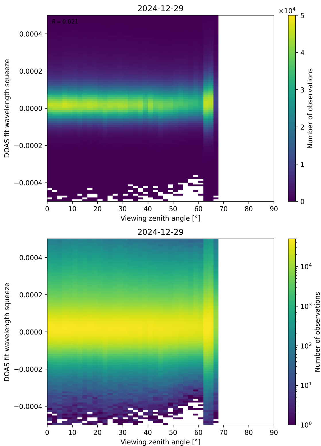
Figure 184: Scatter density plot of “Viewing zenith angle” against “DOAS fit wavelength squeeze” for 2024-12-28 to 2024-12-30.
