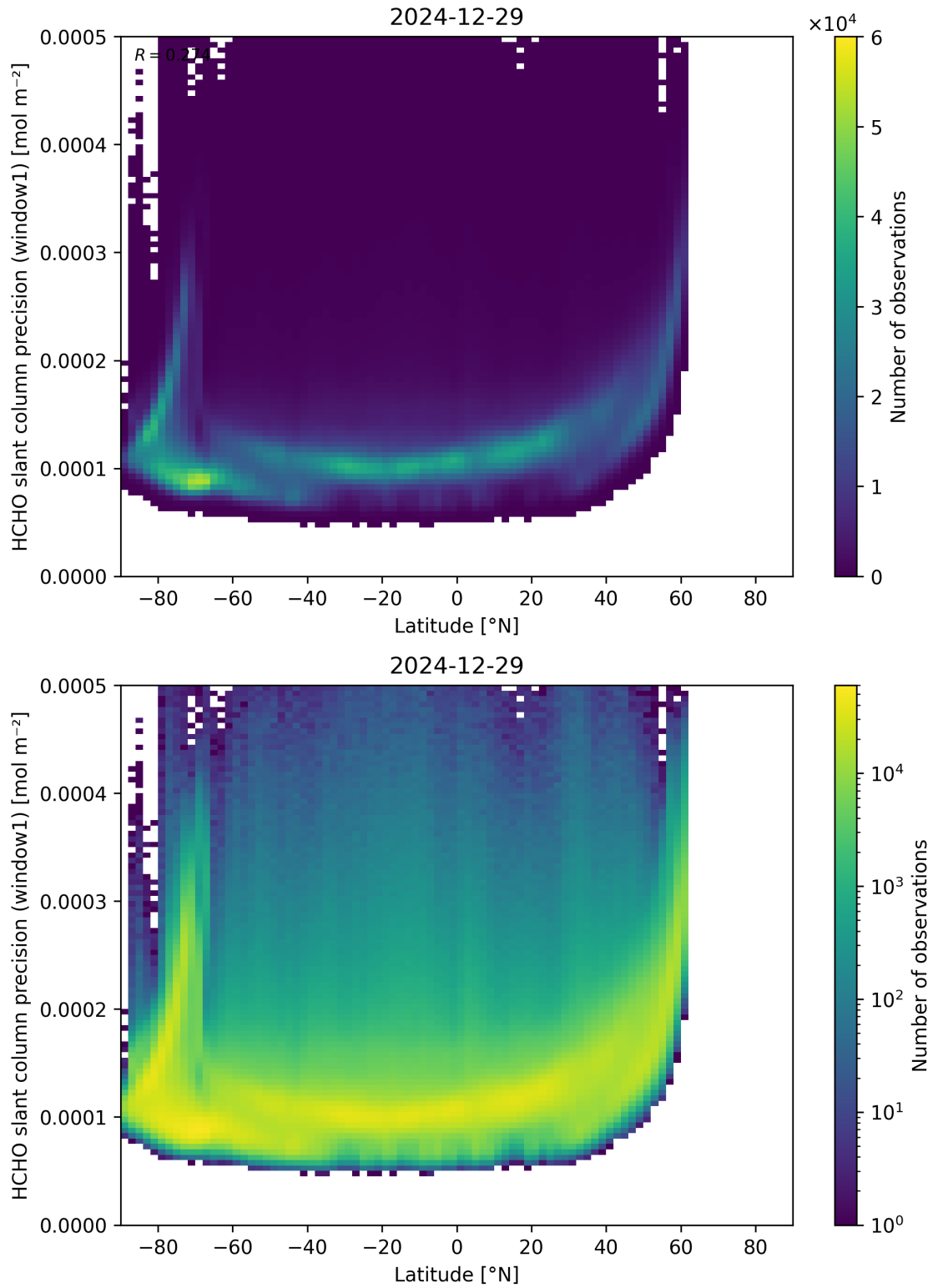
Figure 160: Scatter density plot of “Latitude” against “HCHO slant column precision (window1)” for 2024-12-28 to 2024-12-30.
