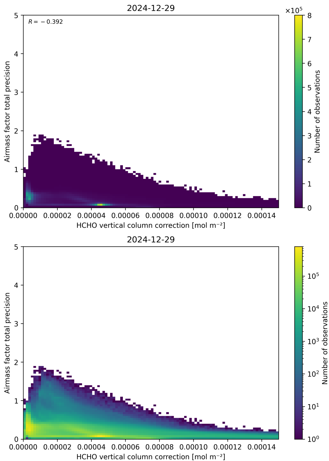
Figure 121: Scatter density plot of “HCHO vertical column correction” against “Airmass factor total precision” for 2024-12-28 to 2024-12-30.
