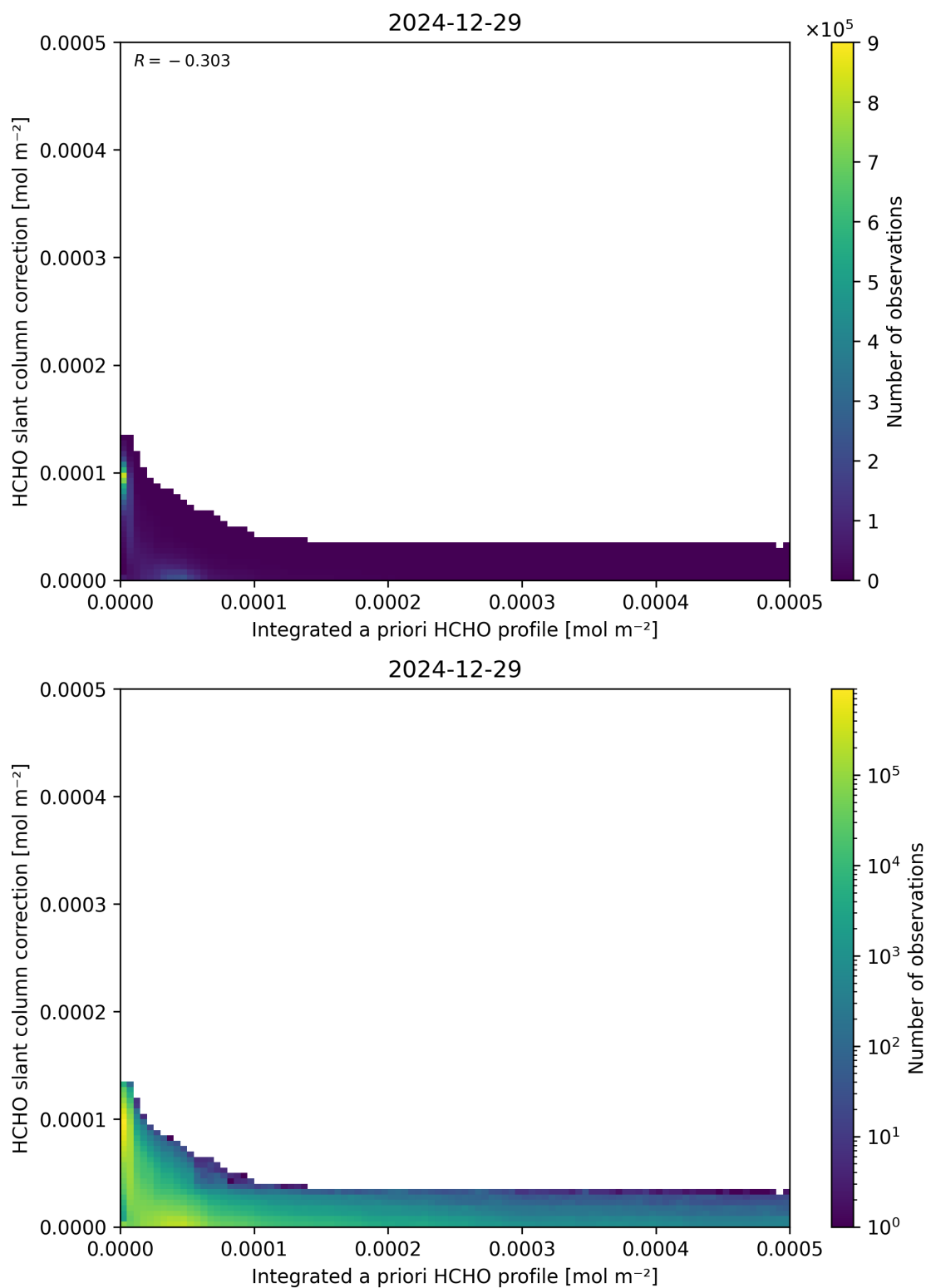
Figure 152: Scatter density plot of “Integrated a priori HCHO profile” against “HCHO slant column correction” for 2024-12-28 to 2024-12-30.
