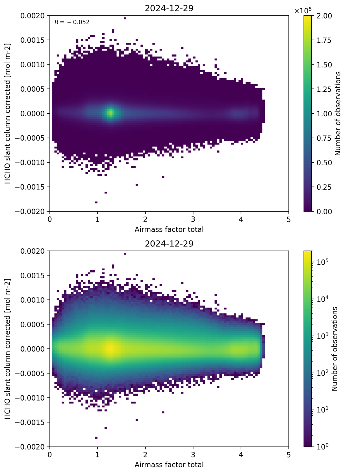
Figure 101: Scatter density plot of “Airmass factor total” against “HCHO slant column corrected” for 2024-12-28 to 2024-12-30.
