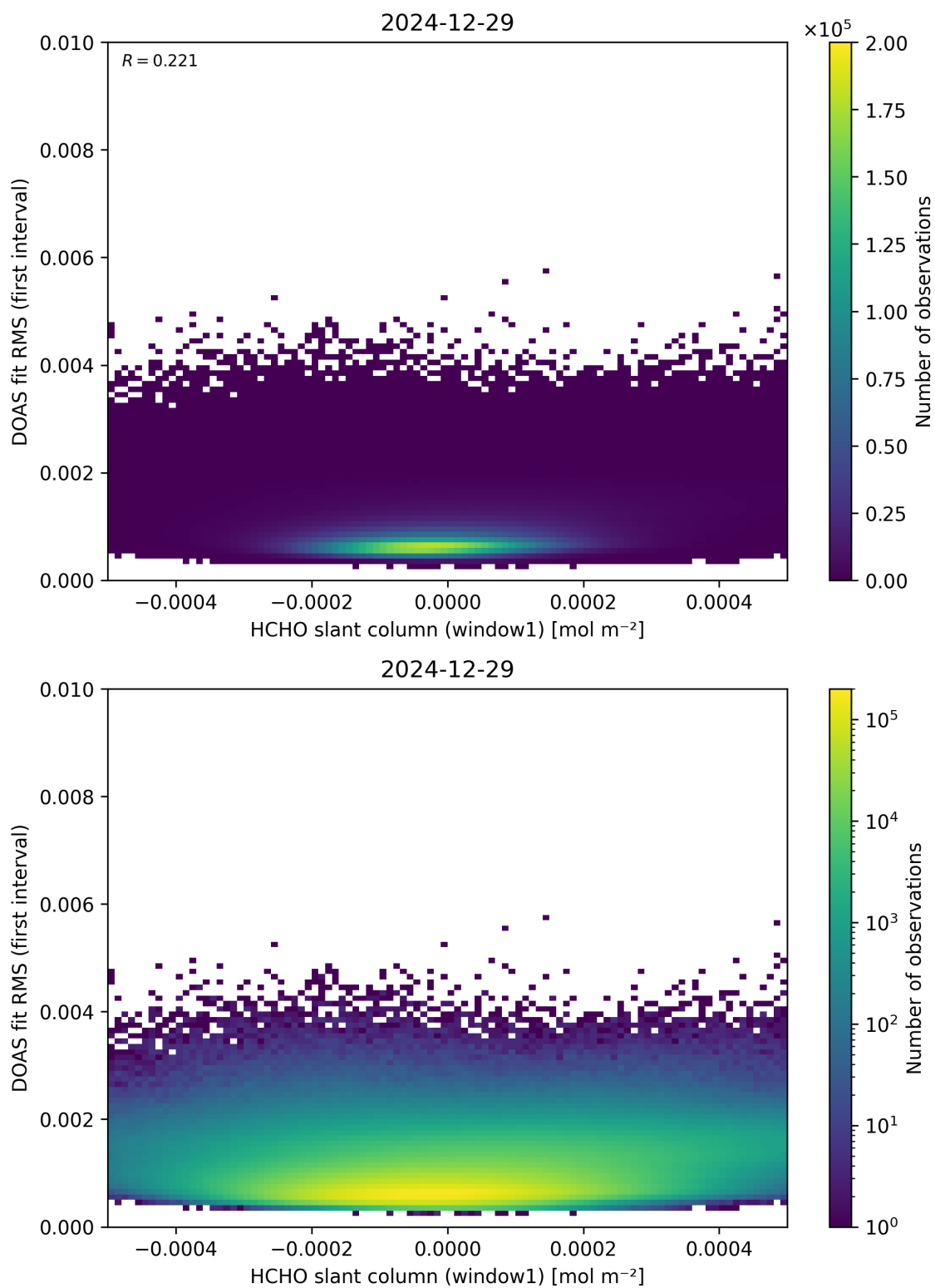
Figure 78: Scatter density plot of “HCHO slant column (window1)” against “DOAS fit RMS (first interval)” for 2024-12-28 to 2024-12-30.
