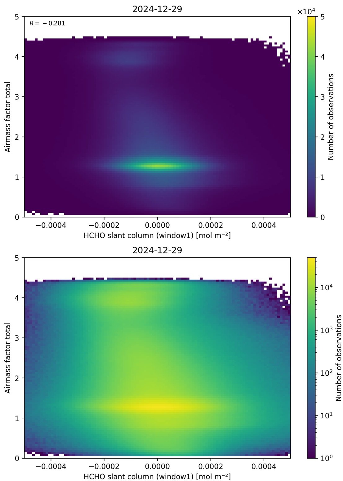
Figure 85: Scatter density plot of “HCHO slant column (window1)” against “Airmass factor total” for 2024-12-28 to 2024-12-30.
