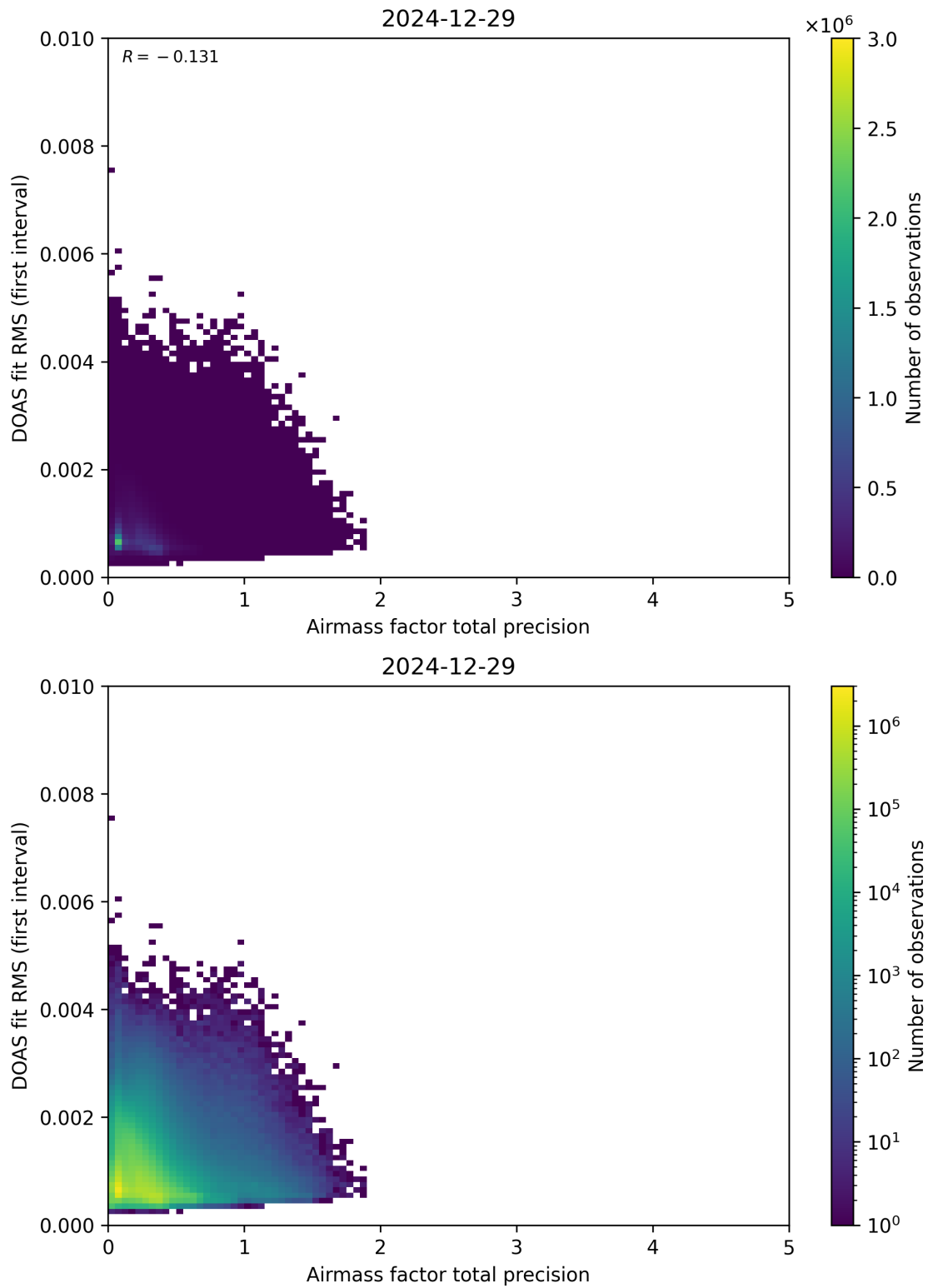
Figure 105: Scatter density plot of “Airmass factor total precision” against “DOAS fit RMS (first interval)” for 2024-12-28 to 2024-12-30.
