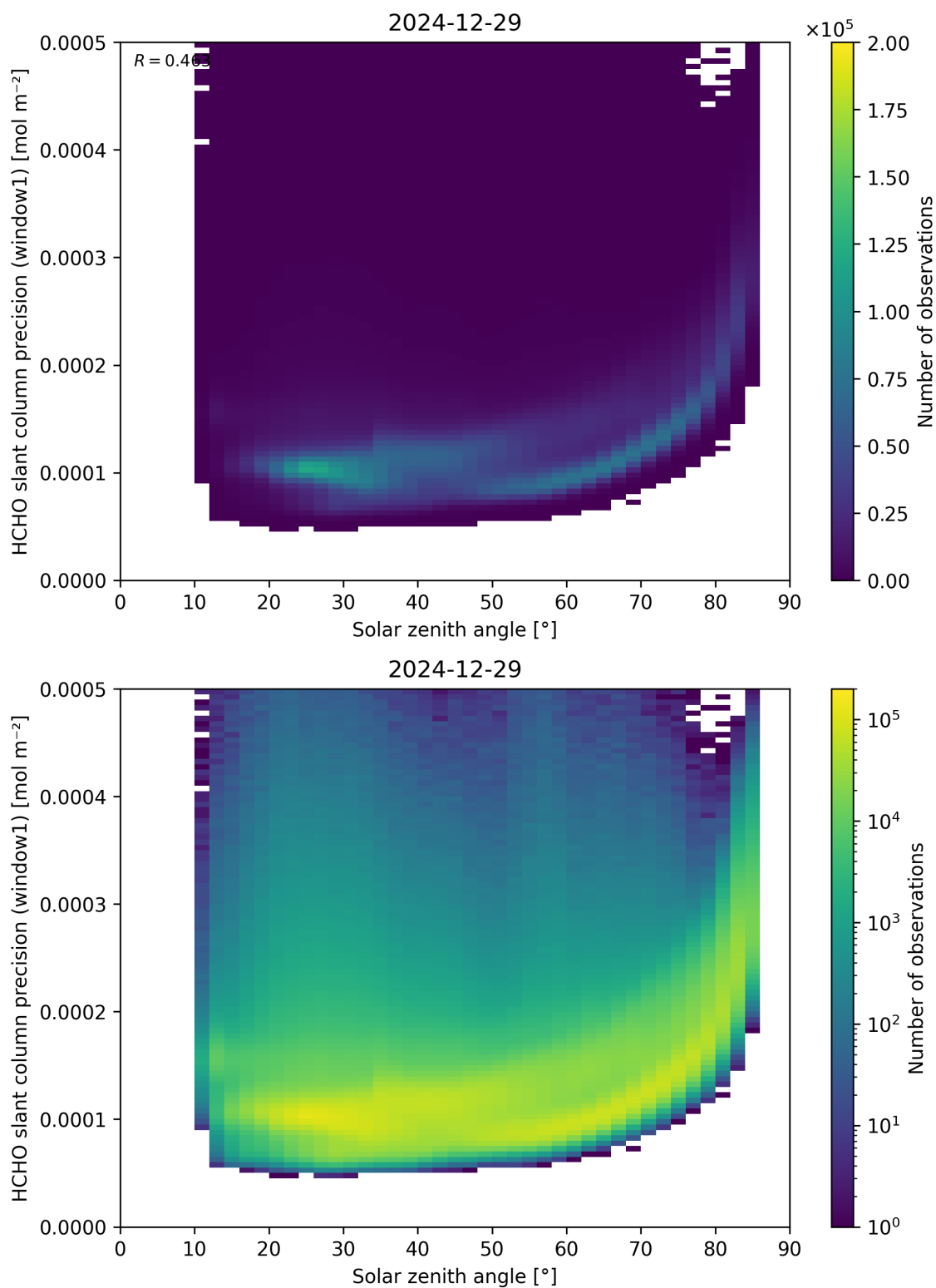
Figure 174: Scatter density plot of “Solar zenith angle” against “HCHO slant column precision (window1)” for 2024-12-28 to 2024-12-30.
