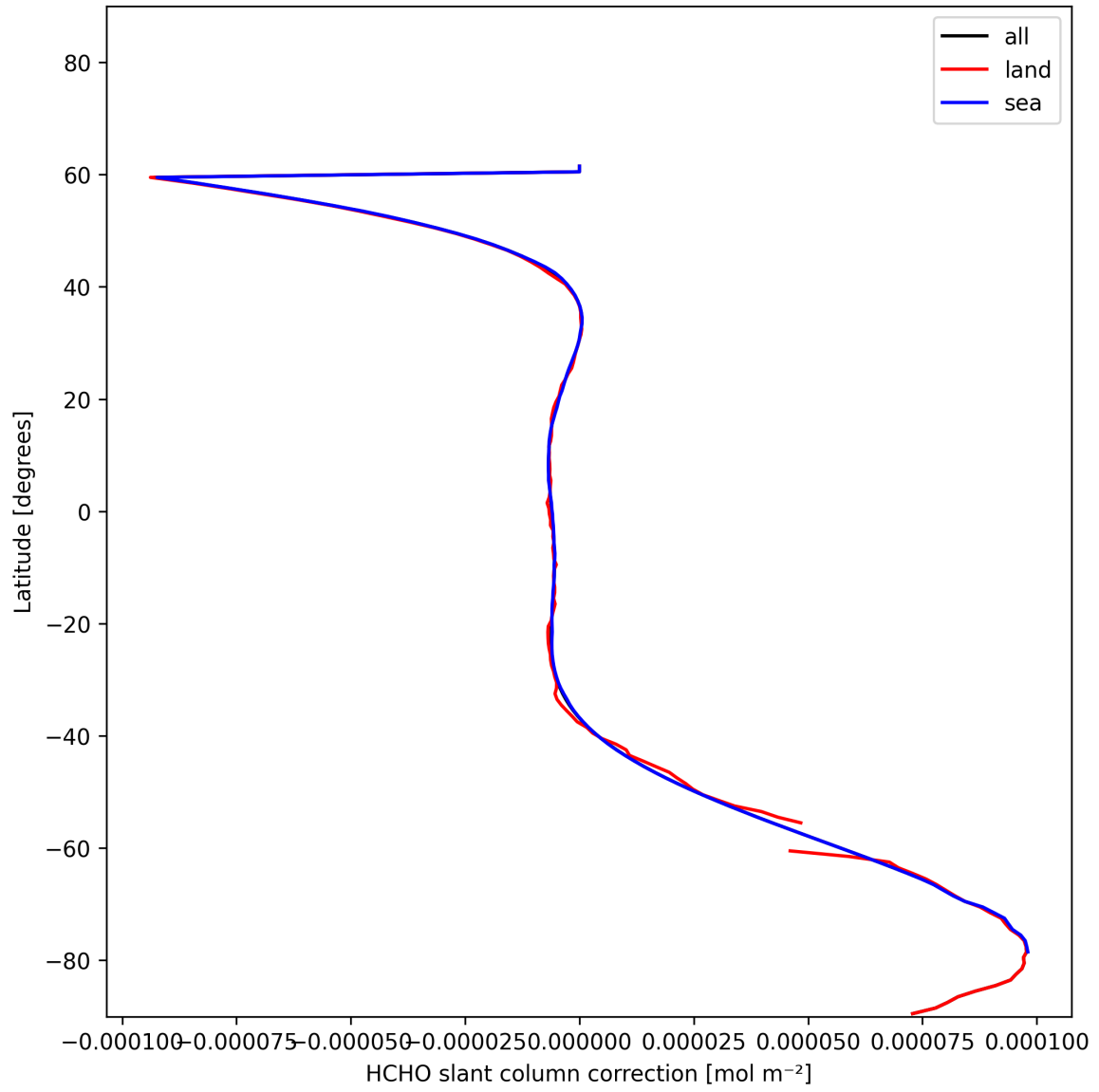
Figure 33: Zonal average of “HCHO slant column correction” for 2024-12-28 to 2024-12-30.
