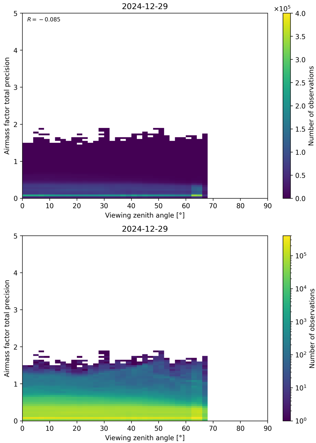
Figure 191: Scatter density plot of “Viewing zenith angle” against “Airmass factor total precision” for 2024-12-28 to 2024-12-30.
