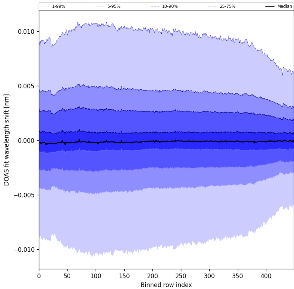
Figure 58: Along track statistics of “DOAS fit wavelength shift” for 2024-12-28 to 2024-12-30
