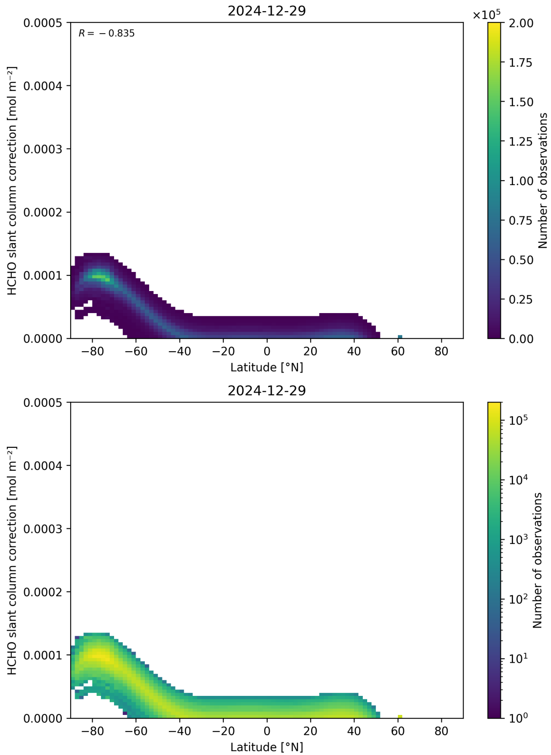
Figure 158: Scatter density plot of “Latitude” against “HCHO slant column correction” for 2024-12-28 to 2024-12-30.
