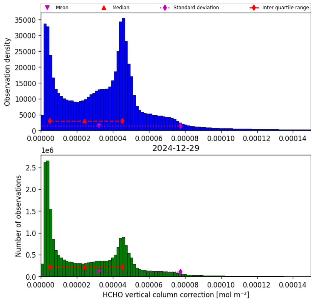
Figure 37: Histogram of “HCHO vertical column correction” for 2024-12-28 to 2024-12-30
