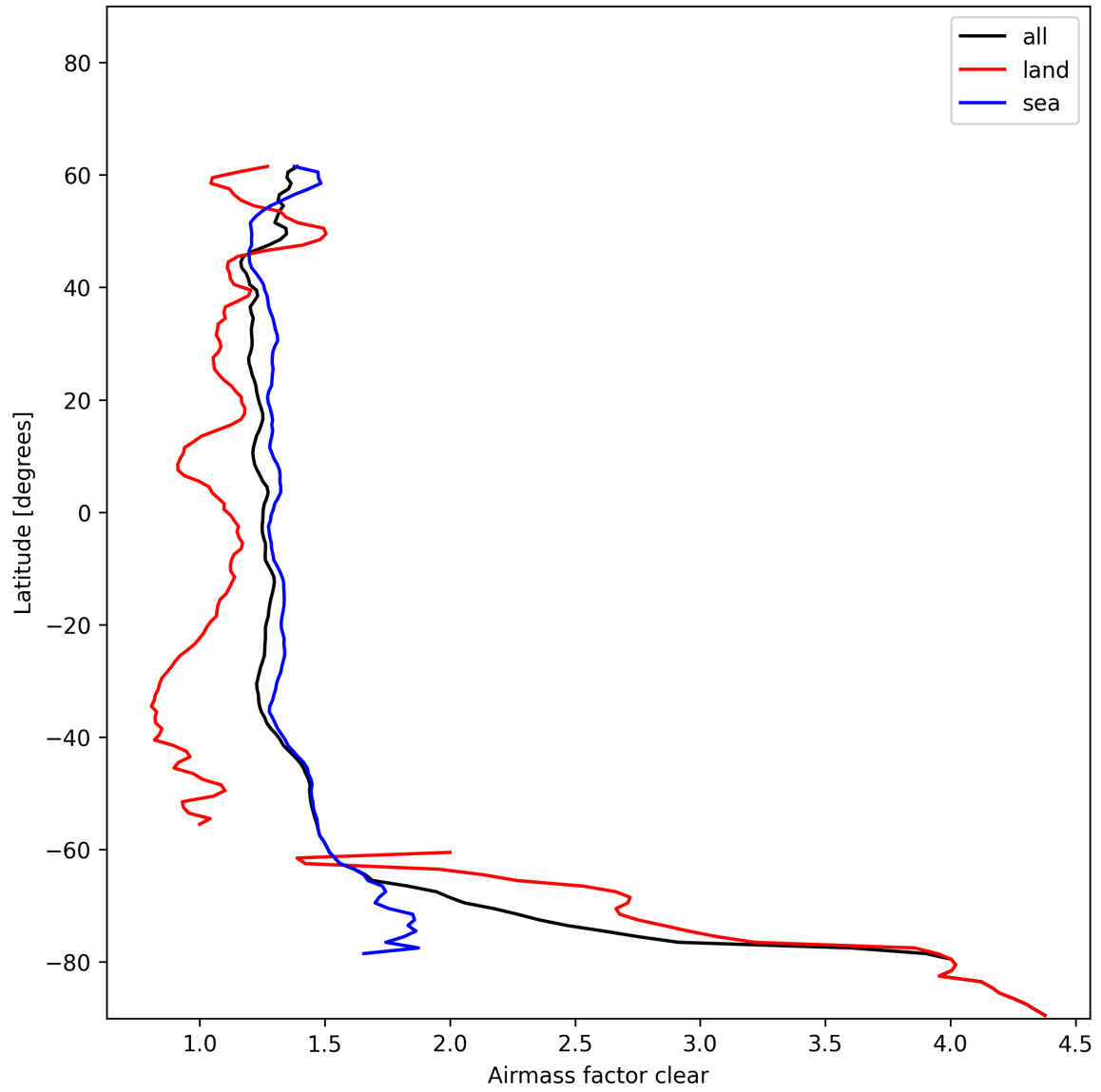
Figure 28: Zonal average of “Airmass factor clear” for 2024-12-28 to 2024-12-30.
