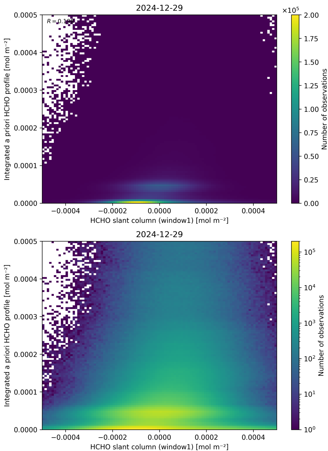
Figure 87: Scatter density plot of “HCHO slant column (window1)” against “Integrated a priori HCHO profile” for 2024-12-28 to 2024-12-30.
