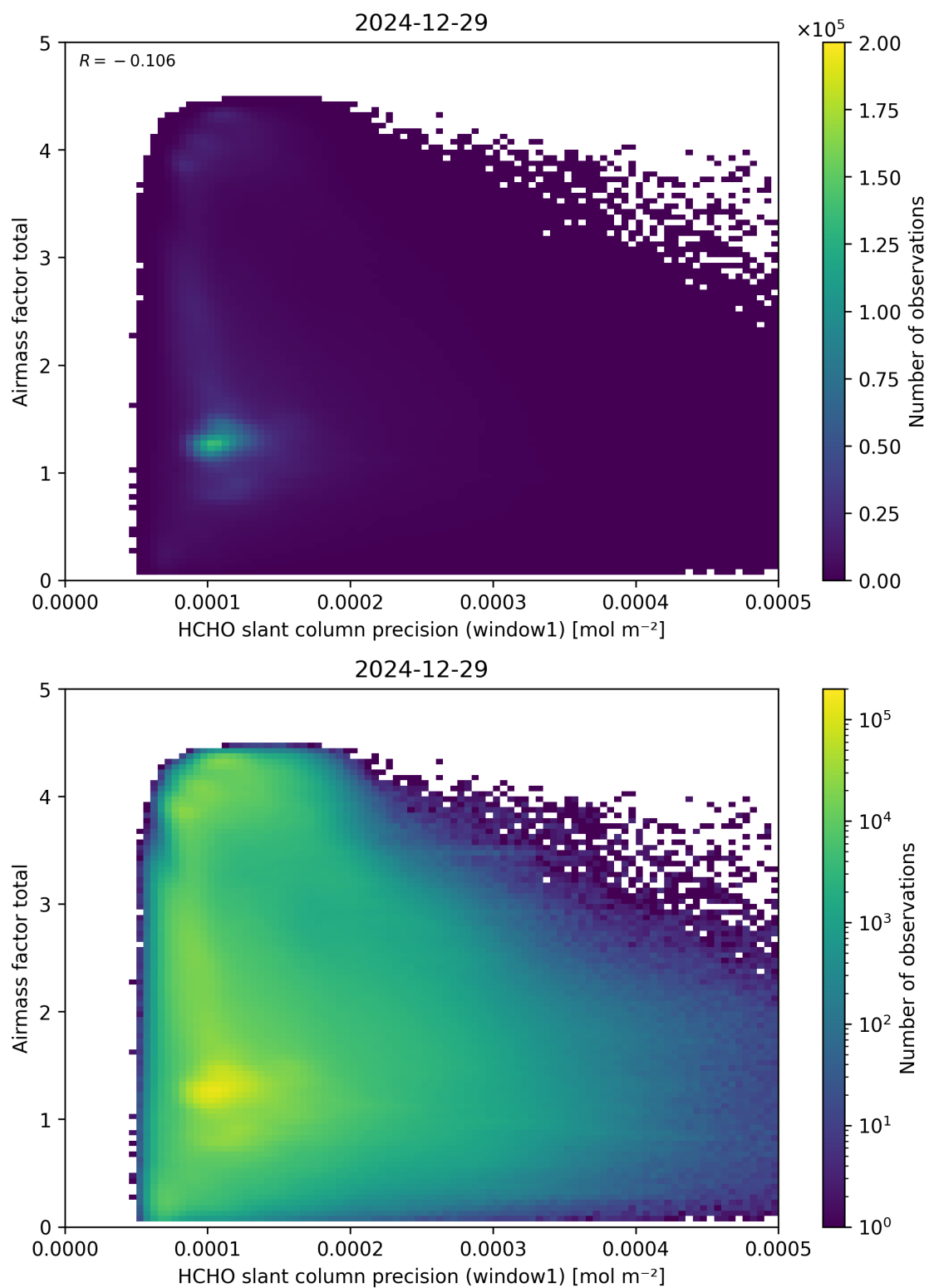
Figure 94: Scatter density plot of “HCHO slant column precision (window1)” against “Airmass factor total” for 2024-12-28 to 2024-12-30.
