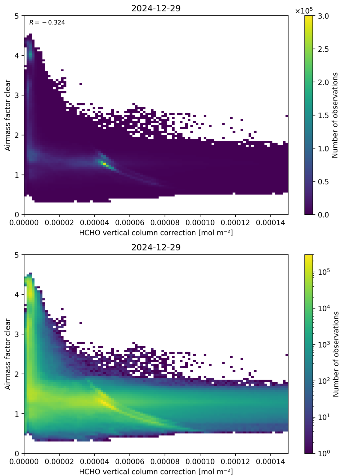
Figure 115: Scatter density plot of “HCHO vertical column correction” against “Airmass factor clear” for 2024-12-28 to 2024-12-30.
