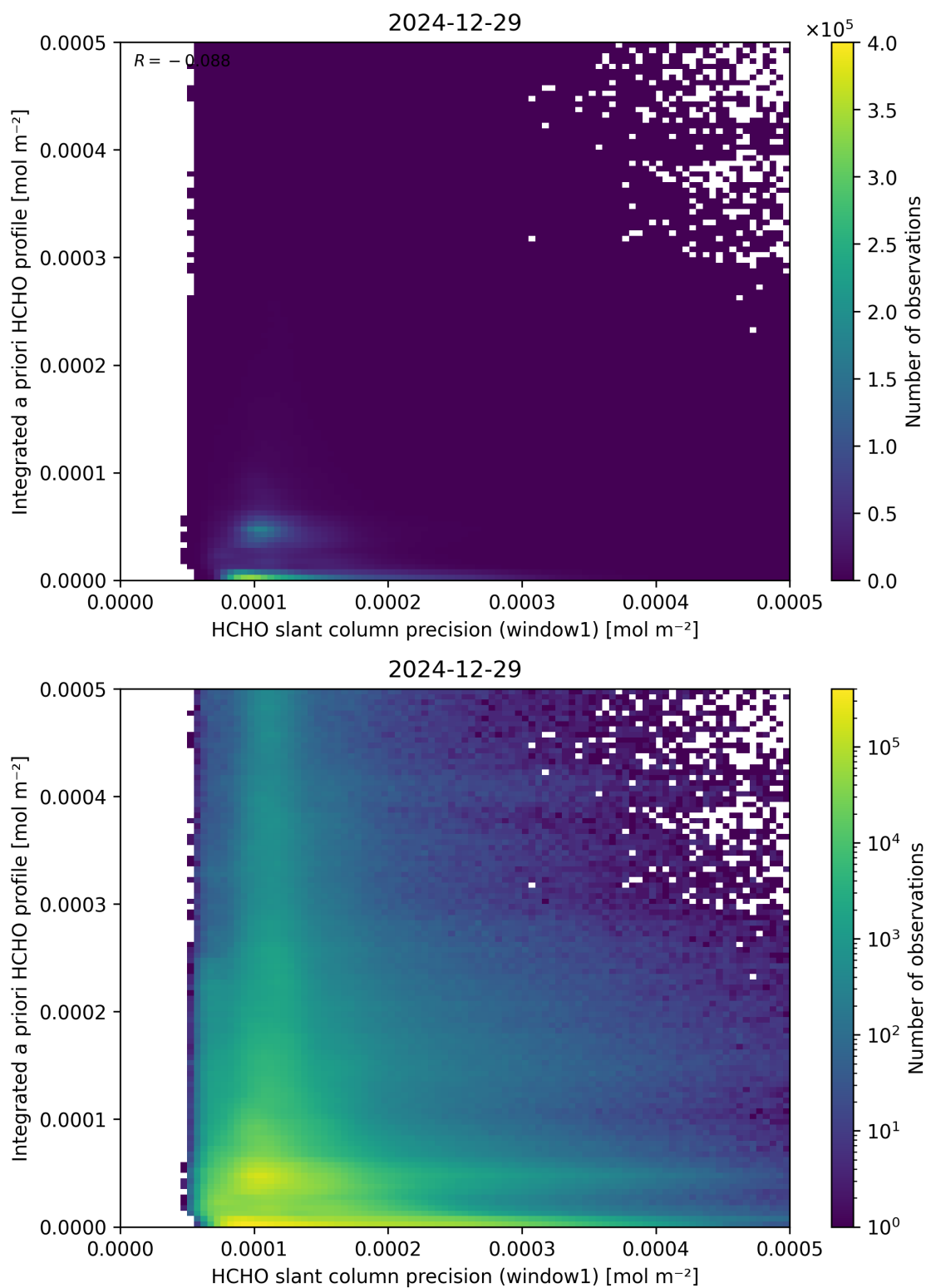
Figure 96: Scatter density plot of “HCHO slant column precision (window1)” against “Integrated a priori HCHO profile” for 2024-12-28 to 2024-12-30.
