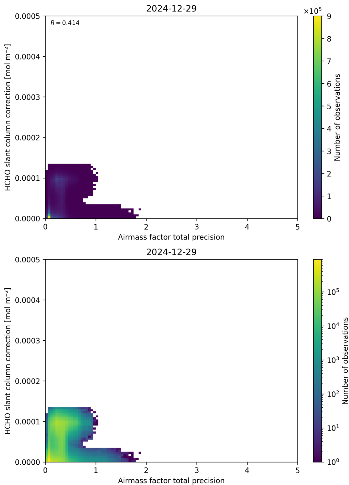
Figure 110: Scatter density plot of “Airmass factor total precision” against “HCHO slant column correction” for 2024-12-28 to 2024-12-30.
