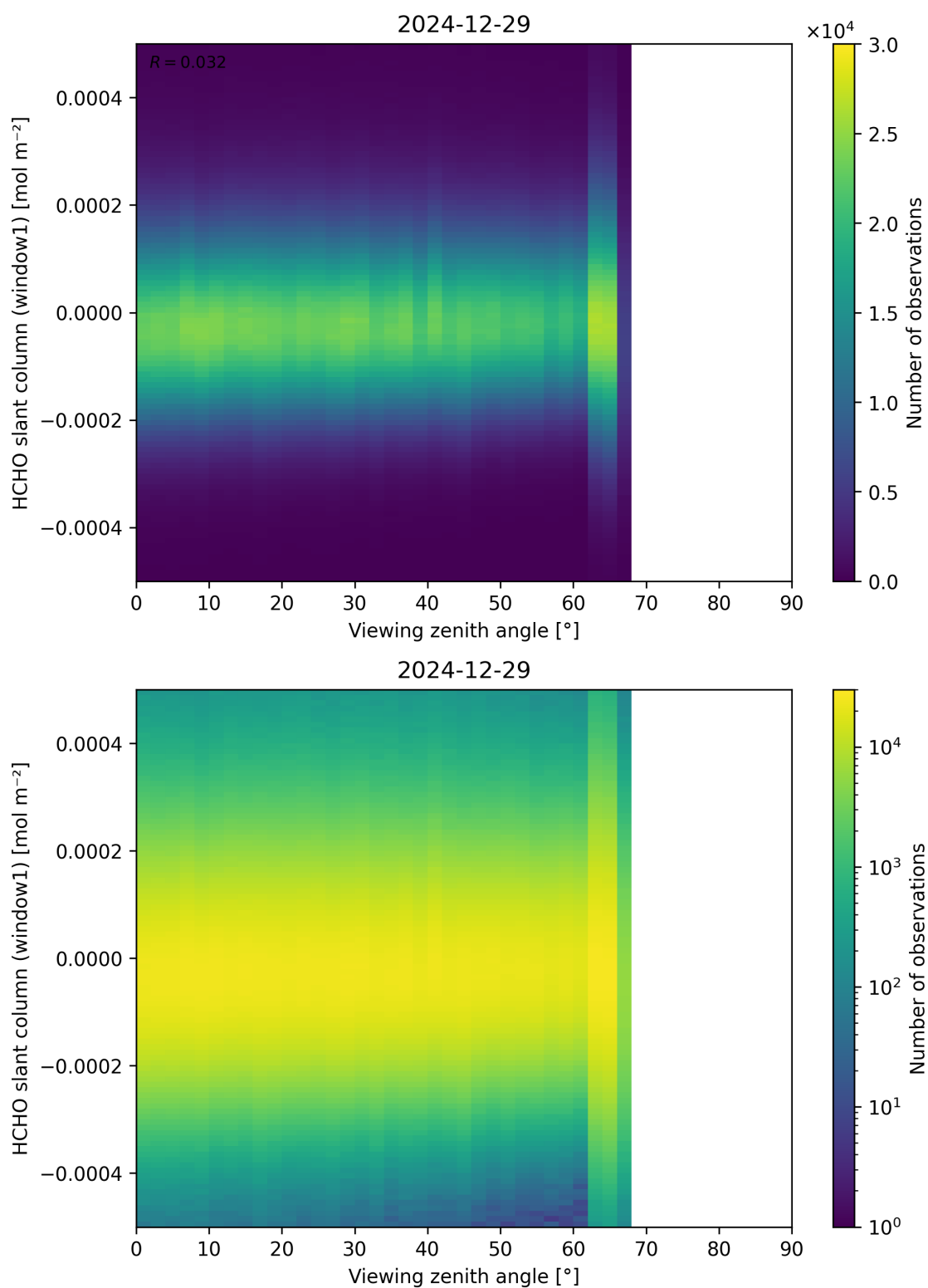
Figure 188: Scatter density plot of “Viewing zenith angle” against “HCHO slant column (window1)” for 2024-12-28 to 2024-12-30.
