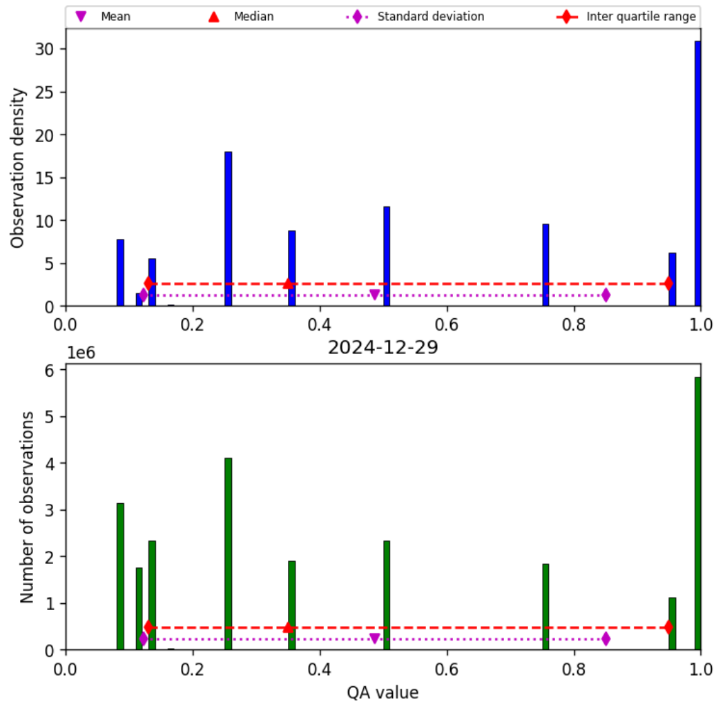
Figure 34: Histogram of “QA value” for 2024-12-28 to 2024-12-30
