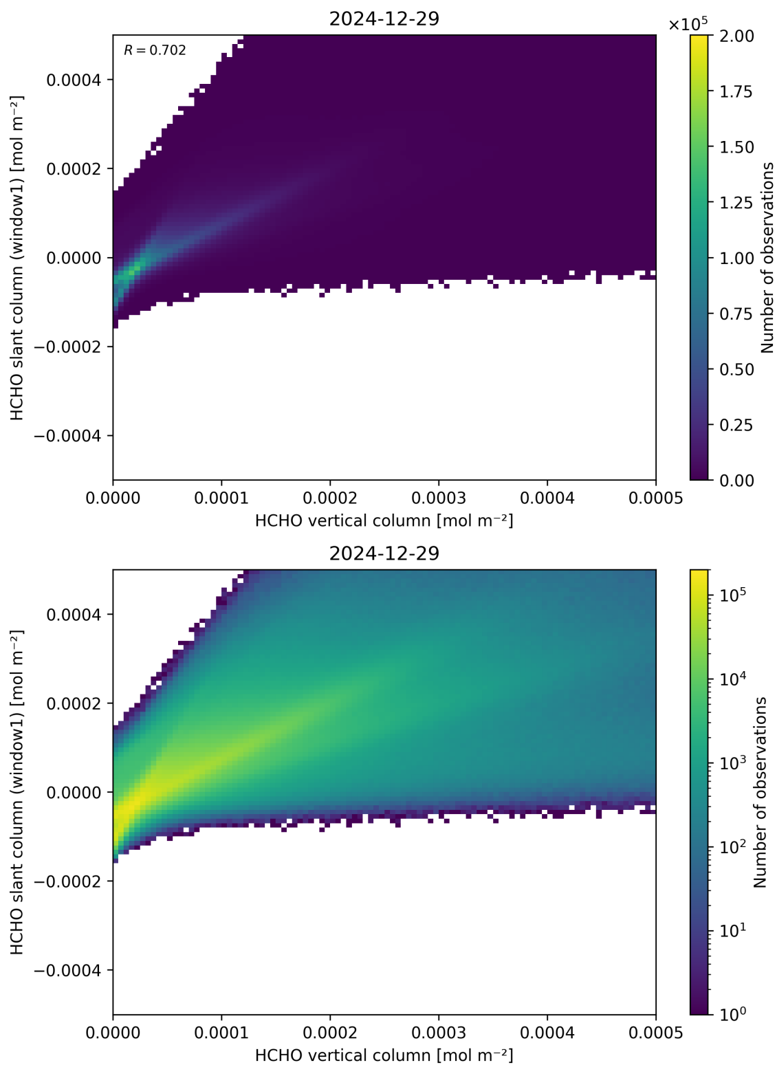
Figure 129: Scatter density plot of “HCHO vertical column” against “HCHO slant column (window1)” for 2024-12-28 to 2024-12-30.
