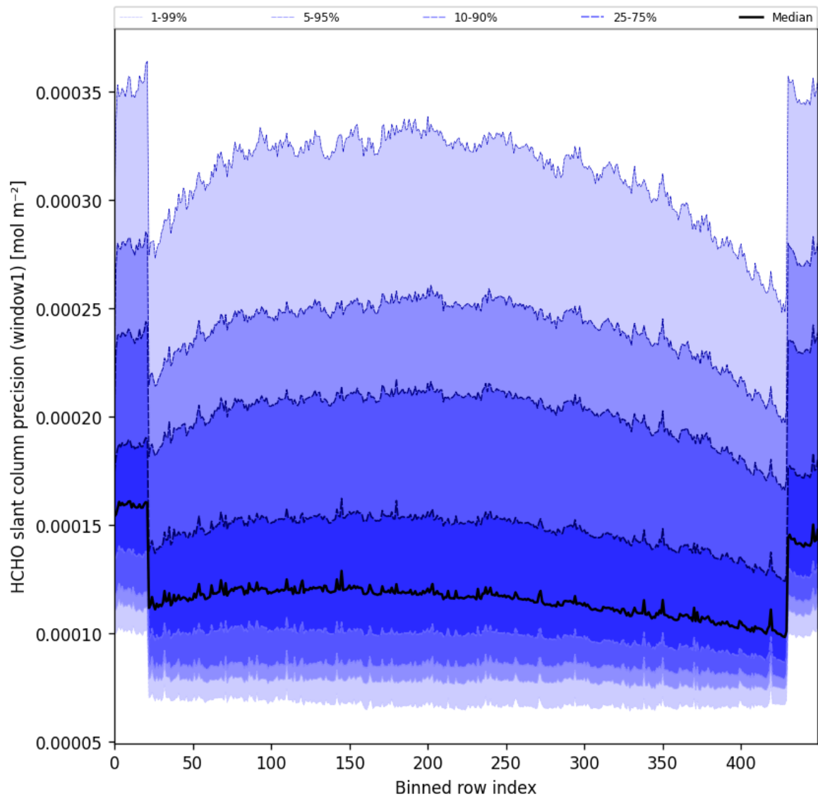
Figure 53: Along track statistics of “HCHO slant column precision (window1)” for 2024-12-28 to 2024-12-30
