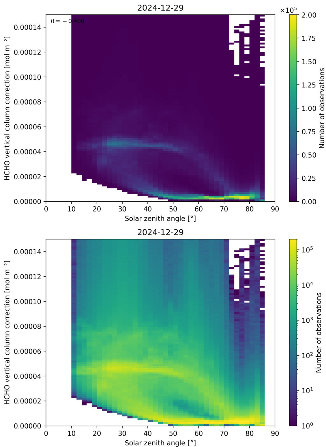
Figure 178: Scatter density plot of “Solar zenith angle” against “HCHO vertical column correction” for 2024-12-28 to 2024-12-30.
