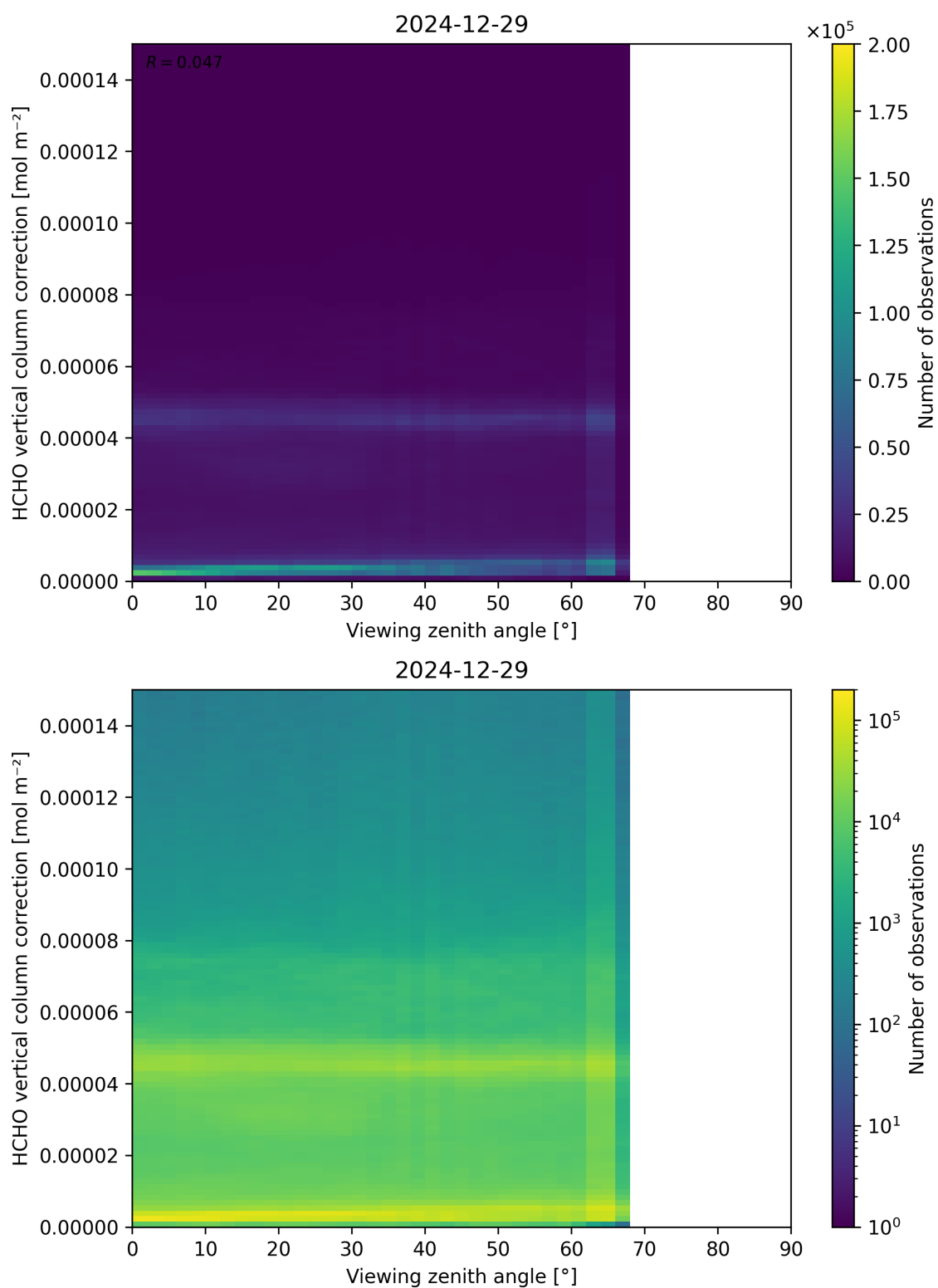
Figure 193: Scatter density plot of “Viewing zenith angle” against “HCHO vertical column correction” for 2024-12-28 to 2024-12-30.
