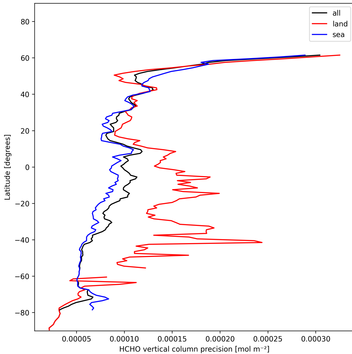
Figure 22: Zonal average of “HCHO vertical column precision” for 2024-12-28 to 2024-12-30.
