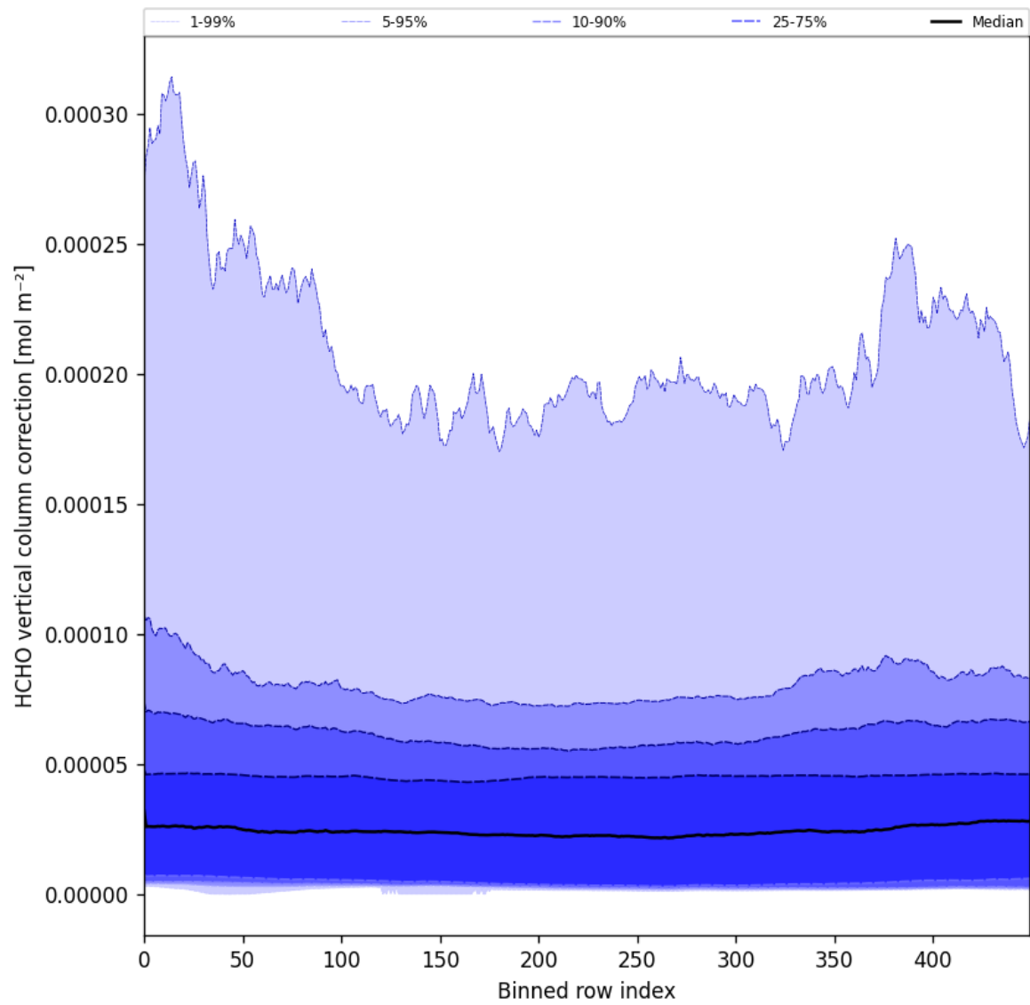
Figure 51: Along track statistics of “HCHO vertical column correction” for 2024-12-28 to 2024-12-30
