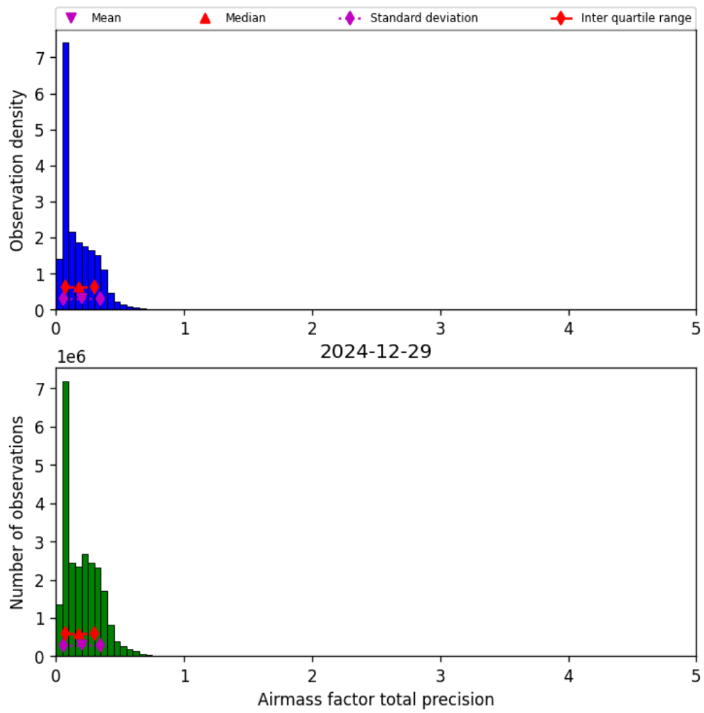
Figure 41: Histogram of “Airmass factor total precision” for 2024-12-28 to 2024-12-30
