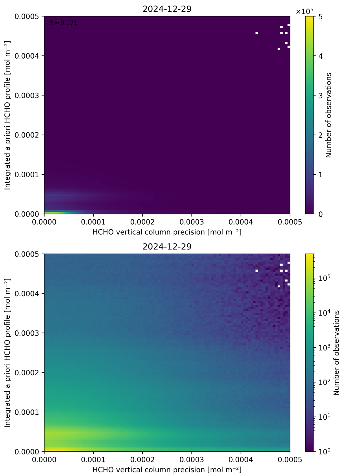
Figure 147: Scatter density plot of “HCHO vertical column precision” against “Integrated a priori HCHO profile” for 2024-12-28 to 2024-12-30.
