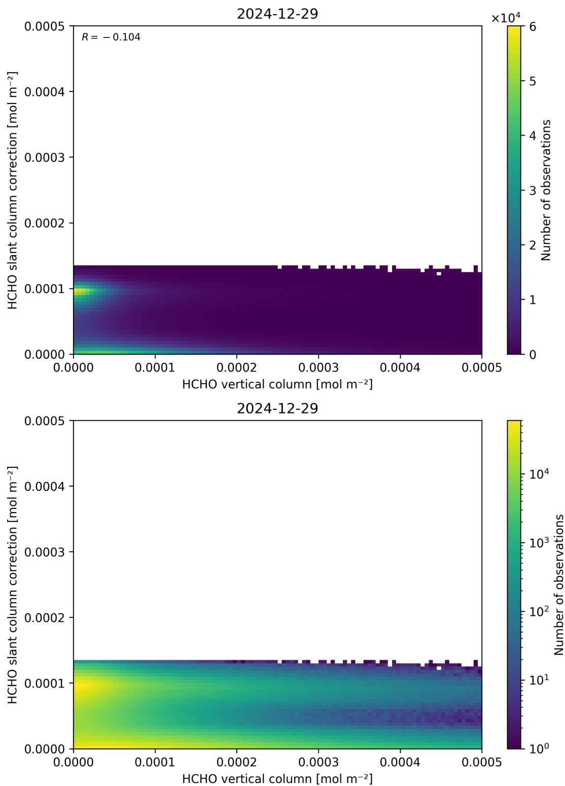
Figure 128: Scatter density plot of “HCHO vertical column” against “HCHO slant column correction” for 2024-12-28 to 2024-12-30.
