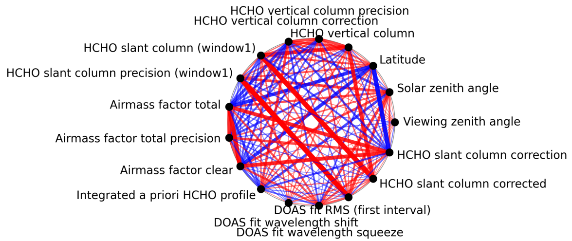
Figure 1: Map of correlation graph for 2024-12-28 to 2024-12-30.
