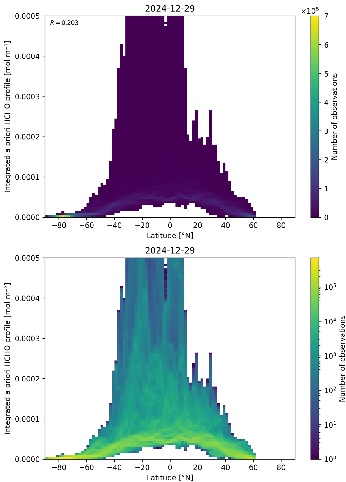
Figure 166: Scatter density plot of “Latitude” against “Integrated a priori HCHO profile” for 2024-12-28 to 2024-12-30.
