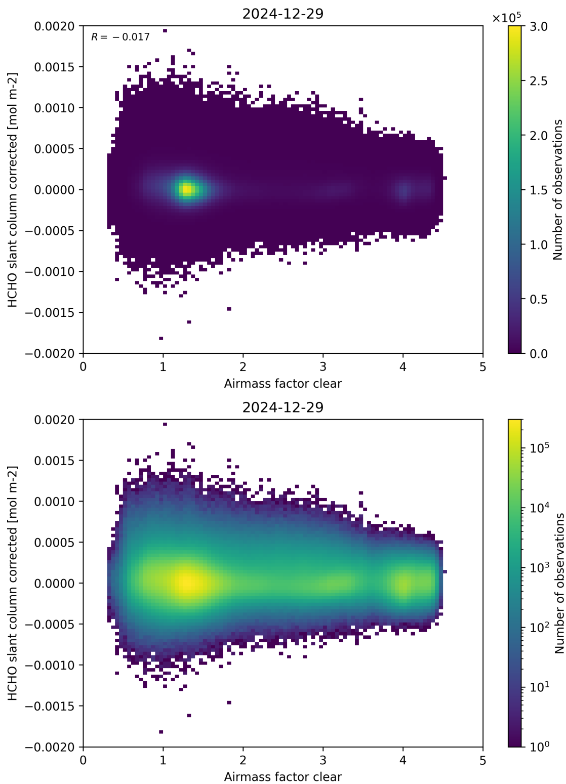
Figure 74: Scatter density plot of “Airmass factor clear” against “HCHO slant column corrected” for 2024-12-28 to 2024-12-30.
