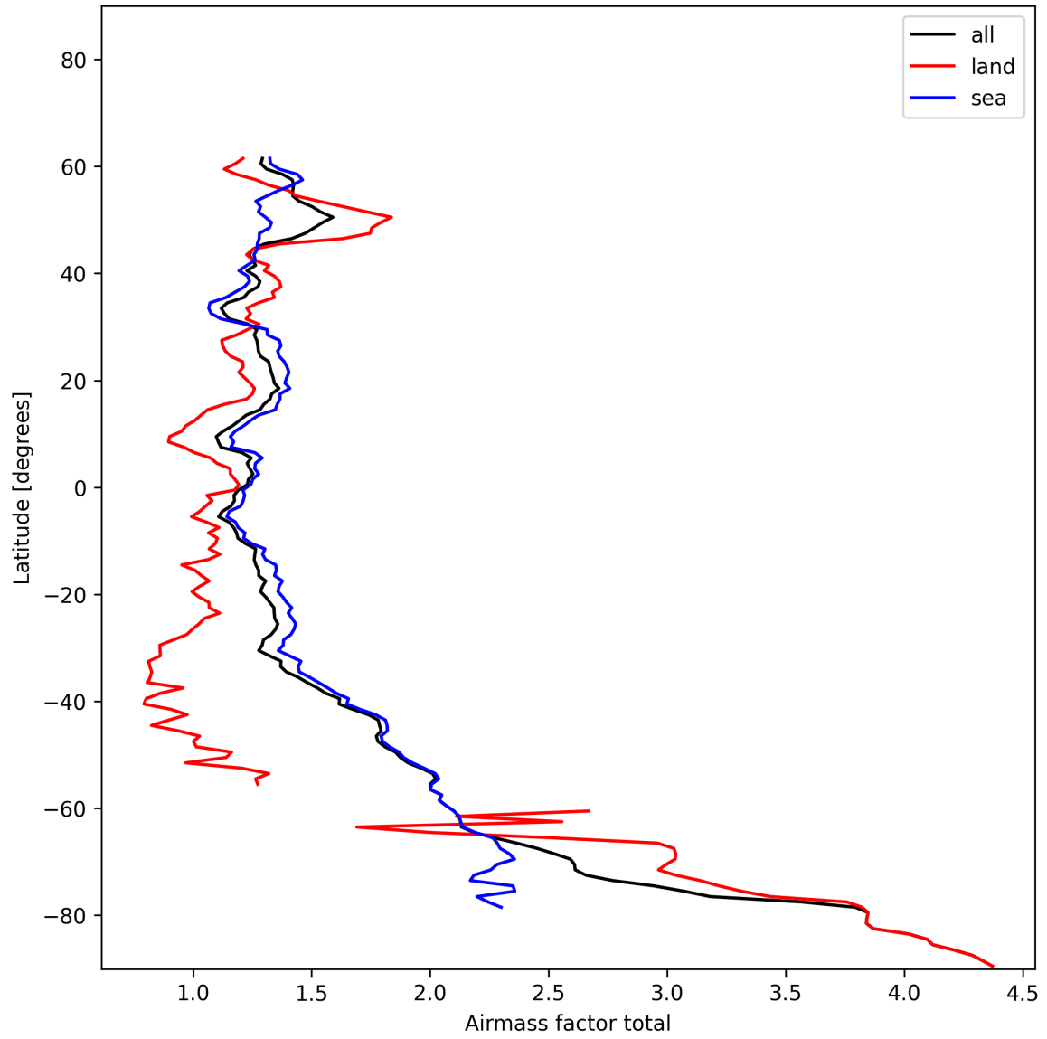
Figure 26: Zonal average of “Airmass factor total” for 2024-12-28 to 2024-12-30.
