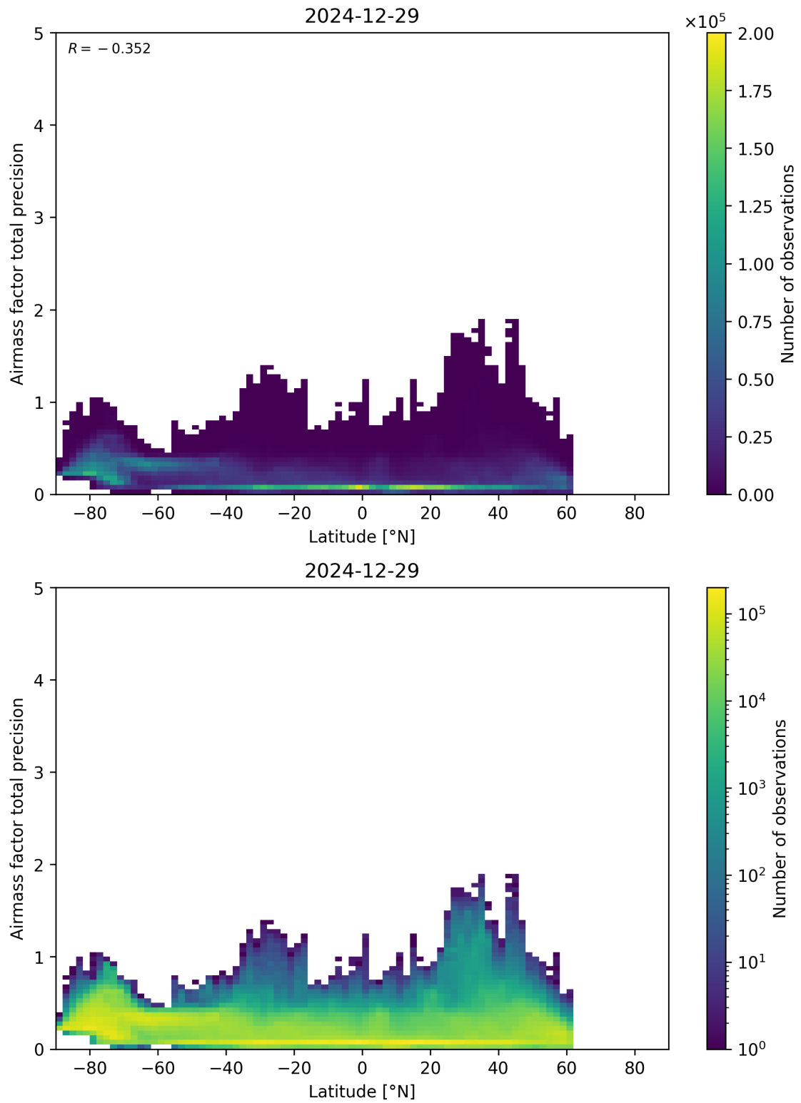
Figure 162: Scatter density plot of “Latitude” against “Airmass factor total precision” for 2024-12-28 to 2024-12-30.
