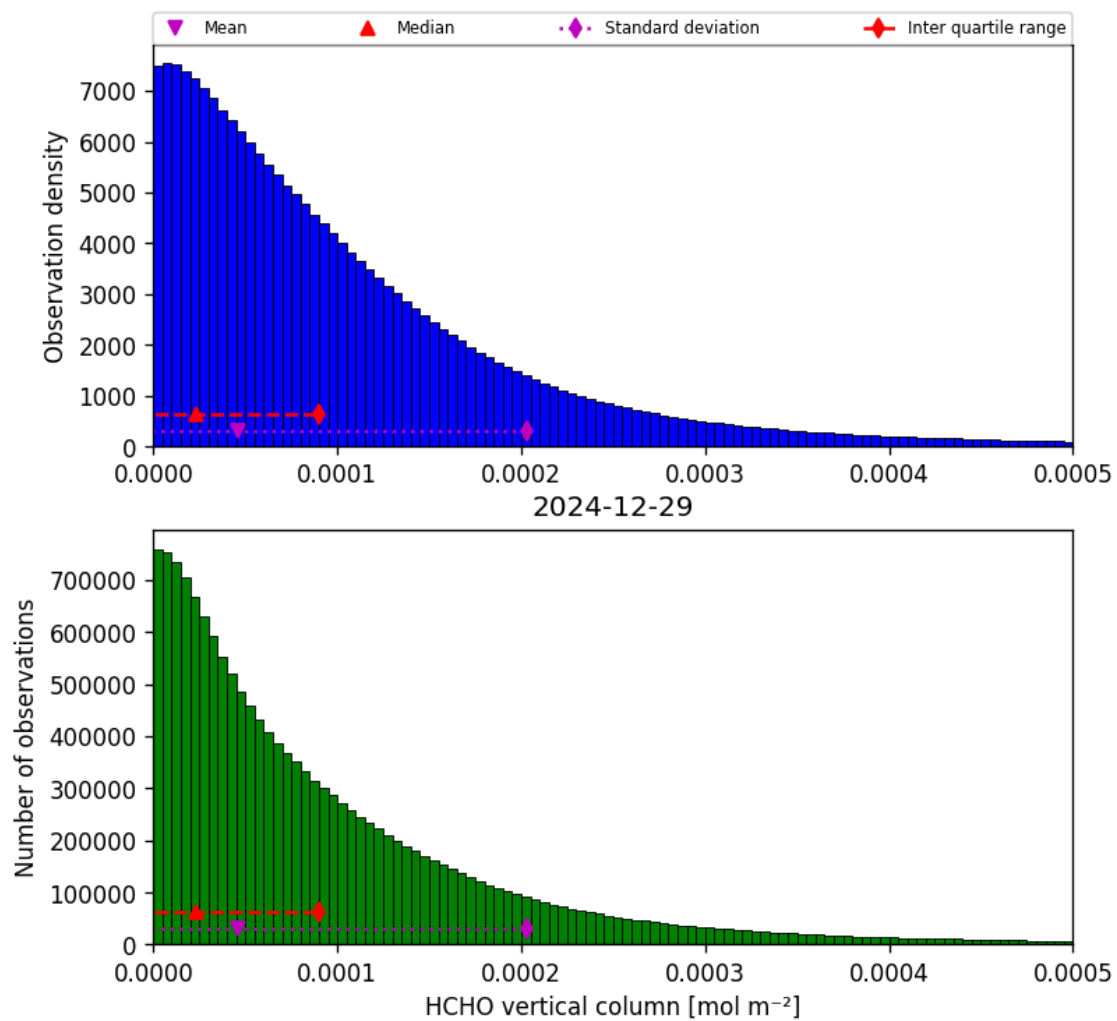
Figure 35: Histogram of “HCHO vertical column” for 2024-12-28 to 2024-12-30
