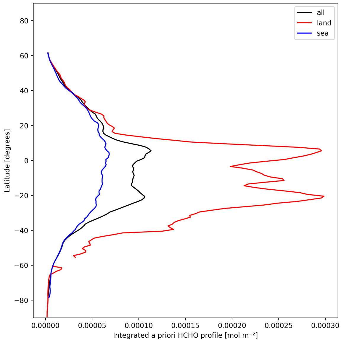
Figure 29: Zonal average of “Integrated a priori HCHO profile” for 2024-12-28 to 2024-12-30.
