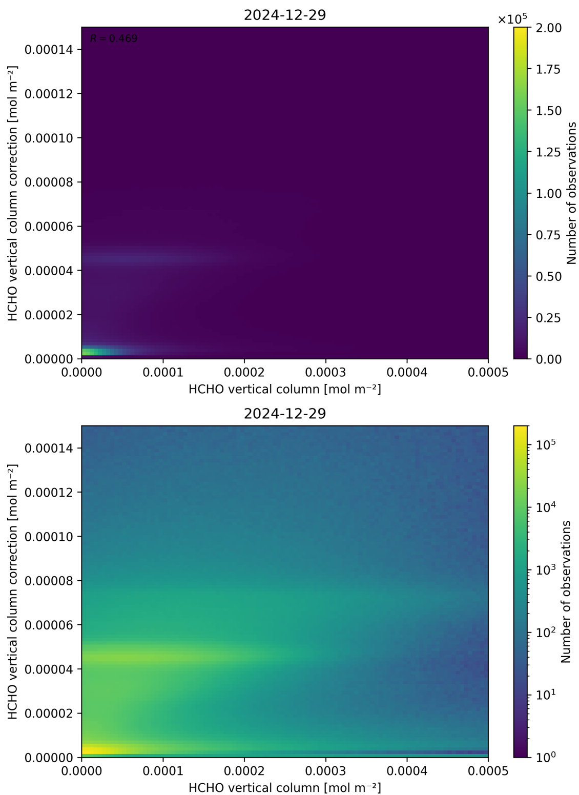
Figure 133: Scatter density plot of “HCHO vertical column” against “HCHO vertical column correction” for 2024-12-28 to 2024-12-30.
