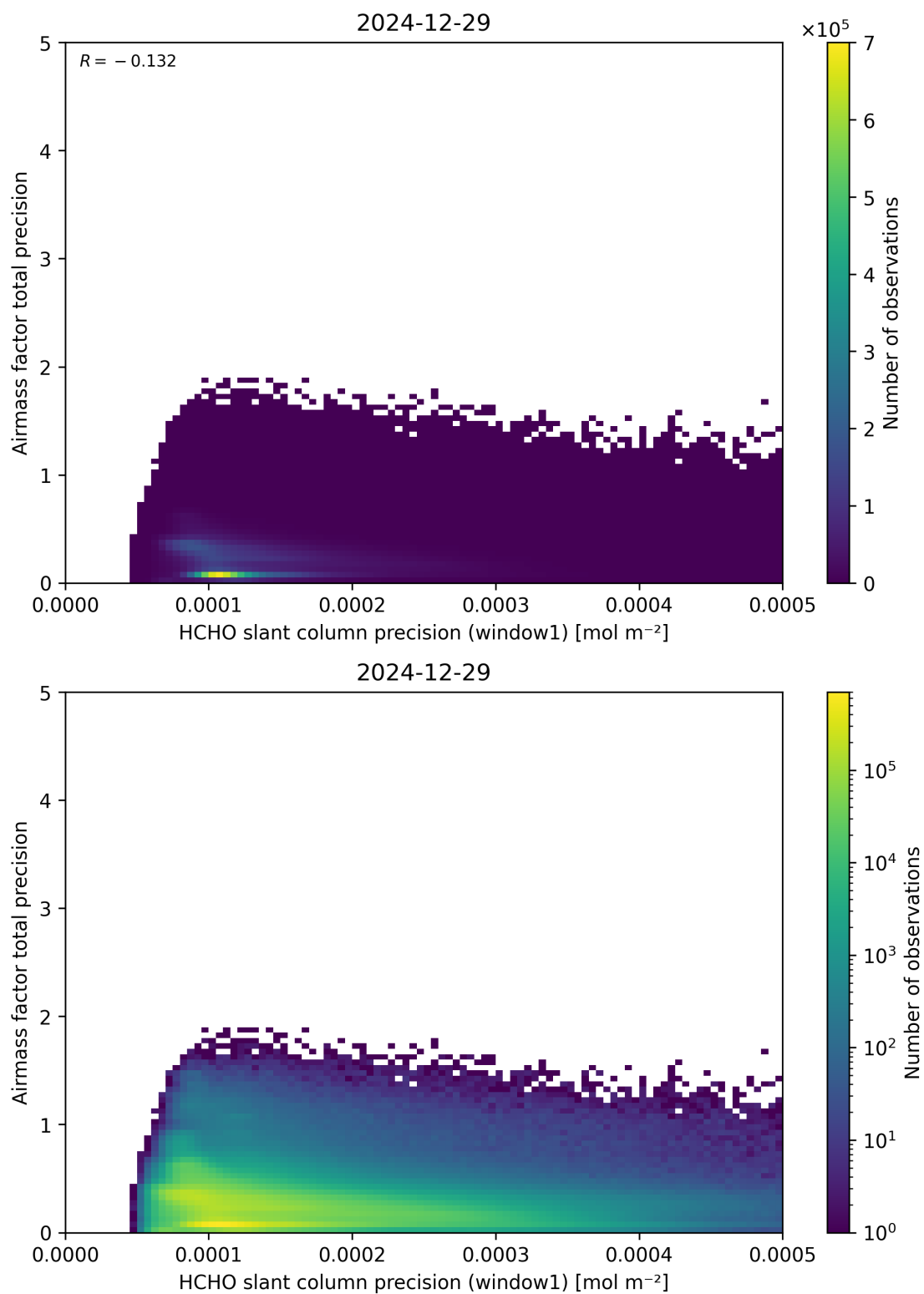
Figure 95: Scatter density plot of “HCHO slant column precision (window1)” against “Airmass factor total precision” for 2024-12-28 to 2024-12-30.
