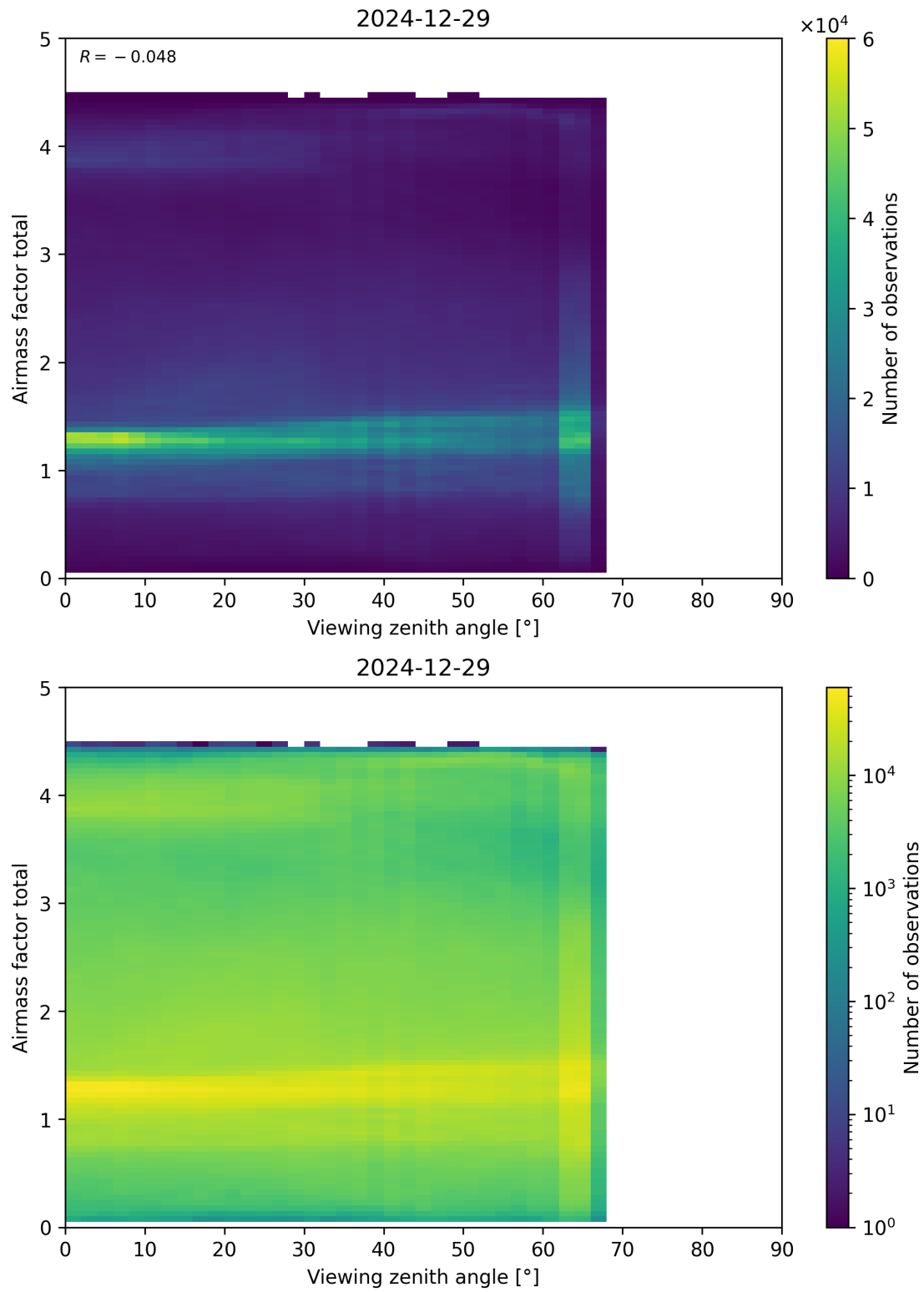
Figure 190: Scatter density plot of “Viewing zenith angle” against “Airmass factor total” for 2024-12-28 to 2024-12-30.
