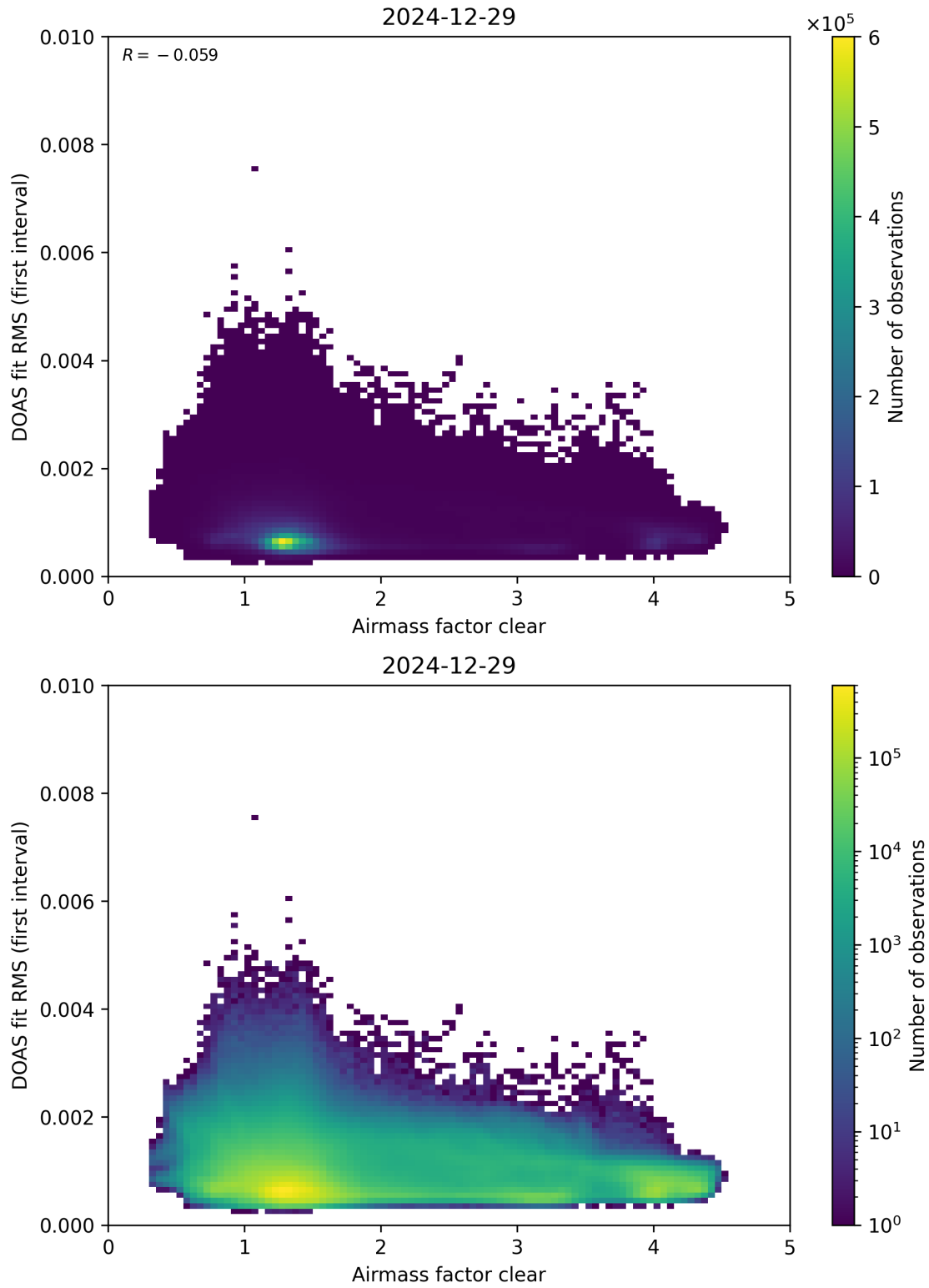
Figure 71: Scatter density plot of “Airmass factor clear” against “DOAS fit RMS (first interval)” for 2024-12-28 to 2024-12-30.
