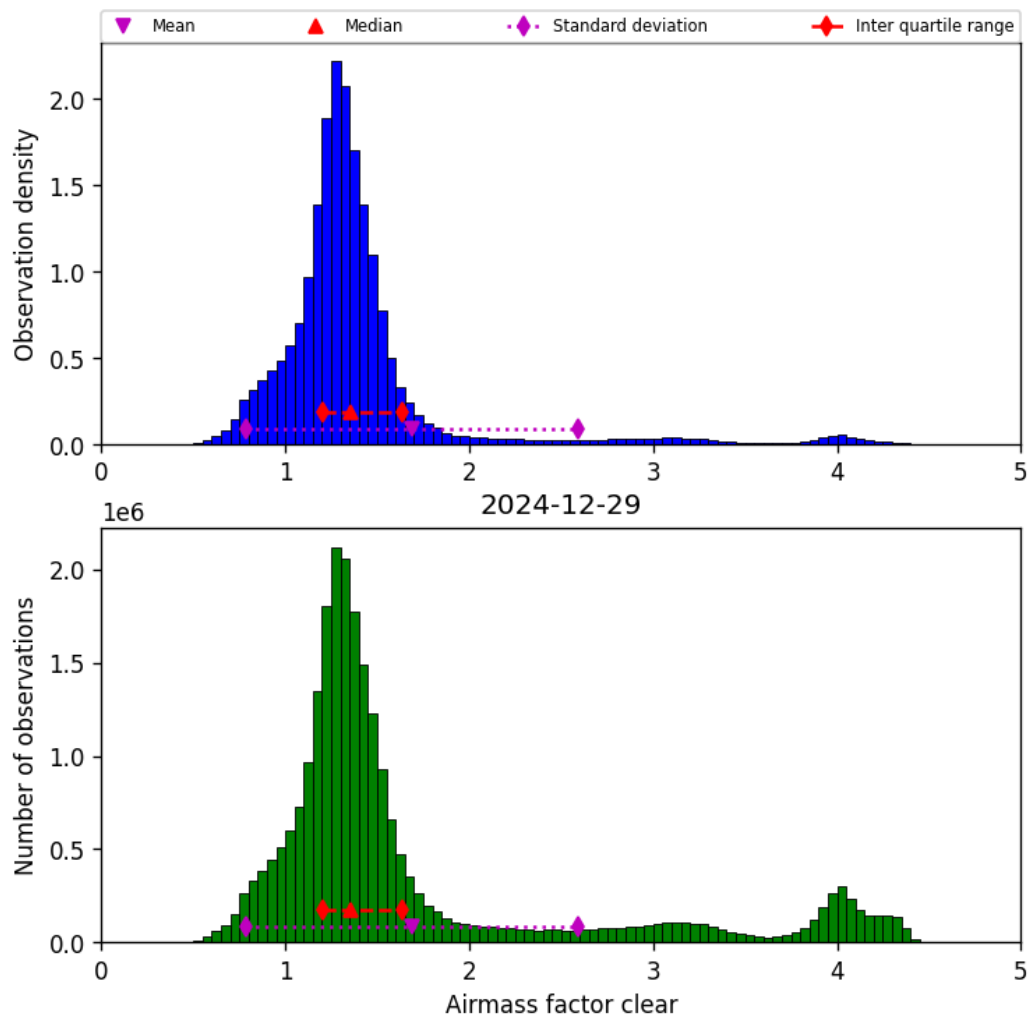
Figure 42: Histogram of “Airmass factor clear” for 2024-12-28 to 2024-12-30
