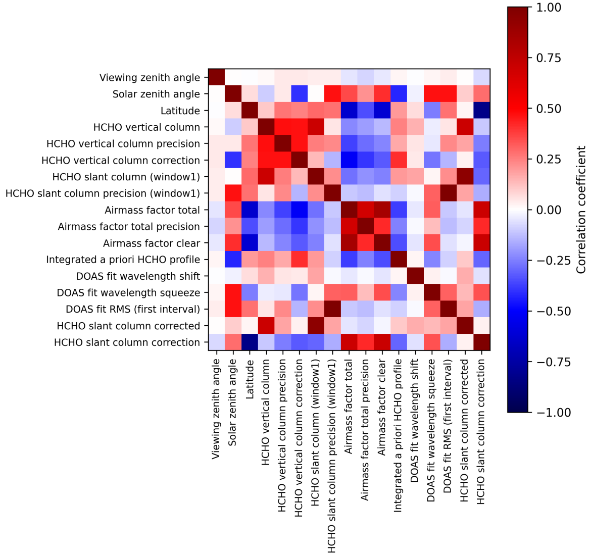
Figure 2: Map of correlation matrix for 2024-12-28 to 2024-12-30.
