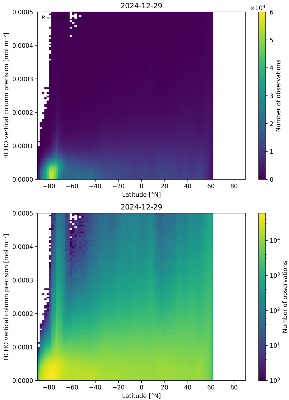
Figure 165: Scatter density plot of “Latitude” against “HCHO vertical column precision” for 2024-12-28 to 2024-12-30.
