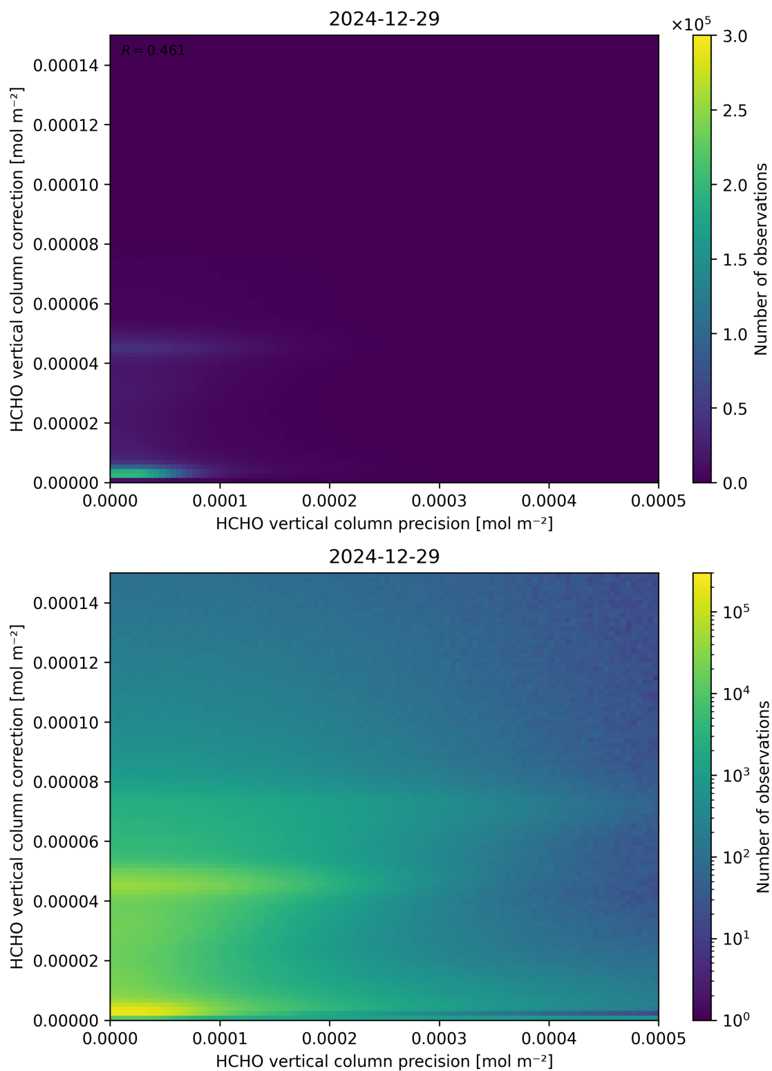
Figure 146: Scatter density plot of “HCHO vertical column precision” against “HCHO vertical column correction” for 2024-12-28 to 2024-12-30.
