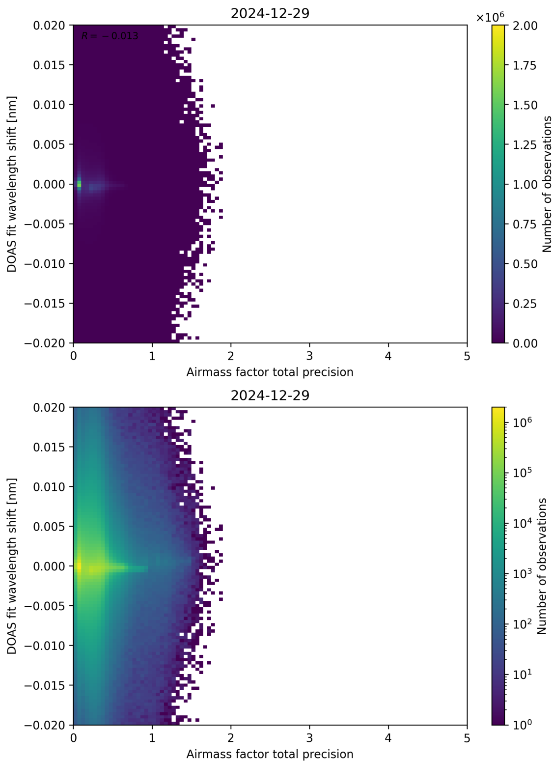
Figure 106: Scatter density plot of “Airmass factor total precision” against “DOAS fit wavelength shift” for 2024-12-28 to 2024-12-30.
