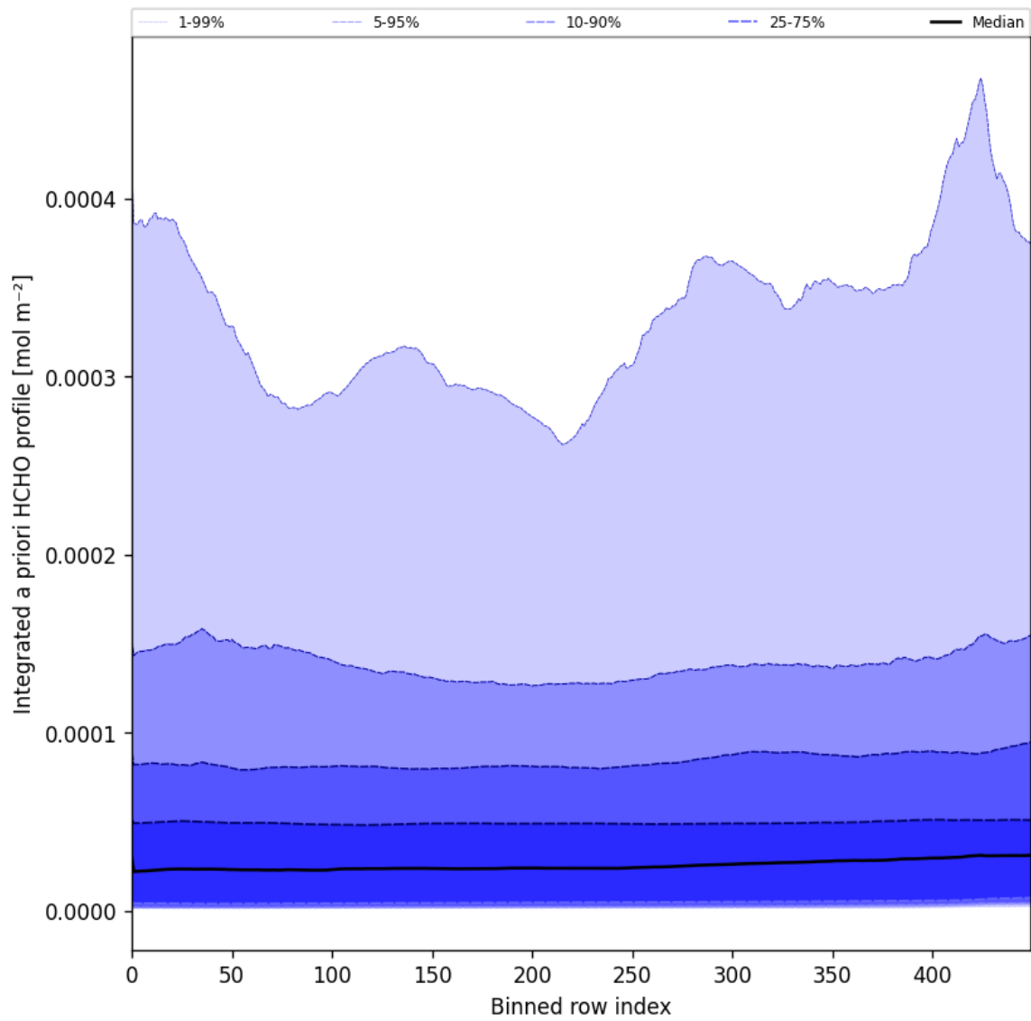
Figure 57: Along track statistics of “Integrated a priori HCHO profile” for 2024-12-28 to 2024-12-30
