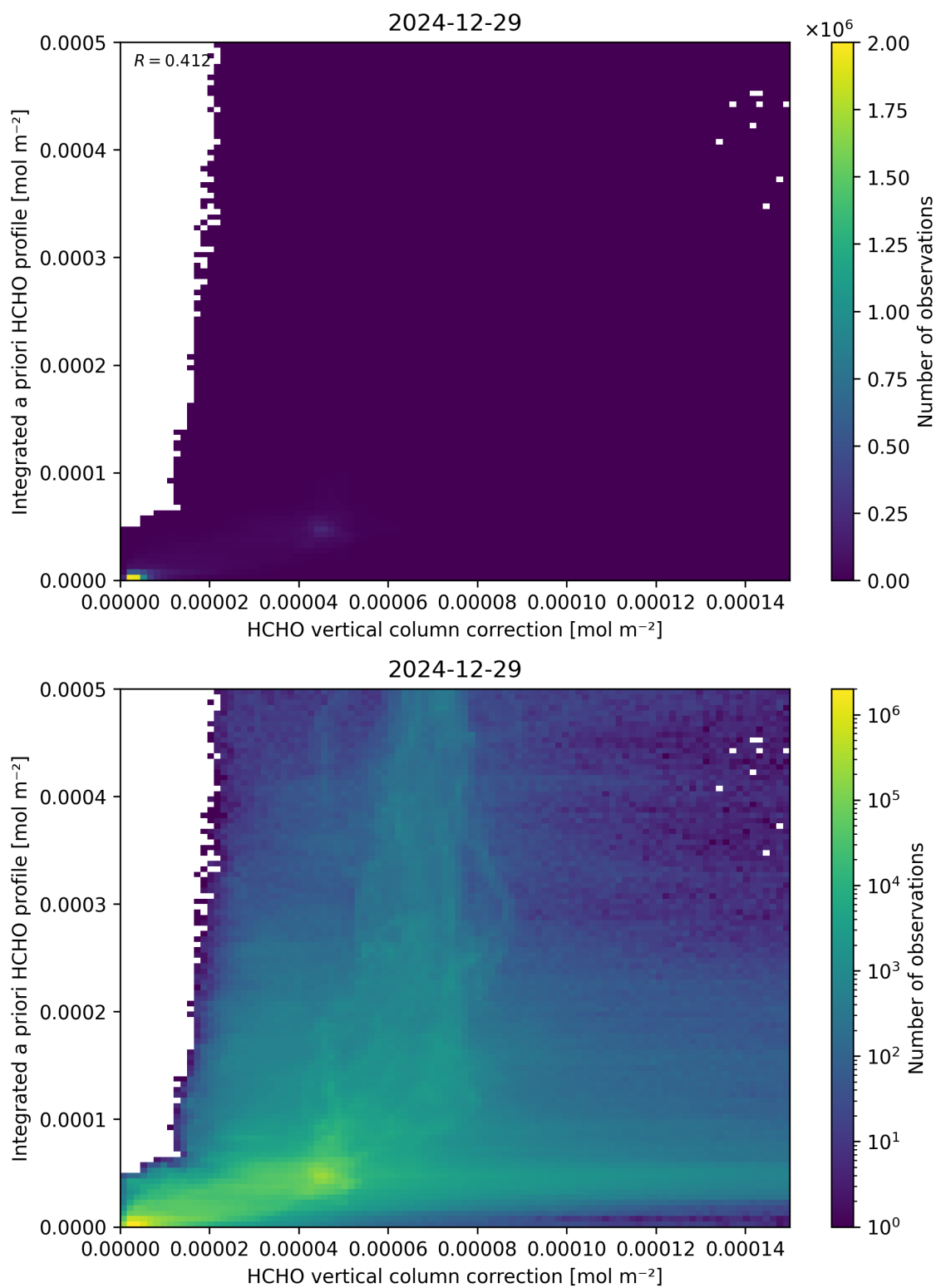
Figure 122: Scatter density plot of “HCHO vertical column correction” against “Integrated a priori HCHO profile” for 2024-12-28 to 2024-12-30.
