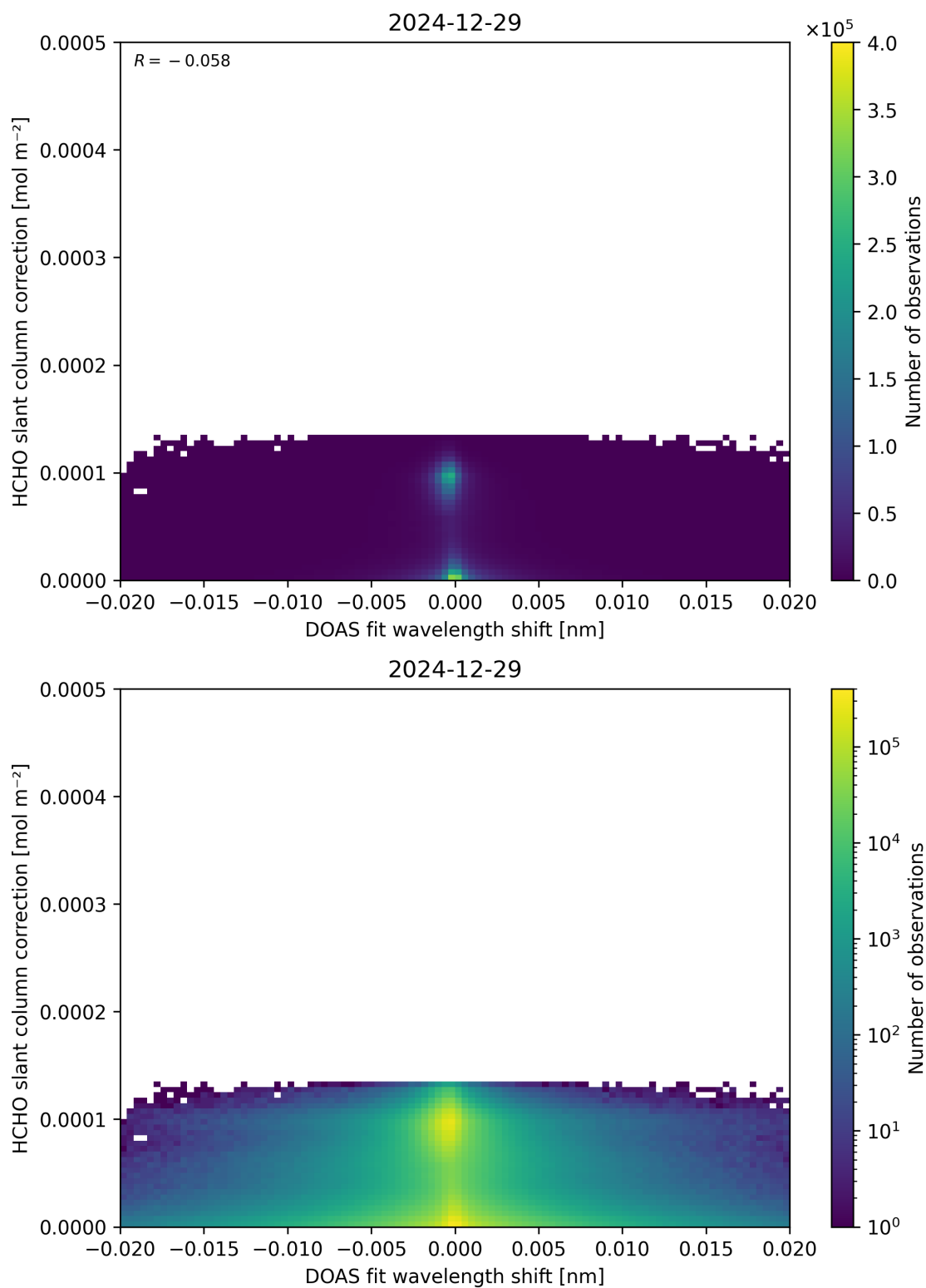
Figure 67: Scatter density plot of “DOAS fit wavelength shift” against “HCHO slant column correction” for 2024-12-28 to 2024-12-30.
