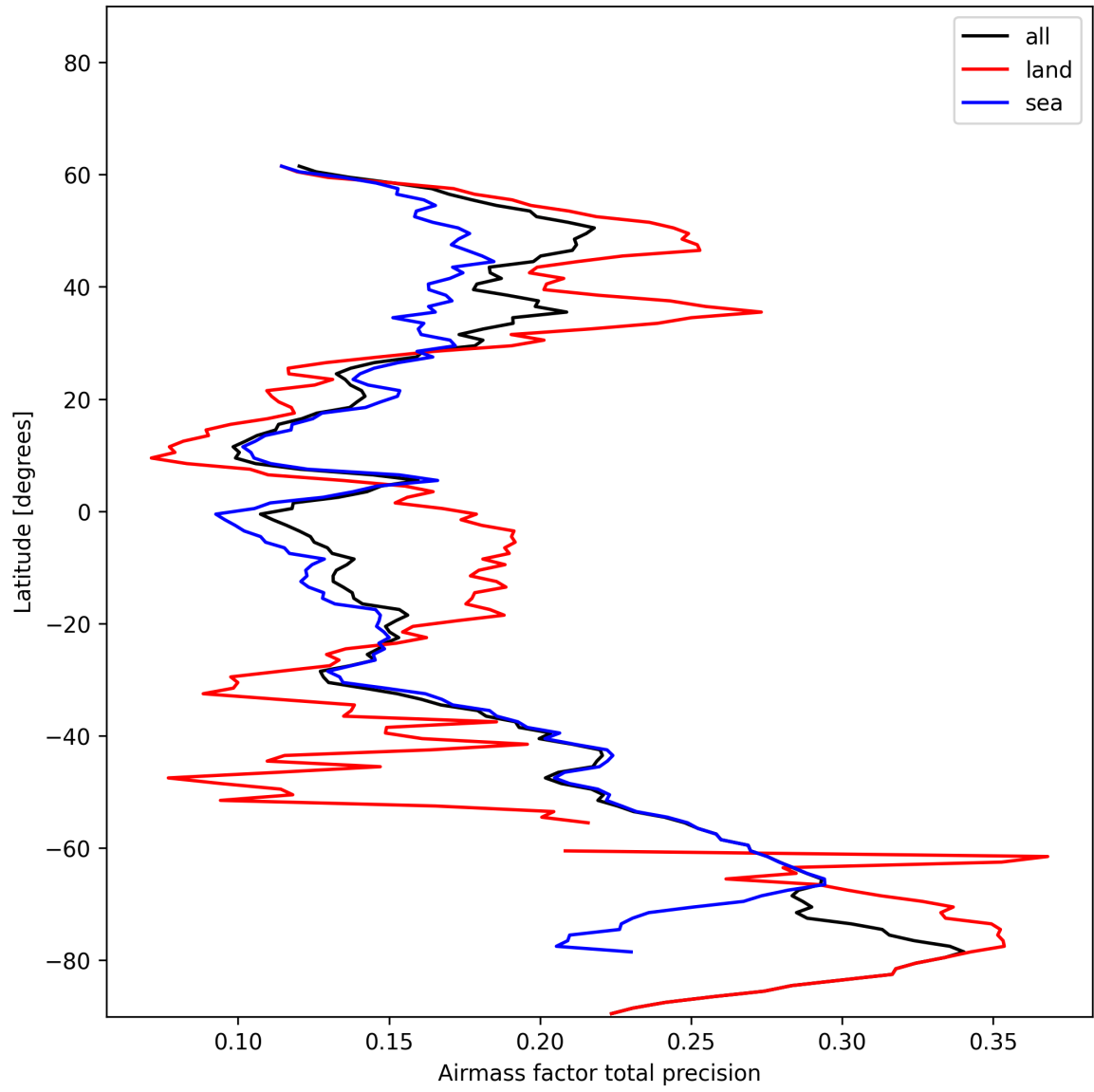
Figure 27: Zonal average of “Airmass factor total precision” for 2024-12-28 to 2024-12-30.
