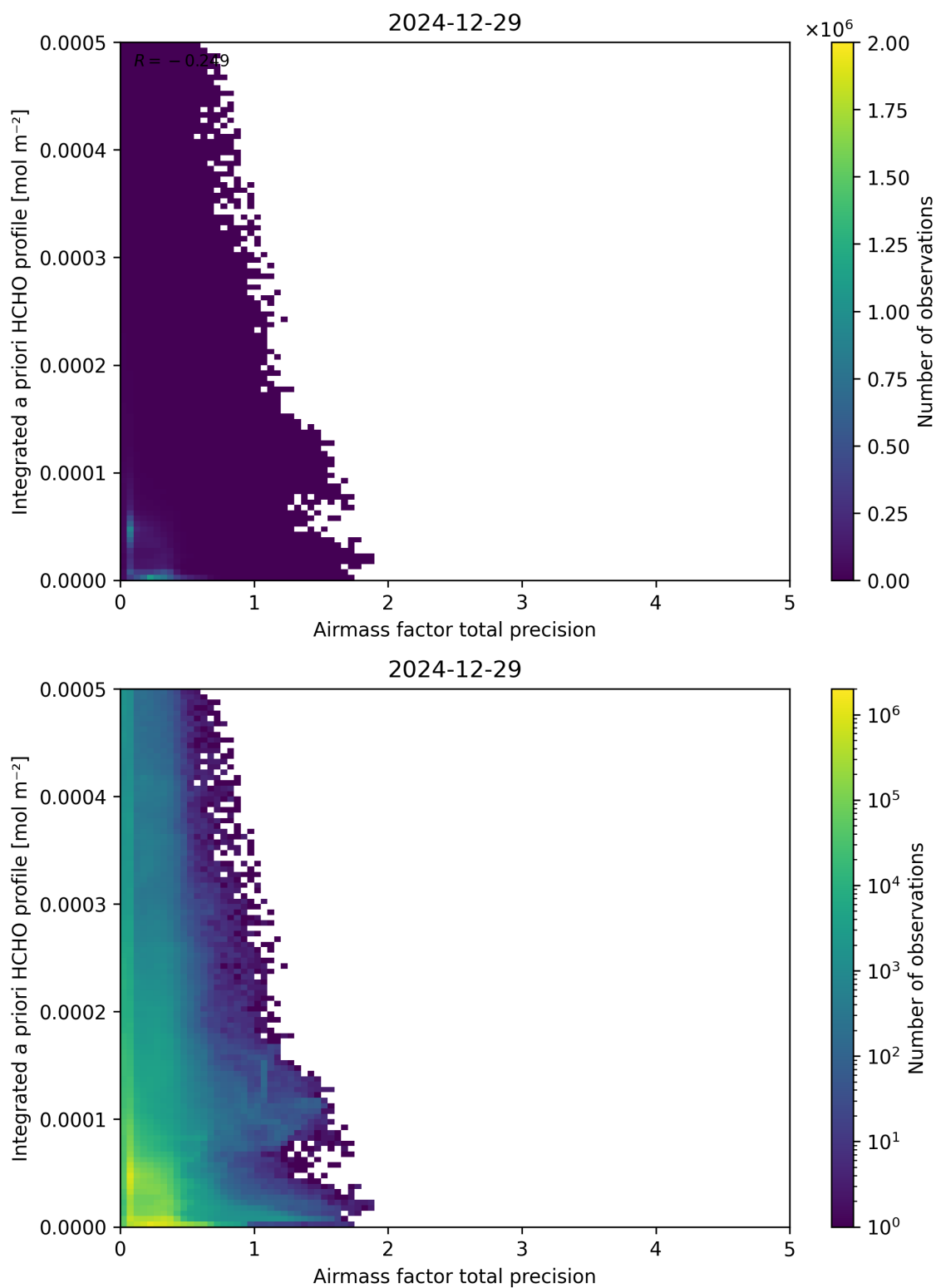
Figure 111: Scatter density plot of “Airmass factor total precision” against “Integrated a priori HCHO profile” for 2024-12-28 to 2024-12-30.
