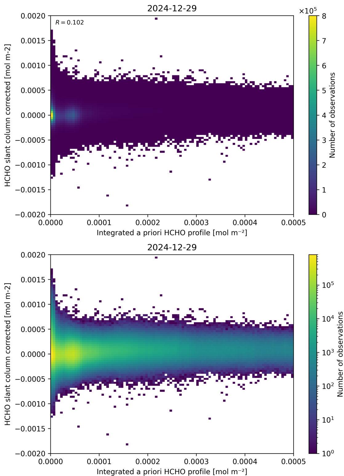
Figure 151: Scatter density plot of “Integrated a priori HCHO profile” against “HCHO slant column corrected” for 2024-12-28 to 2024-12-30.
