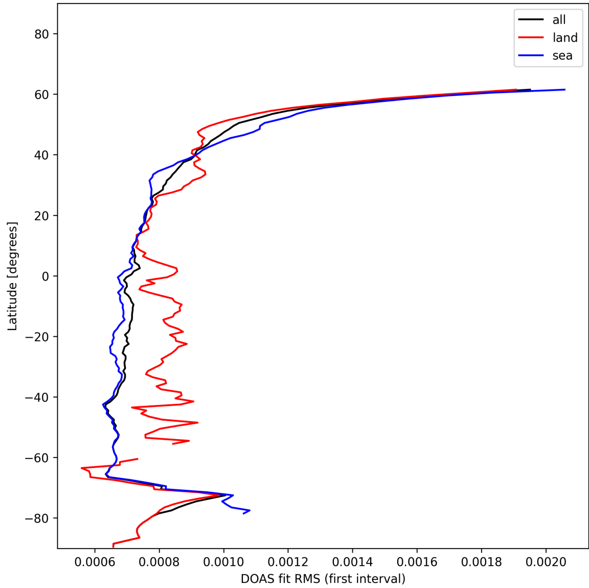
Figure 32: Zonal average of “DOAS fit RMS (first interval)” for 2024-12-28 to 2024-12-30.
