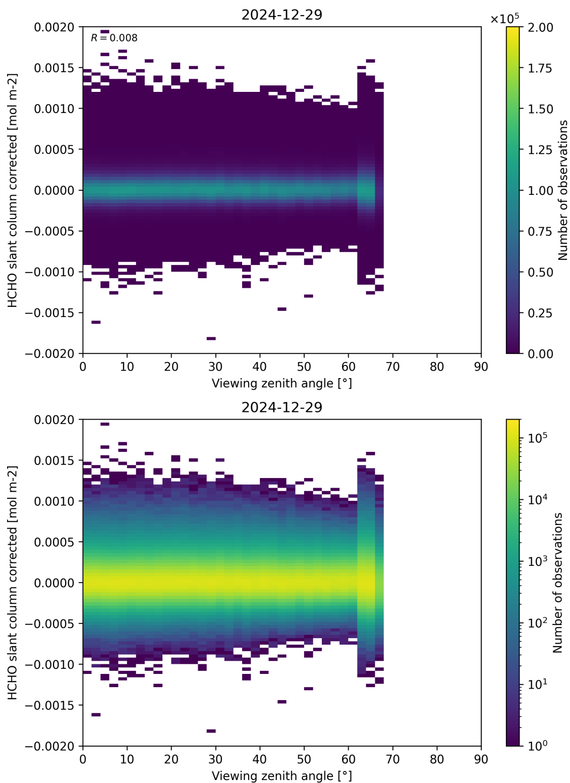
Figure 186: Scatter density plot of “Viewing zenith angle” against “HCHO slant column corrected” for 2024-12-28 to 2024-12-30.
