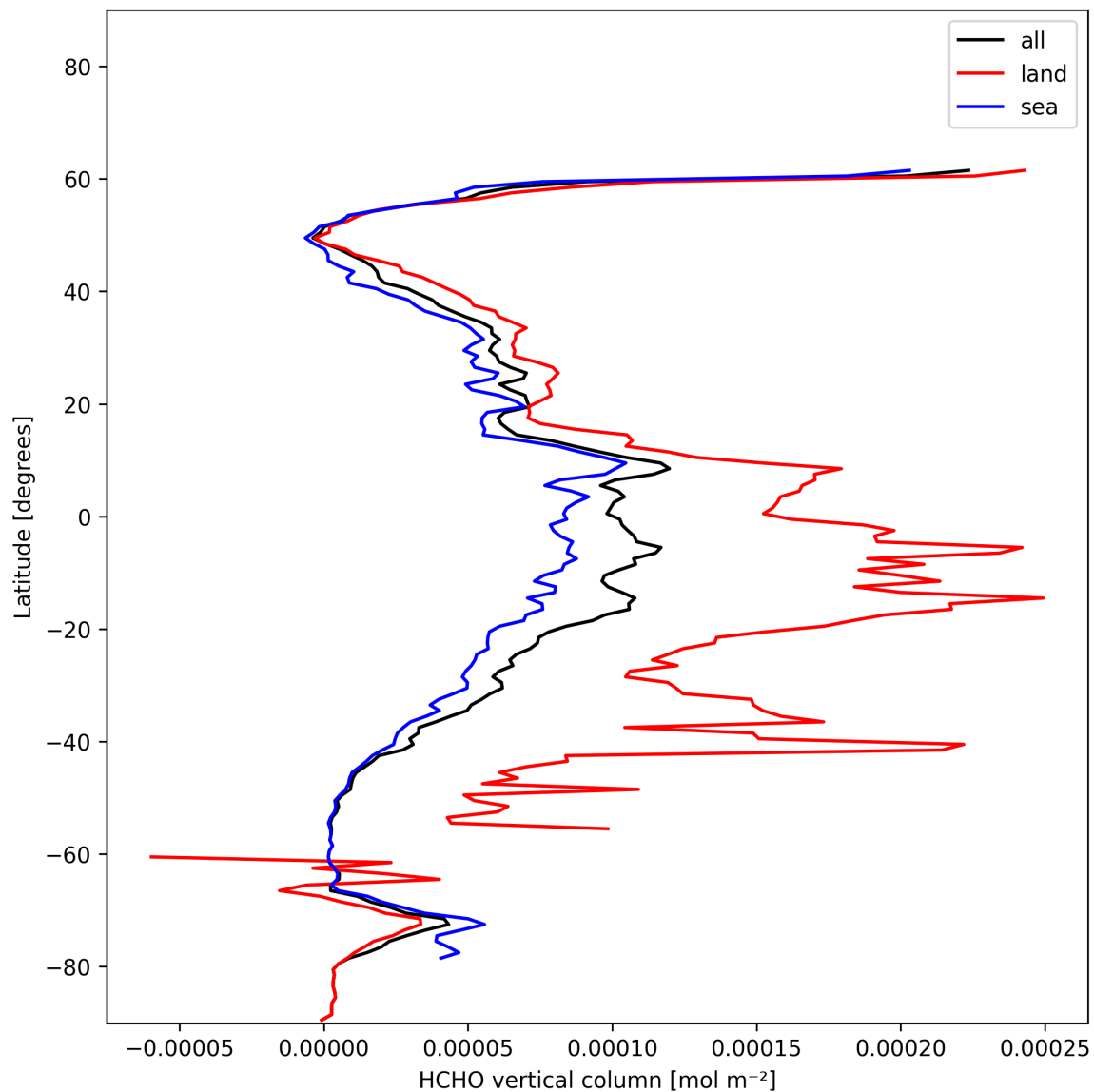
Figure 21: Zonal average of “HCHO vertical column” for 2024-12-28 to 2024-12-30.
