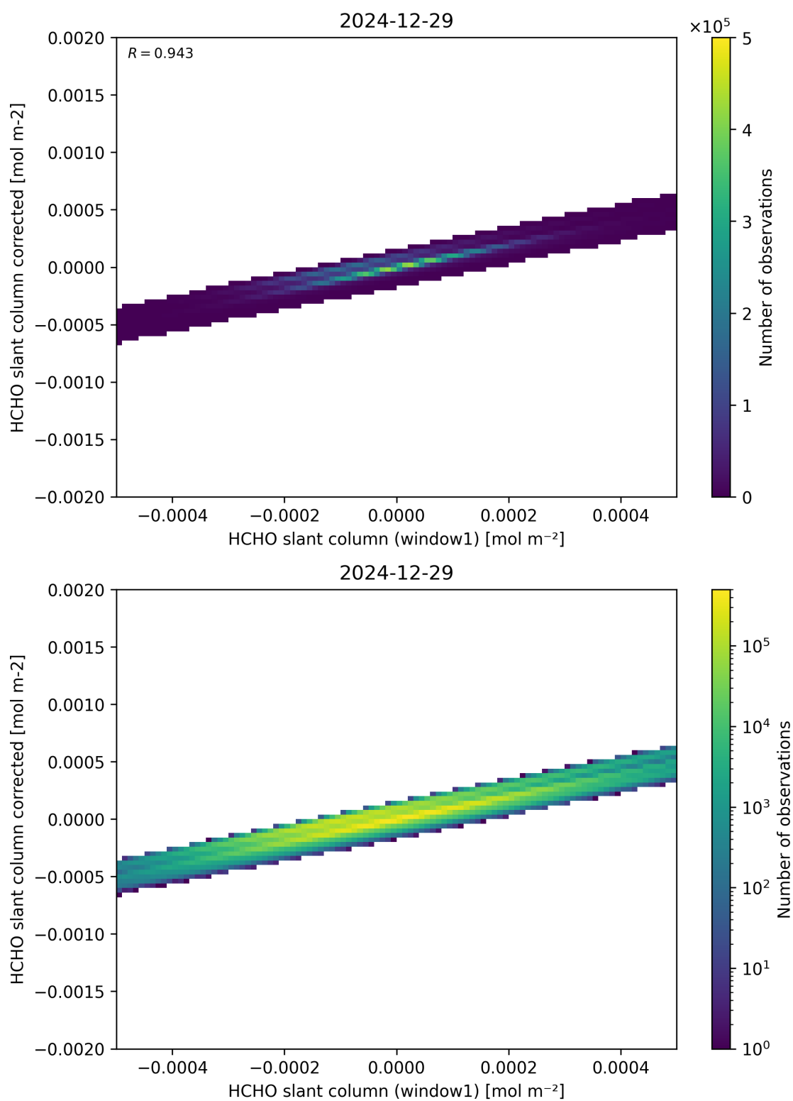
Figure 82: Scatter density plot of “HCHO slant column (window1)” against “HCHO slant column corrected” for 2024-12-28 to 2024-12-30.
