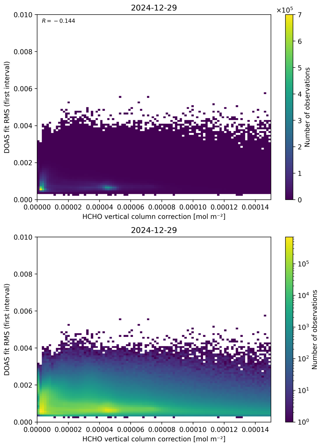
Figure 112: Scatter density plot of “HCHO vertical column correction” against “DOAS fit RMS (first interval)” for 2024-12-28 to 2024-12-30.
