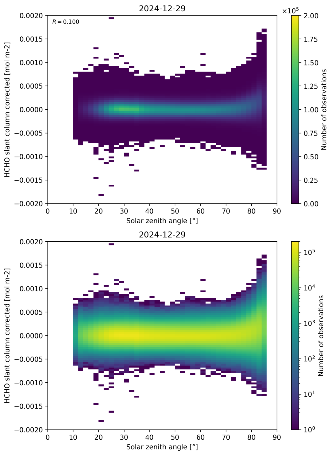
Figure 171: Scatter density plot of “Solar zenith angle” against “HCHO slant column corrected” for 2024-12-28 to 2024-12-30.
