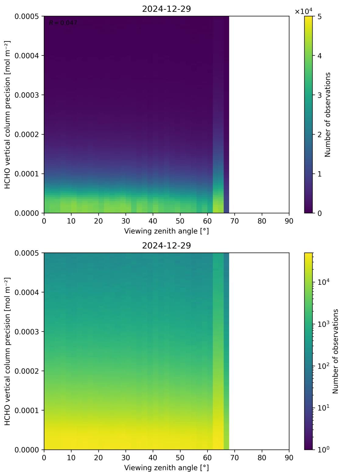
Figure 194: Scatter density plot of “Viewing zenith angle” against “HCHO vertical column precision” for 2024-12-28 to 2024-12-30.
