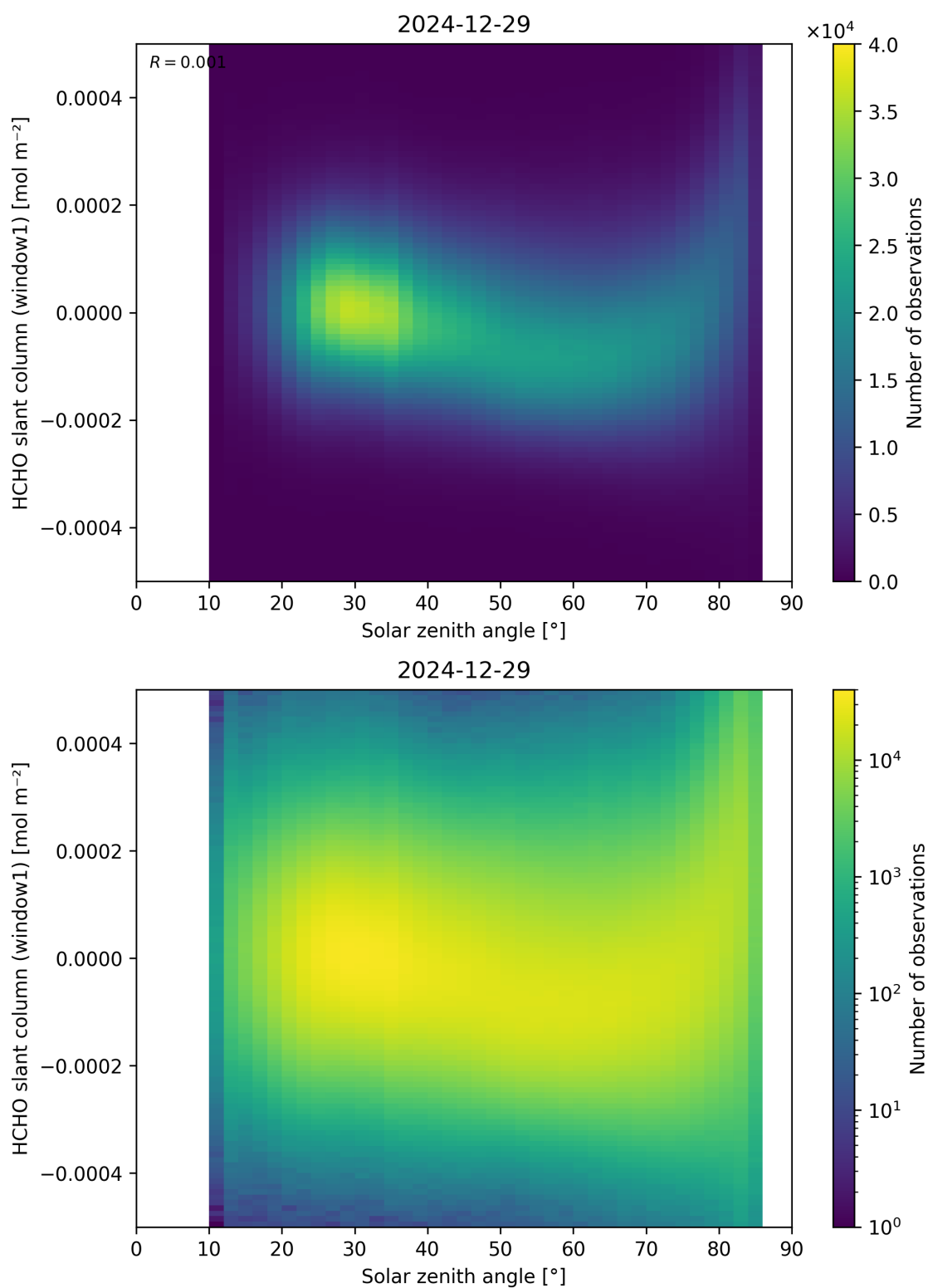
Figure 173: Scatter density plot of “Solar zenith angle” against “HCHO slant column (window1)” for 2024-12-28 to 2024-12-30.
