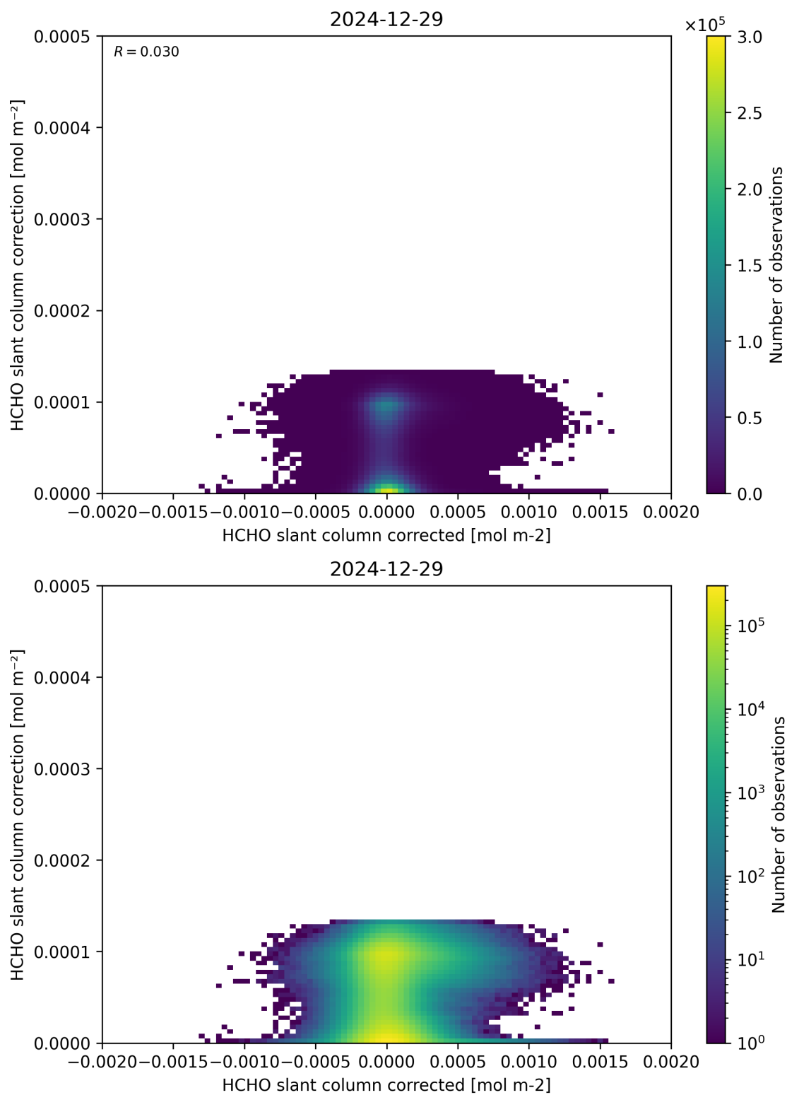
Figure 77: Scatter density plot of “HCHO slant column corrected” against “HCHO slant column correction” for 2024-12-28 to 2024-12-30.
