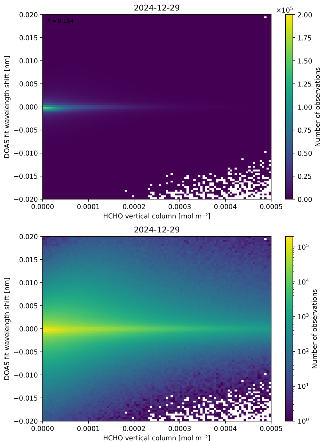
Figure 124: Scatter density plot of “HCHO vertical column” against “DOAS fit wavelength shift” for 2024-12-28 to 2024-12-30.
