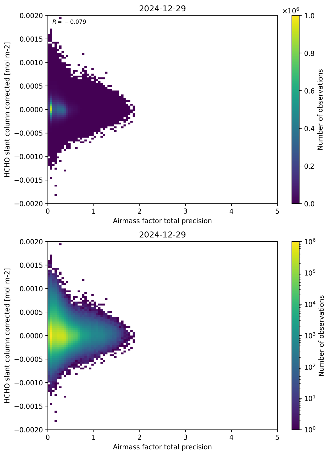
Figure 109: Scatter density plot of “Airmass factor total precision” against “HCHO slant column corrected” for 2024-12-28 to 2024-12-30.
