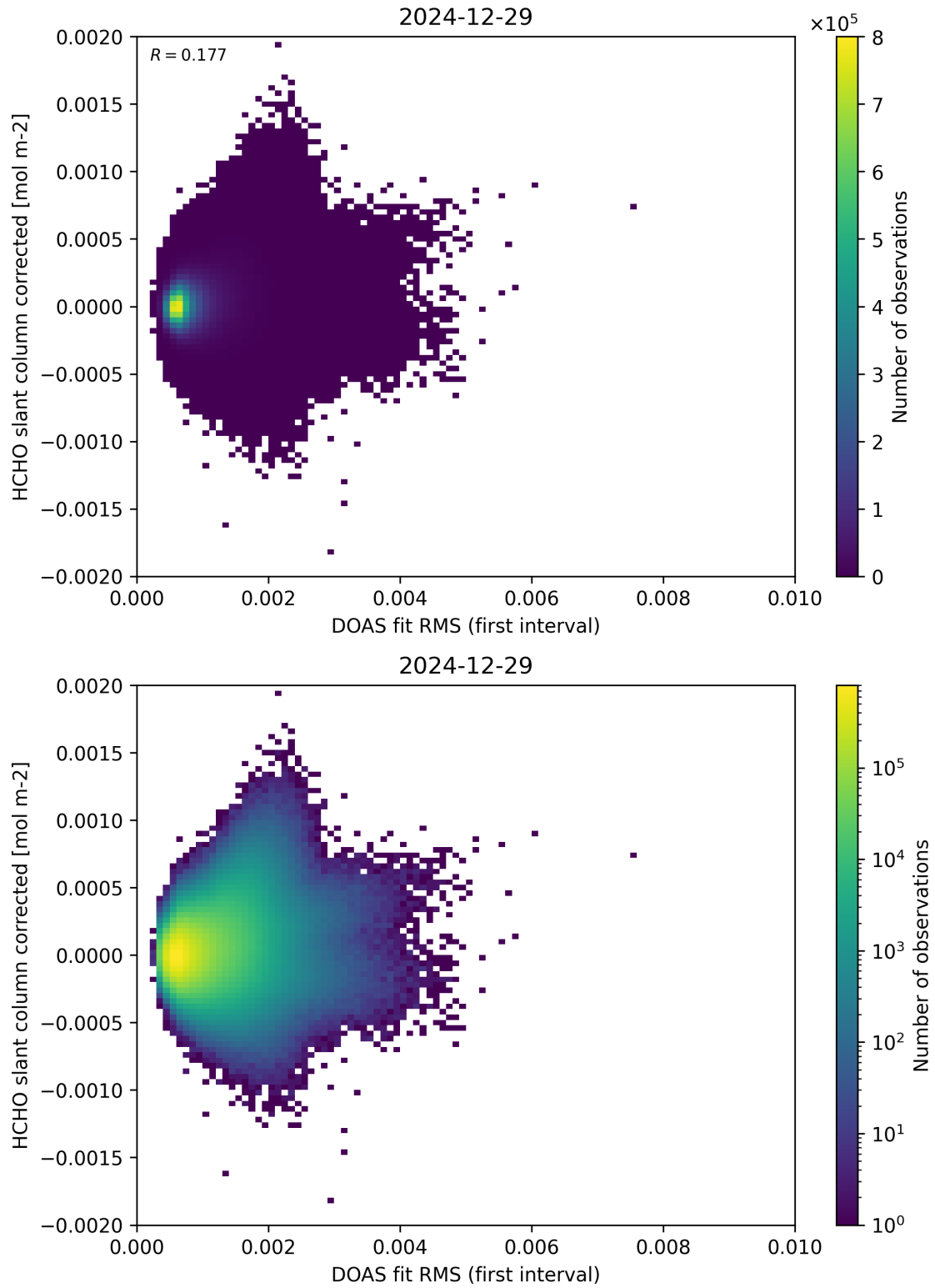
Figure 62: Scatter density plot of “DOAS fit RMS (first interval)” against “HCHO slant column corrected” for 2024-12-28 to 2024-12-30.
