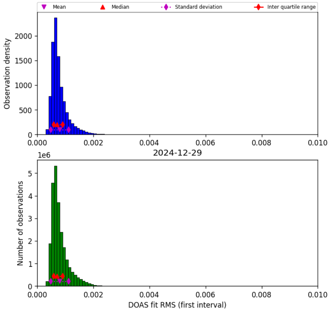
Figure 46: Histogram of “DOAS fit RMS (first interval)” for 2024-12-28 to 2024-12-30
