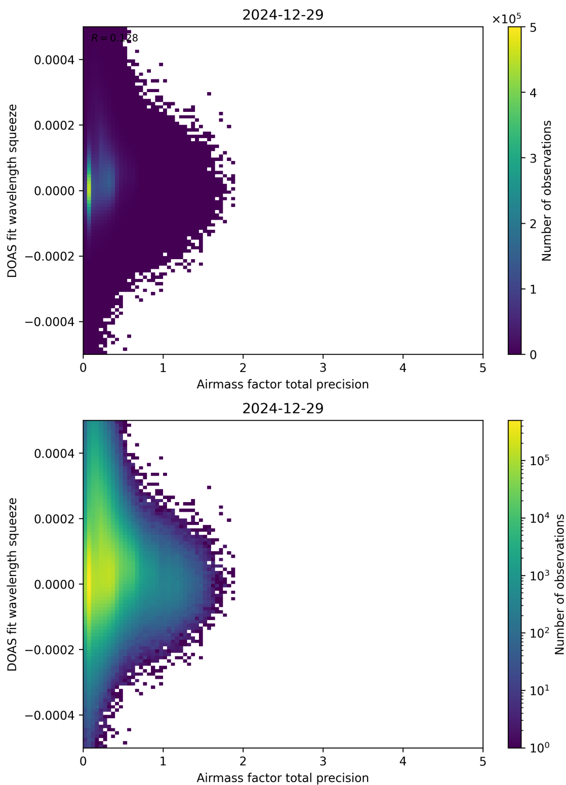
Figure 107: Scatter density plot of “Airmass factor total precision” against “DOAS fit wavelength squeeze” for 2024-12-28 to 2024-12-30.
