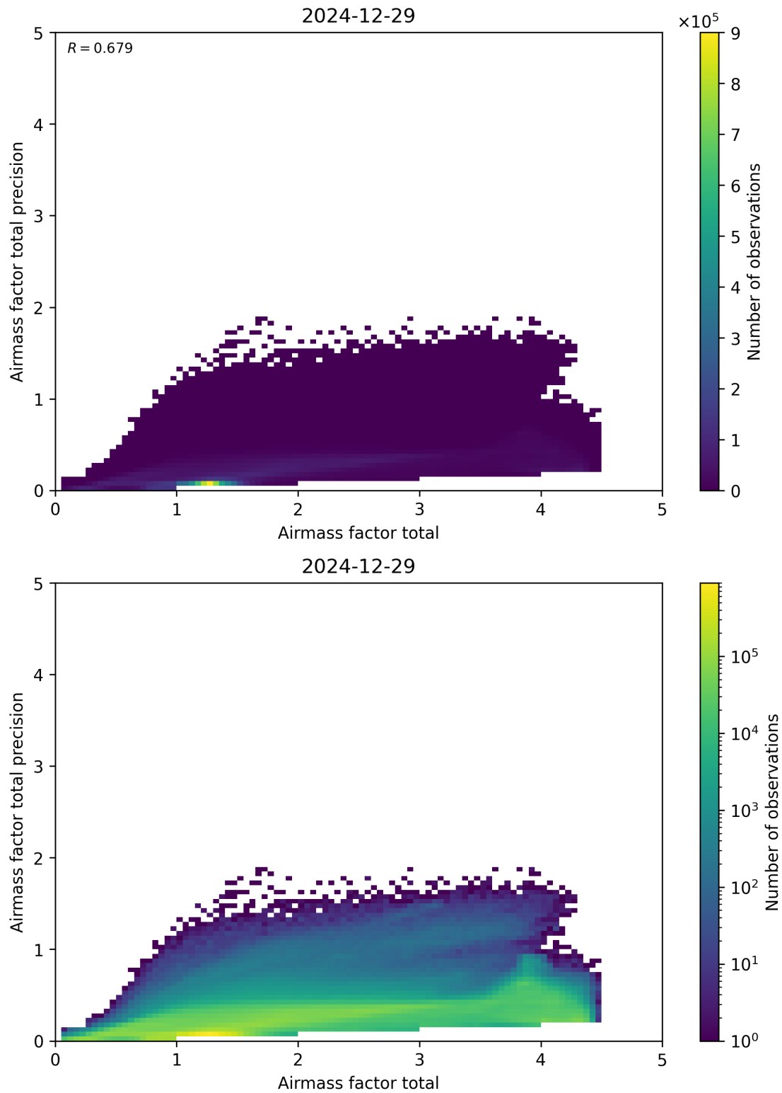
Figure 103: Scatter density plot of “Airmass factor total” against “Airmass factor total precision” for 2024-12-28 to 2024-12-30.
