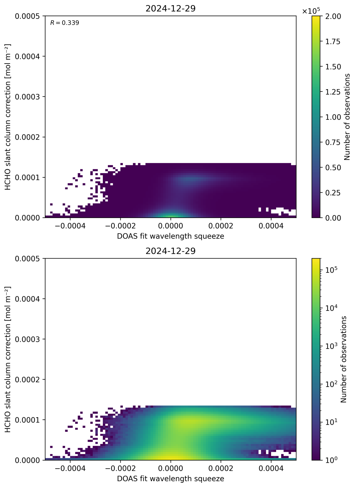
Figure 70: Scatter density plot of “DOAS fit wavelength squeeze” against “HCHO slant column correction” for 2024-12-28 to 2024-12-30.
