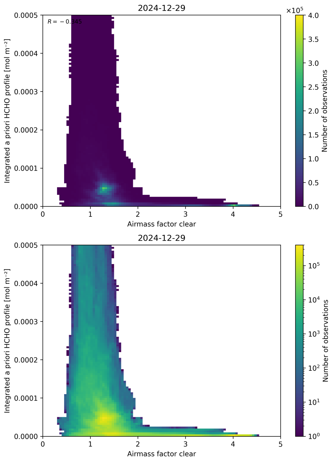
Figure 76: Scatter density plot of “Airmass factor clear” against “Integrated a priori HCHO profile” for 2024-12-28 to 2024-12-30.
