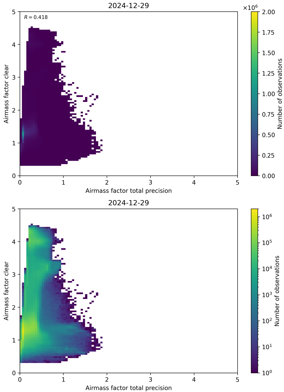
Figure 108: Scatter density plot of “Airmass factor total precision” against “Airmass factor clear” for 2024-12-28 to 2024-12-30.
