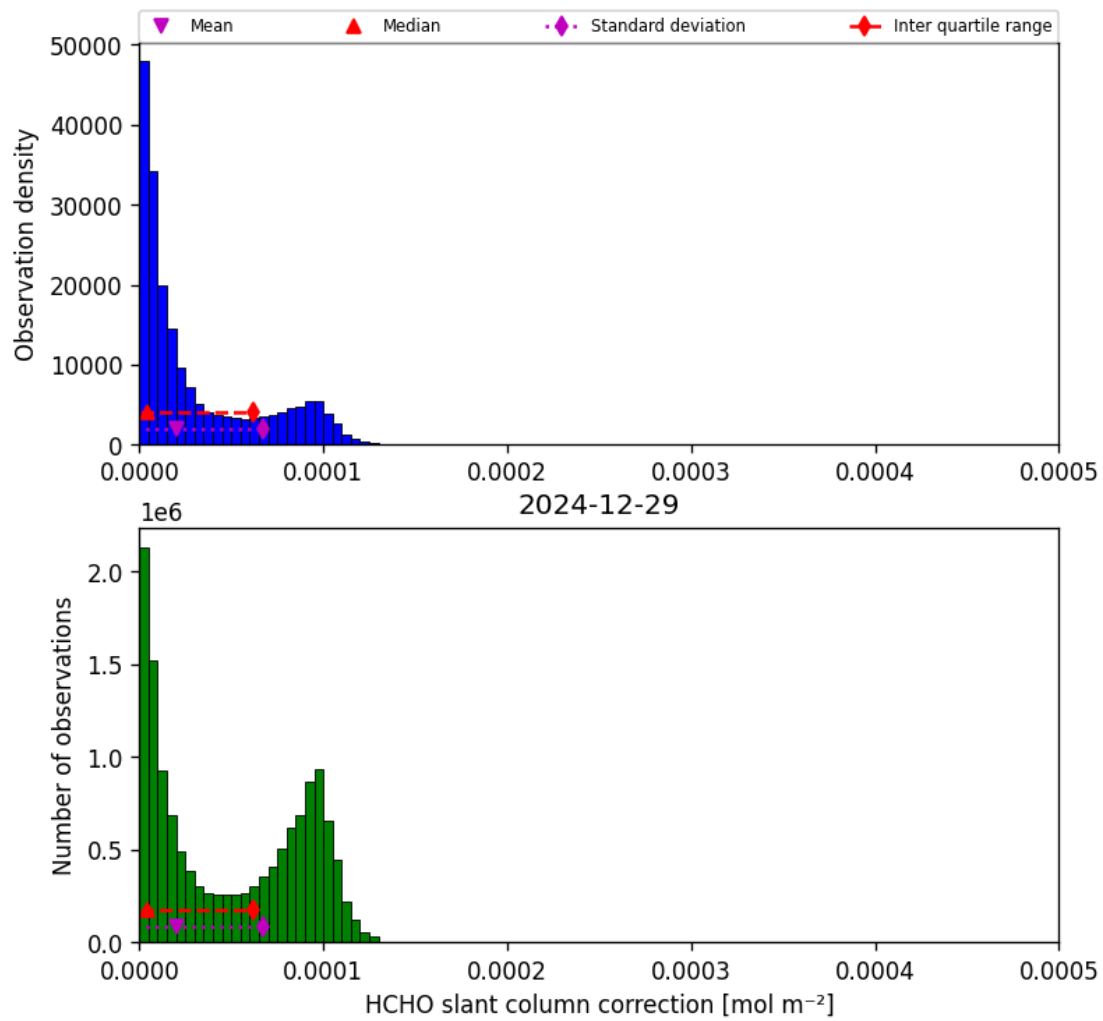
Figure 47: Histogram of “HCHO slant column correction” for 2024-12-28 to 2024-12-30
