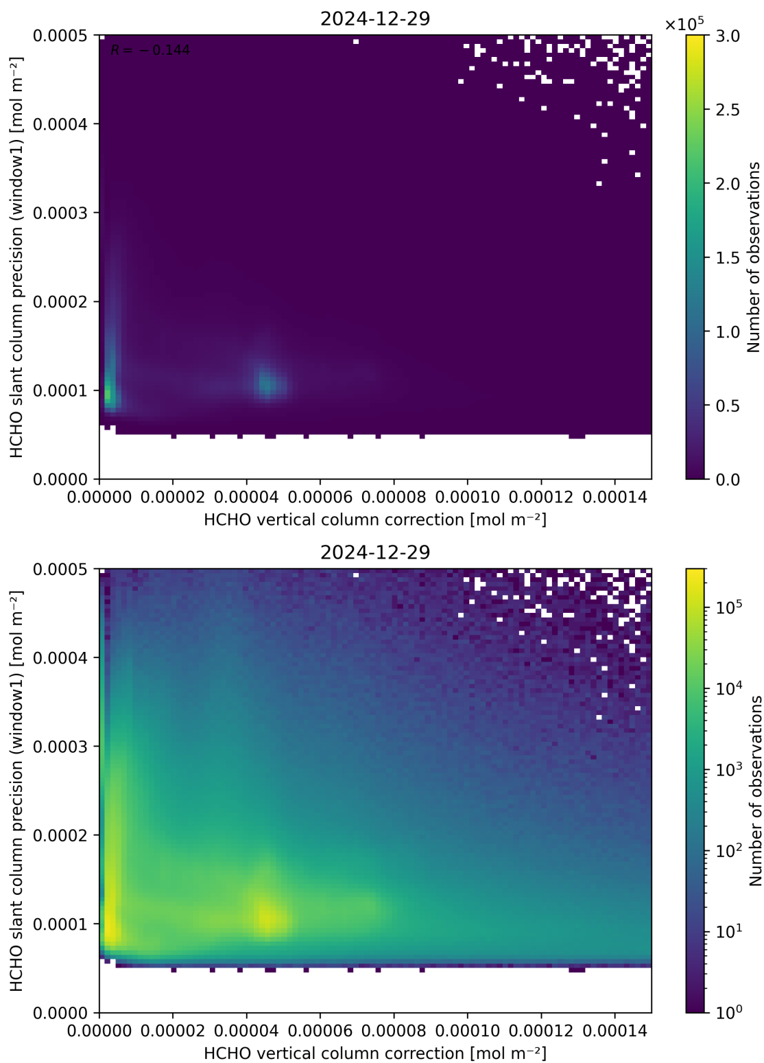
Figure 119: Scatter density plot of “HCHO vertical column correction” against “HCHO slant column precision (window1)” for 2024-12-28 to 2024-12-30.
