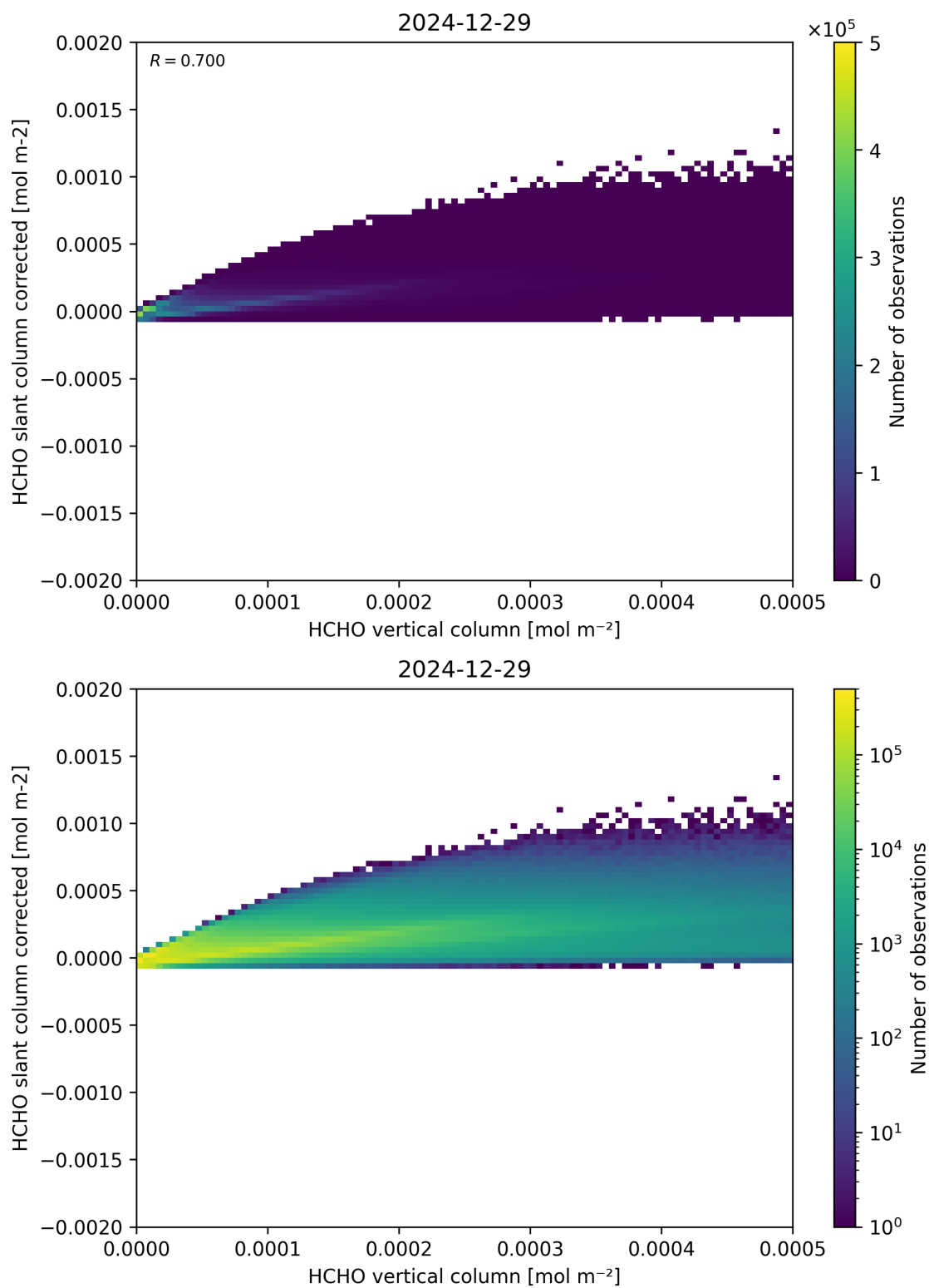
Figure 127: Scatter density plot of “HCHO vertical column” against “HCHO slant column corrected” for 2024-12-28 to 2024-12-30.
