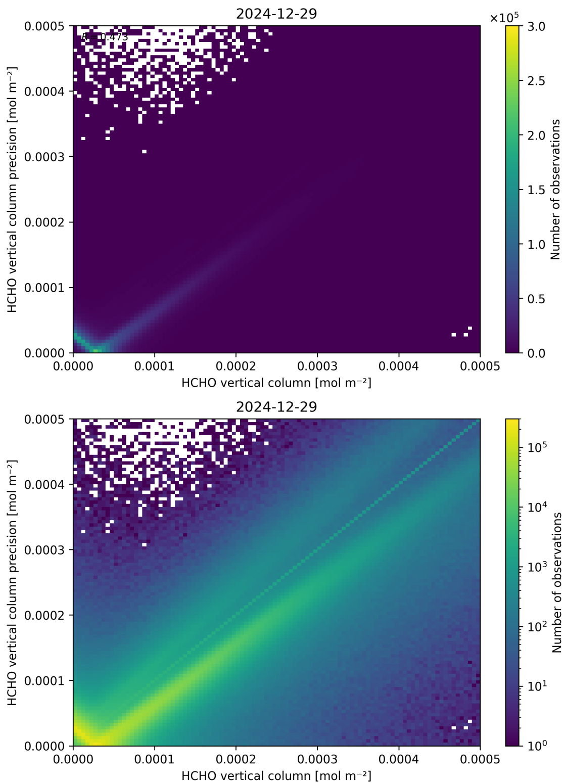
Figure 134: Scatter density plot of “HCHO vertical column” against “HCHO vertical column precision” for 2024-12-28 to 2024-12-30.
