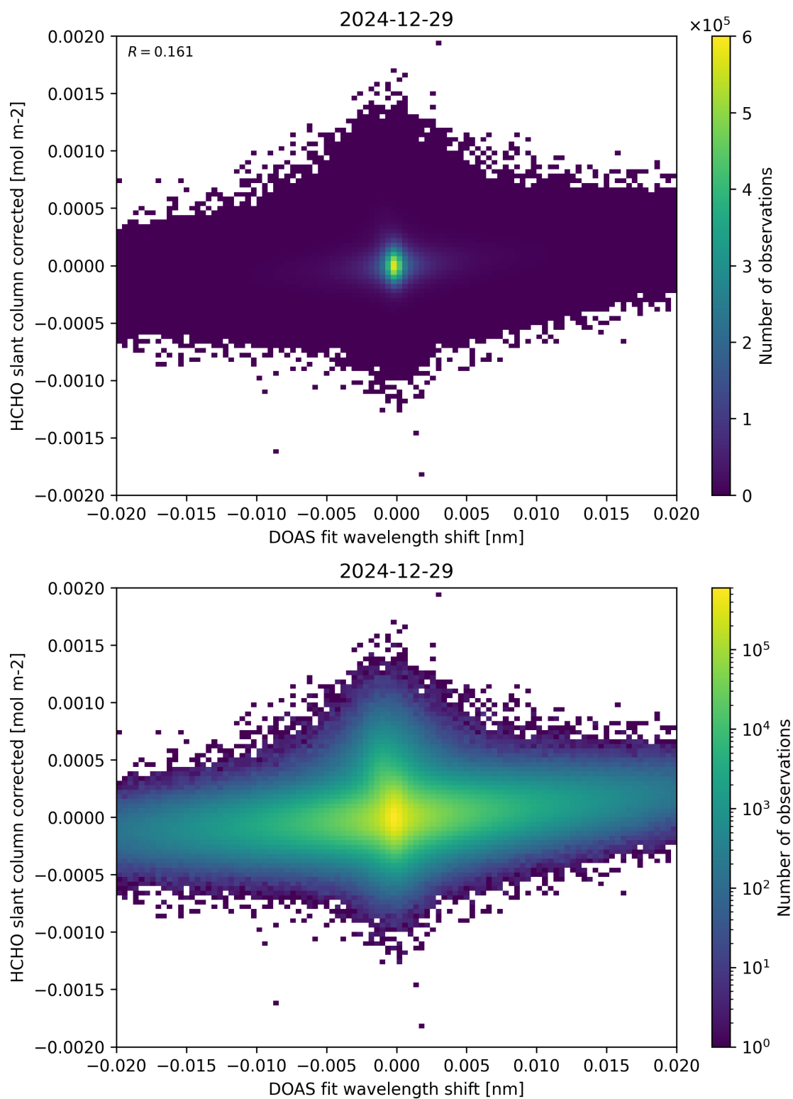
Figure 66: Scatter density plot of “DOAS fit wavelength shift” against “HCHO slant column corrected” for 2024-12-28 to 2024-12-30.
