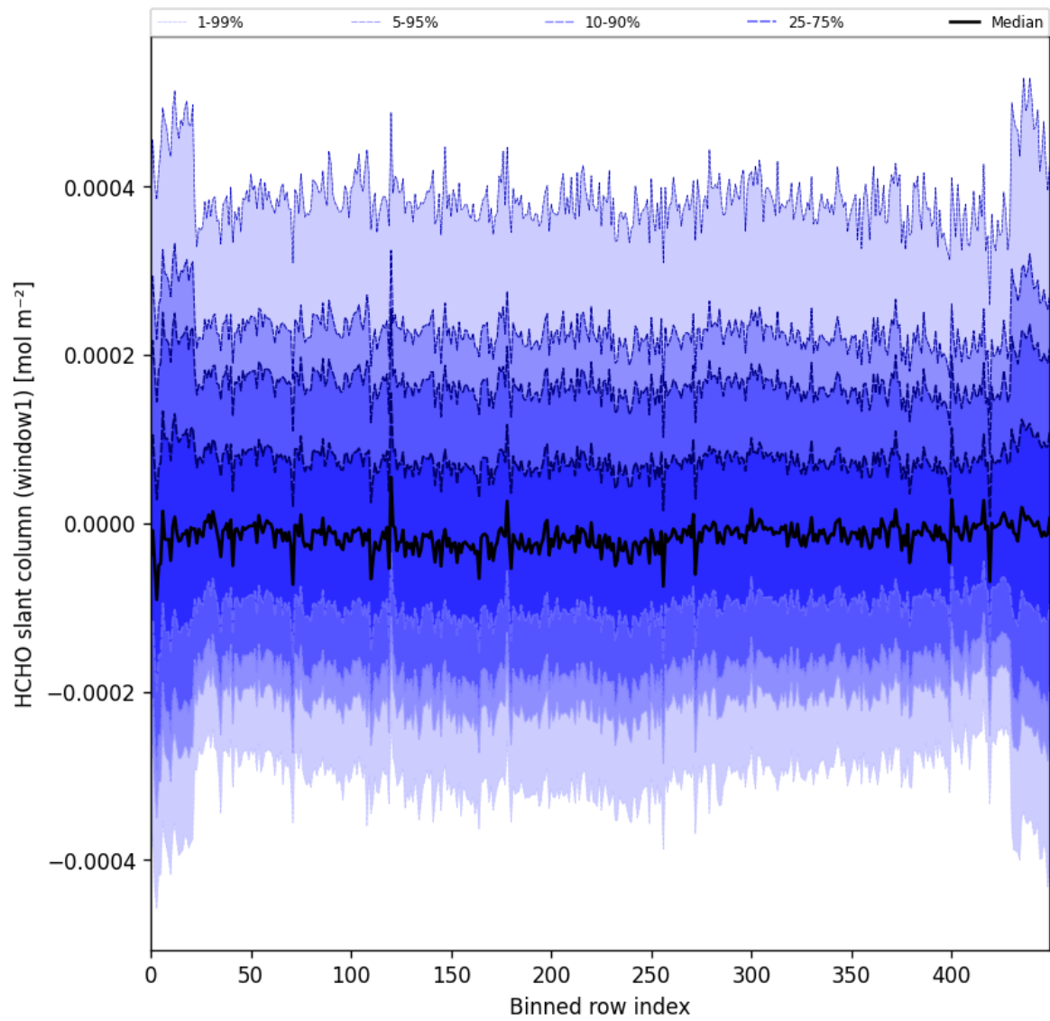
Figure 52: Along track statistics of “HCHO slant column (window1)” for 2024-12-28 to 2024-12-30
