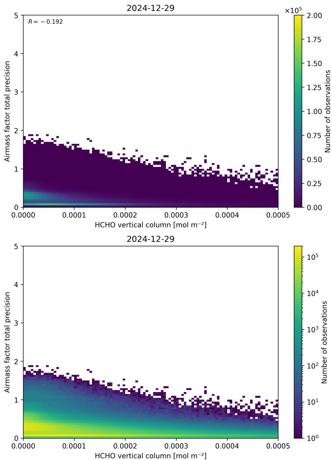
Figure 132: Scatter density plot of “HCHO vertical column” against “Airmass factor total precision” for 2024-12-28 to 2024-12-30.
