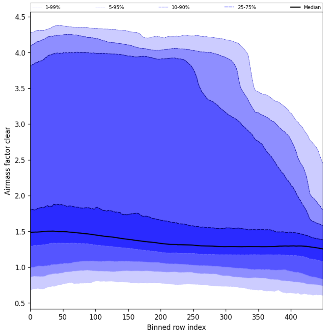
Figure 56: Along track statistics of “Air mass factor clear” for 2024-12-28 to 2024-12-30
