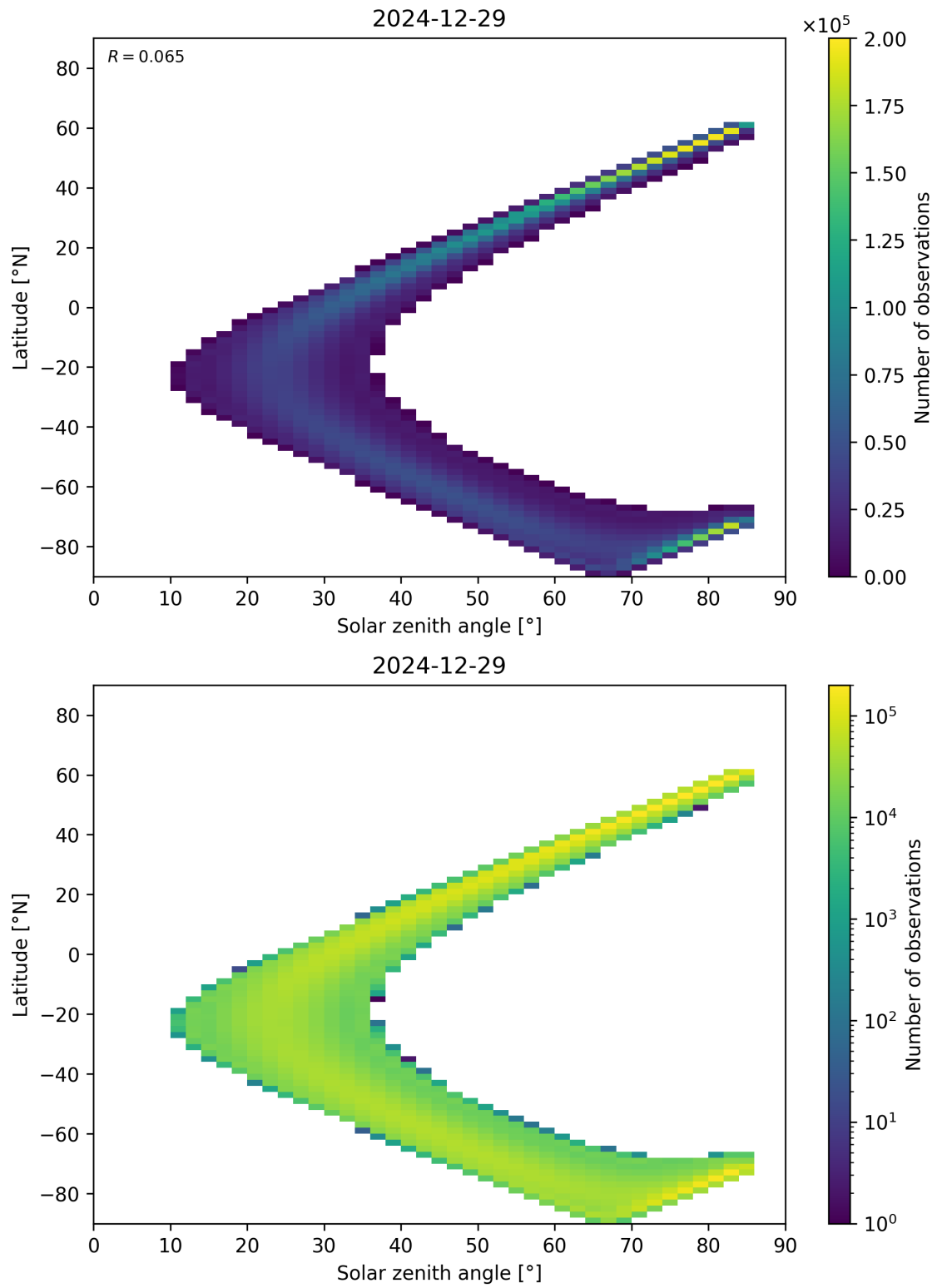
Figure 181: Scatter density plot of “Solar zenith angle” against “Latitude” for 2024-12-28 to 2024-12-30.
