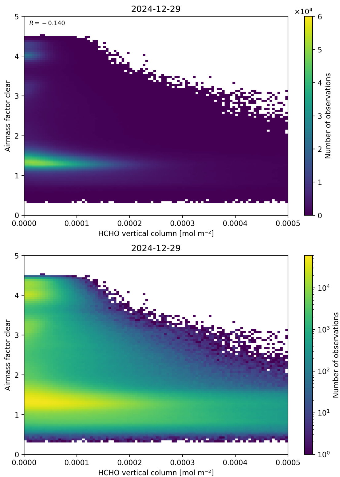
Figure 126: Scatter density plot of “HCHO vertical column” against “Airmass factor clear” for 2024-12-28 to 2024-12-30.
