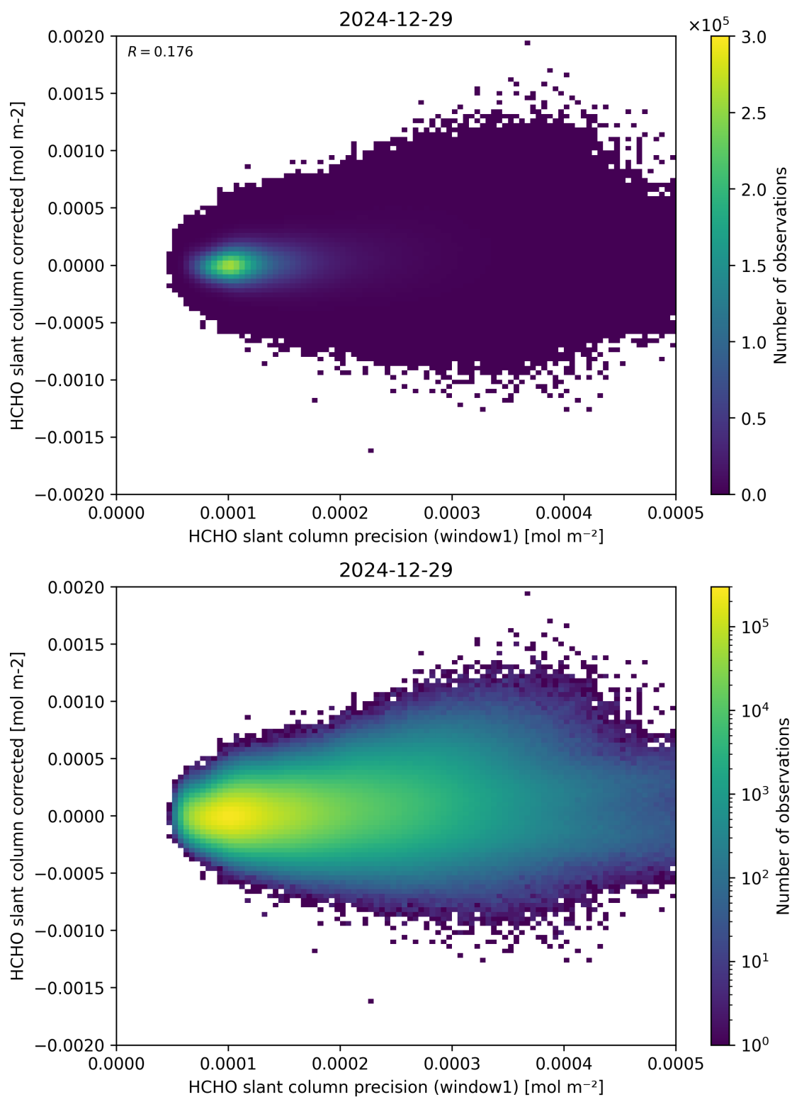
Figure 92: Scatter density plot of “HCHO slant column precision (window1)” against “HCHO slant column corrected” for 2024-12-28 to 2024-12-30.
