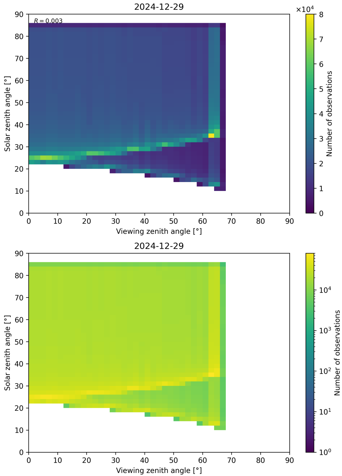
Figure 197: Scatter density plot of “Viewing zenith angle” against “Solar zenith angle” for 2024-12-28 to 2024-12-30.
