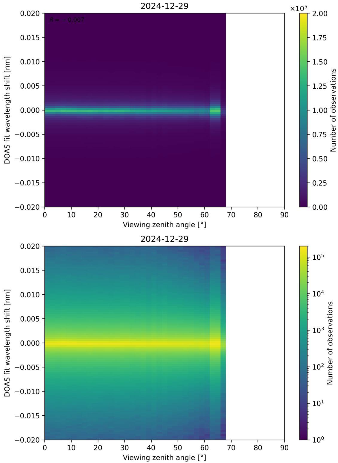
Figure 183: Scatter density plot of “Viewing zenith angle” against “DOAS fit wavelength shift” for 2024-12-28 to 2024-12-30.
