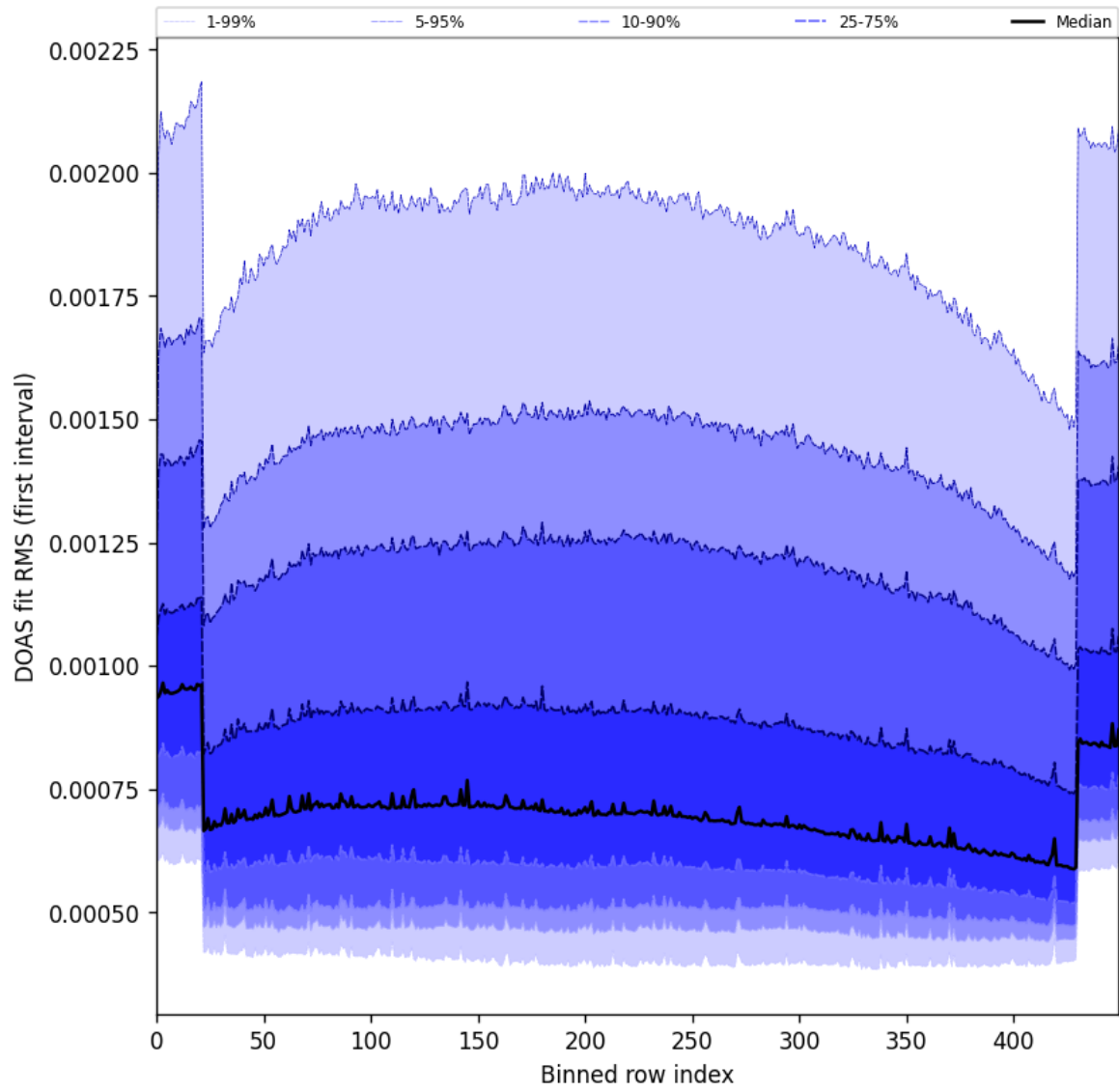
Figure 60: Along track statistics of “DOAS fit RMS (first interval)” for 2024-12-28 to 2024-12-30
