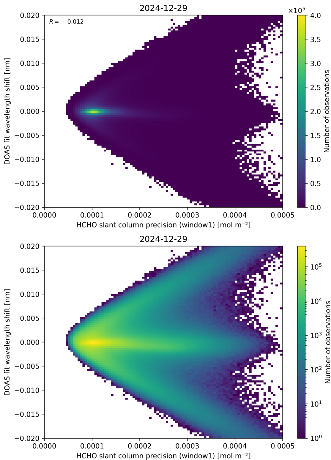
Figure 89: Scatter density plot of “HCHO slant column precision (window1)” against “DOAS fit wavelength shift” for 2024-12-28 to 2024-12-30.
