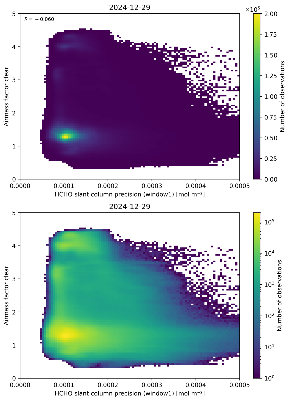
Figure 91: Scatter density plot of “HCHO slant column precision (window1)” against “Airmass factor clear” for 2024-12-28 to 2024-12-30.
