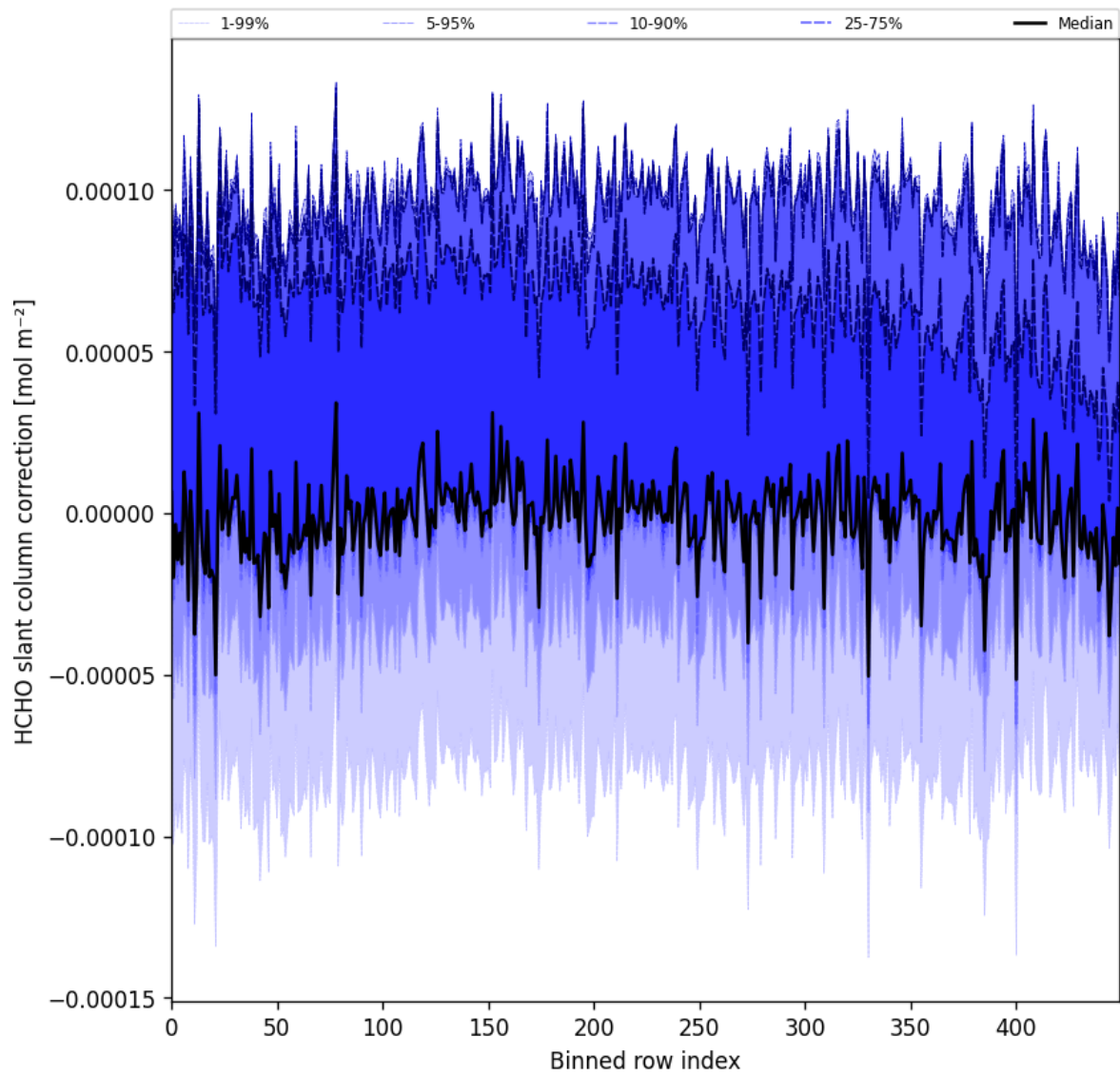
Figure 61: Along track statistics of “HCHO slant column correction” for 2024-12-28 to 2024-12-30
