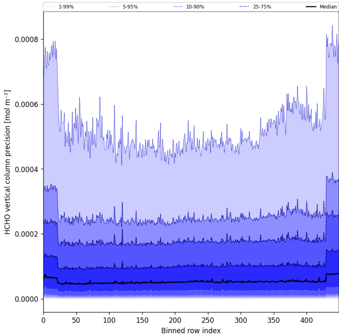
Figure 50: Along track statistics of “HCHO vertical column precision” for 2024-12-28 to 2024-12-30
