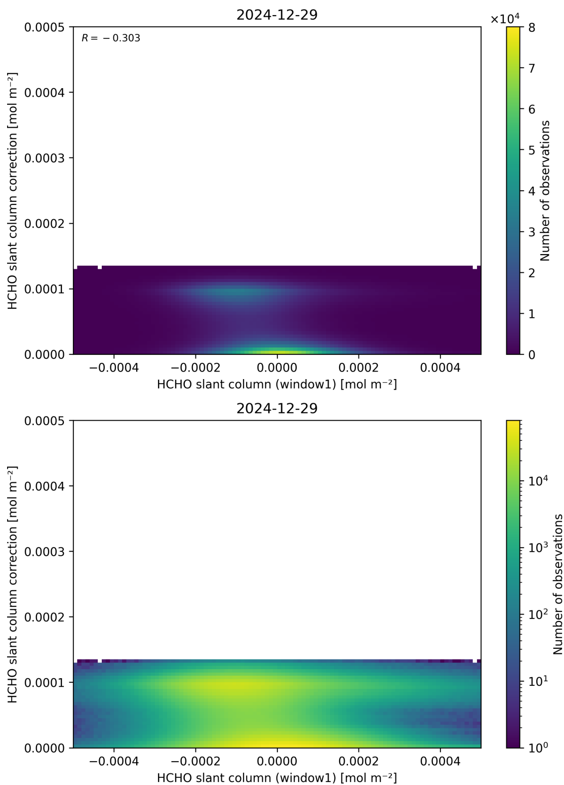
Figure 83: Scatter density plot of “HCHO slant column (window1)” against “HCHO slant column correction” for 2024-12-28 to 2024-12-30.
