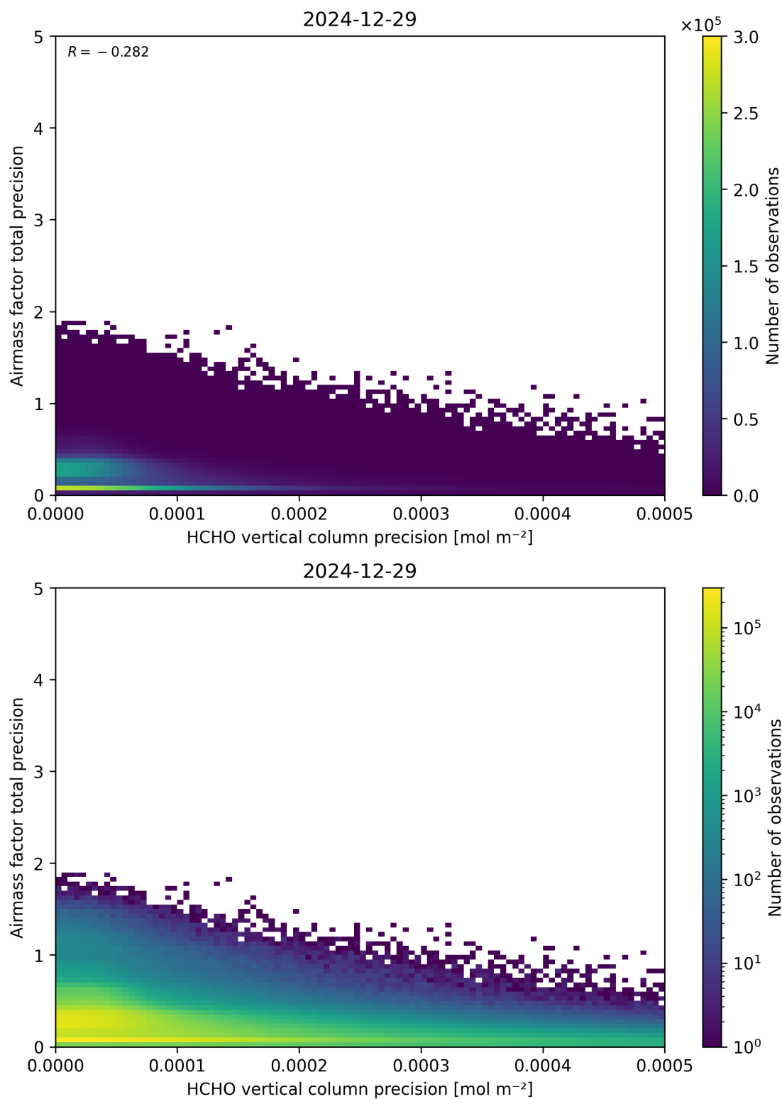
Figure 145: Scatter density plot of “HCHO vertical column precision” against “Airmass factor total precision” for 2024-12-28 to 2024-12-30.
