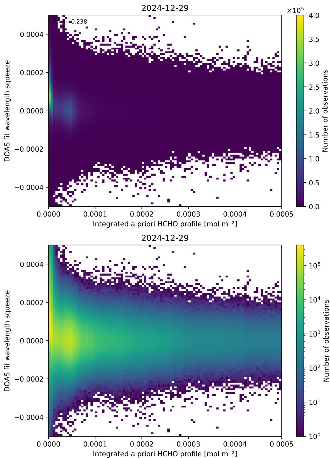
Figure 150: Scatter density plot of “Integrated a priori HCHO profile” against “DOAS fit wavelength squeeze” for 2024-12-28 to 2024-12-30.
