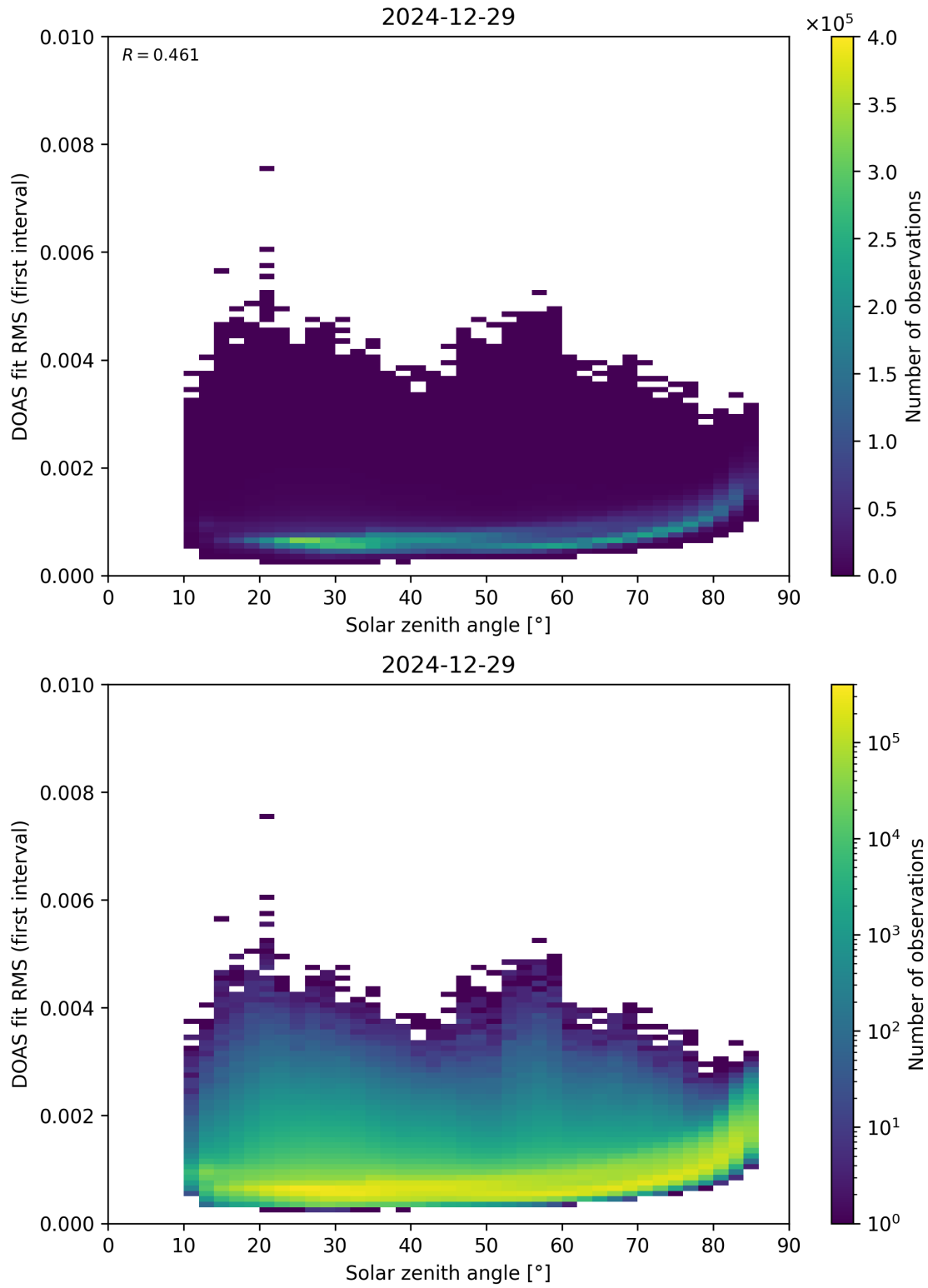
Figure 167: Scatter density plot of “Solar zenith angle” against “DOAS fit RMS (first interval)” for 2024-12-28 to 2024-12-30.
