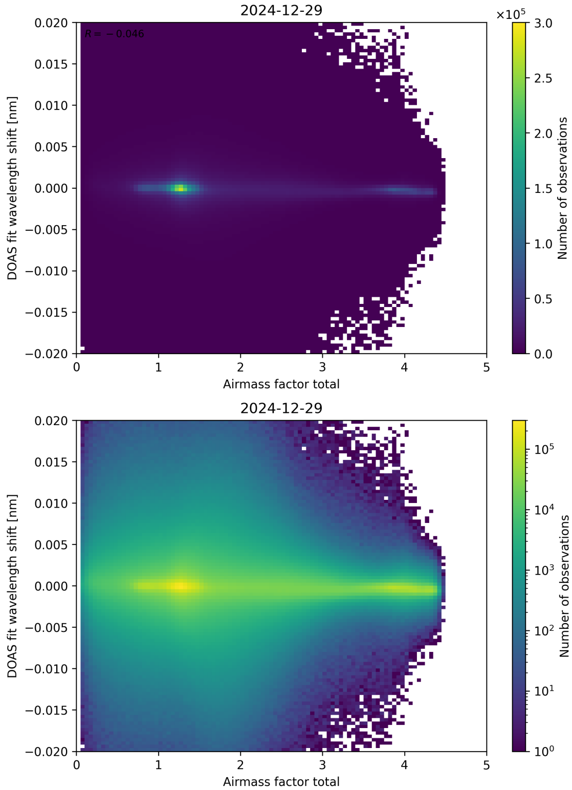
Figure 98: Scatter density plot of “Airmass factor total” against “DOAS fit wavelength shift” for 2024-12-28 to 2024-12-30.
