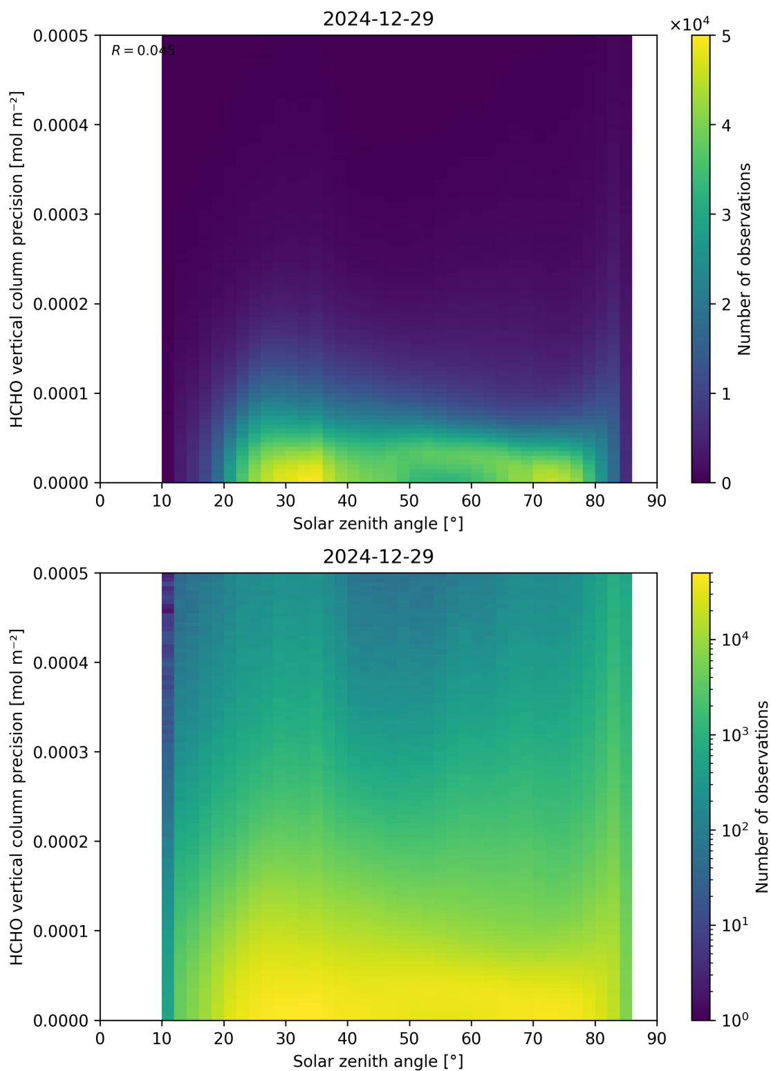
Figure 179: Scatter density plot of “Solar zenith angle” against “HCHO vertical column precision” for 2024-12-28 to 2024-12-30.
