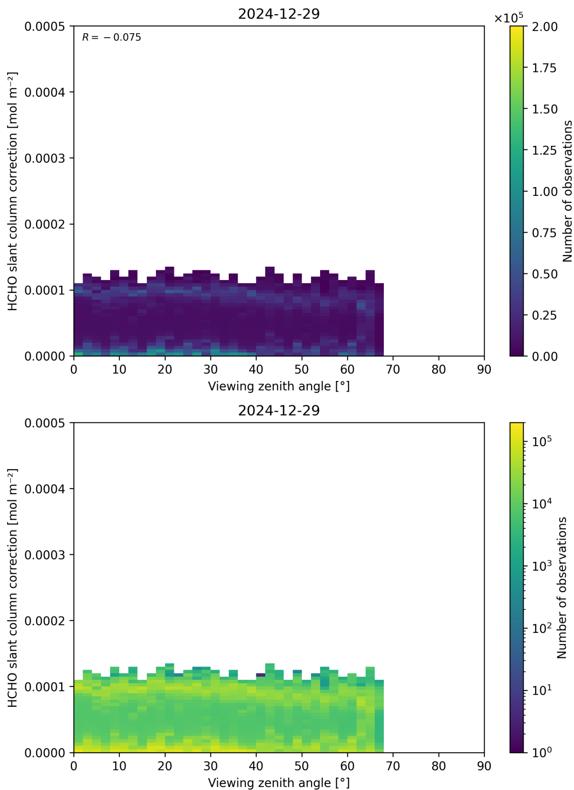
Figure 187: Scatter density plot of “Viewing zenith angle” against “HCHO slant column correction” for 2024-12-28 to 2024-12-30.
