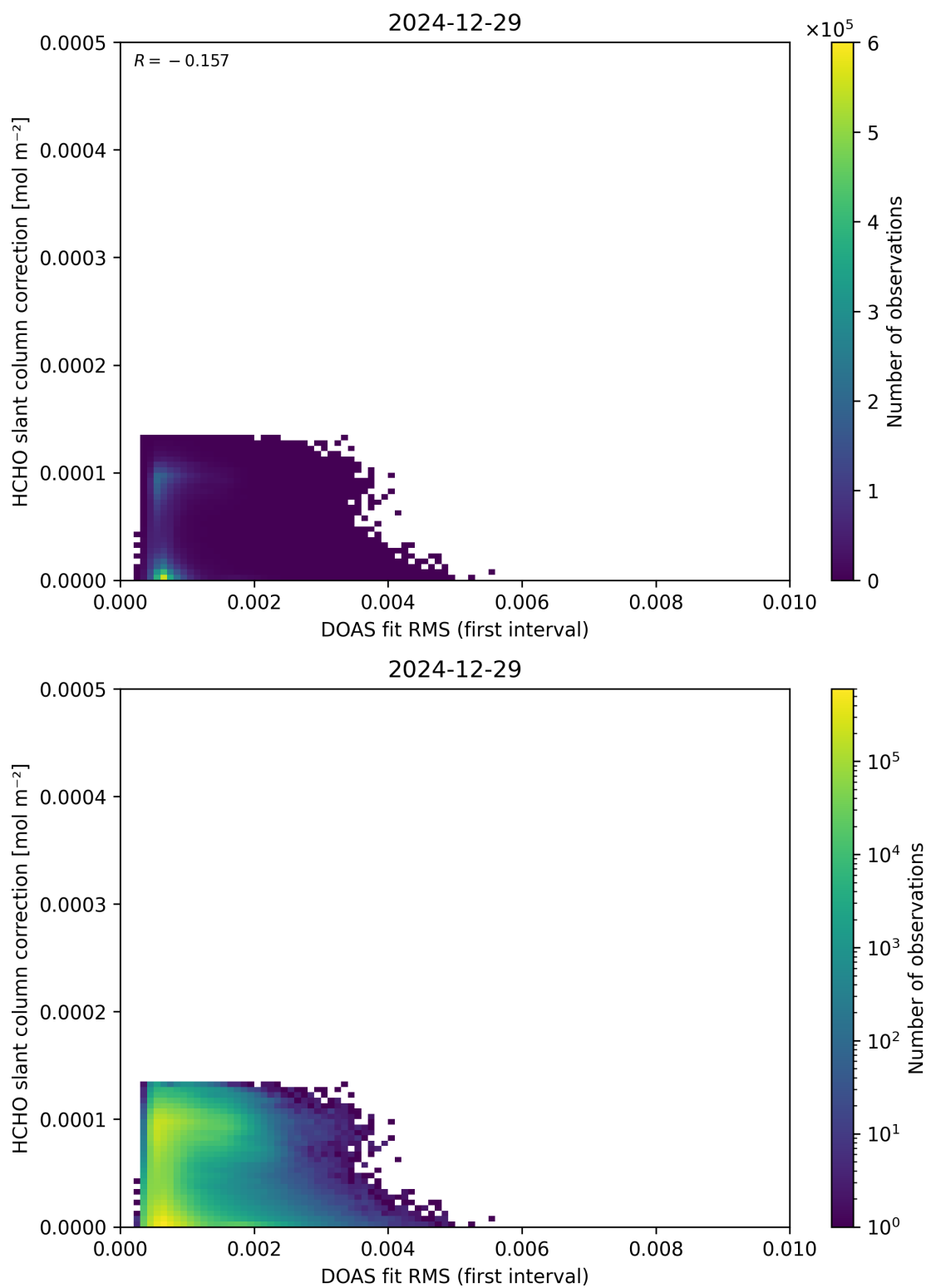
Figure 63: Scatter density plot of “DOAS fit RMS (first interval)” against “HCHO slant column correction” for 2024-12-28 to 2024-12-30.
