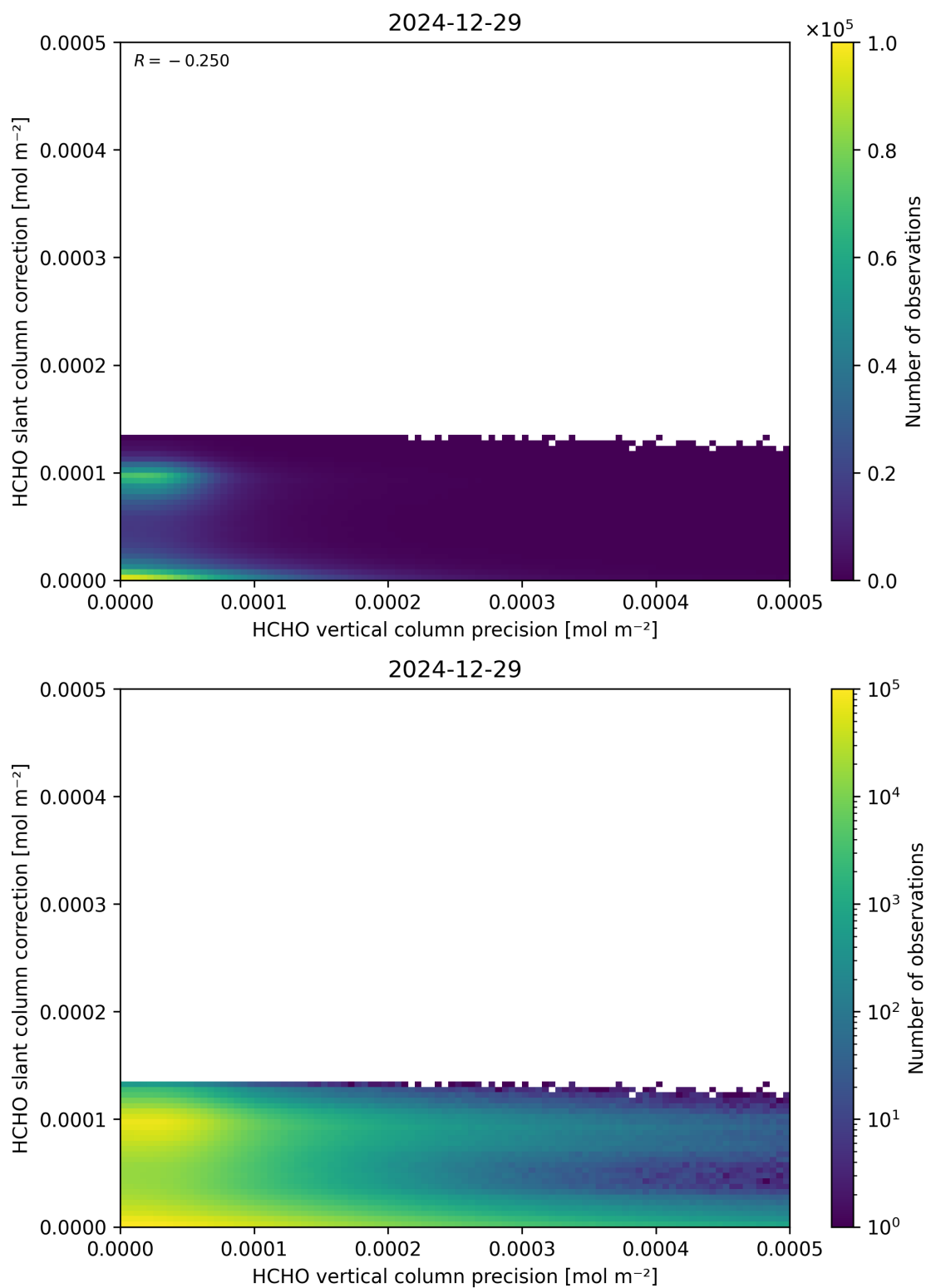
Figure 141: Scatter density plot of “HCHO vertical column precision” against “HCHO slant column correction” for 2024-12-28 to 2024-12-30.
