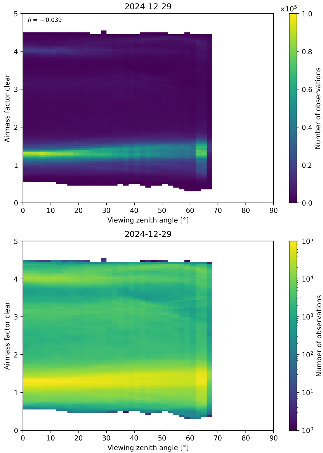
Figure 185: Scatter density plot of “Viewing zenith angle” against “Airmass factor clear” for 2024-12-28 to 2024-12-30.
