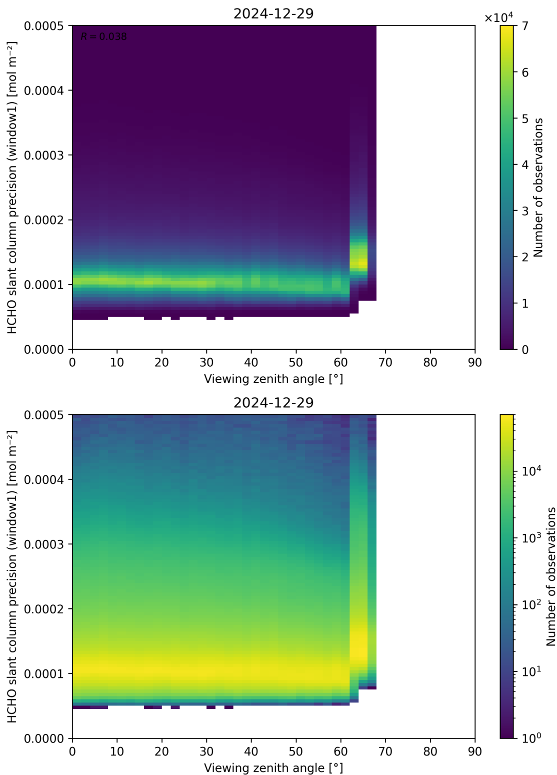
Figure 189: Scatter density plot of “Viewing zenith angle” against “HCHO slant column precision (window1)” for 2024-12-28 to 2024-12-30.
