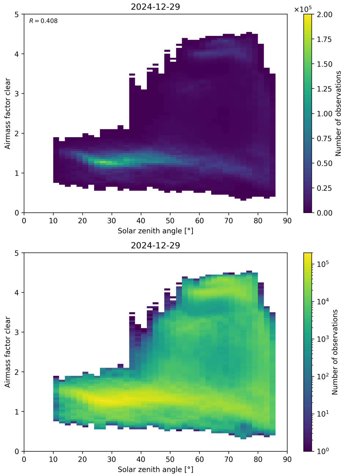
Figure 170: Scatter density plot of “Solar zenith angle” against “Airmass factor clear” for 2024-12-28 to 2024-12-30.
