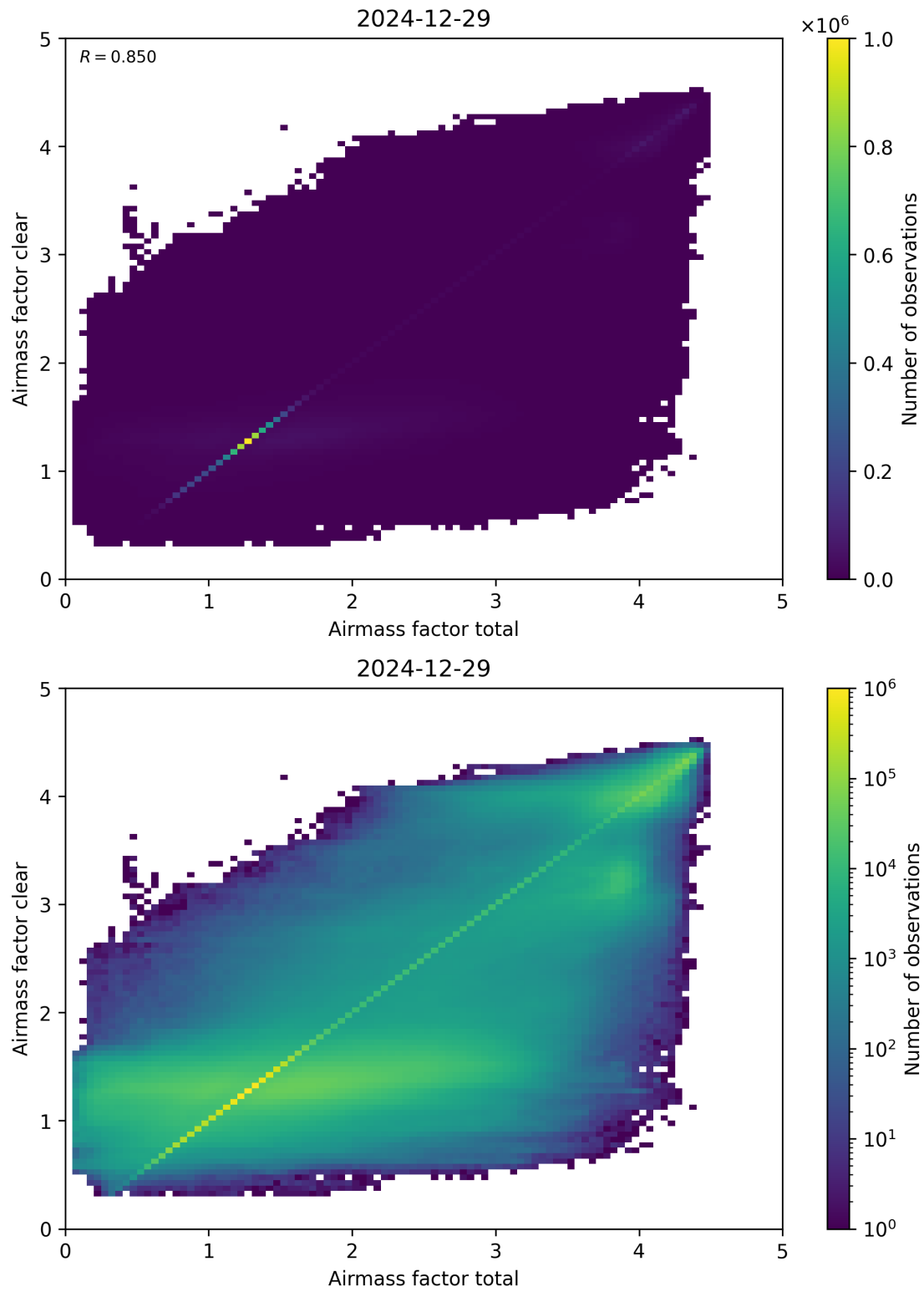
Figure 100: Scatter density plot of “Airmass factor total” against “Airmass factor clear” for 2024-12-28 to 2024-12-30.
