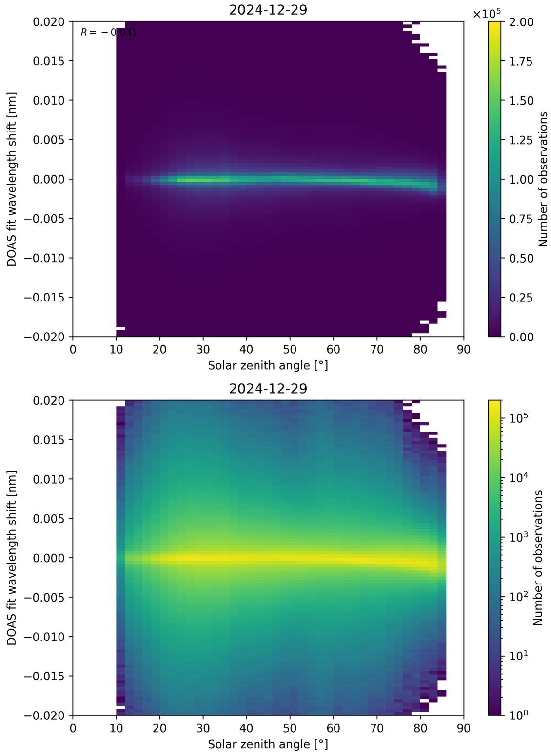
Figure 168: Scatter density plot of “Solar zenith angle” against “DOAS fit wavelength shift” for 2024-12-28 to 2024-12-30.
