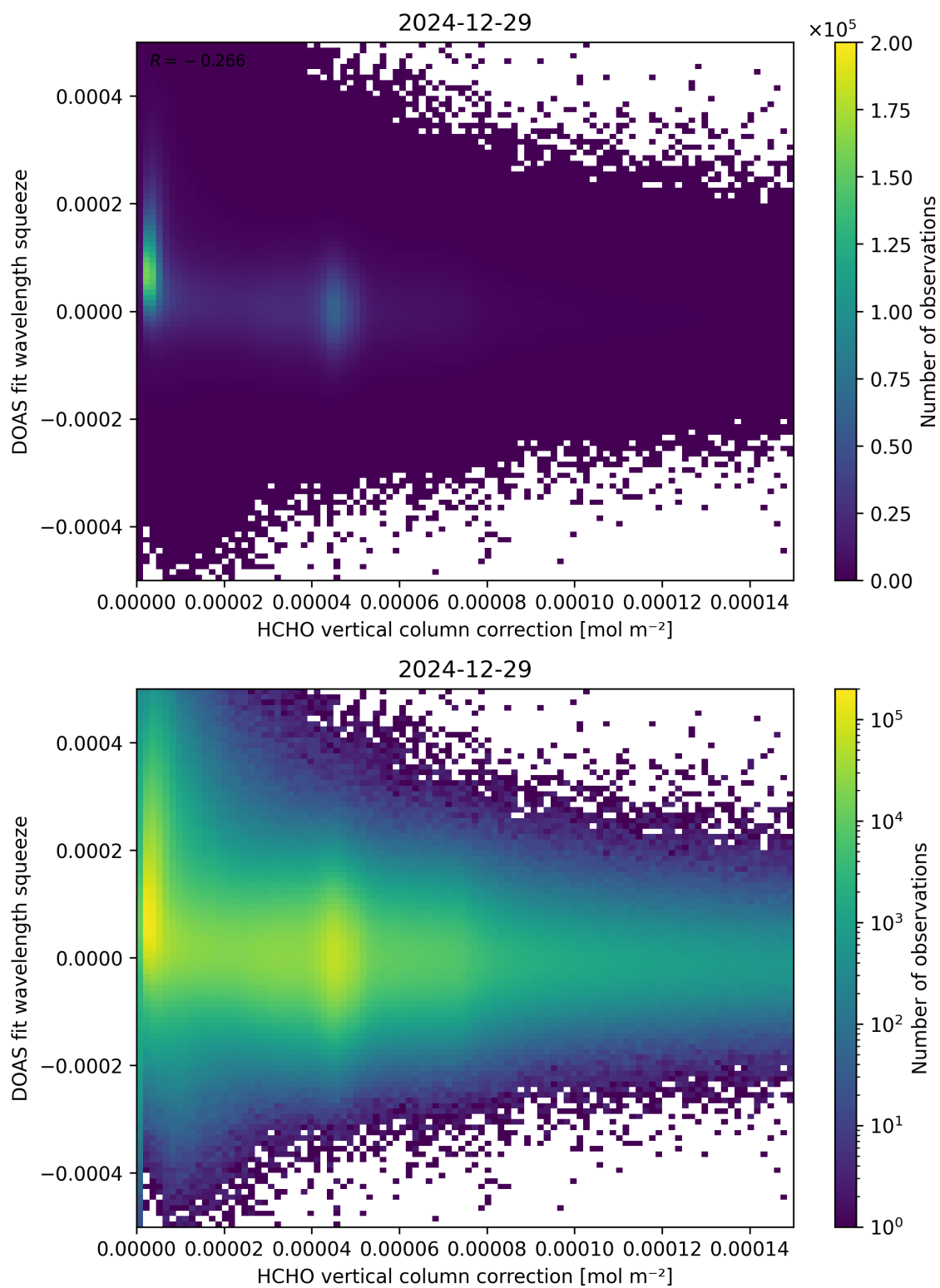
Figure 114: Scatter density plot of “HCHO vertical column correction” against “DOAS fit wavelength squeeze” for 2024-12-28 to 2024-12-30.
