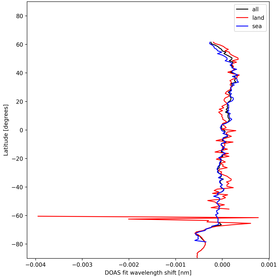
Figure 30: Zonal average of “DOAS fit wavelength shift” for 2024-12-28 to 2024-12-30.
