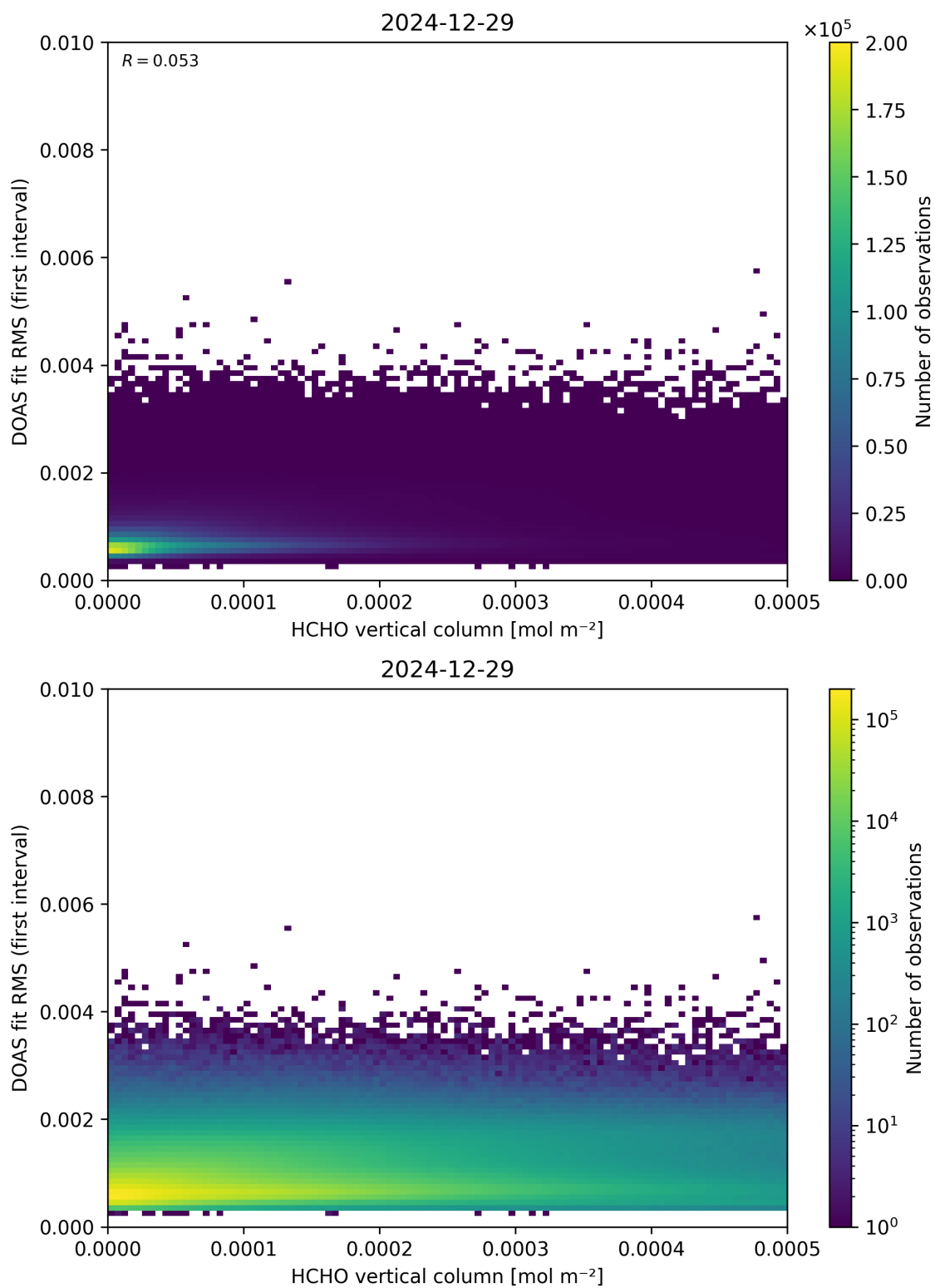
Figure 123: Scatter density plot of “HCHO vertical column” against “DOAS fit RMS (first interval)” for 2024-12-28 to 2024-12-30.
