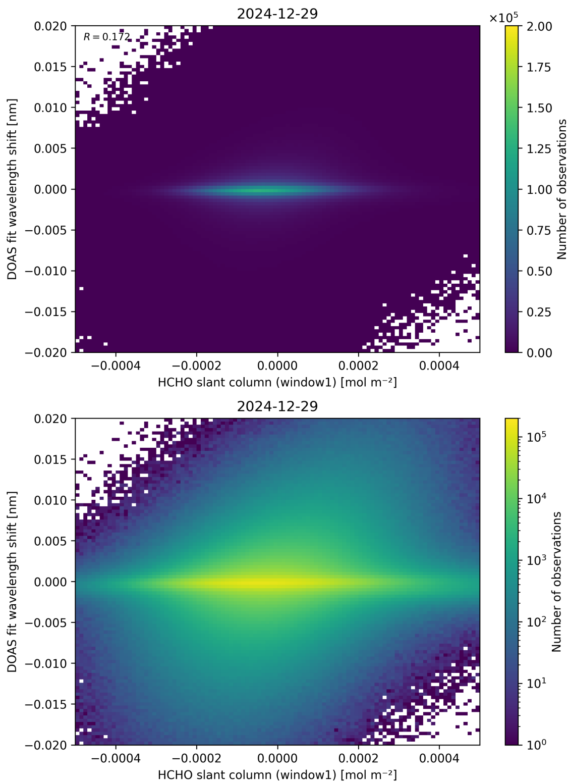
Figure 79: Scatter density plot of “HCHO slant column (window1)” against “DOAS fit wavelength shift” for 2024-12-28 to 2024-12-30.
