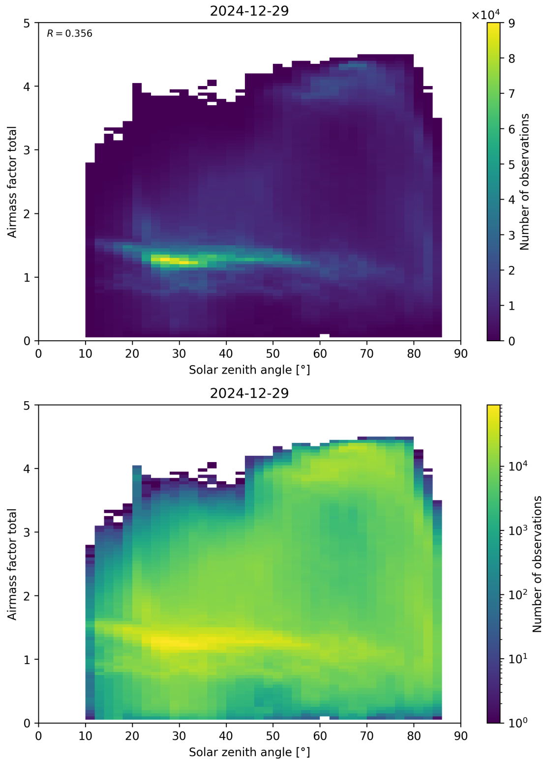
Figure 175: Scatter density plot of “Solar zenith angle” against “Airmass factor total” for 2024-12-28 to 2024-12-30.
