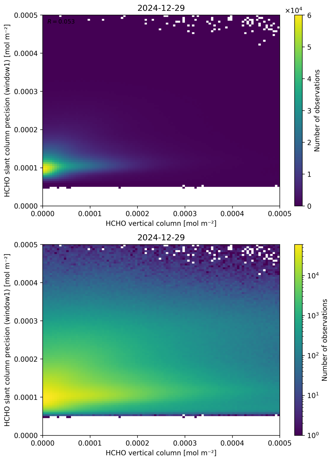
Figure 130: Scatter density plot of “HCHO vertical column” against “HCHO slant column precision (window1)” for 2024-12-28 to 2024-12-30.
