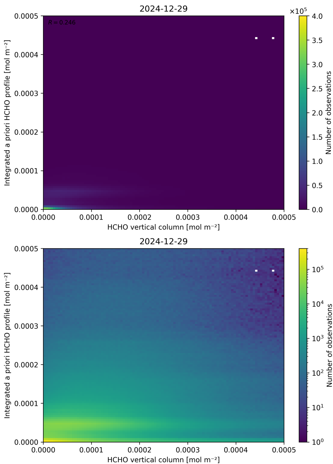
Figure 135: Scatter density plot of “HCHO vertical column” against “Integrated a priori HCHO profile” for 2024-12-28 to 2024-12-30.
