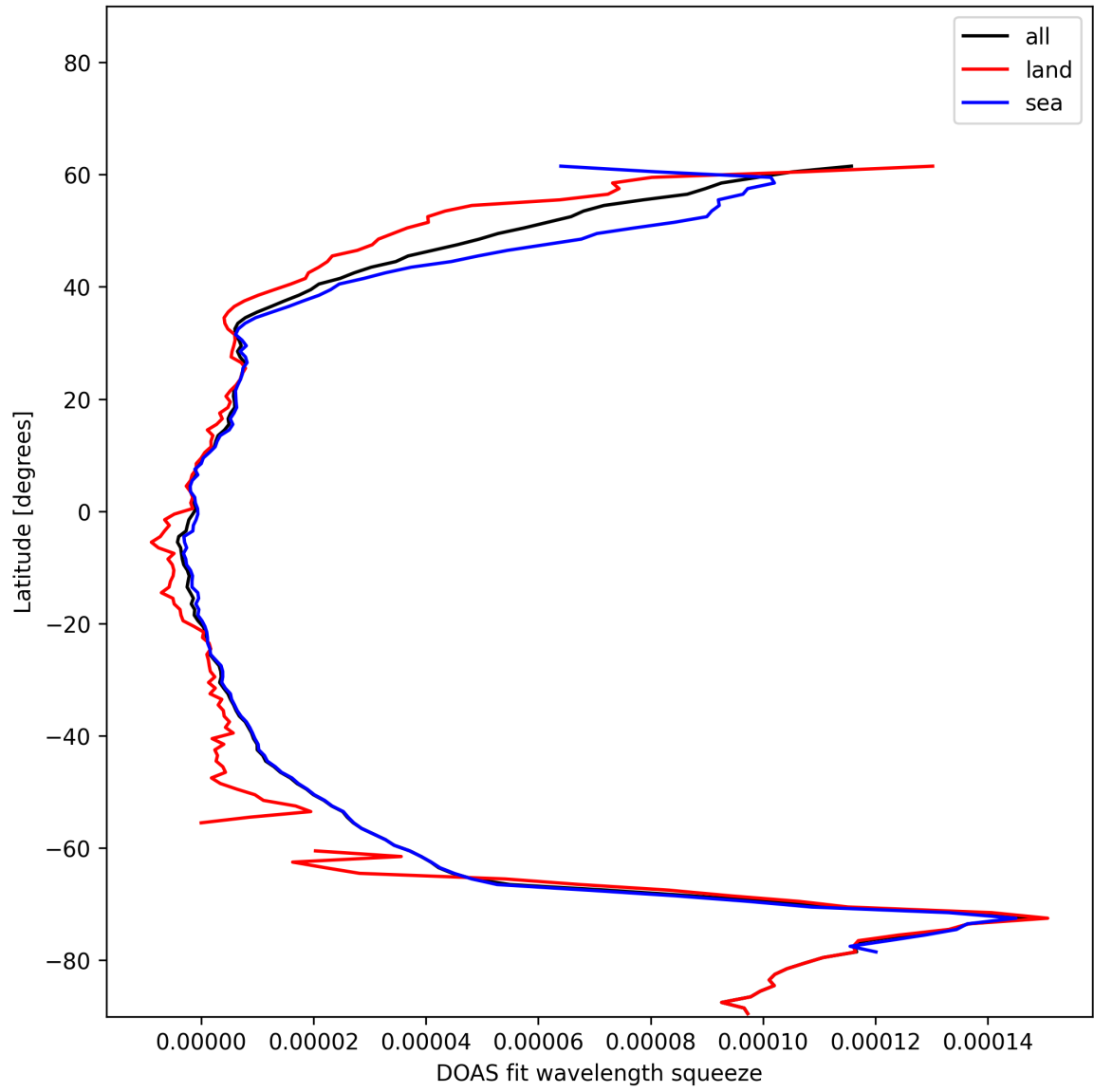
Figure 31: Zonal average of “DOAS fit wavelength squeeze” for 2024-12-28 to 2024-12-30.
