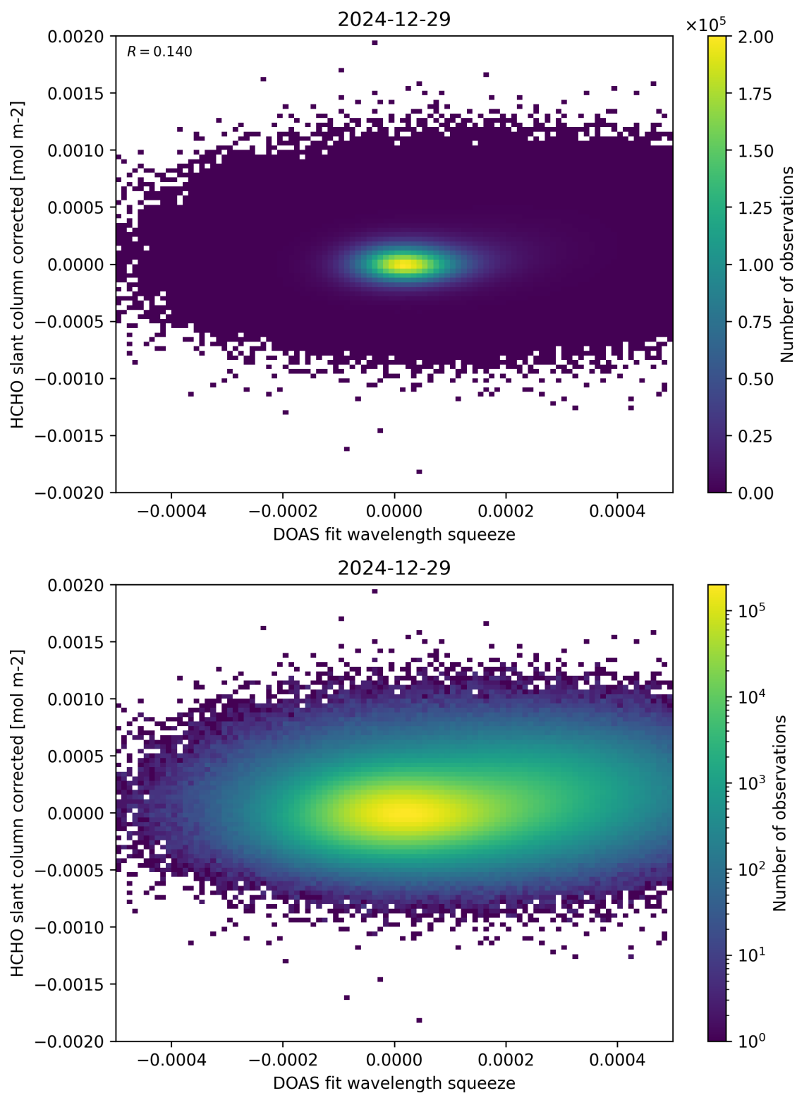
Figure 69: Scatter density plot of “DOAS fit wavelength squeeze” against “HCHO slant column corrected” for 2024-12-28 to 2024-12-30.
