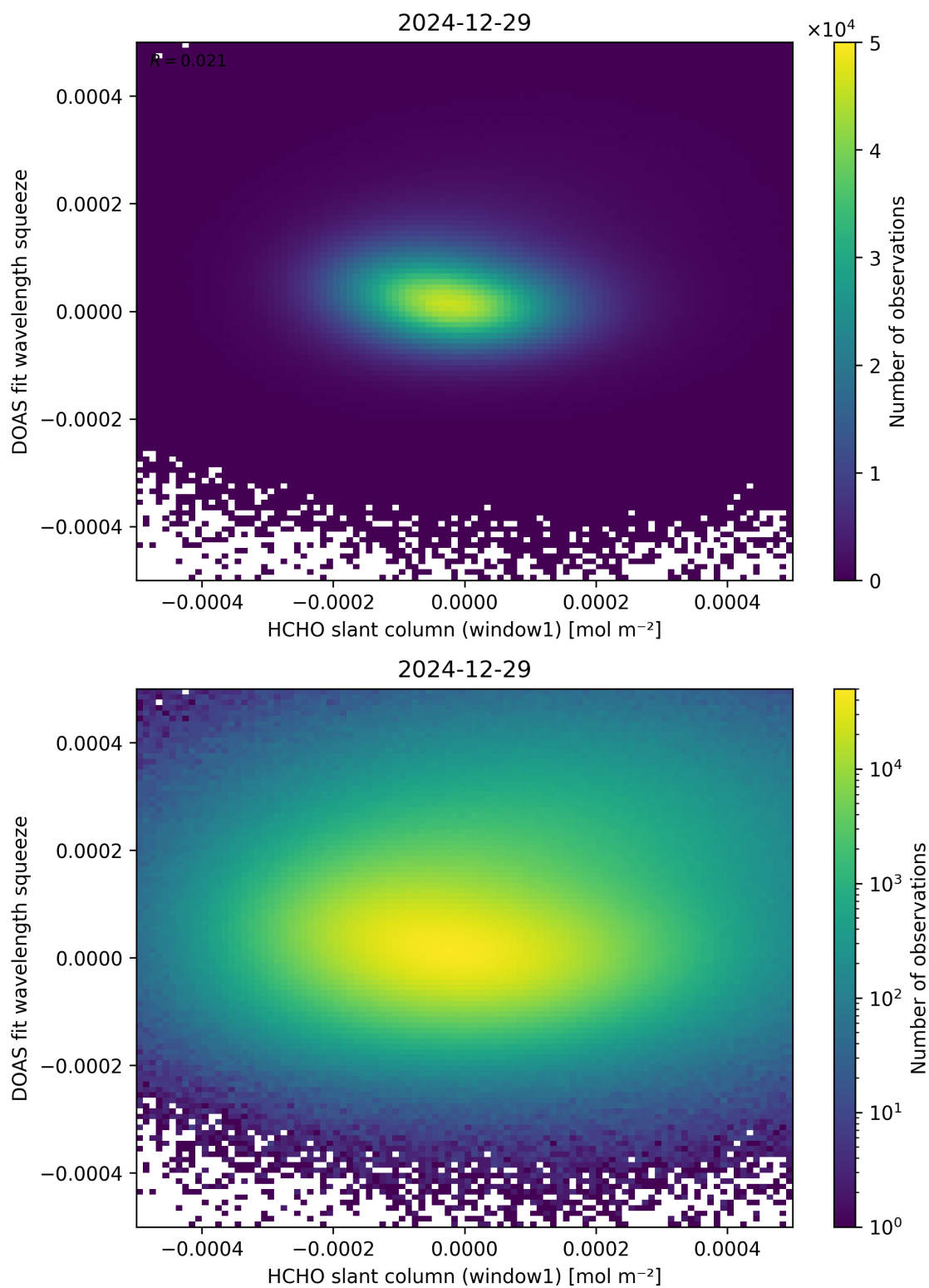
Figure 80: Scatter density plot of “HCHO slant column (window1)” against “DOAS fit wavelength squeeze” for 2024-12-28 to 2024-12-30.
