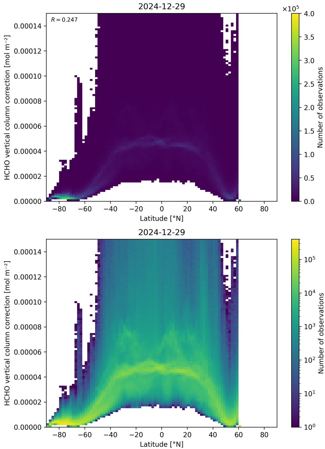
Figure 164: Scatter density plot of “Latitude” against “HCHO vertical column correction” for 2024-12-28 to 2024-12-30.
