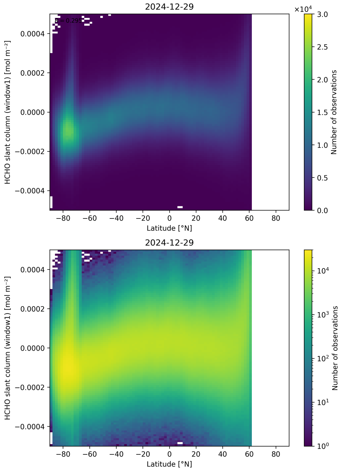
Figure 159: Scatter density plot of “Latitude” against “HCHO slant column (window1)” for 2024-12-28 to 2024-12-30.
