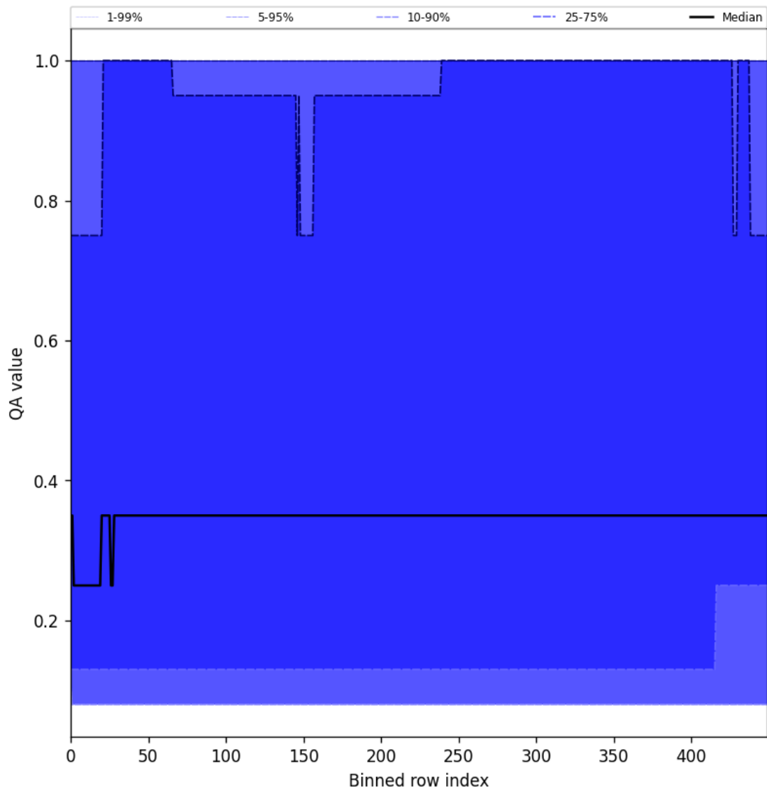
Figure 48: Along track statistics of “QA value” for 2024-12-28 to 2024-12-30
