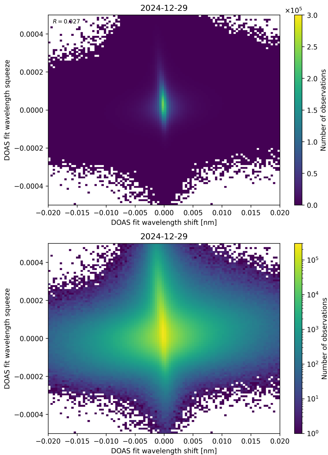
Figure 65: Scatter density plot of “DOAS fit wavelength shift” against “DOAS fit wavelength squeeze” for 2024-12-28 to 2024-12-30.
