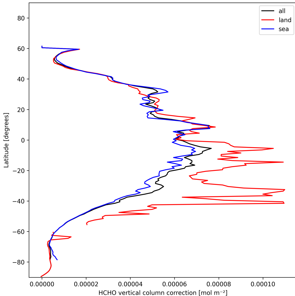
Figure 23: Zonal average of “HCHO vertical column correction” for 2024-12-28 to 2024-12-30.
