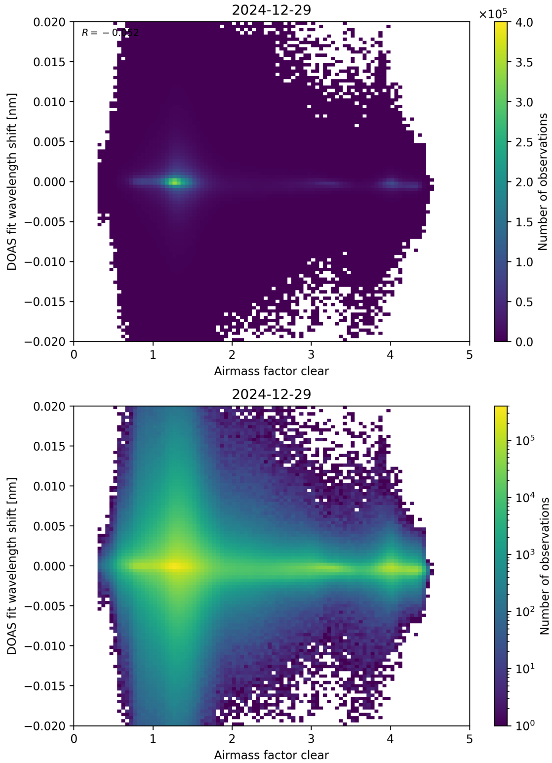
Figure 72: Scatter density plot of “Airmass factor clear” against “DOAS fit wavelength shift” for 2024-12-28 to 2024-12-30.
