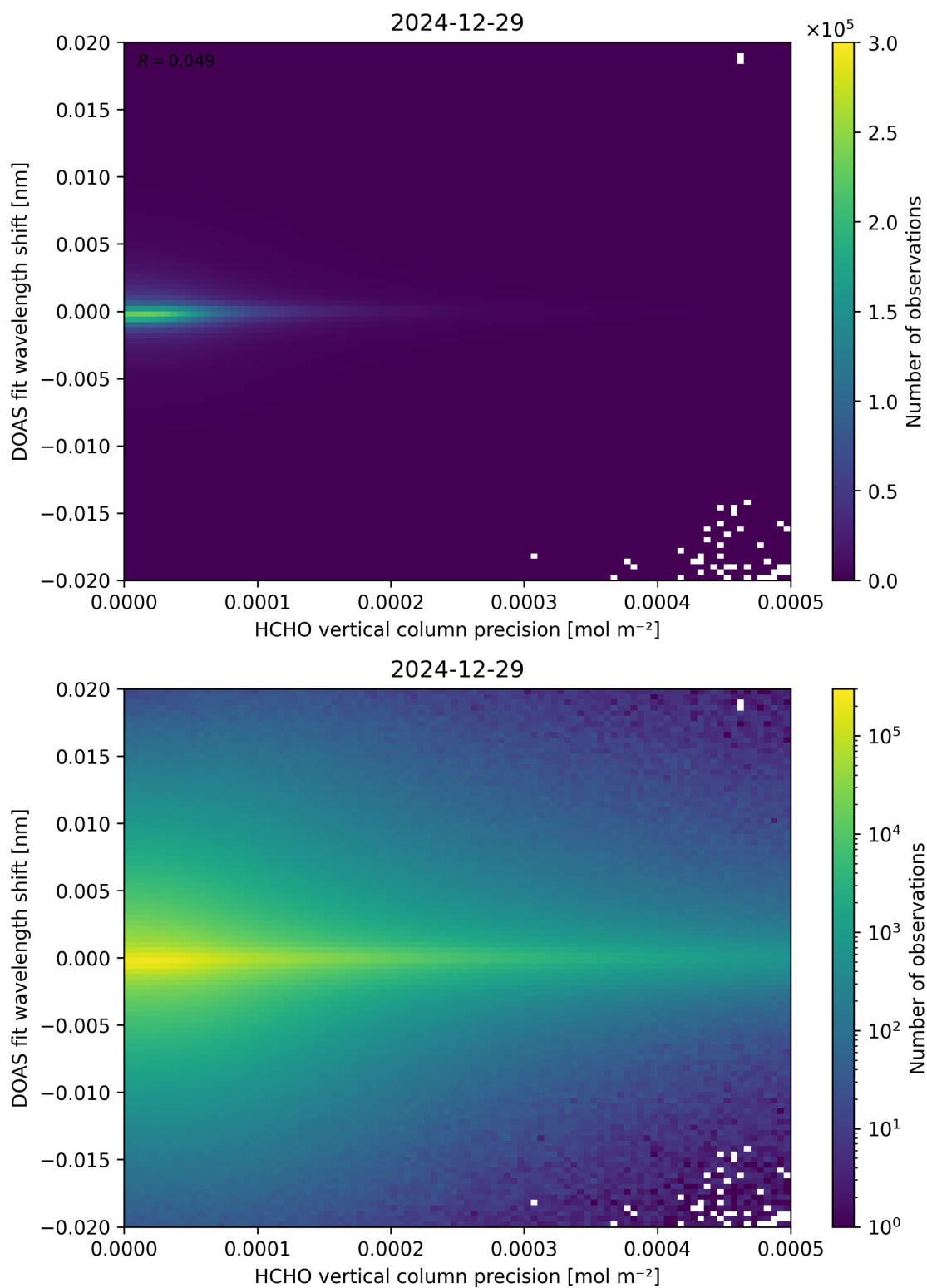
Figure 137: Scatter density plot of “HCHO vertical column precision” against “DOAS fit wavelength shift” for 2024-12-28 to 2024-12-30.
