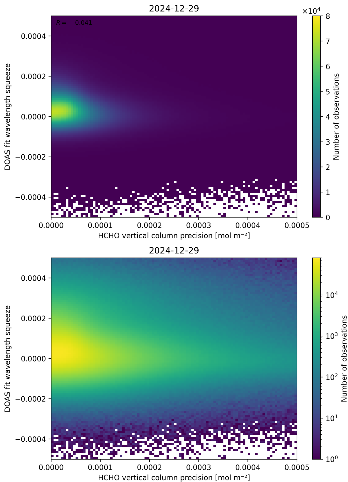
Figure 138: Scatter density plot of “HCHO vertical column precision” against “DOAS fit wavelength squeeze” for 2024-12-28 to 2024-12-30.
