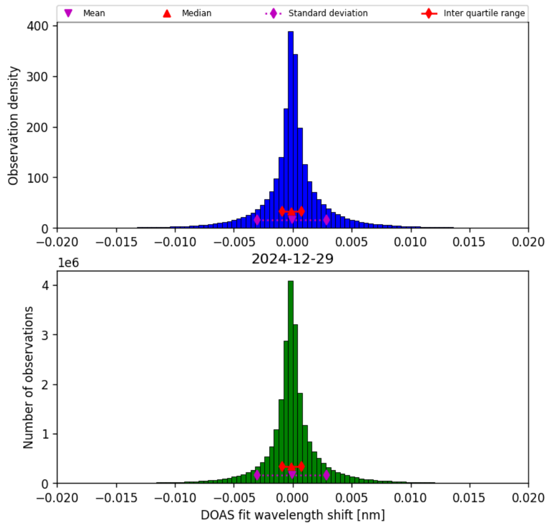
Figure 44: Histogram of “DOAS fit wavelength shift” for 2024-12-28 to 2024-12-30
