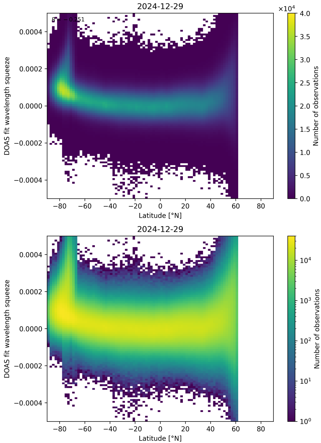
Figure 155: Scatter density plot of “Latitude” against “DOAS fit wavelength squeeze” for 2024-12-28 to 2024-12-30.
