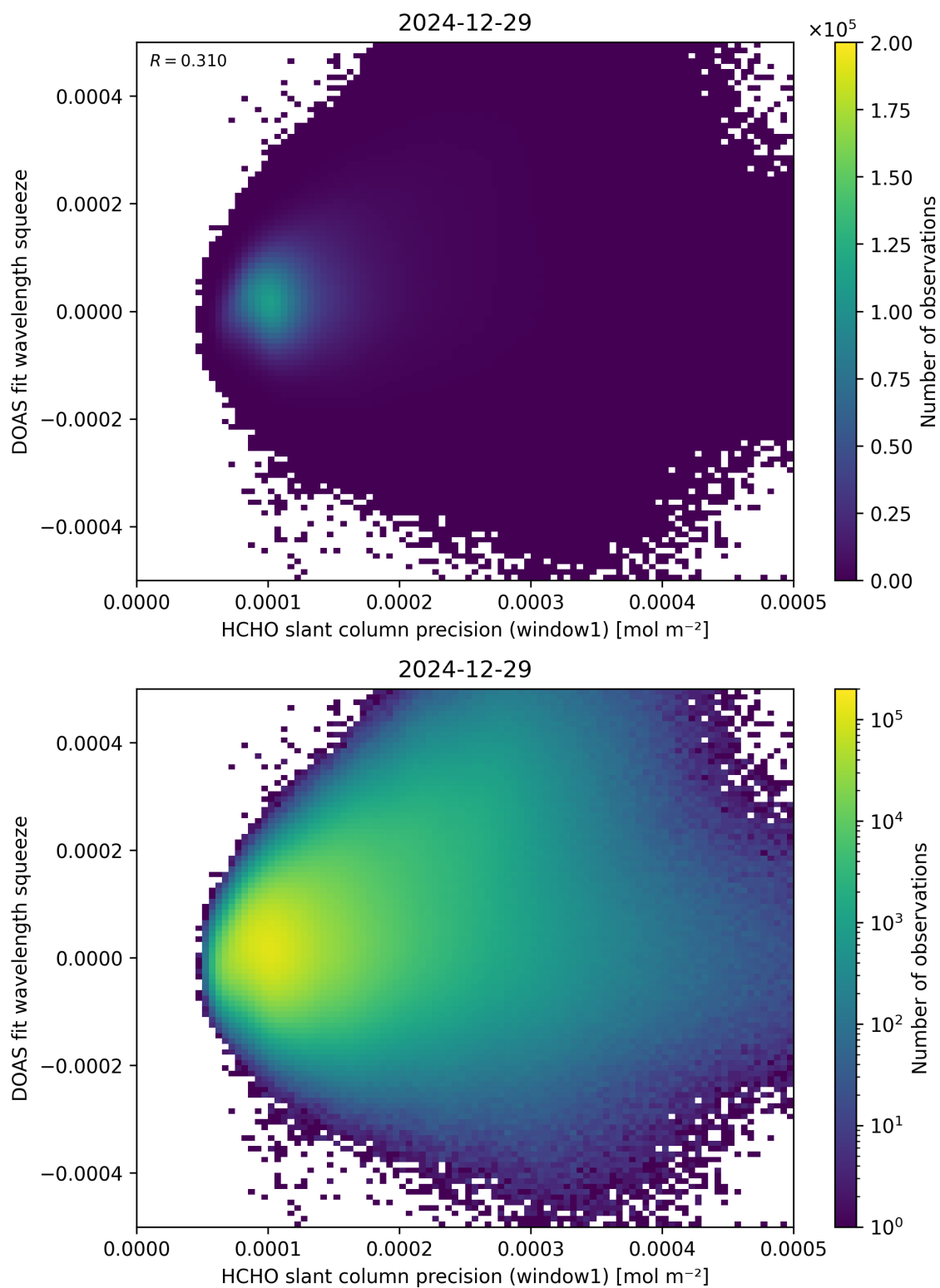
Figure 90: Scatter density plot of “HCHO slant column precision (window1)” against “DOAS fit wavelength squeeze” for 2024-12-28 to 2024-12-30.
