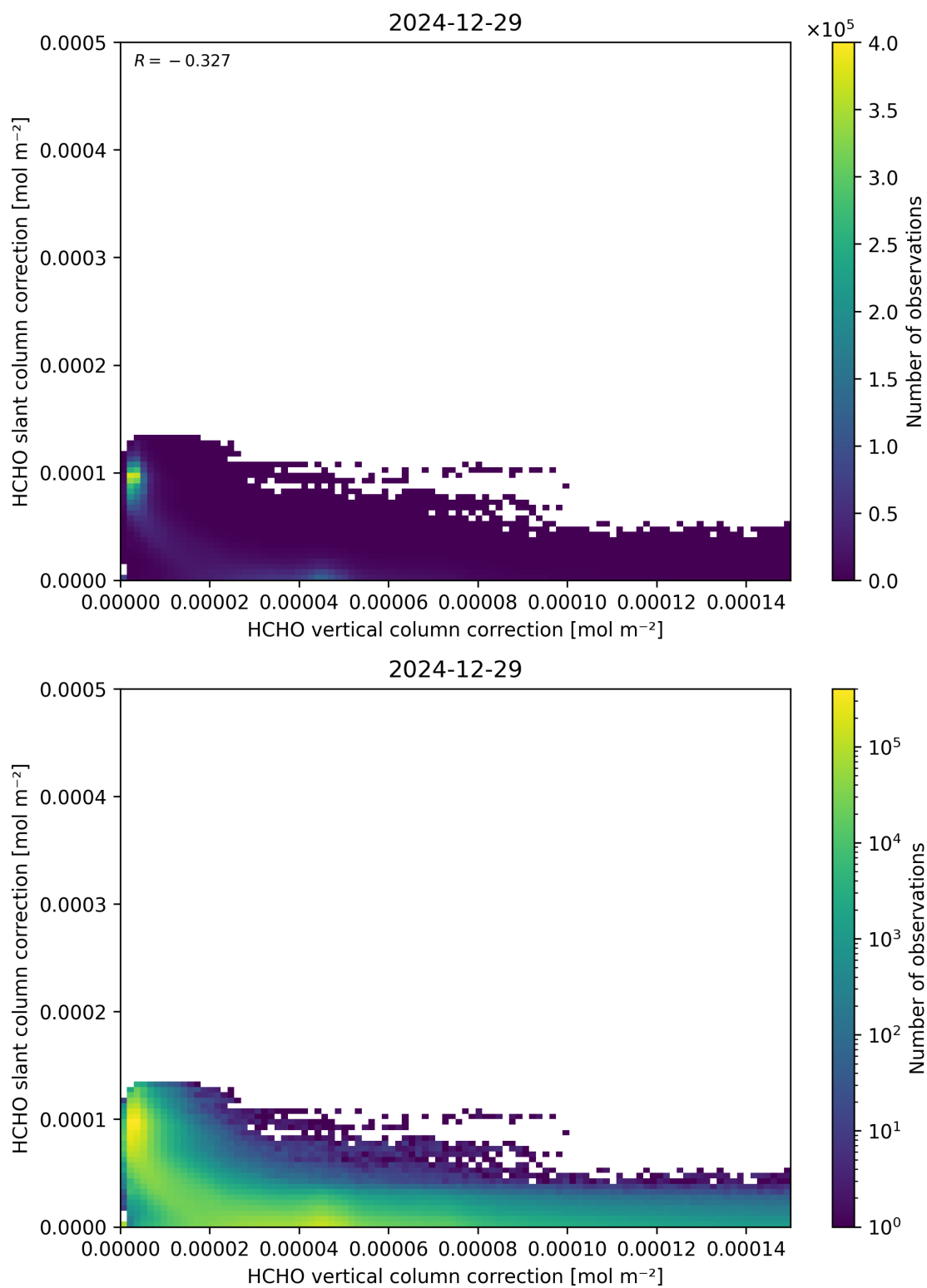
Figure 117: Scatter density plot of “HCHO vertical column correction” against “HCHO slant column correction” for 2024-12-28 to 2024-12-30.
