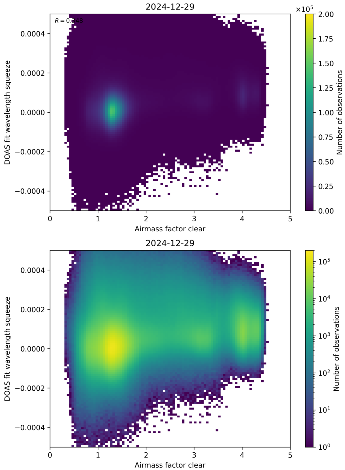
Figure 73: Scatter density plot of “Airmass factor clear” against “DOAS fit wavelength squeeze” for 2024-12-28 to 2024-12-30.
