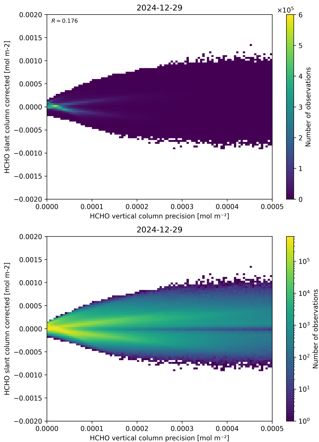
Figure 140: Scatter density plot of “HCHO vertical column precision” against “HCHO slant column corrected” for 2024-12-28 to 2024-12-30.
