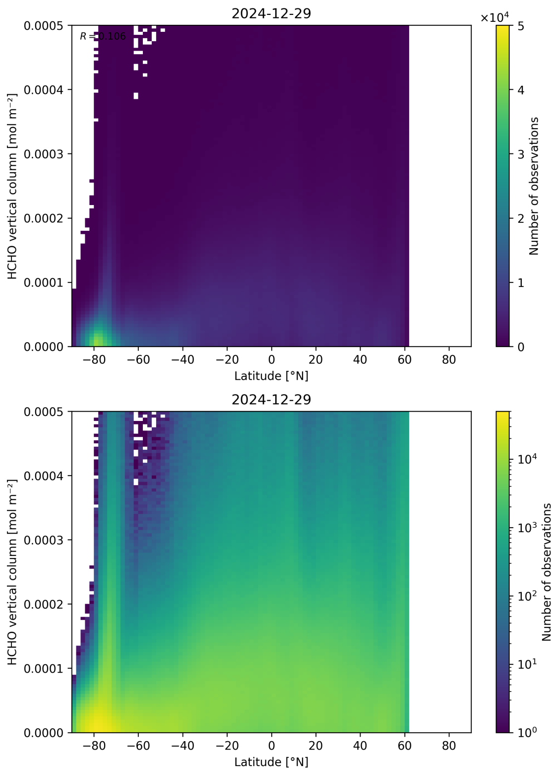
Figure 163: Scatter density plot of “Latitude” against “HCHO vertical column” for 2024-12-28 to 2024-12-30.
