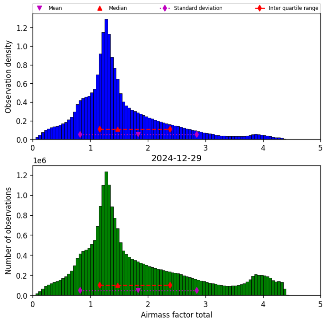
Figure 40: Histogram of “Airmass factor total” for 2024-12-28 to 2024-12-30
