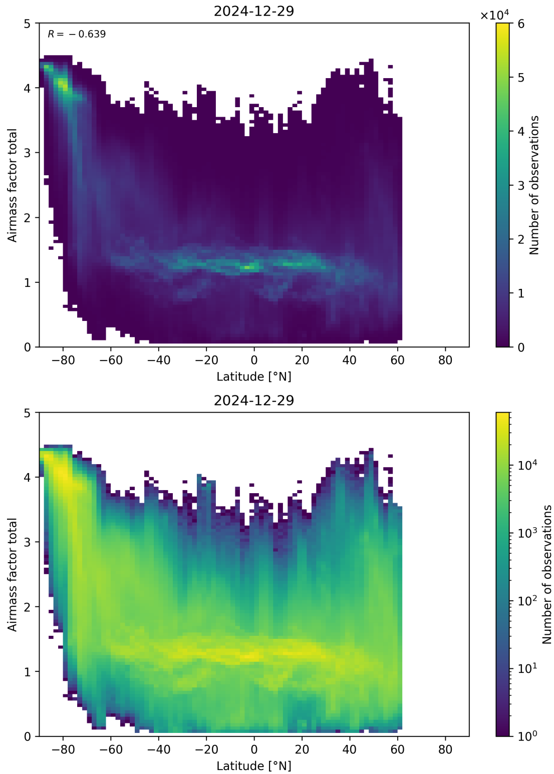
Figure 161: Scatter density plot of “Latitude” against “Airmass factor total” for 2024-12-28 to 2024-12-30.
