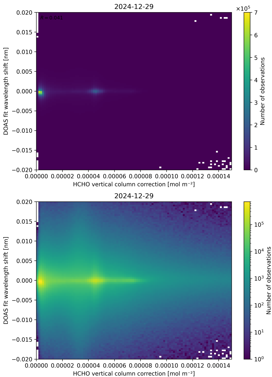
Figure 113: Scatter density plot of “HCHO vertical column correction” against “DOAS fit wavelength shift” for 2024-12-28 to 2024-12-30.
