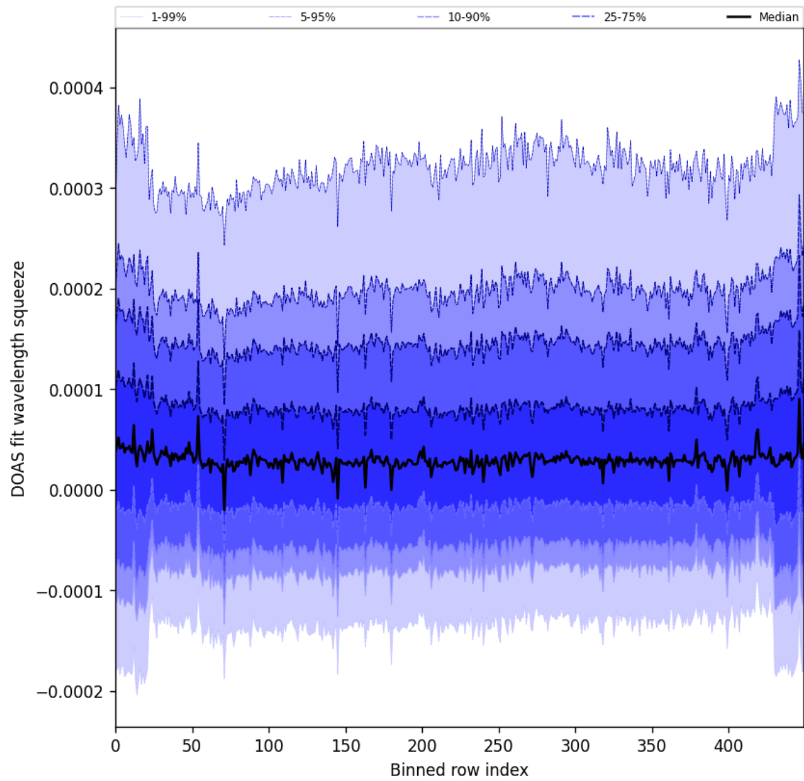
Figure 59: Along track statistics of “DOAS fit wavelength squeeze” for 2024-12-28 to 2024-12-30
