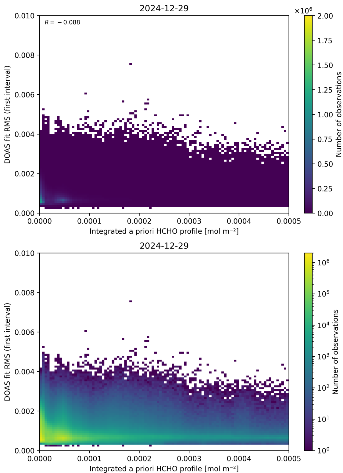
Figure 148: Scatter density plot of “Integrated a priori HCHO profile” against “DOAS fit RMS (first interval)” for 2024-12-28 to 2024-12-30.
