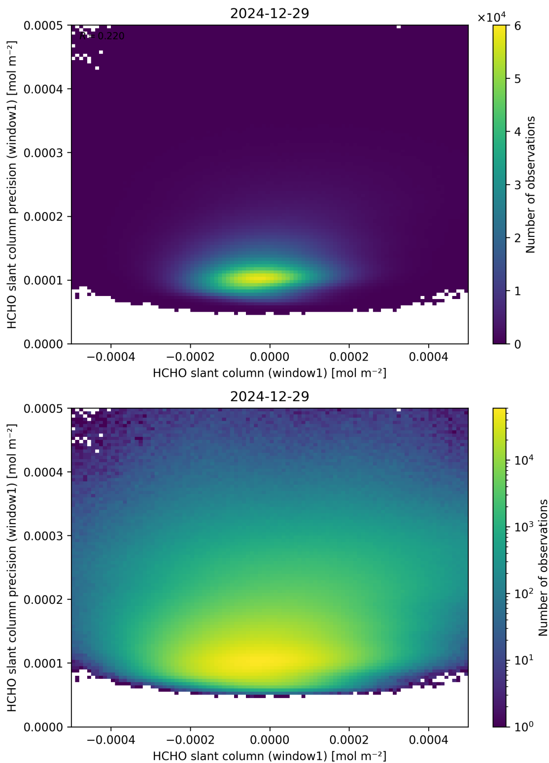
Figure 84: Scatter density plot of “HCHO slant column (window1)” against “HCHO slant column precision (window1)” for 2024-12-28 to 2024-12-30.
