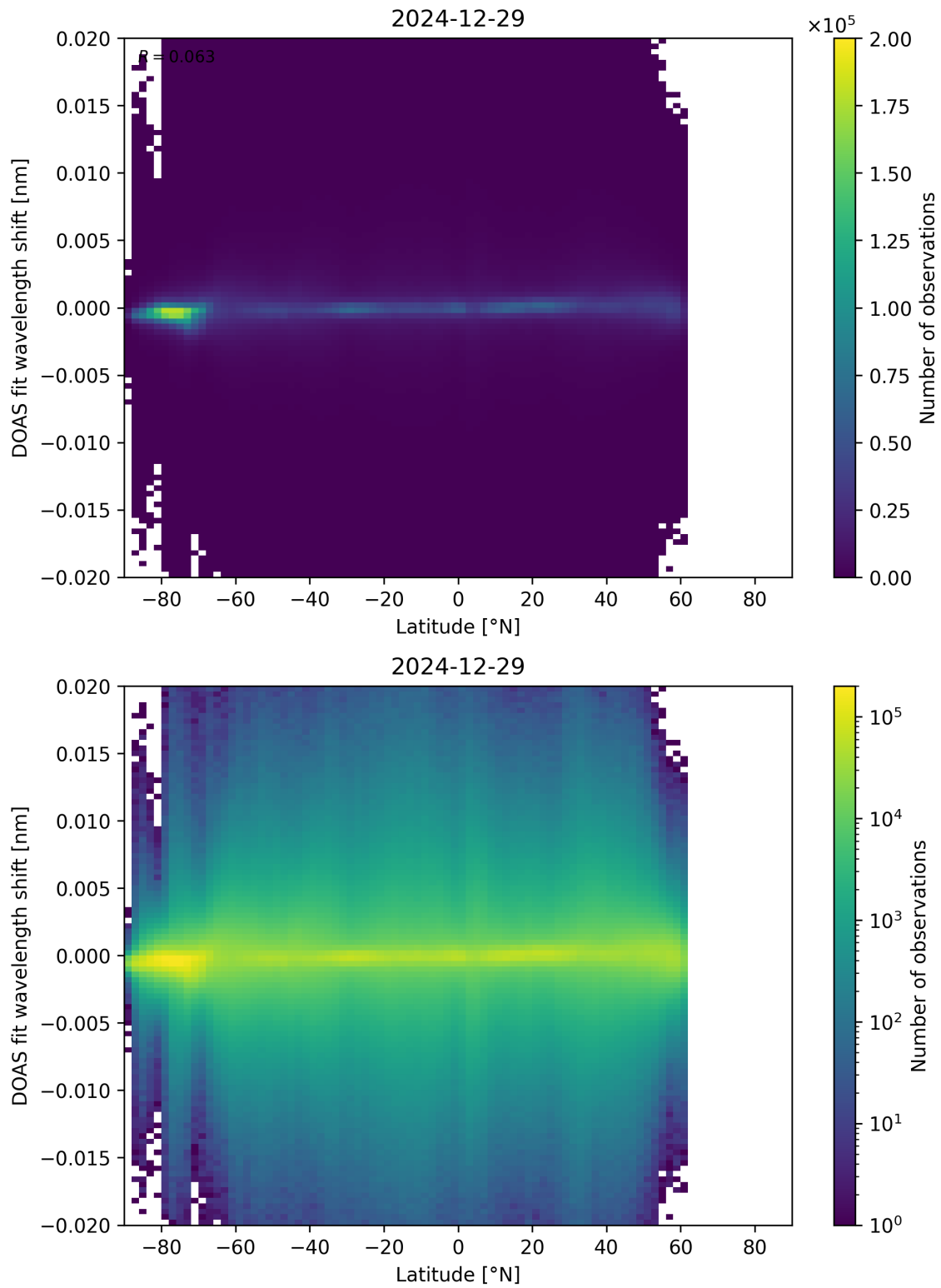
Figure 154: Scatter density plot of “Latitude” against “DOAS fit wavelength shift” for 2024-12-28 to 2024-12-30.
