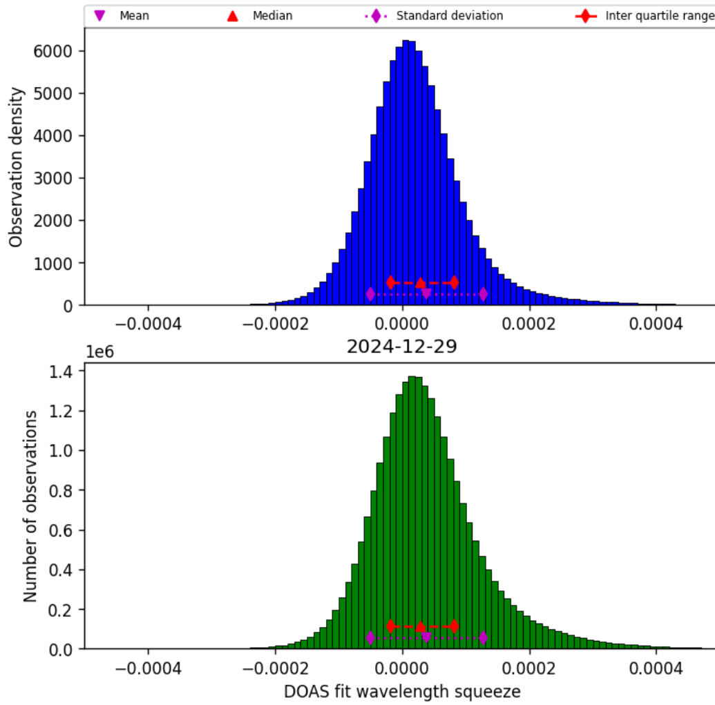
Figure 45: Histogram of “DOAS fit wavelength squeeze” for 2024-12-28 to 2024-12-30
