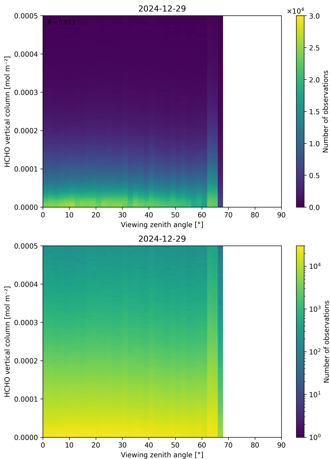
Figure 192: Scatter density plot of “Viewing zenith angle” against “HCHO vertical column” for 2024-12-28 to 2024-12-30.
