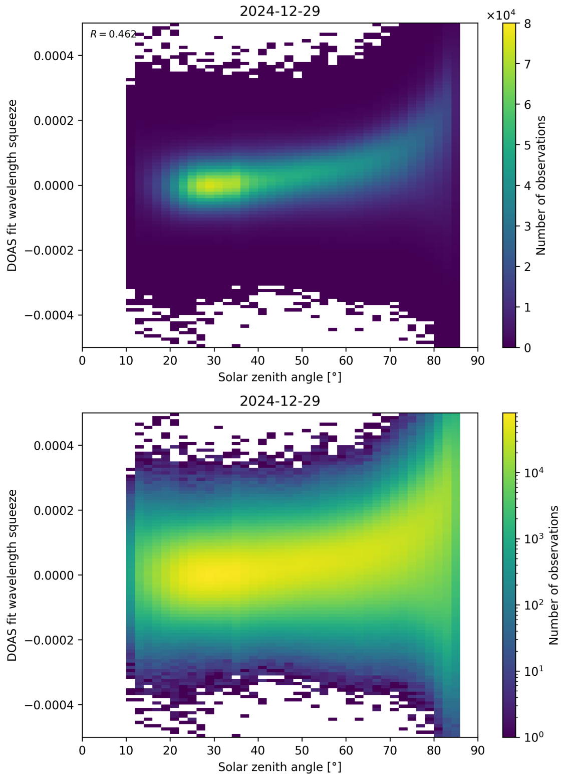
Figure 169: Scatter density plot of “Solar zenith angle” against “DOAS fit wavelength squeeze” for 2024-12-28 to 2024-12-30.
