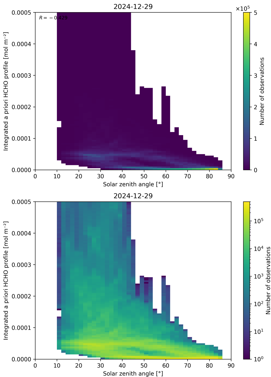
Figure 180: Scatter density plot of “Solar zenith angle” against “Integrated a priori HCHO profile” for 2024-12-28 to 2024-12-30.
