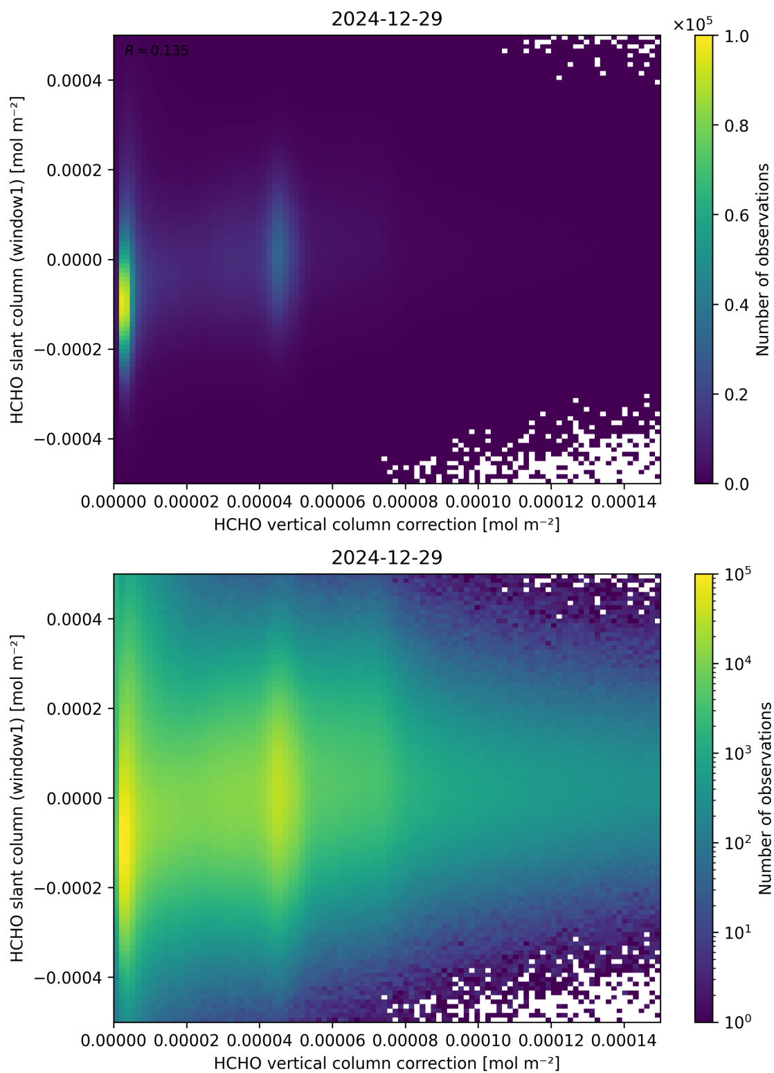
Figure 118: Scatter density plot of “HCHO vertical column correction” against “HCHO slant column (window1)” for 2024-12-28 to 2024-12-30.
