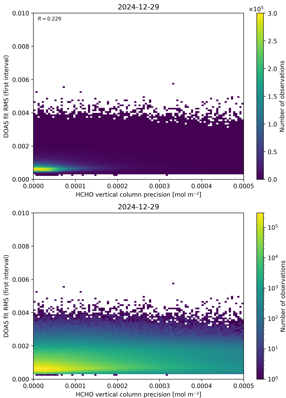
Figure 136: Scatter density plot of “HCHO vertical column precision” against “DOAS fit RMS (first interval)” for 2024-12-28 to 2024-12-30.
