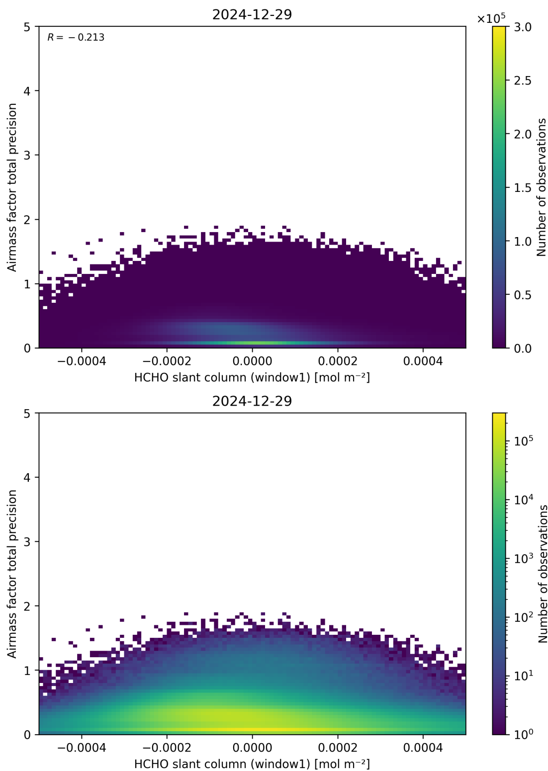
Figure 86: Scatter density plot of “HCHO slant column (window1)” against “Airmass factor total precision” for 2024-12-28 to 2024-12-30.
