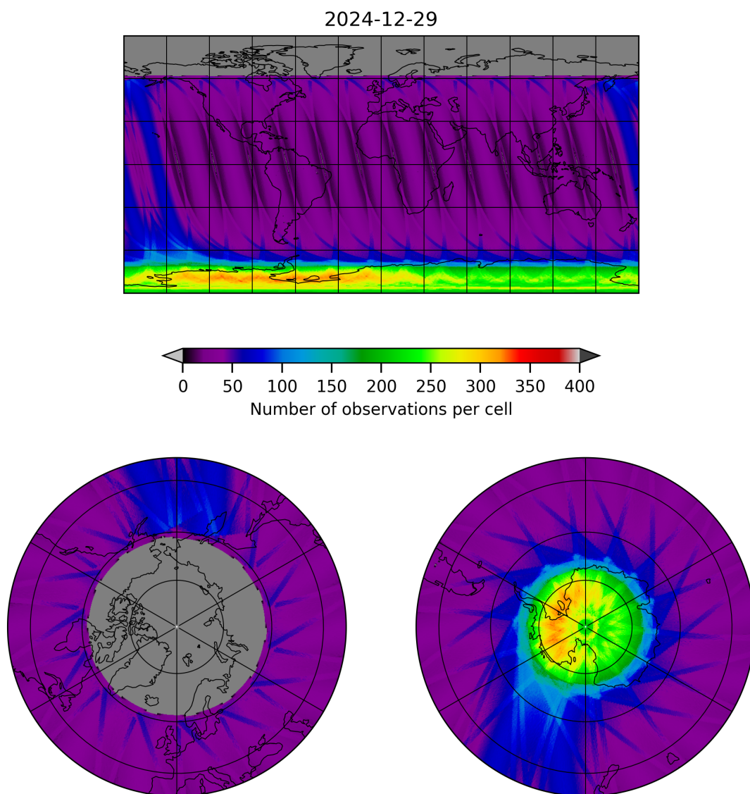
Figure 19: Map of the number of observations for 2024-12-28 to 2024-12-30
