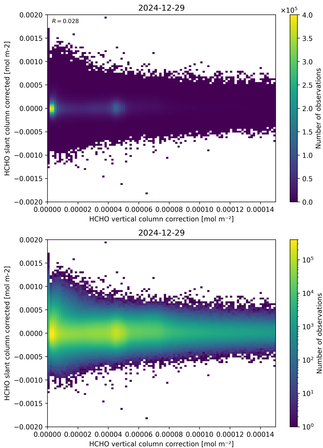
Figure 116: Scatter density plot of “HCHO vertical column correction” against “HCHO slant column corrected” for 2024-12-28 to 2024-12-30.
