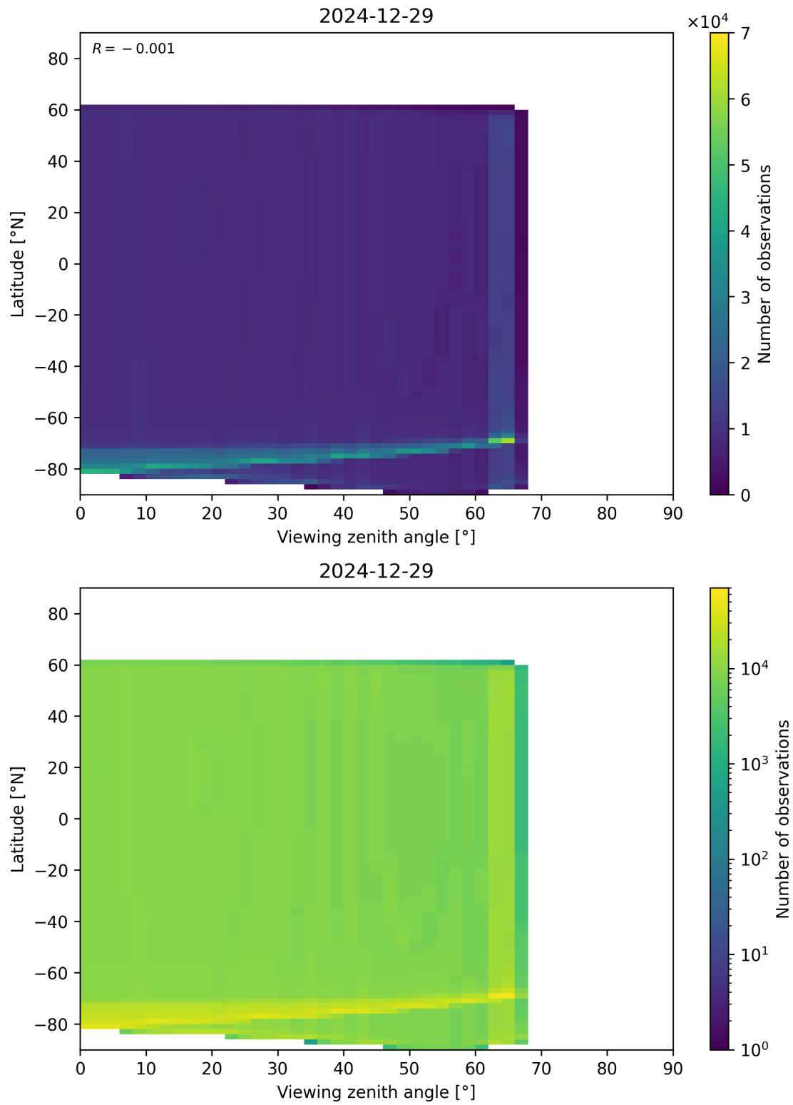
Figure 196: Scatter density plot of “Viewing zenith angle” against “Latitude” for 2024-12-28 to 2024-12-30.
