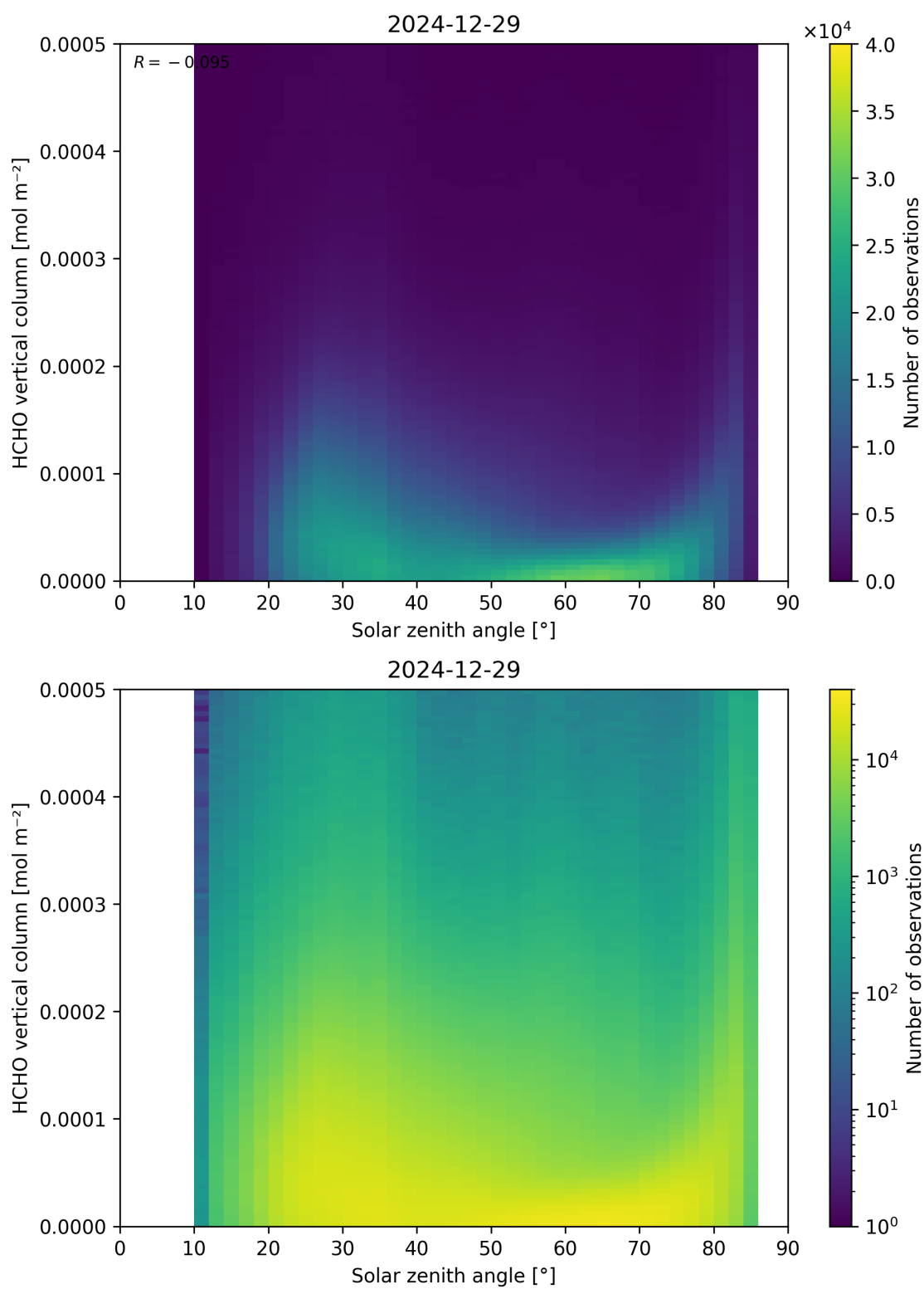
Figure 177: Scatter density plot of “Solar zenith angle” against “HCHO vertical column” for 2024-12-28 to 2024-12-30.
