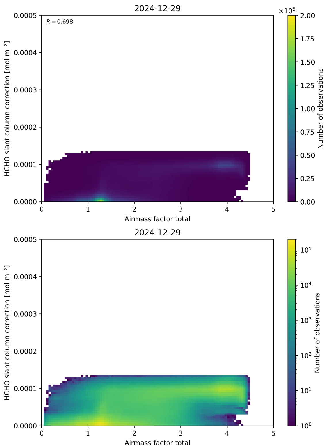
Figure 102: Scatter density plot of “Airmass factor total” against “HCHO slant column correction” for 2024-12-28 to 2024-12-30.
