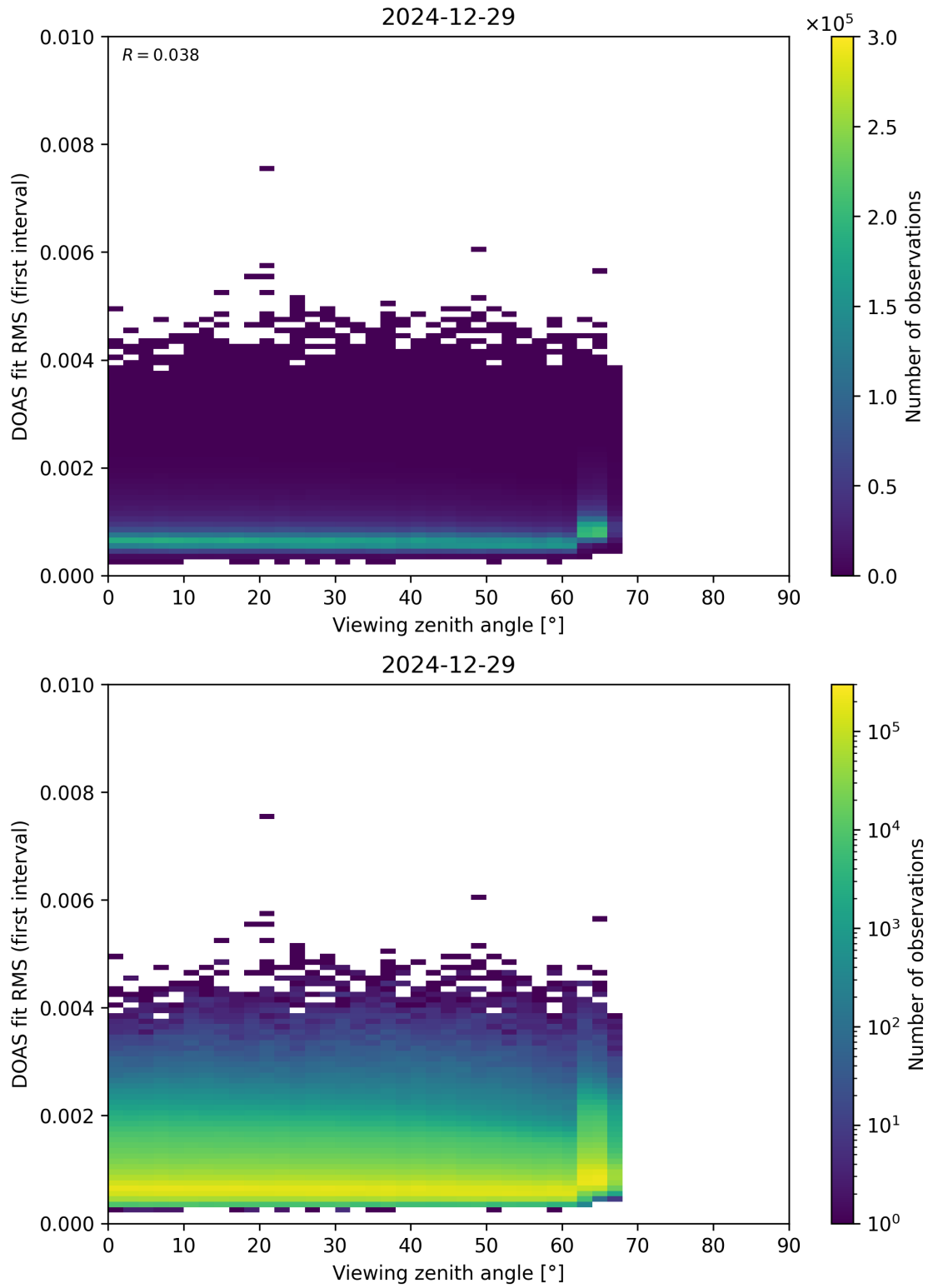
Figure 182: Scatter density plot of “Viewing zenith angle” against “DOAS fit RMS (first interval)” for 2024-12-28 to 2024-12-30.
