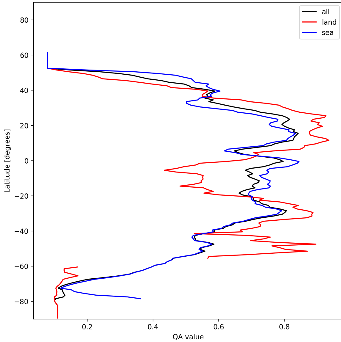
Figure 20: Zonal average of “QA value” for 2024-12-28 to 2024-12-30.
