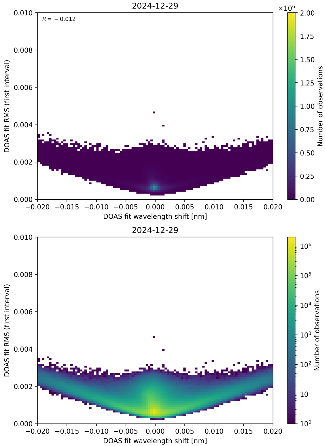
Figure 64: Scatter density plot of “DOAS fit wavelength shift” against “DOAS fit RMS (first interval)” for 2024-12-28 to 2024-12-30.
