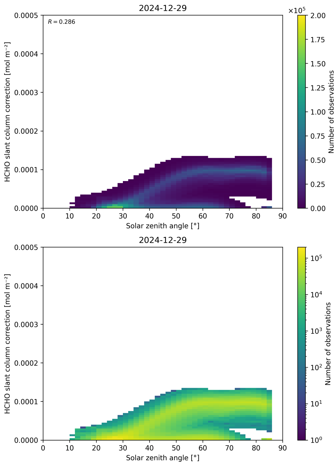
Figure 172: Scatter density plot of “Solar zenith angle” against “HCHO slant column correction” for 2024-12-28 to 2024-12-30.
