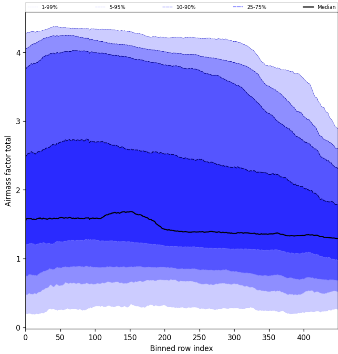
Figure 54: Along track statistics of “Airmass factor total” for 2024-12-28 to 2024-12-30
