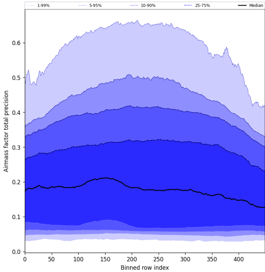
Figure 55: Along track statistics of “Airmass factor total precision” for 2024-12-28 to 2024-12-30
