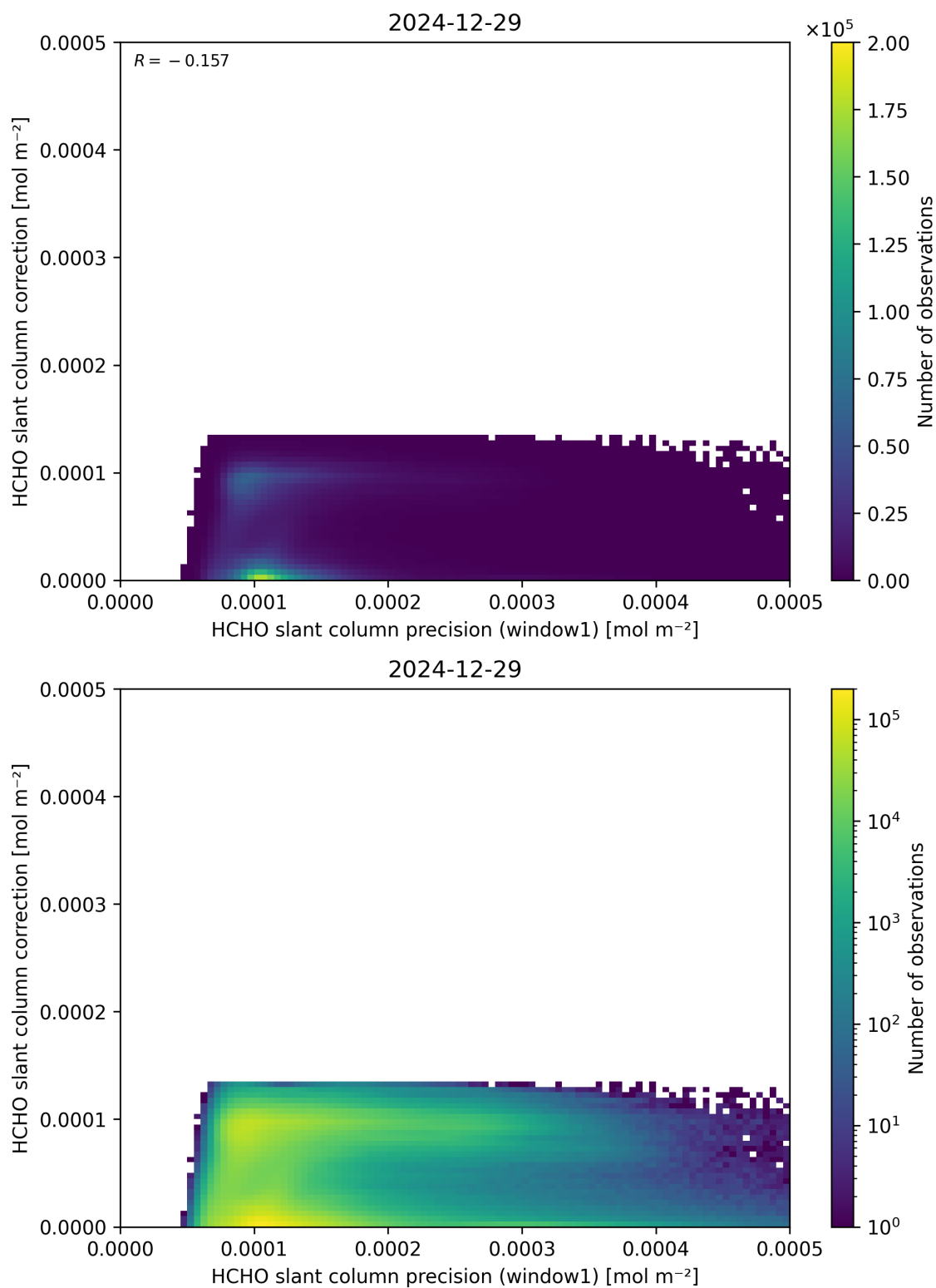
Figure 93: Scatter density plot of “HCHO slant column precision (window1)” against “HCHO slant column correction” for 2024-12-28 to 2024-12-30.
