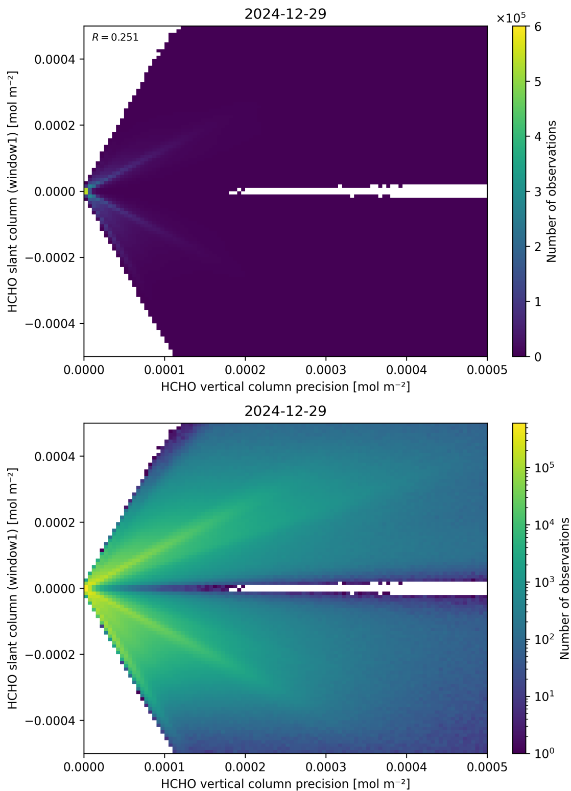
Figure 142: Scatter density plot of “HCHO vertical column precision” against “HCHO slant column (window1)” for 2024-12-28 to 2024-12-30.
