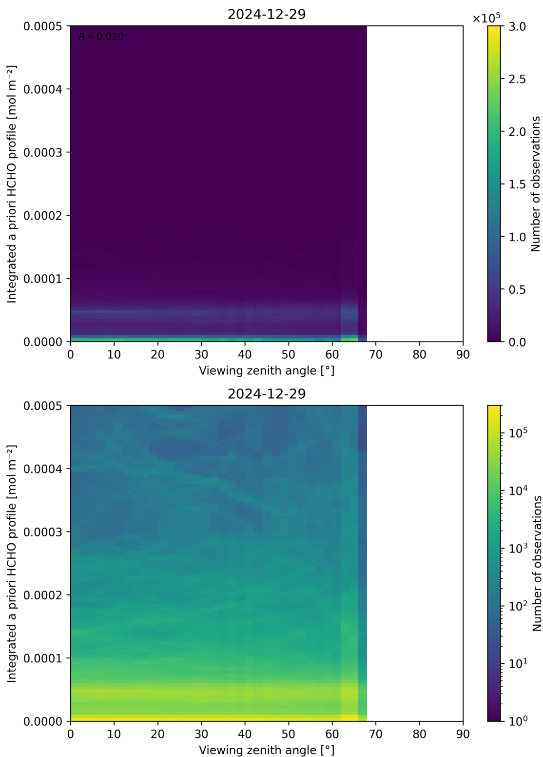
Figure 195: Scatter density plot of “Viewing zenith angle” against “Integrated a priori HCHO profile” for 2024-12-28 to 2024-12-30.
