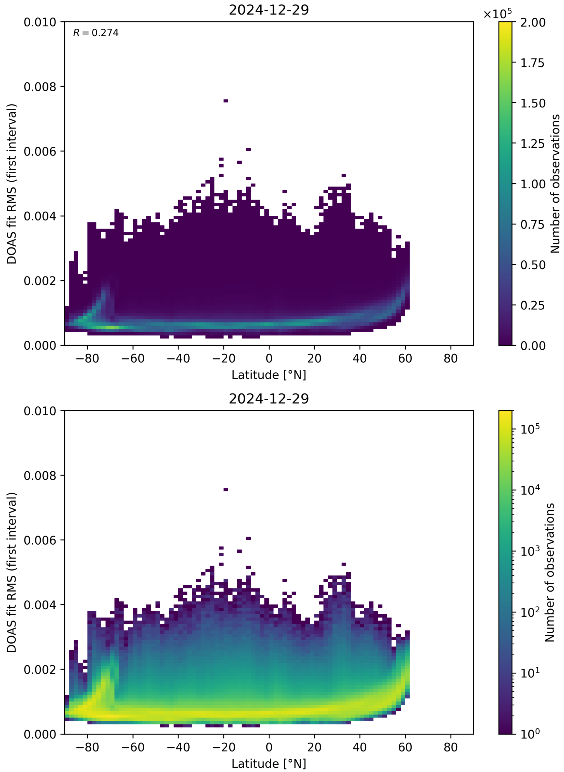
Figure 153: Scatter density plot of “Latitude” against “DOAS fit RMS (first interval)” for 2024-12-28 to 2024-12-30.
