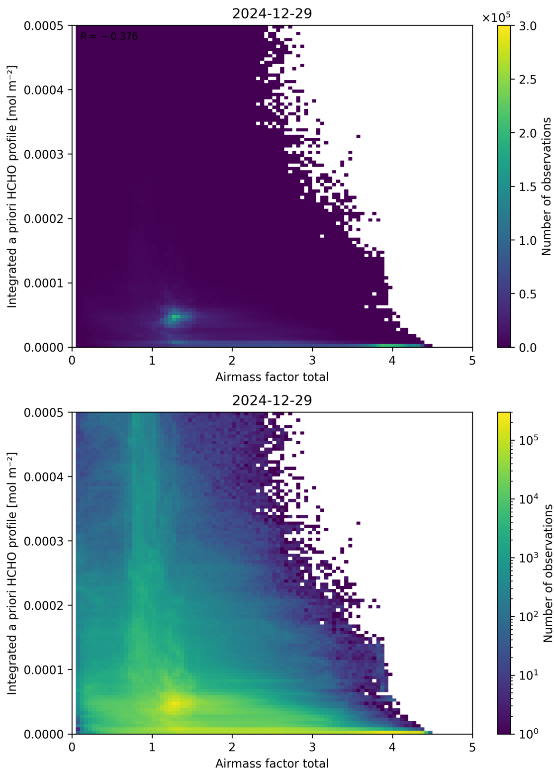
Figure 104: Scatter density plot of “Airmass factor total” against “Integrated a priori HCHO profile” for 2024-12-28 to 2024-12-30.
