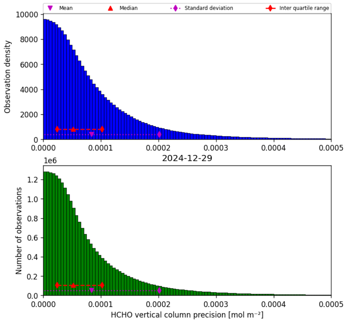
Figure 36: Histogram of “HCHO vertical column precision” for 2024-12-28 to 2024-12-30
