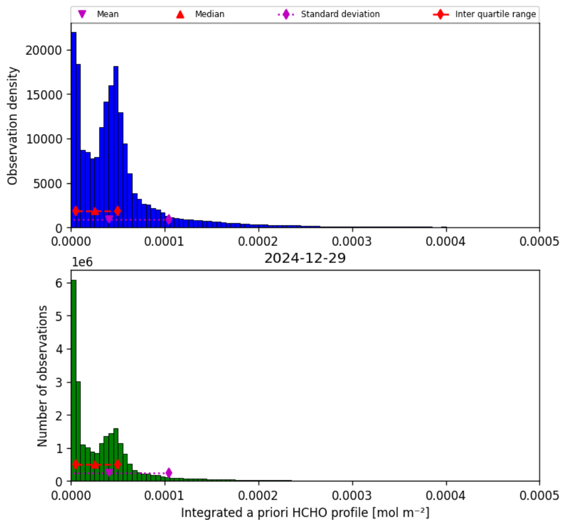
Figure 43: Histogram of “Integrated a priori HCHO profile” for 2024-12-28 to 2024-12-30
