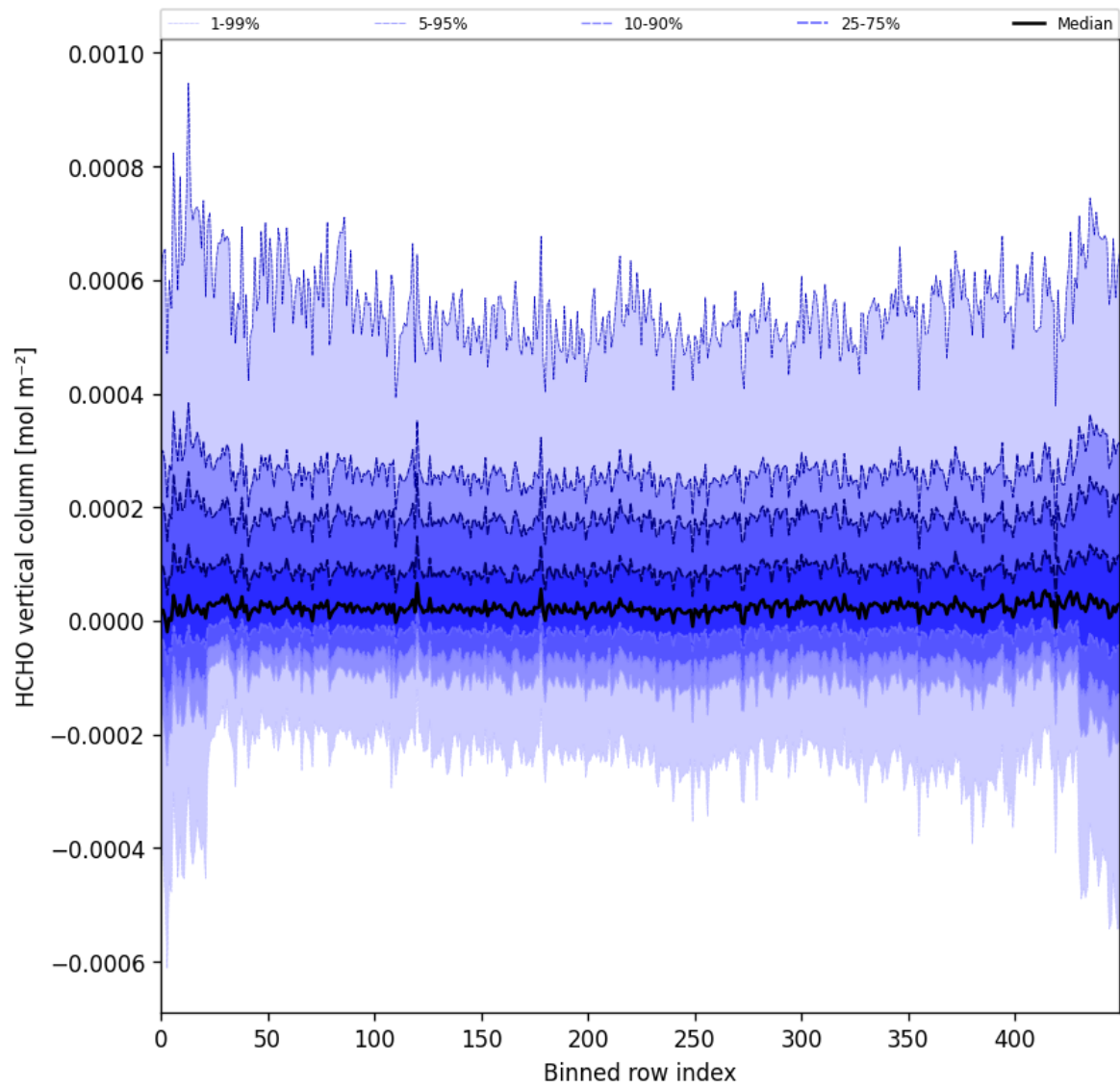
Figure 49: Along track statistics of “HCHO vertical column” for 2024-12-28 to 2024-12-30
