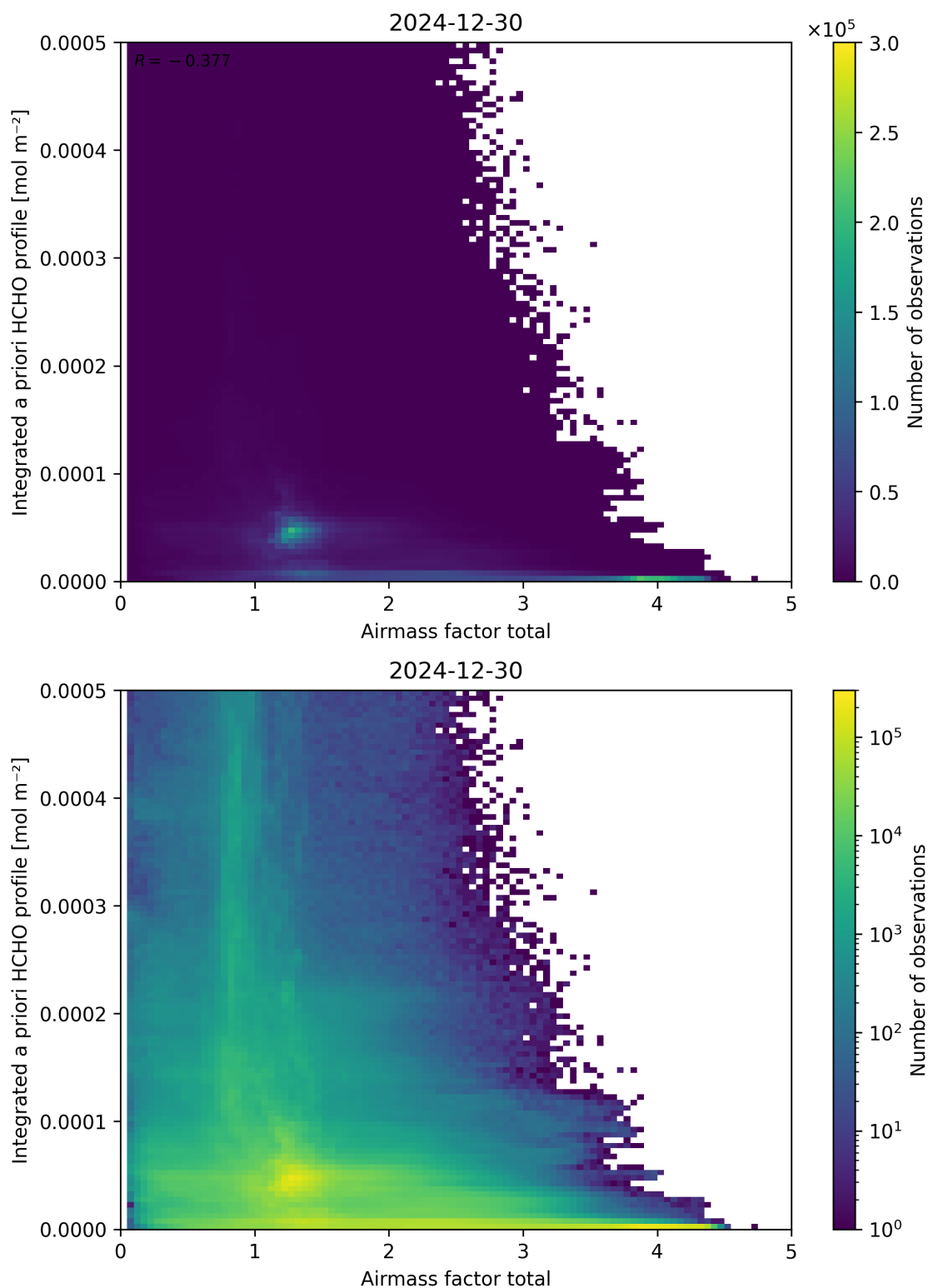
Figure 104: Scatter density plot of “Airmass factor total” against “Integrated a priori HCHO profile” for 2024-12-29 to 2024-12-31.
