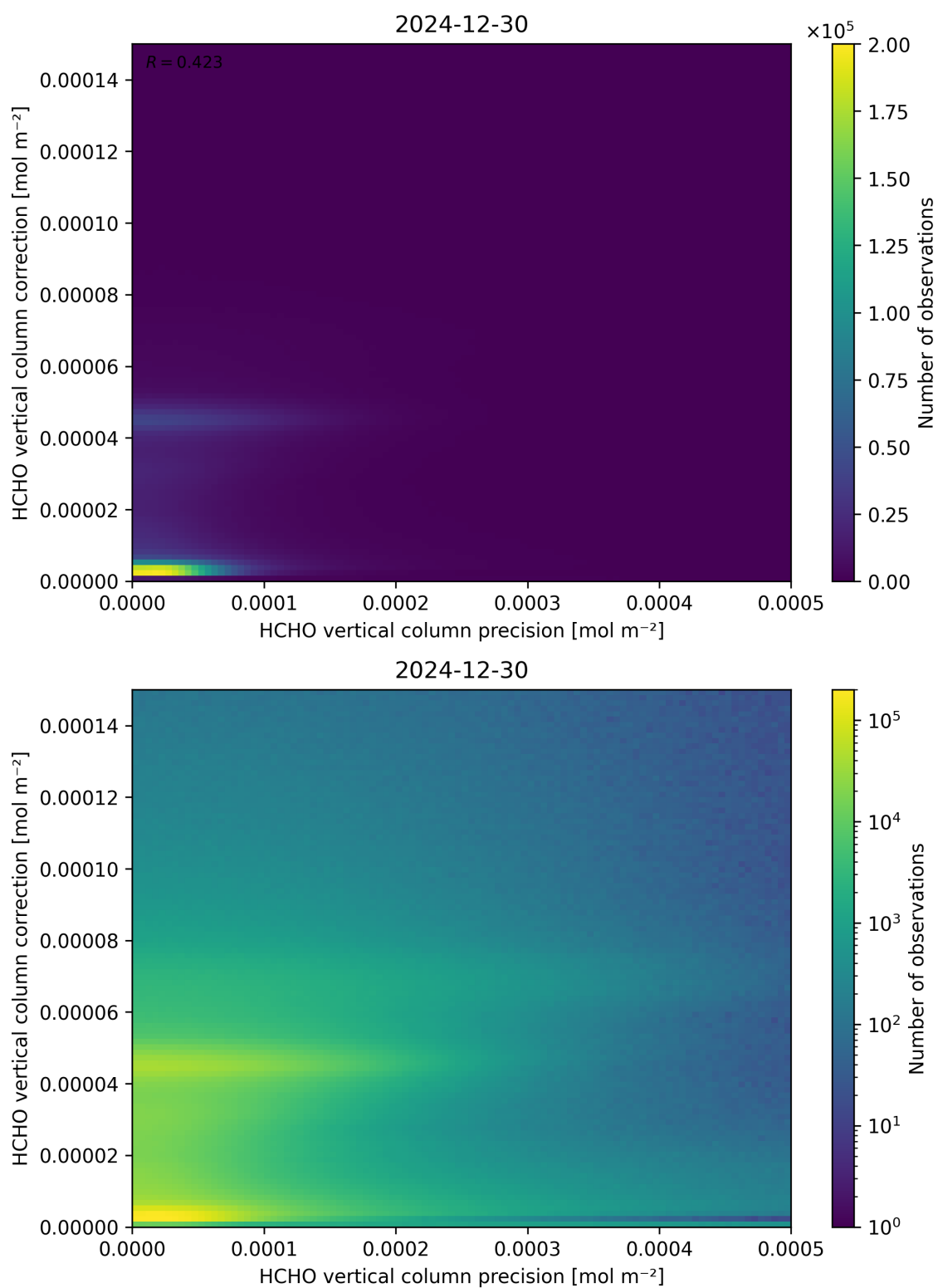
Figure 146: Scatter density plot of “HCHO vertical column precision” against “HCHO vertical column correction” for 2024-12-29 to 2024-12-31.
