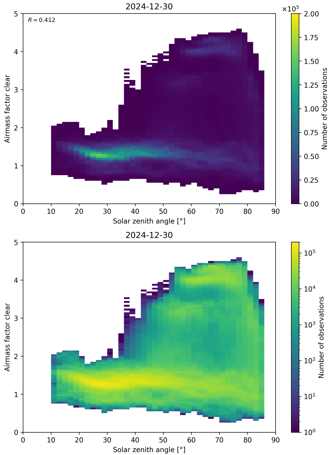
Figure 170: Scatter density plot of “Solar zenith angle” against “Airmass factor clear” for 2024-12-29 to 2024-12-31.
