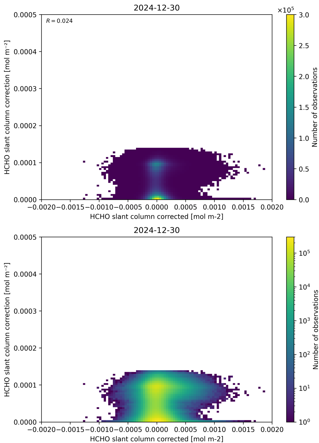
Figure 77: Scatter density plot of “HCHO slant column corrected” against “HCHO slant column correction” for 2024-12-29 to 2024-12-31.
