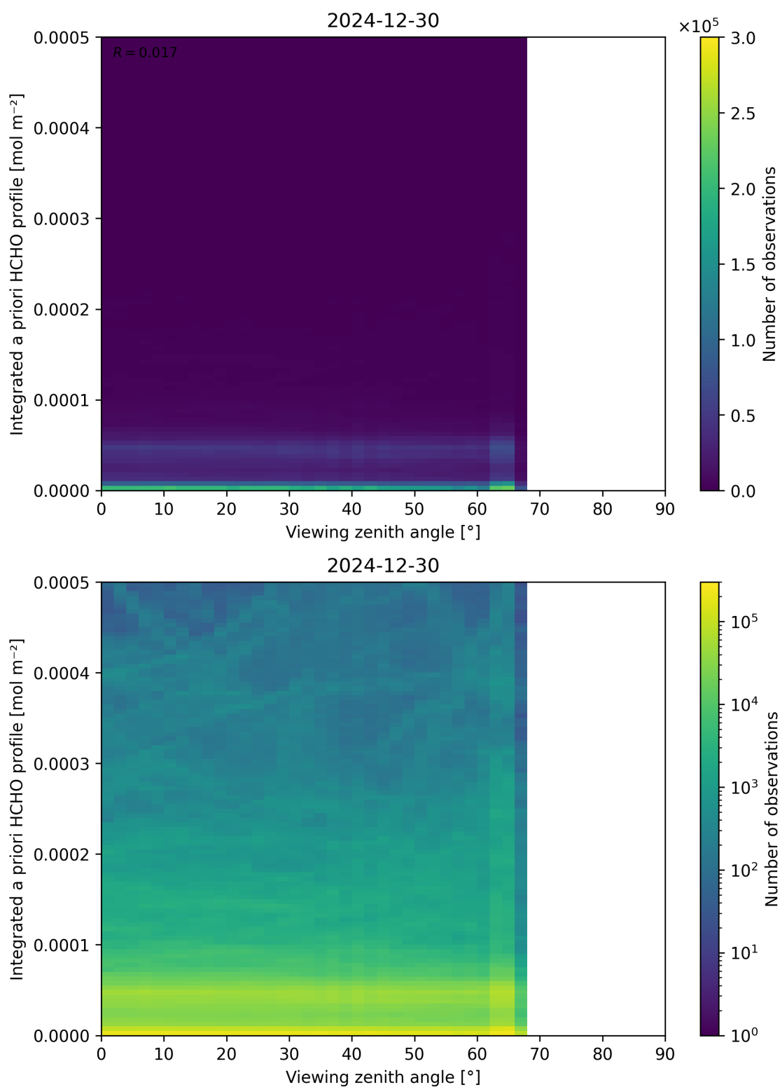
Figure 195: Scatter density plot of “Viewing zenith angle” against “Integrated a priori HCHO profile” for 2024-12-29 to 2024-12-31.
