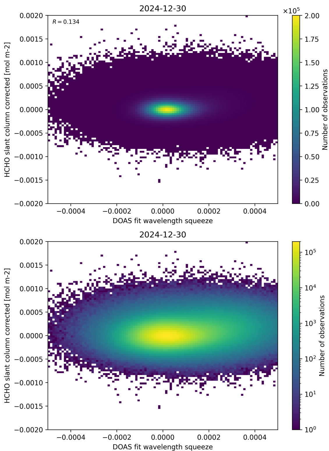
Figure 69: Scatter density plot of “DOAS fit wavelength squeeze” against “HCHO slant column corrected” for 2024-12-29 to 2024-12-31.
