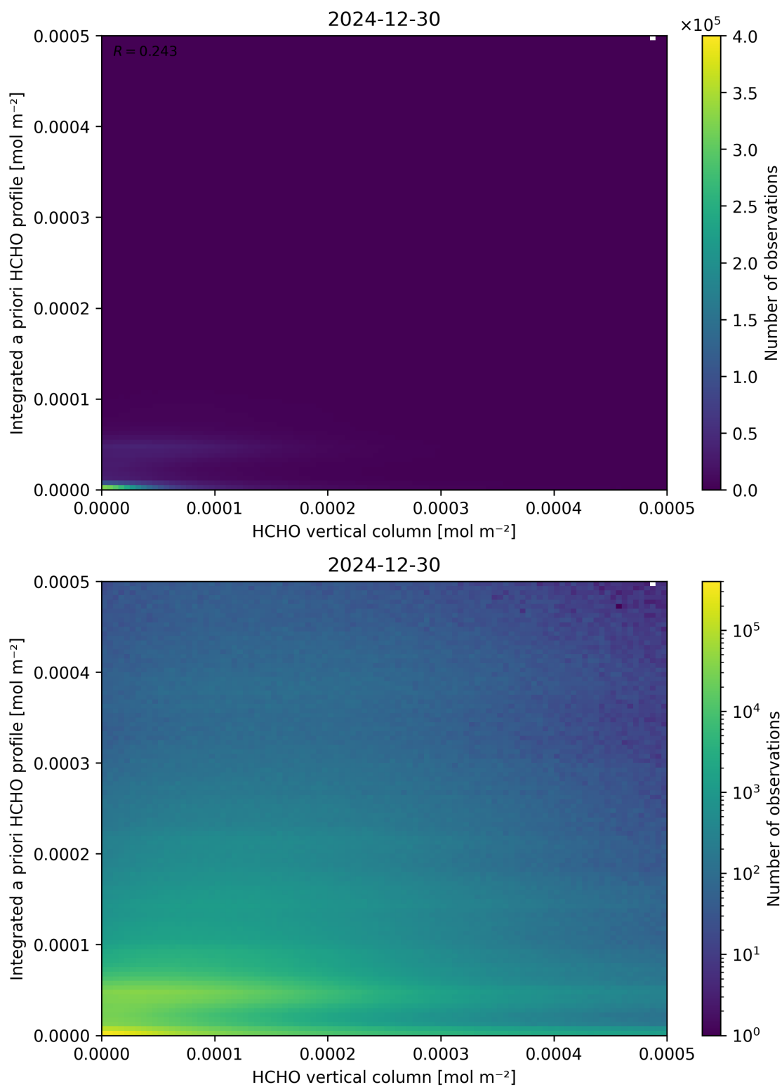
Figure 135: Scatter density plot of “HCHO vertical column” against “Integrated a priori HCHO profile” for 2024-12-29 to 2024-12-31.
