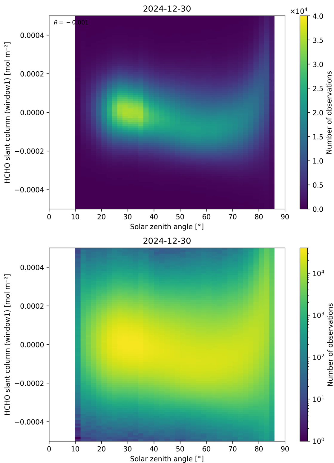
Figure 173: Scatter density plot of “Solar zenith angle” against “HCHO slant column (window1)” for 2024-12-29 to 2024-12-31.
