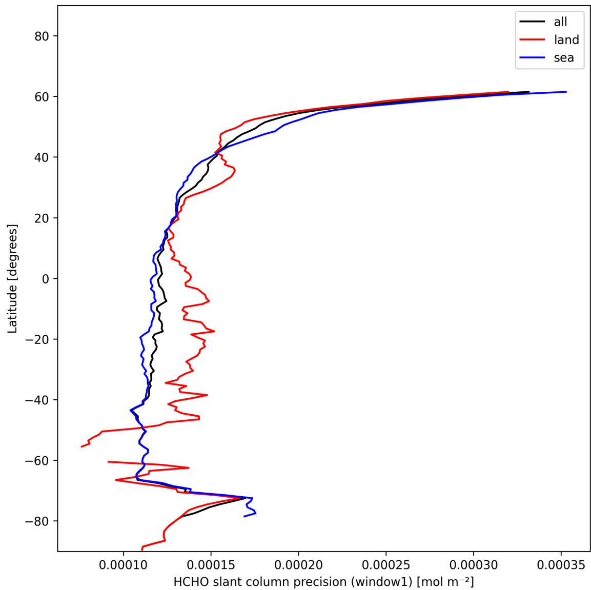
Figure 25: Zonal average of "HCHO slant column precision (window1)" for 2024-12-29 to 2024-12-31.
