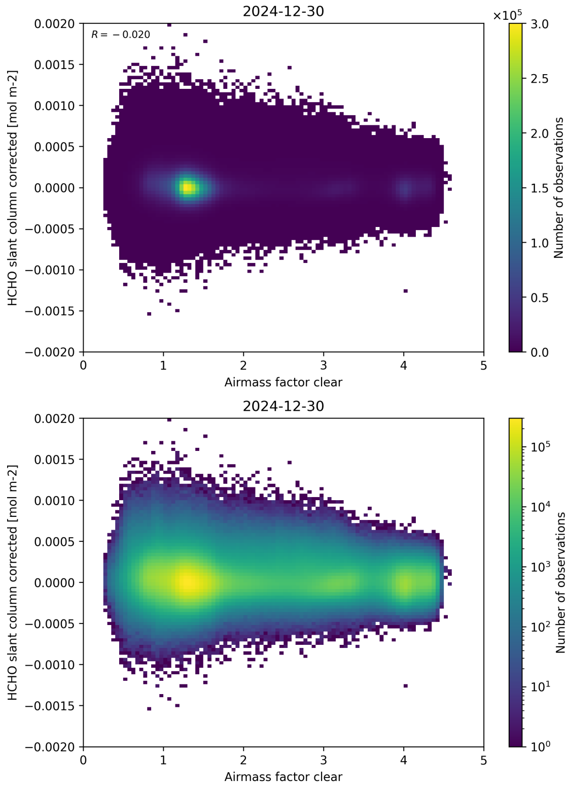
Figure 74: Scatter density plot of “Airmass factor clear” against “HCHO slant column corrected” for 2024-12-29 to 2024-12-31.
