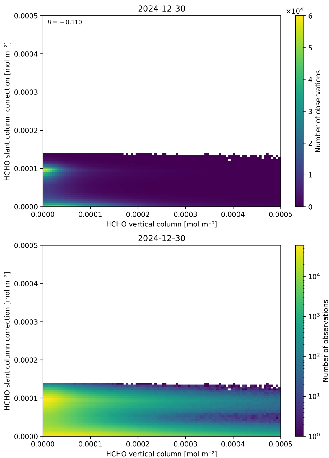
Figure 128: Scatter density plot of “HCHO vertical column” against “HCHO slant column correction” for 2024-12-29 to 2024-12-31.
