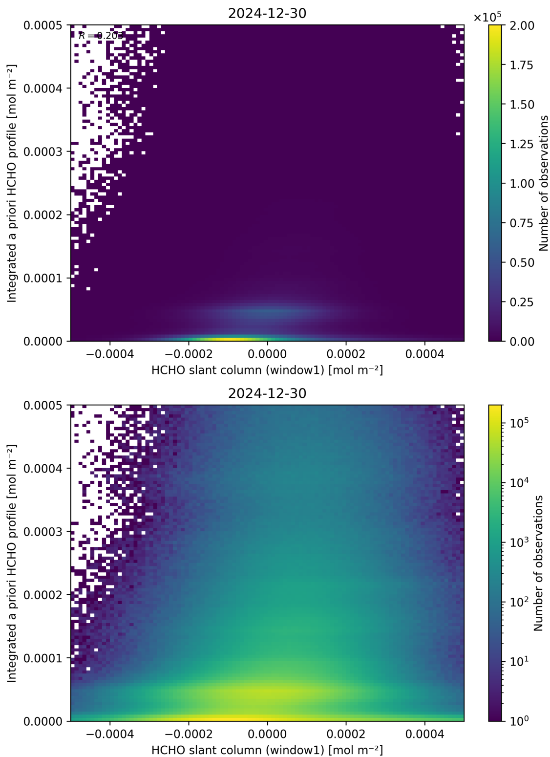
Figure 87: Scatter density plot of “HCHO slant column (window1)” against “Integrated a priori HCHO profile” for 2024-12-29 to 2024-12-31.
