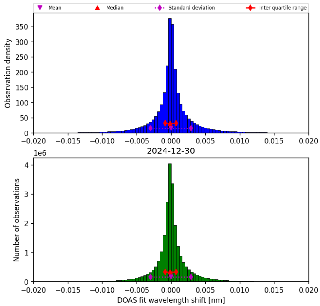
Figure 44: Histogram of “DOAS fit wavelength shift” for 2024-12-29 to 2024-12-31
