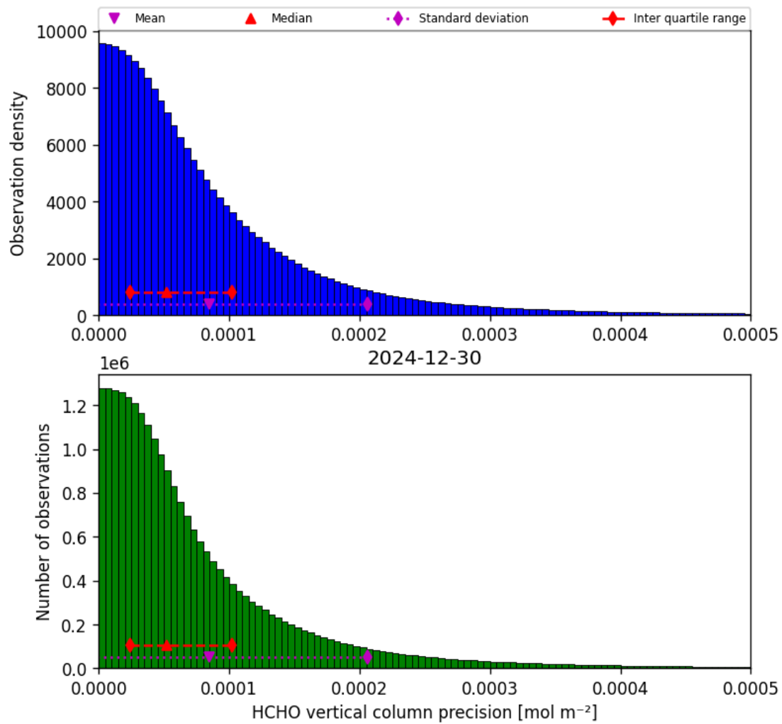
Figure 36: Histogram of “HCHO vertical column precision” for 2024-12-29 to 2024-12-31
