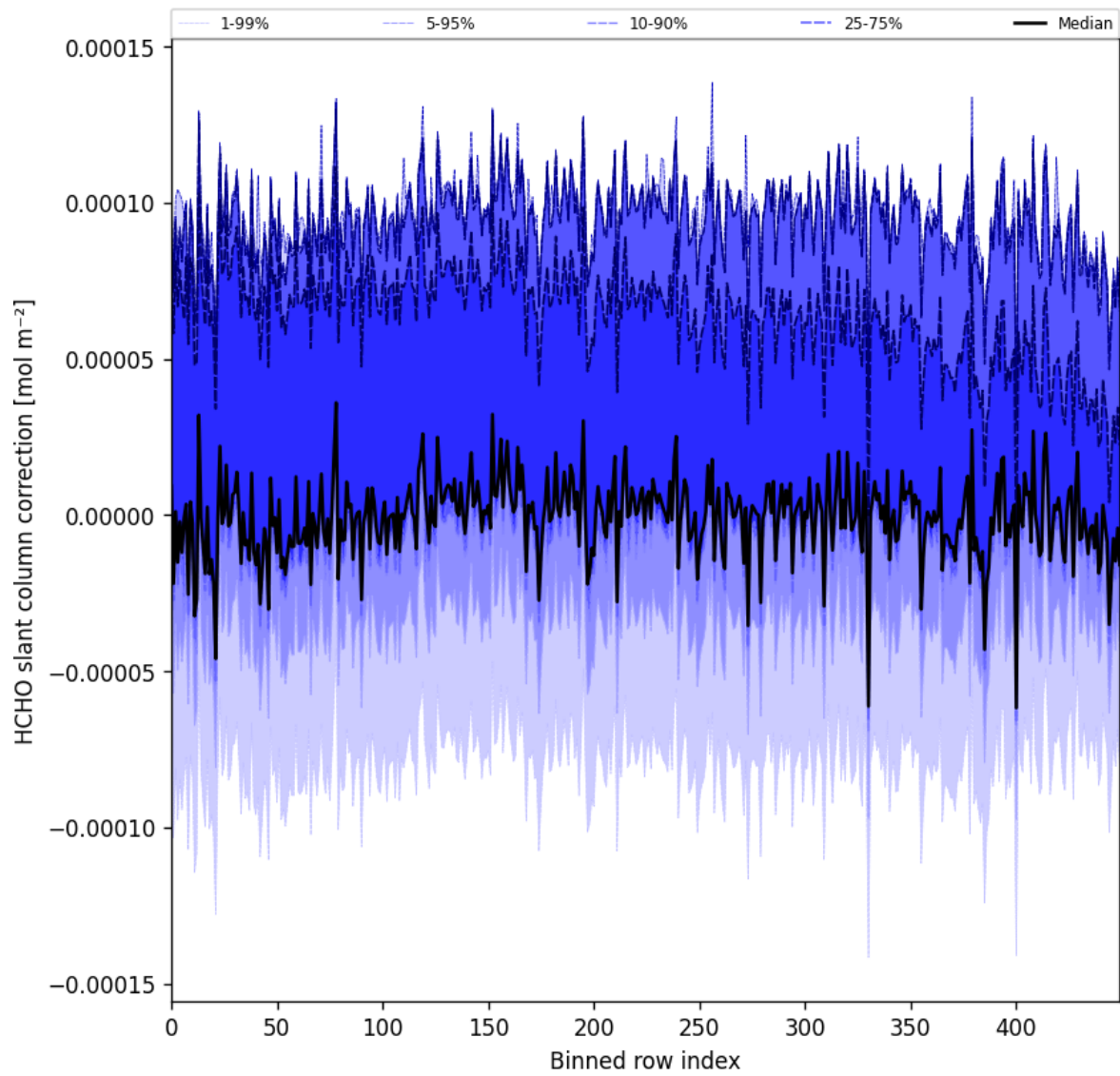
Figure 61: Along track statistics of “HCHO slant column correction” for 2024-12-29 to 2024-12-31
