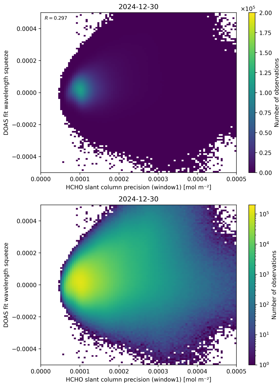
Figure 90: Scatter density plot of “HCHO slant column precision (window1)” against “DOAS fit wavelength squeeze” for 2024-12-29 to 2024-12-31.
