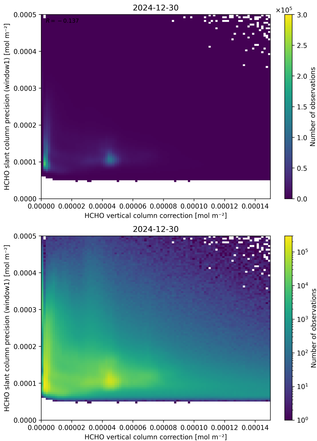
Figure 119: Scatter density plot of “HCHO vertical column correction” against “HCHO slant column precision (window1)” for 2024-12-29 to 2024-12-31.
