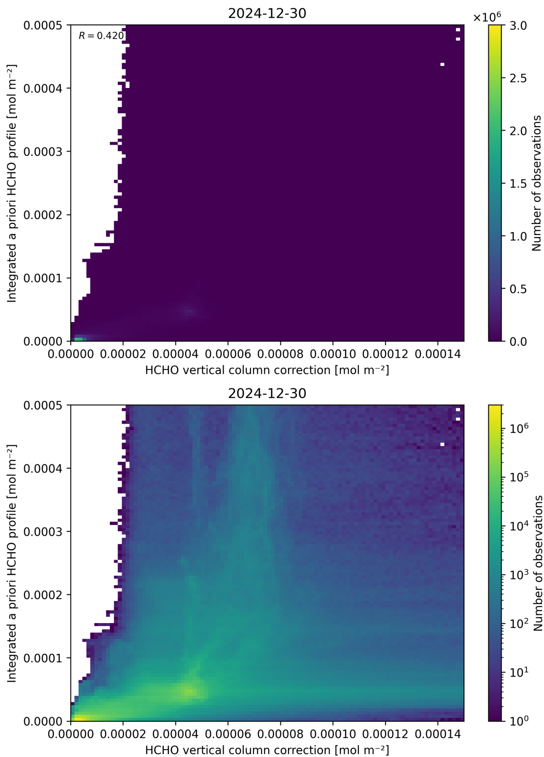
Figure 122: Scatter density plot of “HCHO vertical column correction” against “Integrated a priori HCHO profile” for 2024-12-29 to 2024-12-31.
