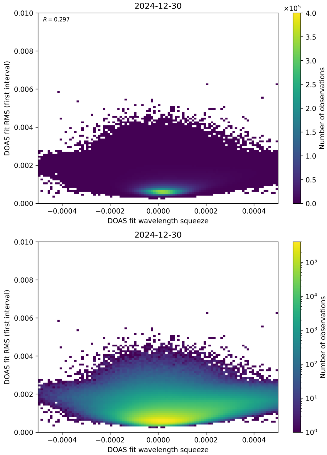
Figure 68: Scatter density plot of “DOAS fit wavelength squeeze” against “DOAS fit RMS (first interval)” for 2024-12-29 to 2024-12-31.
