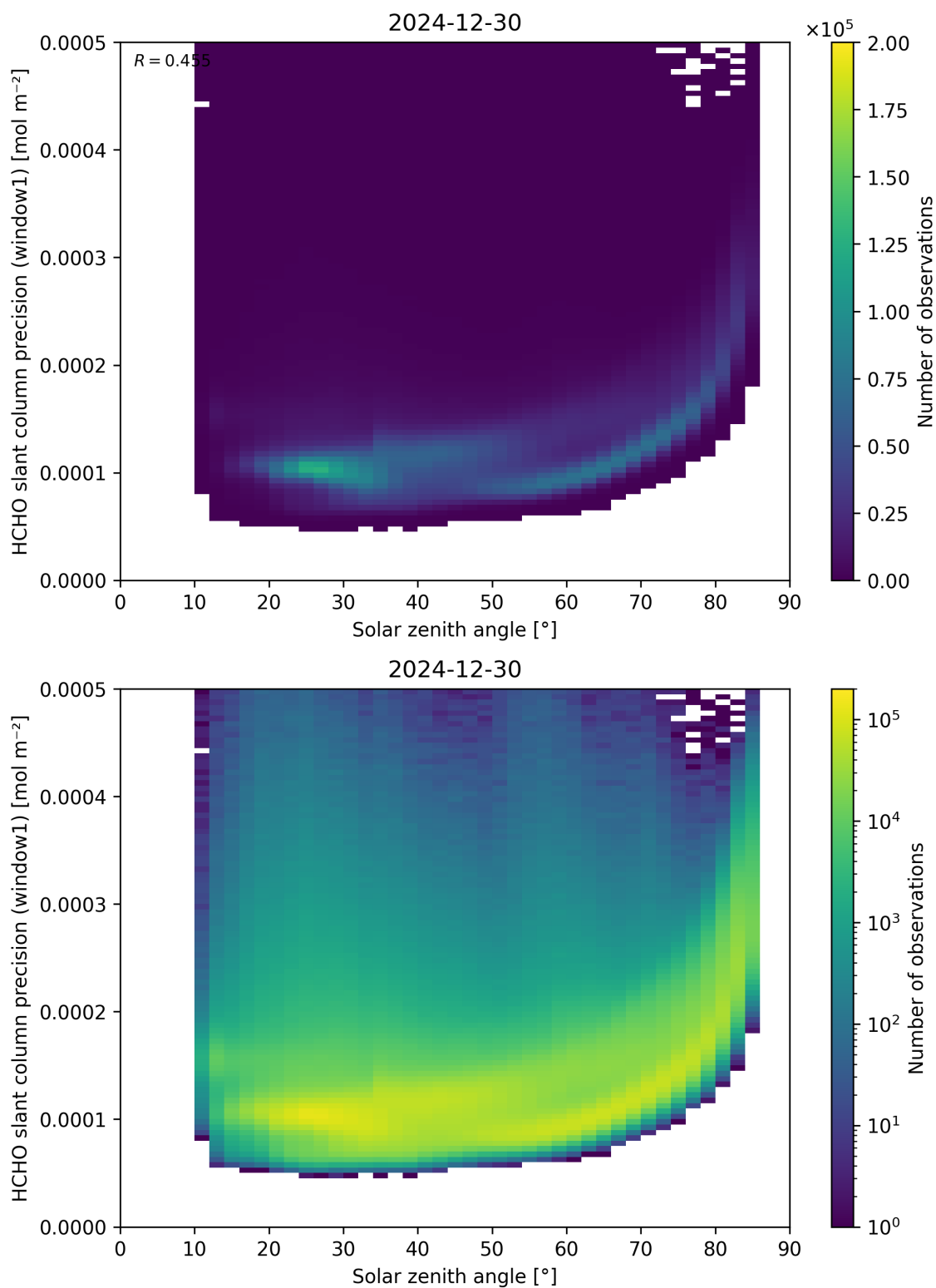
Figure 174: Scatter density plot of “Solar zenith angle” against “HCHO slant column precision (window1)” for 2024-12-29 to 2024-12-31.
