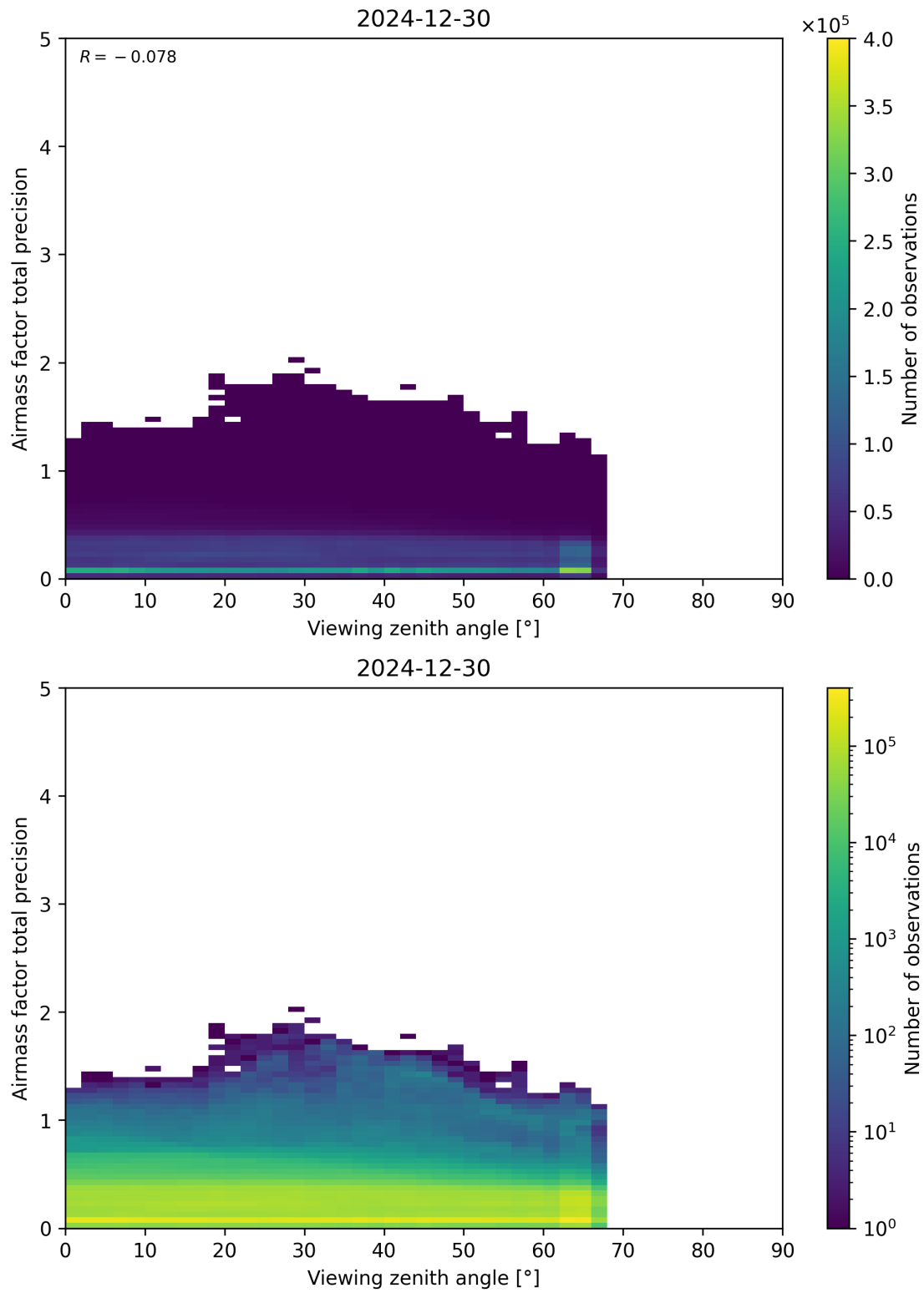
Figure 191: Scatter density plot of “Viewing zenith angle” against “Airmass factor total precision” for 2024-12-29 to 2024-12-31.
