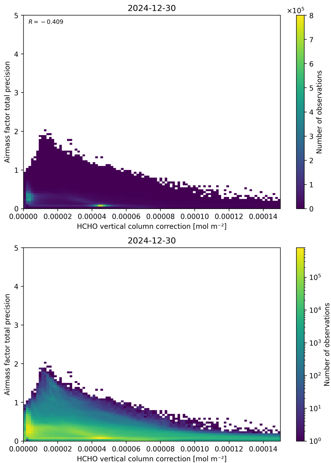
Figure 121: Scatter density plot of “HCHO vertical column correction” against “Airmass factor total precision” for 2024-12-29 to 2024-12-31.
