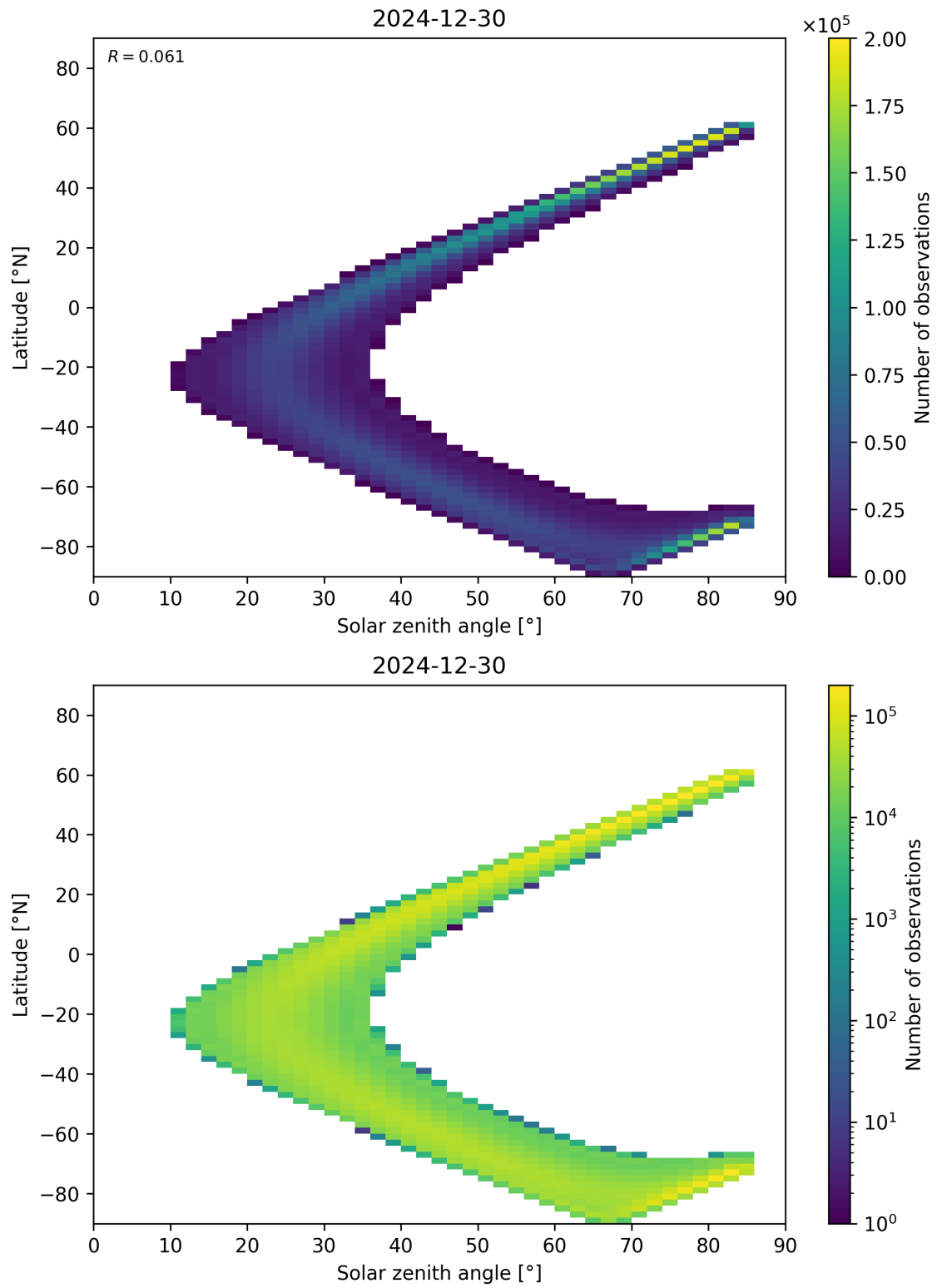
Figure 181: Scatter density plot of “Solar zenith angle” against “Latitude” for 2024-12-29 to 2024-12-31.
