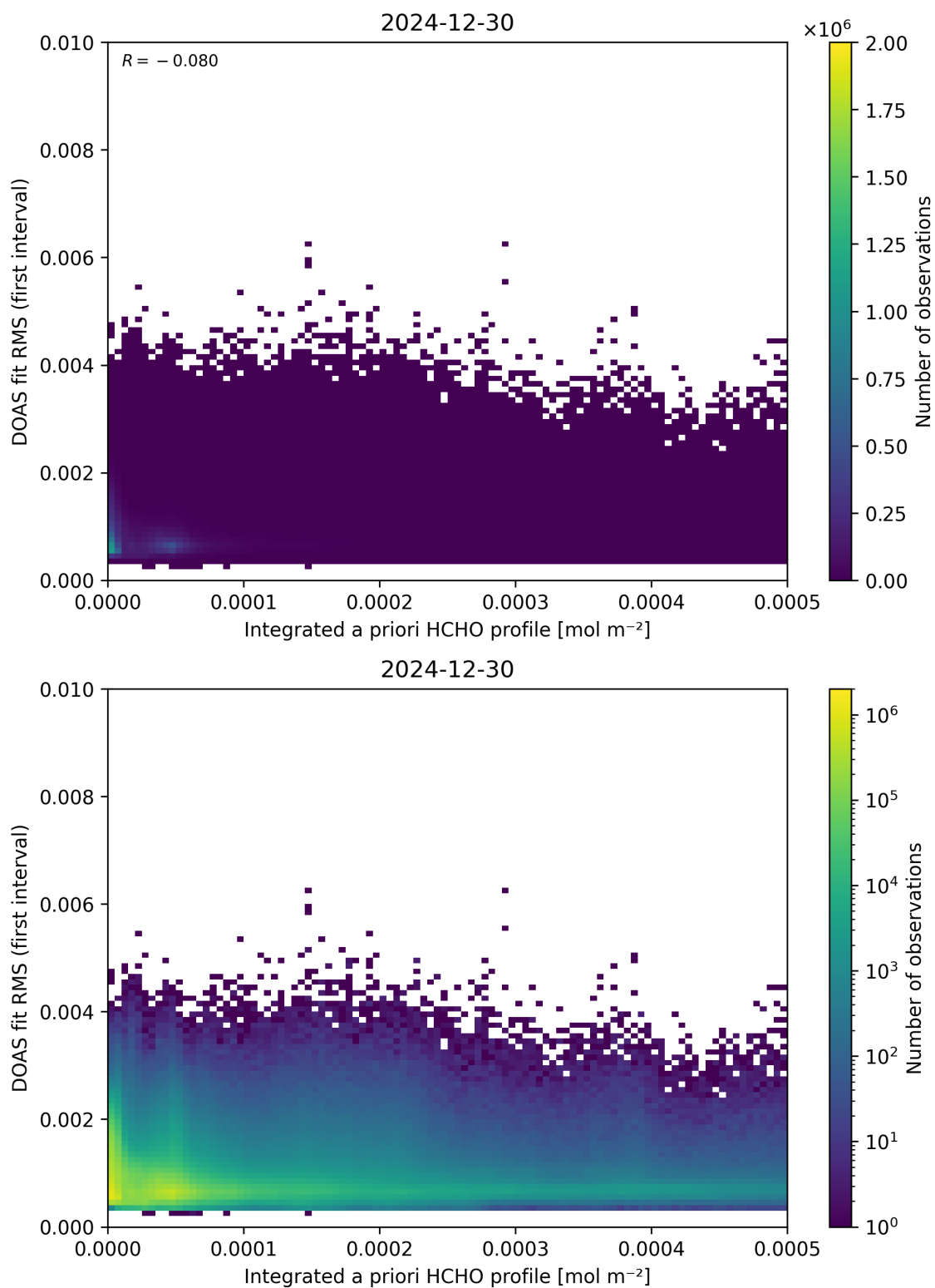
Figure 148: Scatter density plot of “Integrated a priori HCHO profile” against “DOAS fit RMS (first interval)” for 2024-12-29 to 2024-12-31.
