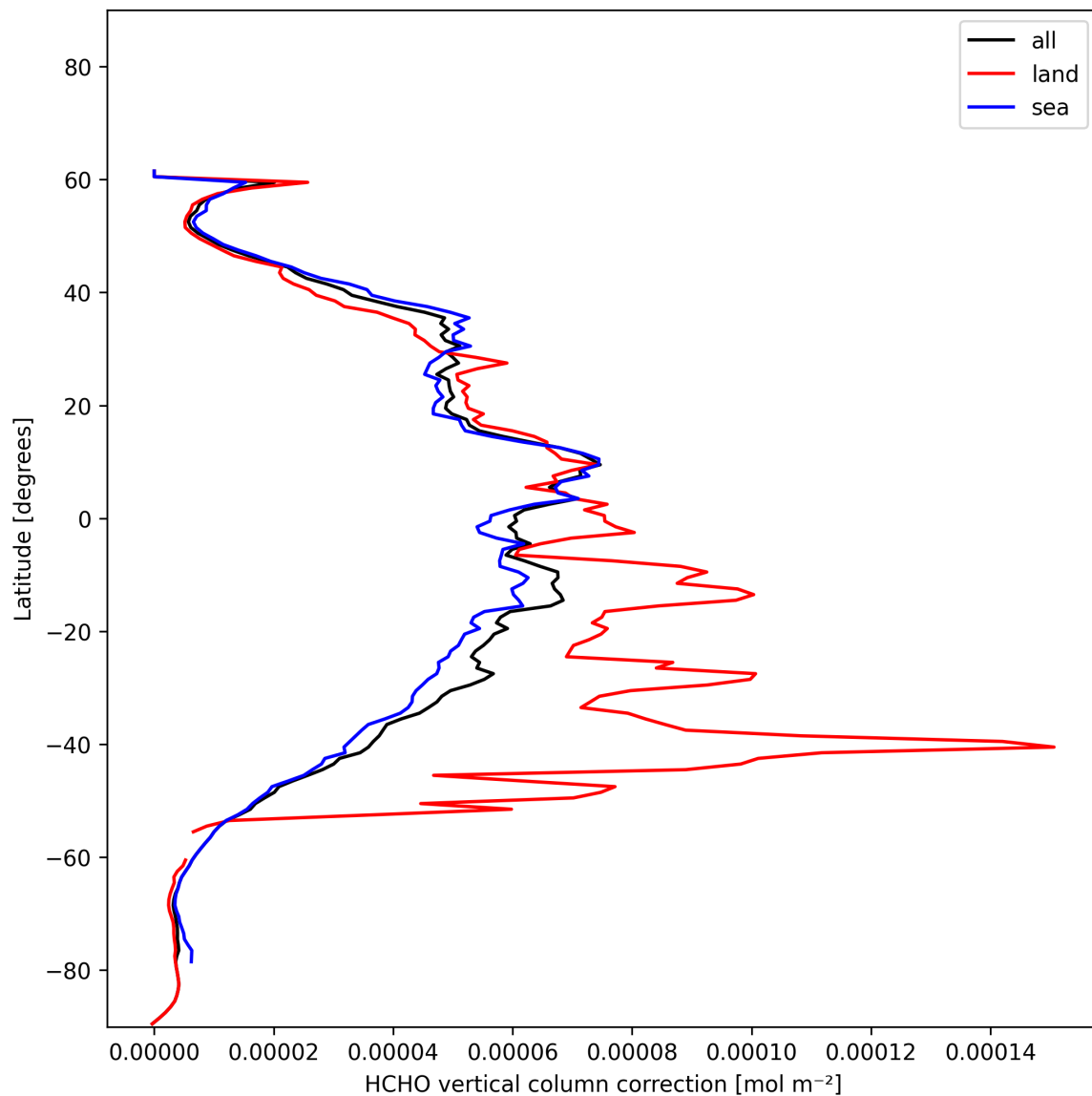
Figure 23: Zonal average of “HCHO vertical column correction” for 2024-12-29 to 2024-12-31.
