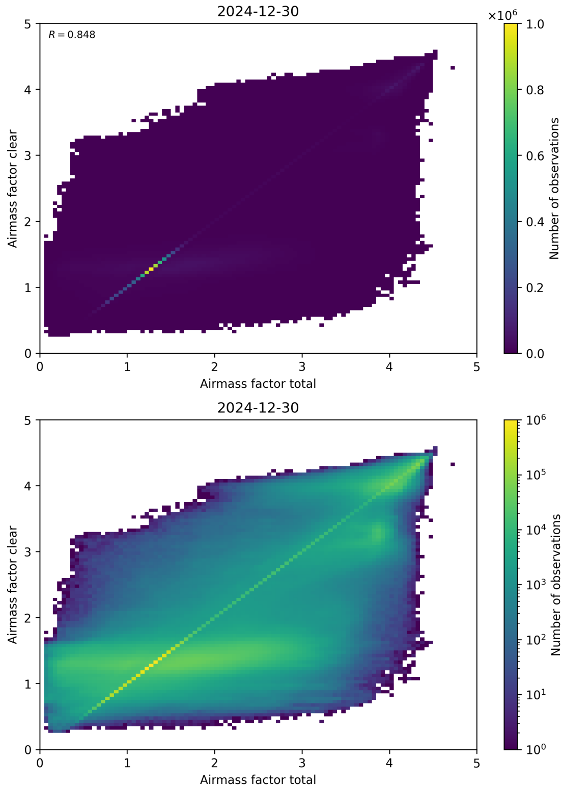
Figure 100: Scatter density plot of “Airmass factor total” against “Airmass factor clear” for 2024-12-29 to 2024-12-31.
