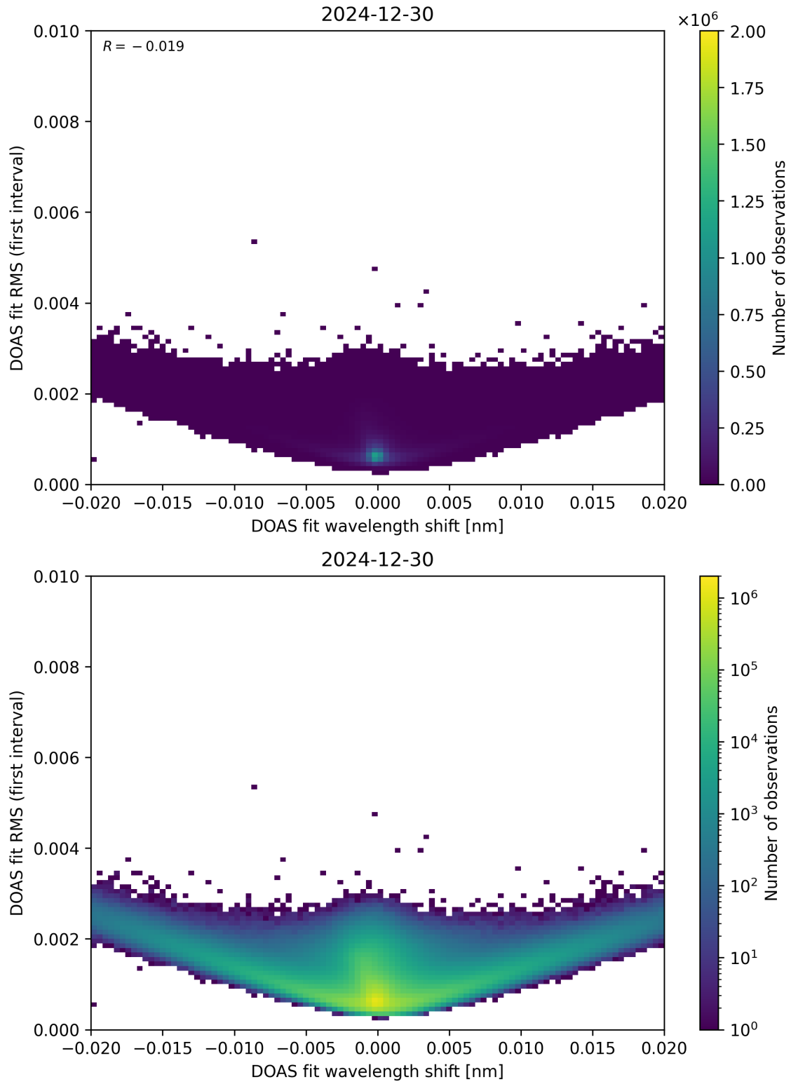
Figure 64: Scatter density plot of “DOAS fit wavelength shift” against “DOAS fit RMS (first interval)” for 2024-12-29 to 2024-12-31.
