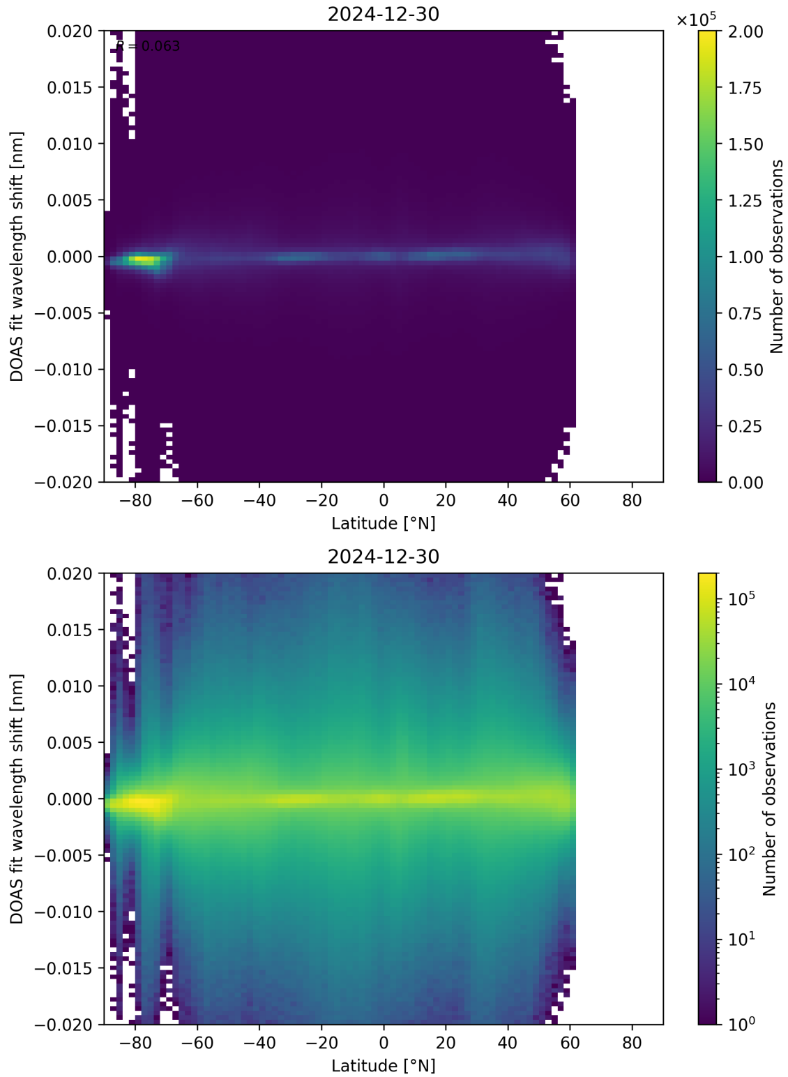
Figure 154: Scatter density plot of “Latitude” against “DOAS fit wavelength shift” for 2024-12-29 to 2024-12-31.
