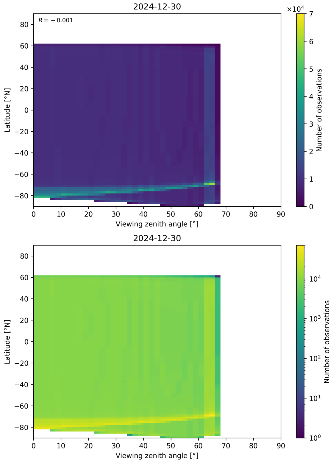
Figure 196: Scatter density plot of “Viewing zenith angle” against “Latitude” for 2024-12-29 to 2024-12-31.
