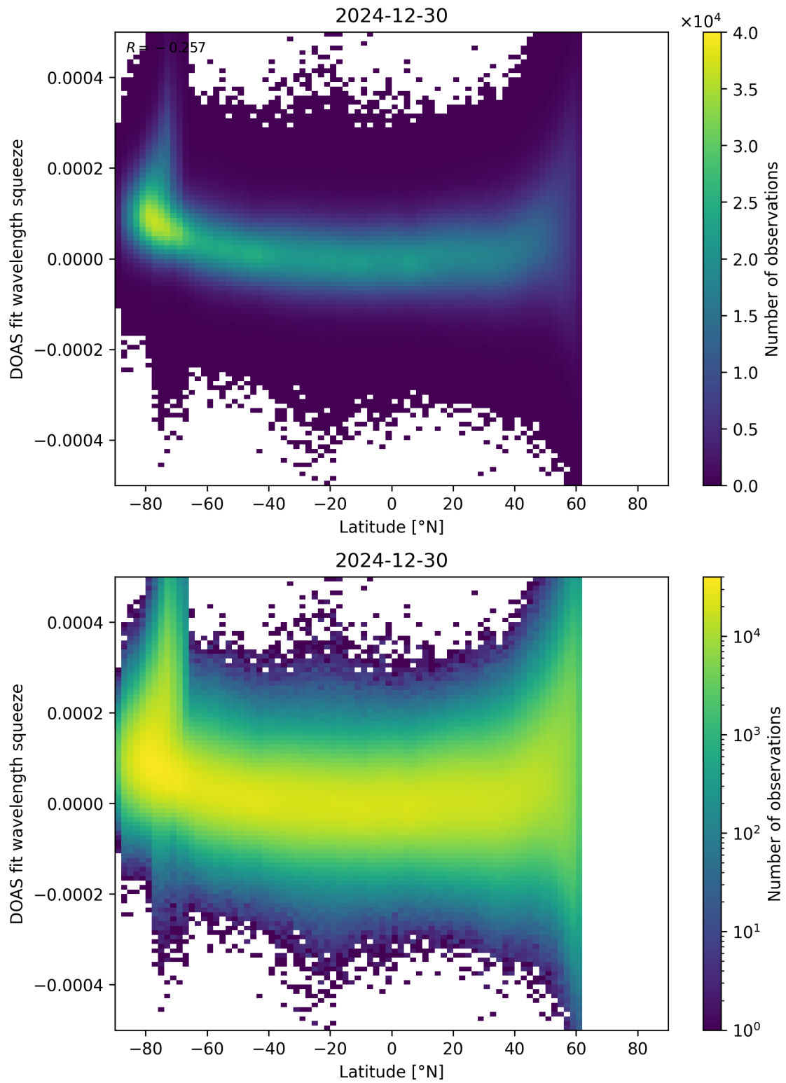
Figure 155: Scatter density plot of “Latitude” against “DOAS fit wavelength squeeze” for 2024-12-29 to 2024-12-31.
