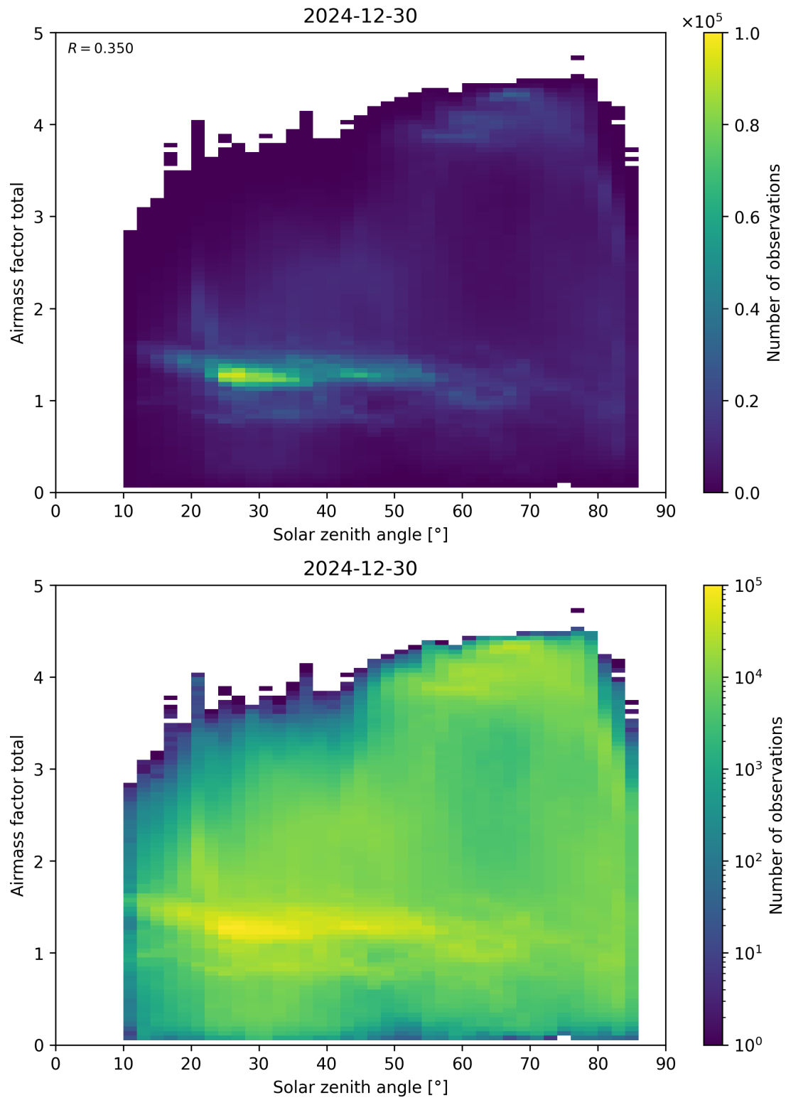
Figure 175: Scatter density plot of “Solar zenith angle” against “Airmass factor total” for 2024-12-29 to 2024-12-31.
