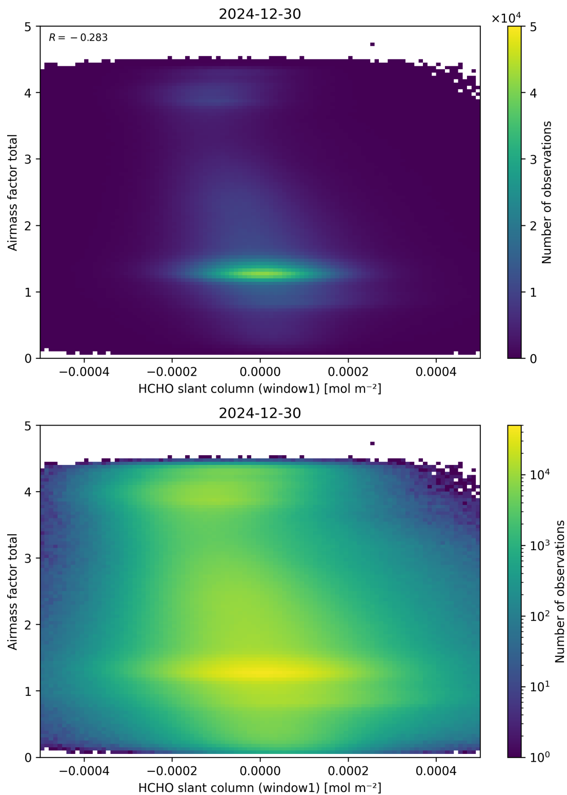
Figure 85: Scatter density plot of “HCHO slant column (window1)” against “Airmass factor total” for 2024-12-29 to 2024-12-31.
