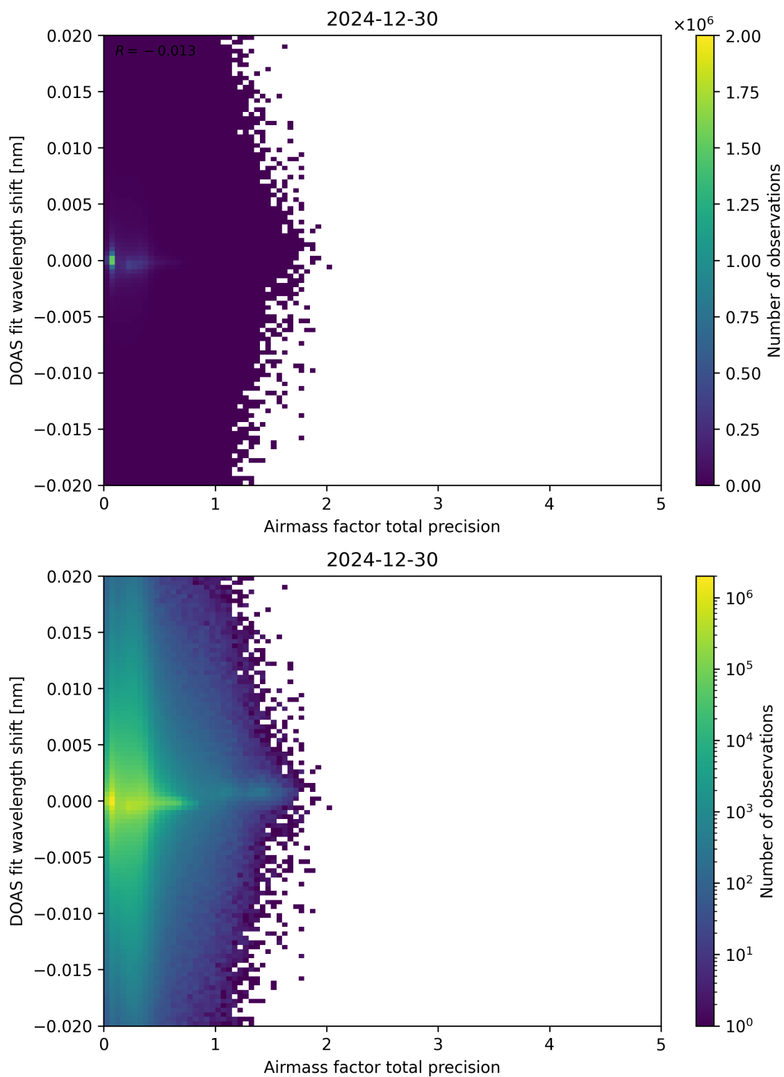
Figure 106: Scatter density plot of “Airmass factor total precision” against “DOAS fit wavelength shift” for 2024-12-29 to 2024-12-31.
