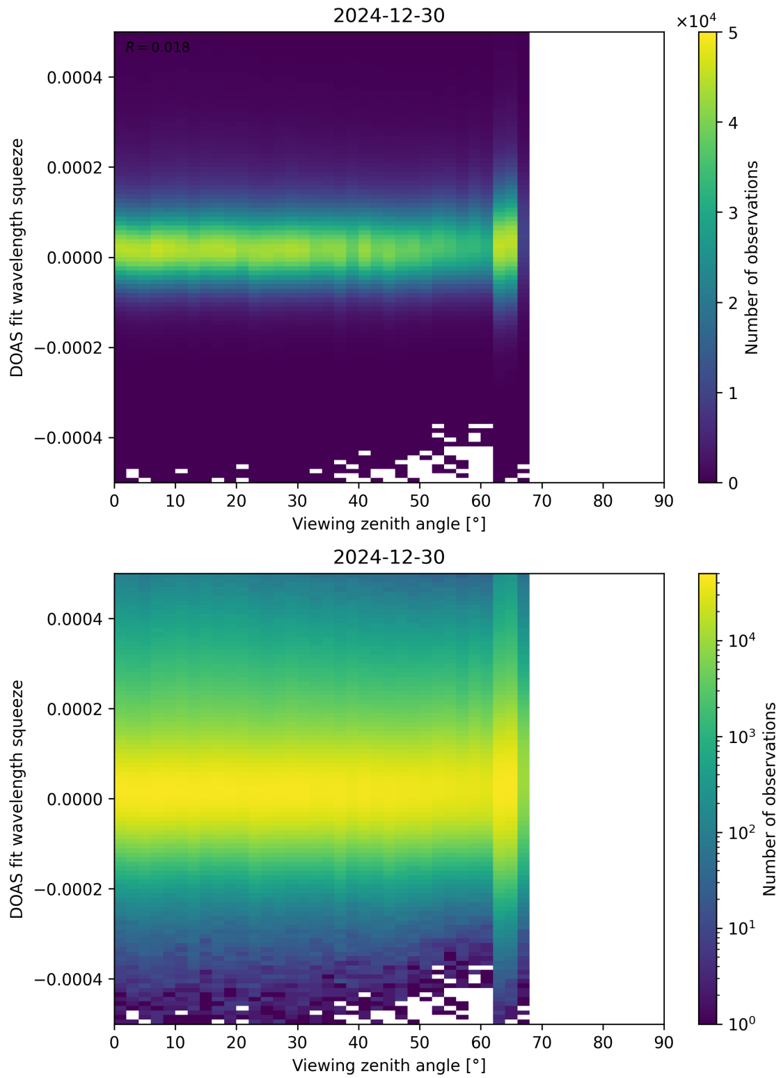
Figure 184: Scatter density plot of “Viewing zenith angle” against “DOAS fit wavelength squeeze” for 2024-12-29 to 2024-12-31.
