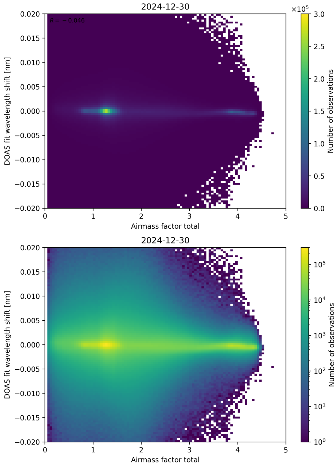
Figure 98: Scatter density plot of “Airmass factor total” against “DOAS fit wavelength shift” for 2024-12-29 to 2024-12-31.
