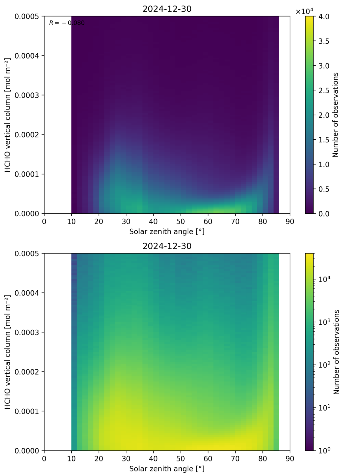
Figure 177: Scatter density plot of “Solar zenith angle” against “HCHO vertical column” for 2024-12-29 to 2024-12-31.
