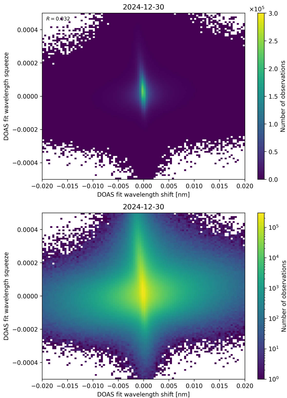
Figure 65: Scatter density plot of “DOAS fit wavelength shift” against “DOAS fit wavelength squeeze” for 2024-12-29 to 2024-12-31.
