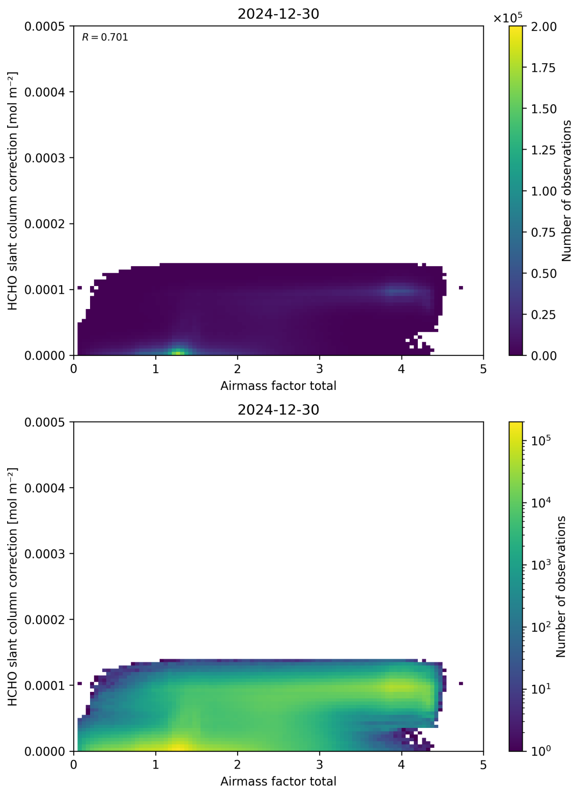
Figure 102: Scatter density plot of “Airmass factor total” against “HCHO slant column correction” for 2024-12-29 to 2024-12-31.
