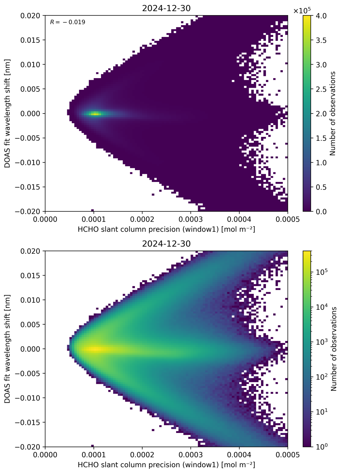
Figure 89: Scatter density plot of “HCHO slant column precision (window1)” against “DOAS fit wavelength shift” for 2024-12-29 to 2024-12-31.
