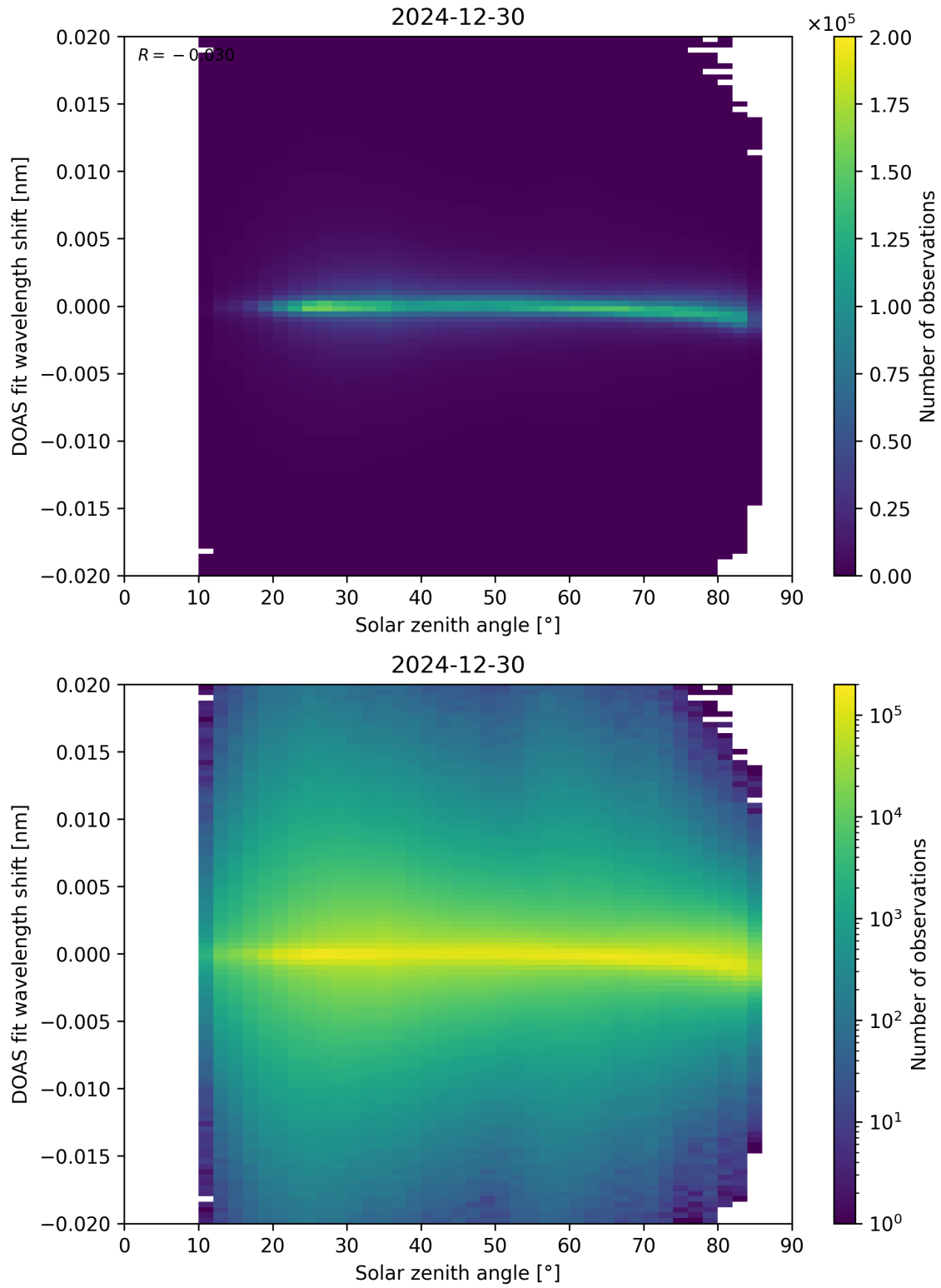
Figure 168: Scatter density plot of “Solar zenith angle” against “DOAS fit wavelength shift” for 2024-12-29 to 2024-12-31.
