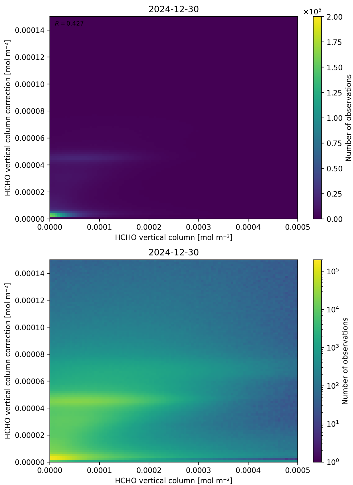
Figure 133: Scatter density plot of “HCHO vertical column” against “HCHO vertical column correction” for 2024-12-29 to 2024-12-31.
