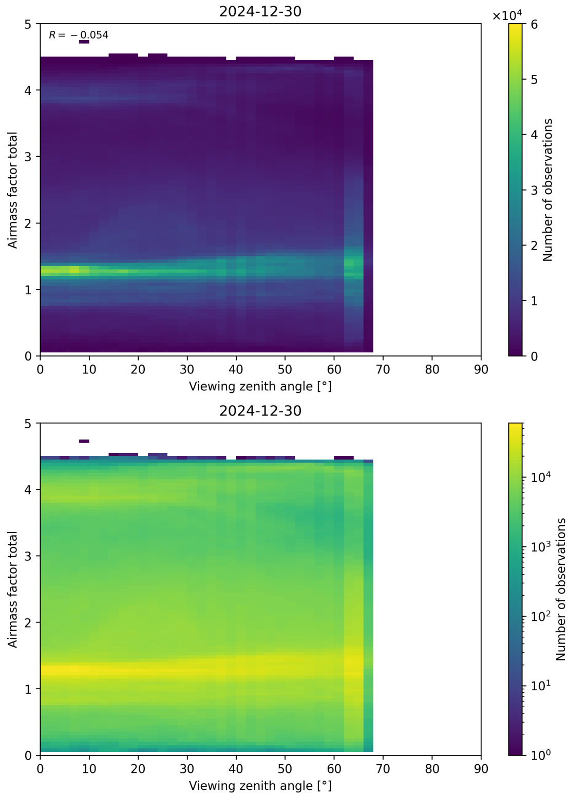
Figure 190: Scatter density plot of “Viewing zenith angle” against “Airmass factor total” for 2024-12-29 to 2024-12-31.
