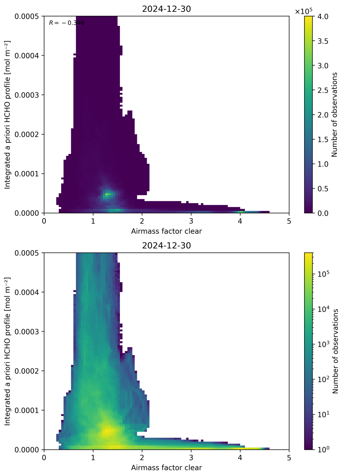
Figure 76: Scatter density plot of “Airmass factor clear” against “Integrated a priori HCHO profile” for 2024-12-29 to 2024-12-31.
