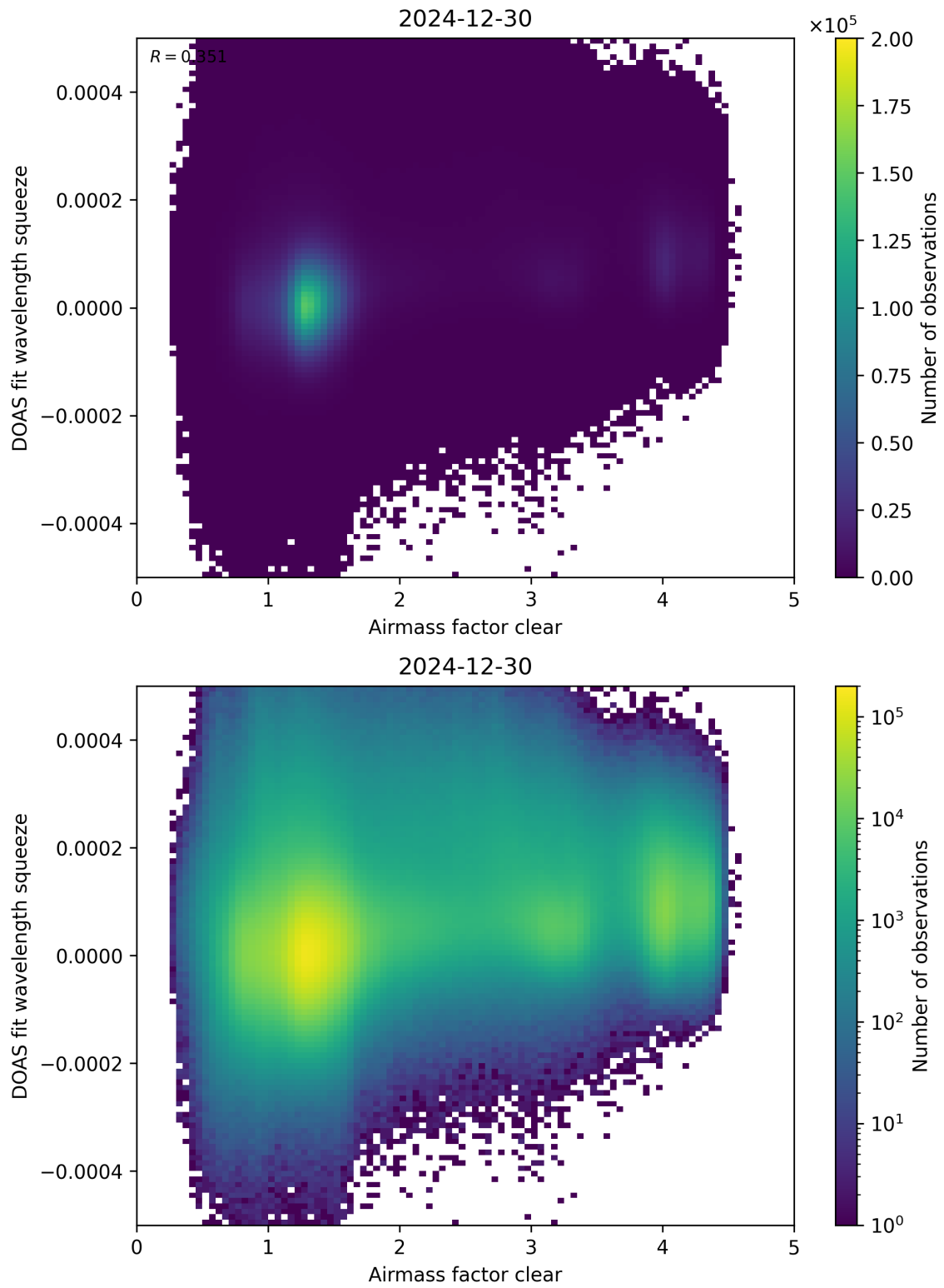
Figure 73: Scatter density plot of “Airmass factor clear” against “DOAS fit wavelength squeeze” for 2024-12-29 to 2024-12-31.
