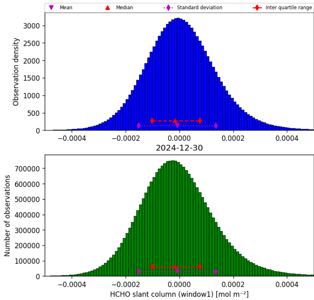
Figure 38: Histogram of “HCHO slant column (window1)” for 2024-12-29 to 2024-12-31
