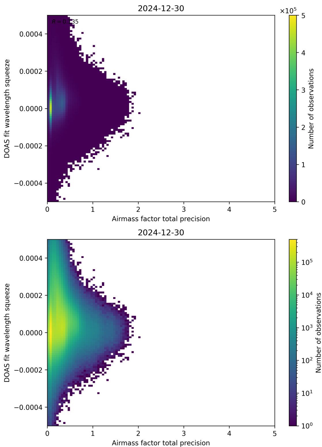
Figure 107: Scatter density plot of “Airmass factor total precision” against “DOAS fit wavelength squeeze” for 2024-12-29 to 2024-12-31.
