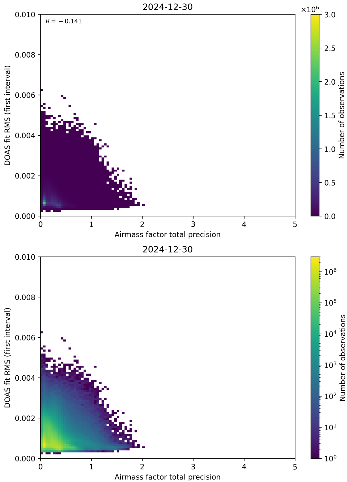
Figure 105: Scatter density plot of “Airmass factor total precision” against “DOAS fit RMS (first interval)” for 2024-12-29 to 2024-12-31.
