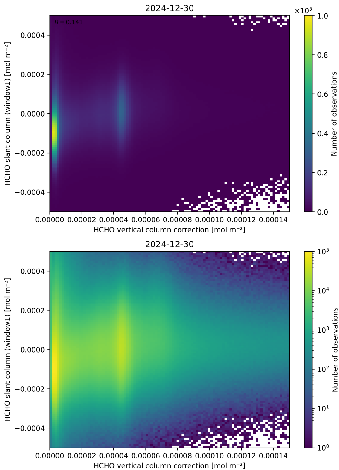
Figure 118: Scatter density plot of “HCHO vertical column correction” against “HCHO slant column (window1)” for 2024-12-29 to 2024-12-31.
