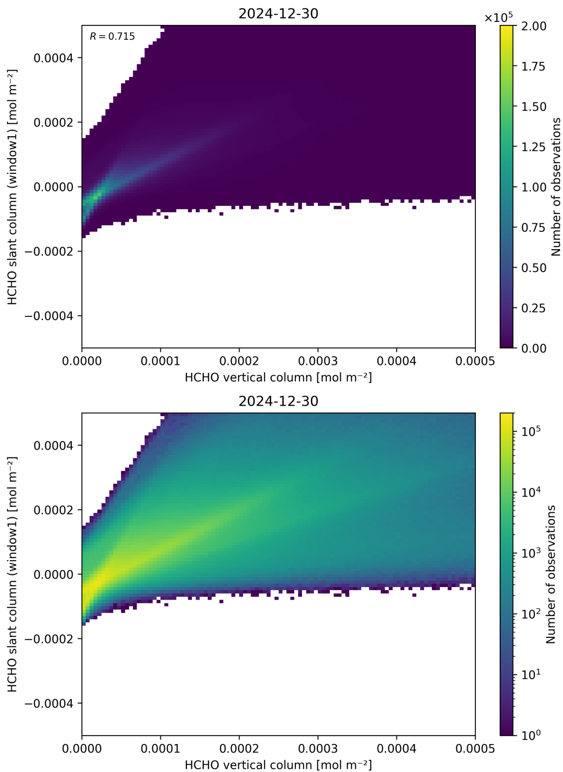
Figure 129: Scatter density plot of “HCHO vertical column” against “HCHO slant column (window1)” for 2024-12-29 to 2024-12-31.
