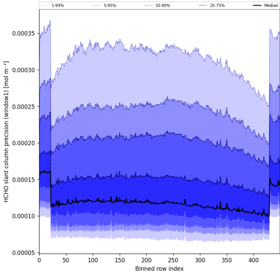
Figure 53: Along track statistics of “HCHO slant column precision (window1)” for 2024-12-29 to 2024-12-31
