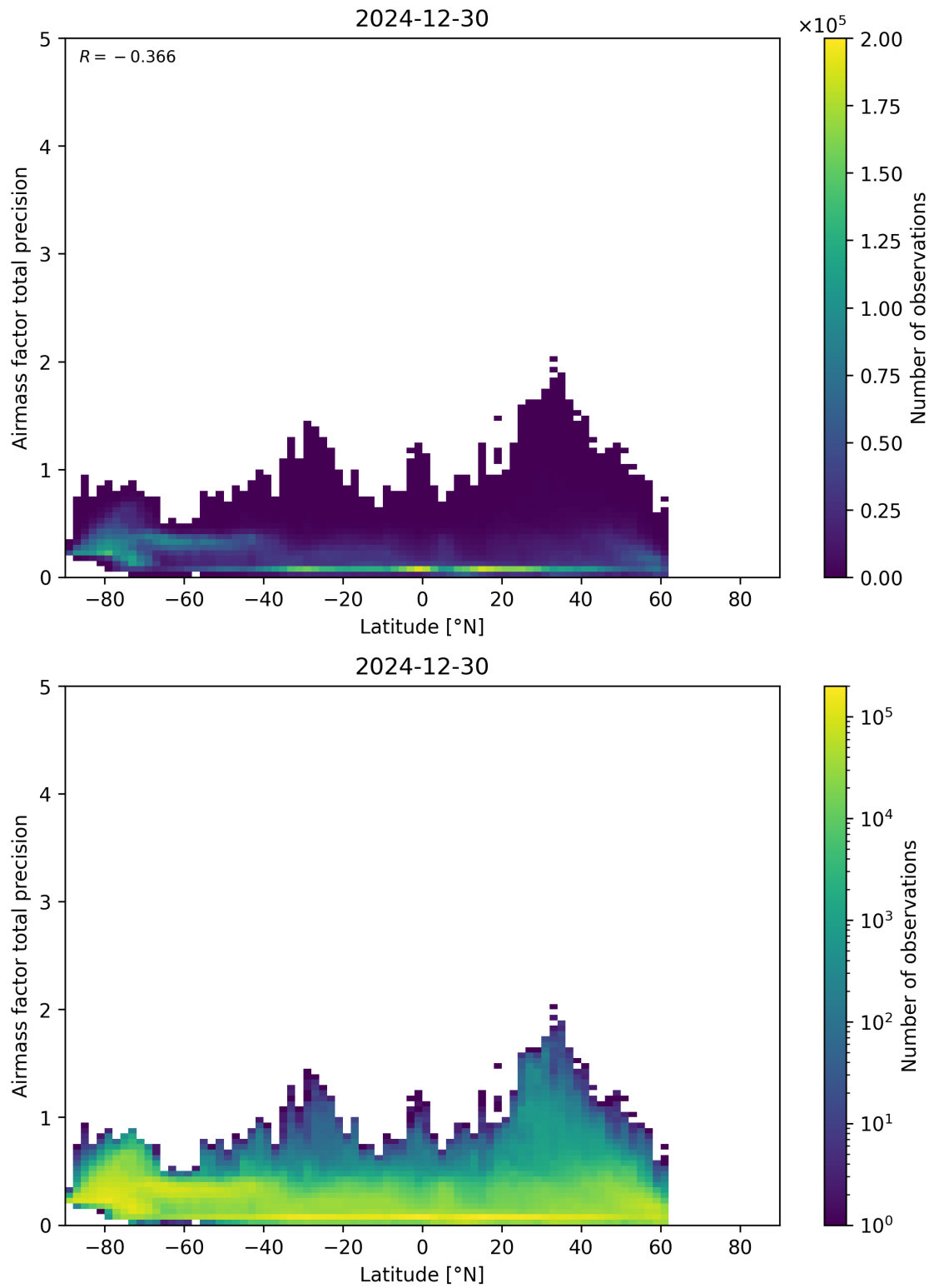
Figure 162: Scatter density plot of “Latitude” against “Airmass factor total precision” for 2024-12-29 to 2024-12-31.
