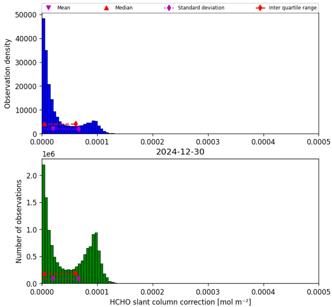
Figure 47: Histogram of “HCHO slant column correction” for 2024-12-29 to 2024-12-31
