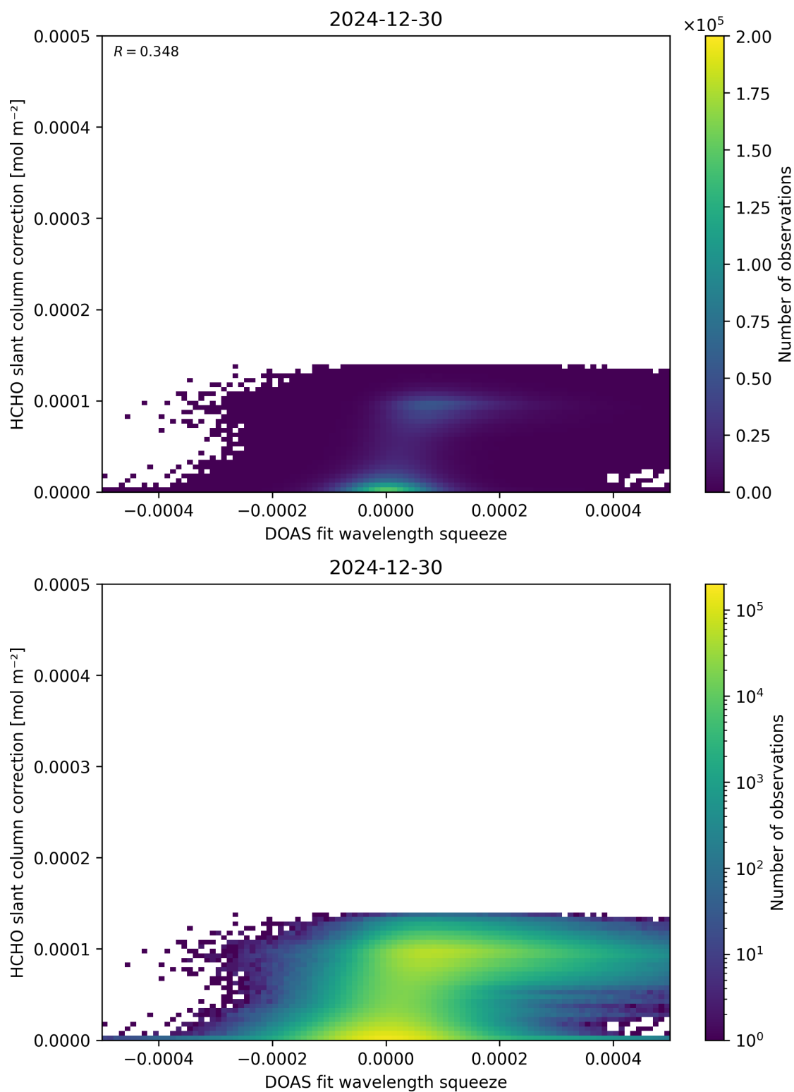
Figure 70: Scatter density plot of “DOAS fit wavelength squeeze” against “HCHO slant column correction” for 2024-12-29 to 2024-12-31.
