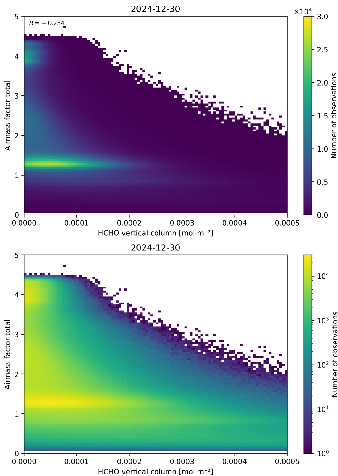
Figure 131: Scatter density plot of “HCHO vertical column” against “Airmass factor total” for 2024-12-29 to 2024-12-31.
