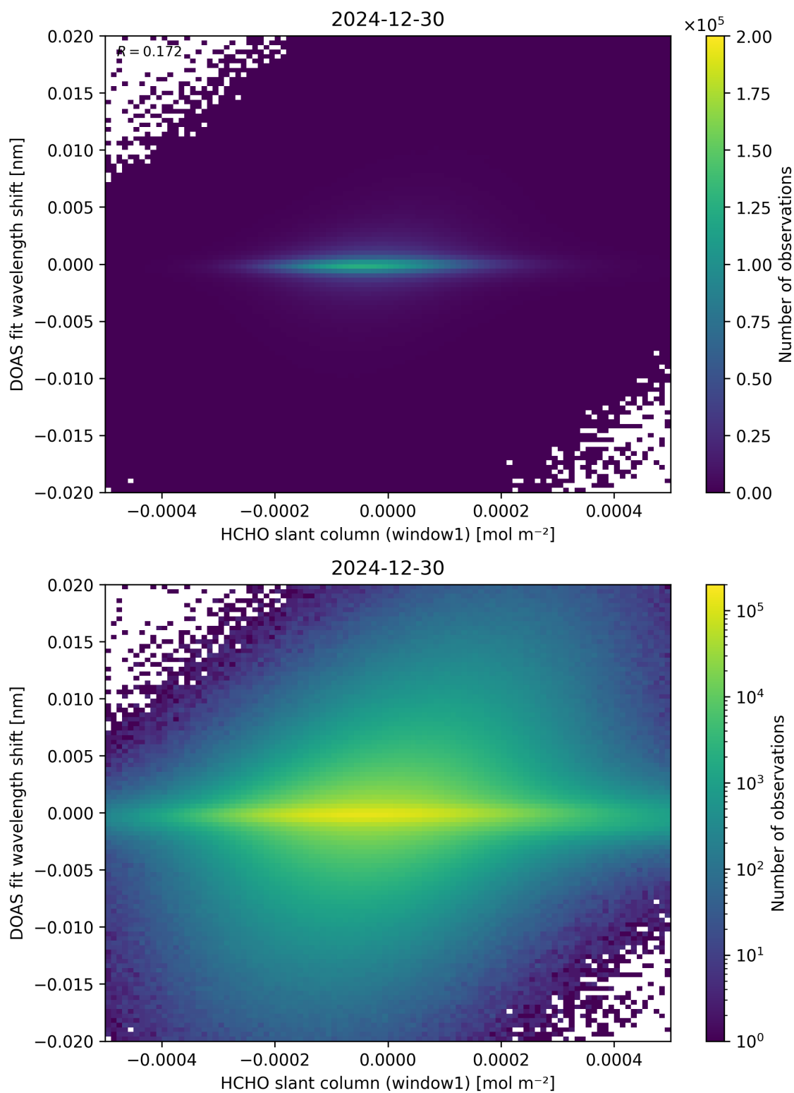
Figure 79: Scatter density plot of “HCHO slant column (window1)” against “DOAS fit wavelength shift” for 2024-12-29 to 2024-12-31.
