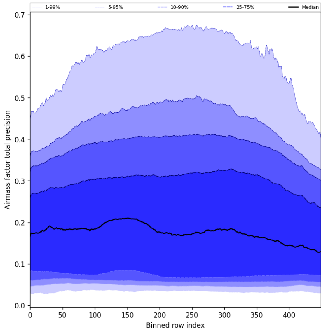
Figure 55: Along track statistics of “Airmass factor total precision” for 2024-12-29 to 2024-12-31
