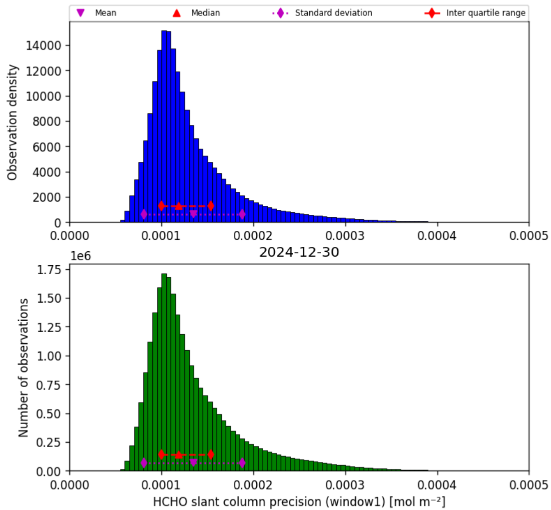
Figure 39: Histogram of “HCHO slant column precision (window1)” for 2024-12-29 to 2024-12-31
