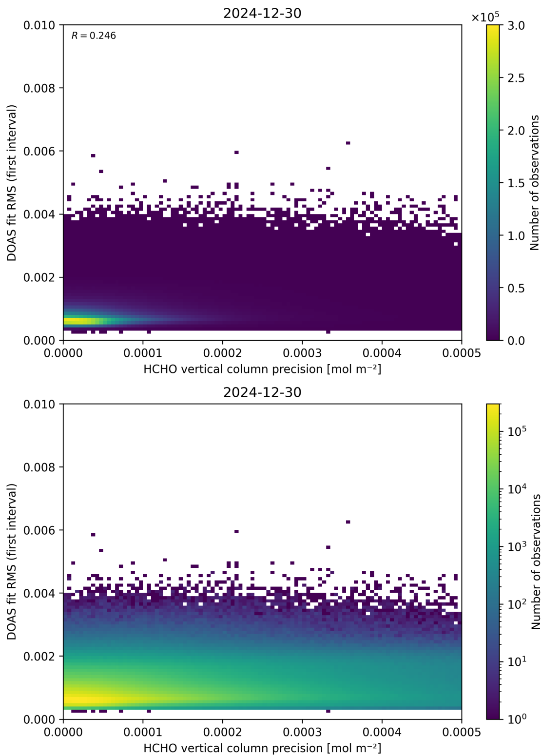
Figure 136: Scatter density plot of “HCHO vertical column precision” against “DOAS fit RMS (first interval)” for 2024-12-29 to 2024-12-31.
