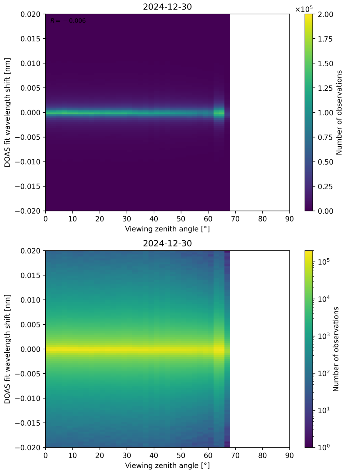
Figure 183: Scatter density plot of “Viewing zenith angle” against “DOAS fit wavelength shift” for 2024-12-29 to 2024-12-31.
