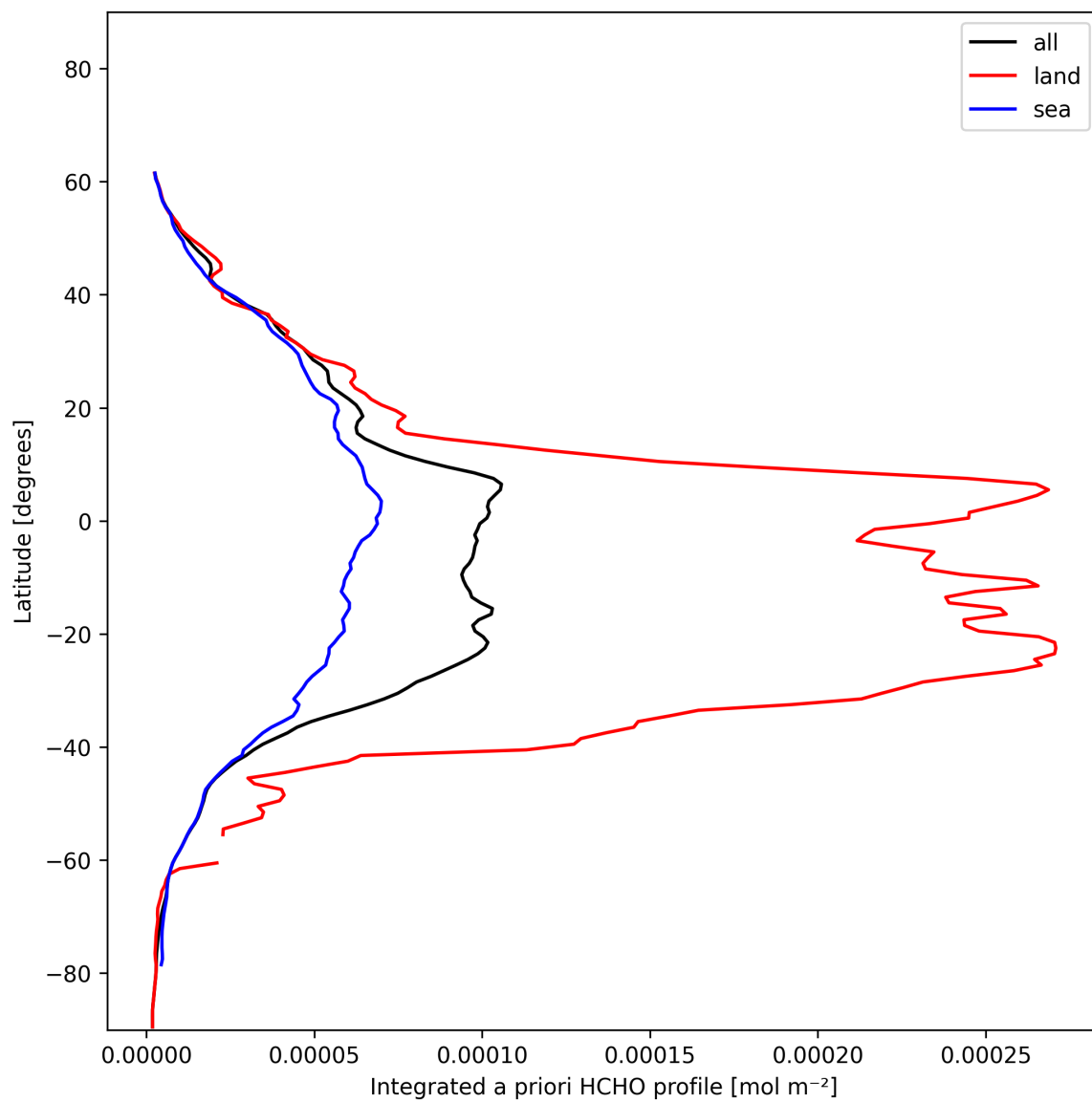
Figure 29: Zonal average of “Integrated a priori HCHO profile” for 2024-12-29 to 2024-12-31.
