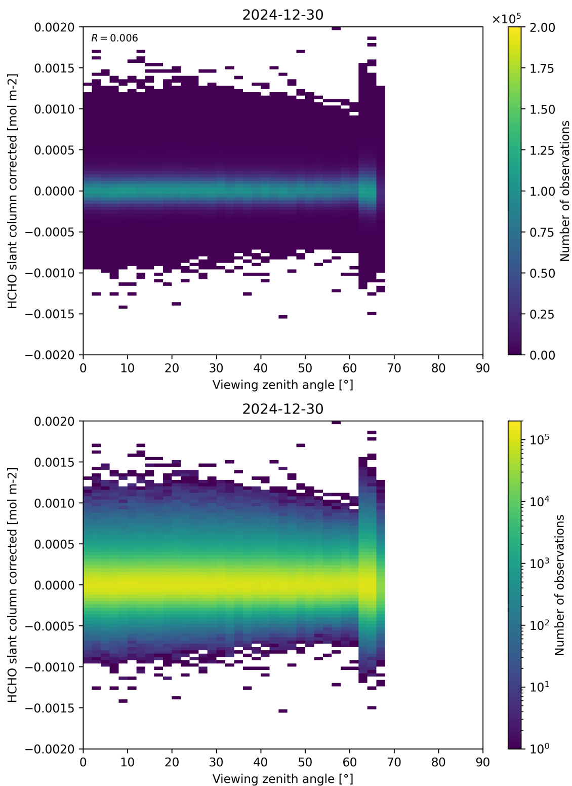
Figure 186: Scatter density plot of “Viewing zenith angle” against “HCHO slant column corrected” for 2024-12-29 to 2024-12-31.
