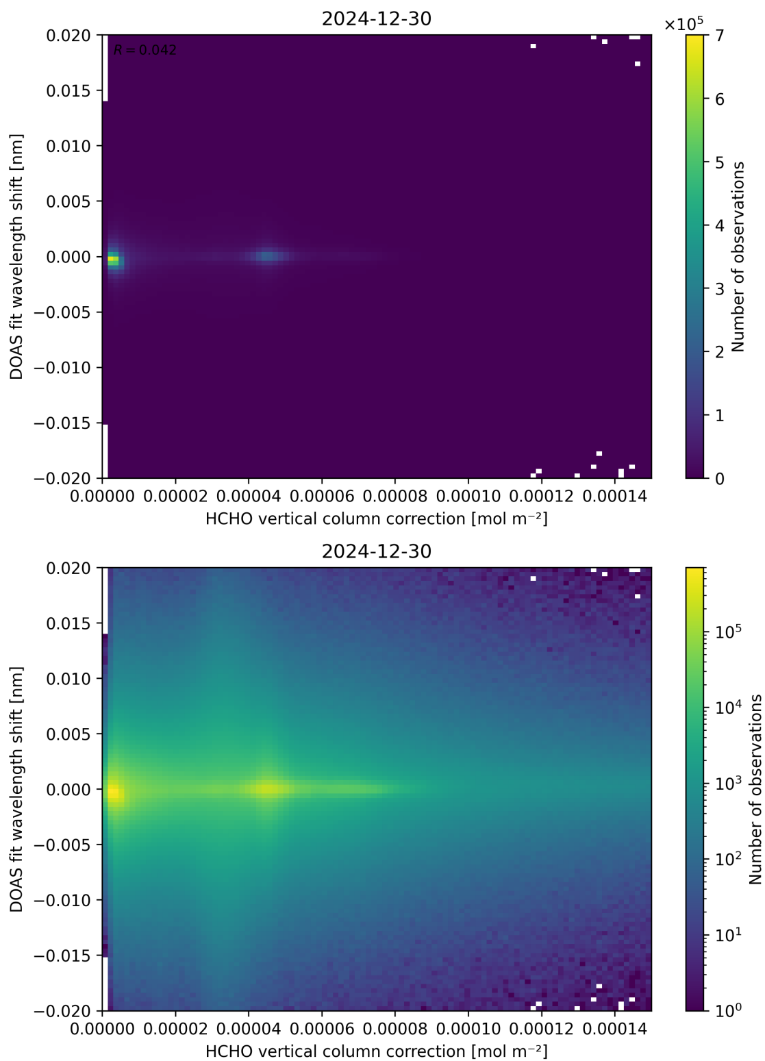
Figure 113: Scatter density plot of “HCHO vertical column correction” against “DOAS fit wavelength shift” for 2024-12-29 to 2024-12-31.
