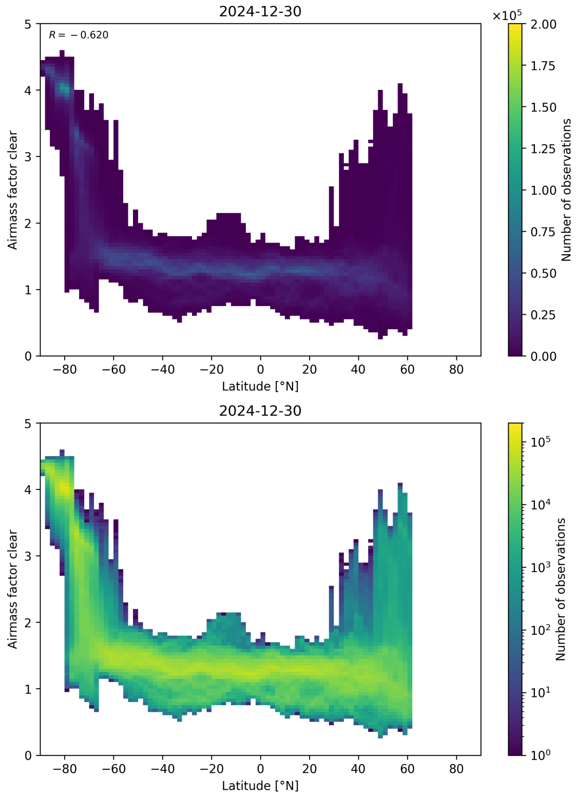
Figure 156: Scatter density plot of “Latitude” against “Airmass factor clear” for 2024-12-29 to 2024-12-31.
