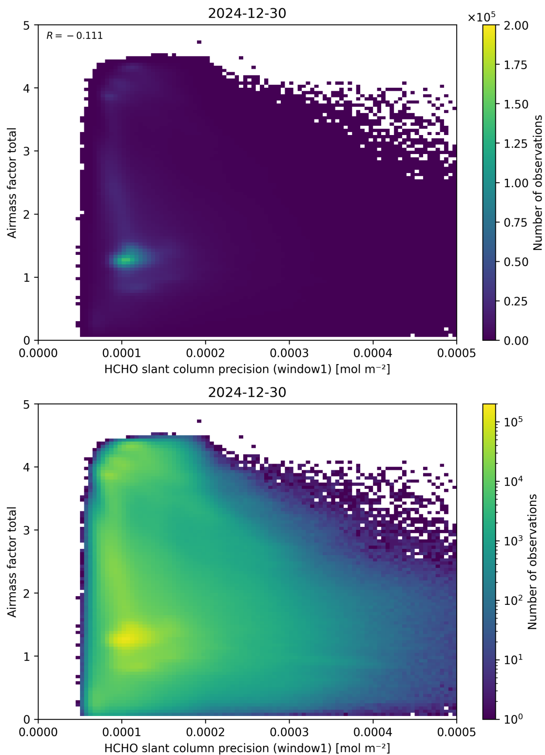
Figure 94: Scatter density plot of “HCHO slant column precision (window1)” against “Airmass factor total” for 2024-12-29 to 2024-12-31.
