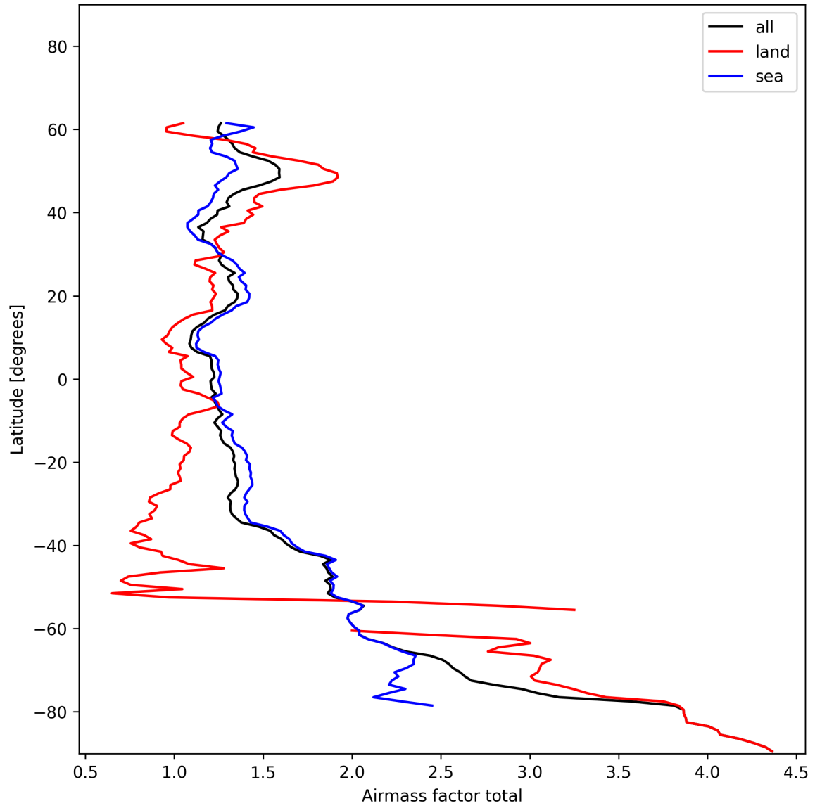
Figure 26: Zonal average of “Airmass factor total” for 2024-12-29 to 2024-12-31.
