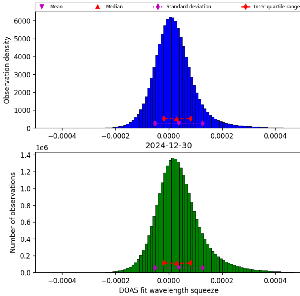
Figure 45: Histogram of “DOAS fit wavelength squeeze” for 2024-12-29 to 2024-12-31
