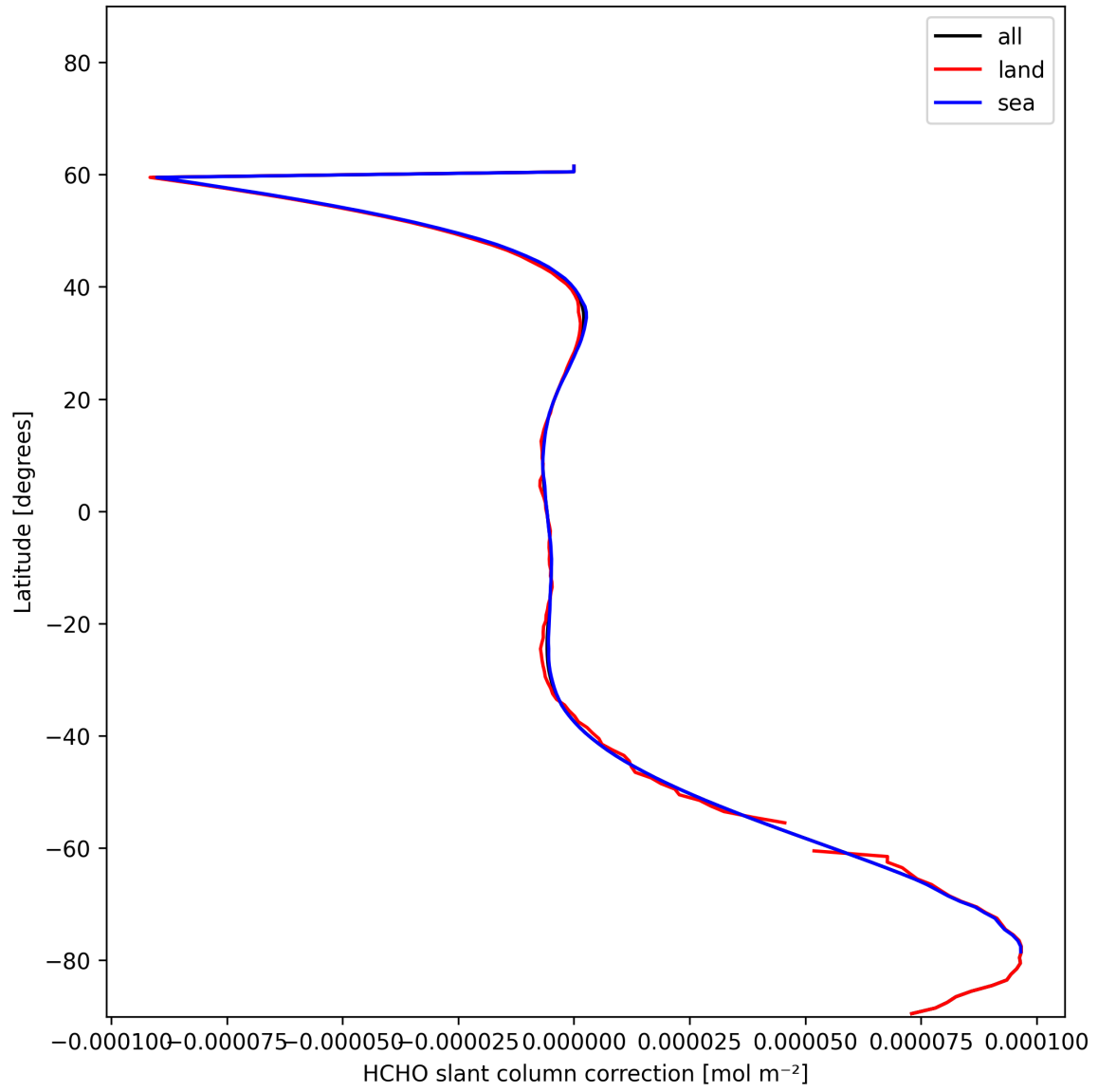
Figure 33: Zonal average of “HCHO slant column correction” for 2024-12-29 to 2024-12-31.
