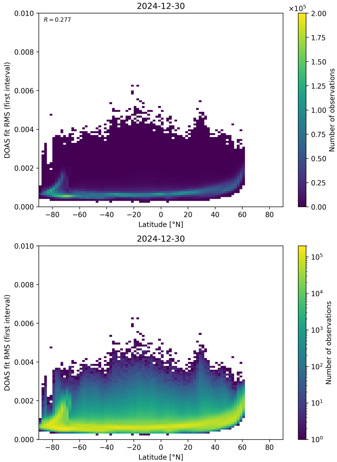
Figure 153: Scatter density plot of “Latitude” against “DOAS fit RMS (first interval)” for 2024-12-29 to 2024-12-31.
