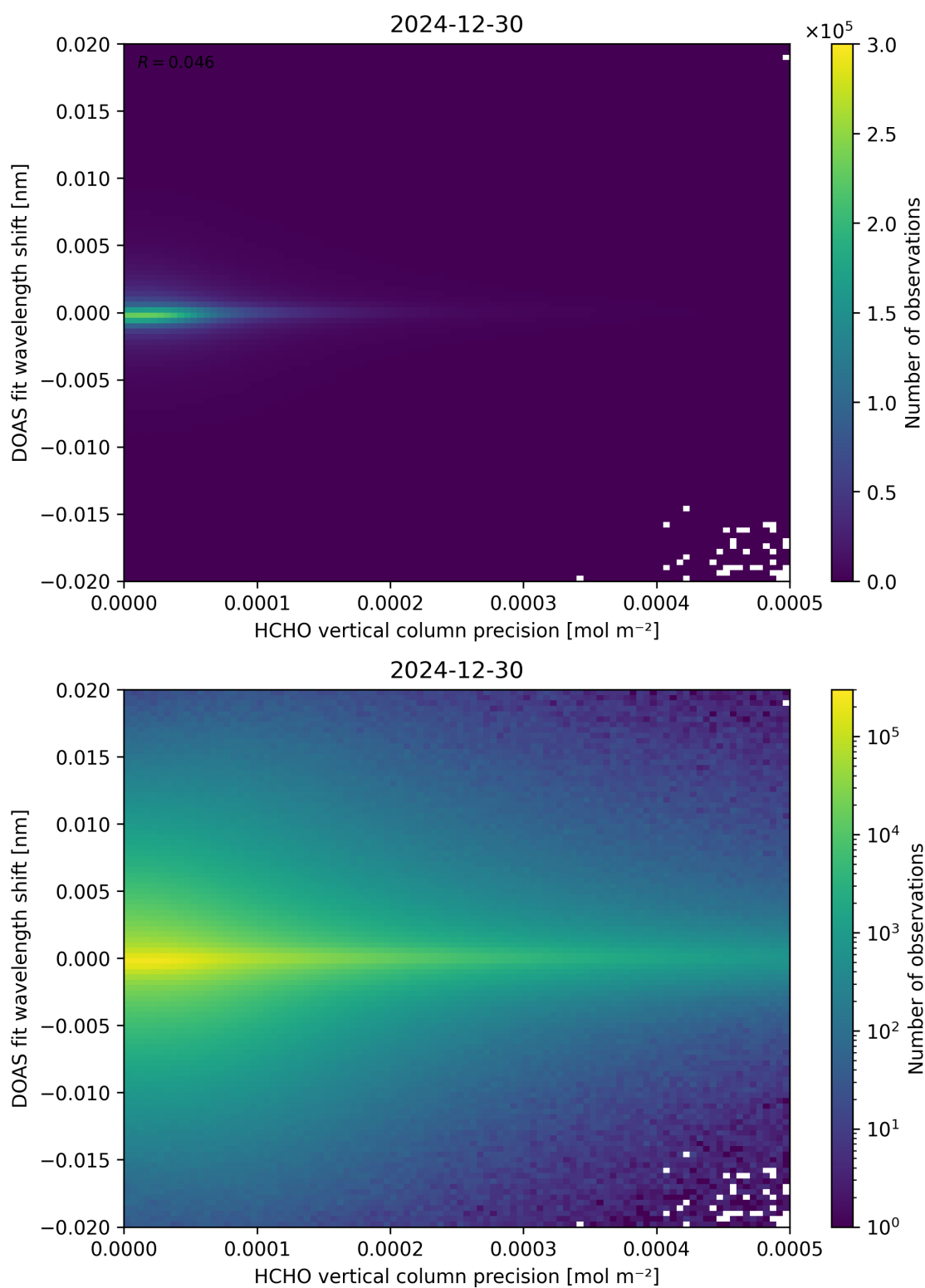
Figure 137: Scatter density plot of “HCHO vertical column precision” against “DOAS fit wavelength shift” for 2024-12-29 to 2024-12-31.
