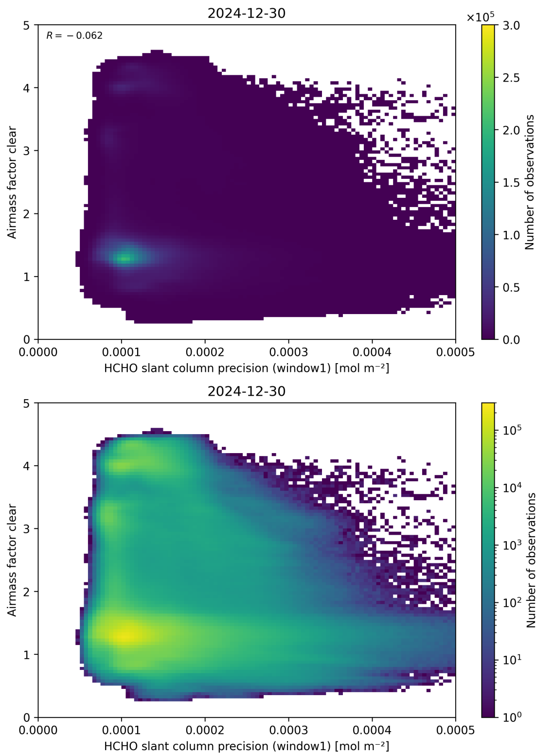
Figure 91: Scatter density plot of “HCHO slant column precision (window1)” against “Airmass factor clear” for 2024-12-29 to 2024-12-31.
