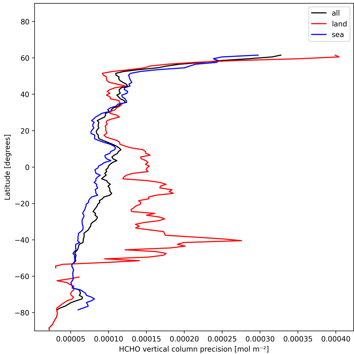
Figure 22: Zonal average of “HCHO vertical column precision” for 2024-12-29 to 2024-12-31.
