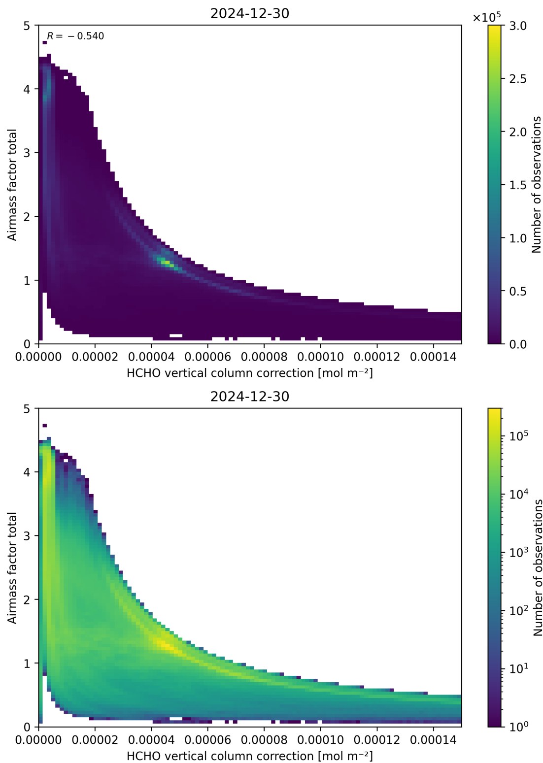
Figure 120: Scatter density plot of “HCHO vertical column correction” against “Airmass factor total” for 2024-12-29 to 2024-12-31.
