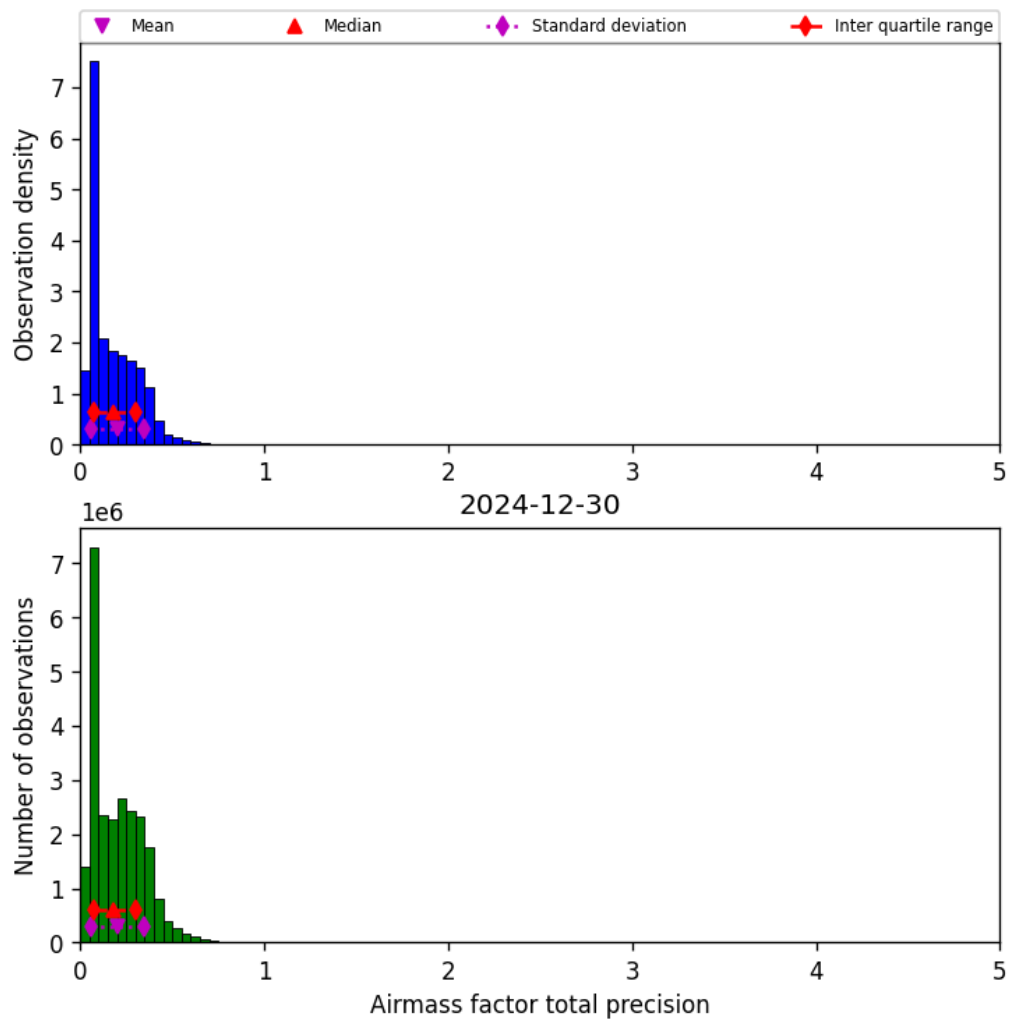
Figure 41: Histogram of “Airmass factor total precision” for 2024-12-29 to 2024-12-31
