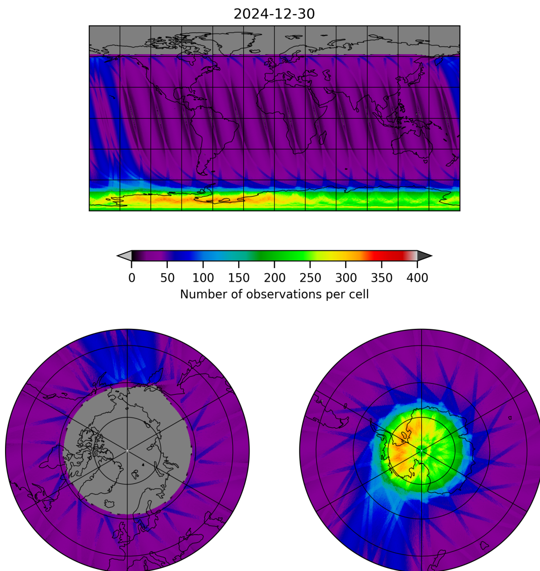
Figure 19: Map of the number of observations for 2024-12-29 to 2024-12-31
