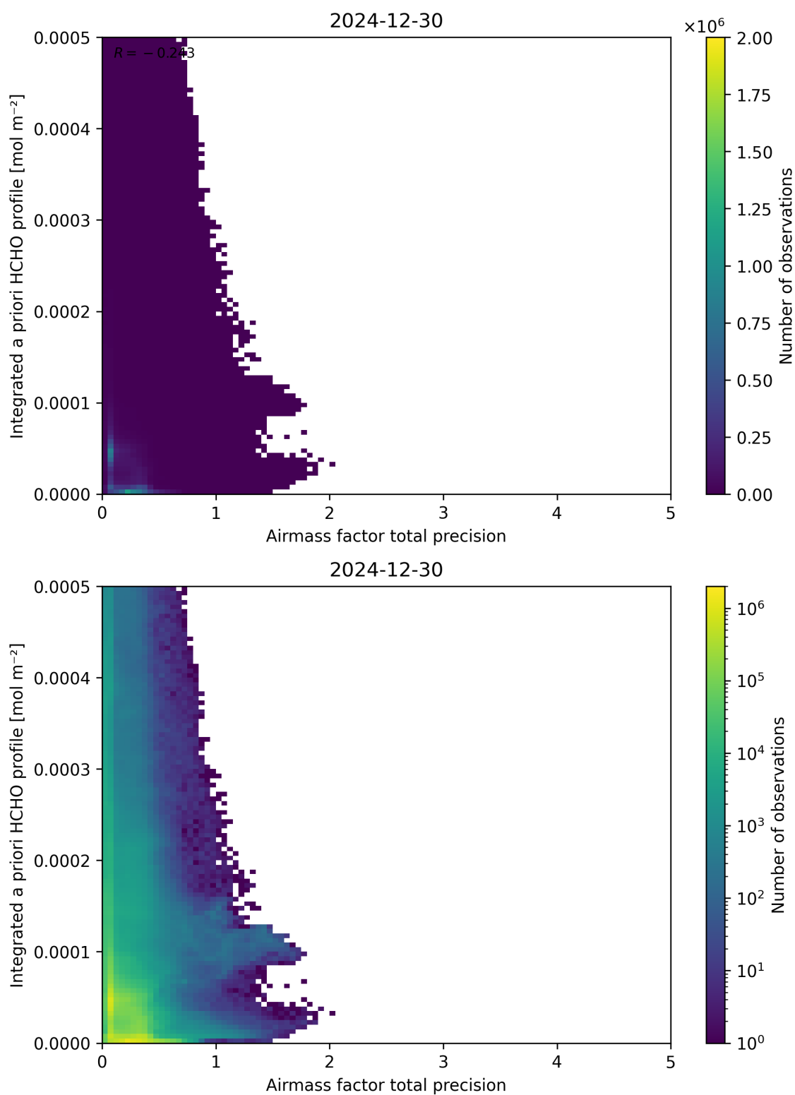
Figure 111: Scatter density plot of “Airmass factor total precision” against “Integrated a priori HCHO profile” for 2024-12-29 to 2024-12-31.
