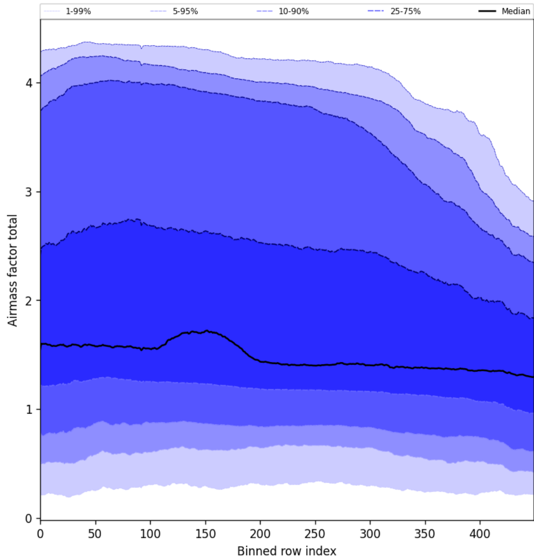
Figure 54: Along track statistics of “Airmass factor total” for 2024-12-29 to 2024-12-31
