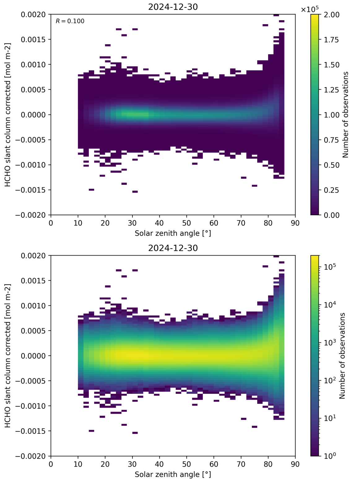
Figure 171: Scatter density plot of “Solar zenith angle” against “HCHO slant column corrected” for 2024-12-29 to 2024-12-31.
