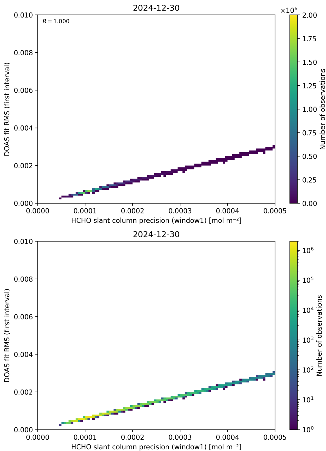
Figure 88: Scatter density plot of “HCHO slant column precision (window1)” against “DOAS fit RMS (first interval)” for 2024-12-29 to 2024-12-31.
