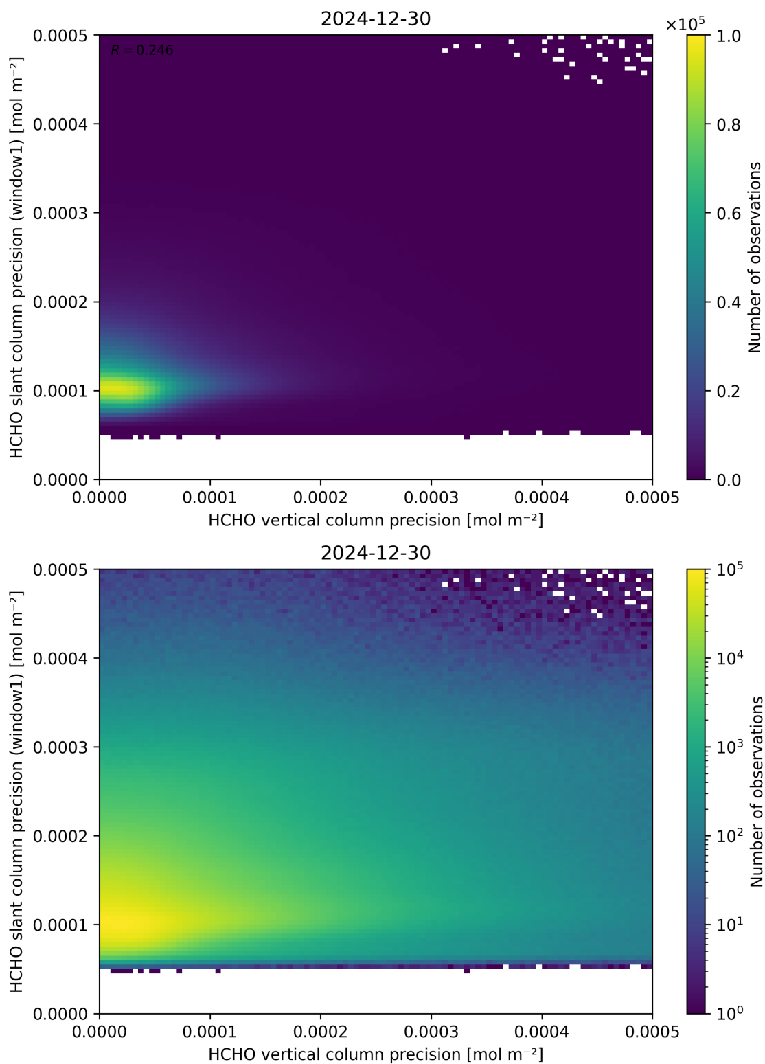
Figure 143: Scatter density plot of “HCHO vertical column precision” against “HCHO slant column precision (window1)” for 2024-12-29 to 2024-12-31.
