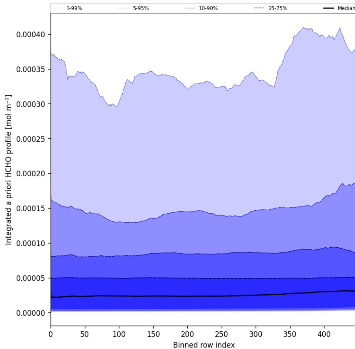
Figure 57: Along track statistics of "Integrated a priori HCHO profile" for 2024-12-29 to 2024-12-31
