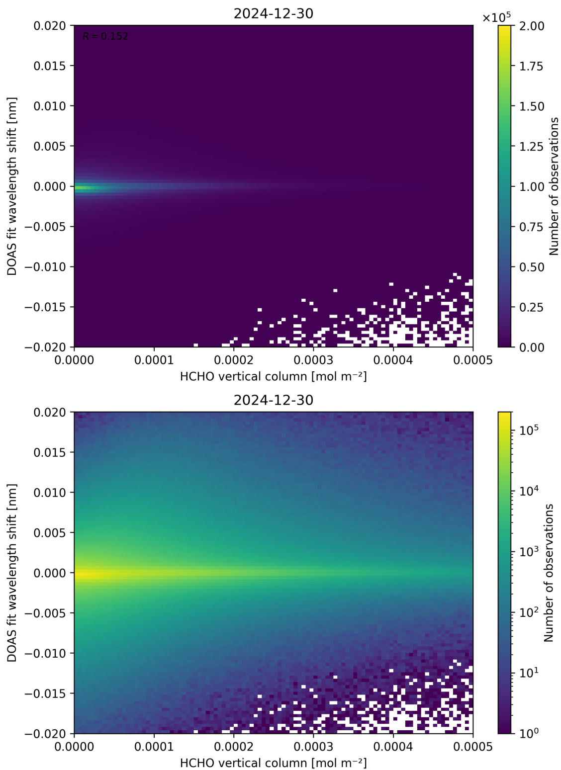
Figure 124: Scatter density plot of “HCHO vertical column” against “DOAS fit wavelength shift” for 2024-12-29 to 2024-12-31.
