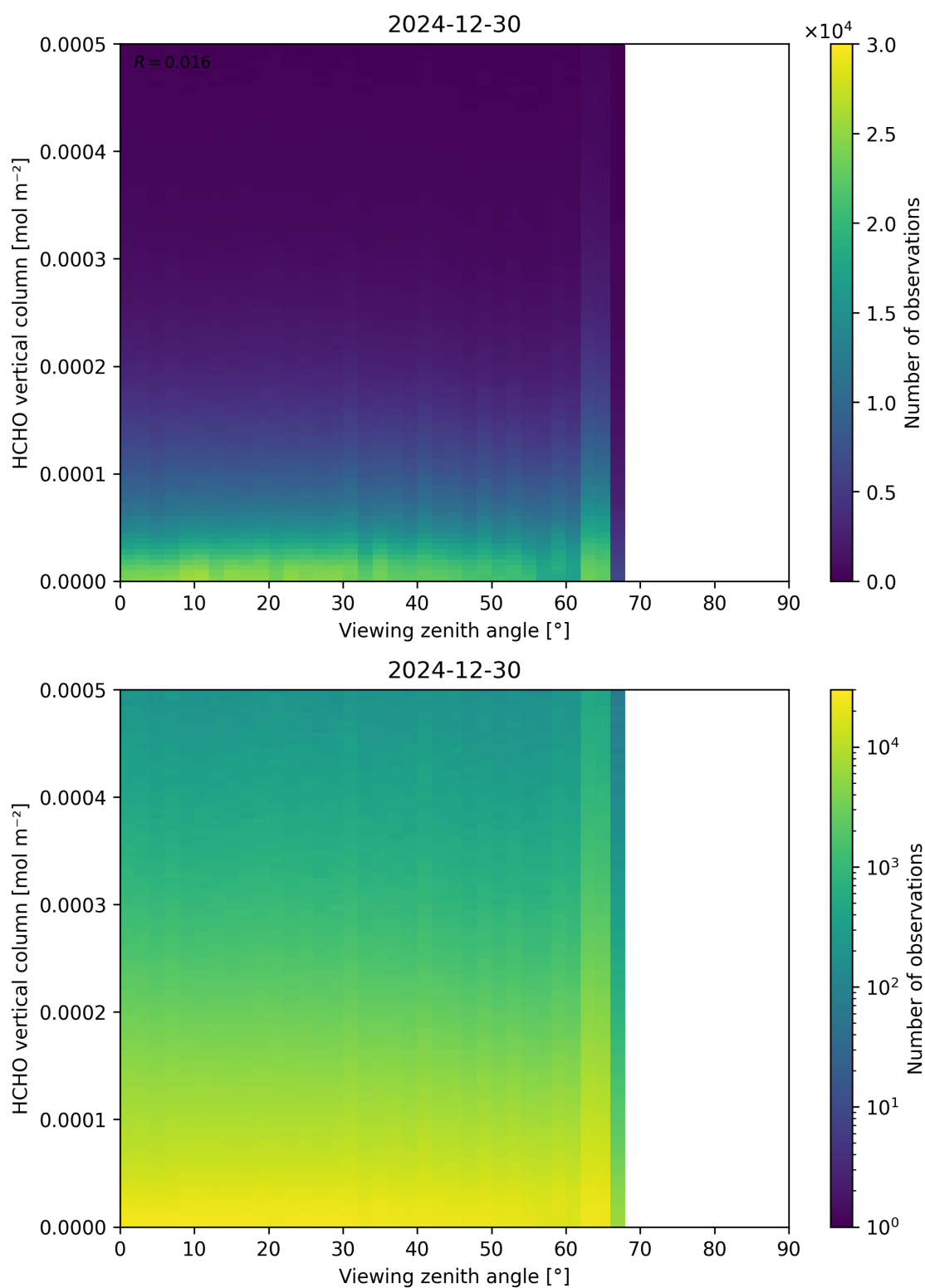
Figure 192: Scatter density plot of “Viewing zenith angle” against “HCHO vertical column” for 2024-12-29 to 2024-12-31.
