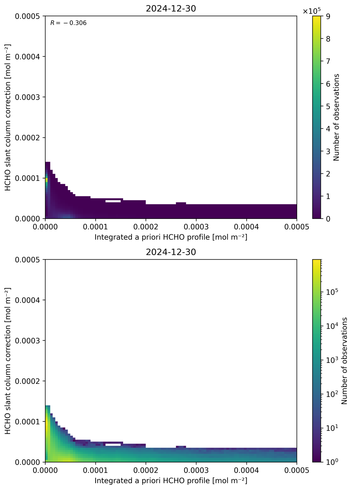
Figure 152: Scatter density plot of “Integrated a priori HCHO profile” against “HCHO slant column correction” for 2024-12-29 to 2024-12-31.
