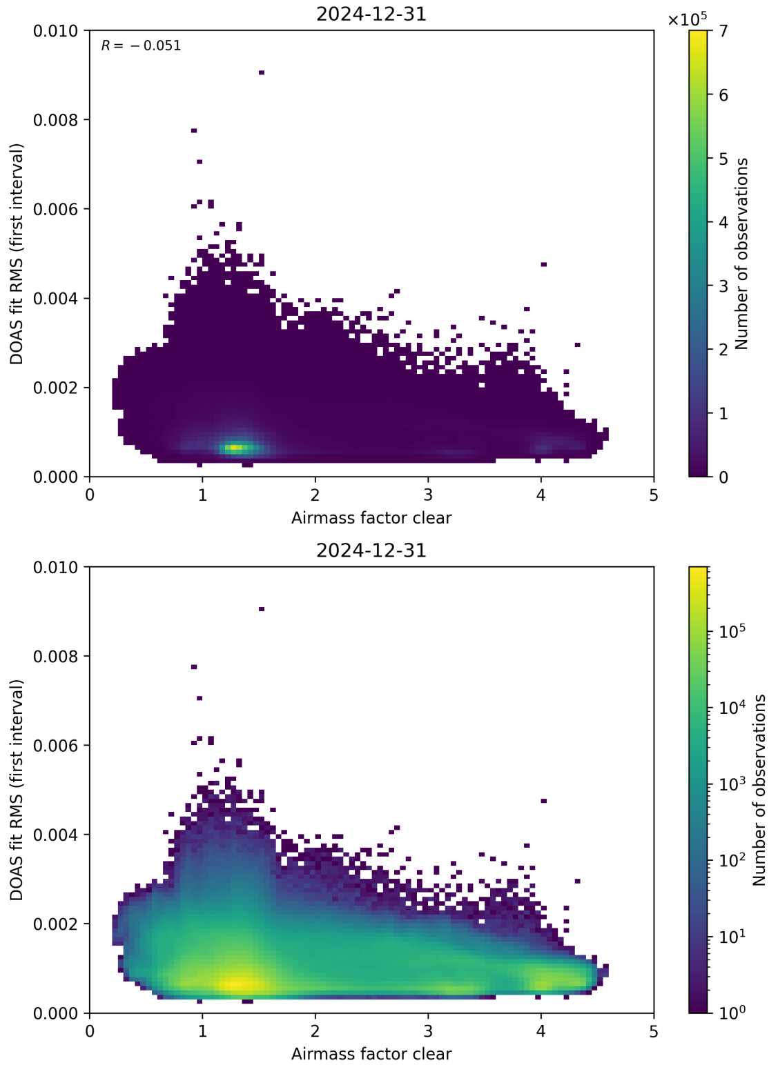
Figure 71: Scatter density plot of “Airmass factor clear” against “DOAS fit RMS (first interval)” for 2024-12-30 to 2025-01-01.
