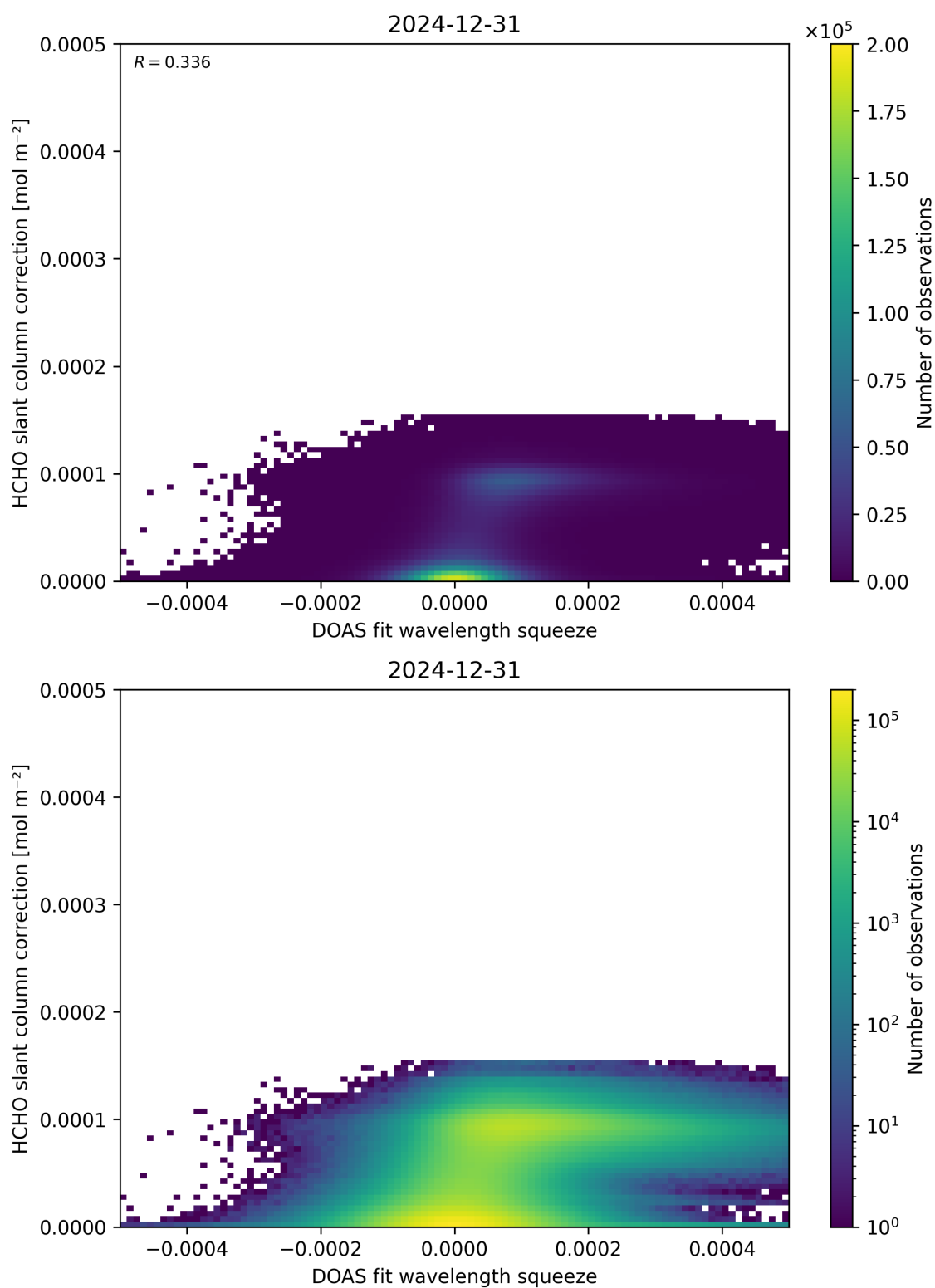
Figure 70: Scatter density plot of “DOAS fit wavelength squeeze” against “HCHO slant column correction” for 2024-12-30 to 2025-01-01.
