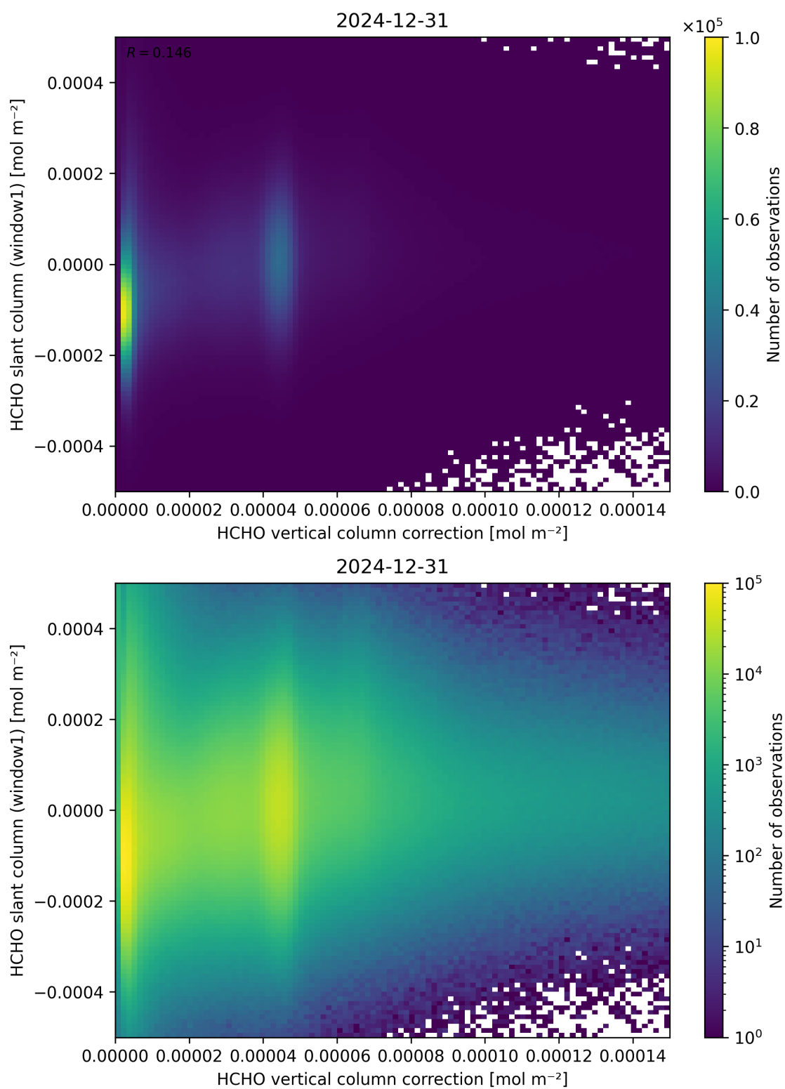
Figure 118: Scatter density plot of “HCHO vertical column correction” against “HCHO slant column (window1)” for 2024-12-30 to 2025-01-01.
