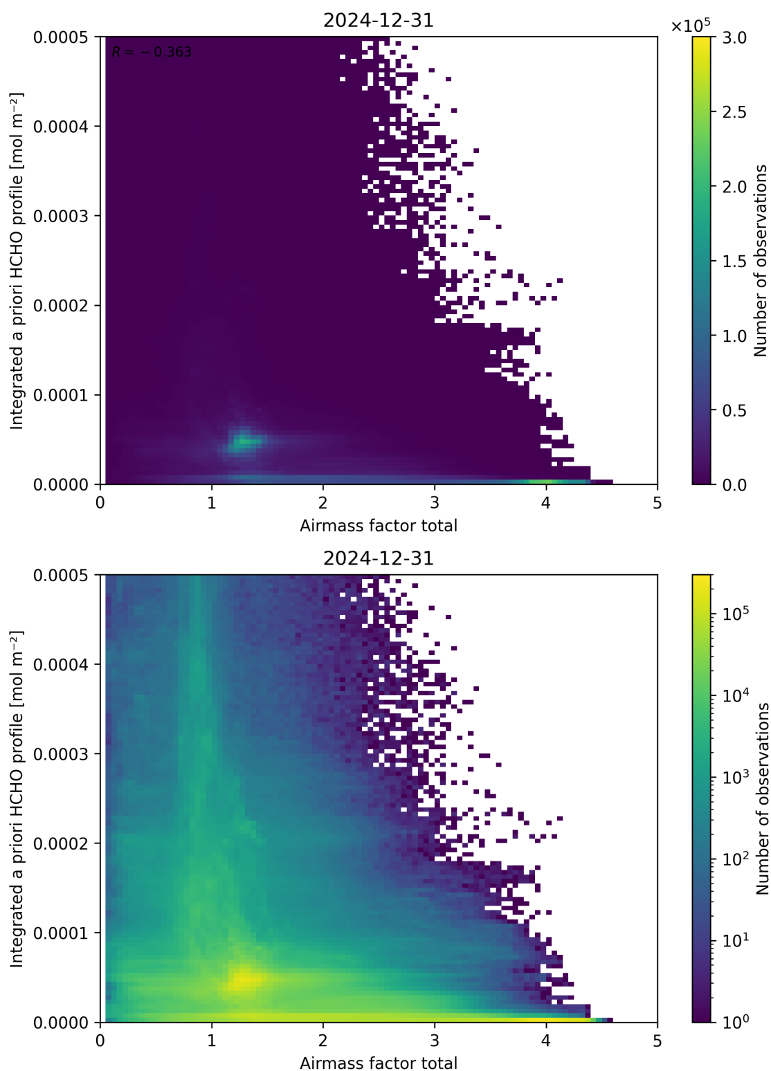
Figure 104: Scatter density plot of “Airmass factor total” against “Integrated a priori HCHO profile” for 2024-12-30 to 2025-01-01.
