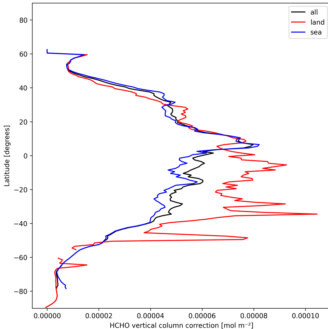
Figure 23: Zonal average of “HCHO vertical column correction” for 2024-12-30 to 2025-01-01.
