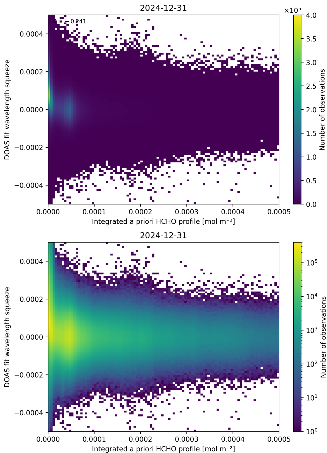
Figure 150: Scatter density plot of “Integrated a priori HCHO profile” against “DOAS fit wavelength squeeze” for 2024-12-30 to 2025-01-01.
