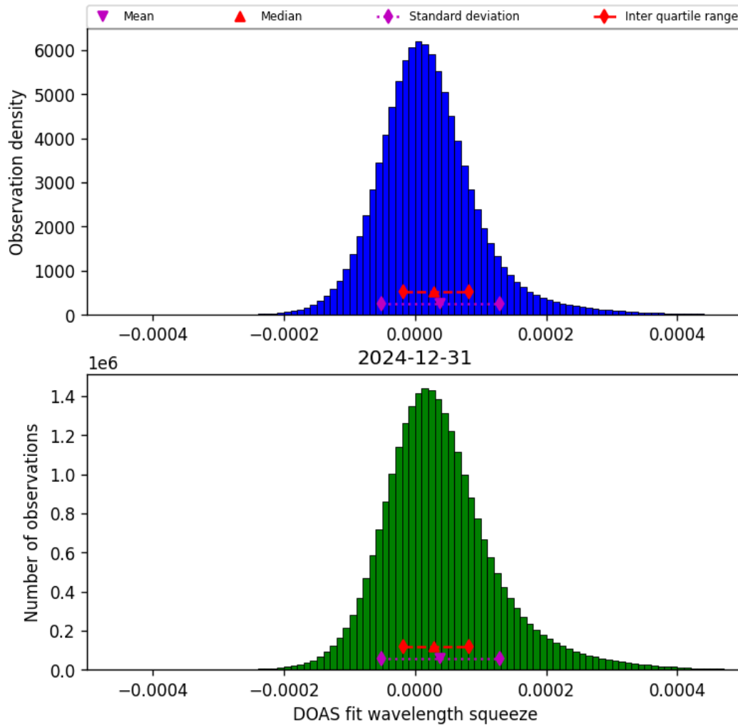
Figure 45: Histogram of “DOAS fit wavelength squeeze” for 2024-12-30 to 2025-01-01
