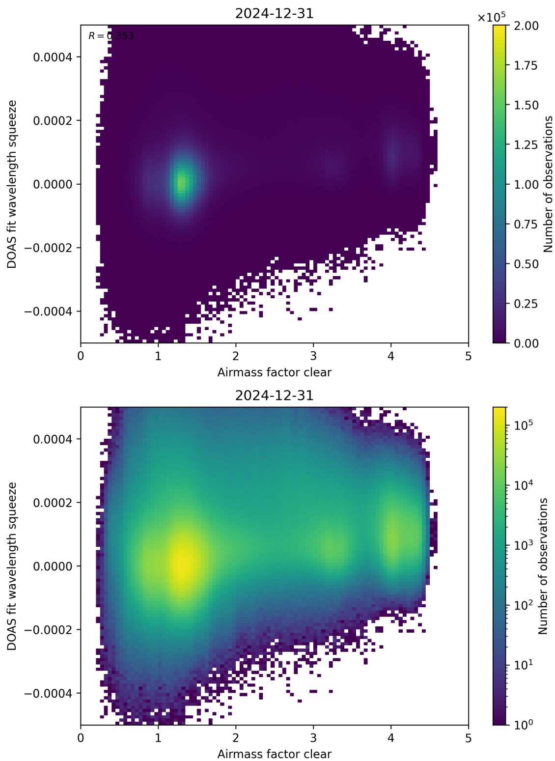
Figure 73: Scatter density plot of “Airmass factor clear” against “DOAS fit wavelength squeeze” for 2024-12-30 to 2025-01-01.
