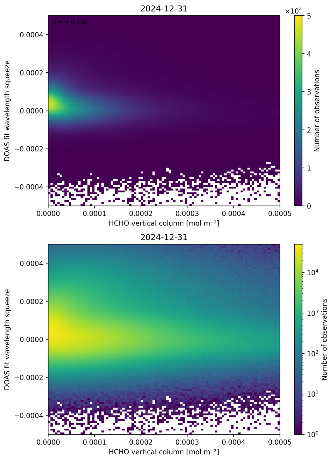
Figure 125: Scatter density plot of “HCHO vertical column” against “DOAS fit wavelength squeeze” for 2024-12-30 to 2025-01-01.
