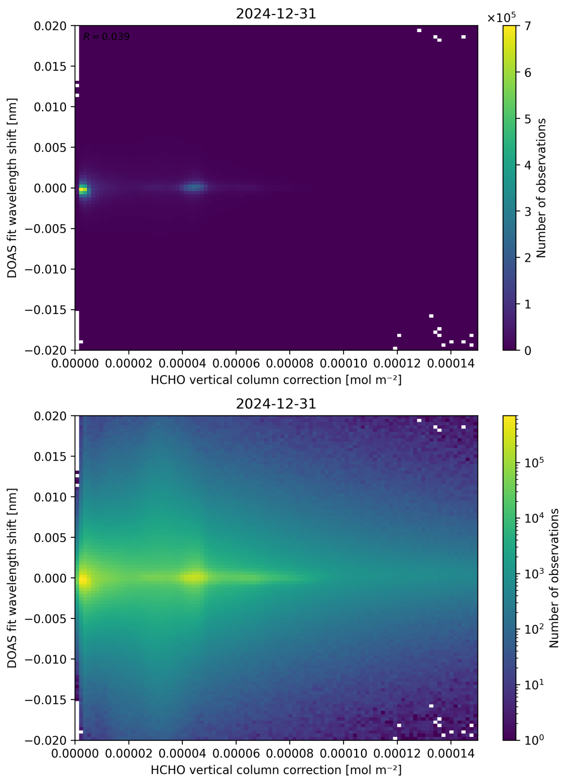
Figure 113: Scatter density plot of “HCHO vertical column correction” against “DOAS fit wavelength shift” for 2024-12-30 to 2025-01-01.
