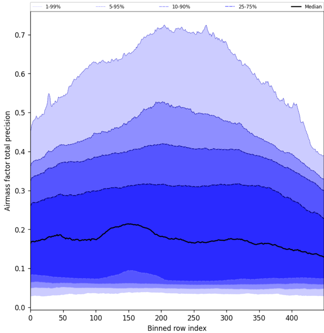
Figure 55: Along track statistics of “Airmass factor total precision” for 2024-12-30 to 2025-01-01
