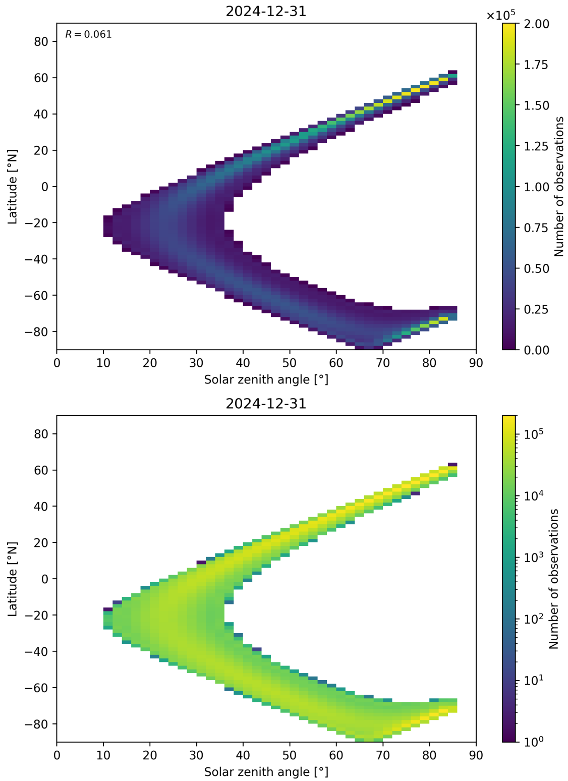
Figure 181: Scatter density plot of “Solar zenith angle” against “Latitude” for 2024-12-30 to 2025-01-01.
