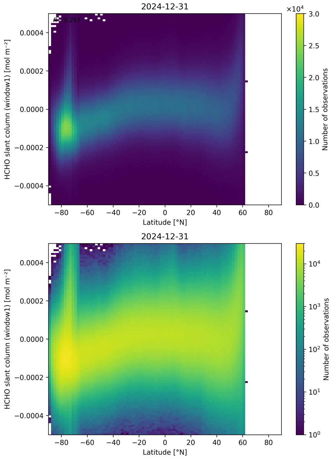
Figure 159: Scatter density plot of “Latitude” against “HCHO slant column (window1)” for 2024-12-30 to 2025-01-01.
