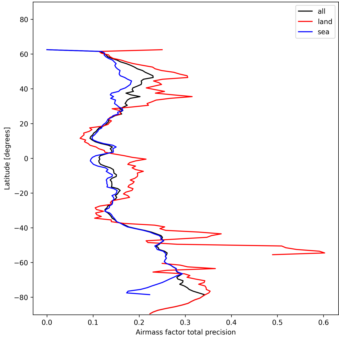
Figure 27: Zonal average of “Airmass factor total precision” for 2024-12-30 to 2025-01-01.
