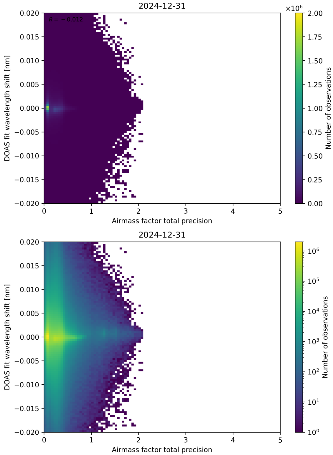
Figure 106: Scatter density plot of “Airmass factor total precision” against “DOAS fit wavelength shift” for 2024-12-30 to 2025-01-01.
