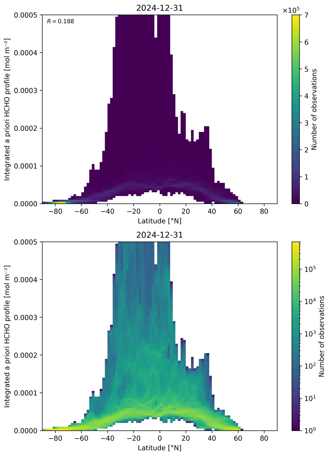
Figure 166: Scatter density plot of “Latitude” against “Integrated a priori HCHO profile” for 2024-12-30 to 2025-01-01.
