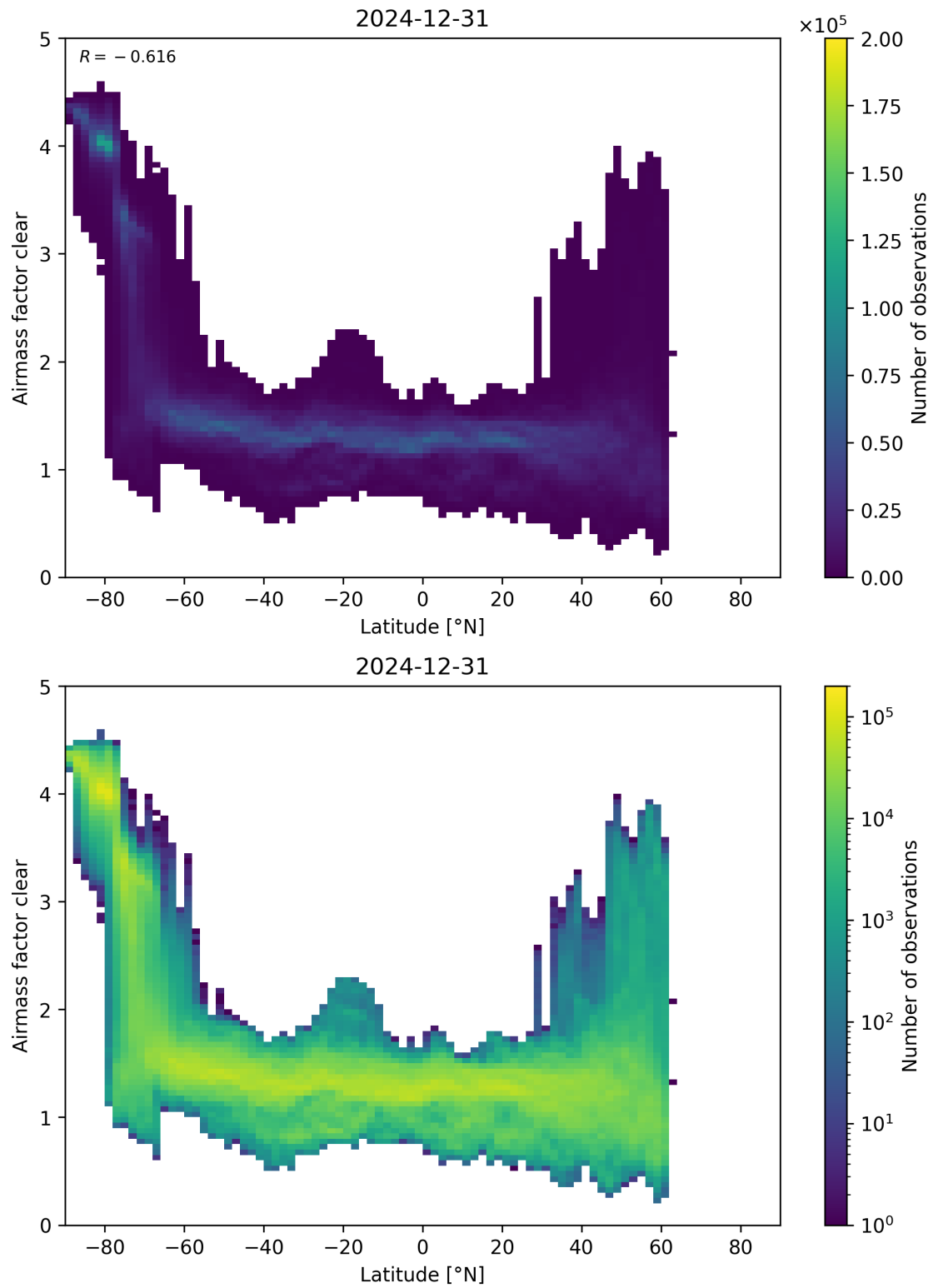
Figure 156: Scatter density plot of “Latitude” against “Airmass factor clear” for 2024-12-30 to 2025-01-01.
