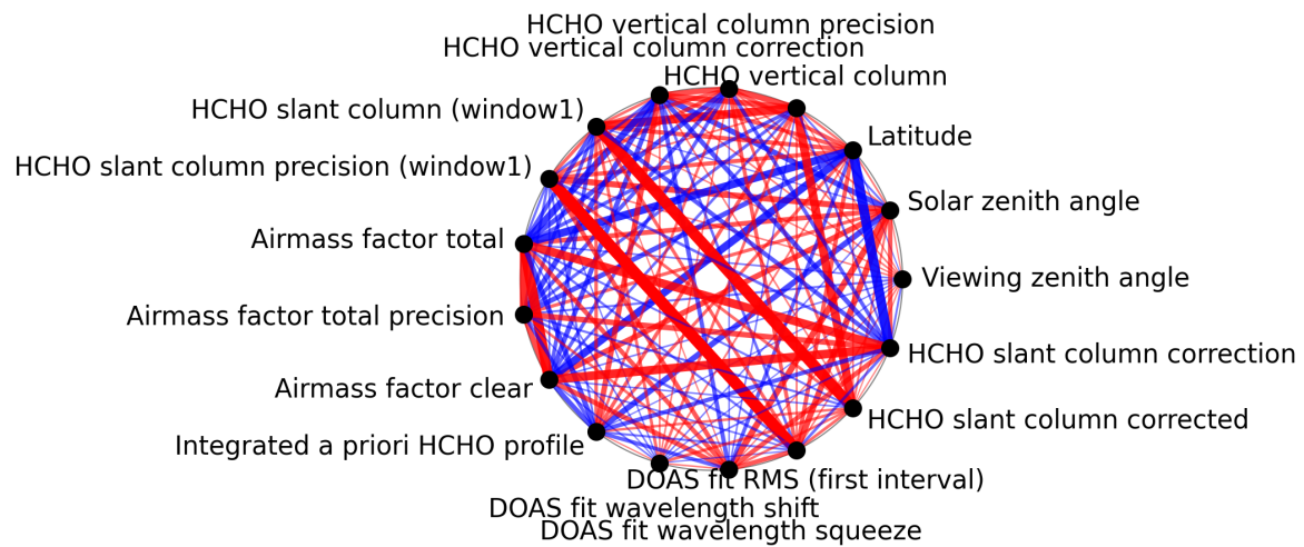
Figure 1: Map of correlation graph for 2024-12-30 to 2025-01-01.
