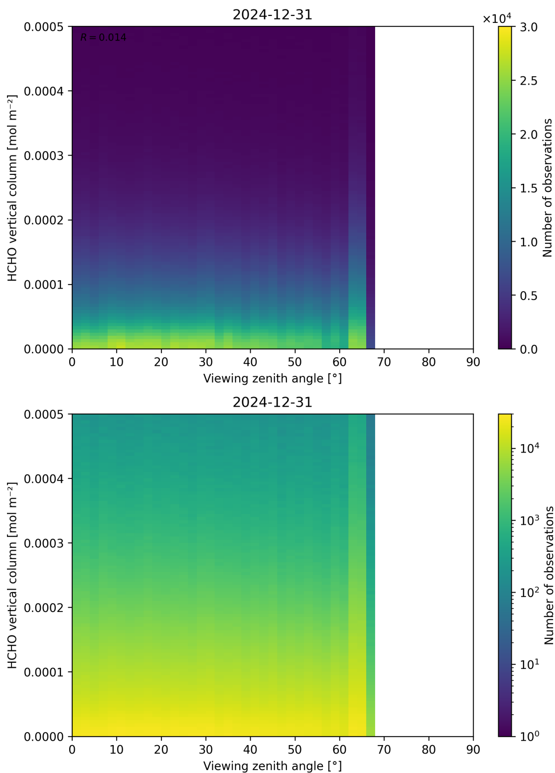
Figure 192: Scatter density plot of “Viewing zenith angle” against “HCHO vertical column” for 2024-12-30 to 2025-01-01.
