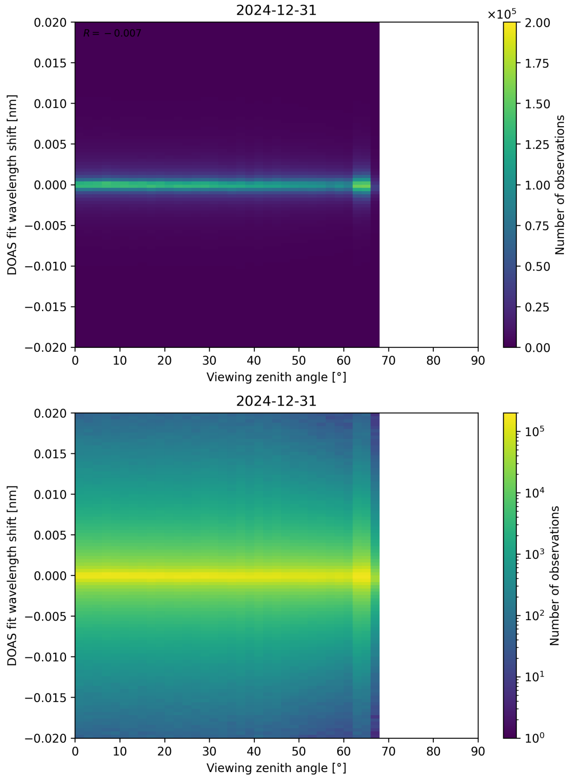
Figure 183: Scatter density plot of “Viewing zenith angle” against “DOAS fit wavelength shift” for 2024-12-30 to 2025-01-01.
