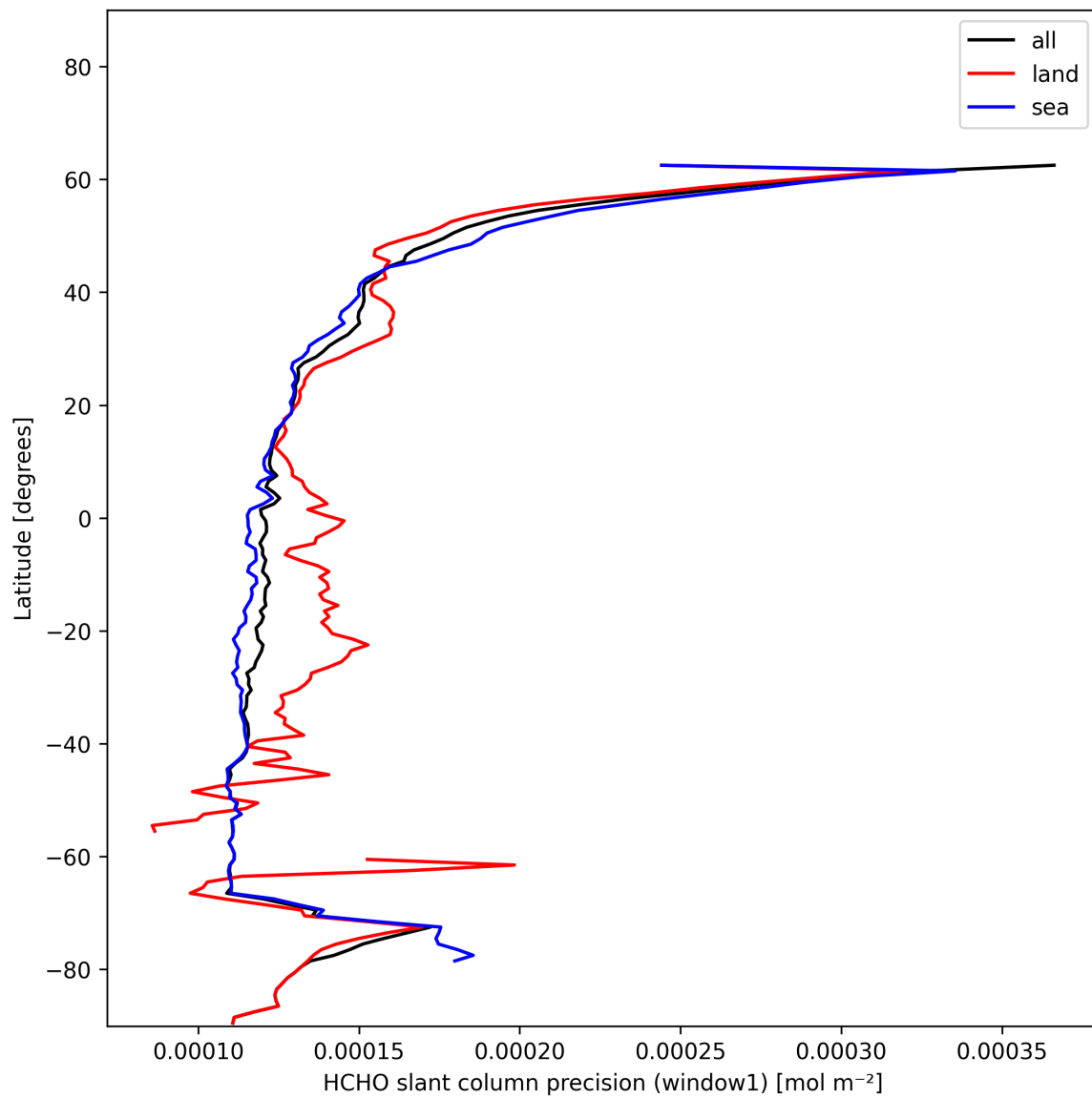
Figure 25: Zonal average of “HCHO slant column precision (window1)” for 2024-12-30 to 2025-01-01.
