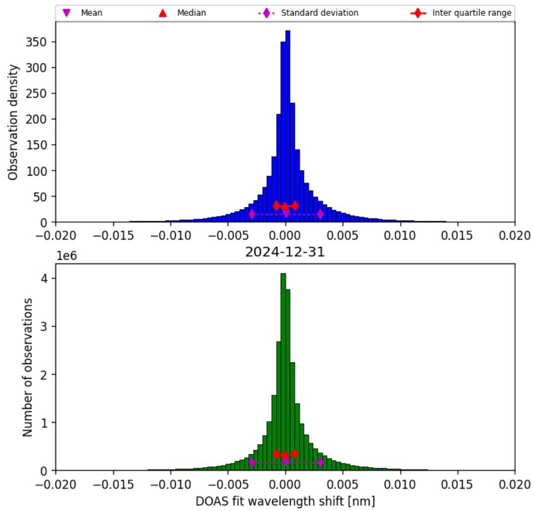
Figure 44: Histogram of “DOAS fit wavelength shift” for 2024-12-30 to 2025-01-01
