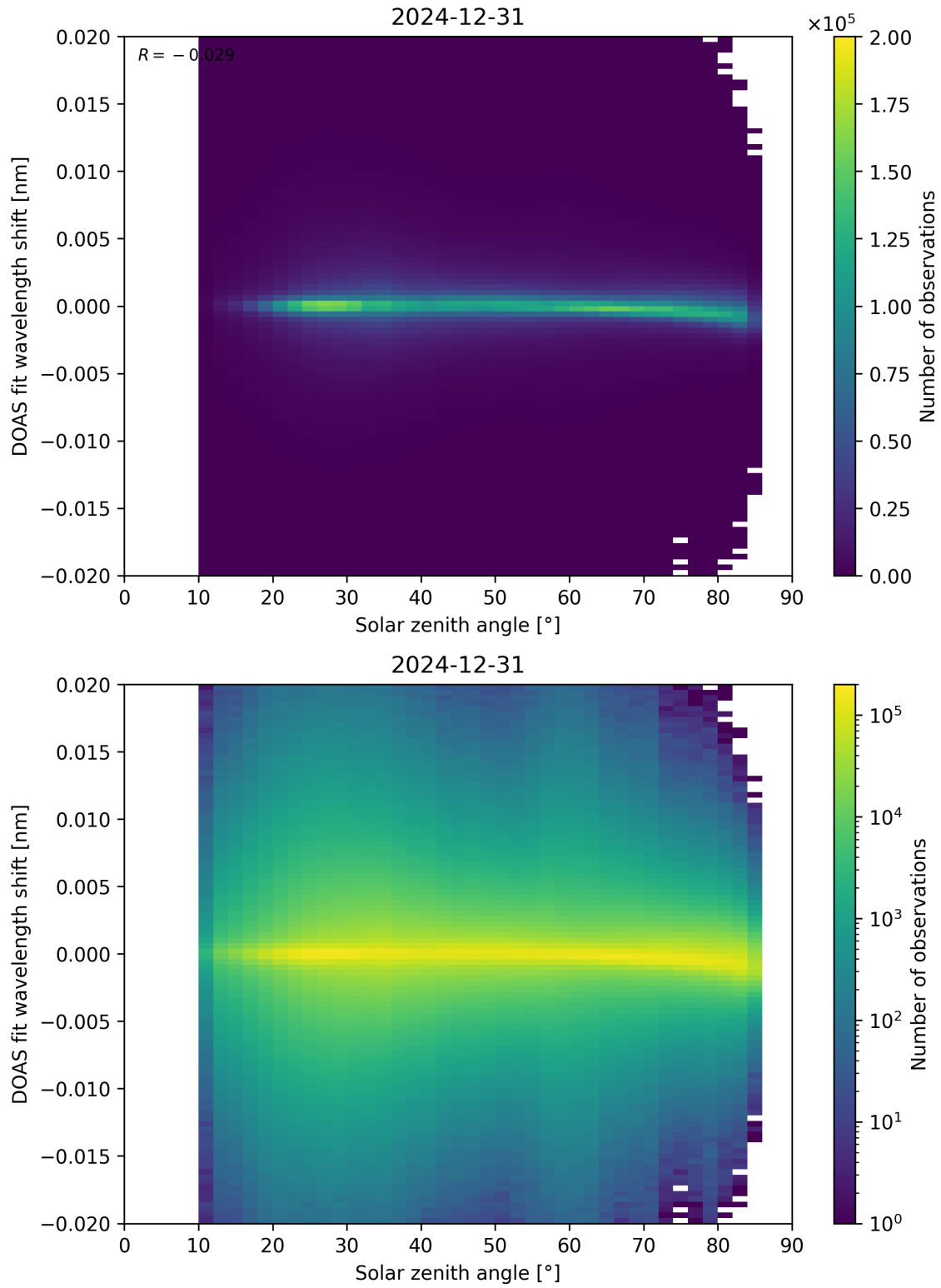
Figure 168: Scatter density plot of “Solar zenith angle” against “DOAS fit wavelength shift” for 2024-12-30 to 2025-01-01.
