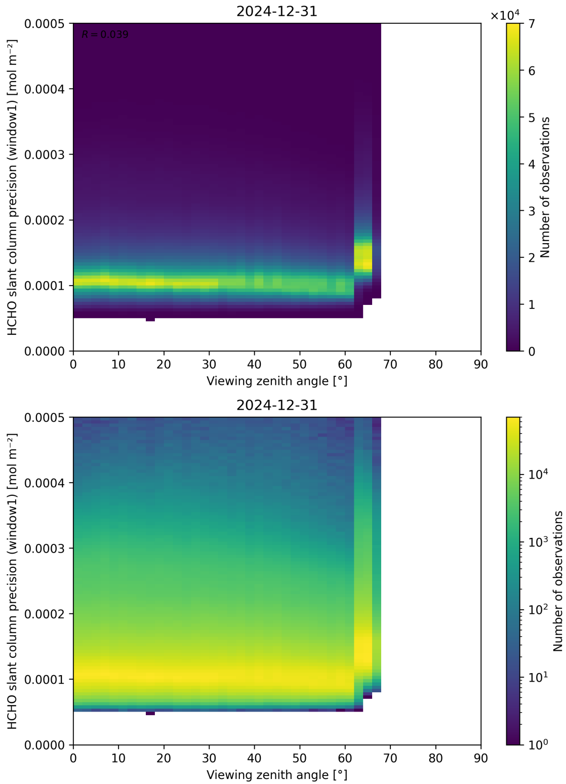
Figure 189: Scatter density plot of “Viewing zenith angle” against “HCHO slant column precision (window1)” for 2024-12-30 to 2025-01-01.
