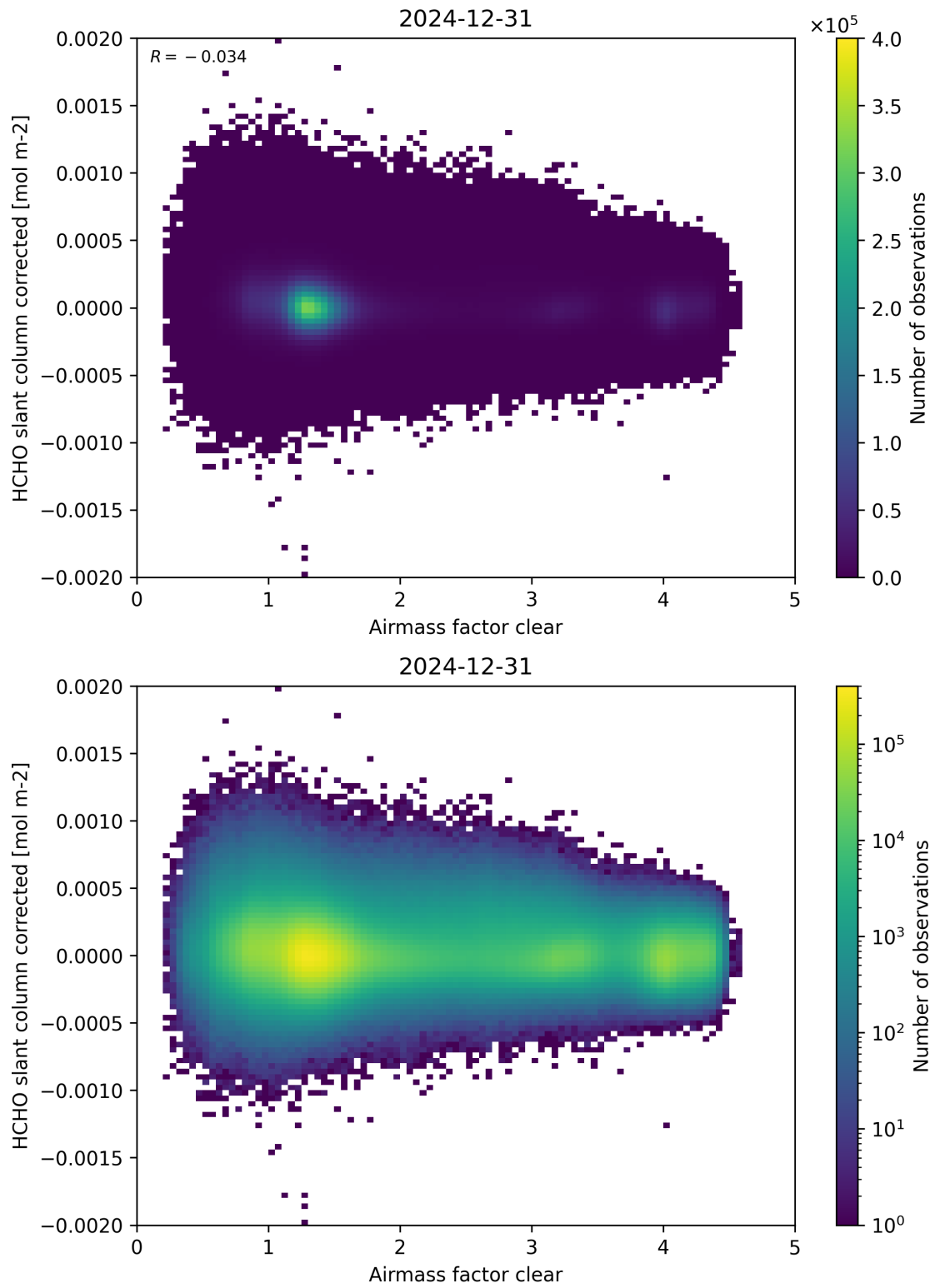
Figure 74: Scatter density plot of “Airmass factor clear” against “HCHO slant column corrected” for 2024-12-30 to 2025-01-01.
