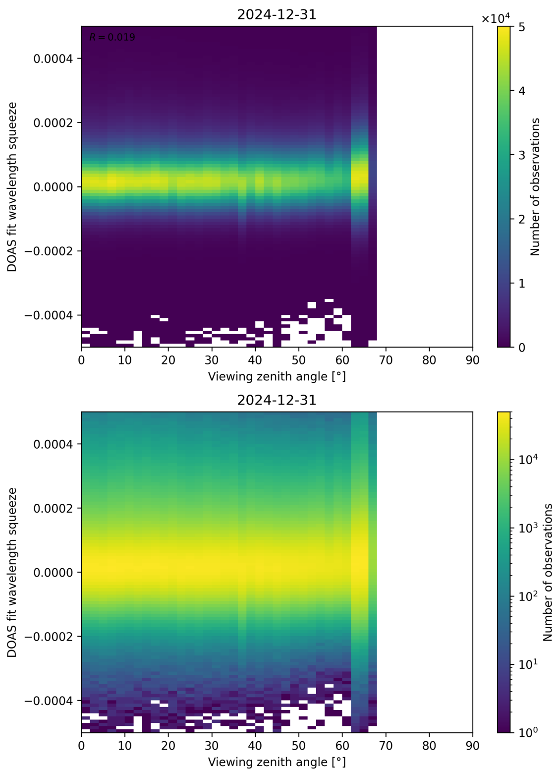
Figure 184: Scatter density plot of “Viewing zenith angle” against “DOAS fit wavelength squeeze” for 2024-12-30 to 2025-01-01.
