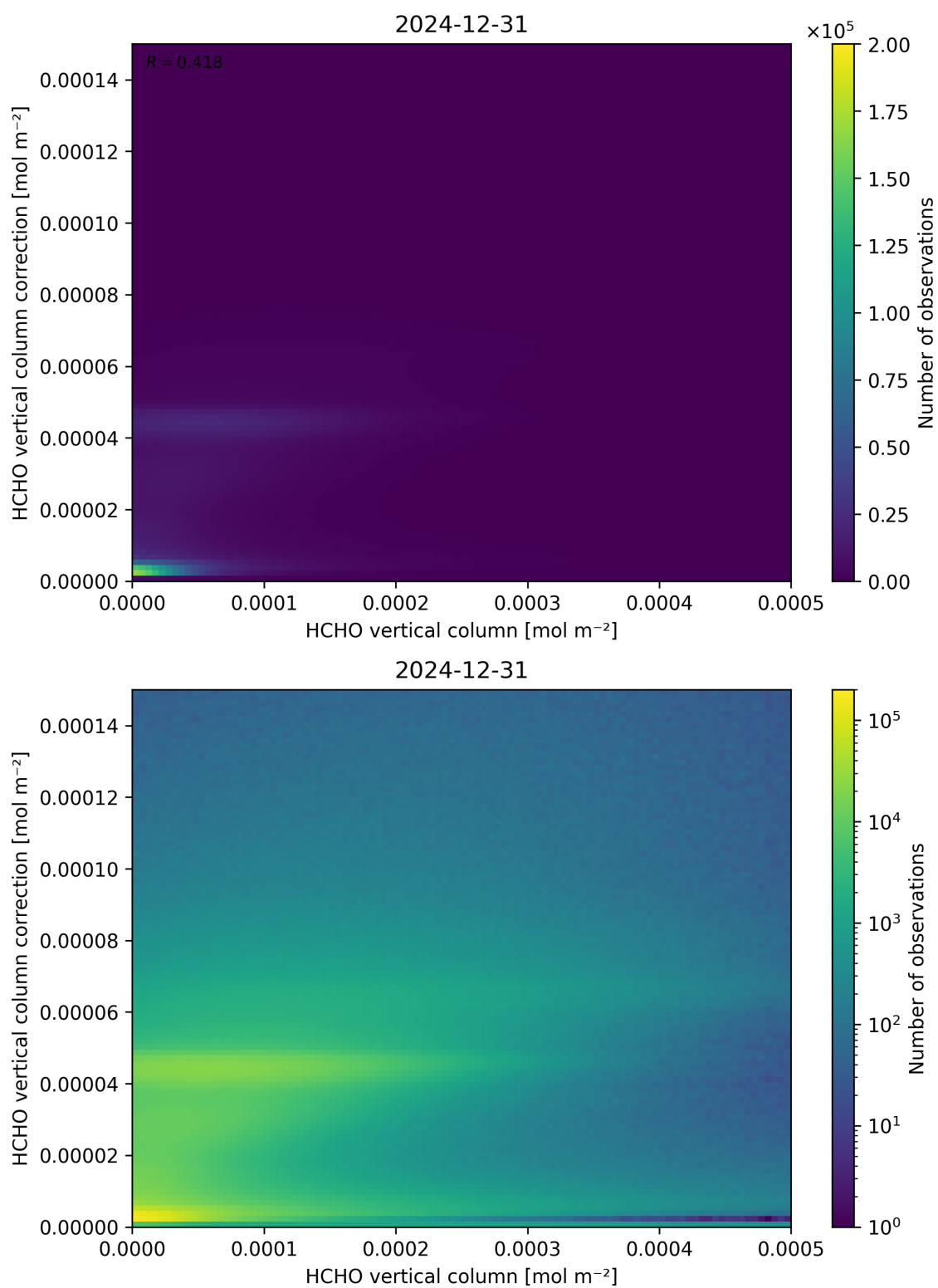
Figure 133: Scatter density plot of “HCHO vertical column” against “HCHO vertical column correction” for 2024-12-30 to 2025-01-01.
