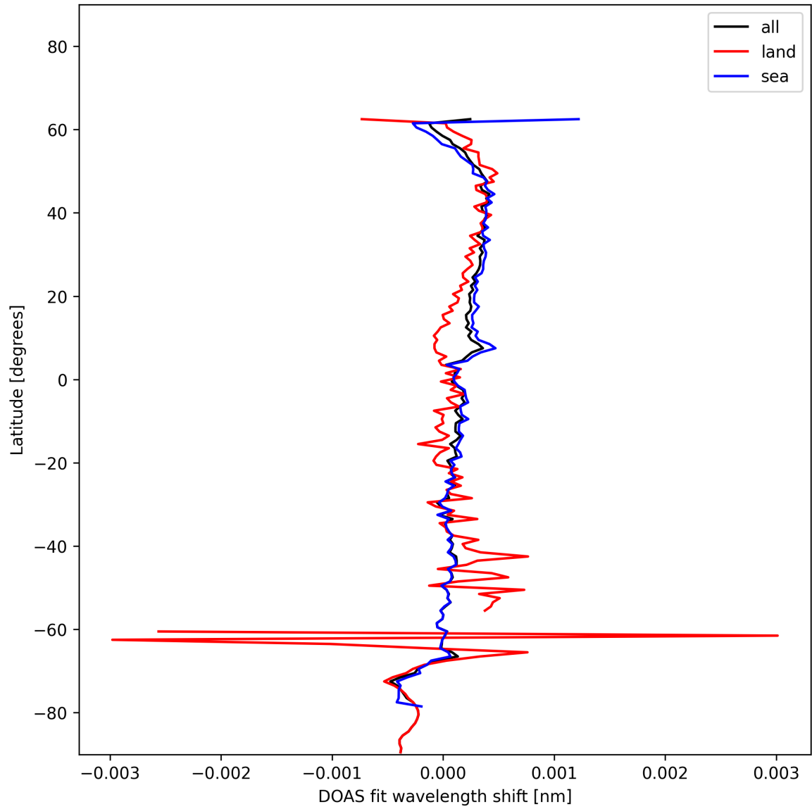
Figure 30: Zonal average of "DOAS fit wavelength shift" for 2024-12-30 to 2025-01-01.
