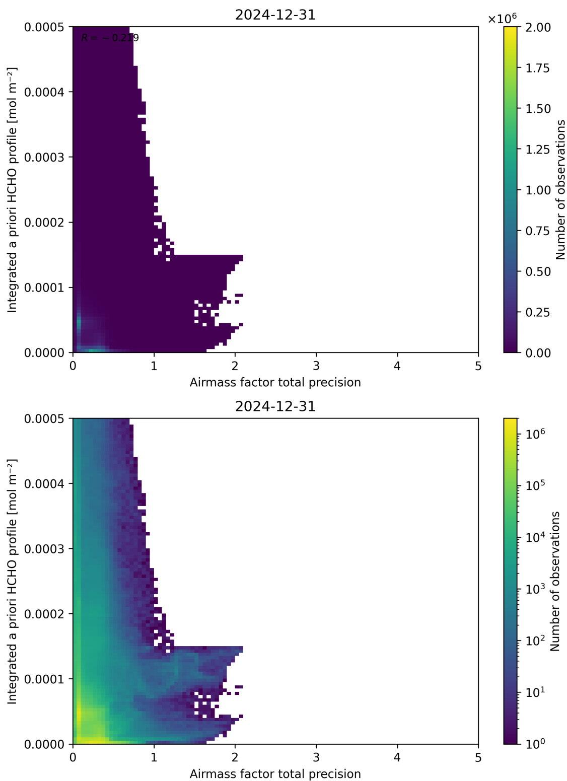
Figure 111: Scatter density plot of “Airmass factor total precision” against “Integrated a priori HCHO profile” for 2024-12-30 to 2025-01-01.
