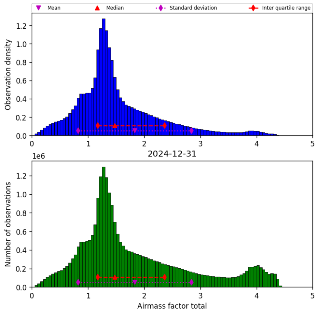
Figure 40: Histogram of “Airmass factor total” for 2024-12-30 to 2025-01-01
