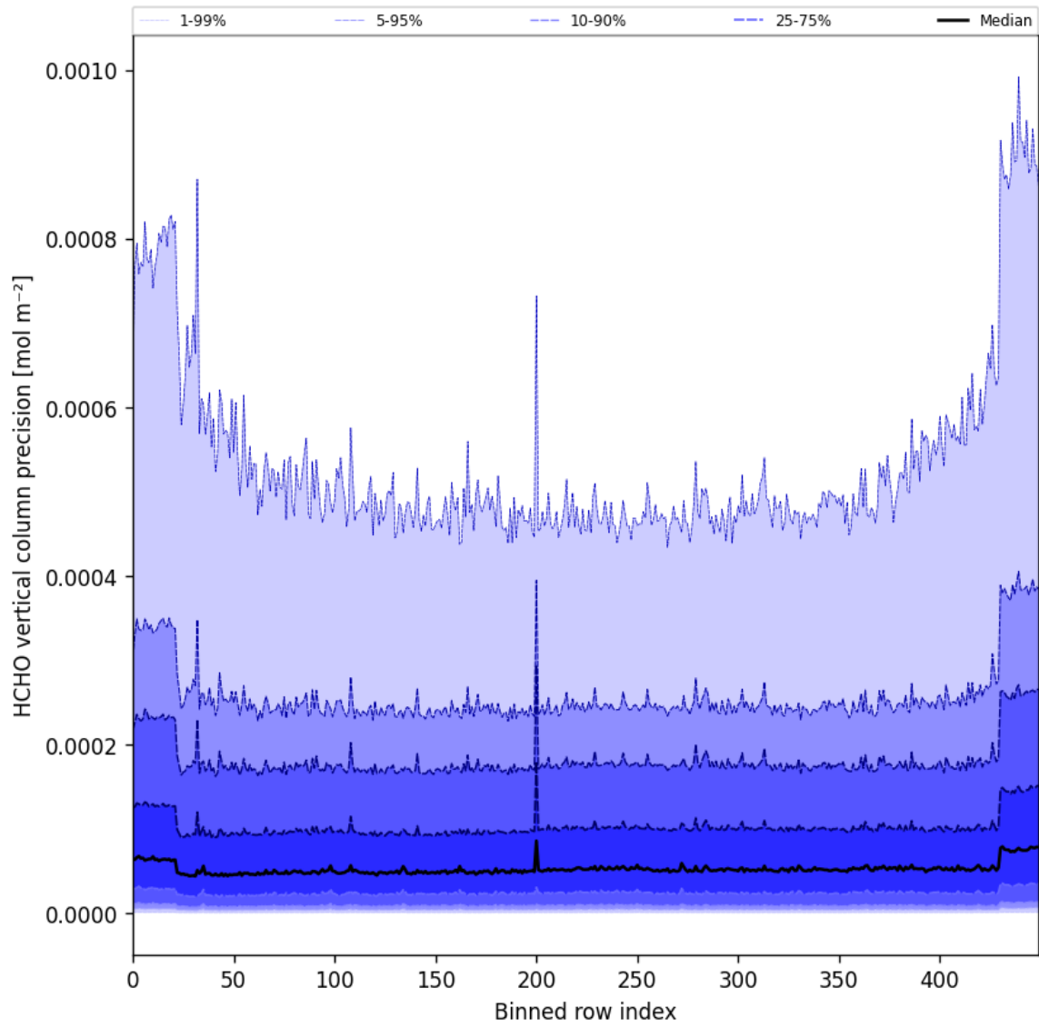
Figure 50: Along track statistics of “HCHO vertical column precision” for 2024-12-30 to 2025-01-01
