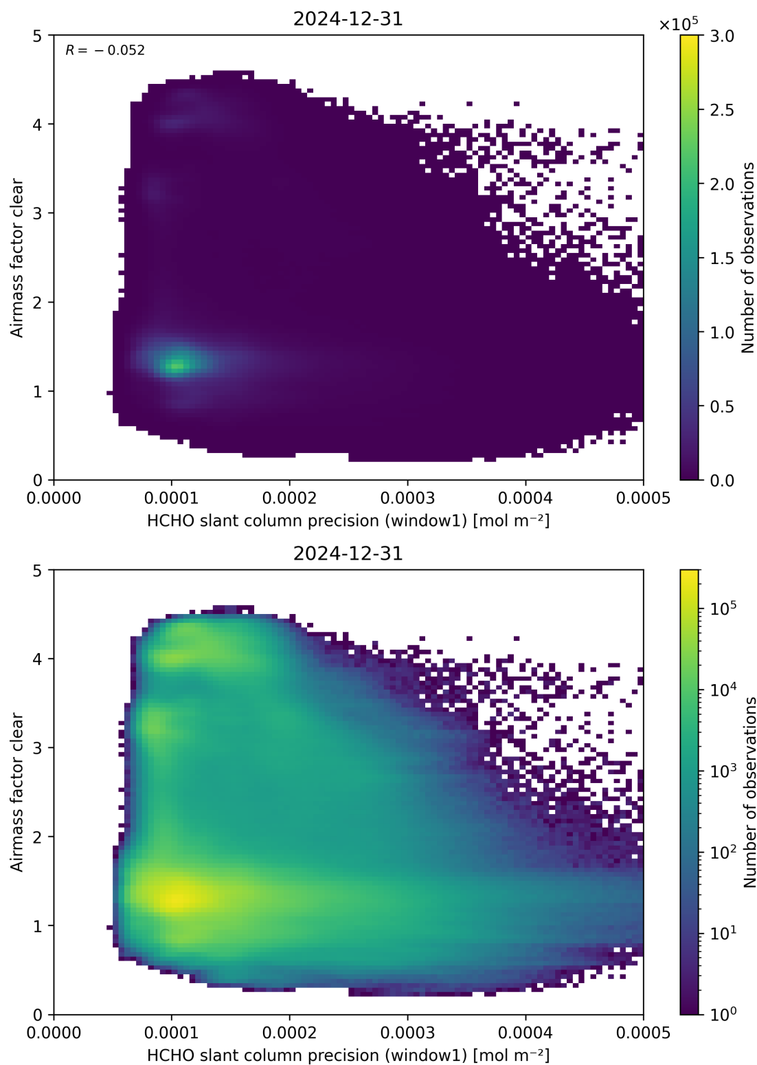
Figure 91: Scatter density plot of “HCHO slant column precision (window1)” against “Airmass factor clear” for 2024-12-30 to 2025-01-01.
