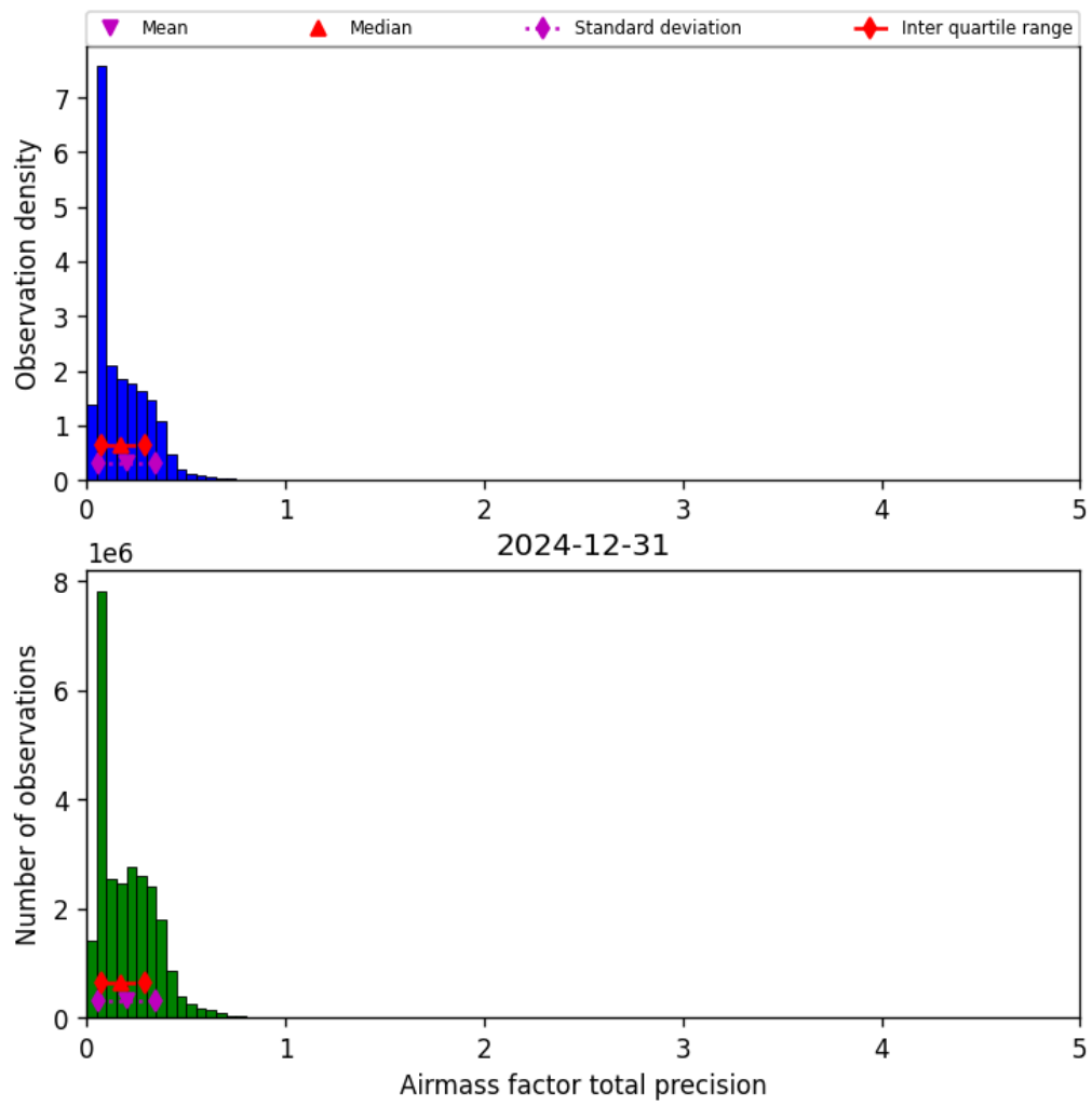
Figure 41: Histogram of “Airmass factor total precision” for 2024-12-30 to 2025-01-01
