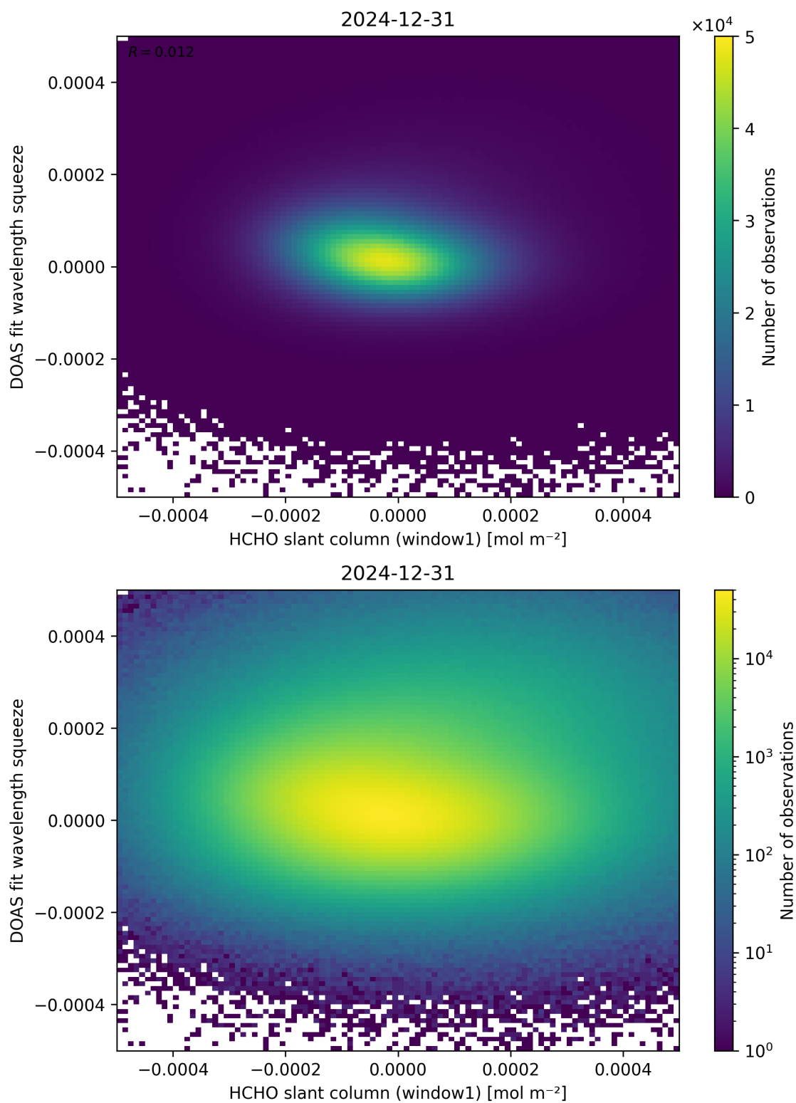
Figure 80: Scatter density plot of “HCHO slant column (window1)” against “DOAS fit wavelength squeeze” for 2024-12-30 to 2025-01-01.
