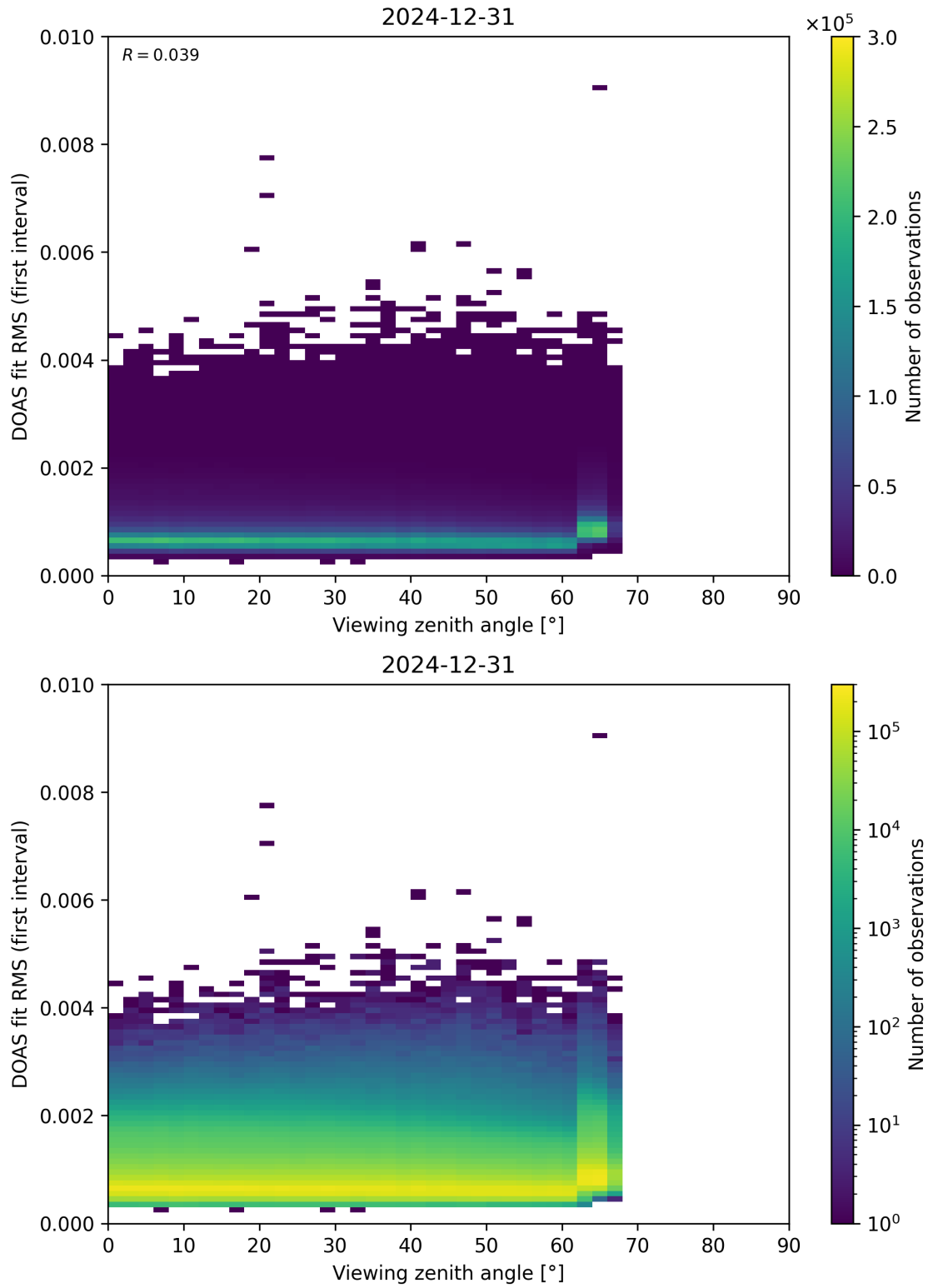
Figure 182: Scatter density plot of “Viewing zenith angle” against “DOAS fit RMS (first interval)” for 2024-12-30 to 2025-01-01.
