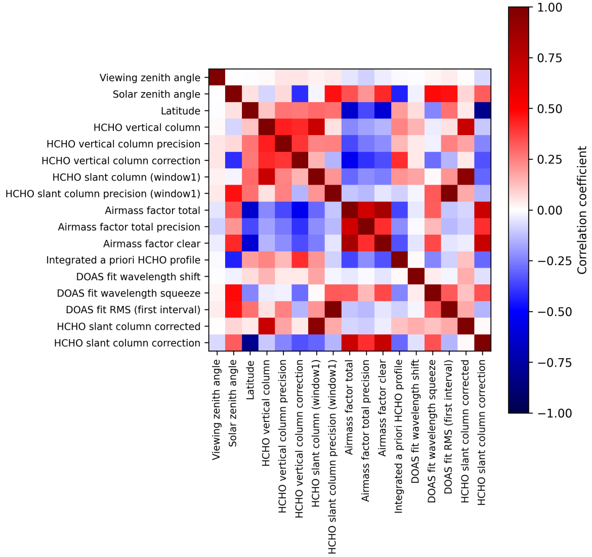
Figure 2: Map of correlation matrix for 2024-12-30 to 2025-01-01.
