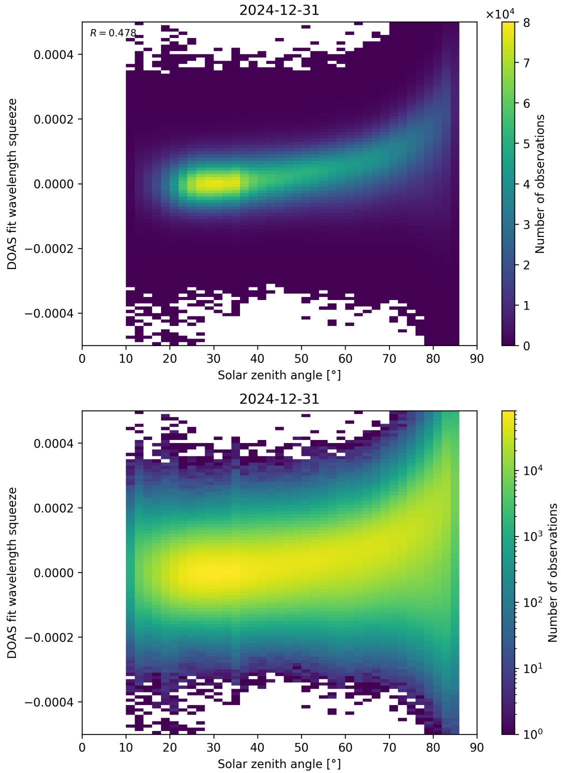
Figure 169: Scatter density plot of “Solar zenith angle” against “DOAS fit wavelength squeeze” for 2024-12-30 to 2025-01-01.
