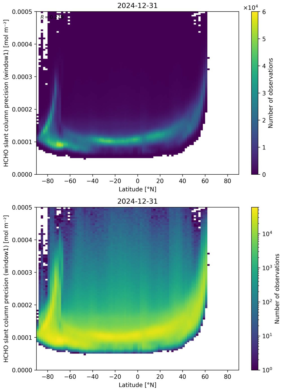
Figure 160: Scatter density plot of “Latitude” against “HCHO slant column precision (window1)” for 2024-12-30 to 2025-01-01.
