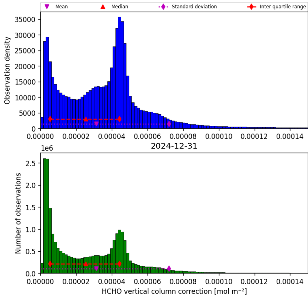
Figure 37: Histogram of “HCHO vertical column correction” for 2024-12-30 to 2025-01-01
