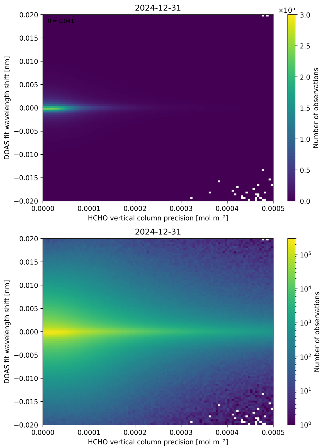
Figure 137: Scatter density plot of “HCHO vertical column precision” against “DOAS fit wavelength shift” for 2024-12-30 to 2025-01-01.
