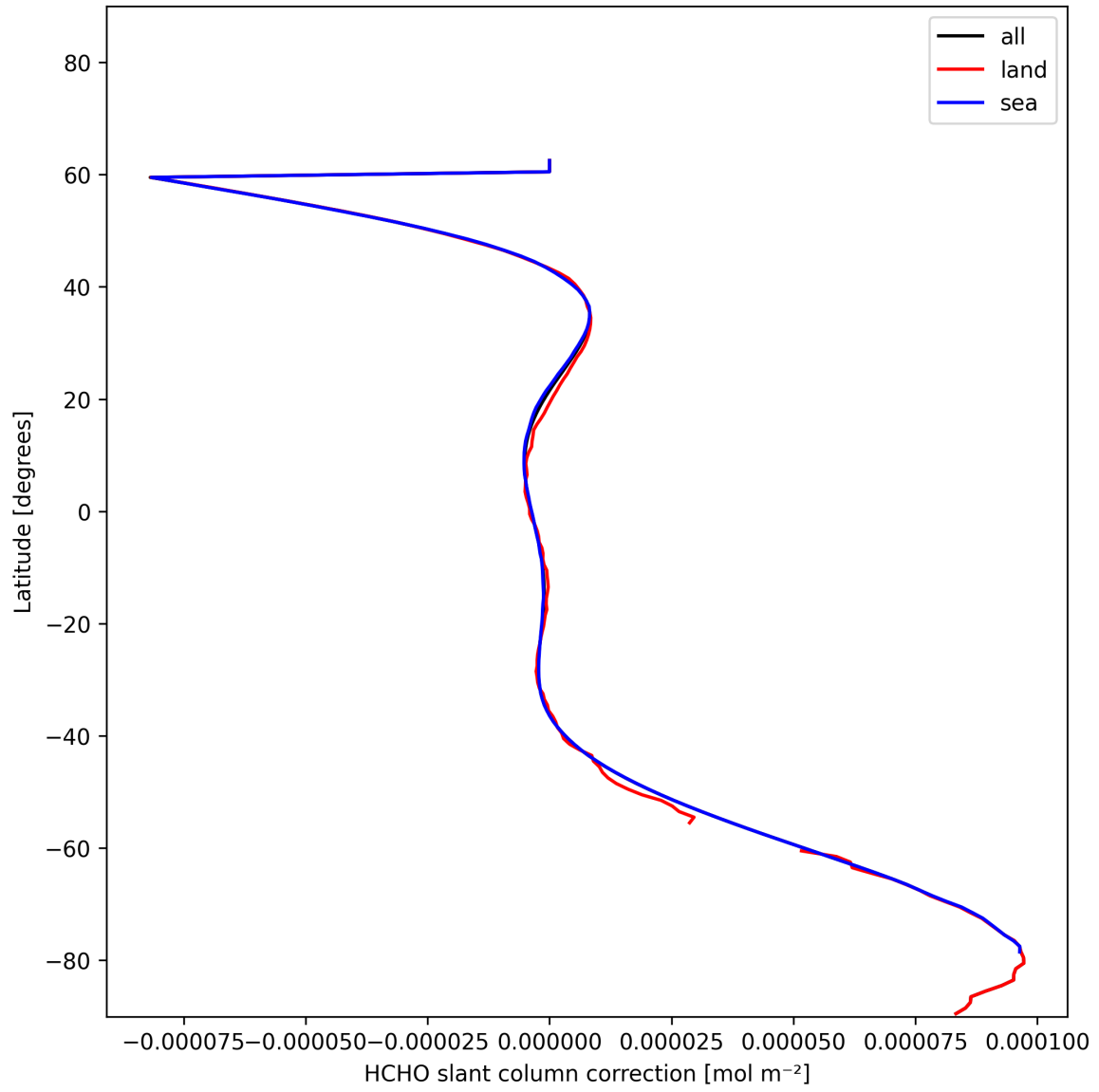
Figure 33: Zonal average of “HCHO slant column correction” for 2024-12-30 to 2025-01-01.
