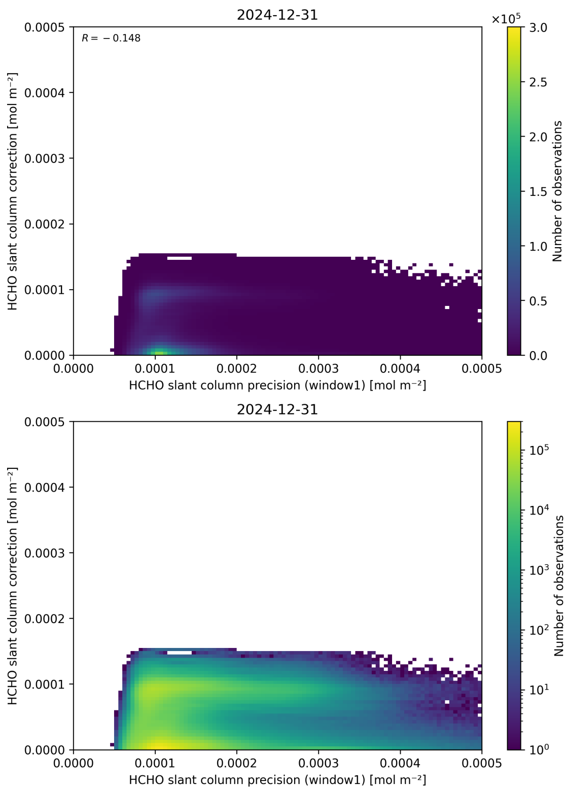
Figure 93: Scatter density plot of “HCHO slant column precision (window1)” against “HCHO slant column correction” for 2024-12-30 to 2025-01-01.
