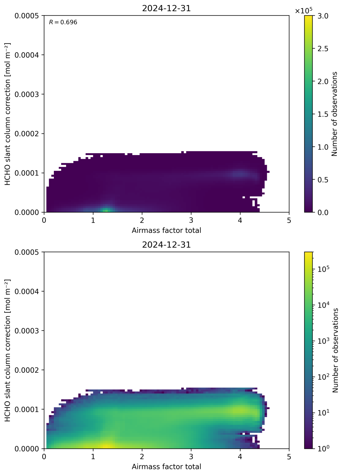
Figure 102: Scatter density plot of “Airmass factor total” against “HCHO slant column correction” for 2024-12-30 to 2025-01-01.
