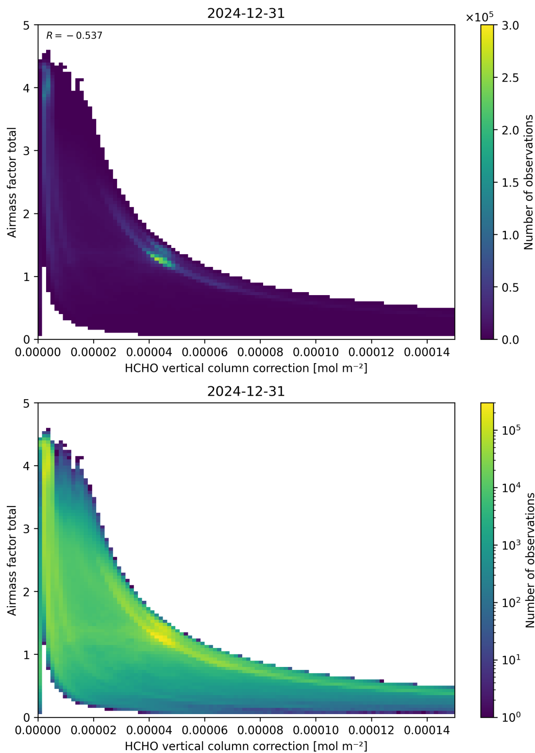
Figure 120: Scatter density plot of “HCHO vertical column correction” against “Airmass factor total” for 2024-12-30 to 2025-01-01.
