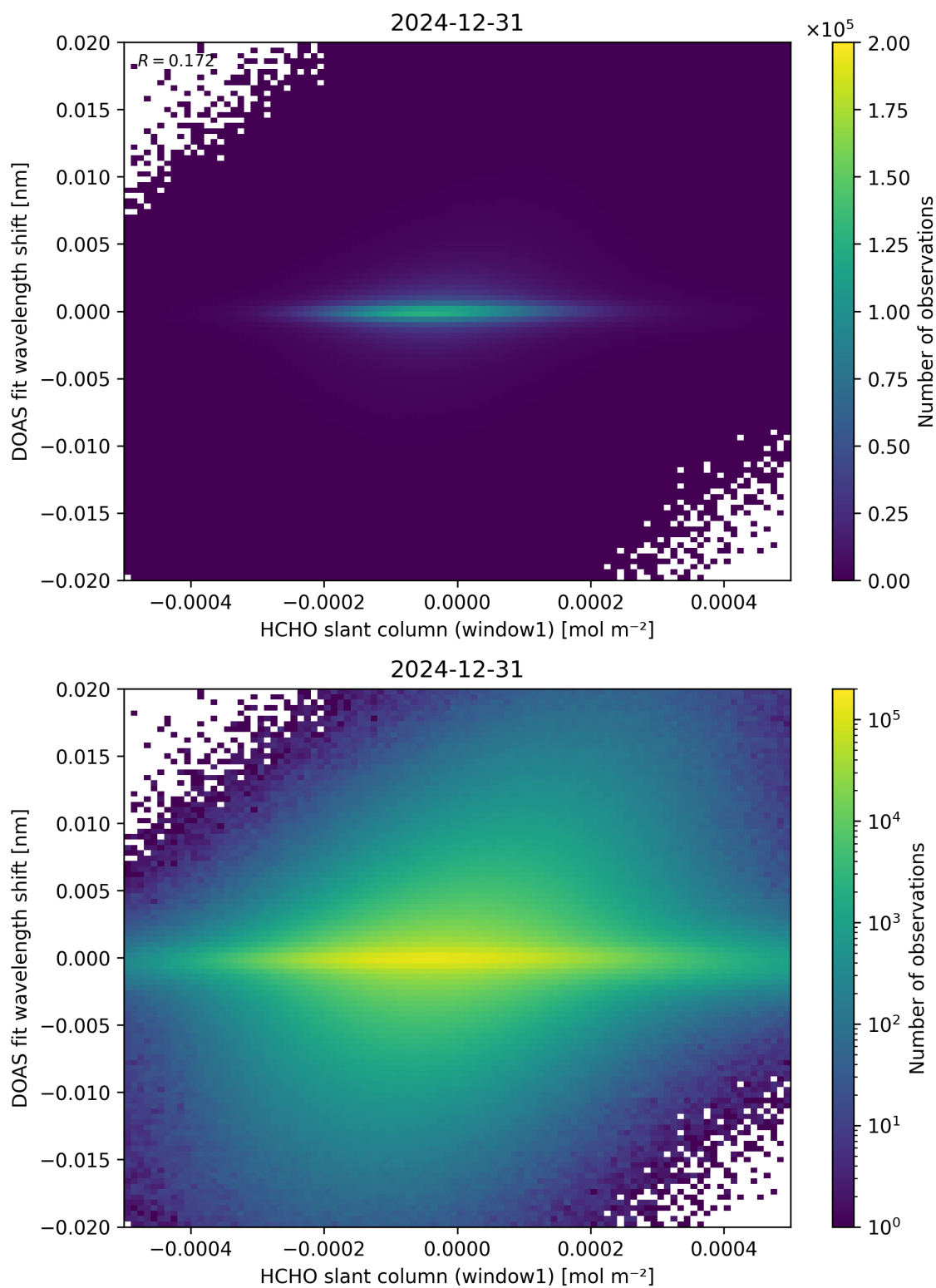
Figure 79: Scatter density plot of “HCHO slant column (window1)” against “DOAS fit wavelength shift” for 2024-12-30 to 2025-01-01.
