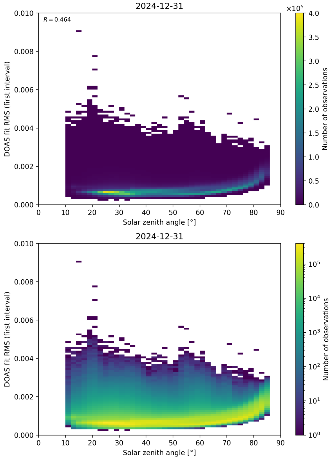
Figure 167: Scatter density plot of “Solar zenith angle” against “DOAS fit RMS (first interval)” for 2024-12-30 to 2025-01-01.
