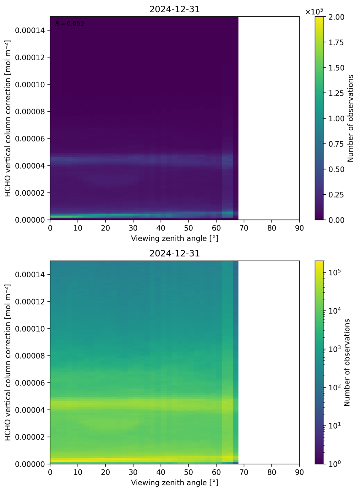
Figure 193: Scatter density plot of “Viewing zenith angle” against “HCHO vertical column correction” for 2024-12-30 to 2025-01-01.
