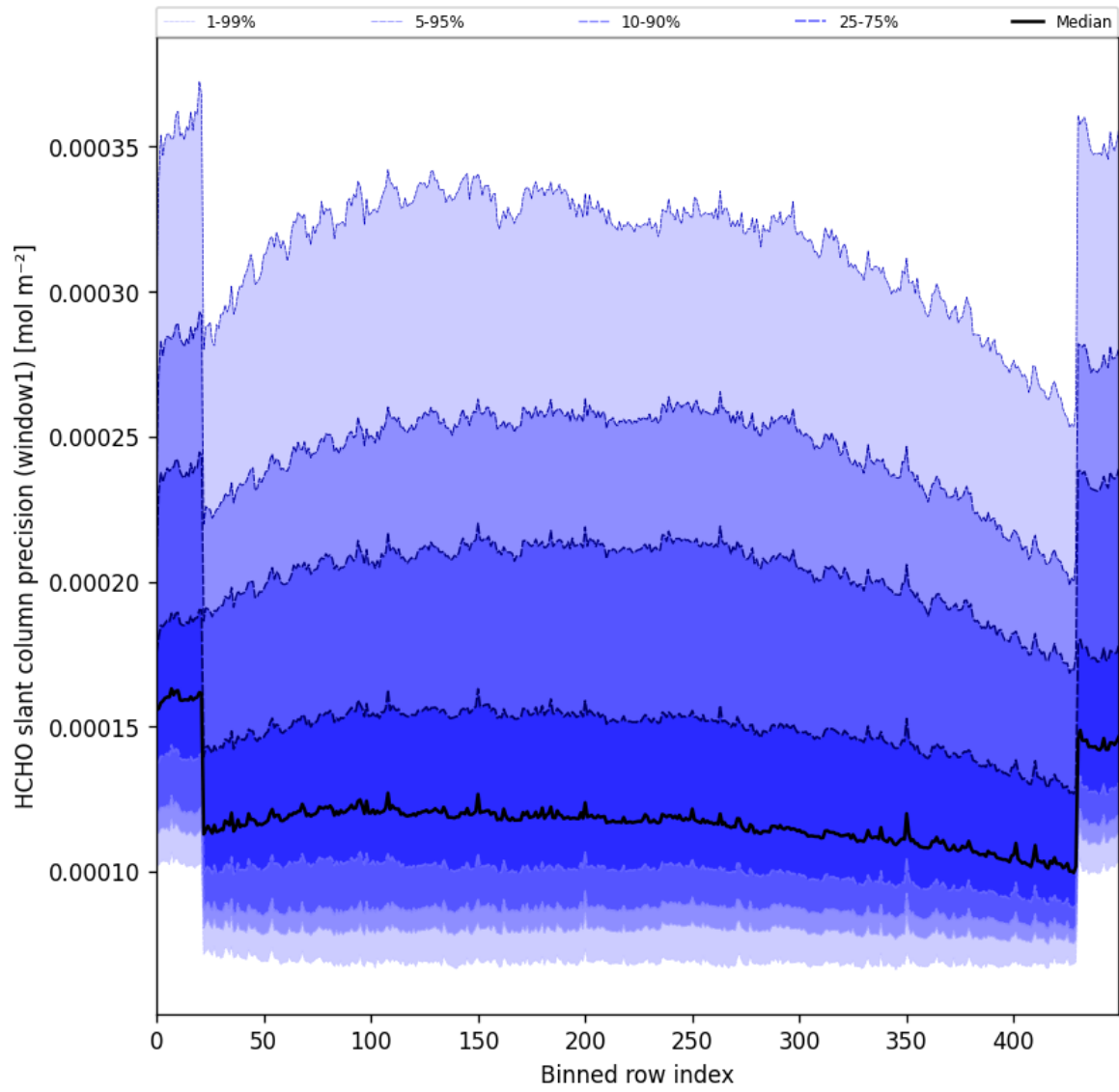
Figure 53: Along track statistics of “HCHO slant column precision (window1)” for 2024-12-30 to 2025-01-01
