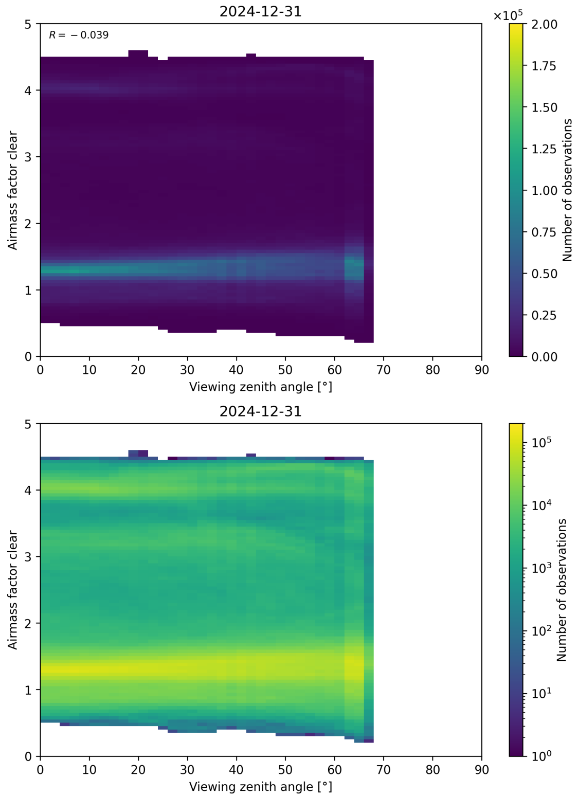
Figure 185: Scatter density plot of “Viewing zenith angle” against “Airmass factor clear” for 2024-12-30 to 2025-01-01.
