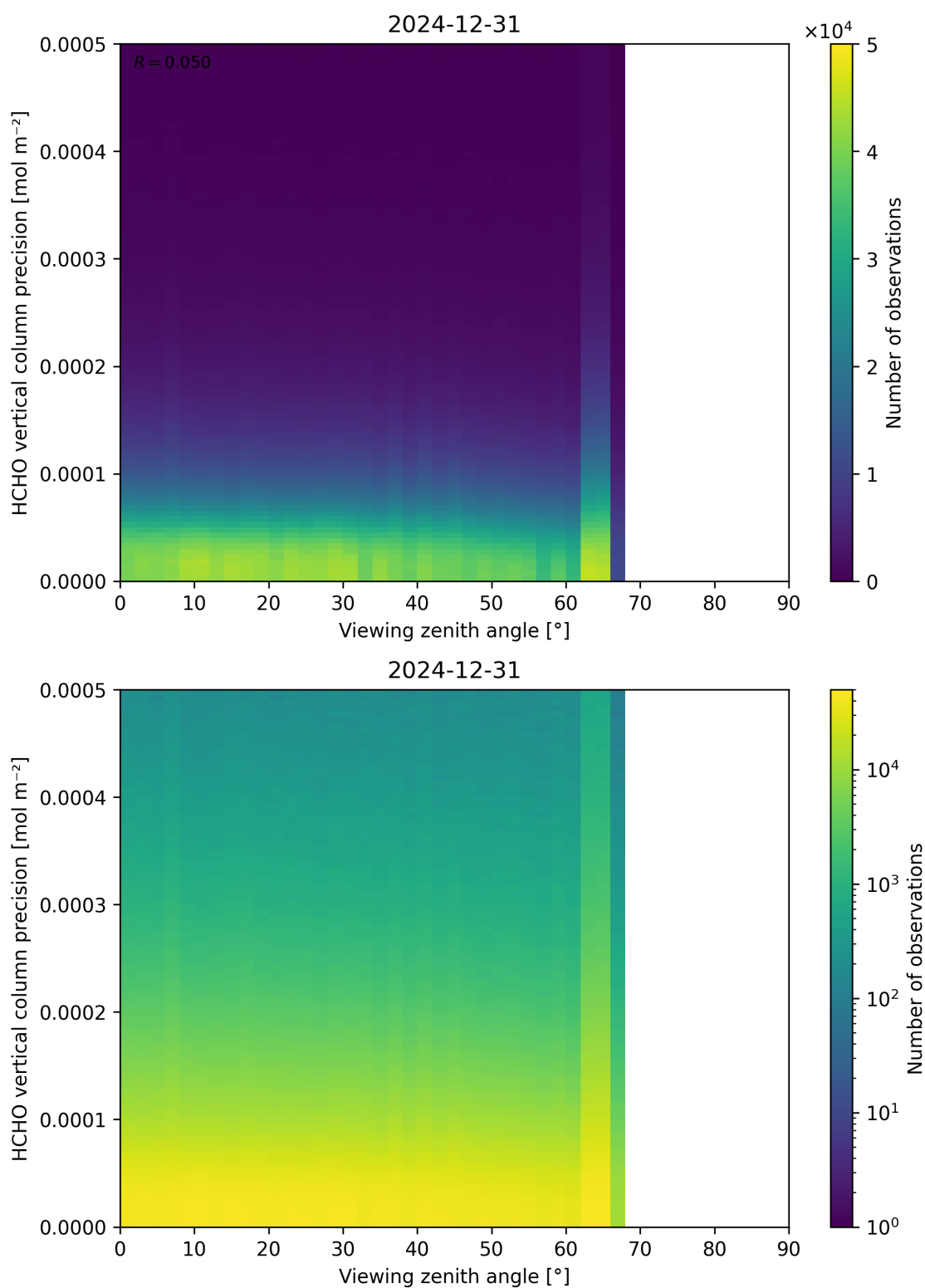
Figure 194: Scatter density plot of “Viewing zenith angle” against “HCHO vertical column precision” for 2024-12-30 to 2025-01-01.
