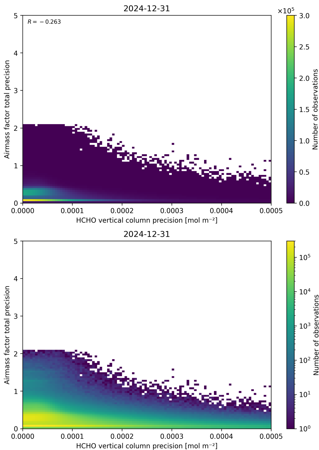
Figure 145: Scatter density plot of “HCHO vertical column precision” against “Airmass factor total precision” for 2024-12-30 to 2025-01-01.
