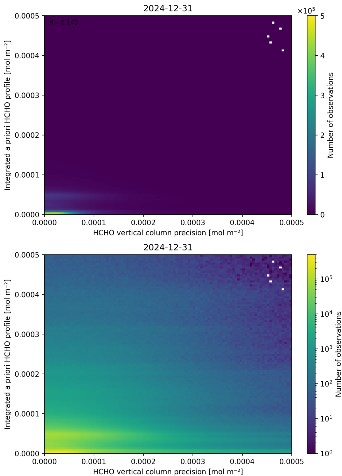
Figure 147: Scatter density plot of “HCHO vertical column precision” against “Integrated a priori HCHO profile” for 2024-12-30 to 2025-01-01.
