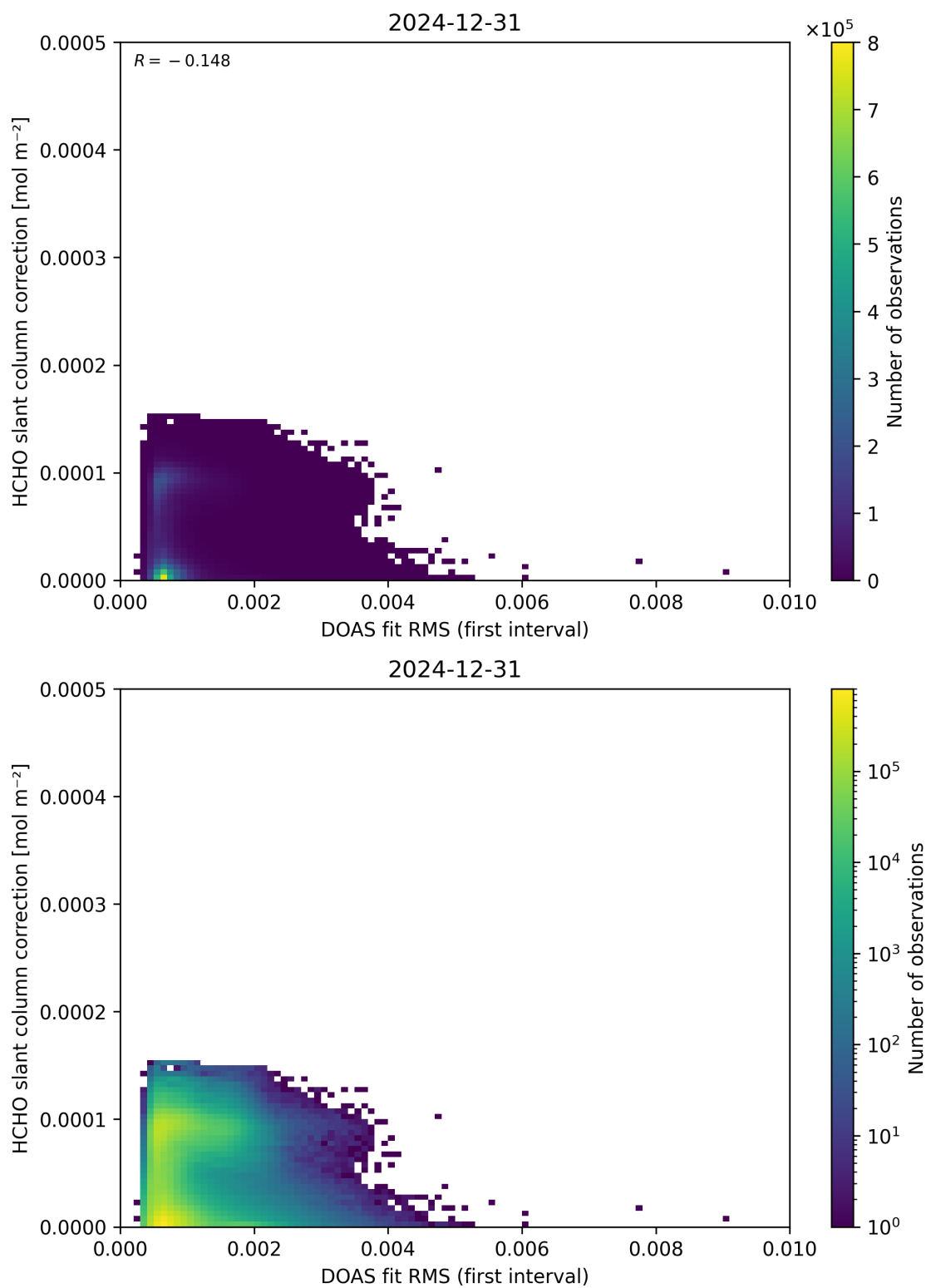
Figure 63: Scatter density plot of “DOAS fit RMS (first interval)” against “HCHO slant column correction” for 2024-12-30 to 2025-01-01.
