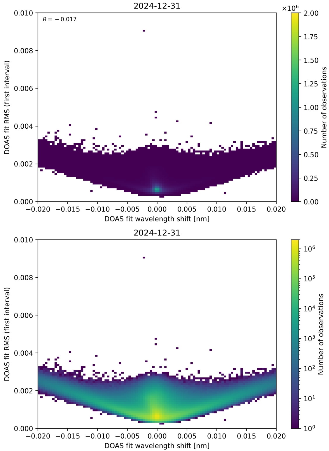
Figure 64: Scatter density plot of “DOAS fit wavelength shift” against “DOAS fit RMS (first interval)” for 2024-12-30 to 2025-01-01.
