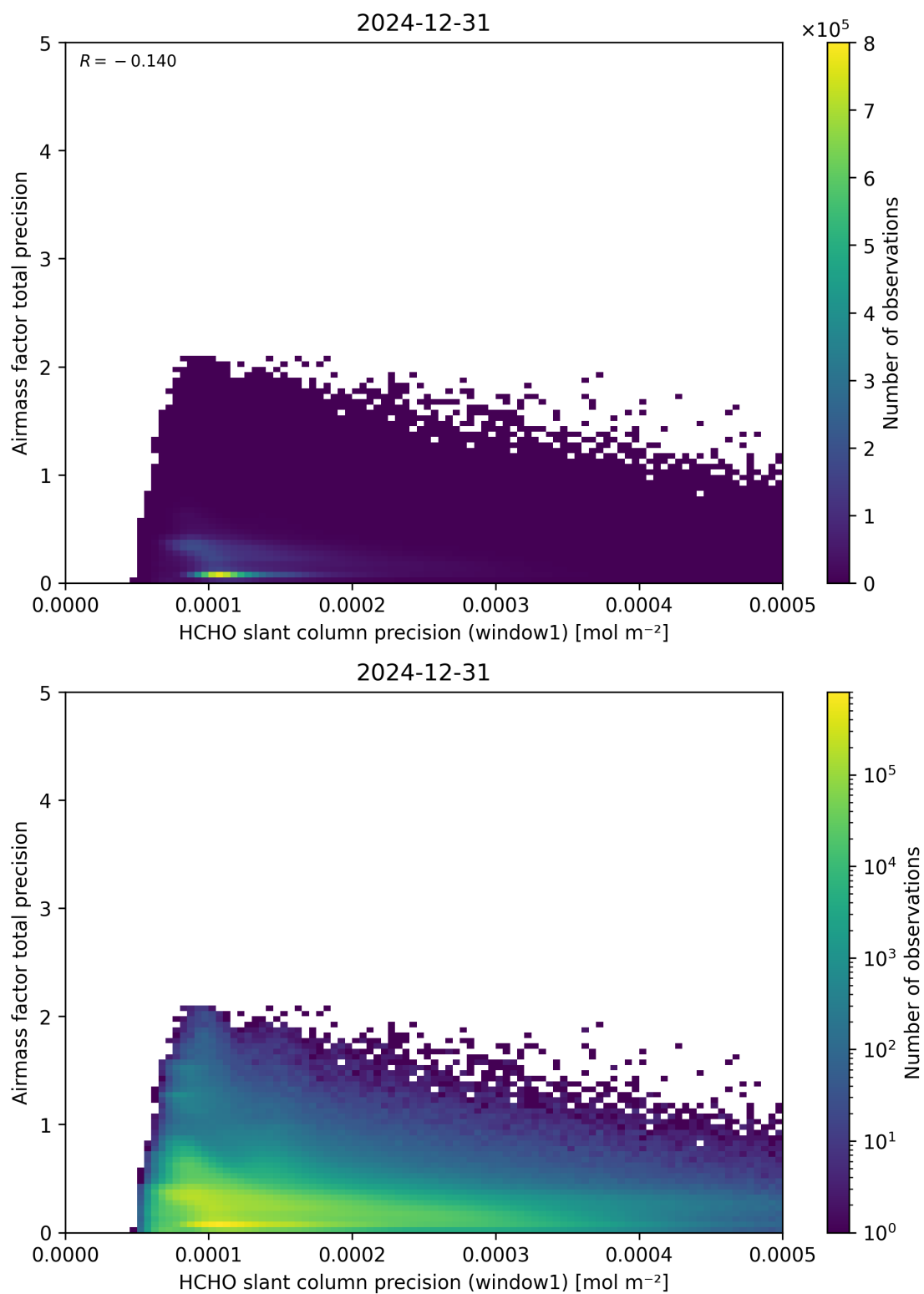
Figure 95: Scatter density plot of “HCHO slant column precision (window1)” against “Airmass factor total precision” for 2024-12-30 to 2025-01-01.
