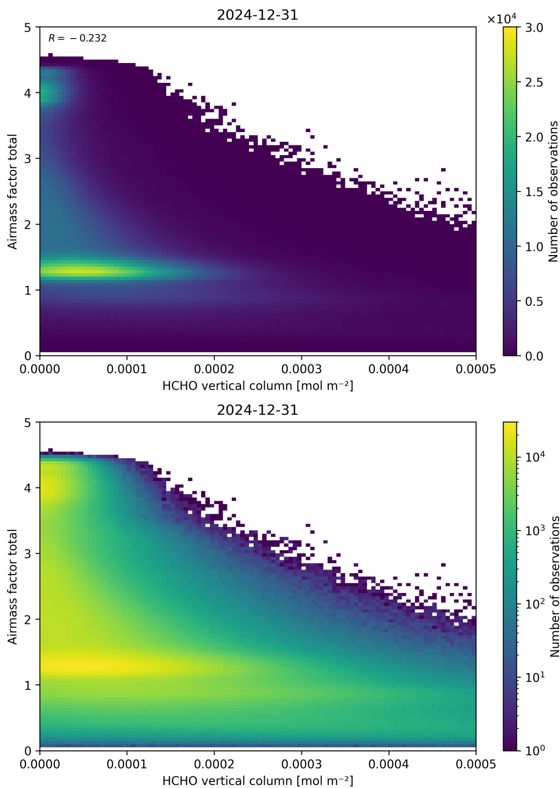
Figure 131: Scatter density plot of “HCHO vertical column” against “Airmass factor total” for 2024-12-30 to 2025-01-01.
