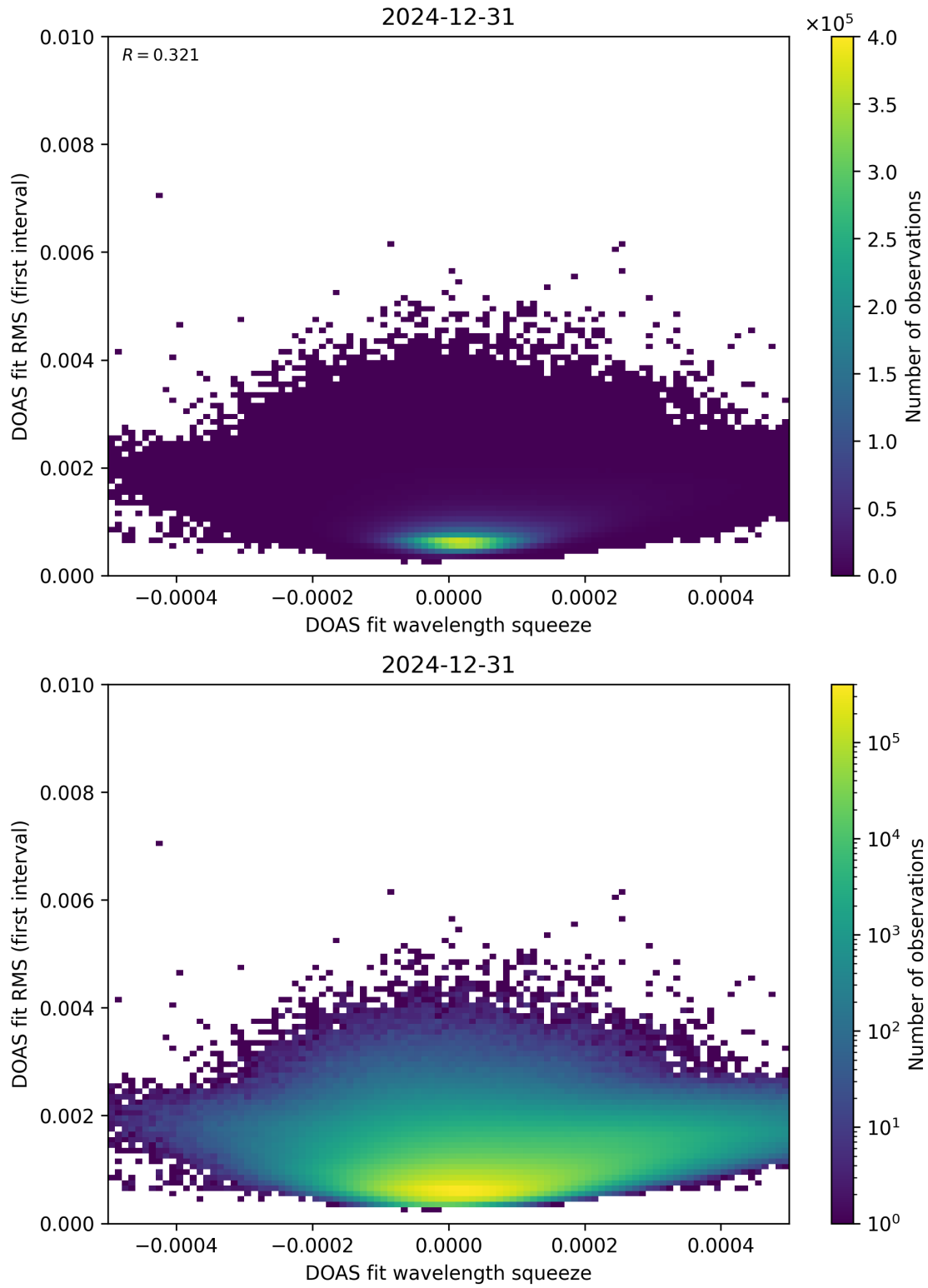
Figure 68: Scatter density plot of “DOAS fit wavelength squeeze” against “DOAS fit RMS (first interval)” for 2024-12-30 to 2025-01-01.
