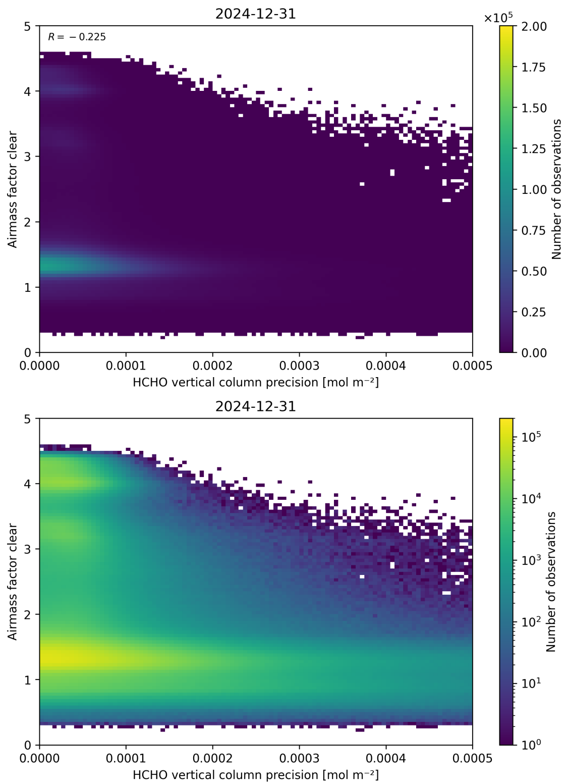
Figure 139: Scatter density plot of “HCHO vertical column precision” against “Airmass factor clear” for 2024-12-30 to 2025-01-01.
