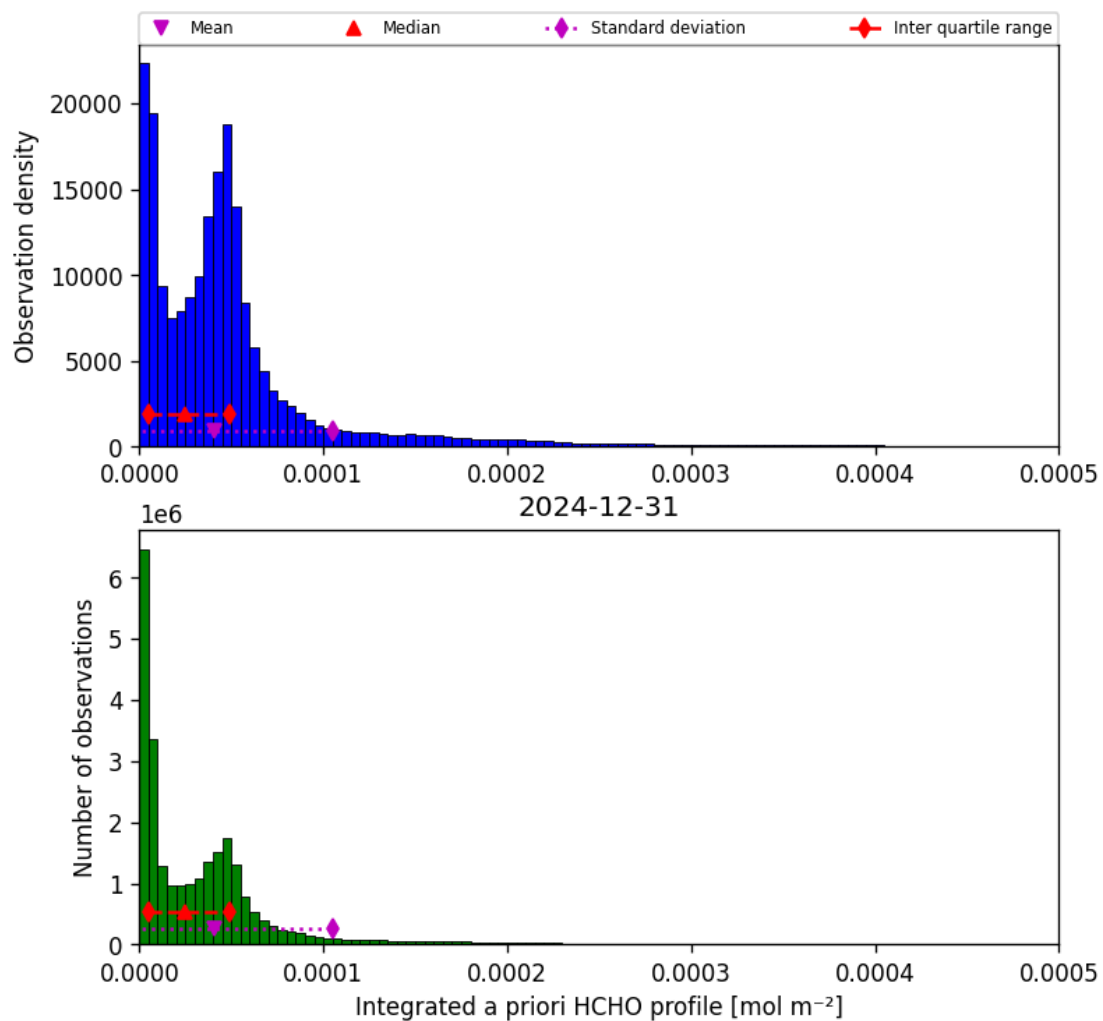
Figure 43: Histogram of “Integrated a priori HCHO profile” for 2024-12-30 to 2025-01-01
