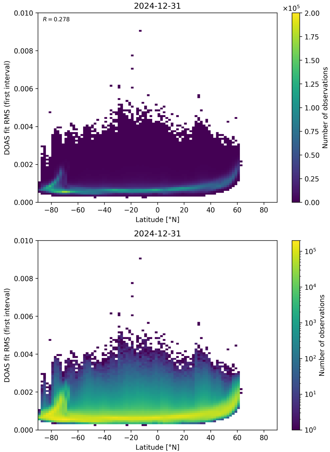
Figure 153: Scatter density plot of “Latitude” against “DOAS fit RMS (first interval)” for 2024-12-30 to 2025-01-01.
