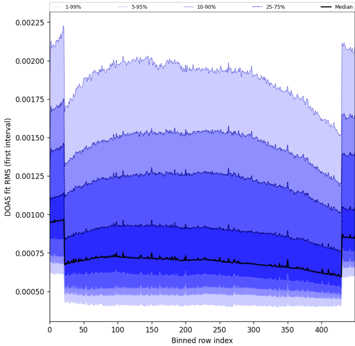
Figure 60: Along track statistics of “DOAS fit RMS (first interval)” for 2024-12-30 to 2025-01-01
