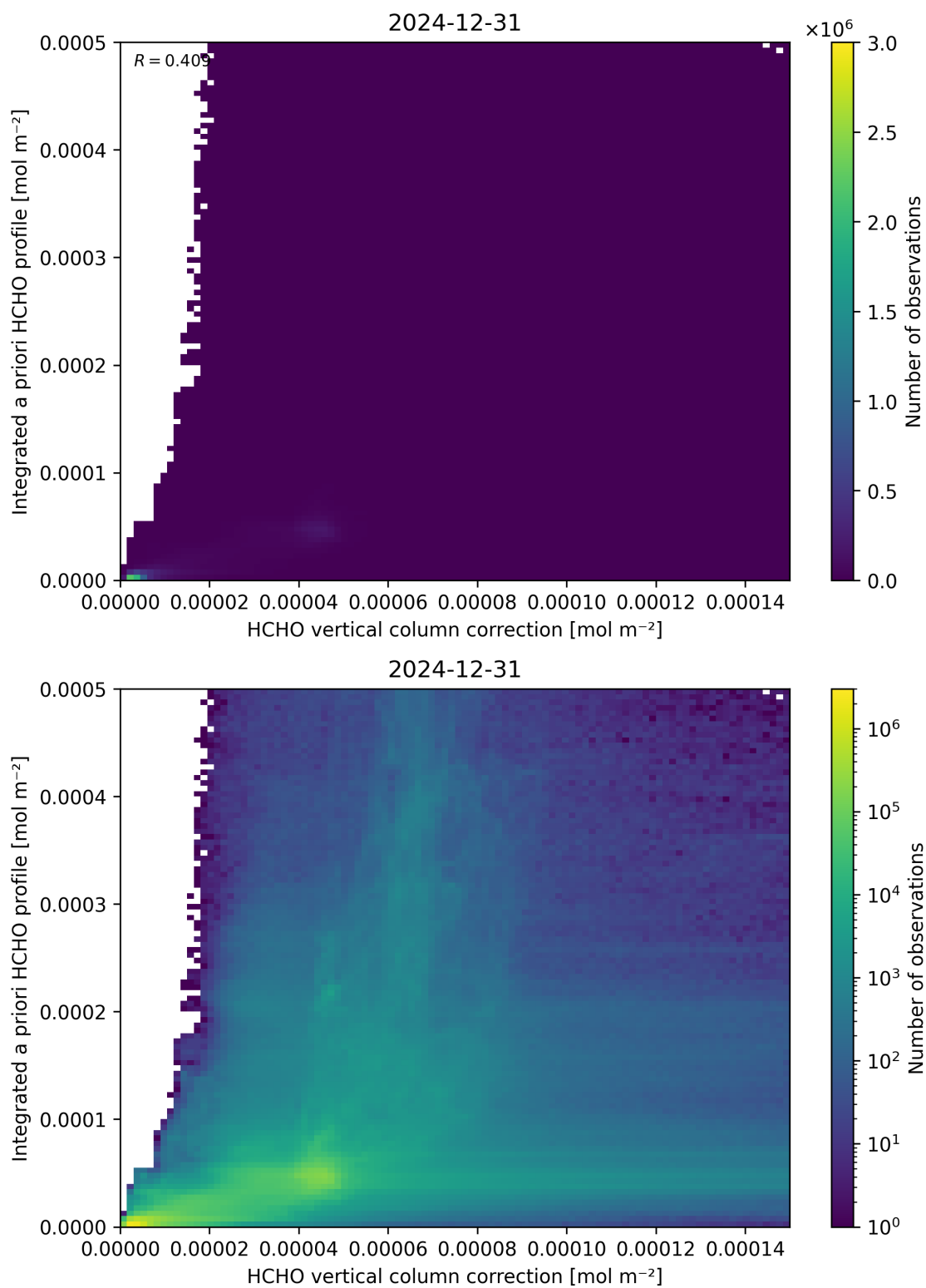
Figure 122: Scatter density plot of “HCHO vertical column correction” against “Integrated a priori HCHO profile” for 2024-12-30 to 2025-01-01.
