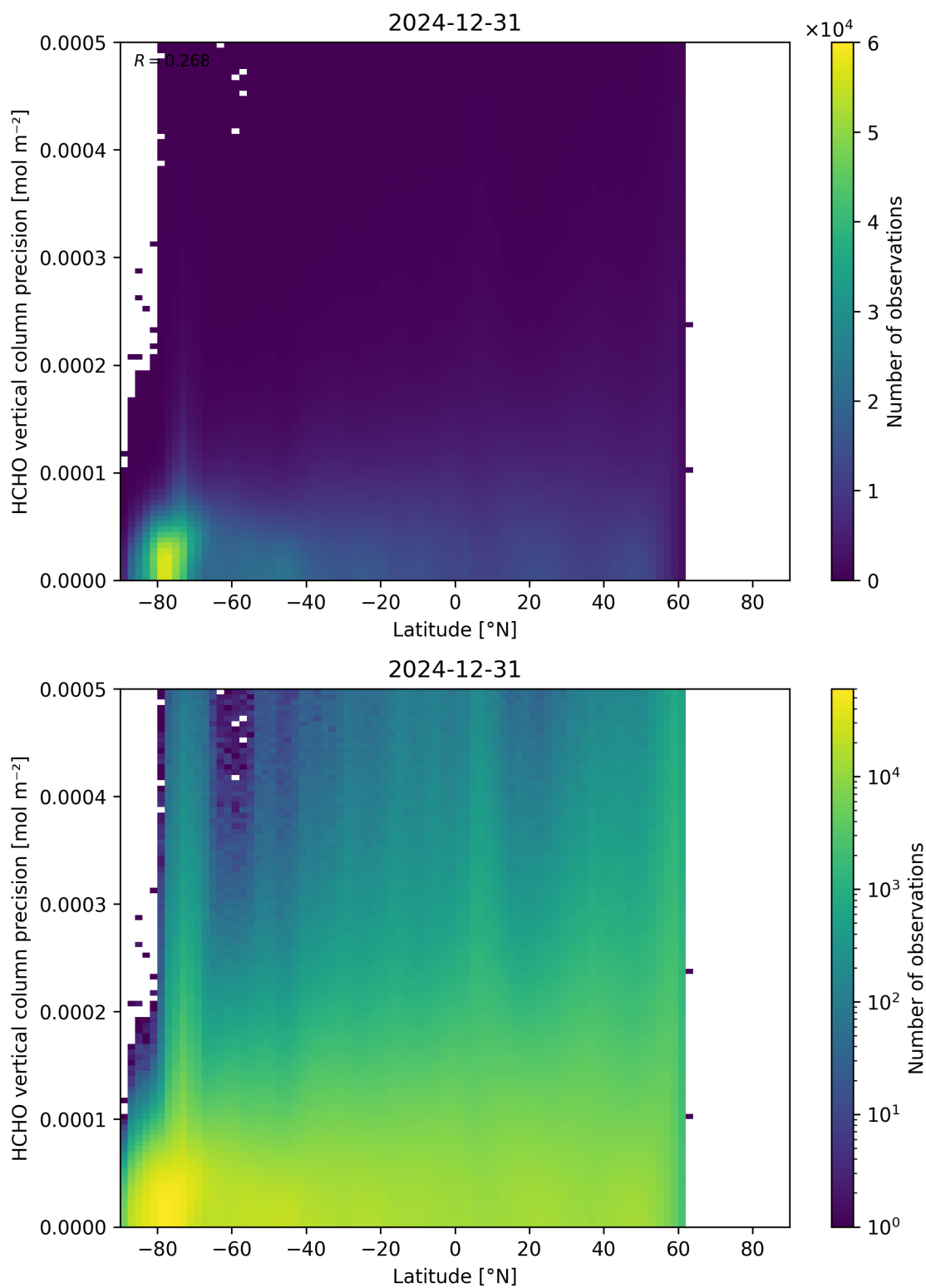
Figure 165: Scatter density plot of “Latitude” against “HCHO vertical column precision” for 2024-12-30 to 2025-01-01.
