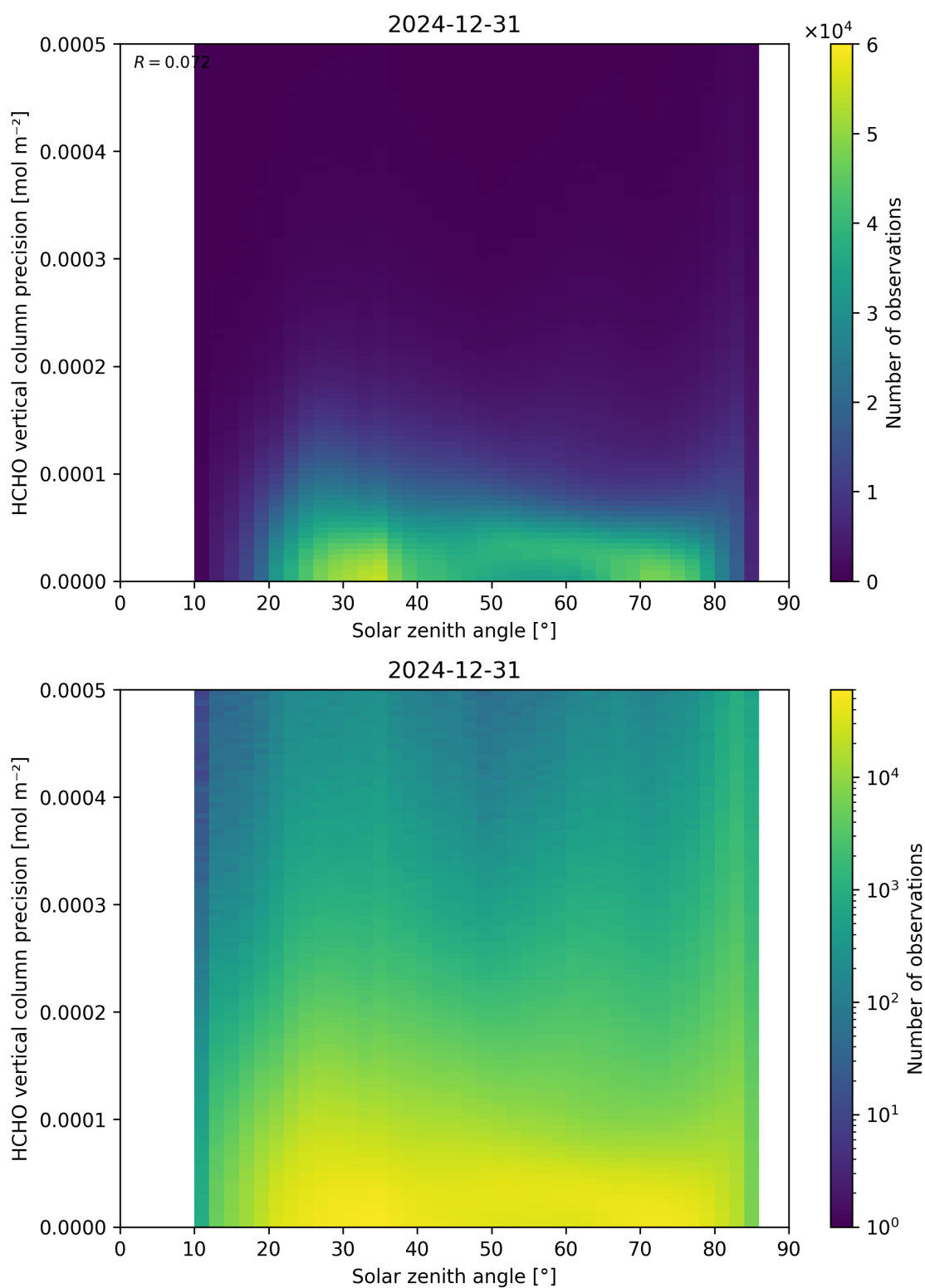
Figure 179: Scatter density plot of “Solar zenith angle” against “HCHO vertical column precision” for 2024-12-30 to 2025-01-01.
