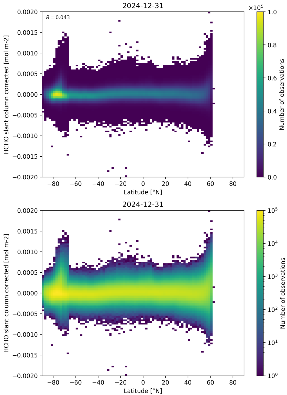
Figure 157: Scatter density plot of “Latitude” against “HCHO slant column corrected” for 2024-12-30 to 2025-01-01.
