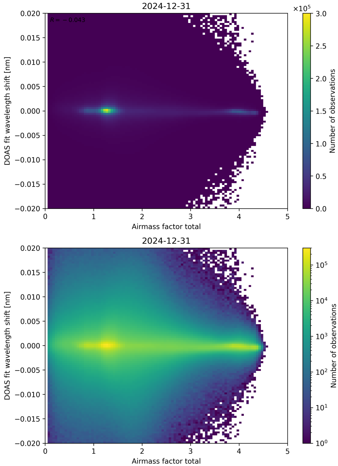
Figure 98: Scatter density plot of “Airmass factor total” against “DOAS fit wavelength shift” for 2024-12-30 to 2025-01-01.
