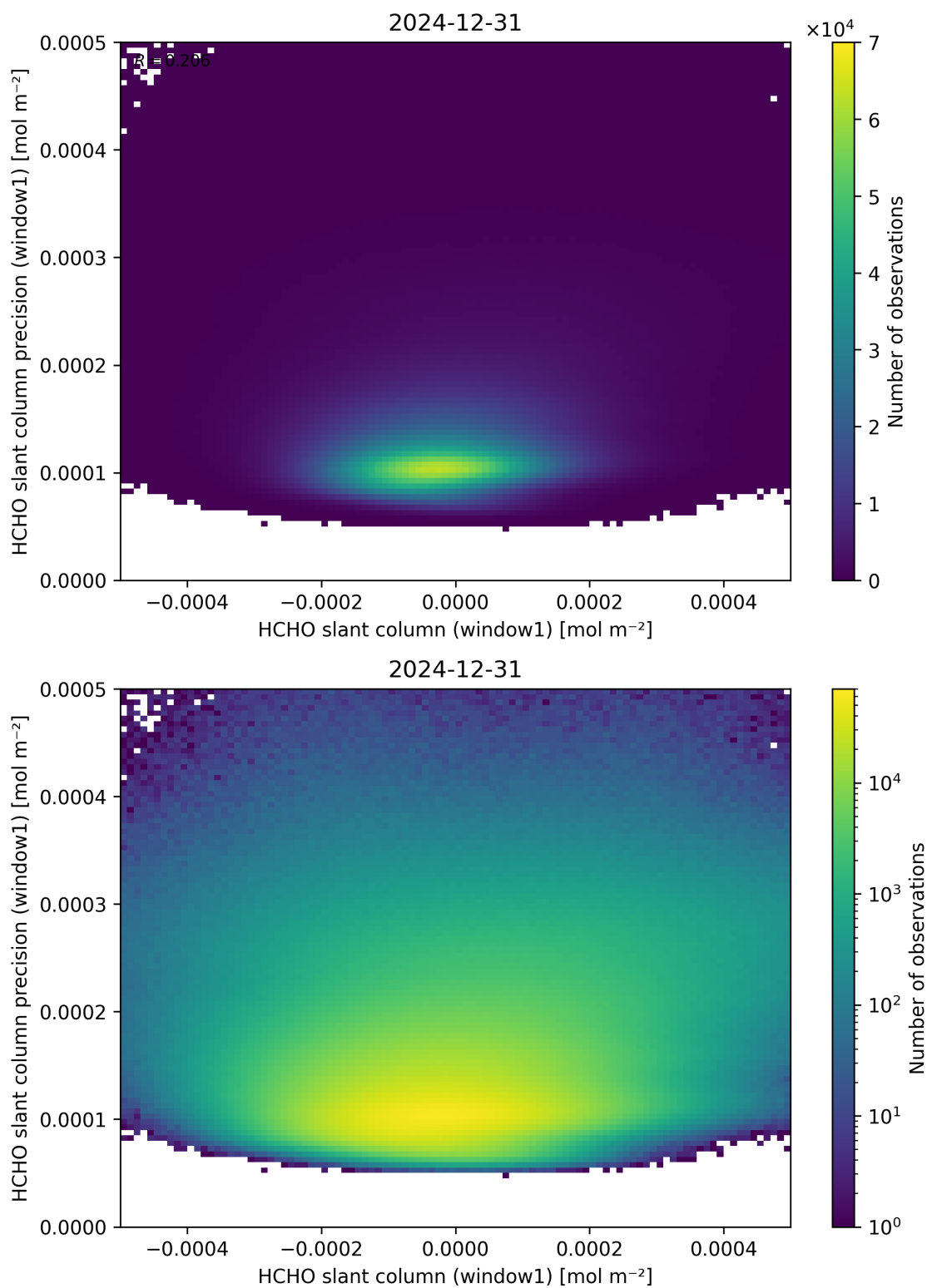
Figure 84: Scatter density plot of “HCHO slant column (window1)” against “HCHO slant column precision (window1)” for 2024-12-30 to 2025-01-01.
