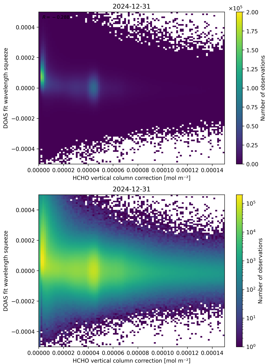
Figure 114: Scatter density plot of “HCHO vertical column correction” against “DOAS fit wavelength squeeze” for 2024-12-30 to 2025-01-01.
