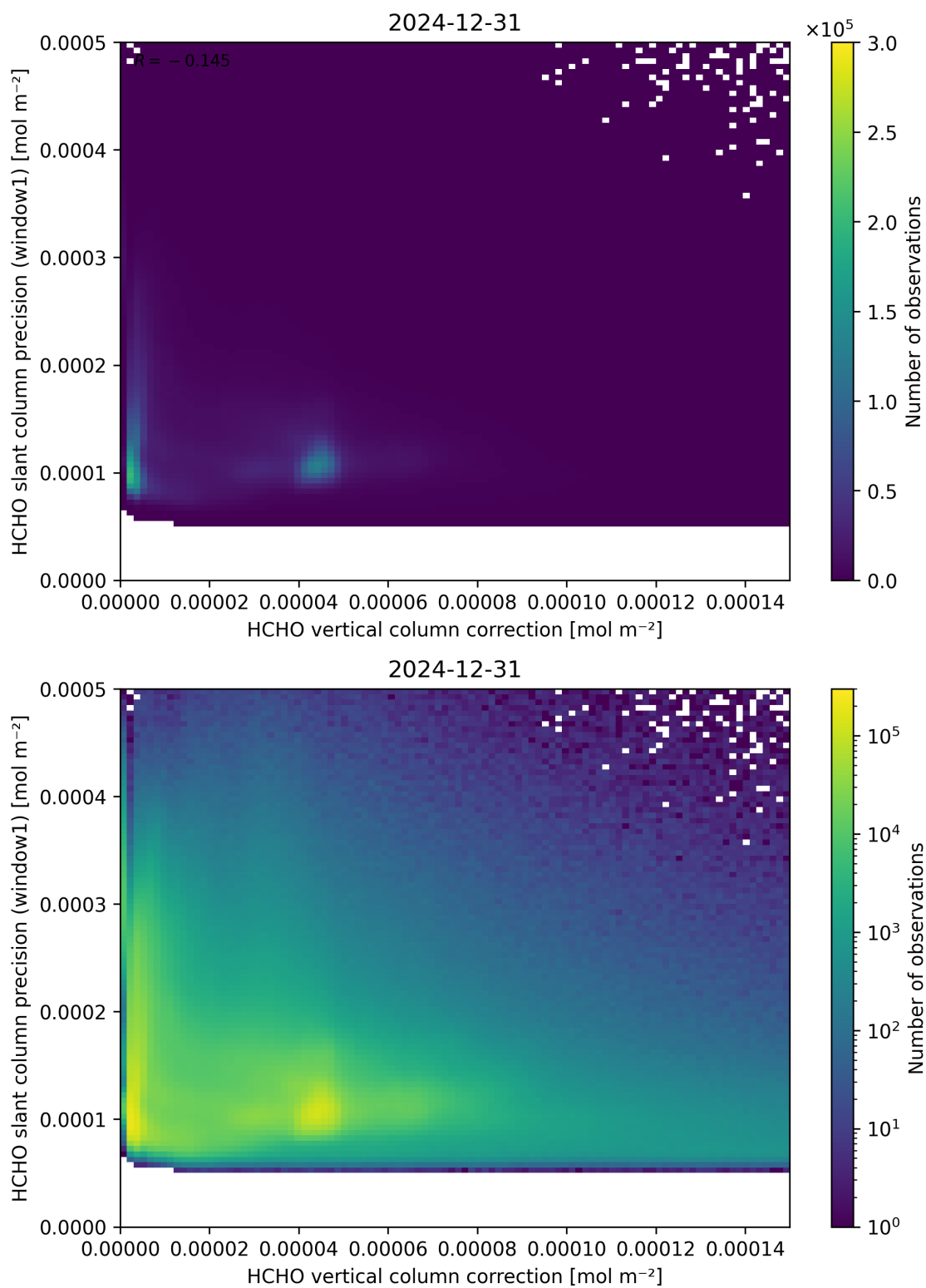
Figure 119: Scatter density plot of “HCHO vertical column correction” against “HCHO slant column precision (window1)” for 2024-12-30 to 2025-01-01.
