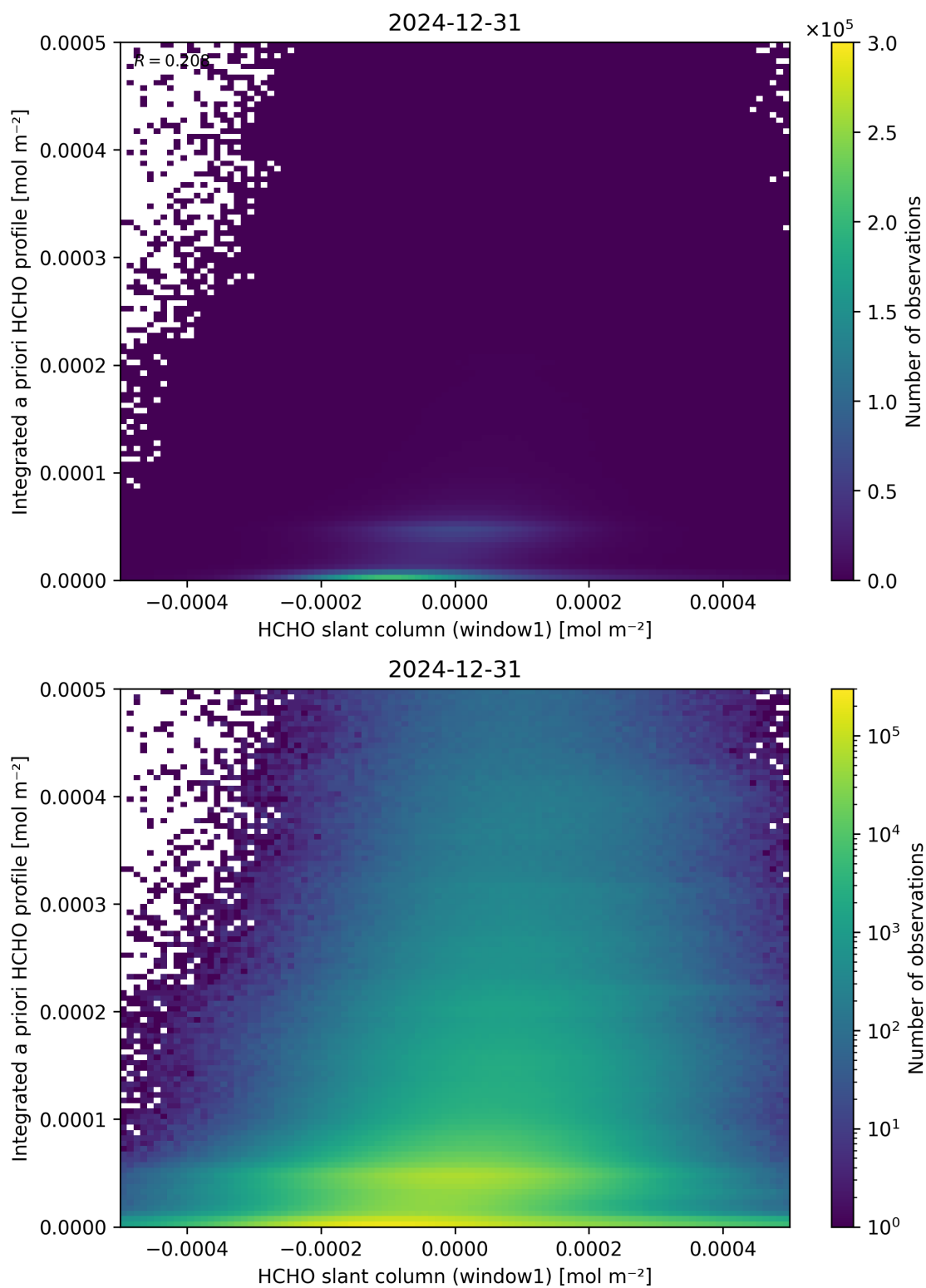
Figure 87: Scatter density plot of “HCHO slant column (window1)” against “Integrated a priori HCHO profile” for 2024-12-30 to 2025-01-01.
