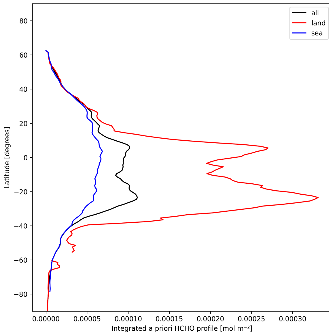
Figure 29: Zonal average of “Integrated a priori HCHO profile” for 2024-12-30 to 2025-01-01.
