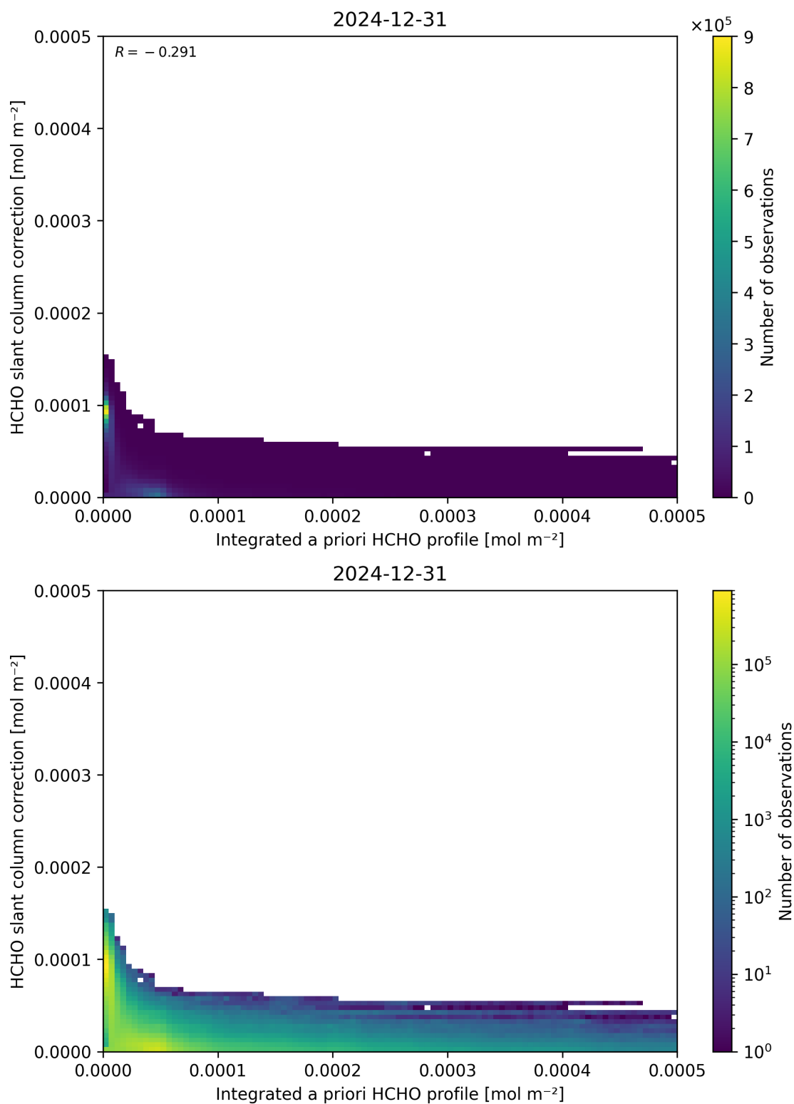
Figure 152: Scatter density plot of “Integrated a priori HCHO profile” against “HCHO slant column correction” for 2024-12-30 to 2025-01-01.
