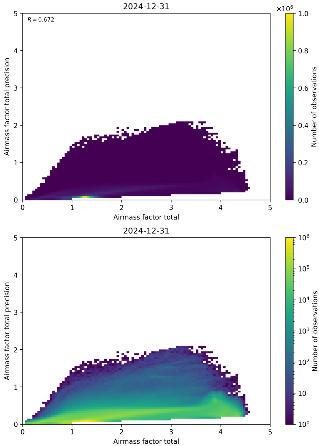
Figure 103: Scatter density plot of “Airmass factor total” against “Airmass factor total precision” for 2024-12-30 to 2025-01-01.
