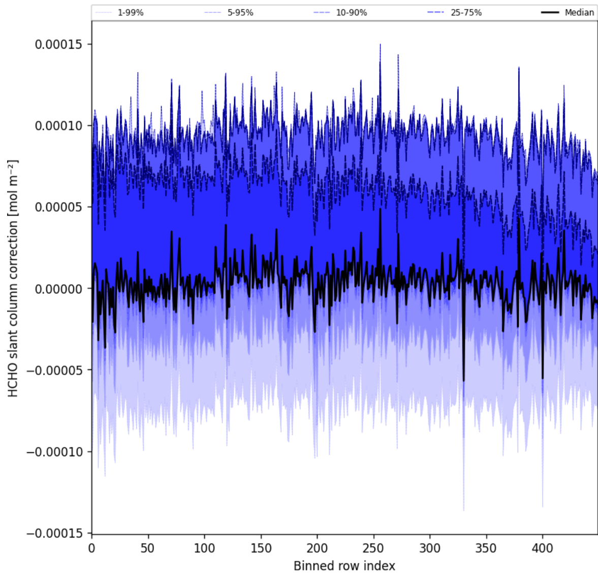
Figure 61: Along track statistics of “HCHO slant column correction” for 2024-12-30 to 2025-01-01
