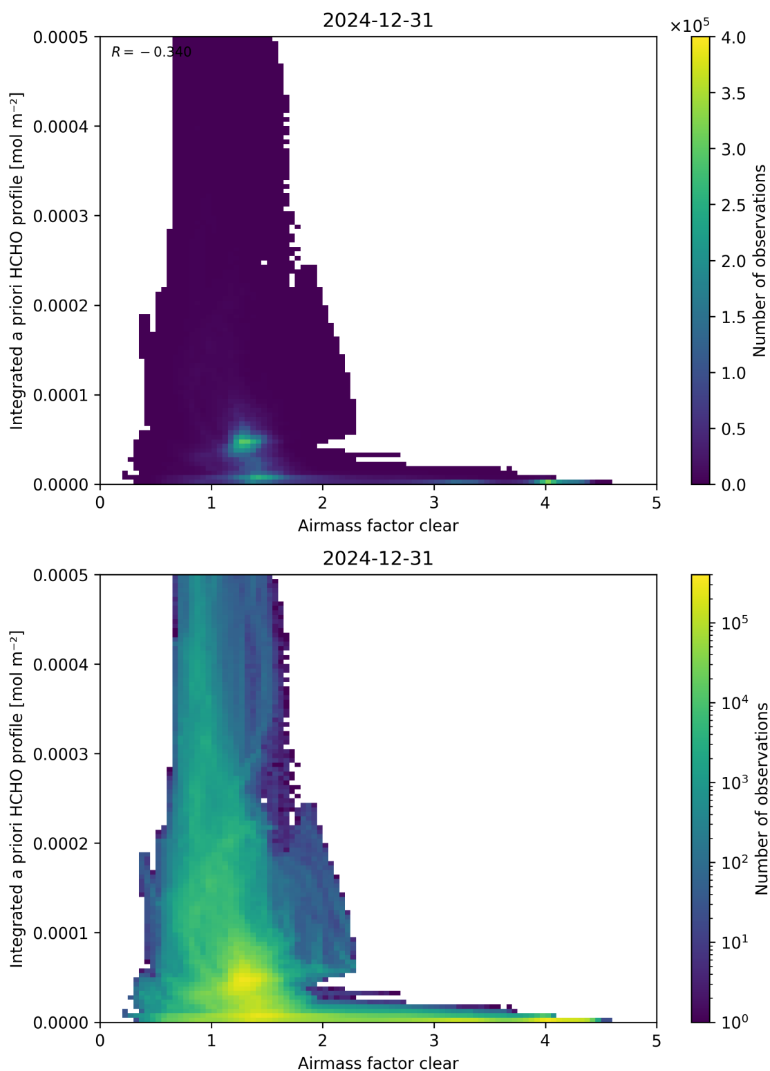
Figure 76: Scatter density plot of “Airmass factor clear” against “Integrated a priori HCHO profile” for 2024-12-30 to 2025-01-01.
