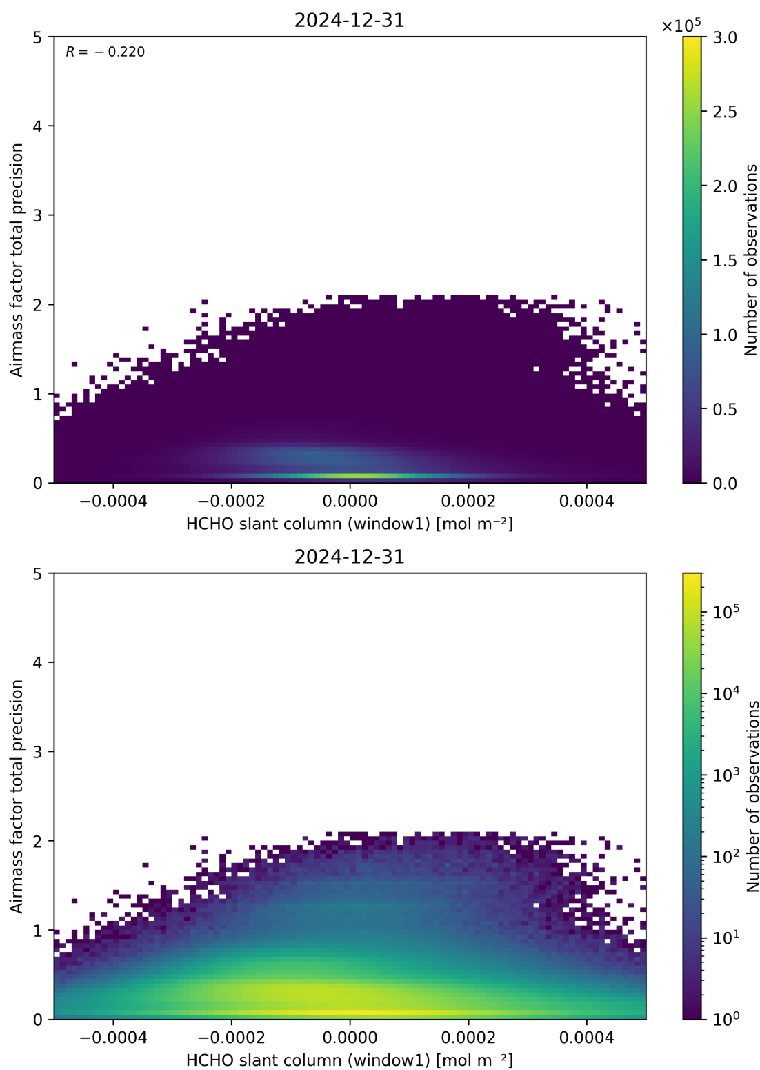
Figure 86: Scatter density plot of “HCHO slant column (window1)” against “Airmass factor total precision” for 2024-12-30 to 2025-01-01.
