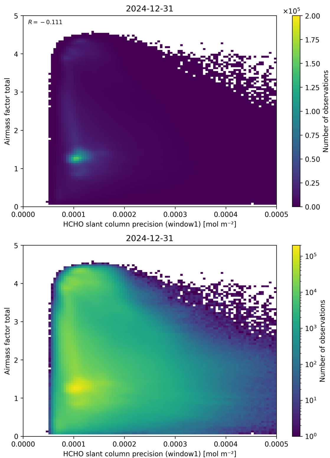
Figure 94: Scatter density plot of “HCHO slant column precision (window1)” against “Airmass factor total” for 2024-12-30 to 2025-01-01.
