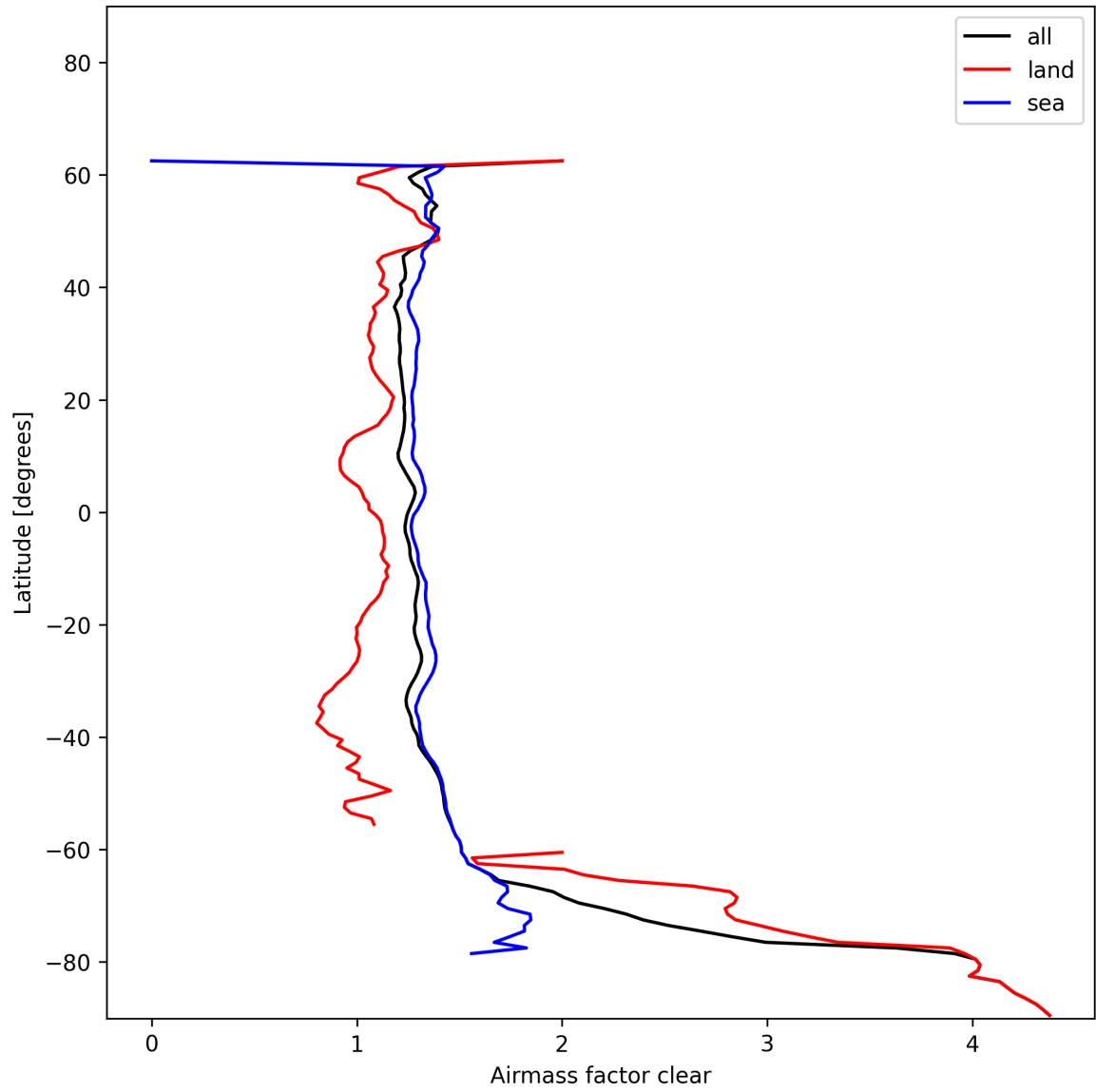
Figure 28: Zonal average of “Airmass factor clear” for 2024-12-30 to 2025-01-01.
