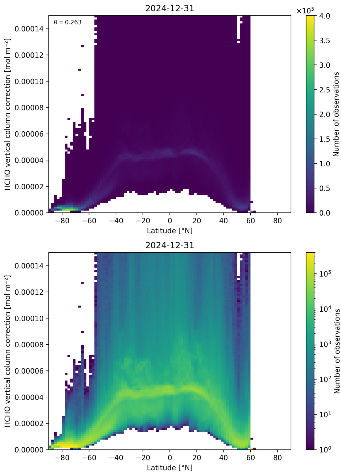
Figure 164: Scatter density plot of “Latitude” against “HCHO vertical column correction” for 2024-12-30 to 2025-01-01.
