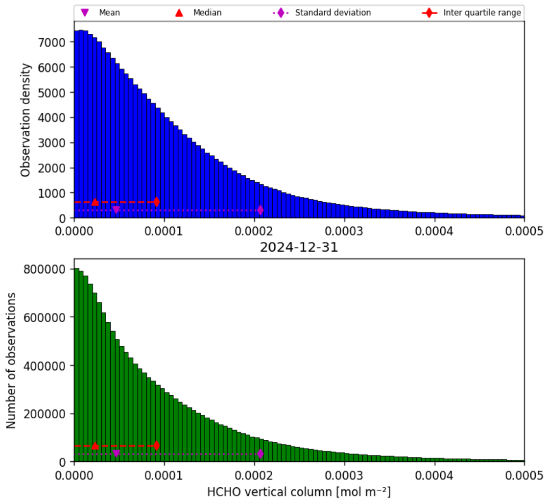
Figure 35: Histogram of “HCHO vertical column” for 2024-12-30 to 2025-01-01
