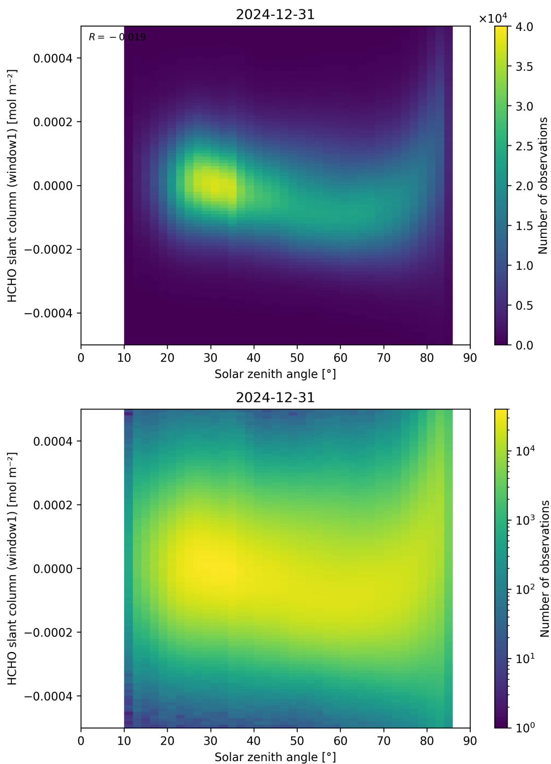
Figure 173: Scatter density plot of “Solar zenith angle” against “HCHO slant column (window1)” for 2024-12-30 to 2025-01-01.
