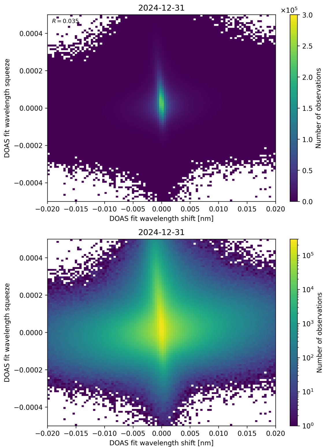
Figure 65: Scatter density plot of “DOAS fit wavelength shift” against “DOAS fit wavelength squeeze” for 2024-12-30 to 2025-01-01.
