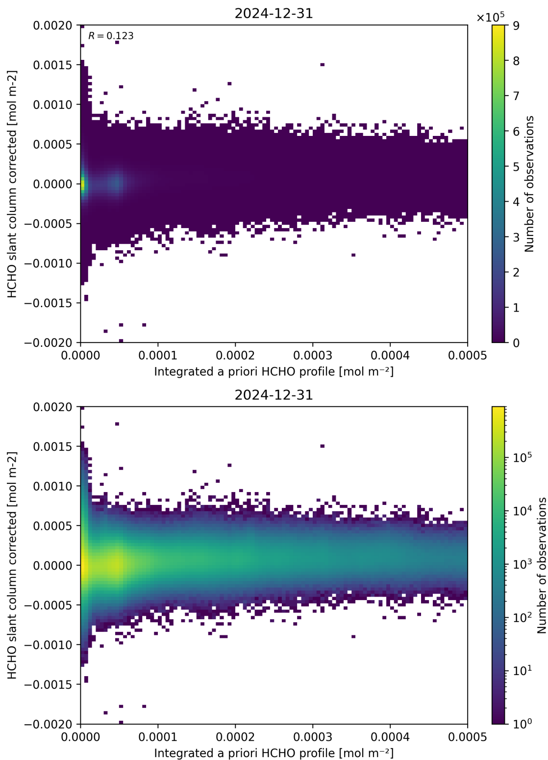
Figure 151: Scatter density plot of “Integrated a priori HCHO profile” against “HCHO slant column corrected” for 2024-12-30 to 2025-01-01.
