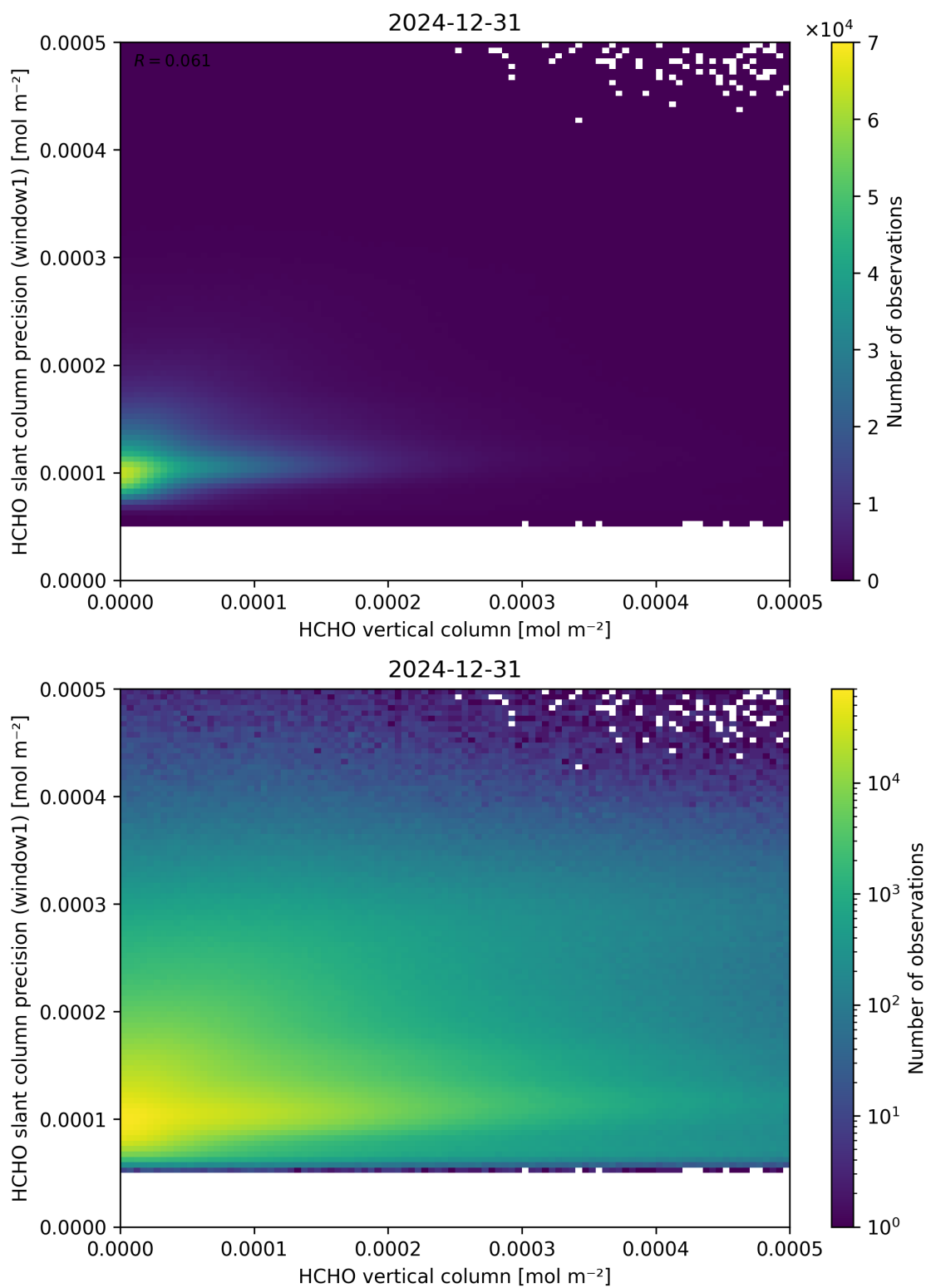
Figure 130: Scatter density plot of “HCHO vertical column” against “HCHO slant column precision (window1)” for 2024-12-30 to 2025-01-01.
