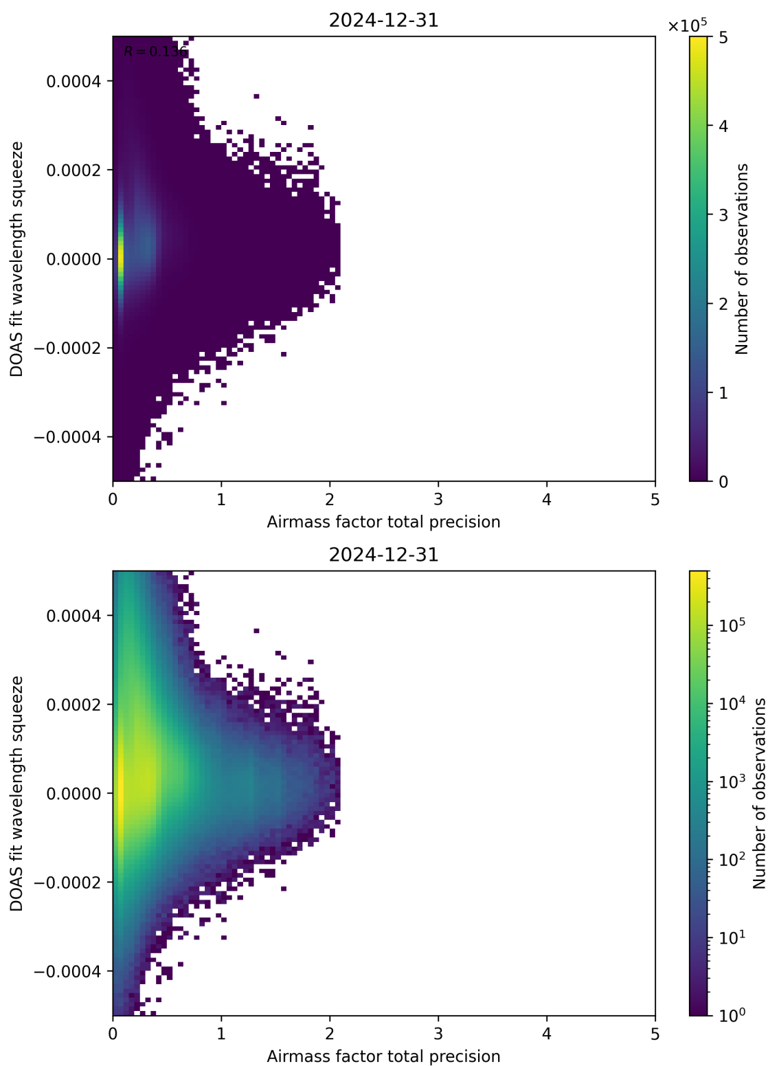
Figure 107: Scatter density plot of “Airmass factor total precision” against “DOAS fit wavelength squeeze” for 2024-12-30 to 2025-01-01.
