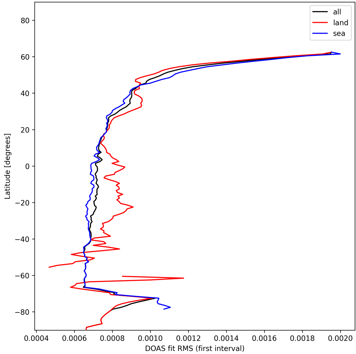
Figure 32: Zonal average of “DOAS fit RMS (first interval)” for 2024-12-30 to 2025-01-01.
