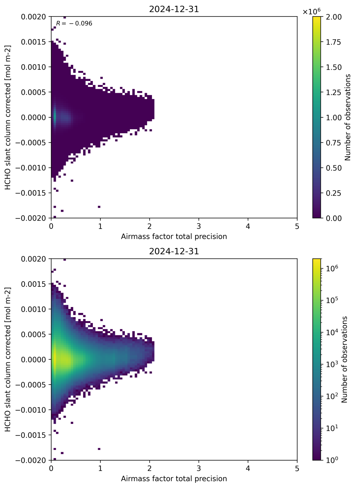
Figure 109: Scatter density plot of “Airmass factor total precision” against “HCHO slant column corrected” for 2024-12-30 to 2025-01-01.
