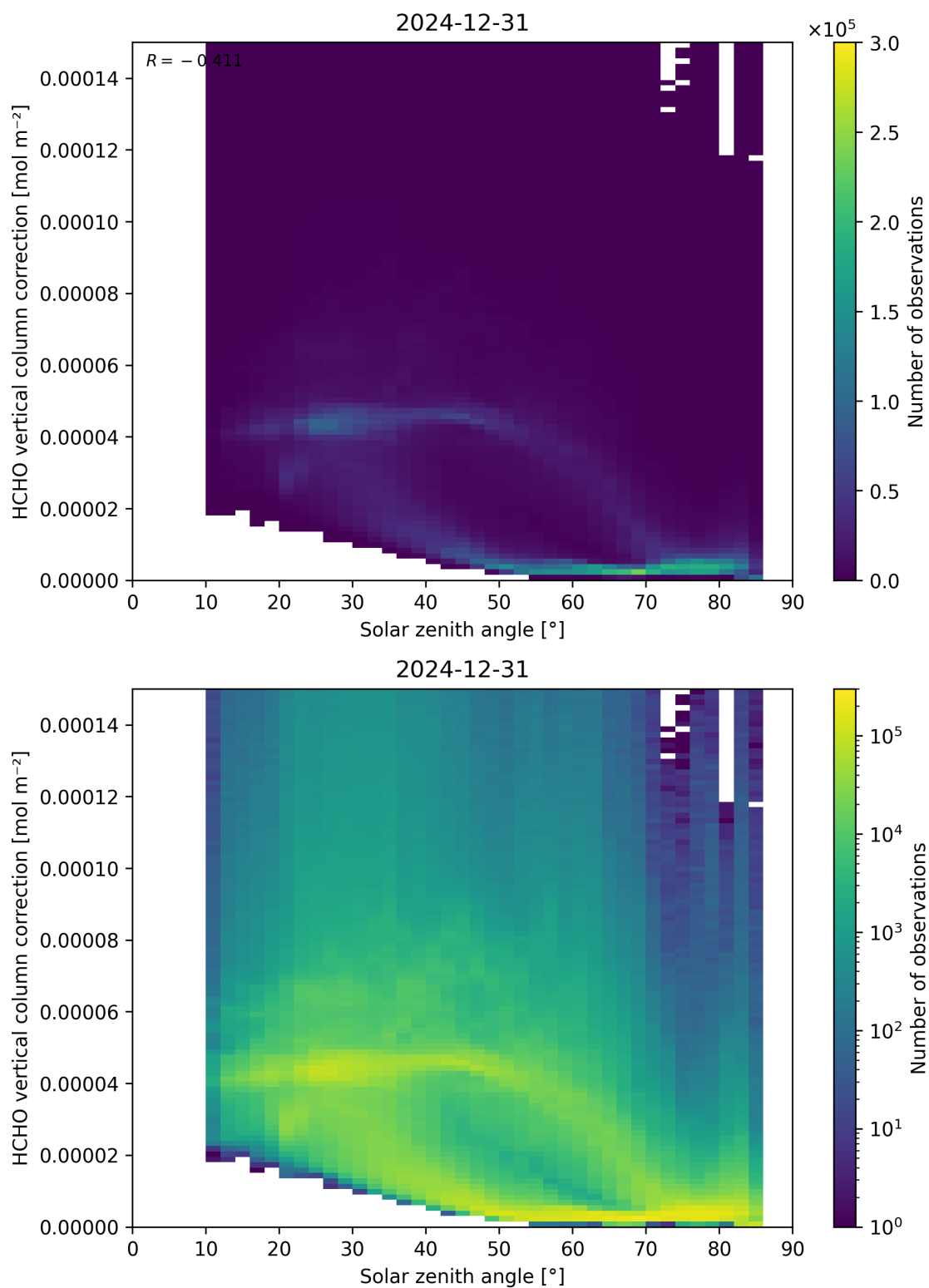
Figure 178: Scatter density plot of “Solar zenith angle” against “HCHO vertical column correction” for 2024-12-30 to 2025-01-01.
