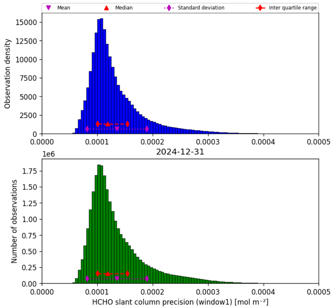
Figure 39: Histogram of “HCHO slant column precision (window1)” for 2024-12-30 to 2025-01-01
