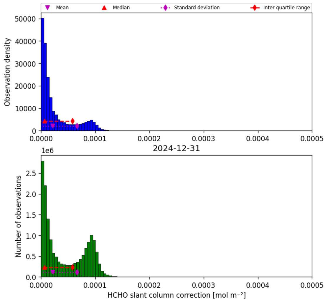
Figure 47: Histogram of “HCHO slant column correction” for 2024-12-30 to 2025-01-01
