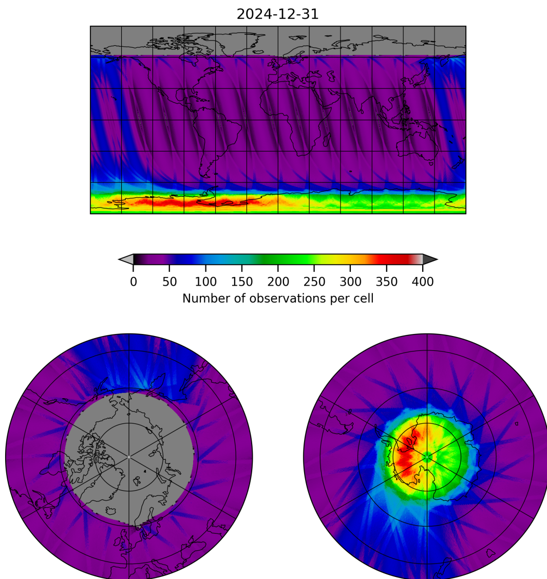
Figure 19: Map of the number of observations for 2024-12-30 to 2025-01-01
