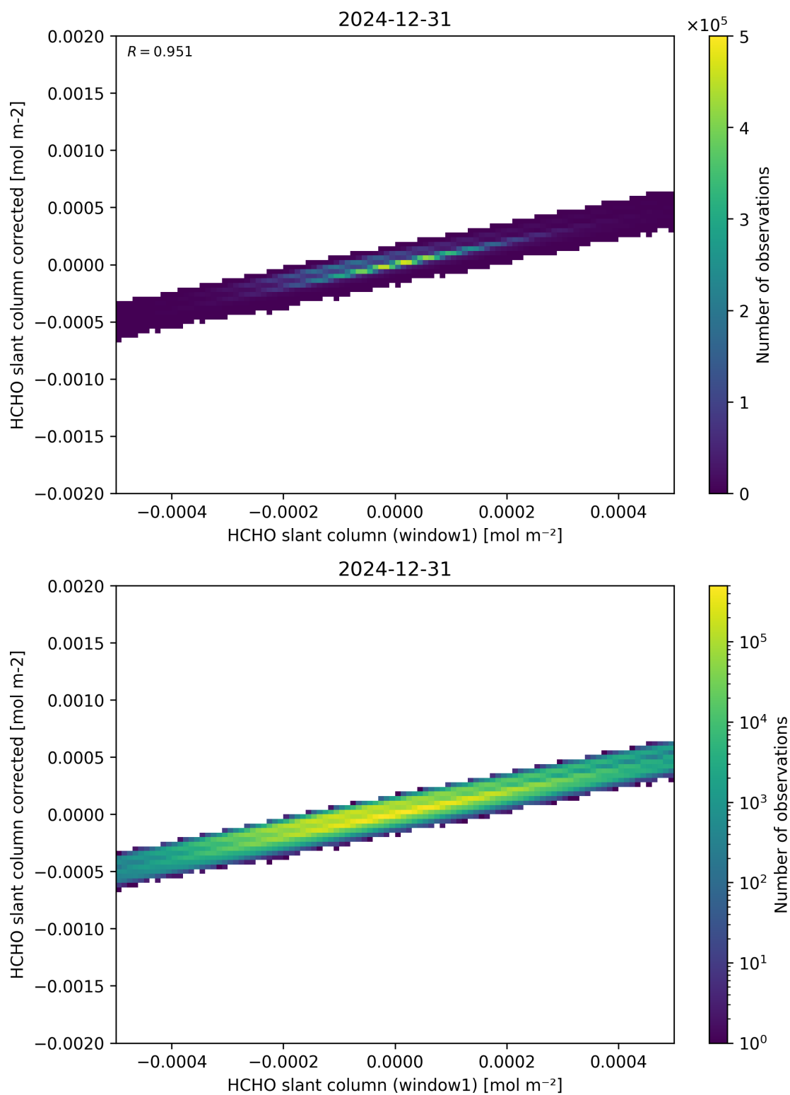
Figure 82: Scatter density plot of “HCHO slant column (window1)” against “HCHO slant column corrected” for 2024-12-30 to 2025-01-01.
