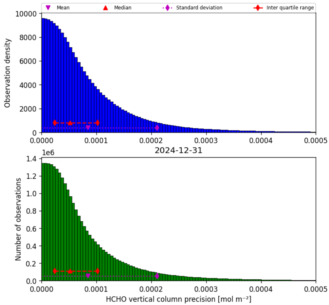
Figure 36: Histogram of “HCHO vertical column precision” for 2024-12-30 to 2025-01-01
