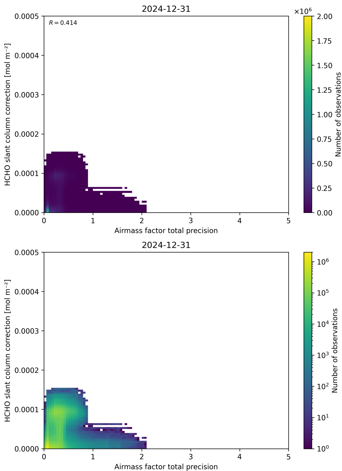
Figure 110: Scatter density plot of “Airmass factor total precision” against “HCHO slant column correction” for 2024-12-30 to 2025-01-01.
