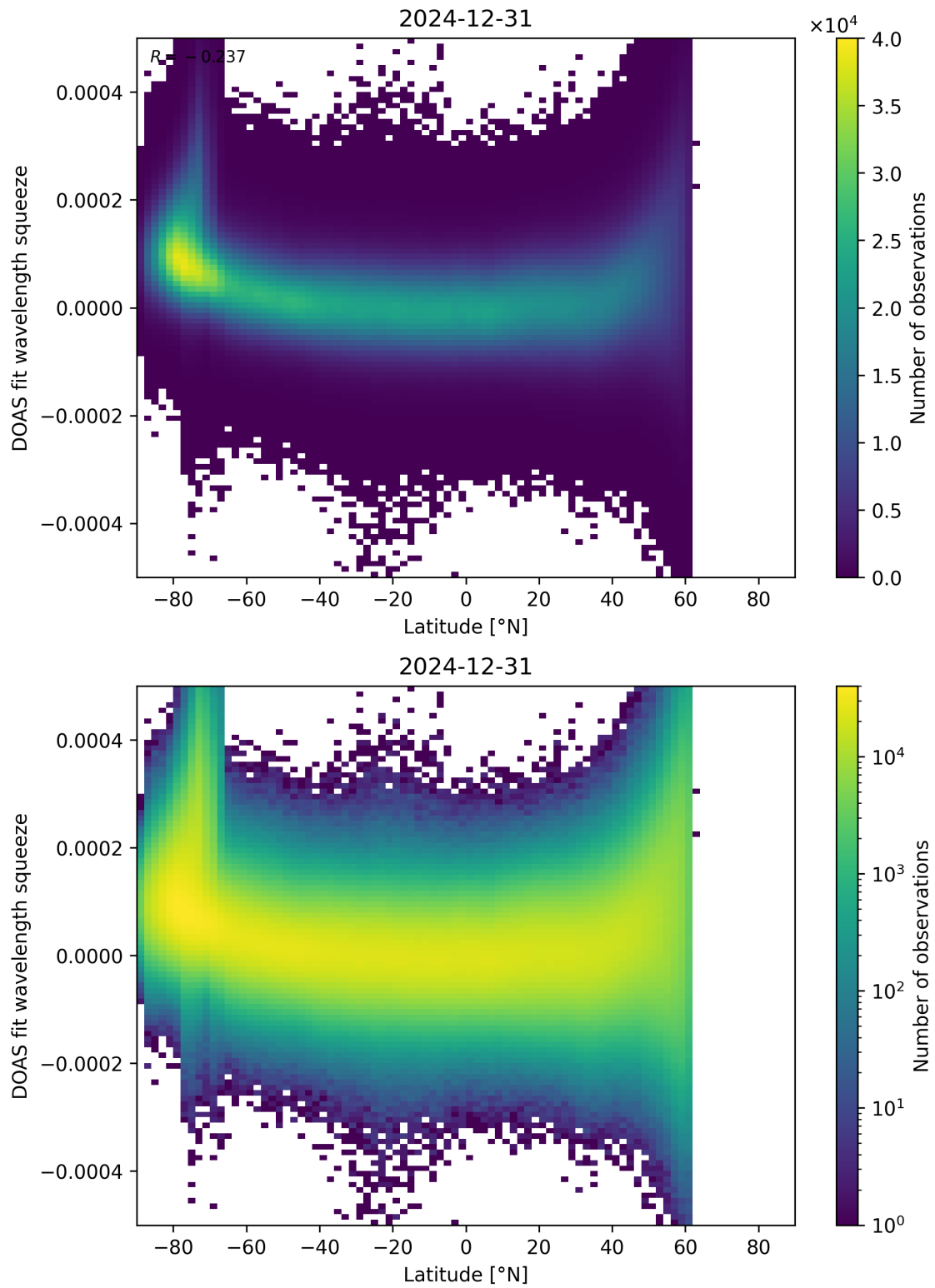
Figure 155: Scatter density plot of “Latitude” against “DOAS fit wavelength squeeze” for 2024-12-30 to 2025-01-01.
