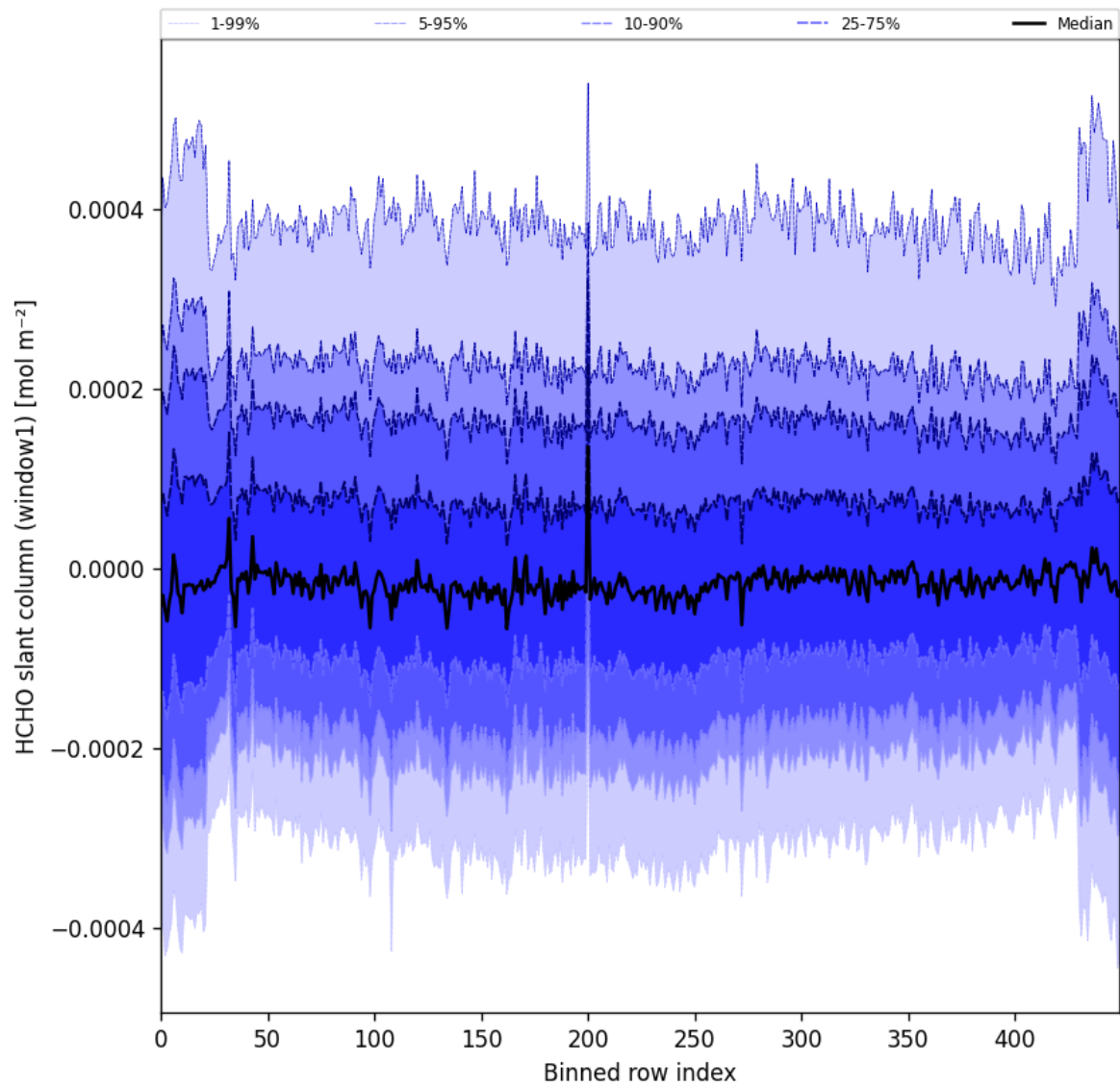
Figure 52: Along track statistics of “HCHO slant column (window1)” for 2024-12-30 to 2025-01-01
