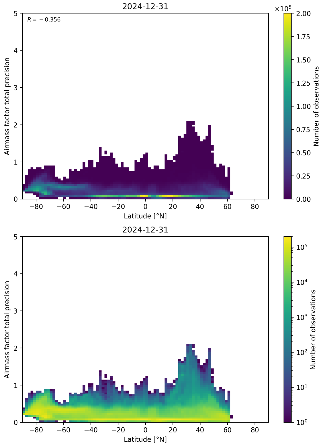
Figure 162: Scatter density plot of “Latitude” against “Airmass factor total precision” for 2024-12-30 to 2025-01-01.
