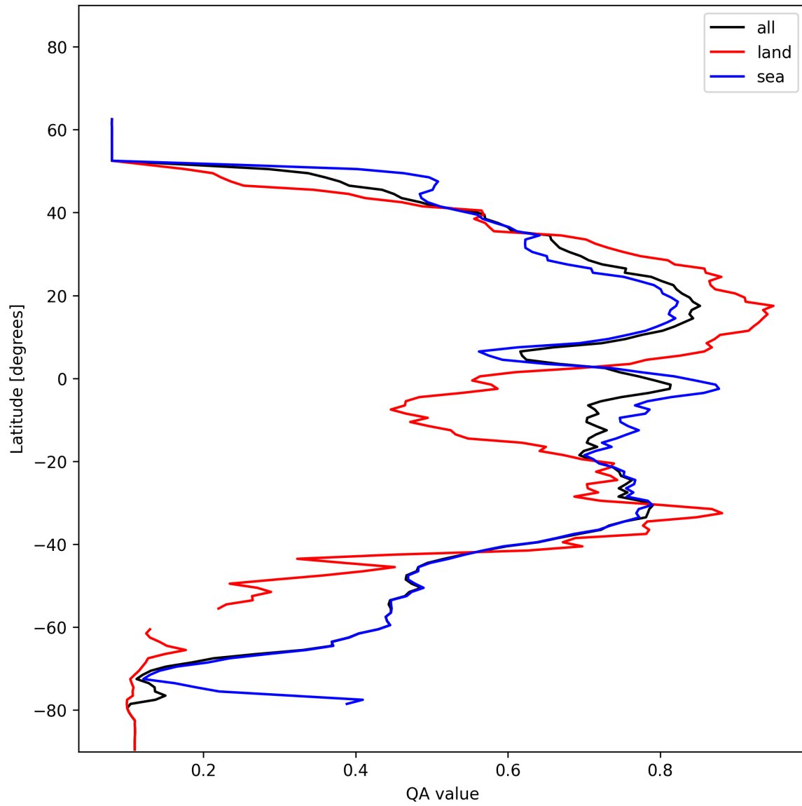
Figure 20: Zonal average of “QA value” for 2024-12-30 to 2025-01-01.
