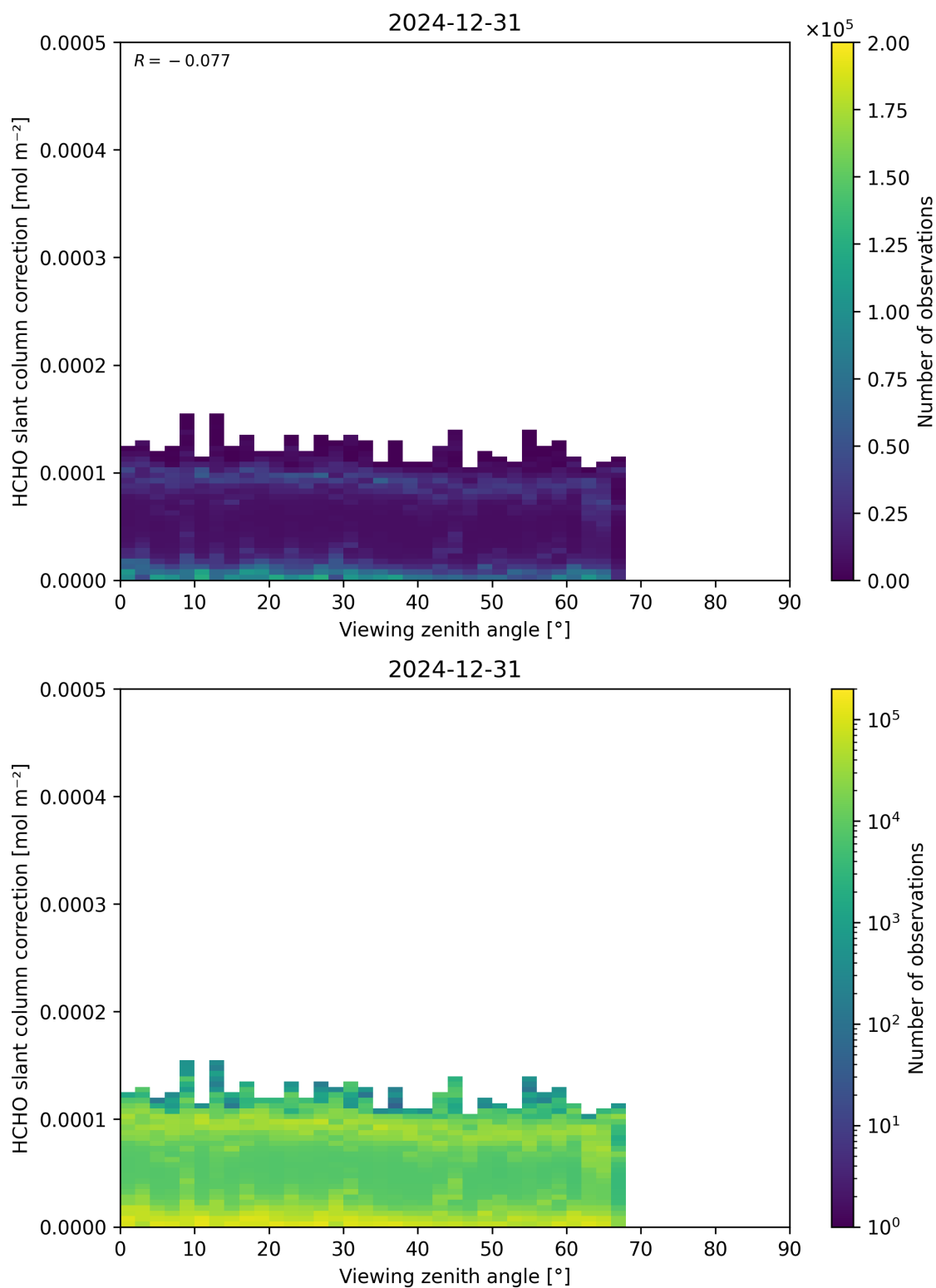
Figure 187: Scatter density plot of “Viewing zenith angle” against “HCHO slant column correction” for 2024-12-30 to 2025-01-01.
