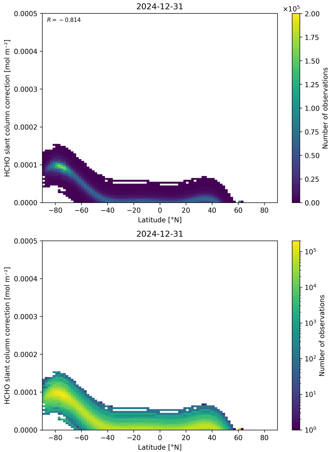
Figure 158: Scatter density plot of “Latitude” against “HCHO slant column correction” for 2024-12-30 to 2025-01-01.
