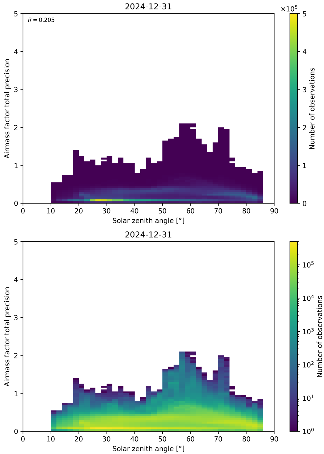
Figure 176: Scatter density plot of “Solar zenith angle” against “Airmass factor total precision” for 2024-12-30 to 2025-01-01.
