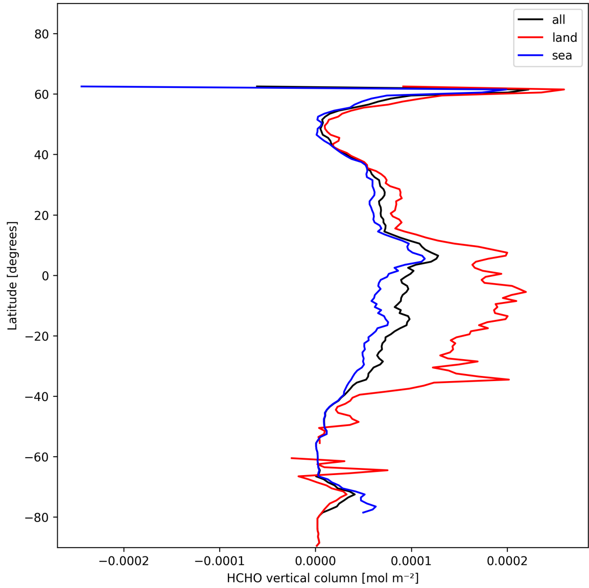
Figure 21: Zonal average of “HCHO vertical column” for 2024-12-30 to 2025-01-01.
