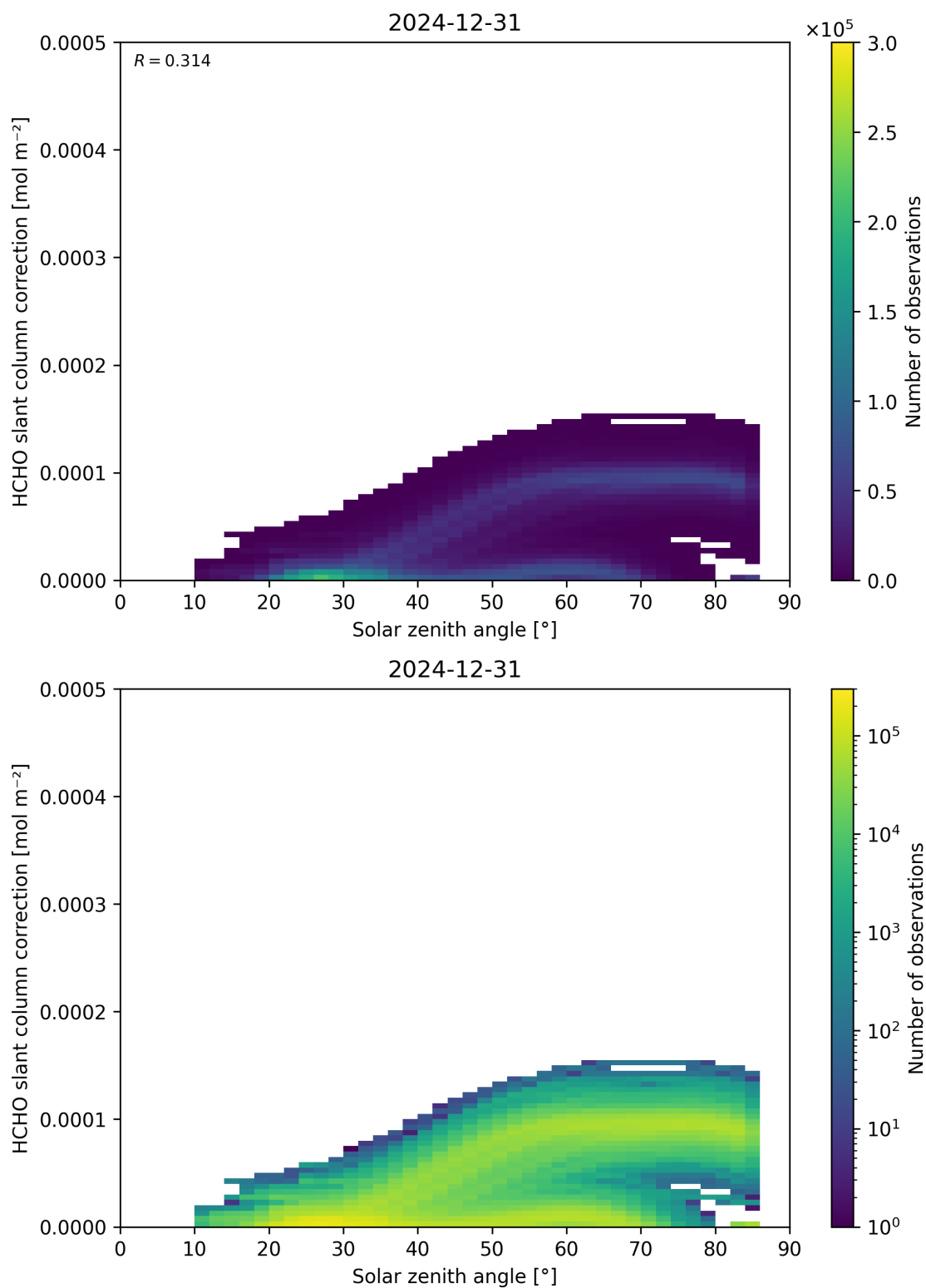
Figure 172: Scatter density plot of “Solar zenith angle” against “HCHO slant column correction” for 2024-12-30 to 2025-01-01.
