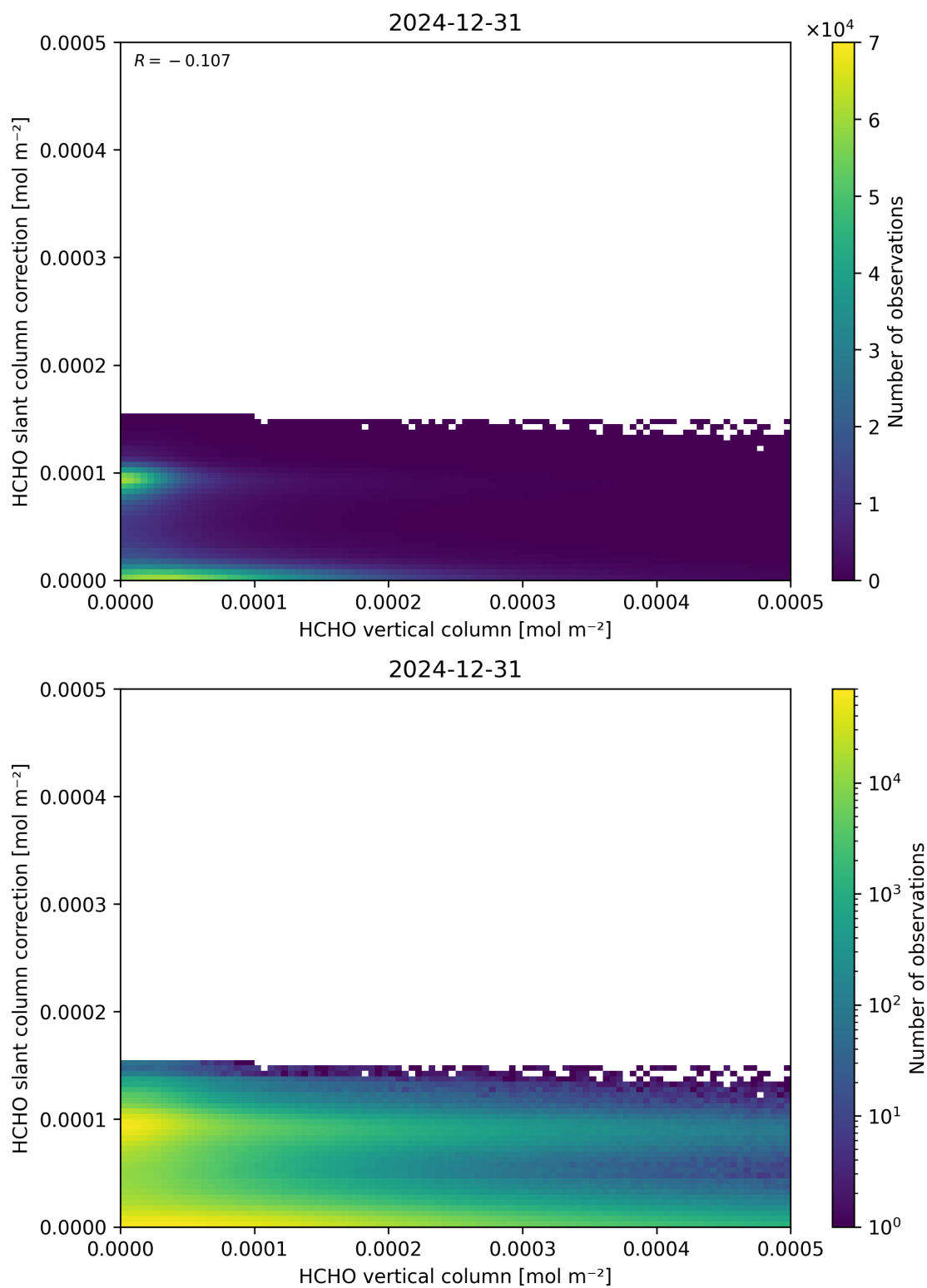
Figure 128: Scatter density plot of “HCHO vertical column” against “HCHO slant column correction” for 2024-12-30 to 2025-01-01.
