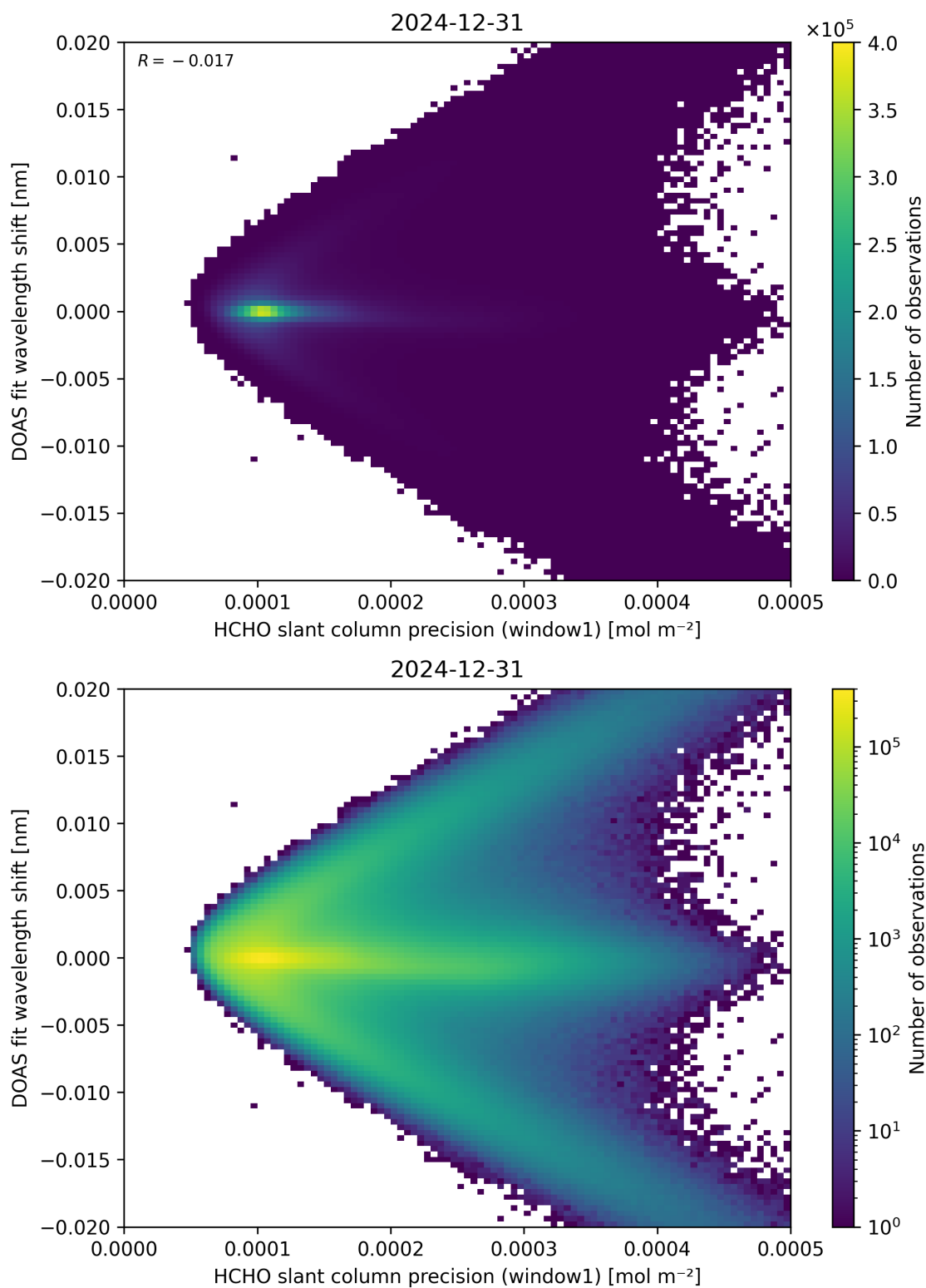
Figure 89: Scatter density plot of “HCHO slant column precision (window1)” against “DOAS fit wavelength shift” for 2024-12-30 to 2025-01-01.
