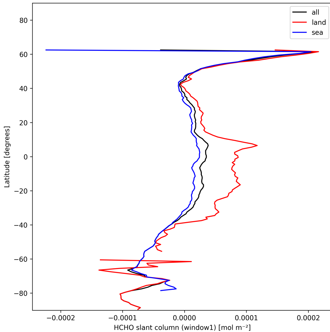
Figure 24: Zonal average of “HCHO slant column (window1)” for 2024-12-30 to 2025-01-01.
