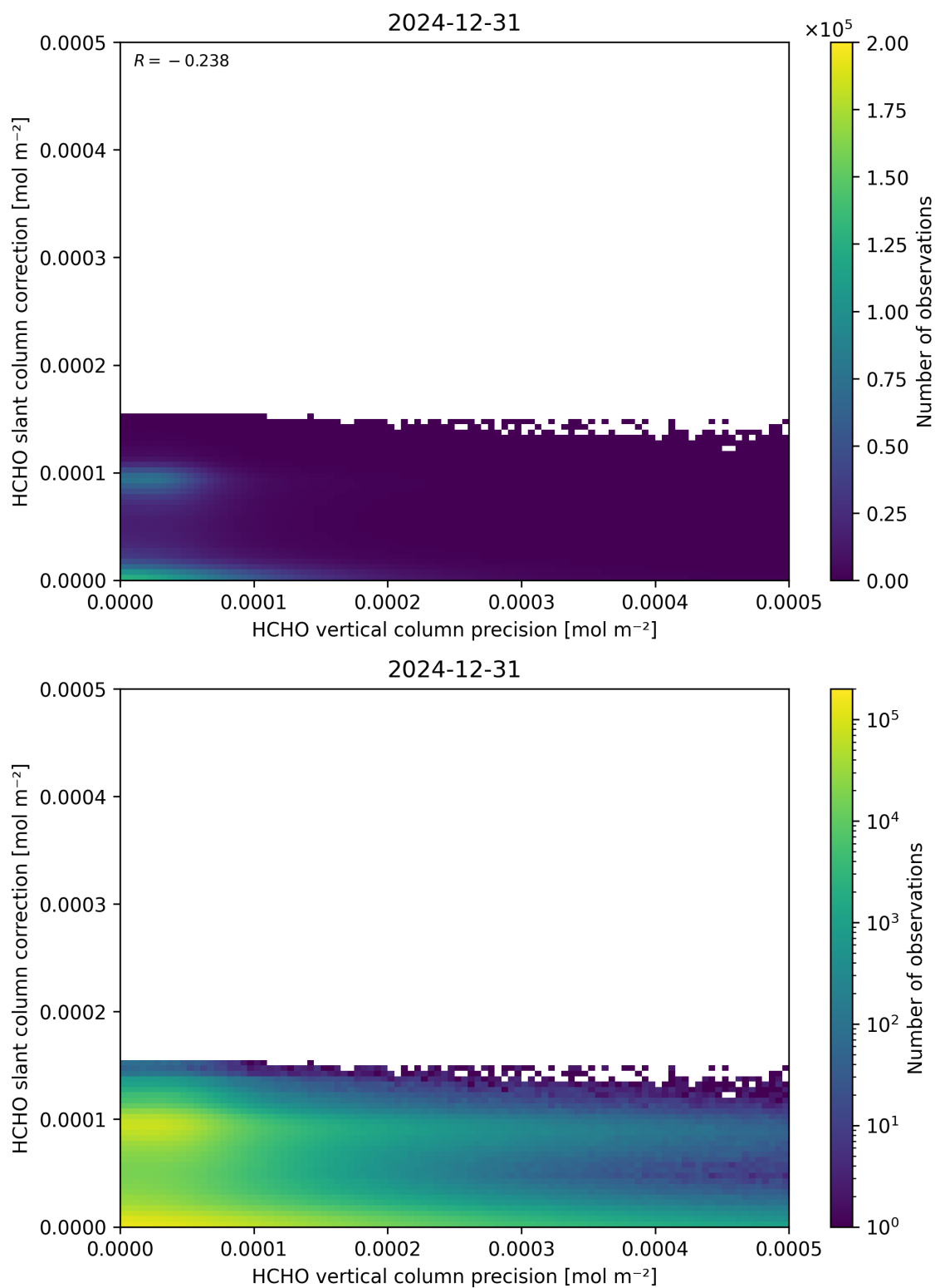
Figure 141: Scatter density plot of “HCHO vertical column precision” against “HCHO slant column correction” for 2024-12-30 to 2025-01-01.
