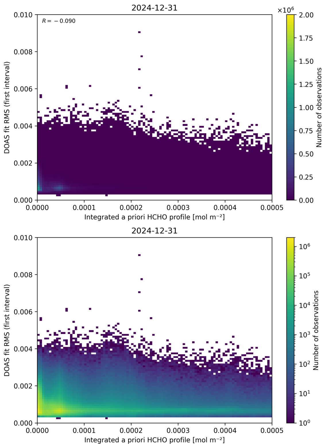
Figure 148: Scatter density plot of “Integrated a priori HCHO profile” against “DOAS fit RMS (first interval)” for 2024-12-30 to 2025-01-01.
