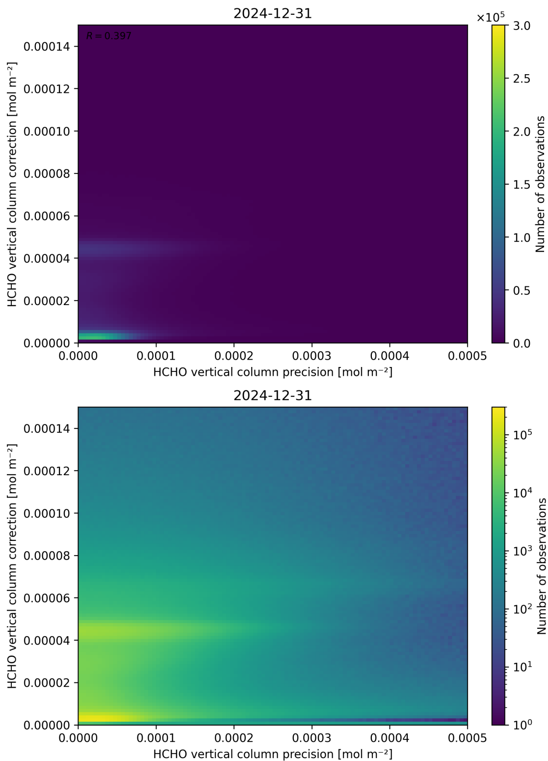
Figure 146: Scatter density plot of “HCHO vertical column precision” against “HCHO vertical column correction” for 2024-12-30 to 2025-01-01.
