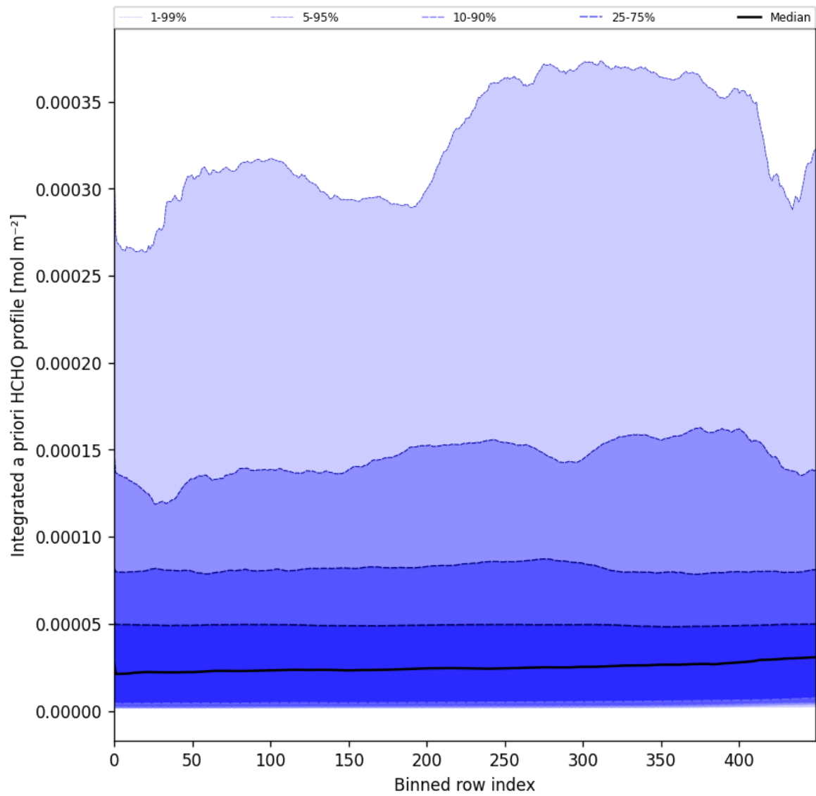
Figure 57: Along track statistics of “Integrated a priori HCHO profile” for 2024-12-30 to 2025-01-01
