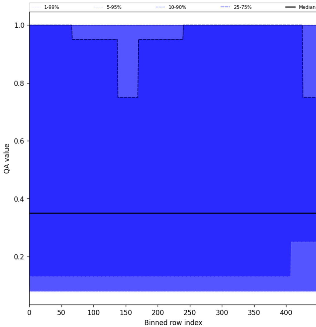
Figure 48: Along track statistics of “QA value” for 2024-12-30 to 2025-01-01
