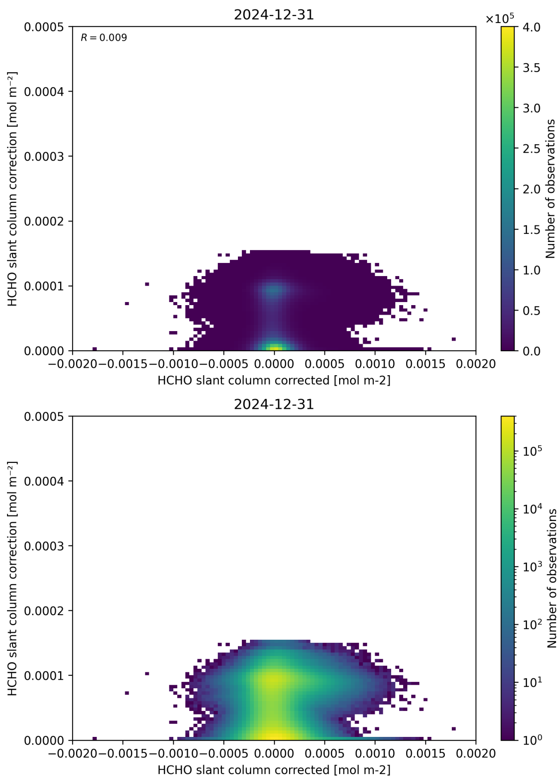
Figure 77: Scatter density plot of “HCHO slant column corrected” against “HCHO slant column correction” for 2024-12-30 to 2025-01-01.
