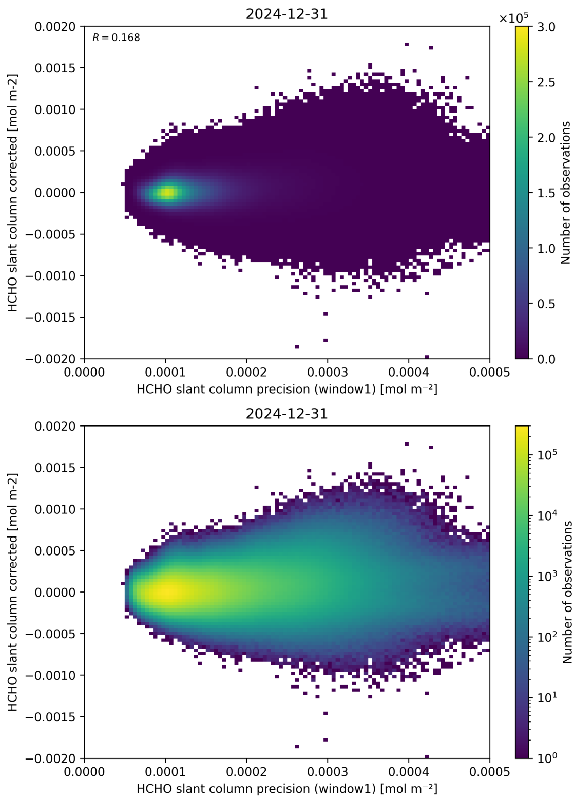
Figure 92: Scatter density plot of “HCHO slant column precision (window1)” against “HCHO slant column corrected” for 2024-12-30 to 2025-01-01.
