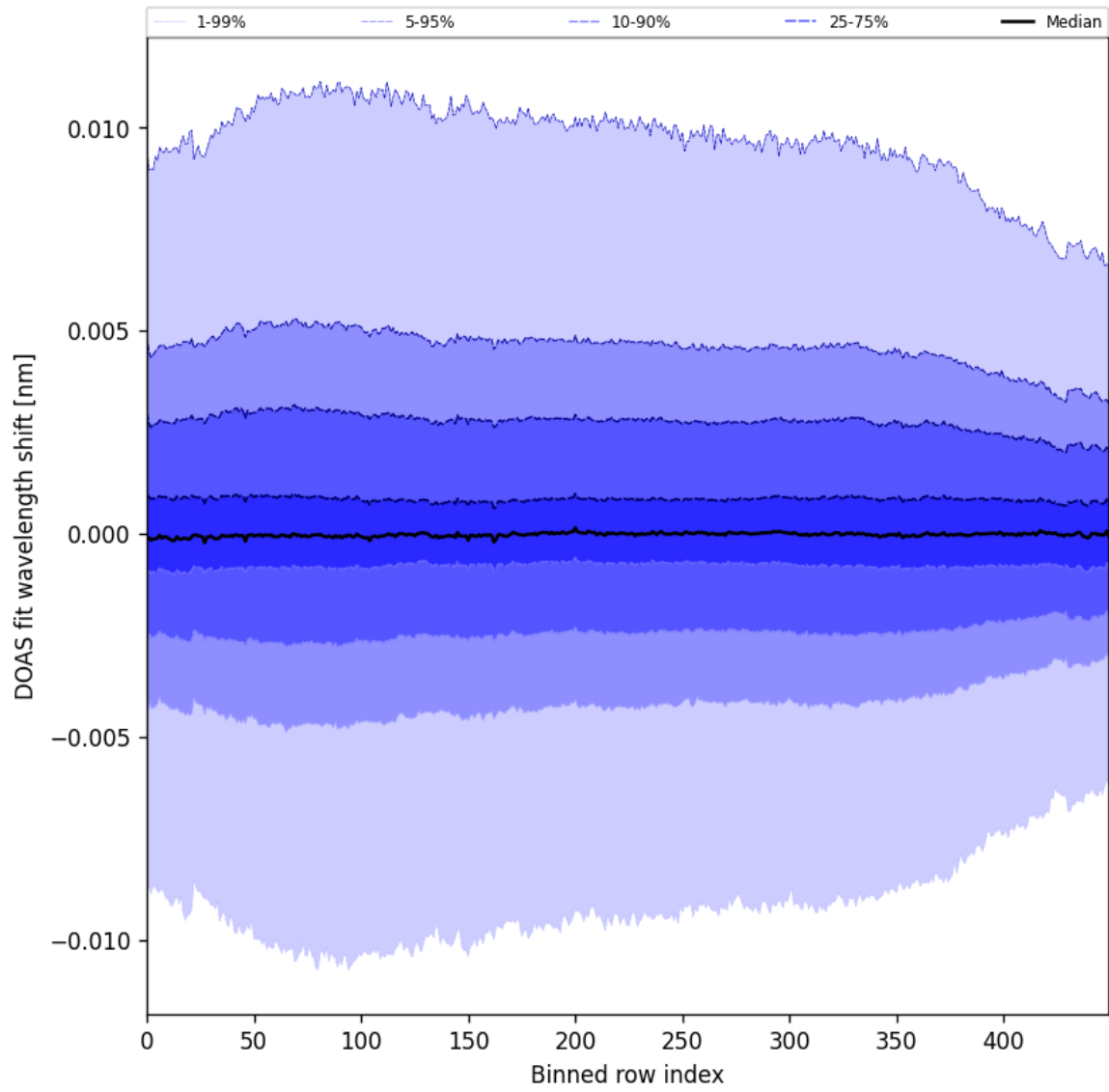
Figure 58: Along track statistics of “DOAS fit wavelength shift” for 2024-12-30 to 2025-01-01
