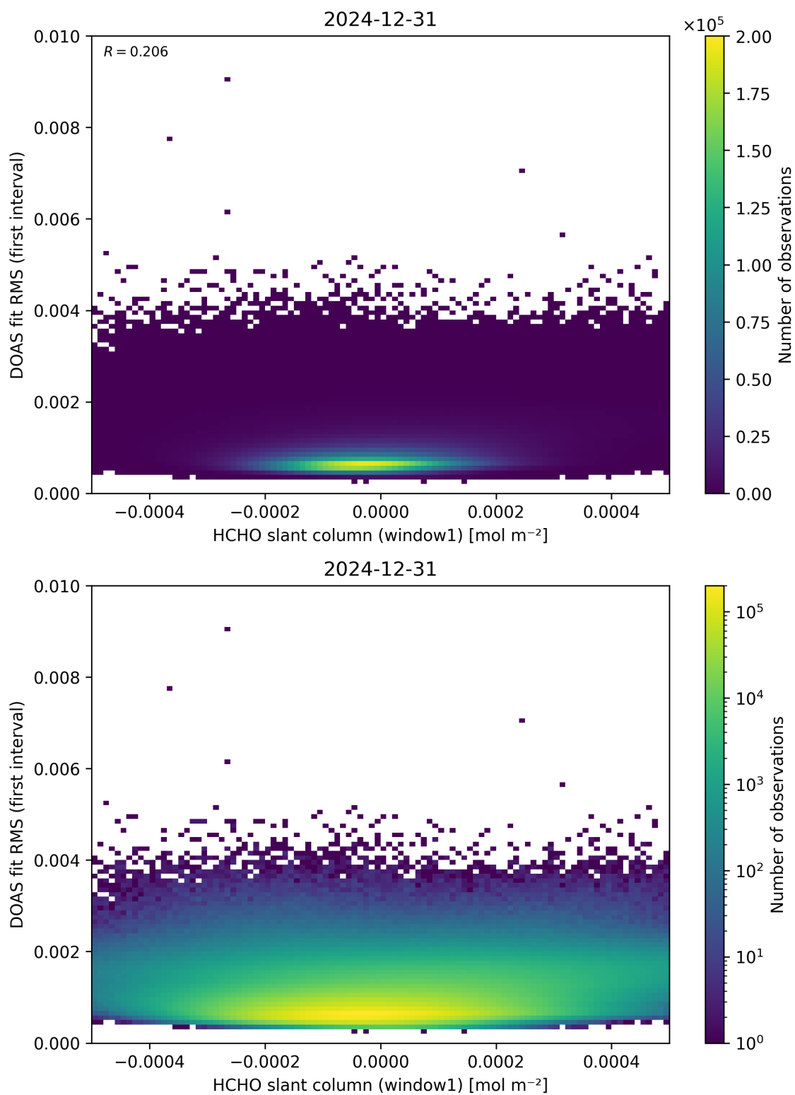
Figure 78: Scatter density plot of “HCHO slant column (window1)” against “DOAS fit RMS (first interval)” for 2024-12-30 to 2025-01-01.
