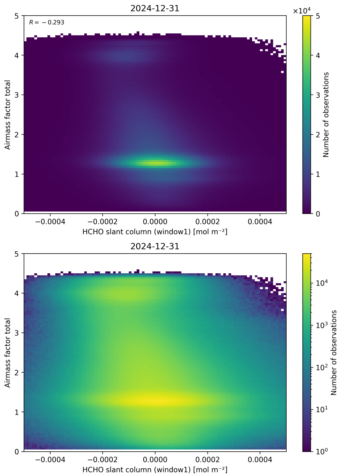
Figure 85: Scatter density plot of “HCHO slant column (window1)” against “Airmass factor total” for 2024-12-30 to 2025-01-01.
