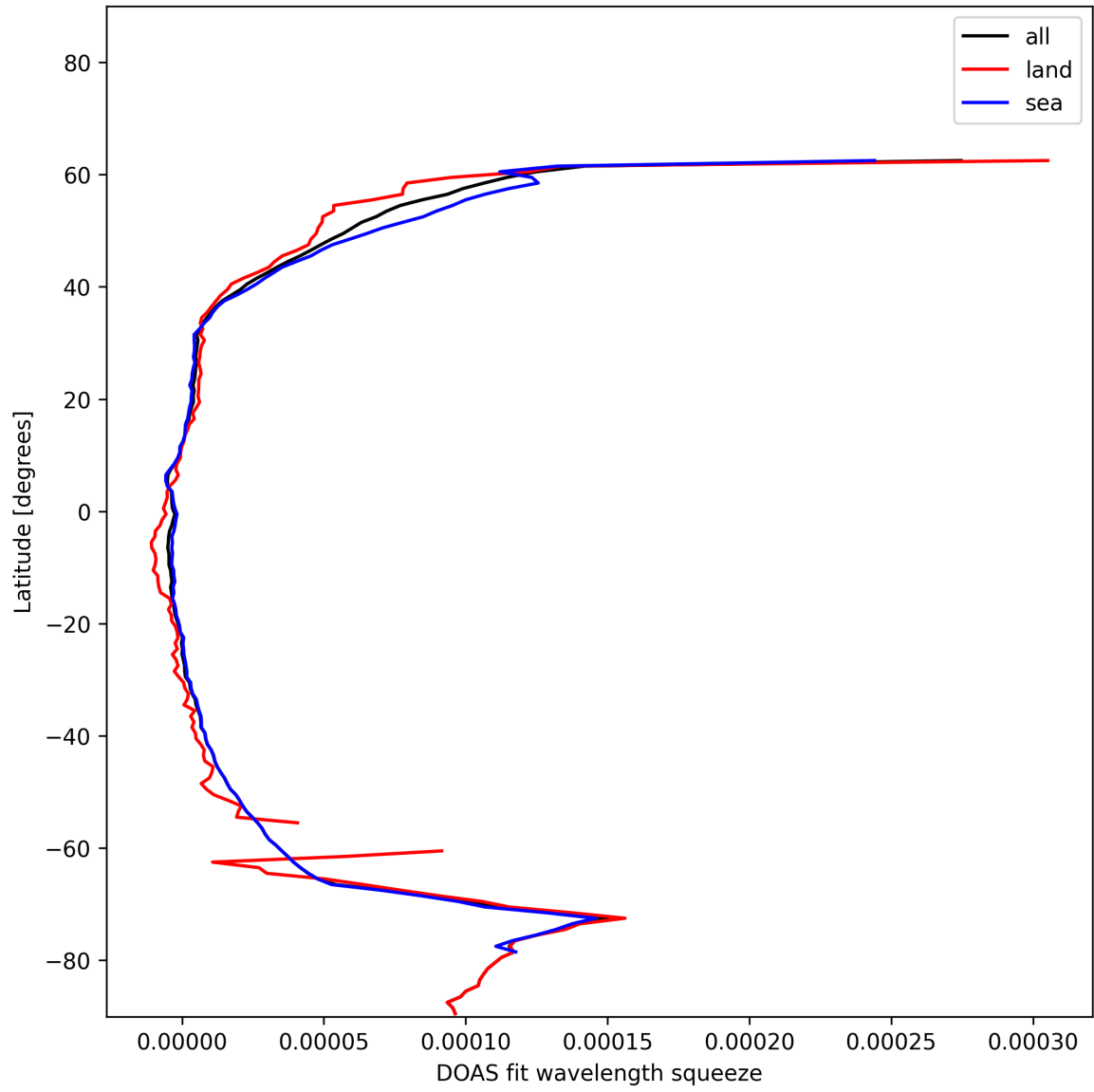
Figure 31: Zonal average of “DOAS fit wavelength squeeze” for 2024-12-30 to 2025-01-01.
