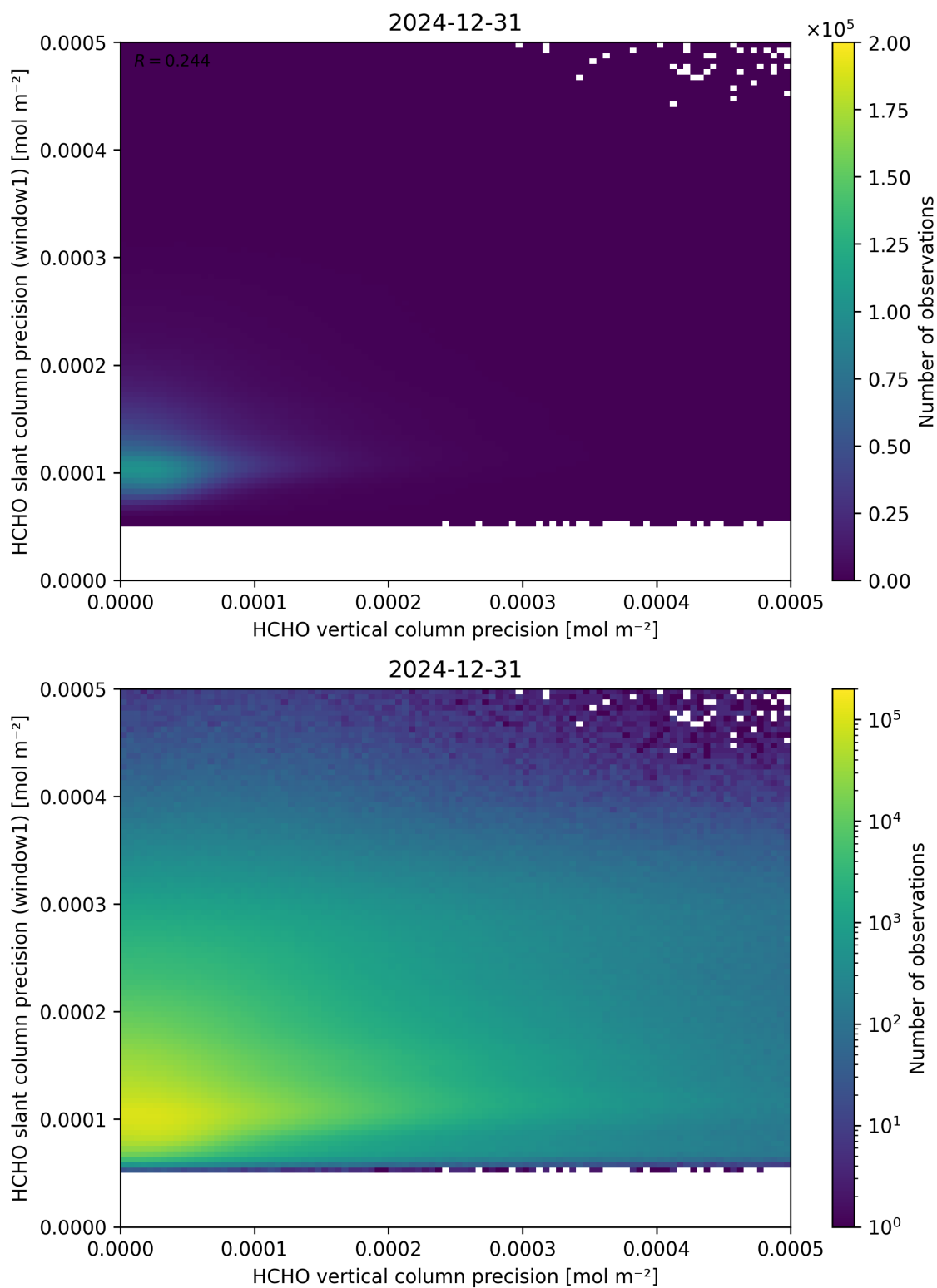
Figure 143: Scatter density plot of “HCHO vertical column precision” against “HCHO slant column precision (window1)” for 2024-12-30 to 2025-01-01.
