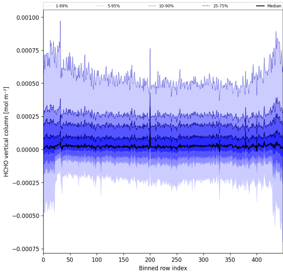
Figure 49: Along track statistics of “HCHO vertical column” for 2024-12-30 to 2025-01-01
