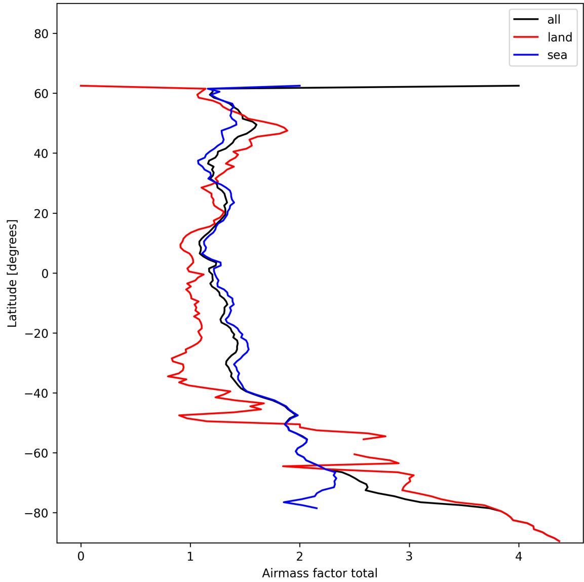
Figure 26: Zonal average of “Airmass factor total” for 2024-12-30 to 2025-01-01.
