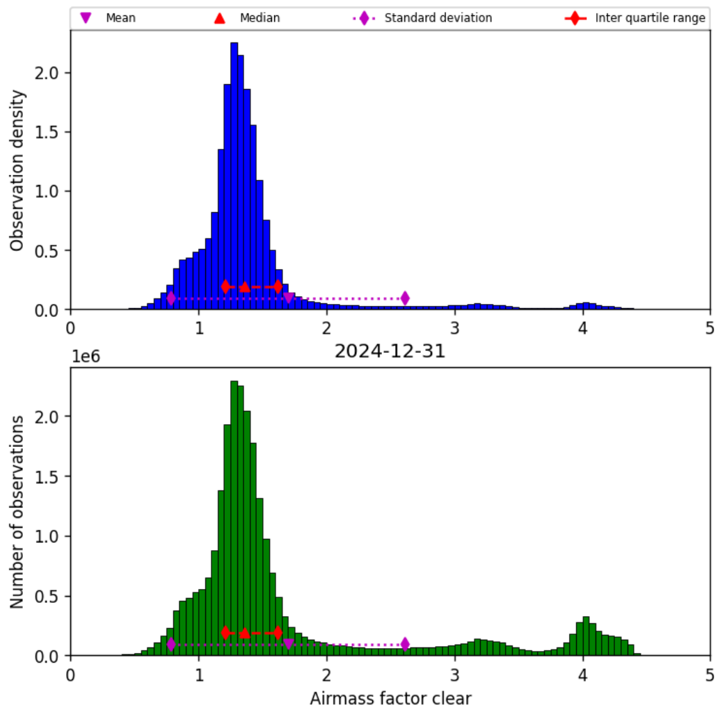
Figure 42: Histogram of “Airmass factor clear” for 2024-12-30 to 2025-01-01
