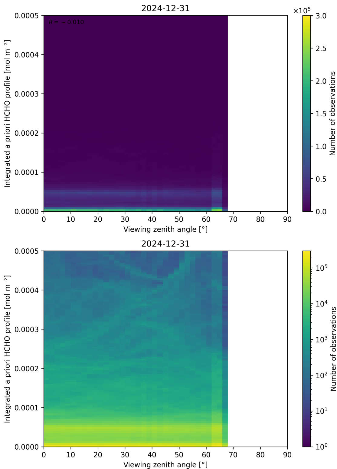
Figure 195: Scatter density plot of “Viewing zenith angle” against “Integrated a priori HCHO profile” for 2024-12-30 to 2025-01-01.
