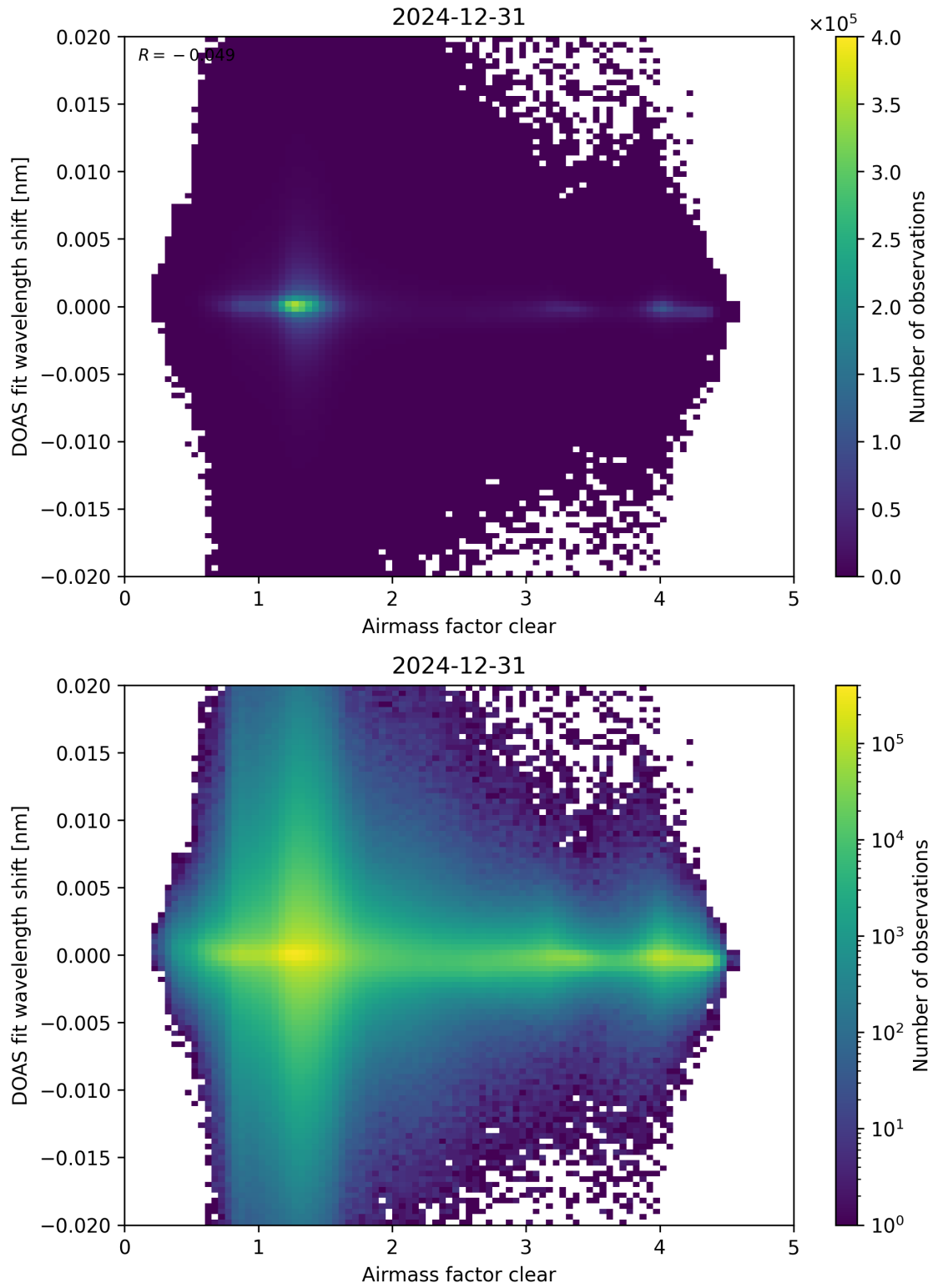
Figure 72: Scatter density plot of “Airmass factor clear” against “DOAS fit wavelength shift” for 2024-12-30 to 2025-01-01.
