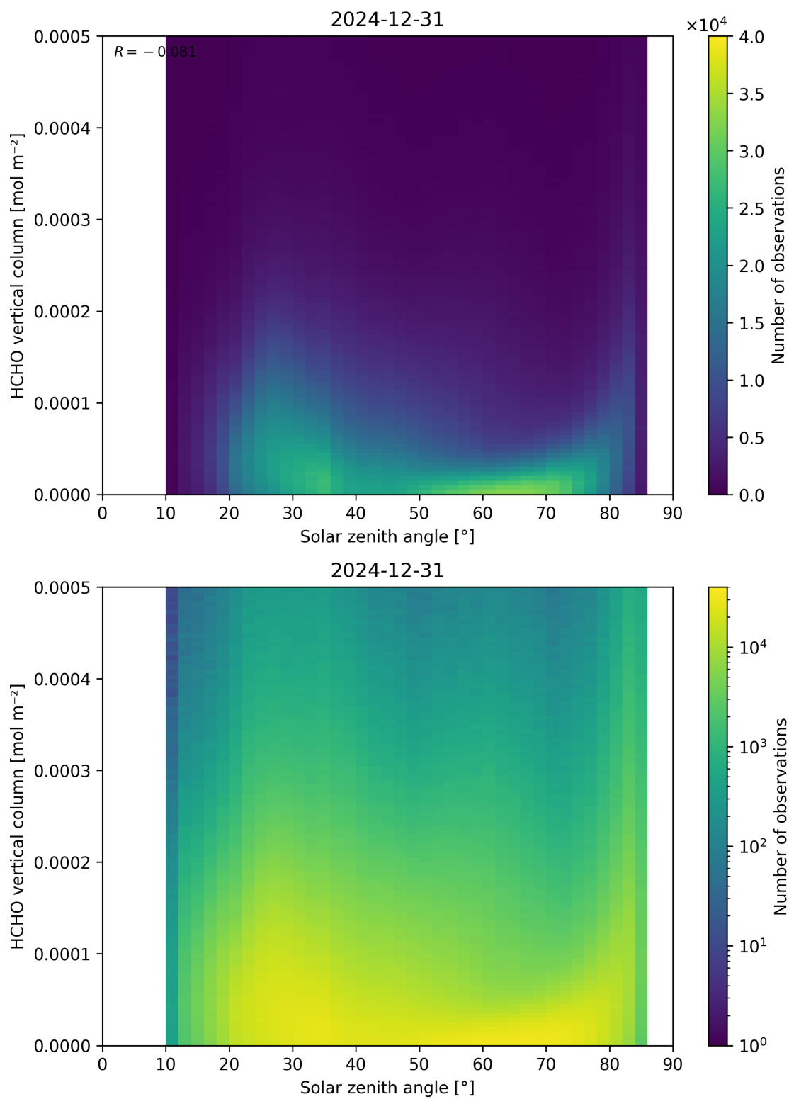
Figure 177: Scatter density plot of “Solar zenith angle” against “HCHO vertical column” for 2024-12-30 to 2025-01-01.
