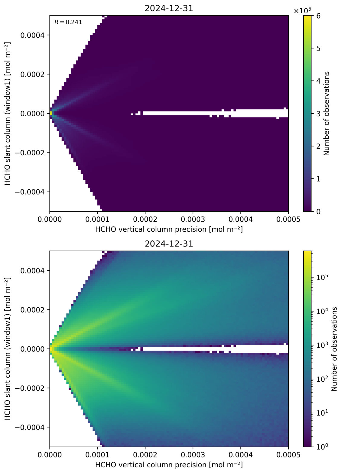
Figure 142: Scatter density plot of “HCHO vertical column precision” against “HCHO slant column (window1)” for 2024-12-30 to 2025-01-01.
