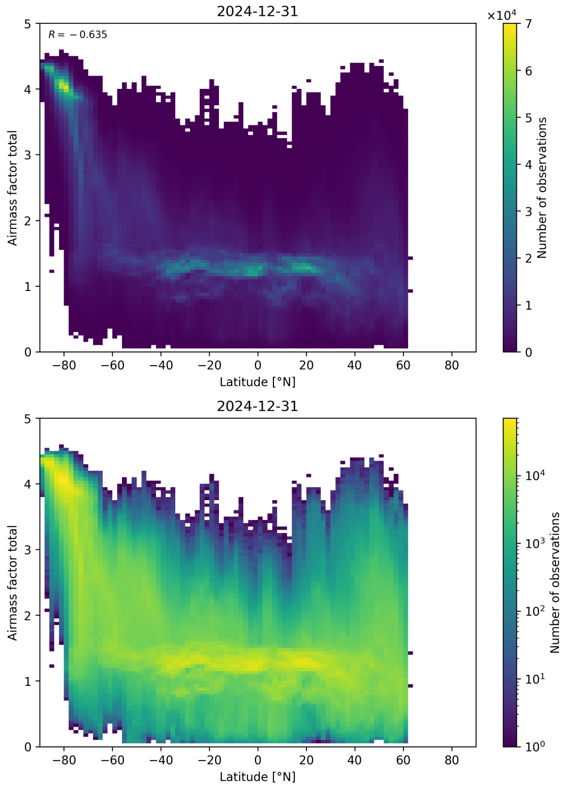
Figure 161: Scatter density plot of “Latitude” against “Airmass factor total” for 2024-12-30 to 2025-01-01.
