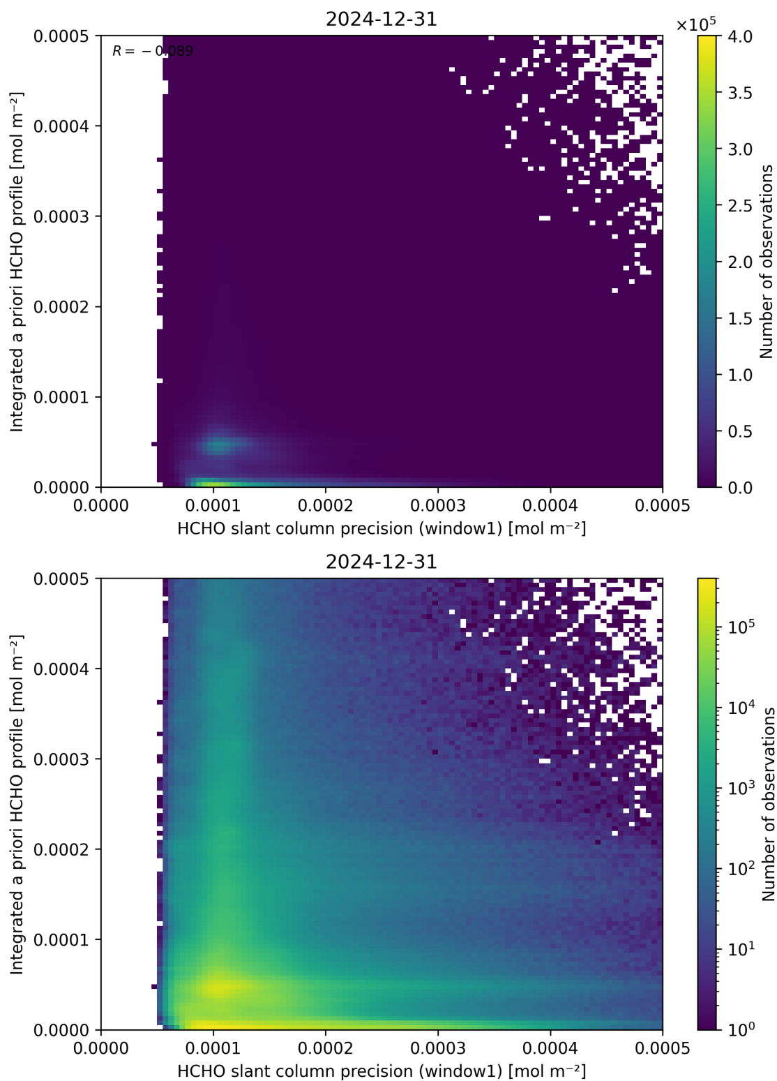
Figure 96: Scatter density plot of “HCHO slant column precision (window1)” against “Integrated a priori HCHO profile” for 2024-12-30 to 2025-01-01.
