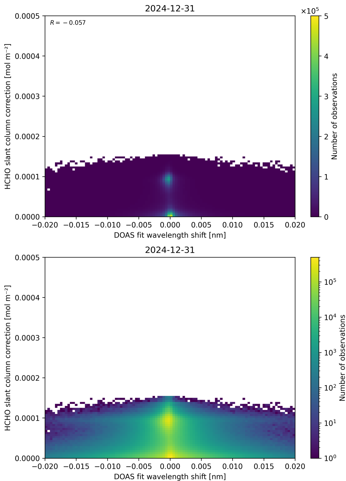
Figure 67: Scatter density plot of “DOAS fit wavelength shift” against “HCHO slant column correction” for 2024-12-30 to 2025-01-01.
