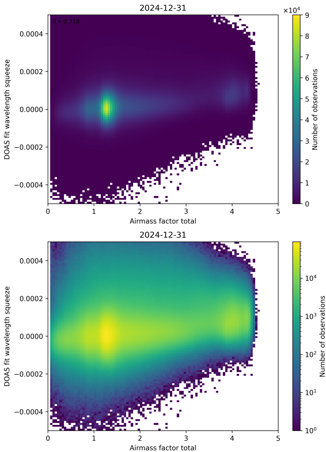
Figure 99: Scatter density plot of “Airmass factor total” against “DOAS fit wavelength squeeze” for 2024-12-30 to 2025-01-01.
