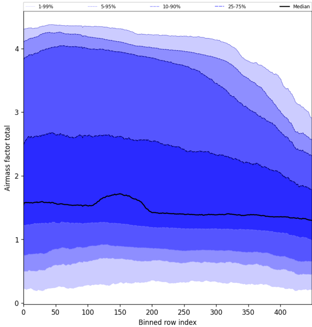
Figure 54: Along track statistics of “Airmass factor total” for 2024-12-30 to 2025-01-01
