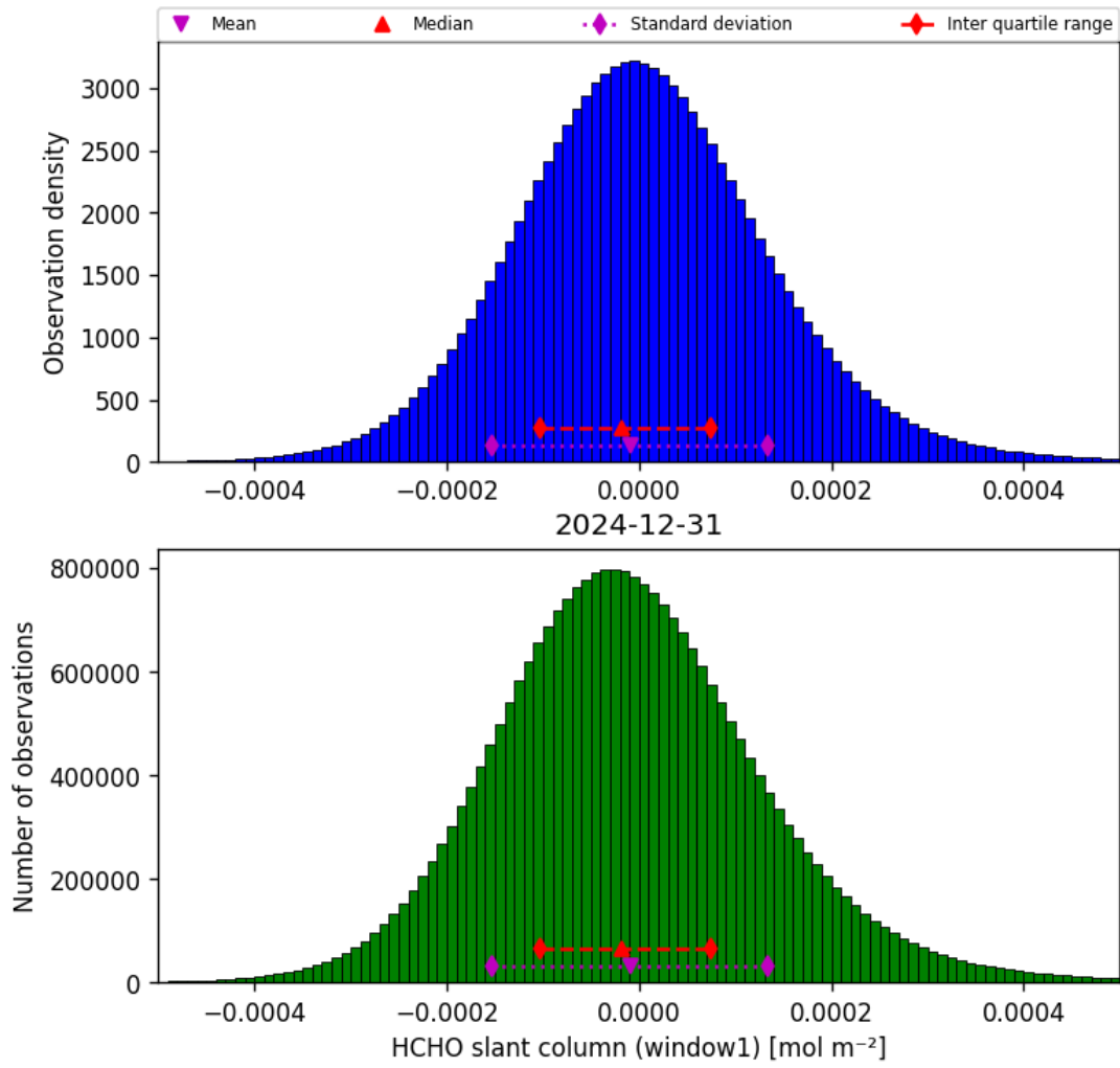
Figure 38: Histogram of “HCHO slant column (window1)” for 2024-12-30 to 2025-01-01
