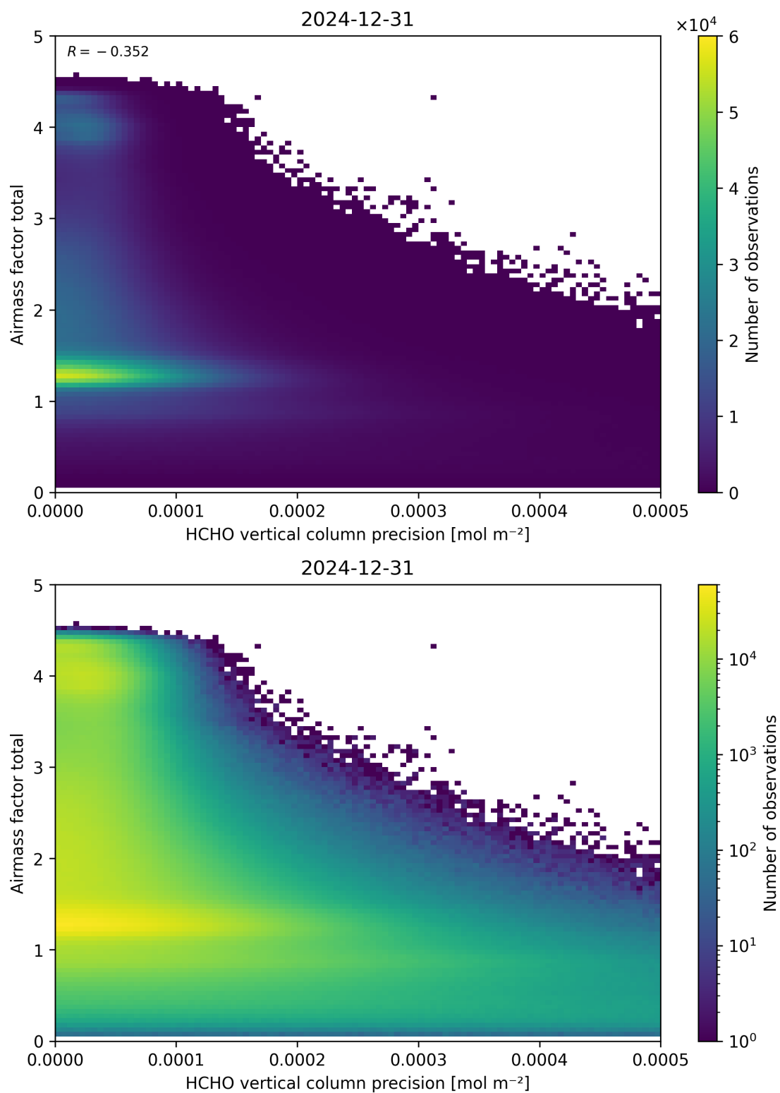
Figure 144: Scatter density plot of “HCHO vertical column precision” against “Airmass factor total” for 2024-12-30 to 2025-01-01.
