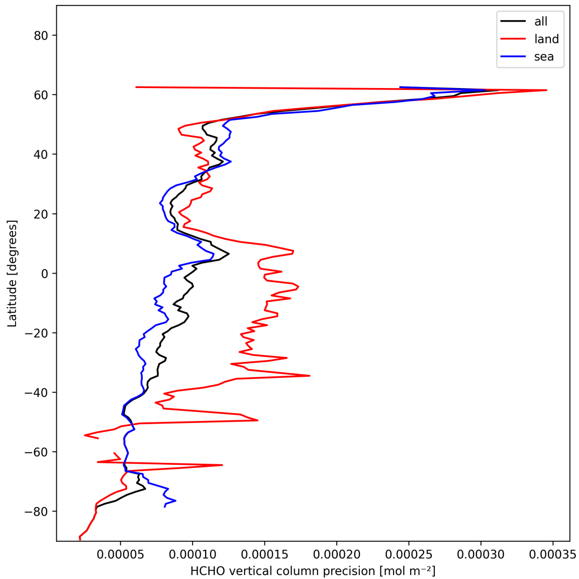
Figure 22: Zonal average of “HCHO vertical column precision” for 2024-12-30 to 2025-01-01.
