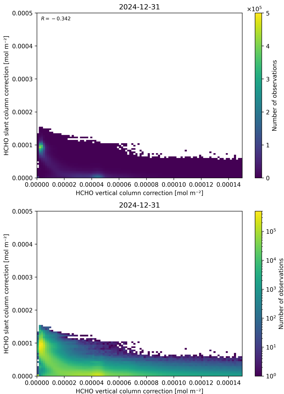
Figure 117: Scatter density plot of “HCHO vertical column correction” against “HCHO slant column correction” for 2024-12-30 to 2025-01-01.
