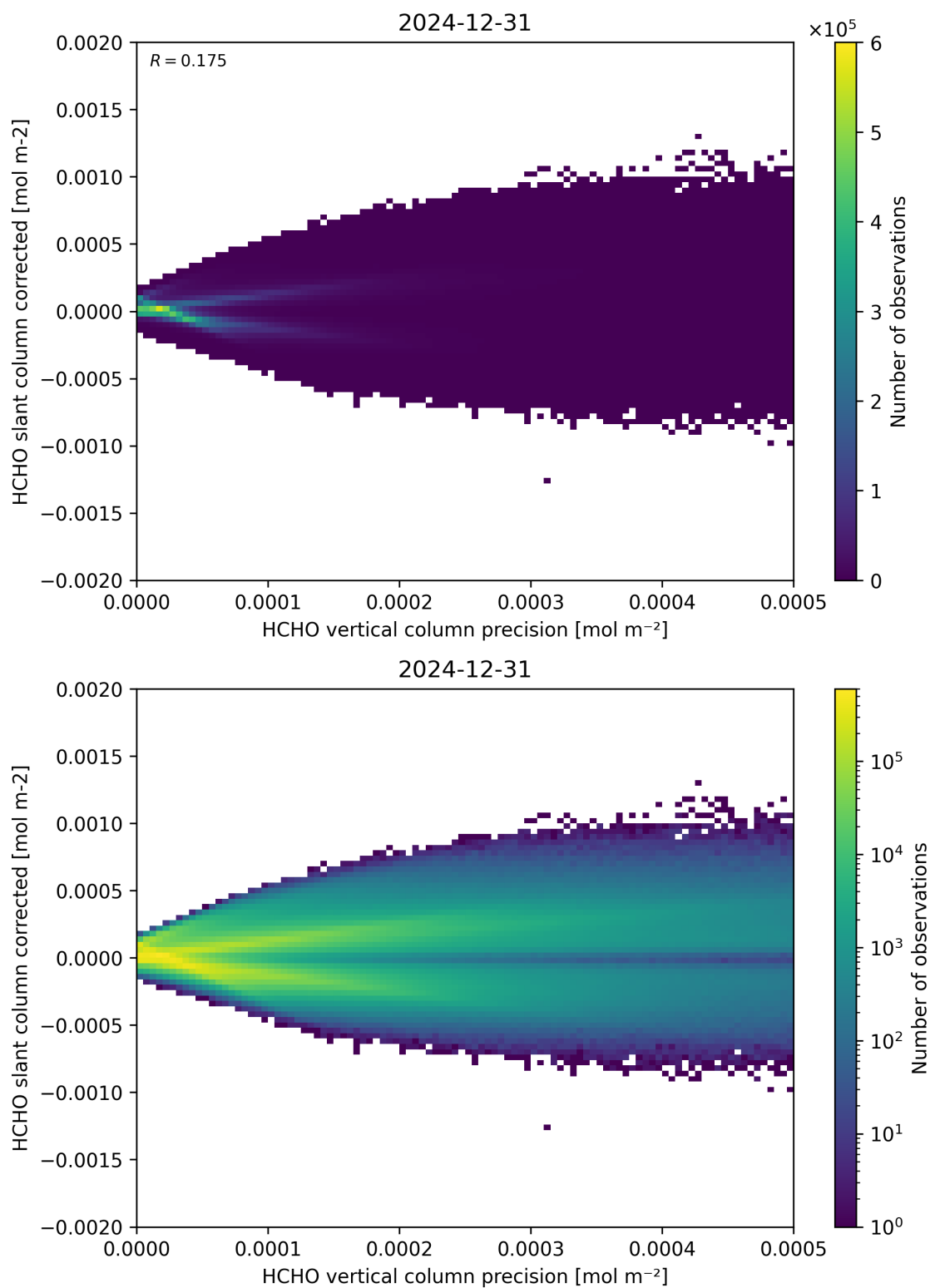
Figure 140: Scatter density plot of “HCHO vertical column precision” against “HCHO slant column corrected” for 2024-12-30 to 2025-01-01.
