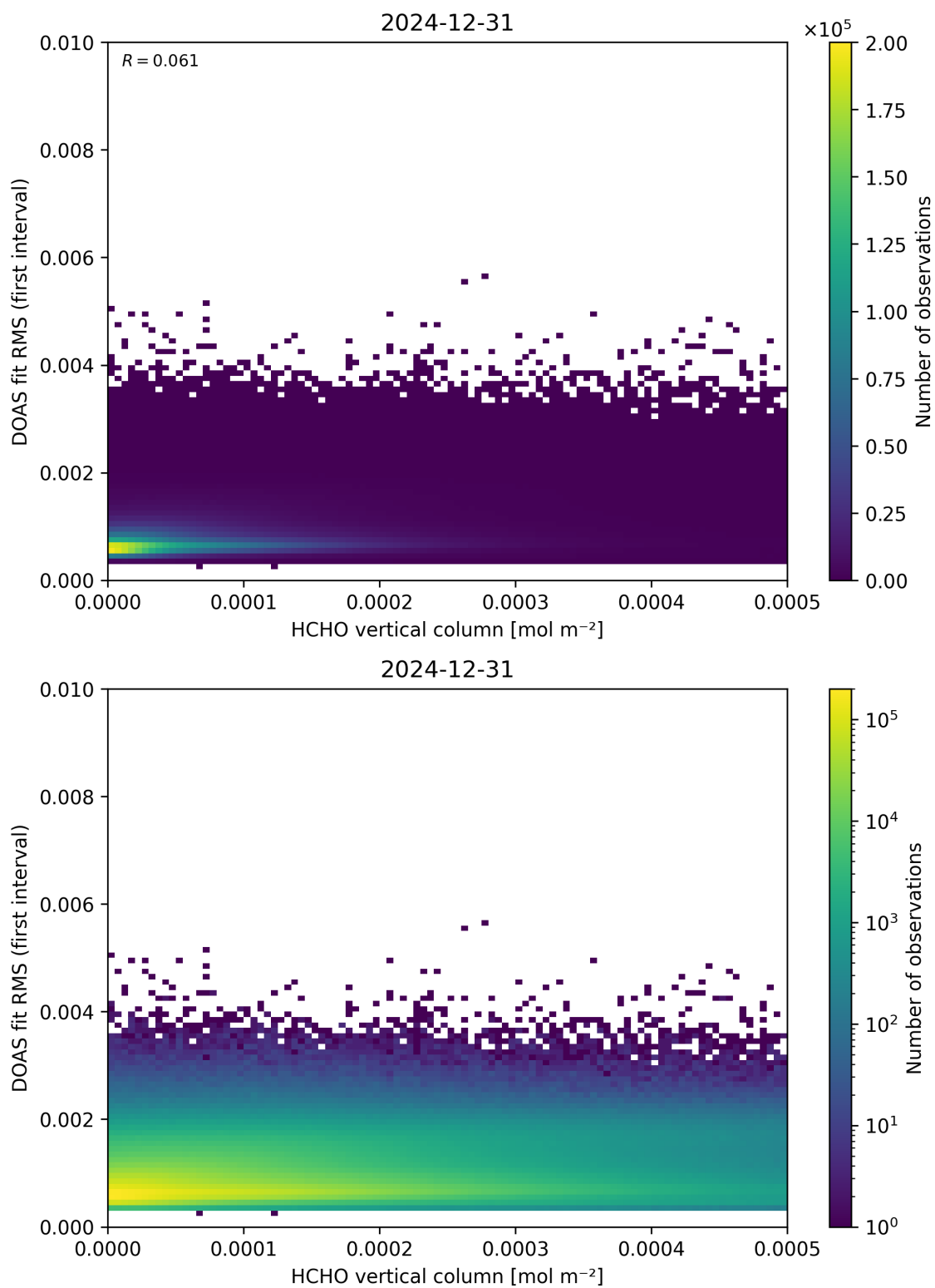
Figure 123: Scatter density plot of “HCHO vertical column” against “DOAS fit RMS (first interval)” for 2024-12-30 to 2025-01-01.
