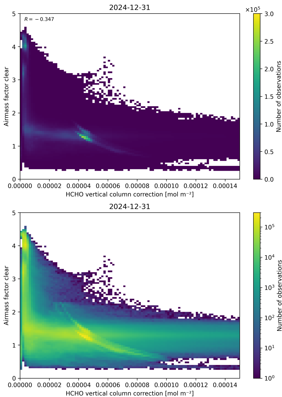
Figure 115: Scatter density plot of “HCHO vertical column correction” against “Airmass factor clear” for 2024-12-30 to 2025-01-01.
