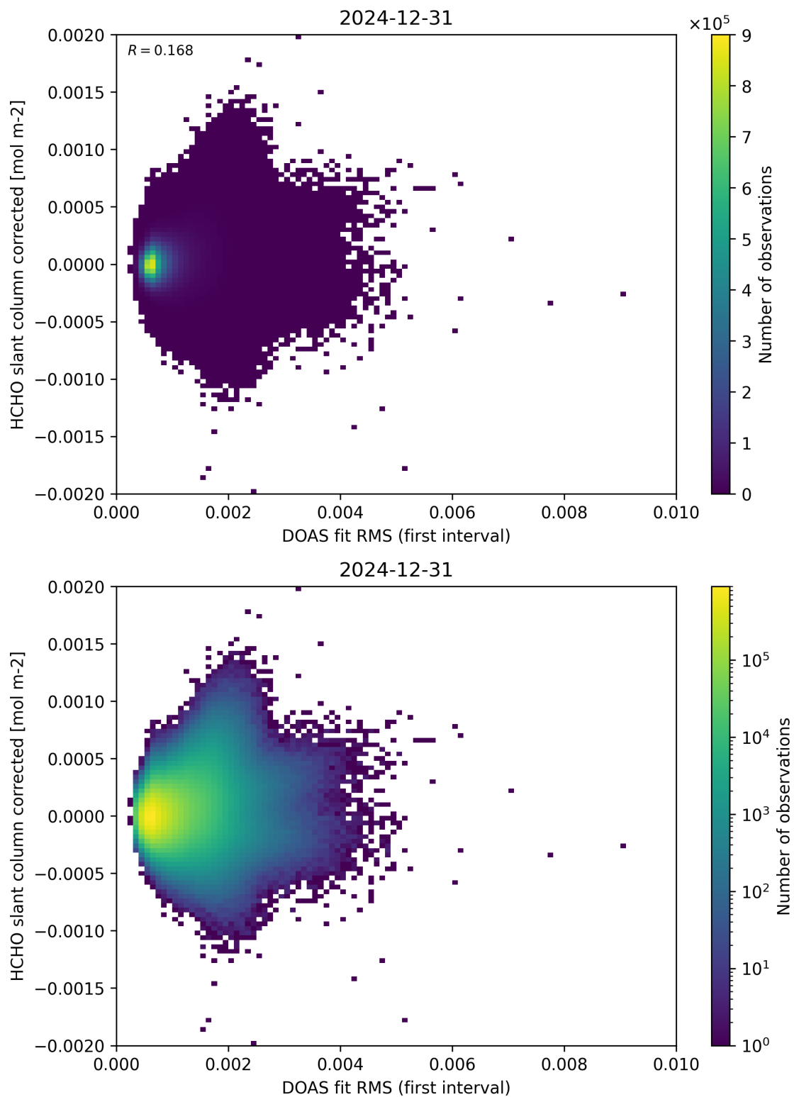
Figure 62: Scatter density plot of “DOAS fit RMS (first interval)” against “HCHO slant column corrected” for 2024-12-30 to 2025-01-01.
