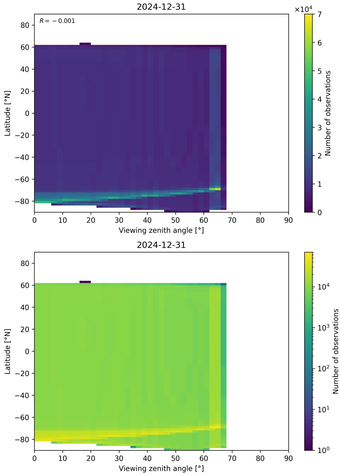
Figure 196: Scatter density plot of “Viewing zenith angle” against “Latitude” for 2024-12-30 to 2025-01-01.
