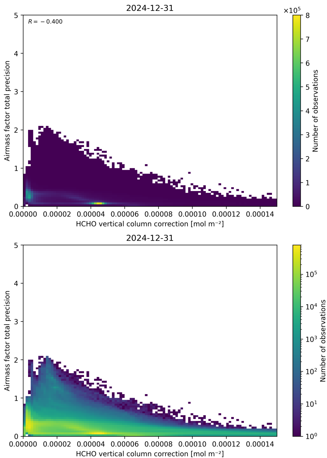
Figure 121: Scatter density plot of “HCHO vertical column correction” against “Airmass factor total precision” for 2024-12-30 to 2025-01-01.
