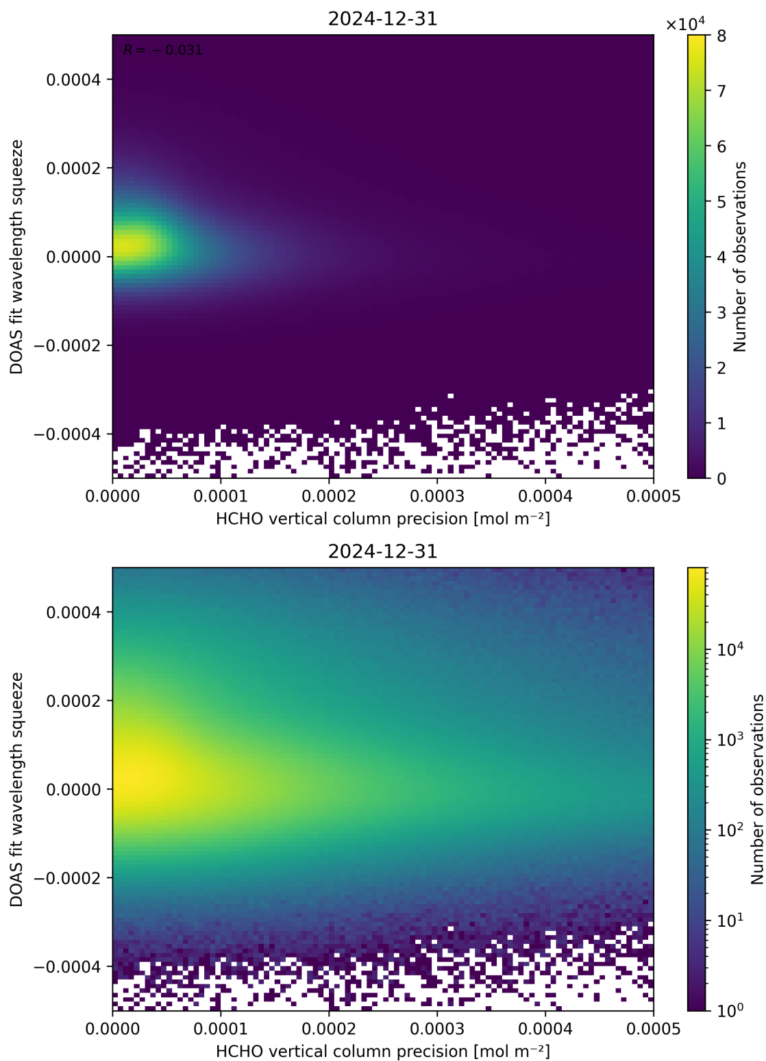
Figure 138: Scatter density plot of “HCHO vertical column precision” against “DOAS fit wavelength squeeze” for 2024-12-30 to 2025-01-01.
