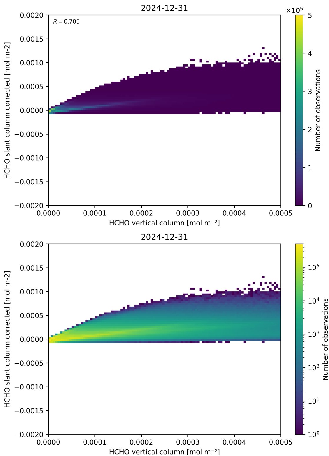
Figure 127: Scatter density plot of “HCHO vertical column” against “HCHO slant column corrected” for 2024-12-30 to 2025-01-01.
