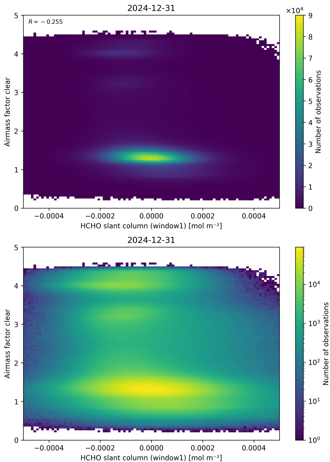
Figure 81: Scatter density plot of “HCHO slant column (window1)” against “Airmass factor clear” for 2024-12-30 to 2025-01-01.
