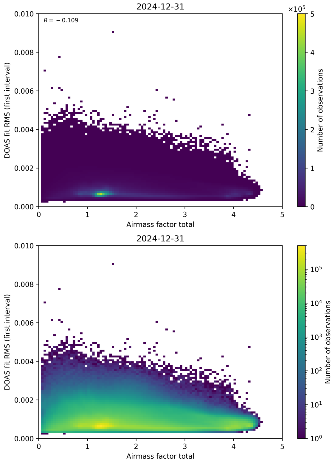
Figure 97: Scatter density plot of “Airmass factor total” against “DOAS fit RMS (first interval)” for 2024-12-30 to 2025-01-01.
