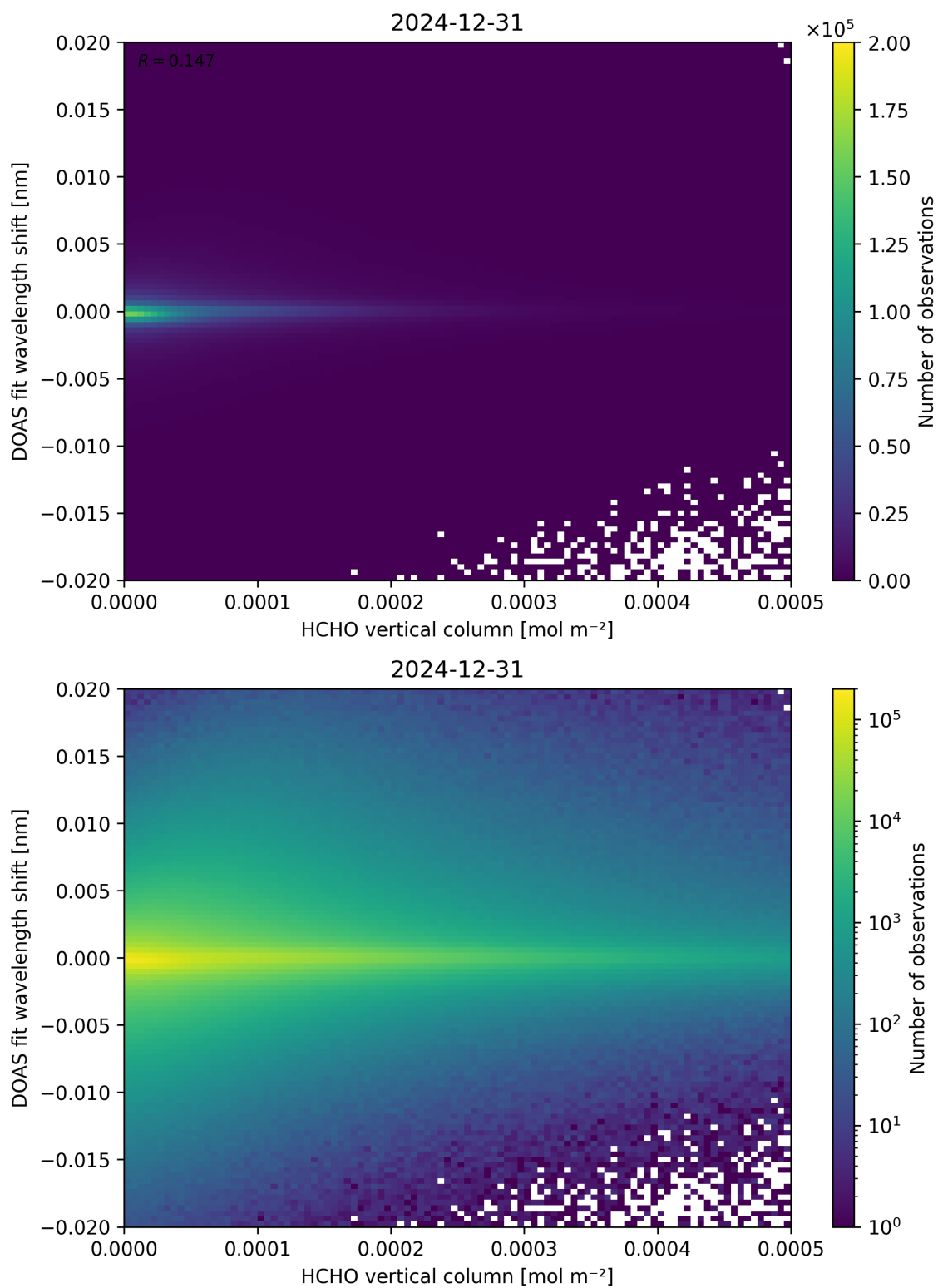
Figure 124: Scatter density plot of “HCHO vertical column” against “DOAS fit wavelength shift” for 2024-12-30 to 2025-01-01.
