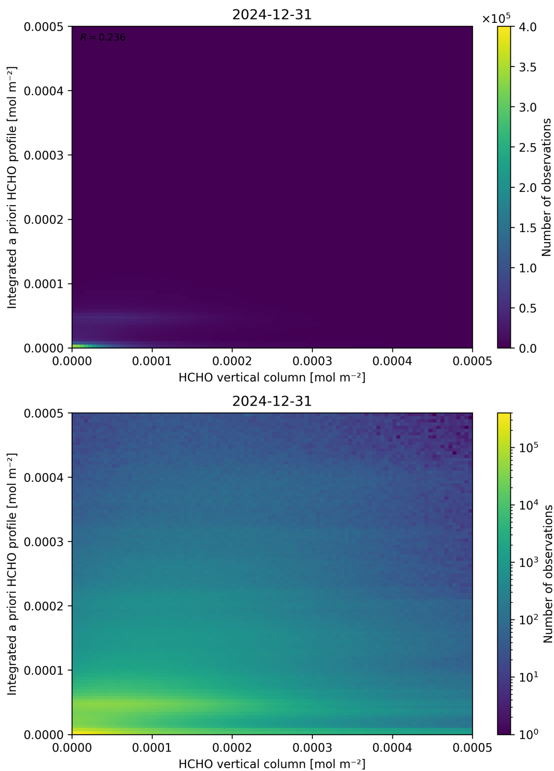
Figure 135: Scatter density plot of “HCHO vertical column” against “Integrated a priori HCHO profile” for 2024-12-30 to 2025-01-01.
