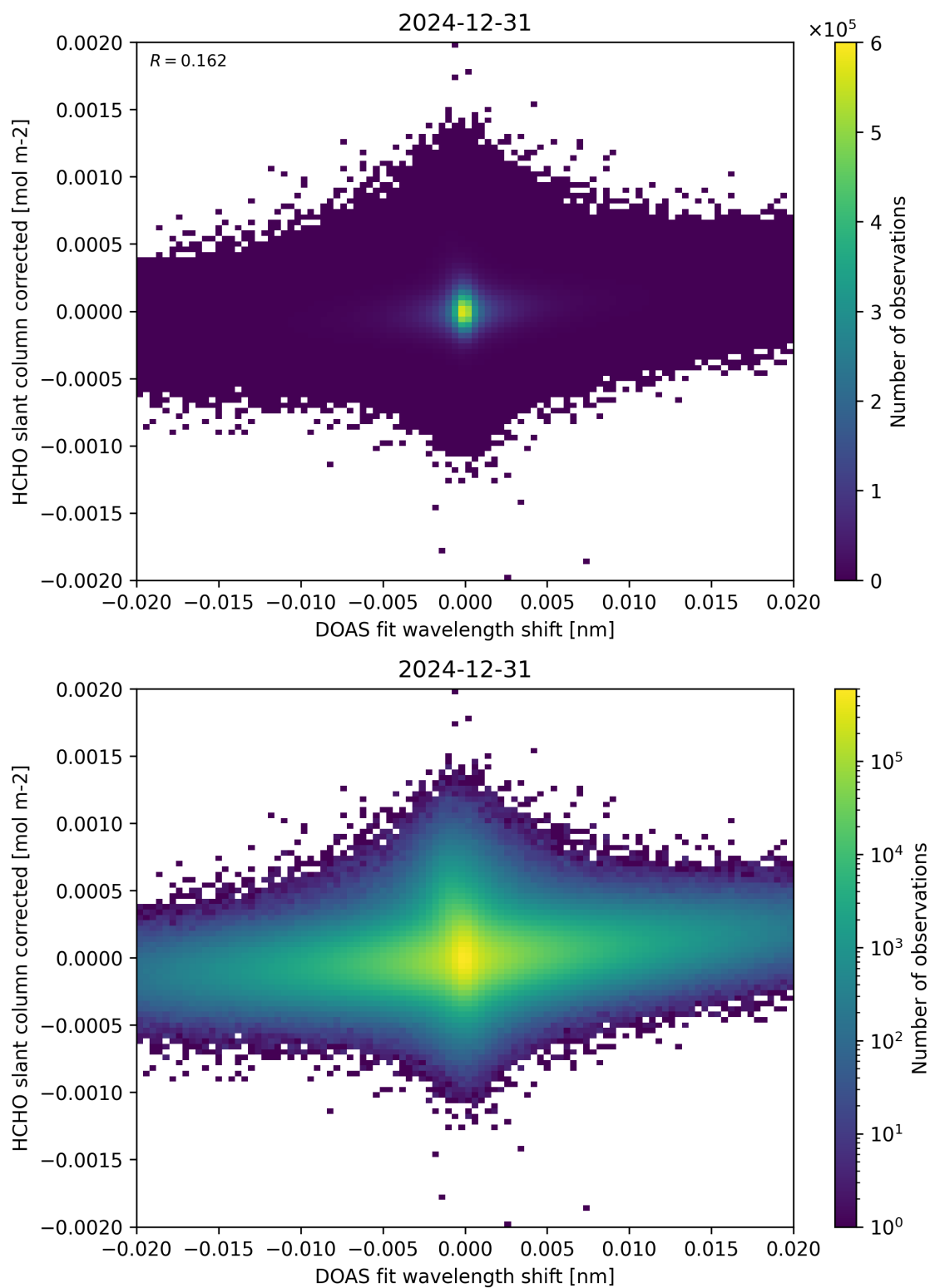
Figure 66: Scatter density plot of “DOAS fit wavelength shift” against “HCHO slant column corrected” for 2024-12-30 to 2025-01-01.
