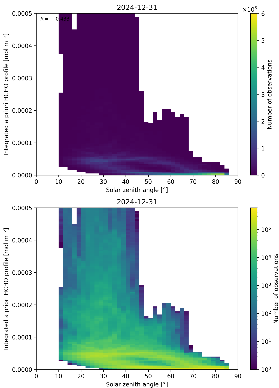
Figure 180: Scatter density plot of “Solar zenith angle” against “Integrated a priori HCHO profile” for 2024-12-30 to 2025-01-01.
