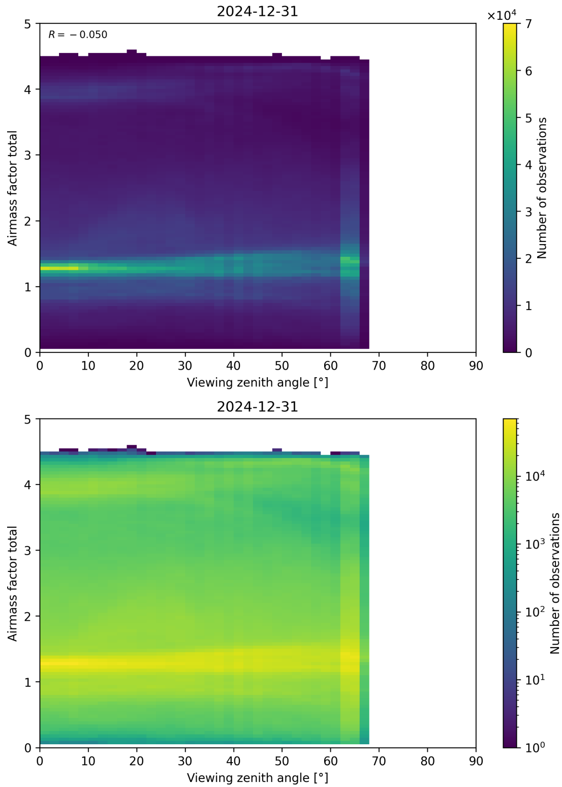
Figure 190: Scatter density plot of “Viewing zenith angle” against “Airmass factor total” for 2024-12-30 to 2025-01-01.
