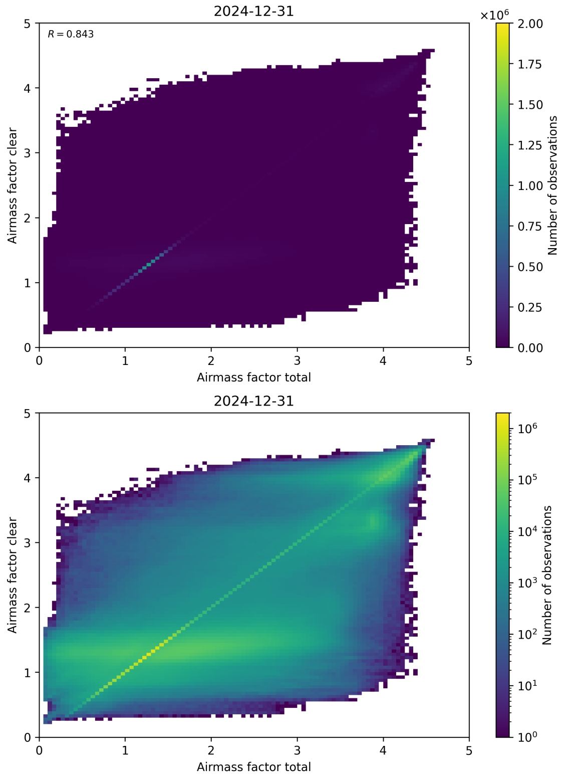
Figure 100: Scatter density plot of “Airmass factor total” against “Airmass factor clear” for 2024-12-30 to 2025-01-01.
