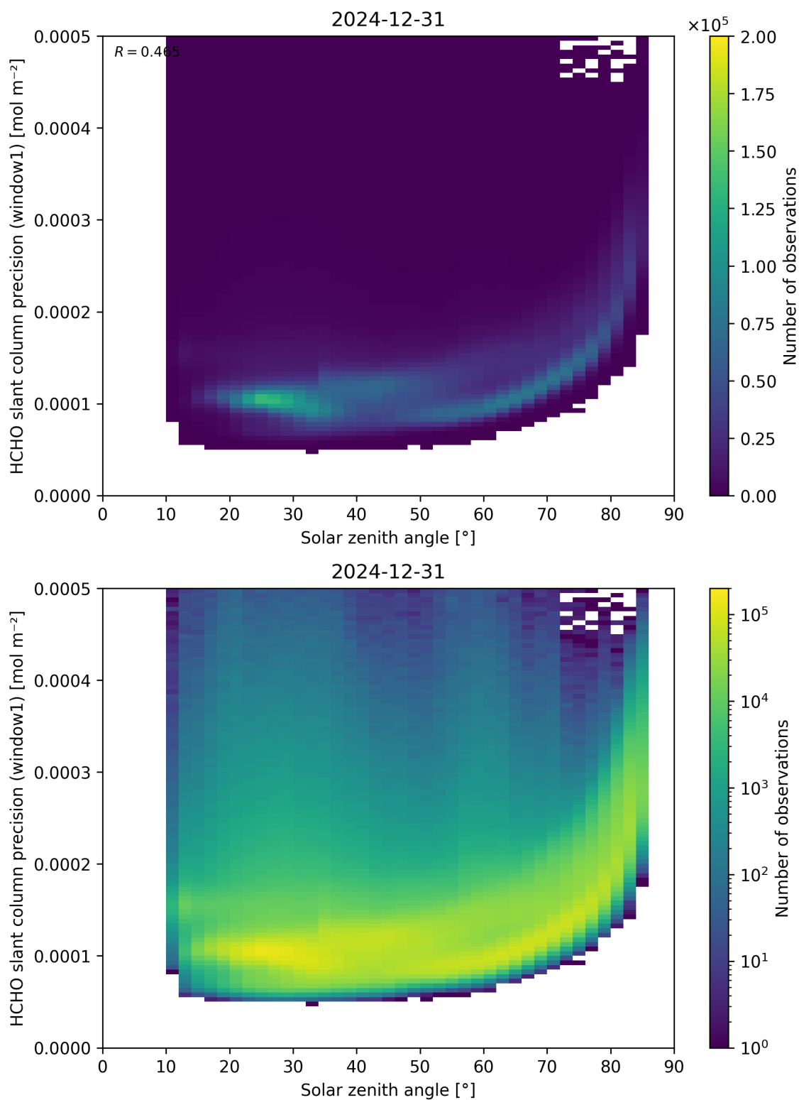
Figure 174: Scatter density plot of “Solar zenith angle” against “HCHO slant column precision (window1)” for 2024-12-30 to 2025-01-01.
