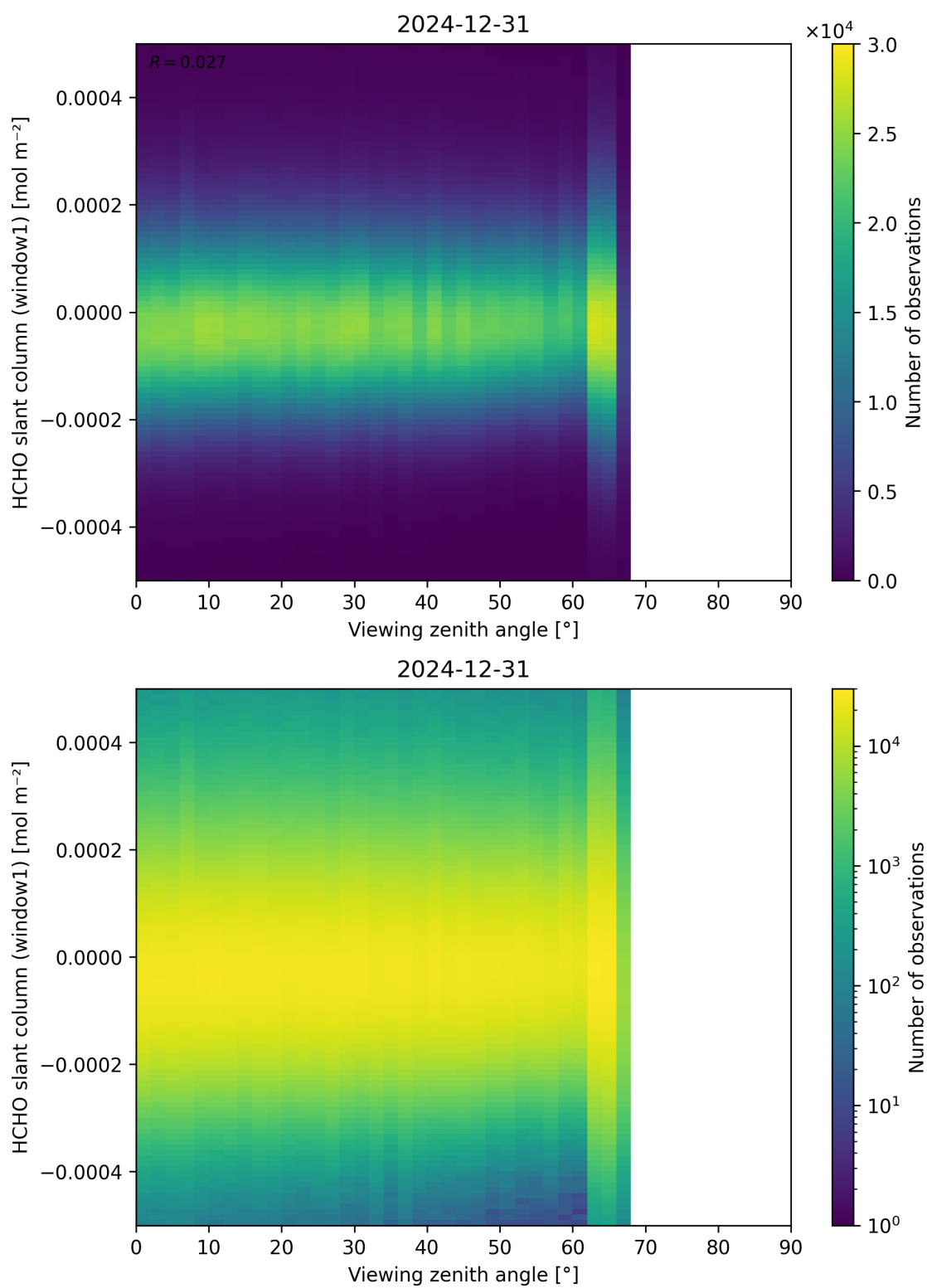
Figure 188: Scatter density plot of “Viewing zenith angle” against “HCHO slant column (window1)” for 2024-12-30 to 2025-01-01.
