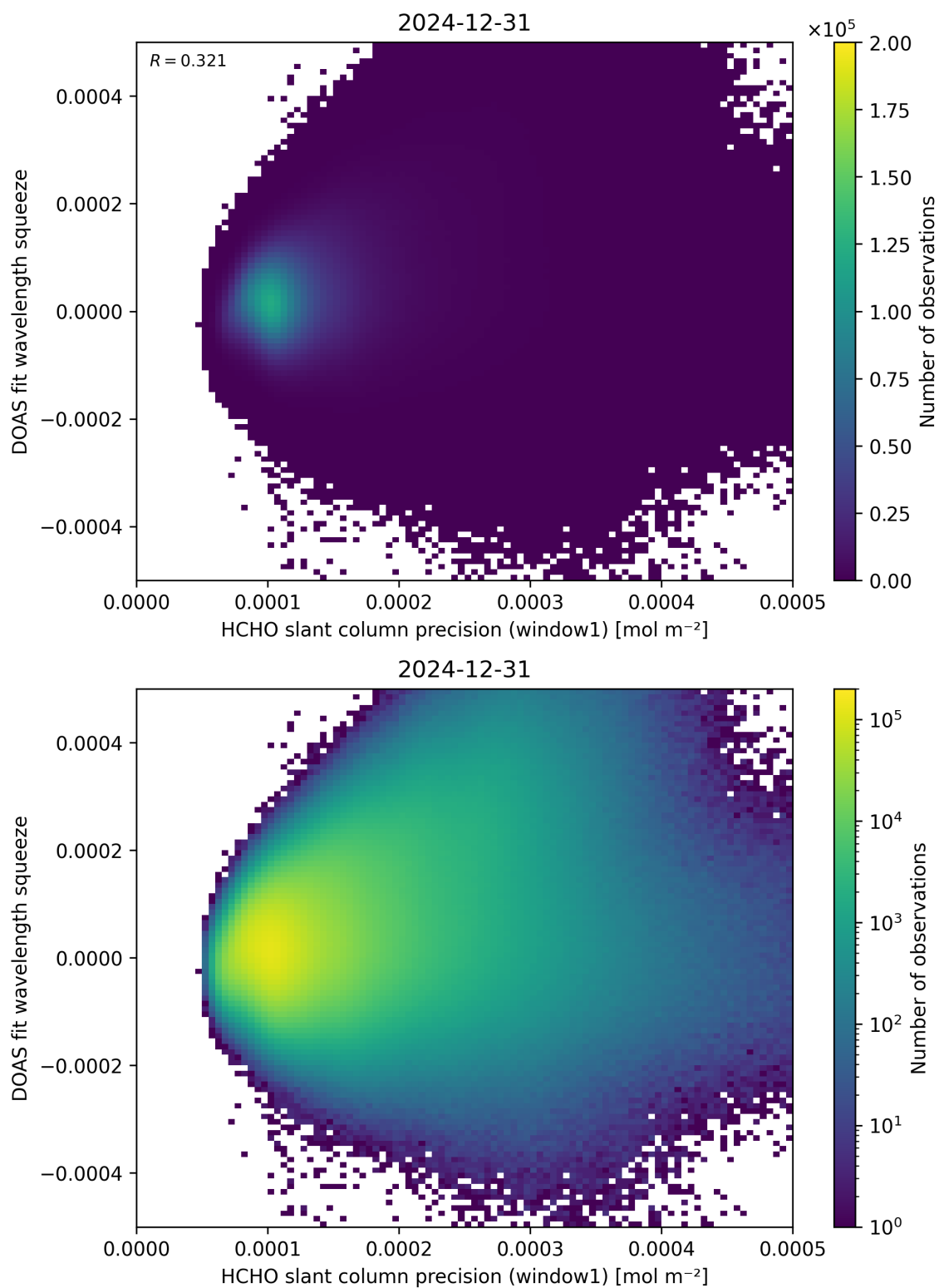
Figure 90: Scatter density plot of “HCHO slant column precision (window1)” against “DOAS fit wavelength squeeze” for 2024-12-30 to 2025-01-01.
