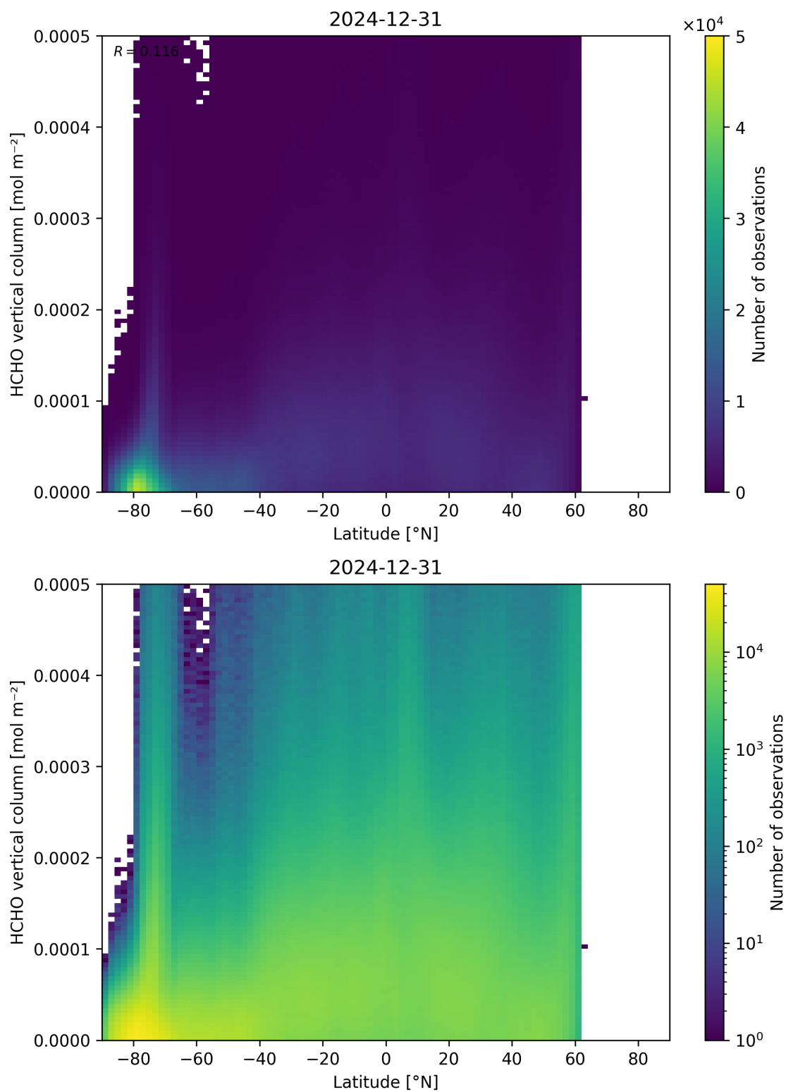
Figure 163: Scatter density plot of “Latitude” against “HCHO vertical column” for 2024-12-30 to 2025-01-01.
