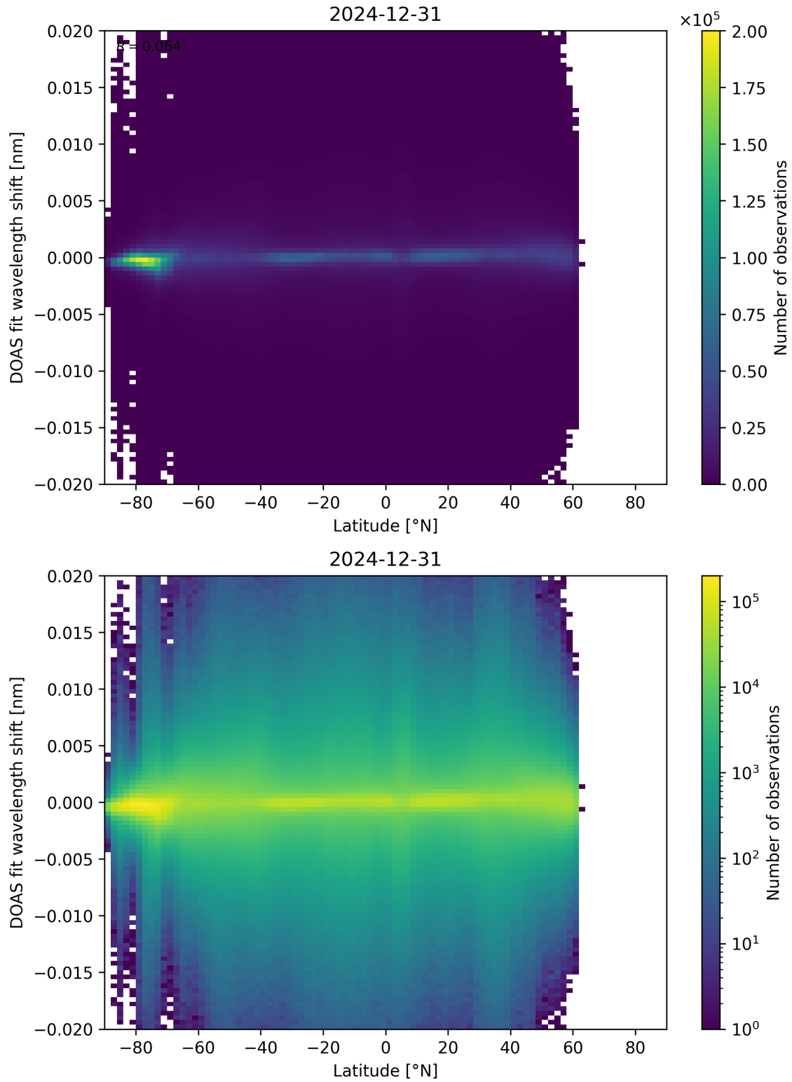
Figure 154: Scatter density plot of “Latitude” against “DOAS fit wavelength shift” for 2024-12-30 to 2025-01-01.
