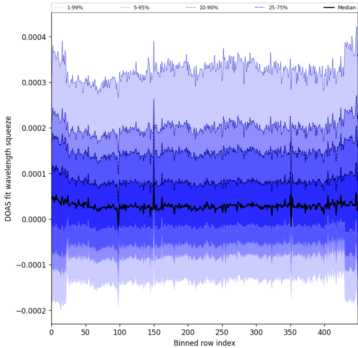
Figure 59: Along track statistics of “DOAS fit wavelength squeeze” for 2024-12-30 to 2025-01-01
