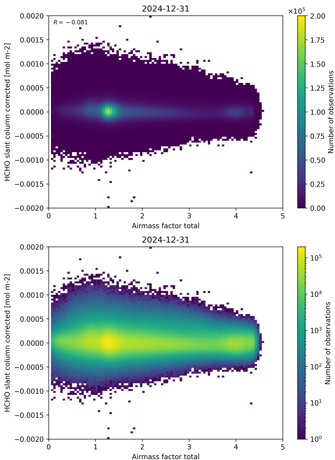
Figure 101: Scatter density plot of “Airmass factor total” against “HCHO slant column corrected” for 2024-12-30 to 2025-01-01.
