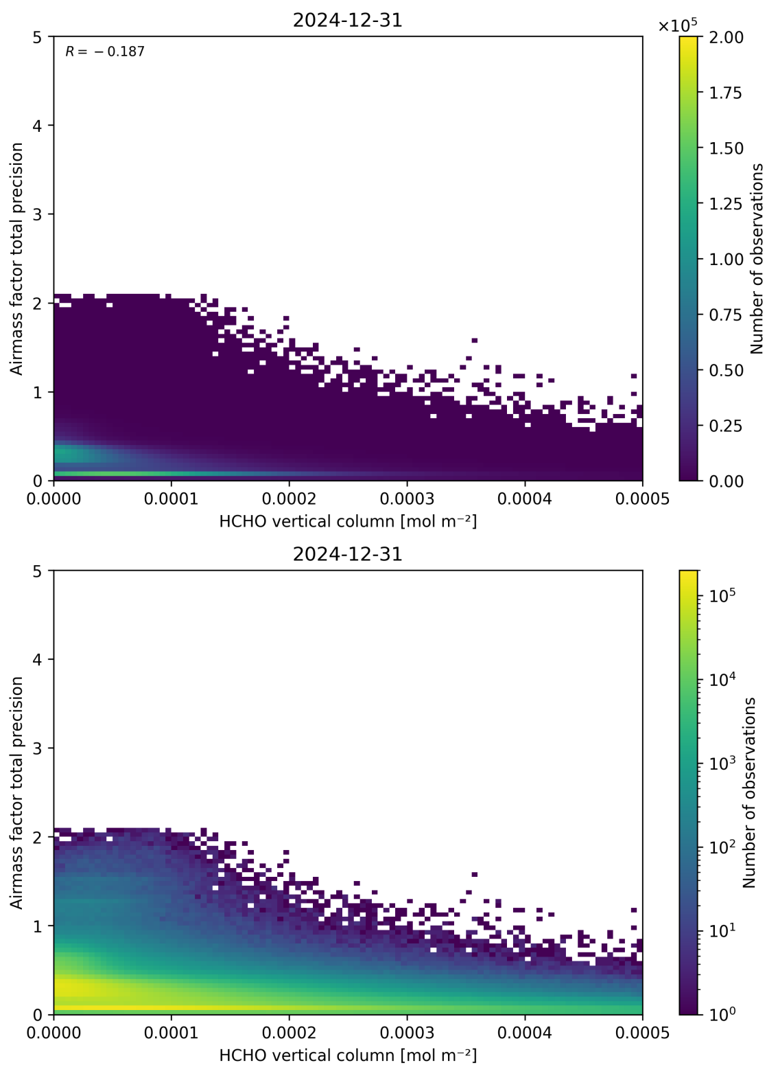
Figure 132: Scatter density plot of “HCHO vertical column” against “Airmass factor total precision” for 2024-12-30 to 2025-01-01.
