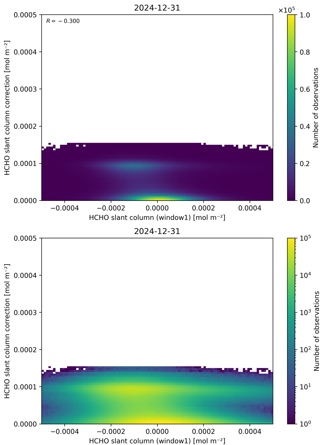
Figure 83: Scatter density plot of “HCHO slant column (window1)” against “HCHO slant column correction” for 2024-12-30 to 2025-01-01.
