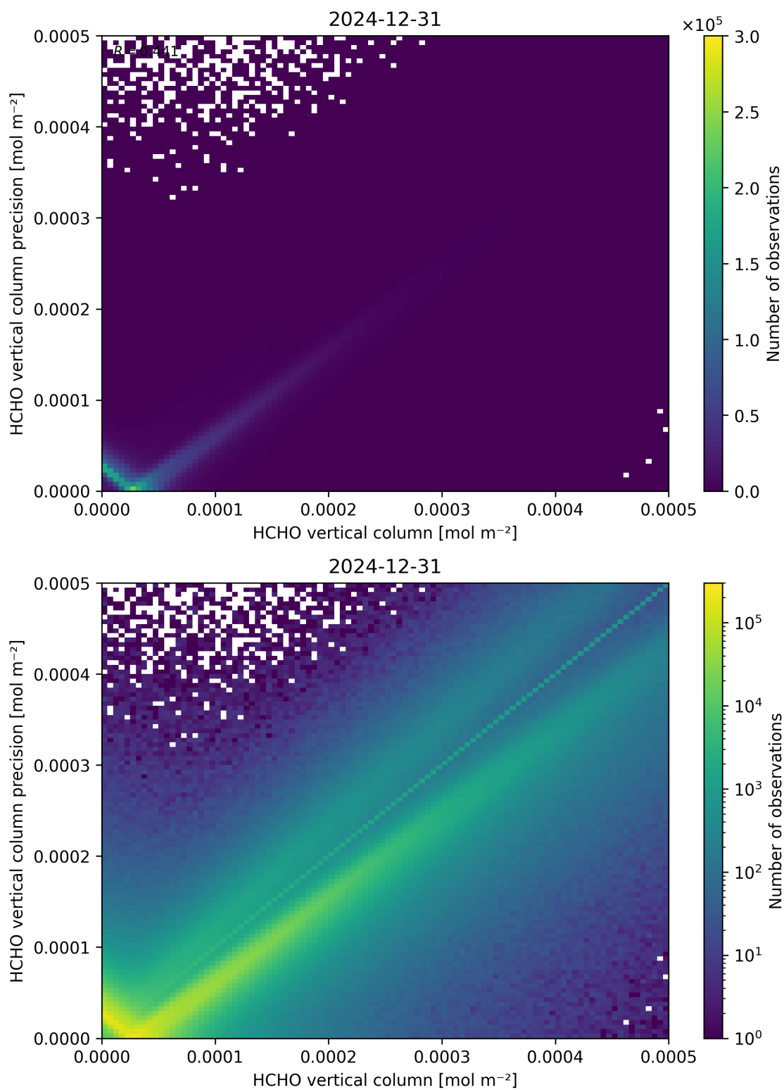
Figure 134: Scatter density plot of “HCHO vertical column” against “HCHO vertical column precision” for 2024-12-30 to 2025-01-01.
