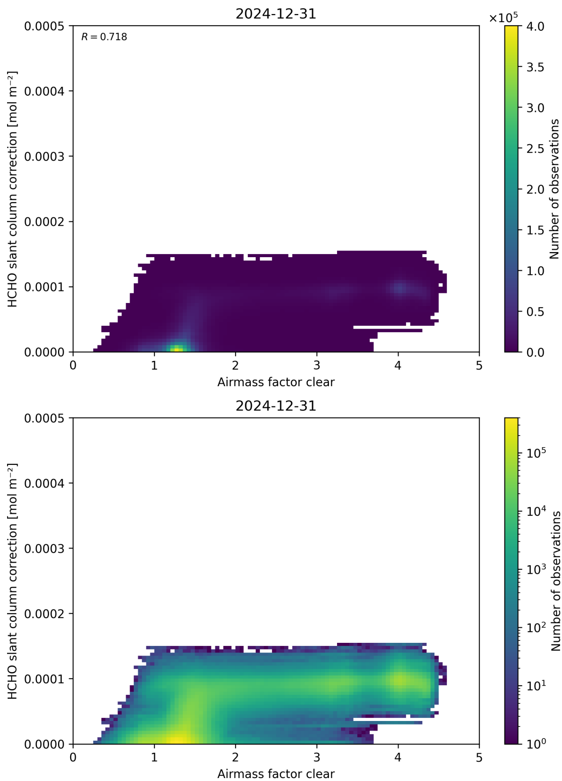
Figure 75: Scatter density plot of “Airmass factor clear” against “HCHO slant column correction” for 2024-12-30 to 2025-01-01.
