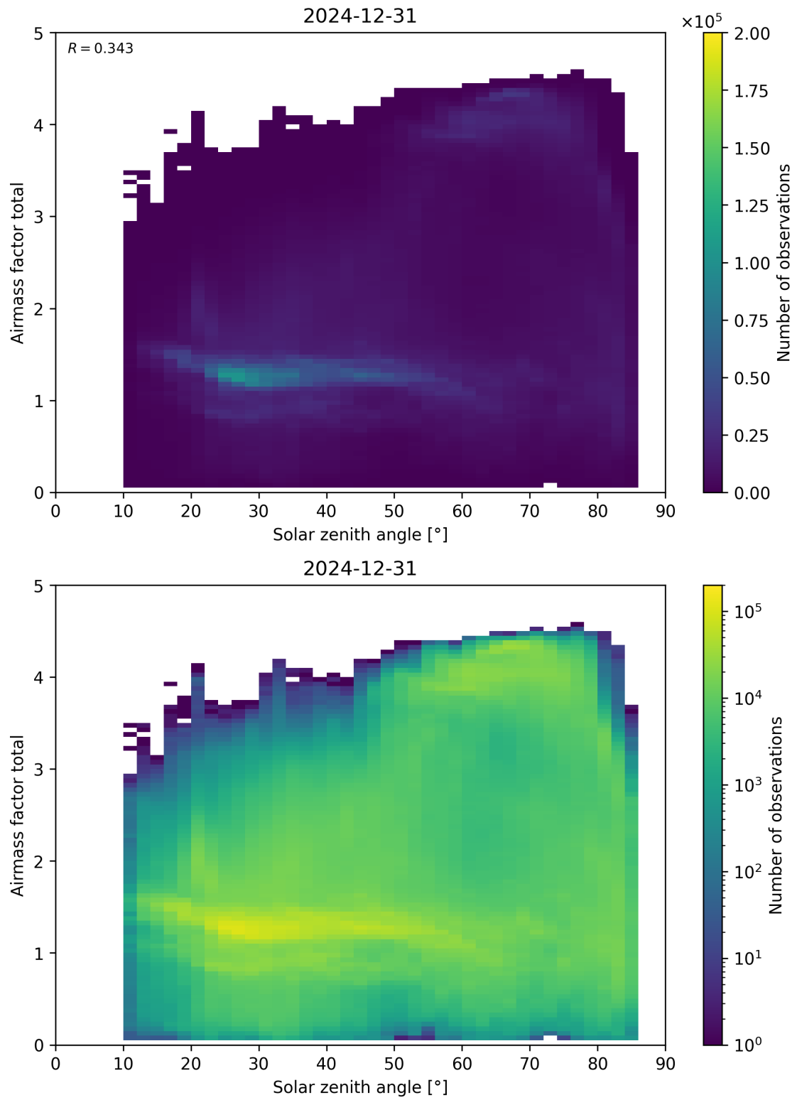
Figure 175: Scatter density plot of “Solar zenith angle” against “Airmass factor total” for 2024-12-30 to 2025-01-01.
