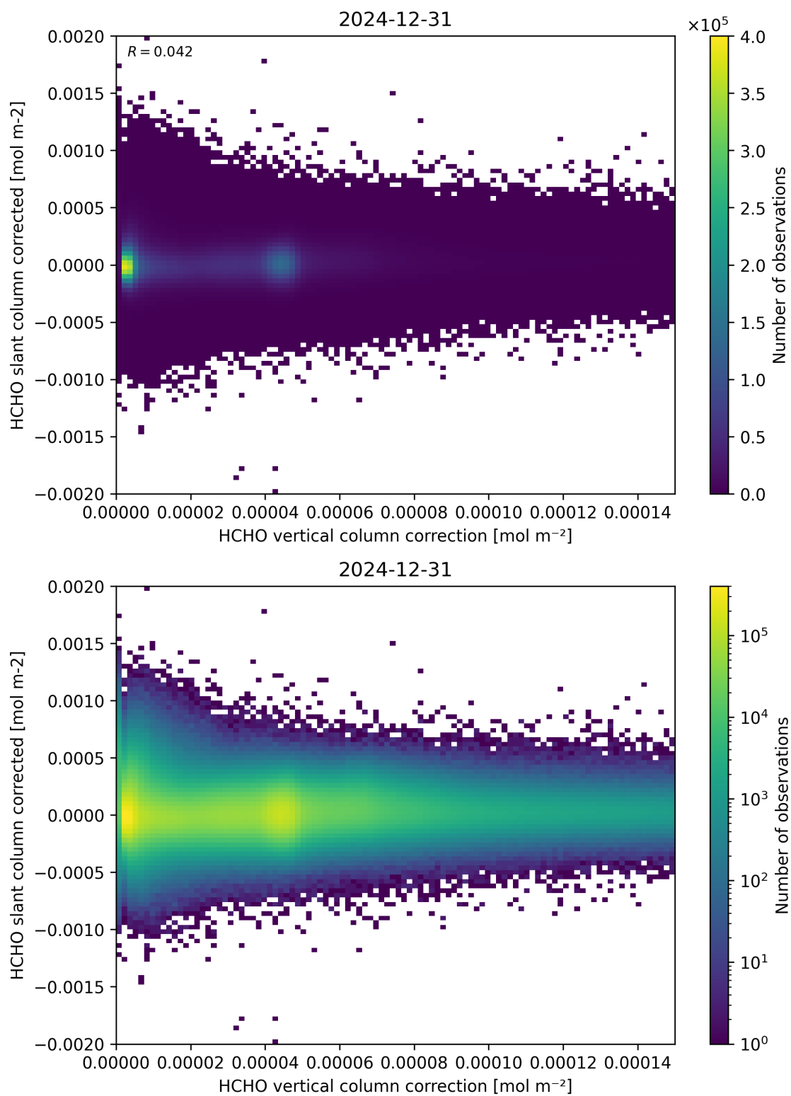
Figure 116: Scatter density plot of “HCHO vertical column correction” against “HCHO slant column corrected” for 2024-12-30 to 2025-01-01.
