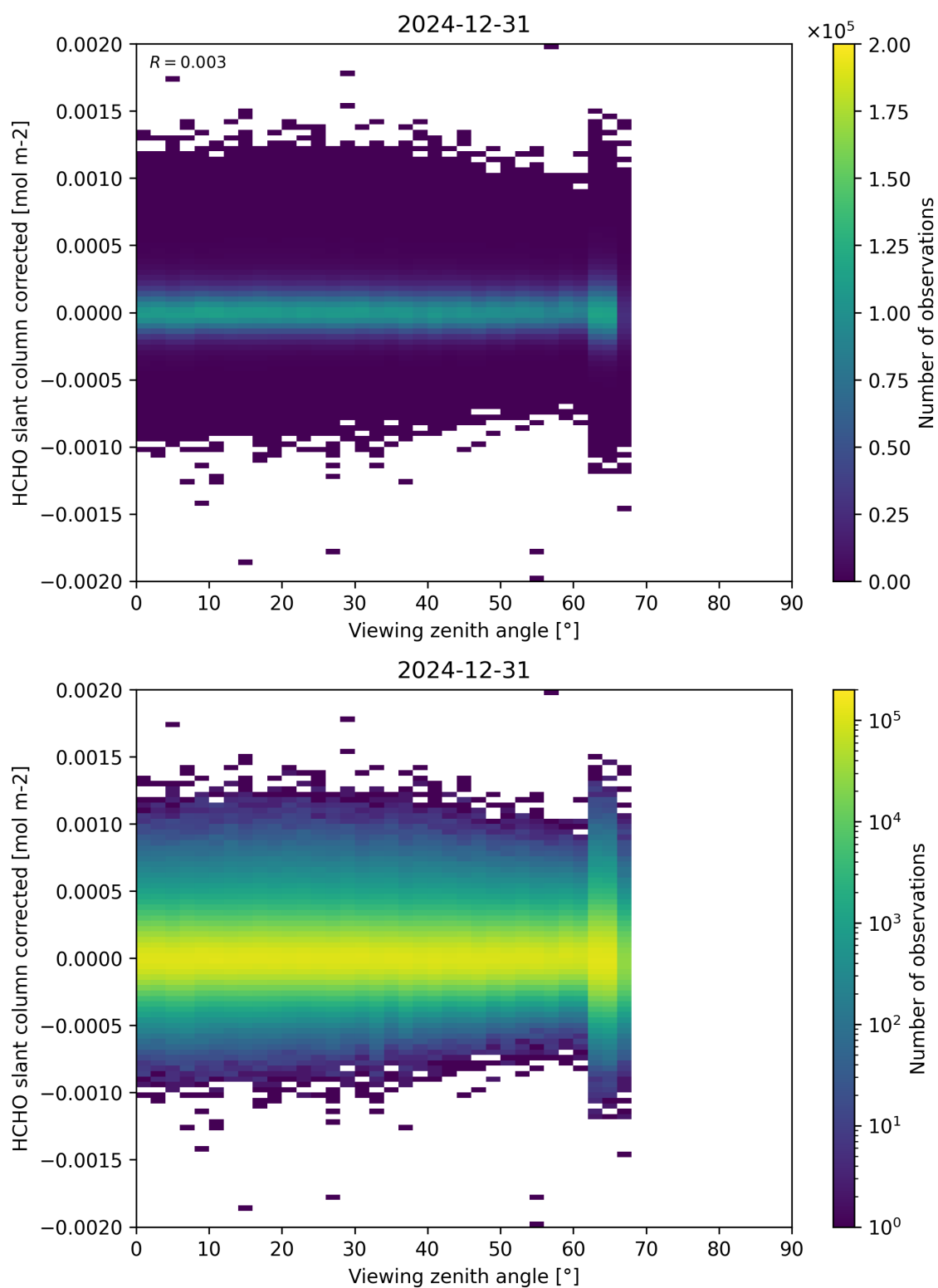
Figure 186: Scatter density plot of “Viewing zenith angle” against “HCHO slant column corrected” for 2024-12-30 to 2025-01-01.
