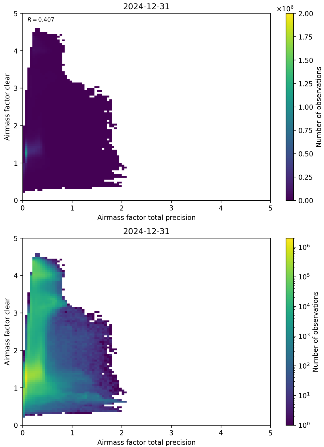
Figure 108: Scatter density plot of “Airmass factor total precision” against “Airmass factor clear” for 2024-12-30 to 2025-01-01.
