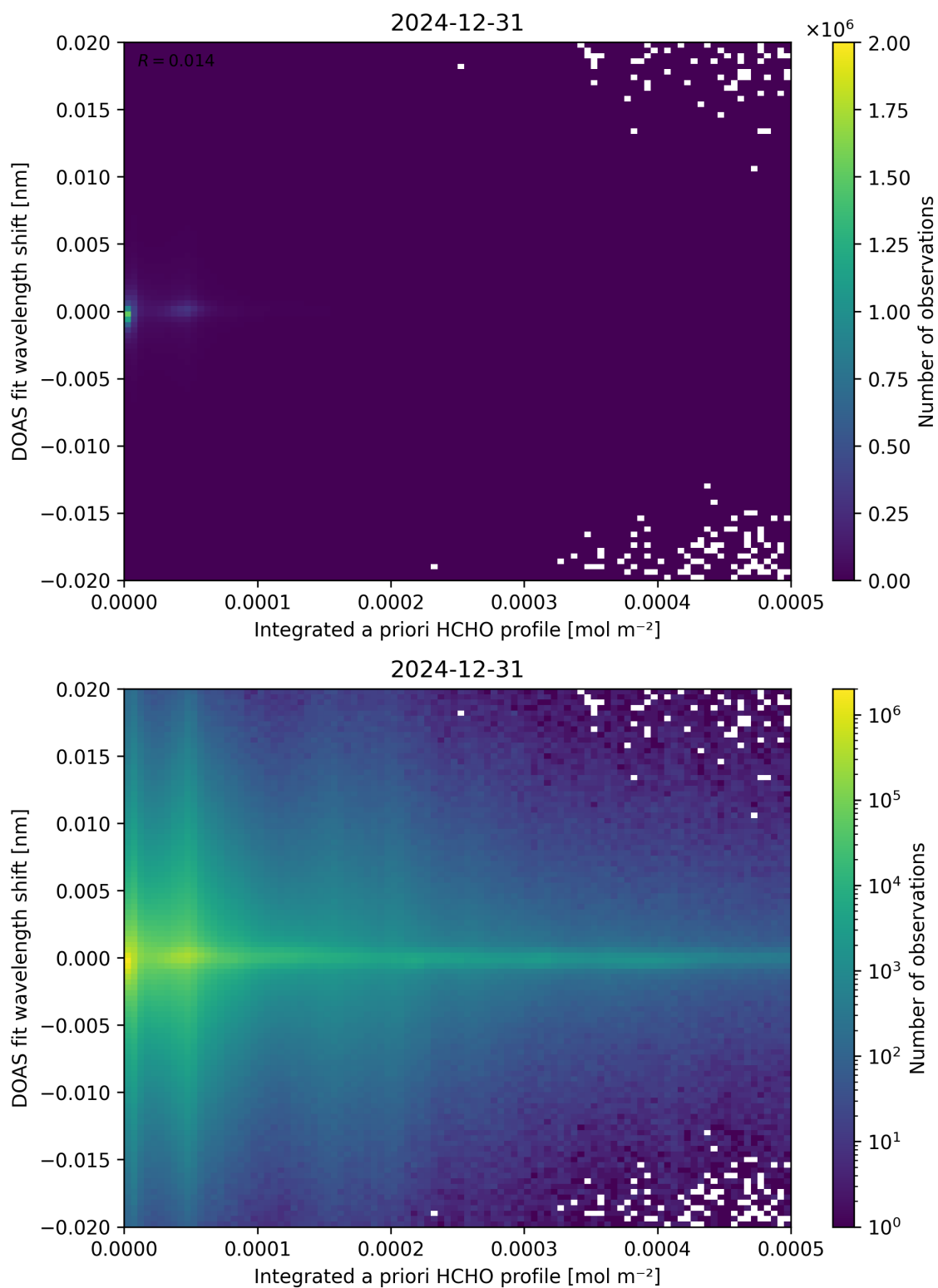
Figure 149: Scatter density plot of “Integrated a priori HCHO profile” against “DOAS fit wavelength shift” for 2024-12-30 to 2025-01-01.
