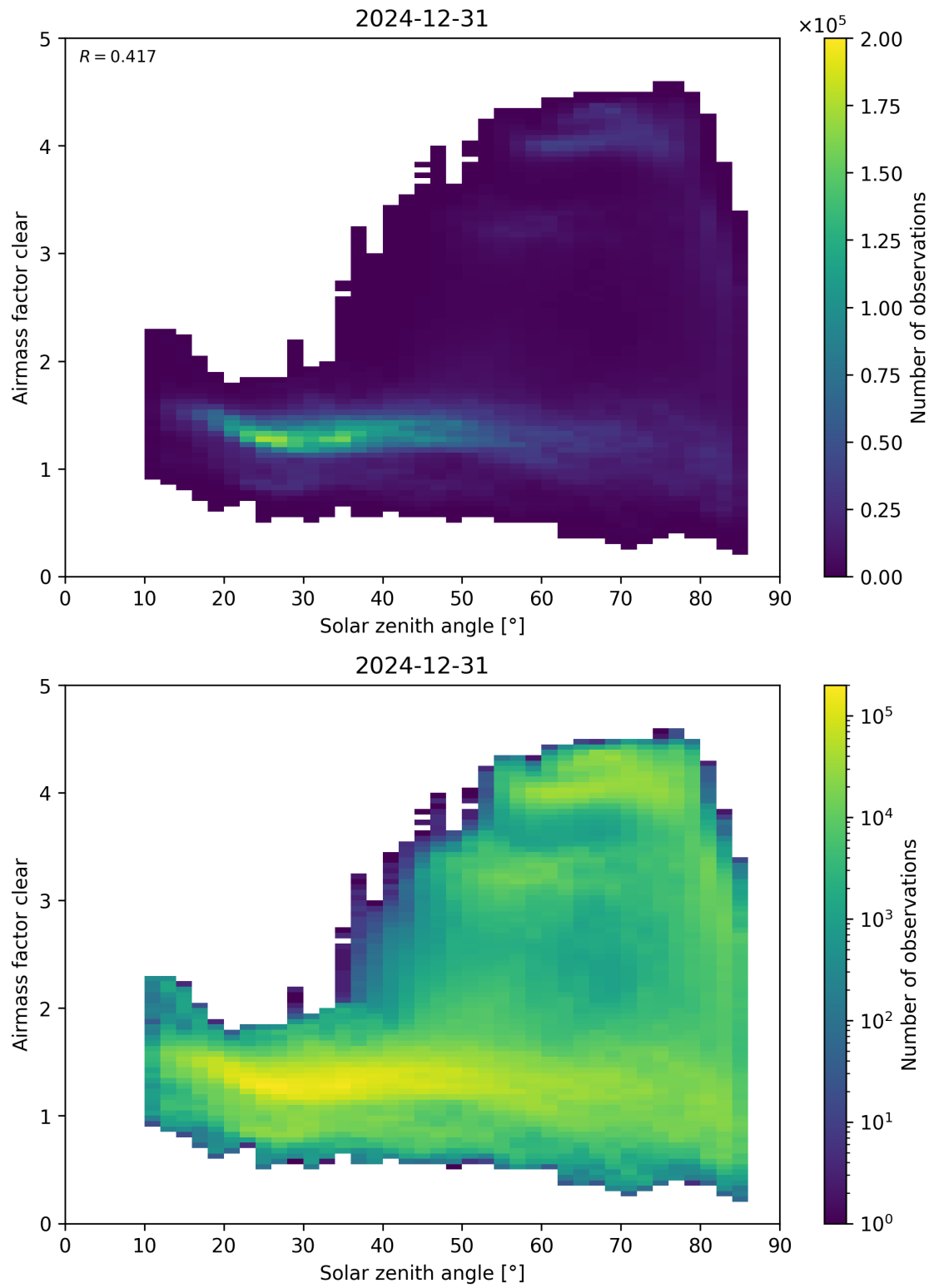
Figure 170: Scatter density plot of “Solar zenith angle” against “Airmass factor clear” for 2024-12-30 to 2025-01-01.
