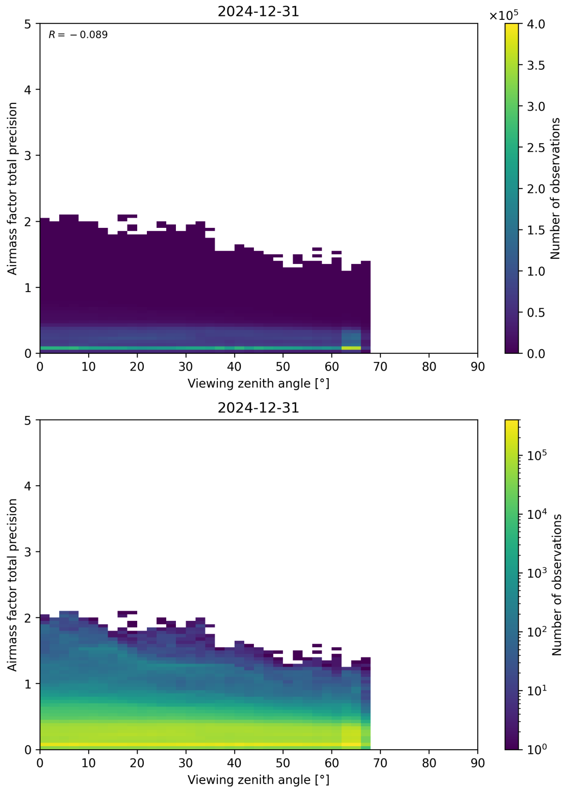
Figure 191: Scatter density plot of “Viewing zenith angle” against “Airmass factor total precision” for 2024-12-30 to 2025-01-01.
