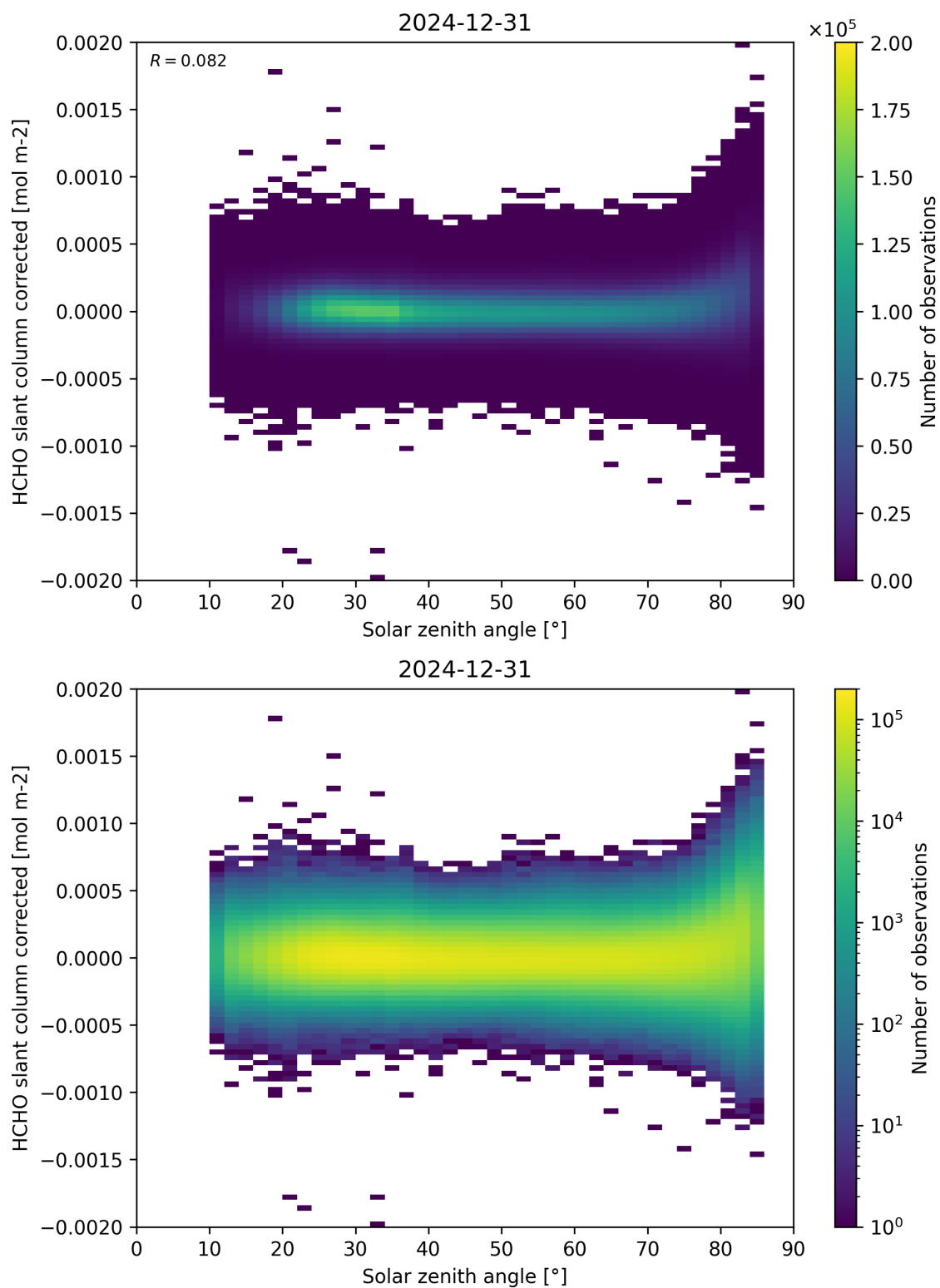
Figure 171: Scatter density plot of “Solar zenith angle” against “HCHO slant column corrected” for 2024-12-30 to 2025-01-01.
