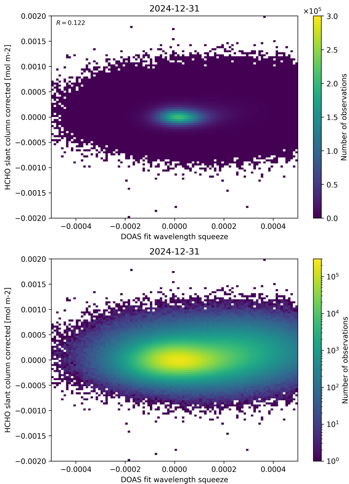
Figure 69: Scatter density plot of “DOAS fit wavelength squeeze” against “HCHO slant column corrected” for 2024-12-30 to 2025-01-01.
