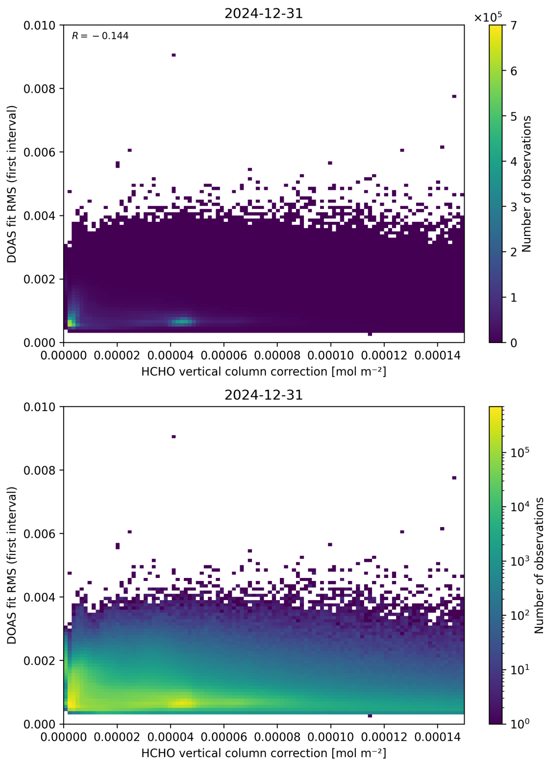
Figure 112: Scatter density plot of “HCHO vertical column correction” against “DOAS fit RMS (first interval)” for 2024-12-30 to 2025-01-01.
