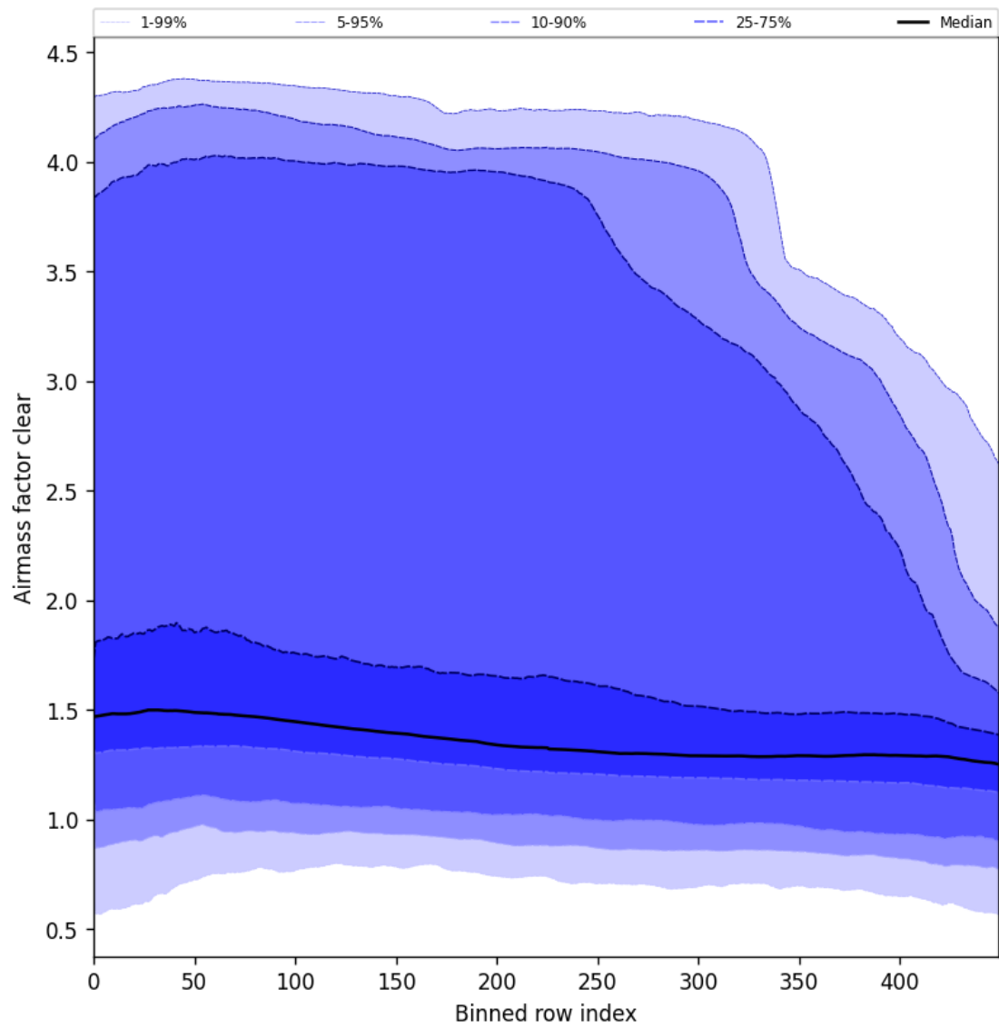
Figure 56: Along track statistics of “Air mass factor clear” for 2024-12-30 to 2025-01-01
