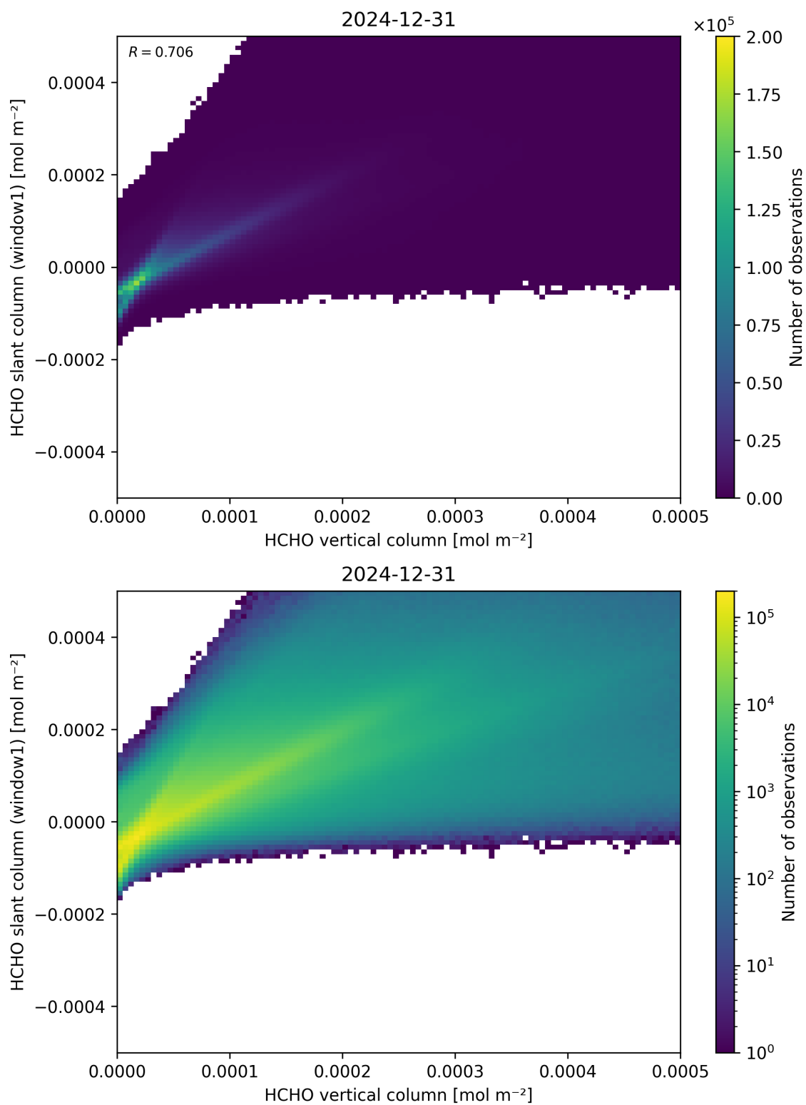
Figure 129: Scatter density plot of “HCHO vertical column” against “HCHO slant column (window1)” for 2024-12-30 to 2025-01-01.
