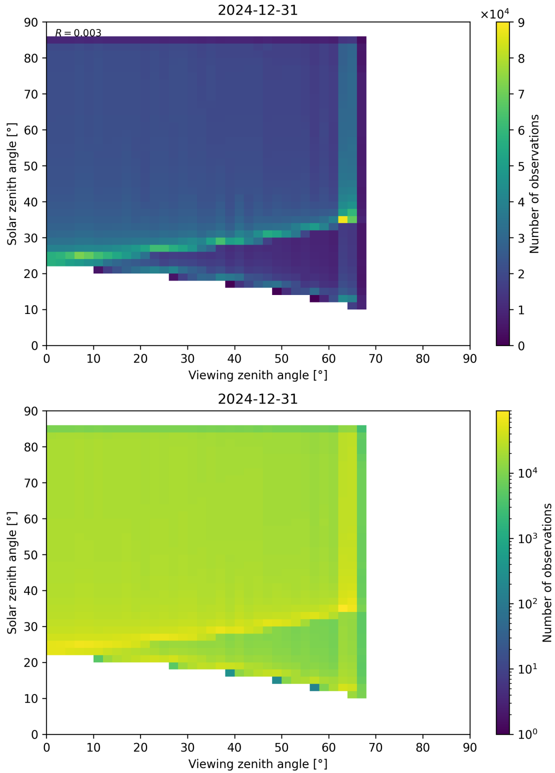
Figure 197: Scatter density plot of “Viewing zenith angle” against “Solar zenith angle” for 2024-12-30 to 2025-01-01.
