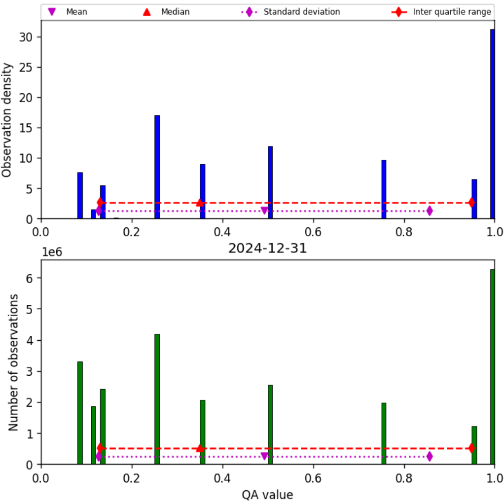
Figure 34: Histogram of “QA value” for 2024-12-30 to 2025-01-01
