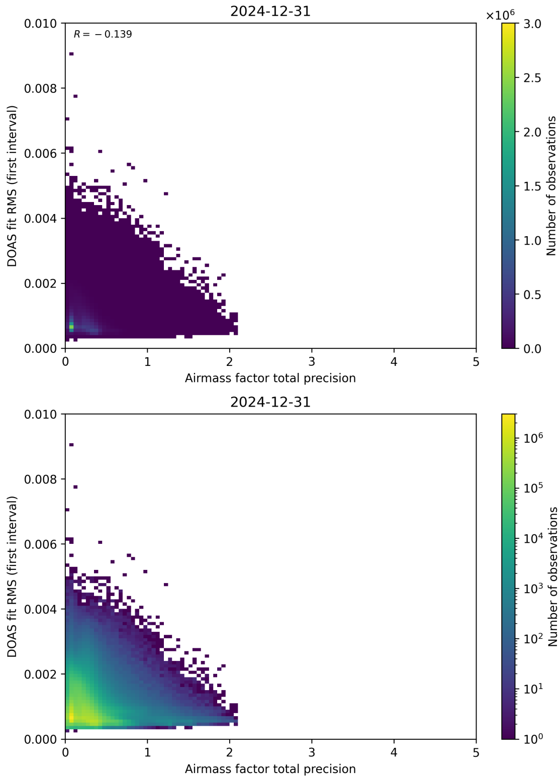
Figure 105: Scatter density plot of “Airmass factor total precision” against “DOAS fit RMS (first interval)” for 2024-12-30 to 2025-01-01.
