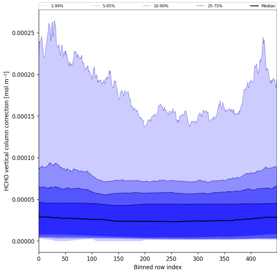
Figure 51: Along track statistics of “HCHO vertical column correction” for 2024-12-30 to 2025-01-01
