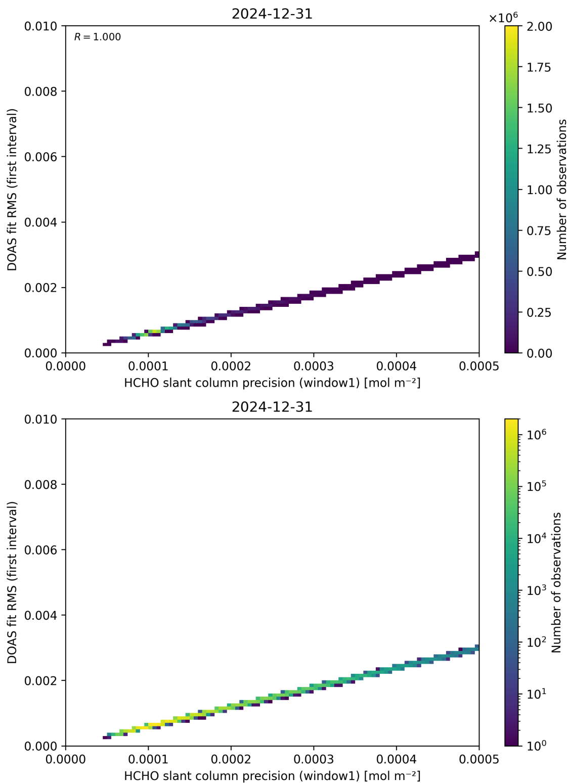
Figure 88: Scatter density plot of “HCHO slant column precision (window1)” against “DOAS fit RMS (first interval)” for 2024-12-30 to 2025-01-01.
