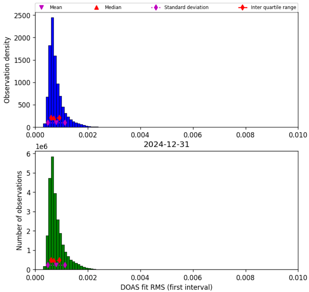
Figure 46: Histogram of “DOAS fit RMS (first interval)” for 2024-12-30 to 2025-01-01
