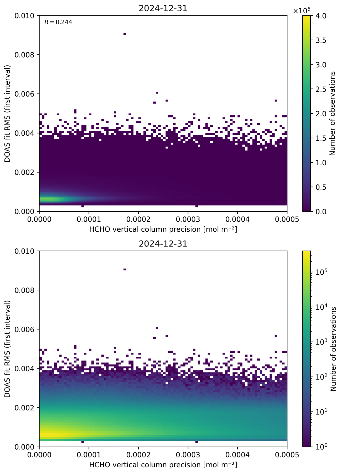
Figure 136: Scatter density plot of “HCHO vertical column precision” against “DOAS fit RMS (first interval)” for 2024-12-30 to 2025-01-01.
