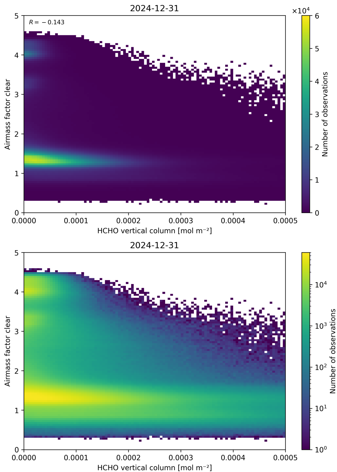
Figure 126: Scatter density plot of “HCHO vertical column” against “Airmass factor clear” for 2024-12-30 to 2025-01-01.
