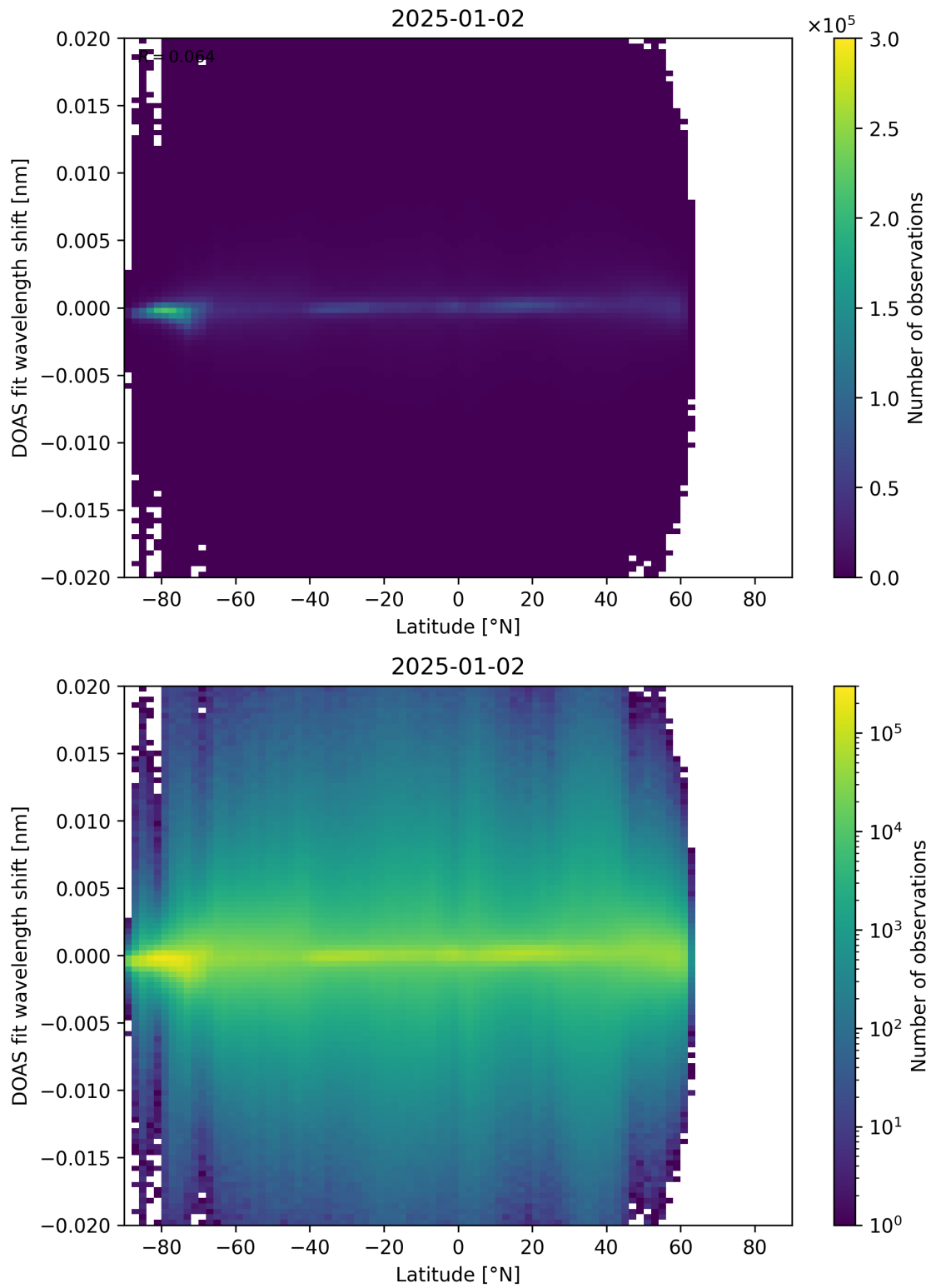
Figure 154: Scatter density plot of “Latitude” against “DOAS fit wavelength shift” for 2025-01-01 to 2025-01-03.
