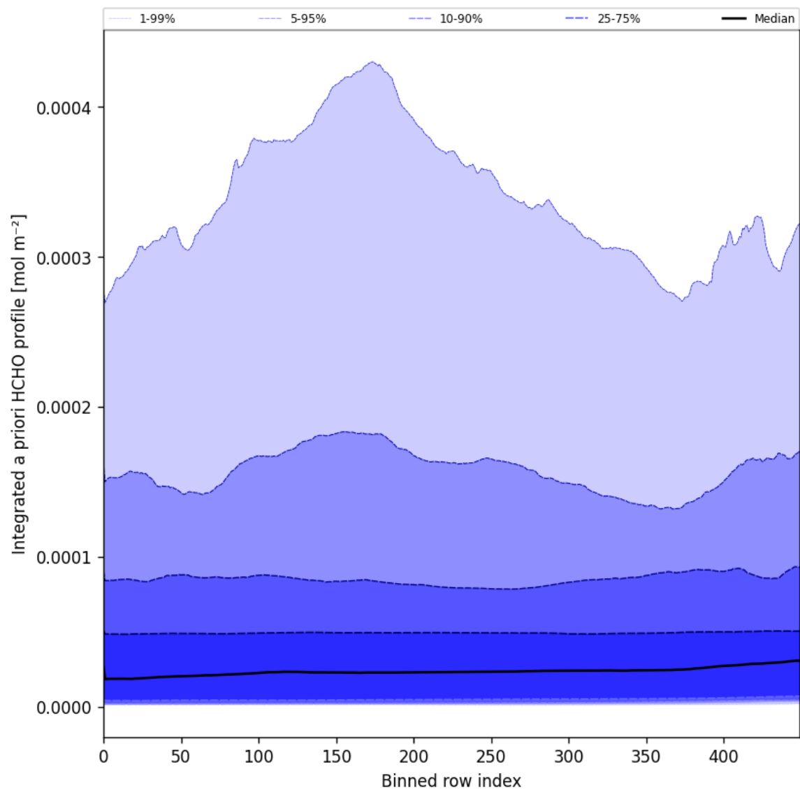
Figure 57: Along track statistics of “Integrated a priori HCHO profile” for 2025-01-01 to 2025-01-03
