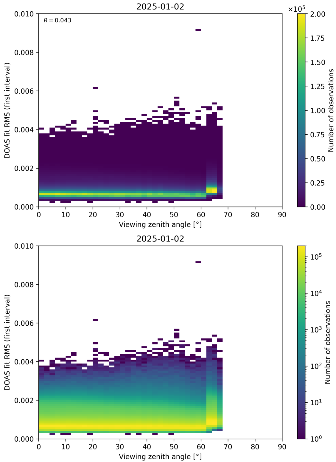
Figure 182: Scatter density plot of “Viewing zenith angle” against “DOAS fit RMS (first interval)” for 2025-01-01 to 2025-01-03.
