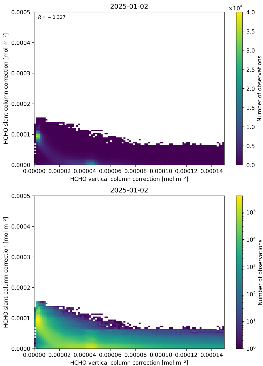
Figure 117: Scatter density plot of “HCHO vertical column correction” against “HCHO slant column correction” for 2025-01-01 to 2025-01-03.
