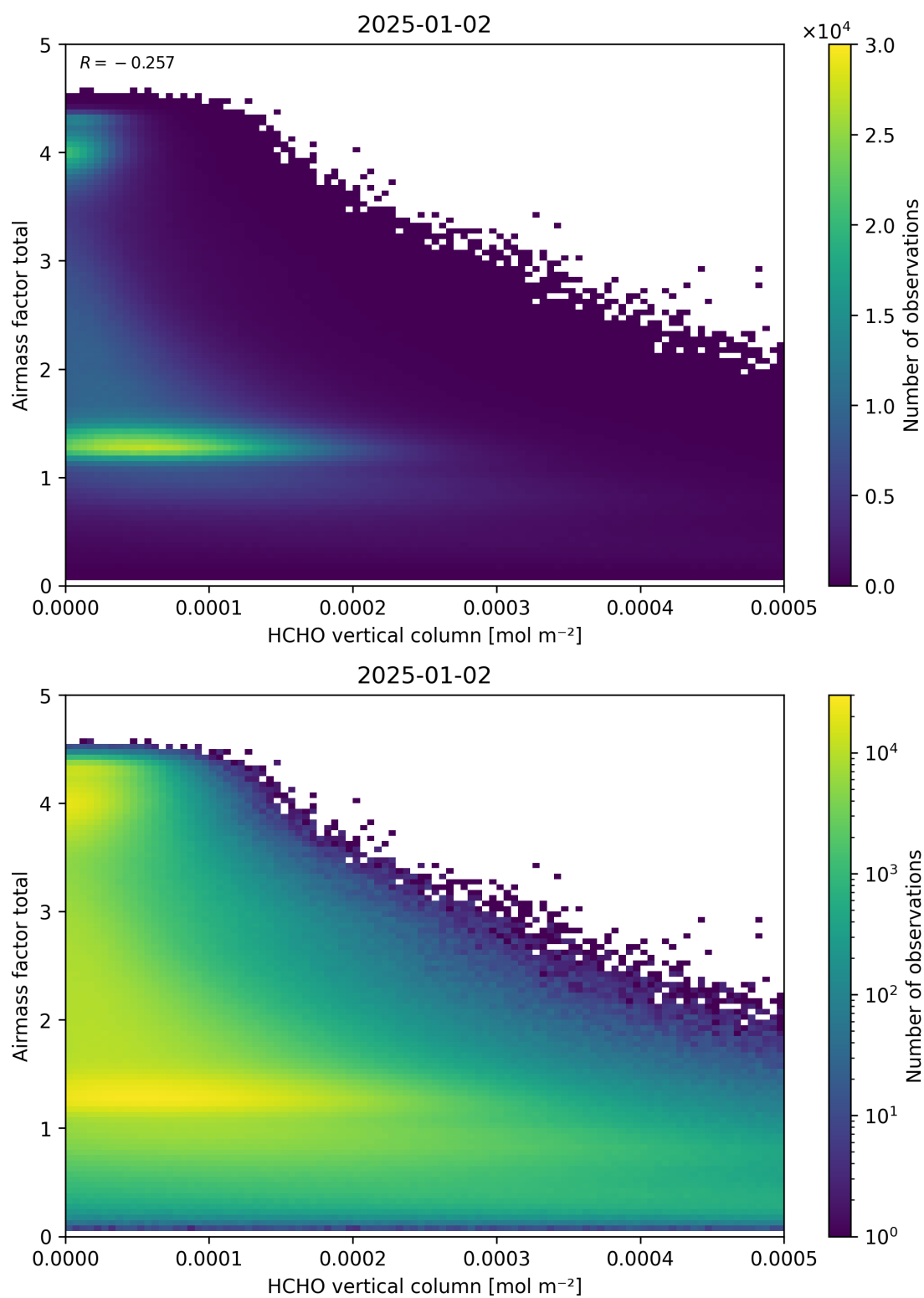
Figure 131: Scatter density plot of “HCHO vertical column” against “Airmass factor total” for 2025-01-01 to 2025-01-03.
