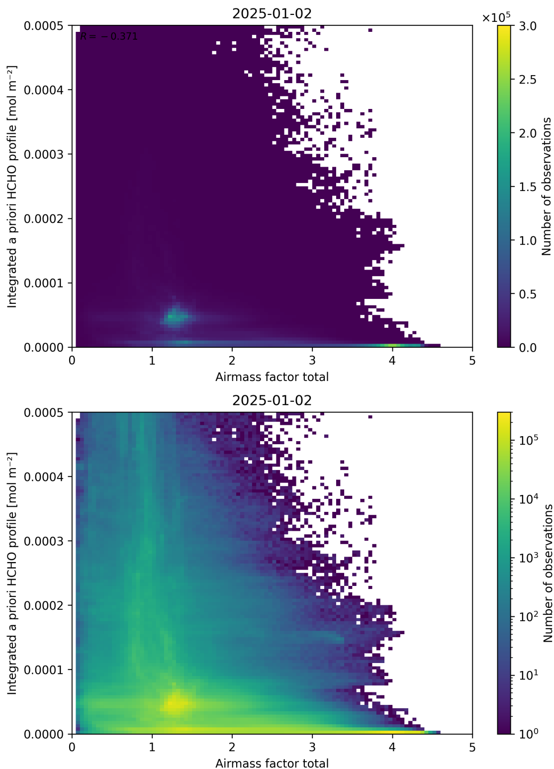
Figure 104: Scatter density plot of “Airmass factor total” against “Integrated a priori HCHO profile” for 2025-01-01 to 2025-01-03.
