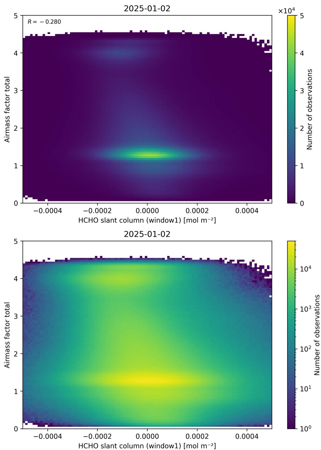
Figure 85: Scatter density plot of “HCHO slant column (window1)” against “Airmass factor total” for 2025-01-01 to 2025-01-03.
