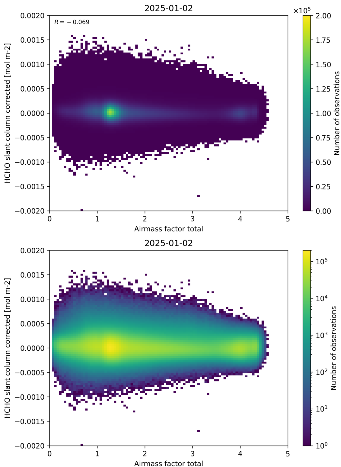
Figure 101: Scatter density plot of “Airmass factor total” against “HCHO slant column corrected” for 2025-01-01 to 2025-01-03.
