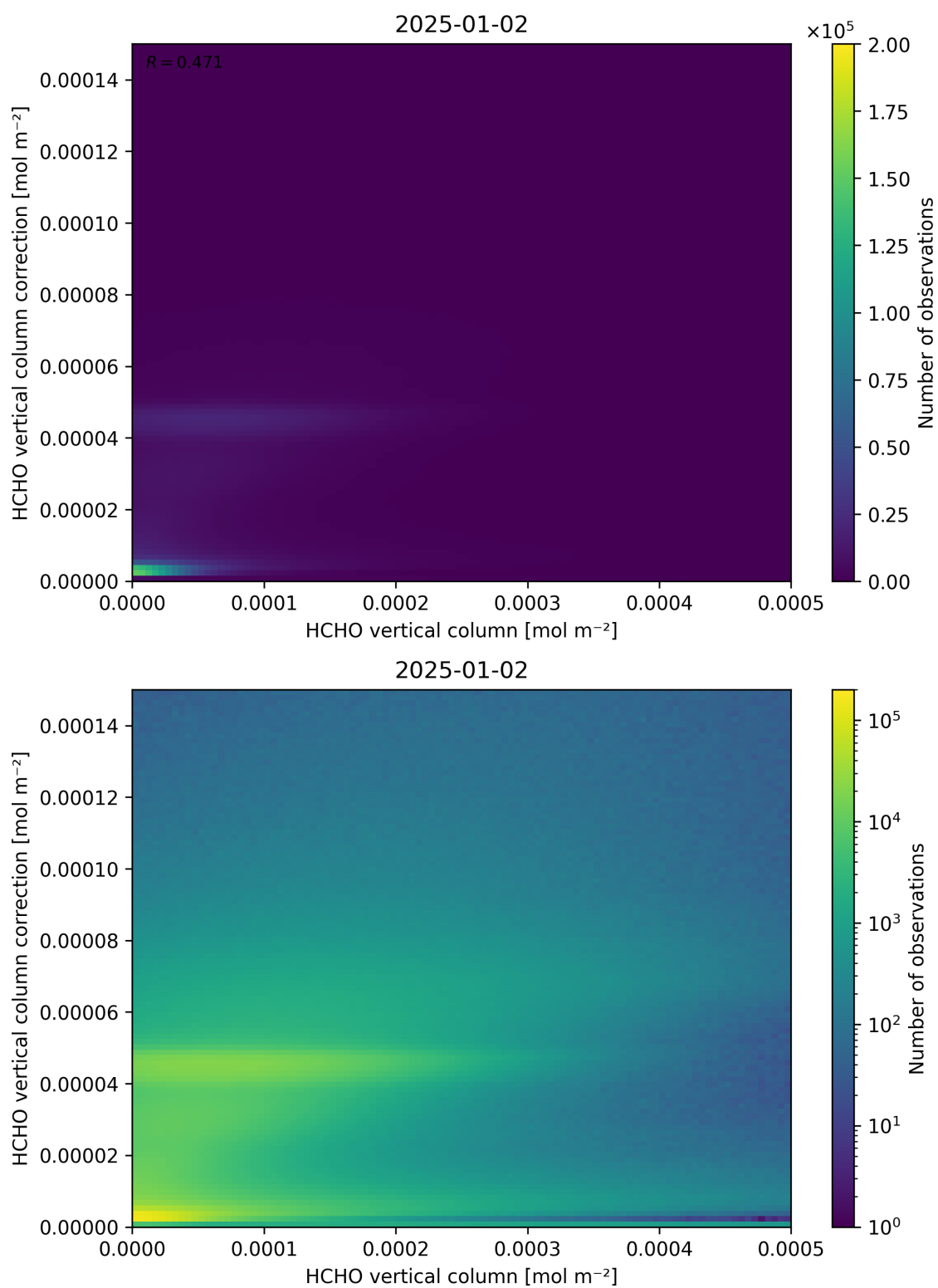
Figure 133: Scatter density plot of “HCHO vertical column” against “HCHO vertical column correction” for 2025-01-01 to 2025-01-03.
