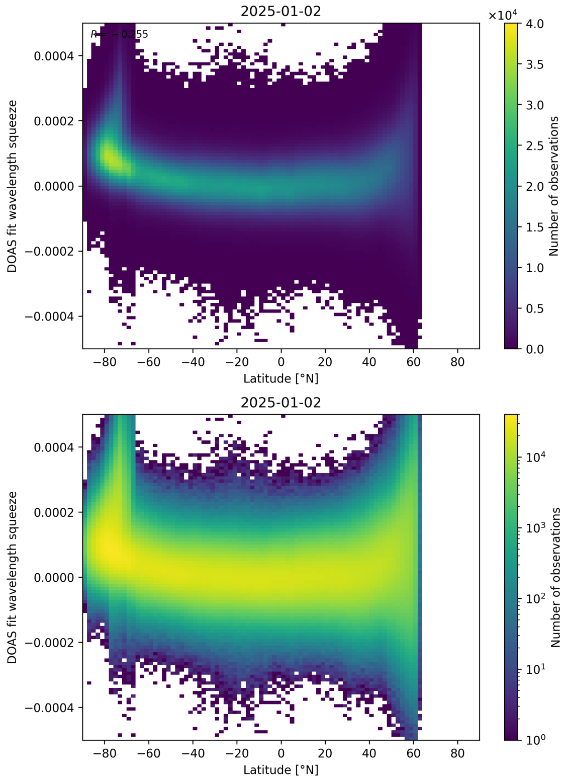
Figure 155: Scatter density plot of “Latitude” against “DOAS fit wavelength squeeze” for 2025-01-01 to 2025-01-03.
