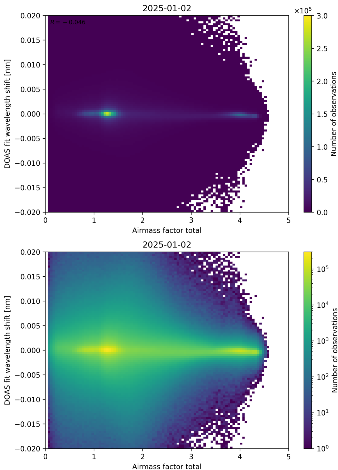
Figure 98: Scatter density plot of “Airmass factor total” against “DOAS fit wavelength shift” for 2025-01-01 to 2025-01-03.
