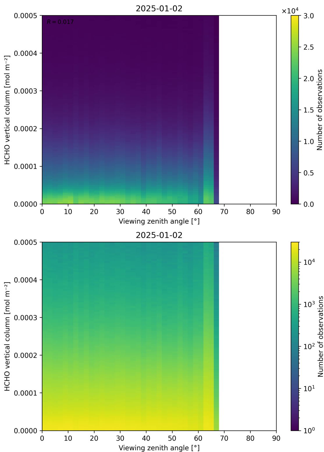
Figure 192: Scatter density plot of “Viewing zenith angle” against “HCHO vertical column” for 2025-01-01 to 2025-01-03.
