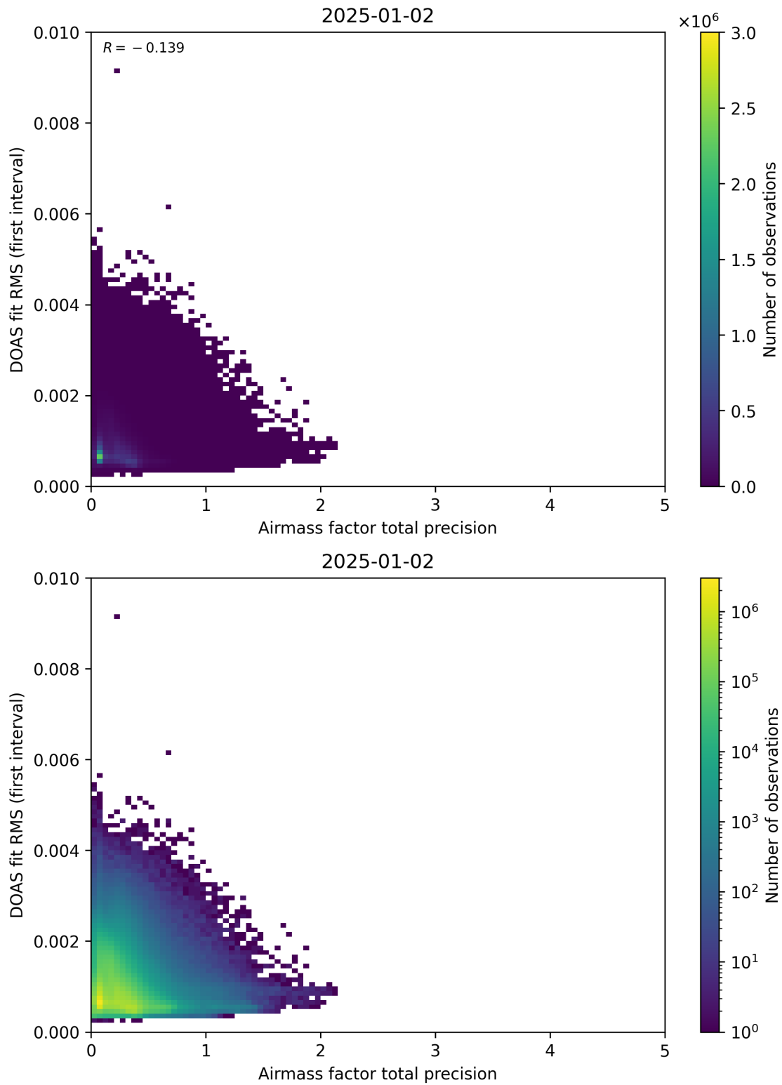
Figure 105: Scatter density plot of “Airmass factor total precision” against “DOAS fit RMS (first interval)” for 2025-01-01 to 2025-01-03.
