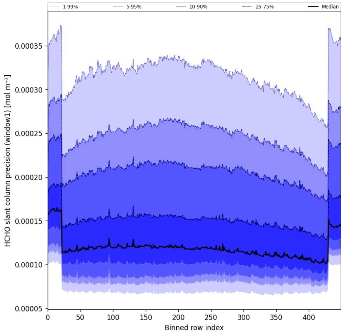
Figure 53: Along track statistics of “HCHO slant column precision (window1)” for 2025-01-01 to 2025-01-03
