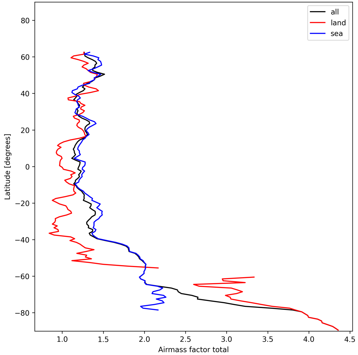
Figure 26: Zonal average of “Airmass factor total” for 2025-01-01 to 2025-01-03.
