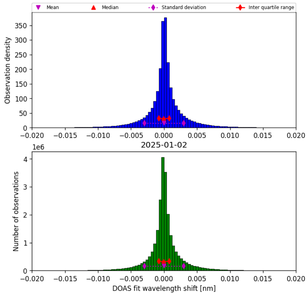
Figure 44: Histogram of “DOAS fit wavelength shift” for 2025-01-01 to 2025-01-03
