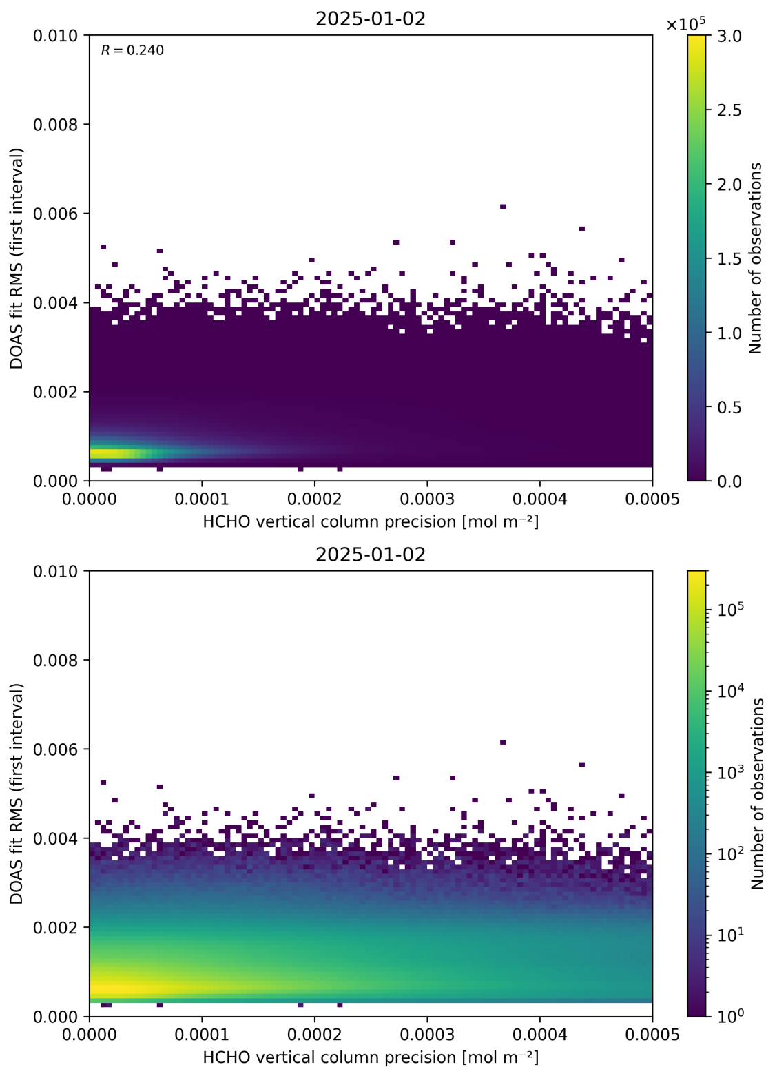
Figure 136: Scatter density plot of “HCHO vertical column precision” against “DOAS fit RMS (first interval)” for 2025-01-01 to 2025-01-03.
