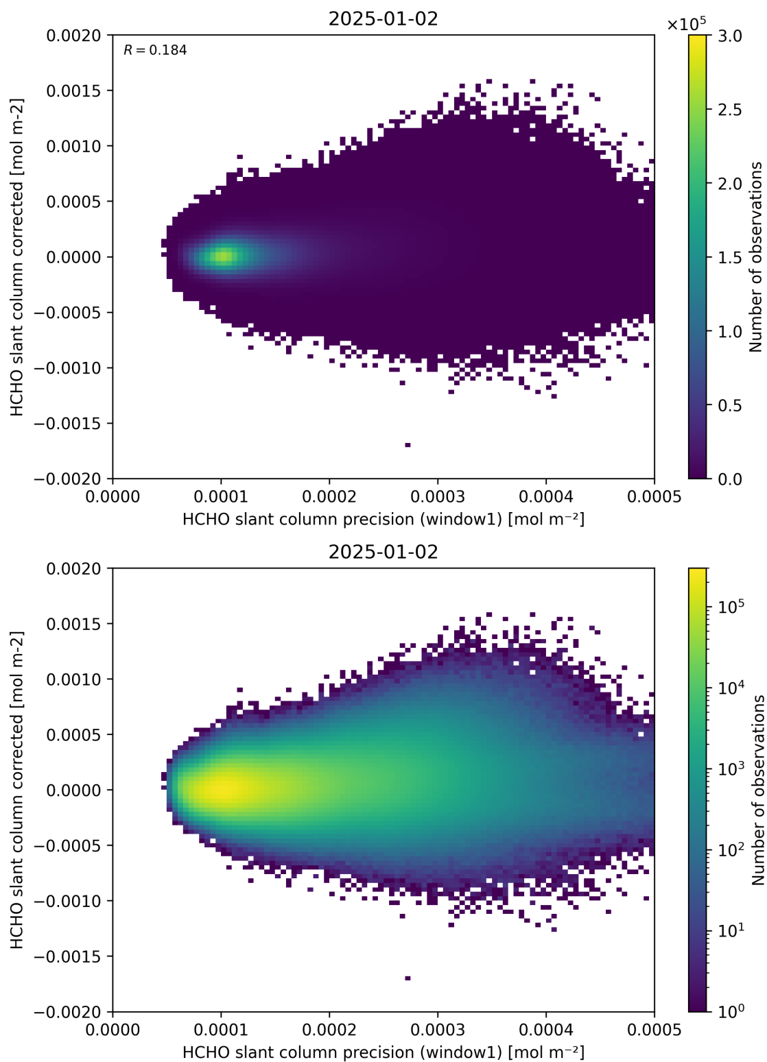
Figure 92: Scatter density plot of “HCHO slant column precision (window1)” against “HCHO slant column corrected” for 2025-01-01 to 2025-01-03.
