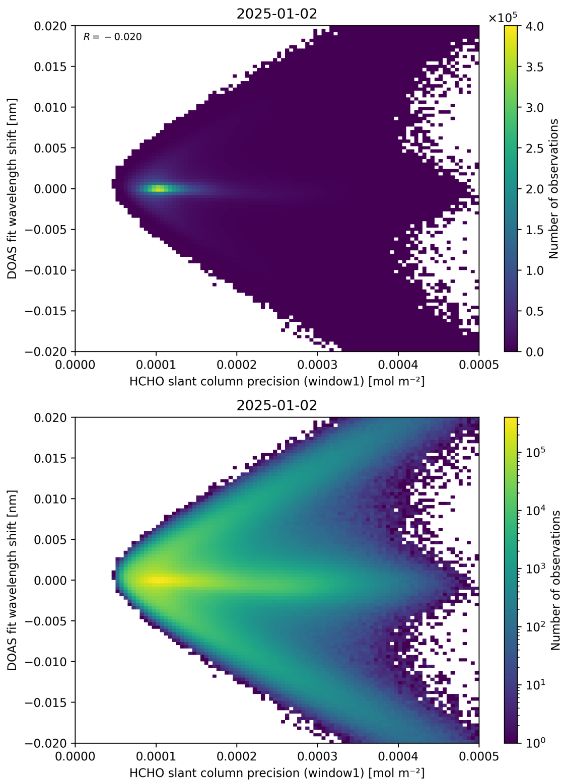
Figure 89: Scatter density plot of “HCHO slant column precision (window1)” against “DOAS fit wavelength shift” for 2025-01-01 to 2025-01-03.
