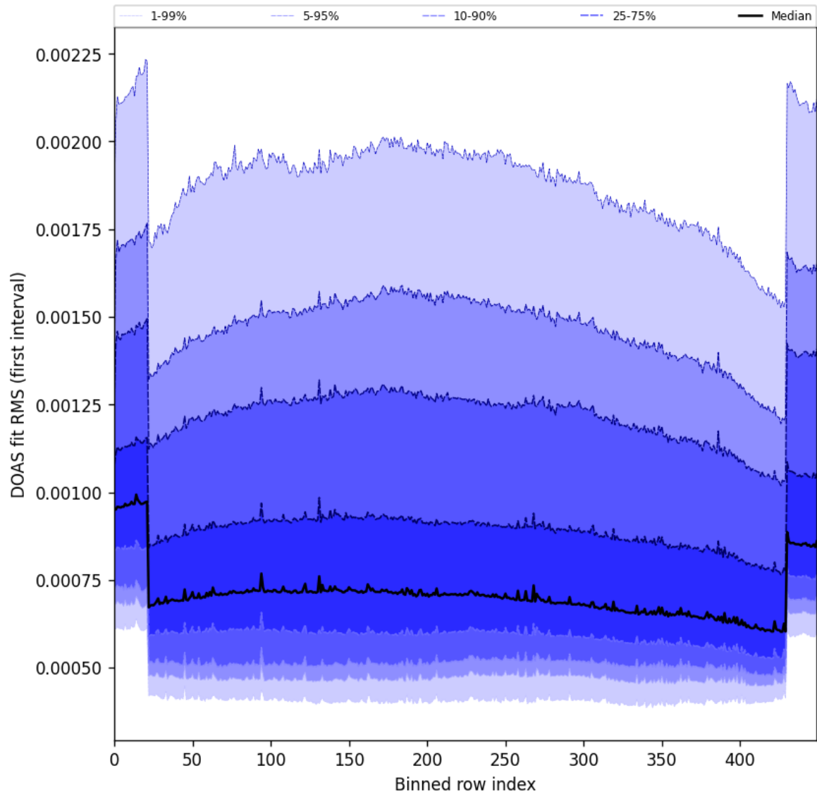
Figure 60: Along track statistics of “DOAS fit RMS (first interval)” for 2025-01-01 to 2025-01-03
