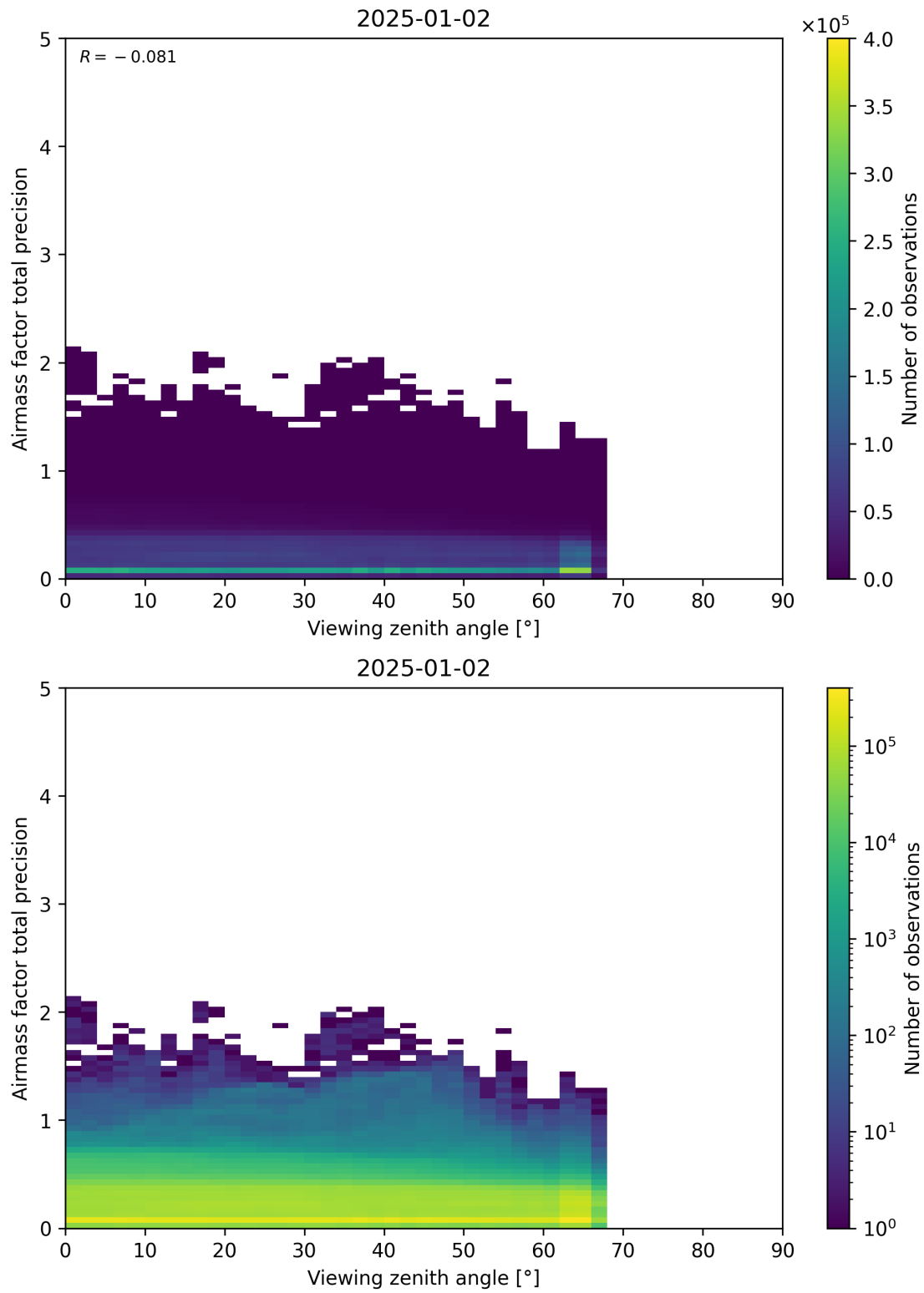
Figure 191: Scatter density plot of “Viewing zenith angle” against “Airmass factor total precision” for 2025-01-01 to 2025-01-03.
