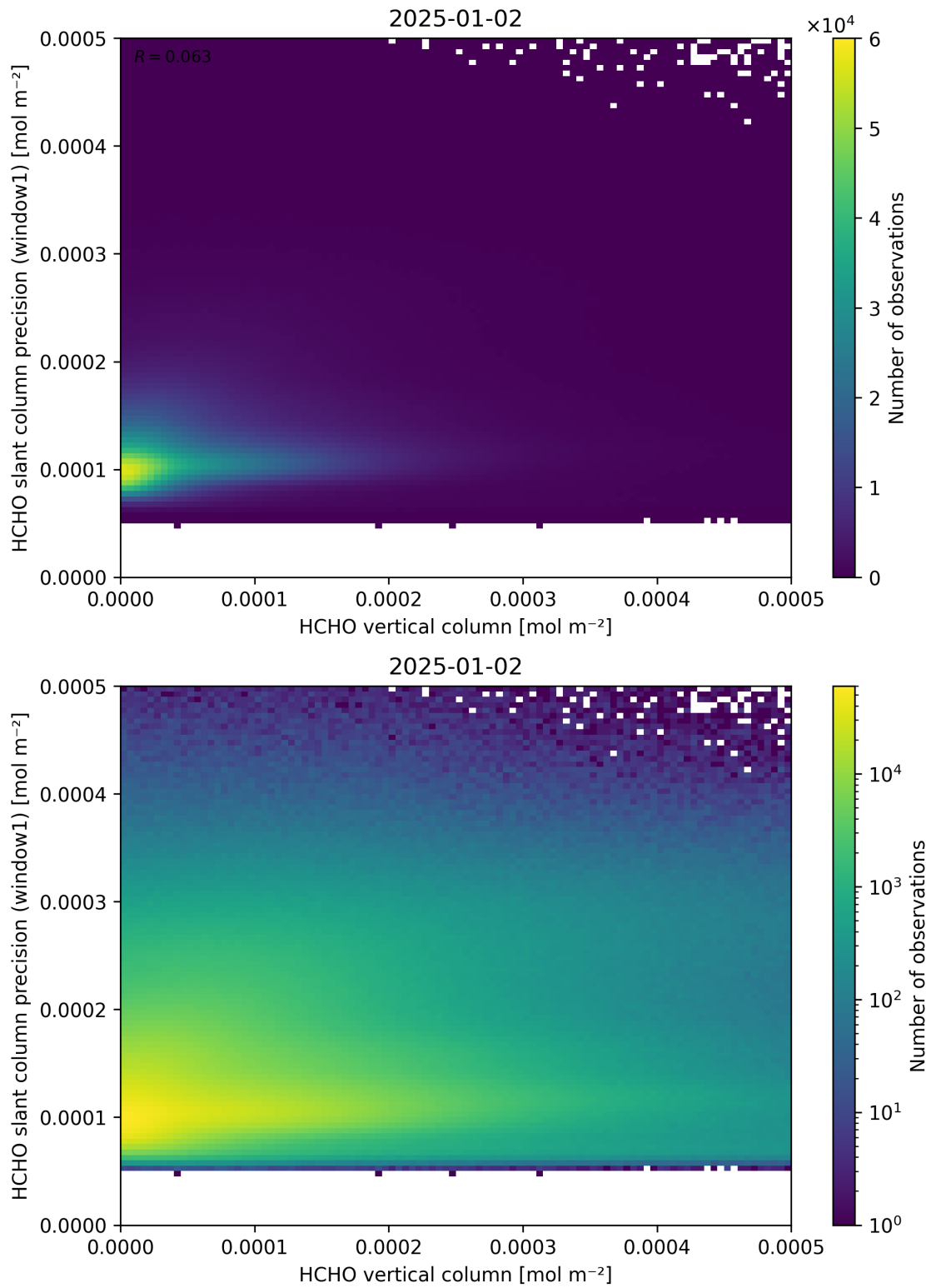
Figure 130: Scatter density plot of “HCHO vertical column” against “HCHO slant column precision (window1)” for 2025-01-01 to 2025-01-03.
