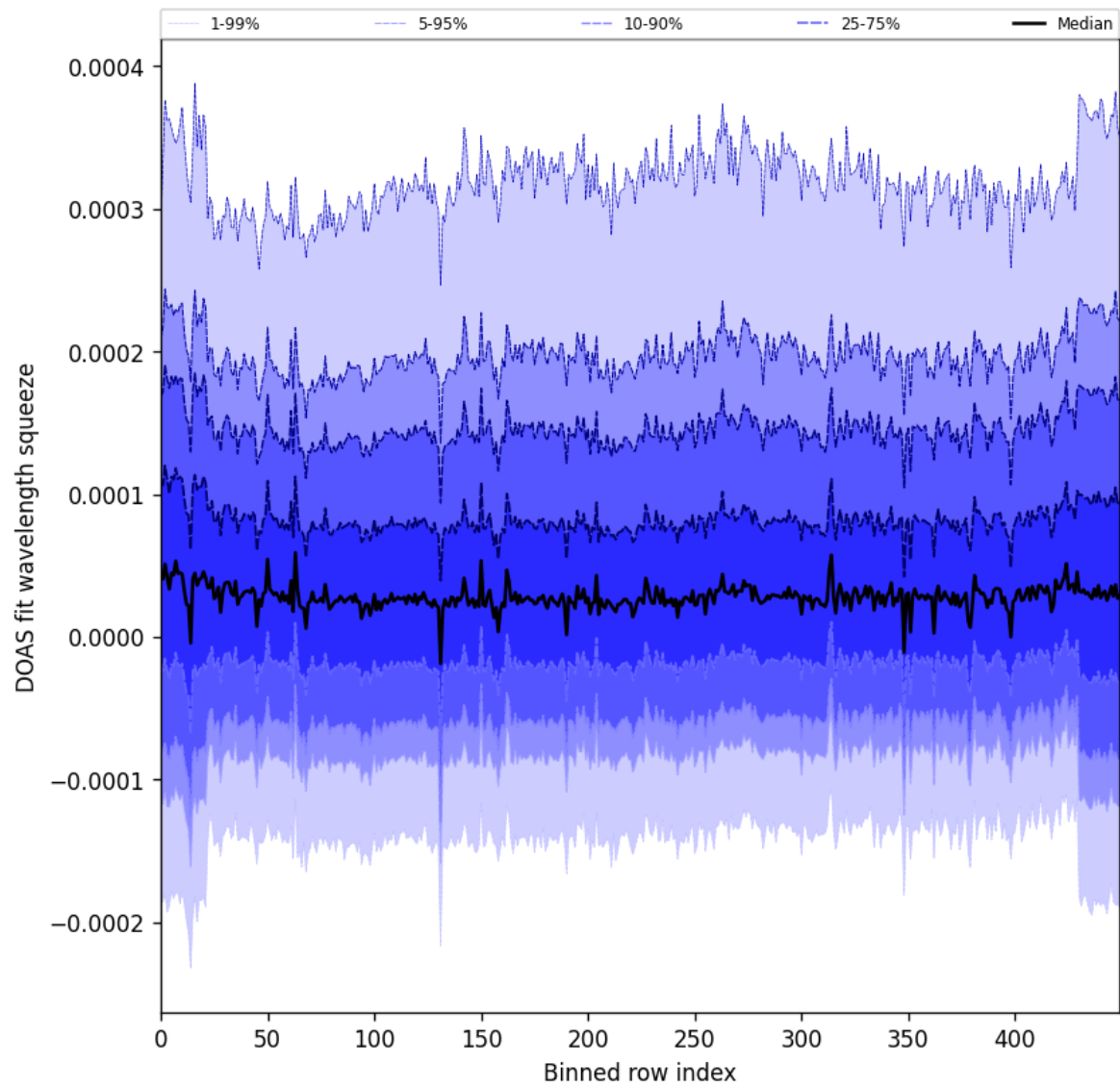
Figure 59: Along track statistics of “DOAS fit wavelength squeeze” for 2025-01-01 to 2025-01-03
