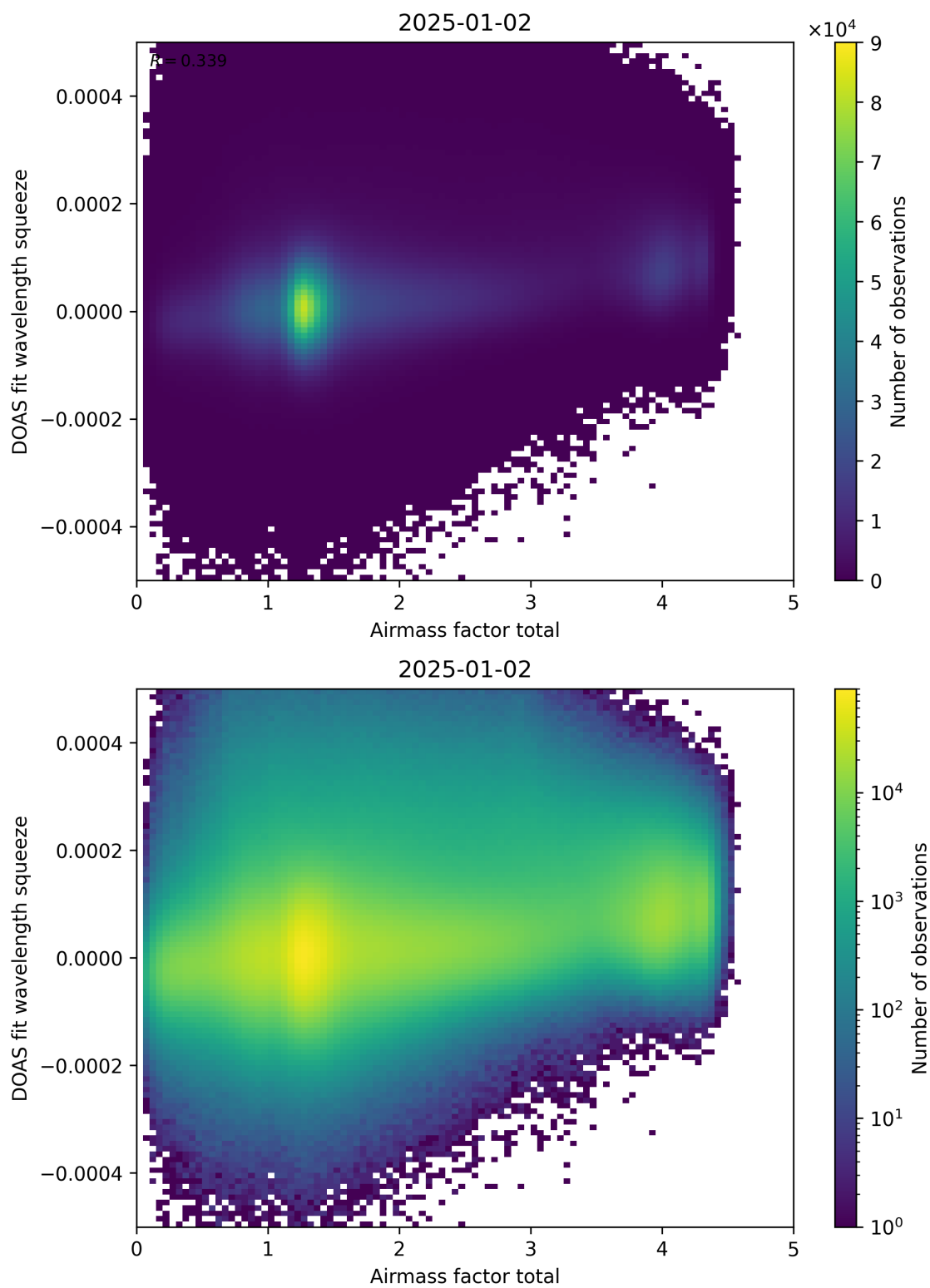
Figure 99: Scatter density plot of “Airmass factor total” against “DOAS fit wavelength squeeze” for 2025-01-01 to 2025-01-03.
