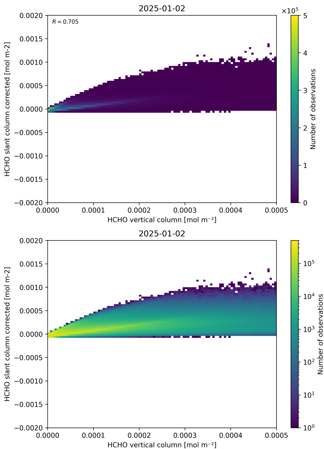
Figure 127: Scatter density plot of “HCHO vertical column” against “HCHO slant column corrected” for 2025-01-01 to 2025-01-03.
