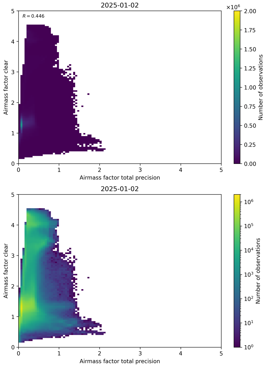
Figure 108: Scatter density plot of “Airmass factor total precision” against “Airmass factor clear” for 2025-01-01 to 2025-01-03.
