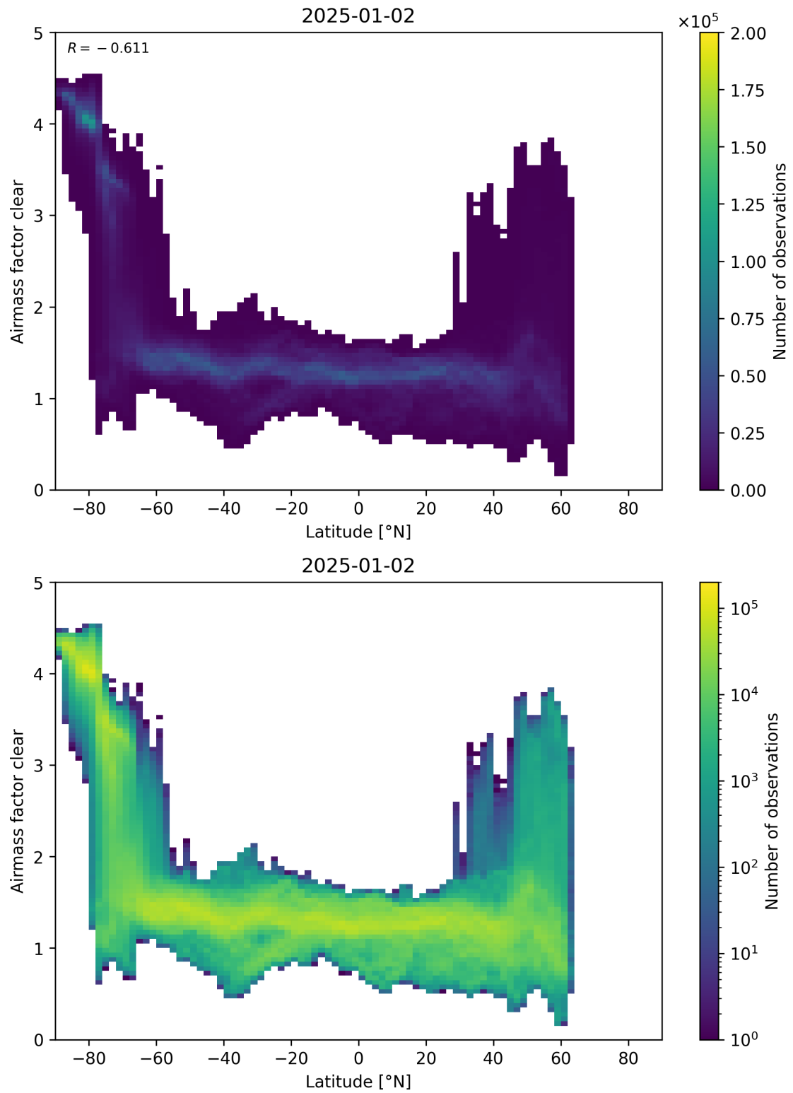
Figure 156: Scatter density plot of “Latitude” against “Airmass factor clear” for 2025-01-01 to 2025-01-03.
