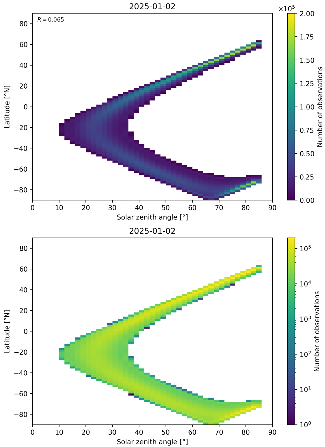
Figure 181: Scatter density plot of “Solar zenith angle” against “Latitude” for 2025-01-01 to 2025-01-03.
