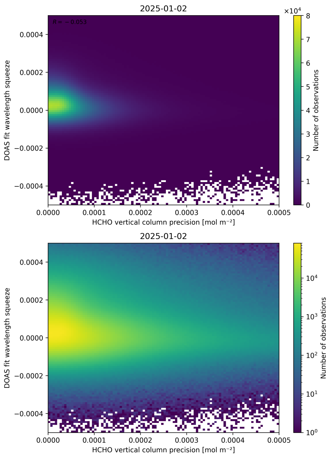
Figure 138: Scatter density plot of “HCHO vertical column precision” against “DOAS fit wavelength squeeze” for 2025-01-01 to 2025-01-03.
