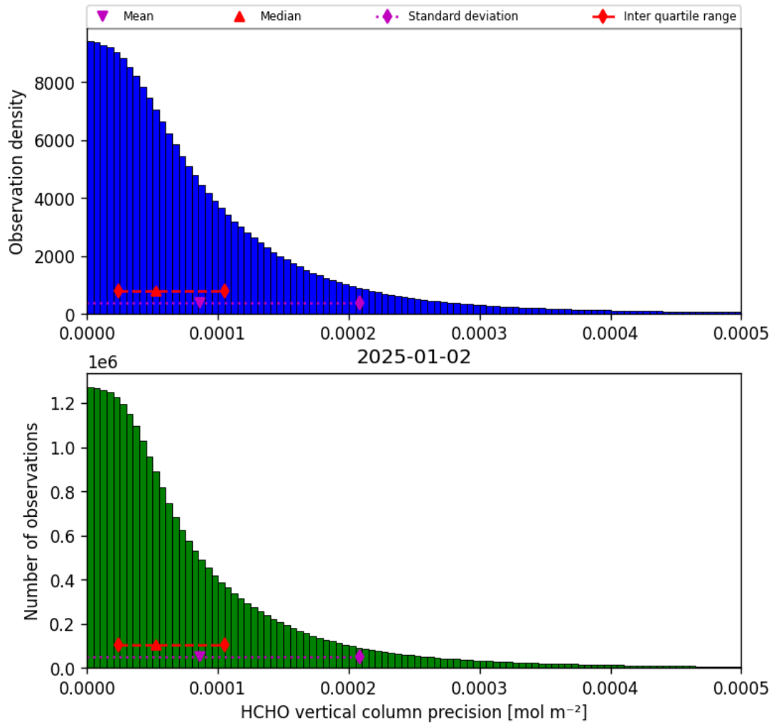
Figure 36: Histogram of “HCHO vertical column precision” for 2025-01-01 to 2025-01-03
