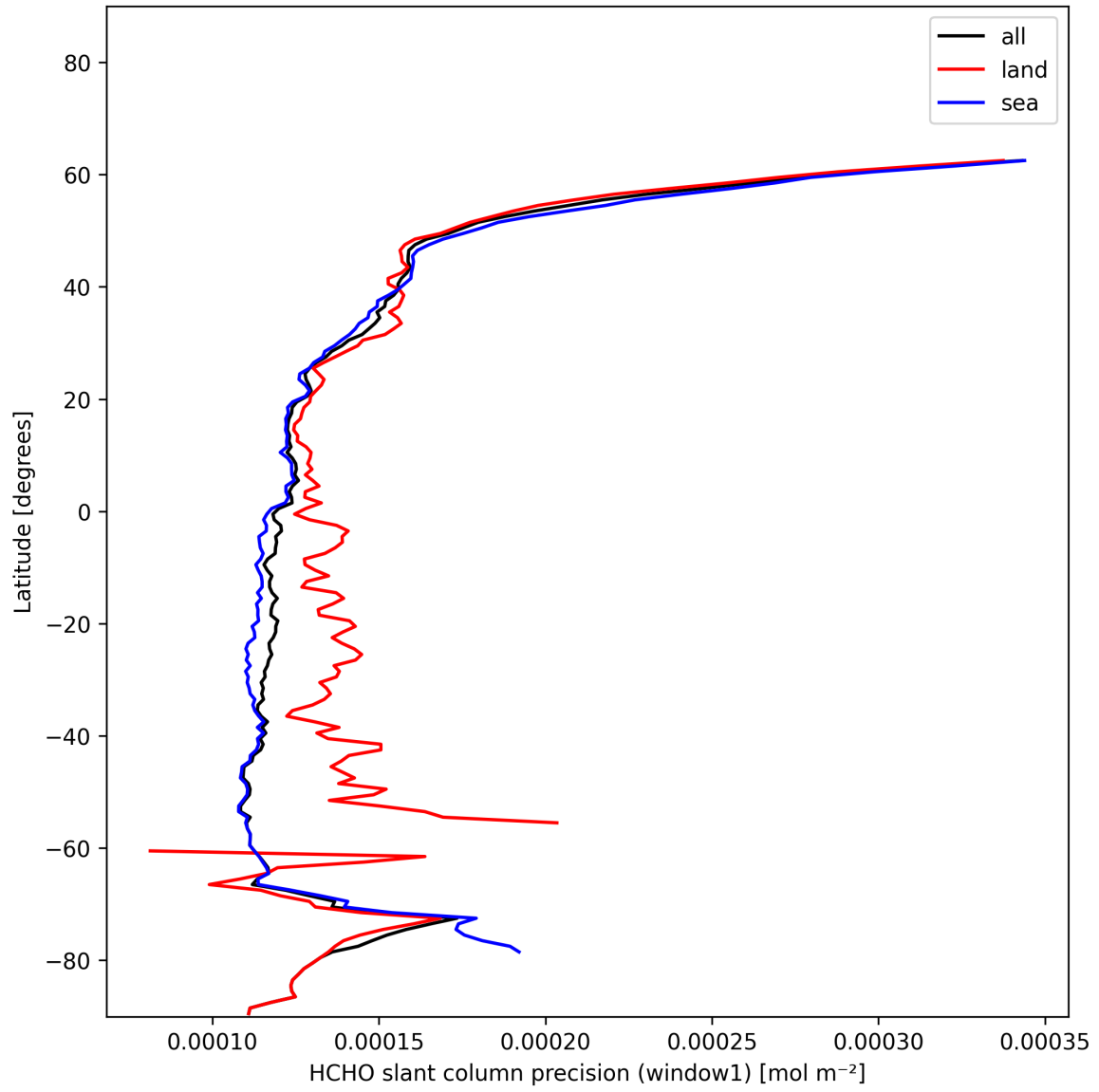
Figure 25: Zonal average of “HCHO slant column precision (window1)” for 2025-01-01 to 2025-01-03.
