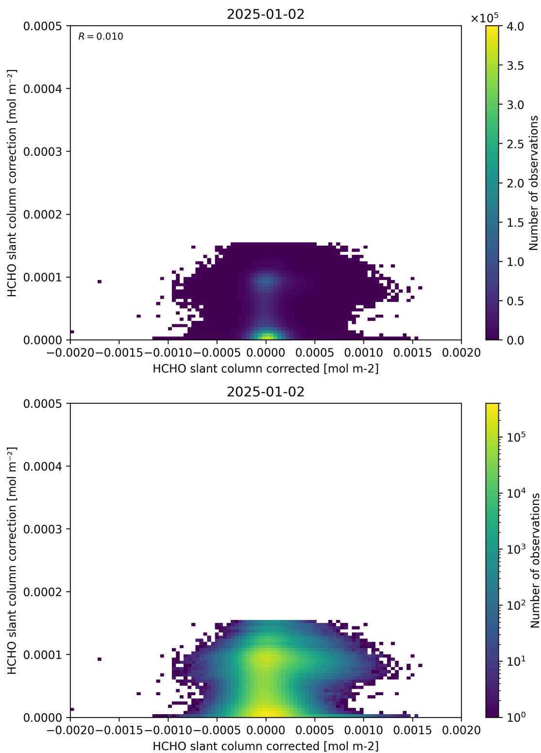
Figure 77: Scatter density plot of “HCHO slant column corrected” against “HCHO slant column correction” for 2025-01-01 to 2025-01-03.
