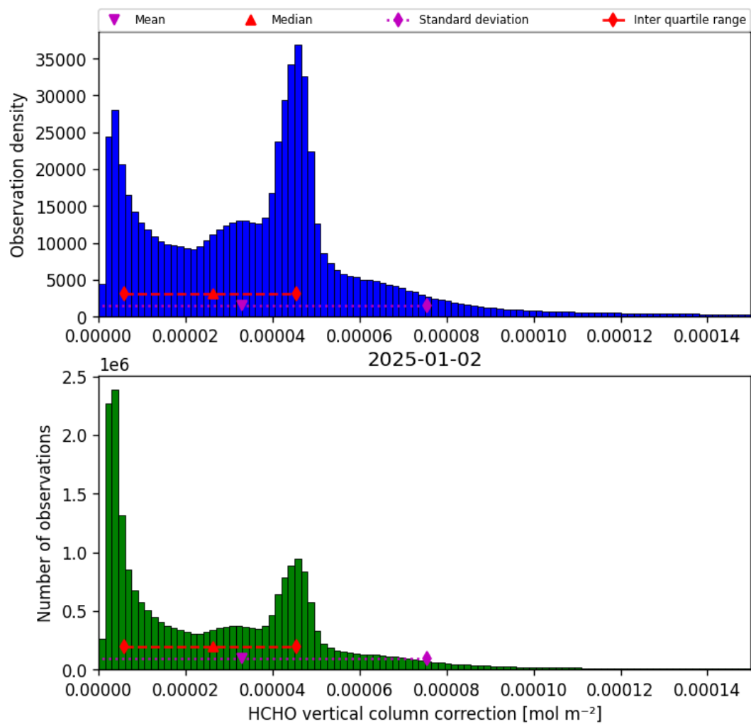
Figure 37: Histogram of “HCHO vertical column correction” for 2025-01-01 to 2025-01-03
