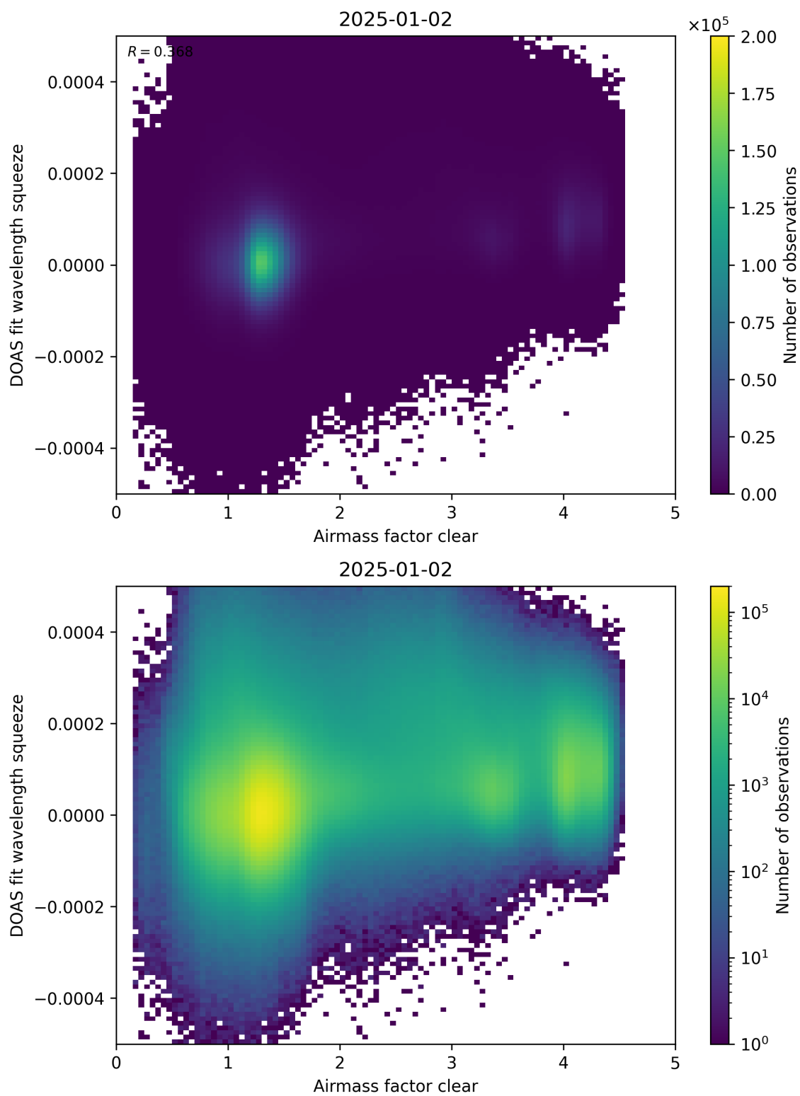
Figure 73: Scatter density plot of “Airmass factor clear” against “DOAS fit wavelength squeeze” for 2025-01-01 to 2025-01-03.
