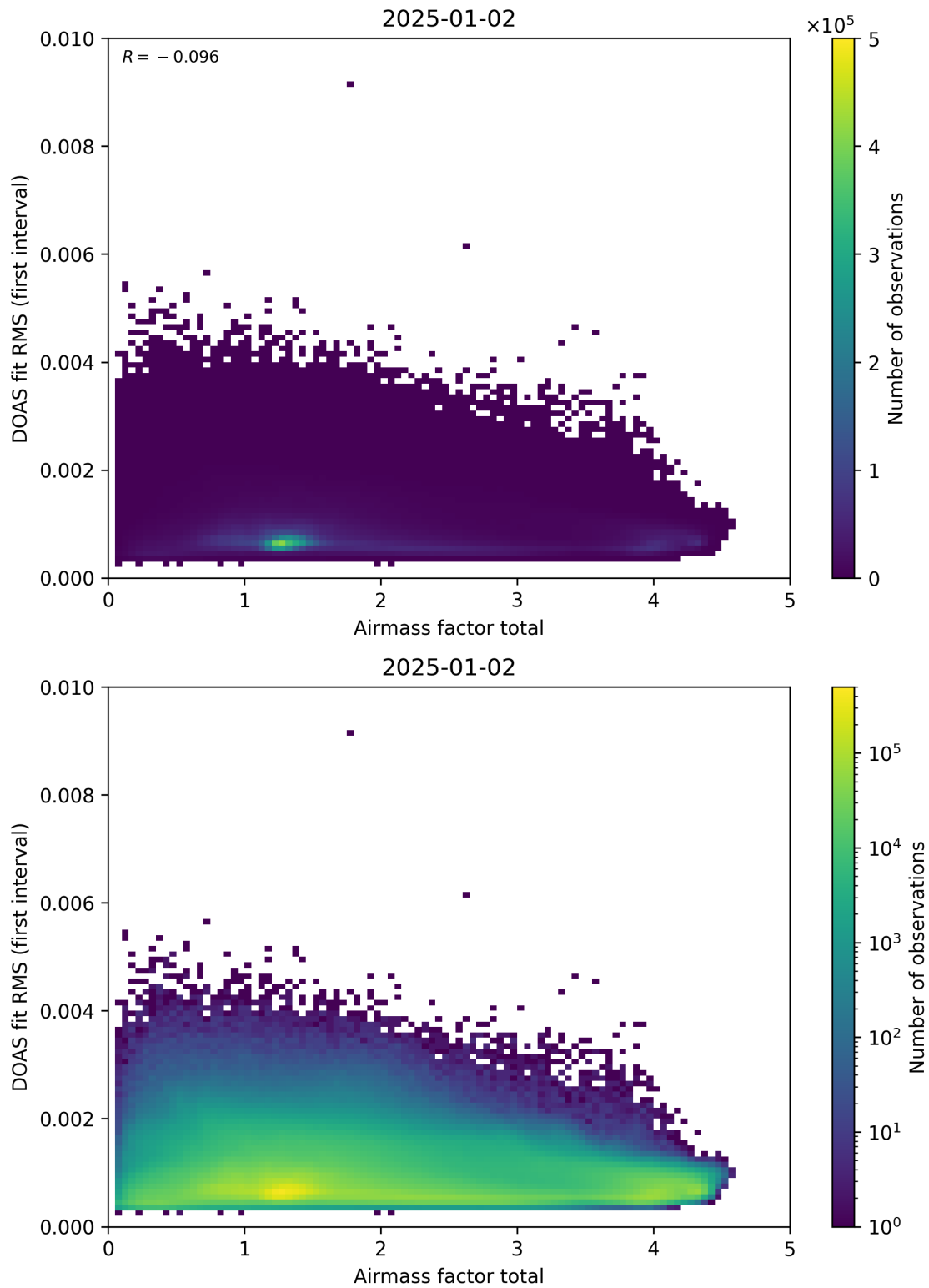
Figure 97: Scatter density plot of “Airmass factor total” against “DOAS fit RMS (first interval)” for 2025-01-01 to 2025-01-03.
