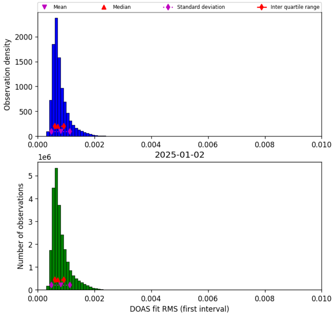
Figure 46: Histogram of “DOAS fit RMS (first interval)” for 2025-01-01 to 2025-01-03
