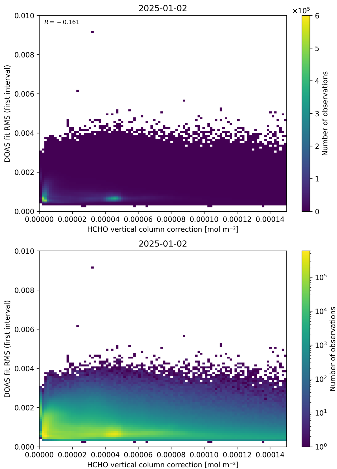
Figure 112: Scatter density plot of “HCHO vertical column correction” against “DOAS fit RMS (first interval)” for 2025-01-01 to 2025-01-03.
