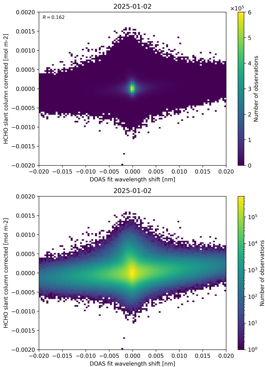
Figure 66: Scatter density plot of “DOAS fit wavelength shift” against “HCHO slant column corrected” for 2025-01-01 to 2025-01-03.
