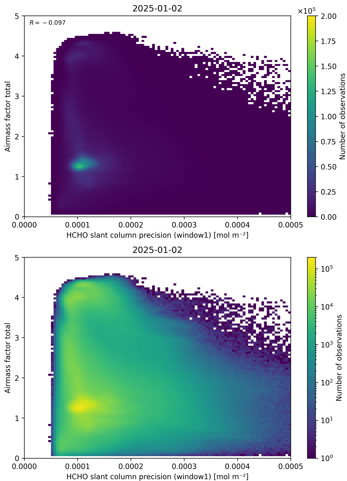
Figure 94: Scatter density plot of “HCHO slant column precision (window1)” against “Airmass factor total” for 2025-01-01 to 2025-01-03.
