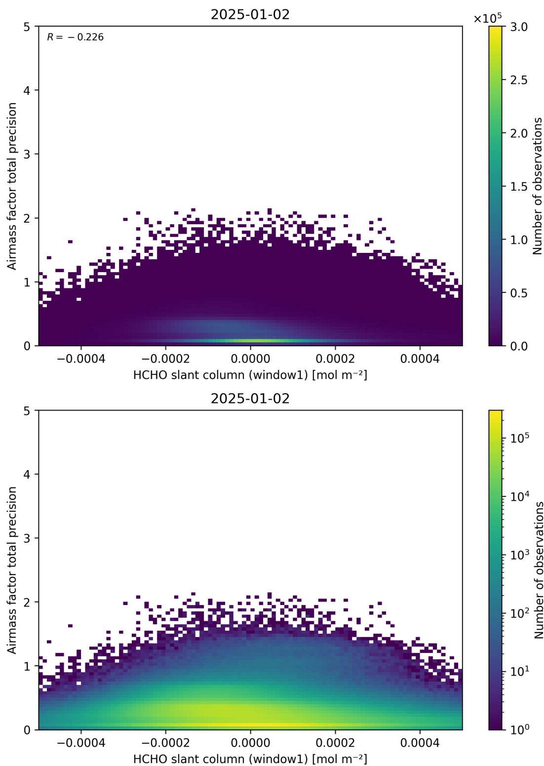
Figure 86: Scatter density plot of “HCHO slant column (window1)” against “Airmass factor total precision” for 2025-01-01 to 2025-01-03.
