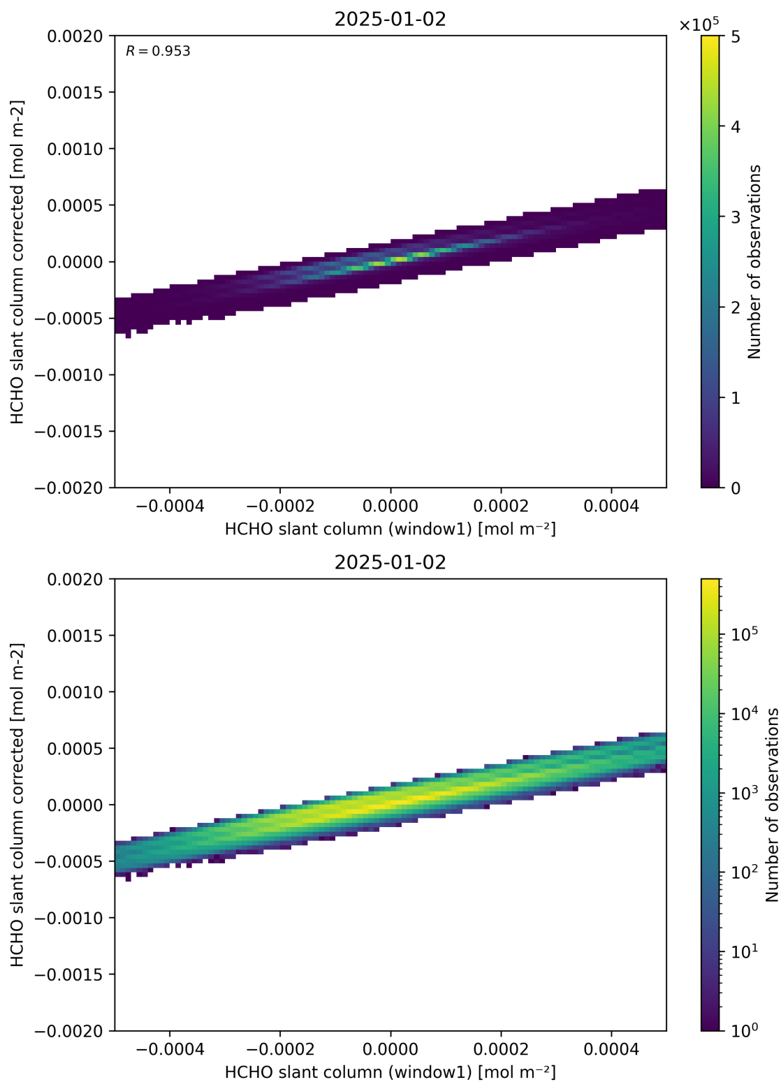
Figure 82: Scatter density plot of “HCHO slant column (window1)” against “HCHO slant column corrected” for 2025-01-01 to 2025-01-03.
