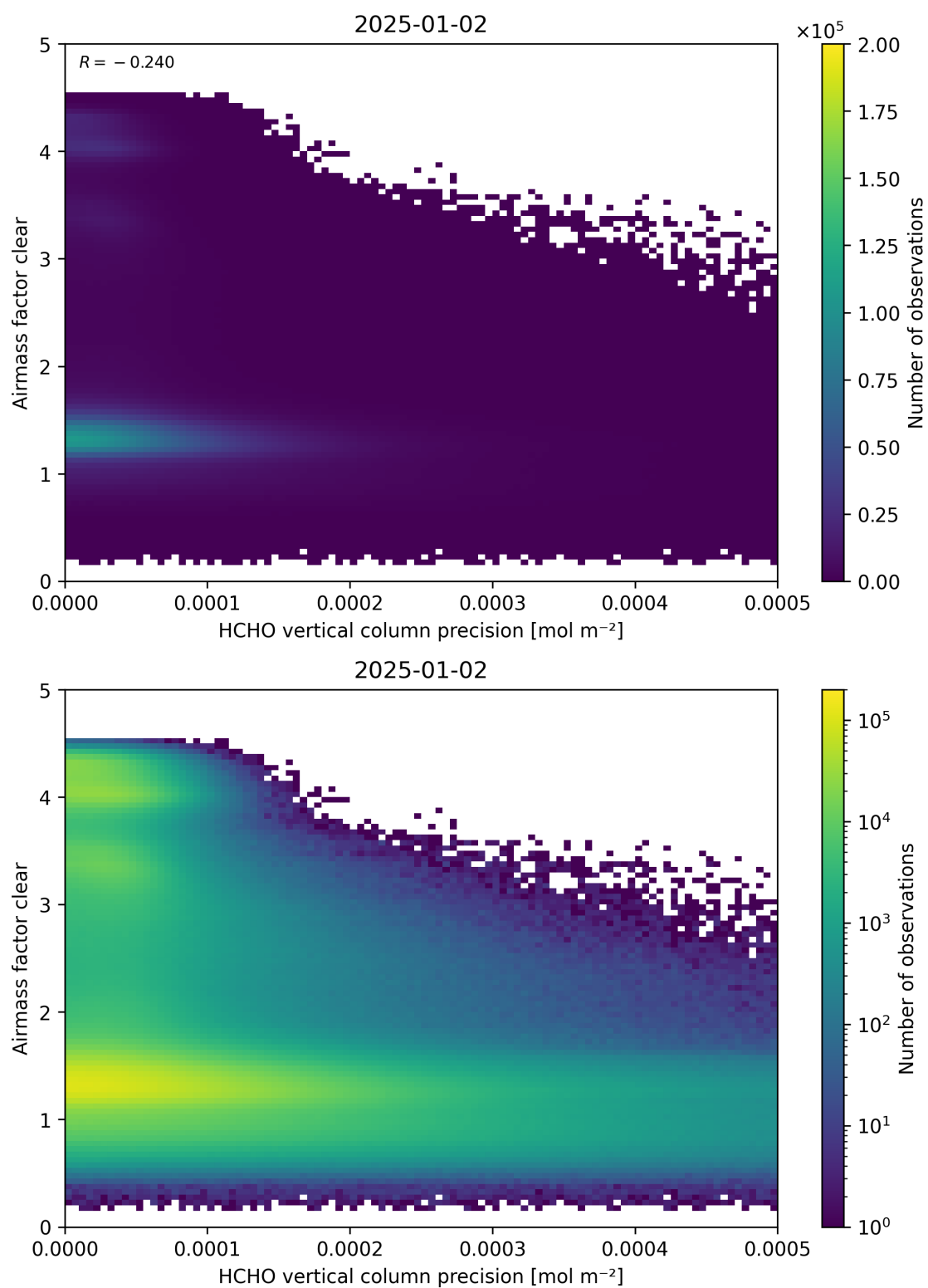
Figure 139: Scatter density plot of “HCHO vertical column precision” against “Airmass factor clear” for 2025-01-01 to 2025-01-03.
