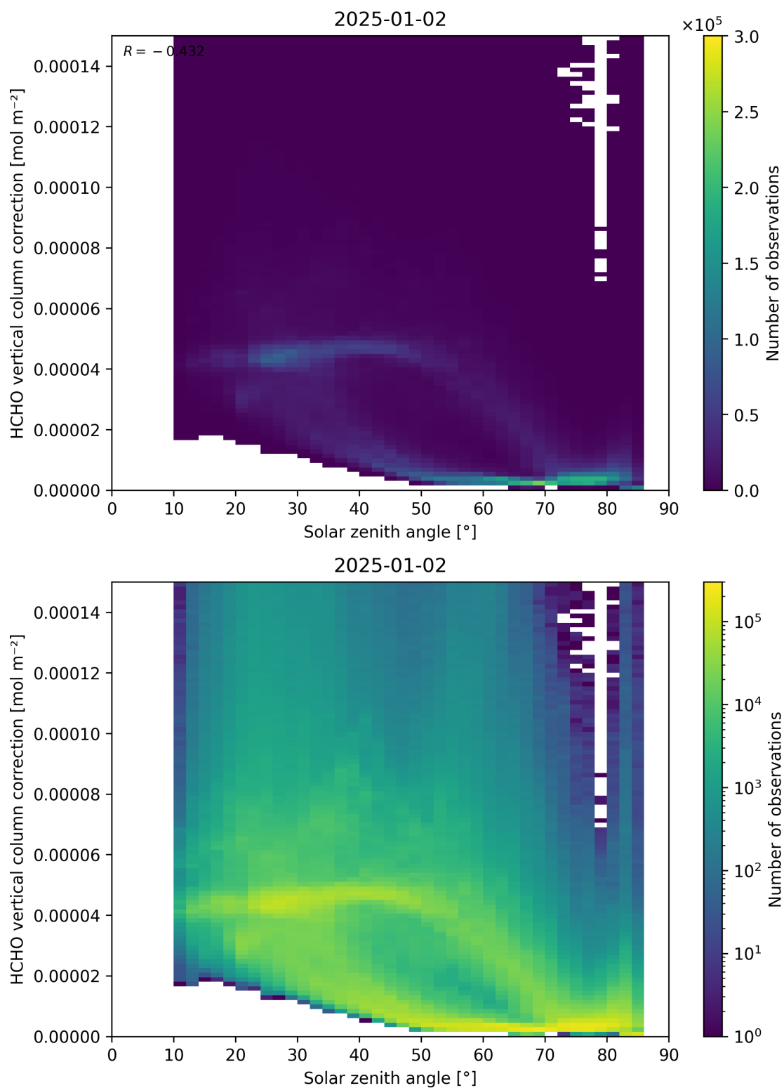
Figure 178: Scatter density plot of “Solar zenith angle” against “HCHO vertical column correction” for 2025-01-01 to 2025-01-03.
