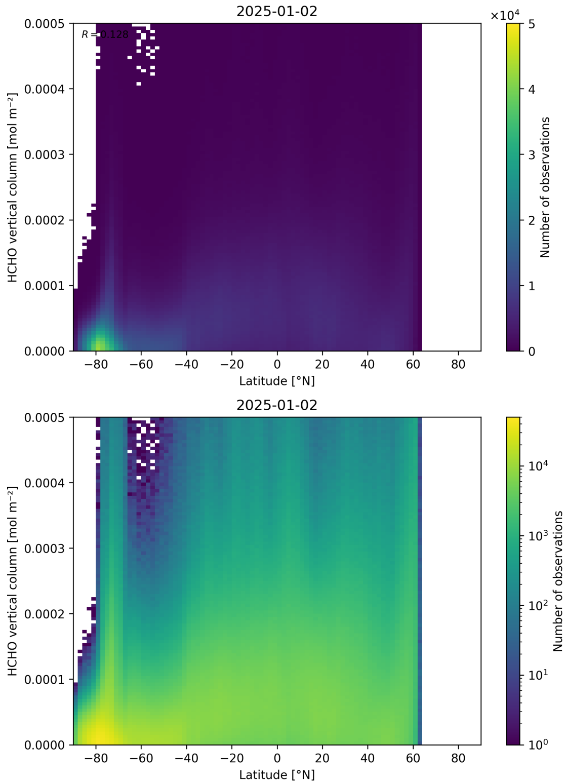
Figure 163: Scatter density plot of “Latitude” against “HCHO vertical column” for 2025-01-01 to 2025-01-03.
