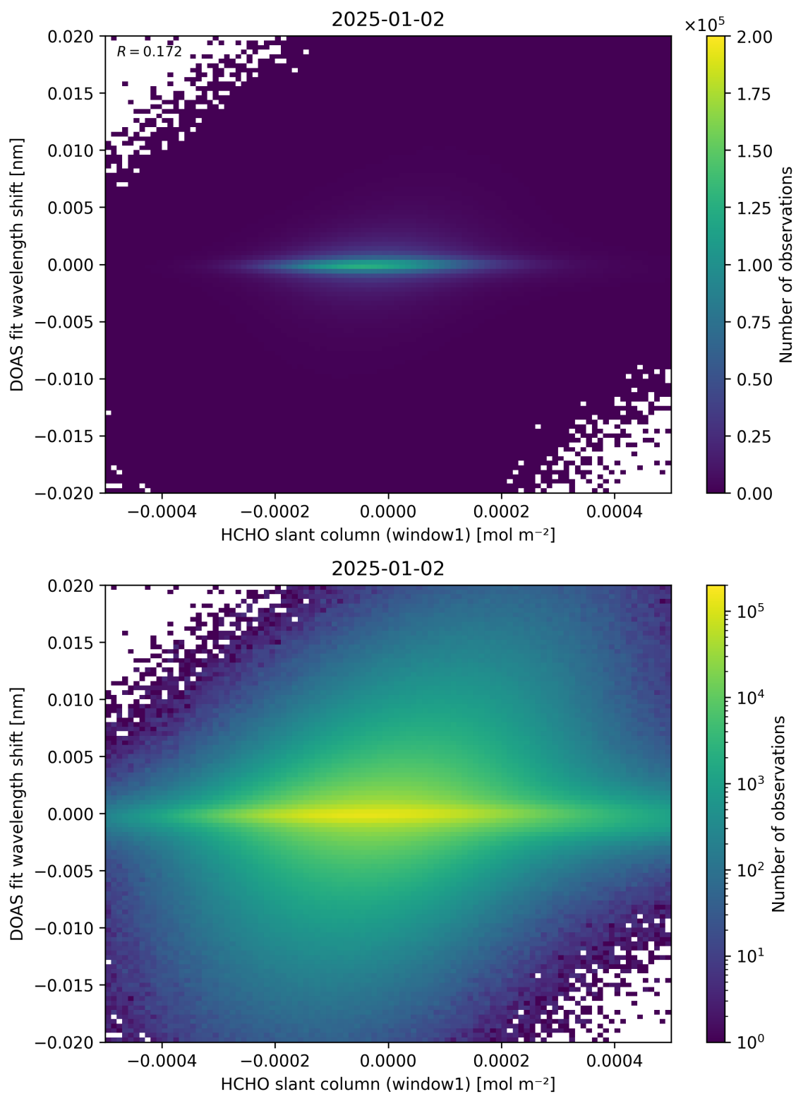
Figure 79: Scatter density plot of “HCHO slant column (window1)” against “DOAS fit wavelength shift” for 2025-01-01 to 2025-01-03.
