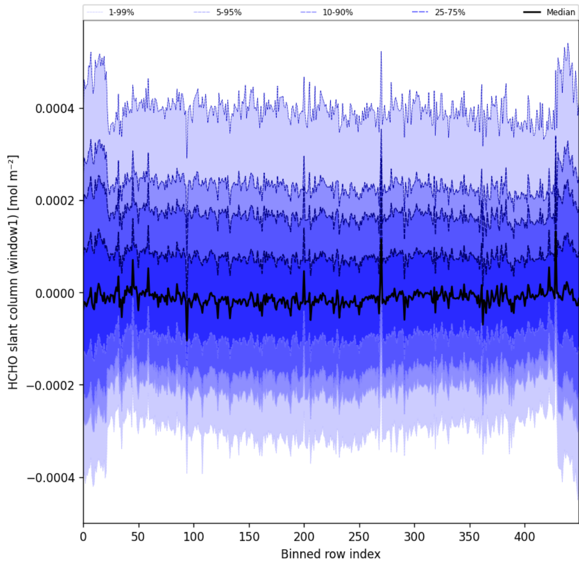
Figure 52: Along track statistics of “HCHO slant column (window1)” for 2025-01-01 to 2025-01-03
