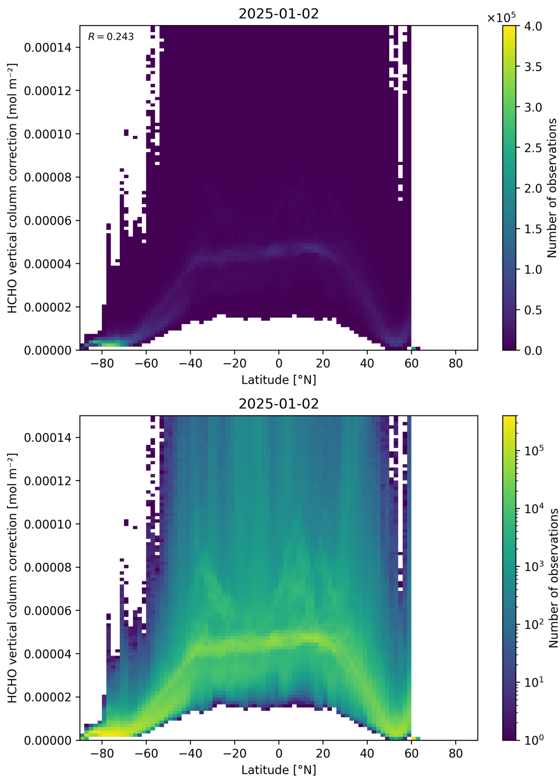
Figure 164: Scatter density plot of “Latitude” against “HCHO vertical column correction” for 2025-01-01 to 2025-01-03.
