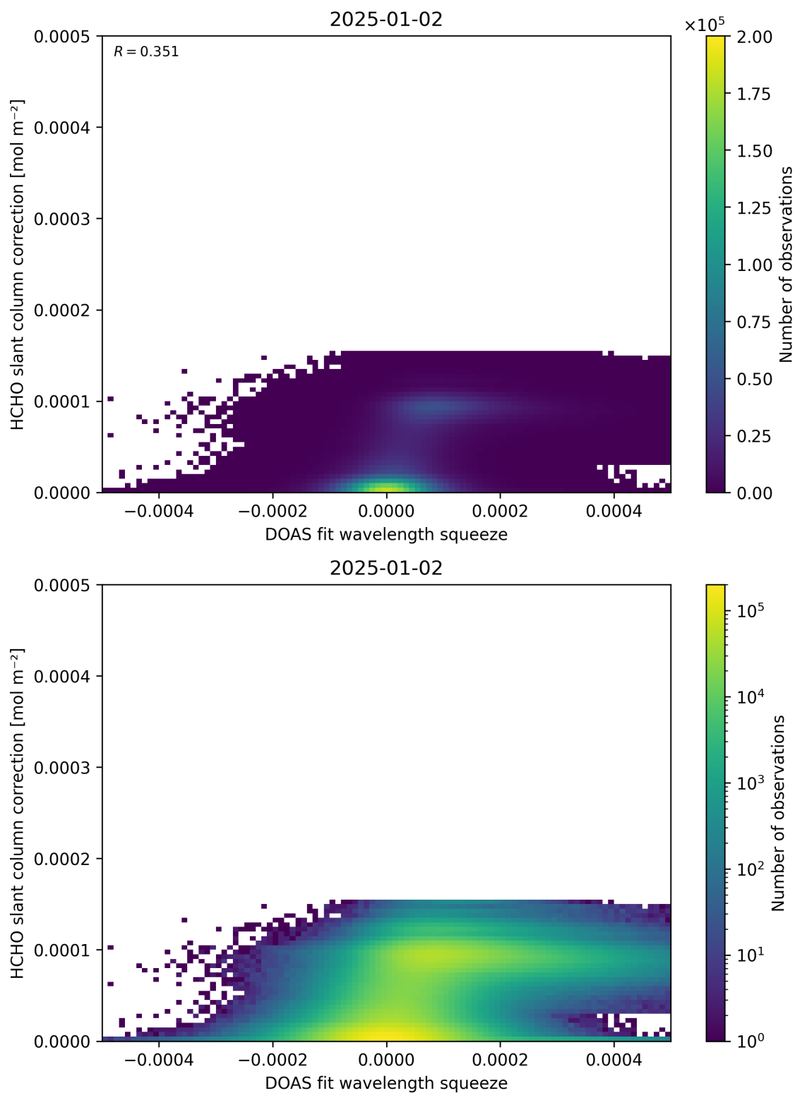
Figure 70: Scatter density plot of “DOAS fit wavelength squeeze” against “HCHO slant column correction” for 2025-01-01 to 2025-01-03.
