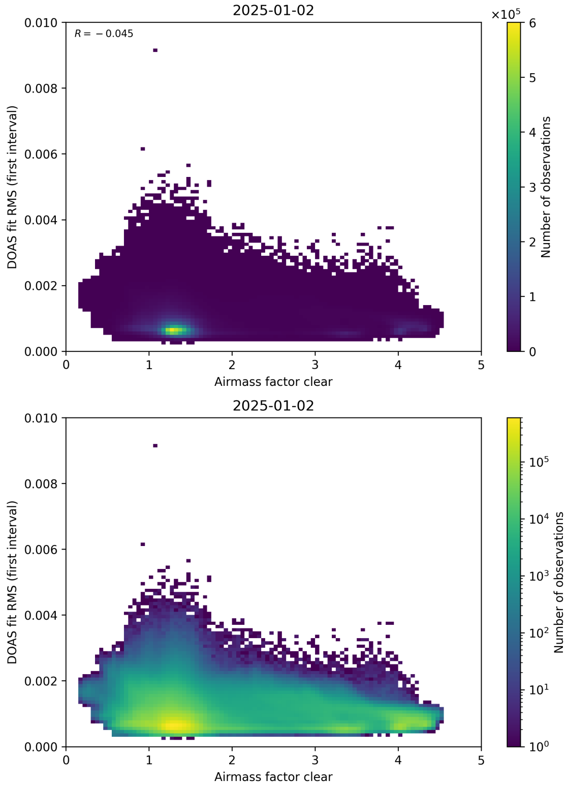
Figure 71: Scatter density plot of “Airmass factor clear” against “DOAS fit RMS (first interval)” for 2025-01-01 to 2025-01-03.
