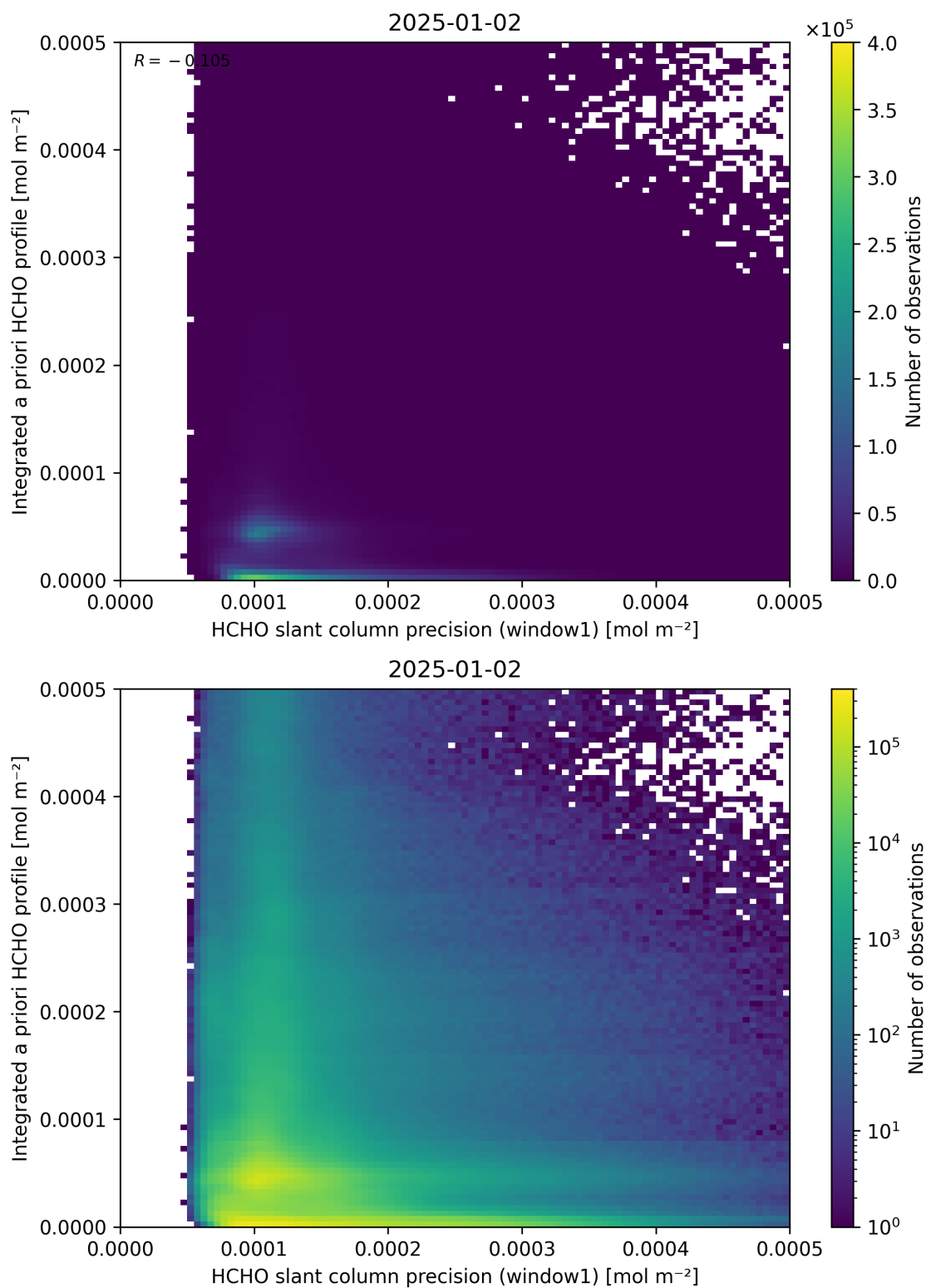
Figure 96: Scatter density plot of “HCHO slant column precision (window1)” against “Integrated a priori HCHO profile” for 2025-01-01 to 2025-01-03.
