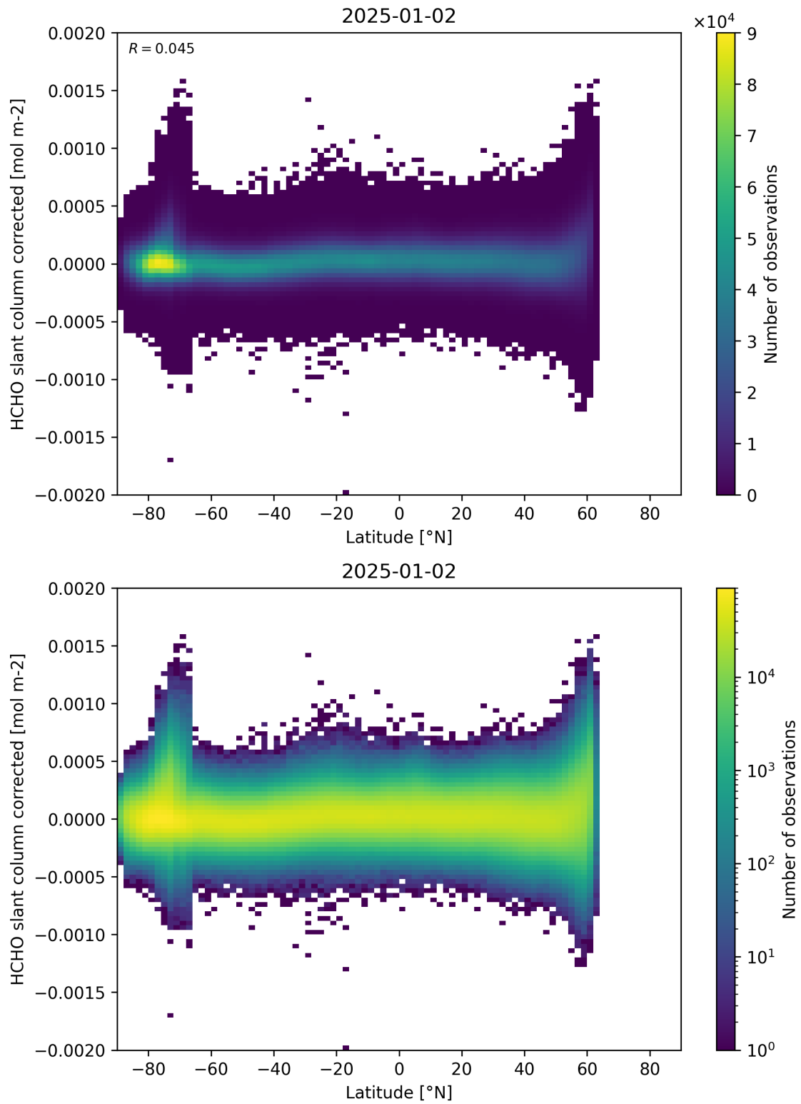
Figure 157: Scatter density plot of “Latitude” against “HCHO slant column corrected” for 2025-01-01 to 2025-01-03.
