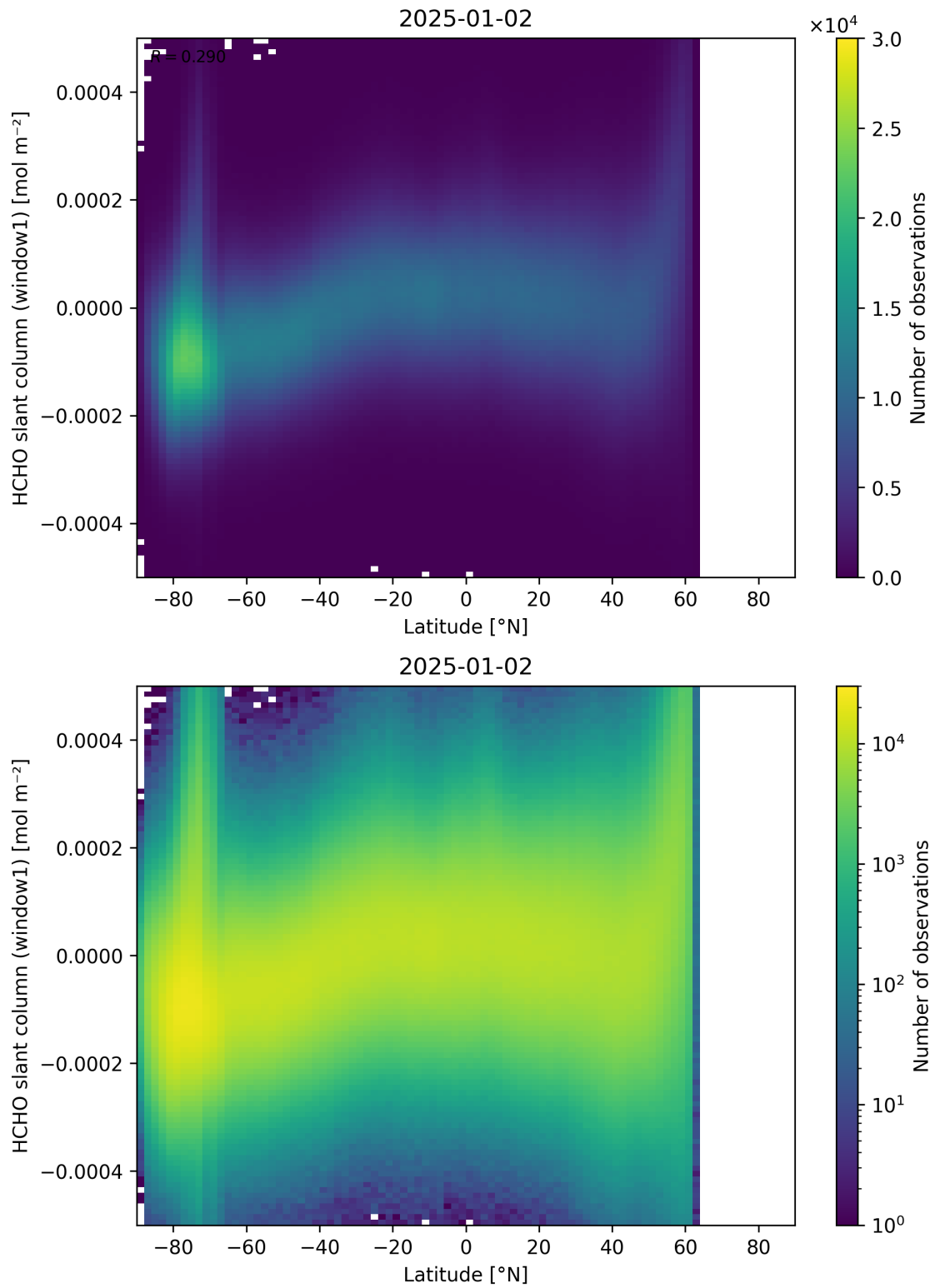
Figure 159: Scatter density plot of “Latitude” against “HCHO slant column (window1)” for 2025-01-01 to 2025-01-03.
