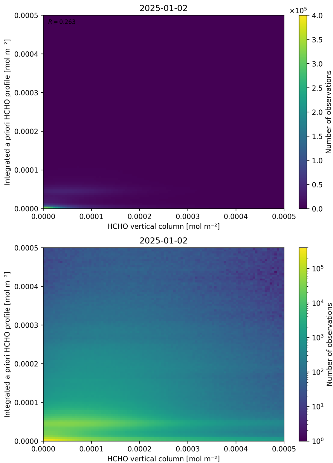
Figure 135: Scatter density plot of “HCHO vertical column” against “Integrated a priori HCHO profile” for 2025-01-01 to 2025-01-03.
