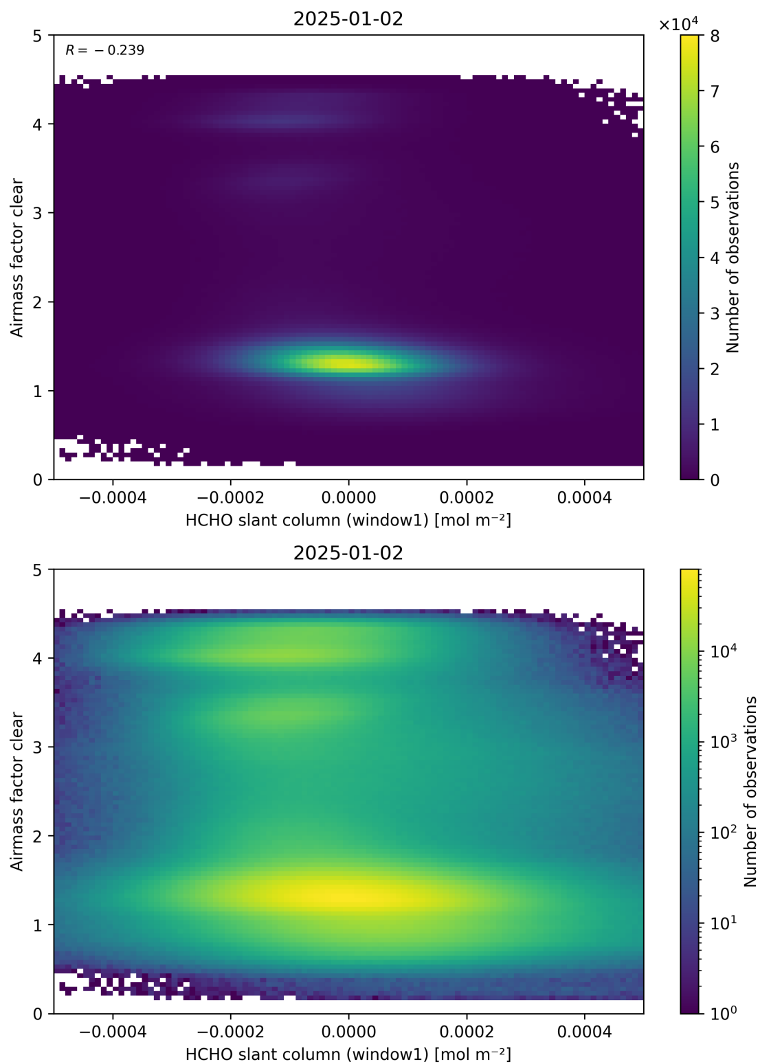
Figure 81: Scatter density plot of “HCHO slant column (window1)” against “Airmass factor clear” for 2025-01-01 to 2025-01-03.
