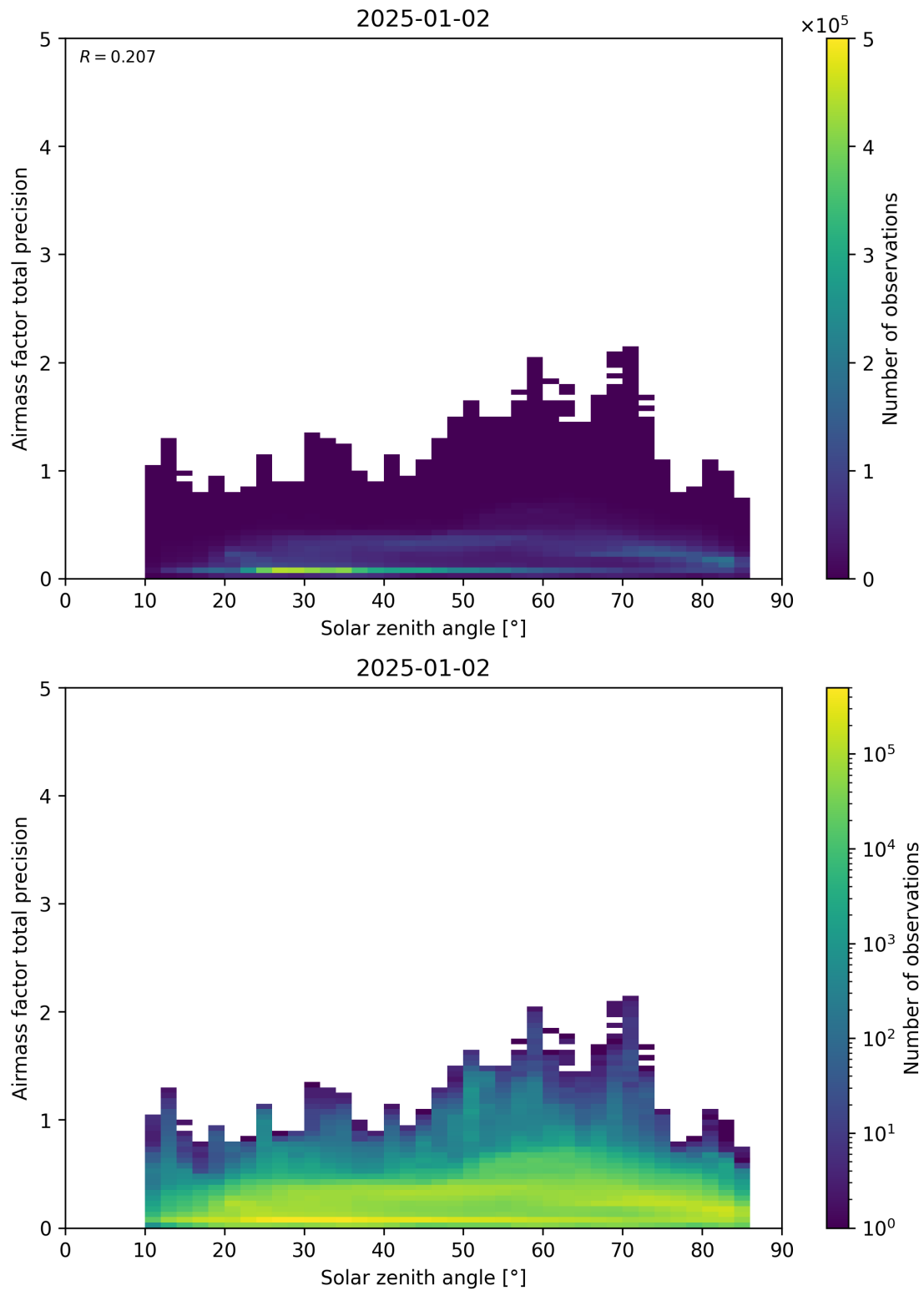
Figure 176: Scatter density plot of “Solar zenith angle” against “Airmass factor total precision” for 2025-01-01 to 2025-01-03.
