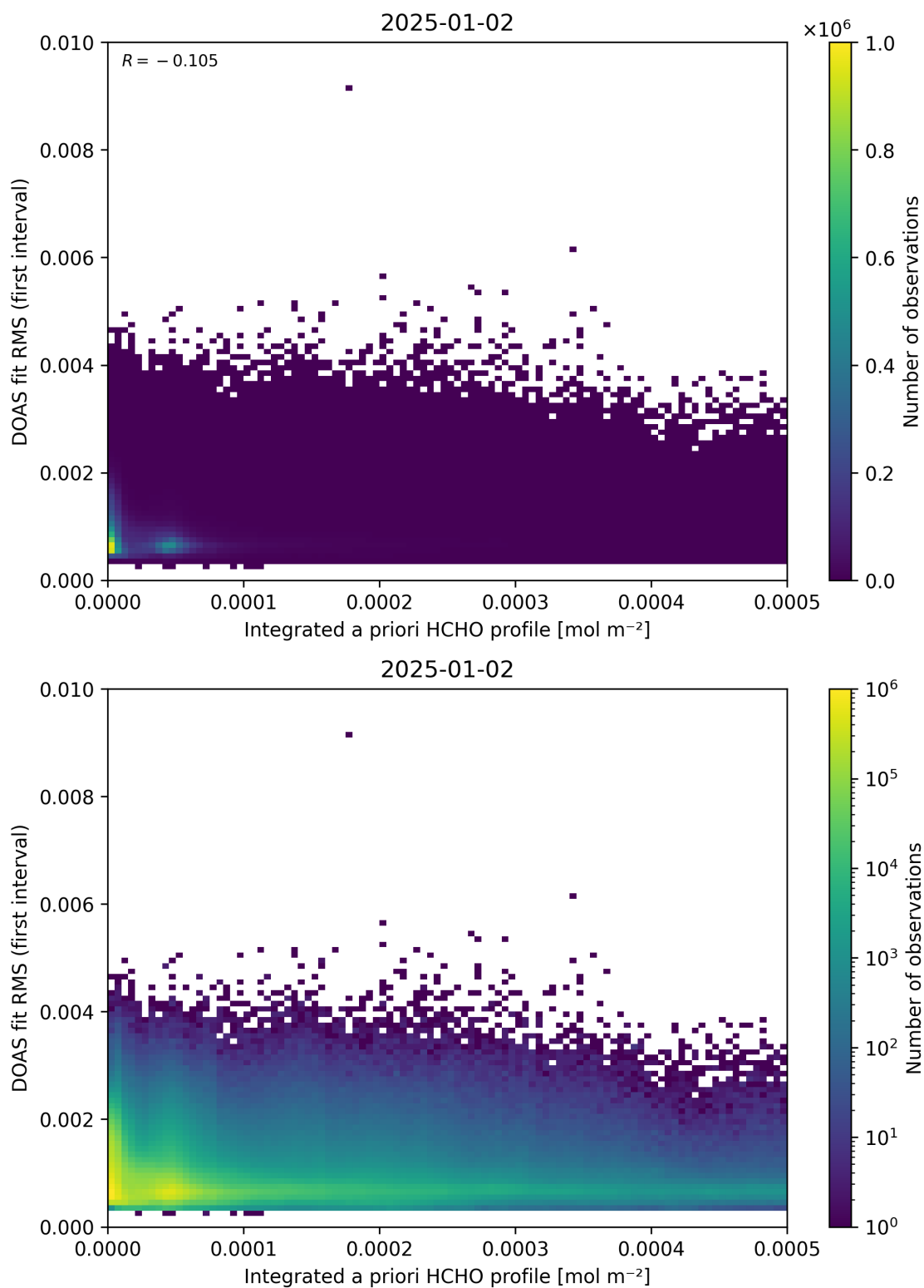
Figure 148: Scatter density plot of “Integrated a priori HCHO profile” against “DOAS fit RMS (first interval)” for 2025-01-01 to 2025-01-03.
