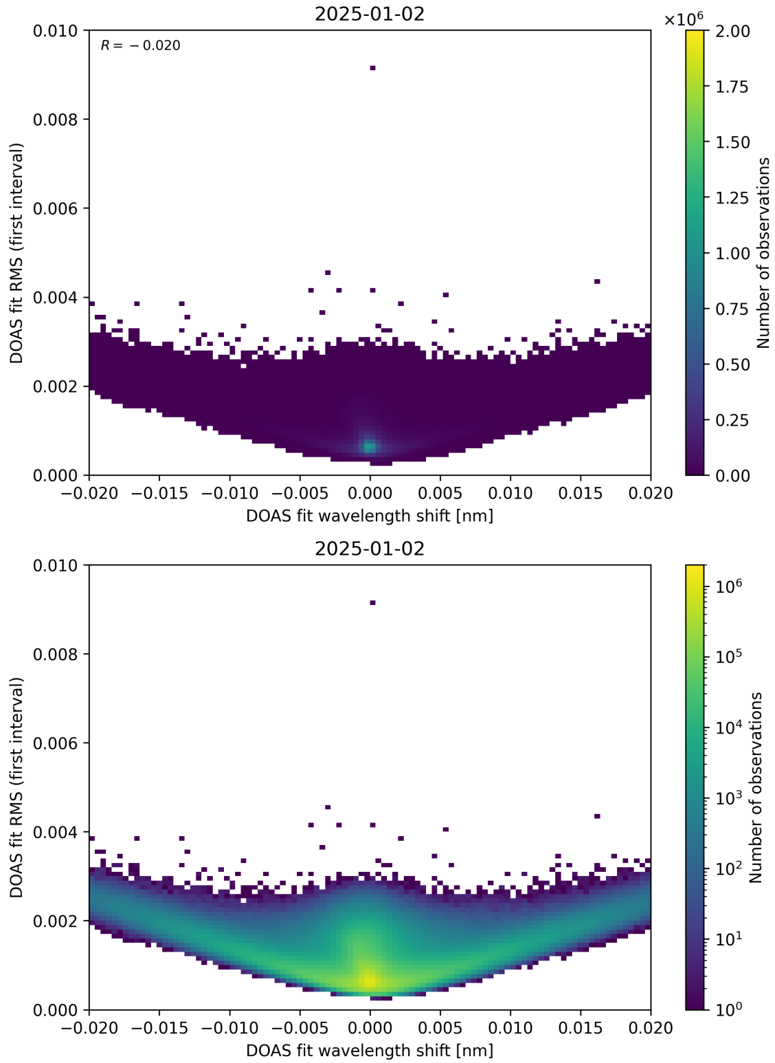
Figure 64: Scatter density plot of “DOAS fit wavelength shift” against “DOAS fit RMS (first interval)” for 2025-01-01 to 2025-01-03.
