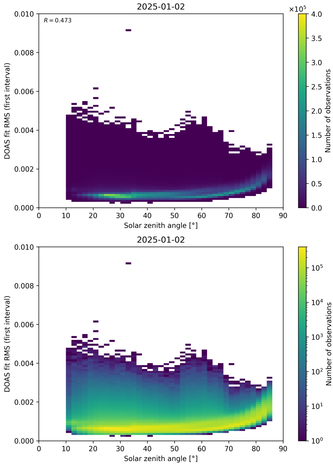
Figure 167: Scatter density plot of “Solar zenith angle” against “DOAS fit RMS (first interval)” for 2025-01-01 to 2025-01-03.
