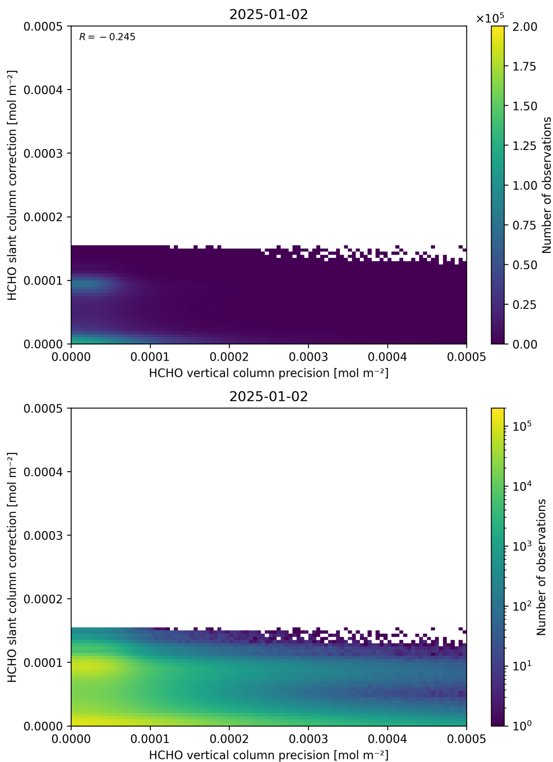
Figure 141: Scatter density plot of “HCHO vertical column precision” against “HCHO slant column correction” for 2025-01-01 to 2025-01-03.
