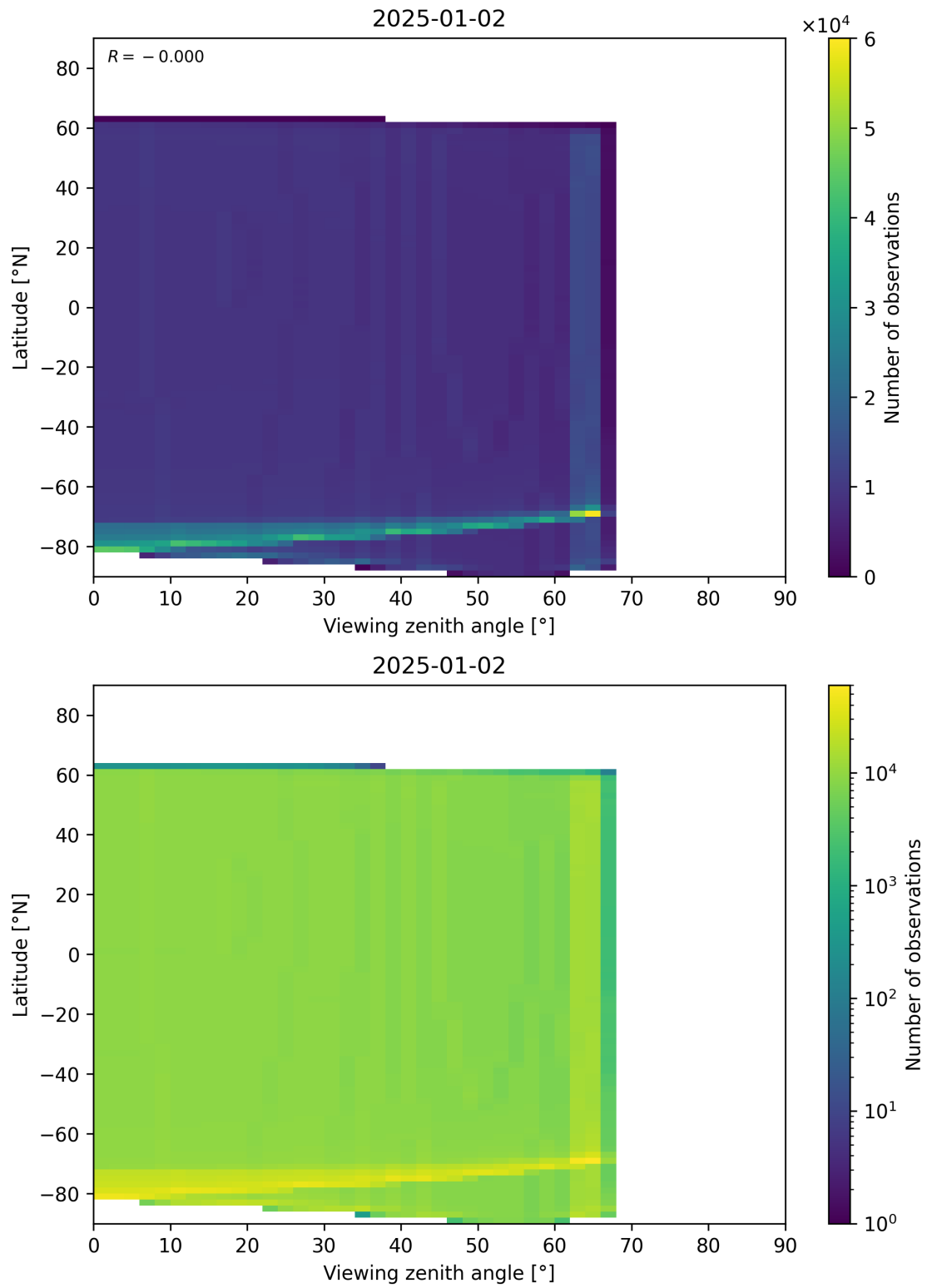
Figure 196: Scatter density plot of “Viewing zenith angle” against “Latitude” for 2025-01-01 to 2025-01-03.
