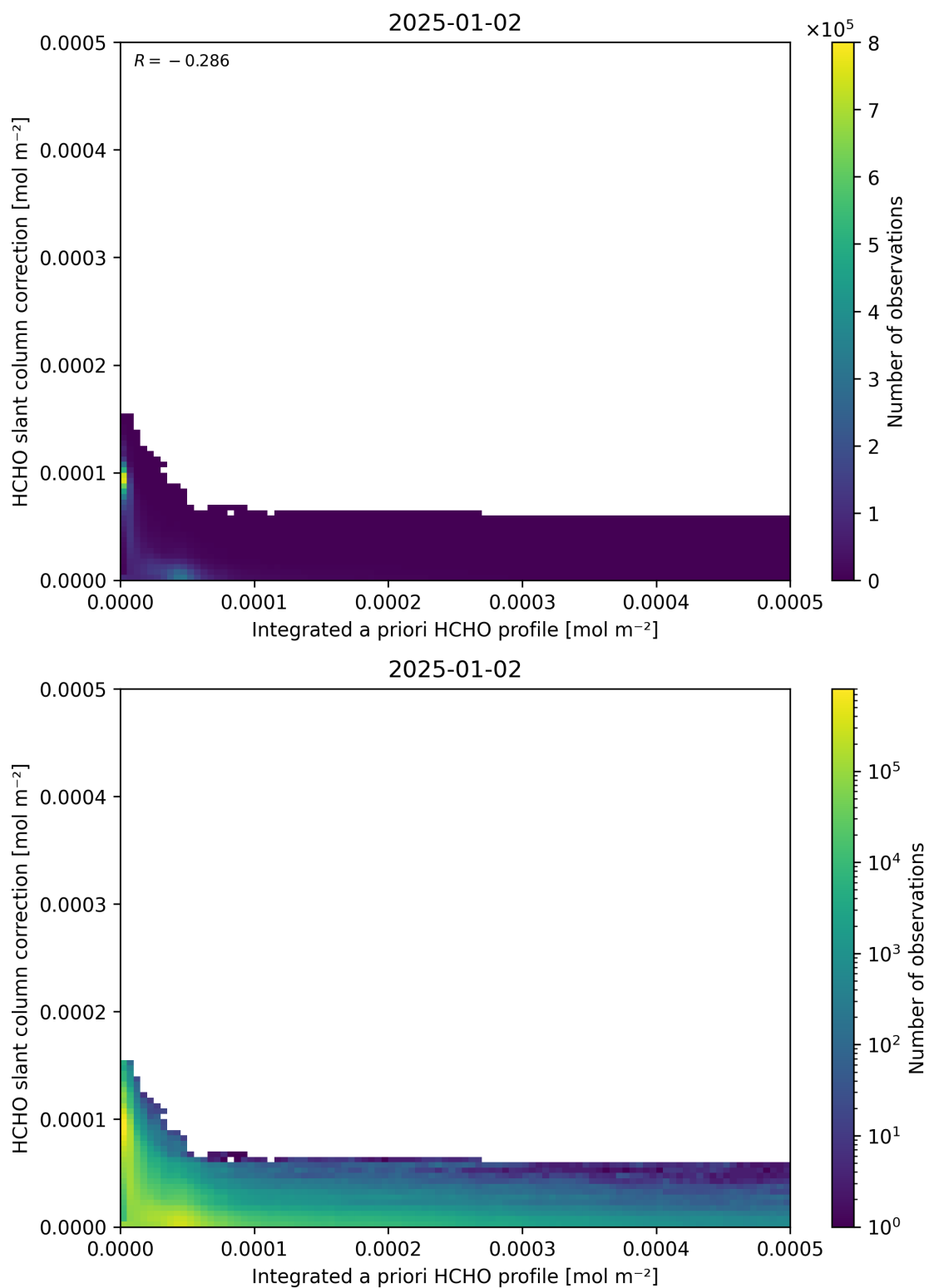
Figure 152: Scatter density plot of “Integrated a priori HCHO profile” against “HCHO slant column correction” for 2025-01-01 to 2025-01-03.
