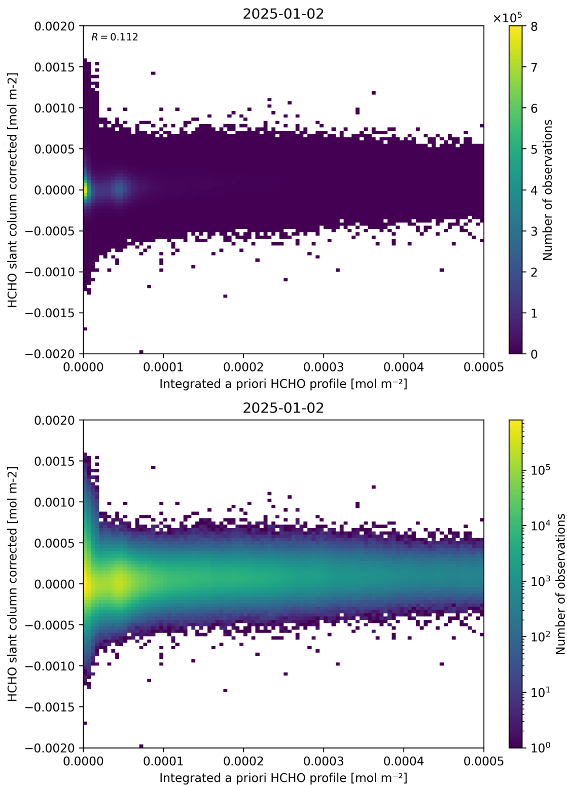
Figure 151: Scatter density plot of “Integrated a priori HCHO profile” against “HCHO slant column corrected” for 2025-01-01 to 2025-01-03.
