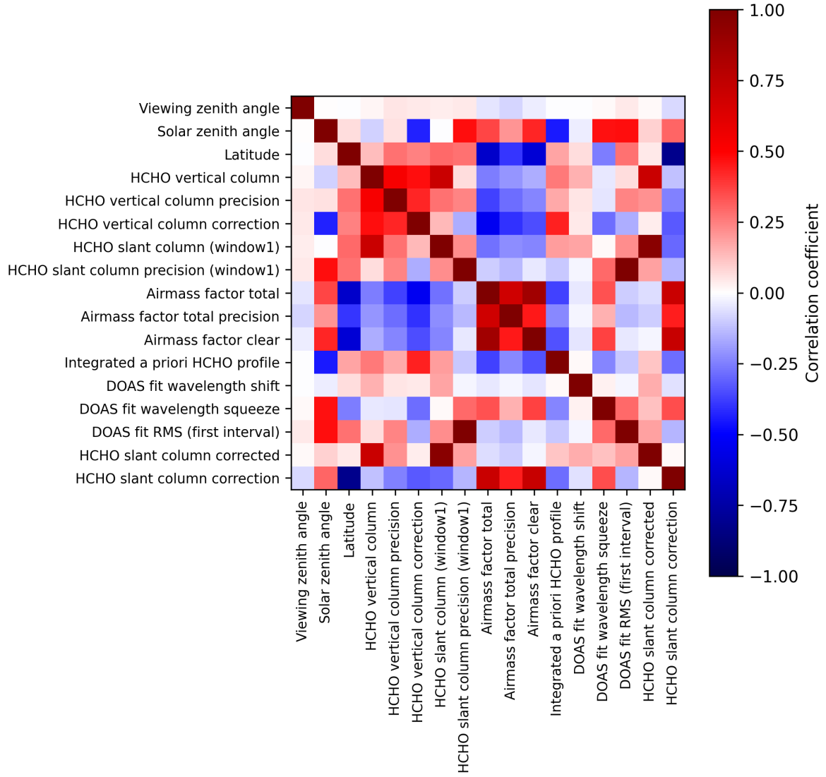
Figure 2: Map of correlation matrix for 2025-01-01 to 2025-01-03.
