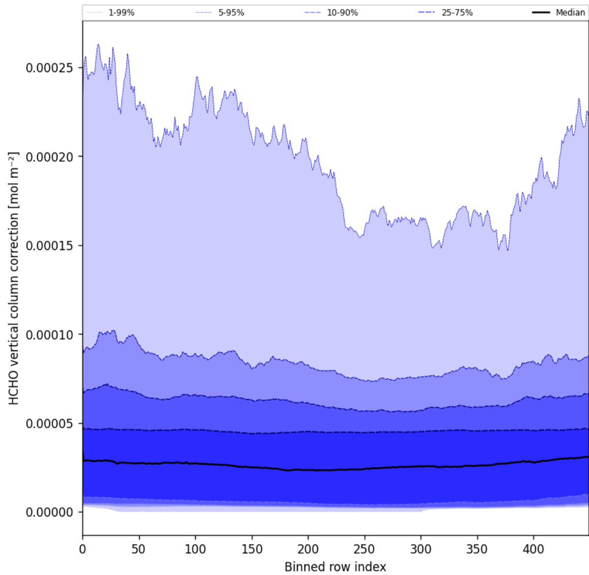
Figure 51: Along track statistics of “HCHO vertical column correction” for 2025-01-01 to 2025-01-03
