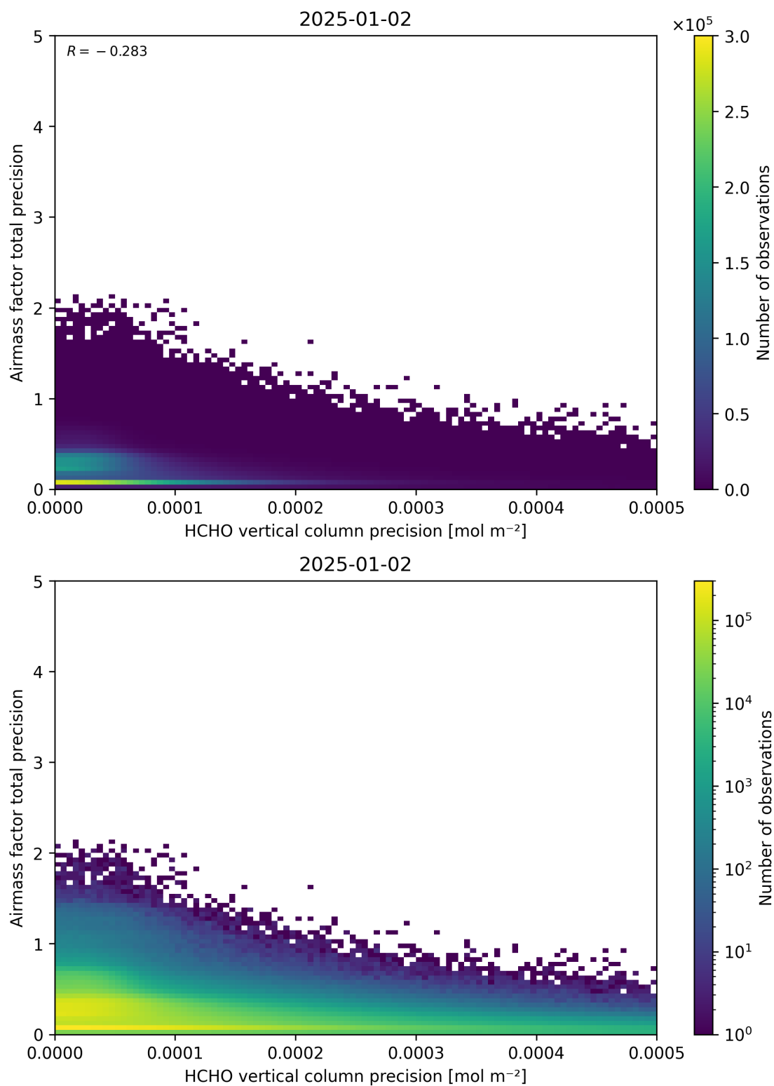
Figure 145: Scatter density plot of “HCHO vertical column precision” against “Airmass factor total precision” for 2025-01-01 to 2025-01-03.
