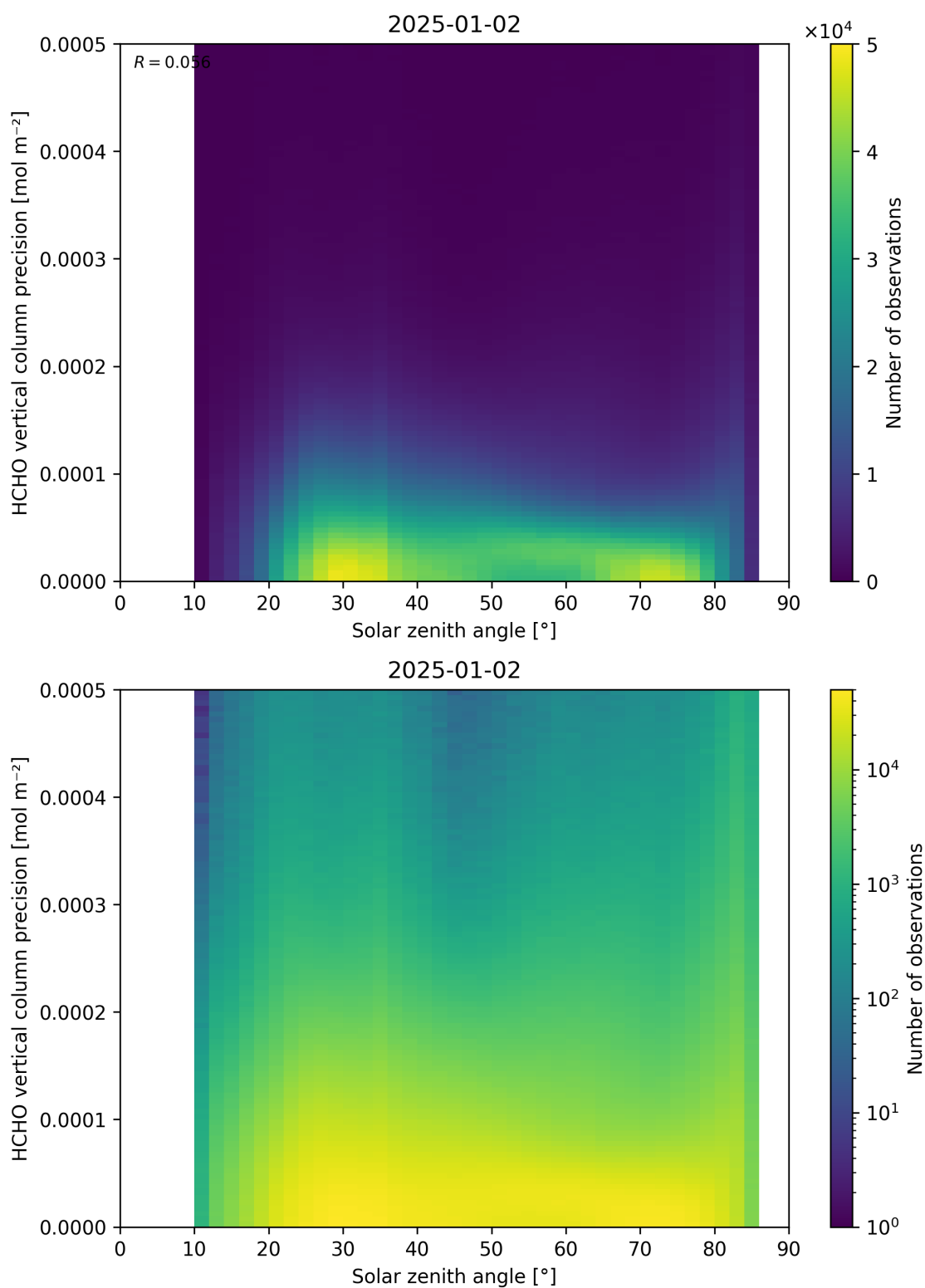
Figure 179: Scatter density plot of “Solar zenith angle” against “HCHO vertical column precision” for 2025-01-01 to 2025-01-03.
