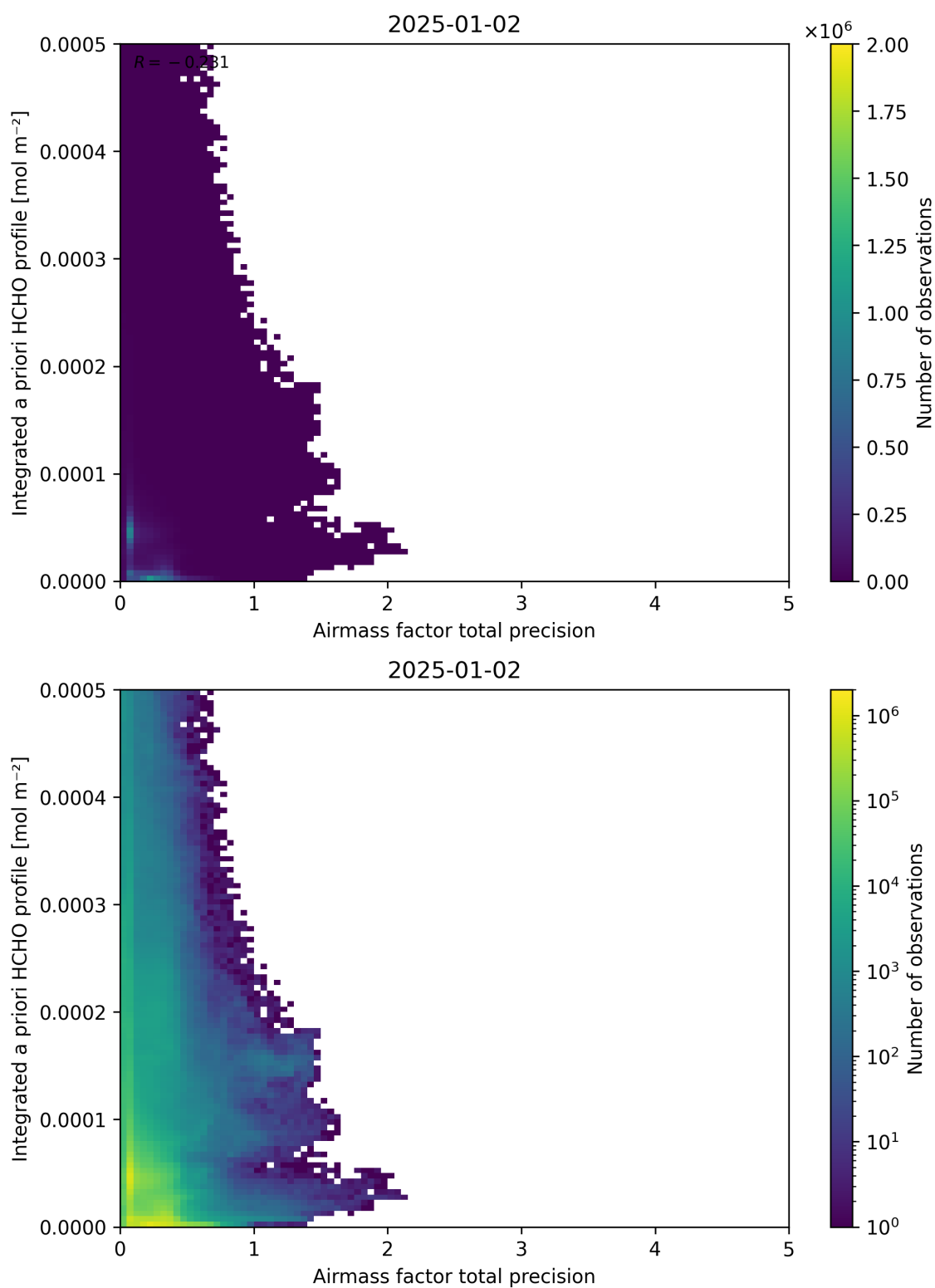
Figure 111: Scatter density plot of “Airmass factor total precision” against “Integrated a priori HCHO profile” for 2025-01-01 to 2025-01-03.
