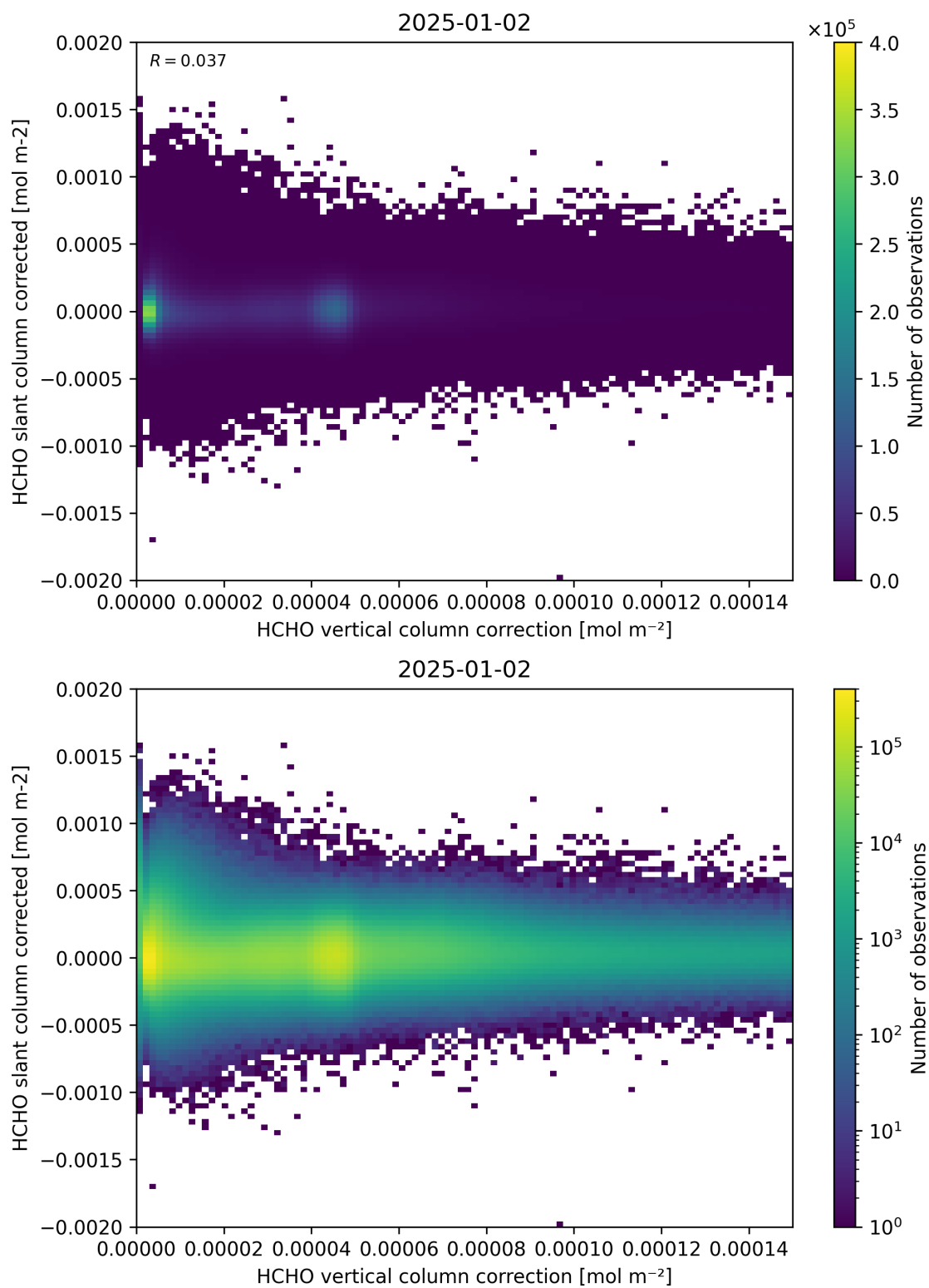
Figure 116: Scatter density plot of “HCHO vertical column correction” against “HCHO slant column corrected” for 2025-01-01 to 2025-01-03.
