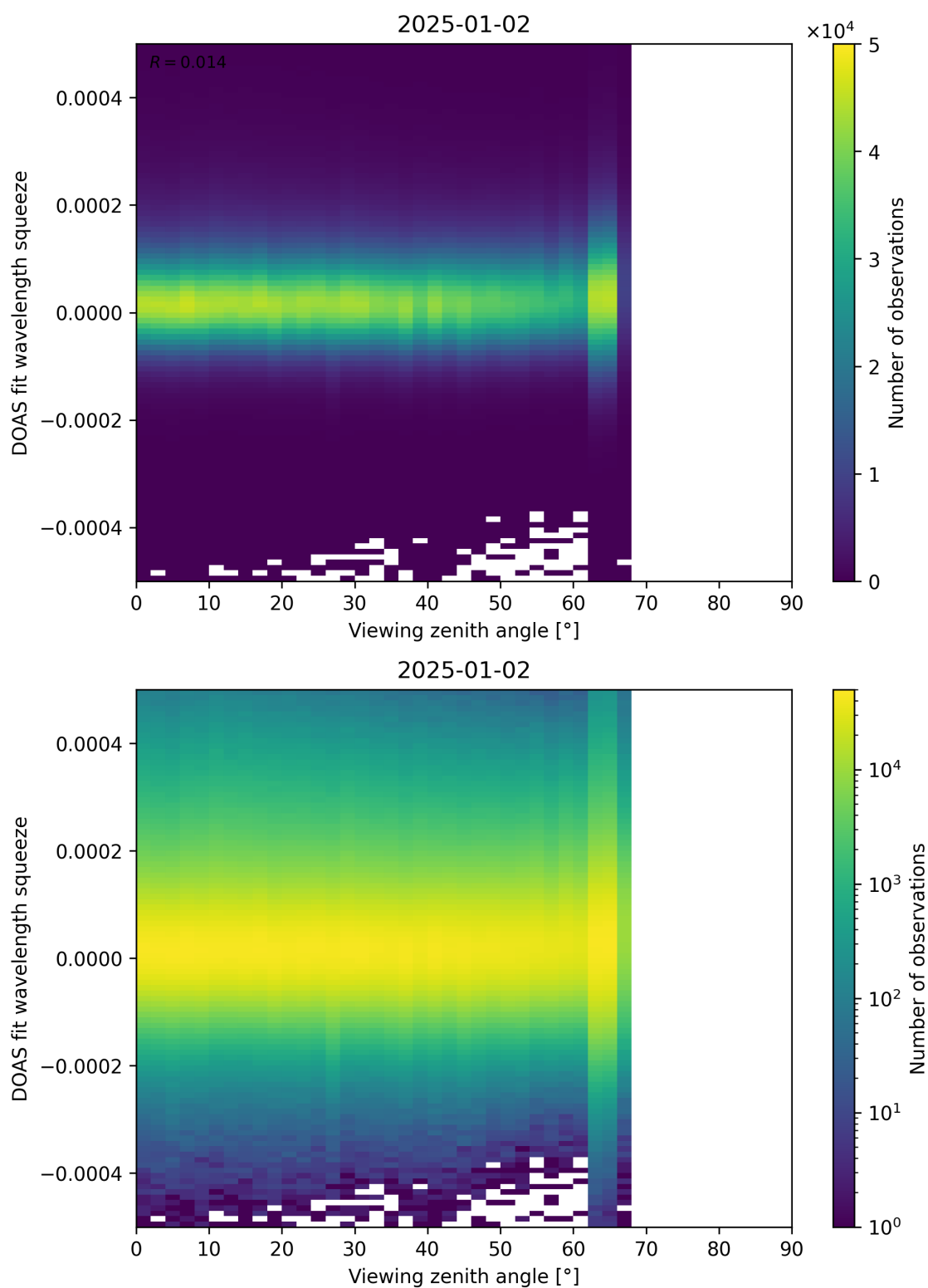
Figure 184: Scatter density plot of “Viewing zenith angle” against “DOAS fit wavelength squeeze” for 2025-01-01 to 2025-01-03.
