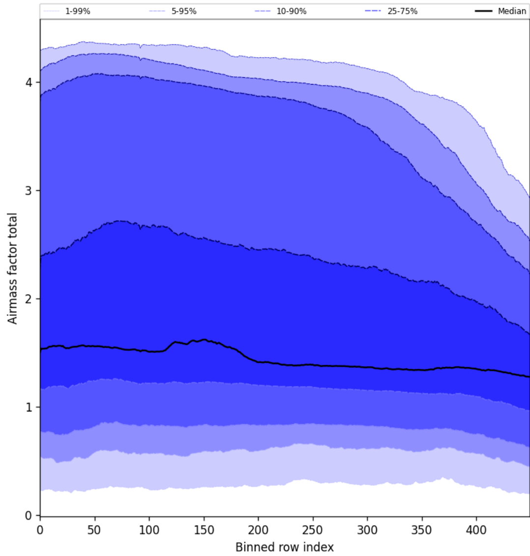
Figure 54: Along track statistics of “Airmass factor total” for 2025-01-01 to 2025-01-03
