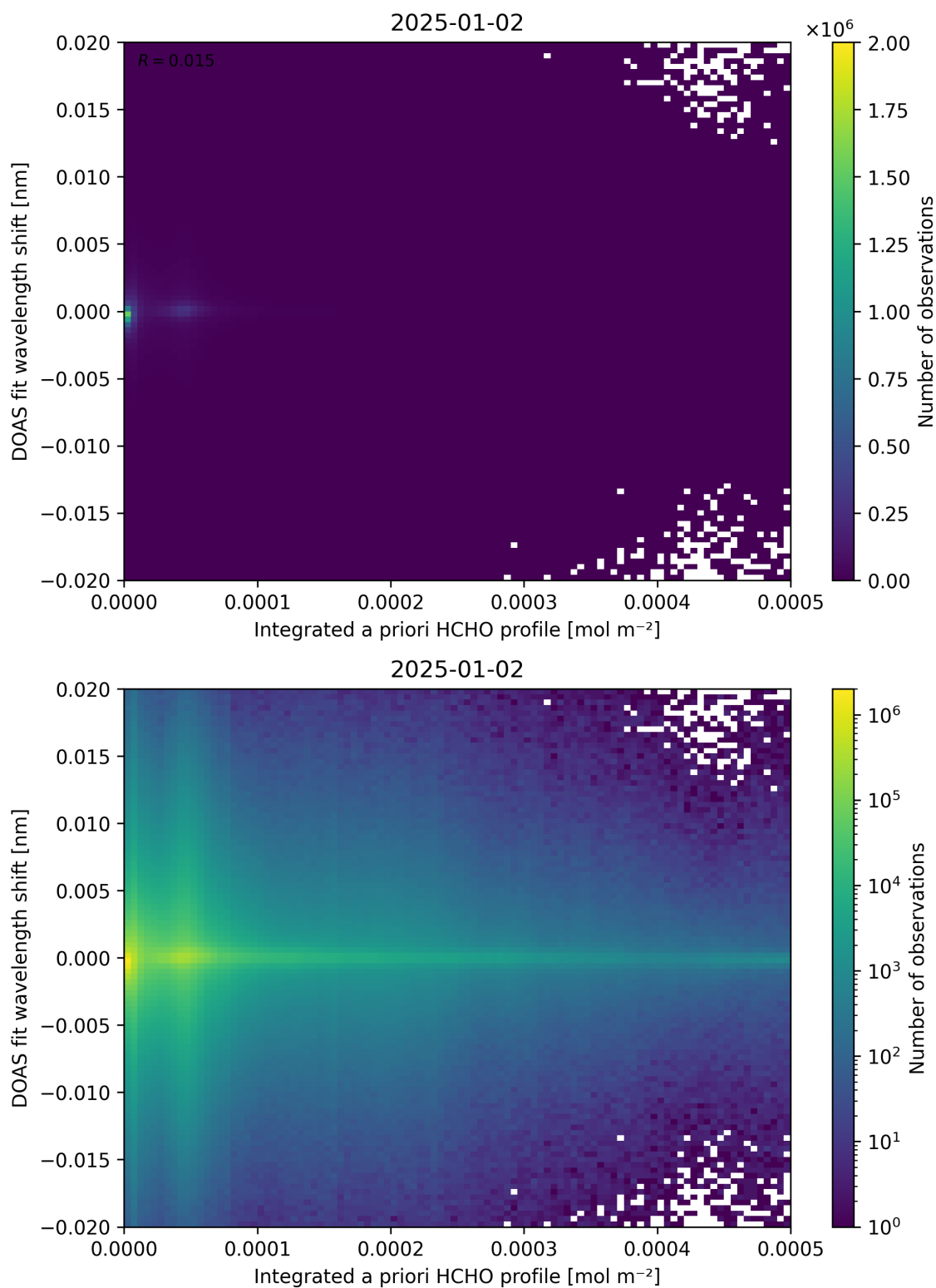
Figure 149: Scatter density plot of “Integrated a priori HCHO profile” against “DOAS fit wavelength shift” for 2025-01-01 to 2025-01-03.
