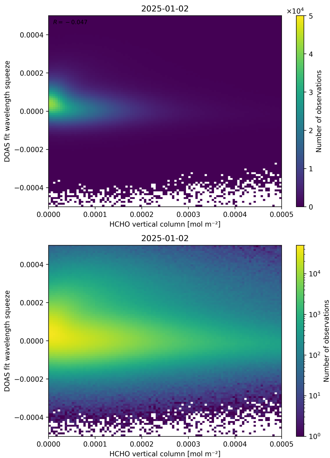
Figure 125: Scatter density plot of “HCHO vertical column” against “DOAS fit wavelength squeeze” for 2025-01-01 to 2025-01-03.
