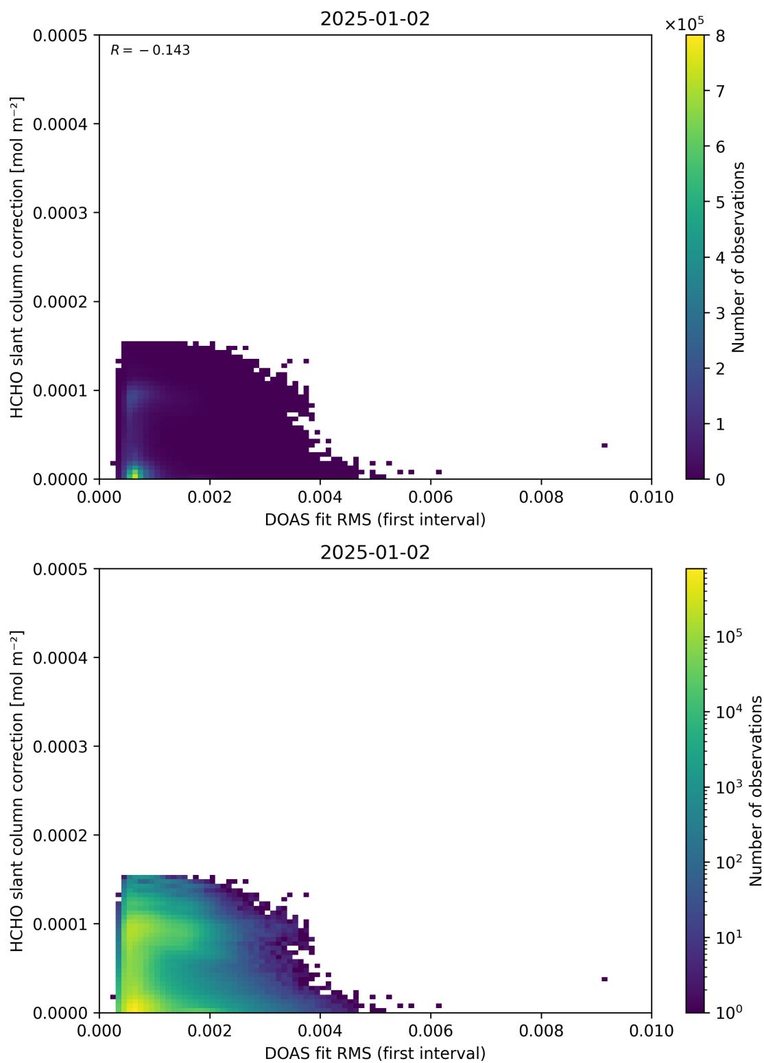
Figure 63: Scatter density plot of “DOAS fit RMS (first interval)” against “HCHO slant column correction” for 2025-01-01 to 2025-01-03.
