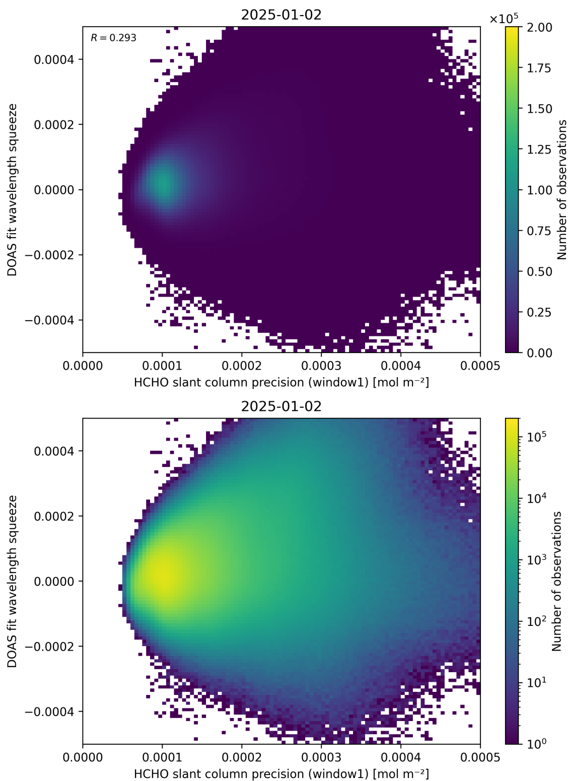
Figure 90: Scatter density plot of “HCHO slant column precision (window1)” against “DOAS fit wavelength squeeze” for 2025-01-01 to 2025-01-03.
