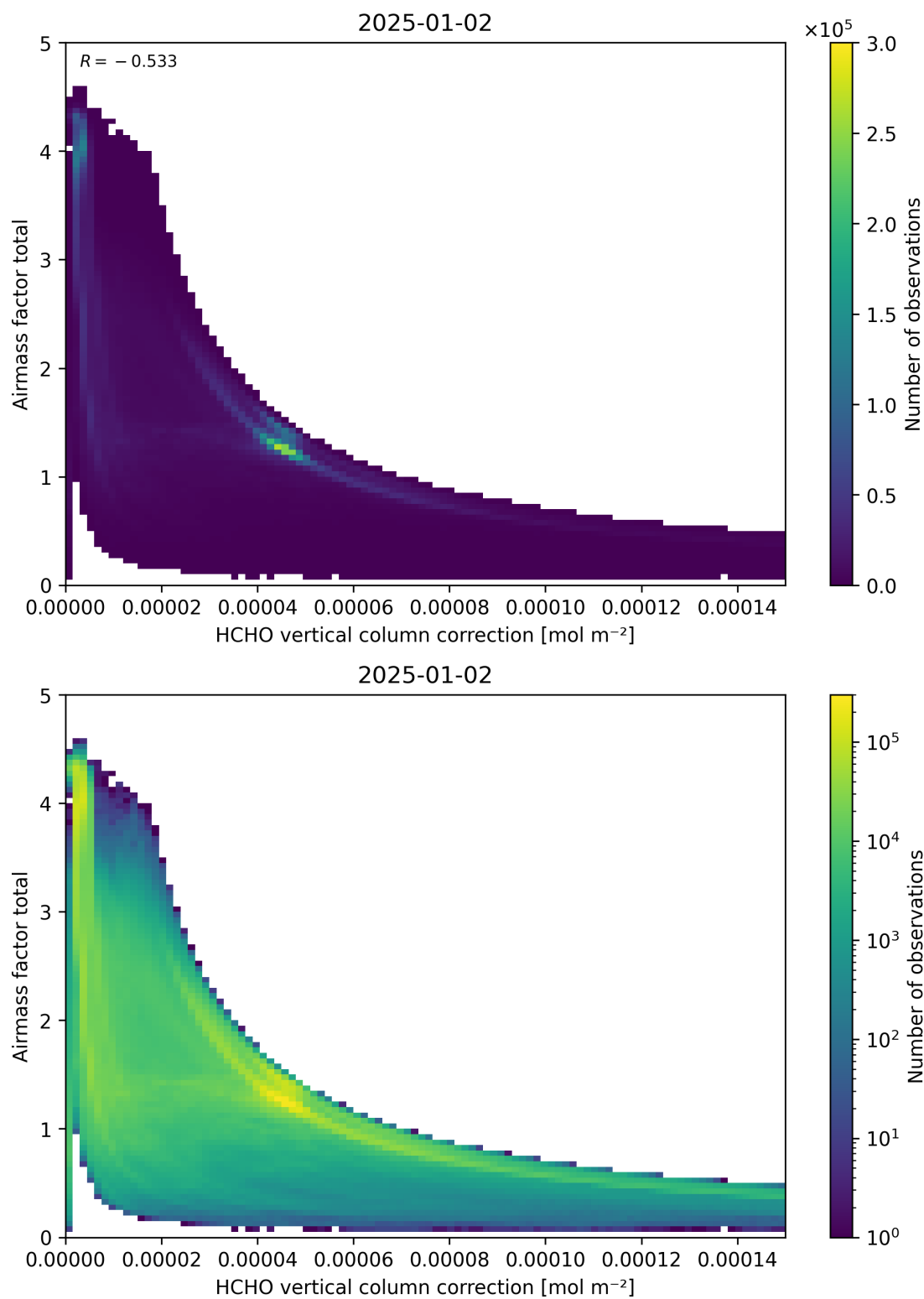
Figure 120: Scatter density plot of “HCHO vertical column correction” against “Airmass factor total” for 2025-01-01 to 2025-01-03.
