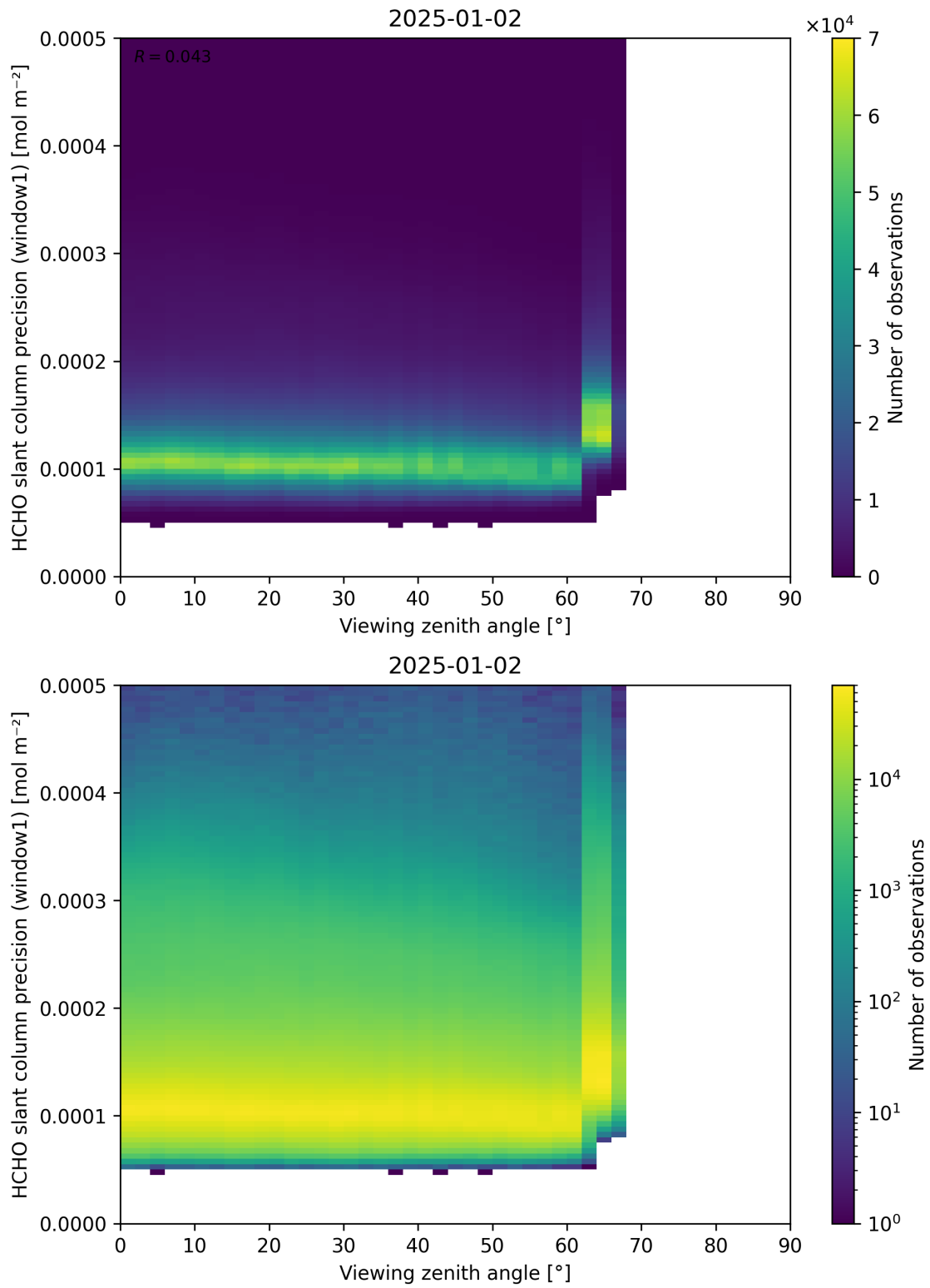
Figure 189: Scatter density plot of “Viewing zenith angle” against “HCHO slant column precision (window1)” for 2025-01-01 to 2025-01-03.
