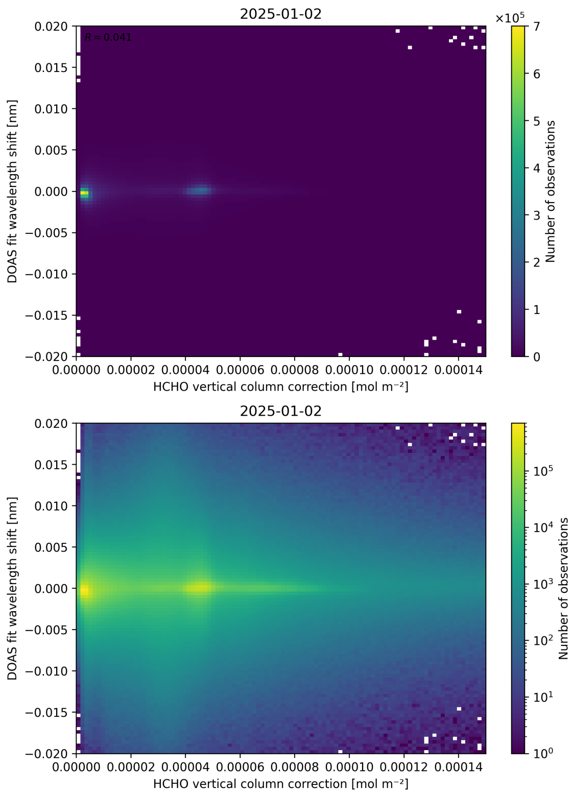
Figure 113: Scatter density plot of “HCHO vertical column correction” against “DOAS fit wavelength shift” for 2025-01-01 to 2025-01-03.
