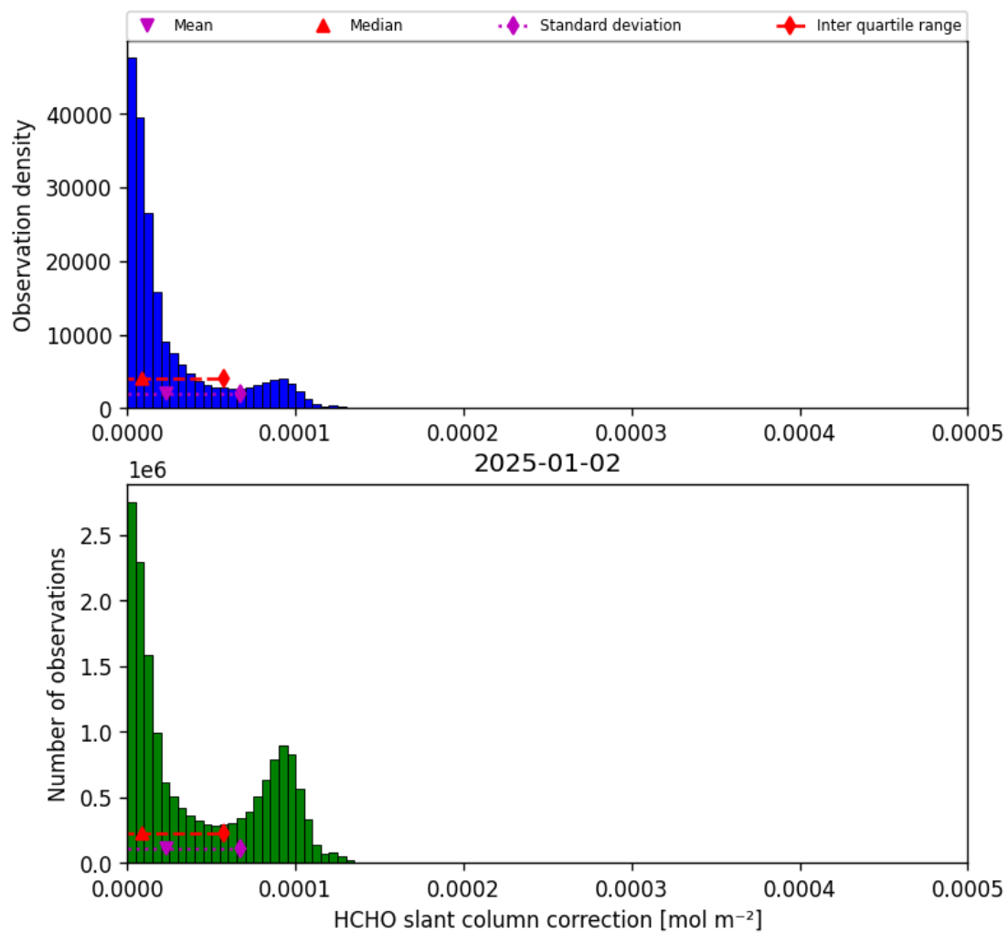
Figure 47: Histogram of “HCHO slant column correction” for 2025-01-01 to 2025-01-03
