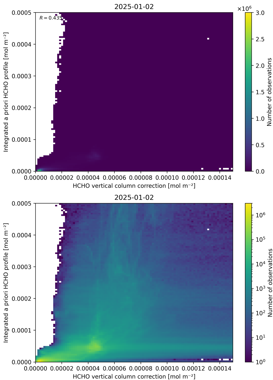
Figure 122: Scatter density plot of “HCHO vertical column correction” against “Integrated a priori HCHO profile” for 2025-01-01 to 2025-01-03.
