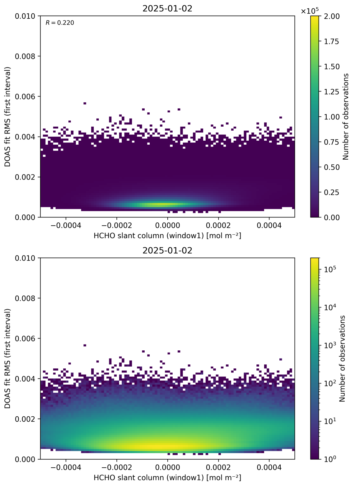
Figure 78: Scatter density plot of “HCHO slant column (window1)” against “DOAS fit RMS (first interval)” for 2025-01-01 to 2025-01-03.
