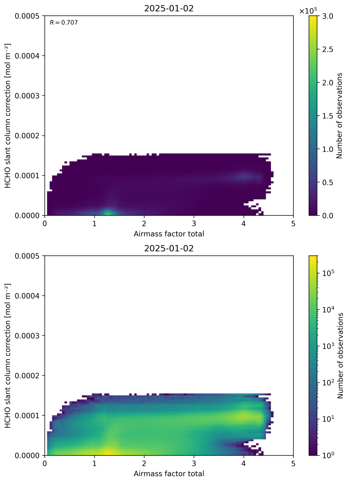
Figure 102: Scatter density plot of “Airmass factor total” against “HCHO slant column correction” for 2025-01-01 to 2025-01-03.
