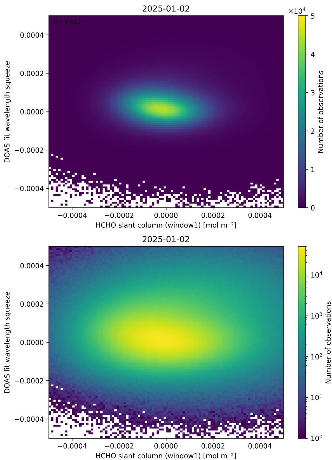
Figure 80: Scatter density plot of “HCHO slant column (window1)” against “DOAS fit wavelength squeeze” for 2025-01-01 to 2025-01-03.
