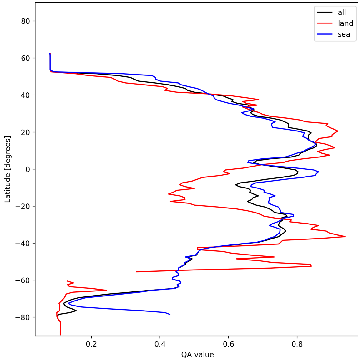
Figure 20: Zonal average of “QA value” for 2025-01-01 to 2025-01-03.
