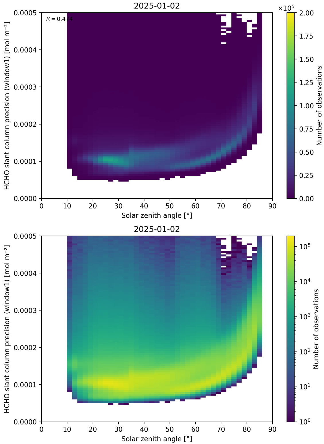
Figure 174: Scatter density plot of “Solar zenith angle” against “HCHO slant column precision (window1)” for 2025-01-01 to 2025-01-03.
