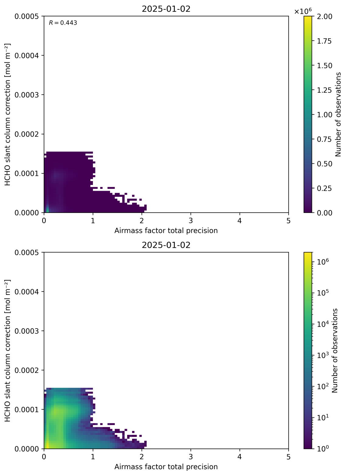
Figure 110: Scatter density plot of “Airmass factor total precision” against “HCHO slant column correction” for 2025-01-01 to 2025-01-03.
