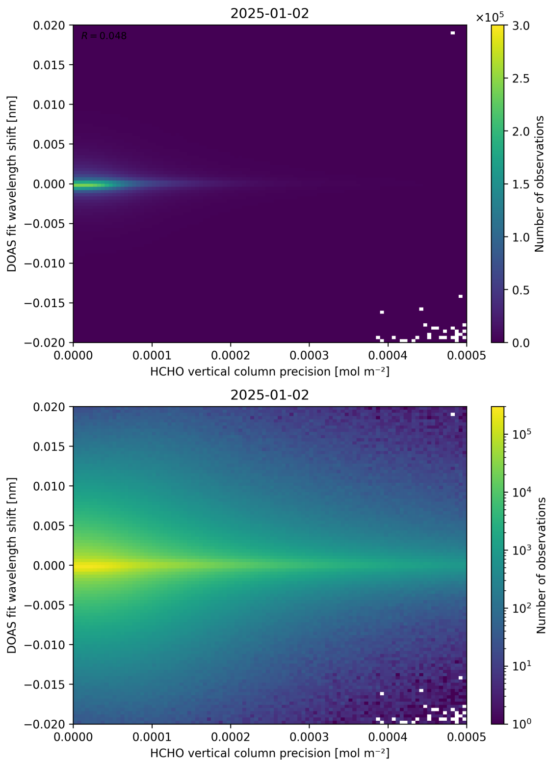
Figure 137: Scatter density plot of “HCHO vertical column precision” against “DOAS fit wavelength shift” for 2025-01-01 to 2025-01-03.
