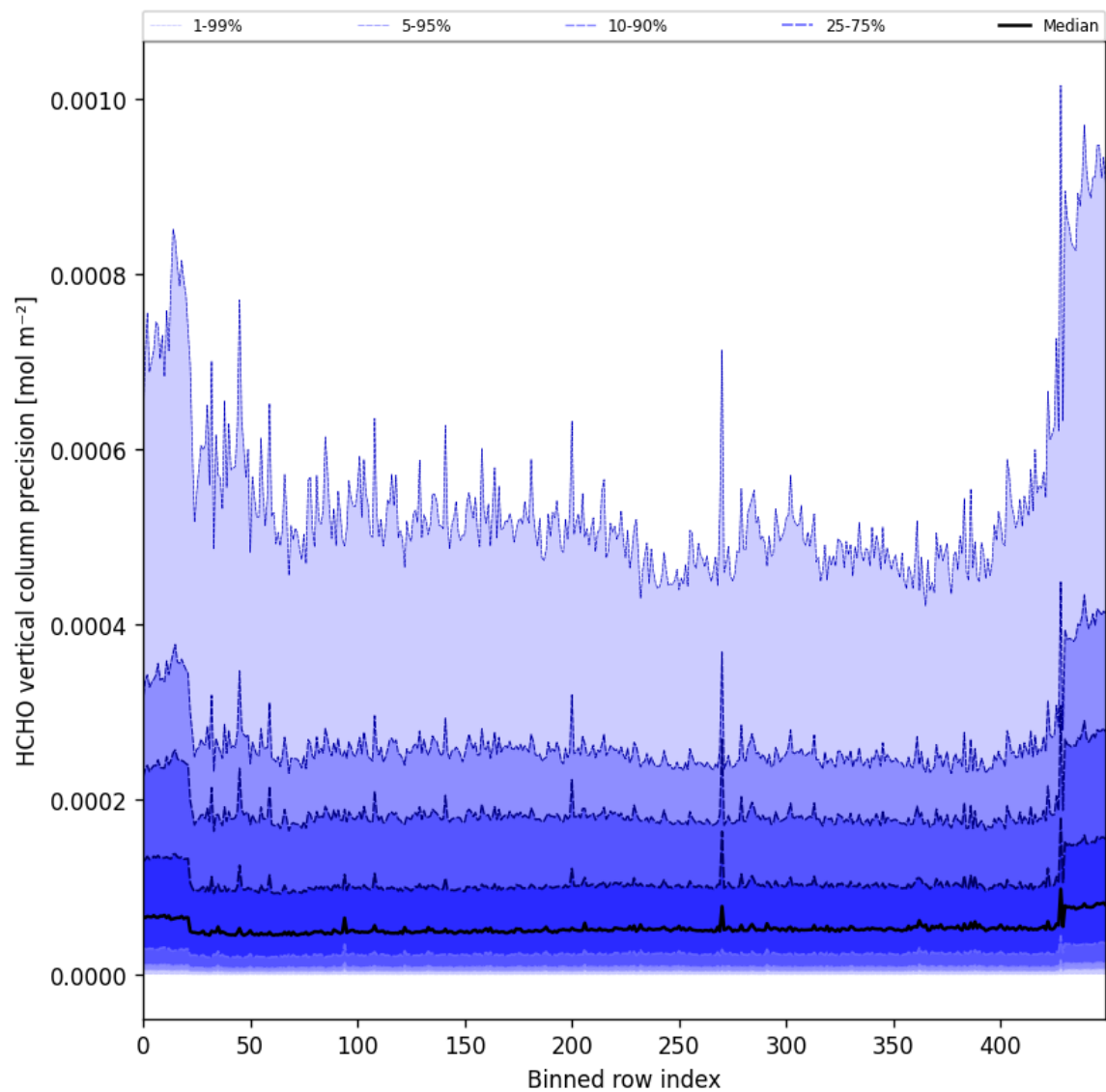
Figure 50: Along track statistics of “HCHO vertical column precision” for 2025-01-01 to 2025-01-03
