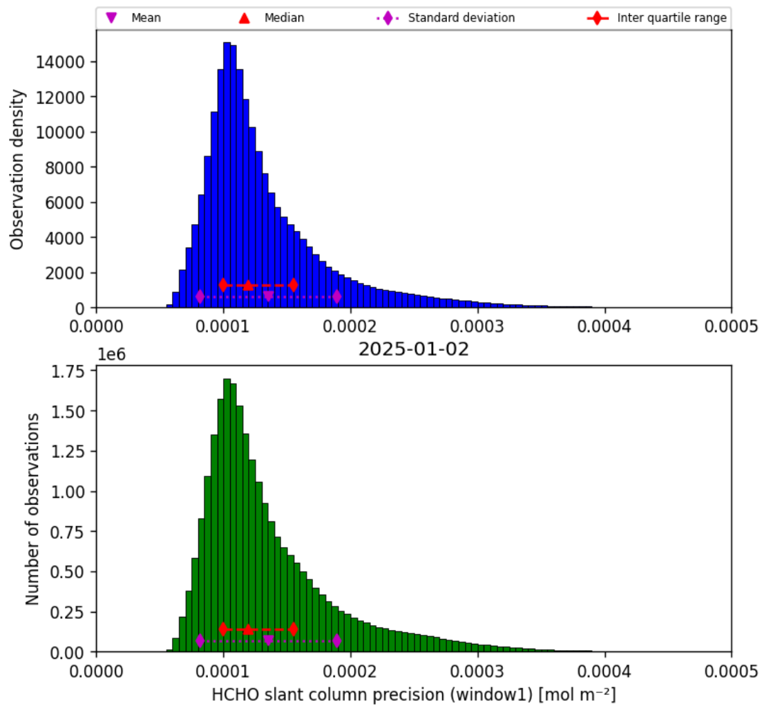
Figure 39: Histogram of “HCHO slant column precision (window1)” for 2025-01-01 to 2025-01-03
