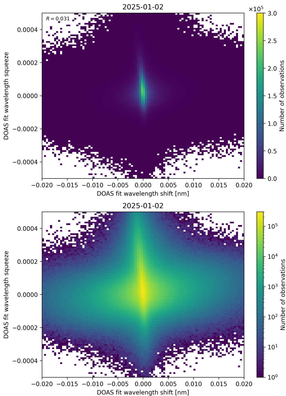
Figure 65: Scatter density plot of “DOAS fit wavelength shift” against “DOAS fit wavelength squeeze” for 2025-01-01 to 2025-01-03.
