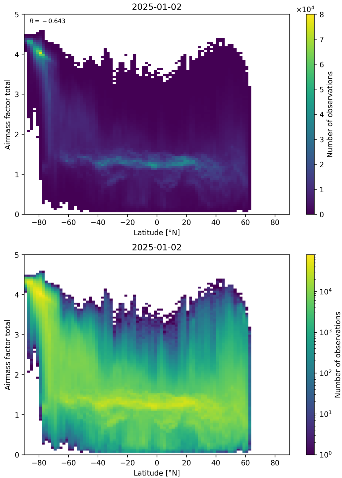
Figure 161: Scatter density plot of “Latitude” against “Airmass factor total” for 2025-01-01 to 2025-01-03.
