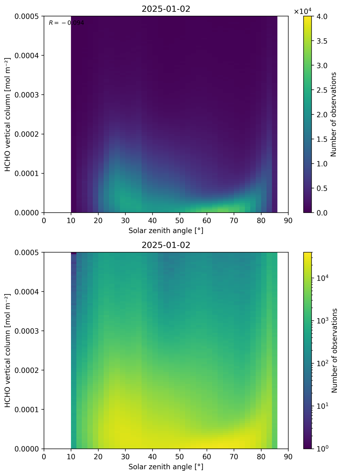
Figure 177: Scatter density plot of “Solar zenith angle” against “HCHO vertical column” for 2025-01-01 to 2025-01-03.
