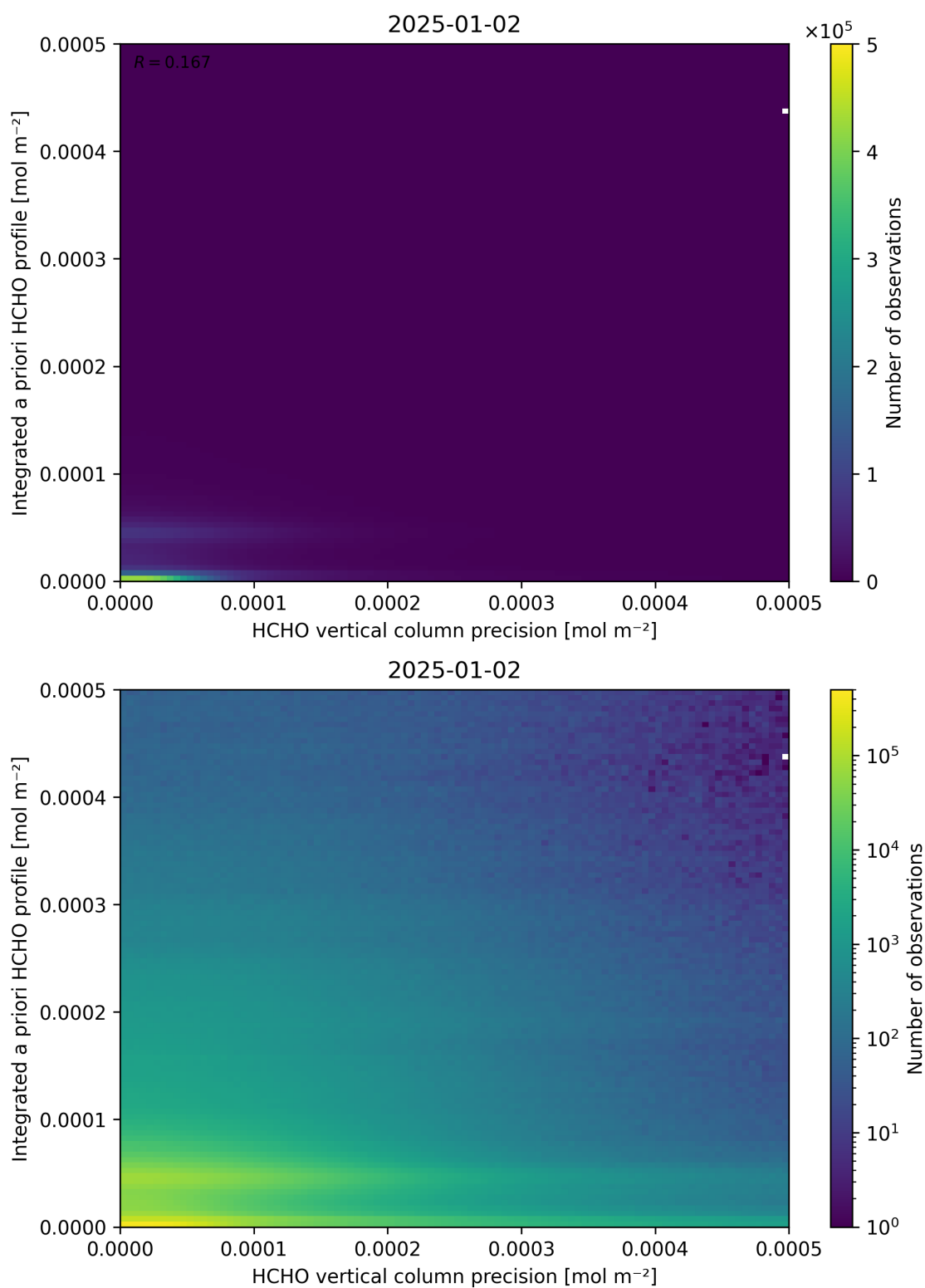
Figure 147: Scatter density plot of “HCHO vertical column precision” against “Integrated a priori HCHO profile” for 2025-01-01 to 2025-01-03.
