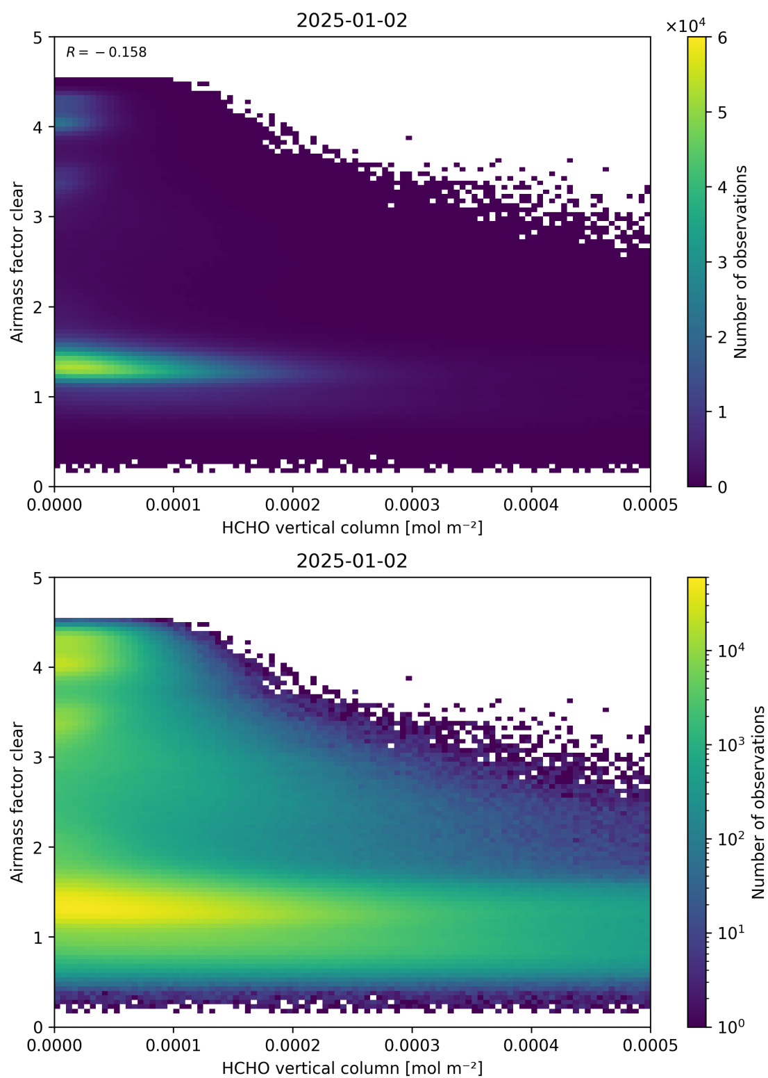
Figure 126: Scatter density plot of “HCHO vertical column” against “Airmass factor clear” for 2025-01-01 to 2025-01-03.
