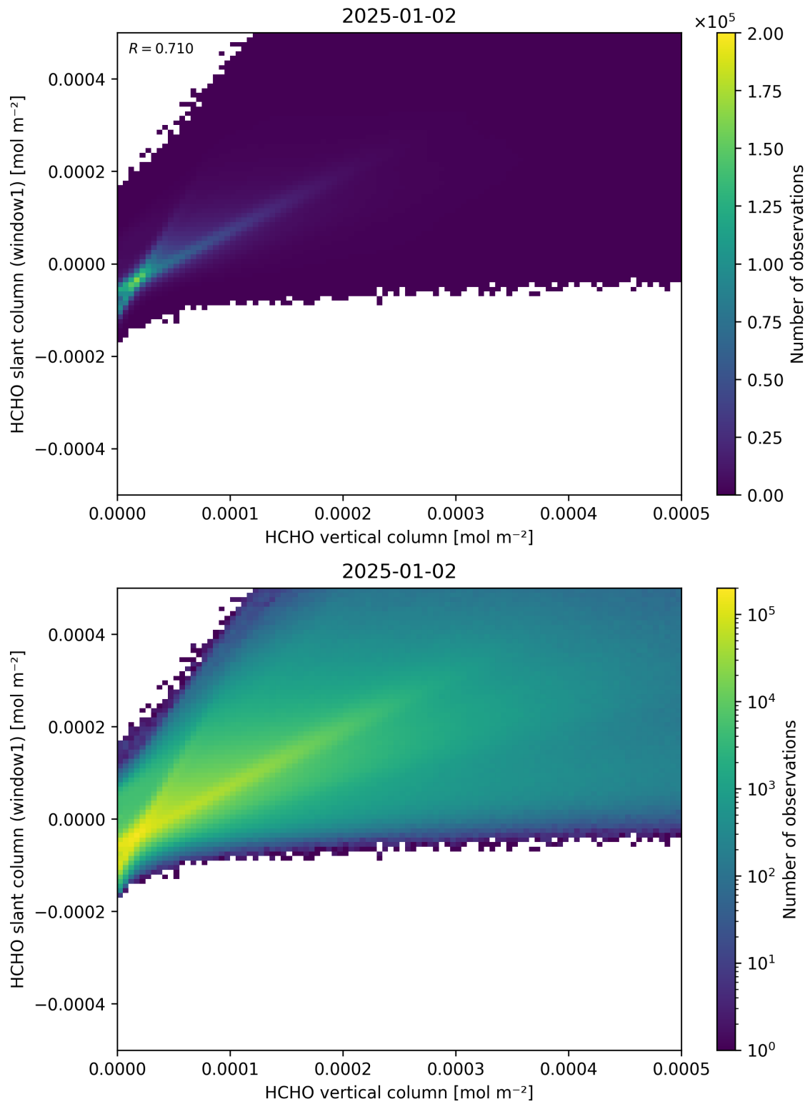
Figure 129: Scatter density plot of “HCHO vertical column” against “HCHO slant column (window1)” for 2025-01-01 to 2025-01-03.
