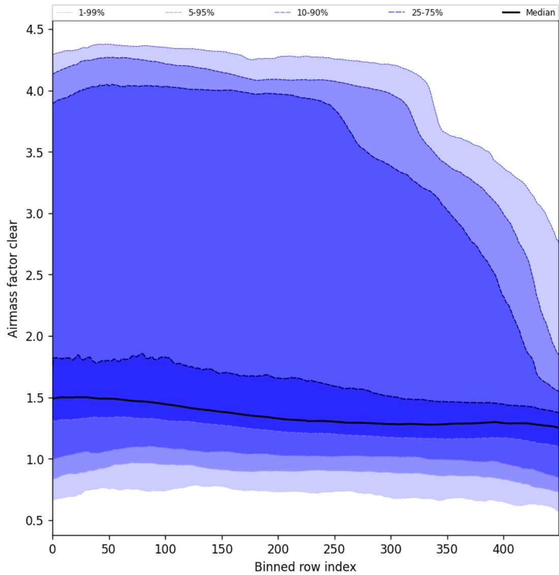
Figure 56: Along track statistics of “Airmass factor clear” for 2025-01-01 to 2025-01-03
