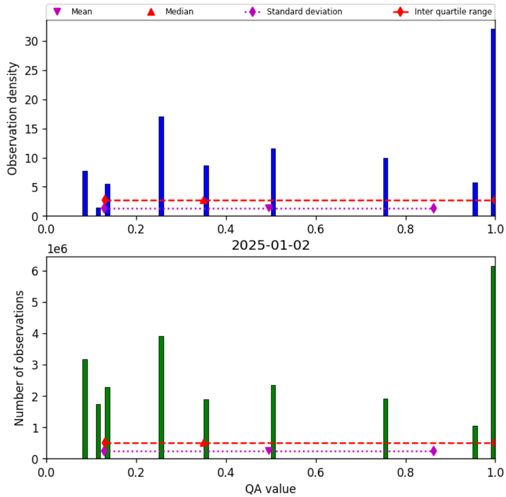
Figure 34: Histogram of “QA value” for 2025-01-01 to 2025-01-03
