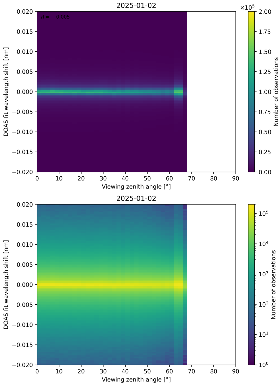
Figure 183: Scatter density plot of “Viewing zenith angle” against “DOAS fit wavelength shift” for 2025-01-01 to 2025-01-03.
