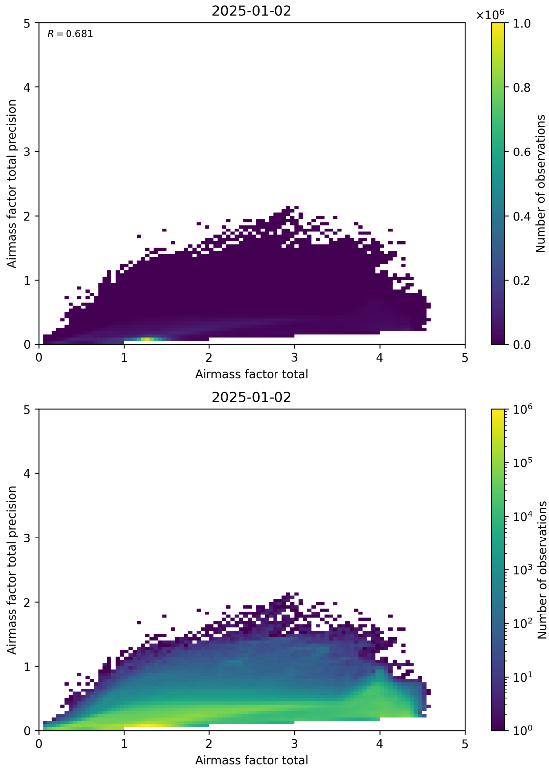
Figure 103: Scatter density plot of “Airmass factor total” against “Airmass factor total precision” for 2025-01-01 to 2025-01-03.
