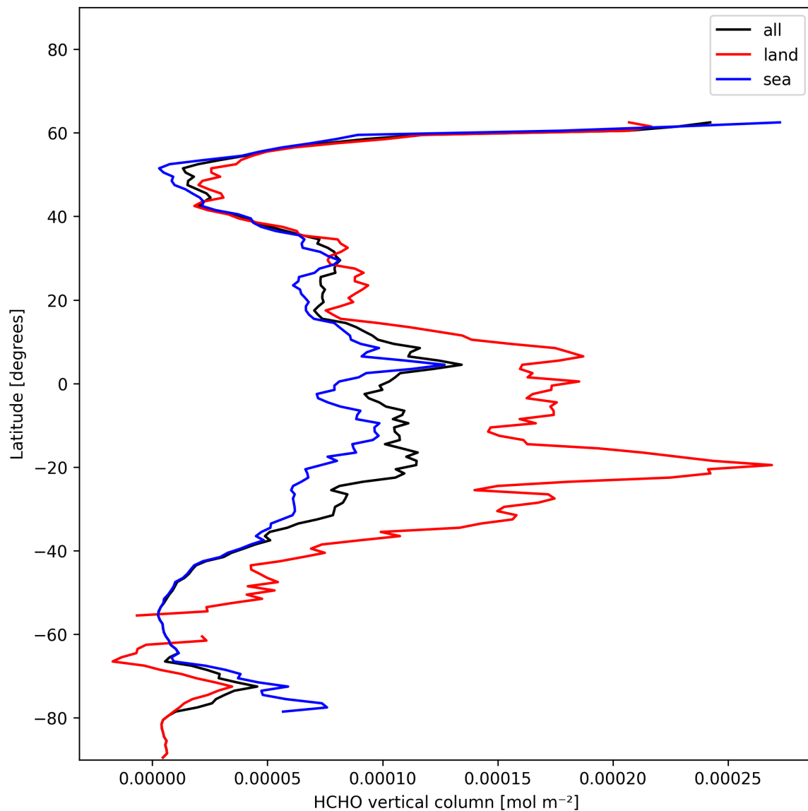
Figure 21: Zonal average of “HCHO vertical column” for 2025-01-01 to 2025-01-03.
