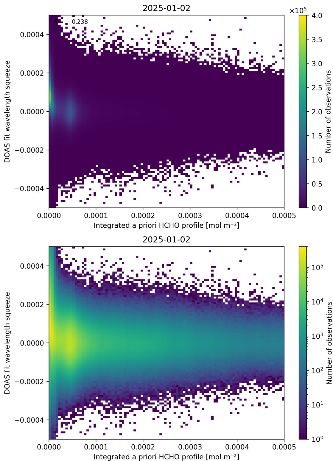
Figure 150: Scatter density plot of “Integrated a priori HCHO profile” against “DOAS fit wavelength squeeze” for 2025-01-01 to 2025-01-03.
