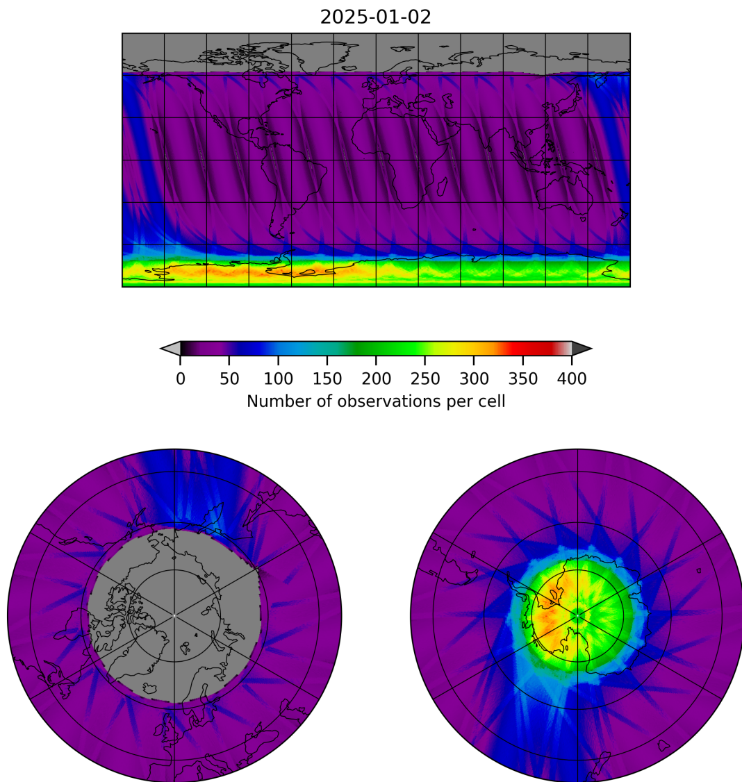
Figure 19: Map of the number of observations for 2025-01-01 to 2025-01-03
