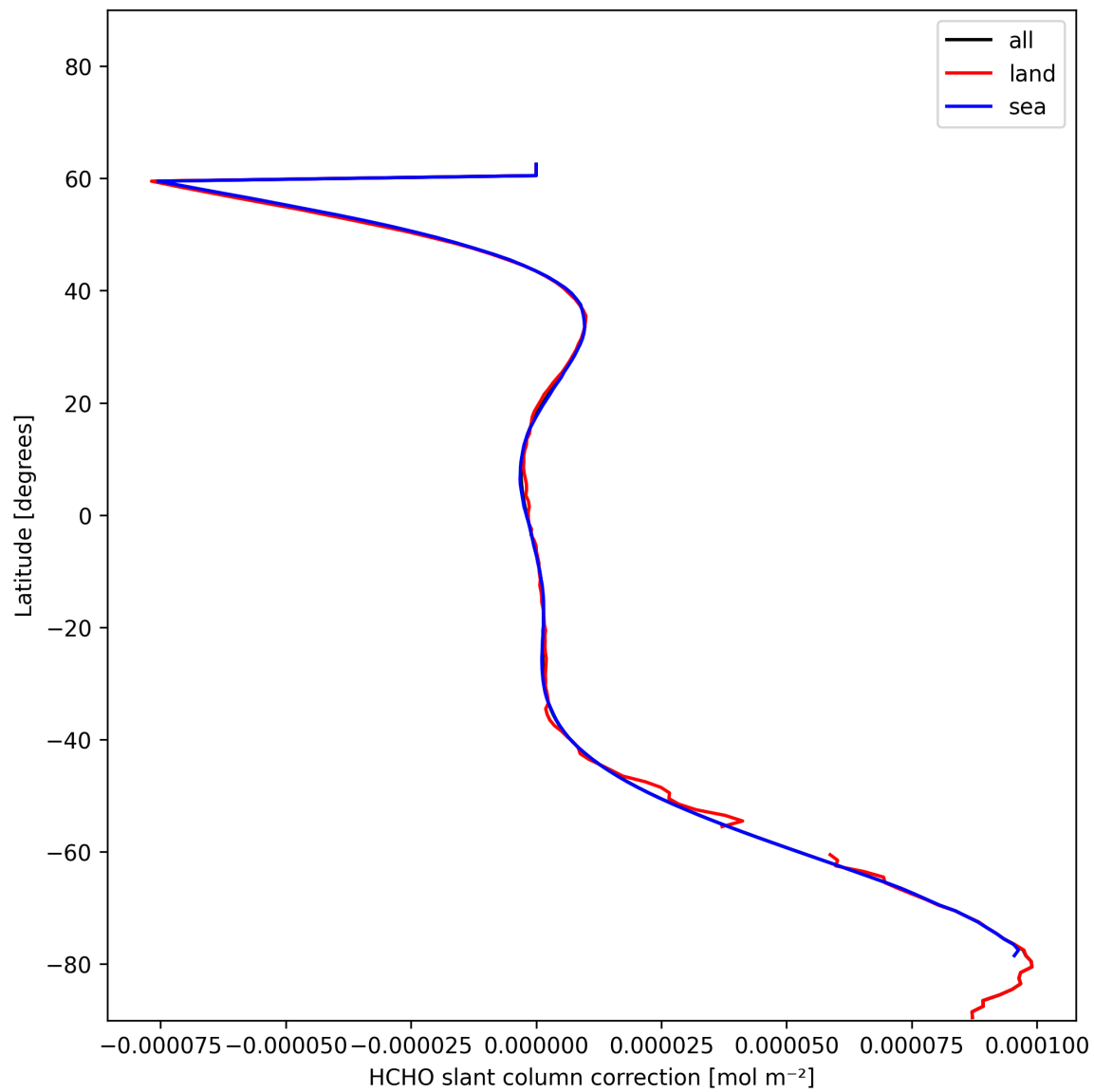
Figure 33: Zonal average of “HCHO slant column correction” for 2025-01-01 to 2025-01-03.
