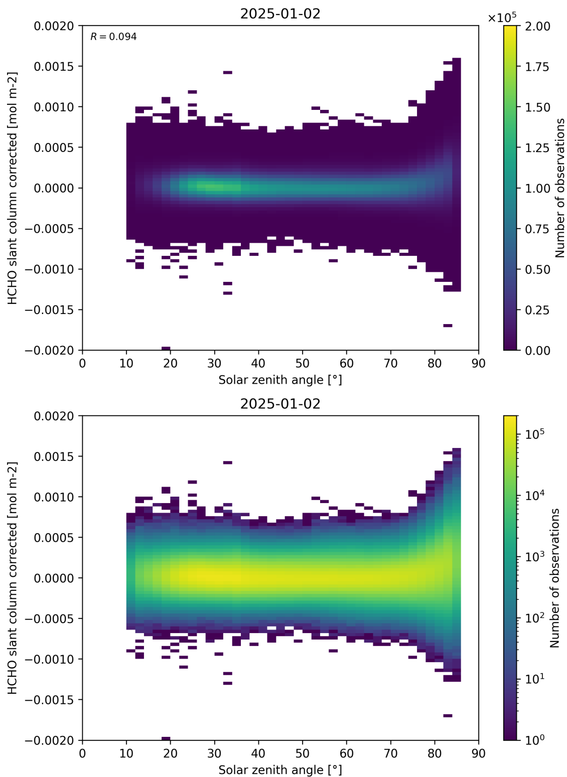
Figure 171: Scatter density plot of “Solar zenith angle” against “HCHO slant column corrected” for 2025-01-01 to 2025-01-03.
