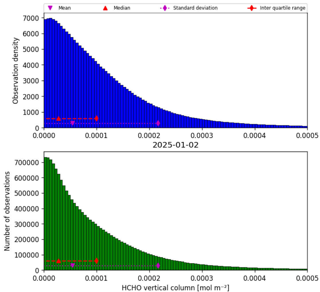
Figure 35: Histogram of “HCHO vertical column” for 2025-01-01 to 2025-01-03
