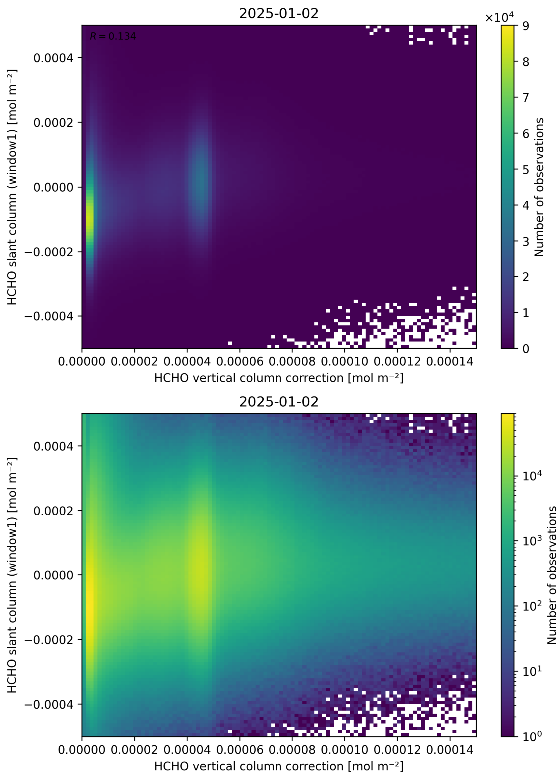
Figure 118: Scatter density plot of “HCHO vertical column correction” against “HCHO slant column (window1)” for 2025-01-01 to 2025-01-03.
