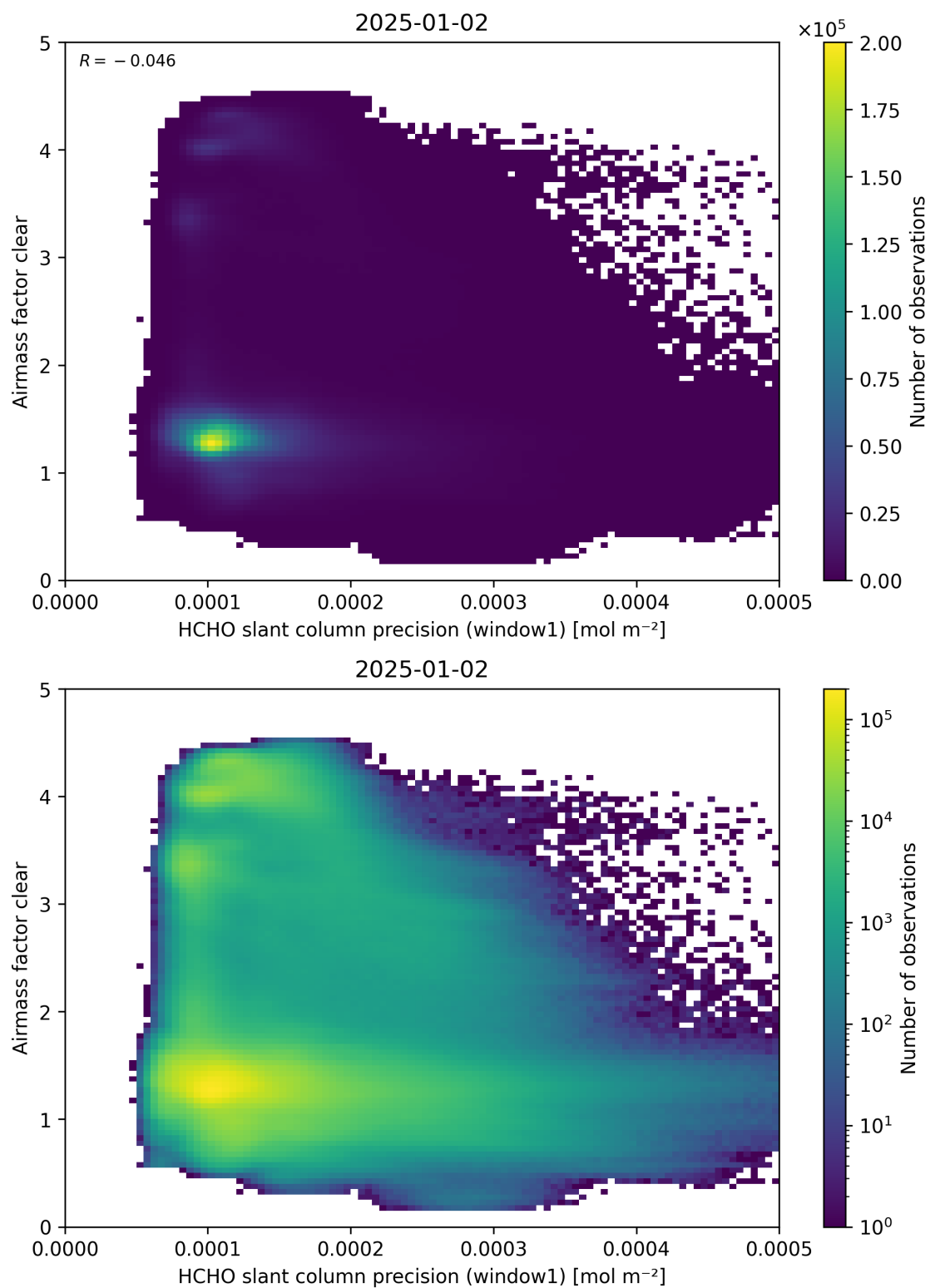
Figure 91: Scatter density plot of “HCHO slant column precision (window1)” against “Airmass factor clear” for 2025-01-01 to 2025-01-03.
