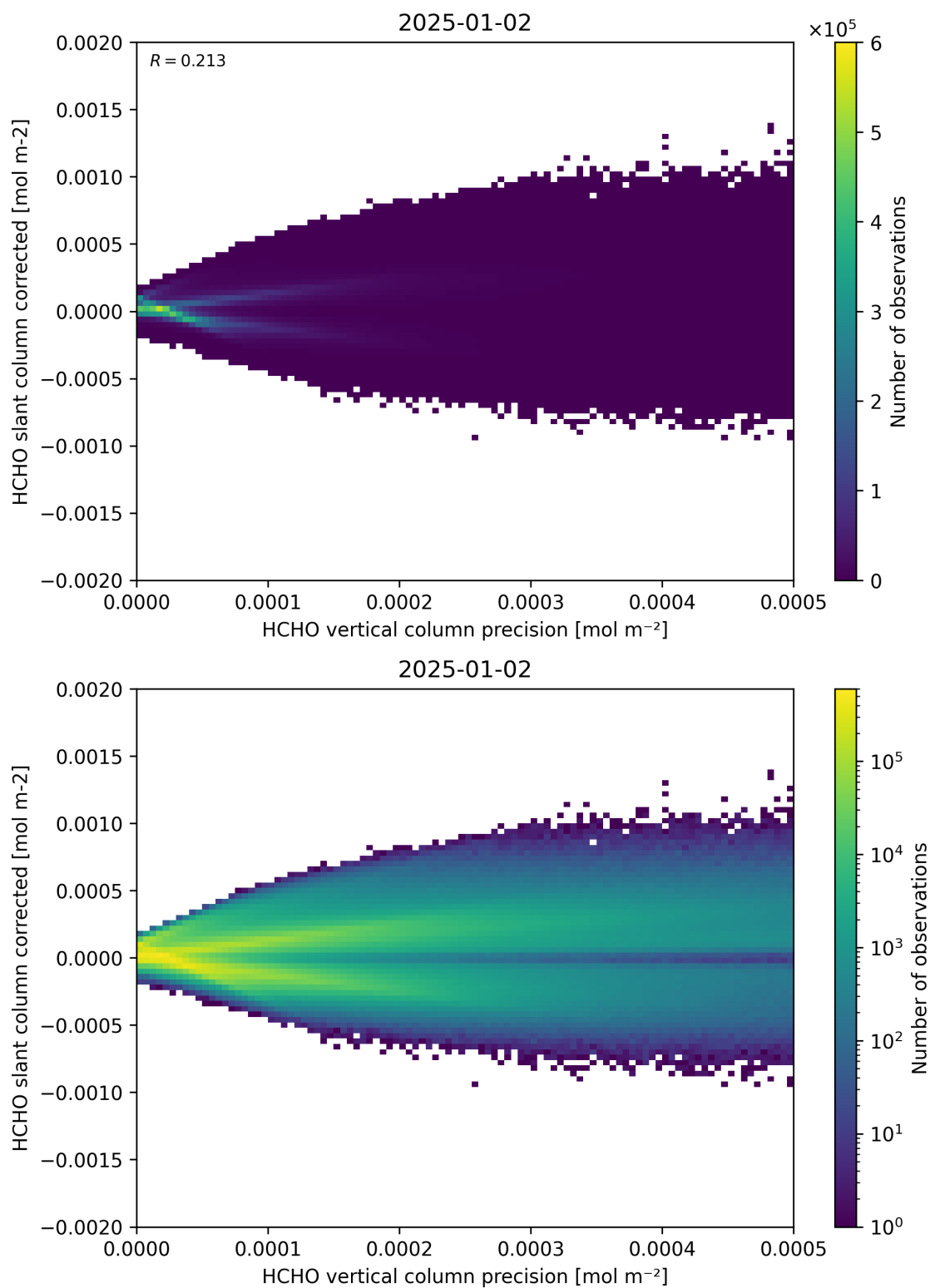
Figure 140: Scatter density plot of “HCHO vertical column precision” against “HCHO slant column corrected” for 2025-01-01 to 2025-01-03.
