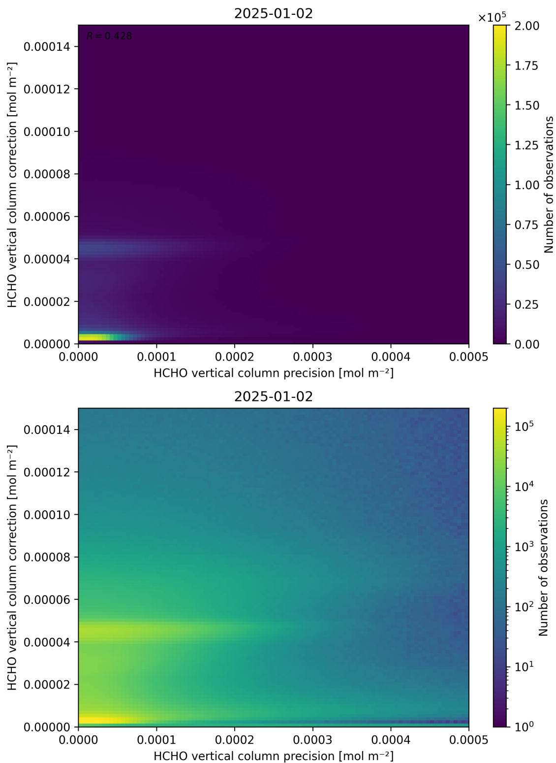
Figure 146: Scatter density plot of “HCHO vertical column precision” against “HCHO vertical column correction” for 2025-01-01 to 2025-01-03.
