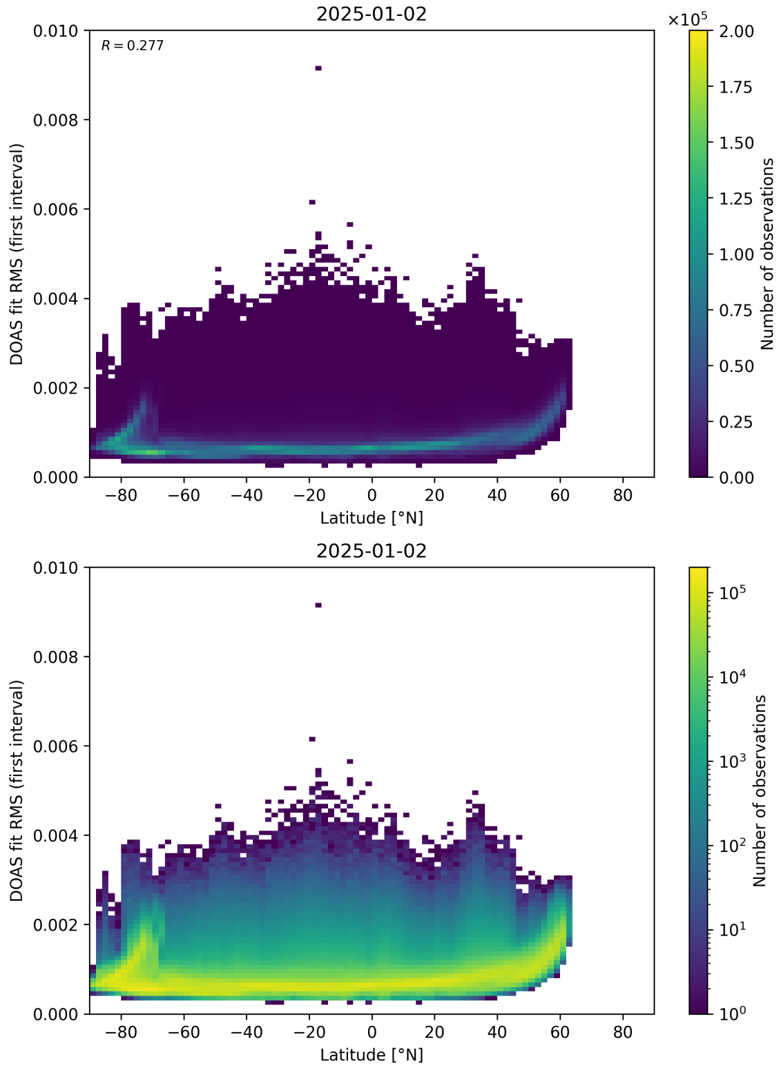
Figure 153: Scatter density plot of “Latitude” against “DOAS fit RMS (first interval)” for 2025-01-01 to 2025-01-03.
