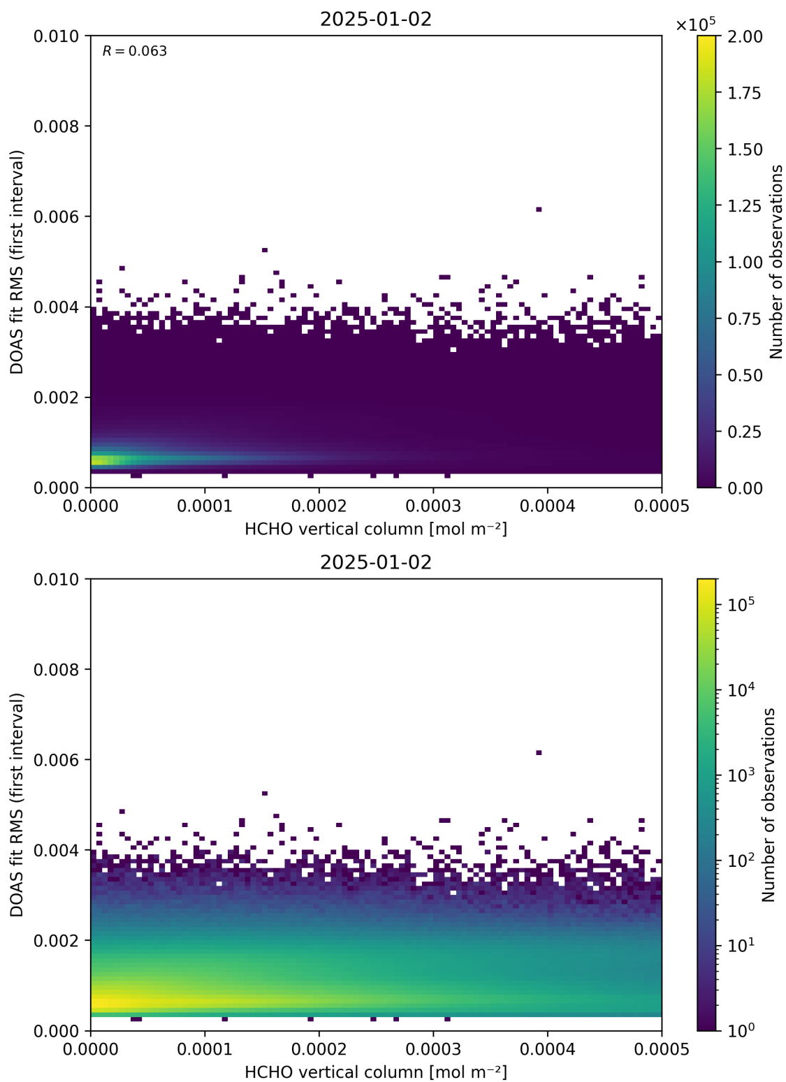
Figure 123: Scatter density plot of “HCHO vertical column” against “DOAS fit RMS (first interval)” for 2025-01-01 to 2025-01-03.
