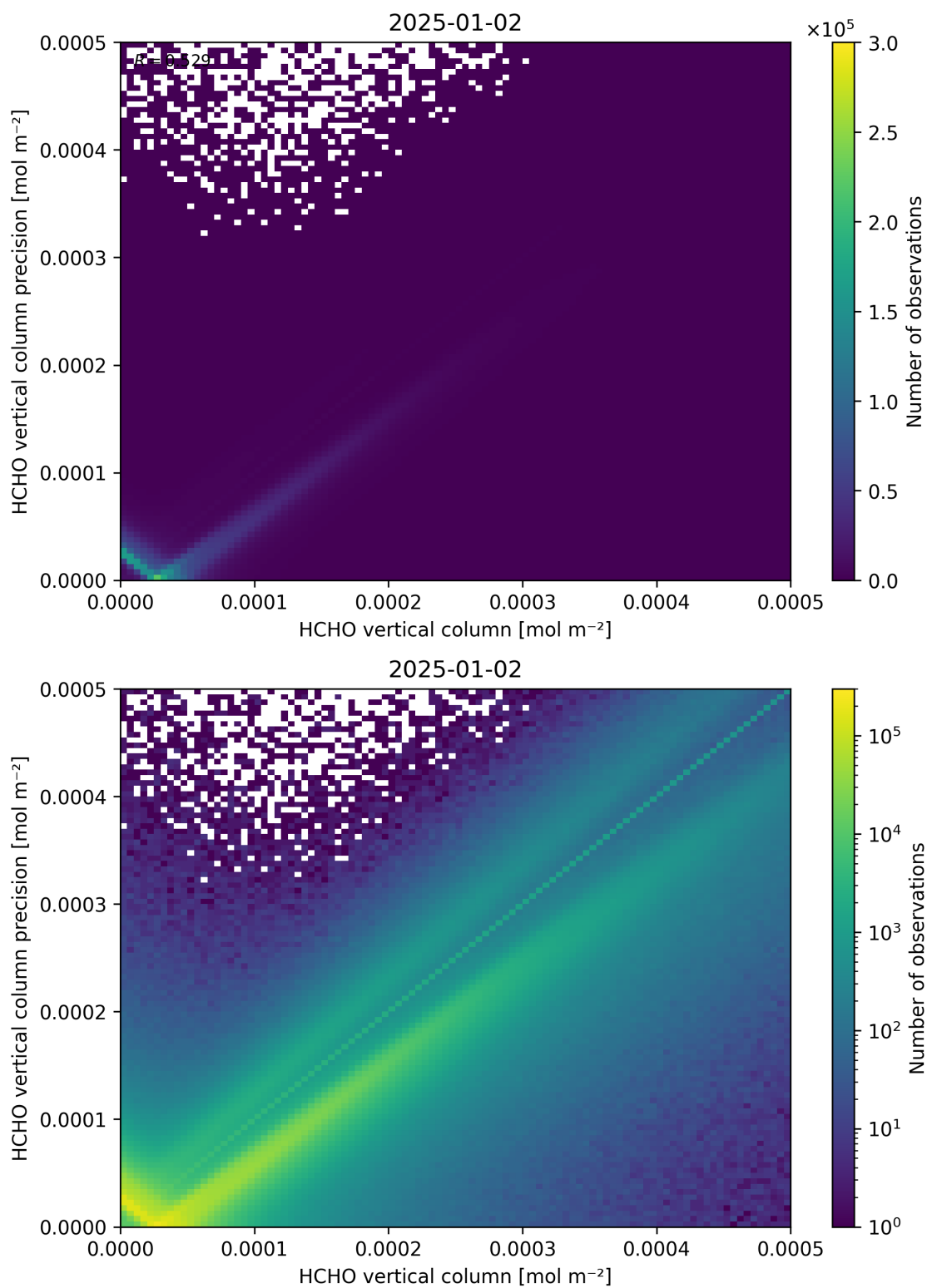
Figure 134: Scatter density plot of “HCHO vertical column” against “HCHO vertical column precision” for 2025-01-01 to 2025-01-03.
