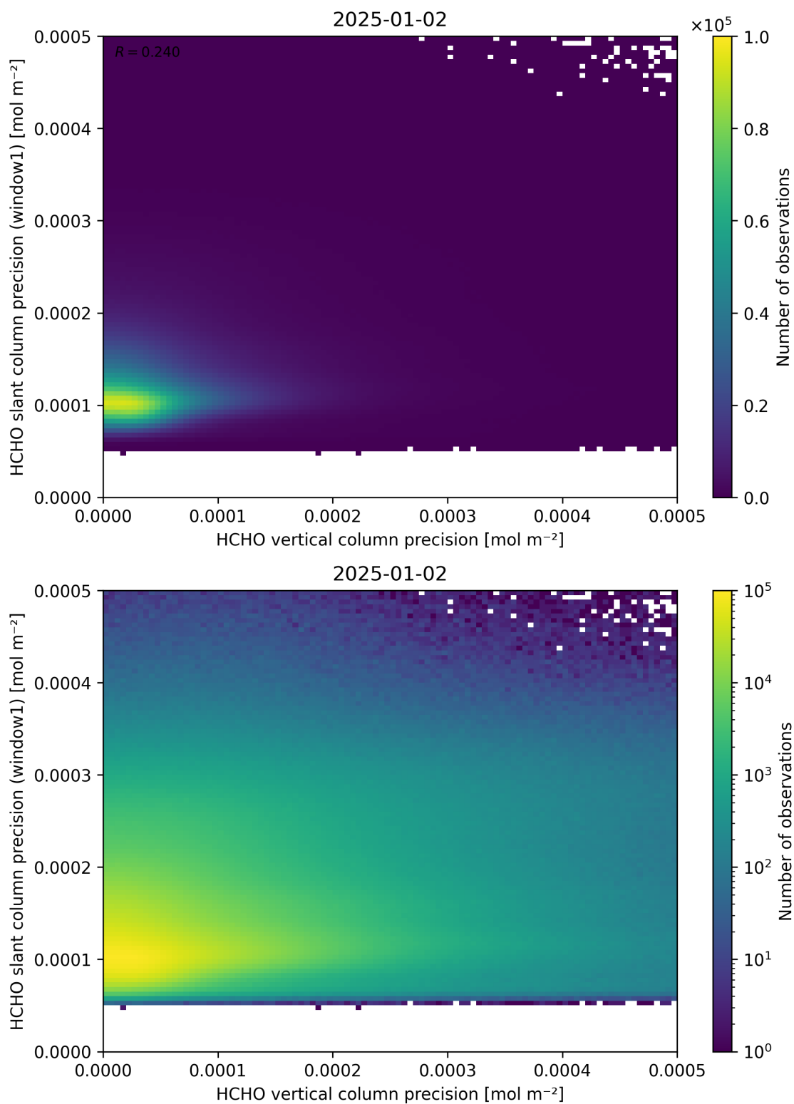
Figure 143: Scatter density plot of “HCHO vertical column precision” against “HCHO slant column precision (window1)” for 2025-01-01 to 2025-01-03.
