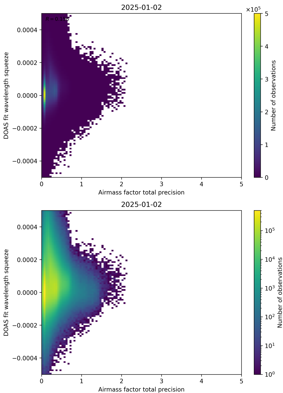
Figure 107: Scatter density plot of “Airmass factor total precision” against “DOAS fit wavelength squeeze” for 2025-01-01 to 2025-01-03.
