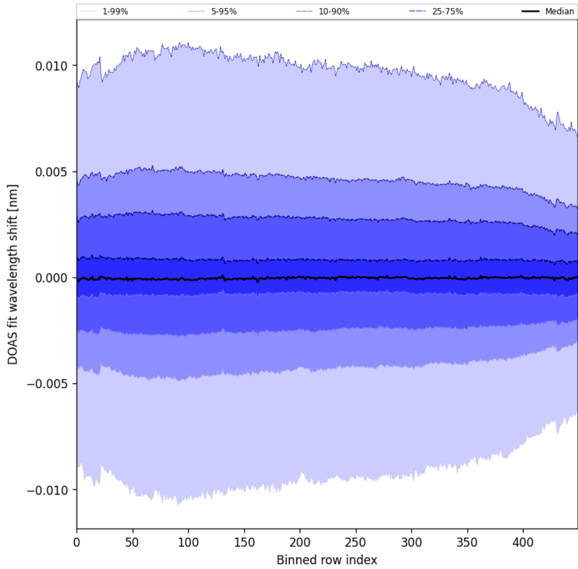
Figure 58: Along track statistics of “DOAS fit wavelength shift” for 2025-01-01 to 2025-01-03
