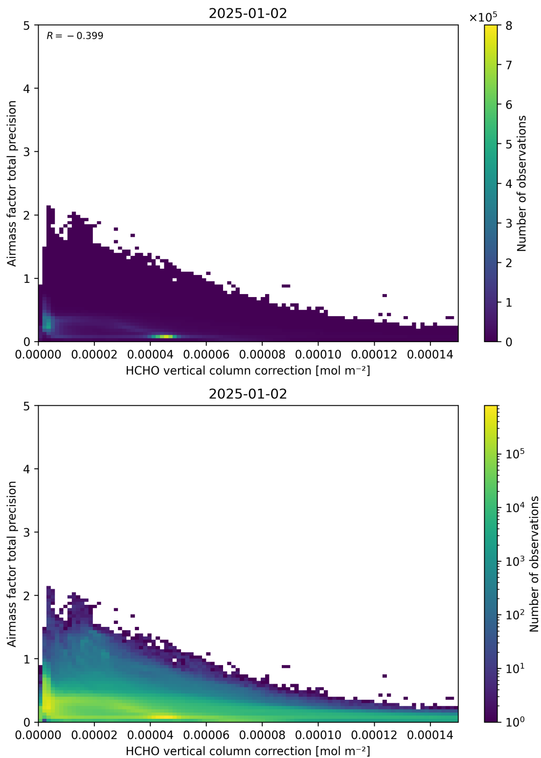
Figure 121: Scatter density plot of “HCHO vertical column correction” against “Airmass factor total precision” for 2025-01-01 to 2025-01-03.
