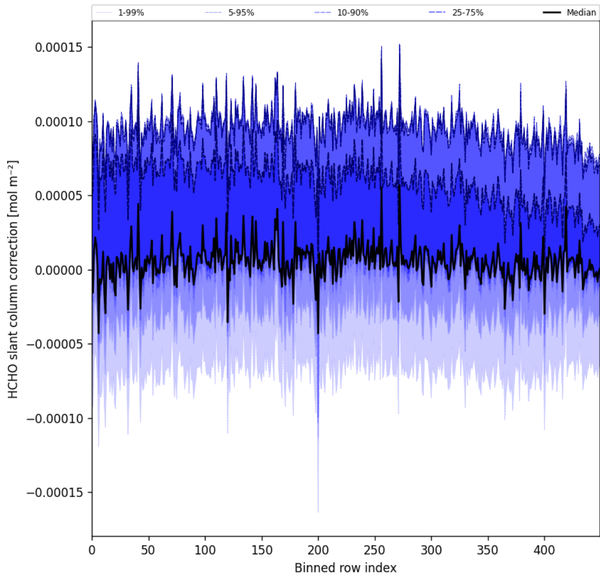
Figure 61: Along track statistics of “HCHO slant column correction” for 2025-01-01 to 2025-01-03
