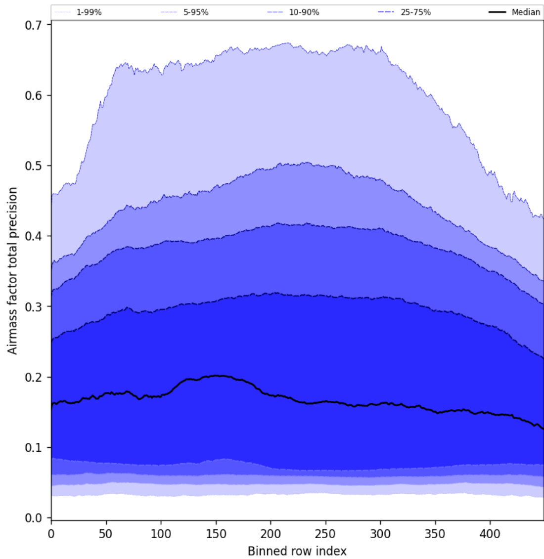
Figure 55: Along track statistics of “Airmass factor total precision” for 2025-01-01 to 2025-01-03
