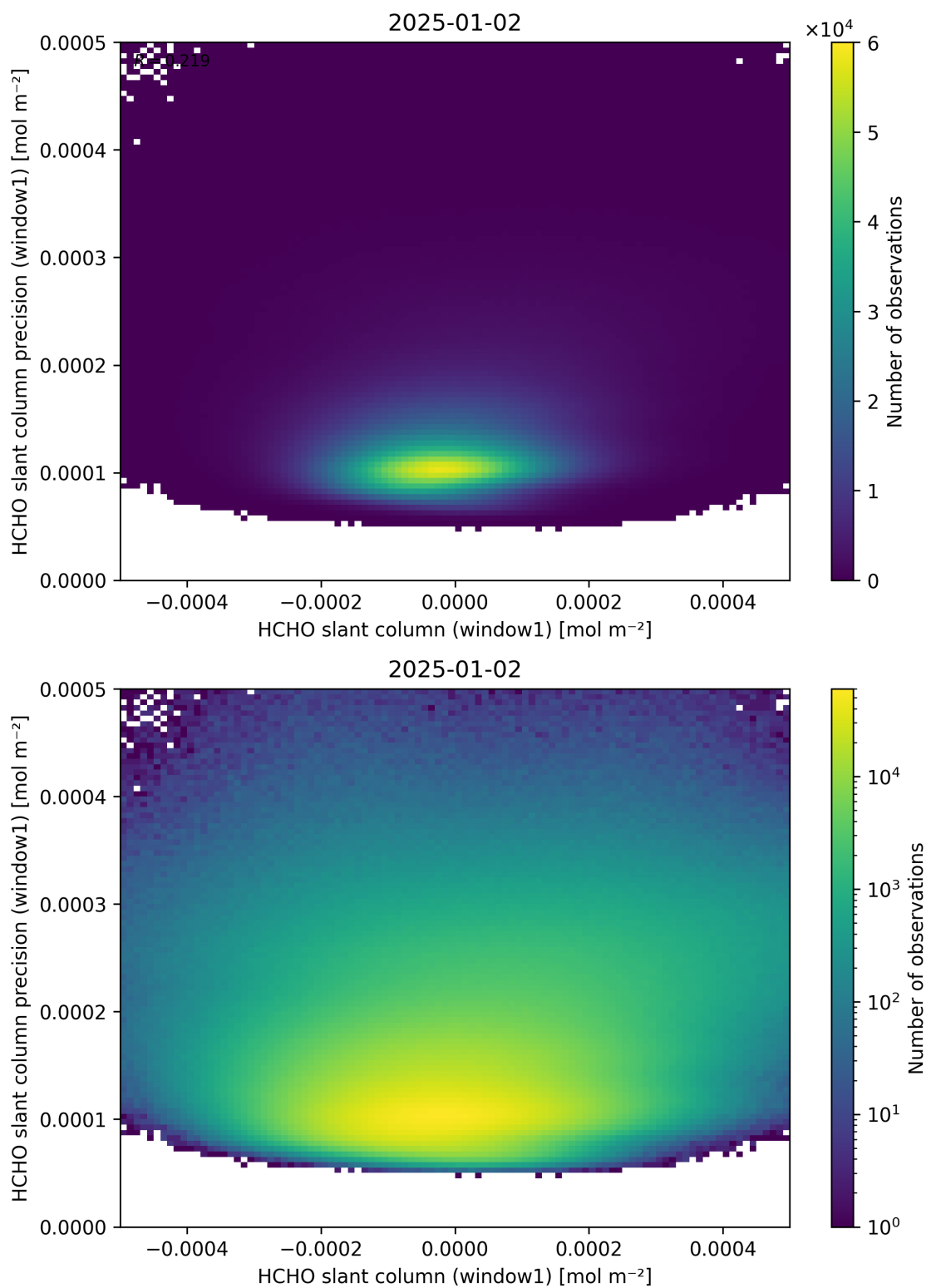
Figure 84: Scatter density plot of “HCHO slant column (window1)” against “HCHO slant column precision (window1)” for 2025-01-01 to 2025-01-03.
