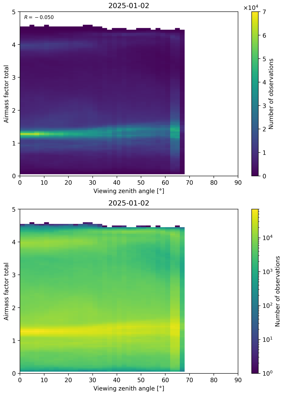
Figure 190: Scatter density plot of “Viewing zenith angle” against “Airmass factor total” for 2025-01-01 to 2025-01-03.
