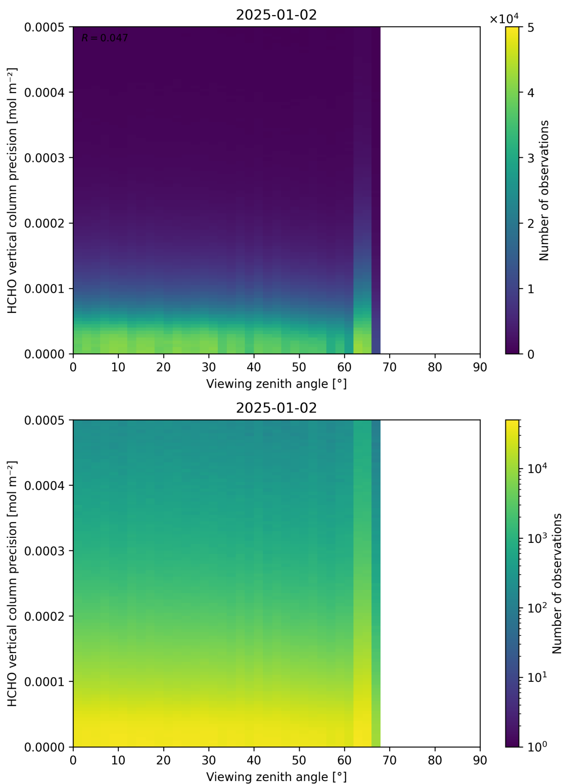
Figure 194: Scatter density plot of “Viewing zenith angle” against “HCHO vertical column precision” for 2025-01-01 to 2025-01-03.
