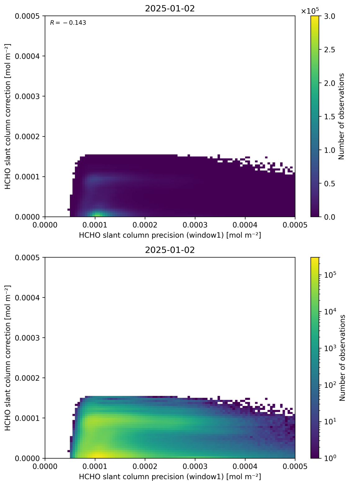
Figure 93: Scatter density plot of “HCHO slant column precision (window1)” against “HCHO slant column correction” for 2025-01-01 to 2025-01-03.
