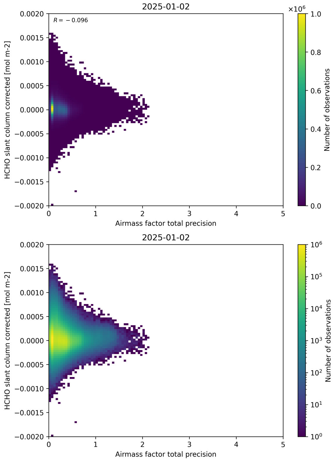
Figure 109: Scatter density plot of “Airmass factor total precision” against “HCHO slant column corrected” for 2025-01-01 to 2025-01-03.
