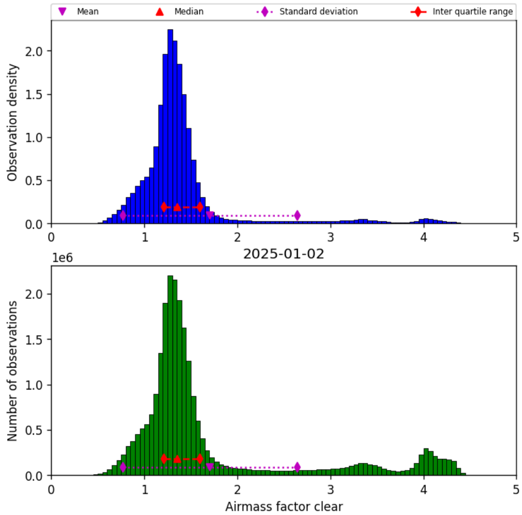
Figure 42: Histogram of “Airmass factor clear” for 2025-01-01 to 2025-01-03
