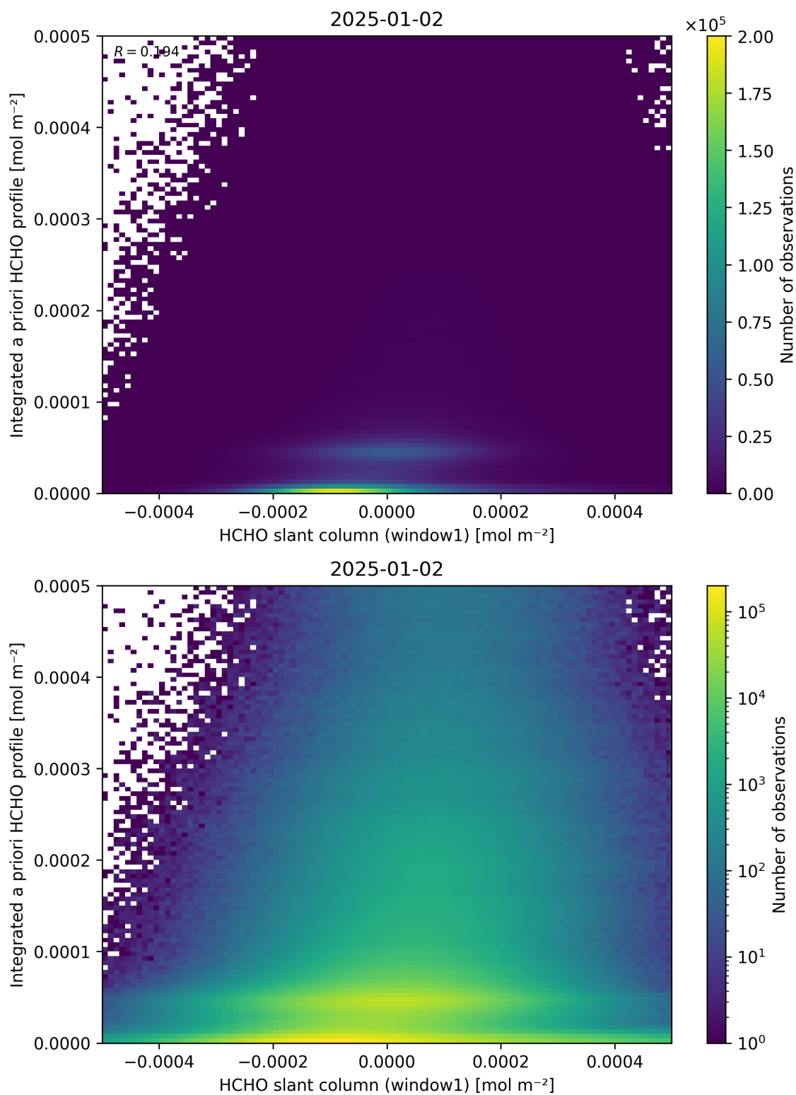
Figure 87: Scatter density plot of “HCHO slant column (window1)” against “Integrated a priori HCHO profile” for 2025-01-01 to 2025-01-03.
