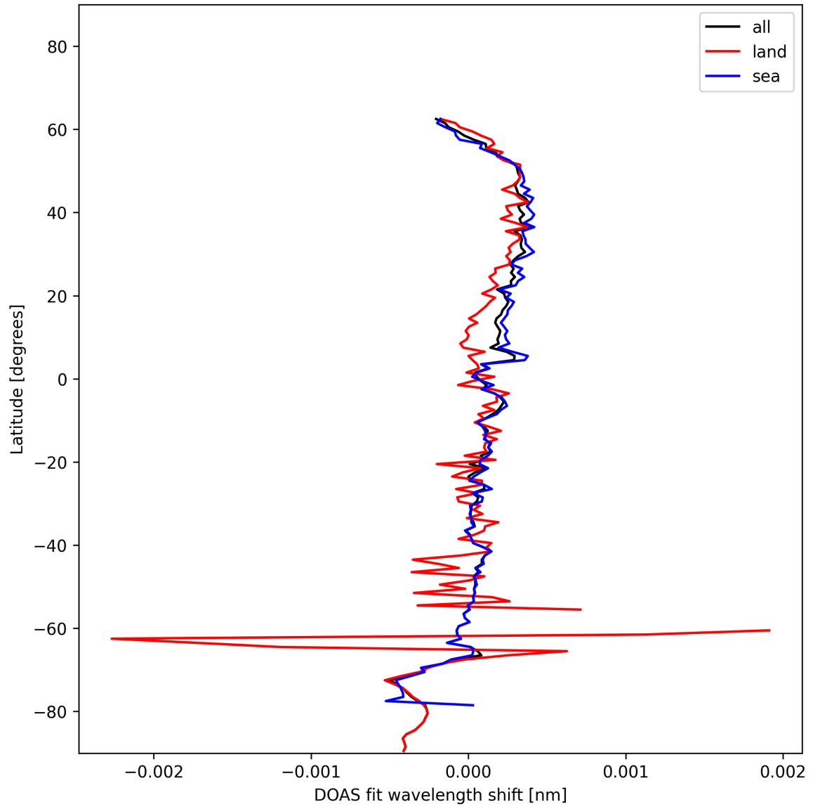
Figure 30: Zonal average of “DOAS fit wavelength shift” for 2025-01-01 to 2025-01-03.
