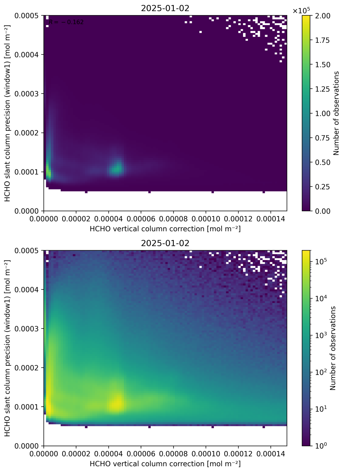
Figure 119: Scatter density plot of “HCHO vertical column correction” against “HCHO slant column precision (window1)” for 2025-01-01 to 2025-01-03.
