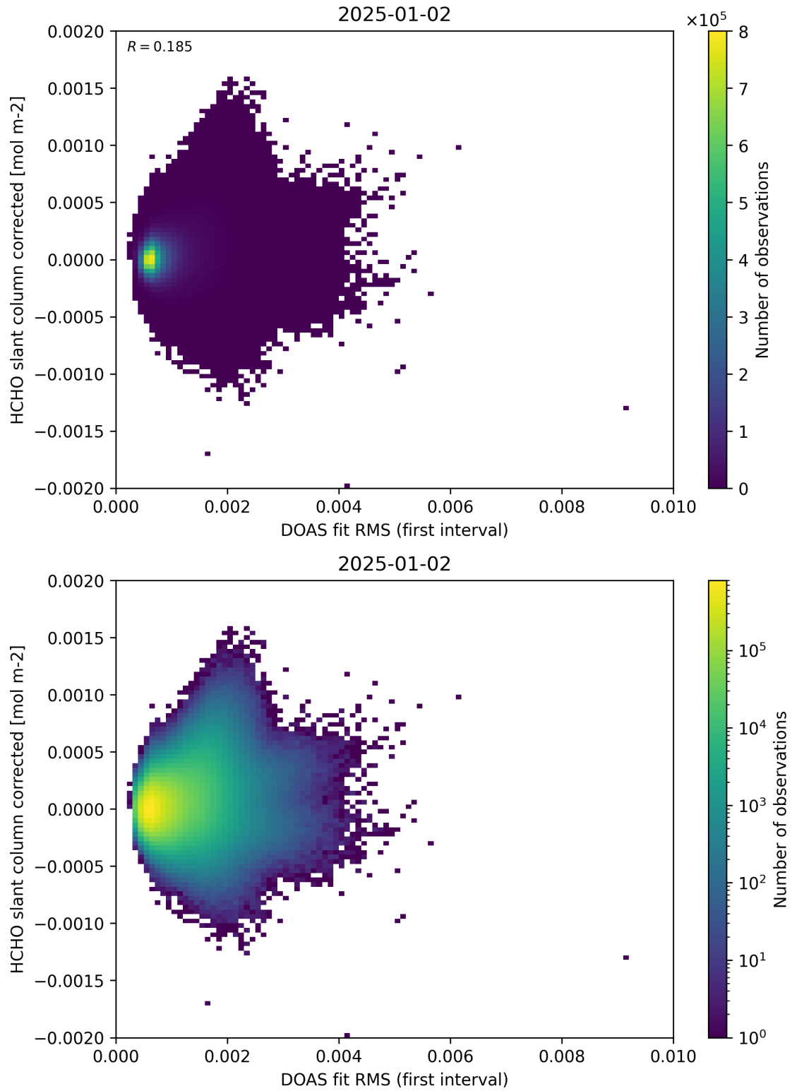
Figure 62: Scatter density plot of “DOAS fit RMS (first interval)” against “HCHO slant column corrected” for 2025-01-01 to 2025-01-03.
