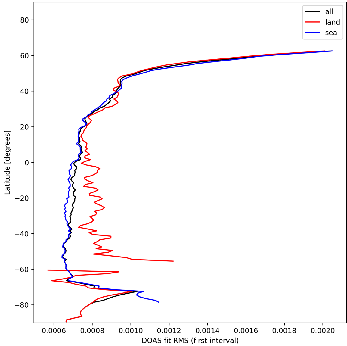
Figure 32: Zonal average of “DOAS fit RMS (first interval)” for 2025-01-01 to 2025-01-03.
