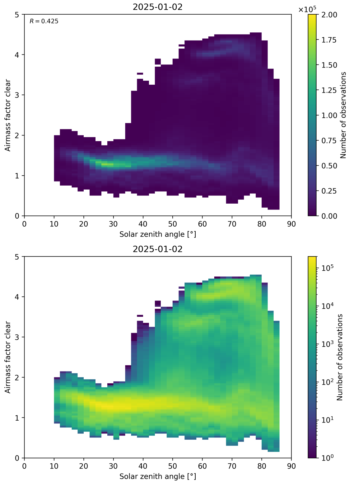
Figure 170: Scatter density plot of “Solar zenith angle” against “Airmass factor clear” for 2025-01-01 to 2025-01-03.
