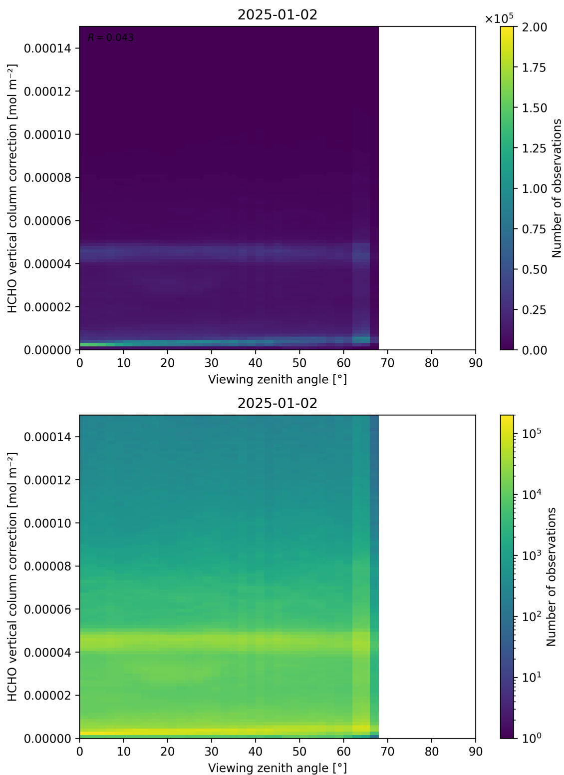
Figure 193: Scatter density plot of “Viewing zenith angle” against “HCHO vertical column correction” for 2025-01-01 to 2025-01-03.
