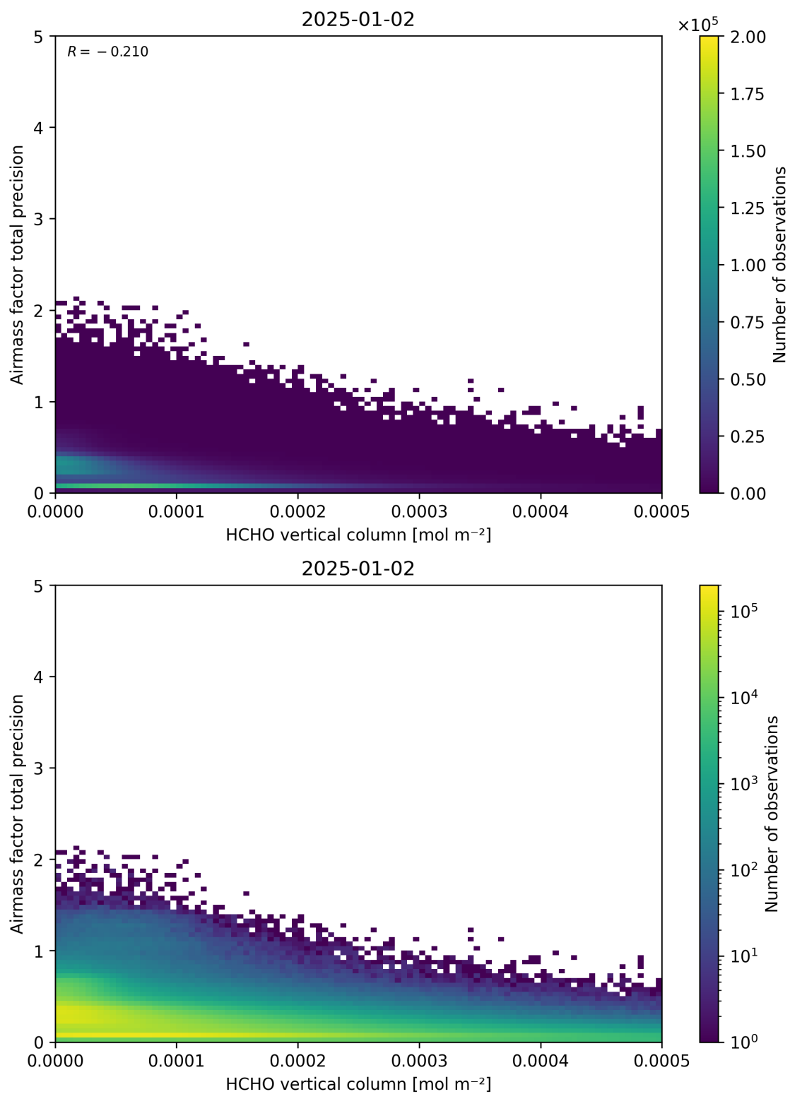
Figure 132: Scatter density plot of “HCHO vertical column” against “Airmass factor total precision” for 2025-01-01 to 2025-01-03.
