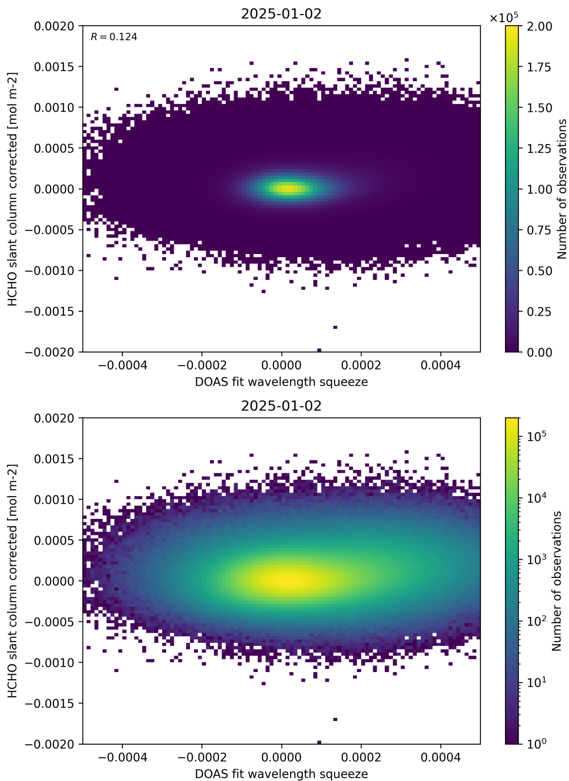
Figure 69: Scatter density plot of “DOAS fit wavelength squeeze” against “HCHO slant column corrected” for 2025-01-01 to 2025-01-03.
