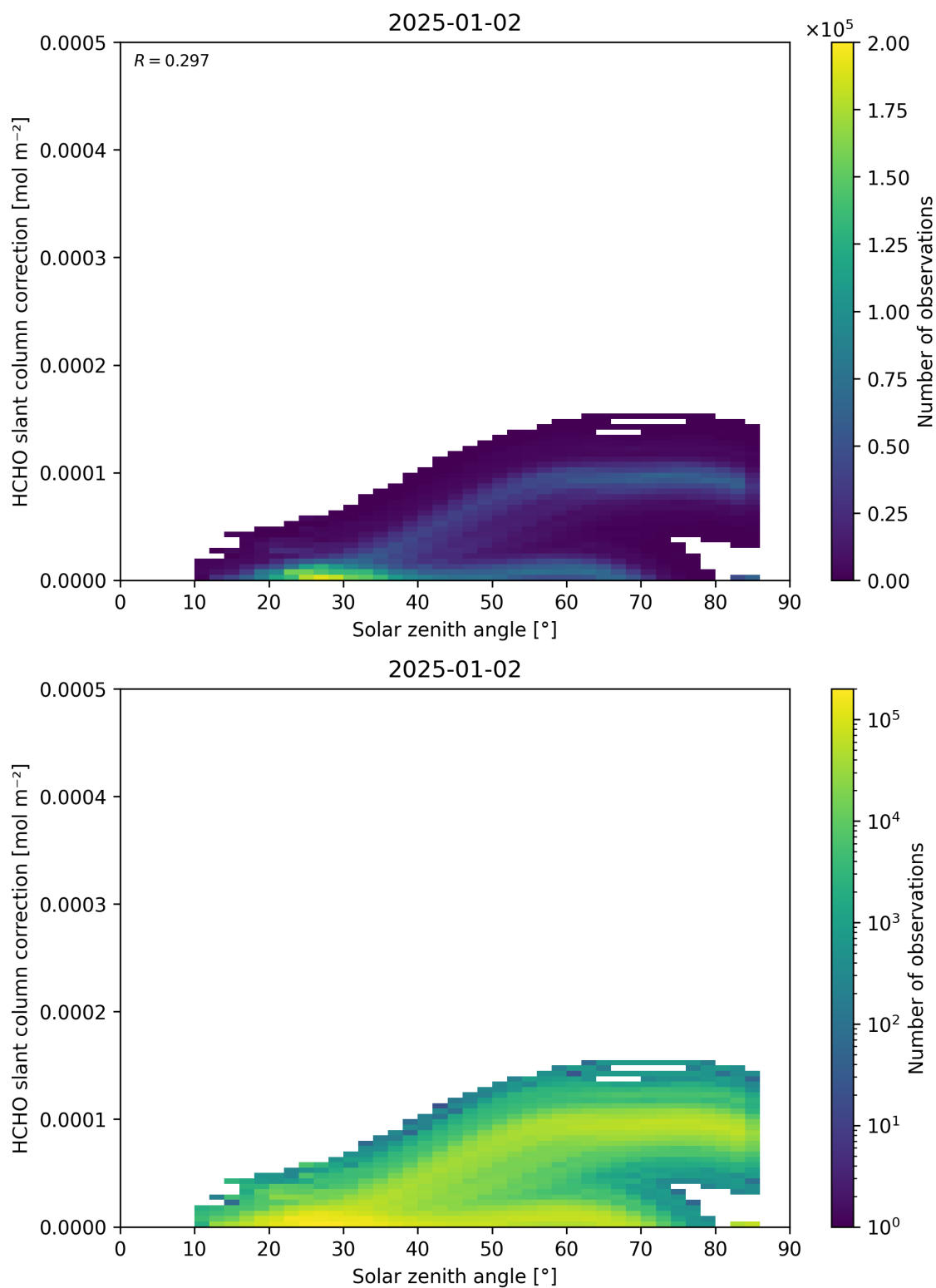
Figure 172: Scatter density plot of “Solar zenith angle” against “HCHO slant column correction” for 2025-01-01 to 2025-01-03.
