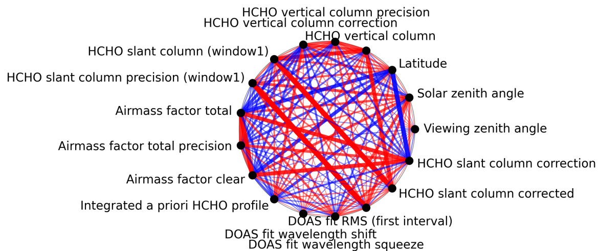
Figure 1: Map of correlation graph for 2025-01-01 to 2025-01-03.
