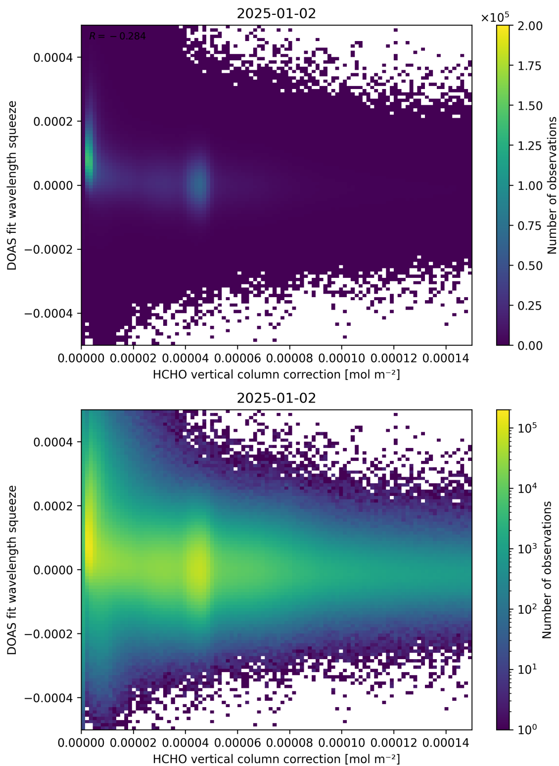
Figure 114: Scatter density plot of “HCHO vertical column correction” against “DOAS fit wavelength squeeze” for 2025-01-01 to 2025-01-03.
