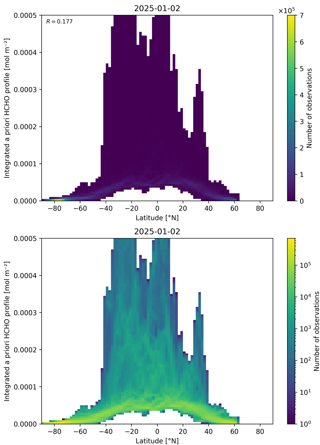
Figure 166: Scatter density plot of “Latitude” against “Integrated a priori HCHO profile” for 2025-01-01 to 2025-01-03.
