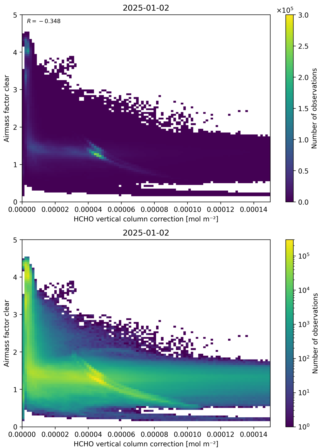
Figure 115: Scatter density plot of “HCHO vertical column correction” against “Airmass factor clear” for 2025-01-01 to 2025-01-03.
