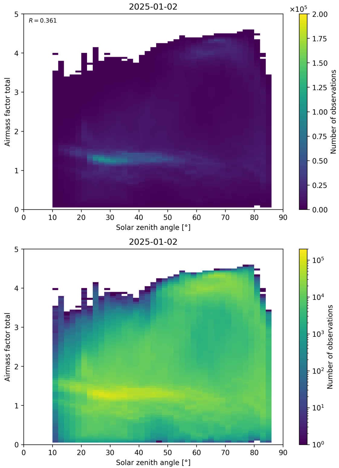
Figure 175: Scatter density plot of “Solar zenith angle” against “Airmass factor total” for 2025-01-01 to 2025-01-03.
