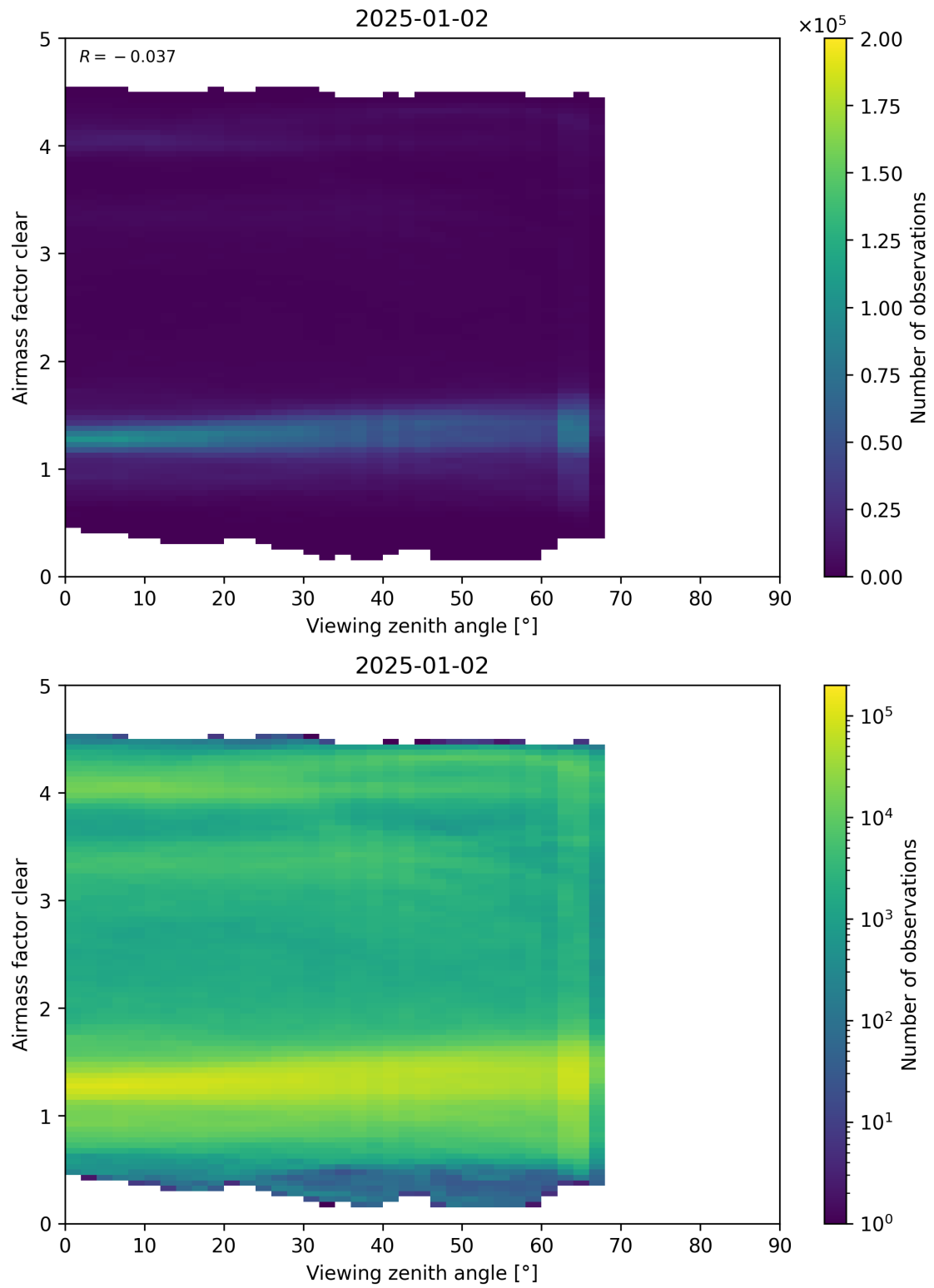
Figure 185: Scatter density plot of “Viewing zenith angle” against “Airmass factor clear” for 2025-01-01 to 2025-01-03.
