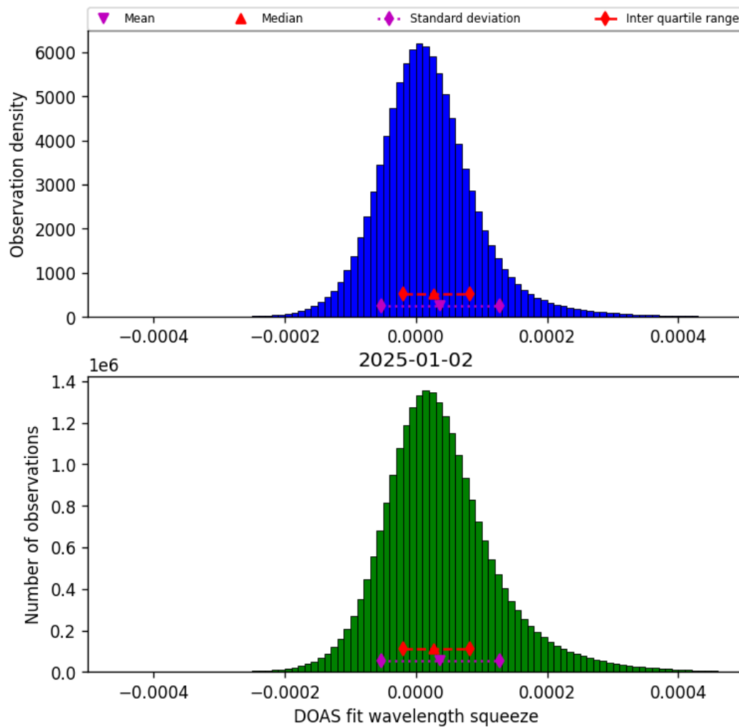
Figure 45: Histogram of “DOAS fit wavelength squeeze” for 2025-01-01 to 2025-01-03
