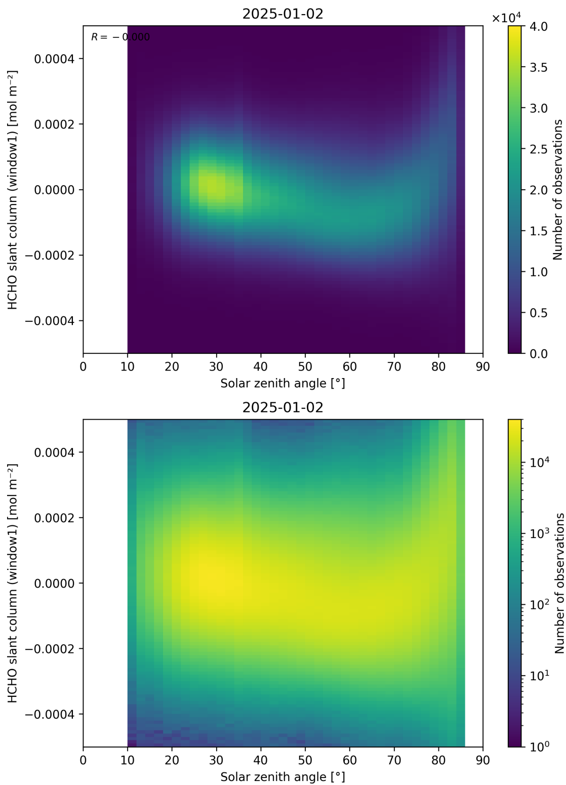
Figure 173: Scatter density plot of “Solar zenith angle” against “HCHO slant column (window1)” for 2025-01-01 to 2025-01-03.
