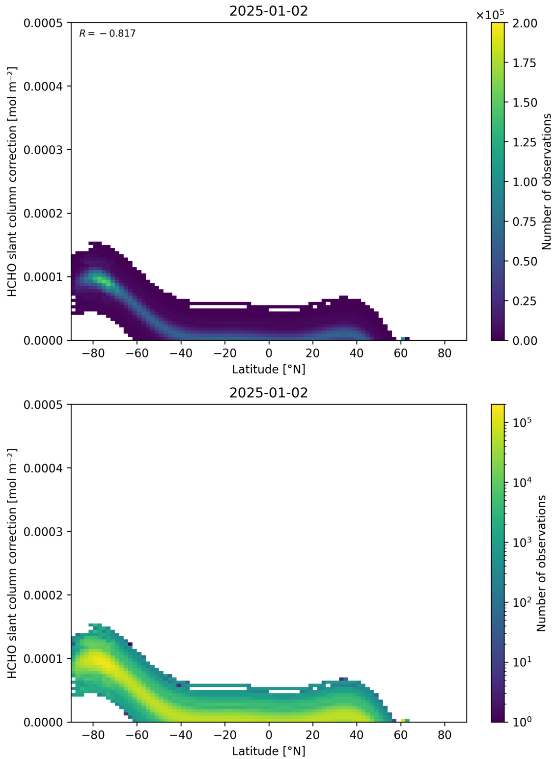
Figure 158: Scatter density plot of “Latitude” against “HCHO slant column correction” for 2025-01-01 to 2025-01-03.
