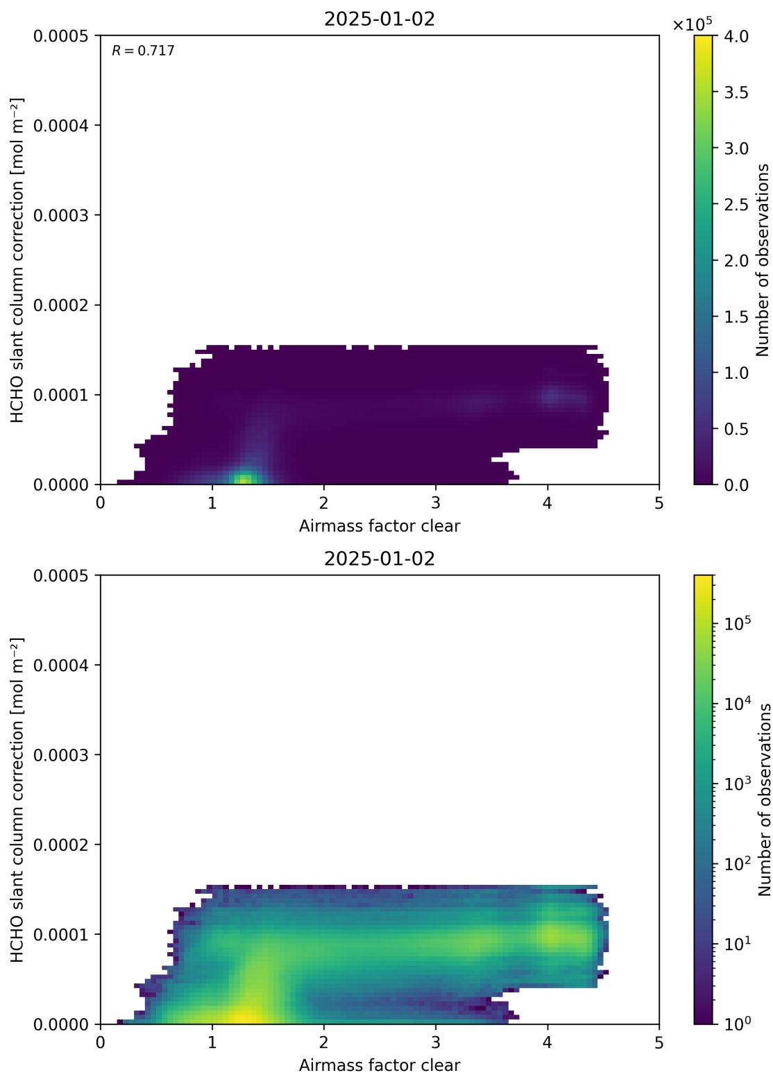
Figure 75: Scatter density plot of “Airmass factor clear” against “HCHO slant column correction” for 2025-01-01 to 2025-01-03.
