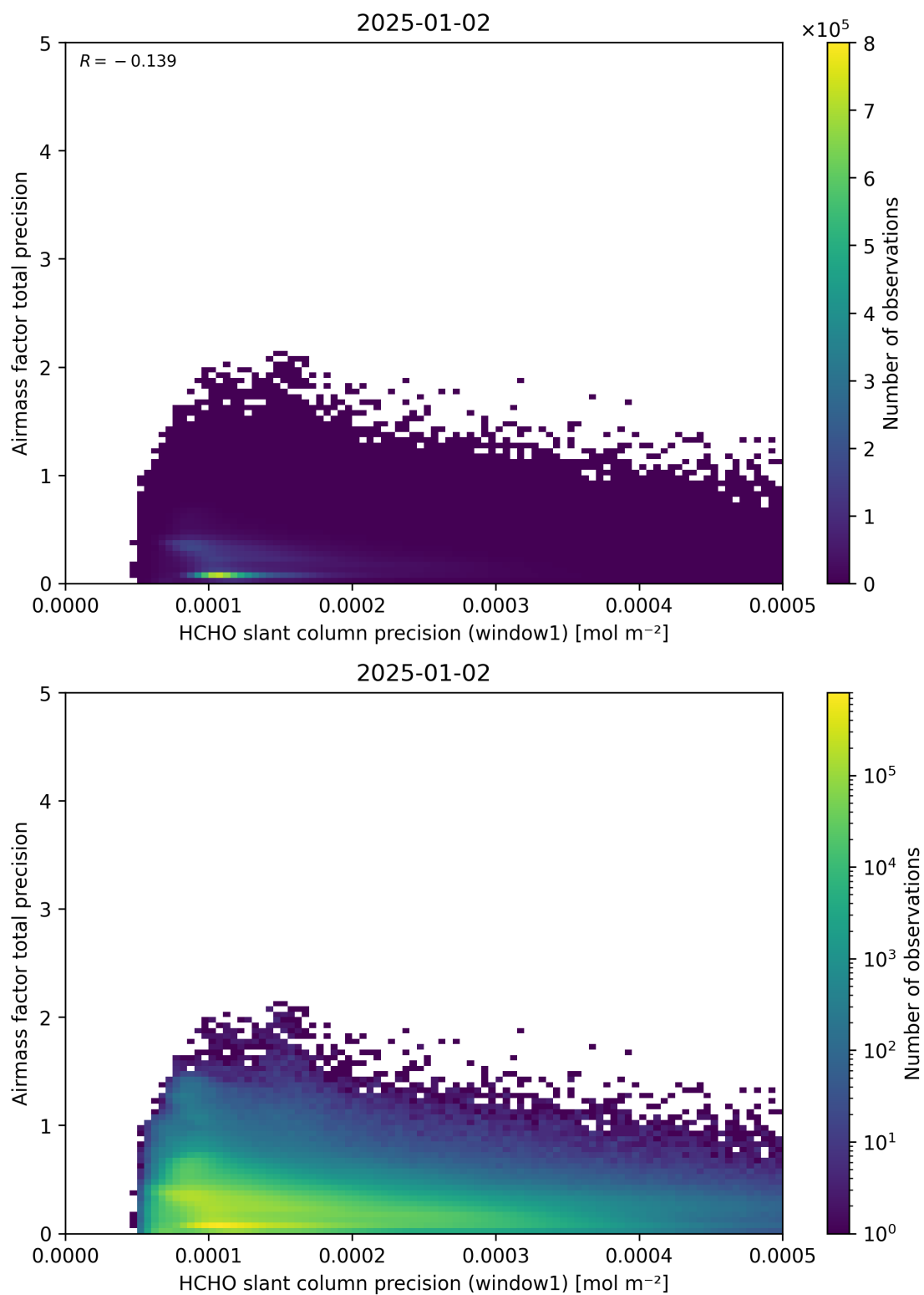
Figure 95: Scatter density plot of “HCHO slant column precision (window1)” against “Airmass factor total precision” for 2025-01-01 to 2025-01-03.
