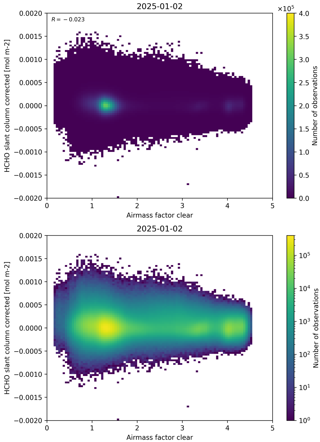
Figure 74: Scatter density plot of “Airmass factor clear” against “HCHO slant column corrected” for 2025-01-01 to 2025-01-03.
