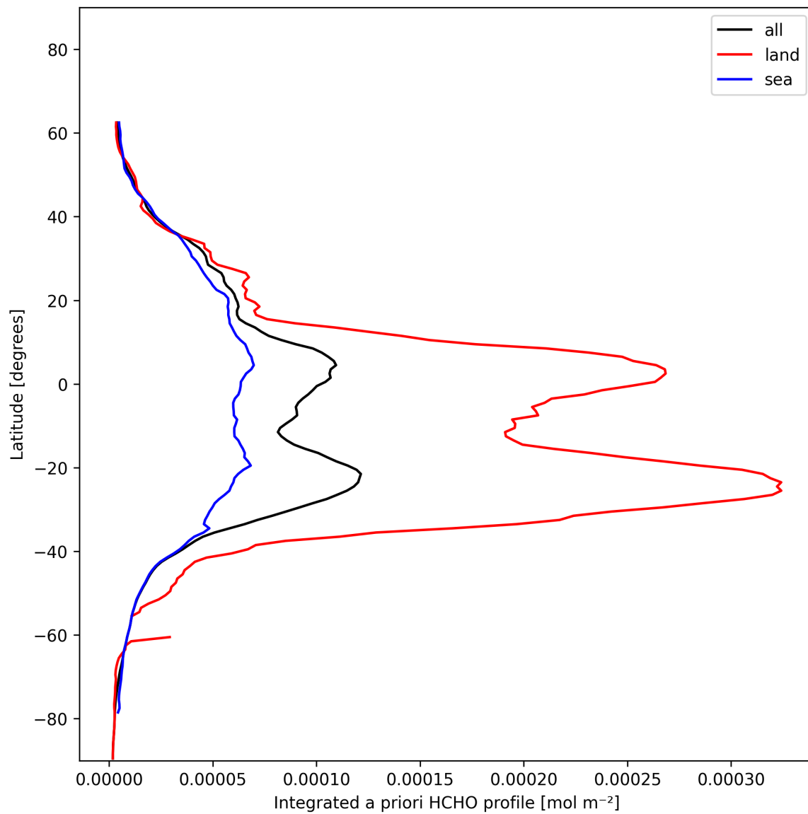
Figure 29: Zonal average of “Integrated a priori HCHO profile” for 2025-01-01 to 2025-01-03.
