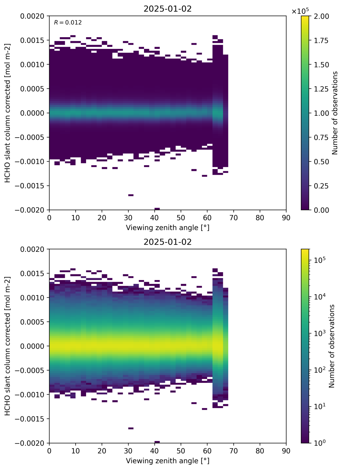
Figure 186: Scatter density plot of “Viewing zenith angle” against “HCHO slant column corrected” for 2025-01-01 to 2025-01-03.
