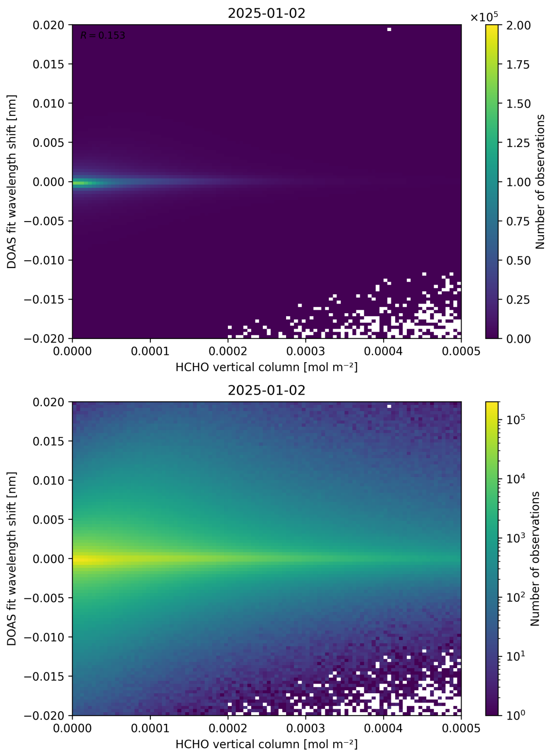
Figure 124: Scatter density plot of “HCHO vertical column” against “DOAS fit wavelength shift” for 2025-01-01 to 2025-01-03.
