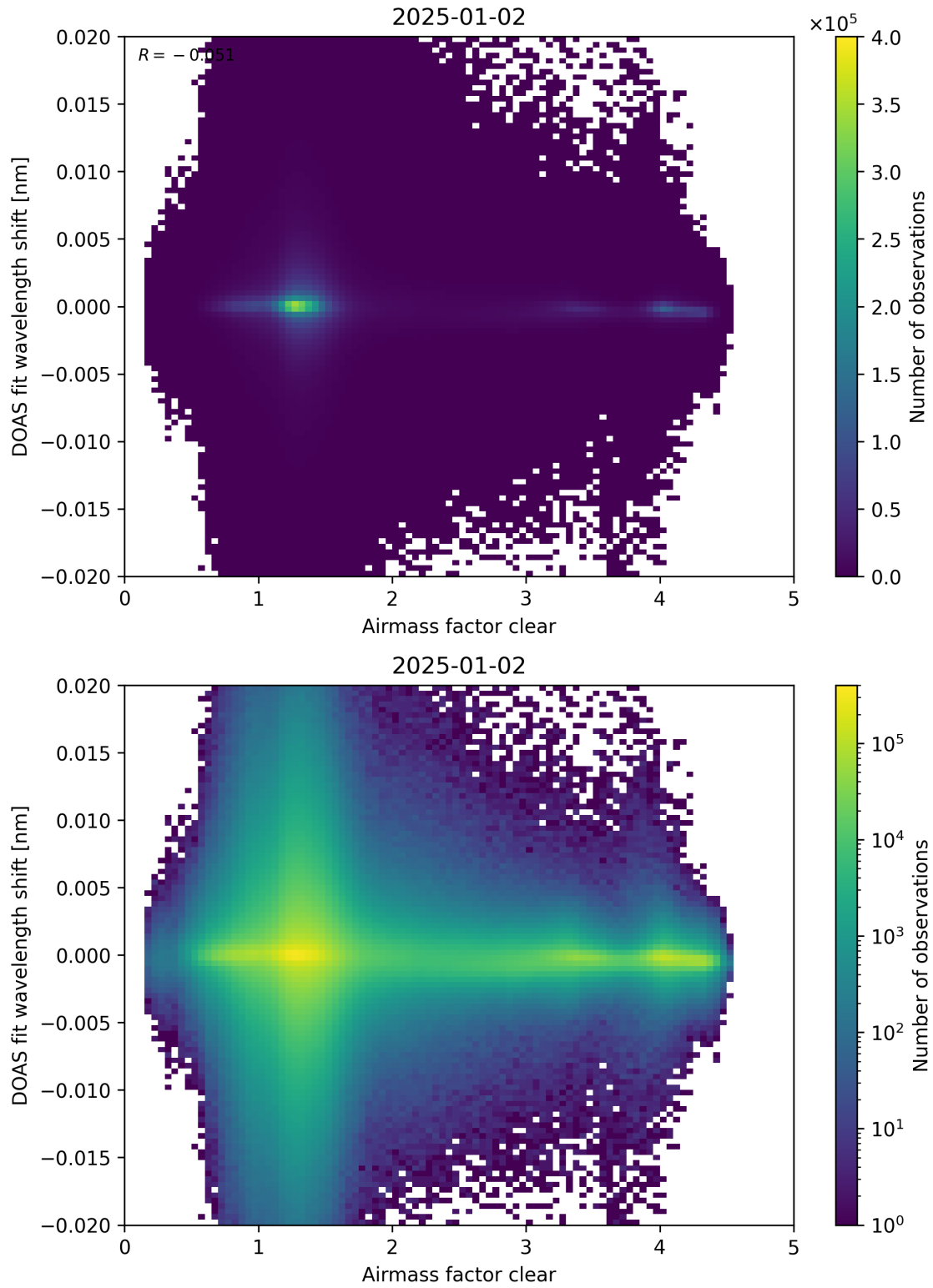
Figure 72: Scatter density plot of “Airmass factor clear” against “DOAS fit wavelength shift” for 2025-01-01 to 2025-01-03.
