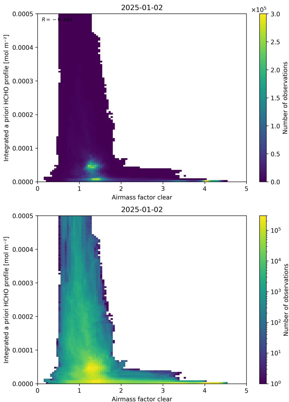
Figure 76: Scatter density plot of “Airmass factor clear” against “Integrated a priori HCHO profile” for 2025-01-01 to 2025-01-03.
