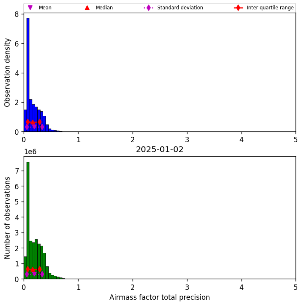
Figure 41: Histogram of “Airmass factor total precision” for 2025-01-01 to 2025-01-03
