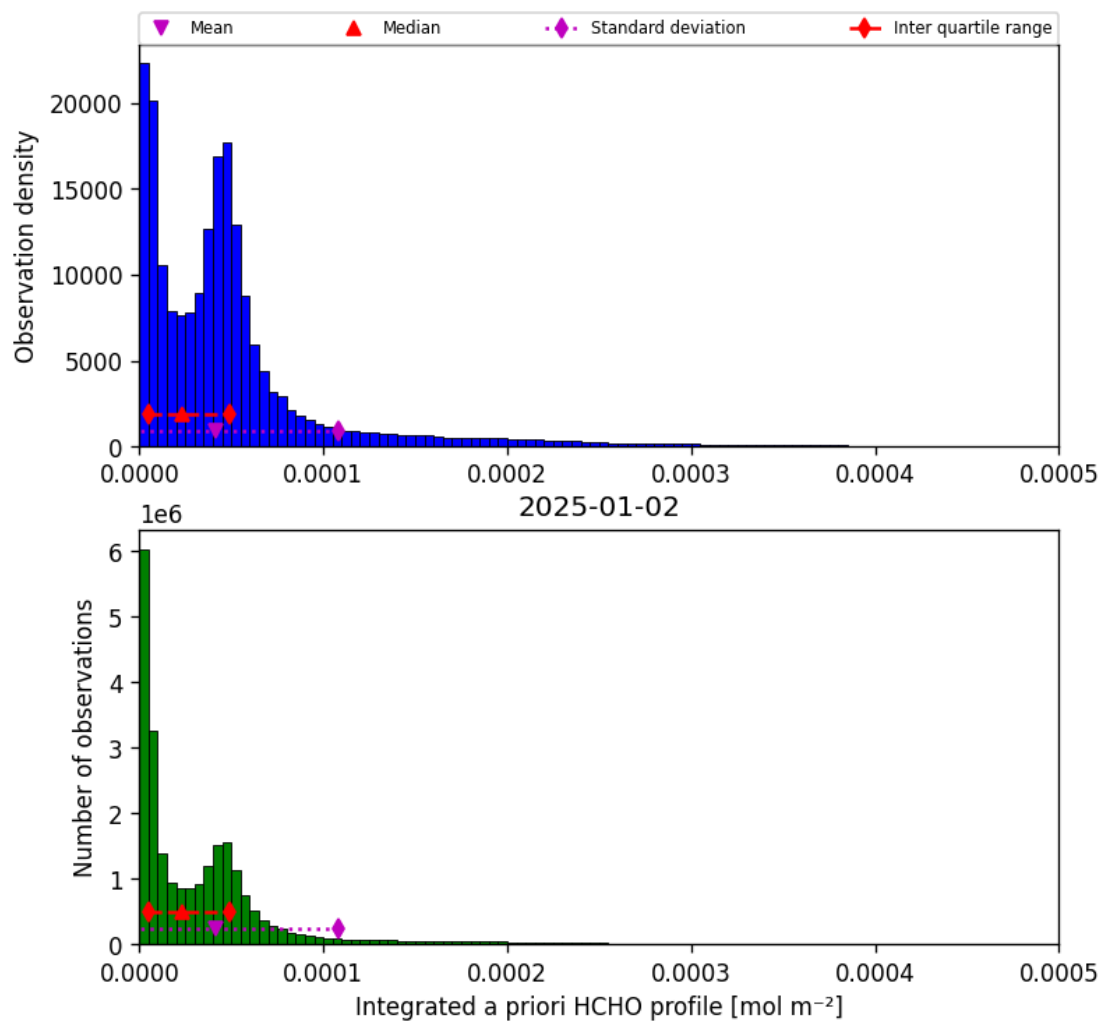
Figure 43: Histogram of “Integrated a priori HCHO profile” for 2025-01-01 to 2025-01-03
