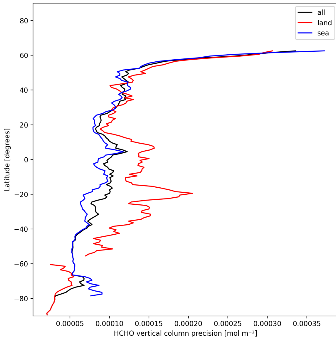
Figure 22: Zonal average of “HCHO vertical column precision” for 2025-01-01 to 2025-01-03.
