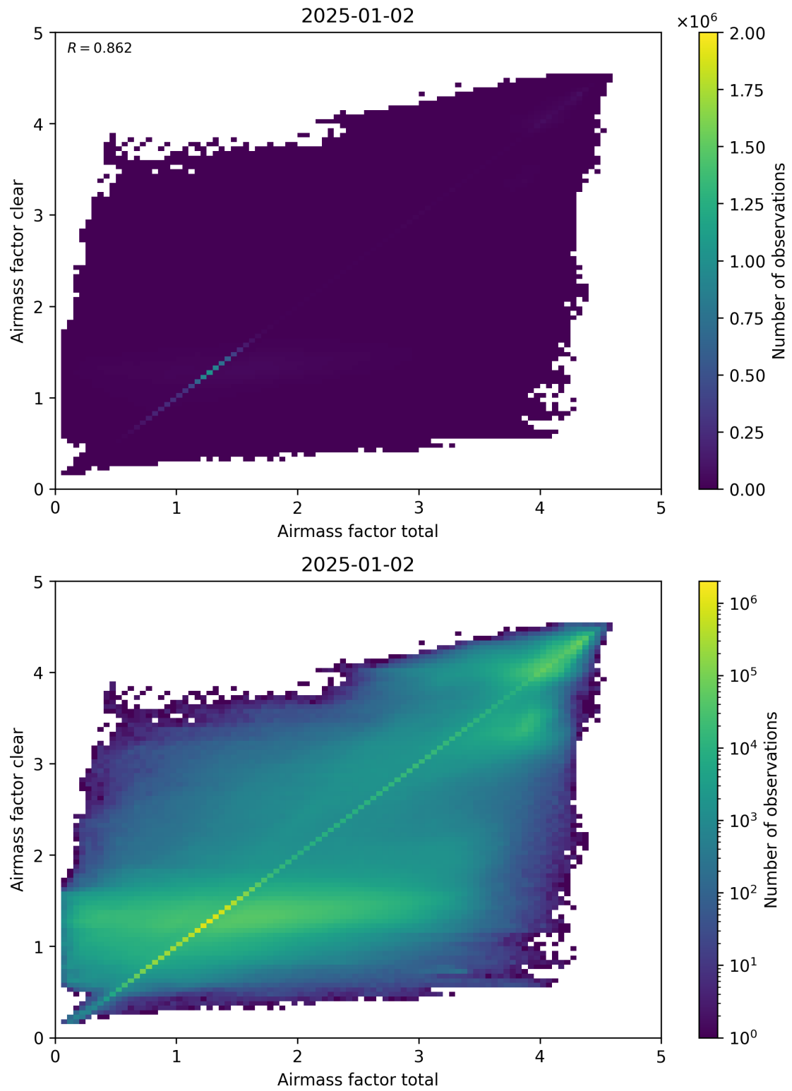
Figure 100: Scatter density plot of “Airmass factor total” against “Airmass factor clear” for 2025-01-01 to 2025-01-03.
