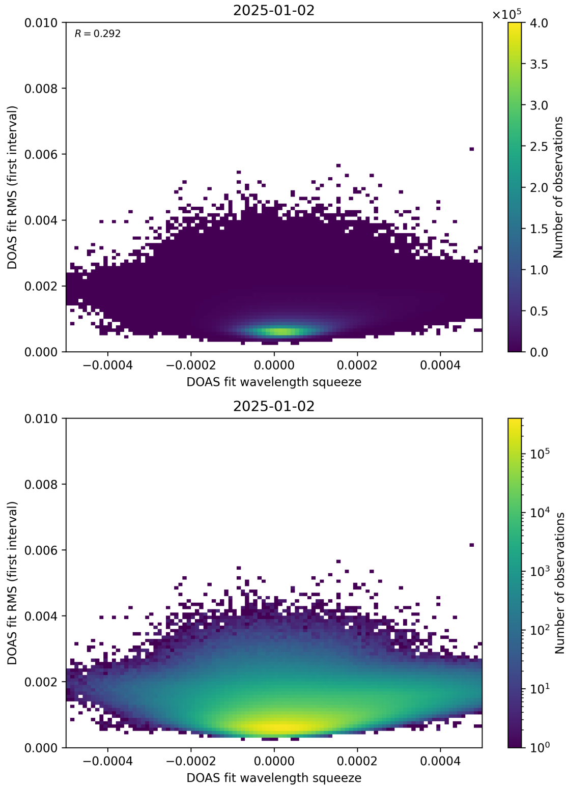
Figure 68: Scatter density plot of “DOAS fit wavelength squeeze” against “DOAS fit RMS (first interval)” for 2025-01-01 to 2025-01-03.
