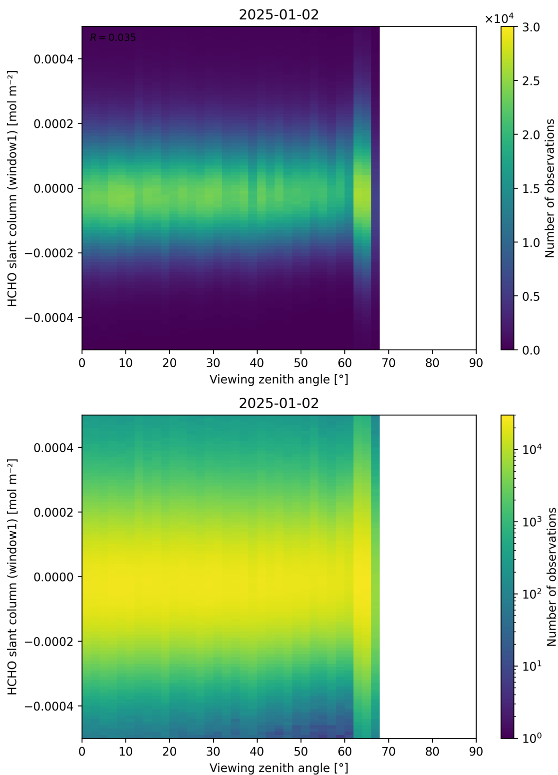
Figure 188: Scatter density plot of “Viewing zenith angle” against “HCHO slant column (window1)” for 2025-01-01 to 2025-01-03.
