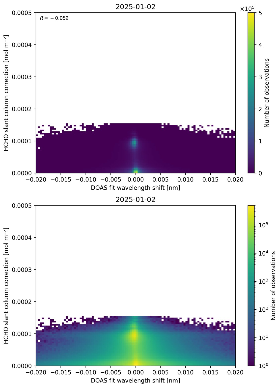
Figure 67: Scatter density plot of “DOAS fit wavelength shift” against “HCHO slant column correction” for 2025-01-01 to 2025-01-03.
