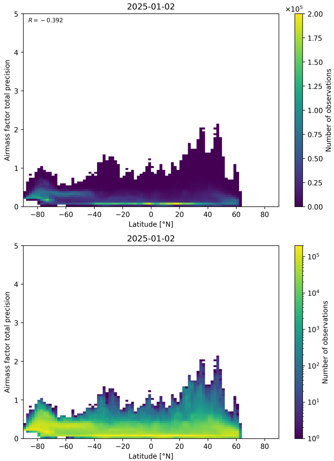
Figure 162: Scatter density plot of “Latitude” against “Airmass factor total precision” for 2025-01-01 to 2025-01-03.
