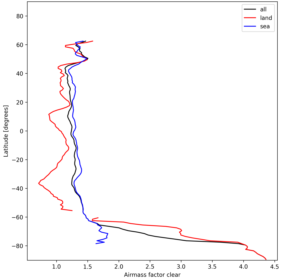
Figure 28: Zonal average of “Airmass factor clear” for 2025-01-01 to 2025-01-03.
