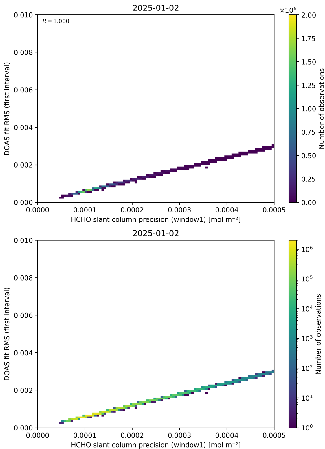
Figure 88: Scatter density plot of “HCHO slant column precision (window1)” against “DOAS fit RMS (first interval)” for 2025-01-01 to 2025-01-03.
