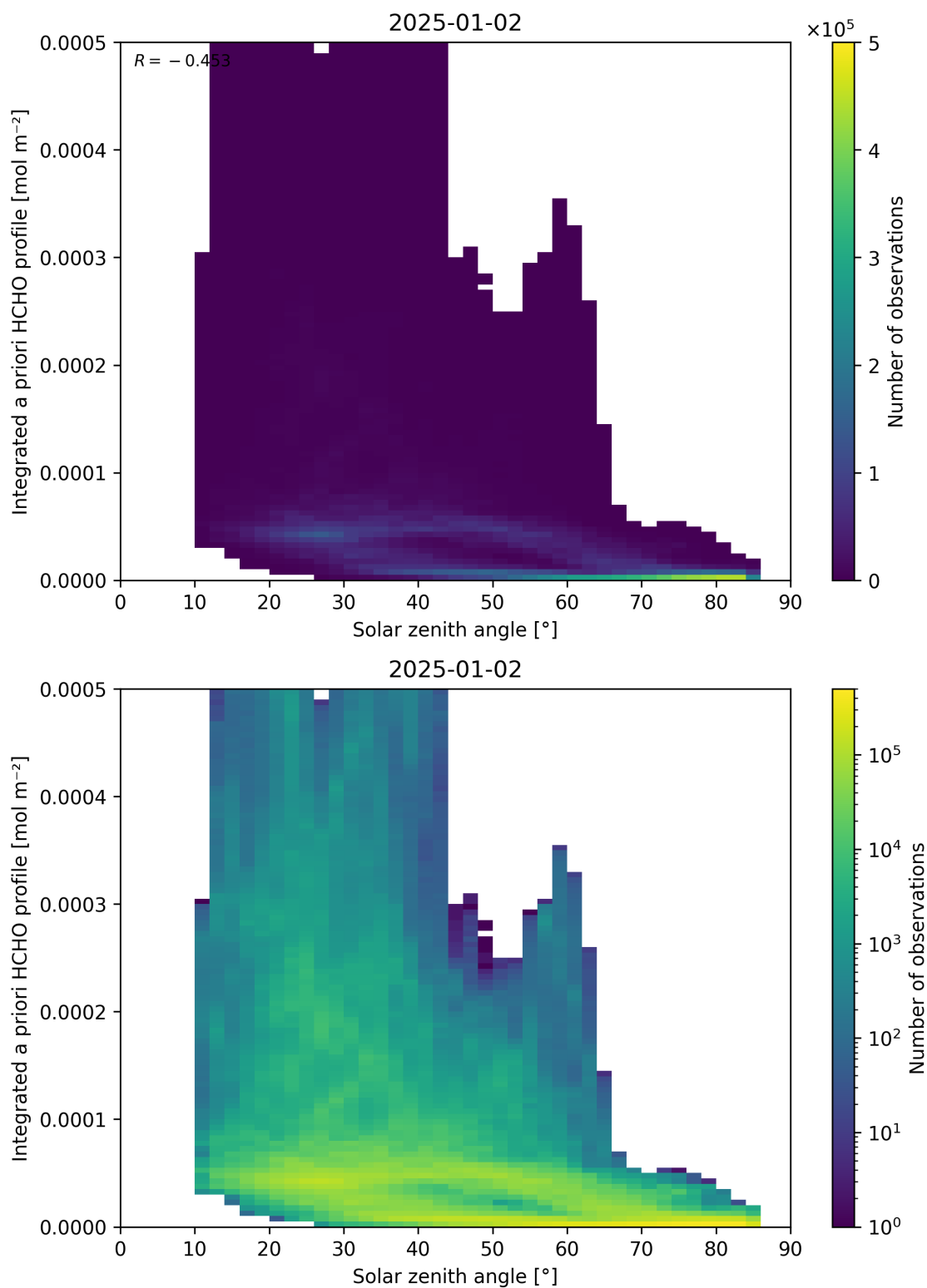
Figure 180: Scatter density plot of “Solar zenith angle” against “Integrated a priori HCHO profile” for 2025-01-01 to 2025-01-03.
