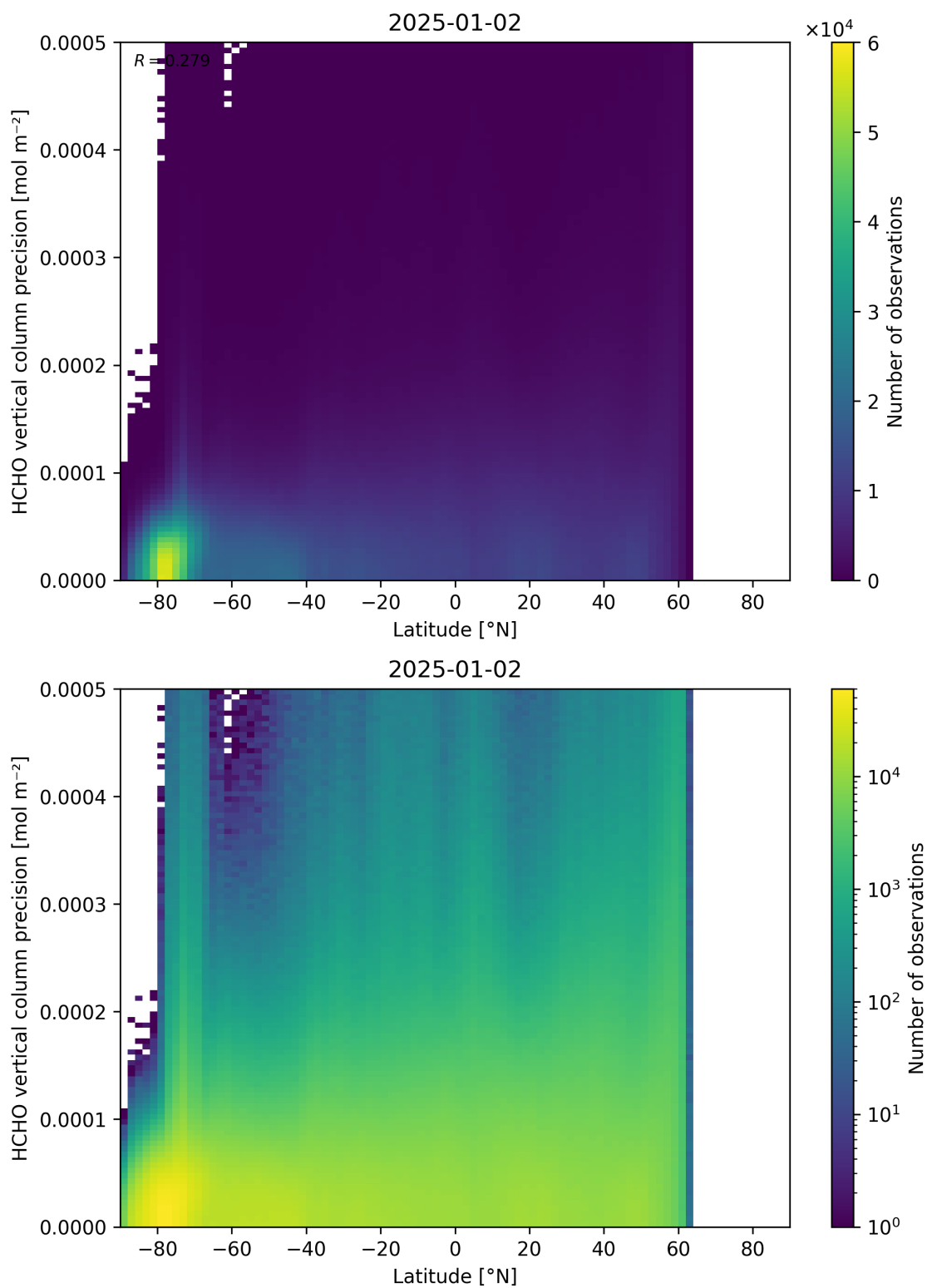
Figure 165: Scatter density plot of “Latitude” against “HCHO vertical column precision” for 2025-01-01 to 2025-01-03.
