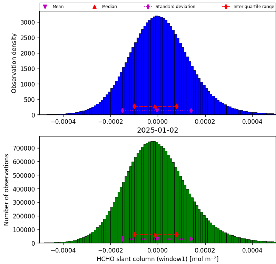
Figure 38: Histogram of “HCHO slant column (window1)” for 2025-01-01 to 2025-01-03
