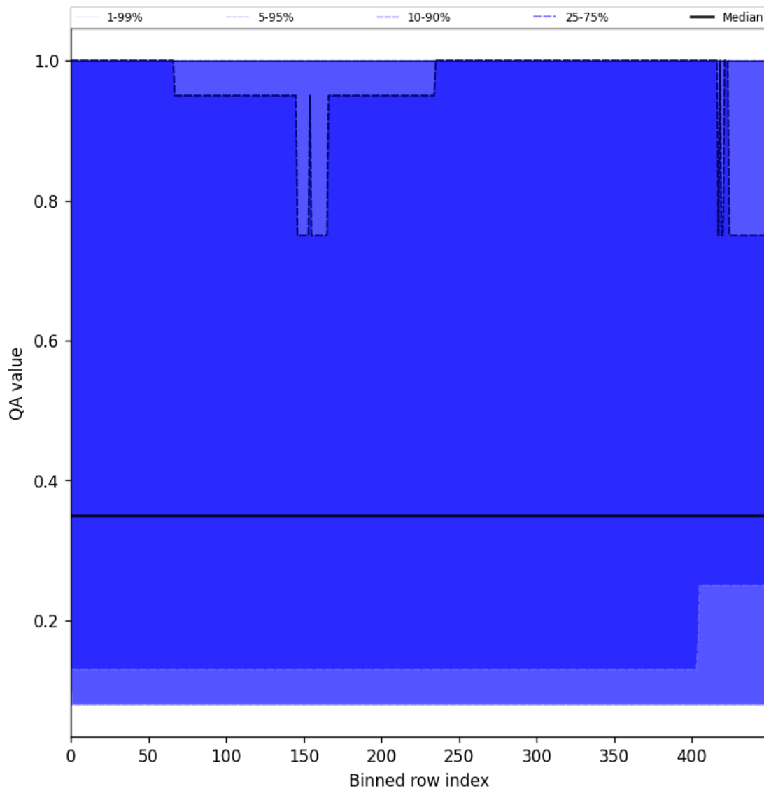
Figure 48: Along track statistics of “QA value” for 2025-01-01 to 2025-01-03
