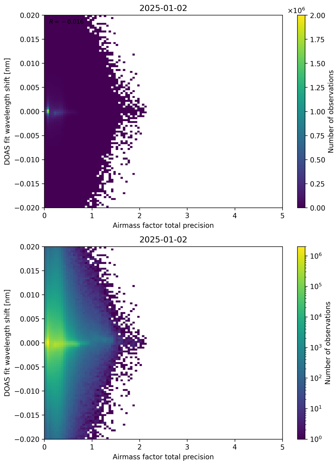
Figure 106: Scatter density plot of “Airmass factor total precision” against “DOAS fit wavelength shift” for 2025-01-01 to 2025-01-03.
