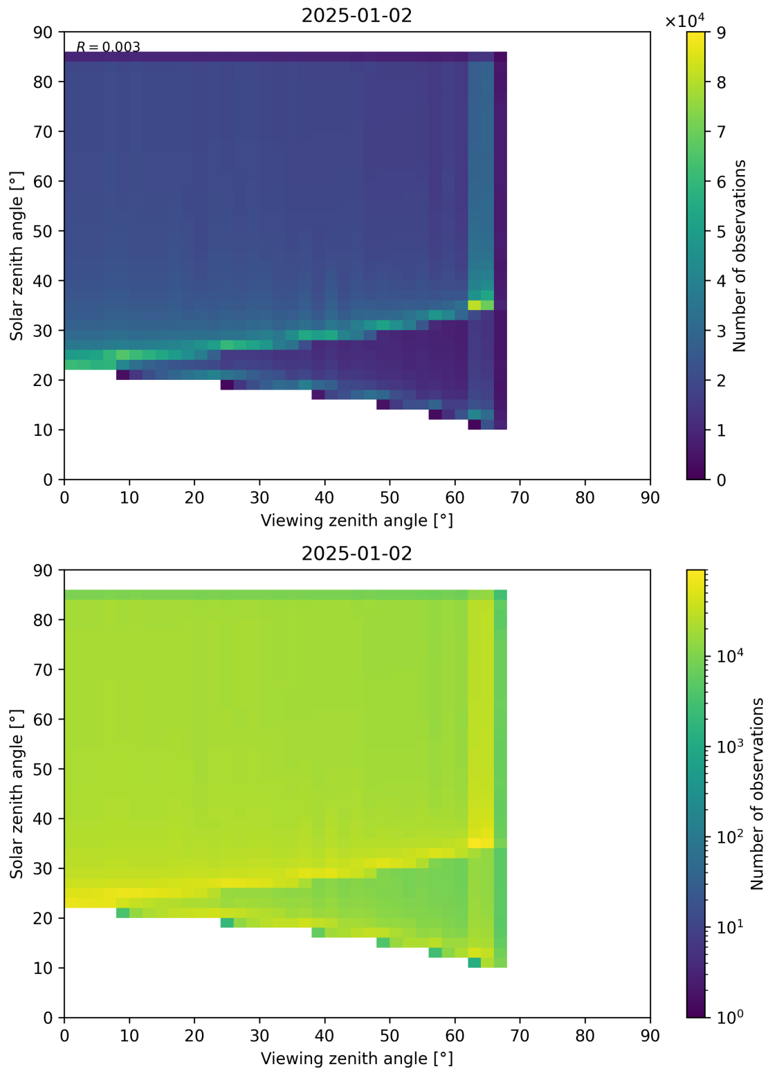
Figure 197: Scatter density plot of “Viewing zenith angle” against “Solar zenith angle” for 2025-01-01 to 2025-01-03.
