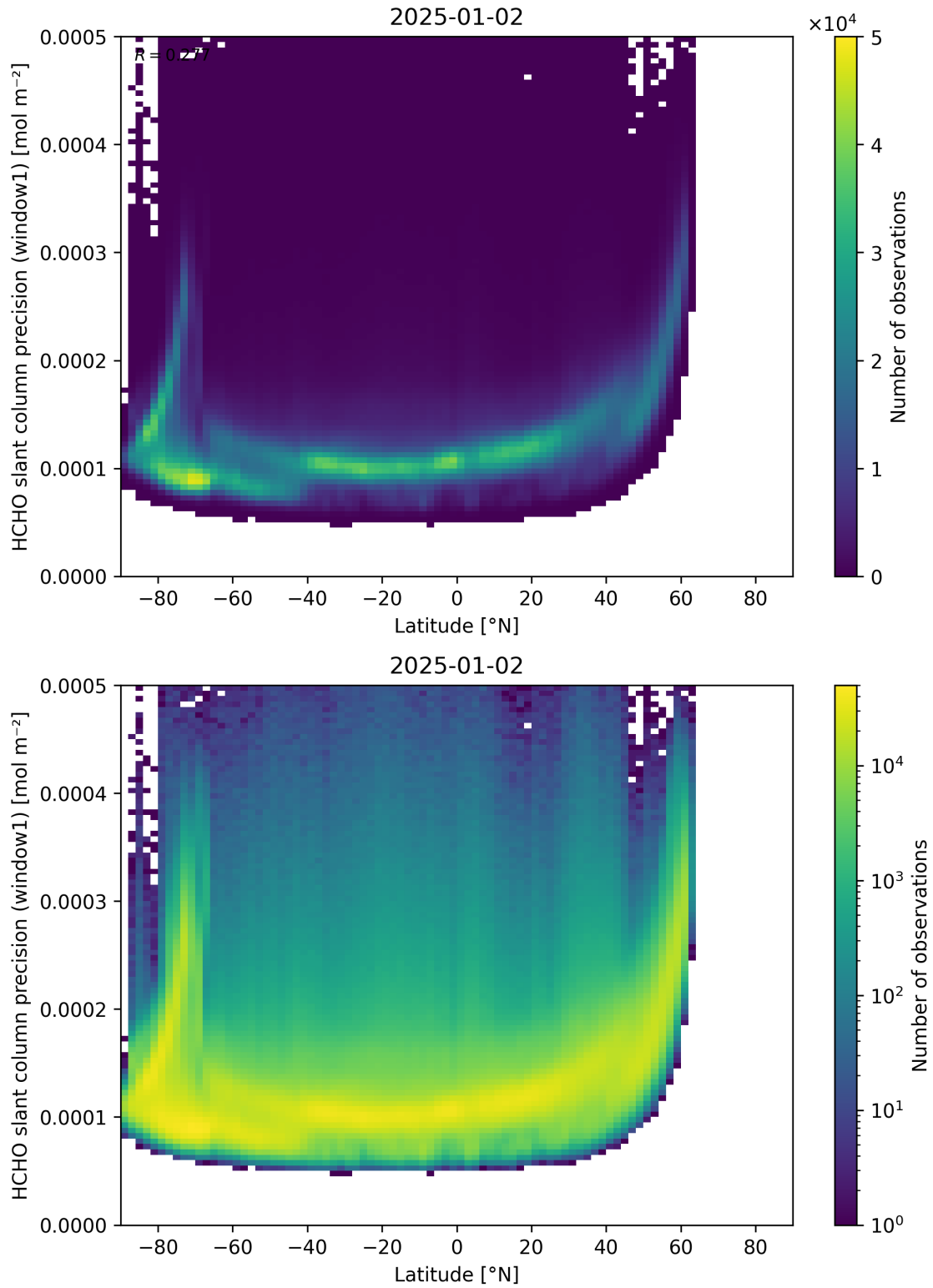
Figure 160: Scatter density plot of “Latitude” against “HCHO slant column precision (window1)” for 2025-01-01 to 2025-01-03.
