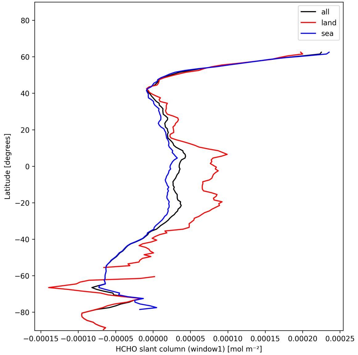
Figure 24: Zonal average of "HCHO slant column (window1)" for 2025-01-01 to 2025-01-03.
