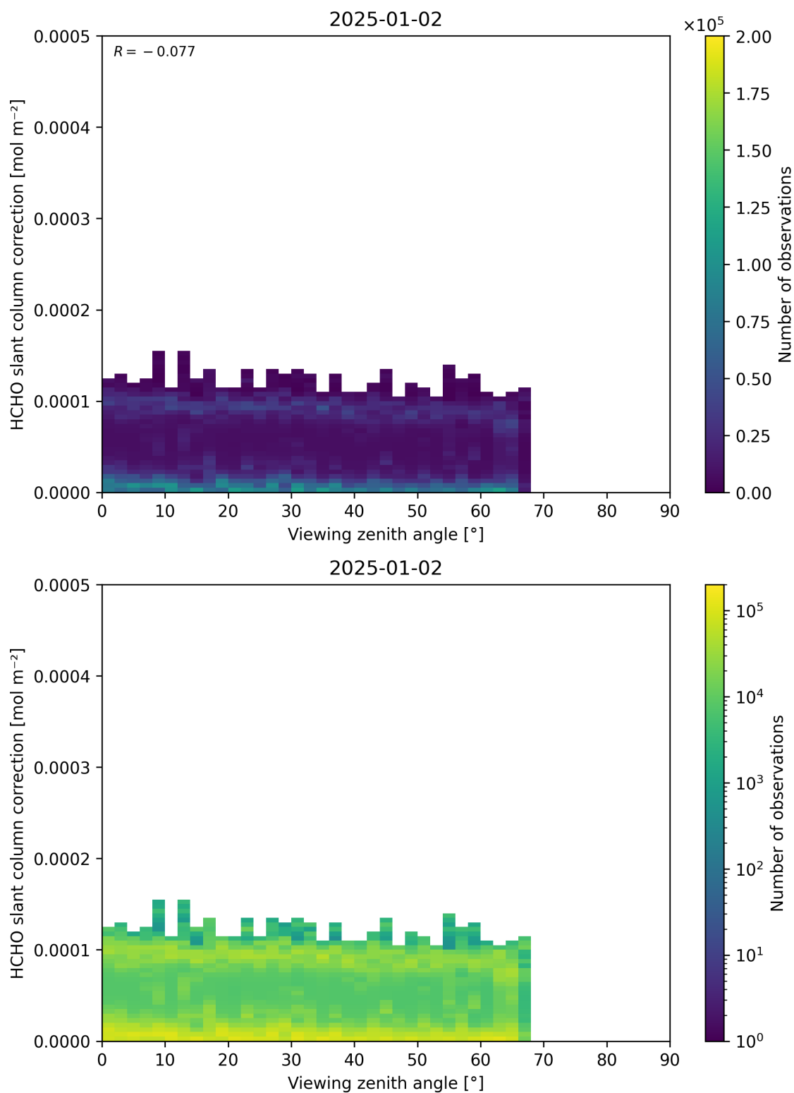
Figure 187: Scatter density plot of “Viewing zenith angle” against “HCHO slant column correction” for 2025-01-01 to 2025-01-03.
