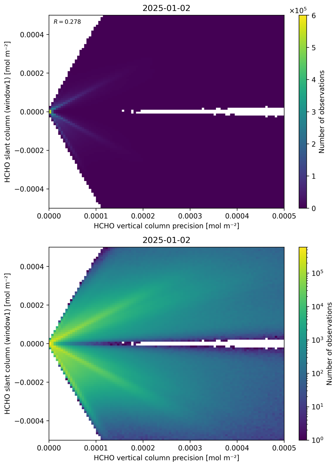
Figure 142: Scatter density plot of “HCHO vertical column precision” against “HCHO slant column (window1)” for 2025-01-01 to 2025-01-03.
