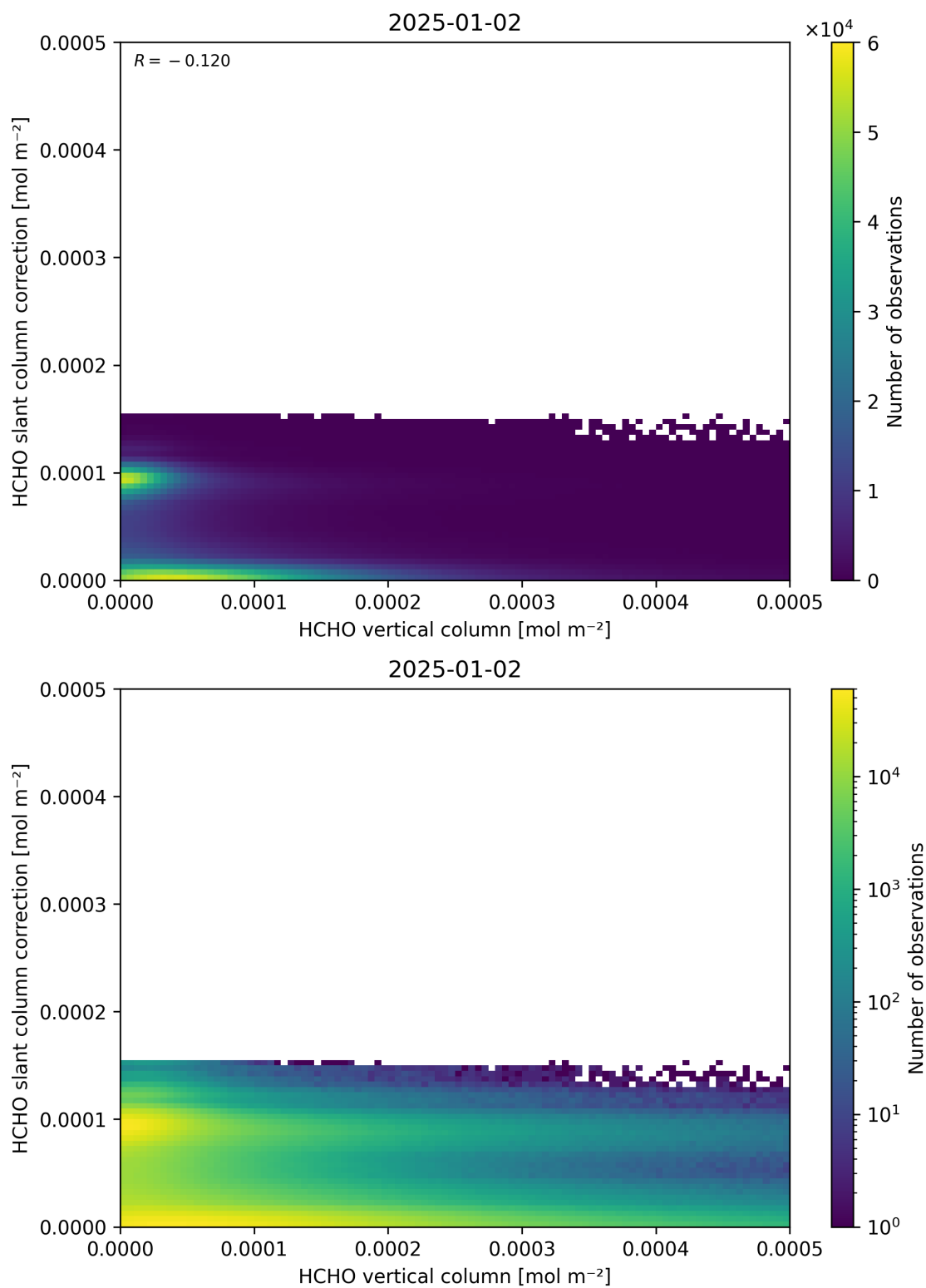
Figure 128: Scatter density plot of “HCHO vertical column” against “HCHO slant column correction” for 2025-01-01 to 2025-01-03.
