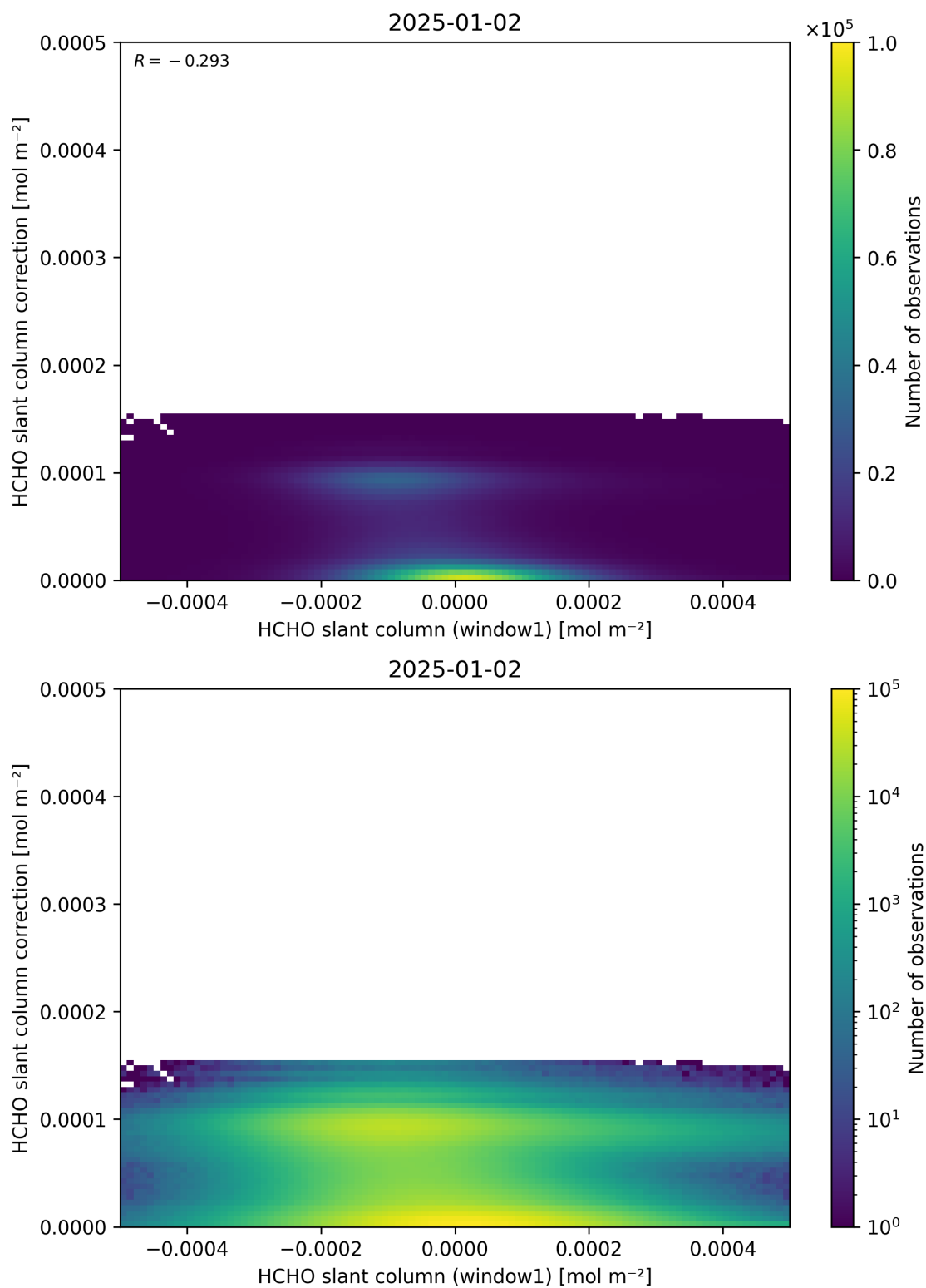
Figure 83: Scatter density plot of “HCHO slant column (window1)” against “HCHO slant column correction” for 2025-01-01 to 2025-01-03.
