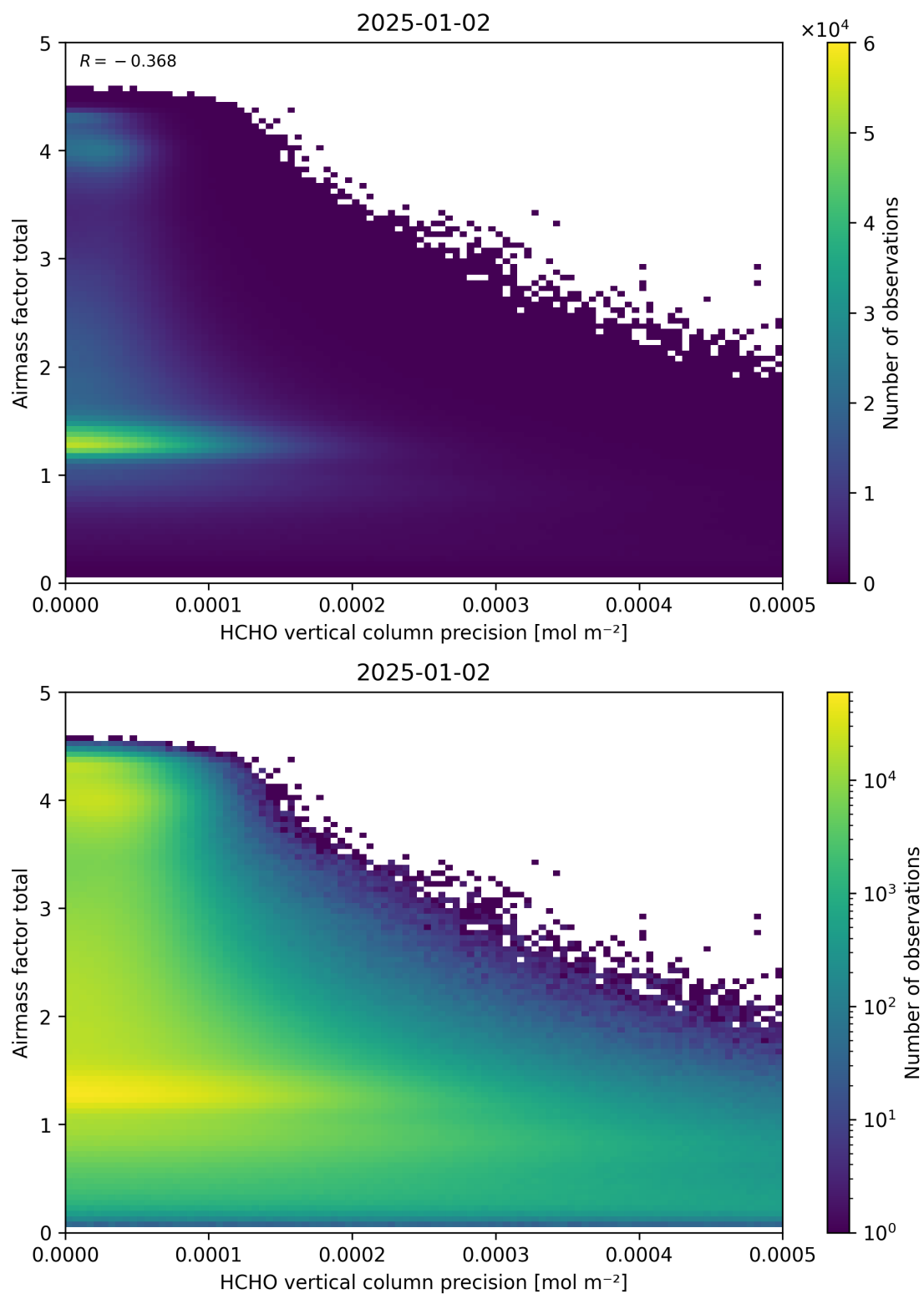
Figure 144: Scatter density plot of “HCHO vertical column precision” against “Airmass factor total” for 2025-01-01 to 2025-01-03.
