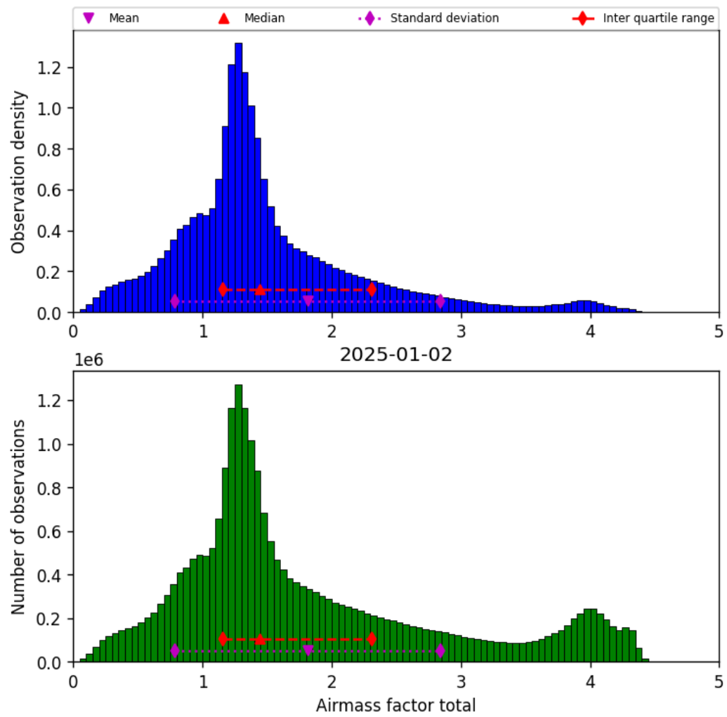
Figure 40: Histogram of “Airmass factor total” for 2025-01-01 to 2025-01-03
