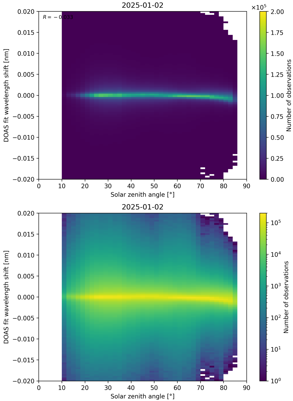
Figure 168: Scatter density plot of “Solar zenith angle” against “DOAS fit wavelength shift” for 2025-01-01 to 2025-01-03.
