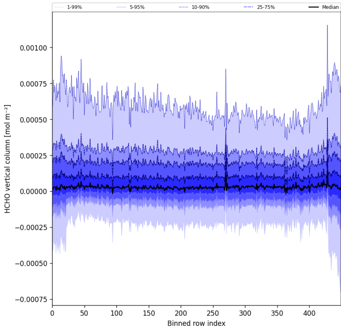
Figure 49: Along track statistics of “HCHO vertical column” for 2025-01-01 to 2025-01-03
