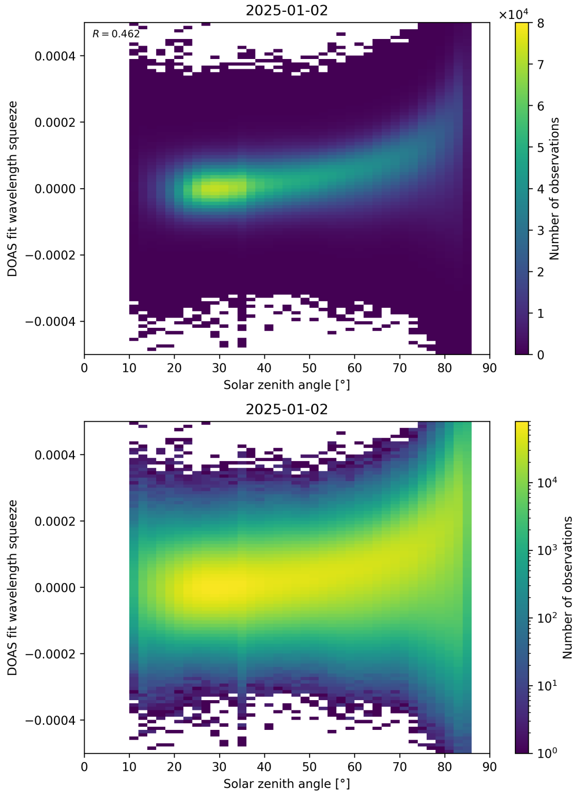
Figure 169: Scatter density plot of “Solar zenith angle” against “DOAS fit wavelength squeeze” for 2025-01-01 to 2025-01-03.
