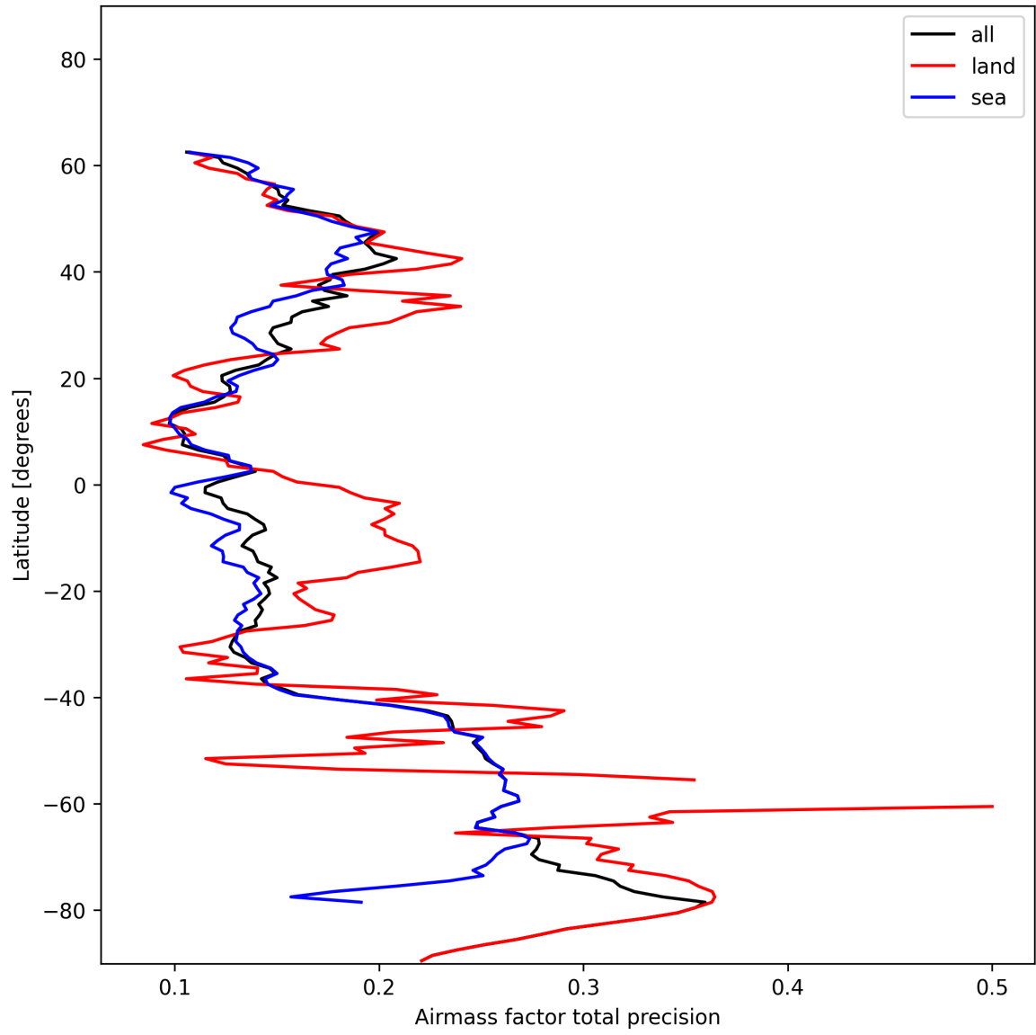
Figure 27: Zonal average of “Airmass factor total precision” for 2025-01-01 to 2025-01-03.
