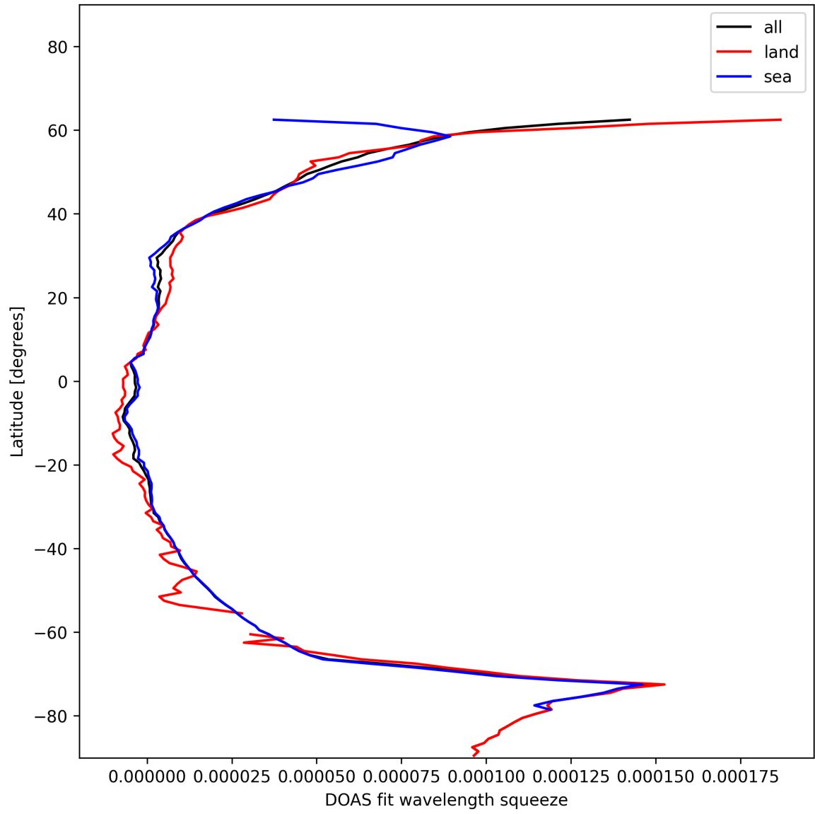
Figure 31: Zonal average of “DOAS fit wavelength squeeze” for 2025-01-01 to 2025-01-03.
