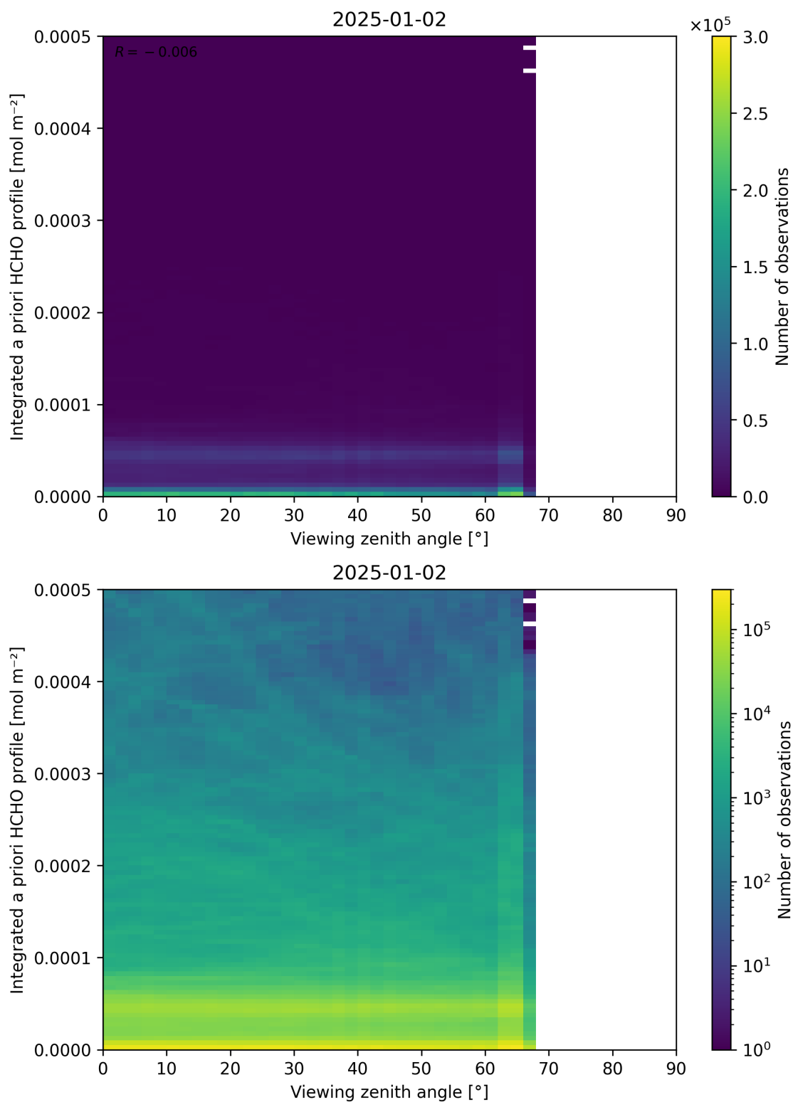
Figure 195: Scatter density plot of “Viewing zenith angle” against “Integrated a priori HCHO profile” for 2025-01-01 to 2025-01-03.
