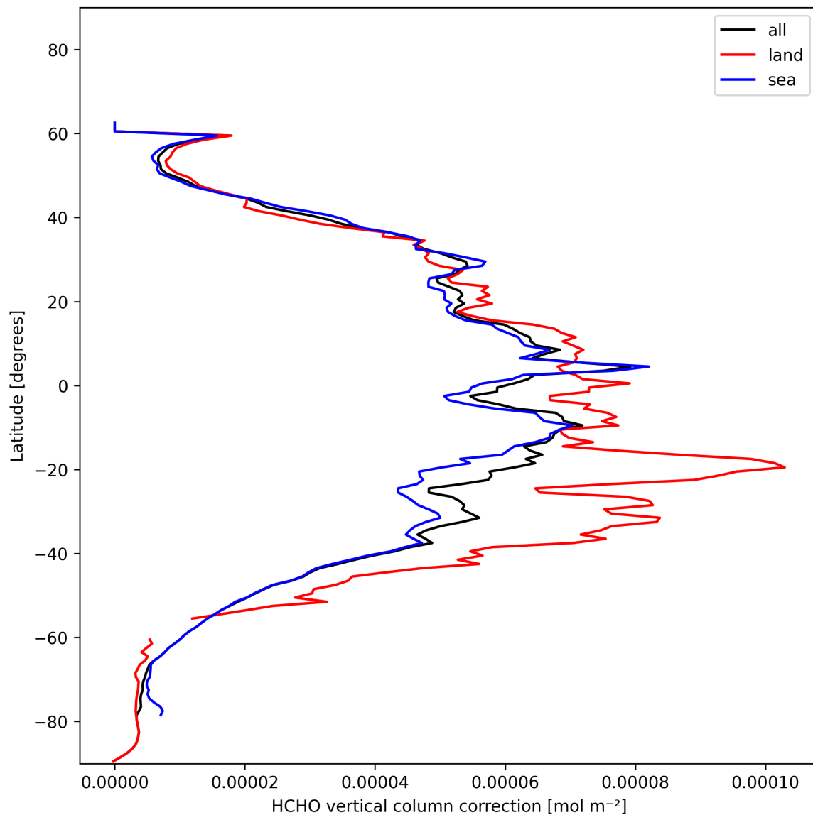
Figure 23: Zonal average of “HCHO vertical column correction” for 2025-01-01 to 2025-01-03.
