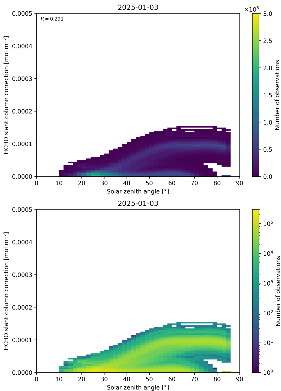
Figure 172: Scatter density plot of “Solar zenith angle” against “HCHO slant column correction” for 2025-01-02 to 2025-01-04.
