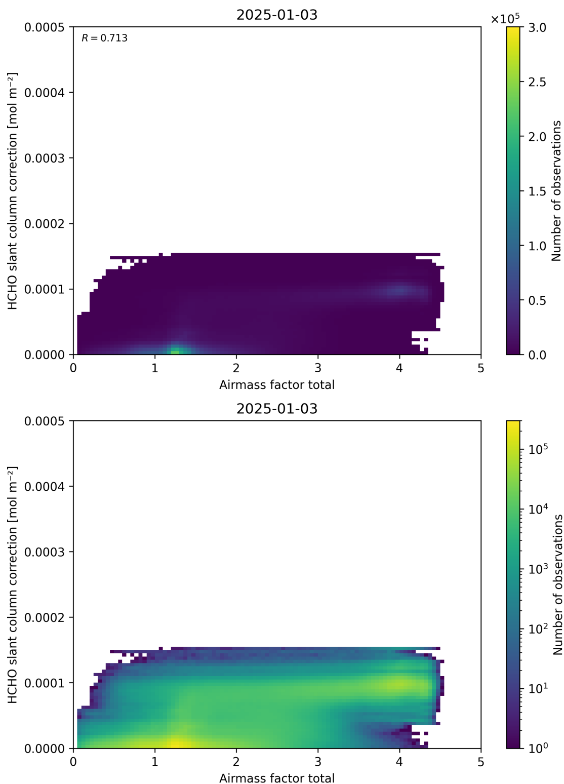
Figure 102: Scatter density plot of “Airmass factor total” against “HCHO slant column correction” for 2025-01-02 to 2025-01-04.
