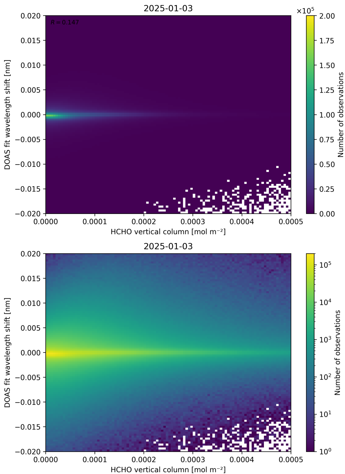
Figure 124: Scatter density plot of “HCHO vertical column” against “DOAS fit wavelength shift” for 2025-01-02 to 2025-01-04.
