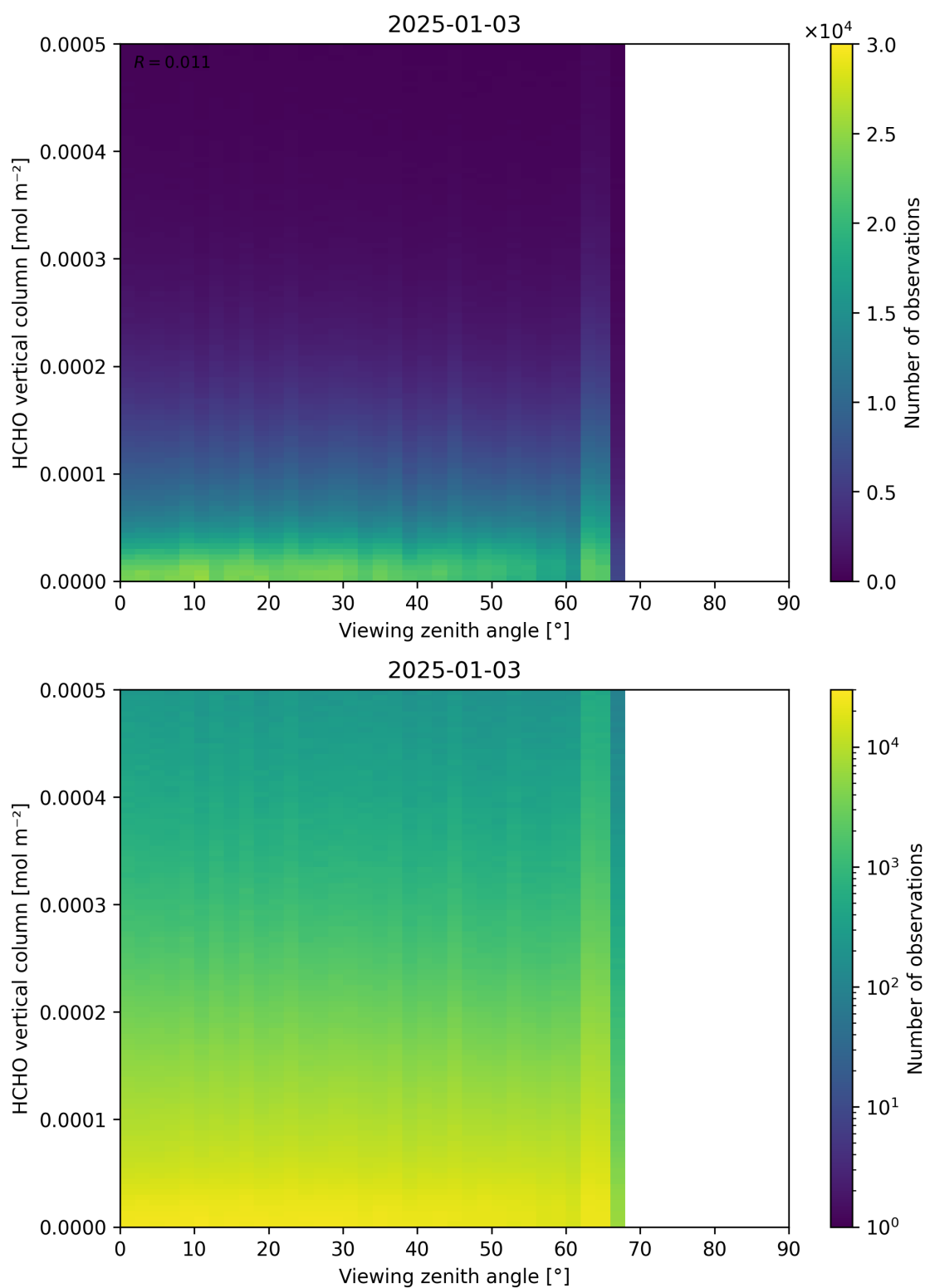
Figure 192: Scatter density plot of “Viewing zenith angle” against “HCHO vertical column” for 2025-01-02 to 2025-01-04.
