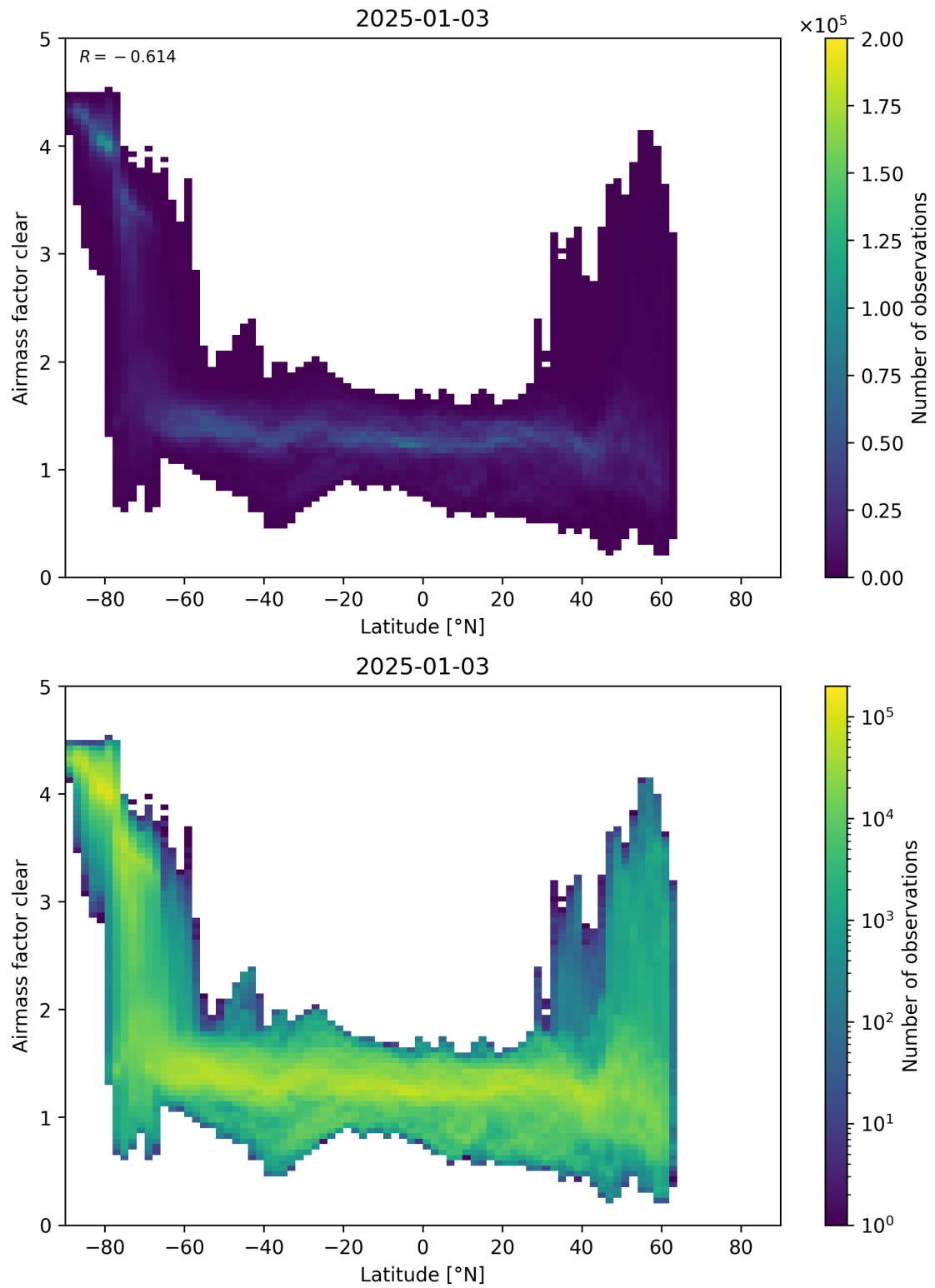
Figure 156: Scatter density plot of “Latitude” against “Airmass factor clear” for 2025-01-02 to 2025-01-04.
