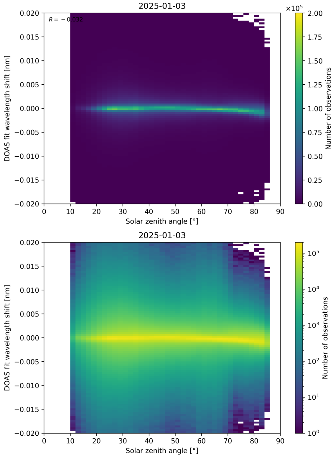
Figure 168: Scatter density plot of “Solar zenith angle” against “DOAS fit wavelength shift” for 2025-01-02 to 2025-01-04.
