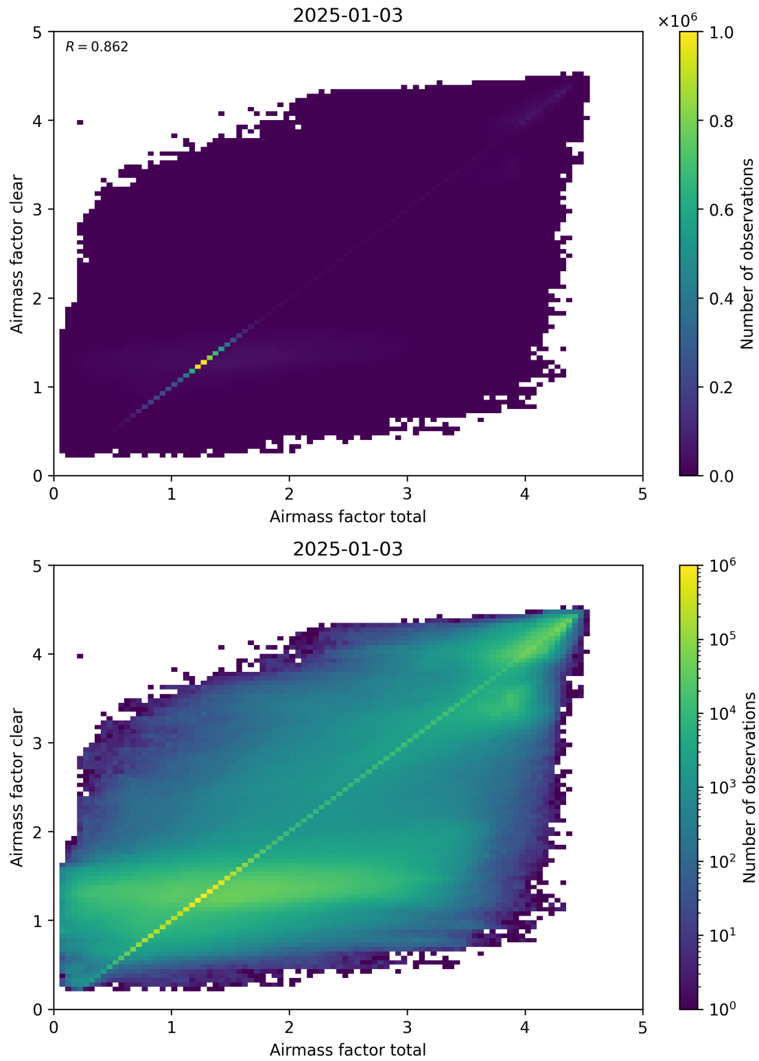
Figure 100: Scatter density plot of “Airmass factor total” against “Airmass factor clear” for 2025-01-02 to 2025-01-04.
