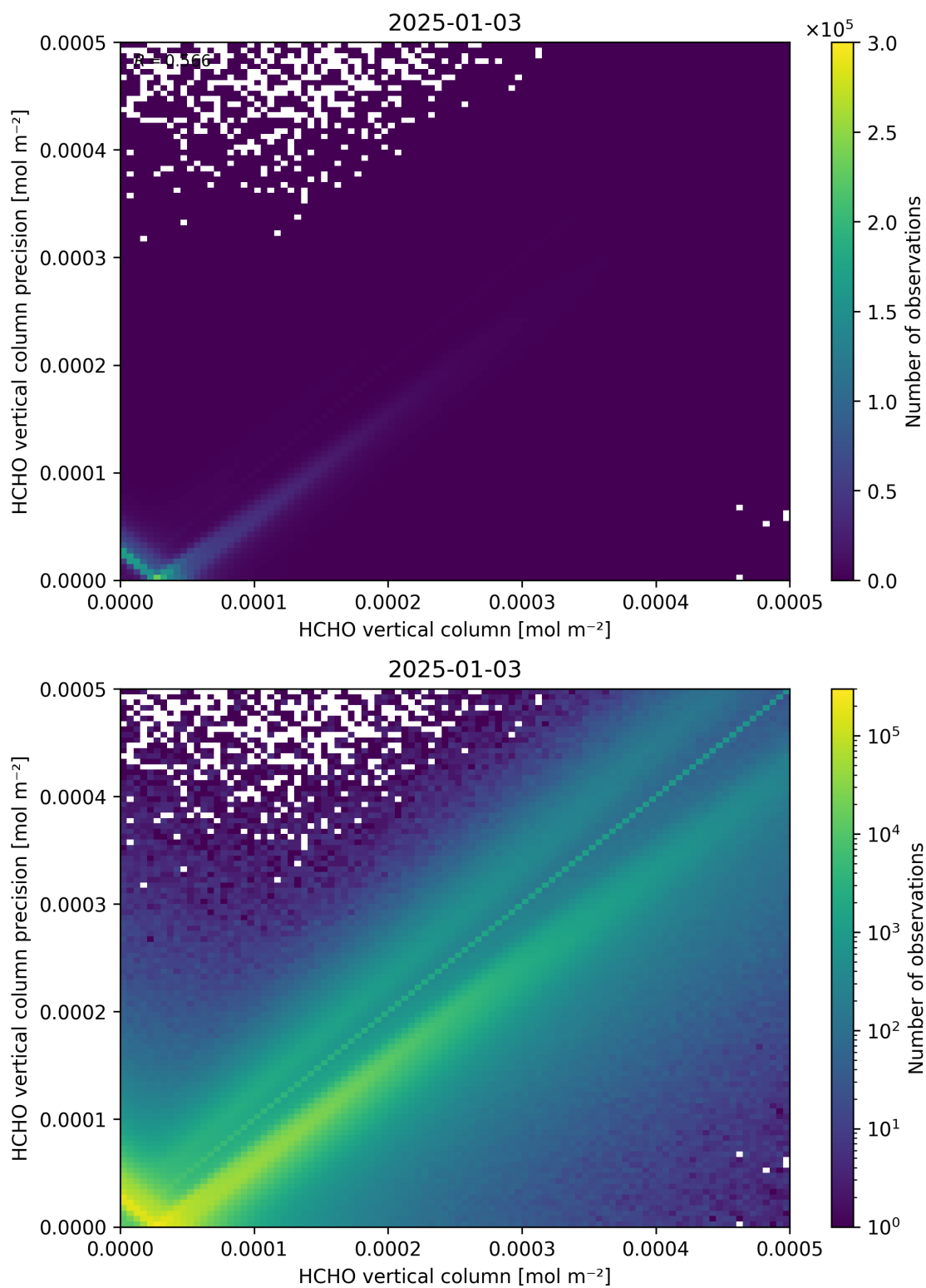
Figure 134: Scatter density plot of “HCHO vertical column” against “HCHO vertical column precision” for 2025-01-02 to 2025-01-04.
