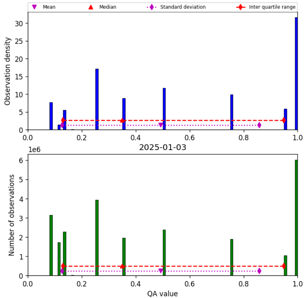
Figure 34: Histogram of “QA value” for 2025-01-02 to 2025-01-04
