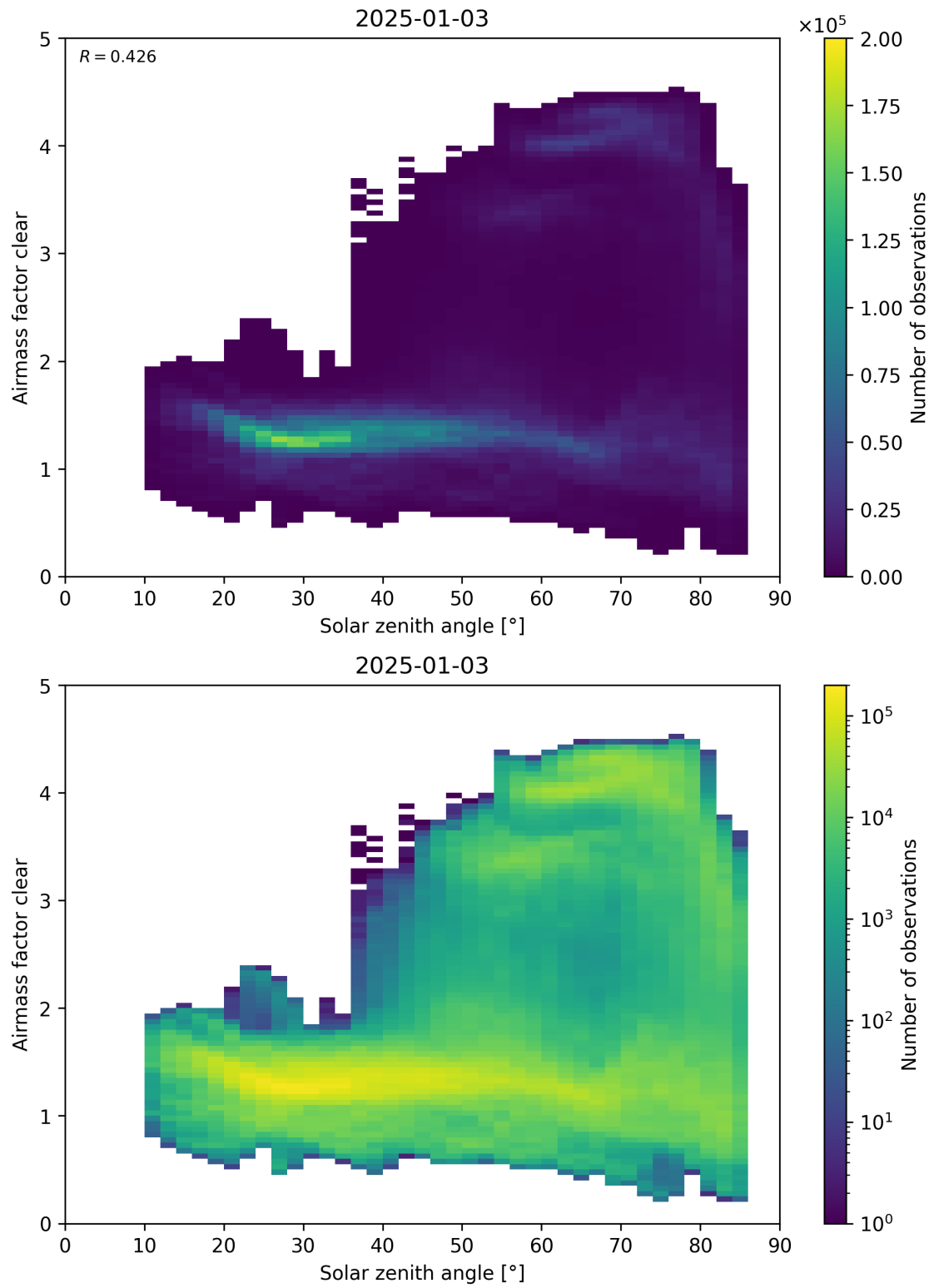
Figure 170: Scatter density plot of “Solar zenith angle” against “Airmass factor clear” for 2025-01-02 to 2025-01-04.
