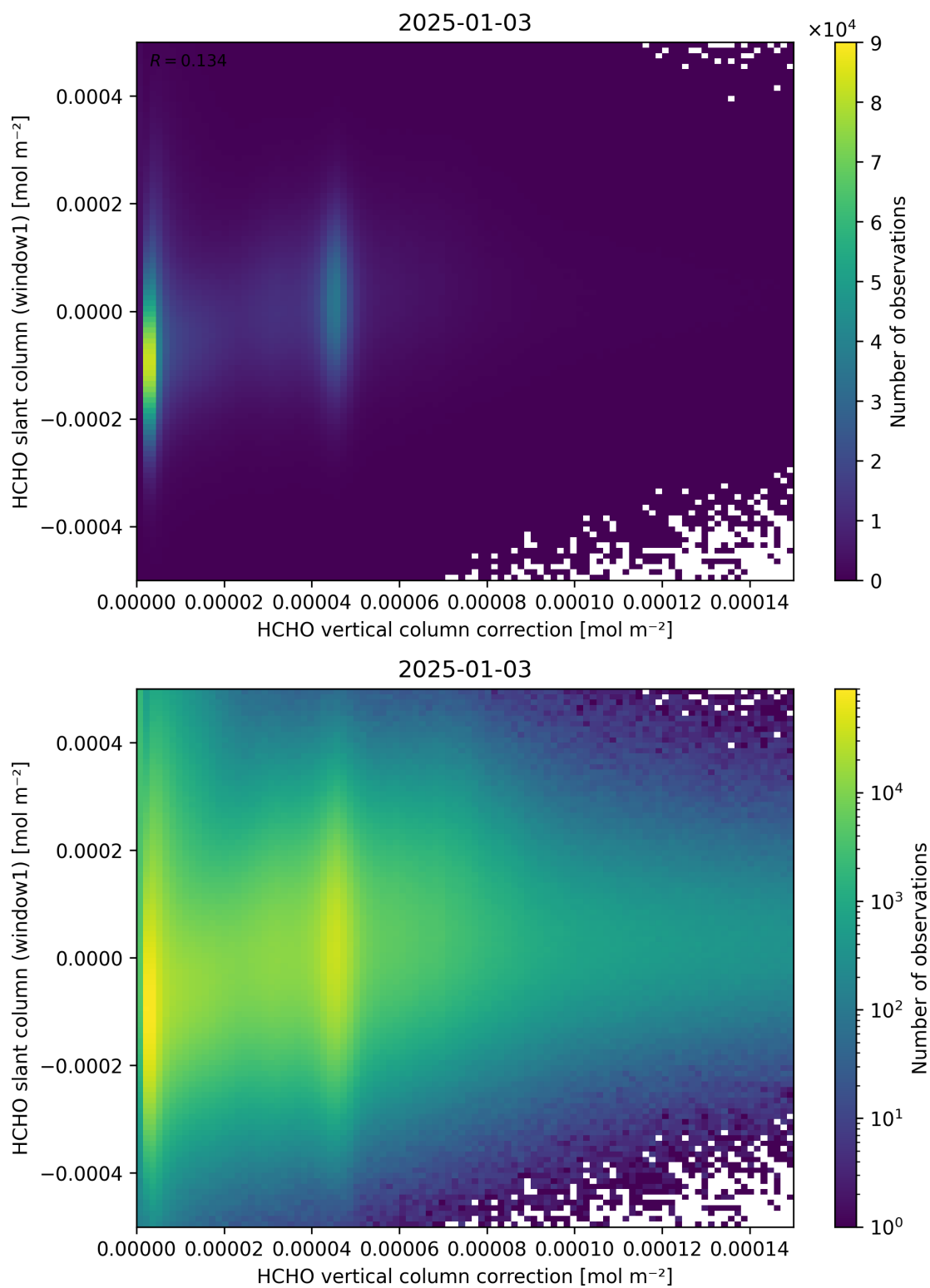
Figure 118: Scatter density plot of “HCHO vertical column correction” against “HCHO slant column (window1)” for 2025-01-02 to 2025-01-04.
