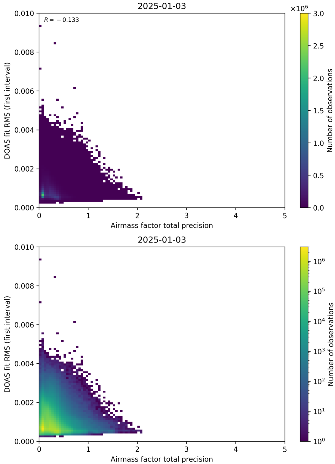
Figure 105: Scatter density plot of “Airmass factor total precision” against “DOAS fit RMS (first interval)” for 2025-01-02 to 2025-01-04.
