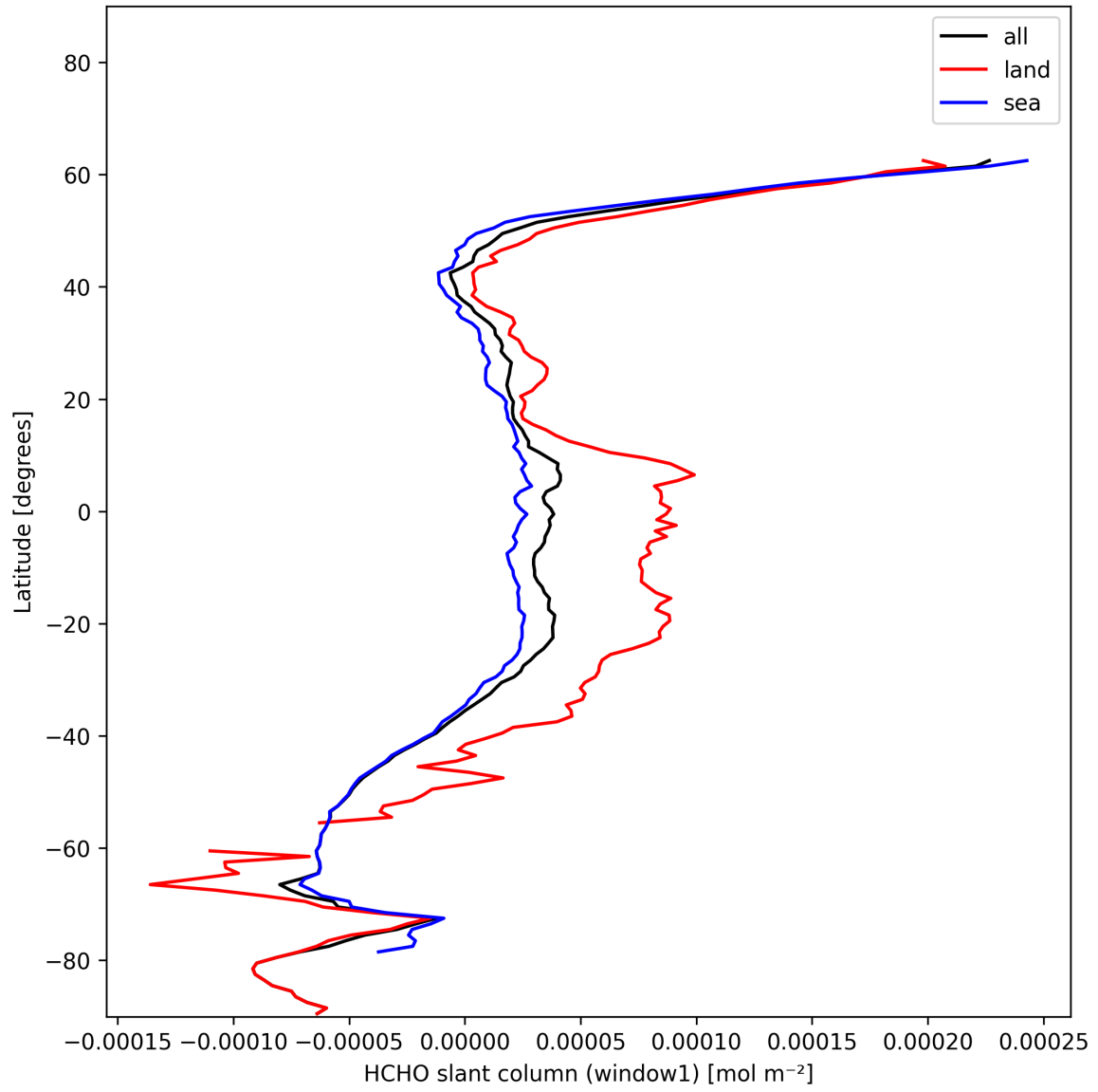
Figure 24: Zonal average of “HCHO slant column (window1)” for 2025-01-02 to 2025-01-04.
