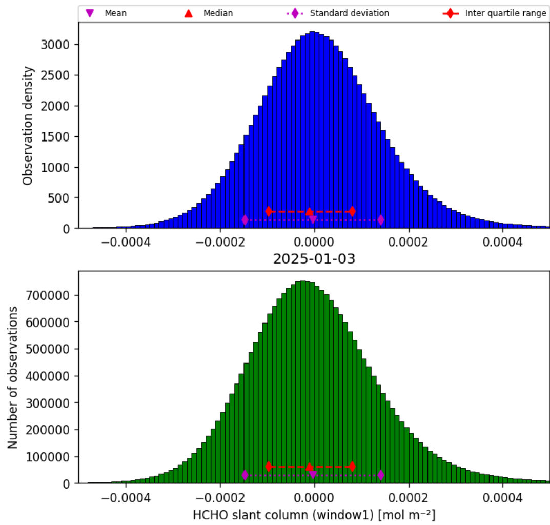
Figure 38: Histogram of “HCHO slant column (window1)” for 2025-01-02 to 2025-01-04
