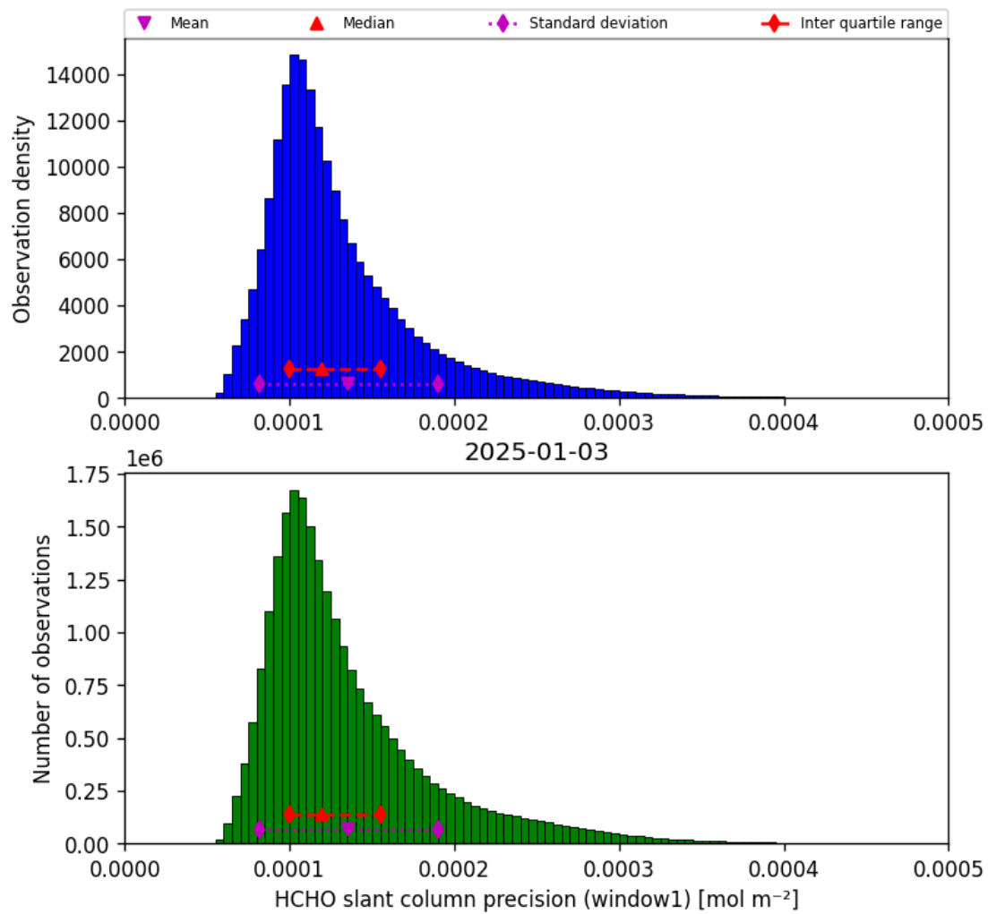
Figure 39: Histogram of “HCHO slant column precision (window1)” for 2025-01-02 to 2025-01-04
