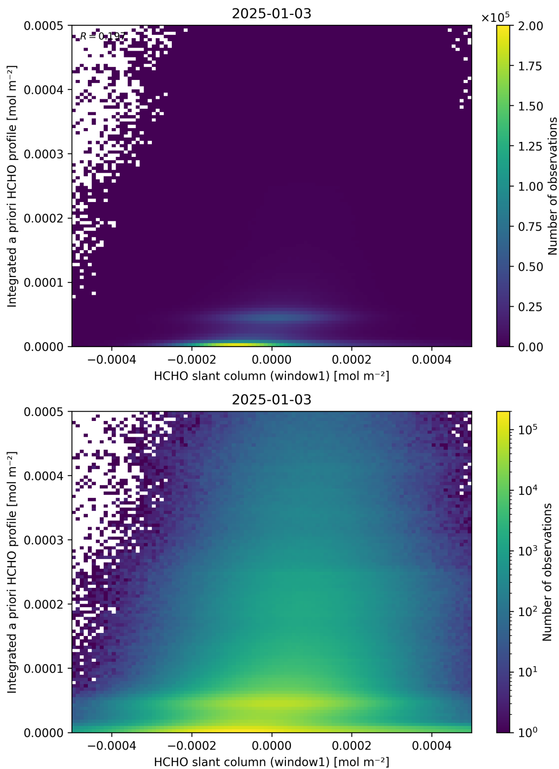
Figure 87: Scatter density plot of “HCHO slant column (window1)” against “Integrated a priori HCHO profile” for 2025-01-02 to 2025-01-04.
