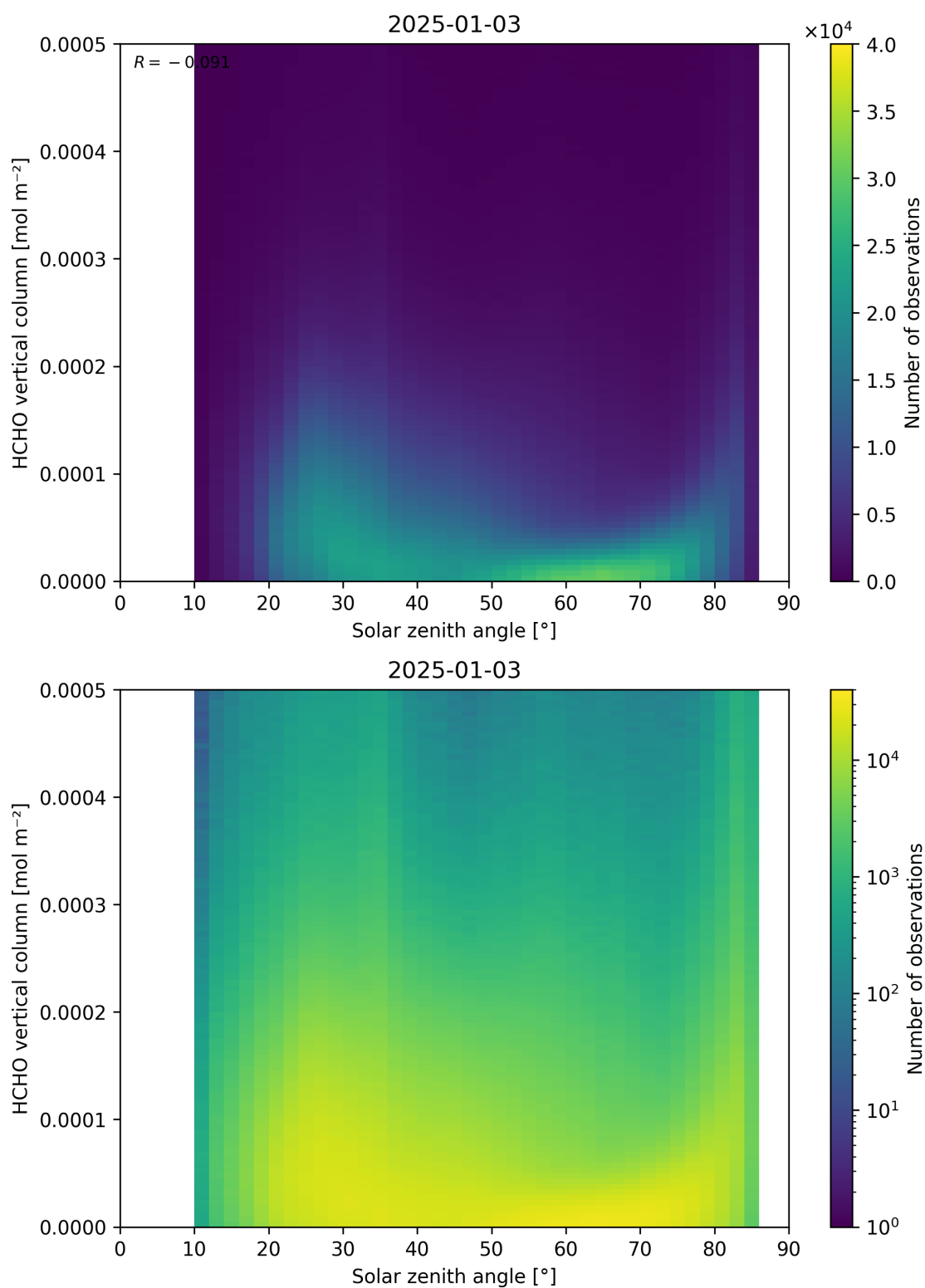
Figure 177: Scatter density plot of “Solar zenith angle” against “HCHO vertical column” for 2025-01-02 to 2025-01-04.
