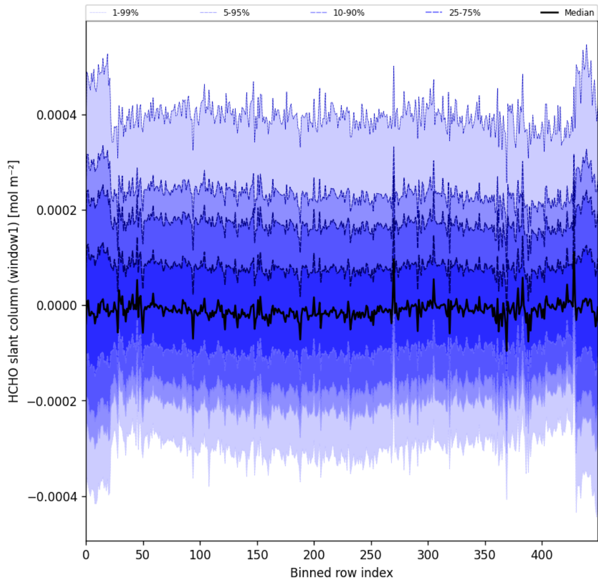
Figure 52: Along track statistics of “HCHO slant column (window1)” for 2025-01-02 to 2025-01-04
