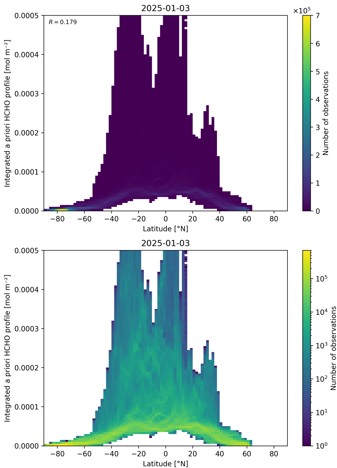
Figure 166: Scatter density plot of “Latitude” against “Integrated a priori HCHO profile” for 2025-01-02 to 2025-01-04.
