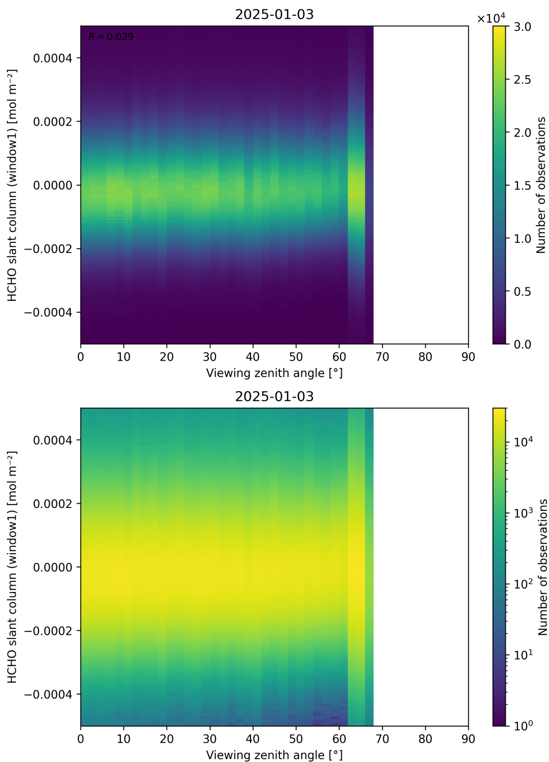
Figure 188: Scatter density plot of “Viewing zenith angle” against “HCHO slant column (window1)” for 2025-01-02 to 2025-01-04.
