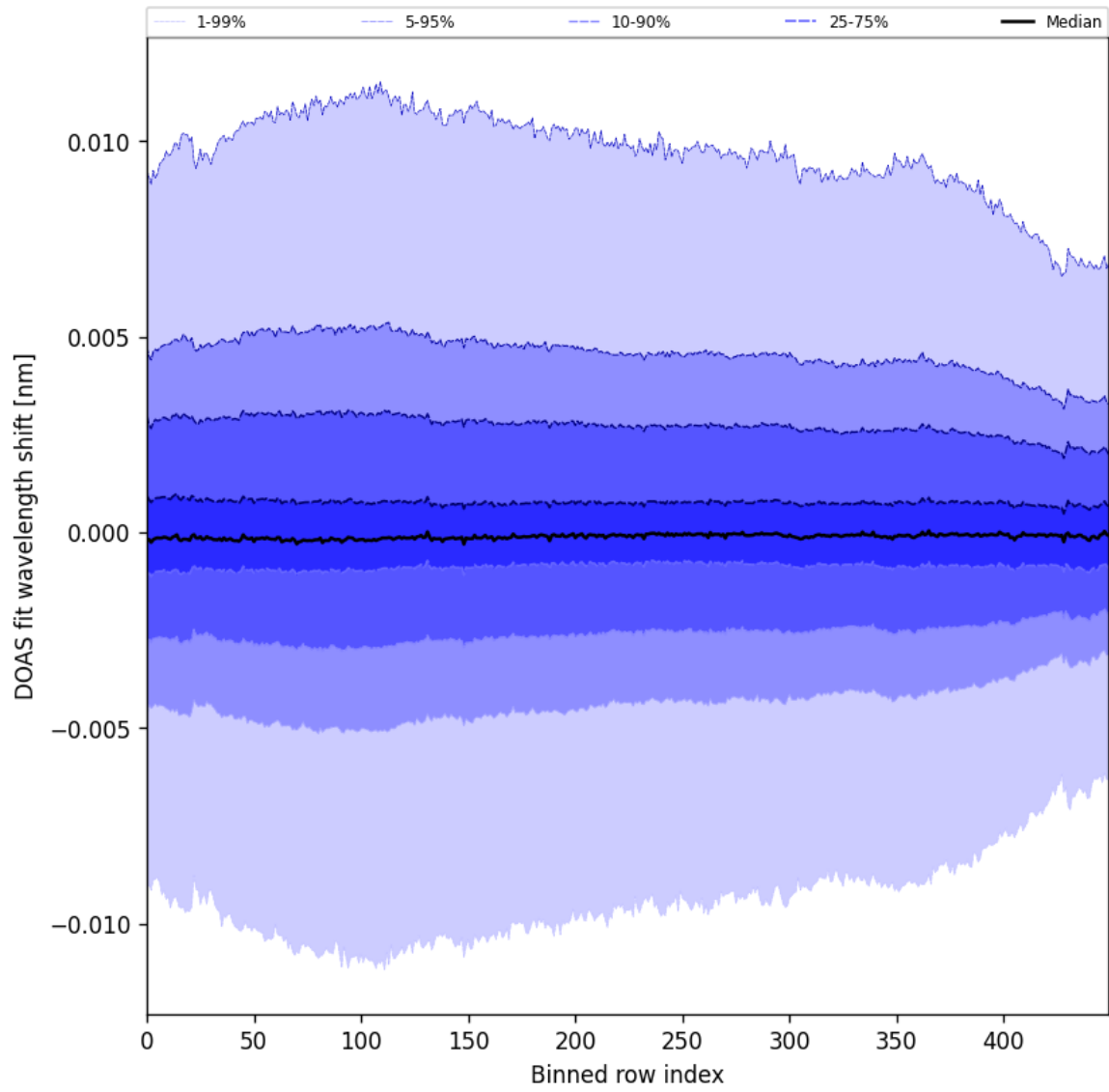
Figure 58: Along track statistics of “DOAS fit wavelength shift” for 2025-01-02 to 2025-01-04
