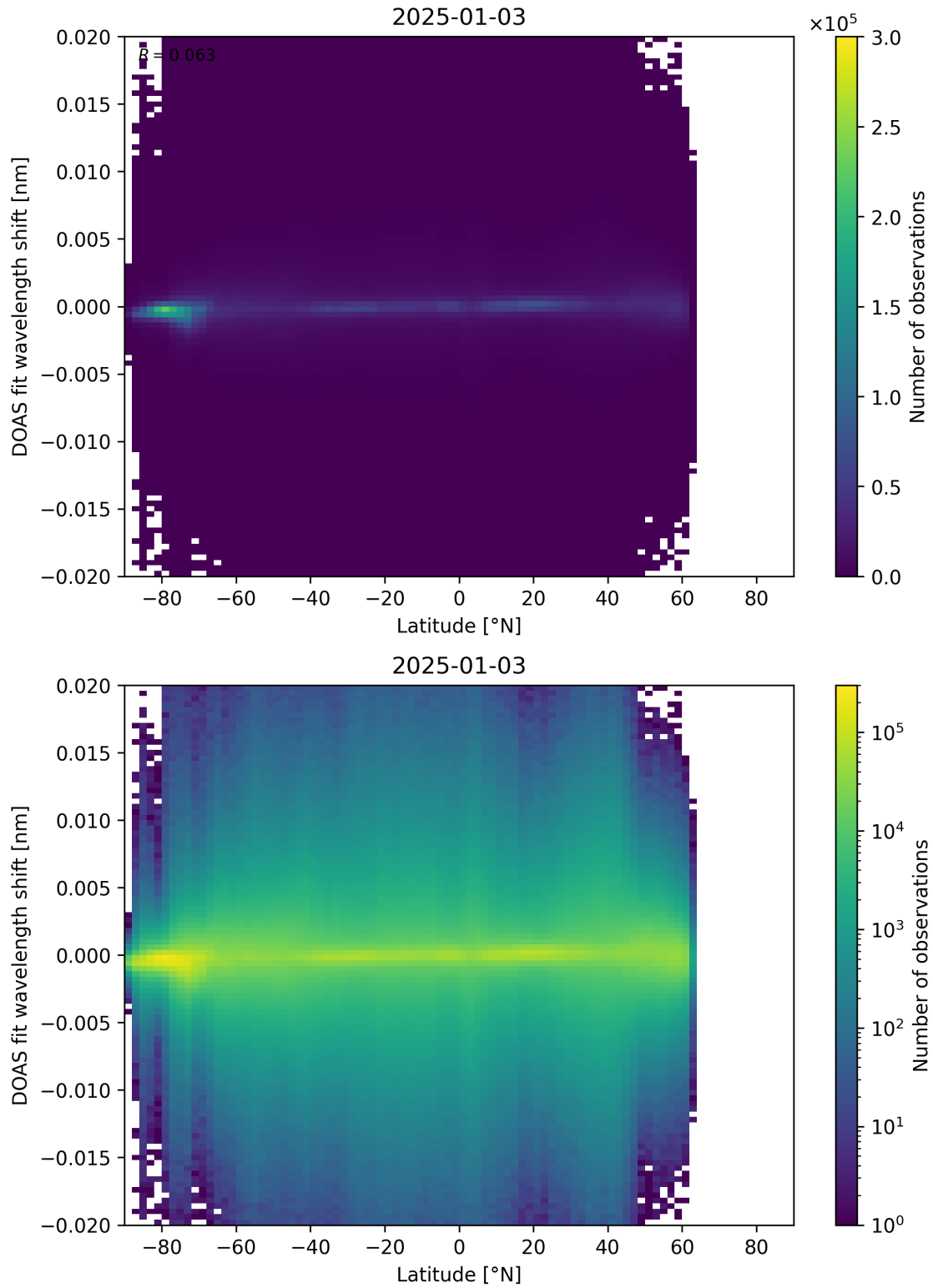
Figure 154: Scatter density plot of “Latitude” against “DOAS fit wavelength shift” for 2025-01-02 to 2025-01-04.
