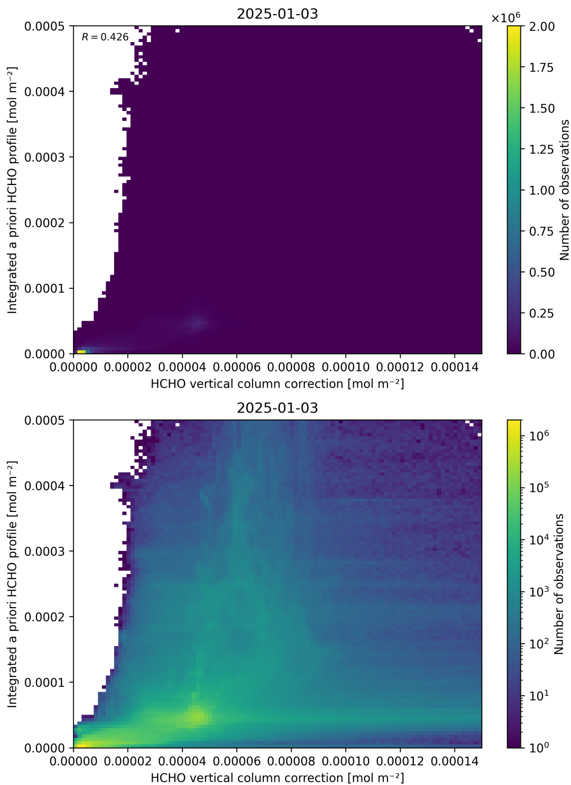
Figure 122: Scatter density plot of “HCHO vertical column correction” against “Integrated a priori HCHO profile” for 2025-01-02 to 2025-01-04.
