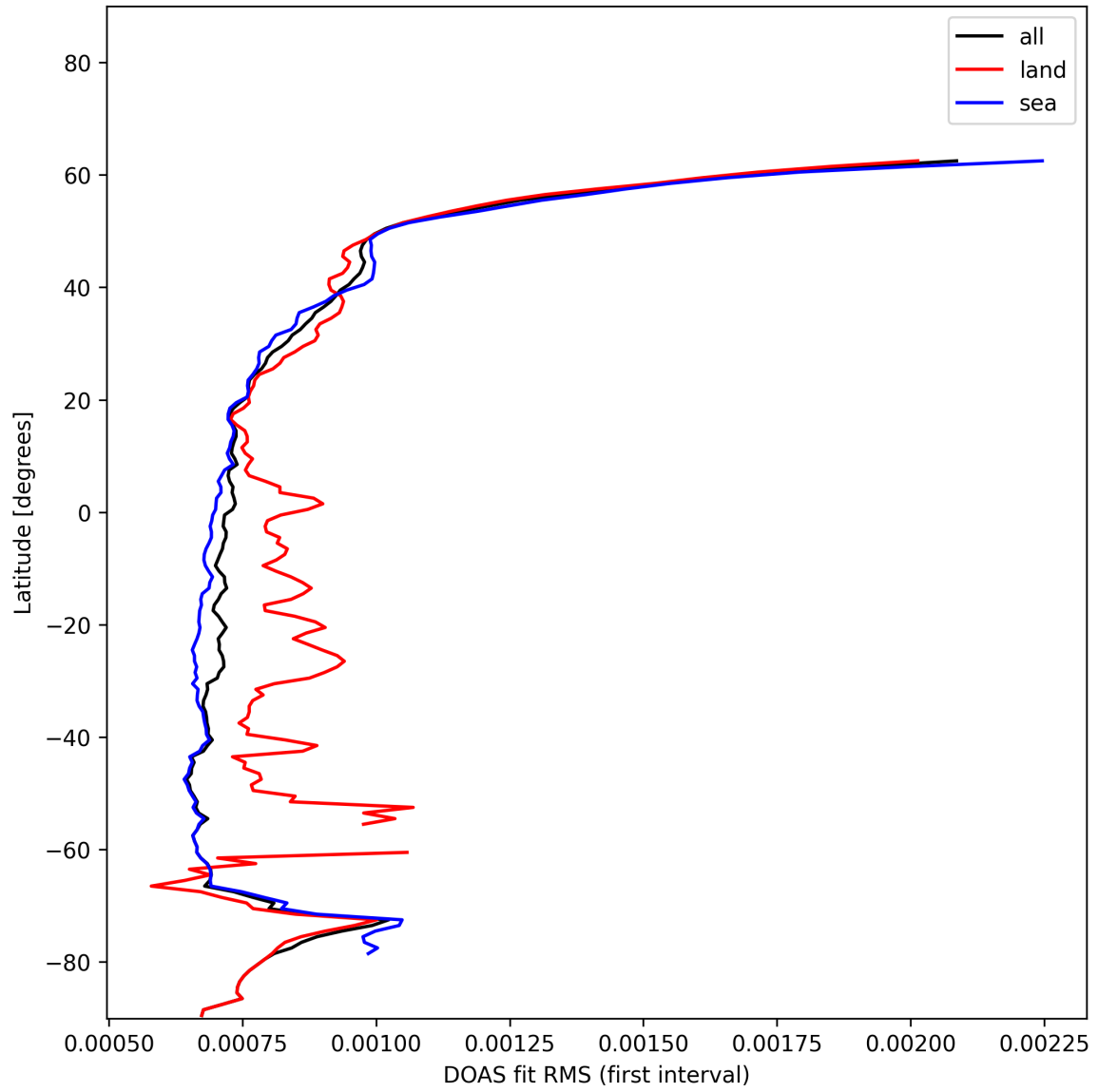
Figure 32: Zonal average of “DOAS fit RMS (first interval)” for 2025-01-02 to 2025-01-04.
