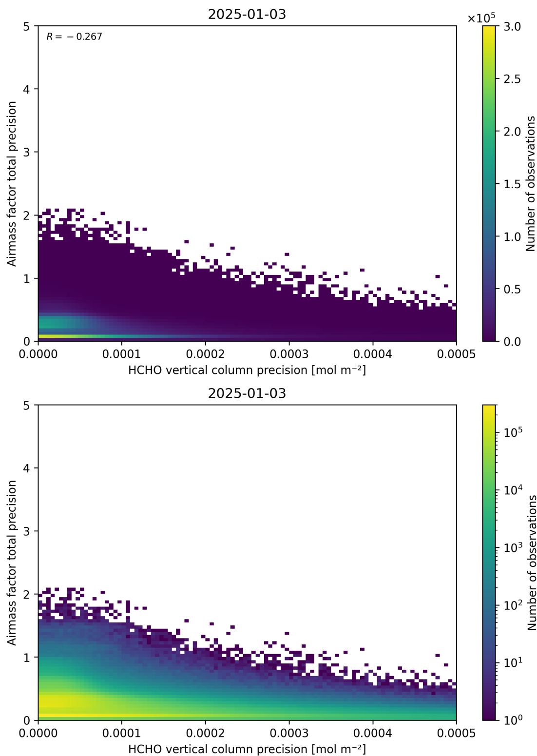
Figure 145: Scatter density plot of “HCHO vertical column precision” against “Airmass factor total precision” for 2025-01-02 to 2025-01-04.
