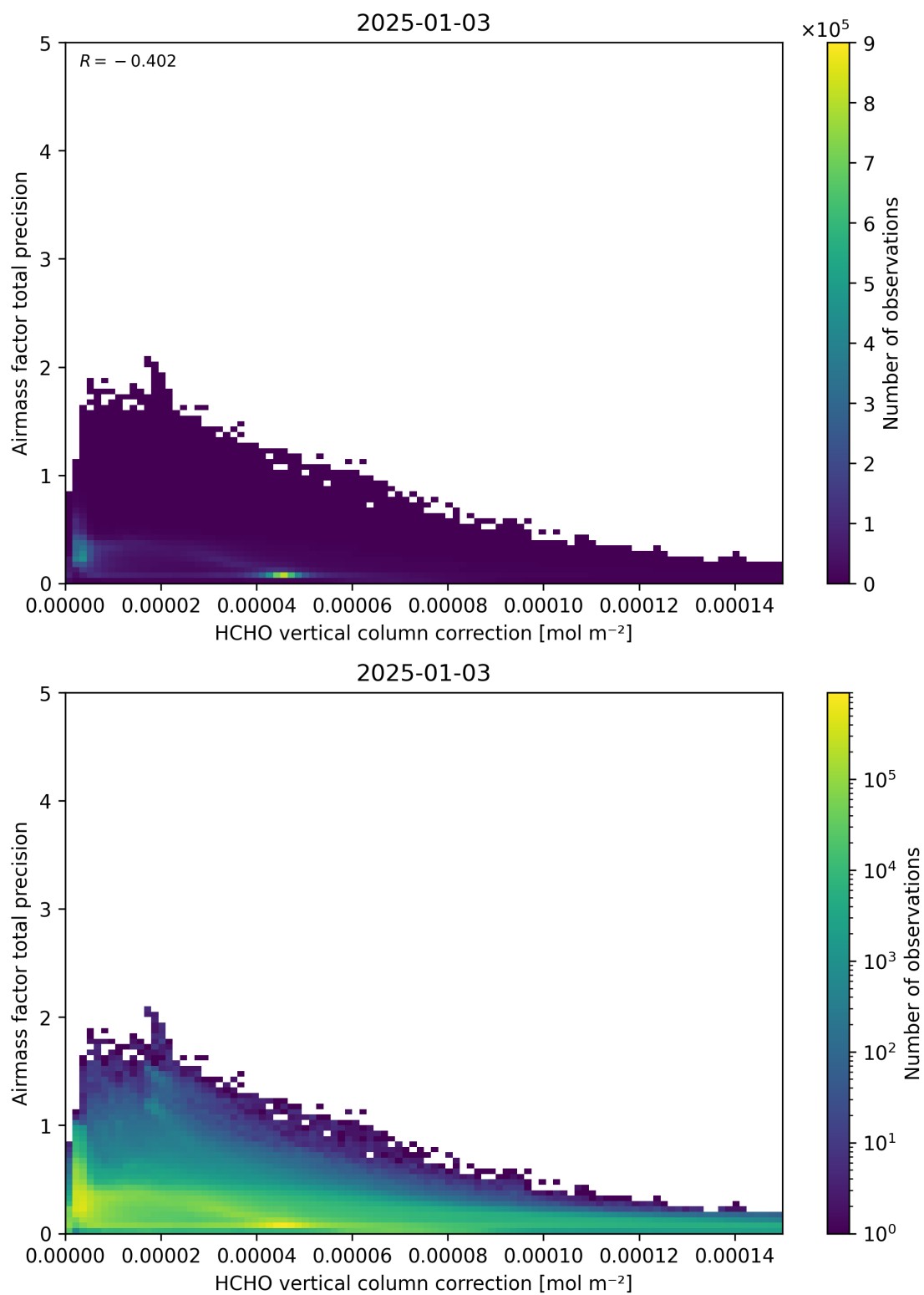
Figure 121: Scatter density plot of “HCHO vertical column correction” against “Airmass factor total precision” for 2025-01-02 to 2025-01-04.
