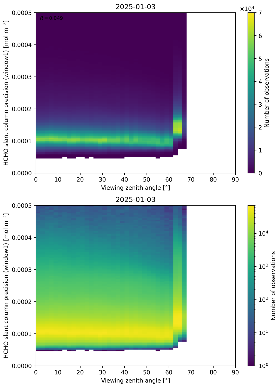
Figure 189: Scatter density plot of “Viewing zenith angle” against “HCHO slant column precision (window1)” for 2025-01-02 to 2025-01-04.
