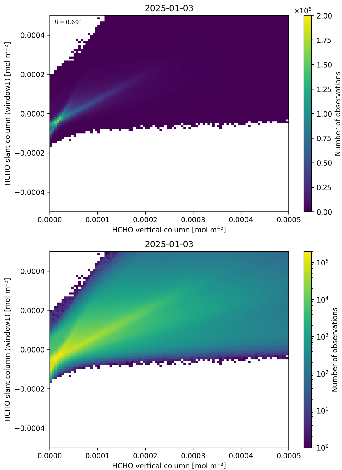
Figure 129: Scatter density plot of “HCHO vertical column” against “HCHO slant column (window1)” for 2025-01-02 to 2025-01-04.
