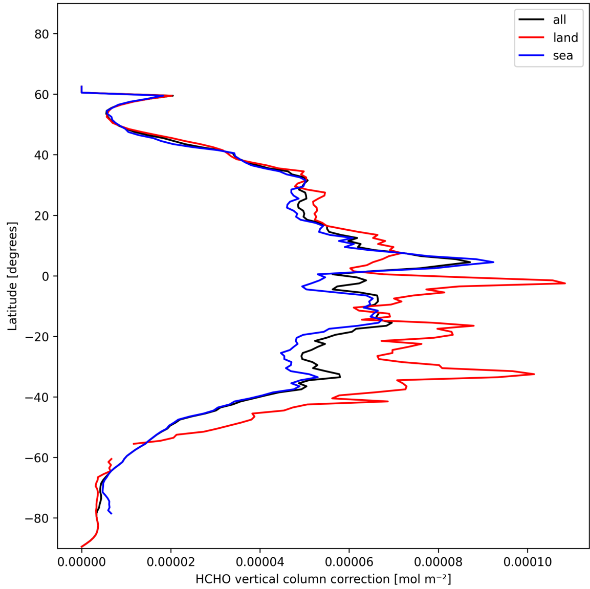
Figure 23: Zonal average of “HCHO vertical column correction” for 2025-01-02 to 2025-01-04.
