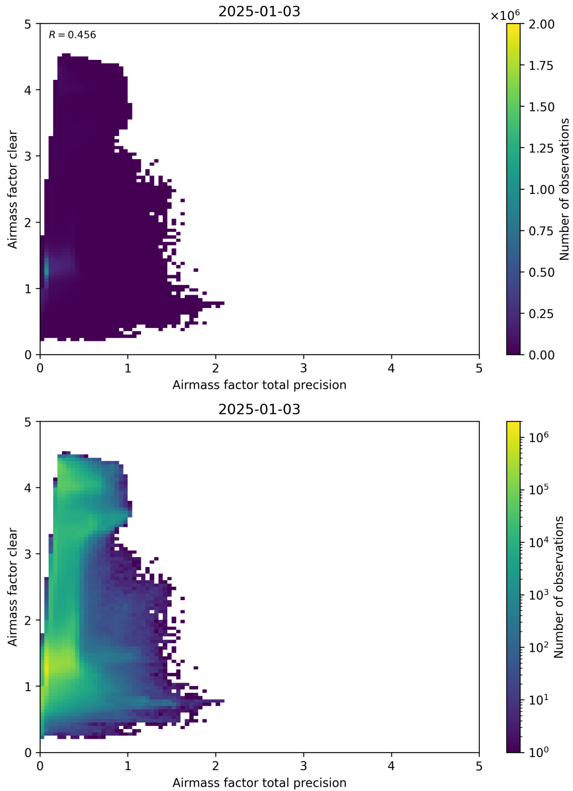
Figure 108: Scatter density plot of “Airmass factor total precision” against “Airmass factor clear” for 2025-01-02 to 2025-01-04.
