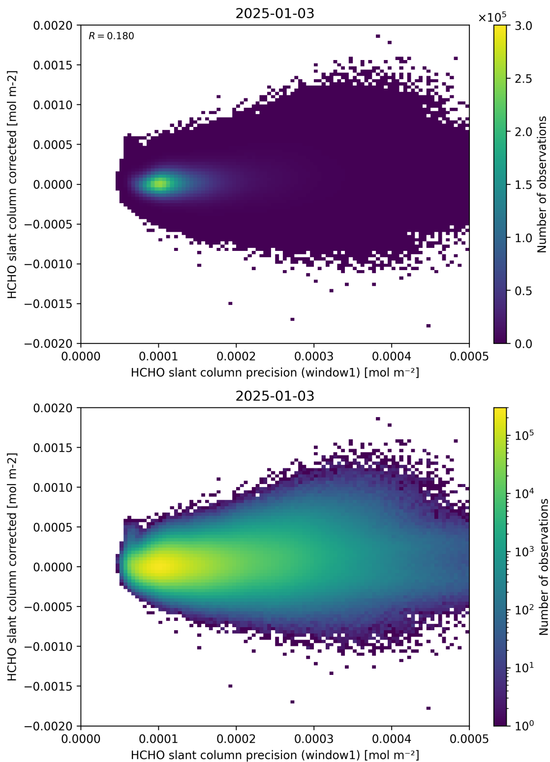
Figure 92: Scatter density plot of “HCHO slant column precision (window1)” against “HCHO slant column corrected” for 2025-01-02 to 2025-01-04.
