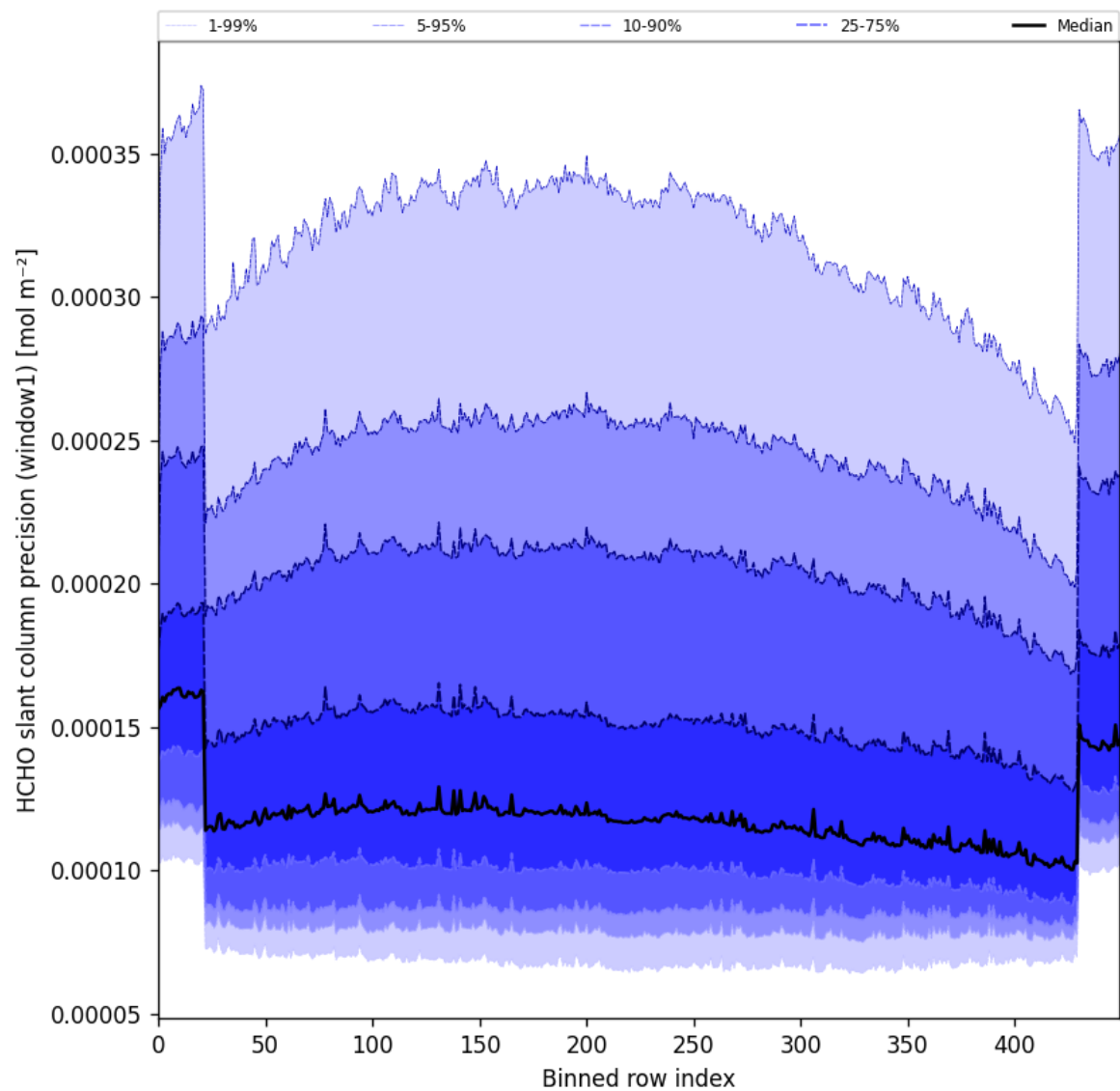
Figure 53: Along track statistics of “HCHO slant column precision (window1)” for 2025-01-02 to 2025-01-04
