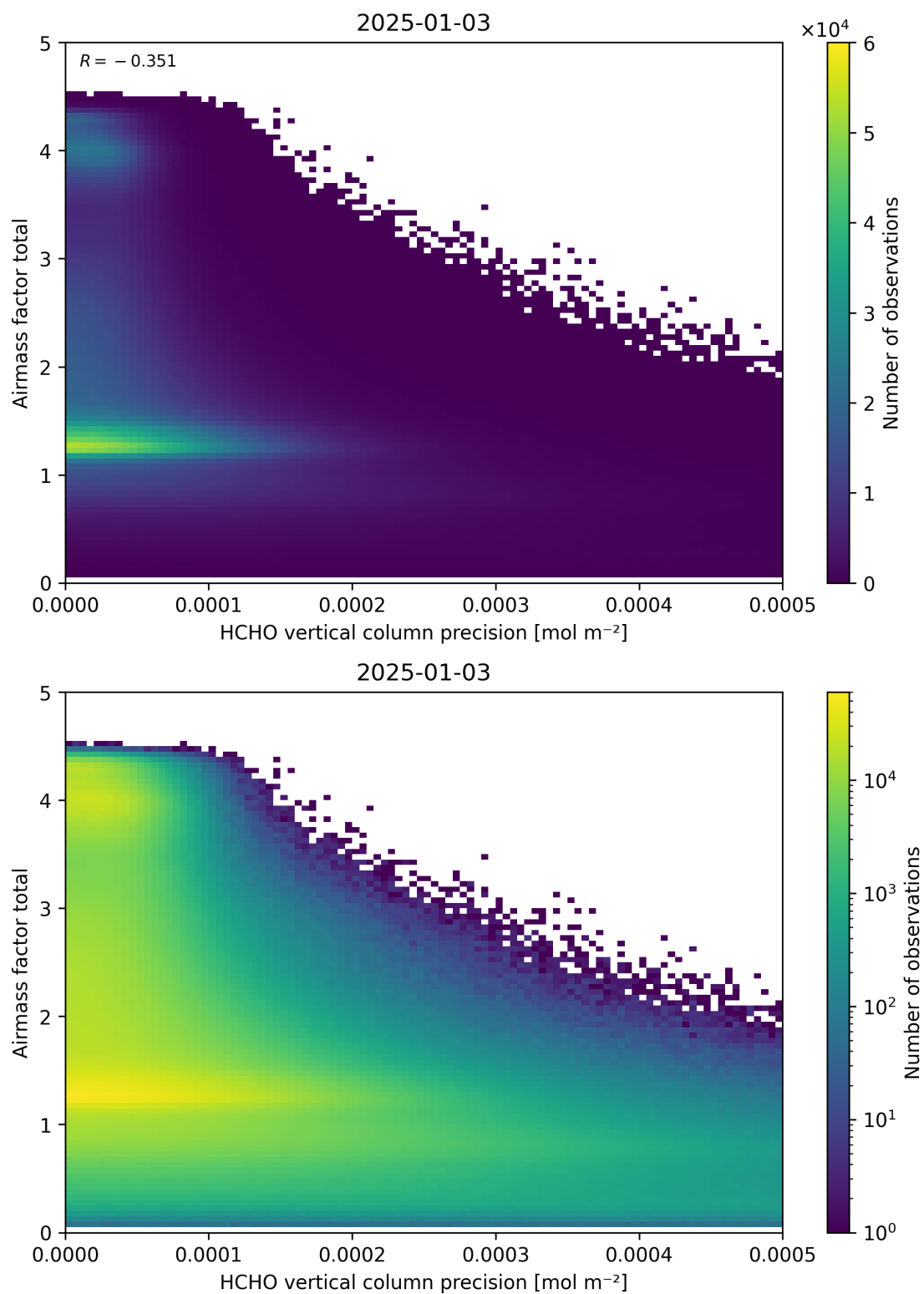
Figure 144: Scatter density plot of “HCHO vertical column precision” against “Airmass factor total” for 2025-01-02 to 2025-01-04.
