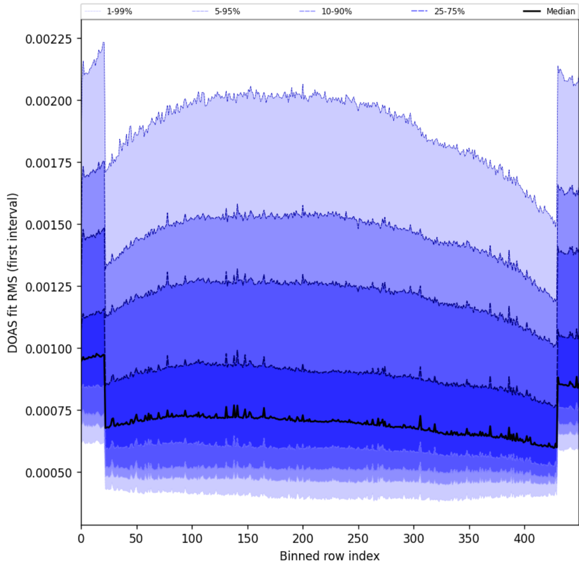
Figure 60: Along track statistics of “DOAS fit RMS (first interval)” for 2025-01-02 to 2025-01-04
