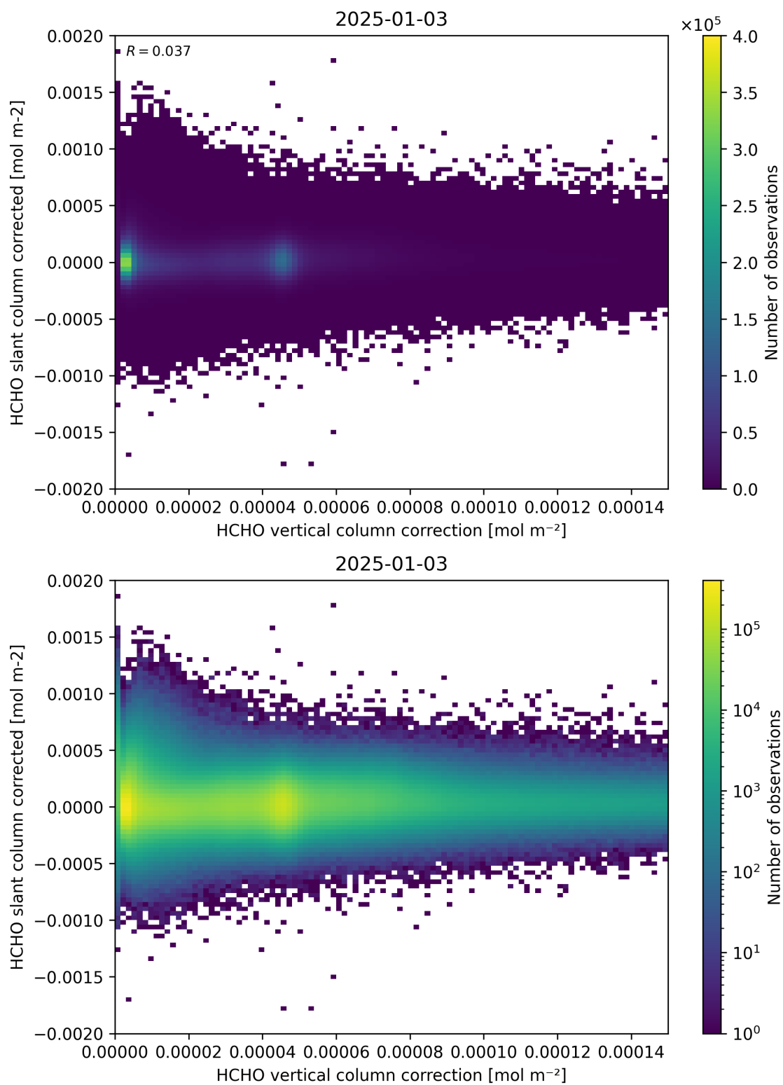
Figure 116: Scatter density plot of “HCHO vertical column correction” against “HCHO slant column corrected” for 2025-01-02 to 2025-01-04.
