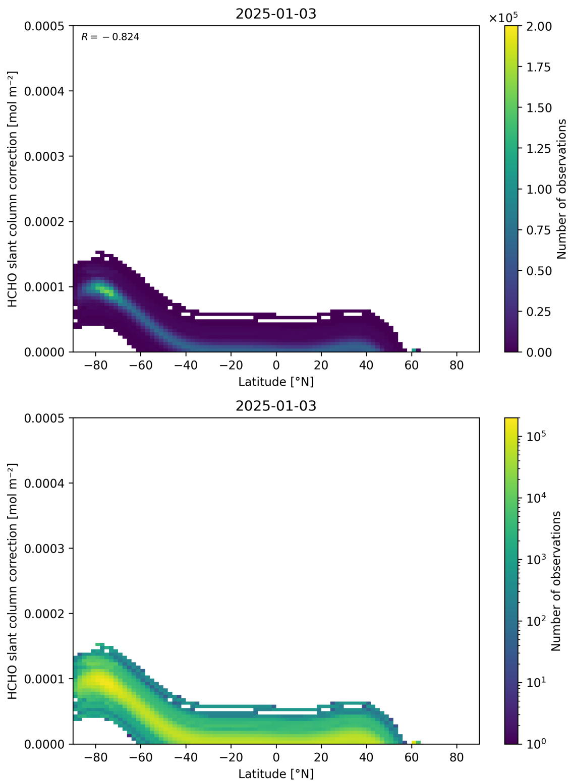
Figure 158: Scatter density plot of “Latitude” against “HCHO slant column correction” for 2025-01-02 to 2025-01-04.
