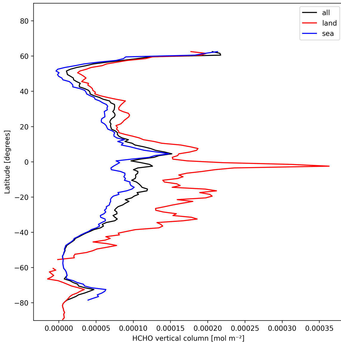
Figure 21: Zonal average of “HCHO vertical column” for 2025-01-02 to 2025-01-04.
