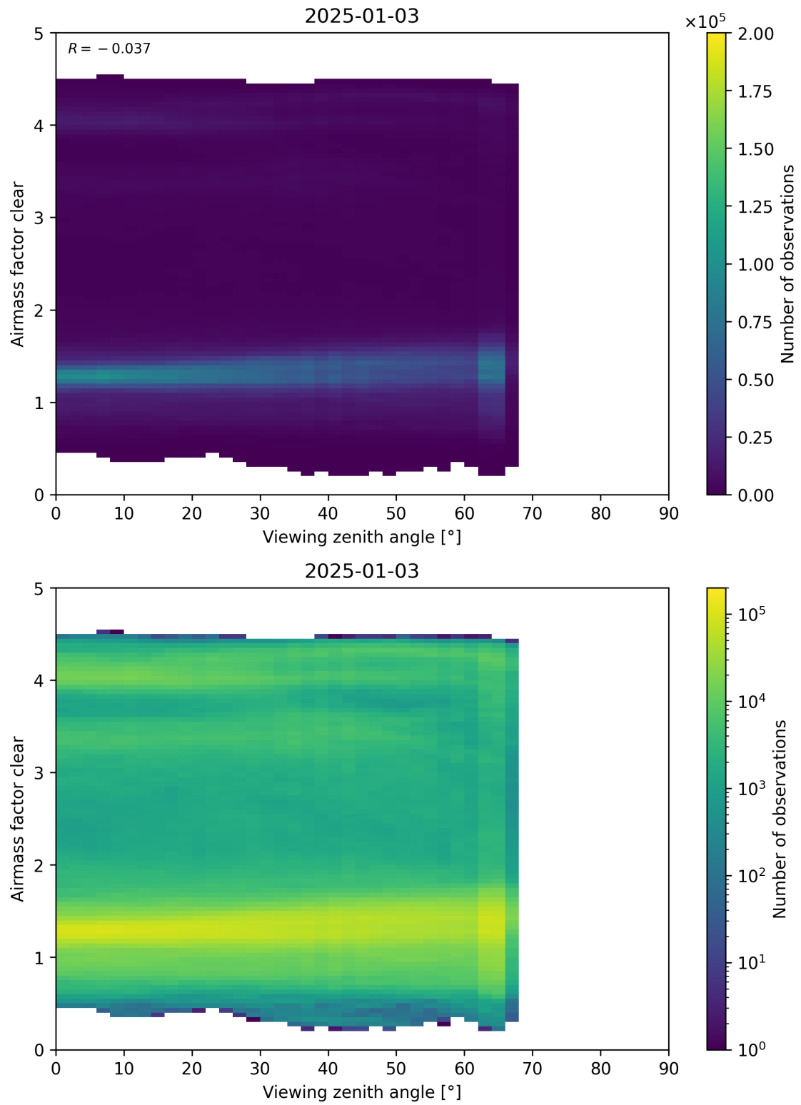
Figure 185: Scatter density plot of “Viewing zenith angle” against “Airmass factor clear” for 2025-01-02 to 2025-01-04.
