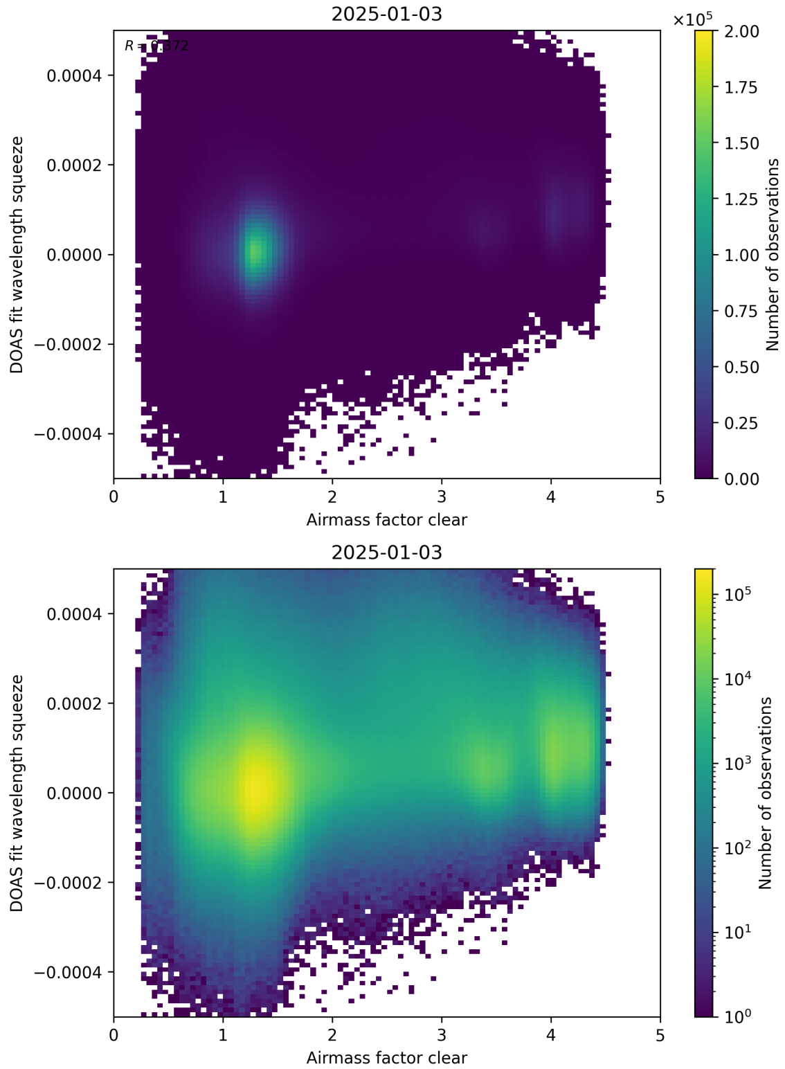
Figure 73: Scatter density plot of “Airmass factor clear” against “DOAS fit wavelength squeeze” for 2025-01-02 to 2025-01-04.
