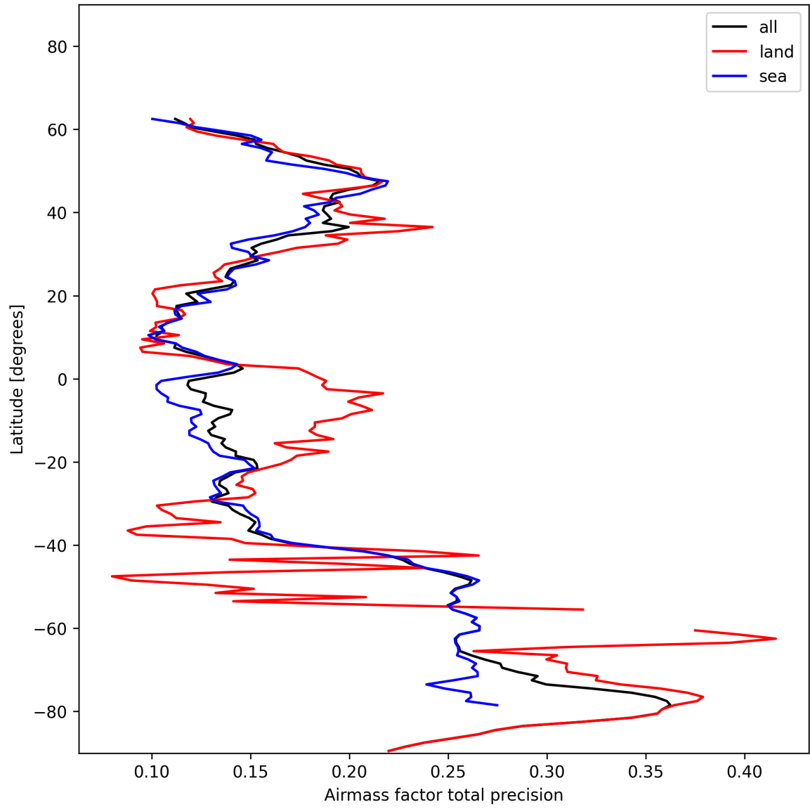
Figure 27: Zonal average of “Airmass factor total precision” for 2025-01-02 to 2025-01-04.
