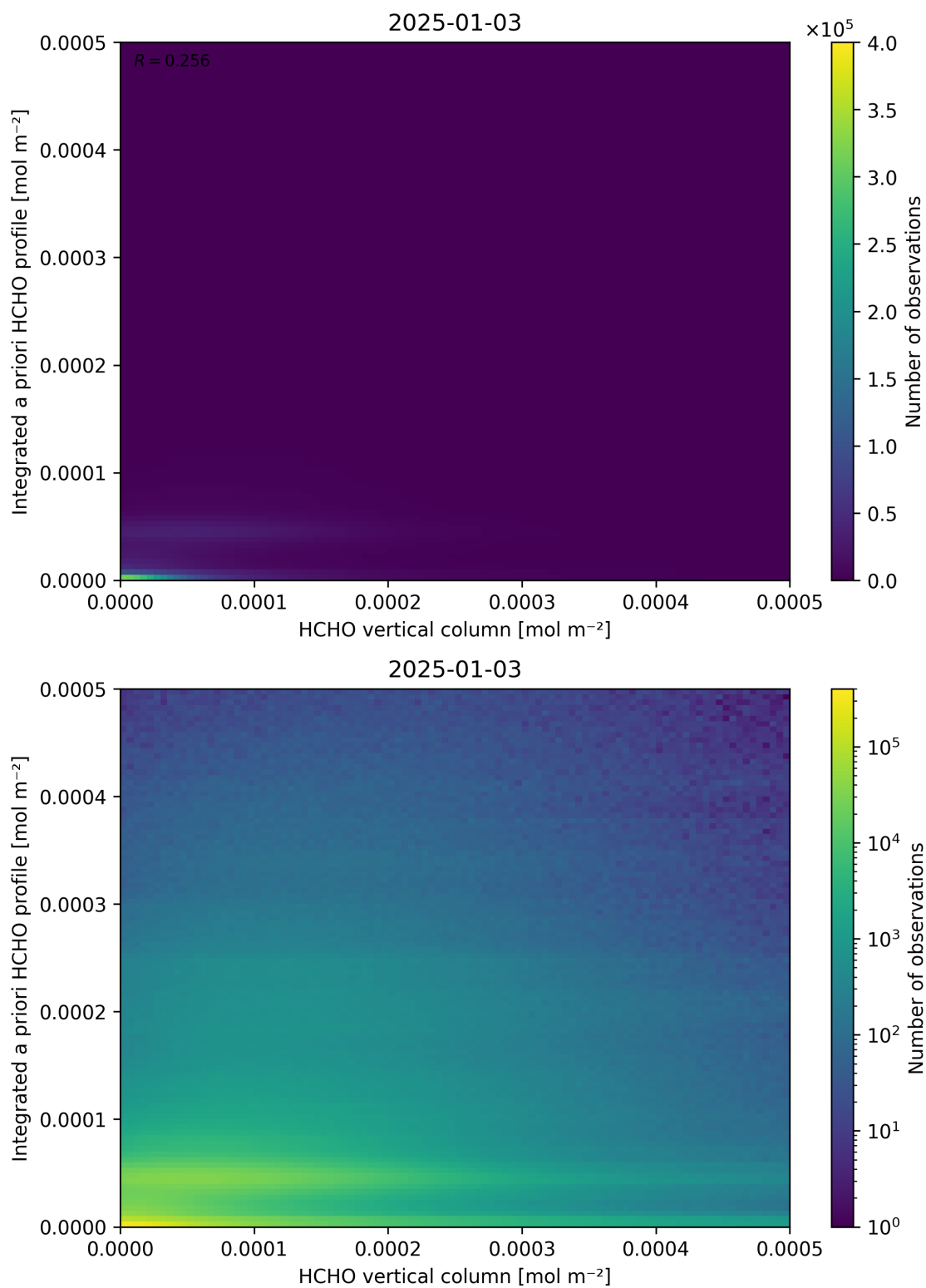
Figure 135: Scatter density plot of “HCHO vertical column” against “Integrated a priori HCHO profile” for 2025-01-02 to 2025-01-04.
