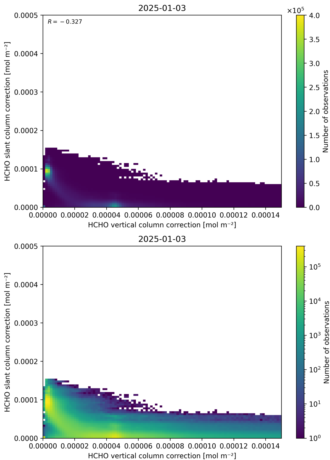
Figure 117: Scatter density plot of “HCHO vertical column correction” against “HCHO slant column correction” for 2025-01-02 to 2025-01-04.
