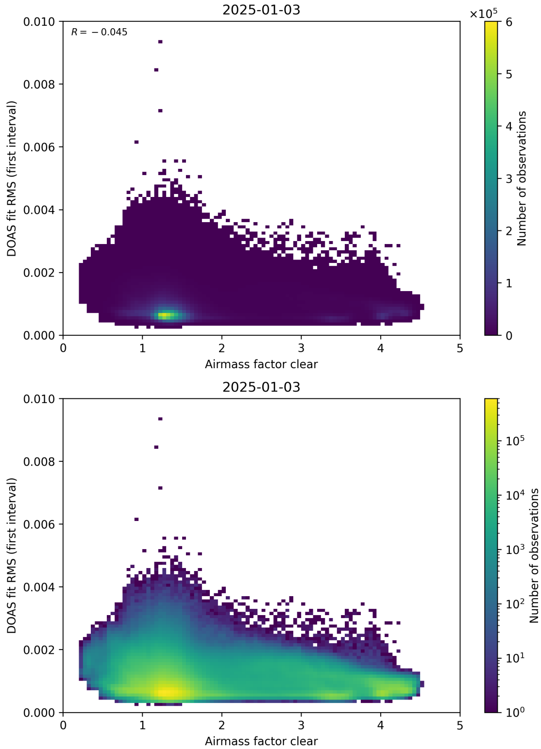
Figure 71: Scatter density plot of “Airmass factor clear” against “DOAS fit RMS (first interval)” for 2025-01-02 to 2025-01-04.
