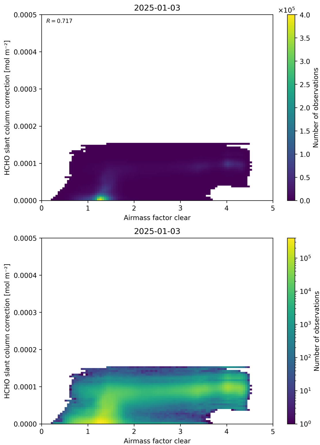
Figure 75: Scatter density plot of “Airmass factor clear” against “HCHO slant column correction” for 2025-01-02 to 2025-01-04.
