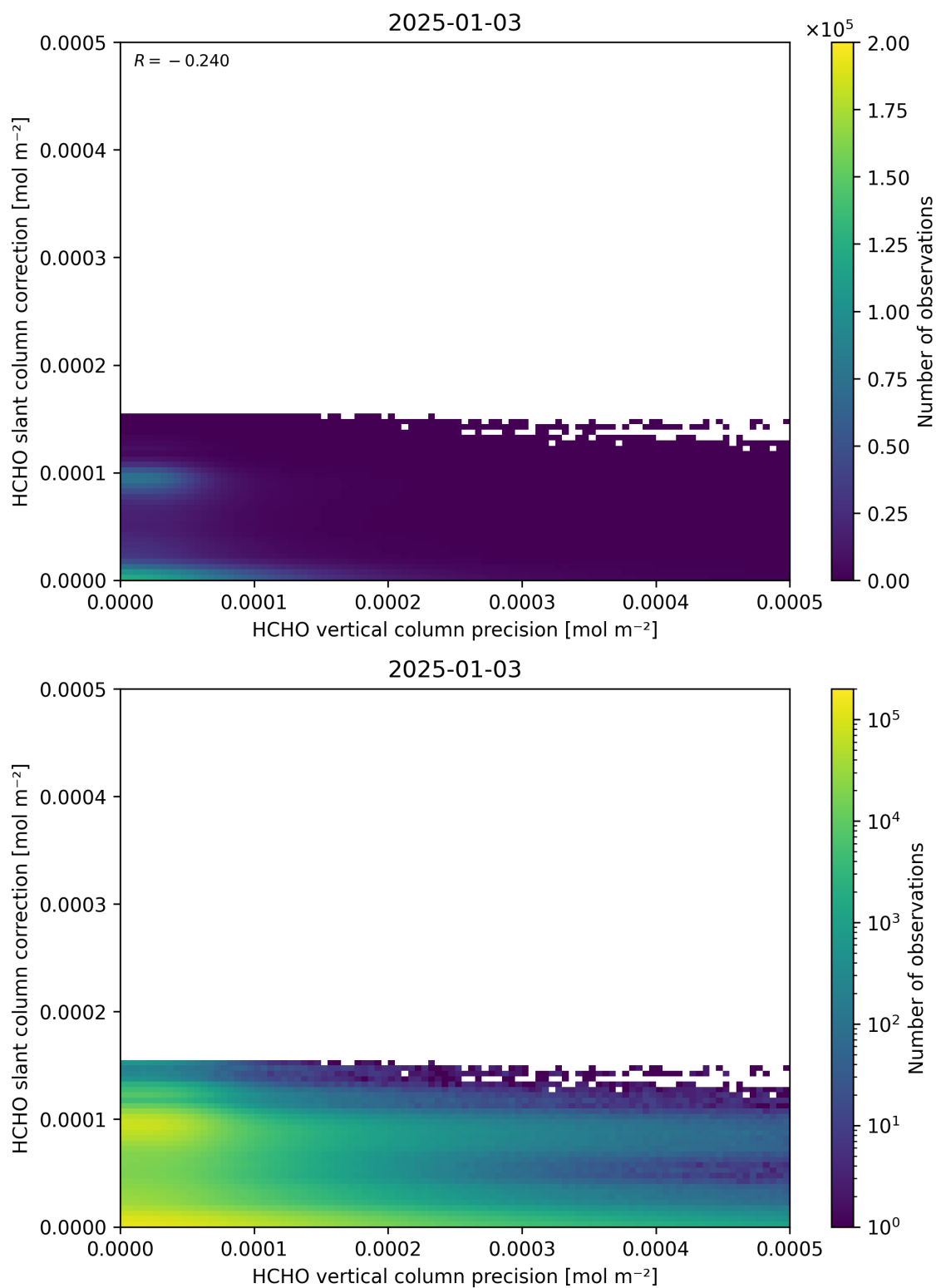
Figure 141: Scatter density plot of “HCHO vertical column precision” against “HCHO slant column correction” for 2025-01-02 to 2025-01-04.
