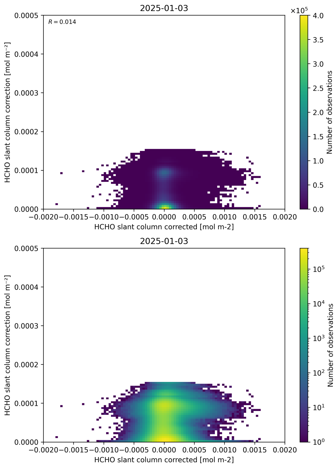
Figure 77: Scatter density plot of “HCHO slant column corrected” against “HCHO slant column correction” for 2025-01-02 to 2025-01-04.
