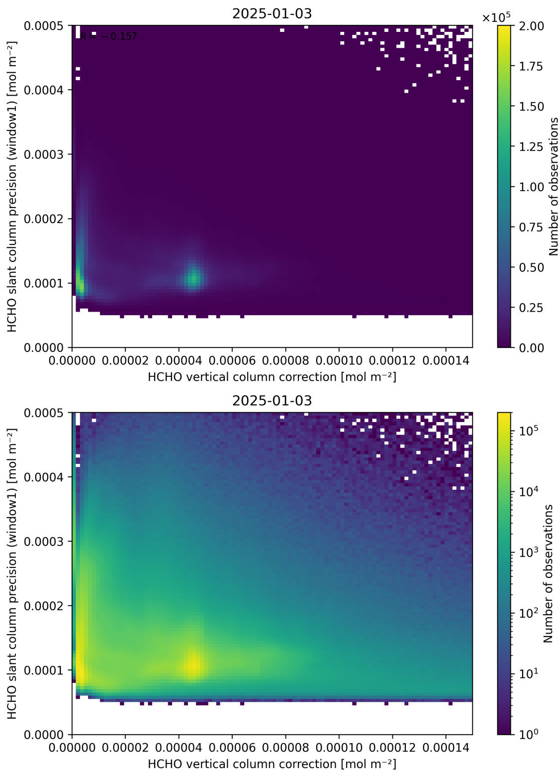
Figure 119: Scatter density plot of “HCHO vertical column correction” against “HCHO slant column precision (window1)” for 2025-01-02 to 2025-01-04.
