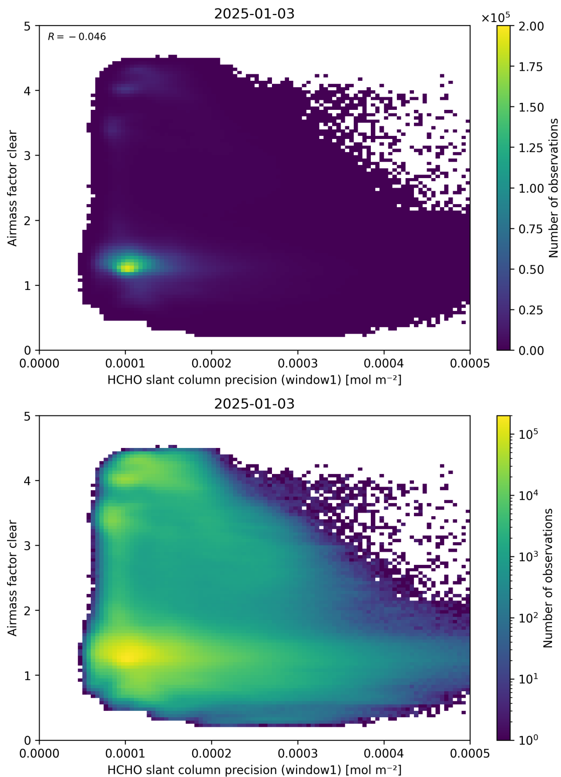
Figure 91: Scatter density plot of “HCHO slant column precision (window1)” against “Airmass factor clear” for 2025-01-02 to 2025-01-04.
