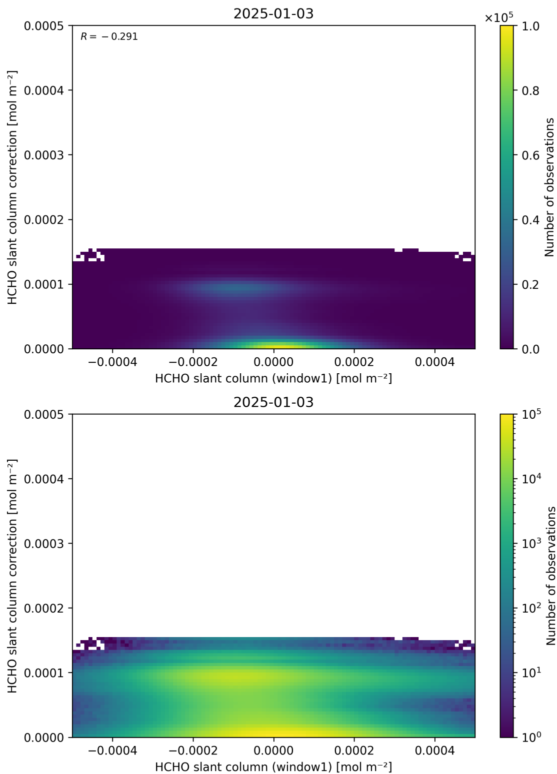
Figure 83: Scatter density plot of “HCHO slant column (window1)” against “HCHO slant column correction” for 2025-01-02 to 2025-01-04.
