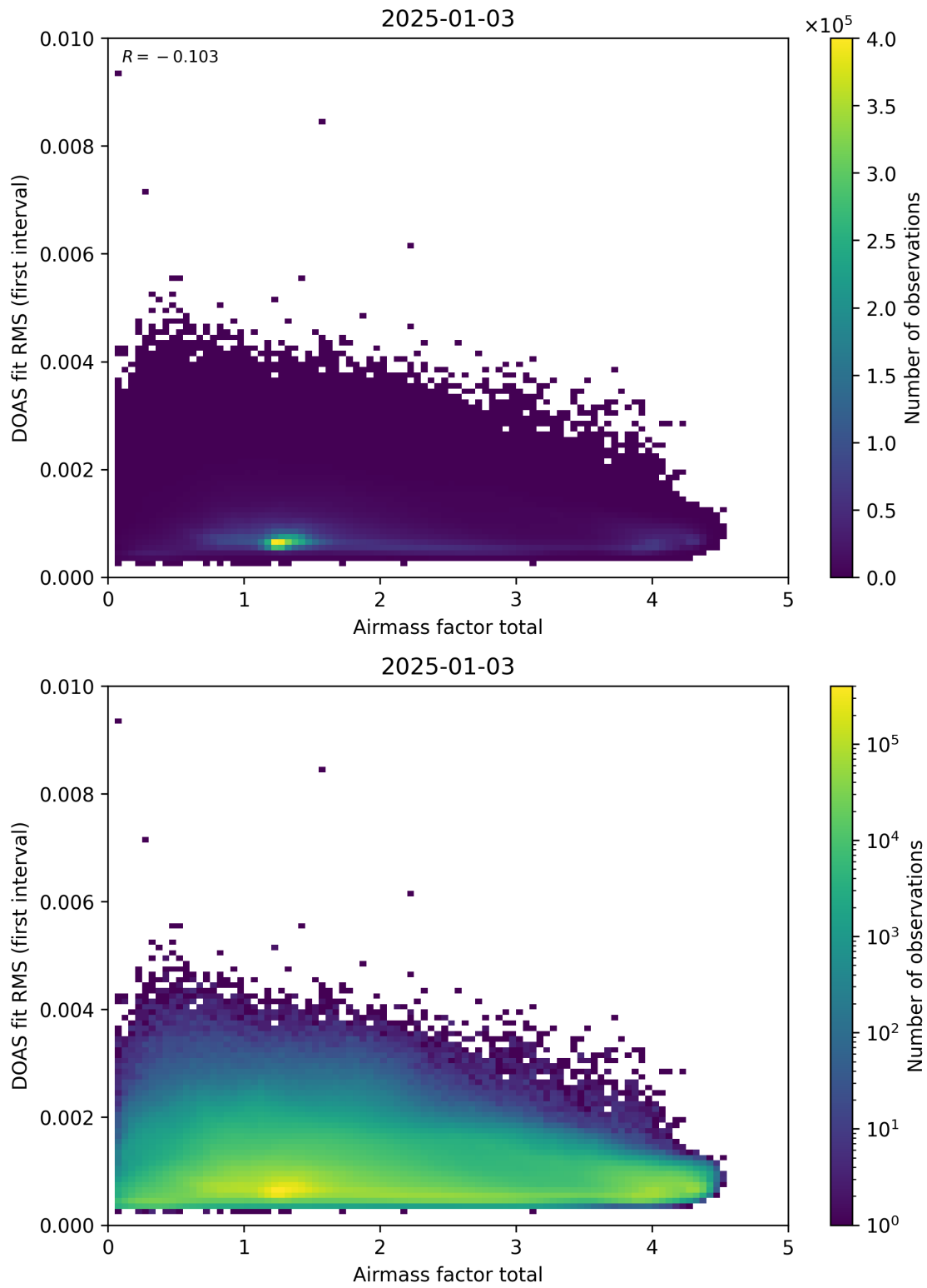
Figure 97: Scatter density plot of “Airmass factor total” against “DOAS fit RMS (first interval)” for 2025-01-02 to 2025-01-04.
