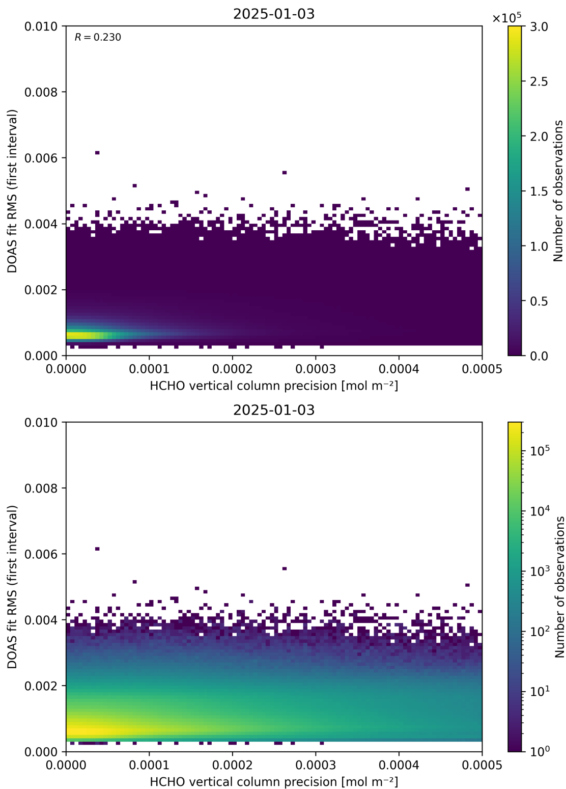
Figure 136: Scatter density plot of “HCHO vertical column precision” against “DOAS fit RMS (first interval)” for 2025-01-02 to 2025-01-04.
