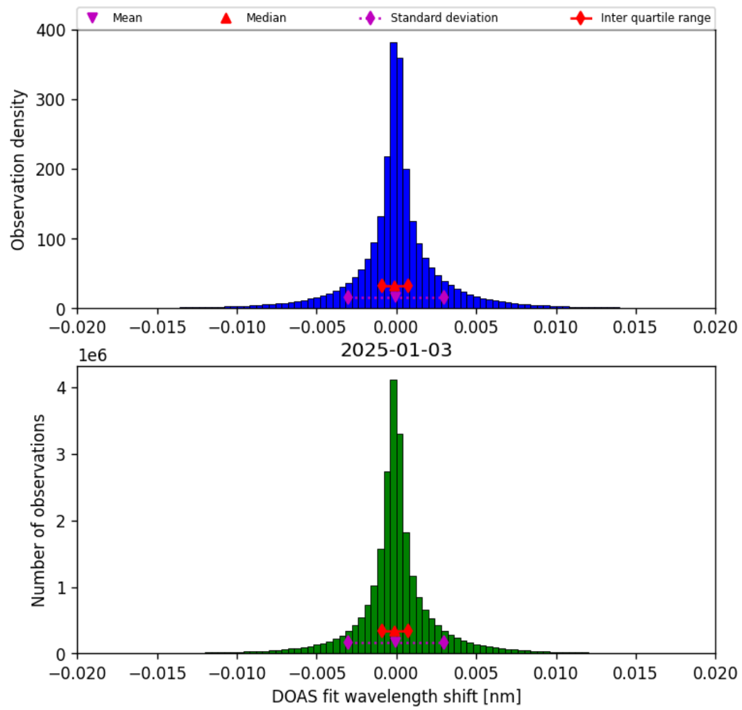
Figure 44: Histogram of “DOAS fit wavelength shift” for 2025-01-02 to 2025-01-04
