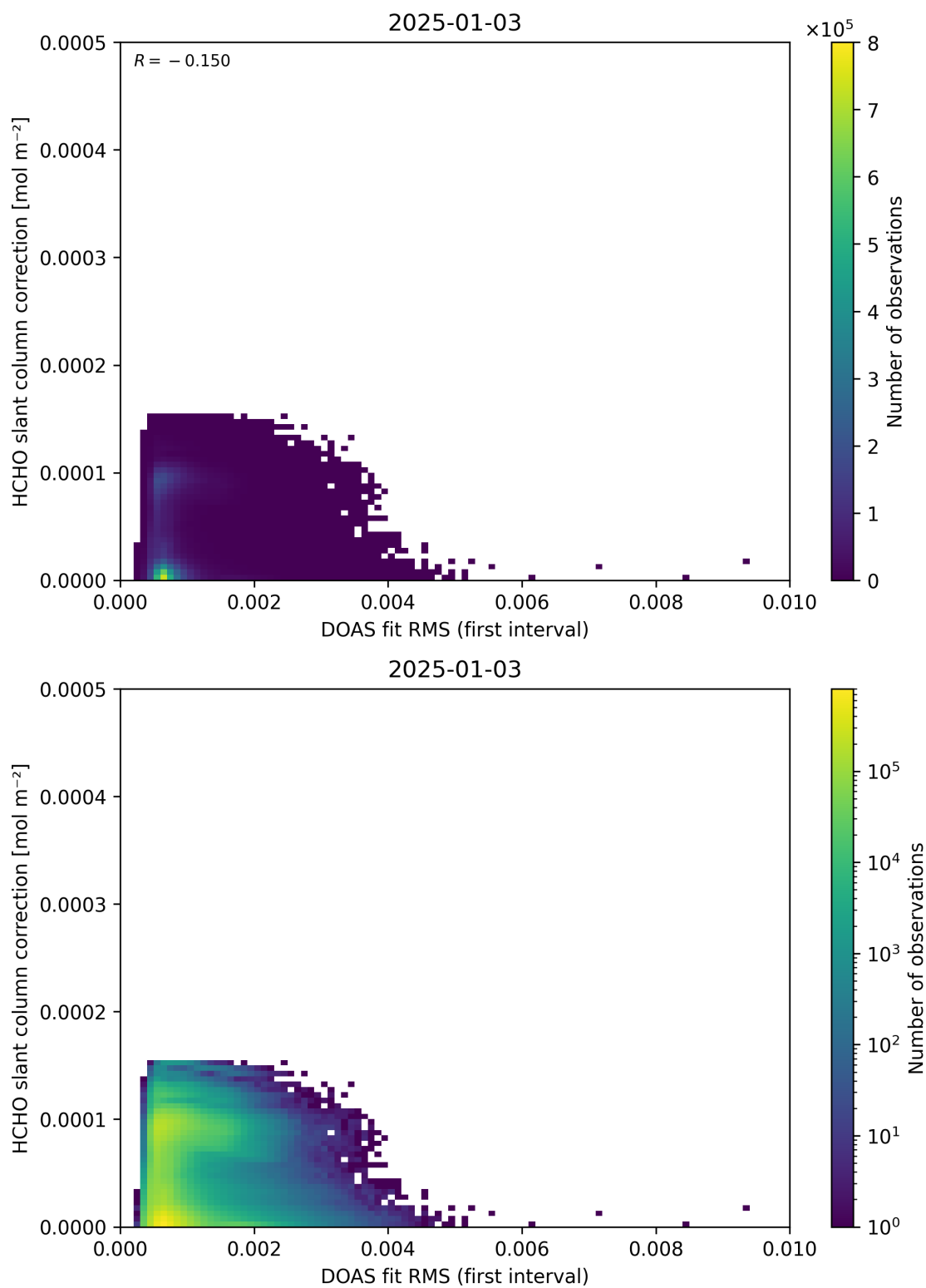
Figure 63: Scatter density plot of “DOAS fit RMS (first interval)” against “HCHO slant column correction” for 2025-01-02 to 2025-01-04.
