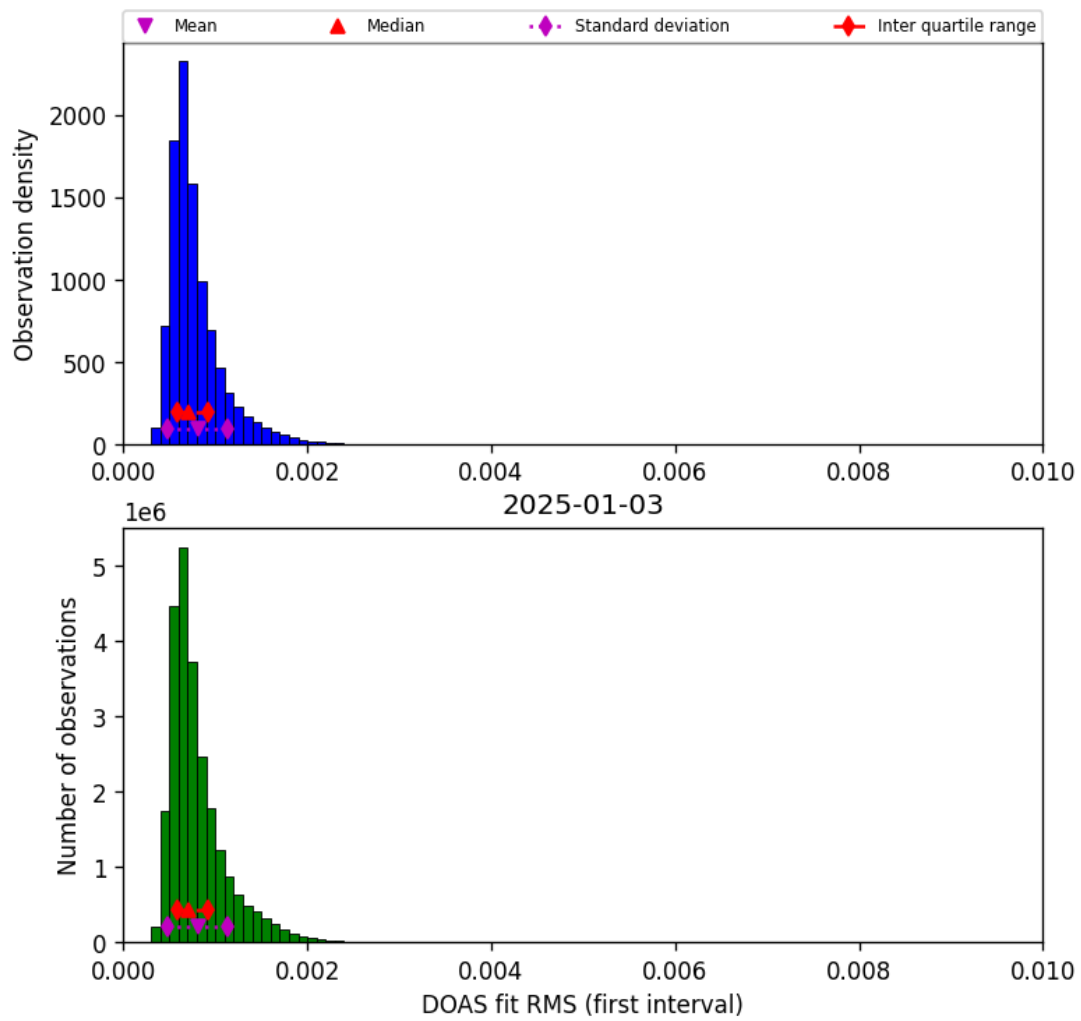
Figure 46: Histogram of “DOAS fit RMS (first interval)” for 2025-01-02 to 2025-01-04
