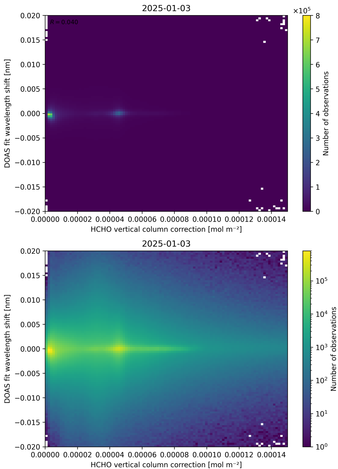
Figure 113: Scatter density plot of “HCHO vertical column correction” against “DOAS fit wavelength shift” for 2025-01-02 to 2025-01-04.
