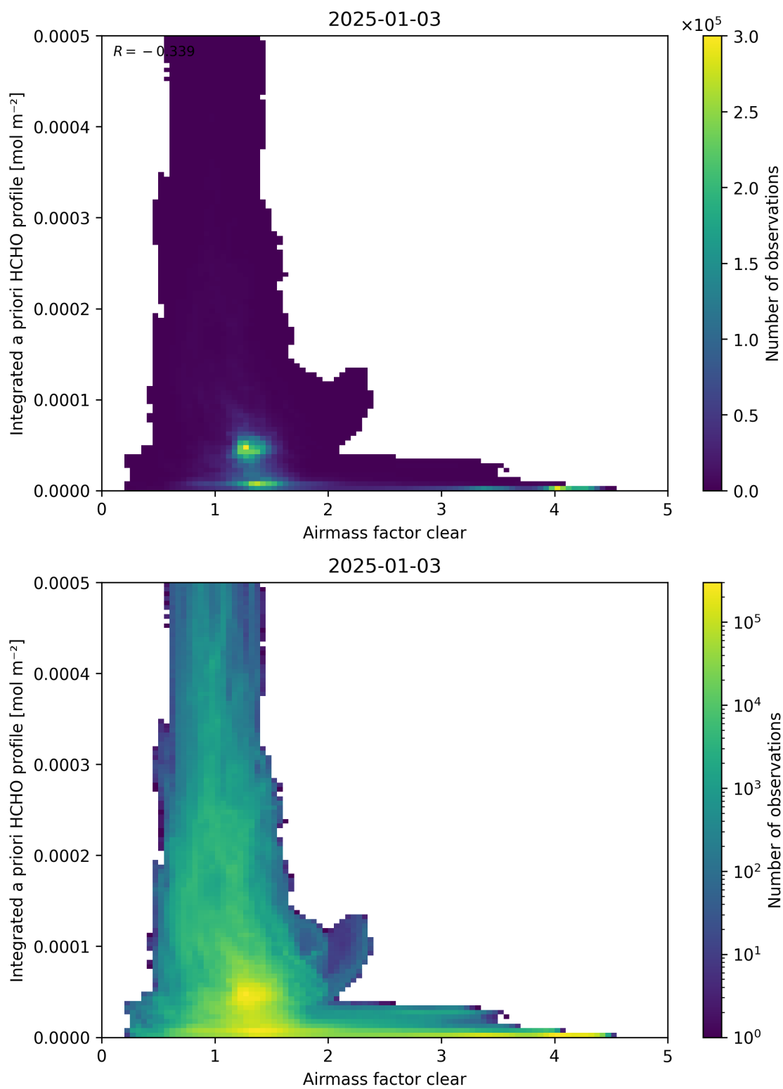
Figure 76: Scatter density plot of “Airmass factor clear” against “Integrated a priori HCHO profile” for 2025-01-02 to 2025-01-04.
