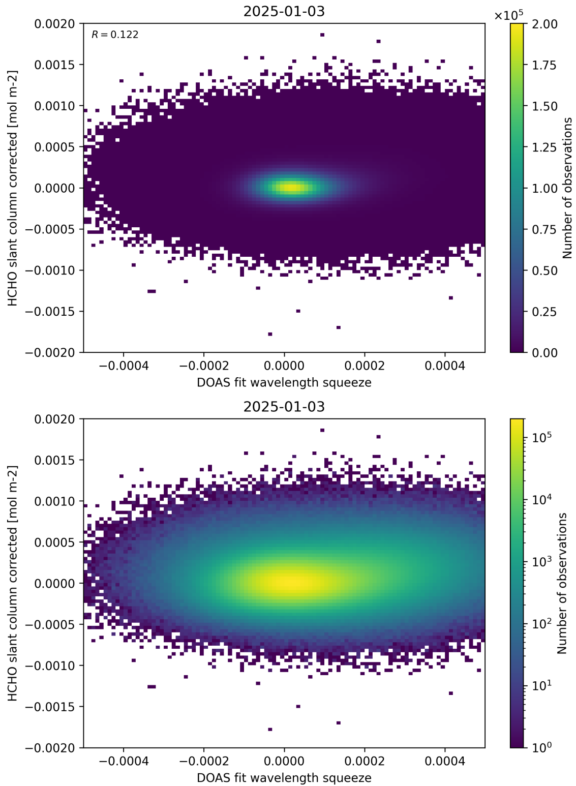
Figure 69: Scatter density plot of “DOAS fit wavelength squeeze” against “HCHO slant column corrected” for 2025-01-02 to 2025-01-04.
