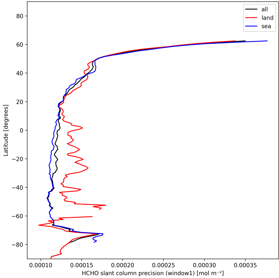
Figure 25: Zonal average of “HCHO slant column precision (window1)” for 2025-01-02 to 2025-01-04.
