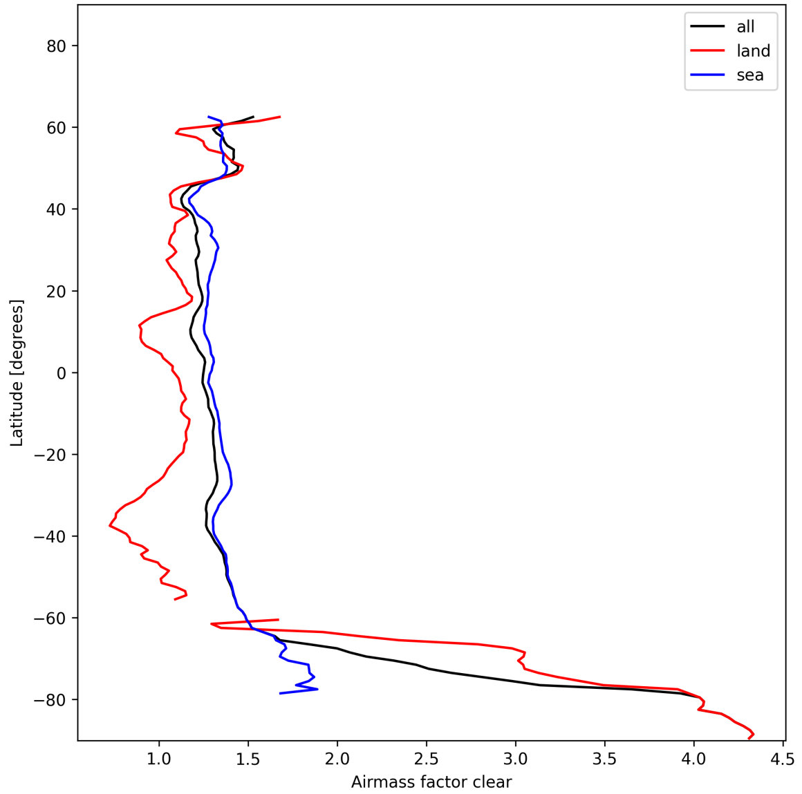
Figure 28: Zonal average of “Airmass factor clear” for 2025-01-02 to 2025-01-04.
