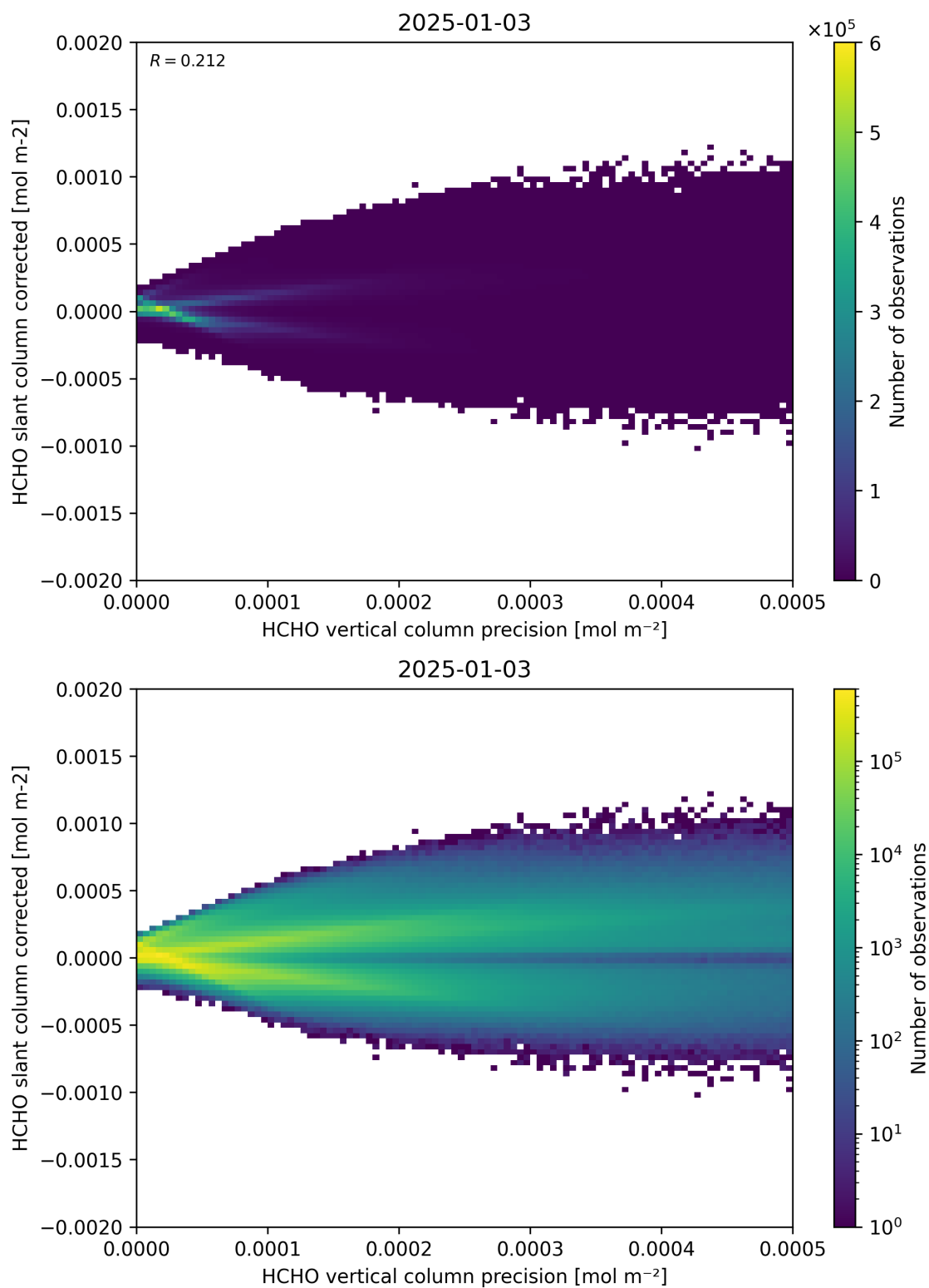
Figure 140: Scatter density plot of “HCHO vertical column precision” against “HCHO slant column corrected” for 2025-01-02 to 2025-01-04.
