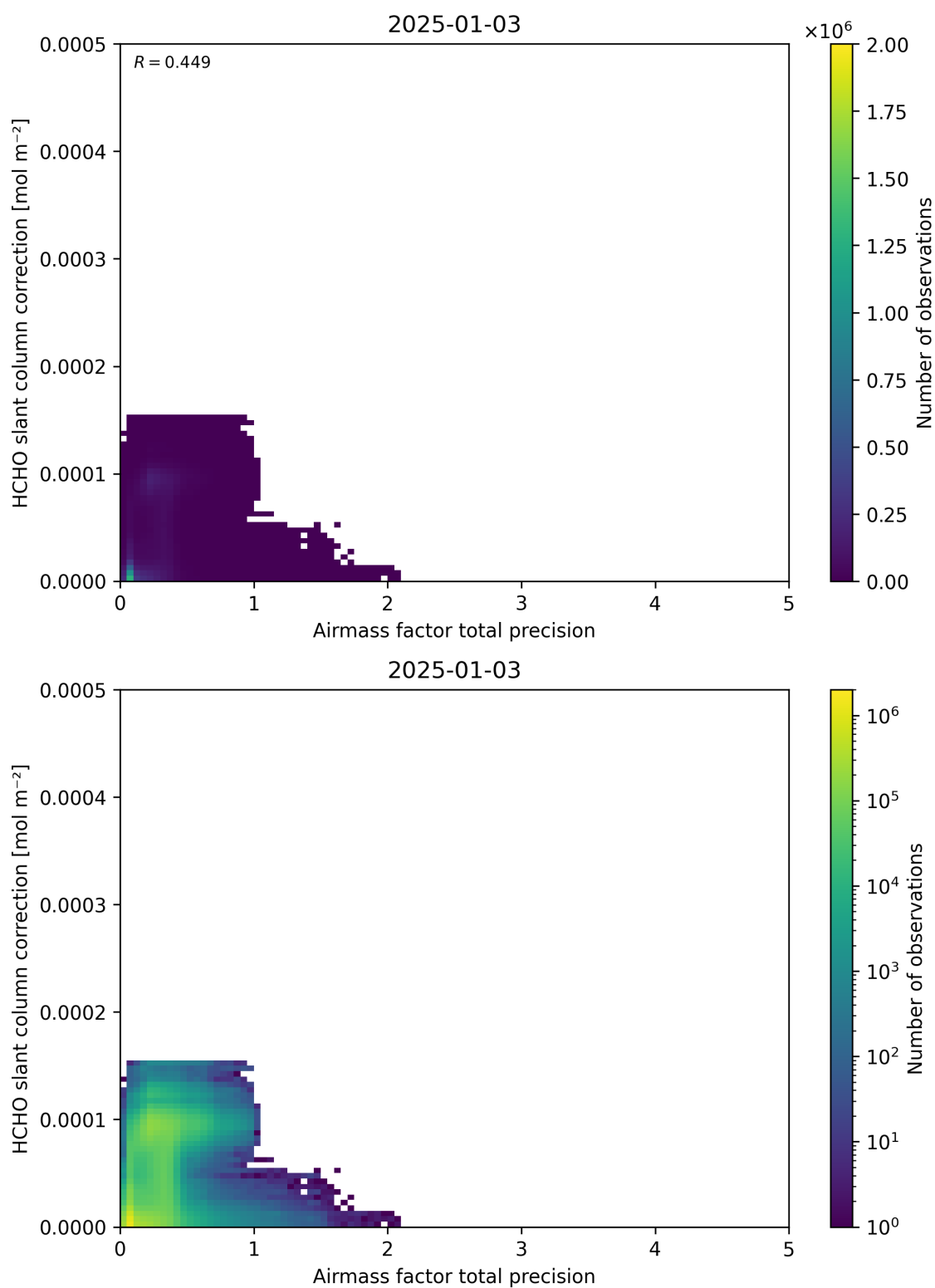
Figure 110: Scatter density plot of “Airmass factor total precision” against “HCHO slant column correction” for 2025-01-02 to 2025-01-04.
