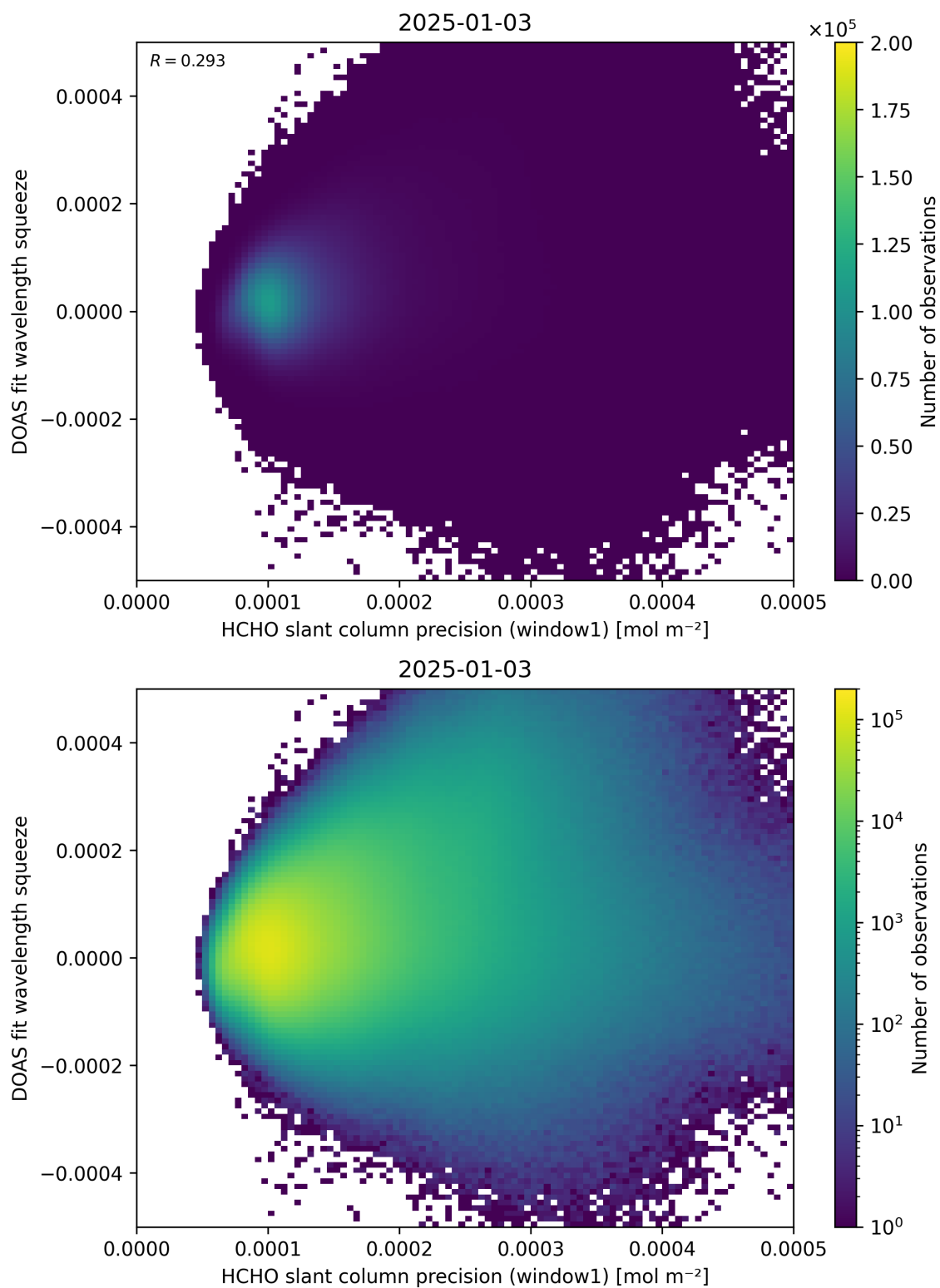
Figure 90: Scatter density plot of “HCHO slant column precision (window1)” against “DOAS fit wavelength squeeze” for 2025-01-02 to 2025-01-04.
