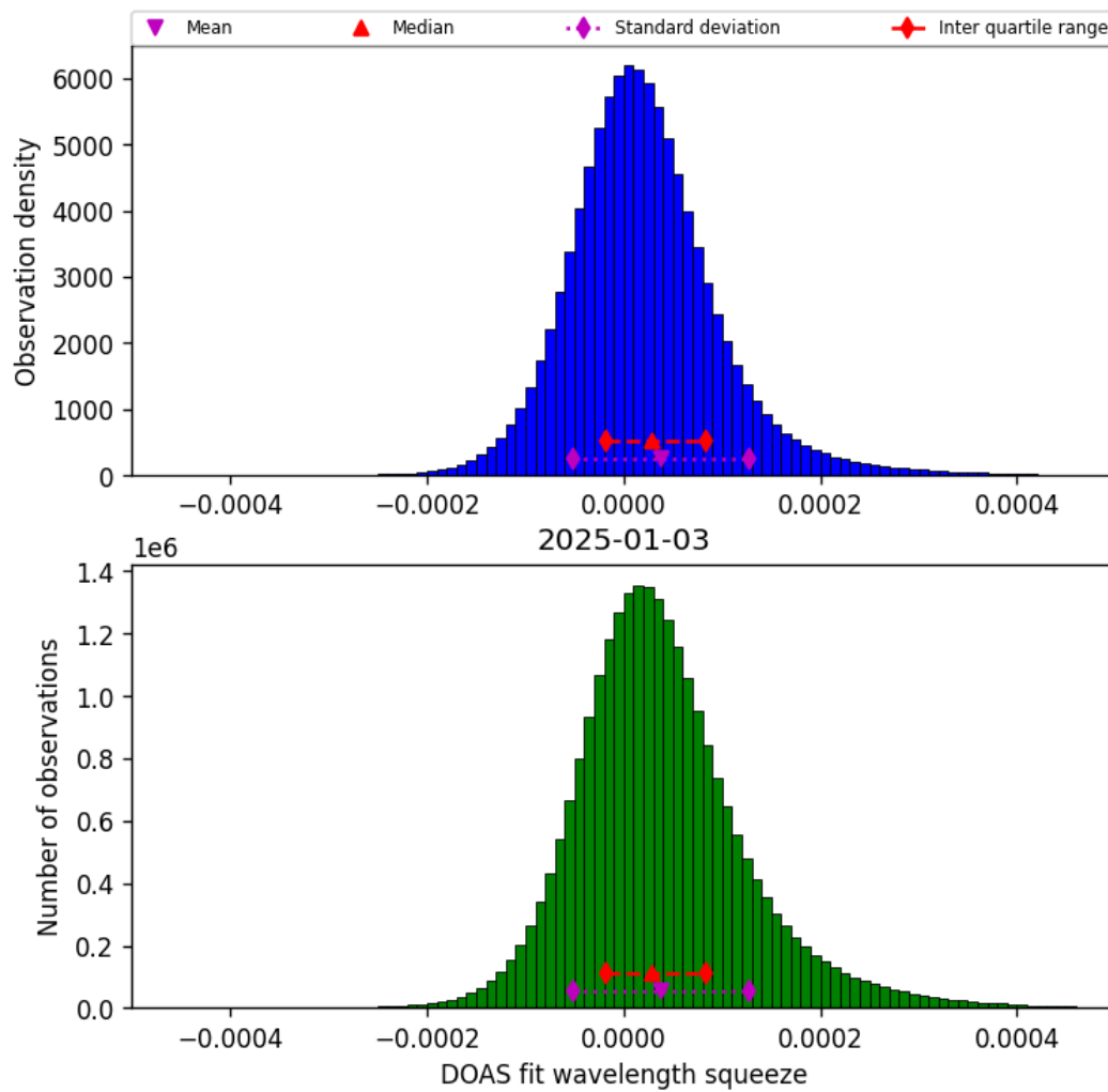
Figure 45: Histogram of “DOAS fit wavelength squeeze” for 2025-01-02 to 2025-01-04
