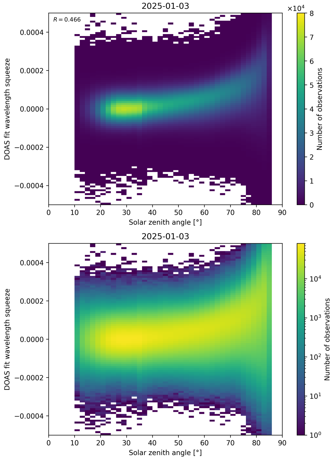
Figure 169: Scatter density plot of “Solar zenith angle” against “DOAS fit wavelength squeeze” for 2025-01-02 to 2025-01-04.
