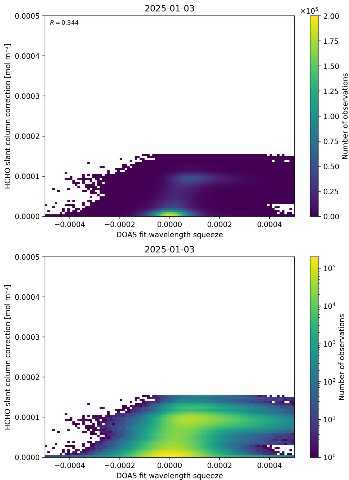
Figure 70: Scatter density plot of “DOAS fit wavelength squeeze” against “HCHO slant column correction” for 2025-01-02 to 2025-01-04.
