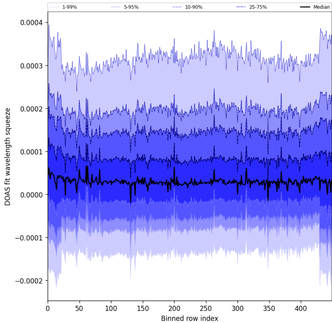
Figure 59: Along track statistics of “DOAS fit wavelength squeeze” for 2025-01-02 to 2025-01-04
