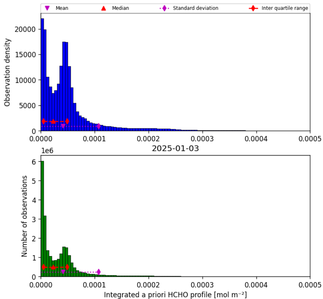
Figure 43: Histogram of “Integrated a priori HCHO profile” for 2025-01-02 to 2025-01-04
