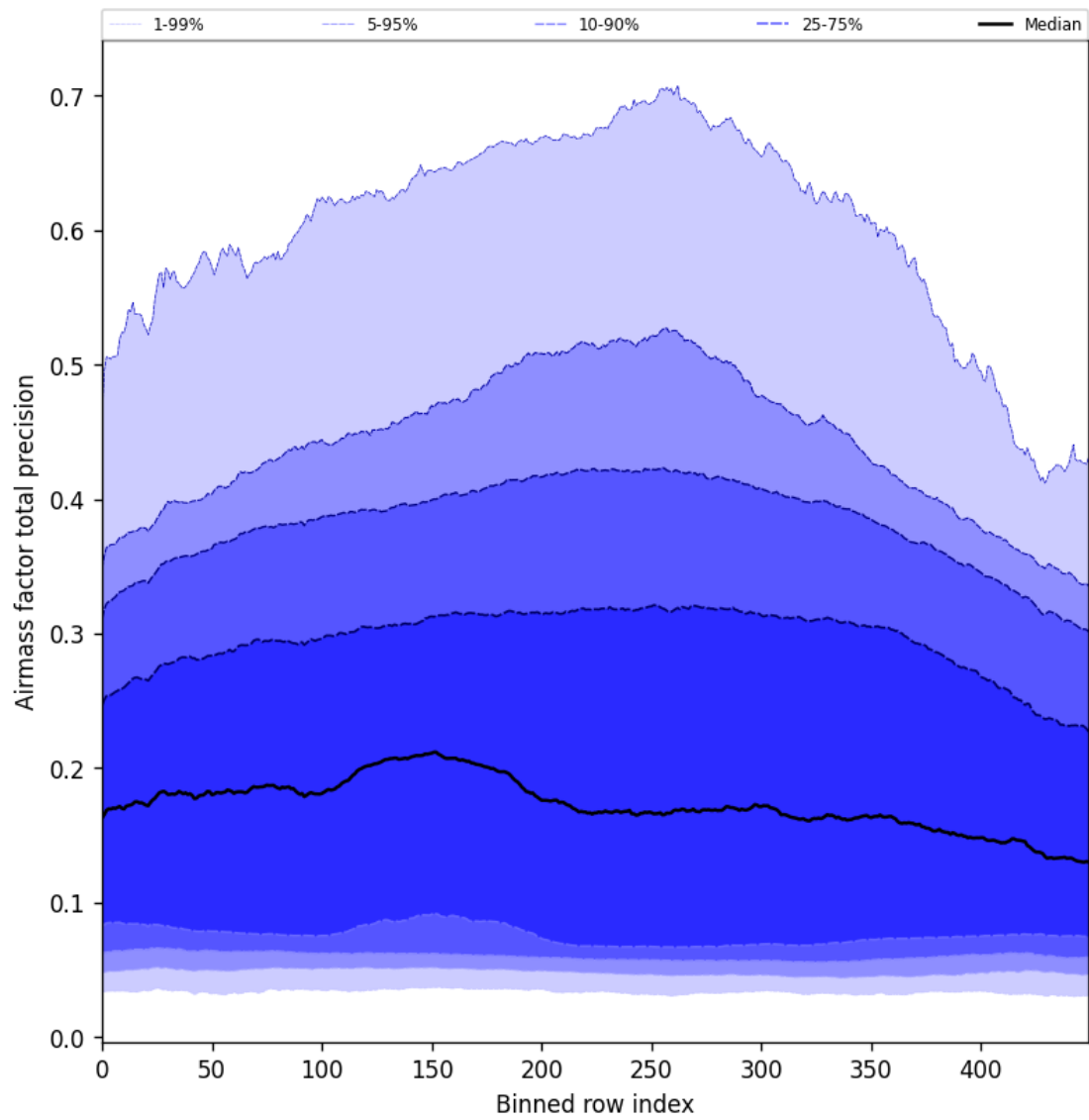
Figure 55: Along track statistics of “Airmass factor total precision” for 2025-01-02 to 2025-01-04
