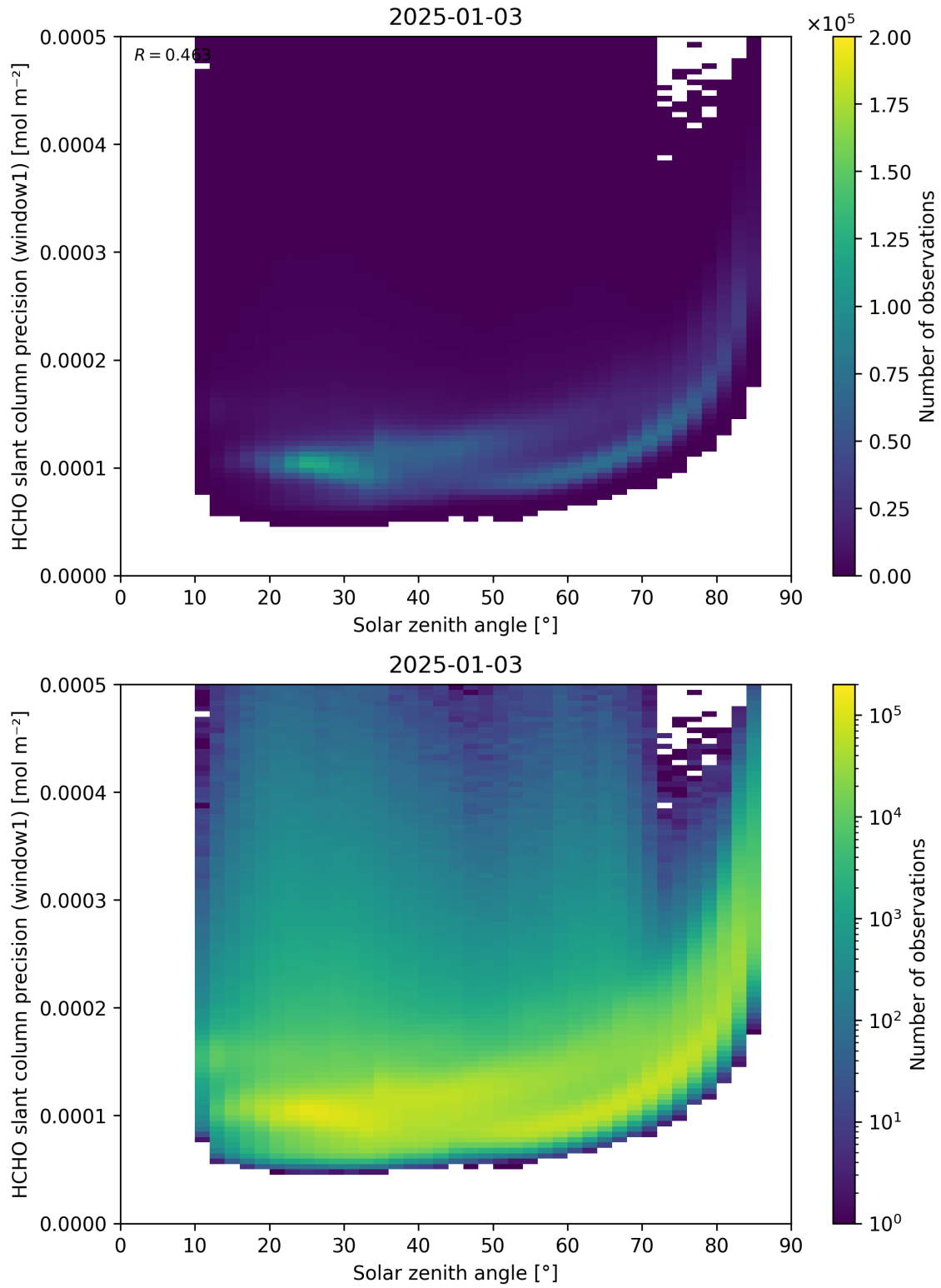
Figure 174: Scatter density plot of “Solar zenith angle” against “HCHO slant column precision (window1)” for 2025-01-02 to 2025-01-04.
