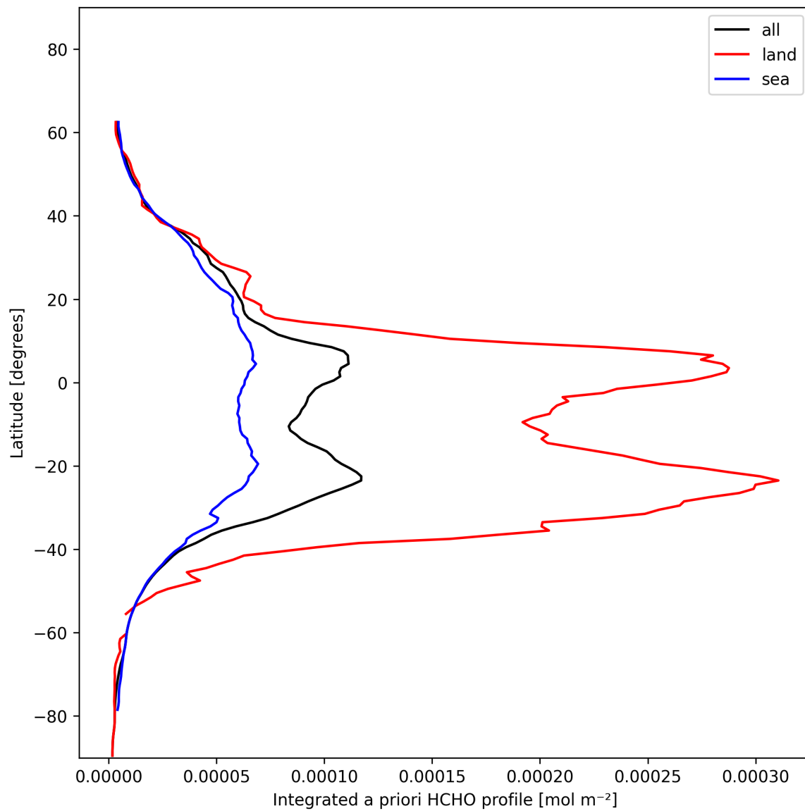
Figure 29: Zonal average of “Integrated a priori HCHO profile” for 2025-01-02 to 2025-01-04.
