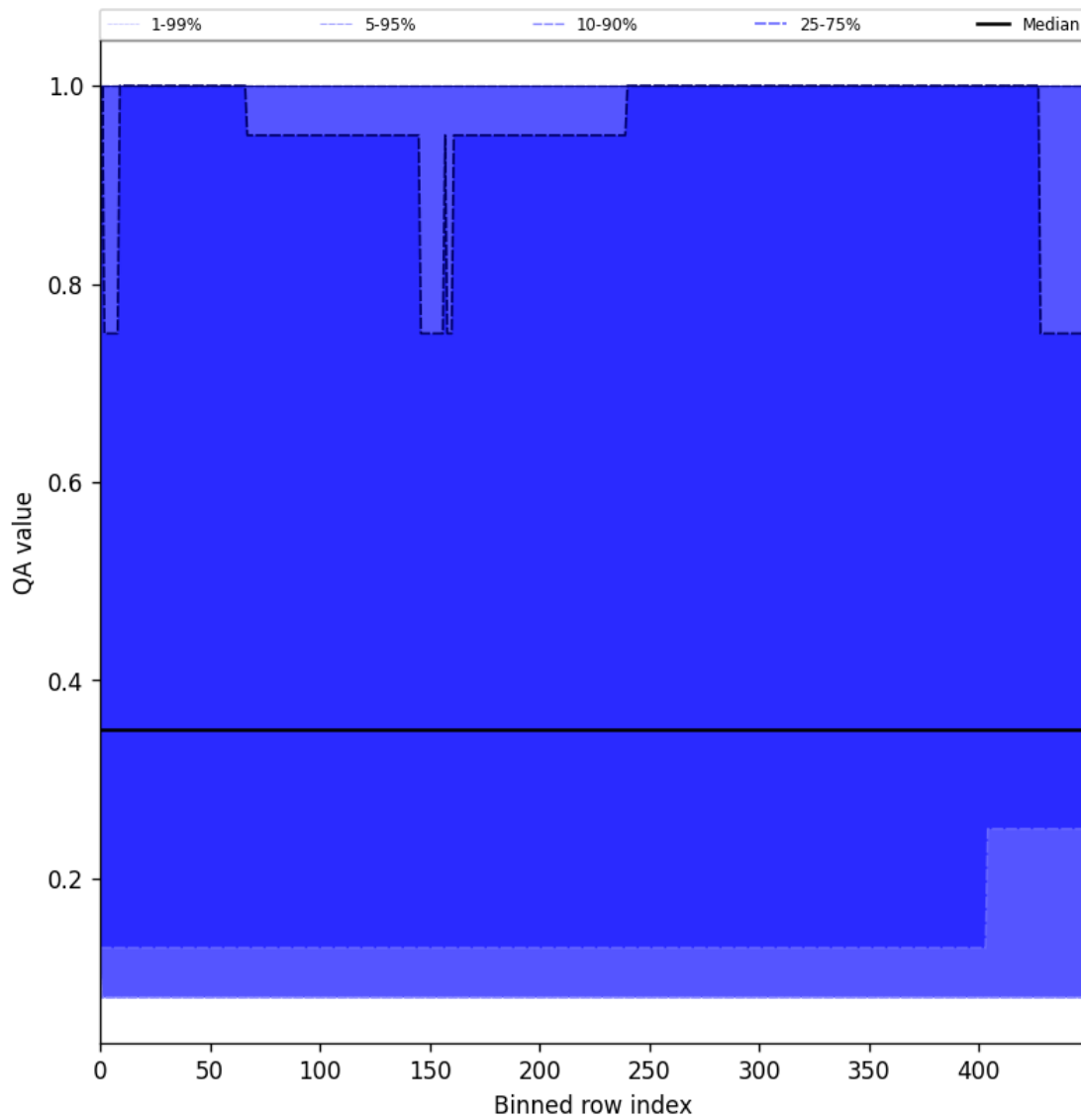
Figure 48: Along track statistics of “QA value” for 2025-01-02 to 2025-01-04
