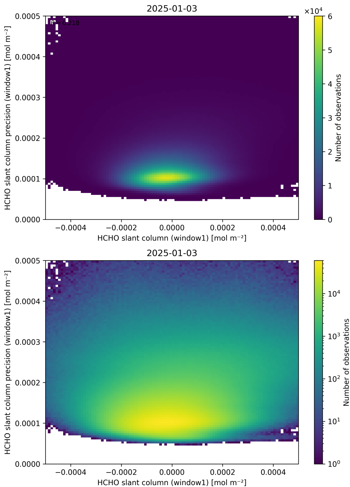
Figure 84: Scatter density plot of “HCHO slant column (window1)” against “HCHO slant column precision (window1)” for 2025-01-02 to 2025-01-04.
