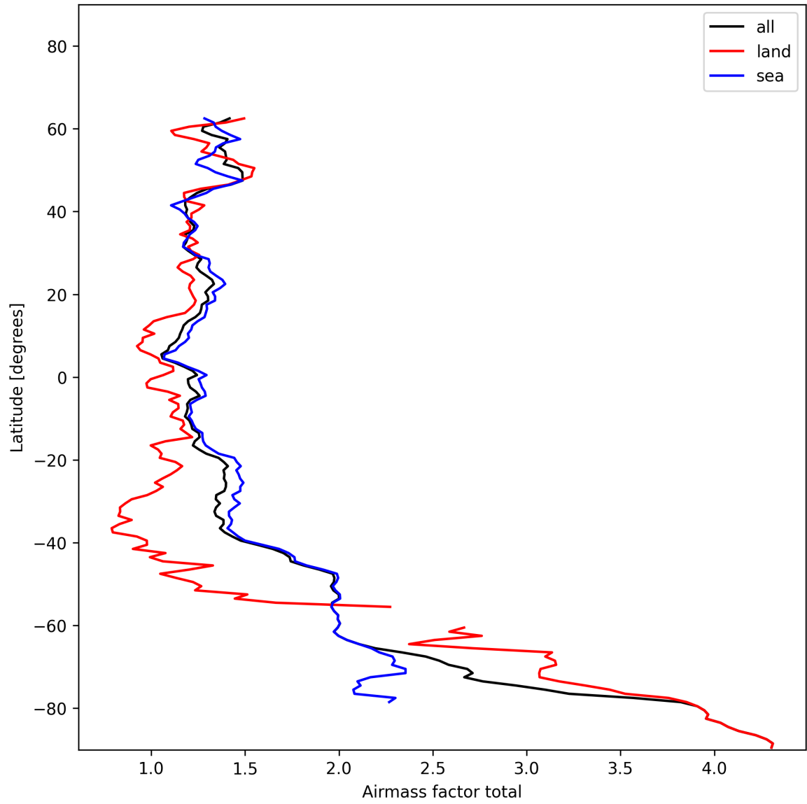
Figure 26: Zonal average of “Airmass factor total” for 2025-01-02 to 2025-01-04.
