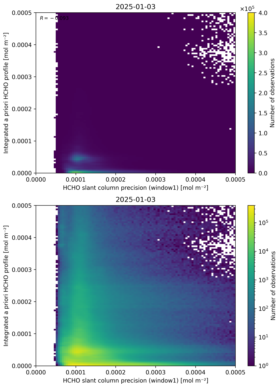
Figure 96: Scatter density plot of “HCHO slant column precision (window1)” against “Integrated a priori HCHO profile” for 2025-01-02 to 2025-01-04.
