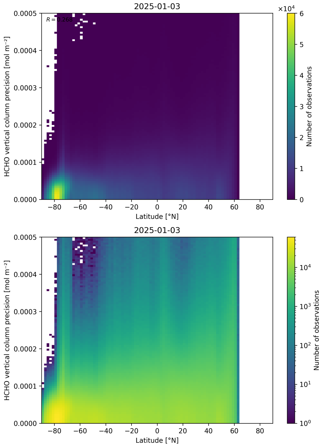
Figure 165: Scatter density plot of “Latitude” against “HCHO vertical column precision” for 2025-01-02 to 2025-01-04.
