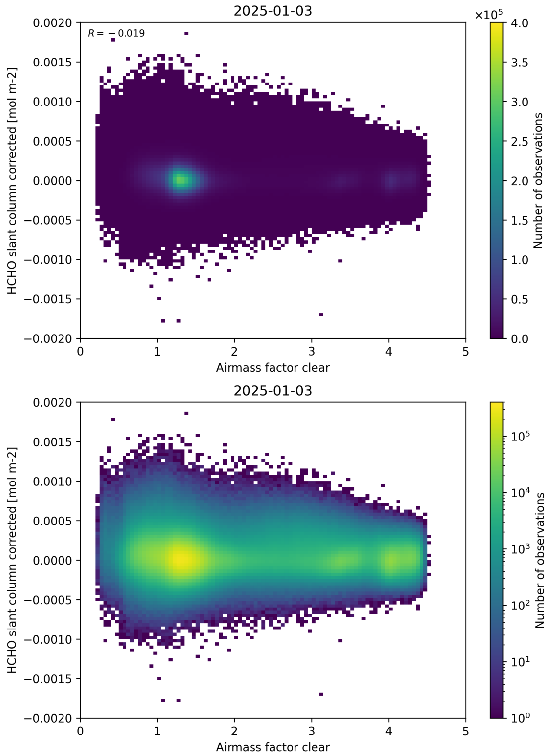
Figure 74: Scatter density plot of “Airmass factor clear” against “HCHO slant column corrected” for 2025-01-02 to 2025-01-04.
