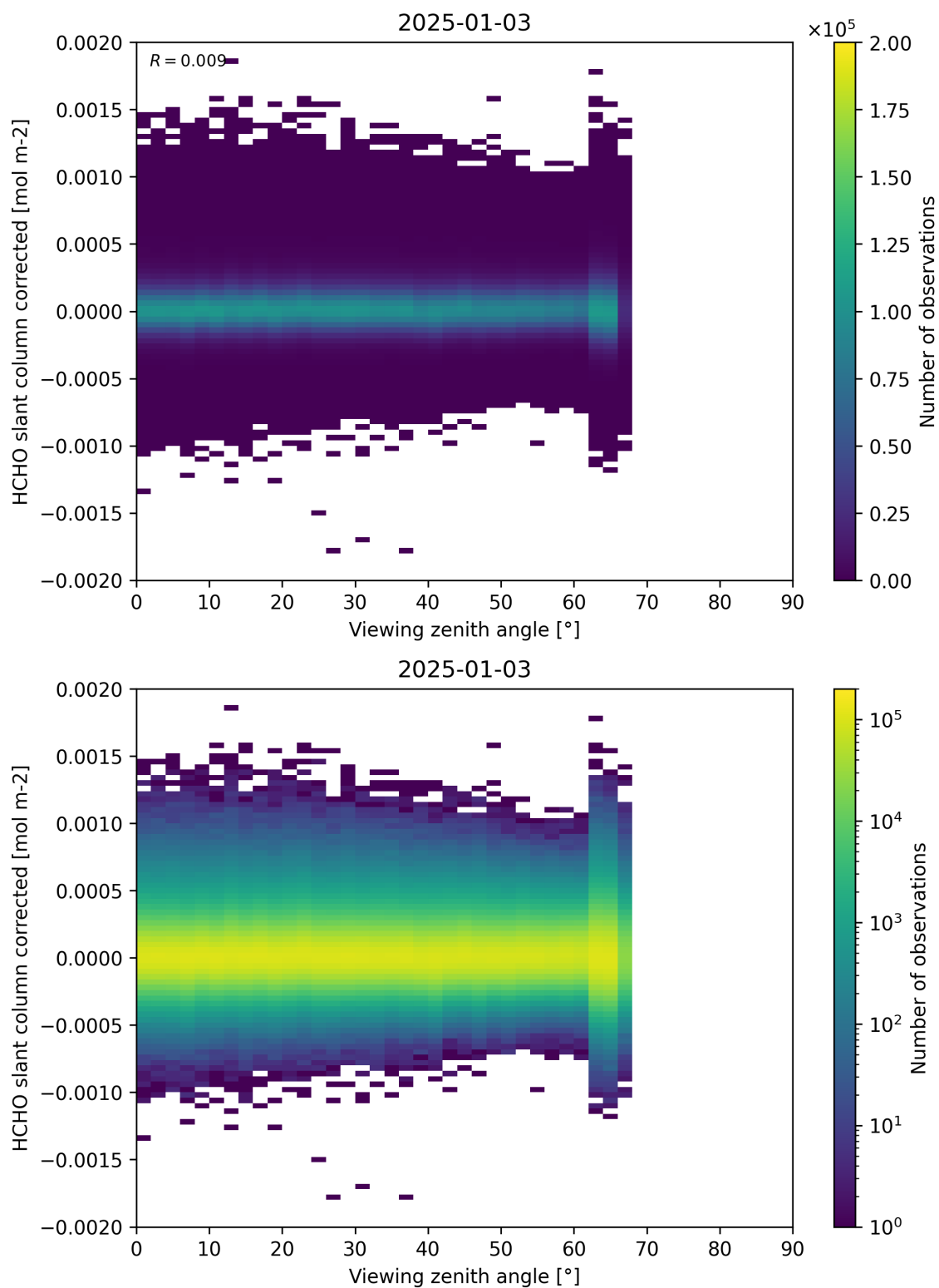
Figure 186: Scatter density plot of “Viewing zenith angle” against “HCHO slant column corrected” for 2025-01-02 to 2025-01-04.
