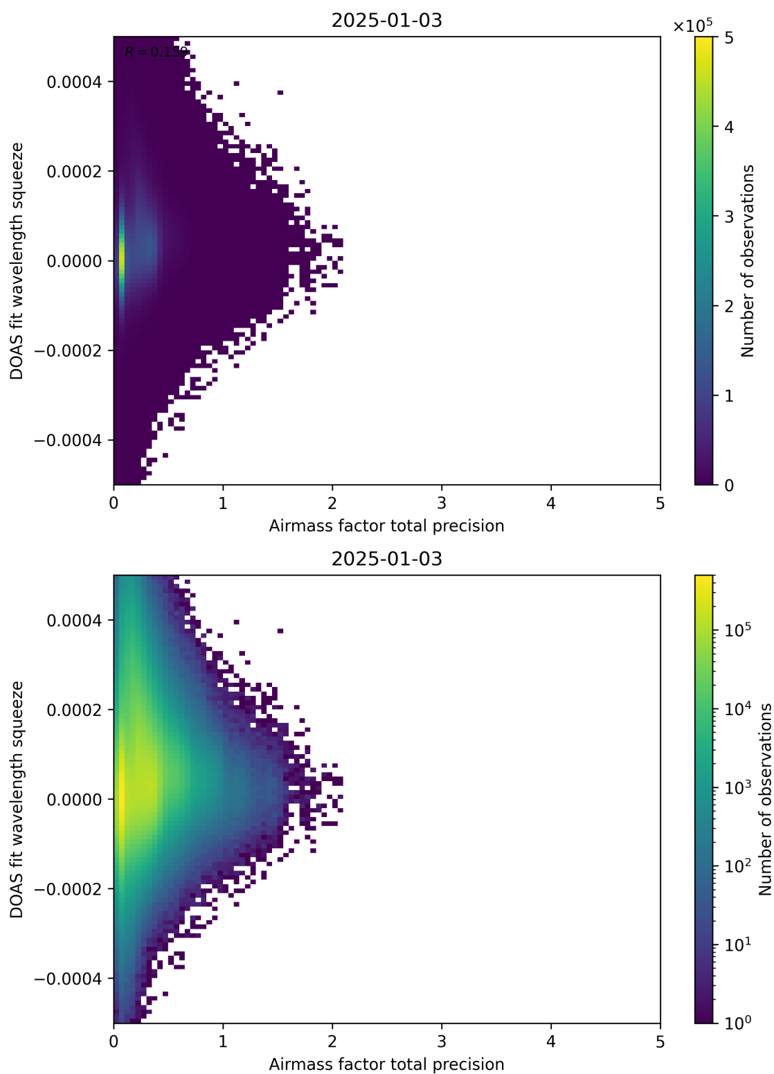
Figure 107: Scatter density plot of “Airmass factor total precision” against “DOAS fit wavelength squeeze” for 2025-01-02 to 2025-01-04.
