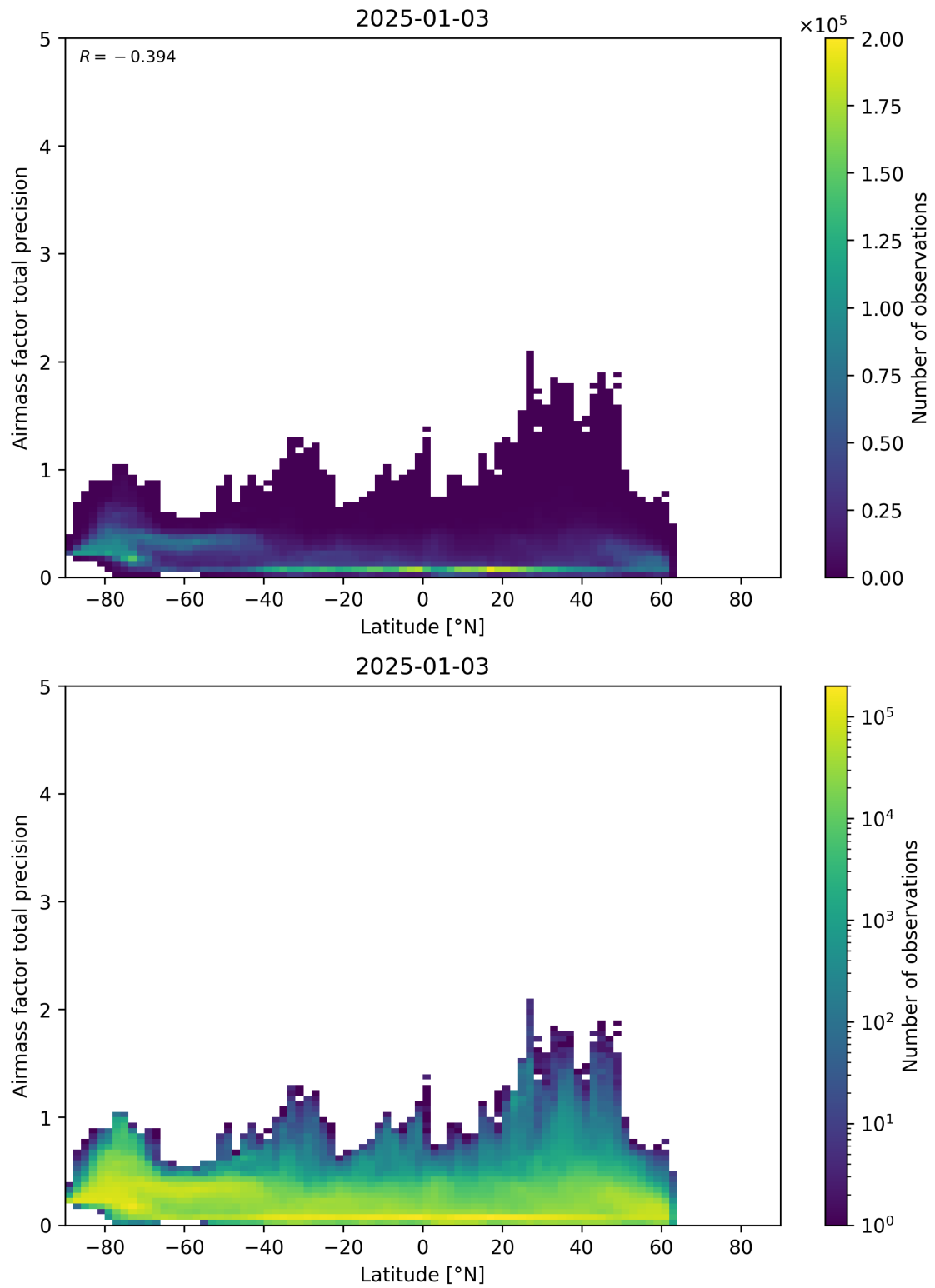
Figure 162: Scatter density plot of “Latitude” against “Airmass factor total precision” for 2025-01-02 to 2025-01-04.
