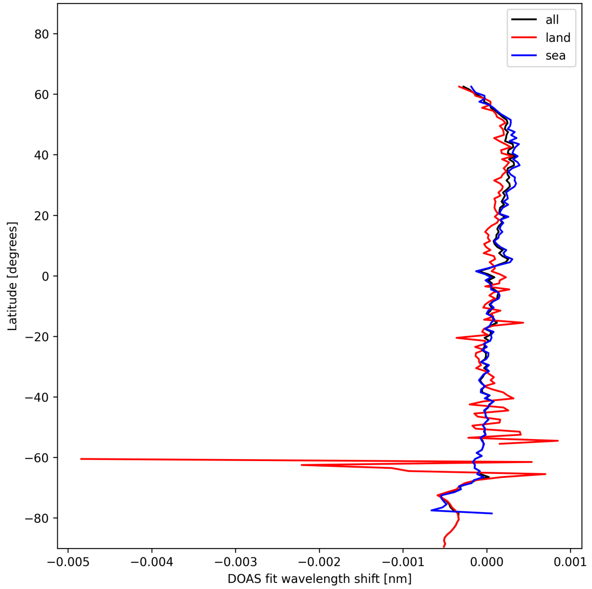
Figure 30: Zonal average of “DOAS fit wavelength shift” for 2025-01-02 to 2025-01-04.
