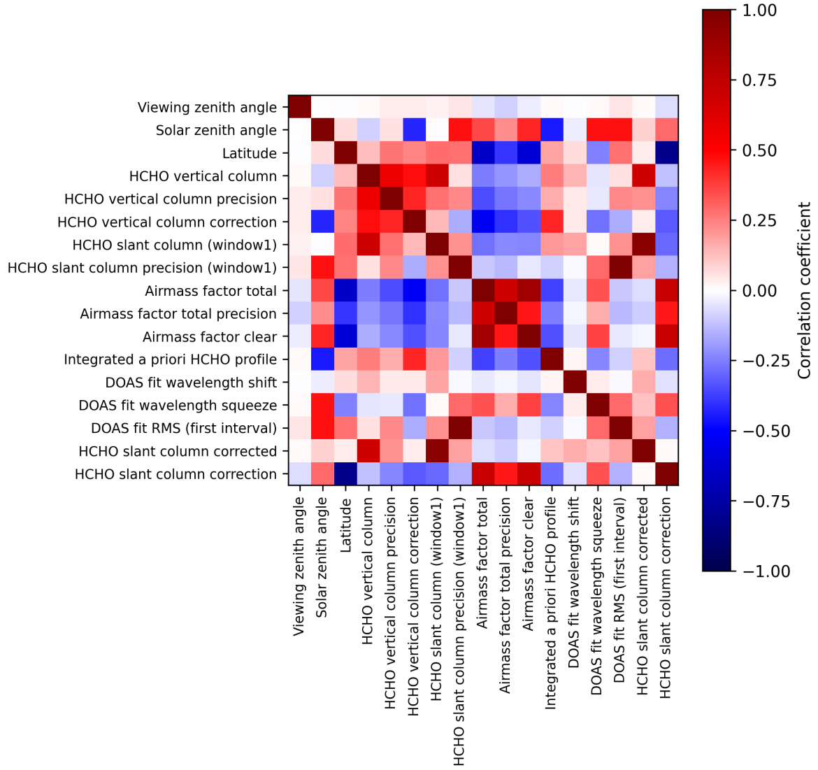
Figure 2: Map of correlation matrix for 2025-01-02 to 2025-01-04.
