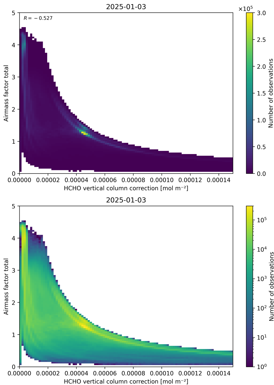
Figure 120: Scatter density plot of “HCHO vertical column correction” against “Airmass factor total” for 2025-01-02 to 2025-01-04.
