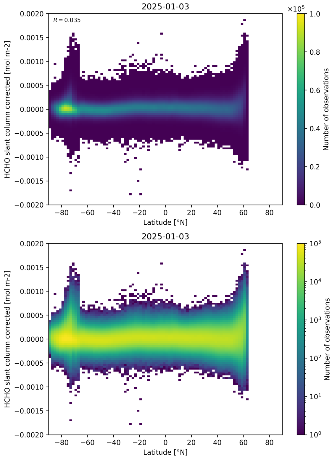
Figure 157: Scatter density plot of “Latitude” against “HCHO slant column corrected” for 2025-01-02 to 2025-01-04.
