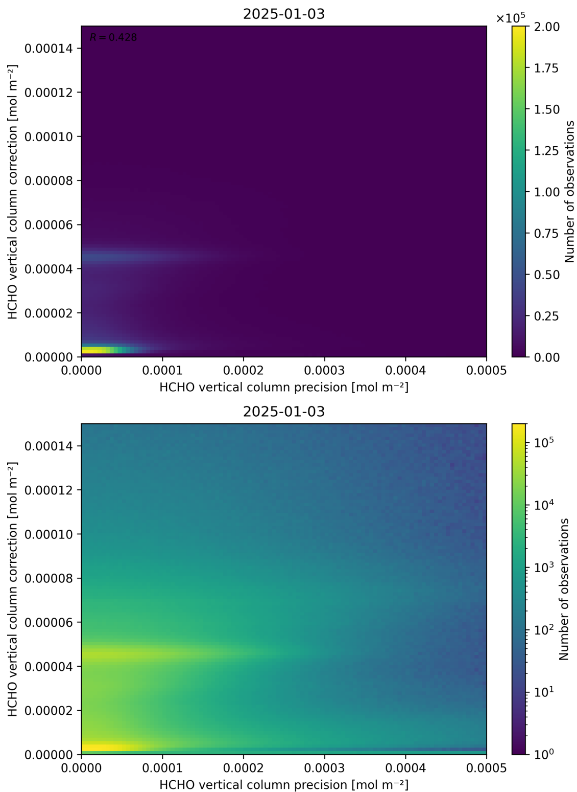
Figure 146: Scatter density plot of “HCHO vertical column precision” against “HCHO vertical column correction” for 2025-01-02 to 2025-01-04.
