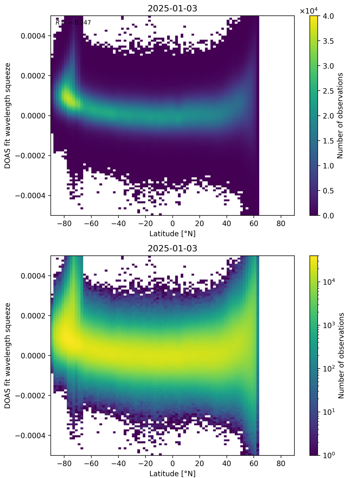
Figure 155: Scatter density plot of “Latitude” against “DOAS fit wavelength squeeze” for 2025-01-02 to 2025-01-04.
