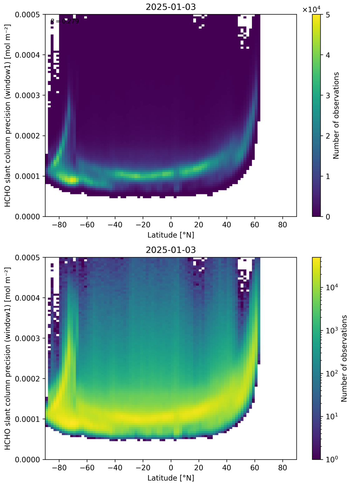
Figure 160: Scatter density plot of “Latitude” against “HCHO slant column precision (window1)” for 2025-01-02 to 2025-01-04.
