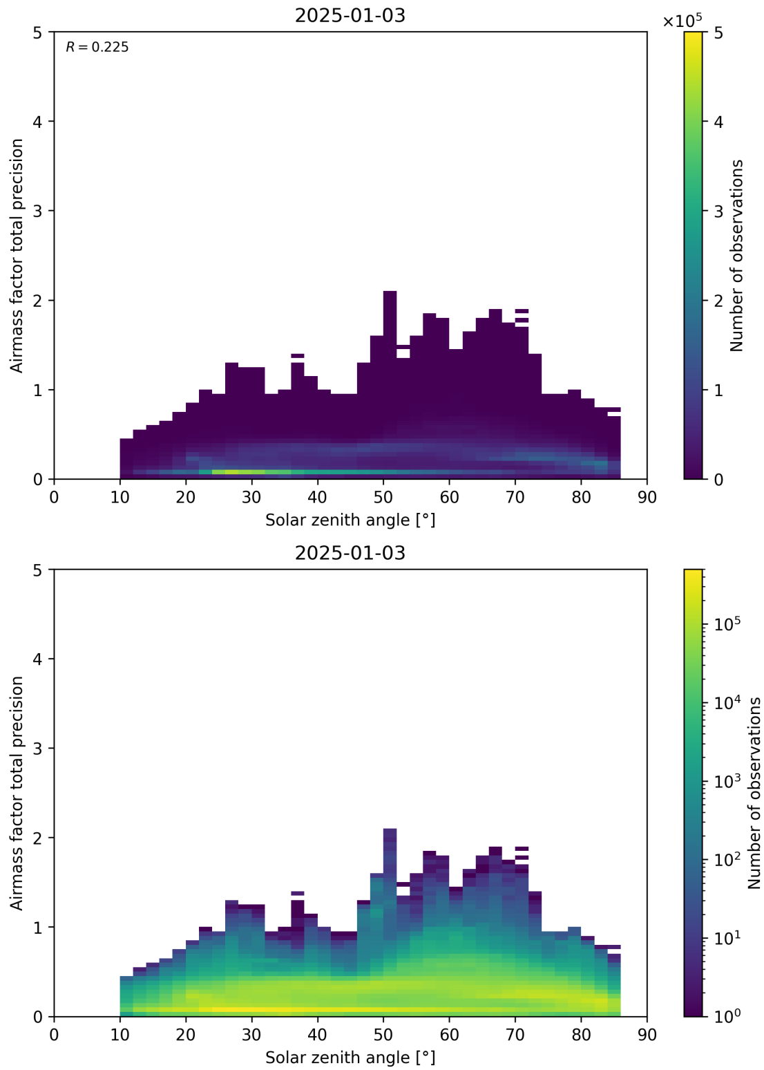
Figure 176: Scatter density plot of “Solar zenith angle” against “Airmass factor total precision” for 2025-01-02 to 2025-01-04.
