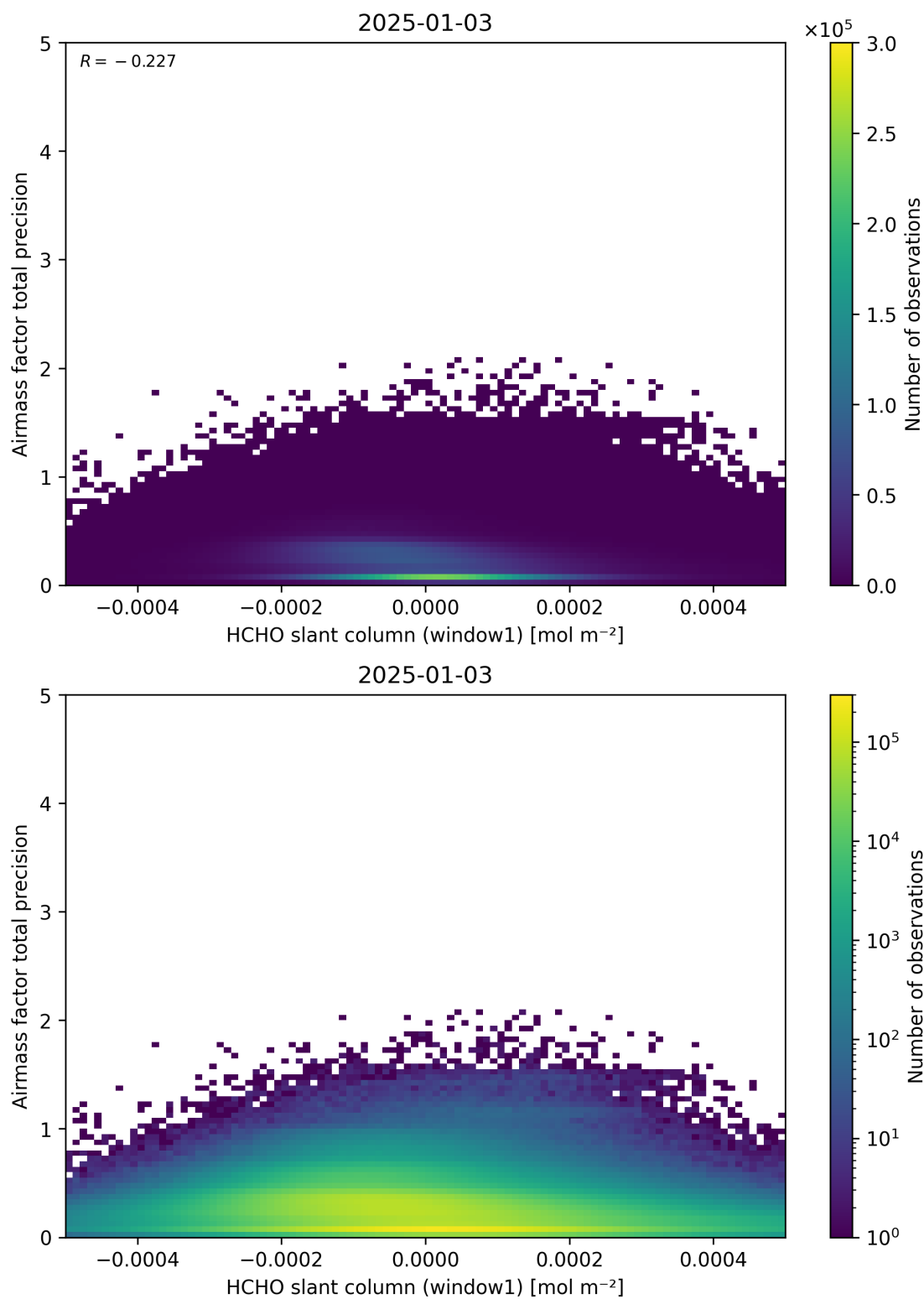
Figure 86: Scatter density plot of “HCHO slant column (window1)” against “Airmass factor total precision” for 2025-01-02 to 2025-01-04.
