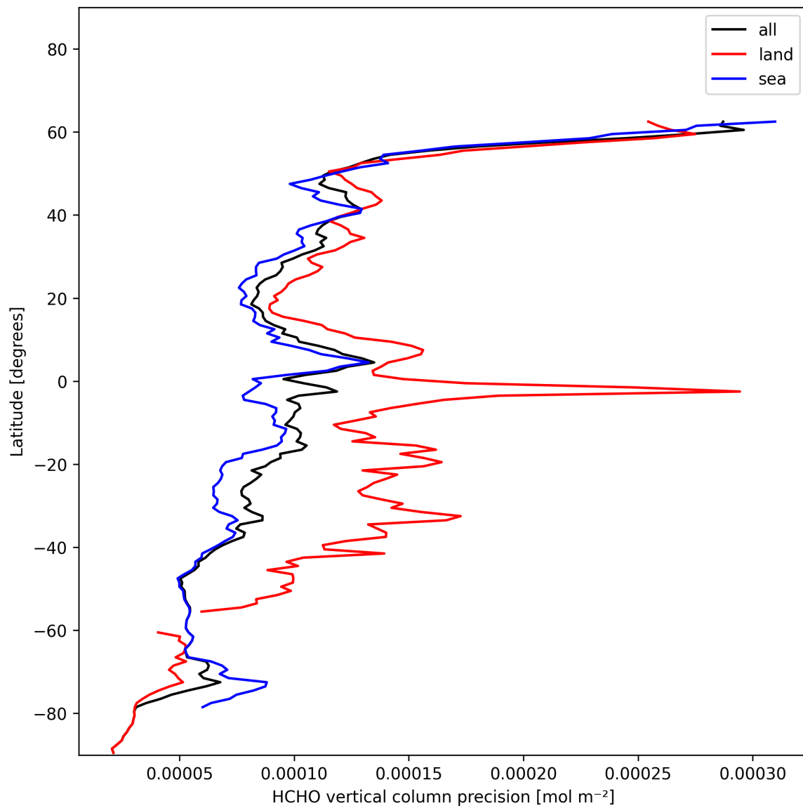
Figure 22: Zonal average of “HCHO vertical column precision” for 2025-01-02 to 2025-01-04.
