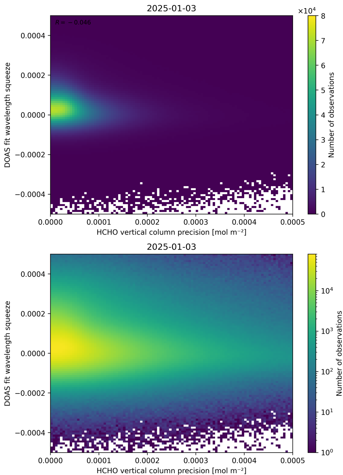
Figure 138: Scatter density plot of “HCHO vertical column precision” against “DOAS fit wavelength squeeze” for 2025-01-02 to 2025-01-04.
