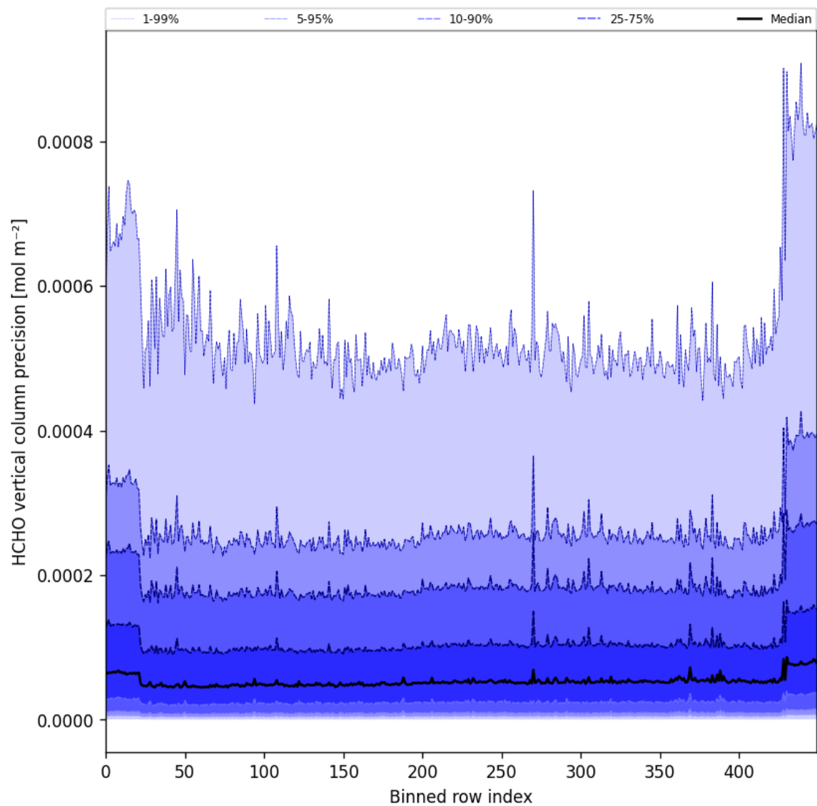
Figure 50: Along track statistics of “HCHO vertical column precision” for 2025-01-02 to 2025-01-04
