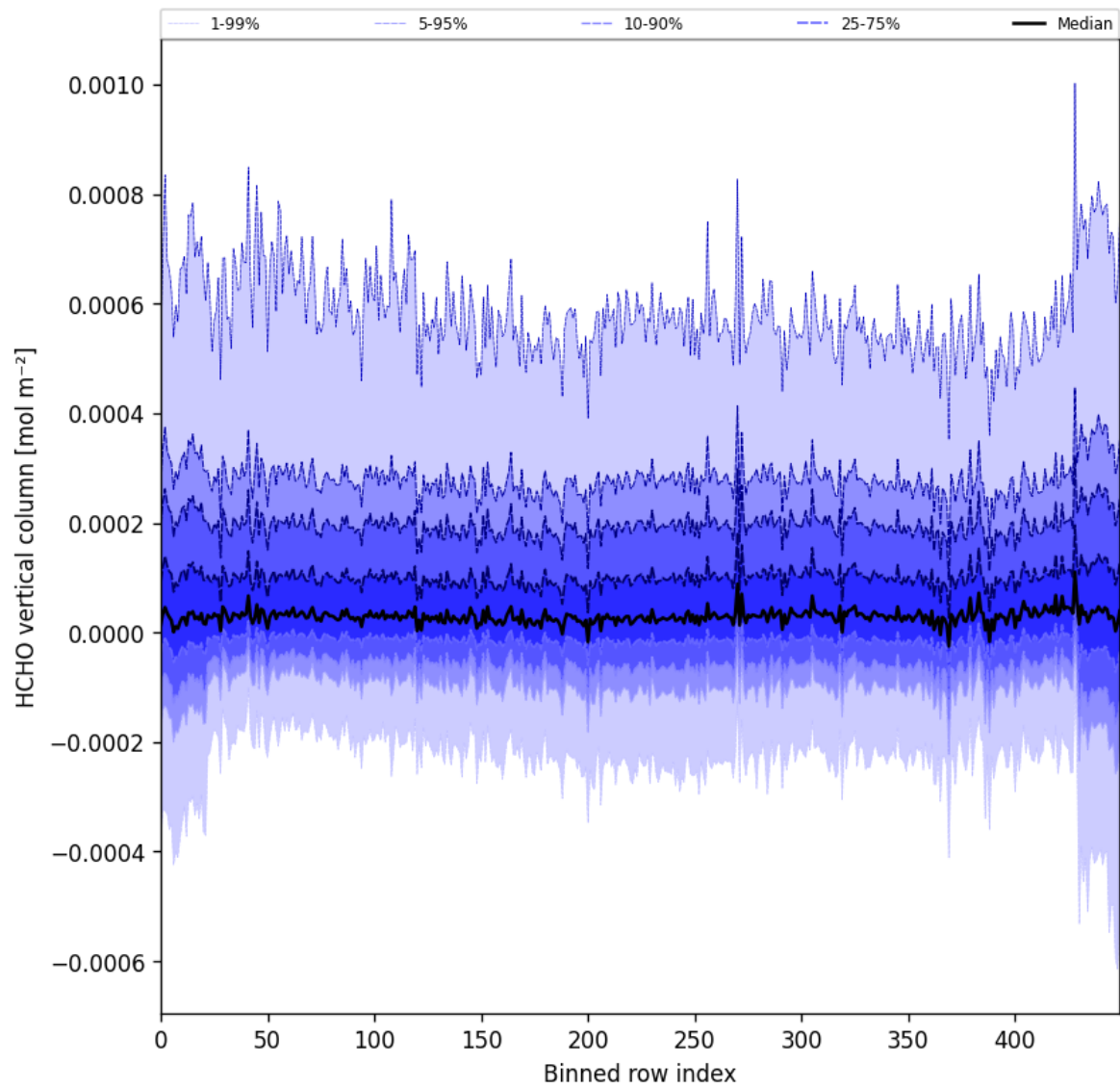
Figure 49: Along track statistics of “HCHO vertical column” for 2025-01-02 to 2025-01-04
