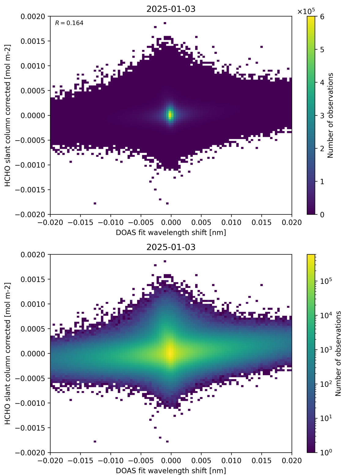
Figure 66: Scatter density plot of “DOAS fit wavelength shift” against “HCHO slant column corrected” for 2025-01-02 to 2025-01-04.
