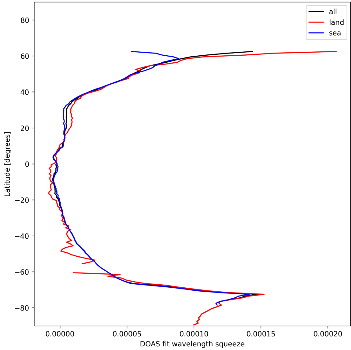
Figure 31: Zonal average of “DOAS fit wavelength squeeze” for 2025-01-02 to 2025-01-04.
