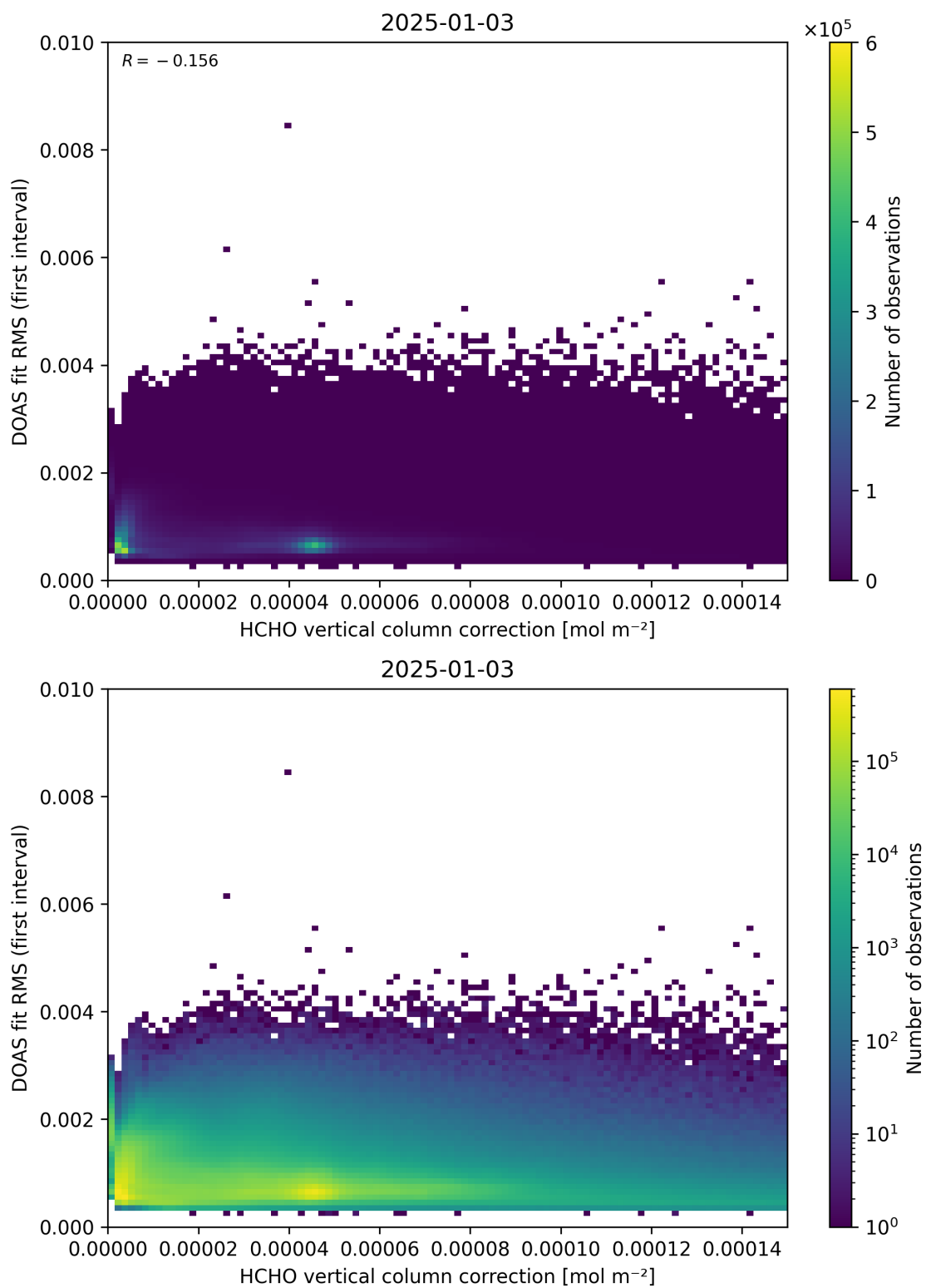
Figure 112: Scatter density plot of “HCHO vertical column correction” against “DOAS fit RMS (first interval)” for 2025-01-02 to 2025-01-04.
