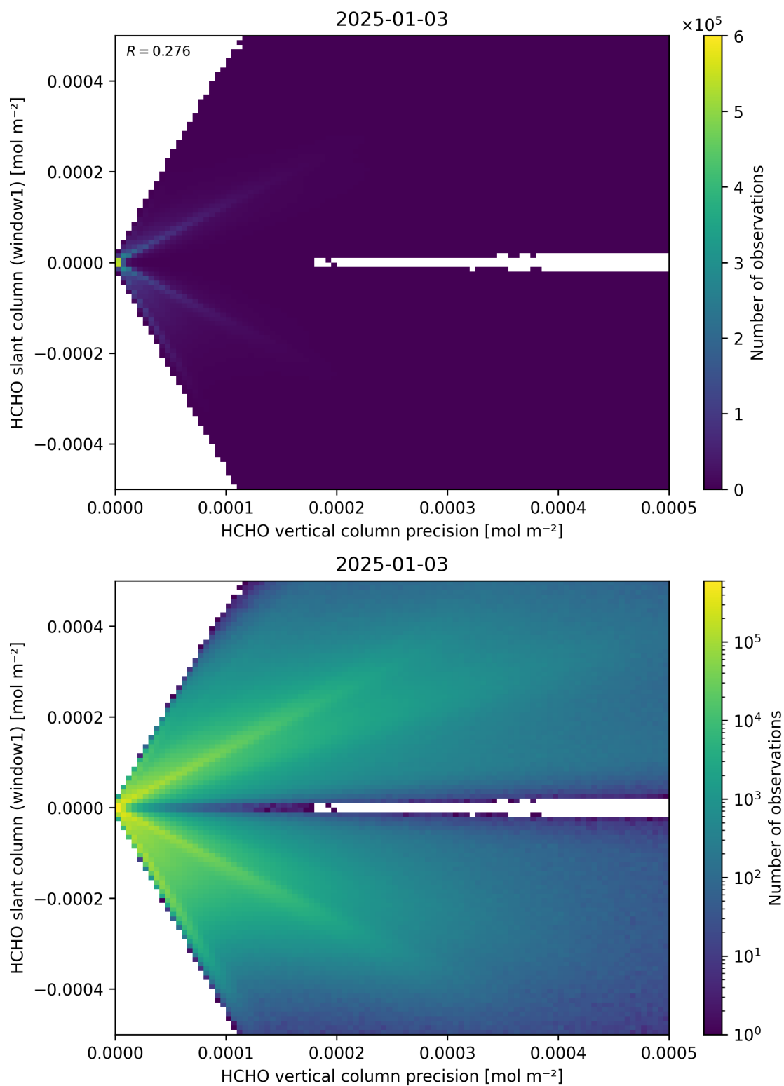
Figure 142: Scatter density plot of “HCHO vertical column precision” against “HCHO slant column (window1)” for 2025-01-02 to 2025-01-04.
