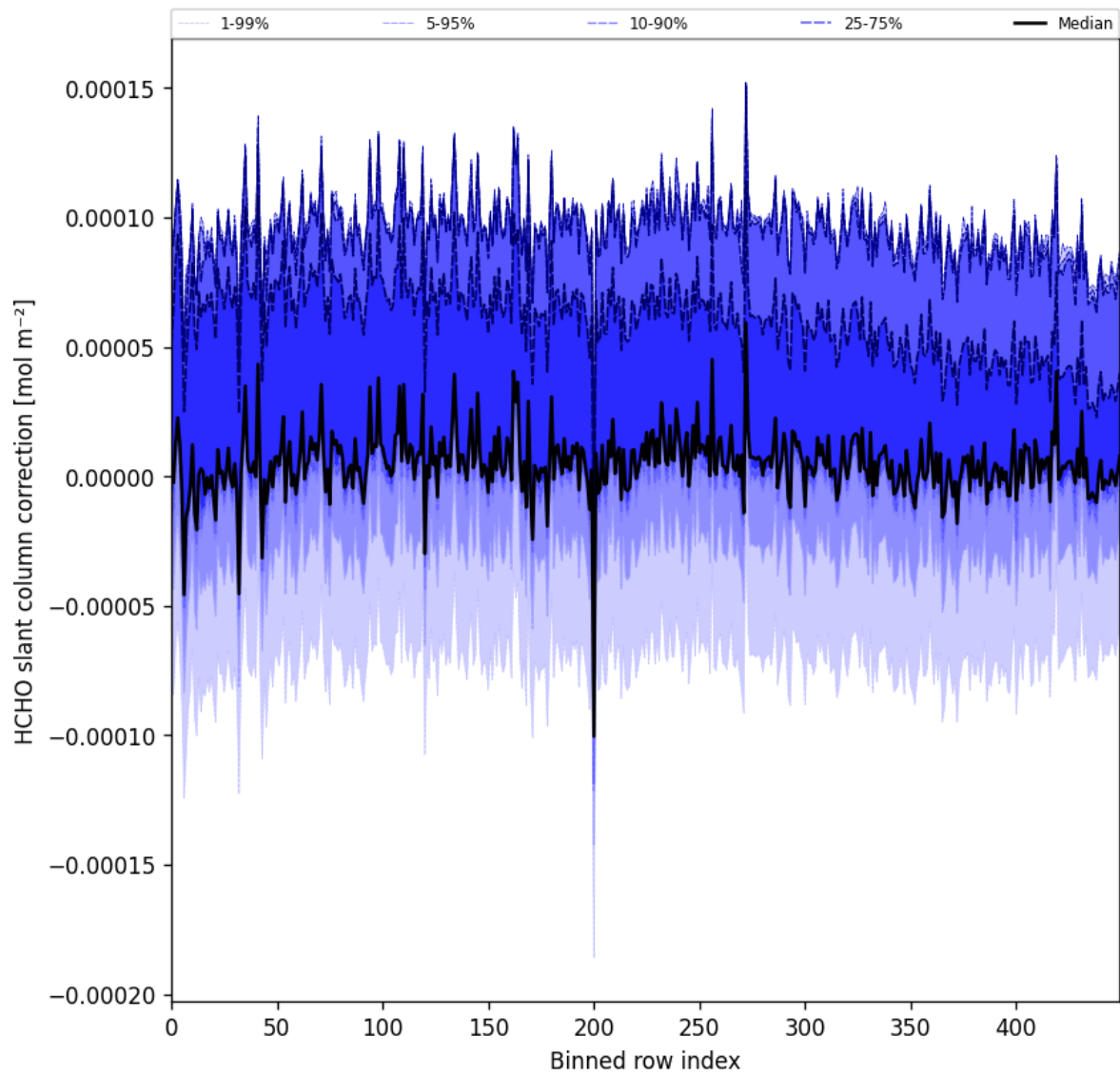
Figure 61: Along track statistics of “HCHO slant column correction” for 2025-01-02 to 2025-01-04
