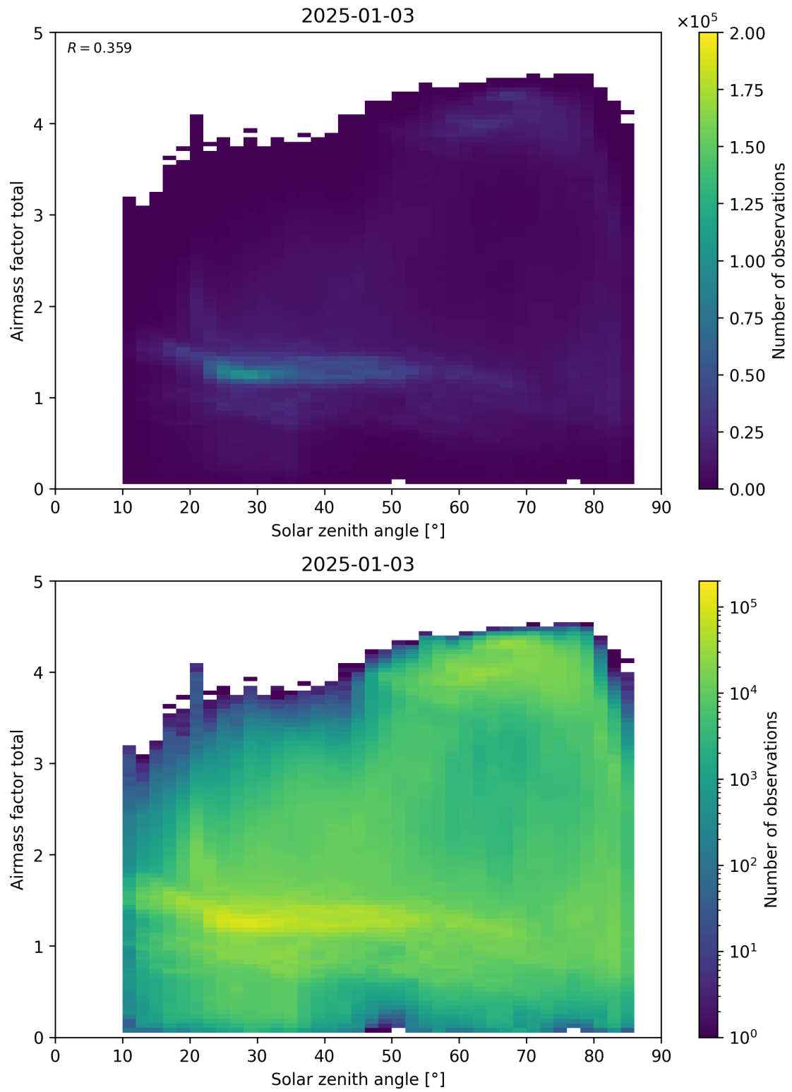
Figure 175: Scatter density plot of “Solar zenith angle” against “Airmass factor total” for 2025-01-02 to 2025-01-04.
