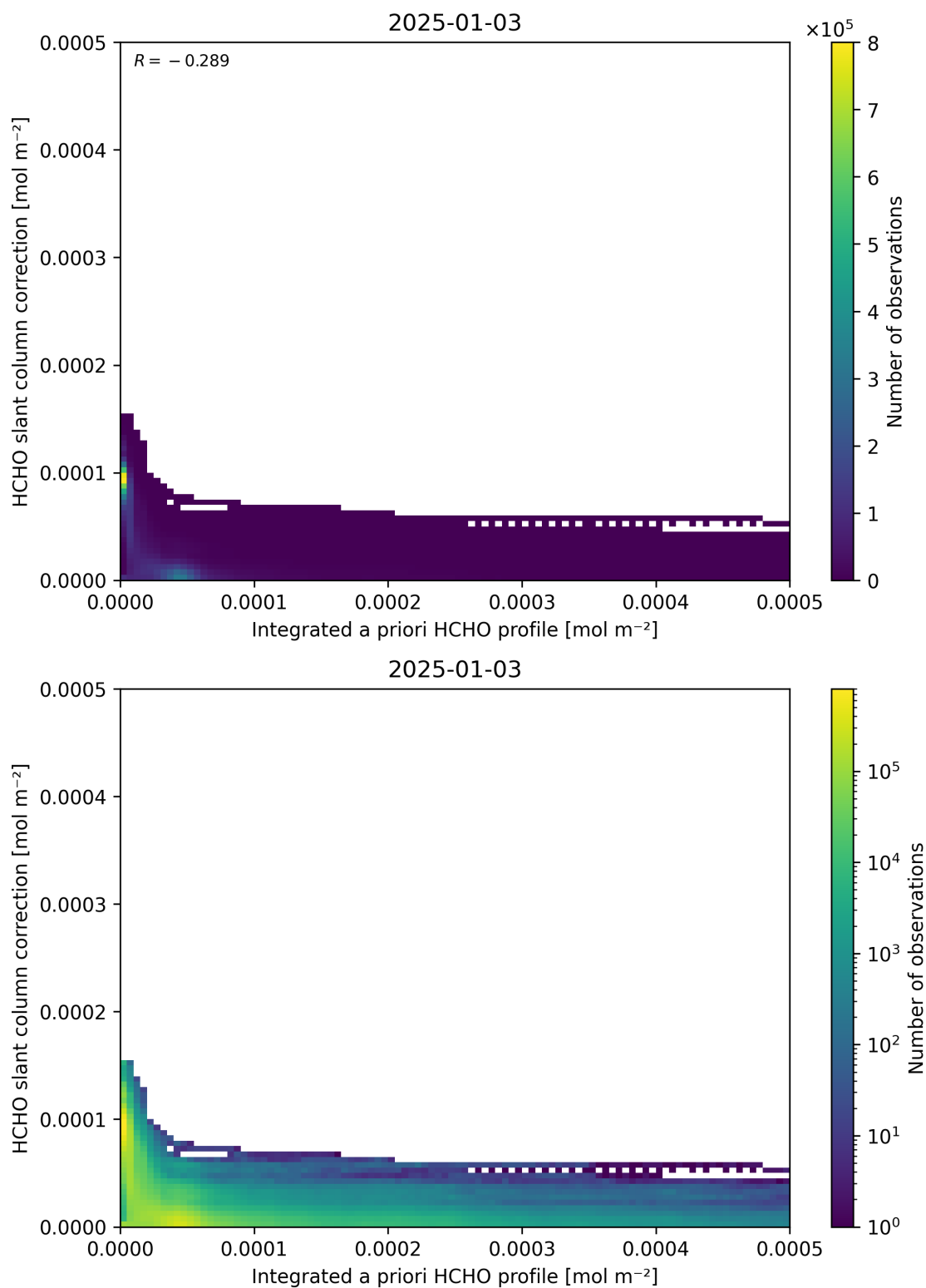
Figure 152: Scatter density plot of “Integrated a priori HCHO profile” against “HCHO slant column correction” for 2025-01-02 to 2025-01-04.
