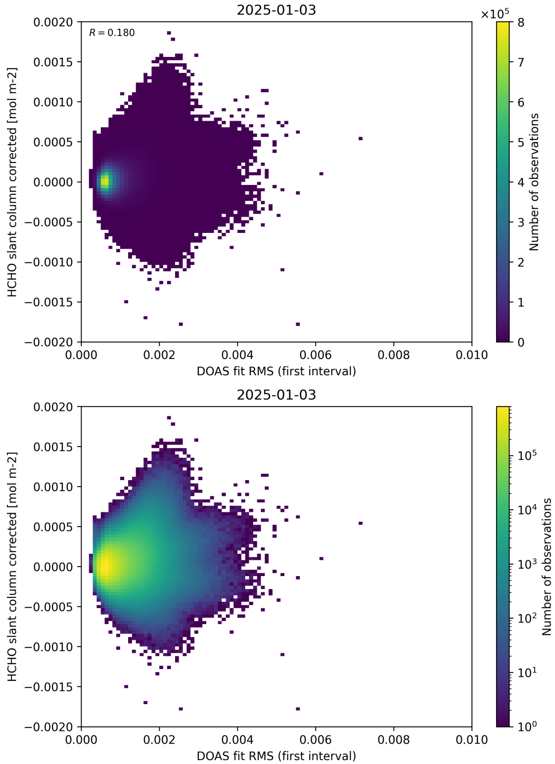
Figure 62: Scatter density plot of “DOAS fit RMS (first interval)” against “HCHO slant column corrected” for 2025-01-02 to 2025-01-04.
