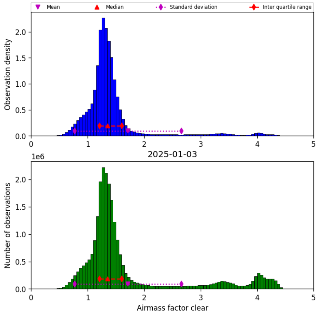
Figure 42: Histogram of “Airmass factor clear” for 2025-01-02 to 2025-01-04
