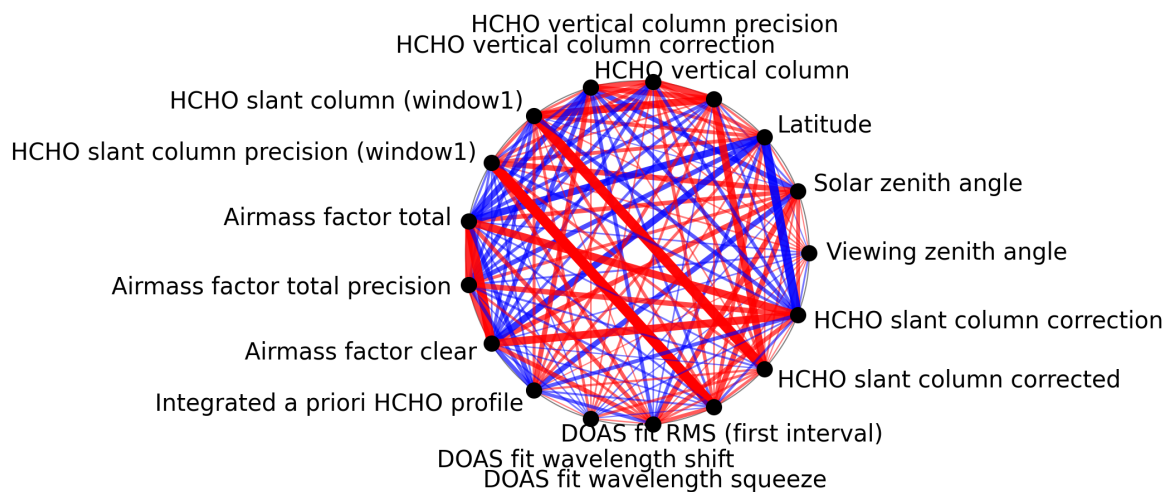
Figure 1: Map of correlation graph for 2025-01-02 to 2025-01-04.
