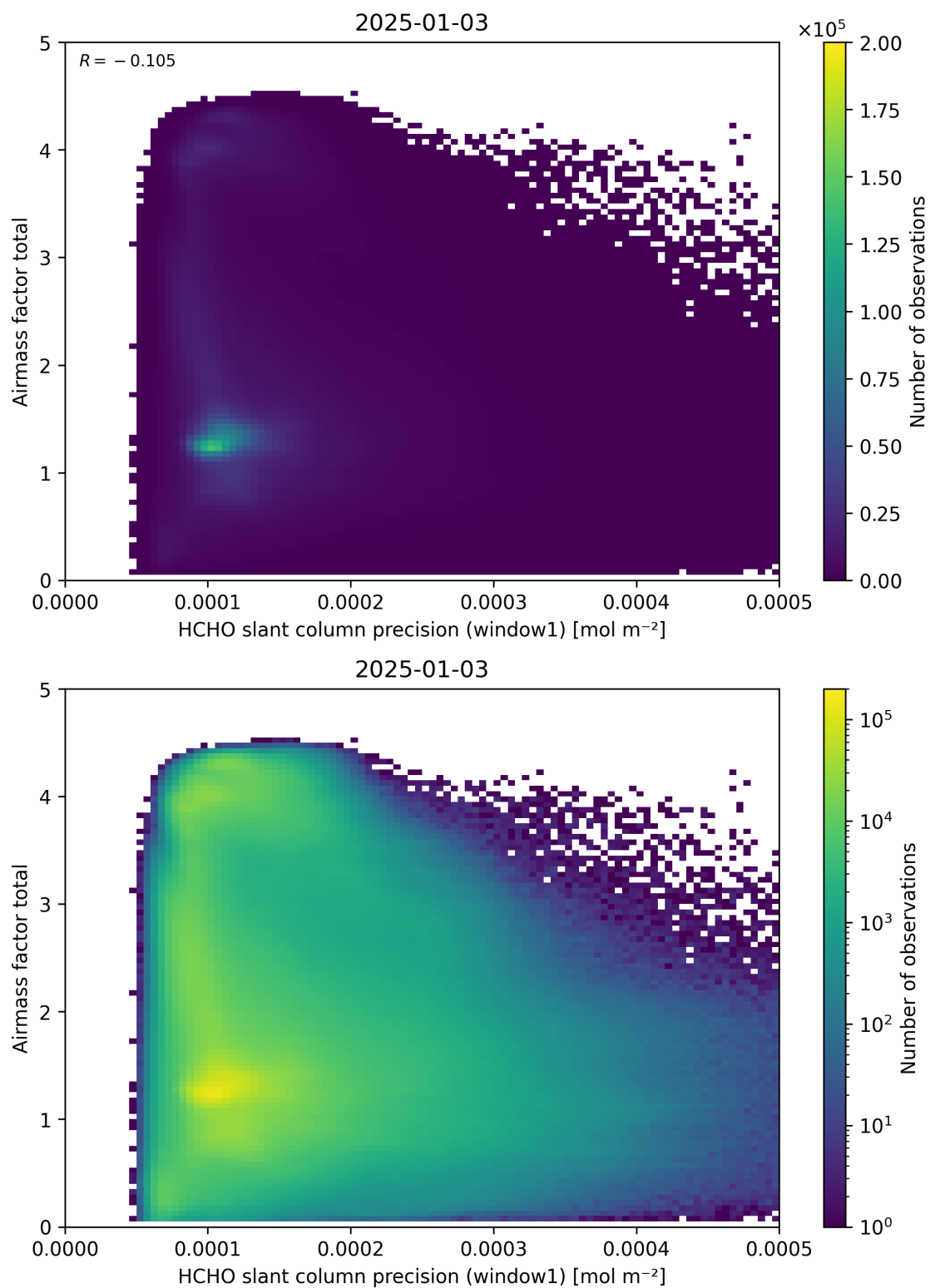
Figure 94: Scatter density plot of “HCHO slant column precision (window1)” against “Airmass factor total” for 2025-01-02 to 2025-01-04.
