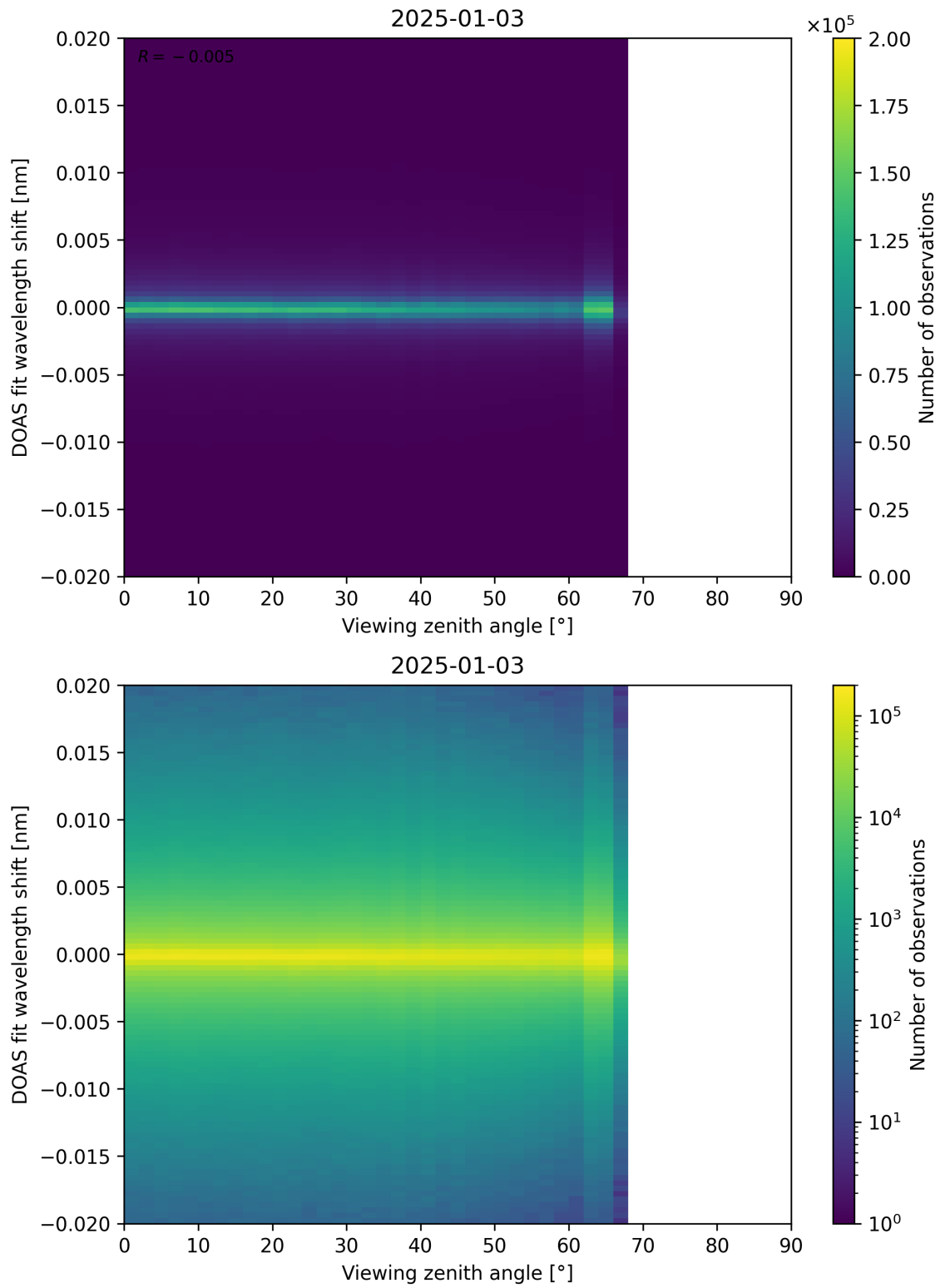
Figure 183: Scatter density plot of “Viewing zenith angle” against “DOAS fit wavelength shift” for 2025-01-02 to 2025-01-04.
