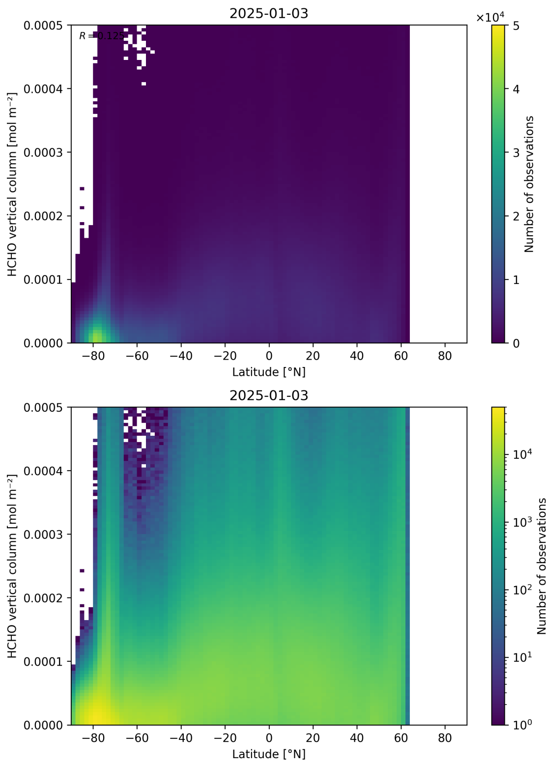
Figure 163: Scatter density plot of “Latitude” against “HCHO vertical column” for 2025-01-02 to 2025-01-04.
