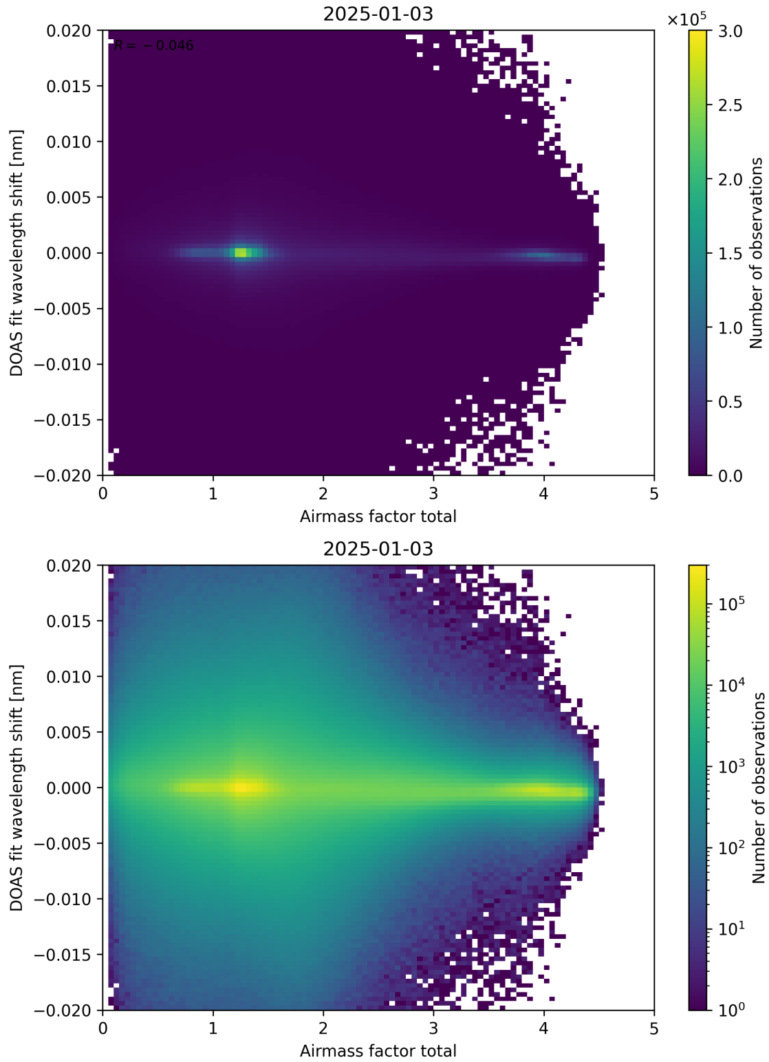
Figure 98: Scatter density plot of “Airmass factor total” against “DOAS fit wavelength shift” for 2025-01-02 to 2025-01-04.
