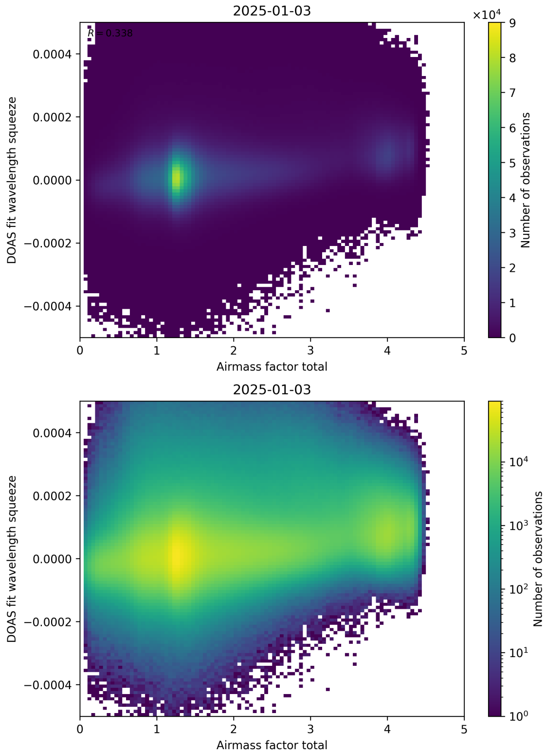
Figure 99: Scatter density plot of “Airmass factor total” against “DOAS fit wavelength squeeze” for 2025-01-02 to 2025-01-04.
