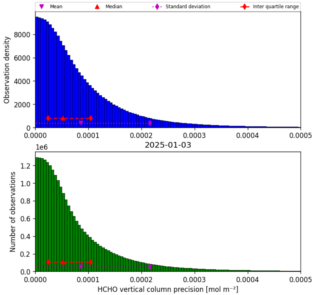
Figure 36: Histogram of “HCHO vertical column precision” for 2025-01-02 to 2025-01-04
