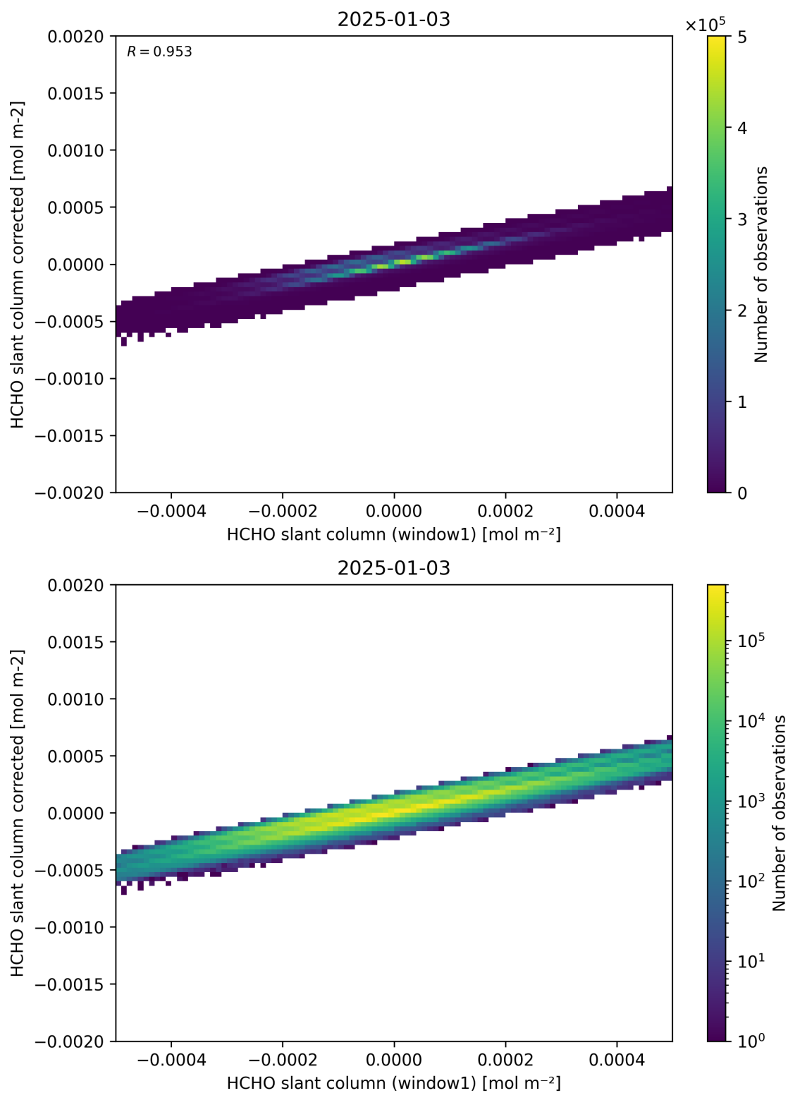
Figure 82: Scatter density plot of “HCHO slant column (window1)” against “HCHO slant column corrected” for 2025-01-02 to 2025-01-04.
