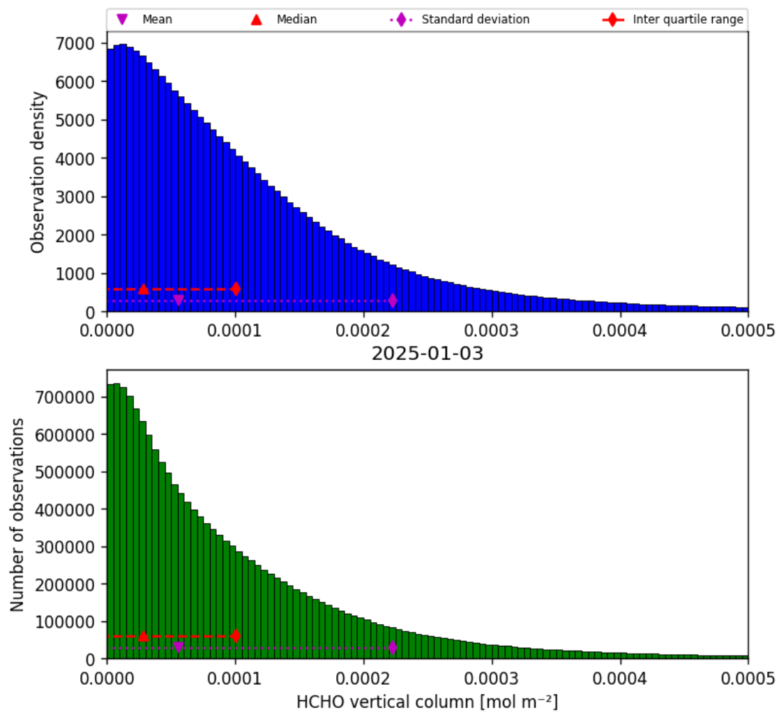
Figure 35: Histogram of “HCHO vertical column” for 2025-01-02 to 2025-01-04
