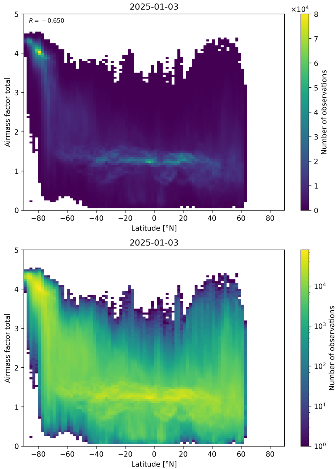
Figure 161: Scatter density plot of “Latitude” against “Airmass factor total” for 2025-01-02 to 2025-01-04.
