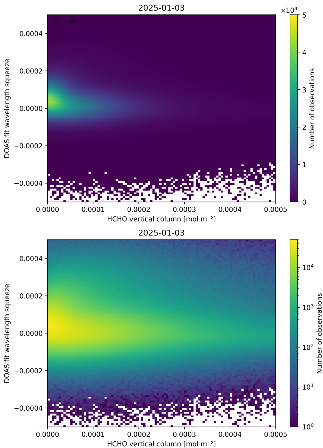
Figure 125: Scatter density plot of “HCHO vertical column” against “DOAS fit wavelength squeeze” for 2025-01-02 to 2025-01-04.
