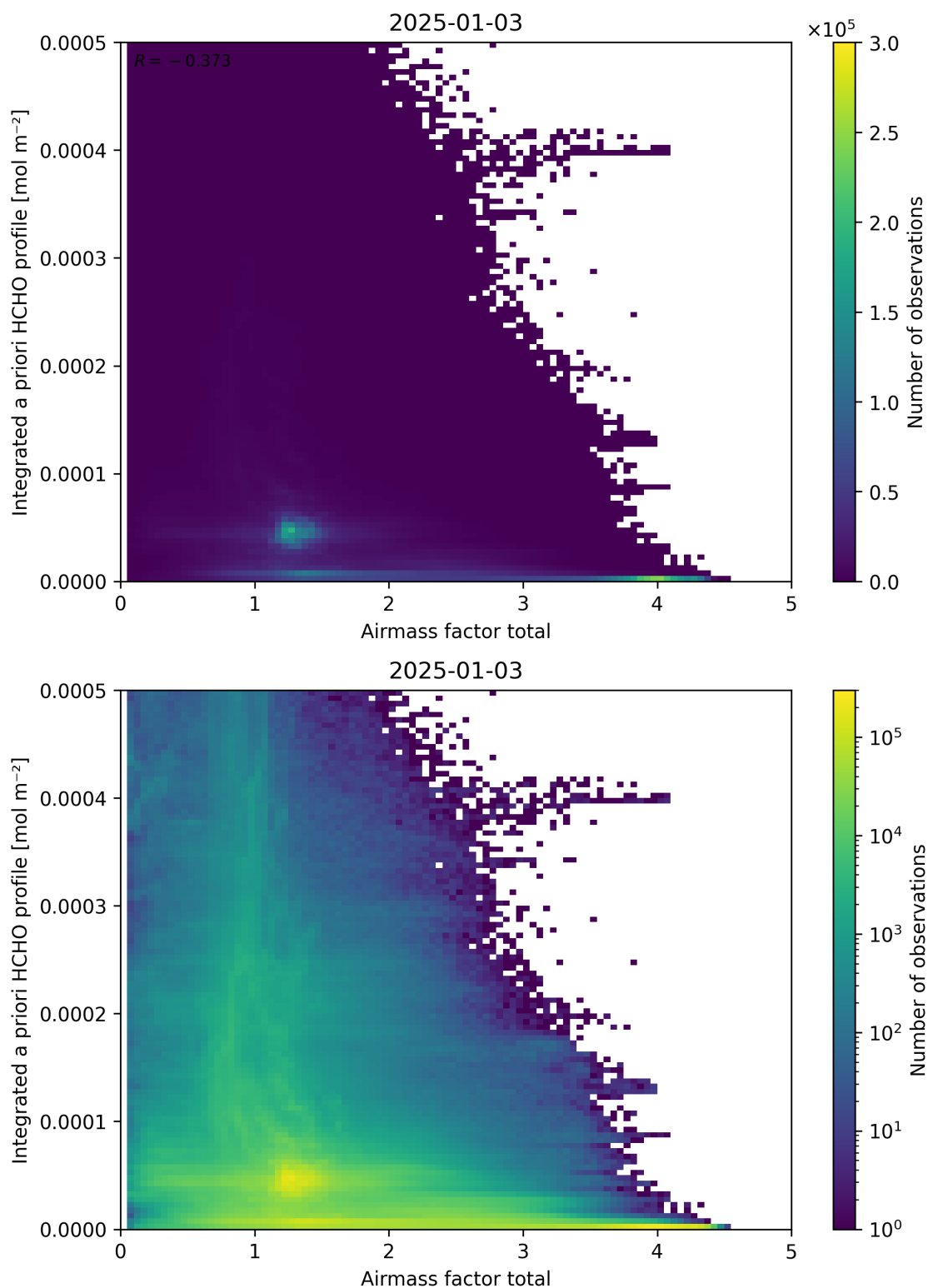
Figure 104: Scatter density plot of “Airmass factor total” against “Integrated a priori HCHO profile” for 2025-01-02 to 2025-01-04.
