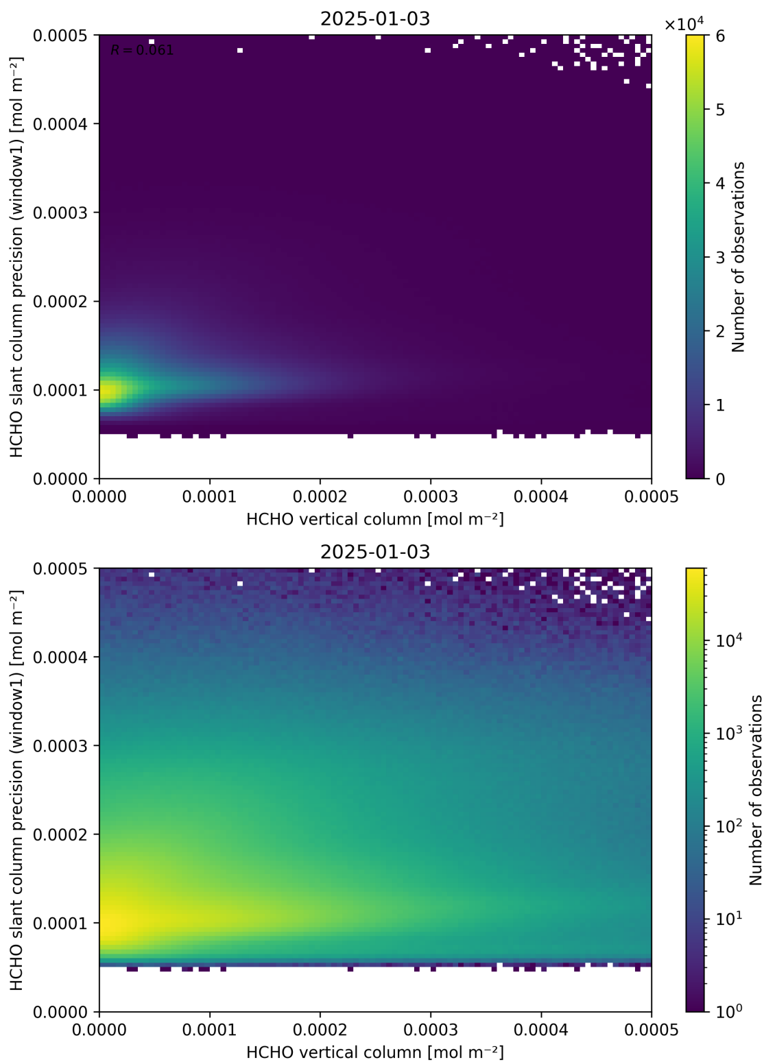
Figure 130: Scatter density plot of “HCHO vertical column” against “HCHO slant column precision (window1)” for 2025-01-02 to 2025-01-04.
