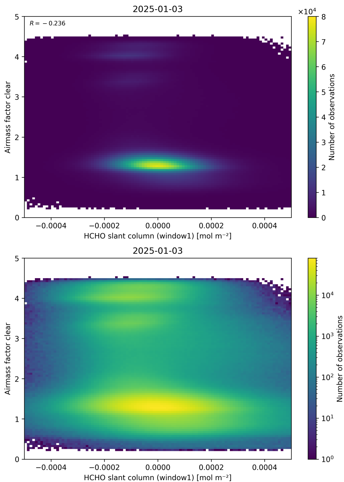
Figure 81: Scatter density plot of “HCHO slant column (window1)” against “Airmass factor clear” for 2025-01-02 to 2025-01-04.
