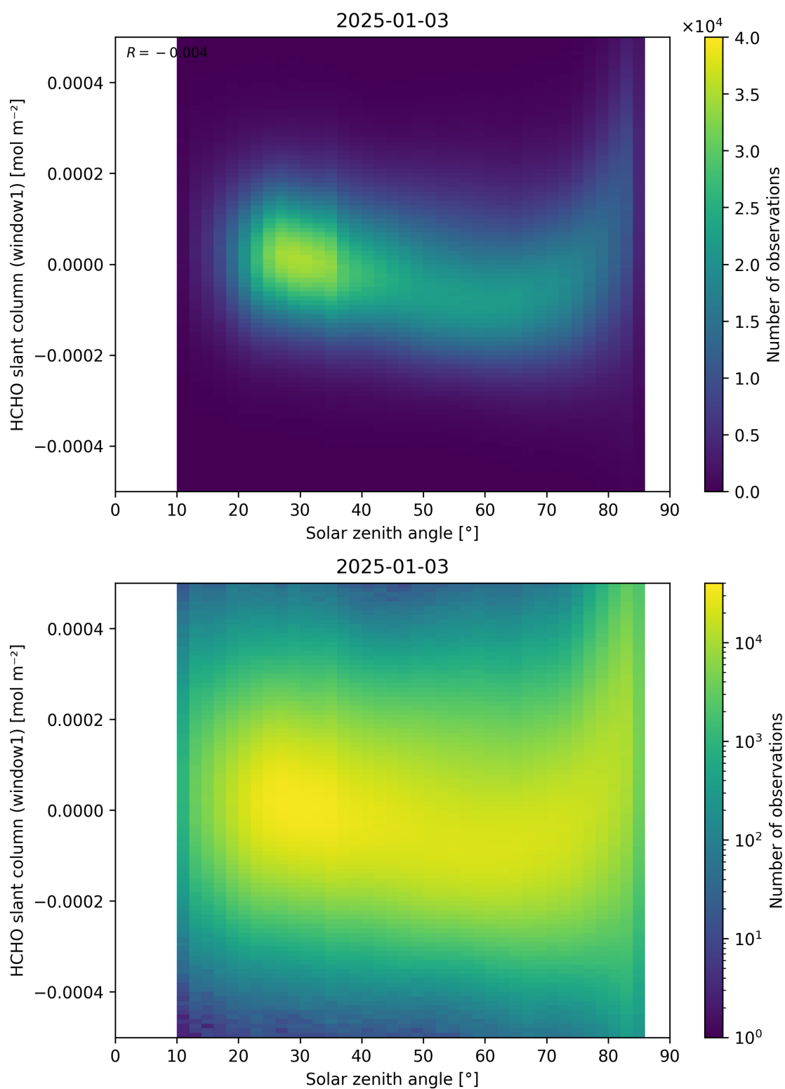
Figure 173: Scatter density plot of “Solar zenith angle” against “HCHO slant column (window1)” for 2025-01-02 to 2025-01-04.
