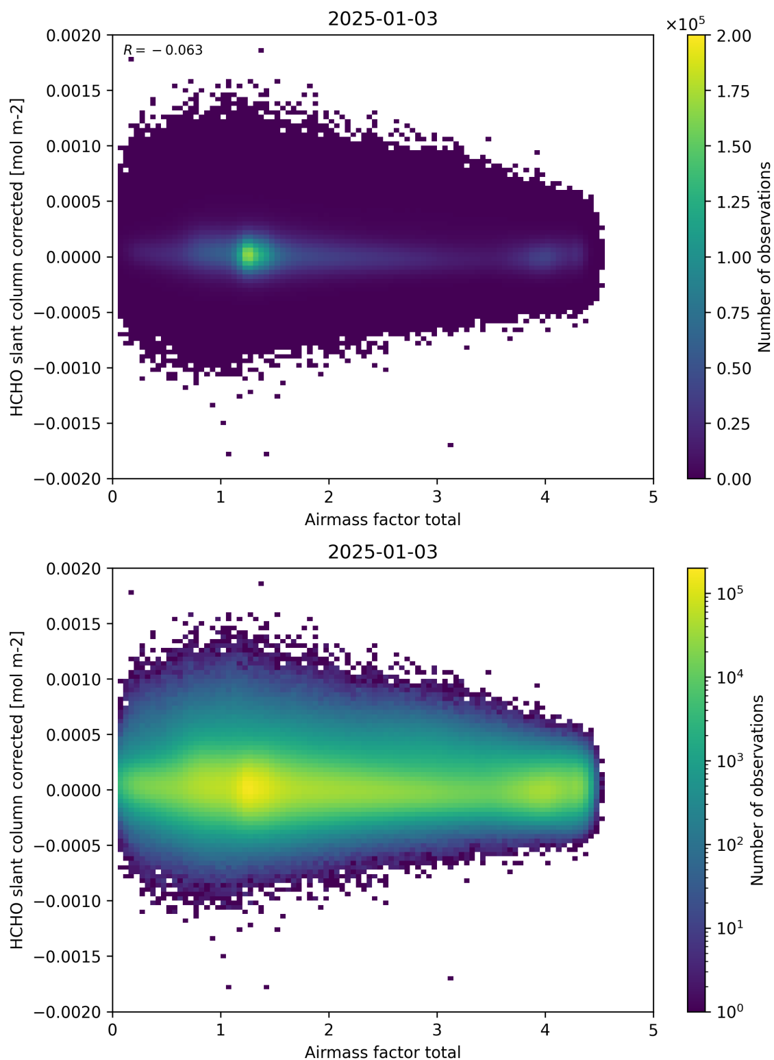
Figure 101: Scatter density plot of “Airmass factor total” against “HCHO slant column corrected” for 2025-01-02 to 2025-01-04.
