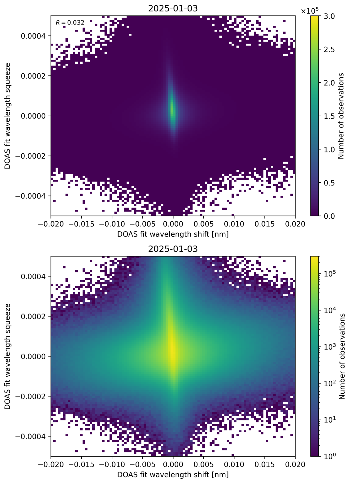
Figure 65: Scatter density plot of “DOAS fit wavelength shift” against “DOAS fit wavelength squeeze” for 2025-01-02 to 2025-01-04.
