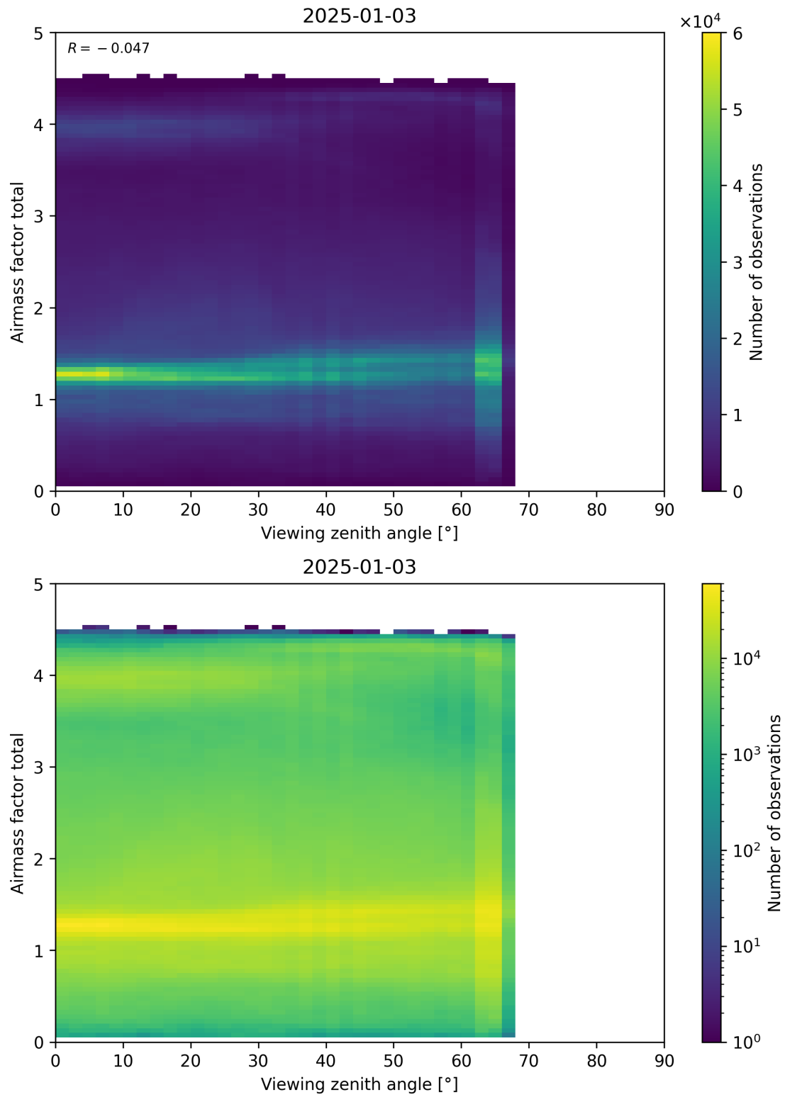
Figure 190: Scatter density plot of “Viewing zenith angle” against “Airmass factor total” for 2025-01-02 to 2025-01-04.
