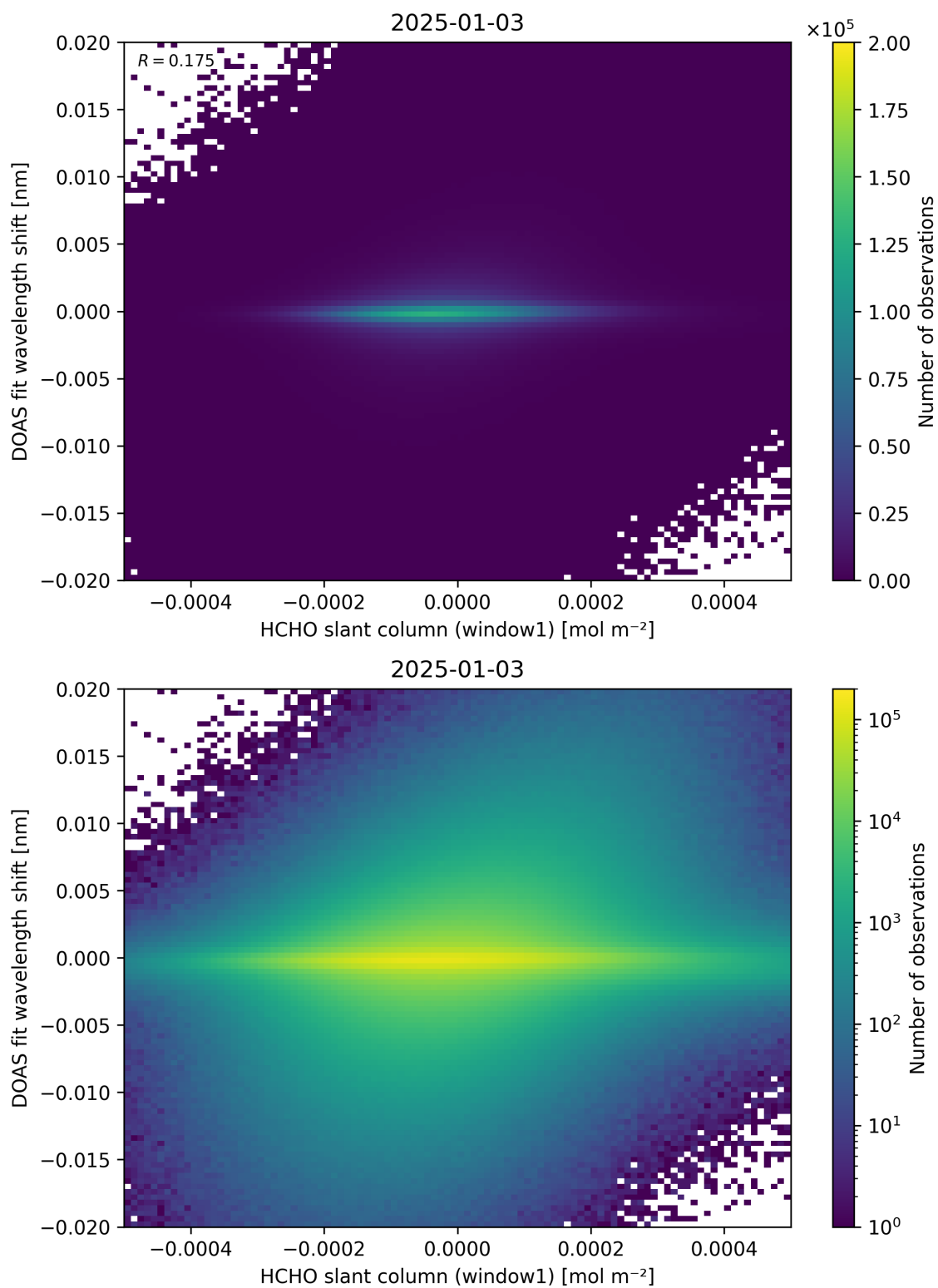
Figure 79: Scatter density plot of “HCHO slant column (window1)” against “DOAS fit wavelength shift” for 2025-01-02 to 2025-01-04.
