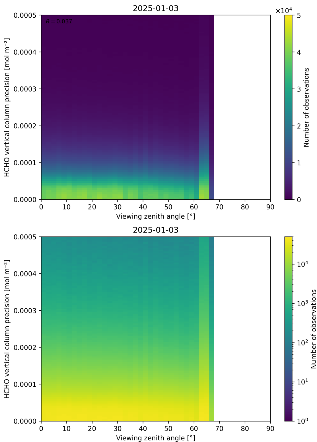
Figure 194: Scatter density plot of “Viewing zenith angle” against “HCHO vertical column precision” for 2025-01-02 to 2025-01-04.
