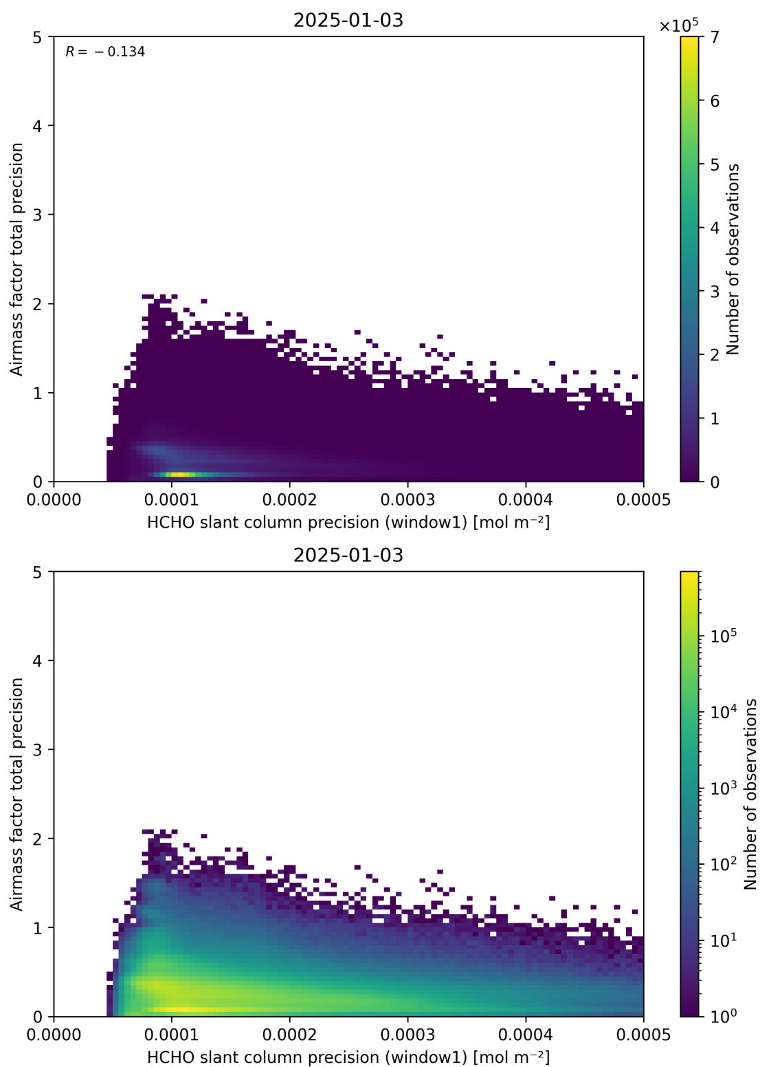
Figure 95: Scatter density plot of “HCHO slant column precision (window1)” against “Airmass factor total precision” for 2025-01-02 to 2025-01-04.
