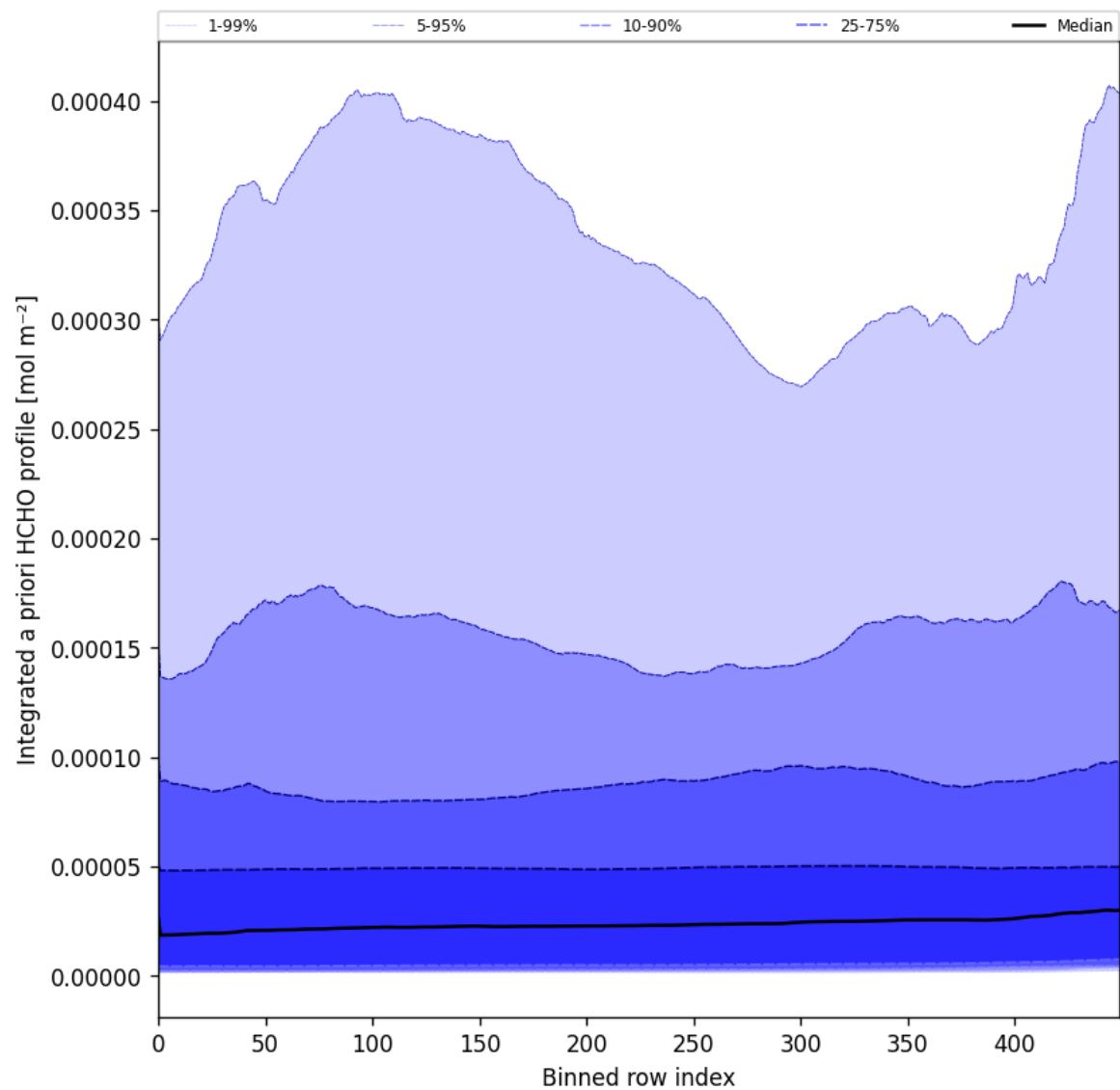
Figure 57: Along track statistics of "Integrated a priori HCHO profile" for 2025-01-02 to 2025-01-04
