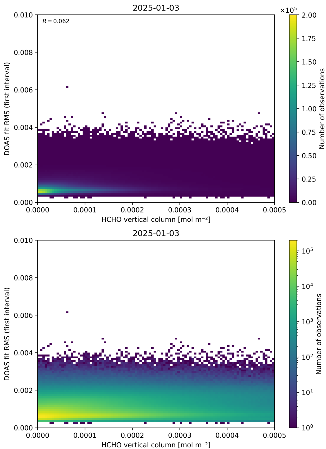
Figure 123: Scatter density plot of “HCHO vertical column” against “DOAS fit RMS (first interval)” for 2025-01-02 to 2025-01-04.
