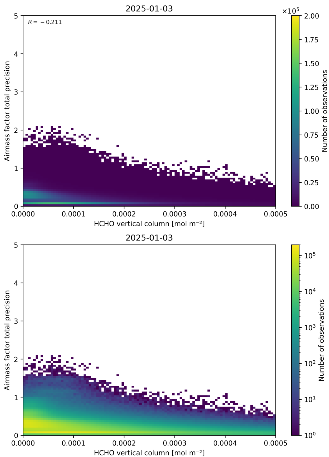
Figure 132: Scatter density plot of “HCHO vertical column” against “Airmass factor total precision” for 2025-01-02 to 2025-01-04.
