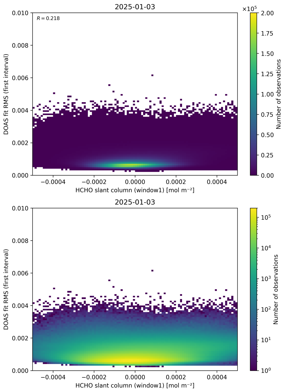
Figure 78: Scatter density plot of “HCHO slant column (window1)” against “DOAS fit RMS (first interval)” for 2025-01-02 to 2025-01-04.
