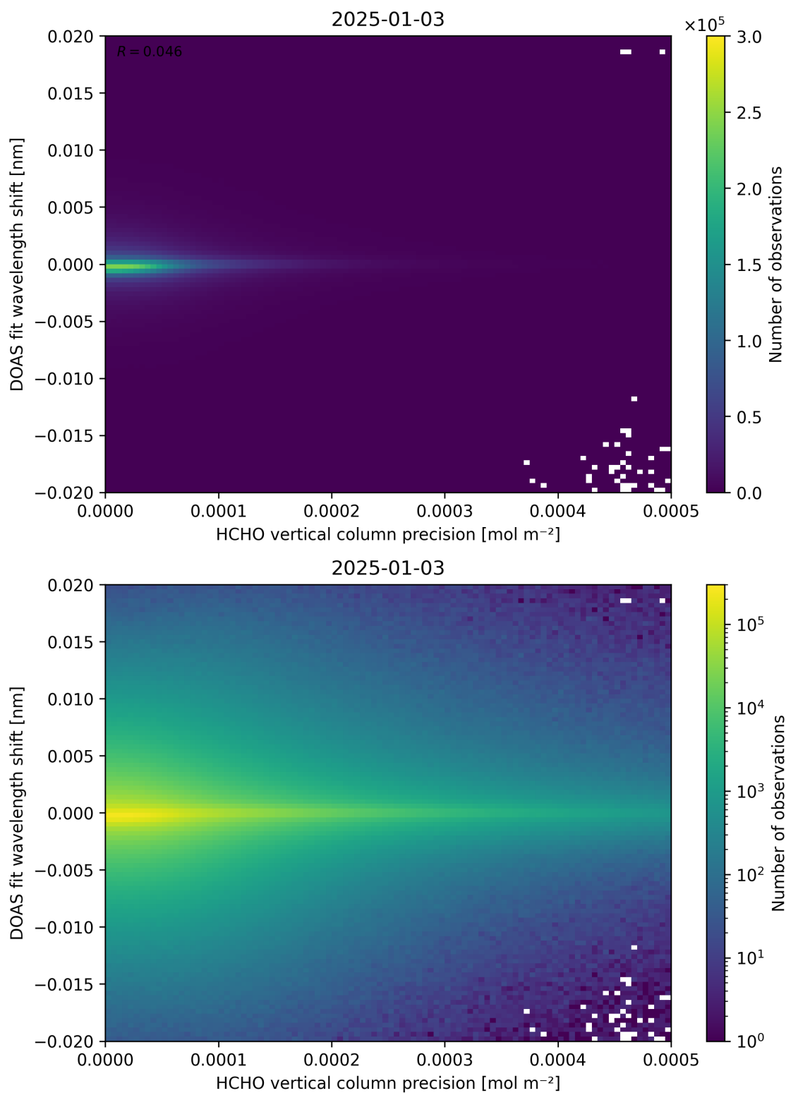
Figure 137: Scatter density plot of “HCHO vertical column precision” against “DOAS fit wavelength shift” for 2025-01-02 to 2025-01-04.
