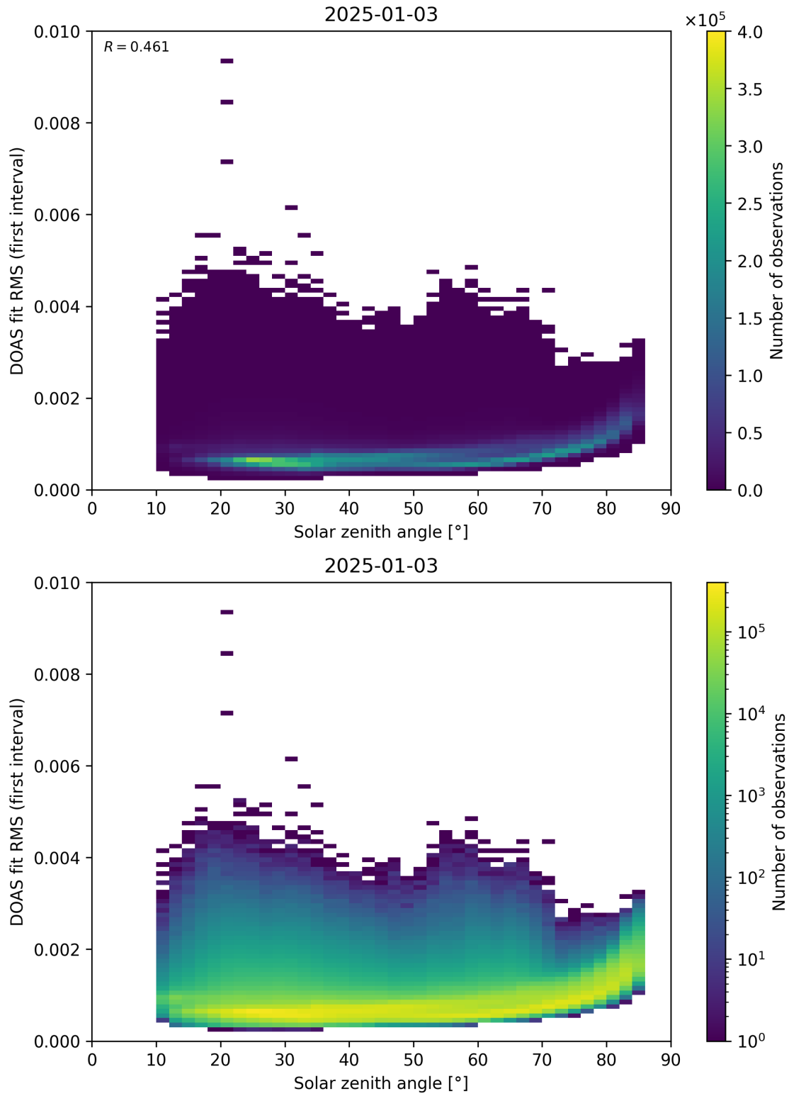
Figure 167: Scatter density plot of “Solar zenith angle” against “DOAS fit RMS (first interval)” for 2025-01-02 to 2025-01-04.
