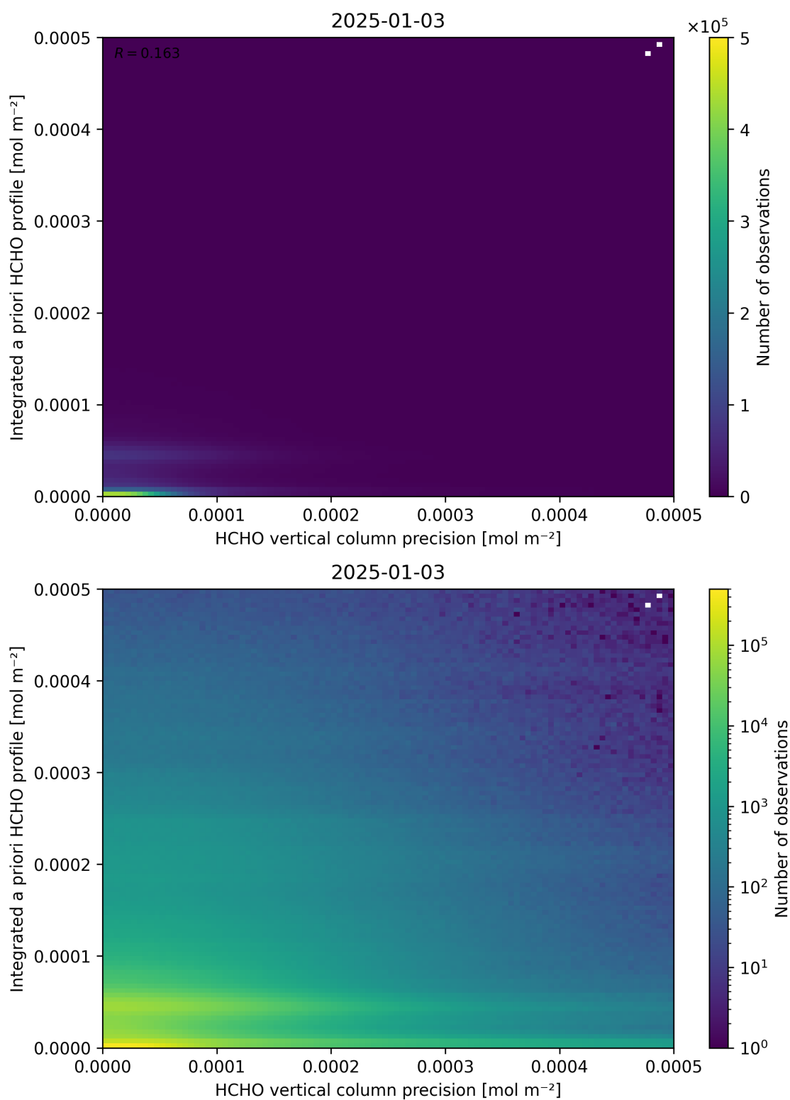
Figure 147: Scatter density plot of “HCHO vertical column precision” against “Integrated a priori HCHO profile” for 2025-01-02 to 2025-01-04.
