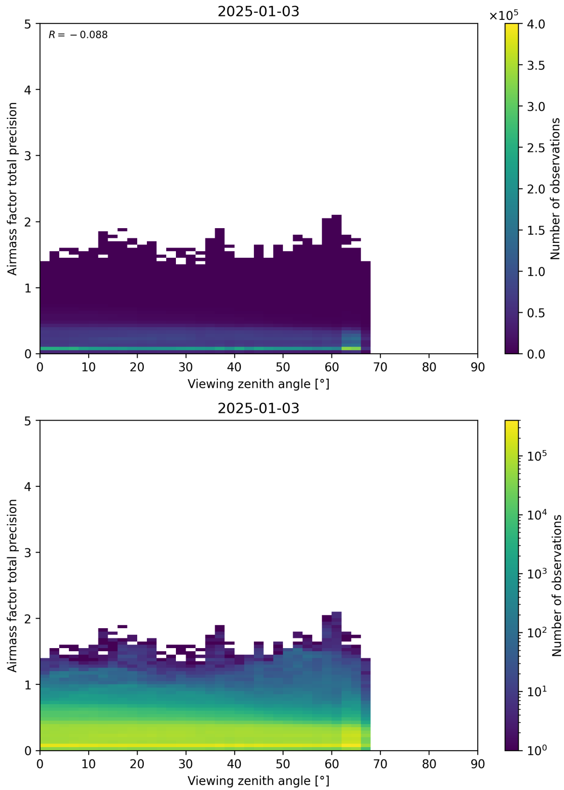
Figure 191: Scatter density plot of “Viewing zenith angle” against “Airmass factor total precision” for 2025-01-02 to 2025-01-04.
