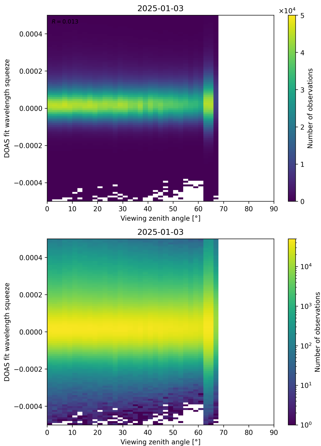
Figure 184: Scatter density plot of “Viewing zenith angle” against “DOAS fit wavelength squeeze” for 2025-01-02 to 2025-01-04.
