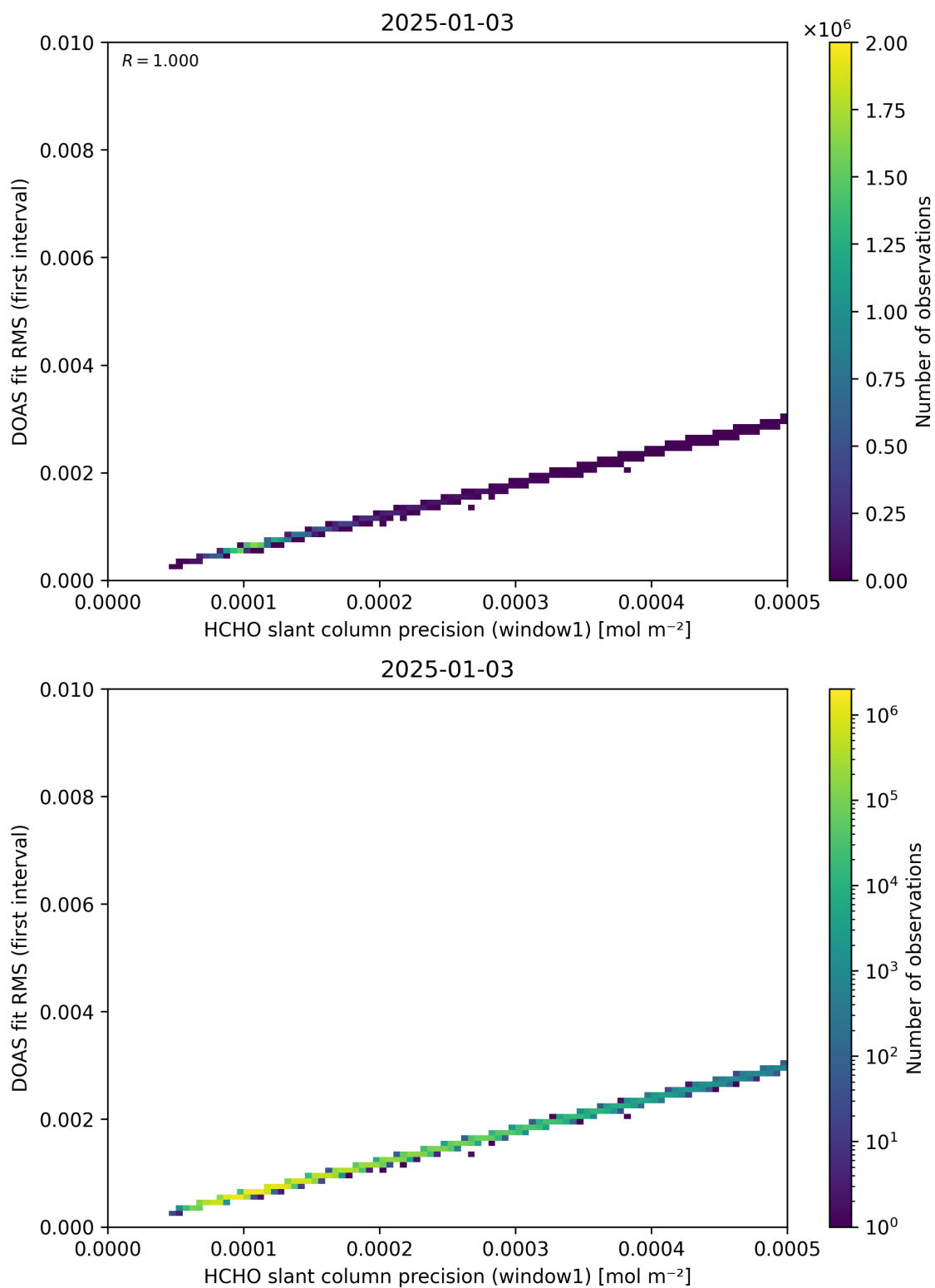
Figure 88: Scatter density plot of “HCHO slant column precision (window1)” against “DOAS fit RMS (first interval)” for 2025-01-02 to 2025-01-04.
