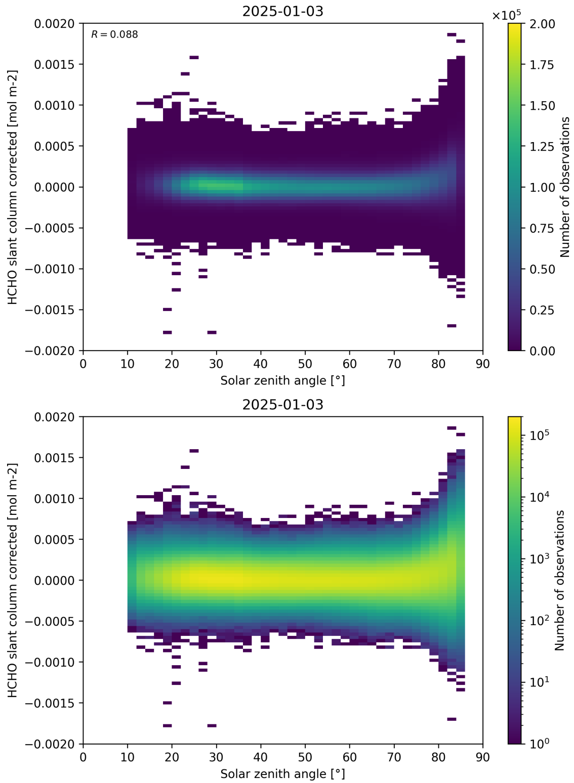
Figure 171: Scatter density plot of “Solar zenith angle” against “HCHO slant column corrected” for 2025-01-02 to 2025-01-04.
