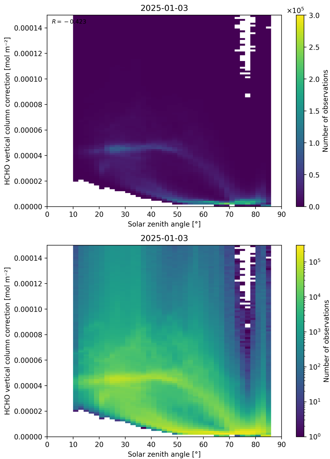
Figure 178: Scatter density plot of “Solar zenith angle” against “HCHO vertical column correction” for 2025-01-02 to 2025-01-04.
