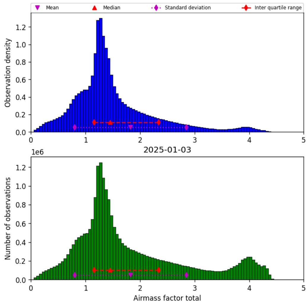
Figure 40: Histogram of “Airmass factor total” for 2025-01-02 to 2025-01-04
