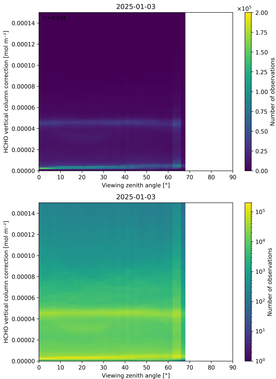
Figure 193: Scatter density plot of “Viewing zenith angle” against “HCHO vertical column correction” for 2025-01-02 to 2025-01-04.
