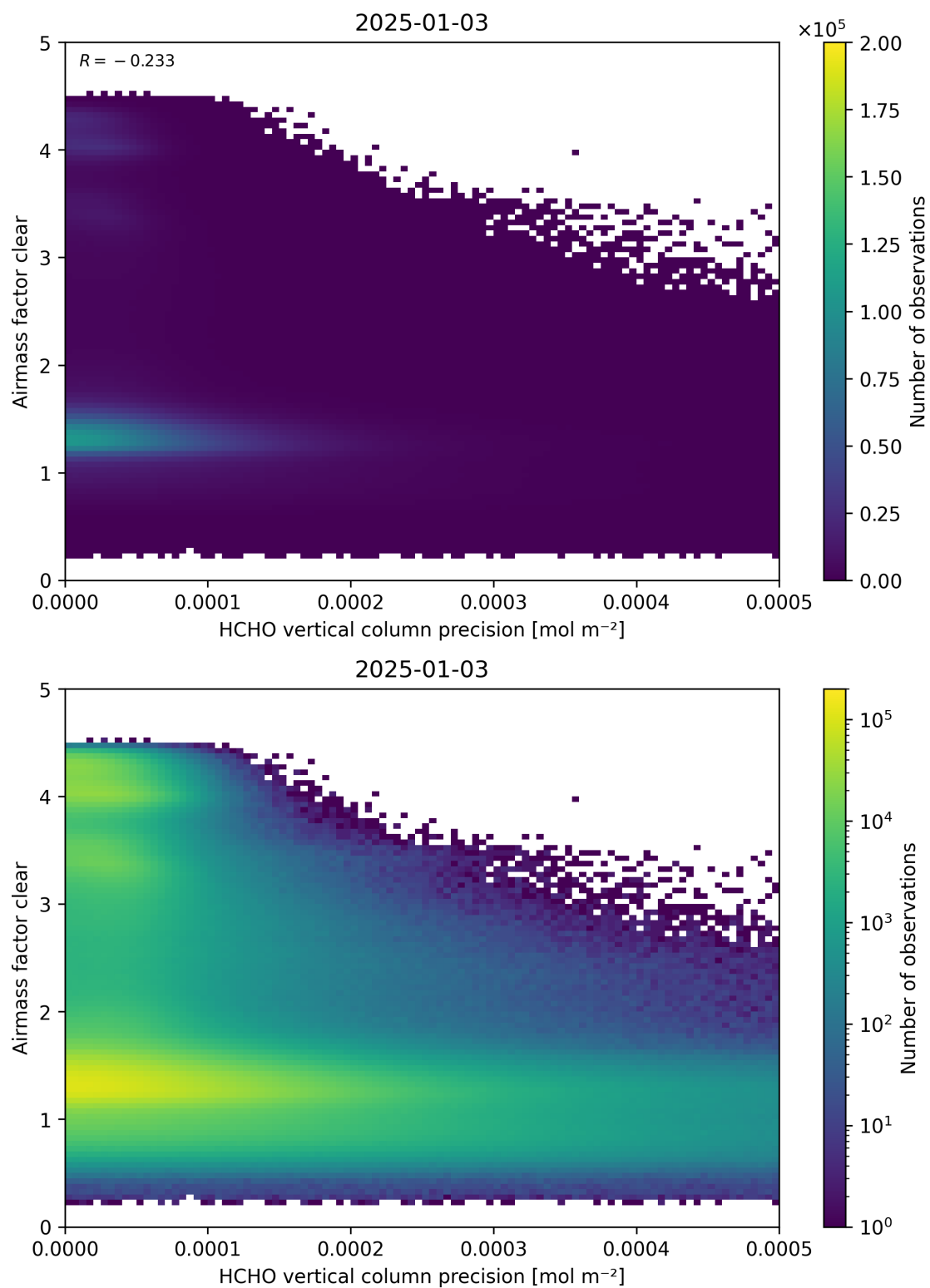
Figure 139: Scatter density plot of “HCHO vertical column precision” against “Airmass factor clear” for 2025-01-02 to 2025-01-04.
