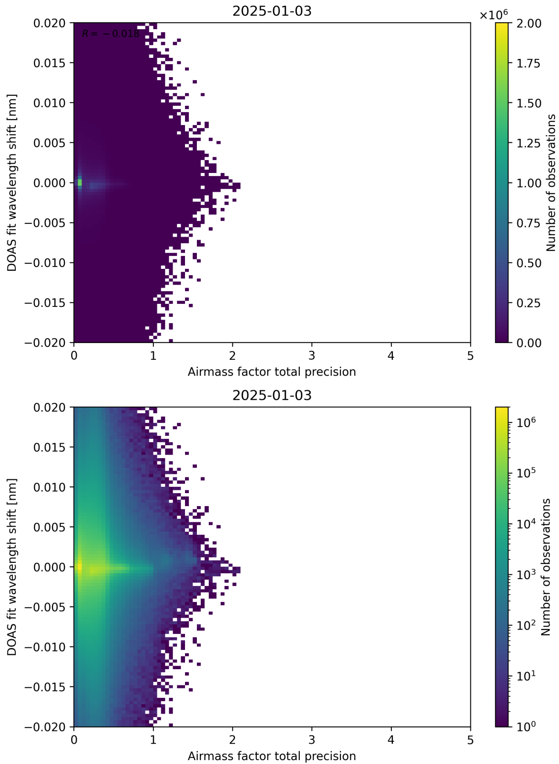
Figure 106: Scatter density plot of “Airmass factor total precision” against “DOAS fit wavelength shift” for 2025-01-02 to 2025-01-04.
