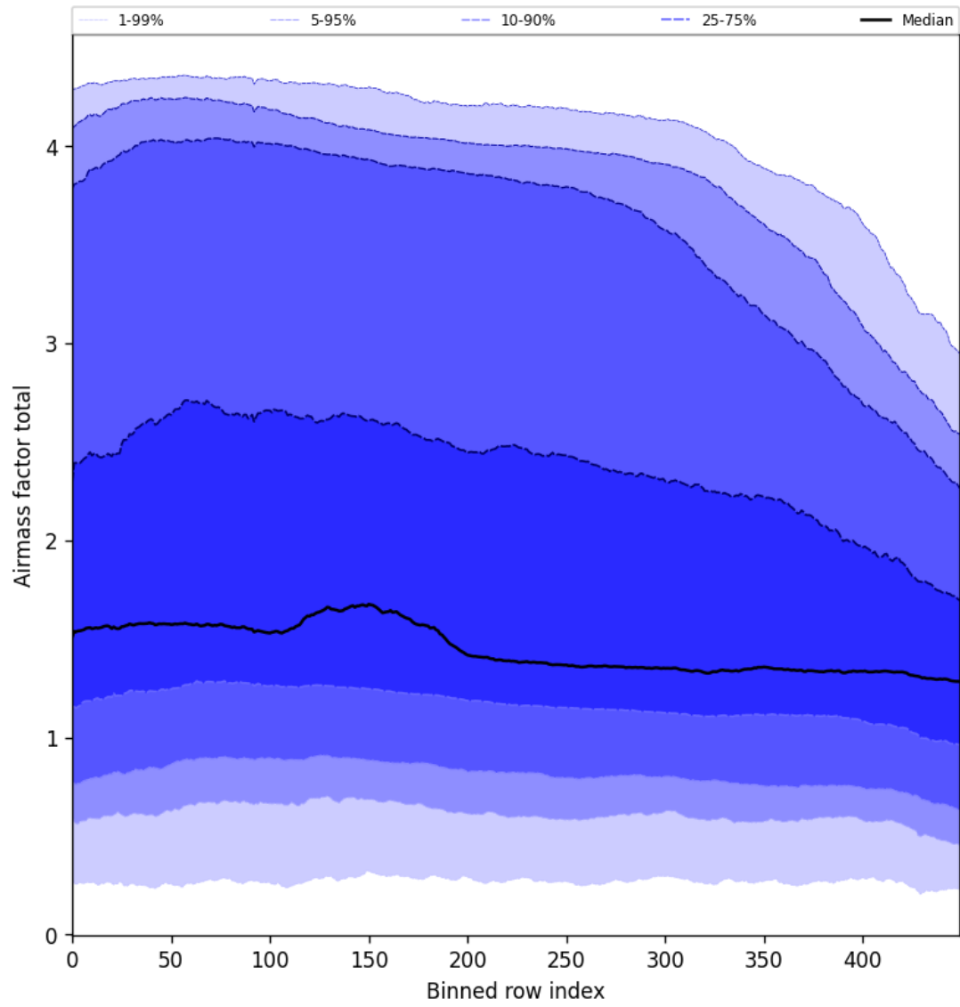
Figure 54: Along track statistics of “Airmass factor total” for 2025-01-02 to 2025-01-04
