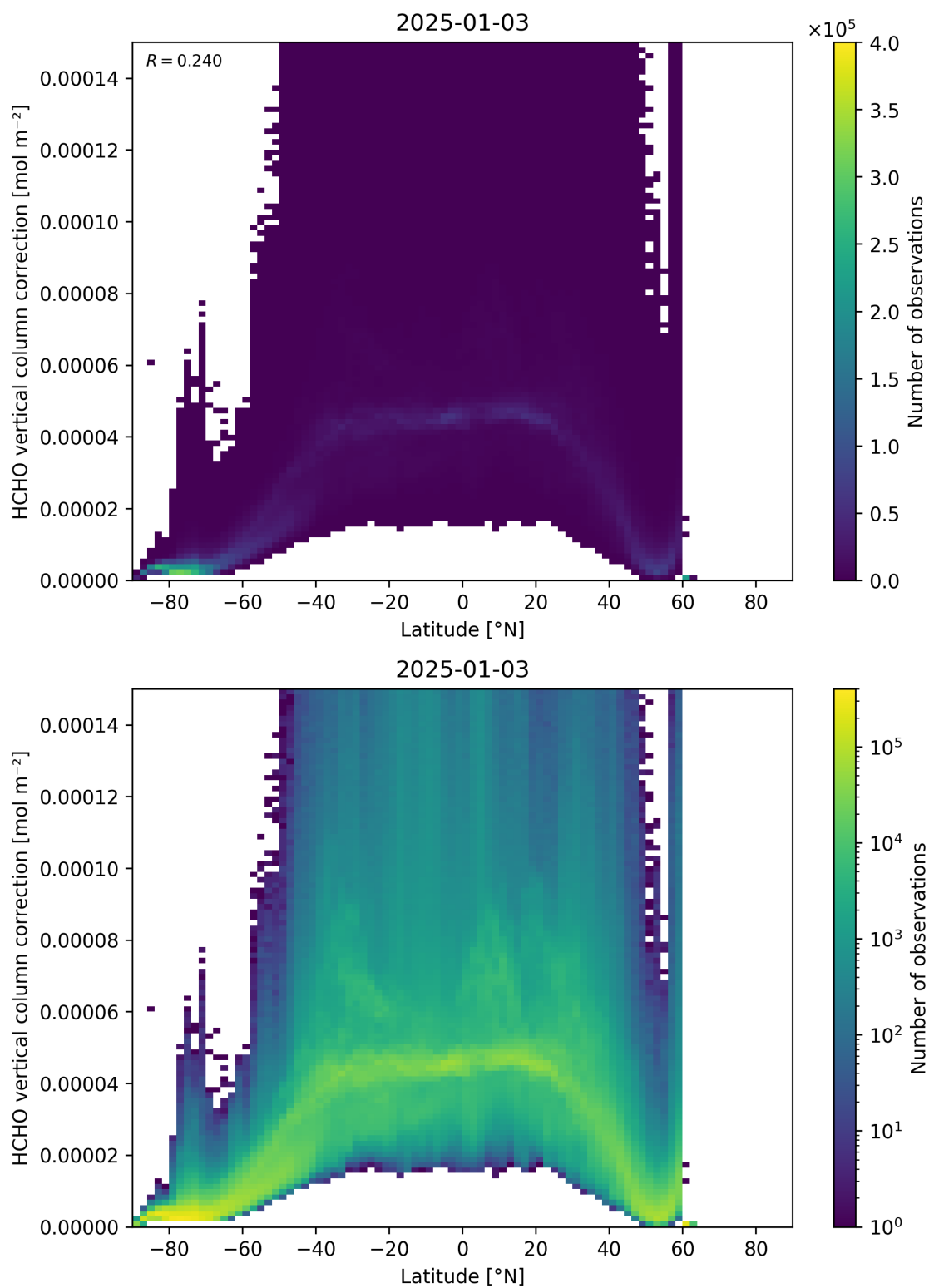
Figure 164: Scatter density plot of “Latitude” against “HCHO vertical column correction” for 2025-01-02 to 2025-01-04.
