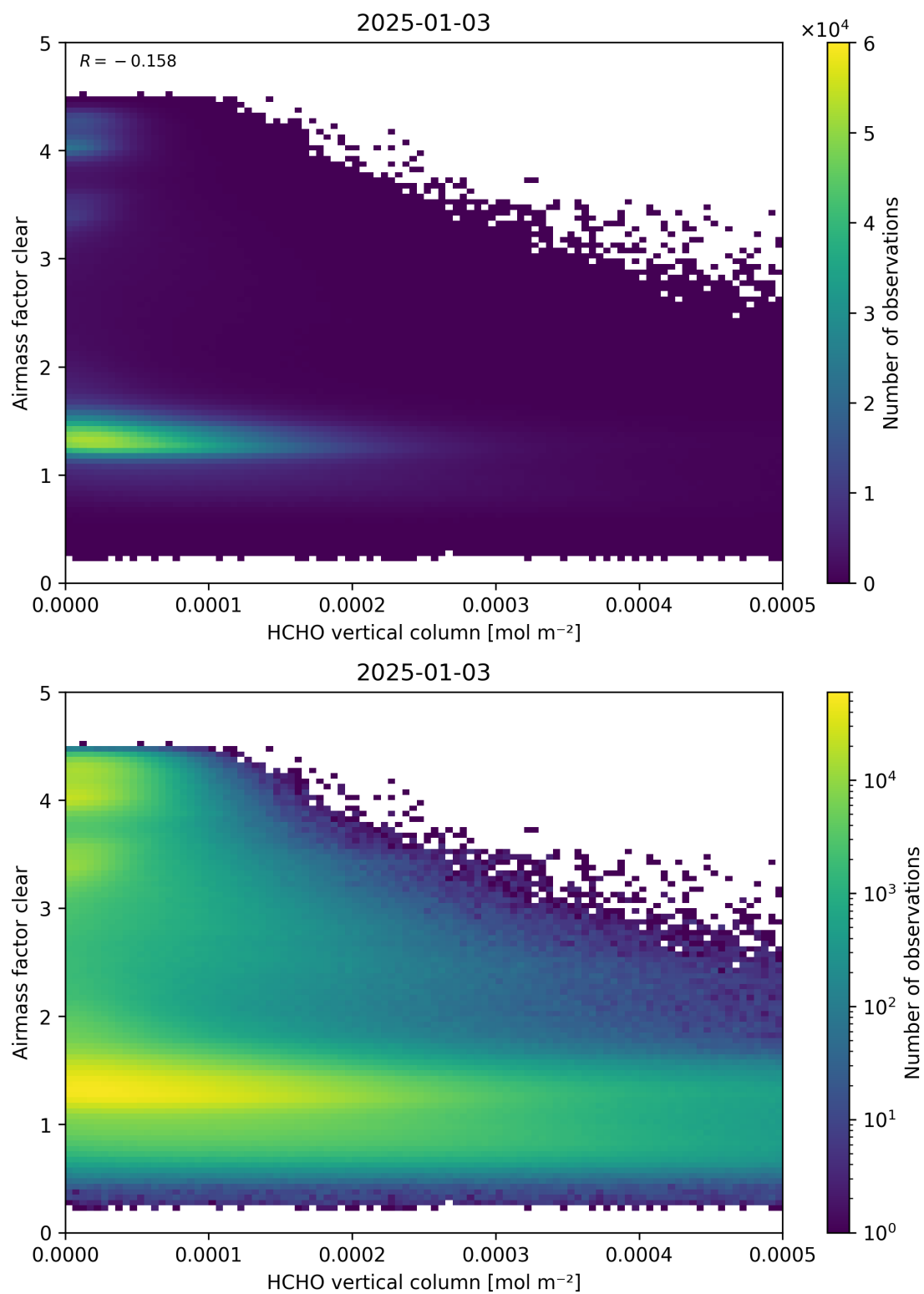
Figure 126: Scatter density plot of “HCHO vertical column” against “Airmass factor clear” for 2025-01-02 to 2025-01-04.
