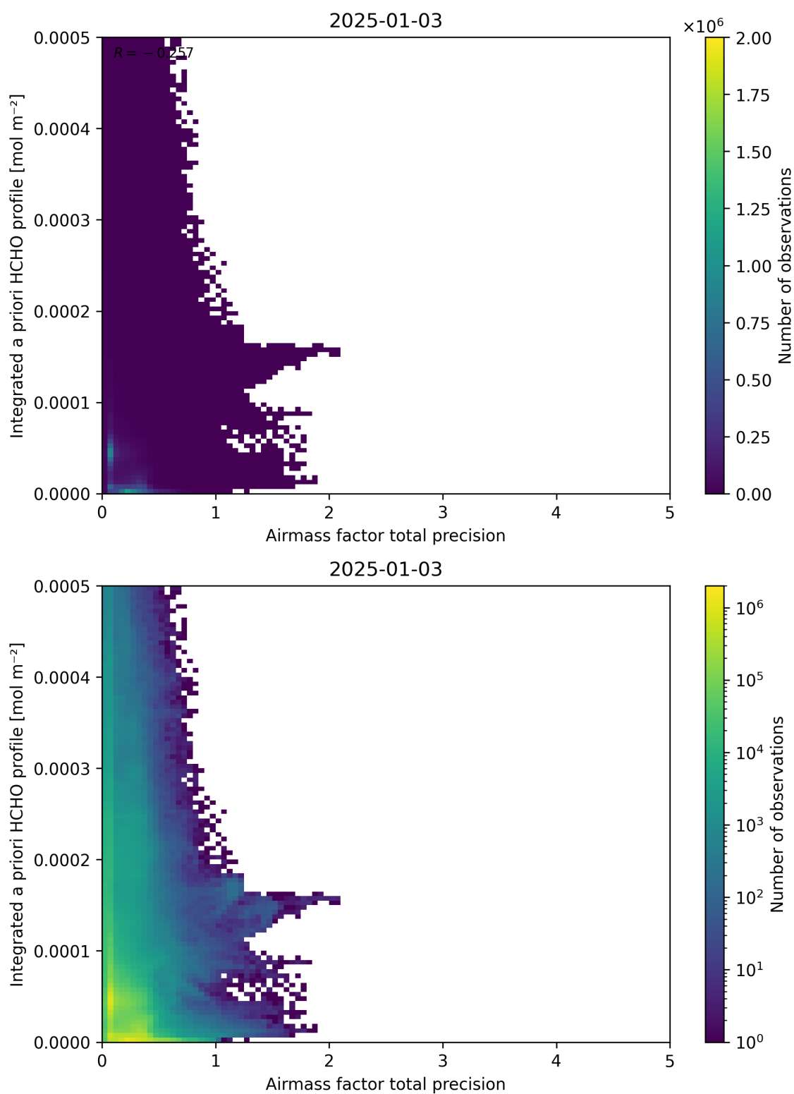
Figure 111: Scatter density plot of “Airmass factor total precision” against “Integrated a priori HCHO profile” for 2025-01-02 to 2025-01-04.
