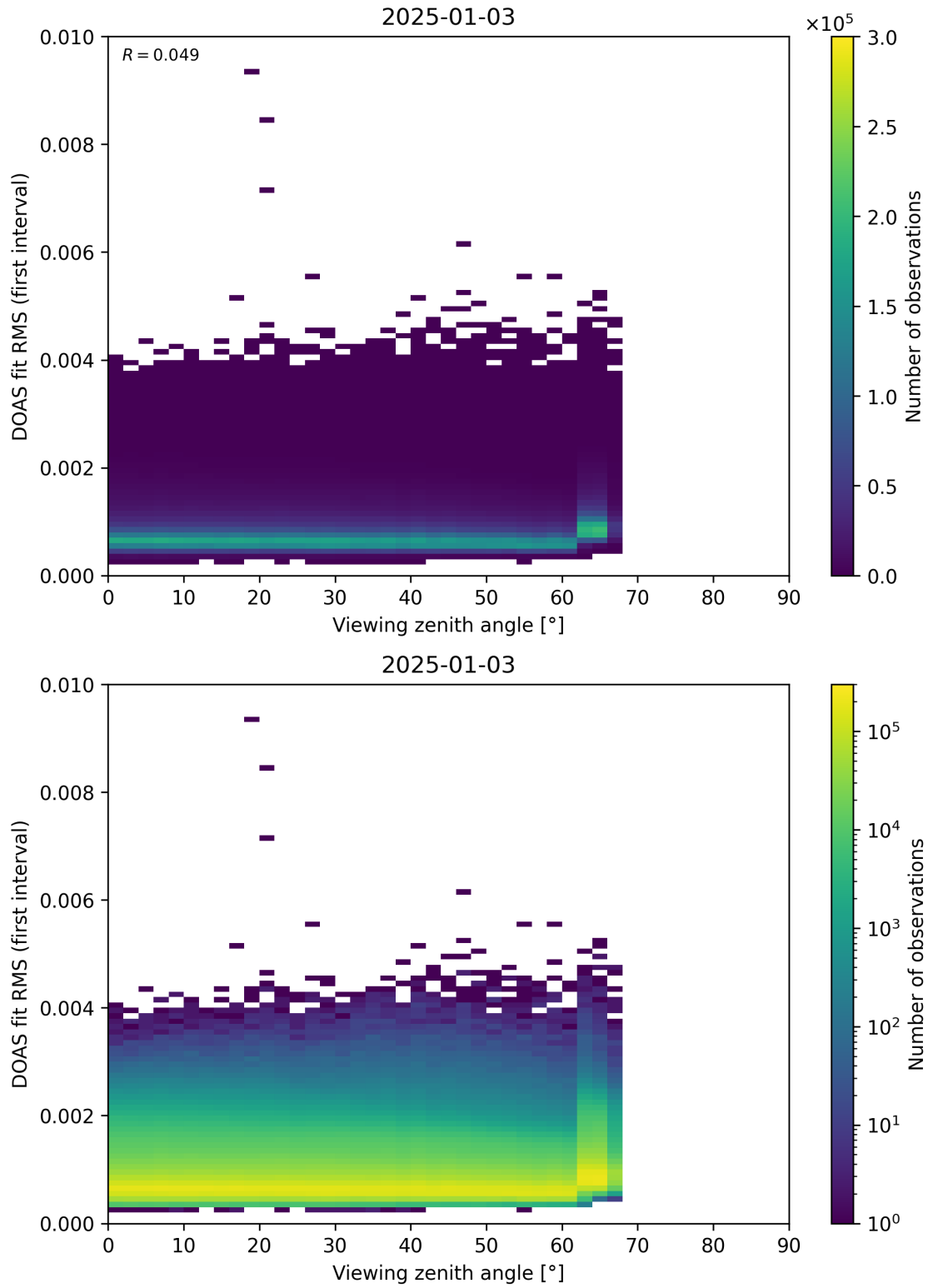
Figure 182: Scatter density plot of “Viewing zenith angle” against “DOAS fit RMS (first interval)” for 2025-01-02 to 2025-01-04.
