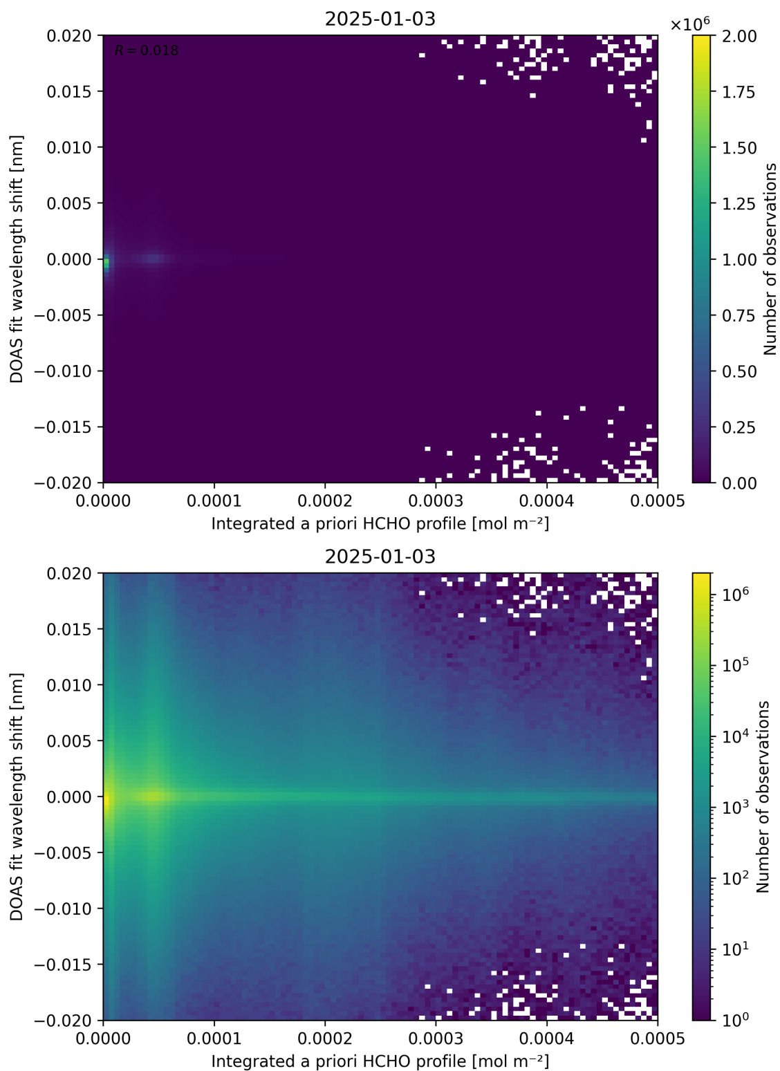
Figure 149: Scatter density plot of “Integrated a priori HCHO profile” against “DOAS fit wavelength shift” for 2025-01-02 to 2025-01-04.
