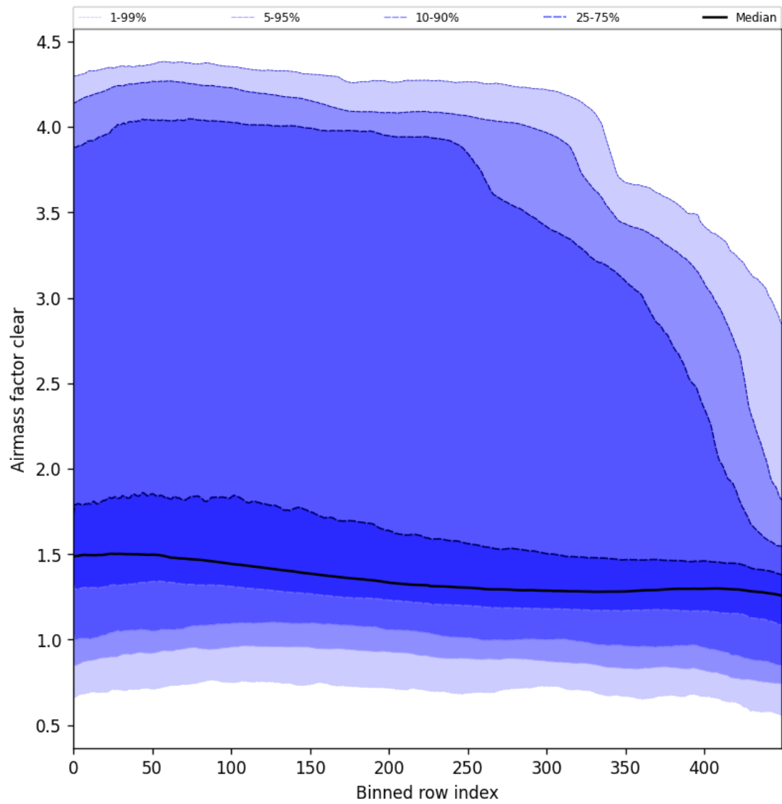
Figure 56: Along track statistics of “Air mass factor clear” for 2025-01-02 to 2025-01-04
