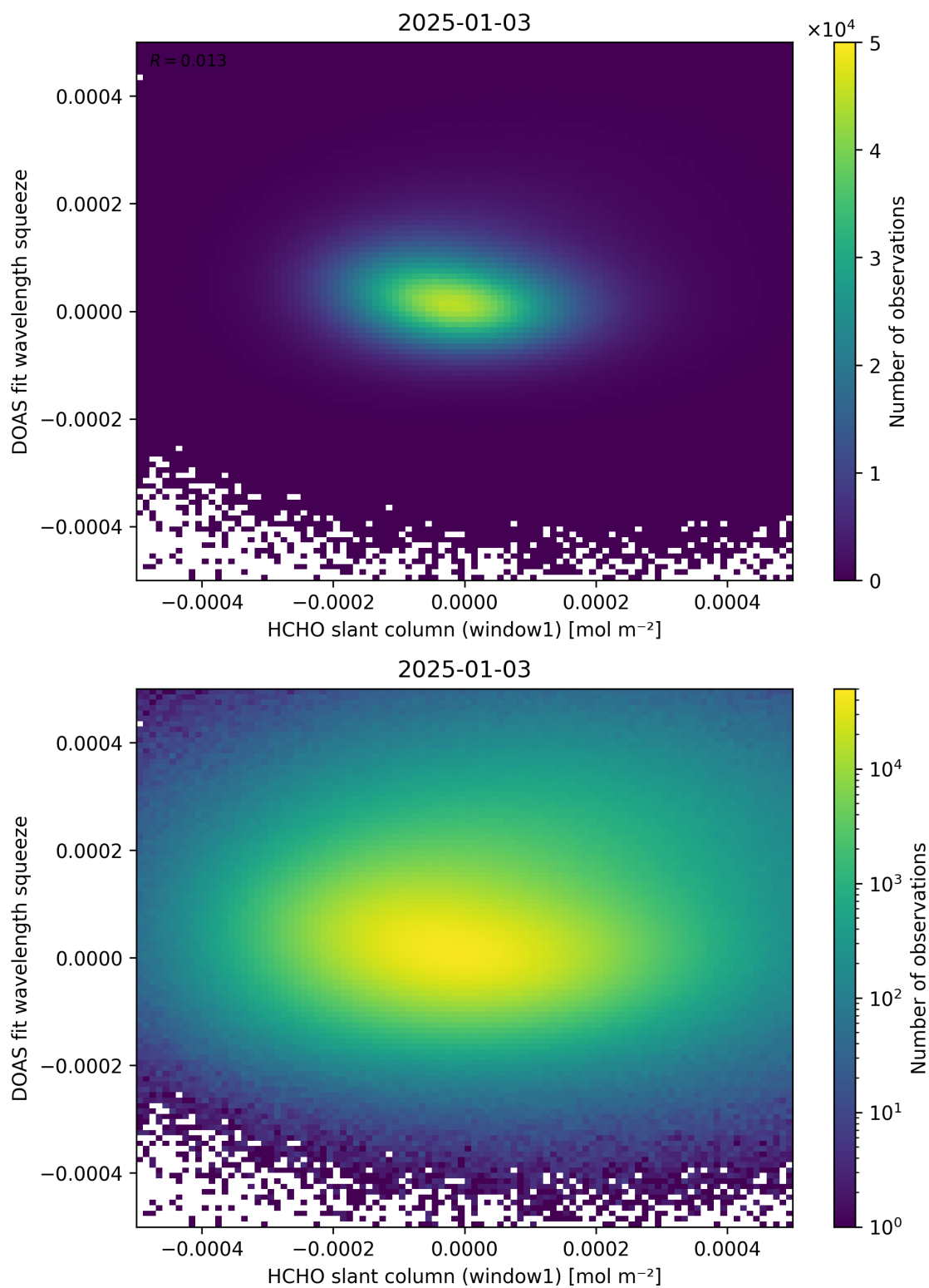
Figure 80: Scatter density plot of “HCHO slant column (window1)” against “DOAS fit wavelength squeeze” for 2025-01-02 to 2025-01-04.
