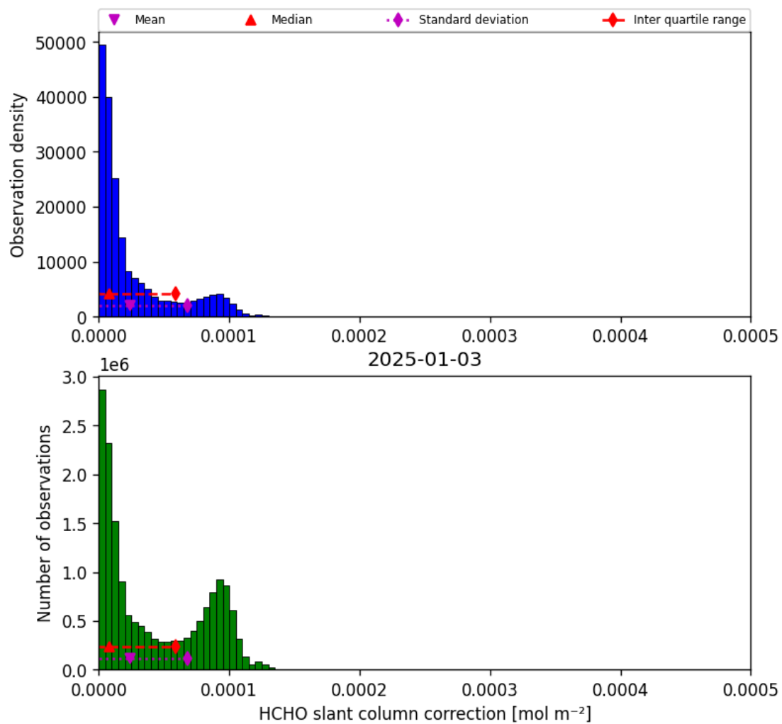
Figure 47: Histogram of “HCHO slant column correction” for 2025-01-02 to 2025-01-04
