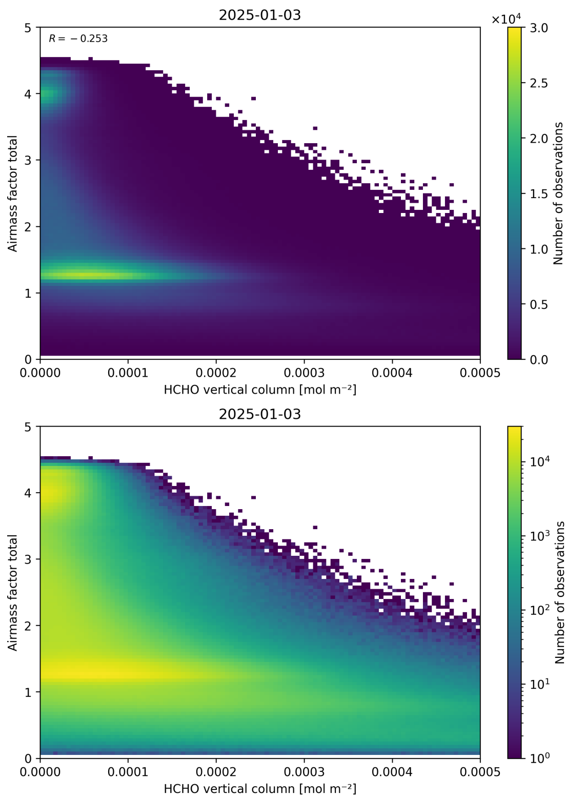
Figure 131: Scatter density plot of “HCHO vertical column” against “Airmass factor total” for 2025-01-02 to 2025-01-04.
