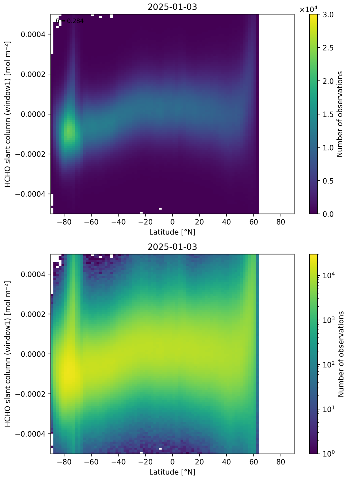
Figure 159: Scatter density plot of “Latitude” against “HCHO slant column (window1)” for 2025-01-02 to 2025-01-04.
