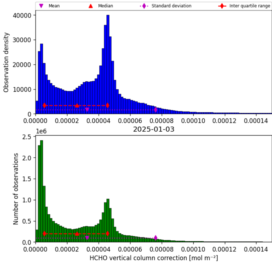
Figure 37: Histogram of “HCHO vertical column correction” for 2025-01-02 to 2025-01-04
