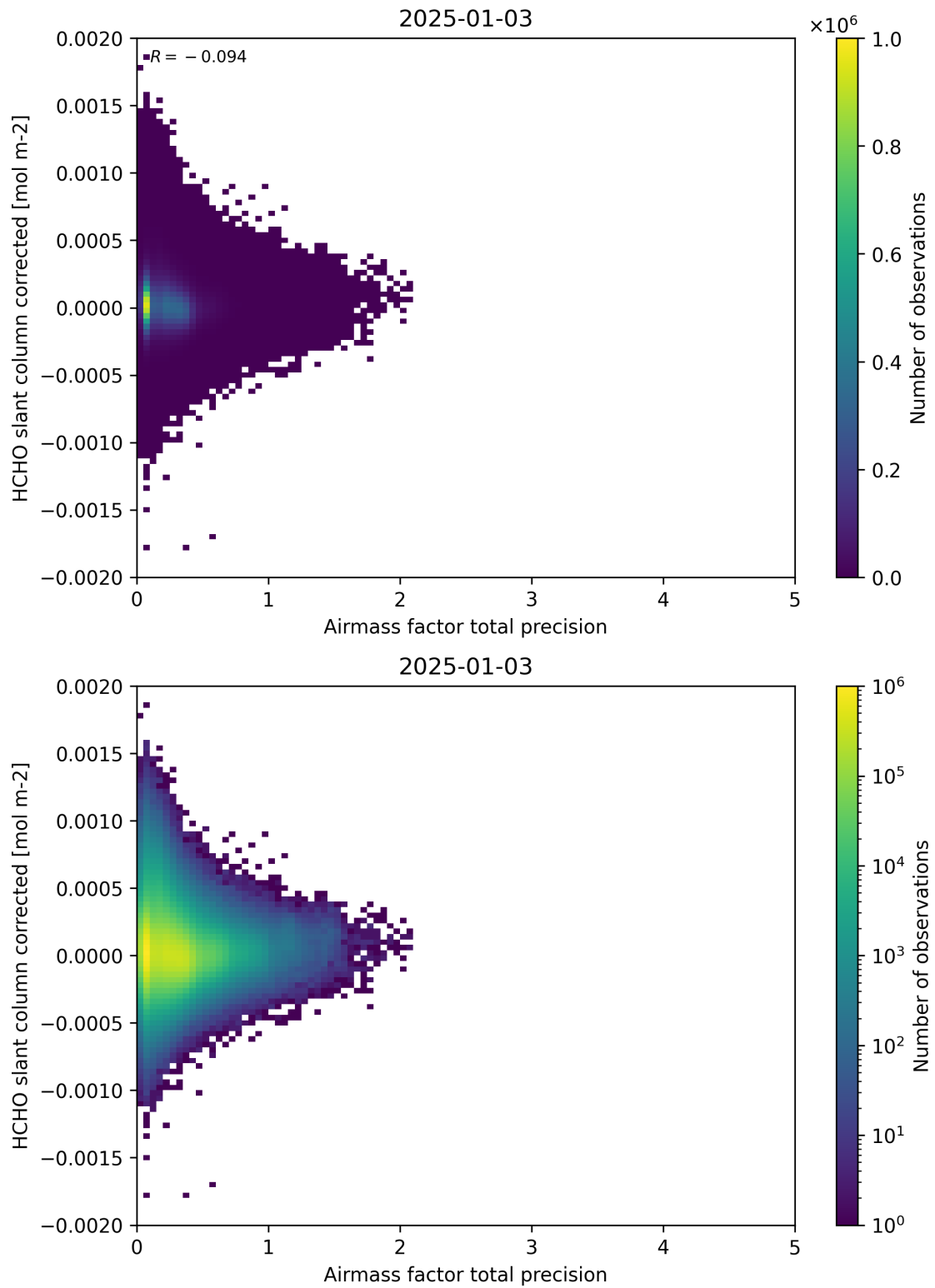
Figure 109: Scatter density plot of “Airmass factor total precision” against “HCHO slant column corrected” for 2025-01-02 to 2025-01-04.
