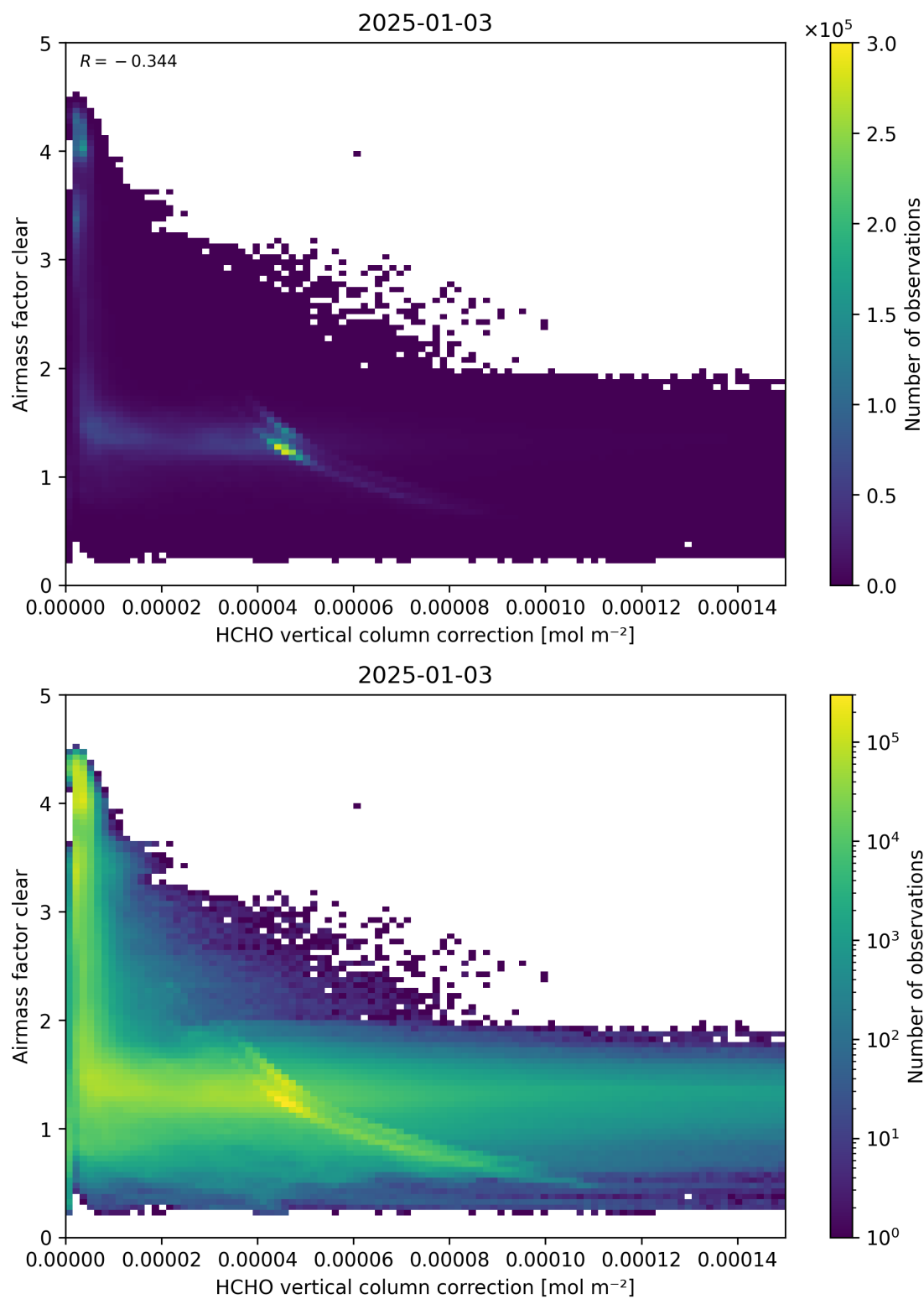
Figure 115: Scatter density plot of “HCHO vertical column correction” against “Airmass factor clear” for 2025-01-02 to 2025-01-04.
