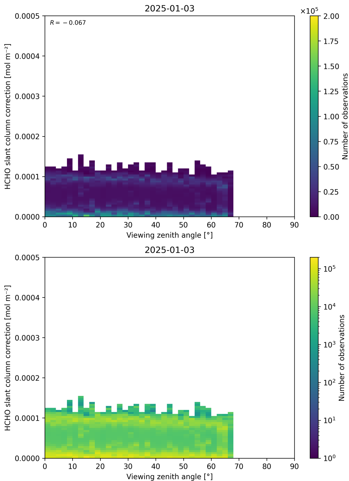
Figure 187: Scatter density plot of “Viewing zenith angle” against “HCHO slant column correction” for 2025-01-02 to 2025-01-04.
