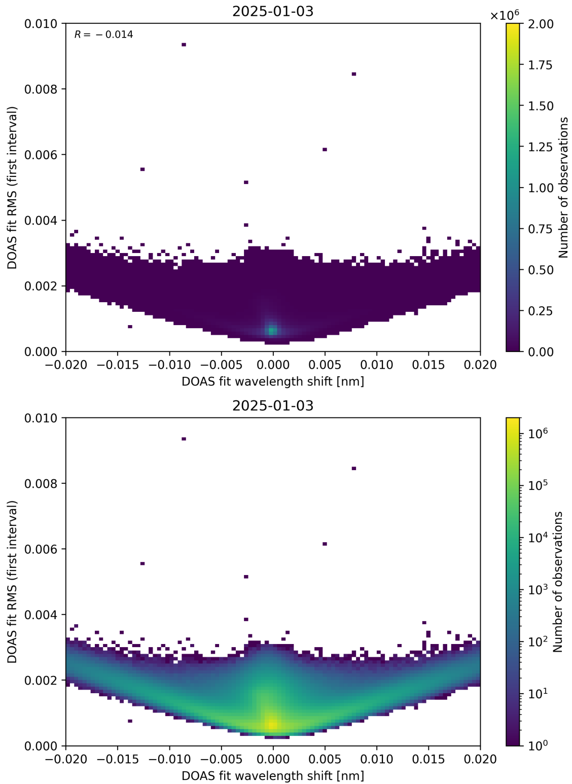
Figure 64: Scatter density plot of “DOAS fit wavelength shift” against “DOAS fit RMS (first interval)” for 2025-01-02 to 2025-01-04.
