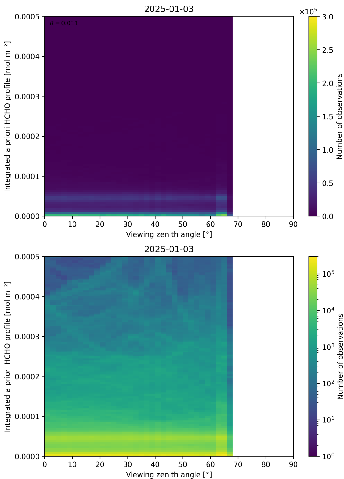
Figure 195: Scatter density plot of “Viewing zenith angle” against “Integrated a priori HCHO profile” for 2025-01-02 to 2025-01-04.
