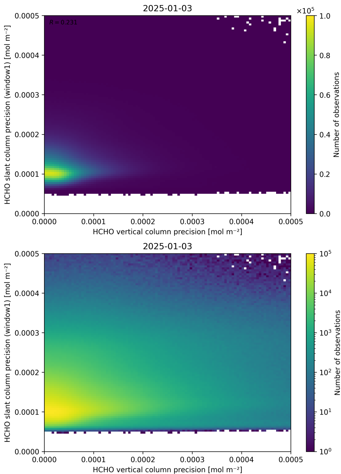
Figure 143: Scatter density plot of “HCHO vertical column precision” against “HCHO slant column precision (window1)” for 2025-01-02 to 2025-01-04.
