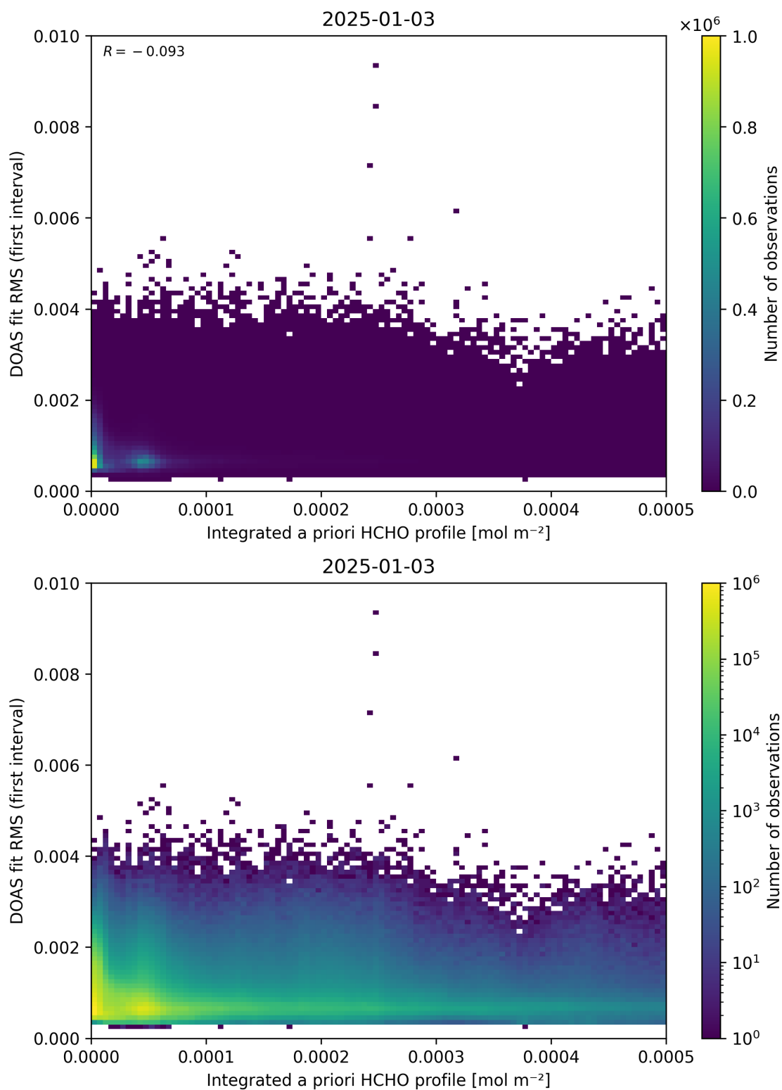
Figure 148: Scatter density plot of “Integrated a priori HCHO profile” against “DOAS fit RMS (first interval)” for 2025-01-02 to 2025-01-04.
