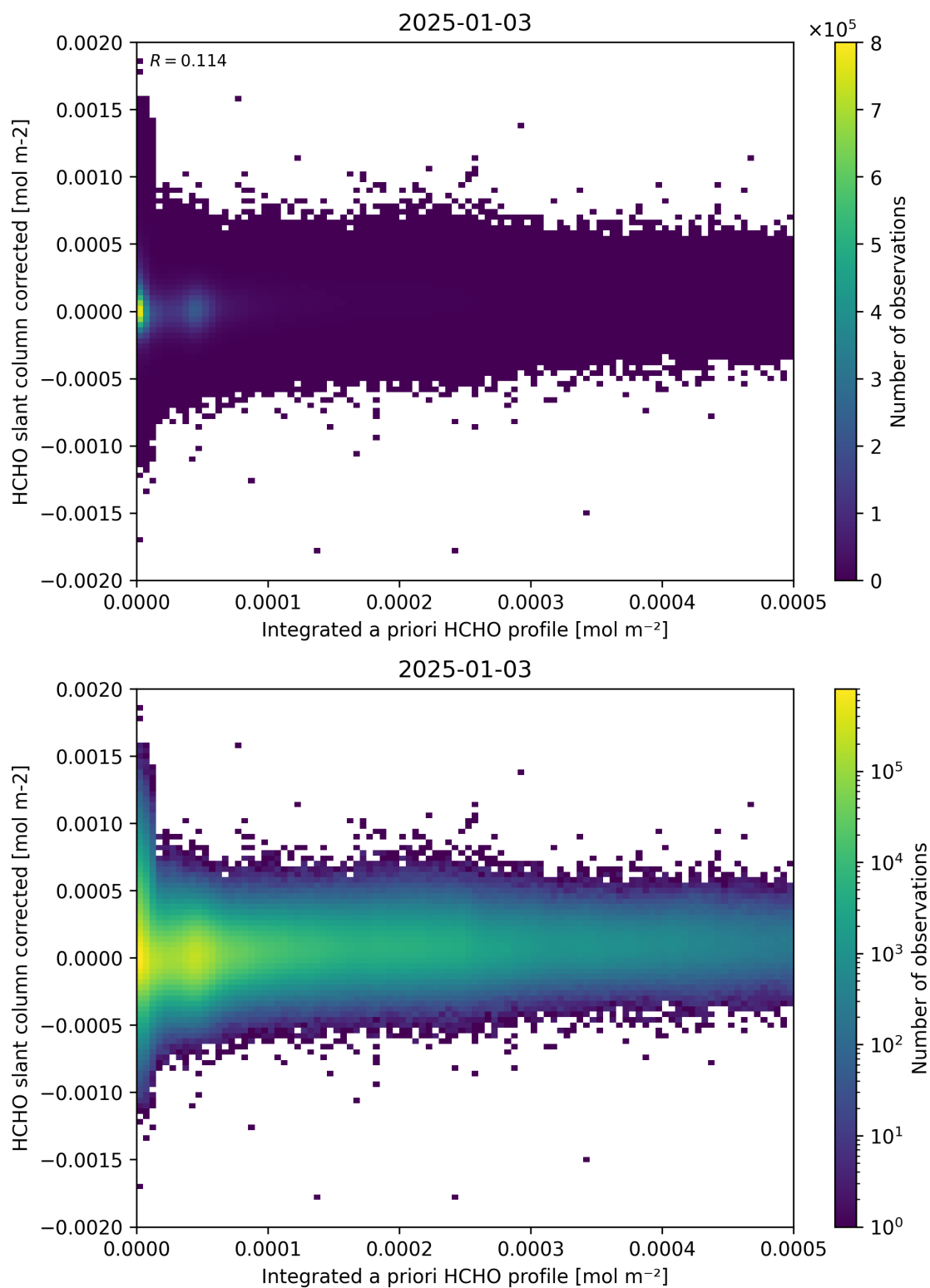
Figure 151: Scatter density plot of “Integrated a priori HCHO profile” against “HCHO slant column corrected” for 2025-01-02 to 2025-01-04.
