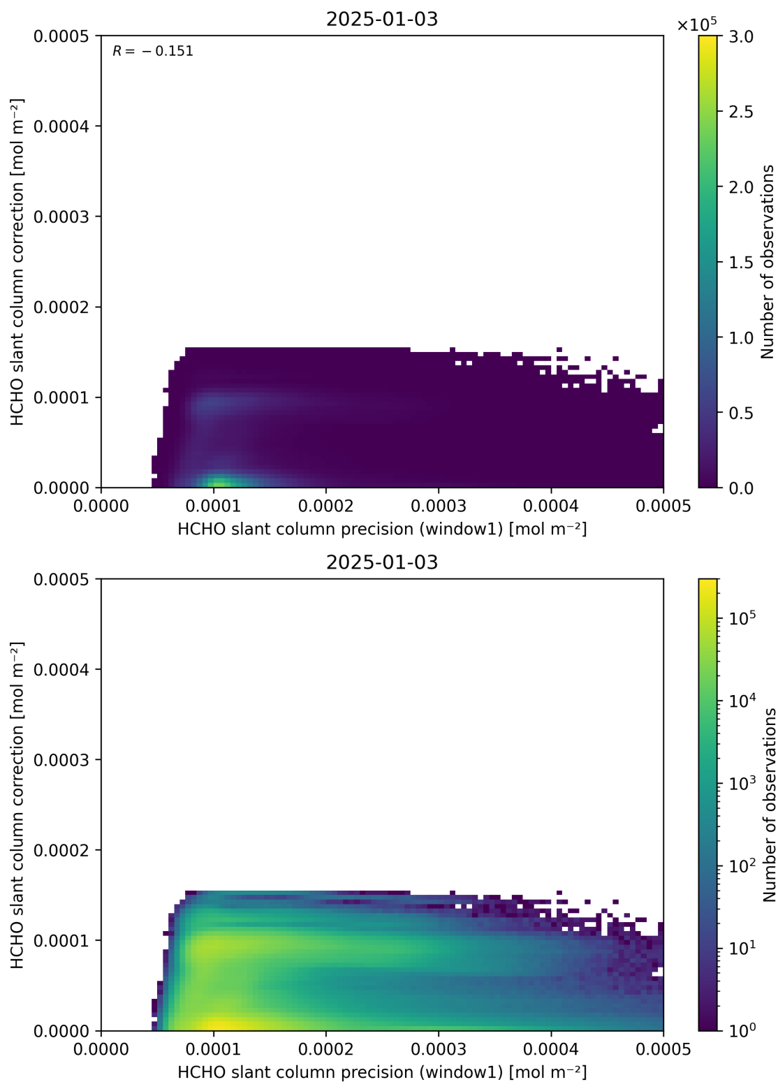
Figure 93: Scatter density plot of “HCHO slant column precision (window1)” against “HCHO slant column correction” for 2025-01-02 to 2025-01-04.
