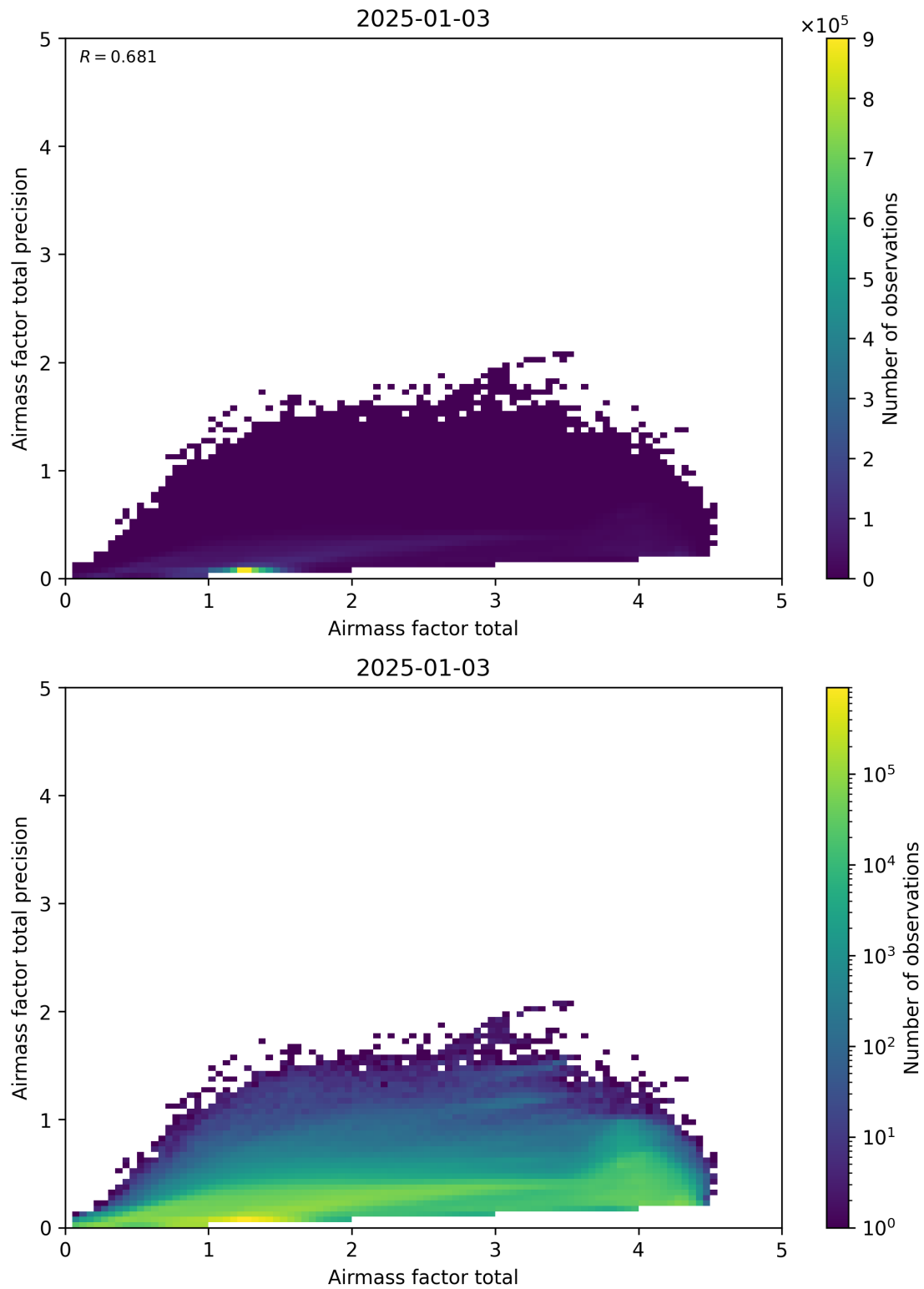
Figure 103: Scatter density plot of “Airmass factor total” against “Airmass factor total precision” for 2025-01-02 to 2025-01-04.
