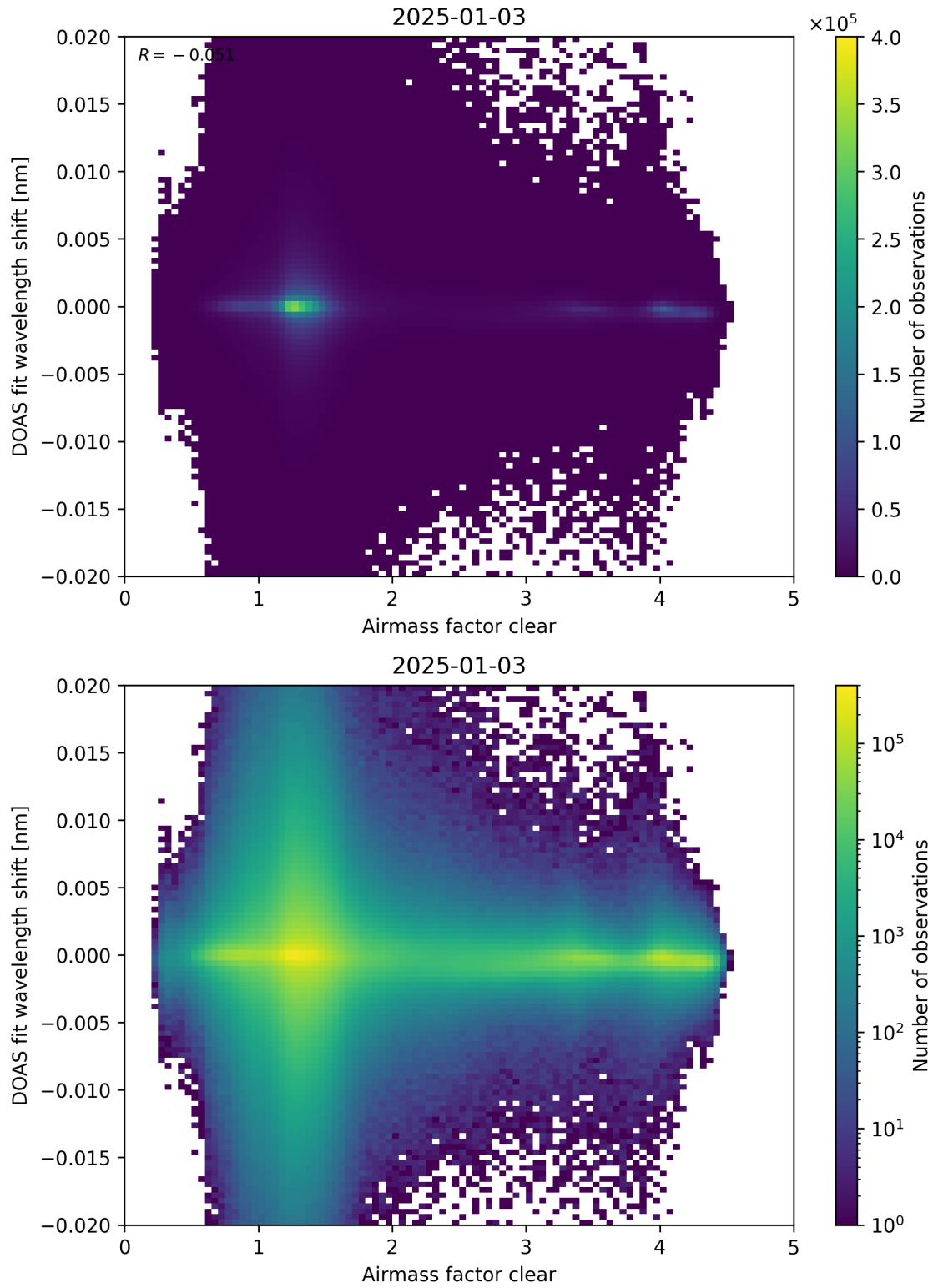
Figure 72: Scatter density plot of “Airmass factor clear” against “DOAS fit wavelength shift” for 2025-01-02 to 2025-01-04.
