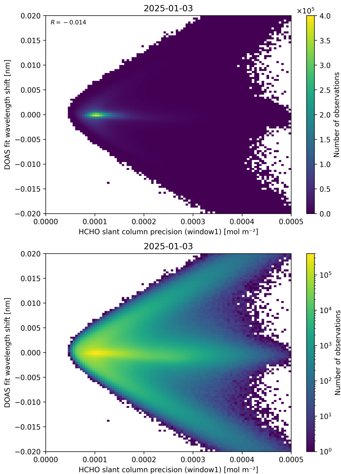
Figure 89: Scatter density plot of “HCHO slant column precision (window1)” against “DOAS fit wavelength shift” for 2025-01-02 to 2025-01-04.
