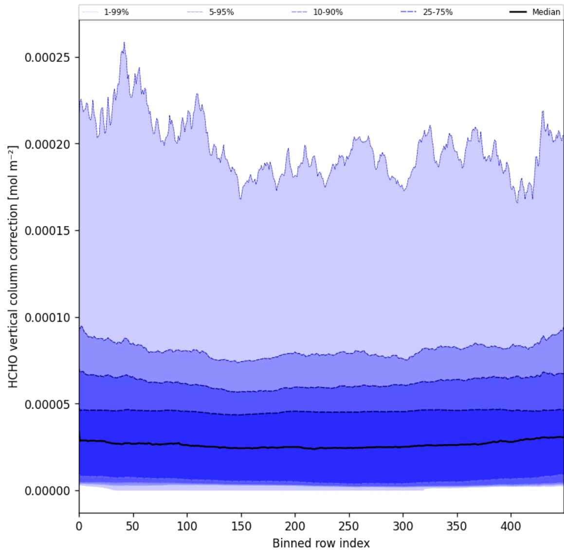
Figure 51: Along track statistics of “HCHO vertical column correction” for 2025-01-02 to 2025-01-04
