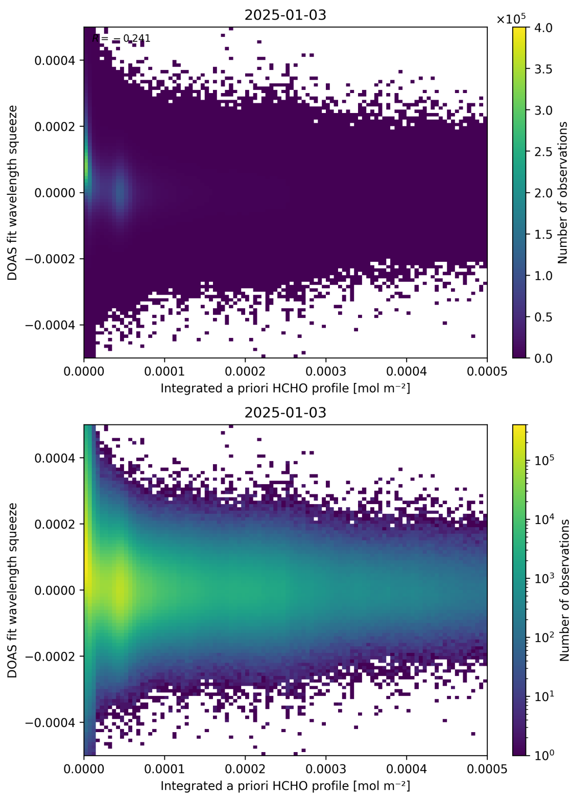
Figure 150: Scatter density plot of “Integrated a priori HCHO profile” against “DOAS fit wavelength squeeze” for 2025-01-02 to 2025-01-04.
