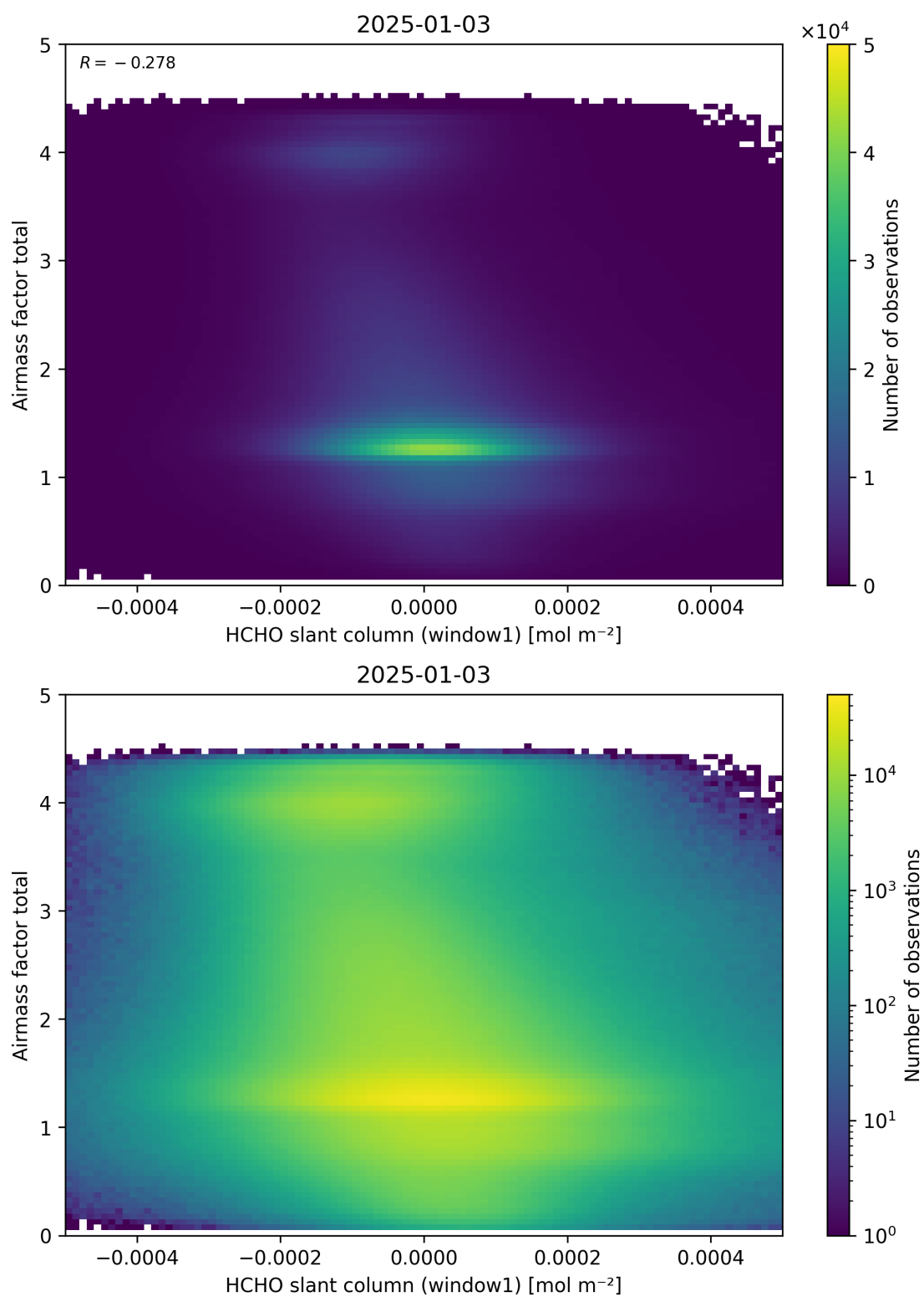
Figure 85: Scatter density plot of “HCHO slant column (window1)” against “Airmass factor total” for 2025-01-02 to 2025-01-04.
