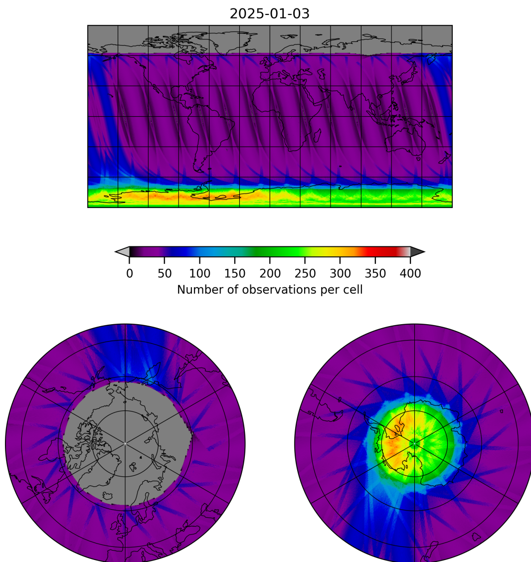
Figure 19: Map of the number of observations for 2025-01-02 to 2025-01-04
