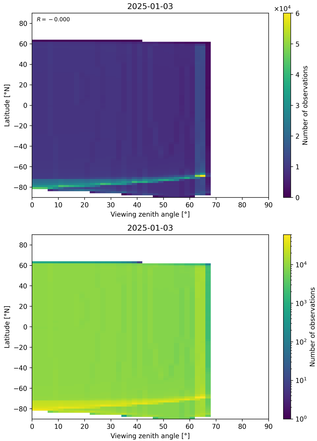
Figure 196: Scatter density plot of “Viewing zenith angle” against “Latitude” for 2025-01-02 to 2025-01-04.
