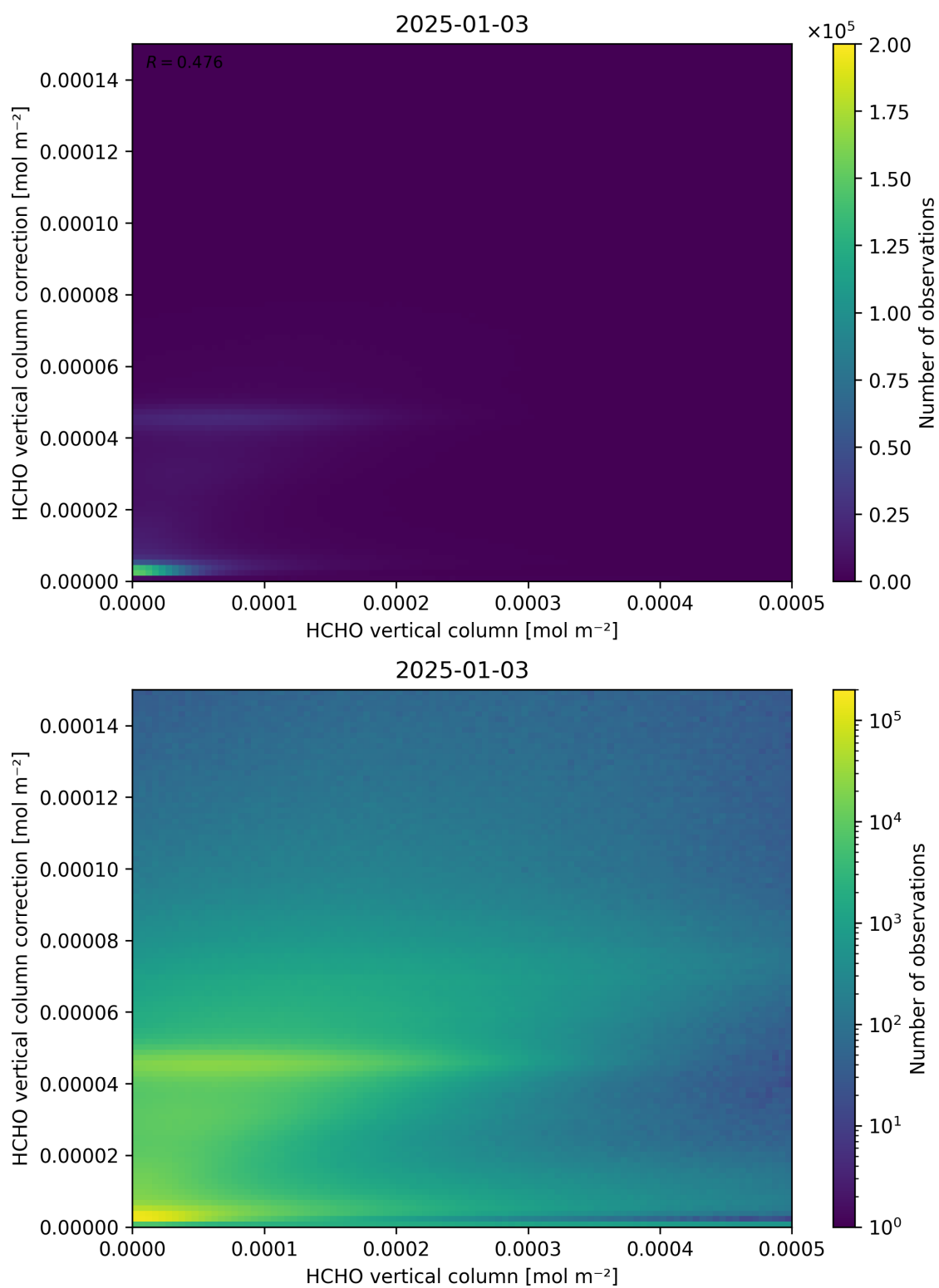
Figure 133: Scatter density plot of “HCHO vertical column” against “HCHO vertical column correction” for 2025-01-02 to 2025-01-04.
