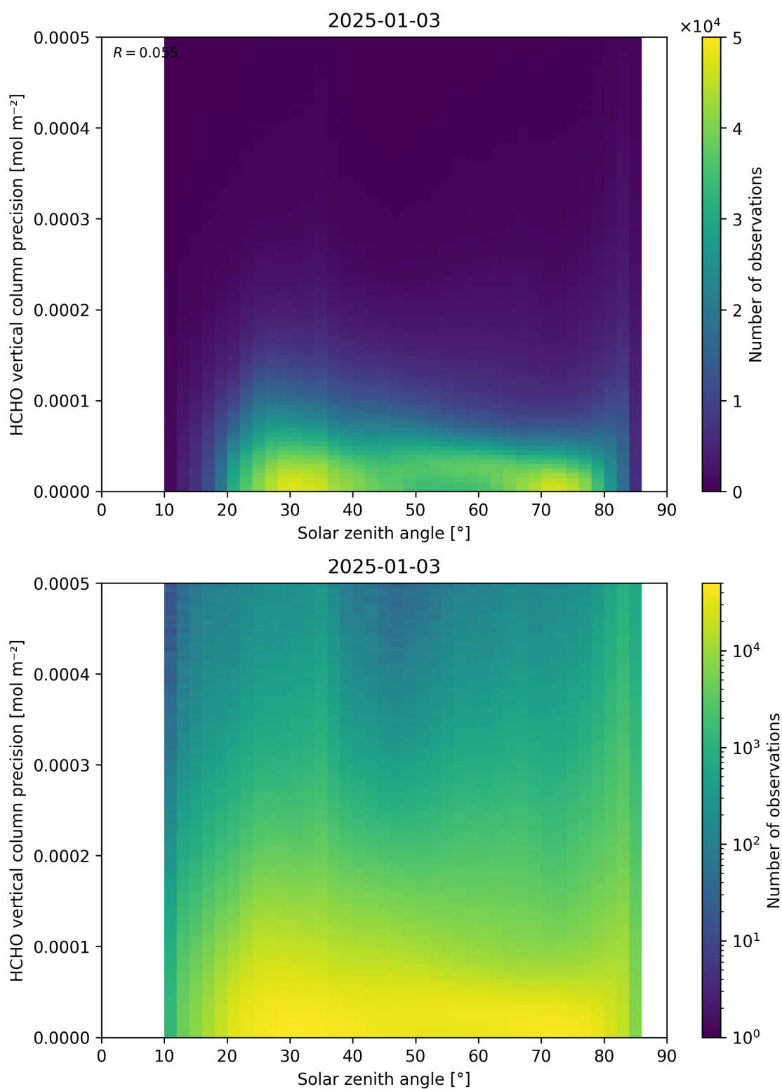
Figure 179: Scatter density plot of “Solar zenith angle” against “HCHO vertical column precision” for 2025-01-02 to 2025-01-04.
