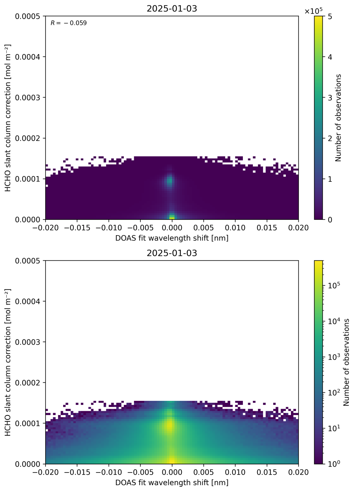
Figure 67: Scatter density plot of “DOAS fit wavelength shift” against “HCHO slant column correction” for 2025-01-02 to 2025-01-04.
