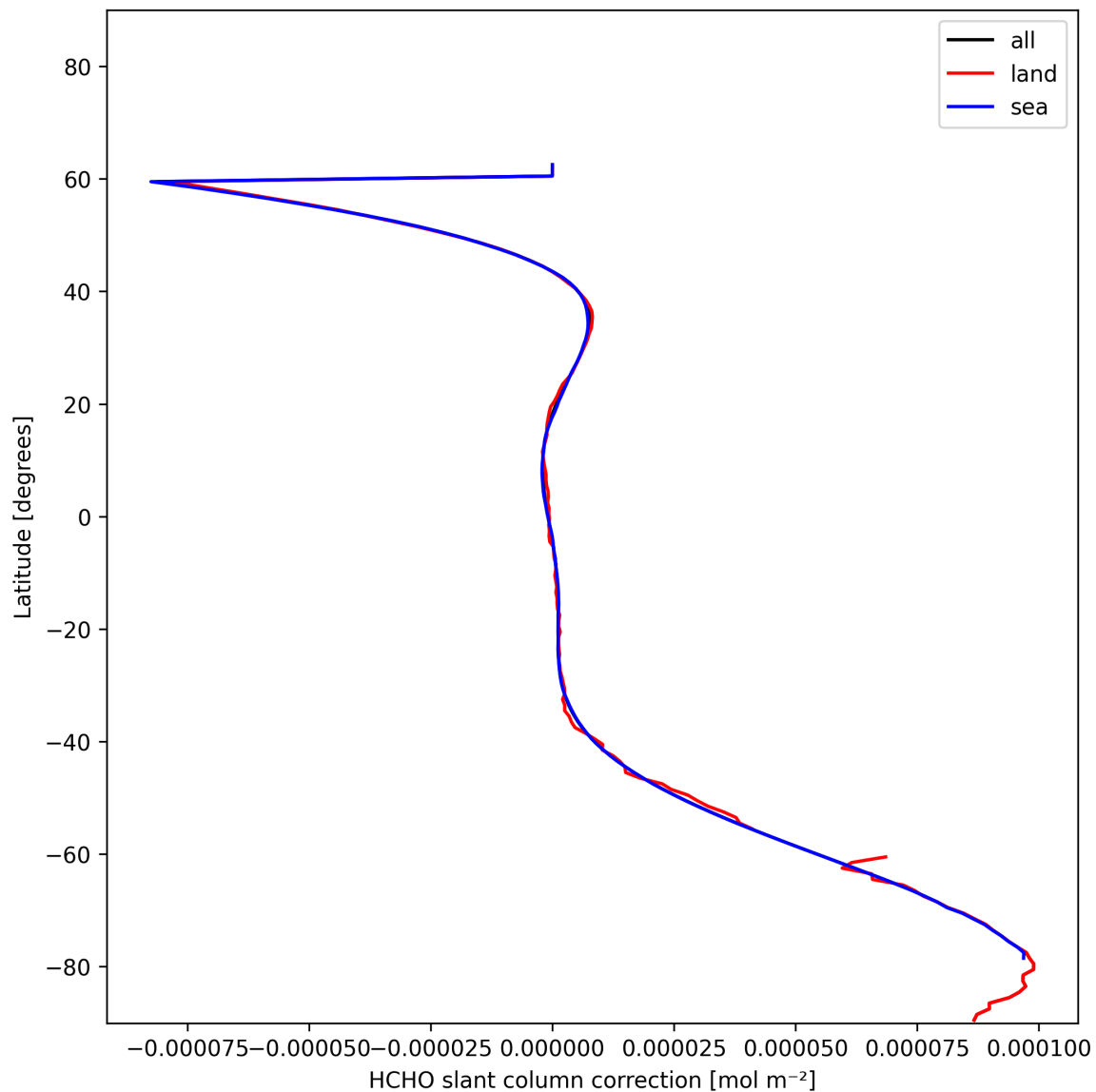
Figure 33: Zonal average of “HCHO slant column correction” for 2025-01-02 to 2025-01-04.
