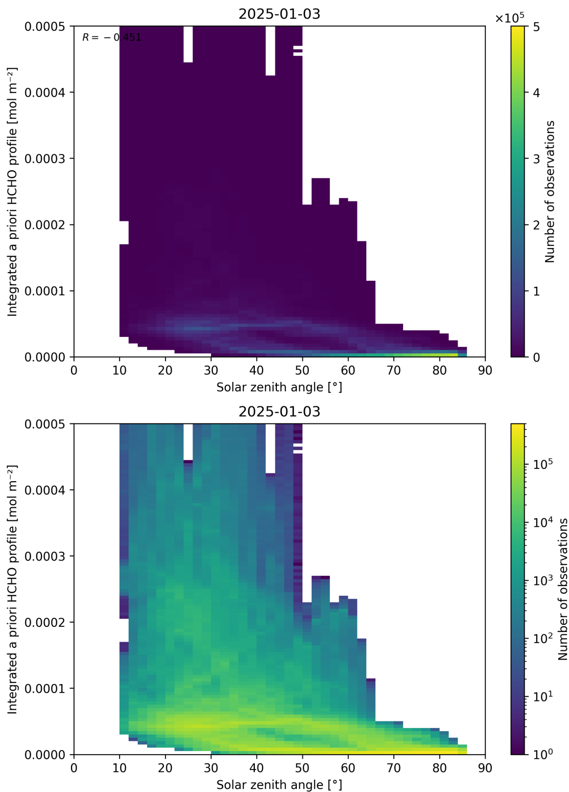
Figure 180: Scatter density plot of “Solar zenith angle” against “Integrated a priori HCHO profile” for 2025-01-02 to 2025-01-04.
