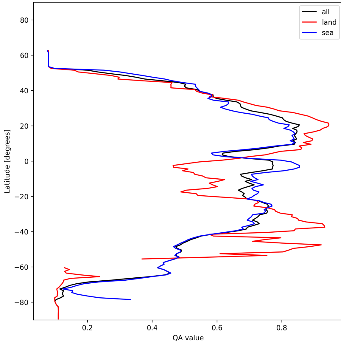
Figure 20: Zonal average of “QA value” for 2025-01-02 to 2025-01-04.
