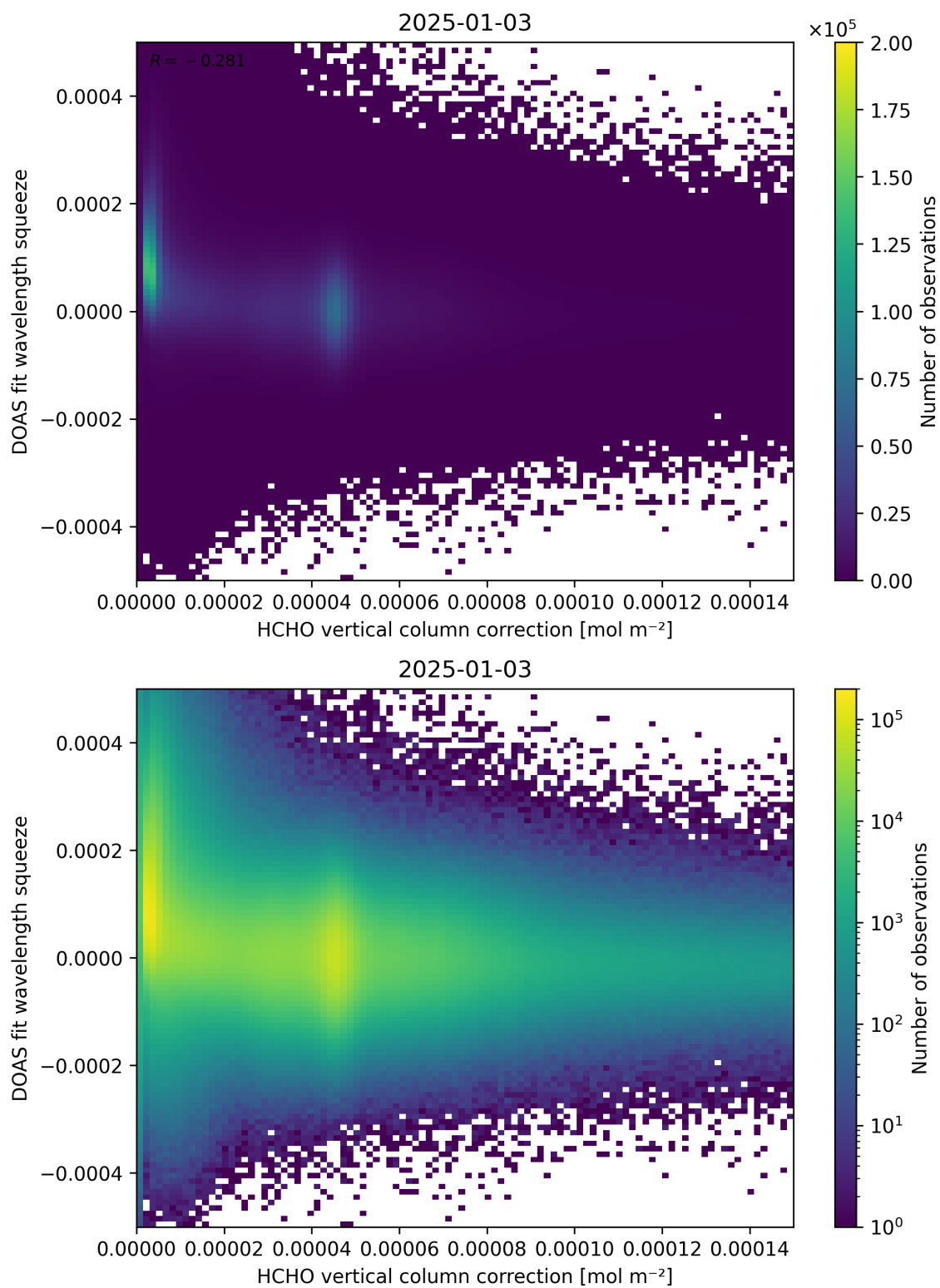
Figure 114: Scatter density plot of “HCHO vertical column correction” against “DOAS fit wavelength squeeze” for 2025-01-02 to 2025-01-04.
