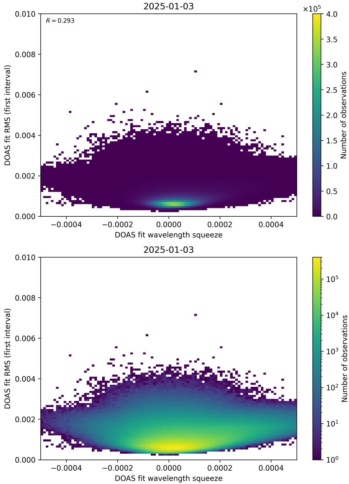
Figure 68: Scatter density plot of “DOAS fit wavelength squeeze” against “DOAS fit RMS (first interval)” for 2025-01-02 to 2025-01-04.
