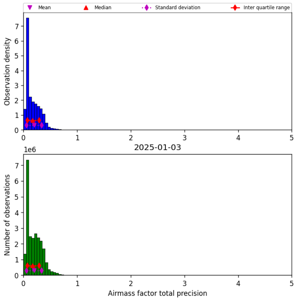
Figure 41: Histogram of “Airmass factor total precision” for 2025-01-02 to 2025-01-04
