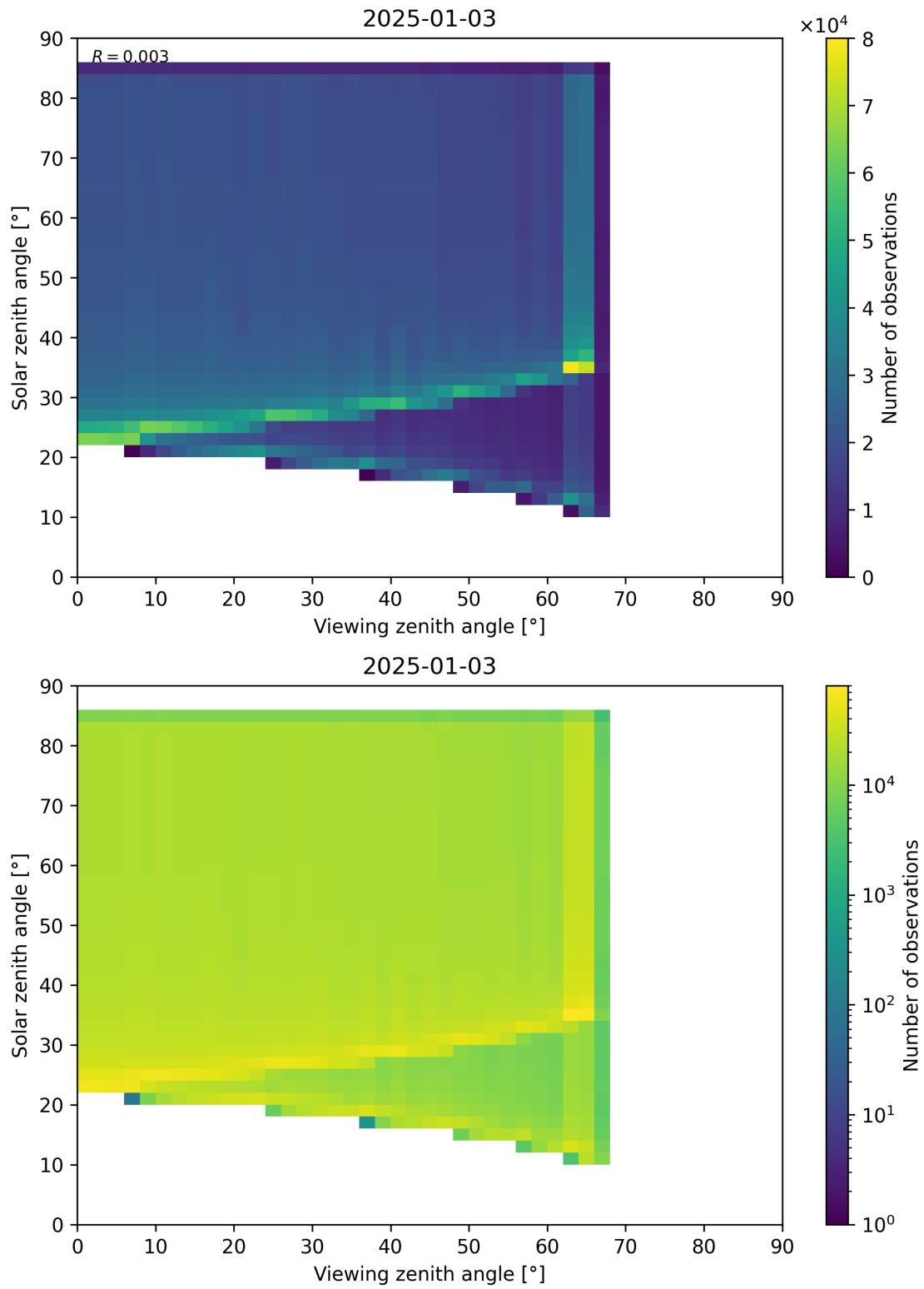
Figure 197: Scatter density plot of “Viewing zenith angle” against “Solar zenith angle” for 2025-01-02 to 2025-01-04.
