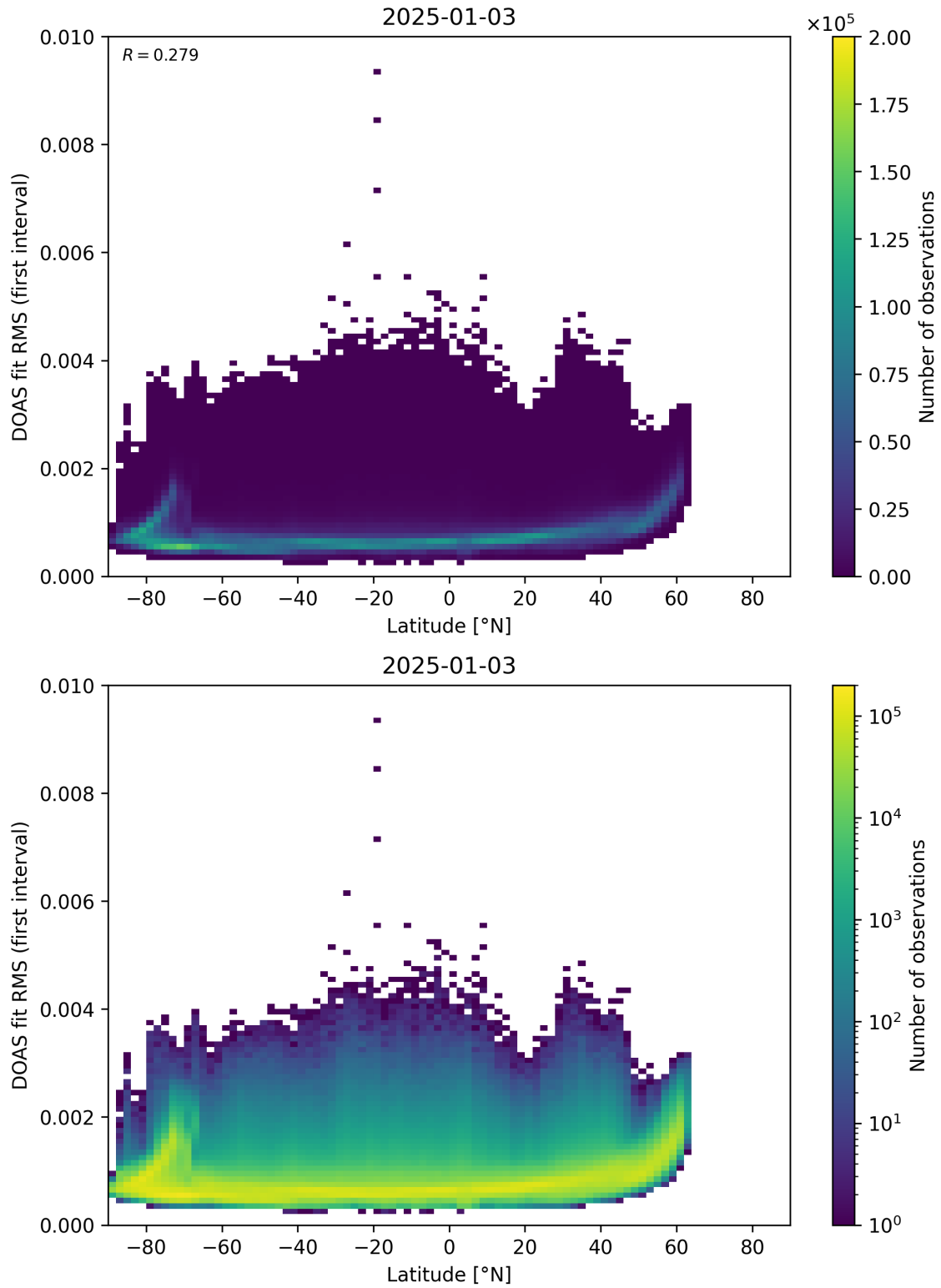
Figure 153: Scatter density plot of “Latitude” against “DOAS fit RMS (first interval)” for 2025-01-02 to 2025-01-04.
