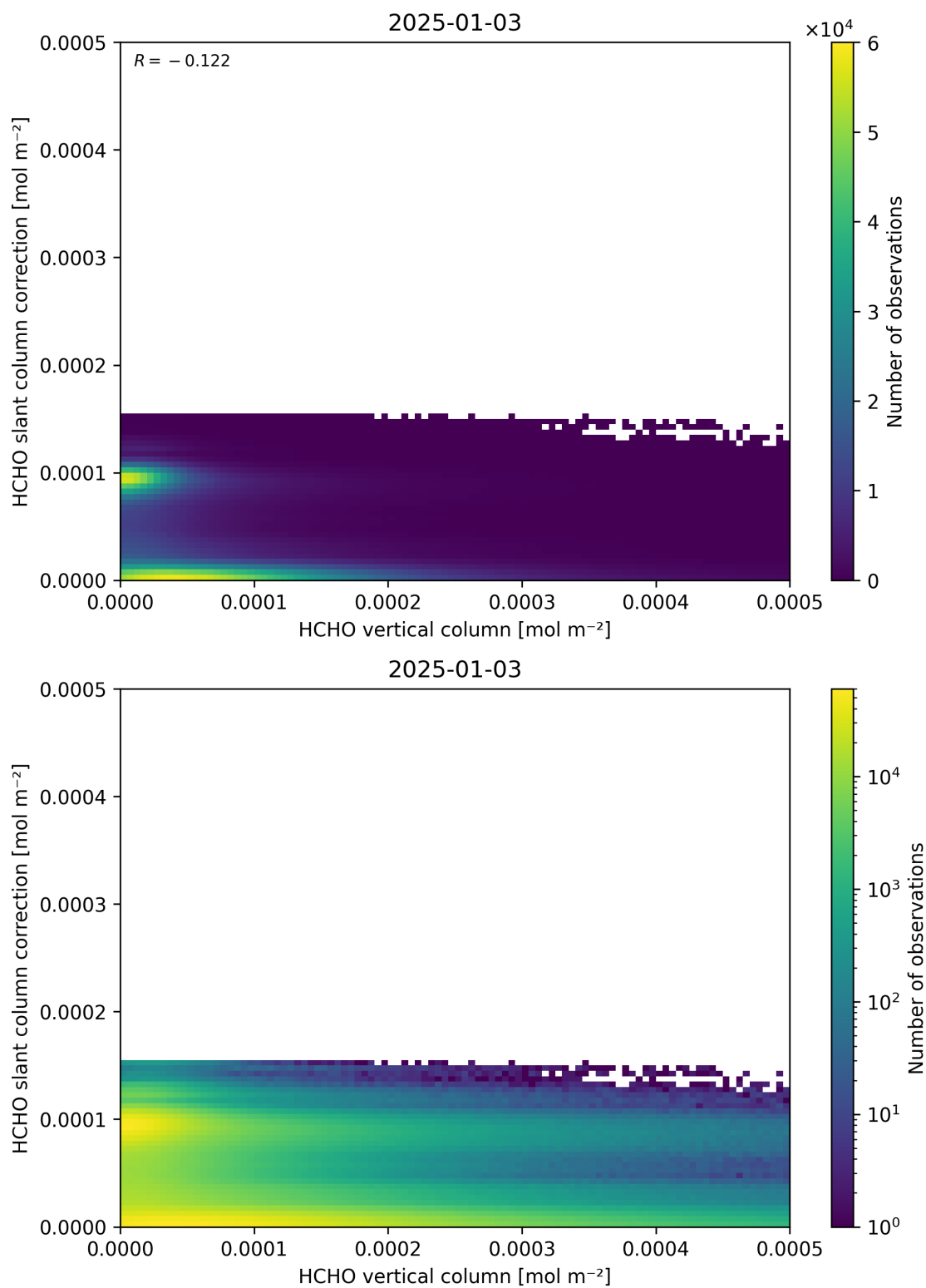
Figure 128: Scatter density plot of “HCHO vertical column” against “HCHO slant column correction” for 2025-01-02 to 2025-01-04.
