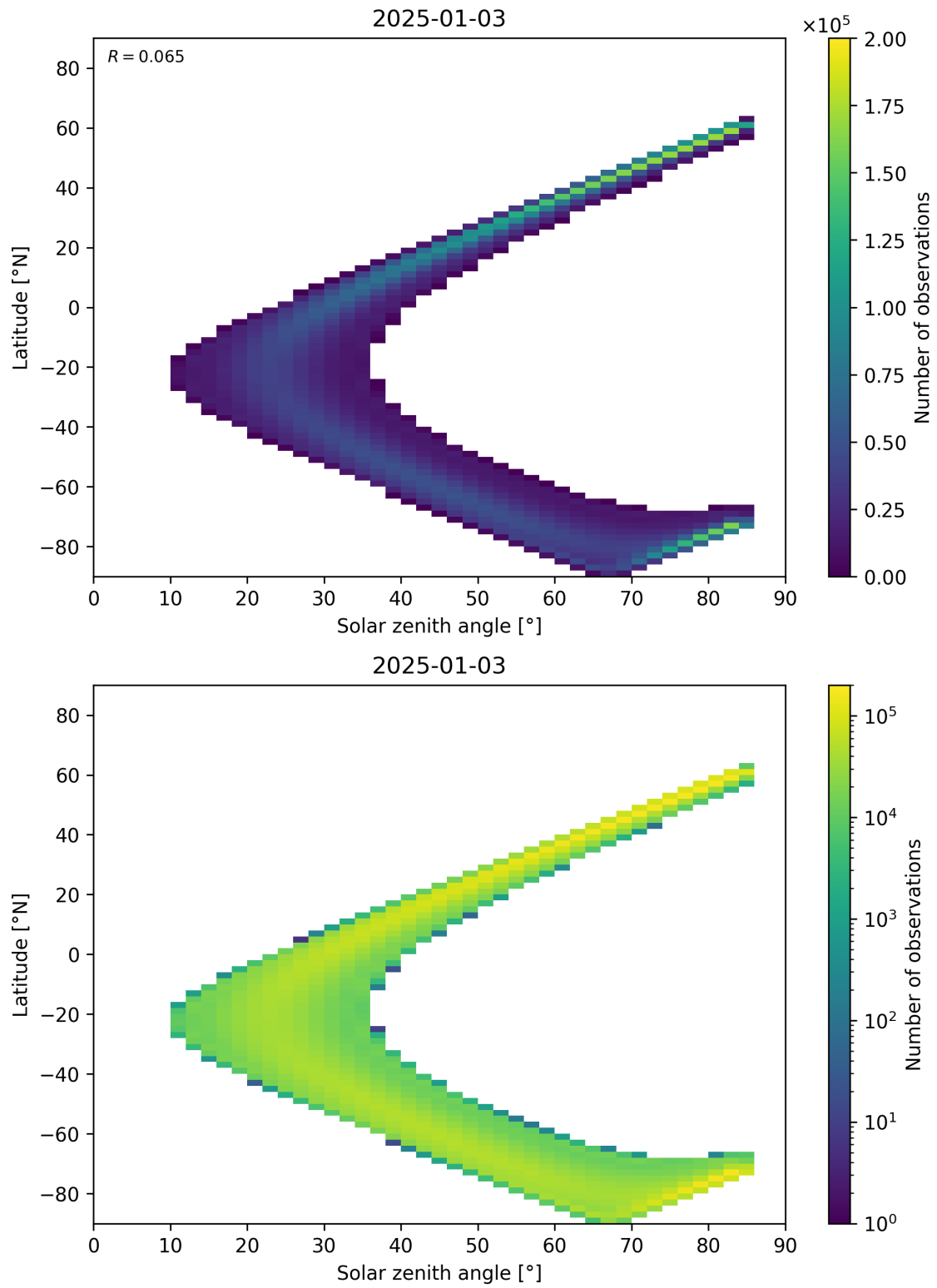
Figure 181: Scatter density plot of “Solar zenith angle” against “Latitude” for 2025-01-02 to 2025-01-04.
