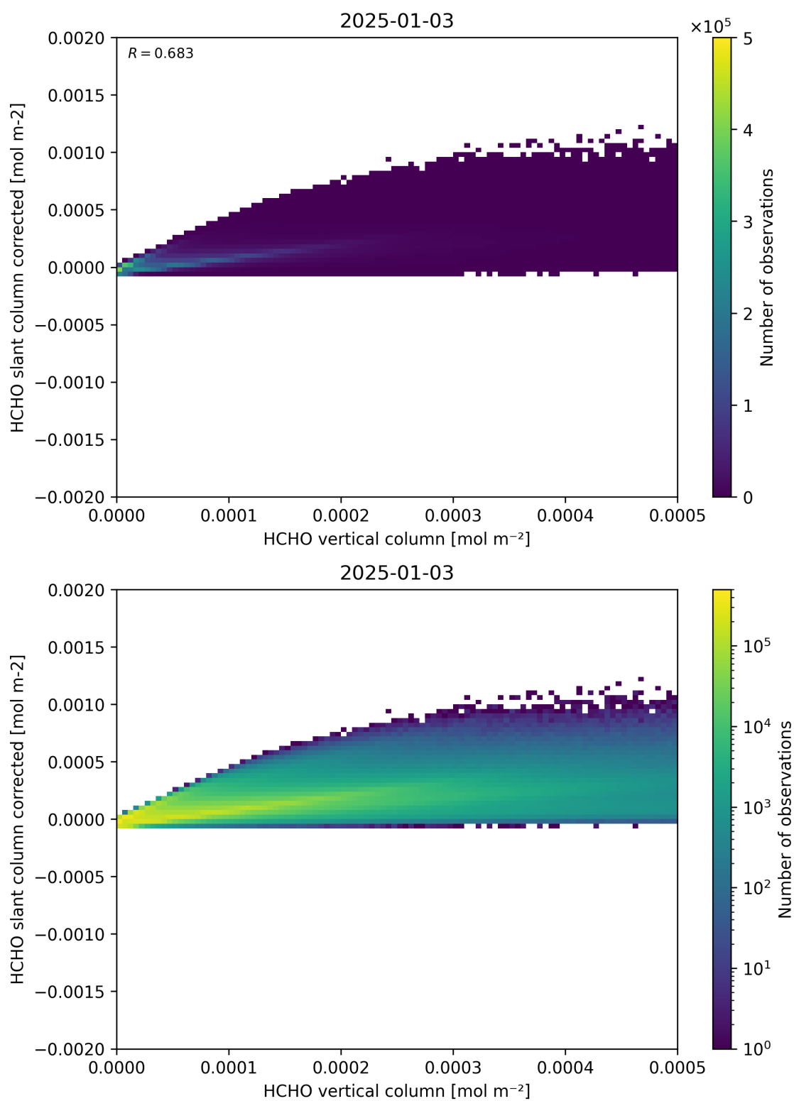
Figure 127: Scatter density plot of “HCHO vertical column” against “HCHO slant column corrected” for 2025-01-02 to 2025-01-04.
