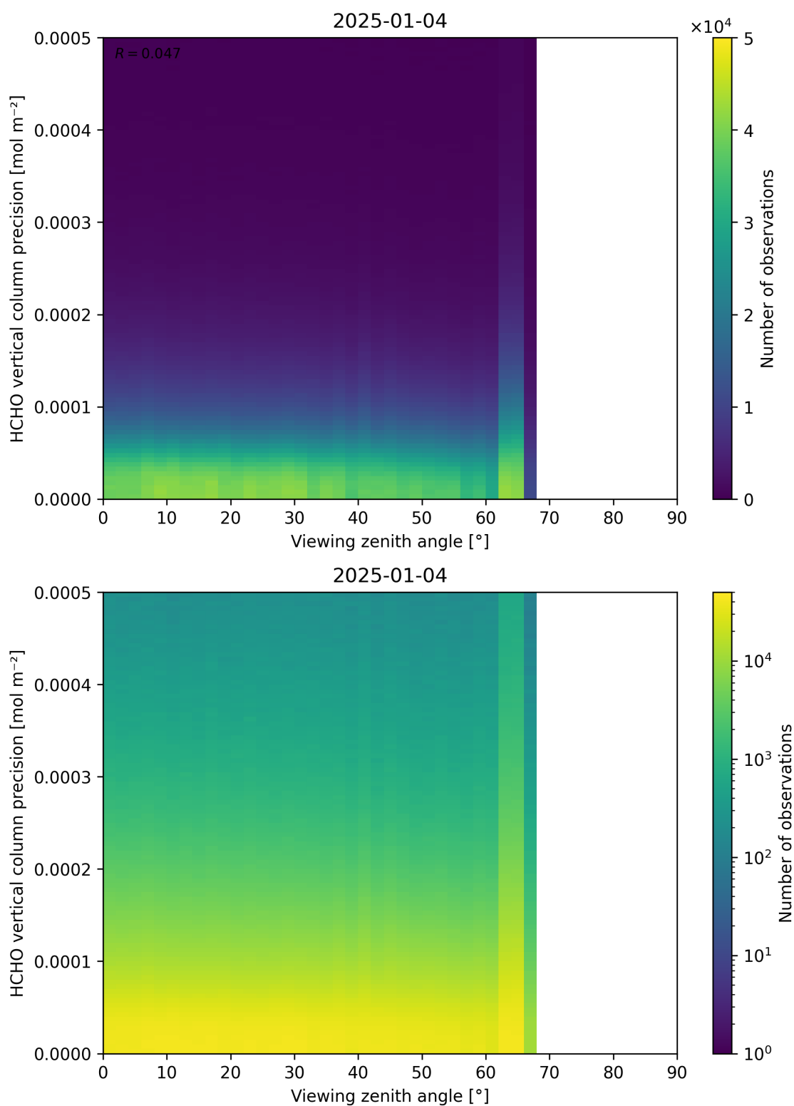
Figure 194: Scatter density plot of “Viewing zenith angle” against “HCHO vertical column precision” for 2025-01-03 to 2025-01-05.
