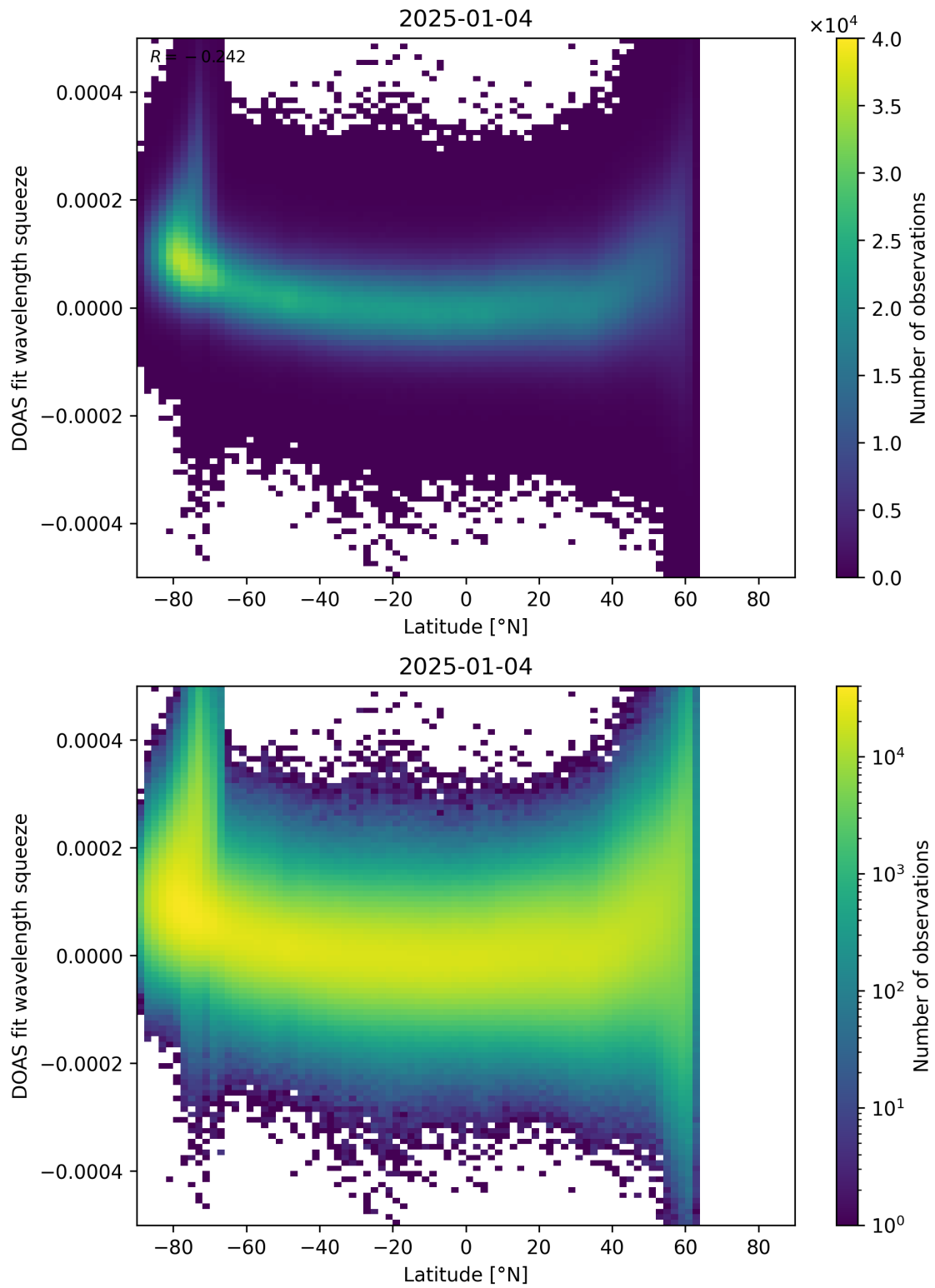
Figure 155: Scatter density plot of “Latitude” against “DOAS fit wavelength squeeze” for 2025-01-03 to 2025-01-05.
