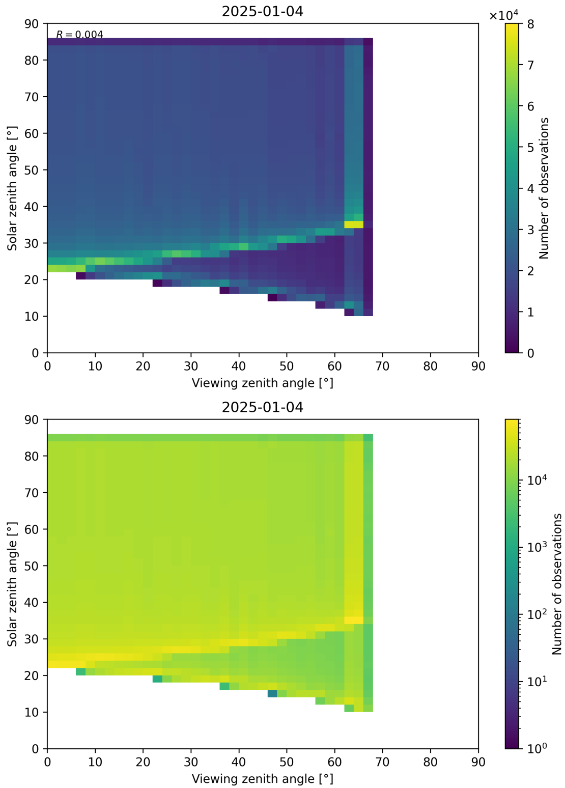
Figure 197: Scatter density plot of “Viewing zenith angle” against “Solar zenith angle” for 2025-01-03 to 2025-01-05.
