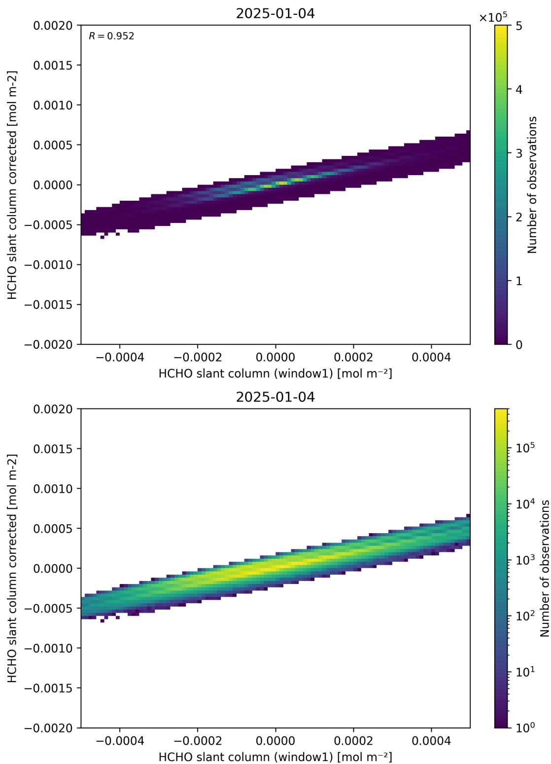
Figure 82: Scatter density plot of “HCHO slant column (window1)” against “HCHO slant column corrected” for 2025-01-03 to 2025-01-05.
