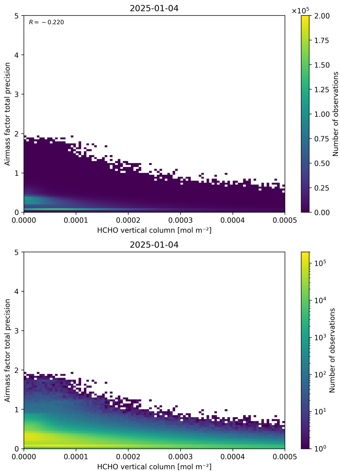
Figure 132: Scatter density plot of “HCHO vertical column” against “Airmass factor total precision” for 2025-01-03 to 2025-01-05.
