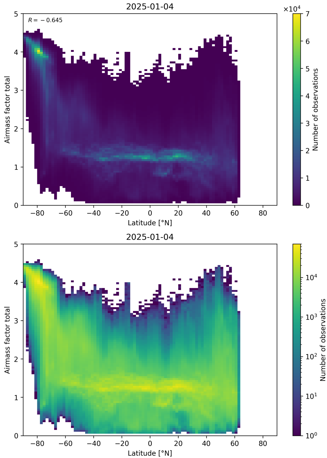
Figure 161: Scatter density plot of “Latitude” against “Airmass factor total” for 2025-01-03 to 2025-01-05.
