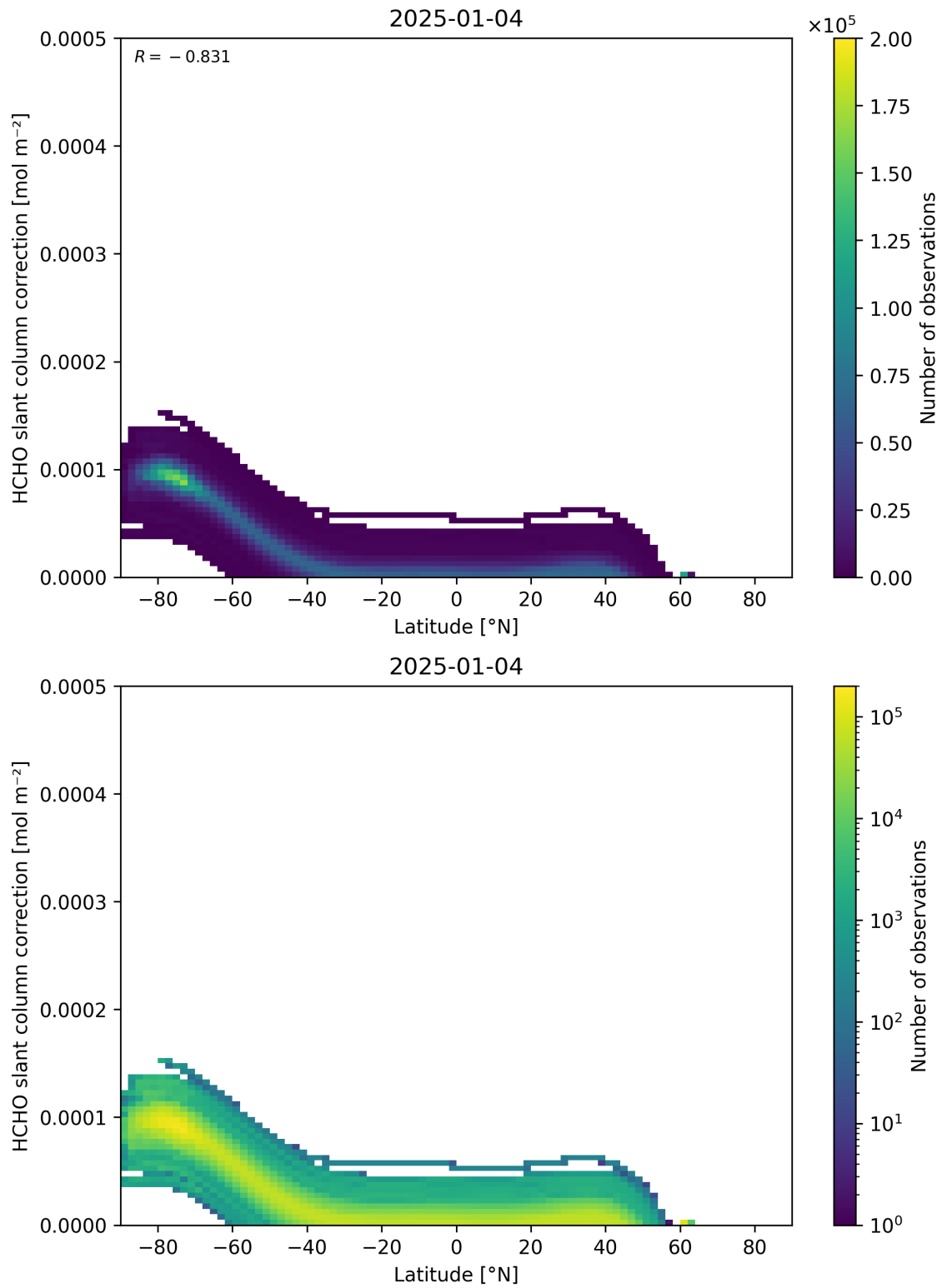
Figure 158: Scatter density plot of “Latitude” against “HCHO slant column correction” for 2025-01-03 to 2025-01-05.
