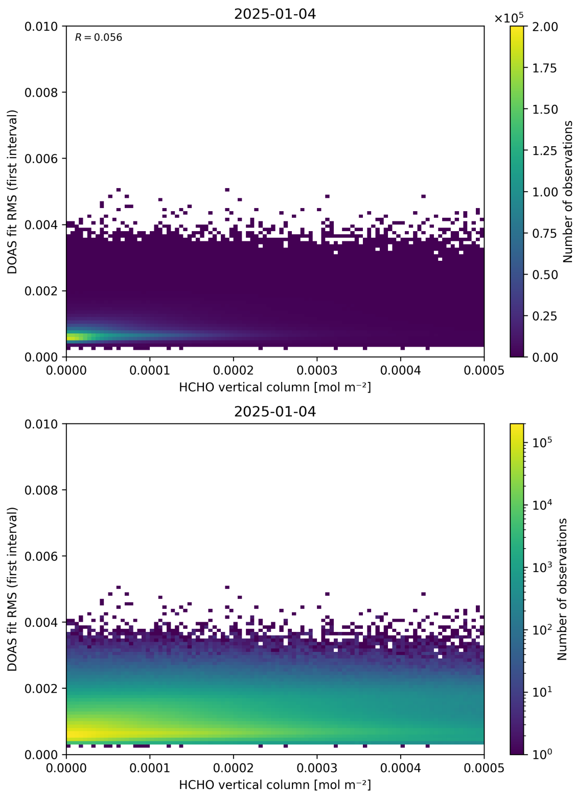
Figure 123: Scatter density plot of “HCHO vertical column” against “DOAS fit RMS (first interval)” for 2025-01-03 to 2025-01-05.
