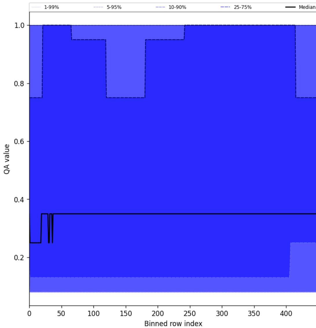
Figure 48: Along track statistics of “QA value” for 2025-01-03 to 2025-01-05
