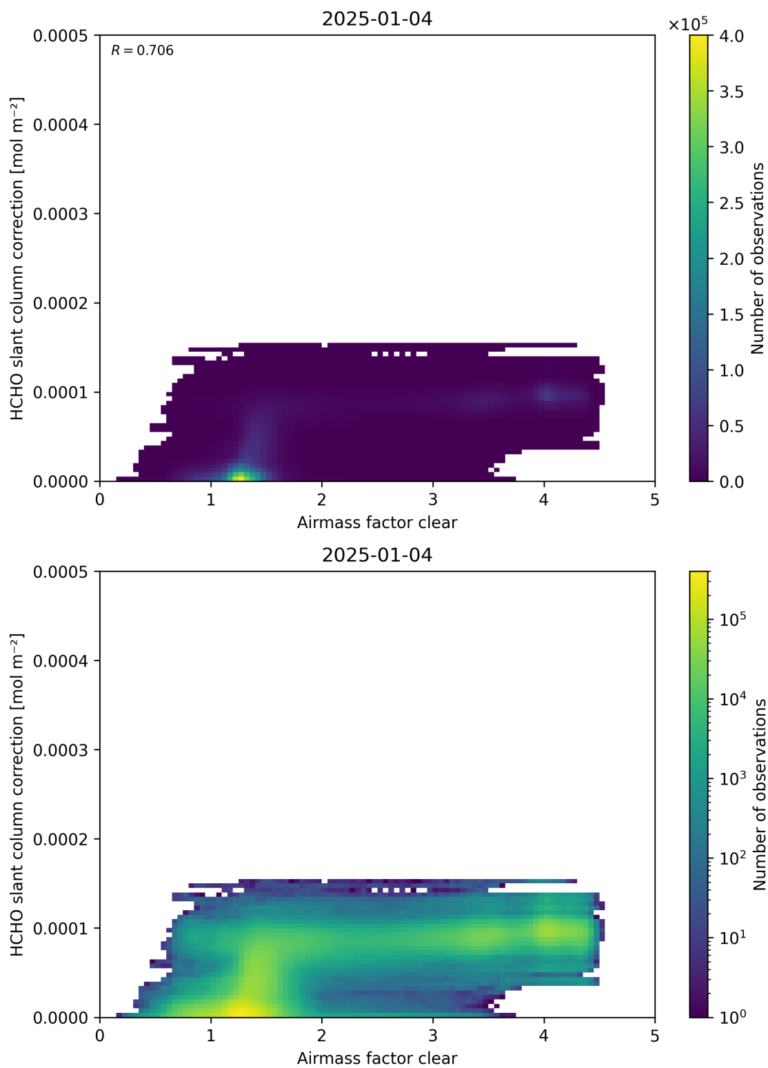
Figure 75: Scatter density plot of “Air mass factor clear” against “HCHO slant column correction” for 2025-01-03 to 2025-01-05.
