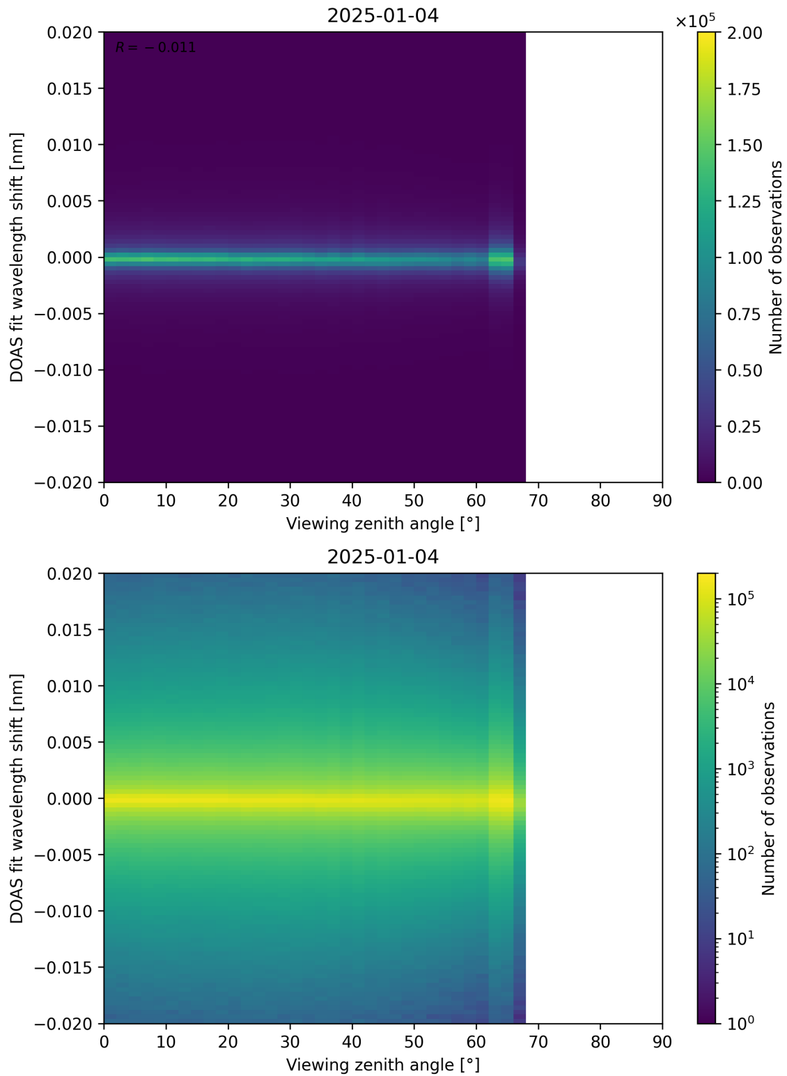
Figure 183: Scatter density plot of “Viewing zenith angle” against “DOAS fit wavelength shift” for 2025-01-03 to 2025-01-05.
