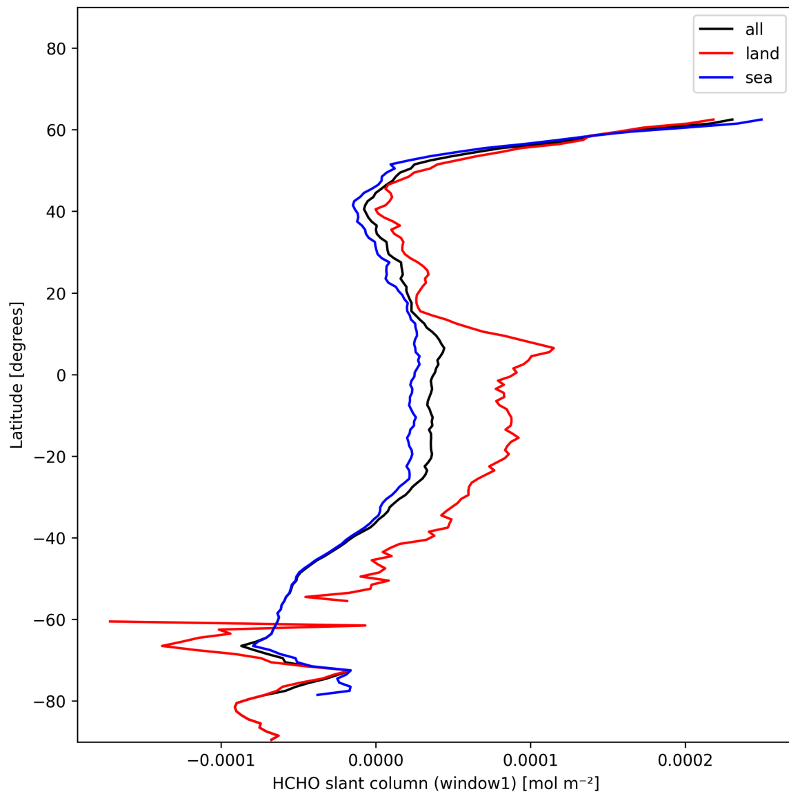
Figure 24: Zonal average of "HCHO slant column (window1)" for 2025-01-03 to 2025-01-05.
