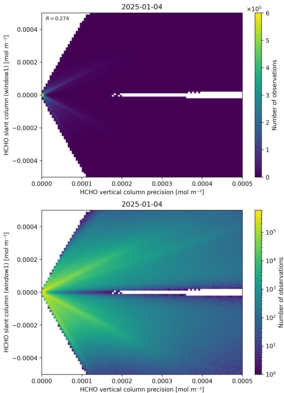
Figure 142: Scatter density plot of “HCHO vertical column precision” against “HCHO slant column (window1)” for 2025-01-03 to 2025-01-05.
