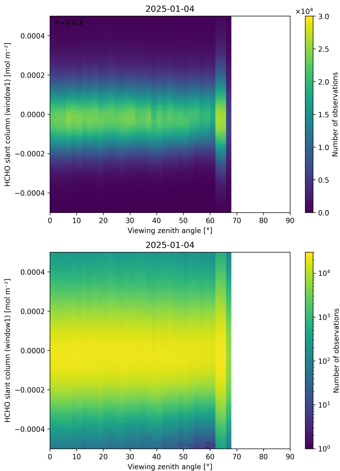
Figure 188: Scatter density plot of “Viewing zenith angle” against “HCHO slant column (window1)” for 2025-01-03 to 2025-01-05.
