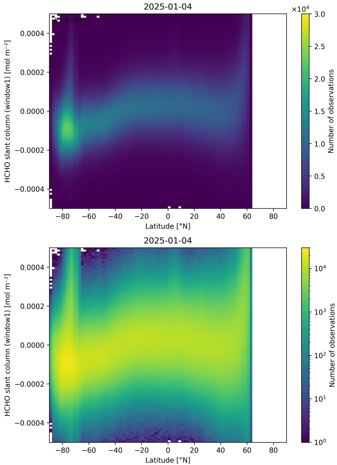
Figure 159: Scatter density plot of “Latitude” against “HCHO slant column (window1)” for 2025-01-03 to 2025-01-05.
