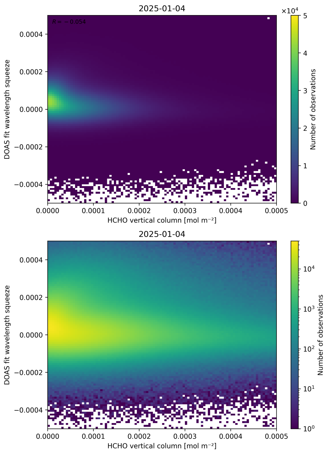
Figure 125: Scatter density plot of “HCHO vertical column” against “DOAS fit wavelength squeeze” for 2025-01-03 to 2025-01-05.
