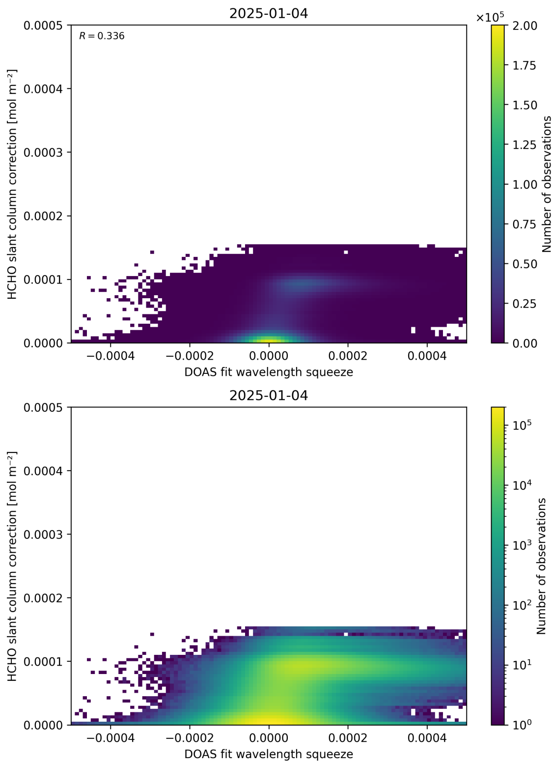
Figure 70: Scatter density plot of “DOAS fit wavelength squeeze” against “HCHO slant column correction” for 2025-01-03 to 2025-01-05.
