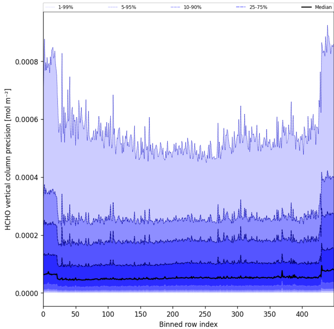
Figure 50: Along track statistics of “HCHO vertical column precision” for 2025-01-03 to 2025-01-05
