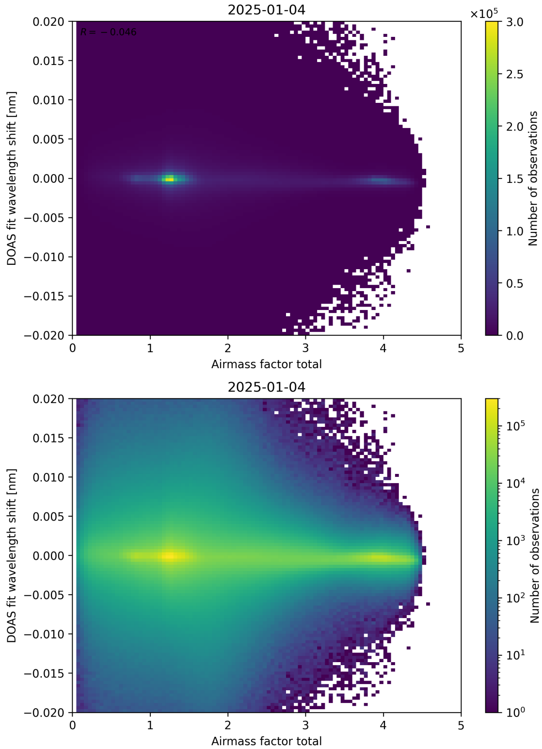
Figure 98: Scatter density plot of “Airmass factor total” against “DOAS fit wavelength shift” for 2025-01-03 to 2025-01-05.
