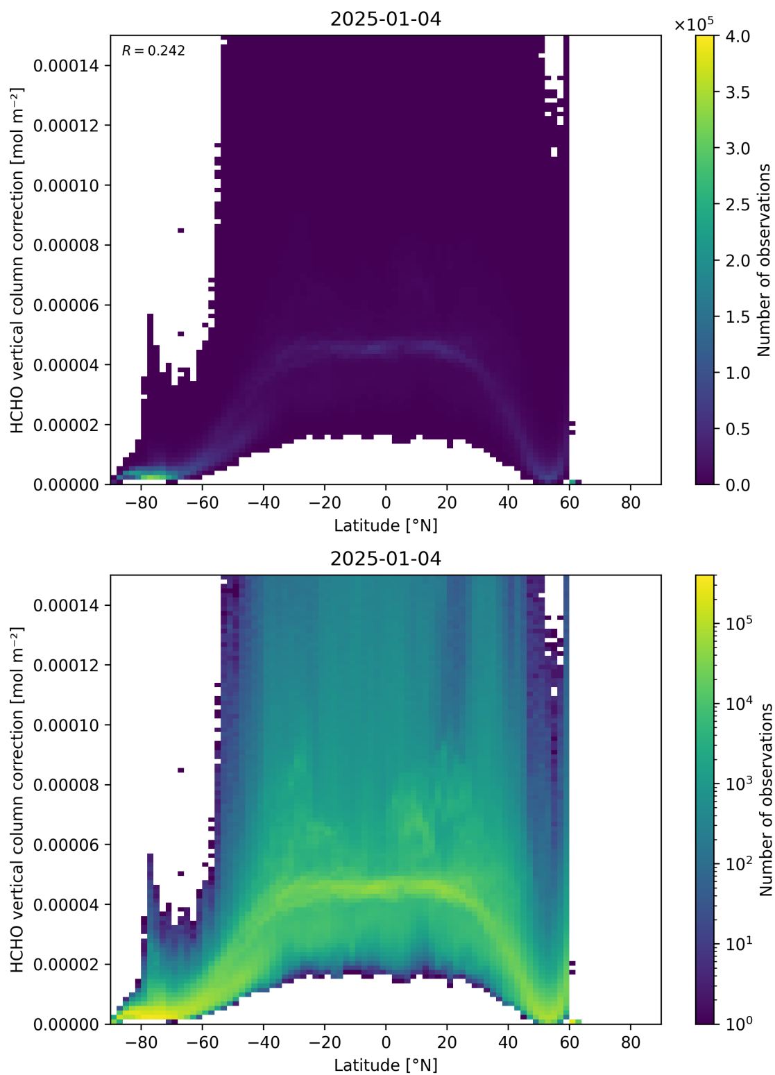
Figure 164: Scatter density plot of “Latitude” against “HCHO vertical column correction” for 2025-01-03 to 2025-01-05.
