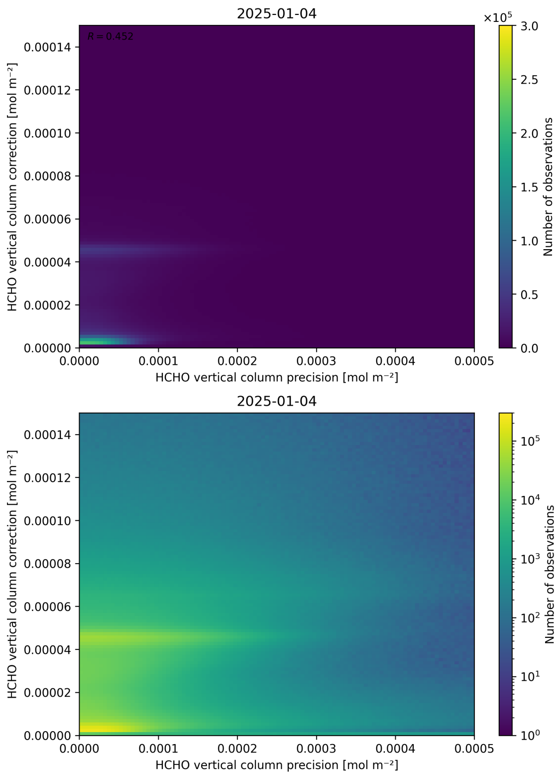
Figure 146: Scatter density plot of “HCHO vertical column precision” against “HCHO vertical column correction” for 2025-01-03 to 2025-01-05.
