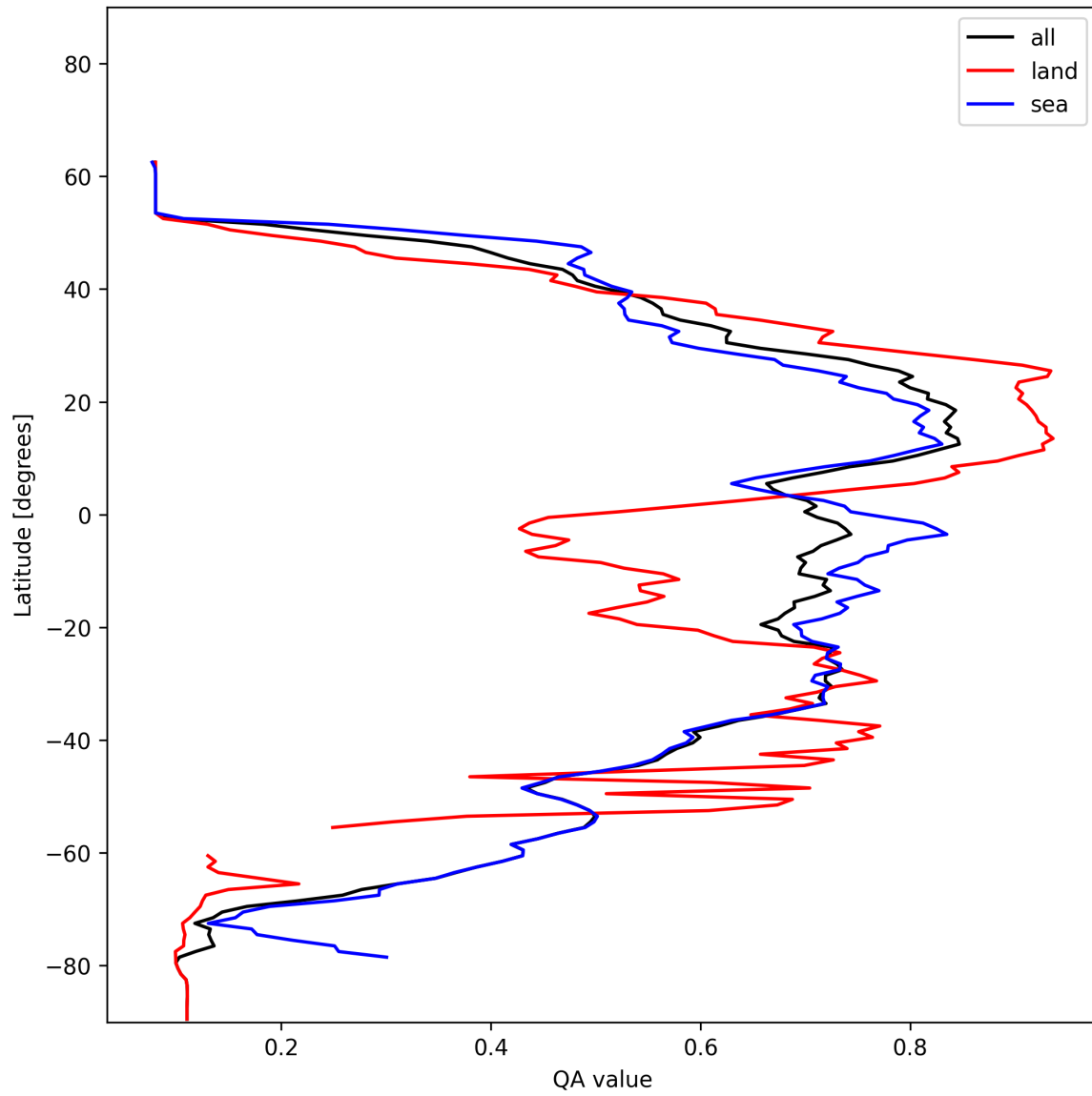
Figure 20: Zonal average of “QA value” for 2025-01-03 to 2025-01-05.
