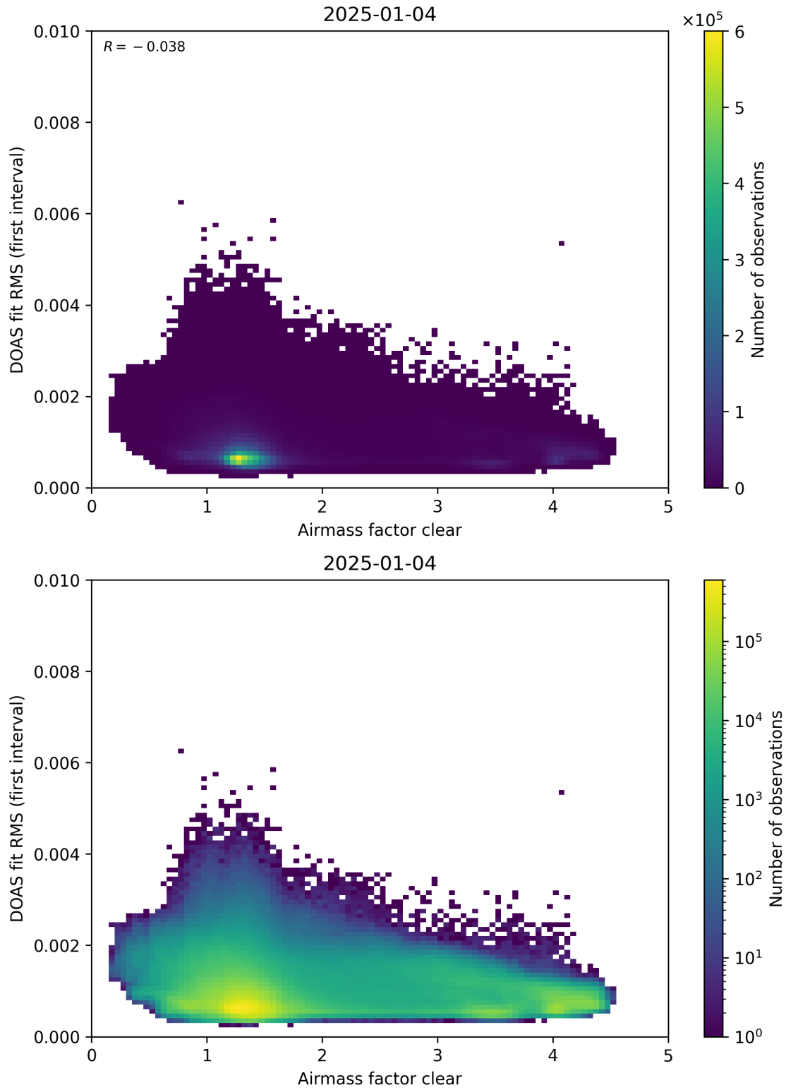
Figure 71: Scatter density plot of “Airmass factor clear” against “DOAS fit RMS (first interval)” for 2025-01-03 to 2025-01-05.
