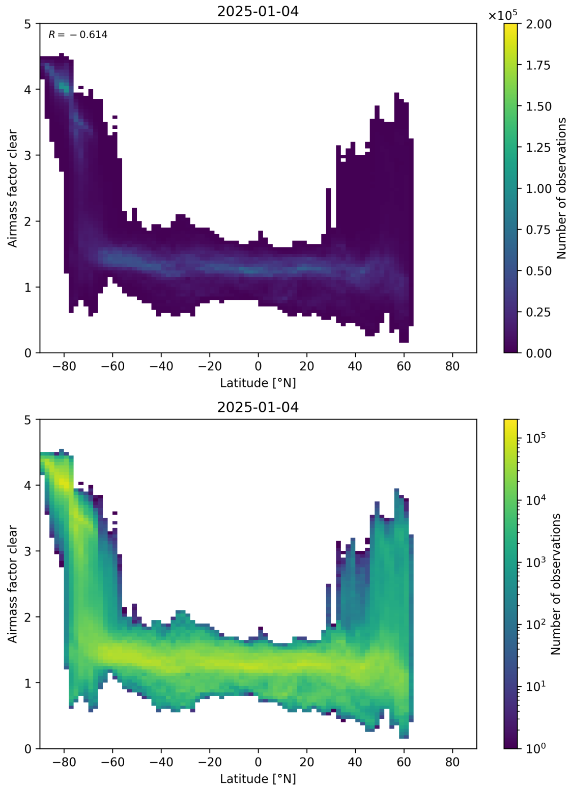
Figure 156: Scatter density plot of “Latitude” against “Airmass factor clear” for 2025-01-03 to 2025-01-05.
