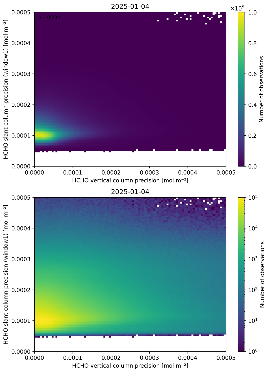
Figure 143: Scatter density plot of “HCHO vertical column precision” against “HCHO slant column precision (window1)” for 2025-01-03 to 2025-01-05.
