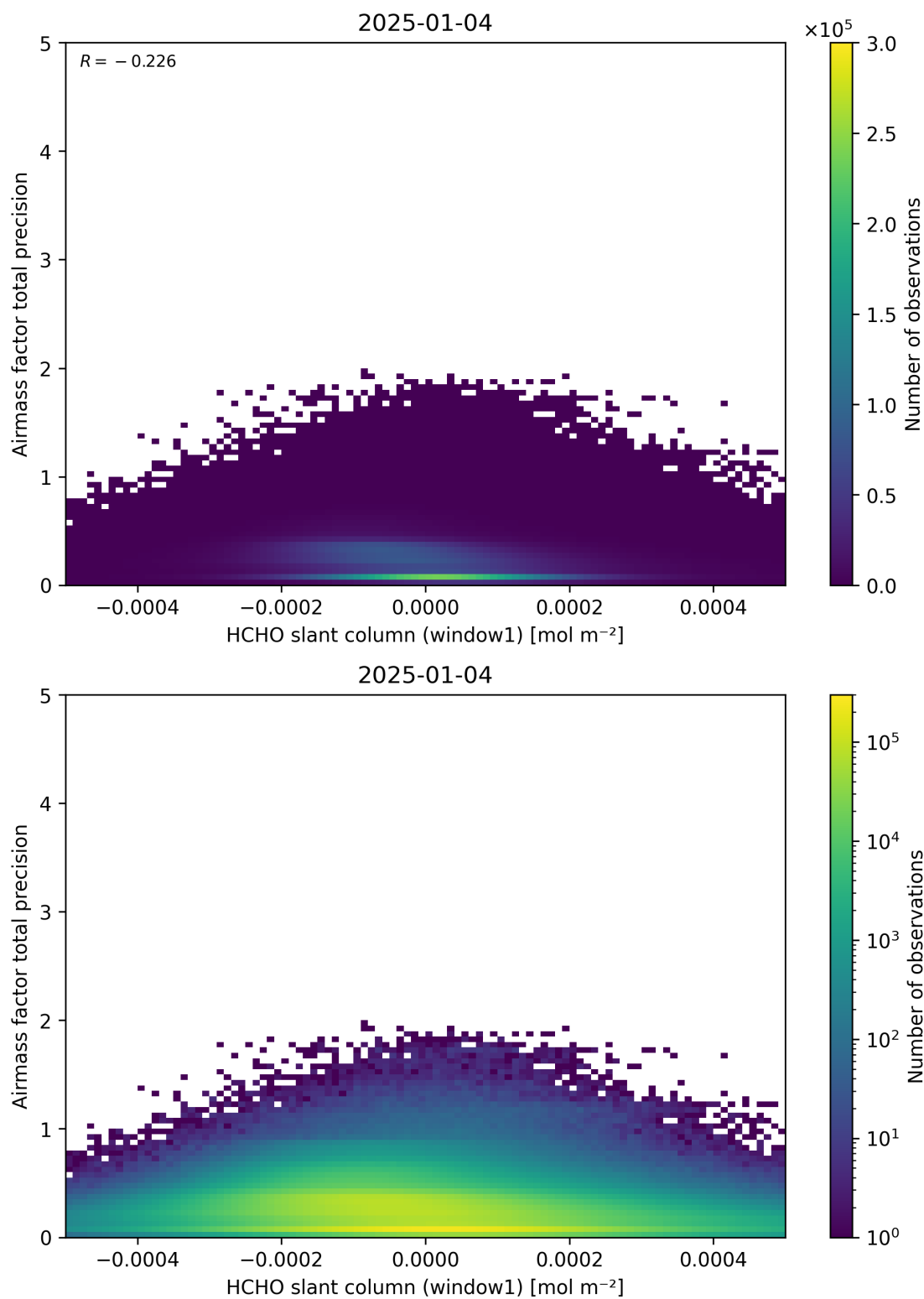
Figure 86: Scatter density plot of “HCHO slant column (window1)” against “Airmass factor total precision” for 2025-01-03 to 2025-01-05.
