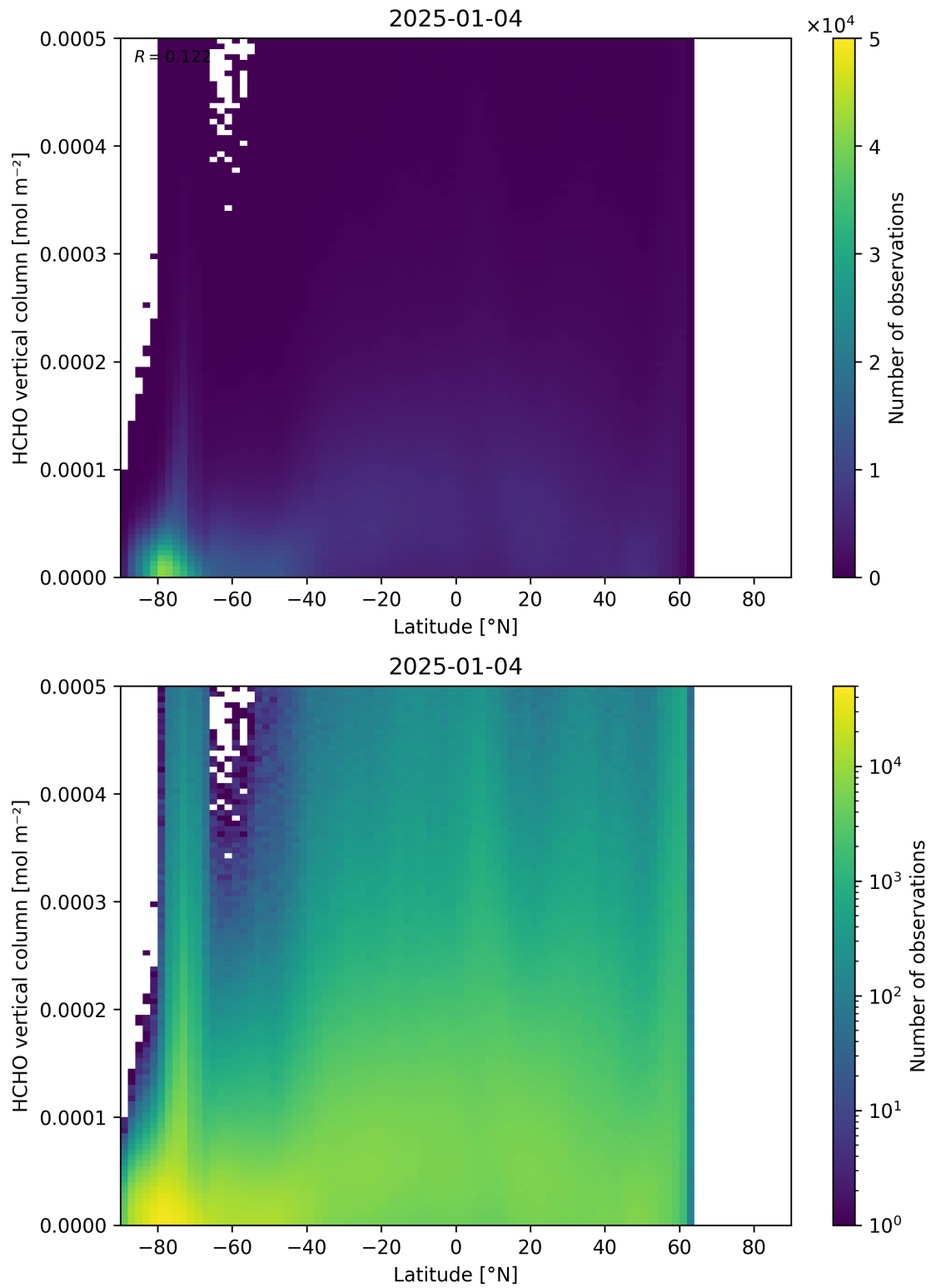
Figure 163: Scatter density plot of “Latitude” against “HCHO vertical column” for 2025-01-03 to 2025-01-05.
