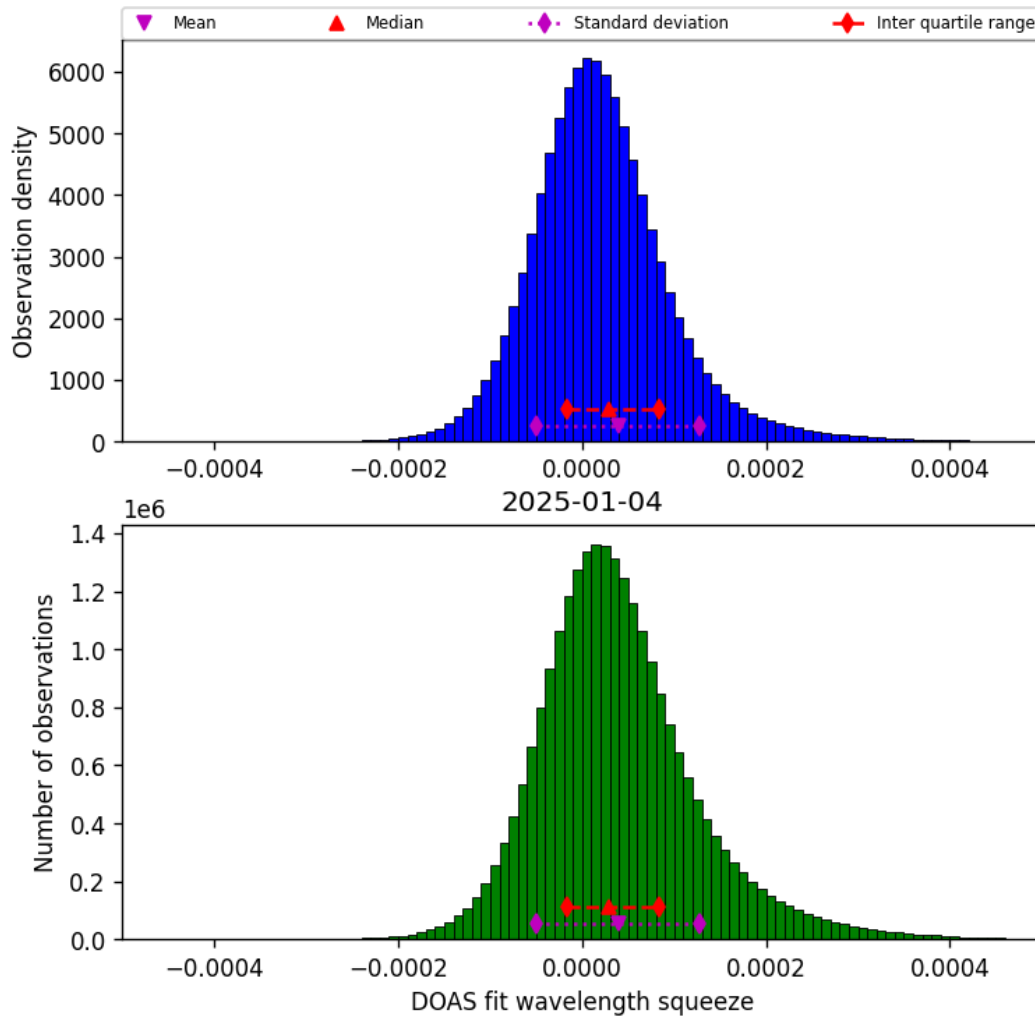
Figure 45: Histogram of “DOAS fit wavelength squeeze” for 2025-01-03 to 2025-01-05
