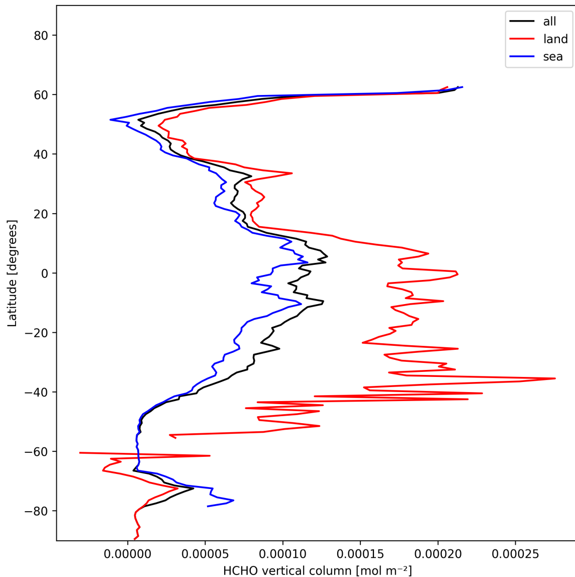
Figure 21: Zonal average of “HCHO vertical column” for 2025-01-03 to 2025-01-05.
