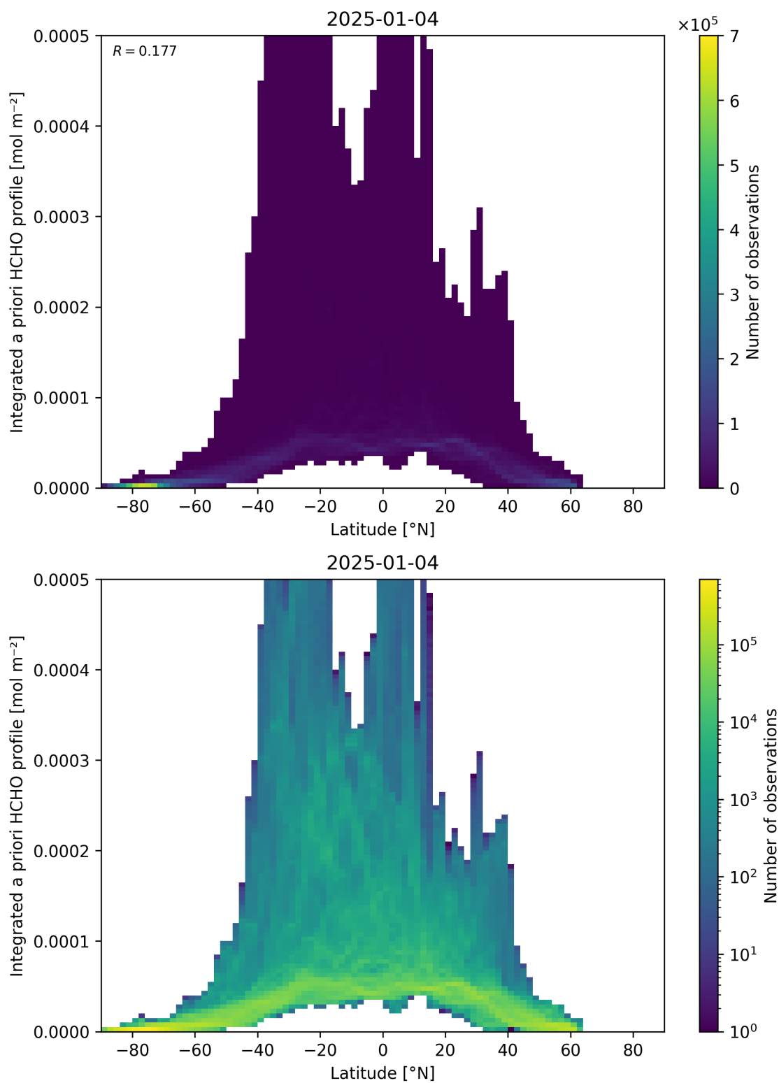
Figure 166: Scatter density plot of “Latitude” against “Integrated a priori HCHO profile” for 2025-01-03 to 2025-01-05.
