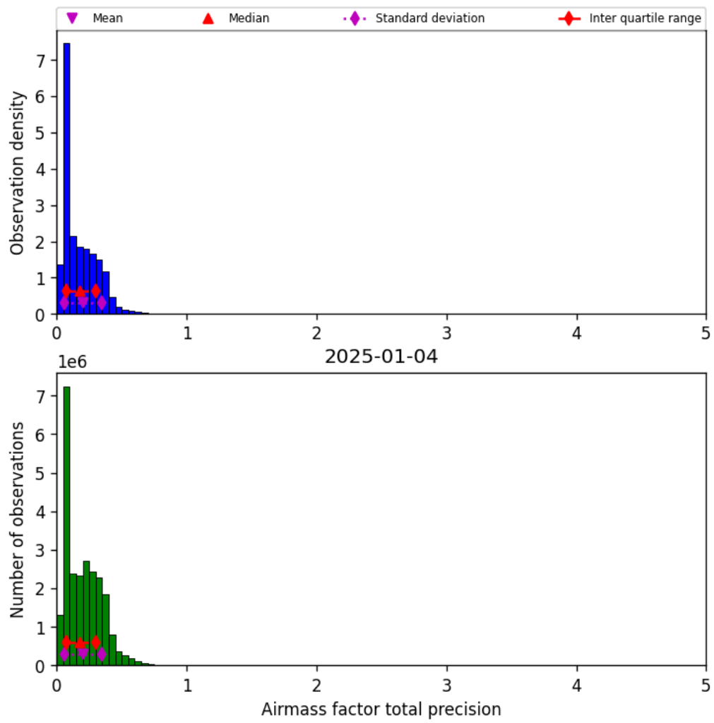
Figure 41: Histogram of “Airmass factor total precision” for 2025-01-03 to 2025-01-05
