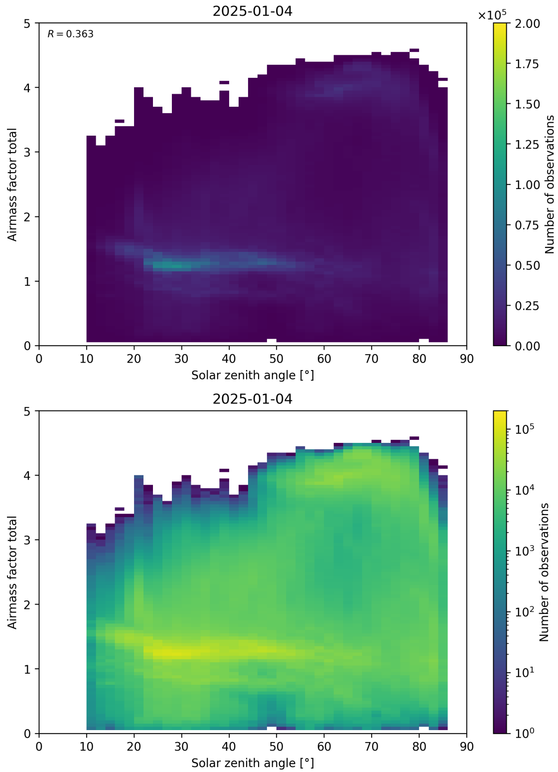
Figure 175: Scatter density plot of “Solar zenith angle” against “Airmass factor total” for 2025-01-03 to 2025-01-05.
