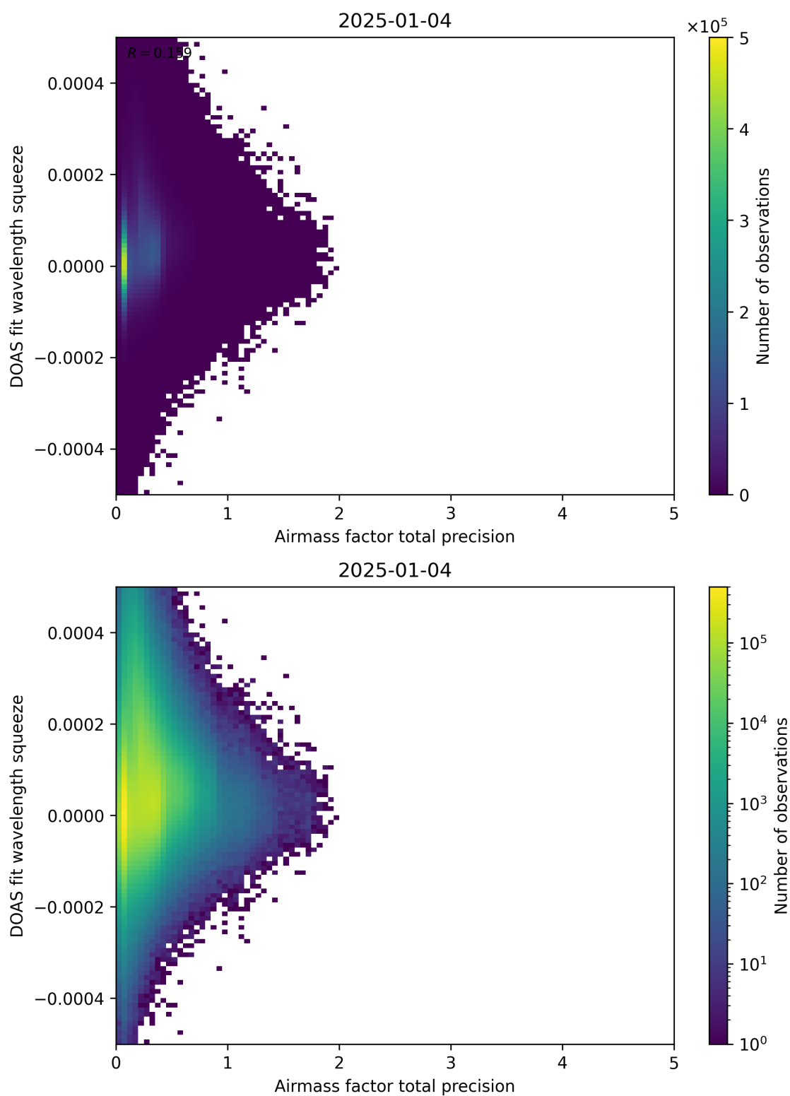
Figure 107: Scatter density plot of “Airmass factor total precision” against “DOAS fit wavelength squeeze” for 2025-01-03 to 2025-01-05.
