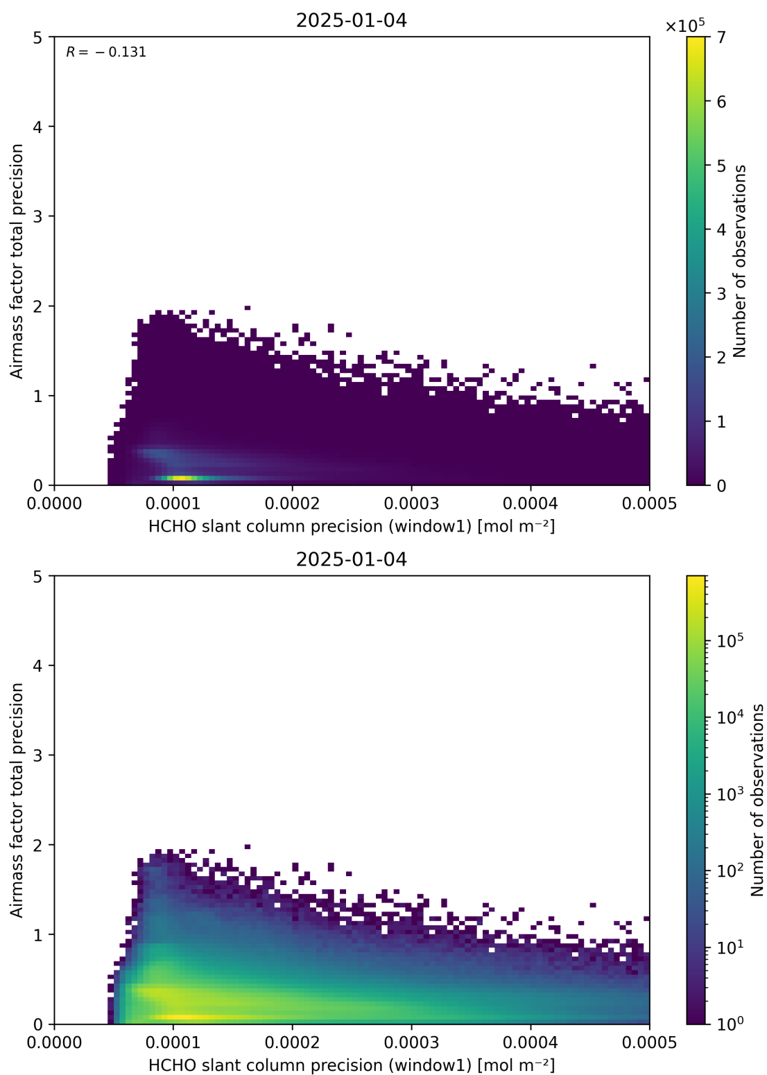
Figure 95: Scatter density plot of “HCHO slant column precision (window1)” against “Airmass factor total precision” for 2025-01-03 to 2025-01-05.
