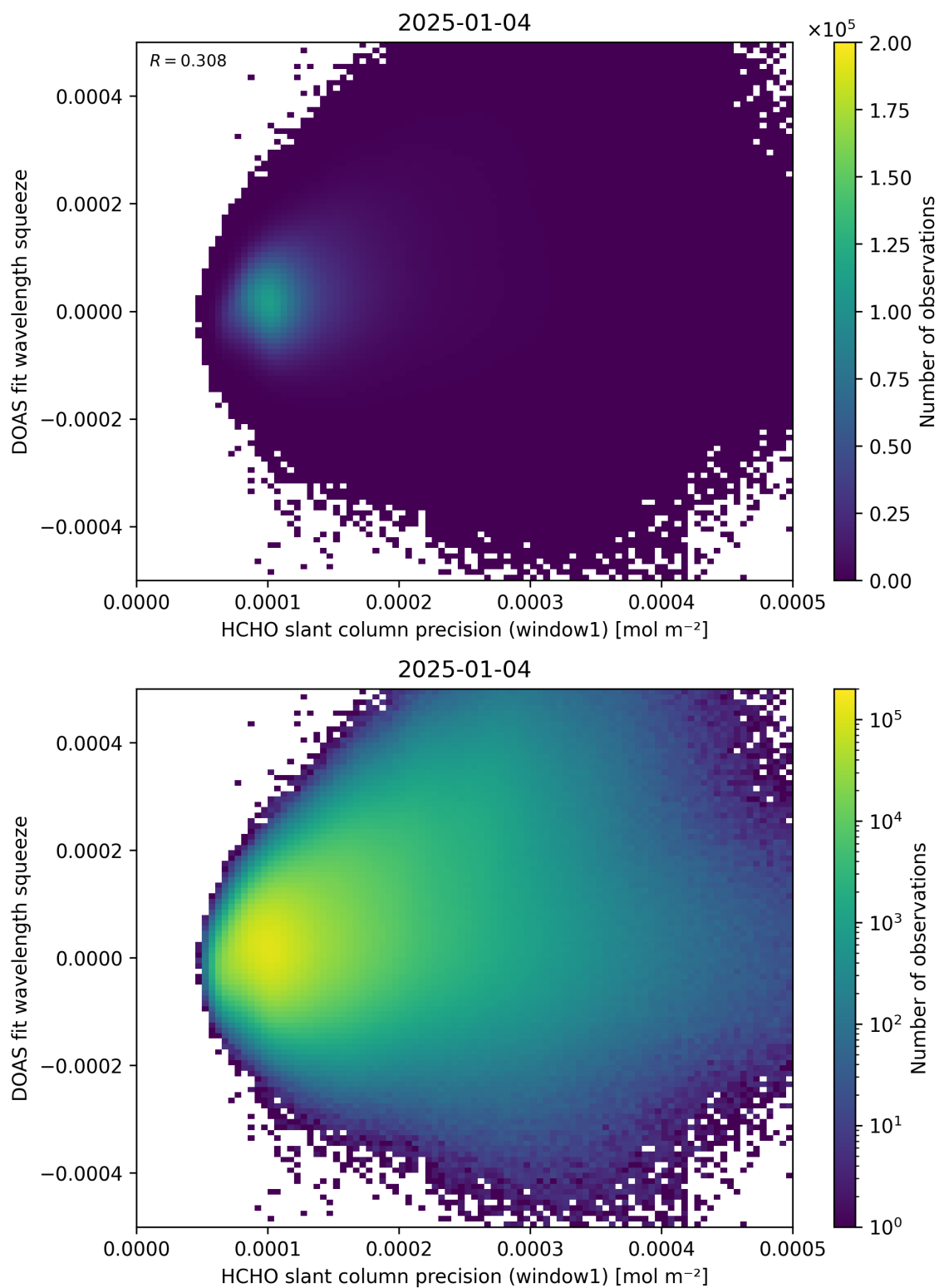
Figure 90: Scatter density plot of “HCHO slant column precision (window1)” against “DOAS fit wavelength squeeze” for 2025-01-03 to 2025-01-05.
