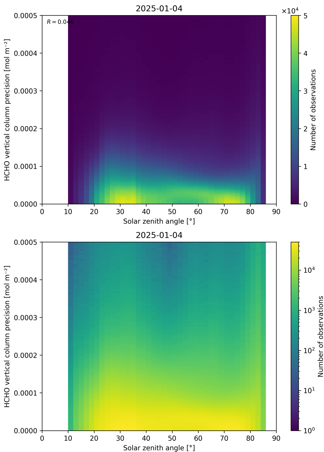
Figure 179: Scatter density plot of “Solar zenith angle” against “HCHO vertical column precision” for 2025-01-03 to 2025-01-05.
