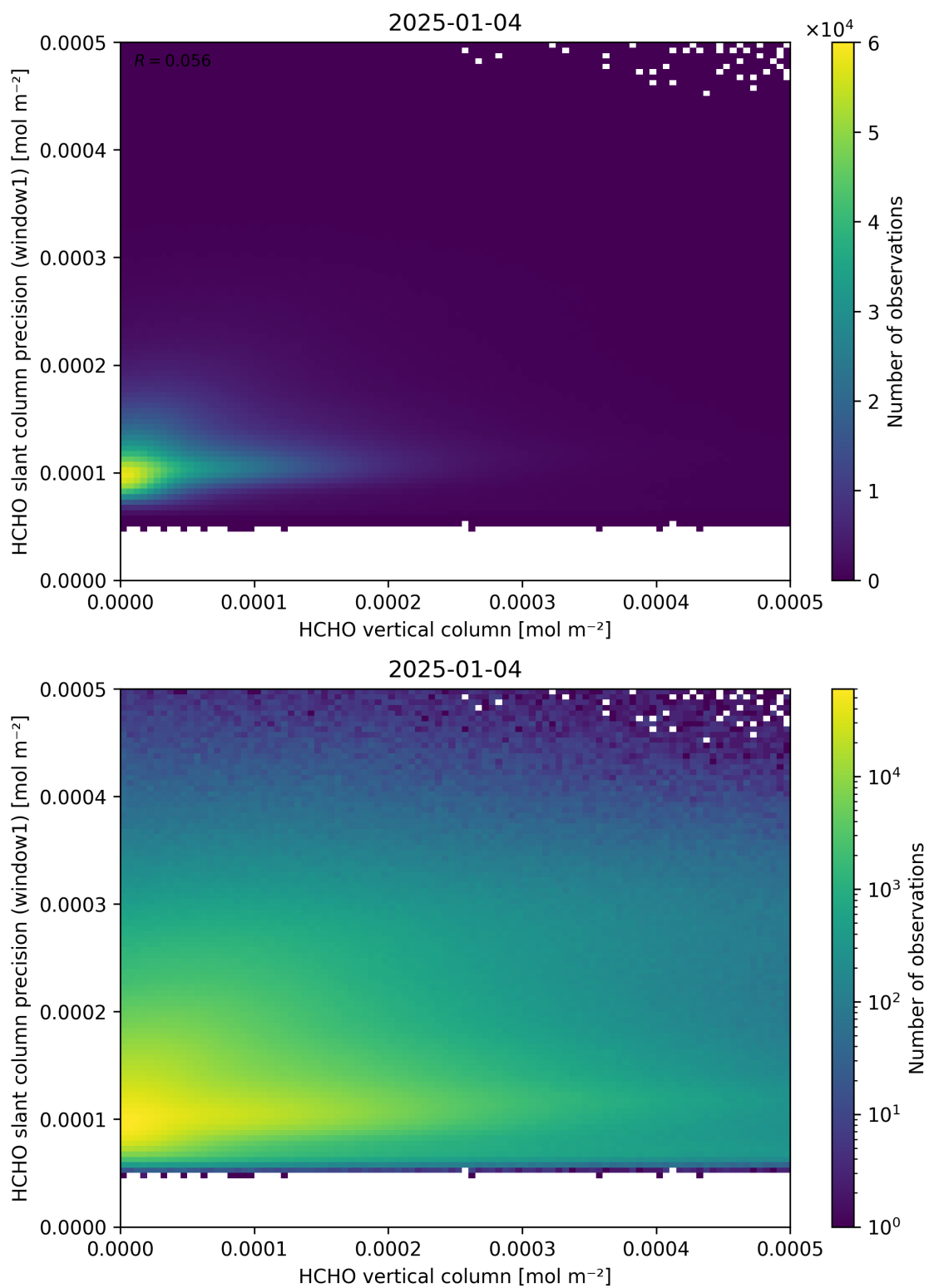
Figure 130: Scatter density plot of “HCHO vertical column” against “HCHO slant column precision (window1)” for 2025-01-03 to 2025-01-05.
