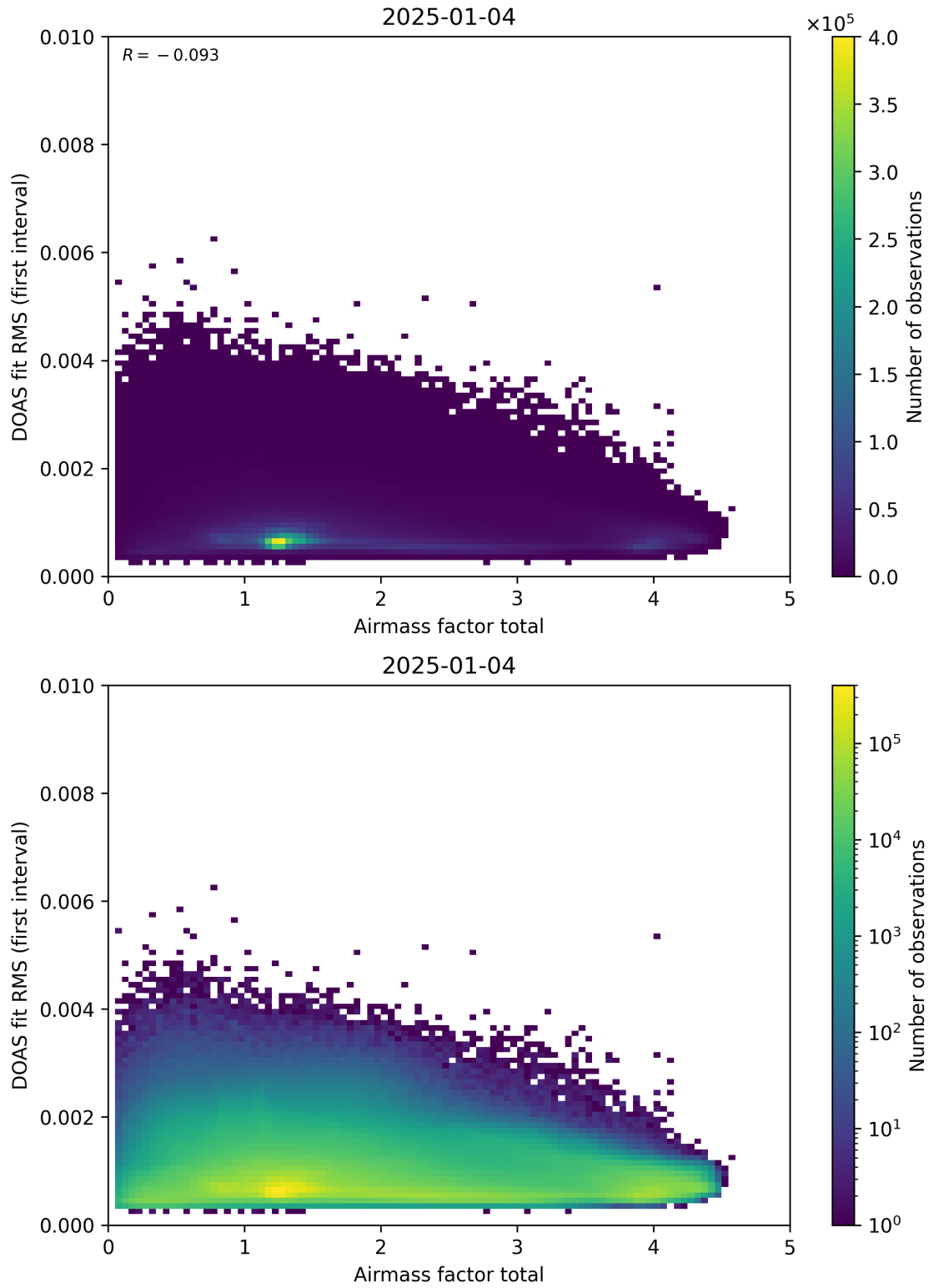
Figure 97: Scatter density plot of “Airmass factor total” against “DOAS fit RMS (first interval)” for 2025-01-03 to 2025-01-05.
