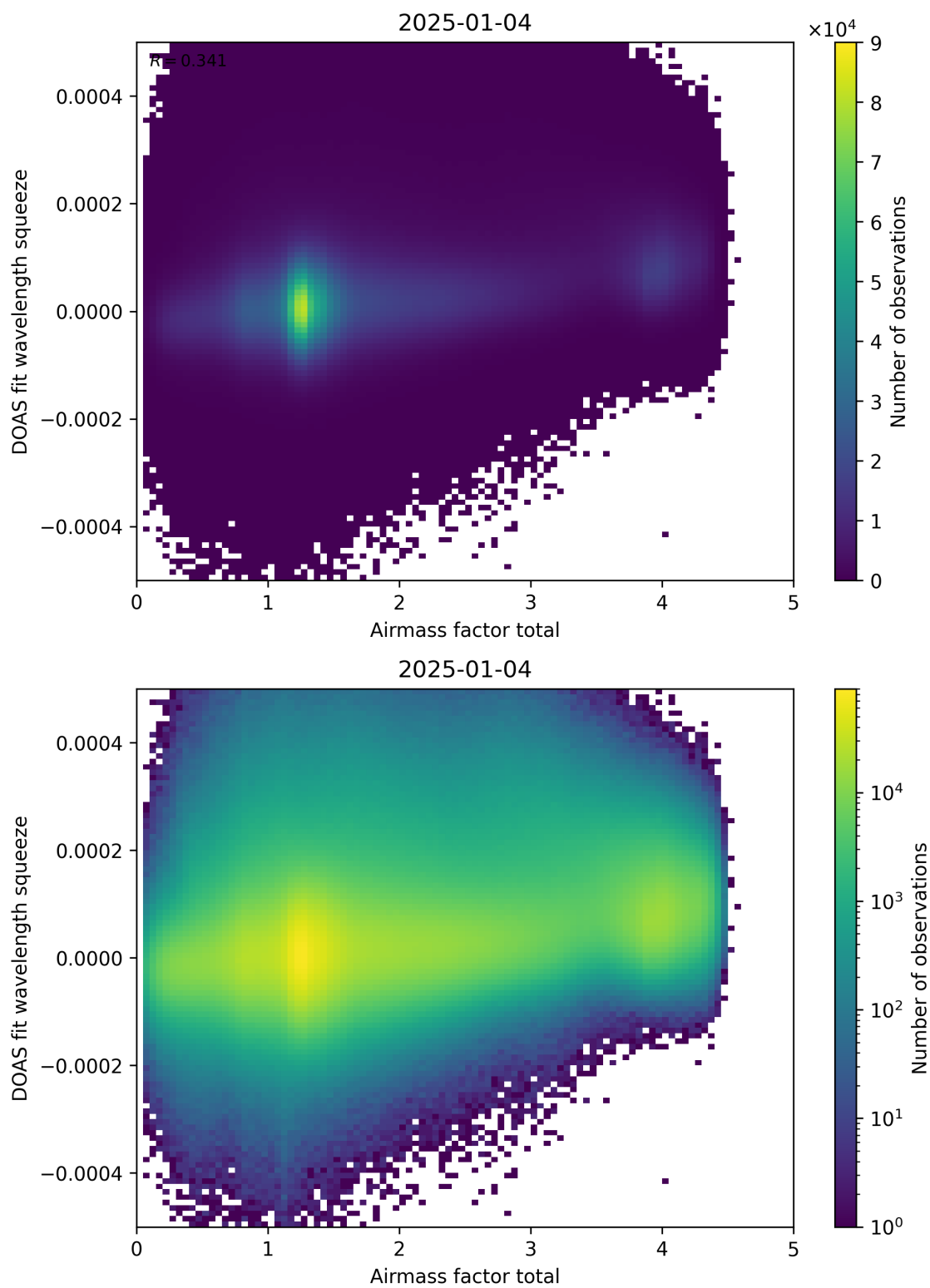
Figure 99: Scatter density plot of “Airmass factor total” against “DOAS fit wavelength squeeze” for 2025-01-03 to 2025-01-05.
