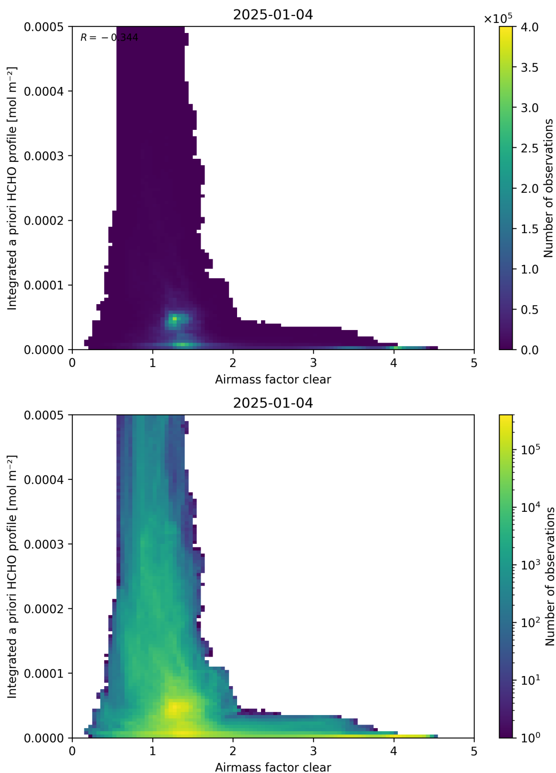
Figure 76: Scatter density plot of “Airmass factor clear” against “Integrated a priori HCHO profile” for 2025-01-03 to 2025-01-05.
