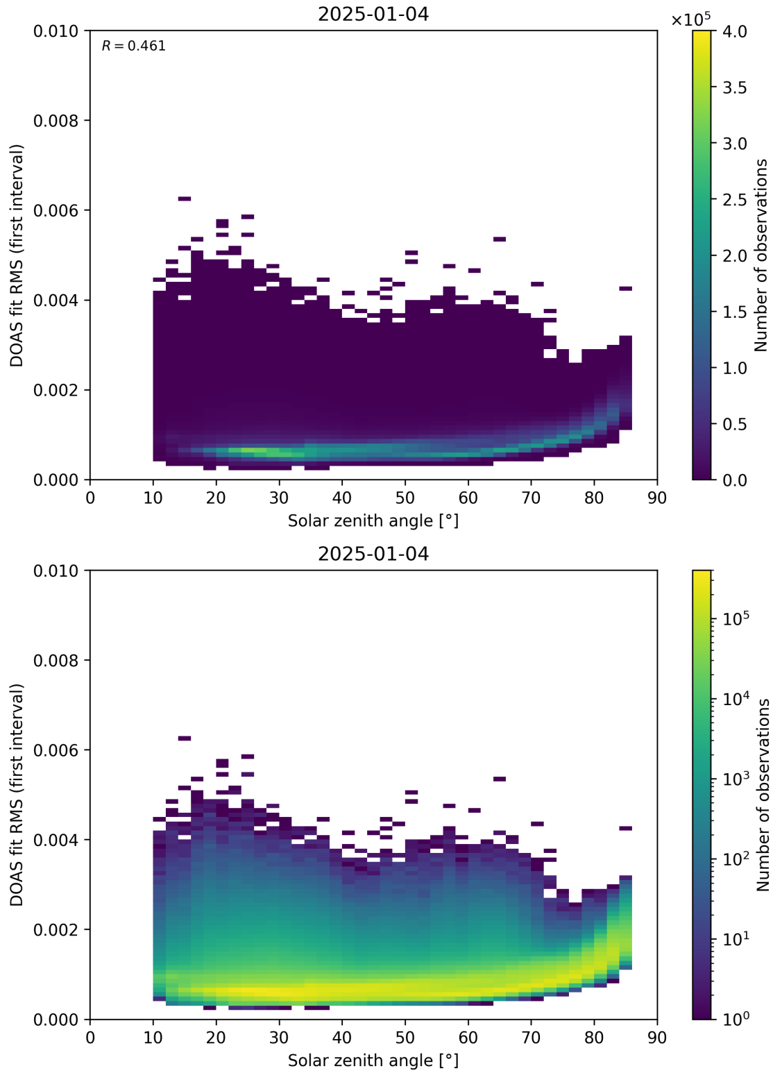
Figure 167: Scatter density plot of “Solar zenith angle” against “DOAS fit RMS (first interval)” for 2025-01-03 to 2025-01-05.
