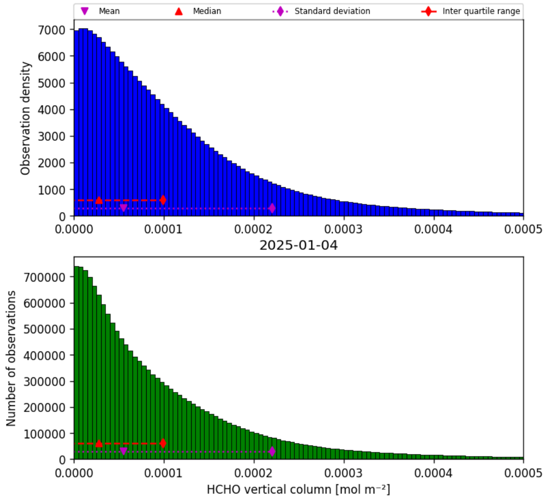
Figure 35: Histogram of “HCHO vertical column” for 2025-01-03 to 2025-01-05
