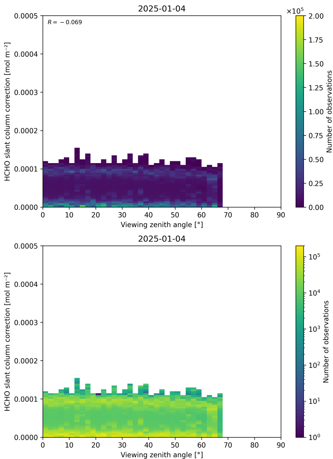
Figure 187: Scatter density plot of “Viewing zenith angle” against “HCHO slant column correction” for 2025-01-03 to 2025-01-05.
