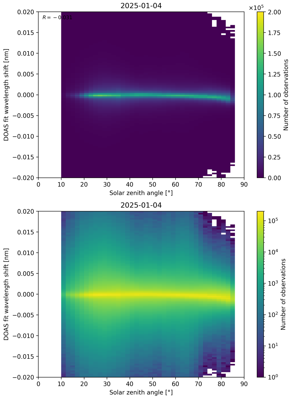
Figure 168: Scatter density plot of “Solar zenith angle” against “DOAS fit wavelength shift” for 2025-01-03 to 2025-01-05.
