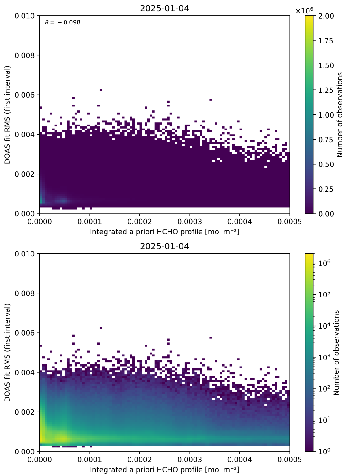
Figure 148: Scatter density plot of “Integrated a priori HCHO profile” against “DOAS fit RMS (first interval)” for 2025-01-03 to 2025-01-05.
