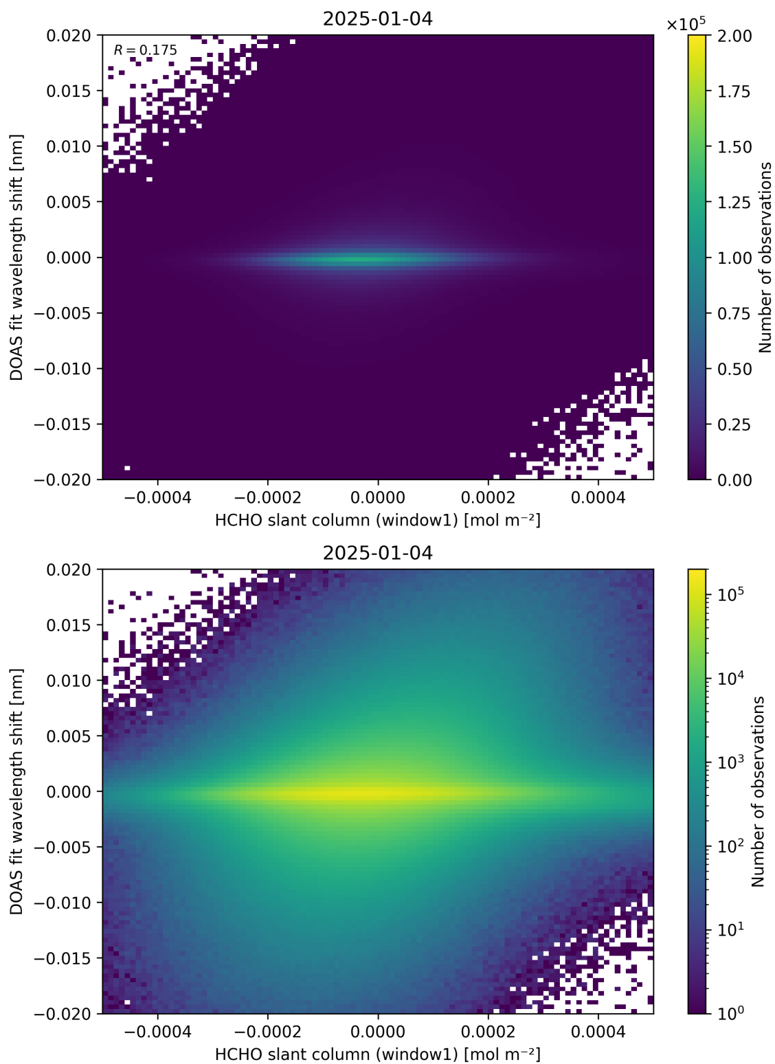
Figure 79: Scatter density plot of “HCHO slant column (window1)” against “DOAS fit wavelength shift” for 2025-01-03 to 2025-01-05.
