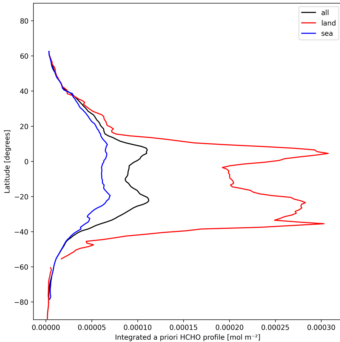
Figure 29: Zonal average of “Integrated a priori HCHO profile” for 2025-01-03 to 2025-01-05.
