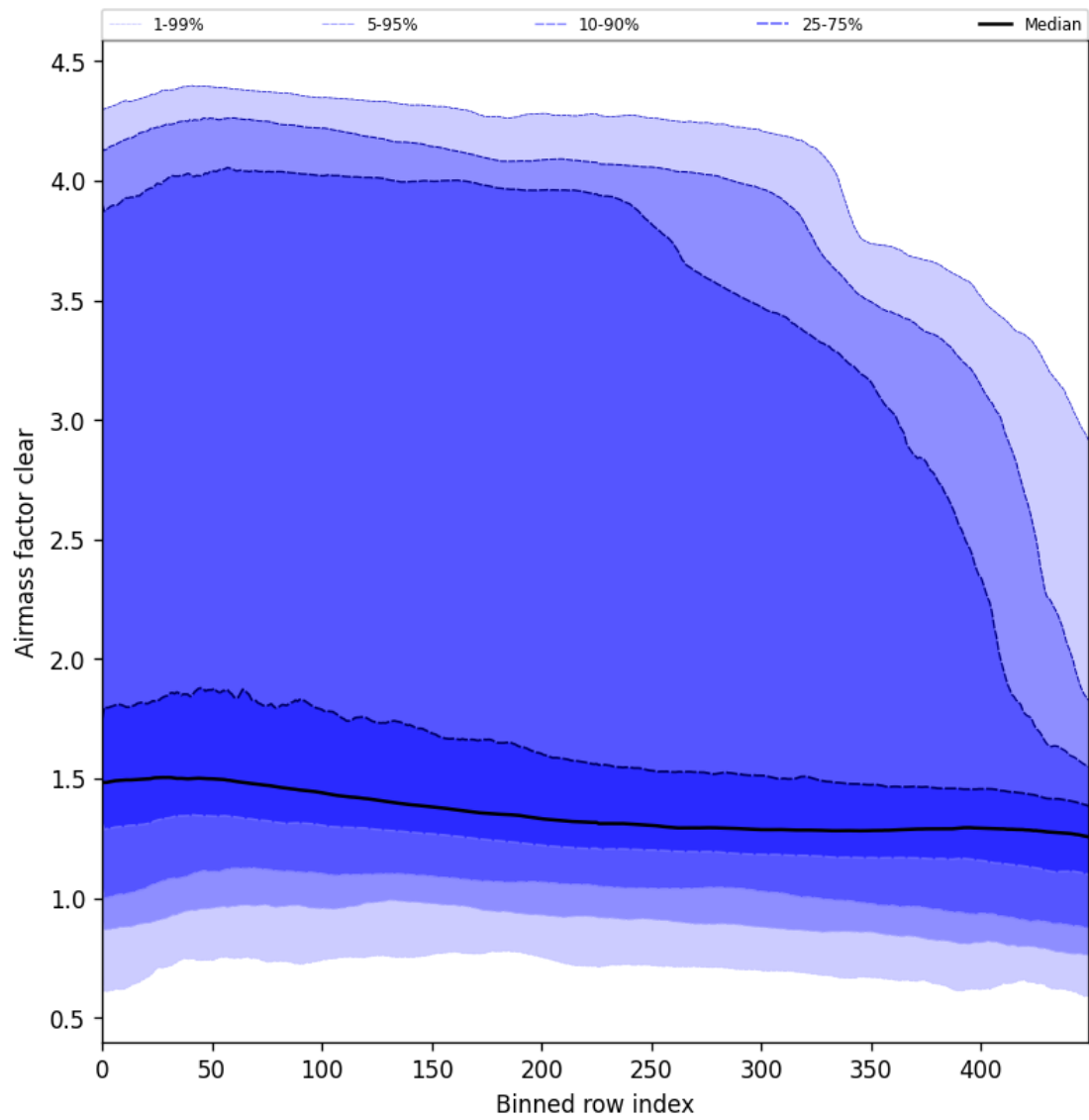
Figure 56: Along track statistics of “Airmass factor clear” for 2025-01-03 to 2025-01-05
