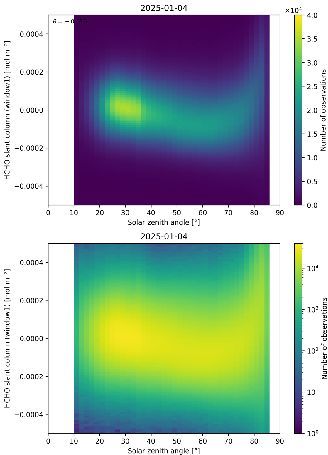
Figure 173: Scatter density plot of “Solar zenith angle” against “HCHO slant column (window1)” for 2025-01-03 to 2025-01-05.
