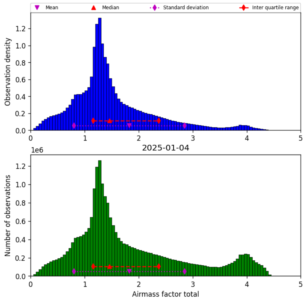
Figure 40: Histogram of “Airmass factor total” for 2025-01-03 to 2025-01-05
