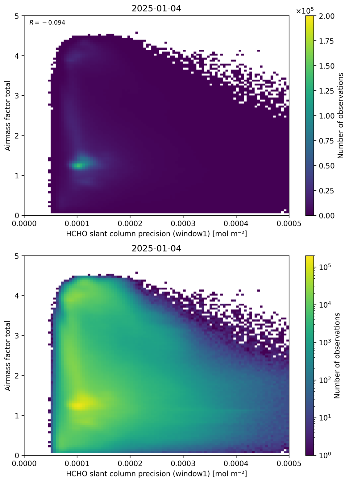
Figure 94: Scatter density plot of “HCHO slant column precision (window1)” against “Airmass factor total” for 2025-01-03 to 2025-01-05.
