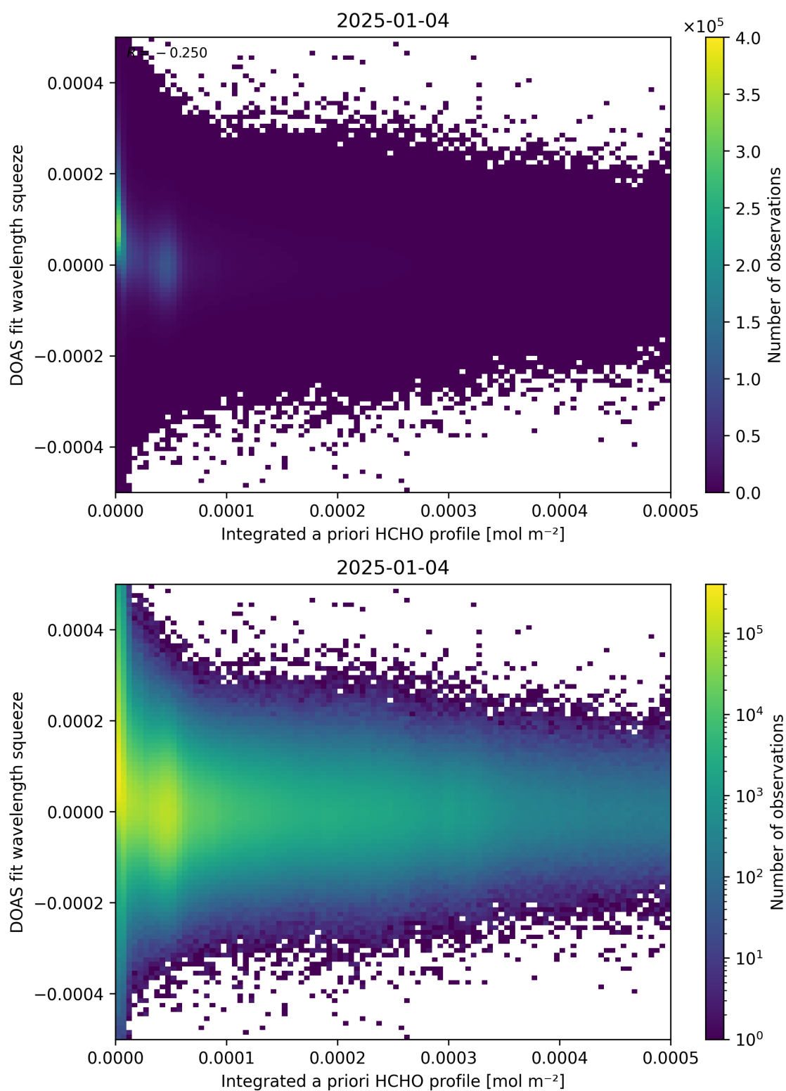
Figure 150: Scatter density plot of “Integrated a priori HCHO profile” against “DOAS fit wavelength squeeze” for 2025-01-03 to 2025-01-05.
