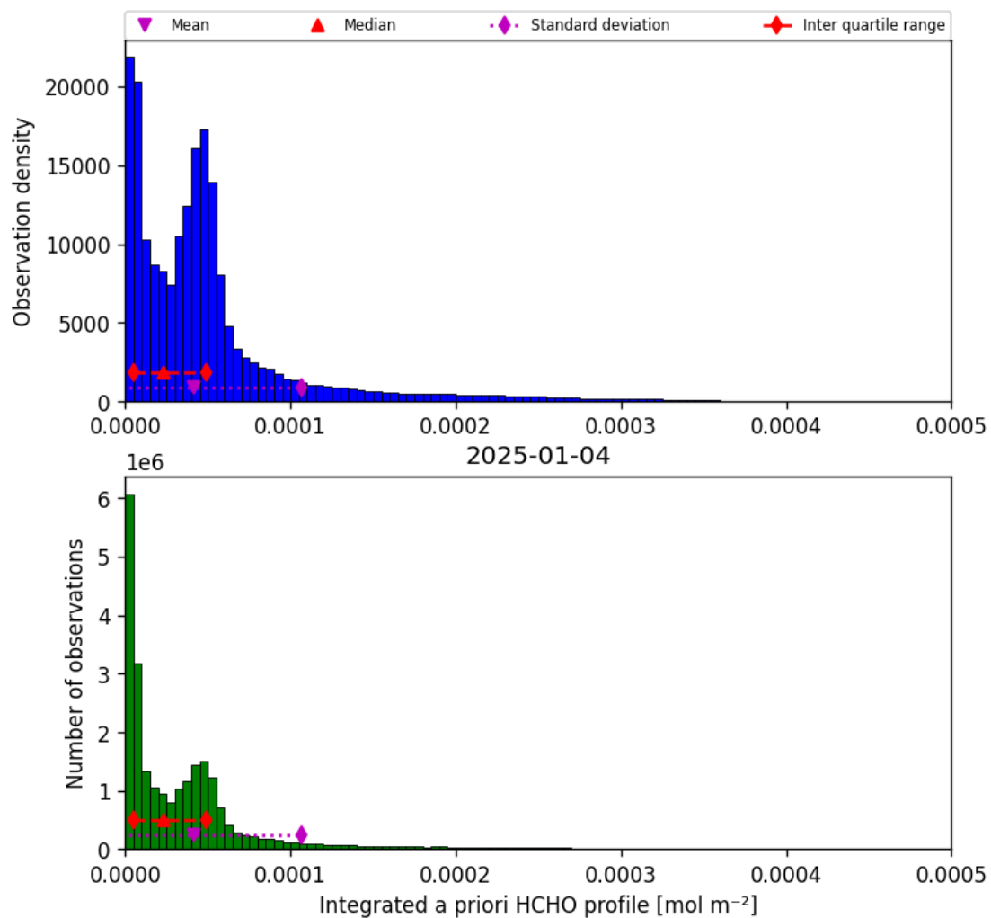
Figure 43: Histogram of “Integrated a priori HCHO profile” for 2025-01-03 to 2025-01-05
