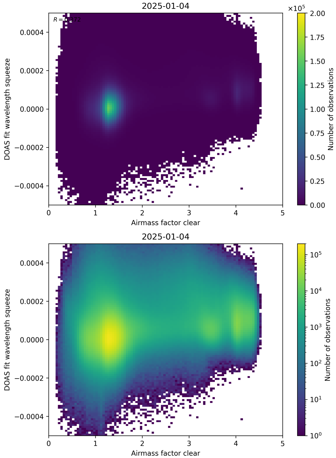
Figure 73: Scatter density plot of “Airmass factor clear” against “DOAS fit wavelength squeeze” for 2025-01-03 to 2025-01-05.
