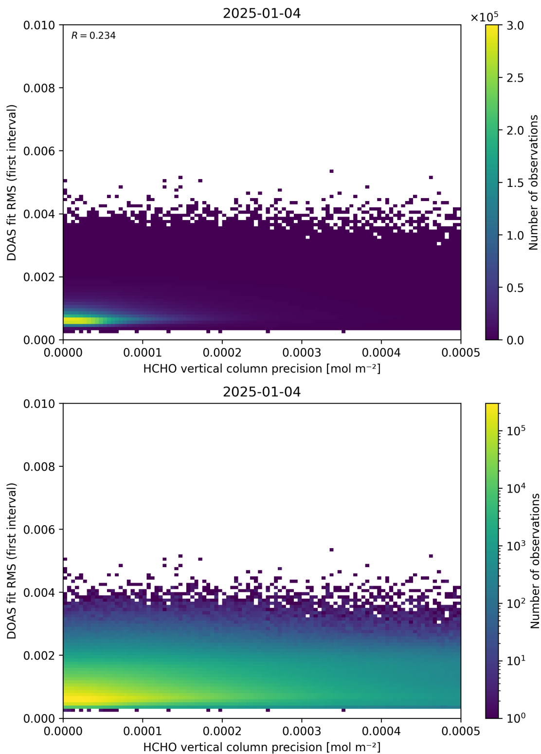
Figure 136: Scatter density plot of “HCHO vertical column precision” against “DOAS fit RMS (first interval)” for 2025-01-03 to 2025-01-05.
