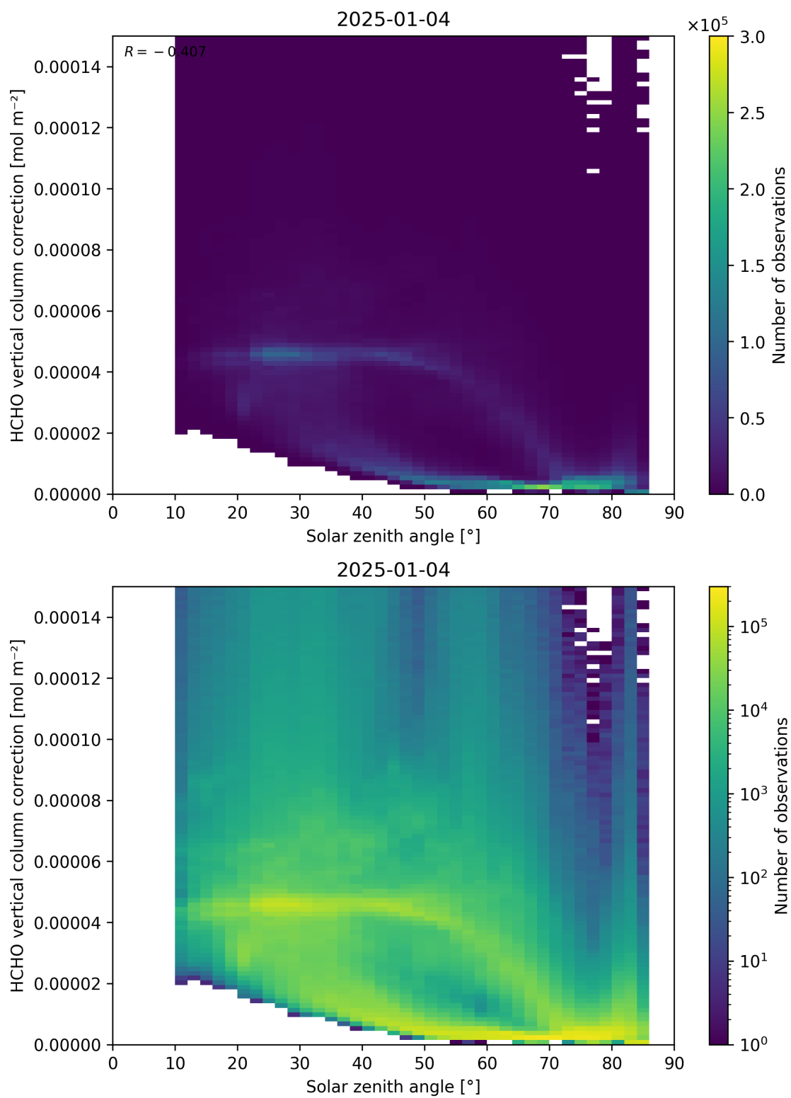
Figure 178: Scatter density plot of “Solar zenith angle” against “HCHO vertical column correction” for 2025-01-03 to 2025-01-05.
