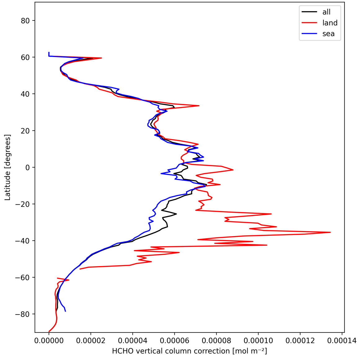
Figure 23: Zonal average of “HCHO vertical column correction” for 2025-01-03 to 2025-01-05.
