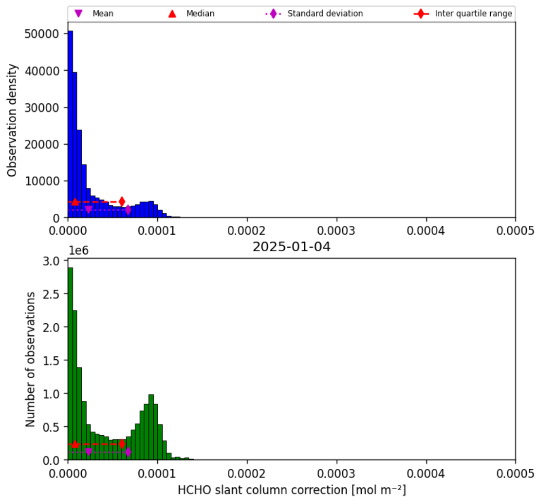
Figure 47: Histogram of “HCHO slant column correction” for 2025-01-03 to 2025-01-05
