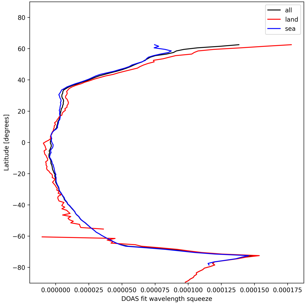
Figure 31: Zonal average of “DOAS fit wavelength squeeze” for 2025-01-03 to 2025-01-05.
