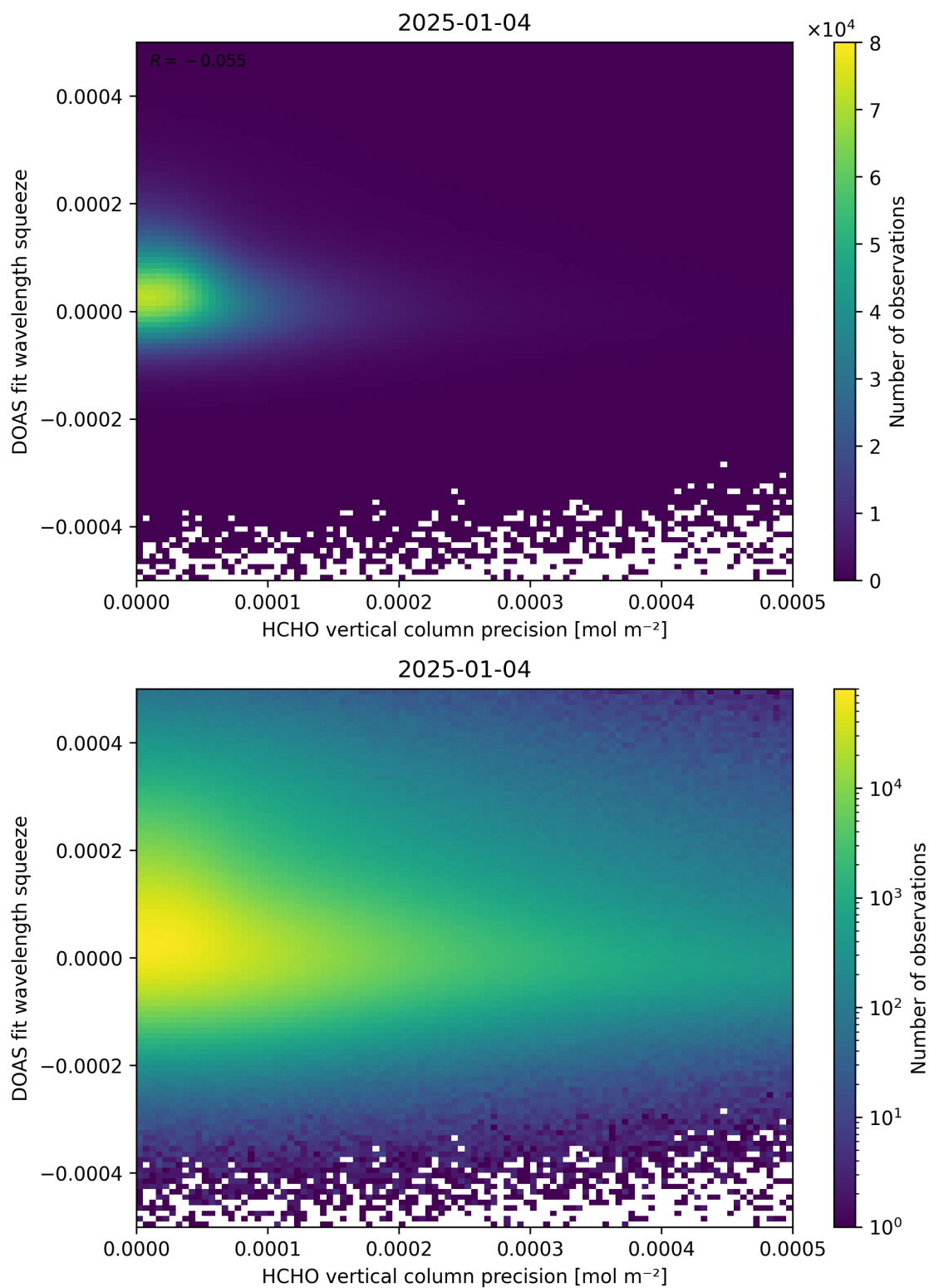
Figure 138: Scatter density plot of “HCHO vertical column precision” against “DOAS fit wavelength squeeze” for 2025-01-03 to 2025-01-05.
