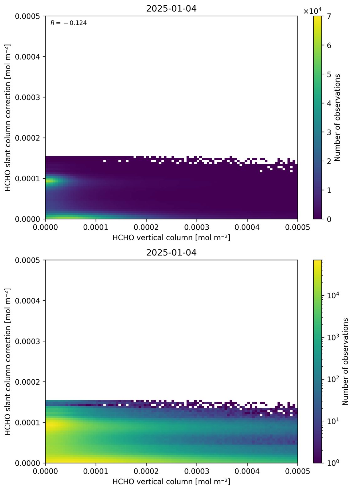
Figure 128: Scatter density plot of “HCHO vertical column” against “HCHO slant column correction” for 2025-01-03 to 2025-01-05.
