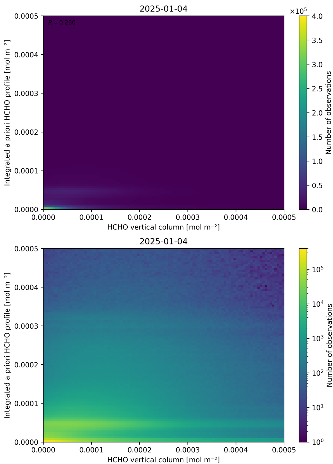
Figure 135: Scatter density plot of “HCHO vertical column” against “Integrated a priori HCHO profile” for 2025-01-03 to 2025-01-05.
