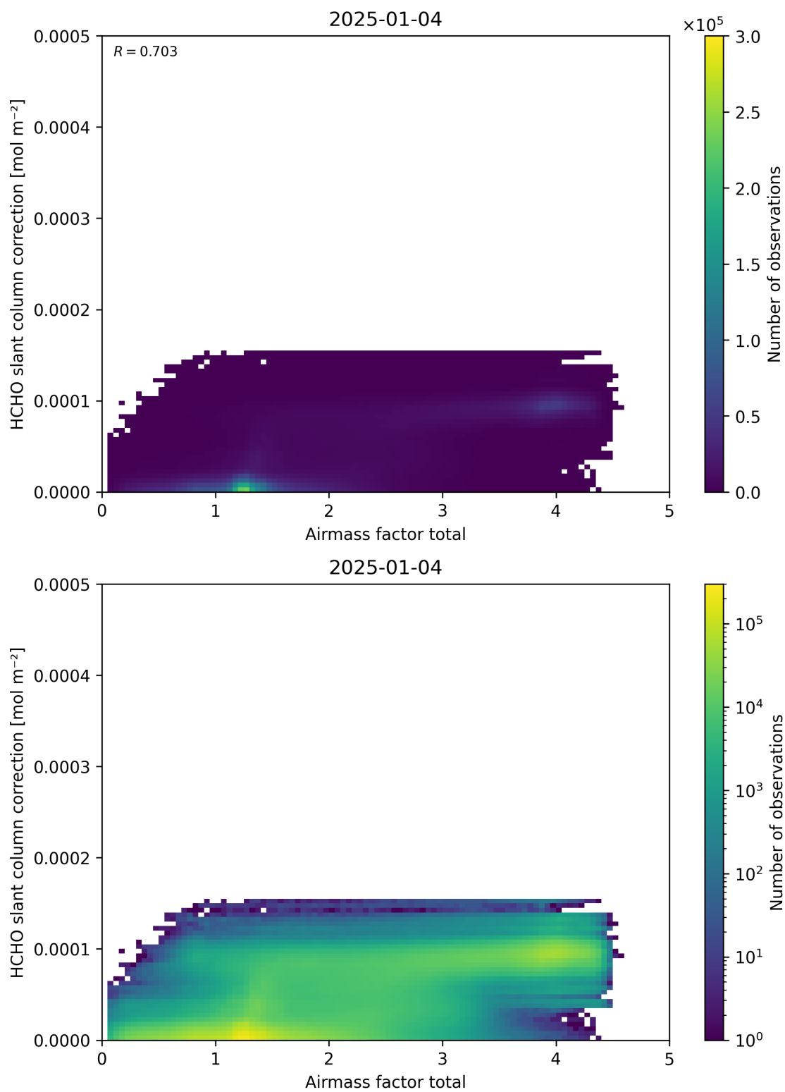
Figure 102: Scatter density plot of “Airmass factor total” against “HCHO slant column correction” for 2025-01-03 to 2025-01-05.
