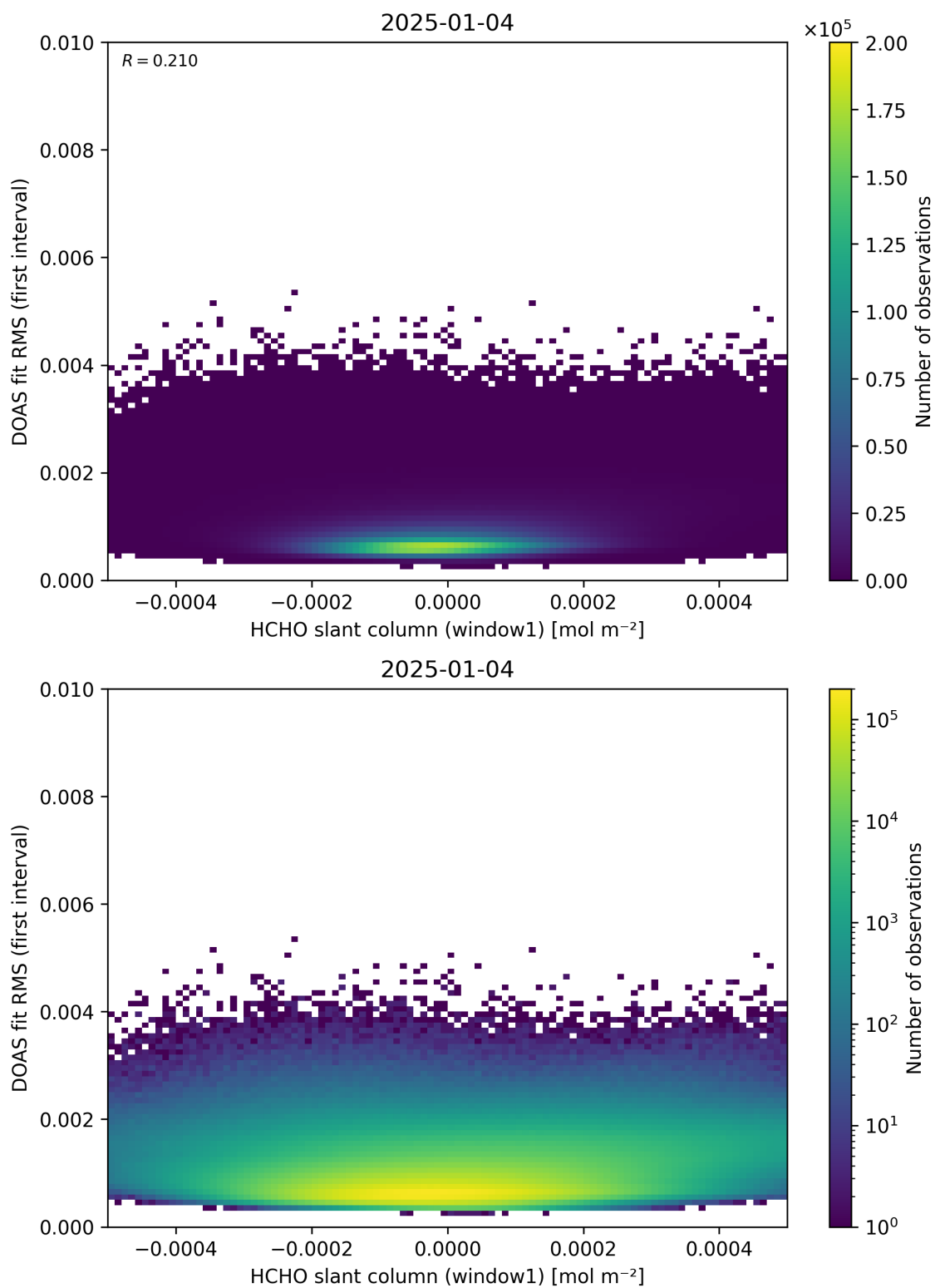
Figure 78: Scatter density plot of “HCHO slant column (window1)” against “DOAS fit RMS (first interval)” for 2025-01-03 to 2025-01-05.
