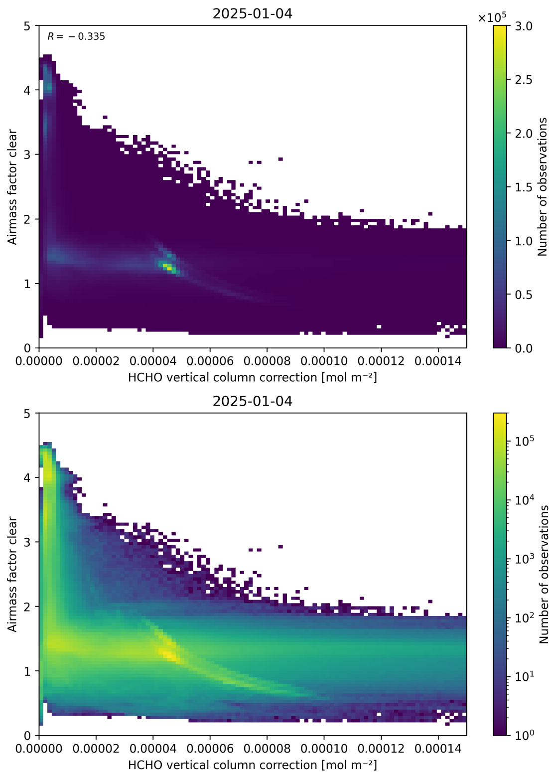
Figure 115: Scatter density plot of “HCHO vertical column correction” against “Airmass factor clear” for 2025-01-03 to 2025-01-05.
