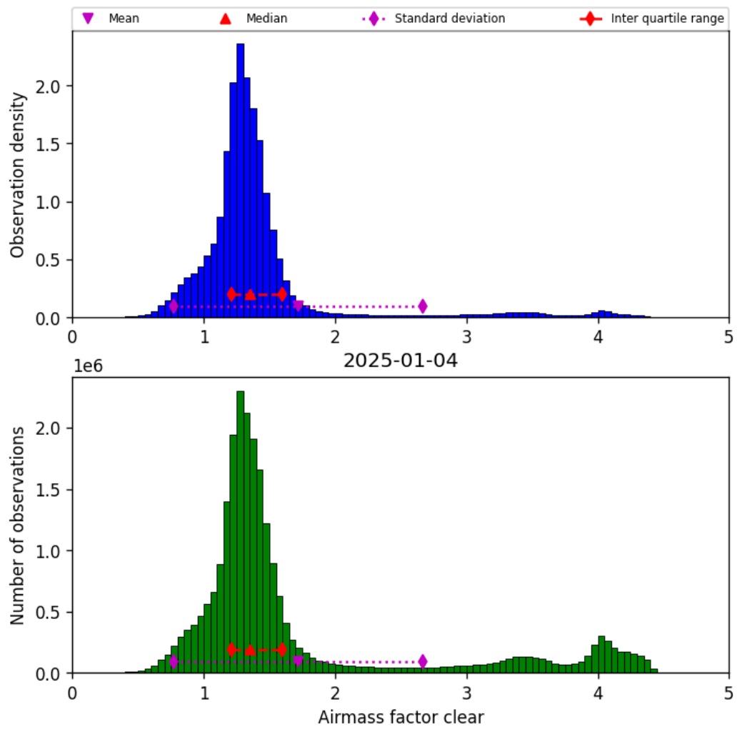
Figure 42: Histogram of “Airmass factor clear” for 2025-01-03 to 2025-01-05
