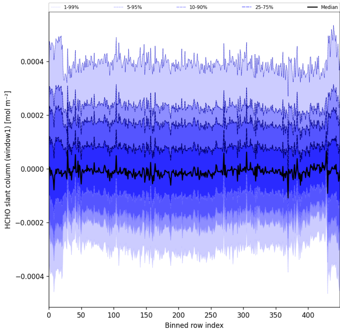
Figure 52: Along track statistics of “HCHO slant column (window1)” for 2025-01-03 to 2025-01-05
