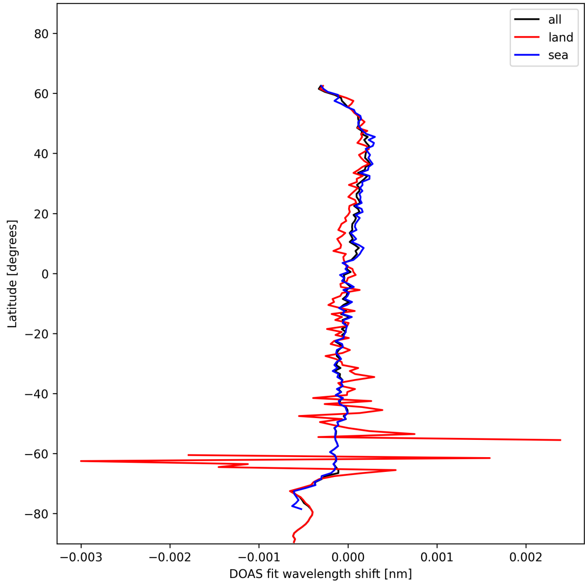
Figure 30: Zonal average of “DOAS fit wavelength shift” for 2025-01-03 to 2025-01-05.
