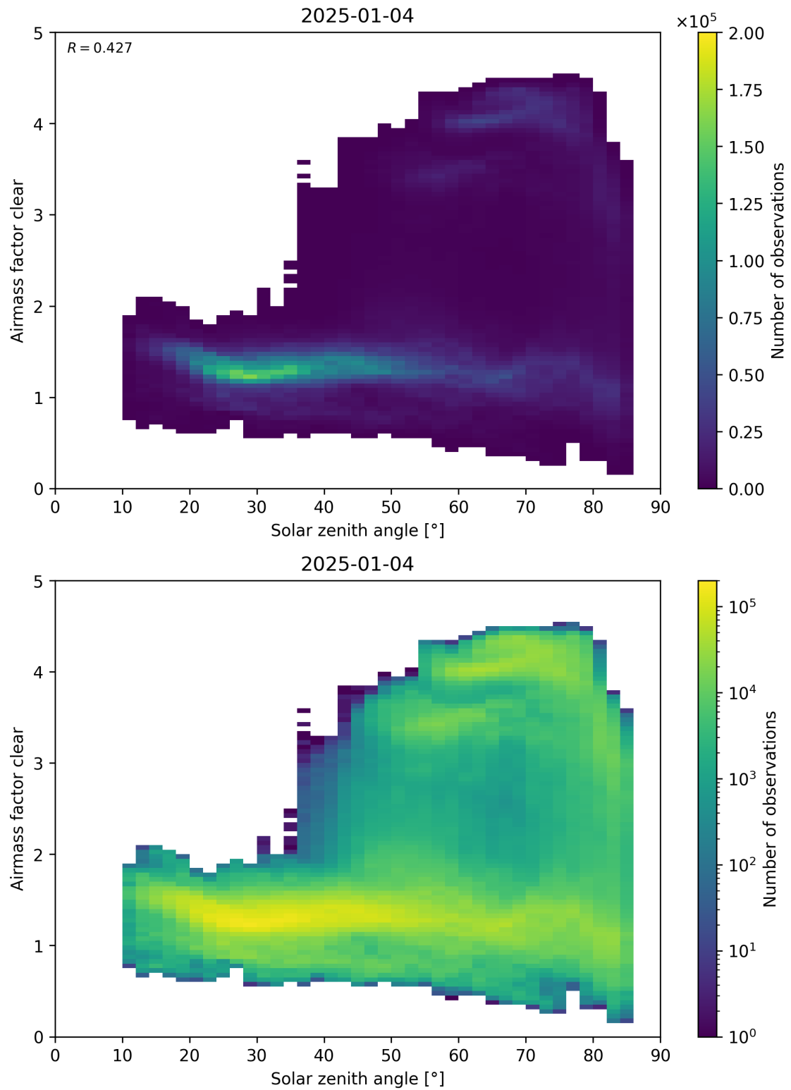
Figure 170: Scatter density plot of “Solar zenith angle” against “Airmass factor clear” for 2025-01-03 to 2025-01-05.
