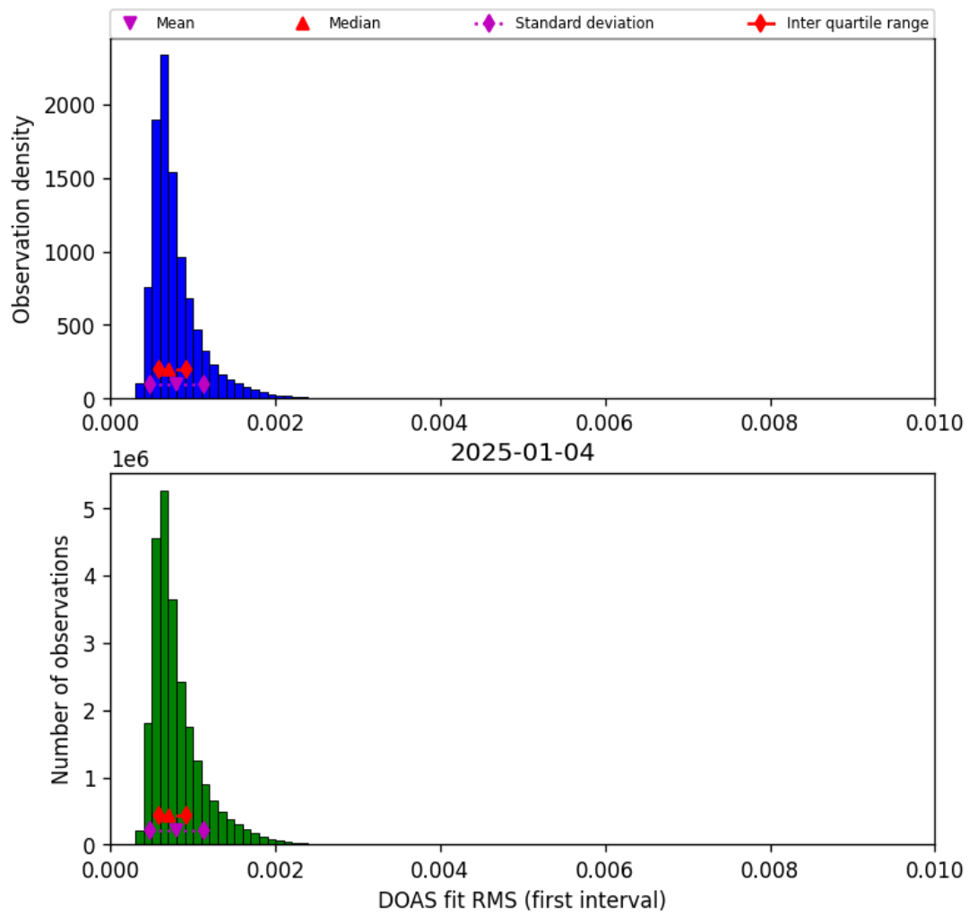
Figure 46: Histogram of “DOAS fit RMS (first interval)” for 2025-01-03 to 2025-01-05
