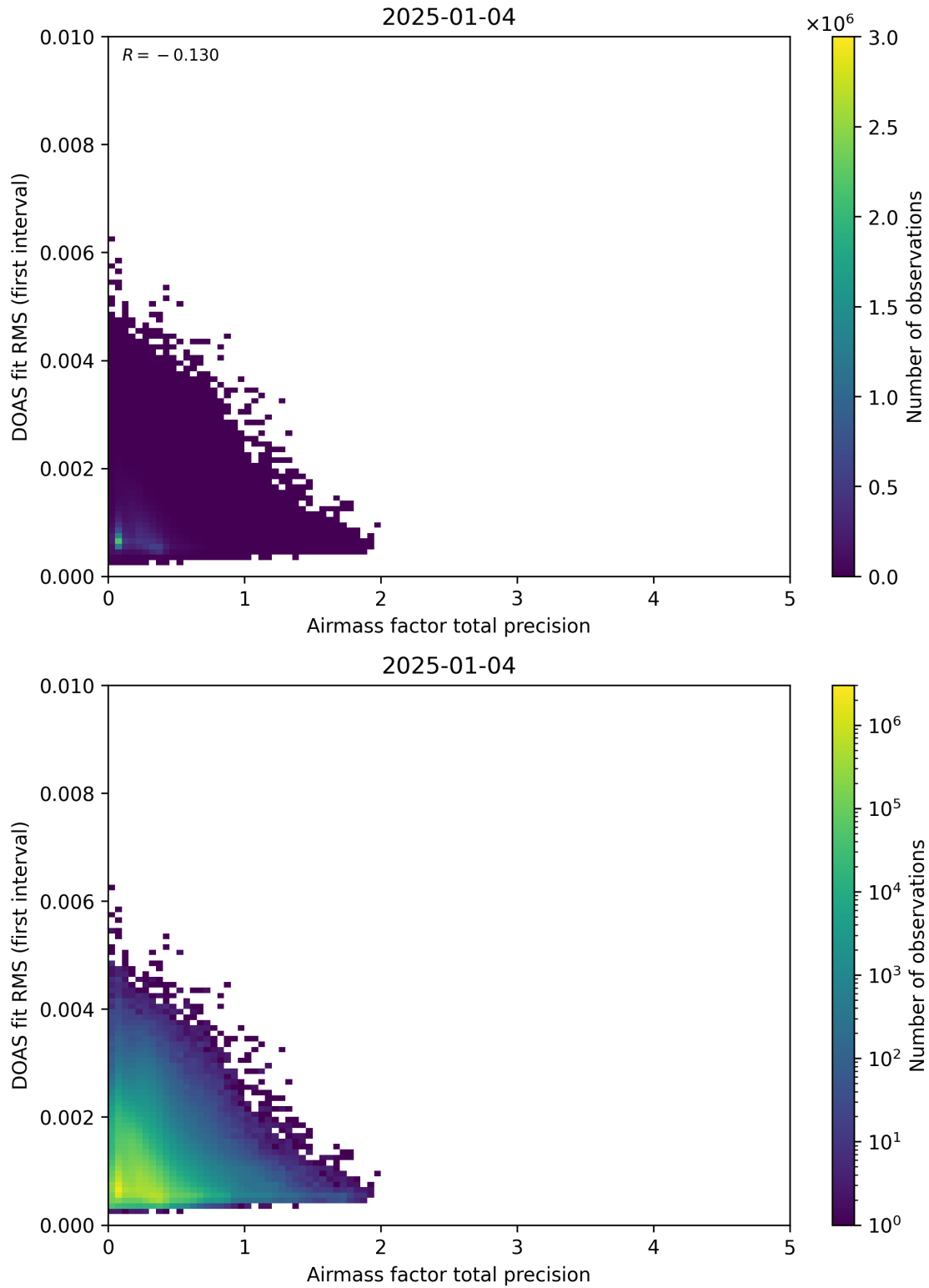
Figure 105: Scatter density plot of “Airmass factor total precision” against “DOAS fit RMS (first interval)” for 2025-01-03 to 2025-01-05.
