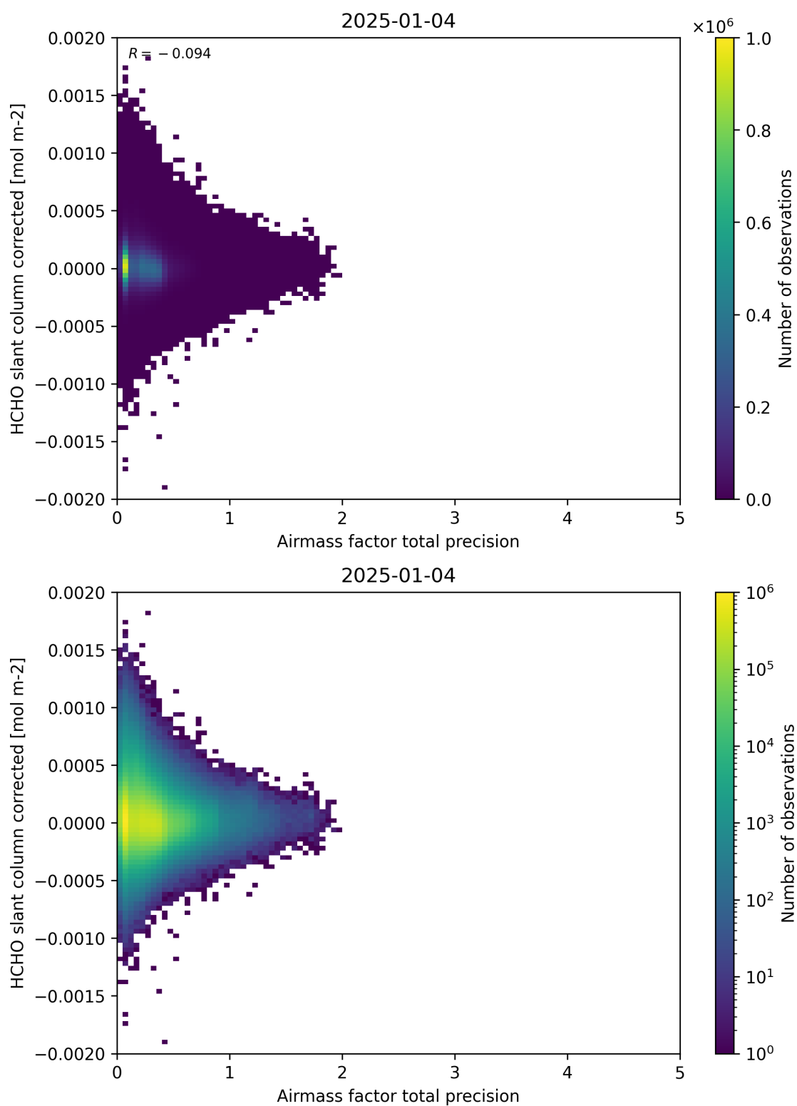
Figure 109: Scatter density plot of “Airmass factor total precision” against “HCHO slant column corrected” for 2025-01-03 to 2025-01-05.
