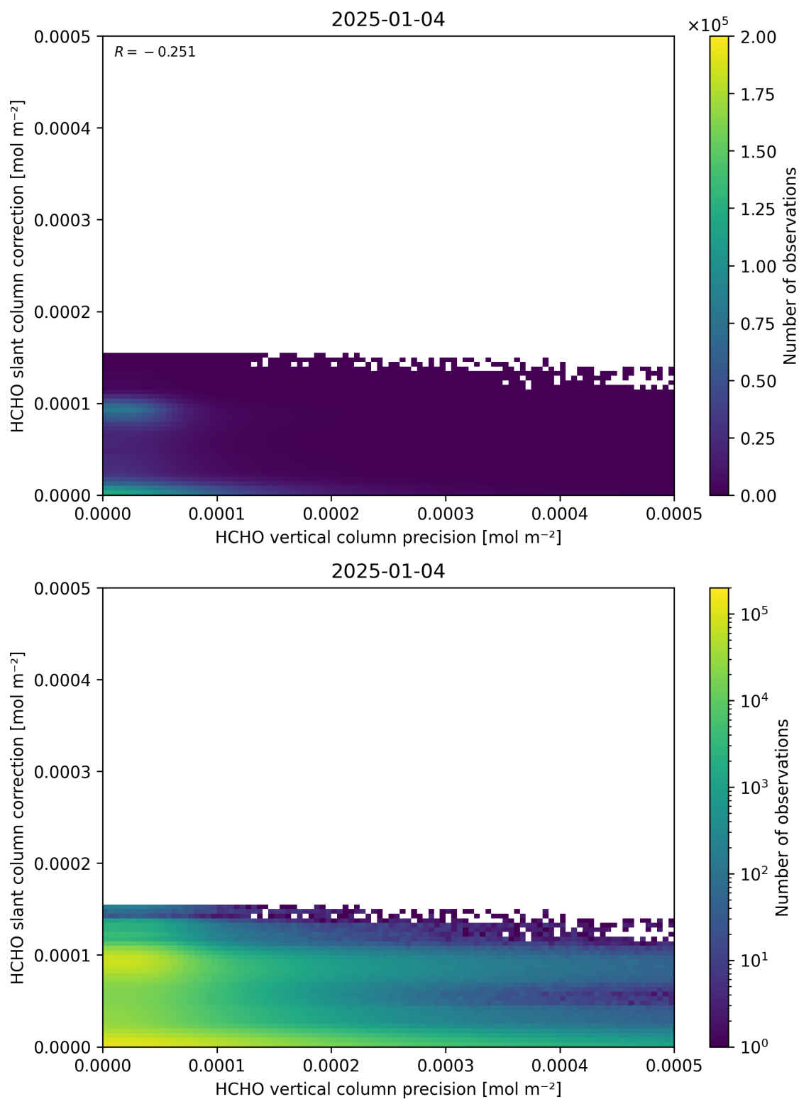
Figure 141: Scatter density plot of “HCHO vertical column precision” against “HCHO slant column correction” for 2025-01-03 to 2025-01-05.
