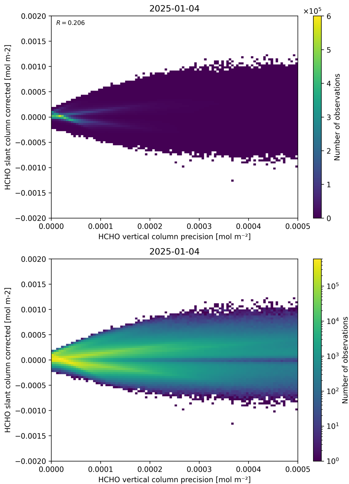
Figure 140: Scatter density plot of “HCHO vertical column precision” against “HCHO slant column corrected” for 2025-01-03 to 2025-01-05.
