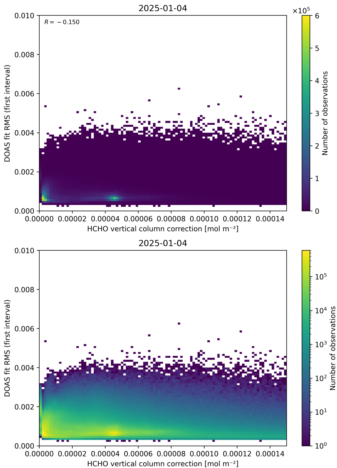
Figure 112: Scatter density plot of “HCHO vertical column correction” against “DOAS fit RMS (first interval)” for 2025-01-03 to 2025-01-05.
