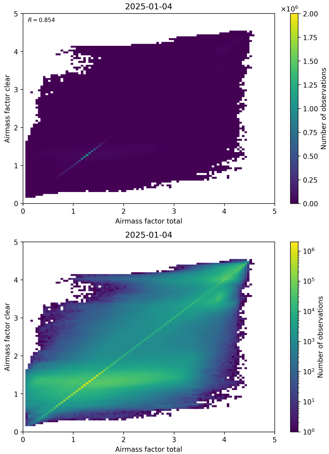
Figure 100: Scatter density plot of “Airmass factor total” against “Airmass factor clear” for 2025-01-03 to 2025-01-05.
