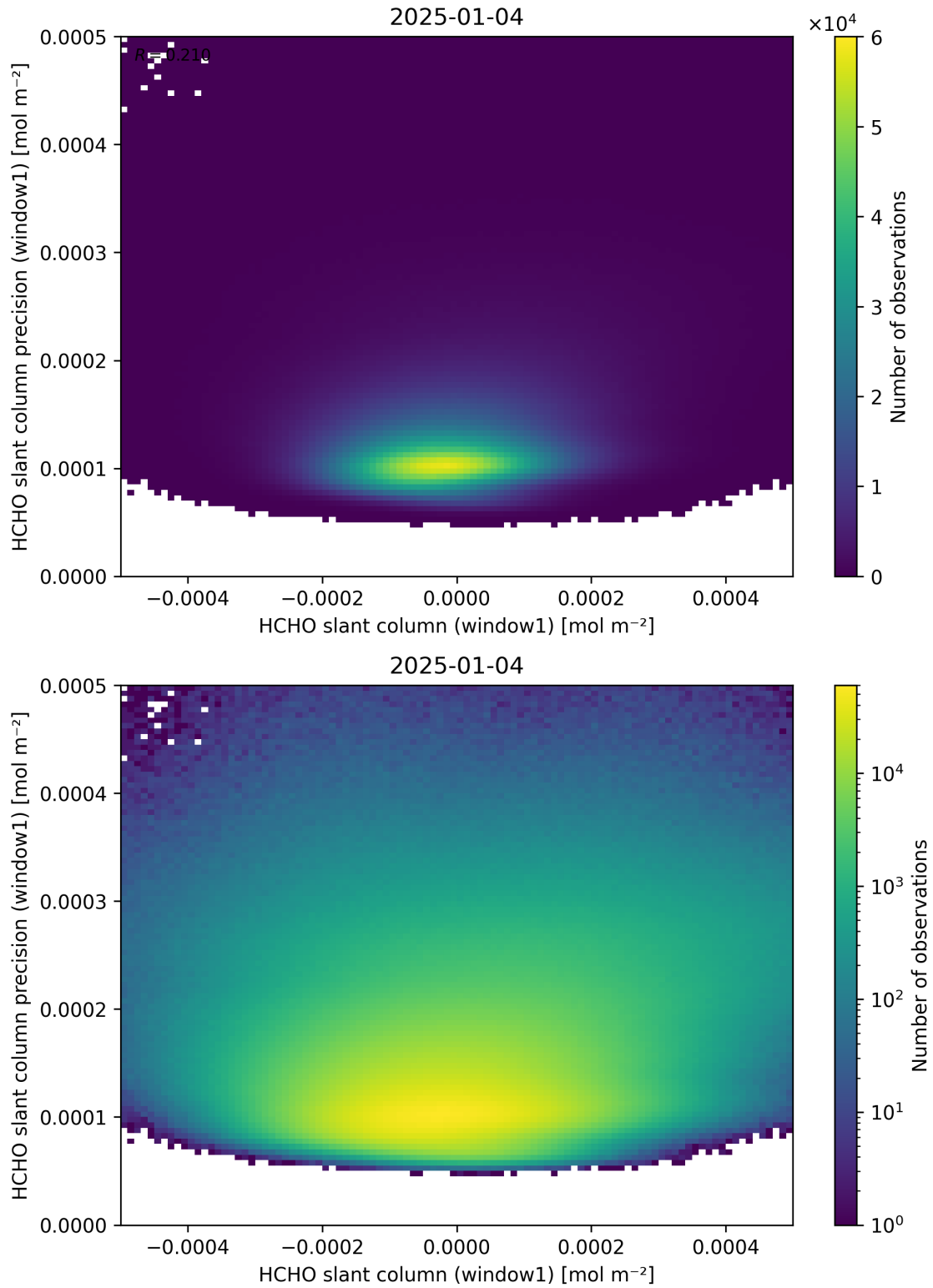
Figure 84: Scatter density plot of “HCHO slant column (window1)” against “HCHO slant column precision (window1)” for 2025-01-03 to 2025-01-05.
