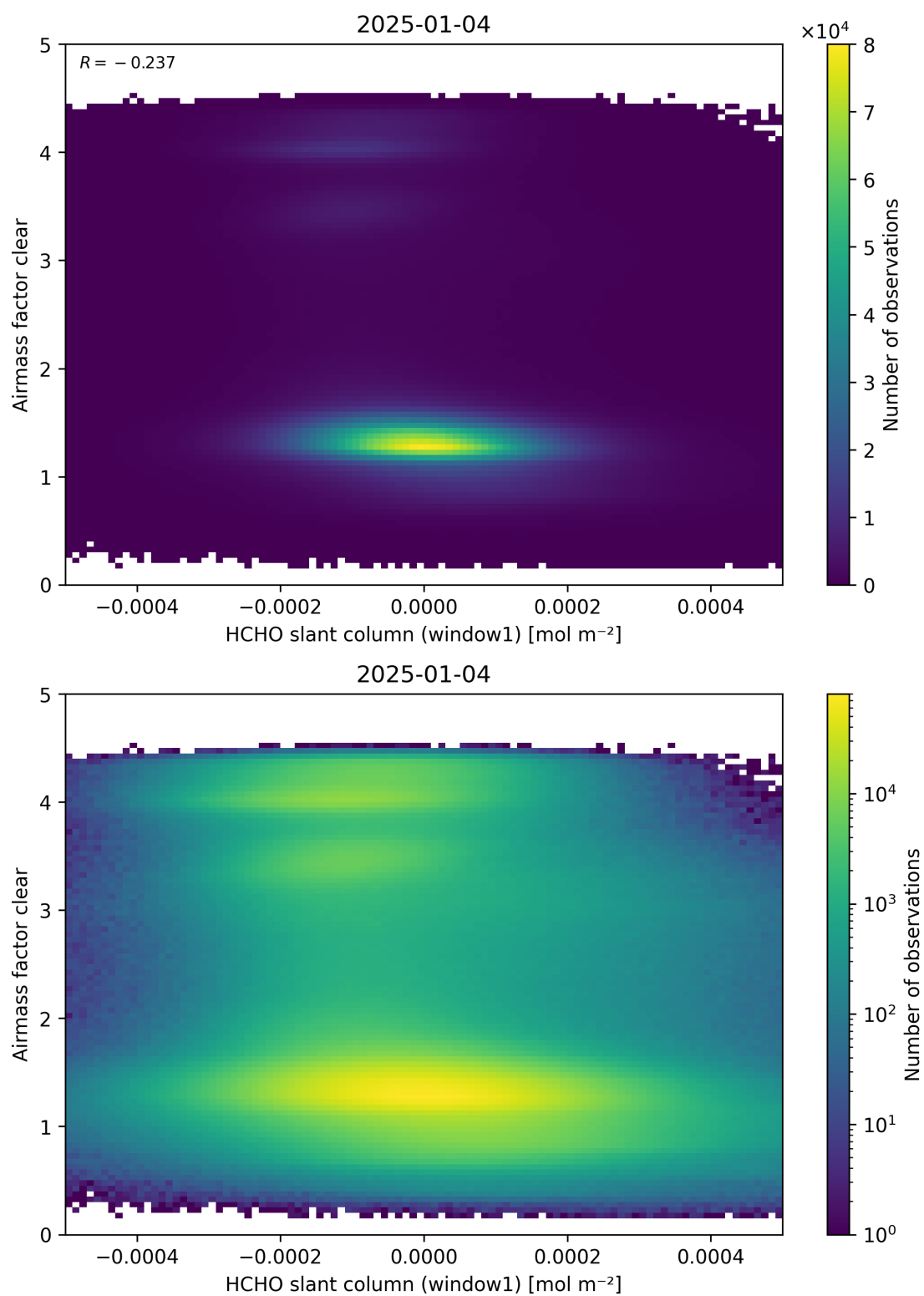
Figure 81: Scatter density plot of “HCHO slant column (window1)” against “Airmass factor clear” for 2025-01-03 to 2025-01-05.
