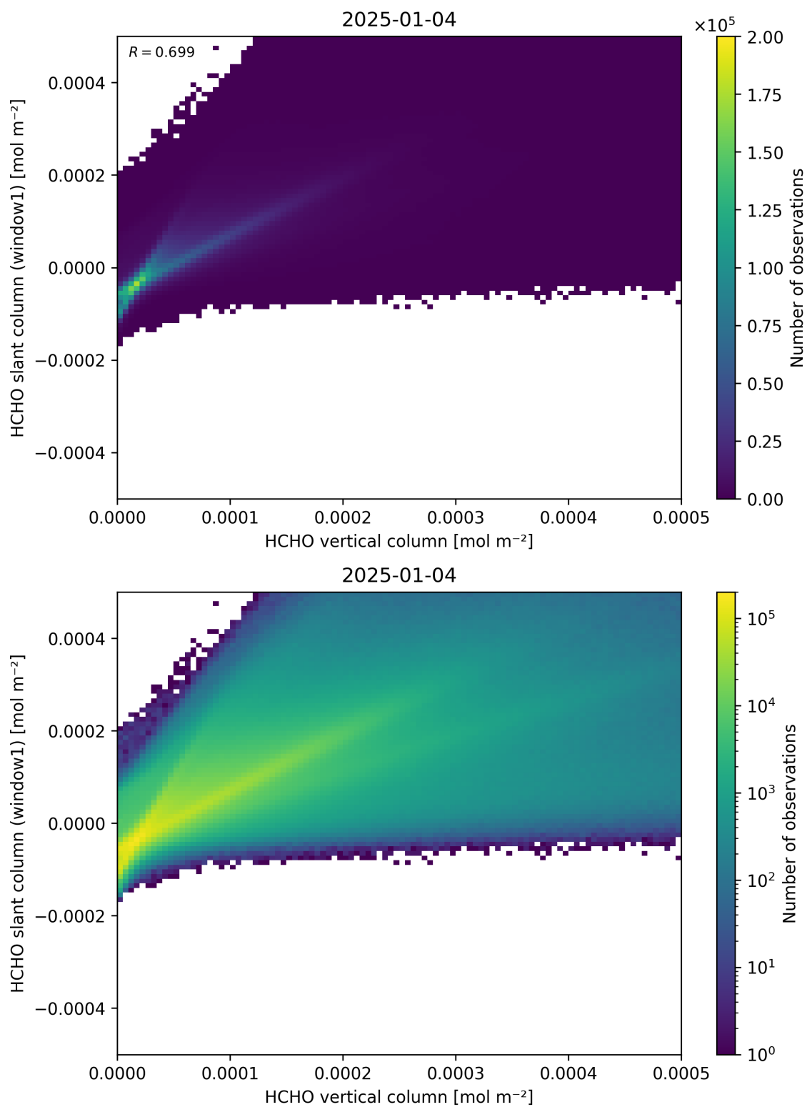
Figure 129: Scatter density plot of “HCHO vertical column” against “HCHO slant column (window1)” for 2025-01-03 to 2025-01-05.
