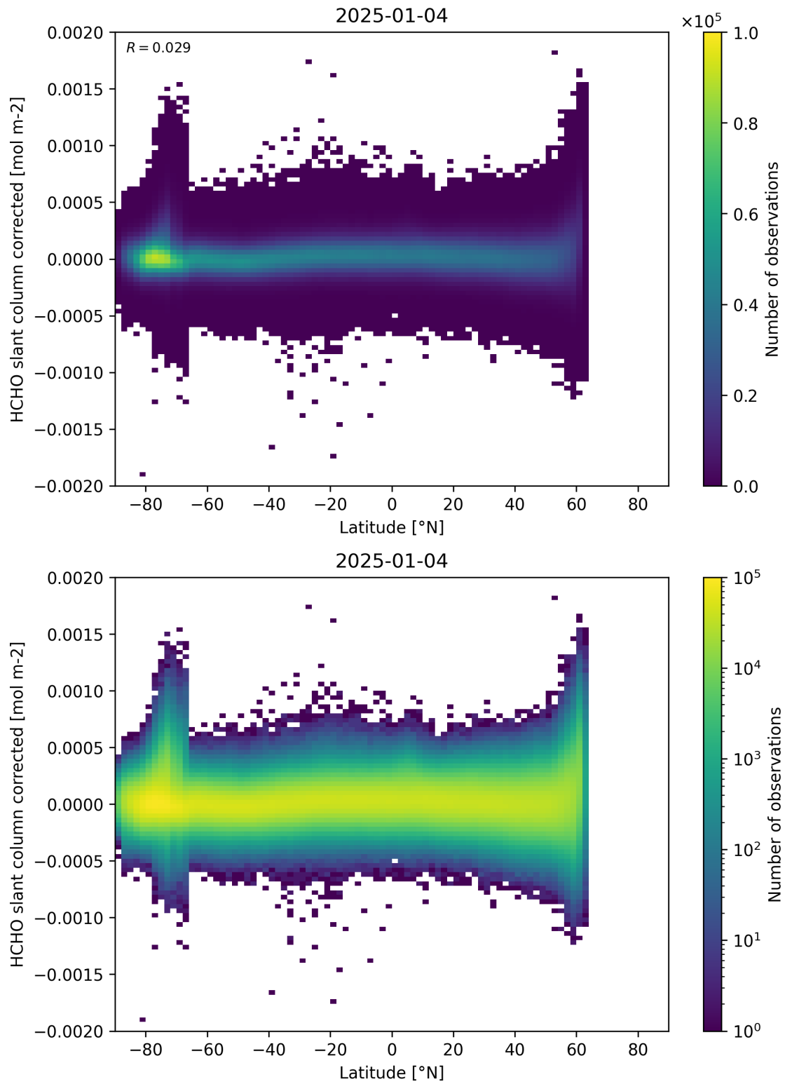
Figure 157: Scatter density plot of “Latitude” against “HCHO slant column corrected” for 2025-01-03 to 2025-01-05.
