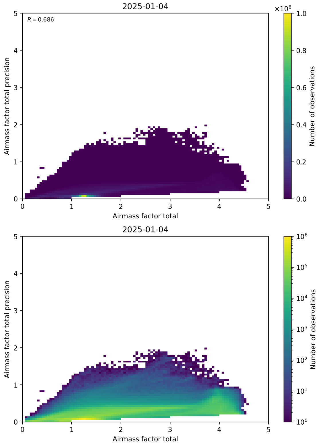
Figure 103: Scatter density plot of “Airmass factor total” against “Airmass factor total precision” for 2025-01-03 to 2025-01-05.
