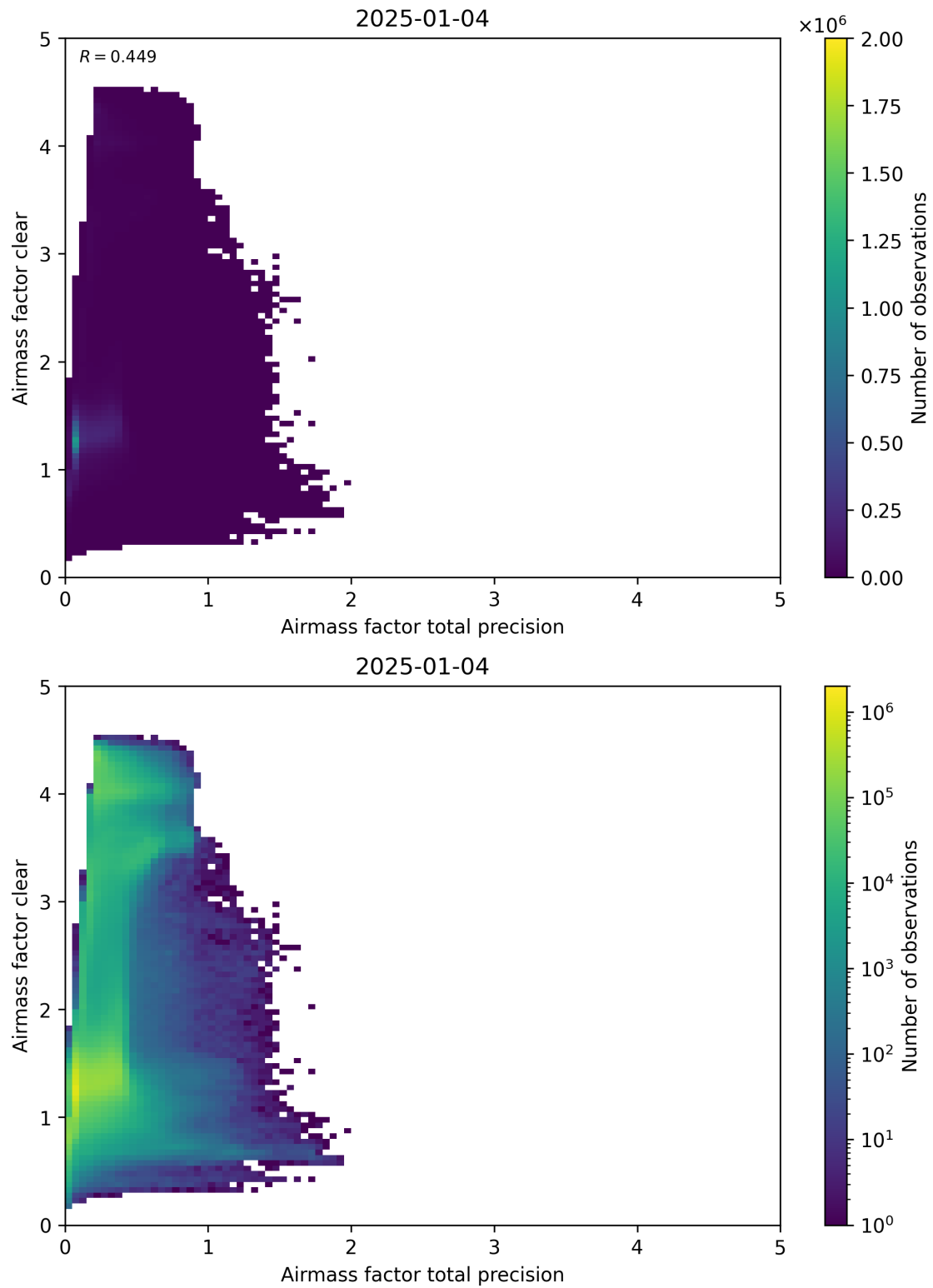
Figure 108: Scatter density plot of “Airmass factor total precision” against “Airmass factor clear” for 2025-01-03 to 2025-01-05.
