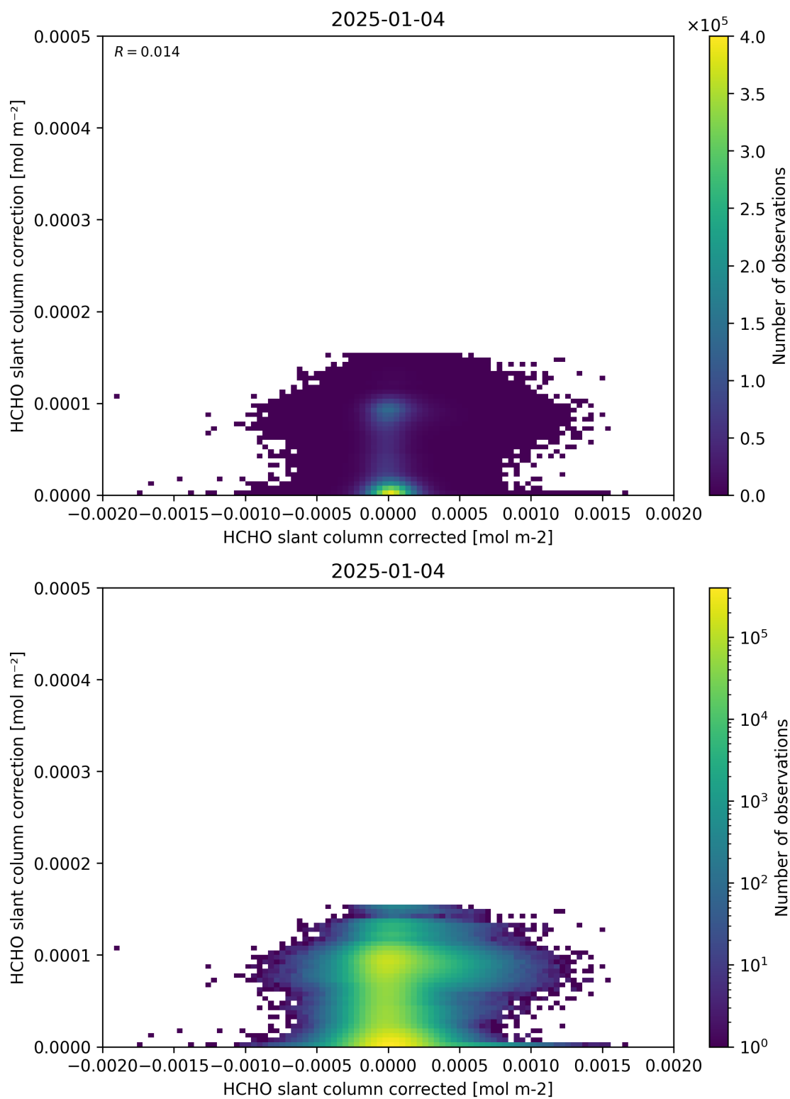
Figure 77: Scatter density plot of “HCHO slant column corrected” against “HCHO slant column correction” for 2025-01-03 to 2025-01-05.
