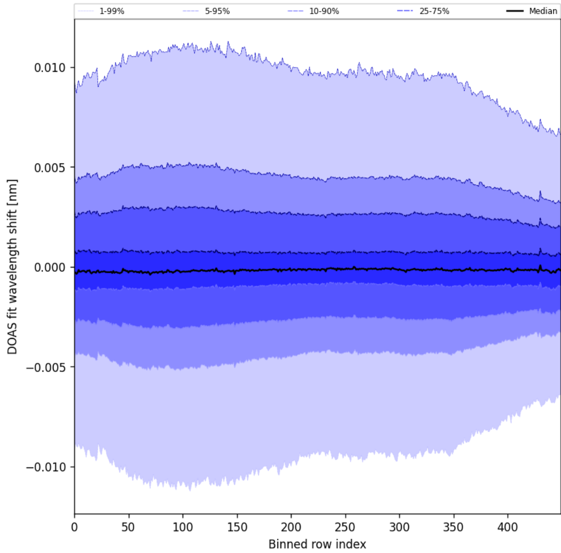
Figure 58: Along track statistics of “DOAS fit wavelength shift” for 2025-01-03 to 2025-01-05
