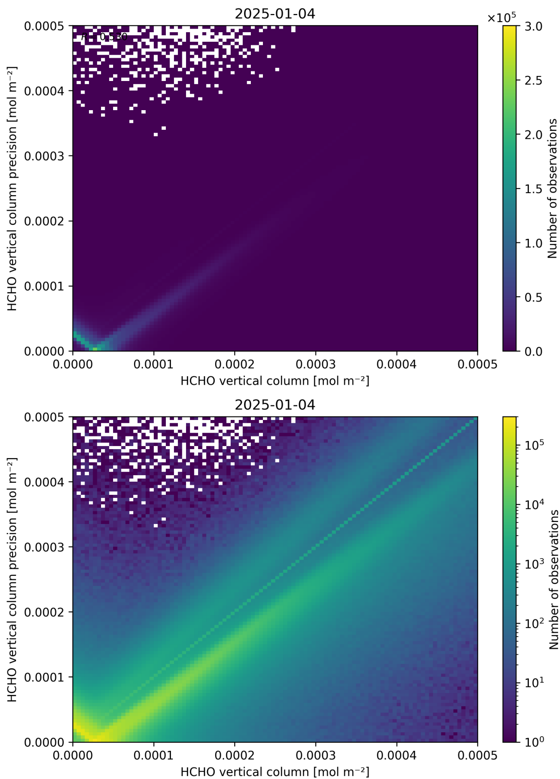
Figure 134: Scatter density plot of “HCHO vertical column” against “HCHO vertical column precision” for 2025-01-03 to 2025-01-05.
