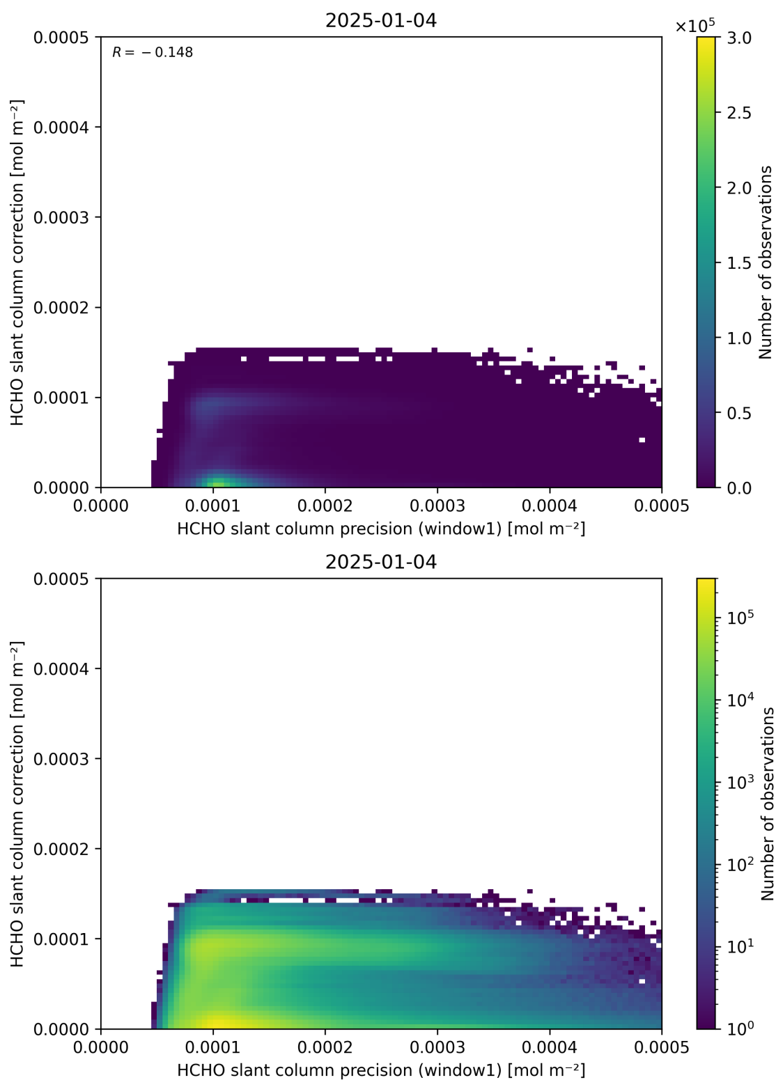
Figure 93: Scatter density plot of “HCHO slant column precision (window1)” against “HCHO slant column correction” for 2025-01-03 to 2025-01-05.
