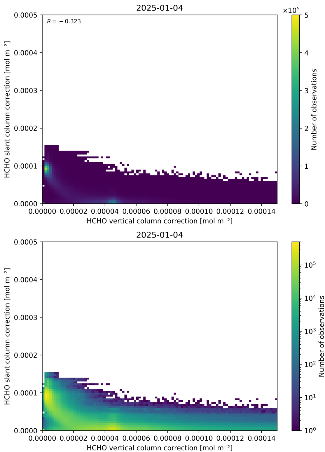
Figure 117: Scatter density plot of “HCHO vertical column correction” against “HCHO slant column correction” for 2025-01-03 to 2025-01-05.
