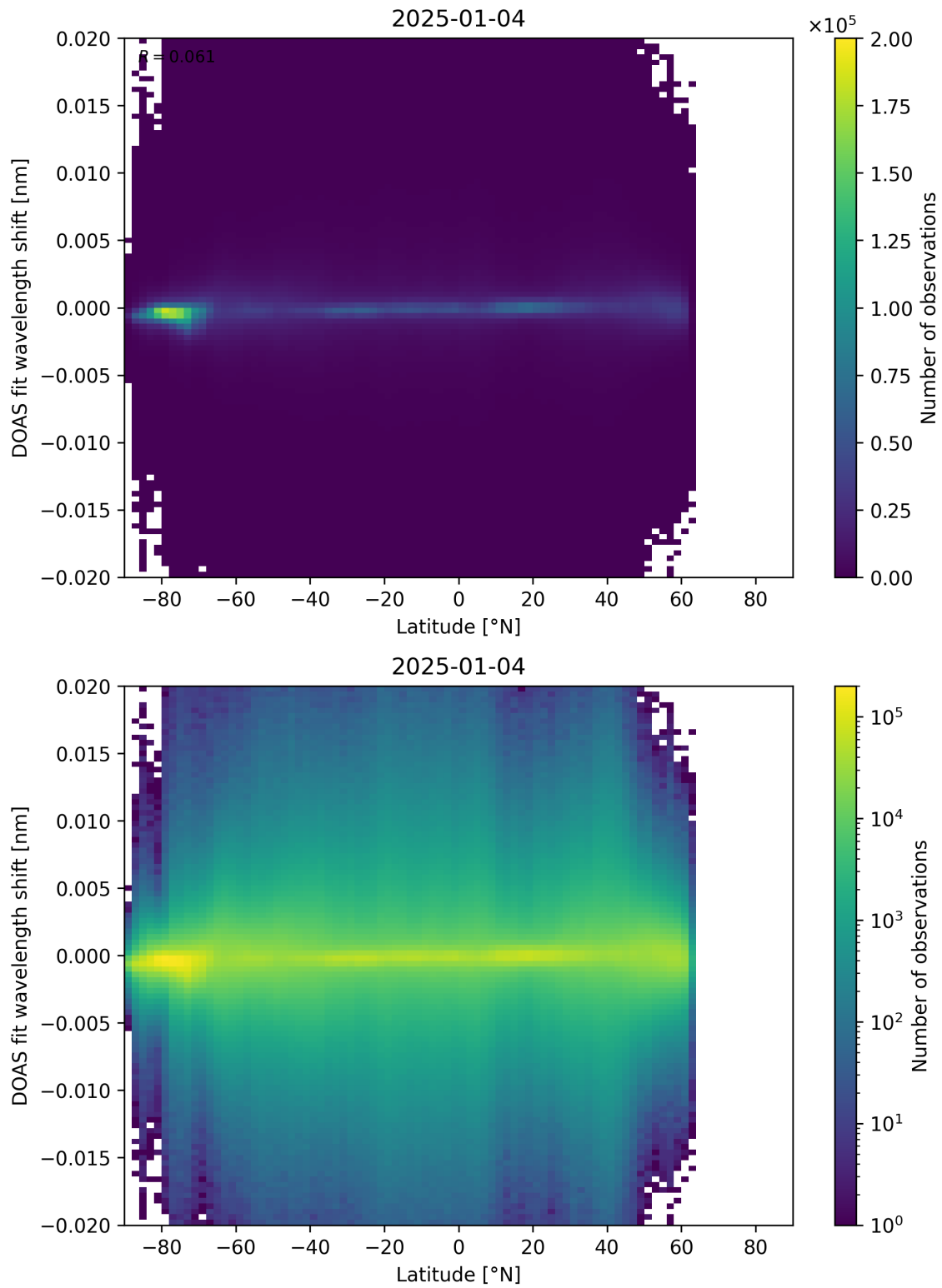
Figure 154: Scatter density plot of “Latitude” against “DOAS fit wavelength shift” for 2025-01-03 to 2025-01-05.
