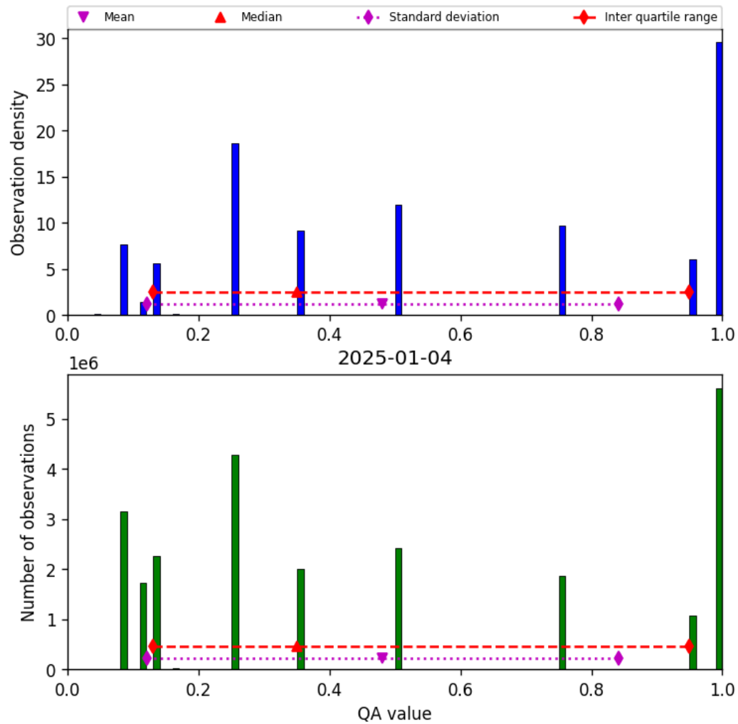
Figure 34: Histogram of “QA value” for 2025-01-03 to 2025-01-05
