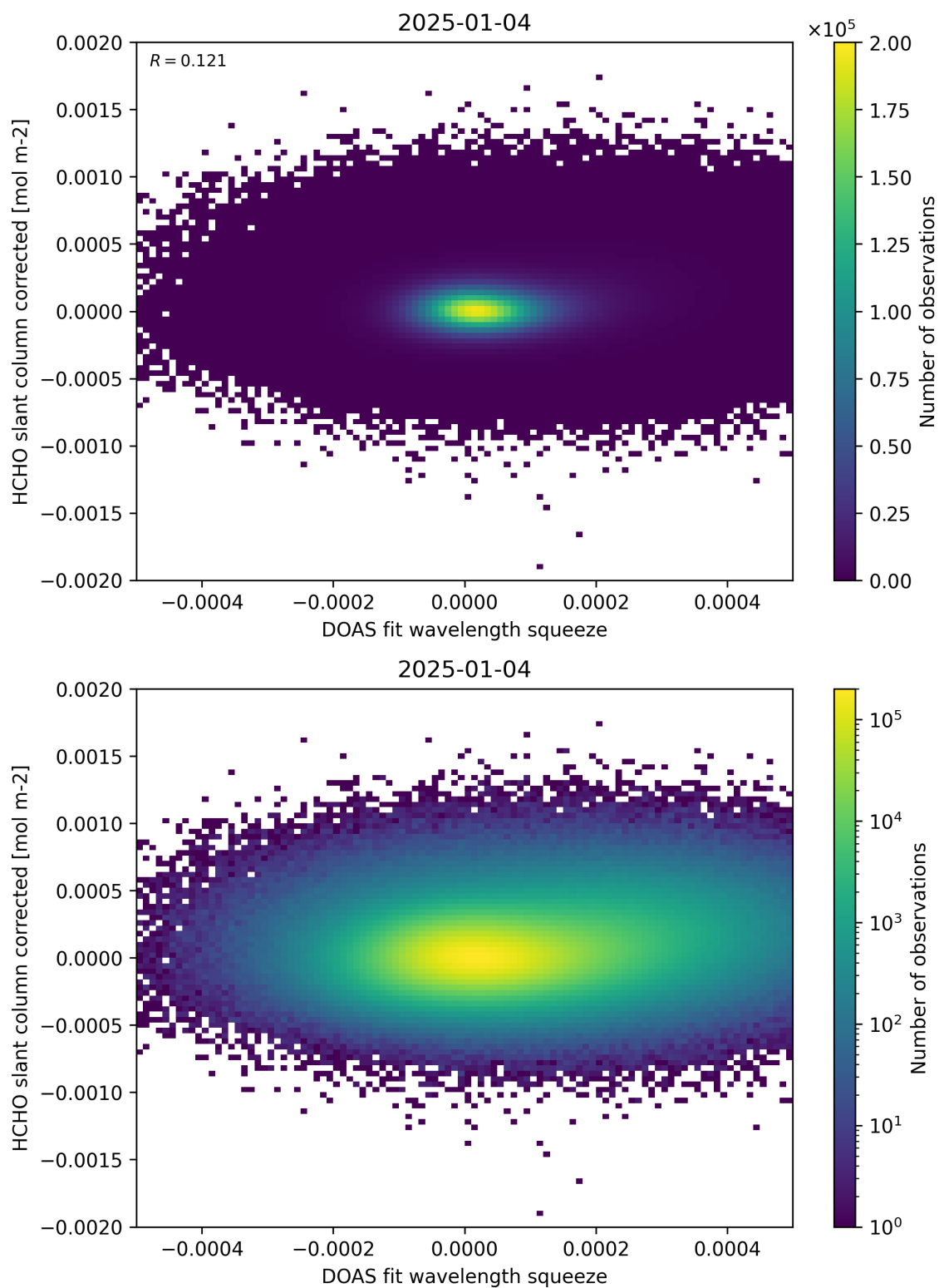
Figure 69: Scatter density plot of “DOAS fit wavelength squeeze” against “HCHO slant column corrected” for 2025-01-03 to 2025-01-05.
