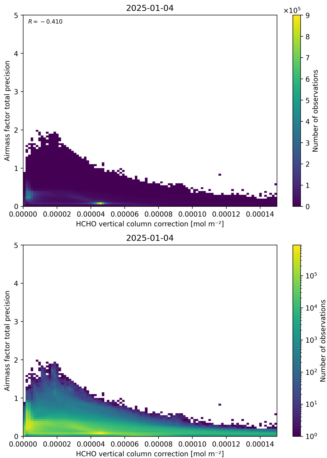
Figure 121: Scatter density plot of “HCHO vertical column correction” against “Airmass factor total precision” for 2025-01-03 to 2025-01-05.
