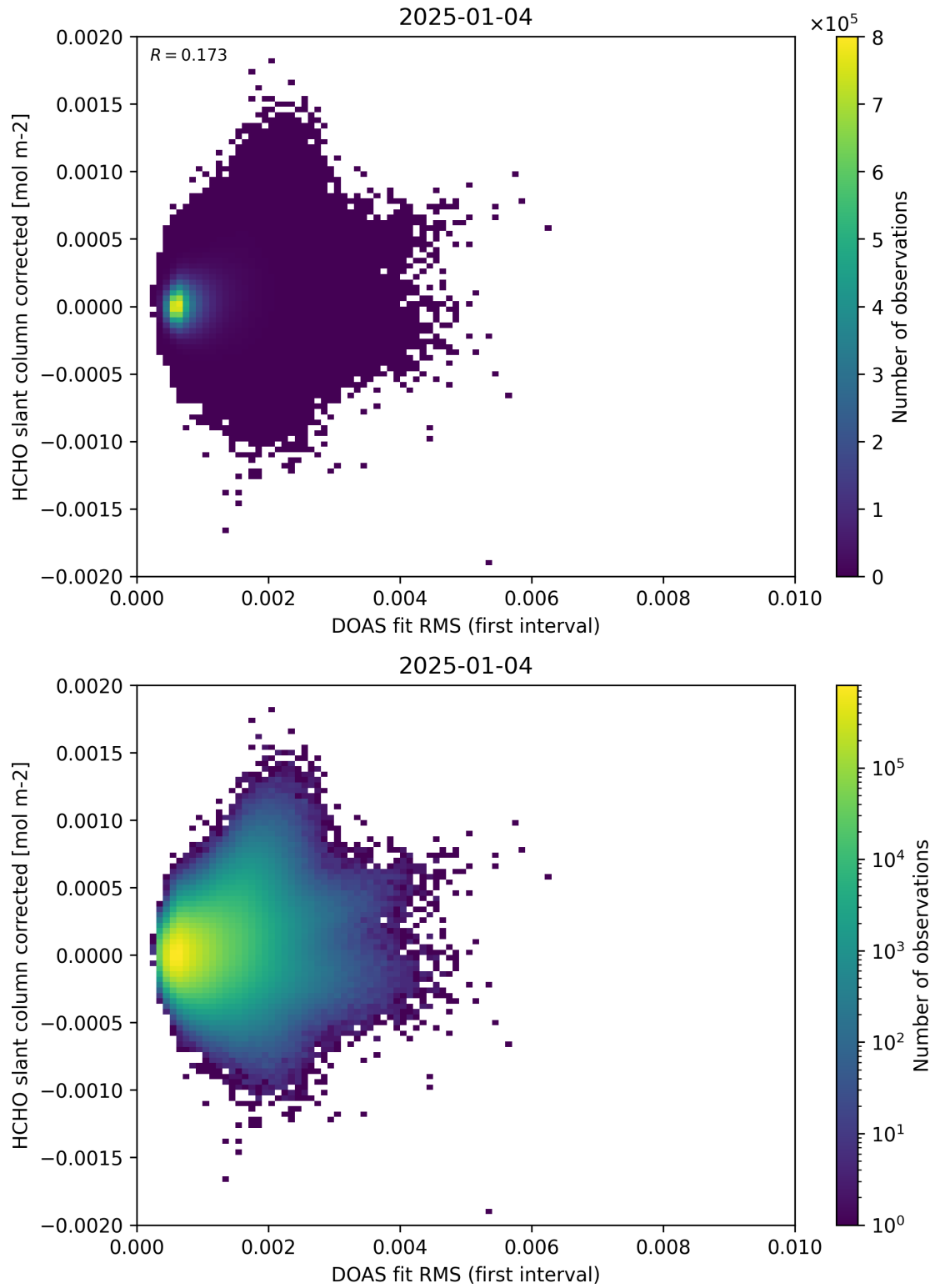
Figure 62: Scatter density plot of “DOAS fit RMS (first interval)” against “HCHO slant column corrected” for 2025-01-03 to 2025-01-05.
