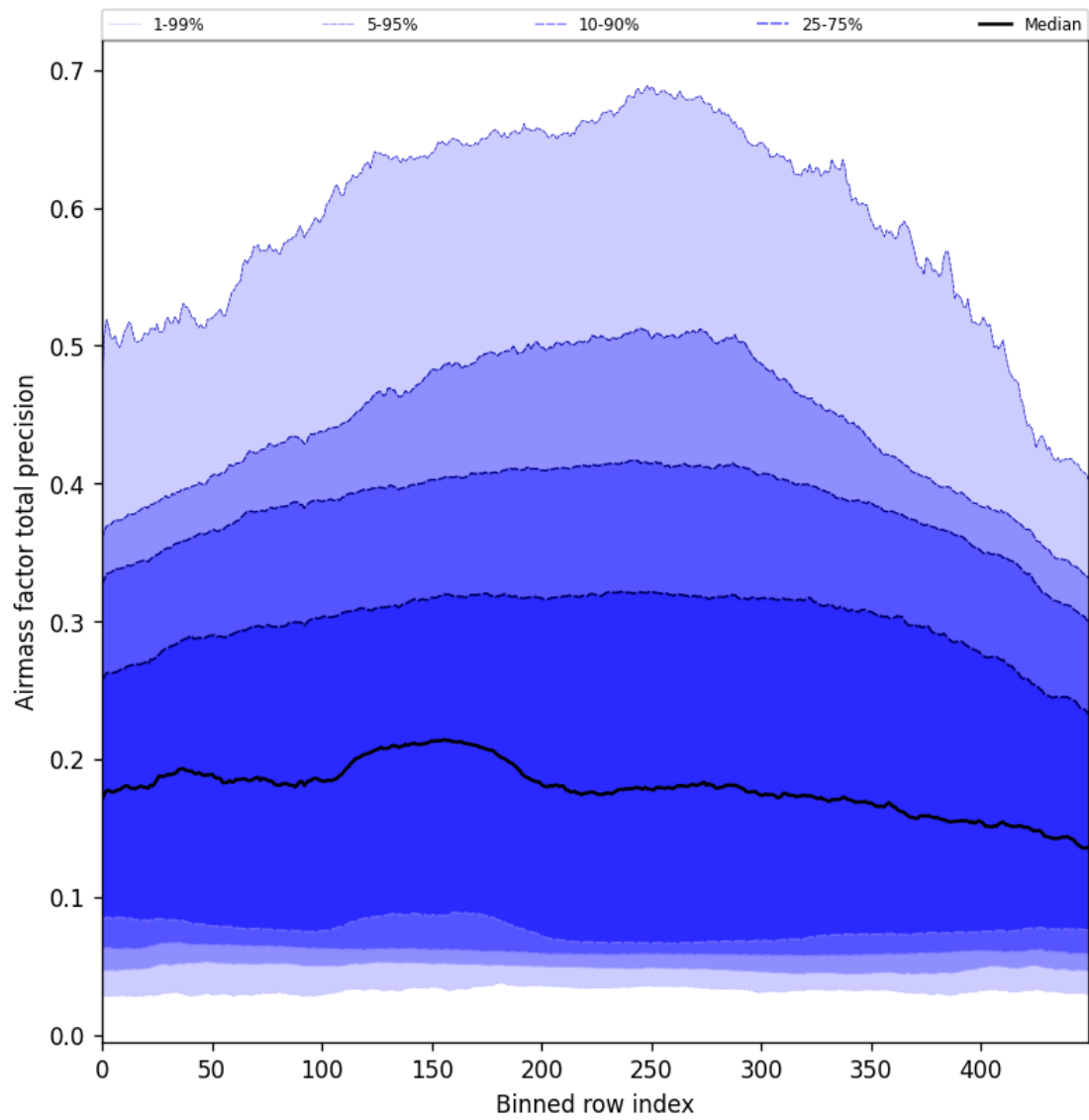
Figure 55: Along track statistics of “Airmass factor total precision” for 2025-01-03 to 2025-01-05
