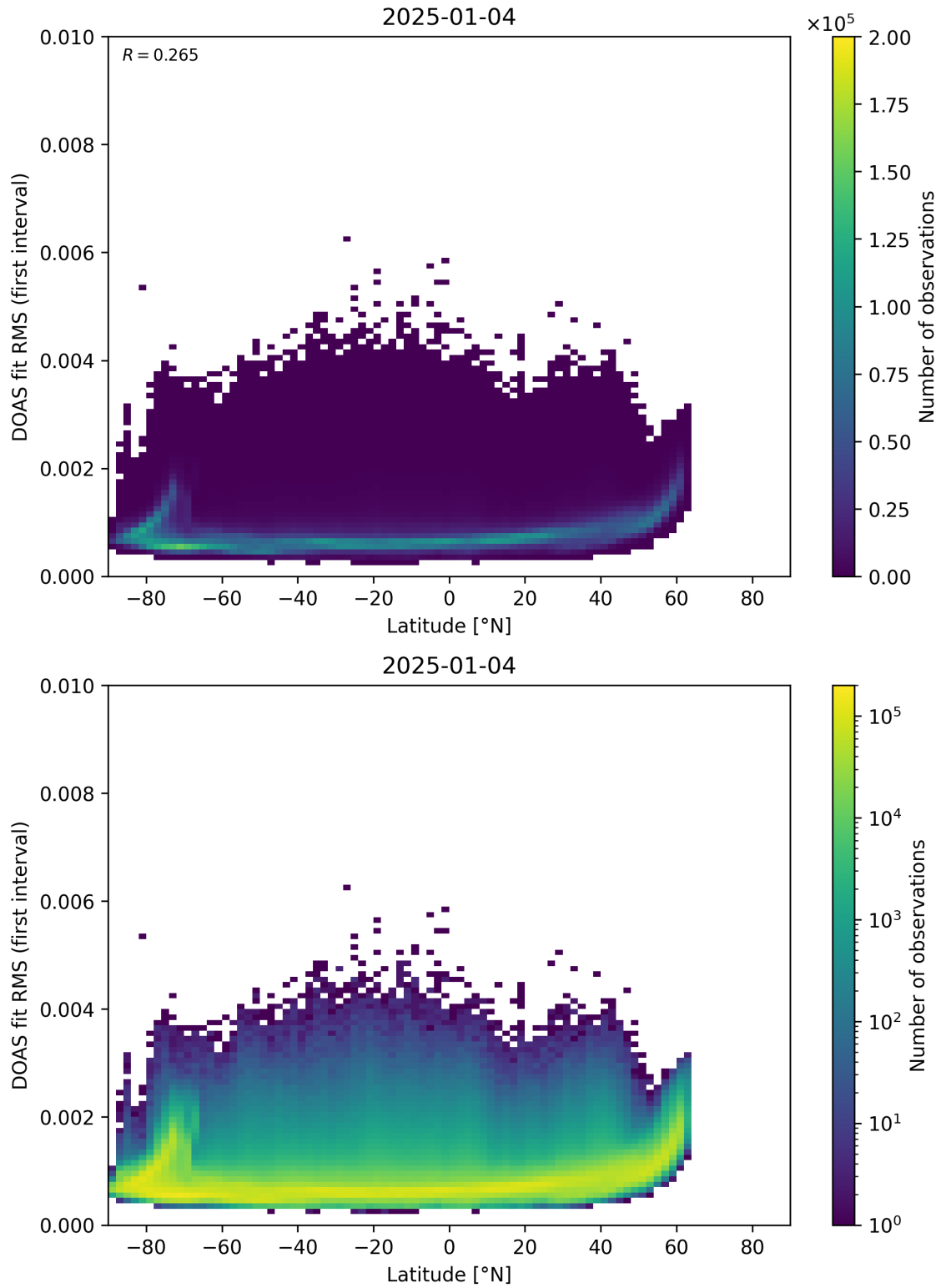
Figure 153: Scatter density plot of “Latitude” against “DOAS fit RMS (first interval)” for 2025-01-03 to 2025-01-05.
