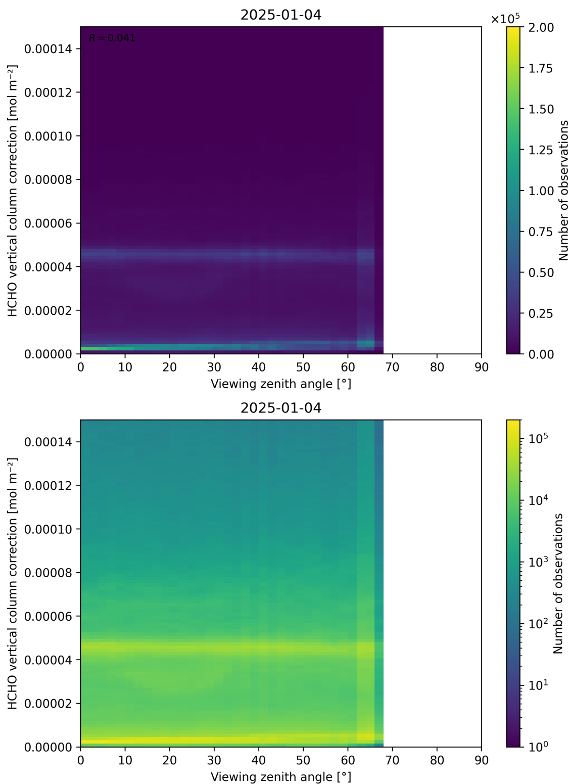
Figure 193: Scatter density plot of “Viewing zenith angle” against “HCHO vertical column correction” for 2025-01-03 to 2025-01-05.
