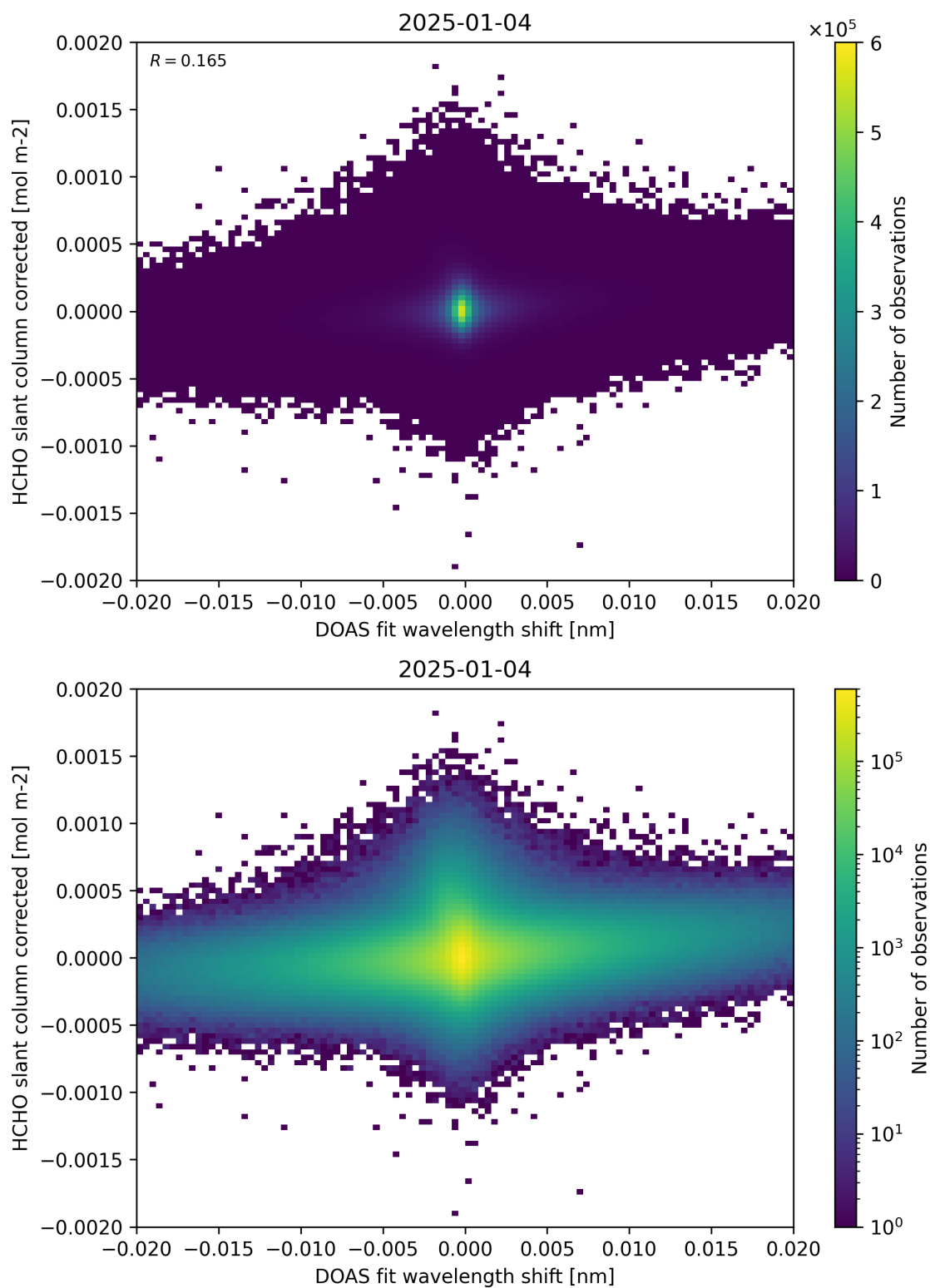
Figure 66: Scatter density plot of “DOAS fit wavelength shift” against “HCHO slant column corrected” for 2025-01-03 to 2025-01-05.
