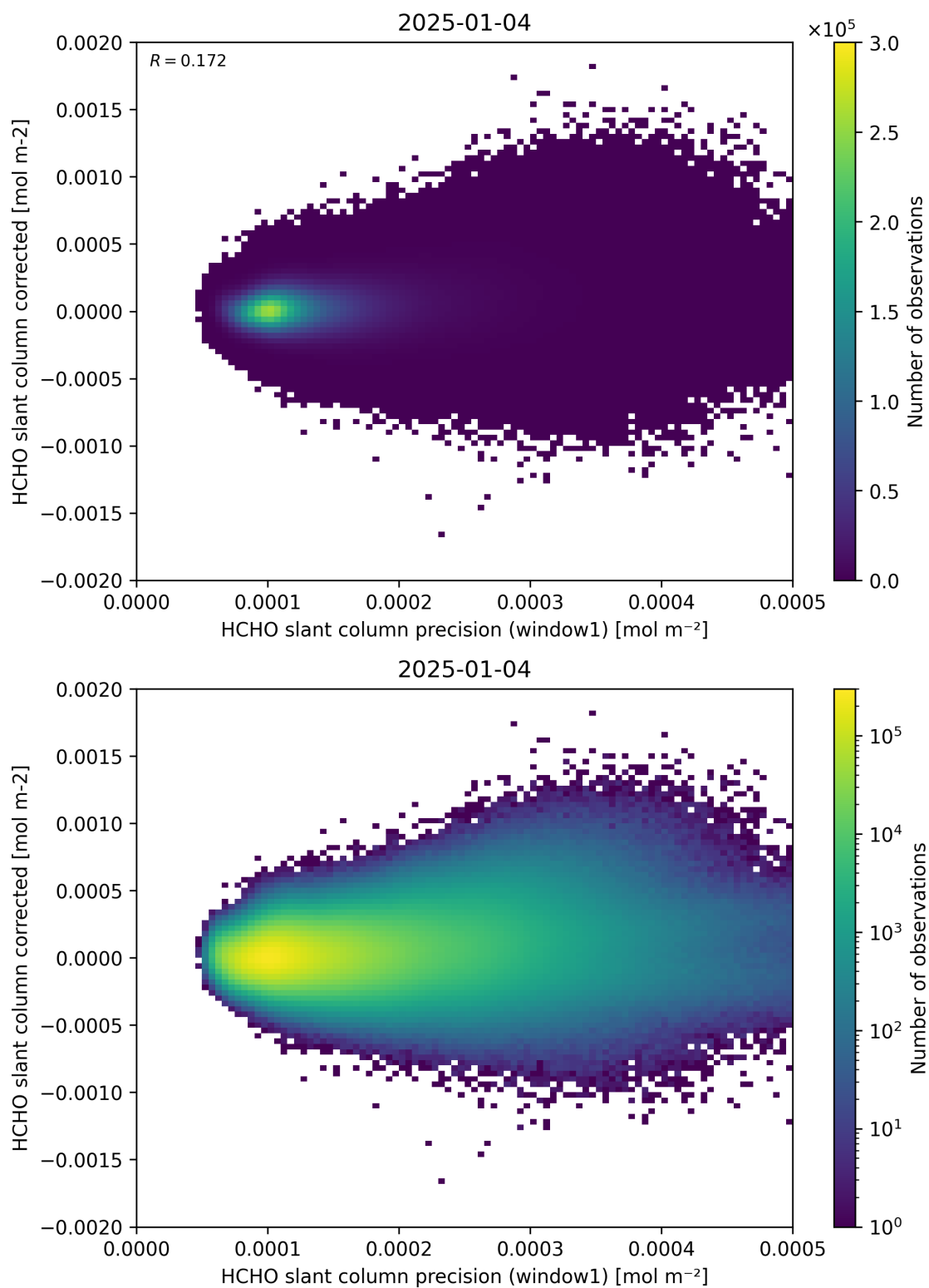
Figure 92: Scatter density plot of “HCHO slant column precision (window1)” against “HCHO slant column corrected” for 2025-01-03 to 2025-01-05.
