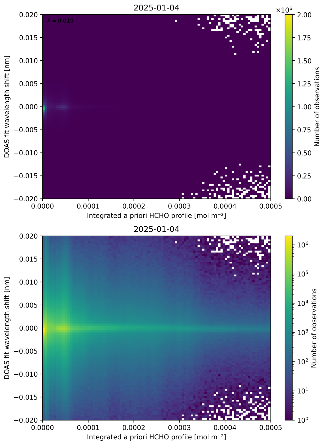
Figure 149: Scatter density plot of “Integrated a priori HCHO profile” against “DOAS fit wavelength shift” for 2025-01-03 to 2025-01-05.
