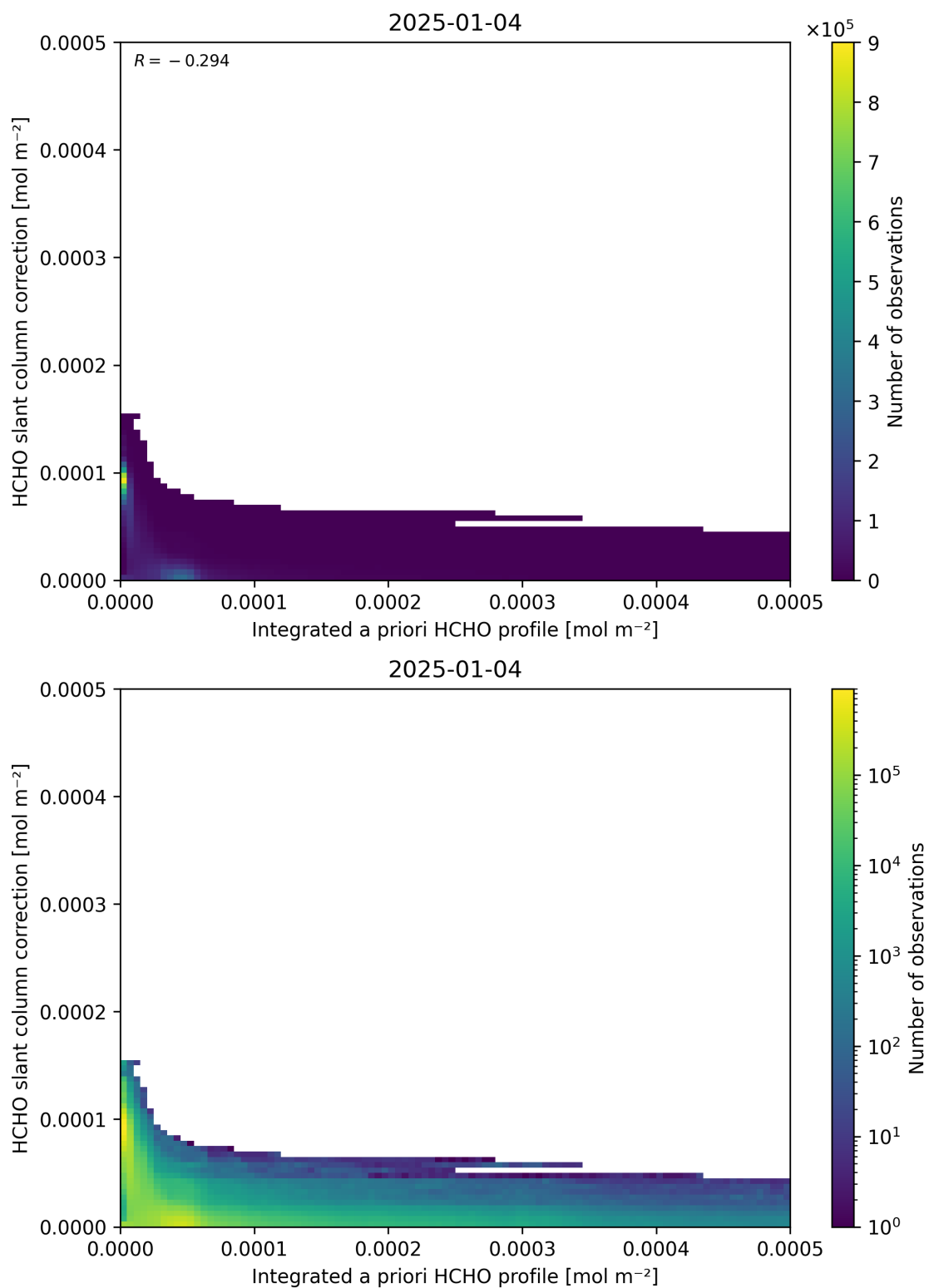
Figure 152: Scatter density plot of “Integrated a priori HCHO profile” against “HCHO slant column correction” for 2025-01-03 to 2025-01-05.
