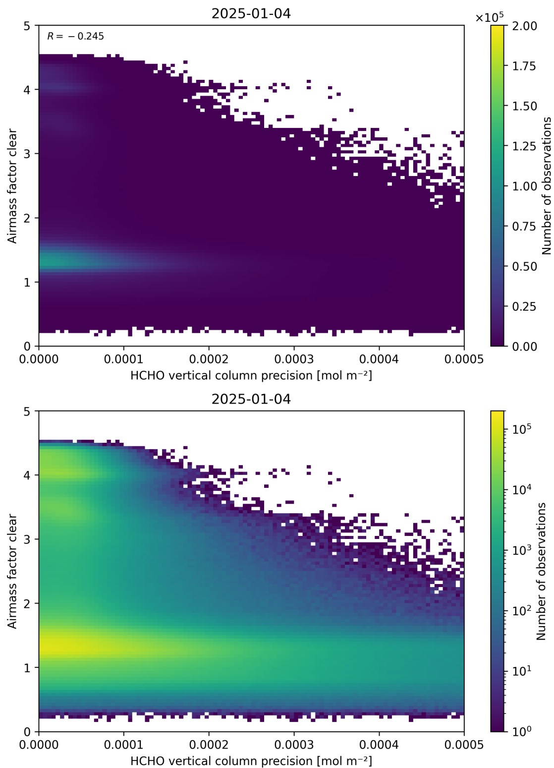
Figure 139: Scatter density plot of “HCHO vertical column precision” against “Airmass factor clear” for 2025-01-03 to 2025-01-05.
