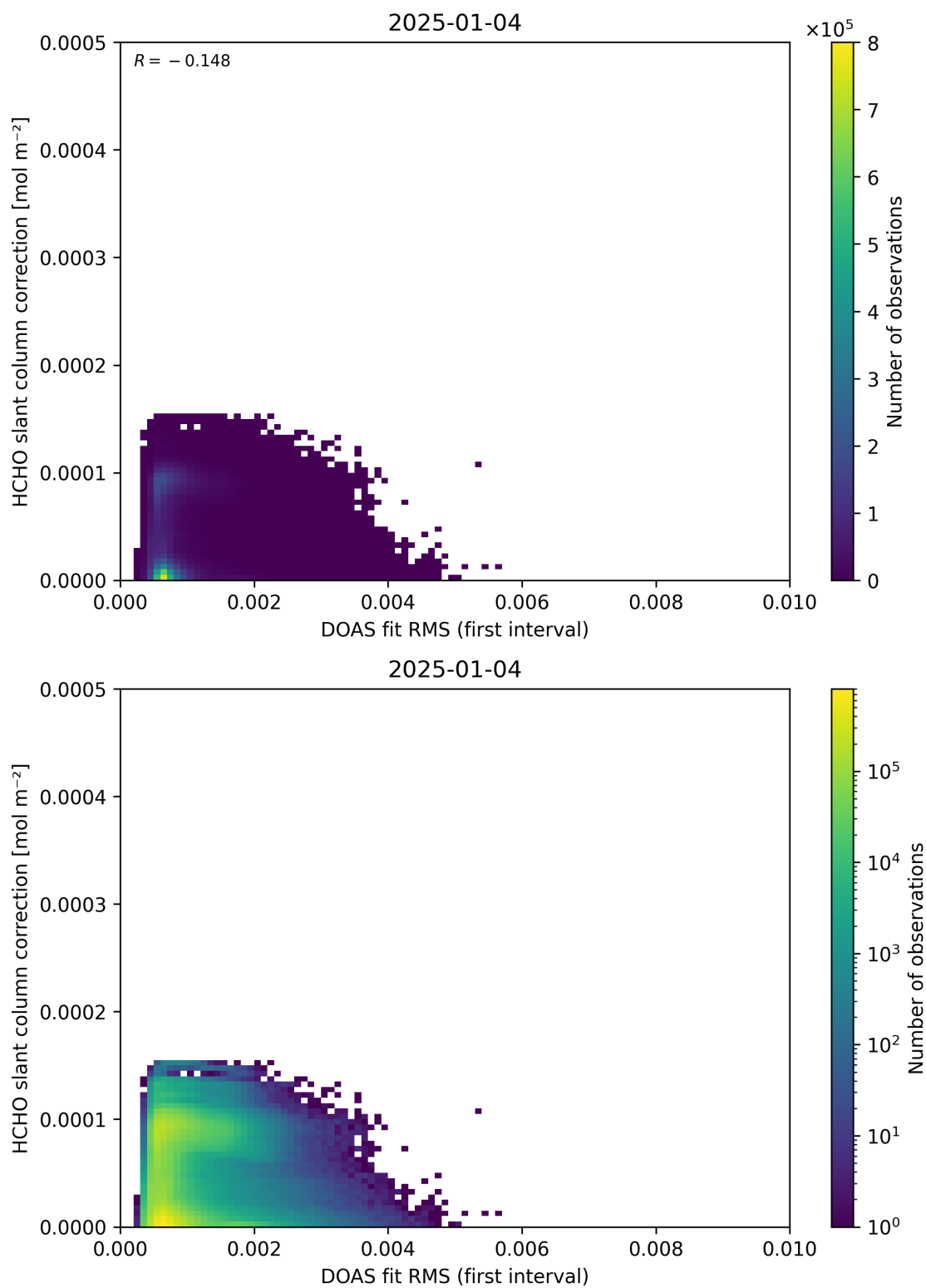
Figure 63: Scatter density plot of “DOAS fit RMS (first interval)” against “HCHO slant column correction” for 2025-01-03 to 2025-01-05.
