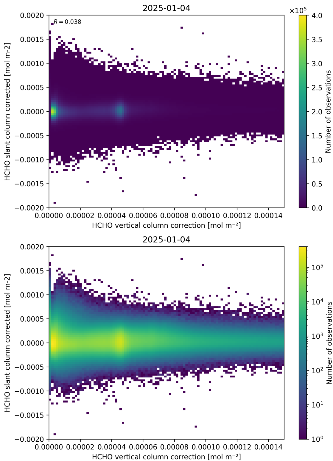
Figure 116: Scatter density plot of “HCHO vertical column correction” against “HCHO slant column corrected” for 2025-01-03 to 2025-01-05.
