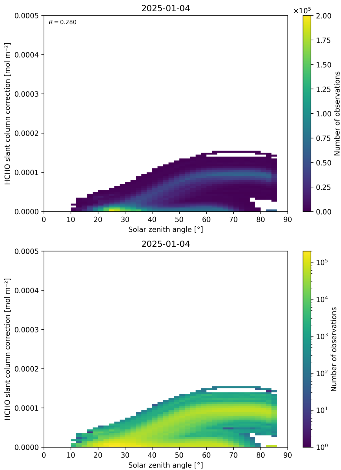
Figure 172: Scatter density plot of “Solar zenith angle” against “HCHO slant column correction” for 2025-01-03 to 2025-01-05.
