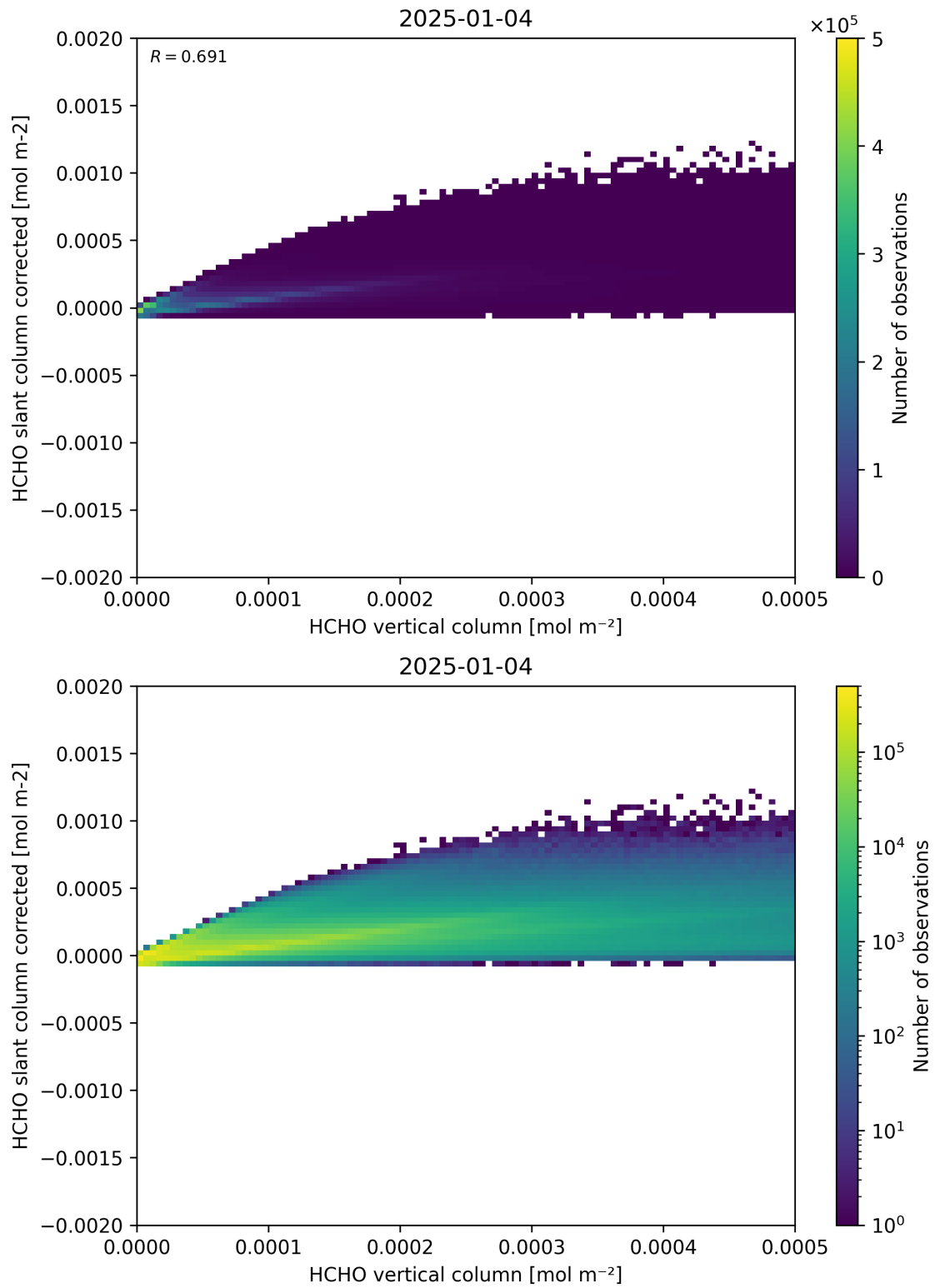
Figure 127: Scatter density plot of “HCHO vertical column” against “HCHO slant column corrected” for 2025-01-03 to 2025-01-05.
