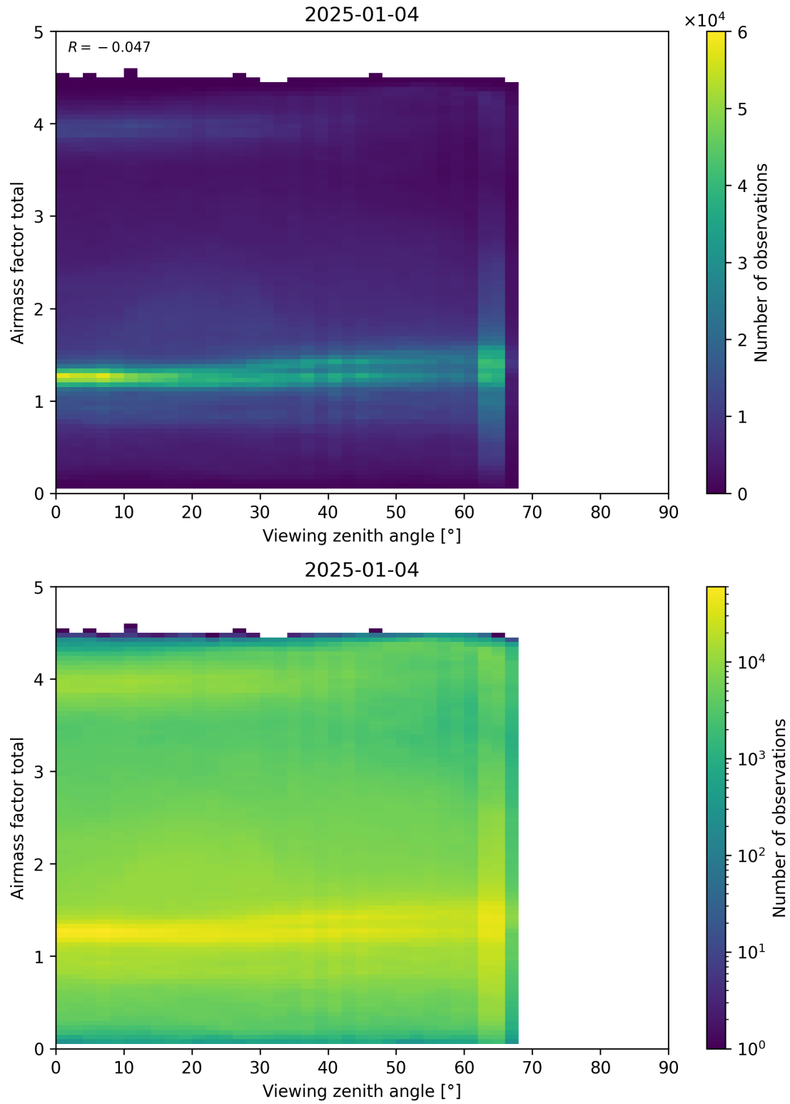
Figure 190: Scatter density plot of “Viewing zenith angle” against “Airmass factor total” for 2025-01-03 to 2025-01-05.
