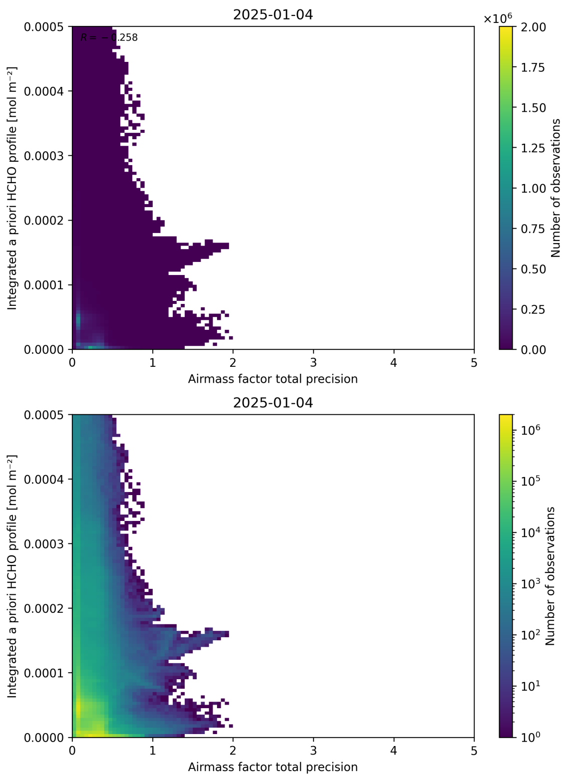
Figure 111: Scatter density plot of “Airmass factor total precision” against “Integrated a priori HCHO profile” for 2025-01-03 to 2025-01-05.
