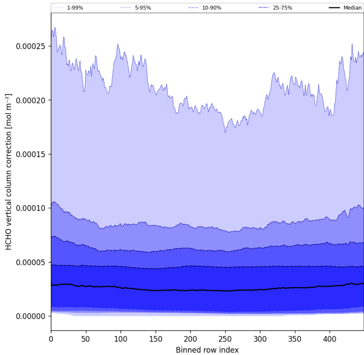
Figure 51: Along track statistics of “HCHO vertical column correction” for 2025-01-03 to 2025-01-05
