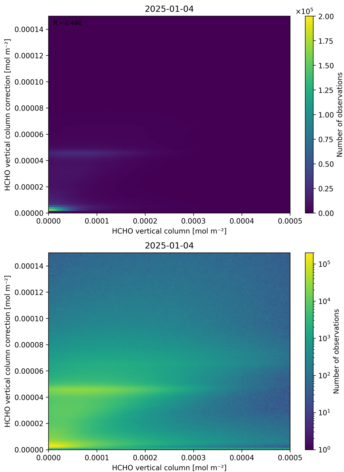
Figure 133: Scatter density plot of “HCHO vertical column” against “HCHO vertical column correction” for 2025-01-03 to 2025-01-05.
