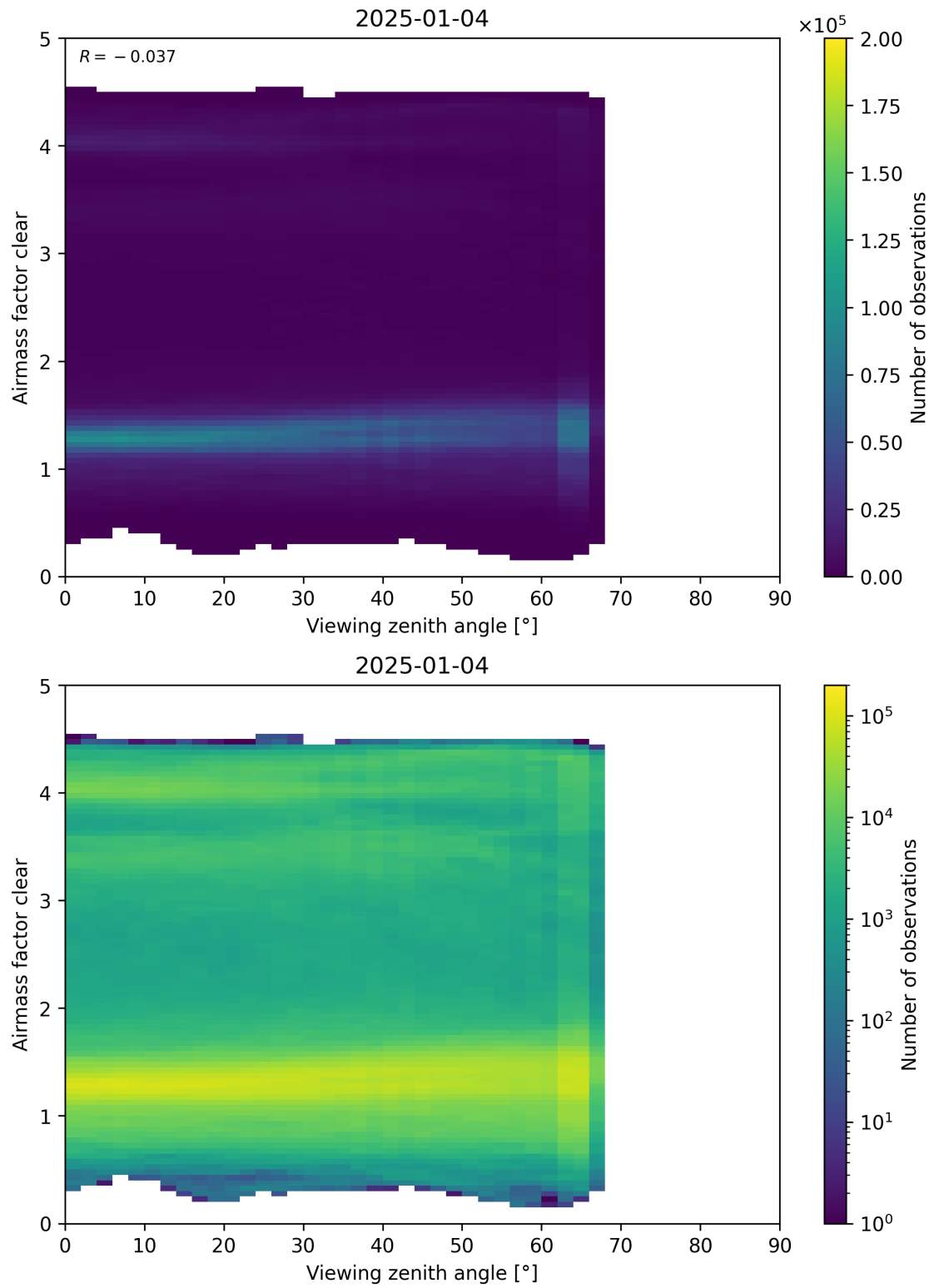
Figure 185: Scatter density plot of “Viewing zenith angle” against “Airmass factor clear” for 2025-01-03 to 2025-01-05.
