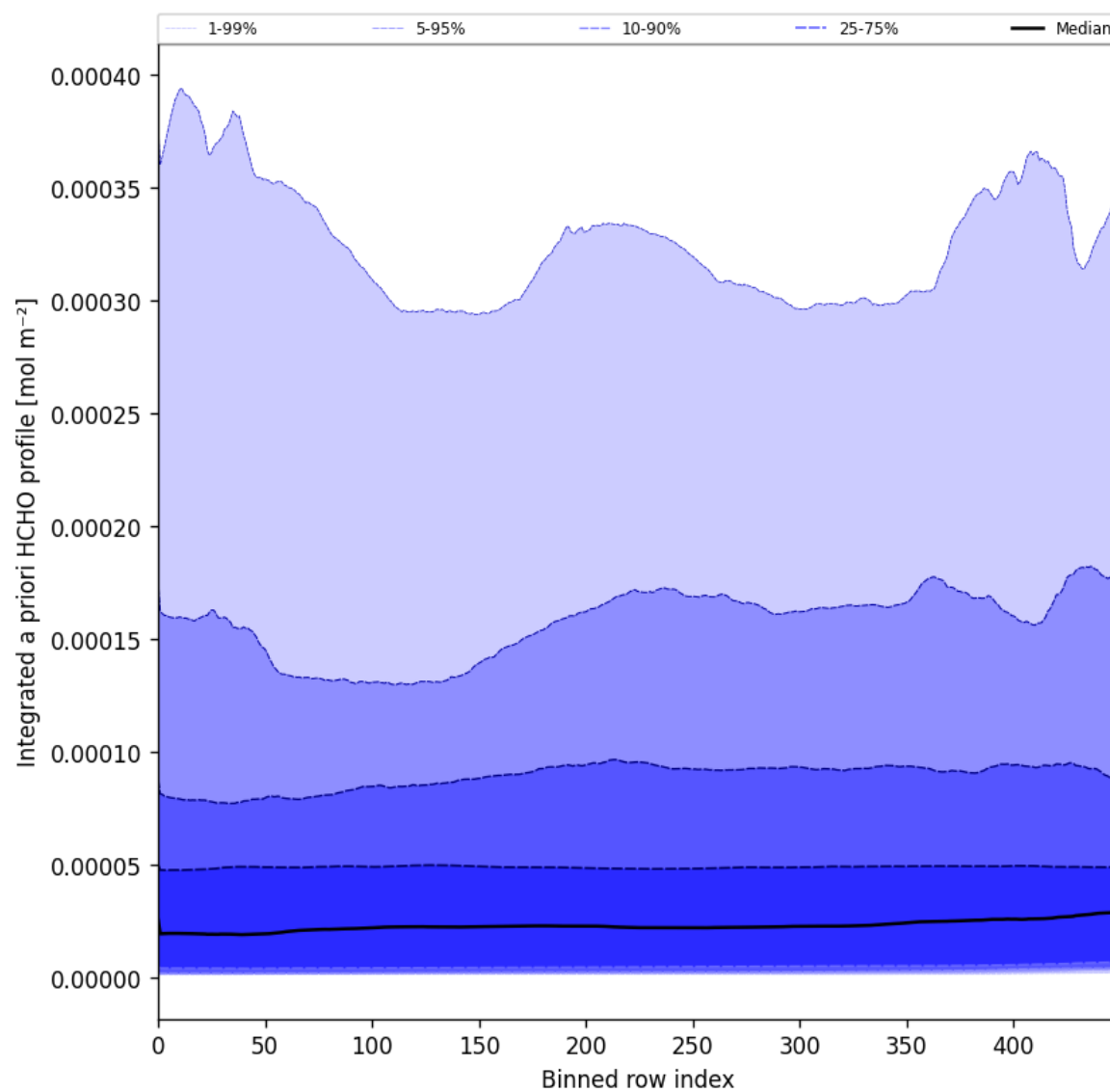
Figure 57: Along track statistics of "Integrated a priori HCHO profile" for 2025-01-03 to 2025-01-05
