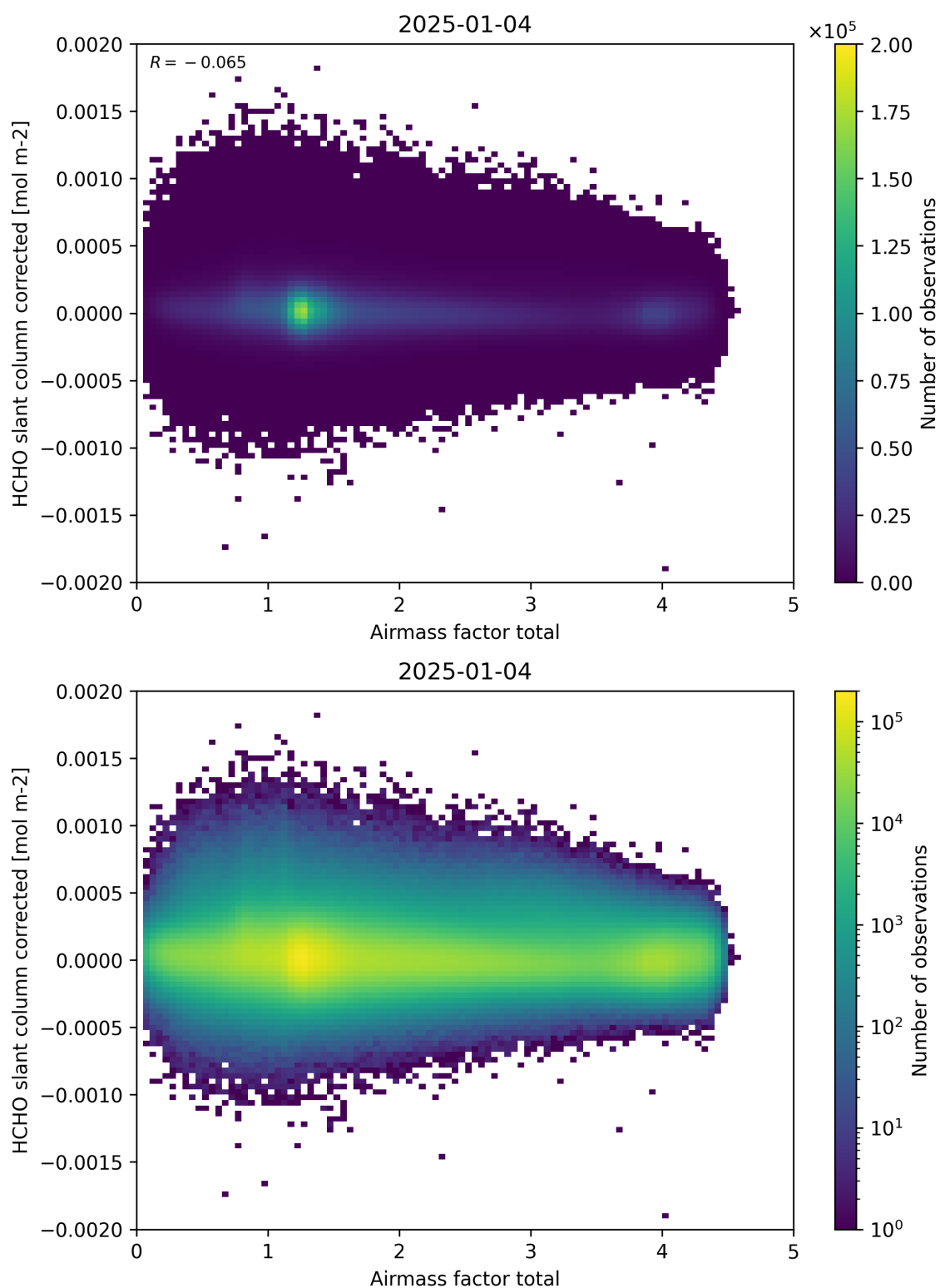
Figure 101: Scatter density plot of “Airmass factor total” against “HCHO slant column corrected” for 2025-01-03 to 2025-01-05.
