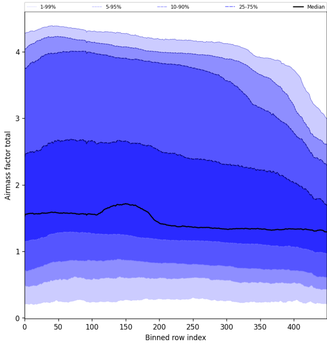
Figure 54: Along track statistics of “Airmass factor total” for 2025-01-03 to 2025-01-05
