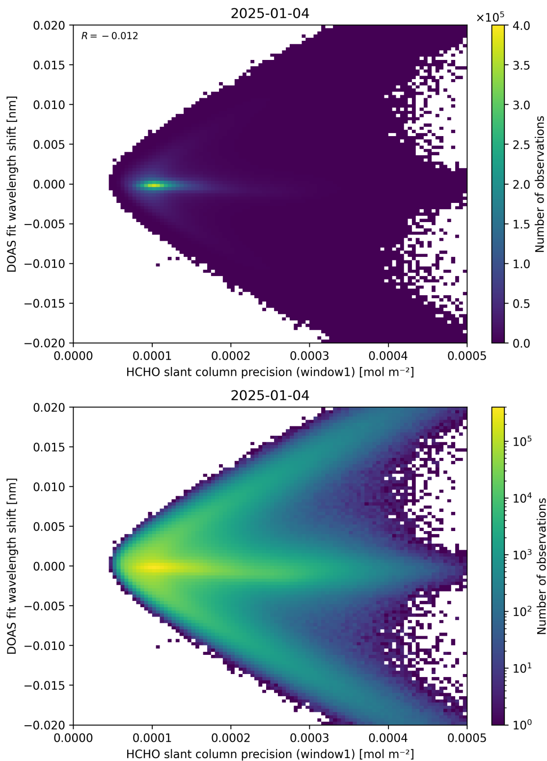
Figure 89: Scatter density plot of “HCHO slant column precision (window1)” against “DOAS fit wavelength shift” for 2025-01-03 to 2025-01-05.
