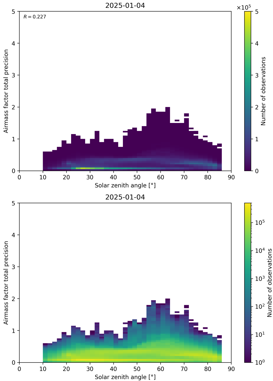
Figure 176: Scatter density plot of “Solar zenith angle” against “Airmass factor total precision” for 2025-01-03 to 2025-01-05.
