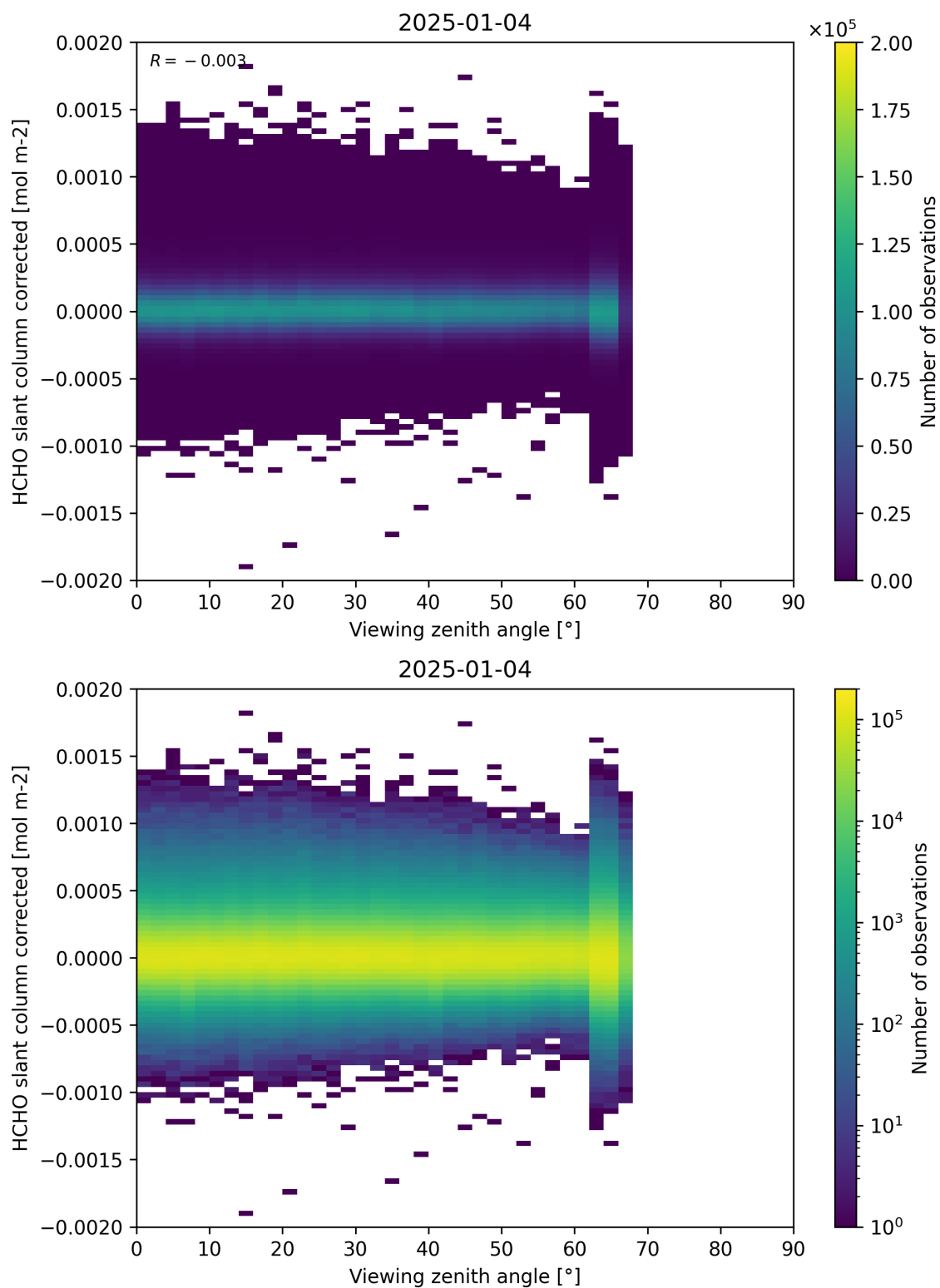
Figure 186: Scatter density plot of “Viewing zenith angle” against “HCHO slant column corrected” for 2025-01-03 to 2025-01-05.
