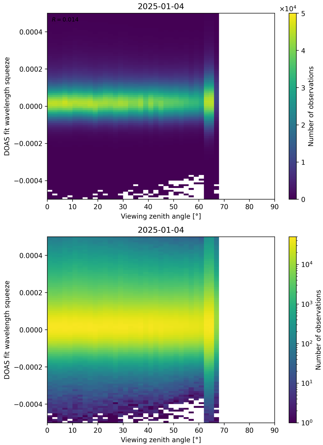
Figure 184: Scatter density plot of “Viewing zenith angle” against “DOAS fit wavelength squeeze” for 2025-01-03 to 2025-01-05.
