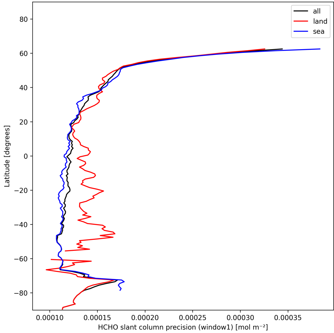
Figure 25: Zonal average of “HCHO slant column precision (window1)” for 2025-01-03 to 2025-01-05.
