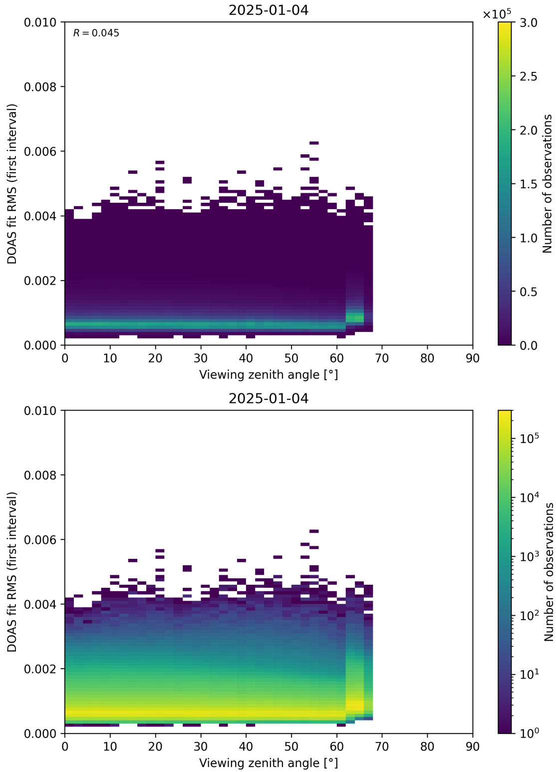
Figure 182: Scatter density plot of “Viewing zenith angle” against “DOAS fit RMS (first interval)” for 2025-01-03 to 2025-01-05.
