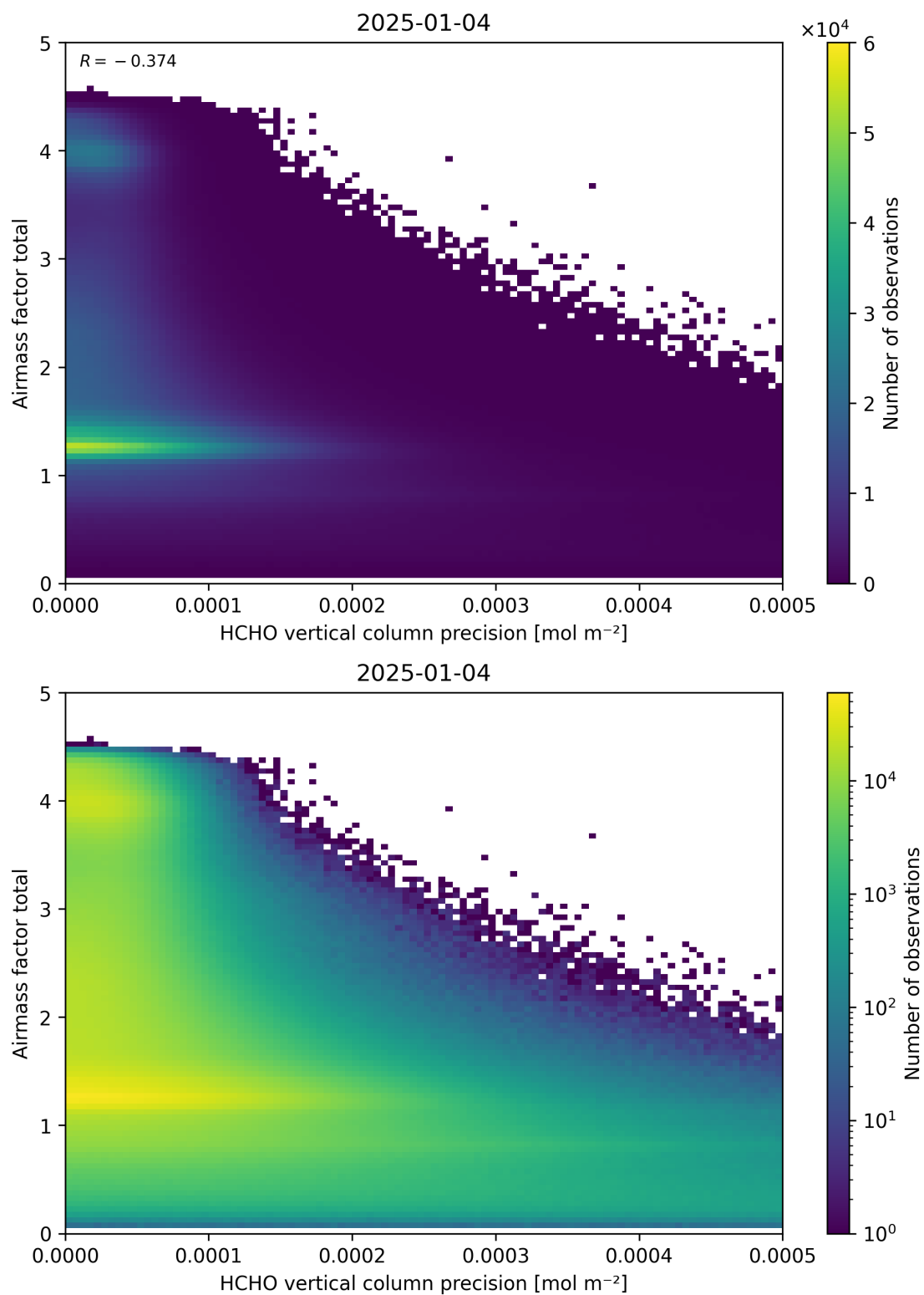
Figure 144: Scatter density plot of “HCHO vertical column precision” against “Airmass factor total” for 2025-01-03 to 2025-01-05.
