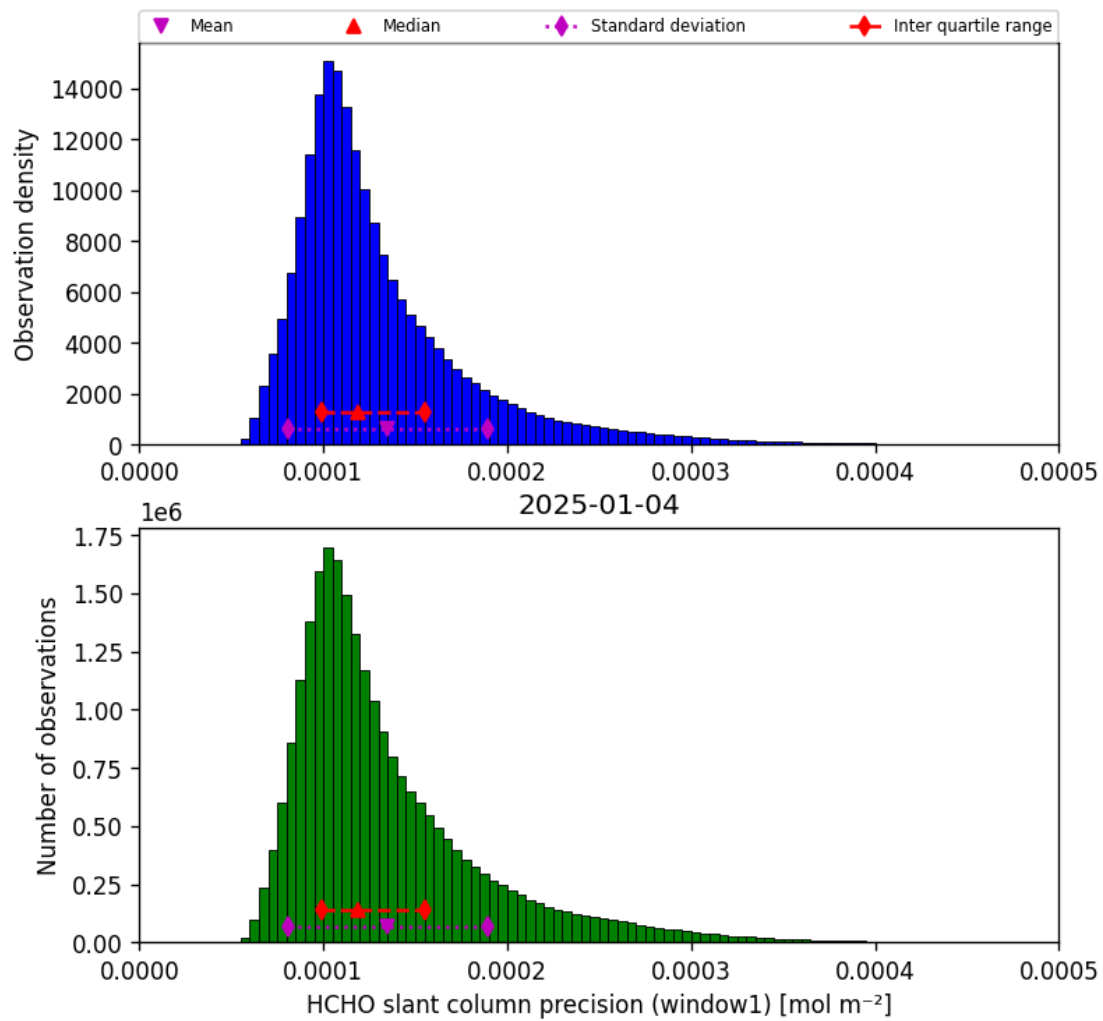
Figure 39: Histogram of “HCHO slant column precision (window1)” for 2025-01-03 to 2025-01-05
