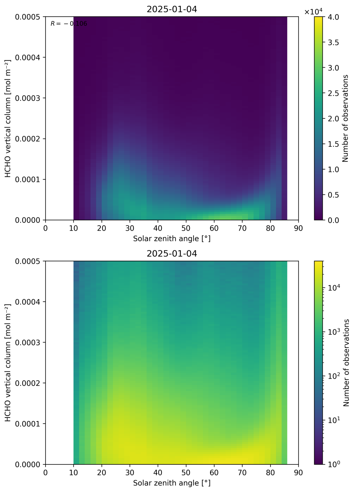
Figure 177: Scatter density plot of “Solar zenith angle” against “HCHO vertical column” for 2025-01-03 to 2025-01-05.
