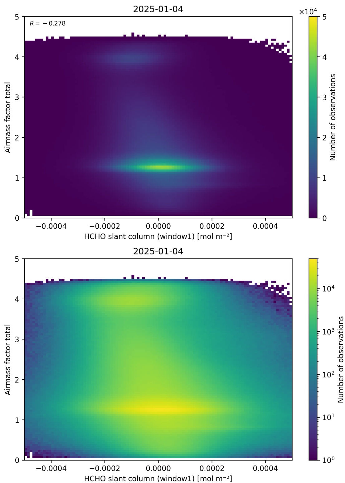
Figure 85: Scatter density plot of “HCHO slant column (window1)” against “Airmass factor total” for 2025-01-03 to 2025-01-05.
