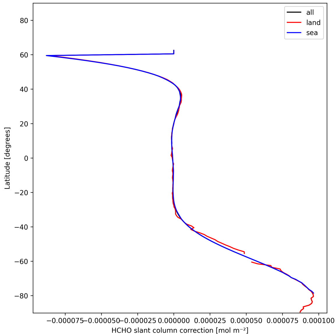
Figure 33: Zonal average of “HCHO slant column correction” for 2025-01-03 to 2025-01-05.
