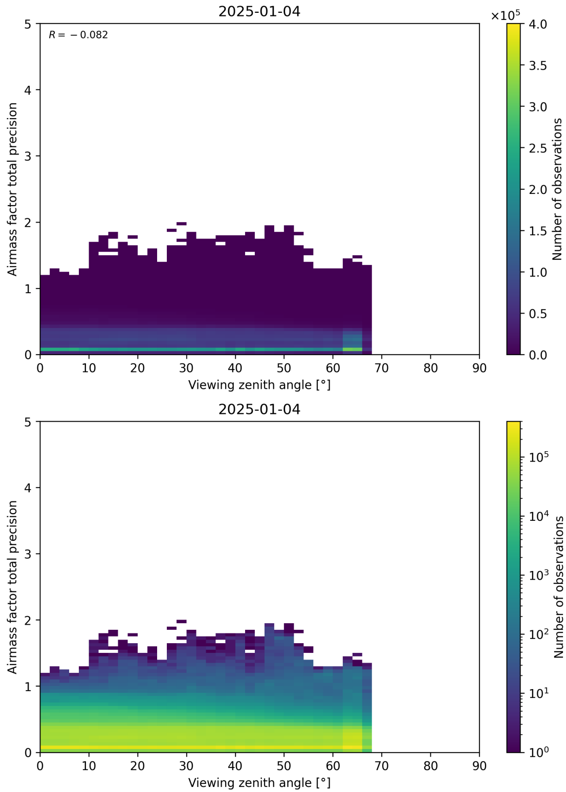
Figure 191: Scatter density plot of “Viewing zenith angle” against “Airmass factor total precision” for 2025-01-03 to 2025-01-05.
