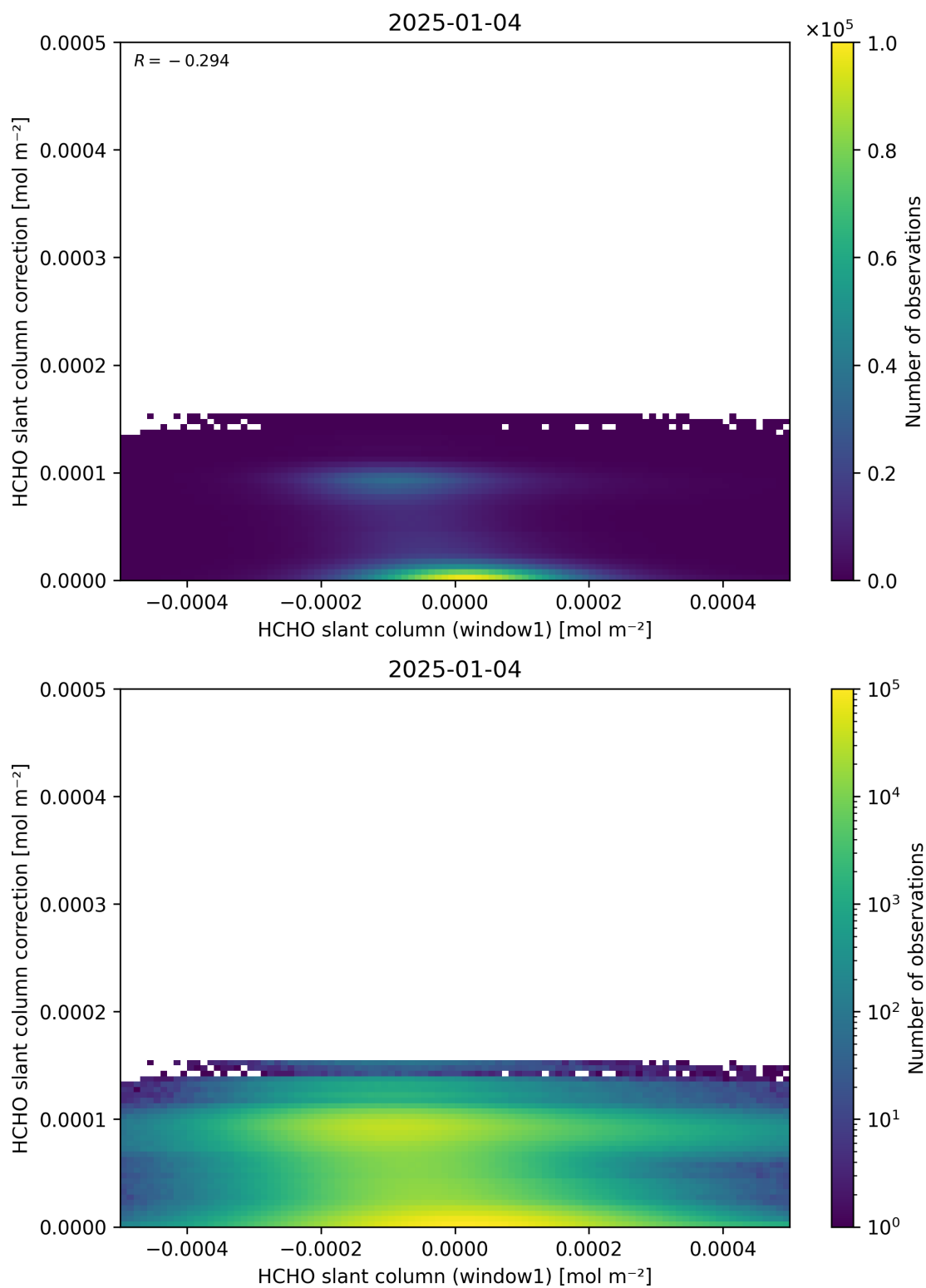
Figure 83: Scatter density plot of “HCHO slant column (window1)” against “HCHO slant column correction” for 2025-01-03 to 2025-01-05.
