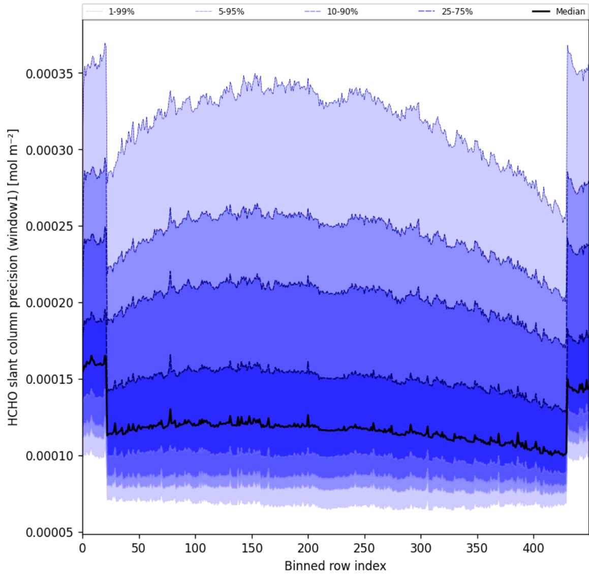
Figure 53: Along track statistics of “HCHO slant column precision (window1)” for 2025-01-03 to 2025-01-05
