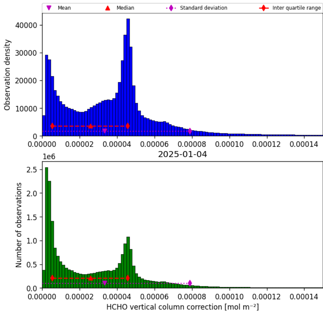
Figure 37: Histogram of “HCHO vertical column correction” for 2025-01-03 to 2025-01-05
