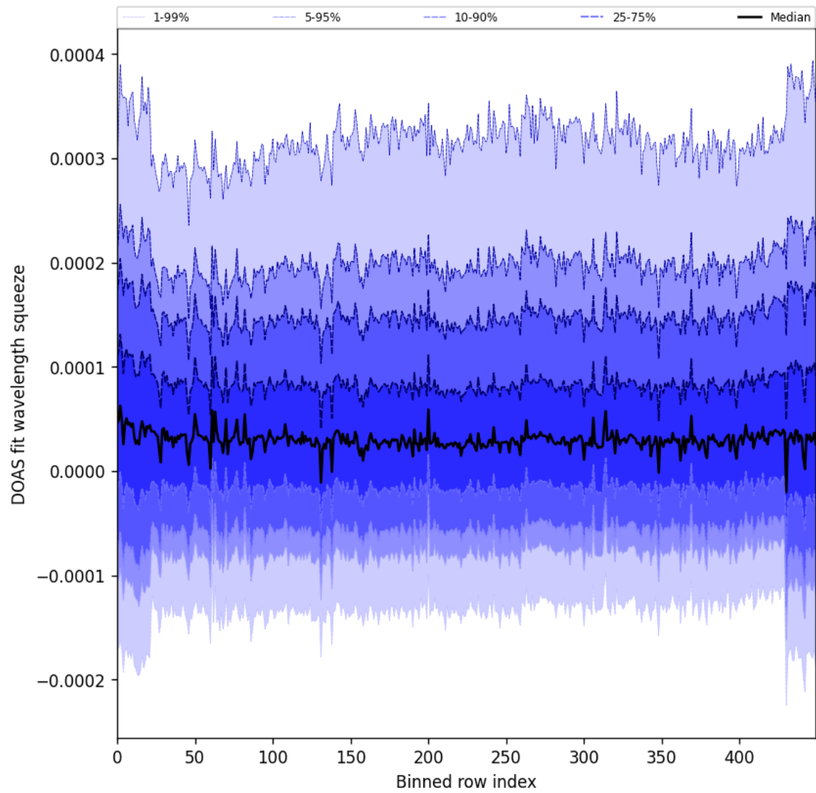
Figure 59: Along track statistics of “DOAS fit wavelength squeeze” for 2025-01-03 to 2025-01-05
