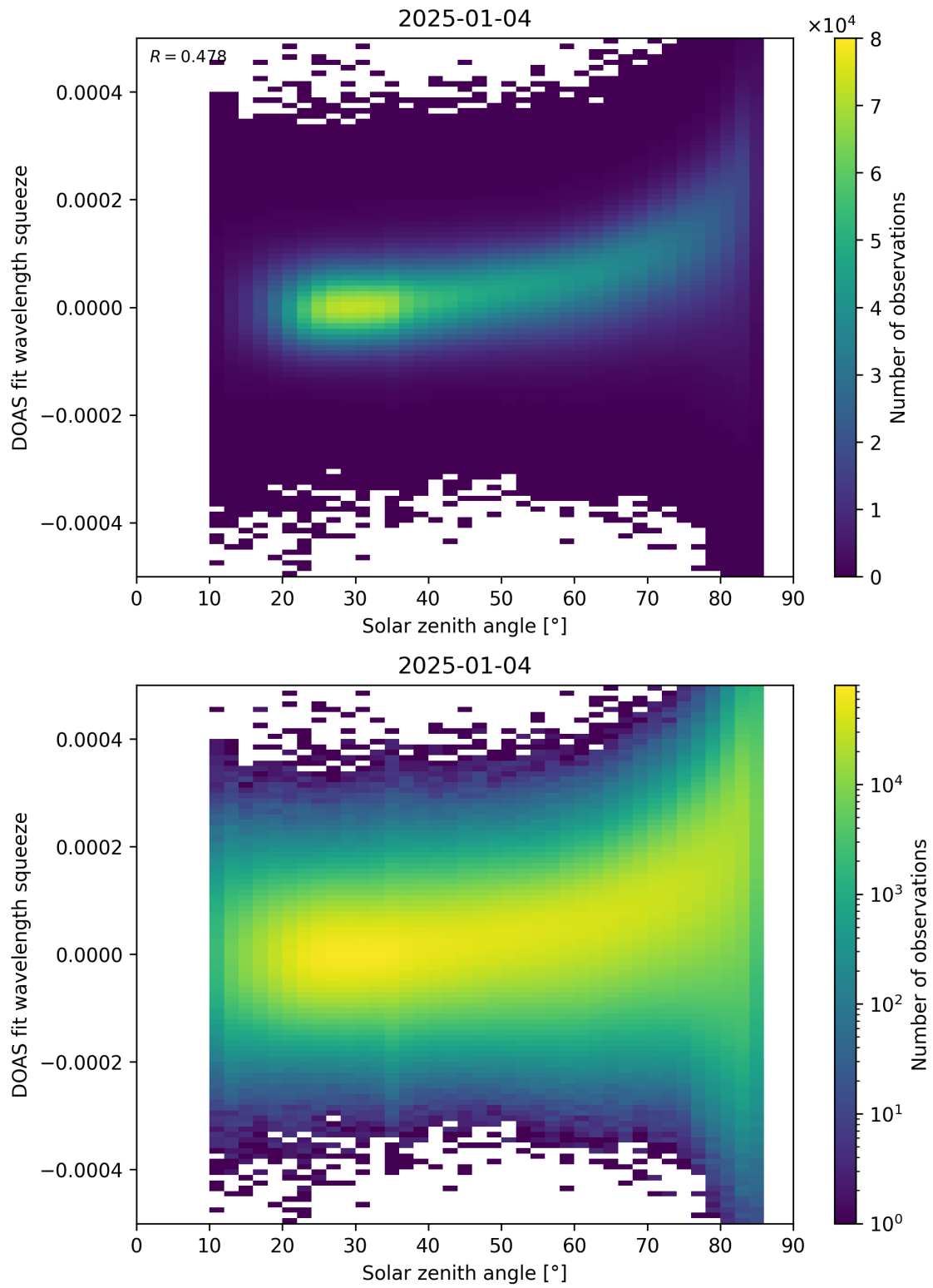
Figure 169: Scatter density plot of “Solar zenith angle” against “DOAS fit wavelength squeeze” for 2025-01-03 to 2025-01-05.
