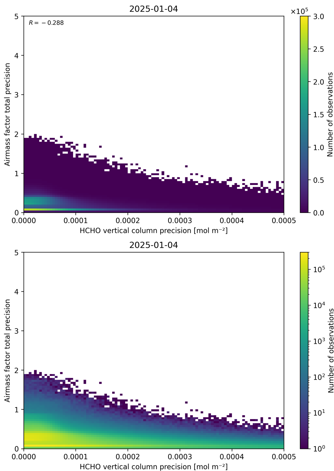
Figure 145: Scatter density plot of “HCHO vertical column precision” against “Airmass factor total precision” for 2025-01-03 to 2025-01-05.
