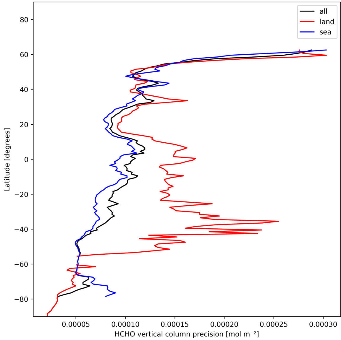
Figure 22: Zonal average of “HCHO vertical column precision” for 2025-01-03 to 2025-01-05.
