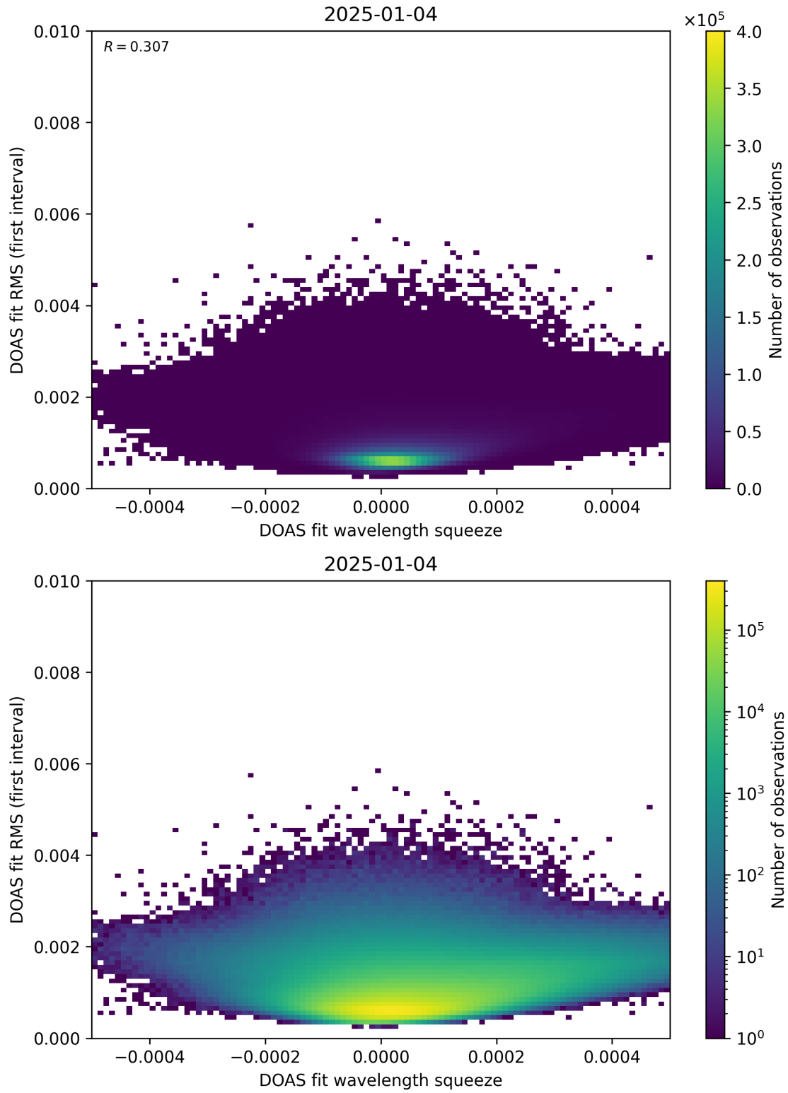
Figure 68: Scatter density plot of “DOAS fit wavelength squeeze” against “DOAS fit RMS (first interval)” for 2025-01-03 to 2025-01-05.
