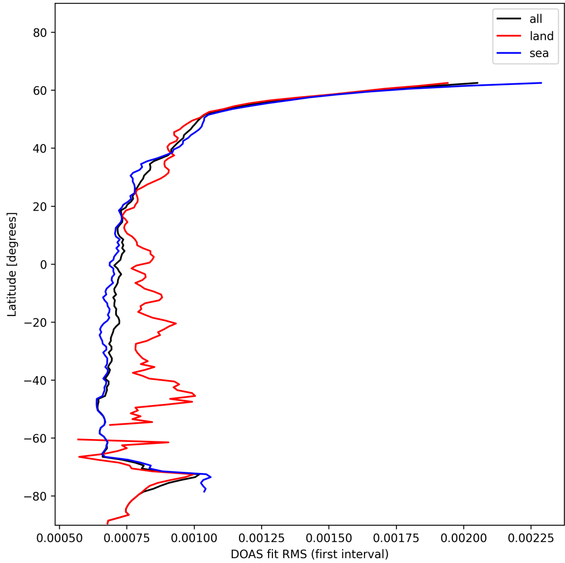
Figure 32: Zonal average of “DOAS fit RMS (first interval)” for 2025-01-03 to 2025-01-05.
