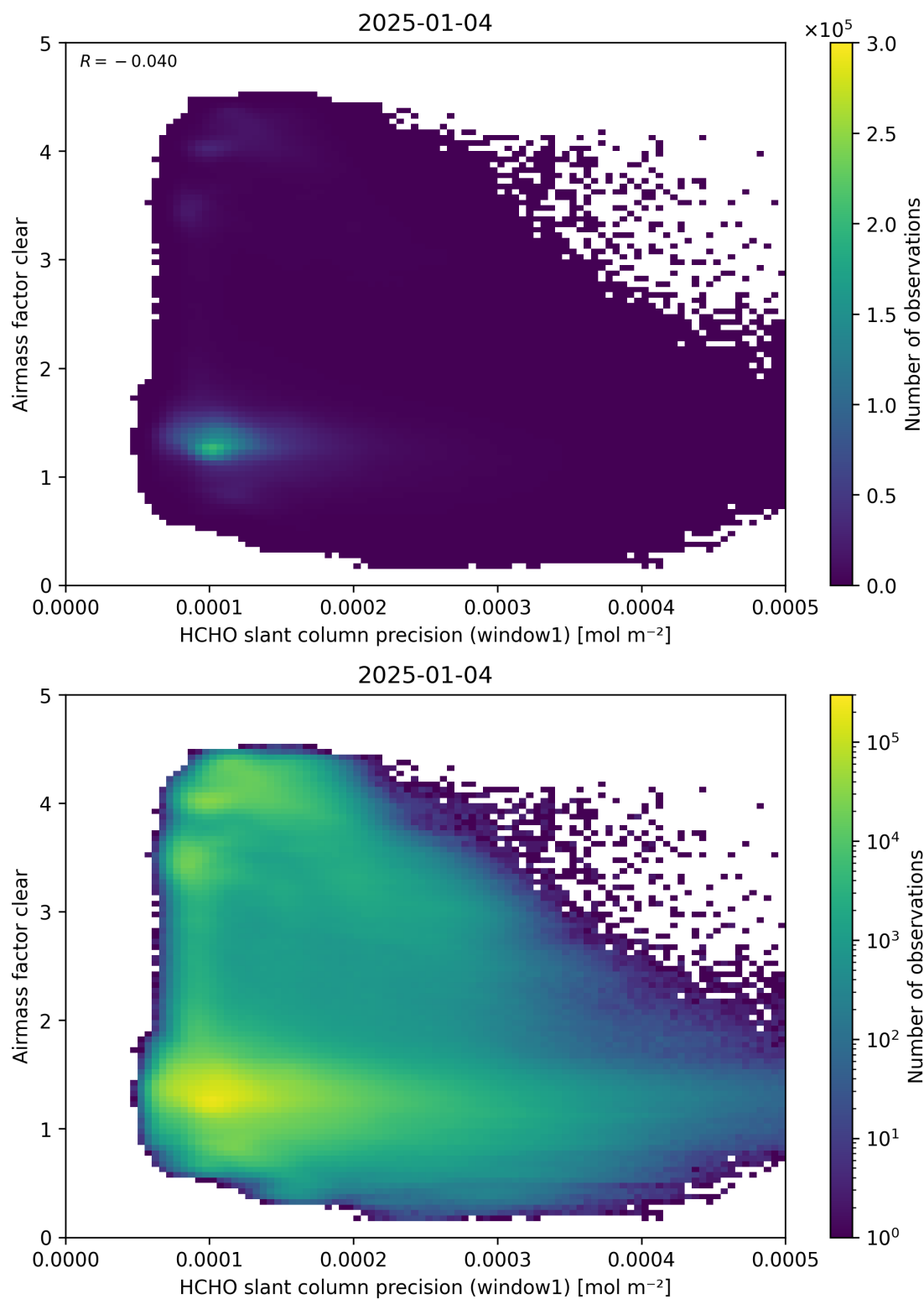
Figure 91: Scatter density plot of “HCHO slant column precision (window1)” against “Airmass factor clear” for 2025-01-03 to 2025-01-05.
