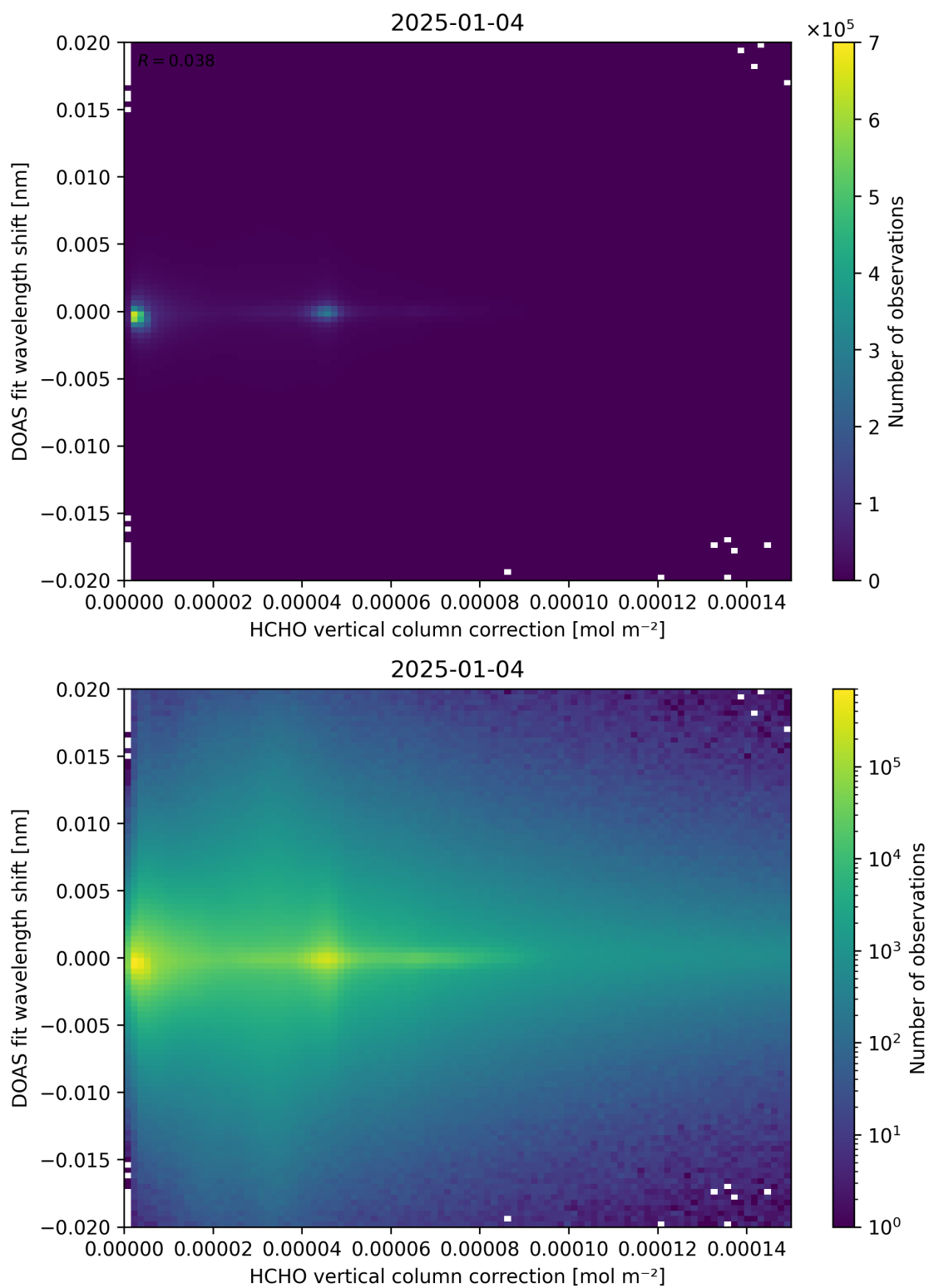
Figure 113: Scatter density plot of “HCHO vertical column correction” against “DOAS fit wavelength shift” for 2025-01-03 to 2025-01-05.
