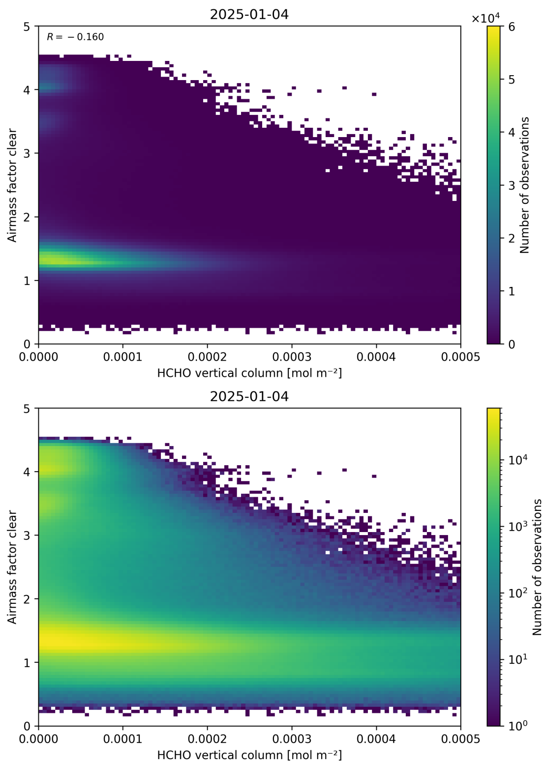
Figure 126: Scatter density plot of “HCHO vertical column” against “Airmass factor clear” for 2025-01-03 to 2025-01-05.
