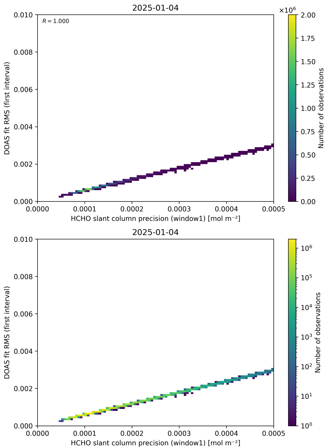
Figure 88: Scatter density plot of “HCHO slant column precision (window1)” against “DOAS fit RMS (first interval)” for 2025-01-03 to 2025-01-05.
