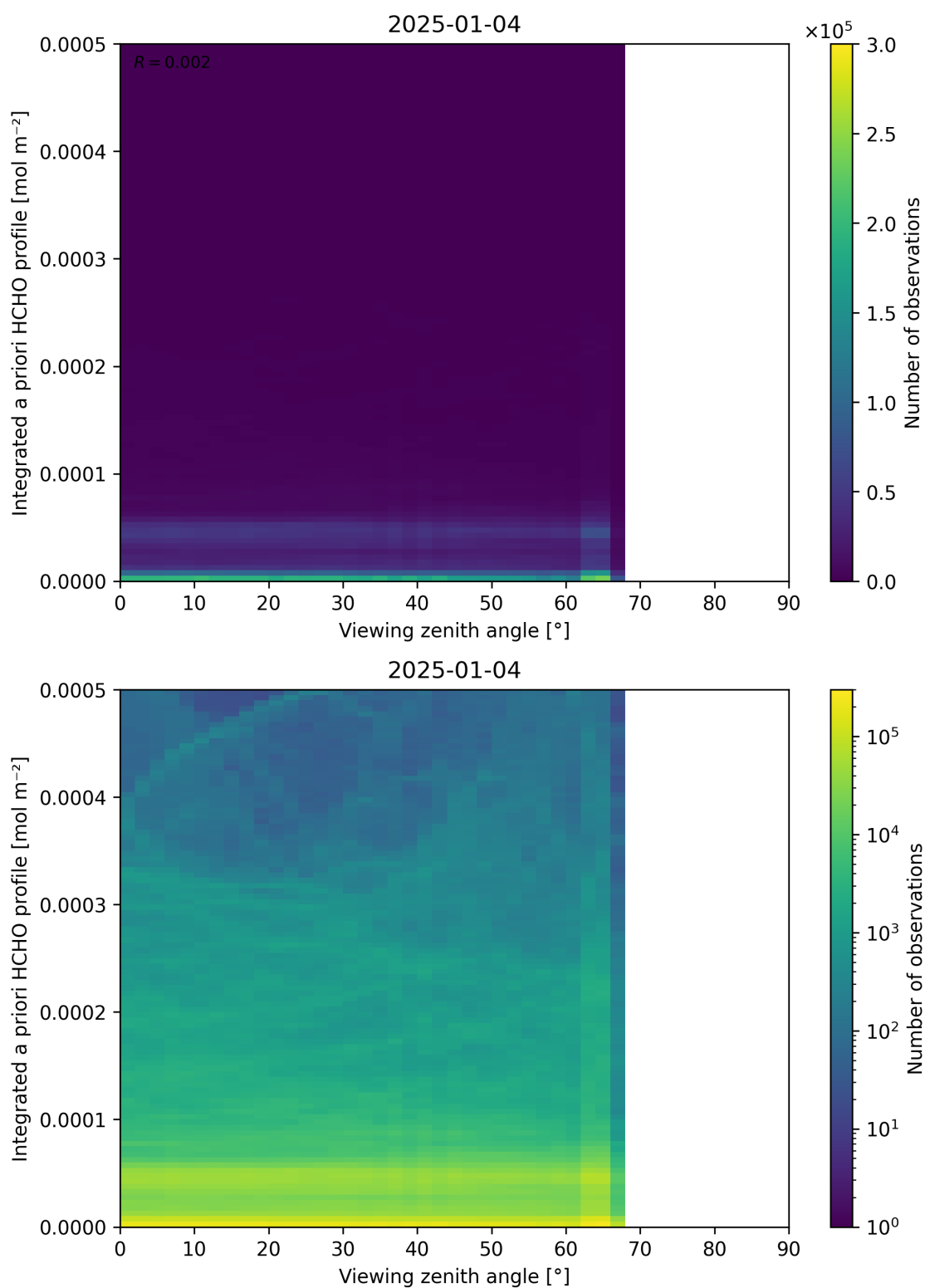
Figure 195: Scatter density plot of “Viewing zenith angle” against “Integrated a priori HCHO profile” for 2025-01-03 to 2025-01-05.
