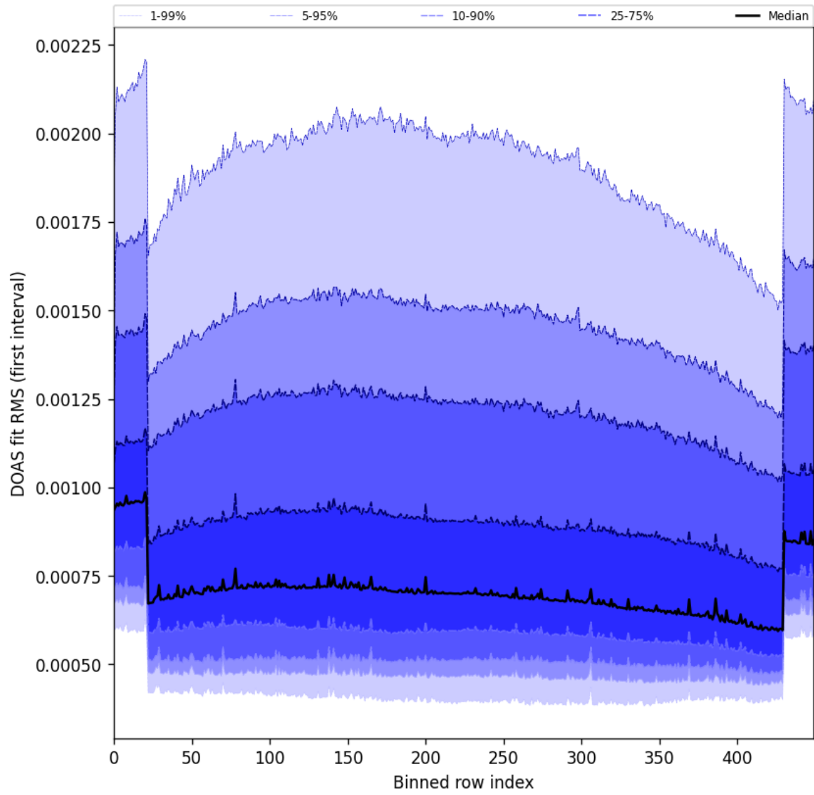
Figure 60: Along track statistics of “DOAS fit RMS (first interval)” for 2025-01-03 to 2025-01-05
