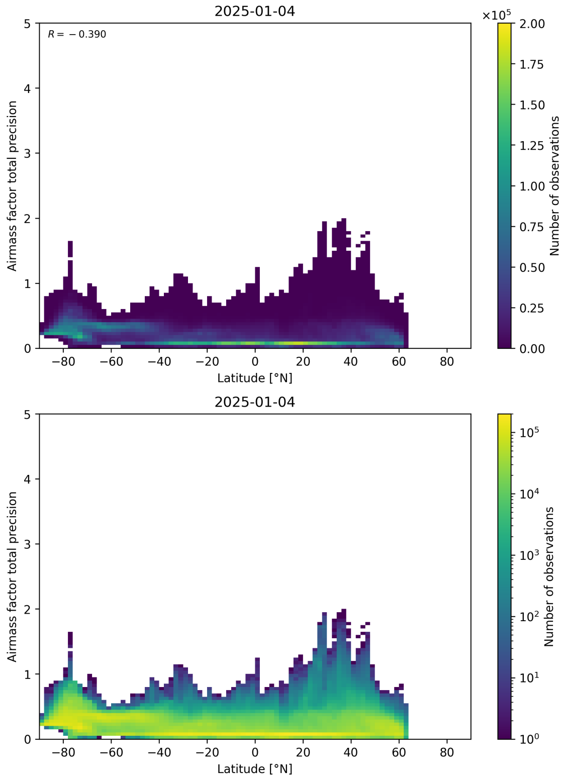
Figure 162: Scatter density plot of “Latitude” against “Airmass factor total precision” for 2025-01-03 to 2025-01-05.
