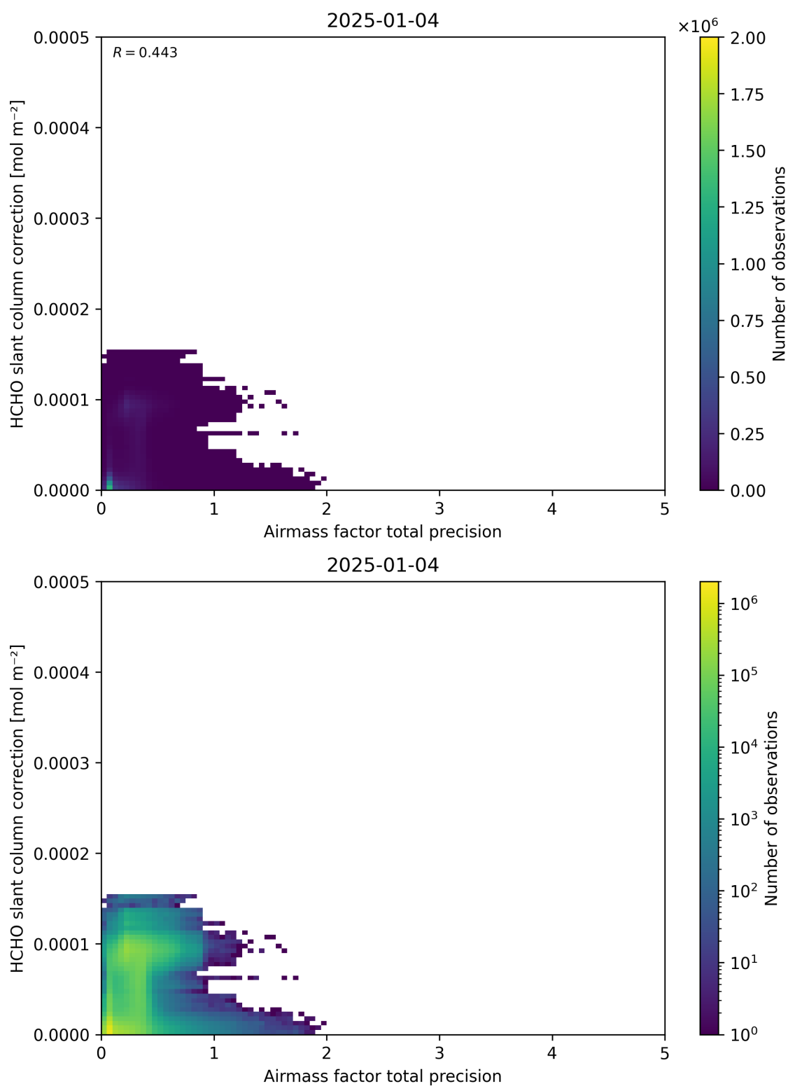
Figure 110: Scatter density plot of “Airmass factor total precision” against “HCHO slant column correction” for 2025-01-03 to 2025-01-05.
