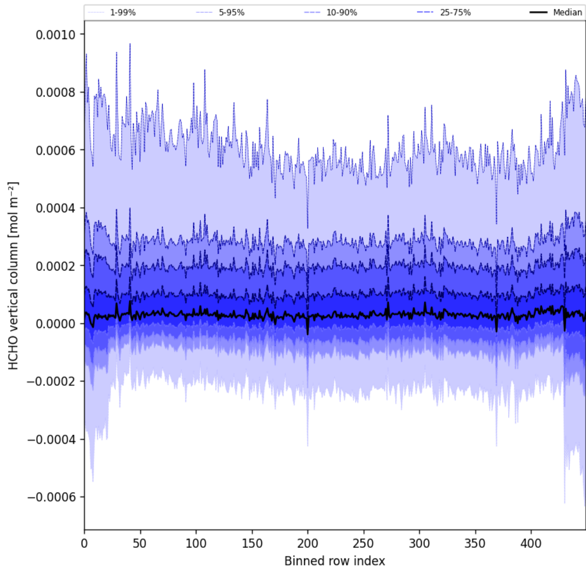
Figure 49: Along track statistics of “HCHO vertical column” for 2025-01-03 to 2025-01-05
