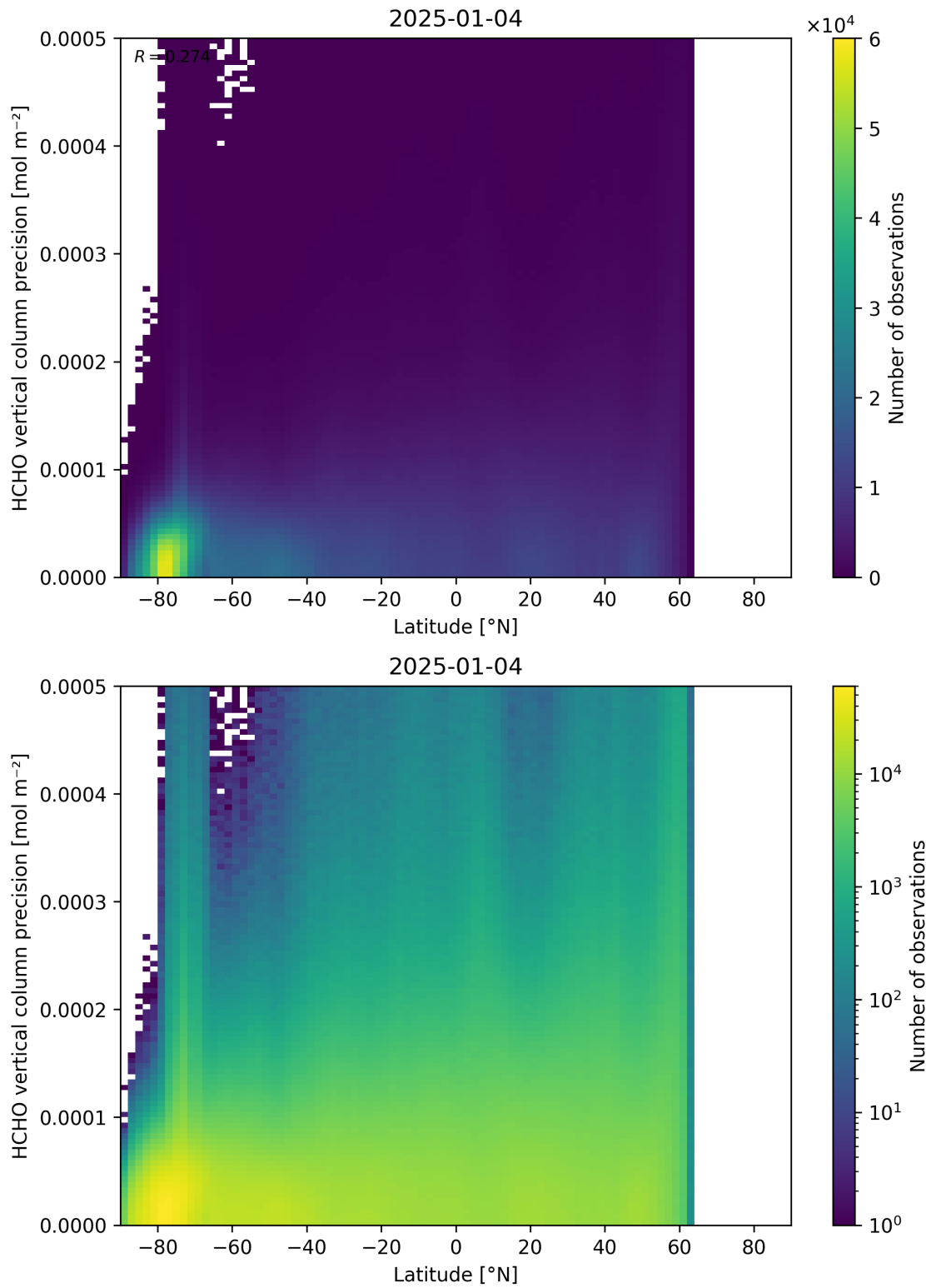
Figure 165: Scatter density plot of “Latitude” against “HCHO vertical column precision” for 2025-01-03 to 2025-01-05.
