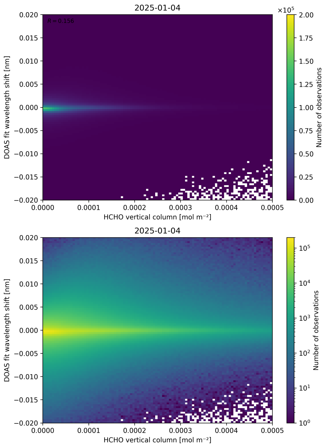
Figure 124: Scatter density plot of “HCHO vertical column” against “DOAS fit wavelength shift” for 2025-01-03 to 2025-01-05.
