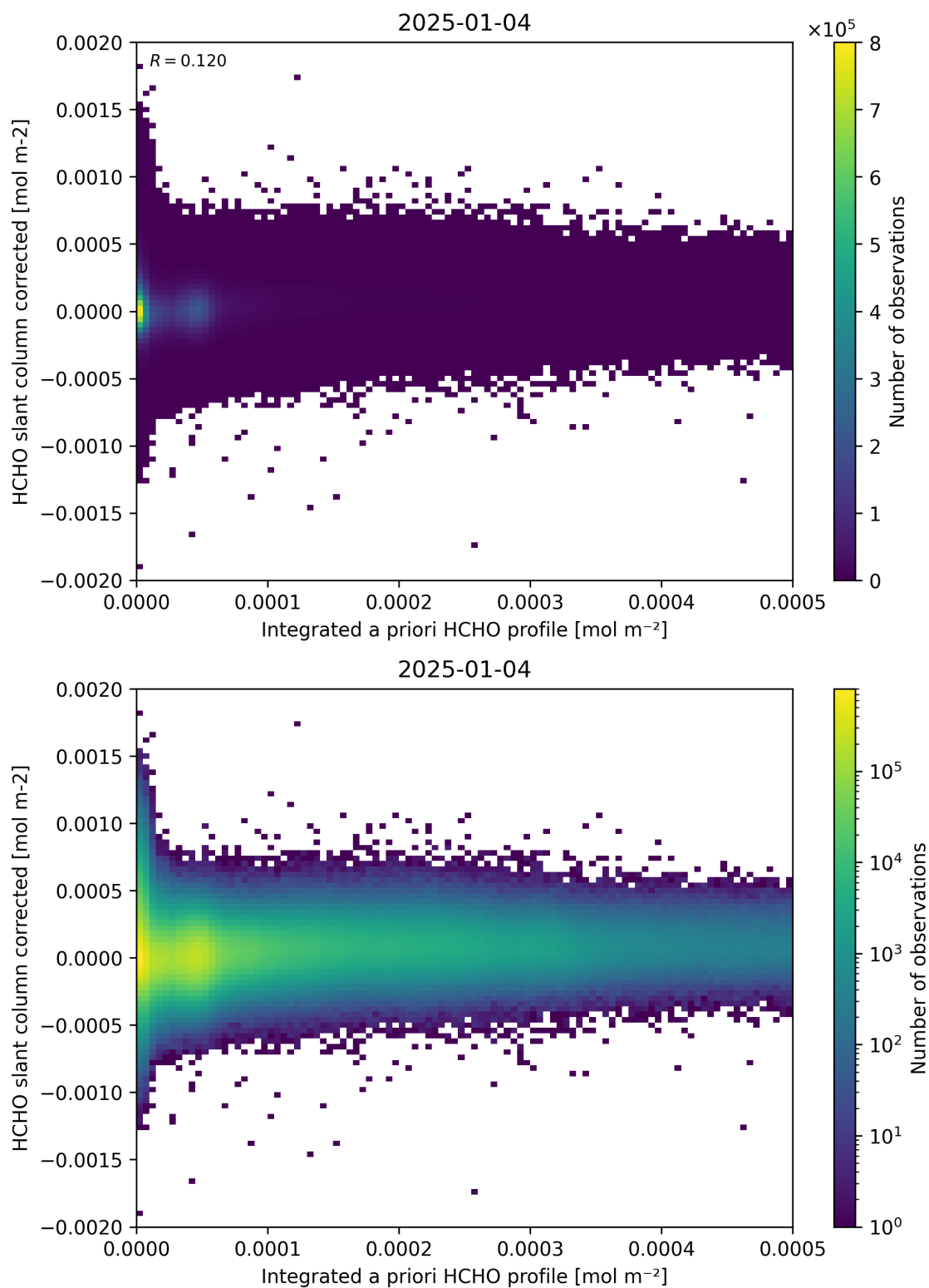
Figure 151: Scatter density plot of “Integrated a priori HCHO profile” against “HCHO slant column corrected” for 2025-01-03 to 2025-01-05.
