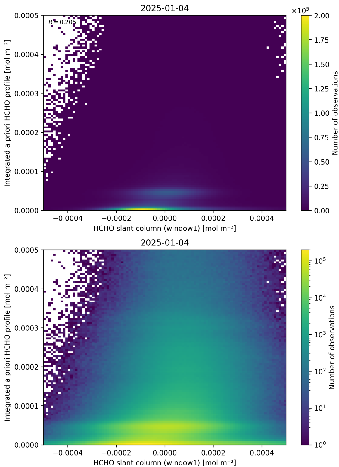
Figure 87: Scatter density plot of “HCHO slant column (window1)” against “Integrated a priori HCHO profile” for 2025-01-03 to 2025-01-05.
