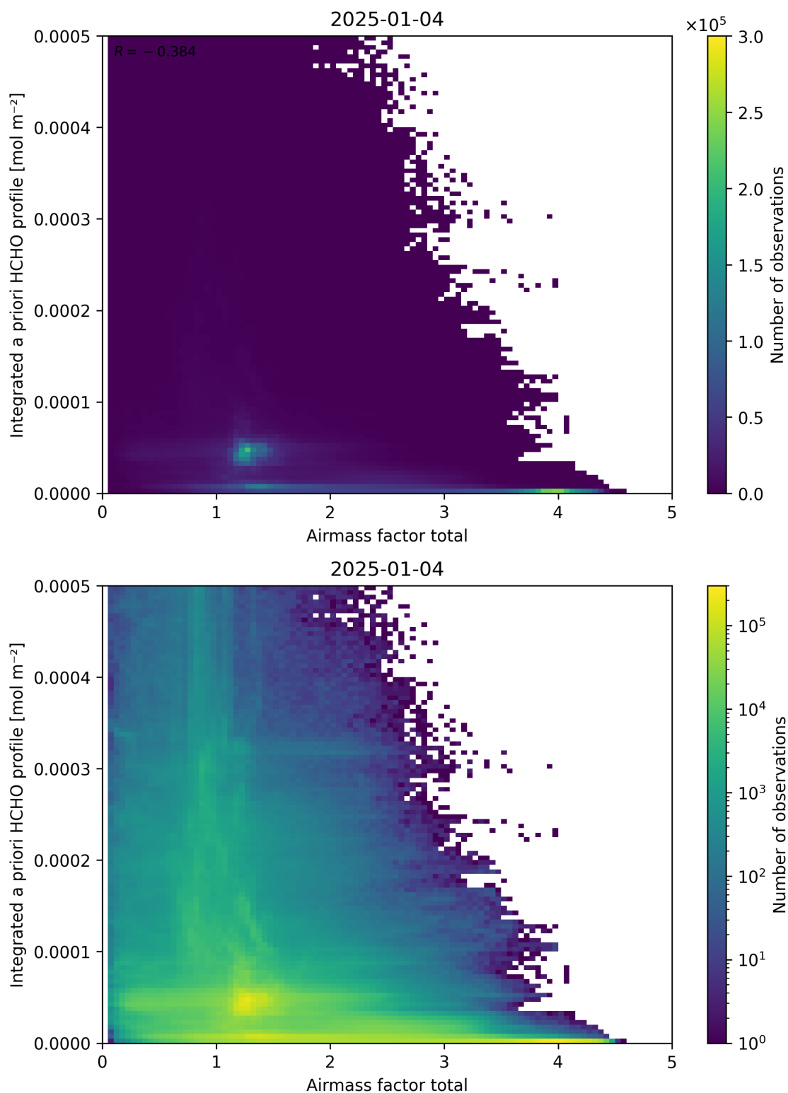
Figure 104: Scatter density plot of “Airmass factor total” against “Integrated a priori HCHO profile” for 2025-01-03 to 2025-01-05.
