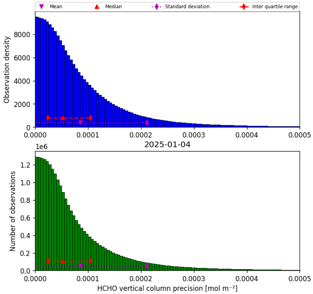
Figure 36: Histogram of “HCHO vertical column precision” for 2025-01-03 to 2025-01-05
