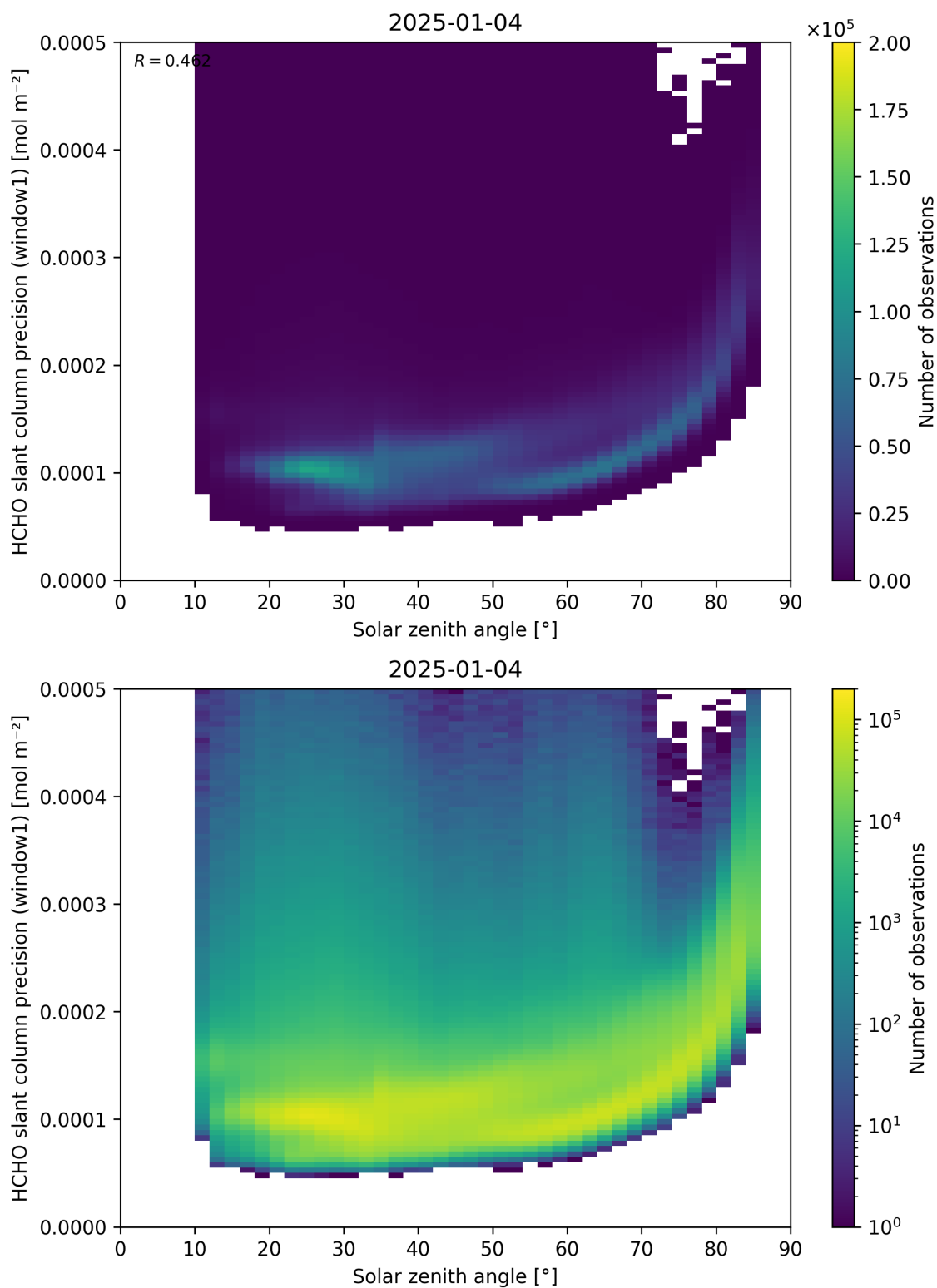
Figure 174: Scatter density plot of “Solar zenith angle” against “HCHO slant column precision (window1)” for 2025-01-03 to 2025-01-05.
