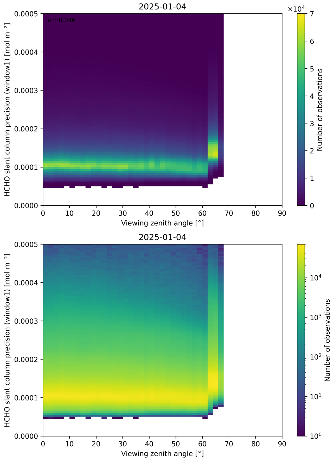
Figure 189: Scatter density plot of “Viewing zenith angle” against “HCHO slant column precision (window1)” for 2025-01-03 to 2025-01-05.
