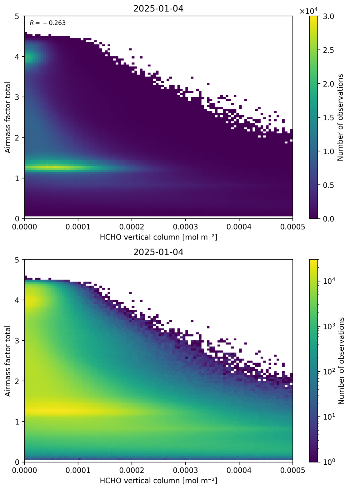
Figure 131: Scatter density plot of “HCHO vertical column” against “Airmass factor total” for 2025-01-03 to 2025-01-05.
