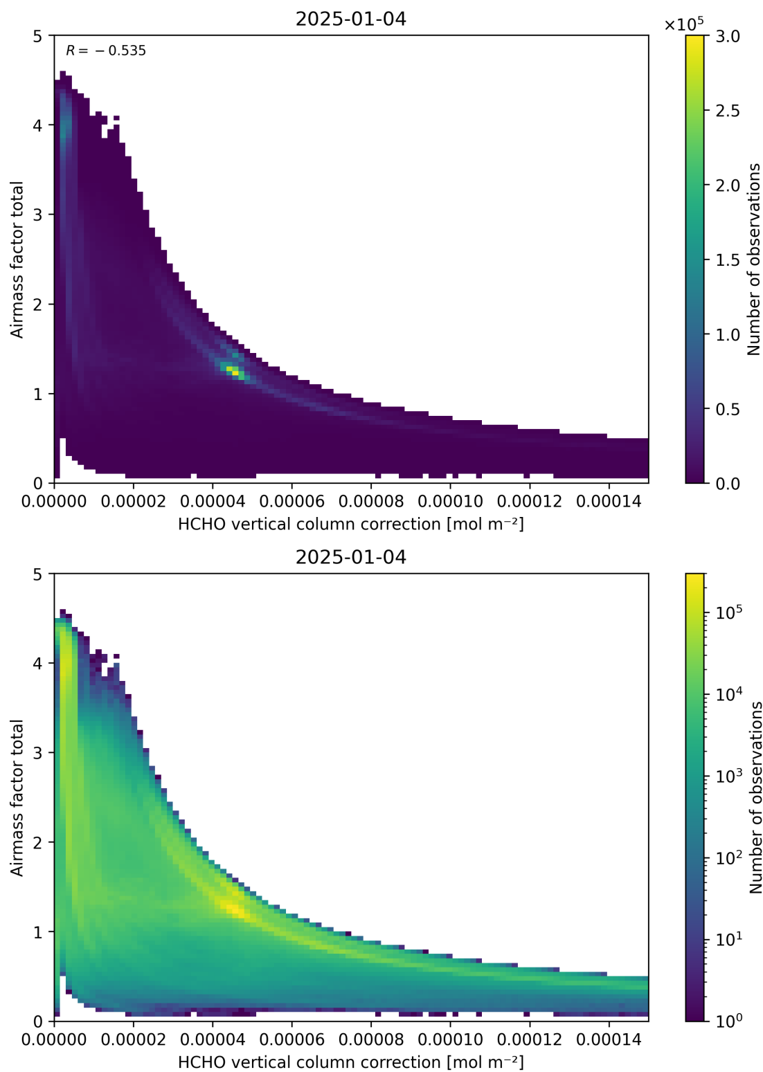
Figure 120: Scatter density plot of “HCHO vertical column correction” against “Airmass factor total” for 2025-01-03 to 2025-01-05.
