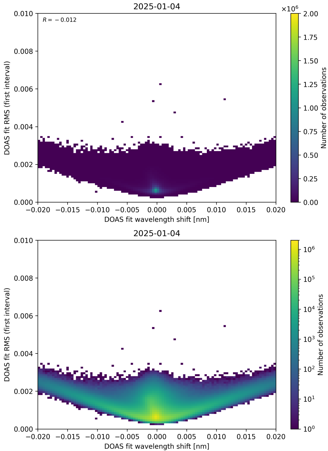
Figure 64: Scatter density plot of “DOAS fit wavelength shift” against “DOAS fit RMS (first interval)” for 2025-01-03 to 2025-01-05.
