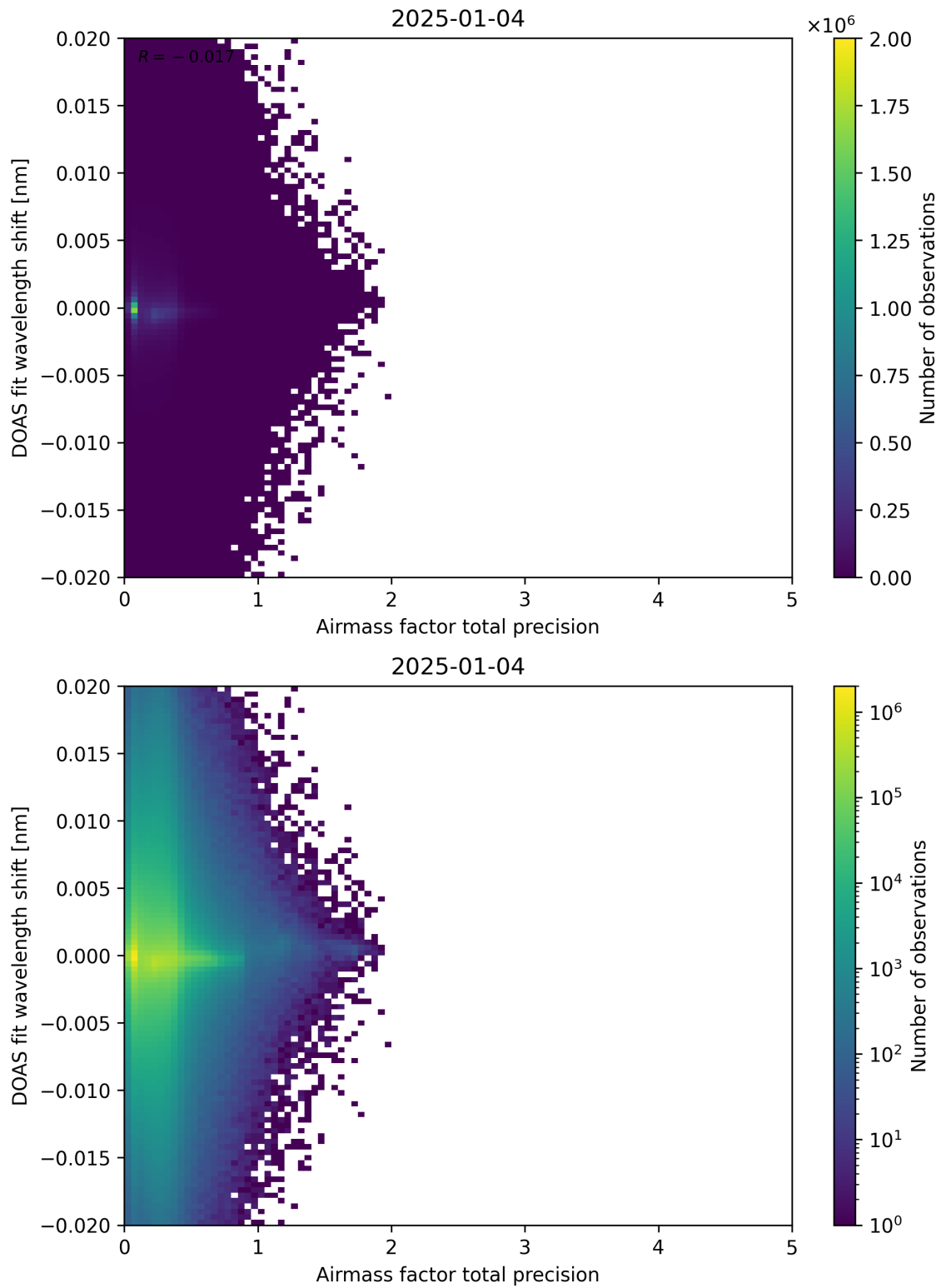
Figure 106: Scatter density plot of “Airmass factor total precision” against “DOAS fit wavelength shift” for 2025-01-03 to 2025-01-05.
