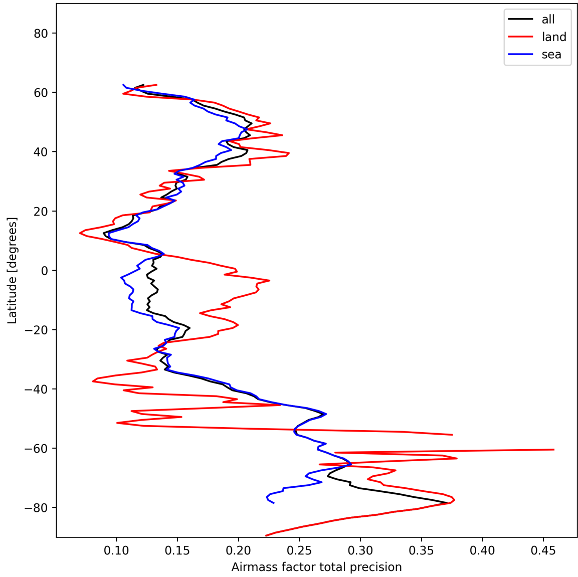
Figure 27: Zonal average of “Airmass factor total precision” for 2025-01-03 to 2025-01-05.
