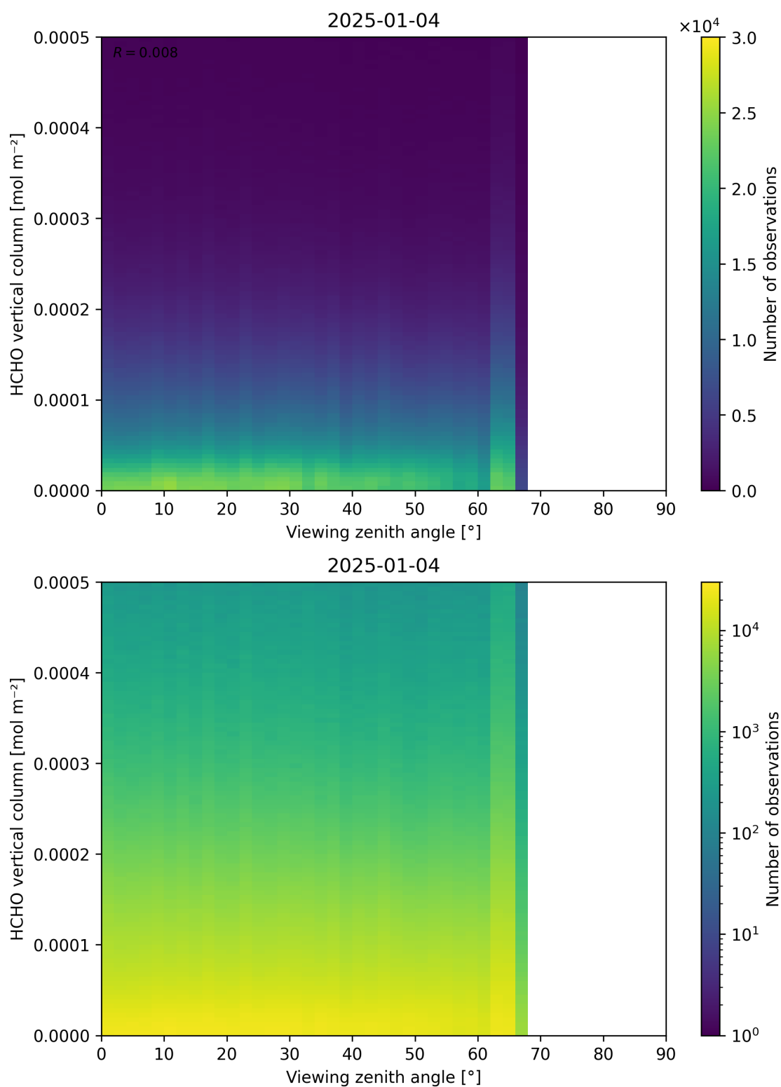
Figure 192: Scatter density plot of “Viewing zenith angle” against “HCHO vertical column” for 2025-01-03 to 2025-01-05.
