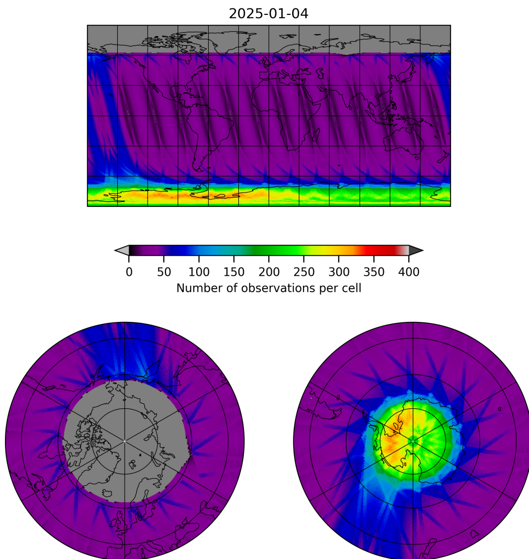
Figure 19: Map of the number of observations for 2025-01-03 to 2025-01-05
