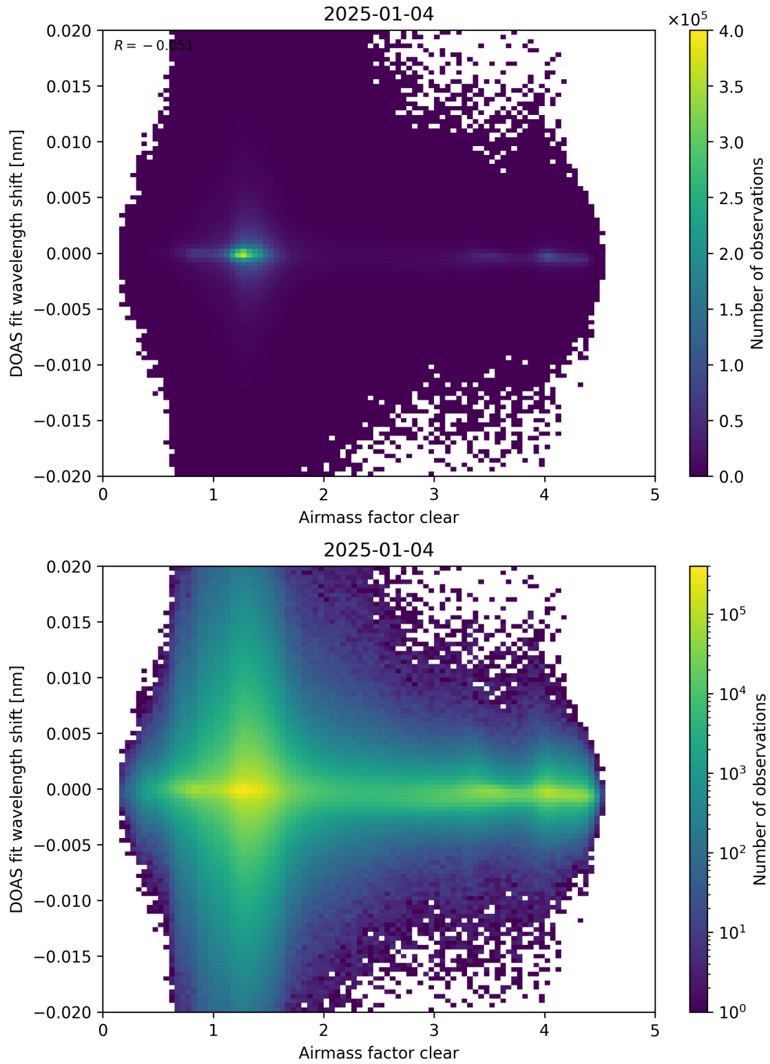
Figure 72: Scatter density plot of “Airmass factor clear” against “DOAS fit wavelength shift” for 2025-01-03 to 2025-01-05.
