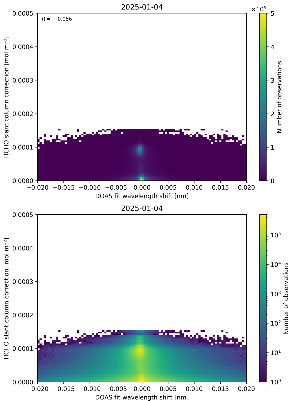
Figure 67: Scatter density plot of “DOAS fit wavelength shift” against “HCHO slant column correction” for 2025-01-03 to 2025-01-05.
