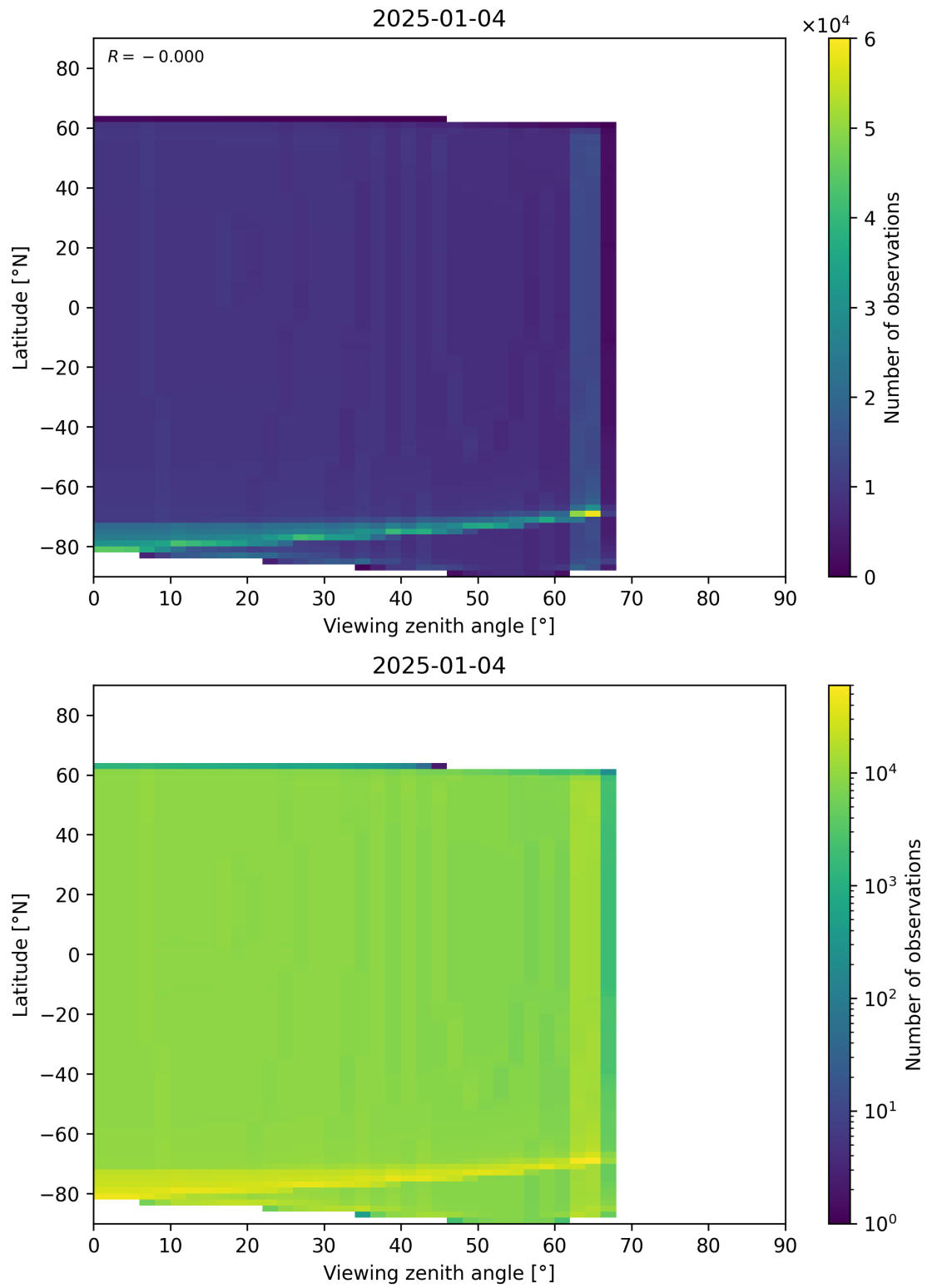
Figure 196: Scatter density plot of “Viewing zenith angle” against “Latitude” for 2025-01-03 to 2025-01-05.
