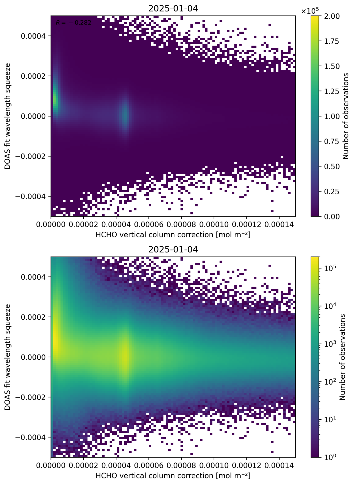
Figure 114: Scatter density plot of “HCHO vertical column correction” against “DOAS fit wavelength squeeze” for 2025-01-03 to 2025-01-05.
