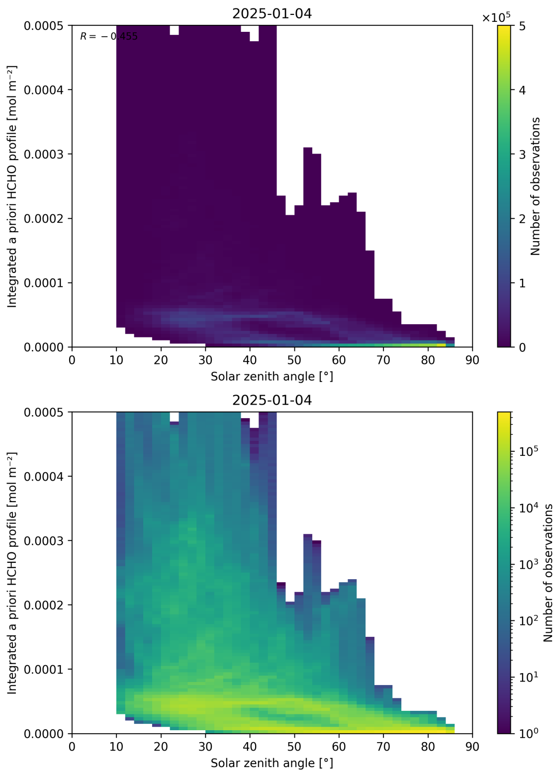
Figure 180: Scatter density plot of “Solar zenith angle” against “Integrated a priori HCHO profile” for 2025-01-03 to 2025-01-05.
