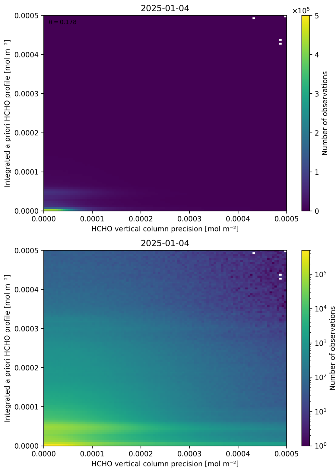
Figure 147: Scatter density plot of “HCHO vertical column precision” against “Integrated a priori HCHO profile” for 2025-01-03 to 2025-01-05.
