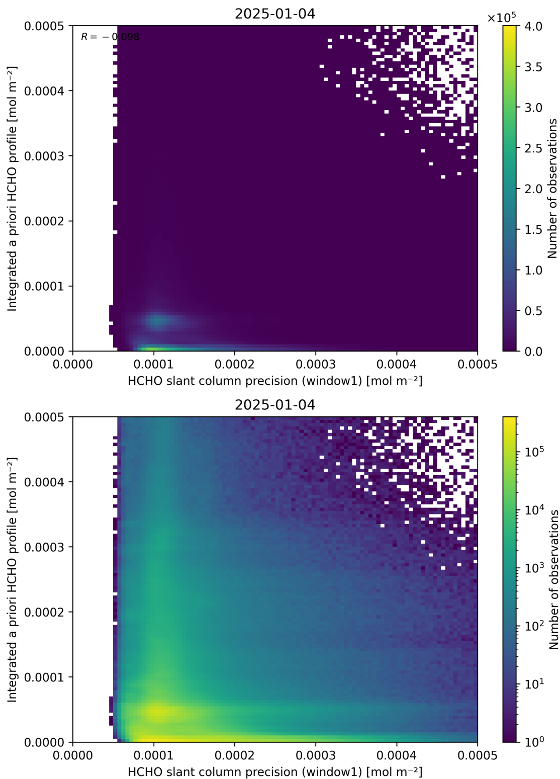
Figure 96: Scatter density plot of “HCHO slant column precision (window1)” against “Integrated a priori HCHO profile” for 2025-01-03 to 2025-01-05.
