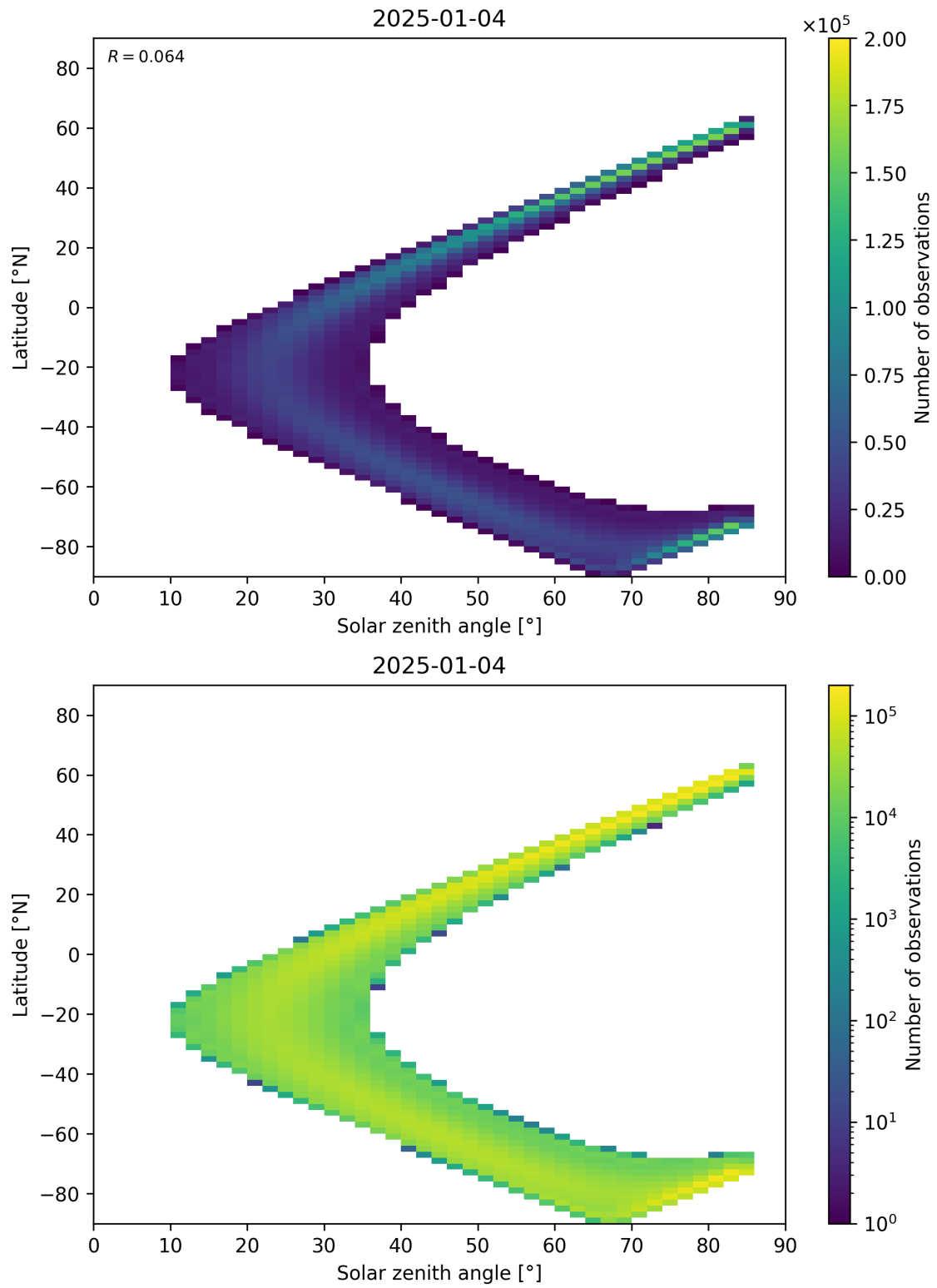
Figure 181: Scatter density plot of “Solar zenith angle” against “Latitude” for 2025-01-03 to 2025-01-05.
