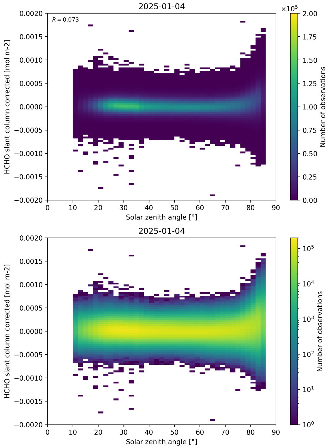
Figure 171: Scatter density plot of “Solar zenith angle” against “HCHO slant column corrected” for 2025-01-03 to 2025-01-05.
