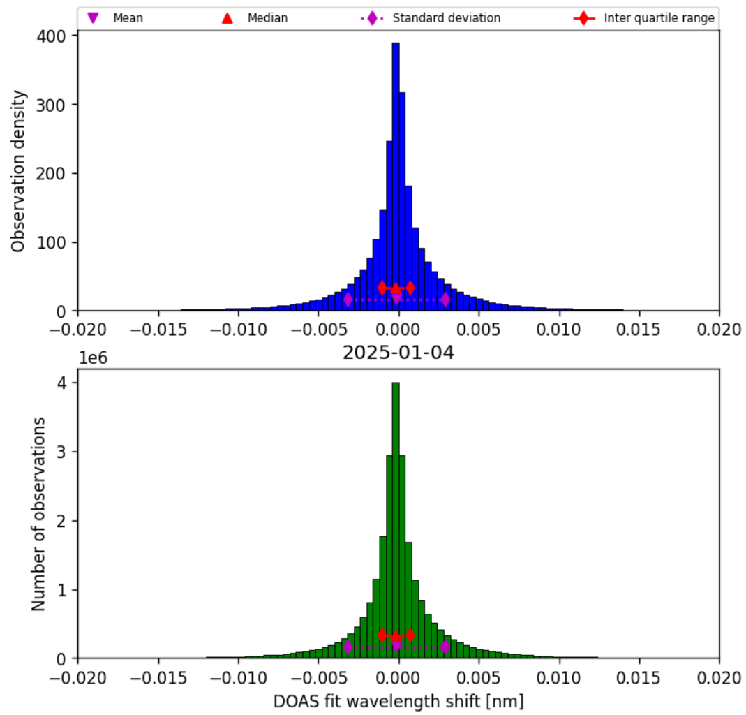
Figure 44: Histogram of “DOAS fit wavelength shift” for 2025-01-03 to 2025-01-05
