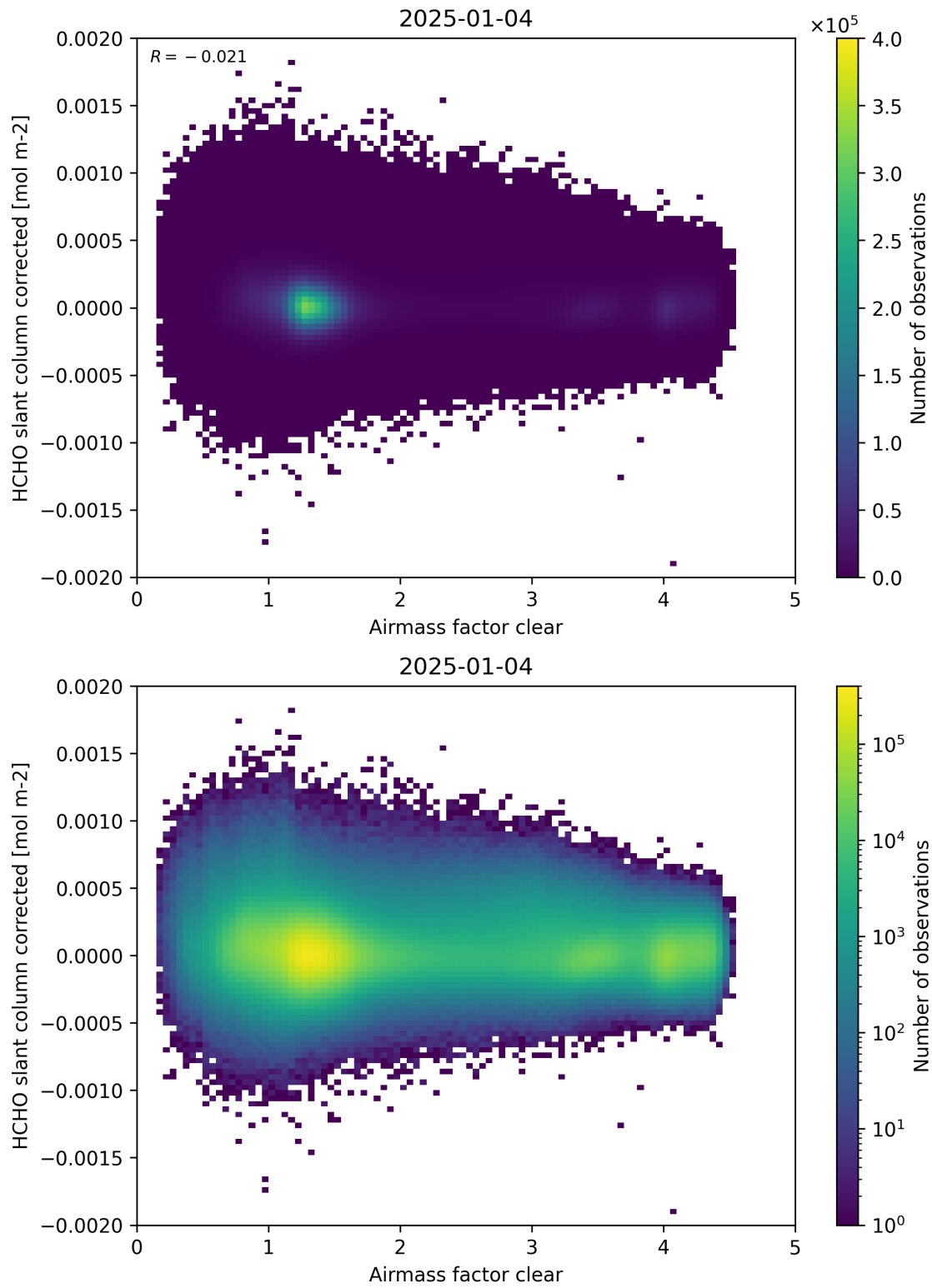
Figure 74: Scatter density plot of “Airmass factor clear” against “HCHO slant column corrected” for 2025-01-03 to 2025-01-05.
