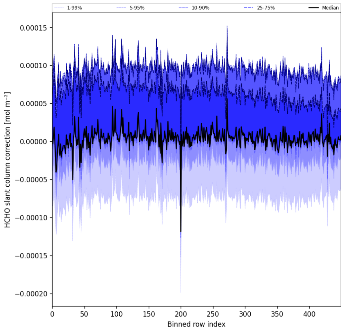
Figure 61: Along track statistics of “HCHO slant column correction” for 2025-01-03 to 2025-01-05
