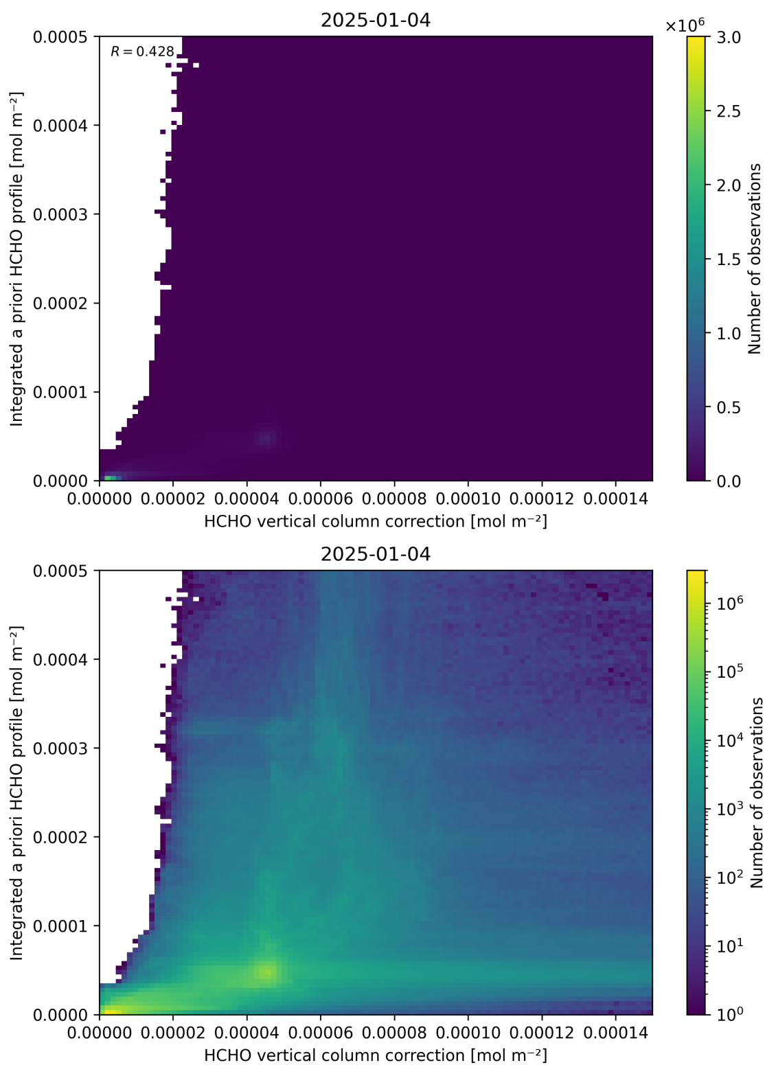
Figure 122: Scatter density plot of “HCHO vertical column correction” against “Integrated a priori HCHO profile” for 2025-01-03 to 2025-01-05.
