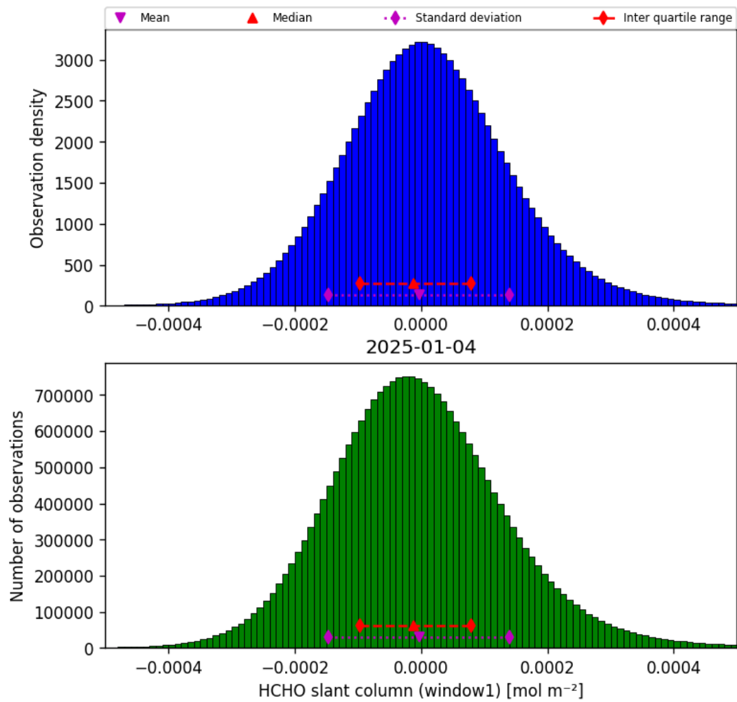
Figure 38: Histogram of “HCHO slant column (window1)” for 2025-01-03 to 2025-01-05
