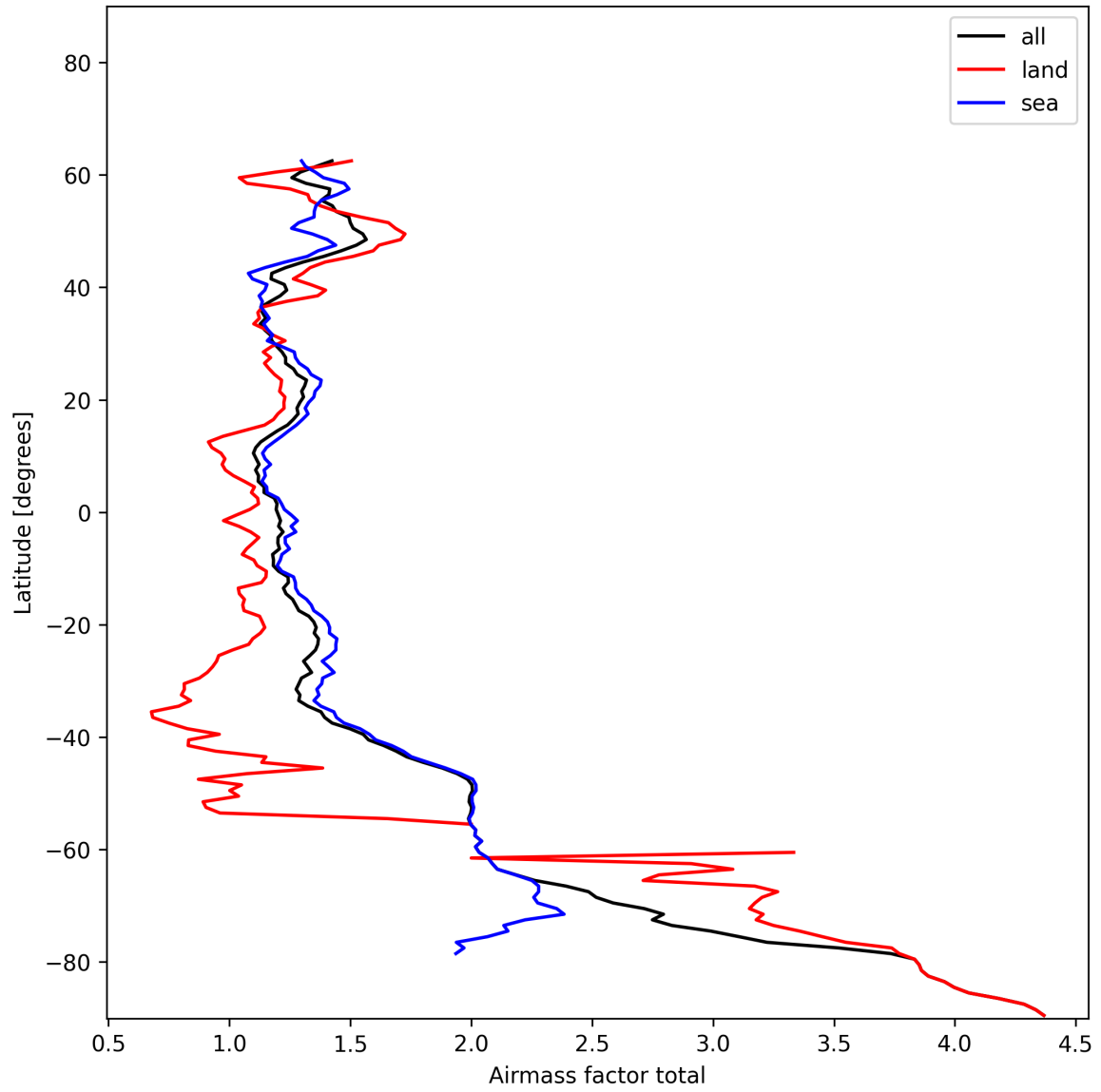
Figure 26: Zonal average of “Airmass factor total” for 2025-01-03 to 2025-01-05.
