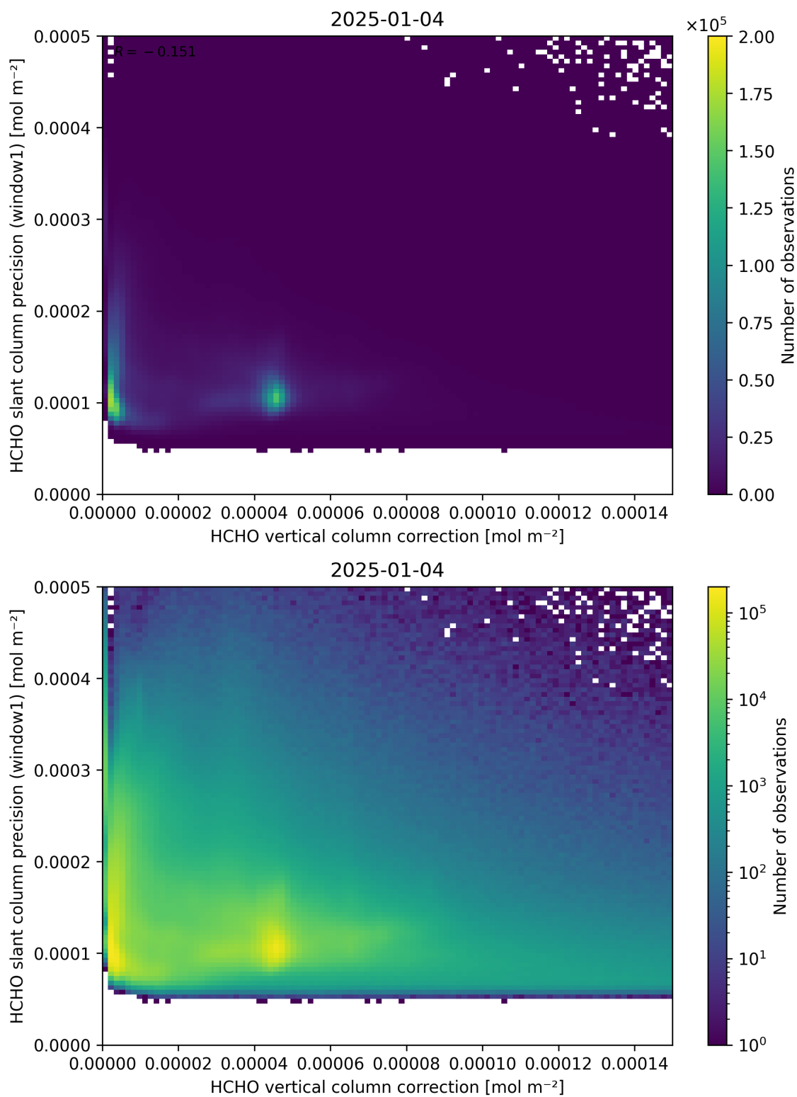
Figure 119: Scatter density plot of “HCHO vertical column correction” against “HCHO slant column precision (window1)” for 2025-01-03 to 2025-01-05.
