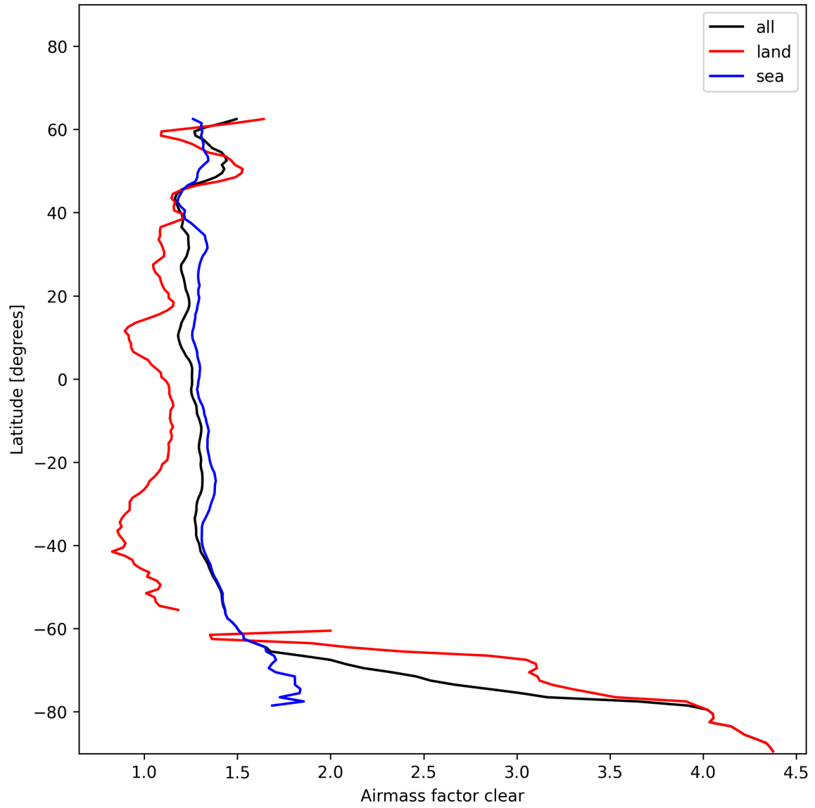
Figure 28: Zonal average of “Airmass factor clear” for 2025-01-03 to 2025-01-05.
