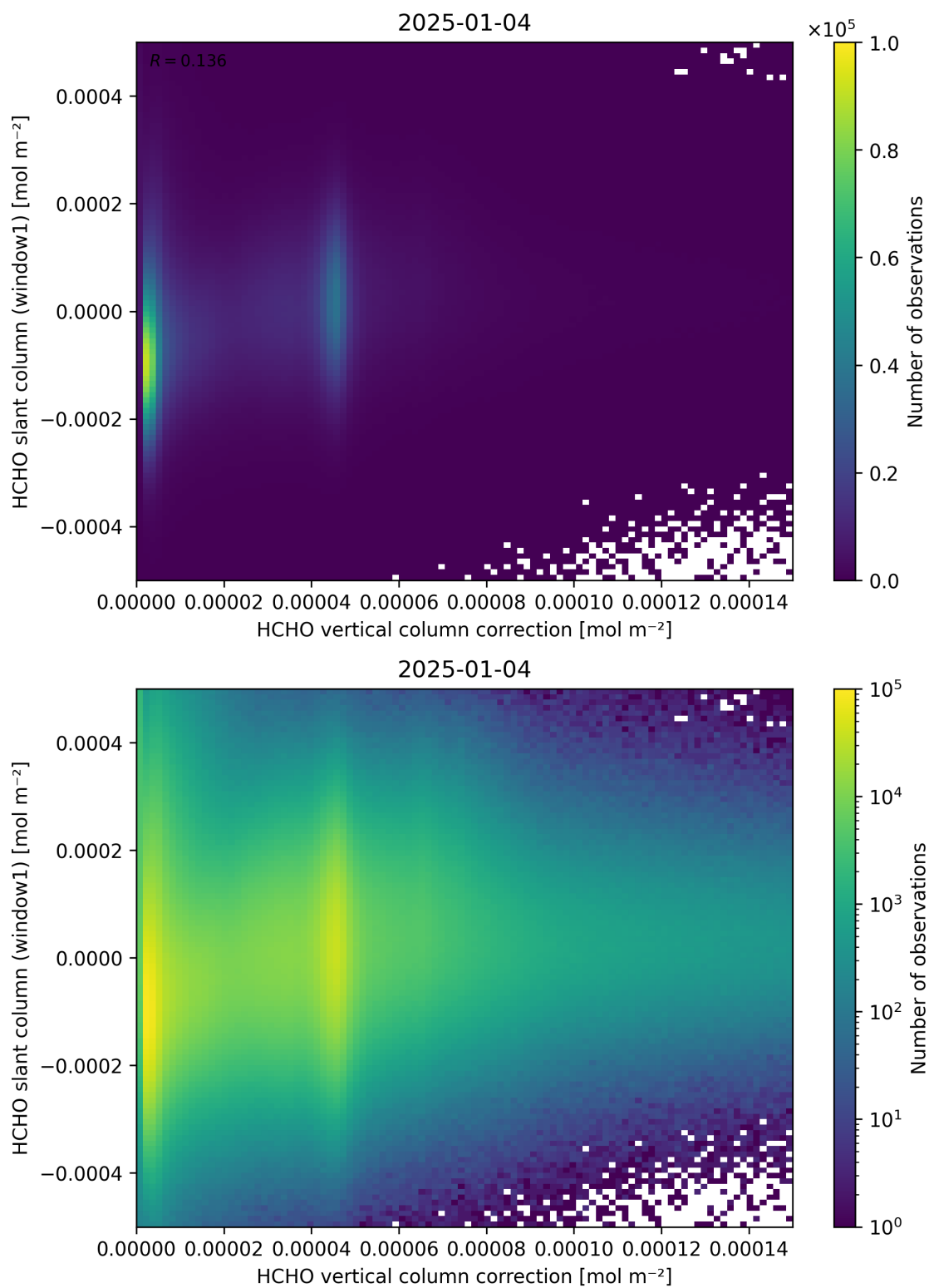
Figure 118: Scatter density plot of “HCHO vertical column correction” against “HCHO slant column (window1)” for 2025-01-03 to 2025-01-05.
