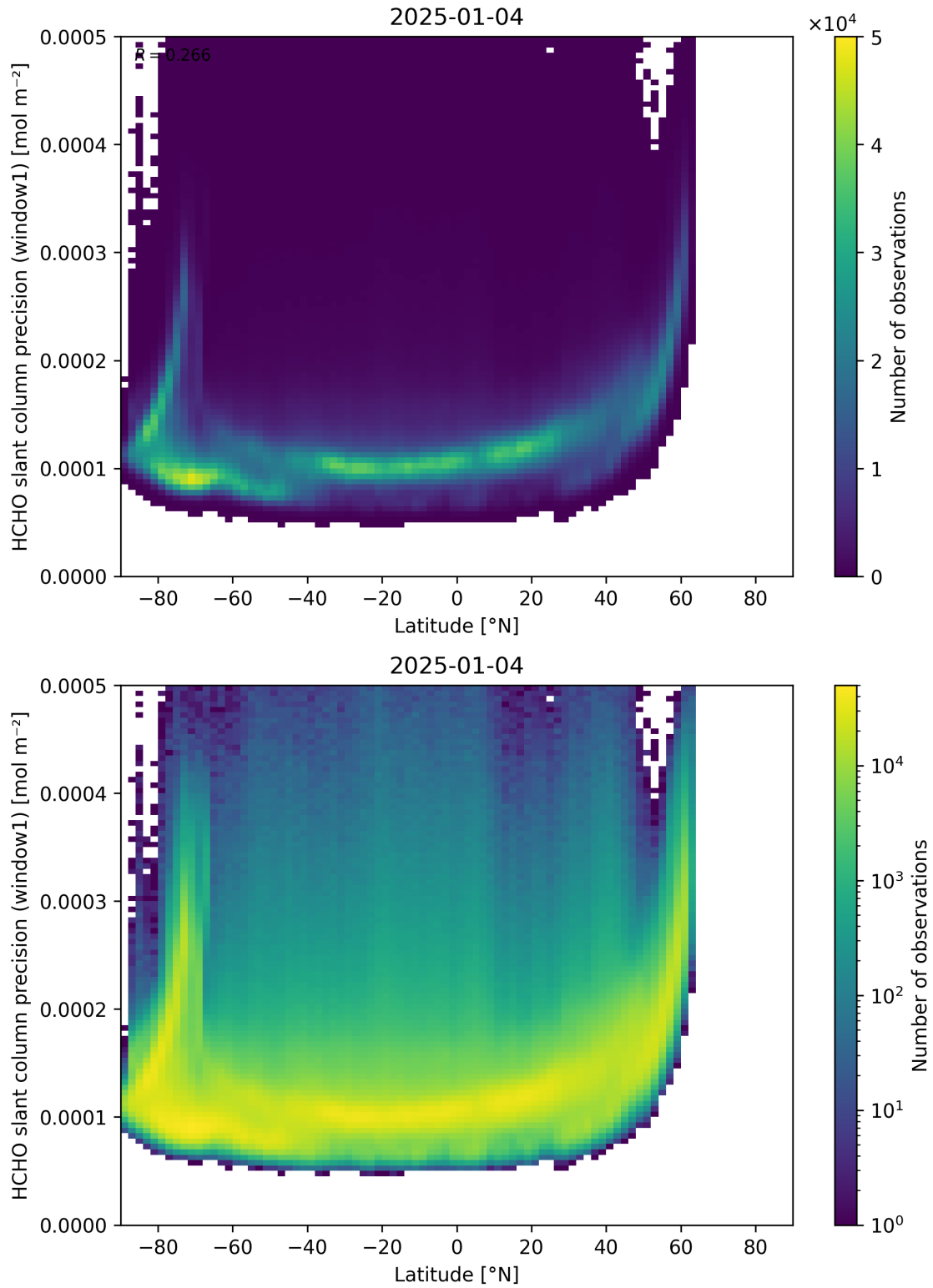
Figure 160: Scatter density plot of “Latitude” against “HCHO slant column precision (window1)” for 2025-01-03 to 2025-01-05.
