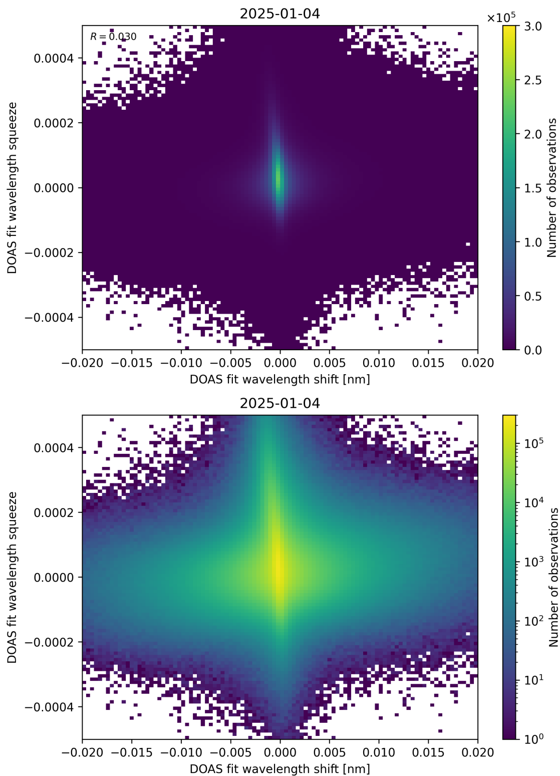
Figure 65: Scatter density plot of “DOAS fit wavelength shift” against “DOAS fit wavelength squeeze” for 2025-01-03 to 2025-01-05.
