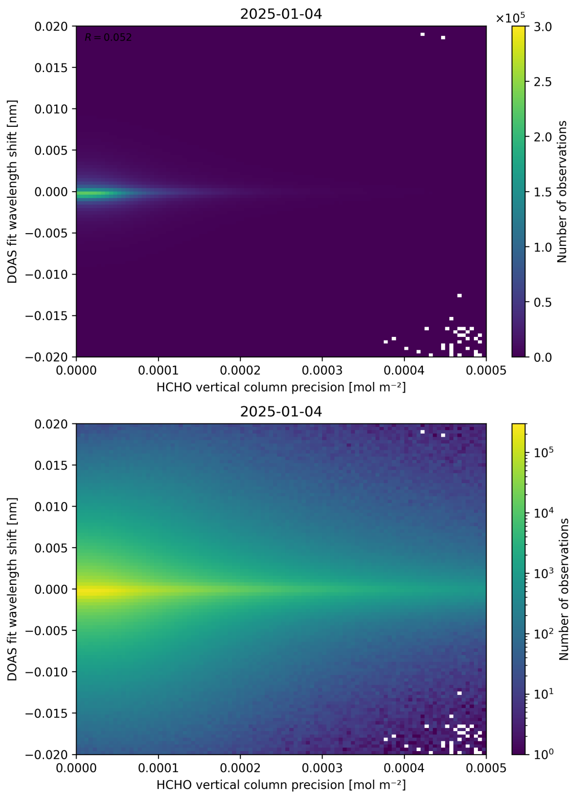
Figure 137: Scatter density plot of “HCHO vertical column precision” against “DOAS fit wavelength shift” for 2025-01-03 to 2025-01-05.
