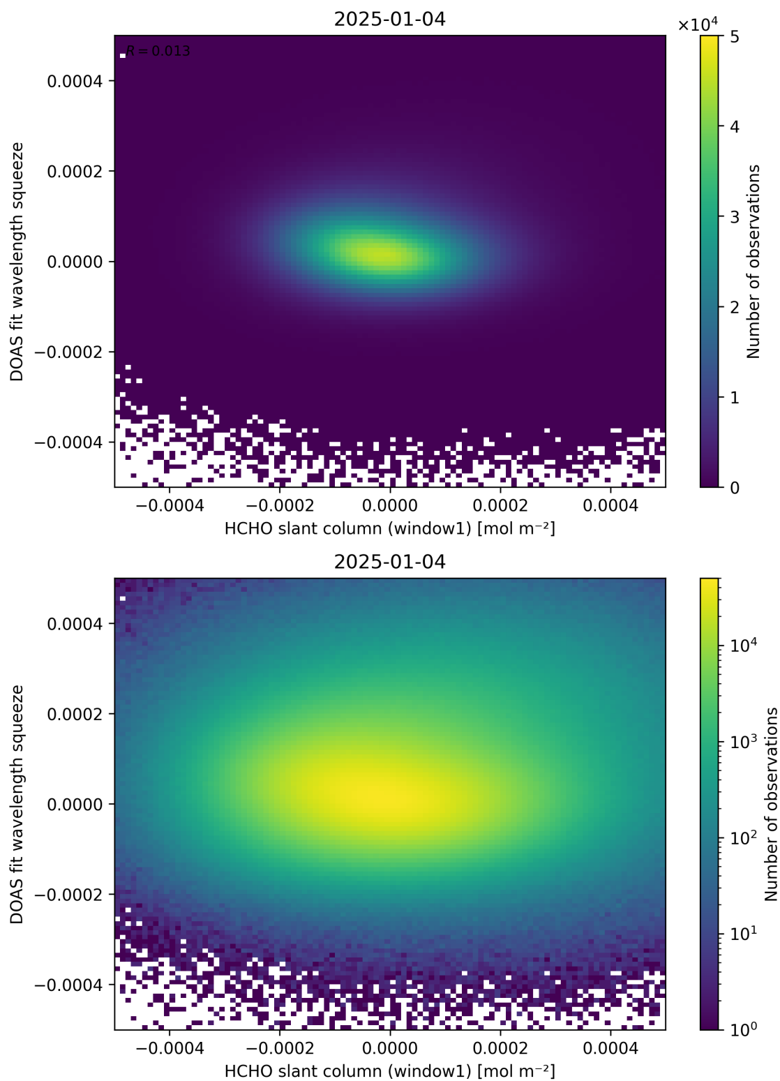
Figure 80: Scatter density plot of “HCHO slant column (window1)” against “DOAS fit wavelength squeeze” for 2025-01-03 to 2025-01-05.
