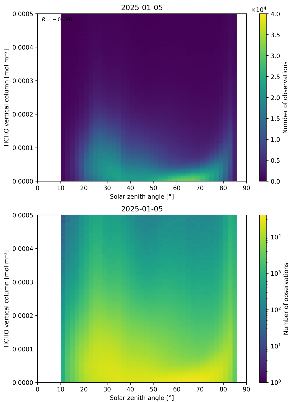
Figure 177: Scatter density plot of “Solar zenith angle” against “HCHO vertical column” for 2025-01-04 to 2025-01-06.
