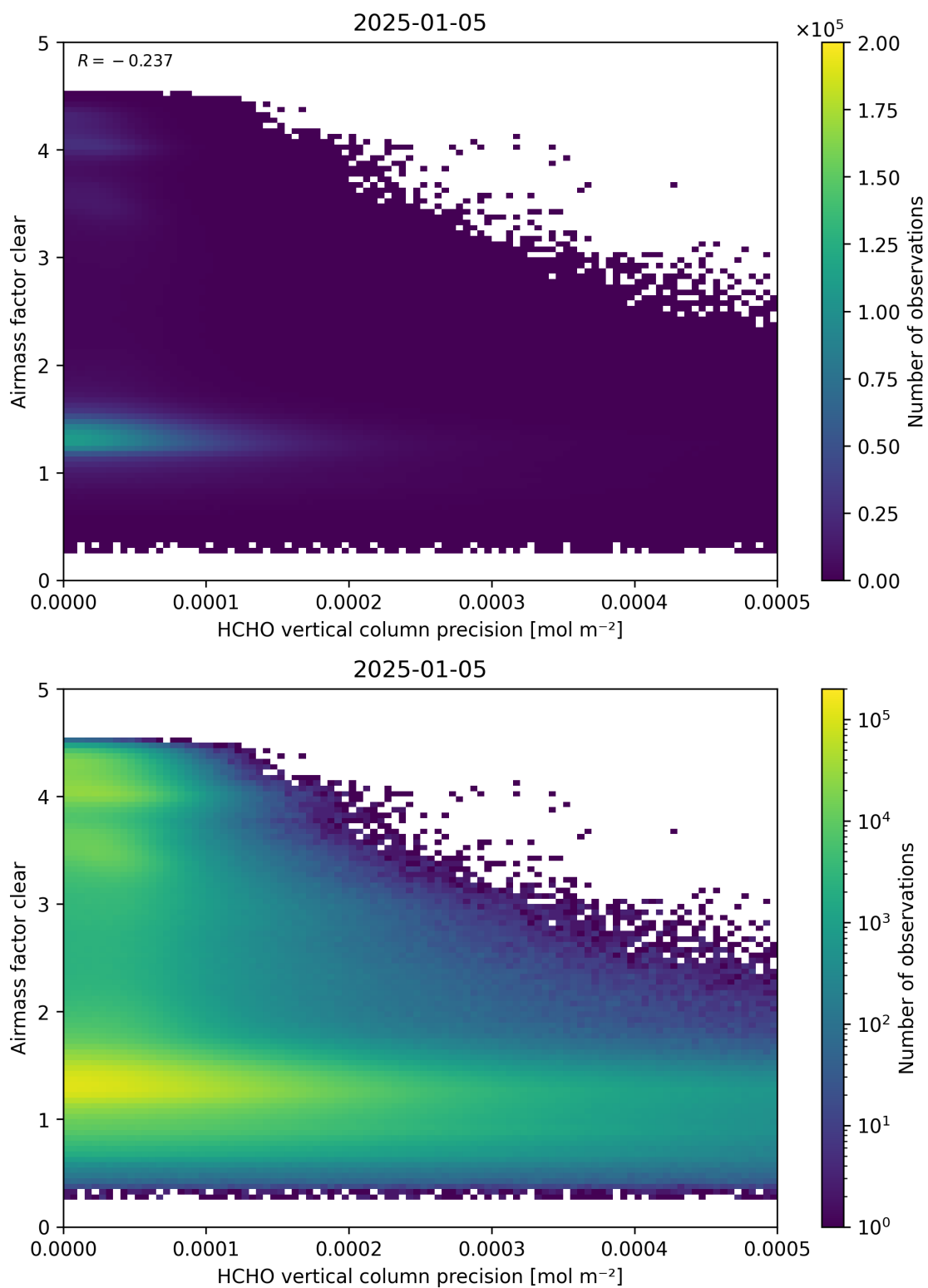
Figure 139: Scatter density plot of “HCHO vertical column precision” against “Airmass factor clear” for 2025-01-04 to 2025-01-06.
