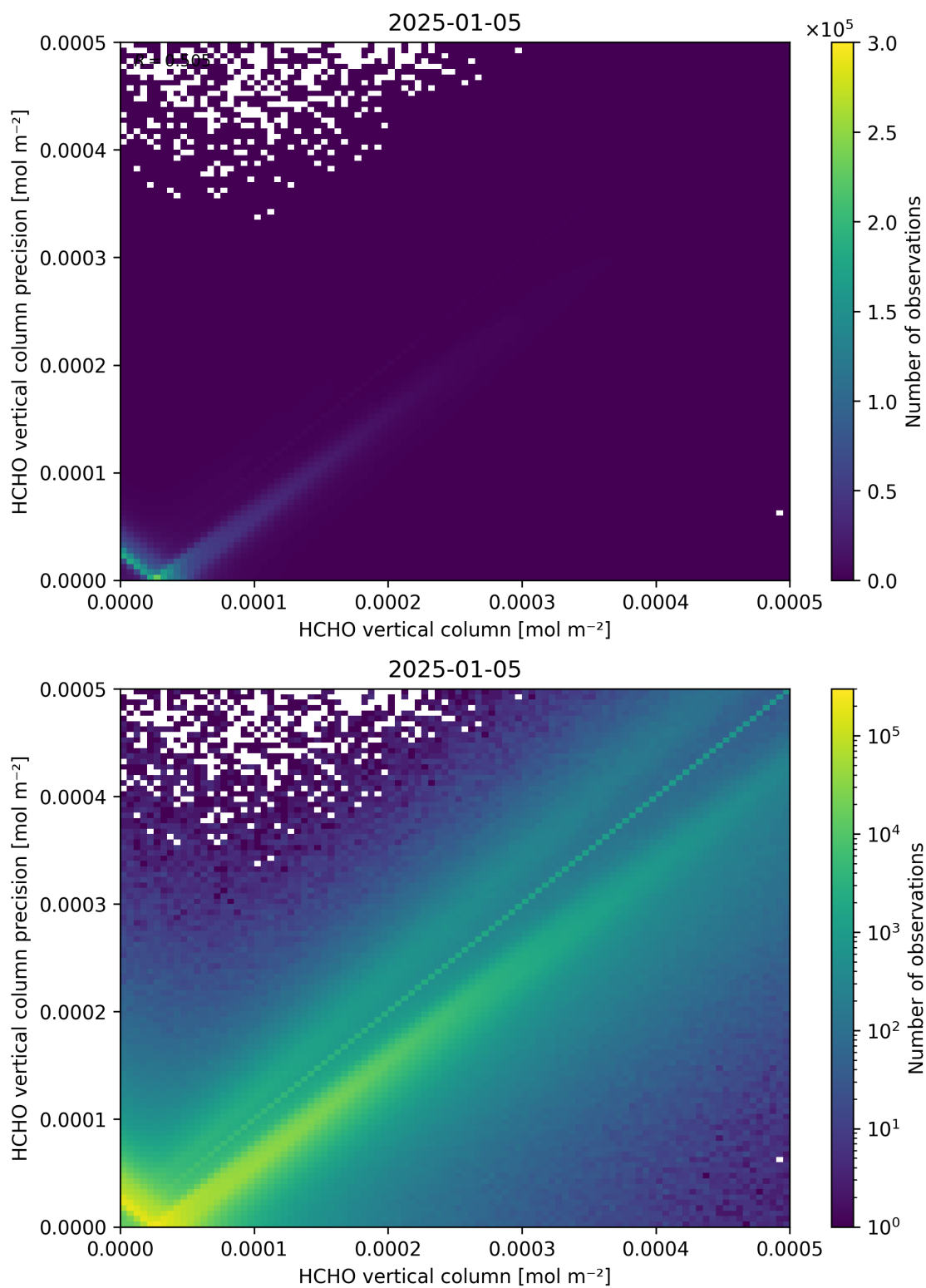
Figure 134: Scatter density plot of “HCHO vertical column” against “HCHO vertical column precision” for 2025-01-04 to 2025-01-06.
