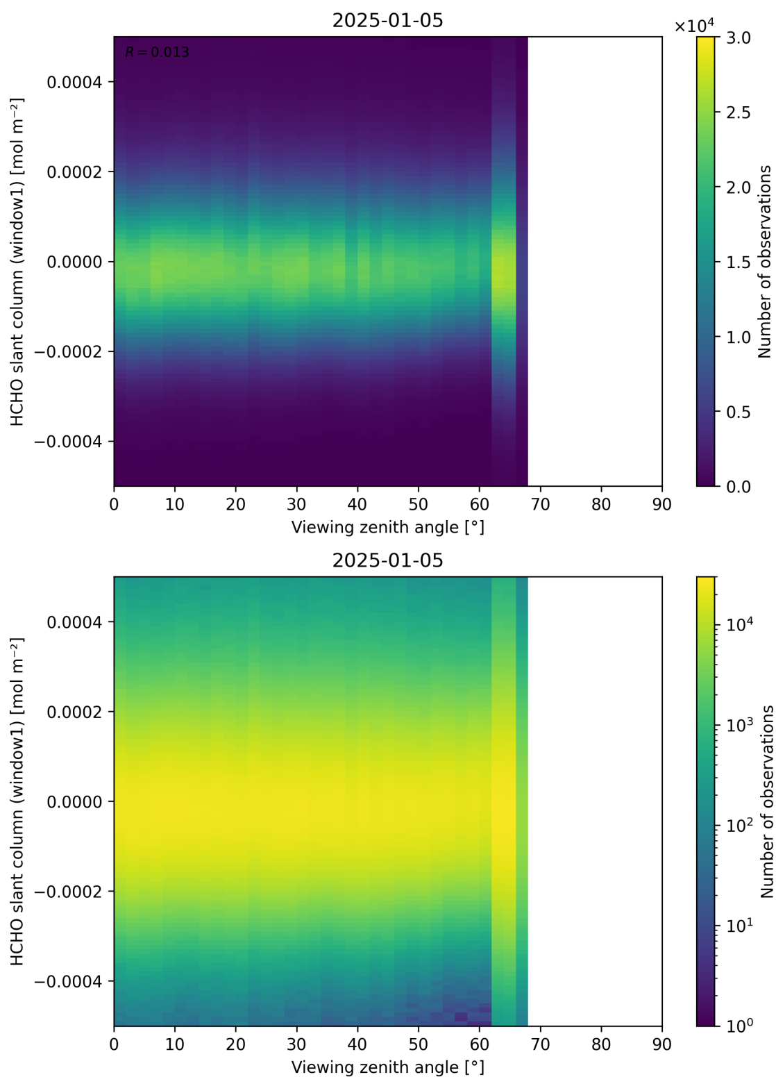
Figure 188: Scatter density plot of “Viewing zenith angle” against “HCHO slant column (window1)” for 2025-01-04 to 2025-01-06.
