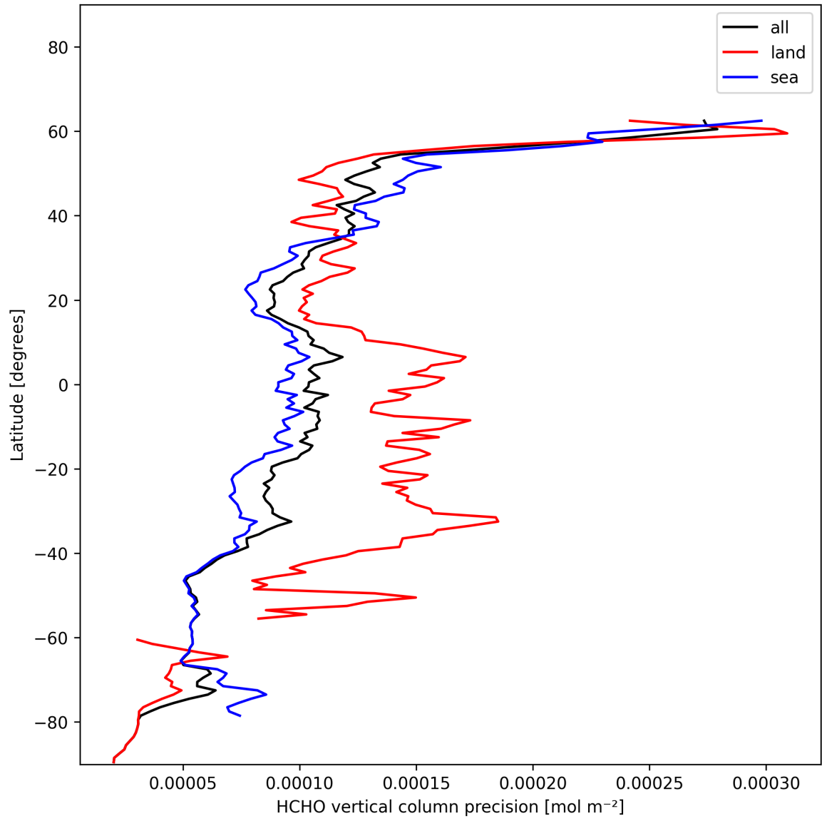
Figure 22: Zonal average of “HCHO vertical column precision” for 2025-01-04 to 2025-01-06.
