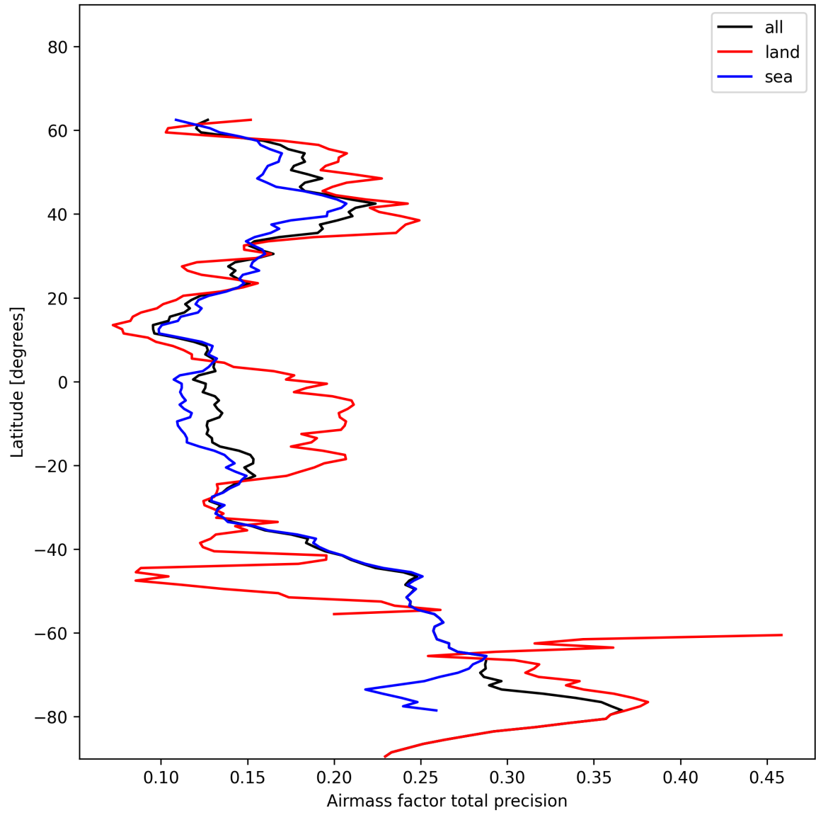
Figure 27: Zonal average of “Airmass factor total precision” for 2025-01-04 to 2025-01-06.
