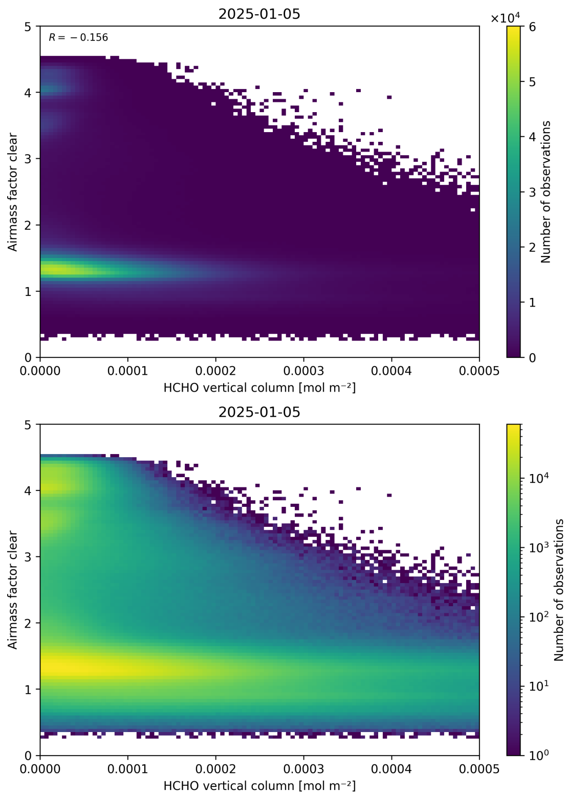
Figure 126: Scatter density plot of “HCHO vertical column” against “Airmass factor clear” for 2025-01-04 to 2025-01-06.
