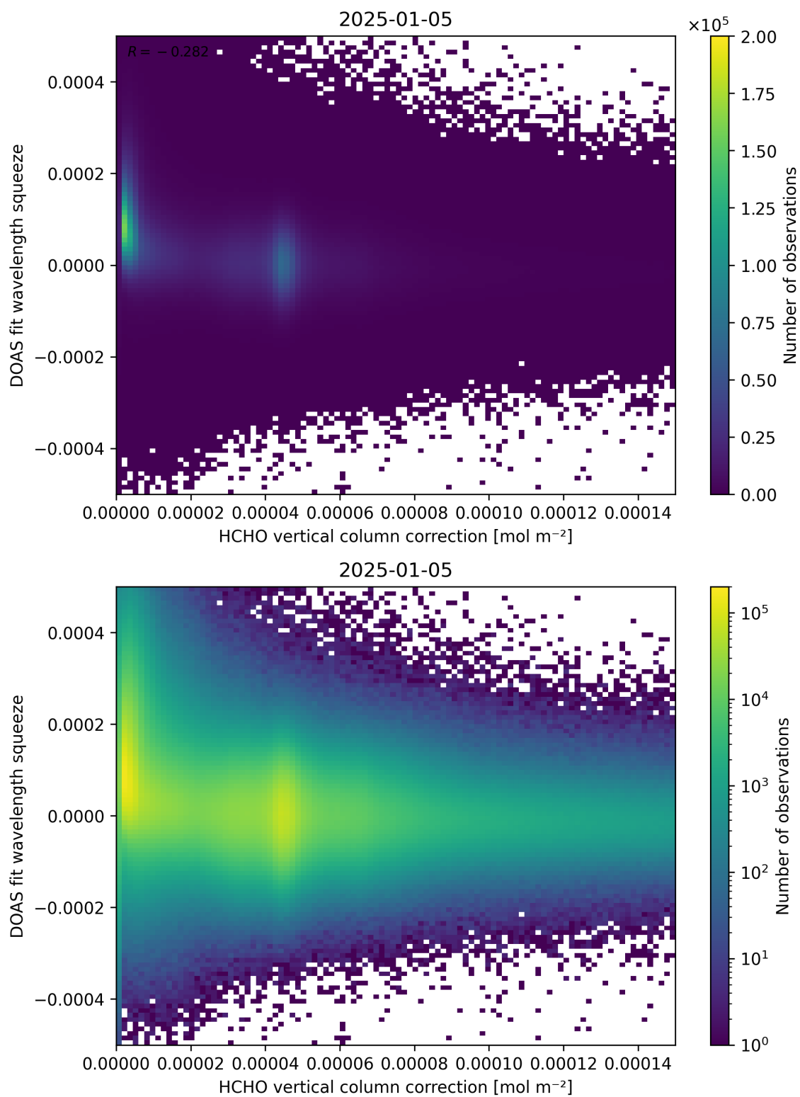
Figure 114: Scatter density plot of “HCHO vertical column correction” against “DOAS fit wavelength squeeze” for 2025-01-04 to 2025-01-06.
