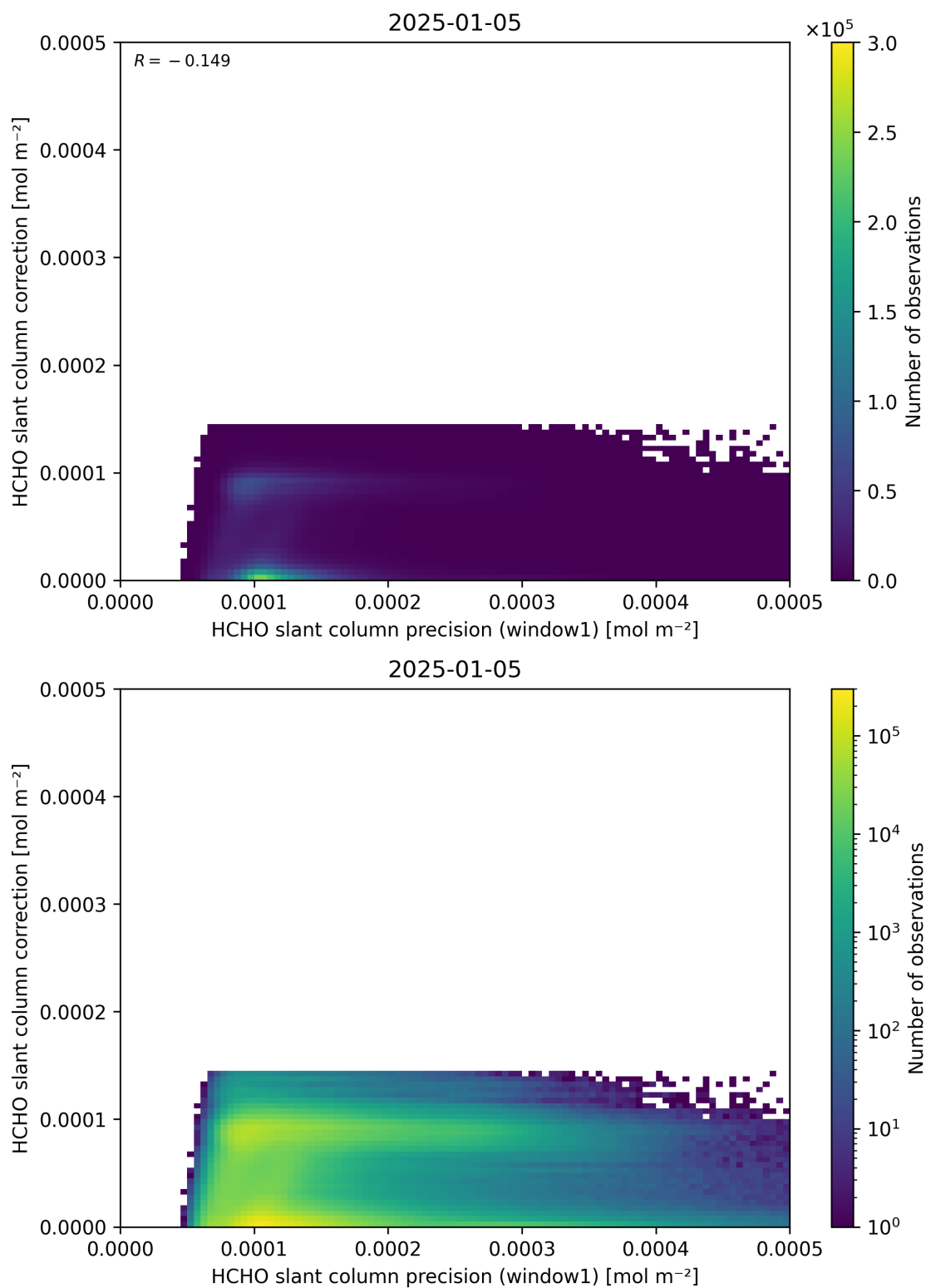
Figure 93: Scatter density plot of “HCHO slant column precision (window1)” against “HCHO slant column correction” for 2025-01-04 to 2025-01-06.
