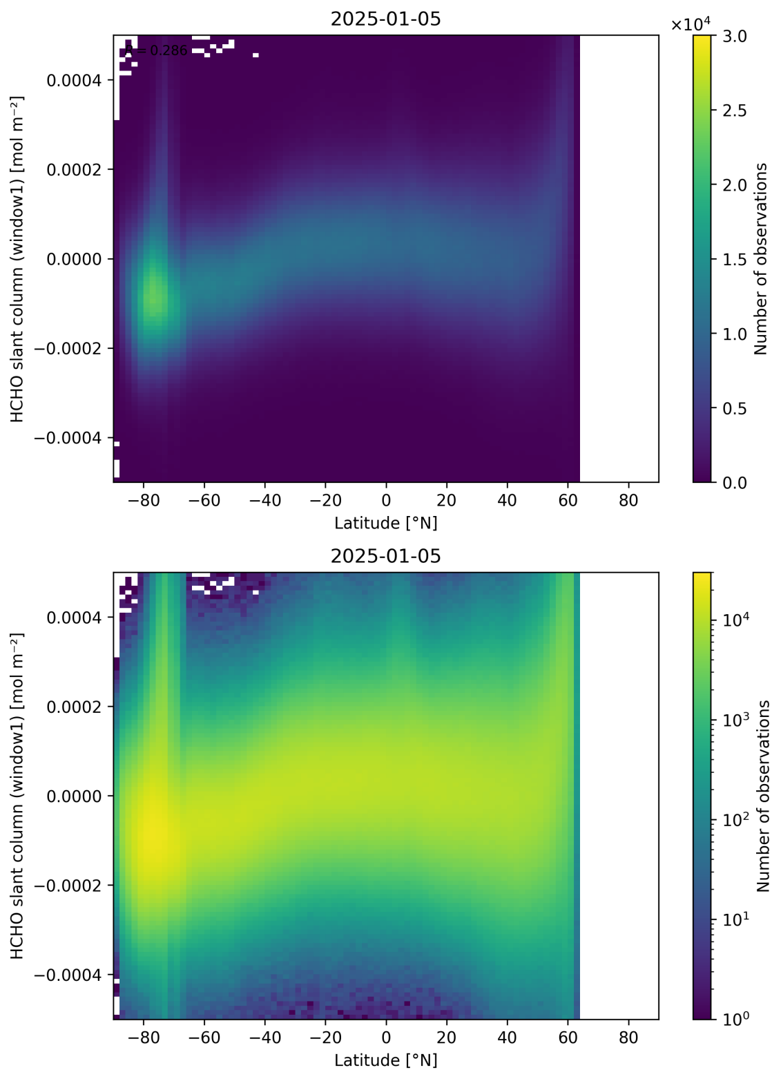
Figure 159: Scatter density plot of “Latitude” against “HCHO slant column (window1)” for 2025-01-04 to 2025-01-06.
