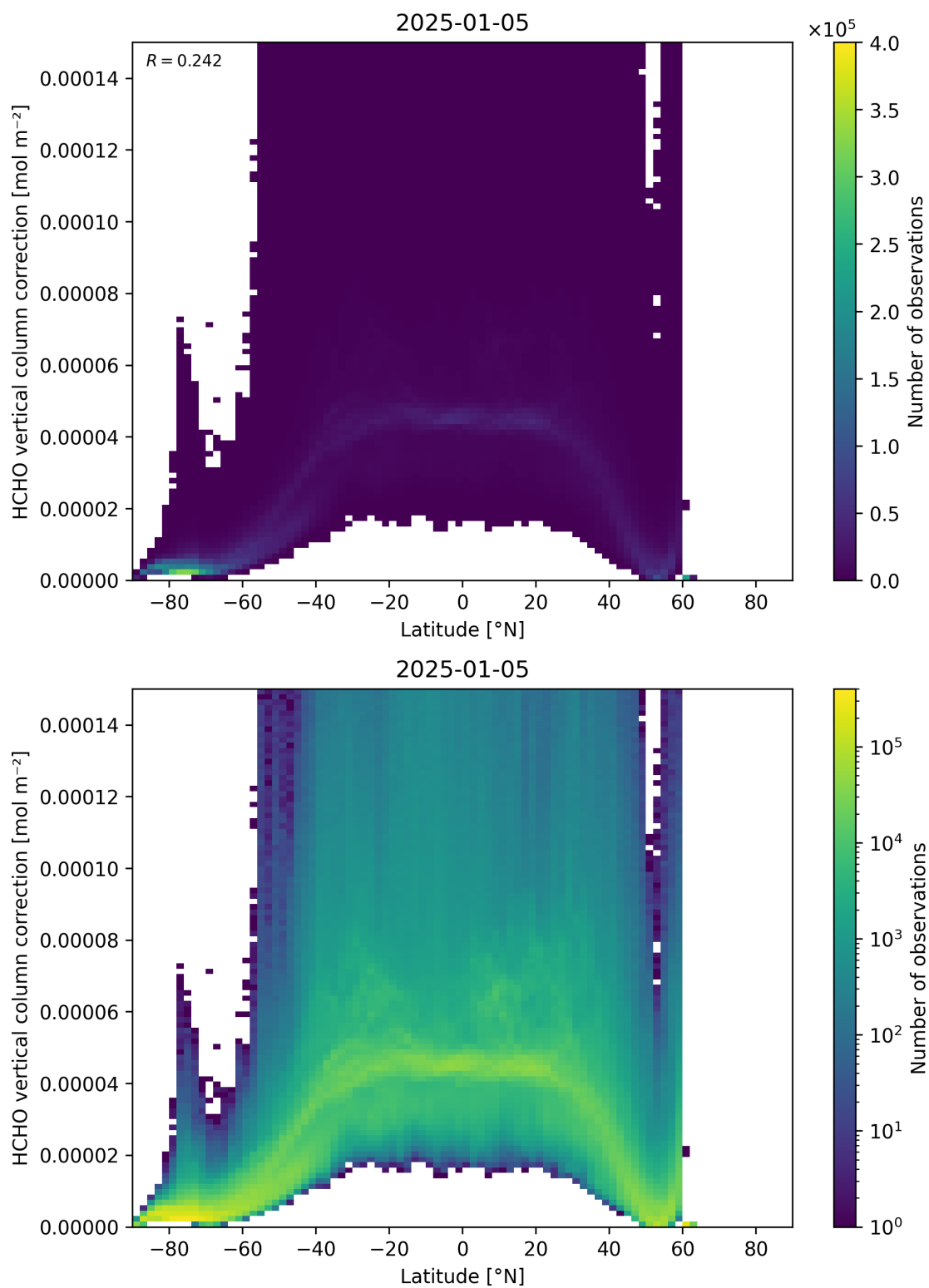
Figure 164: Scatter density plot of “Latitude” against “HCHO vertical column correction” for 2025-01-04 to 2025-01-06.
