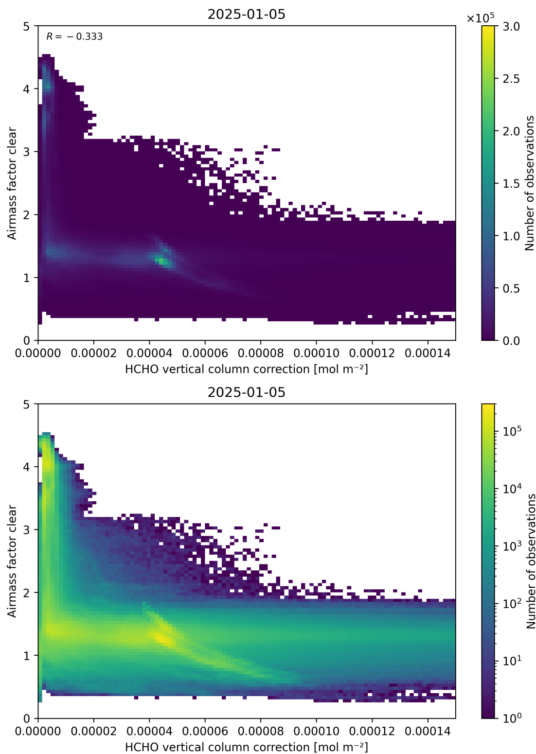
Figure 115: Scatter density plot of “HCHO vertical column correction” against “Airmass factor clear” for 2025-01-04 to 2025-01-06.
