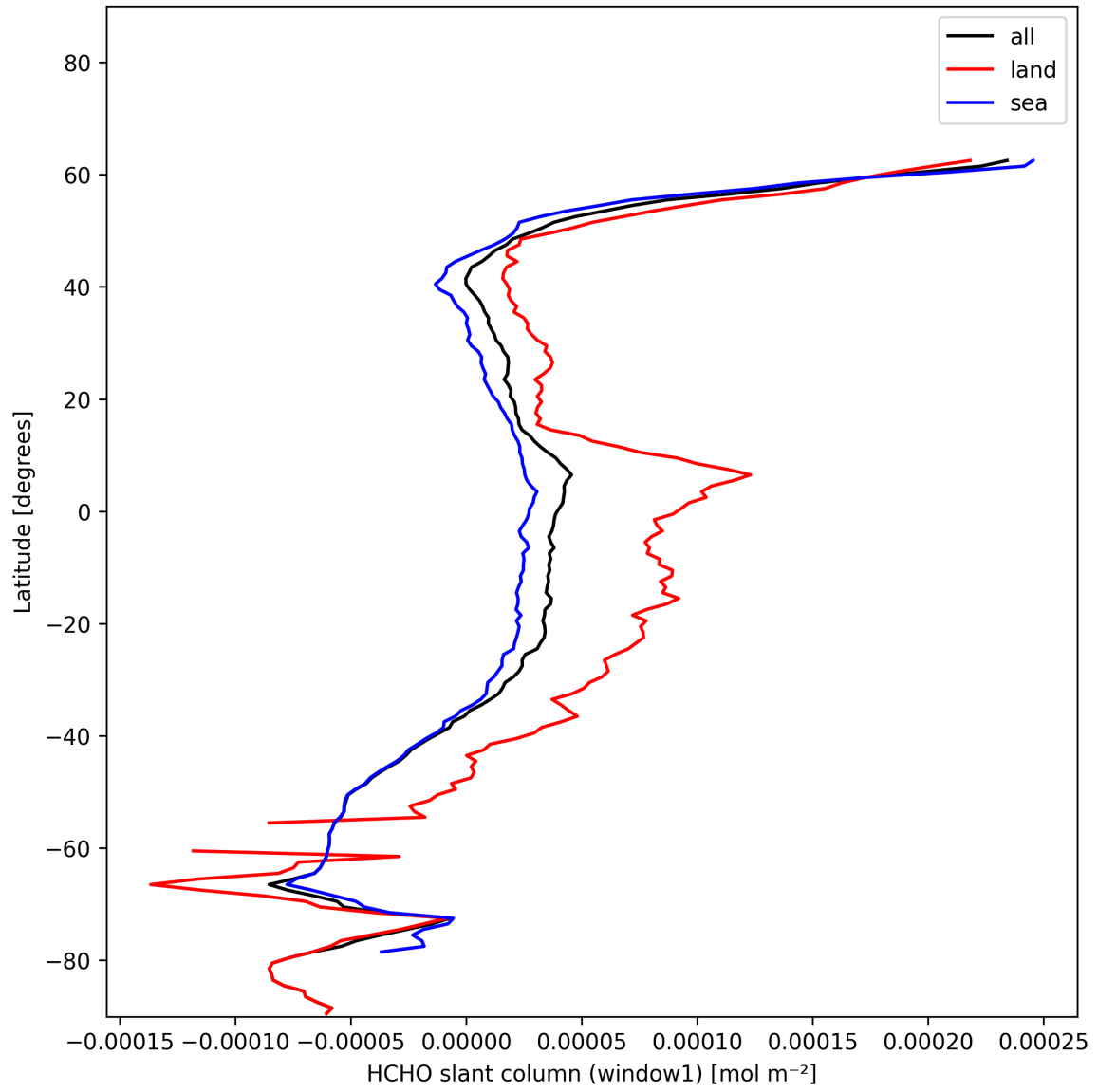
Figure 24: Zonal average of "HCHO slant column (window1)" for 2025-01-04 to 2025-01-06.
