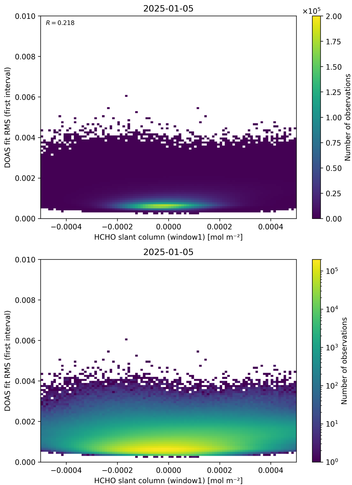
Figure 78: Scatter density plot of “HCHO slant column (window1)” against “DOAS fit RMS (first interval)” for 2025-01-04 to 2025-01-06.
