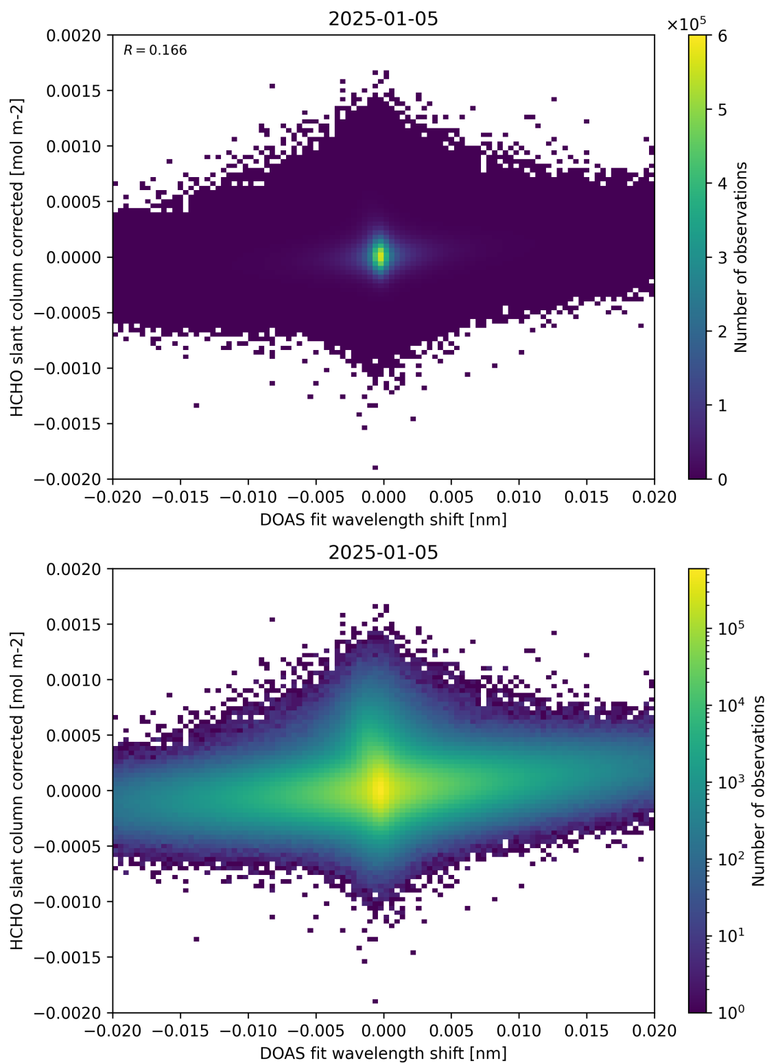
Figure 66: Scatter density plot of “DOAS fit wavelength shift” against “HCHO slant column corrected” for 2025-01-04 to 2025-01-06.
