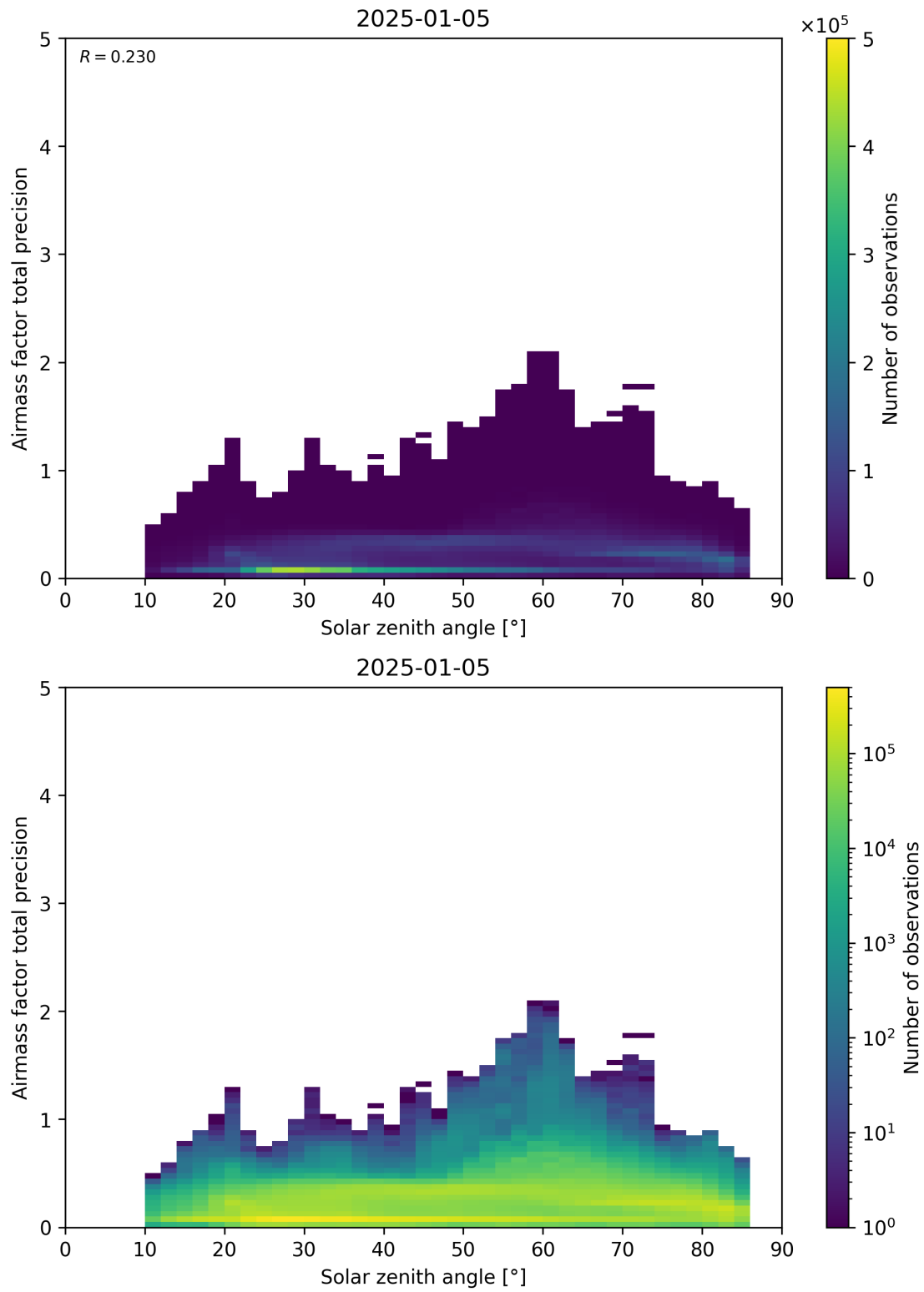
Figure 176: Scatter density plot of “Solar zenith angle” against “Airmass factor total precision” for 2025-01-04 to 2025-01-06.
