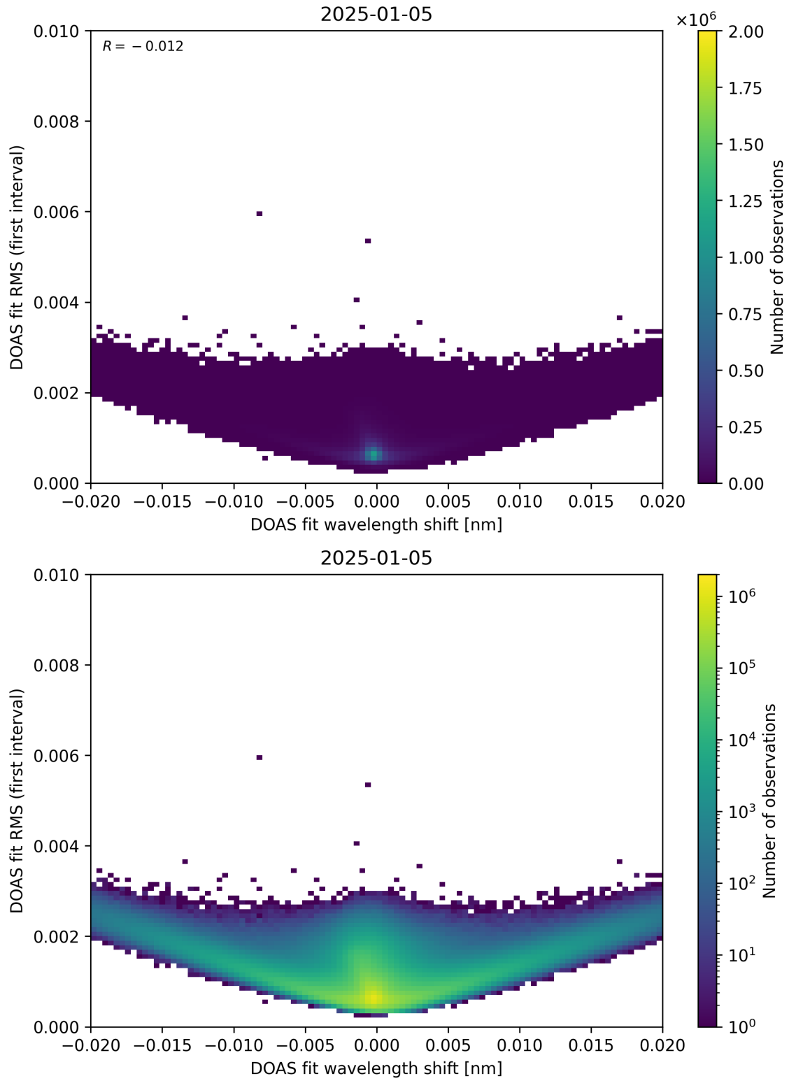
Figure 64: Scatter density plot of “DOAS fit wavelength shift” against “DOAS fit RMS (first interval)” for 2025-01-04 to 2025-01-06.
