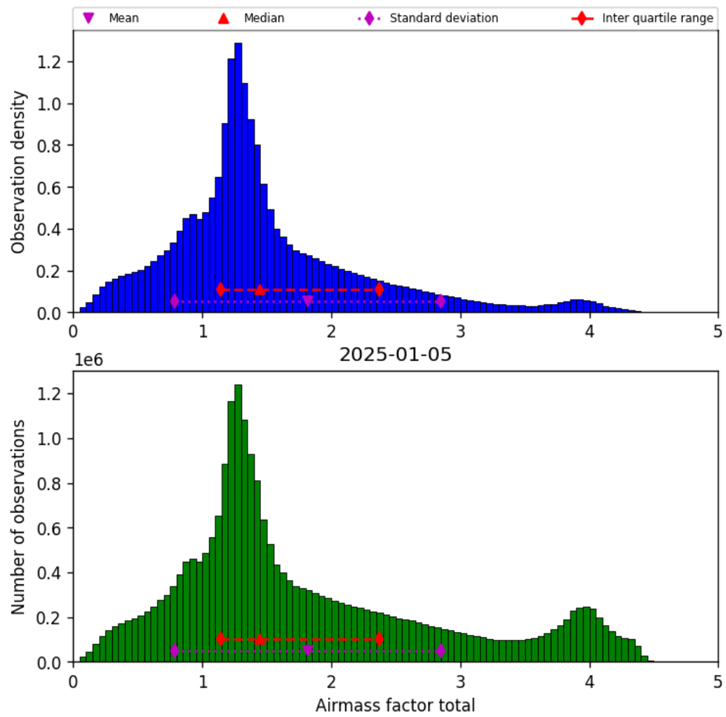
Figure 40: Histogram of “Airmass factor total” for 2025-01-04 to 2025-01-06
