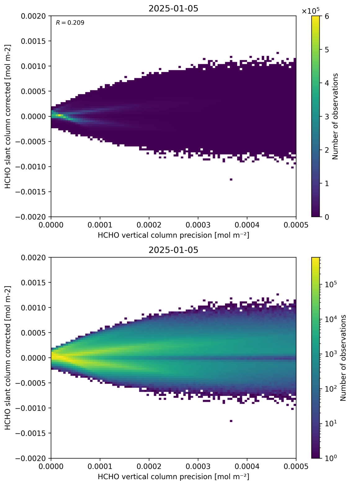
Figure 140: Scatter density plot of “HCHO vertical column precision” against “HCHO slant column corrected” for 2025-01-04 to 2025-01-06.
