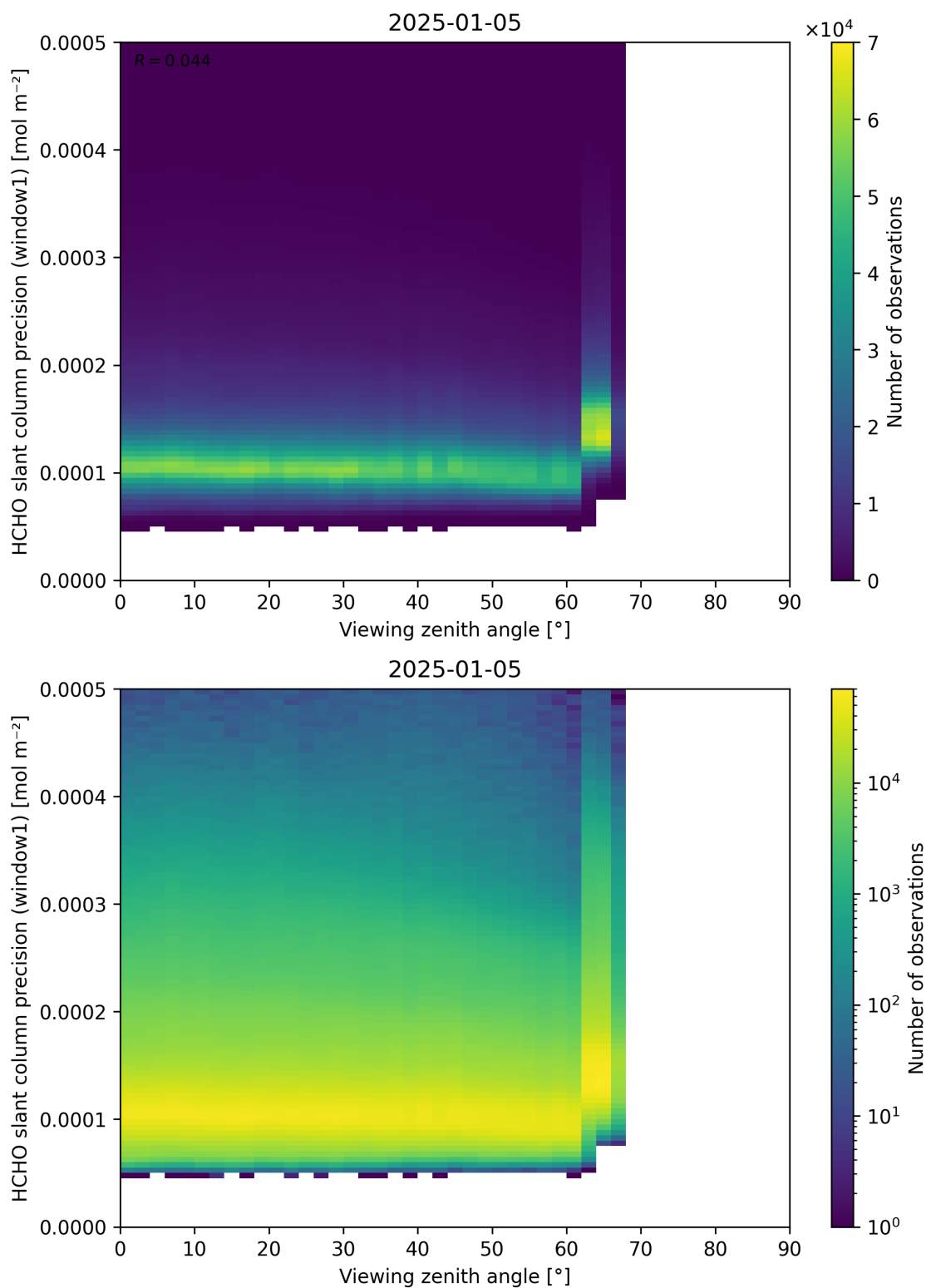
Figure 189: Scatter density plot of “Viewing zenith angle” against “HCHO slant column precision (window1)” for 2025-01-04 to 2025-01-06.
