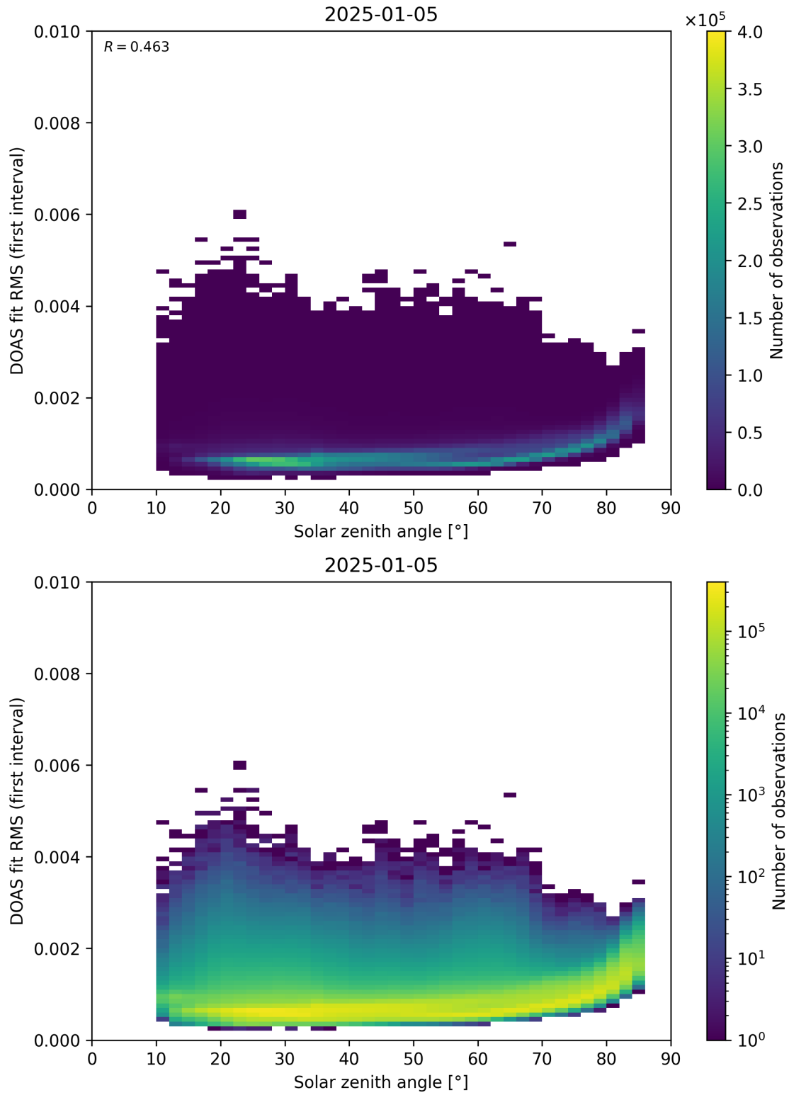
Figure 167: Scatter density plot of “Solar zenith angle” against “DOAS fit RMS (first interval)” for 2025-01-04 to 2025-01-06.
