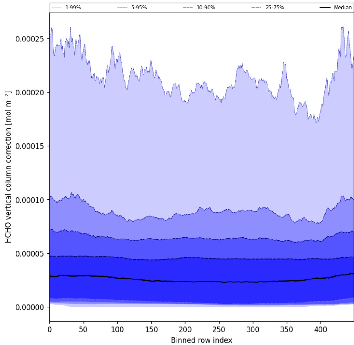
Figure 51: Along track statistics of “HCHO vertical column correction” for 2025-01-04 to 2025-01-06
