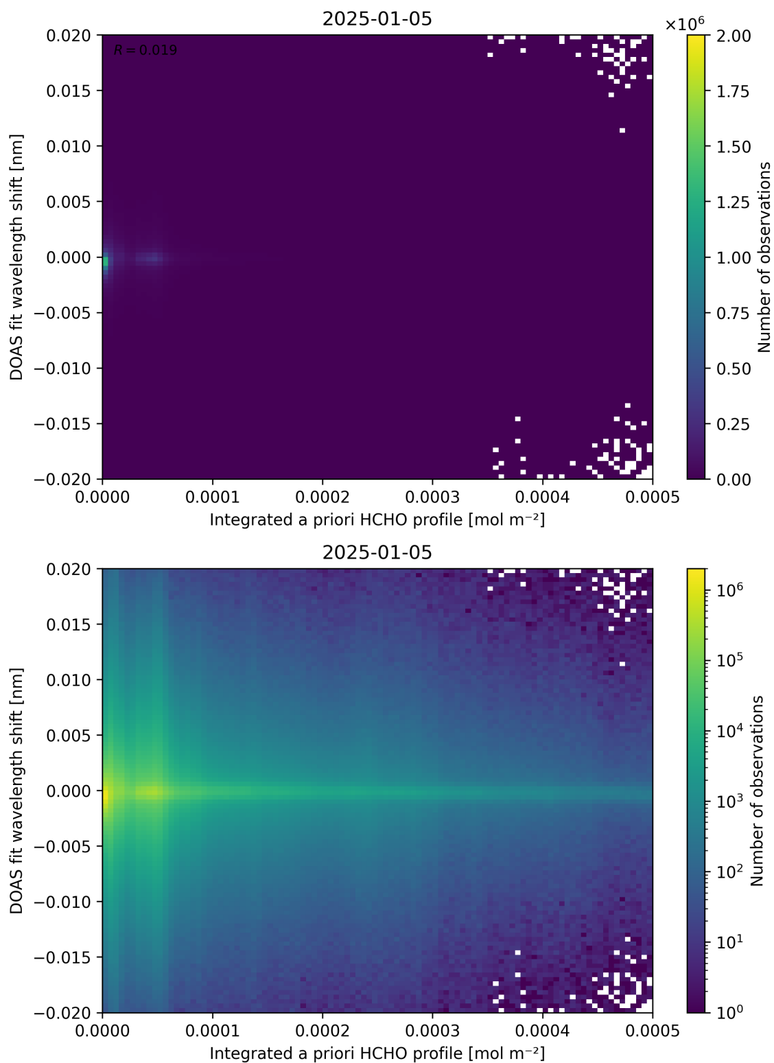
Figure 149: Scatter density plot of “Integrated a priori HCHO profile” against “DOAS fit wavelength shift” for 2025-01-04 to 2025-01-06.
