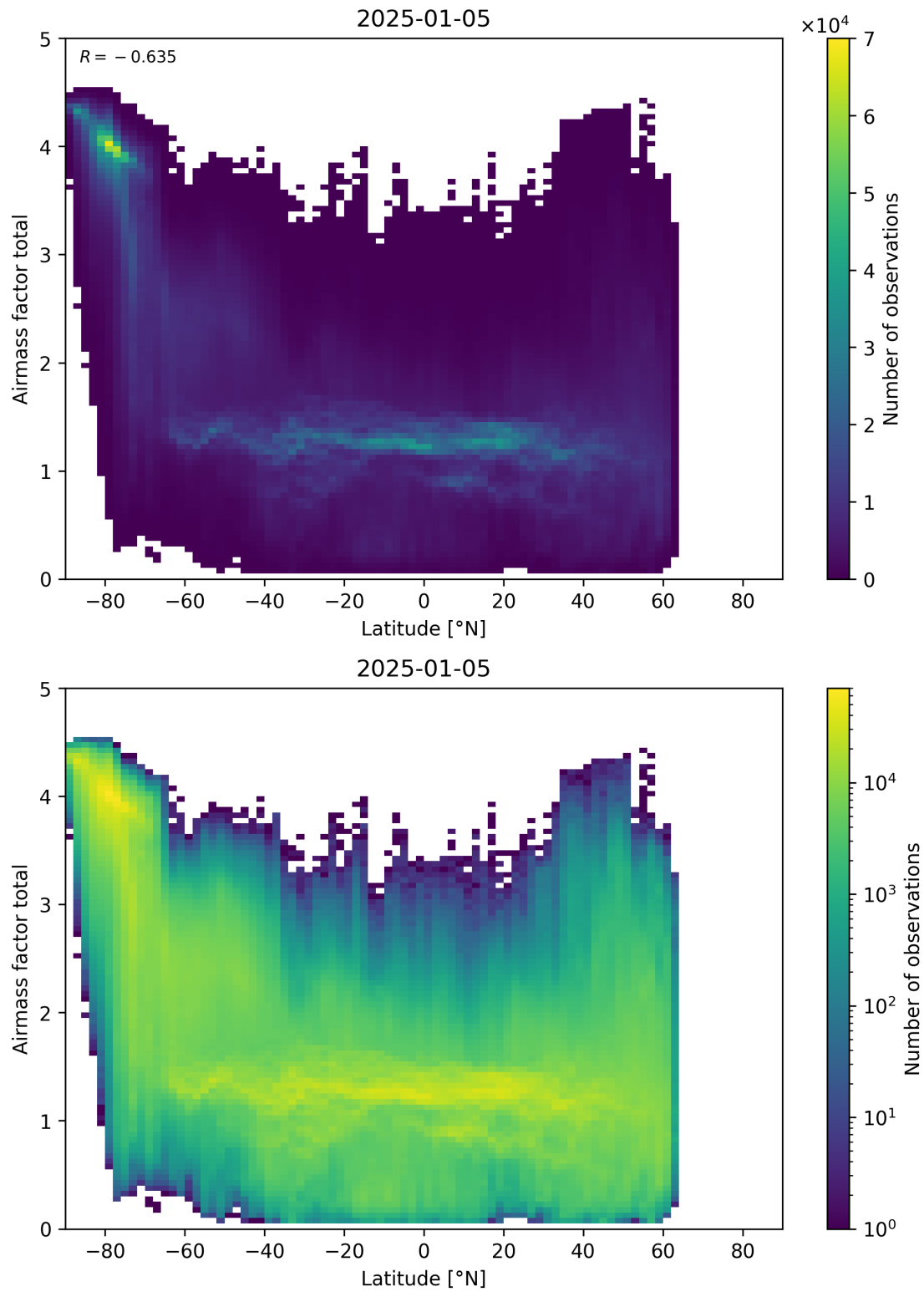
Figure 161: Scatter density plot of “Latitude” against “Airmass factor total” for 2025-01-04 to 2025-01-06.
