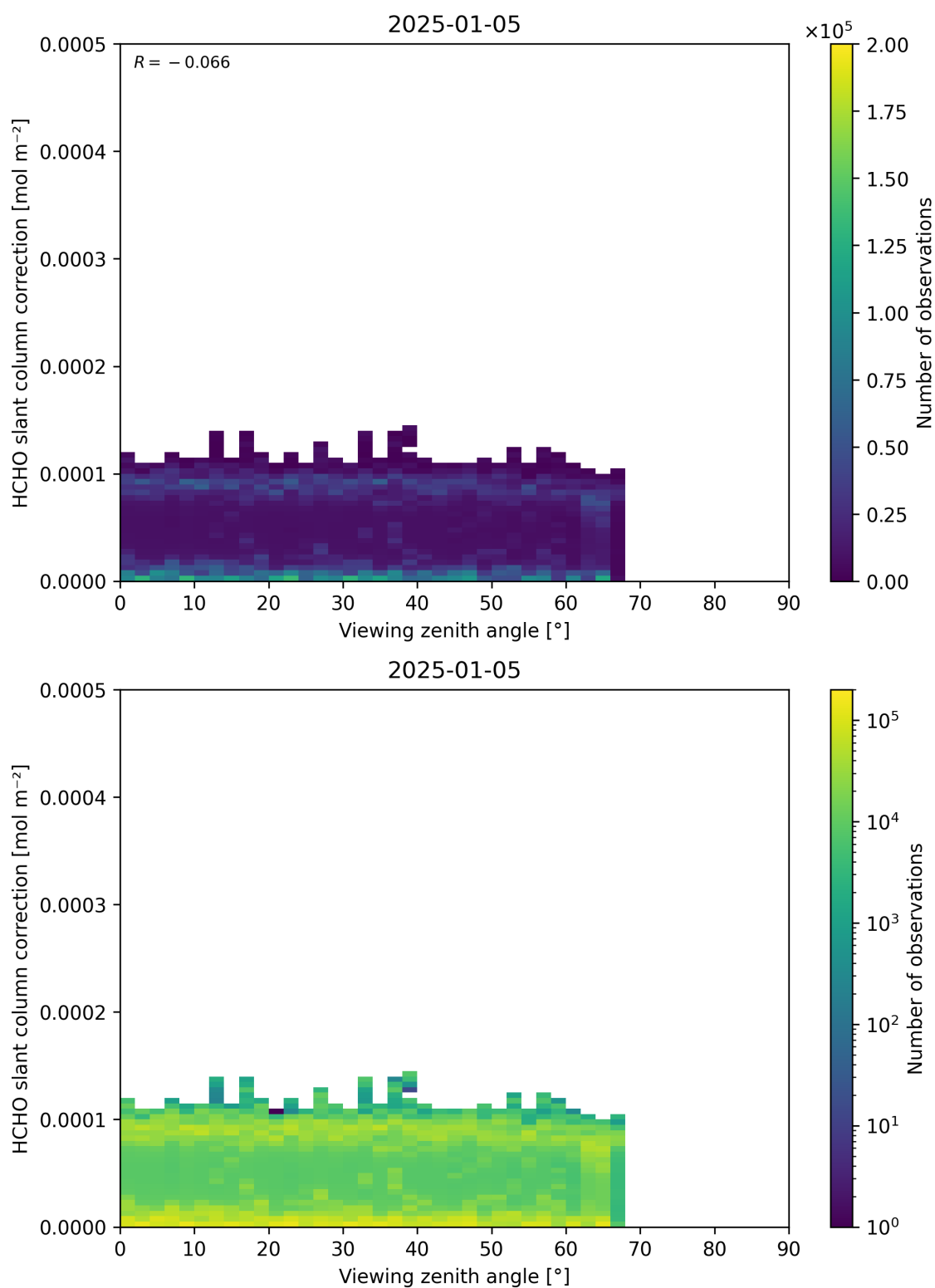
Figure 187: Scatter density plot of “Viewing zenith angle” against “HCHO slant column correction” for 2025-01-04 to 2025-01-06.
