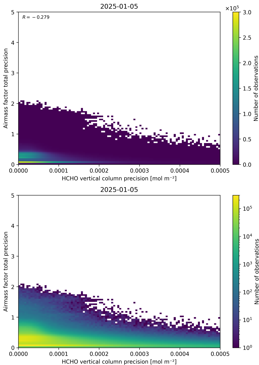
Figure 145: Scatter density plot of “HCHO vertical column precision” against “Airmass factor total precision” for 2025-01-04 to 2025-01-06.
