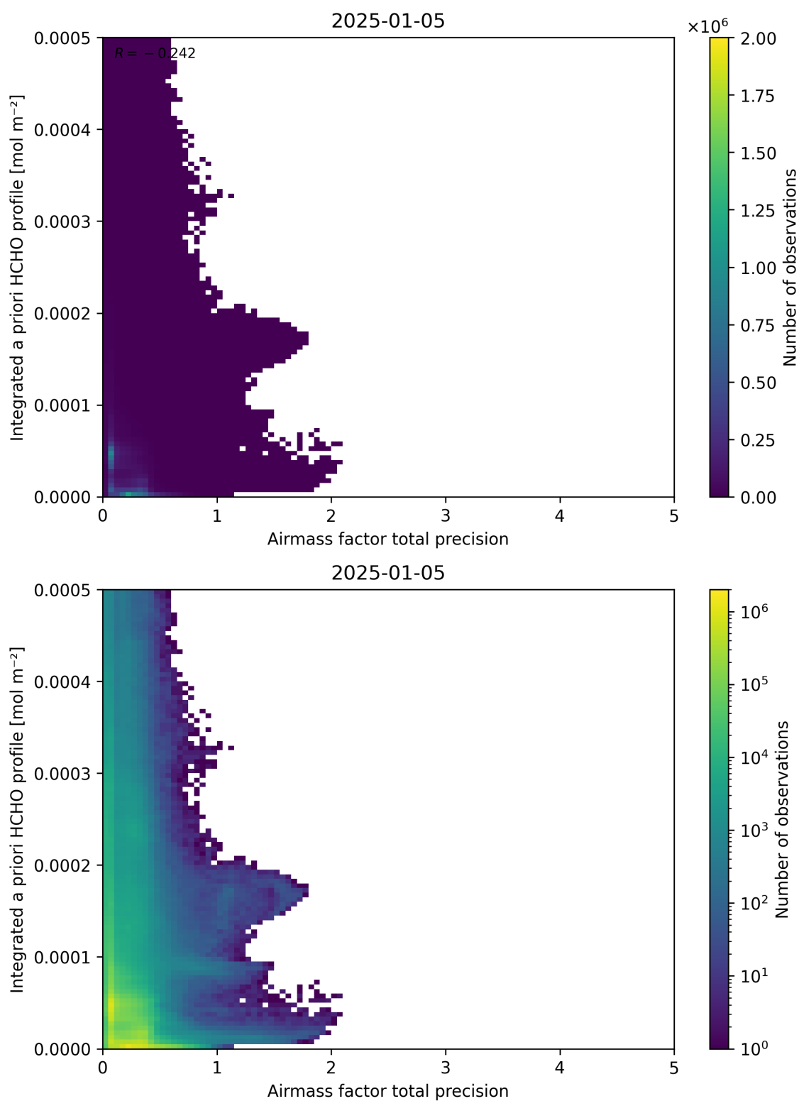
Figure 111: Scatter density plot of “Airmass factor total precision” against “Integrated a priori HCHO profile” for 2025-01-04 to 2025-01-06.
