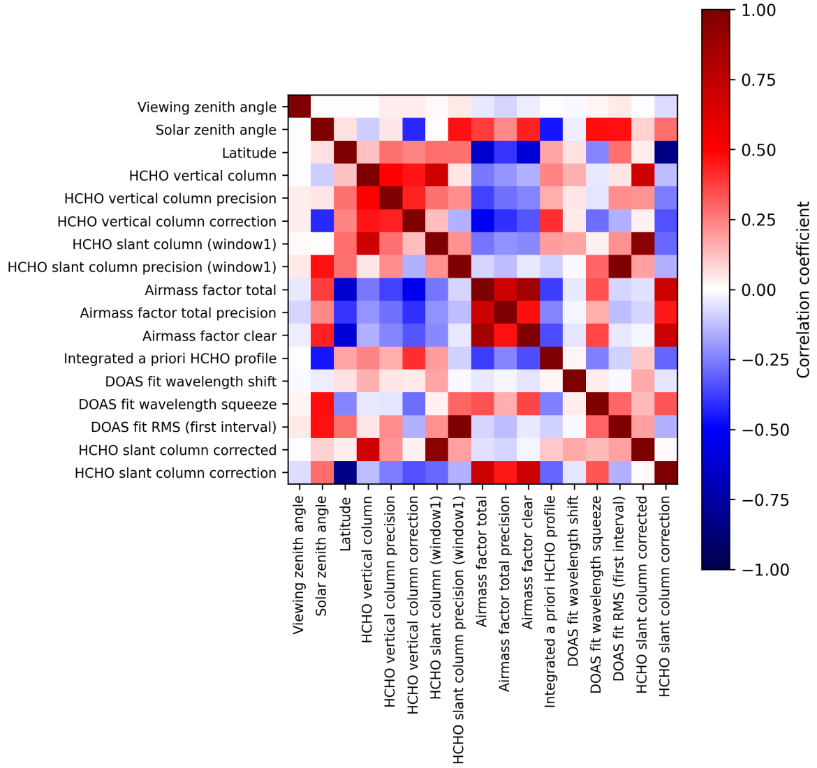
Figure 2: Map of correlation matrix for 2025-01-04 to 2025-01-06.
