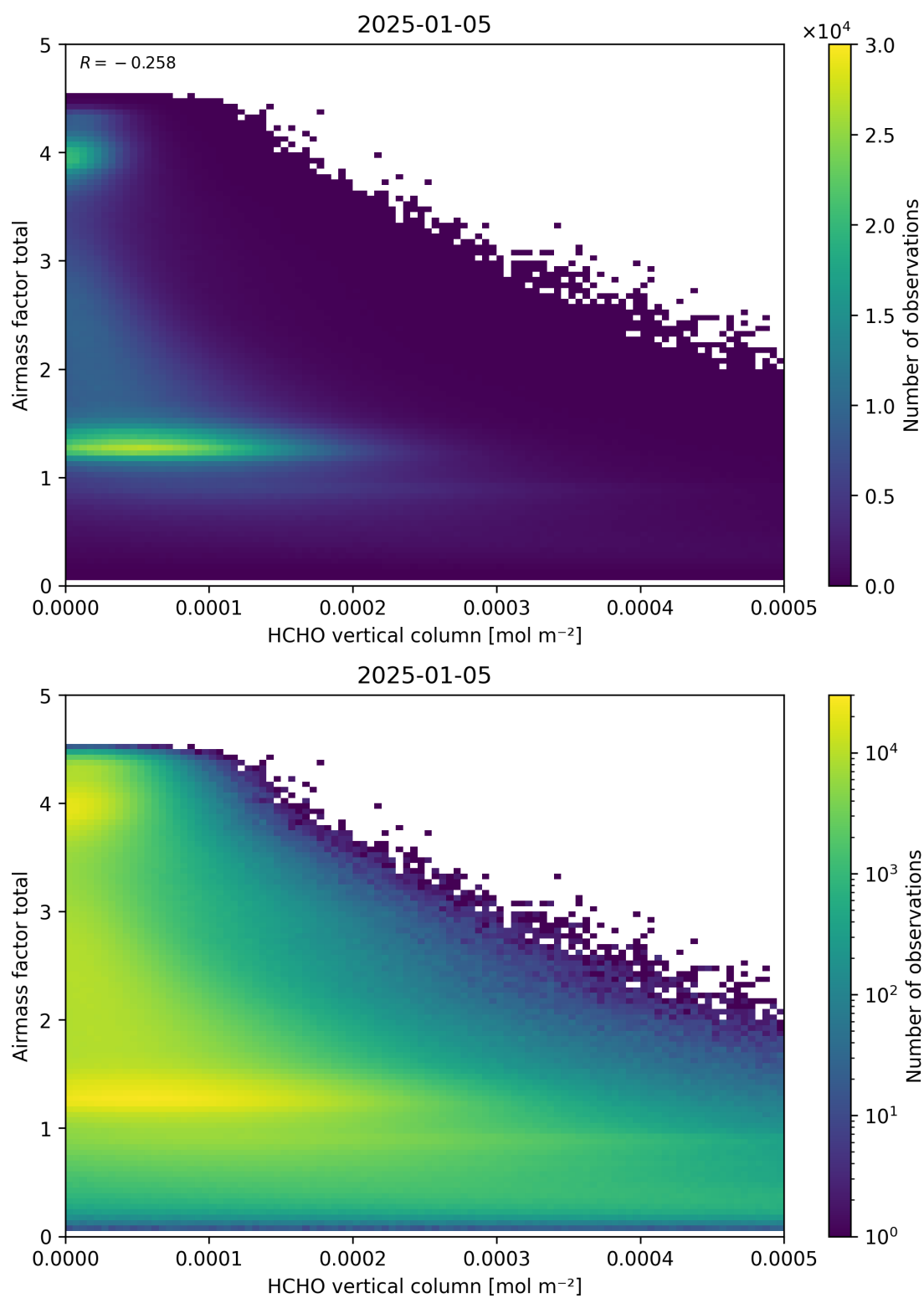
Figure 131: Scatter density plot of “HCHO vertical column” against “Airmass factor total” for 2025-01-04 to 2025-01-06.
