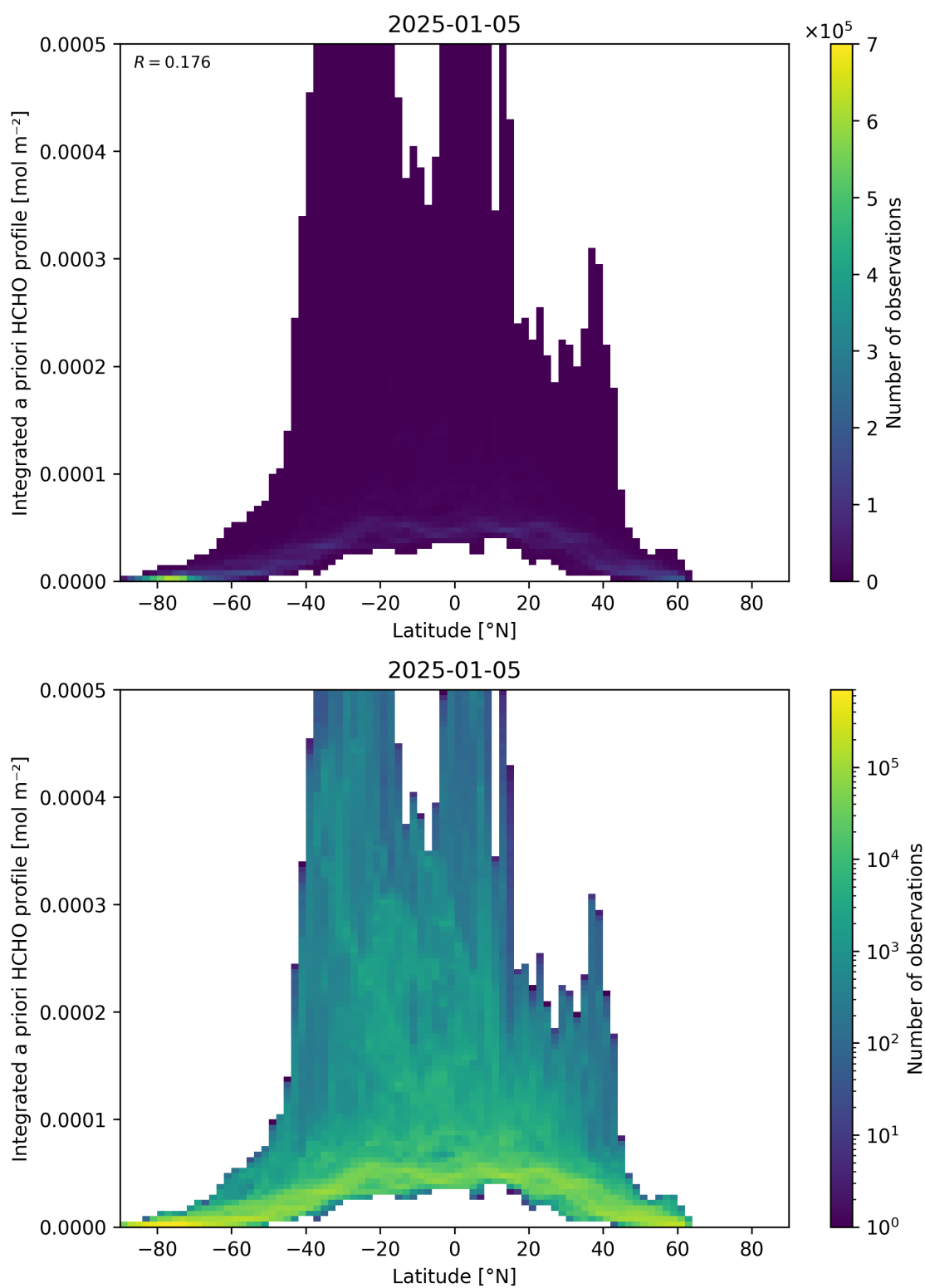
Figure 166: Scatter density plot of “Latitude” against “Integrated a priori HCHO profile” for 2025-01-04 to 2025-01-06.
