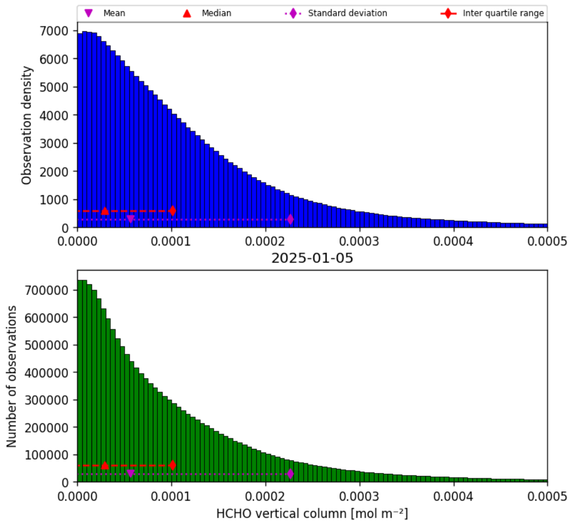
Figure 35: Histogram of “HCHO vertical column” for 2025-01-04 to 2025-01-06
