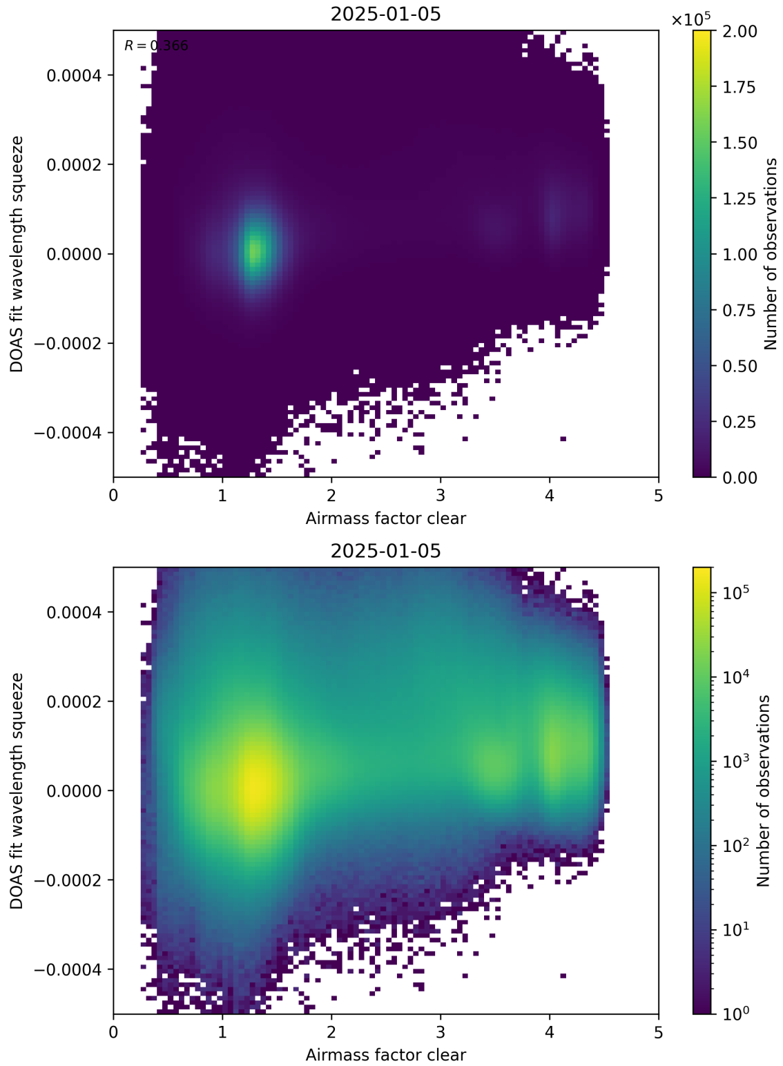
Figure 73: Scatter density plot of “Airmass factor clear” against “DOAS fit wavelength squeeze” for 2025-01-04 to 2025-01-06.
