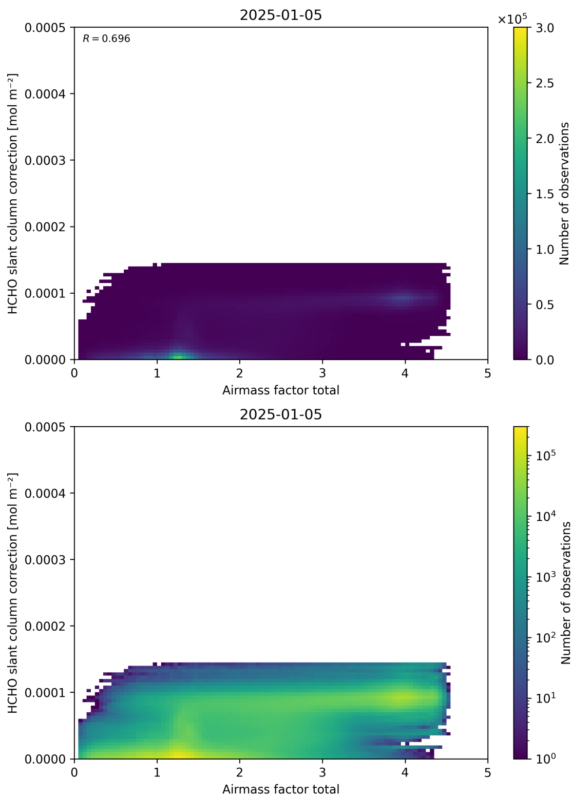
Figure 102: Scatter density plot of “Airmass factor total” against “HCHO slant column correction” for 2025-01-04 to 2025-01-06.
