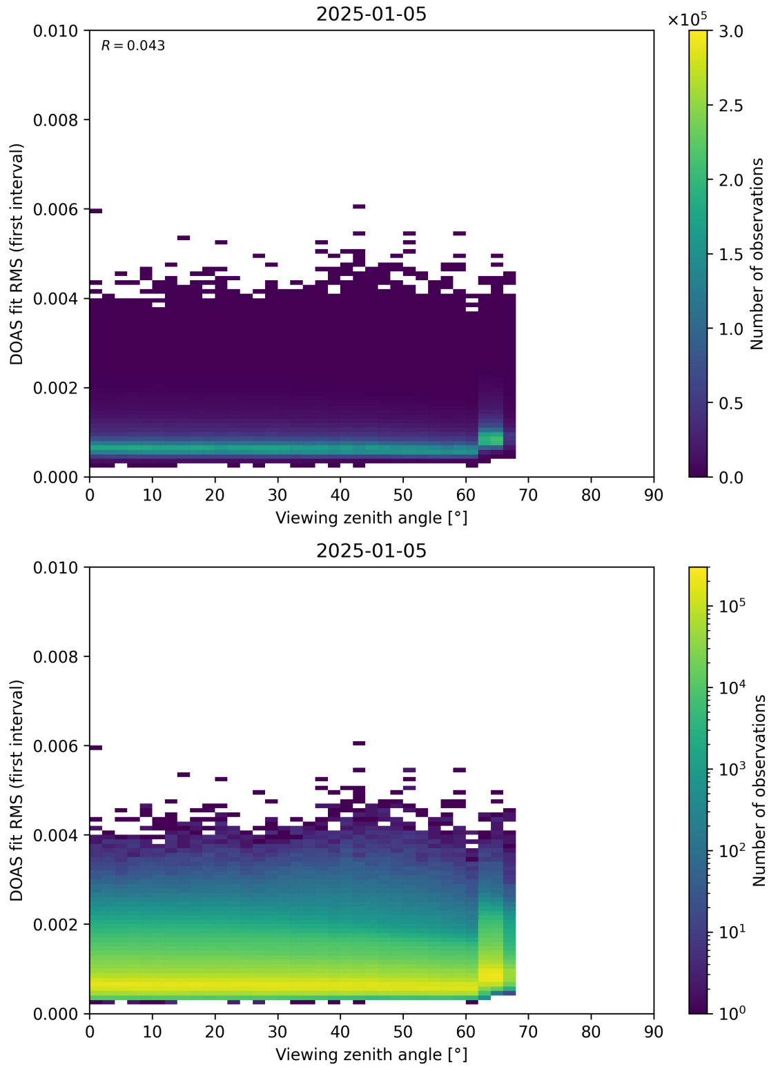
Figure 182: Scatter density plot of “Viewing zenith angle” against “DOAS fit RMS (first interval)” for 2025-01-04 to 2025-01-06.
