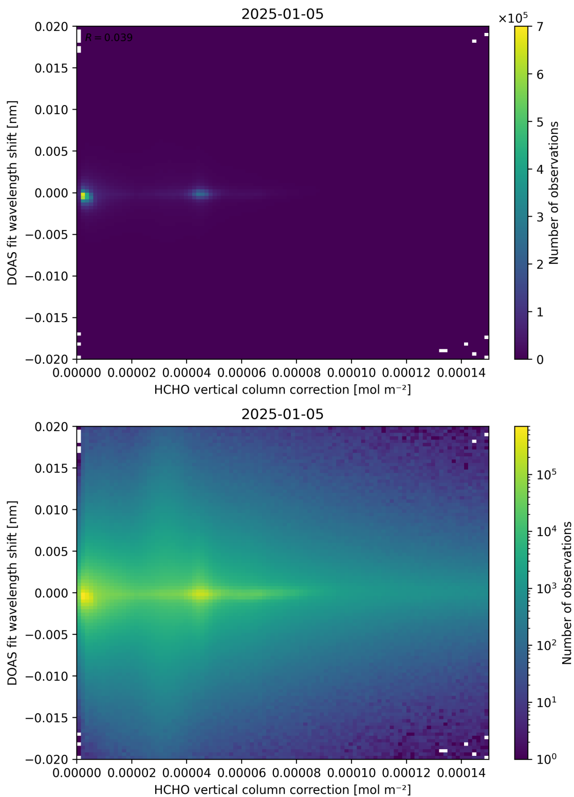
Figure 113: Scatter density plot of “HCHO vertical column correction” against “DOAS fit wavelength shift” for 2025-01-04 to 2025-01-06.
