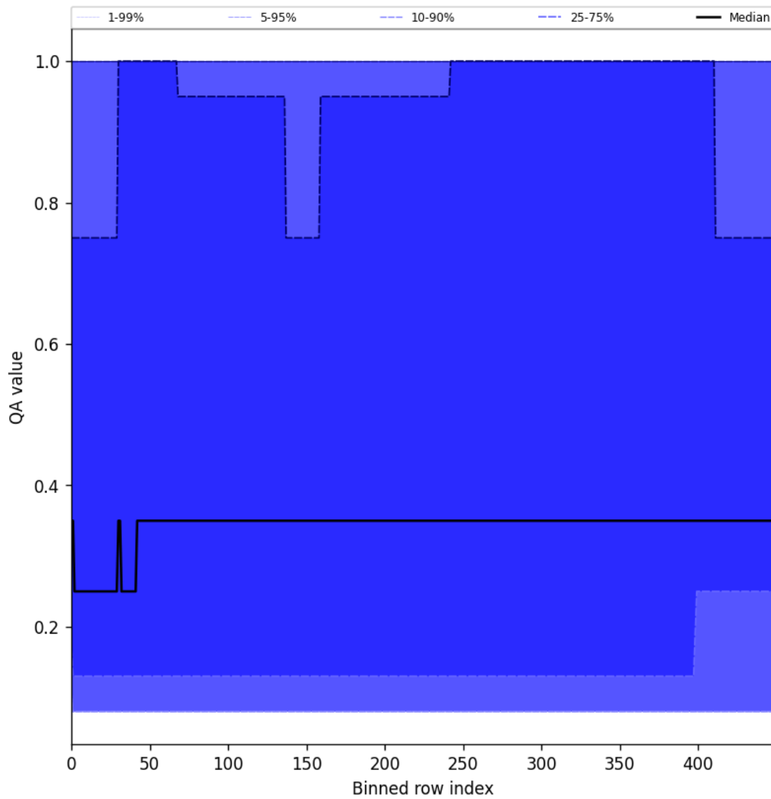
Figure 48: Along track statistics of “QA value” for 2025-01-04 to 2025-01-06
