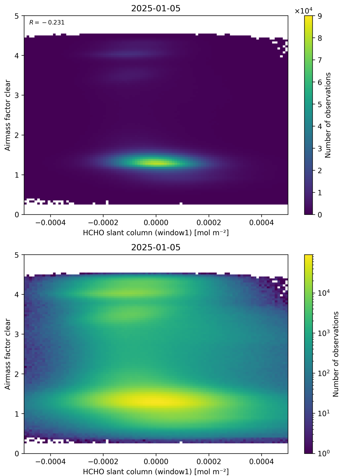
Figure 81: Scatter density plot of “HCHO slant column (window1)” against “Airmass factor clear” for 2025-01-04 to 2025-01-06.
