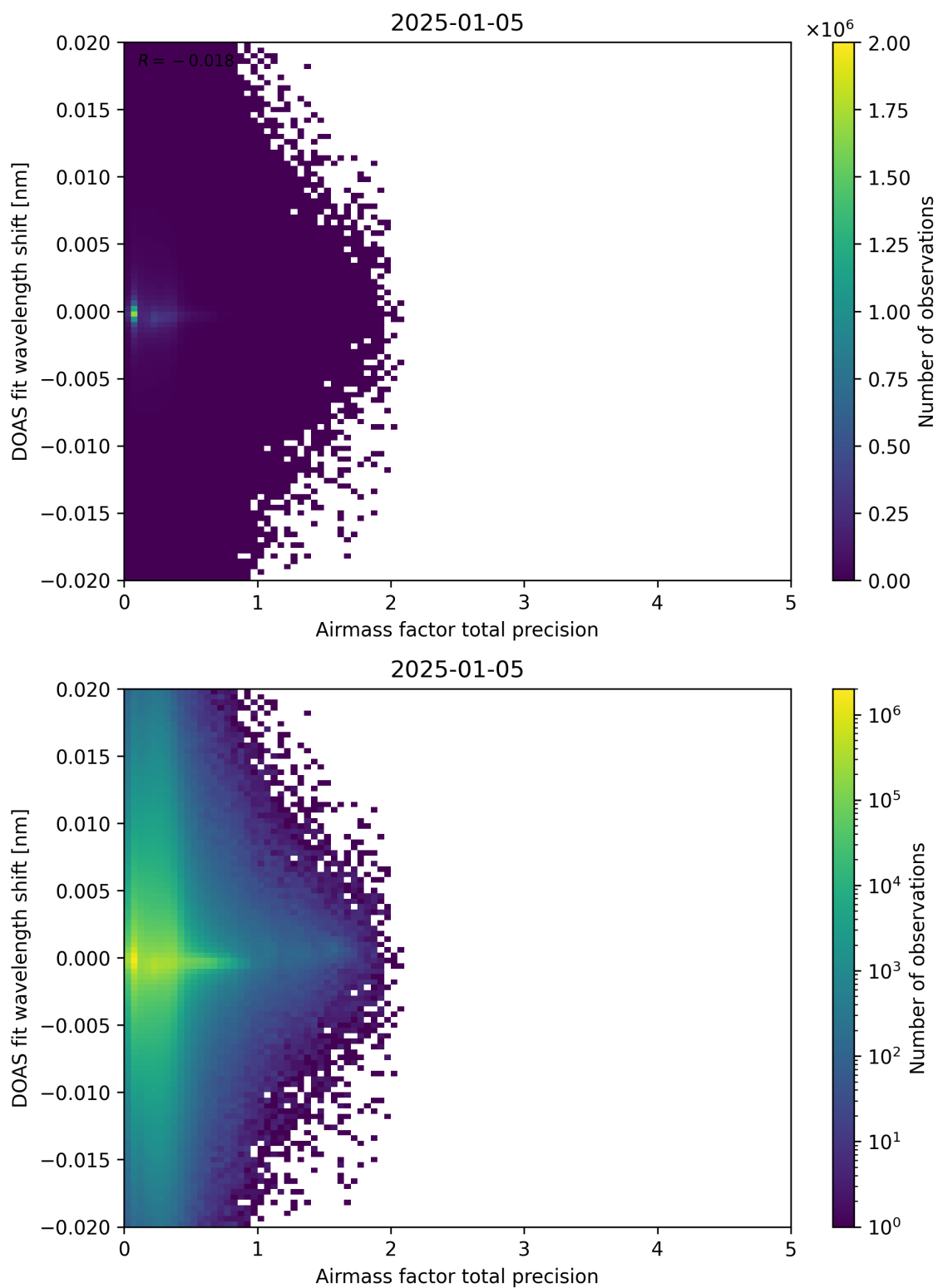
Figure 106: Scatter density plot of “Airmass factor total precision” against “DOAS fit wavelength shift” for 2025-01-04 to 2025-01-06.
