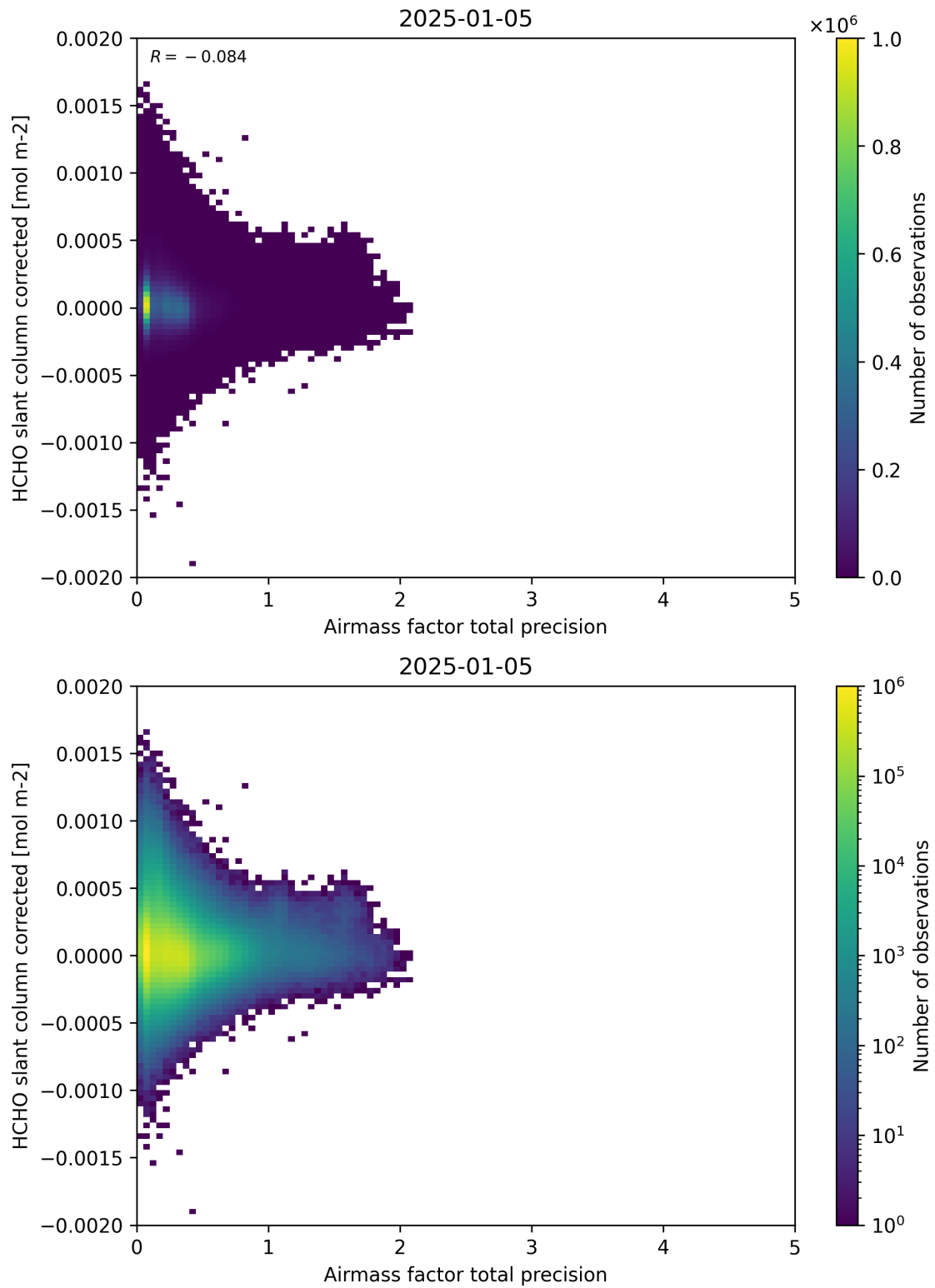
Figure 109: Scatter density plot of “Airmass factor total precision” against “HCHO slant column corrected” for 2025-01-04 to 2025-01-06.
