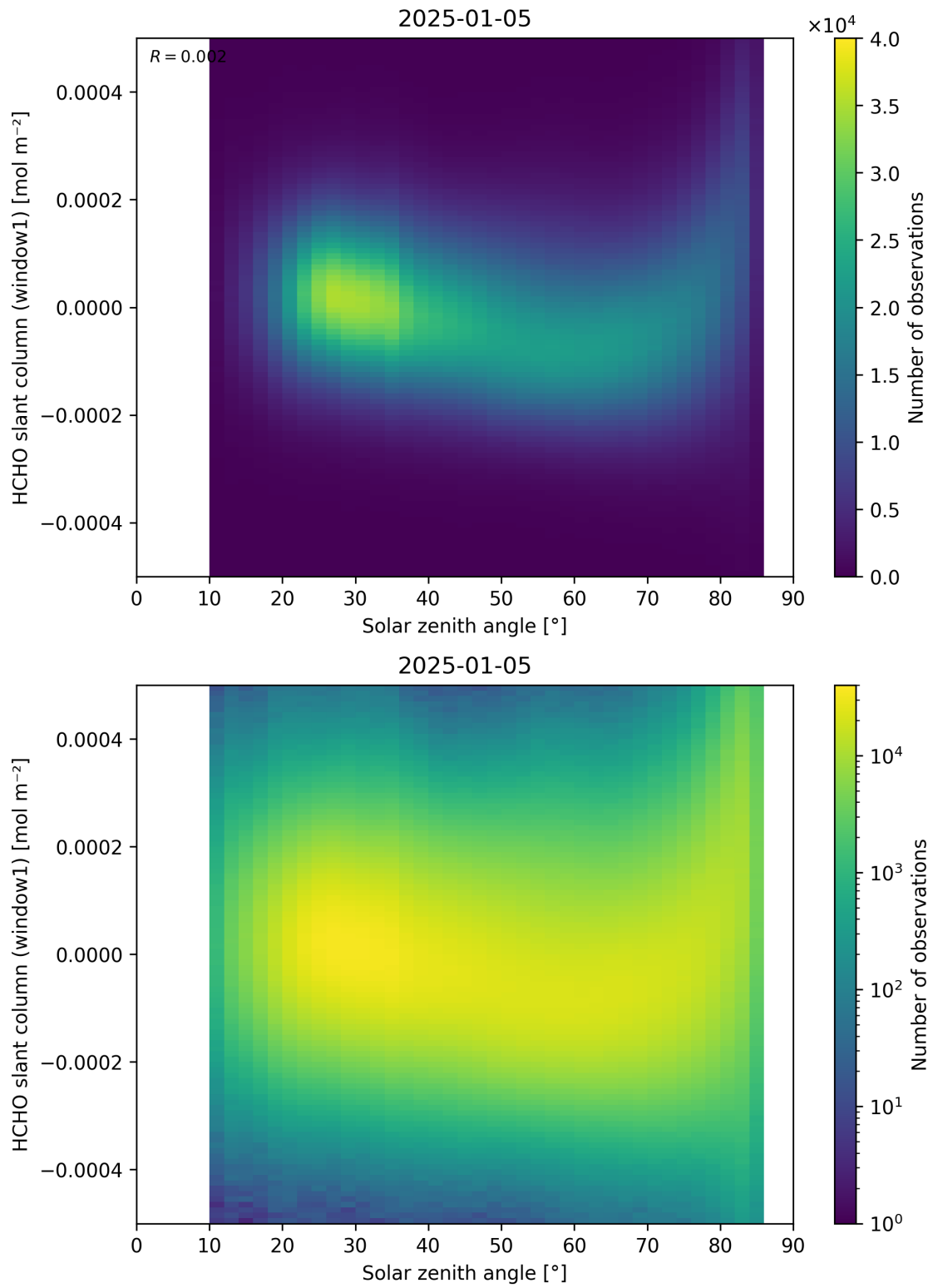
Figure 173: Scatter density plot of “Solar zenith angle” against “HCHO slant column (window1)” for 2025-01-04 to 2025-01-06.
