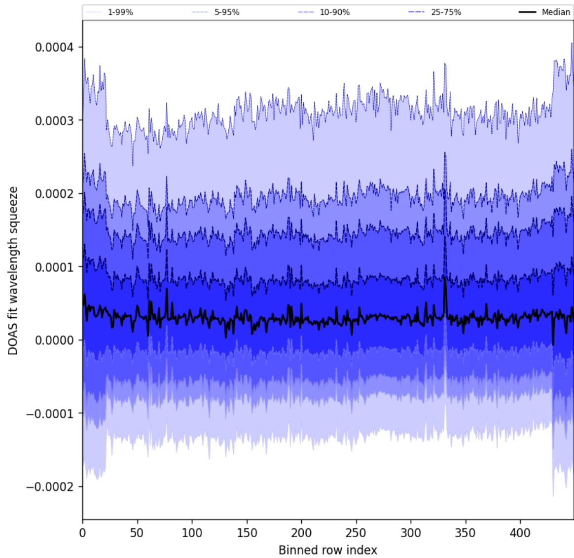
Figure 59: Along track statistics of “DOAS fit wavelength squeeze” for 2025-01-04 to 2025-01-06
