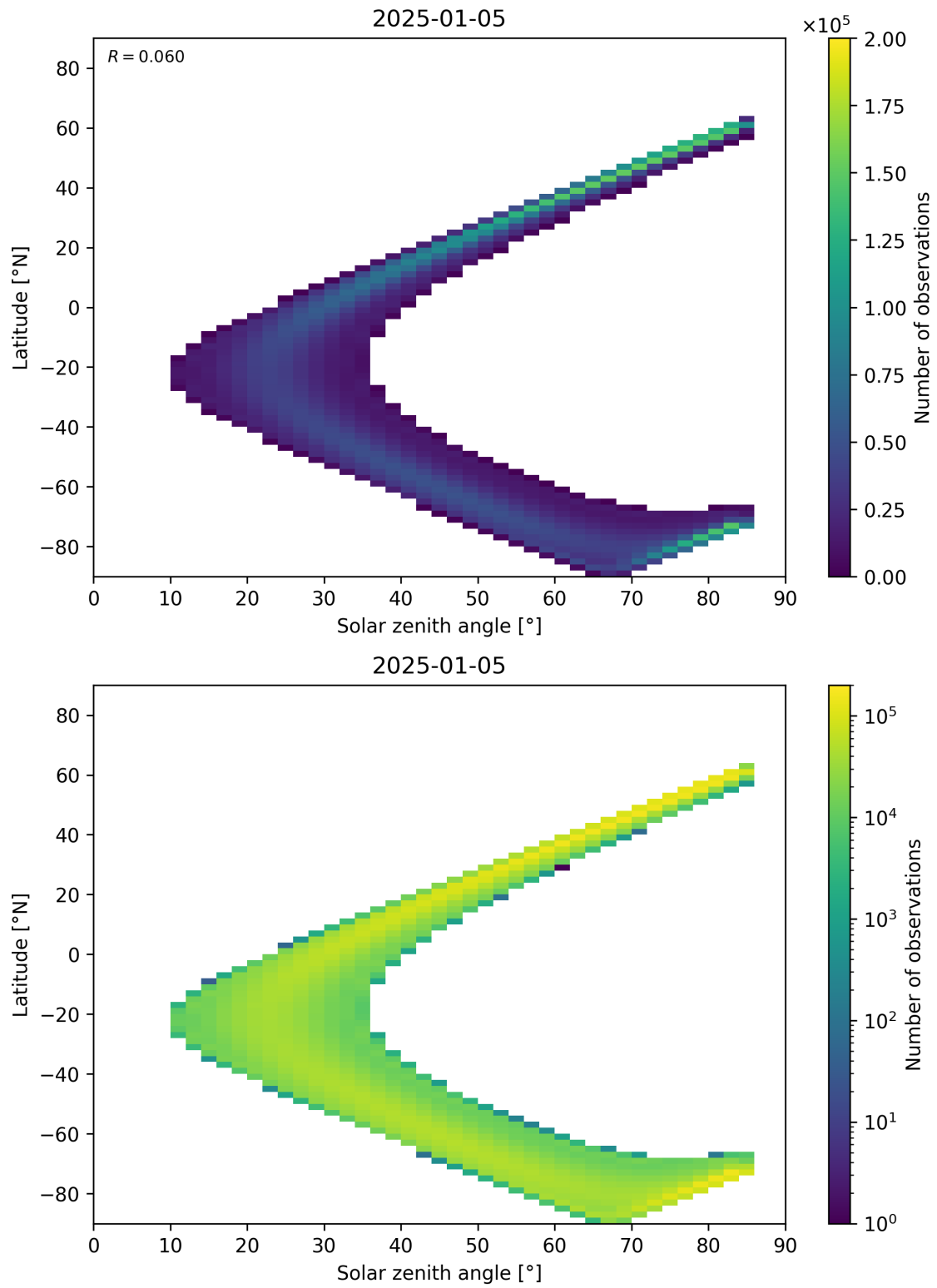
Figure 181: Scatter density plot of “Solar zenith angle” against “Latitude” for 2025-01-04 to 2025-01-06.
