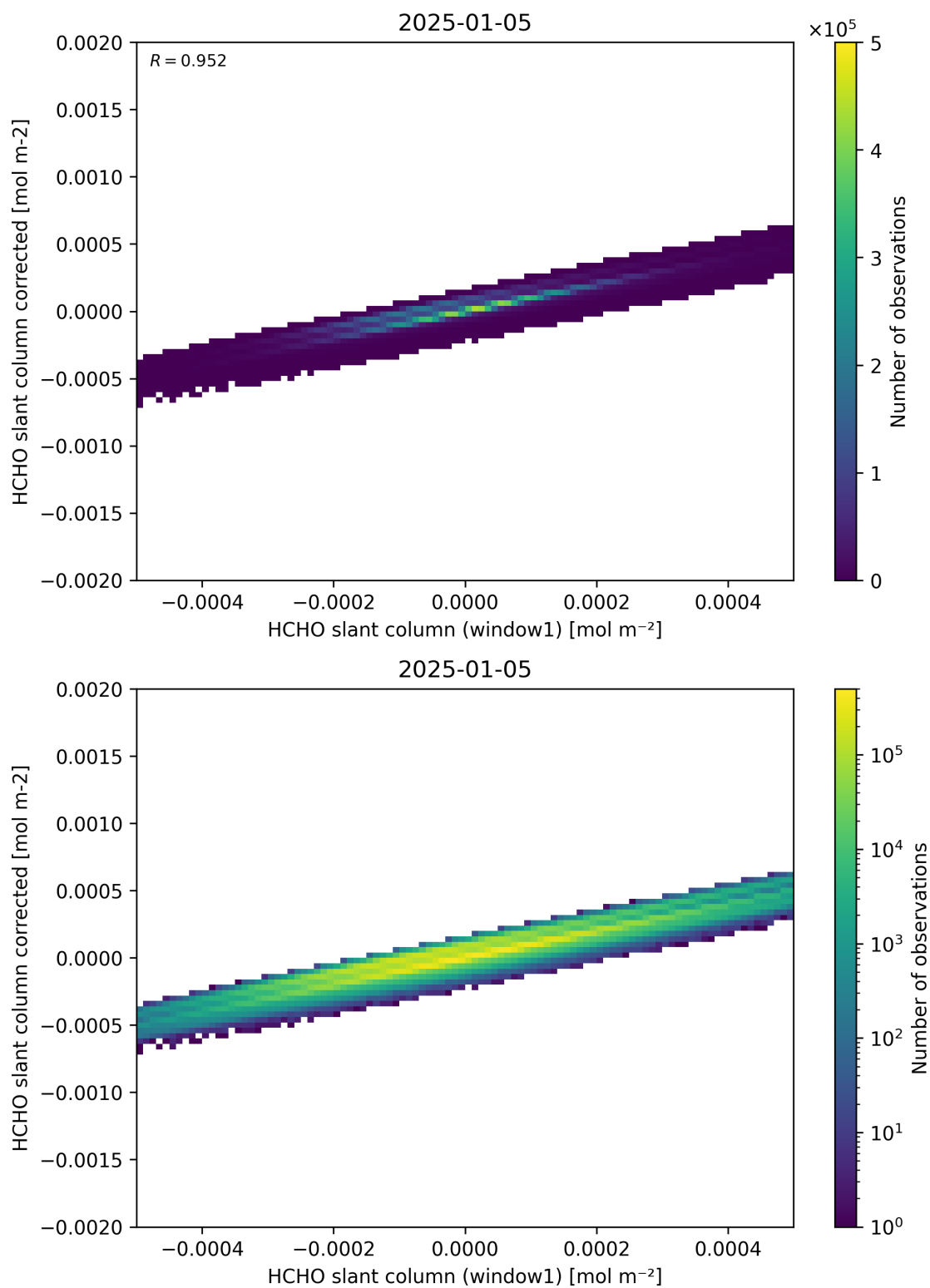
Figure 82: Scatter density plot of “HCHO slant column (window1)” against “HCHO slant column corrected” for 2025-01-04 to 2025-01-06.
