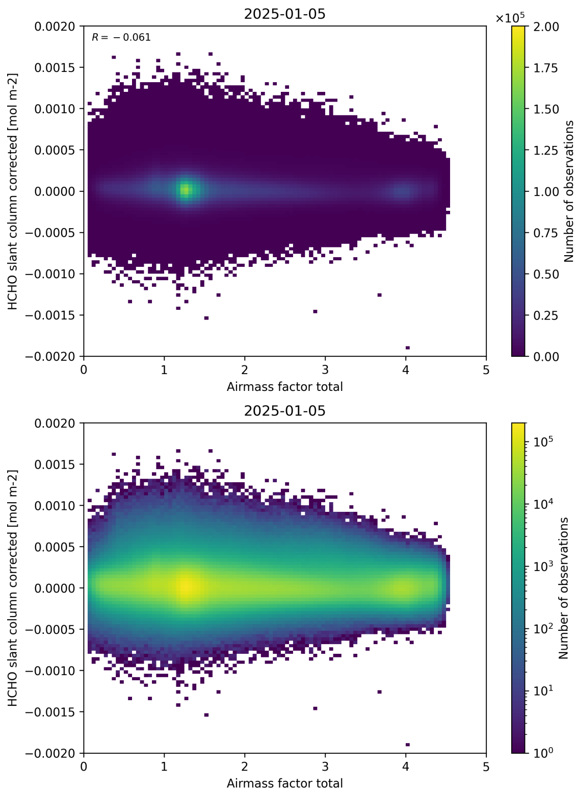
Figure 101: Scatter density plot of “Airmass factor total” against “HCHO slant column corrected” for 2025-01-04 to 2025-01-06.
