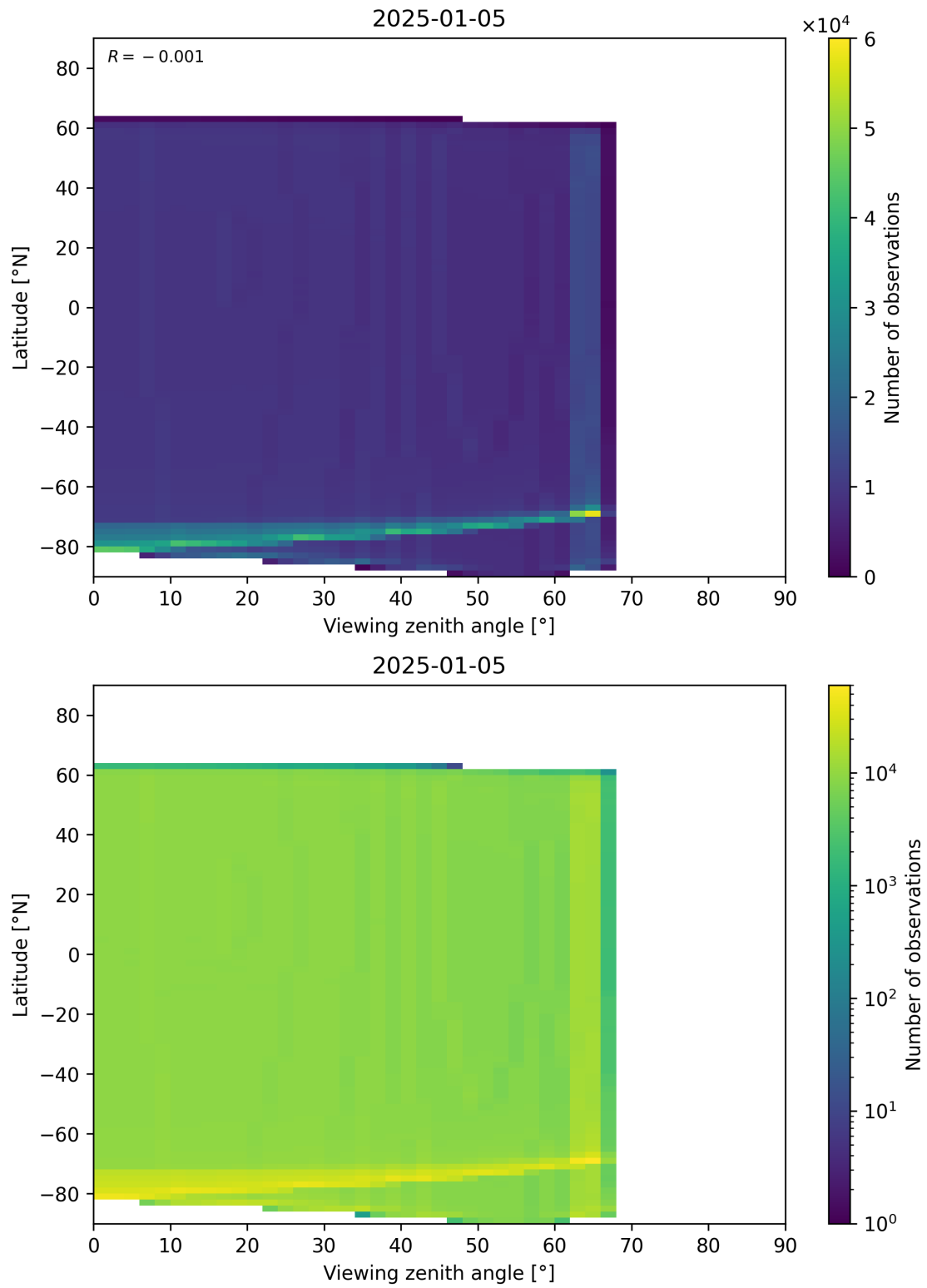
Figure 196: Scatter density plot of “Viewing zenith angle” against “Latitude” for 2025-01-04 to 2025-01-06.
