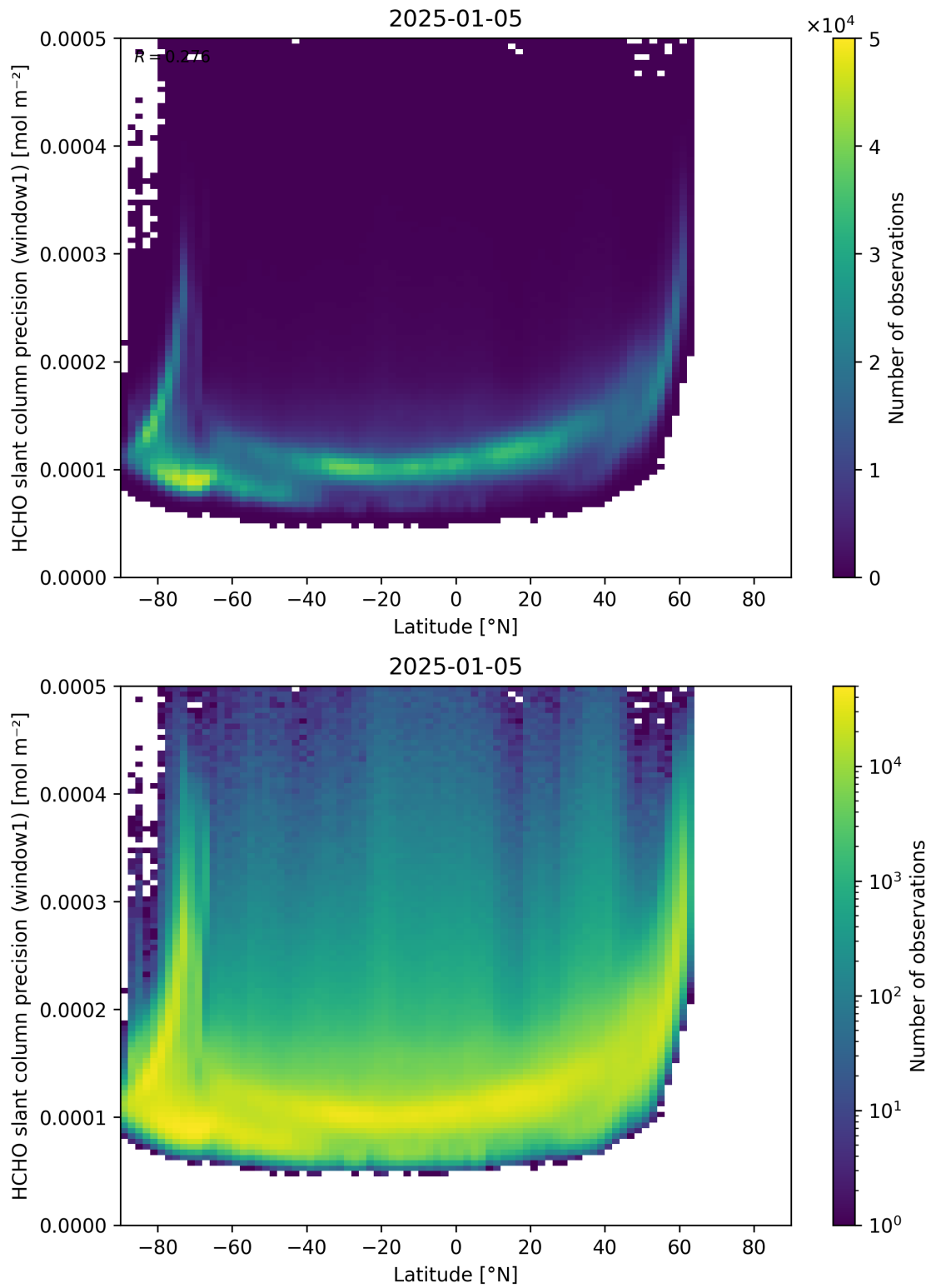
Figure 160: Scatter density plot of “Latitude” against “HCHO slant column precision (window1)” for 2025-01-04 to 2025-01-06.
