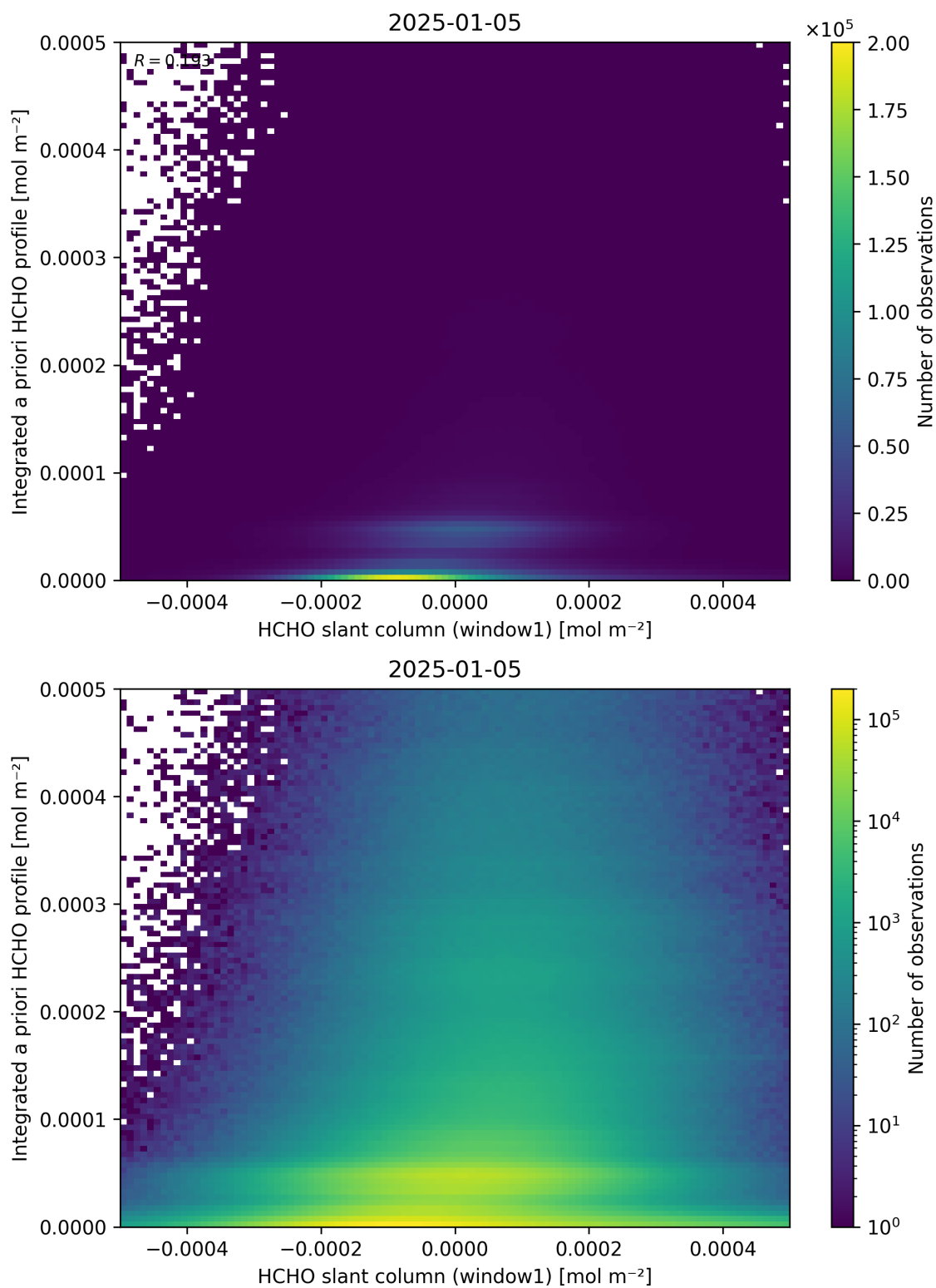
Figure 87: Scatter density plot of “HCHO slant column (window1)” against “Integrated a priori HCHO profile” for 2025-01-04 to 2025-01-06.
