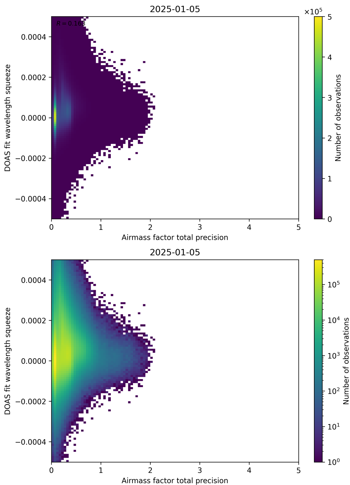
Figure 107: Scatter density plot of “Airmass factor total precision” against “DOAS fit wavelength squeeze” for 2025-01-04 to 2025-01-06.
