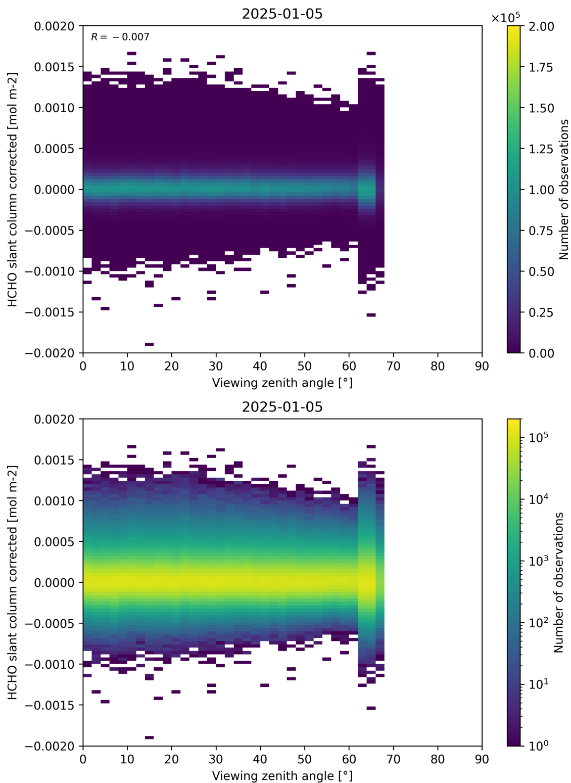
Figure 186: Scatter density plot of “Viewing zenith angle” against “HCHO slant column corrected” for 2025-01-04 to 2025-01-06.
