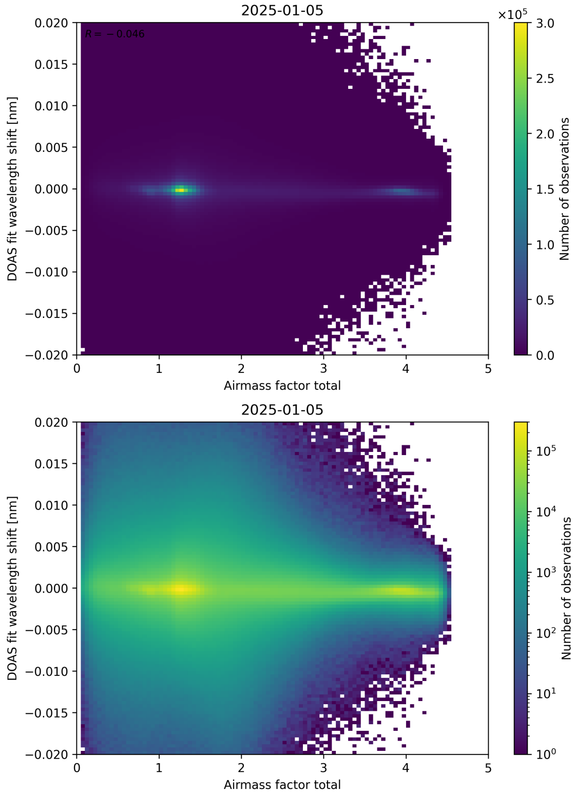
Figure 98: Scatter density plot of “Airmass factor total” against “DOAS fit wavelength shift” for 2025-01-04 to 2025-01-06.
