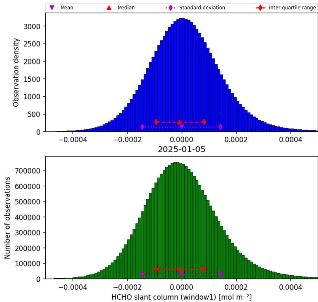
Figure 38: Histogram of “HCHO slant column (window1)” for 2025-01-04 to 2025-01-06
