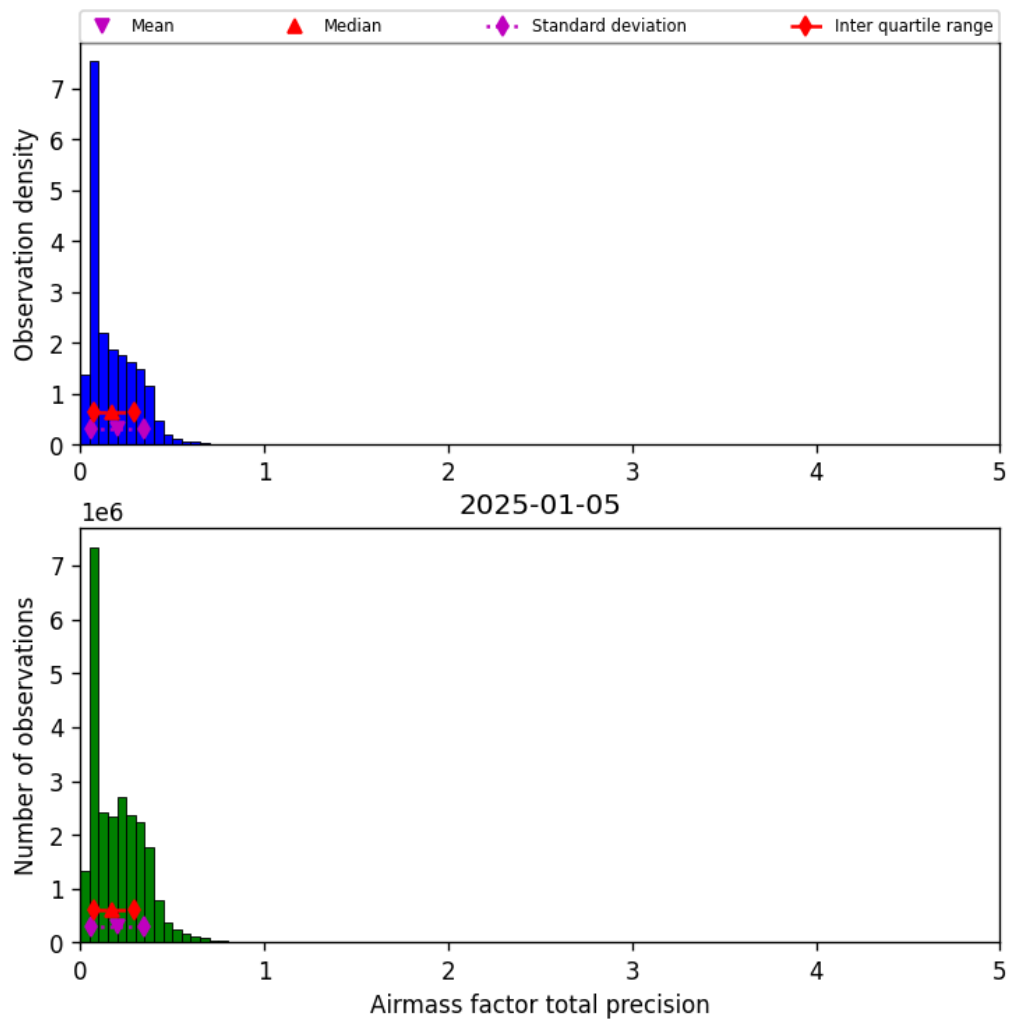
Figure 41: Histogram of “Airmass factor total precision” for 2025-01-04 to 2025-01-06
