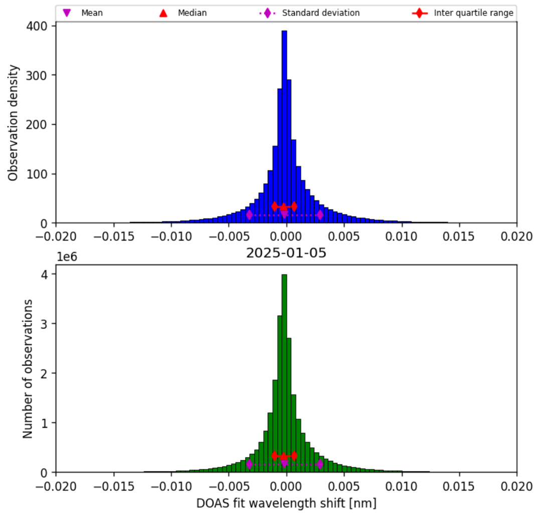
Figure 44: Histogram of “DOAS fit wavelength shift” for 2025-01-04 to 2025-01-06
