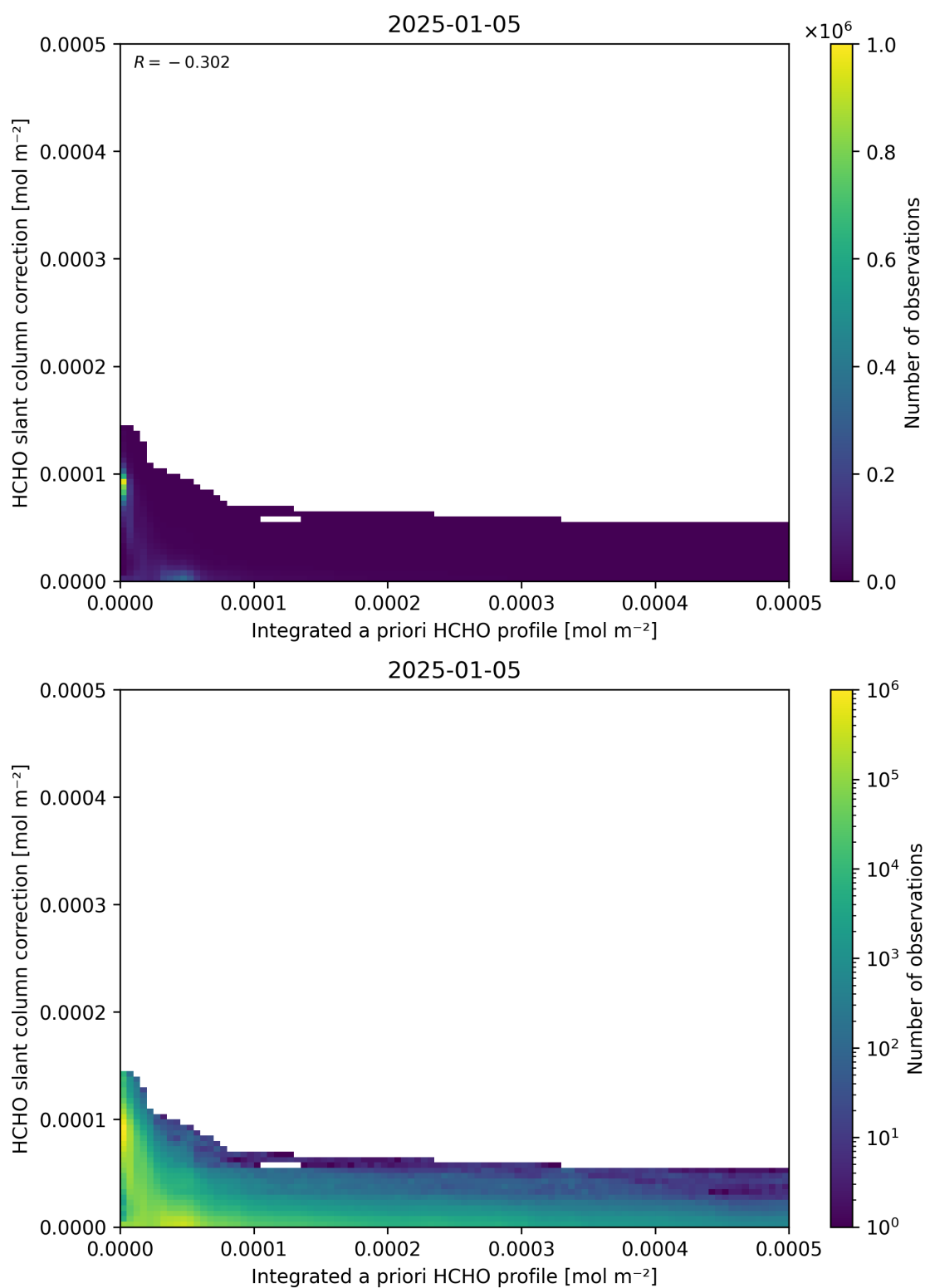
Figure 152: Scatter density plot of “Integrated a priori HCHO profile” against “HCHO slant column correction” for 2025-01-04 to 2025-01-06.
