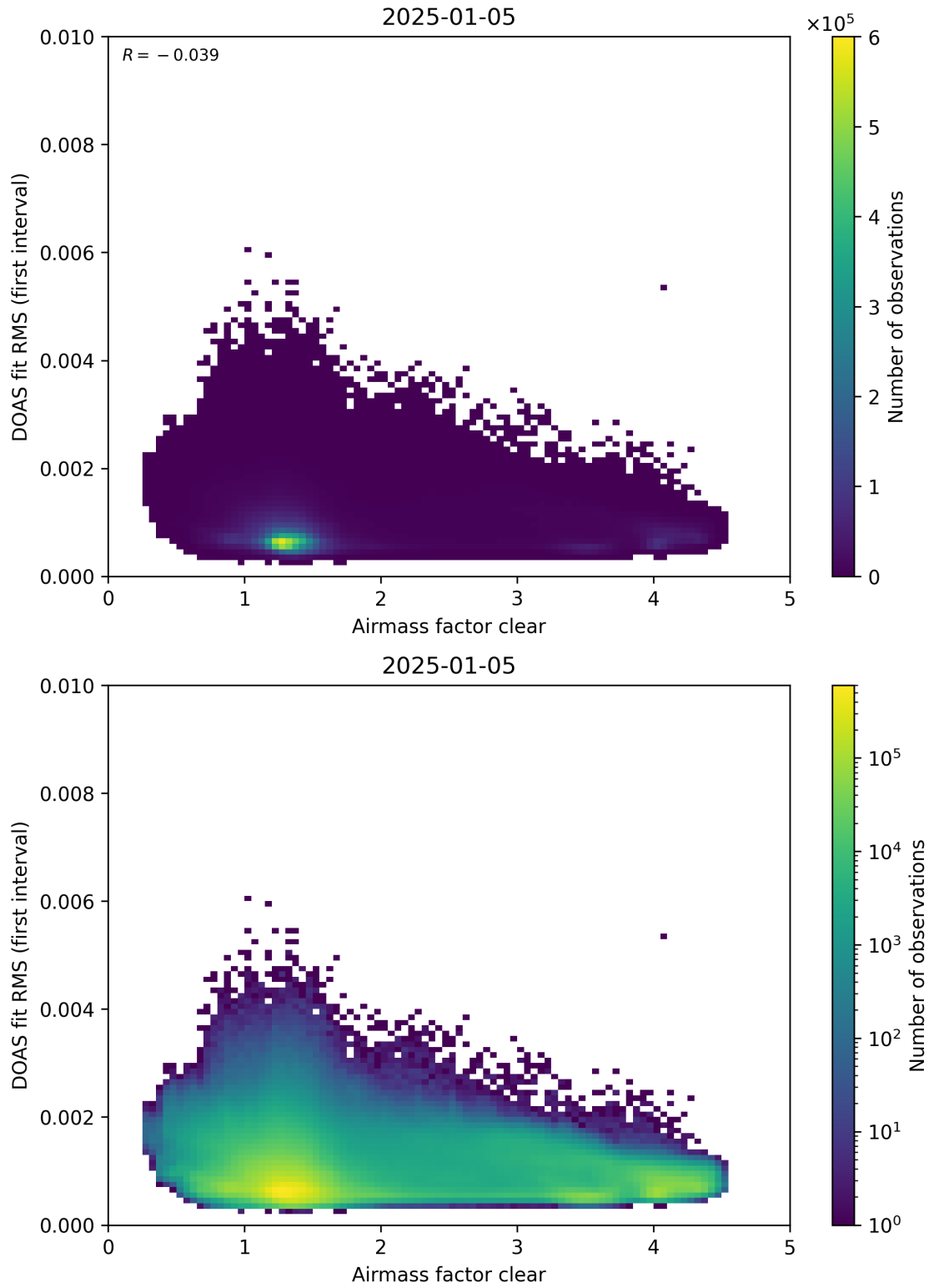
Figure 71: Scatter density plot of “Airmass factor clear” against “DOAS fit RMS (first interval)” for 2025-01-04 to 2025-01-06.
