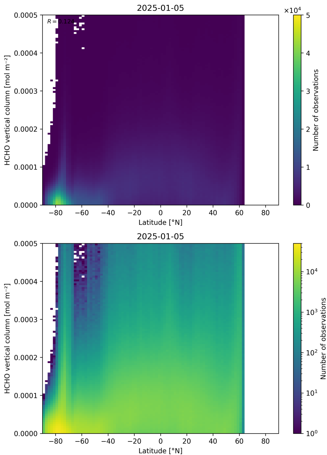
Figure 163: Scatter density plot of “Latitude” against “HCHO vertical column” for 2025-01-04 to 2025-01-06.
