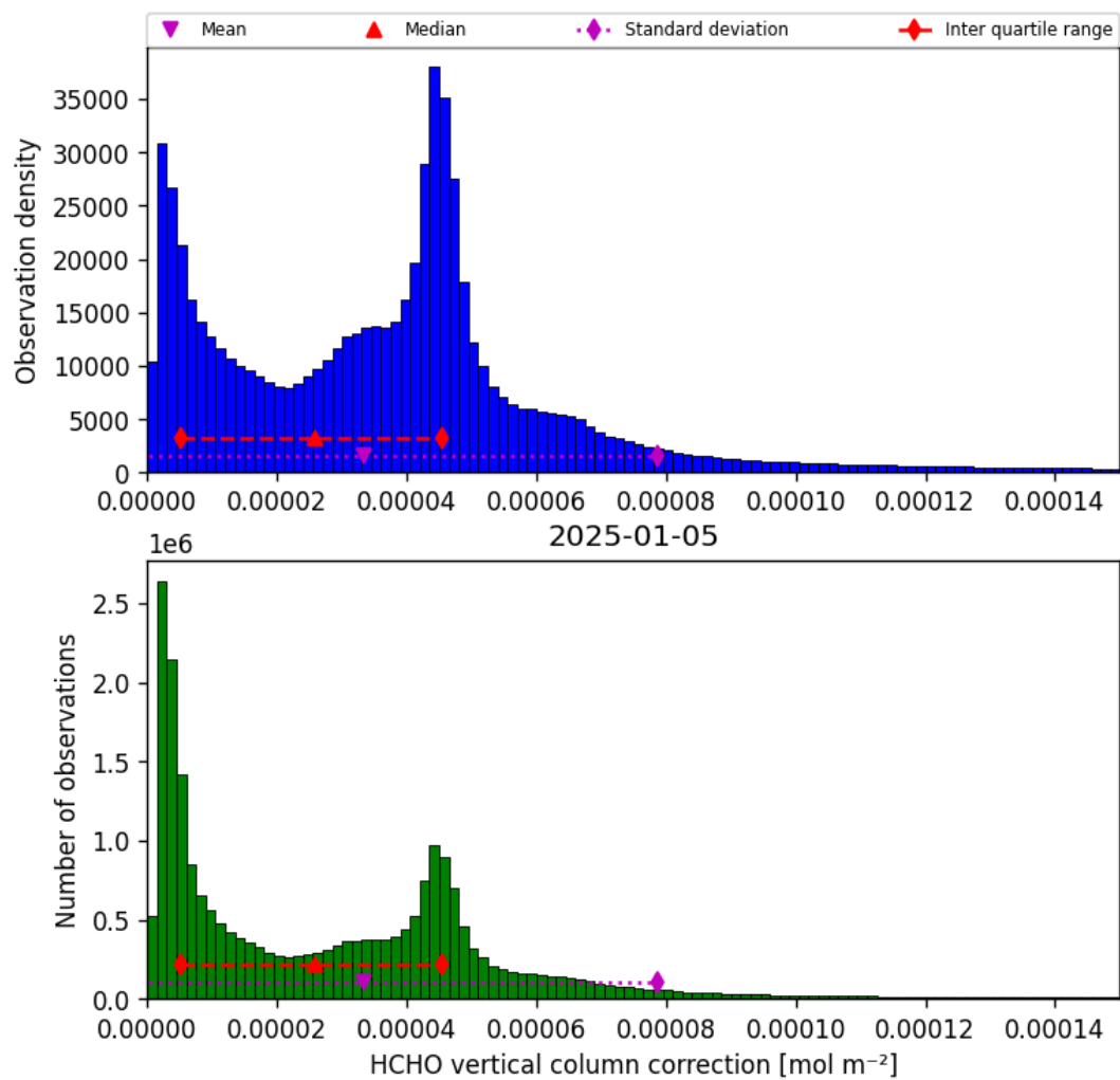
Figure 37: Histogram of “HCHO vertical column correction” for 2025-01-04 to 2025-01-06
