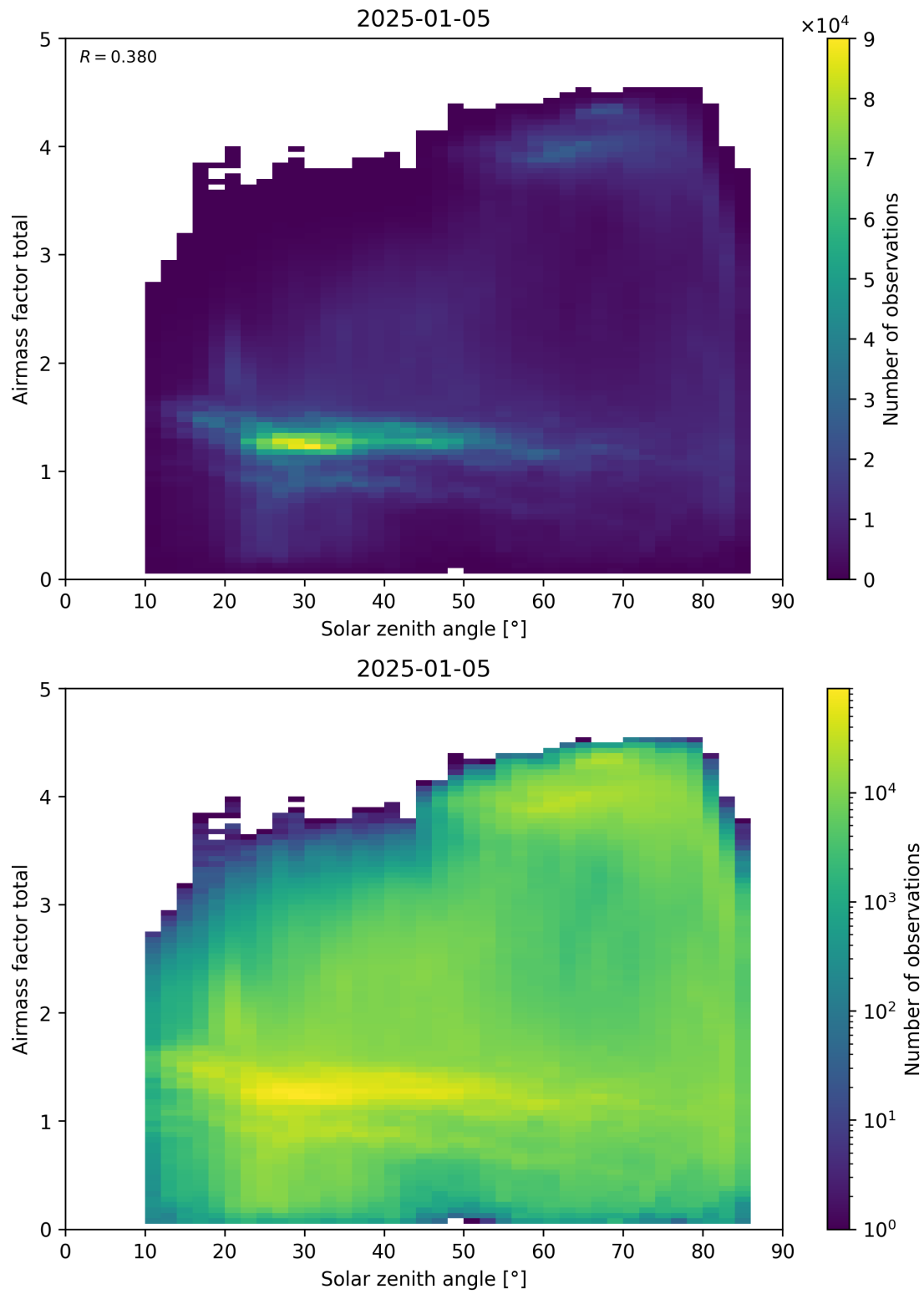
Figure 175: Scatter density plot of “Solar zenith angle” against “Airmass factor total” for 2025-01-04 to 2025-01-06.
