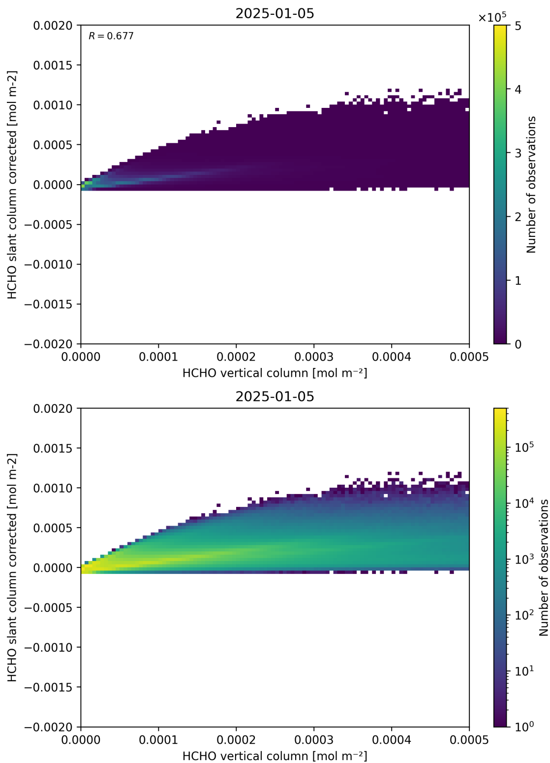
Figure 127: Scatter density plot of “HCHO vertical column” against “HCHO slant column corrected” for 2025-01-04 to 2025-01-06.
