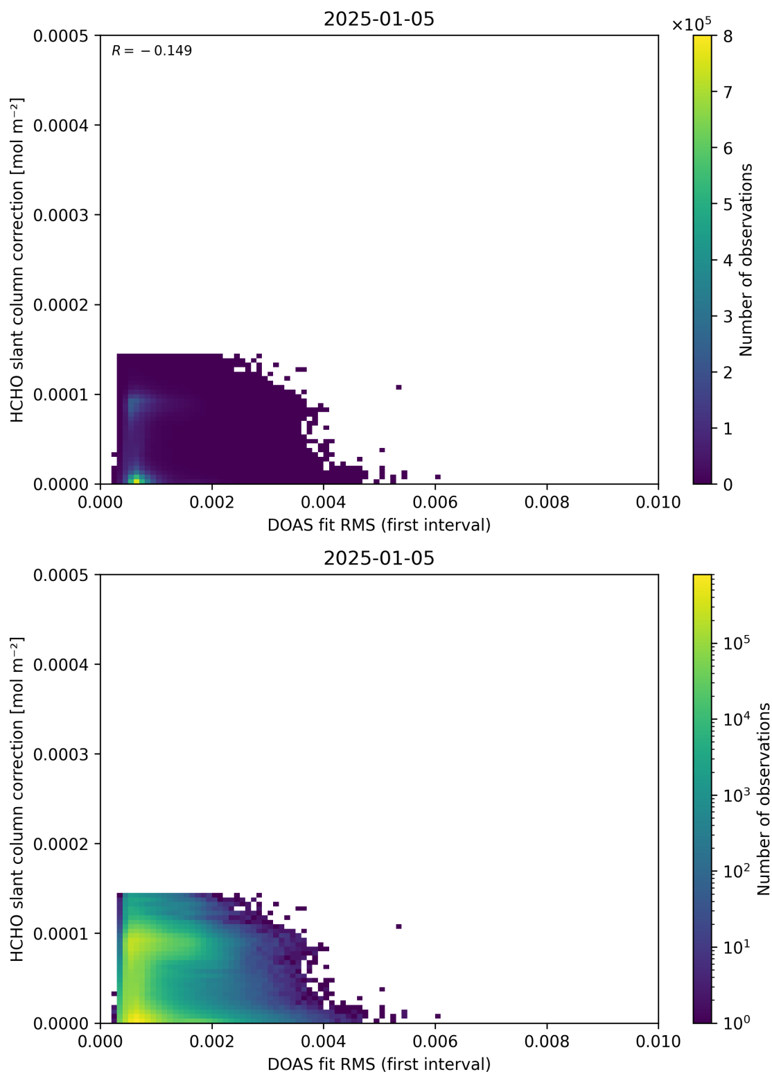
Figure 63: Scatter density plot of “DOAS fit RMS (first interval)” against “HCHO slant column correction” for 2025-01-04 to 2025-01-06.
