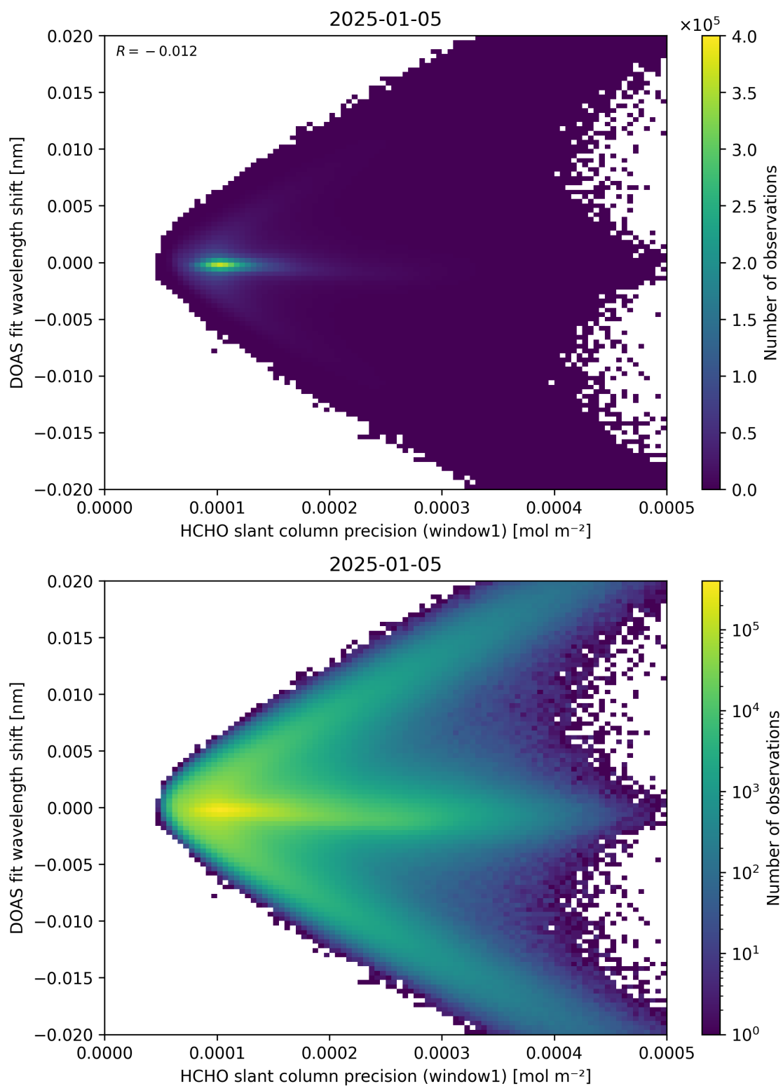
Figure 89: Scatter density plot of “HCHO slant column precision (window1)” against “DOAS fit wavelength shift” for 2025-01-04 to 2025-01-06.
