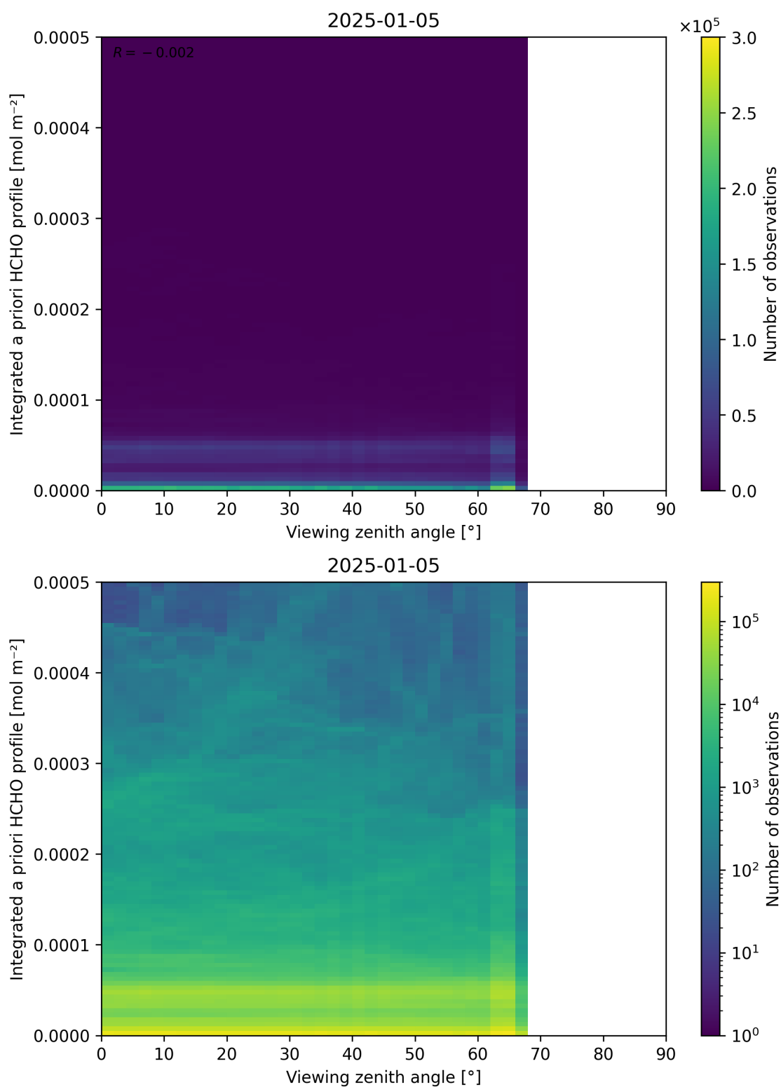
Figure 195: Scatter density plot of “Viewing zenith angle” against “Integrated a priori HCHO profile” for 2025-01-04 to 2025-01-06.
