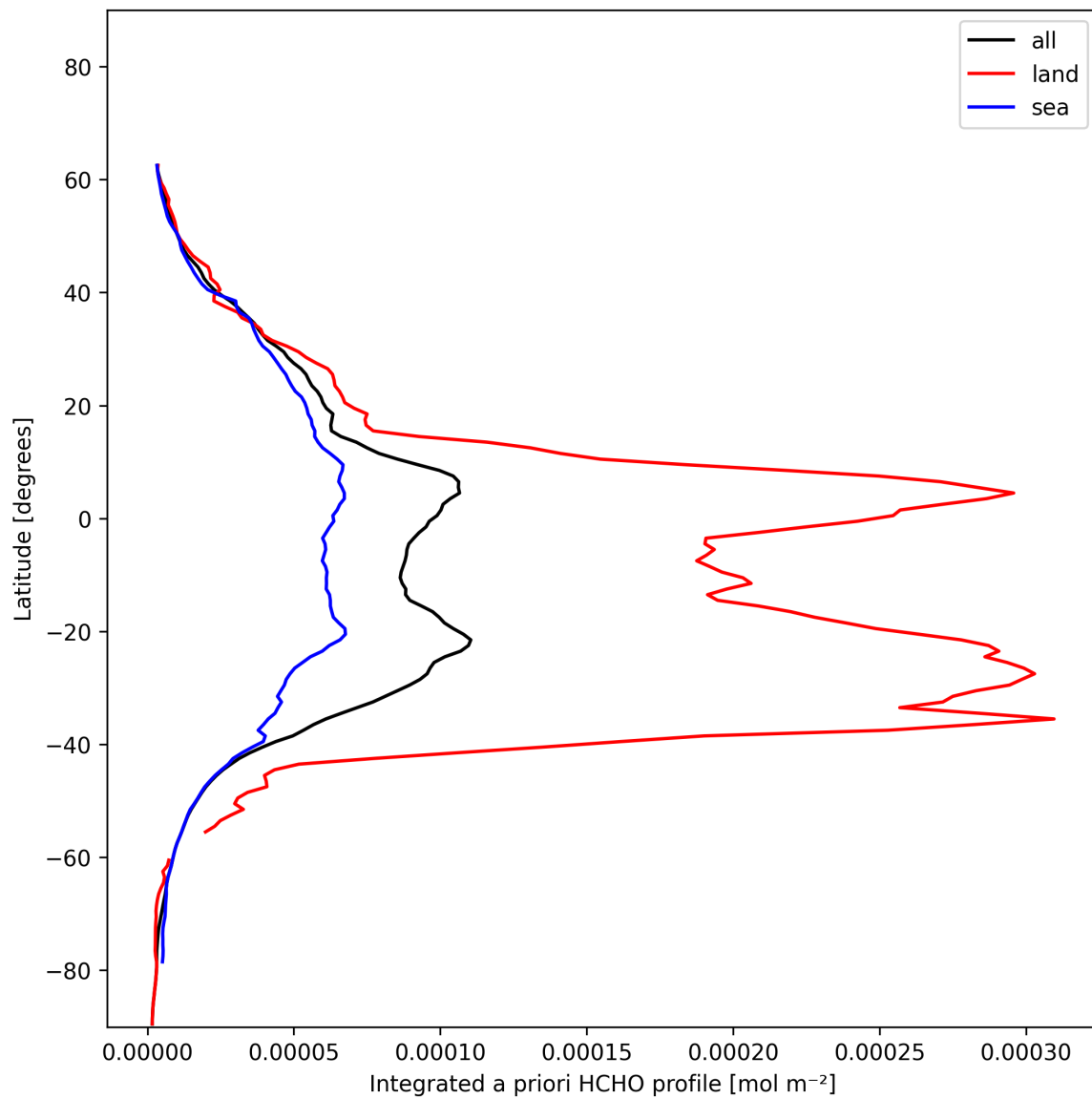
Figure 29: Zonal average of “Integrated a priori HCHO profile” for 2025-01-04 to 2025-01-06.
