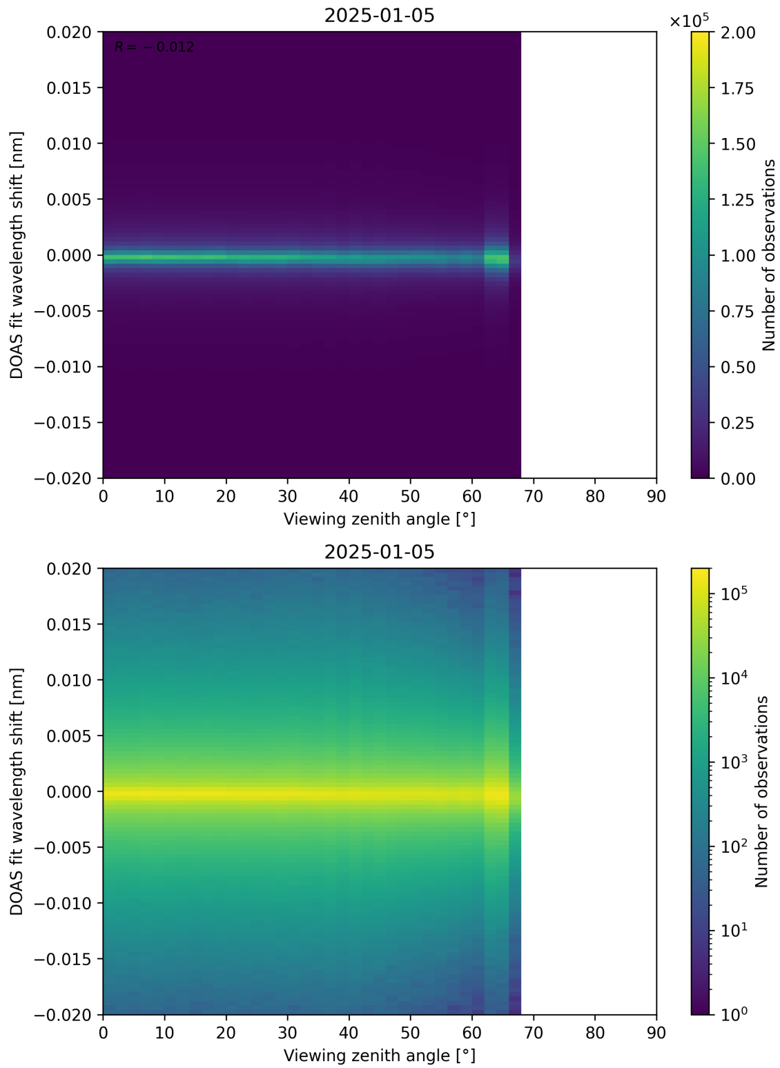
Figure 183: Scatter density plot of “Viewing zenith angle” against “DOAS fit wavelength shift” for 2025-01-04 to 2025-01-06.
