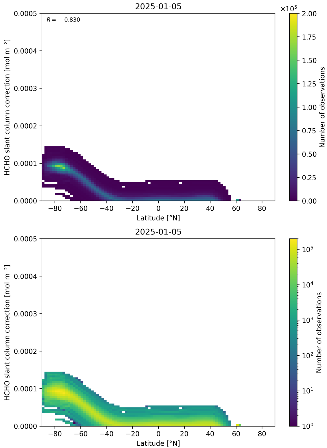
Figure 158: Scatter density plot of “Latitude” against “HCHO slant column correction” for 2025-01-04 to 2025-01-06.
