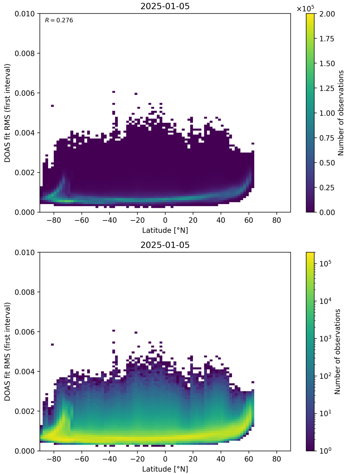
Figure 153: Scatter density plot of “Latitude” against “DOAS fit RMS (first interval)” for 2025-01-04 to 2025-01-06.
