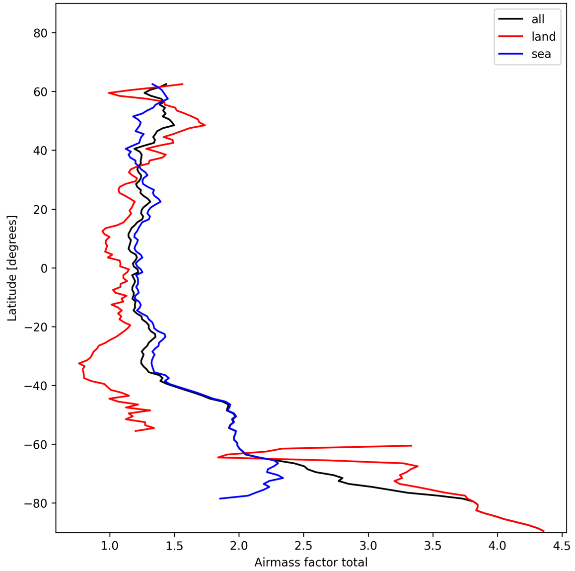
Figure 26: Zonal average of “Airmass factor total” for 2025-01-04 to 2025-01-06.
