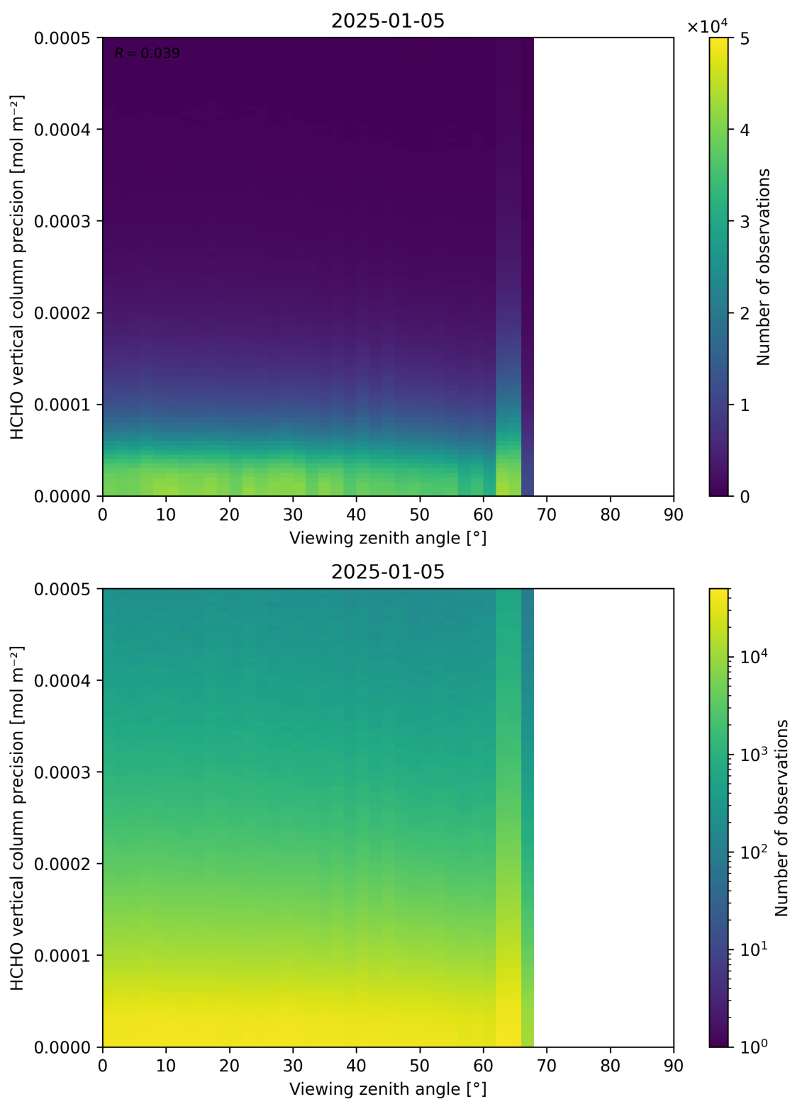
Figure 194: Scatter density plot of “Viewing zenith angle” against “HCHO vertical column precision” for 2025-01-04 to 2025-01-06.
