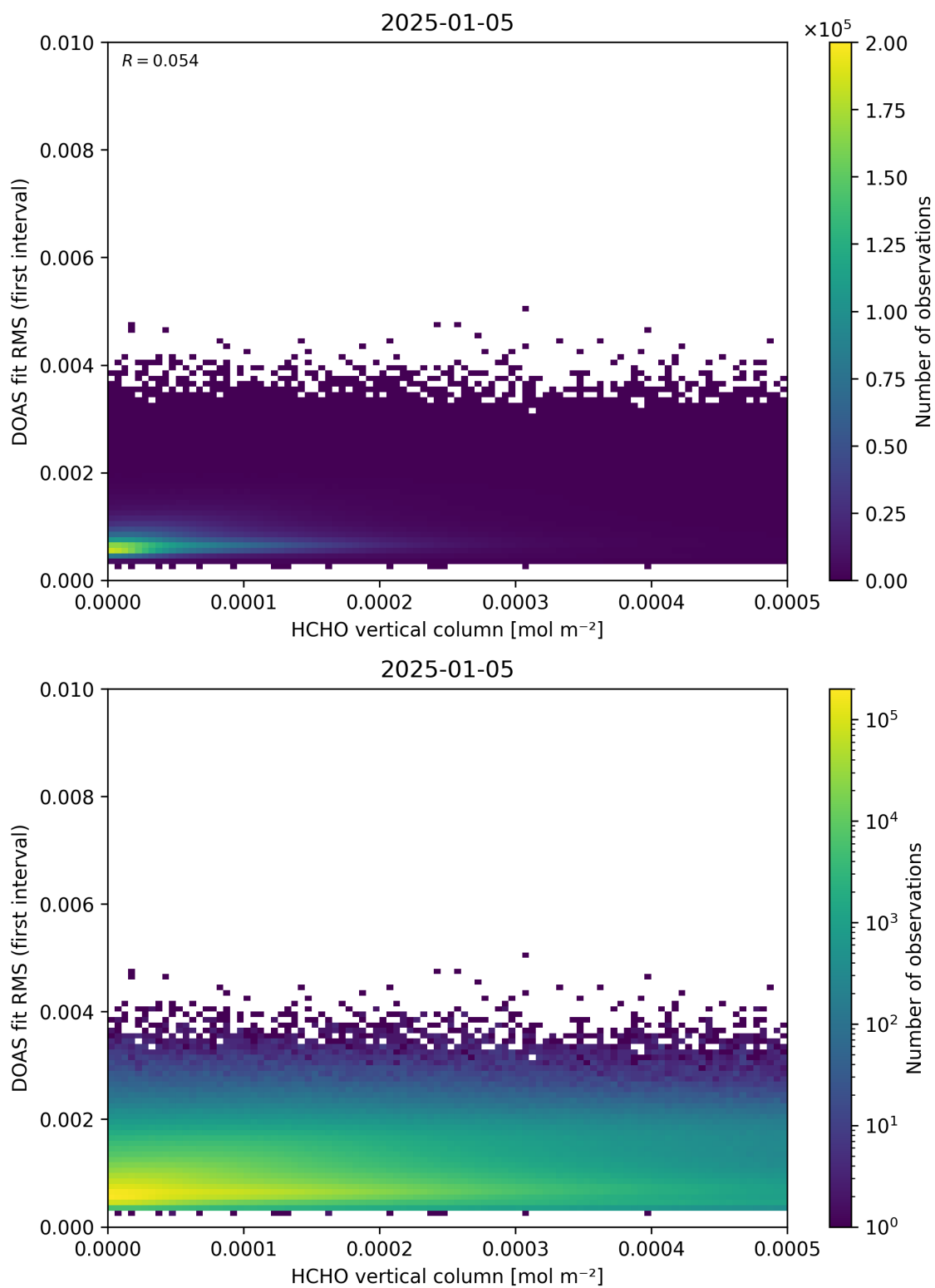
Figure 123: Scatter density plot of “HCHO vertical column” against “DOAS fit RMS (first interval)” for 2025-01-04 to 2025-01-06.
