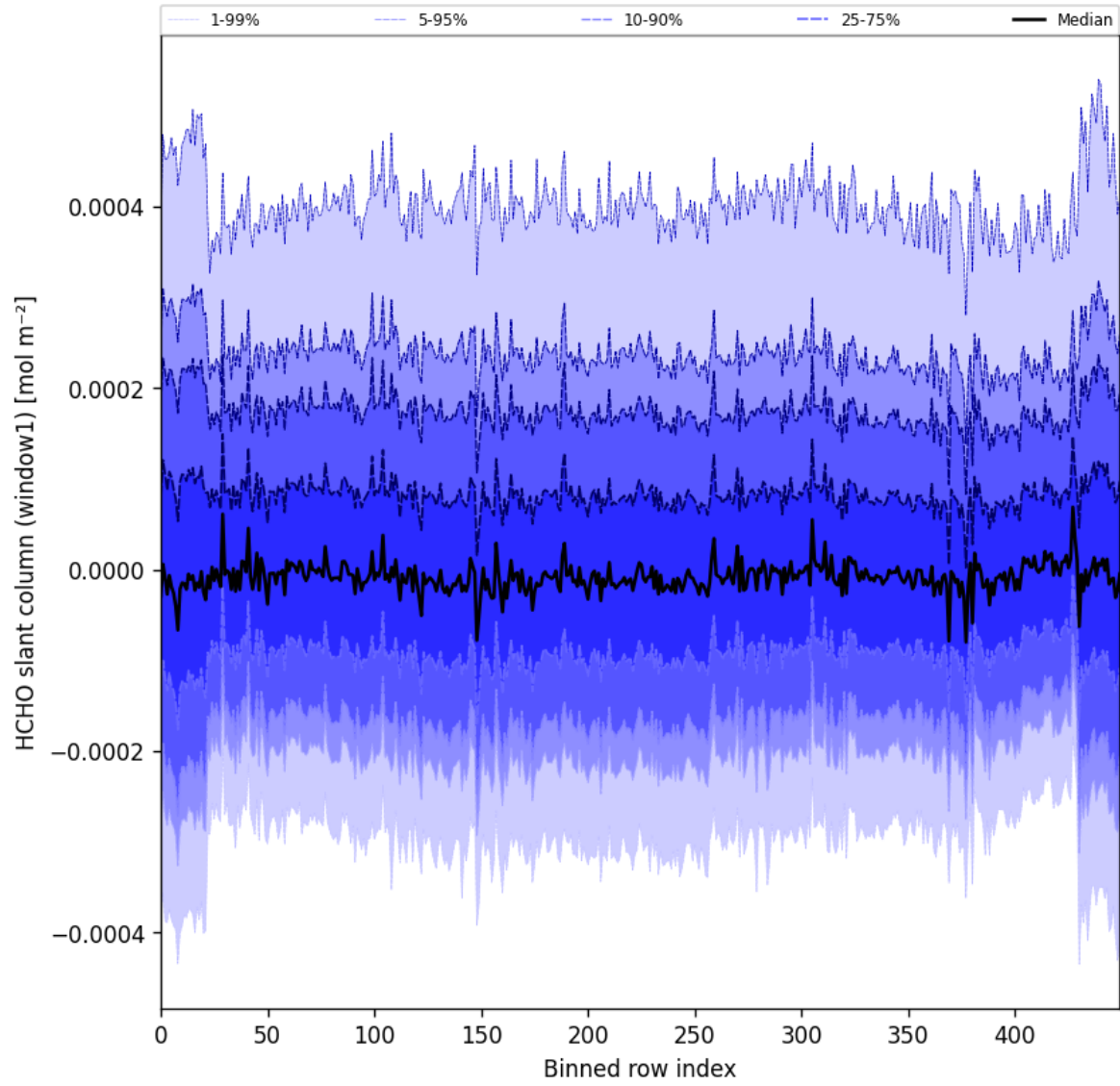
Figure 52: Along track statistics of “HCHO slant column (window1)” for 2025-01-04 to 2025-01-06
