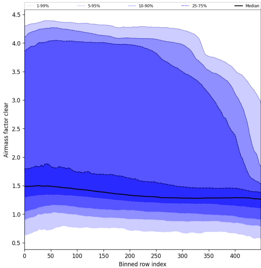
Figure 56: Along track statistics of “Airmass factor clear” for 2025-01-04 to 2025-01-06
