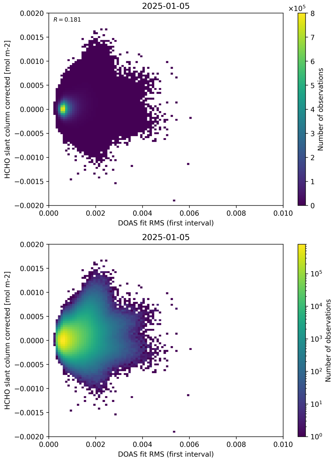
Figure 62: Scatter density plot of “DOAS fit RMS (first interval)” against “HCHO slant column corrected” for 2025-01-04 to 2025-01-06.
