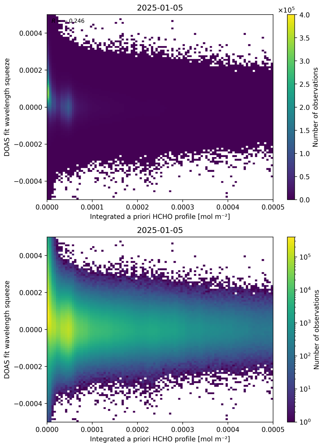
Figure 150: Scatter density plot of “Integrated a priori HCHO profile” against “DOAS fit wavelength squeeze” for 2025-01-04 to 2025-01-06.
