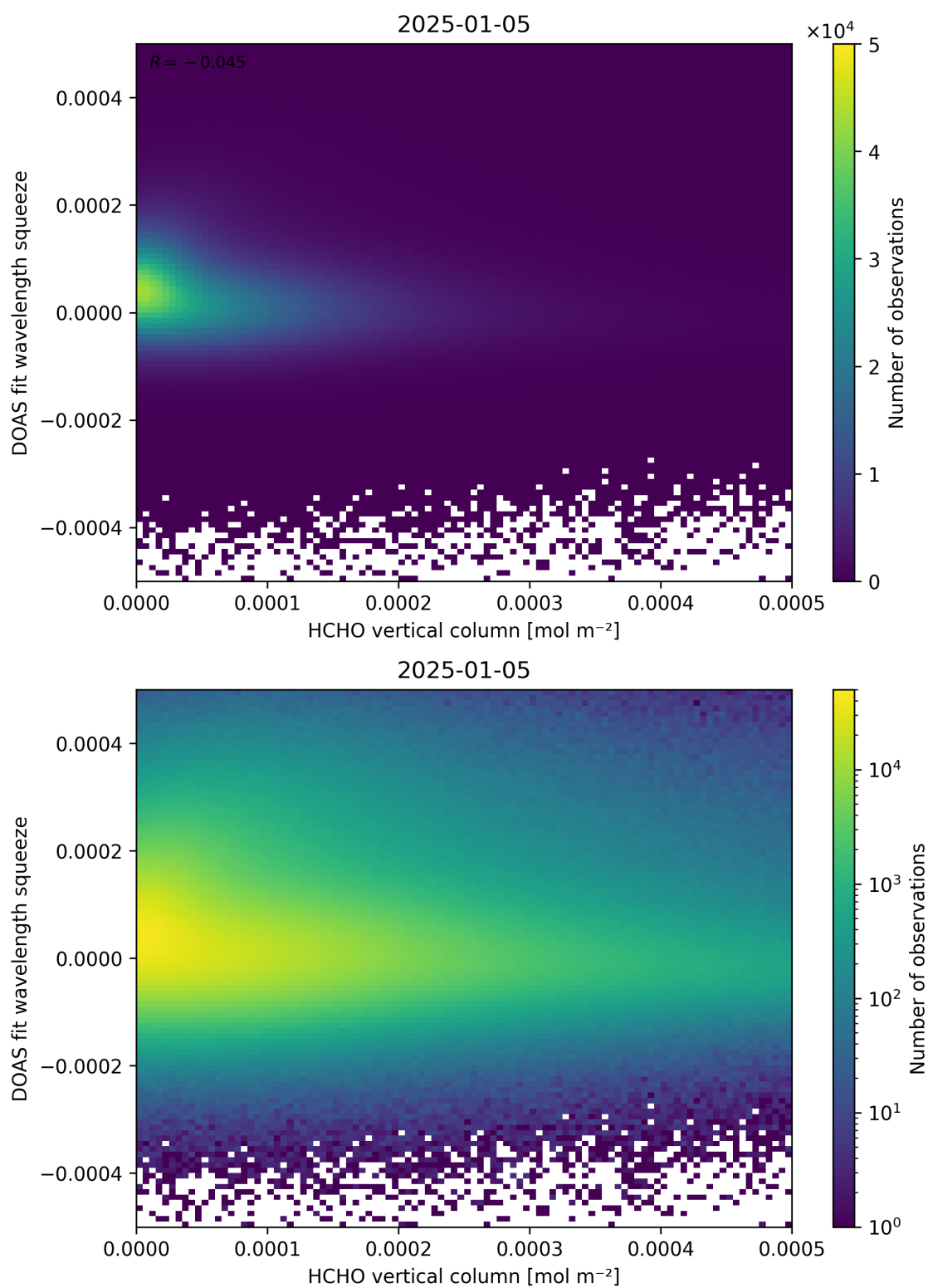
Figure 125: Scatter density plot of “HCHO vertical column” against “DOAS fit wavelength squeeze” for 2025-01-04 to 2025-01-06.
