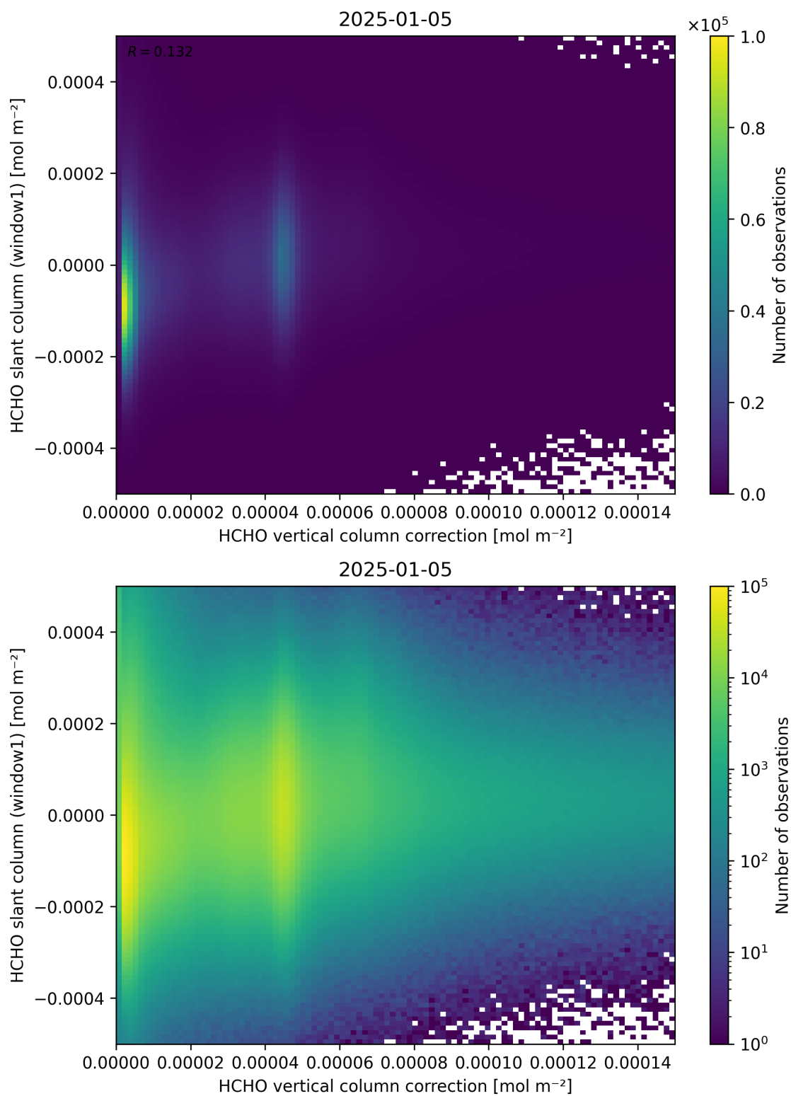
Figure 118: Scatter density plot of “HCHO vertical column correction” against “HCHO slant column (window1)” for 2025-01-04 to 2025-01-06.
