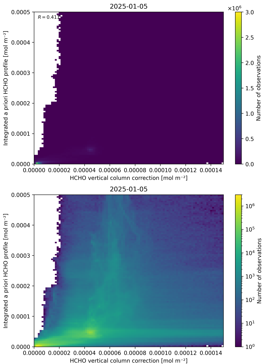
Figure 122: Scatter density plot of “HCHO vertical column correction” against “Integrated a priori HCHO profile” for 2025-01-04 to 2025-01-06.
