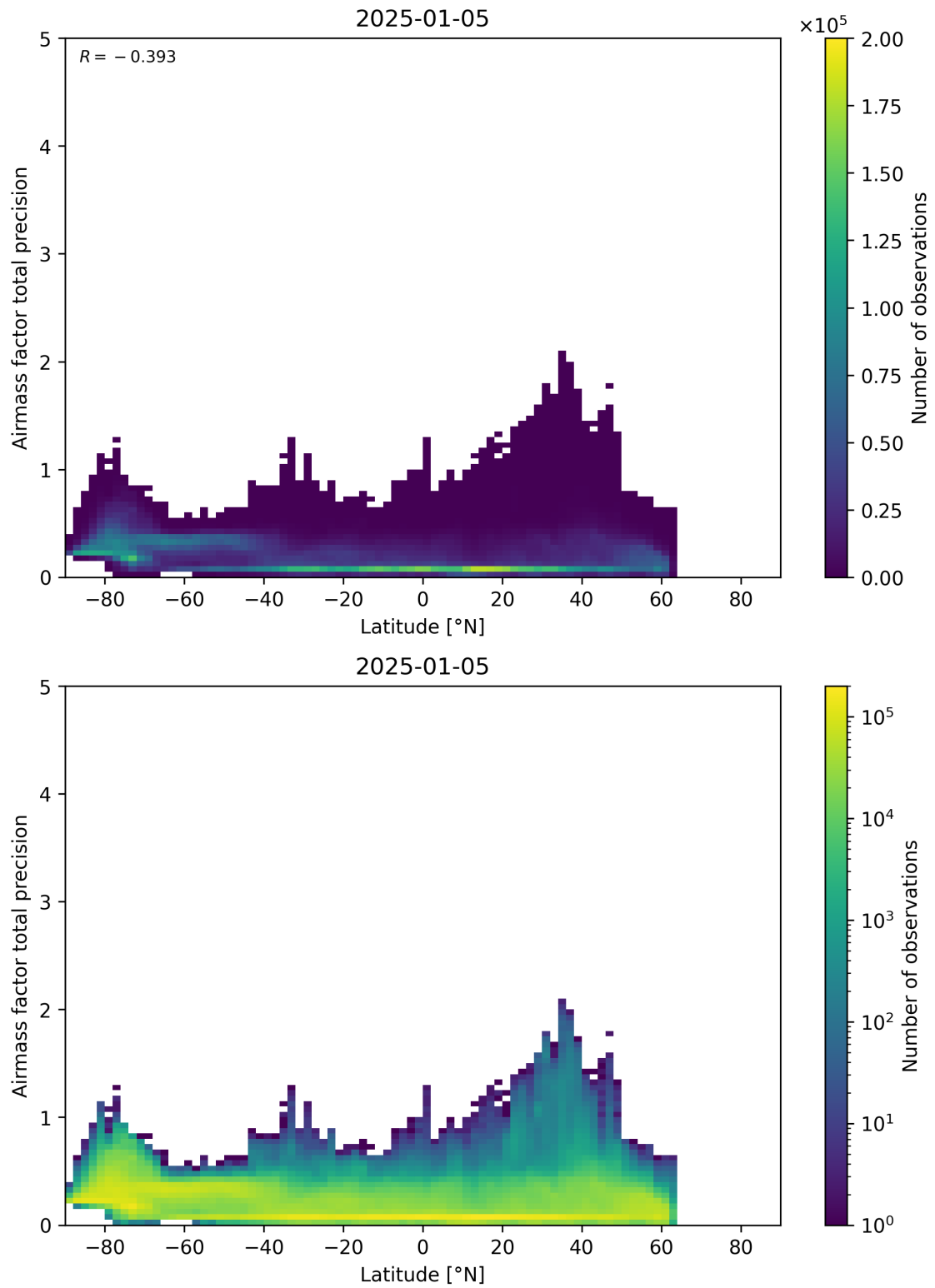
Figure 162: Scatter density plot of “Latitude” against “Airmass factor total precision” for 2025-01-04 to 2025-01-06.
