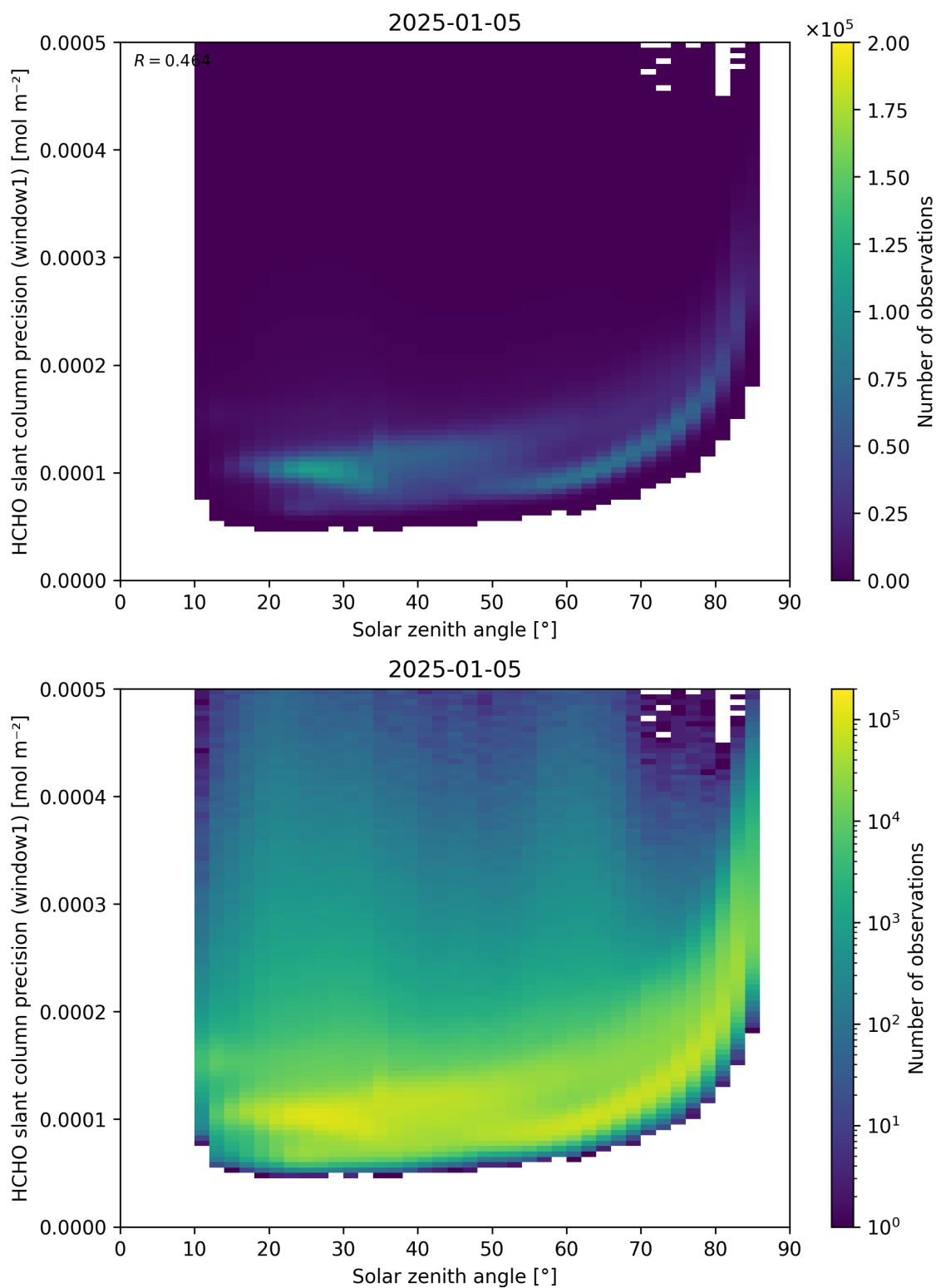
Figure 174: Scatter density plot of “Solar zenith angle” against “HCHO slant column precision (window1)” for 2025-01-04 to 2025-01-06.
