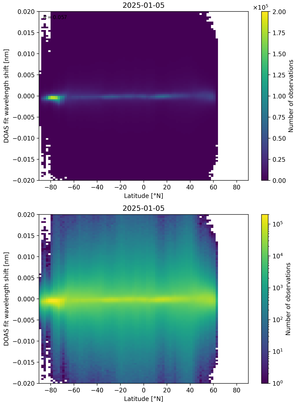
Figure 154: Scatter density plot of “Latitude” against “DOAS fit wavelength shift” for 2025-01-04 to 2025-01-06.
