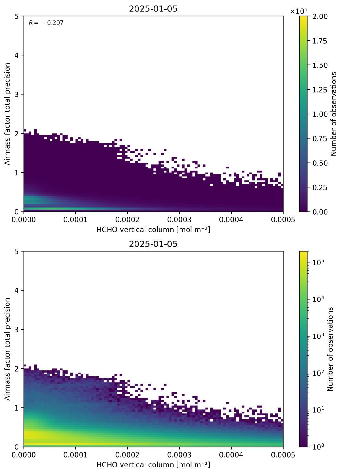
Figure 132: Scatter density plot of “HCHO vertical column” against “Airmass factor total precision” for 2025-01-04 to 2025-01-06.
