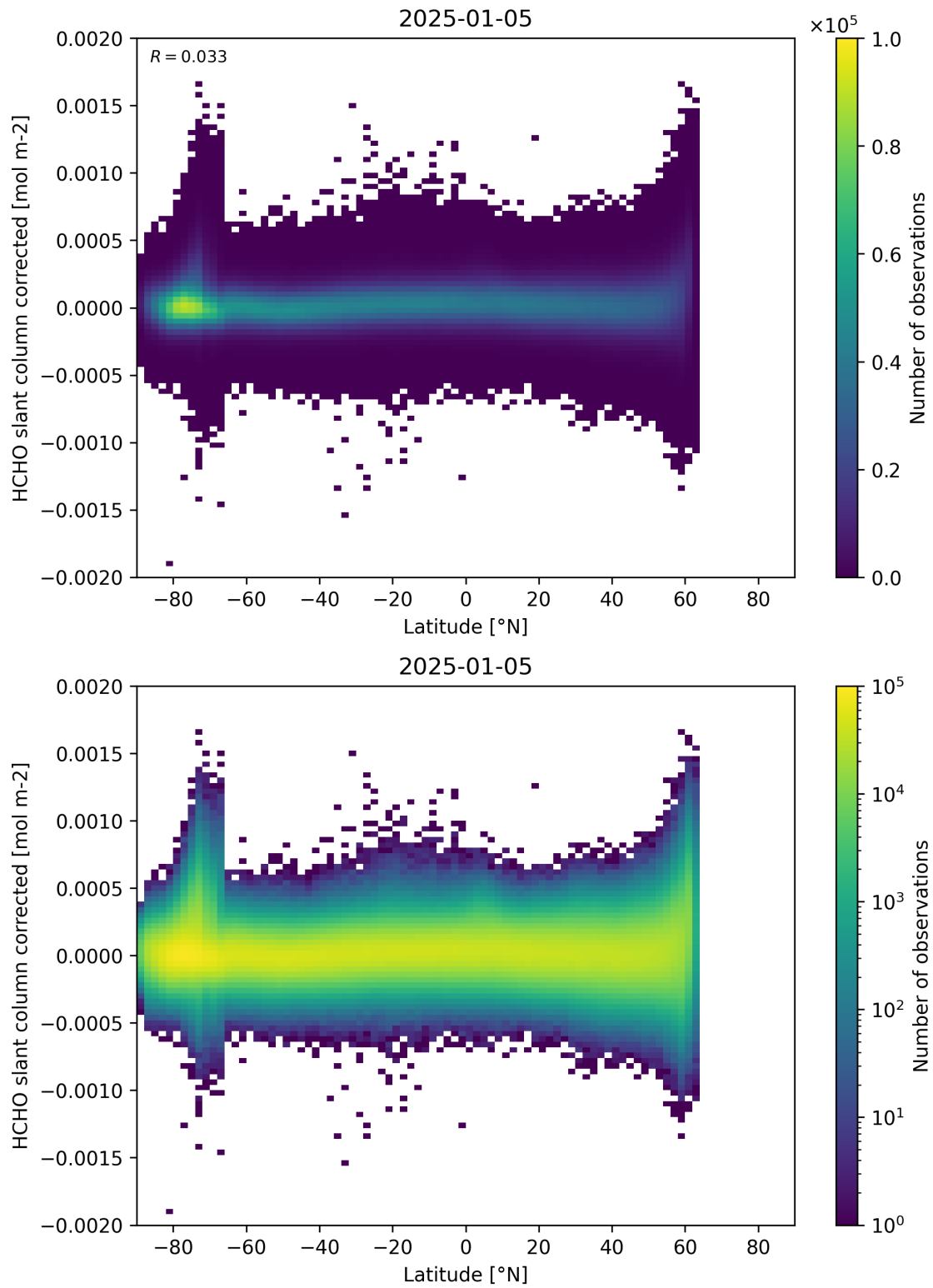
Figure 157: Scatter density plot of “Latitude” against “HCHO slant column corrected” for 2025-01-04 to 2025-01-06.
