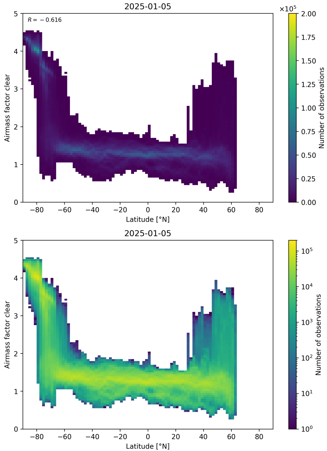
Figure 156: Scatter density plot of “Latitude” against “Airmass factor clear” for 2025-01-04 to 2025-01-06.
