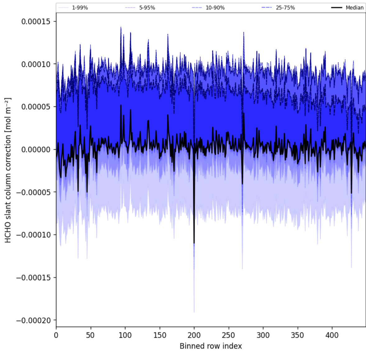
Figure 61: Along track statistics of “HCHO slant column correction” for 2025-01-04 to 2025-01-06
