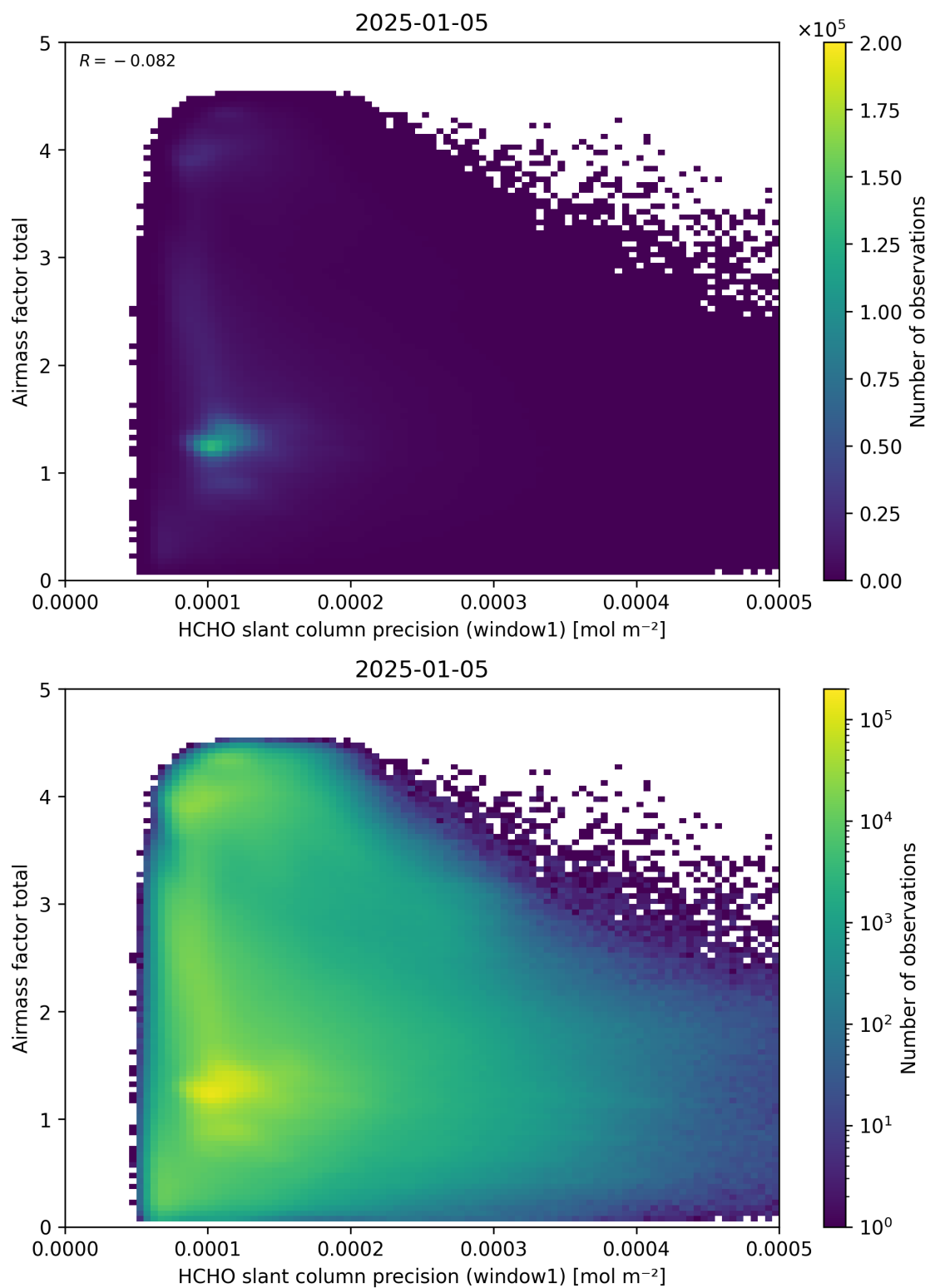
Figure 94: Scatter density plot of “HCHO slant column precision (window1)” against “Airmass factor total” for 2025-01-04 to 2025-01-06.
