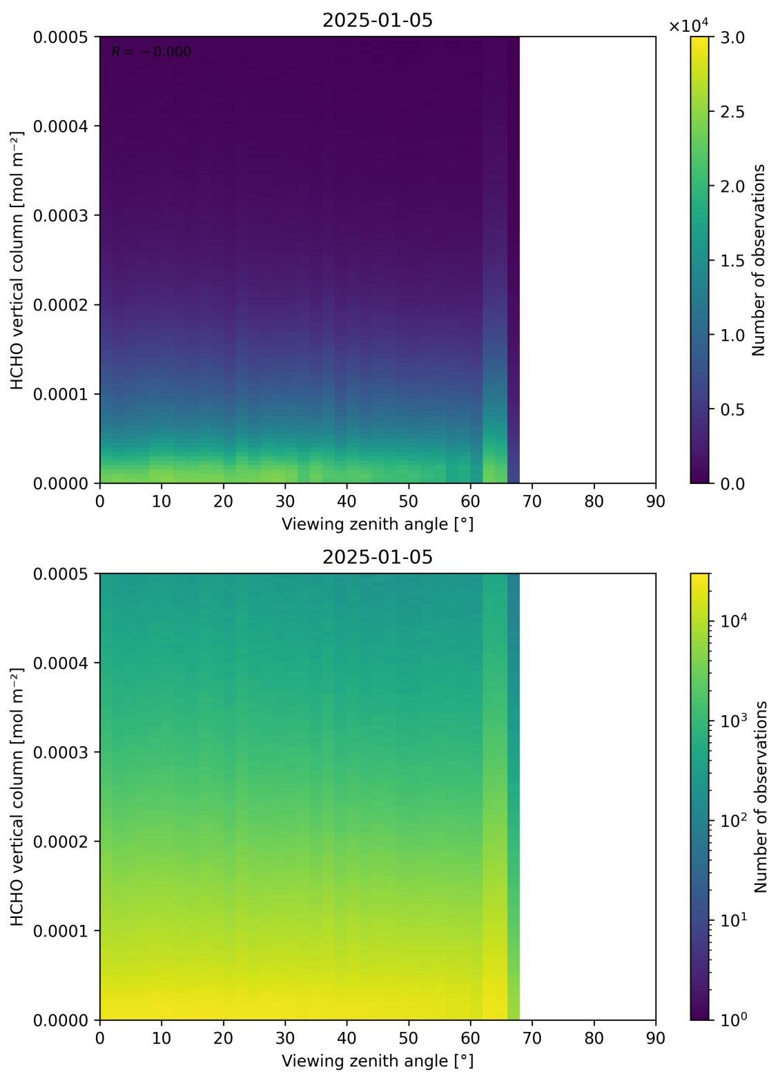
Figure 192: Scatter density plot of “Viewing zenith angle” against “HCHO vertical column” for 2025-01-04 to 2025-01-06.
