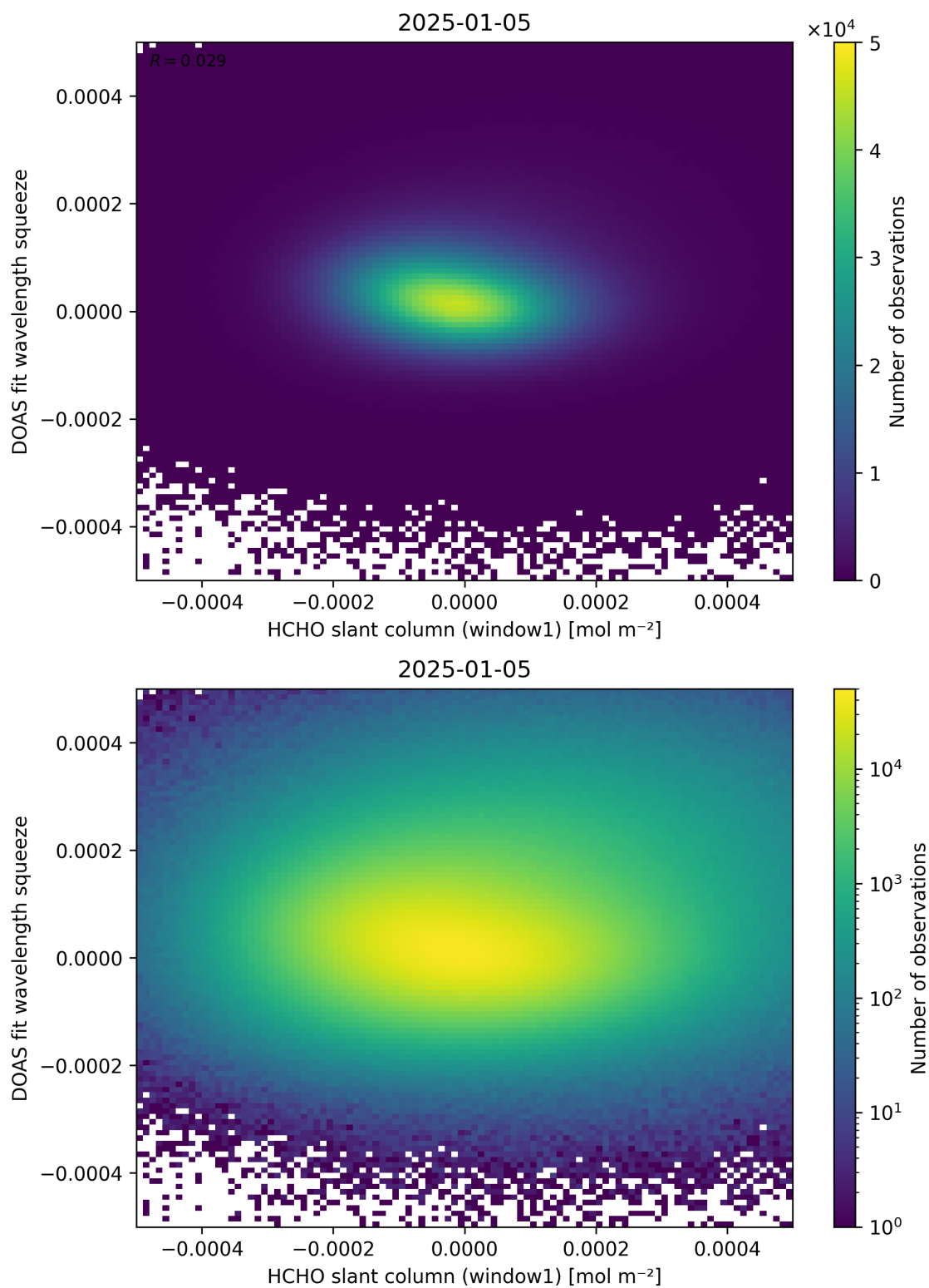
Figure 80: Scatter density plot of “HCHO slant column (window1)” against “DOAS fit wavelength squeeze” for 2025-01-04 to 2025-01-06.
