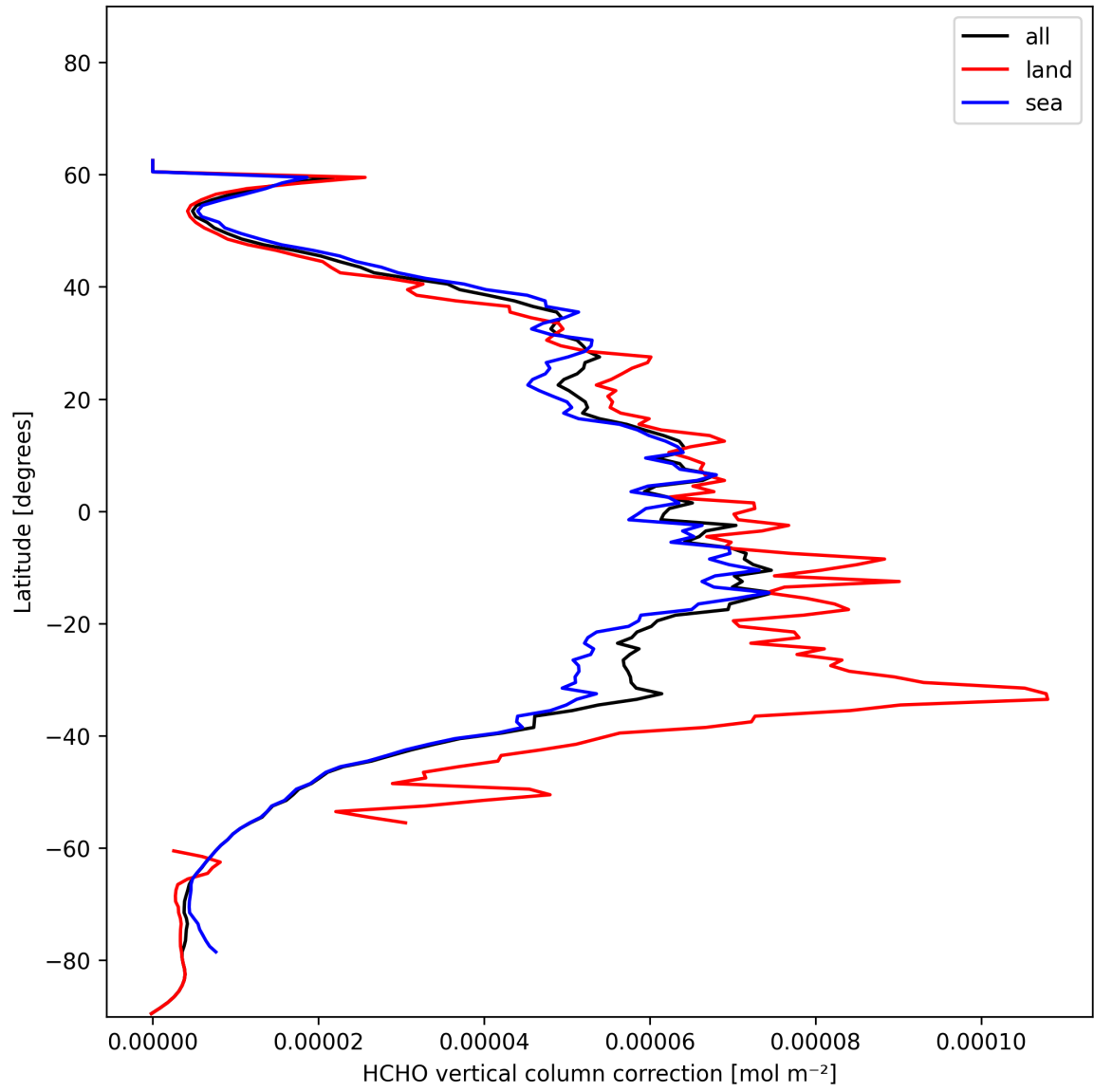
Figure 23: Zonal average of “HCHO vertical column correction” for 2025-01-04 to 2025-01-06.
