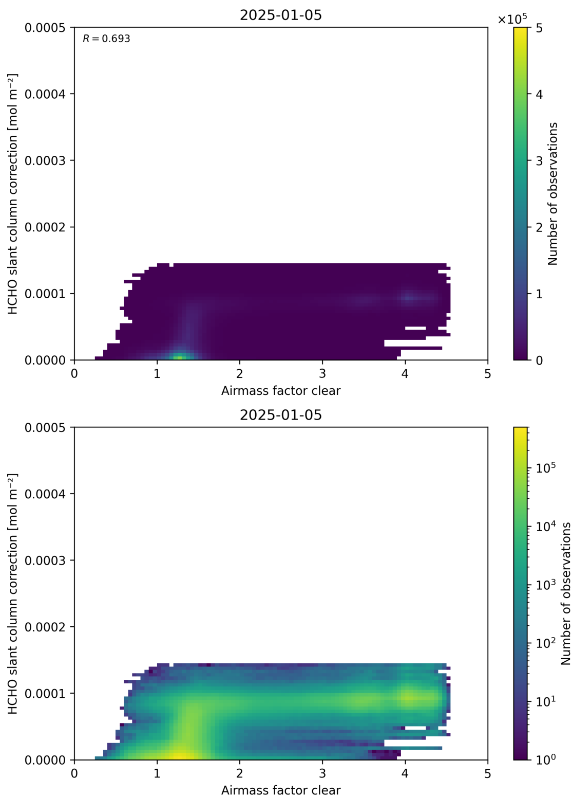
Figure 75: Scatter density plot of “Airmass factor clear” against “HCHO slant column correction” for 2025-01-04 to 2025-01-06.
