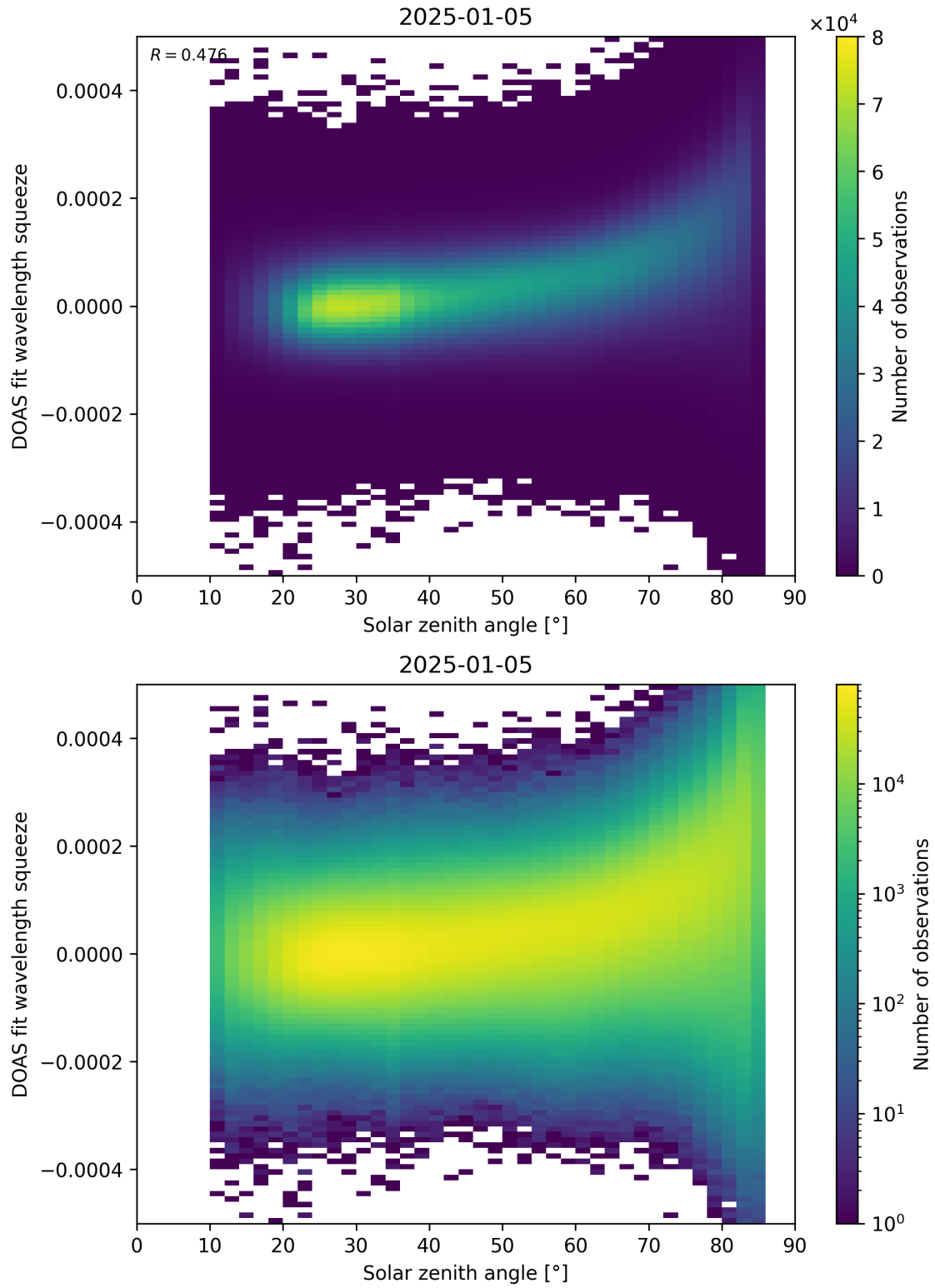
Figure 169: Scatter density plot of “Solar zenith angle” against “DOAS fit wavelength squeeze” for 2025-01-04 to 2025-01-06.
