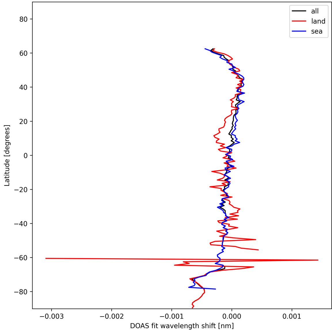
Figure 30: Zonal average of “DOAS fit wavelength shift” for 2025-01-04 to 2025-01-06.
