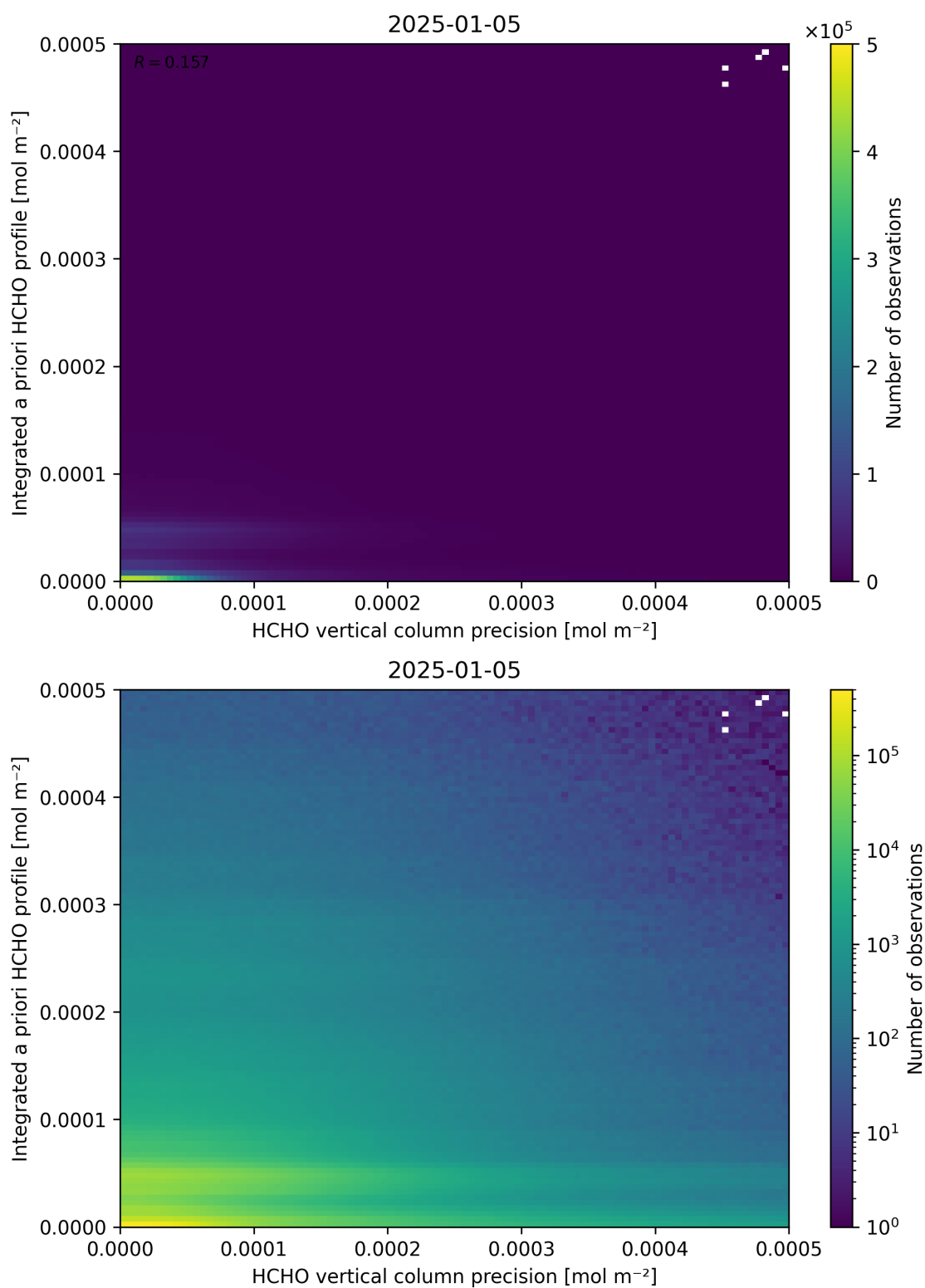
Figure 147: Scatter density plot of “HCHO vertical column precision” against “Integrated a priori HCHO profile” for 2025-01-04 to 2025-01-06.
