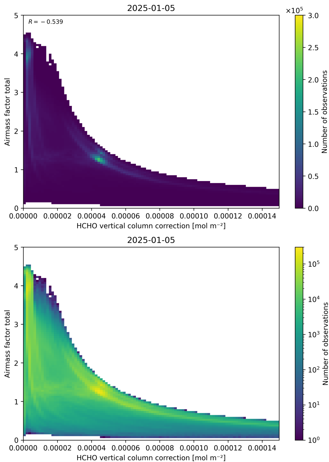
Figure 120: Scatter density plot of “HCHO vertical column correction” against “Airmass factor total” for 2025-01-04 to 2025-01-06.
