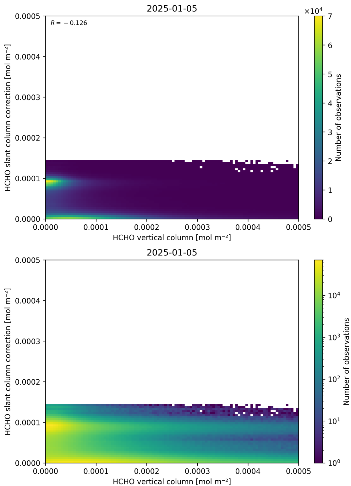
Figure 128: Scatter density plot of “HCHO vertical column” against “HCHO slant column correction” for 2025-01-04 to 2025-01-06.
