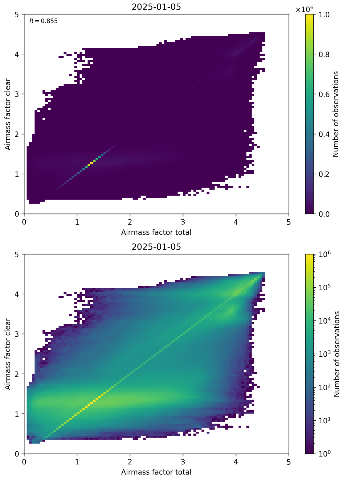
Figure 100: Scatter density plot of “Airmass factor total” against “Airmass factor clear” for 2025-01-04 to 2025-01-06.
