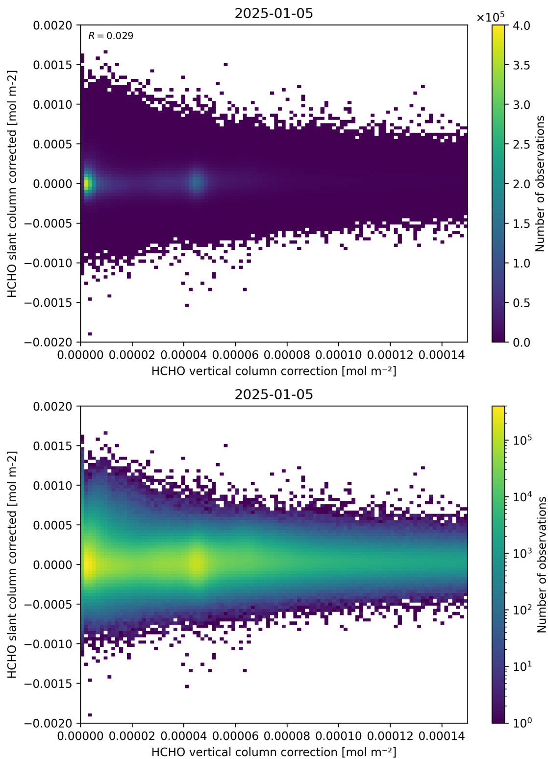
Figure 116: Scatter density plot of “HCHO vertical column correction” against “HCHO slant column corrected” for 2025-01-04 to 2025-01-06.
