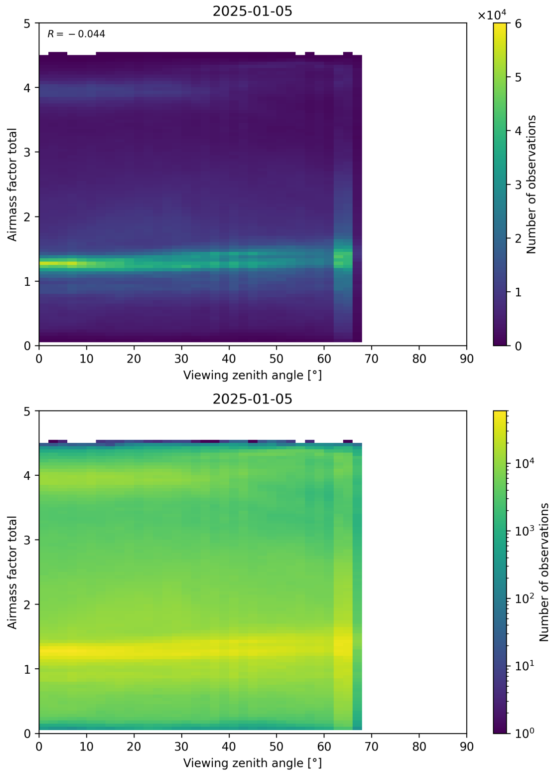
Figure 190: Scatter density plot of “Viewing zenith angle” against “Airmass factor total” for 2025-01-04 to 2025-01-06.
