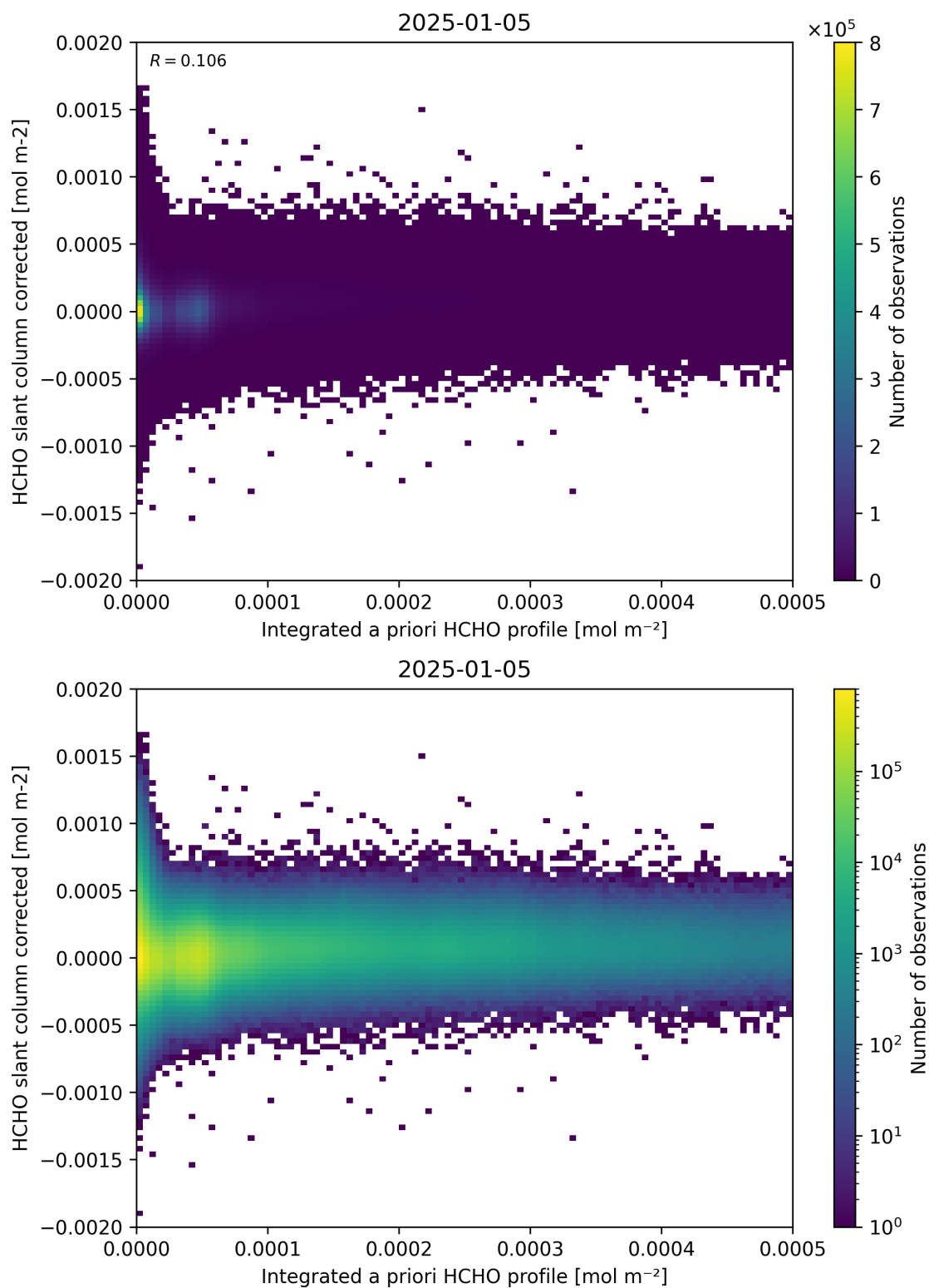
Figure 151: Scatter density plot of “Integrated a priori HCHO profile” against “HCHO slant column corrected” for 2025-01-04 to 2025-01-06.
