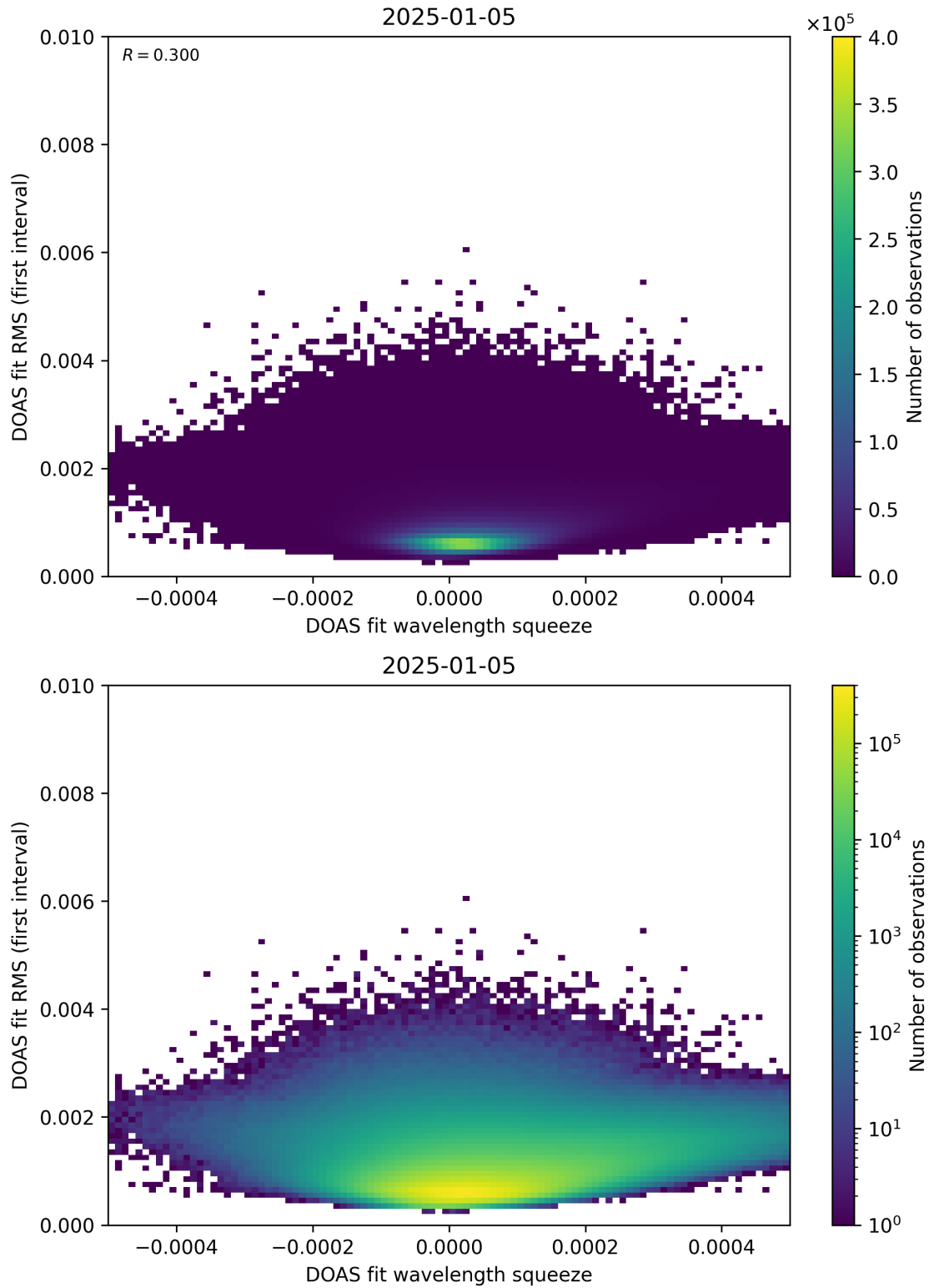
Figure 68: Scatter density plot of “DOAS fit wavelength squeeze” against “DOAS fit RMS (first interval)” for 2025-01-04 to 2025-01-06.
