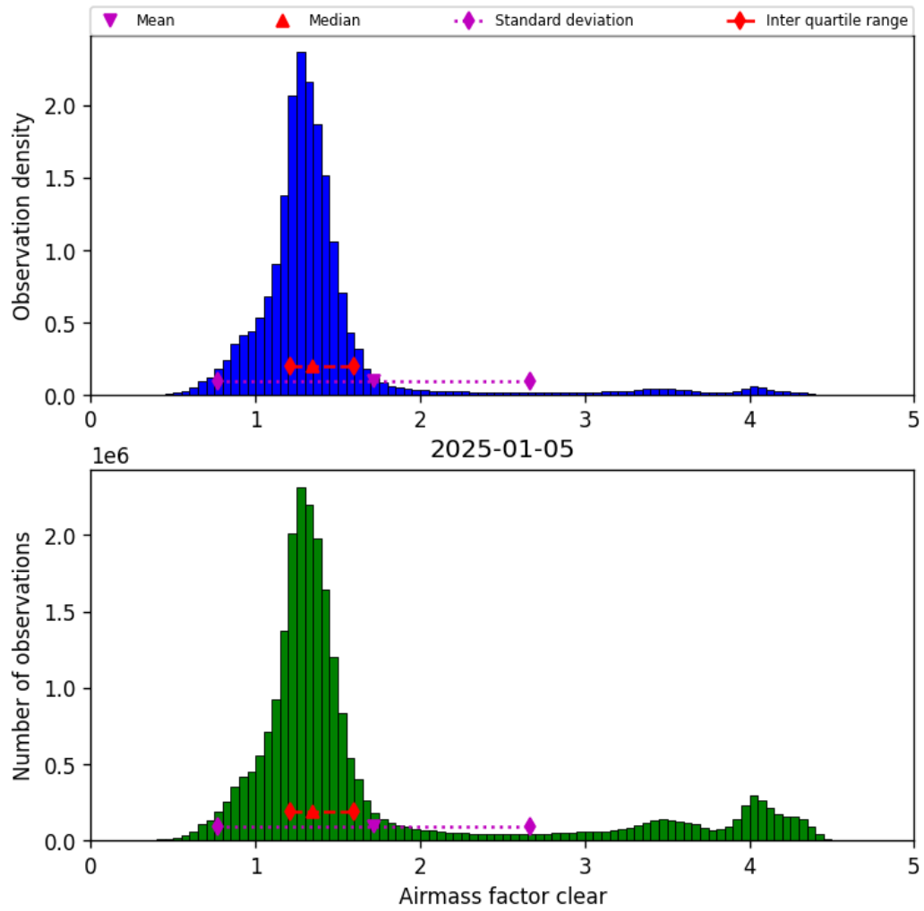
Figure 42: Histogram of “Airmass factor clear” for 2025-01-04 to 2025-01-06
