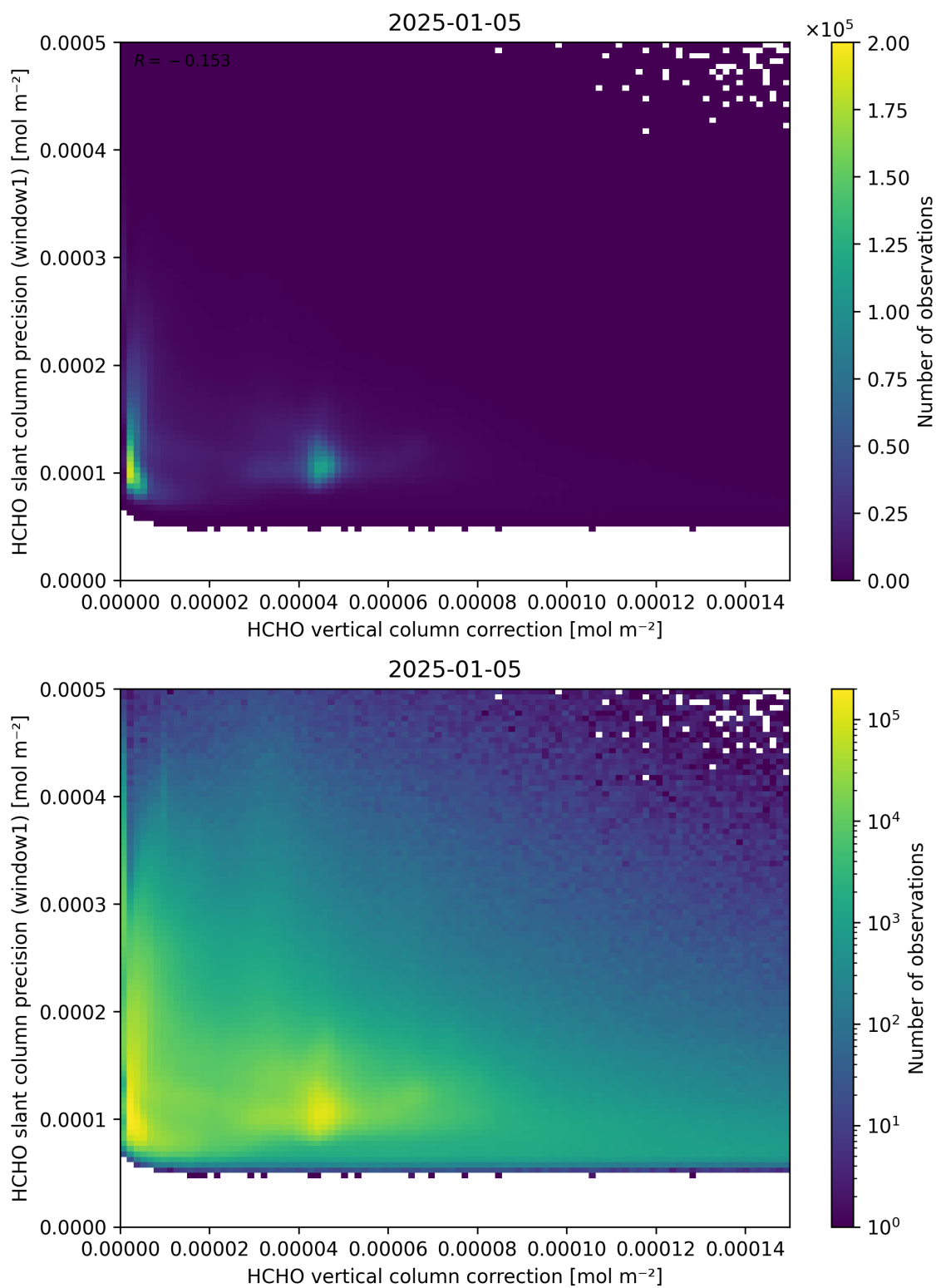
Figure 119: Scatter density plot of “HCHO vertical column correction” against “HCHO slant column precision (window1)” for 2025-01-04 to 2025-01-06.
