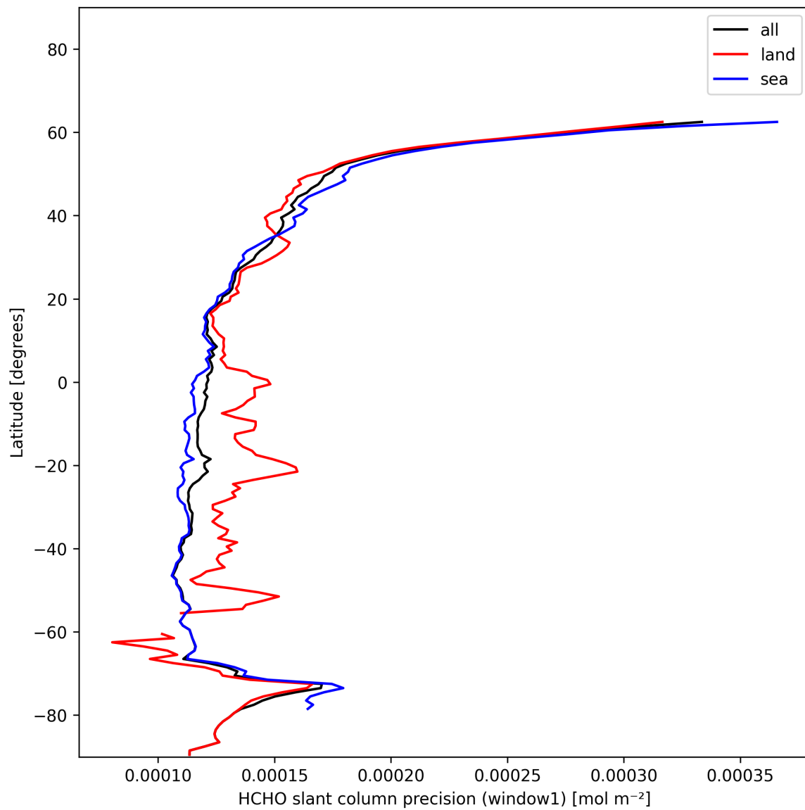
Figure 25: Zonal average of “HCHO slant column precision (window1)” for 2025-01-04 to 2025-01-06.
