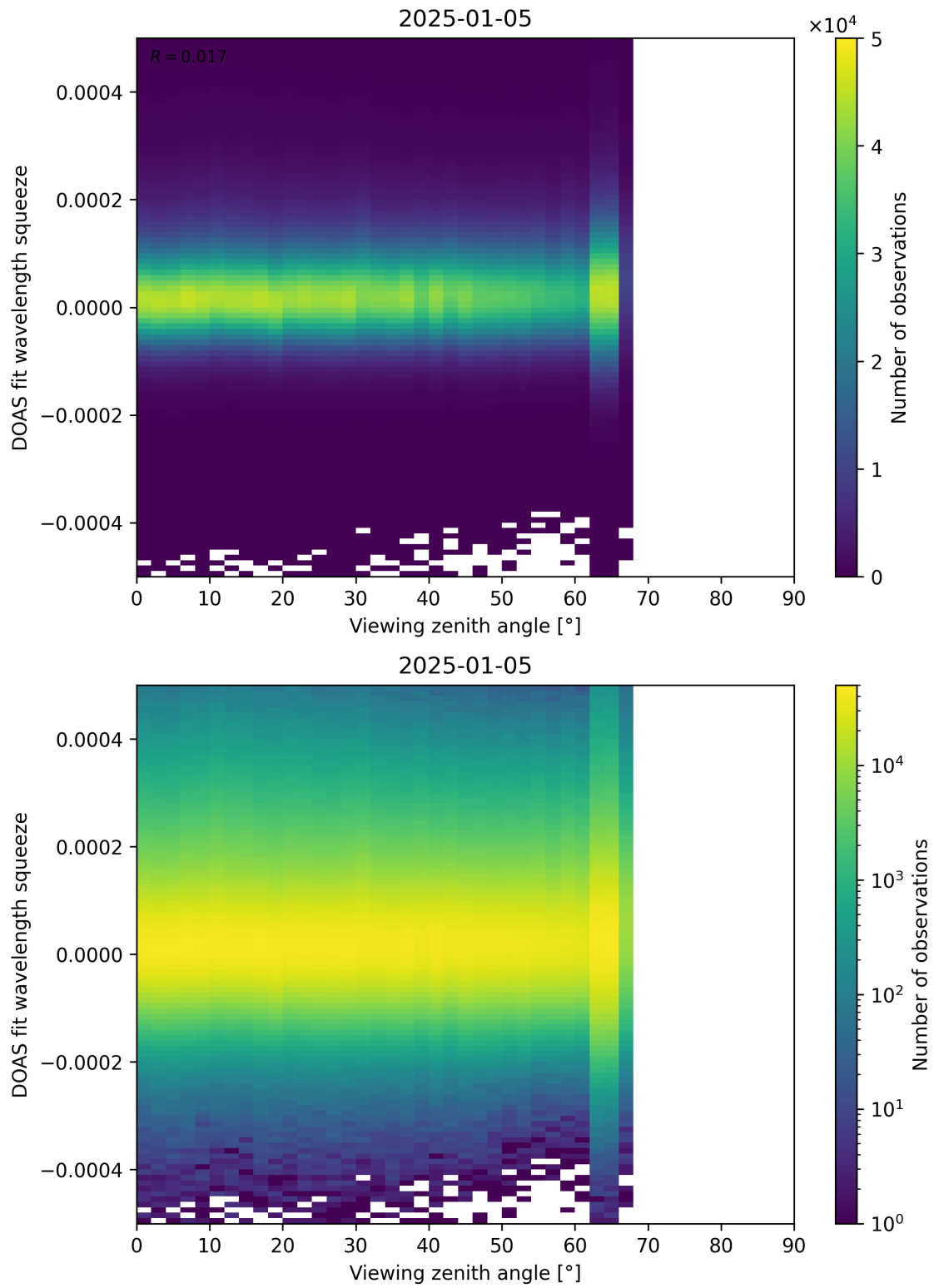
Figure 184: Scatter density plot of “Viewing zenith angle” against “DOAS fit wavelength squeeze” for 2025-01-04 to 2025-01-06.
