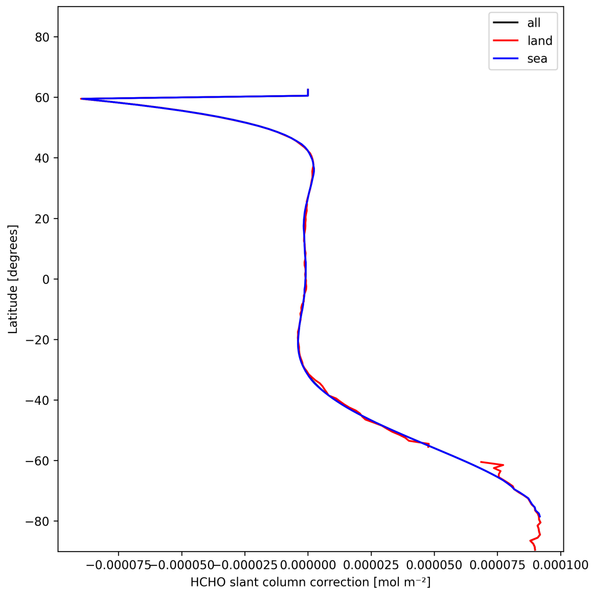
Figure 33: Zonal average of “HCHO slant column correction” for 2025-01-04 to 2025-01-06.
