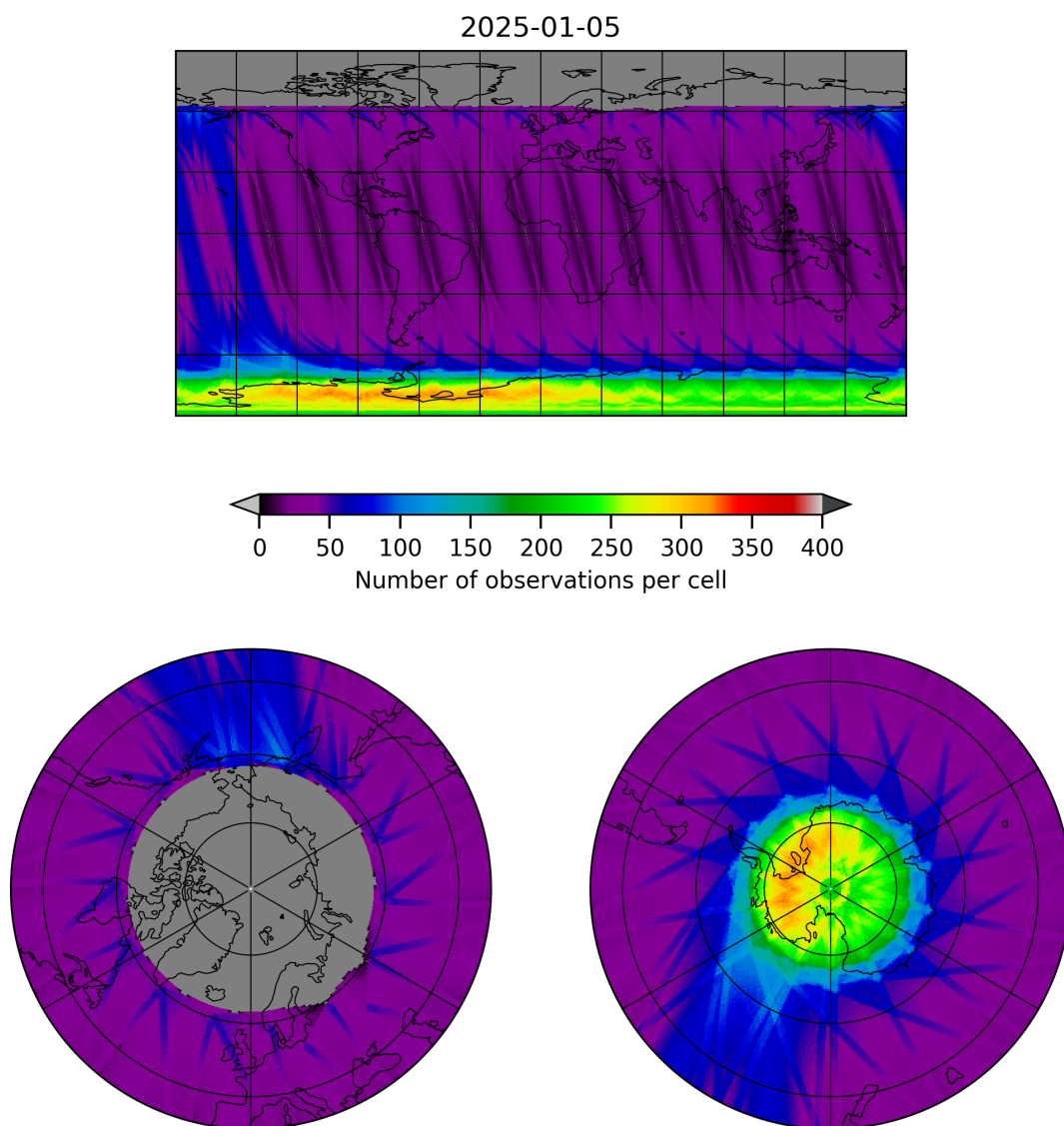
Figure 19: Map of the number of observations for 2025-01-04 to 2025-01-06
