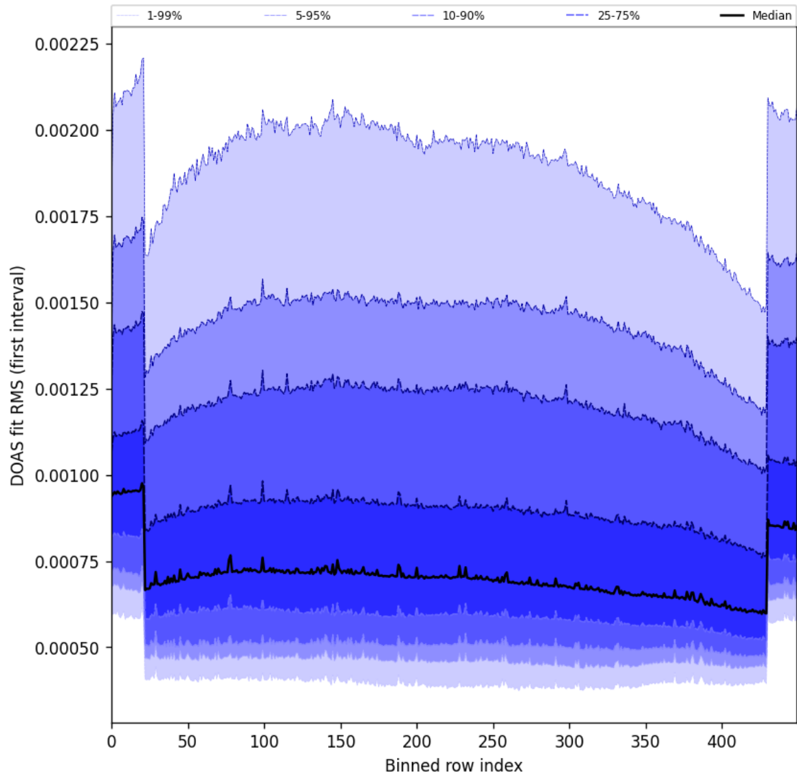
Figure 60: Along track statistics of “DOAS fit RMS (first interval)” for 2025-01-04 to 2025-01-06
