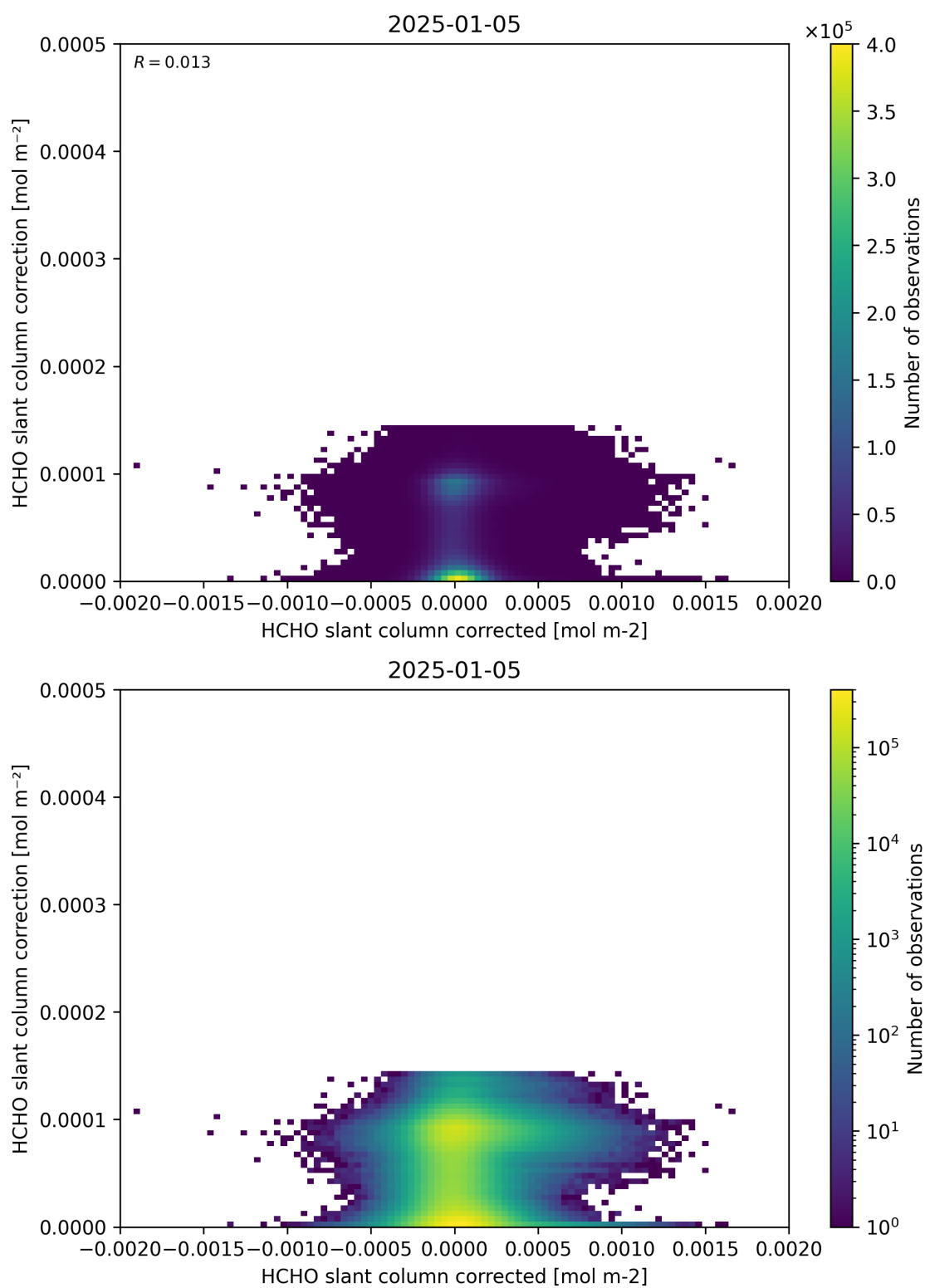
Figure 77: Scatter density plot of “HCHO slant column corrected” against “HCHO slant column correction” for 2025-01-04 to 2025-01-06.
