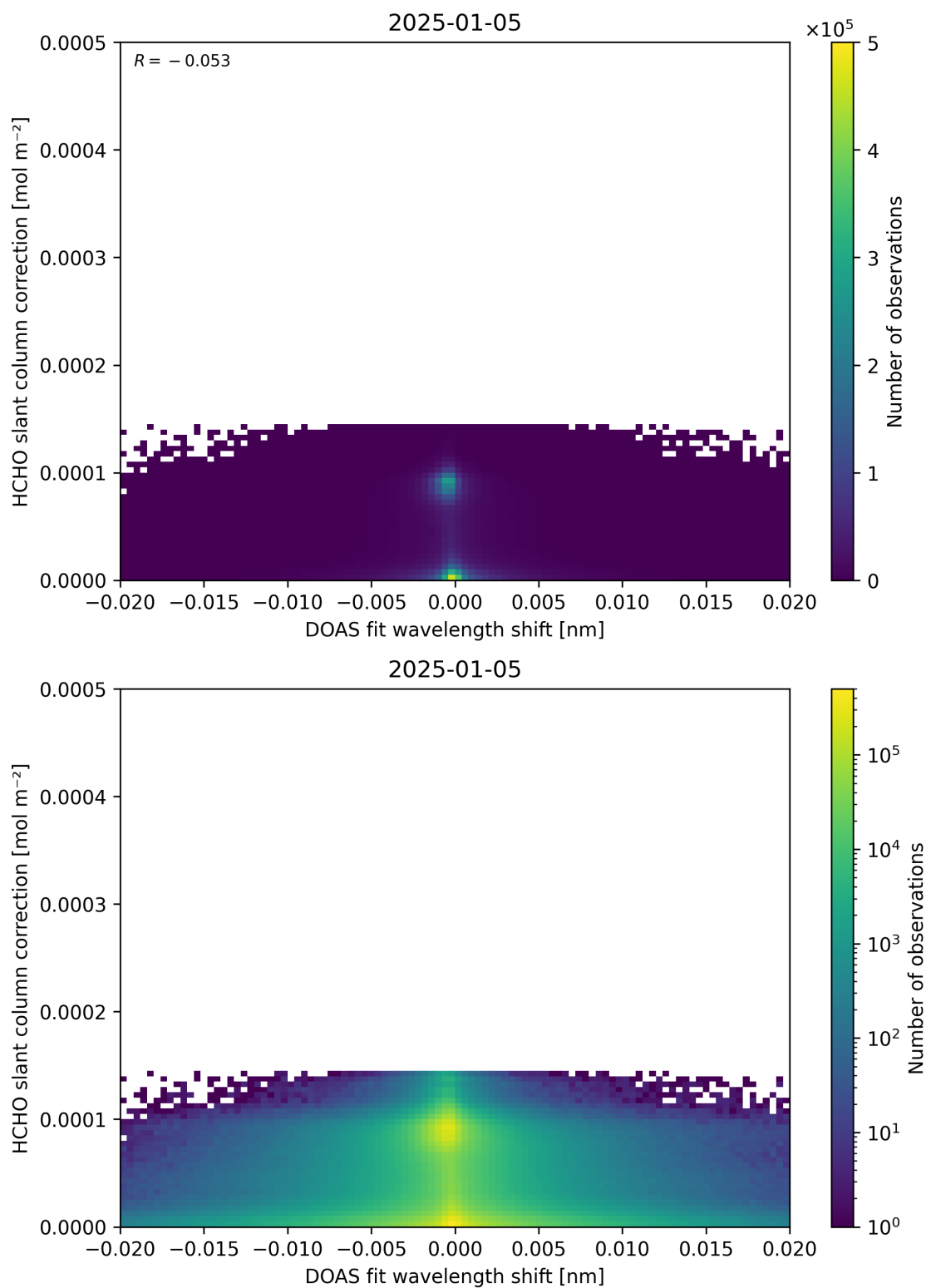
Figure 67: Scatter density plot of “DOAS fit wavelength shift” against “HCHO slant column correction” for 2025-01-04 to 2025-01-06.
