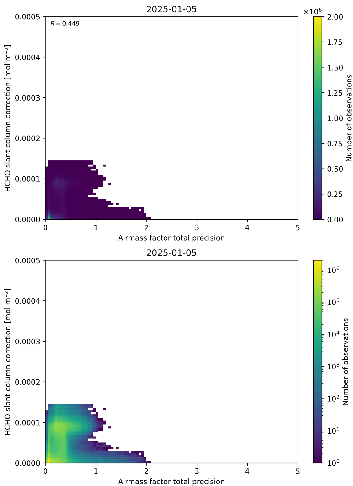
Figure 110: Scatter density plot of “Airmass factor total precision” against “HCHO slant column correction” for 2025-01-04 to 2025-01-06.
