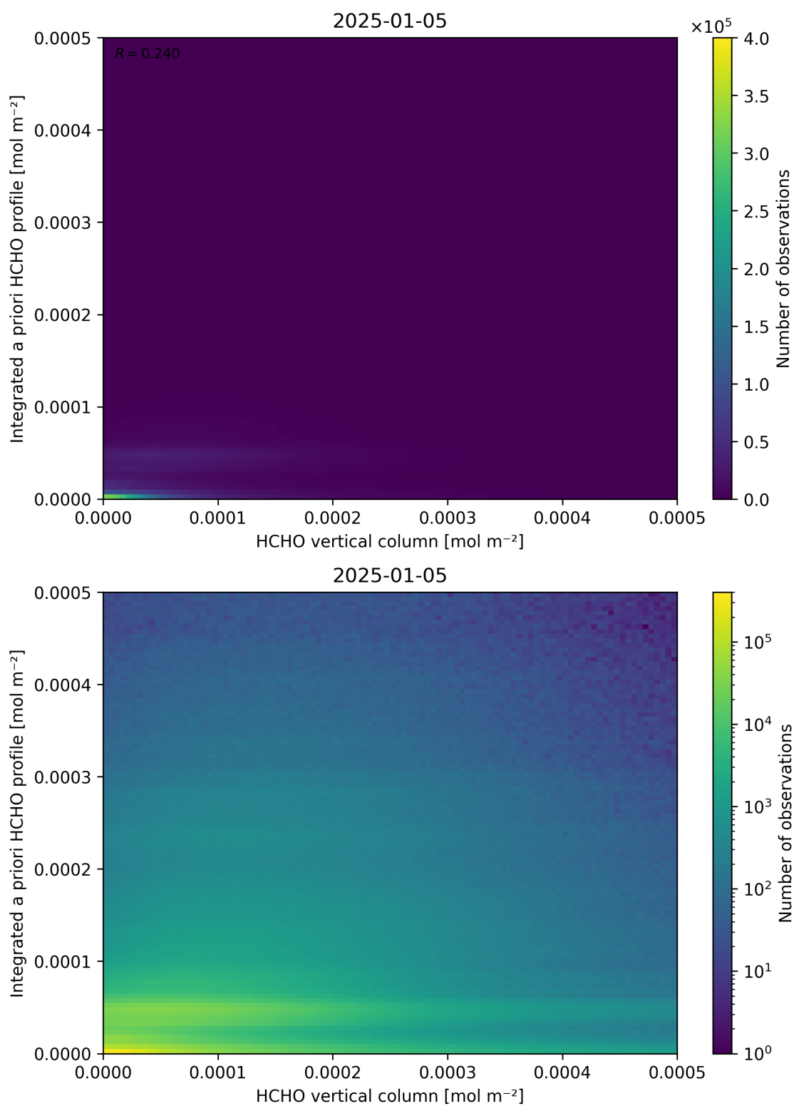
Figure 135: Scatter density plot of “HCHO vertical column” against “Integrated a priori HCHO profile” for 2025-01-04 to 2025-01-06.
