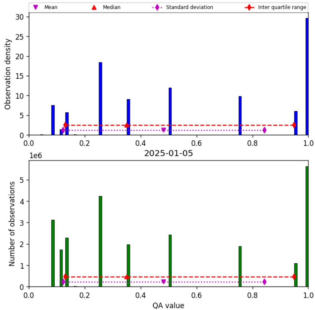
Figure 34: Histogram of “QA value” for 2025-01-04 to 2025-01-06
