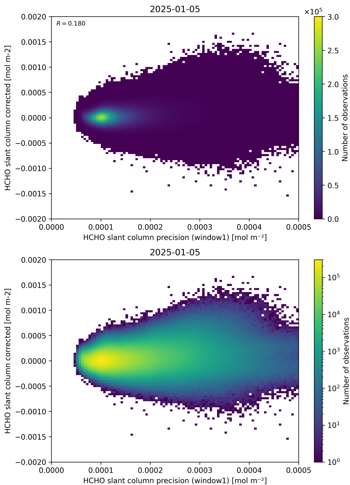
Figure 92: Scatter density plot of “HCHO slant column precision (window1)” against “HCHO slant column corrected” for 2025-01-04 to 2025-01-06.
