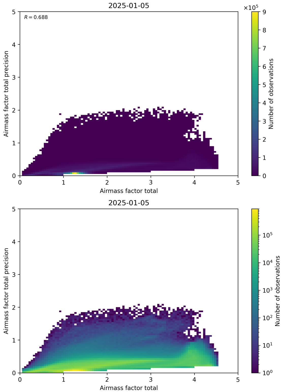
Figure 103: Scatter density plot of “Airmass factor total” against “Airmass factor total precision” for 2025-01-04 to 2025-01-06.
