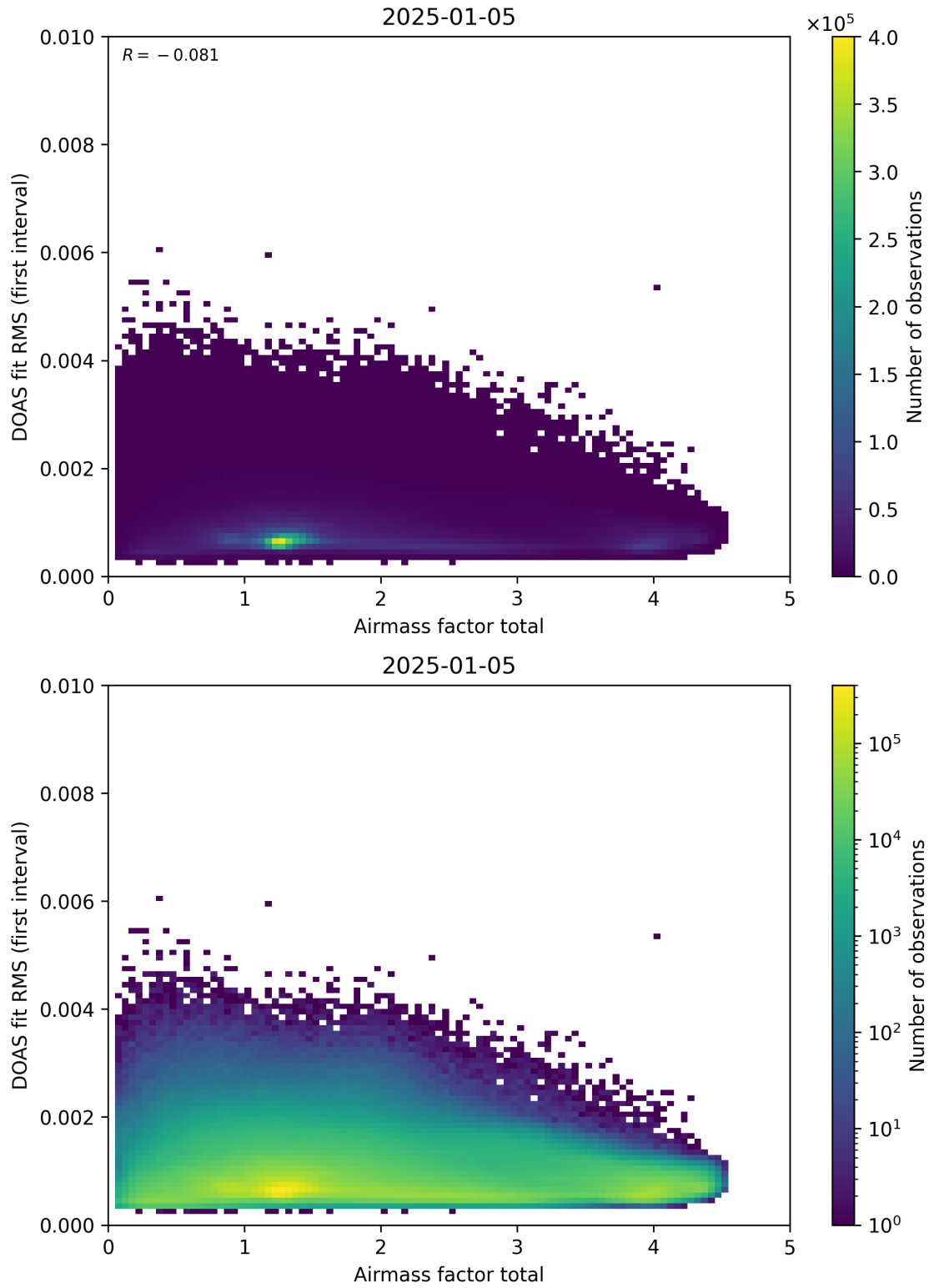
Figure 97: Scatter density plot of “Airmass factor total” against “DOAS fit RMS (first interval)” for 2025-01-04 to 2025-01-06.
