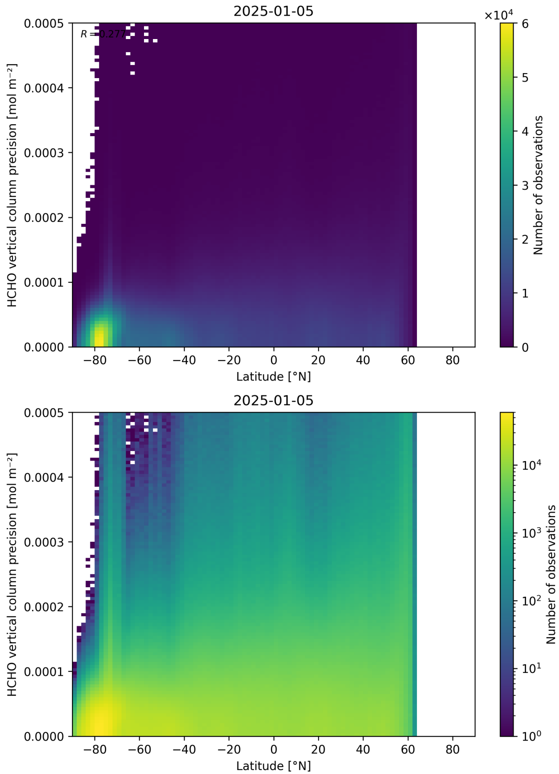
Figure 165: Scatter density plot of “Latitude” against “HCHO vertical column precision” for 2025-01-04 to 2025-01-06.
