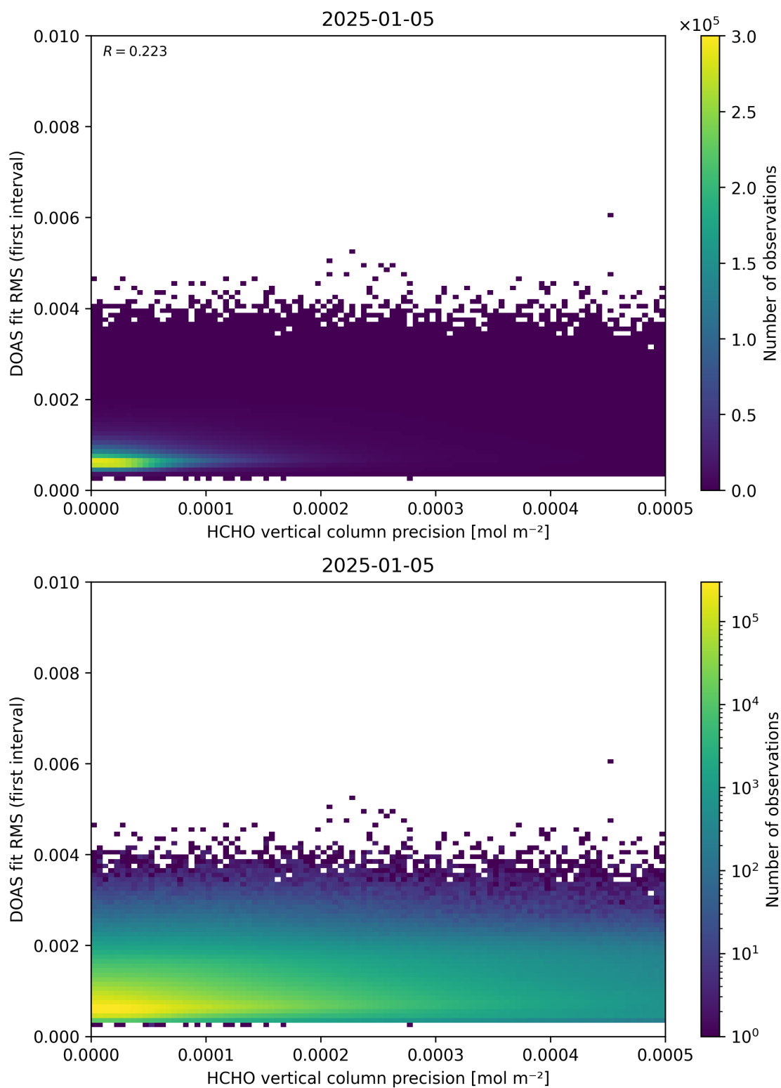
Figure 136: Scatter density plot of “HCHO vertical column precision” against “DOAS fit RMS (first interval)” for 2025-01-04 to 2025-01-06.
