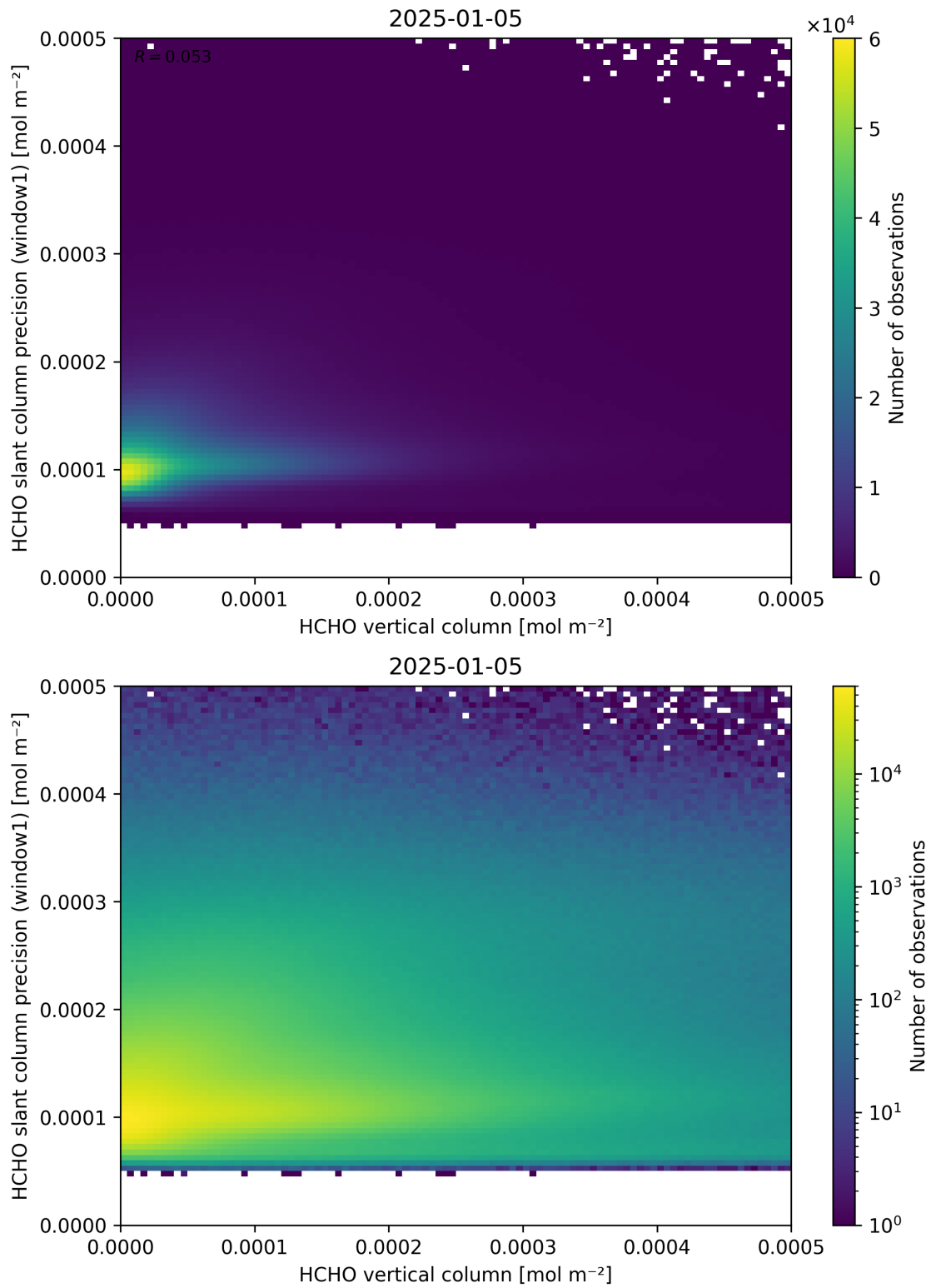
Figure 130: Scatter density plot of “HCHO vertical column” against “HCHO slant column precision (window1)” for 2025-01-04 to 2025-01-06.
