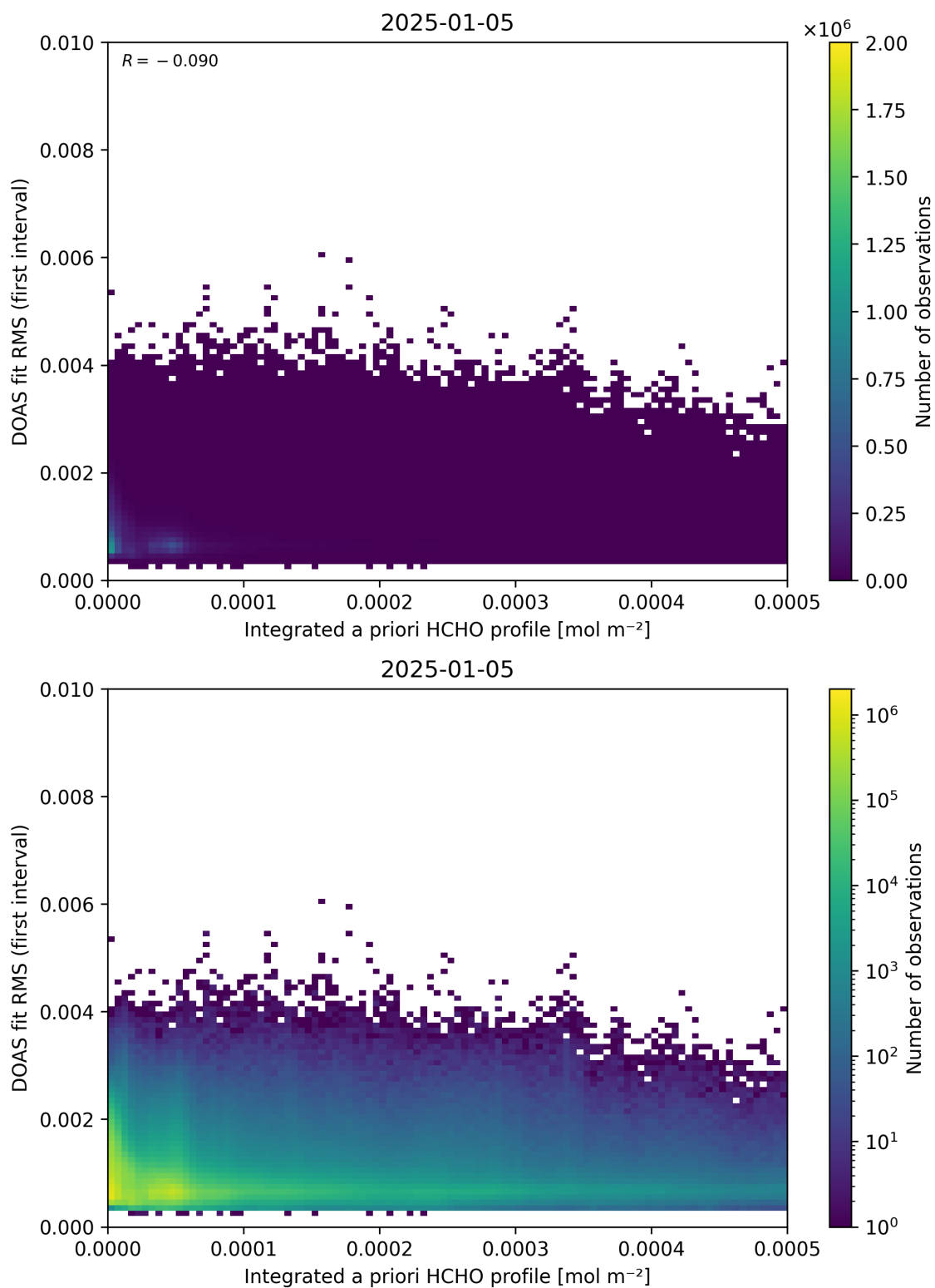
Figure 148: Scatter density plot of “Integrated a priori HCHO profile” against “DOAS fit RMS (first interval)” for 2025-01-04 to 2025-01-06.
