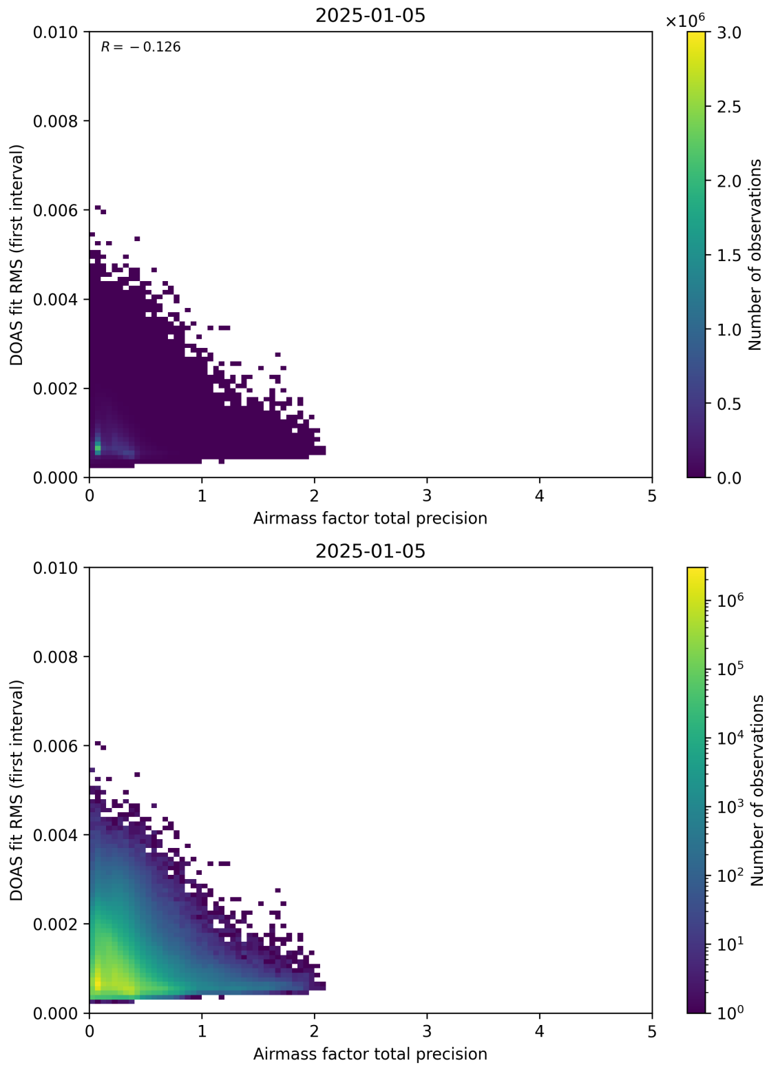
Figure 105: Scatter density plot of “Airmass factor total precision” against “DOAS fit RMS (first interval)” for 2025-01-04 to 2025-01-06.
