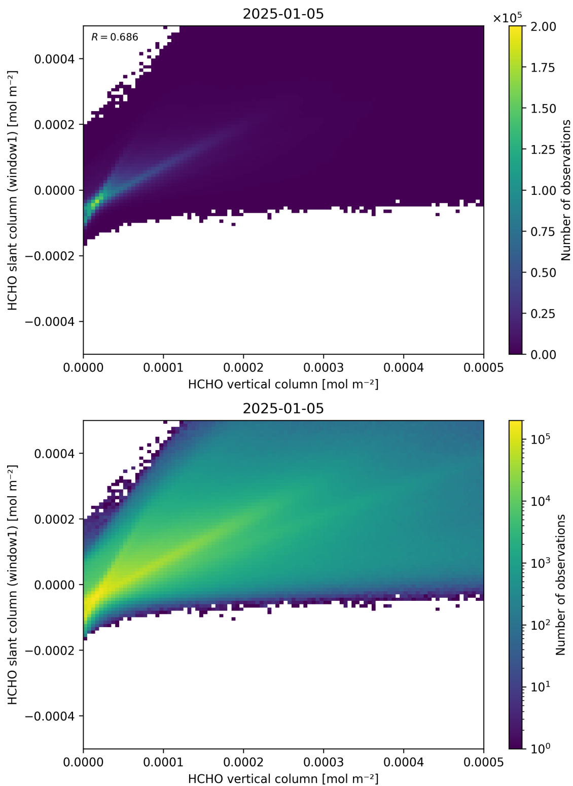
Figure 129: Scatter density plot of “HCHO vertical column” against “HCHO slant column (window1)” for 2025-01-04 to 2025-01-06.
