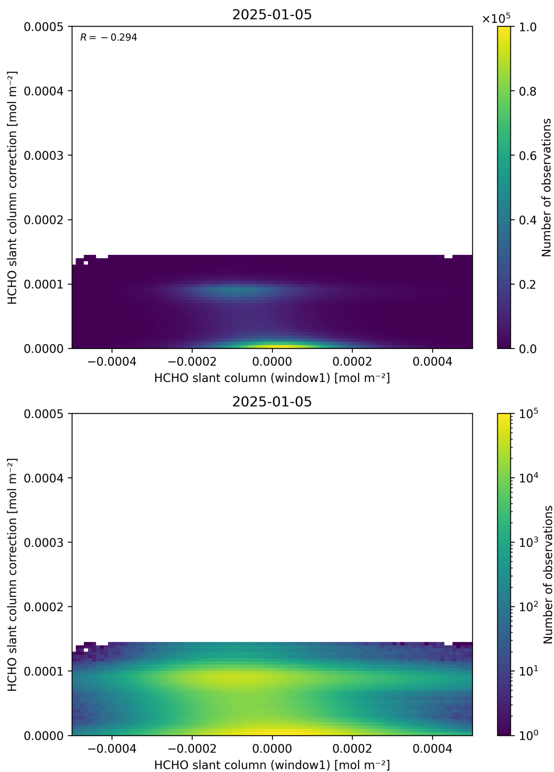
Figure 83: Scatter density plot of “HCHO slant column (window1)” against “HCHO slant column correction” for 2025-01-04 to 2025-01-06.
