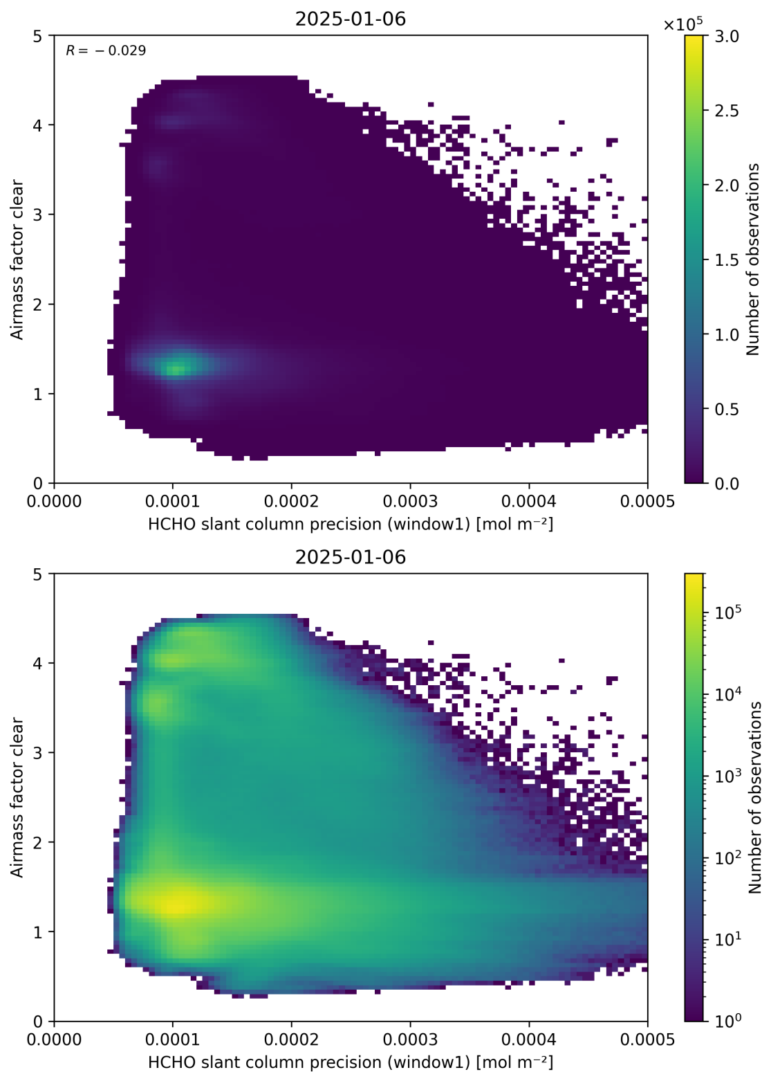
Figure 91: Scatter density plot of “HCHO slant column precision (window1)” against “Airmass factor clear” for 2025-01-05 to 2025-01-07.
