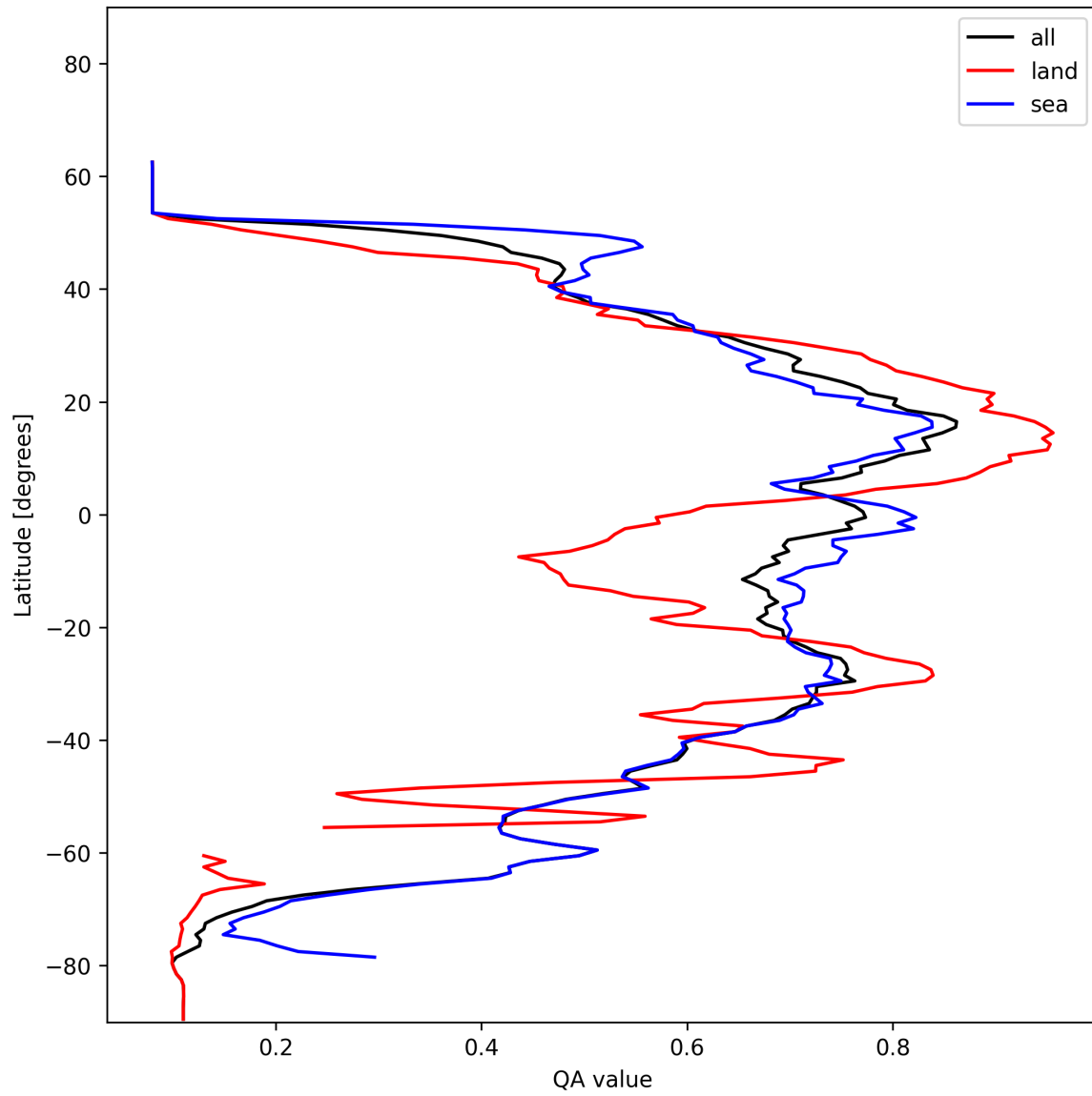
Figure 20: Zonal average of “QA value” for 2025-01-05 to 2025-01-07.
