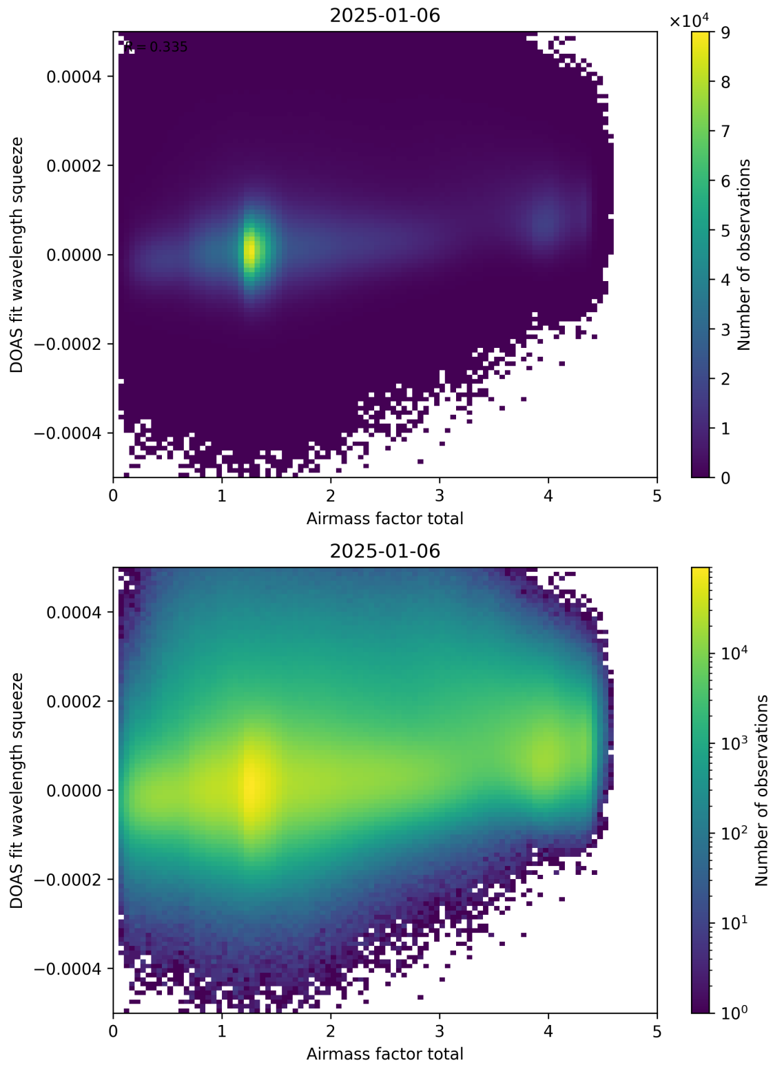
Figure 99: Scatter density plot of “Airmass factor total” against “DOAS fit wavelength squeeze” for 2025-01-05 to 2025-01-07.
