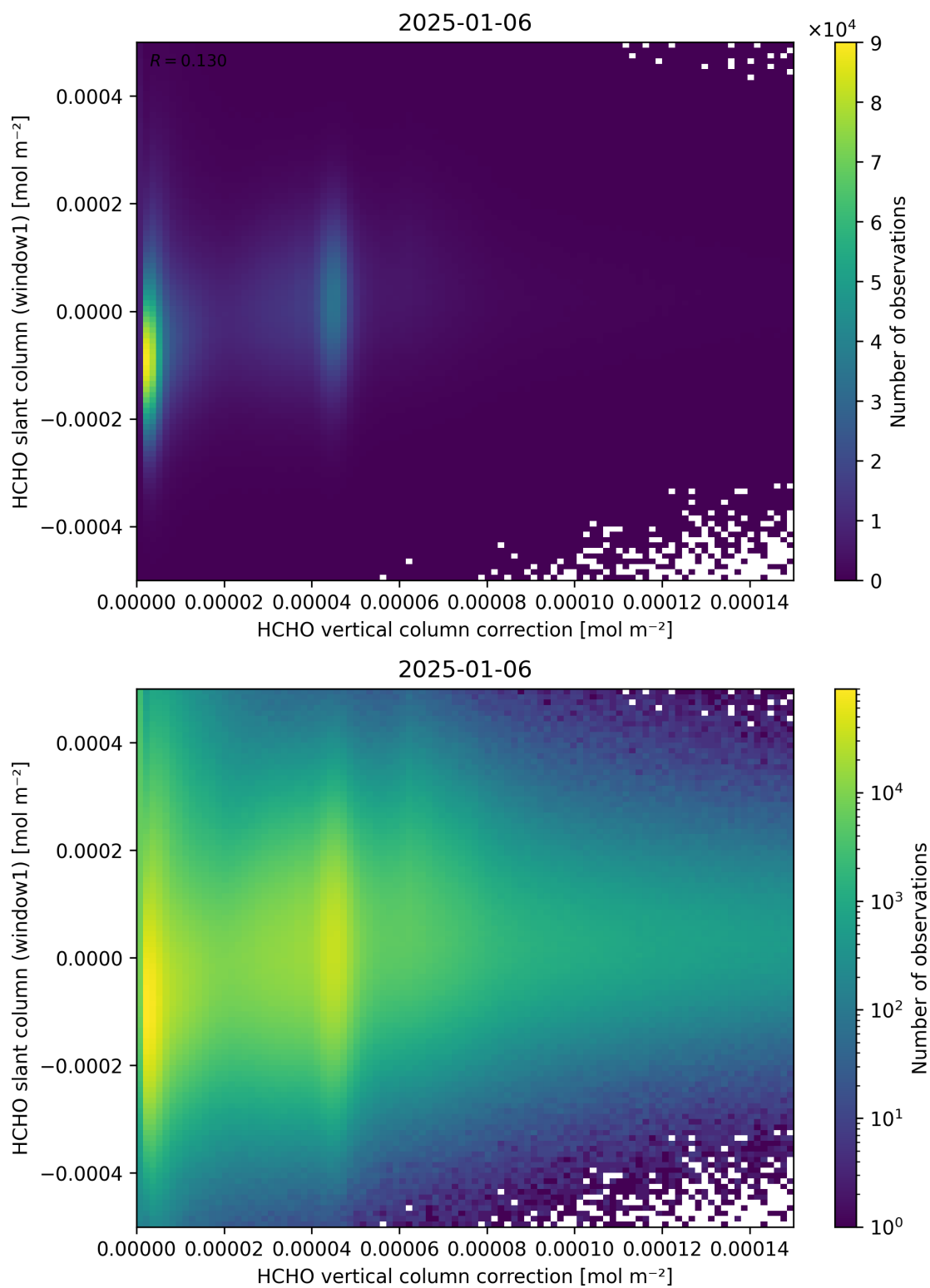
Figure 118: Scatter density plot of “HCHO vertical column correction” against “HCHO slant column (window1)” for 2025-01-05 to 2025-01-07.
