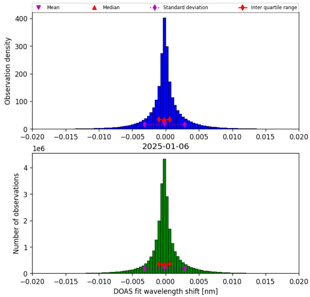
Figure 44: Histogram of “DOAS fit wavelength shift” for 2025-01-05 to 2025-01-07
