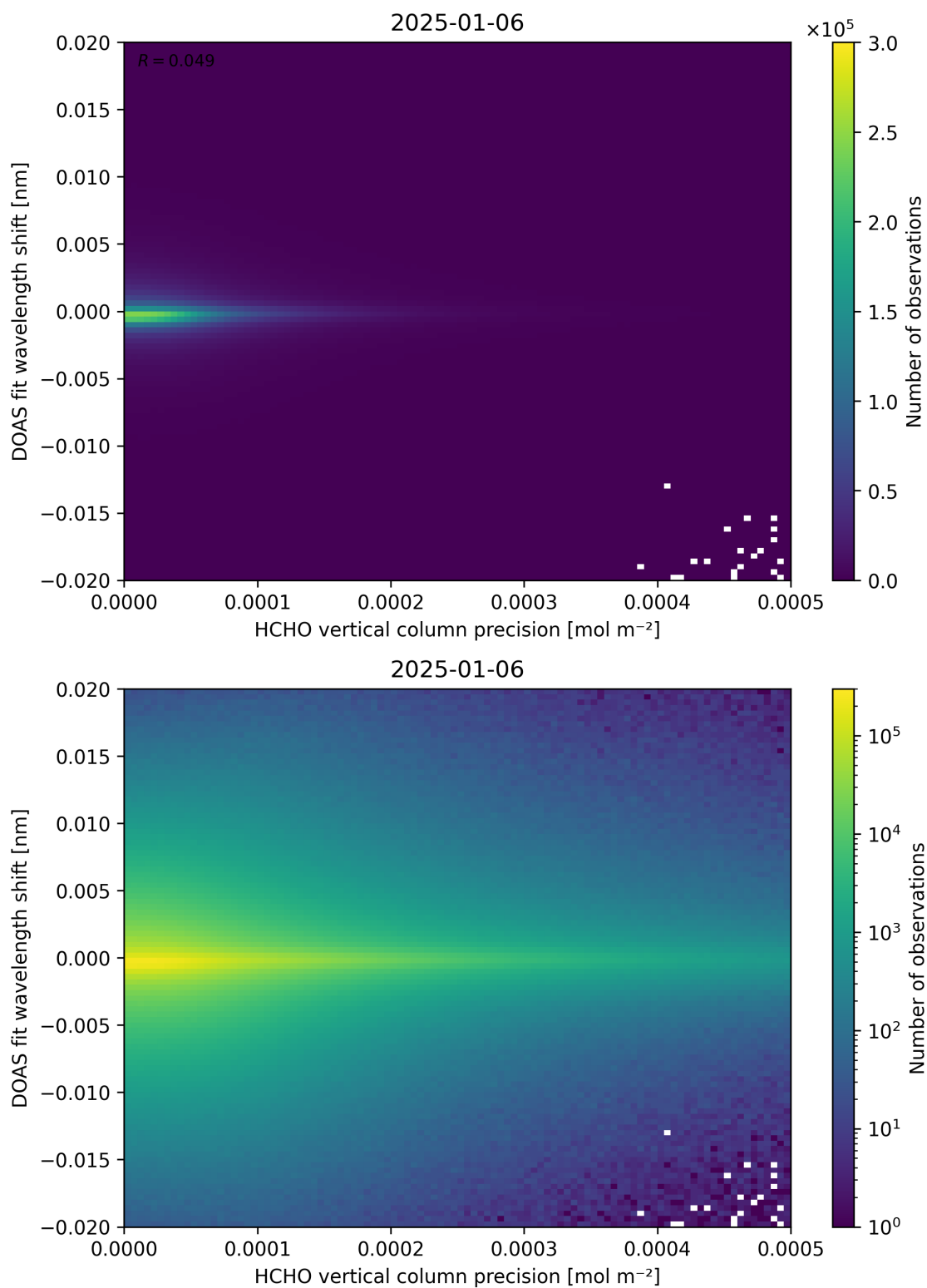
Figure 137: Scatter density plot of “HCHO vertical column precision” against “DOAS fit wavelength shift” for 2025-01-05 to 2025-01-07.
