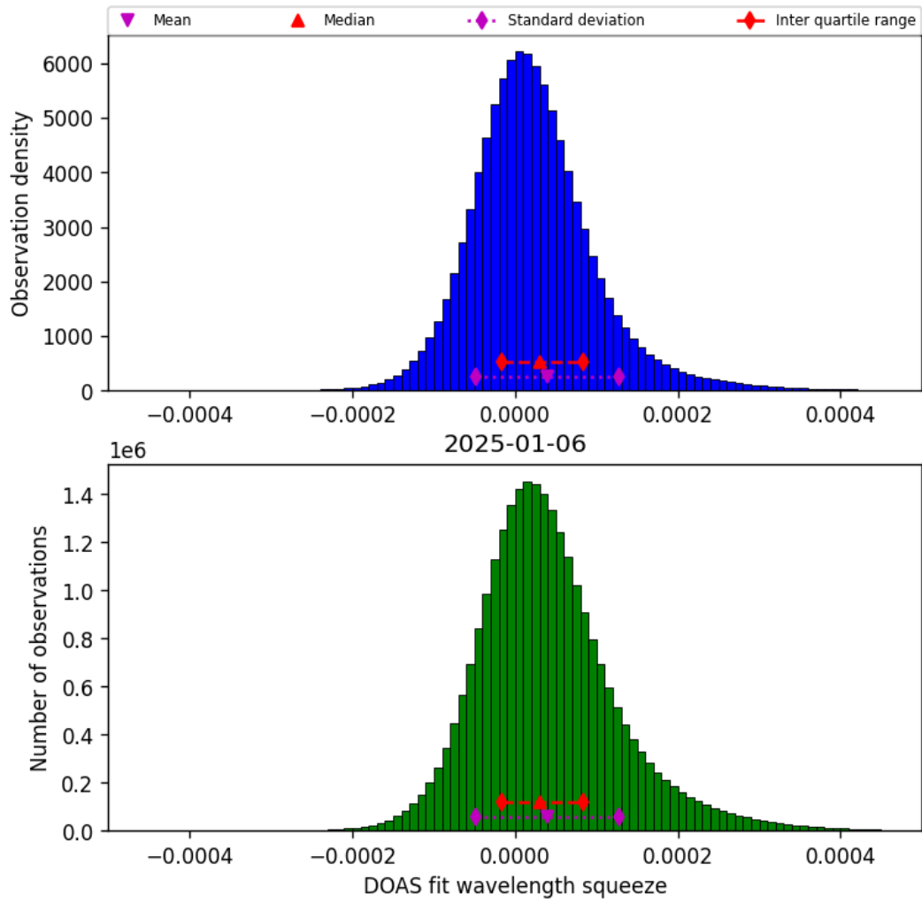
Figure 45: Histogram of “DOAS fit wavelength squeeze” for 2025-01-05 to 2025-01-07
