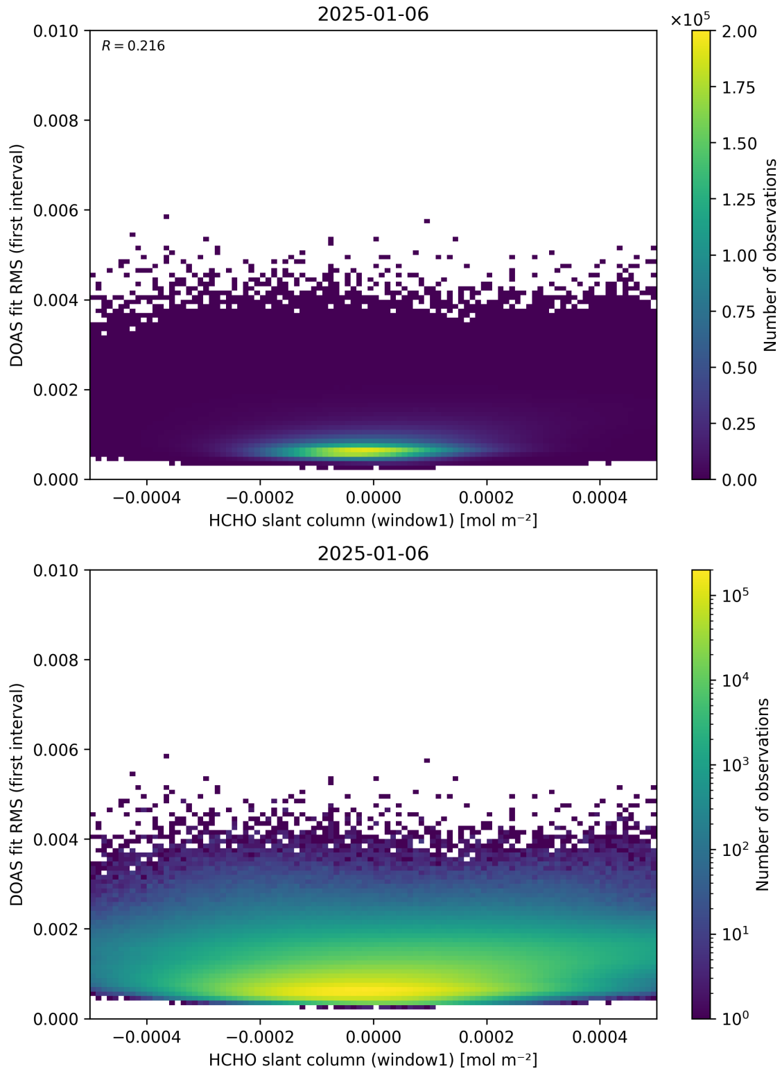
Figure 78: Scatter density plot of “HCHO slant column (window1)” against “DOAS fit RMS (first interval)” for 2025-01-05 to 2025-01-07.
