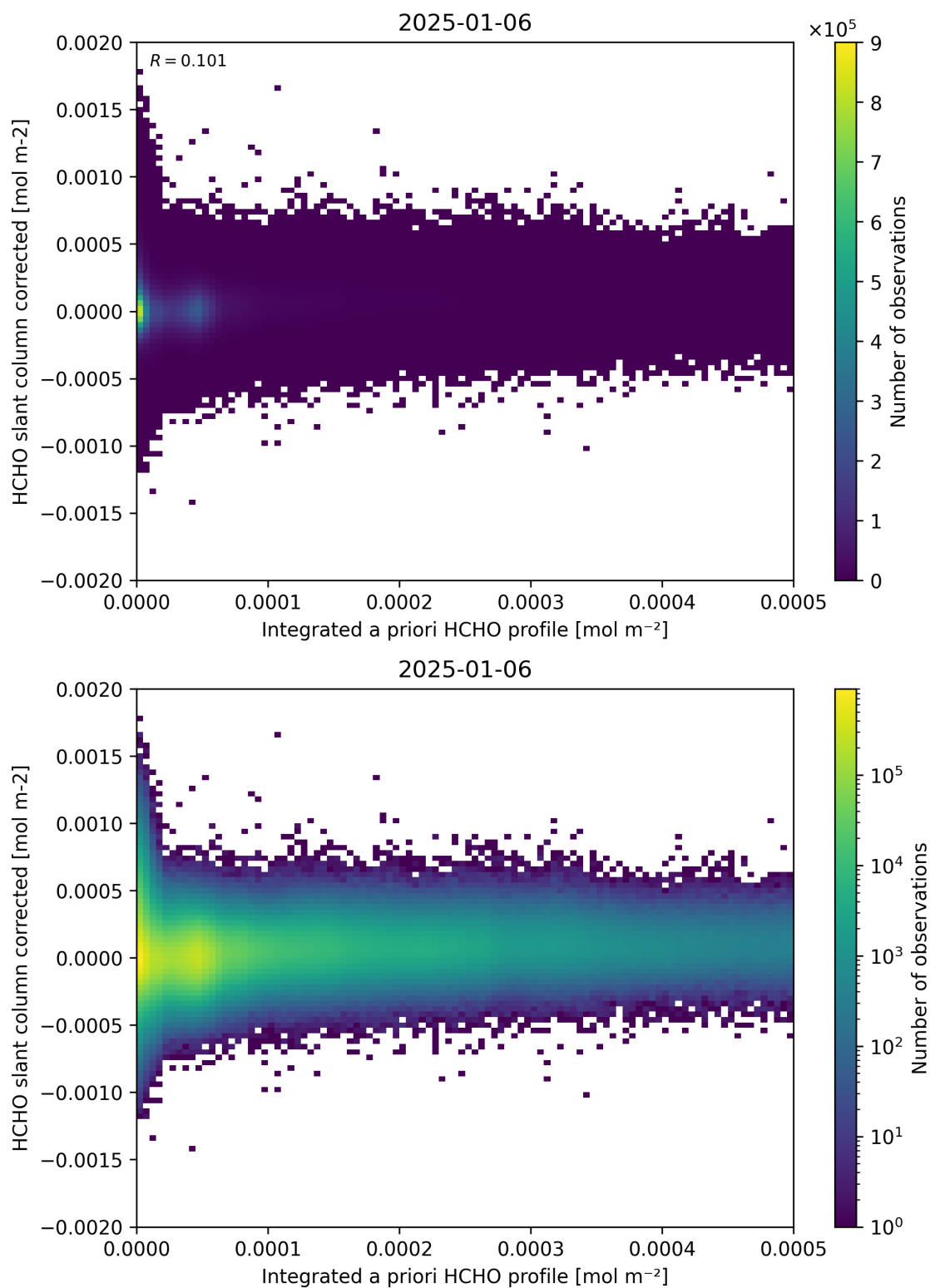
Figure 151: Scatter density plot of “Integrated a priori HCHO profile” against “HCHO slant column corrected” for 2025-01-05 to 2025-01-07.
