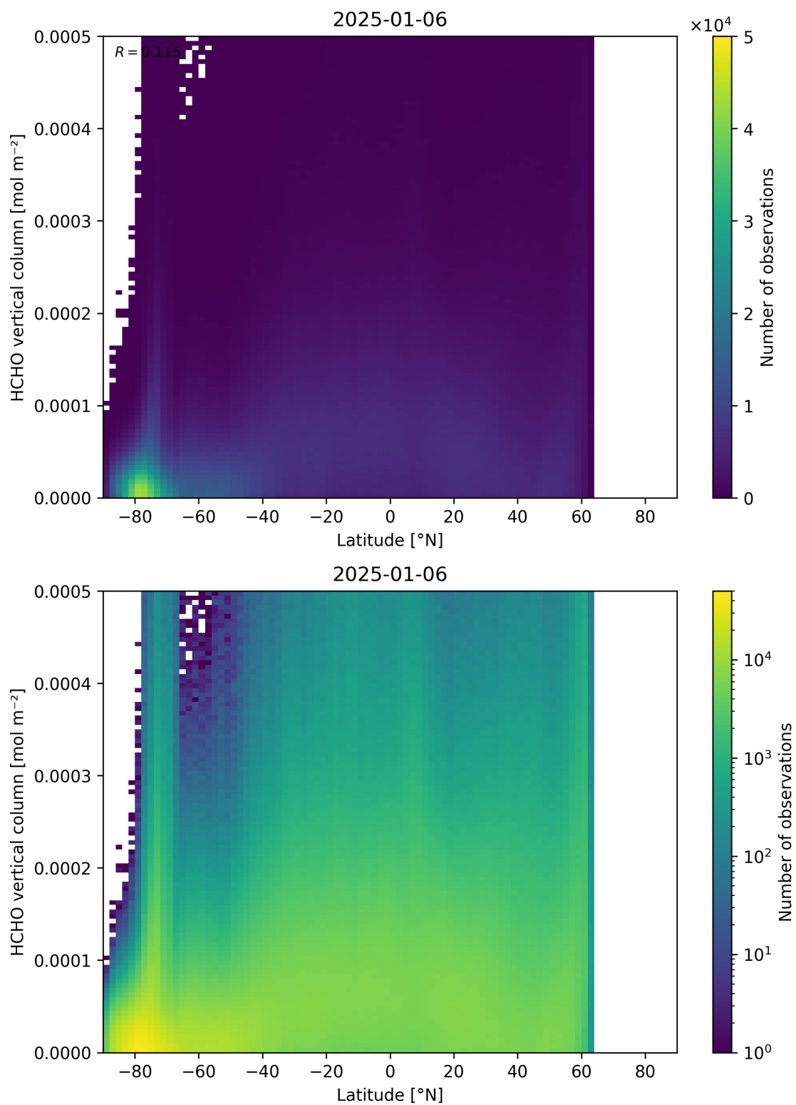
Figure 163: Scatter density plot of “Latitude” against “HCHO vertical column” for 2025-01-05 to 2025-01-07.
