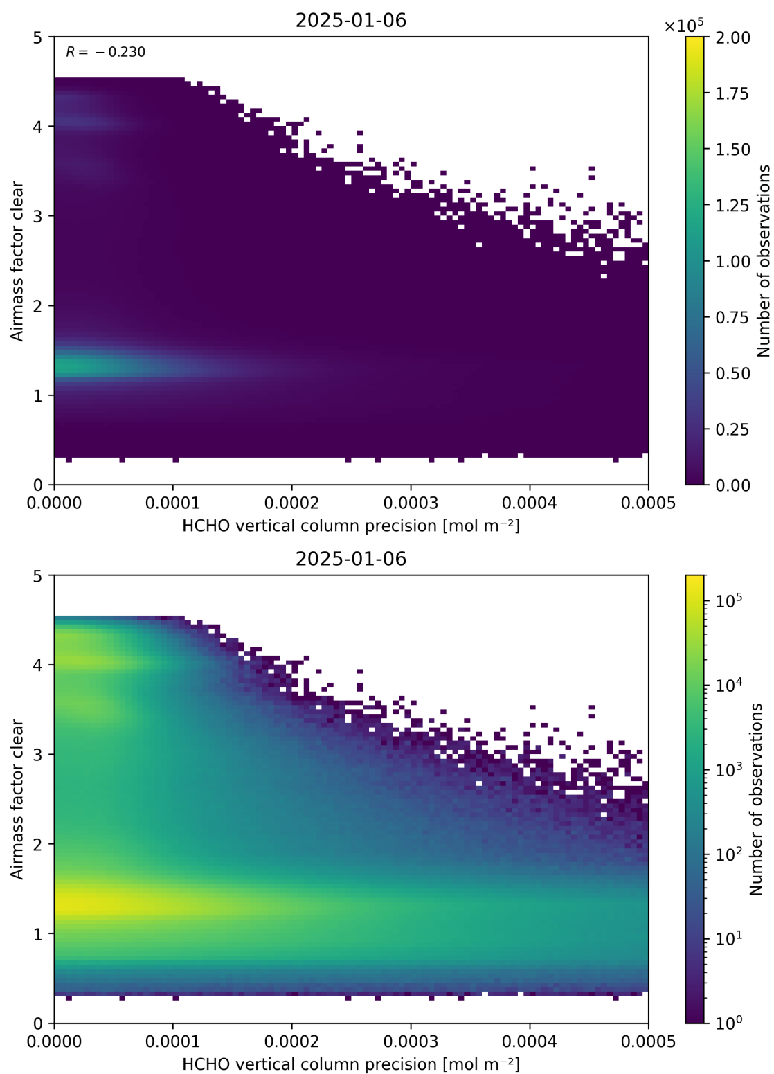
Figure 139: Scatter density plot of “HCHO vertical column precision” against “Airmass factor clear” for 2025-01-05 to 2025-01-07.
