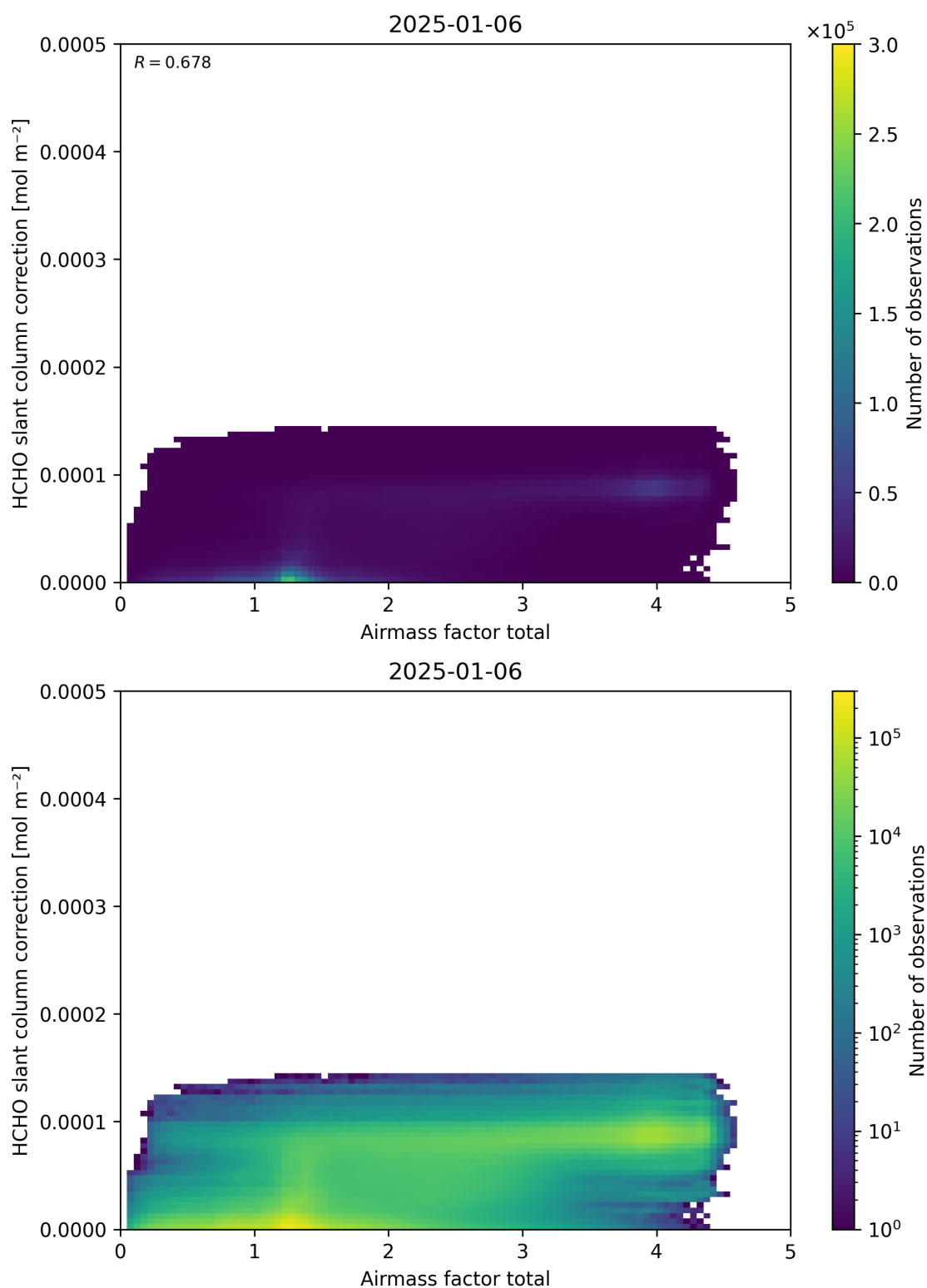
Figure 102: Scatter density plot of “Airmass factor total” against “HCHO slant column correction” for 2025-01-05 to 2025-01-07.
