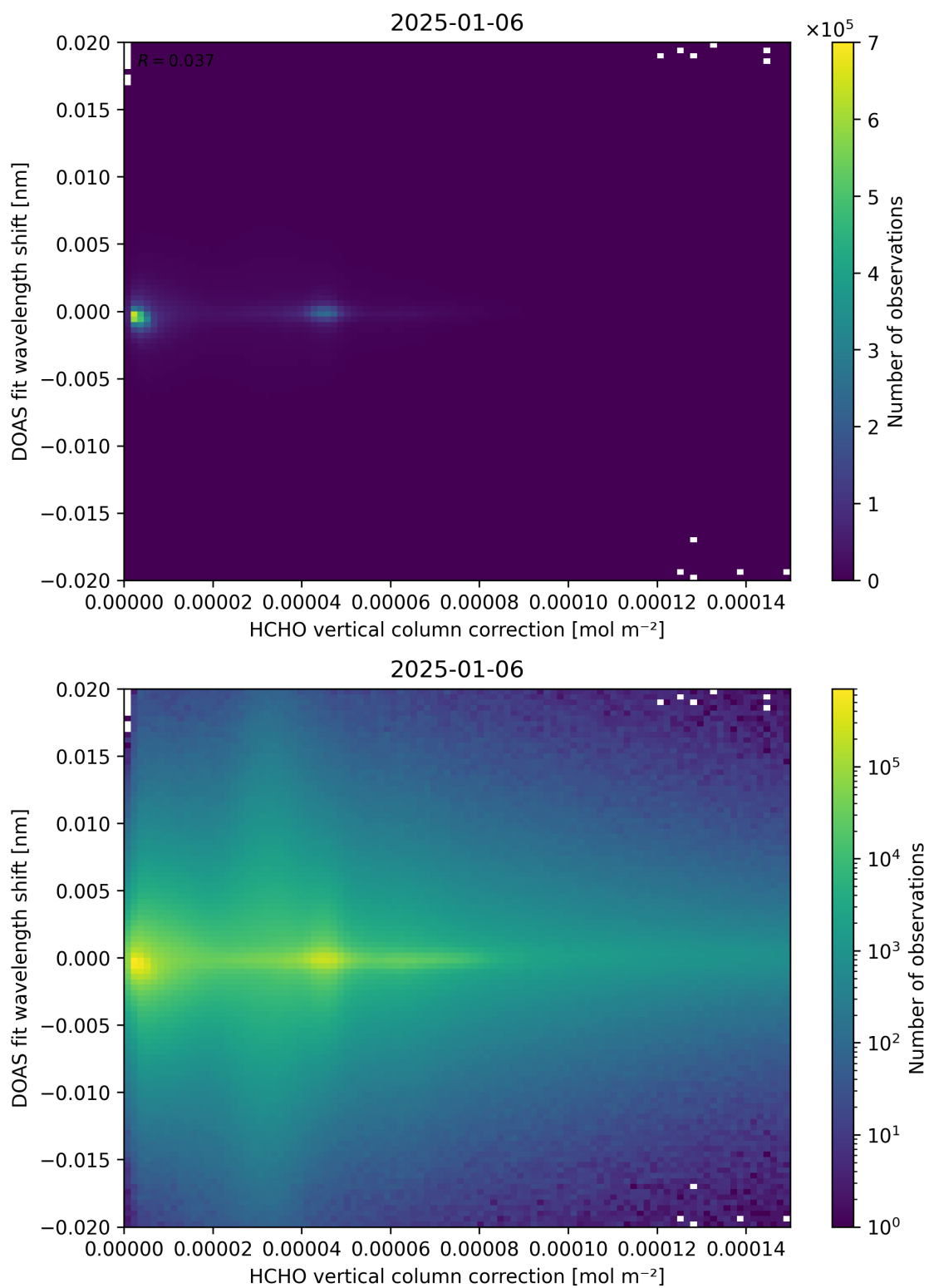
Figure 113: Scatter density plot of “HCHO vertical column correction” against “DOAS fit wavelength shift” for 2025-01-05 to 2025-01-07.
