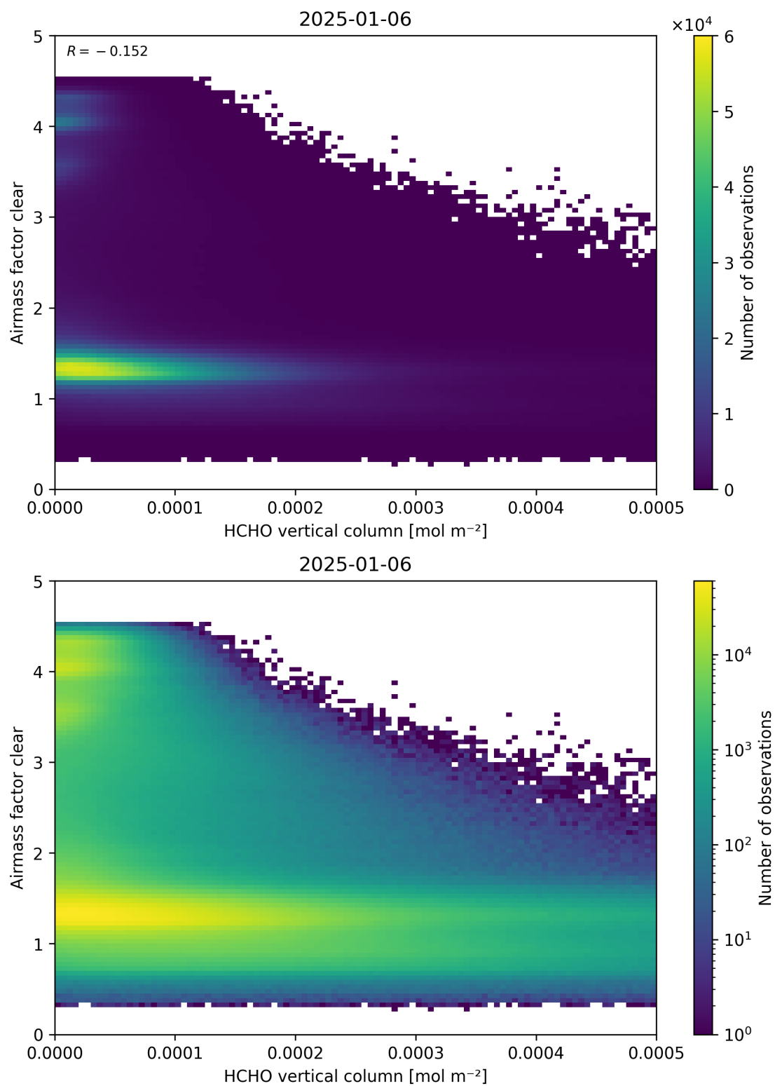
Figure 126: Scatter density plot of “HCHO vertical column” against “Airmass factor clear” for 2025-01-05 to 2025-01-07.
