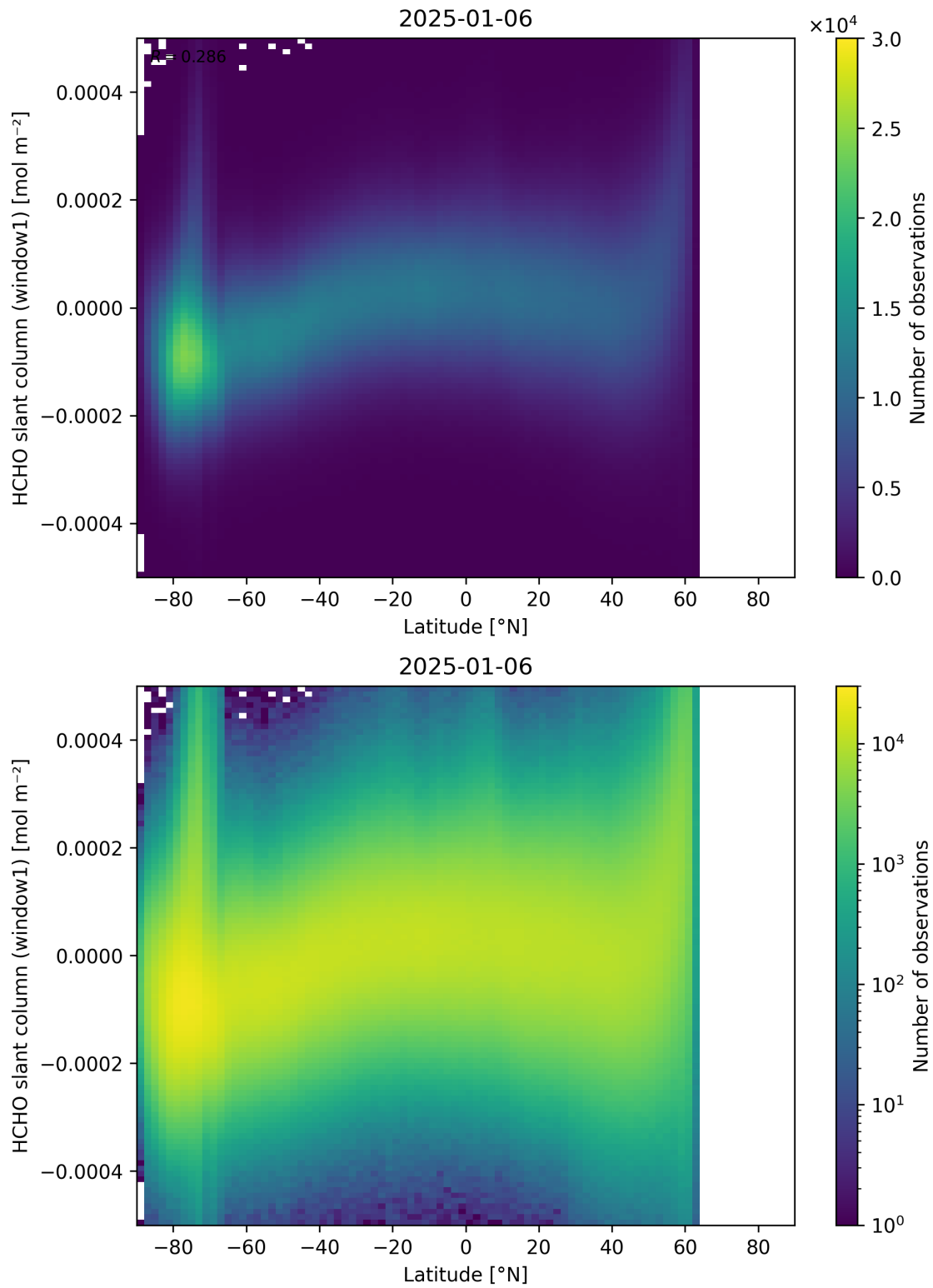
Figure 159: Scatter density plot of “Latitude” against “HCHO slant column (window1)” for 2025-01-05 to 2025-01-07.
