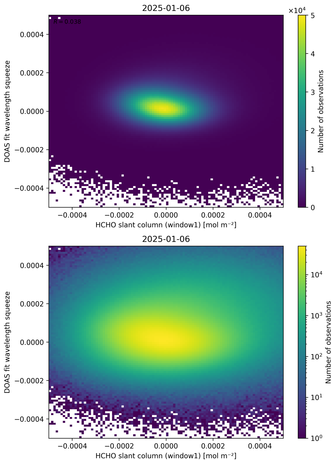
Figure 80: Scatter density plot of “HCHO slant column (window1)” against “DOAS fit wavelength squeeze” for 2025-01-05 to 2025-01-07.
