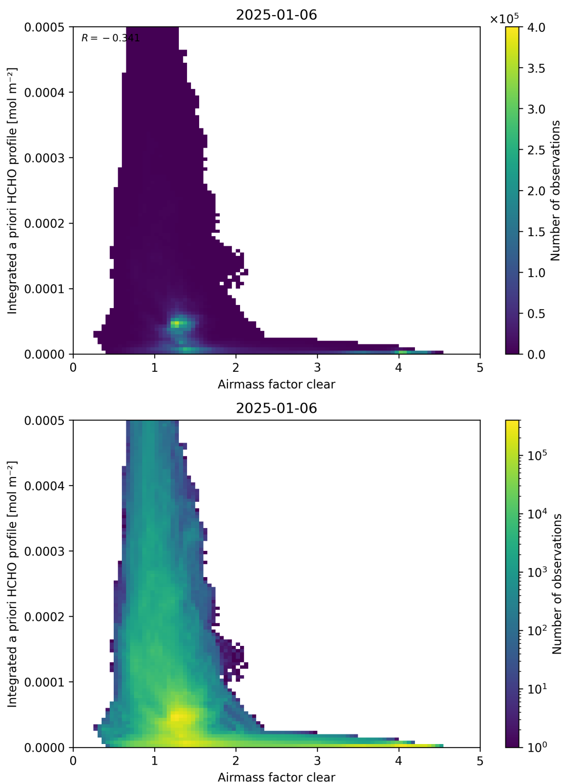
Figure 76: Scatter density plot of “Airmass factor clear” against “Integrated a priori HCHO profile” for 2025-01-05 to 2025-01-07.
