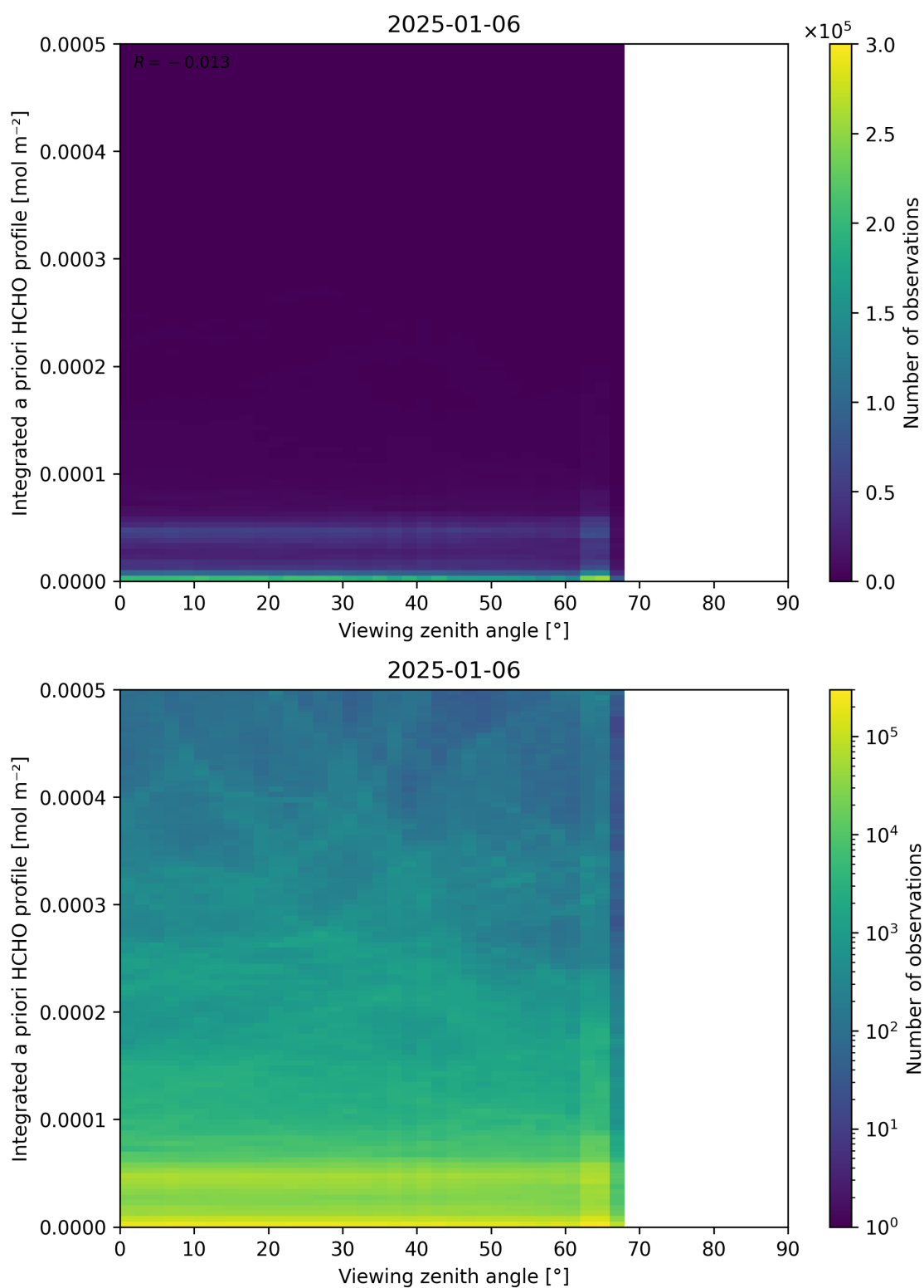
Figure 195: Scatter density plot of “Viewing zenith angle” against “Integrated a priori HCHO profile” for 2025-01-05 to 2025-01-07.
