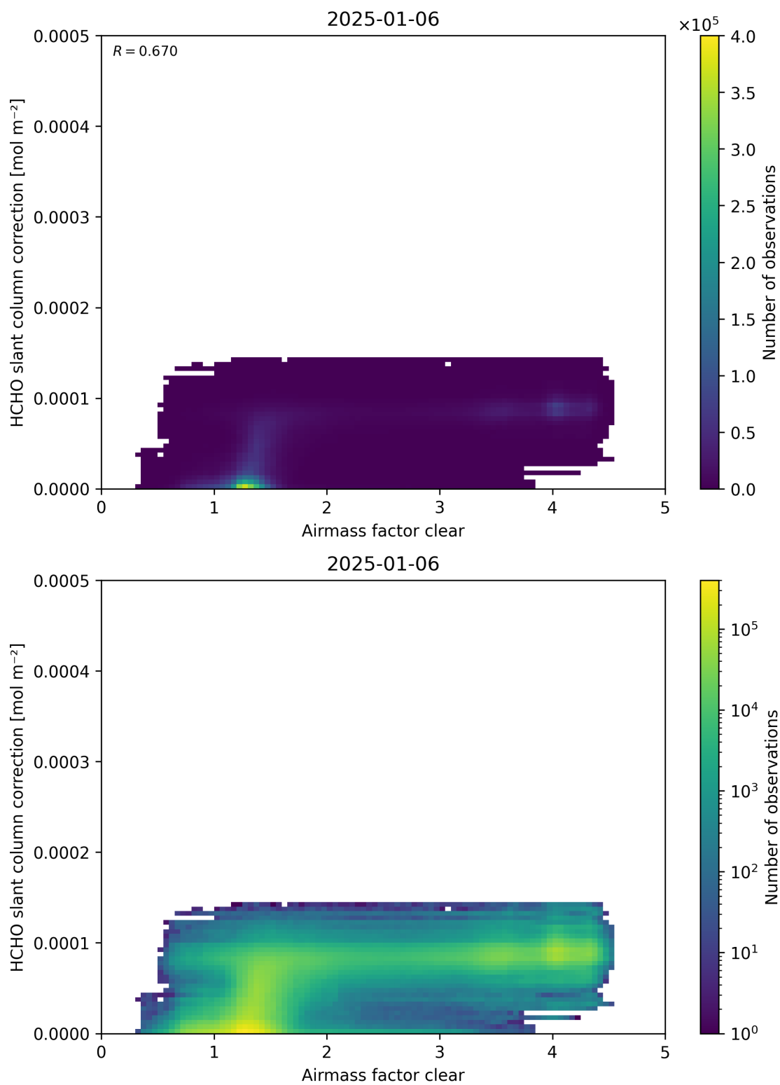
Figure 75: Scatter density plot of “Airmass factor clear” against “HCHO slant column correction” for 2025-01-05 to 2025-01-07.
