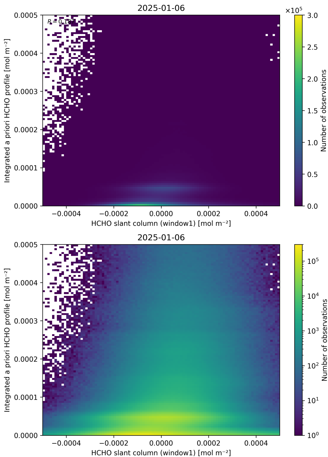
Figure 87: Scatter density plot of “HCHO slant column (window1)” against “Integrated a priori HCHO profile” for 2025-01-05 to 2025-01-07.
