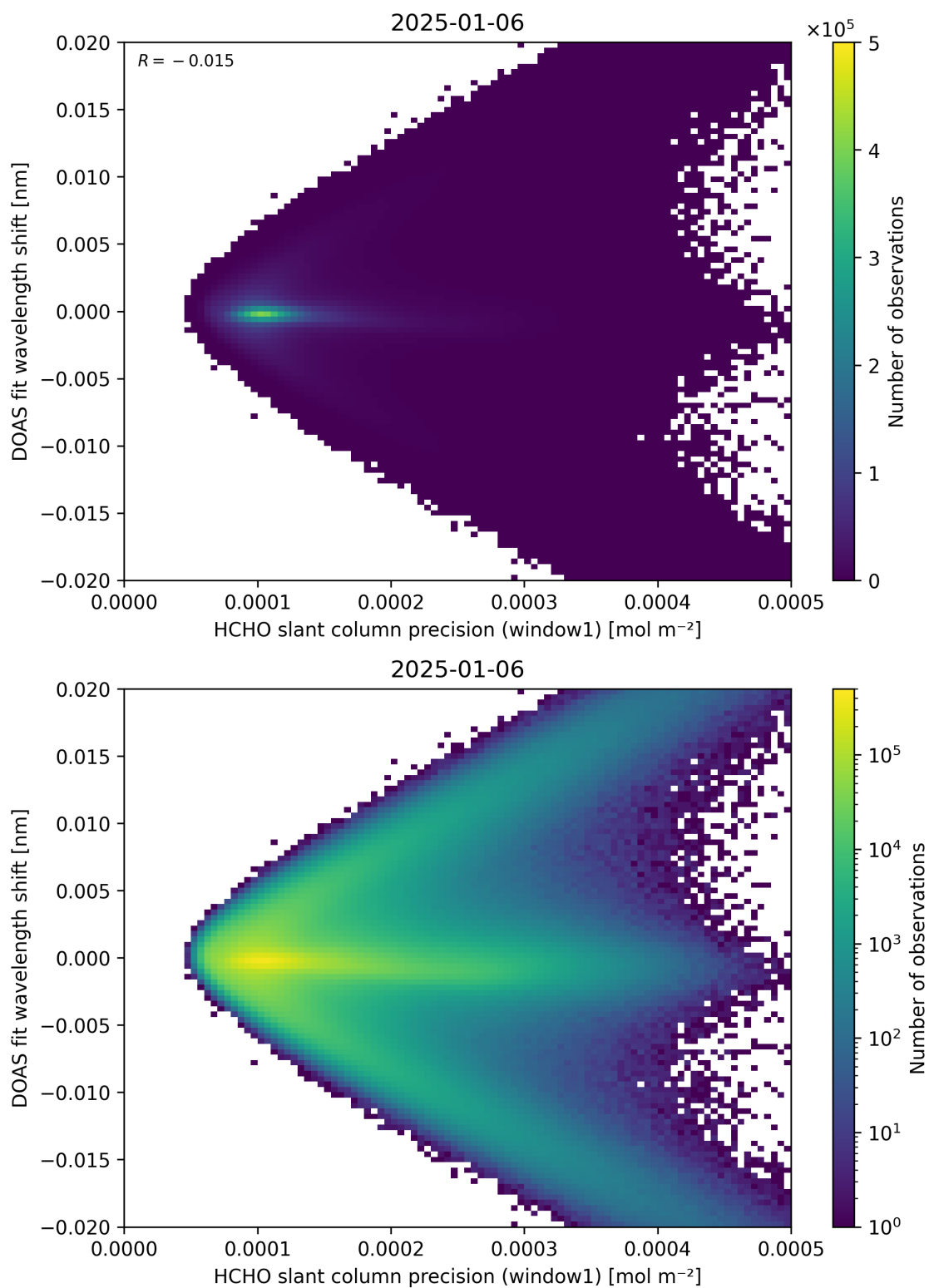
Figure 89: Scatter density plot of “HCHO slant column precision (window1)” against “DOAS fit wavelength shift” for 2025-01-05 to 2025-01-07.
