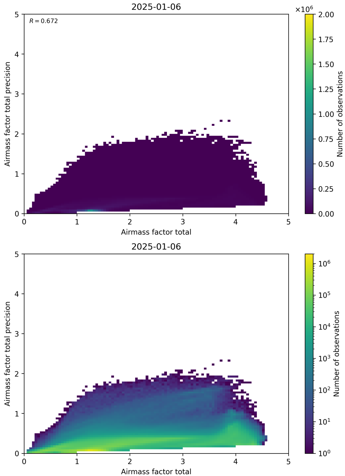
Figure 103: Scatter density plot of “Airmass factor total” against “Airmass factor total precision” for 2025-01-05 to 2025-01-07.
