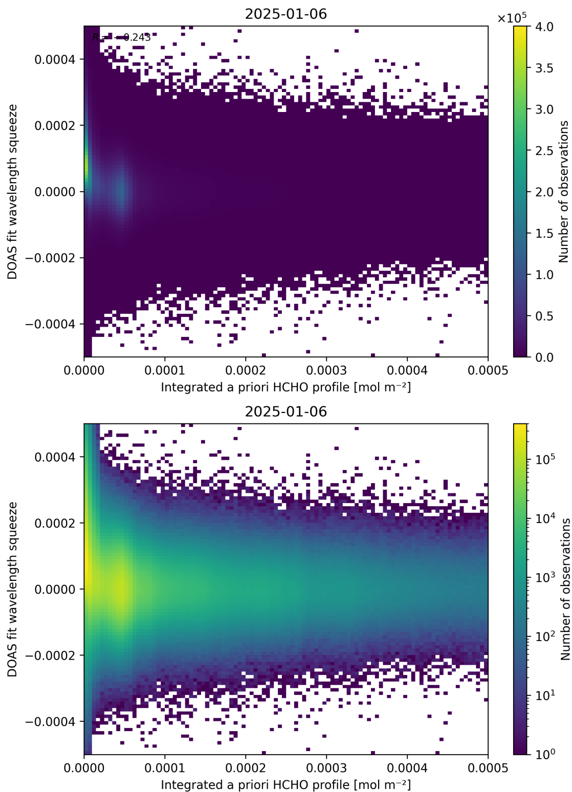
Figure 150: Scatter density plot of “Integrated a priori HCHO profile” against “DOAS fit wavelength squeeze” for 2025-01-05 to 2025-01-07.
