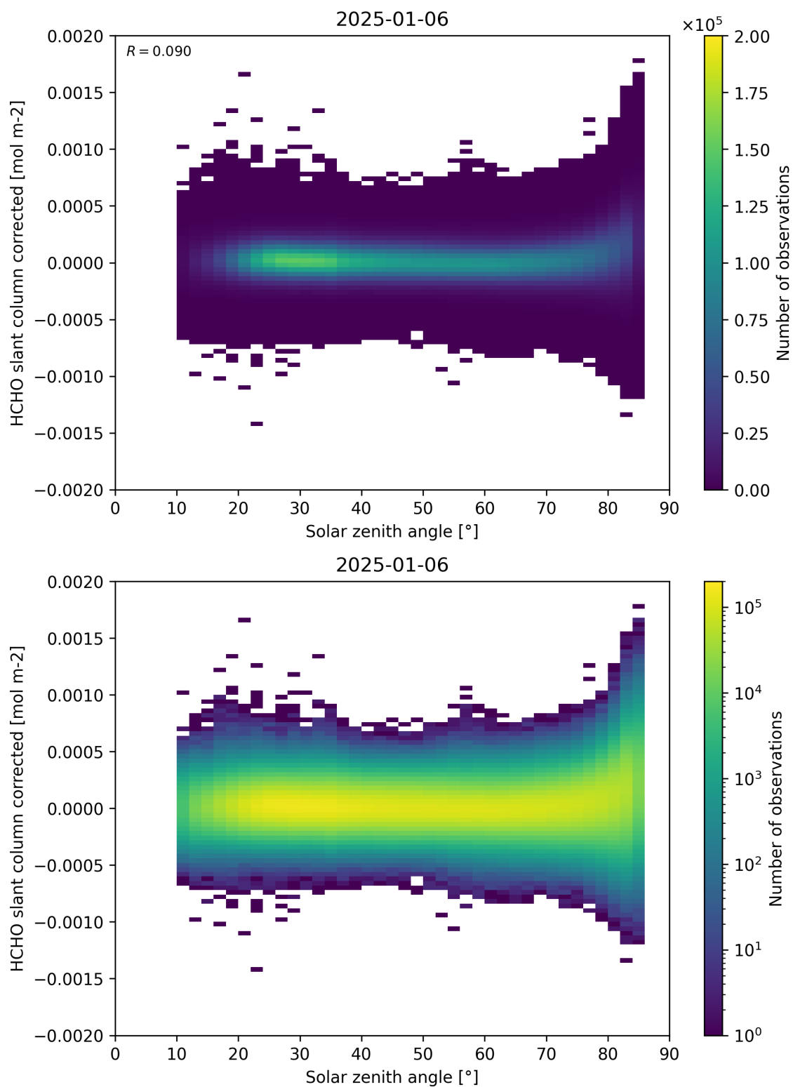
Figure 171: Scatter density plot of “Solar zenith angle” against “HCHO slant column corrected” for 2025-01-05 to 2025-01-07.
