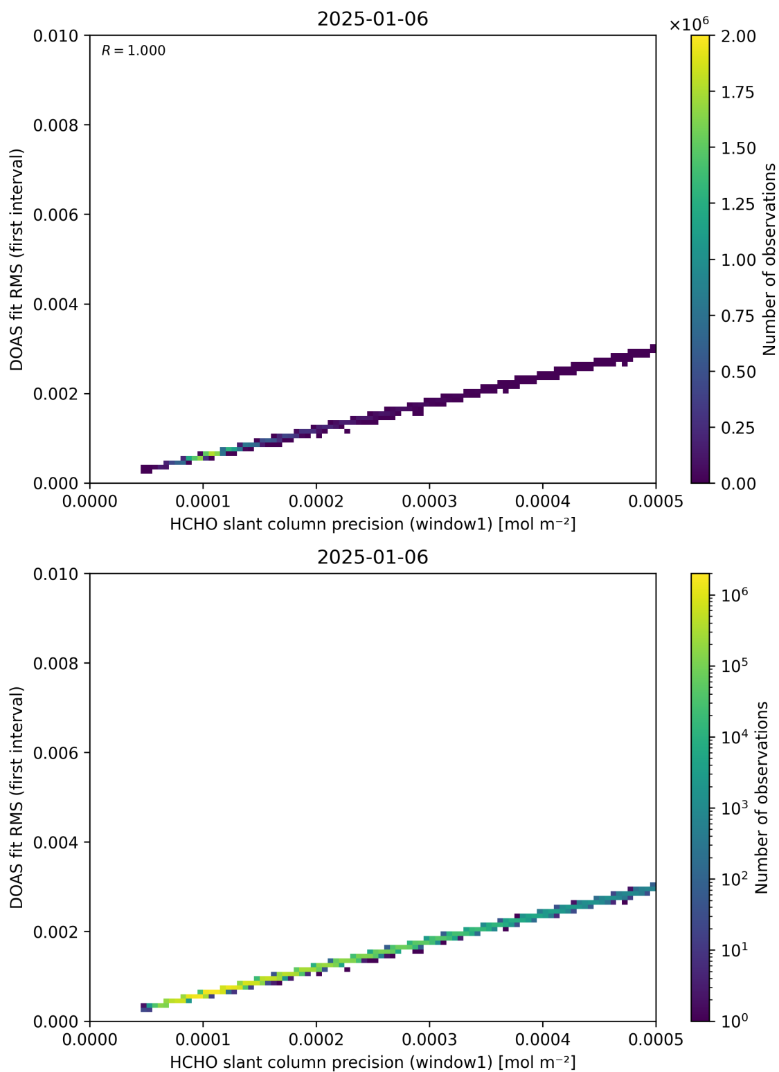
Figure 88: Scatter density plot of “HCHO slant column precision (window1)” against “DOAS fit RMS (first interval)” for 2025-01-05 to 2025-01-07.
