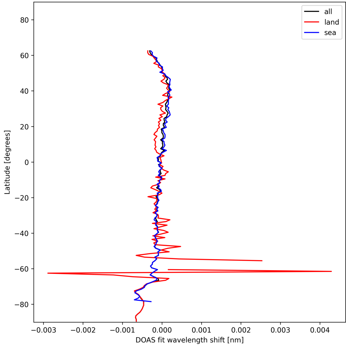
Figure 30: Zonal average of “DOAS fit wavelength shift” for 2025-01-05 to 2025-01-07.
