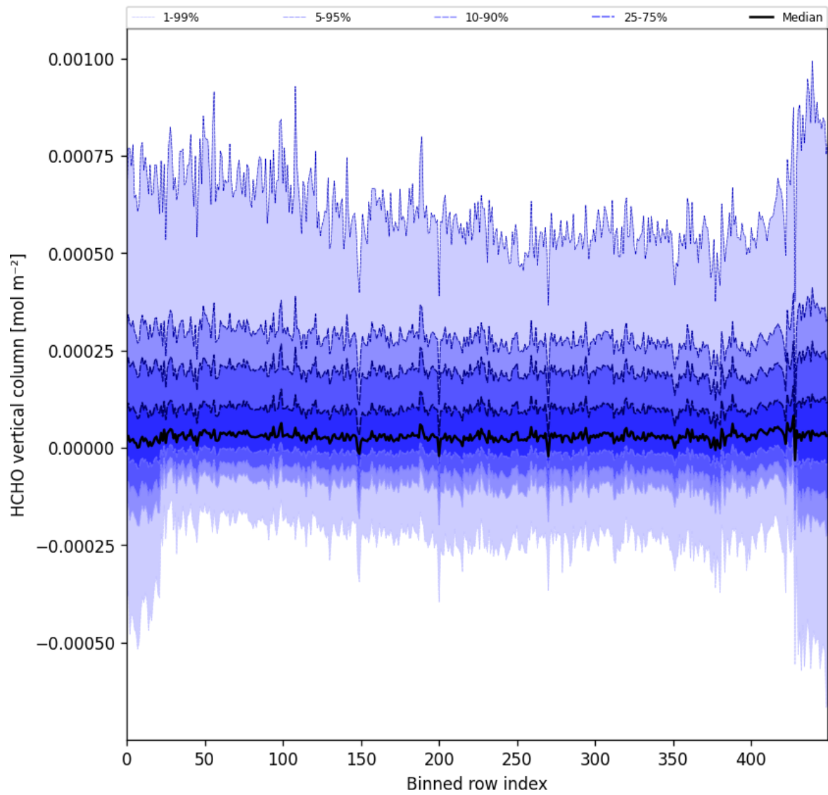
Figure 49: Along track statistics of “HCHO vertical column” for 2025-01-05 to 2025-01-07
