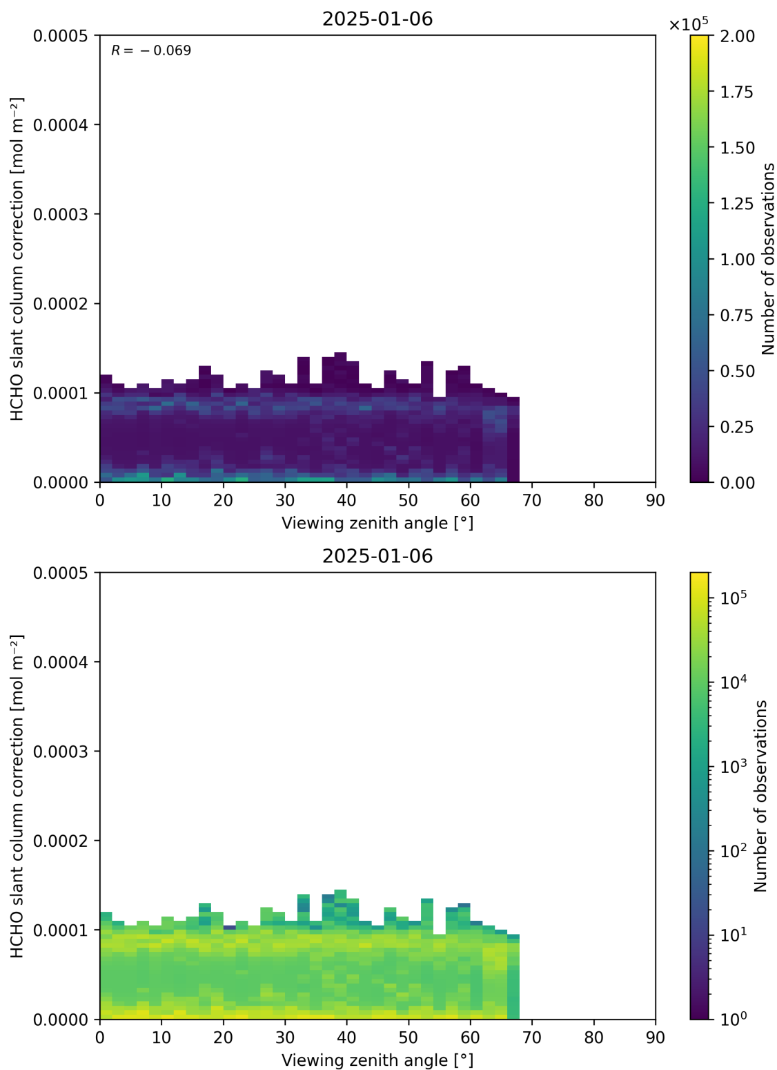
Figure 187: Scatter density plot of “Viewing zenith angle” against “HCHO slant column correction” for 2025-01-05 to 2025-01-07.
