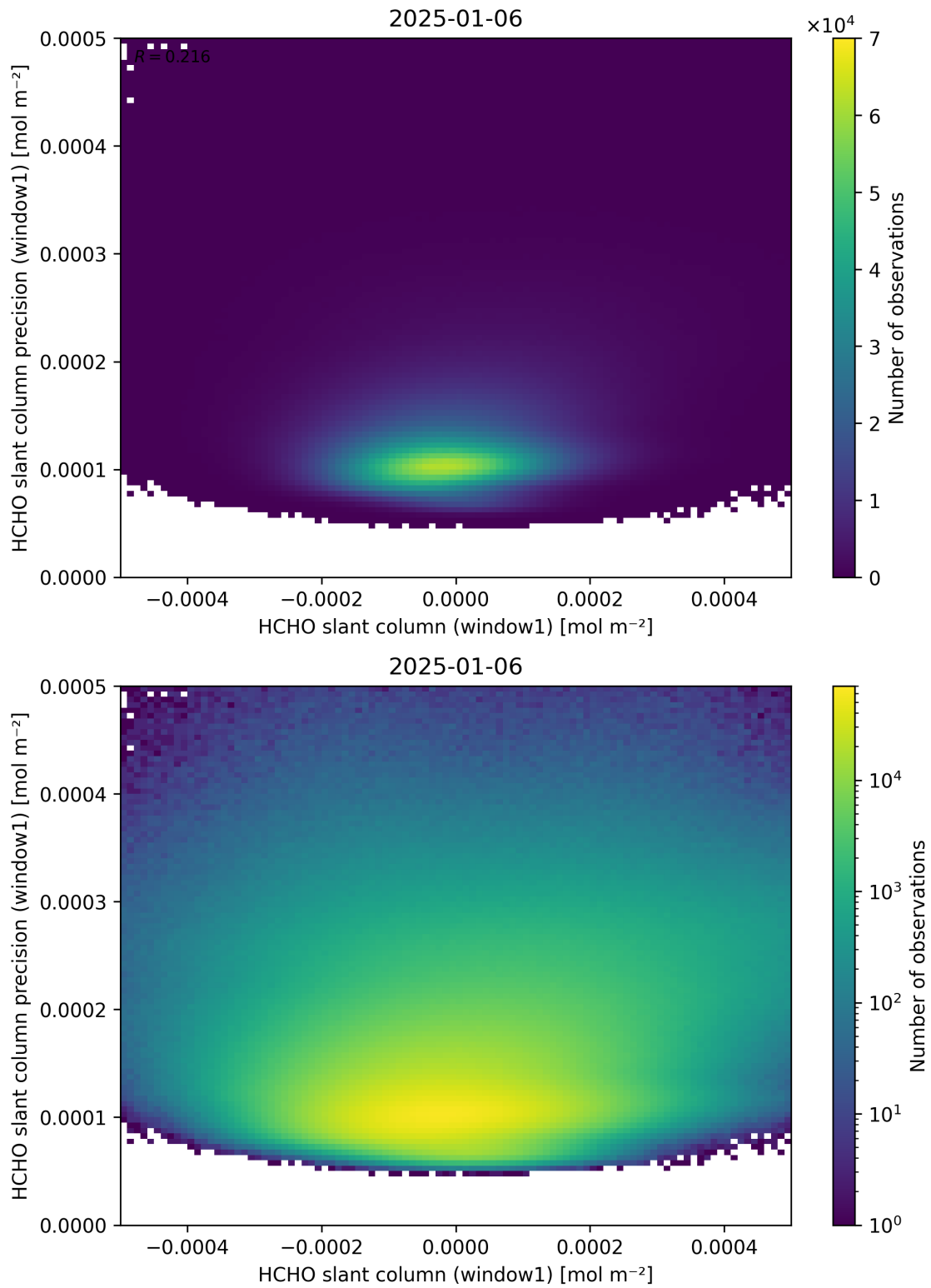
Figure 84: Scatter density plot of “HCHO slant column (window1)” against “HCHO slant column precision (window1)” for 2025-01-05 to 2025-01-07.
