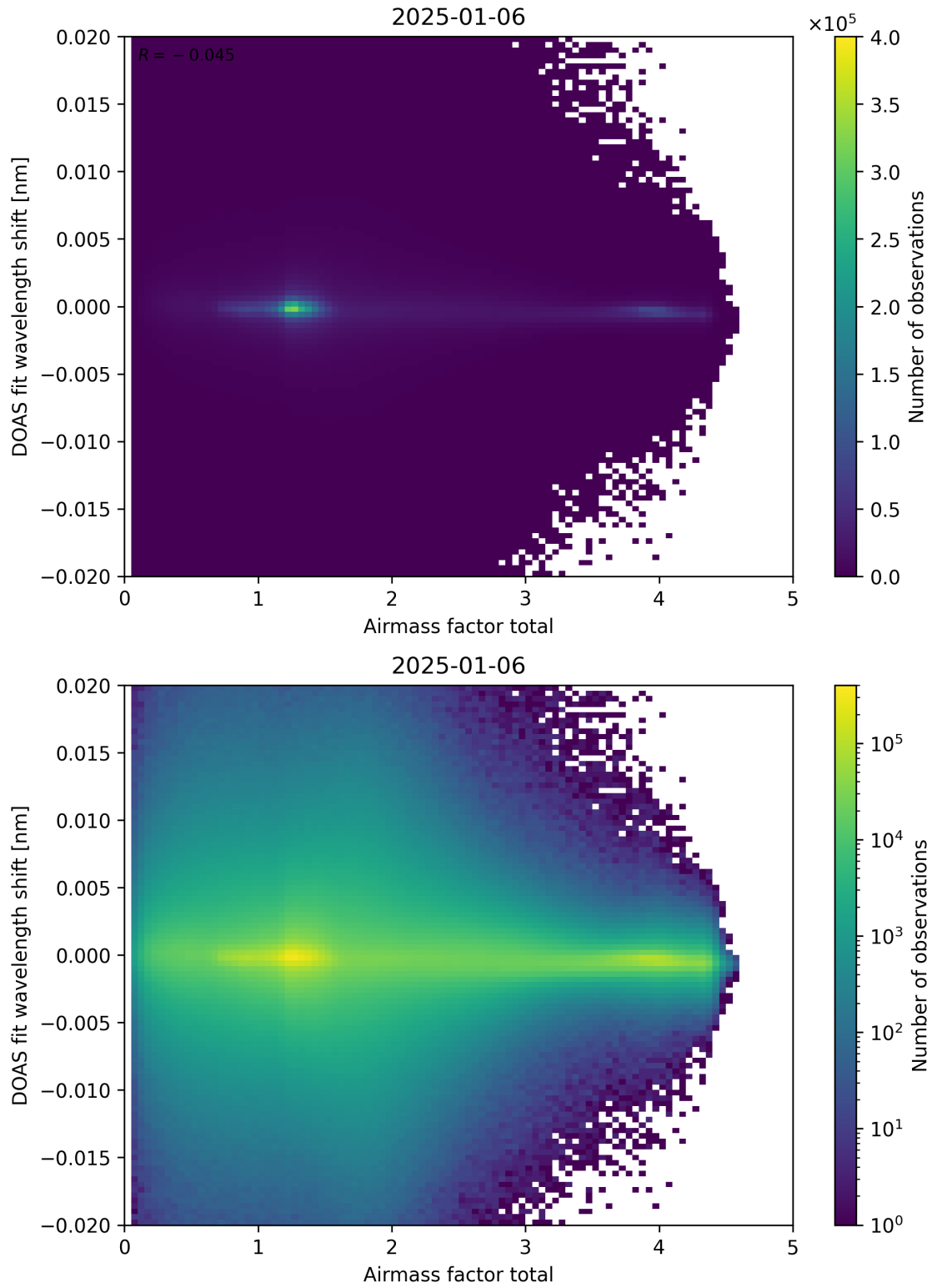
Figure 98: Scatter density plot of “Airmass factor total” against “DOAS fit wavelength shift” for 2025-01-05 to 2025-01-07.
