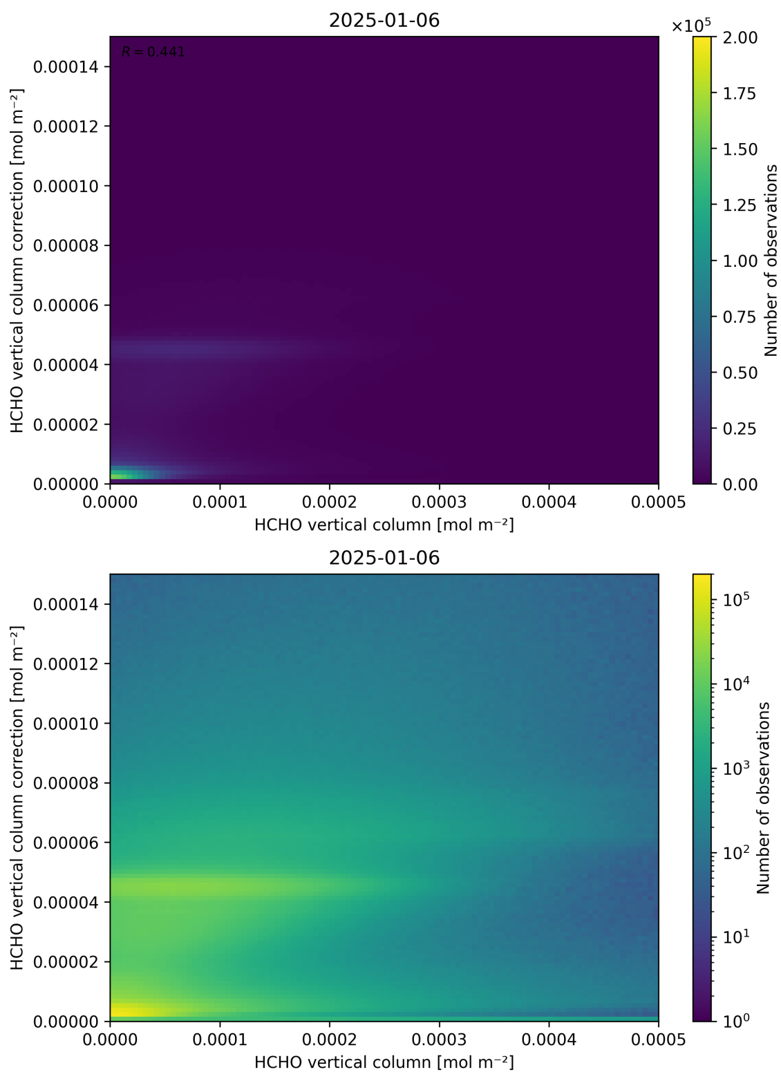
Figure 133: Scatter density plot of “HCHO vertical column” against “HCHO vertical column correction” for 2025-01-05 to 2025-01-07.
