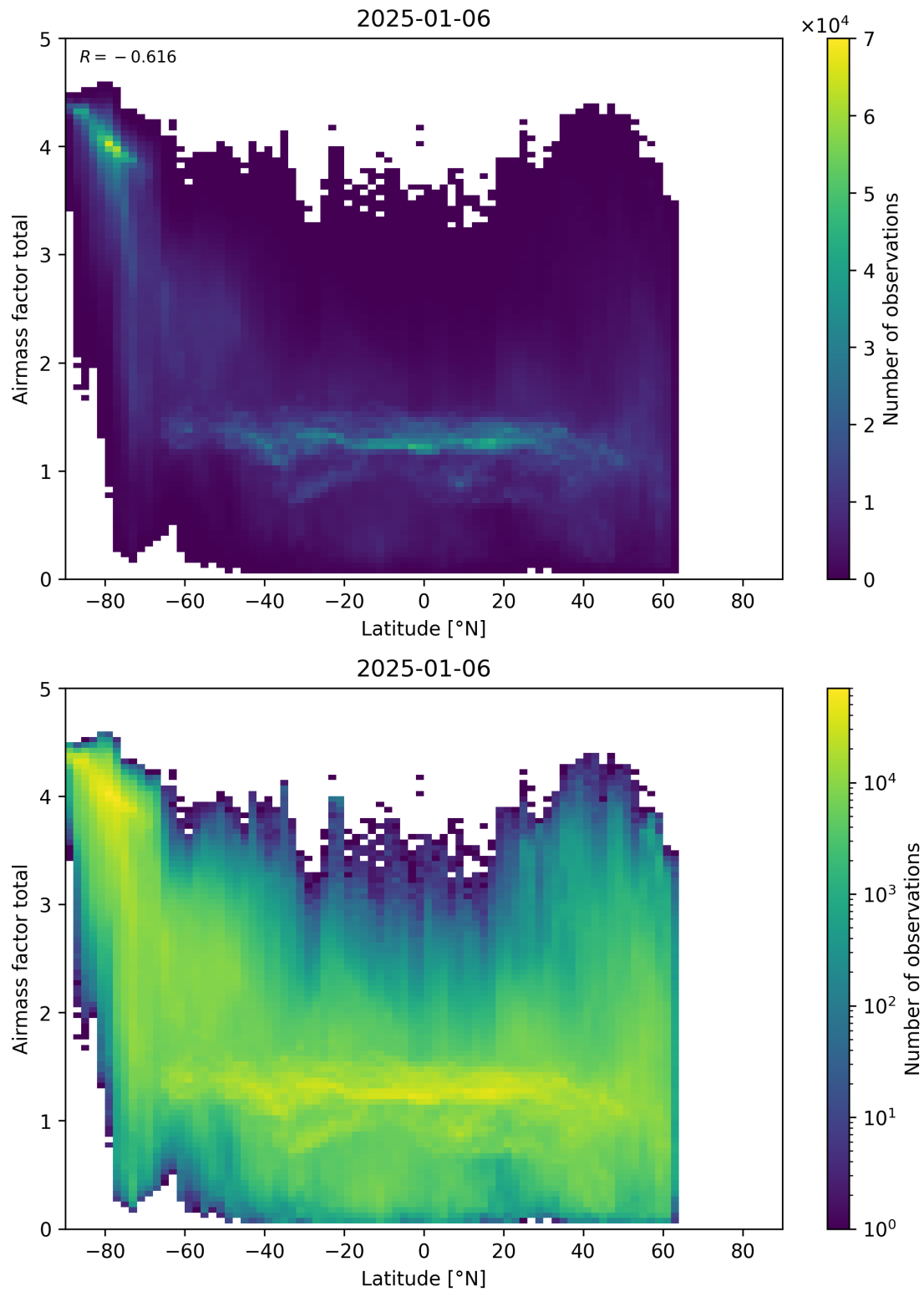
Figure 161: Scatter density plot of “Latitude” against “Airmass factor total” for 2025-01-05 to 2025-01-07.
