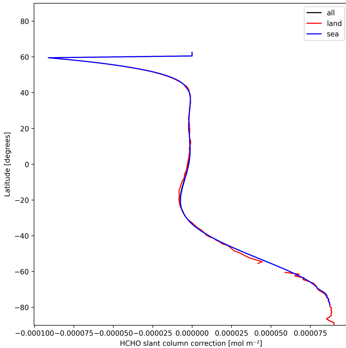
Figure 33: Zonal average of “HCHO slant column correction” for 2025-01-05 to 2025-01-07.
