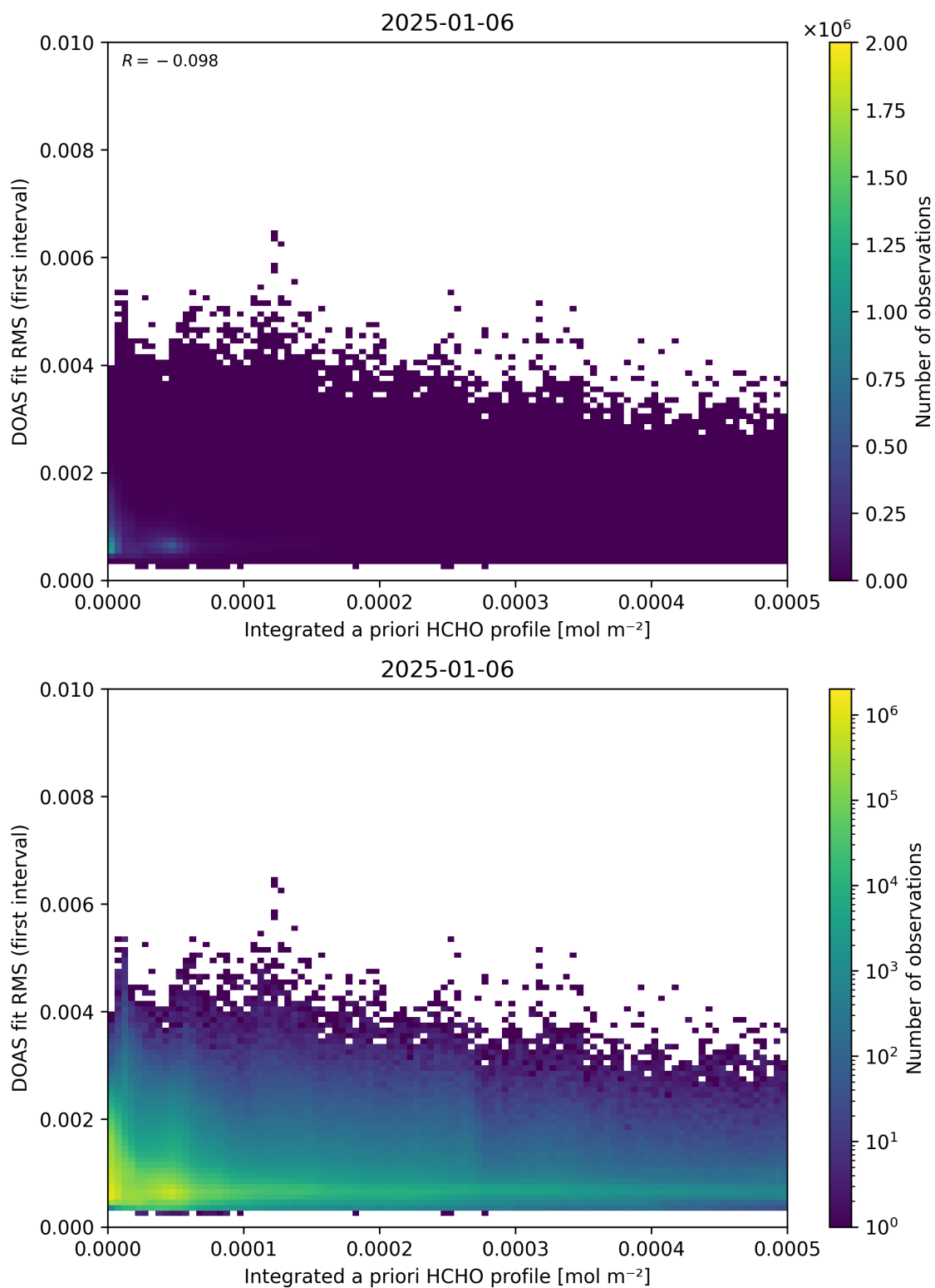
Figure 148: Scatter density plot of “Integrated a priori HCHO profile” against “DOAS fit RMS (first interval)” for 2025-01-05 to 2025-01-07.
