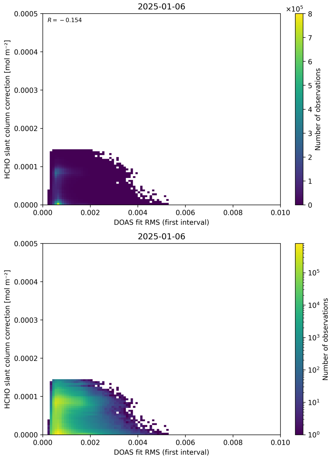
Figure 63: Scatter density plot of “DOAS fit RMS (first interval)” against “HCHO slant column correction” for 2025-01-05 to 2025-01-07.
