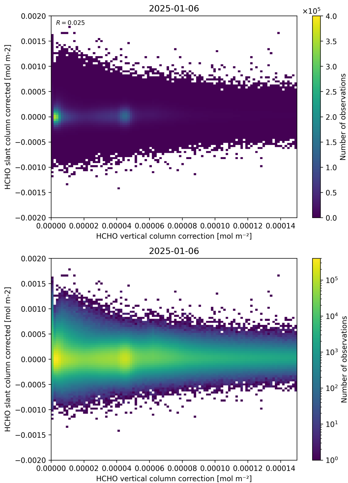
Figure 116: Scatter density plot of “HCHO vertical column correction” against “HCHO slant column corrected” for 2025-01-05 to 2025-01-07.
