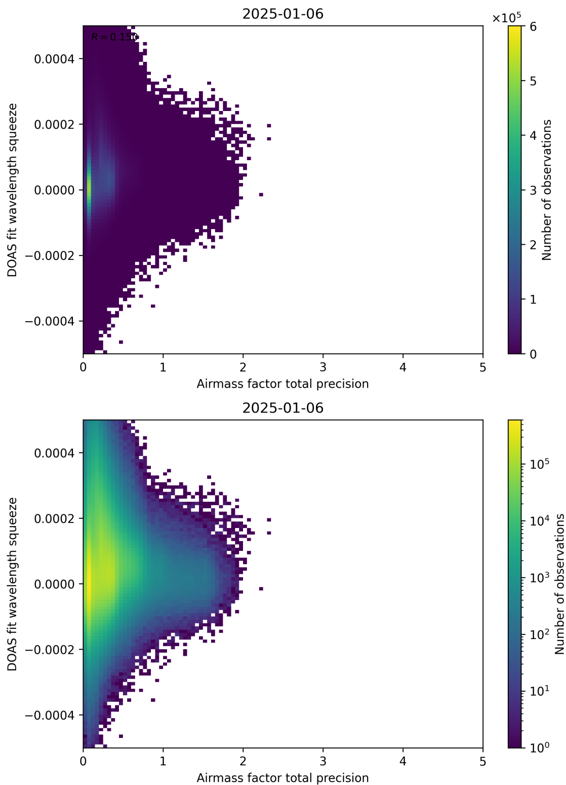
Figure 107: Scatter density plot of “Airmass factor total precision” against “DOAS fit wavelength squeeze” for 2025-01-05 to 2025-01-07.
