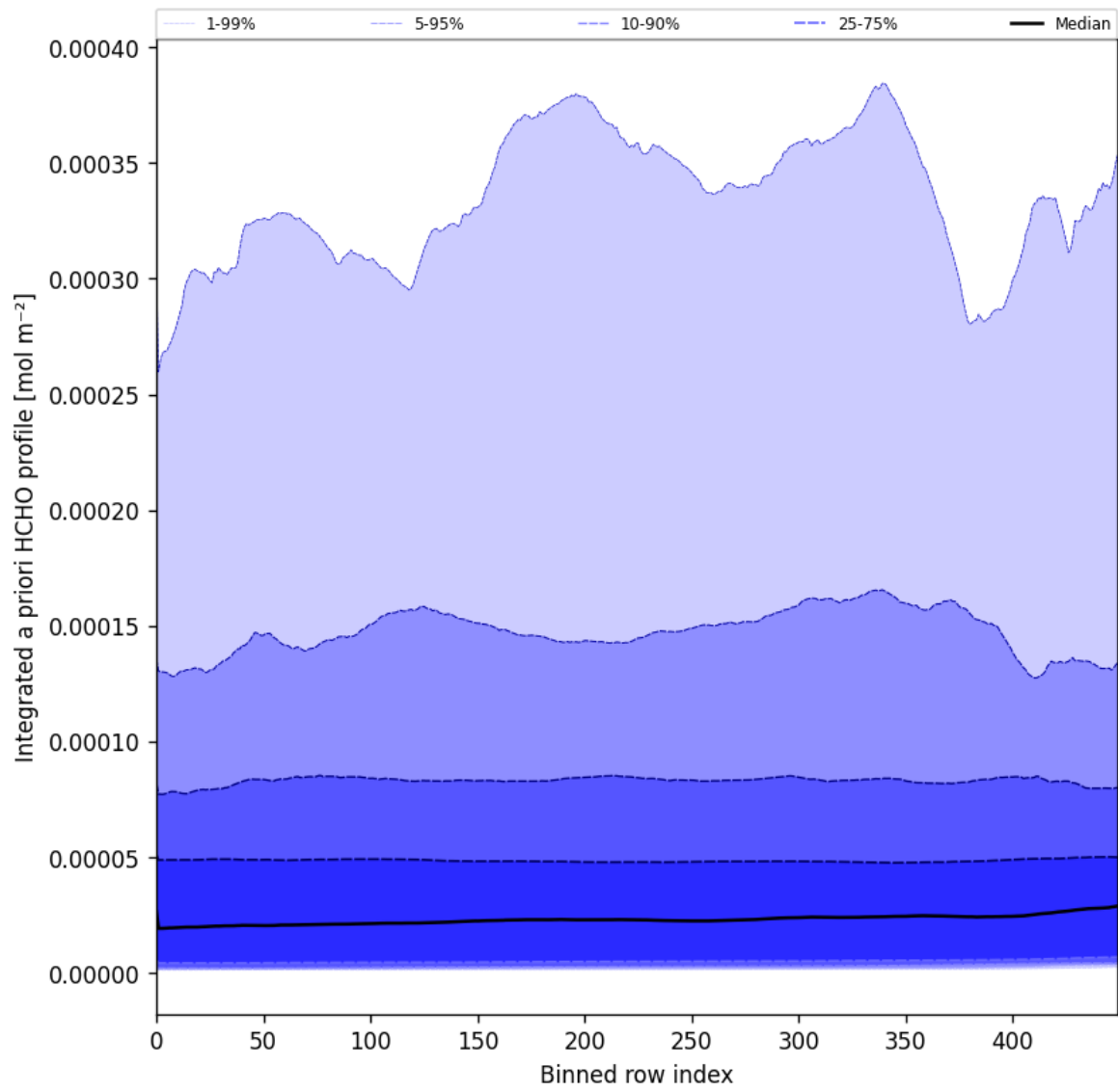
Figure 57: Along track statistics of "Integrated a priori HCHO profile" for 2025-01-05 to 2025-01-07
