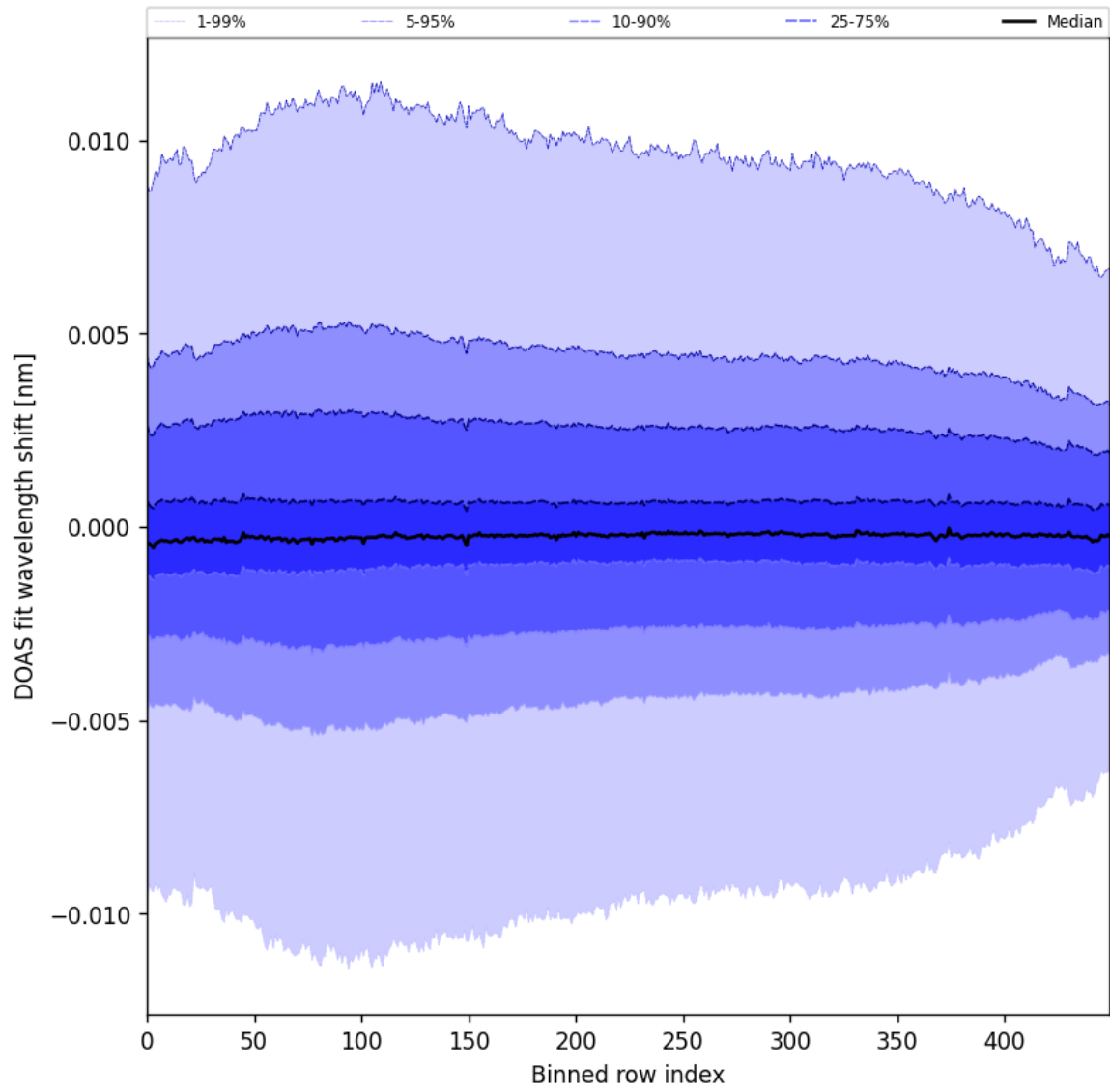
Figure 58: Along track statistics of “DOAS fit wavelength shift” for 2025-01-05 to 2025-01-07
