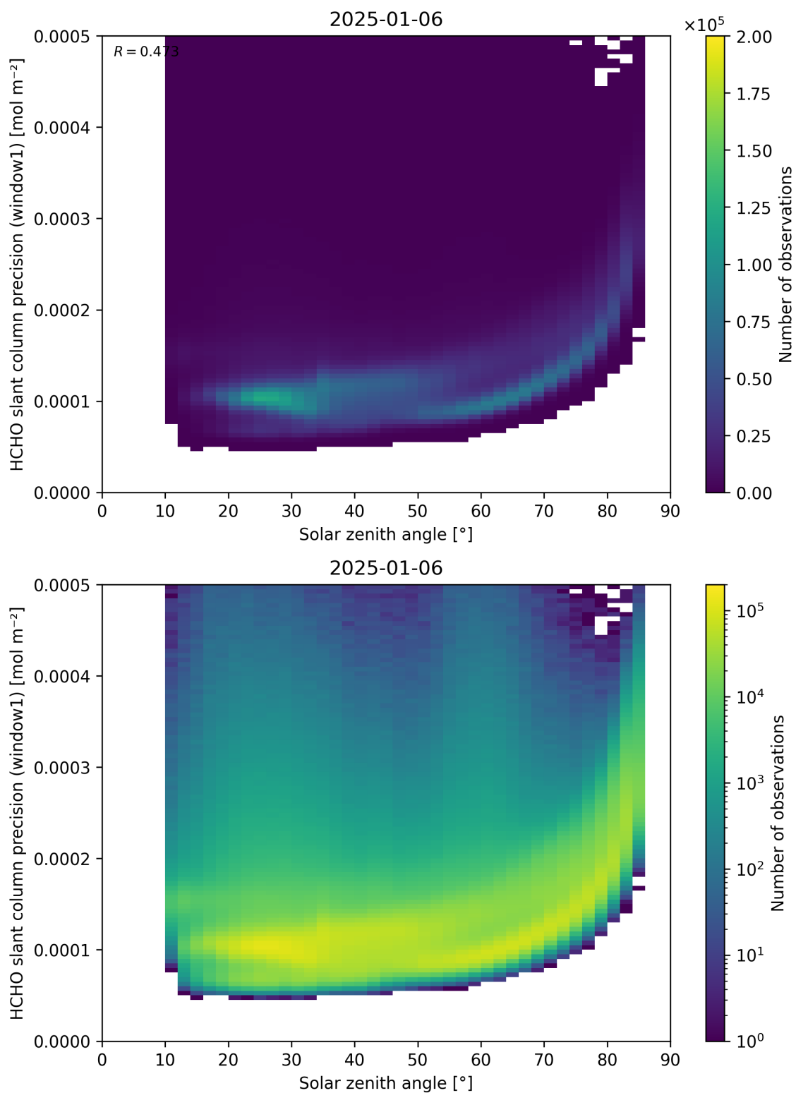
Figure 174: Scatter density plot of “Solar zenith angle” against “HCHO slant column precision (window1)” for 2025-01-05 to 2025-01-07.
