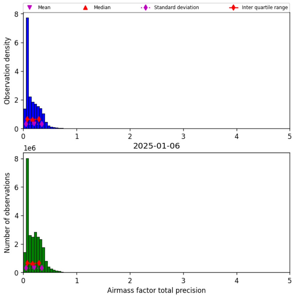
Figure 41: Histogram of “Airmass factor total precision” for 2025-01-05 to 2025-01-07
