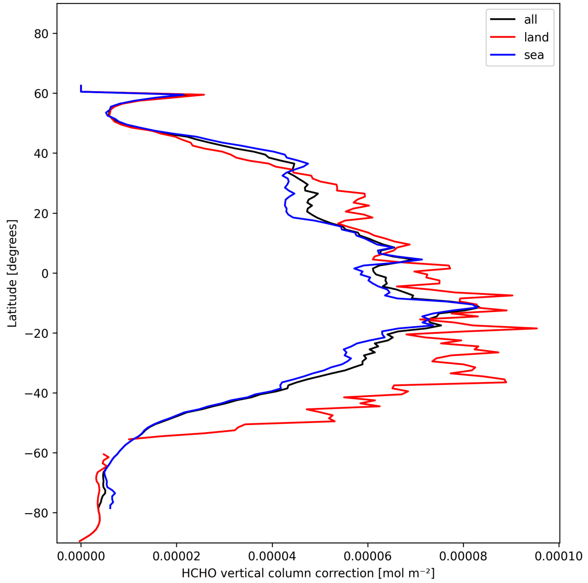
Figure 23: Zonal average of “HCHO vertical column correction” for 2025-01-05 to 2025-01-07.
