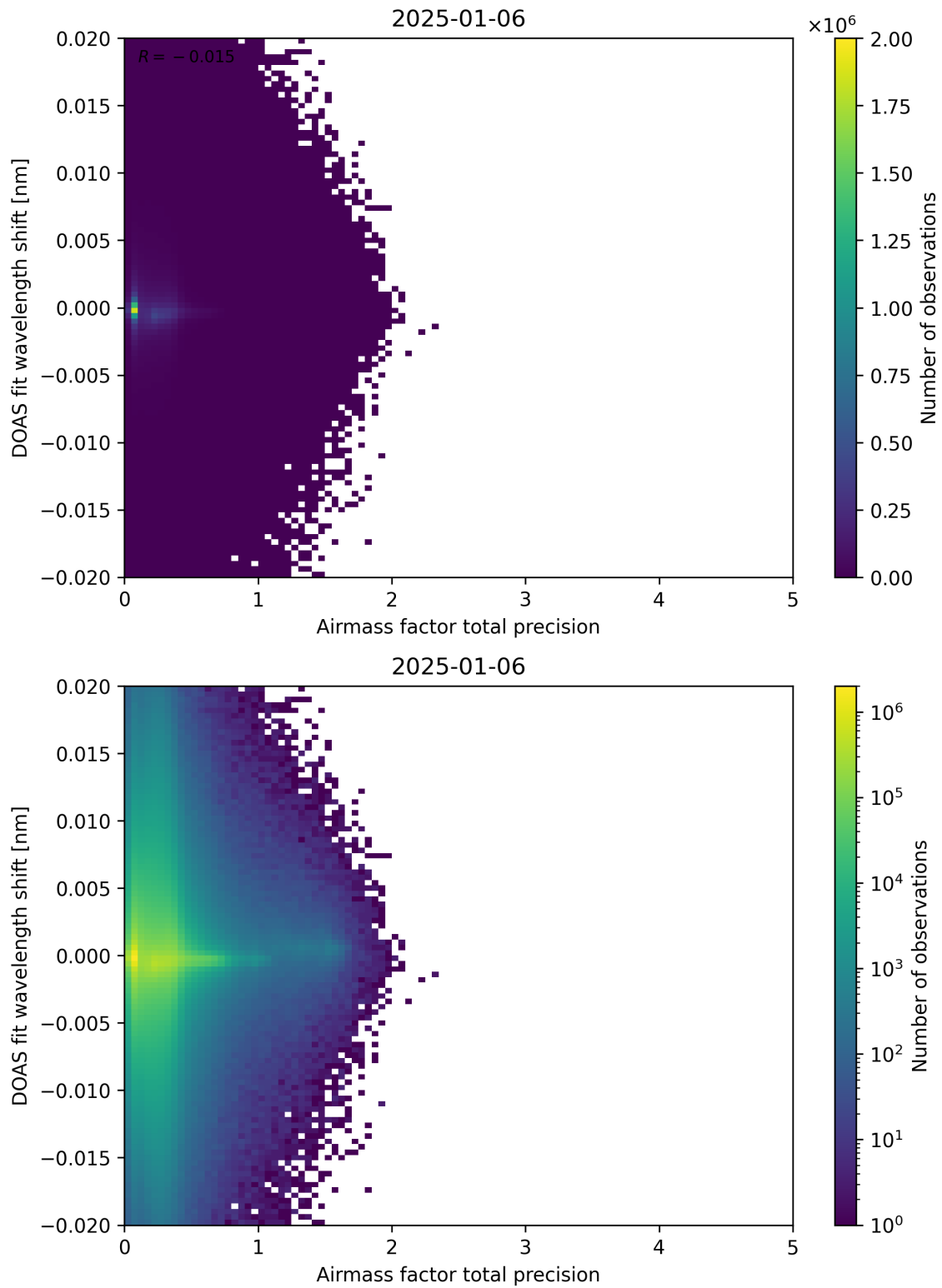
Figure 106: Scatter density plot of “Airmass factor total precision” against “DOAS fit wavelength shift” for 2025-01-05 to 2025-01-07.
