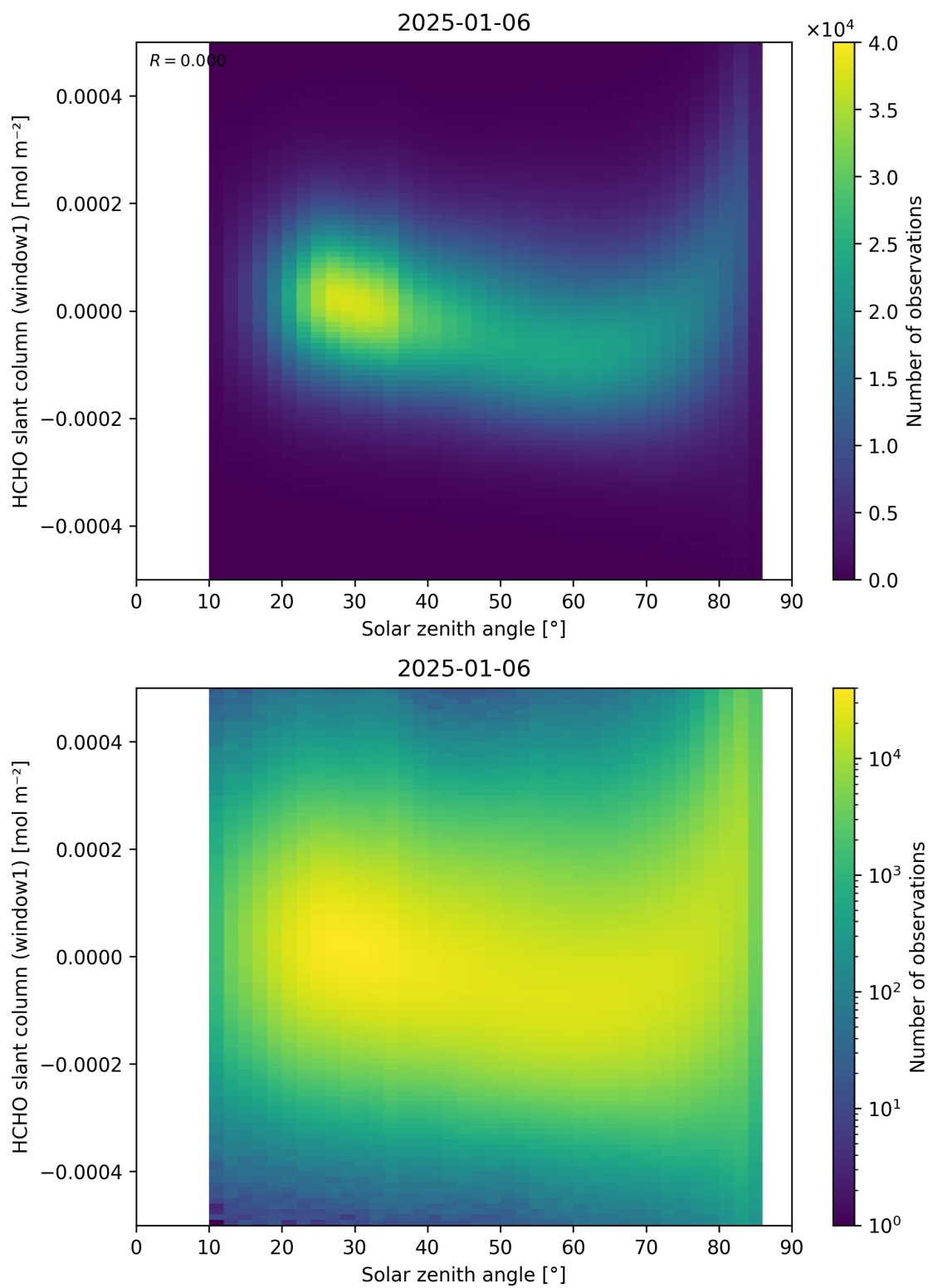
Figure 173: Scatter density plot of “Solar zenith angle” against “HCHO slant column (window1)” for 2025-01-05 to 2025-01-07.
