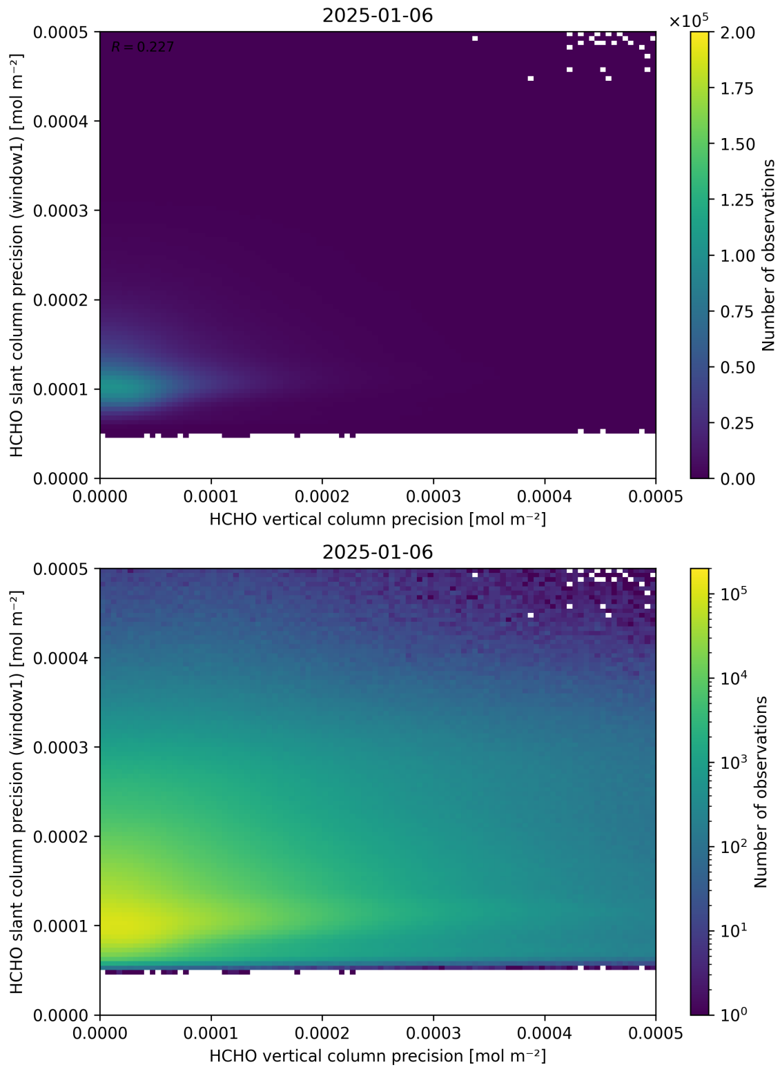
Figure 143: Scatter density plot of “HCHO vertical column precision” against “HCHO slant column precision (window1)” for 2025-01-05 to 2025-01-07.
