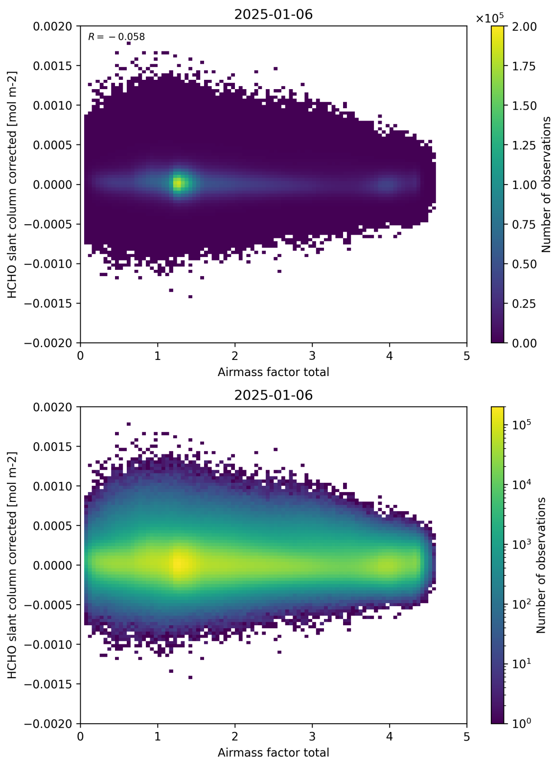
Figure 101: Scatter density plot of “Airmass factor total” against “HCHO slant column corrected” for 2025-01-05 to 2025-01-07.
