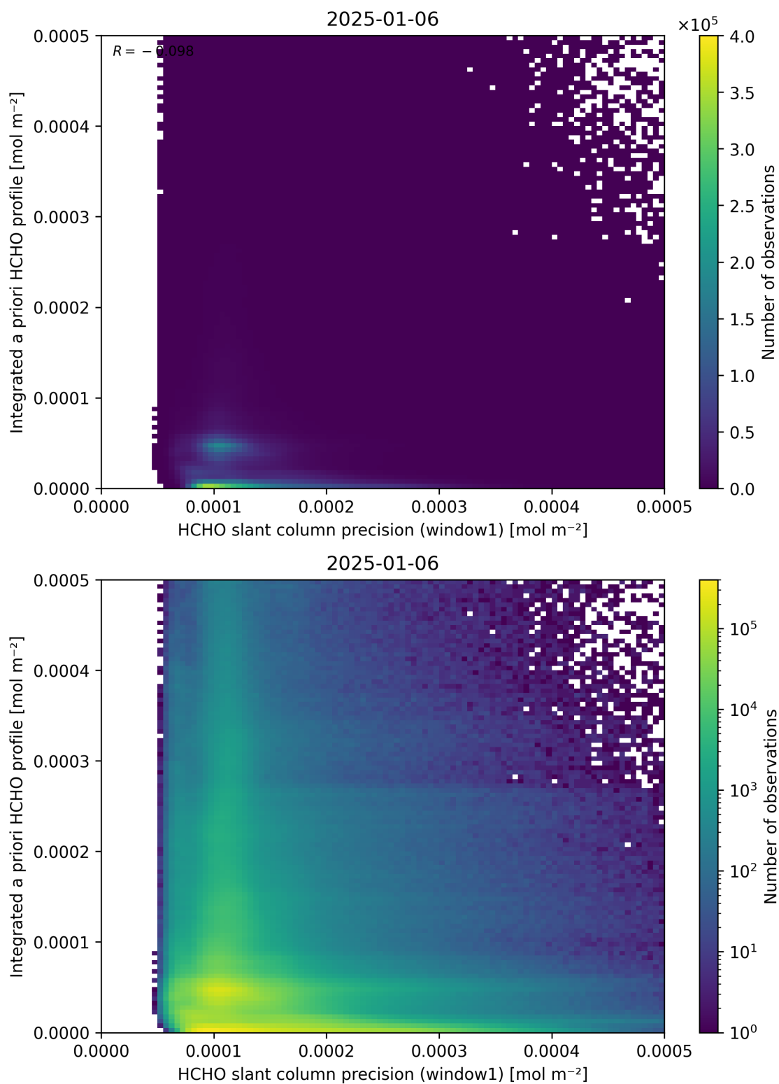
Figure 96: Scatter density plot of “HCHO slant column precision (window1)” against “Integrated a priori HCHO profile” for 2025-01-05 to 2025-01-07.
