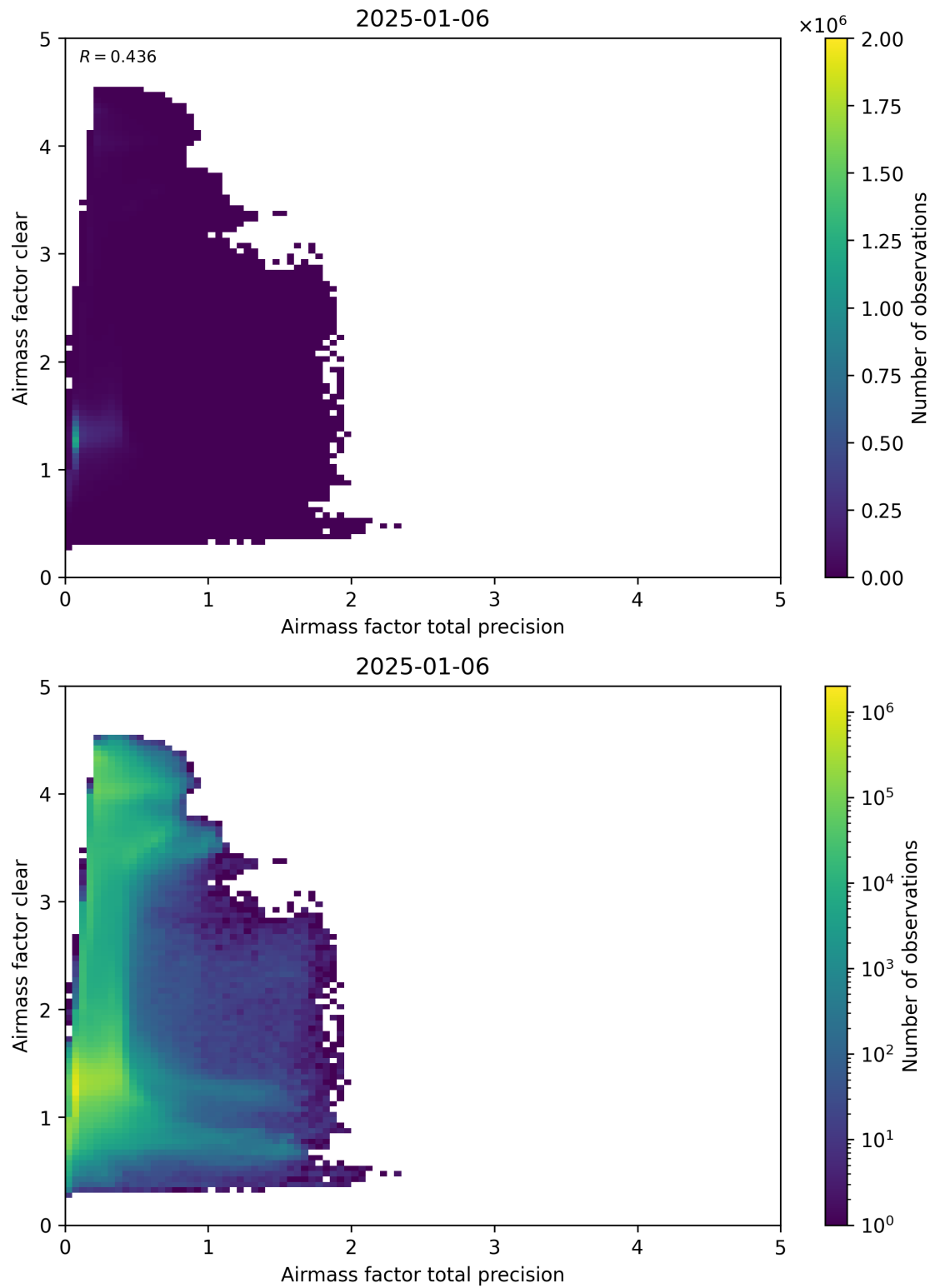
Figure 108: Scatter density plot of “Airmass factor total precision” against “Airmass factor clear” for 2025-01-05 to 2025-01-07.
