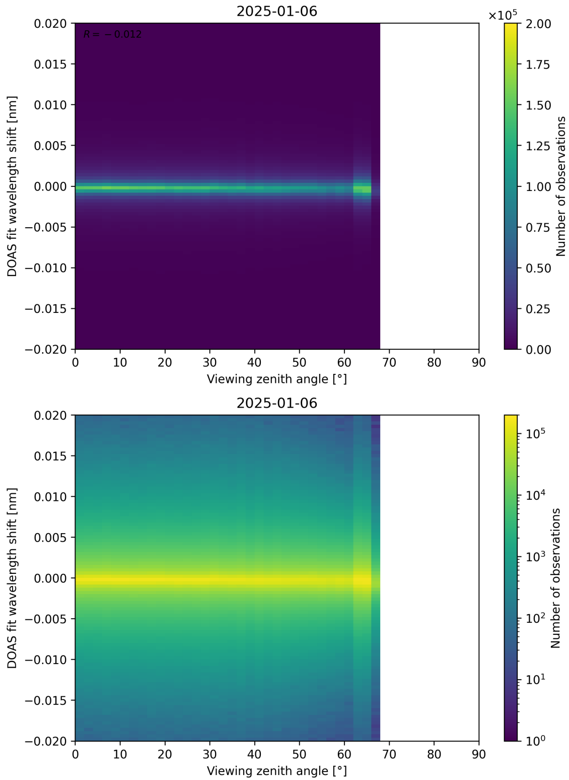
Figure 183: Scatter density plot of “Viewing zenith angle” against “DOAS fit wavelength shift” for 2025-01-05 to 2025-01-07.
