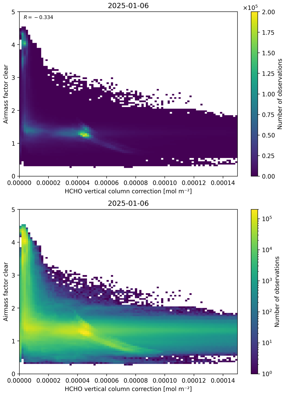
Figure 115: Scatter density plot of “HCHO vertical column correction” against “Airmass factor clear” for 2025-01-05 to 2025-01-07.
