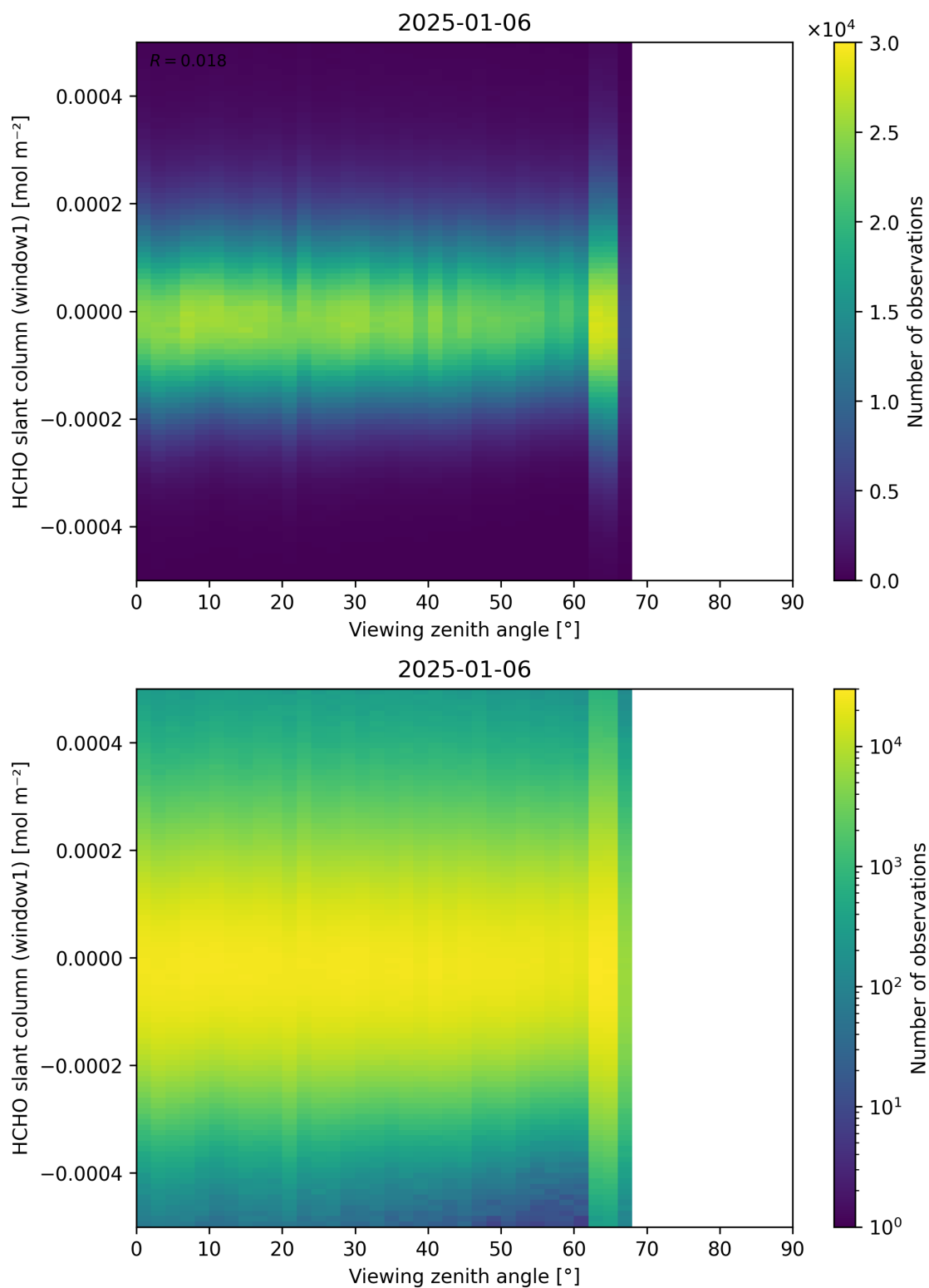
Figure 188: Scatter density plot of “Viewing zenith angle” against “HCHO slant column (window1)” for 2025-01-05 to 2025-01-07.
