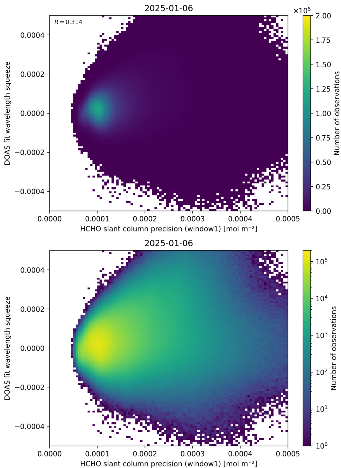
Figure 90: Scatter density plot of “HCHO slant column precision (window1)” against “DOAS fit wavelength squeeze” for 2025-01-05 to 2025-01-07.
