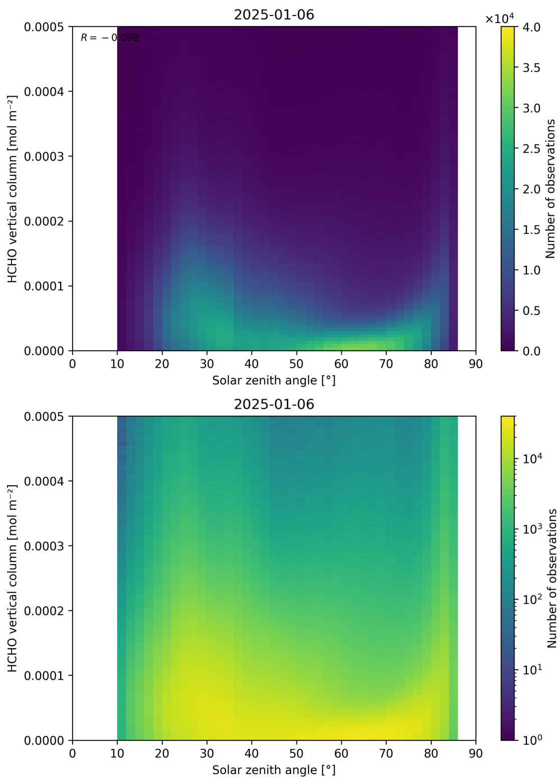
Figure 177: Scatter density plot of “Solar zenith angle” against “HCHO vertical column” for 2025-01-05 to 2025-01-07.
