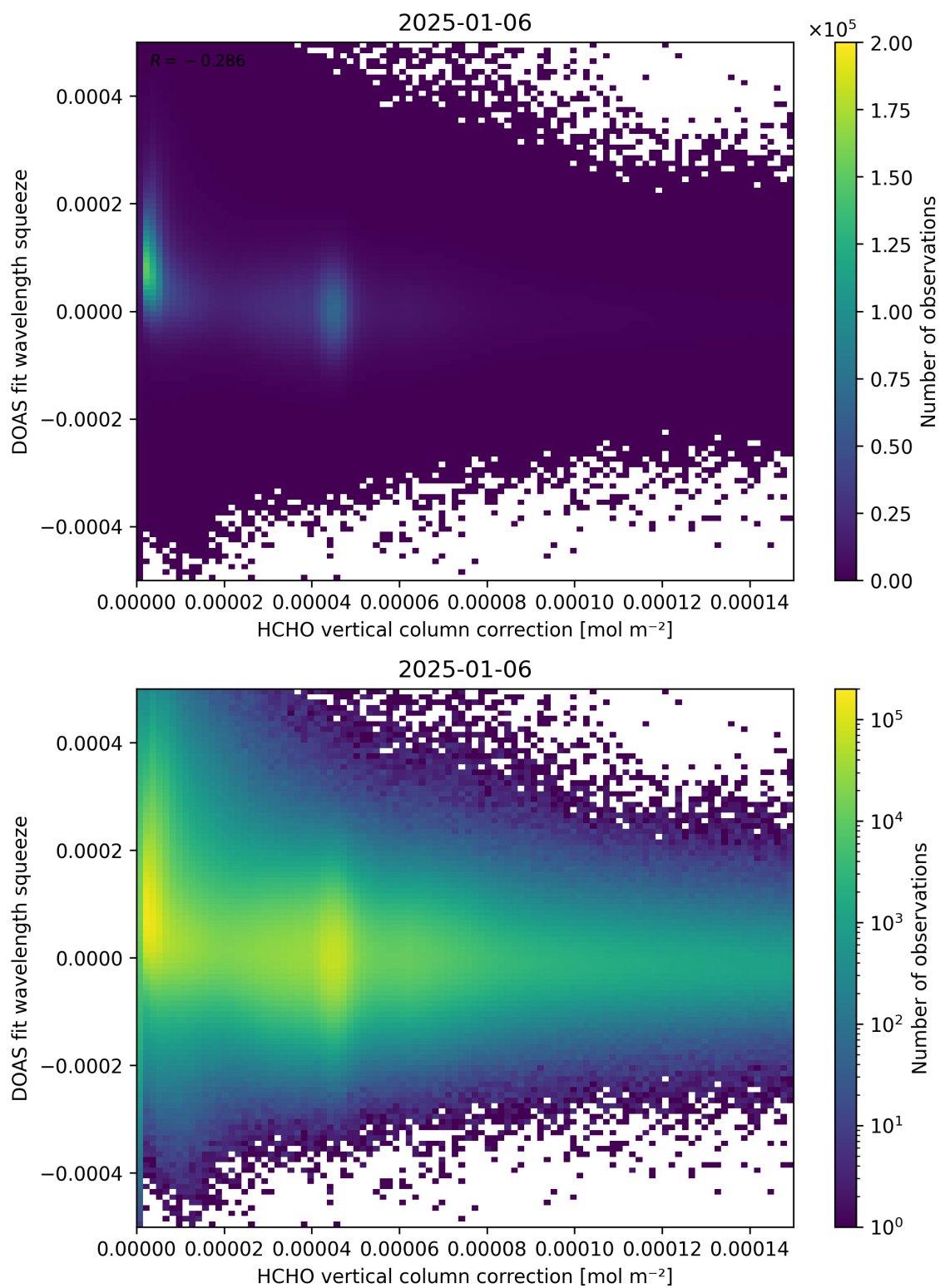
Figure 114: Scatter density plot of “HCHO vertical column correction” against “DOAS fit wavelength squeeze” for 2025-01-05 to 2025-01-07.
