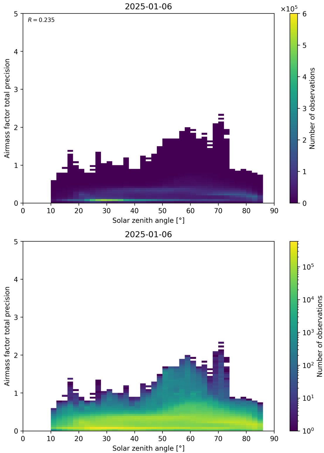
Figure 176: Scatter density plot of “Solar zenith angle” against “Airmass factor total precision” for 2025-01-05 to 2025-01-07.
