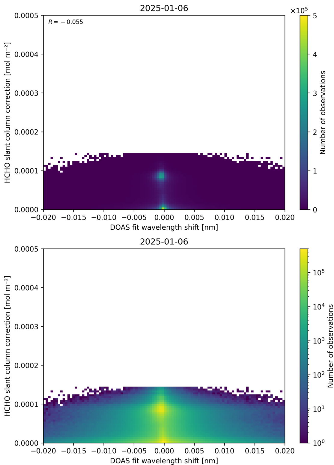
Figure 67: Scatter density plot of “DOAS fit wavelength shift” against “HCHO slant column correction” for 2025-01-05 to 2025-01-07.
