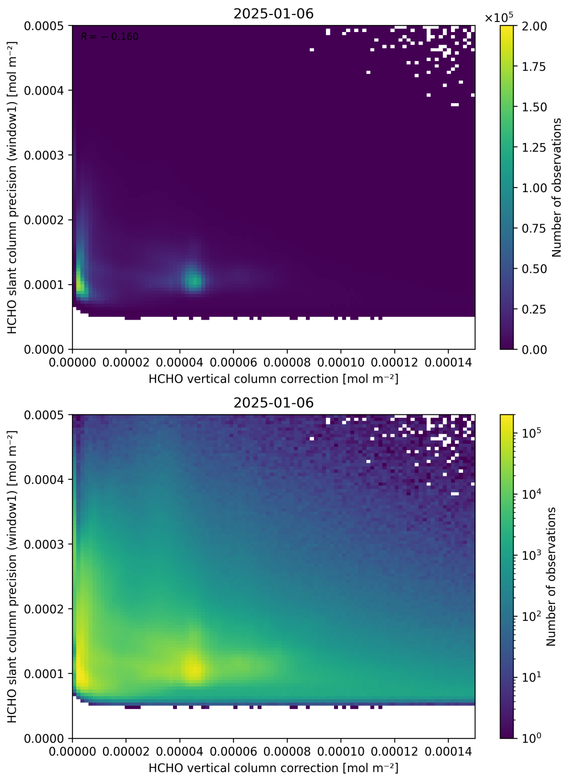
Figure 119: Scatter density plot of “HCHO vertical column correction” against “HCHO slant column precision (window1)” for 2025-01-05 to 2025-01-07.
