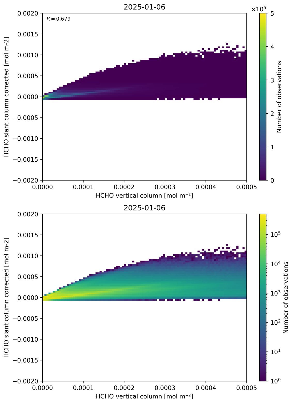
Figure 127: Scatter density plot of “HCHO vertical column” against “HCHO slant column corrected” for 2025-01-05 to 2025-01-07.
