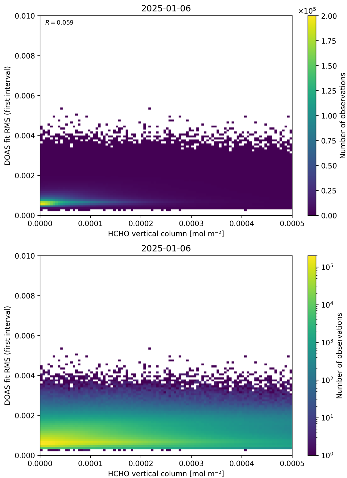
Figure 123: Scatter density plot of “HCHO vertical column” against “DOAS fit RMS (first interval)” for 2025-01-05 to 2025-01-07.
