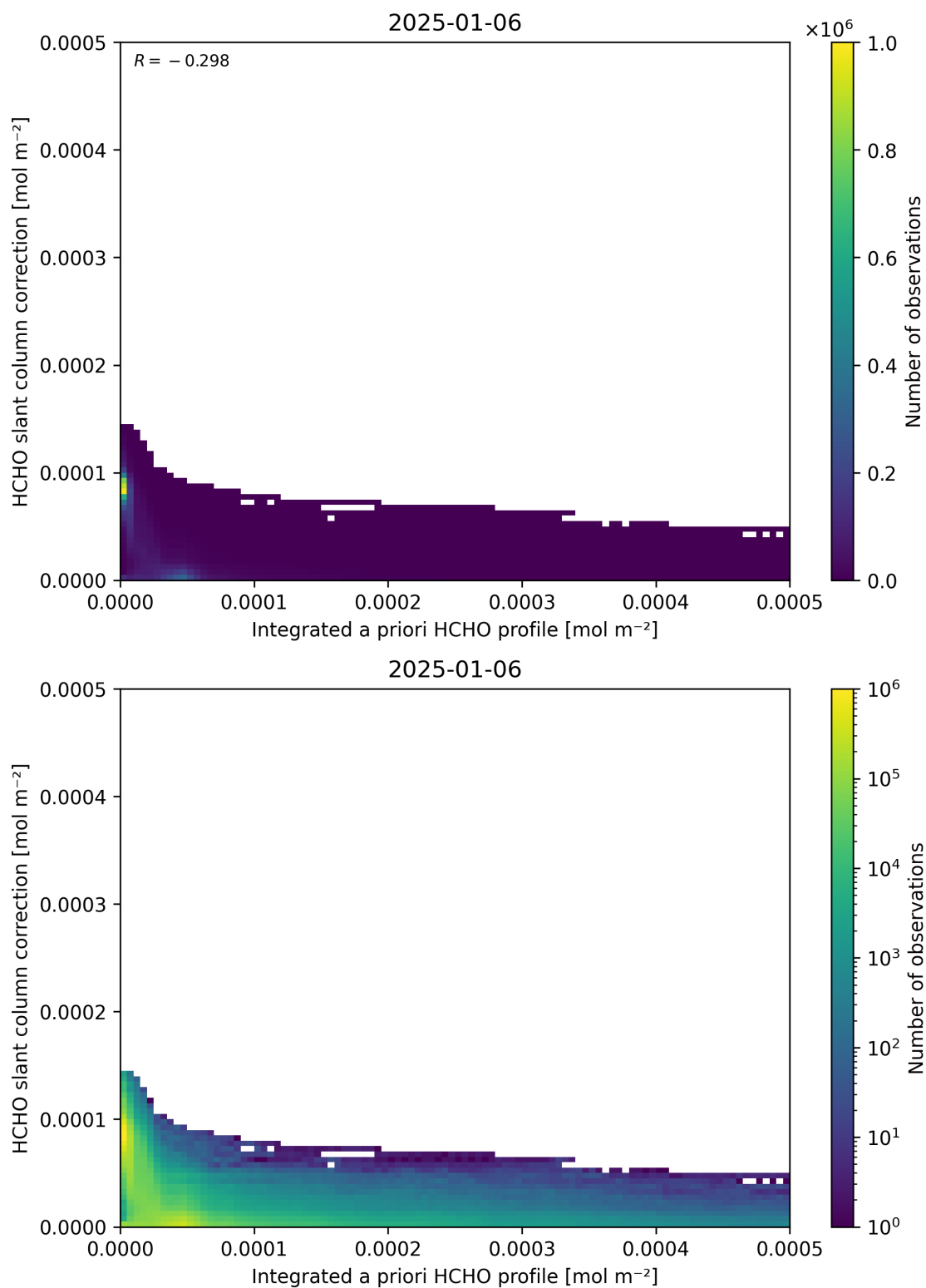
Figure 152: Scatter density plot of “Integrated a priori HCHO profile” against “HCHO slant column correction” for 2025-01-05 to 2025-01-07.
