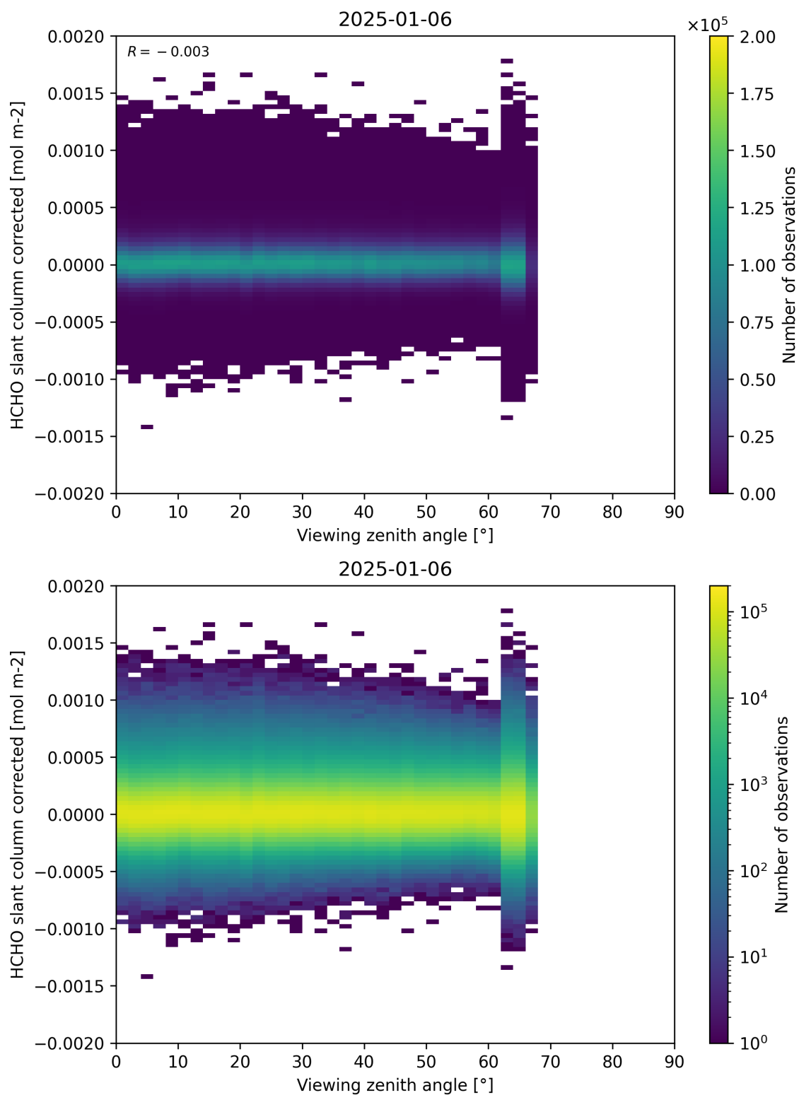
Figure 186: Scatter density plot of “Viewing zenith angle” against “HCHO slant column corrected” for 2025-01-05 to 2025-01-07.
