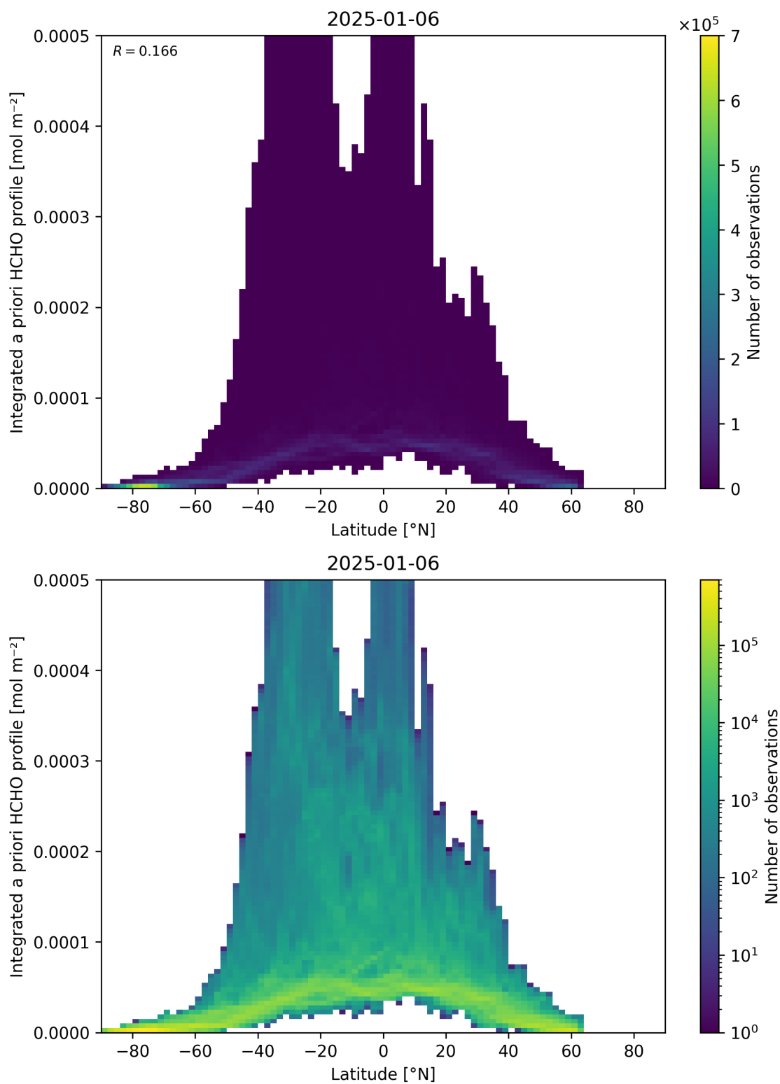
Figure 166: Scatter density plot of “Latitude” against “Integrated a priori HCHO profile” for 2025-01-05 to 2025-01-07.
