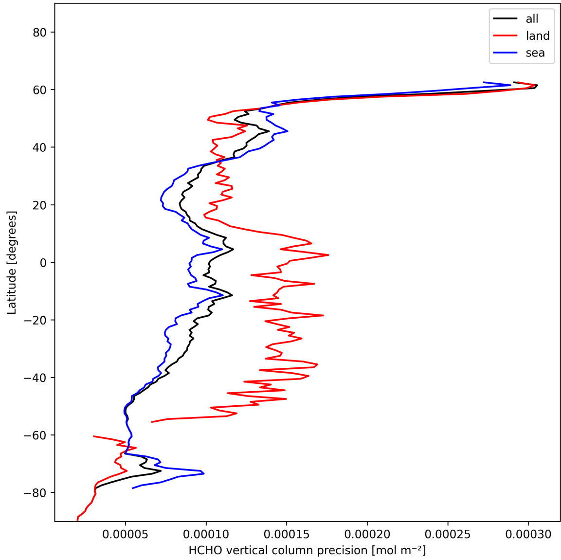
Figure 22: Zonal average of “HCHO vertical column precision” for 2025-01-05 to 2025-01-07.
