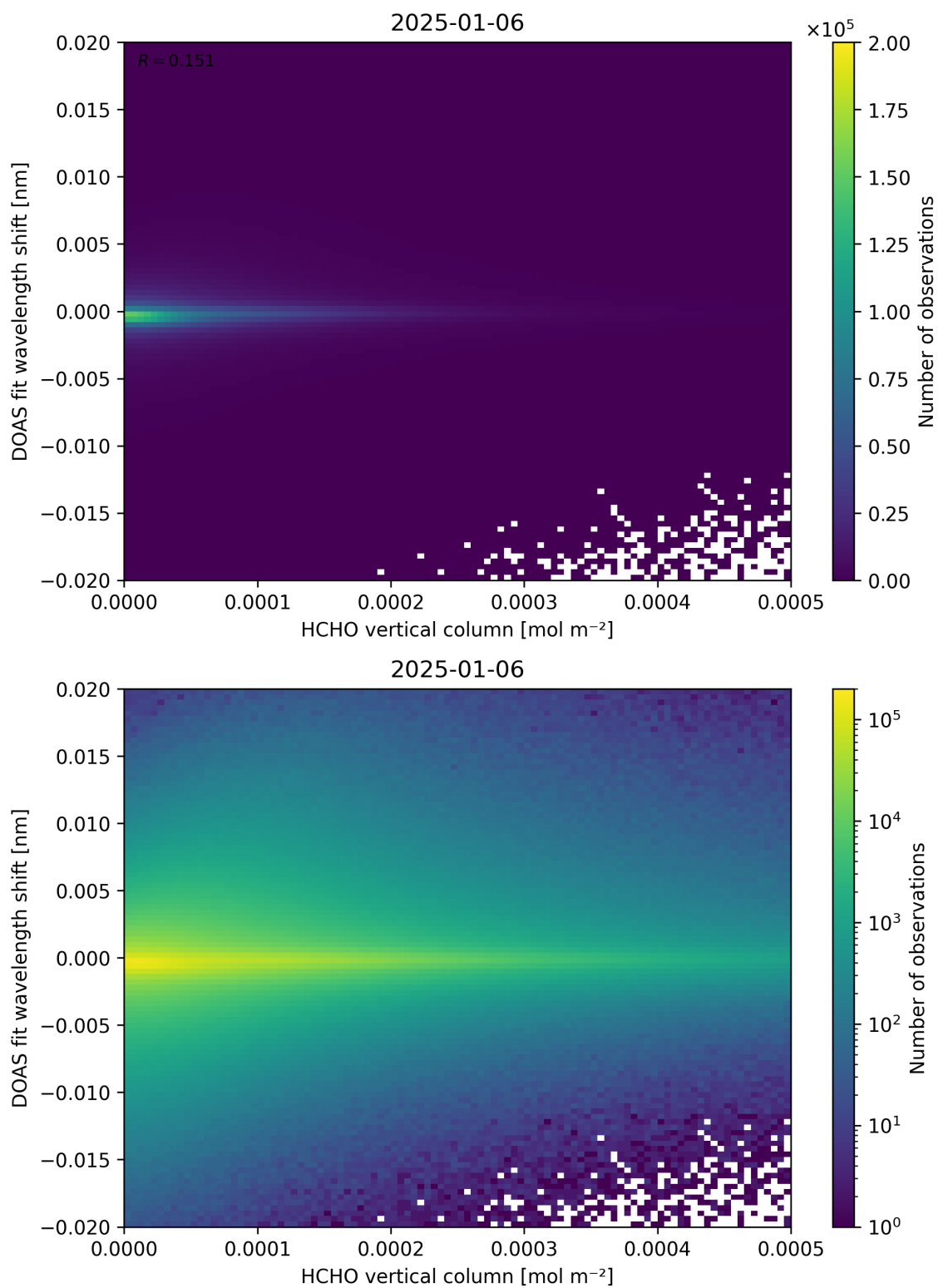
Figure 124: Scatter density plot of “HCHO vertical column” against “DOAS fit wavelength shift” for 2025-01-05 to 2025-01-07.
