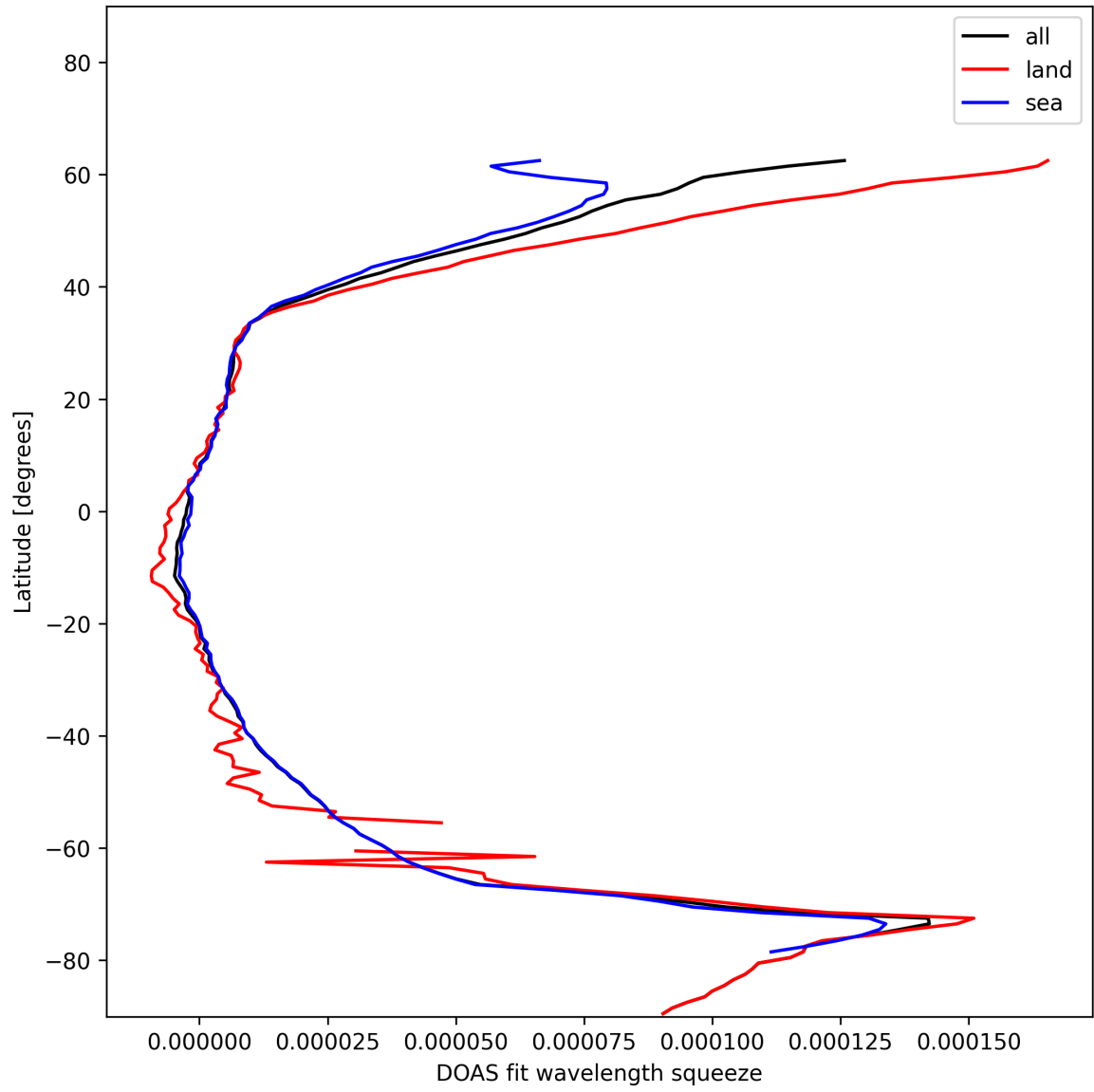
Figure 31: Zonal average of “DOAS fit wavelength squeeze” for 2025-01-05 to 2025-01-07.
