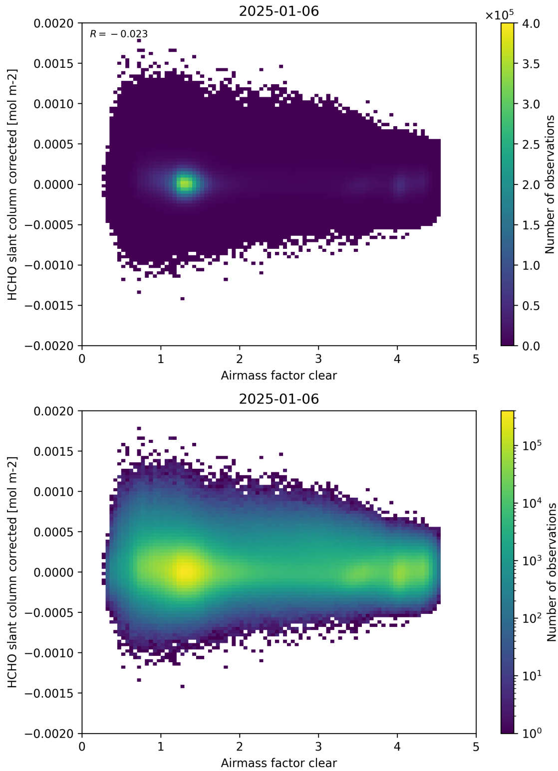
Figure 74: Scatter density plot of “Airmass factor clear” against “HCHO slant column corrected” for 2025-01-05 to 2025-01-07.
