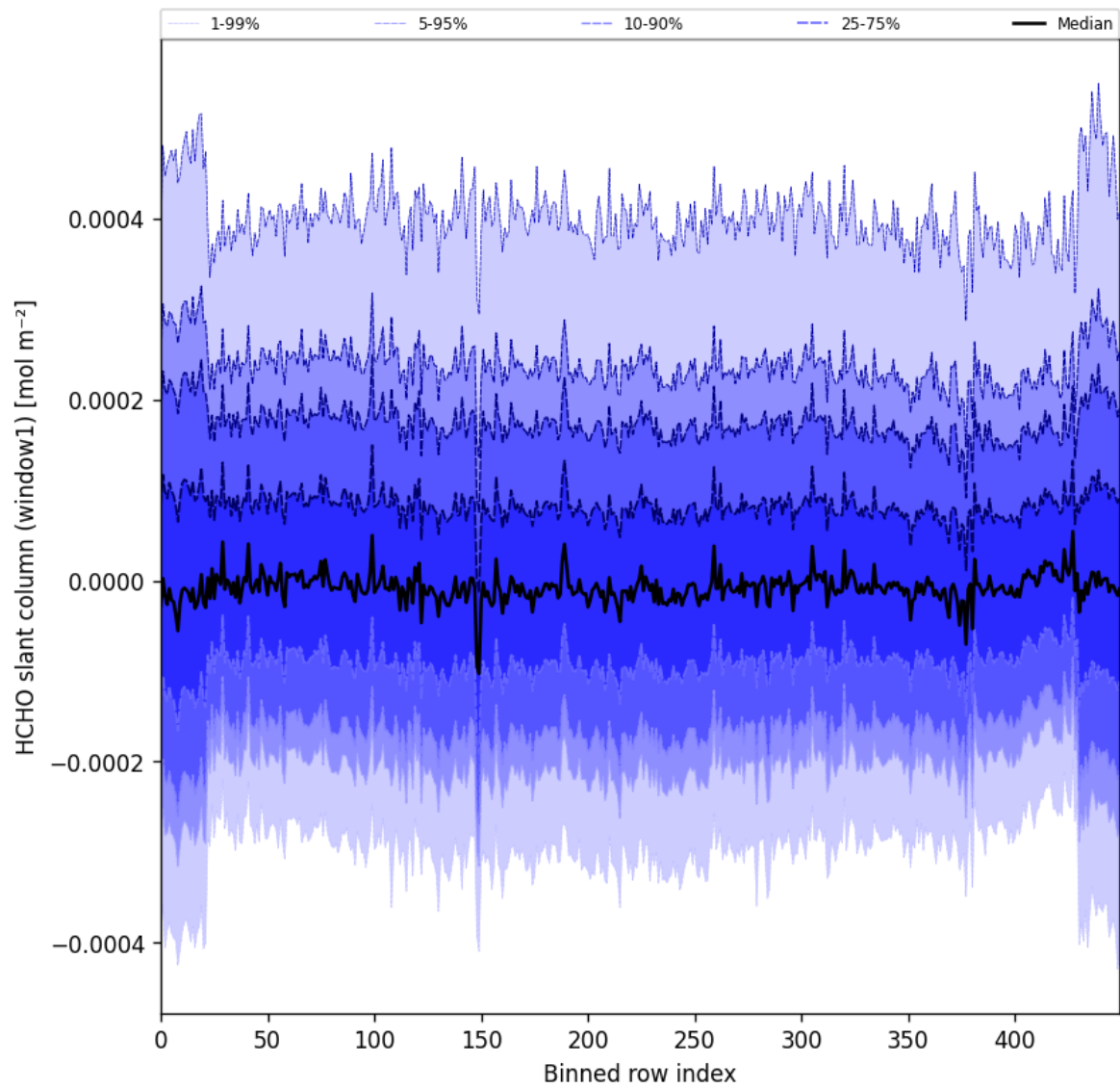
Figure 52: Along track statistics of “HCHO slant column (window1)” for 2025-01-05 to 2025-01-07
