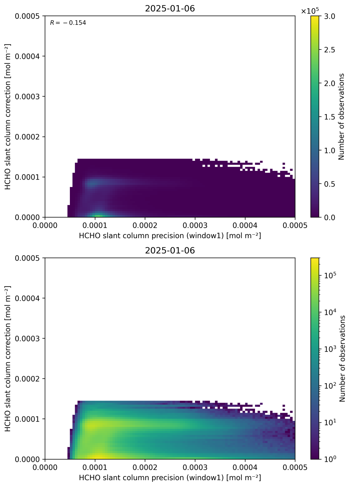
Figure 93: Scatter density plot of “HCHO slant column precision (window1)” against “HCHO slant column correction” for 2025-01-05 to 2025-01-07.
