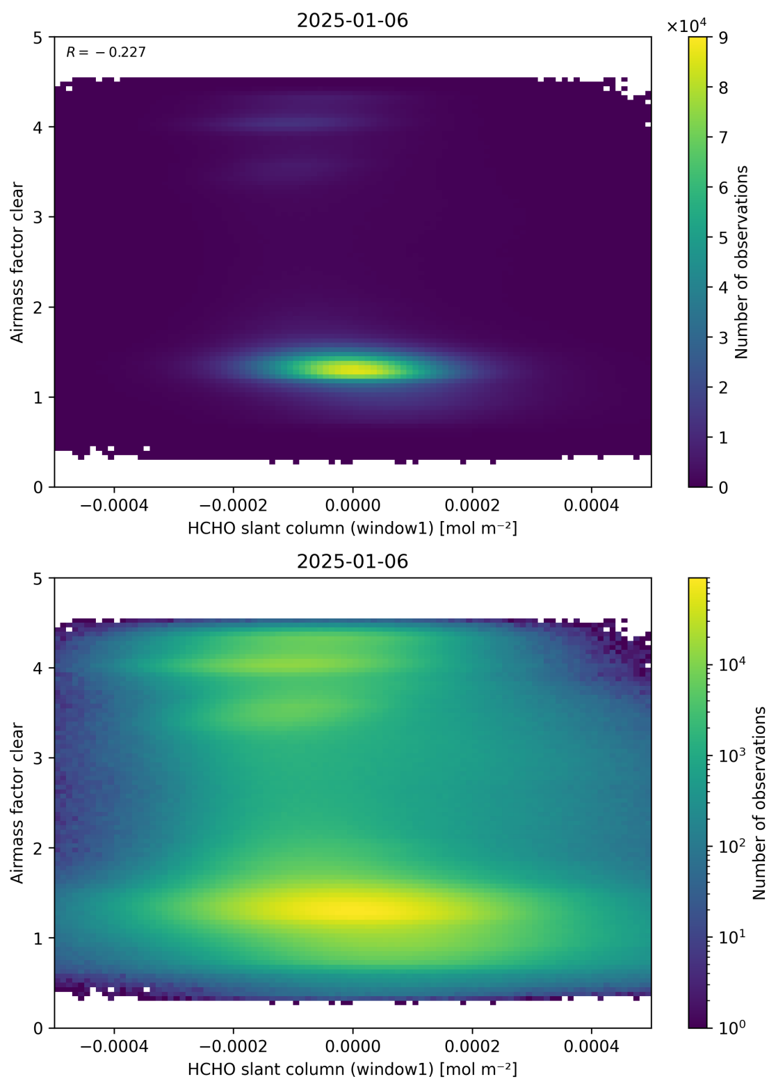
Figure 81: Scatter density plot of “HCHO slant column (window1)” against “Airmass factor clear” for 2025-01-05 to 2025-01-07.
