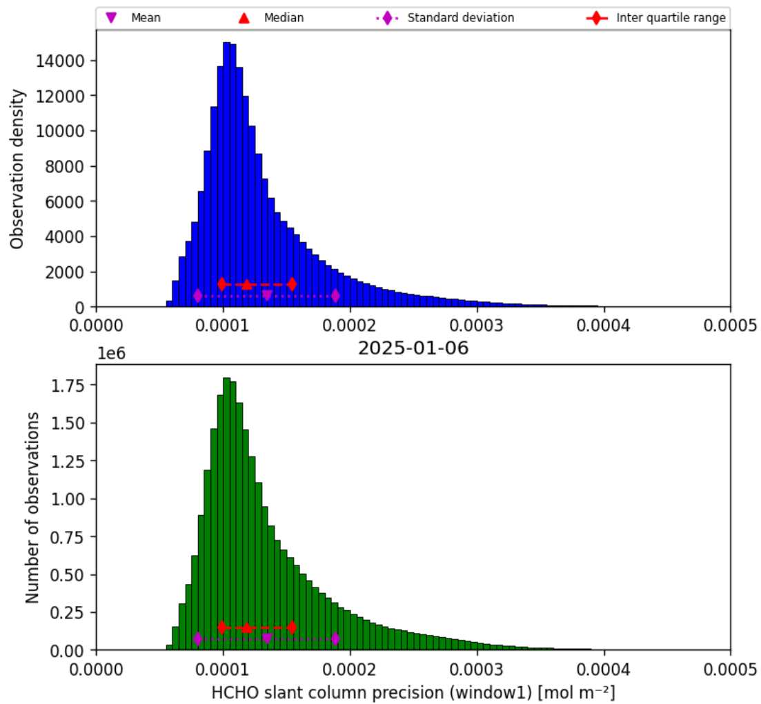
Figure 39: Histogram of “HCHO slant column precision (window1)” for 2025-01-05 to 2025-01-07
