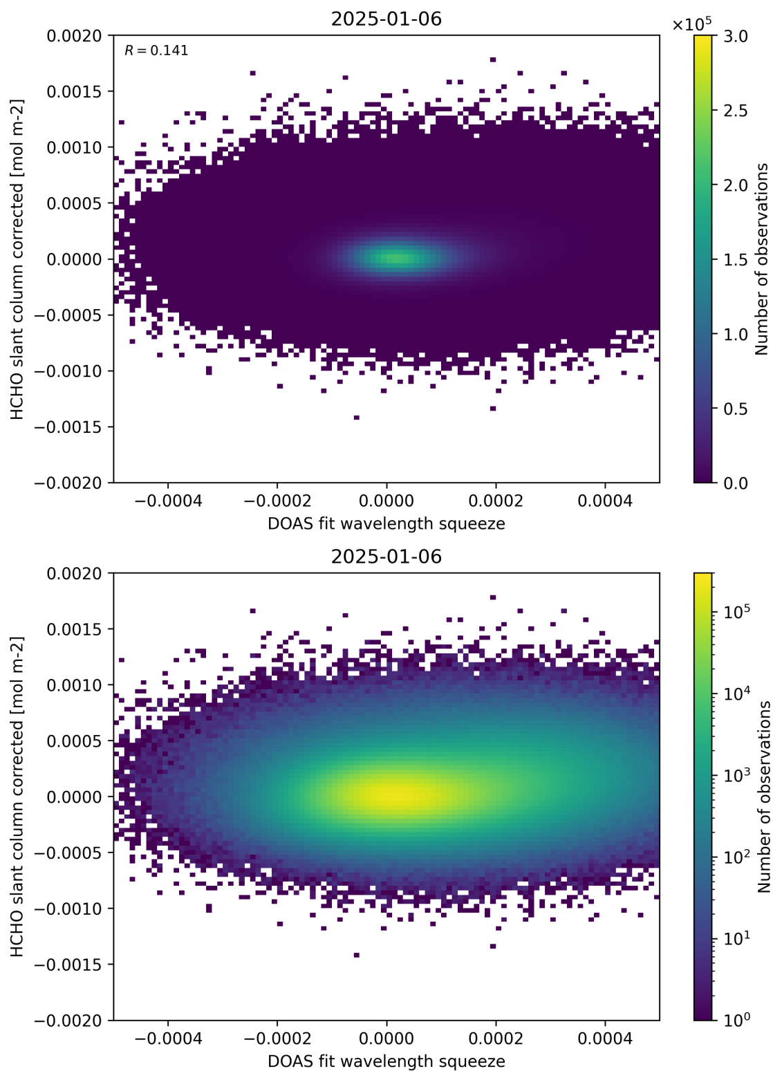
Figure 69: Scatter density plot of “DOAS fit wavelength squeeze” against “HCHO slant column corrected” for 2025-01-05 to 2025-01-07.
