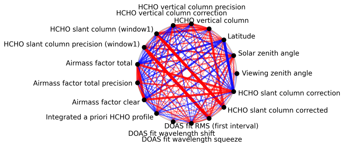
Figure 1: Map of correlation graph for 2025-01-05 to 2025-01-07.
