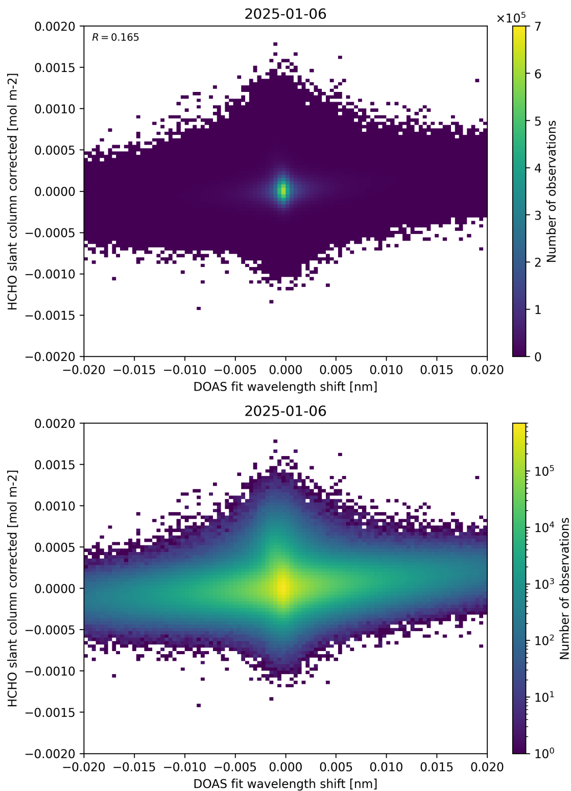
Figure 66: Scatter density plot of “DOAS fit wavelength shift” against “HCHO slant column corrected” for 2025-01-05 to 2025-01-07.
