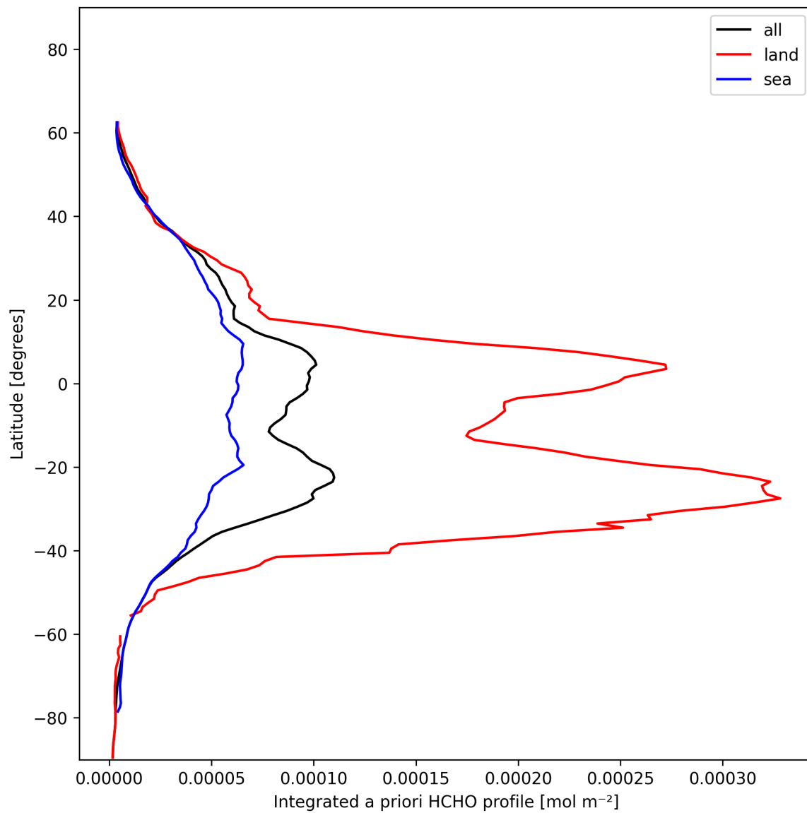
Figure 29: Zonal average of “Integrated a priori HCHO profile” for 2025-01-05 to 2025-01-07.
