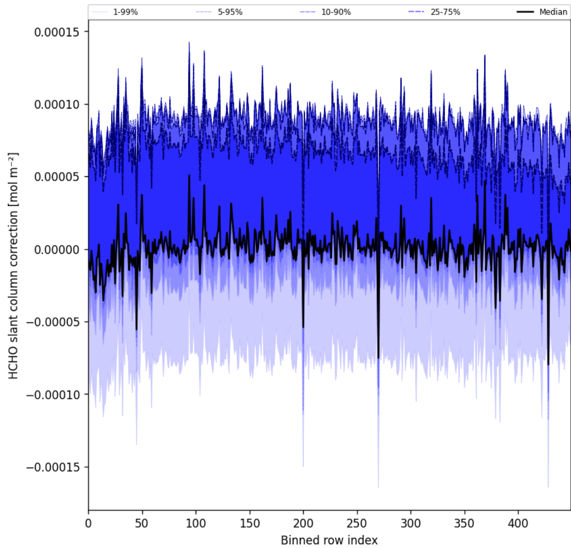
Figure 61: Along track statistics of “HCHO slant column correction” for 2025-01-05 to 2025-01-07
