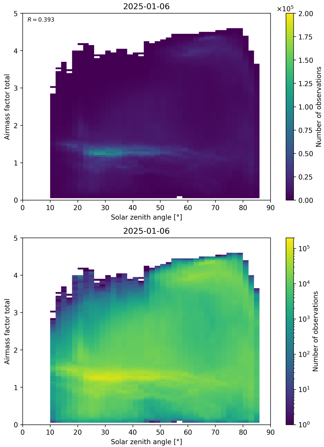
Figure 175: Scatter density plot of “Solar zenith angle” against “Airmass factor total” for 2025-01-05 to 2025-01-07.
