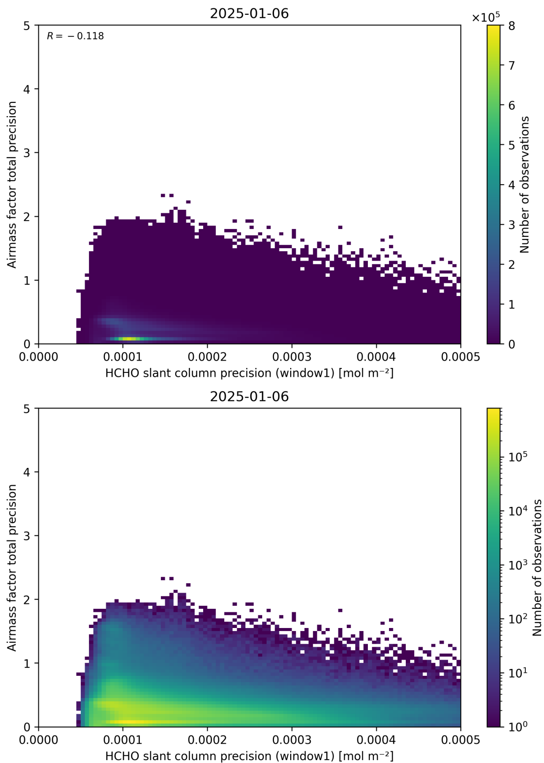
Figure 95: Scatter density plot of “HCHO slant column precision (window1)” against “Airmass factor total precision” for 2025-01-05 to 2025-01-07.
