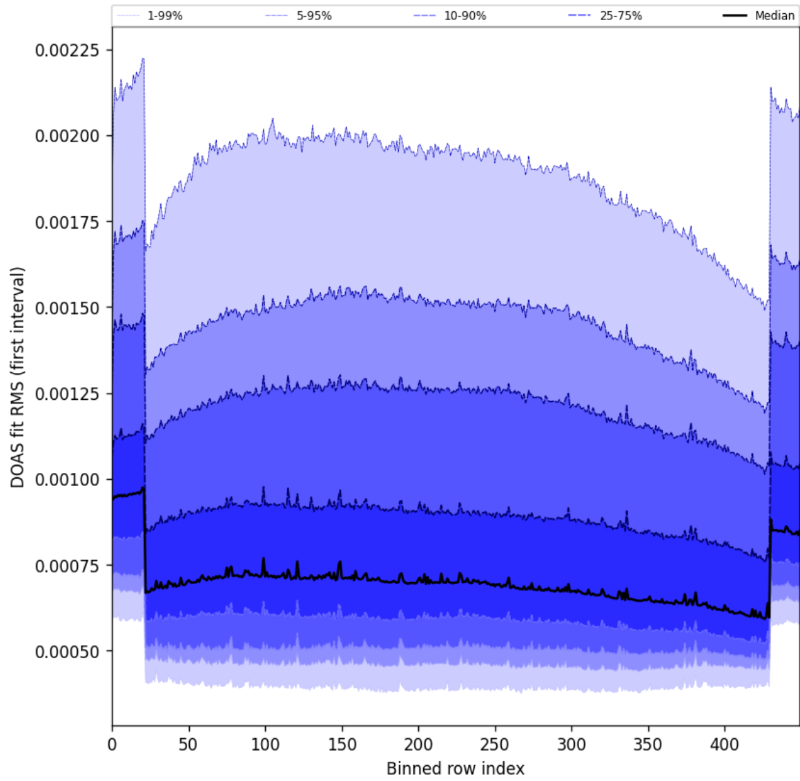
Figure 60: Along track statistics of “DOAS fit RMS (first interval)” for 2025-01-05 to 2025-01-07
