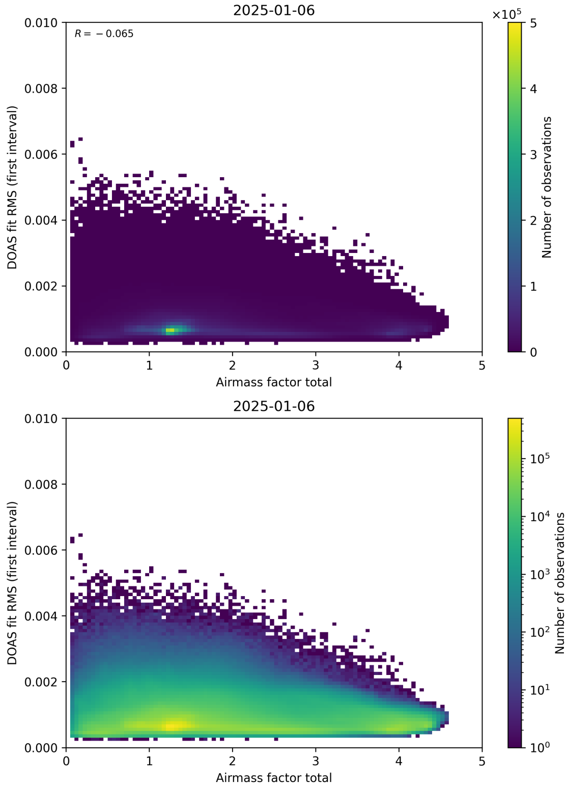
Figure 97: Scatter density plot of “Airmass factor total” against “DOAS fit RMS (first interval)” for 2025-01-05 to 2025-01-07.
