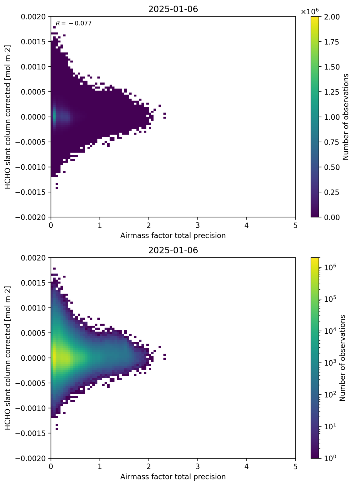
Figure 109: Scatter density plot of “Airmass factor total precision” against “HCHO slant column corrected” for 2025-01-05 to 2025-01-07.
