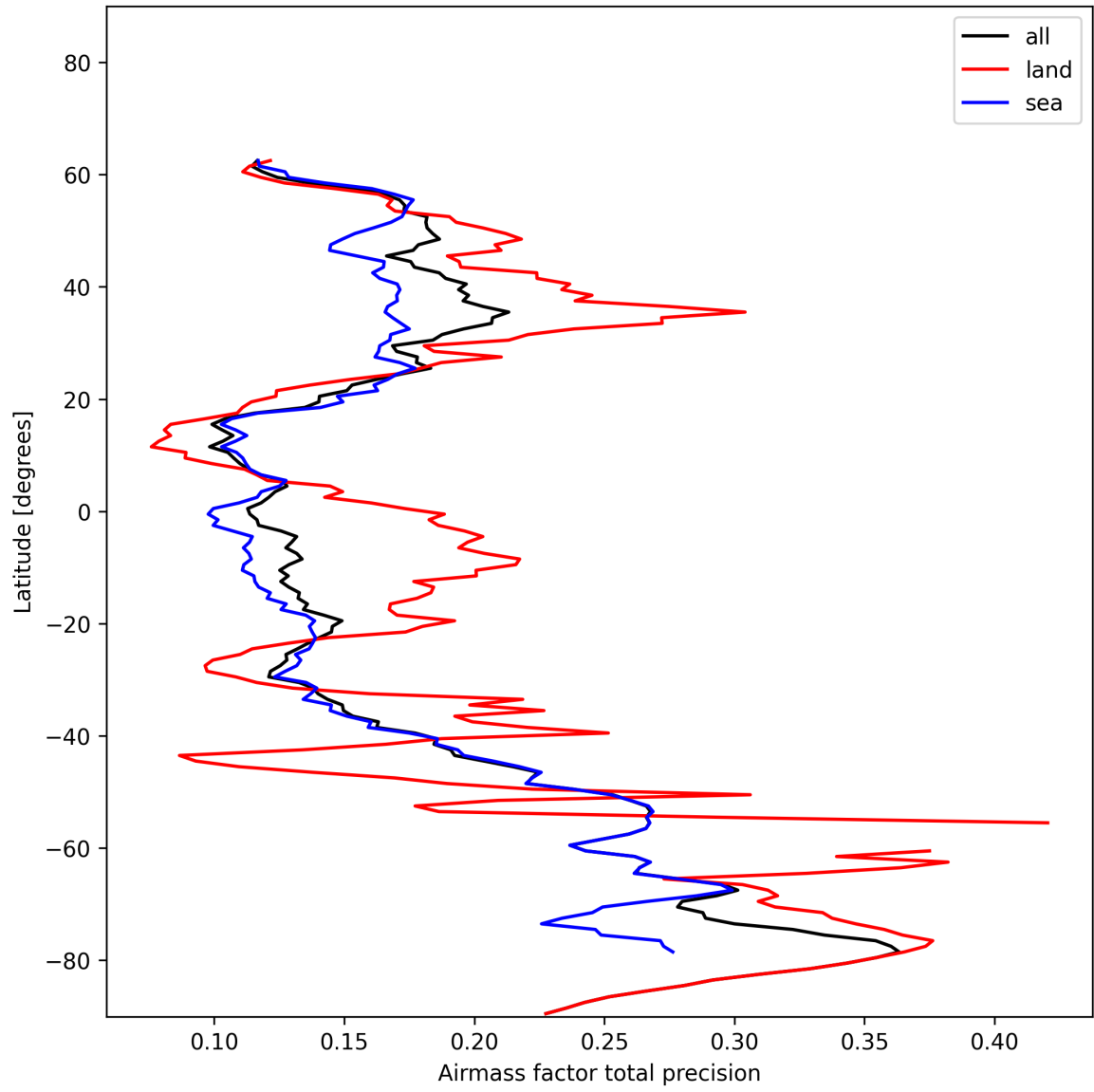
Figure 27: Zonal average of “Airmass factor total precision” for 2025-01-05 to 2025-01-07.
