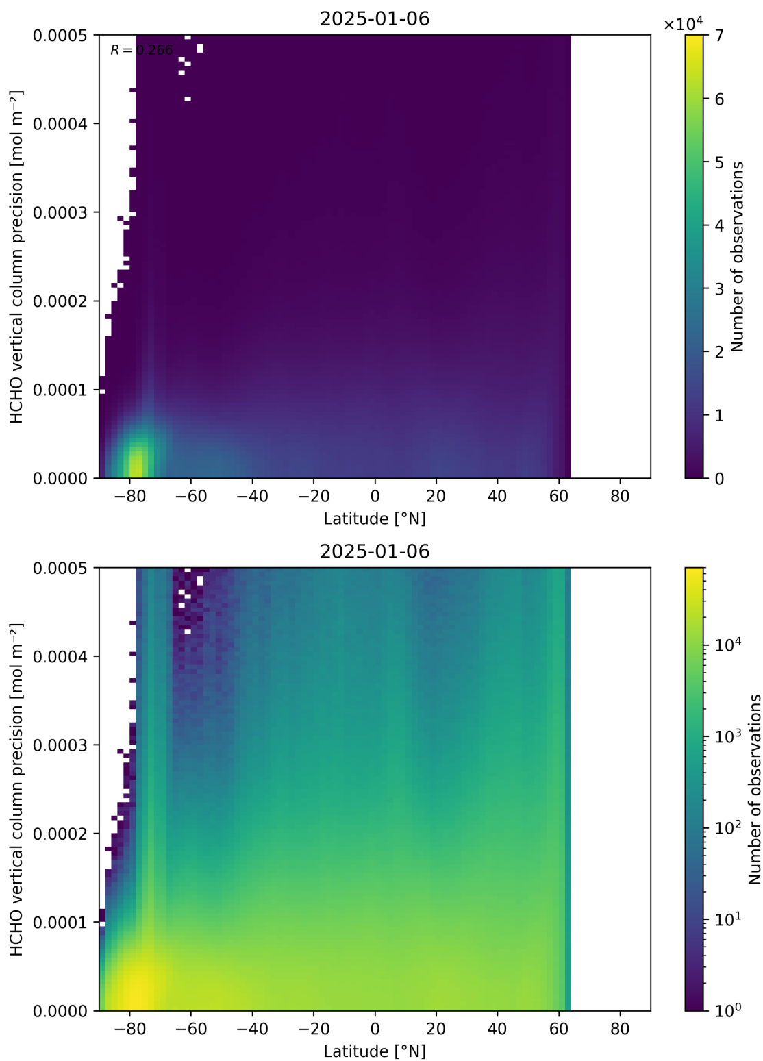
Figure 165: Scatter density plot of “Latitude” against “HCHO vertical column precision” for 2025-01-05 to 2025-01-07.
