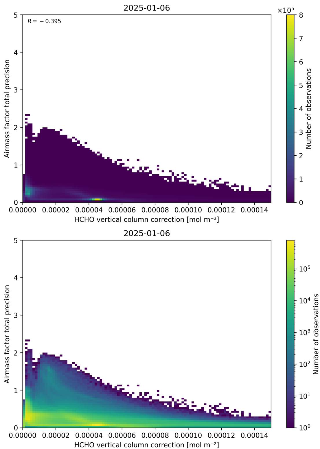
Figure 121: Scatter density plot of “HCHO vertical column correction” against “Airmass factor total precision” for 2025-01-05 to 2025-01-07.
