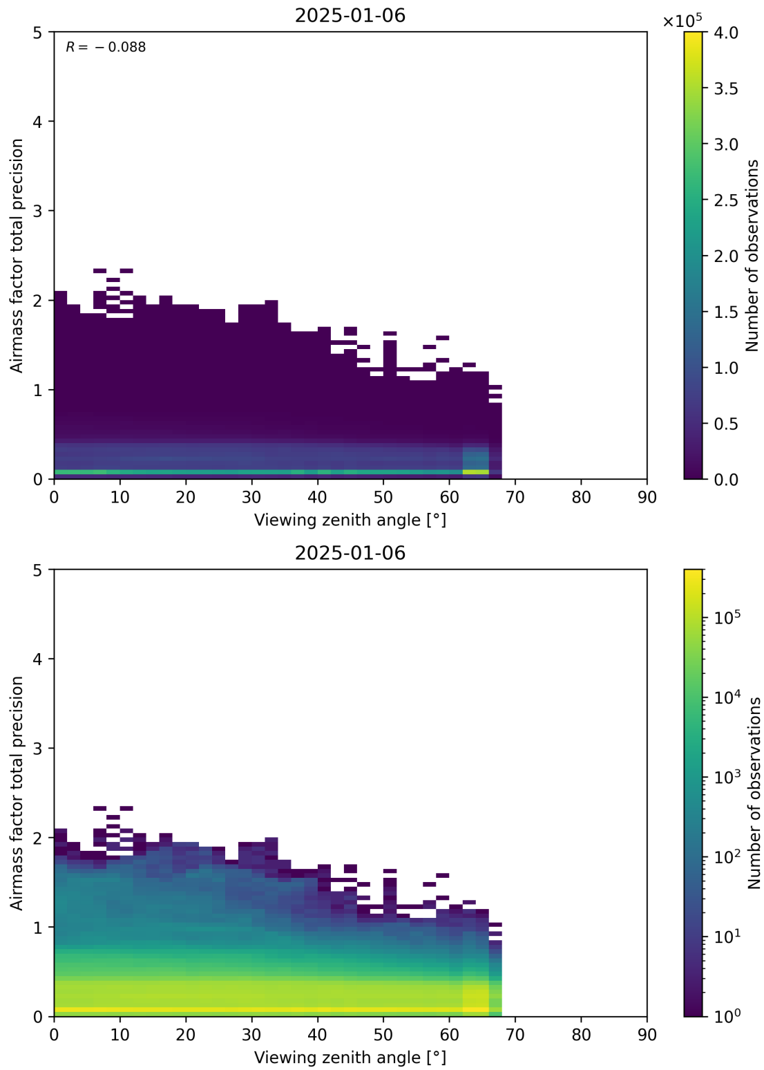
Figure 191: Scatter density plot of “Viewing zenith angle” against “Airmass factor total precision” for 2025-01-05 to 2025-01-07.
