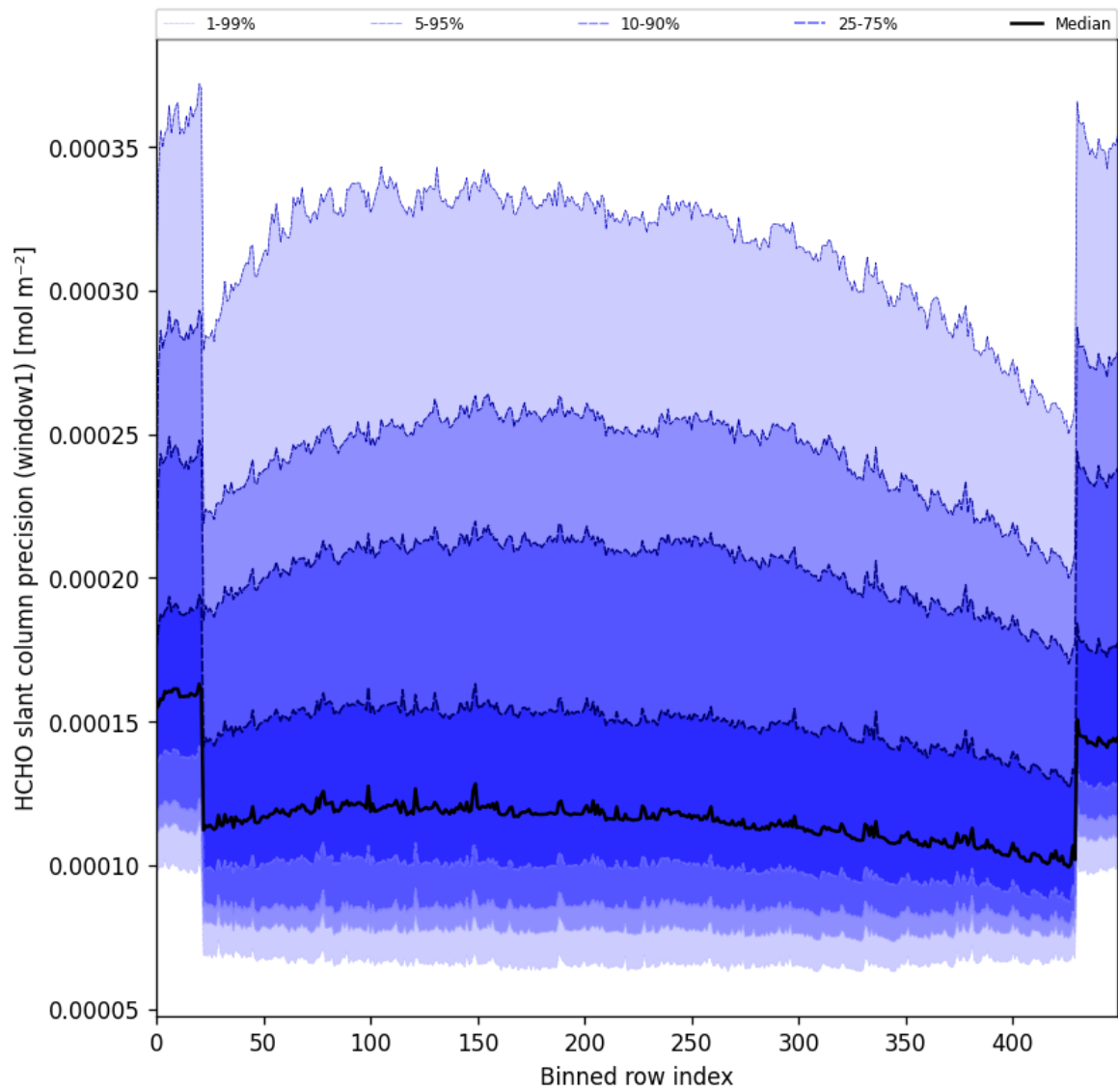
Figure 53: Along track statistics of “HCHO slant column precision (window1)” for 2025-01-05 to 2025-01-07
