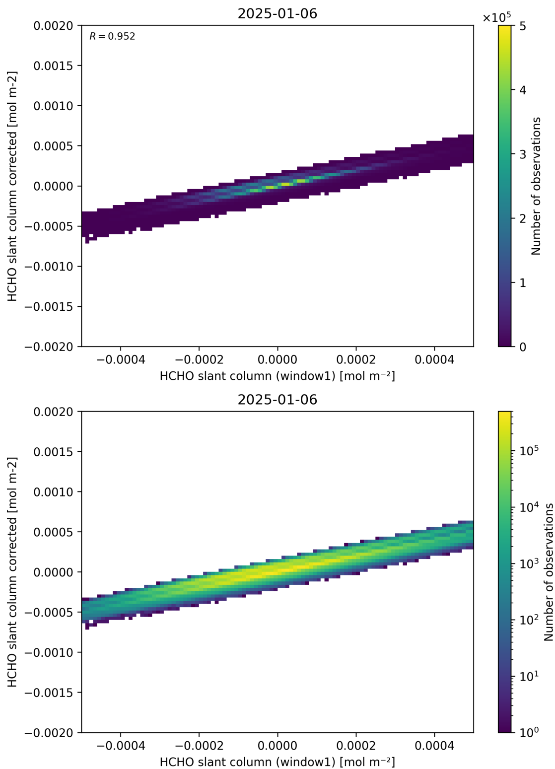
Figure 82: Scatter density plot of “HCHO slant column (window1)” against “HCHO slant column corrected” for 2025-01-05 to 2025-01-07.
