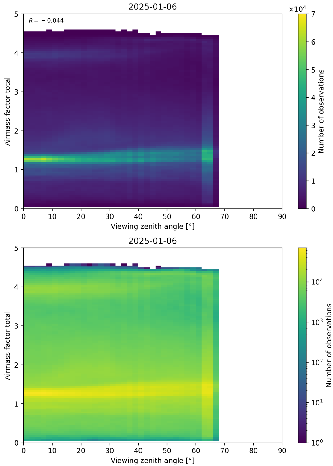
Figure 190: Scatter density plot of “Viewing zenith angle” against “Airmass factor total” for 2025-01-05 to 2025-01-07.
