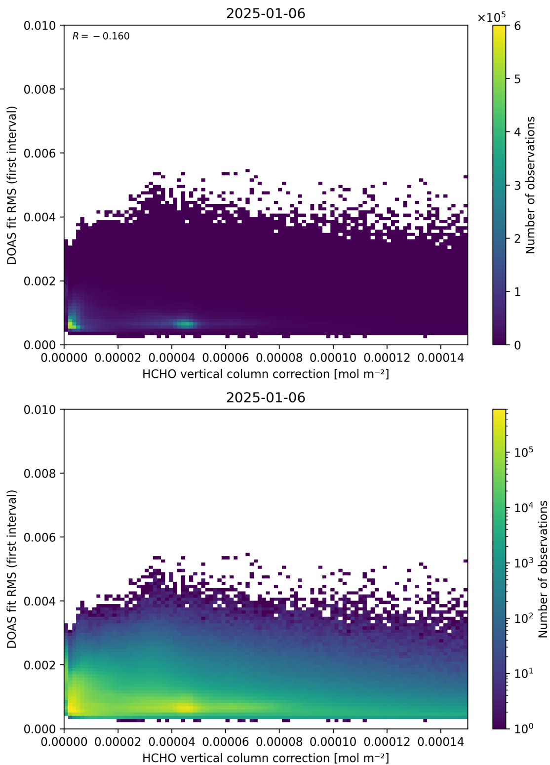
Figure 112: Scatter density plot of “HCHO vertical column correction” against “DOAS fit RMS (first interval)” for 2025-01-05 to 2025-01-07.
