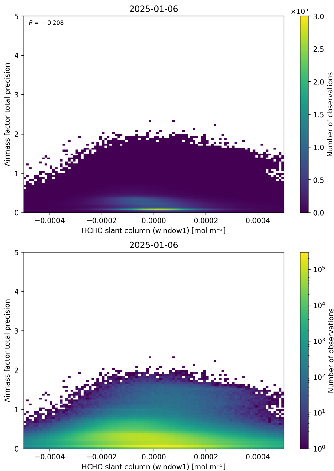
Figure 86: Scatter density plot of “HCHO slant column (window1)” against “Airmass factor total precision” for 2025-01-05 to 2025-01-07.
