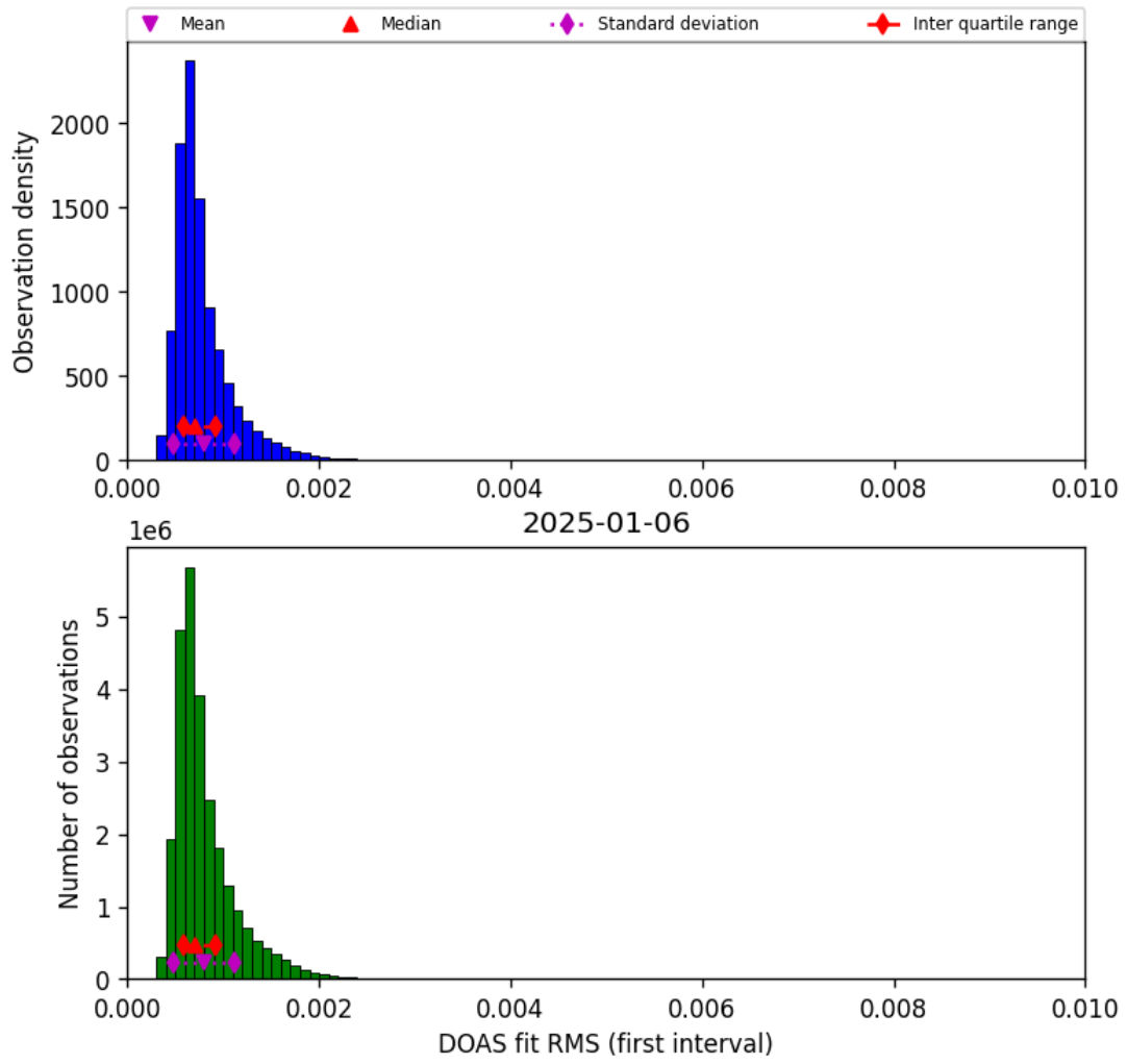
Figure 46: Histogram of “DOAS fit RMS (first interval)” for 2025-01-05 to 2025-01-07
