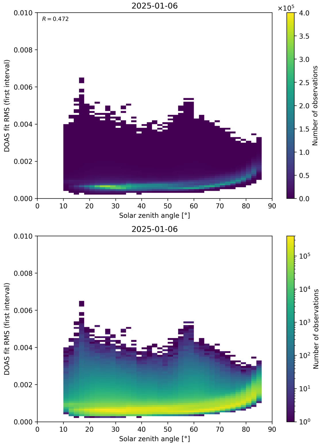
Figure 167: Scatter density plot of “Solar zenith angle” against “DOAS fit RMS (first interval)” for 2025-01-05 to 2025-01-07.
