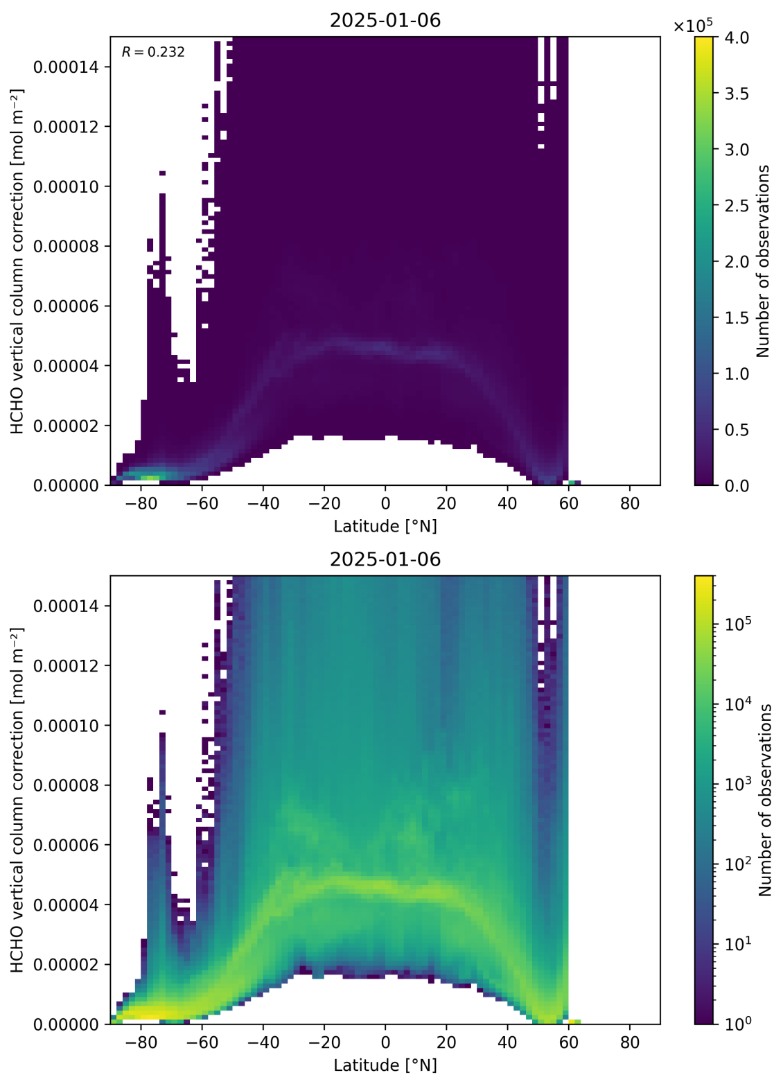
Figure 164: Scatter density plot of “Latitude” against “HCHO vertical column correction” for 2025-01-05 to 2025-01-07.
