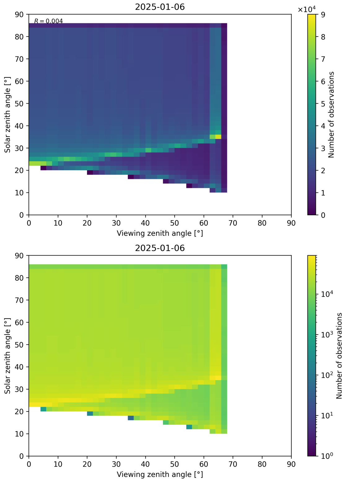
Figure 197: Scatter density plot of “Viewing zenith angle” against “Solar zenith angle” for 2025-01-05 to 2025-01-07.
