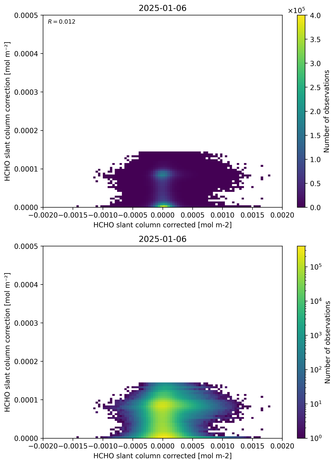
Figure 77: Scatter density plot of “HCHO slant column corrected” against “HCHO slant column correction” for 2025-01-05 to 2025-01-07.
