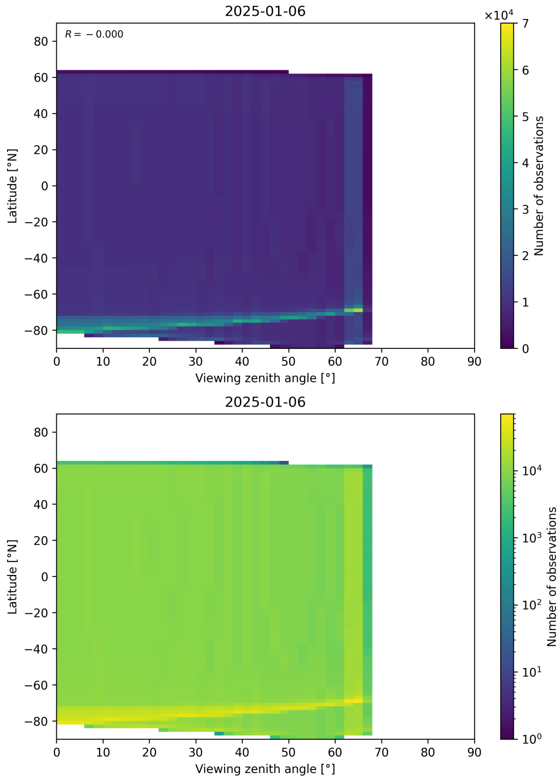
Figure 196: Scatter density plot of “Viewing zenith angle” against “Latitude” for 2025-01-05 to 2025-01-07.
