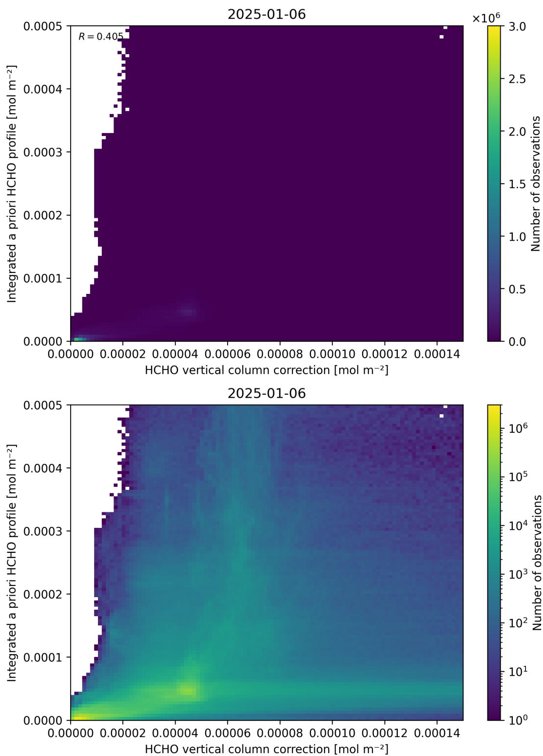
Figure 122: Scatter density plot of “HCHO vertical column correction” against “Integrated a priori HCHO profile” for 2025-01-05 to 2025-01-07.
