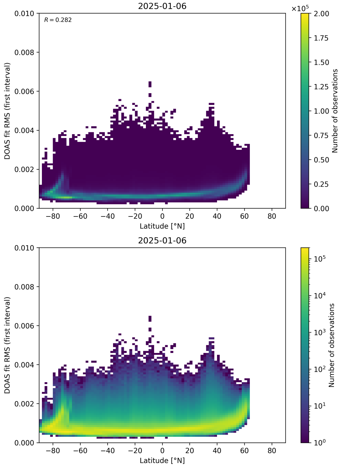
Figure 153: Scatter density plot of “Latitude” against “DOAS fit RMS (first interval)” for 2025-01-05 to 2025-01-07.
