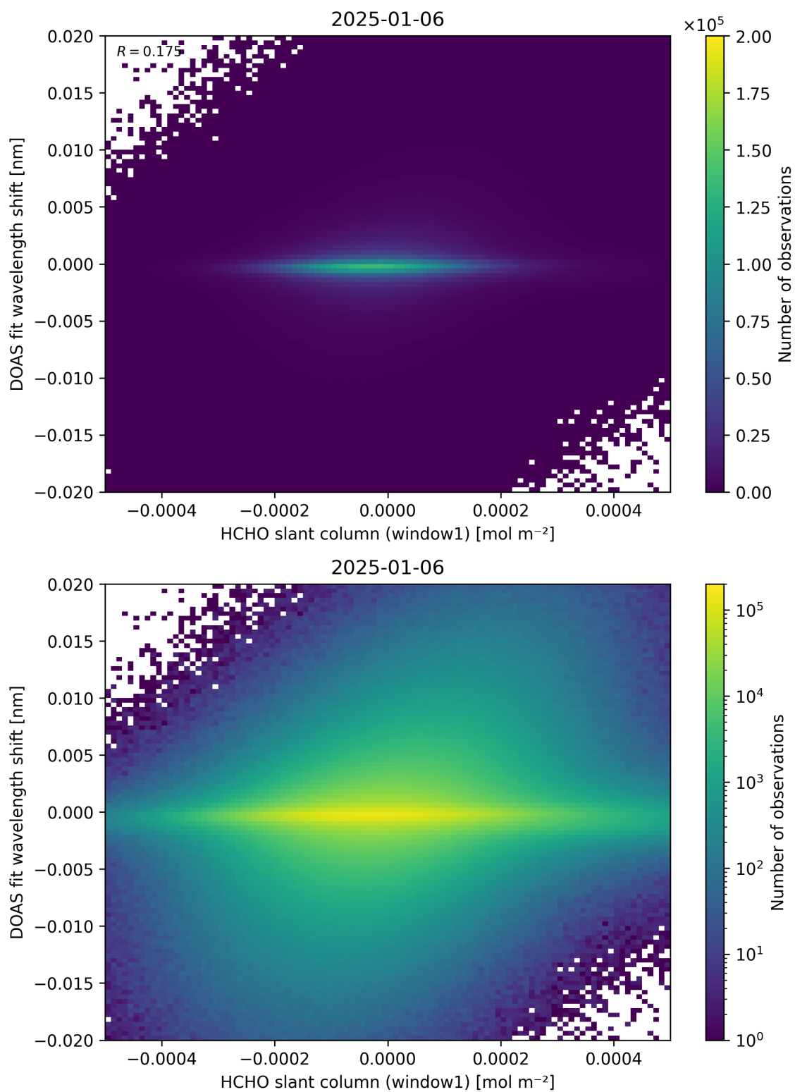
Figure 79: Scatter density plot of “HCHO slant column (window1)” against “DOAS fit wavelength shift” for 2025-01-05 to 2025-01-07.
