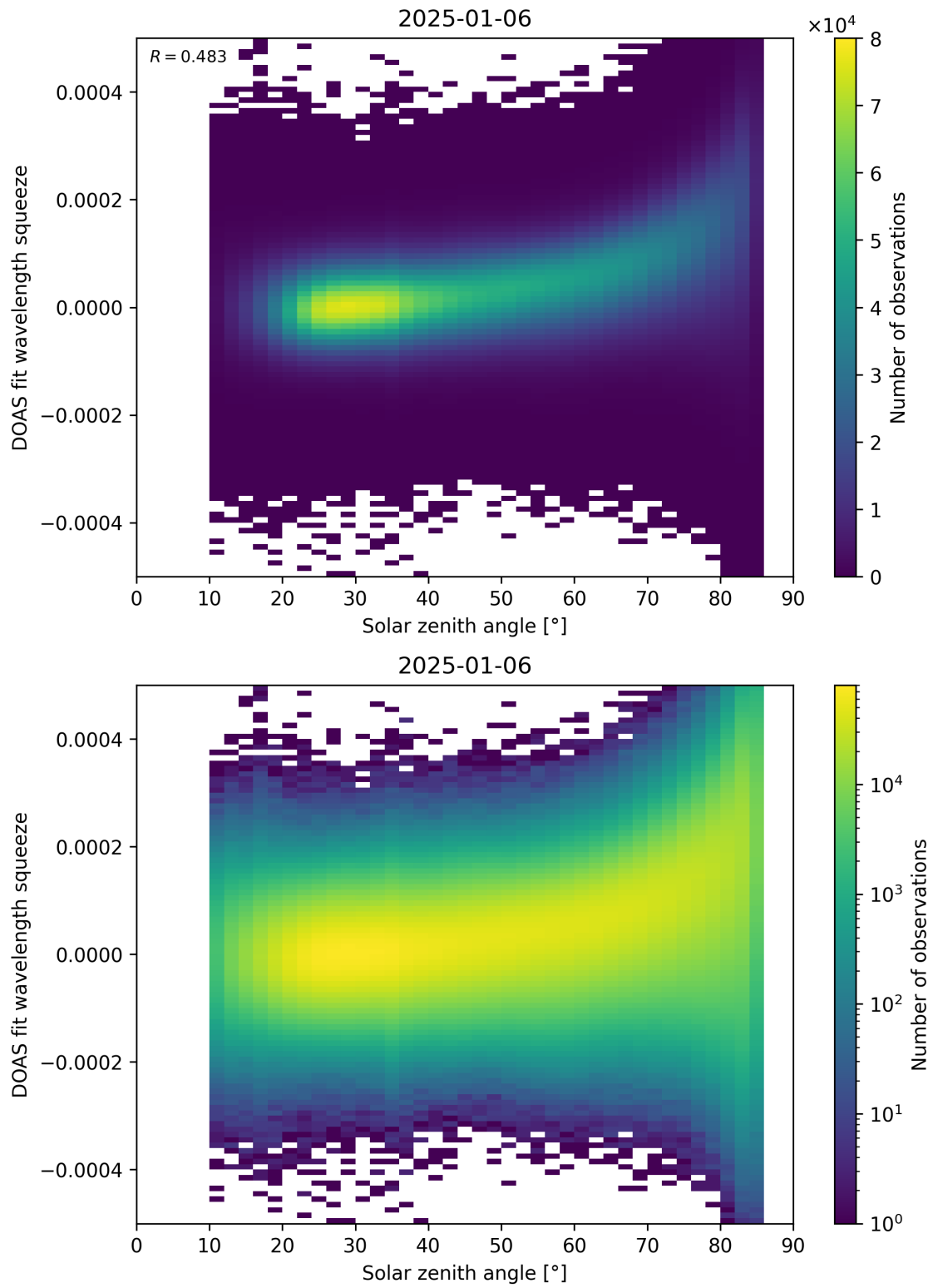
Figure 169: Scatter density plot of “Solar zenith angle” against “DOAS fit wavelength squeeze” for 2025-01-05 to 2025-01-07.
