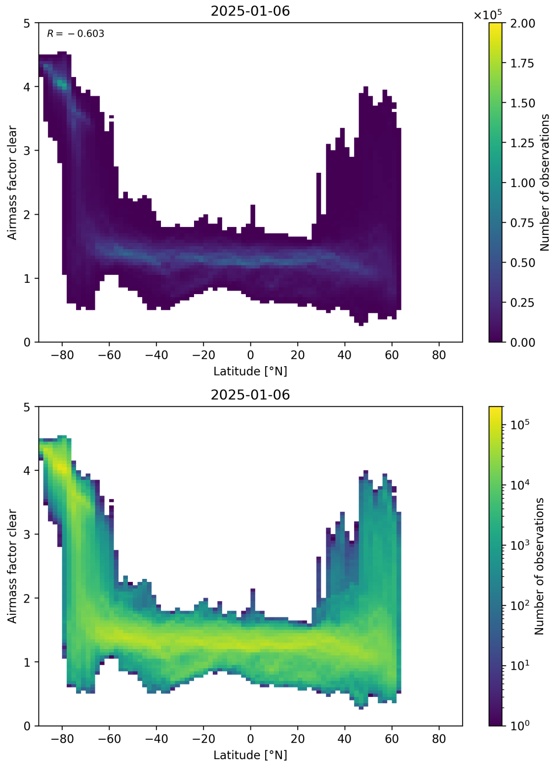
Figure 156: Scatter density plot of “Latitude” against “Airmass factor clear” for 2025-01-05 to 2025-01-07.
