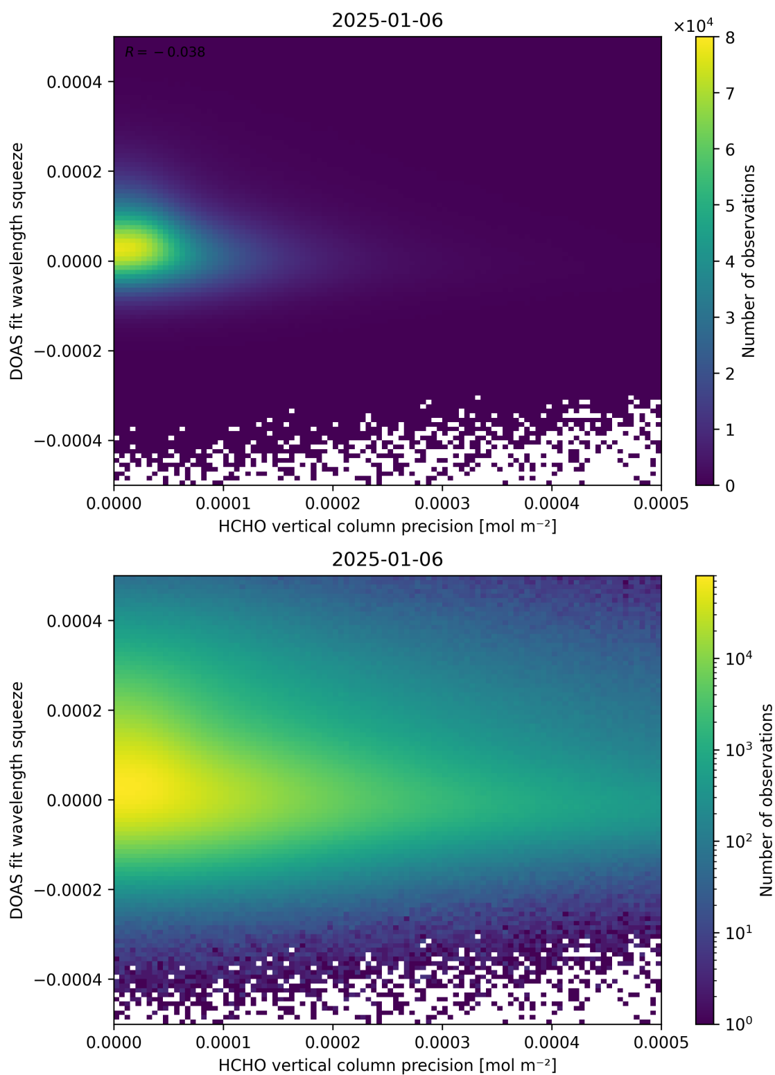
Figure 138: Scatter density plot of “HCHO vertical column precision” against “DOAS fit wavelength squeeze” for 2025-01-05 to 2025-01-07.
