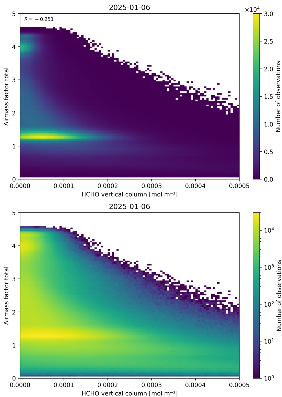
Figure 131: Scatter density plot of “HCHO vertical column” against “Airmass factor total” for 2025-01-05 to 2025-01-07.
