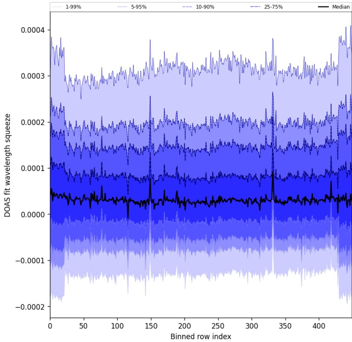
Figure 59: Along track statistics of “DOAS fit wavelength squeeze” for 2025-01-05 to 2025-01-07
