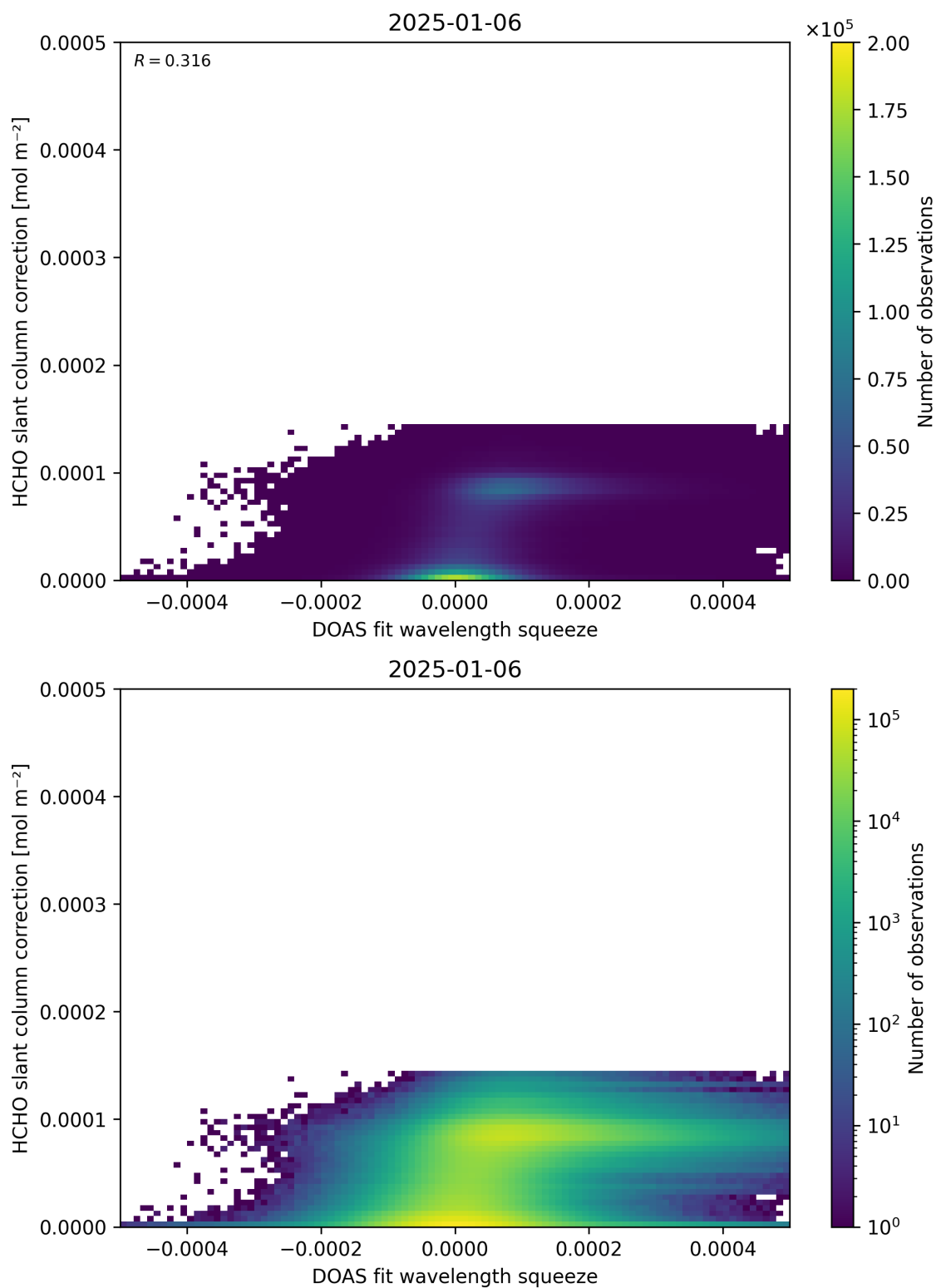
Figure 70: Scatter density plot of “DOAS fit wavelength squeeze” against “HCHO slant column correction” for 2025-01-05 to 2025-01-07.
