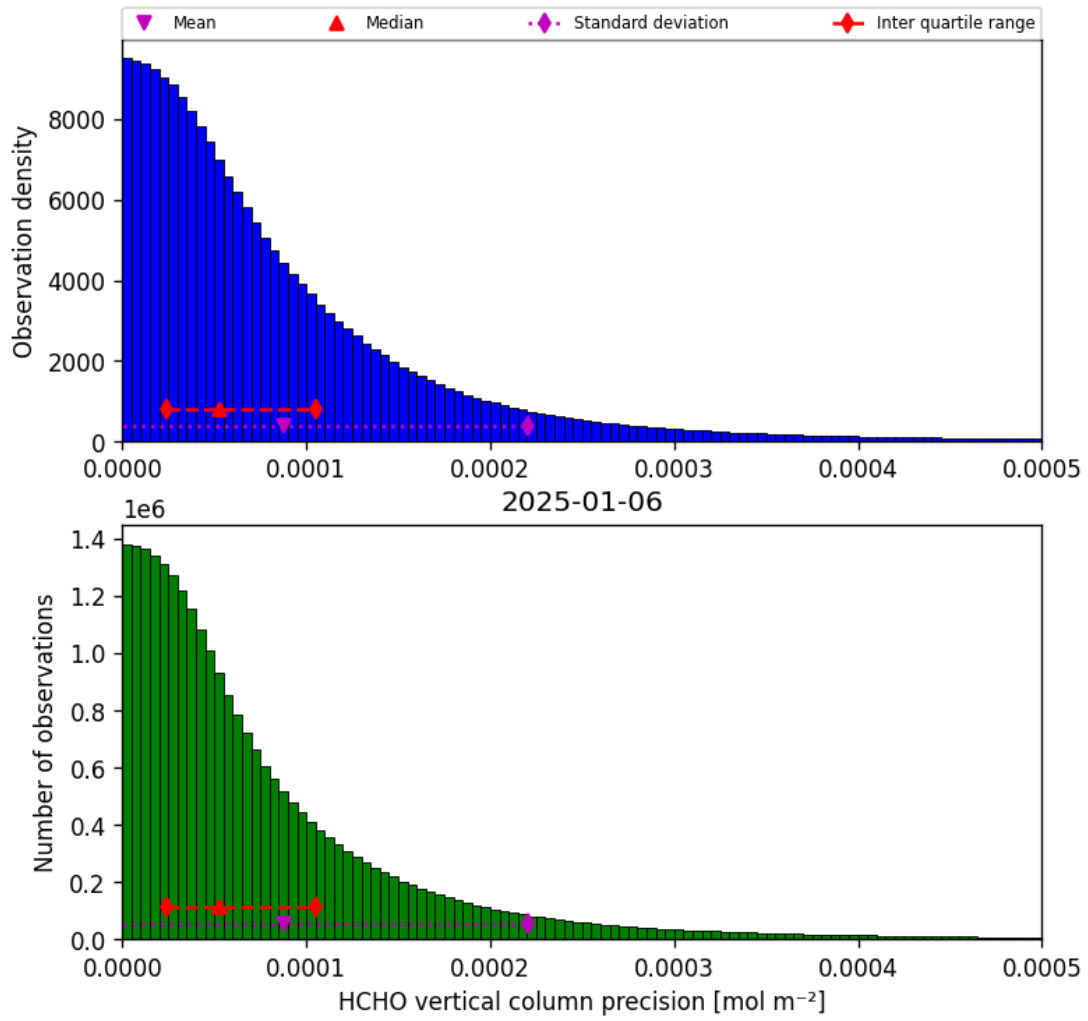
Figure 36: Histogram of “HCHO vertical column precision” for 2025-01-05 to 2025-01-07
