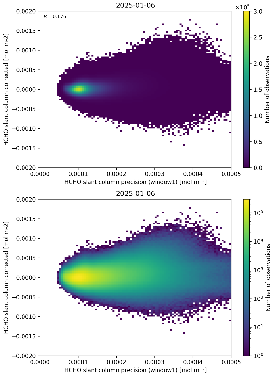
Figure 92: Scatter density plot of “HCHO slant column precision (window1)” against “HCHO slant column corrected” for 2025-01-05 to 2025-01-07.
