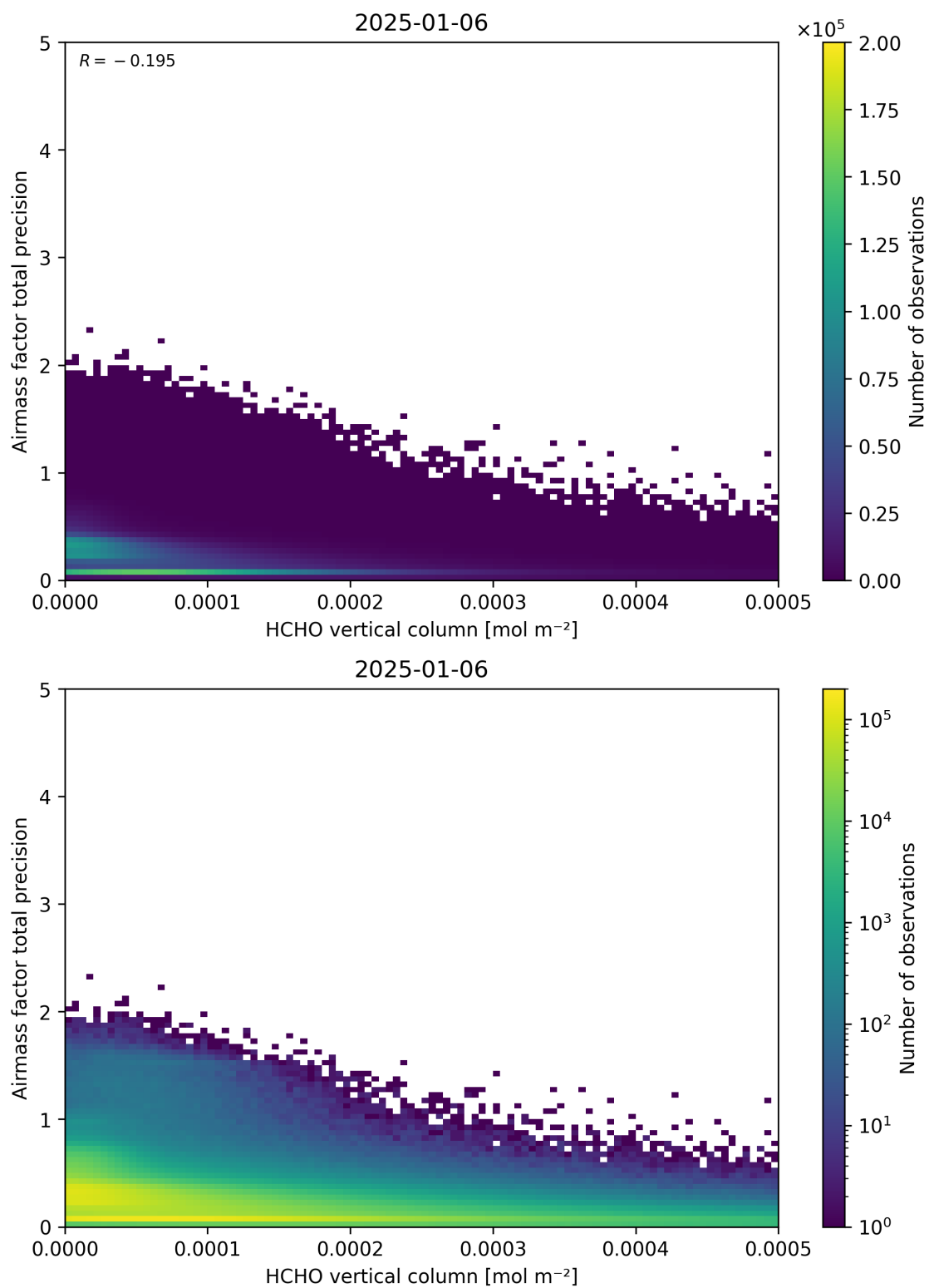
Figure 132: Scatter density plot of “HCHO vertical column” against “Airmass factor total precision” for 2025-01-05 to 2025-01-07.
