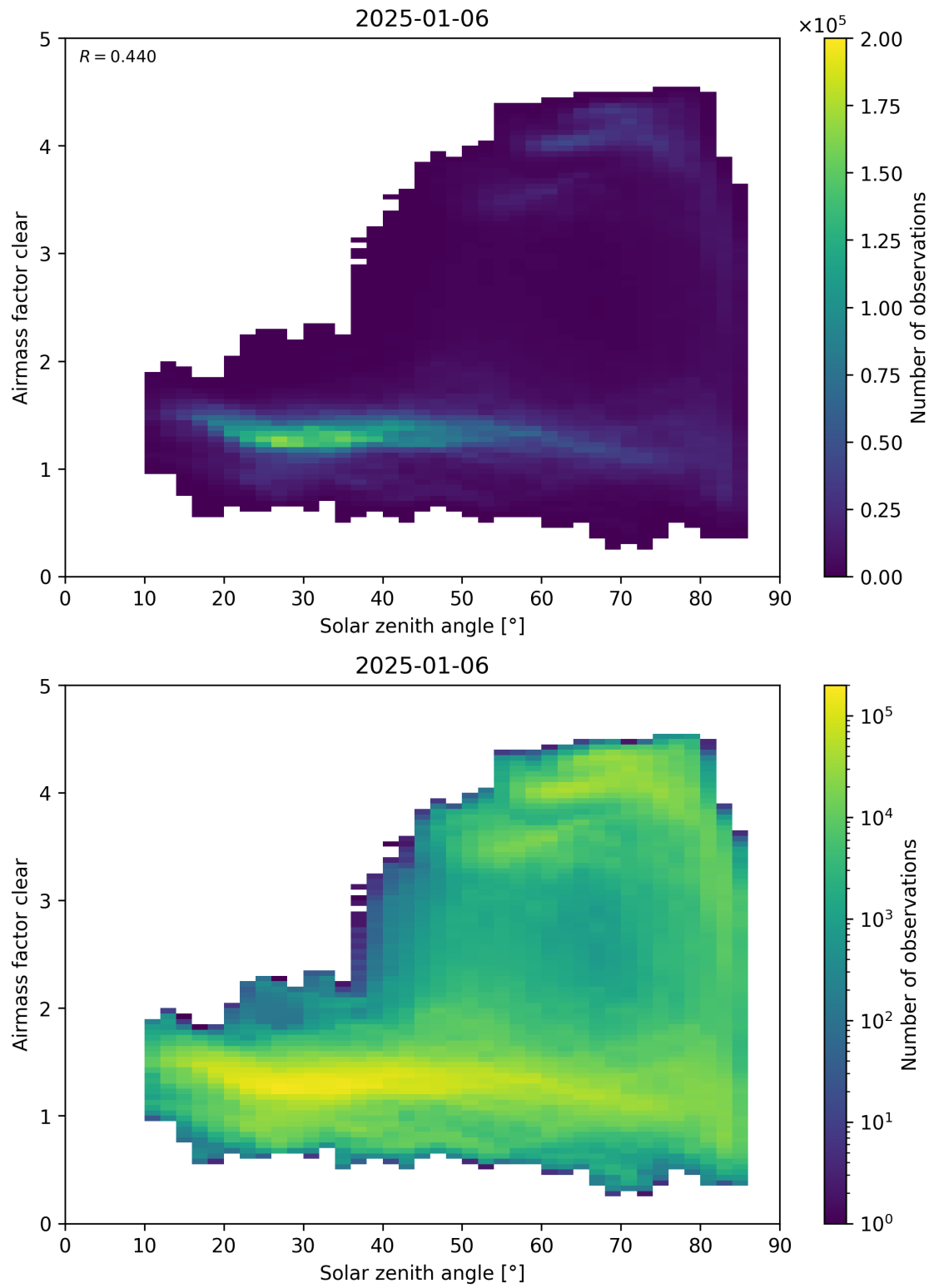
Figure 170: Scatter density plot of “Solar zenith angle” against “Airmass factor clear” for 2025-01-05 to 2025-01-07.
