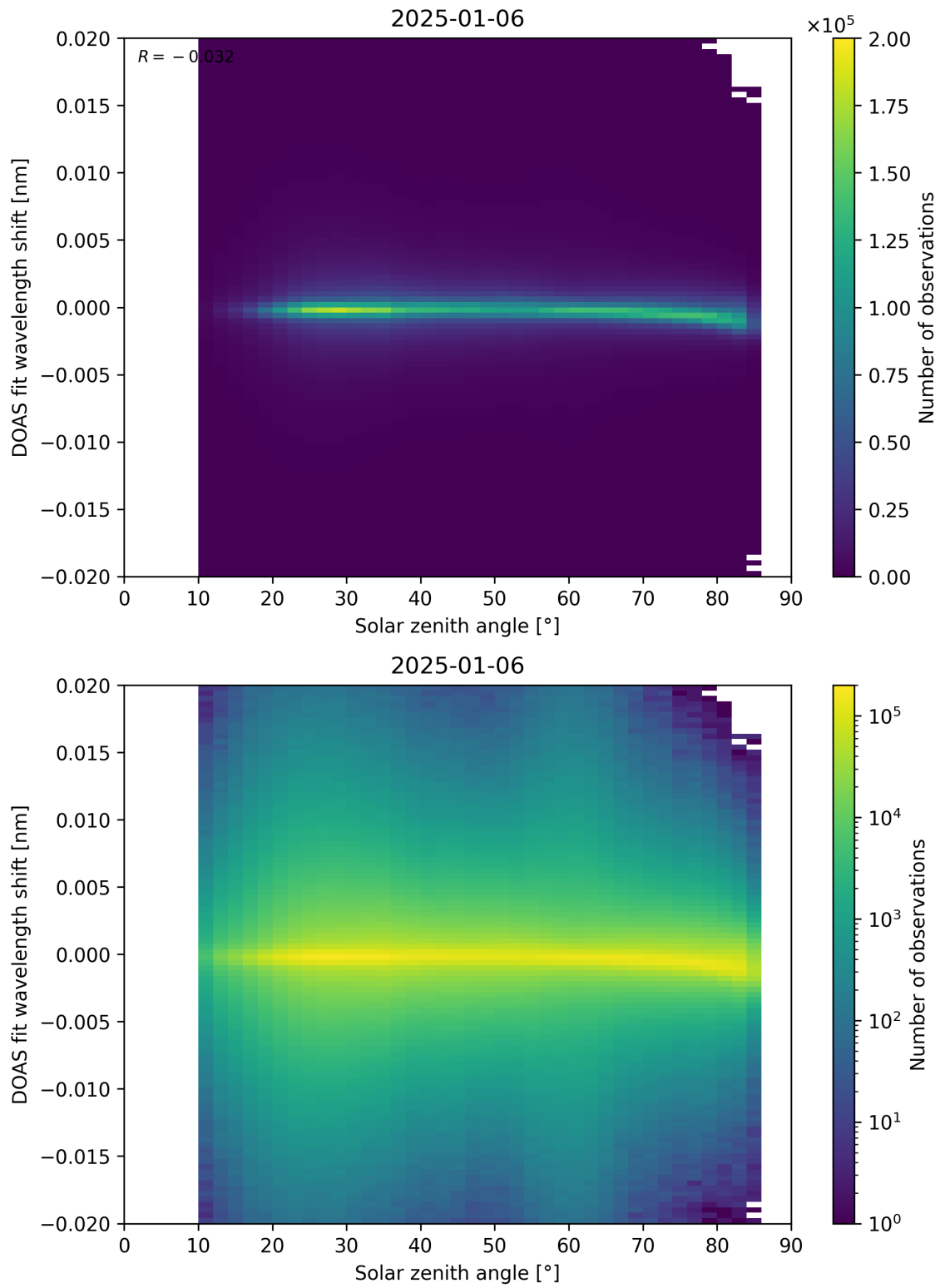
Figure 168: Scatter density plot of “Solar zenith angle” against “DOAS fit wavelength shift” for 2025-01-05 to 2025-01-07.
