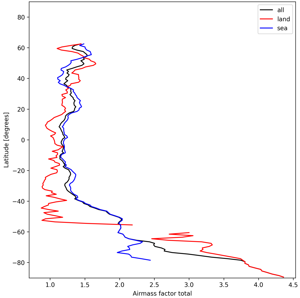
Figure 26: Zonal average of “Airmass factor total” for 2025-01-05 to 2025-01-07.
