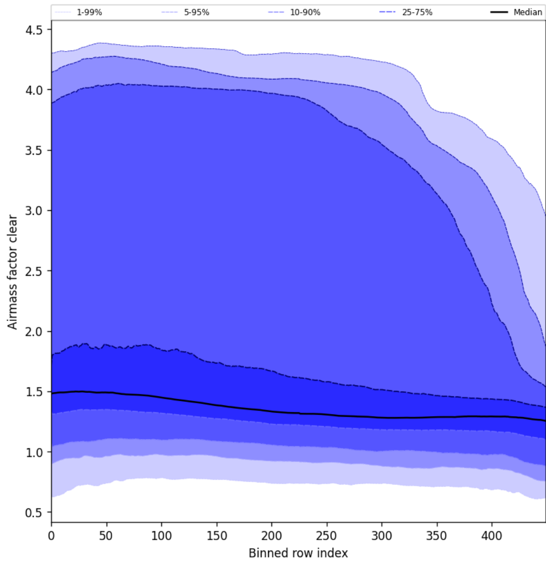
Figure 56: Along track statistics of “Airmass factor clear” for 2025-01-05 to 2025-01-07
