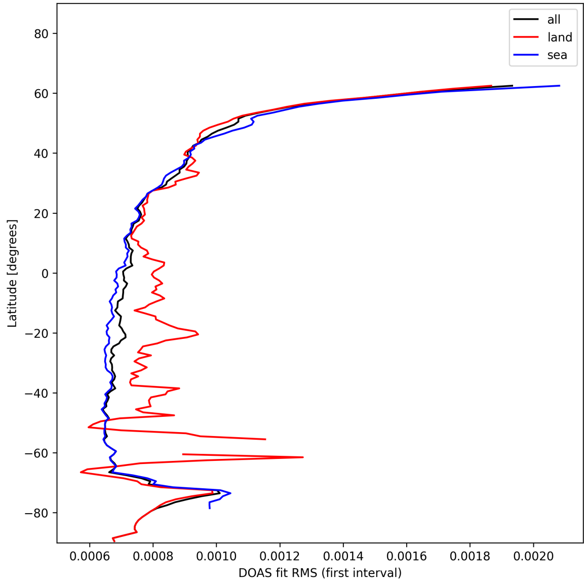
Figure 32: Zonal average of “DOAS fit RMS (first interval)” for 2025-01-05 to 2025-01-07.
