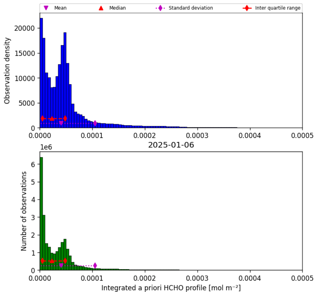
Figure 43: Histogram of “Integrated a priori HCHO profile” for 2025-01-05 to 2025-01-07
