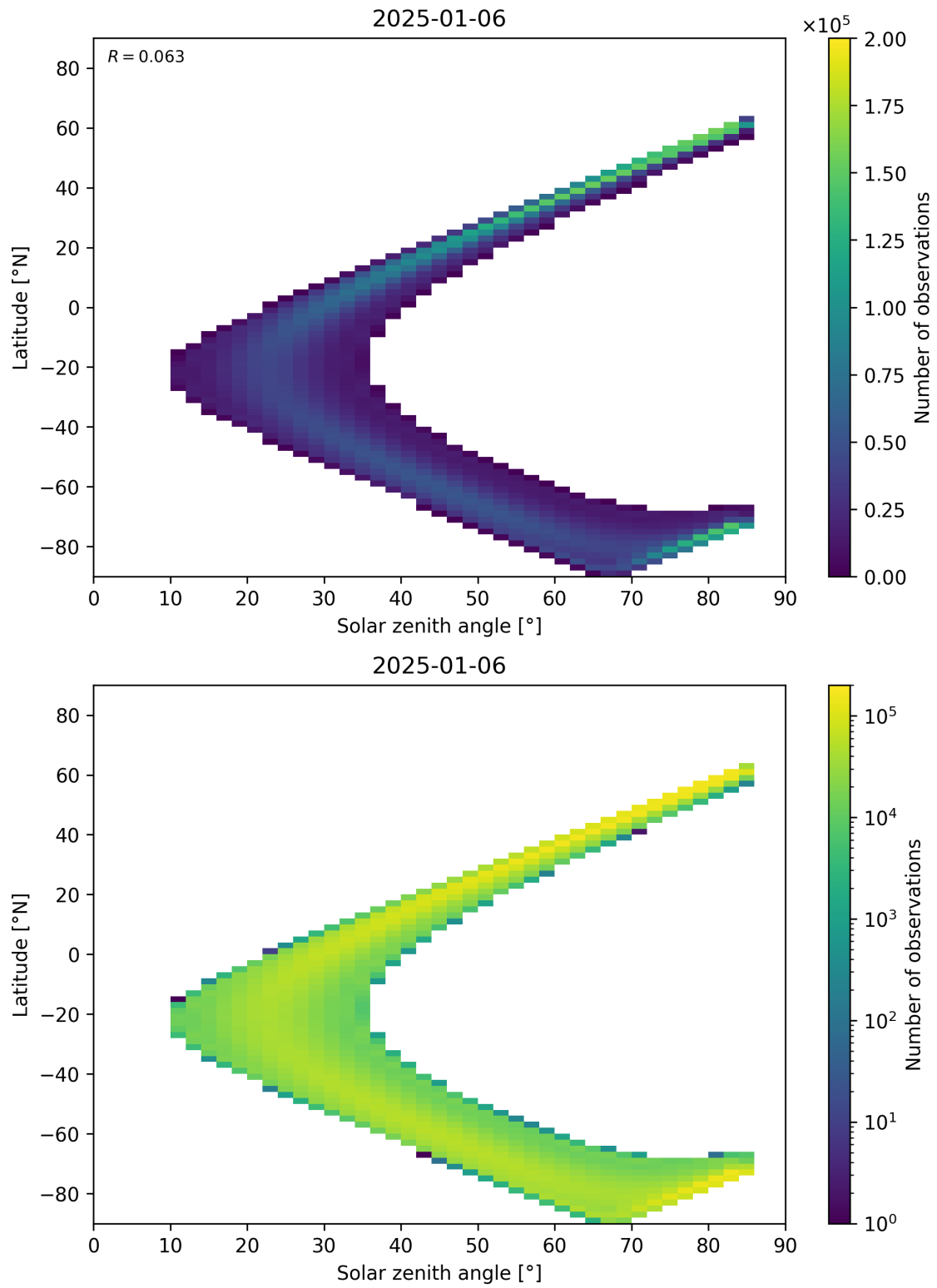
Figure 181: Scatter density plot of “Solar zenith angle” against “Latitude” for 2025-01-05 to 2025-01-07.
