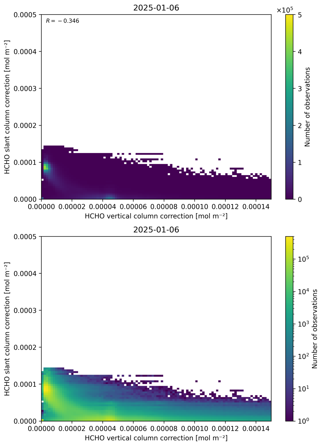
Figure 117: Scatter density plot of “HCHO vertical column correction” against “HCHO slant column correction” for 2025-01-05 to 2025-01-07.
