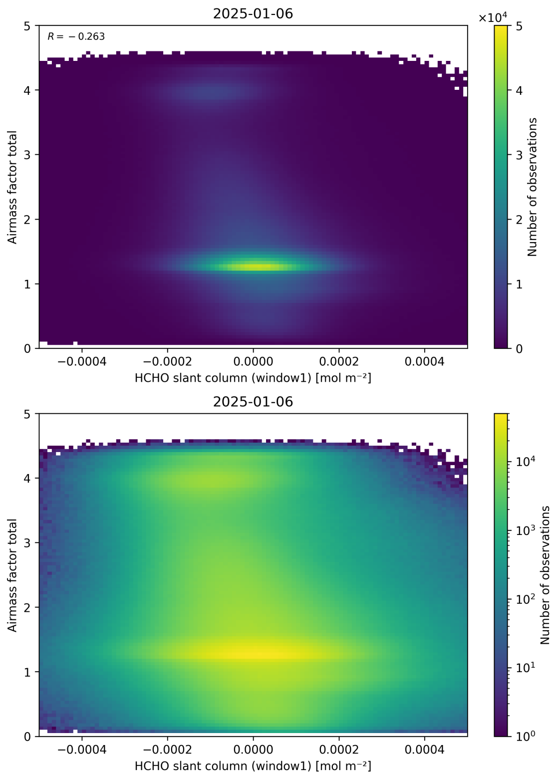
Figure 85: Scatter density plot of “HCHO slant column (window1)” against “Airmass factor total” for 2025-01-05 to 2025-01-07.
