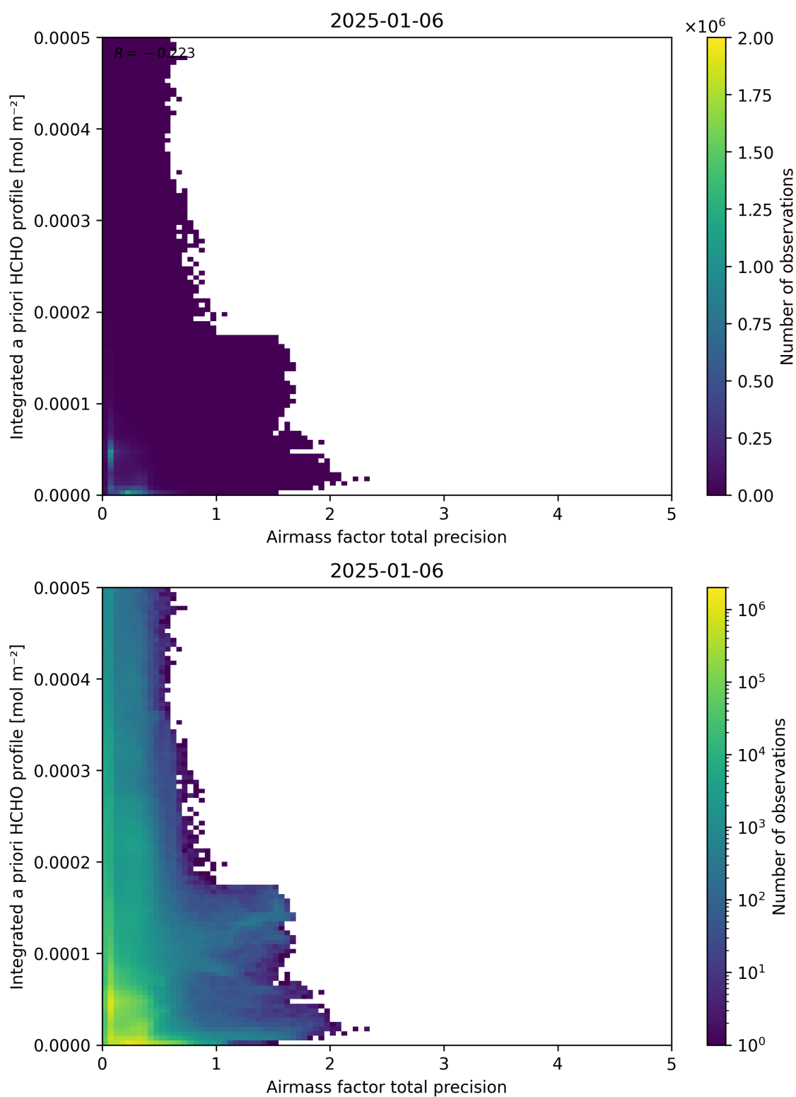
Figure 111: Scatter density plot of “Airmass factor total precision” against “Integrated a priori HCHO profile” for 2025-01-05 to 2025-01-07.
