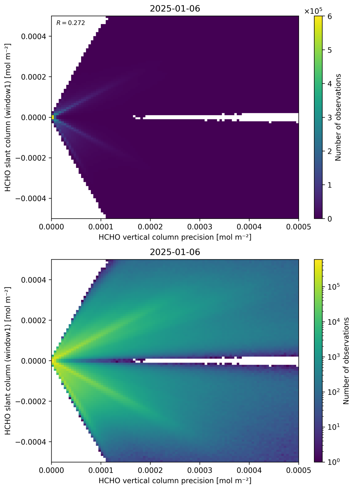
Figure 142: Scatter density plot of “HCHO vertical column precision” against “HCHO slant column (window1)” for 2025-01-05 to 2025-01-07.
