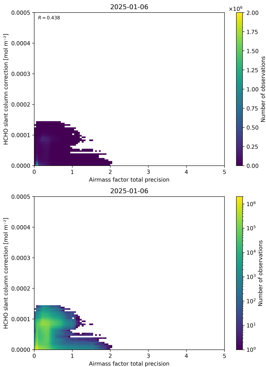
Figure 110: Scatter density plot of “Airmass factor total precision” against “HCHO slant column correction” for 2025-01-05 to 2025-01-07.
