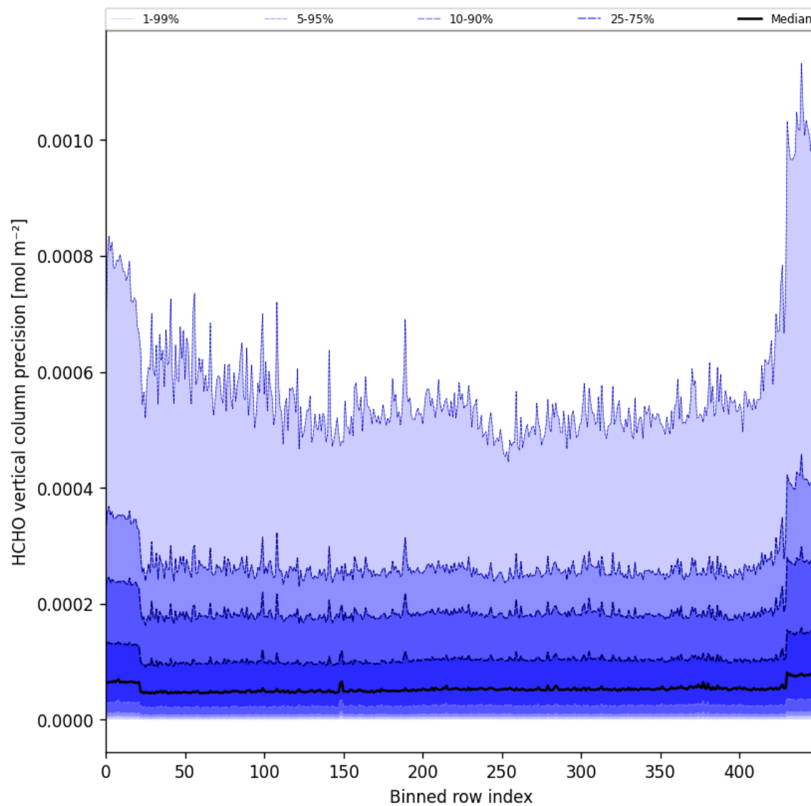
Figure 50: Along track statistics of “HCHO vertical column precision” for 2025-01-05 to 2025-01-07
