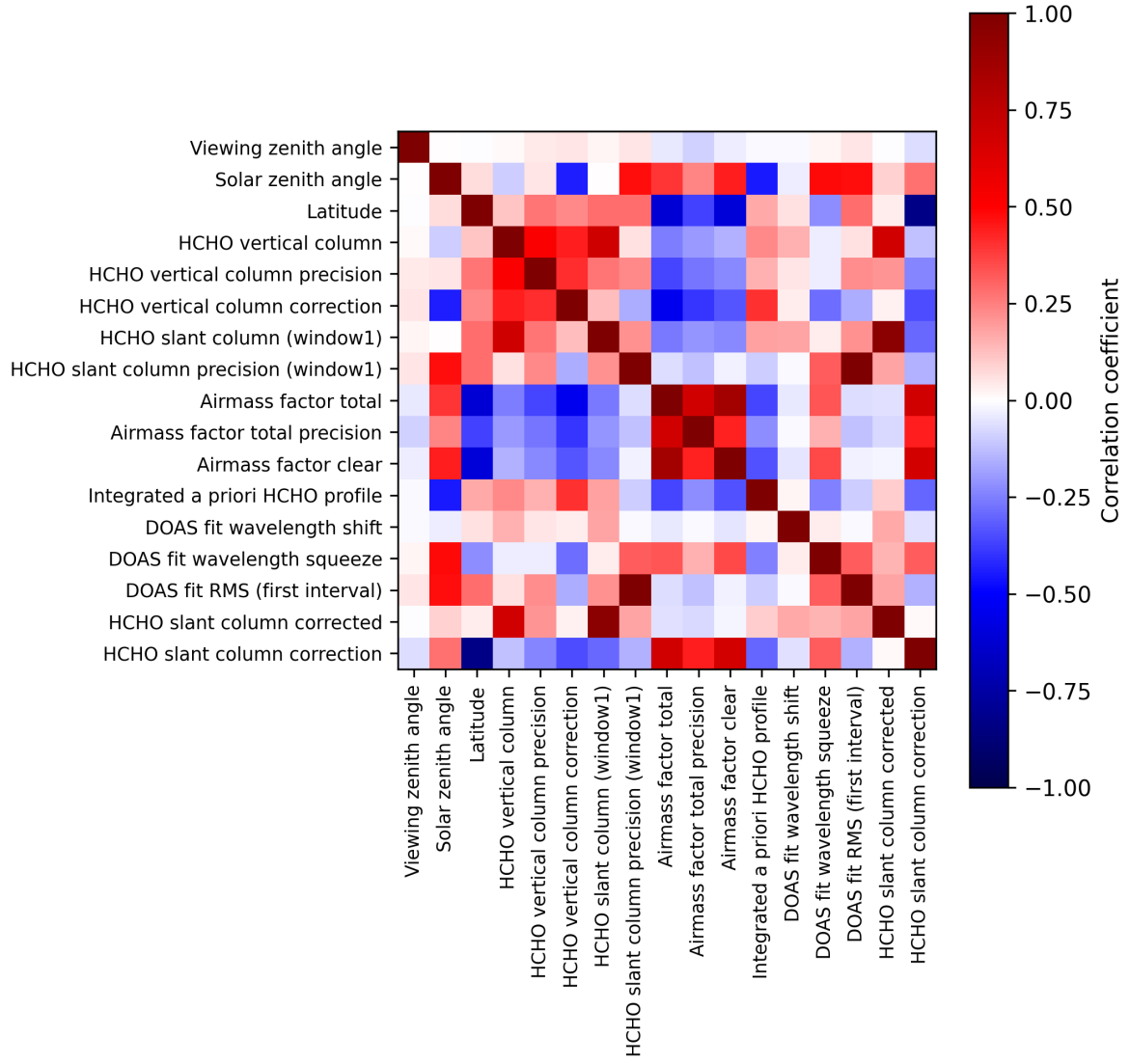
Figure 2: Map of correlation matrix for 2025-01-05 to 2025-01-07.
