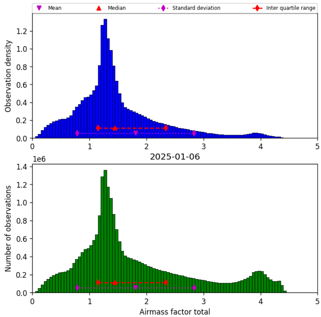
Figure 40: Histogram of “Airmass factor total” for 2025-01-05 to 2025-01-07
