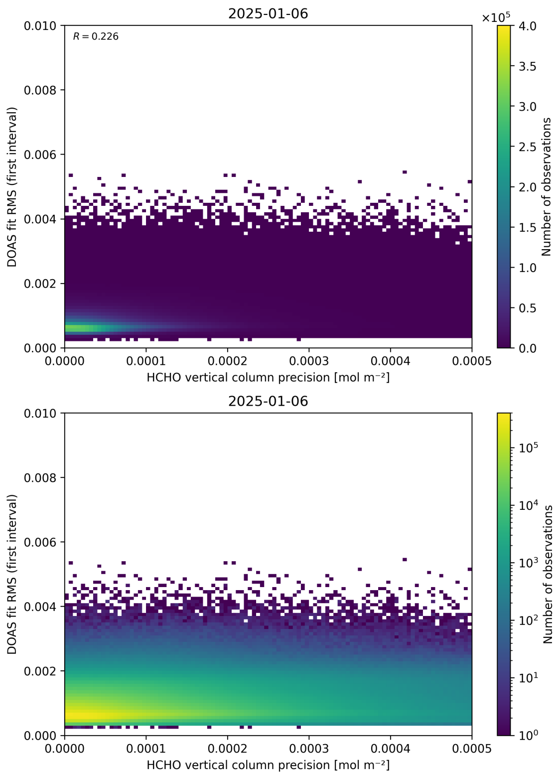
Figure 136: Scatter density plot of “HCHO vertical column precision” against “DOAS fit RMS (first interval)” for 2025-01-05 to 2025-01-07.
