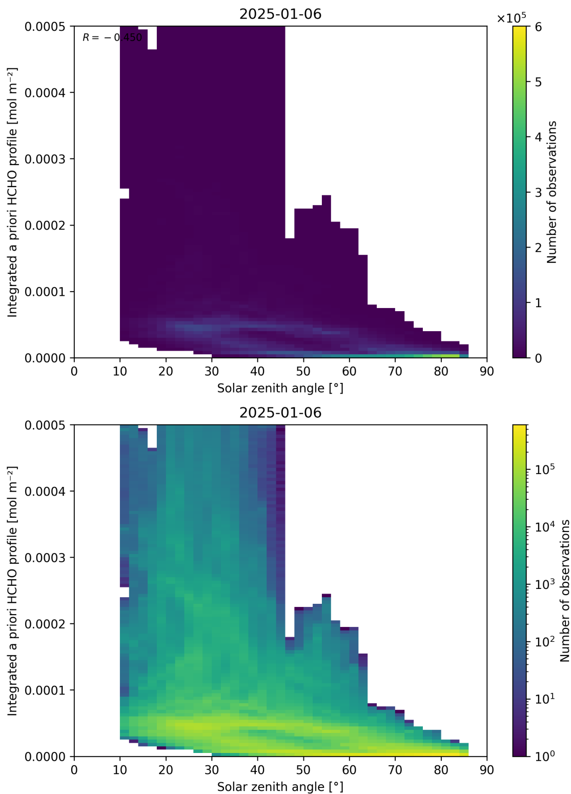
Figure 180: Scatter density plot of “Solar zenith angle” against “Integrated a priori HCHO profile” for 2025-01-05 to 2025-01-07.
