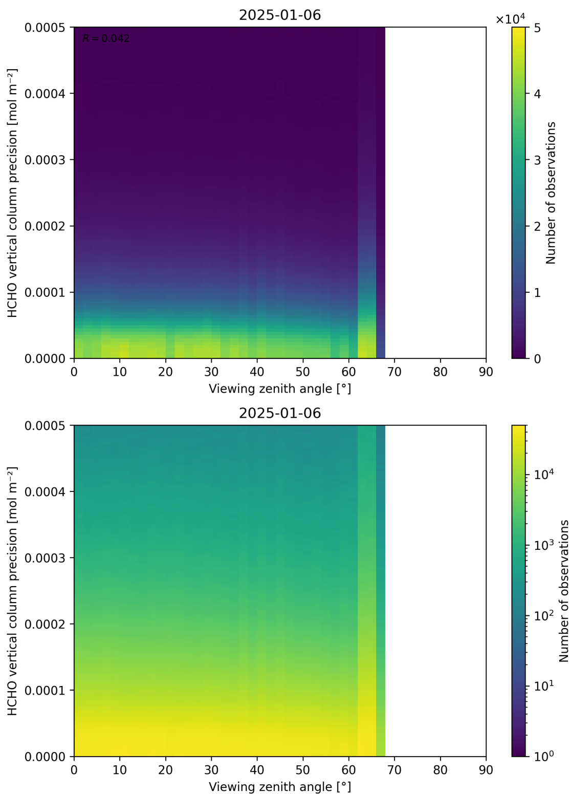
Figure 194: Scatter density plot of “Viewing zenith angle” against “HCHO vertical column precision” for 2025-01-05 to 2025-01-07.
