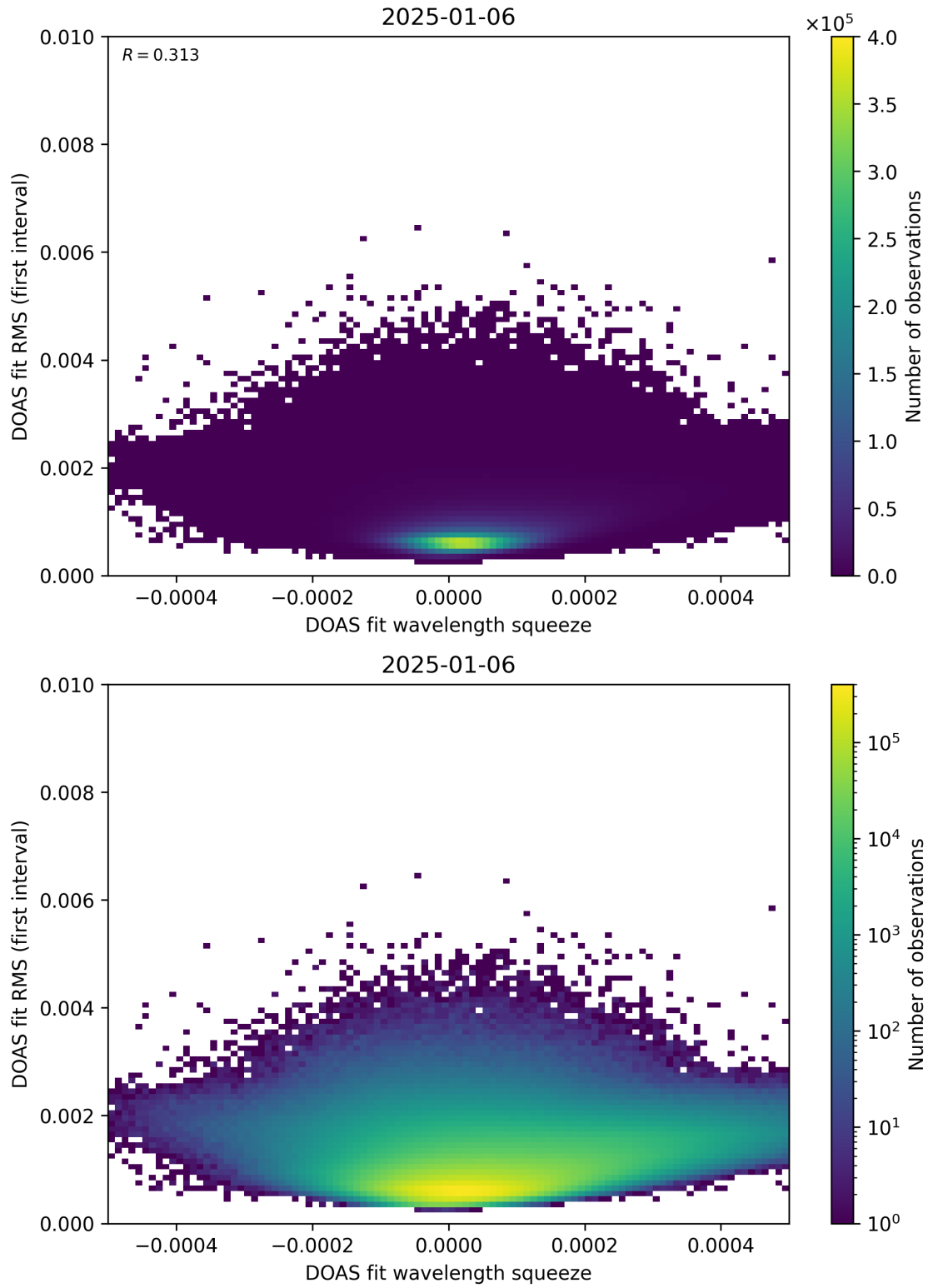
Figure 68: Scatter density plot of “DOAS fit wavelength squeeze” against “DOAS fit RMS (first interval)” for 2025-01-05 to 2025-01-07.
