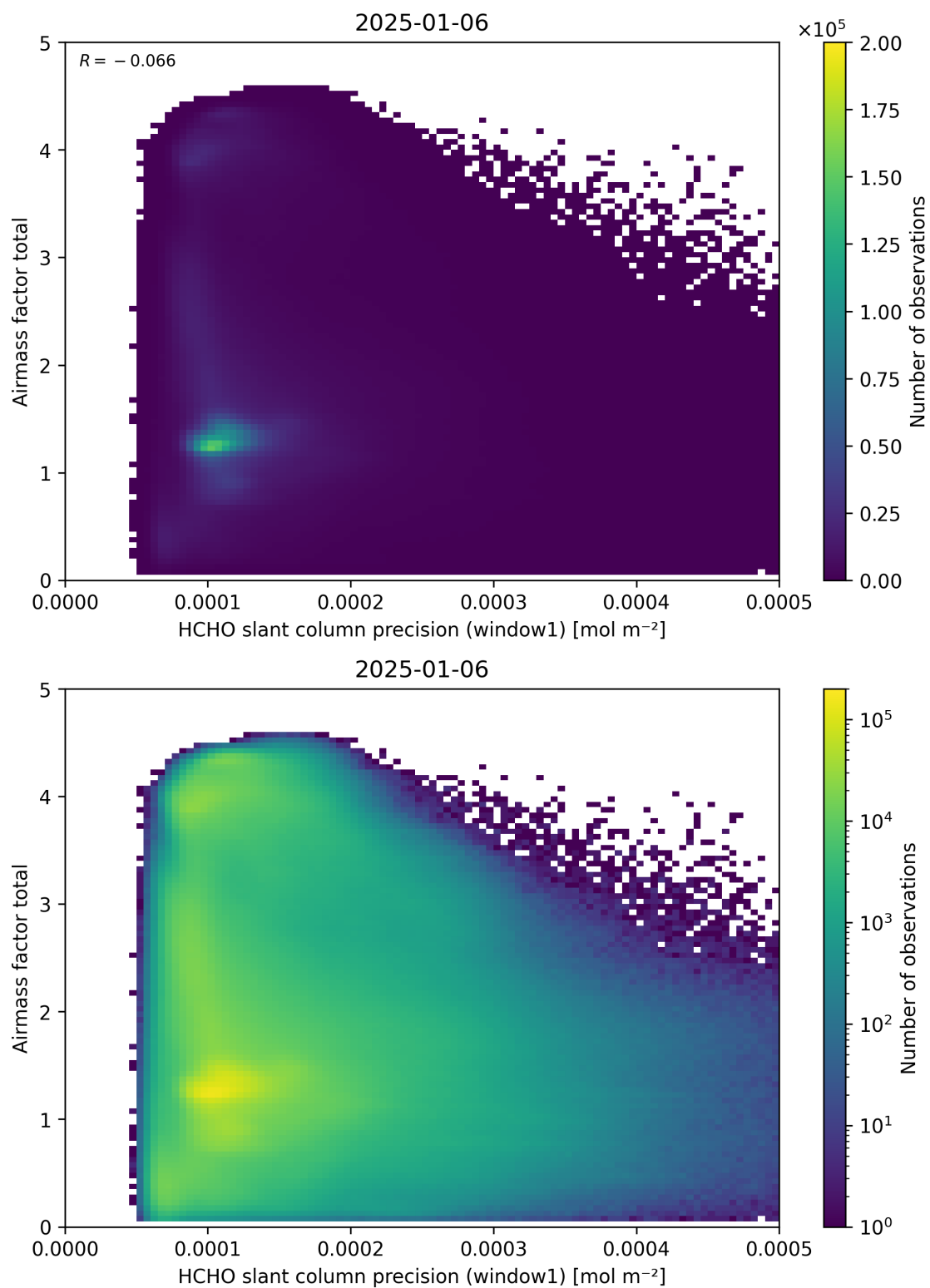
Figure 94: Scatter density plot of “HCHO slant column precision (window1)” against “Airmass factor total” for 2025-01-05 to 2025-01-07.
