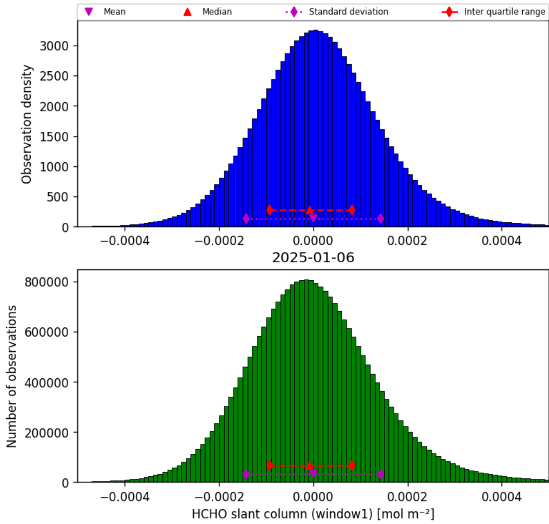
Figure 38: Histogram of “HCHO slant column (window1)” for 2025-01-05 to 2025-01-07
