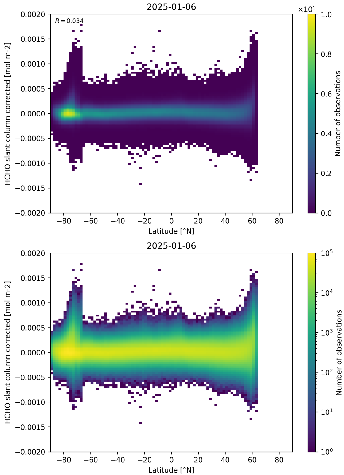
Figure 157: Scatter density plot of “Latitude” against “HCHO slant column corrected” for 2025-01-05 to 2025-01-07.
