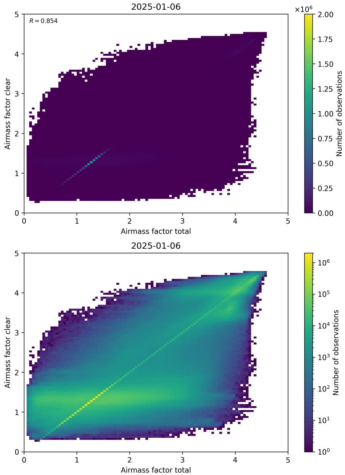
Figure 100: Scatter density plot of “Airmass factor total” against “Airmass factor clear” for 2025-01-05 to 2025-01-07.
