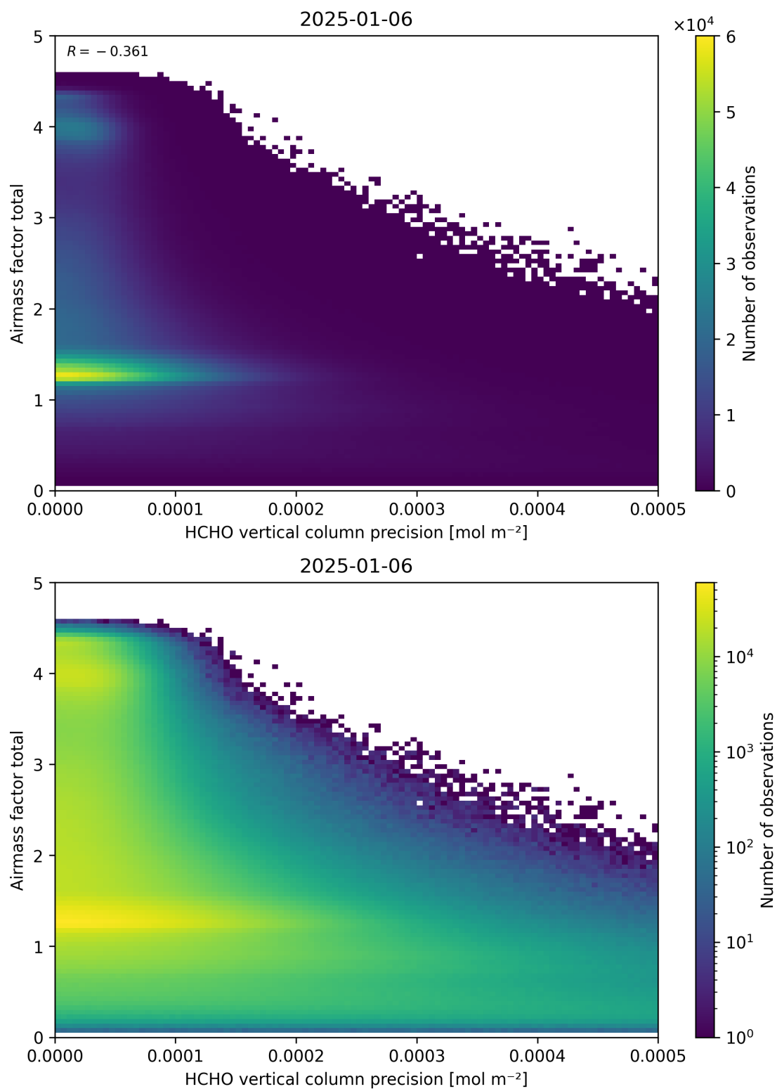
Figure 144: Scatter density plot of “HCHO vertical column precision” against “Airmass factor total” for 2025-01-05 to 2025-01-07.
