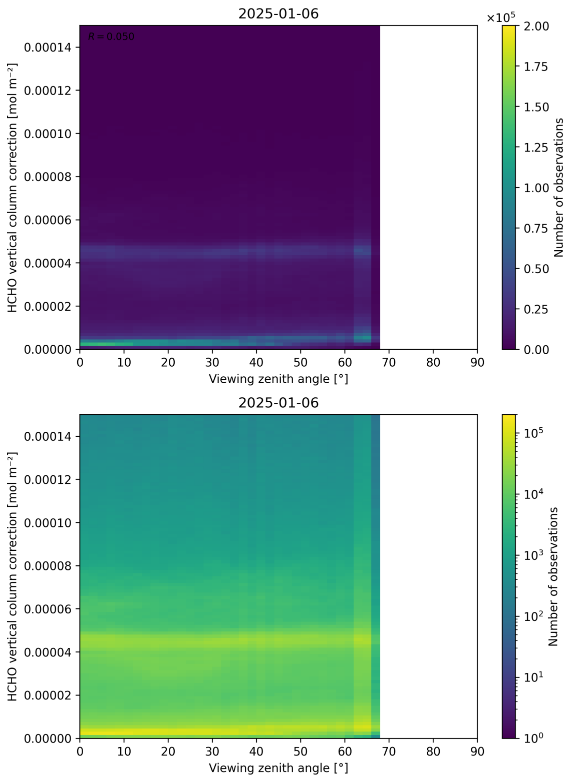
Figure 193: Scatter density plot of “Viewing zenith angle” against “HCHO vertical column correction” for 2025-01-05 to 2025-01-07.
