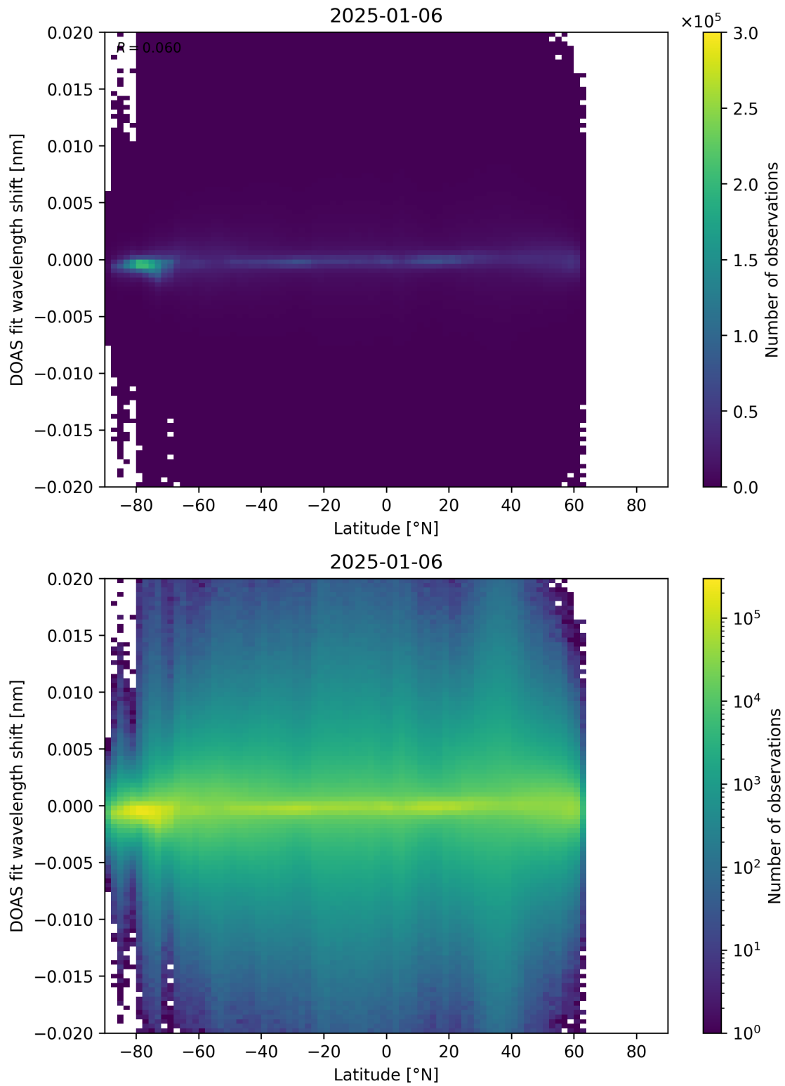
Figure 154: Scatter density plot of “Latitude” against “DOAS fit wavelength shift” for 2025-01-05 to 2025-01-07.
