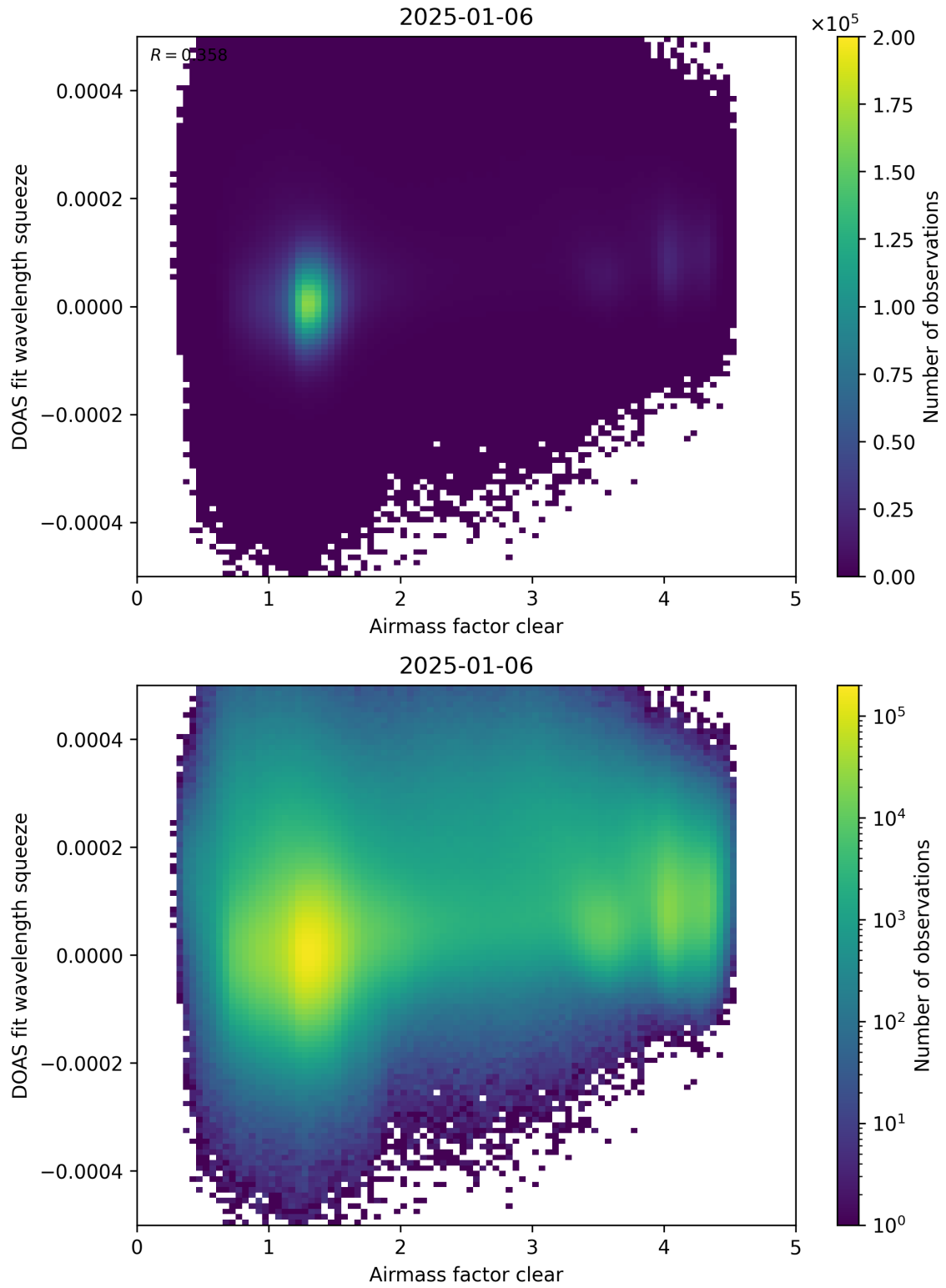
Figure 73: Scatter density plot of “Airmass factor clear” against “DOAS fit wavelength squeeze” for 2025-01-05 to 2025-01-07.
