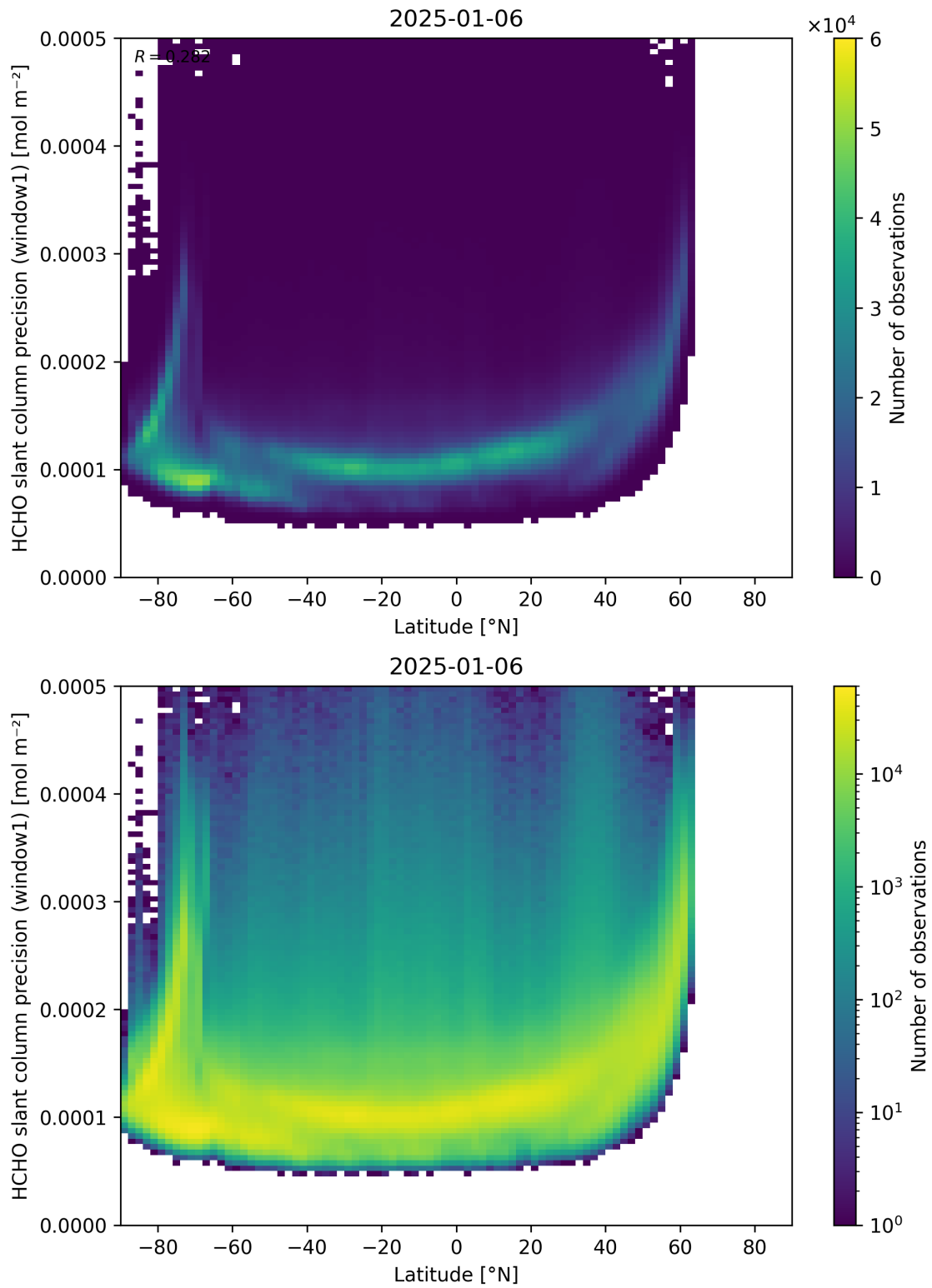
Figure 160: Scatter density plot of “Latitude” against “HCHO slant column precision (window1)” for 2025-01-05 to 2025-01-07.
