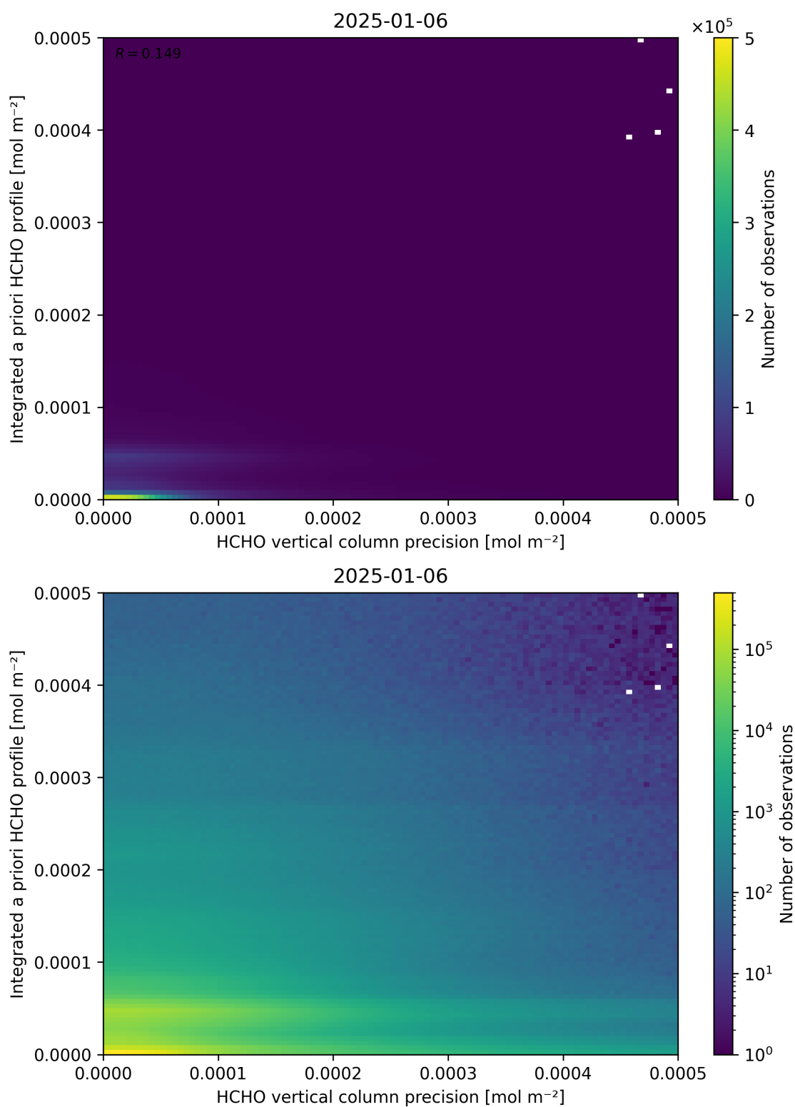
Figure 147: Scatter density plot of “HCHO vertical column precision” against “Integrated a priori HCHO profile” for 2025-01-05 to 2025-01-07.
