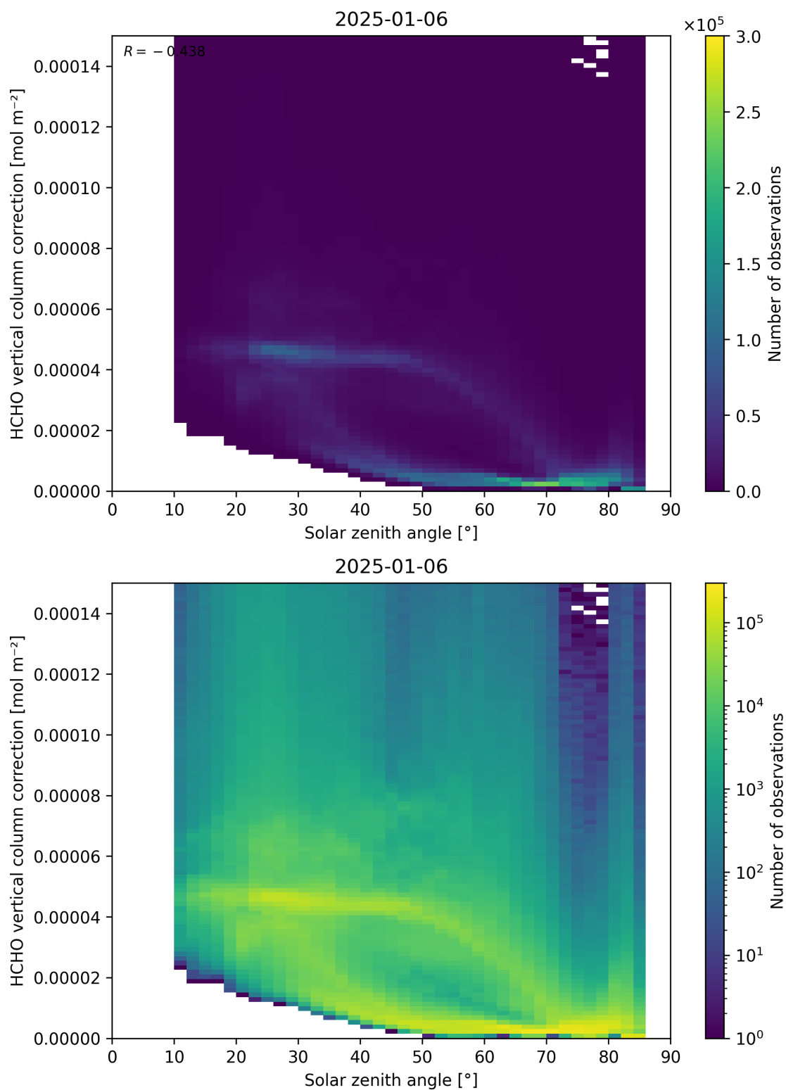
Figure 178: Scatter density plot of “Solar zenith angle” against “HCHO vertical column correction” for 2025-01-05 to 2025-01-07.
