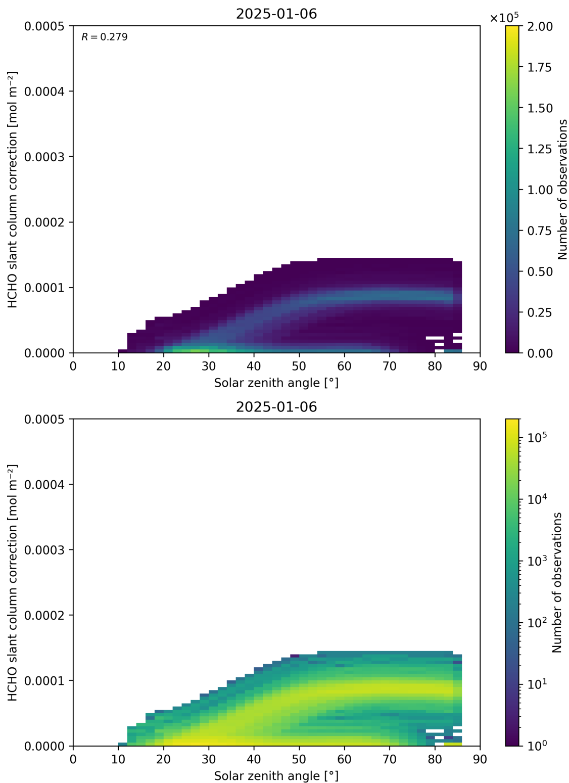
Figure 172: Scatter density plot of “Solar zenith angle” against “HCHO slant column correction” for 2025-01-05 to 2025-01-07.
