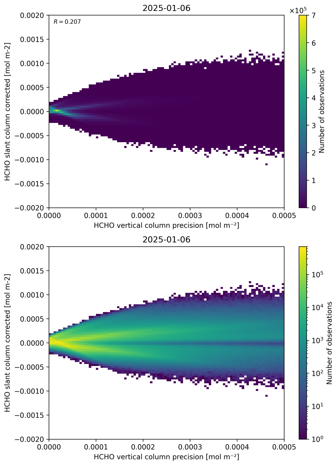
Figure 140: Scatter density plot of “HCHO vertical column precision” against “HCHO slant column corrected” for 2025-01-05 to 2025-01-07.
