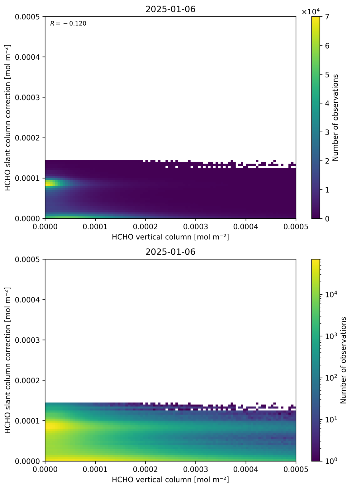
Figure 128: Scatter density plot of “HCHO vertical column” against “HCHO slant column correction” for 2025-01-05 to 2025-01-07.
