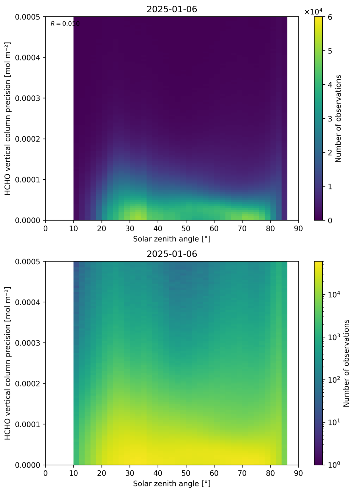
Figure 179: Scatter density plot of “Solar zenith angle” against “HCHO vertical column precision” for 2025-01-05 to 2025-01-07.
