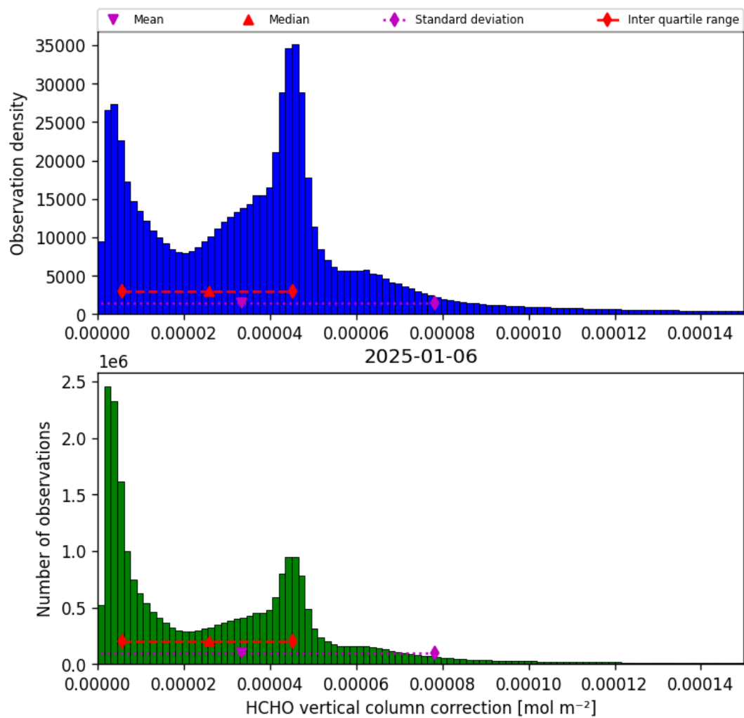
Figure 37: Histogram of “HCHO vertical column correction” for 2025-01-05 to 2025-01-07
