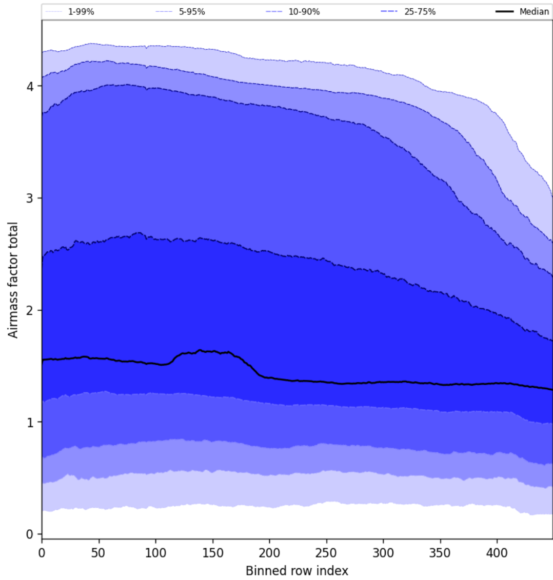
Figure 54: Along track statistics of “Airmass factor total” for 2025-01-05 to 2025-01-07
