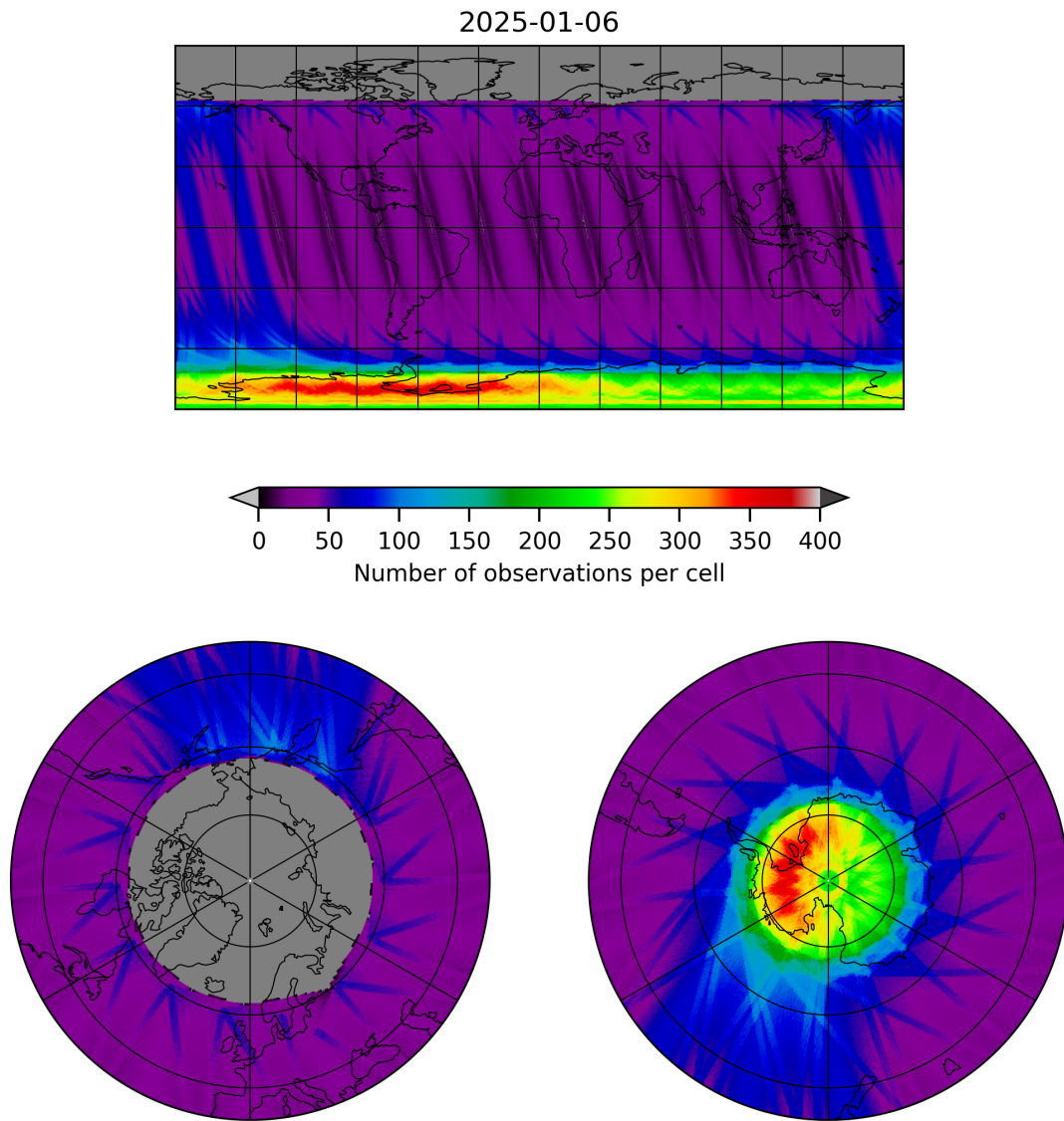
Figure 19: Map of the number of observations for 2025-01-05 to 2025-01-07
