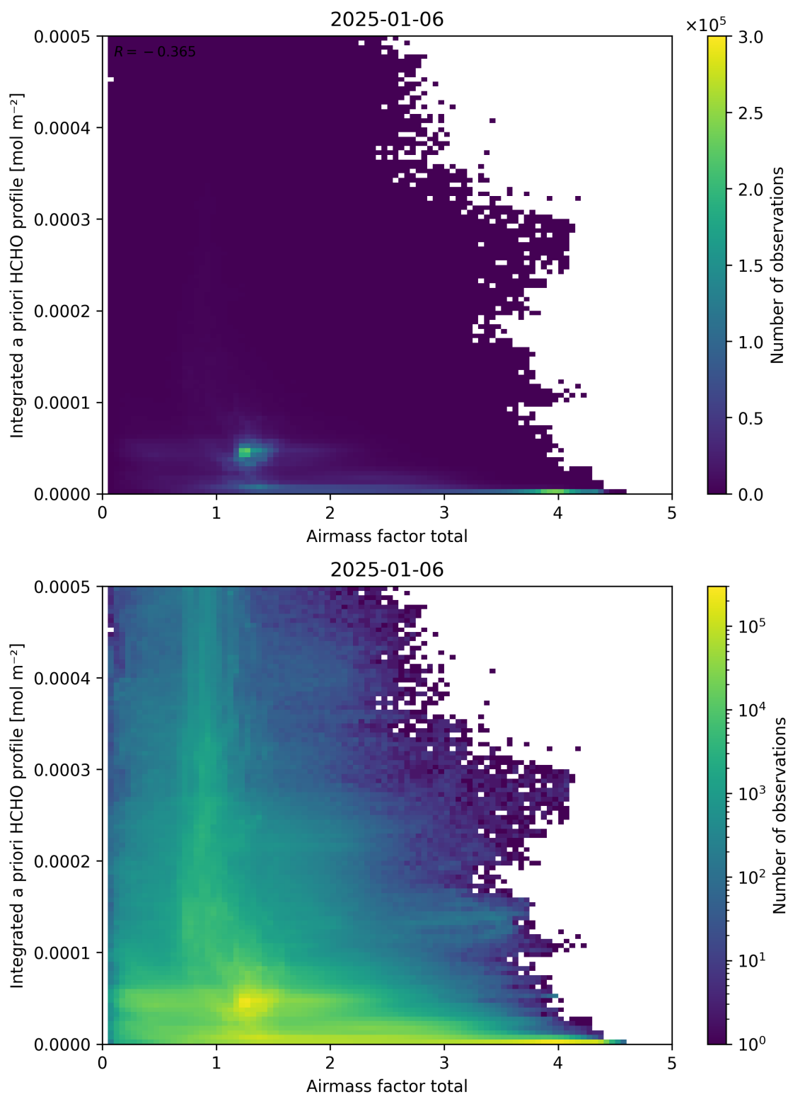
Figure 104: Scatter density plot of “Airmass factor total” against “Integrated a priori HCHO profile” for 2025-01-05 to 2025-01-07.
