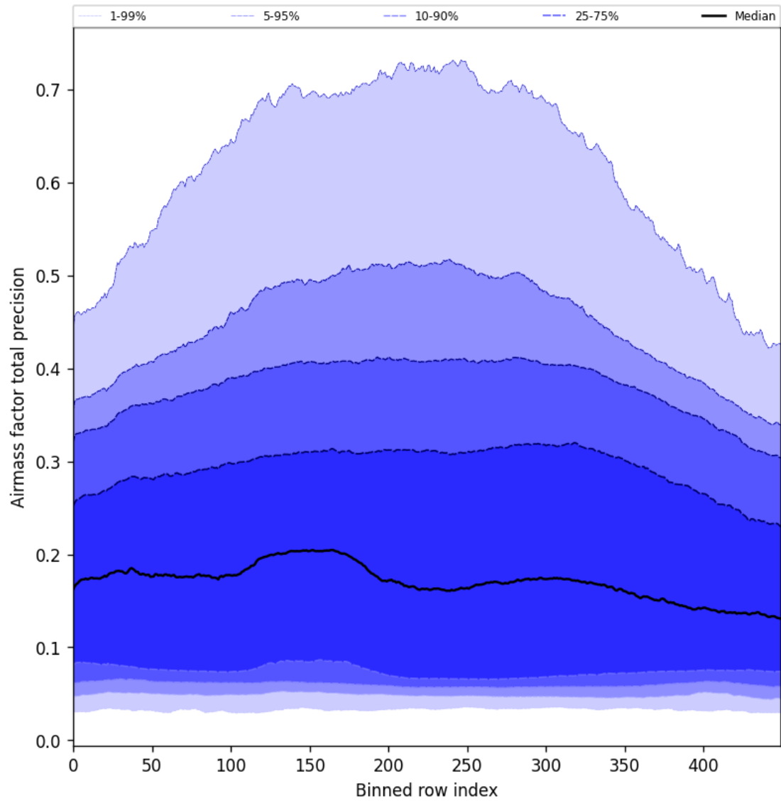
Figure 55: Along track statistics of “Airmass factor total precision” for 2025-01-05 to 2025-01-07
