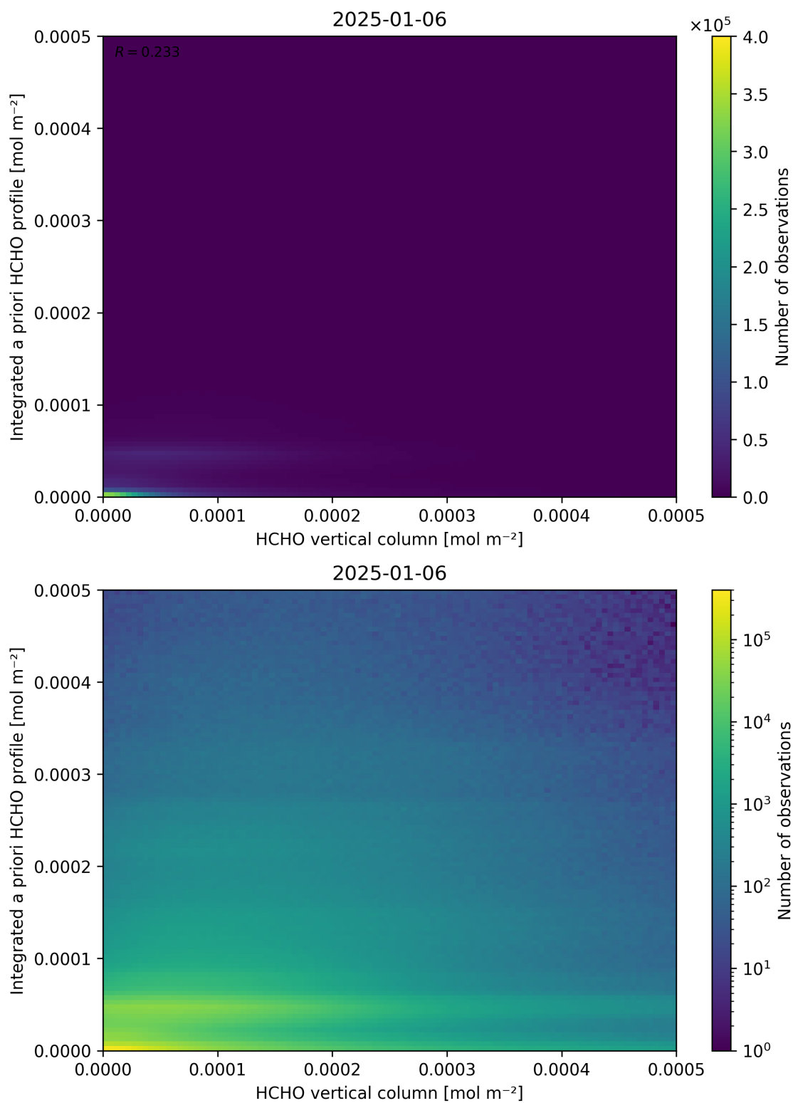
Figure 135: Scatter density plot of “HCHO vertical column” against “Integrated a priori HCHO profile” for 2025-01-05 to 2025-01-07.
