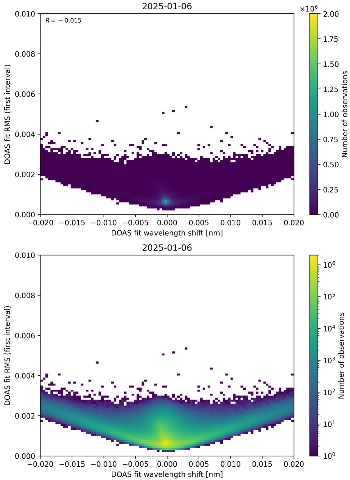
Figure 64: Scatter density plot of “DOAS fit wavelength shift” against “DOAS fit RMS (first interval)” for 2025-01-05 to 2025-01-07.
