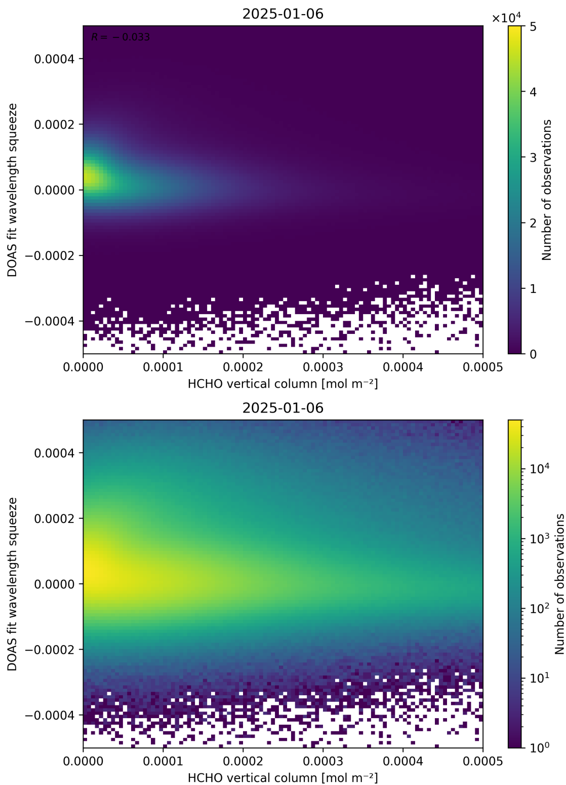
Figure 125: Scatter density plot of “HCHO vertical column” against “DOAS fit wavelength squeeze” for 2025-01-05 to 2025-01-07.
