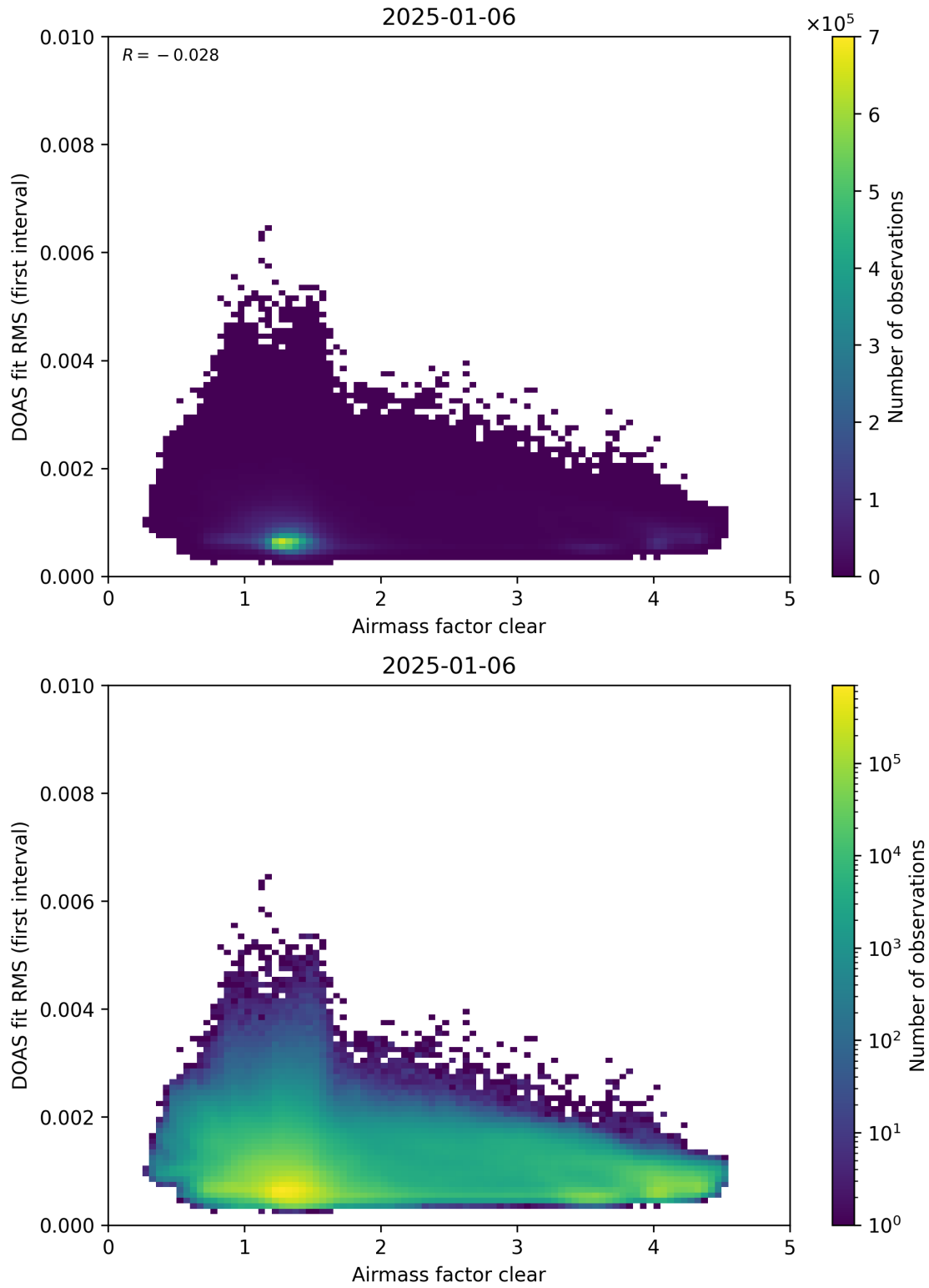
Figure 71: Scatter density plot of “Airmass factor clear” against “DOAS fit RMS (first interval)” for 2025-01-05 to 2025-01-07.
