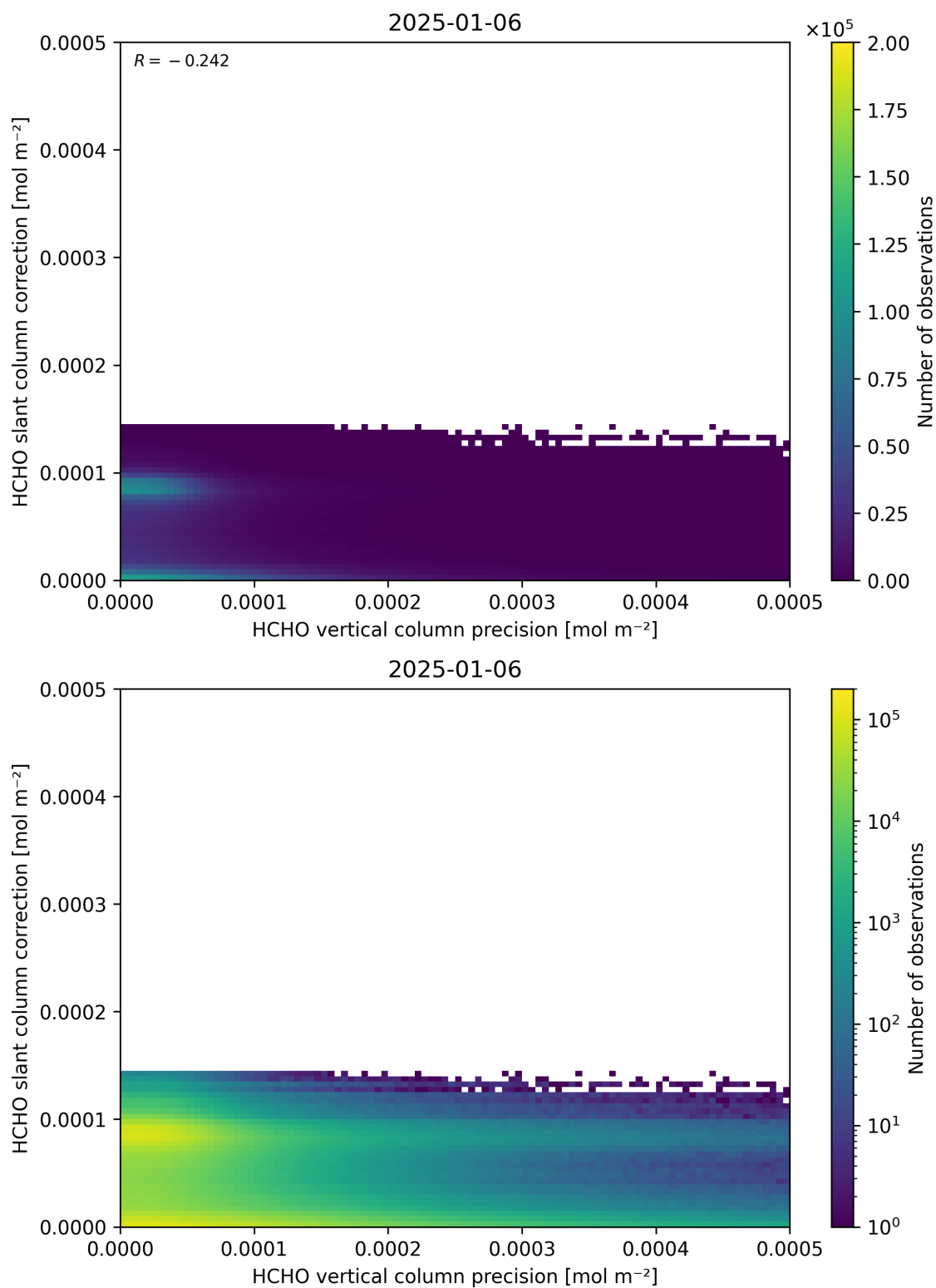
Figure 141: Scatter density plot of “HCHO vertical column precision” against “HCHO slant column correction” for 2025-01-05 to 2025-01-07.
