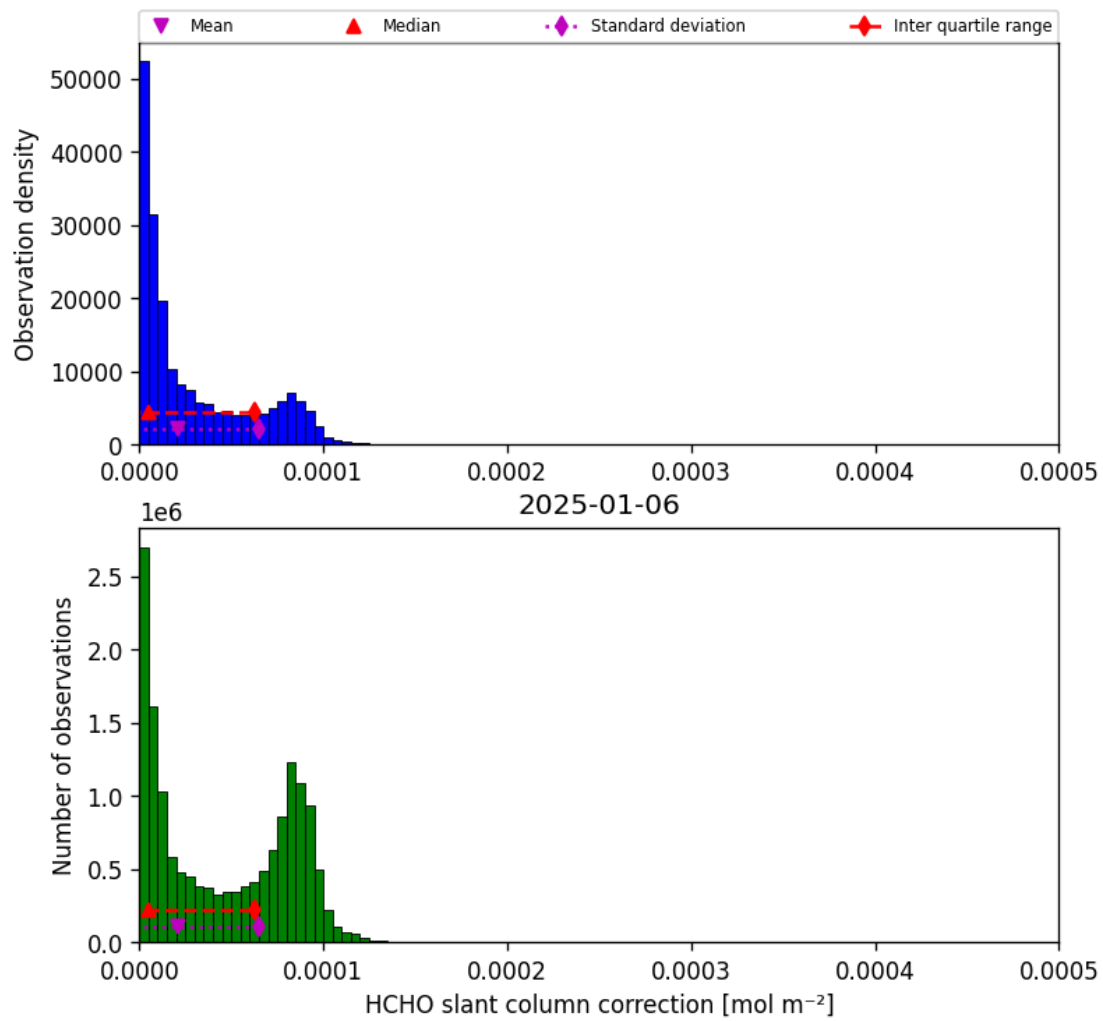
Figure 47: Histogram of “HCHO slant column correction” for 2025-01-05 to 2025-01-07
