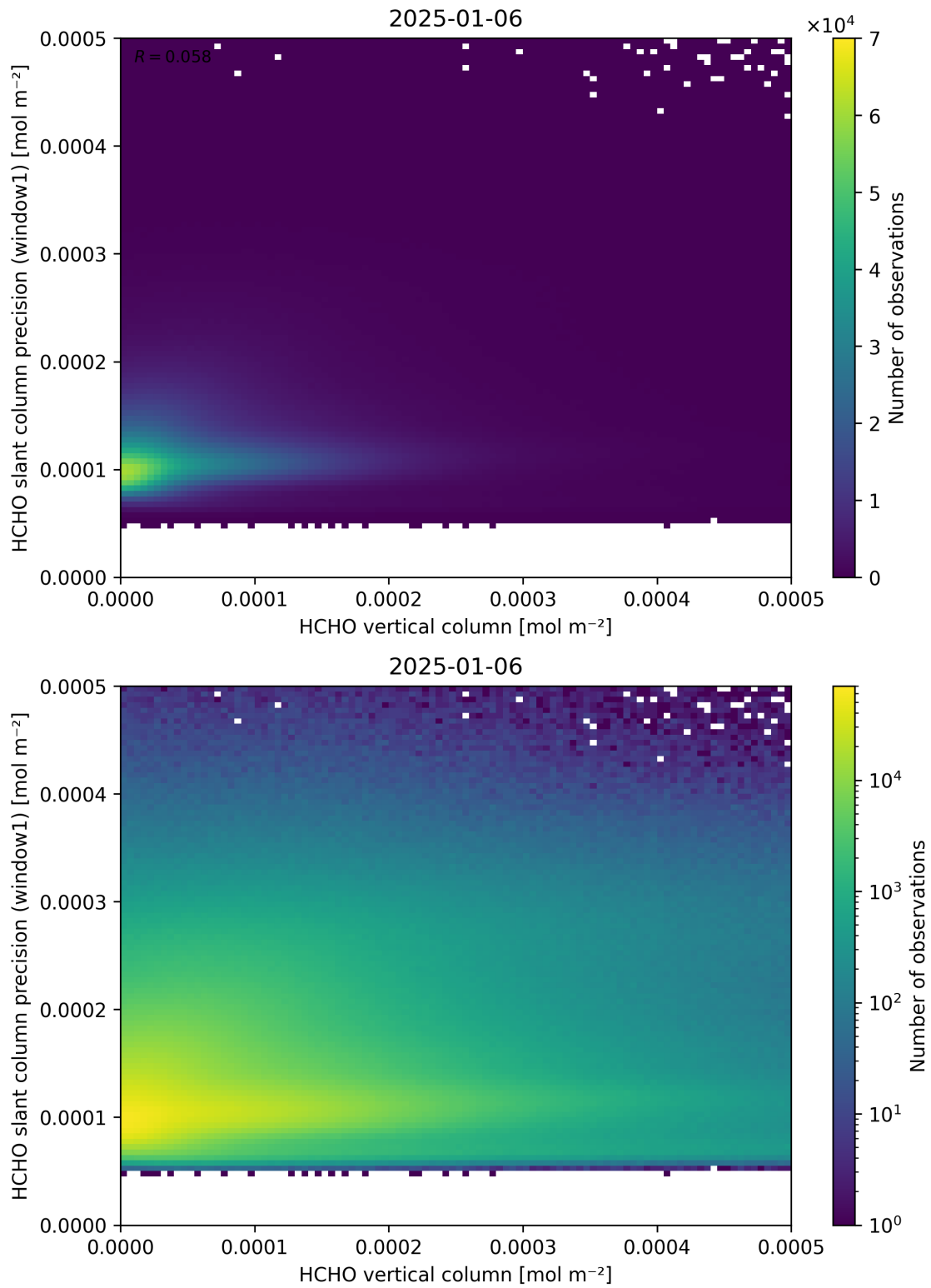
Figure 130: Scatter density plot of “HCHO vertical column” against “HCHO slant column precision (window1)” for 2025-01-05 to 2025-01-07.
