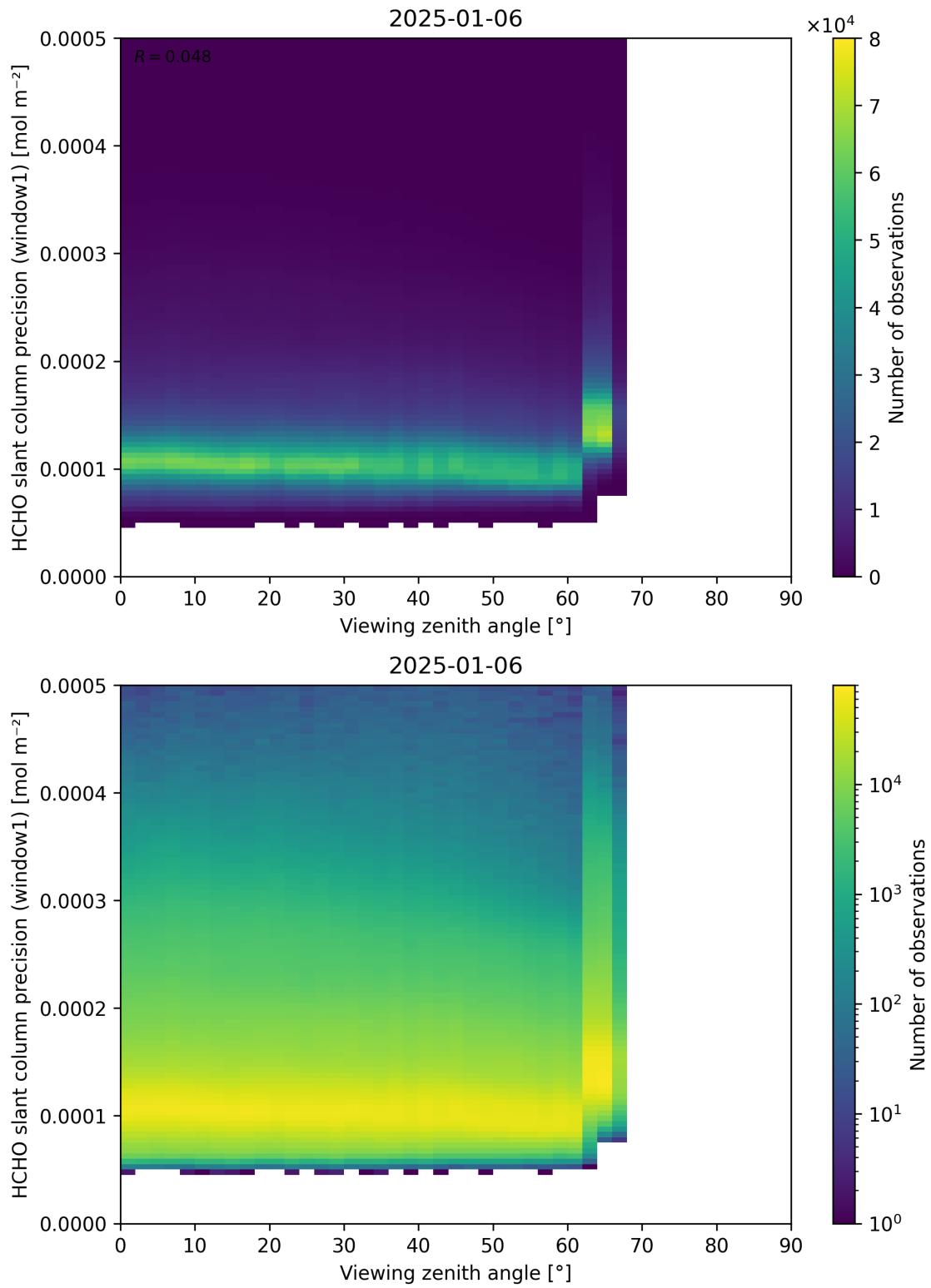
Figure 189: Scatter density plot of “Viewing zenith angle” against “HCHO slant column precision (window1)” for 2025-01-05 to 2025-01-07.
