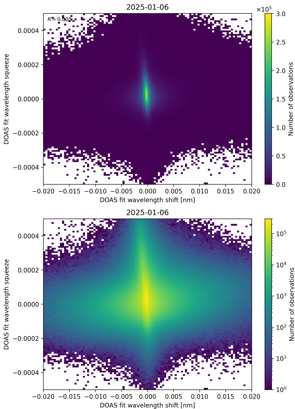
Figure 65: Scatter density plot of “DOAS fit wavelength shift” against “DOAS fit wavelength squeeze” for 2025-01-05 to 2025-01-07.
