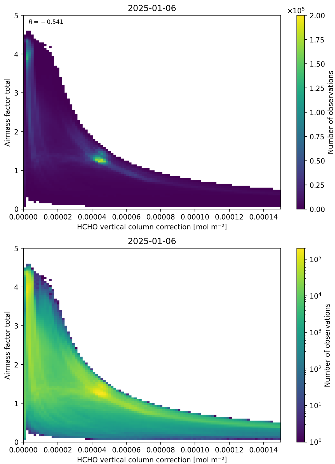
Figure 120: Scatter density plot of “HCHO vertical column correction” against “Airmass factor total” for 2025-01-05 to 2025-01-07.
