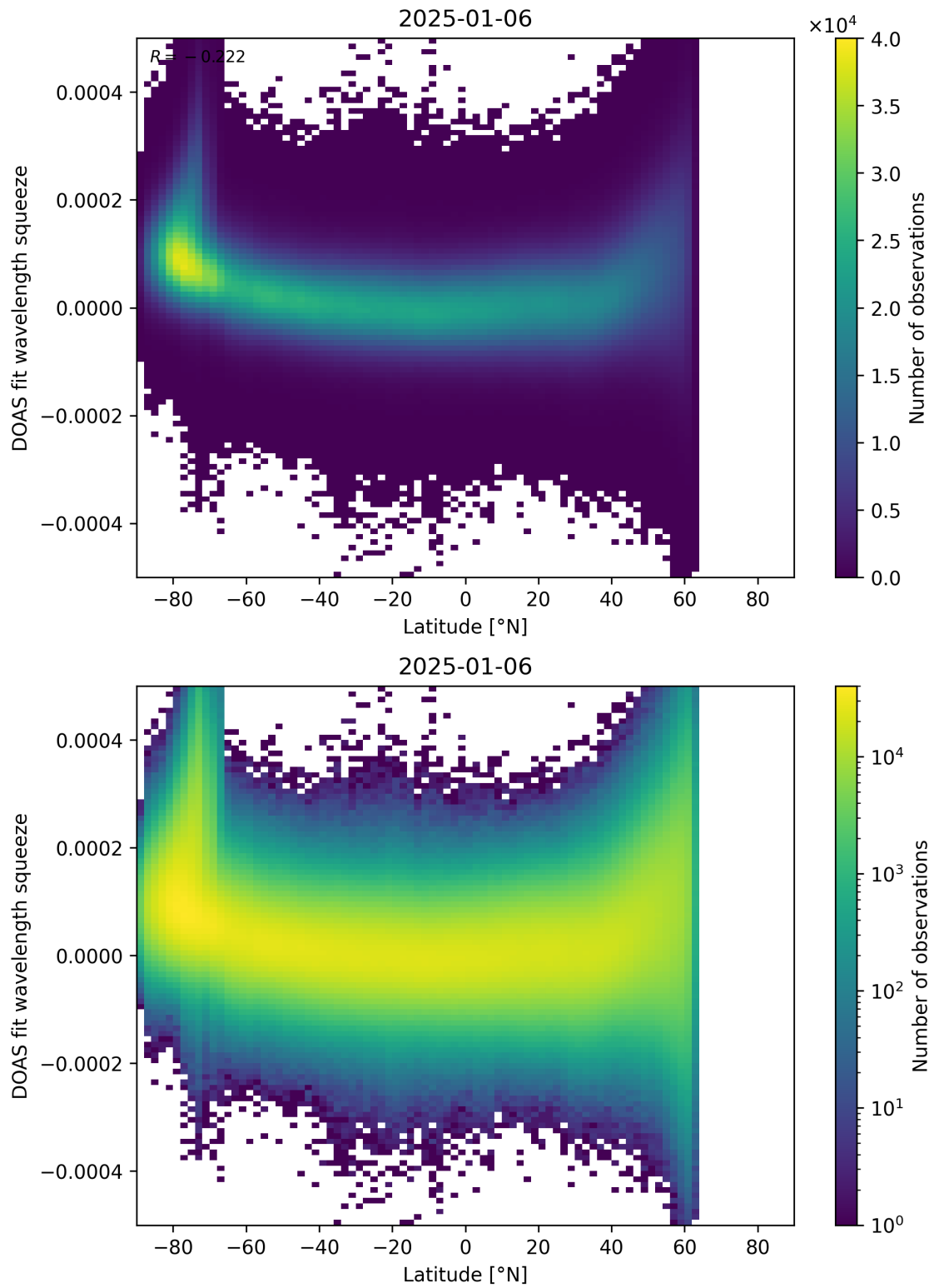
Figure 155: Scatter density plot of “Latitude” against “DOAS fit wavelength squeeze” for 2025-01-05 to 2025-01-07.
