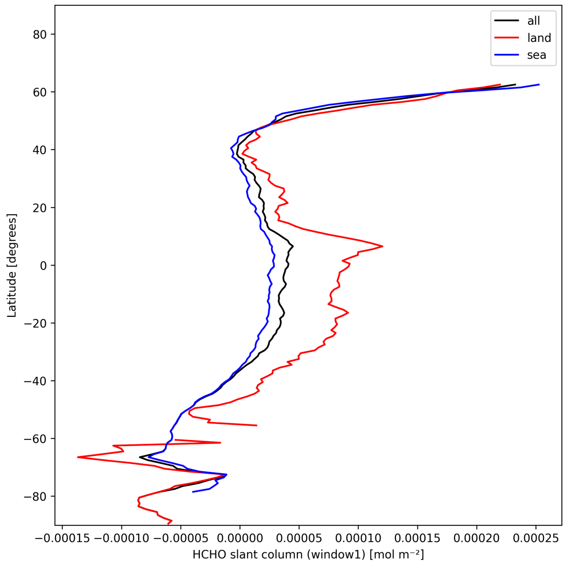
Figure 24: Zonal average of “HCHO slant column (window1)” for 2025-01-05 to 2025-01-07.
