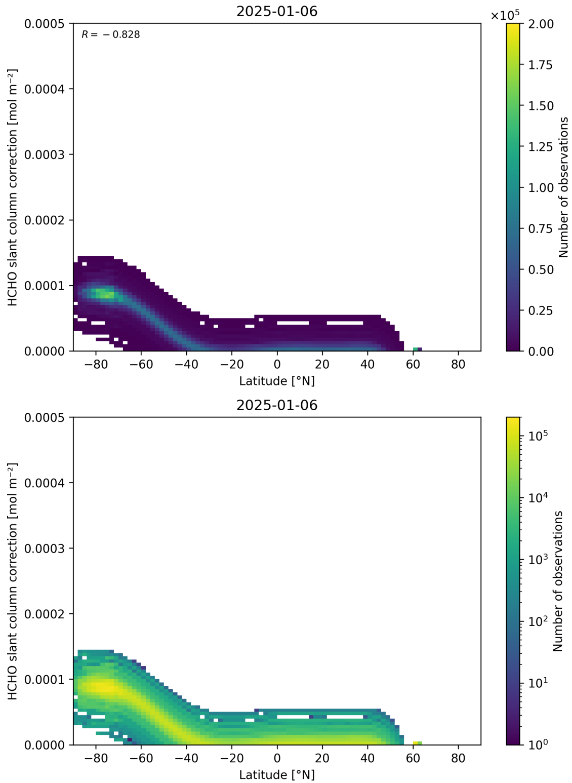
Figure 158: Scatter density plot of “Latitude” against “HCHO slant column correction” for 2025-01-05 to 2025-01-07.
