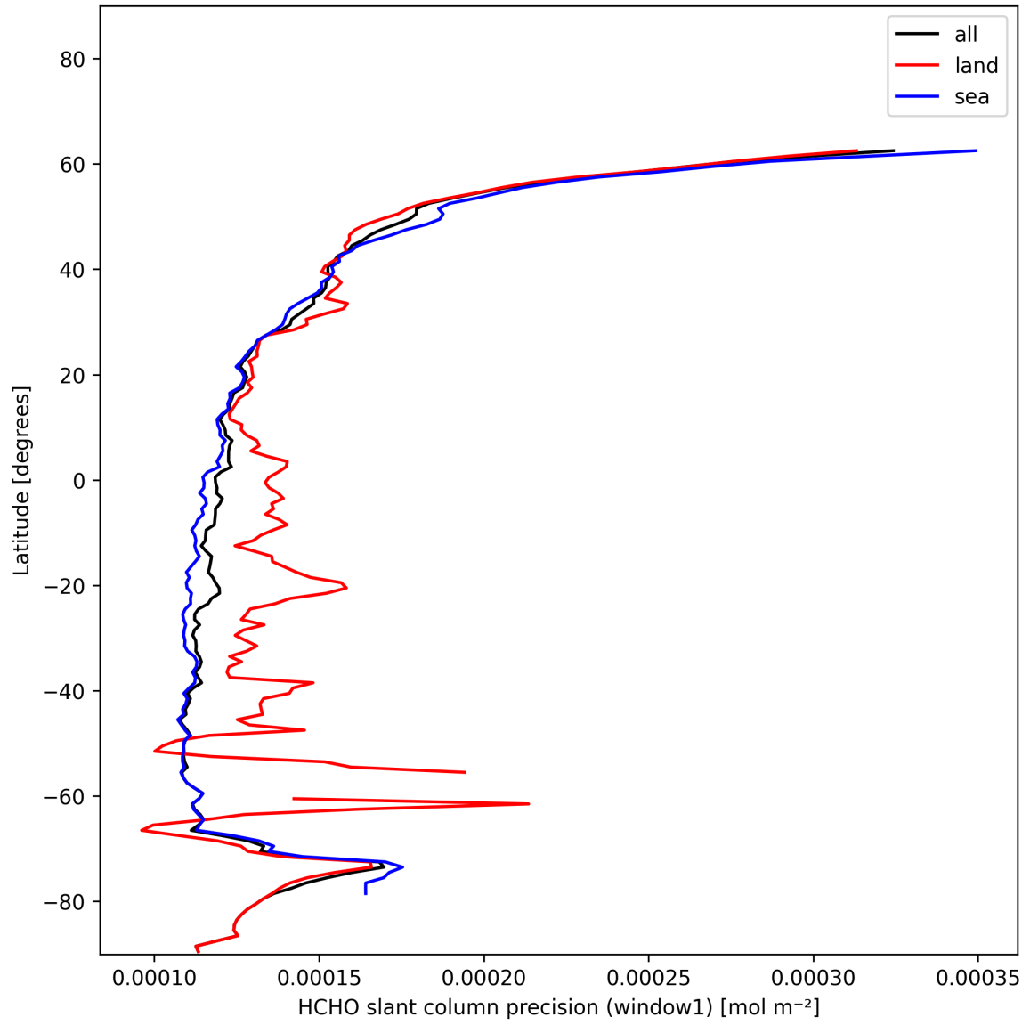
Figure 25: Zonal average of "HCHO slant column precision (window1)" for 2025-01-05 to 2025-01-07.
