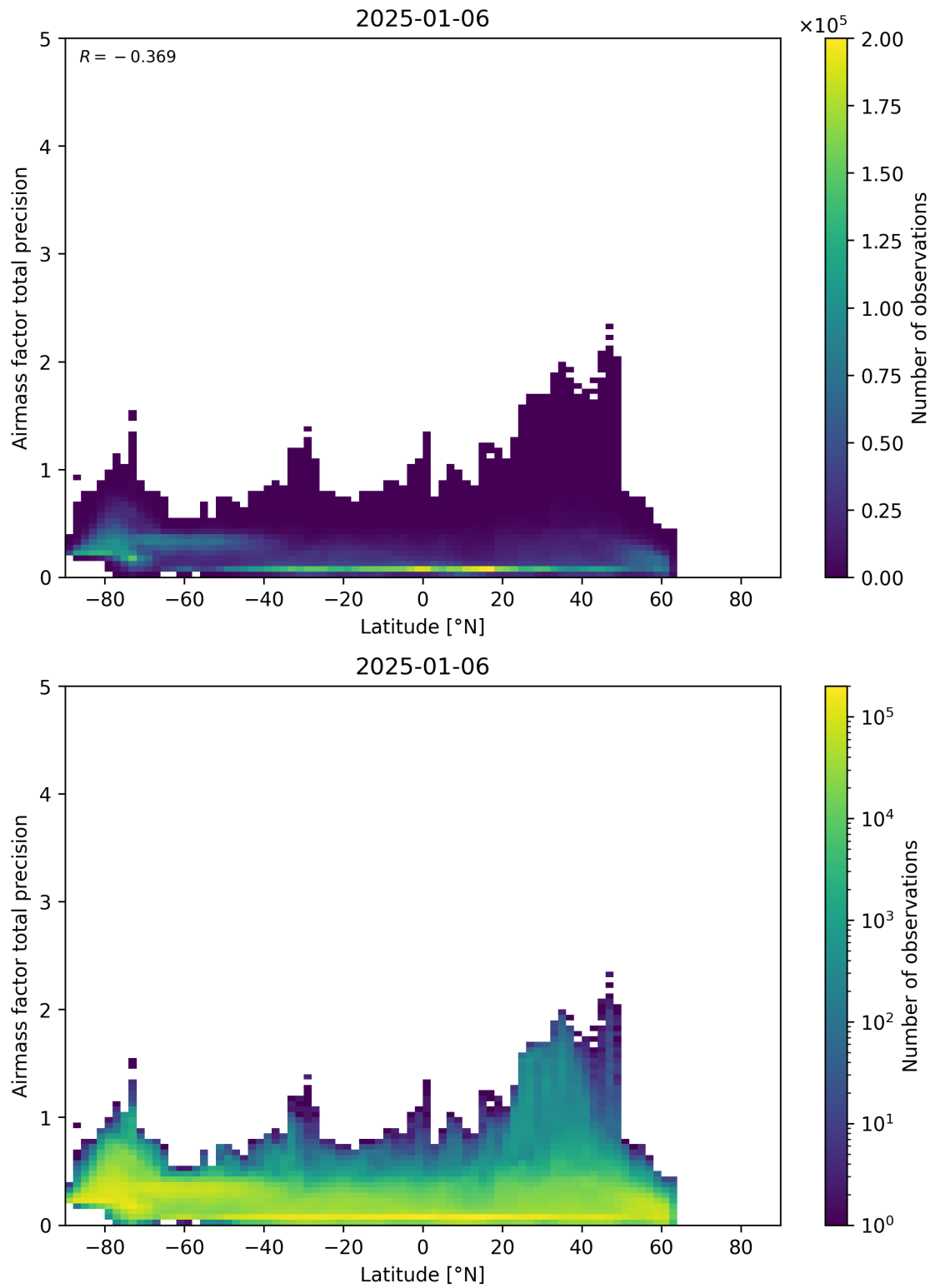
Figure 162: Scatter density plot of “Latitude” against “Airmass factor total precision” for 2025-01-05 to 2025-01-07.
