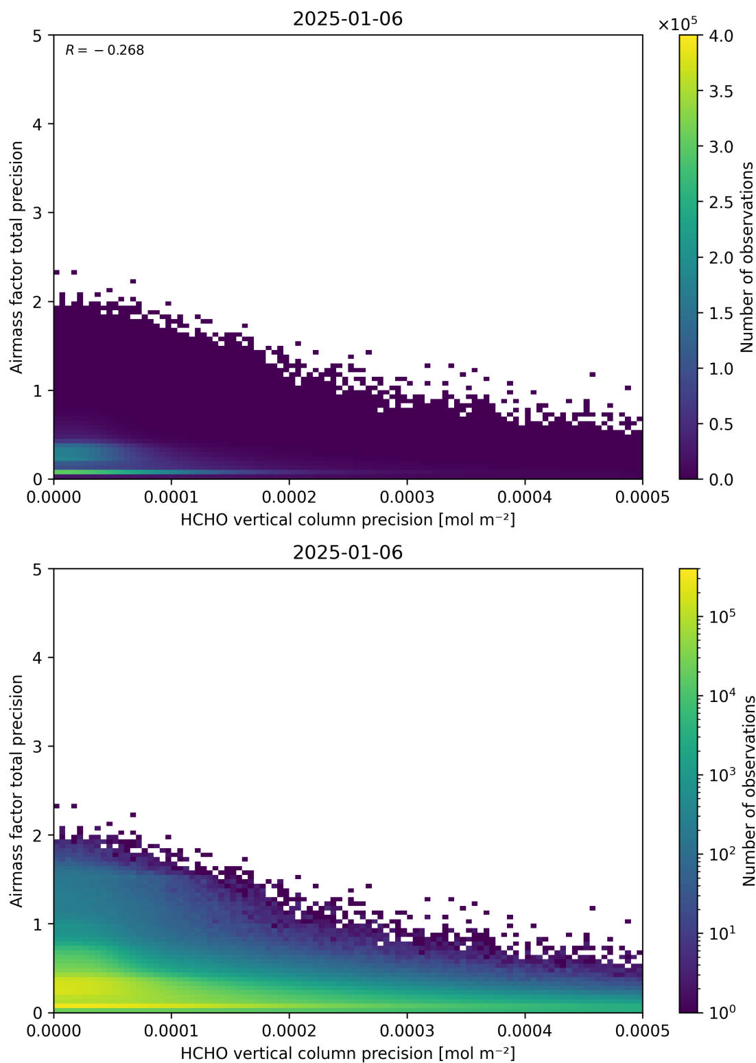
Figure 145: Scatter density plot of “HCHO vertical column precision” against “Airmass factor total precision” for 2025-01-05 to 2025-01-07.
