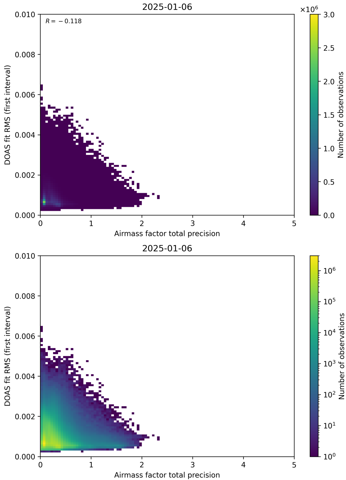
Figure 105: Scatter density plot of “Airmass factor total precision” against “DOAS fit RMS (first interval)” for 2025-01-05 to 2025-01-07.
