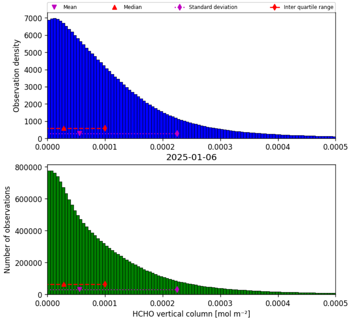
Figure 35: Histogram of “HCHO vertical column” for 2025-01-05 to 2025-01-07
