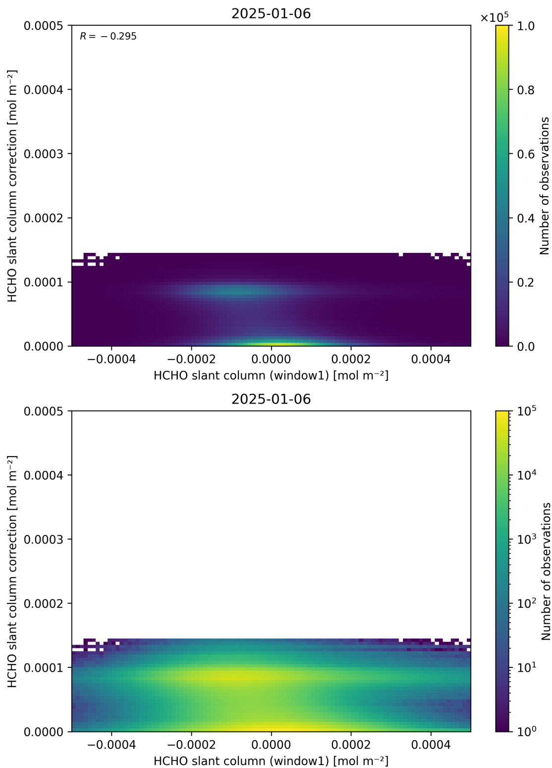
Figure 83: Scatter density plot of “HCHO slant column (window1)” against “HCHO slant column correction” for 2025-01-05 to 2025-01-07.
