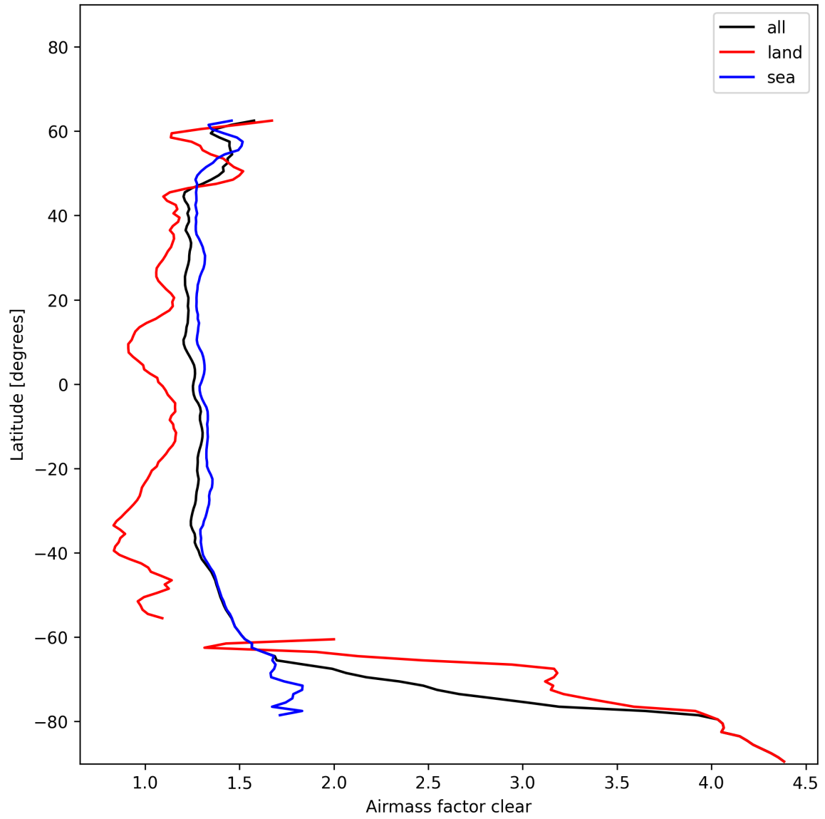
Figure 28: Zonal average of “Airmass factor clear” for 2025-01-05 to 2025-01-07.
