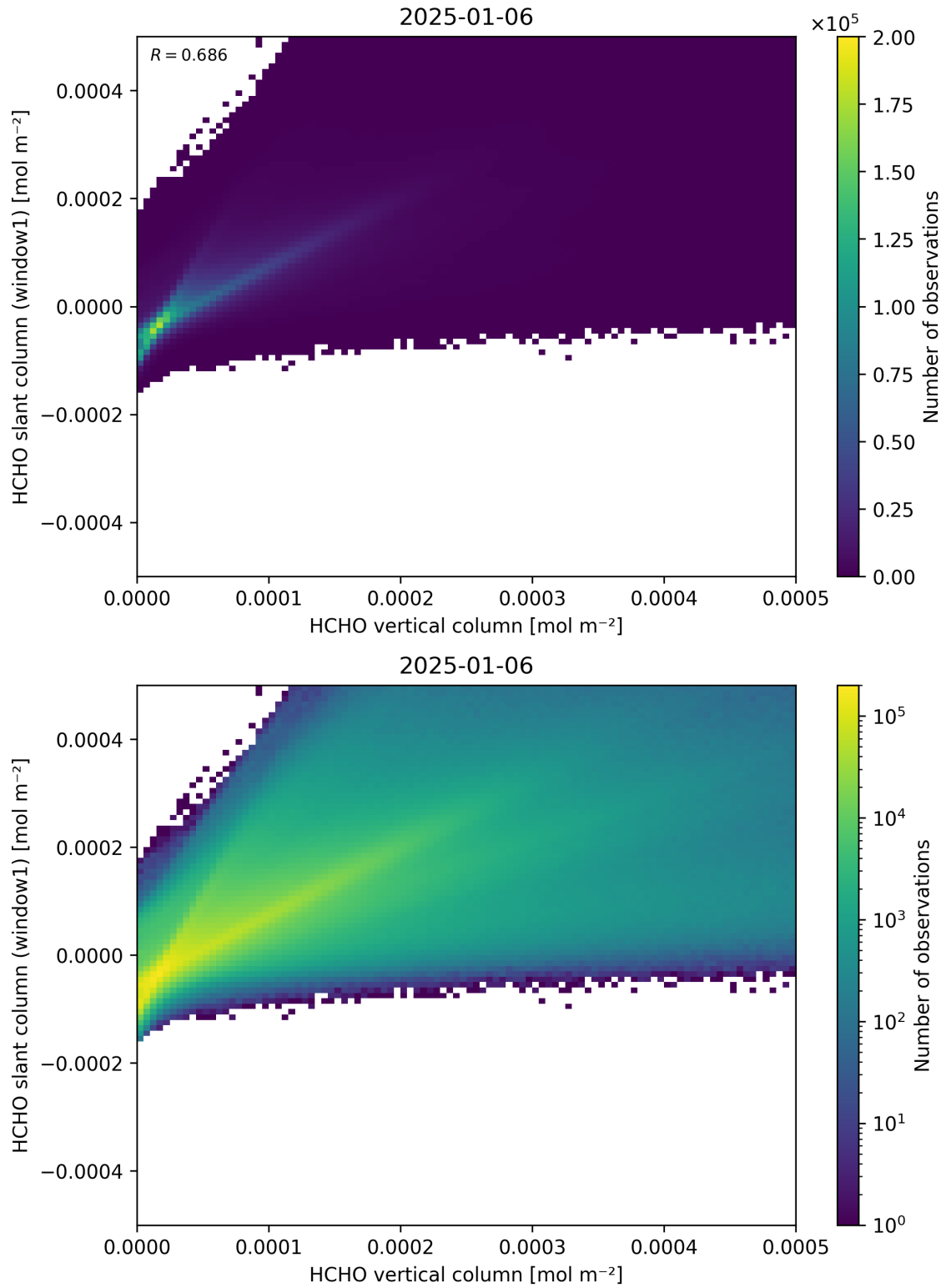
Figure 129: Scatter density plot of “HCHO vertical column” against “HCHO slant column (window1)” for 2025-01-05 to 2025-01-07.
