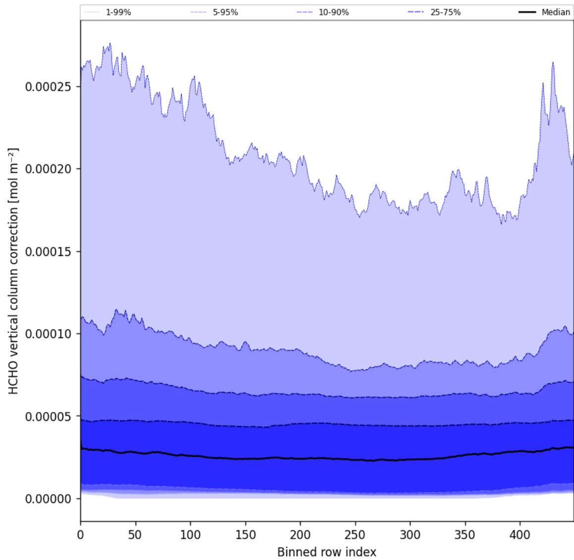
Figure 51: Along track statistics of “HCHO vertical column correction” for 2025-01-05 to 2025-01-07
