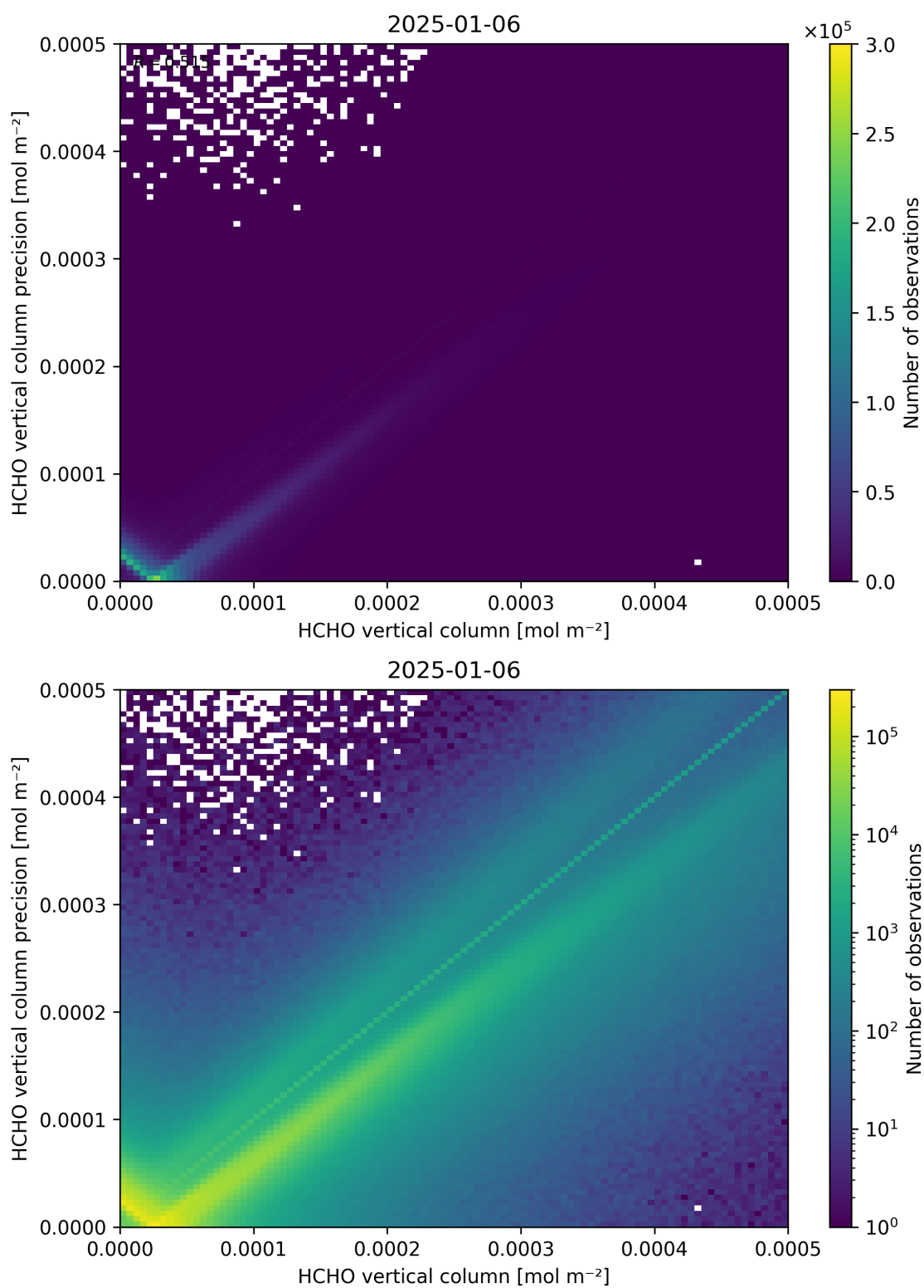
Figure 134: Scatter density plot of “HCHO vertical column” against “HCHO vertical column precision” for 2025-01-05 to 2025-01-07.
