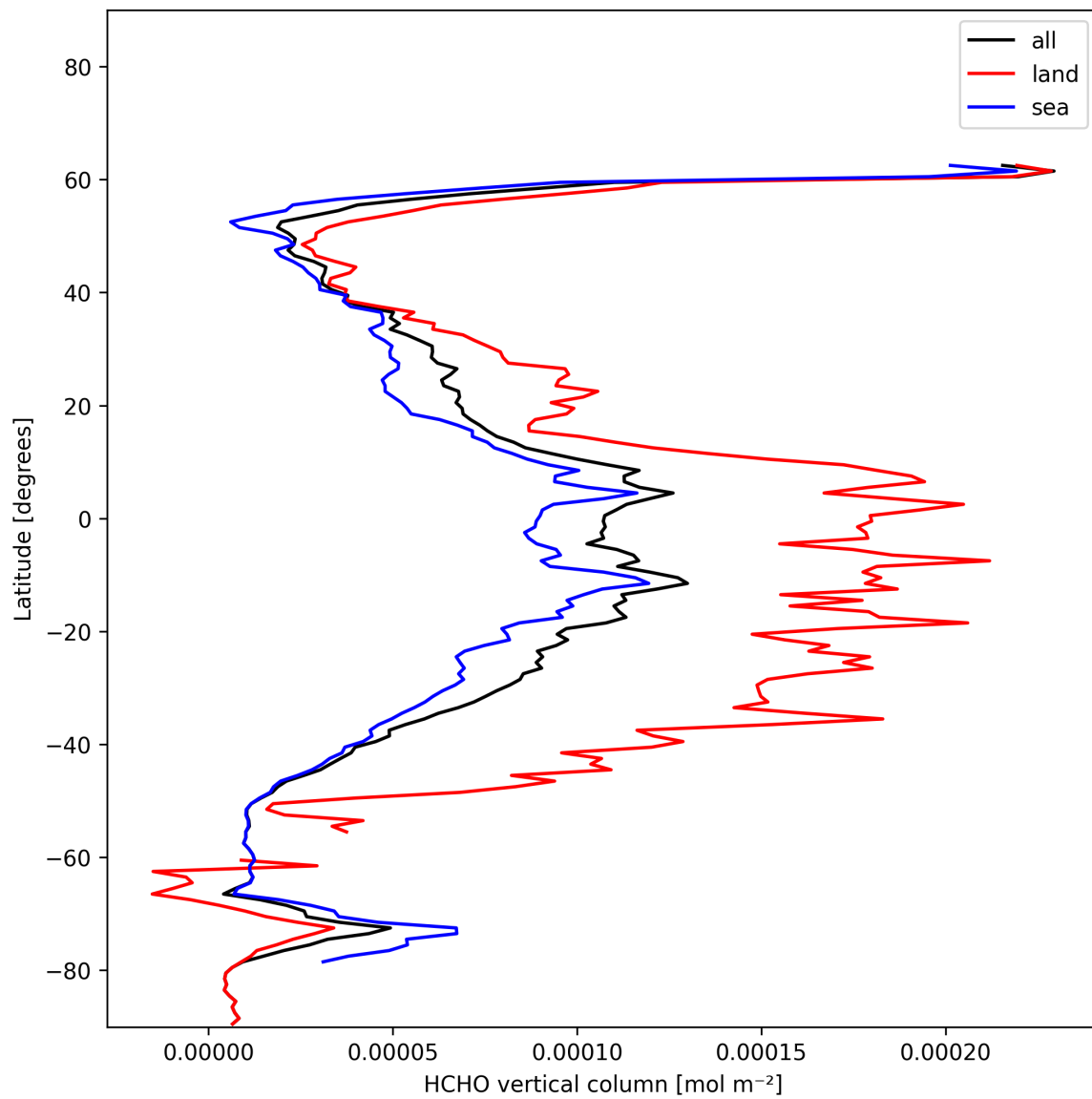
Figure 21: Zonal average of “HCHO vertical column” for 2025-01-05 to 2025-01-07.
