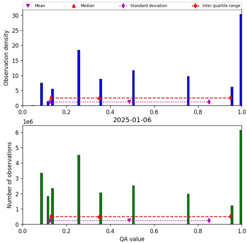
Figure 34: Histogram of “QA value” for 2025-01-05 to 2025-01-07
