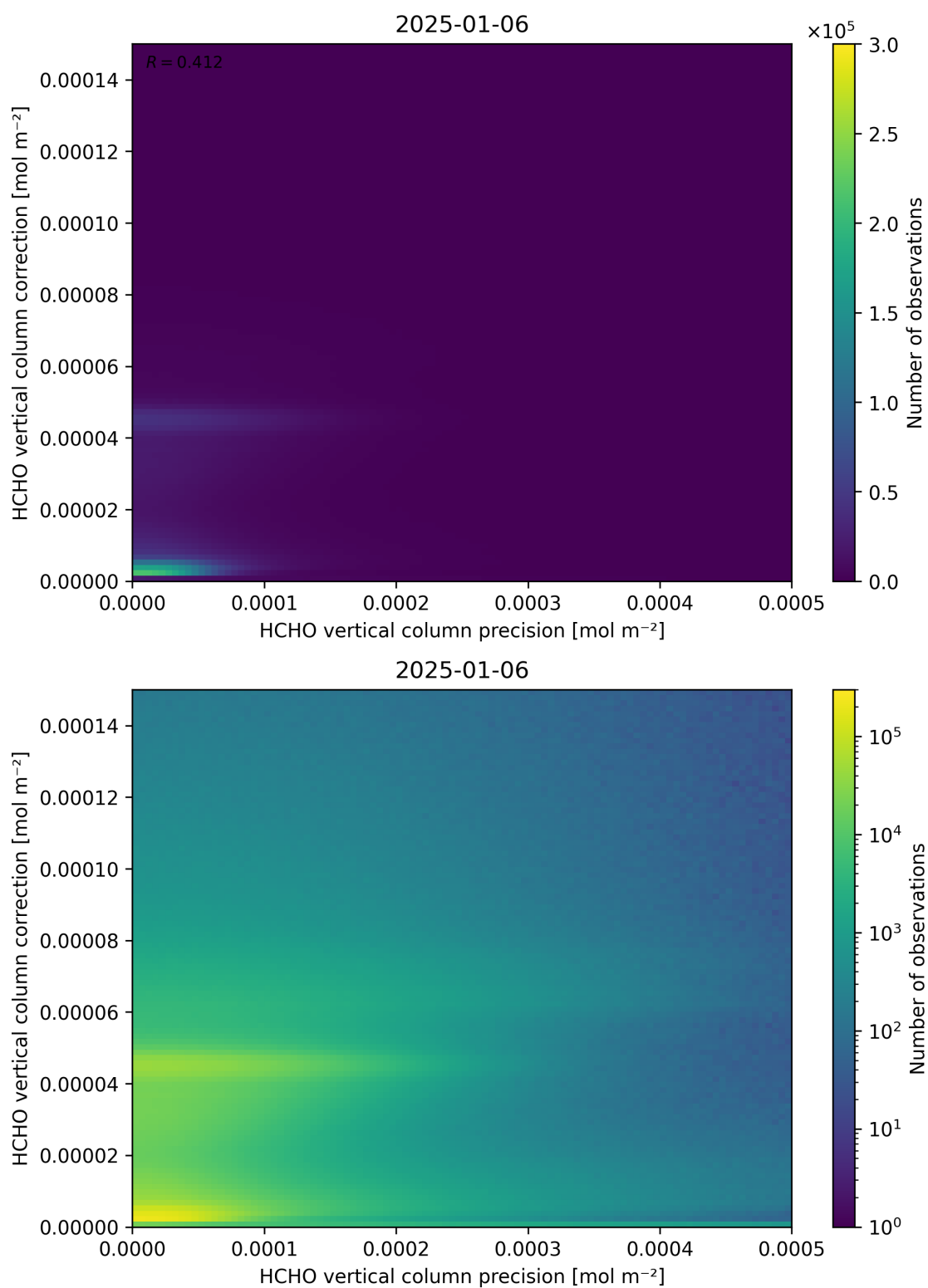
Figure 146: Scatter density plot of “HCHO vertical column precision” against “HCHO vertical column correction” for 2025-01-05 to 2025-01-07.
