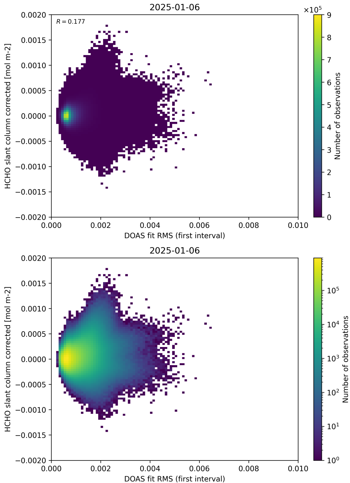
Figure 62: Scatter density plot of “DOAS fit RMS (first interval)” against “HCHO slant column corrected” for 2025-01-05 to 2025-01-07.
