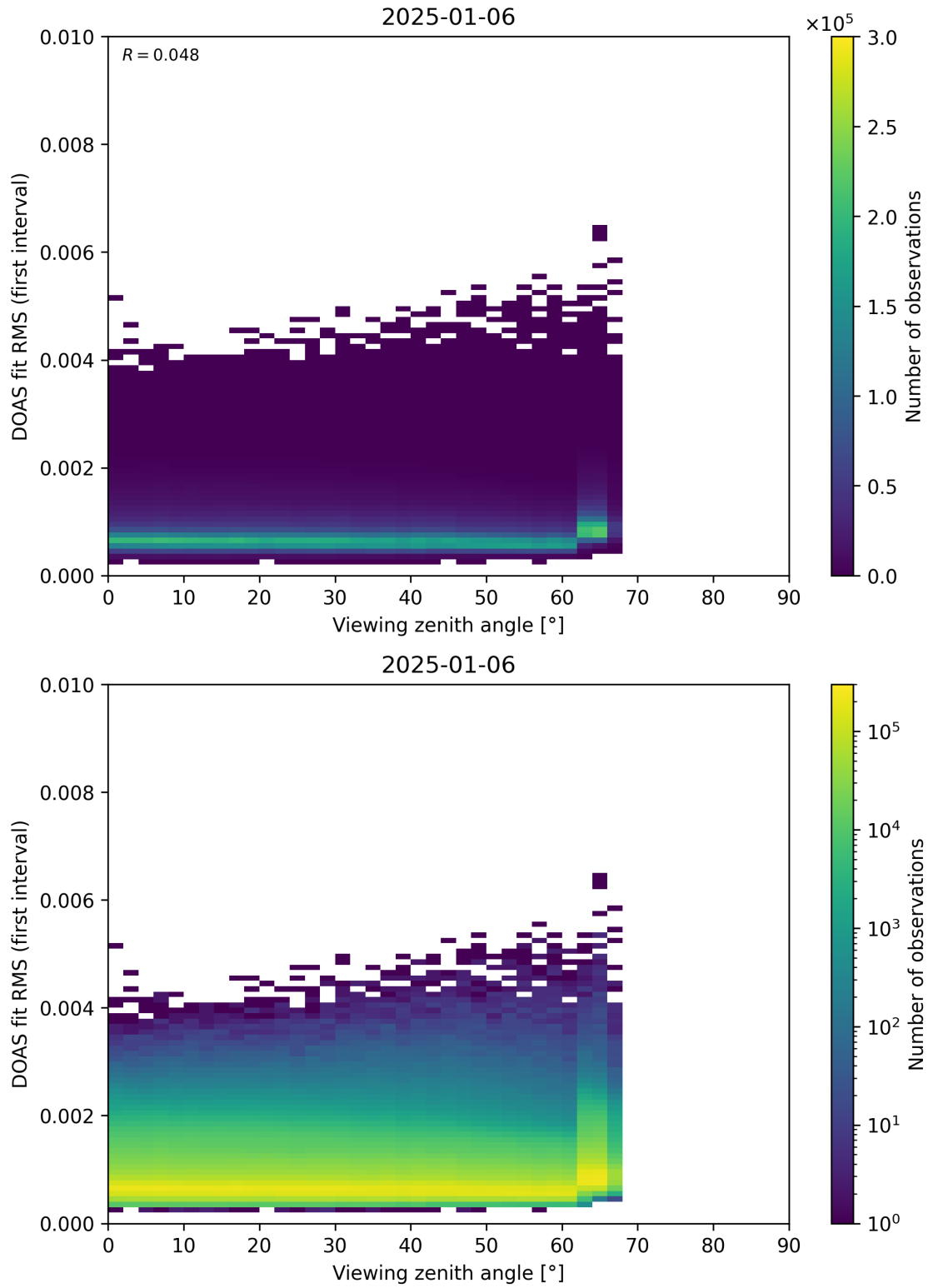
Figure 182: Scatter density plot of “Viewing zenith angle” against “DOAS fit RMS (first interval)” for 2025-01-05 to 2025-01-07.
