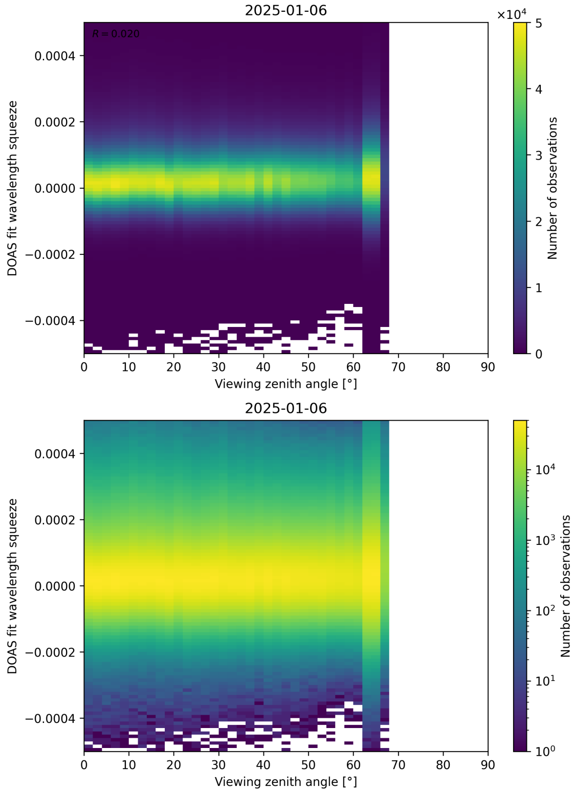
Figure 184: Scatter density plot of “Viewing zenith angle” against “DOAS fit wavelength squeeze” for 2025-01-05 to 2025-01-07.
