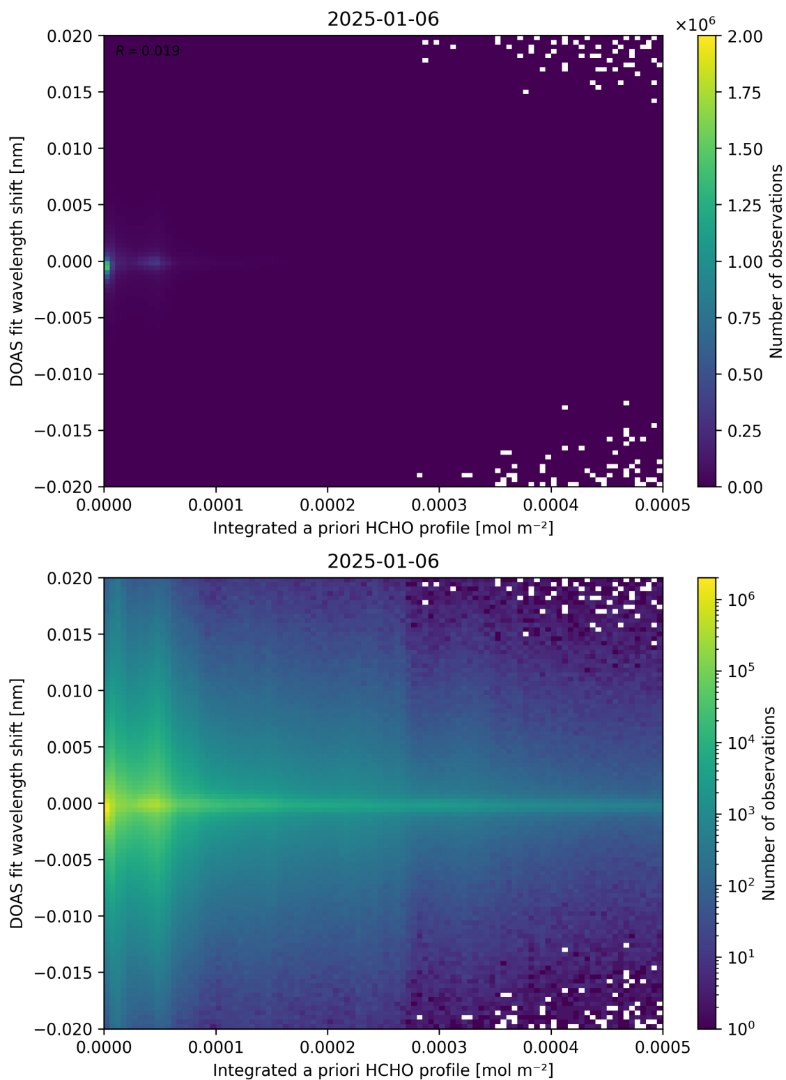
Figure 149: Scatter density plot of “Integrated a priori HCHO profile” against “DOAS fit wavelength shift” for 2025-01-05 to 2025-01-07.
