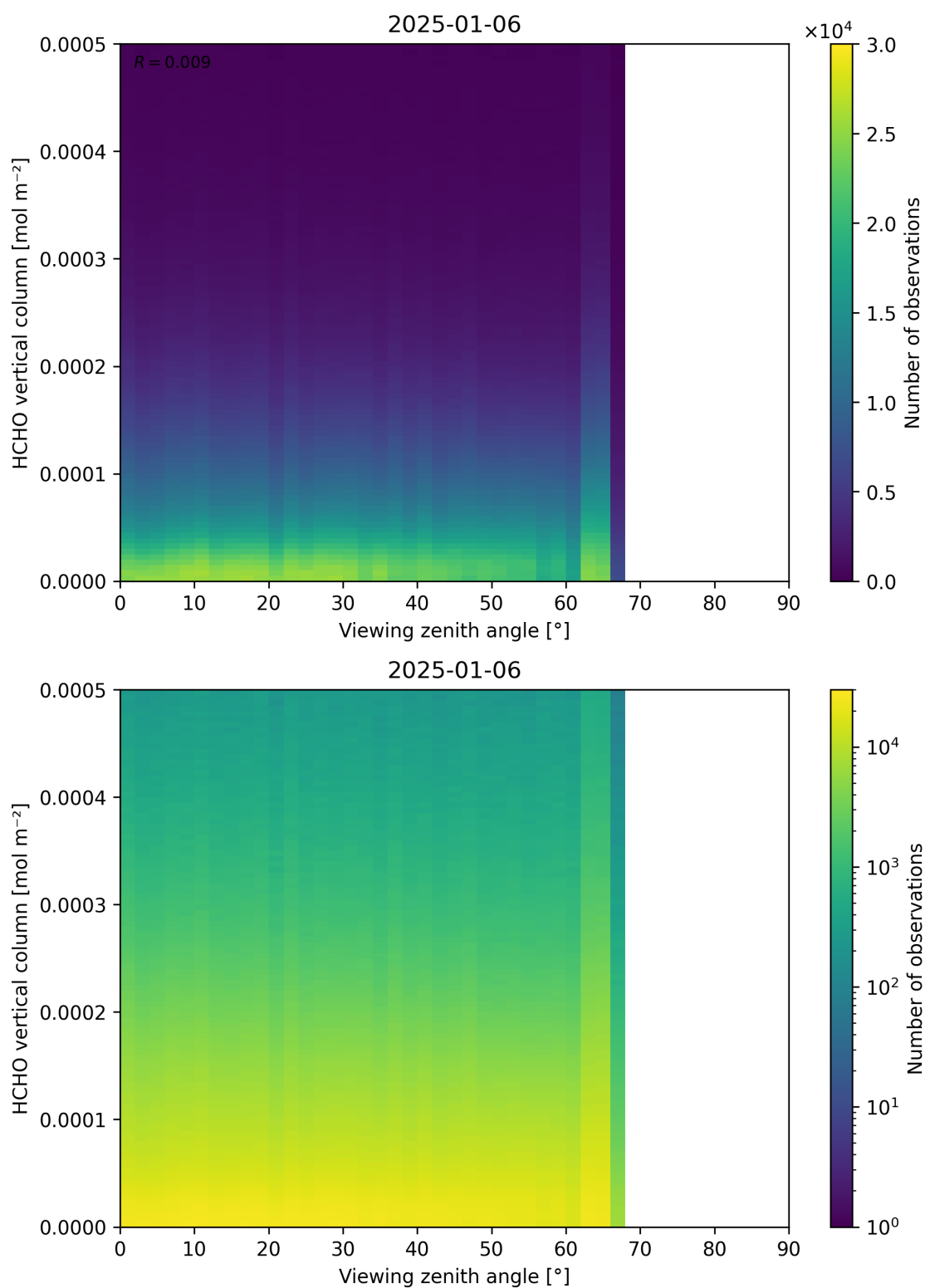
Figure 192: Scatter density plot of “Viewing zenith angle” against “HCHO vertical column” for 2025-01-05 to 2025-01-07.
