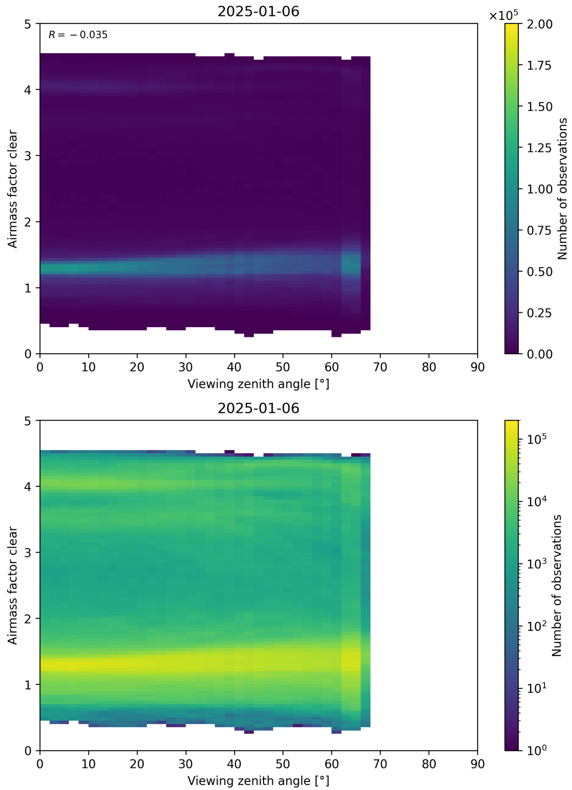
Figure 185: Scatter density plot of “Viewing zenith angle” against “Airmass factor clear” for 2025-01-05 to 2025-01-07.
