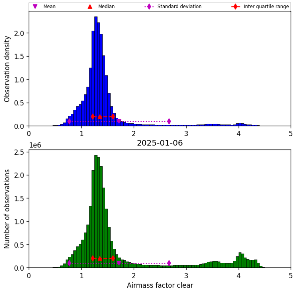
Figure 42: Histogram of “Airmass factor clear” for 2025-01-05 to 2025-01-07
