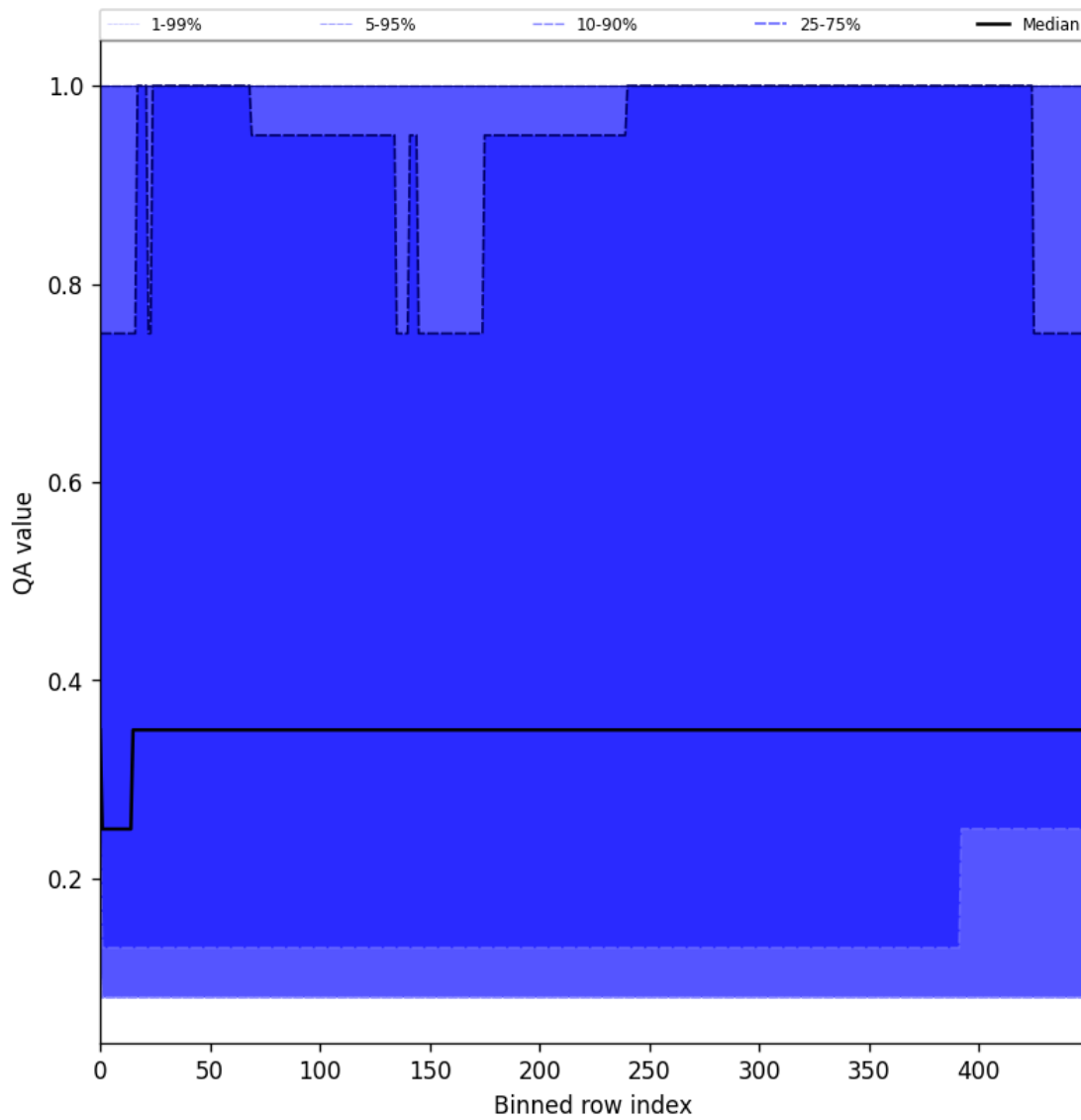
Figure 48: Along track statistics of “QA value” for 2025-01-05 to 2025-01-07
