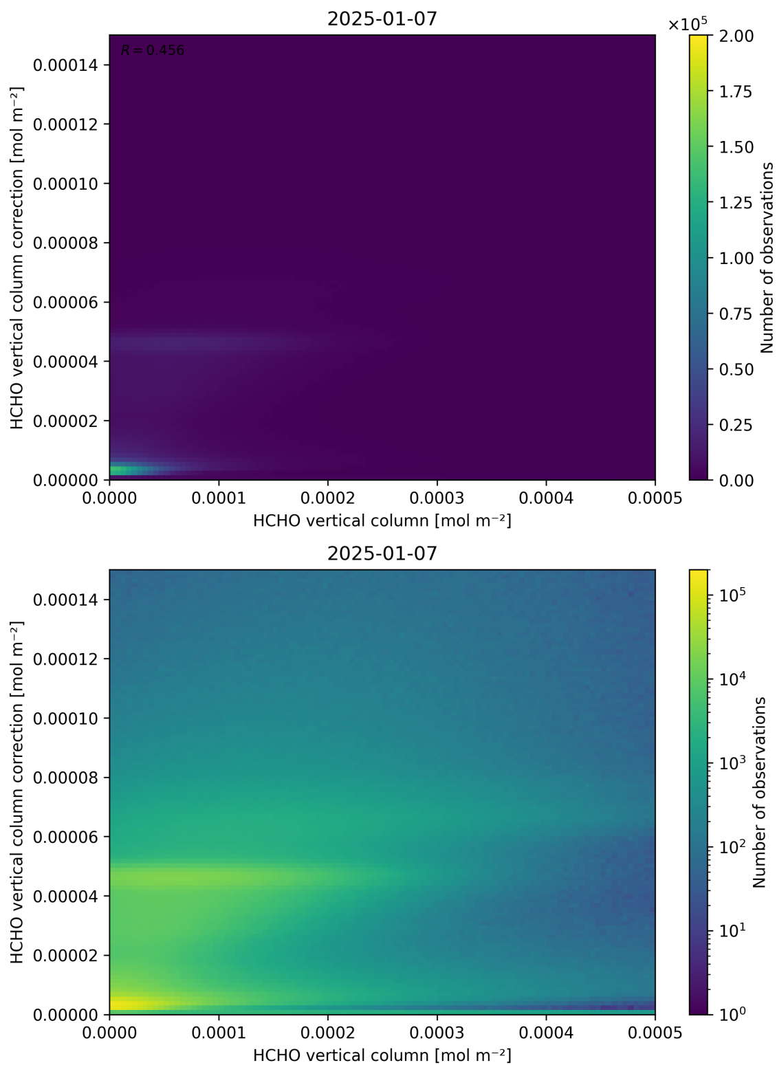
Figure 133: Scatter density plot of “HCHO vertical column” against “HCHO vertical column correction” for 2025-01-07 to 2025-01-08.
