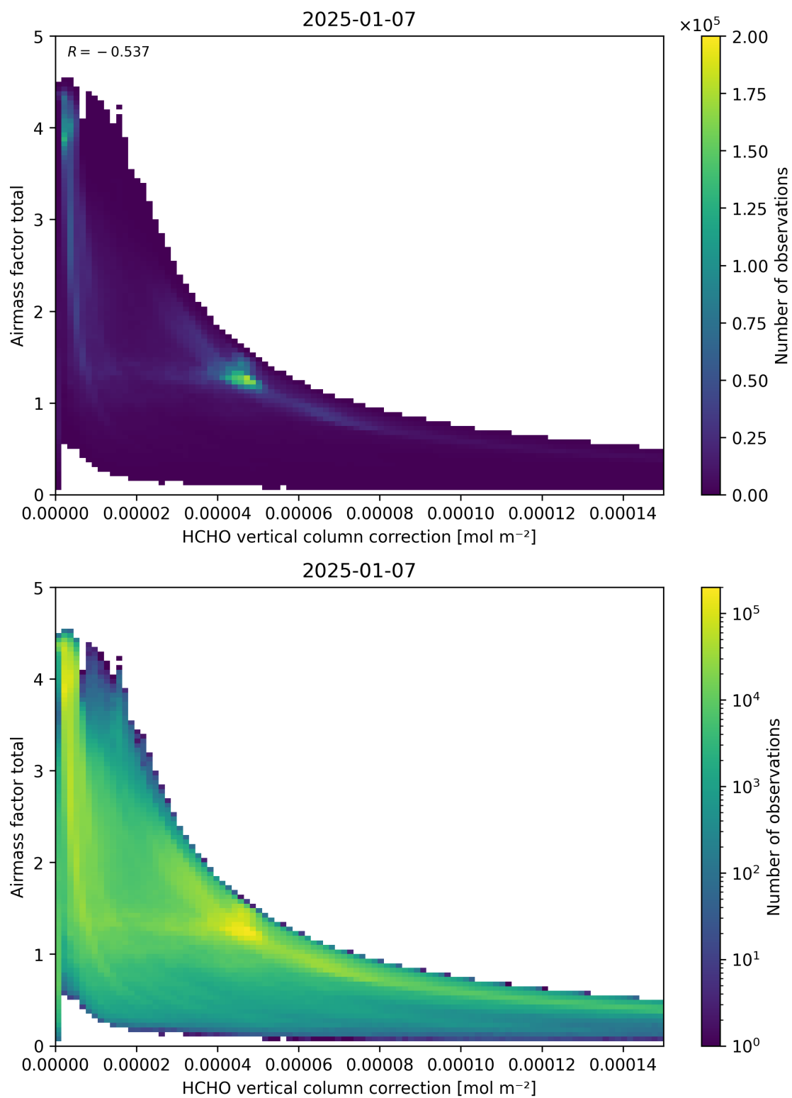
Figure 120: Scatter density plot of “HCHO vertical column correction” against “Airmass factor total” for 2025-01-07 to 2025-01-08.
