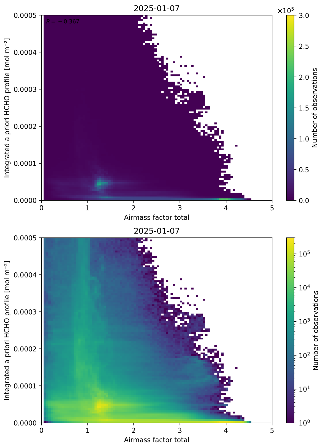
Figure 104: Scatter density plot of “Airmass factor total” against “Integrated a priori HCHO profile” for 2025-01-07 to 2025-01-08.
