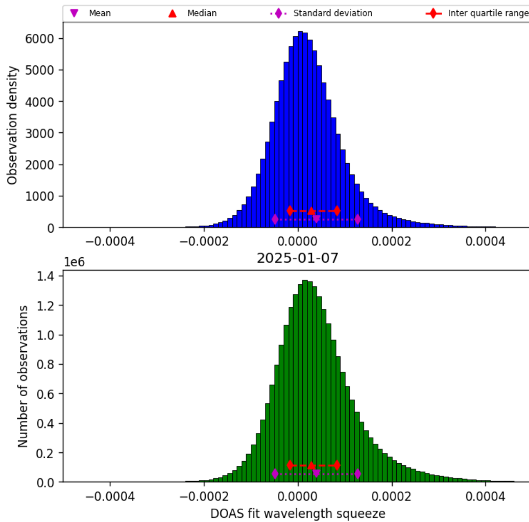
Figure 45: Histogram of “DOAS fit wavelength squeeze” for 2025-01-07 to 2025-01-08
