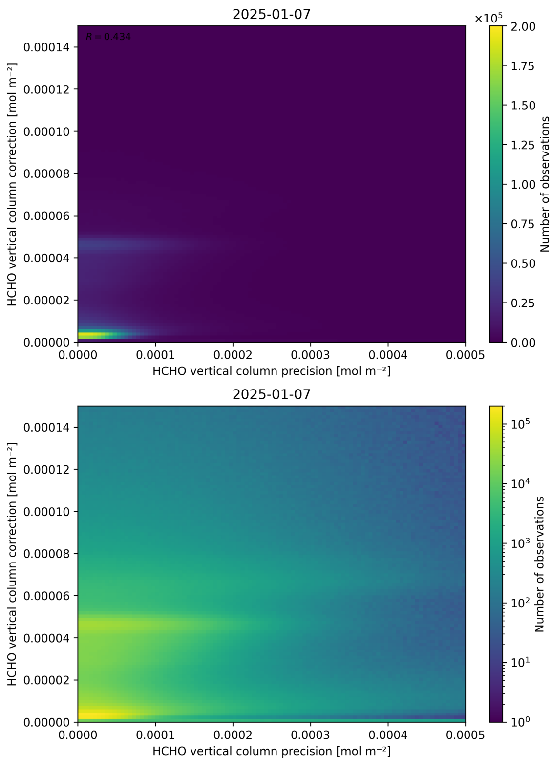
Figure 146: Scatter density plot of “HCHO vertical column precision” against “HCHO vertical column correction” for 2025-01-07 to 2025-01-08.
