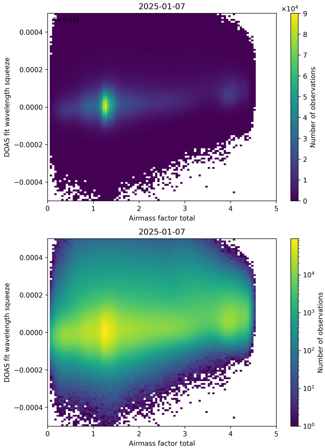
Figure 99: Scatter density plot of “Airmass factor total” against “DOAS fit wavelength squeeze” for 2025-01-07 to 2025-01-08.
