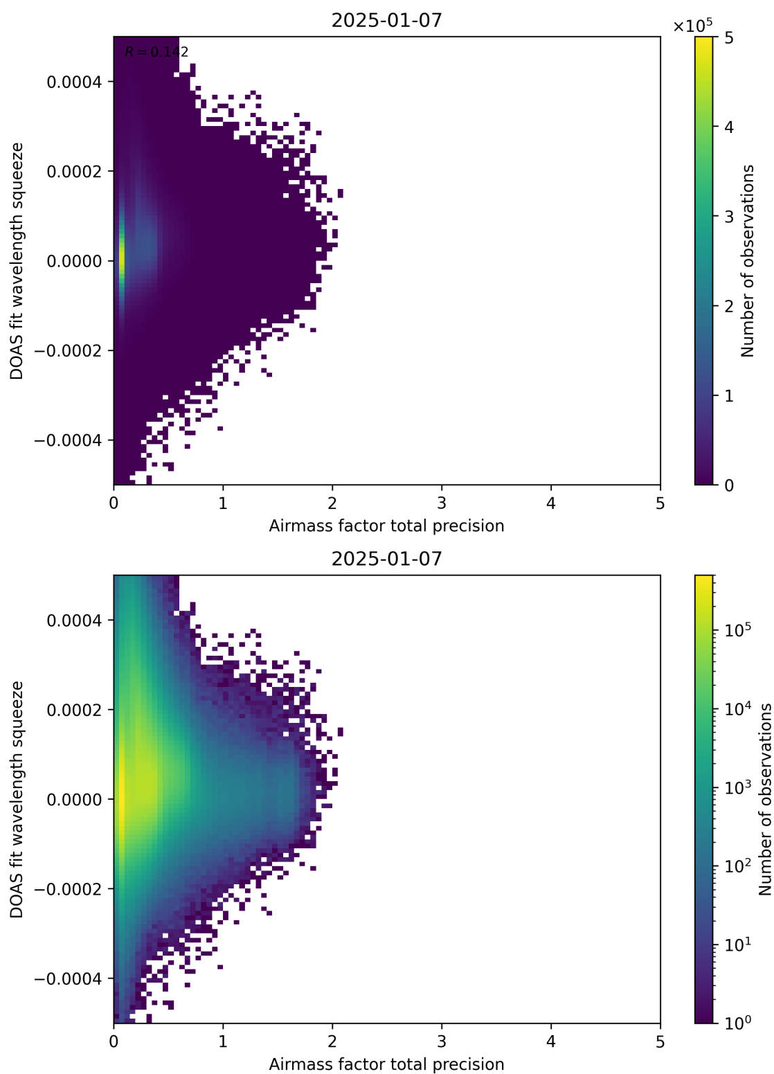
Figure 107: Scatter density plot of “Airmass factor total precision” against “DOAS fit wavelength squeeze” for 2025-01-07 to 2025-01-08.
