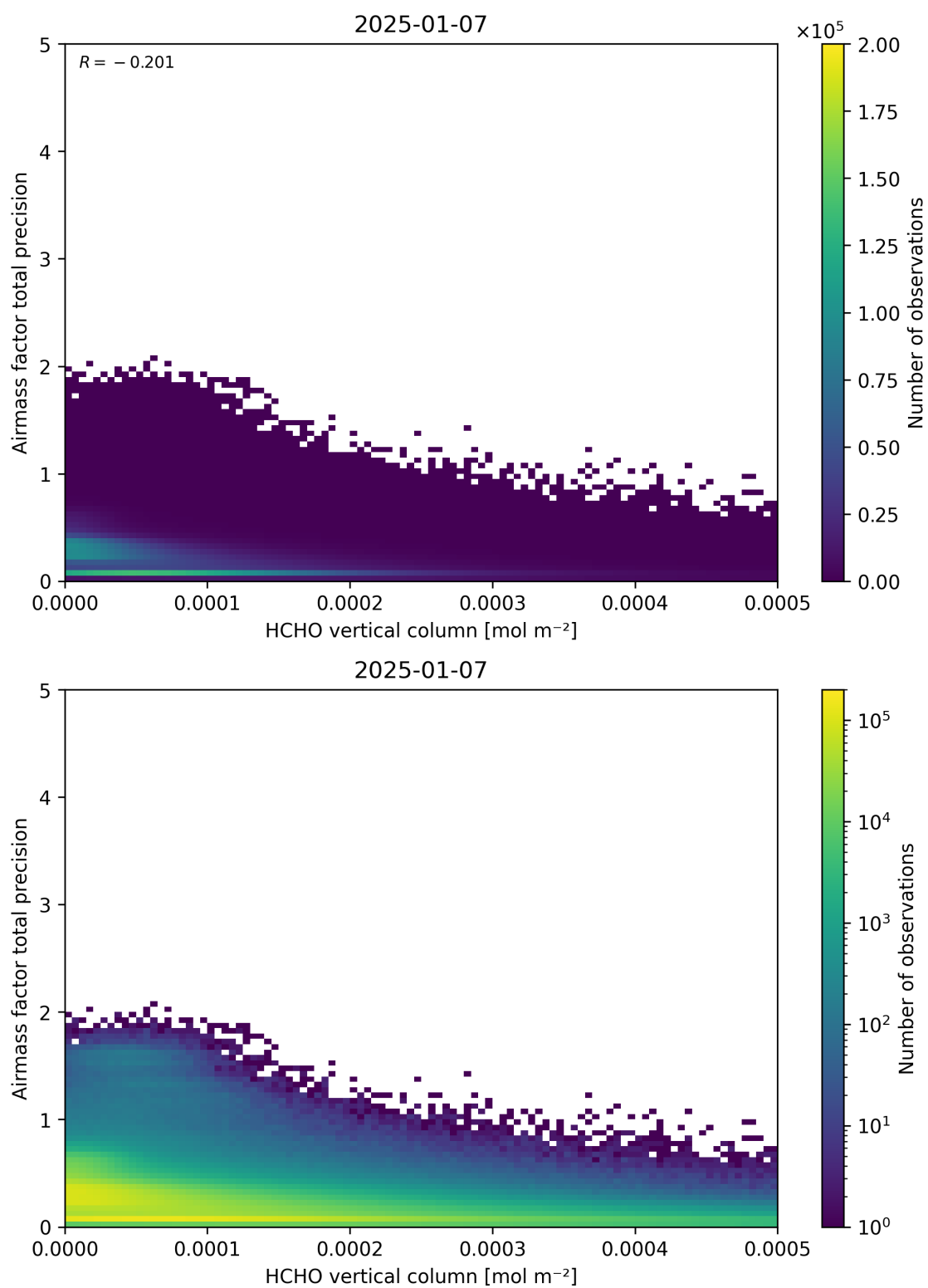
Figure 132: Scatter density plot of “HCHO vertical column” against “Airmass factor total precision” for 2025-01-07 to 2025-01-08.
