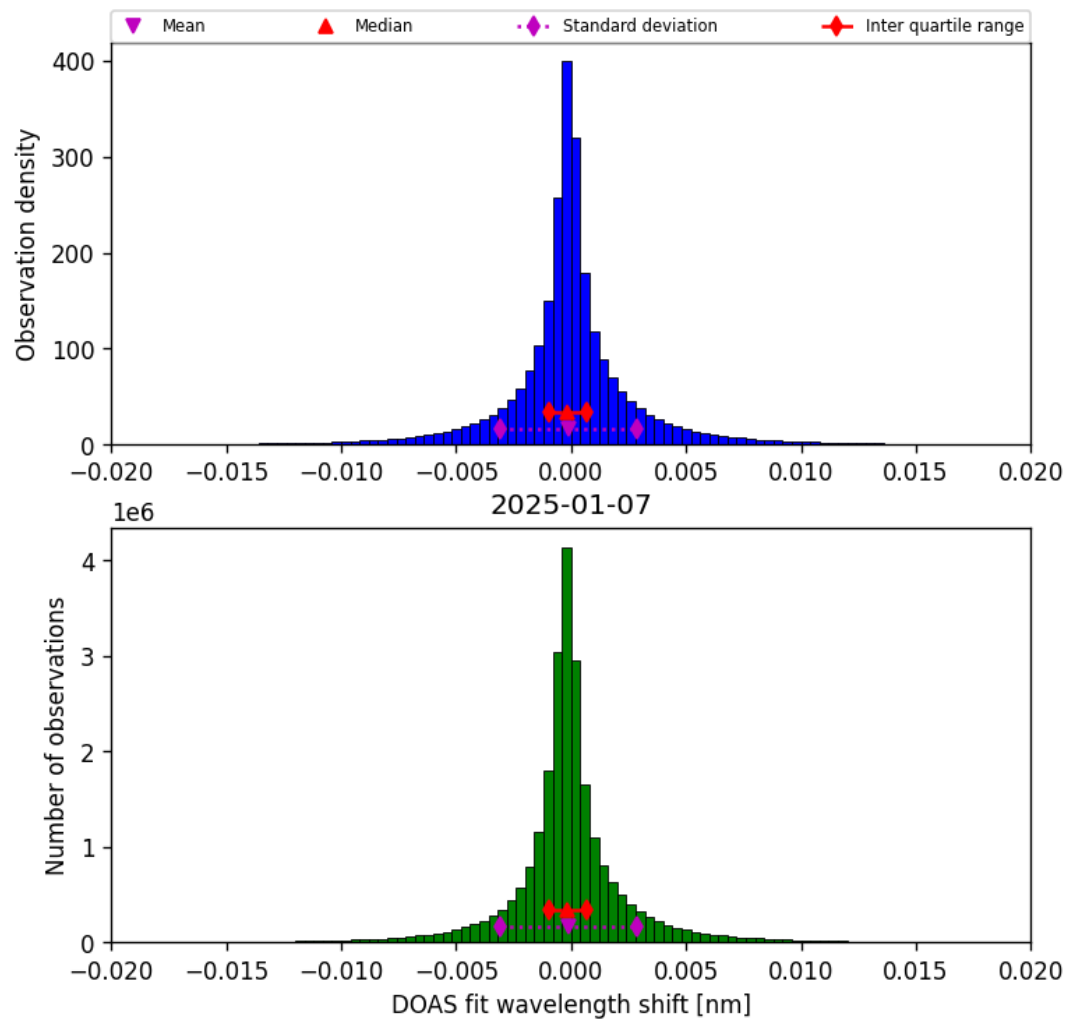
Figure 44: Histogram of “DOAS fit wavelength shift” for 2025-01-07 to 2025-01-08
