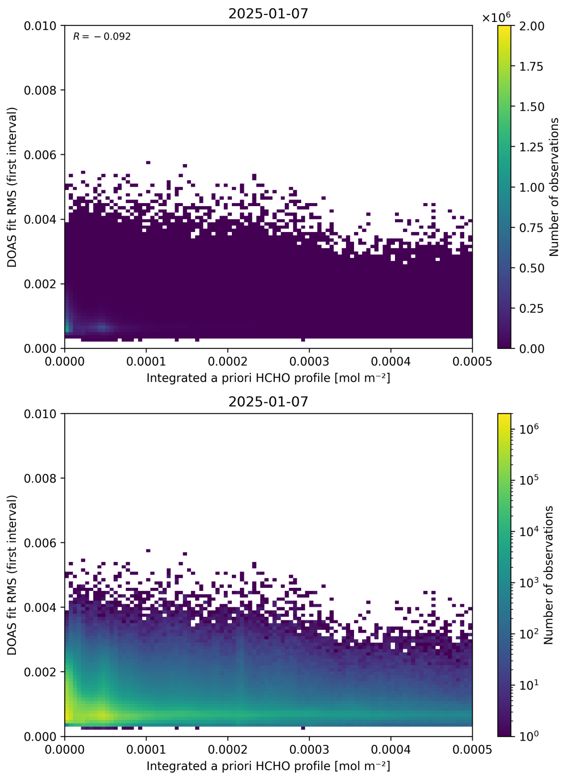
Figure 148: Scatter density plot of “Integrated a priori HCHO profile” against “DOAS fit RMS (first interval)” for 2025-01-07 to 2025-01-08.
