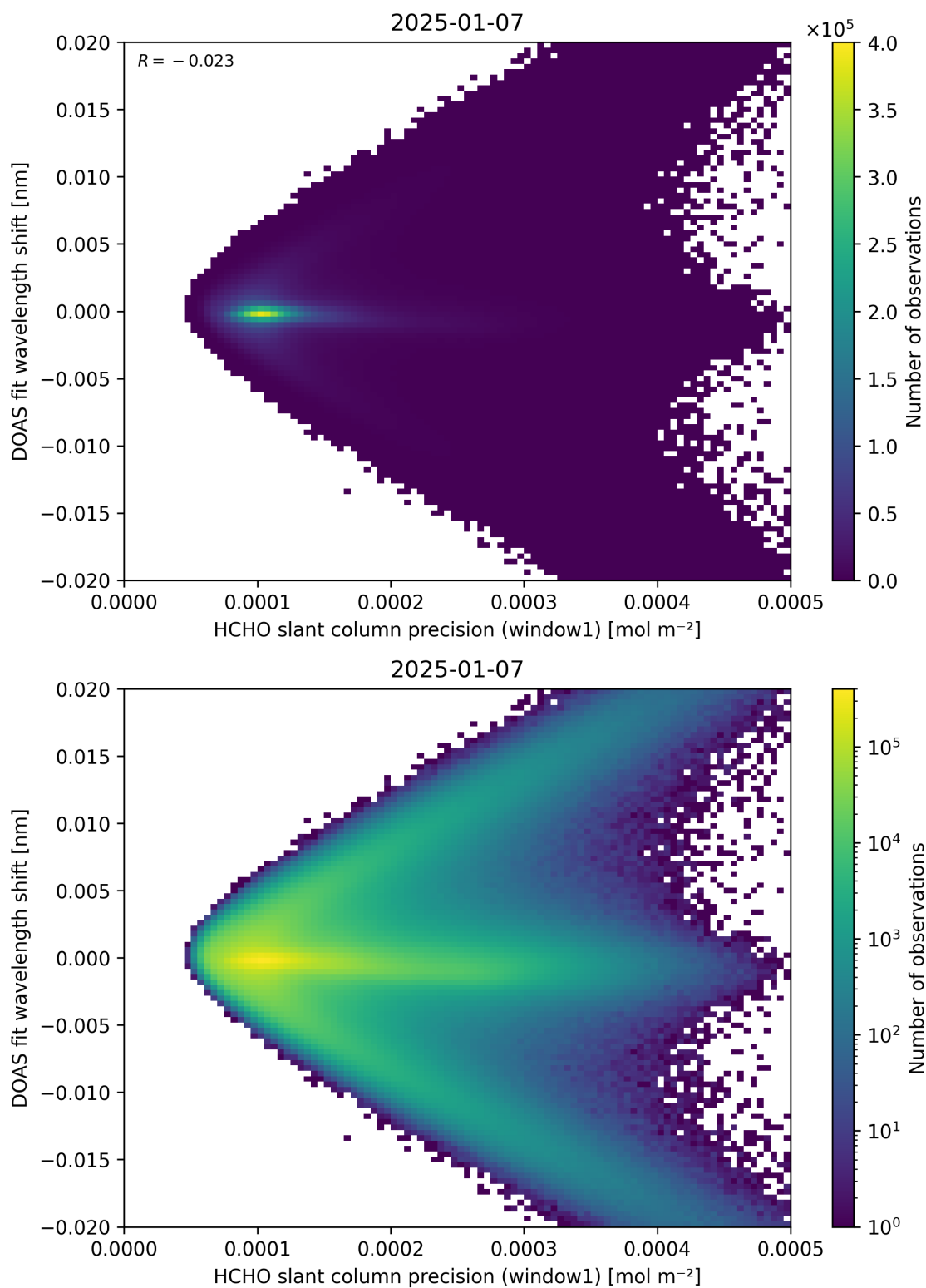
Figure 89: Scatter density plot of “HCHO slant column precision (window1)” against “DOAS fit wavelength shift” for 2025-01-07 to 2025-01-08.
