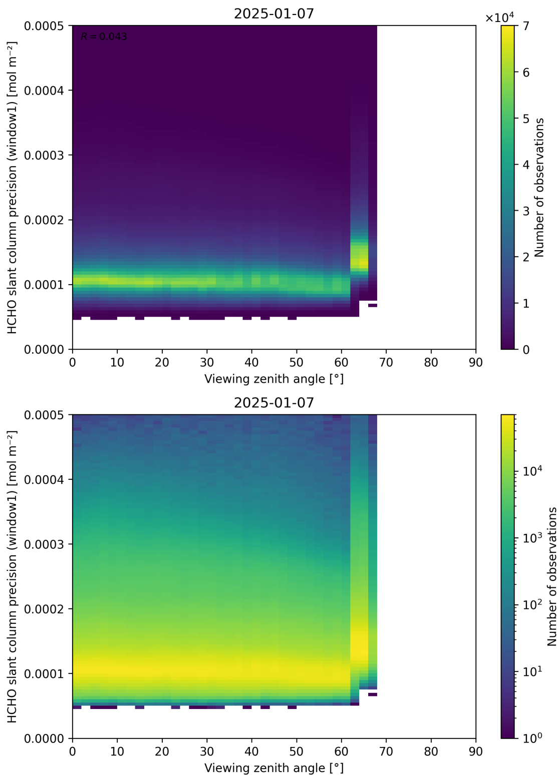
Figure 189: Scatter density plot of “Viewing zenith angle” against “HCHO slant column precision (window1)” for 2025-01-07 to 2025-01-08.
