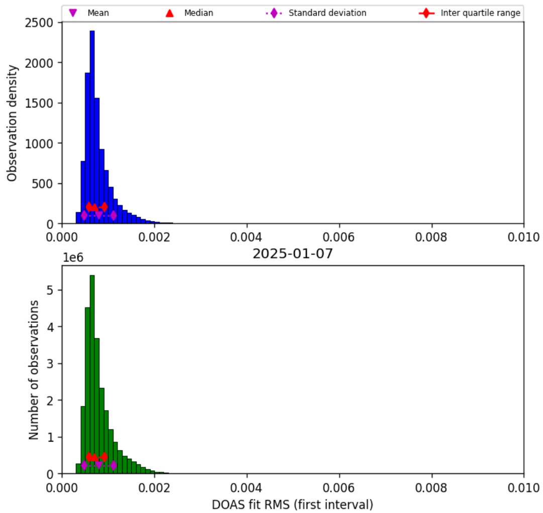
Figure 46: Histogram of “DOAS fit RMS (first interval)” for 2025-01-07 to 2025-01-08
