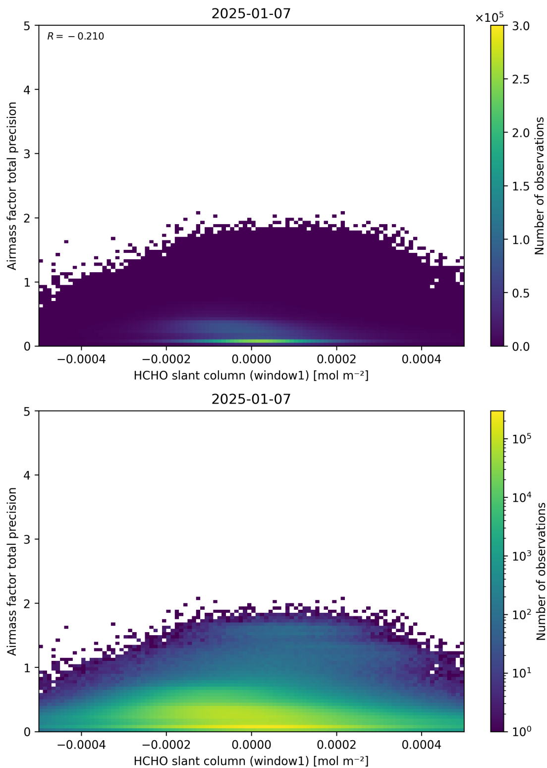
Figure 86: Scatter density plot of “HCHO slant column (window1)” against “Airmass factor total precision” for 2025-01-07 to 2025-01-08.
