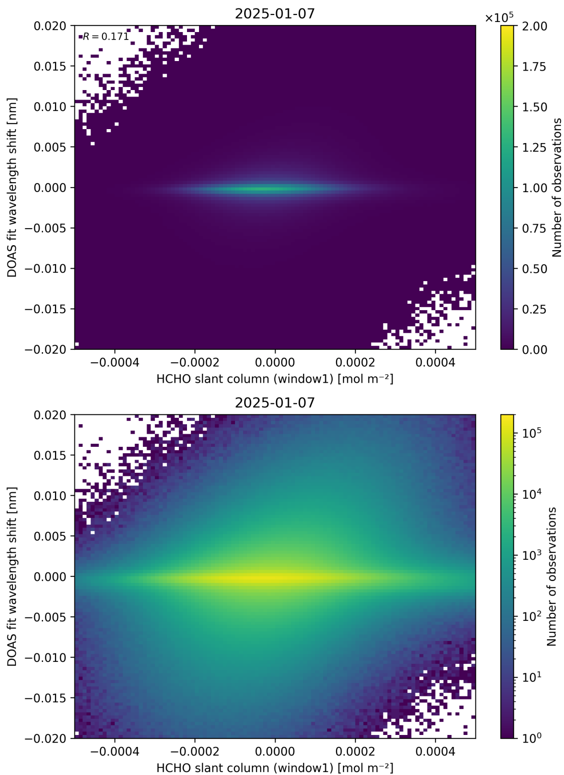
Figure 79: Scatter density plot of “HCHO slant column (window1)” against “DOAS fit wavelength shift” for 2025-01-07 to 2025-01-08.
