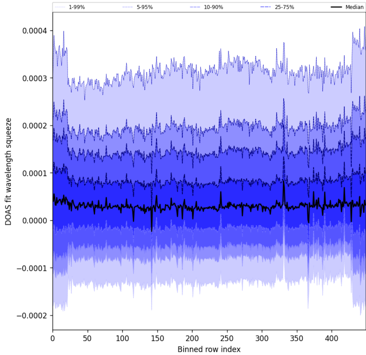
Figure 59: Along track statistics of “DOAS fit wavelength squeeze” for 2025-01-07 to 2025-01-08
