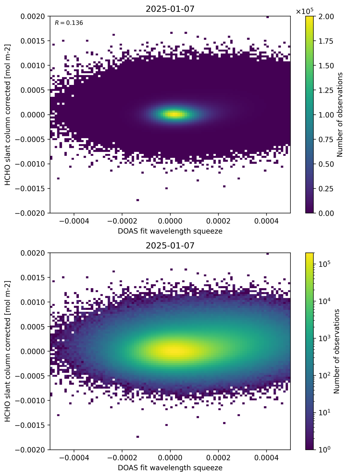
Figure 69: Scatter density plot of “DOAS fit wavelength squeeze” against “HCHO slant column corrected” for 2025-01-07 to 2025-01-08.
