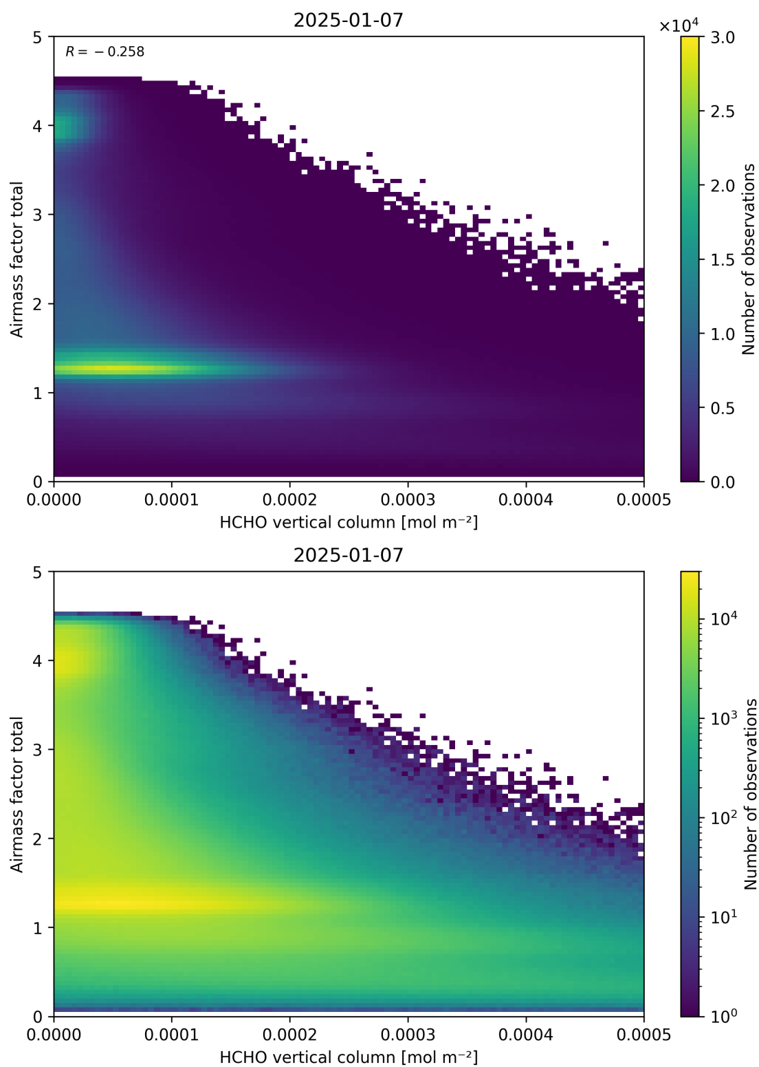
Figure 131: Scatter density plot of “HCHO vertical column” against “Airmass factor total” for 2025-01-07 to 2025-01-08.
