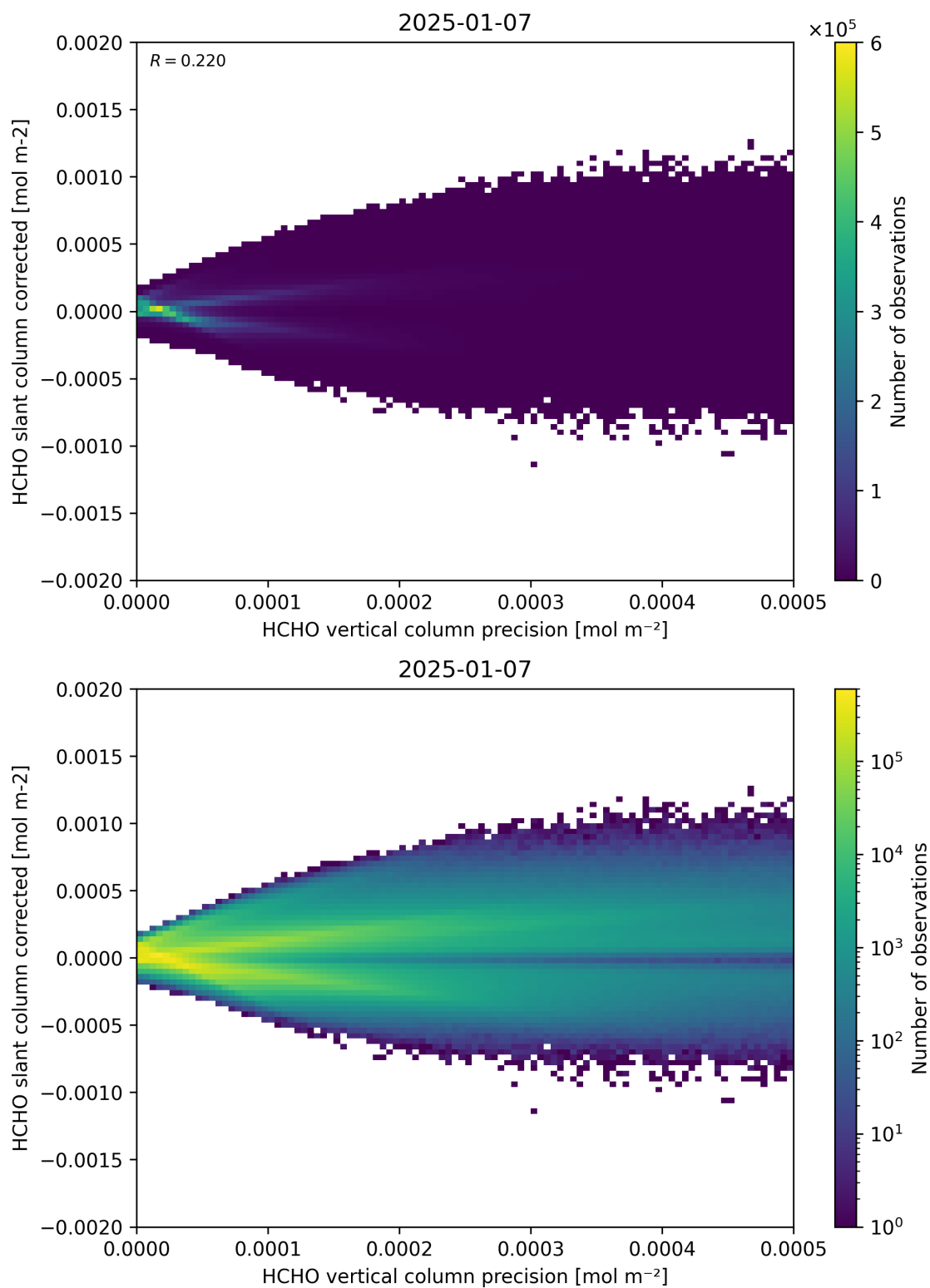
Figure 140: Scatter density plot of “HCHO vertical column precision” against “HCHO slant column corrected” for 2025-01-07 to 2025-01-08.
