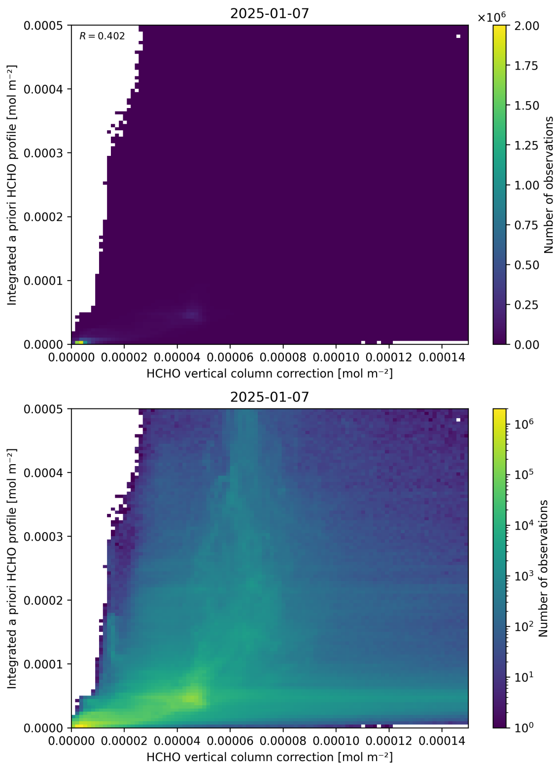
Figure 122: Scatter density plot of “HCHO vertical column correction” against “Integrated a priori HCHO profile” for 2025-01-07 to 2025-01-08.
