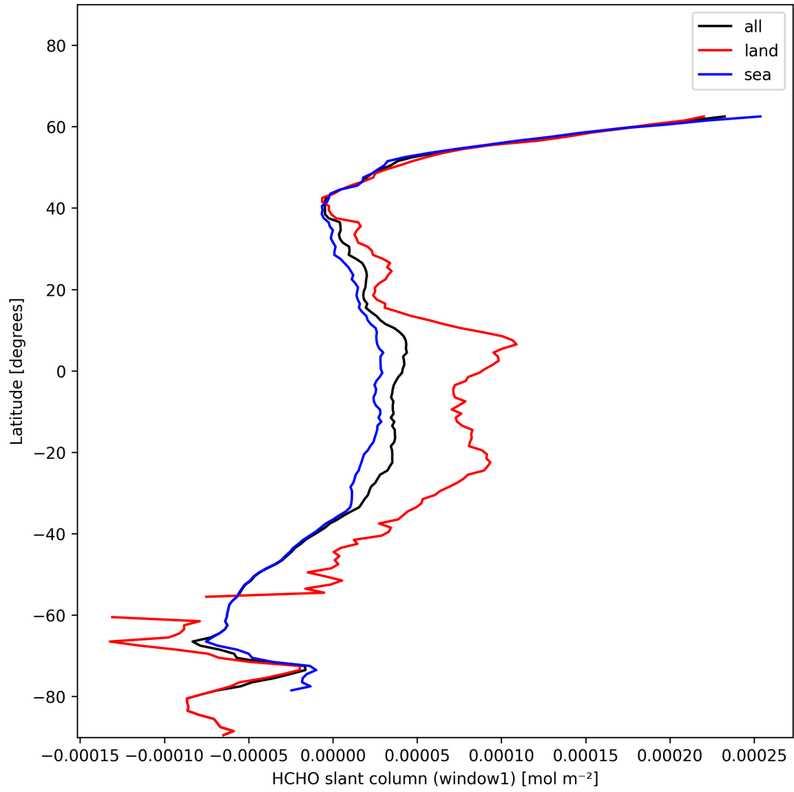
Figure 24: Zonal average of “HCHO slant column (window1)” for 2025-01-07 to 2025-01-08.
