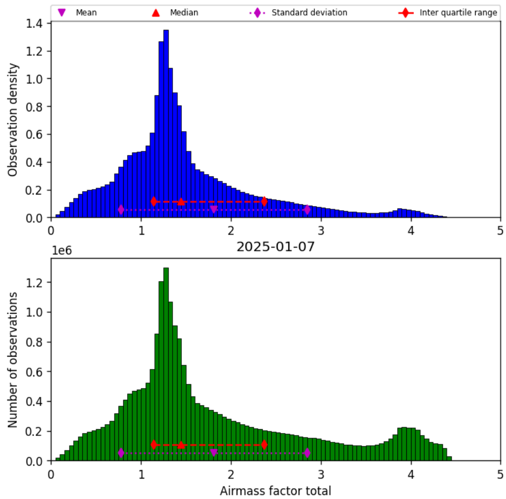
Figure 40: Histogram of “Airmass factor total” for 2025-01-07 to 2025-01-08
