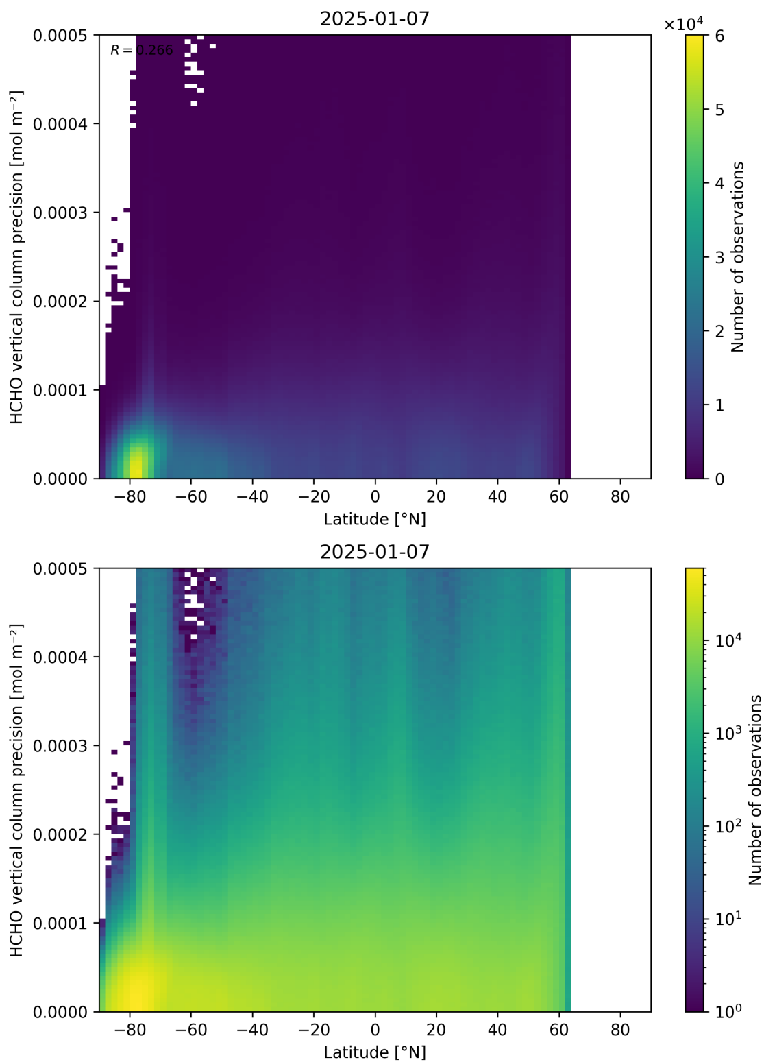
Figure 165: Scatter density plot of “Latitude” against “HCHO vertical column precision” for 2025-01-07 to 2025-01-08.
