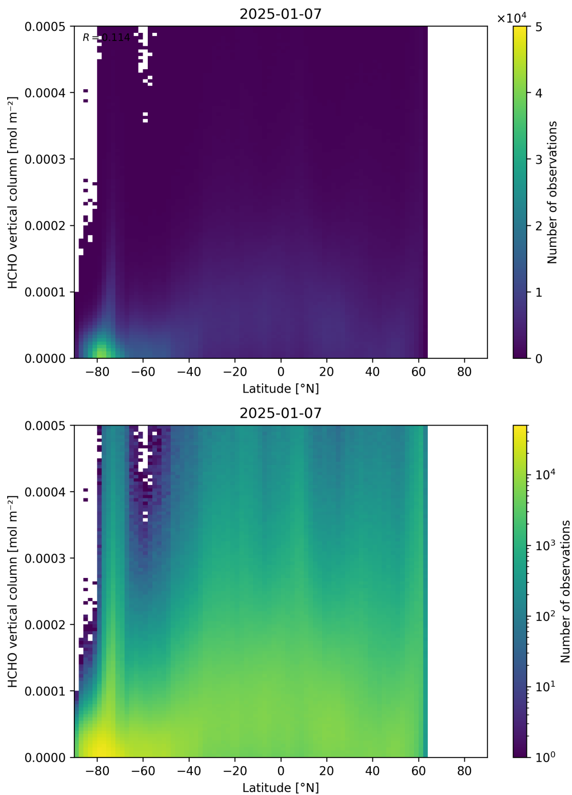
Figure 163: Scatter density plot of “Latitude” against “HCHO vertical column” for 2025-01-07 to 2025-01-08.
