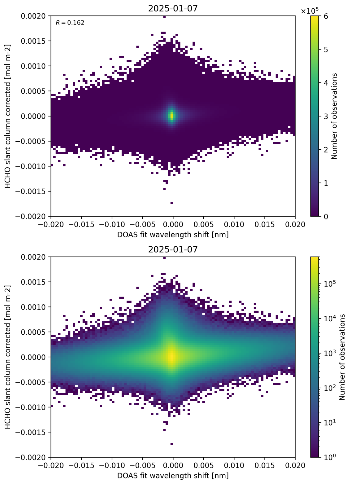
Figure 66: Scatter density plot of “DOAS fit wavelength shift” against “HCHO slant column corrected” for 2025-01-07 to 2025-01-08.
