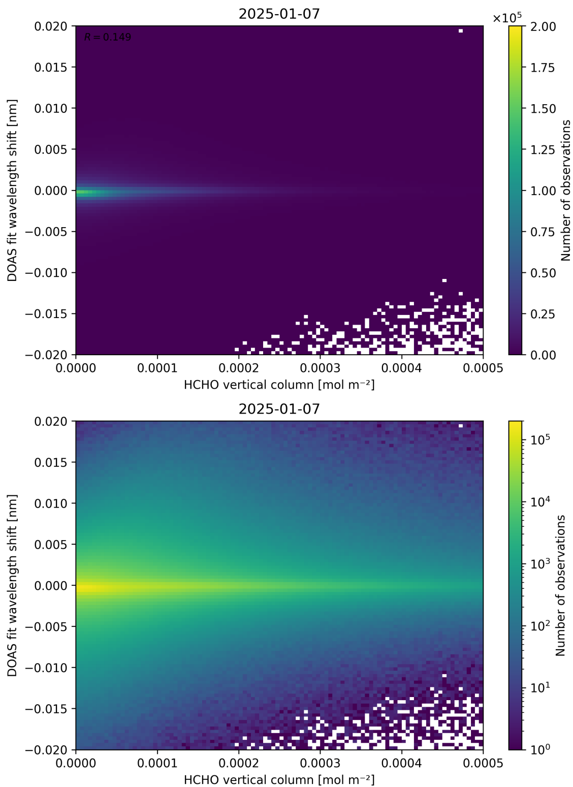
Figure 124: Scatter density plot of “HCHO vertical column” against “DOAS fit wavelength shift” for 2025-01-07 to 2025-01-08.
