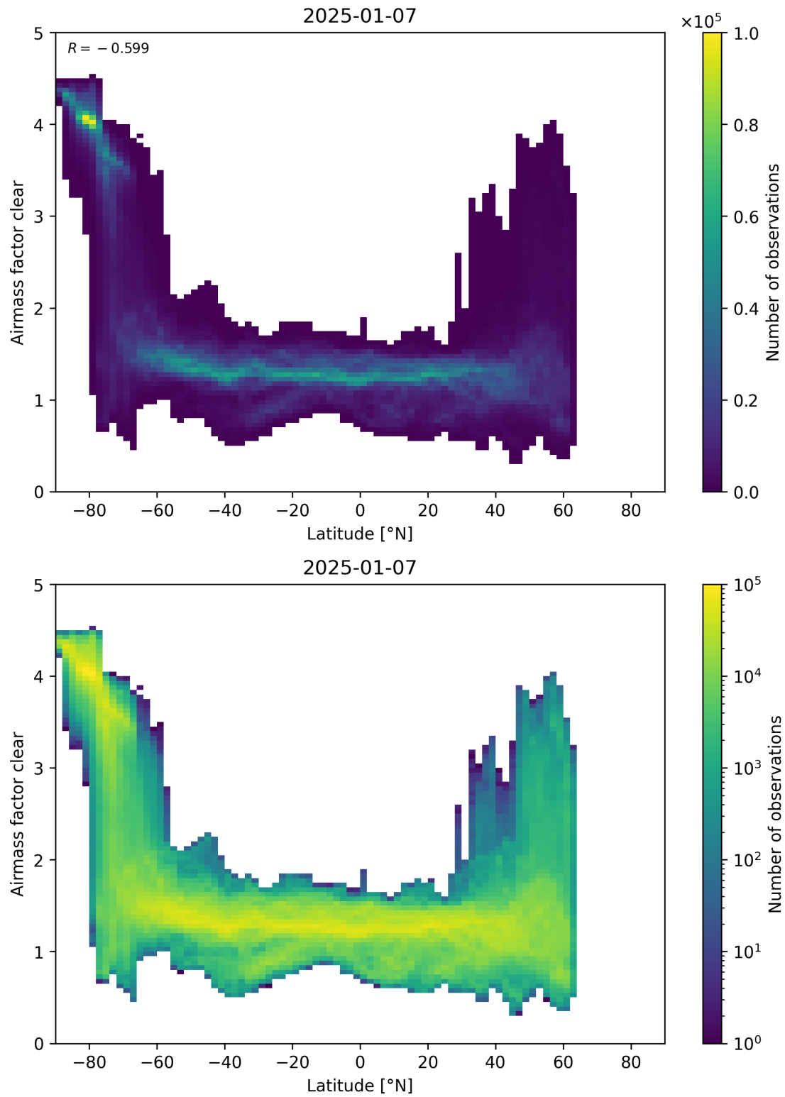
Figure 156: Scatter density plot of “Latitude” against “Airmass factor clear” for 2025-01-07 to 2025-01-08.
