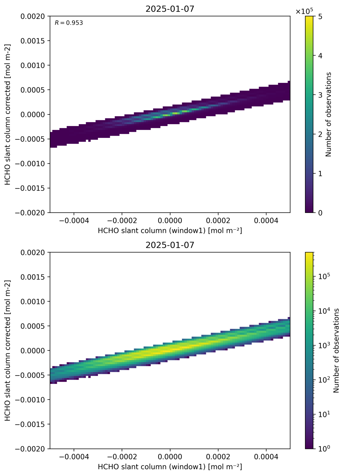
Figure 82: Scatter density plot of “HCHO slant column (window1)” against “HCHO slant column corrected” for 2025-01-07 to 2025-01-08.
