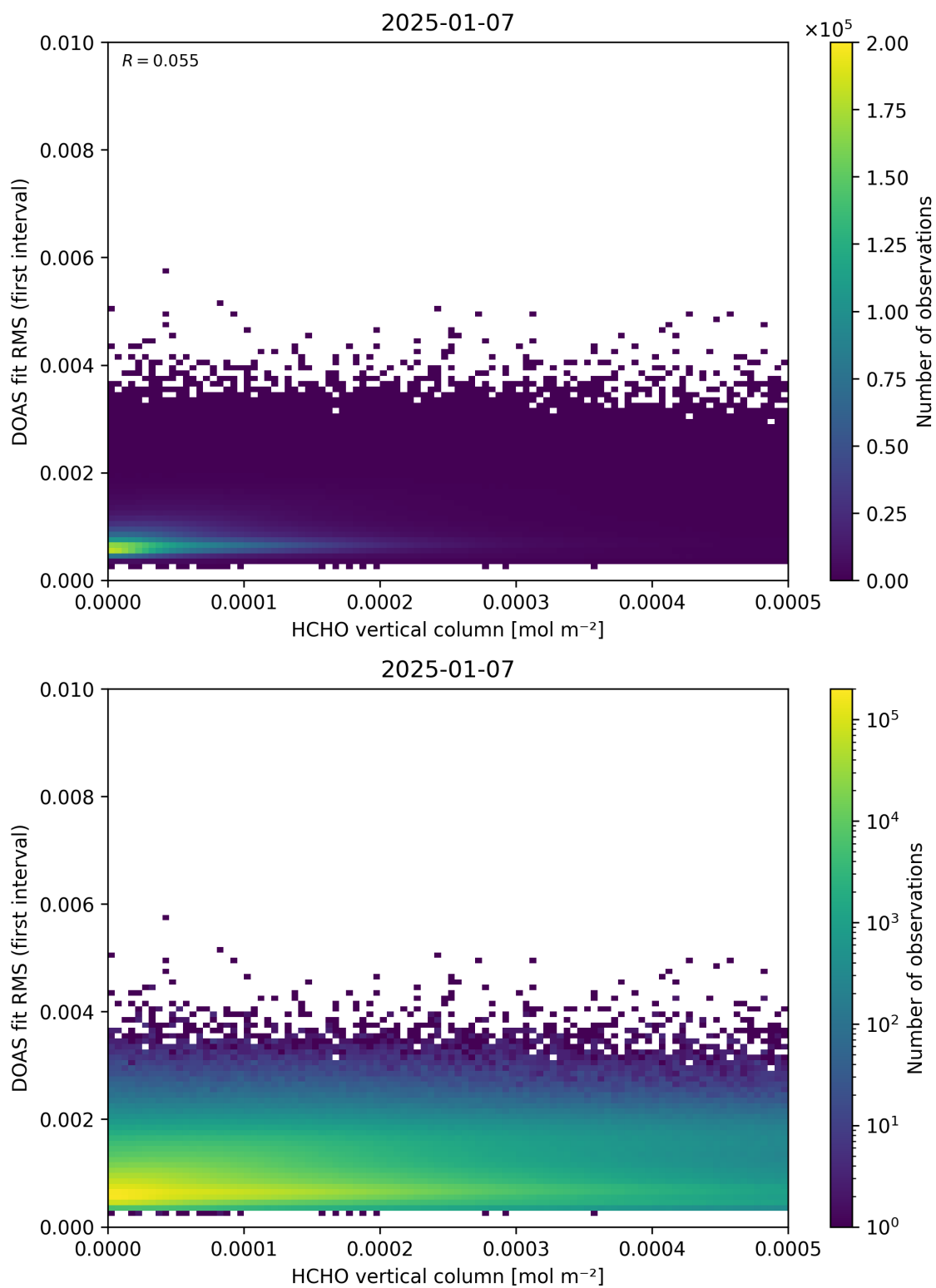
Figure 123: Scatter density plot of “HCHO vertical column” against “DOAS fit RMS (first interval)” for 2025-01-07 to 2025-01-08.
