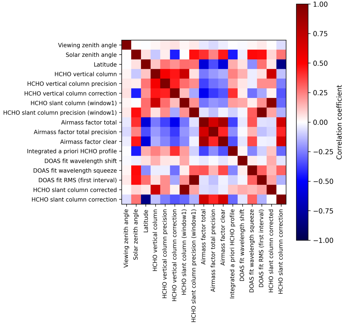
Figure 2: Map of correlation matrix for 2025-01-07 to 2025-01-08.
