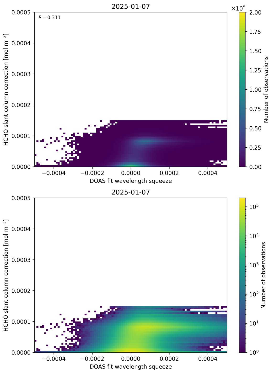
Figure 70: Scatter density plot of “DOAS fit wavelength squeeze” against “HCHO slant column correction” for 2025-01-07 to 2025-01-08.
