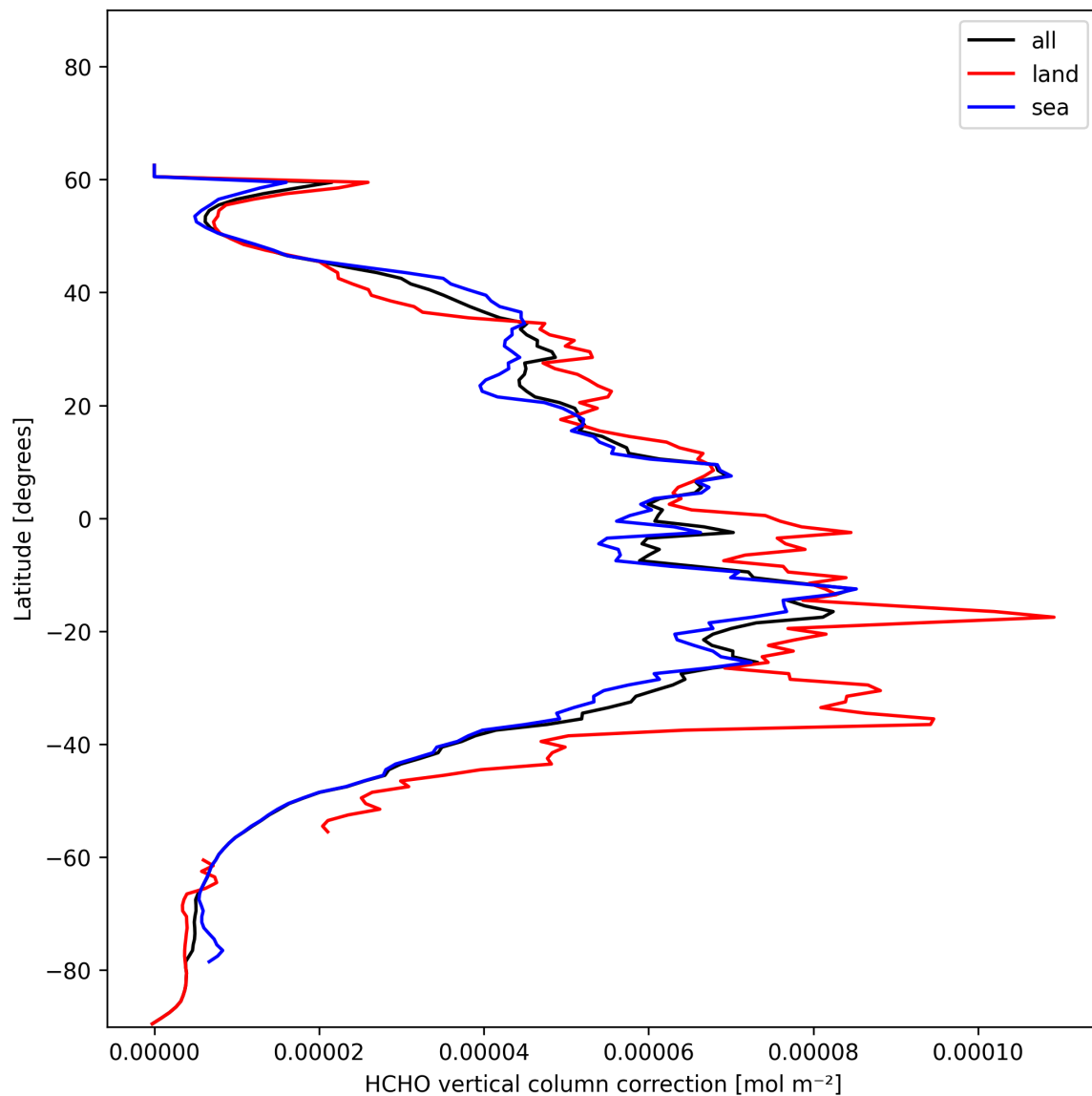
Figure 23: Zonal average of “HCHO vertical column correction” for 2025-01-07 to 2025-01-08.
