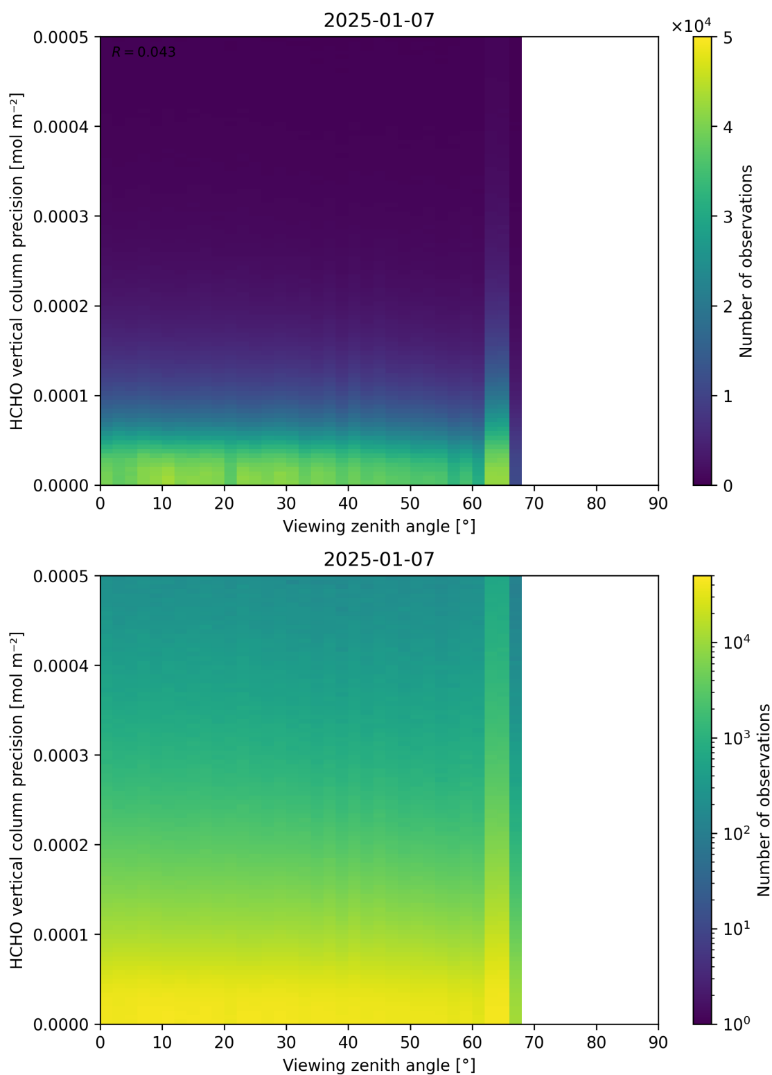
Figure 194: Scatter density plot of “Viewing zenith angle” against “HCHO vertical column precision” for 2025-01-07 to 2025-01-08.
