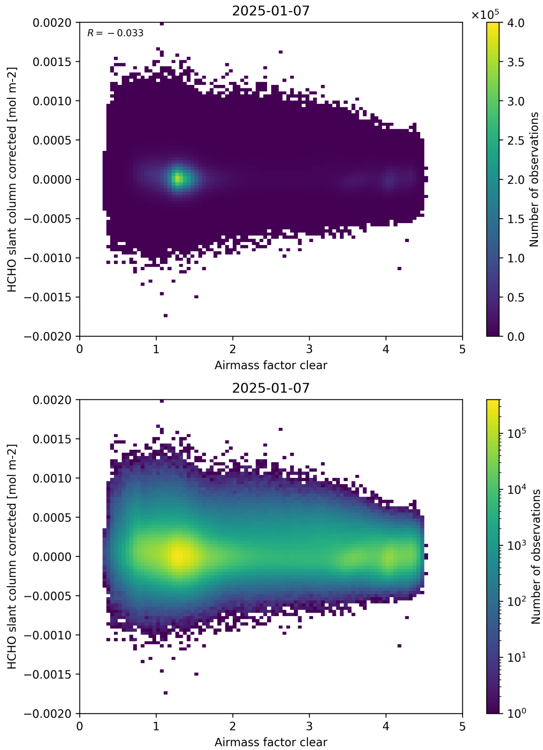
Figure 74: Scatter density plot of “Airmass factor clear” against “HCHO slant column corrected” for 2025-01-07 to 2025-01-08.
