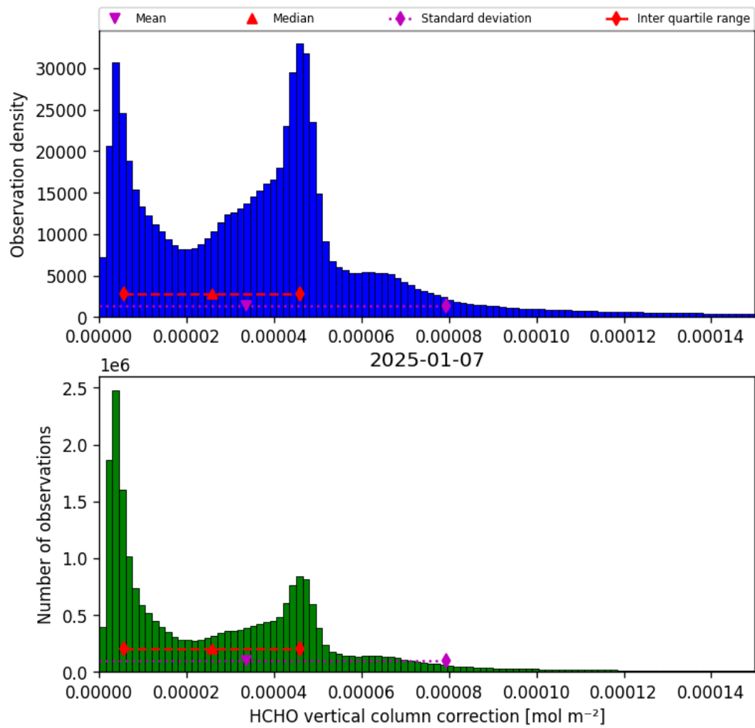
Figure 37: Histogram of “HCHO vertical column correction” for 2025-01-07 to 2025-01-08
