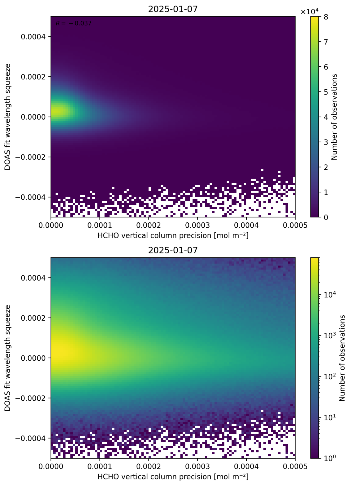
Figure 138: Scatter density plot of “HCHO vertical column precision” against “DOAS fit wavelength squeeze” for 2025-01-07 to 2025-01-08.
