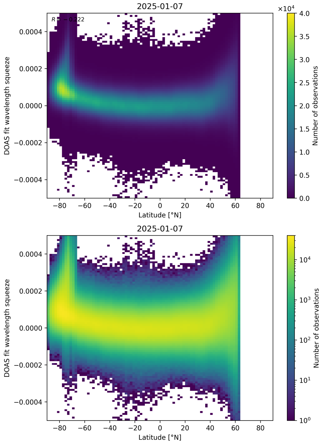
Figure 155: Scatter density plot of “Latitude” against “DOAS fit wavelength squeeze” for 2025-01-07 to 2025-01-08.
