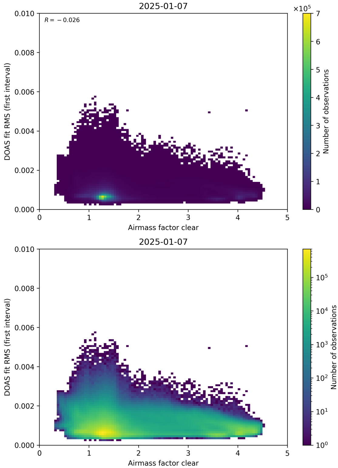
Figure 71: Scatter density plot of “Airmass factor clear” against “DOAS fit RMS (first interval)” for 2025-01-07 to 2025-01-08.
