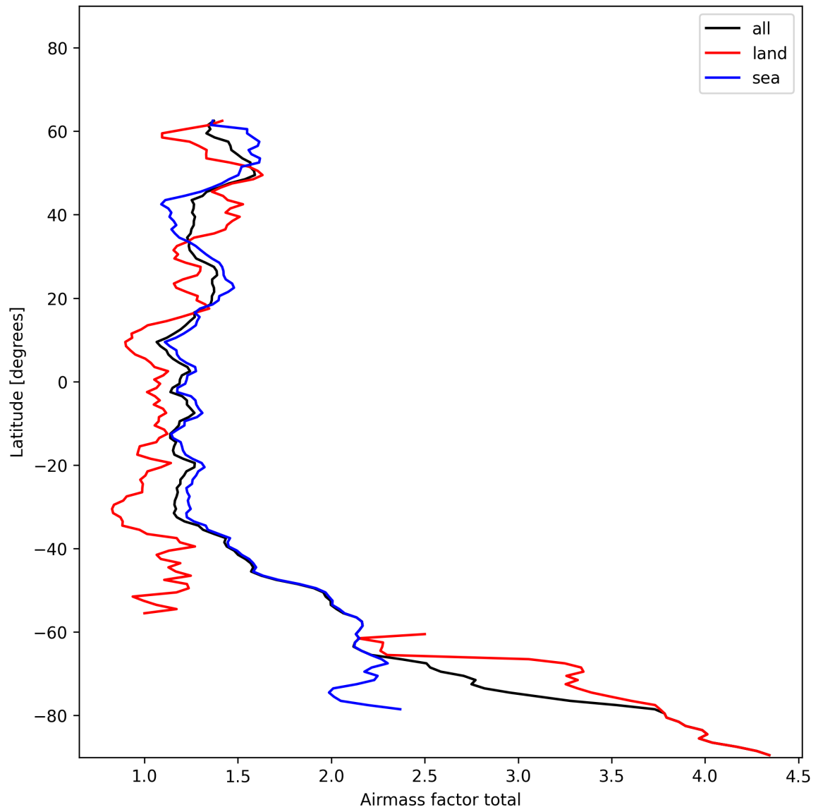
Figure 26: Zonal average of “Airmass factor total” for 2025-01-07 to 2025-01-08.
