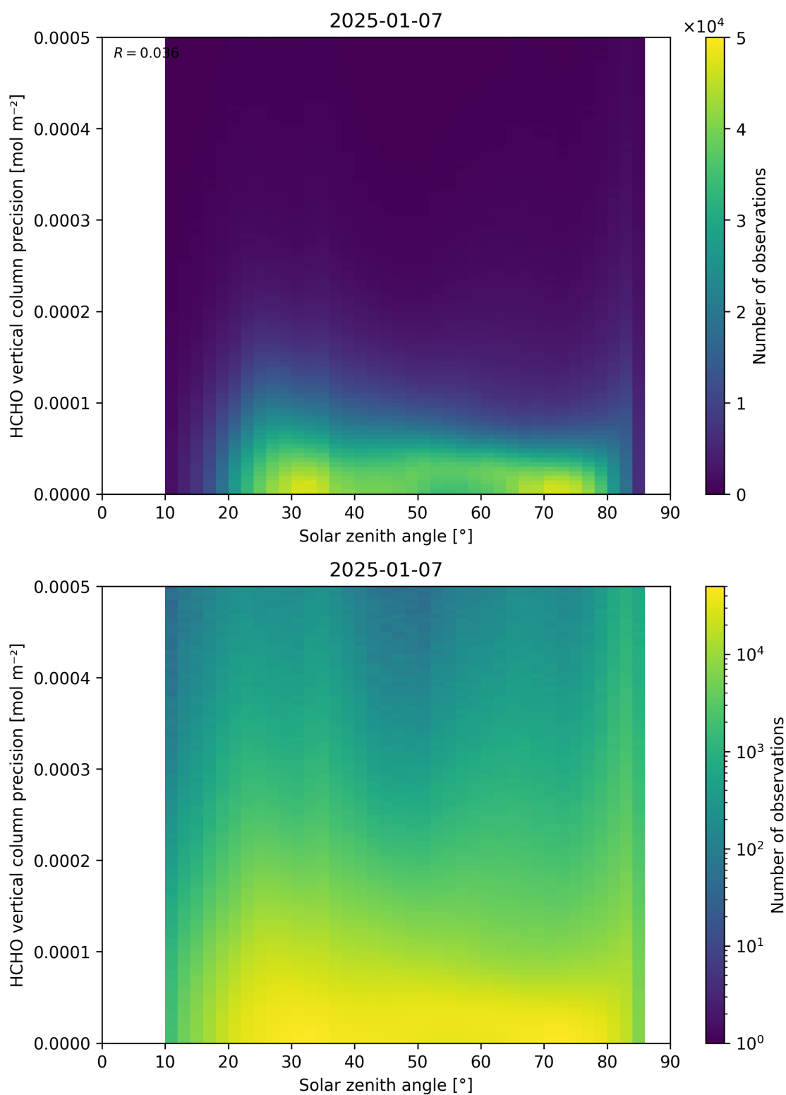
Figure 179: Scatter density plot of “Solar zenith angle” against “HCHO vertical column precision” for 2025-01-07 to 2025-01-08.
