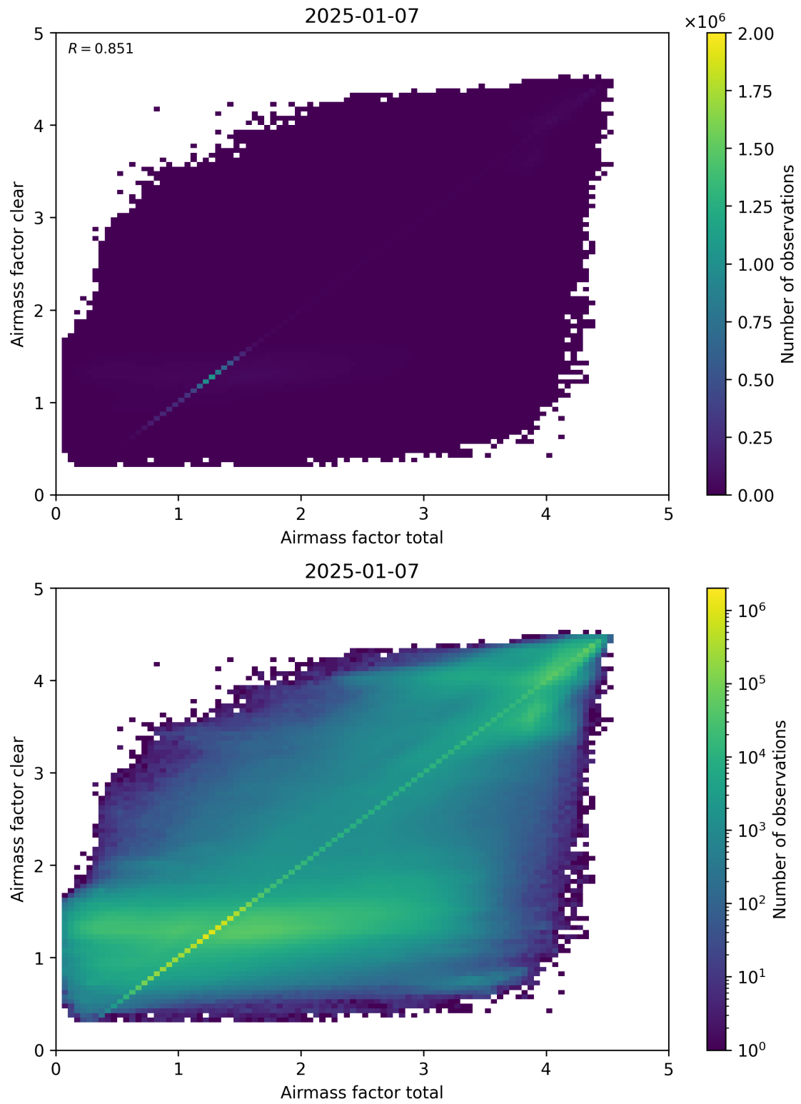
Figure 100: Scatter density plot of “Airmass factor total” against “Airmass factor clear” for 2025-01-07 to 2025-01-08.
