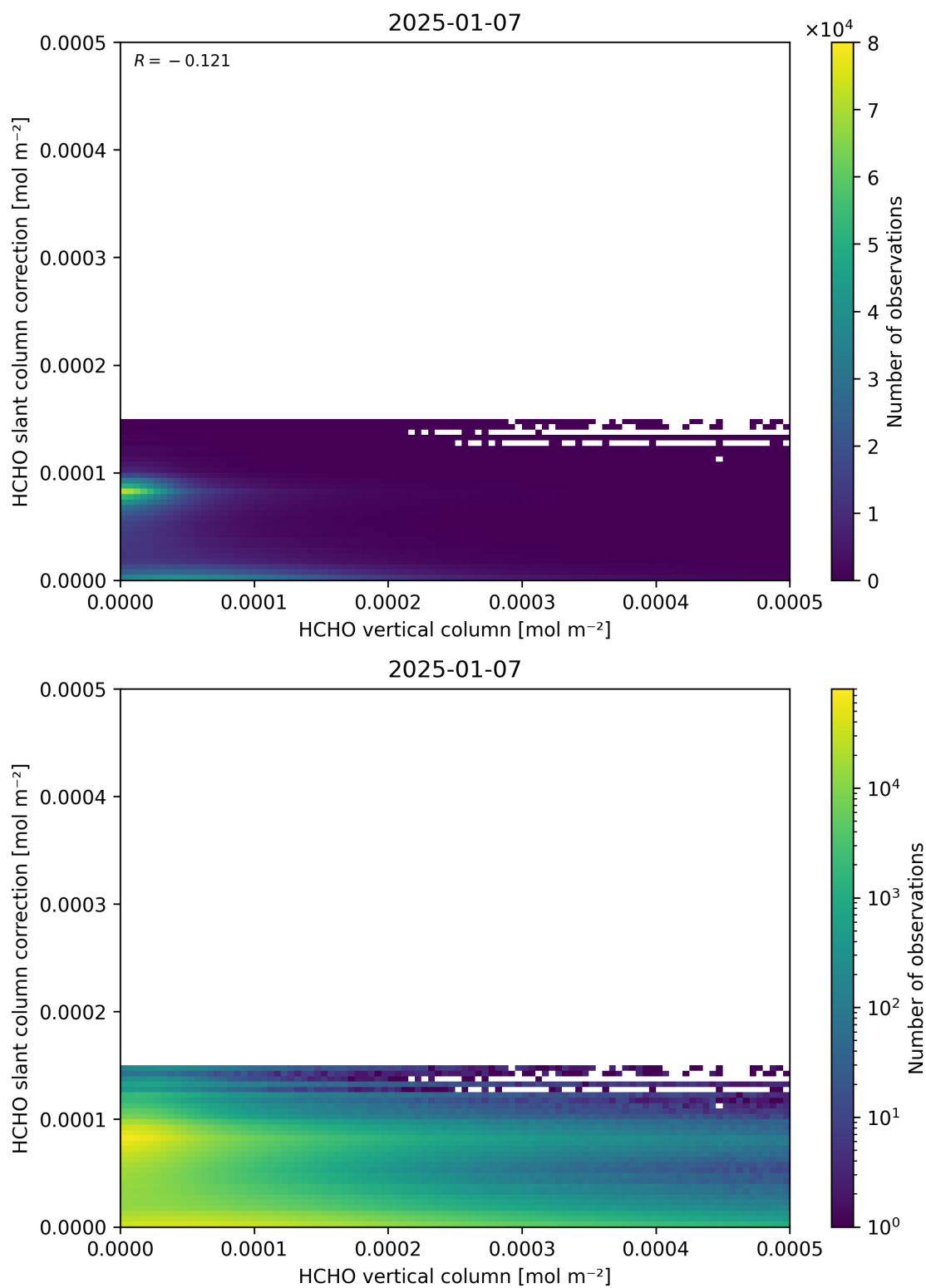
Figure 128: Scatter density plot of “HCHO vertical column” against “HCHO slant column correction” for 2025-01-07 to 2025-01-08.
