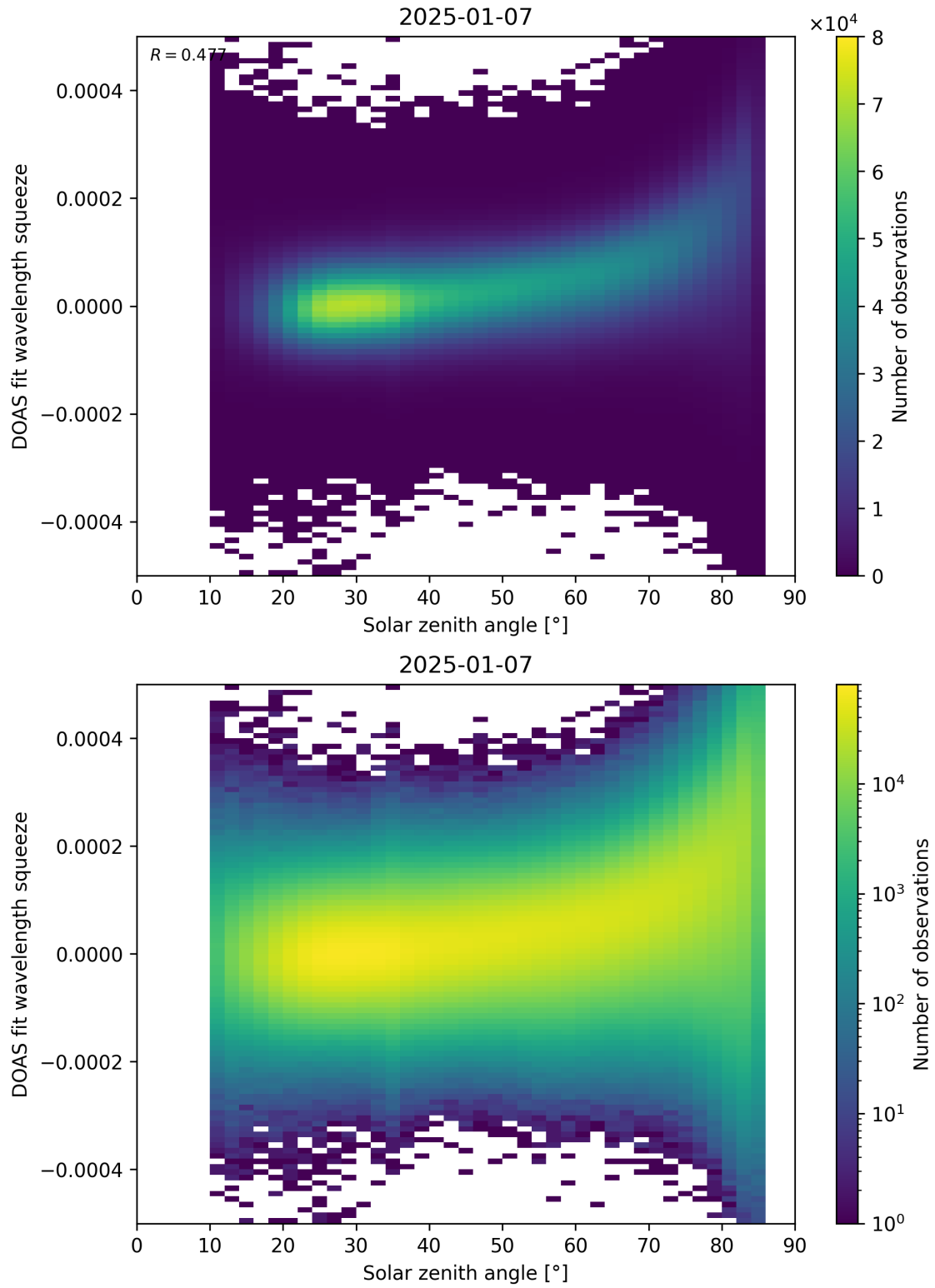
Figure 169: Scatter density plot of “Solar zenith angle” against “DOAS fit wavelength squeeze” for 2025-01-07 to 2025-01-08.
