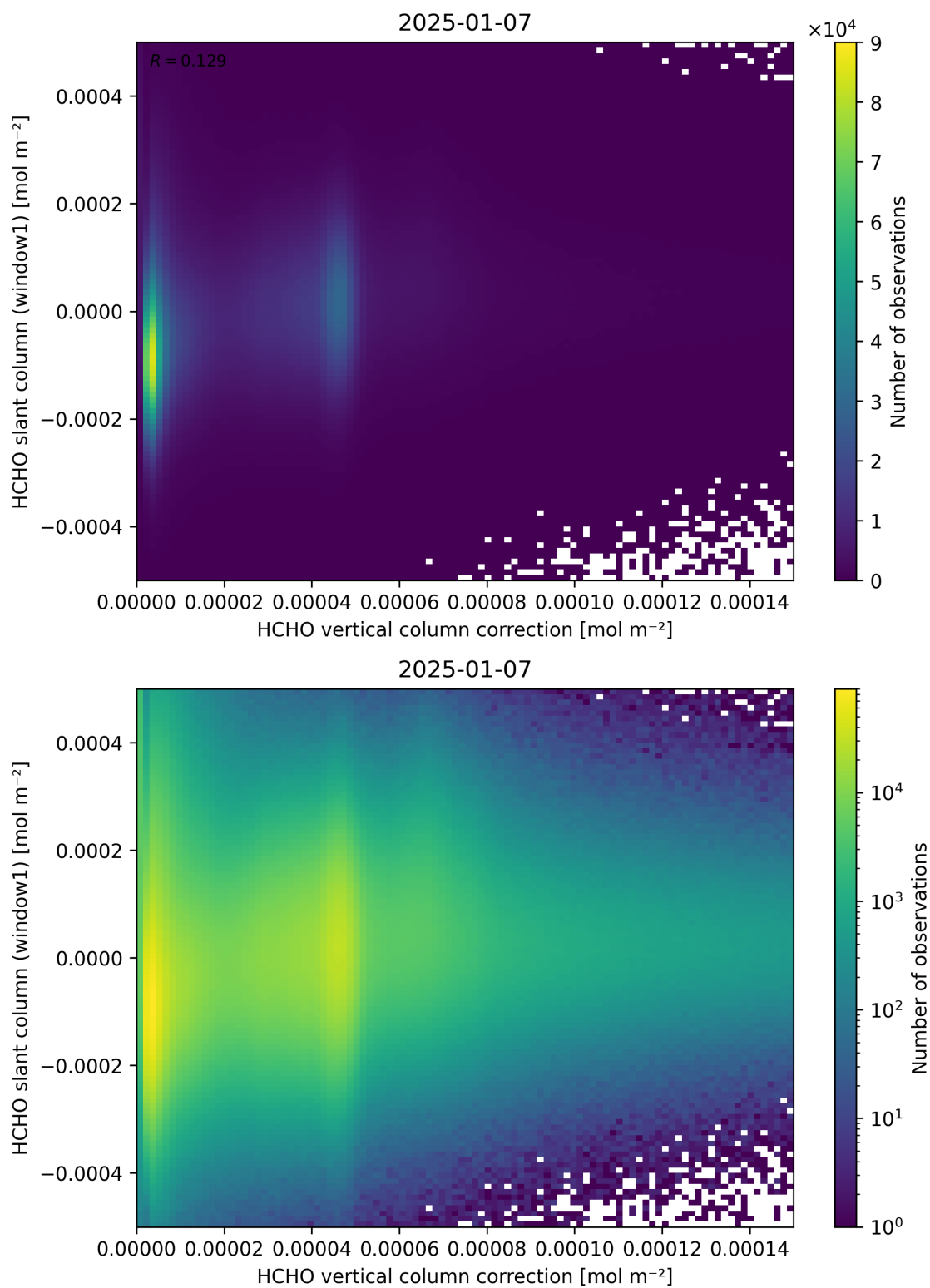
Figure 118: Scatter density plot of “HCHO vertical column correction” against “HCHO slant column (window1)” for 2025-01-07 to 2025-01-08.
