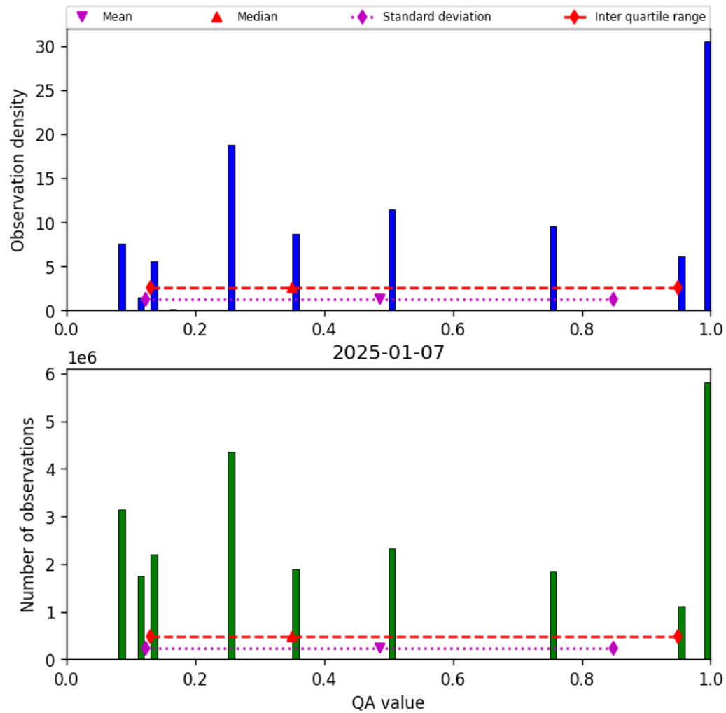
Figure 34: Histogram of “QA value” for 2025-01-07 to 2025-01-08
