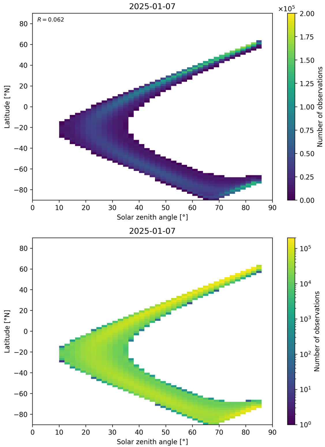
Figure 181: Scatter density plot of “Solar zenith angle” against “Latitude” for 2025-01-07 to 2025-01-08.
