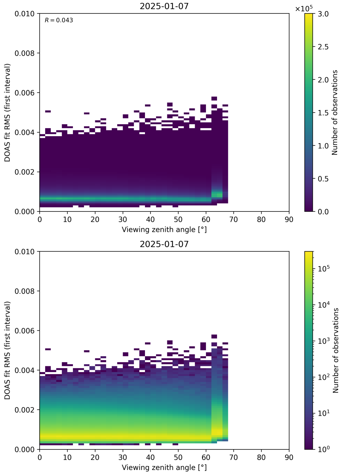
Figure 182: Scatter density plot of “Viewing zenith angle” against “DOAS fit RMS (first interval)” for 2025-01-07 to 2025-01-08.
