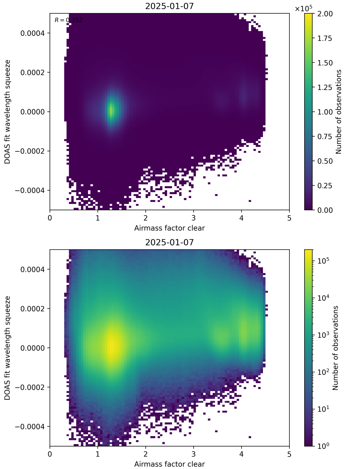
Figure 73: Scatter density plot of “Airmass factor clear” against “DOAS fit wavelength squeeze” for 2025-01-07 to 2025-01-08.
