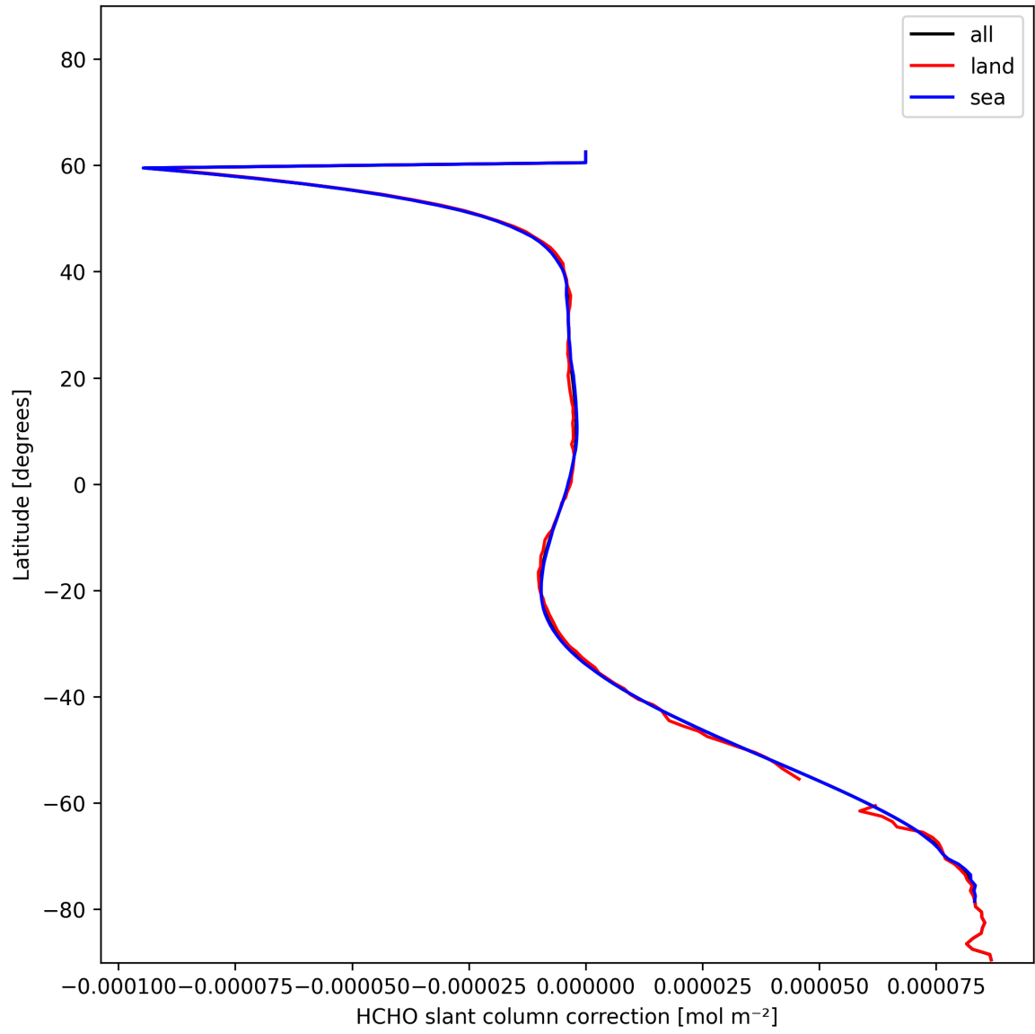
Figure 33: Zonal average of “HCHO slant column correction” for 2025-01-07 to 2025-01-08.
