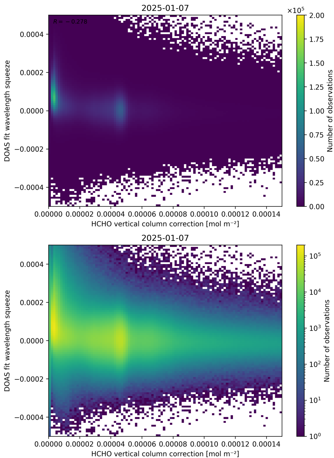
Figure 114: Scatter density plot of “HCHO vertical column correction” against “DOAS fit wavelength squeeze” for 2025-01-07 to 2025-01-08.
