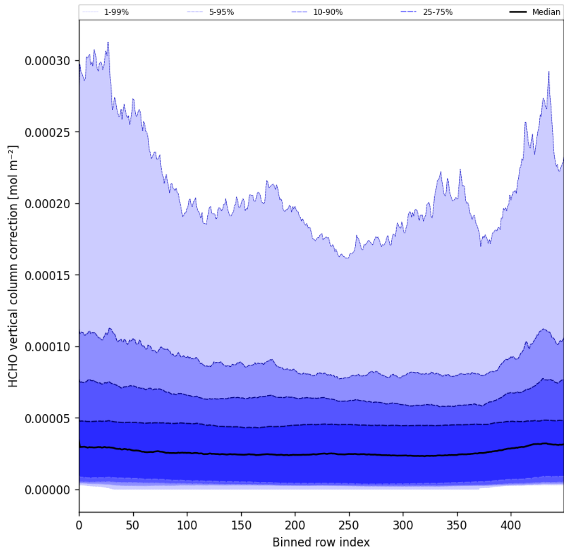
Figure 51: Along track statistics of “HCHO vertical column correction” for 2025-01-07 to 2025-01-08
