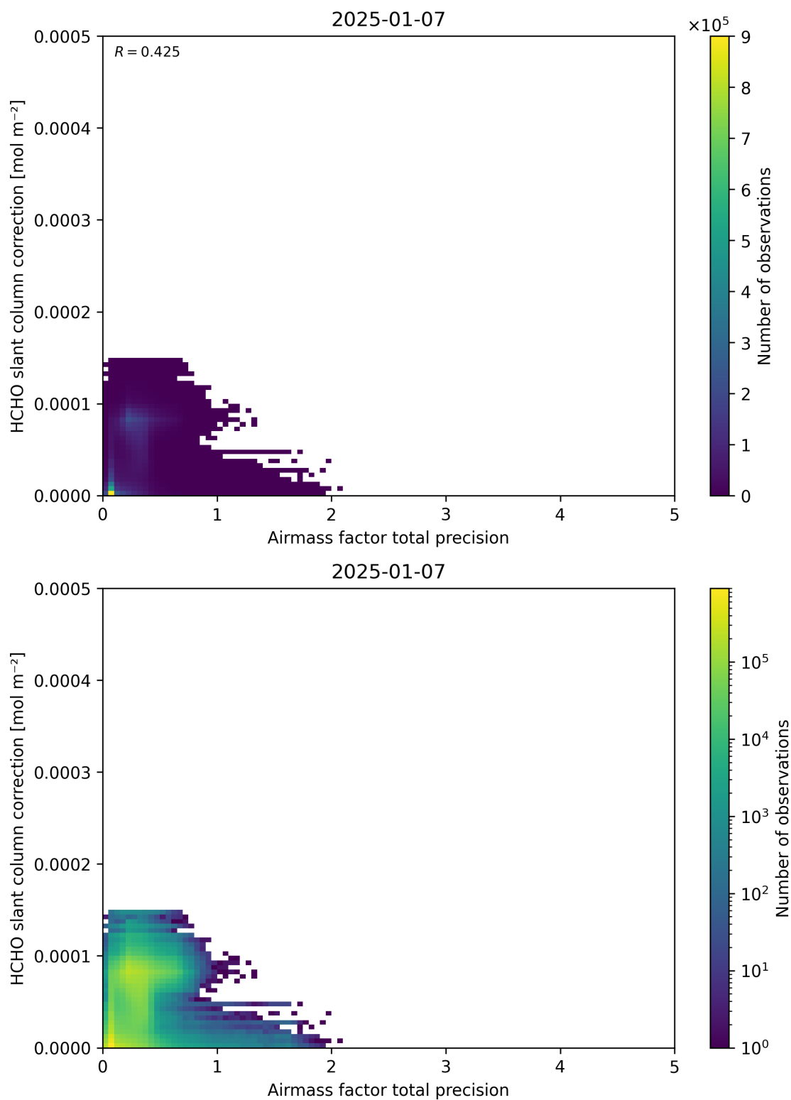
Figure 110: Scatter density plot of “Airmass factor total precision” against “HCHO slant column correction” for 2025-01-07 to 2025-01-08.
