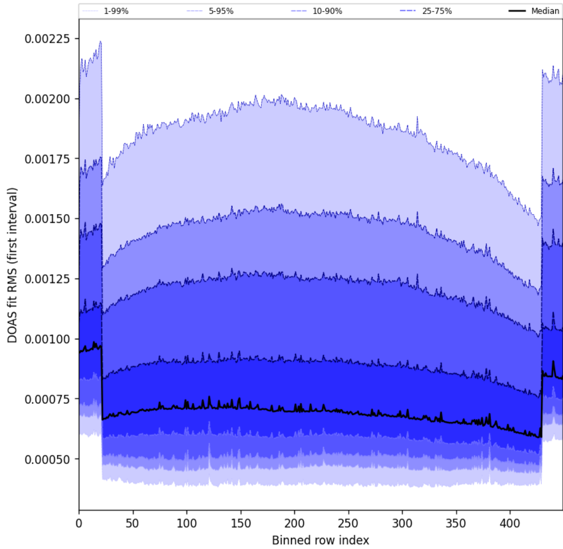
Figure 60: Along track statistics of “DOAS fit RMS (first interval)” for 2025-01-07 to 2025-01-08
