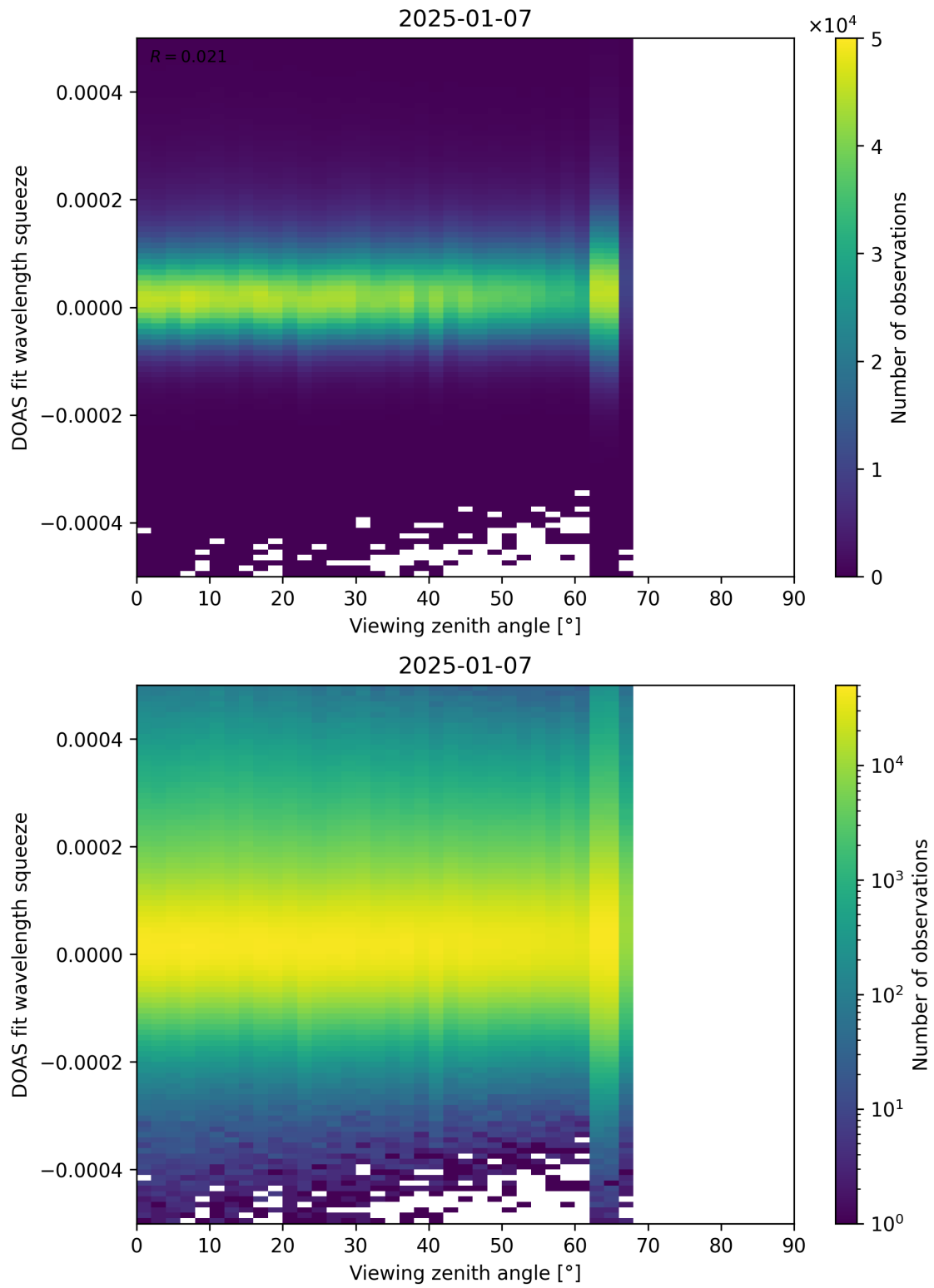
Figure 184: Scatter density plot of “Viewing zenith angle” against “DOAS fit wavelength squeeze” for 2025-01-07 to 2025-01-08.
