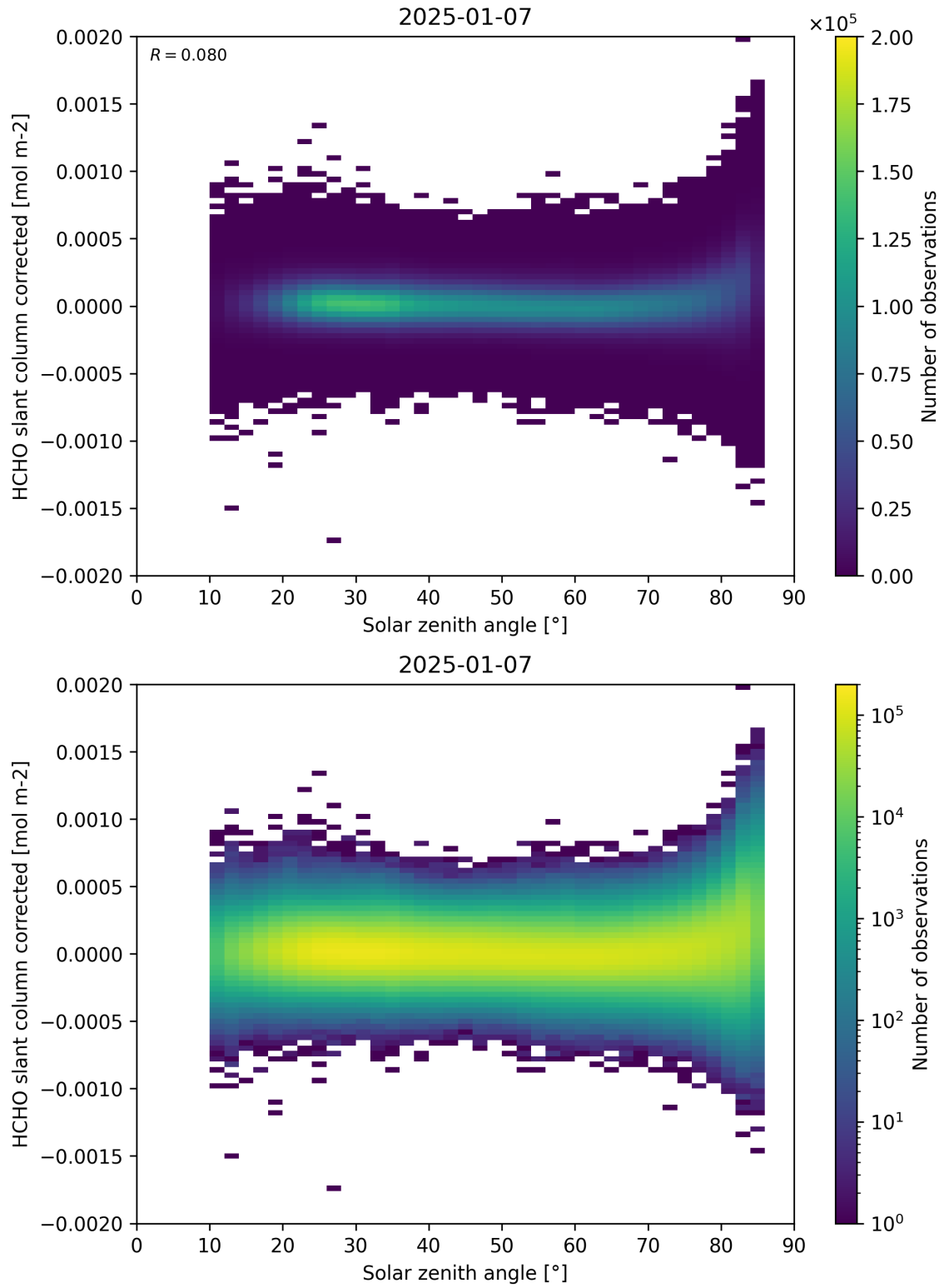
Figure 171: Scatter density plot of “Solar zenith angle” against “HCHO slant column corrected” for 2025-01-07 to 2025-01-08.
