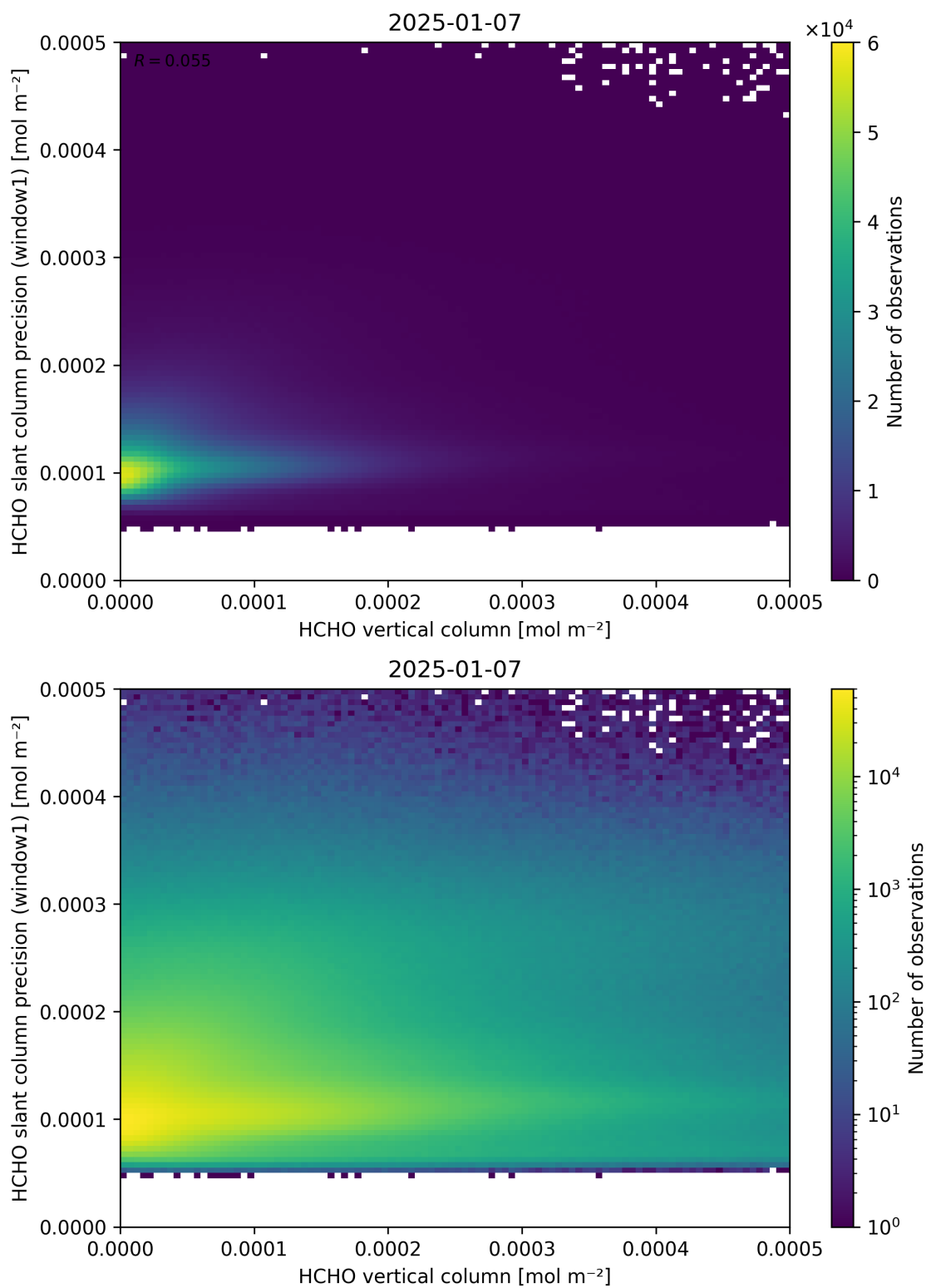
Figure 130: Scatter density plot of “HCHO vertical column” against “HCHO slant column precision (window1)” for 2025-01-07 to 2025-01-08.
