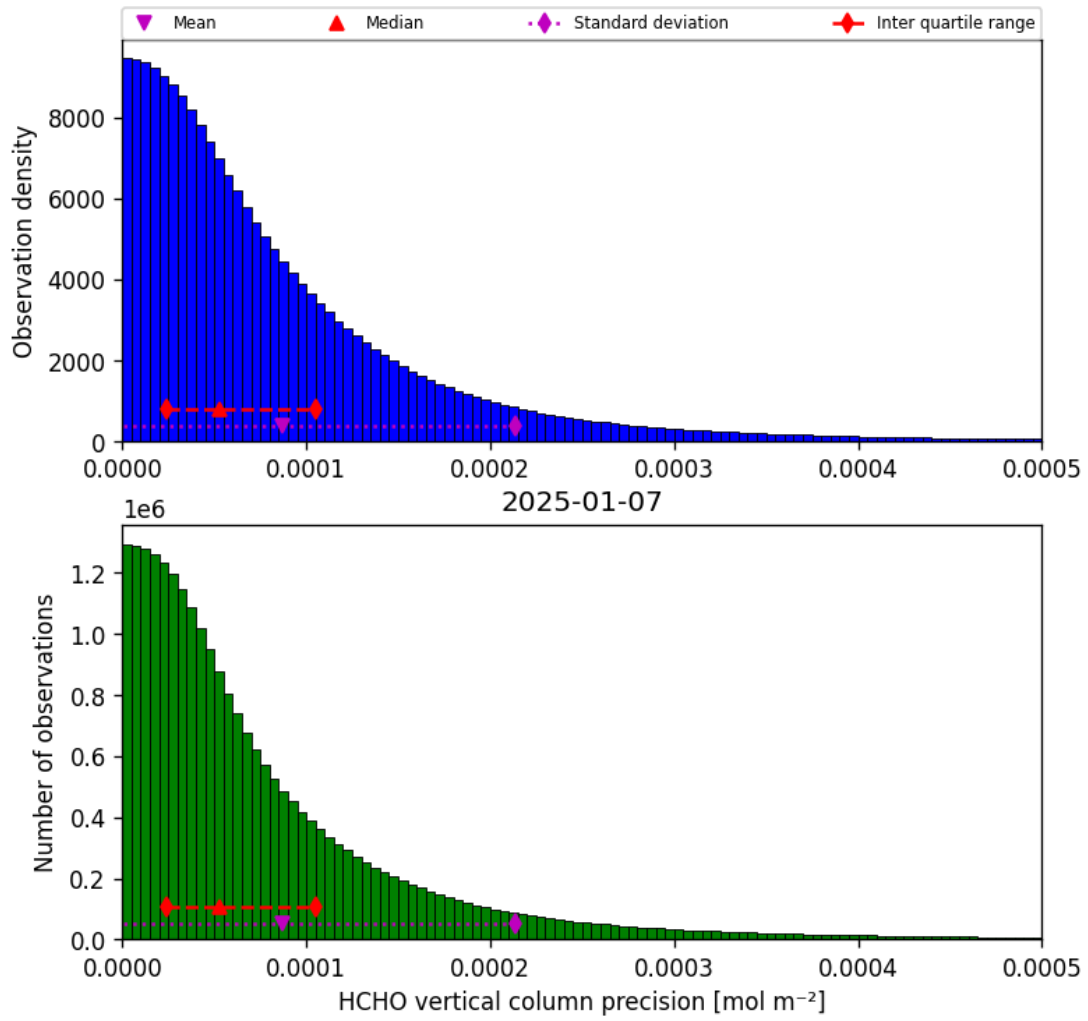
Figure 36: Histogram of “HCHO vertical column precision” for 2025-01-07 to 2025-01-08
