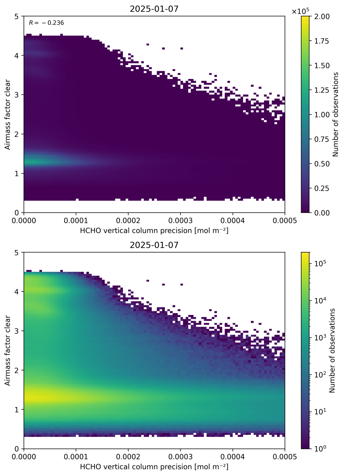
Figure 139: Scatter density plot of “HCHO vertical column precision” against “Airmass factor clear” for 2025-01-07 to 2025-01-08.
