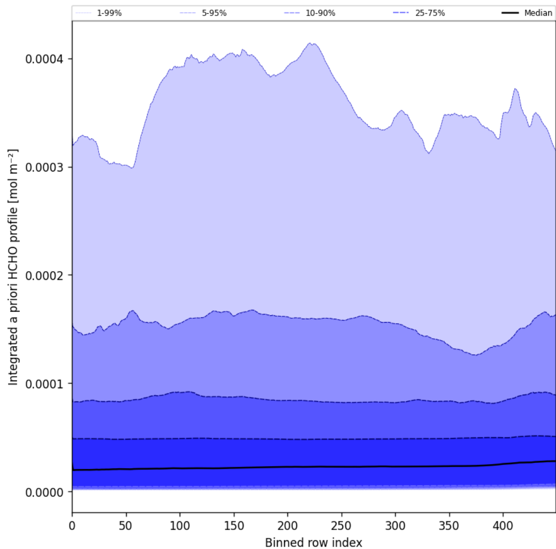
Figure 57: Along track statistics of “Integrated a priori HCHO profile” for 2025-01-07 to 2025-01-08
