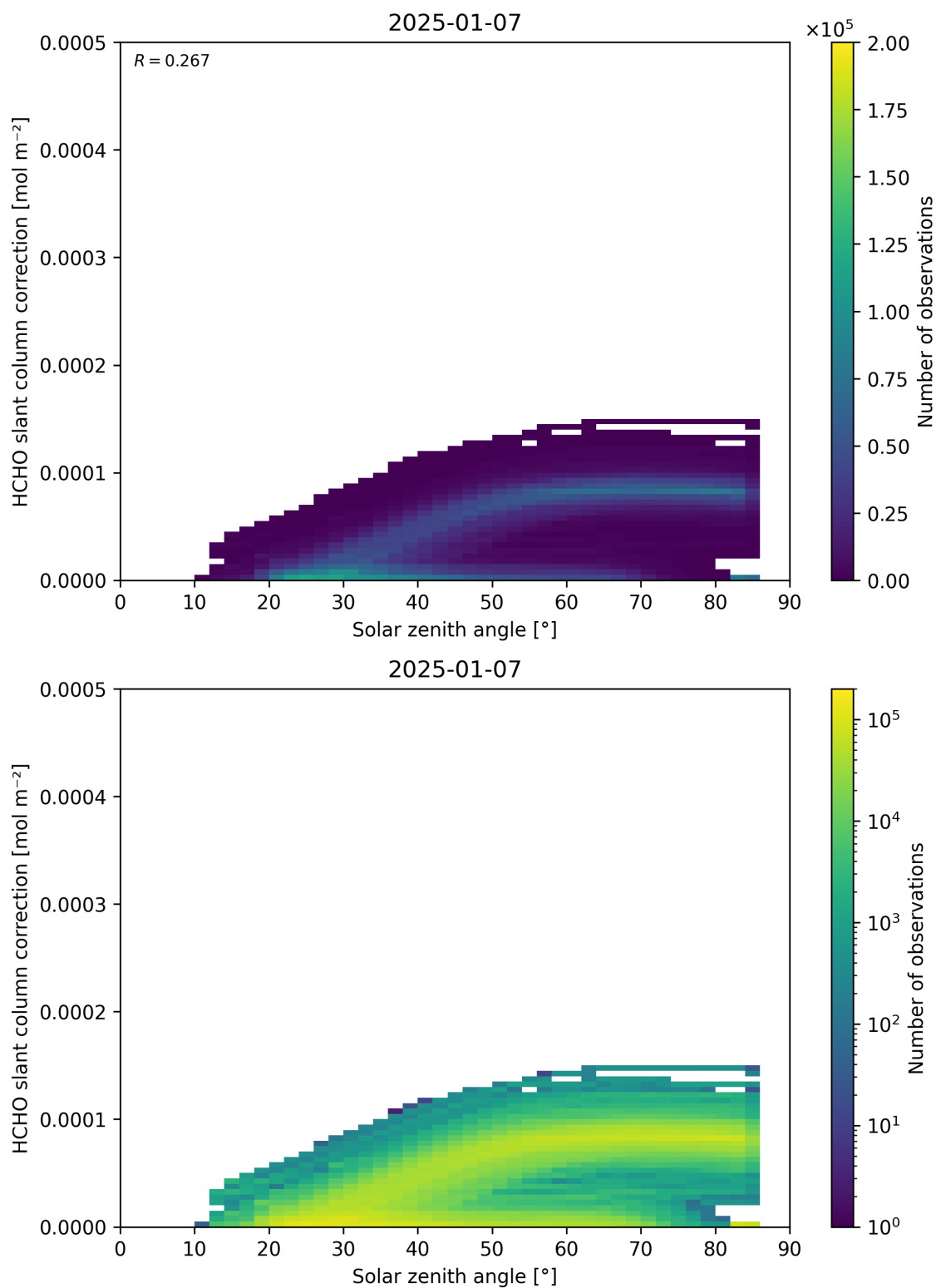
Figure 172: Scatter density plot of “Solar zenith angle” against “HCHO slant column correction” for 2025-01-07 to 2025-01-08.
