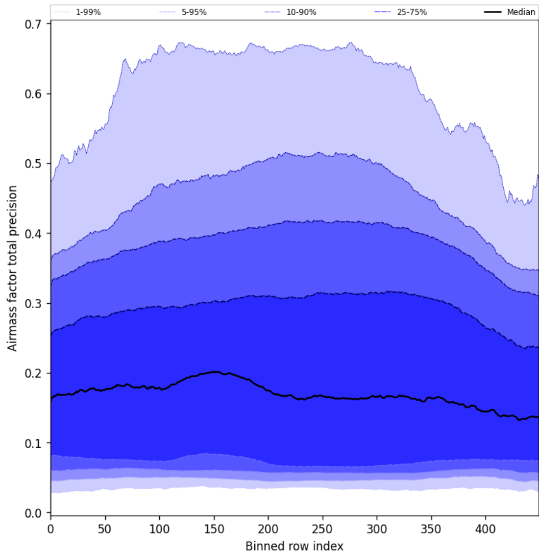
Figure 55: Along track statistics of “Airmass factor total precision” for 2025-01-07 to 2025-01-08
