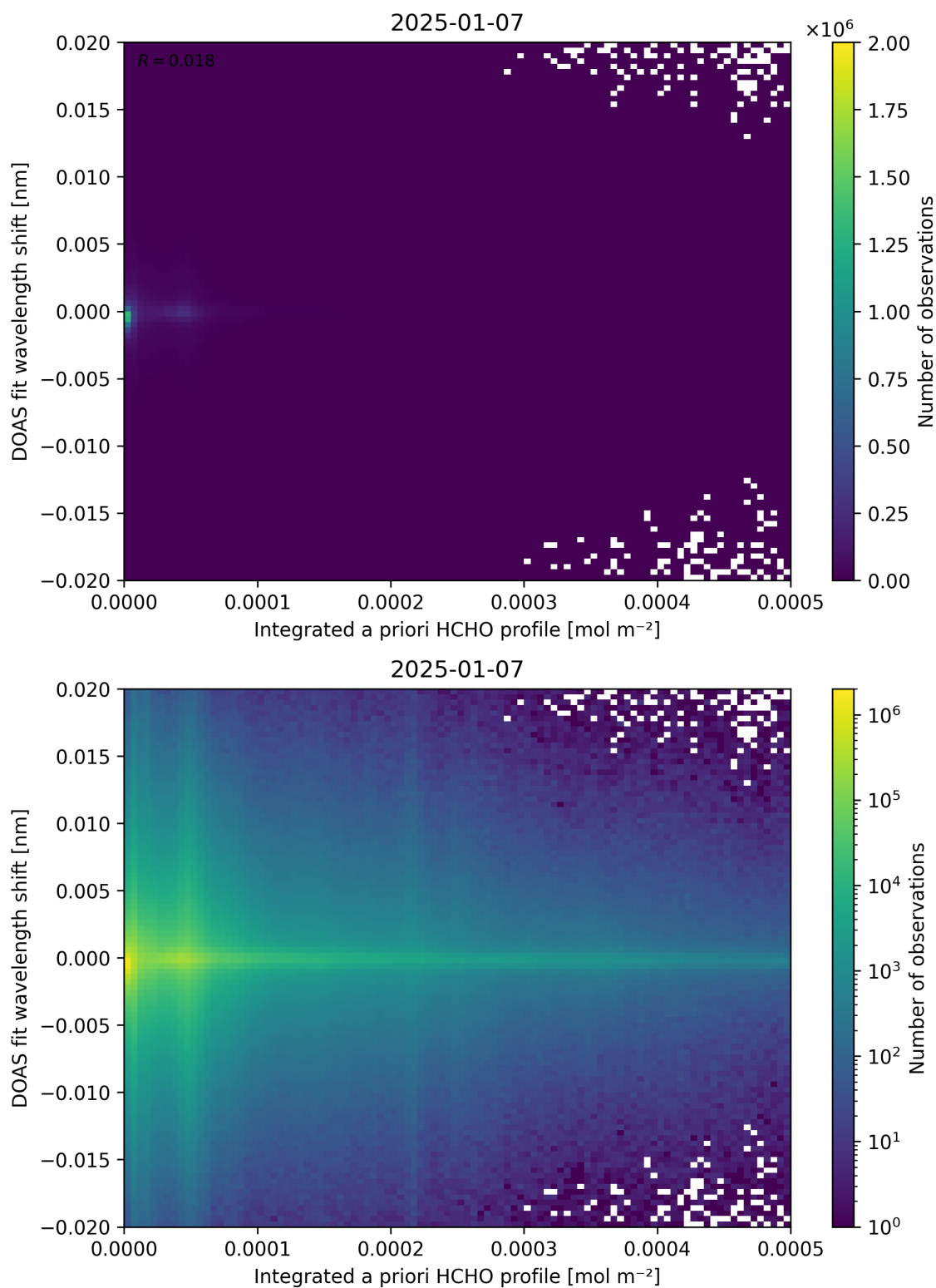
Figure 149: Scatter density plot of “Integrated a priori HCHO profile” against “DOAS fit wavelength shift” for 2025-01-07 to 2025-01-08.
