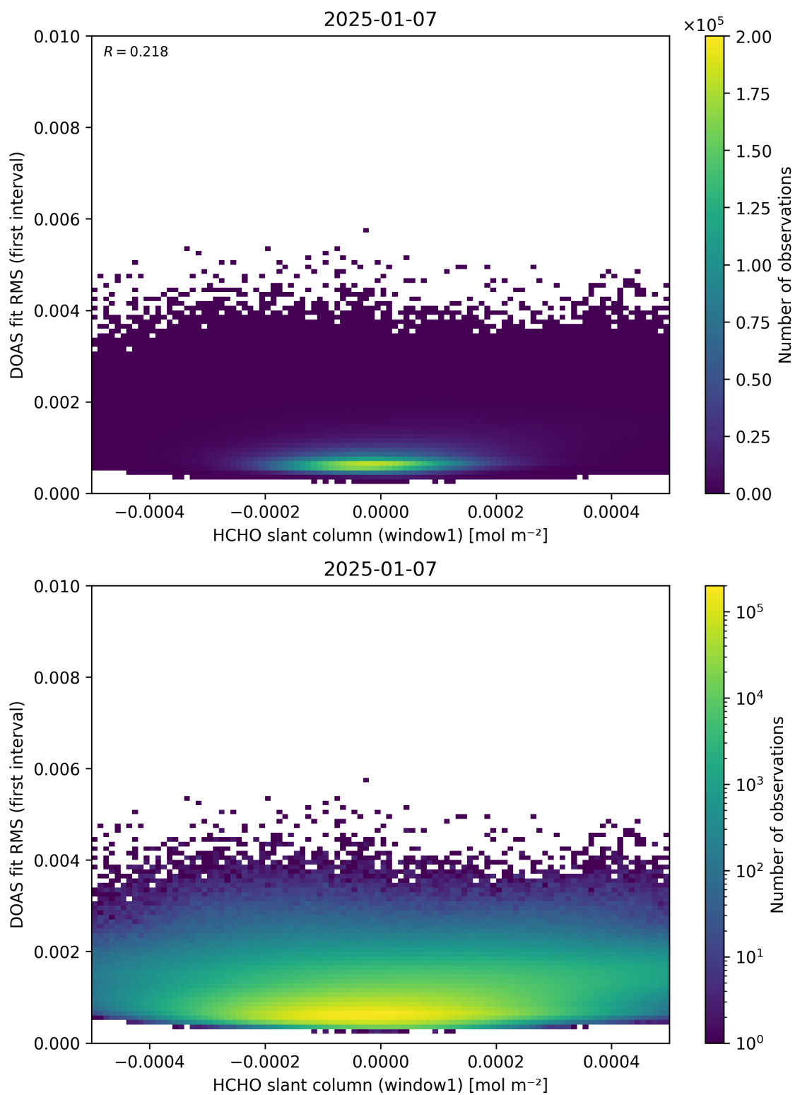
Figure 78: Scatter density plot of “HCHO slant column (window1)” against “DOAS fit RMS (first interval)” for 2025-01-07 to 2025-01-08.
