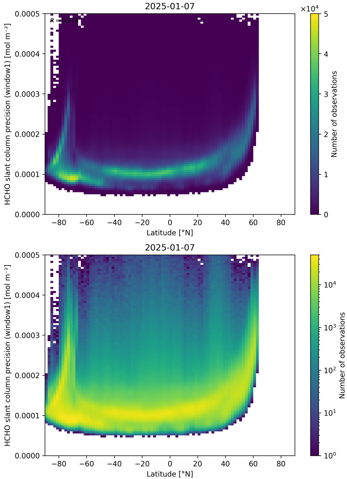
Figure 160: Scatter density plot of “Latitude” against “HCHO slant column precision (window1)” for 2025-01-07 to 2025-01-08.
