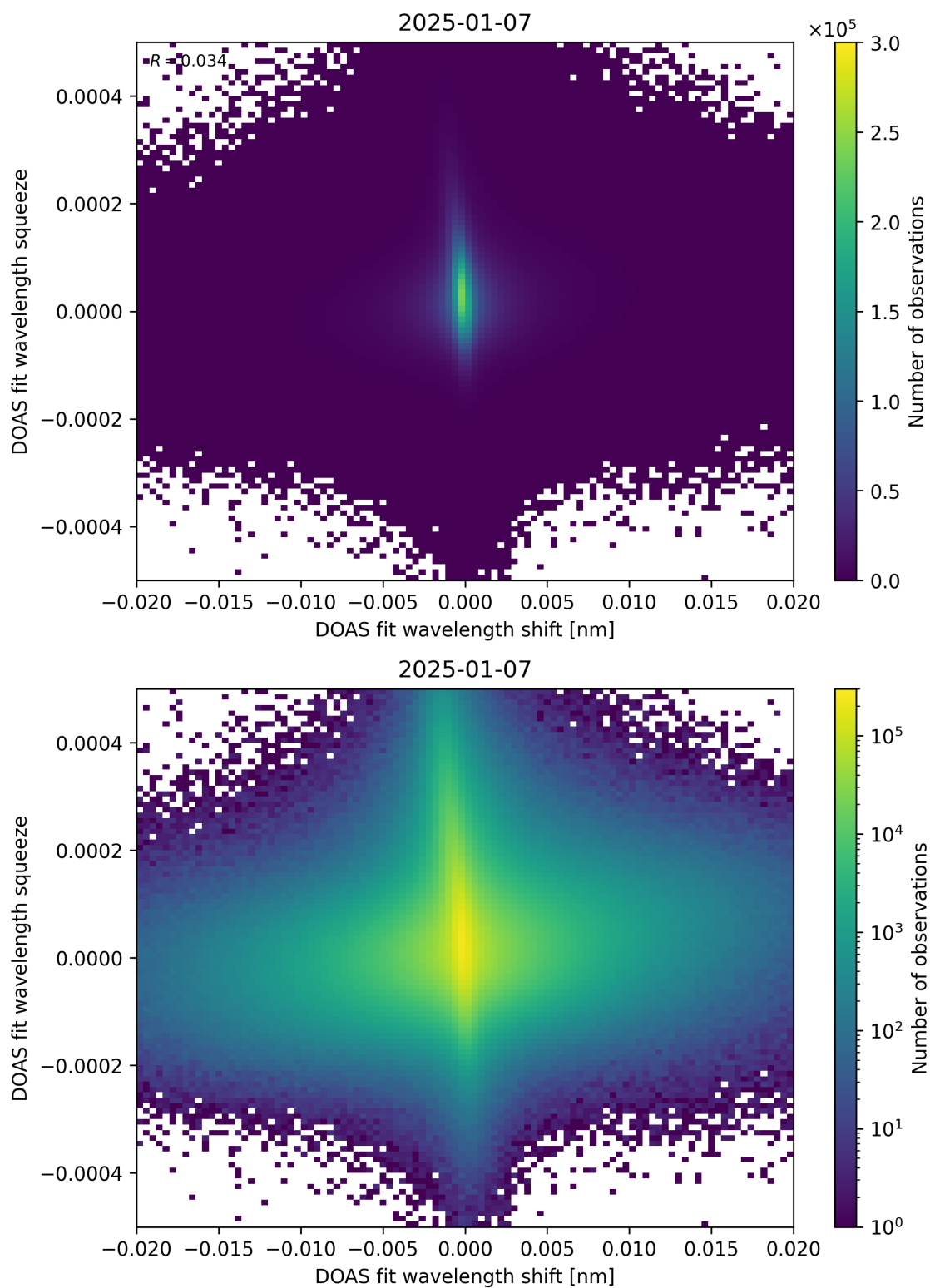
Figure 65: Scatter density plot of “DOAS fit wavelength shift” against “DOAS fit wavelength squeeze” for 2025-01-07 to 2025-01-08.
