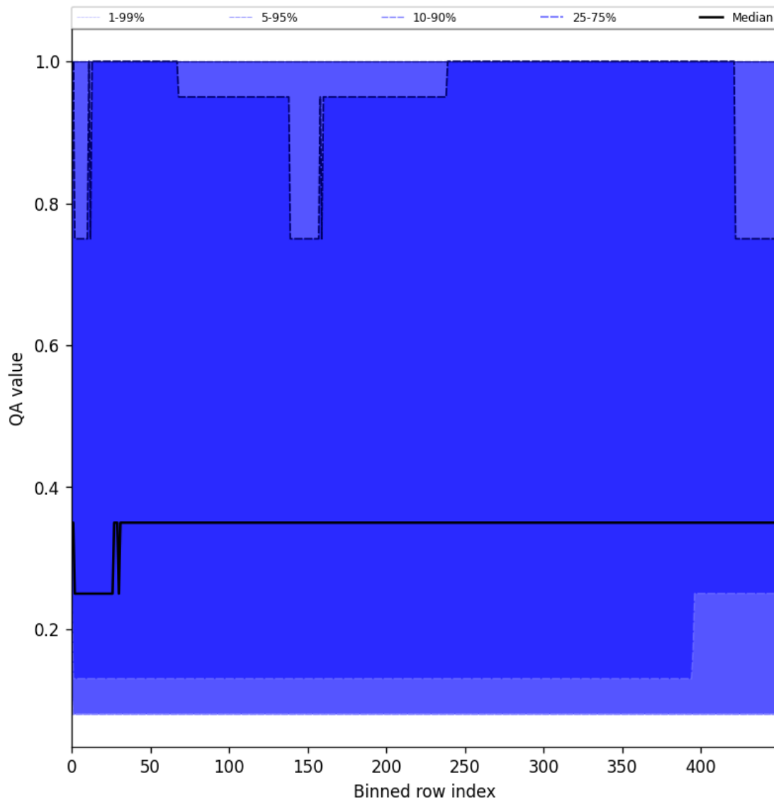
Figure 48: Along track statistics of “QA value” for 2025-01-07 to 2025-01-08
