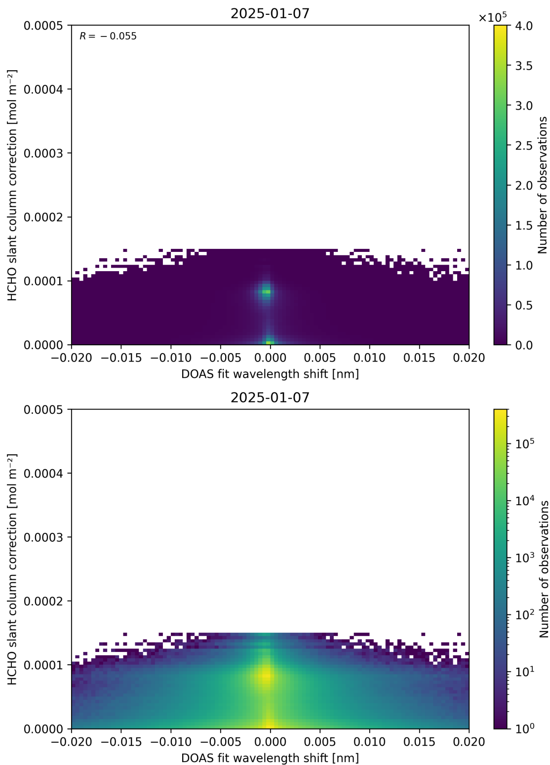
Figure 67: Scatter density plot of “DOAS fit wavelength shift” against “HCHO slant column correction” for 2025-01-07 to 2025-01-08.
