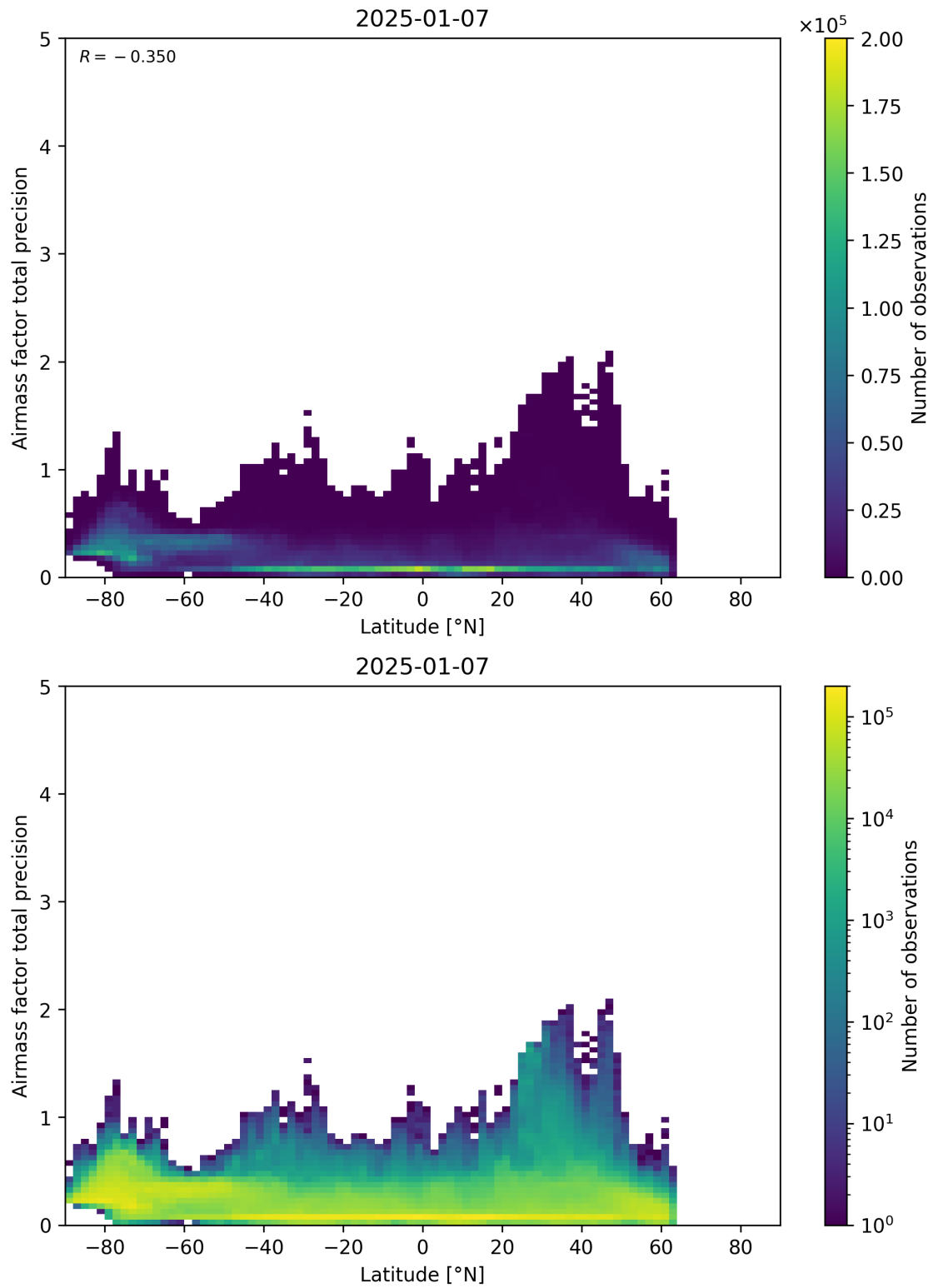
Figure 162: Scatter density plot of “Latitude” against “Airmass factor total precision” for 2025-01-07 to 2025-01-08.
