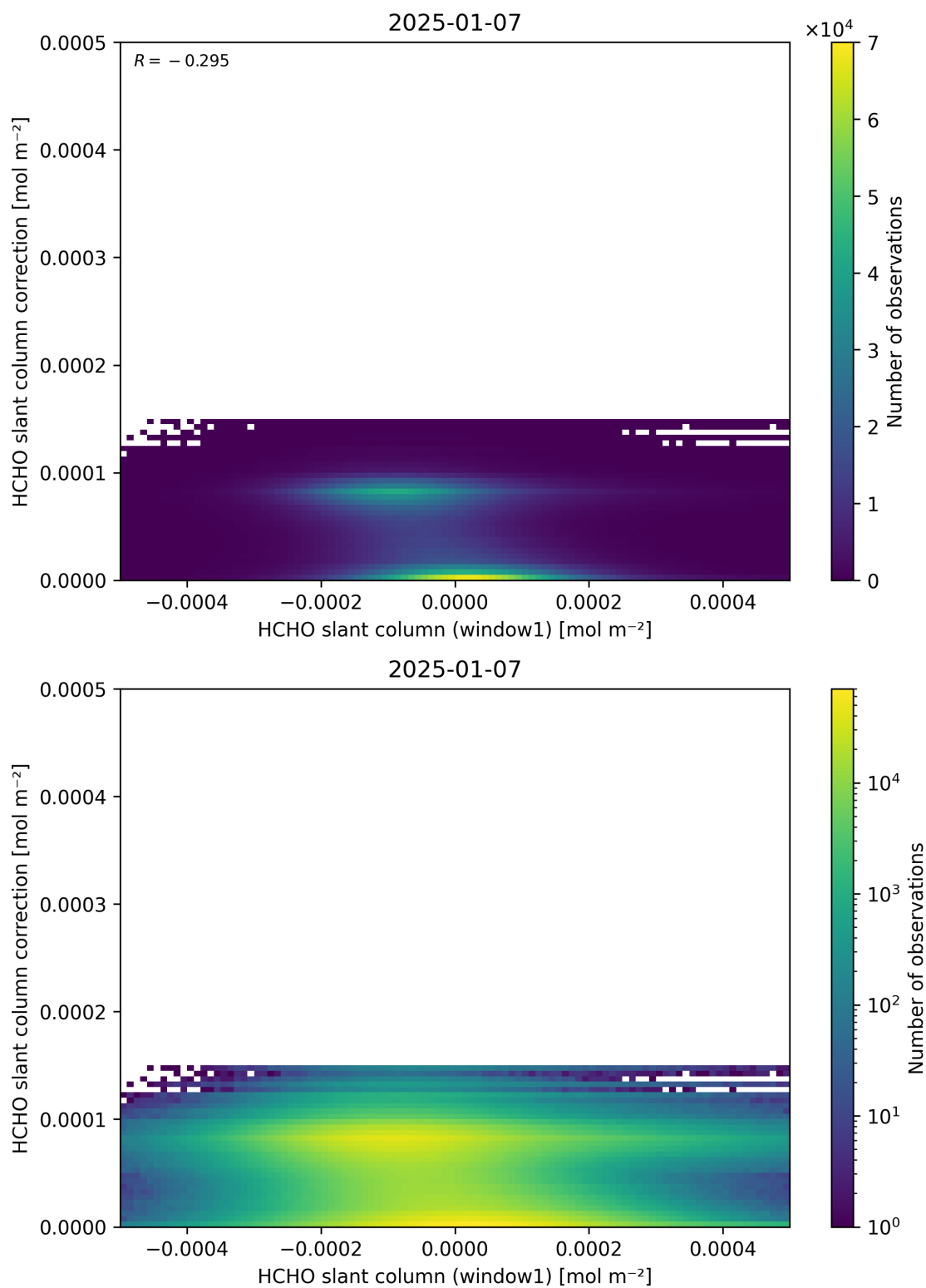
Figure 83: Scatter density plot of “HCHO slant column (window1)” against “HCHO slant column correction” for 2025-01-07 to 2025-01-08.
