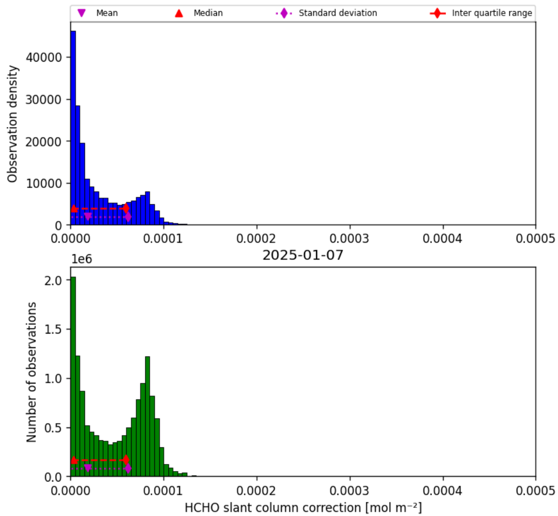
Figure 47: Histogram of “HCHO slant column correction” for 2025-01-07 to 2025-01-08
