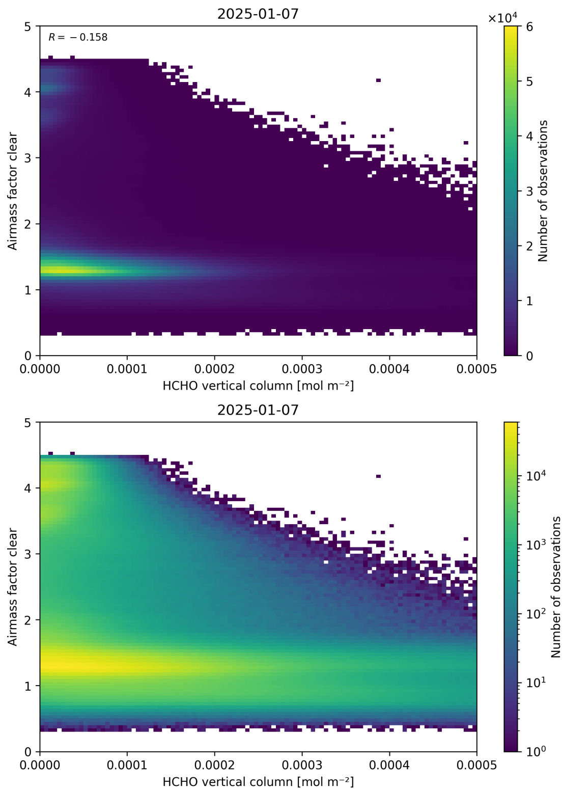
Figure 126: Scatter density plot of “HCHO vertical column” against “Airmass factor clear” for 2025-01-07 to 2025-01-08.
