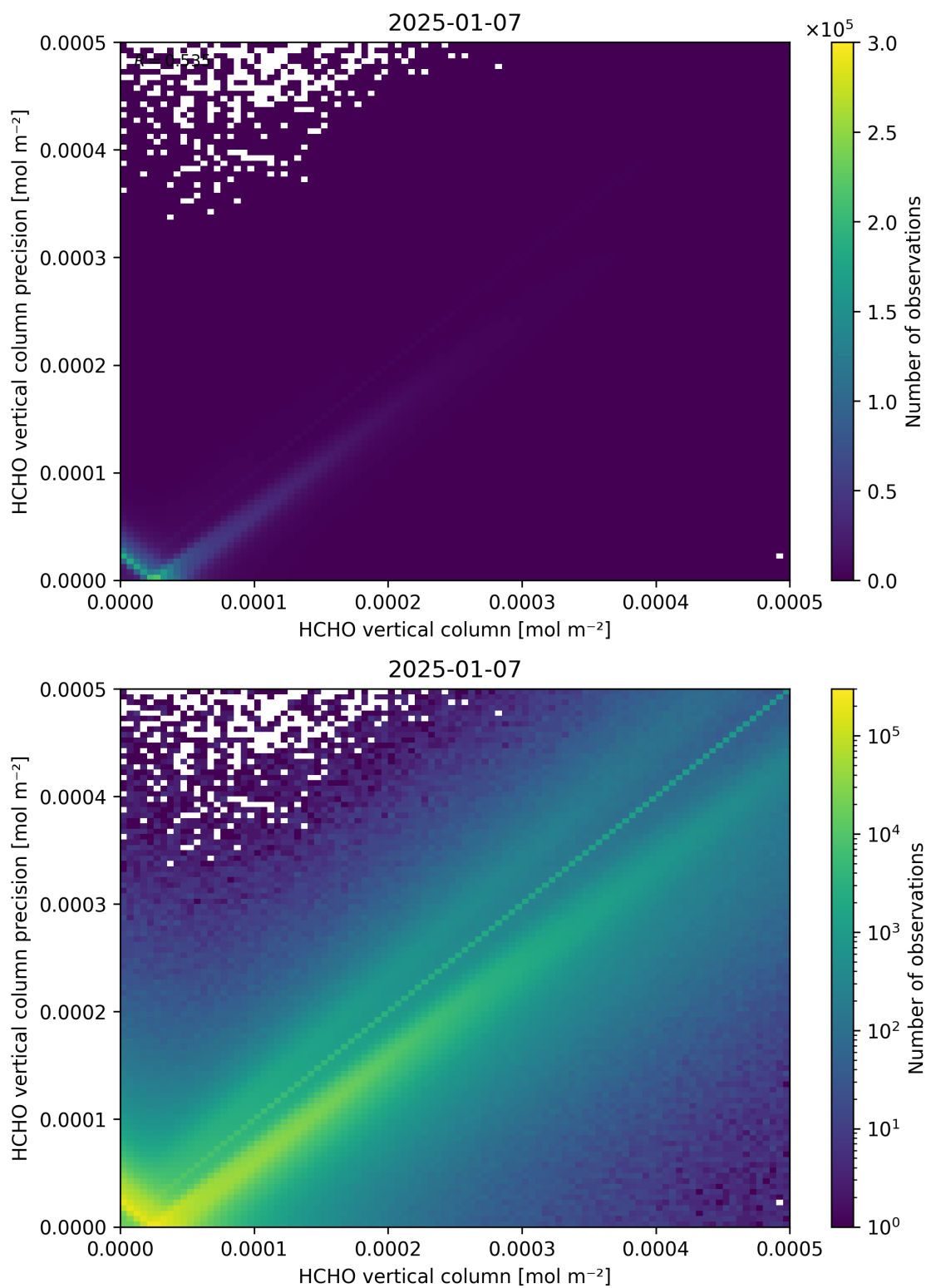
Figure 134: Scatter density plot of “HCHO vertical column” against “HCHO vertical column precision” for 2025-01-07 to 2025-01-08.
