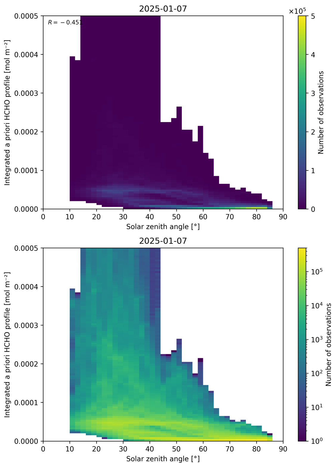
Figure 180: Scatter density plot of “Solar zenith angle” against “Integrated a priori HCHO profile” for 2025-01-07 to 2025-01-08.
