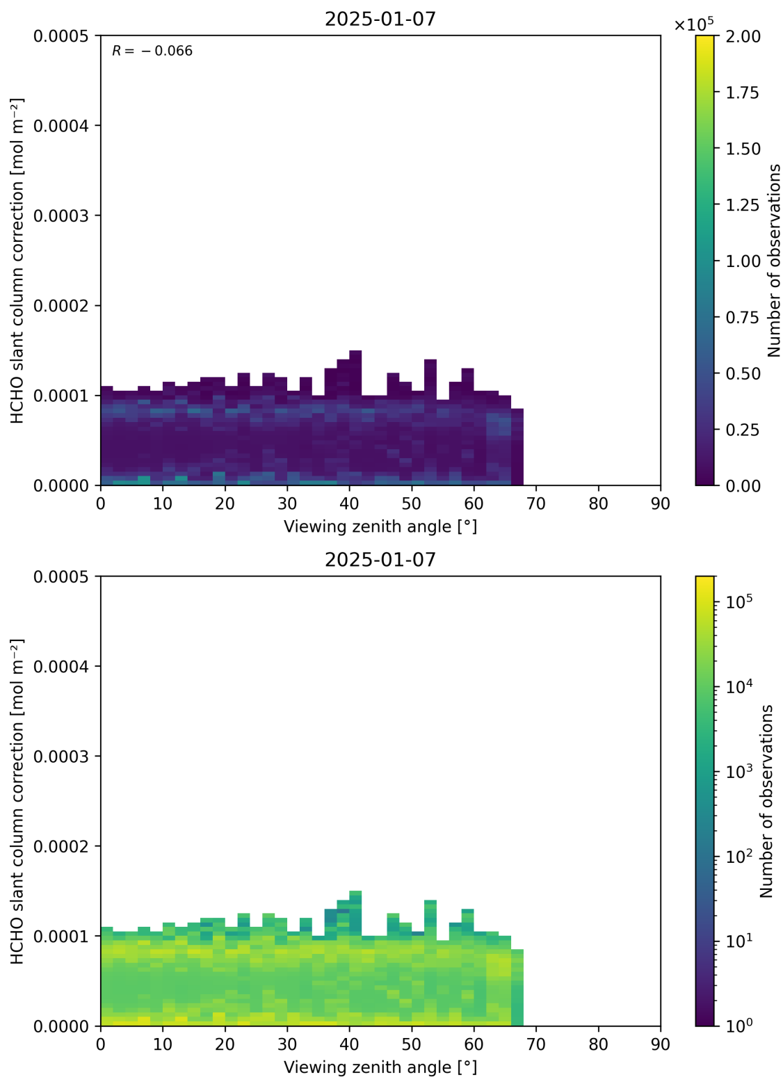
Figure 187: Scatter density plot of “Viewing zenith angle” against “HCHO slant column correction” for 2025-01-07 to 2025-01-08.
