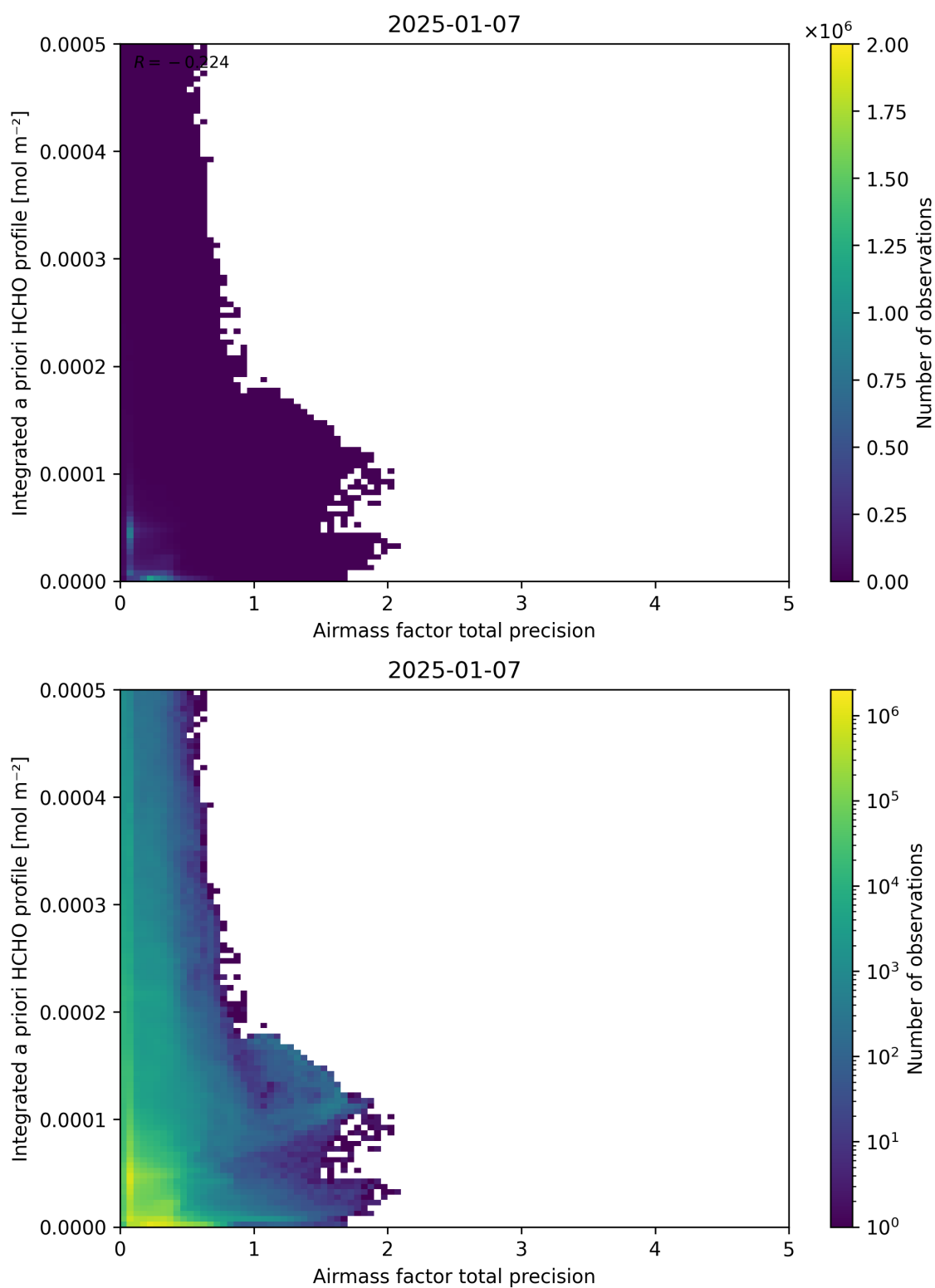
Figure 111: Scatter density plot of “Airmass factor total precision” against “Integrated a priori HCHO profile” for 2025-01-07 to 2025-01-08.
