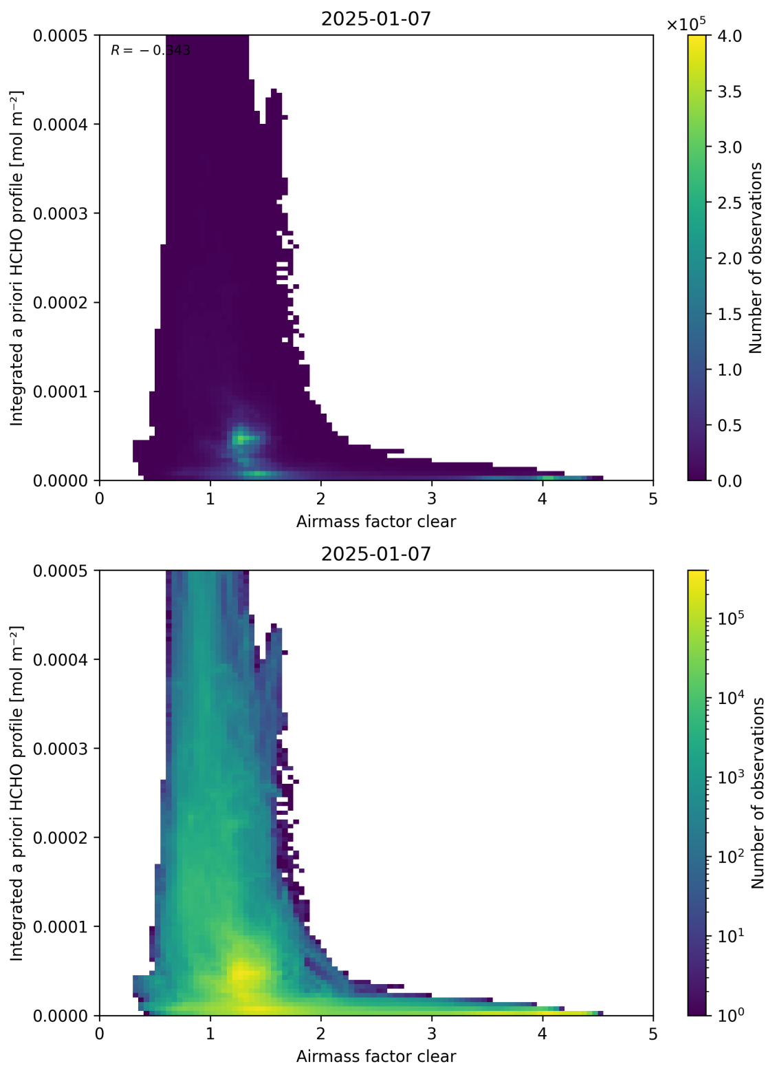
Figure 76: Scatter density plot of “Airmass factor clear” against “Integrated a priori HCHO profile” for 2025-01-07 to 2025-01-08.
