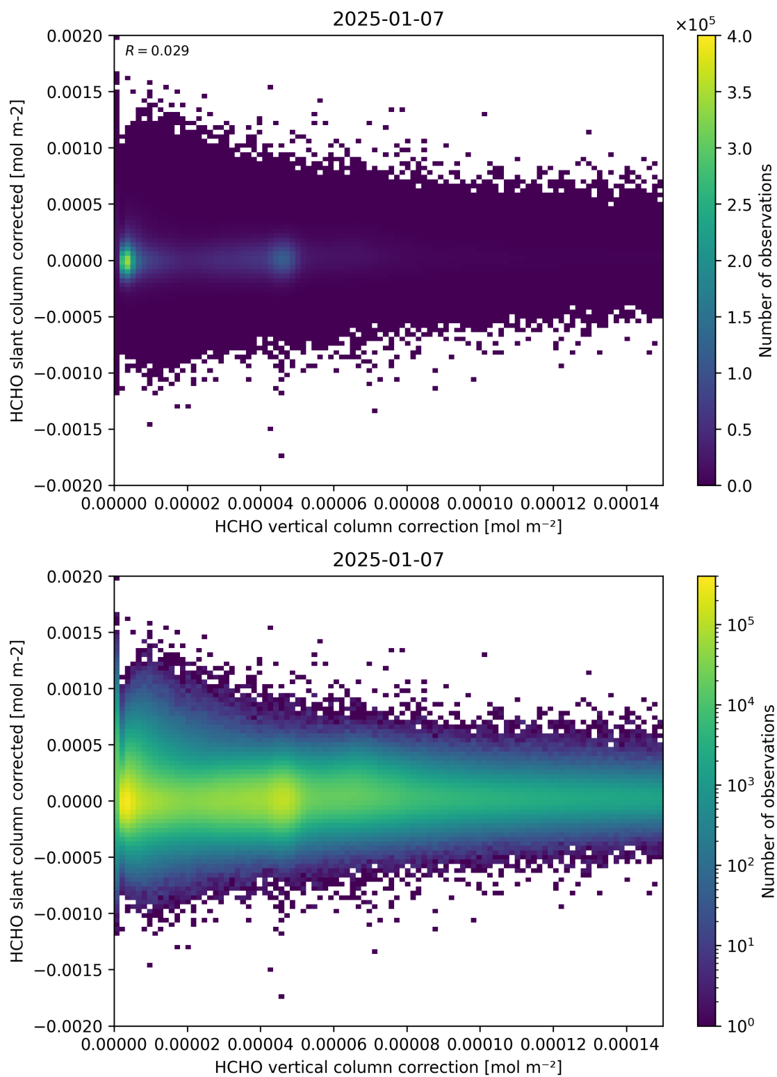
Figure 116: Scatter density plot of “HCHO vertical column correction” against “HCHO slant column corrected” for 2025-01-07 to 2025-01-08.
