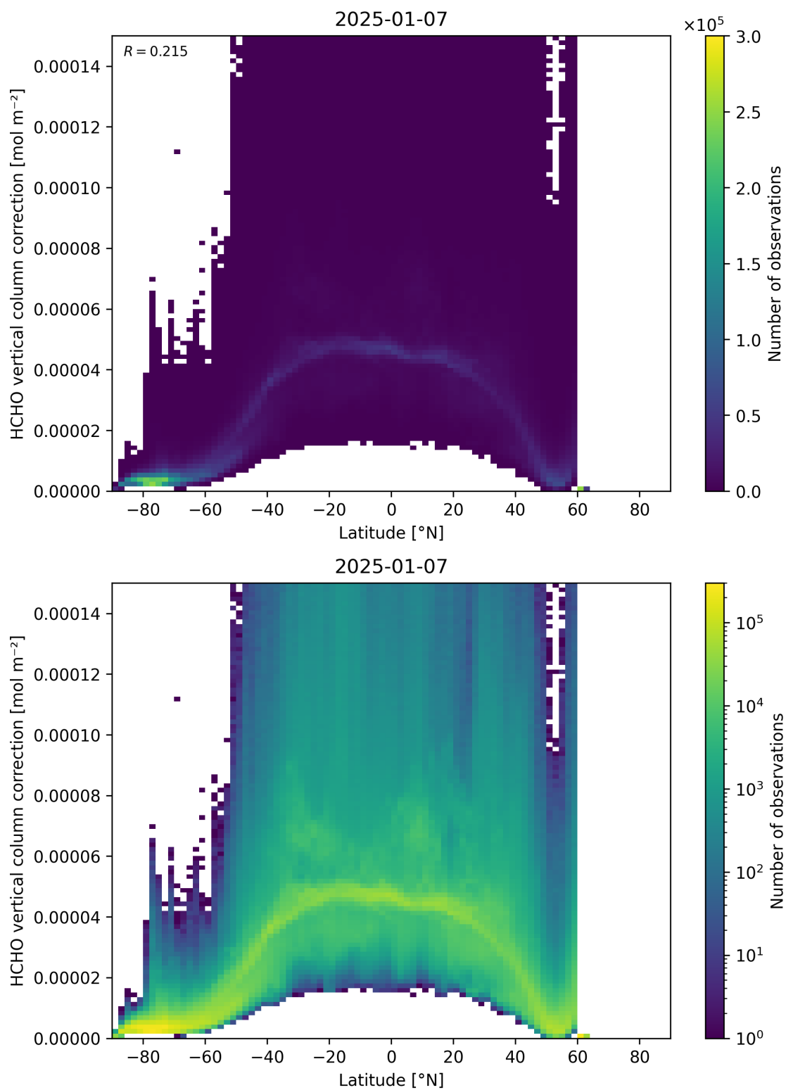
Figure 164: Scatter density plot of “Latitude” against “HCHO vertical column correction” for 2025-01-07 to 2025-01-08.
