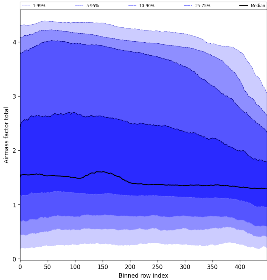
Figure 54: Along track statistics of “Airmass factor total” for 2025-01-07 to 2025-01-08
