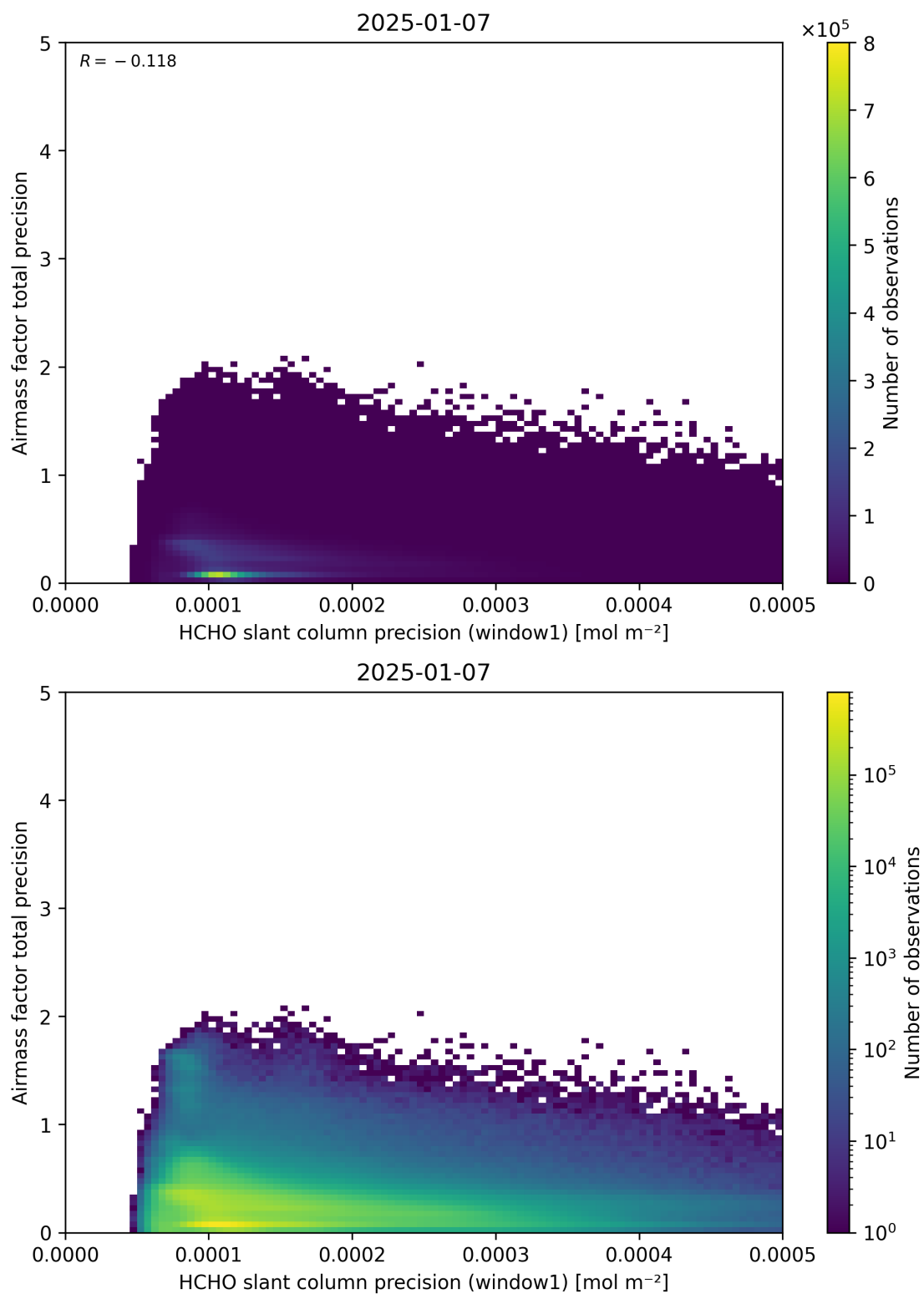
Figure 95: Scatter density plot of “HCHO slant column precision (window1)” against “Airmass factor total precision” for 2025-01-07 to 2025-01-08.
