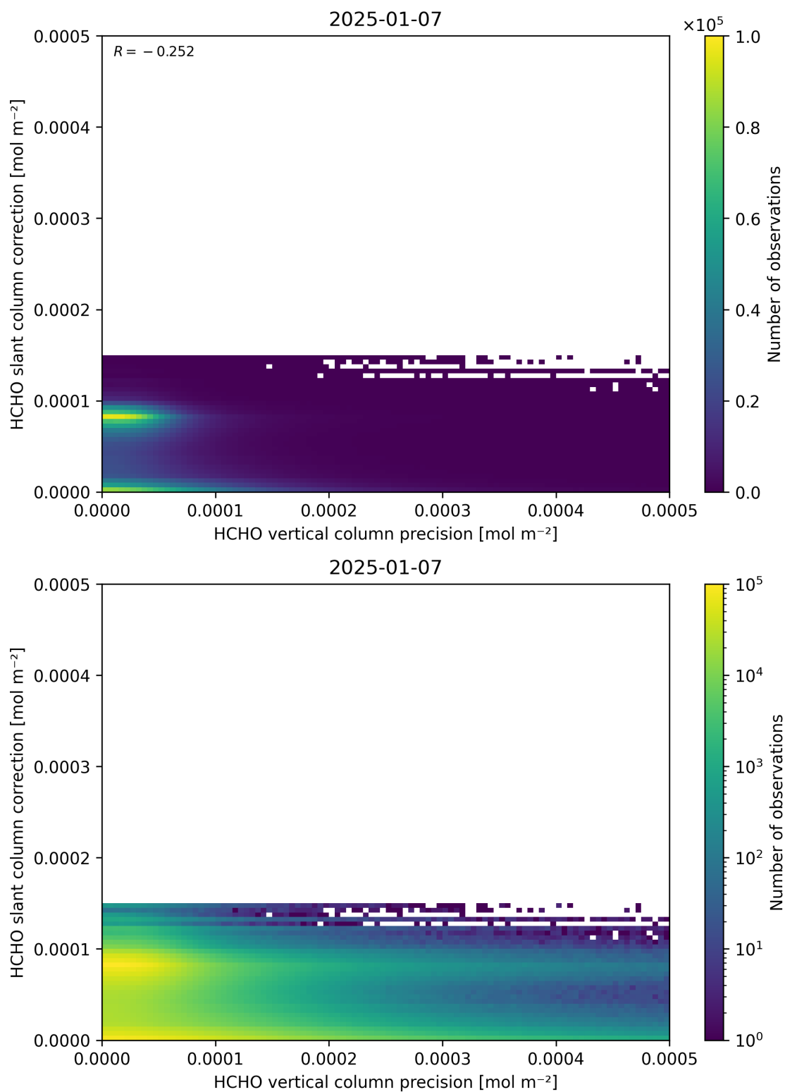
Figure 141: Scatter density plot of “HCHO vertical column precision” against “HCHO slant column correction” for 2025-01-07 to 2025-01-08.
