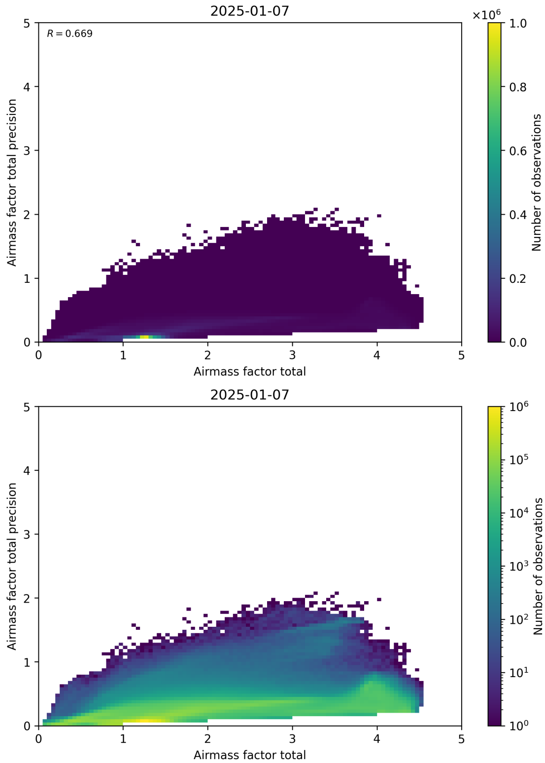
Figure 103: Scatter density plot of “Airmass factor total” against “Airmass factor total precision” for 2025-01-07 to 2025-01-08.
