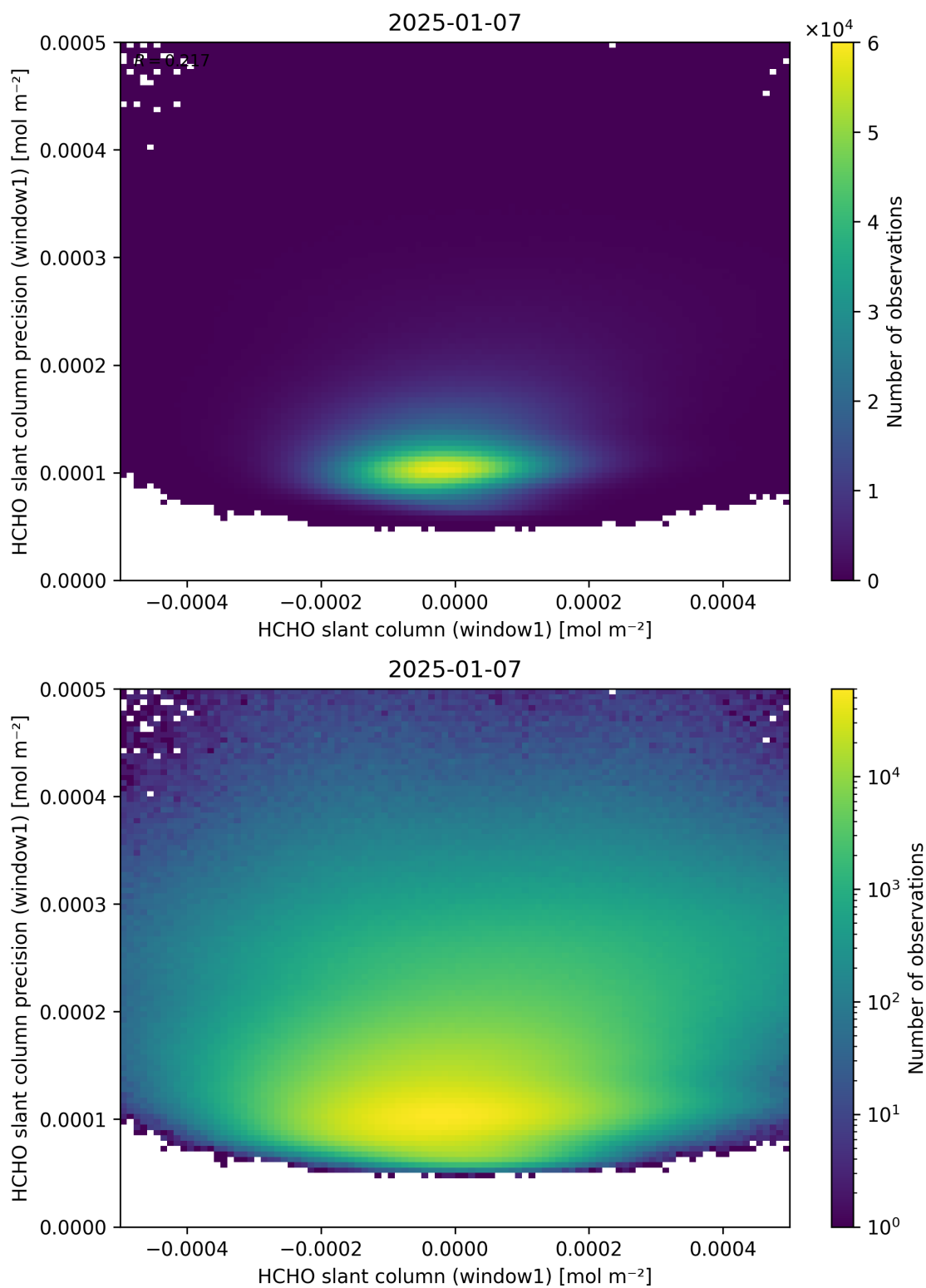
Figure 84: Scatter density plot of “HCHO slant column (window1)” against “HCHO slant column precision (window1)” for 2025-01-07 to 2025-01-08.
