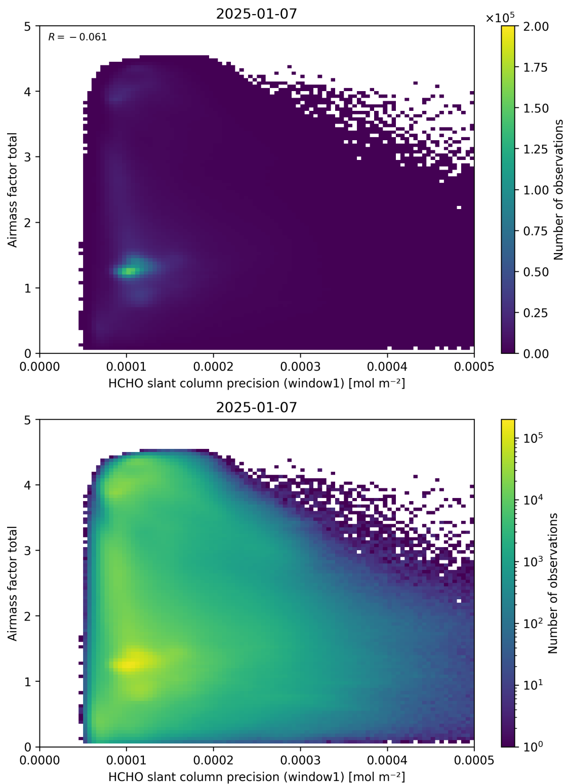
Figure 94: Scatter density plot of “HCHO slant column precision (window1)” against “Airmass factor total” for 2025-01-07 to 2025-01-08.
