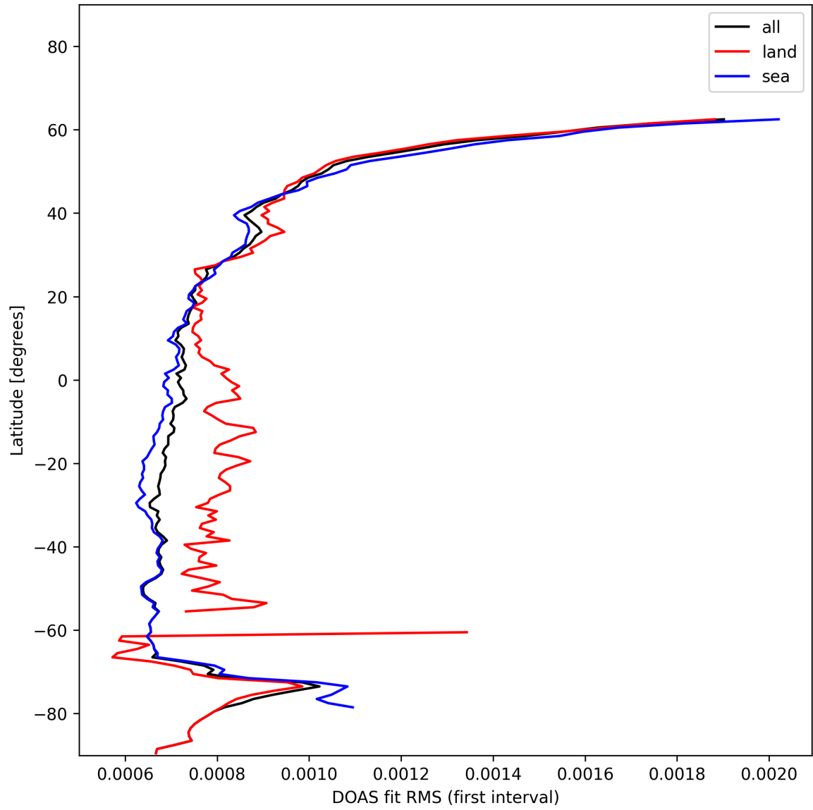
Figure 32: Zonal average of “DOAS fit RMS (first interval)” for 2025-01-07 to 2025-01-08.
