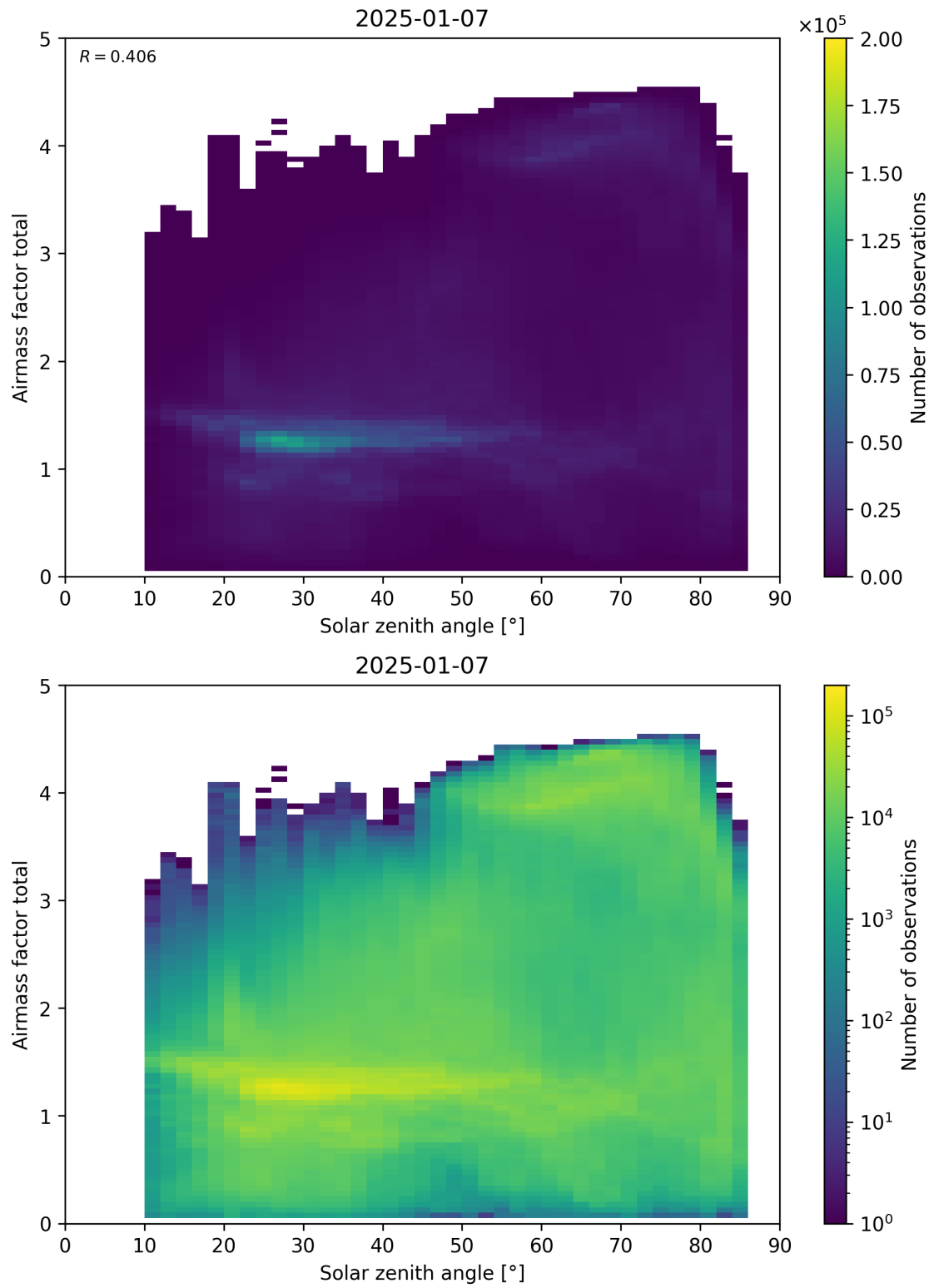
Figure 175: Scatter density plot of “Solar zenith angle” against “Airmass factor total” for 2025-01-07 to 2025-01-08.
