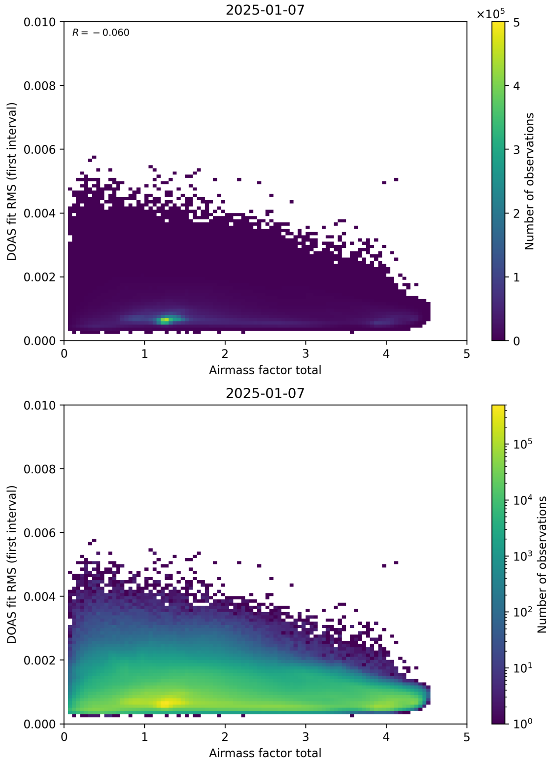
Figure 97: Scatter density plot of “Airmass factor total” against “DOAS fit RMS (first interval)” for 2025-01-07 to 2025-01-08.
