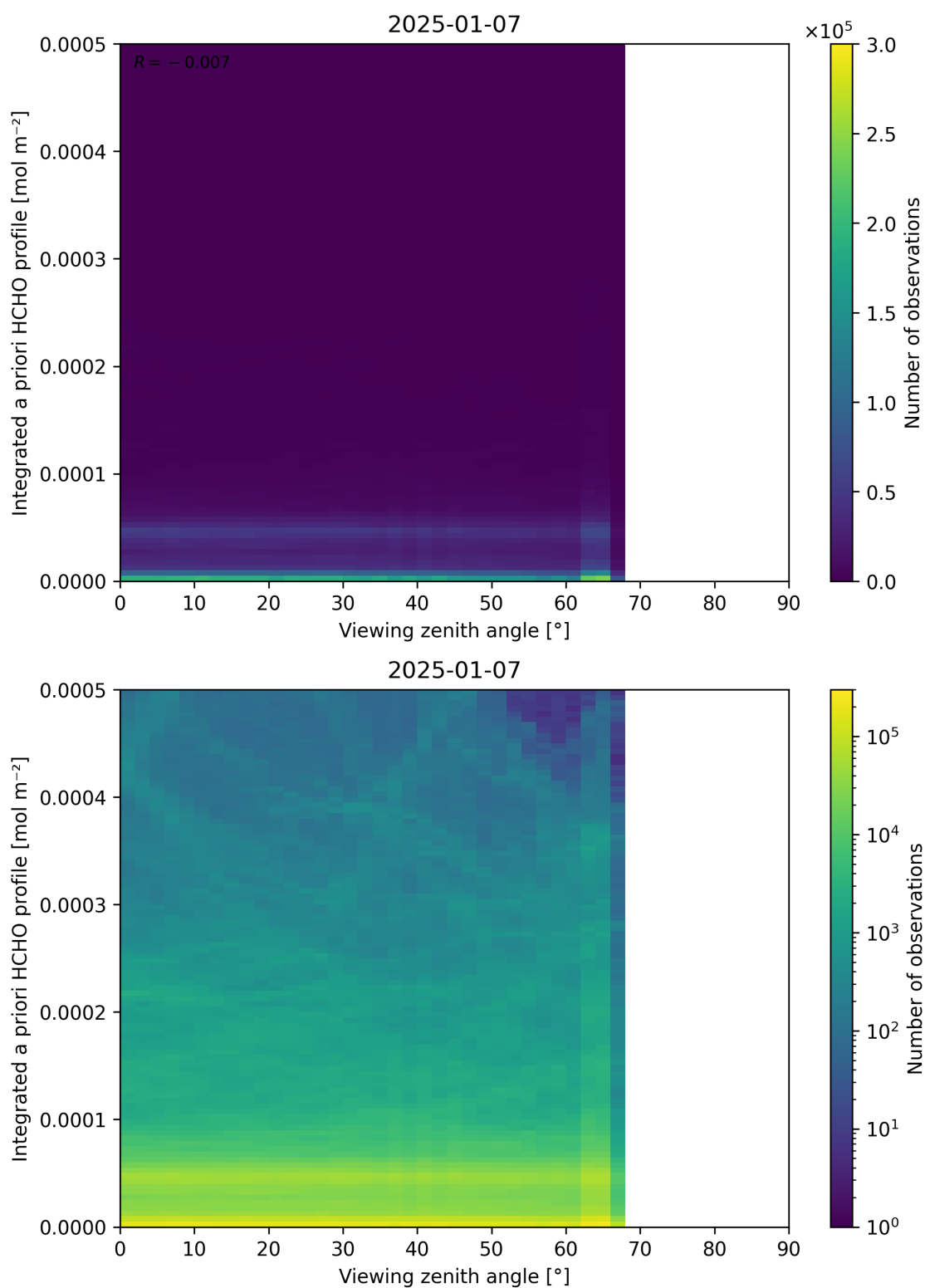
Figure 195: Scatter density plot of “Viewing zenith angle” against “Integrated a priori HCHO profile” for 2025-01-07 to 2025-01-08.
