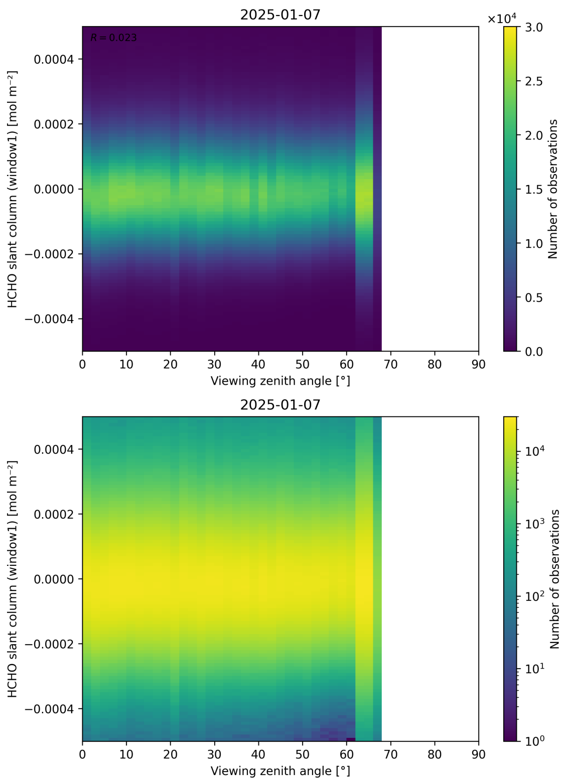
Figure 188: Scatter density plot of “Viewing zenith angle” against “HCHO slant column (window1)” for 2025-01-07 to 2025-01-08.
