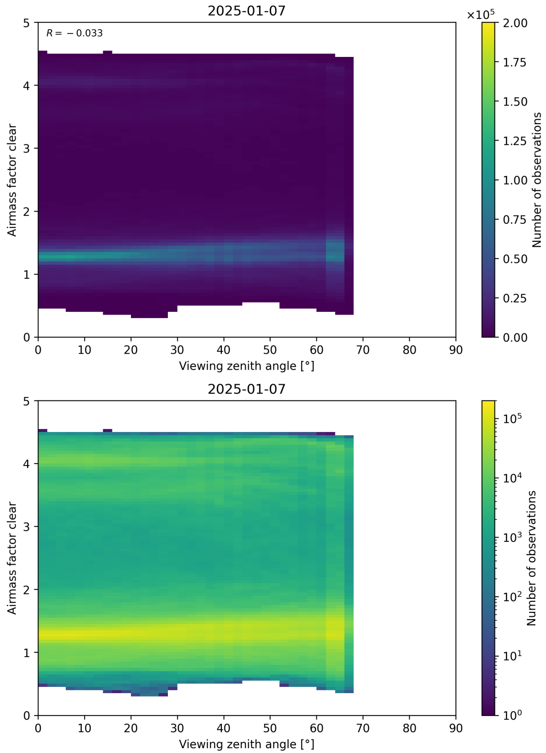
Figure 185: Scatter density plot of “Viewing zenith angle” against “Airmass factor clear” for 2025-01-07 to 2025-01-08.
