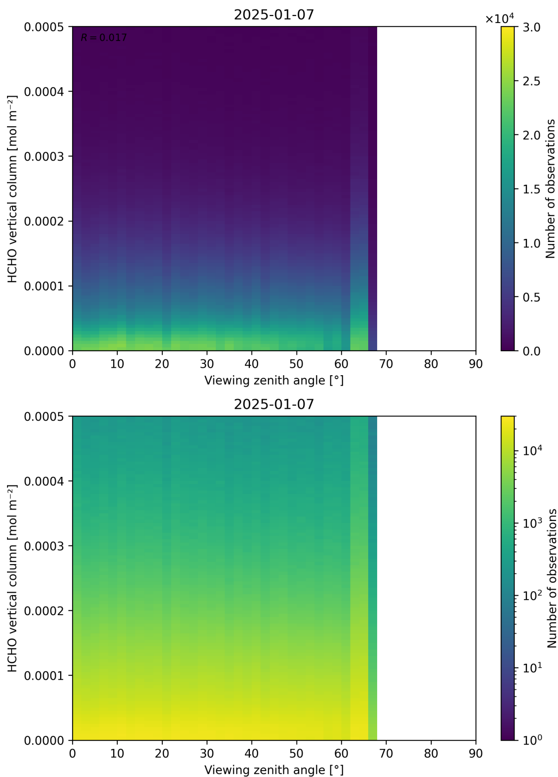
Figure 192: Scatter density plot of “Viewing zenith angle” against “HCHO vertical column” for 2025-01-07 to 2025-01-08.
