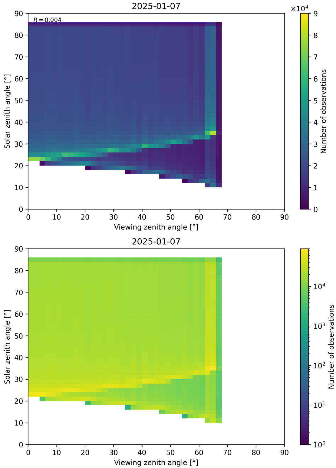
Figure 197: Scatter density plot of “Viewing zenith angle” against “Solar zenith angle” for 2025-01-07 to 2025-01-08.
