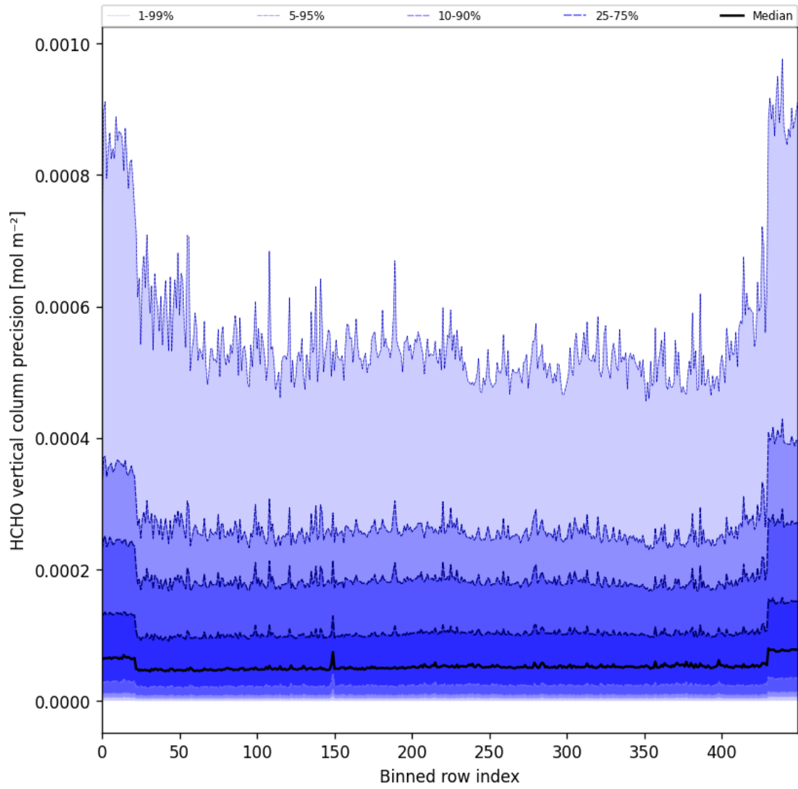
Figure 50: Along track statistics of “HCHO vertical column precision” for 2025-01-07 to 2025-01-08
