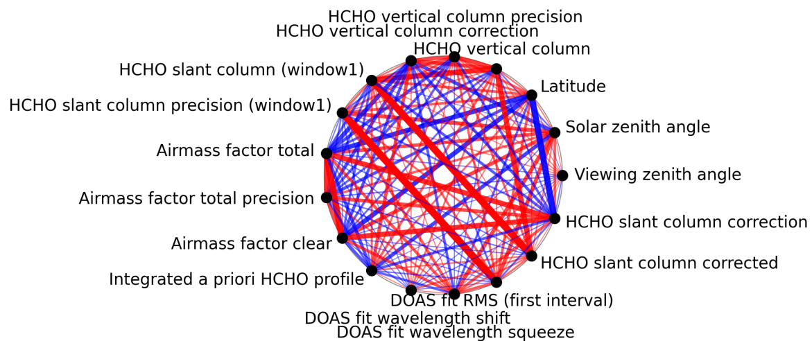
Figure 1: Map of correlation graph for 2025-01-07 to 2025-01-08.
