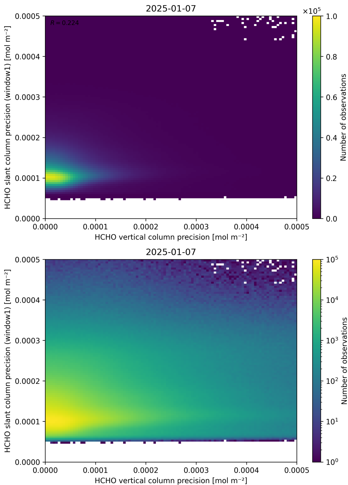
Figure 143: Scatter density plot of “HCHO vertical column precision” against “HCHO slant column precision (window1)” for 2025-01-07 to 2025-01-08.
