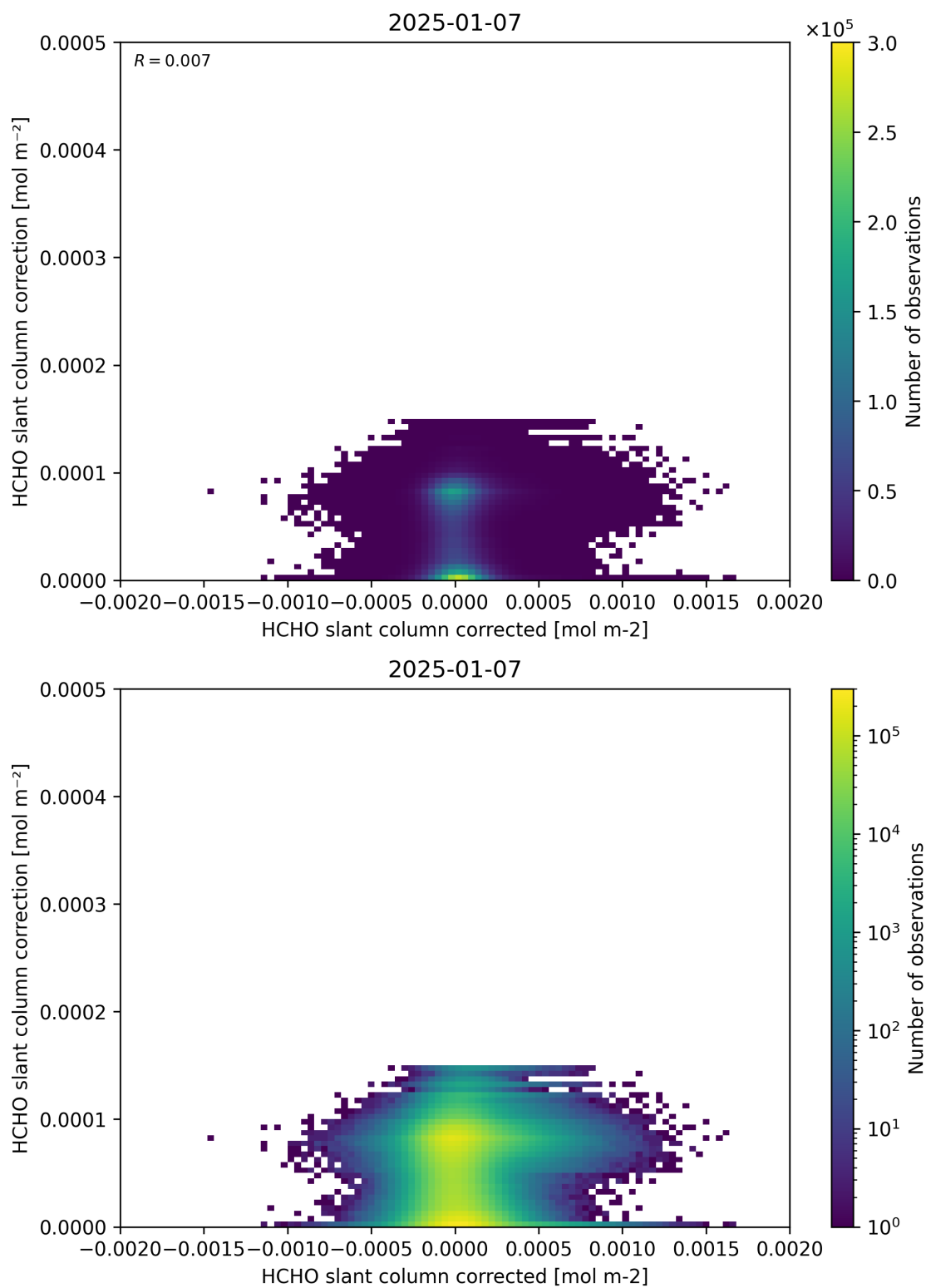
Figure 77: Scatter density plot of “HCHO slant column corrected” against “HCHO slant column correction” for 2025-01-07 to 2025-01-08.
