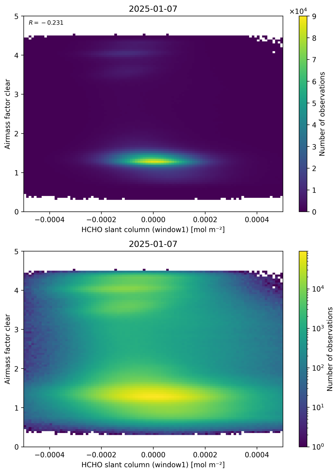
Figure 81: Scatter density plot of “HCHO slant column (window1)” against “Airmass factor clear” for 2025-01-07 to 2025-01-08.
