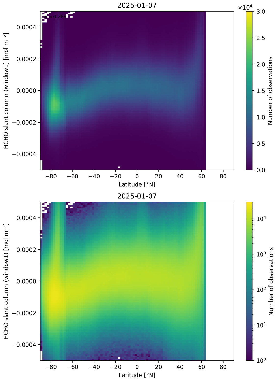
Figure 159: Scatter density plot of “Latitude” against “HCHO slant column (window1)” for 2025-01-07 to 2025-01-08.
