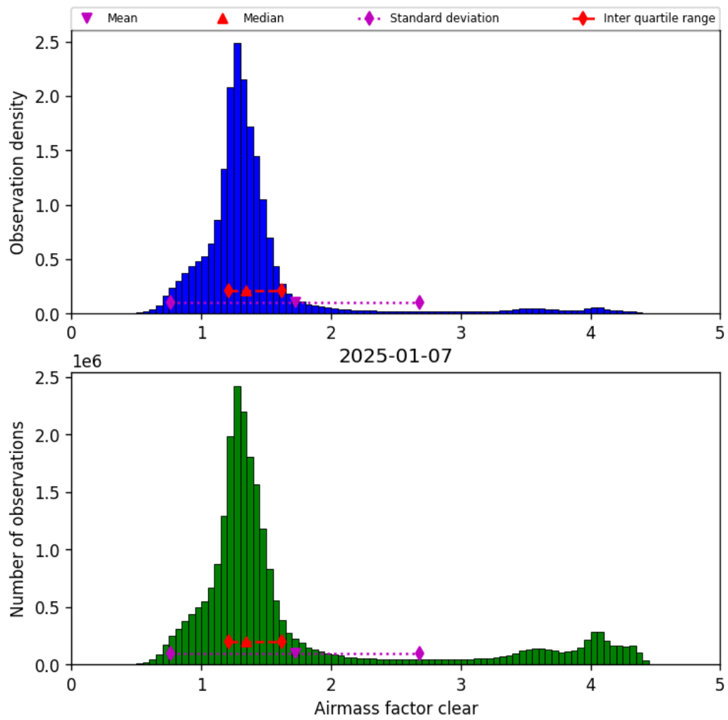
Figure 42: Histogram of “Airmass factor clear” for 2025-01-07 to 2025-01-08
