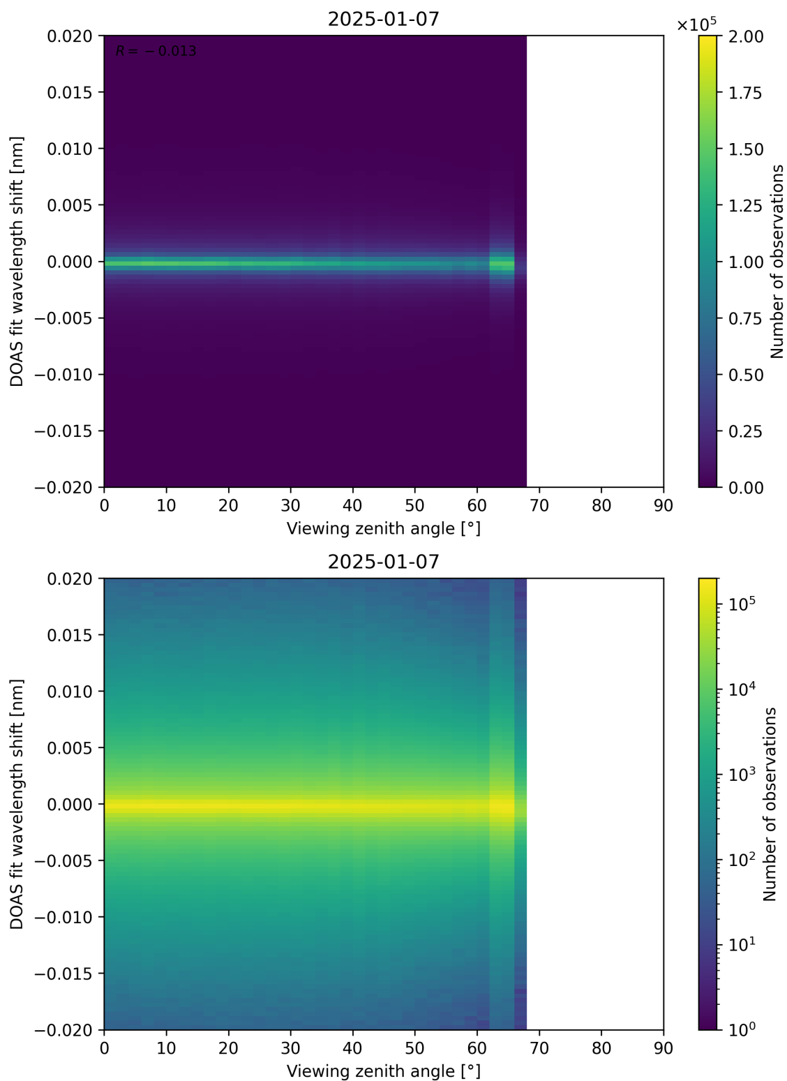
Figure 183: Scatter density plot of “Viewing zenith angle” against “DOAS fit wavelength shift” for 2025-01-07 to 2025-01-08.
