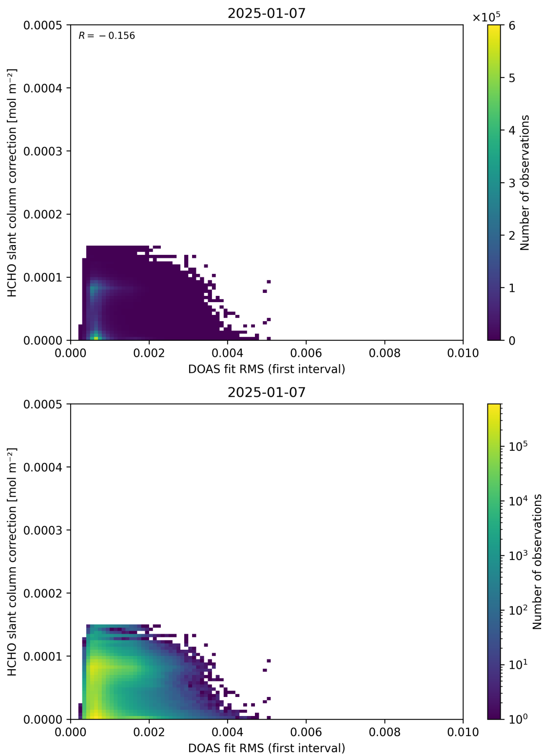
Figure 63: Scatter density plot of “DOAS fit RMS (first interval)” against “HCHO slant column correction” for 2025-01-07 to 2025-01-08.
