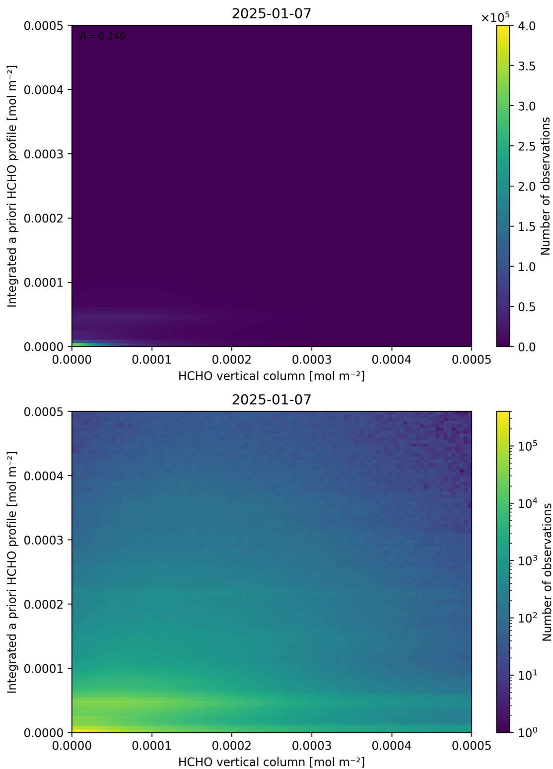
Figure 135: Scatter density plot of “HCHO vertical column” against “Integrated a priori HCHO profile” for 2025-01-07 to 2025-01-08.
