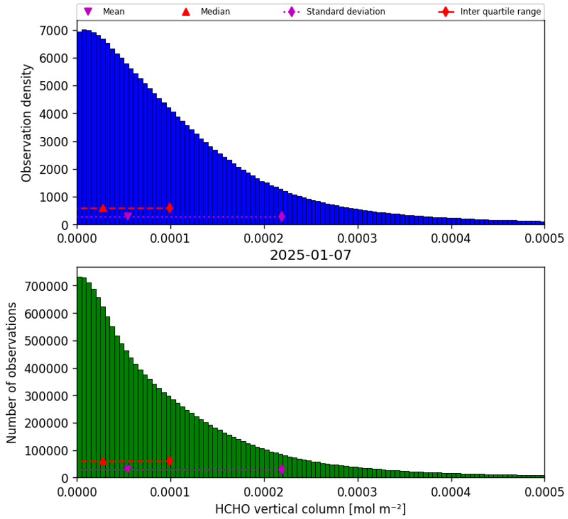
Figure 35: Histogram of “HCHO vertical column” for 2025-01-07 to 2025-01-08
