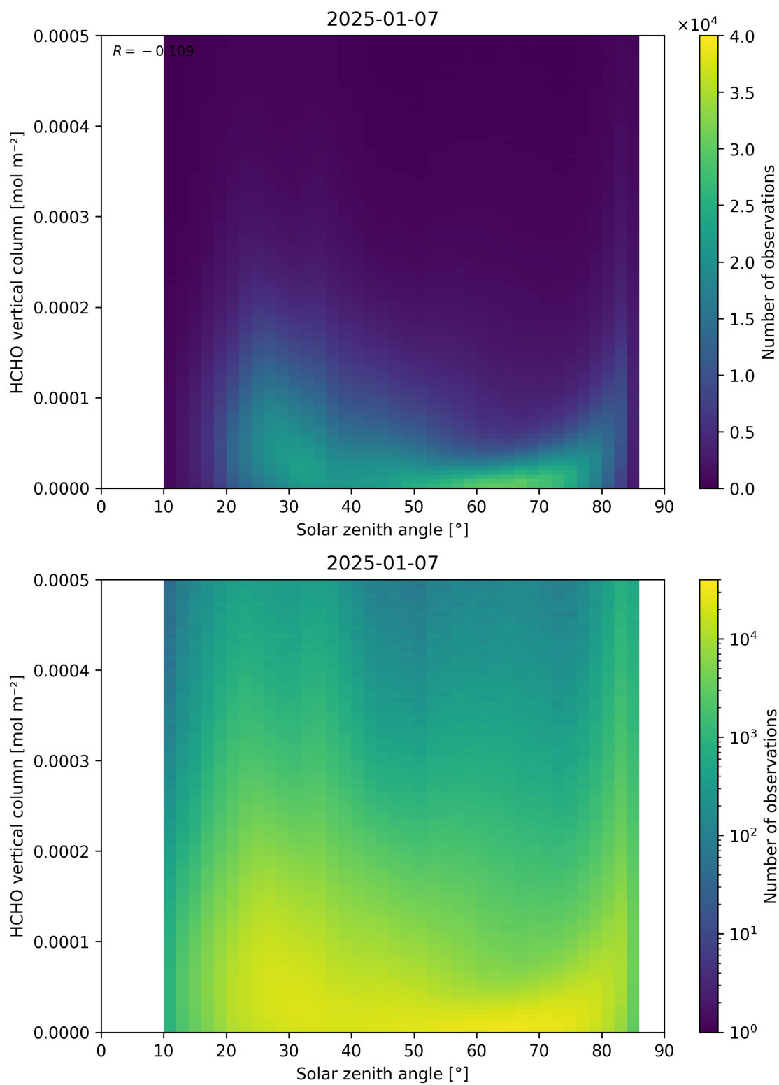
Figure 177: Scatter density plot of “Solar zenith angle” against “HCHO vertical column” for 2025-01-07 to 2025-01-08.
