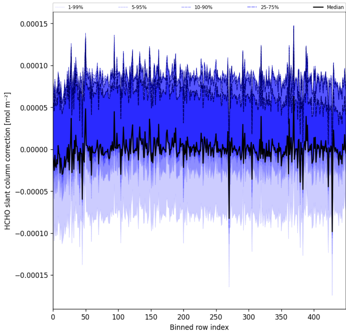
Figure 61: Along track statistics of “HCHO slant column correction” for 2025-01-07 to 2025-01-08
