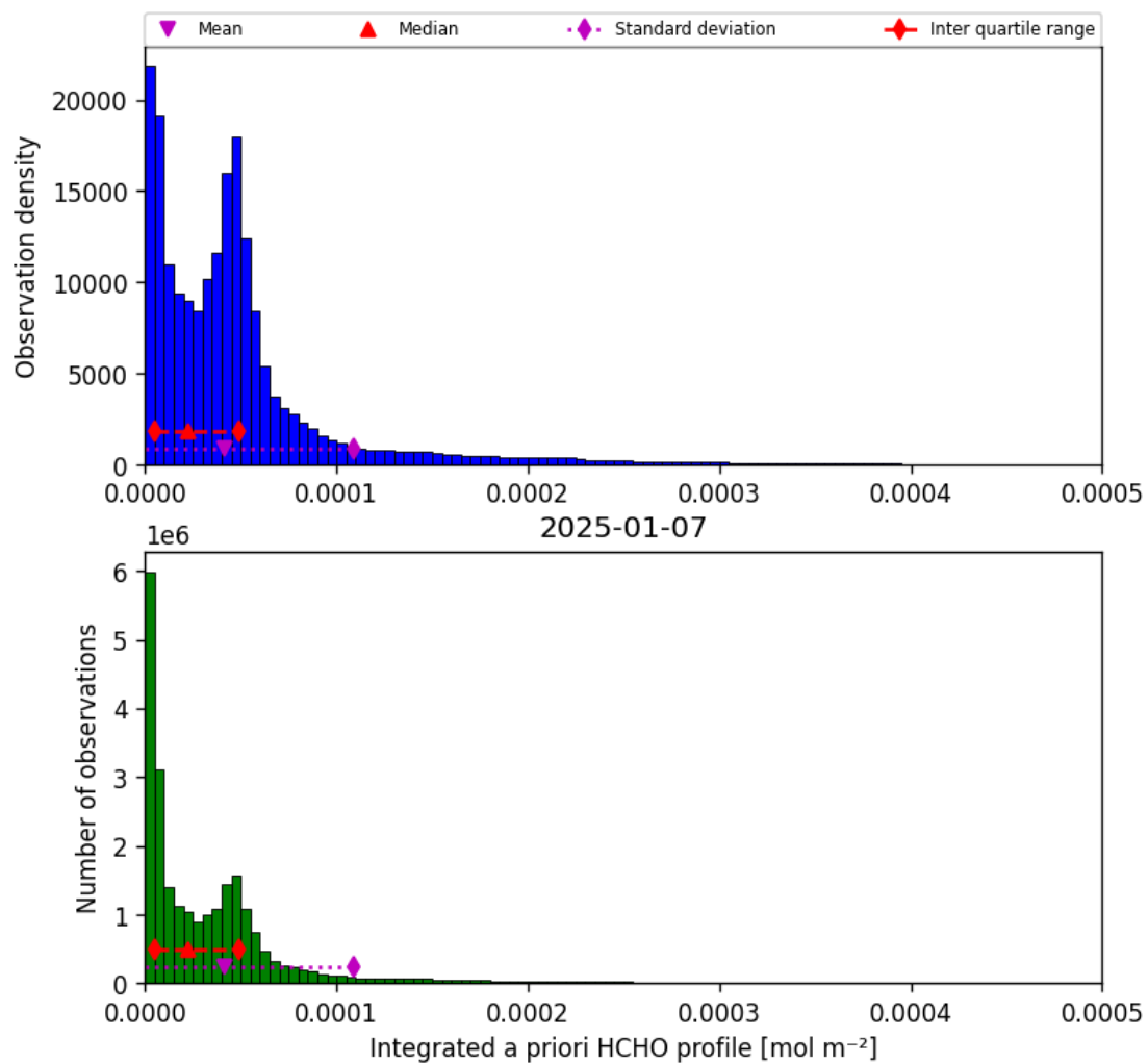
Figure 43: Histogram of “Integrated a priori HCHO profile” for 2025-01-07 to 2025-01-08
