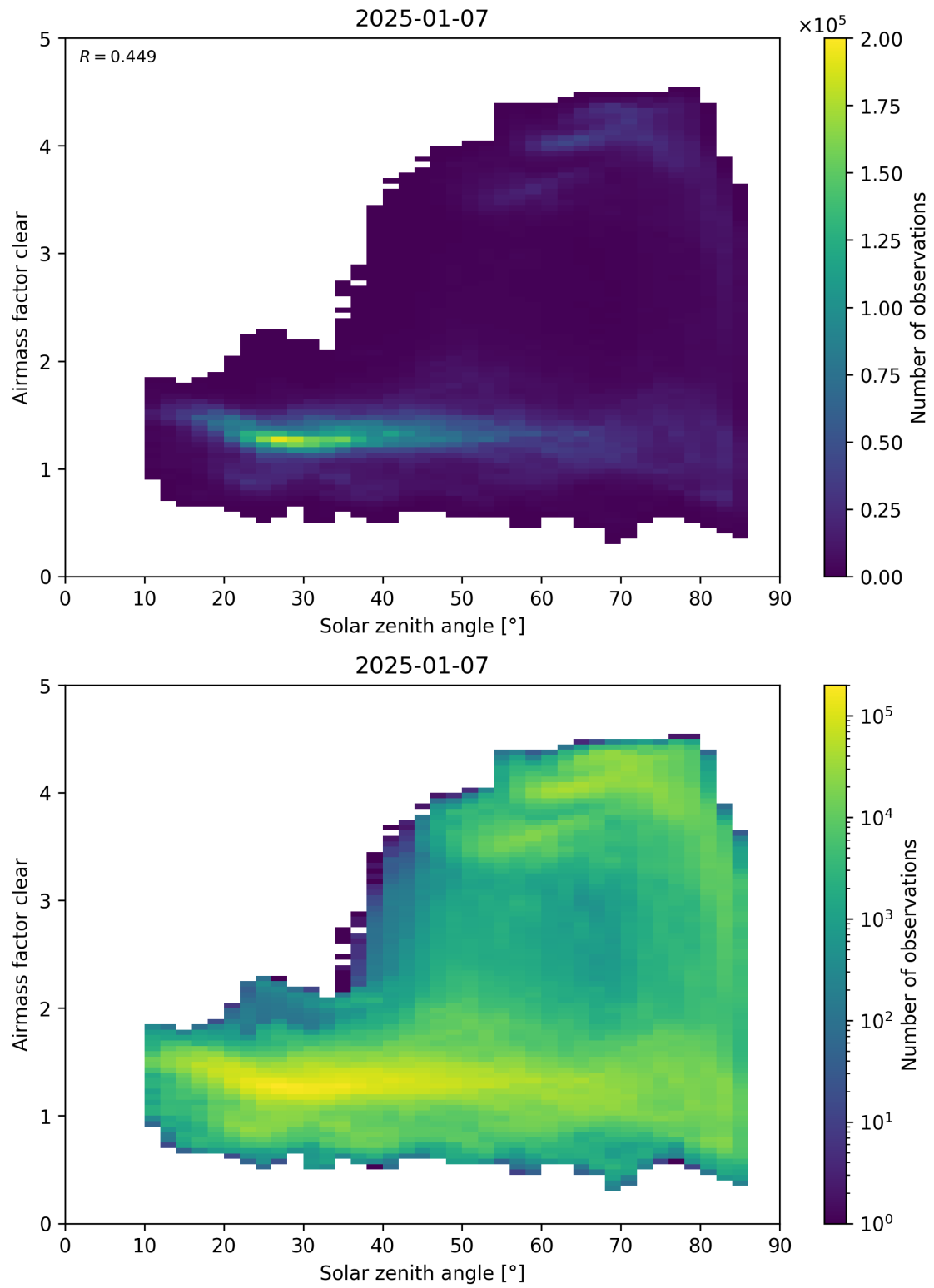
Figure 170: Scatter density plot of “Solar zenith angle” against “Airmass factor clear” for 2025-01-07 to 2025-01-08.
