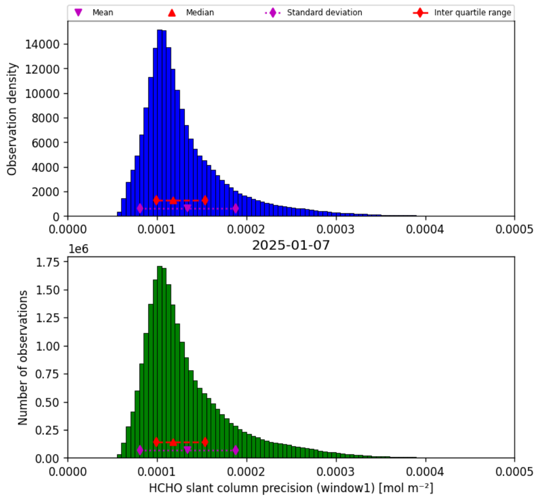
Figure 39: Histogram of “HCHO slant column precision (window1)” for 2025-01-07 to 2025-01-08
