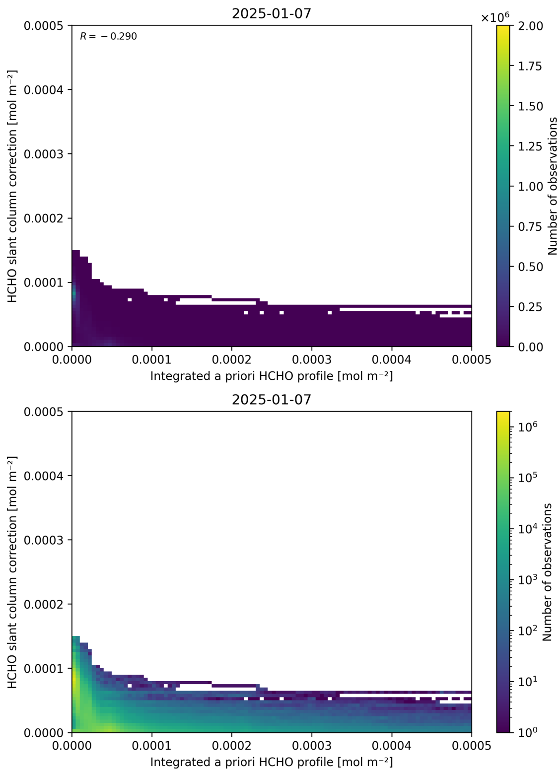
Figure 152: Scatter density plot of “Integrated a priori HCHO profile” against “HCHO slant column correction” for 2025-01-07 to 2025-01-08.
