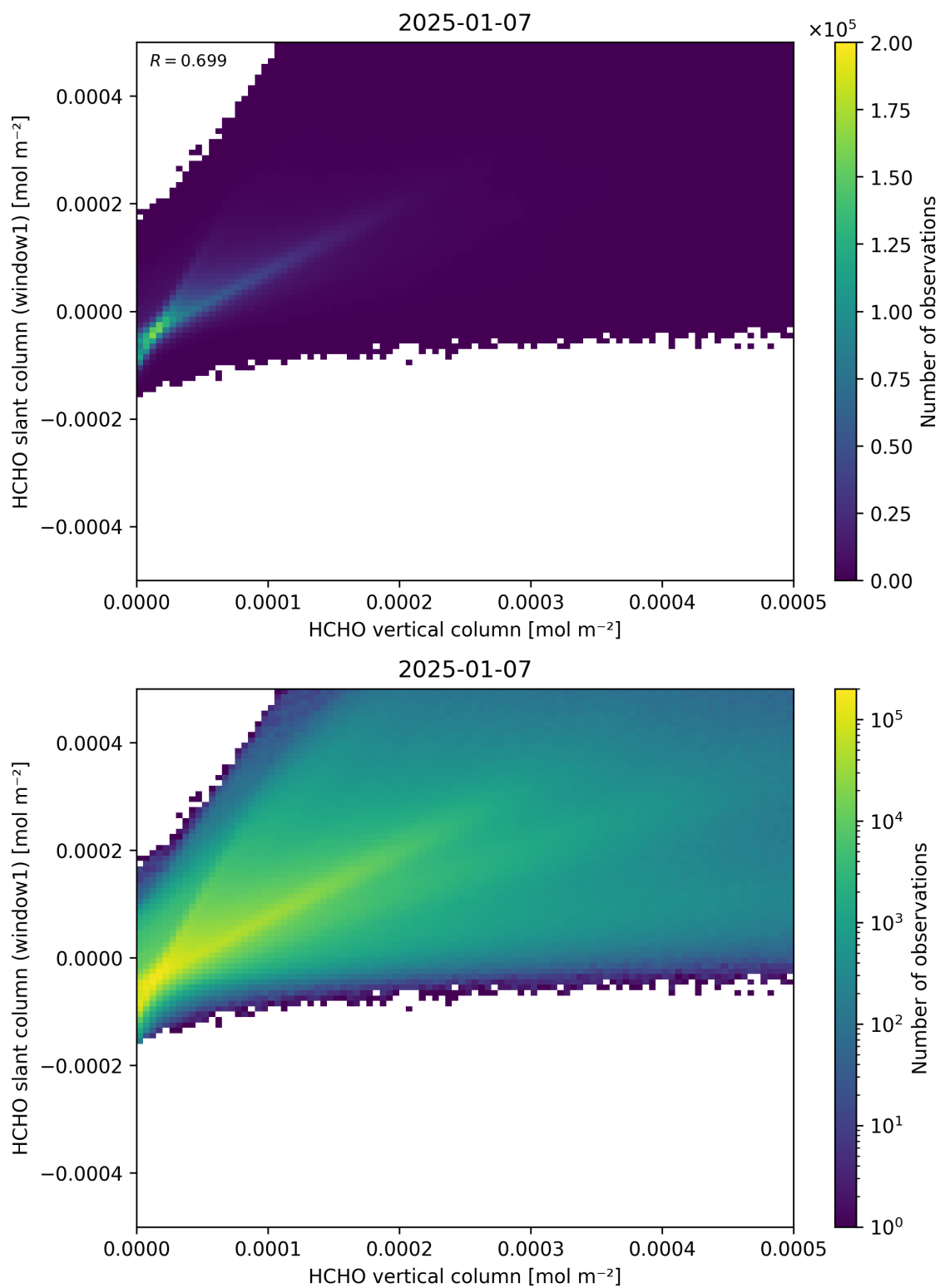
Figure 129: Scatter density plot of “HCHO vertical column” against “HCHO slant column (window1)” for 2025-01-07 to 2025-01-08.
