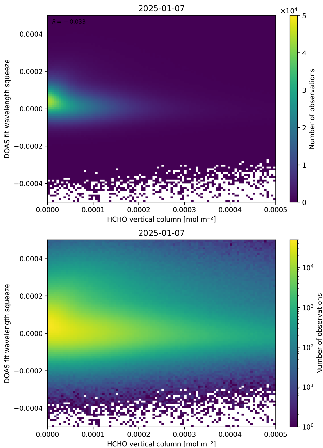
Figure 125: Scatter density plot of “HCHO vertical column” against “DOAS fit wavelength squeeze” for 2025-01-07 to 2025-01-08.
