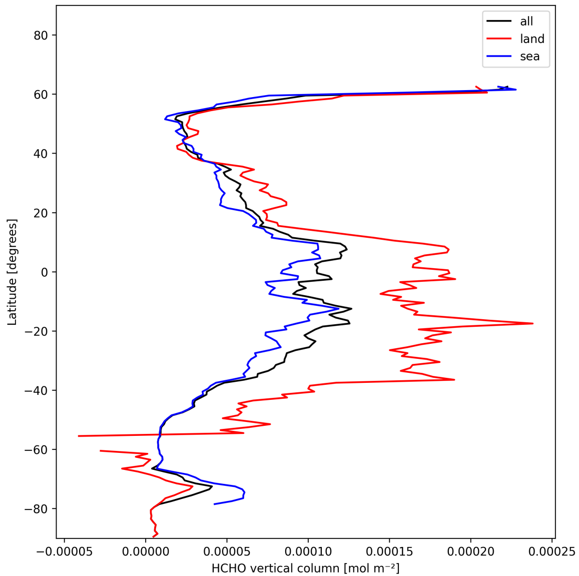
Figure 21: Zonal average of “HCHO vertical column” for 2025-01-07 to 2025-01-08.
