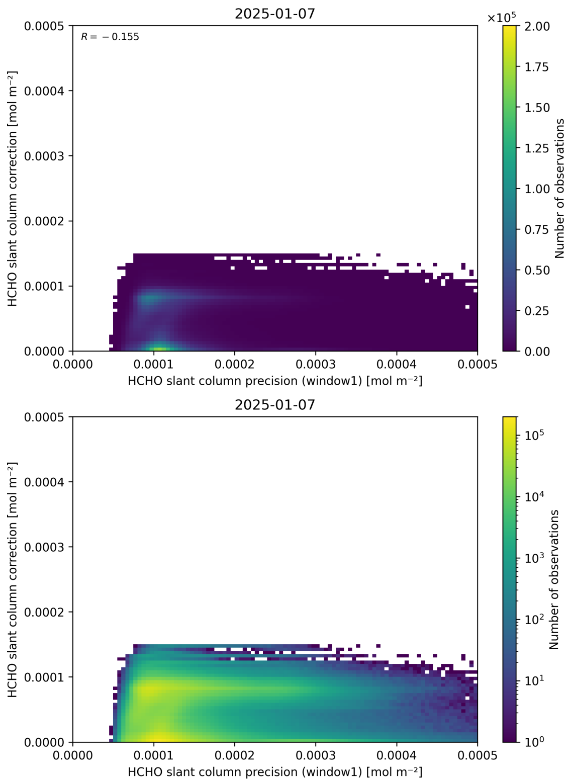
Figure 93: Scatter density plot of “HCHO slant column precision (window1)” against “HCHO slant column correction” for 2025-01-07 to 2025-01-08.
