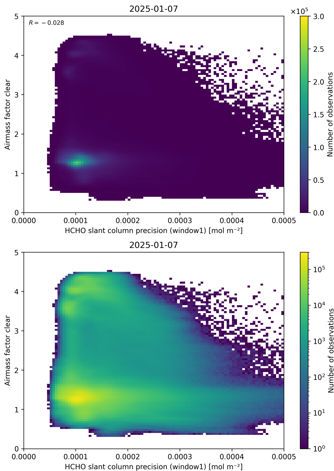
Figure 91: Scatter density plot of “HCHO slant column precision (window1)” against “Airmass factor clear” for 2025-01-07 to 2025-01-08.
