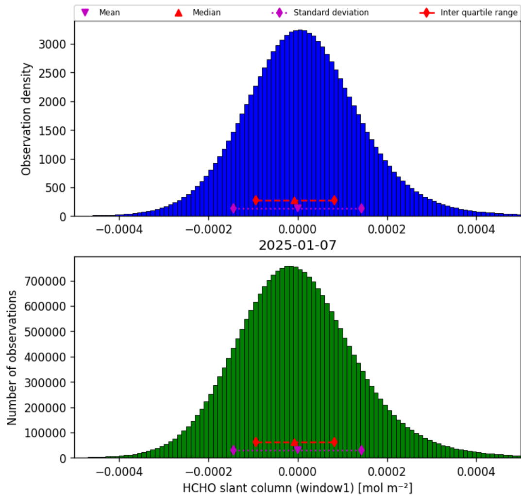
Figure 38: Histogram of “HCHO slant column (window1)” for 2025-01-07 to 2025-01-08
