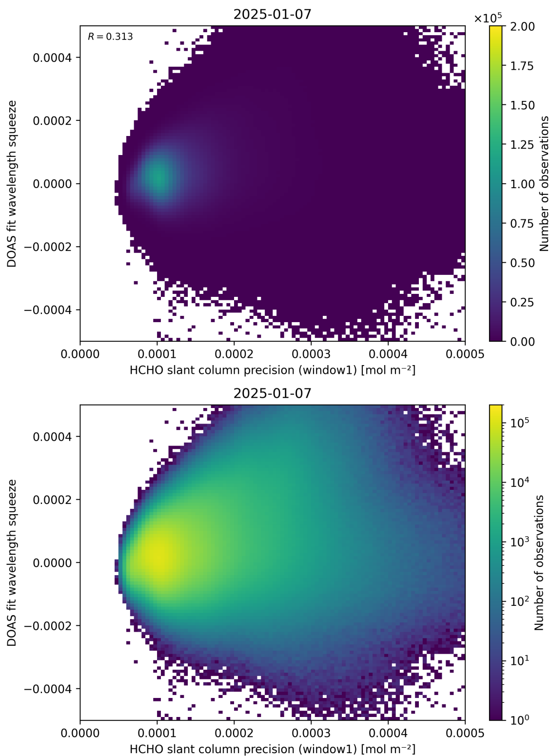
Figure 90: Scatter density plot of “HCHO slant column precision (window1)” against “DOAS fit wavelength squeeze” for 2025-01-07 to 2025-01-08.
