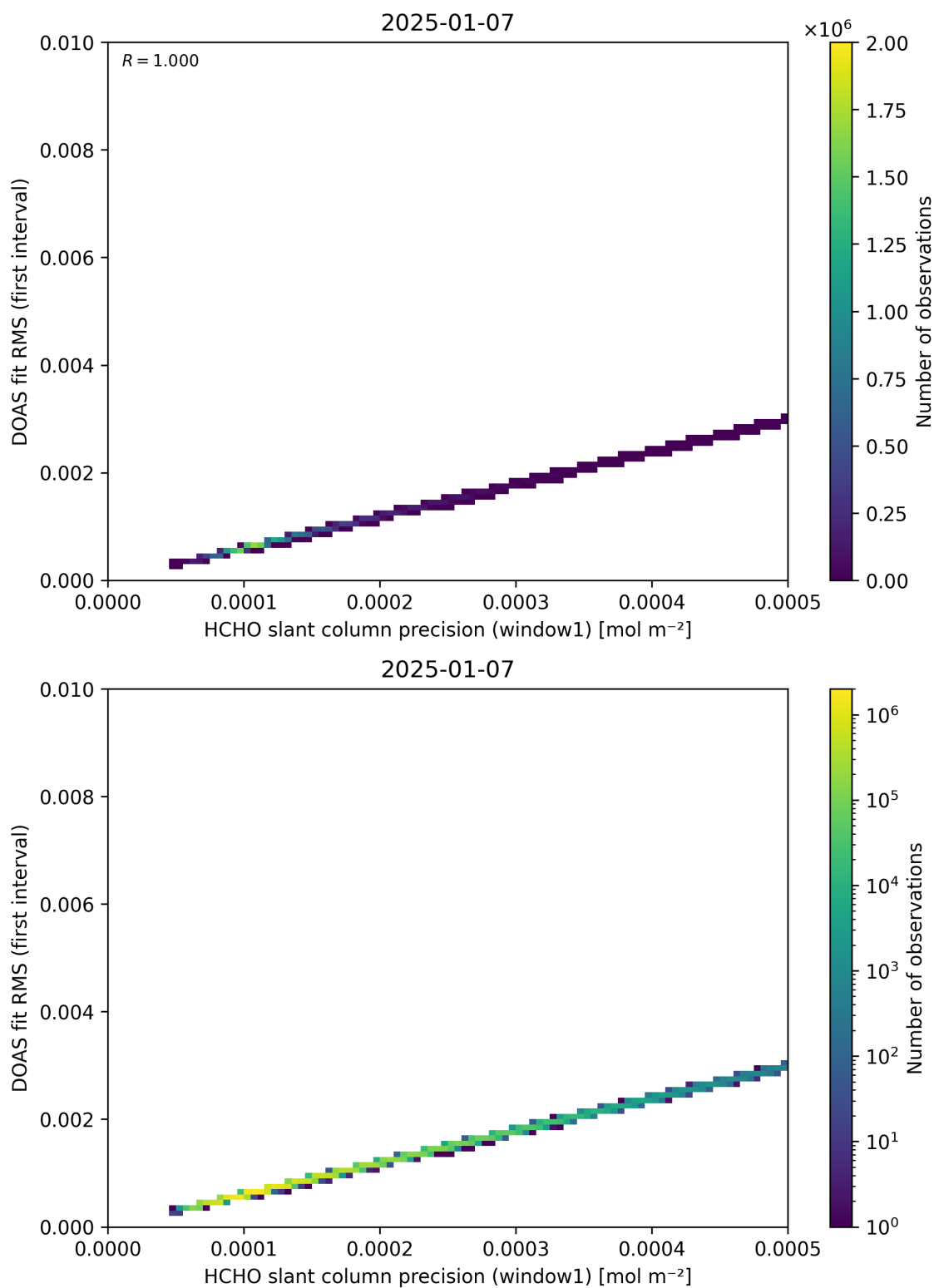
Figure 88: Scatter density plot of “HCHO slant column precision (window1)” against “DOAS fit RMS (first interval)” for 2025-01-07 to 2025-01-08.
