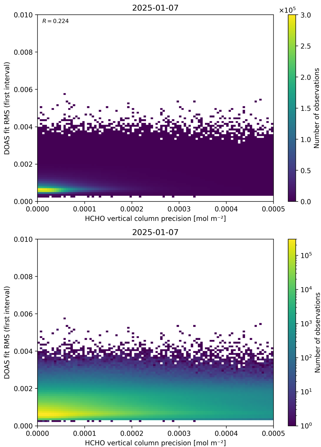
Figure 136: Scatter density plot of “HCHO vertical column precision” against “DOAS fit RMS (first interval)” for 2025-01-07 to 2025-01-08.
