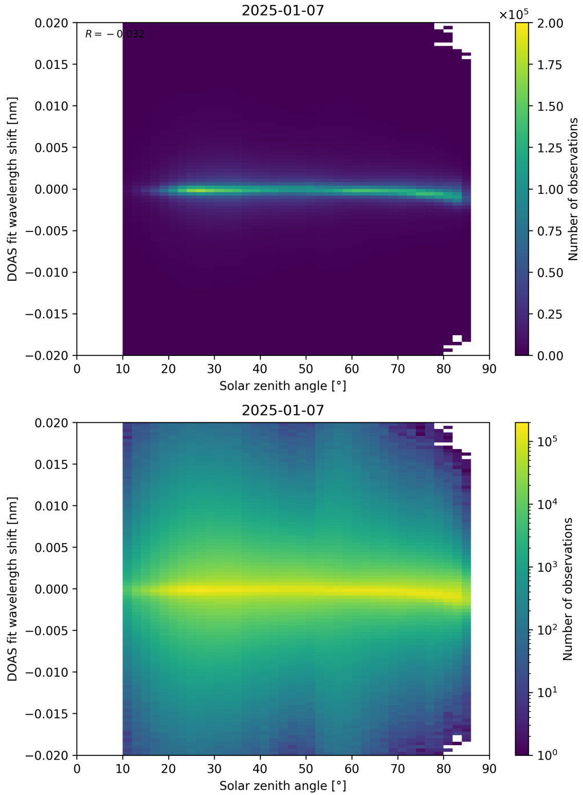
Figure 168: Scatter density plot of “Solar zenith angle” against “DOAS fit wavelength shift” for 2025-01-07 to 2025-01-08.
