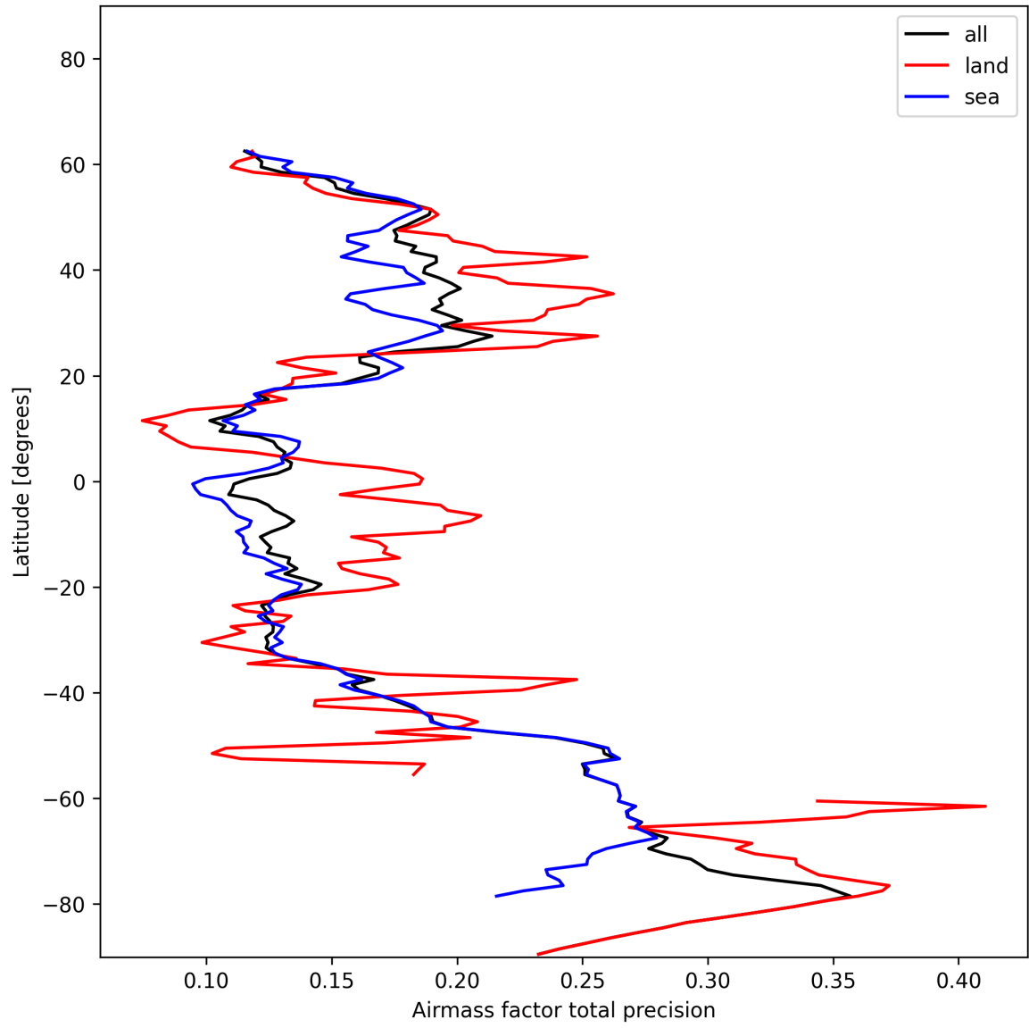
Figure 27: Zonal average of “Airmass factor total precision” for 2025-01-07 to 2025-01-08.
