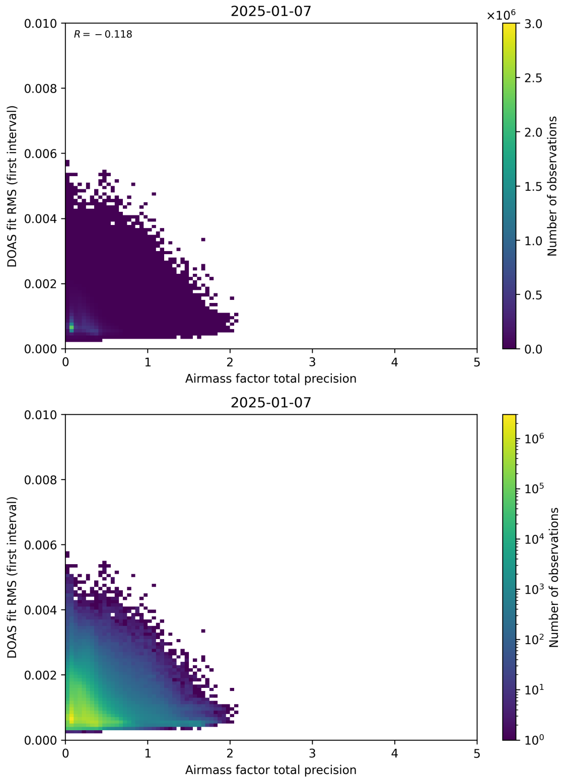
Figure 105: Scatter density plot of “Airmass factor total precision” against “DOAS fit RMS (first interval)” for 2025-01-07 to 2025-01-08.
