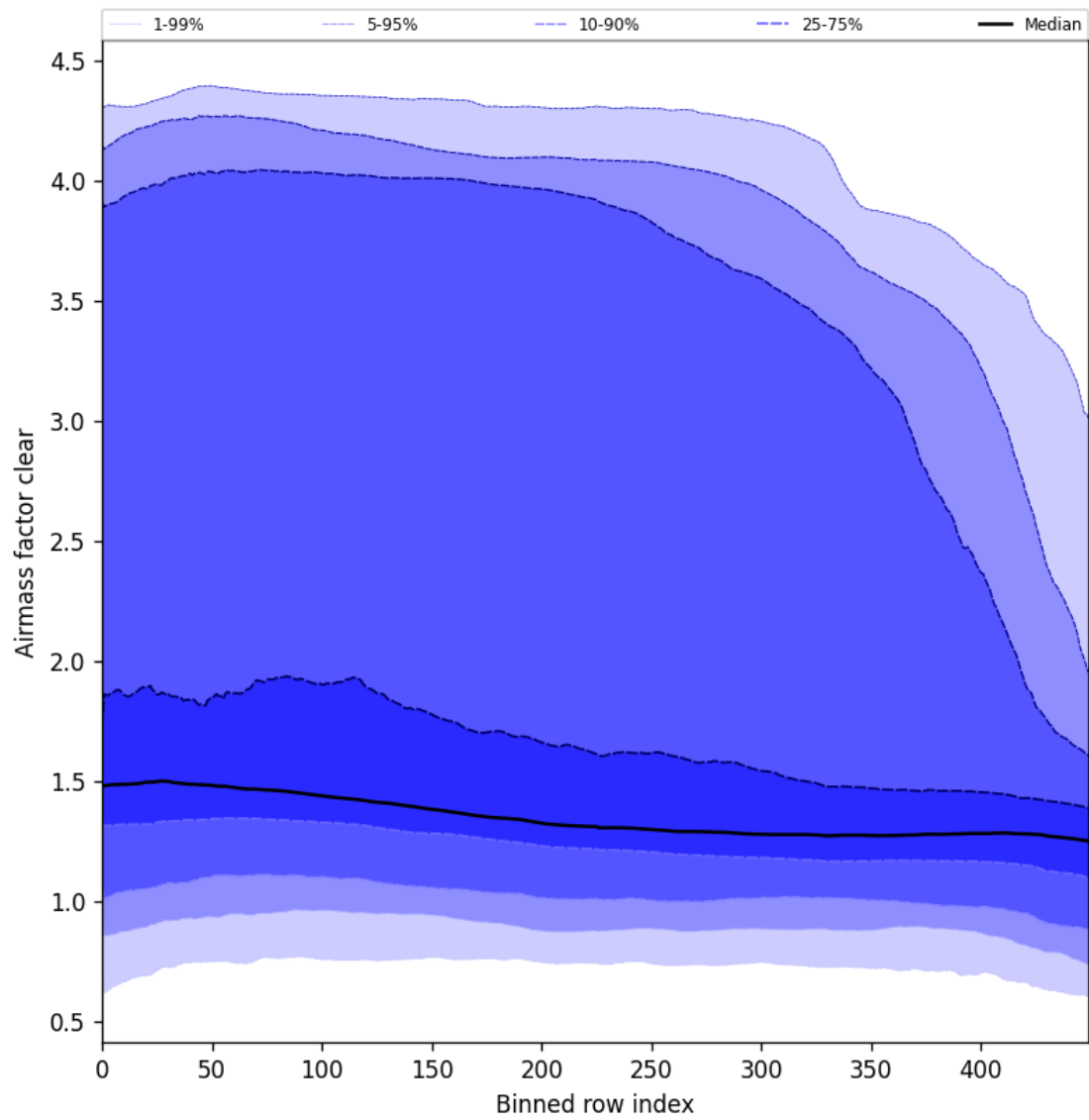
Figure 56: Along track statistics of “Air mass factor clear” for 2025-01-07 to 2025-01-08
