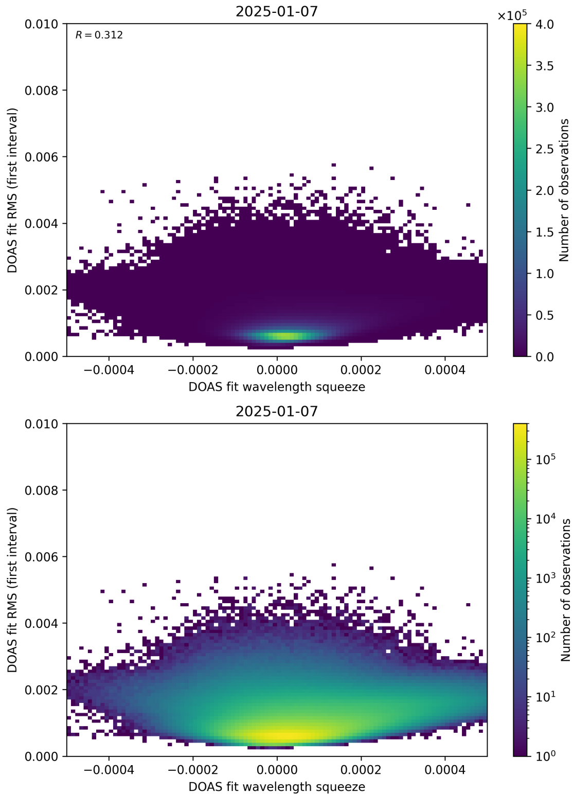
Figure 68: Scatter density plot of “DOAS fit wavelength squeeze” against “DOAS fit RMS (first interval)” for 2025-01-07 to 2025-01-08.
