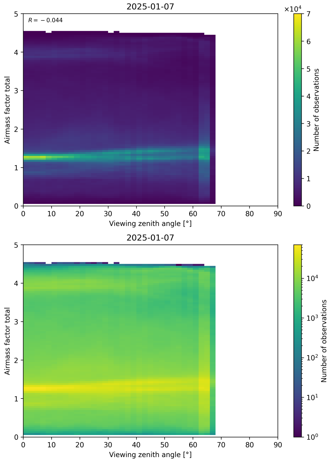
Figure 190: Scatter density plot of “Viewing zenith angle” against “Airmass factor total” for 2025-01-07 to 2025-01-08.
