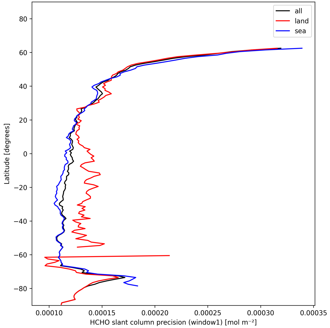
Figure 25: Zonal average of “HCHO slant column precision (window1)” for 2025-01-07 to 2025-01-08.
