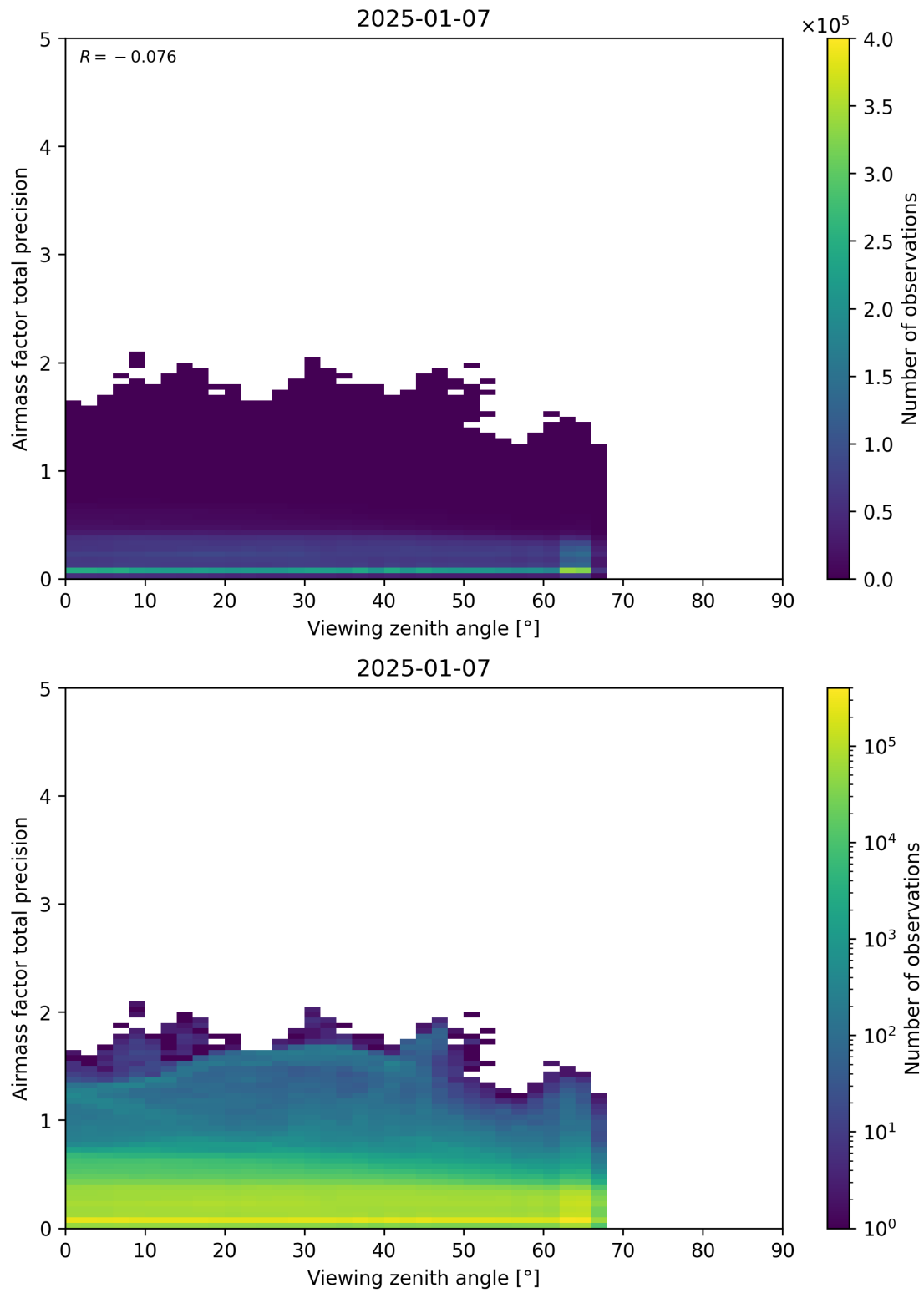
Figure 191: Scatter density plot of “Viewing zenith angle” against “Airmass factor total precision” for 2025-01-07 to 2025-01-08.
