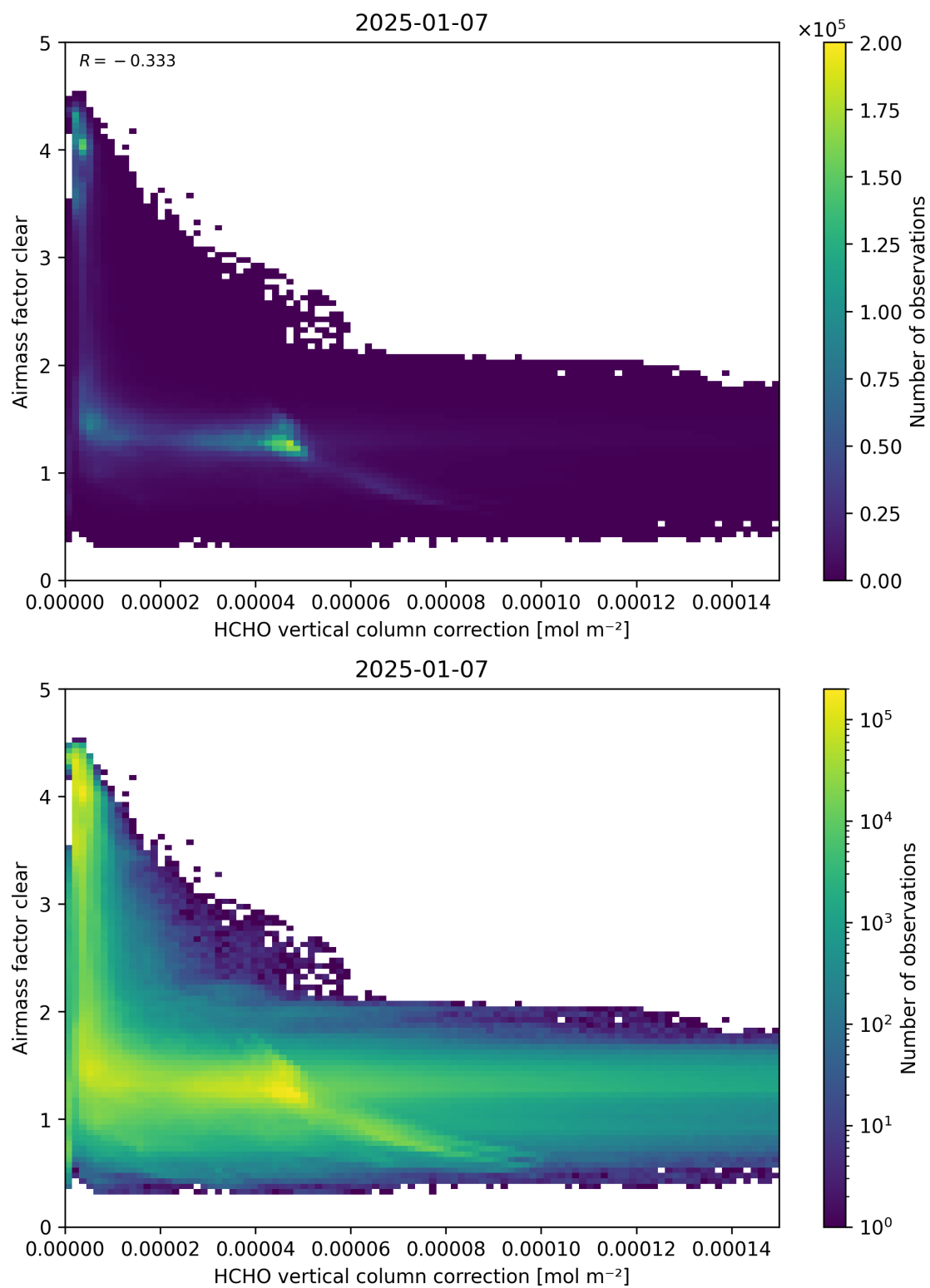
Figure 115: Scatter density plot of “HCHO vertical column correction” against “Airmass factor clear” for 2025-01-07 to 2025-01-08.
