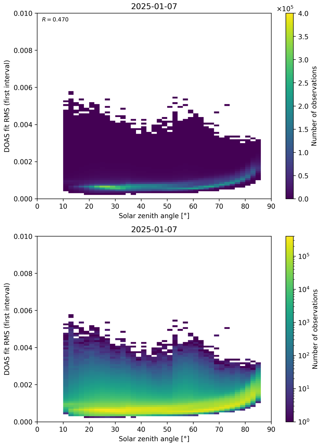
Figure 167: Scatter density plot of “Solar zenith angle” against “DOAS fit RMS (first interval)” for 2025-01-07 to 2025-01-08.
