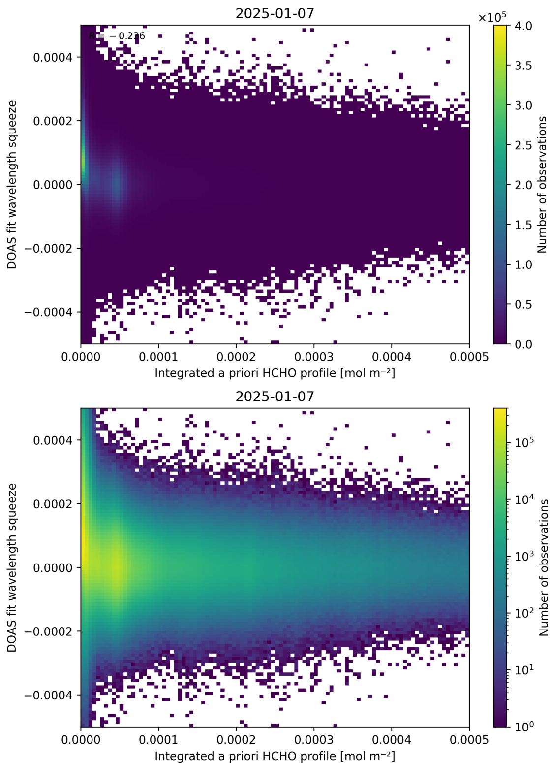
Figure 150: Scatter density plot of “Integrated a priori HCHO profile” against “DOAS fit wavelength squeeze” for 2025-01-07 to 2025-01-08.
