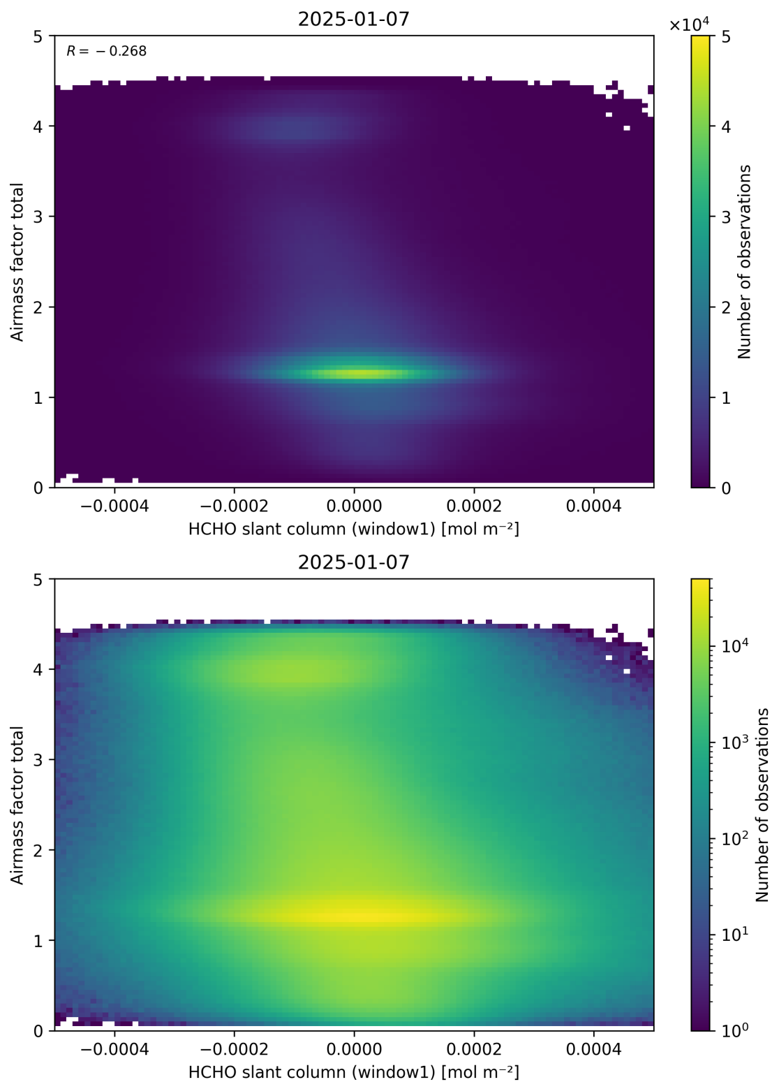
Figure 85: Scatter density plot of “HCHO slant column (window1)” against “Airmass factor total” for 2025-01-07 to 2025-01-08.
