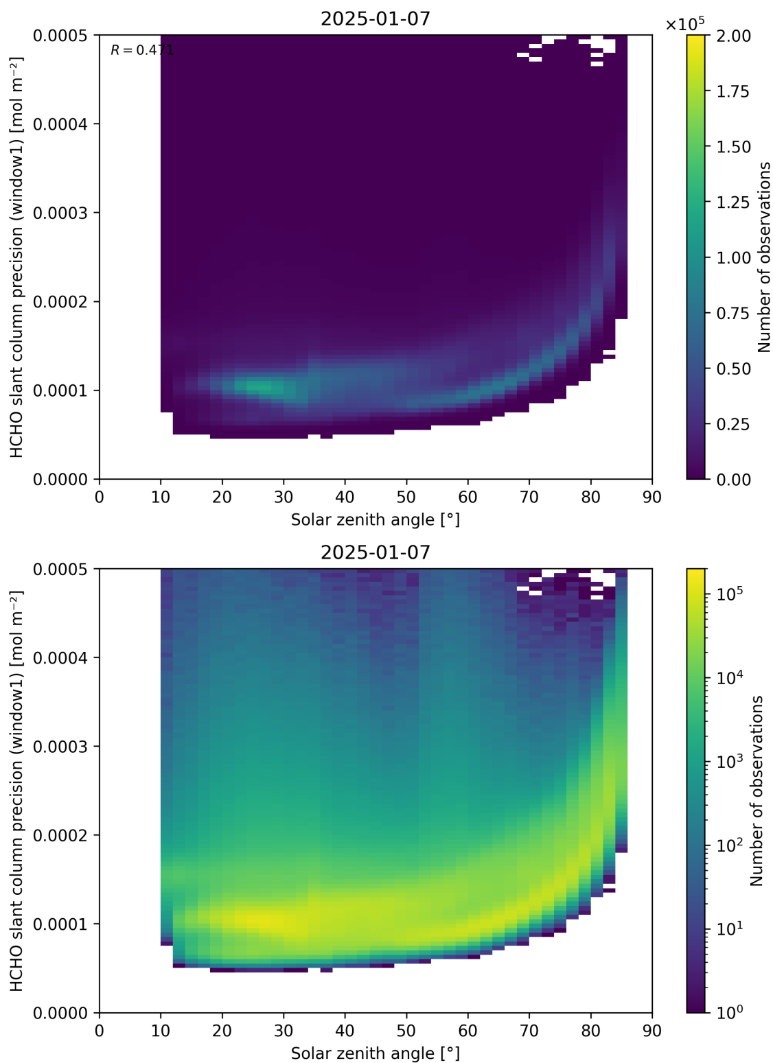
Figure 174: Scatter density plot of “Solar zenith angle” against “HCHO slant column precision (window1)” for 2025-01-07 to 2025-01-08.
