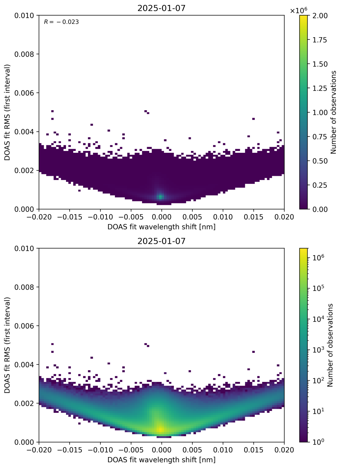
Figure 64: Scatter density plot of “DOAS fit wavelength shift” against “DOAS fit RMS (first interval)” for 2025-01-07 to 2025-01-08.
