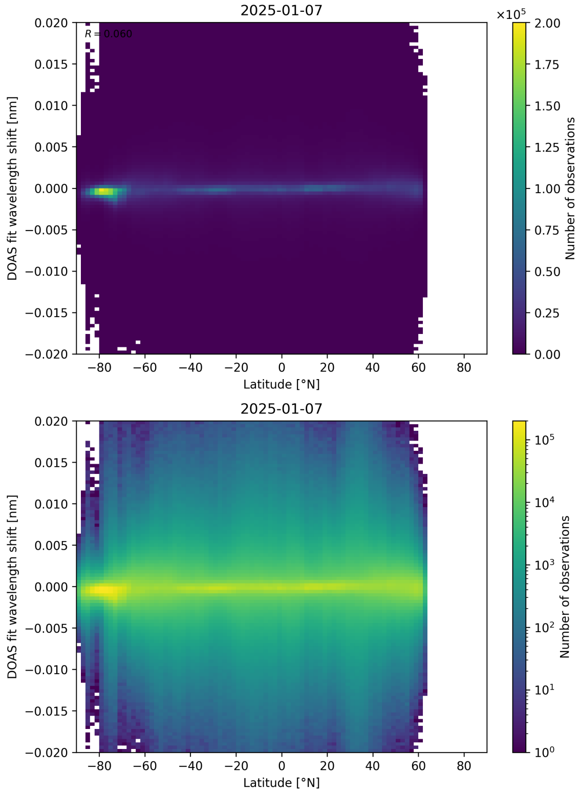
Figure 154: Scatter density plot of “Latitude” against “DOAS fit wavelength shift” for 2025-01-07 to 2025-01-08.
