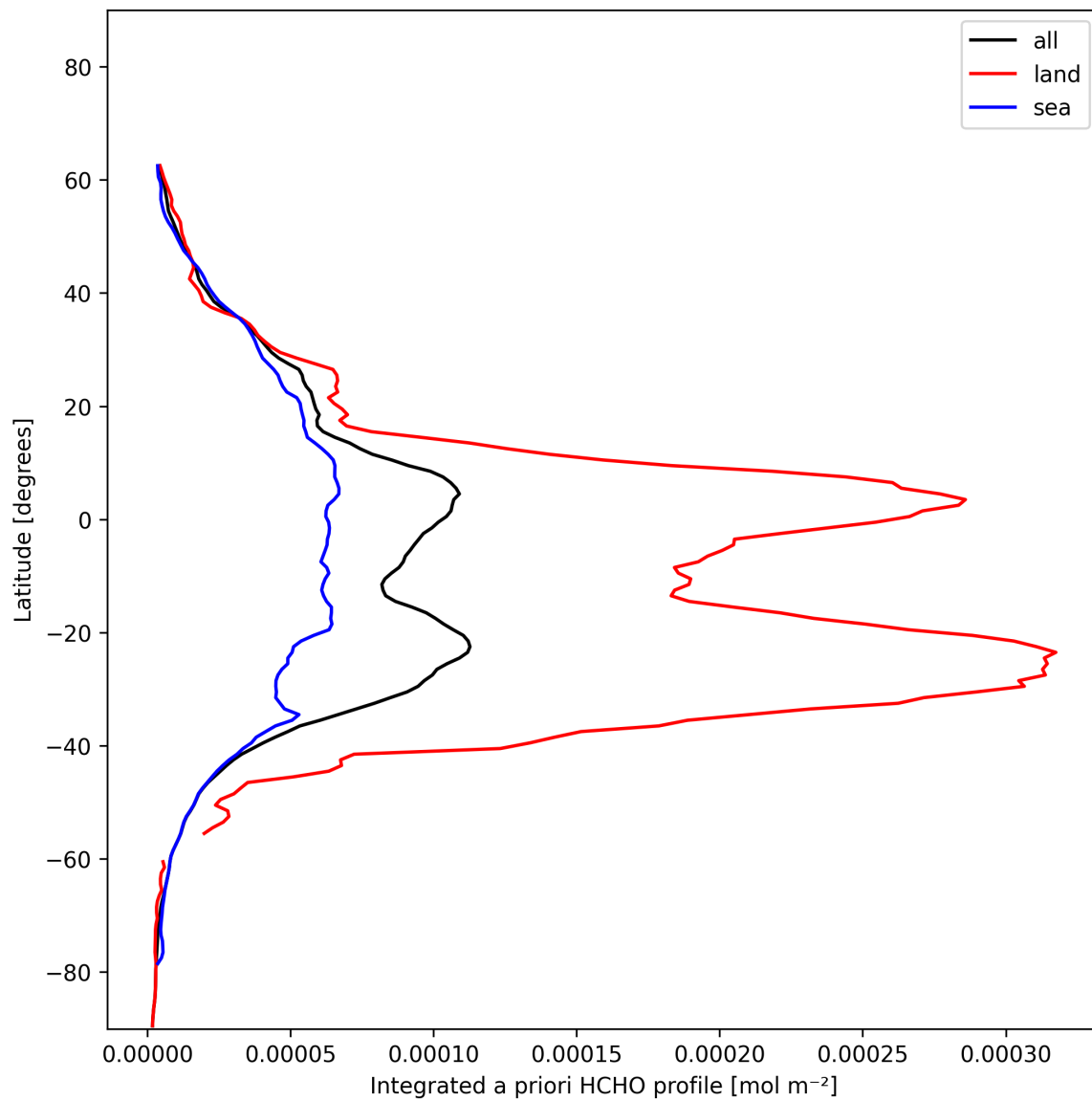
Figure 29: Zonal average of “Integrated a priori HCHO profile” for 2025-01-07 to 2025-01-08.
