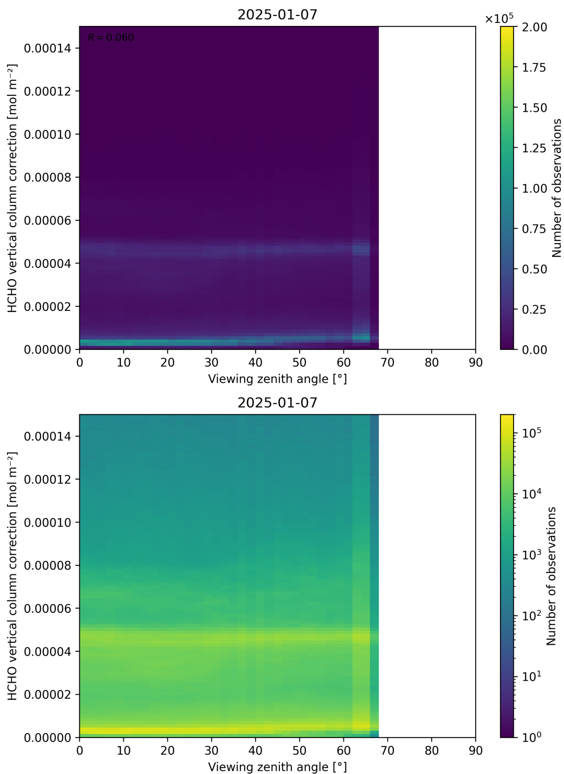
Figure 193: Scatter density plot of “Viewing zenith angle” against “HCHO vertical column correction” for 2025-01-07 to 2025-01-08.
