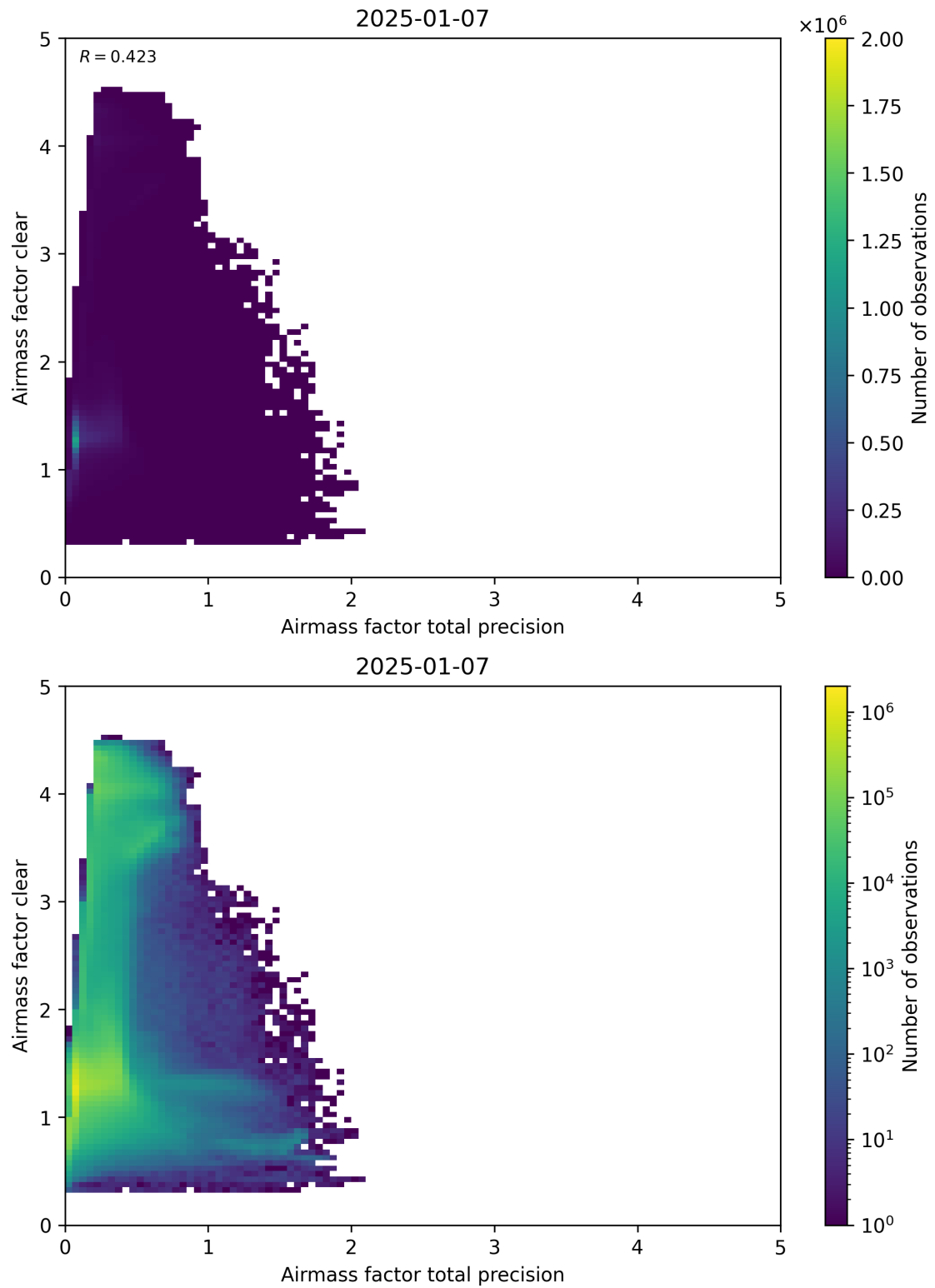
Figure 108: Scatter density plot of “Airmass factor total precision” against “Airmass factor clear” for 2025-01-07 to 2025-01-08.
