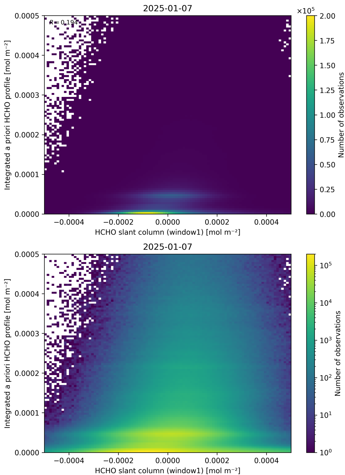
Figure 87: Scatter density plot of “HCHO slant column (window1)” against “Integrated a priori HCHO profile” for 2025-01-07 to 2025-01-08.
