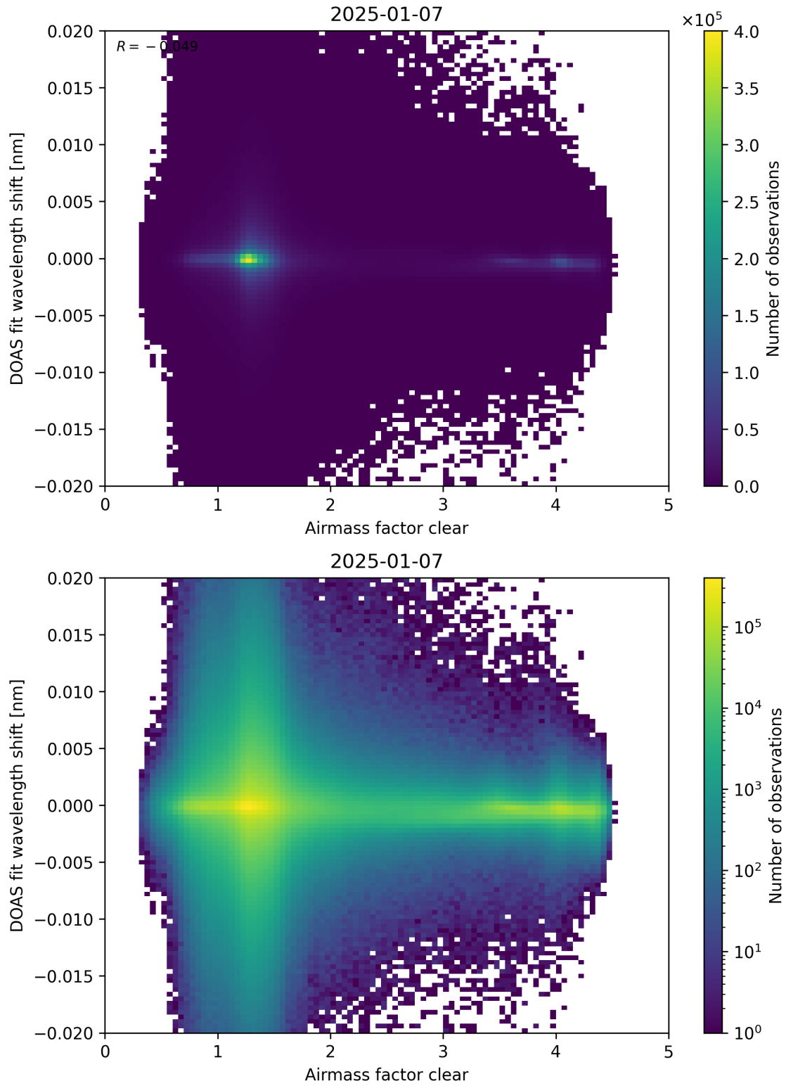
Figure 72: Scatter density plot of “Airmass factor clear” against “DOAS fit wavelength shift” for 2025-01-07 to 2025-01-08.
