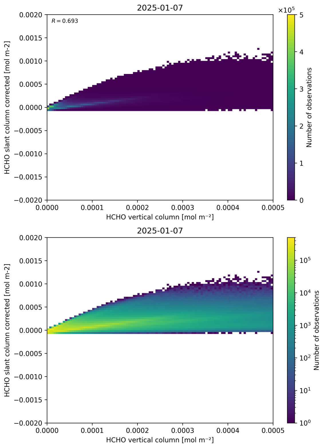
Figure 127: Scatter density plot of “HCHO vertical column” against “HCHO slant column corrected” for 2025-01-07 to 2025-01-08.
