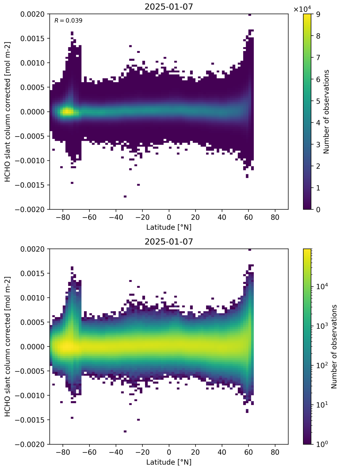
Figure 157: Scatter density plot of “Latitude” against “HCHO slant column corrected” for 2025-01-07 to 2025-01-08.
