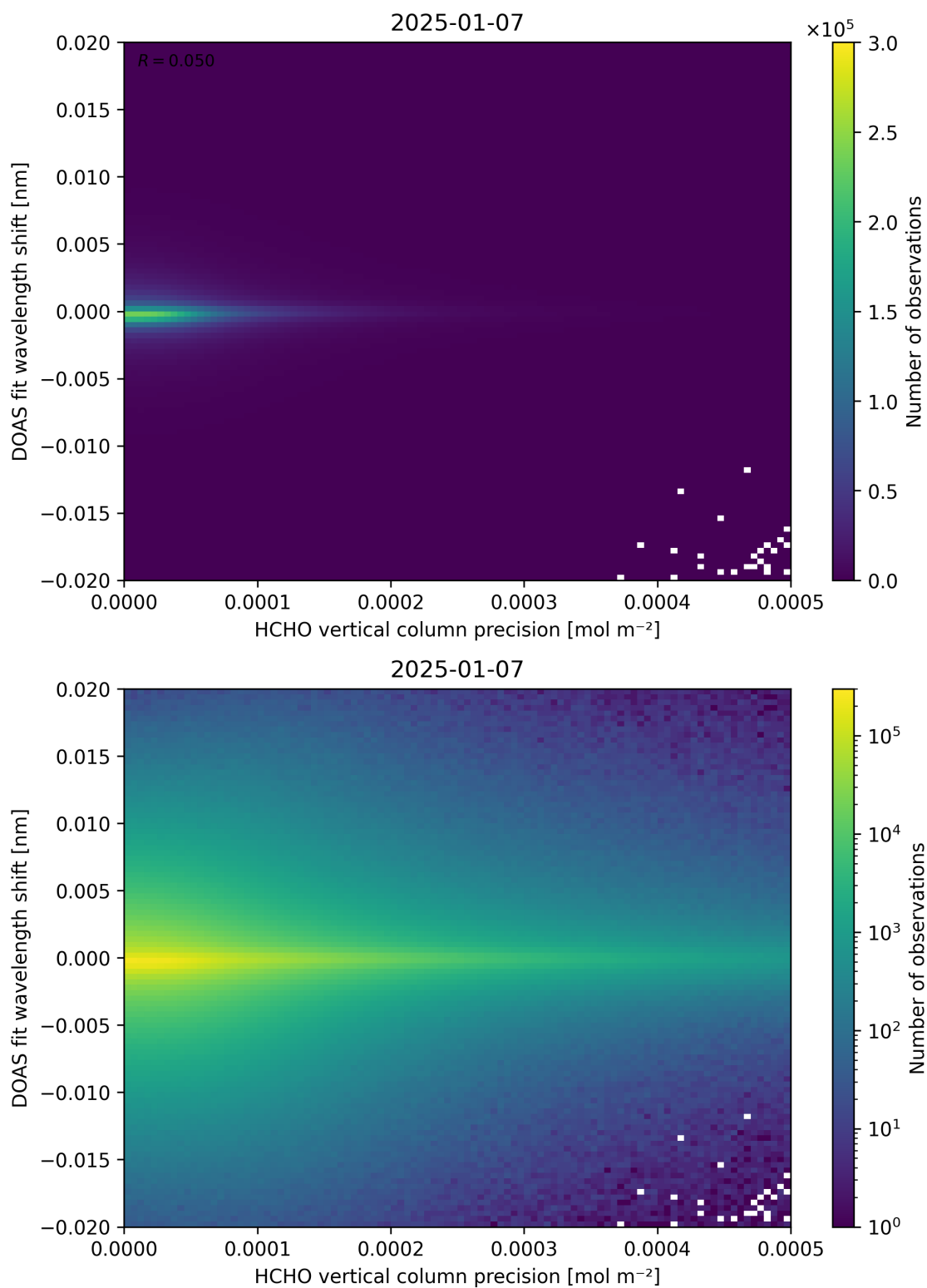
Figure 137: Scatter density plot of “HCHO vertical column precision” against “DOAS fit wavelength shift” for 2025-01-07 to 2025-01-08.
