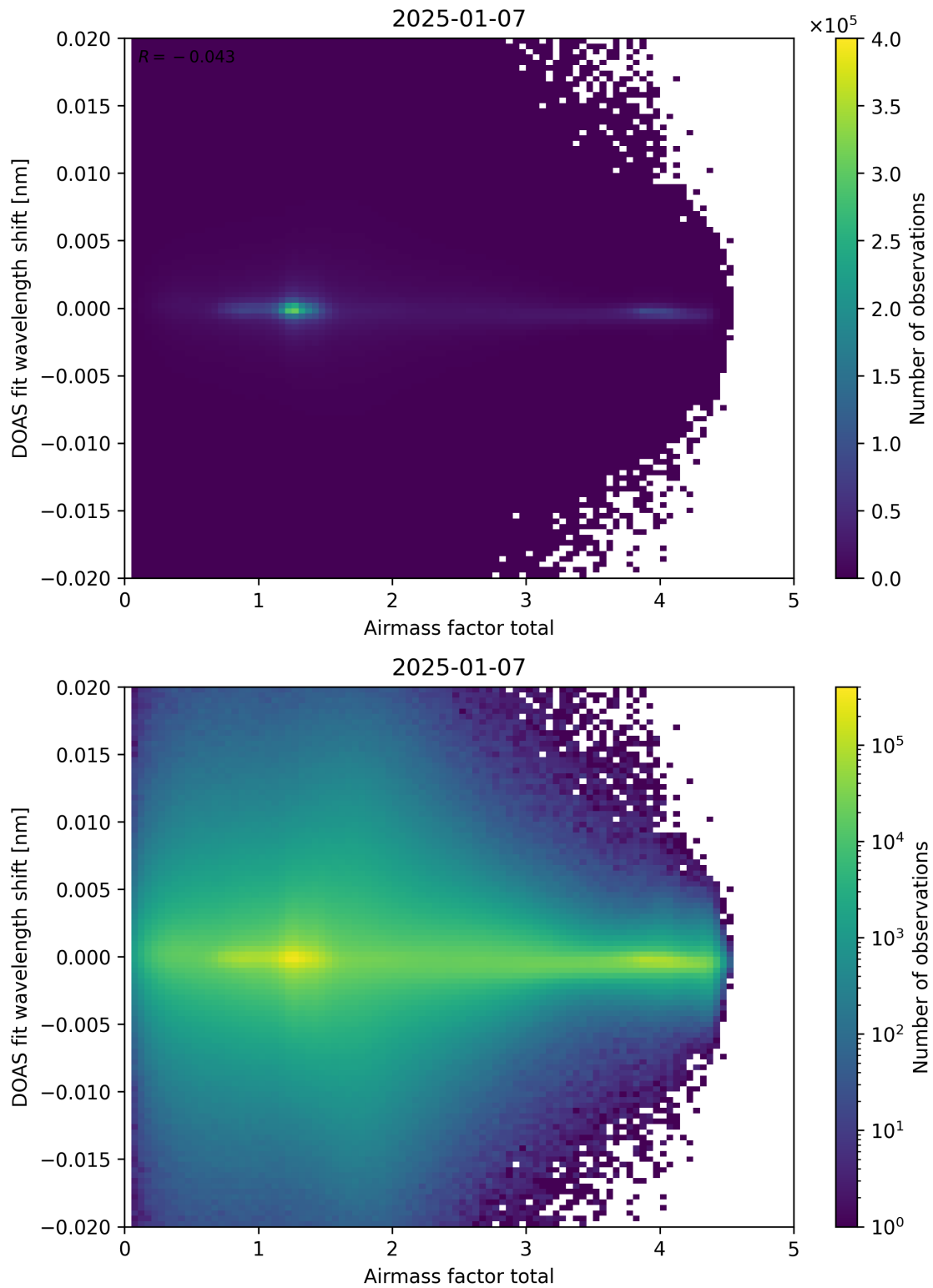
Figure 98: Scatter density plot of “Airmass factor total” against “DOAS fit wavelength shift” for 2025-01-07 to 2025-01-08.
