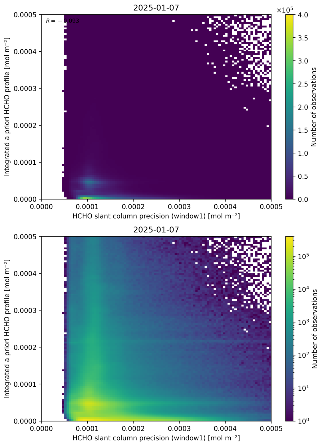
Figure 96: Scatter density plot of “HCHO slant column precision (window1)” against “Integrated a priori HCHO profile” for 2025-01-07 to 2025-01-08.
