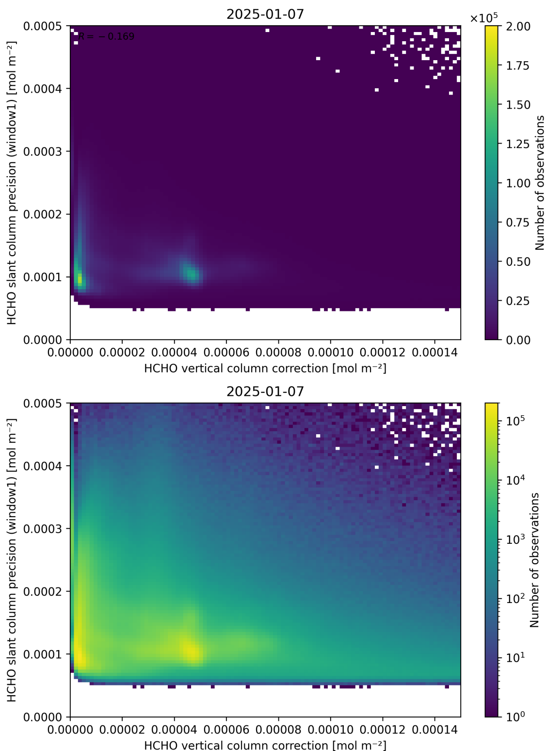
Figure 119: Scatter density plot of “HCHO vertical column correction” against “HCHO slant column precision (window1)” for 2025-01-07 to 2025-01-08.
