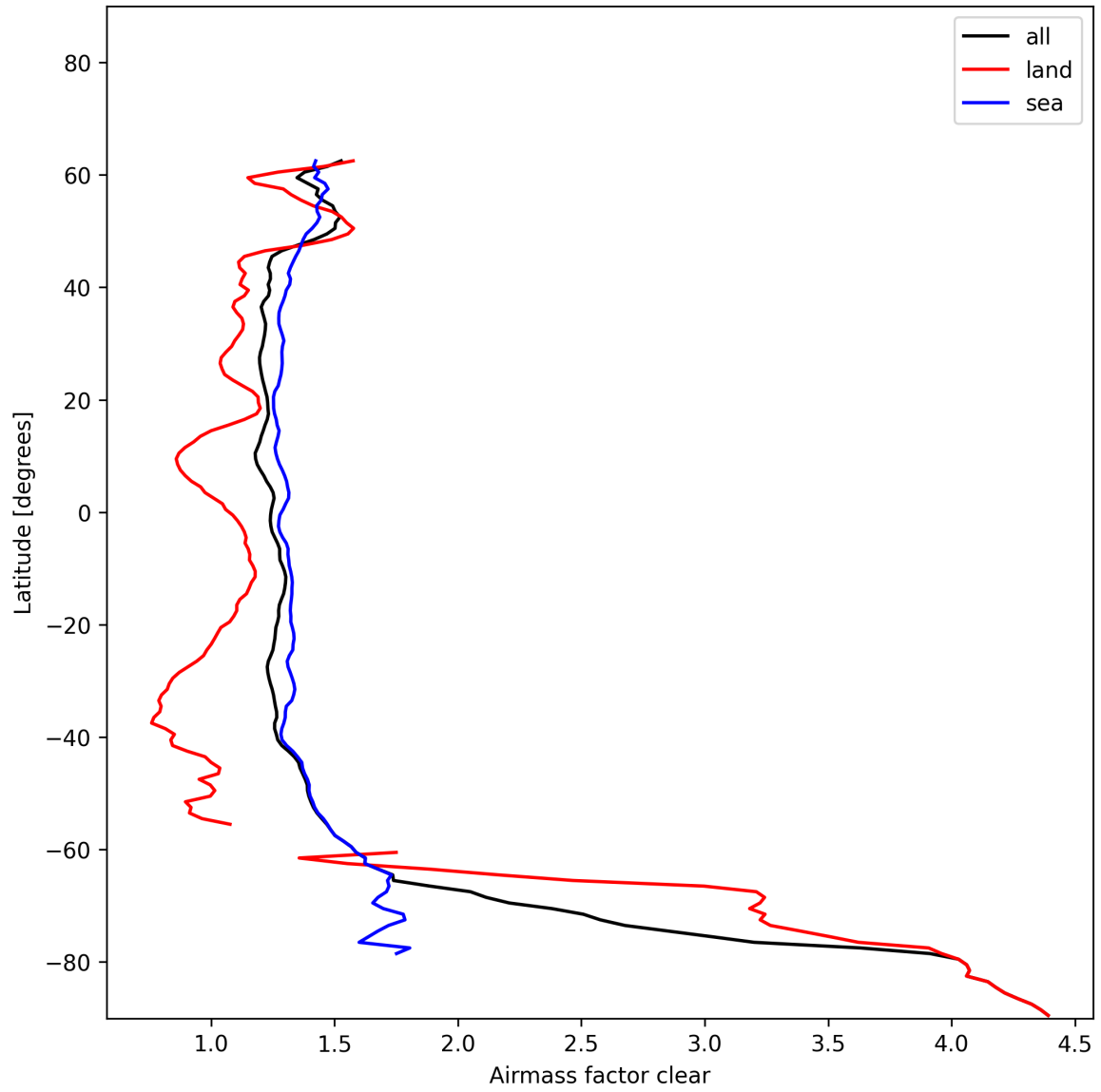
Figure 28: Zonal average of “Airmass factor clear” for 2025-01-07 to 2025-01-08.
