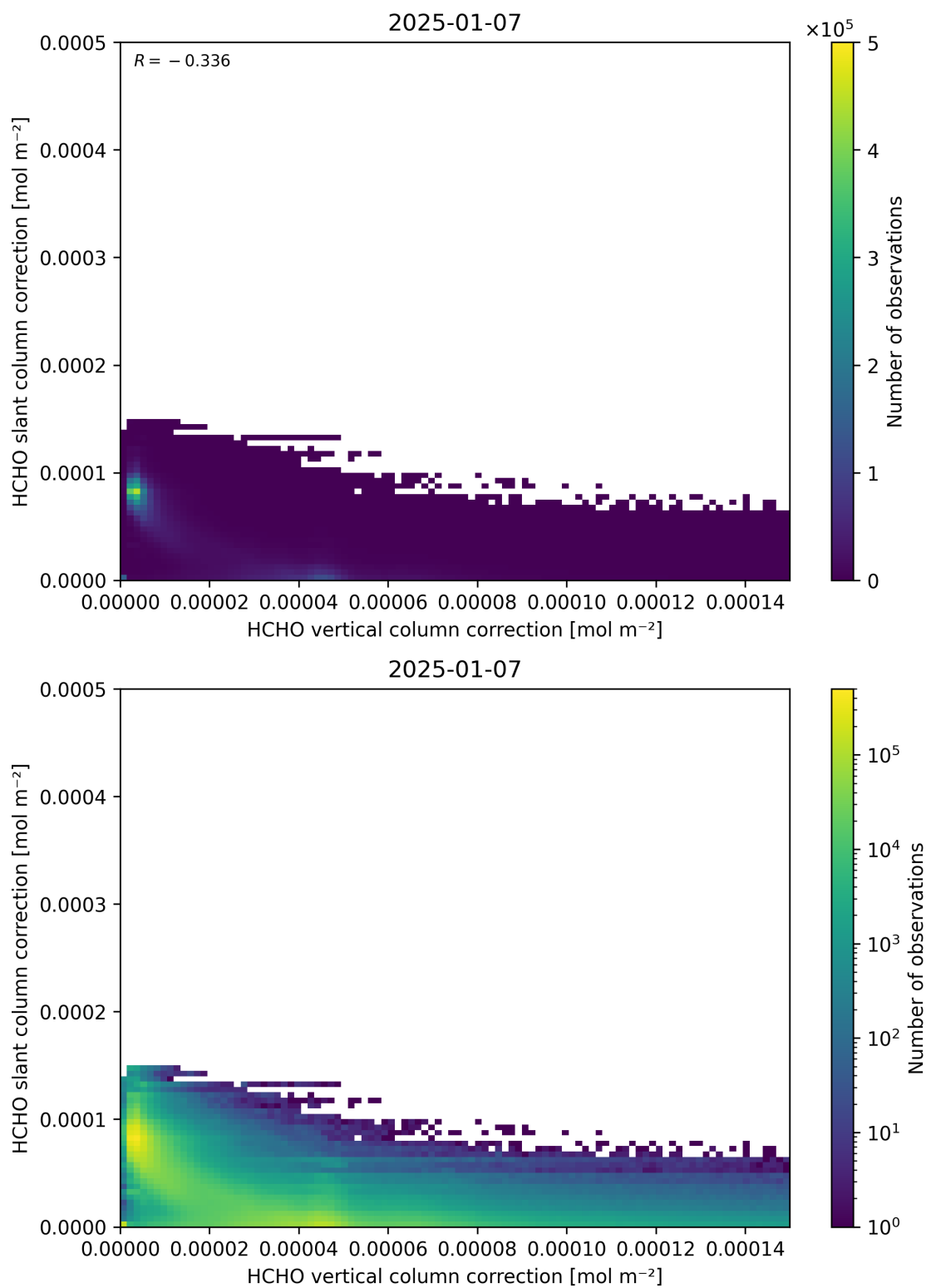
Figure 117: Scatter density plot of “HCHO vertical column correction” against “HCHO slant column correction” for 2025-01-07 to 2025-01-08.
