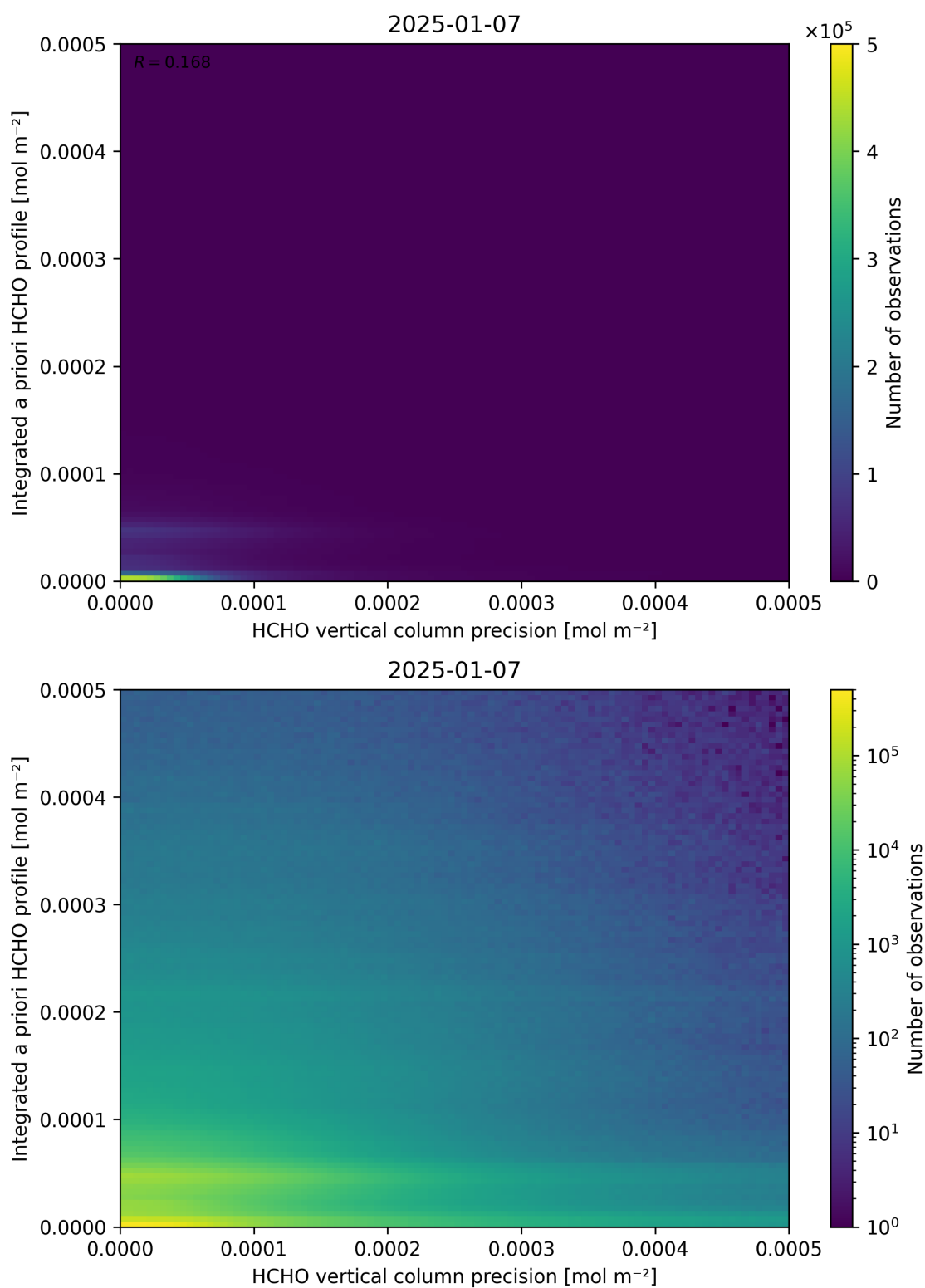
Figure 147: Scatter density plot of “HCHO vertical column precision” against “Integrated a priori HCHO profile” for 2025-01-07 to 2025-01-08.
