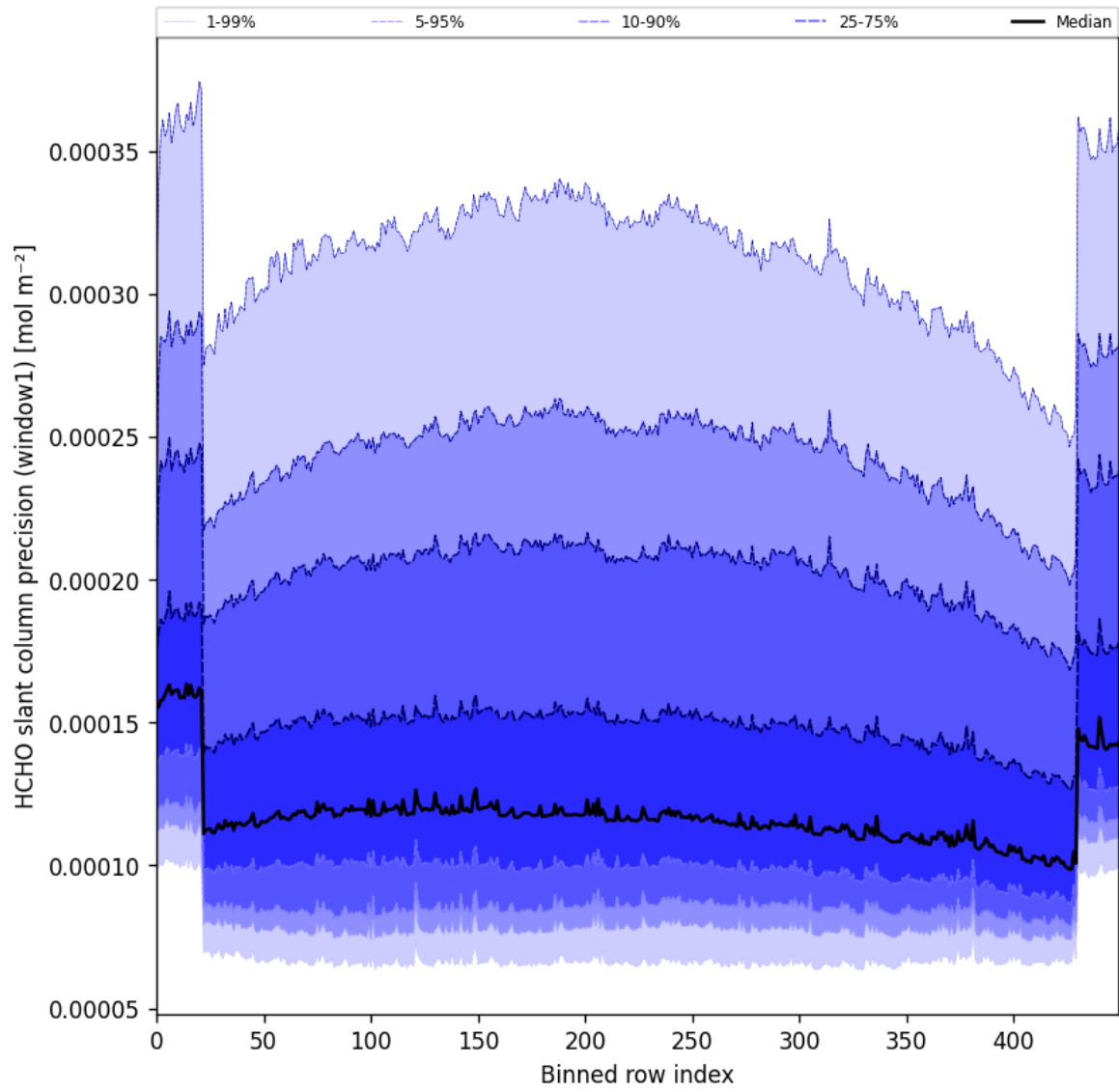
Figure 53: Along track statistics of “HCHO slant column precision (window1)” for 2025-01-07 to 2025-01-08
