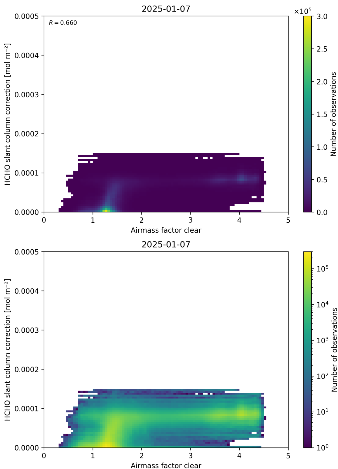
Figure 75: Scatter density plot of “Air mass factor clear” against “HCHO slant column correction” for 2025-01-07 to 2025-01-08.
