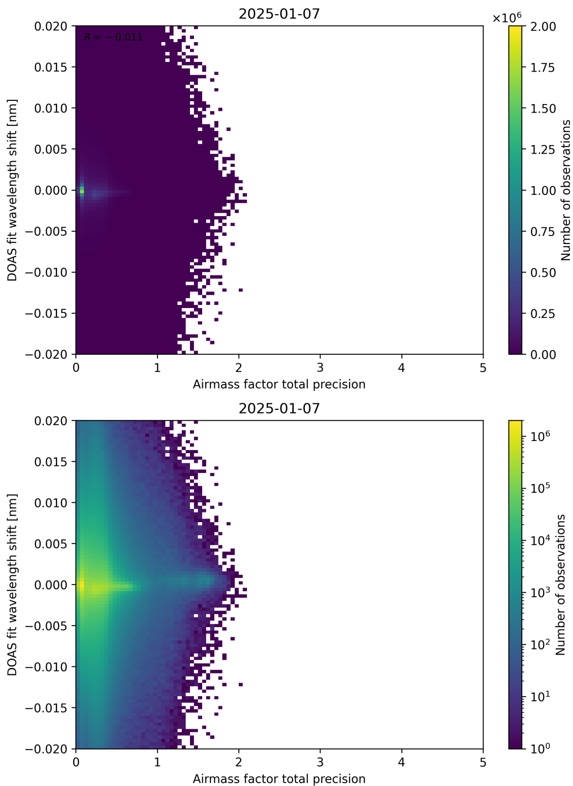
Figure 106: Scatter density plot of “Airmass factor total precision” against “DOAS fit wavelength shift” for 2025-01-07 to 2025-01-08.
