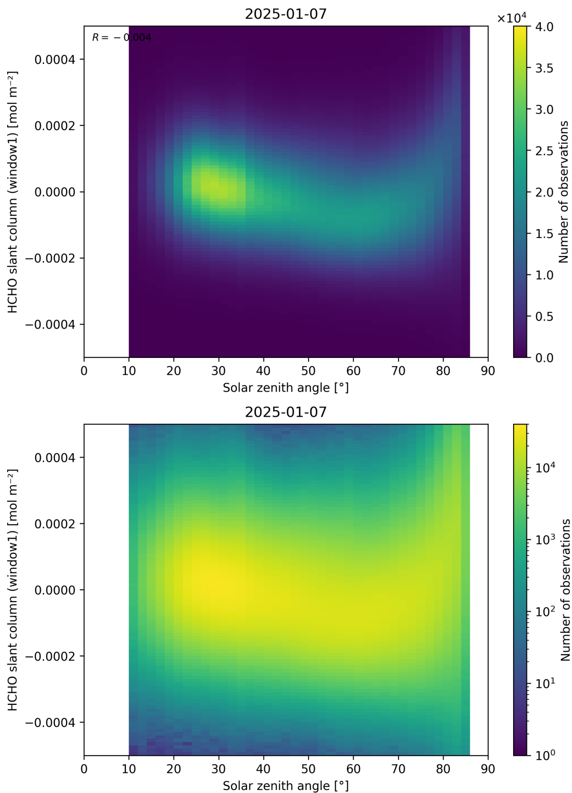
Figure 173: Scatter density plot of “Solar zenith angle” against “HCHO slant column (window1)” for 2025-01-07 to 2025-01-08.
