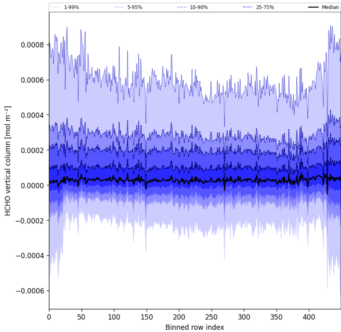
Figure 49: Along track statistics of “HCHO vertical column” for 2025-01-07 to 2025-01-08
