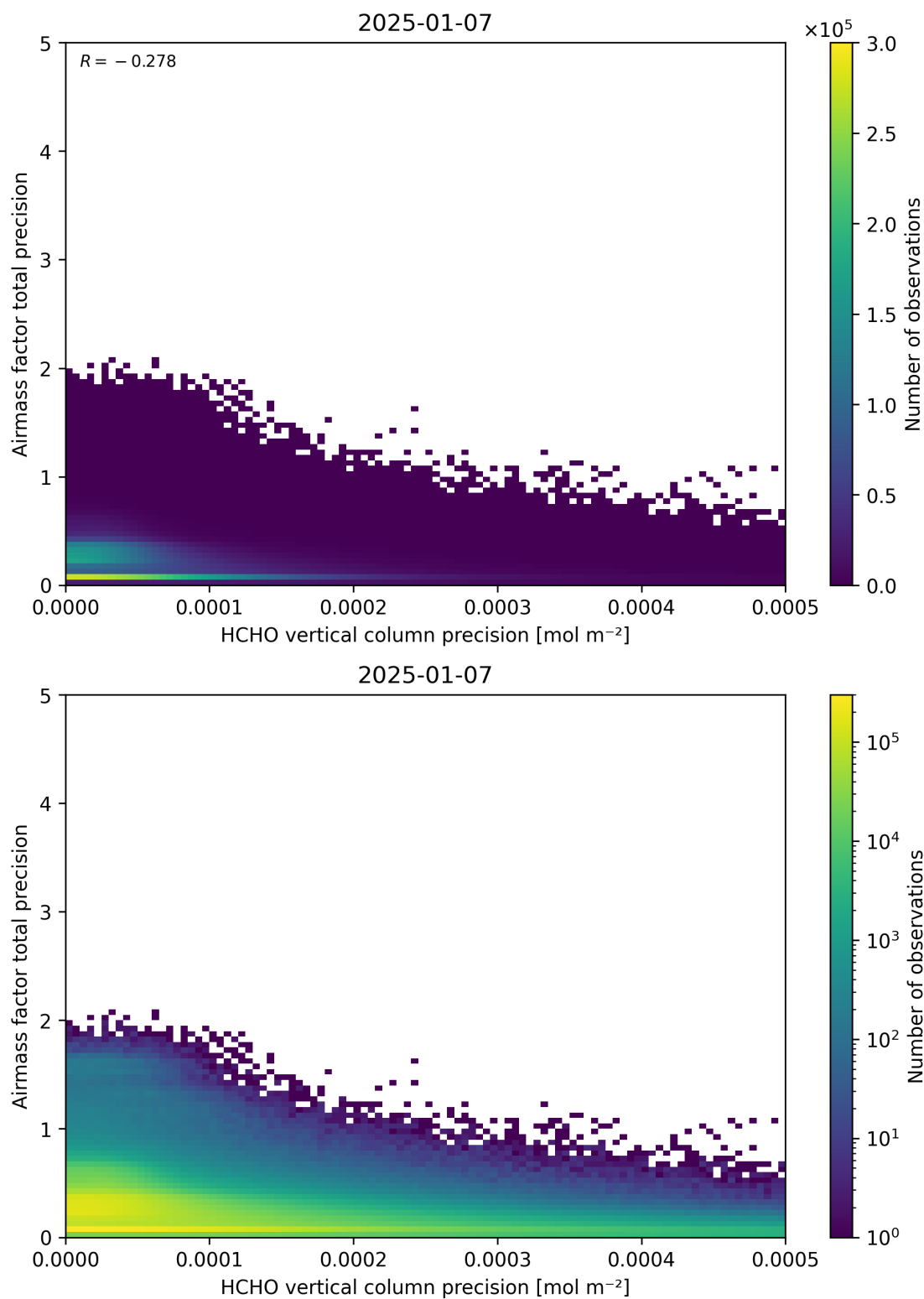
Figure 145: Scatter density plot of “HCHO vertical column precision” against “Airmass factor total precision” for 2025-01-07 to 2025-01-08.
