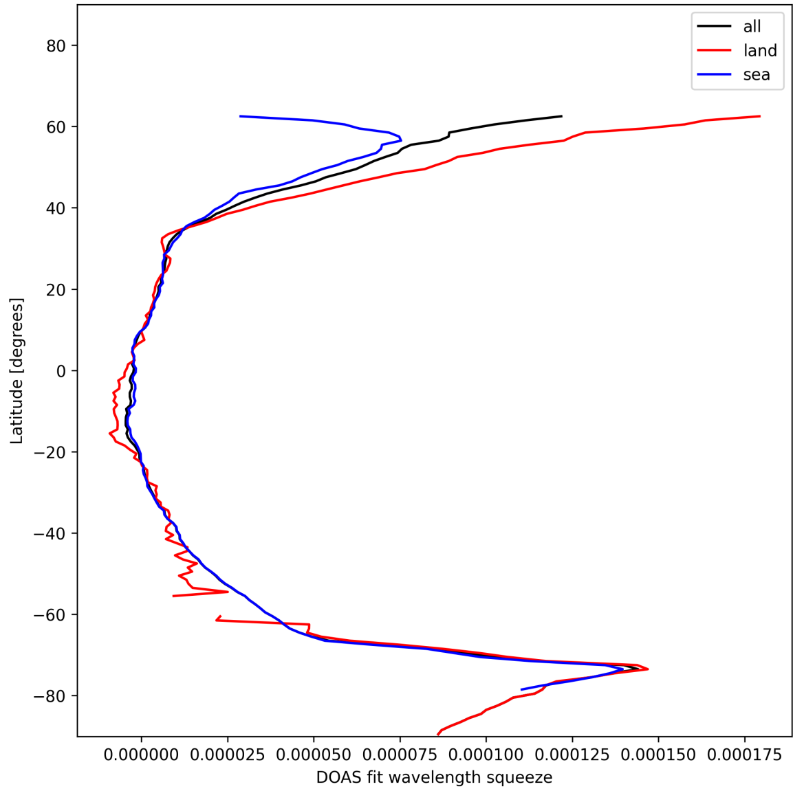
Figure 31: Zonal average of “DOAS fit wavelength squeeze” for 2025-01-07 to 2025-01-08.
