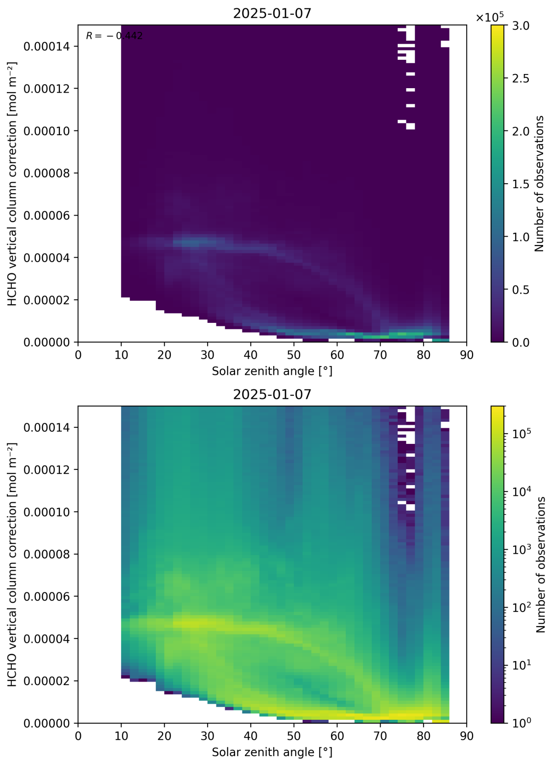
Figure 178: Scatter density plot of “Solar zenith angle” against “HCHO vertical column correction” for 2025-01-07 to 2025-01-08.
