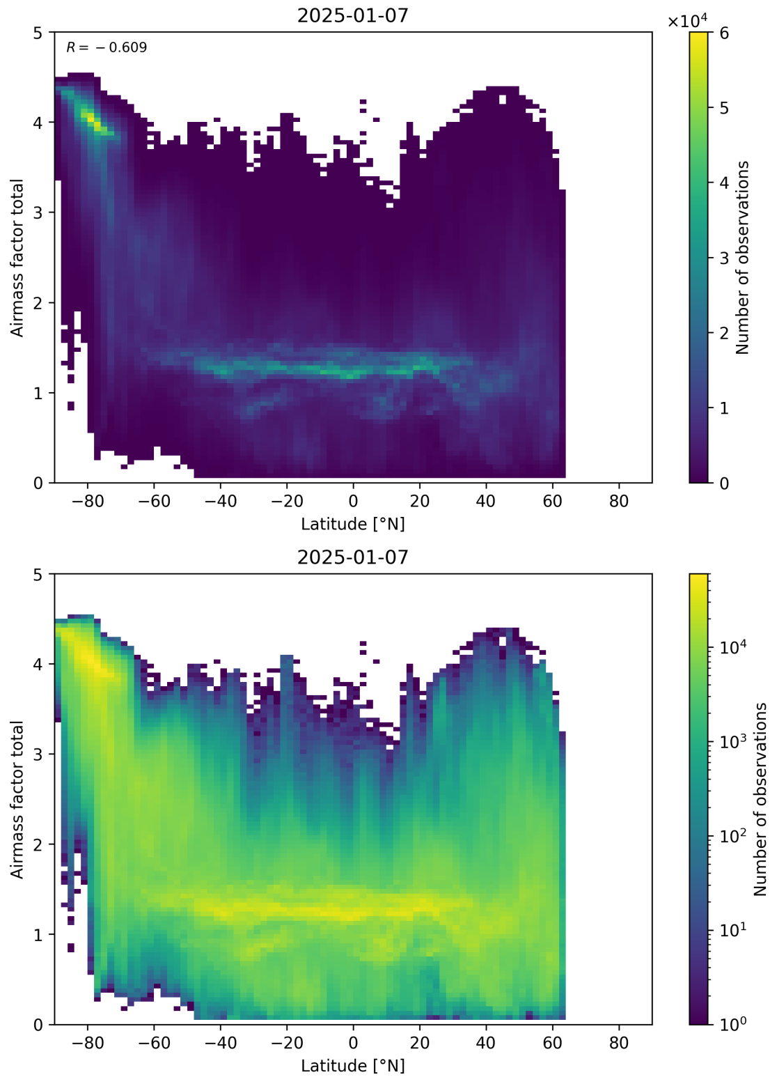
Figure 161: Scatter density plot of “Latitude” against “Airmass factor total” for 2025-01-07 to 2025-01-08.
