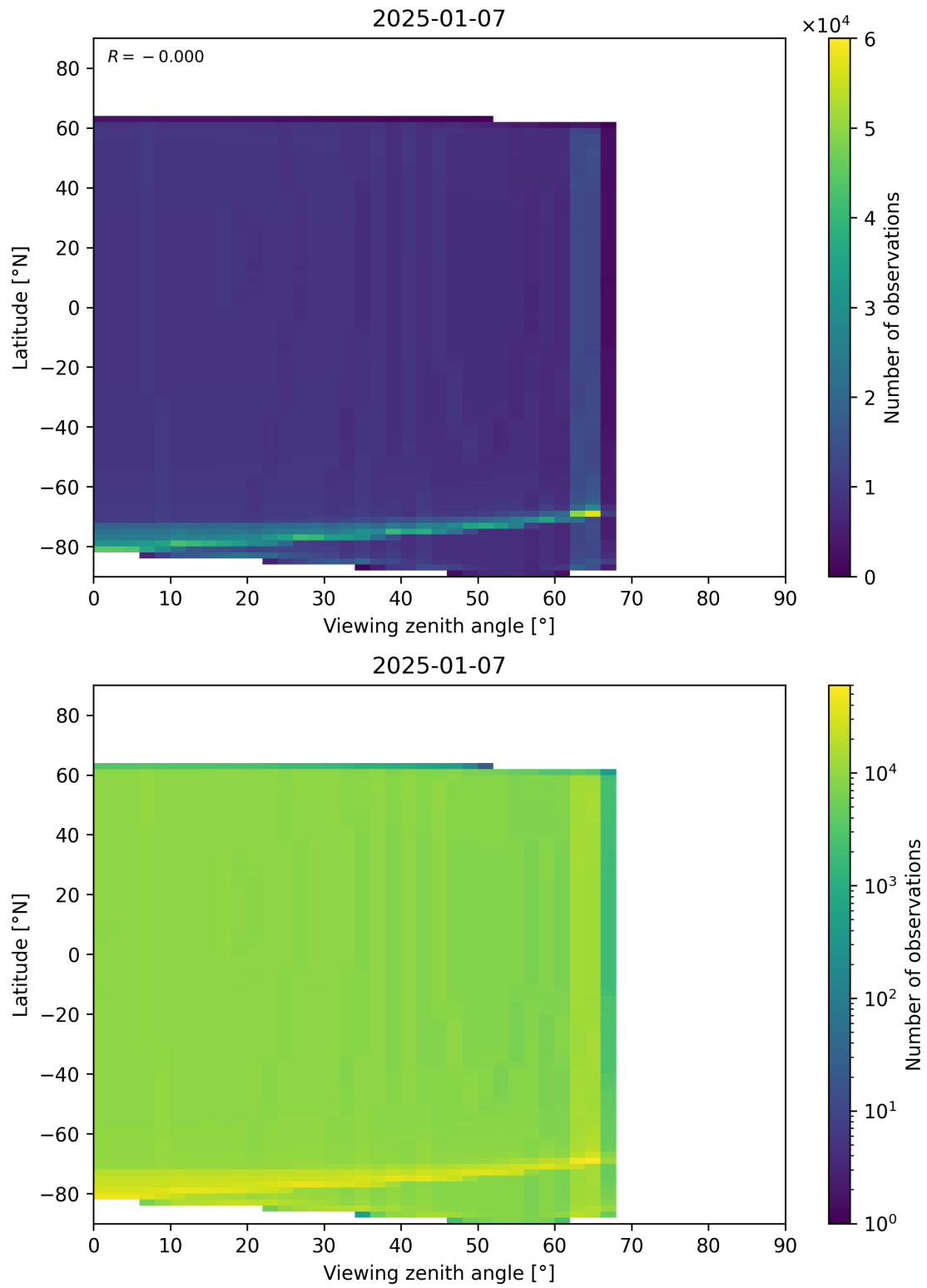
Figure 196: Scatter density plot of “Viewing zenith angle” against “Latitude” for 2025-01-07 to 2025-01-08.
