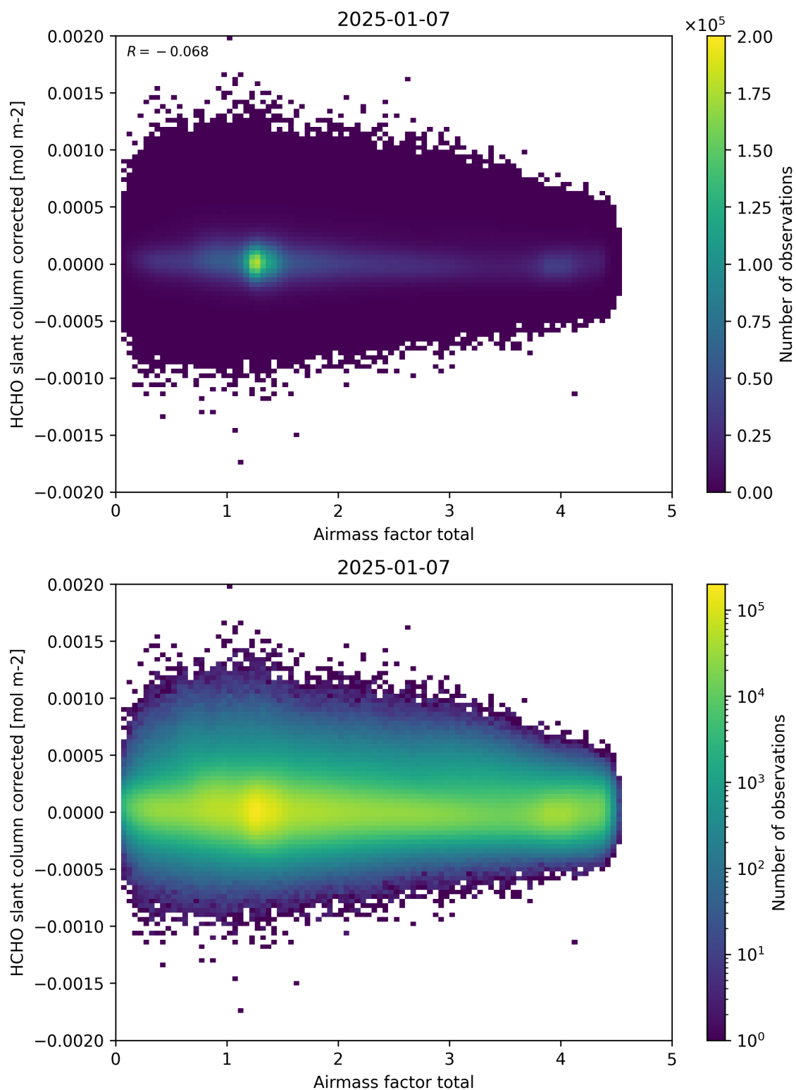
Figure 101: Scatter density plot of “Airmass factor total” against “HCHO slant column corrected” for 2025-01-07 to 2025-01-08.
