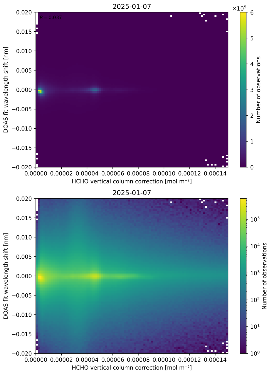
Figure 113: Scatter density plot of “HCHO vertical column correction” against “DOAS fit wavelength shift” for 2025-01-07 to 2025-01-08.
