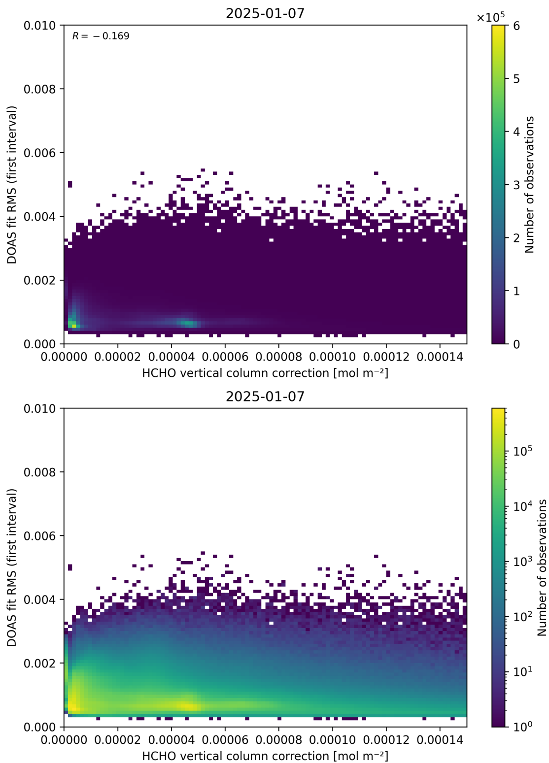
Figure 112: Scatter density plot of “HCHO vertical column correction” against “DOAS fit RMS (first interval)” for 2025-01-07 to 2025-01-08.
