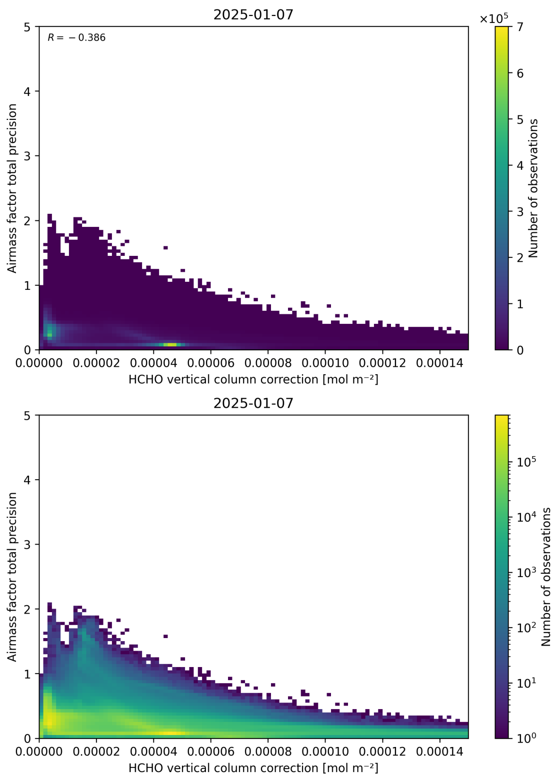
Figure 121: Scatter density plot of “HCHO vertical column correction” against “Airmass factor total precision” for 2025-01-07 to 2025-01-08.
