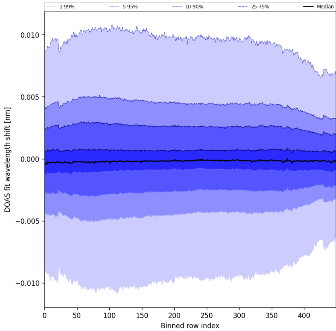
Figure 58: Along track statistics of “DOAS fit wavelength shift” for 2025-01-07 to 2025-01-08
