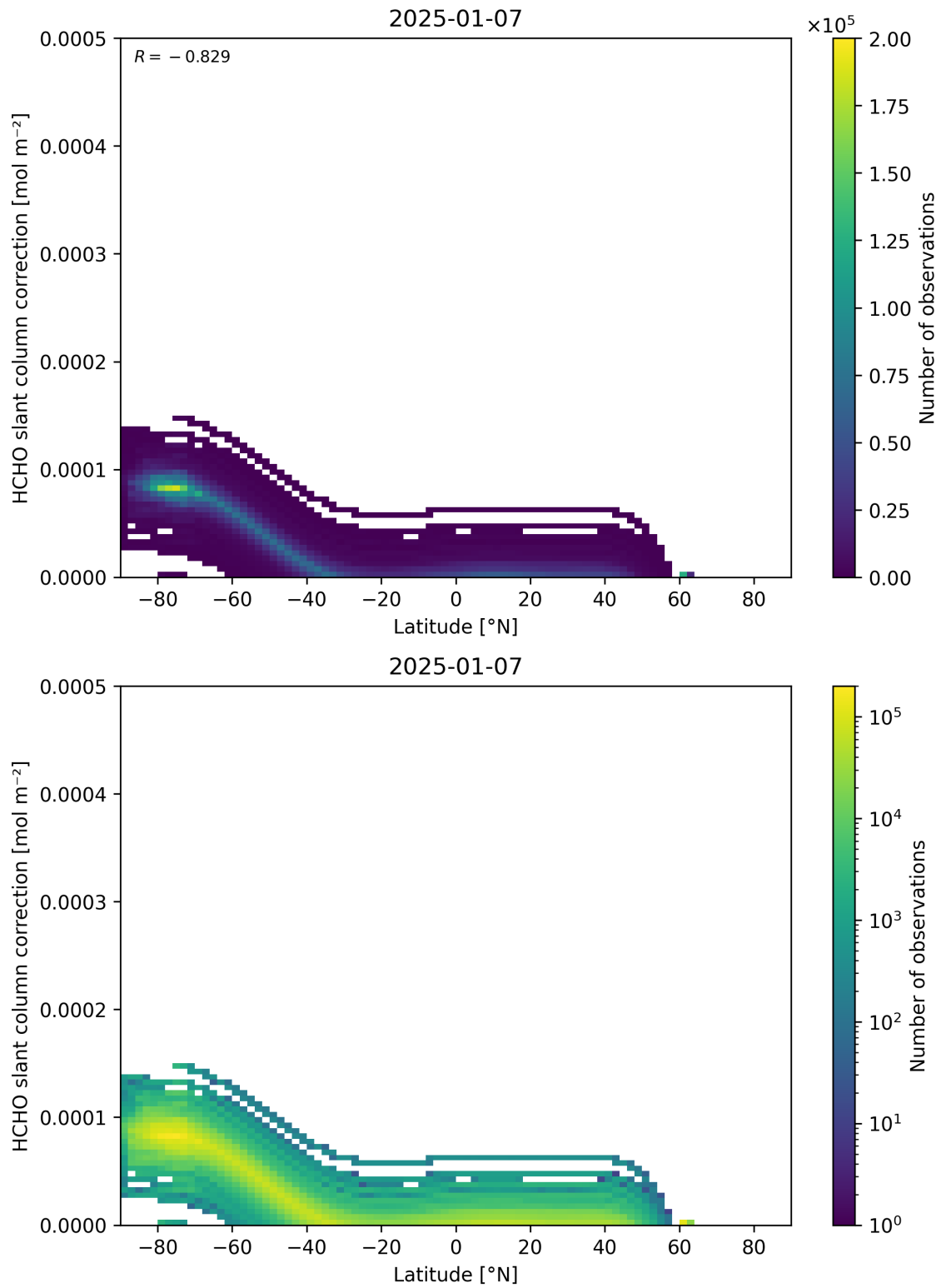
Figure 158: Scatter density plot of “Latitude” against “HCHO slant column correction” for 2025-01-07 to 2025-01-08.
