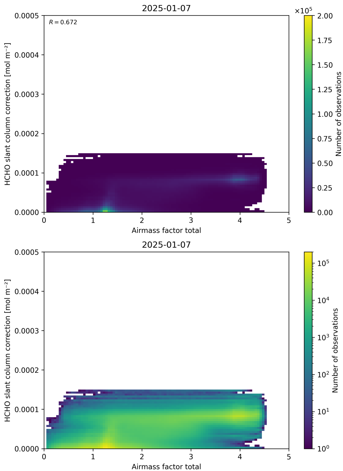
Figure 102: Scatter density plot of “Airmass factor total” against “HCHO slant column correction” for 2025-01-07 to 2025-01-08.
