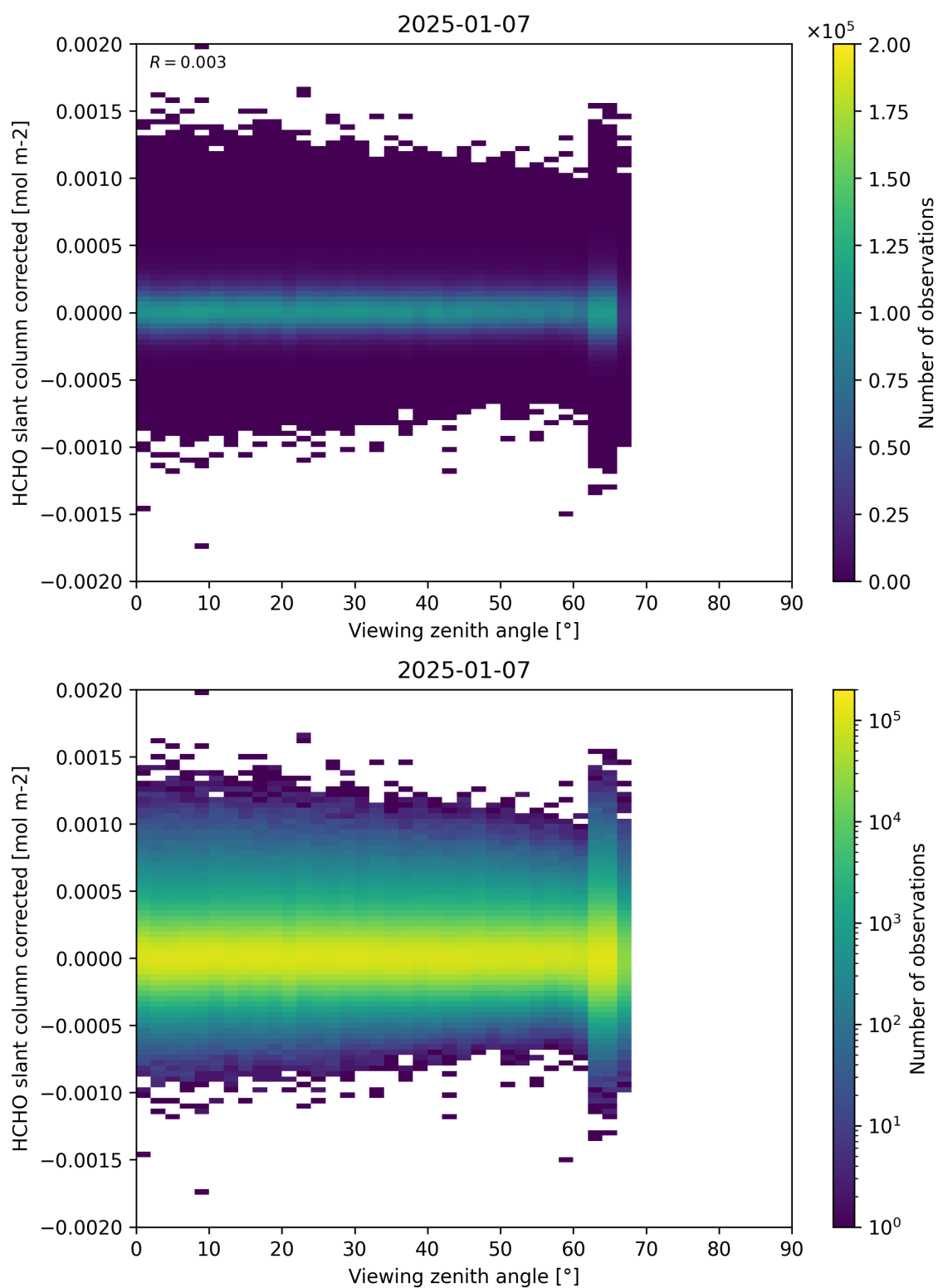
Figure 186: Scatter density plot of “Viewing zenith angle” against “HCHO slant column corrected” for 2025-01-07 to 2025-01-08.
