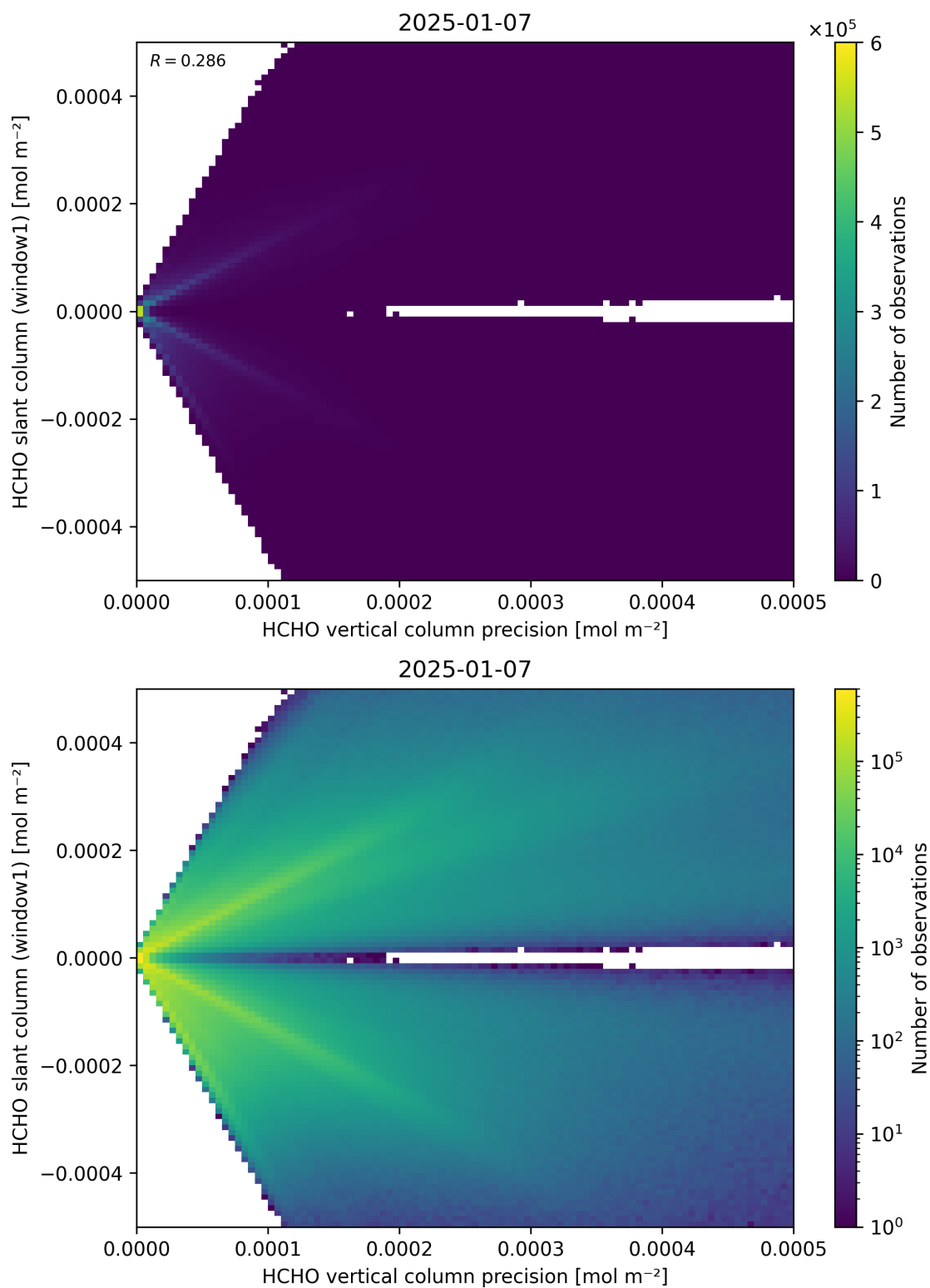
Figure 142: Scatter density plot of “HCHO vertical column precision” against “HCHO slant column (window1)” for 2025-01-07 to 2025-01-08.
