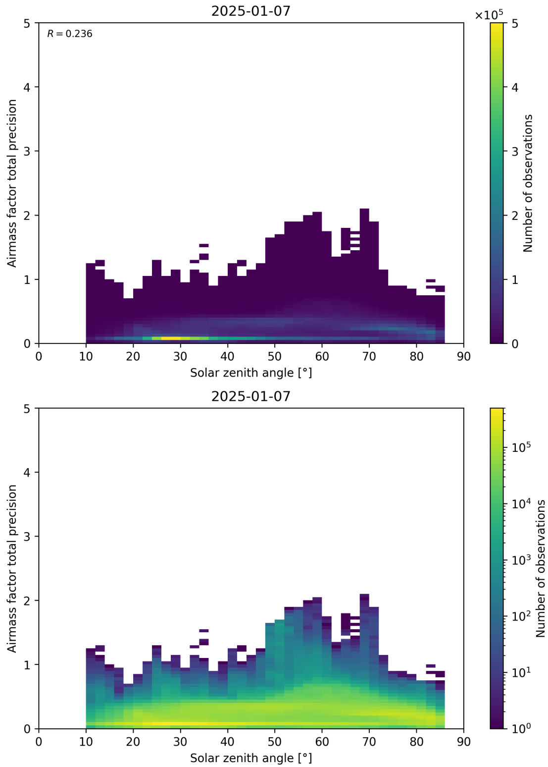
Figure 176: Scatter density plot of “Solar zenith angle” against “Airmass factor total precision” for 2025-01-07 to 2025-01-08.
