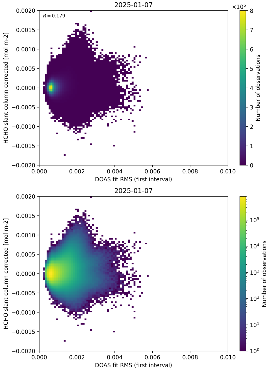
Figure 62: Scatter density plot of “DOAS fit RMS (first interval)” against “HCHO slant column corrected” for 2025-01-07 to 2025-01-08.
