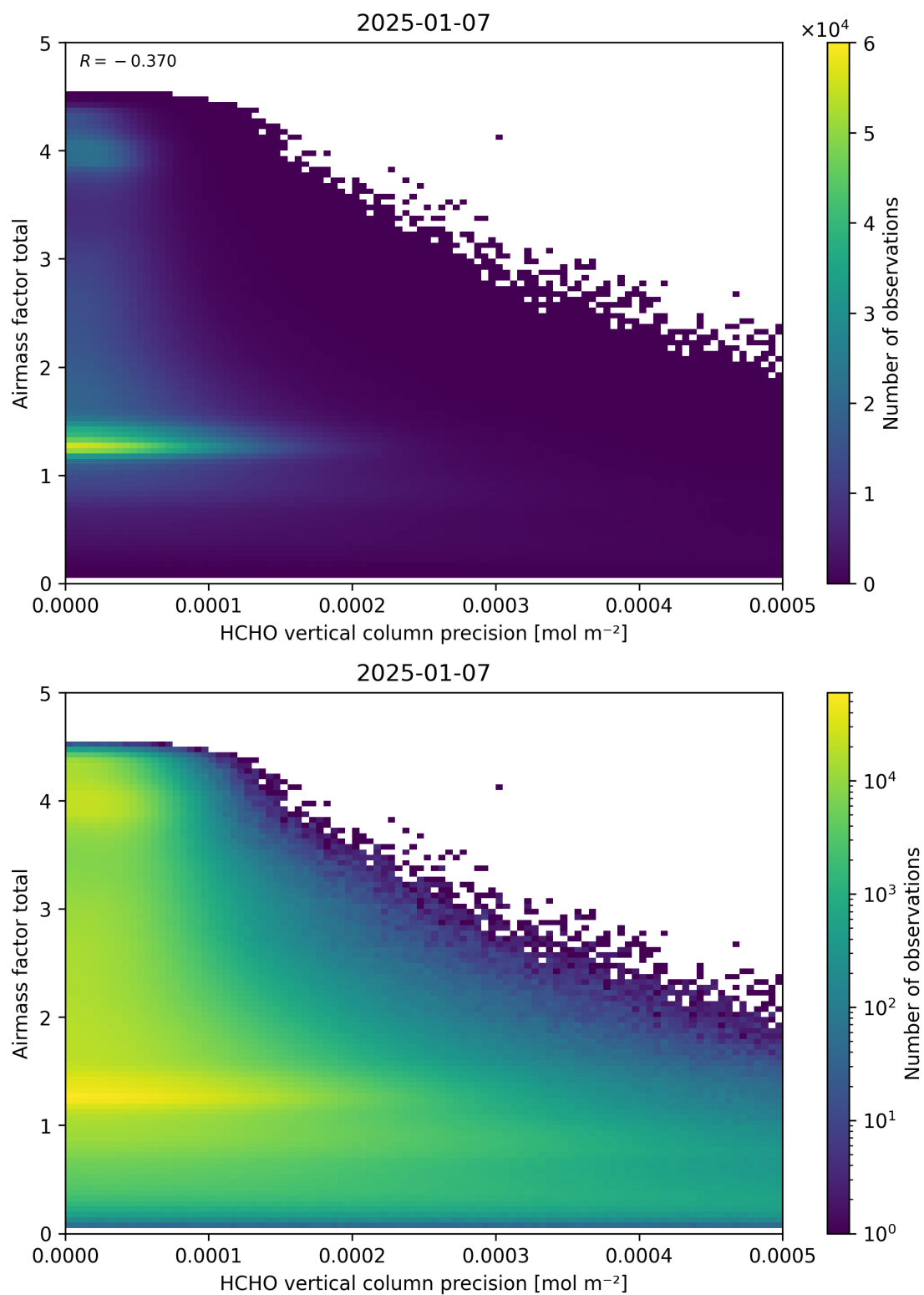
Figure 144: Scatter density plot of “HCHO vertical column precision” against “Airmass factor total” for 2025-01-07 to 2025-01-08.
