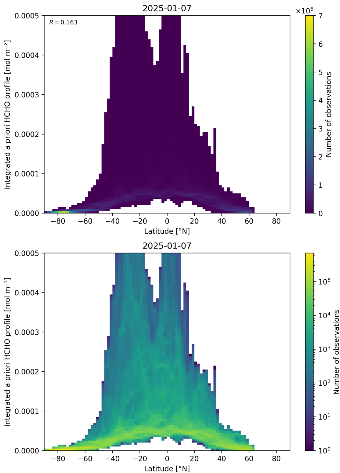
Figure 166: Scatter density plot of “Latitude” against “Integrated a priori HCHO profile” for 2025-01-07 to 2025-01-08.
