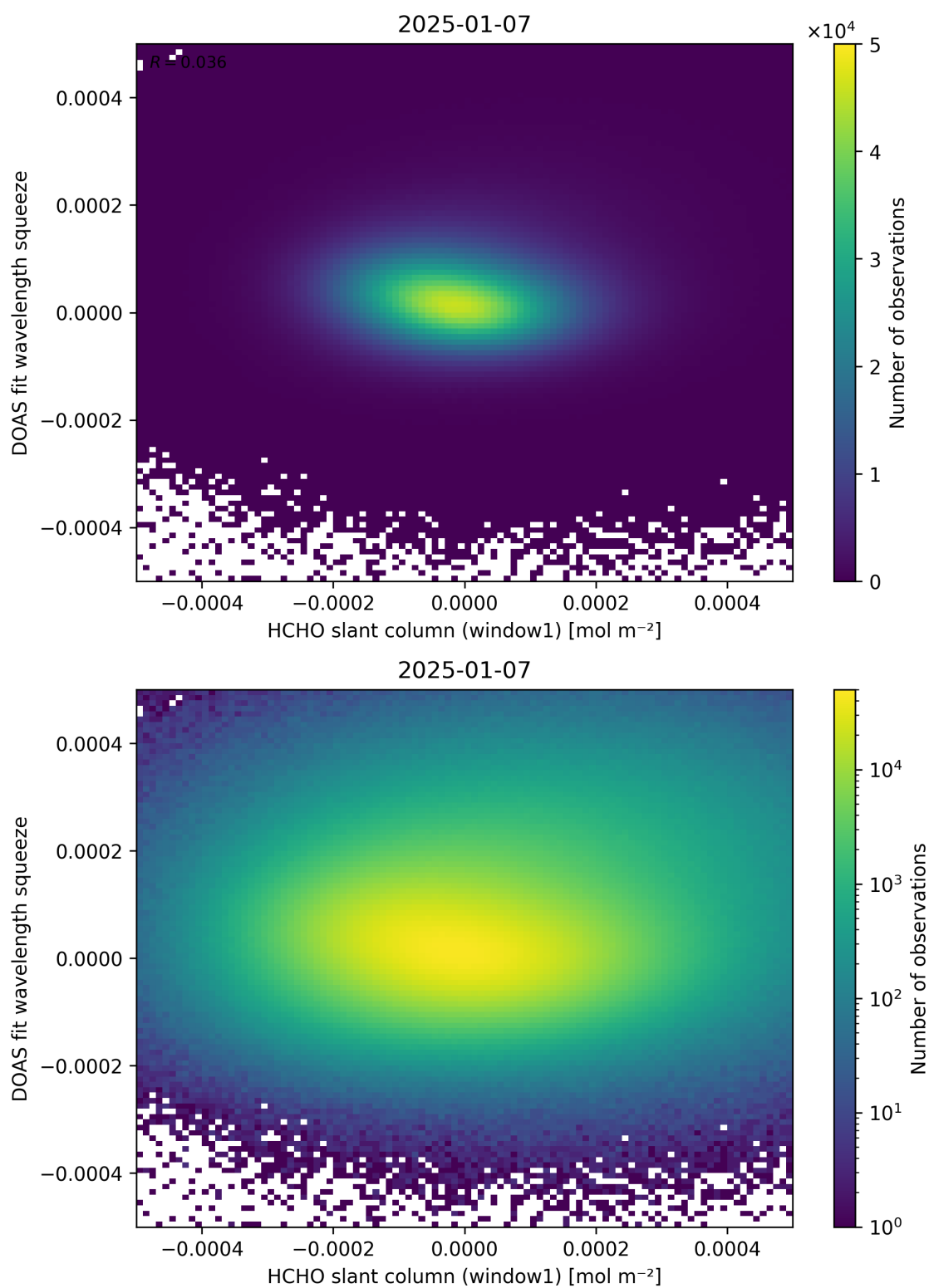
Figure 80: Scatter density plot of “HCHO slant column (window1)” against “DOAS fit wavelength squeeze” for 2025-01-07 to 2025-01-08.
