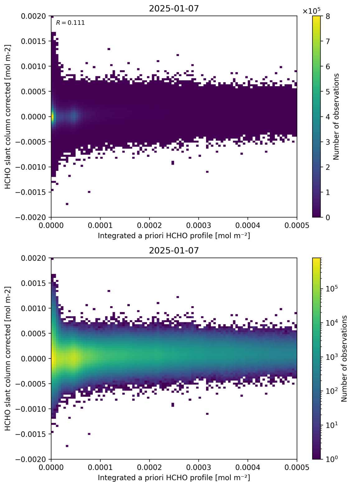
Figure 151: Scatter density plot of “Integrated a priori HCHO profile” against “HCHO slant column corrected” for 2025-01-07 to 2025-01-08.
