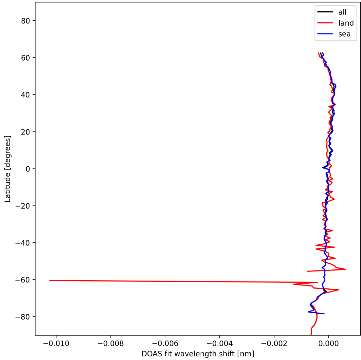
Figure 30: Zonal average of “DOAS fit wavelength shift” for 2025-01-07 to 2025-01-08.
