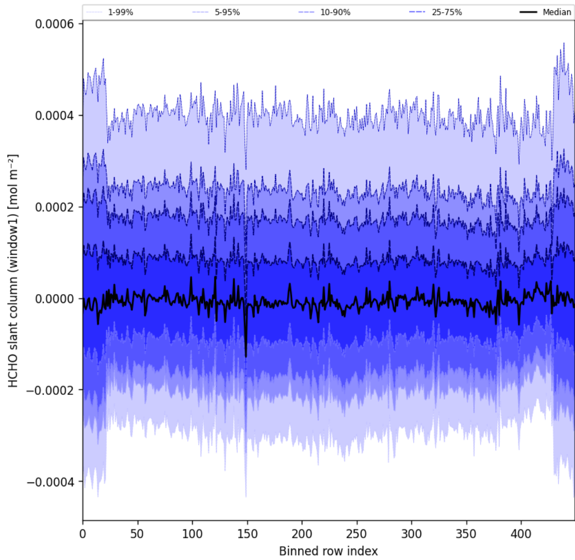
Figure 52: Along track statistics of “HCHO slant column (window1)” for 2025-01-07 to 2025-01-08
