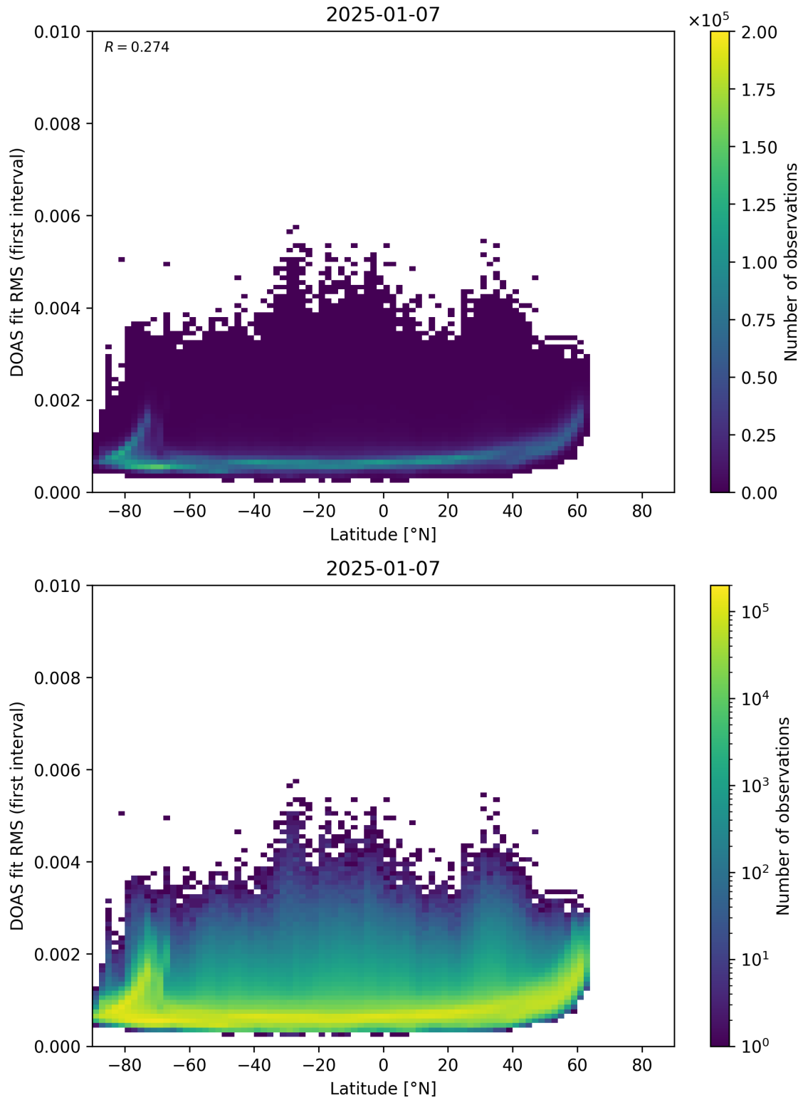
Figure 153: Scatter density plot of “Latitude” against “DOAS fit RMS (first interval)” for 2025-01-07 to 2025-01-08.
