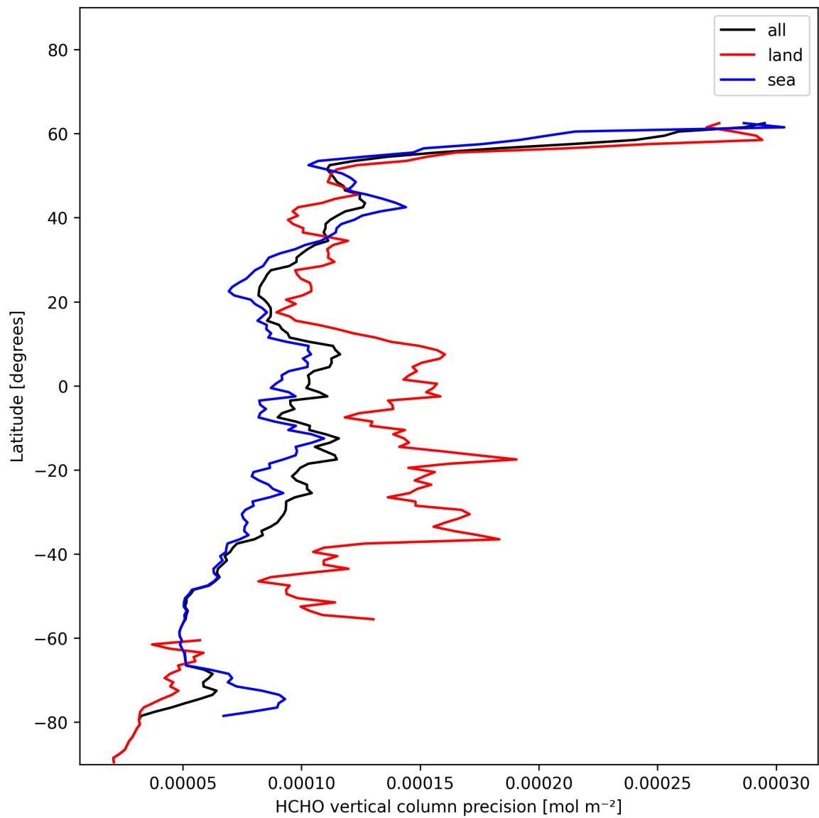
Figure 22: Zonal average of “HCHO vertical column precision” for 2025-01-07 to 2025-01-08.
