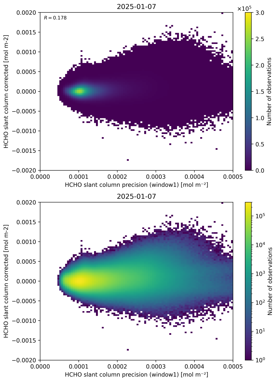
Figure 92: Scatter density plot of “HCHO slant column precision (window1)” against “HCHO slant column corrected” for 2025-01-07 to 2025-01-08.
