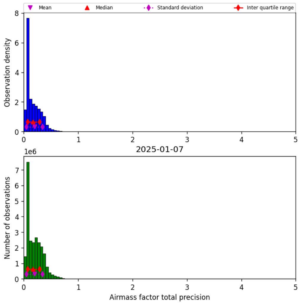
Figure 41: Histogram of “Airmass factor total precision” for 2025-01-07 to 2025-01-08
