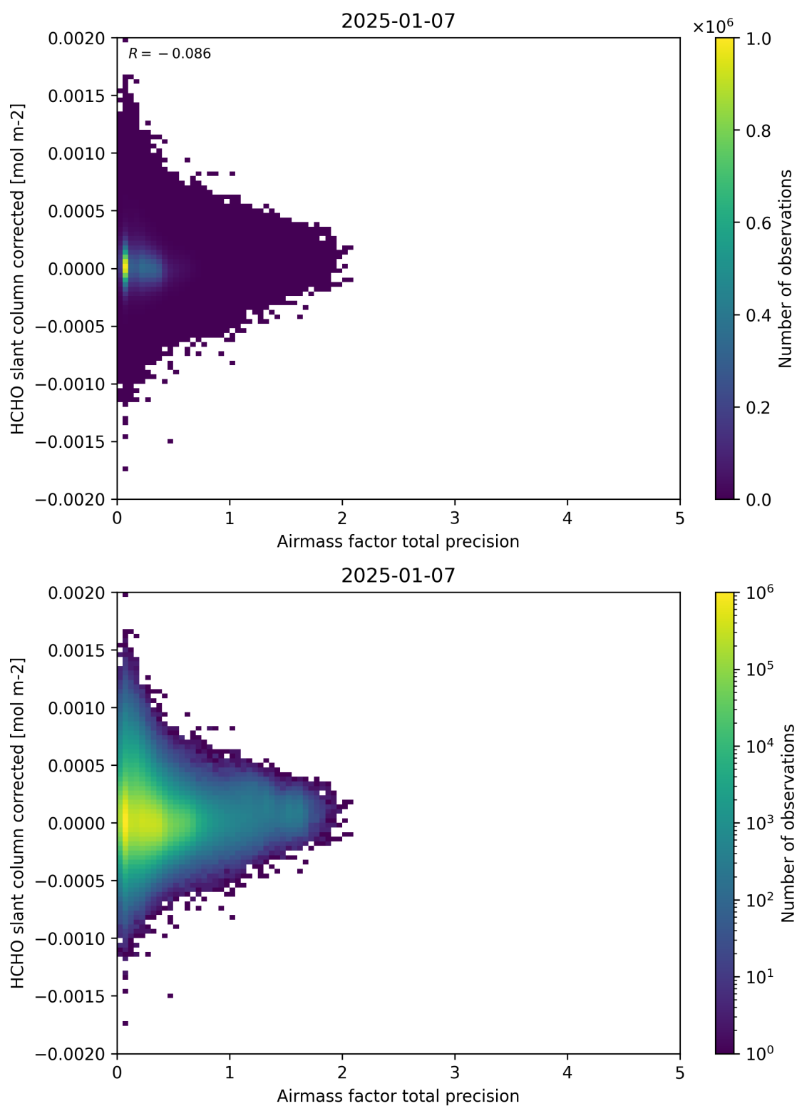
Figure 109: Scatter density plot of “Airmass factor total precision” against “HCHO slant column corrected” for 2025-01-07 to 2025-01-08.
